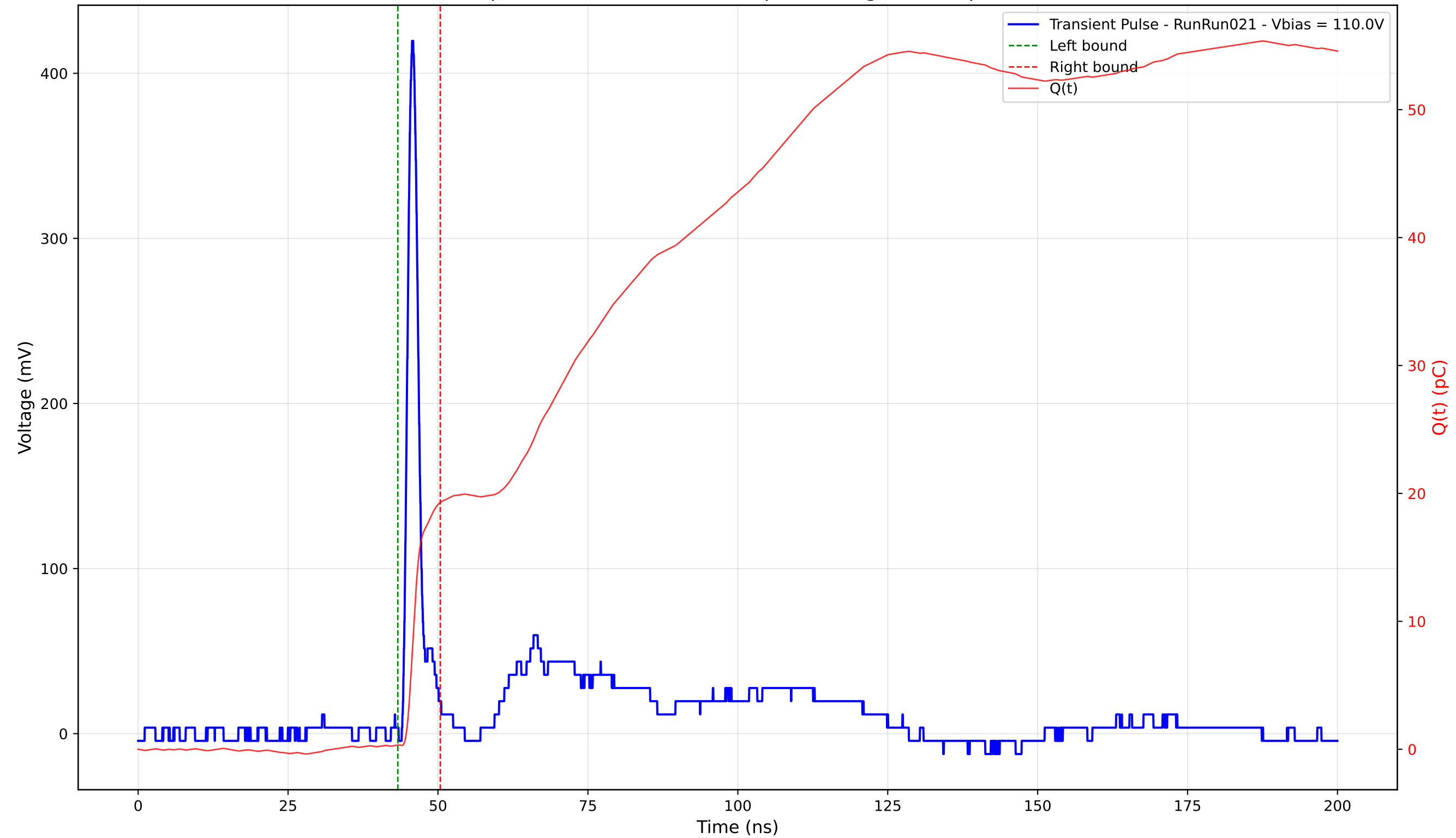
Transient Pulse - Sample: 4003 - Position: 180.0 \mu\text{m} - Charge: 18.96 pC - Rise Time: 1.10 ns
