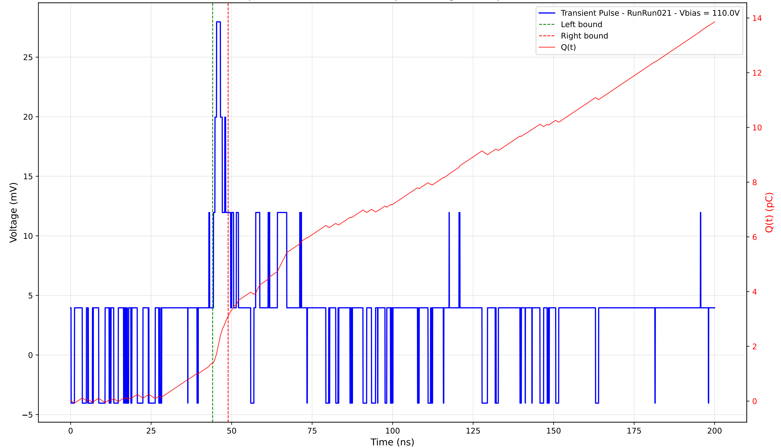
Transient Pulse - Sample: 4003 - Position: 355.0 \mu\text{m} - Charge: 1.71 pC - Rise Time: 0.00 ns (N/A)
