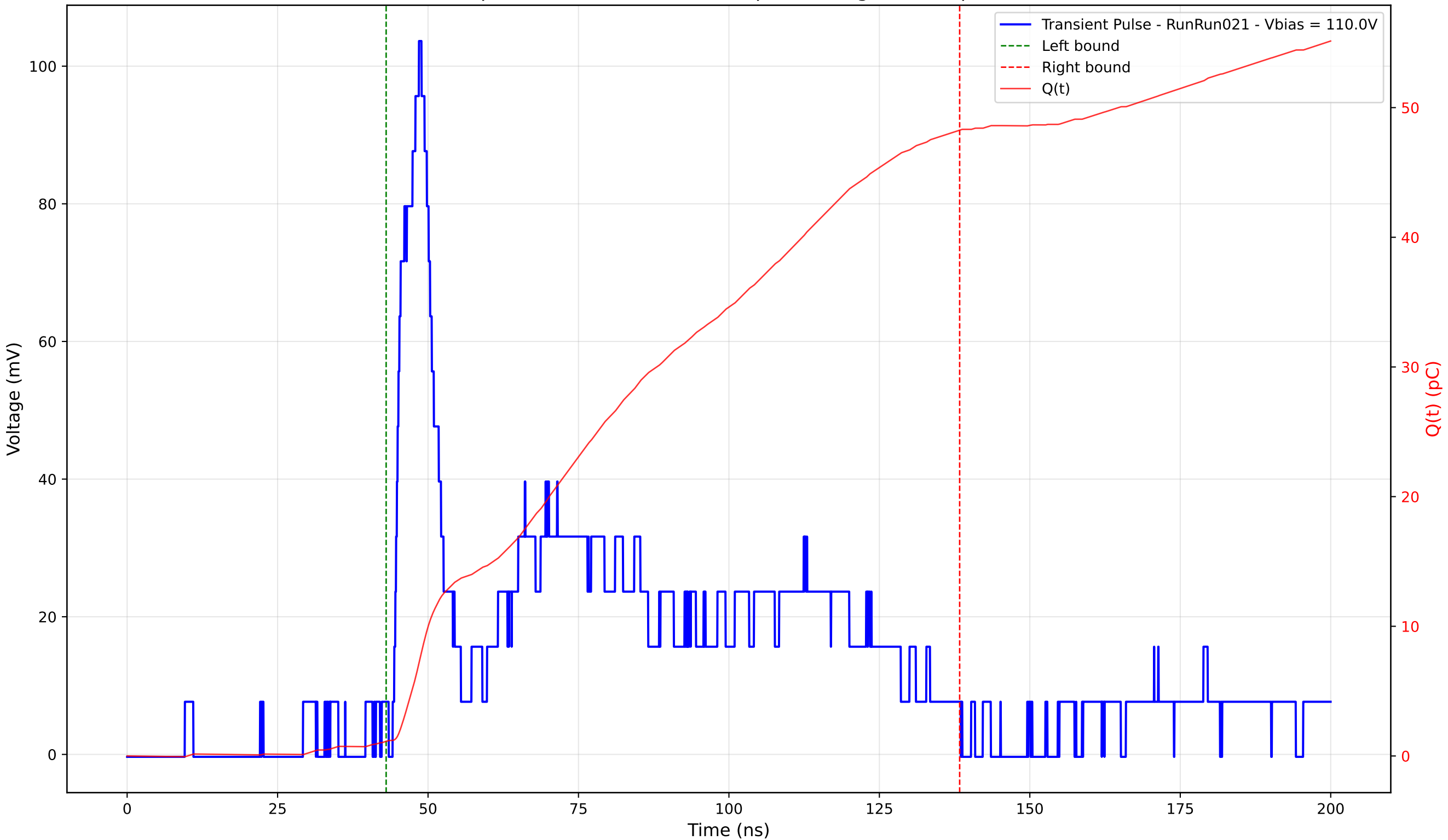
Transient Pulse - Sample: 4003 - Position: 265.0 \mu\text{m} - Charge: 47.14 pC - Rise Time: 3.53 ns
