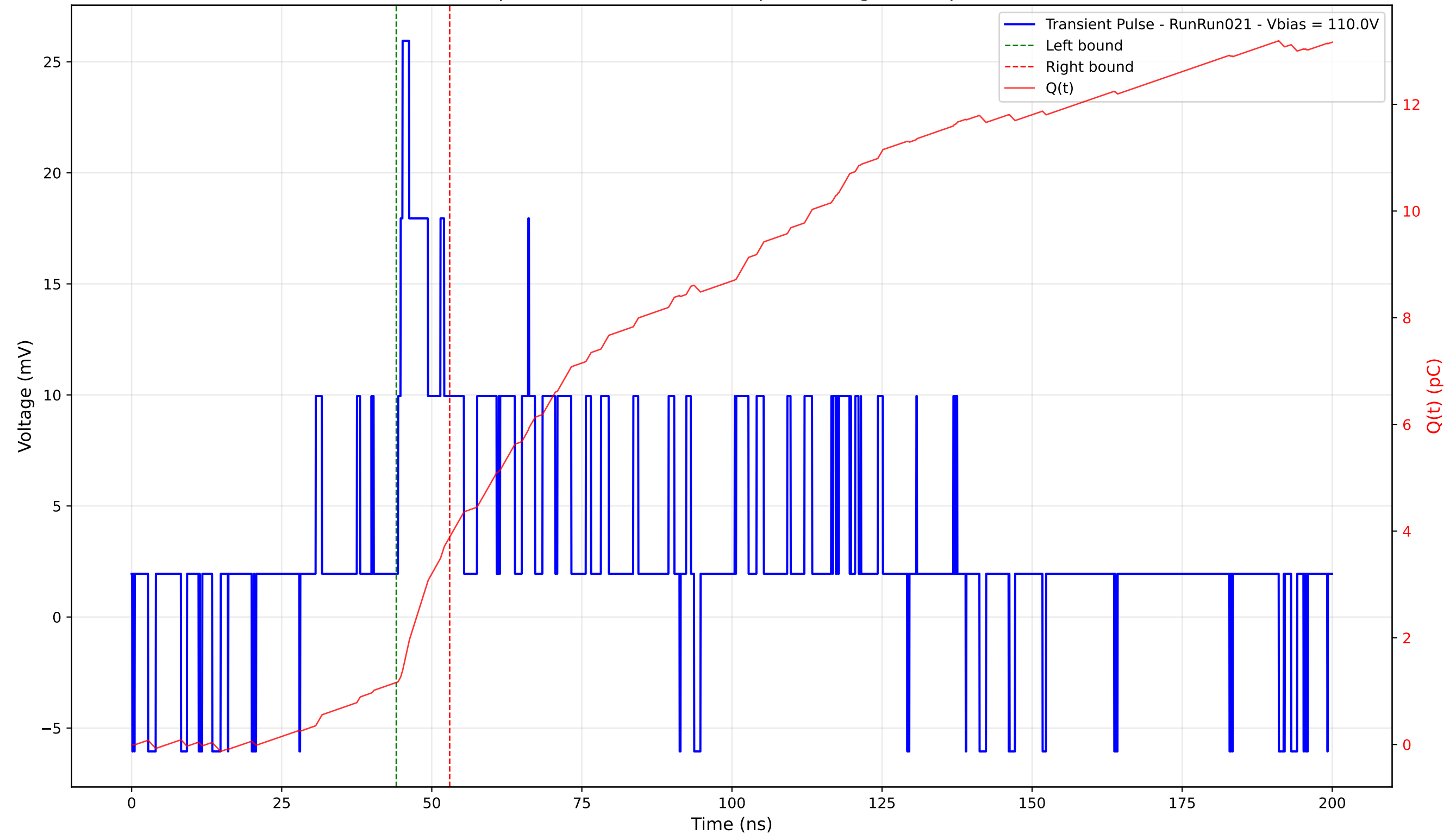
Transient Pulse - Sample: 4003 - Position: 65.0 \mu\text{m} - Charge: 2.73 pC - Rise Time: 0.76 ns
