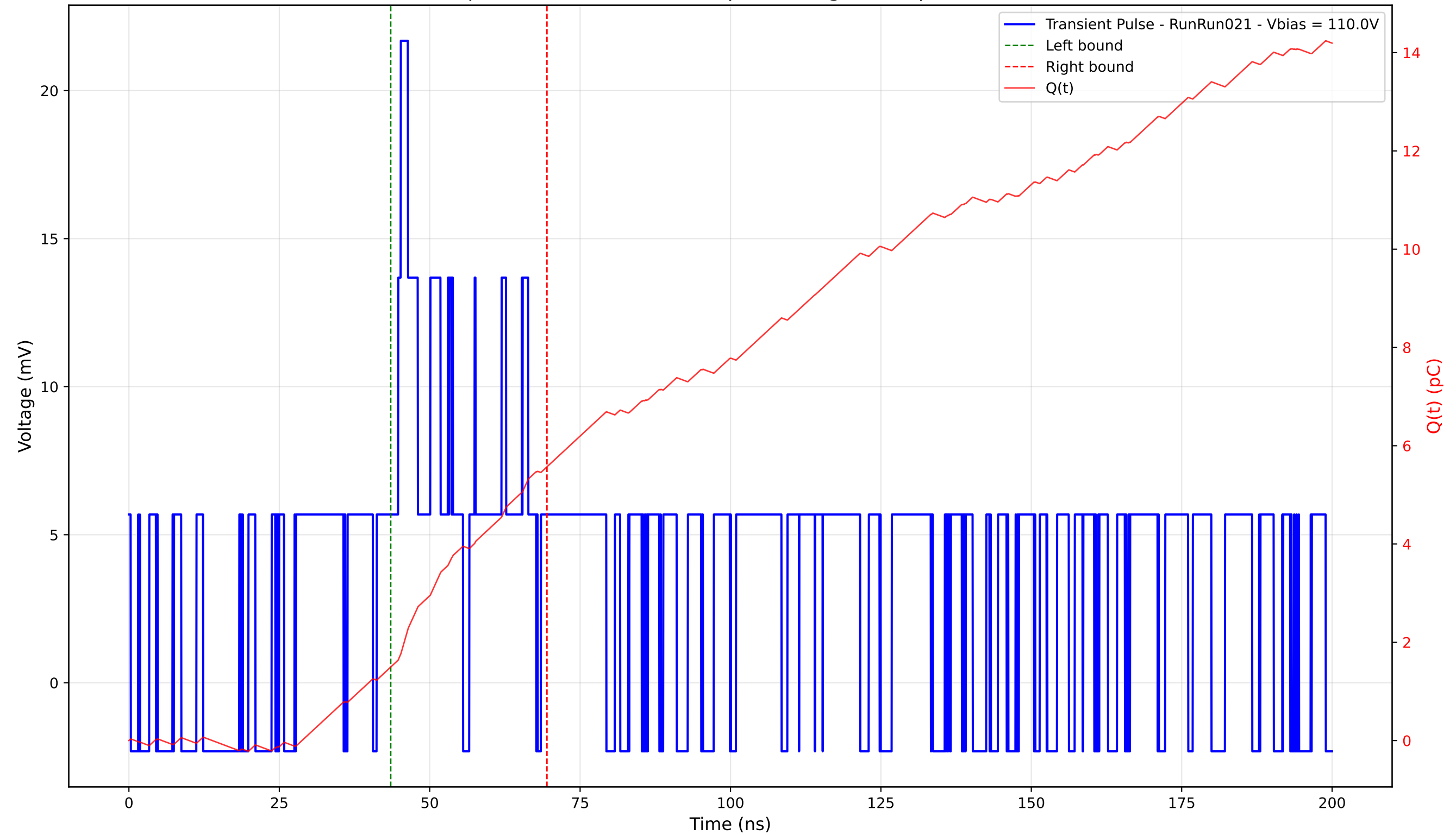
Transient Pulse - Sample: 4003 - Position: 75.0 \mu\text{m} - Charge: 4.07 pC - Rise Time: 0.00 ns (N/A)
