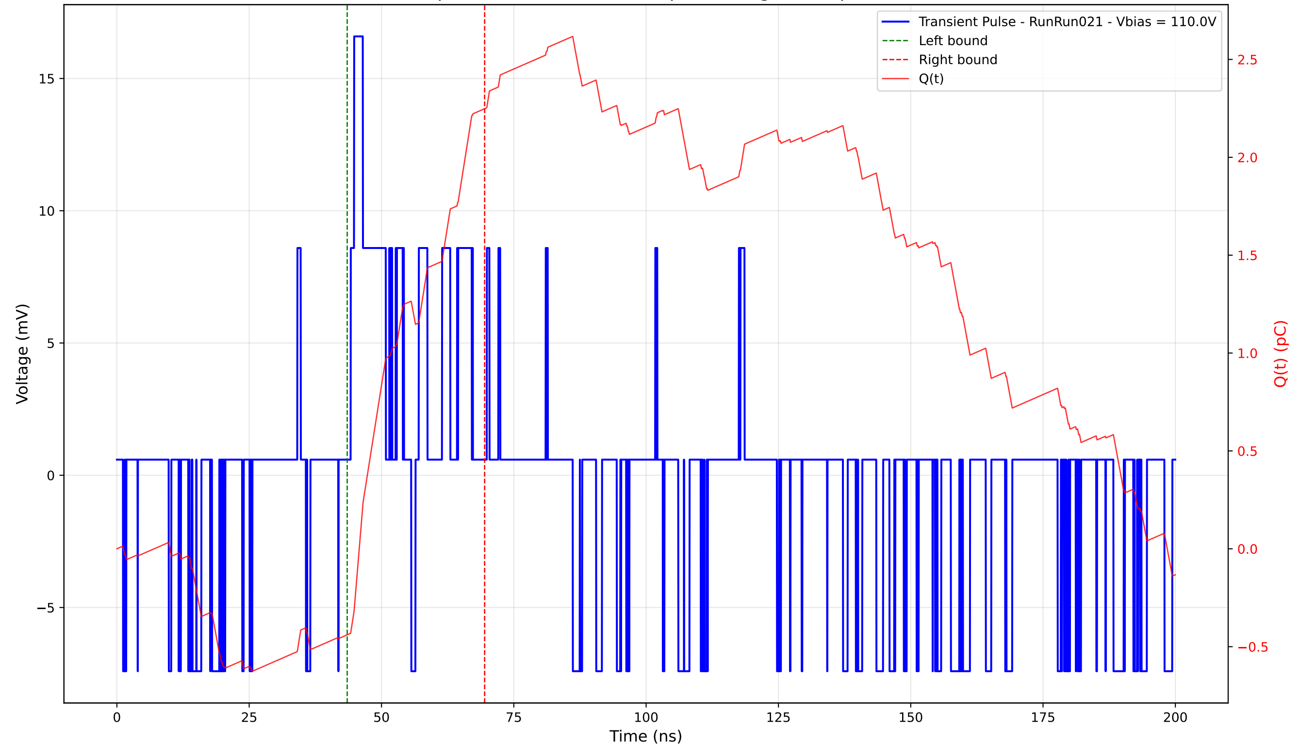
Transient Pulse - Sample: 4003 - Position: 70.0 \mu\text{m} - Charge: 2.69 pC - Rise Time: 0.66 ns
