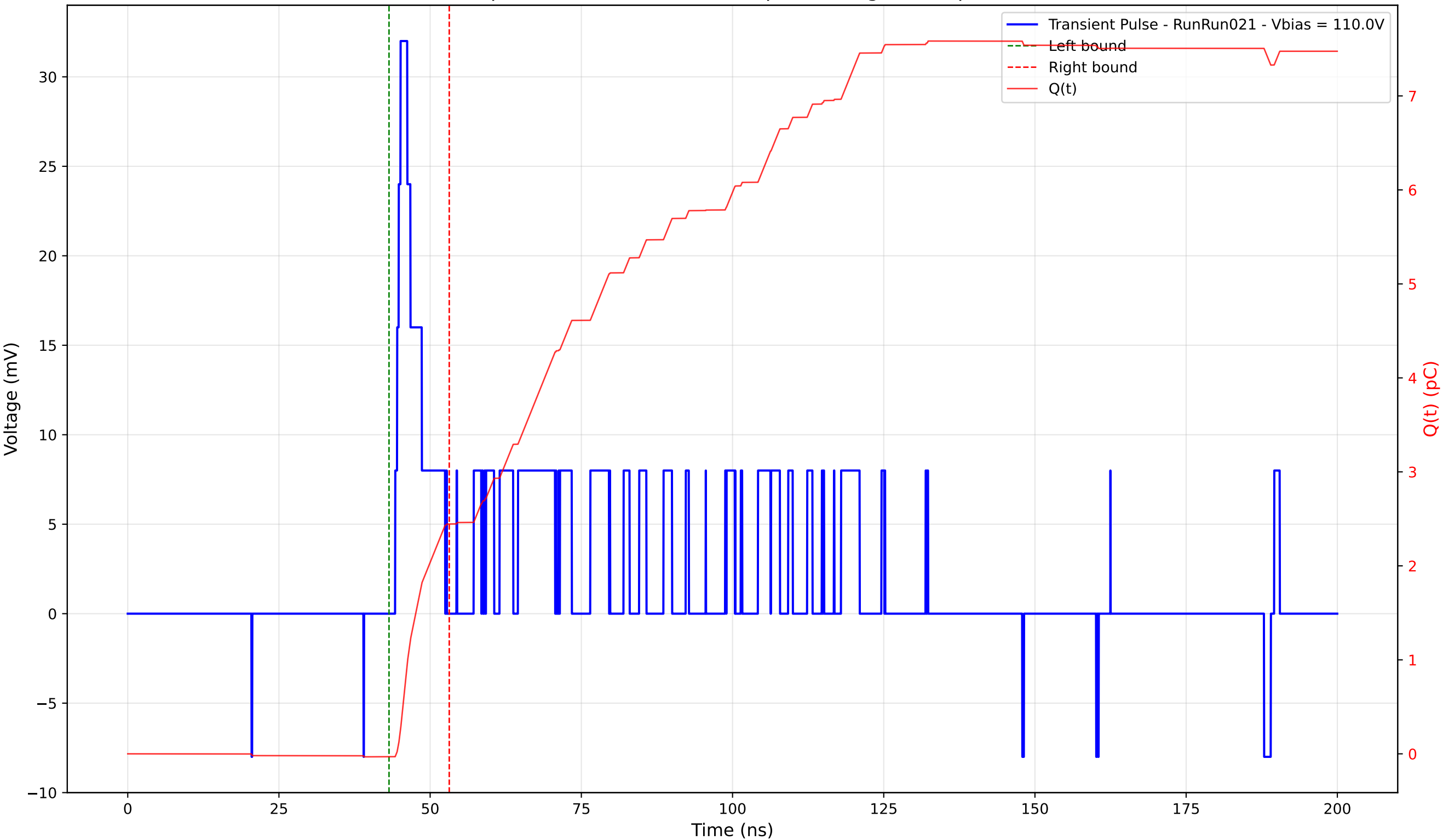
Transient Pulse - Sample: 4003 - Position: 315.0 \mu\text{m} - Charge: 2.48 pC - Rise Time: 0.89 ns
