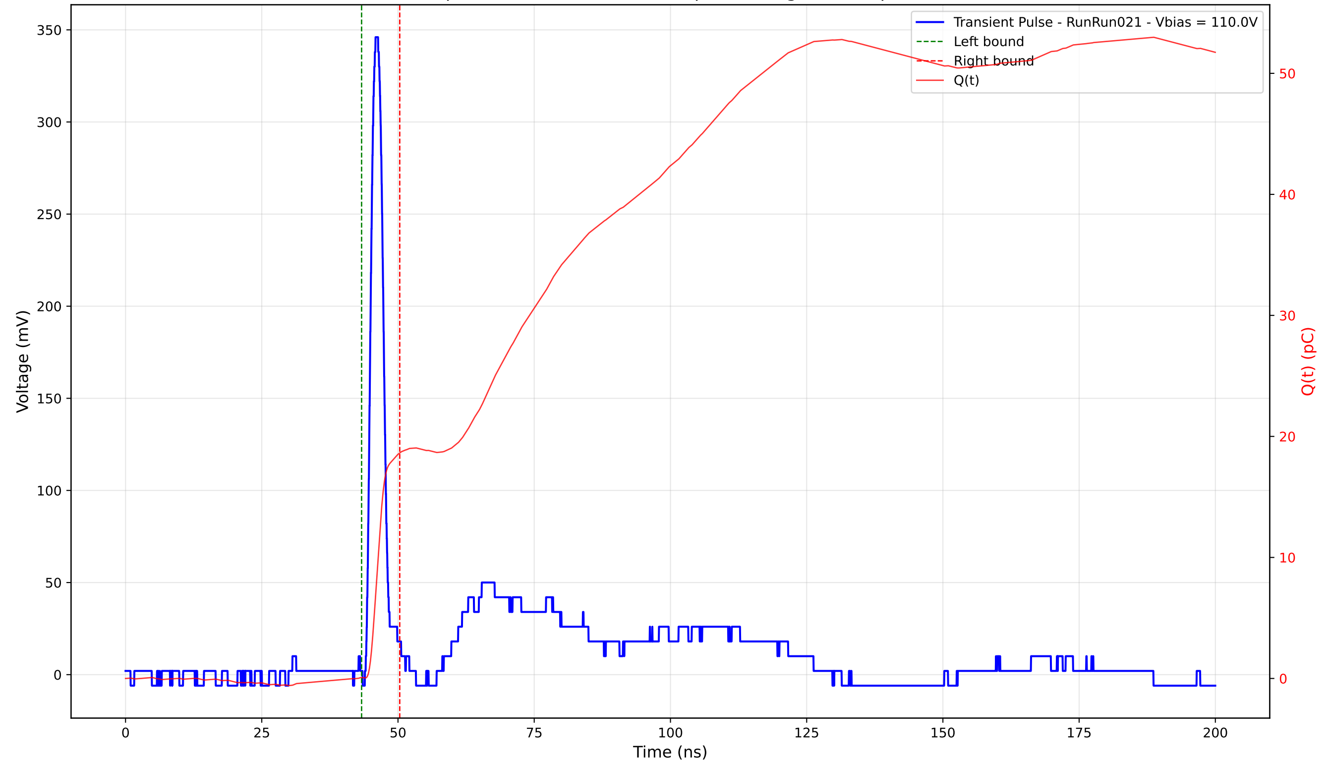
Transient Pulse - Sample: 4003 - Position: 210.0 \mu\text{m} - Charge: 18.56 pC - Rise Time: 1.18 ns
