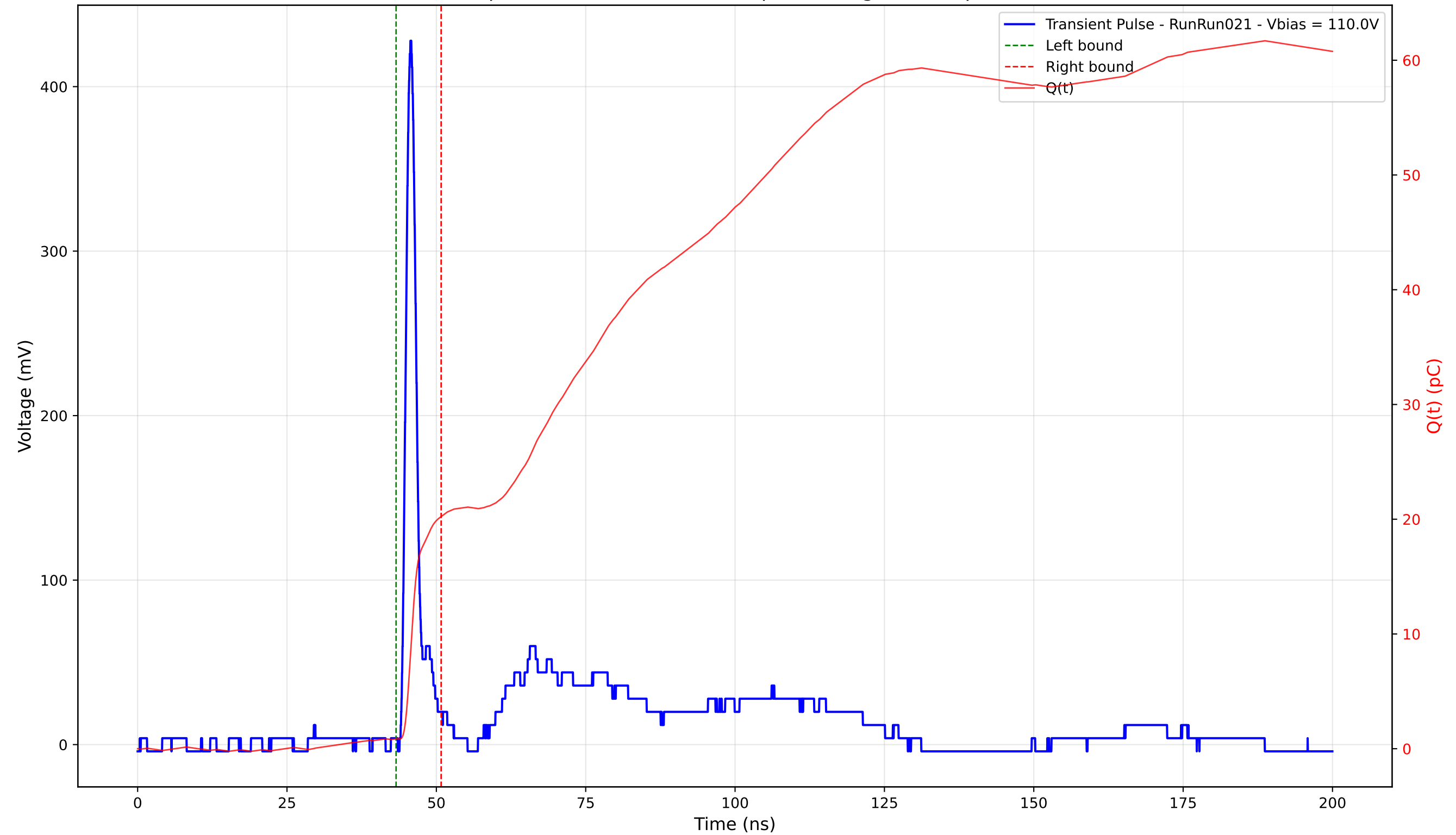
Transient Pulse - Sample: 4003 - Position: 175.0 \mu\text{m} - Charge: 19.37 pC - Rise Time: 1.08 ns
