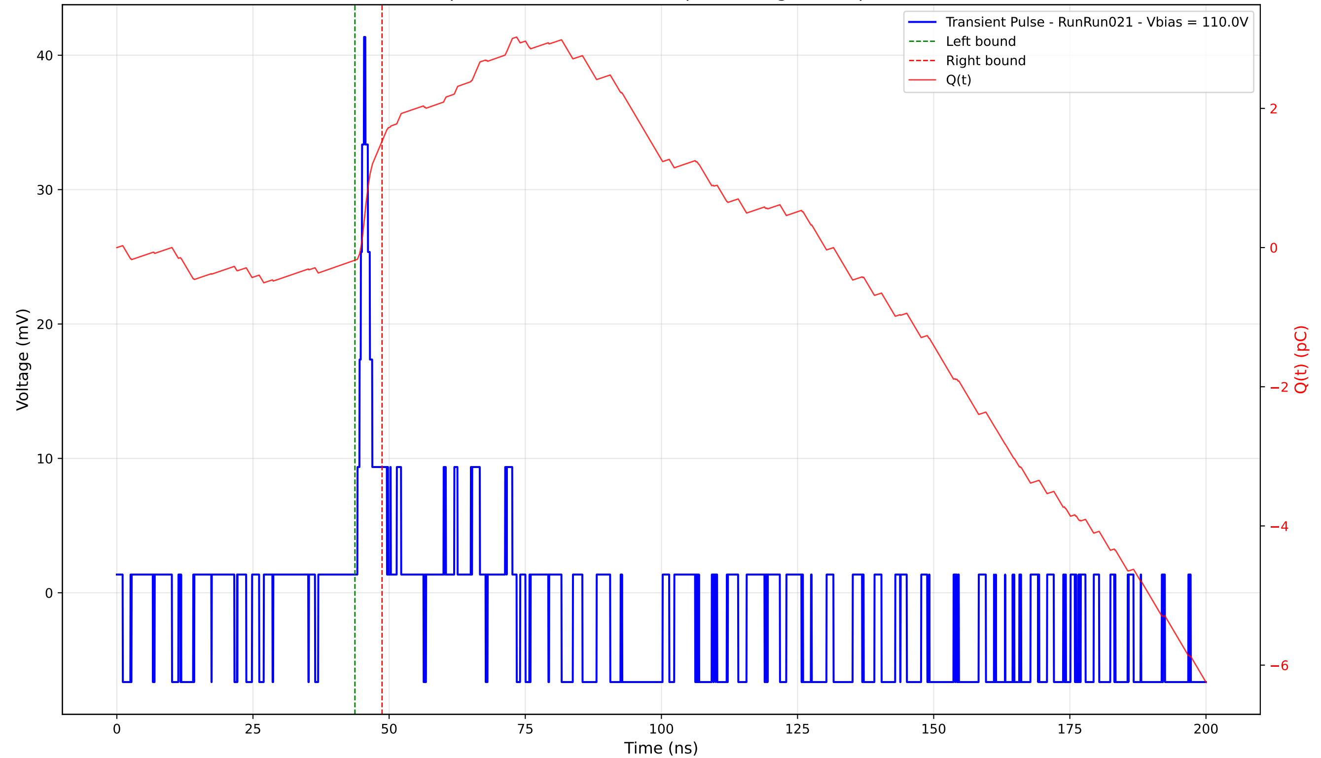
Transient Pulse - Sample: 4003 - Position: 85.0 \mu\text{m} - Charge: 1.71 pC - Rise Time: 1.21 ns
