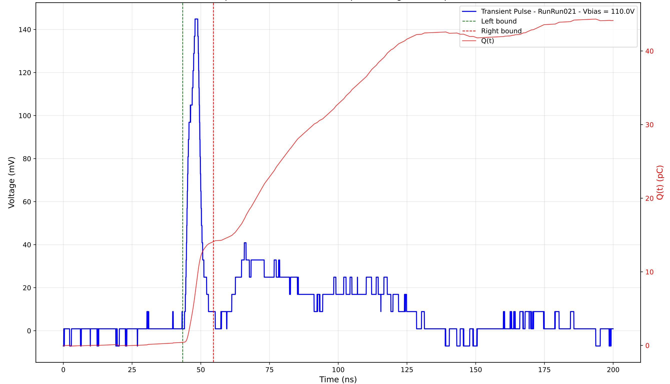
Transient Pulse - Sample: 4003 - Position: 260.0 \mu\text{m} - Charge: 13.69 pC - Rise Time: 3.27 ns
