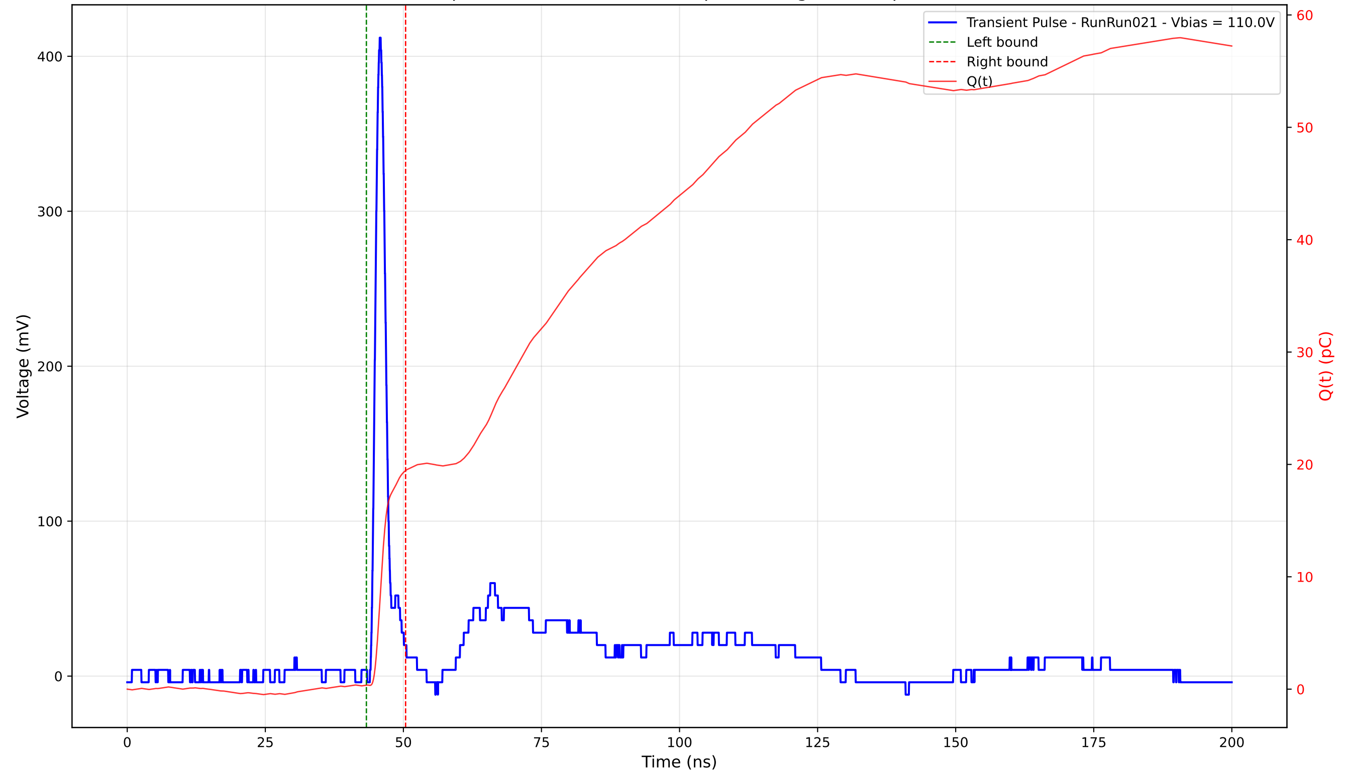
Transient Pulse - Sample: 4003 - Position: 185.0 \mu\text{m} - Charge: 19.09 pC - Rise Time: 1.09 ns
