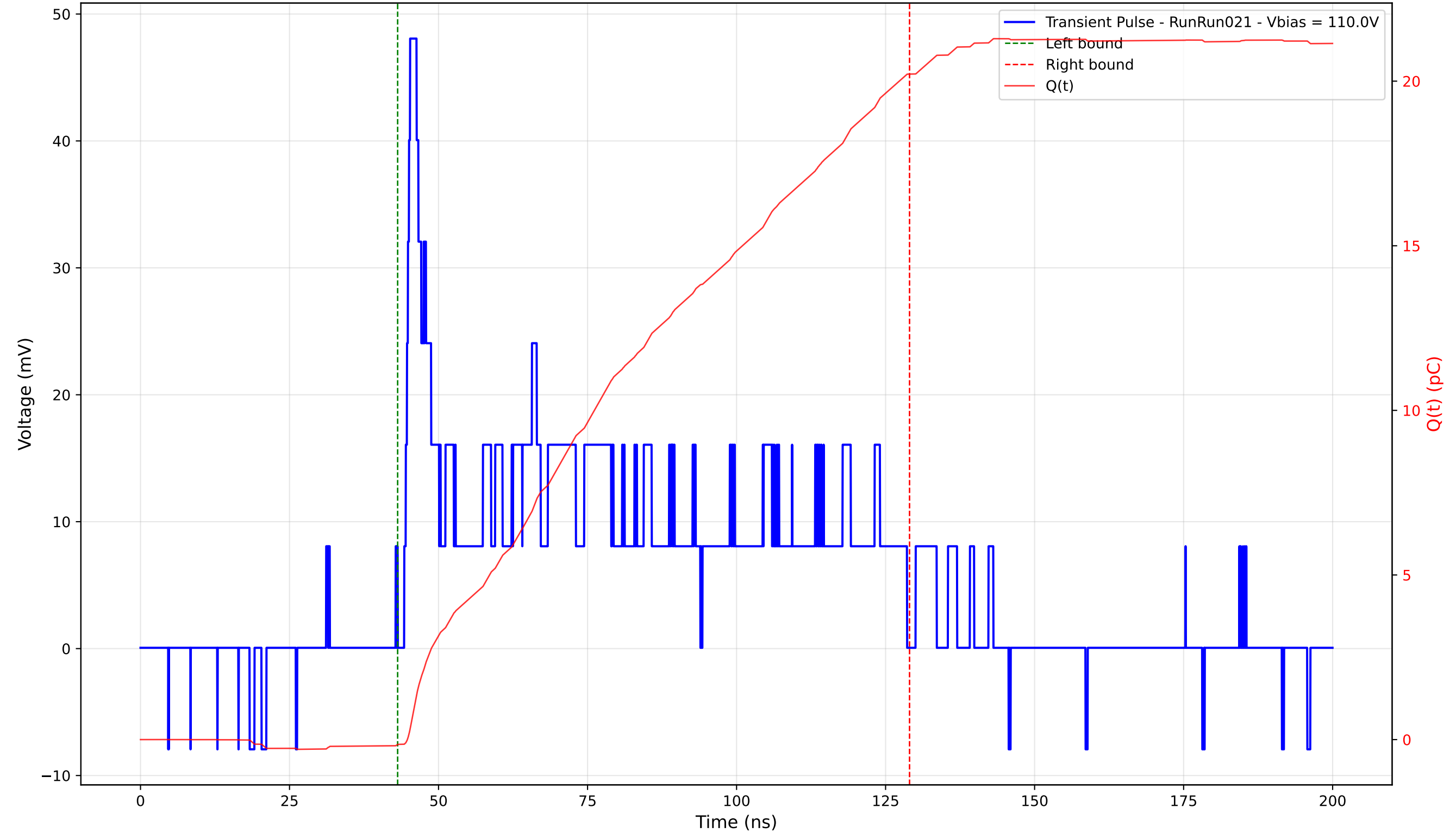
Transient Pulse - Sample: 4003 - Position: 280.0 \mu\text{m} - Charge: 20.36 pC - Rise Time: 0.99 ns
