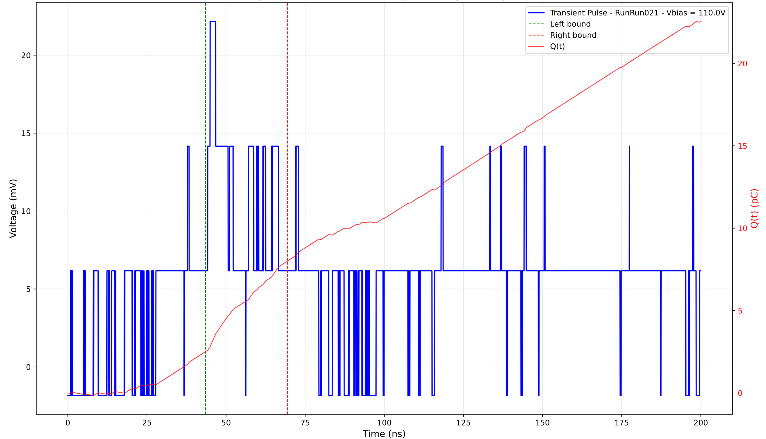
Transient Pulse - Sample: 4003 - Position: 420.0 \mu\text{m} - Charge: 5.50 pC - Rise Time: 8.22 ns
