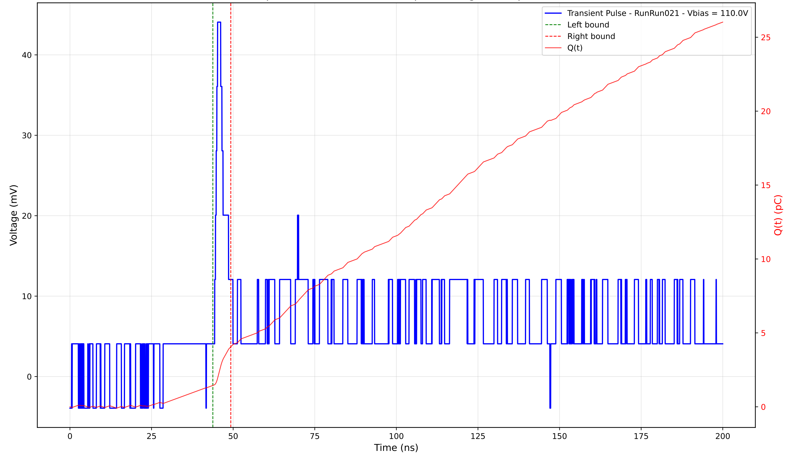
Transient Pulse - Sample: 4003 - Position: 300.0 \mu\text{m} - Charge: 2.62 pC - Rise Time: 0.90 ns
