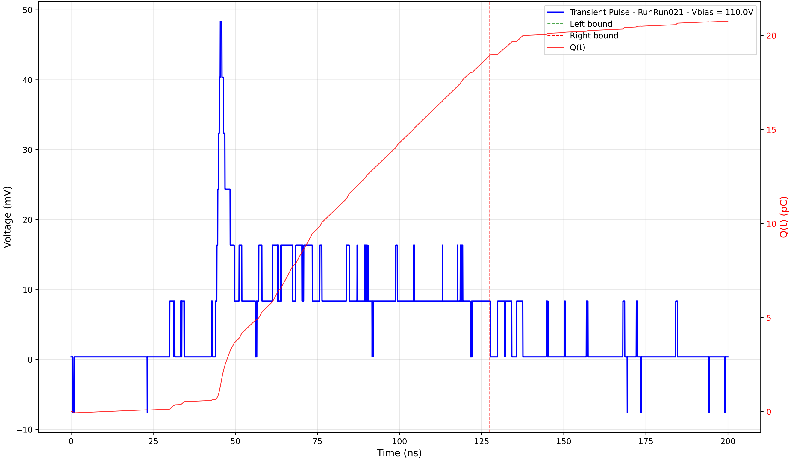
Transient Pulse - Sample: 4003 - Position: 285.0 \mu\text{m} - Charge: 18.30 pC - Rise Time: 1.47 ns
