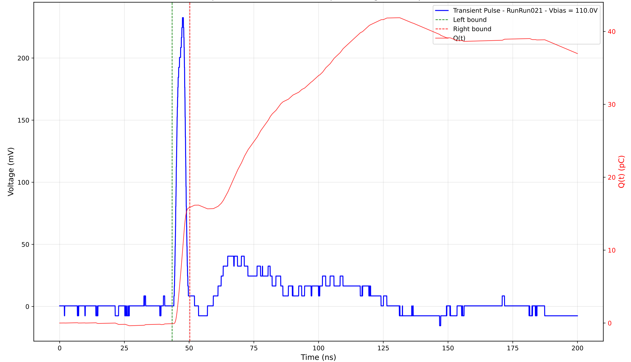
Transient Pulse - Sample: 4003 - Position: 245.0 \mu\text{m} - Charge: 15.95 pC - Rise Time: 2.62 ns
