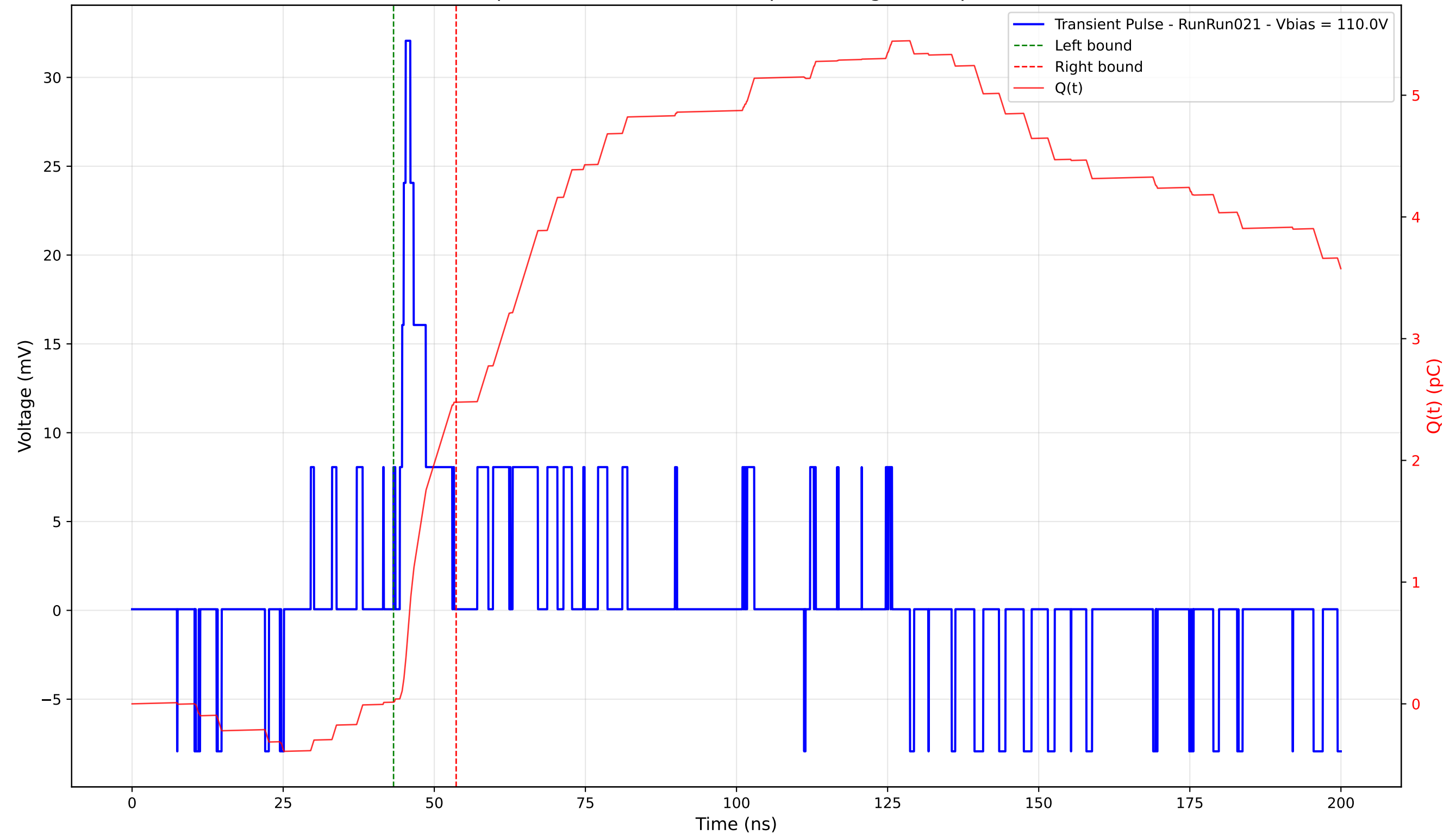
Transient Pulse - Sample: 4003 - Position: 380.0 \mu\text{m} - Charge: 2.46 pC - Rise Time: 0.97 ns
