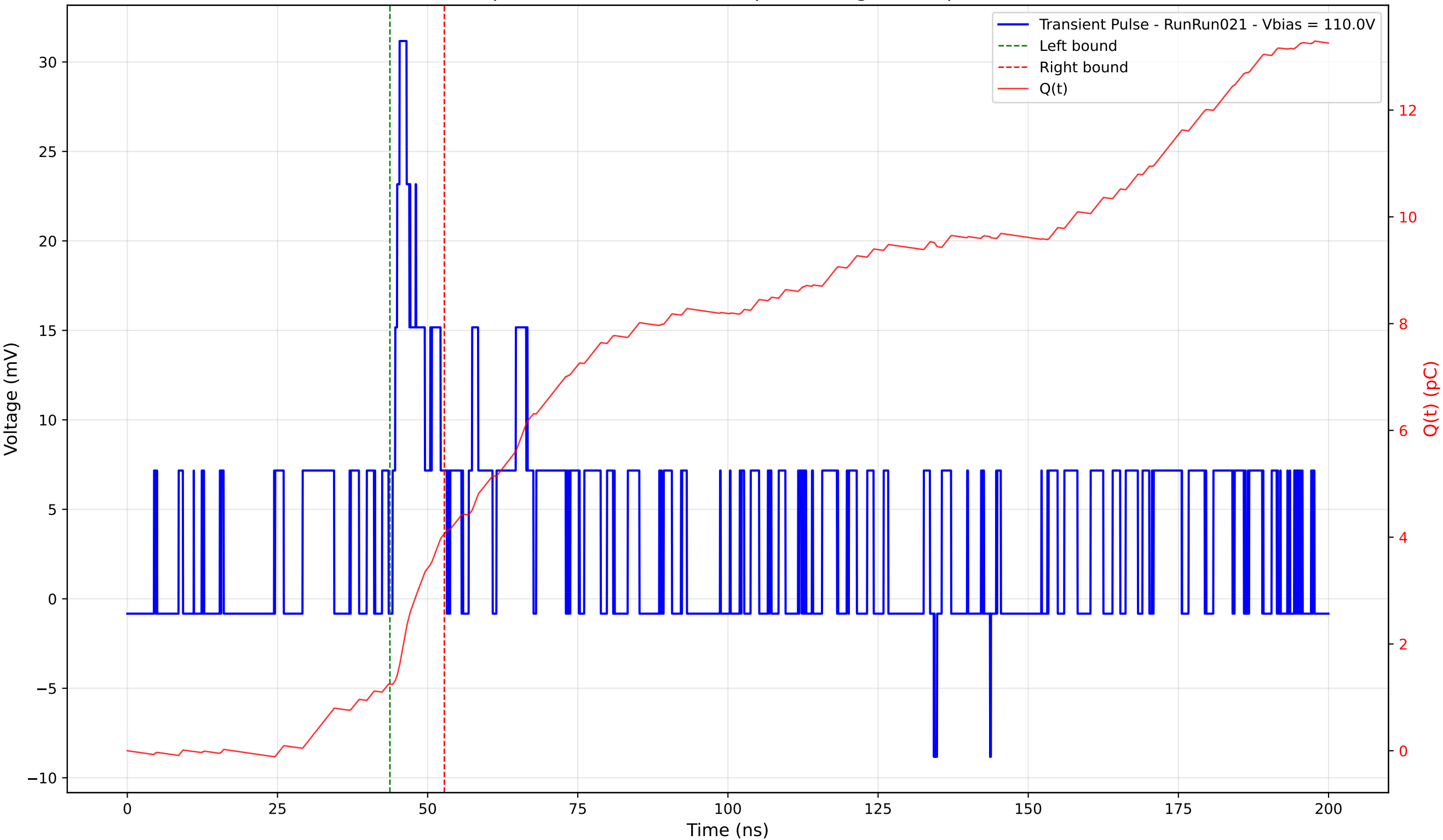
Transient Pulse - Sample: 4003 - Position: 45.0 \mu\text{m} - Charge: 2.82 pC - Rise Time: 1.17 ns
