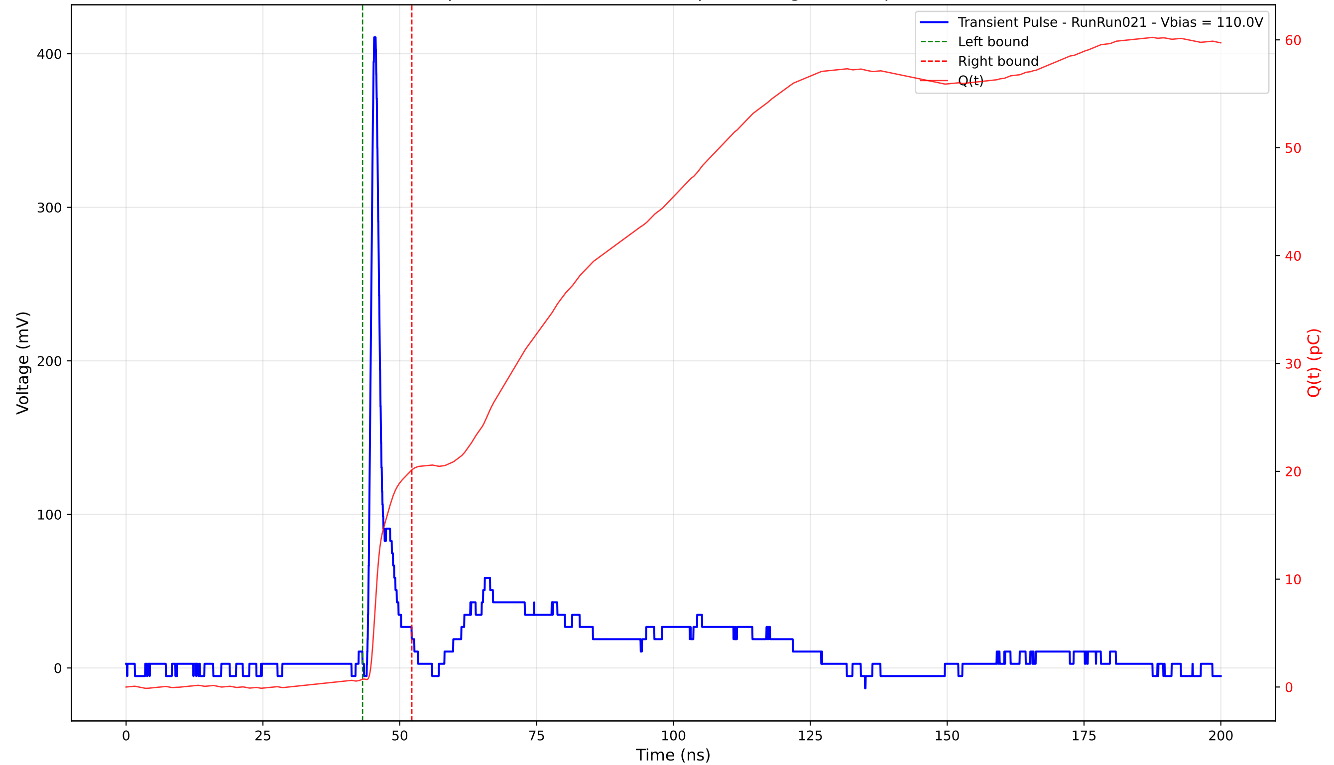
Transient Pulse - Sample: 4003 - Position: 125.0 \mu\text{m} - Charge: 19.41 pC - Rise Time: 0.90 ns
