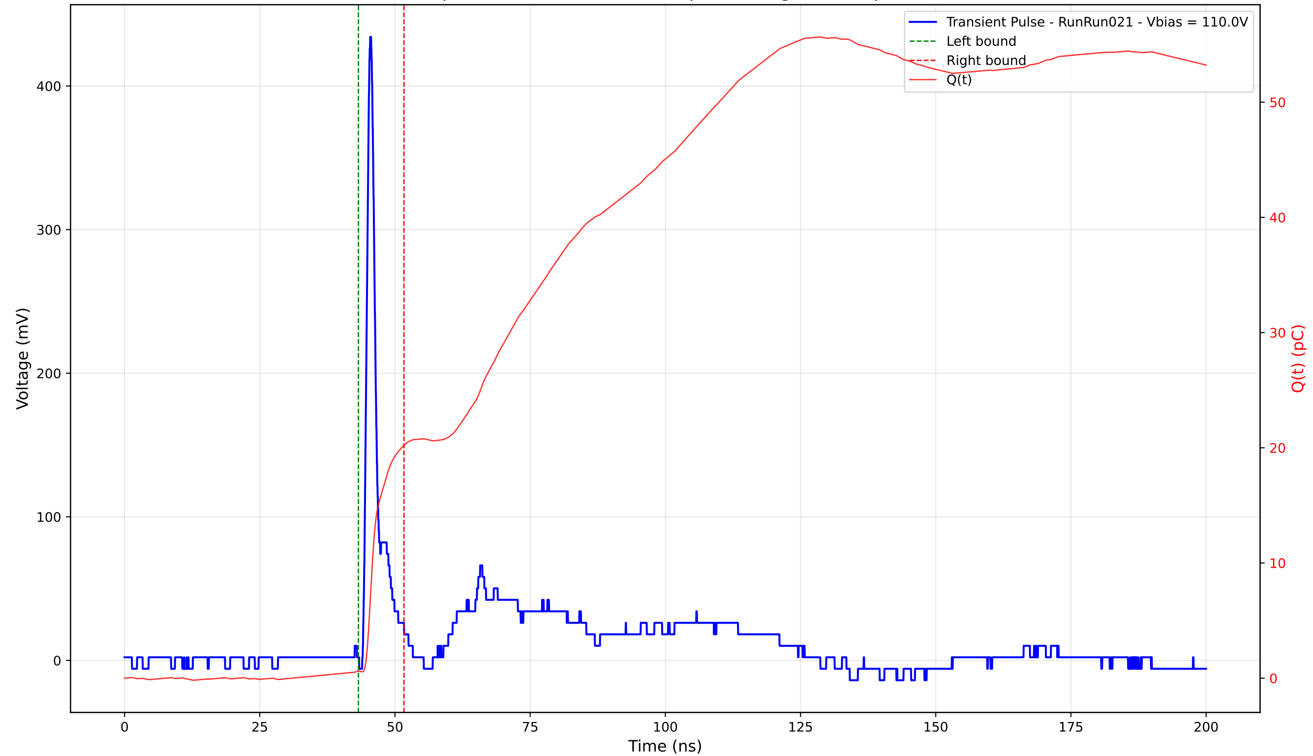
Transient Pulse - Sample: 4003 - Position: 135.0 \mu\text{m} - Charge: 19.63 pC - Rise Time: 0.94 ns
