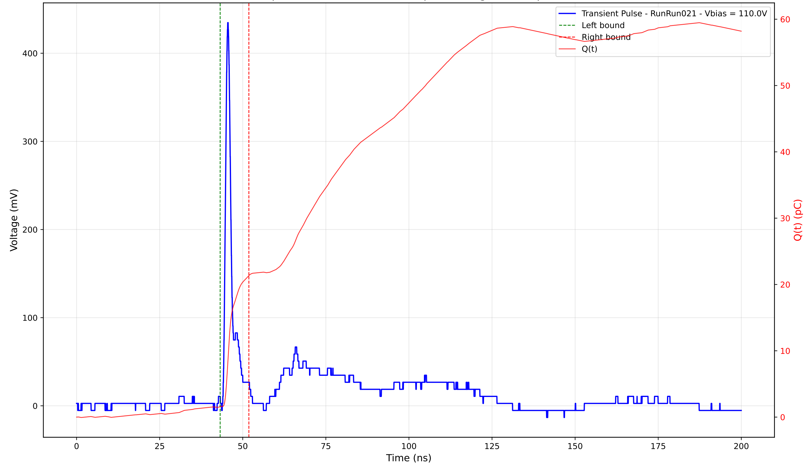
Transient Pulse - Sample: 4003 - Position: 145.0 \mu\text{m} - Charge: 19.75 pC - Rise Time: 0.96 ns
