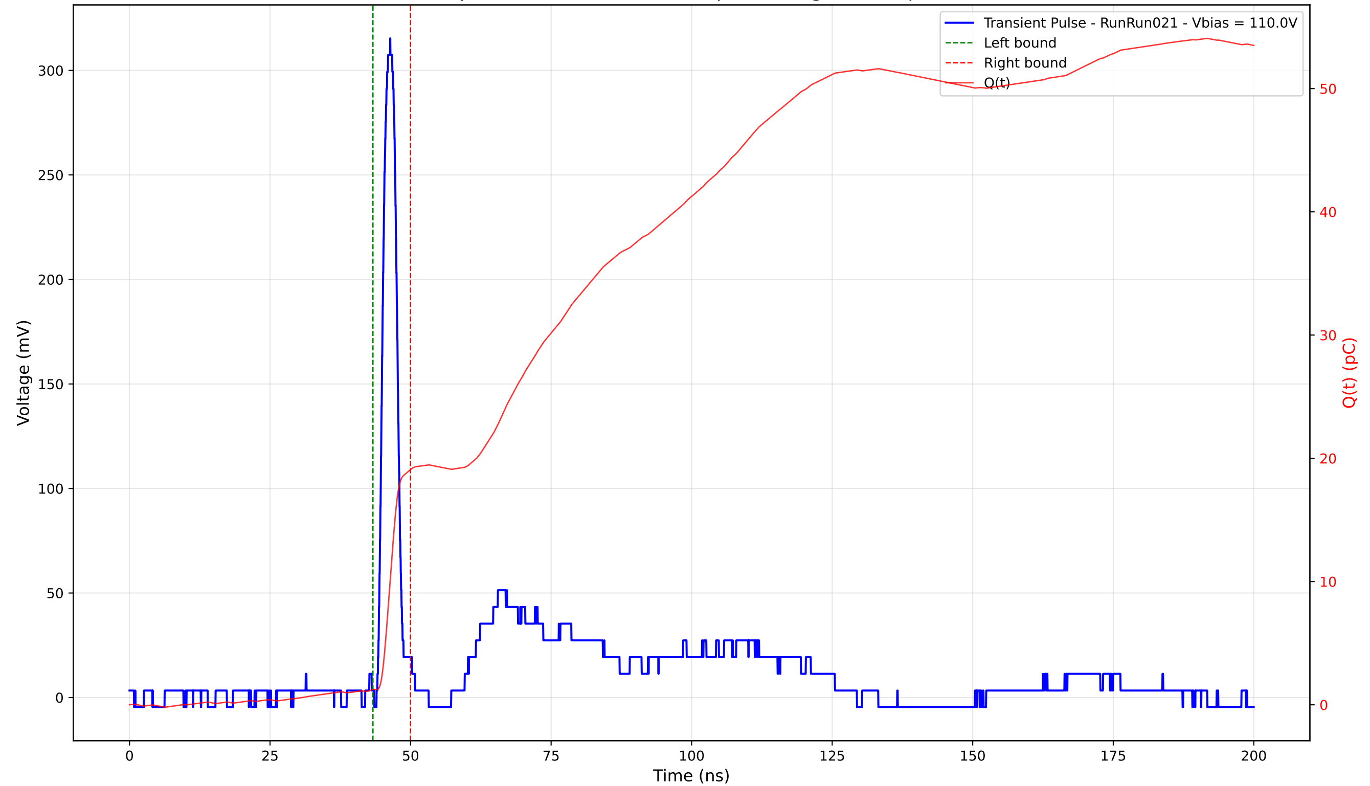
Transient Pulse - Sample: 4003 - Position: 220.0 \mu\text{m} - Charge: 17.84 pC - Rise Time: 1.37 ns
