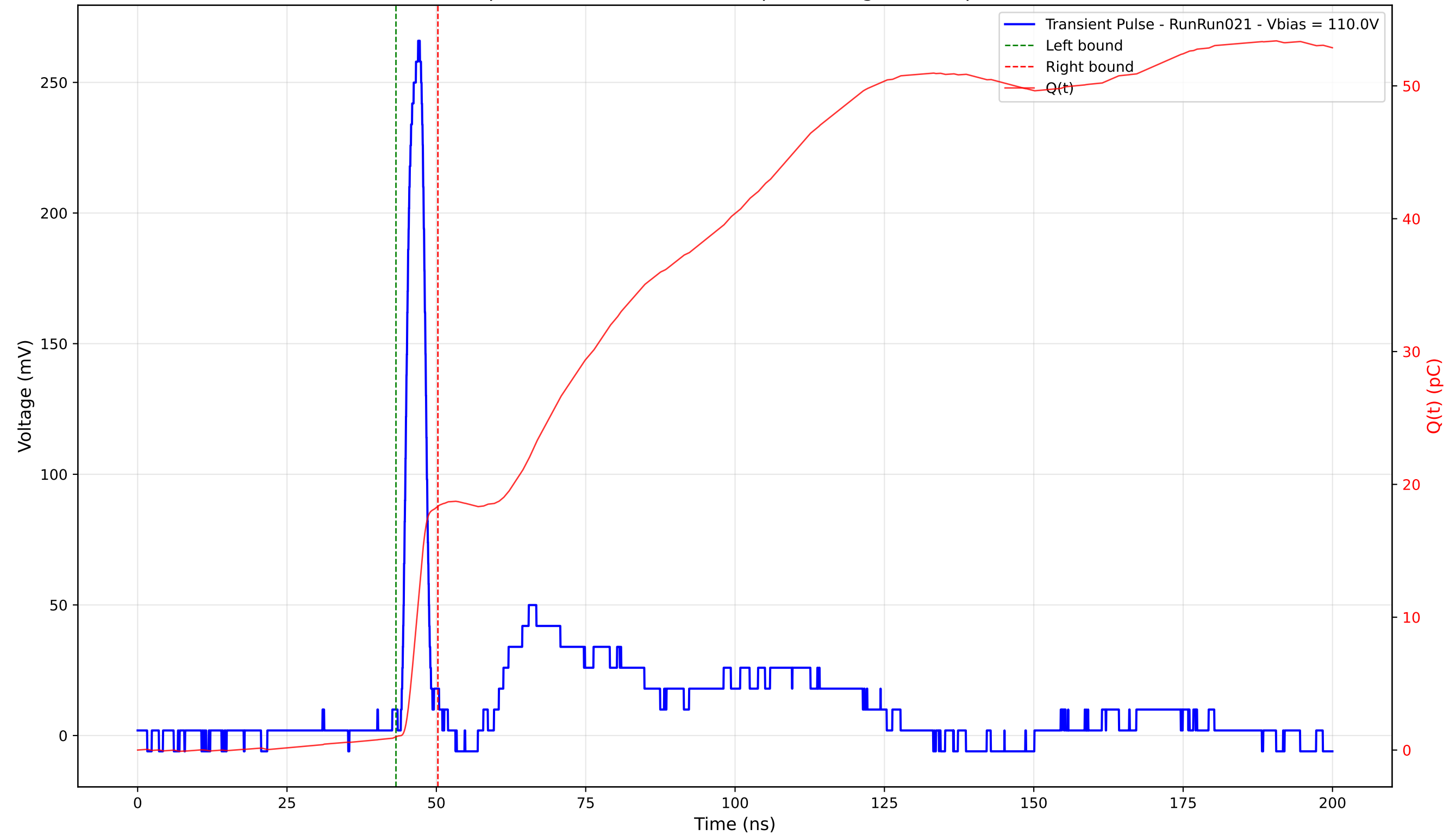
Transient Pulse - Sample: 4003 - Position: 235.0 \mu\text{m} - Charge: 17.35 pC - Rise Time: 1.58 ns
