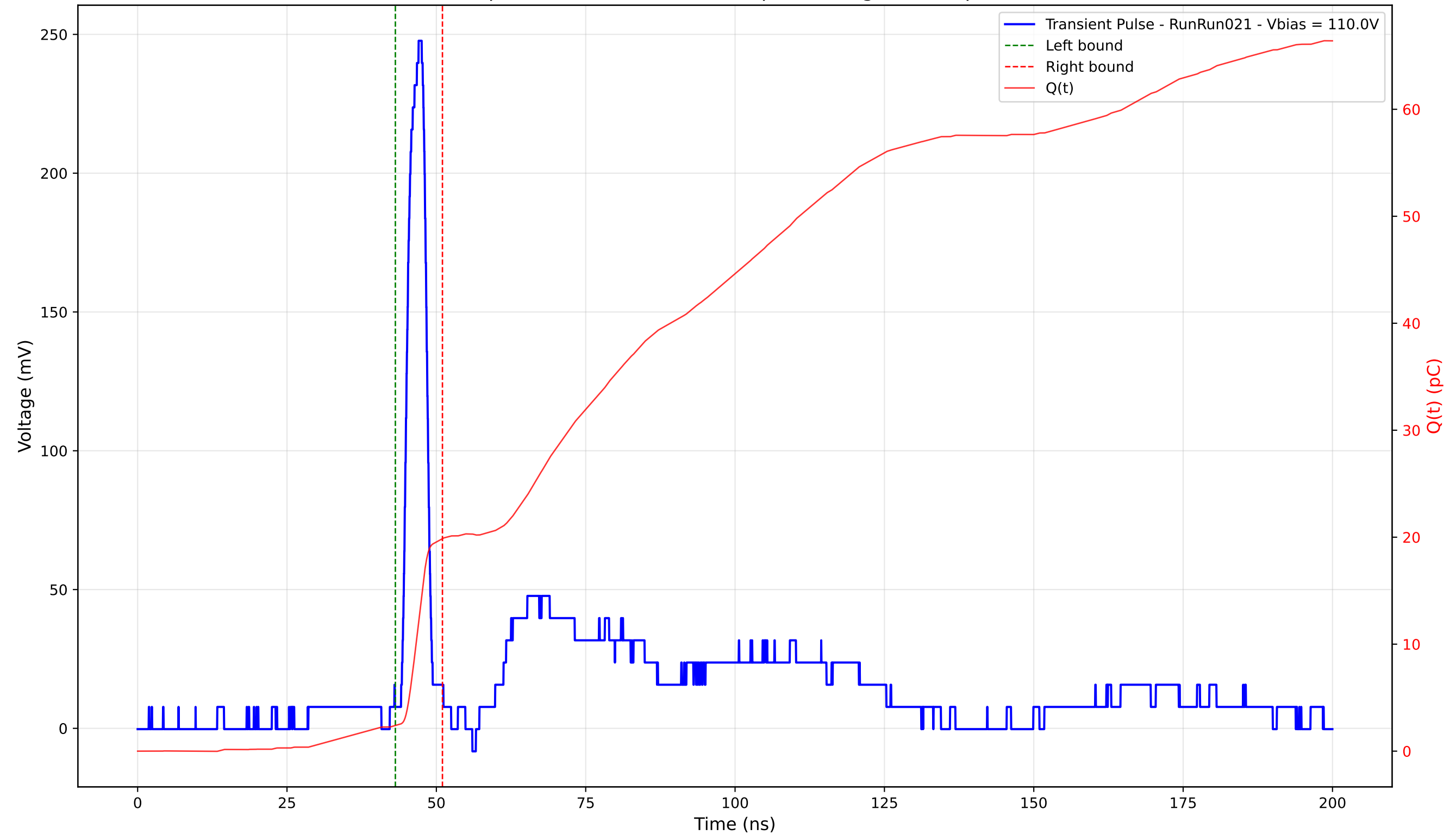
Transient Pulse - Sample: 4003 - Position: 240.0 \mu\text{m} - Charge: 17.47 pC - Rise Time: 1.72 ns
