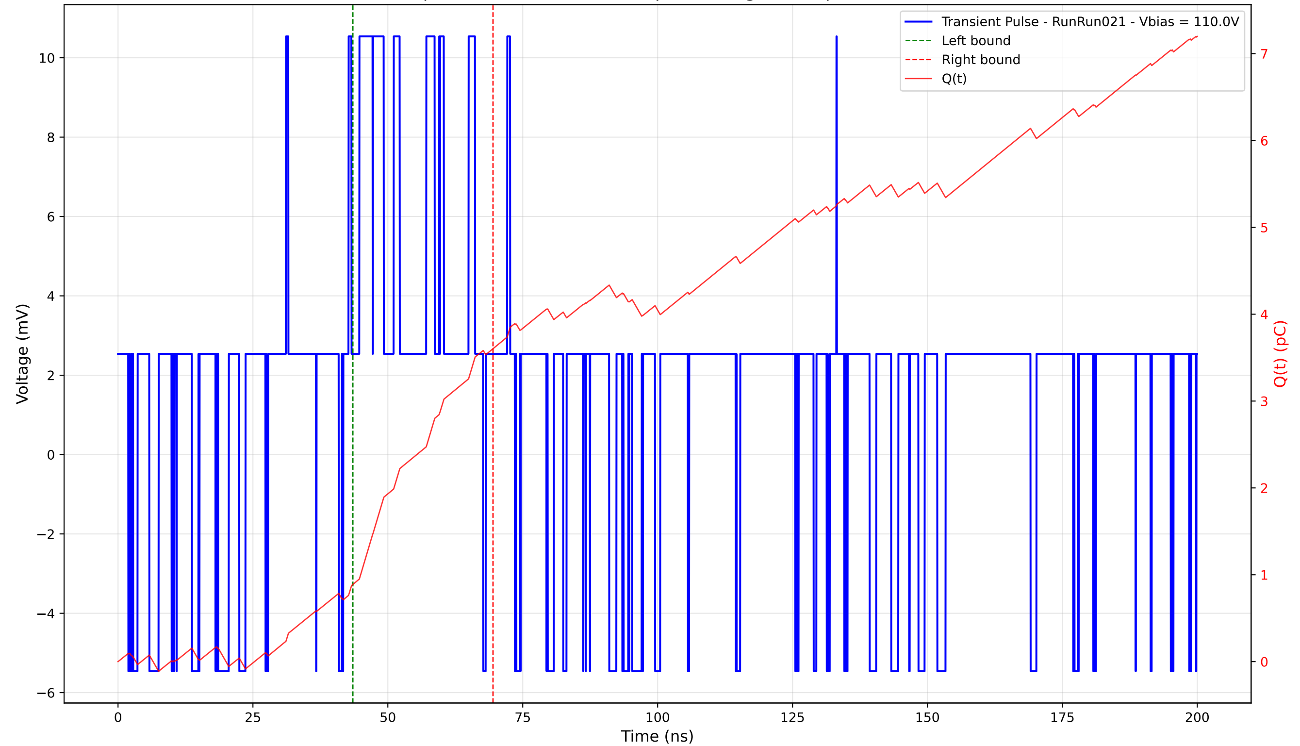
Transient Pulse - Sample: 4003 - Position: 10.0 \mu\text{m} - Charge: 2.71 pC - Rise Time: 0.00 ns (N/A)
