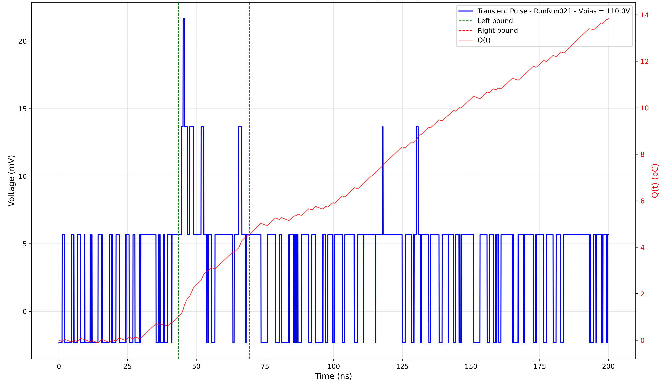
Transient Pulse - Sample: 4003 - Position: 5.0 \mu\text{m} - Charge: 3.54 pC - Rise Time: 0.00 ns (N/A)
