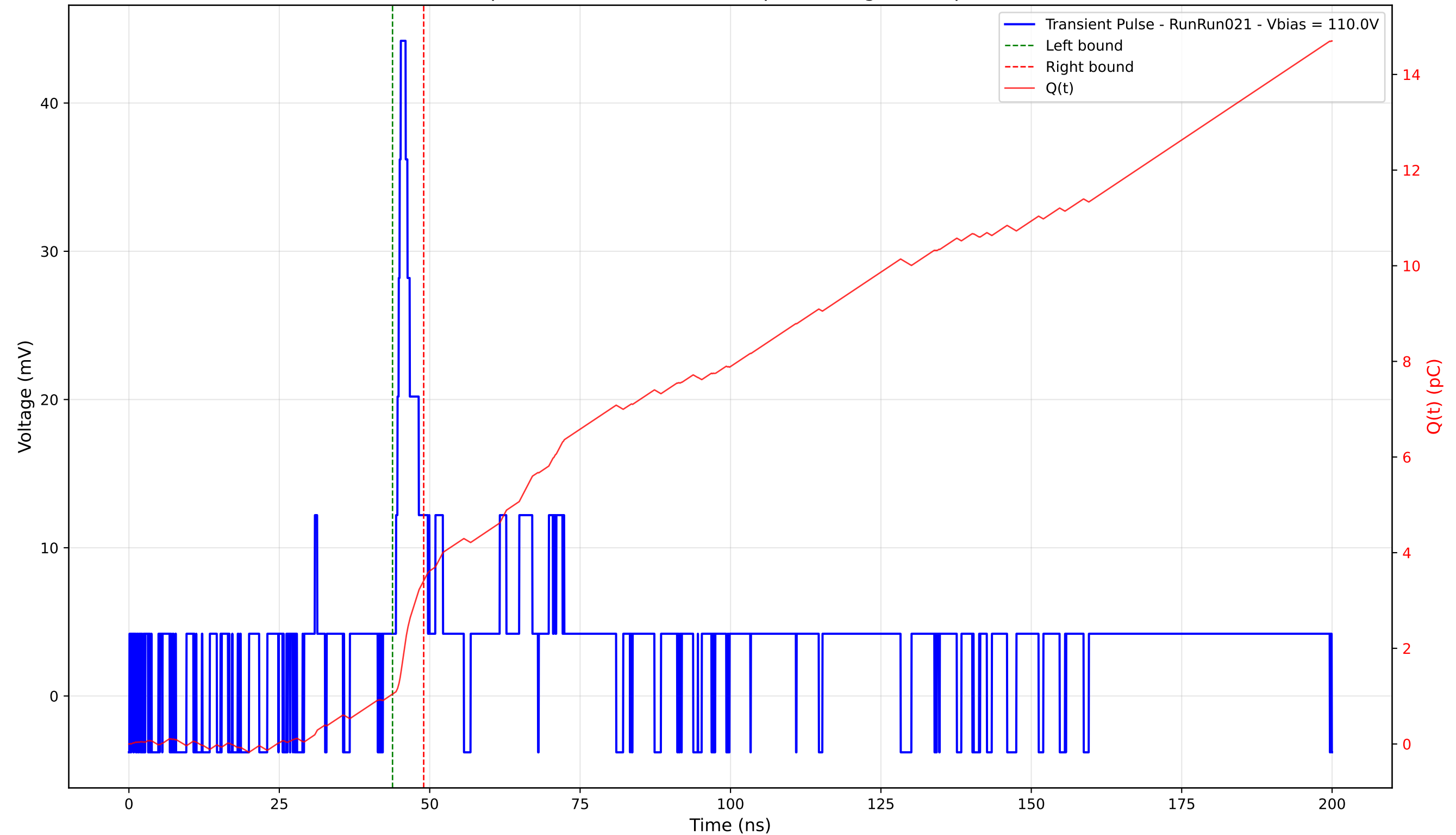
Transient Pulse - Sample: 4003 - Position: 395.0 \mu\text{m} - Charge: 2.37 pC - Rise Time: 0.80 ns
