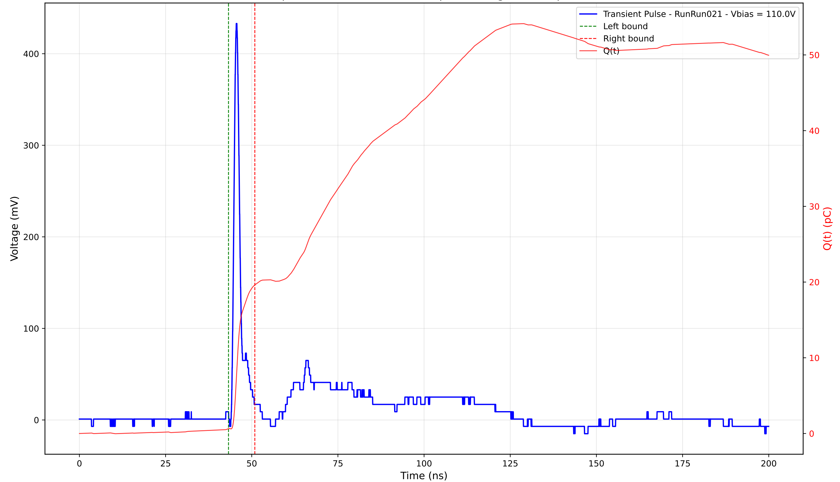
Transient Pulse - Sample: 4003 - Position: 155.0 \mu\text{m} - Charge: 18.98 pC - Rise Time: 0.97 ns
