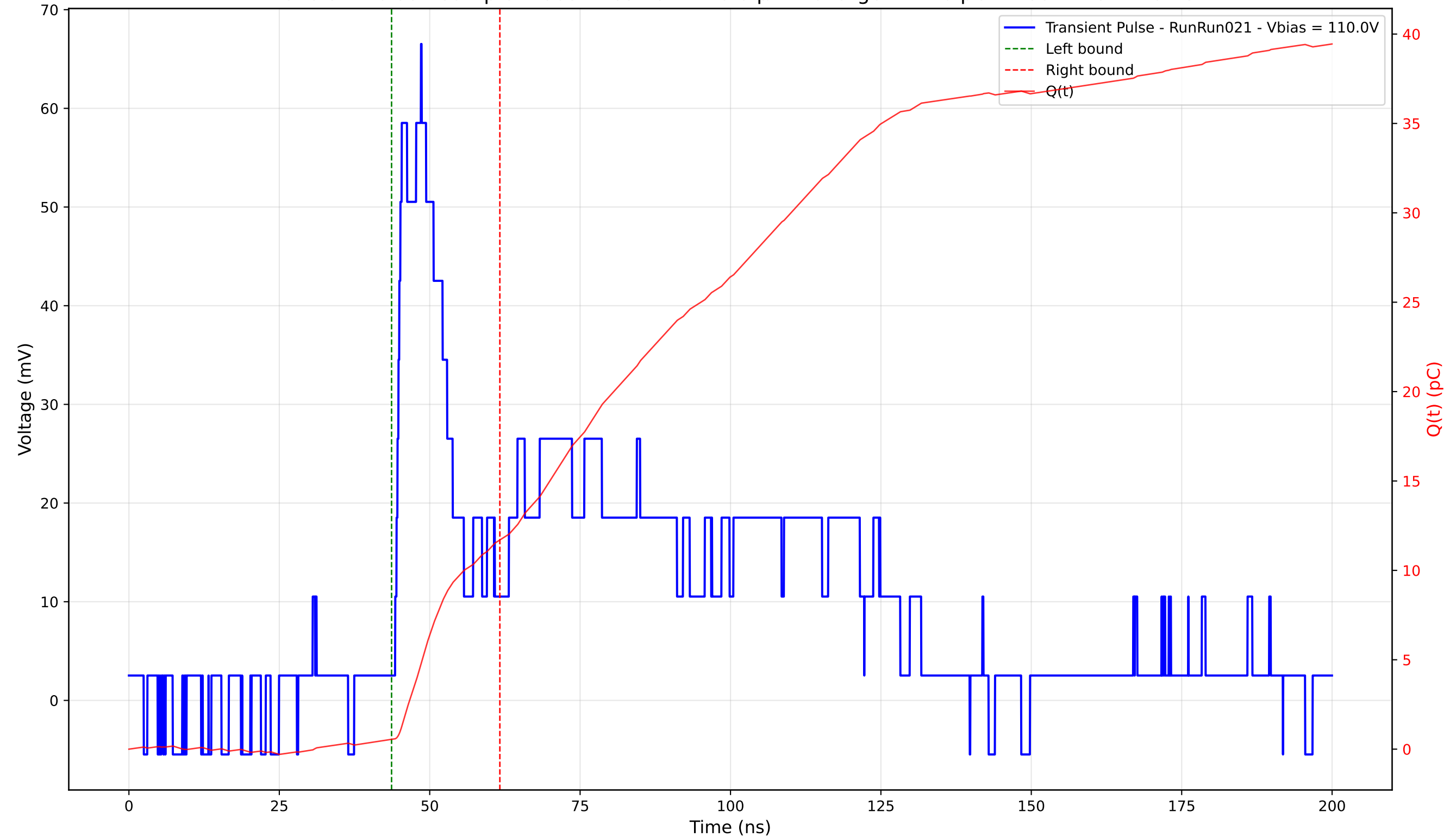
Transient Pulse - Sample: 4003 - Position: 270.0 \mu\text{m} - Charge: 11.16 pC - Rise Time: 4.29 ns
