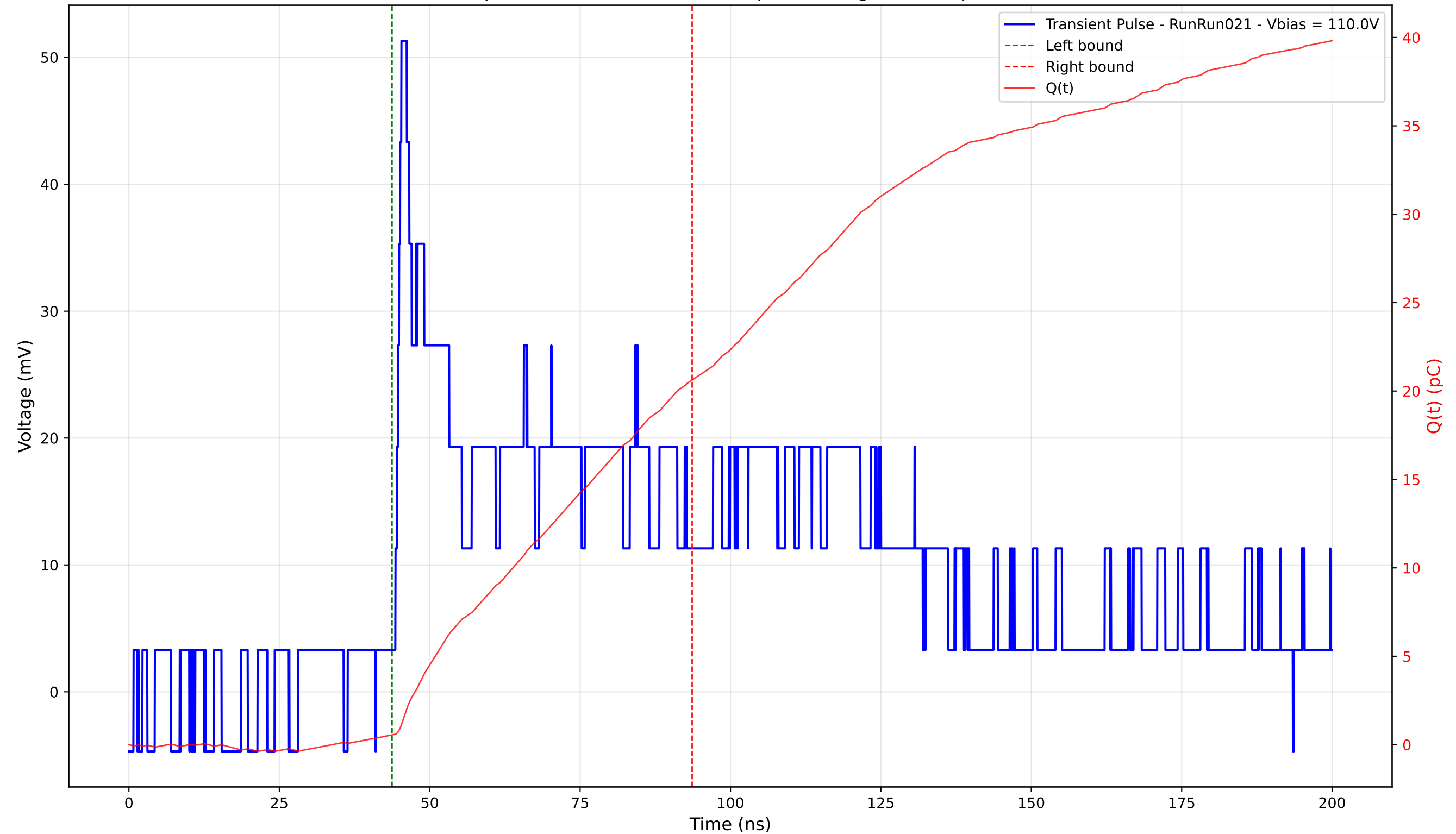
Transient Pulse - Sample: 4003 - Position: 275.0 \mu\text{m} - Charge: 20.08 pC - Rise Time: 1.00 ns
