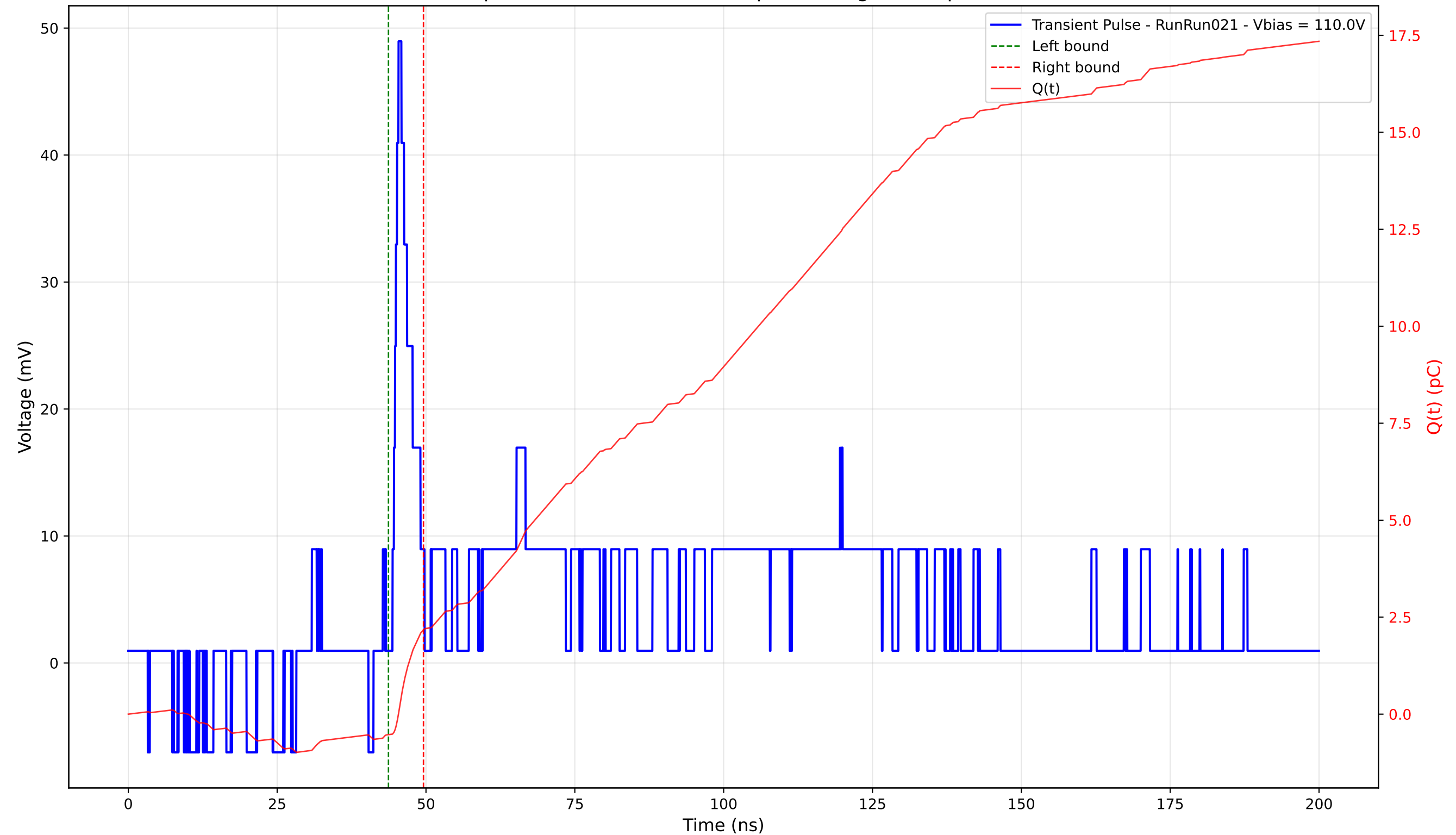
Transient Pulse - Sample: 4003 - Position: 290.0 \mu\text{m} - Charge: 2.70 pC - Rise Time: 1.01 ns
