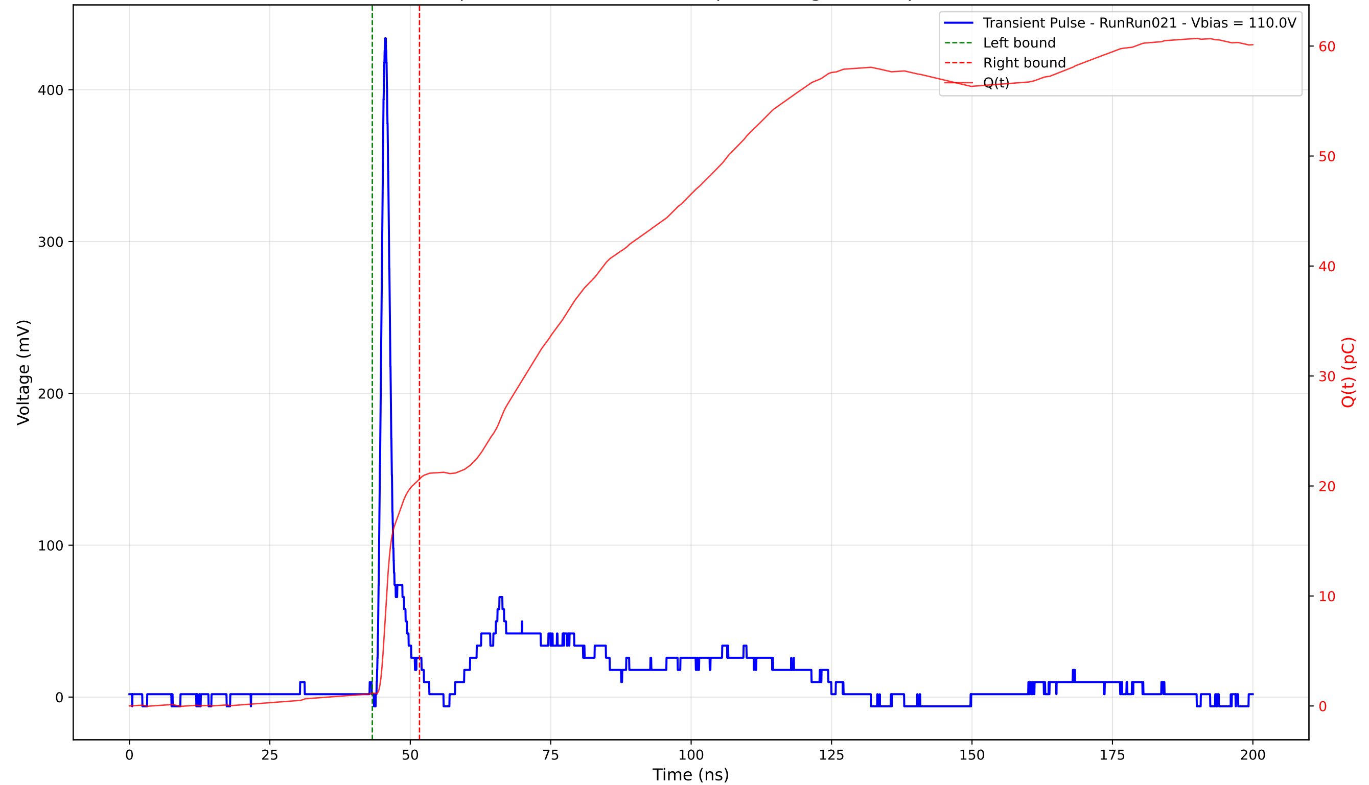
Transient Pulse - Sample: 4003 - Position: 150.0 \mu\text{m} - Charge: 19.48 pC - Rise Time: 0.98 ns
