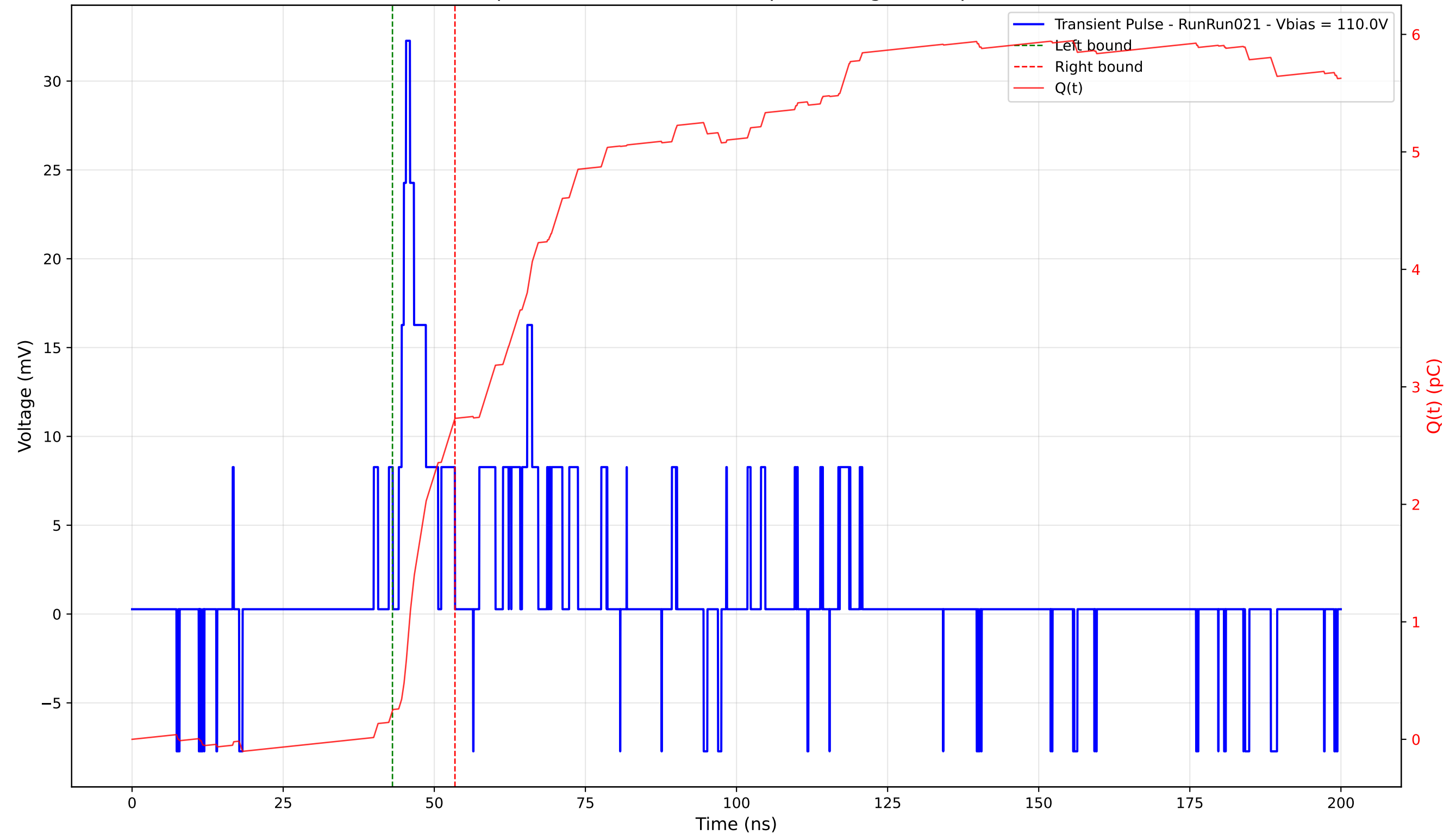
Transient Pulse - Sample: 4003 - Position: 320.0 \mu\text{m} - Charge: 2.49 pC - Rise Time: 1.21 ns
