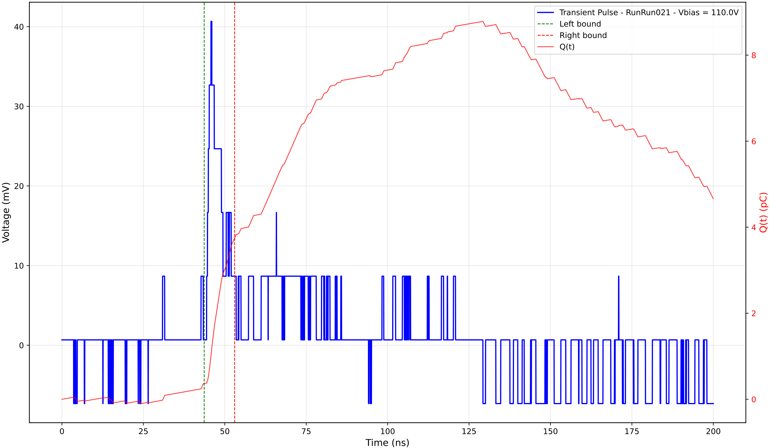
Transient Pulse - Sample: 4003 - Position: 55.0 \mu\text{m} - Charge: 3.39 pC - Rise Time: 1.35 ns
