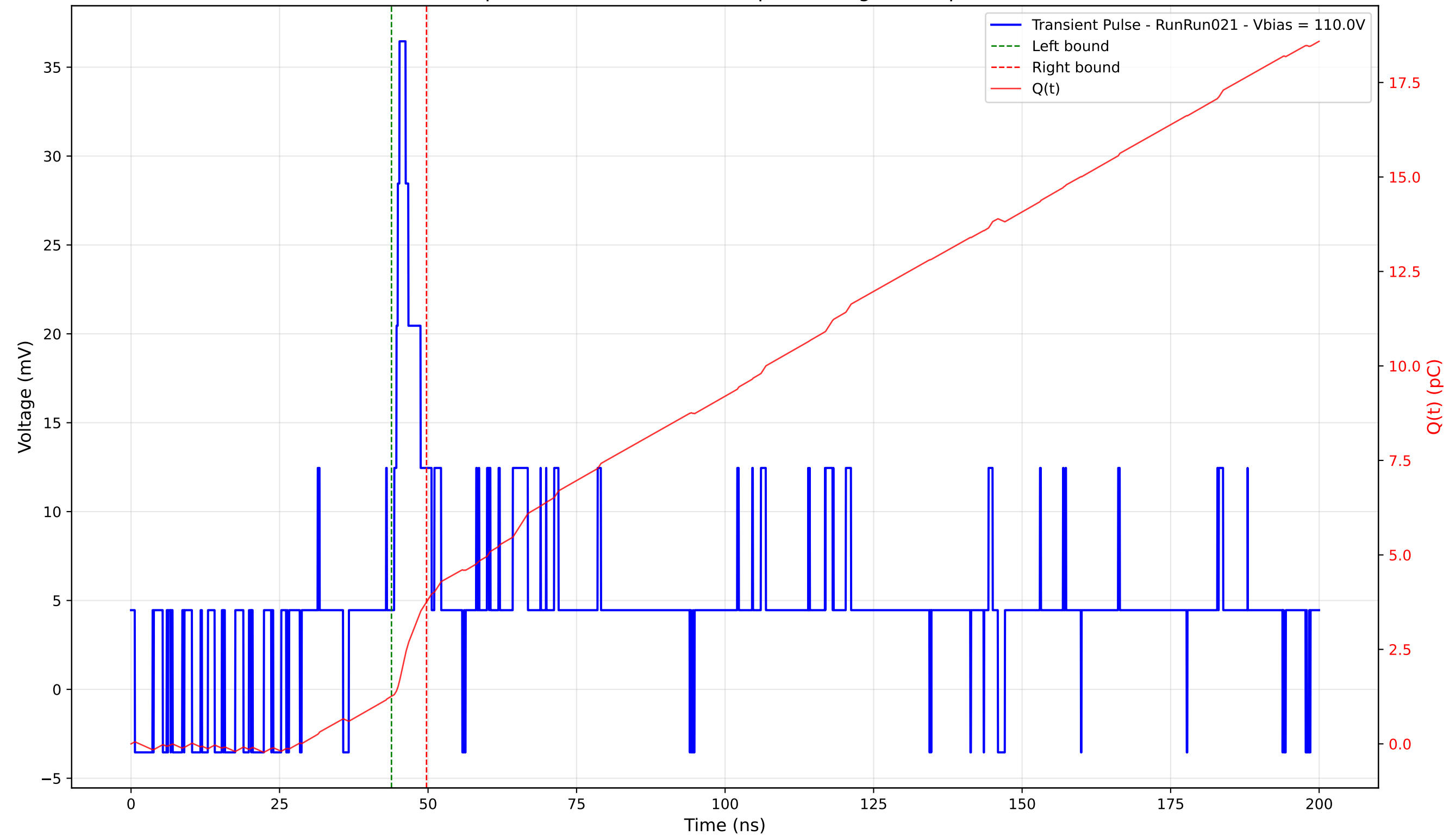
Transient Pulse - Sample: 4003 - Position: 310.0 \mu\text{m} - Charge: 2.50 pC - Rise Time: 8.54 ns
