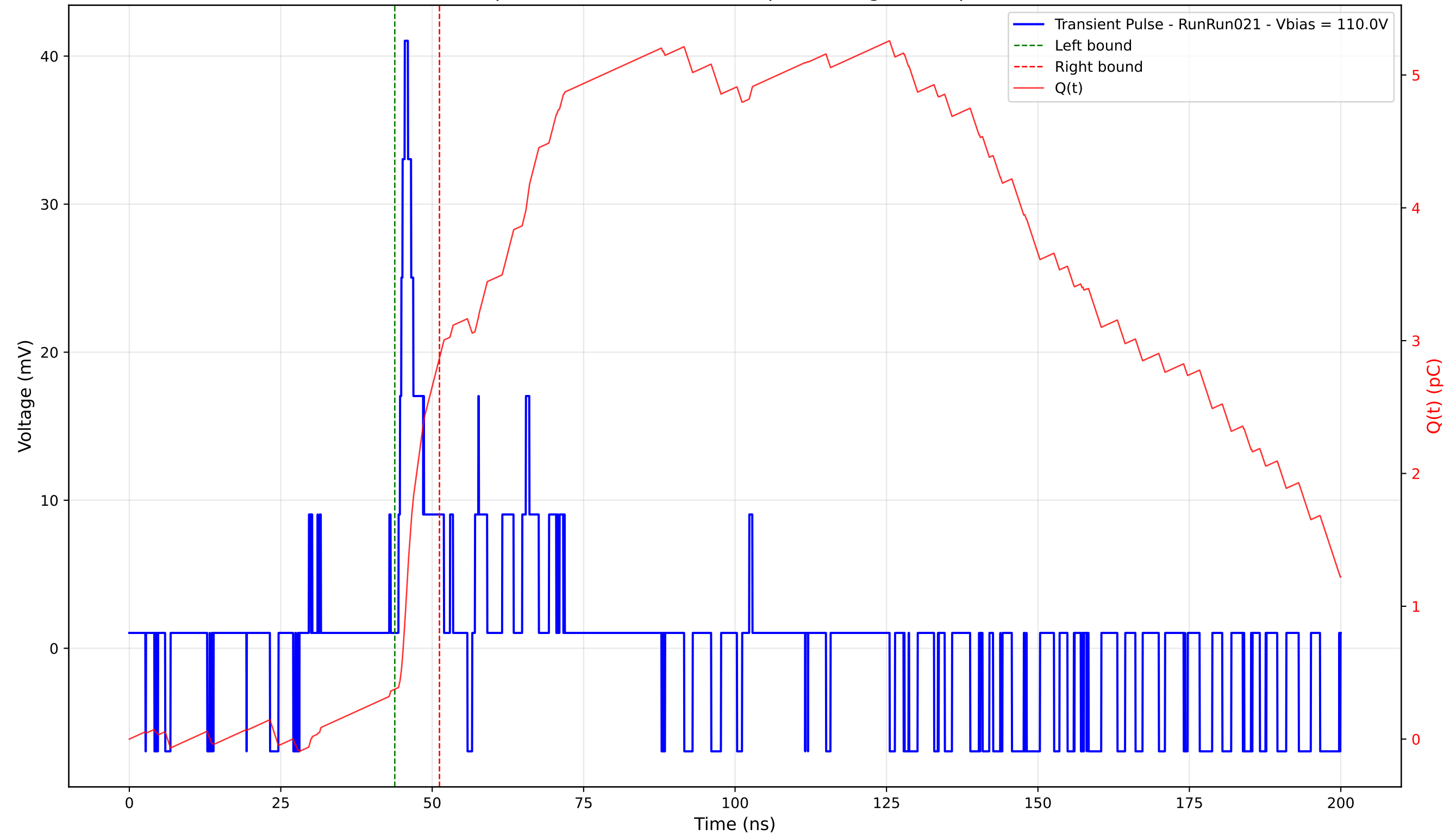
Transient Pulse - Sample: 4003 - Position: 385.0 \mu\text{m} - Charge: 2.50 pC - Rise Time: 1.03 ns
