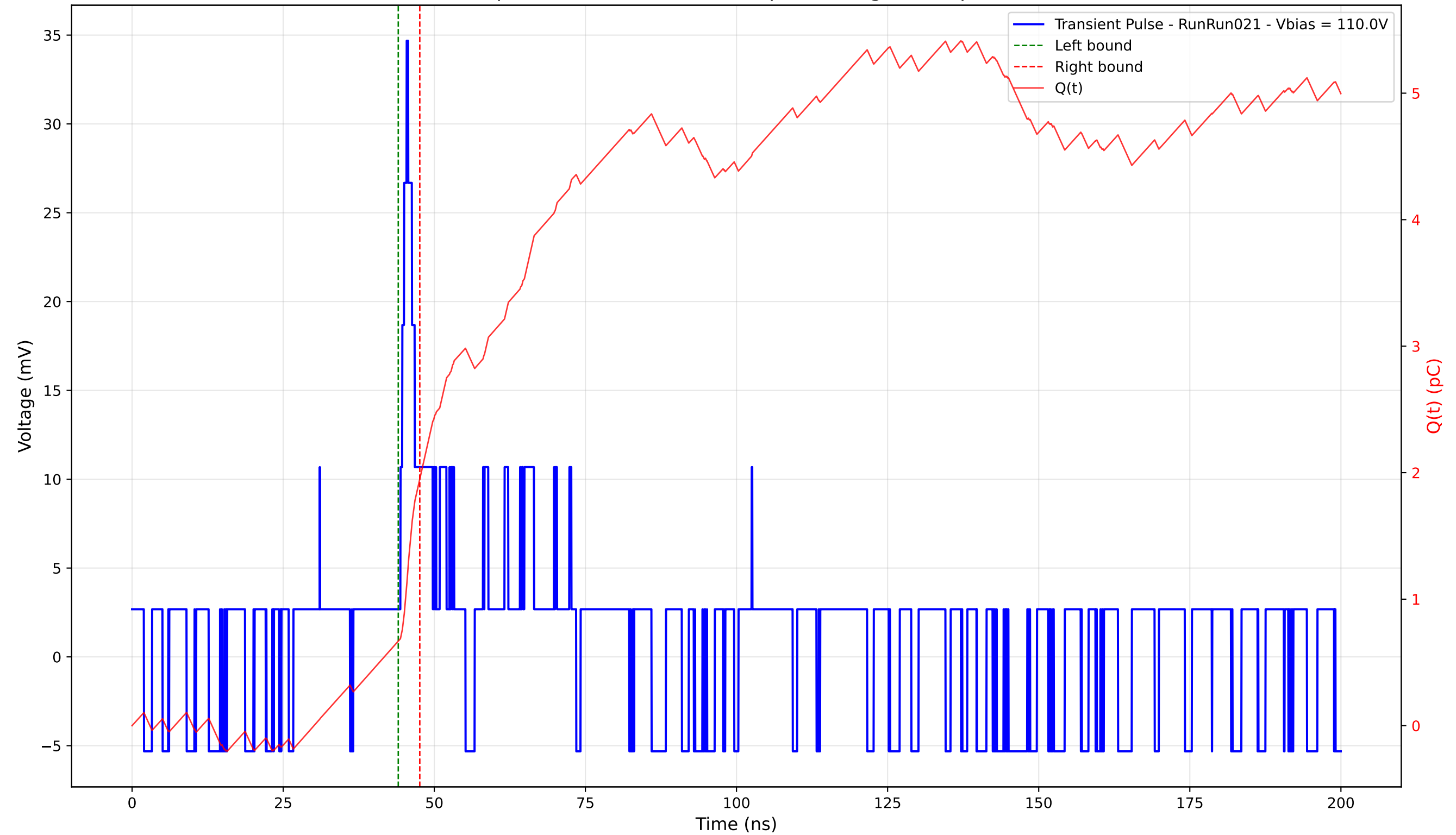
Transient Pulse - Sample: 4003 - Position: 375.0 \mu\text{m} - Charge: 1.28 pC - Rise Time: 1.04 ns
