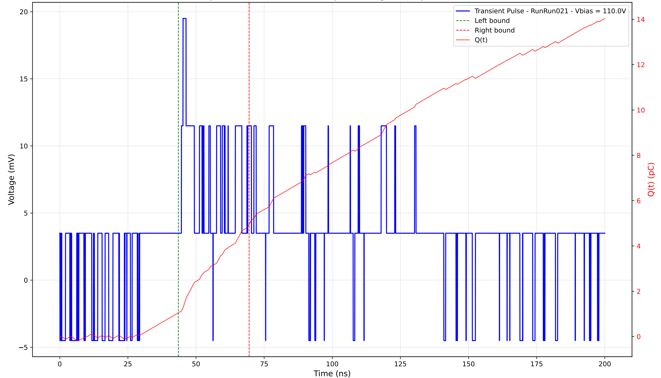
Transient Pulse - Sample: 4003 - Position: 425.0 \mu\text{m} - Charge: 3.91 pC - Rise Time: 0.00 ns (N/A)
