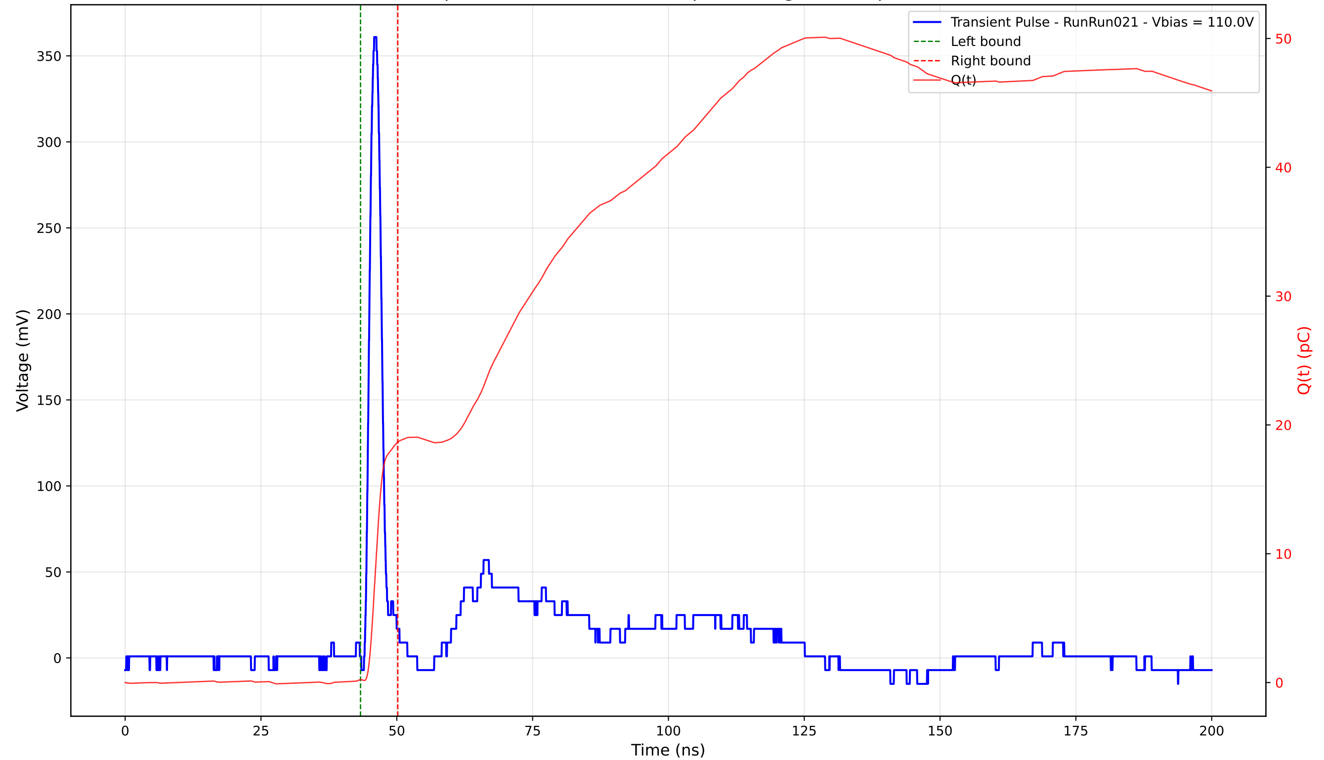
Transient Pulse - Sample: 4003 - Position: 205.0 \mu\text{m} - Charge: 18.44 pC - Rise Time: 1.17 ns
