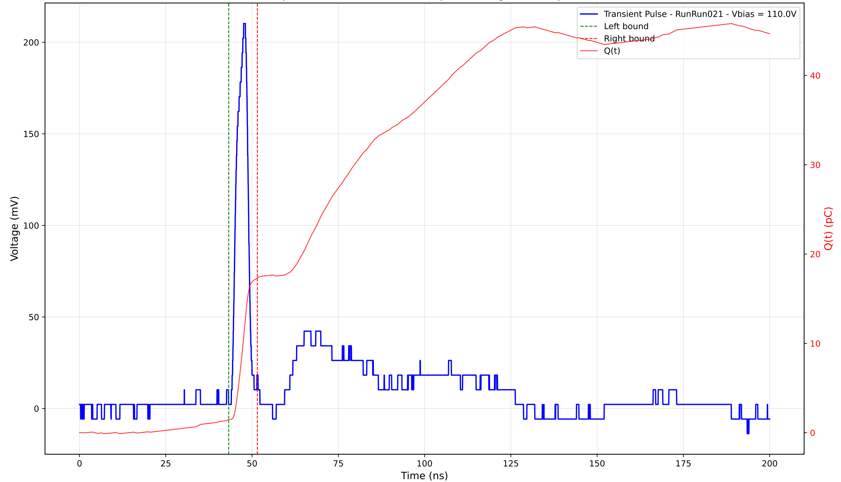
Transient Pulse - Sample: 4003 - Position: 250.0 \mu\text{m} - Charge: 15.85 pC - Rise Time: 2.77 ns
