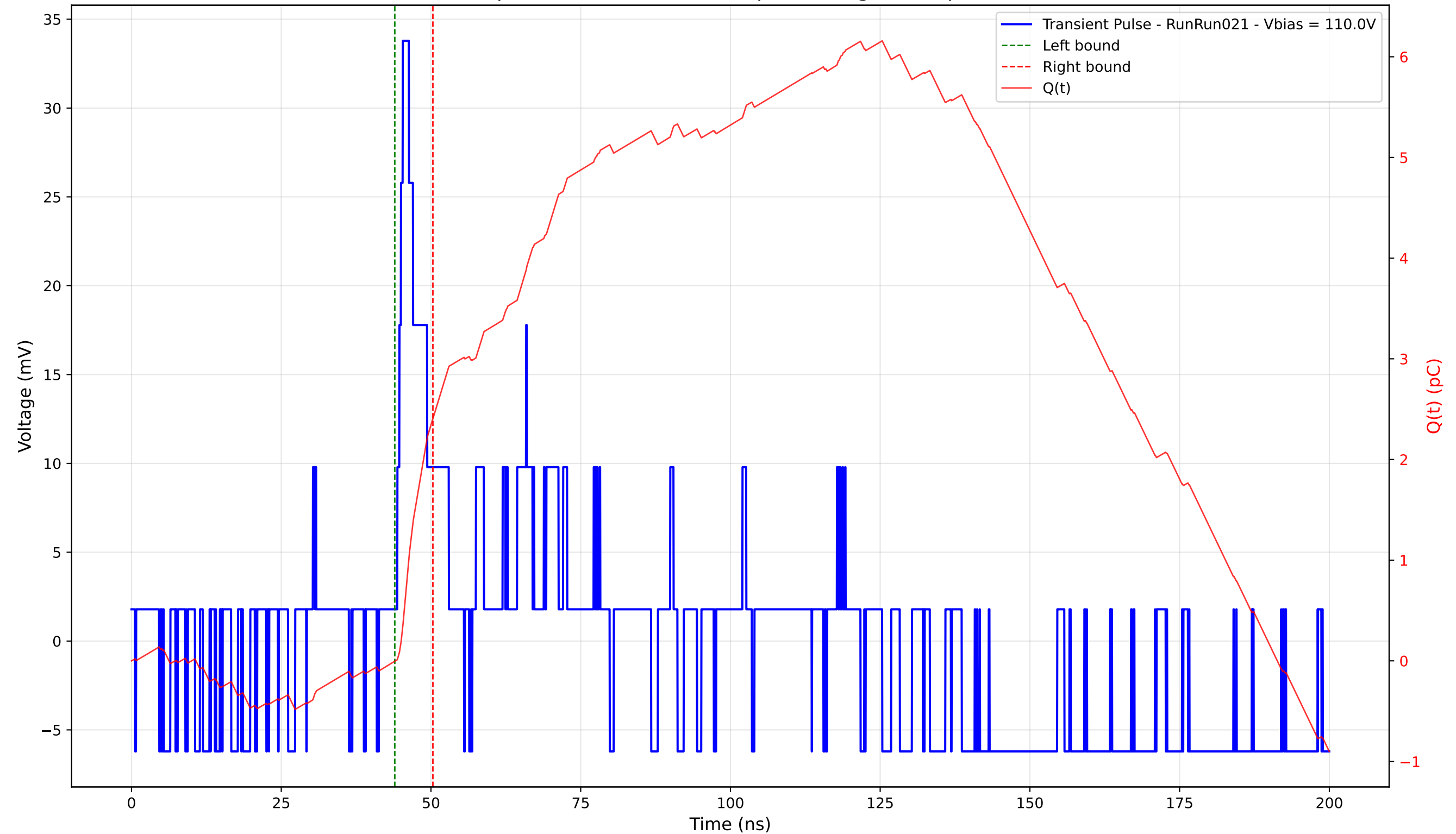
Transient Pulse - Sample: 4003 - Position: 50.0 \mu\text{m} - Charge: 2.41 pC - Rise Time: 0.92 ns
