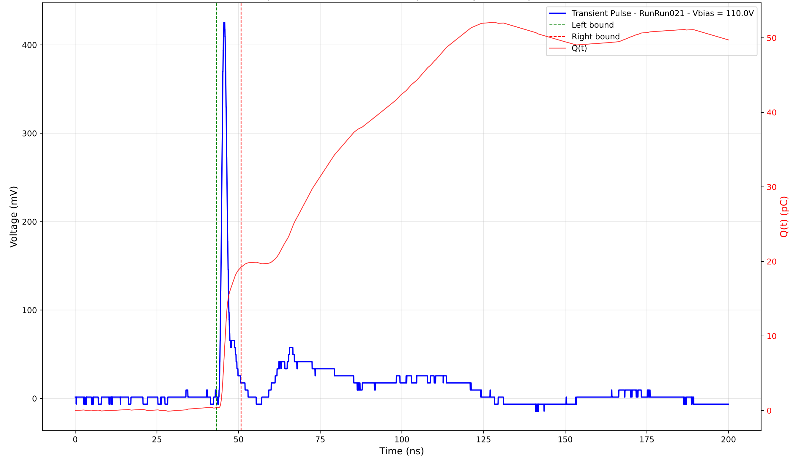
Transient Pulse - Sample: 4003 - Position: 160.0 \mu\text{m} - Charge: 18.81 pC - Rise Time: 0.98 ns
