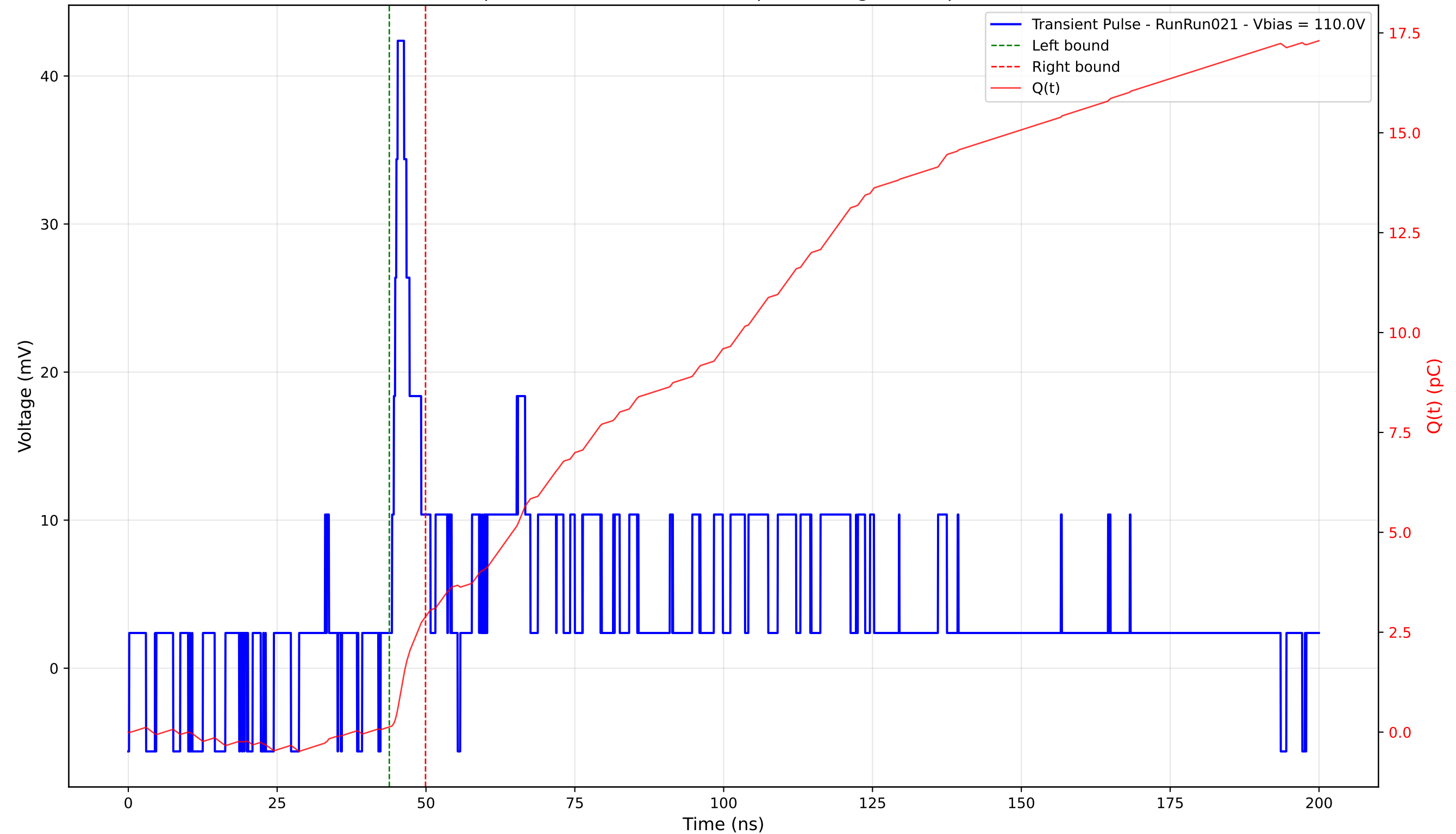
Transient Pulse - Sample: 4003 - Position: 295.0 \mu\text{m} - Charge: 2.76 pC - Rise Time: 0.96 ns
