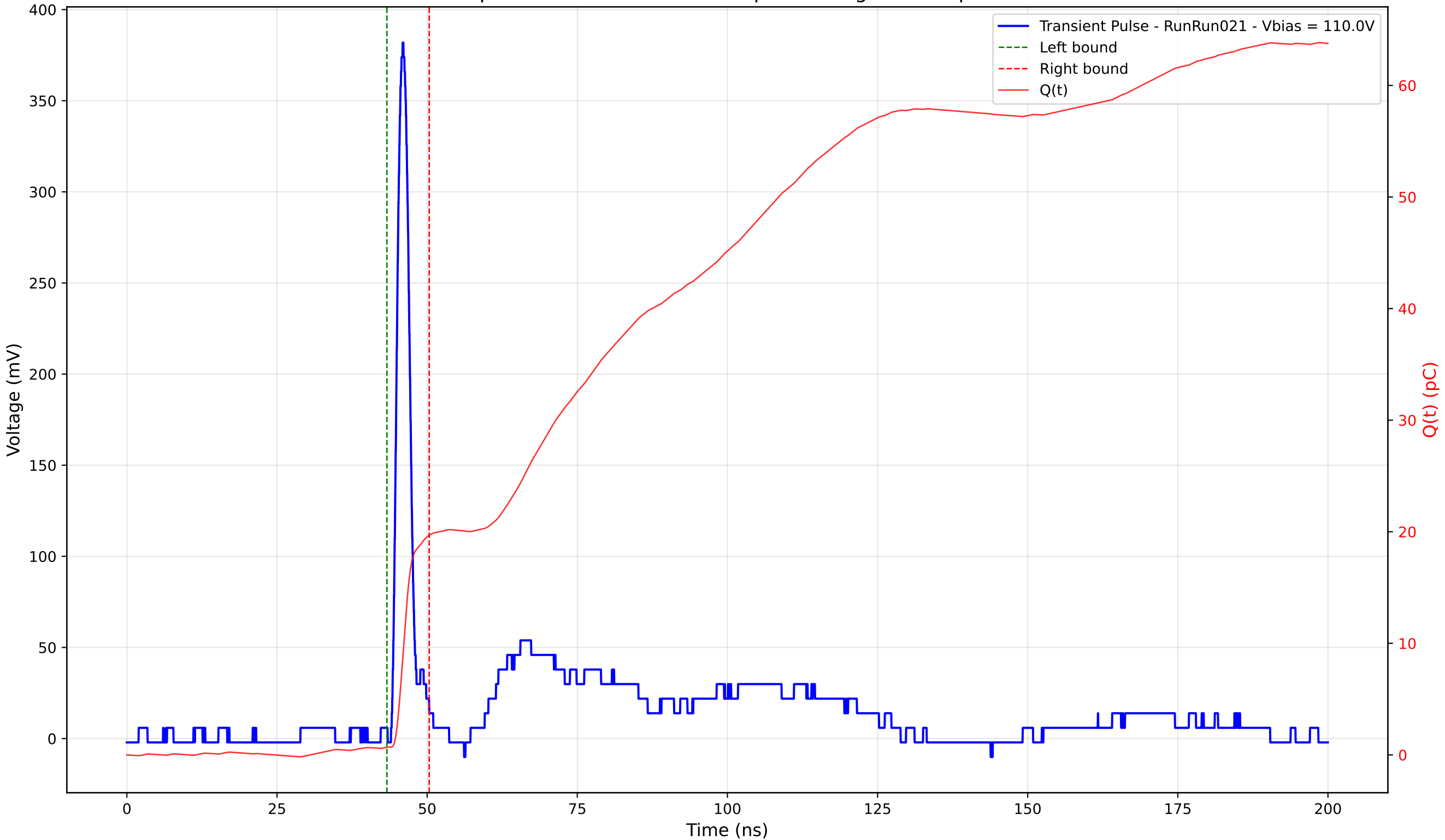
Transient Pulse - Sample: 4003 - Position: 200.0 \mu\text{m} - Charge: 19.00 pC - Rise Time: 1.20 ns
