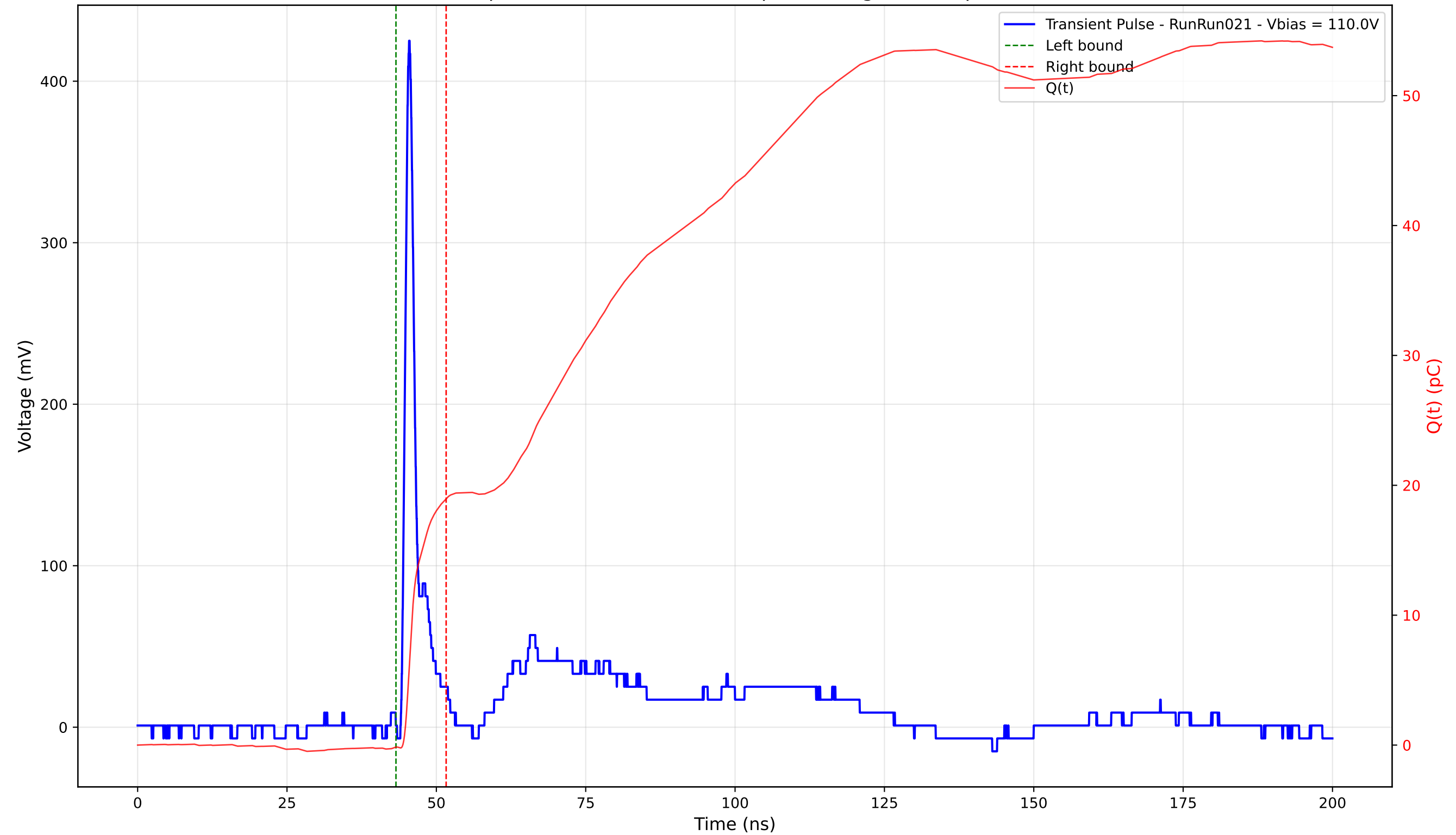
Transient Pulse - Sample: 4003 - Position: 130.0 \mu\text{m} - Charge: 19.11 pC - Rise Time: 0.92 ns
