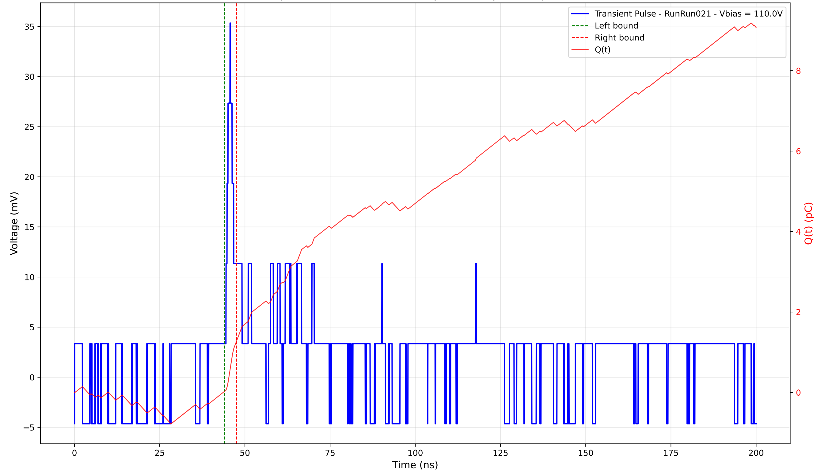
Transient Pulse - Sample: 4003 - Position: 345.0 \mu\text{m} - Charge: 1.26 pC - Rise Time: 1.20 ns
