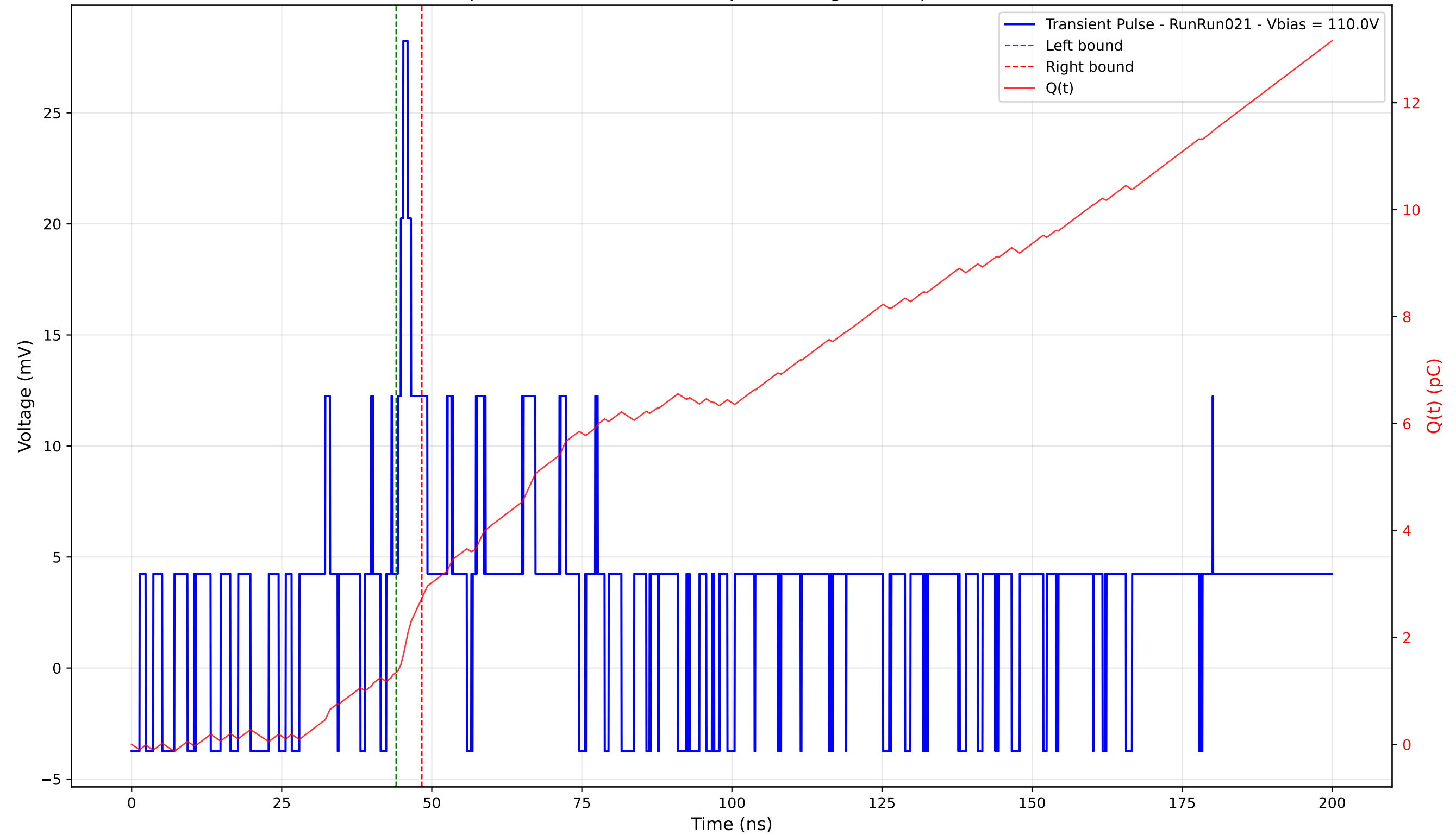
Transient Pulse - Sample: 4003 - Position: 80.0 \mu\text{m} - Charge: 1.39 pC - Rise Time: 0.00 ns (N/A)
