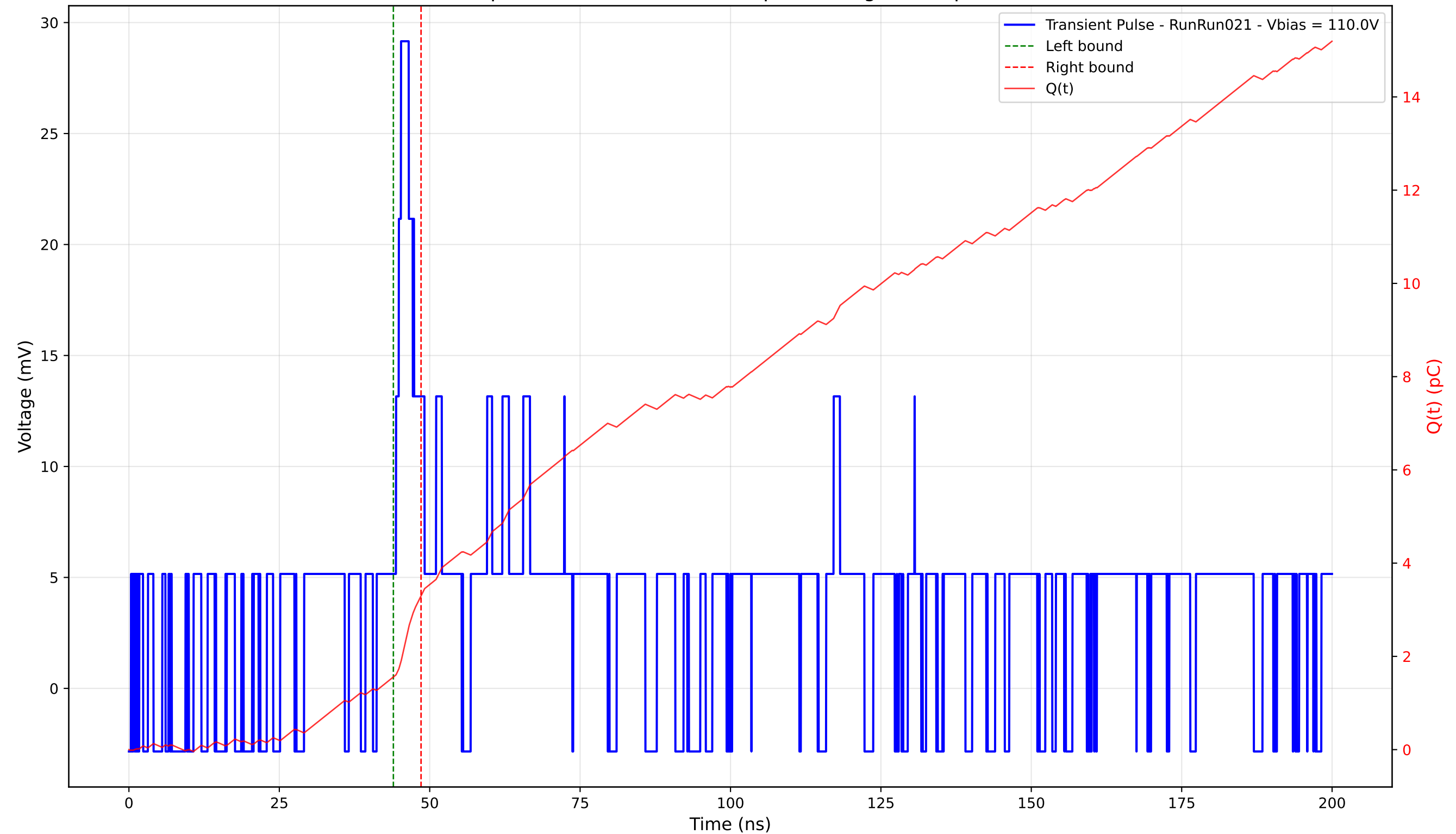
Transient Pulse - Sample: 4003 - Position: 360.0 \mu\text{m} - Charge: 1.74 pC - Rise Time: 4.06 ns
