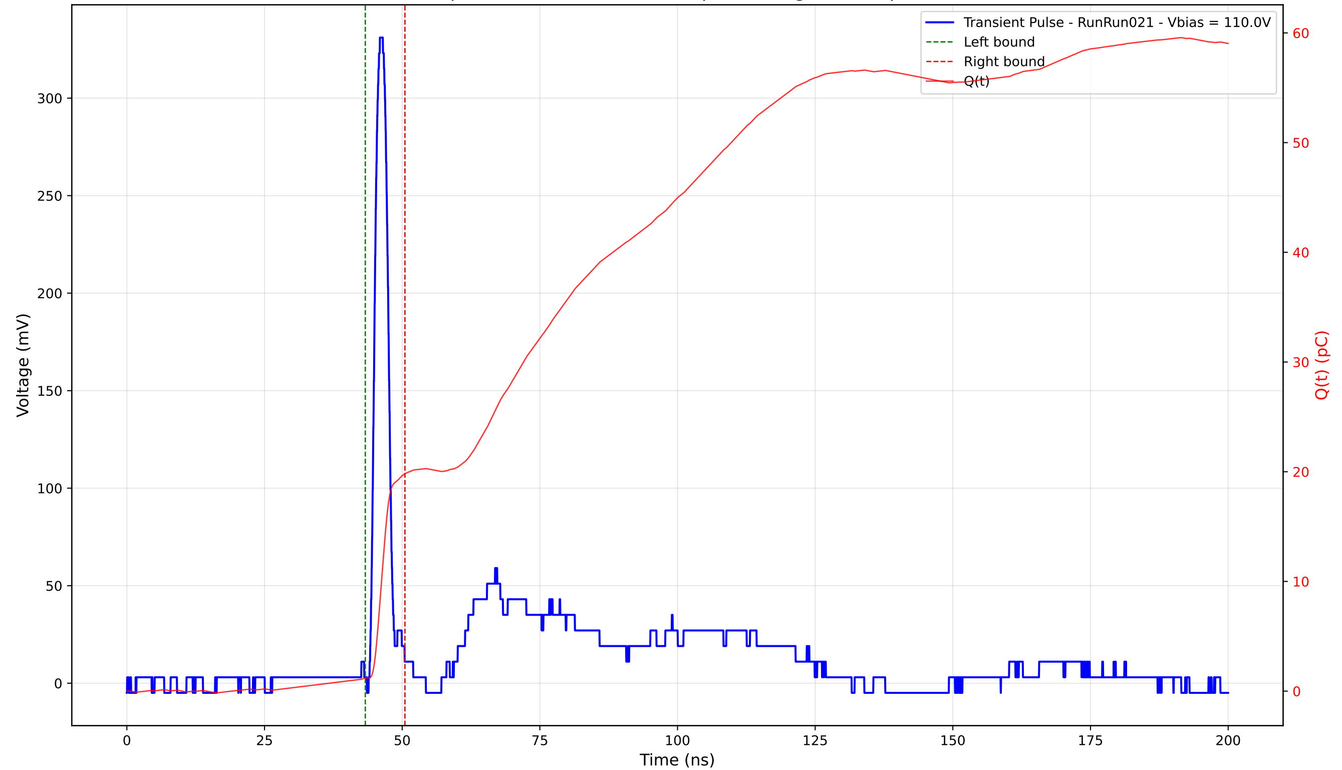
Transient Pulse - Sample: 4003 - Position: 215.0 \mu\text{m} - Charge: 18.63 pC - Rise Time: 1.20 ns
