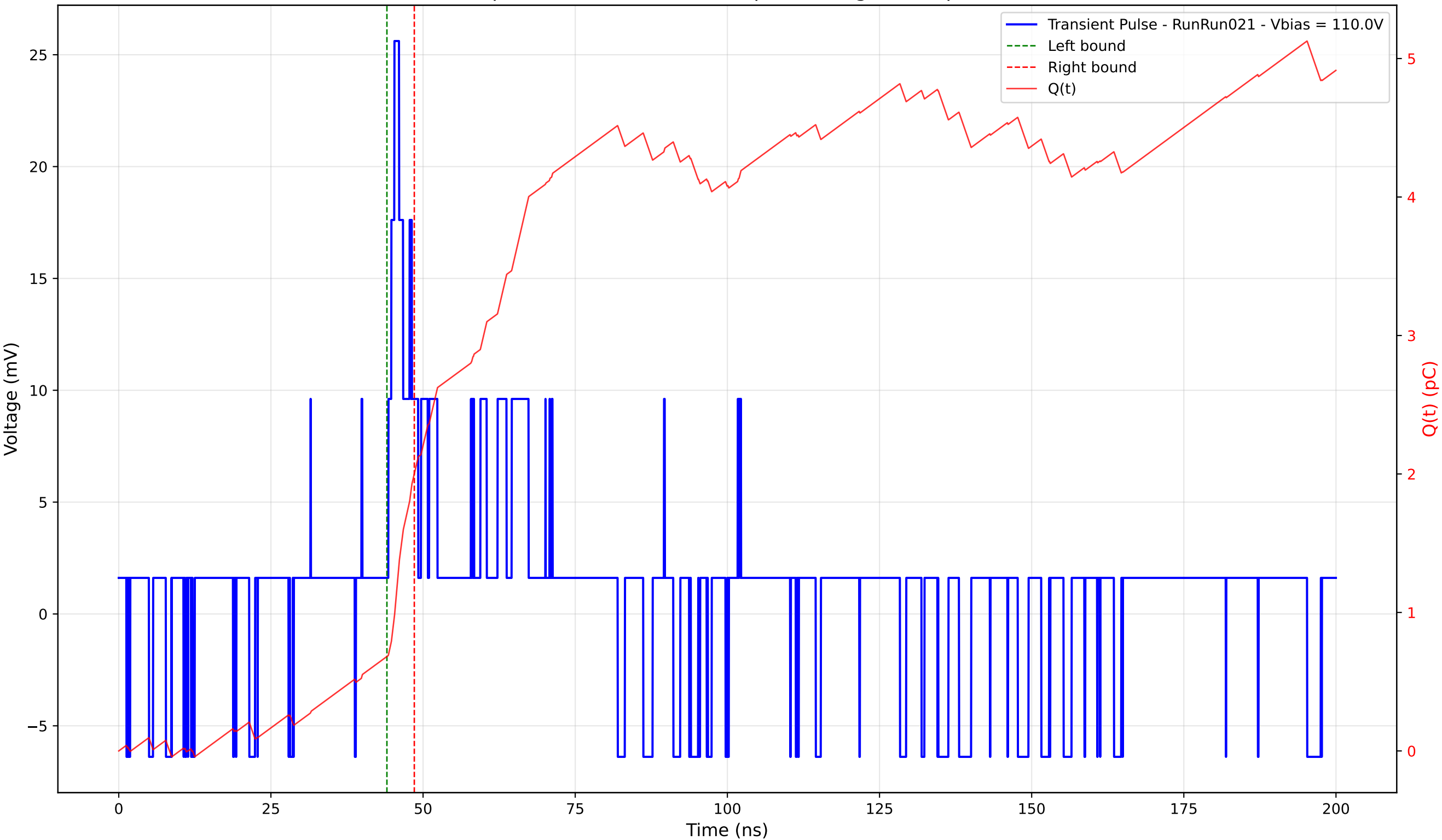
Transient Pulse - Sample: 4003 - Position: 30.0 \mu\text{m} - Charge: 1.32 pC - Rise Time: 1.00 ns
