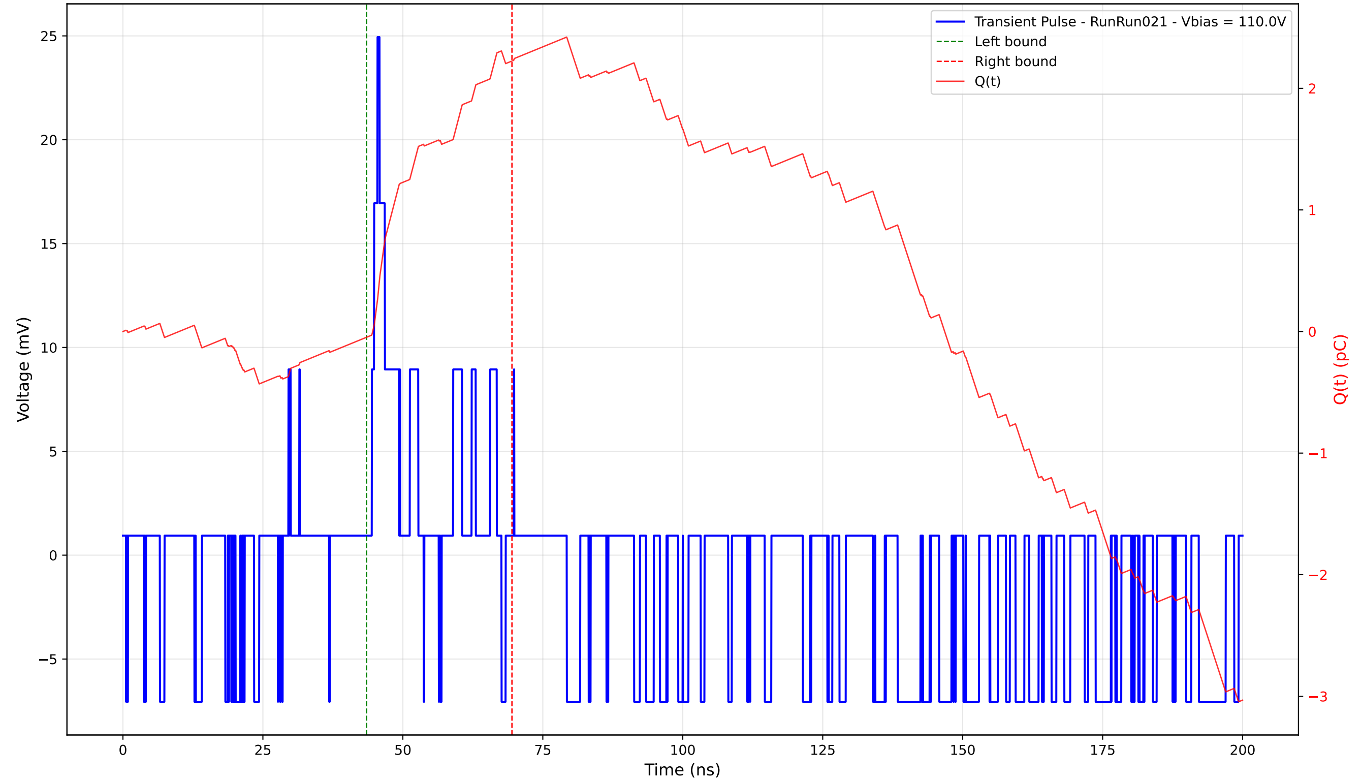
Transient Pulse - Sample: 4003 - Position: 25.0 \mu\text{m} - Charge: 2.27 pC - Rise Time: 1.02 ns
