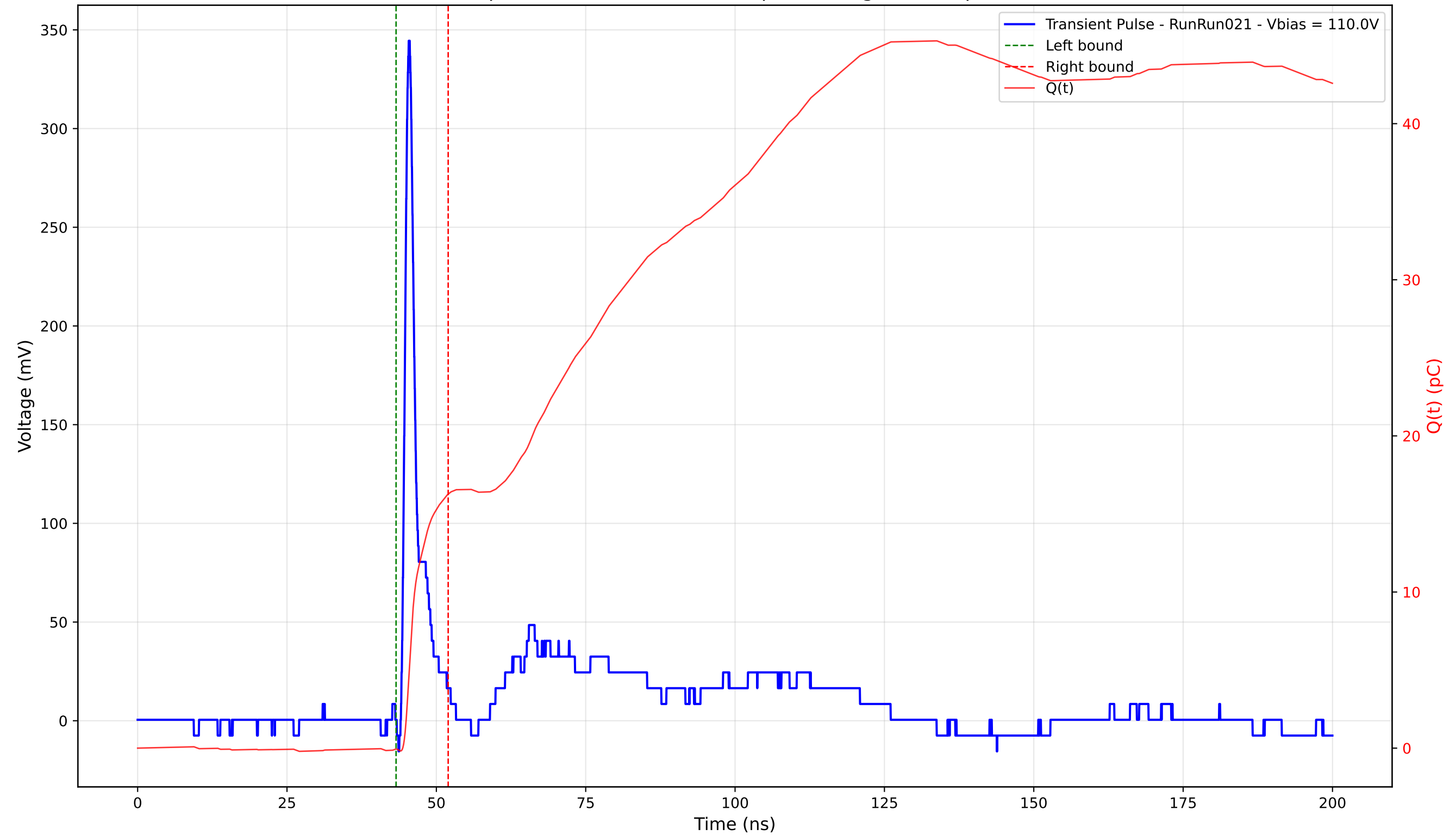
Transient Pulse - Sample: 4003 - Position: 115.0 \mu\text{m} - Charge: 16.33 pC - Rise Time: 0.88 ns
