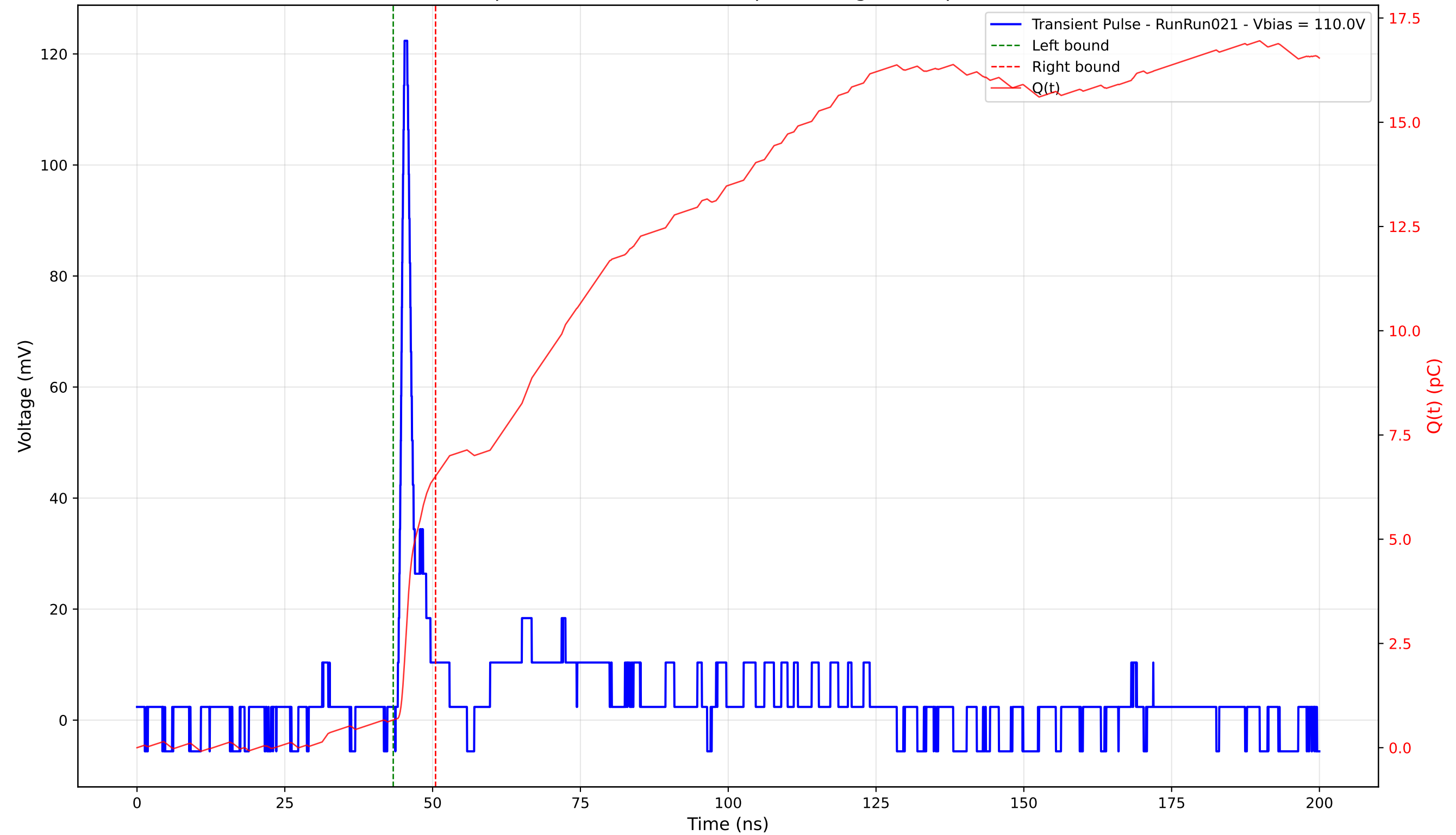
Transient Pulse - Sample: 4003 - Position: 95.0 \mu\text{m} - Charge: 5.85 pC - Rise Time: 0.90 ns
