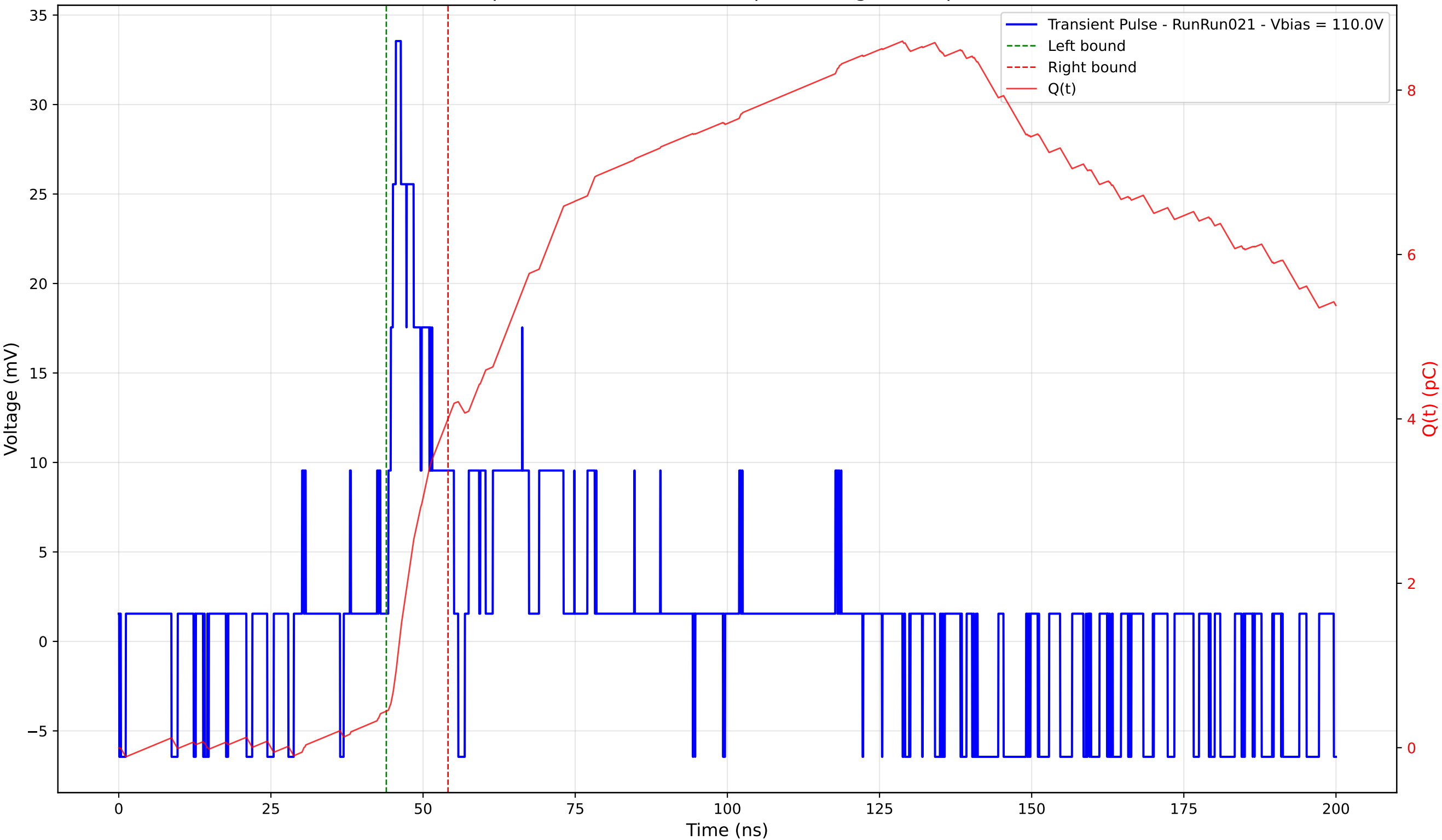
Transient Pulse - Sample: 4003 - Position: 60.0 \mu\text{m} - Charge: 3.56 pC - Rise Time: 1.24 ns
