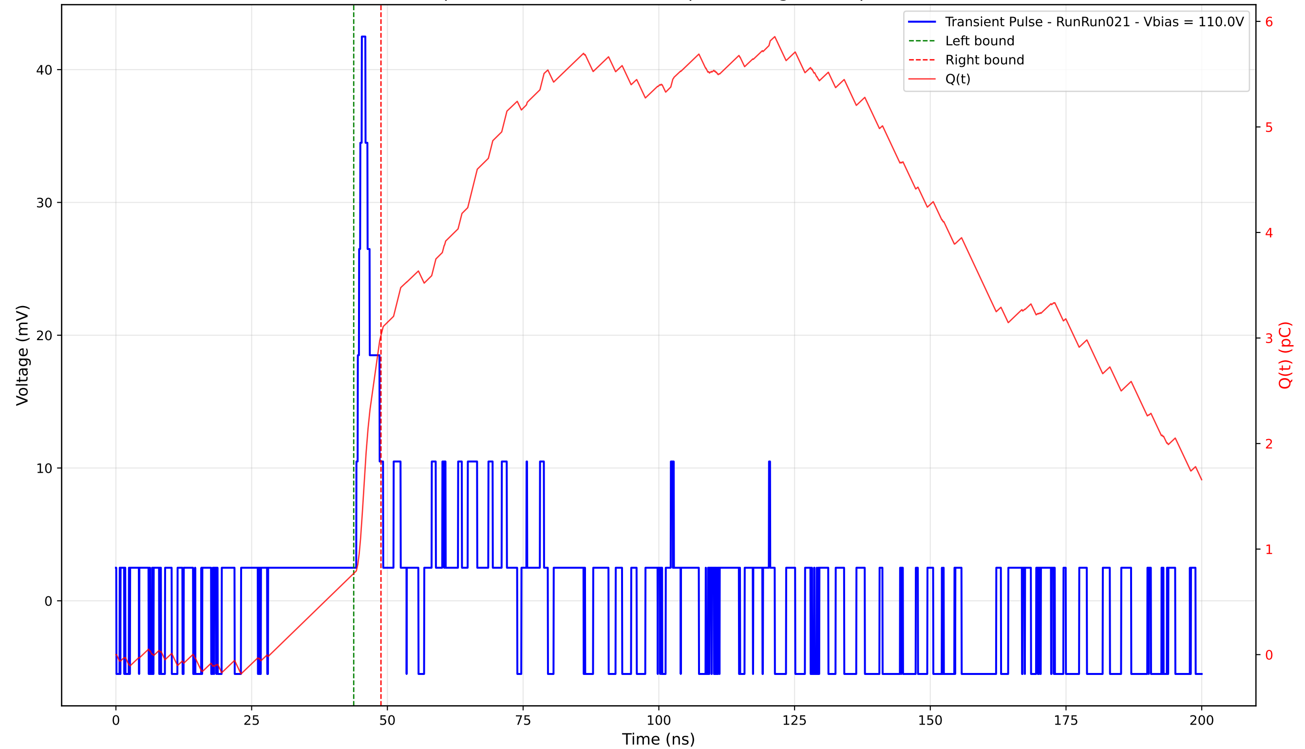
Transient Pulse - Sample: 4003 - Position: 400.0 \mu\text{m} - Charge: 2.26 pC - Rise Time: 1.02 ns
