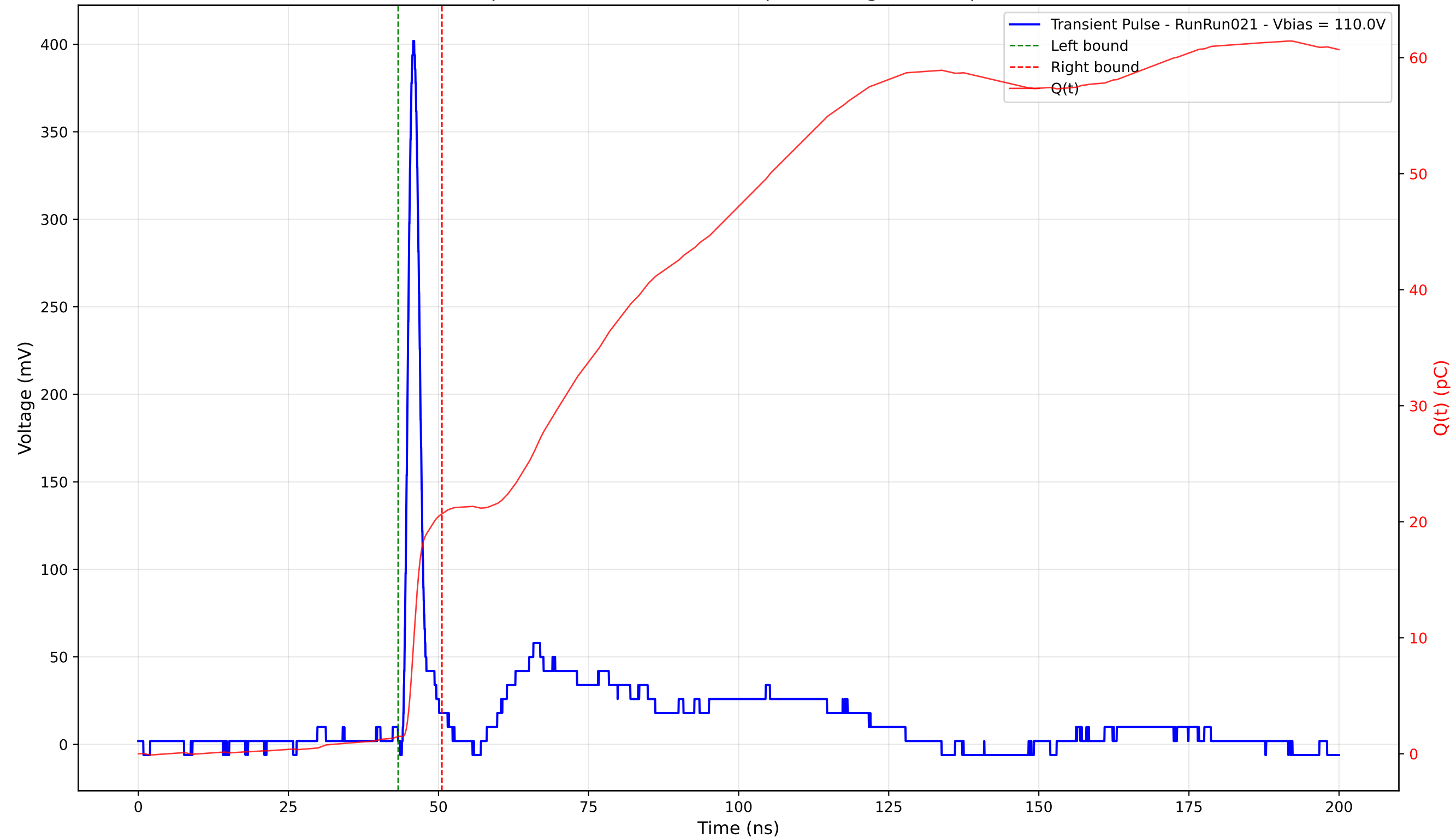
Transient Pulse - Sample: 4003 - Position: 190.0 \mu\text{m} - Charge: 19.18 pC - Rise Time: 1.14 ns
