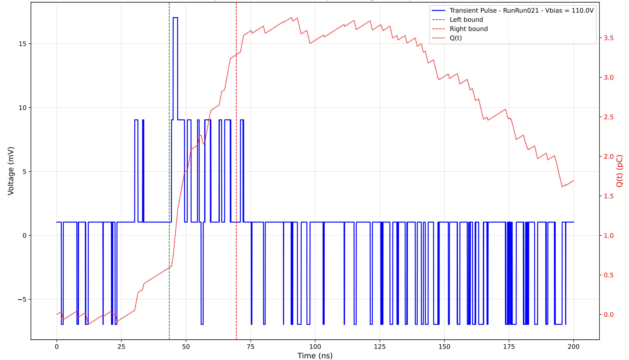
Transient Pulse - Sample: 4003 - Position: 15.0 \mu\text{m} - Charge: 2.69 pC - Rise Time: 0.66 ns
