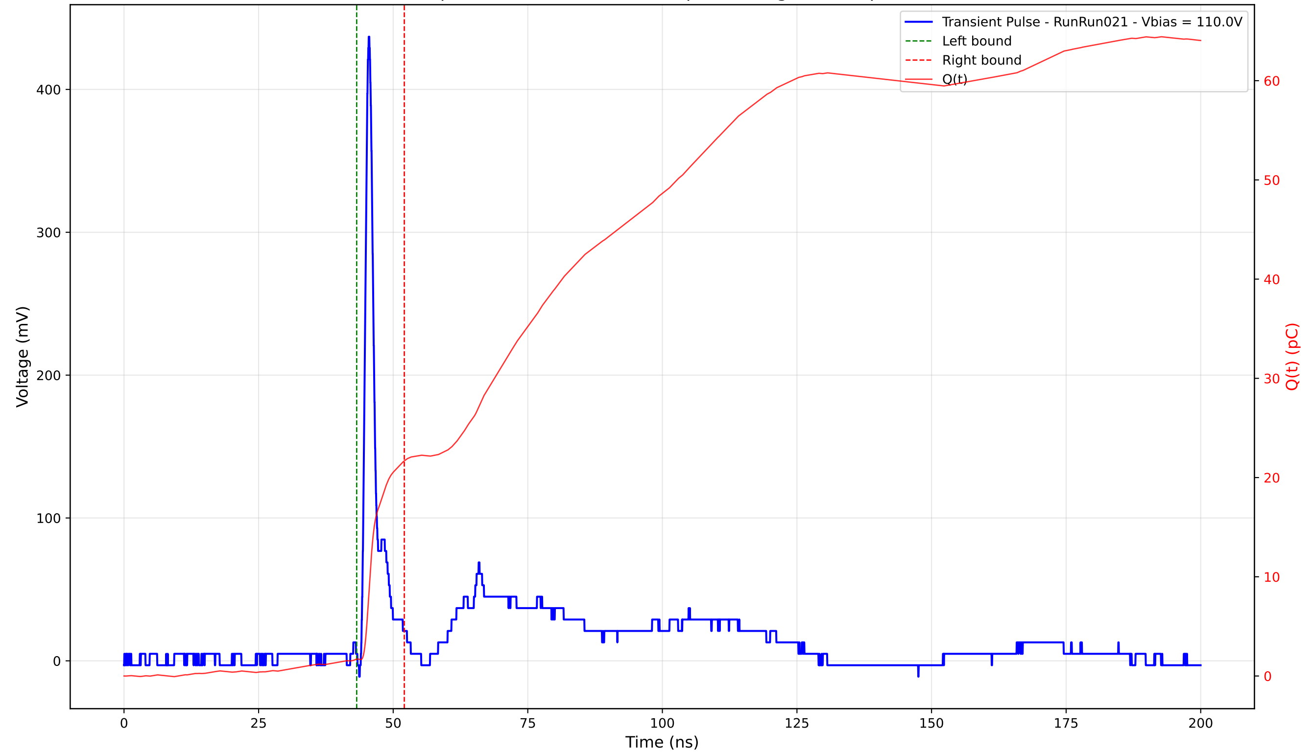
Transient Pulse - Sample: 4003 - Position: 140.0 \mu\text{m} - Charge: 19.97 pC - Rise Time: 0.96 ns
