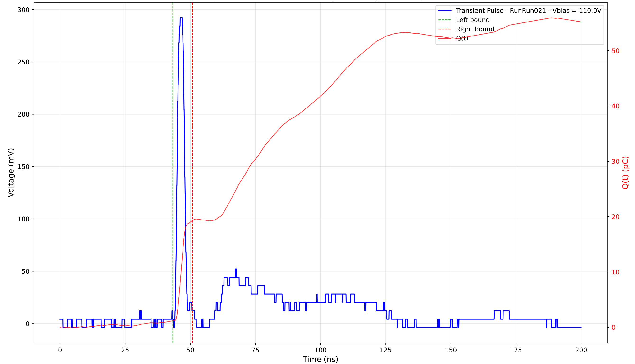
Transient Pulse - Sample: 4003 - Position: 225.0 \mu\text{m} - Charge: 18.12 pC - Rise Time: 1.28 ns
