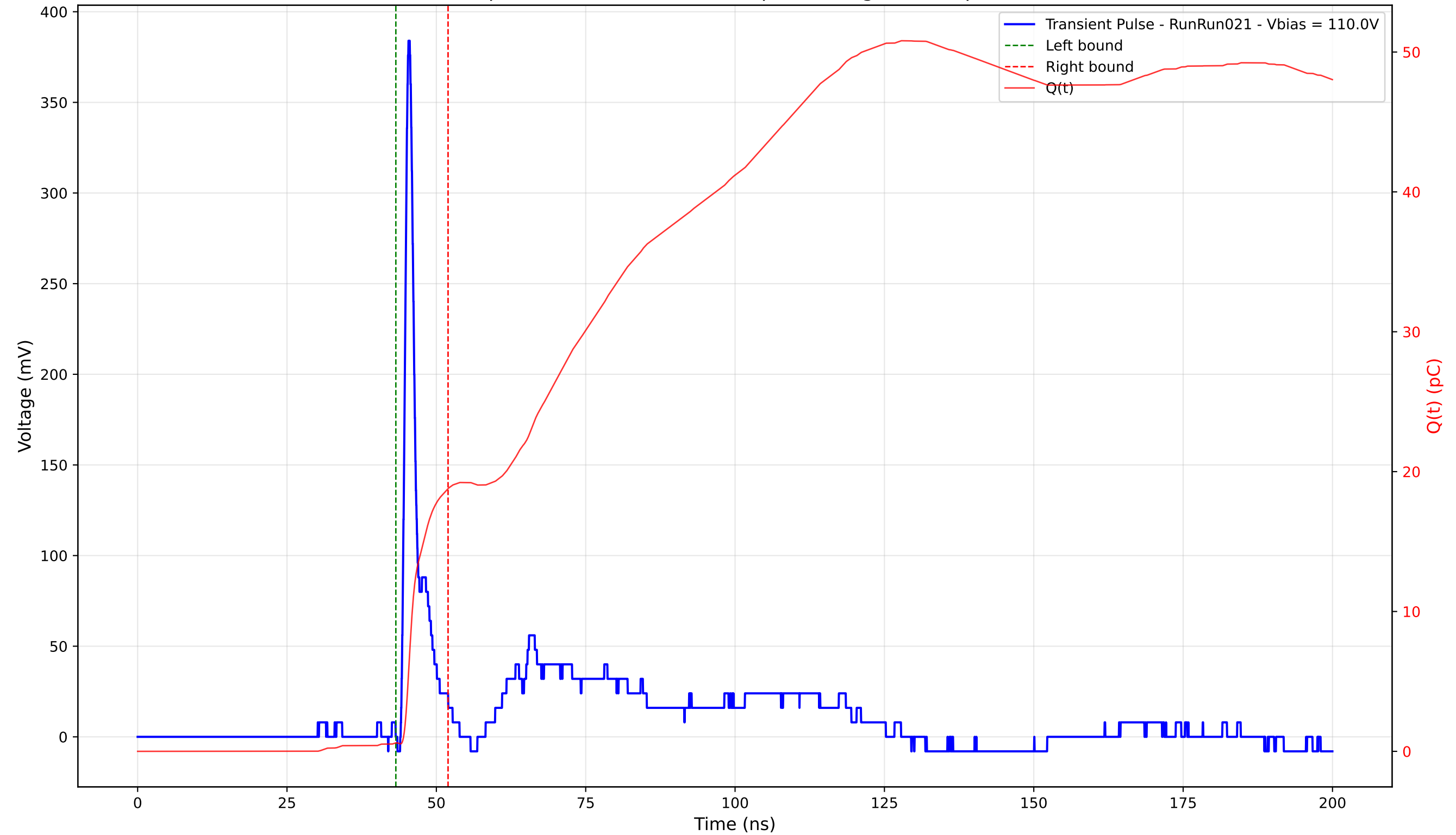
Transient Pulse - Sample: 4003 - Position: 120.0 \mu\text{m} - Charge: 18.19 pC - Rise Time: 0.90 ns
