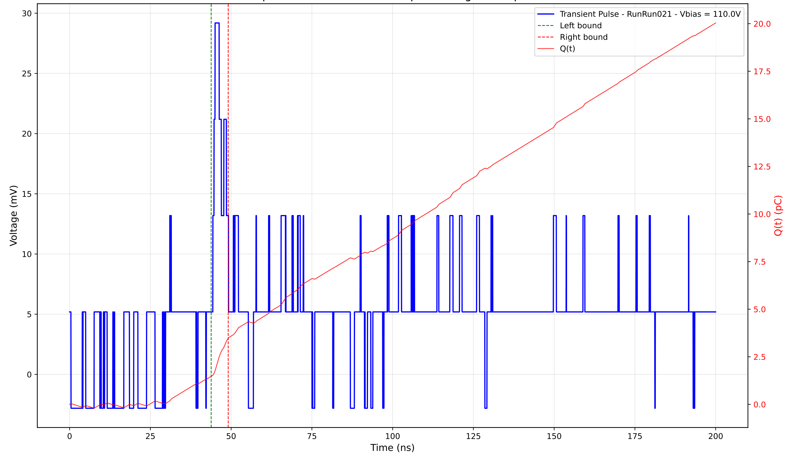
Transient Pulse - Sample: 4003 - Position: 325.0 \mu\text{m} - Charge: 2.01 pC - Rise Time: 2.72 ns
