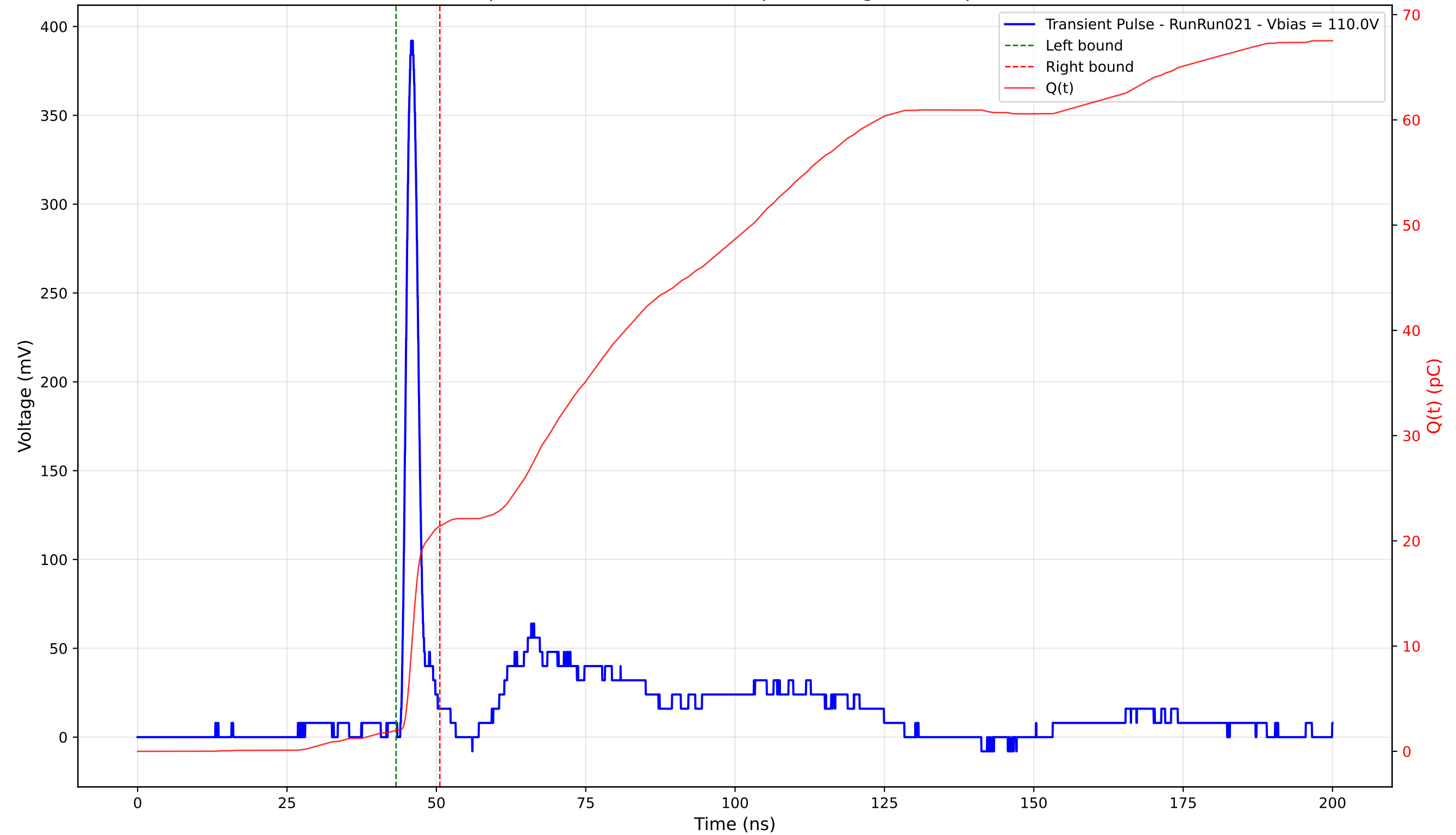
Transient Pulse - Sample: 4003 - Position: 195.0 \mu\text{m} - Charge: 19.41 pC - Rise Time: 1.18 ns
