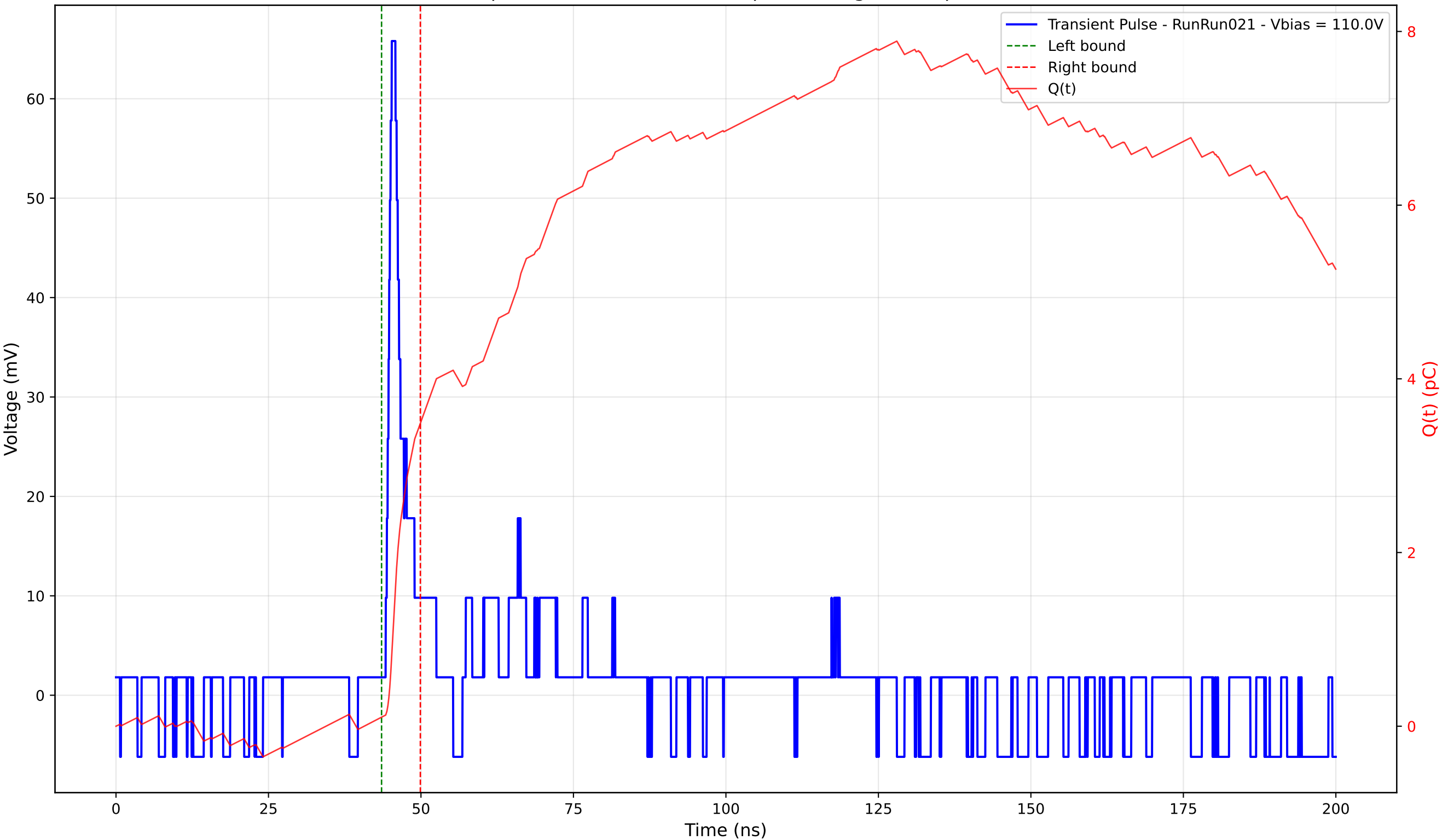
Transient Pulse - Sample: 4003 - Position: 90.0 \mu\text{m} - Charge: 3.39 pC - Rise Time: 0.99 ns
