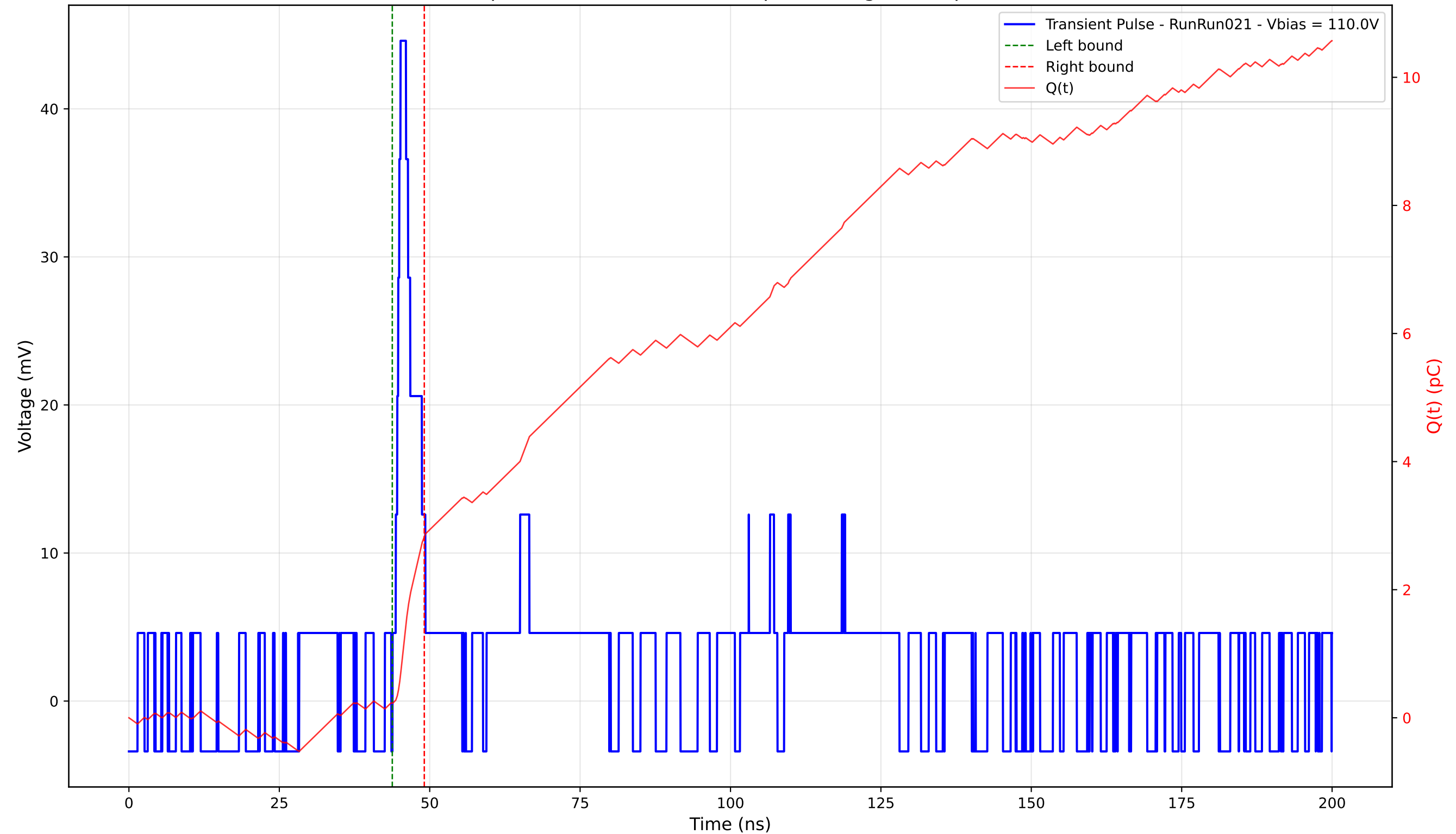
Transient Pulse - Sample: 4003 - Position: 390.0 \mu\text{m} - Charge: 2.60 pC - Rise Time: 1.32 ns
