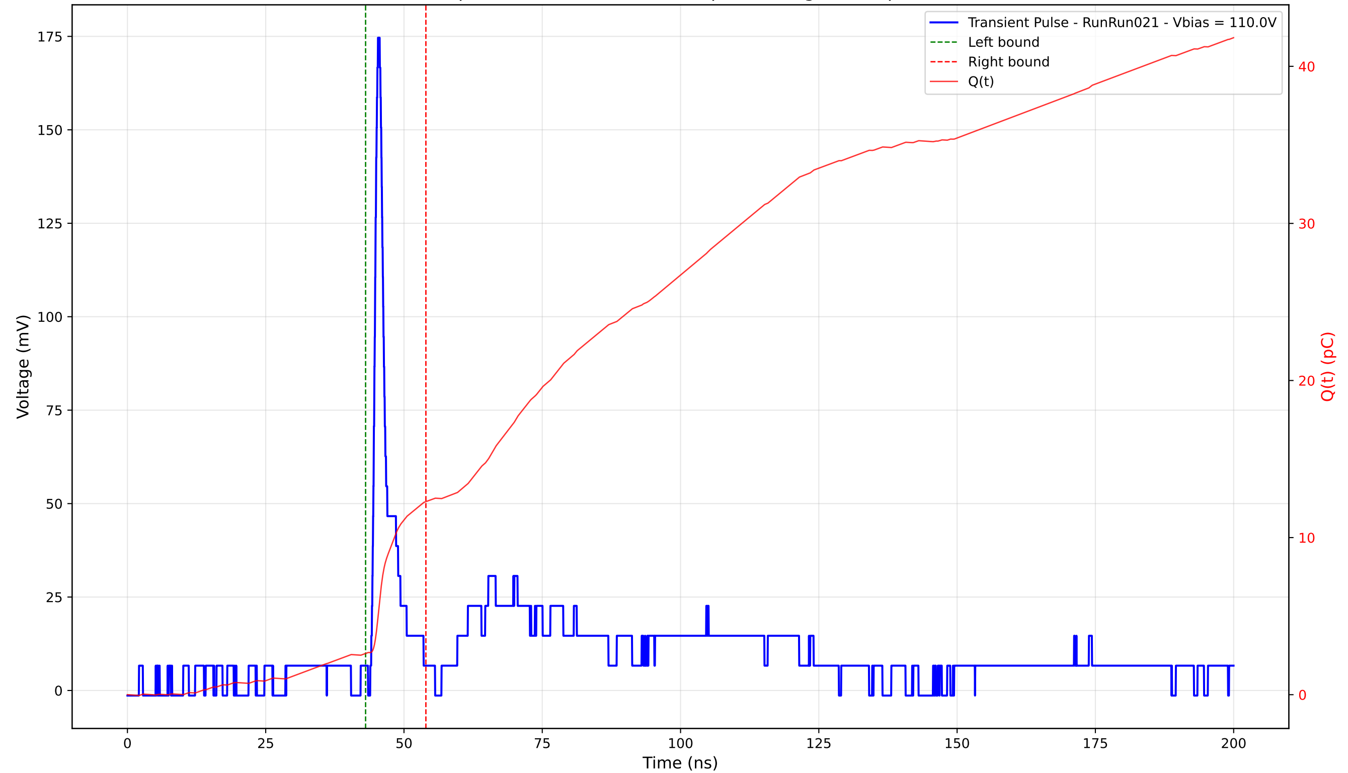
Transient Pulse - Sample: 4003 - Position: 100.0 \mu\text{m} - Charge: 9.66 pC - Rise Time: 0.91 ns
