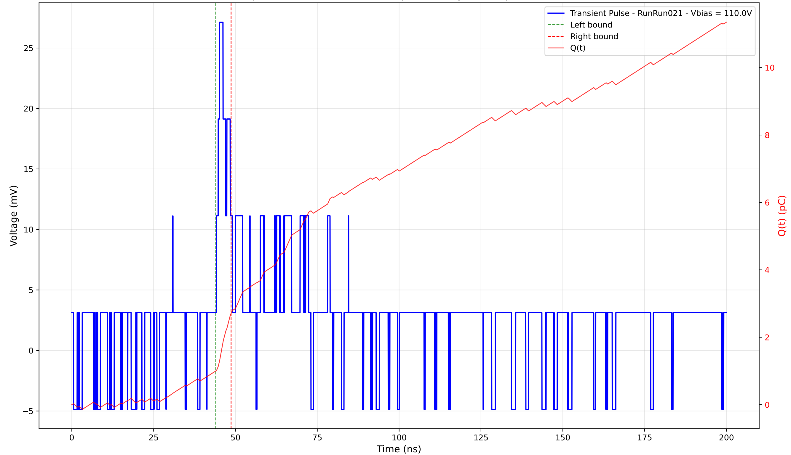
Transient Pulse - Sample: 4003 - Position: 335.0 \mu\text{m} - Charge: 1.71 pC - Rise Time: 0.00 ns (N/A)
