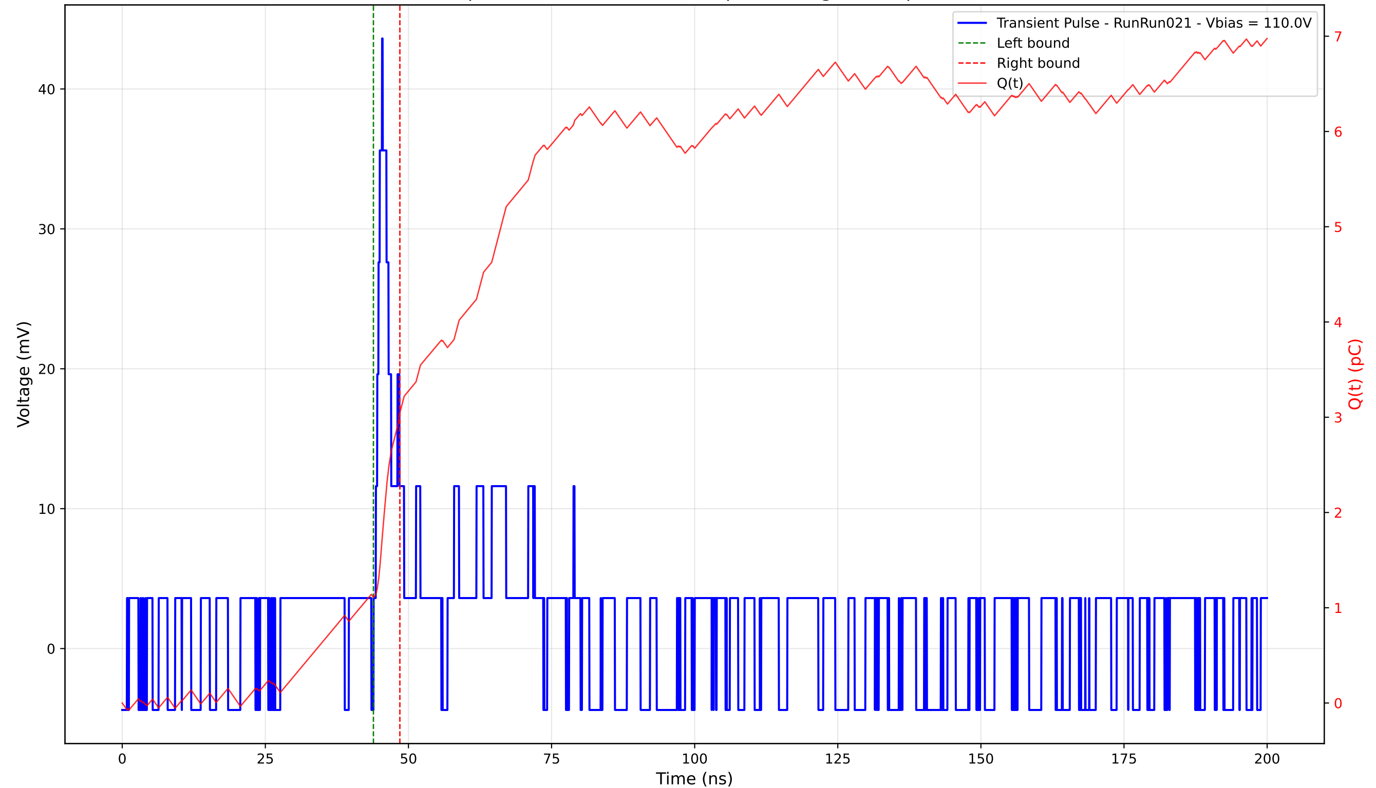
Transient Pulse - Sample: 4003 - Position: 405.0 \mu\text{m} - Charge: 1.94 pC - Rise Time: 1.10 ns
