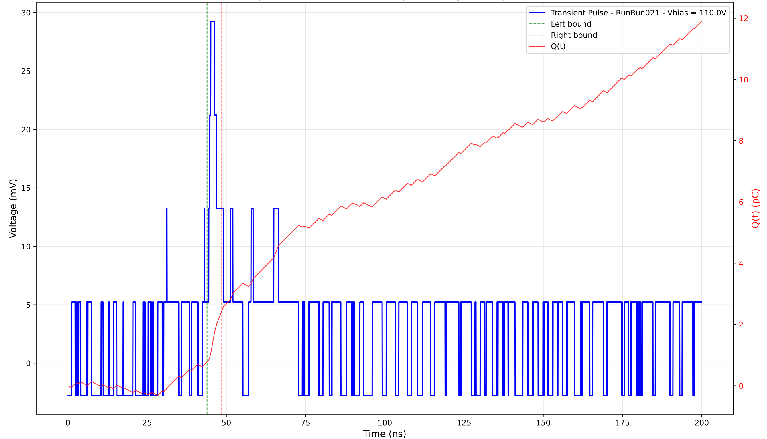
Transient Pulse - Sample: 4003 - Position: 410.0 \mu\text{m} - Charge: 1.67 pC - Rise Time: 2.70 ns
