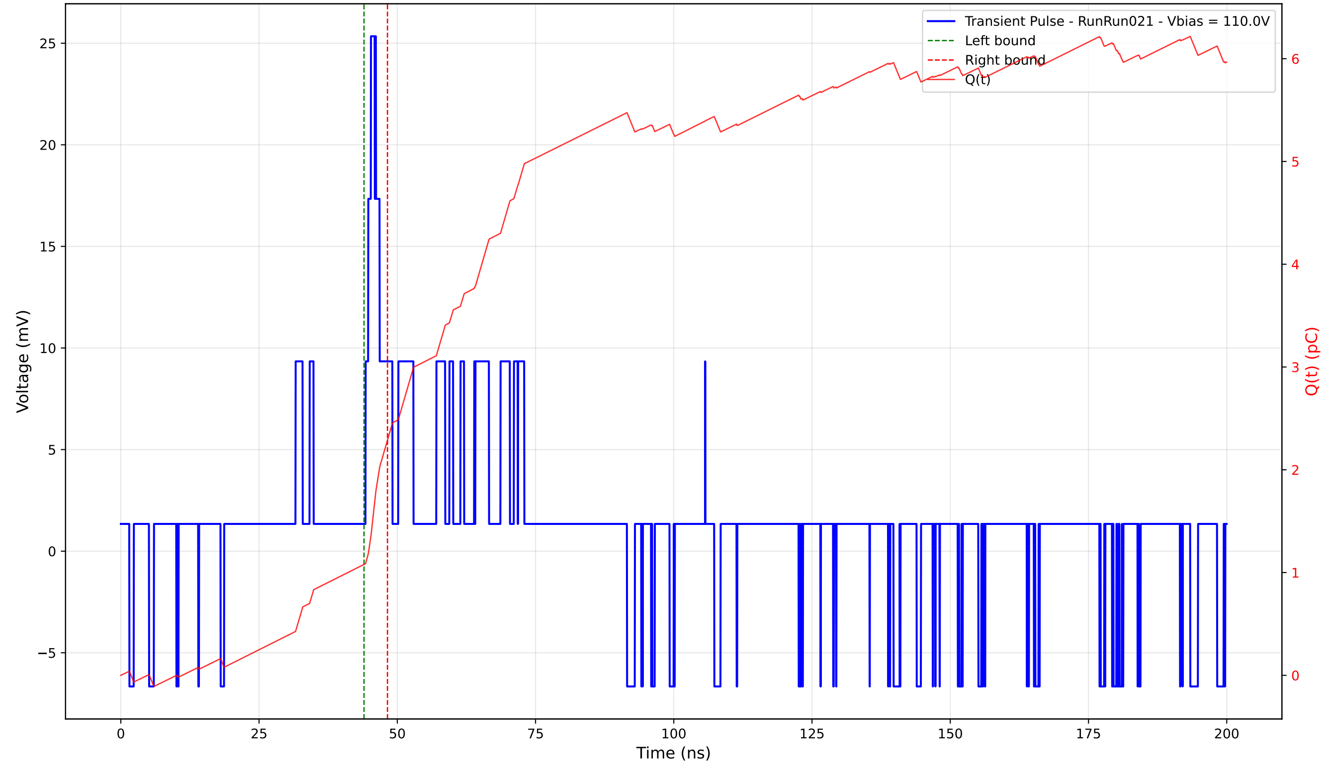
Transient Pulse - Sample: 4003 - Position: 415.0 \mu\text{m} - Charge: 1.21 pC - Rise Time: 0.98 ns
