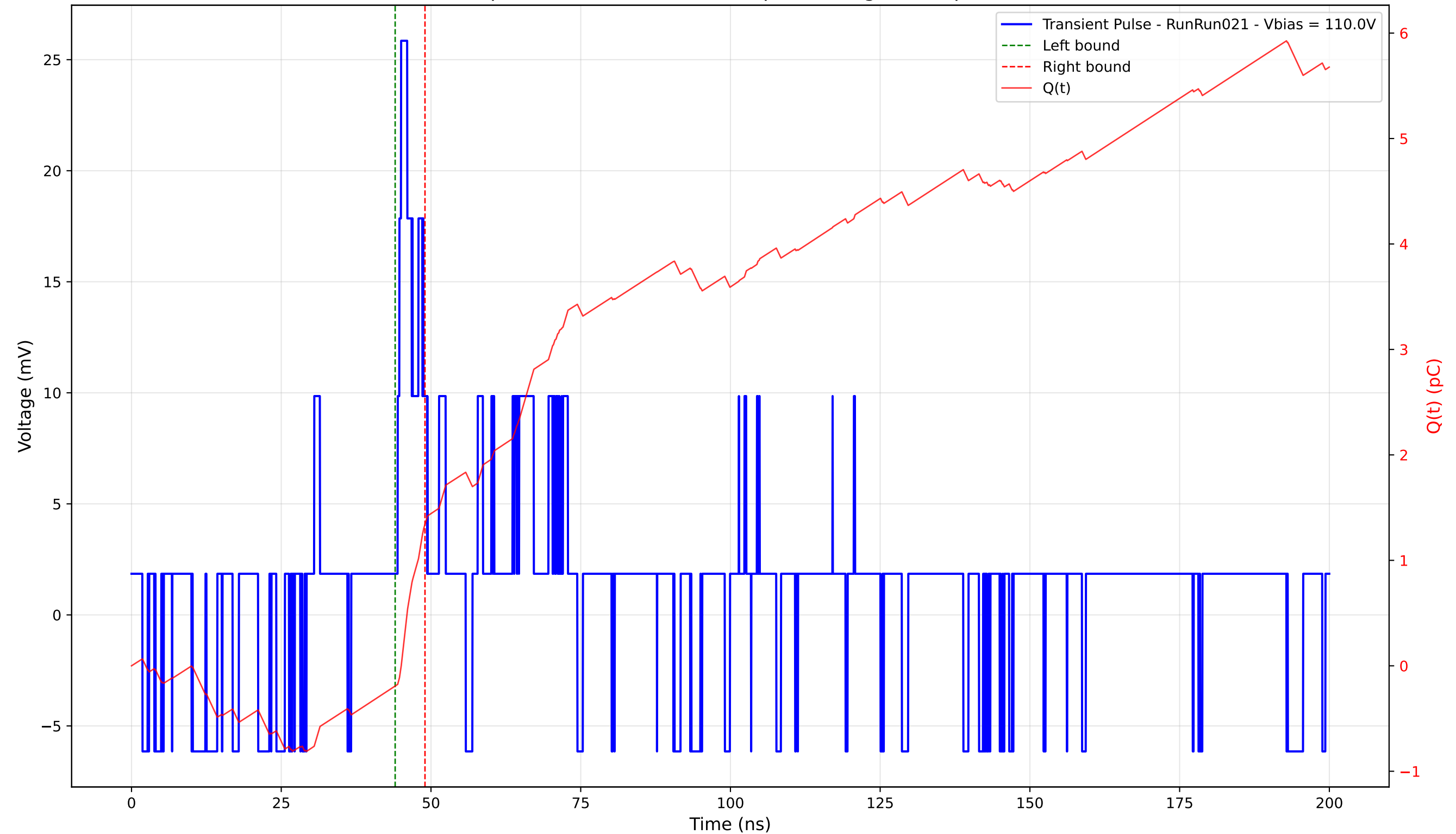
Transient Pulse - Sample: 4003 - Position: 370.0 \mu\text{m} - Charge: 1.54 pC - Rise Time: 0.58 ns
