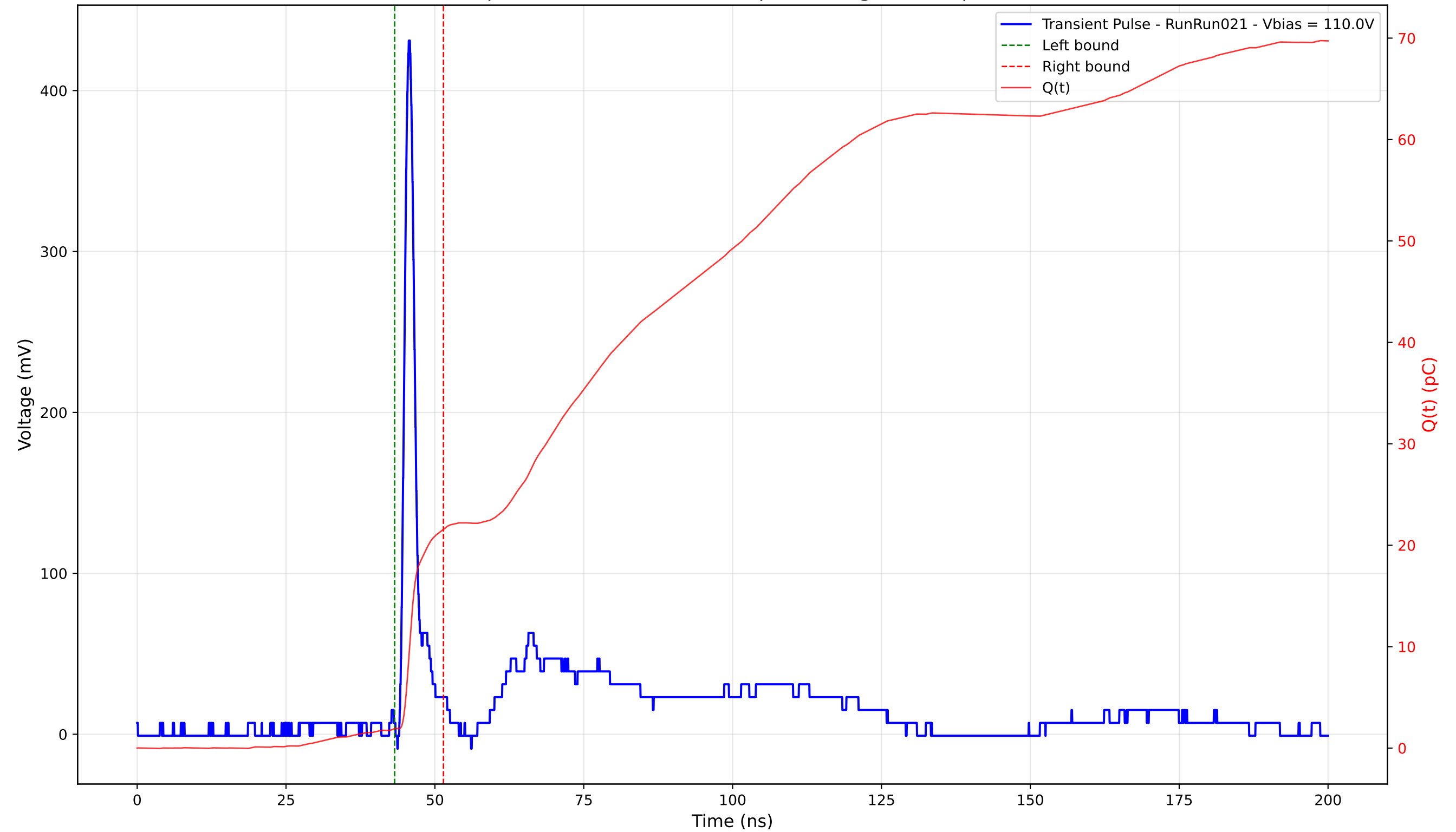
Transient Pulse - Sample: 4003 - Position: 170.0 \mu\text{m} - Charge: 19.65 pC - Rise Time: 1.04 ns
