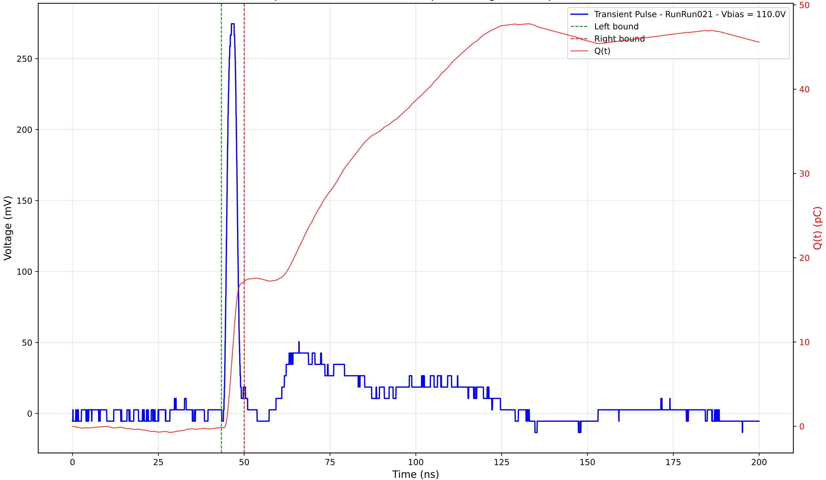
Transient Pulse - Sample: 4003 - Position: 230.0 \mu\text{m} - Charge: 17.33 pC - Rise Time: 1.32 ns
