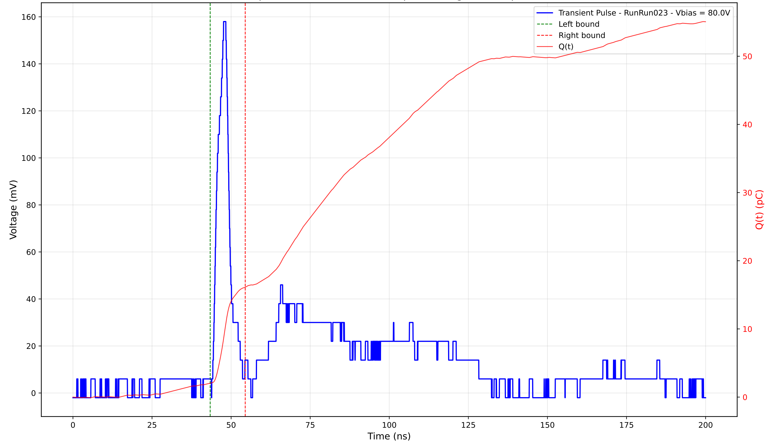
Transient Pulse - Sample: 4003 - Position: 230.0 \mu\text{m} - Charge: 14.06 pC - Rise Time: 3.00 ns
