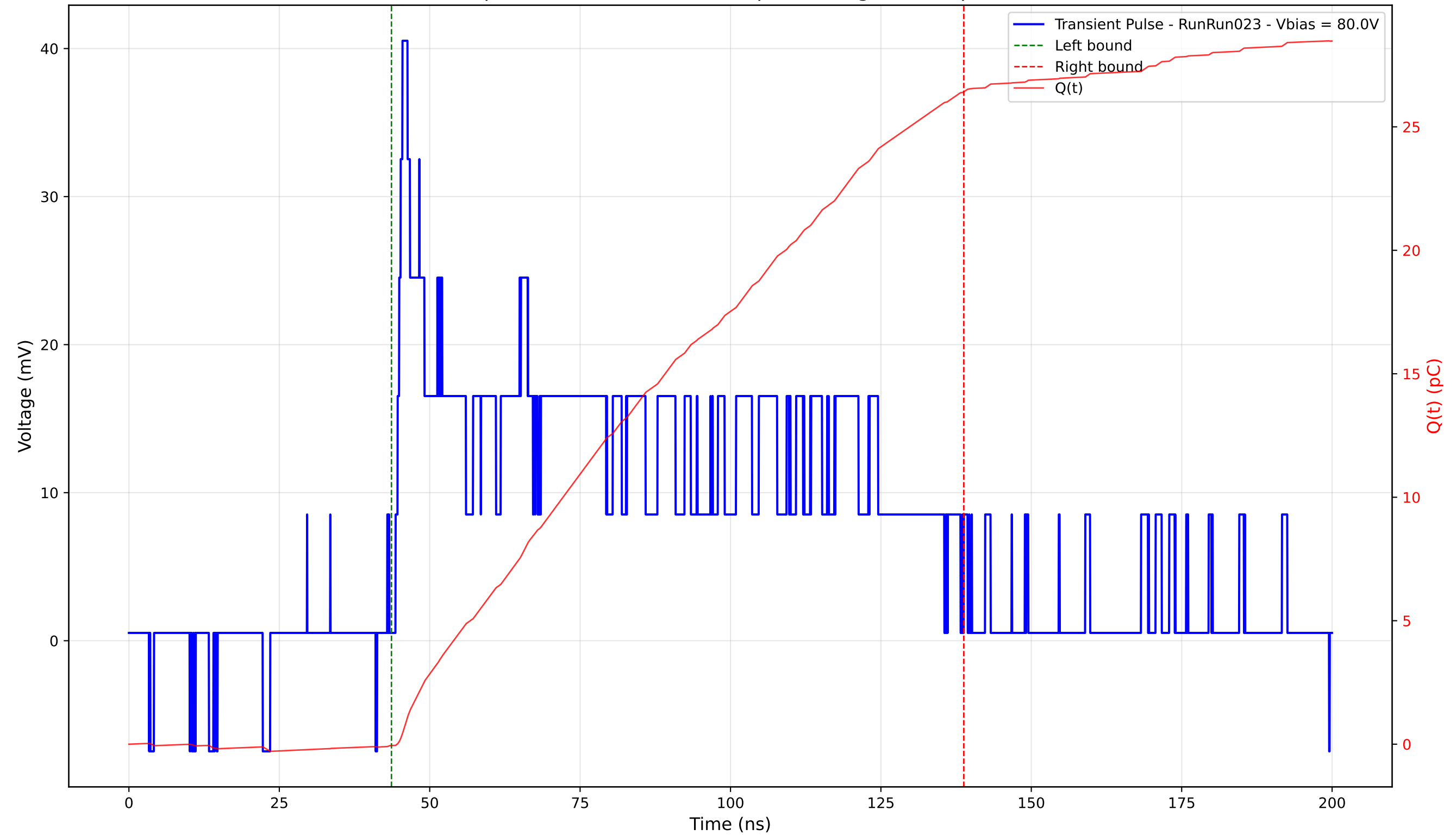
Transient Pulse - Sample: 4003 - Position: 250.0 \mu\text{m} - Charge: 26.48 pC - Rise Time: 1.15 ns
