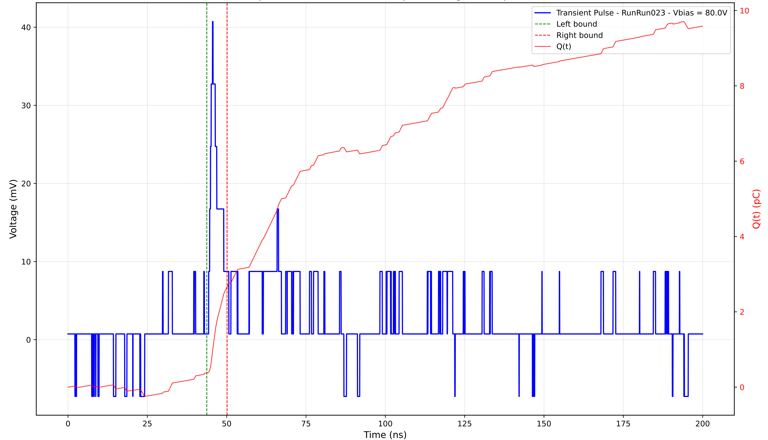
Transient Pulse - Sample: 4003 - Position: 290.0 \mu\text{m} - Charge: 2.28 pC - Rise Time: 1.23 ns
