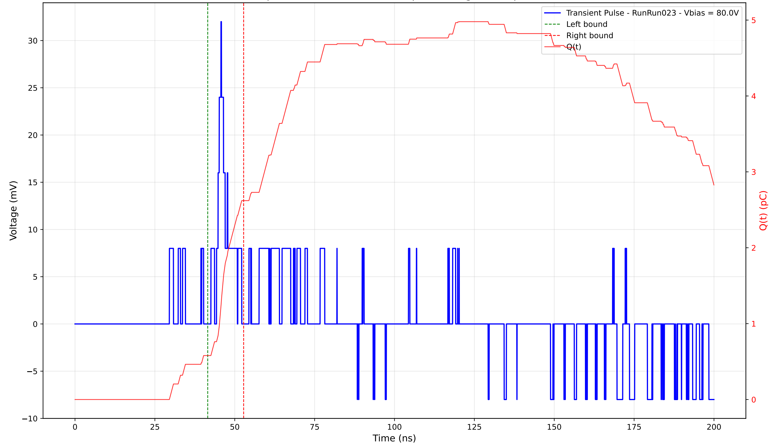
Transient Pulse - Sample: 4003 - Position: 330.0 \mu\text{m} - Charge: 2.04 pC - Rise Time: 1.39 ns
