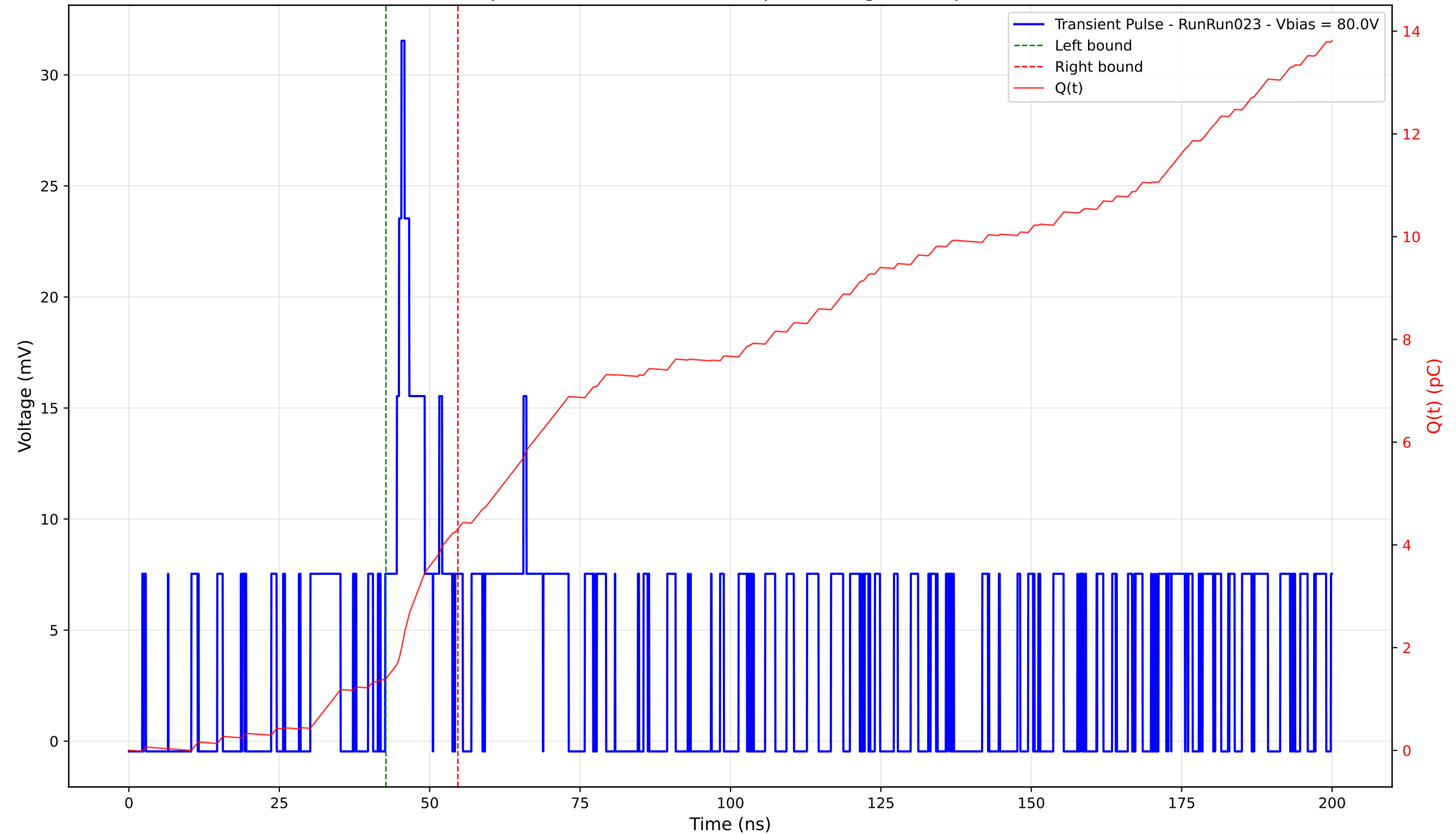
Transient Pulse - Sample: 4003 - Position: 325.0 \mu\text{m} - Charge: 2.92 pC - Rise Time: 2.71 ns
