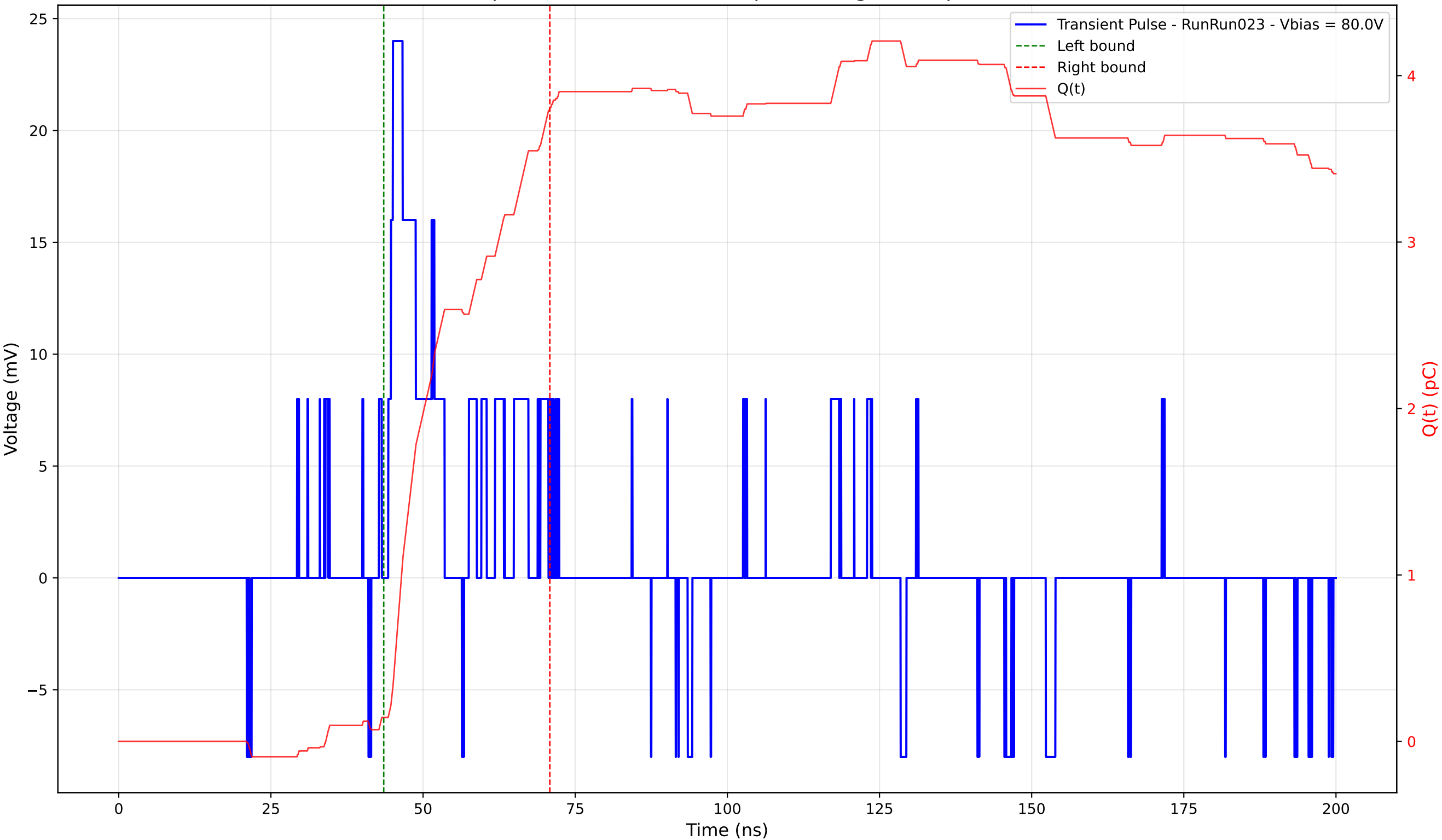
Transient Pulse - Sample: 4003 - Position: 50.0 \mu\text{m} - Charge: 3.66 pC - Rise Time: 0.77 ns
