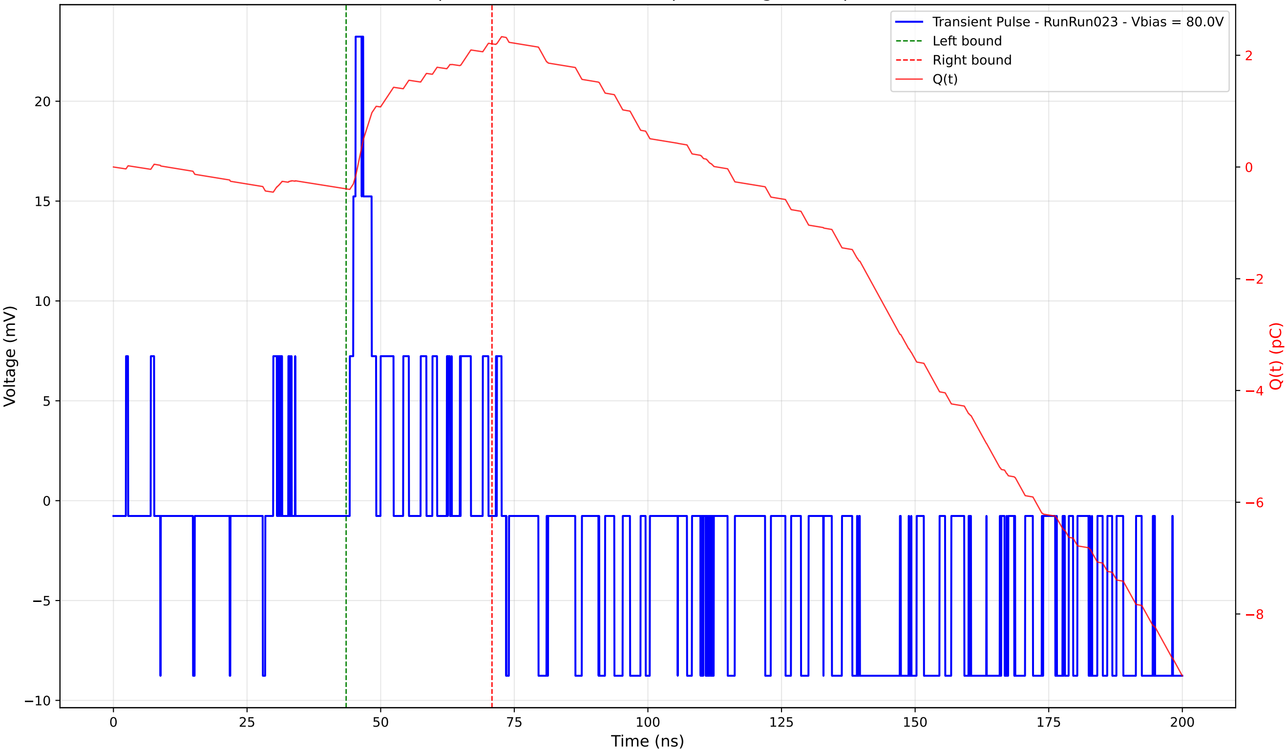
Transient Pulse - Sample: 4003 - Position: 45.0 \mu\text{m} - Charge: 2.60 pC - Rise Time: 1.10 ns
