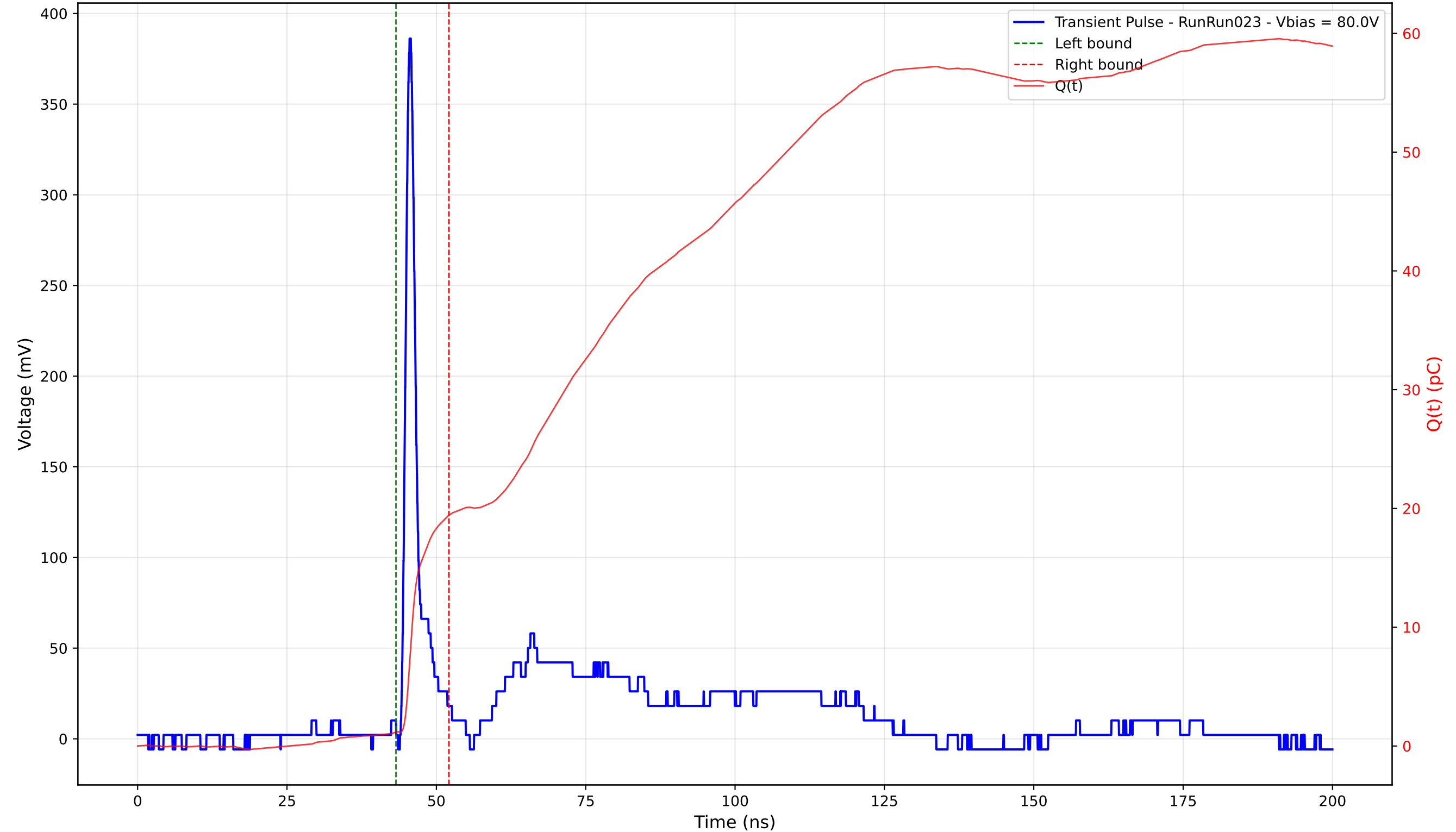
Transient Pulse - Sample: 4003 - Position: 145.0 \mu\text{m} - Charge: 18.24 pC - Rise Time: 1.01 ns
