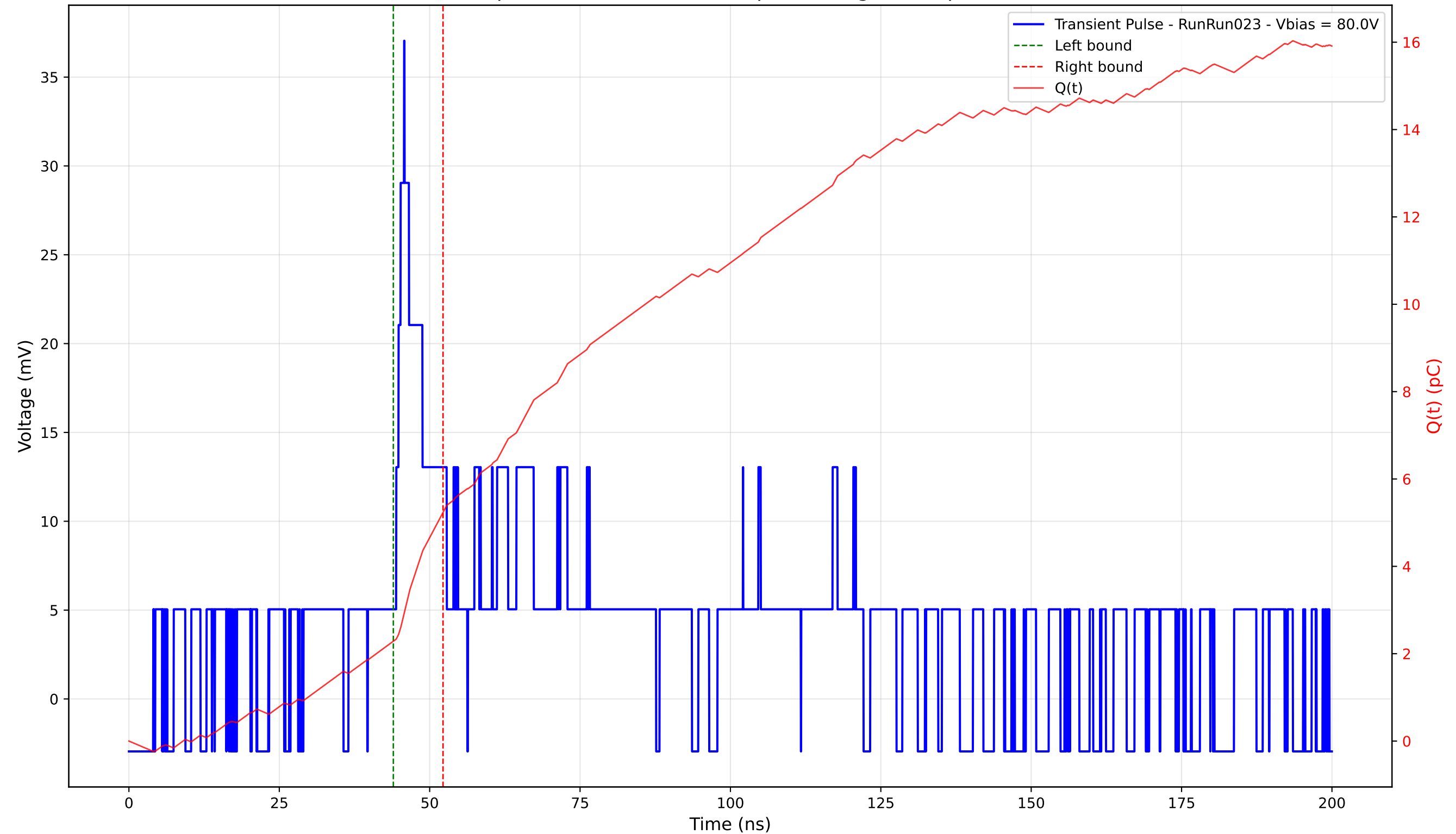
Transient Pulse - Sample: 4003 - Position: 60.0 \mu\text{m} - Charge: 2.95 pC - Rise Time: 6.03 ns
