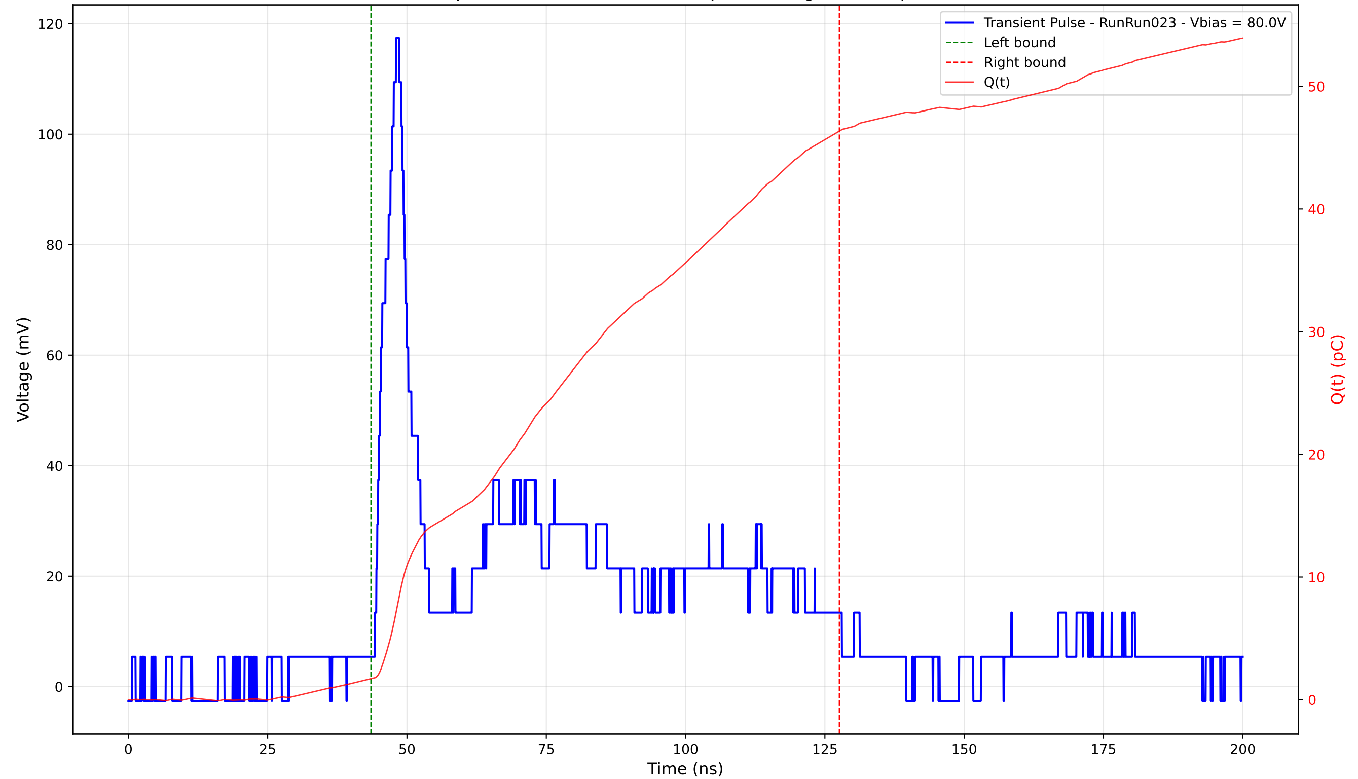
Transient Pulse - Sample: 4003 - Position: 235.0 \mu\text{m} - Charge: 44.66 pC - Rise Time: 3.36 ns
