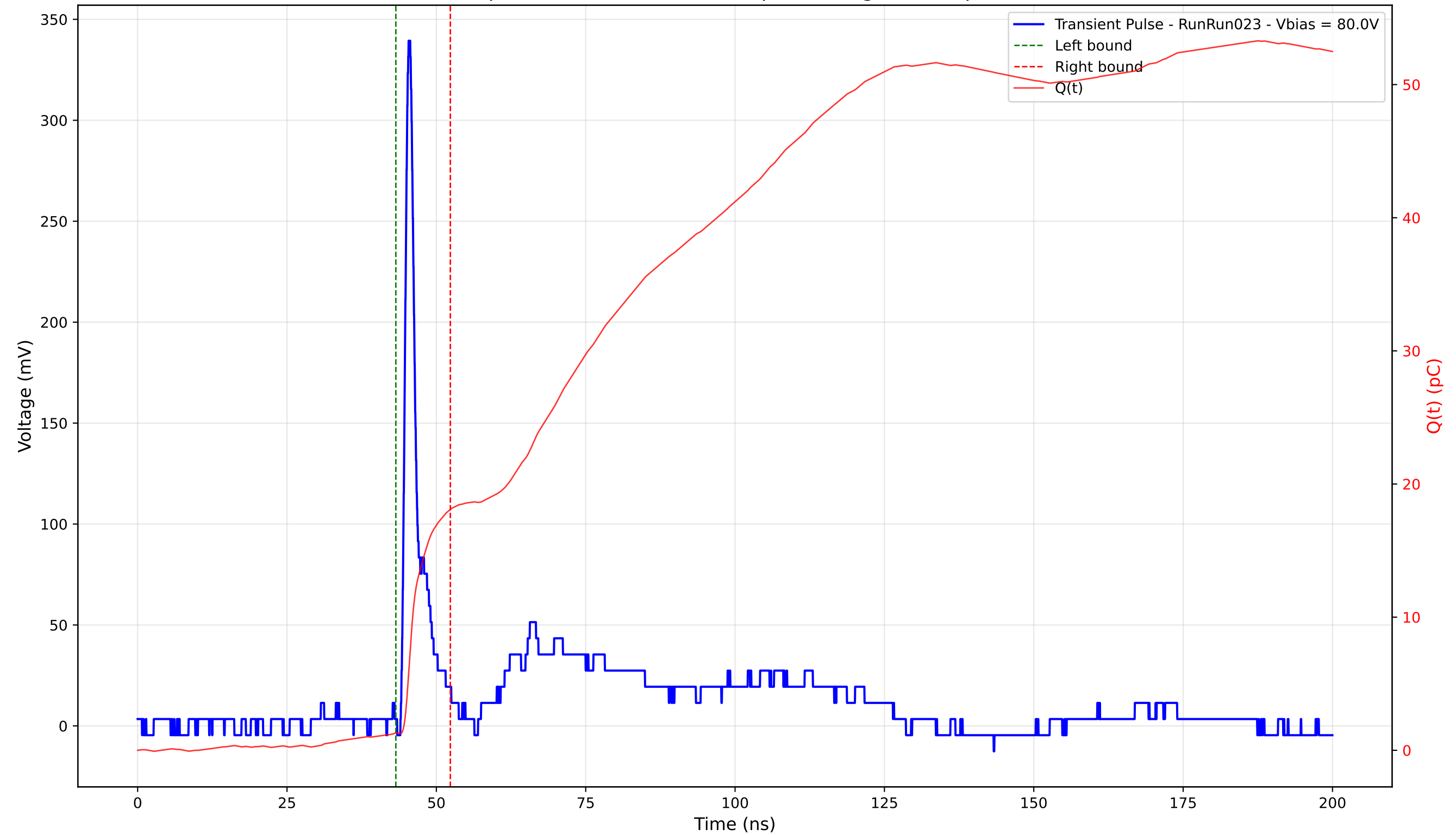
Transient Pulse - Sample: 4003 - Position: 120.0 \mu\text{m} - Charge: 16.80 pC - Rise Time: 0.90 ns
