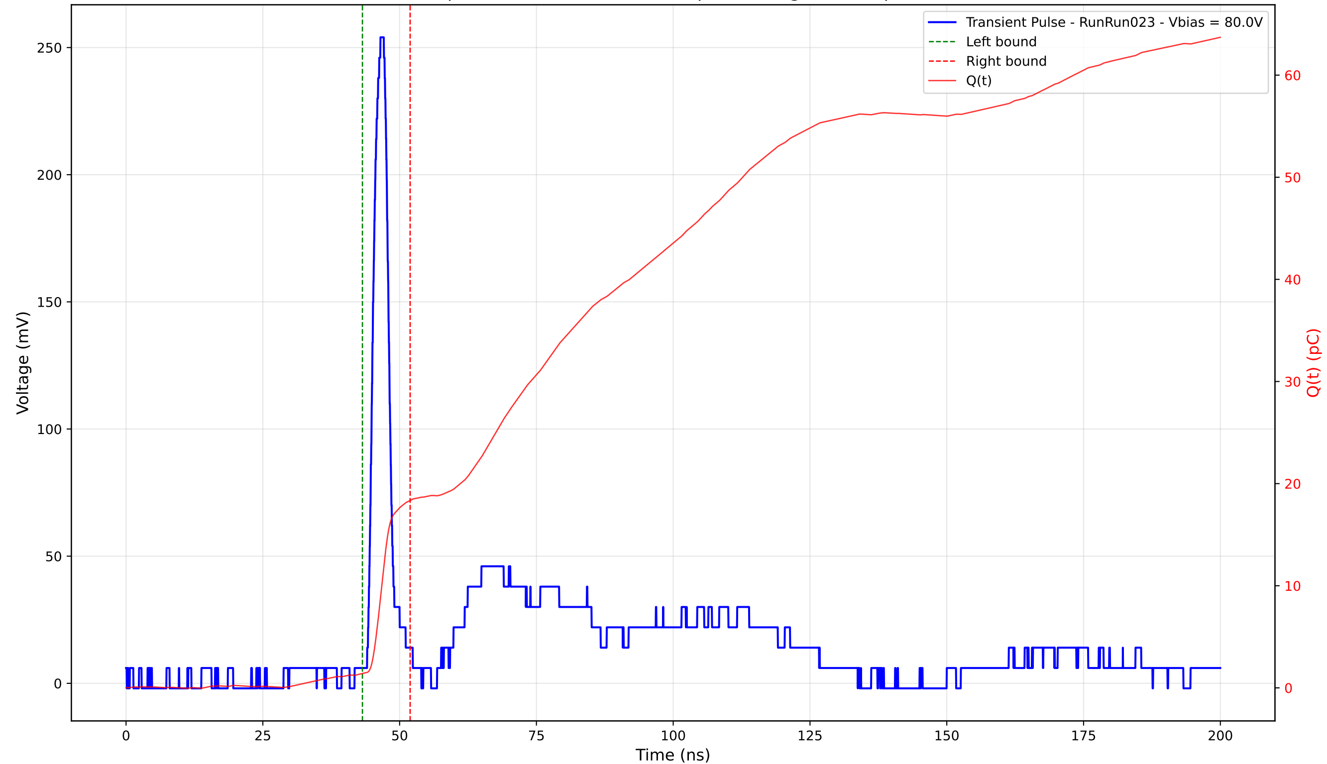
Transient Pulse - Sample: 4003 - Position: 210.0 \mu\text{m} - Charge: 16.96 pC - Rise Time: 1.63 ns
