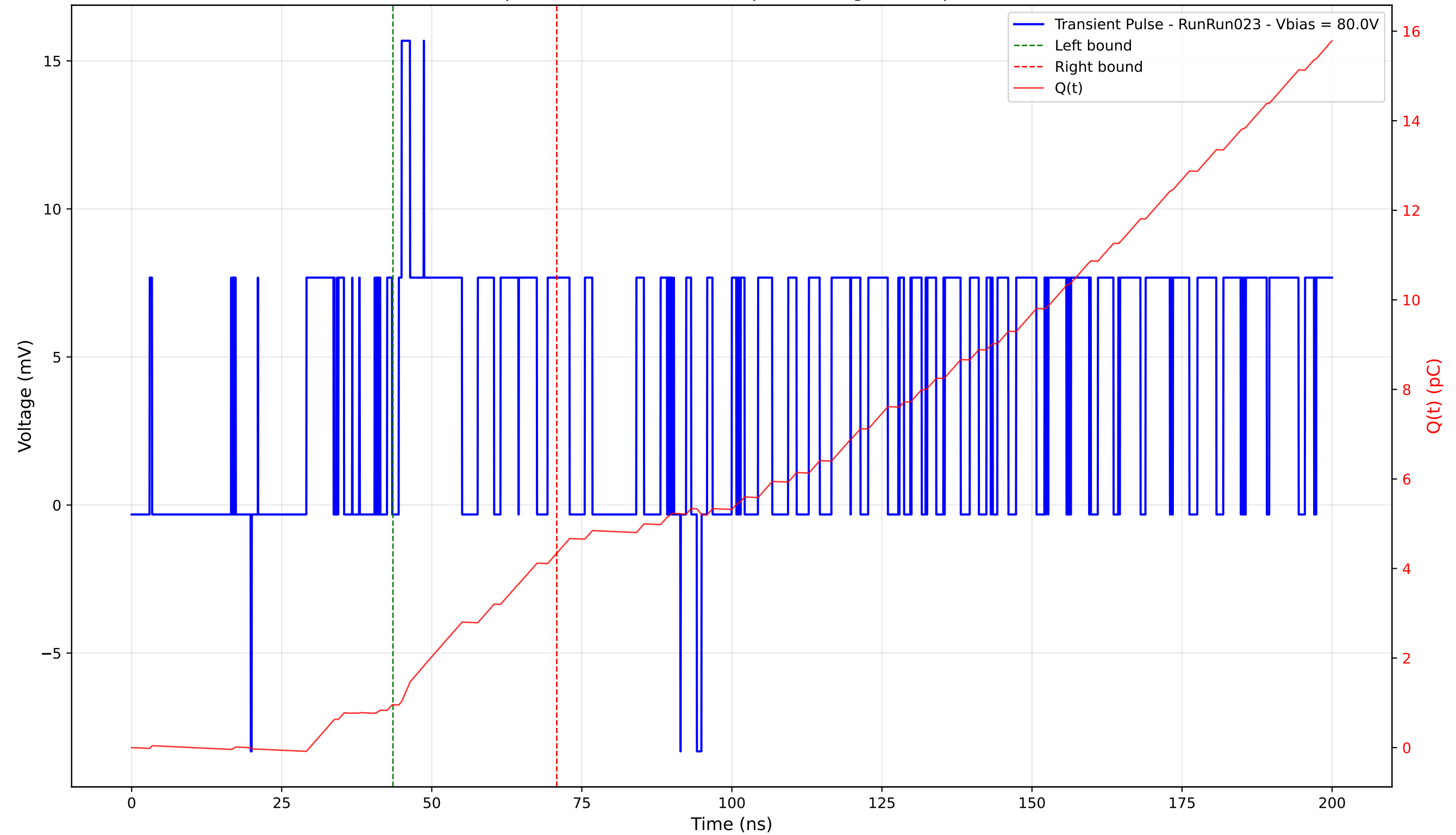
Transient Pulse - Sample: 4003 - Position: 0.0 \mu\text{m} - Charge: 3.39 pC - Rise Time: 0.50 ns
