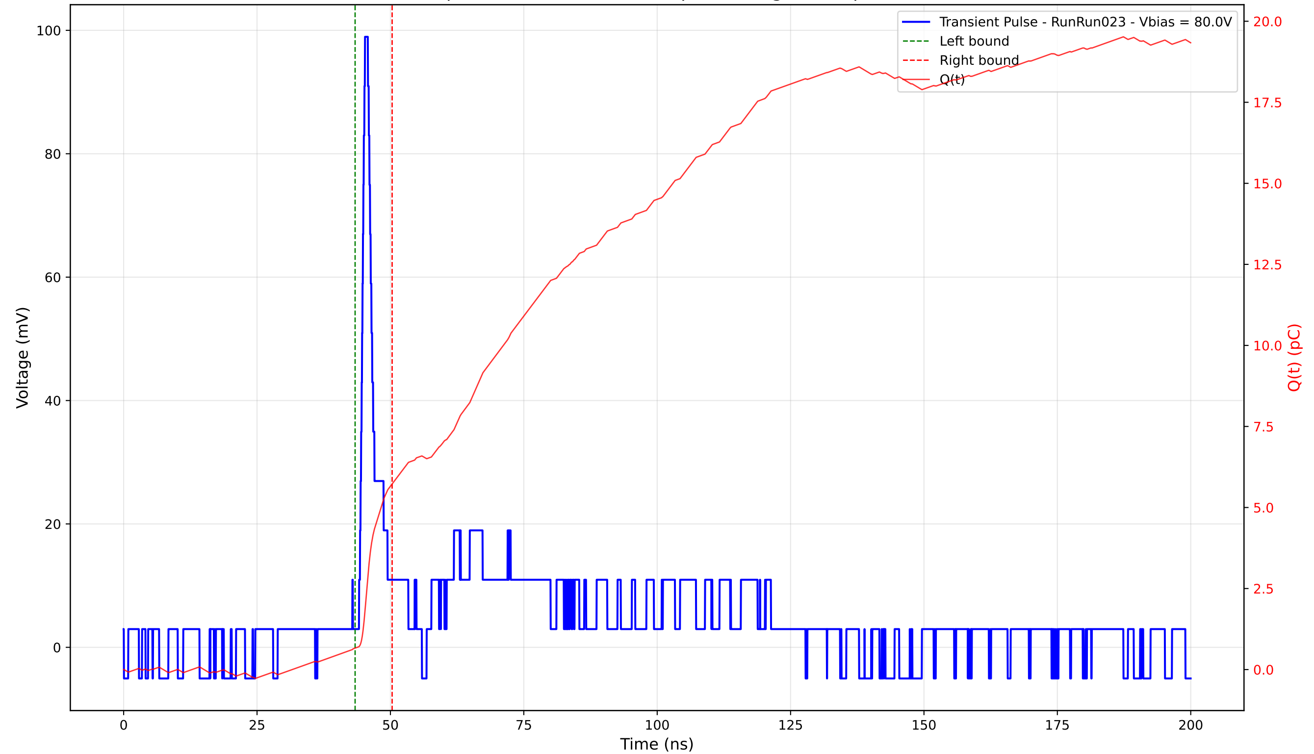
Transient Pulse - Sample: 4003 - Position: 95.0 \mu\text{m} - Charge: 5.06 pC - Rise Time: 1.00 ns
