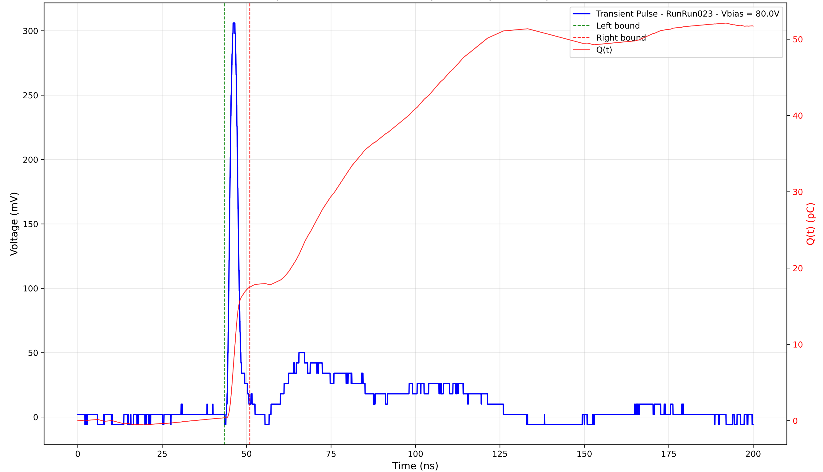
Transient Pulse - Sample: 4003 - Position: 195.0 \mu\text{m} - Charge: 17.11 pC - Rise Time: 1.33 ns
