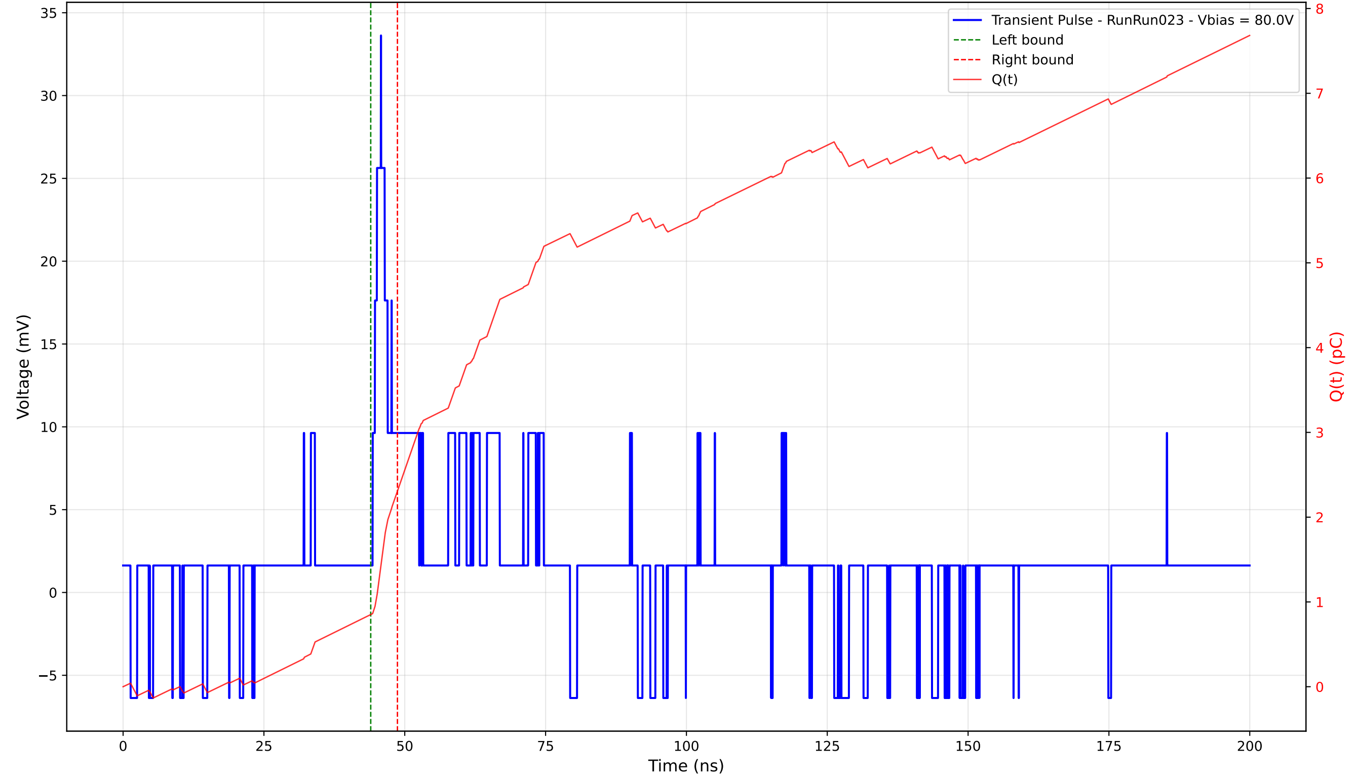
Transient Pulse - Sample: 4003 - Position: 315.0 \mu\text{m} - Charge: 1.46 pC - Rise Time: 1.48 ns
