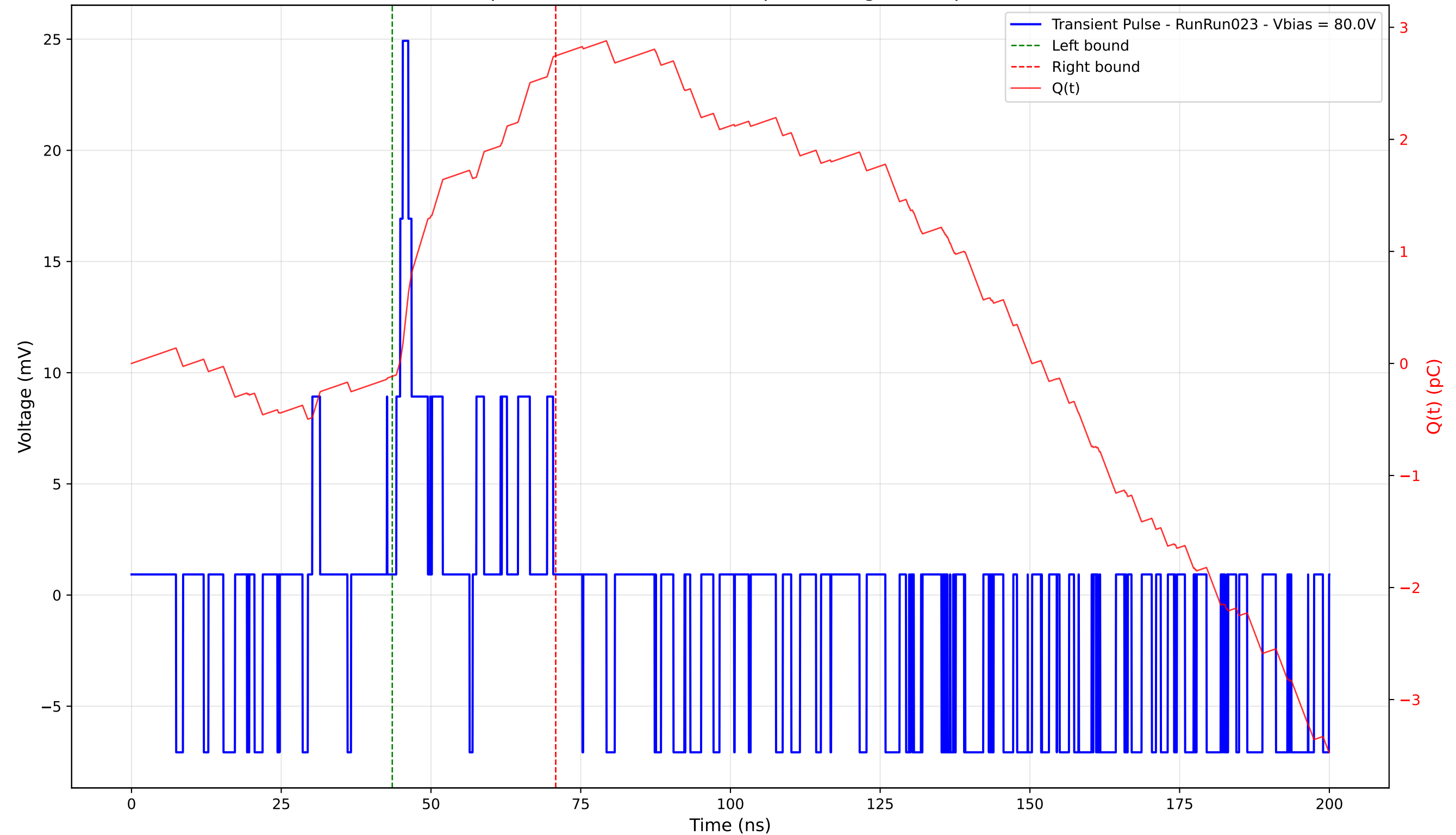
Transient Pulse - Sample: 4003 - Position: 335.0 \mu\text{m} - Charge: 2.86 pC - Rise Time: 1.08 ns
