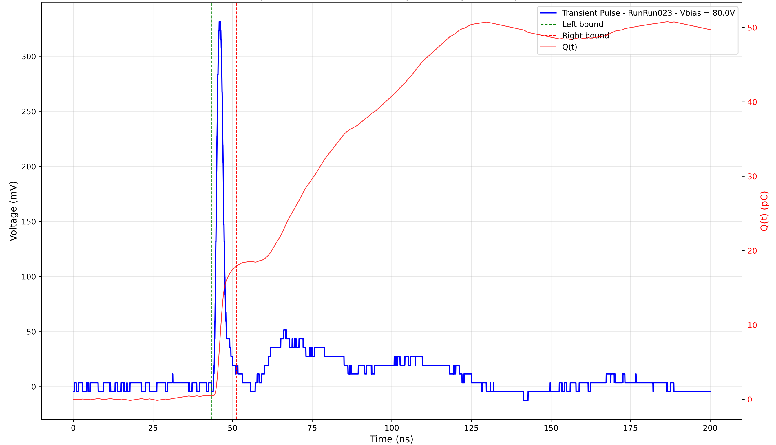
Transient Pulse - Sample: 4003 - Position: 185.0 \mu\text{m} - Charge: 17.35 pC - Rise Time: 1.17 ns
