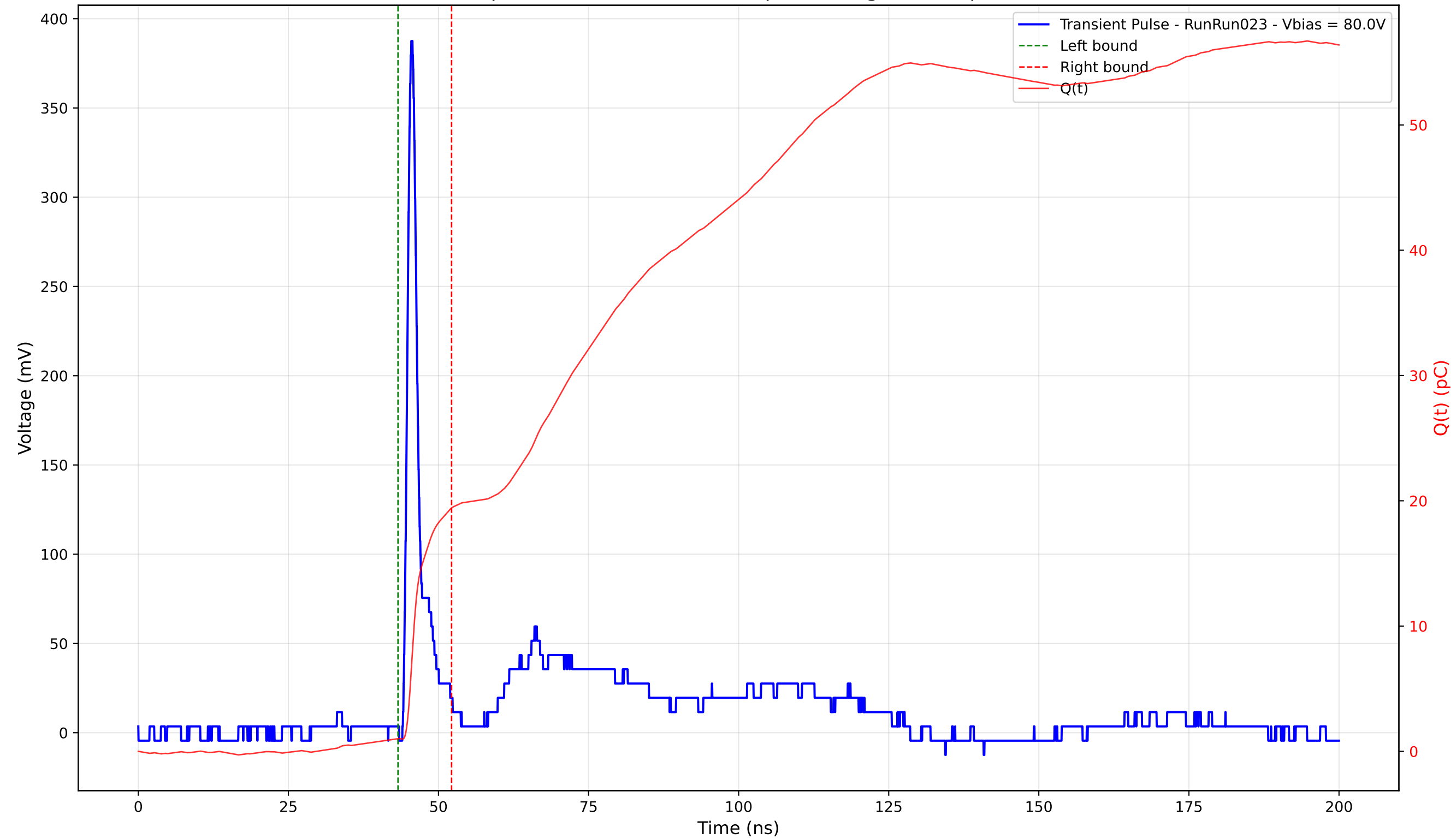
Transient Pulse - Sample: 4003 - Position: 140.0 \mu\text{m} - Charge: 18.41 pC - Rise Time: 0.98 ns
