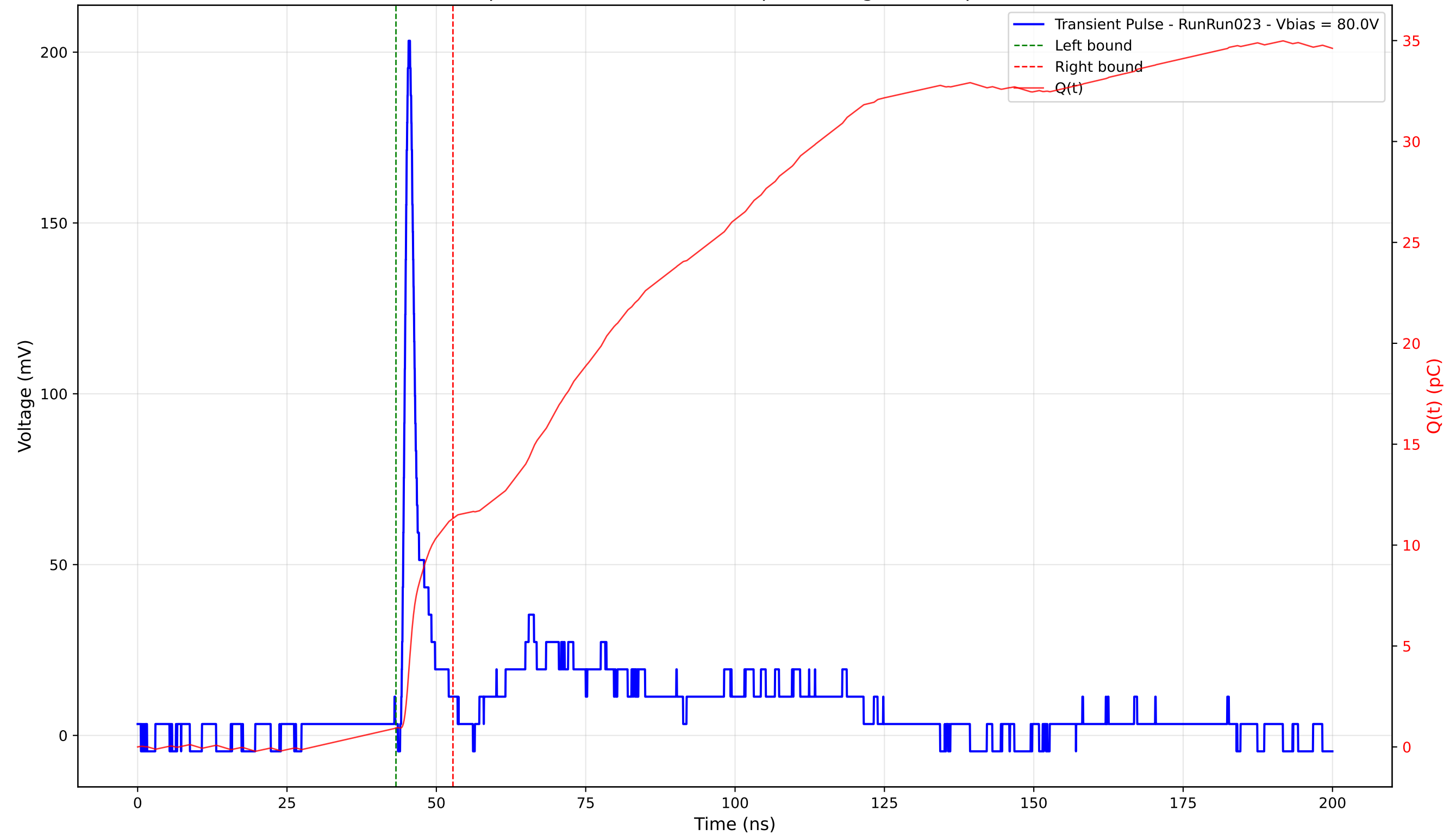
Transient Pulse - Sample: 4003 - Position: 105.0 \mu\text{m} - Charge: 10.38 pC - Rise Time: 0.92 ns
