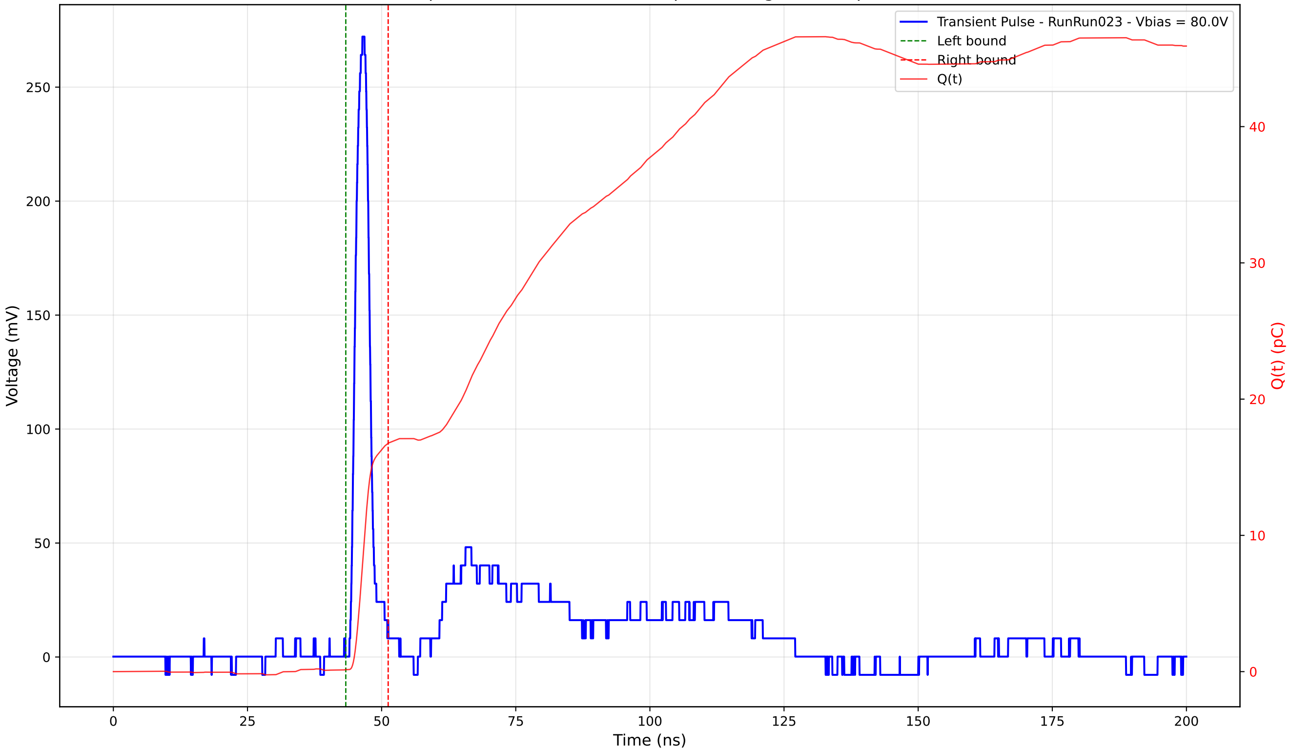
Transient Pulse - Sample: 4003 - Position: 205.0 \mu\text{m} - Charge: 16.62 pC - Rise Time: 1.49 ns
