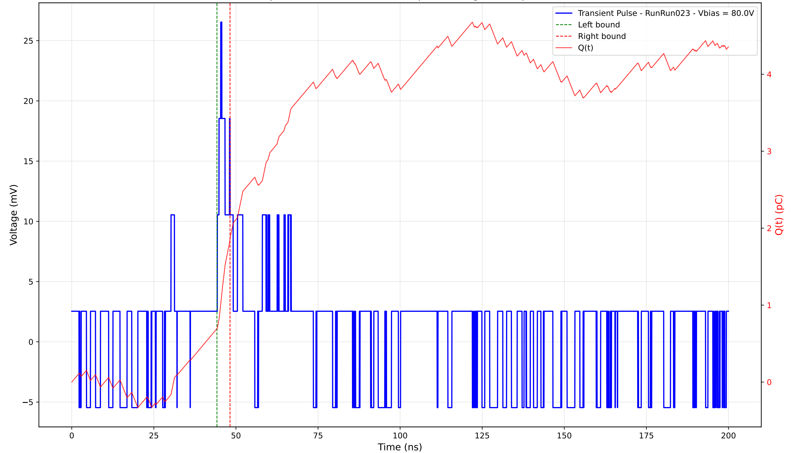
Transient Pulse - Sample: 4003 - Position: 355.0 \mu\text{m} - Charge: 1.17 pC - Rise Time: 1.06 ns
