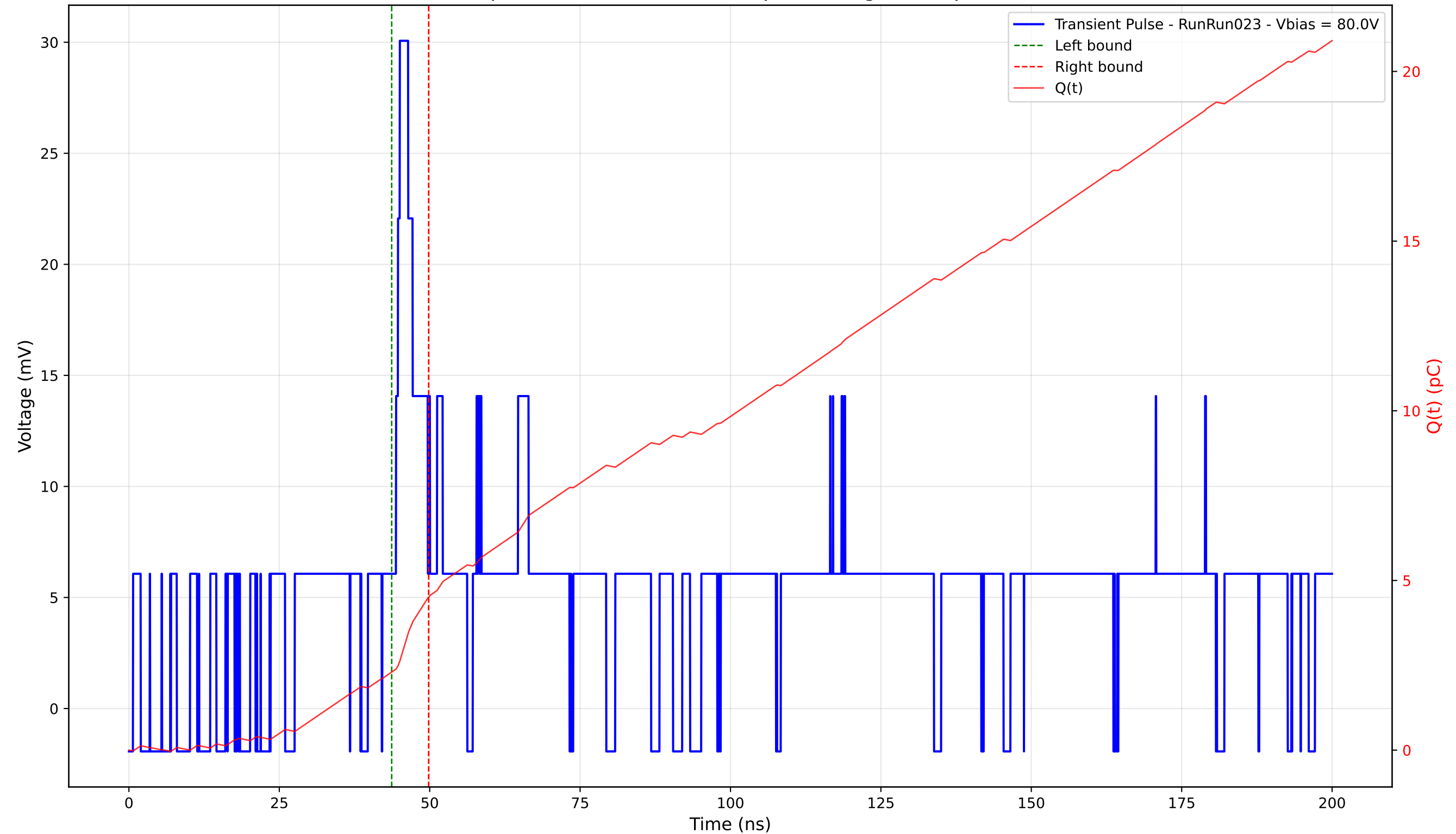
Transient Pulse - Sample: 4003 - Position: 305.0 \mu\text{m} - Charge: 2.20 pC - Rise Time: 2.91 ns
