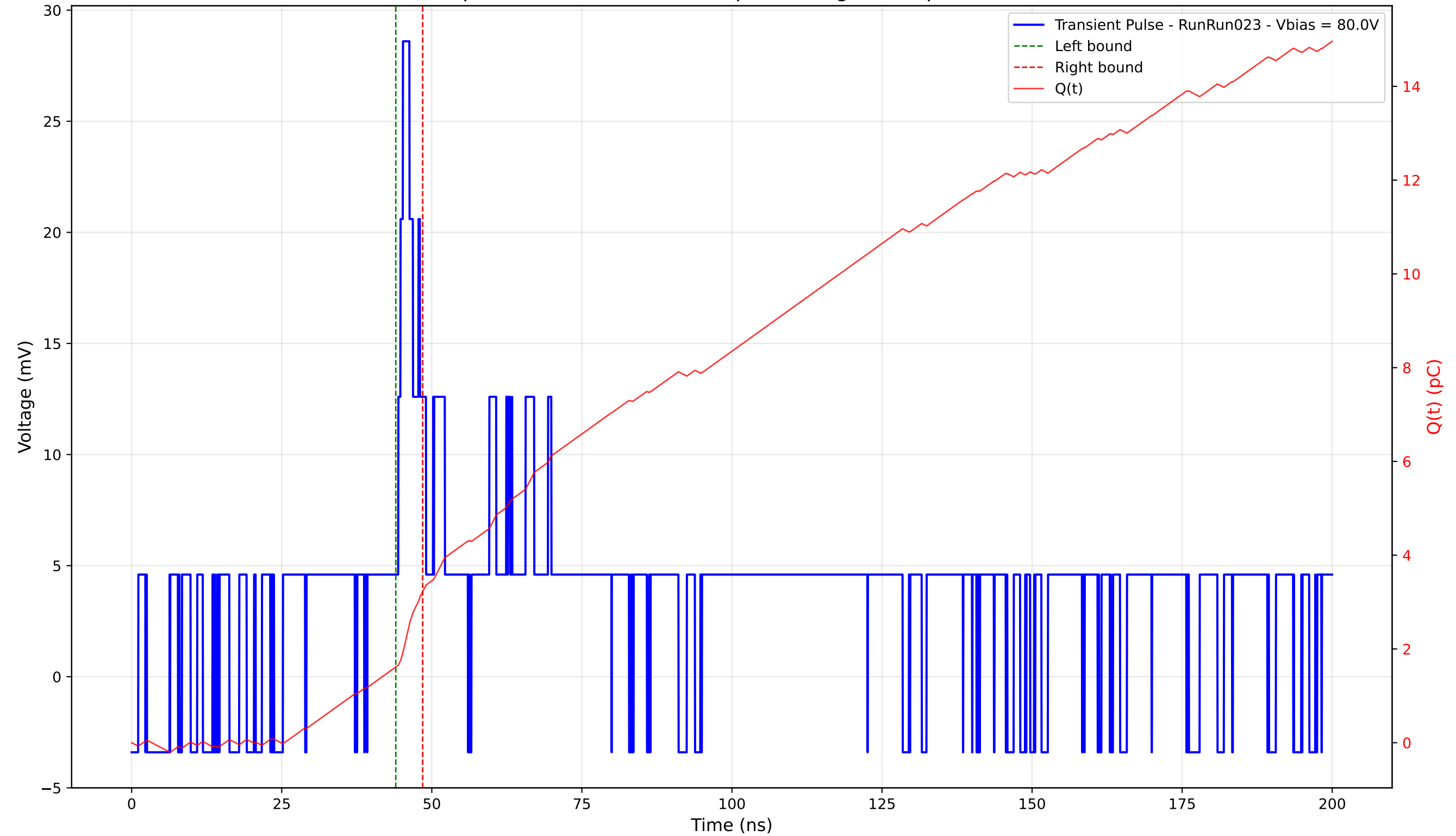
Transient Pulse - Sample: 4003 - Position: 320.0 \mu\text{m} - Charge: 1.61 pC - Rise Time: 0.00 ns (N/A)
