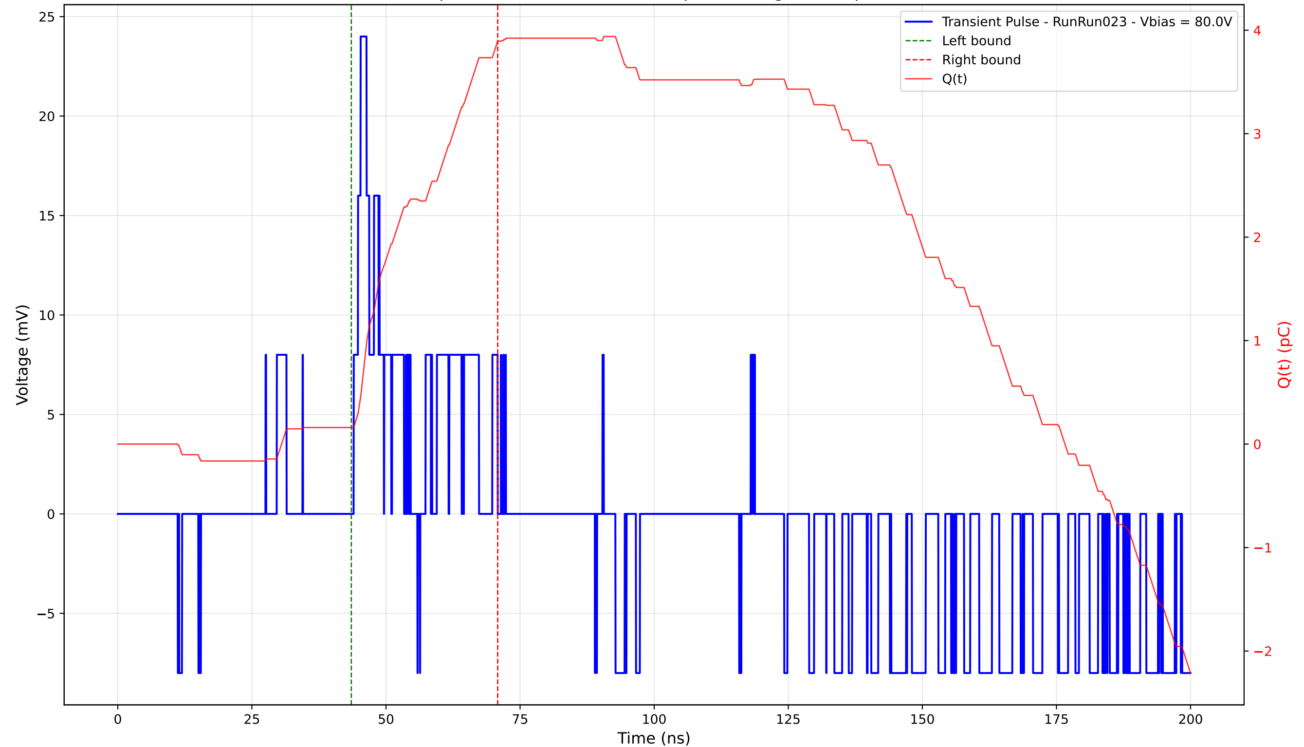
Transient Pulse - Sample: 4003 - Position: 360.0 \mu\text{m} - Charge: 3.73 pC - Rise Time: 1.29 ns
