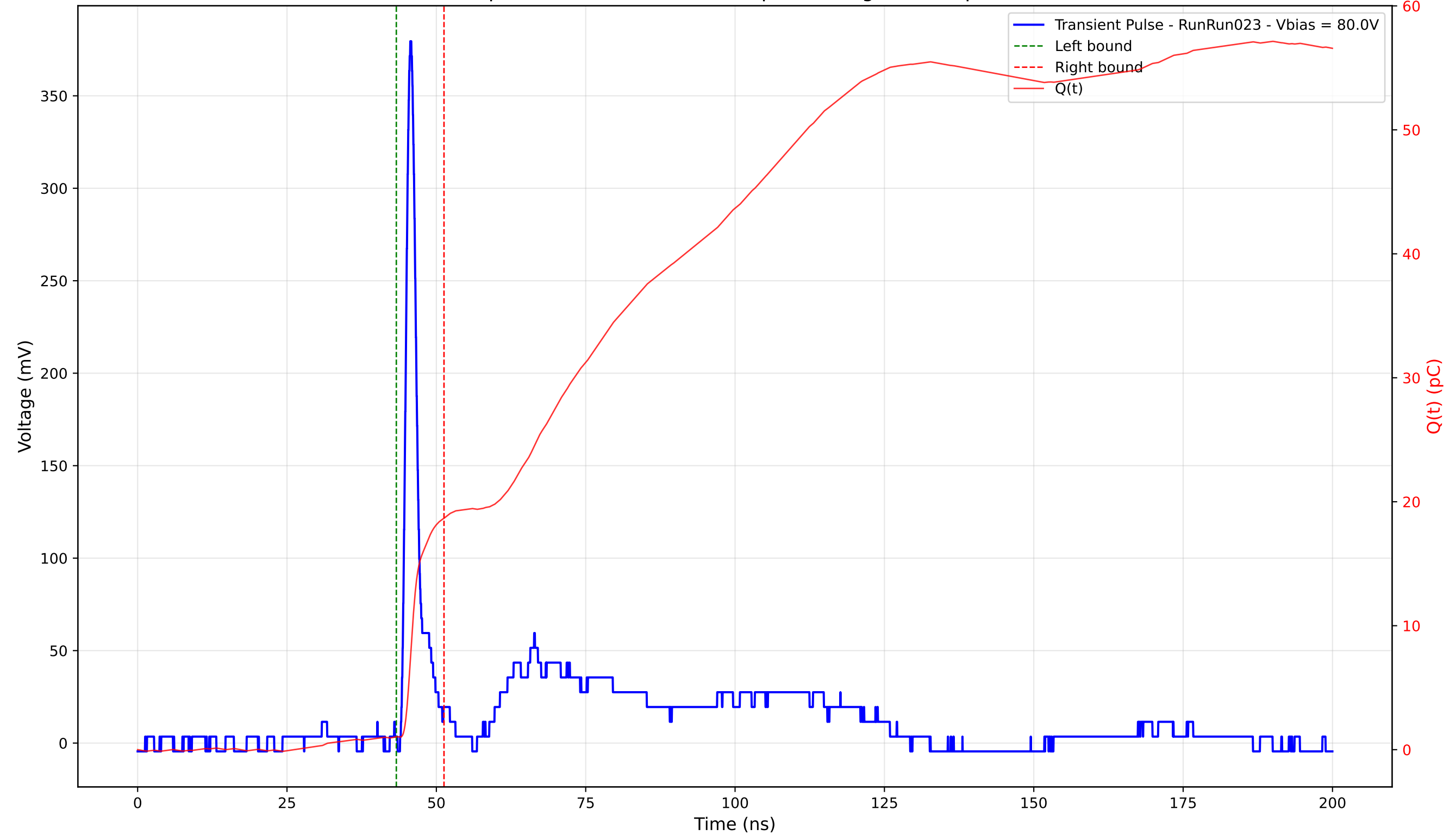
Transient Pulse - Sample: 4003 - Position: 160.0 \mu\text{m} - Charge: 17.63 pC - Rise Time: 1.07 ns
