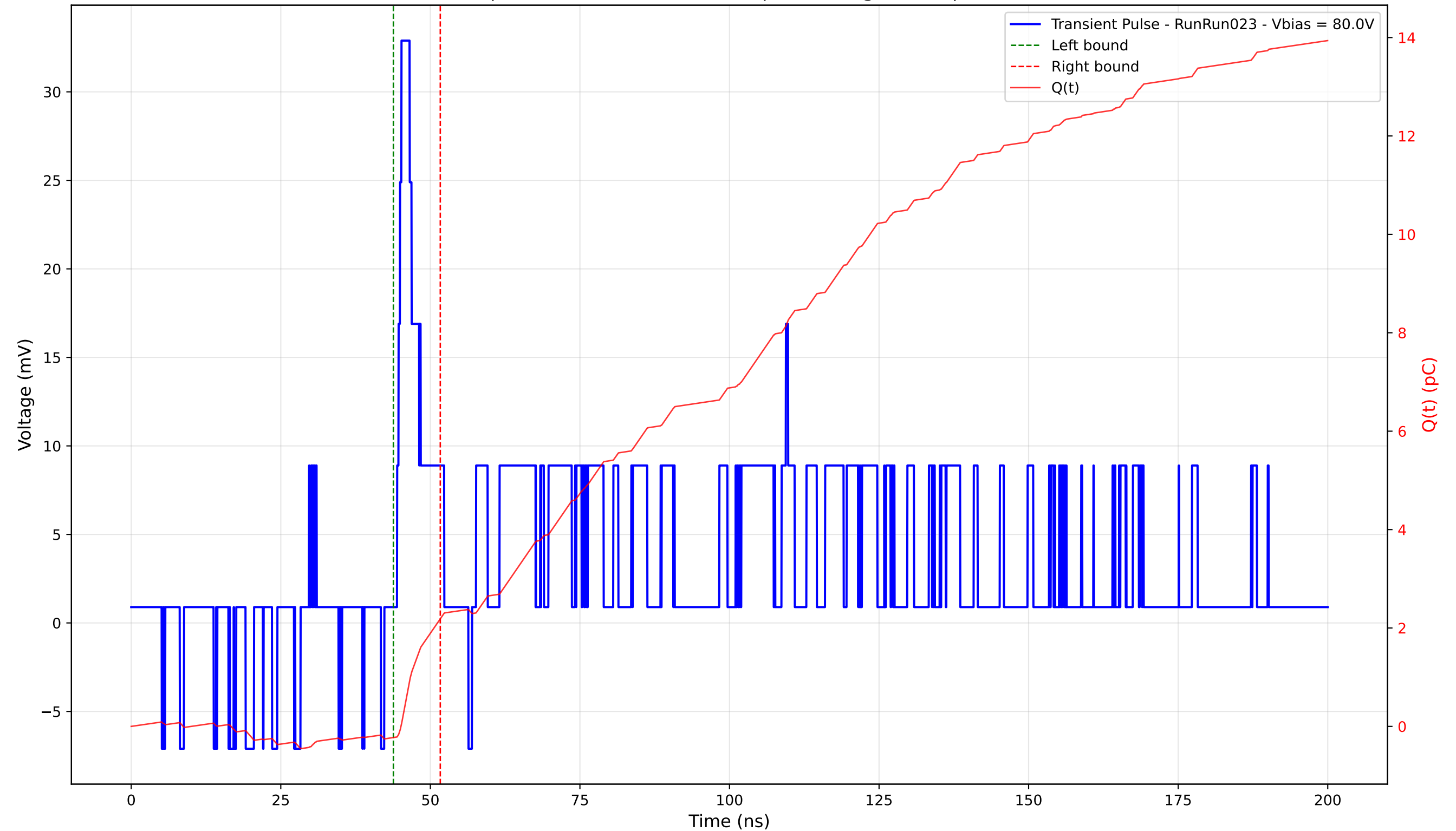
Transient Pulse - Sample: 4003 - Position: 275.0 \mu\text{m} - Charge: 2.42 pC - Rise Time: 0.73 ns
