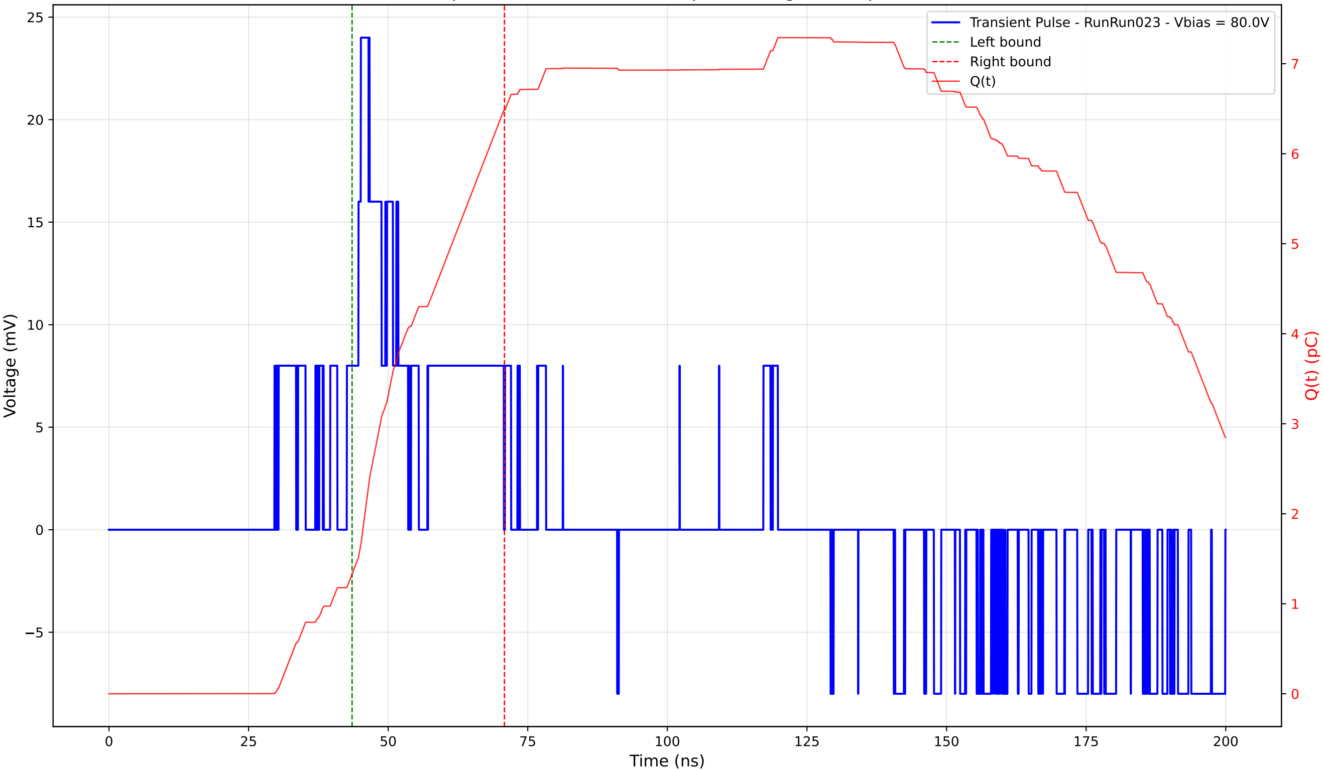
Transient Pulse - Sample: 4003 - Position: 65.0 \mu\text{m} - Charge: 5.15 pC - Rise Time: 2.51 ns
