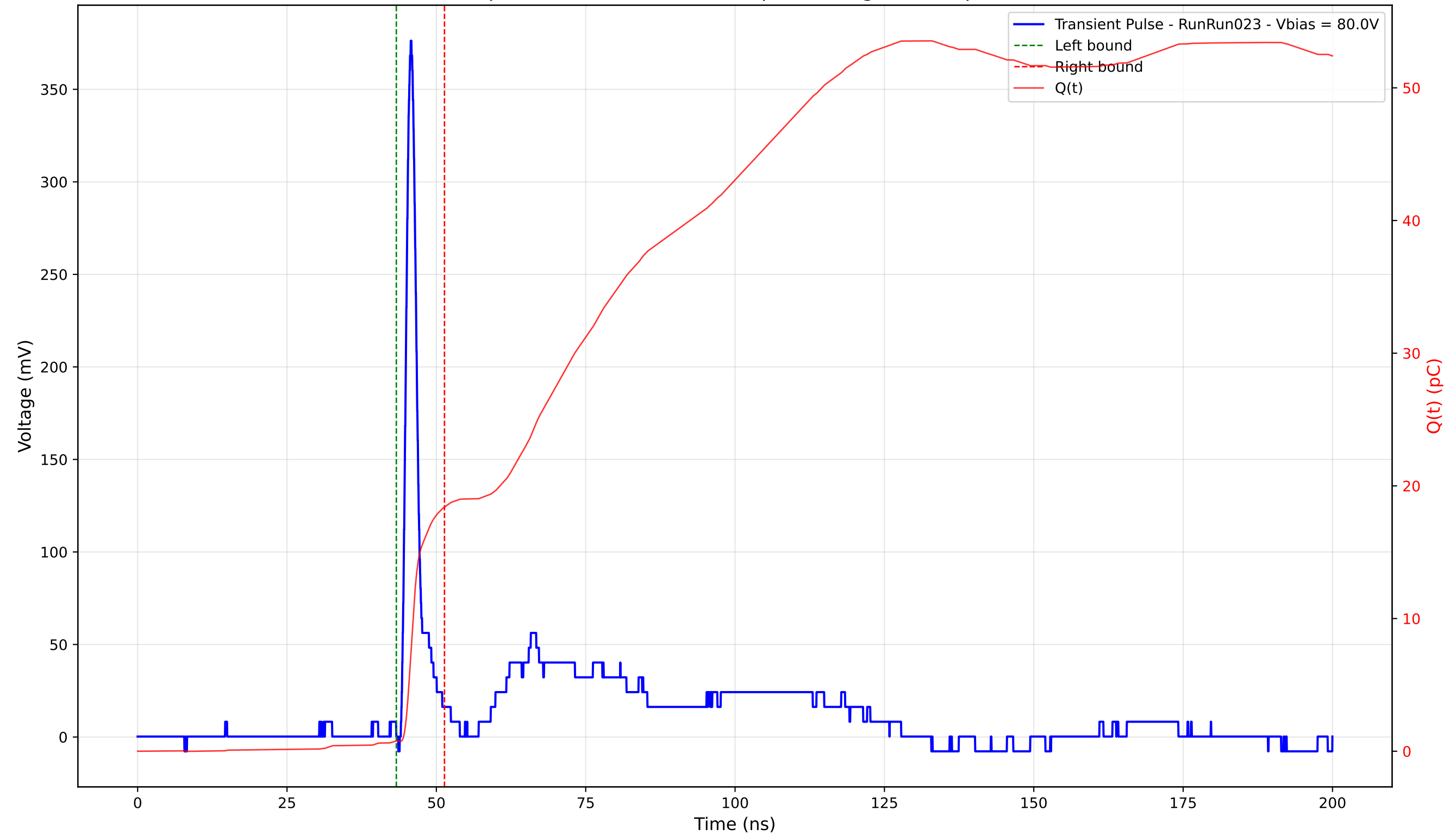
Transient Pulse - Sample: 4003 - Position: 165.0 \mu\text{m} - Charge: 17.62 pC - Rise Time: 1.11 ns
