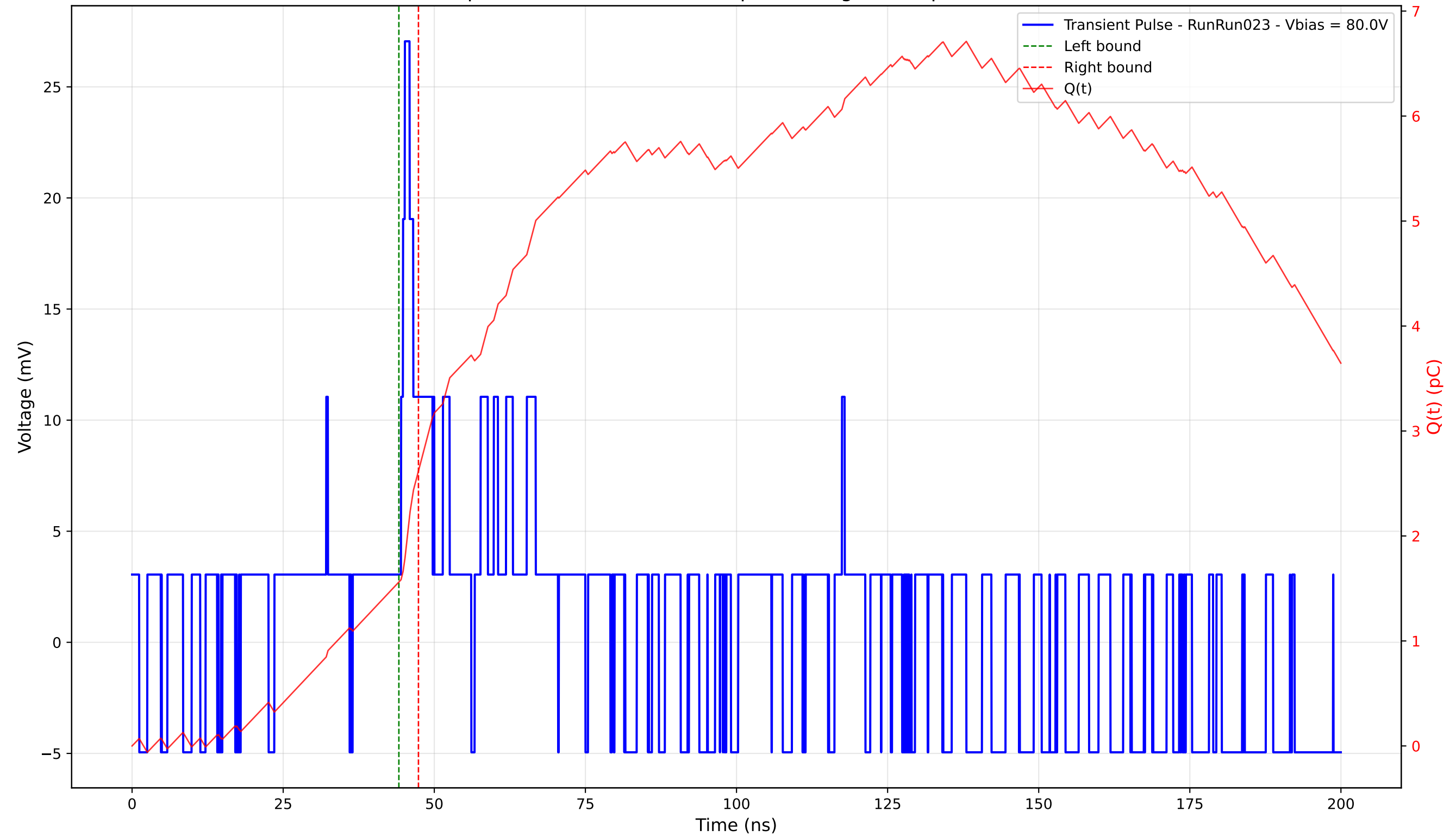
Transient Pulse - Sample: 4003 - Position: 415.0 \mu\text{m} - Charge: 1.06 pC - Rise Time: 0.00 ns (N/A)
