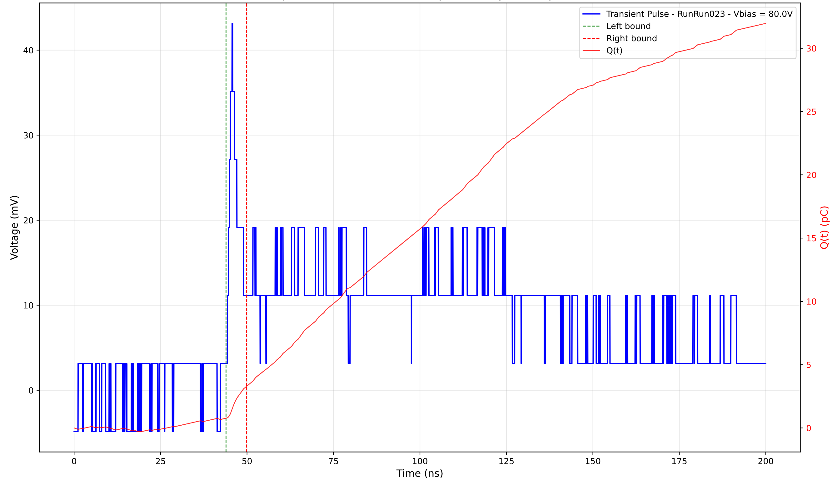
Transient Pulse - Sample: 4003 - Position: 255.0 \mu\text{m} - Charge: 2.51 pC - Rise Time: 1.38 ns
