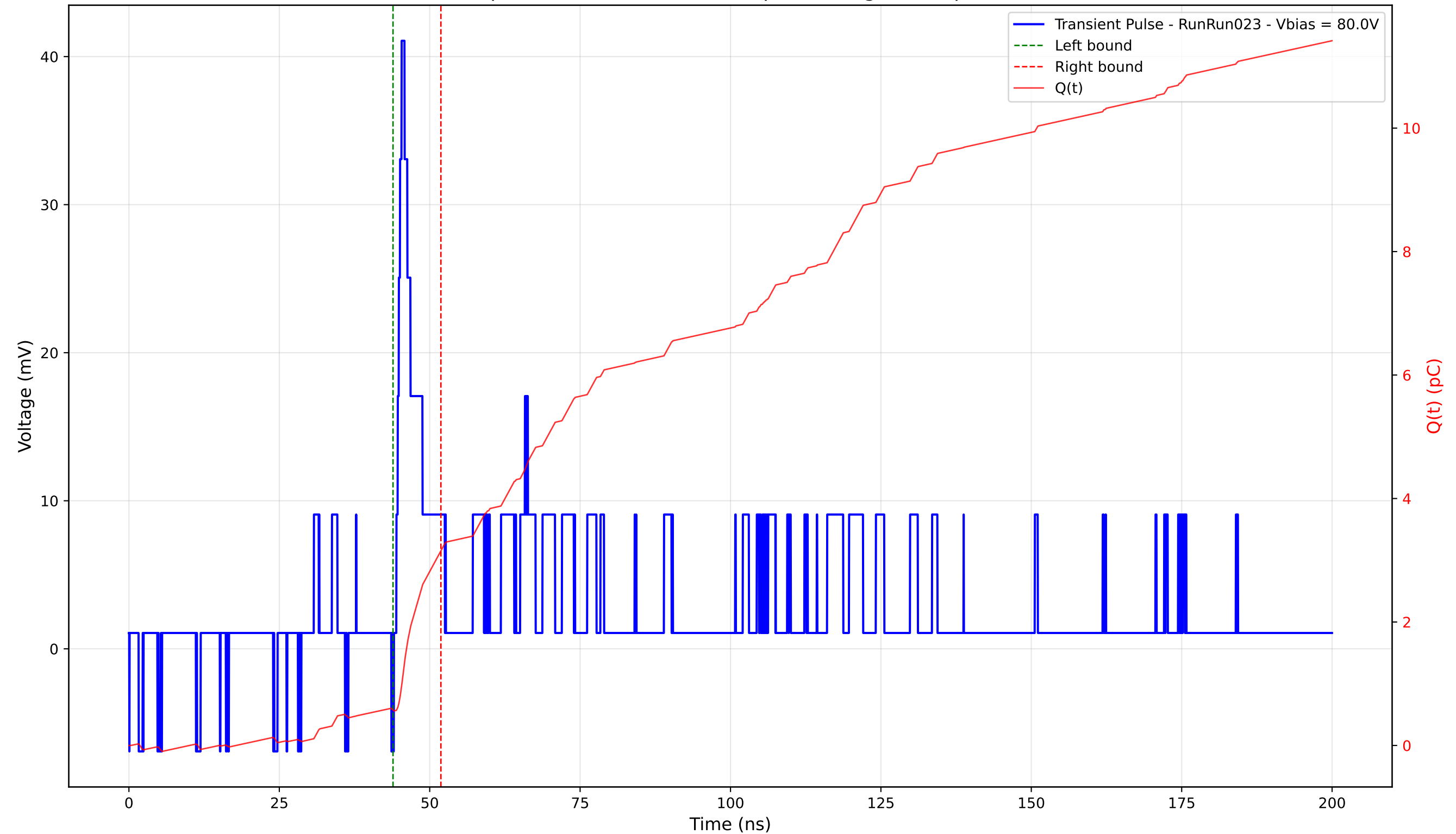
Transient Pulse - Sample: 4003 - Position: 280.0 \mu\text{m} - Charge: 2.58 pC - Rise Time: 0.87 ns
