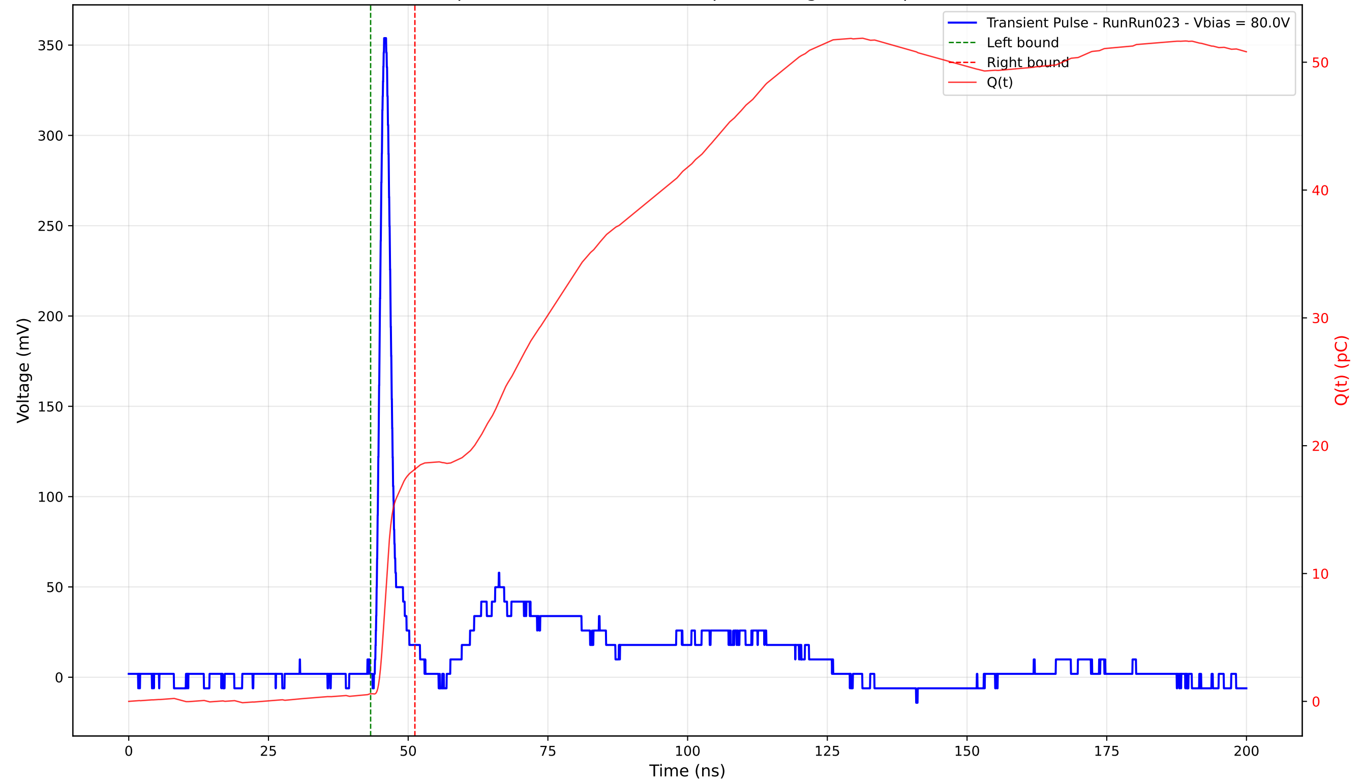
Transient Pulse - Sample: 4003 - Position: 175.0 \mu\text{m} - Charge: 17.57 pC - Rise Time: 1.12 ns
