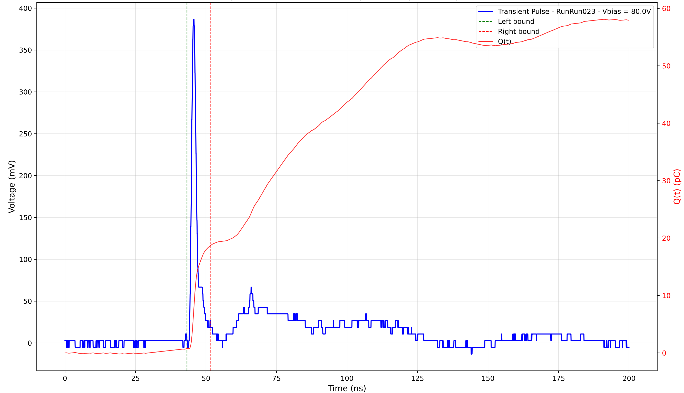
Transient Pulse - Sample: 4003 - Position: 150.0 \mu\text{m} - Charge: 17.86 pC - Rise Time: 1.01 ns
