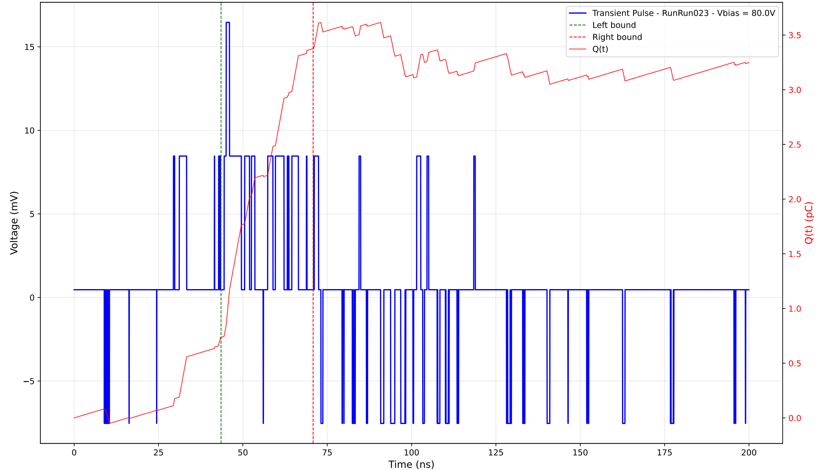
Transient Pulse - Sample: 4003 - Position: 15.0 \mu\text{m} - Charge: 2.64 pC - Rise Time: 0.62 ns
