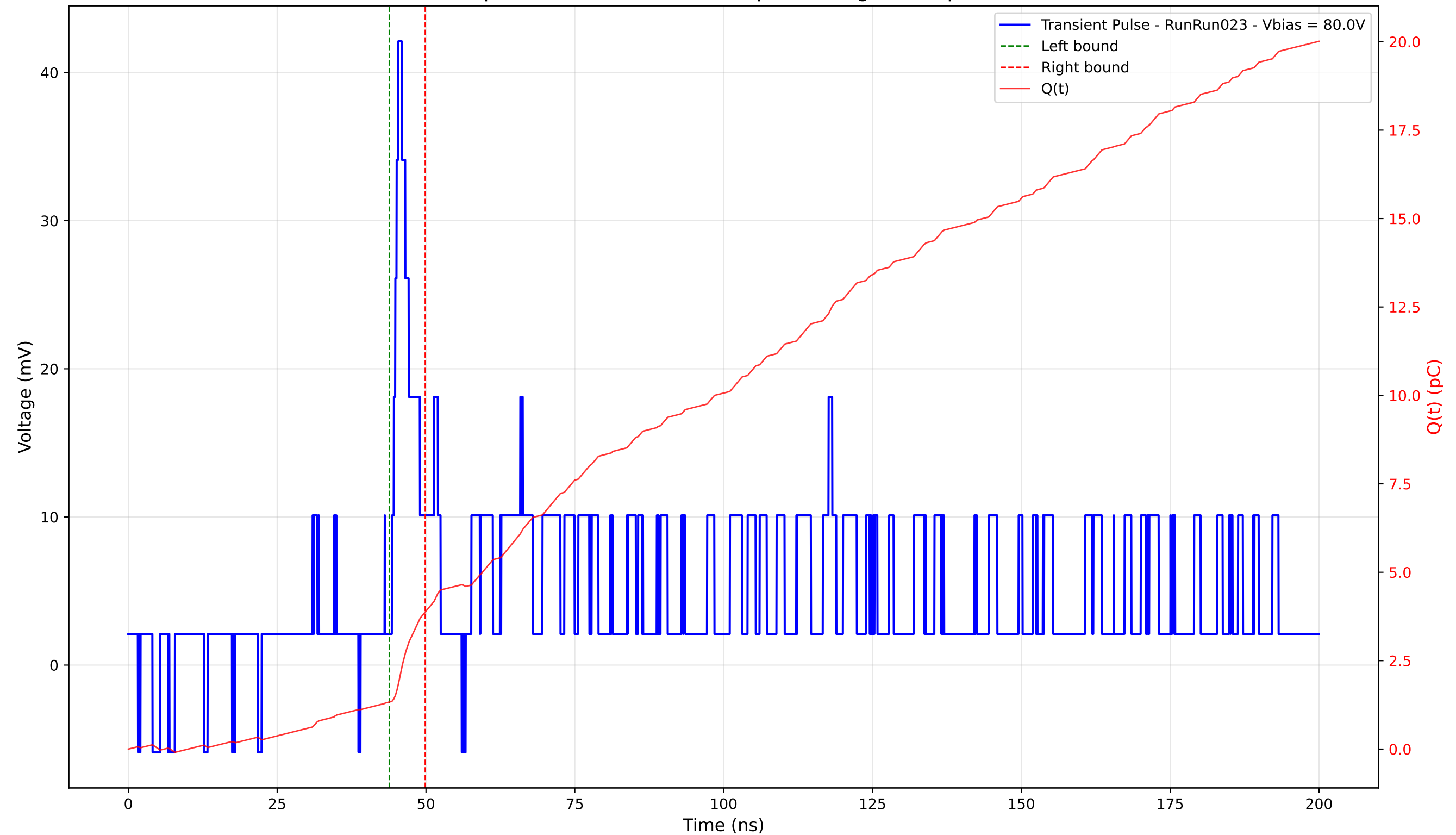
Transient Pulse - Sample: 4003 - Position: 270.0 \mu\text{m} - Charge: 2.54 pC - Rise Time: 1.07 ns
