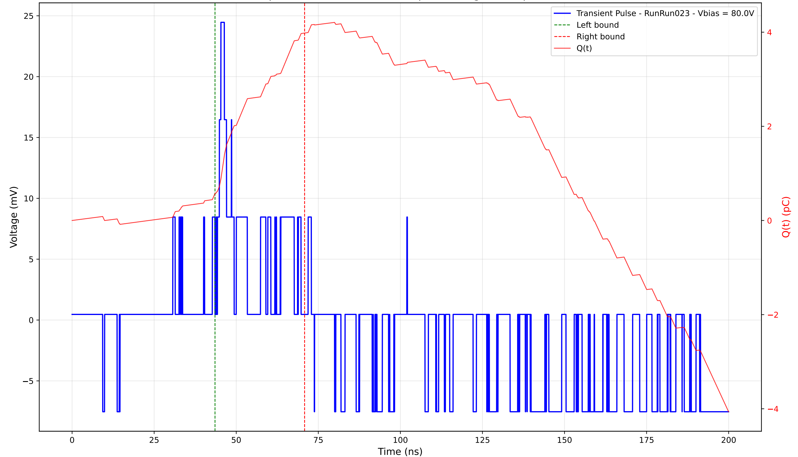
Transient Pulse - Sample: 4003 - Position: 340.0 \mu\text{m} - Charge: 3.40 pC - Rise Time: 1.06 ns
