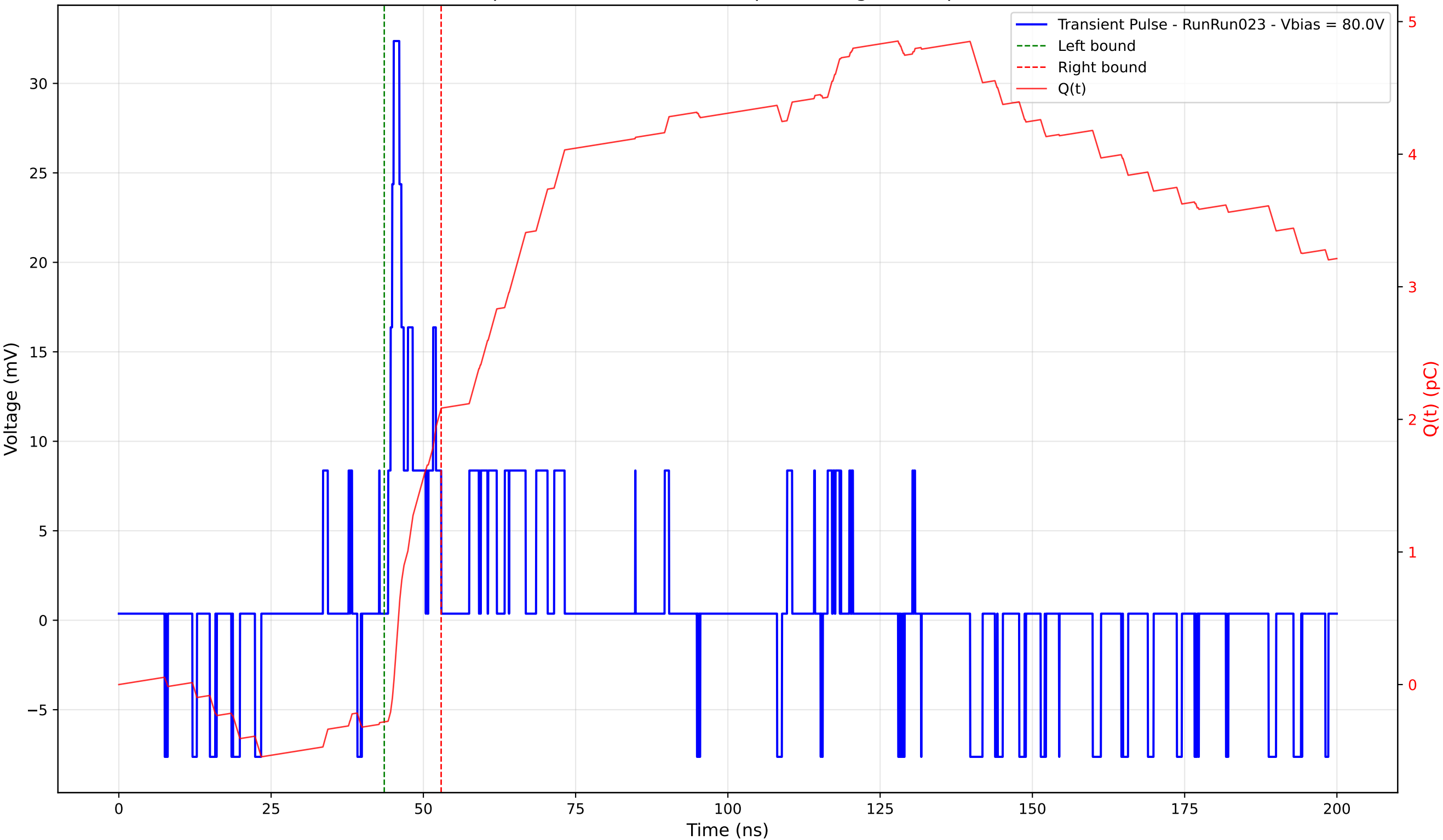
Transient Pulse - Sample: 4003 - Position: 85.0 \mu\text{m} - Charge: 2.36 pC - Rise Time: 0.91 ns
