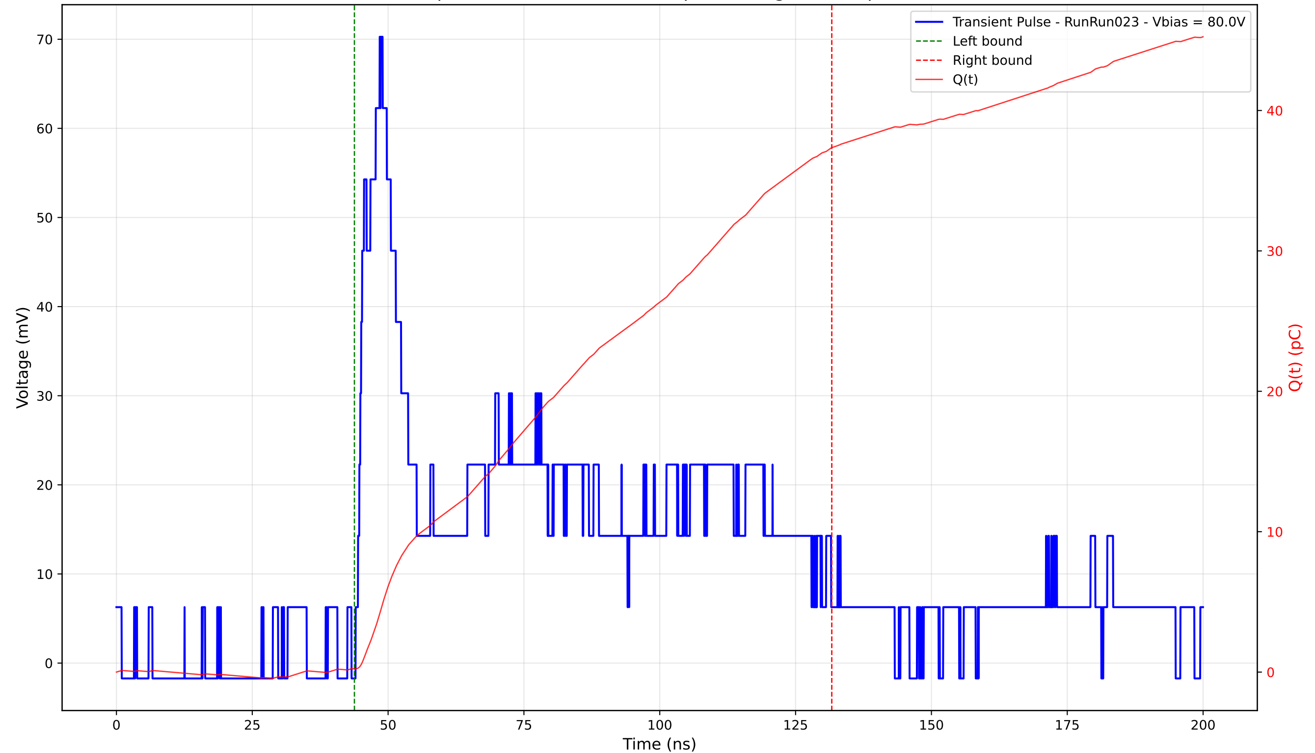
Transient Pulse - Sample: 4003 - Position: 240.0 \mu\text{m} - Charge: 37.13 pC - Rise Time: 4.00 ns
