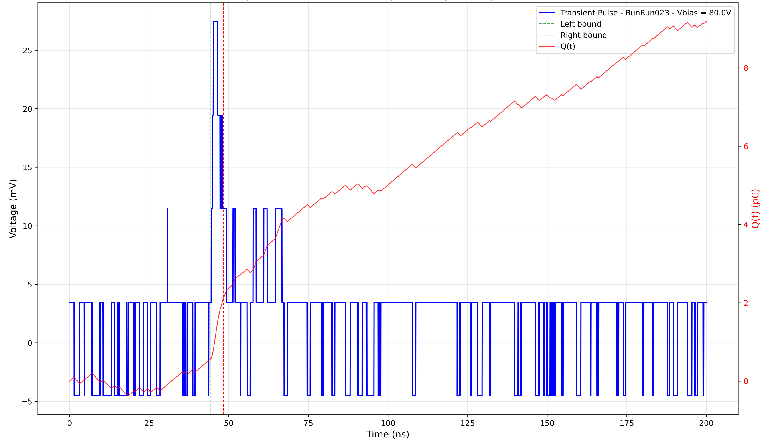
Transient Pulse - Sample: 4003 - Position: 385.0 \mu\text{m} - Charge: 1.57 pC - Rise Time: 0.00 ns (N/A)
