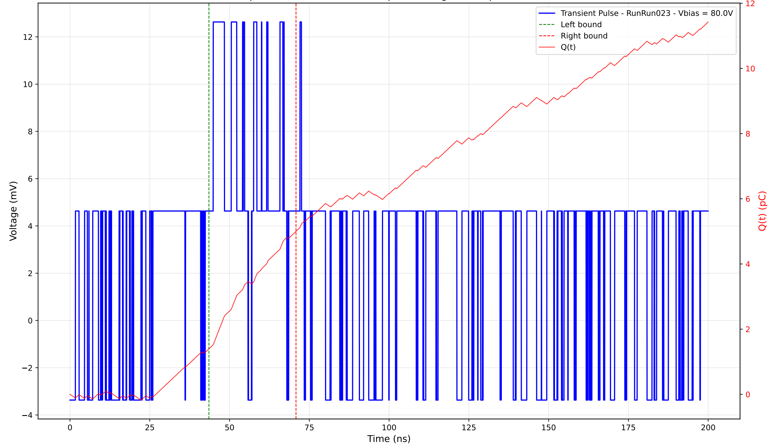
Transient Pulse - Sample: 4003 - Position: 75.0 \mu\text{m} - Charge: 3.60 pC - Rise Time: 0.00 ns (N/A)
