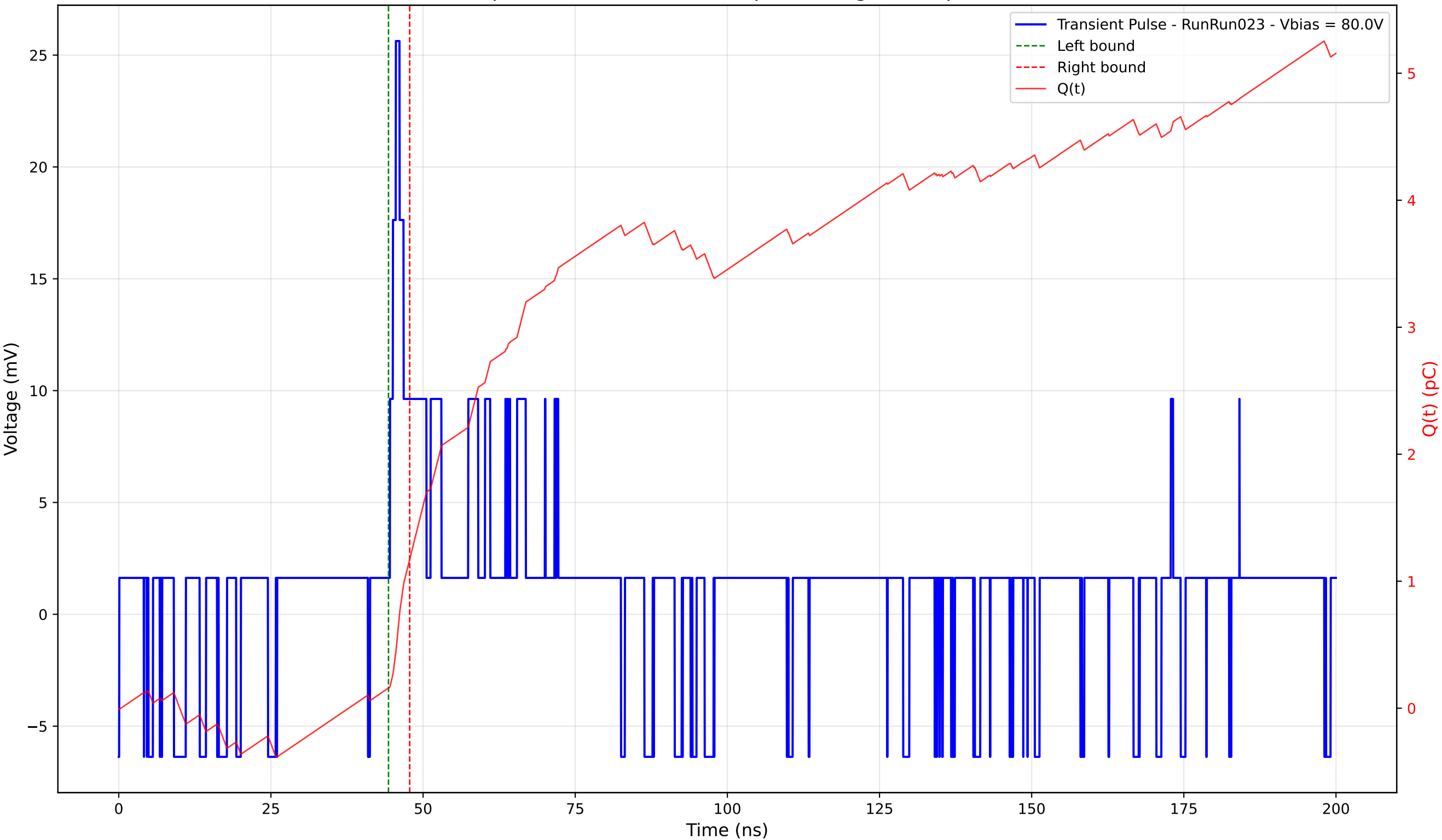
Transient Pulse - Sample: 4003 - Position: 30.0 \mu\text{m} - Charge: 1.01 pC - Rise Time: 0.98 ns
