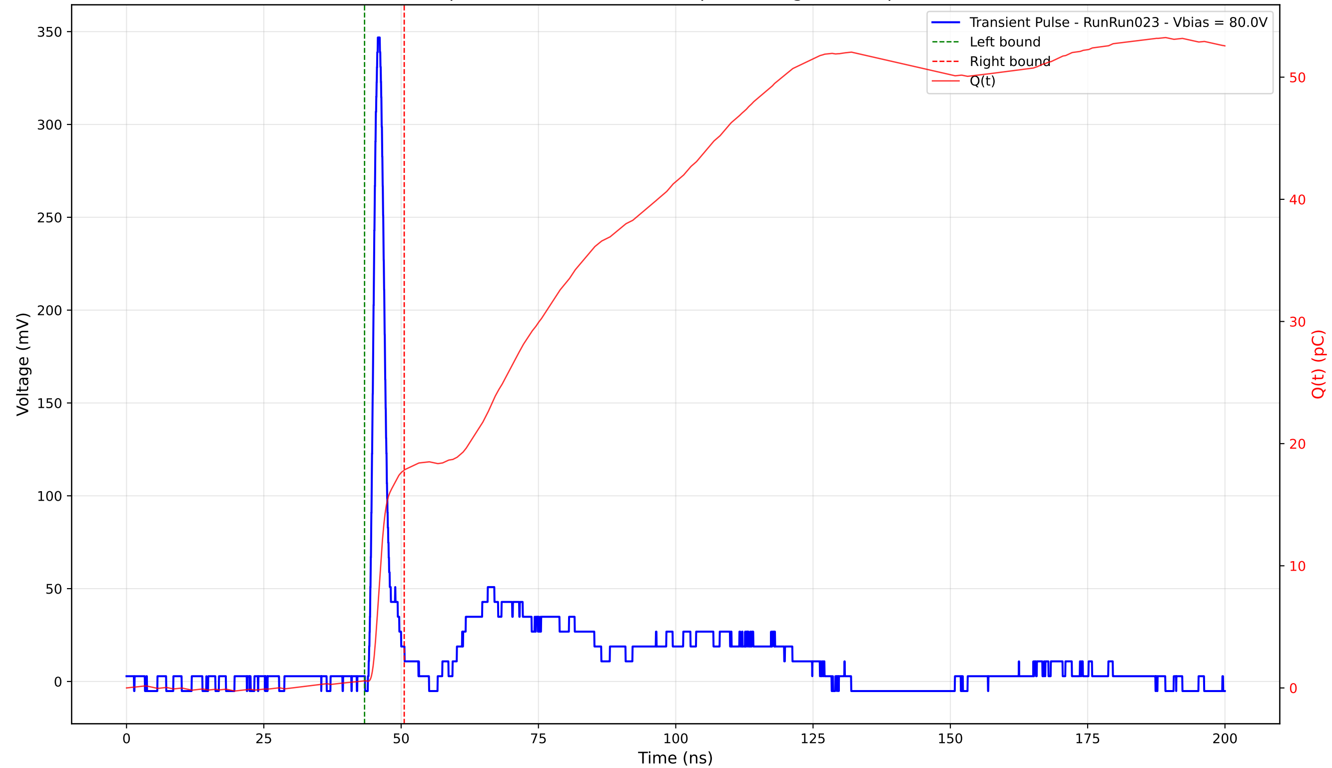
Transient Pulse - Sample: 4003 - Position: 180.0 \mu\text{m} - Charge: 17.25 pC - Rise Time: 1.16 ns
