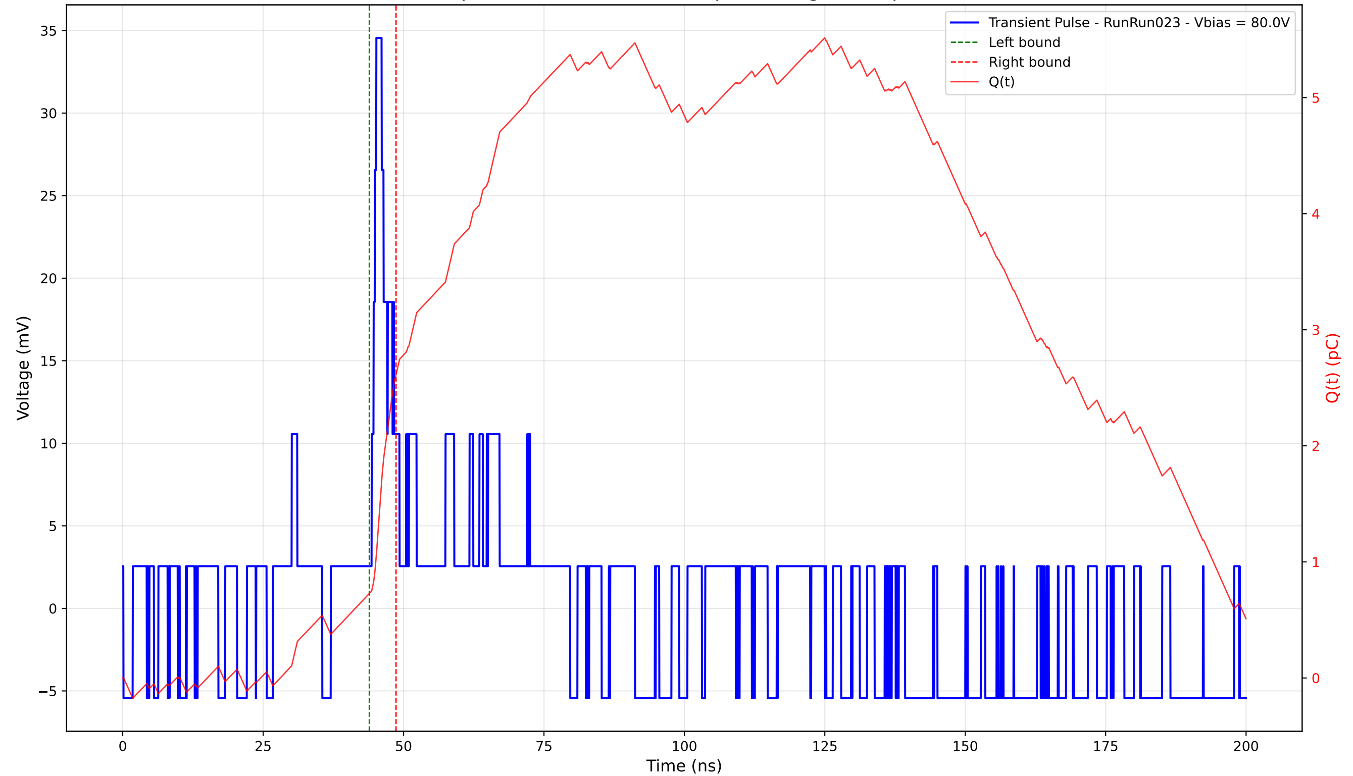
Transient Pulse - Sample: 4003 - Position: 390.0 \mu\text{m} - Charge: 1.89 pC - Rise Time: 0.84 ns
