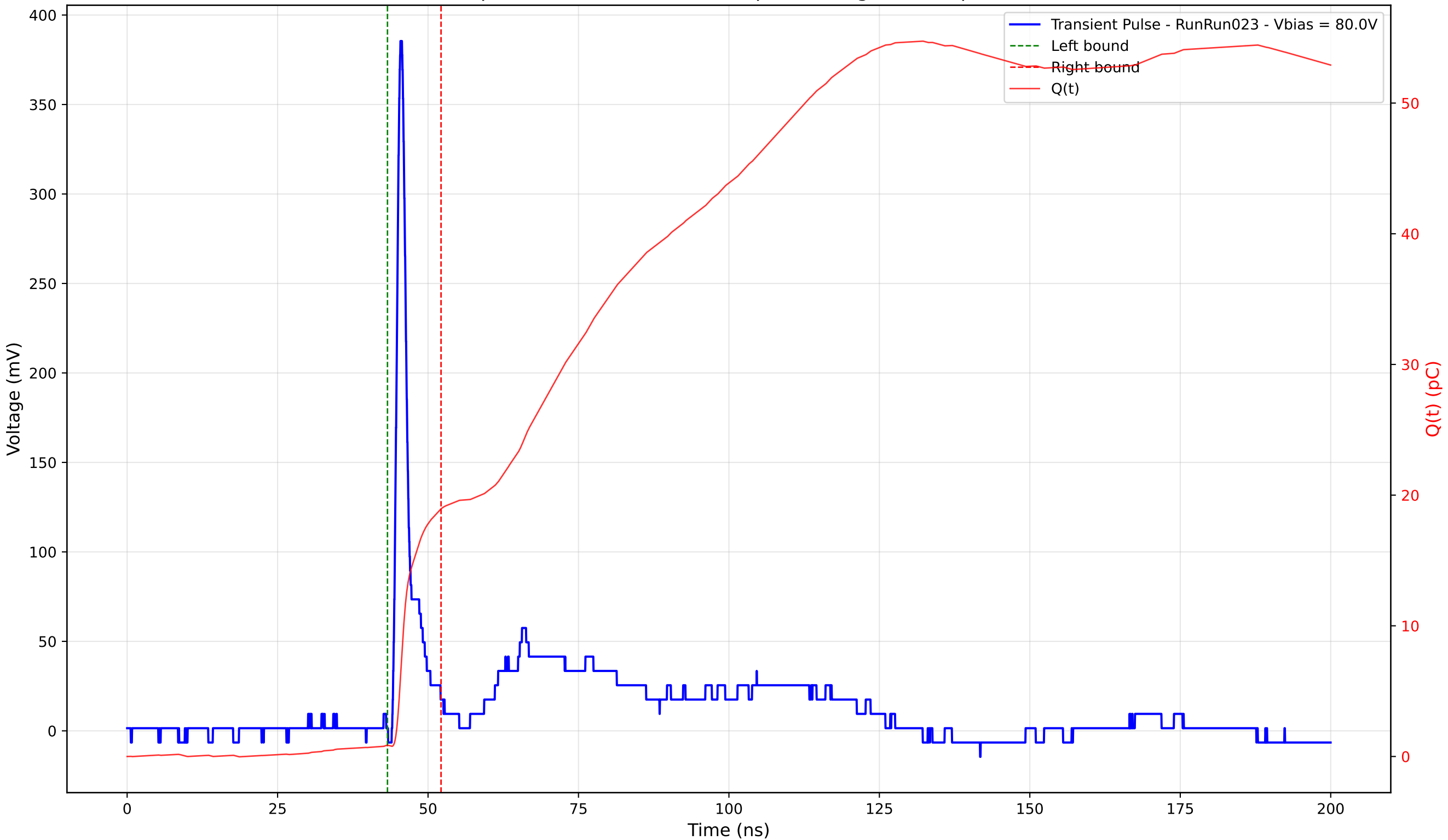
Transient Pulse - Sample: 4003 - Position: 135.0 \mu\text{m} - Charge: 18.10 pC - Rise Time: 0.97 ns
