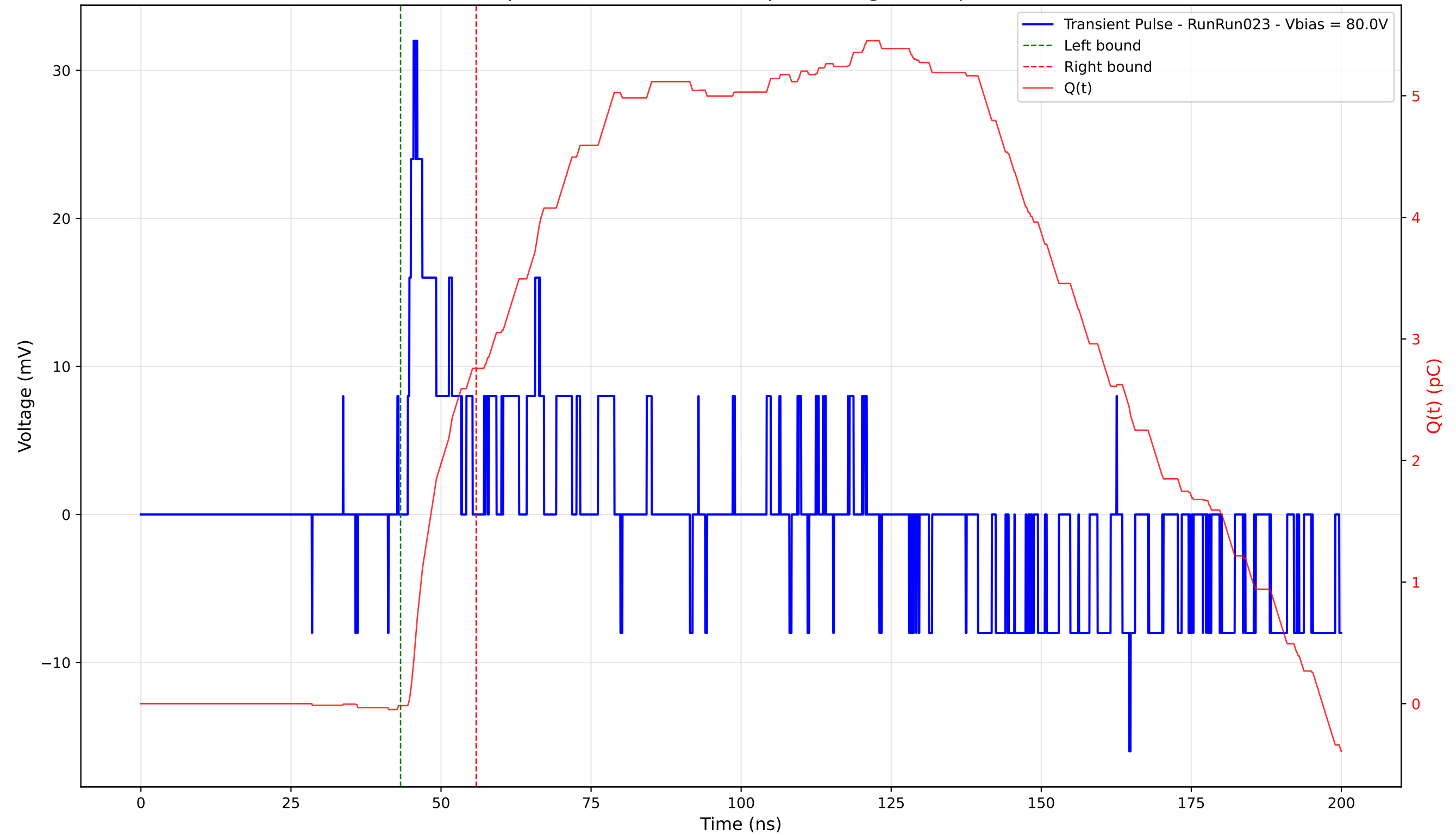
Transient Pulse - Sample: 4003 - Position: 55.0 \mu\text{m} - Charge: 2.77 pC - Rise Time: 0.97 ns
