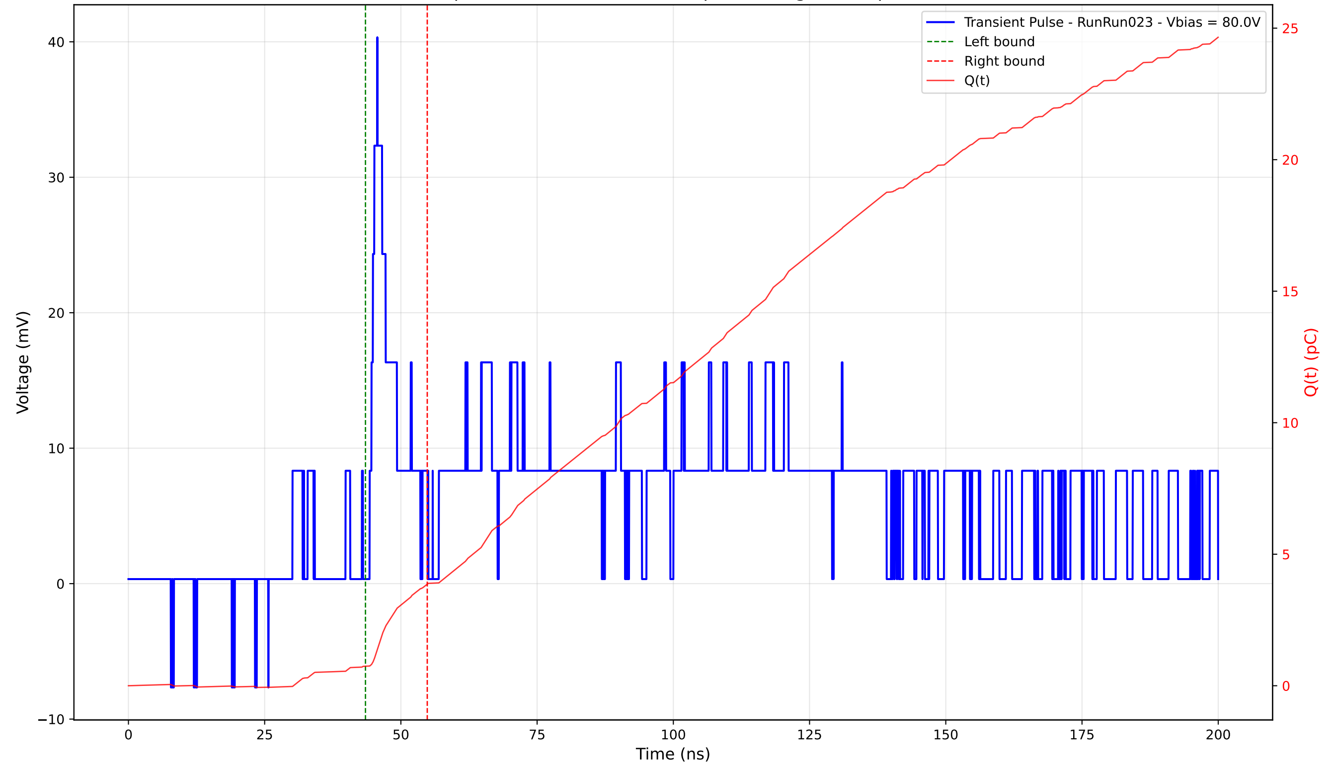
Transient Pulse - Sample: 4003 - Position: 260.0 \mu\text{m} - Charge: 3.12 pC - Rise Time: 1.41 ns
