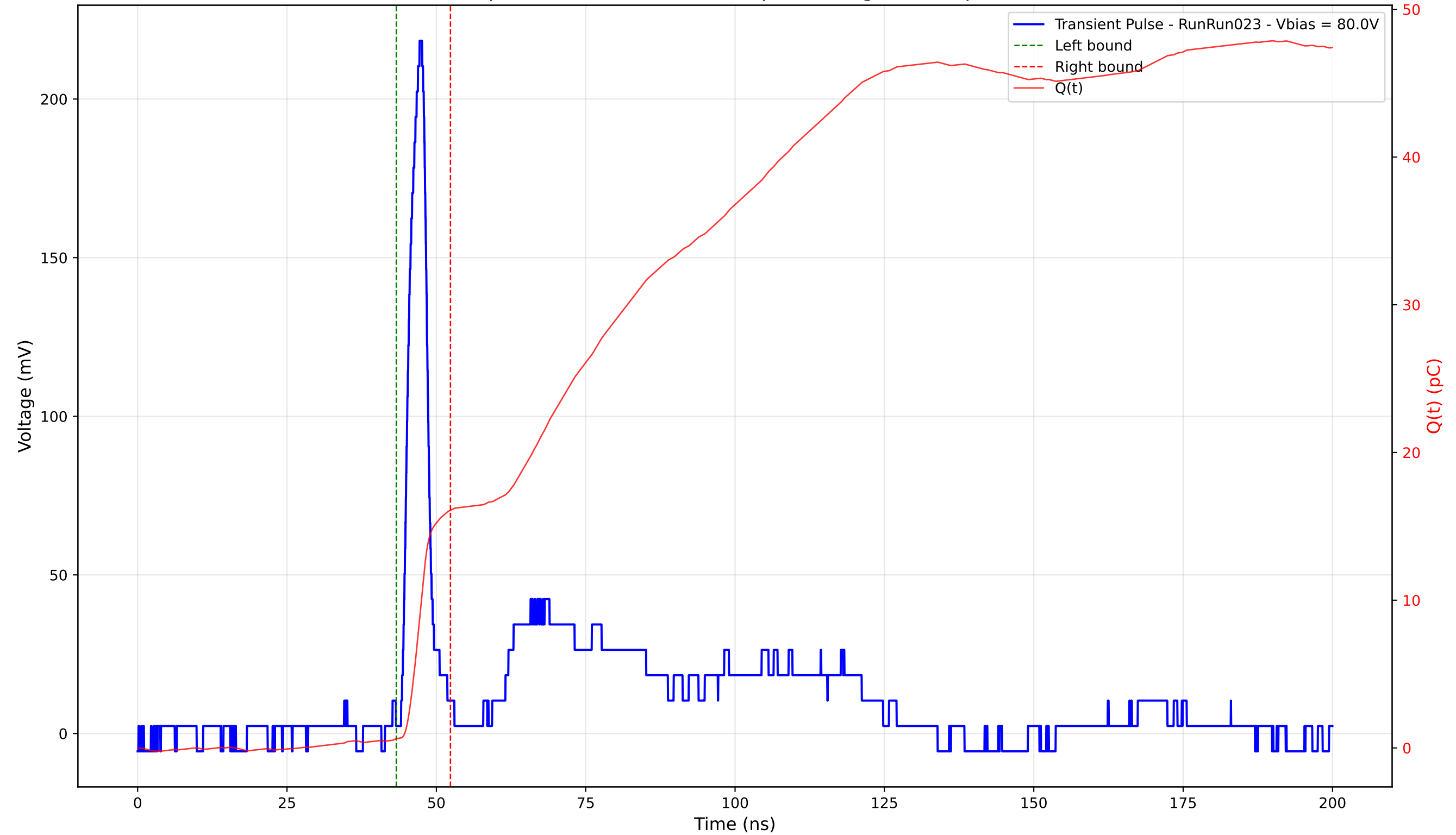
Transient Pulse - Sample: 4003 - Position: 220.0 \mu\text{m} - Charge: 15.46 pC - Rise Time: 2.31 ns
