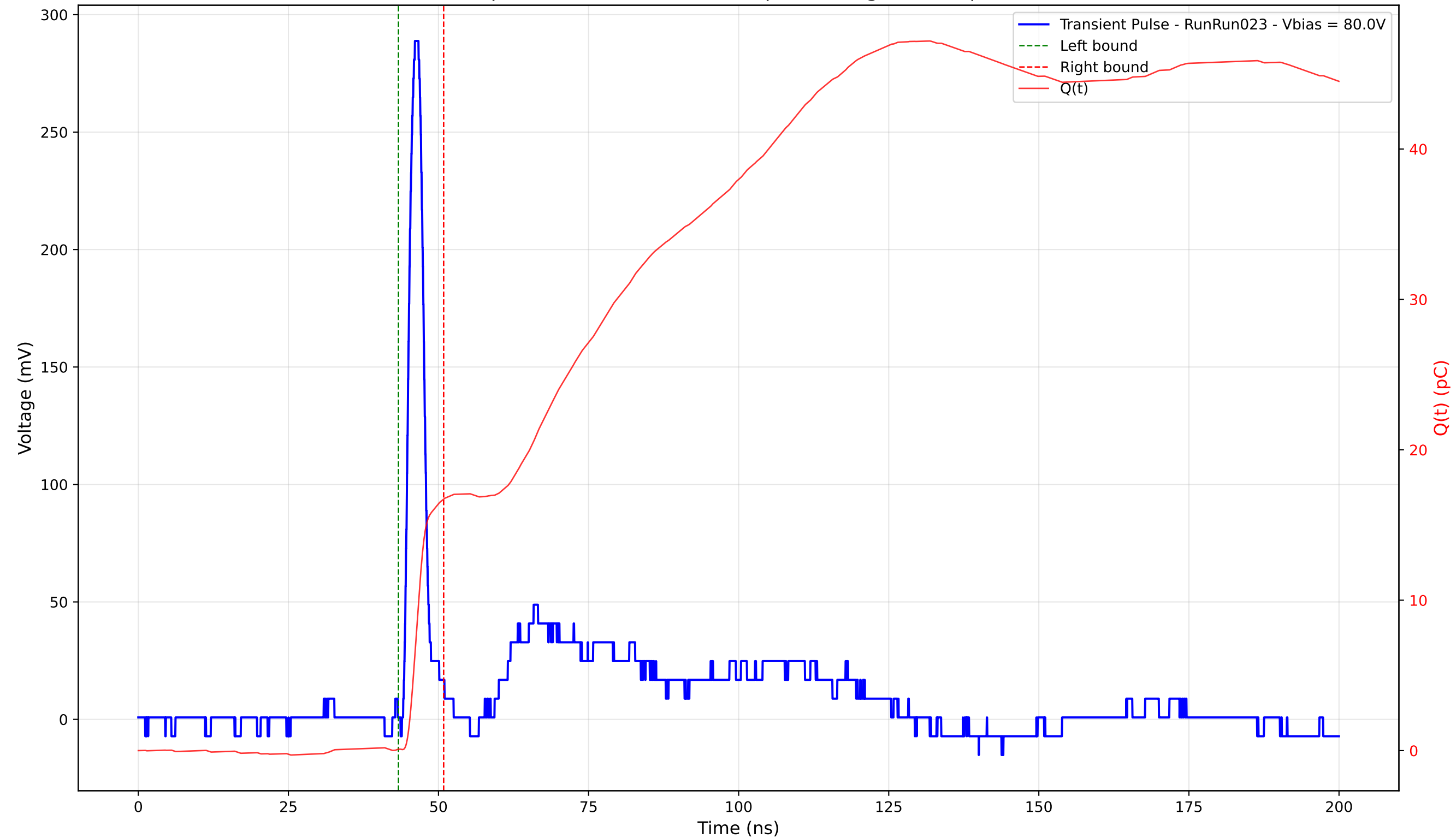
Transient Pulse - Sample: 4003 - Position: 200.0 \mu\text{m} - Charge: 16.63 pC - Rise Time: 1.35 ns
