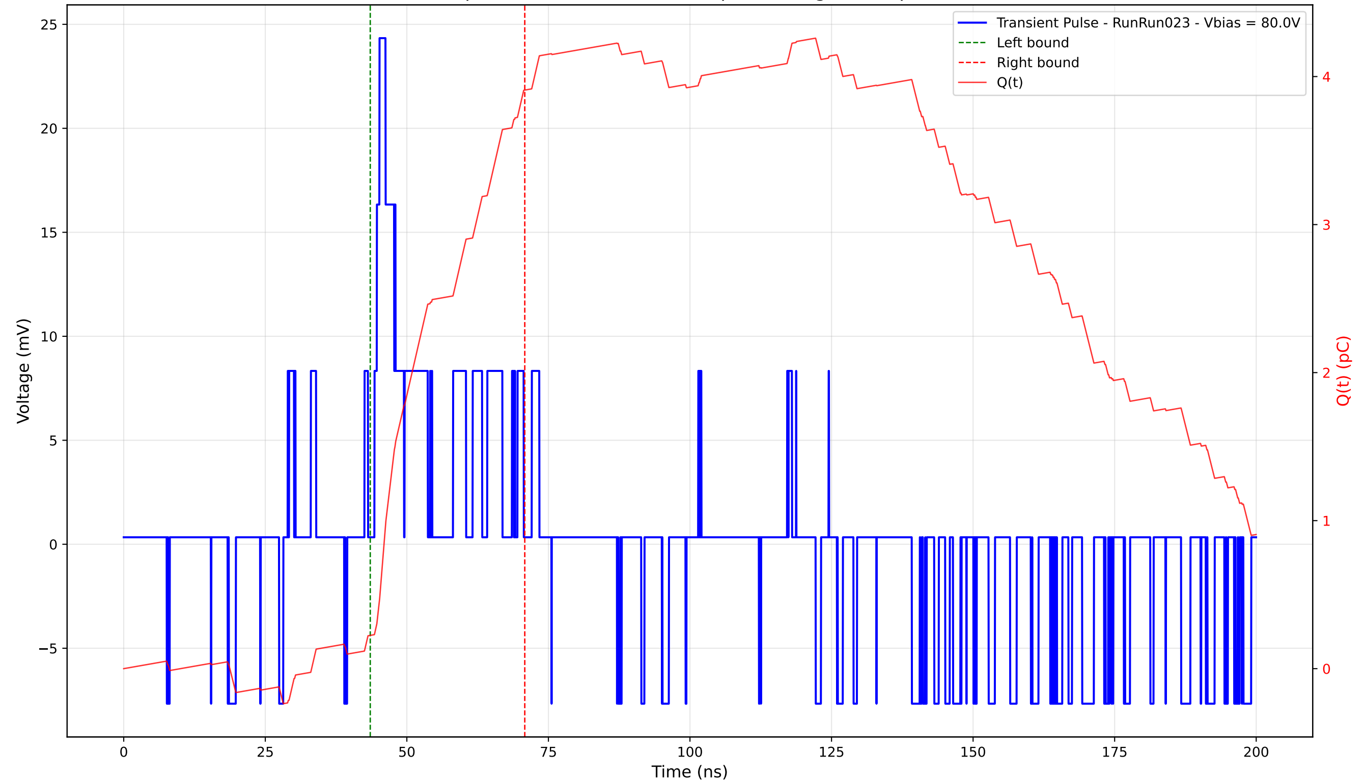
Transient Pulse - Sample: 4003 - Position: 375.0 \mu\text{m} - Charge: 3.68 pC - Rise Time: 0.89 ns
