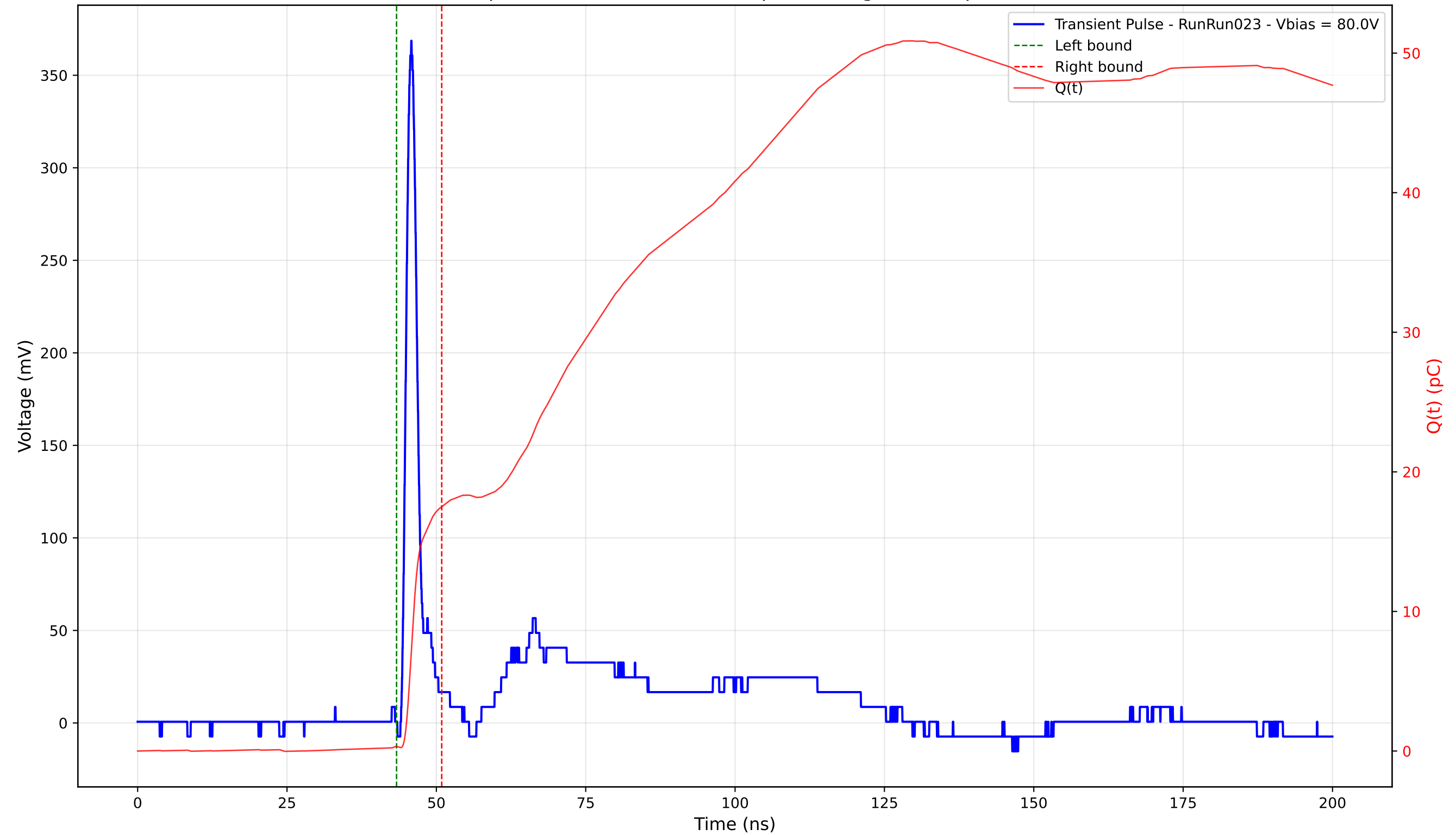
Transient Pulse - Sample: 4003 - Position: 170.0 \mu\text{m} - Charge: 17.19 pC - Rise Time: 1.11 ns
