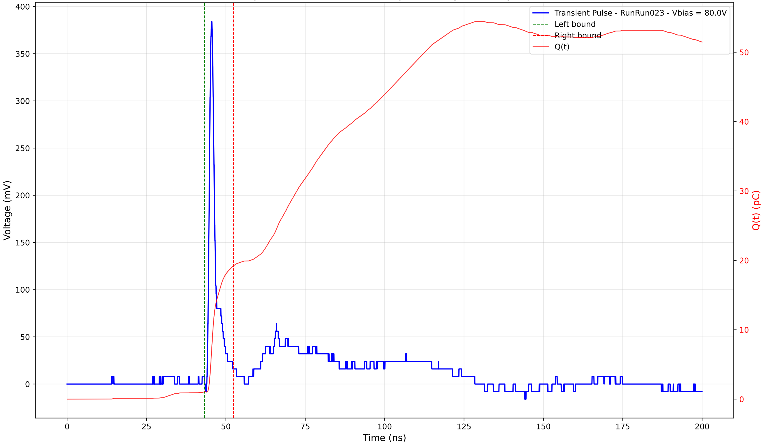
Transient Pulse - Sample: 4003 - Position: 130.0 \mu\text{m} - Charge: 18.14 pC - Rise Time: 0.96 ns
