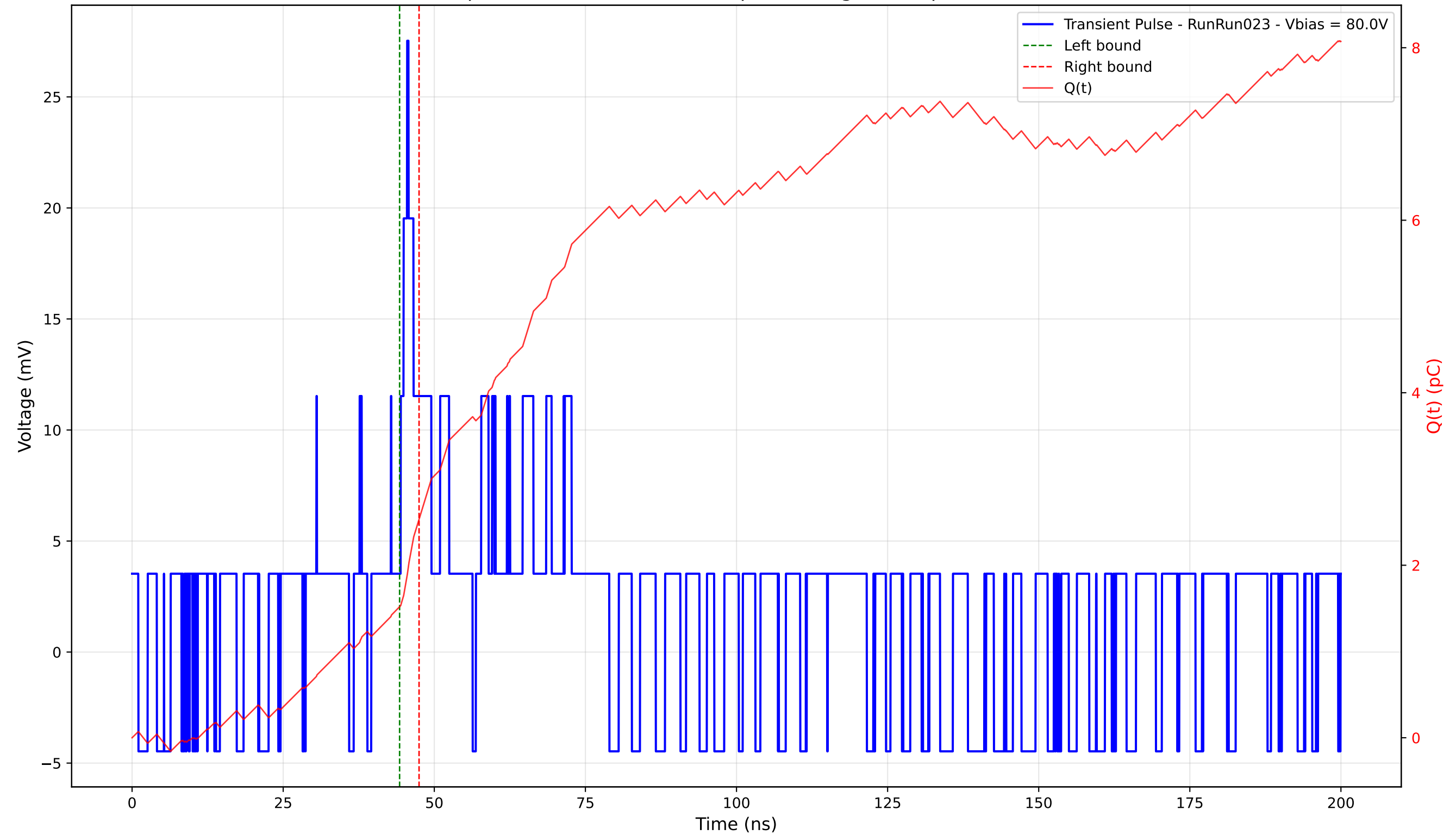
Transient Pulse - Sample: 4003 - Position: 345.0 \mu\text{m} - Charge: 1.02 pC - Rise Time: 0.00 ns (N/A)
