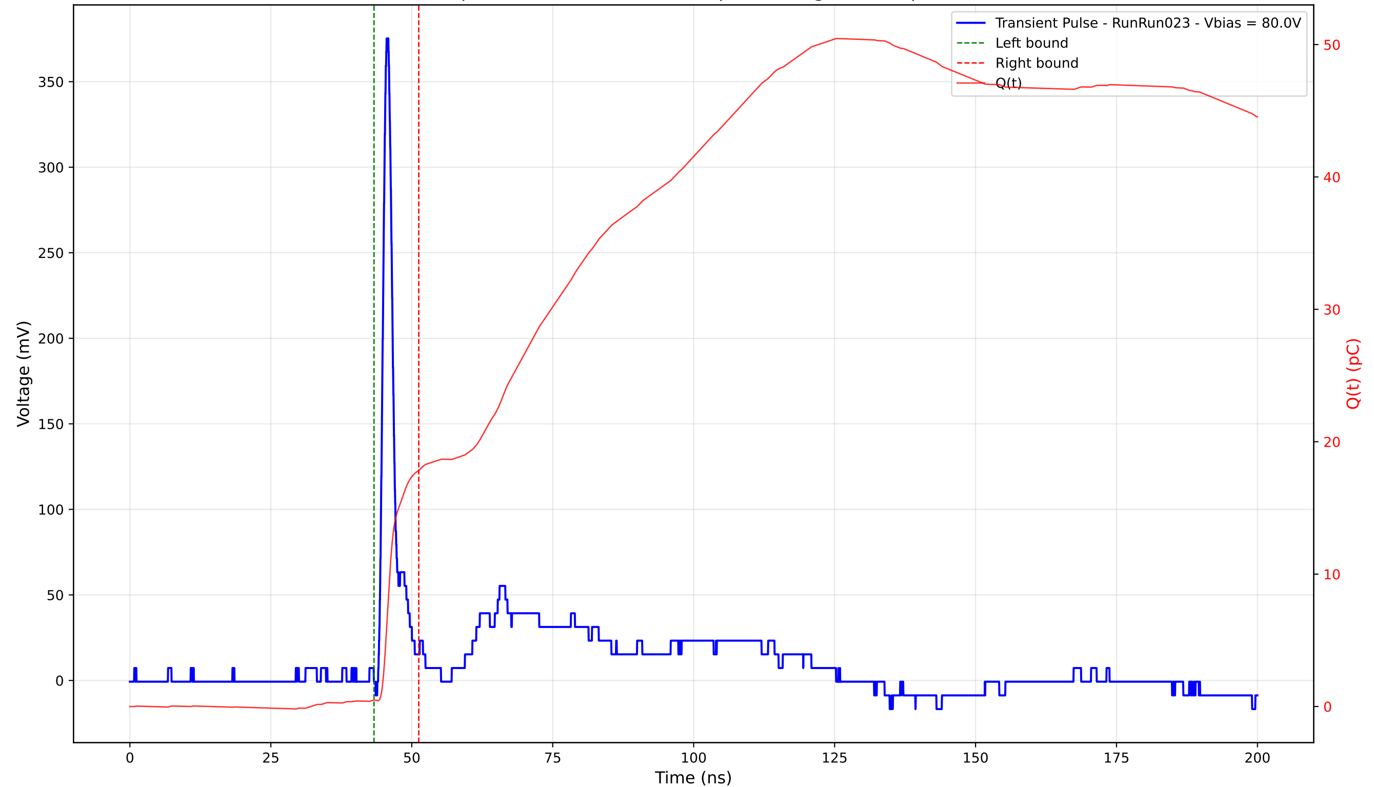
Transient Pulse - Sample: 4003 - Position: 155.0 \mu\text{m} - Charge: 17.33 pC - Rise Time: 1.02 ns
