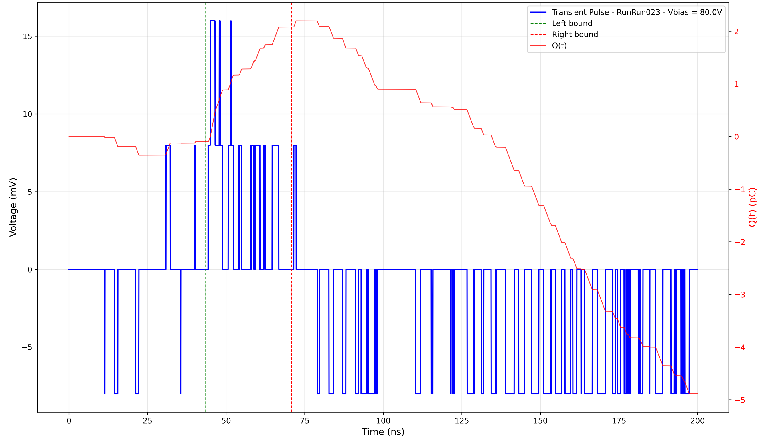
Transient Pulse - Sample: 4003 - Position: 20.0 \mu\text{m} - Charge: 2.18 pC - Rise Time: 0.60 ns
