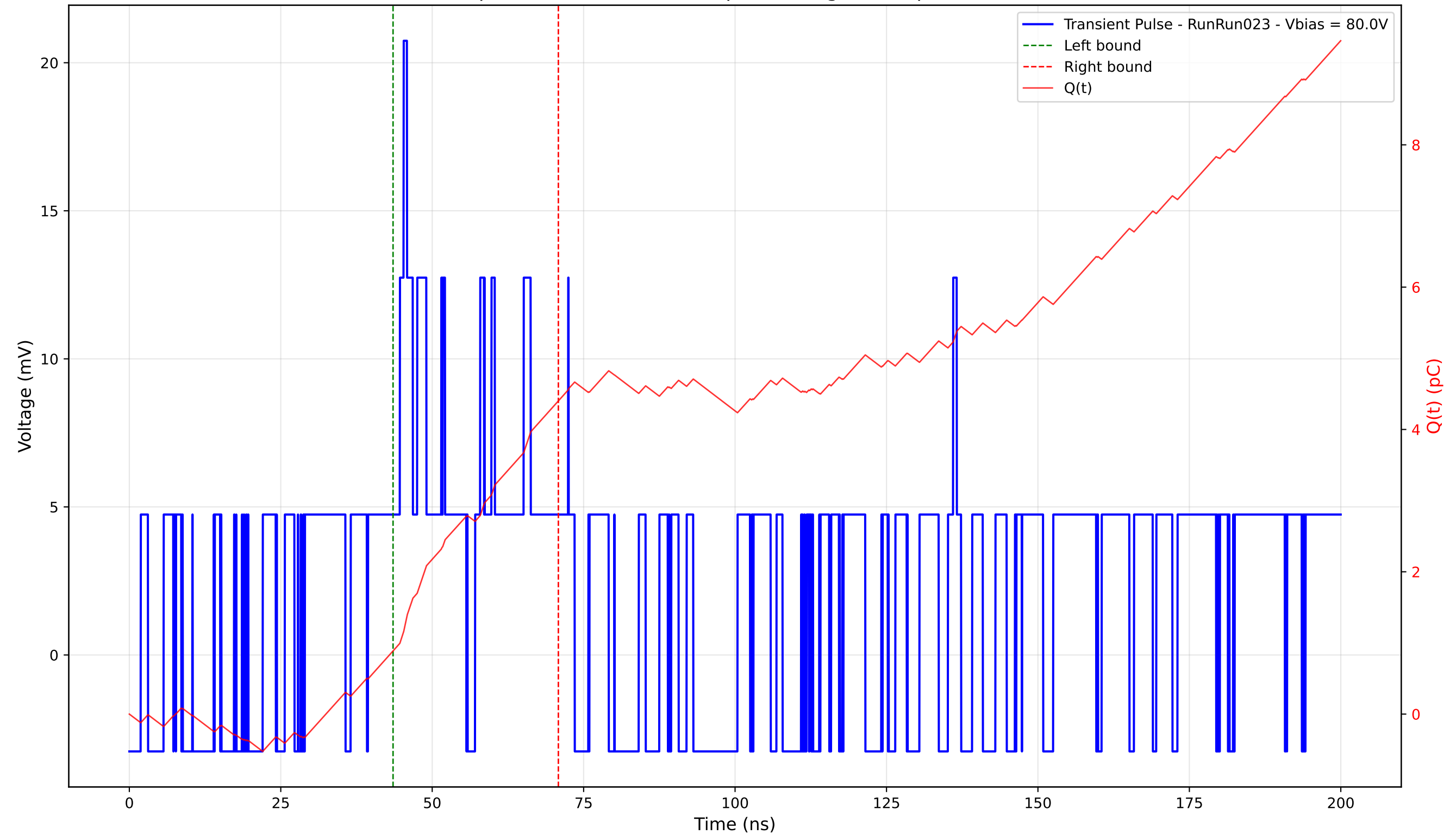
Transient Pulse - Sample: 4003 - Position: 5.0 \mu\text{m} - Charge: 3.51 pC - Rise Time: 0.00 ns (N/A)
