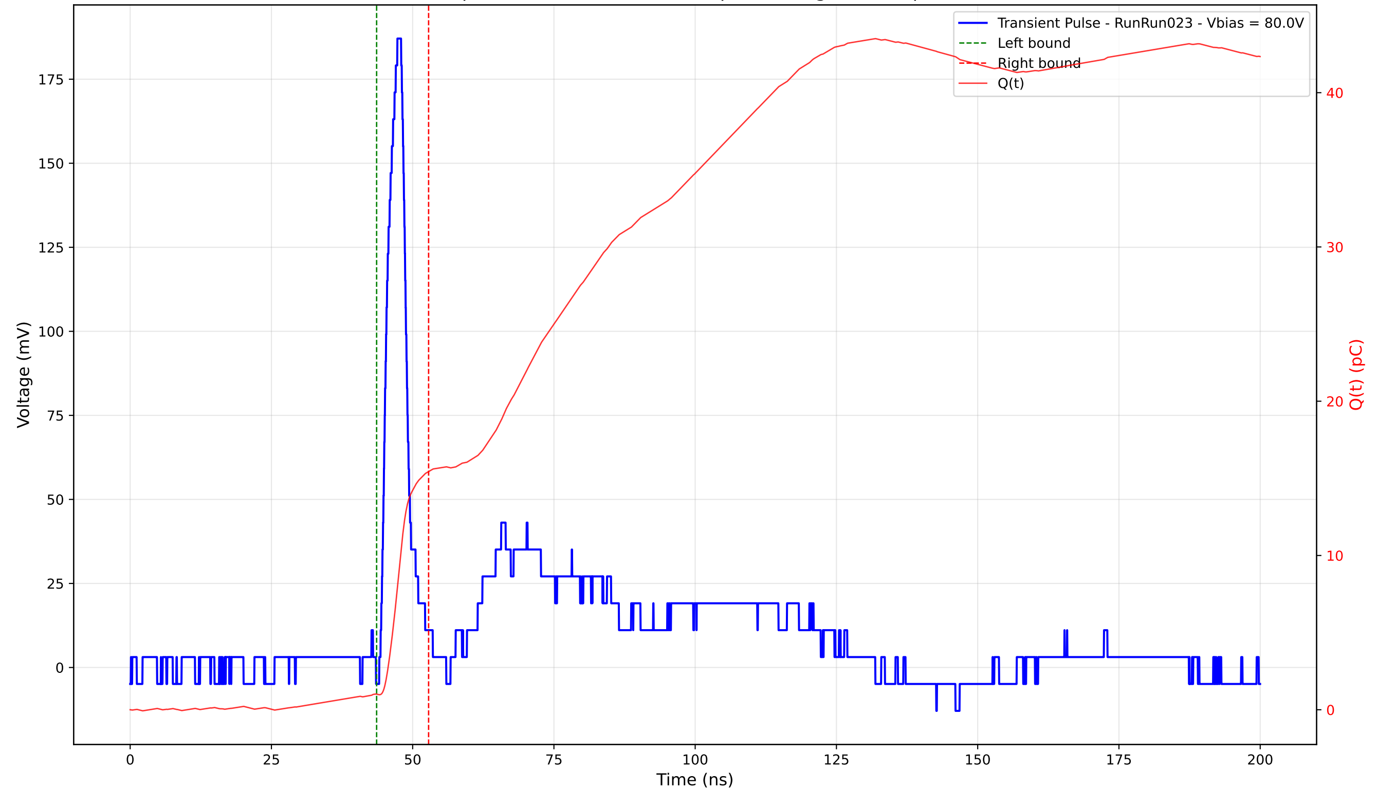
Transient Pulse - Sample: 4003 - Position: 225.0 \mu\text{m} - Charge: 14.43 pC - Rise Time: 2.34 ns
