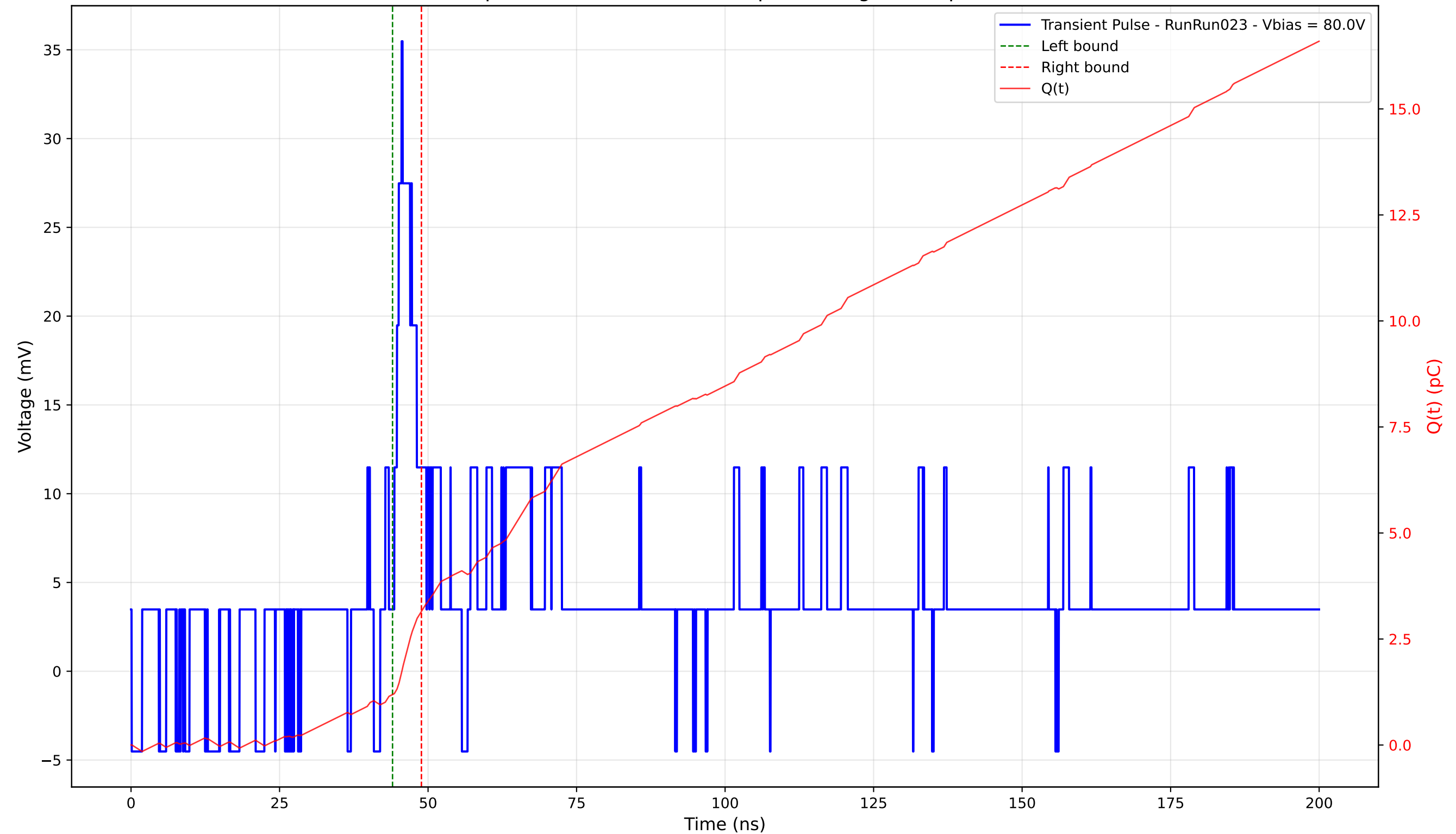
Transient Pulse - Sample: 4003 - Position: 300.0 \mu\text{m} - Charge: 1.96 pC - Rise Time: 1.24 ns
