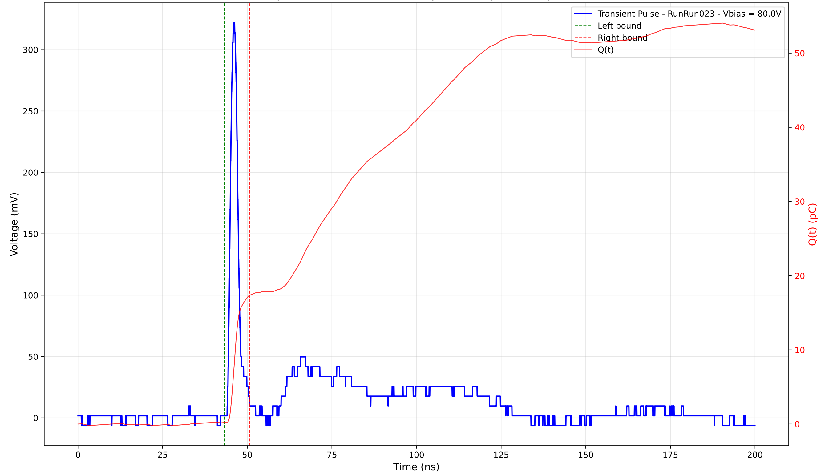
Transient Pulse - Sample: 4003 - Position: 190.0 \mu\text{m} - Charge: 17.18 pC - Rise Time: 1.24 ns
