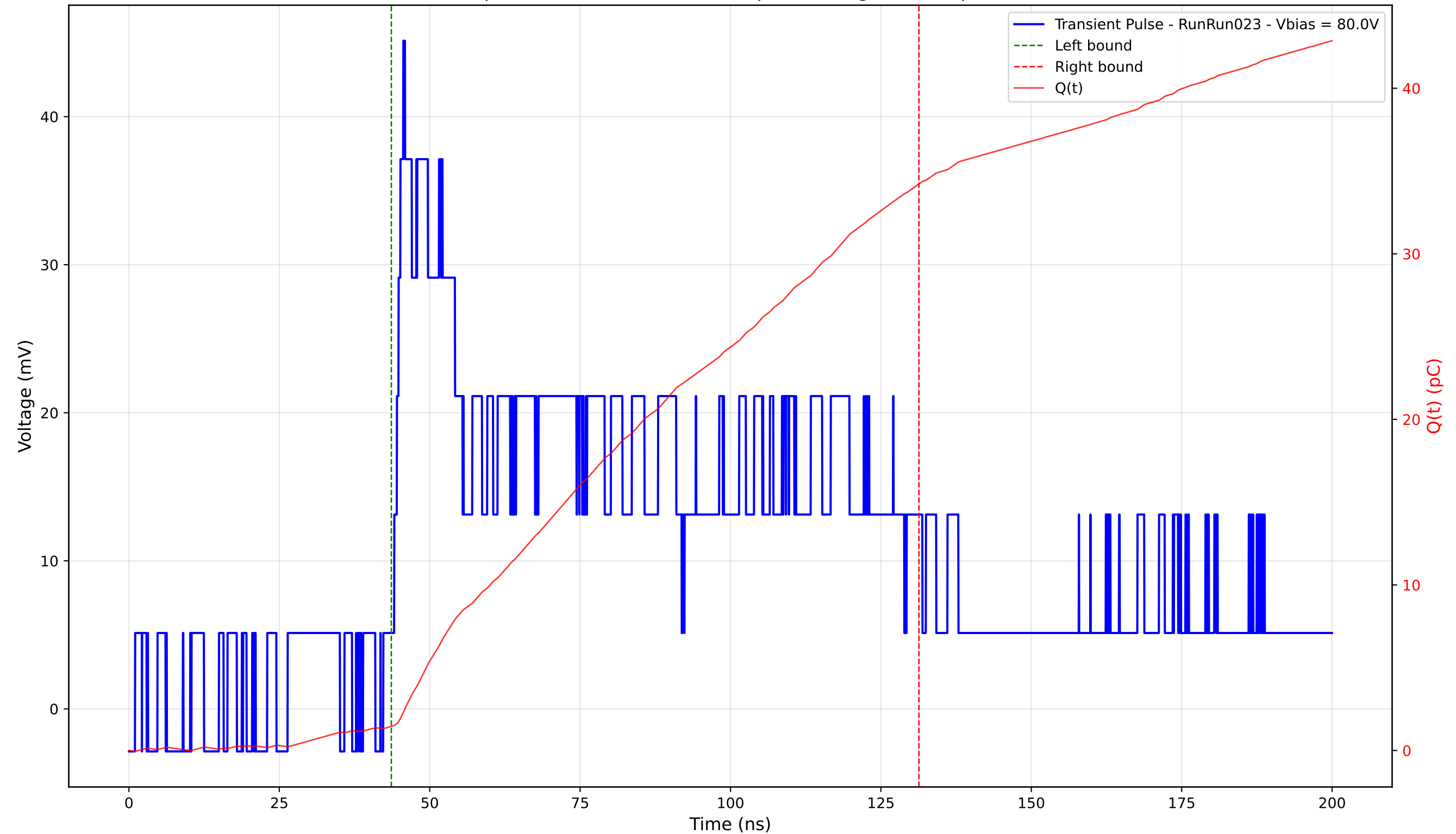
Transient Pulse - Sample: 4003 - Position: 245.0 \mu\text{m} - Charge: 32.77 pC - Rise Time: 3.33 ns
