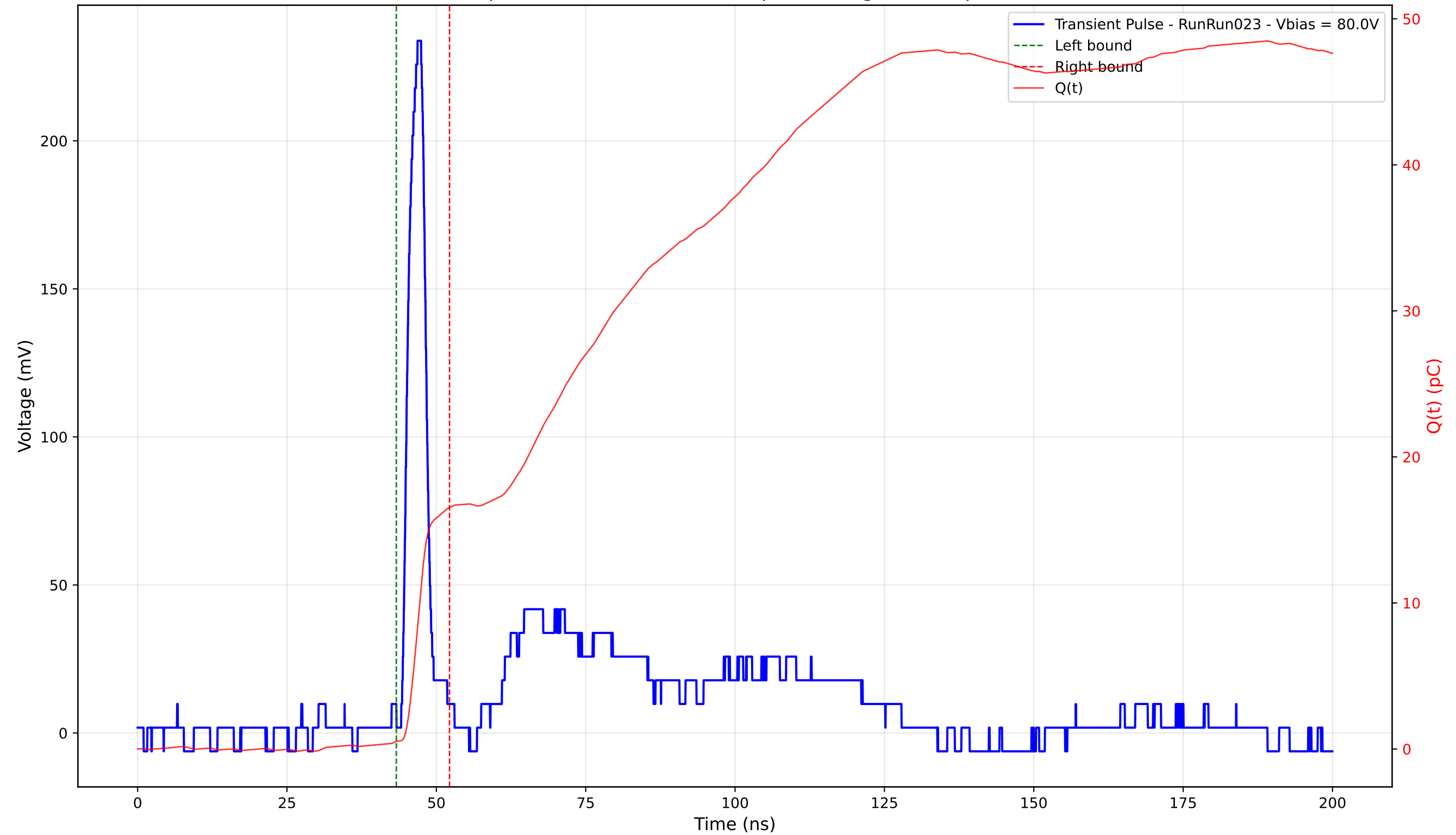
Transient Pulse - Sample: 4003 - Position: 215.0 \mu\text{m} - Charge: 16.00 pC - Rise Time: 2.01 ns
