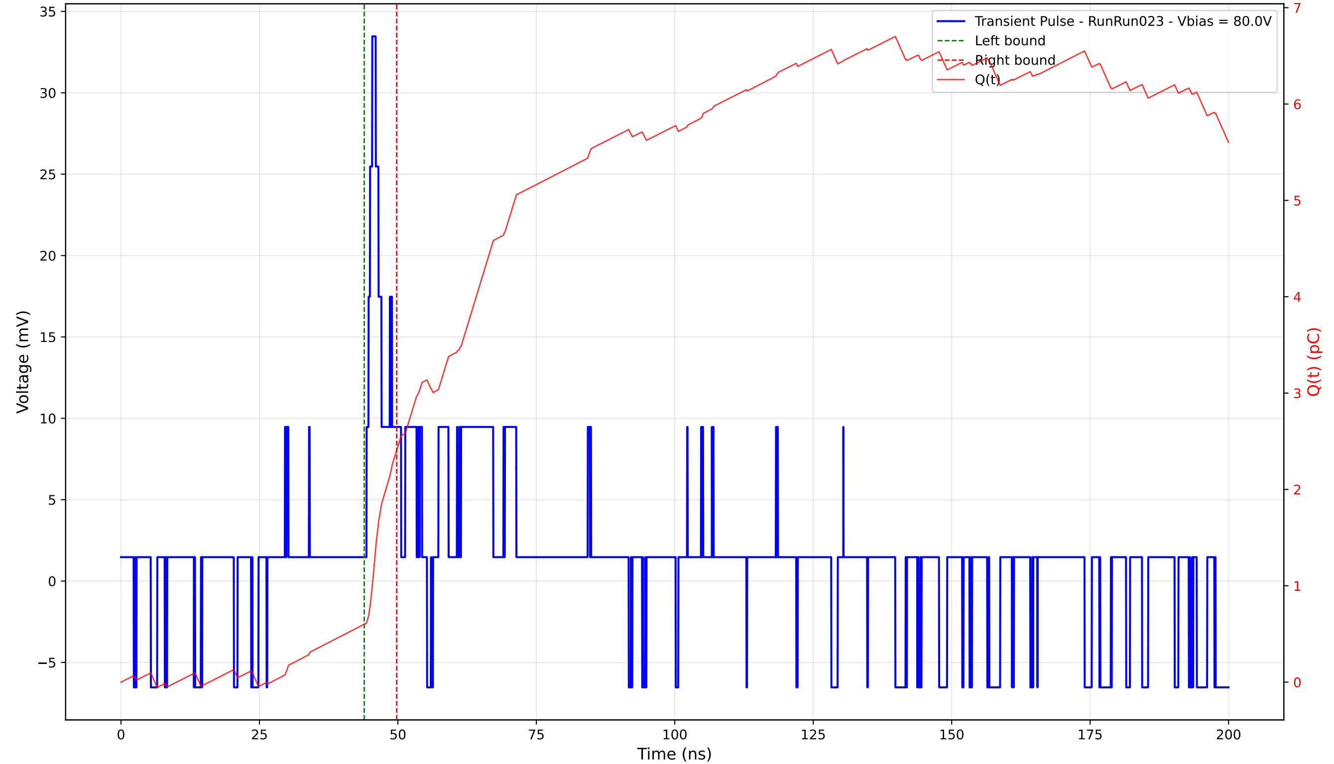
Transient Pulse - Sample: 4003 - Position: 405.0 \mu\text{m} - Charge: 1.81 pC - Rise Time: 1.04 ns
