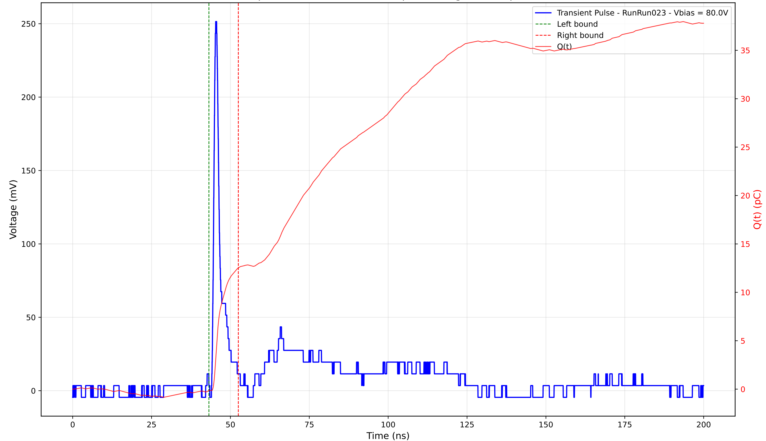
Transient Pulse - Sample: 4003 - Position: 110.0 \mu\text{m} - Charge: 12.65 pC - Rise Time: 0.89 ns
