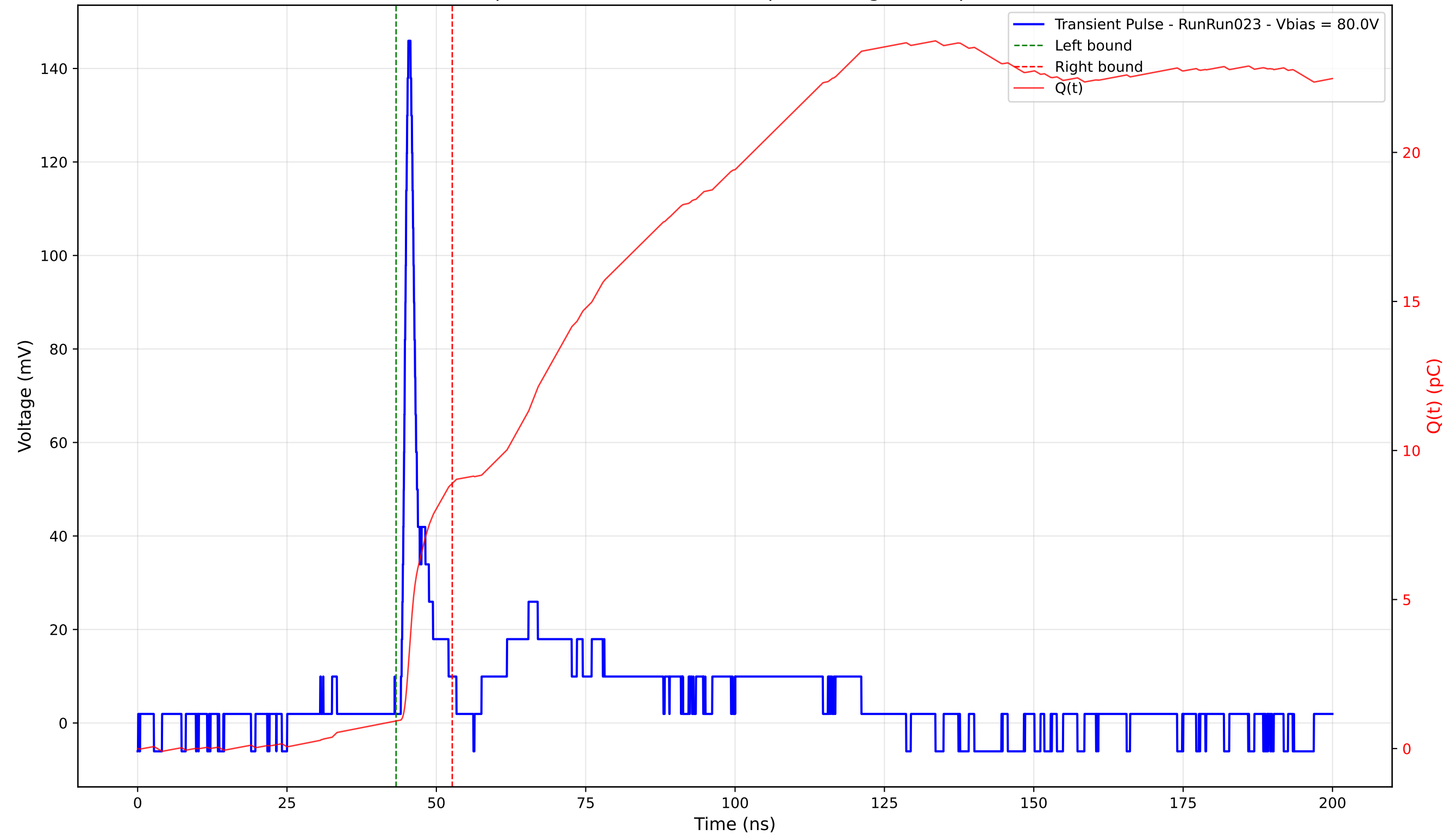
Transient Pulse - Sample: 4003 - Position: 100.0 \mu\text{m} - Charge: 7.97 pC - Rise Time: 0.99 ns
