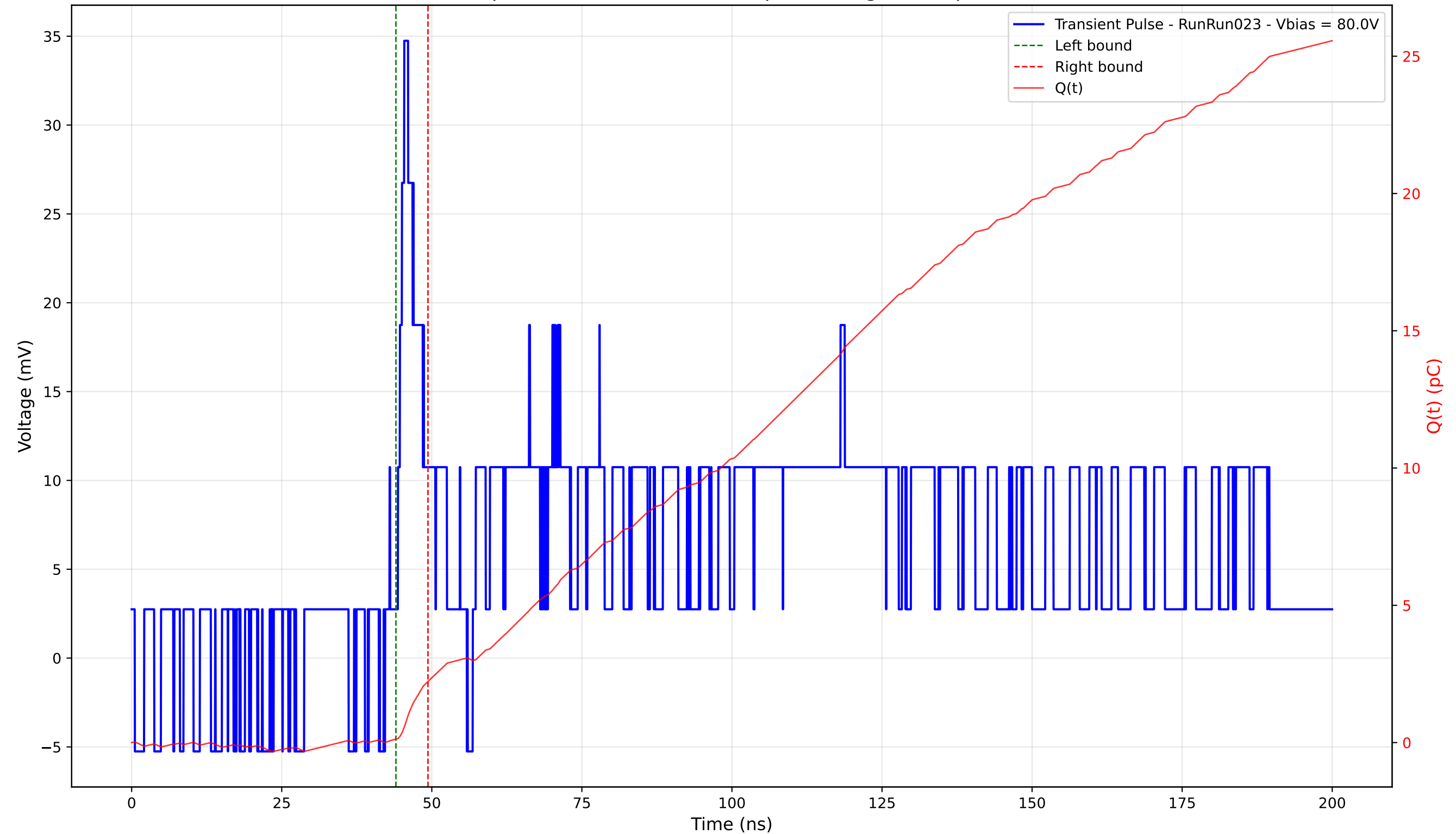
Transient Pulse - Sample: 4003 - Position: 265.0 \mu\text{m} - Charge: 2.11 pC - Rise Time: 1.06 ns
