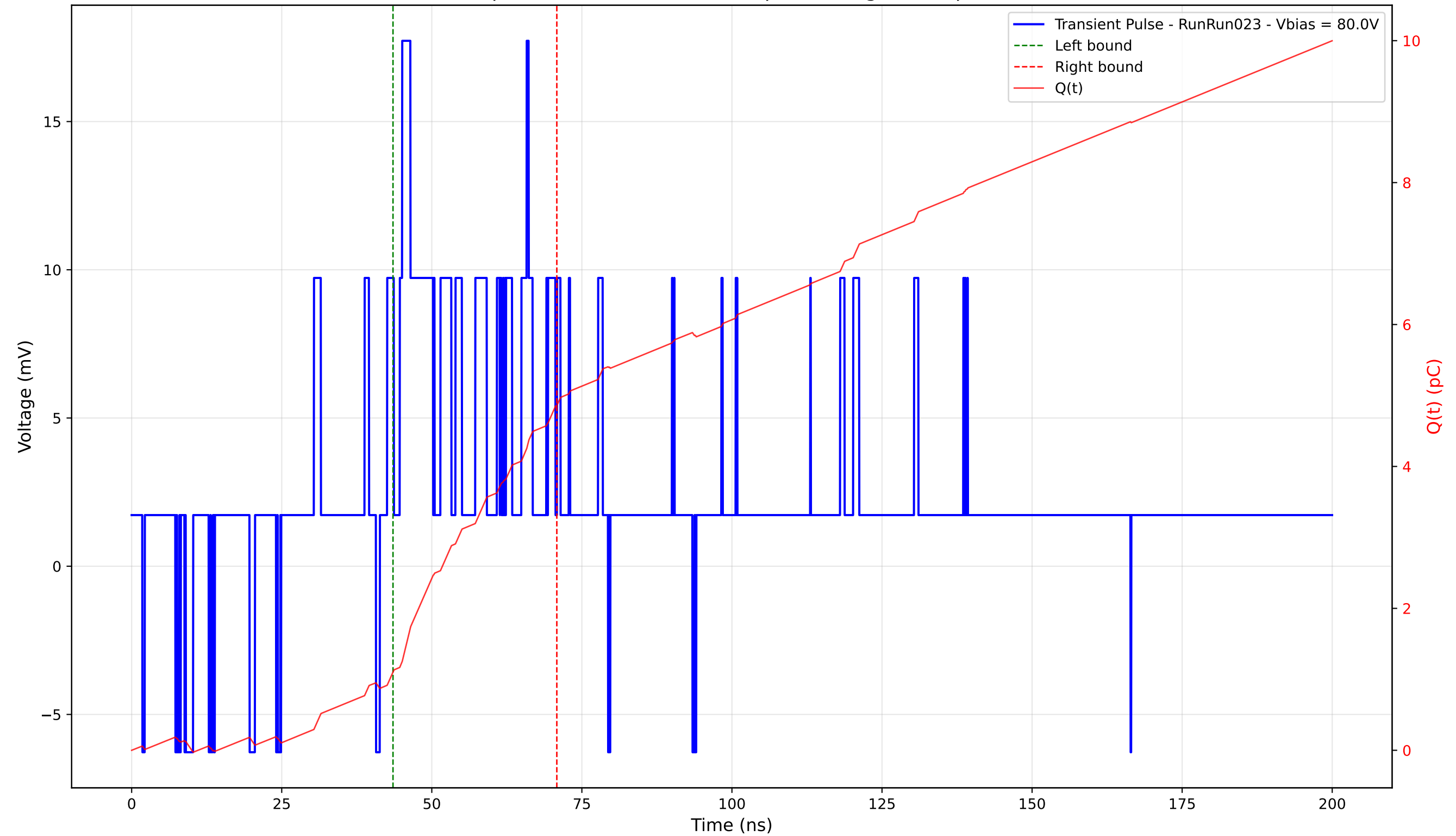
Transient Pulse - Sample: 4003 - Position: 425.0 \mu\text{m} - Charge: 3.75 pC - Rise Time: 0.42 ns
