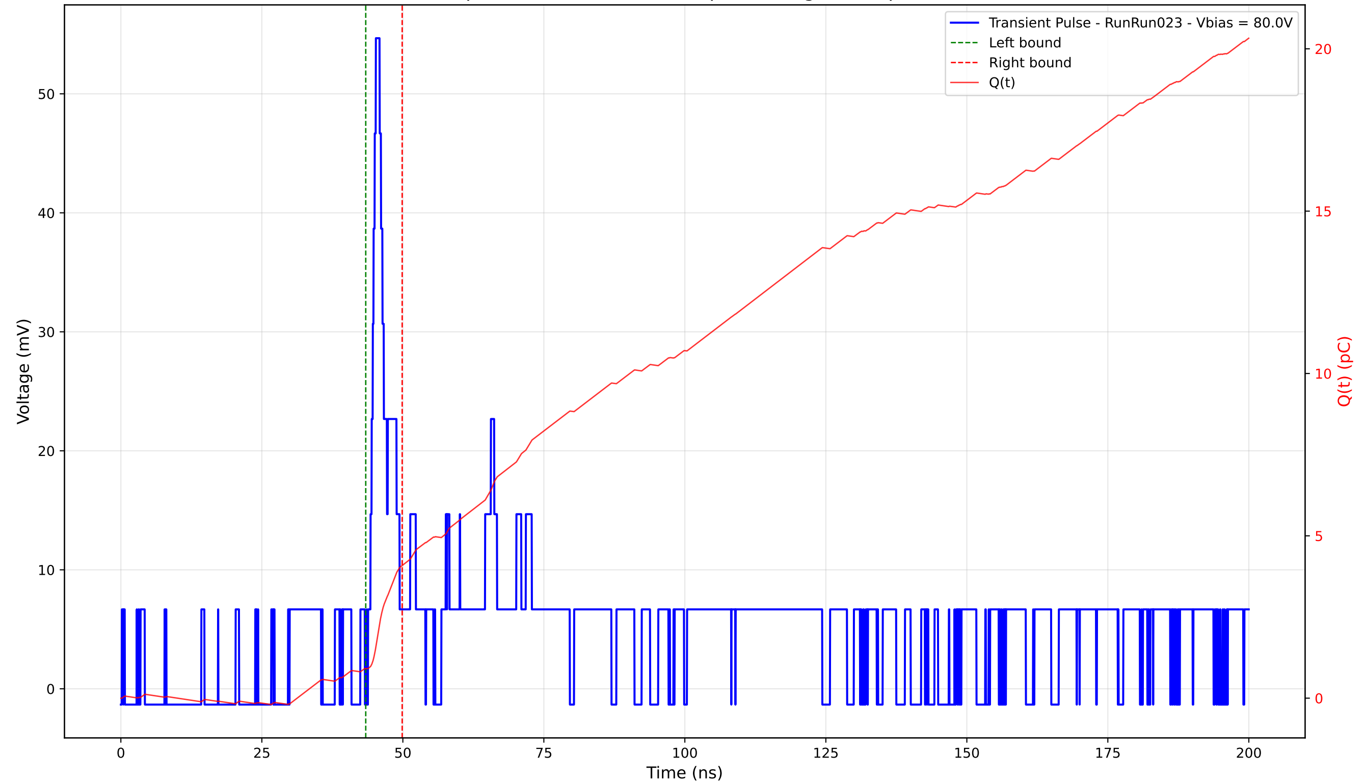
Transient Pulse - Sample: 4003 - Position: 90.0 \mu\text{m} - Charge: 3.17 pC - Rise Time: 1.38 ns
