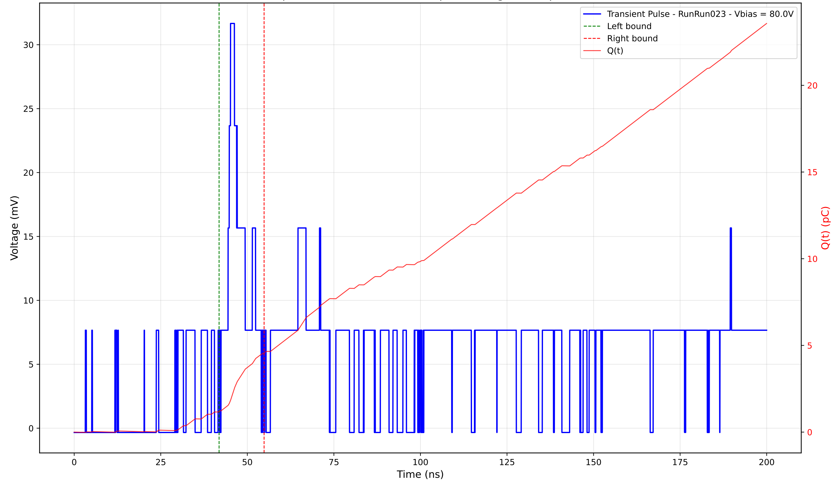
Transient Pulse - Sample: 4003 - Position: 310.0 \mu\text{m} - Charge: 3.38 pC - Rise Time: 2.75 ns
