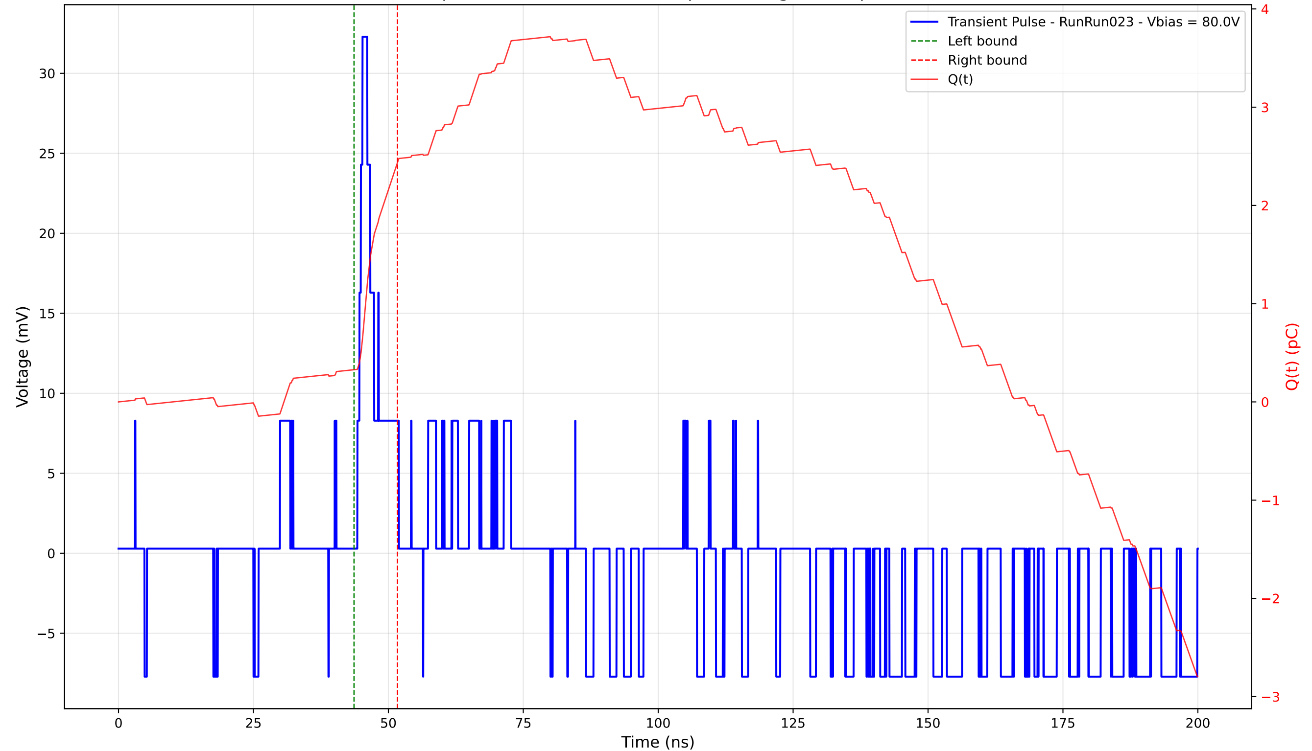
Transient Pulse - Sample: 4003 - Position: 395.0 \mu\text{m} - Charge: 2.11 pC - Rise Time: 0.95 ns
