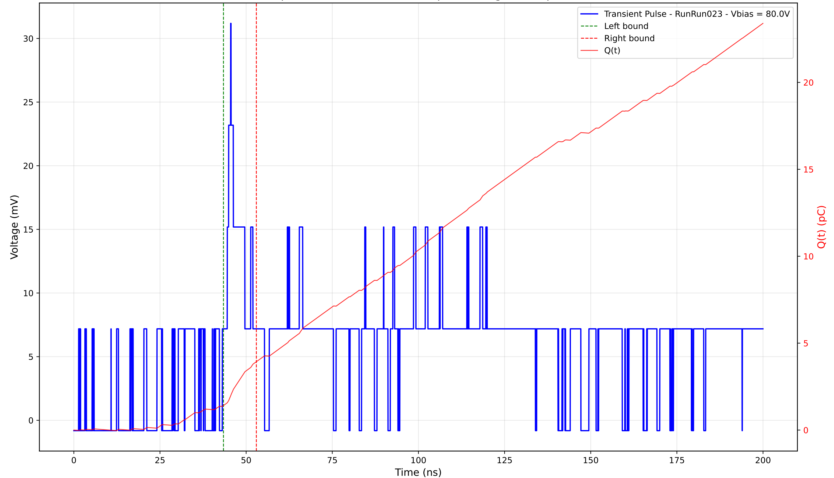
Transient Pulse - Sample: 4003 - Position: 350.0 \mu\text{m} - Charge: 2.53 pC - Rise Time: 2.43 ns
