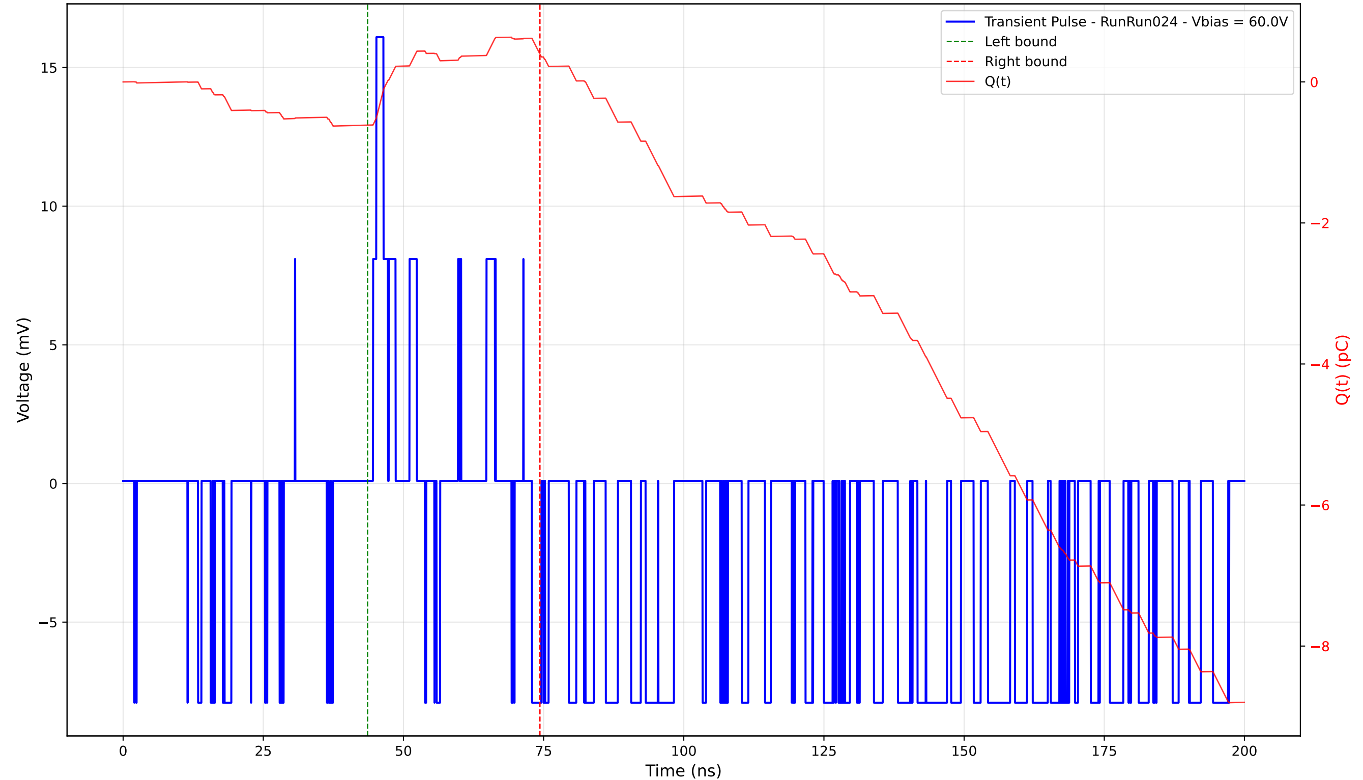
Transient Pulse - Sample: 4003 - Position: 415.0 \mu\text{m} - Charge: 1.01 pC - Rise Time: 0.60 ns
