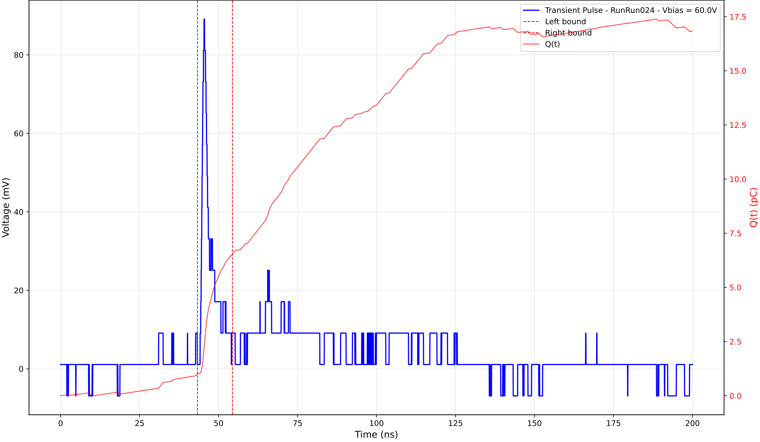
Transient Pulse - Sample: 4003 - Position: 95.0 \mu\text{m} - Charge: 5.53 pC - Rise Time: 1.06 ns
