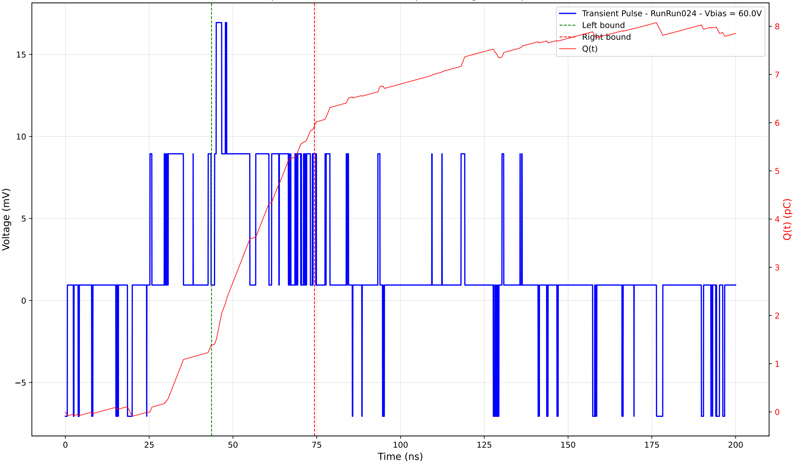
Transient Pulse - Sample: 4003 - Position: 70.0 \mu\text{m} - Charge: 4.55 pC - Rise Time: 0.50 ns
