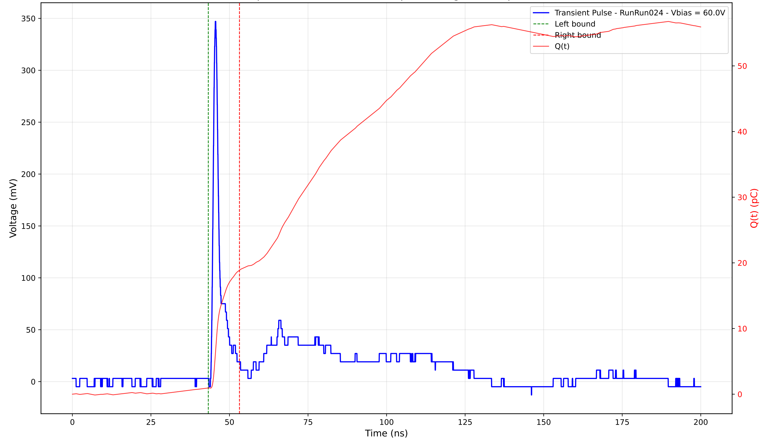
Transient Pulse - Sample: 4003 - Position: 130.0 \mu\text{m} - Charge: 17.94 pC - Rise Time: 0.98 ns
