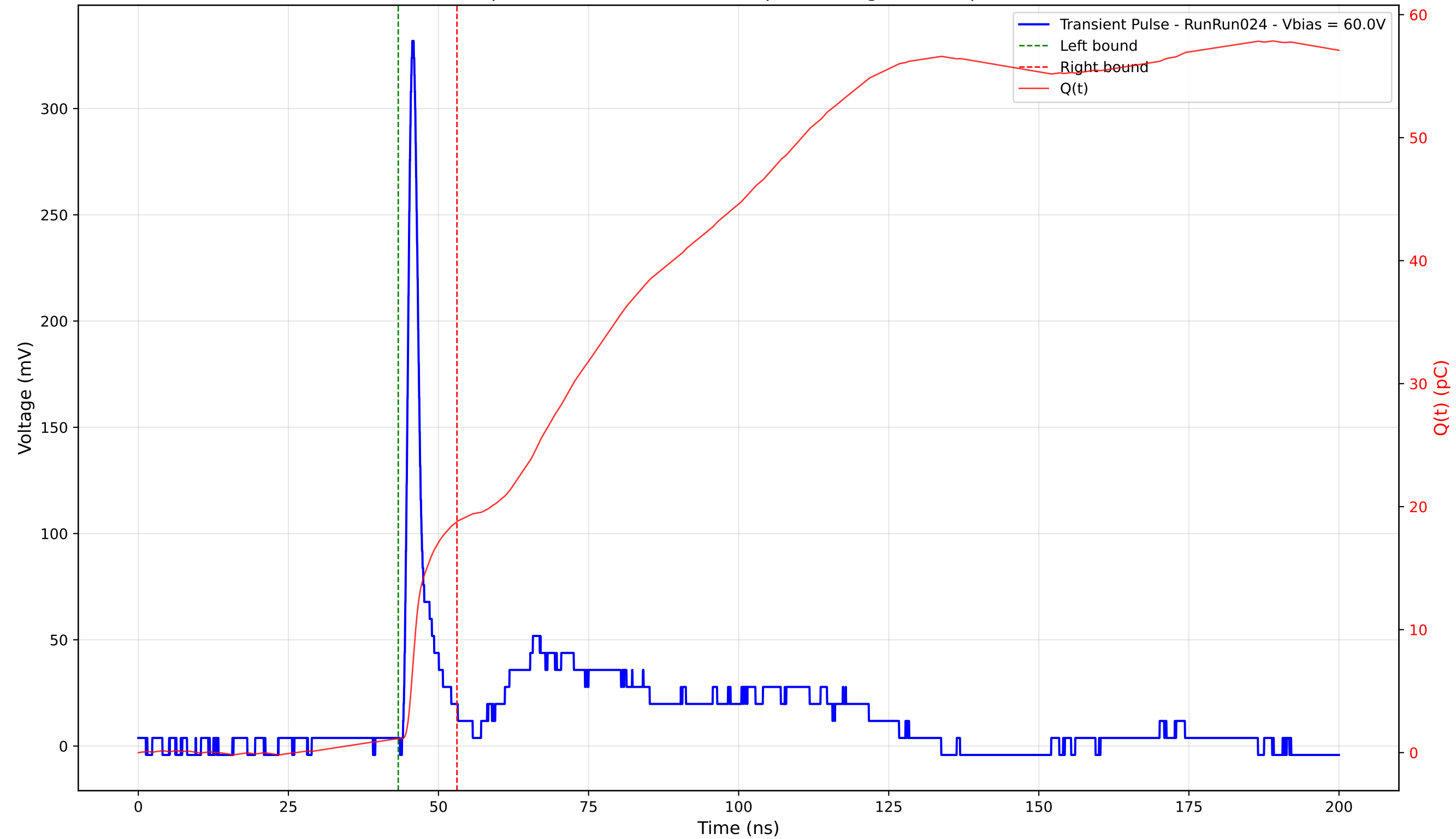
Transient Pulse - Sample: 4003 - Position: 150.0 \mu\text{m} - Charge: 17.63 pC - Rise Time: 1.05 ns
