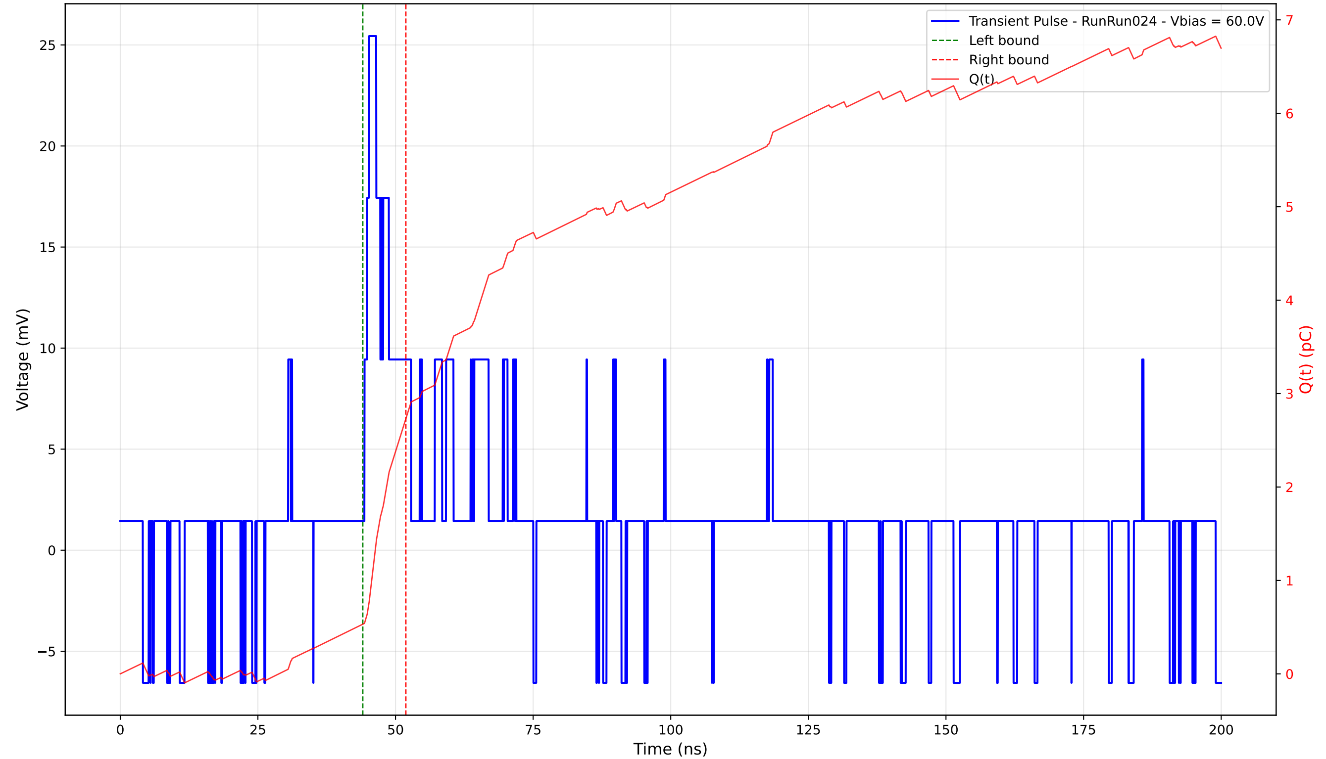
Transient Pulse - Sample: 4003 - Position: 295.0 \mu\text{m} - Charge: 2.20 pC - Rise Time: 0.84 ns
