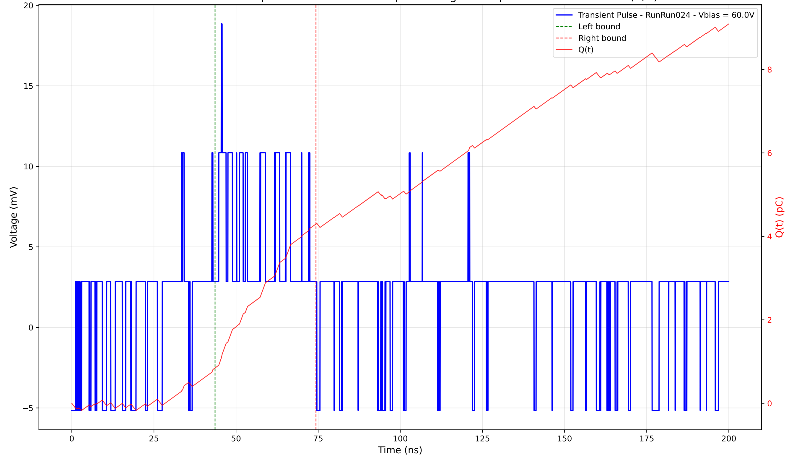
Transient Pulse - Sample: 4003 - Position: 5.0 \mu\text{m} - Charge: 3.45 pC - Rise Time: 0.00 ns (N/A)
