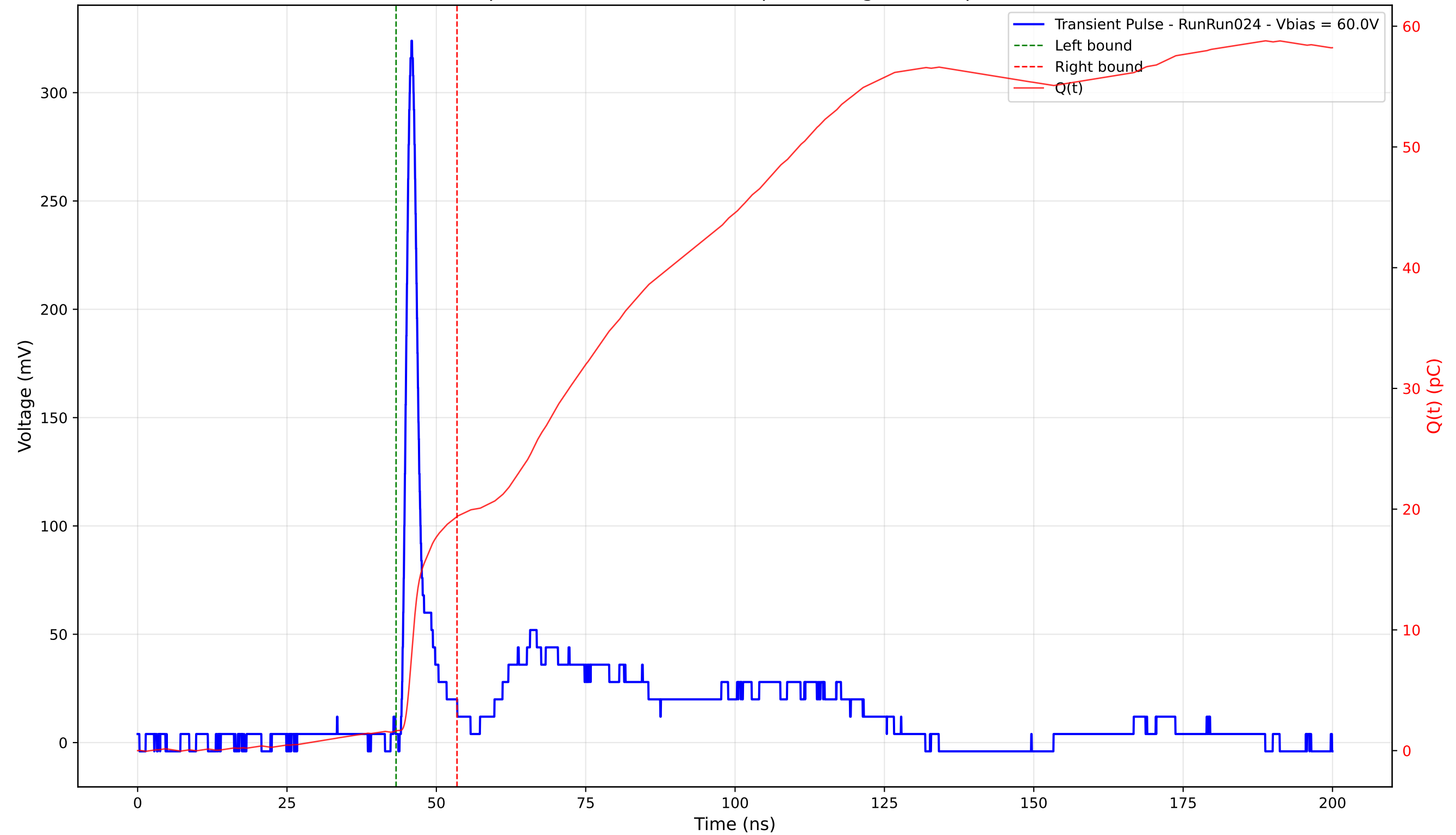
Transient Pulse - Sample: 4003 - Position: 160.0 \mu\text{m} - Charge: 17.75 pC - Rise Time: 1.15 ns
