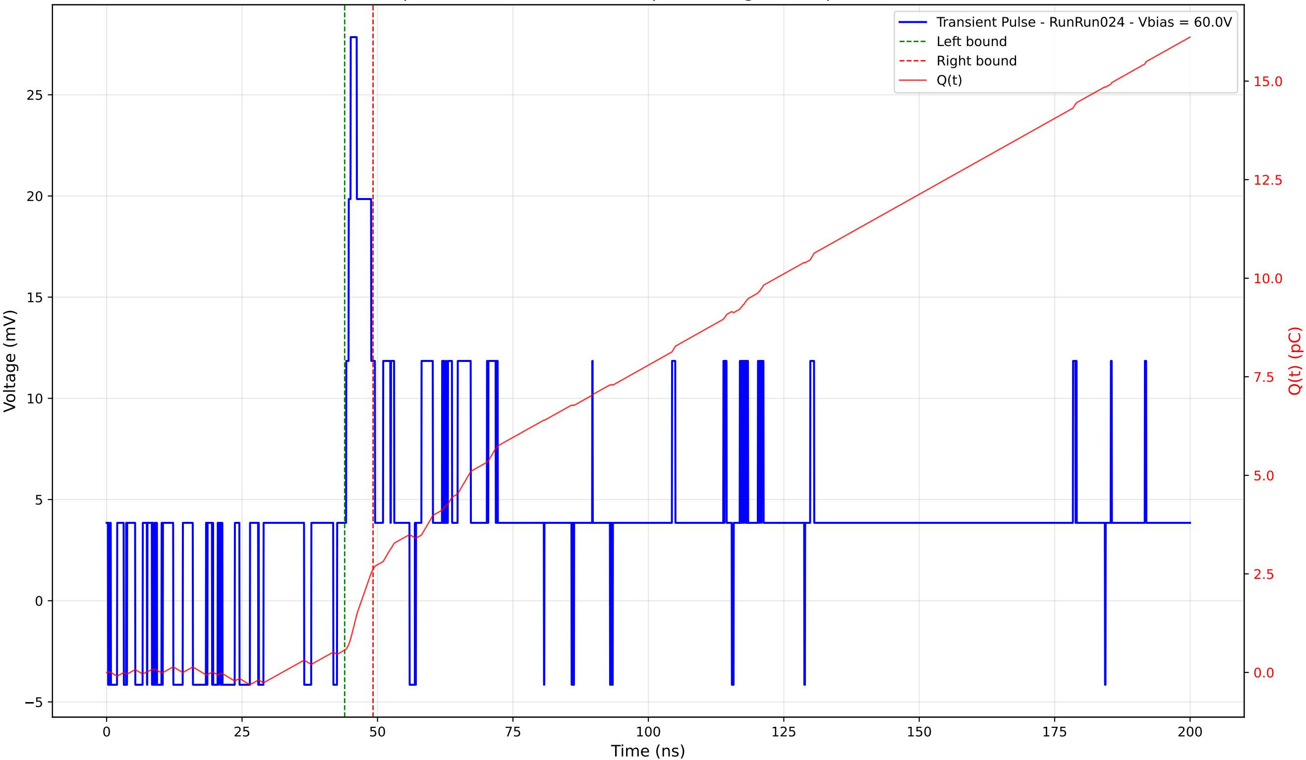
Transient Pulse - Sample: 4003 - Position: 260.0 \mu\text{m} - Charge: 2.05 pC - Rise Time: 0.00 ns (N/A)
