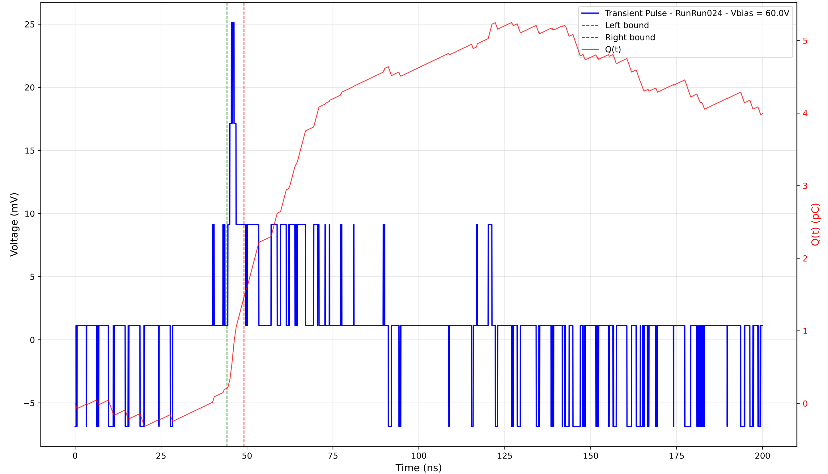
Transient Pulse - Sample: 4003 - Position: 365.0 \mu\text{m} - Charge: 1.26 pC - Rise Time: 1.06 ns
