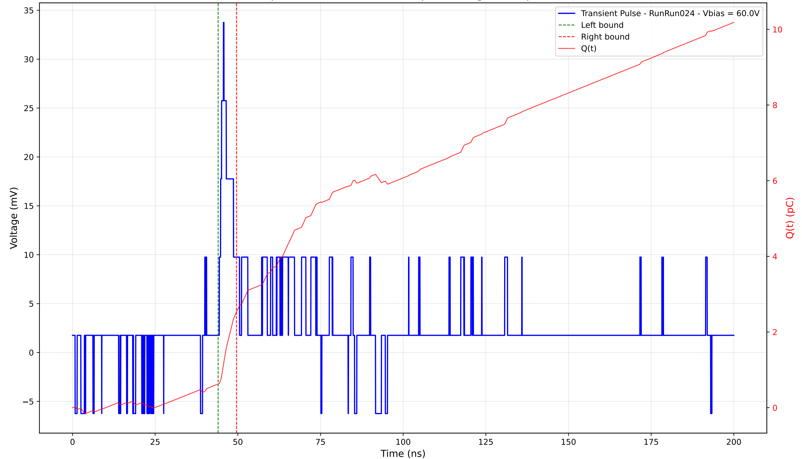
Transient Pulse - Sample: 4003 - Position: 265.0 \mu\text{m} - Charge: 1.90 pC - Rise Time: 1.26 ns
