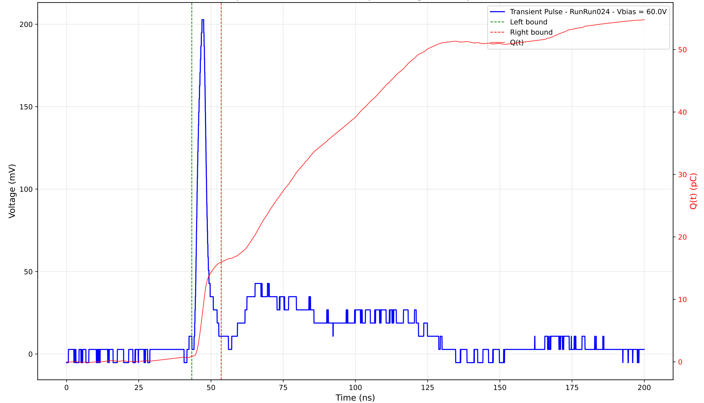
Transient Pulse - Sample: 4003 - Position: 200.0 \mu\text{m} - Charge: 15.07 pC - Rise Time: 2.04 ns
