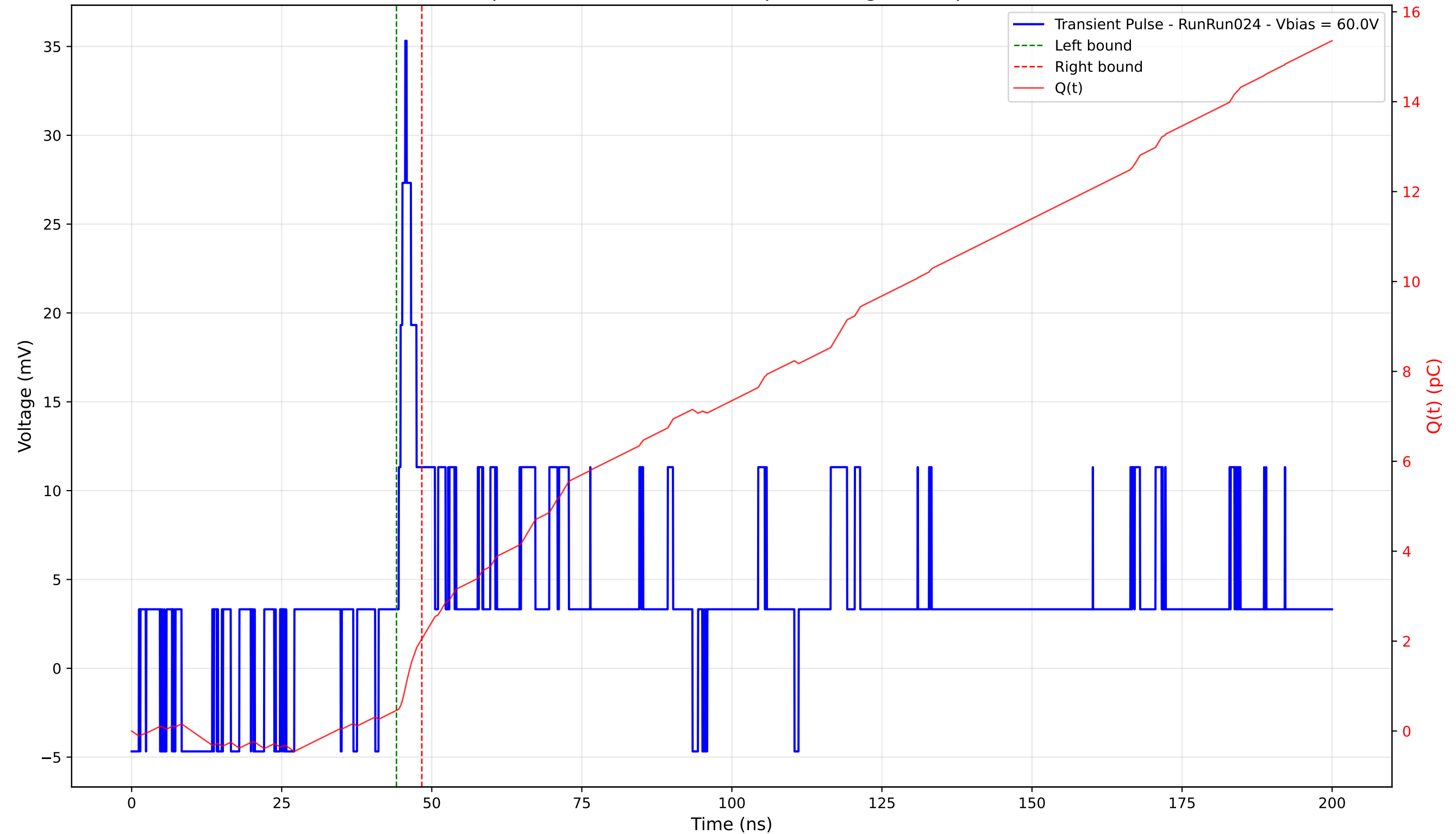
Transient Pulse - Sample: 4003 - Position: 275.0 \mu\text{m} - Charge: 1.59 pC - Rise Time: 1.10 ns
