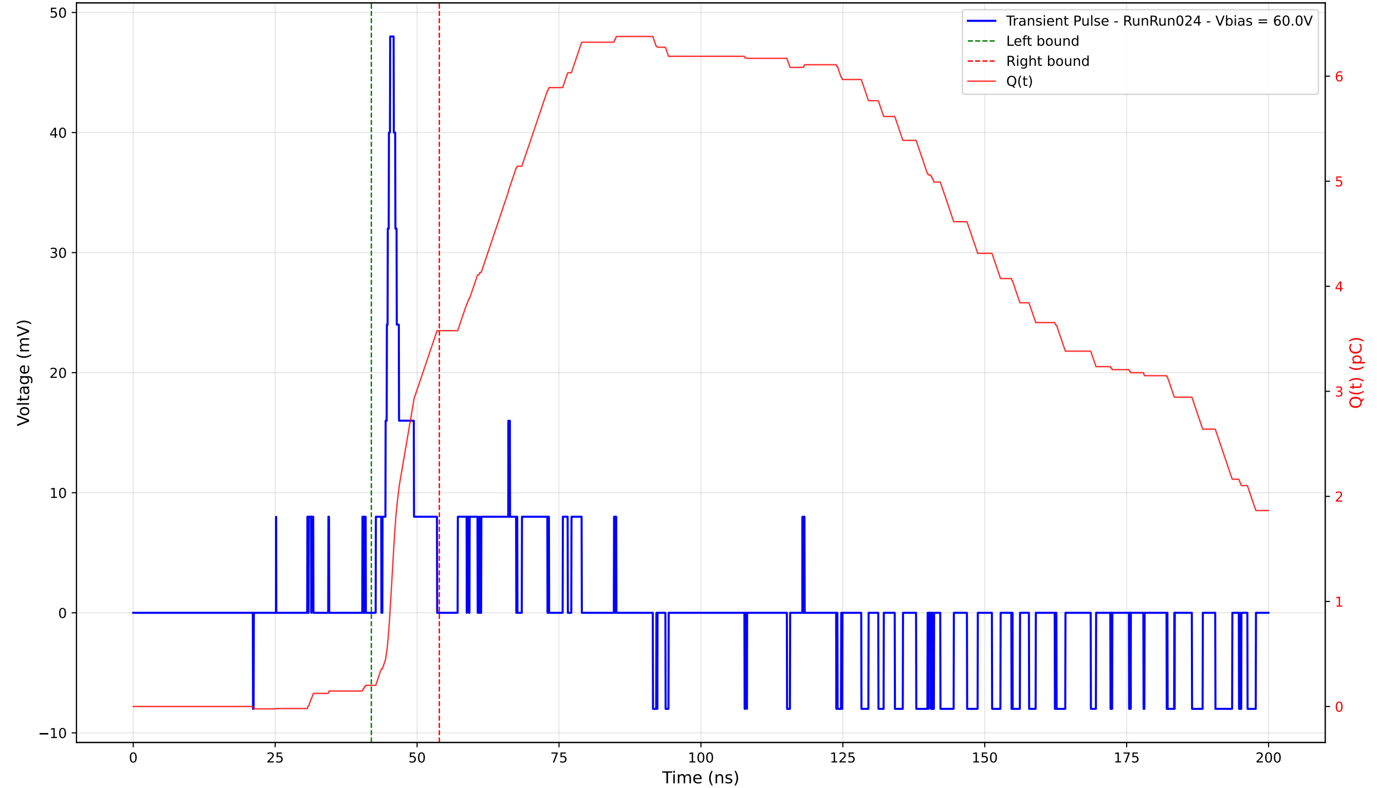
Transient Pulse - Sample: 4003 - Position: 90.0 \mu\text{m} - Charge: 3.38 pC - Rise Time: 1.35 ns
