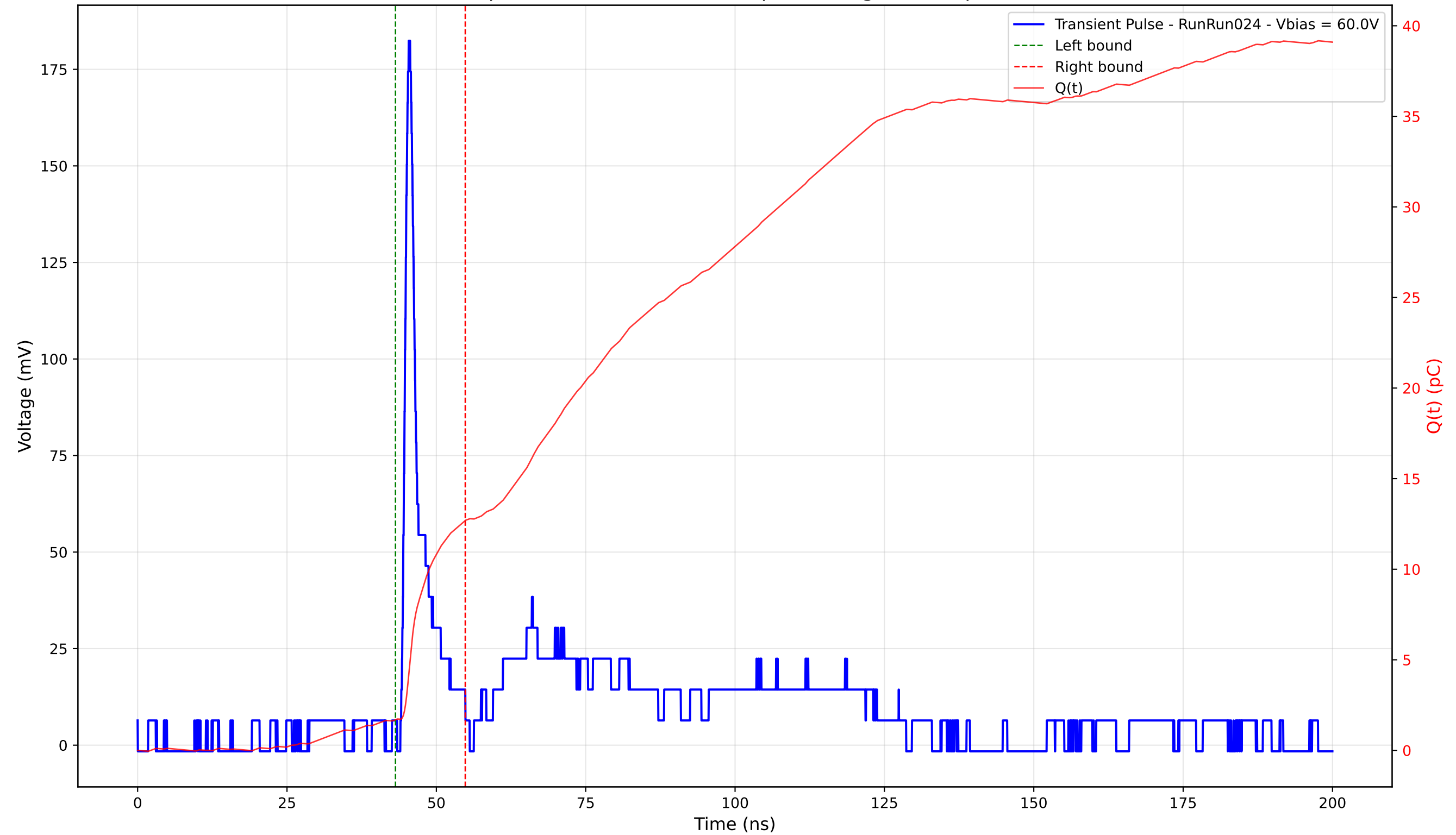
Transient Pulse - Sample: 4003 - Position: 105.0 \mu\text{m} - Charge: 11.00 pC - Rise Time: 0.93 ns
