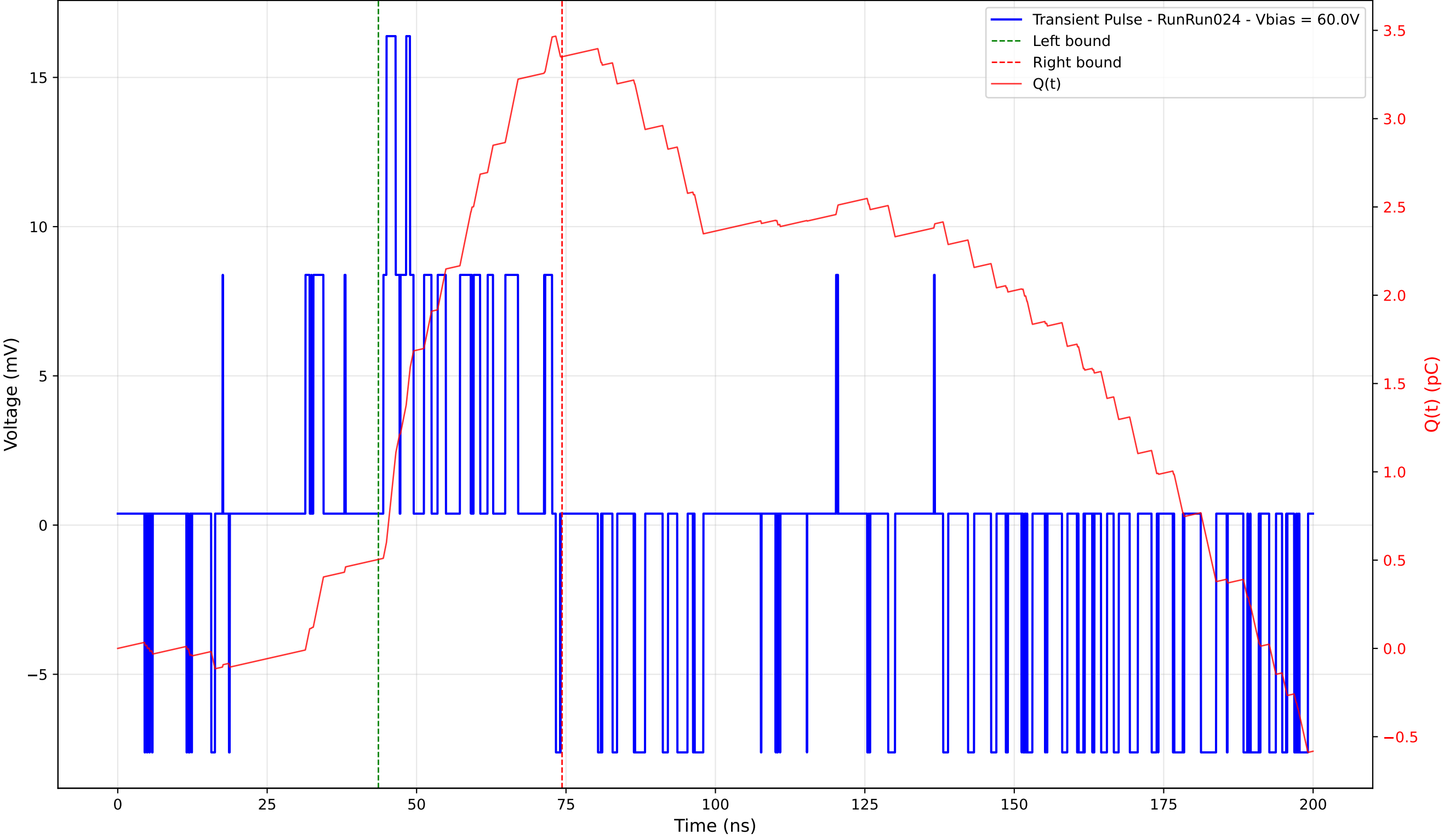
Transient Pulse - Sample: 4003 - Position: 80.0 \mu\text{m} - Charge: 2.85 pC - Rise Time: 0.54 ns
