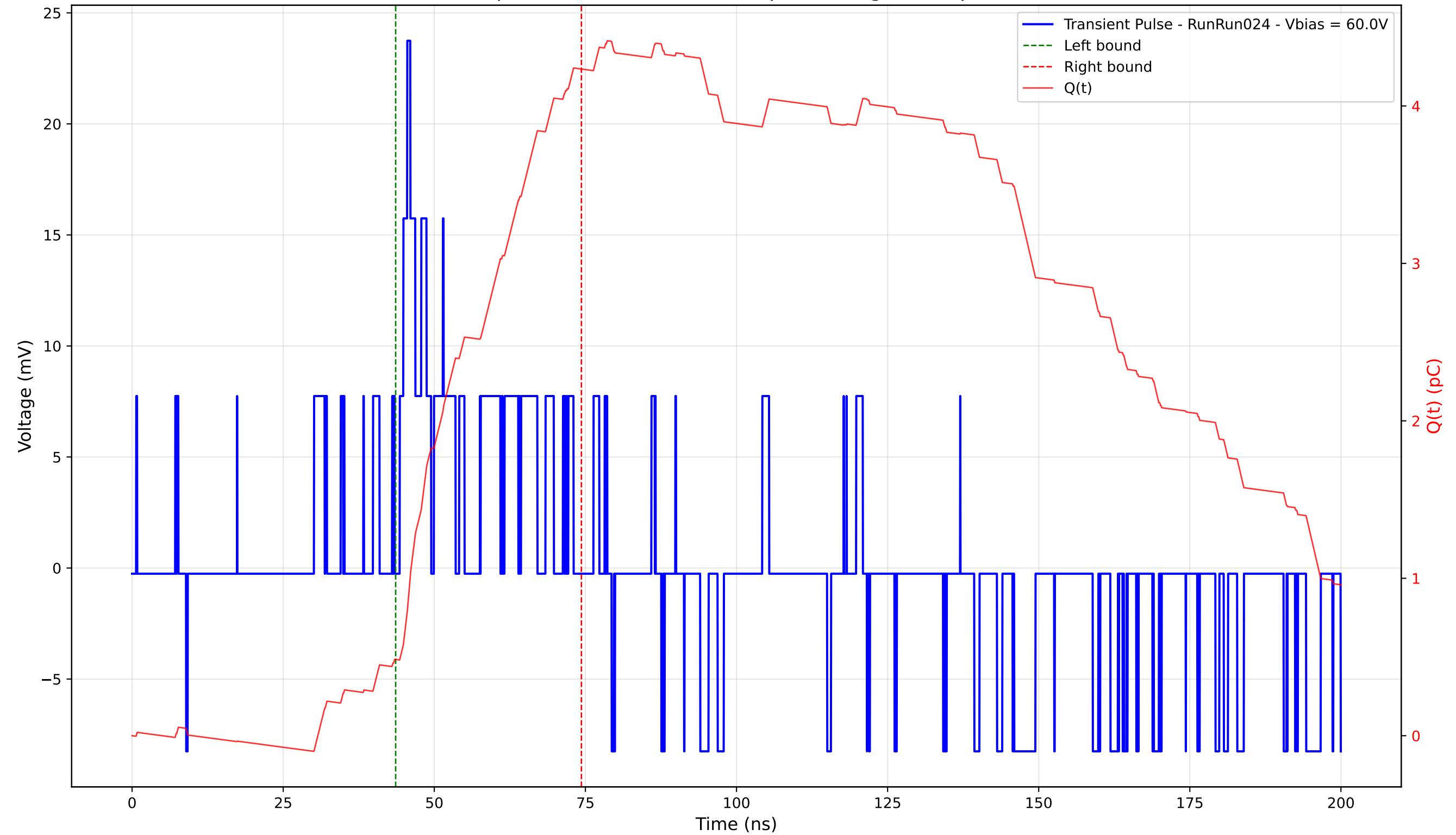
Transient Pulse - Sample: 4003 - Position: 330.0 \mu\text{m} - Charge: 3.75 pC - Rise Time: 1.25 ns
