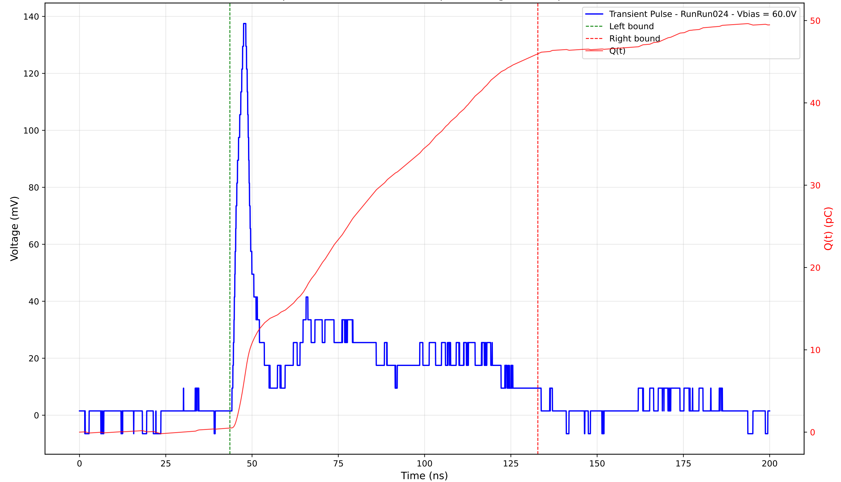
Transient Pulse - Sample: 4003 - Position: 210.0 \mu\text{m} - Charge: 45.49 pC - Rise Time: 2.83 ns
