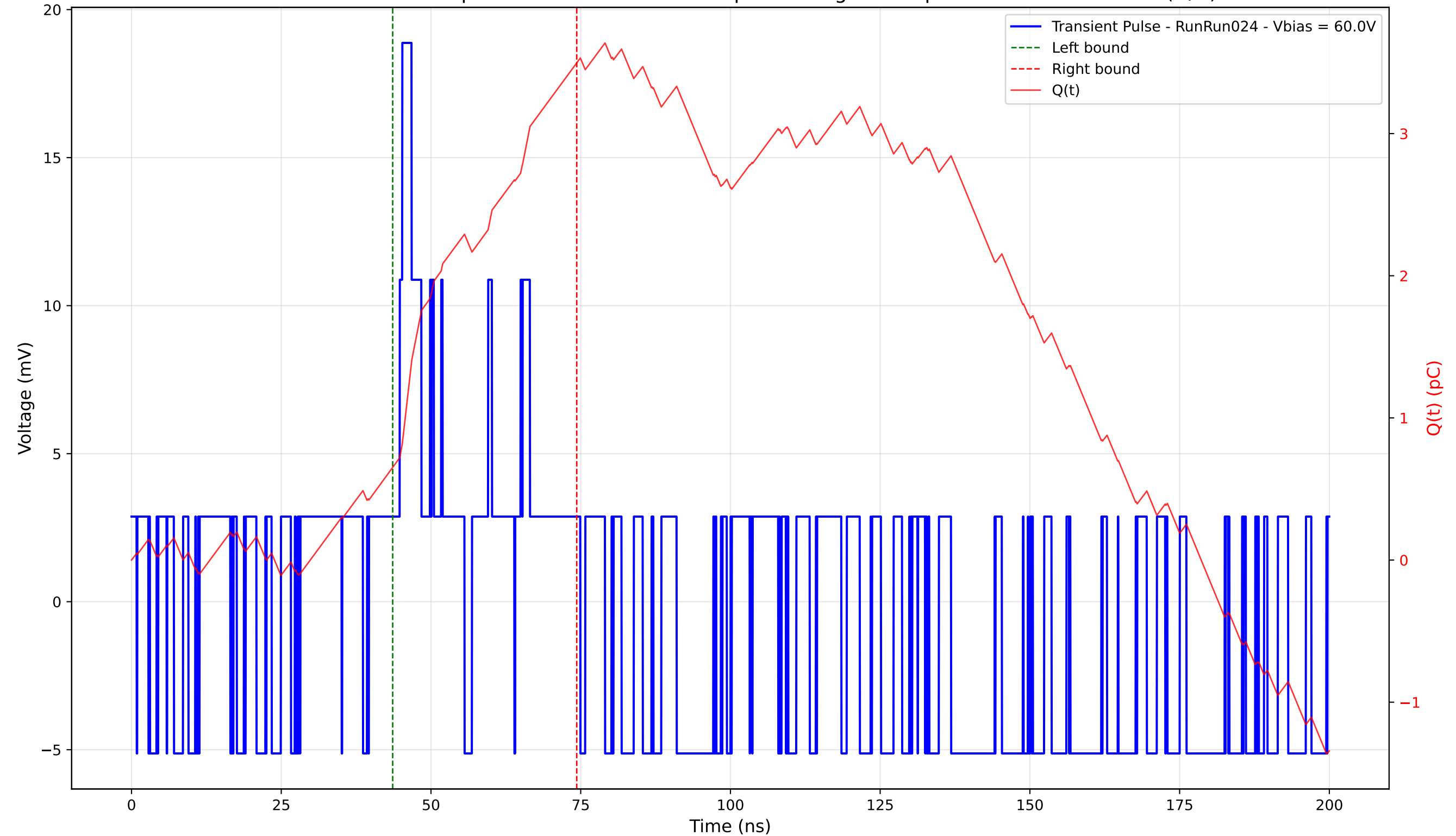
Transient Pulse - Sample: 4003 - Position: 375.0 \mu\text{m} - Charge: 2.85 pC - Rise Time: 0.00 ns (N/A)
