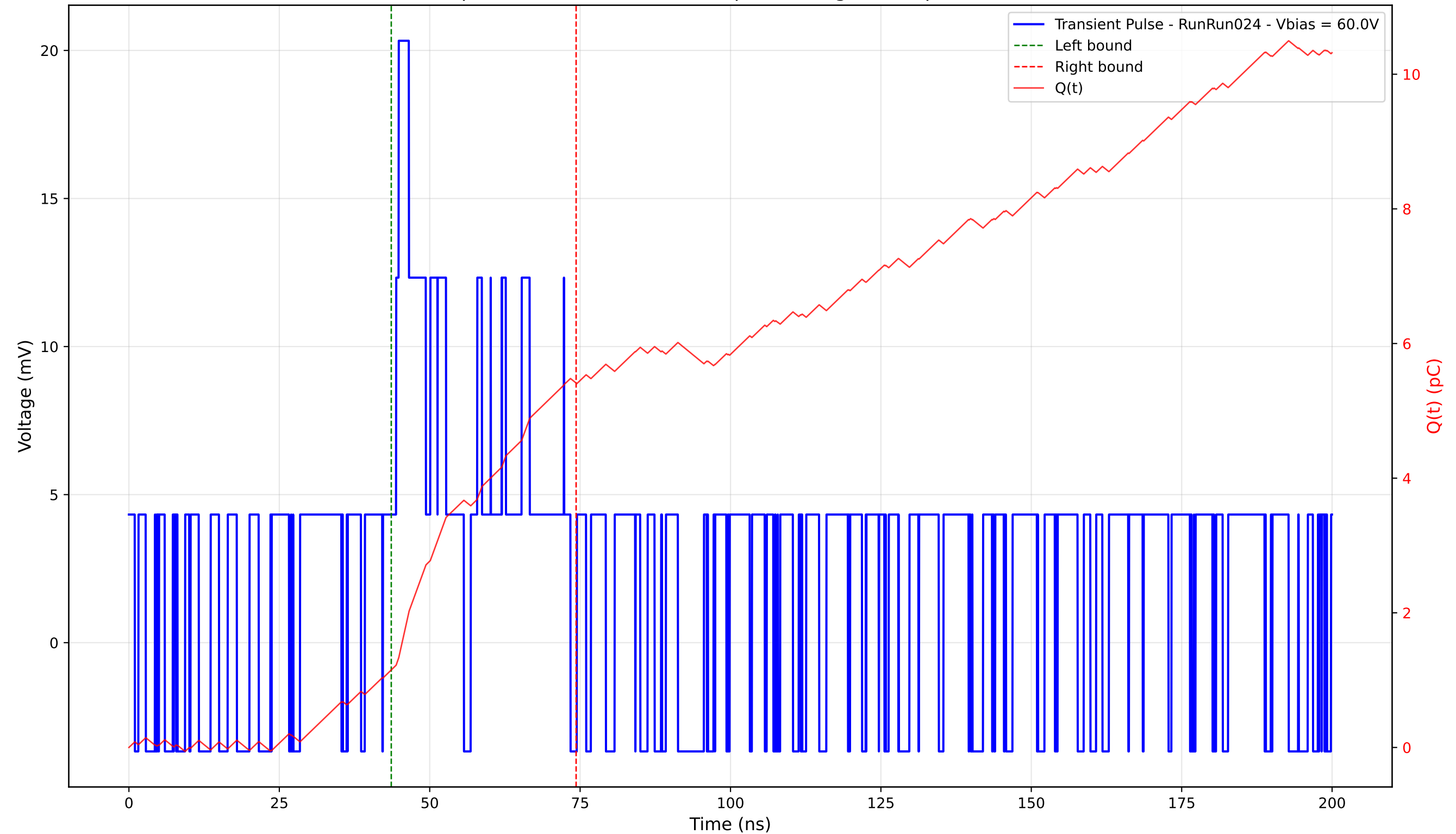
Transient Pulse - Sample: 4003 - Position: 370.0 \mu\text{m} - Charge: 4.26 pC - Rise Time: 0.00 ns (N/A)
