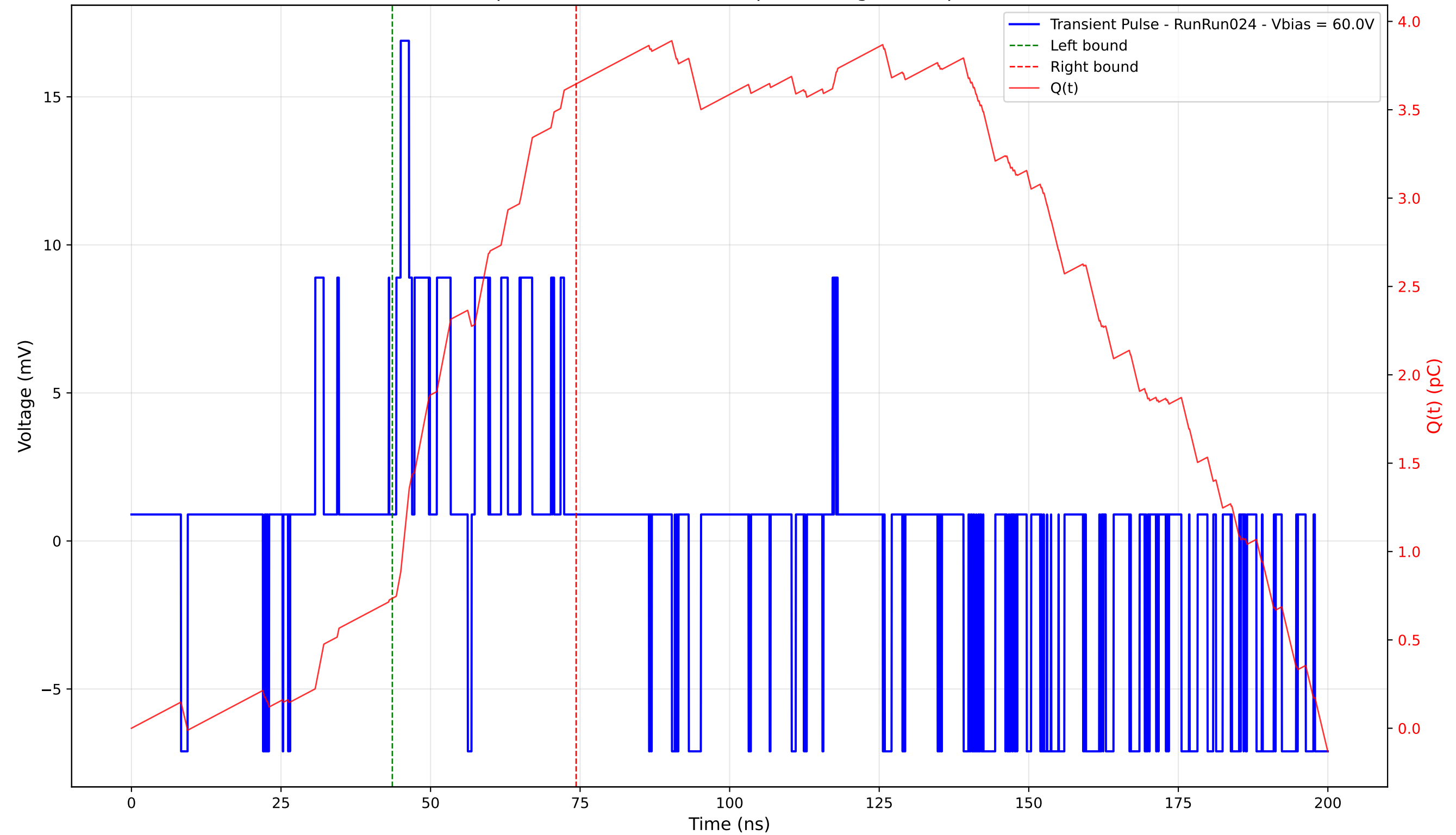
Transient Pulse - Sample: 4003 - Position: 20.0 \mu\text{m} - Charge: 2.91 pC - Rise Time: 0.74 ns
