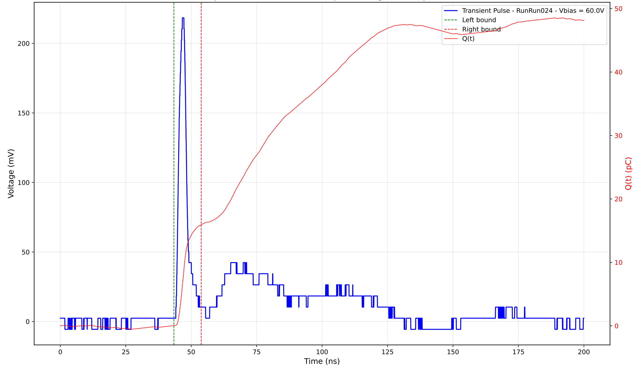
Transient Pulse - Sample: 4003 - Position: 195.0 \mu\text{m} - Charge: 15.91 pC - Rise Time: 1.83 ns
