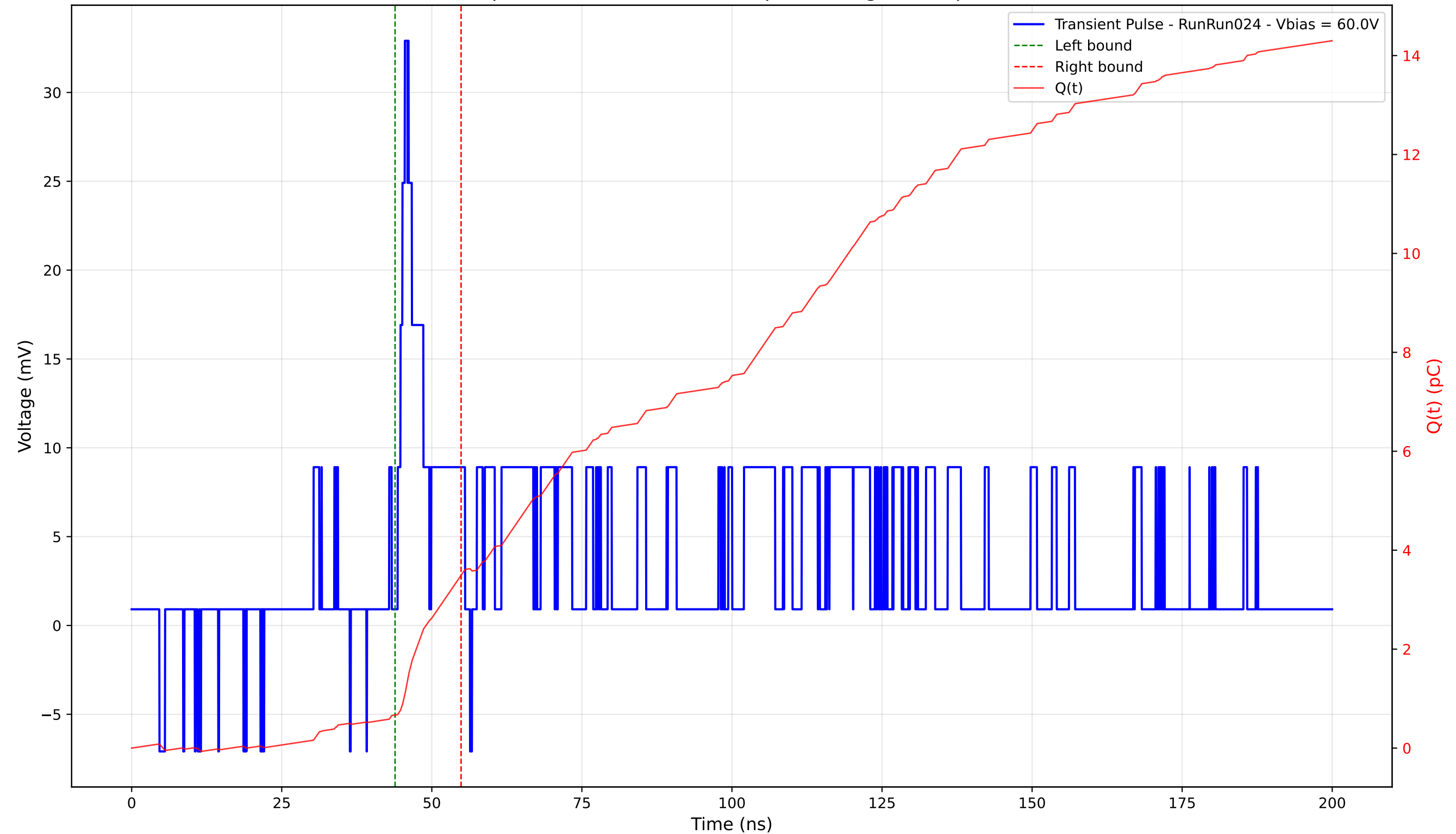
Transient Pulse - Sample: 4003 - Position: 250.0 \mu\text{m} - Charge: 2.83 pC - Rise Time: 1.19 ns
