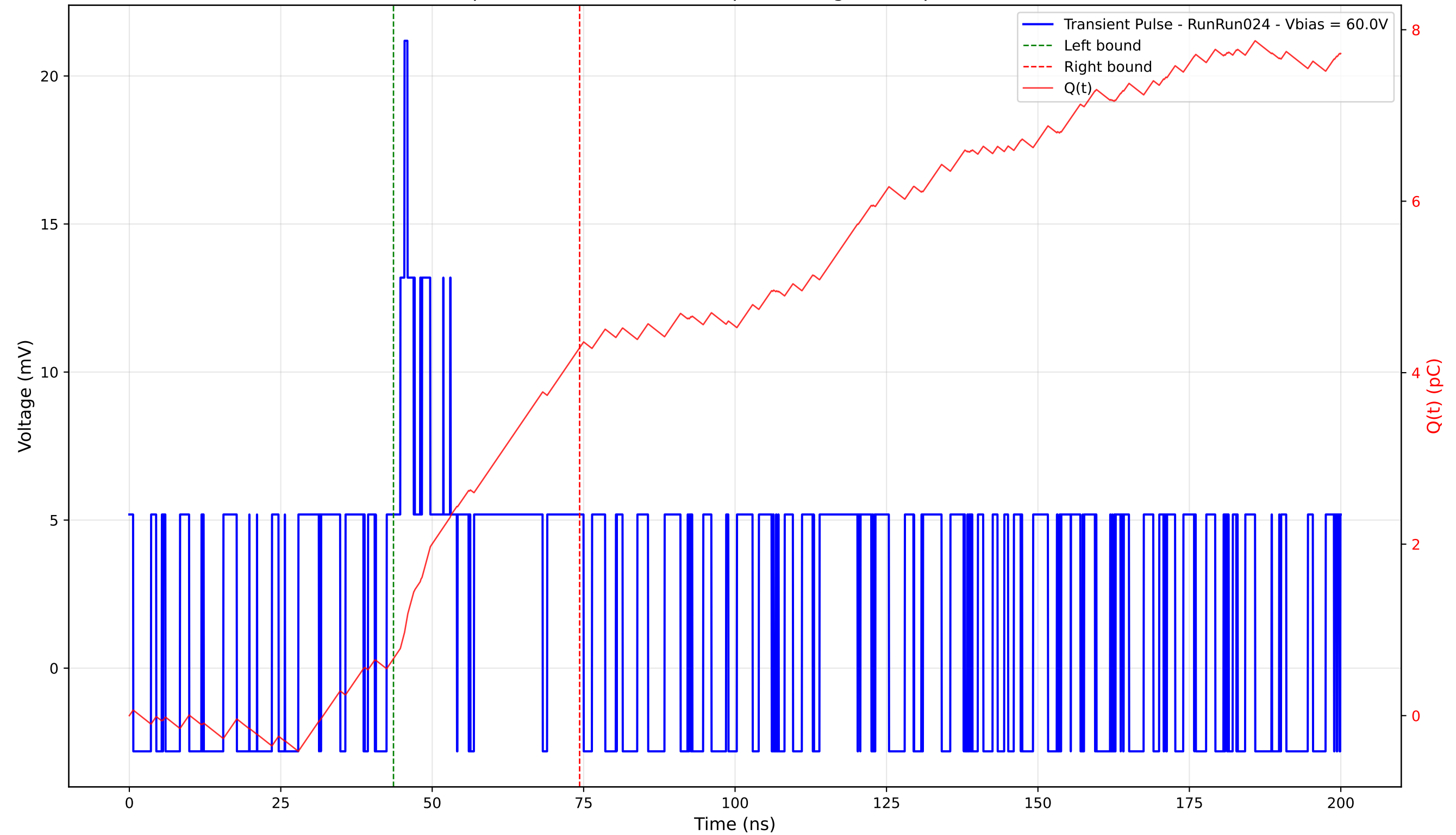
Transient Pulse - Sample: 4003 - Position: 75.0 \mu\text{m} - Charge: 3.62 pC - Rise Time: 0.00 ns (N/A)
