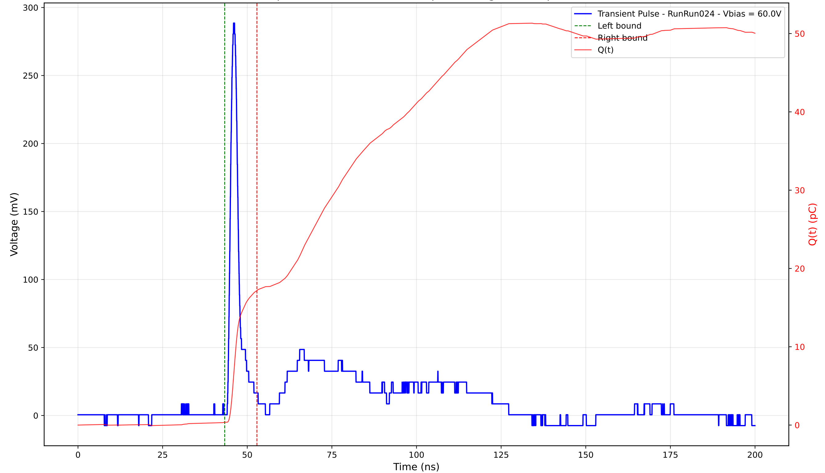
Transient Pulse - Sample: 4003 - Position: 175.0 \mu\text{m} - Charge: 16.84 pC - Rise Time: 1.27 ns
