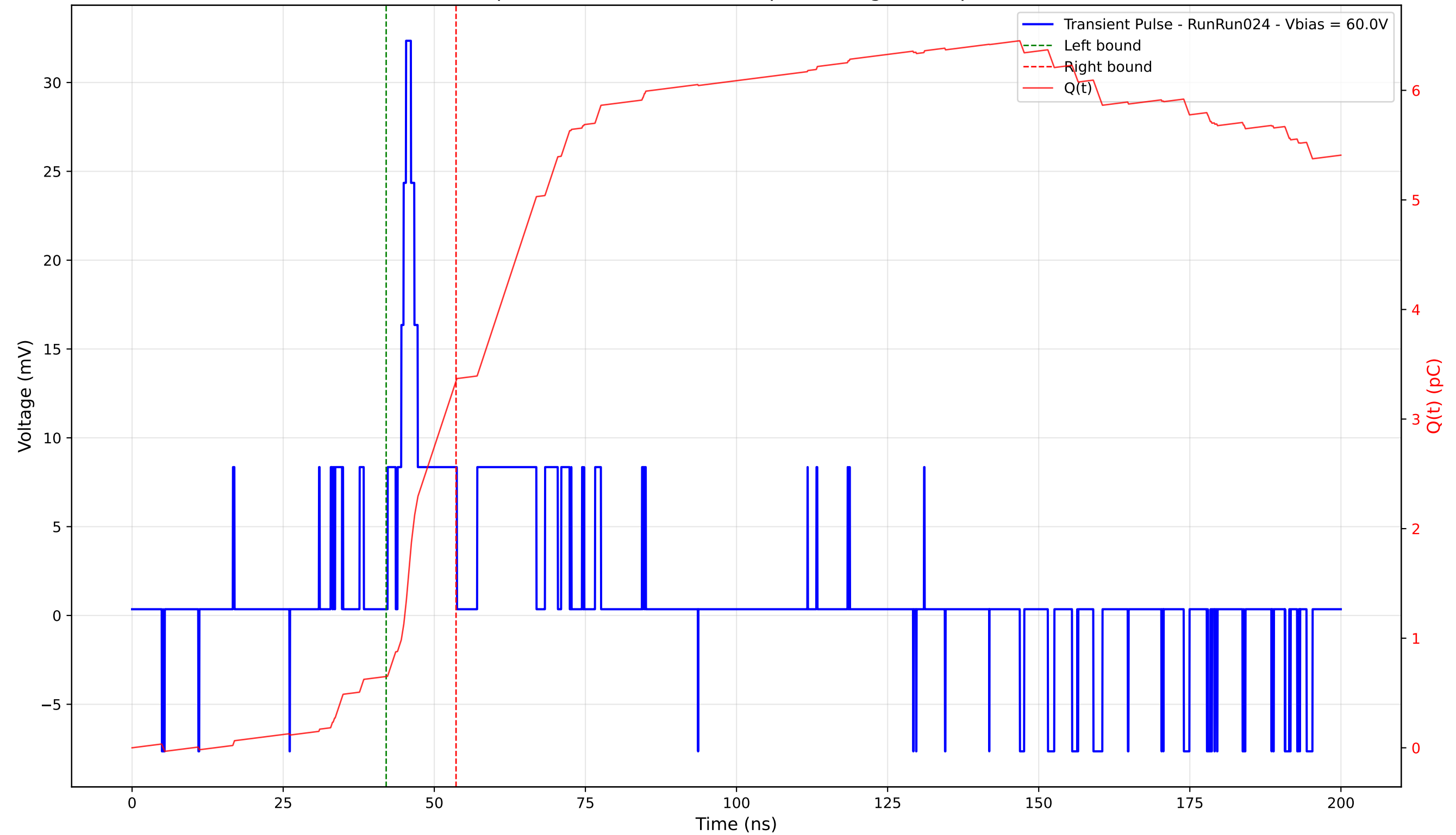
Transient Pulse - Sample: 4003 - Position: 395.0 \mu\text{m} - Charge: 2.70 pC - Rise Time: 1.41 ns
