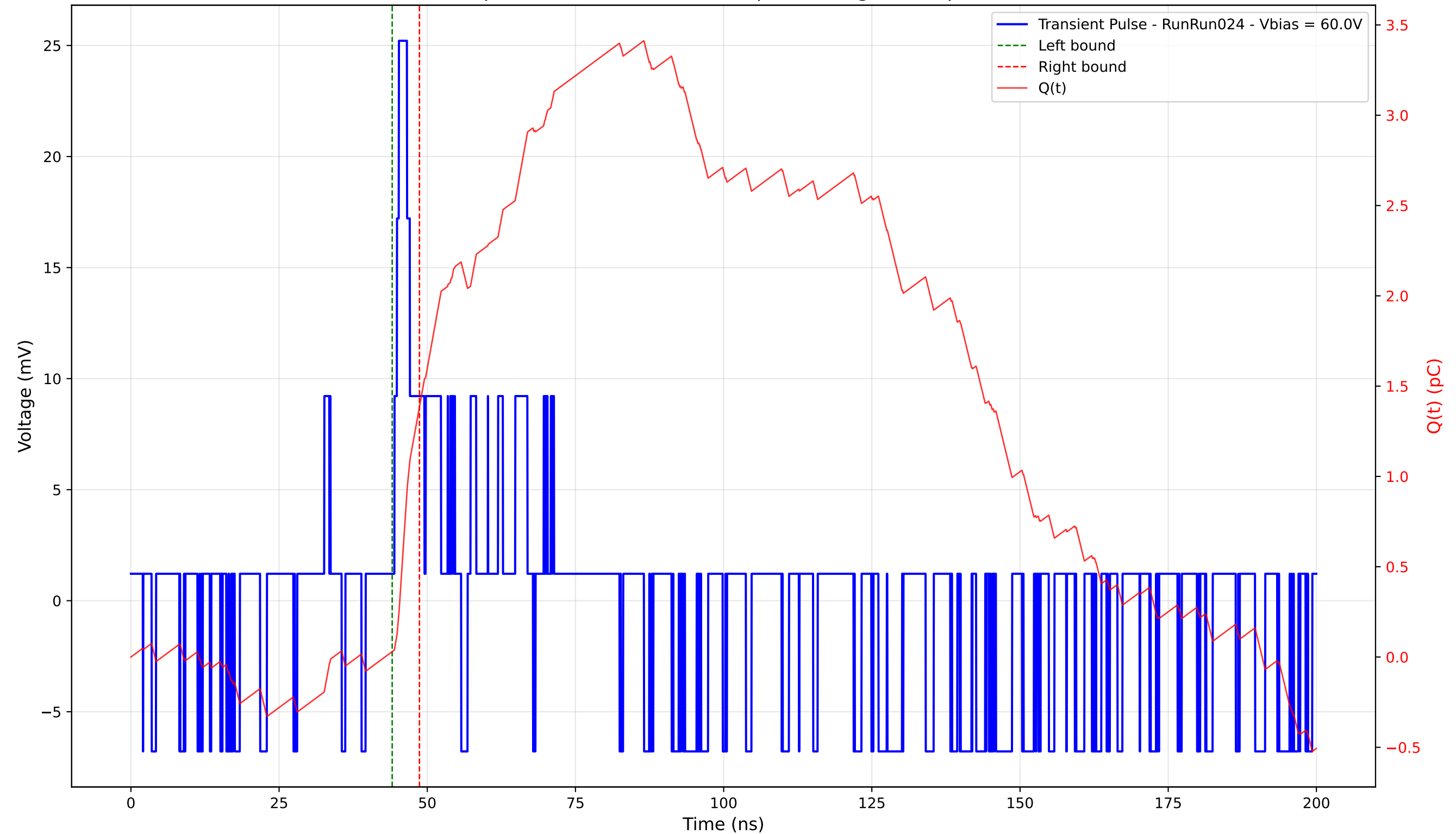
Transient Pulse - Sample: 4003 - Position: 300.0 \mu\text{m} - Charge: 1.36 pC - Rise Time: 0.76 ns
