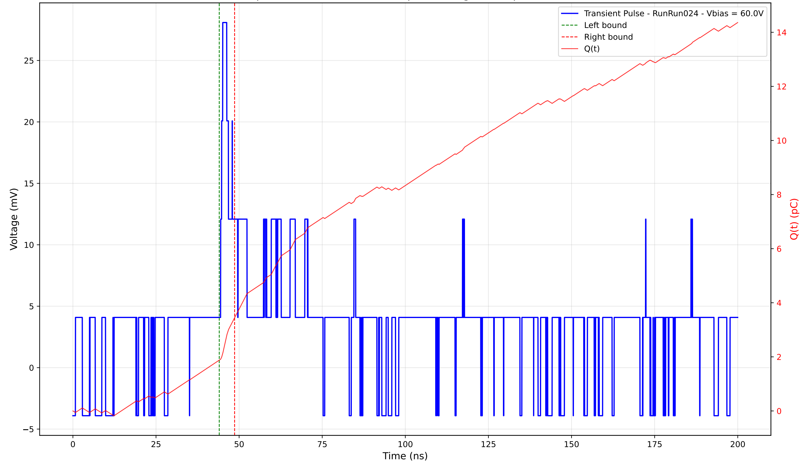
Transient Pulse - Sample: 4003 - Position: 405.0 \mu\text{m} - Charge: 1.58 pC - Rise Time: 0.00 ns (N/A)
