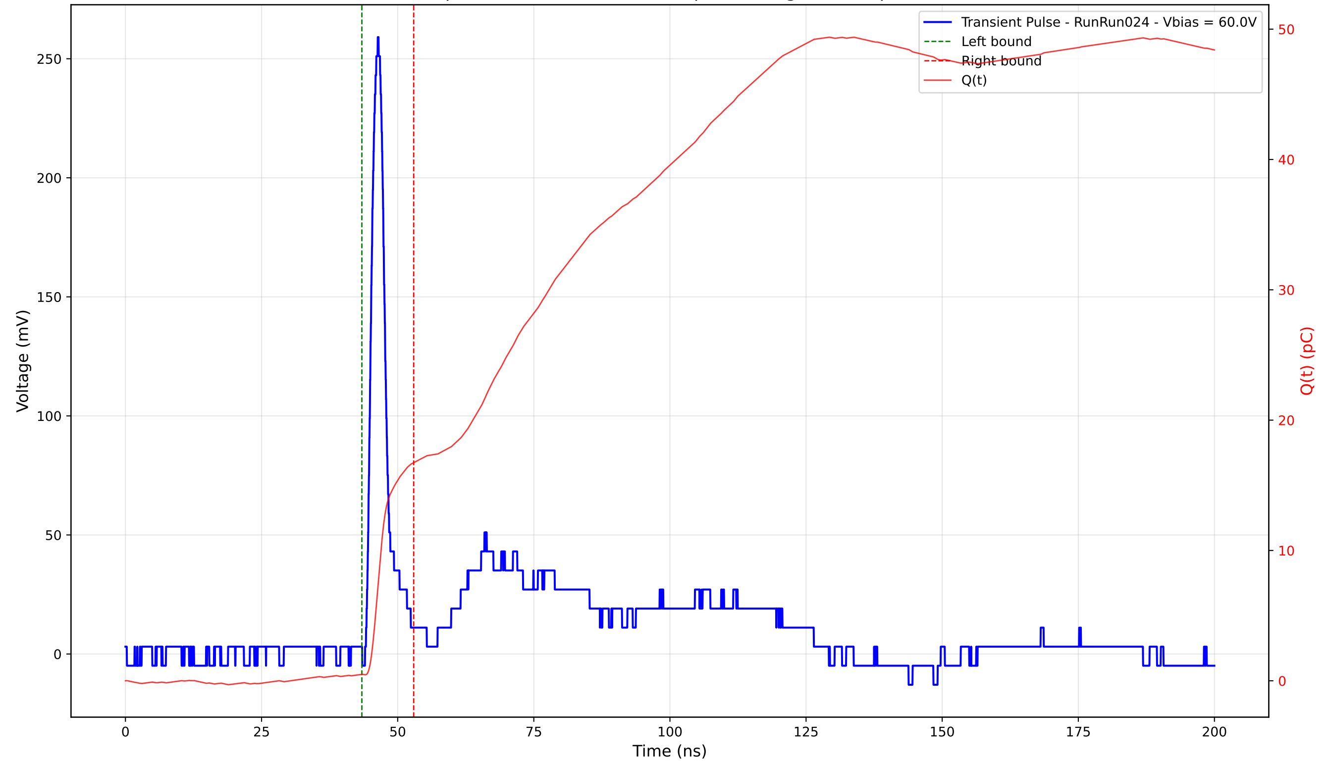
Transient Pulse - Sample: 4003 - Position: 185.0 \mu\text{m} - Charge: 16.24 pC - Rise Time: 1.44 ns
