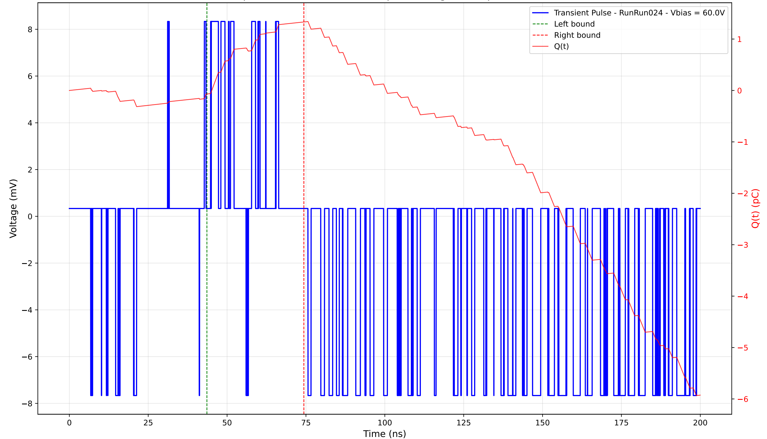
Transient Pulse - Sample: 4003 - Position: 425.0 \mu\text{m} - Charge: 1.40 pC - Rise Time: 0.00 ns (N/A)
