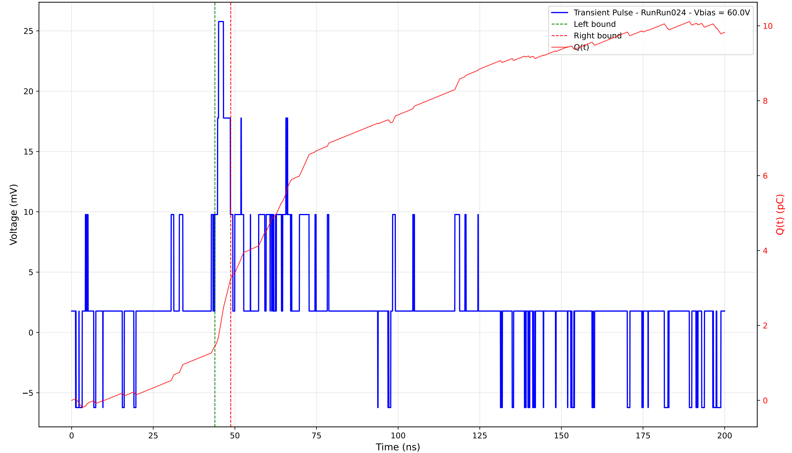
Transient Pulse - Sample: 4003 - Position: 290.0 \mu\text{m} - Charge: 1.82 pC - Rise Time: 1.16 ns
