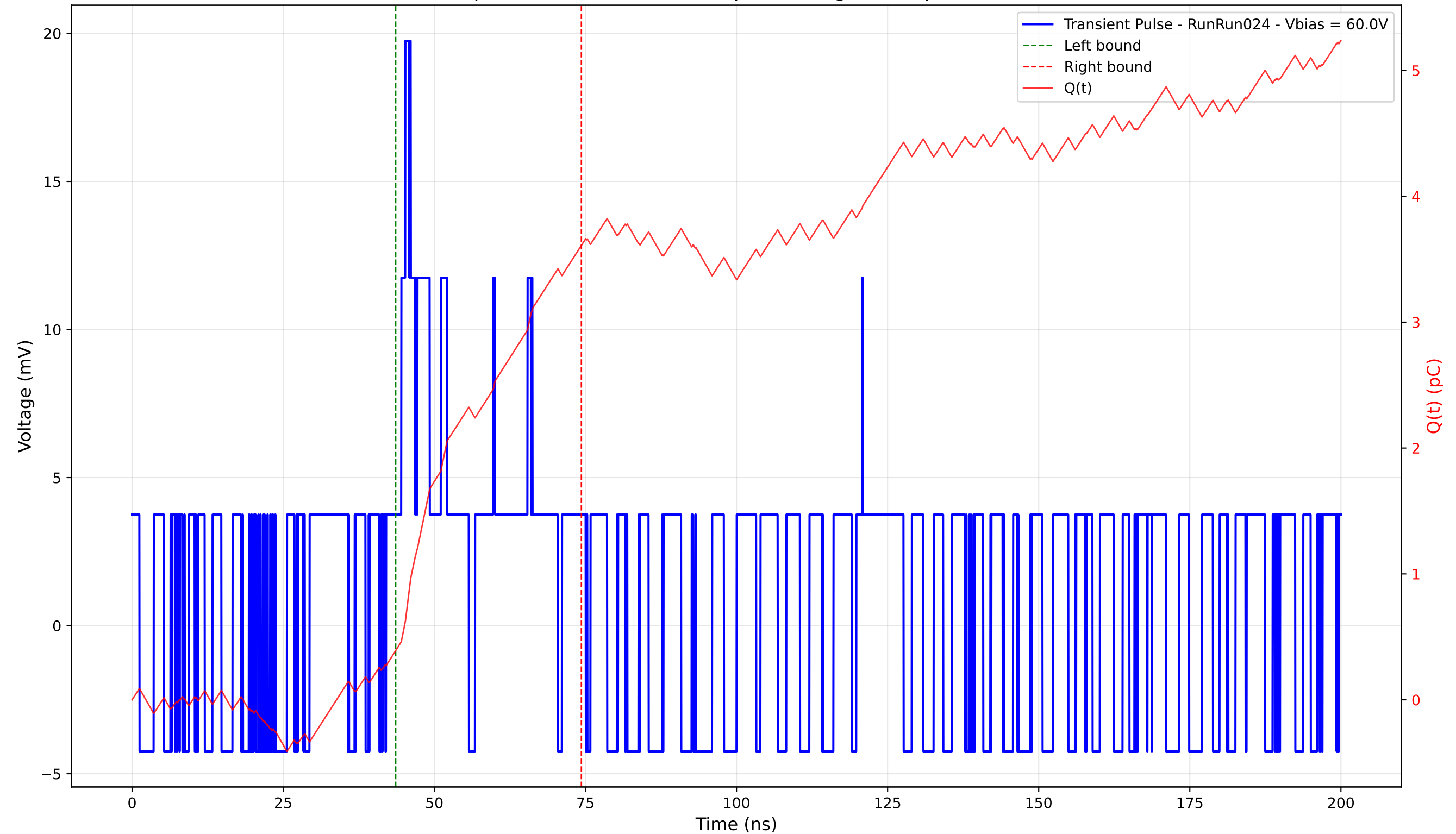
Transient Pulse - Sample: 4003 - Position: 30.0 \mu\text{m} - Charge: 3.22 pC - Rise Time: 0.00 ns (N/A)
