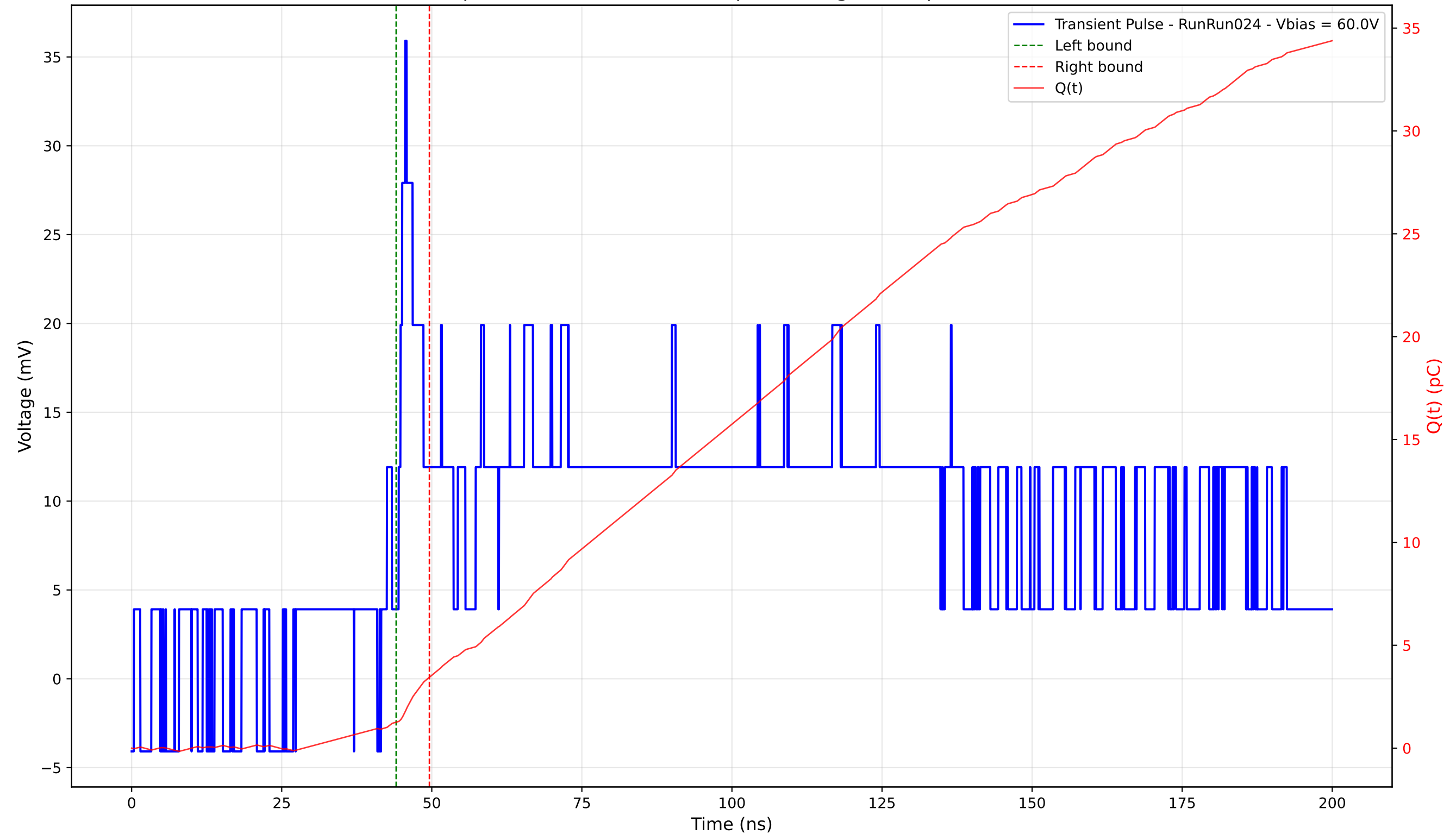
Transient Pulse - Sample: 4003 - Position: 240.0 \mu\text{m} - Charge: 2.19 pC - Rise Time: 0.00 ns (N/A)
