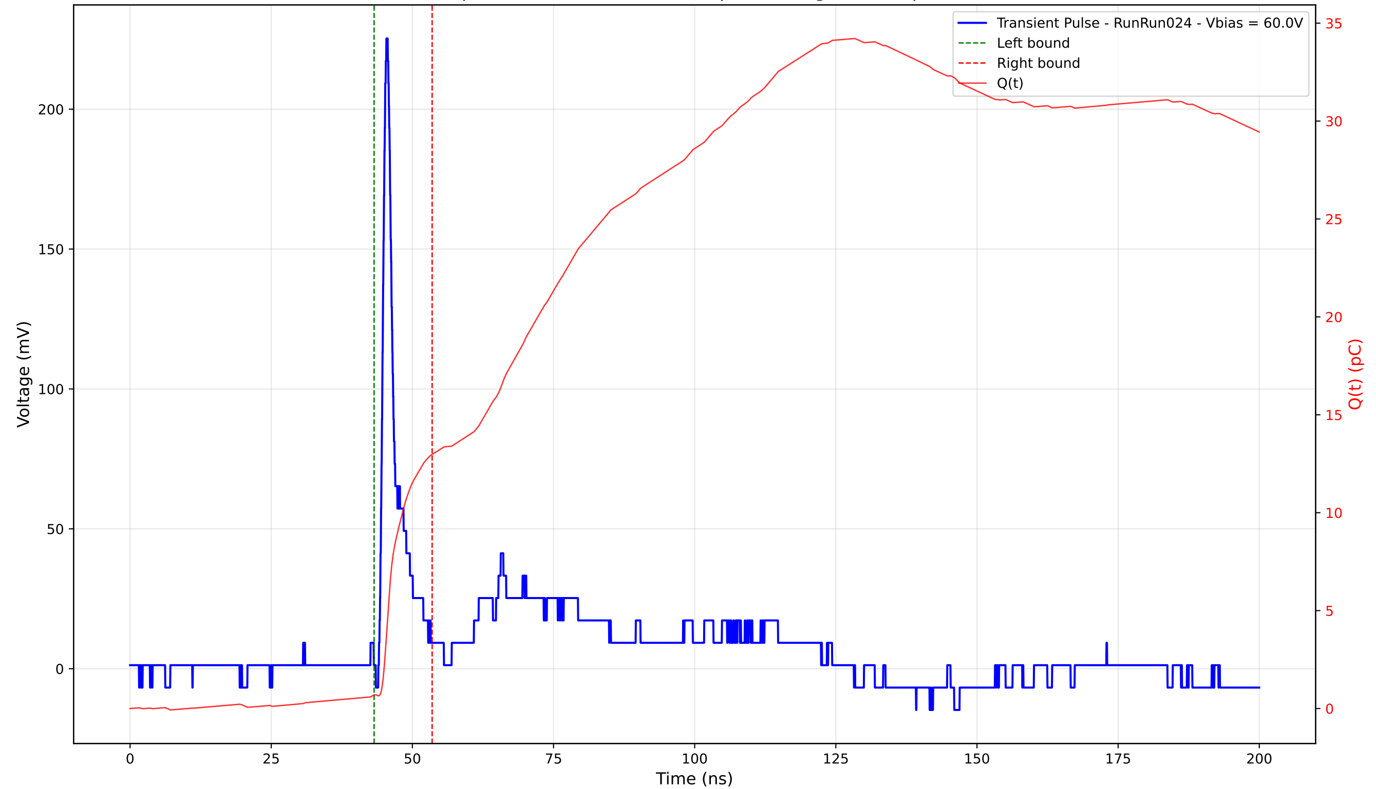
Transient Pulse - Sample: 4003 - Position: 110.0 \mu\text{m} - Charge: 12.28 pC - Rise Time: 0.95 ns
