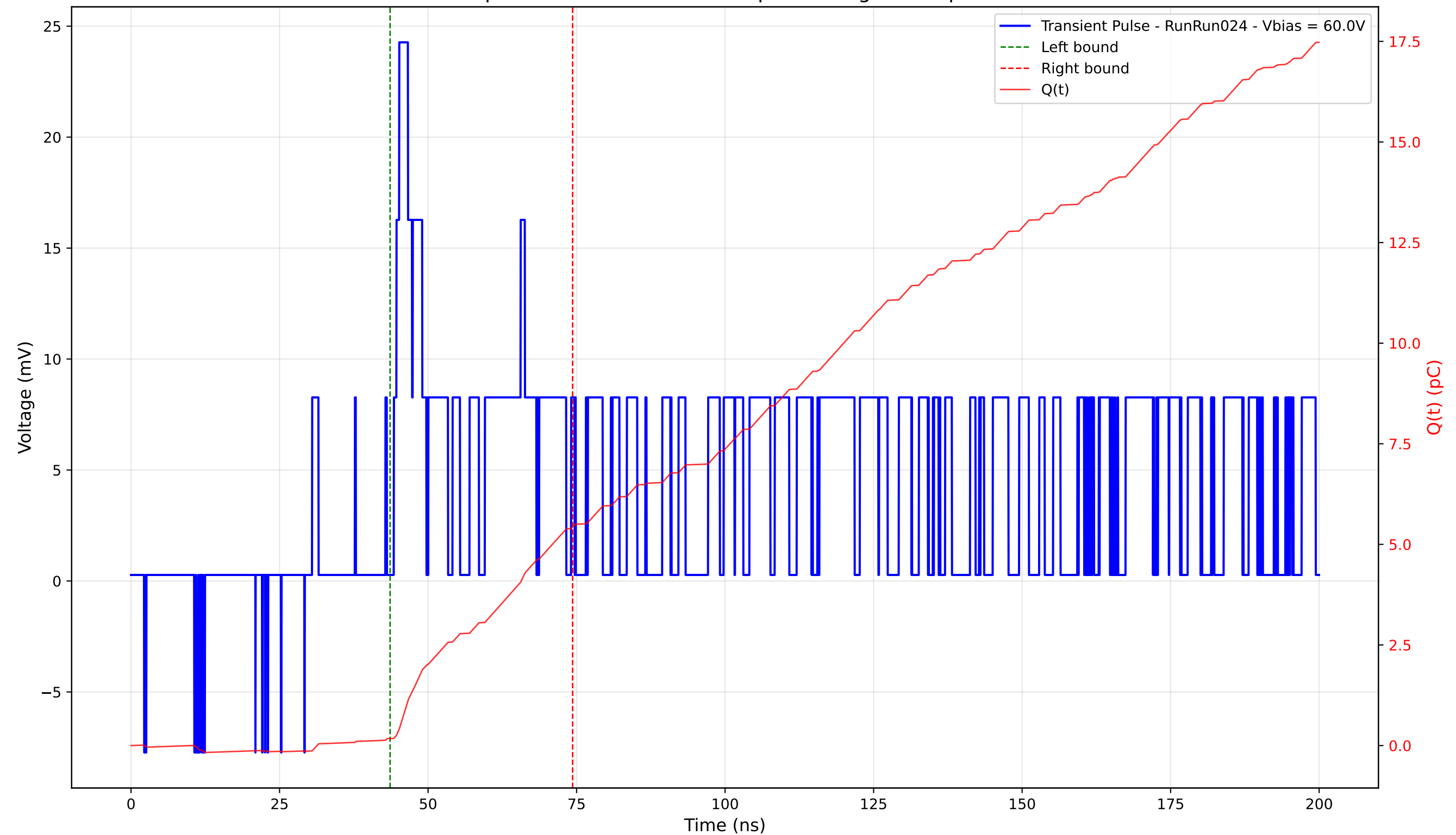
Transient Pulse - Sample: 4003 - Position: 245.0 \mu\text{m} - Charge: 5.26 pC - Rise Time: 0.91 ns
