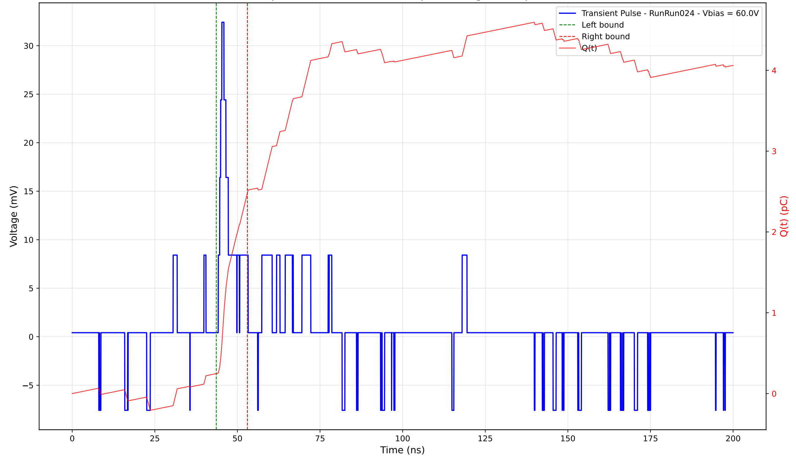
Transient Pulse - Sample: 4003 - Position: 285.0 \mu\text{m} - Charge: 2.24 pC - Rise Time: 1.09 ns
