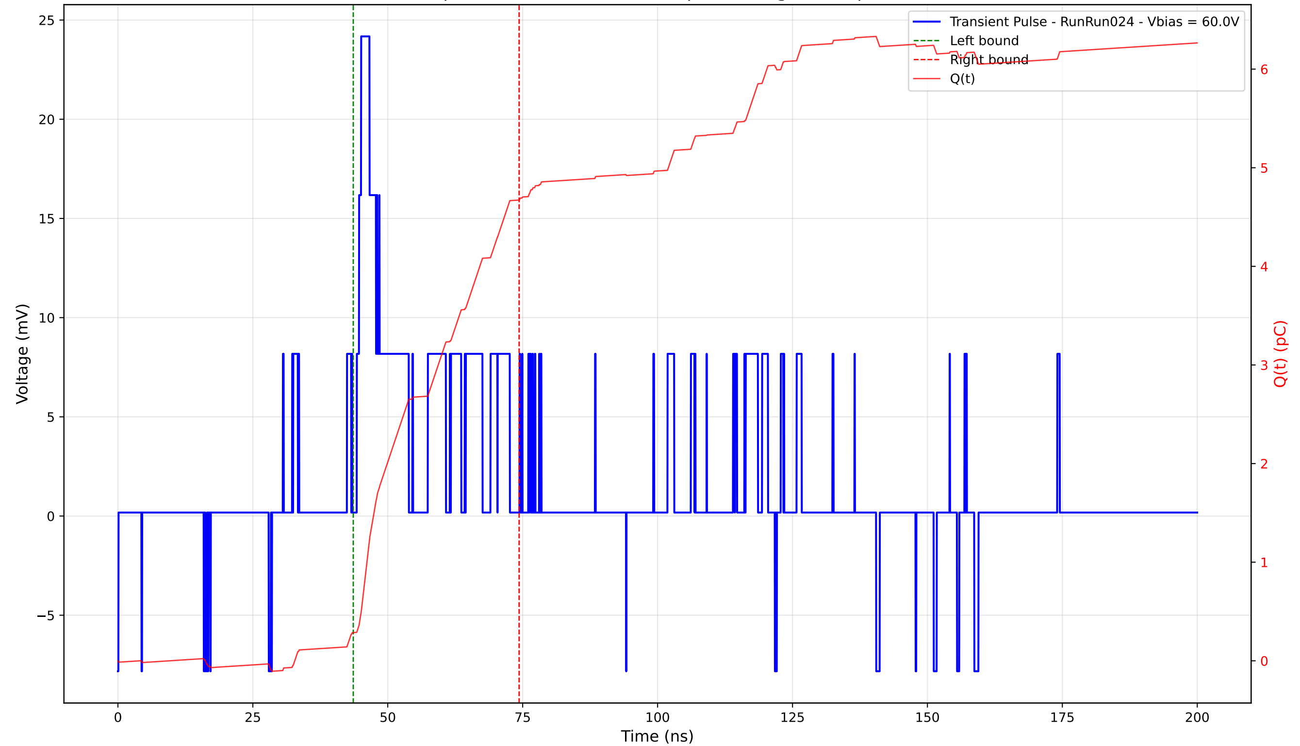
Transient Pulse - Sample: 4003 - Position: 270.0 \mu\text{m} - Charge: 4.39 pC - Rise Time: 0.81 ns
