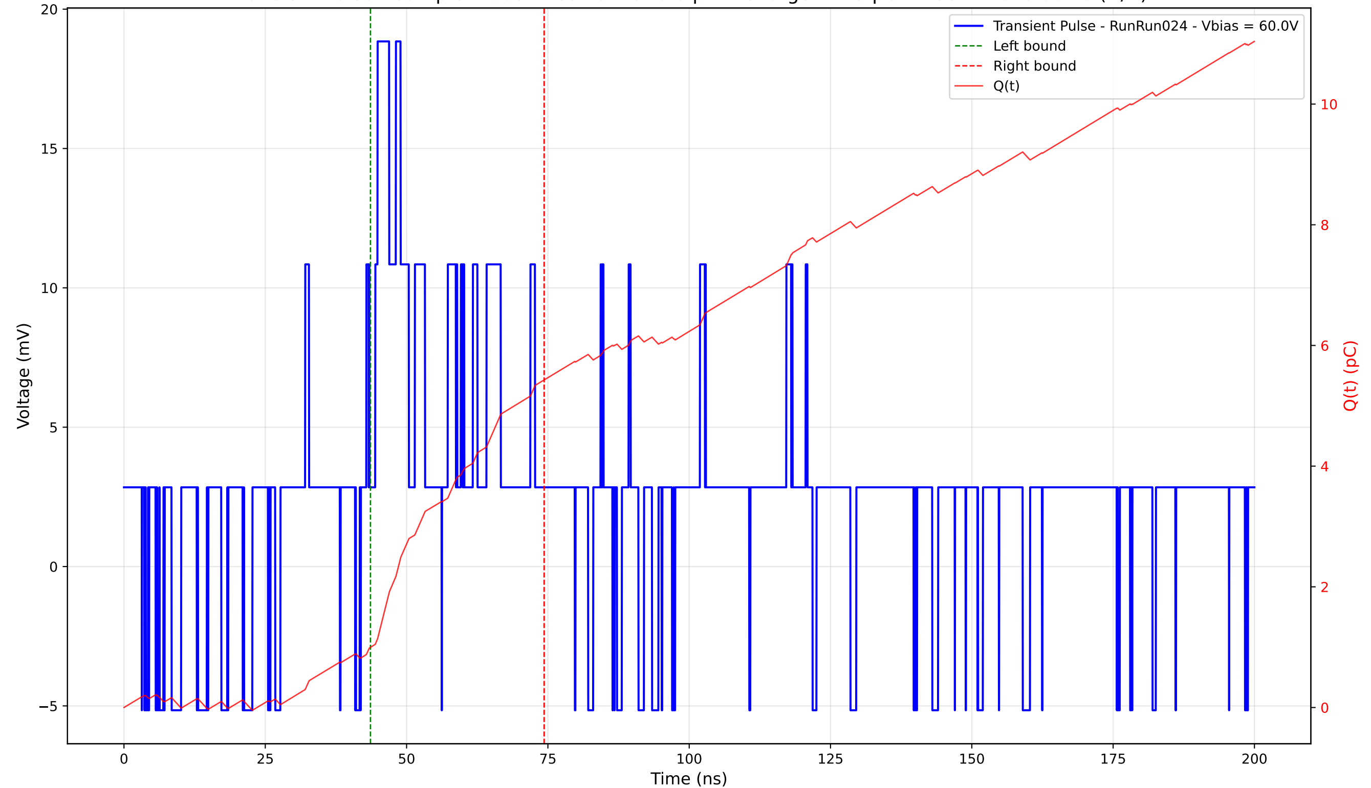
Transient Pulse - Sample: 4003 - Position: 310.0 \mu\text{m} - Charge: 4.43 pC - Rise Time: 0.00 ns (N/A)
