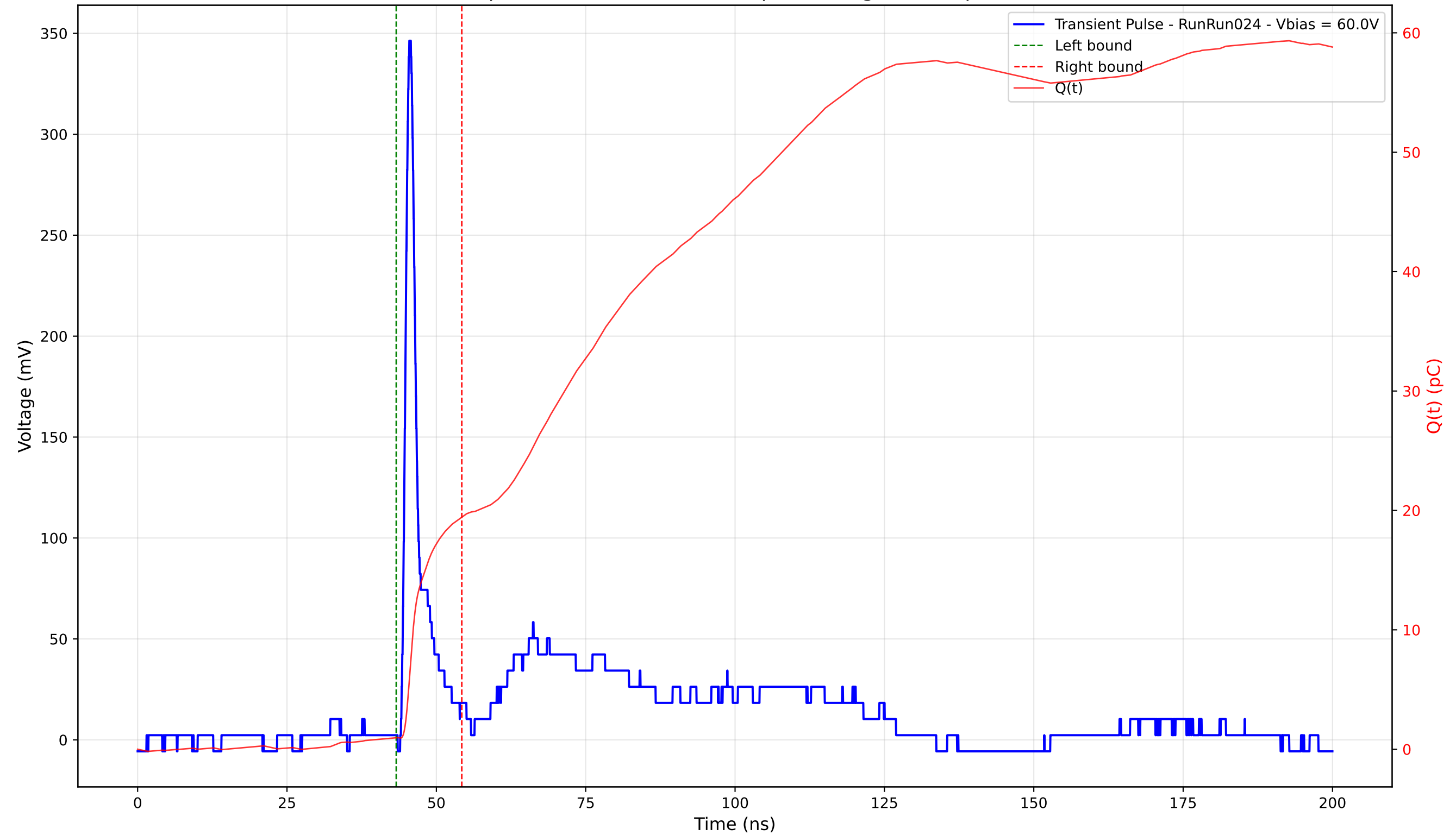
Transient Pulse - Sample: 4003 - Position: 135.0 \mu\text{m} - Charge: 18.46 pC - Rise Time: 0.98 ns
