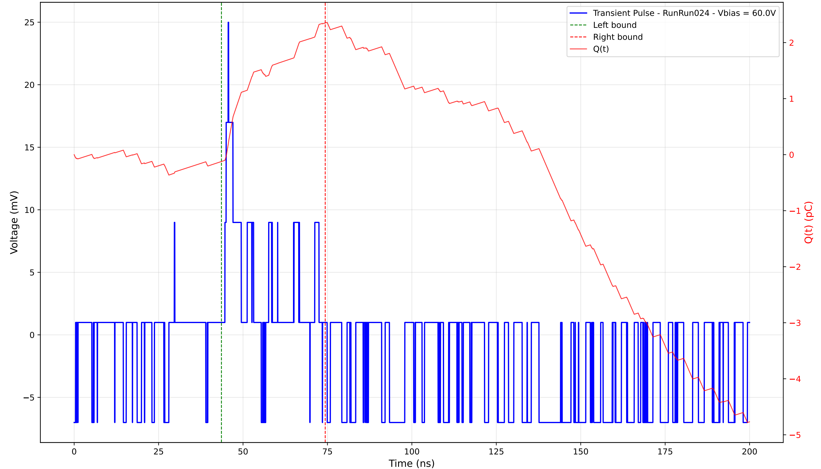
Transient Pulse - Sample: 4003 - Position: 410.0 \mu\text{m} - Charge: 2.47 pC - Rise Time: 0.98 ns
