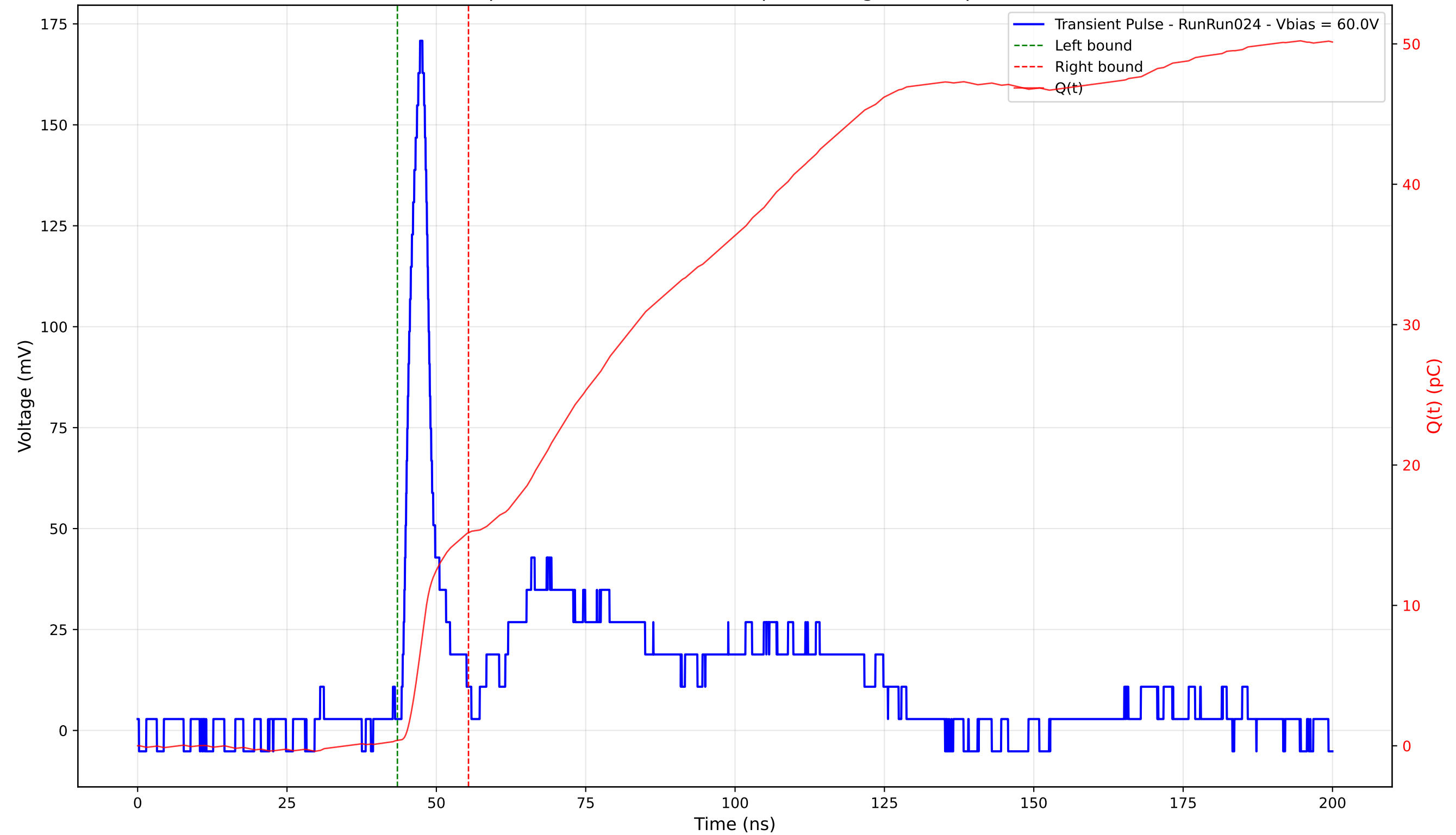
Transient Pulse - Sample: 4003 - Position: 205.0 \mu\text{m} - Charge: 14.80 pC - Rise Time: 2.40 ns
