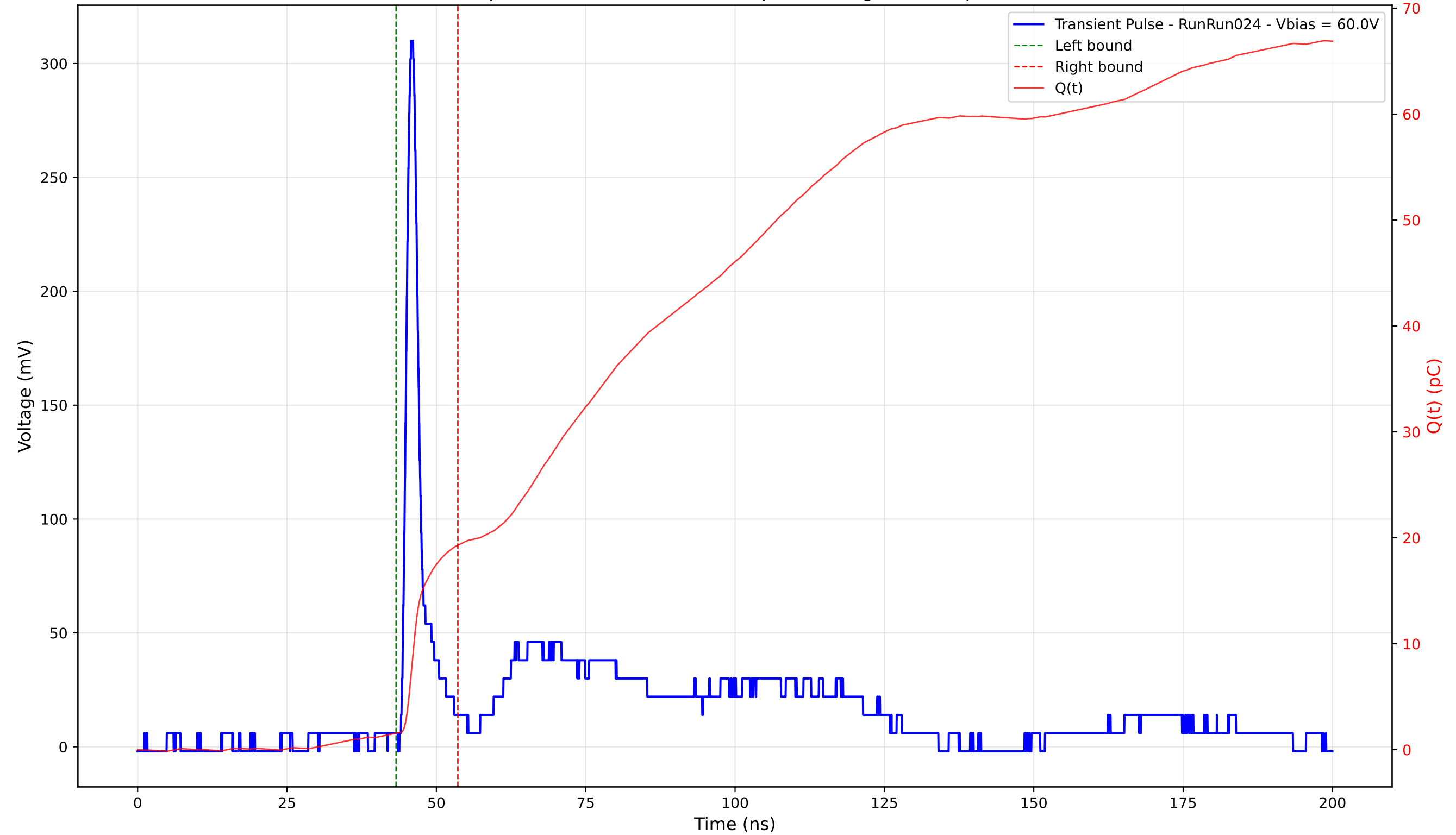
Transient Pulse - Sample: 4003 - Position: 165.0 \mu\text{m} - Charge: 17.74 pC - Rise Time: 1.18 ns
