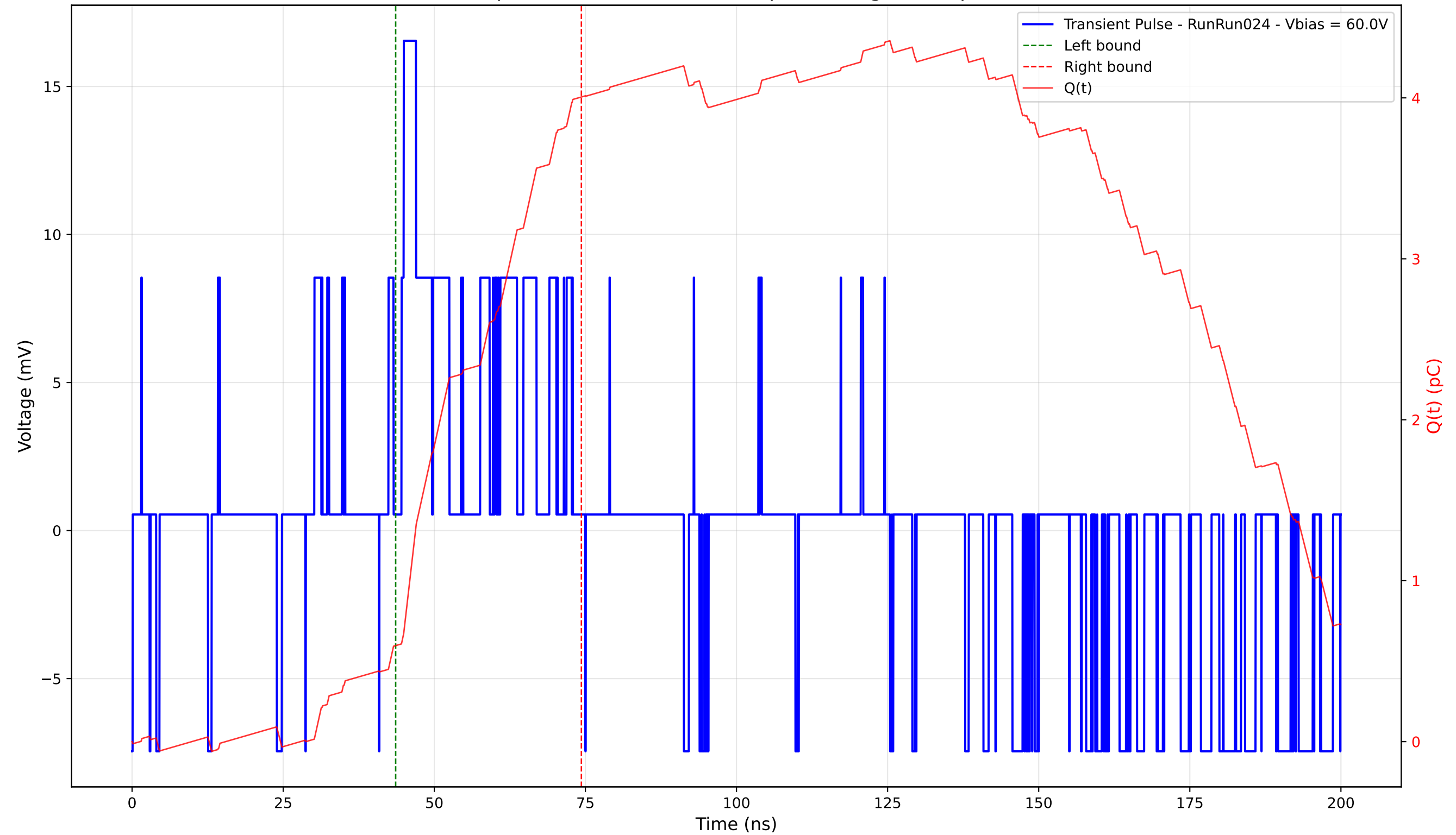
Transient Pulse - Sample: 4003 - Position: 350.0 \mu\text{m} - Charge: 3.41 pC - Rise Time: 0.38 ns
