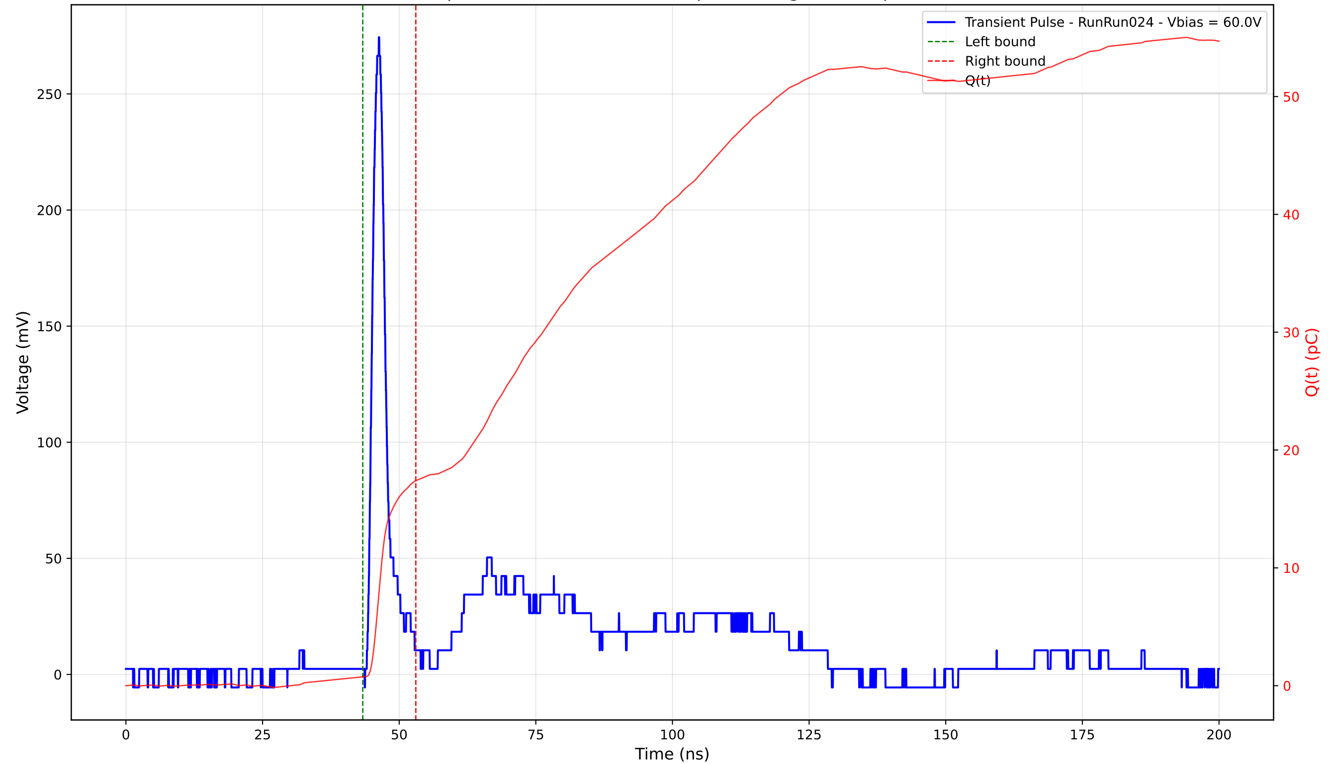
Transient Pulse - Sample: 4003 - Position: 180.0 \mu\text{m} - Charge: 16.64 pC - Rise Time: 1.38 ns
