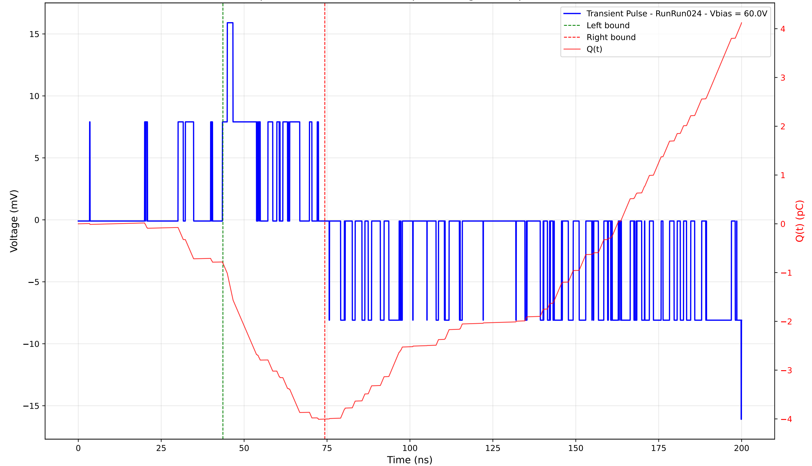
Transient Pulse - Sample: 4003 - Position: 420.0 \mu\text{m} - Charge: 3.20 pC - Rise Time: 0.00 ns (N/A)
