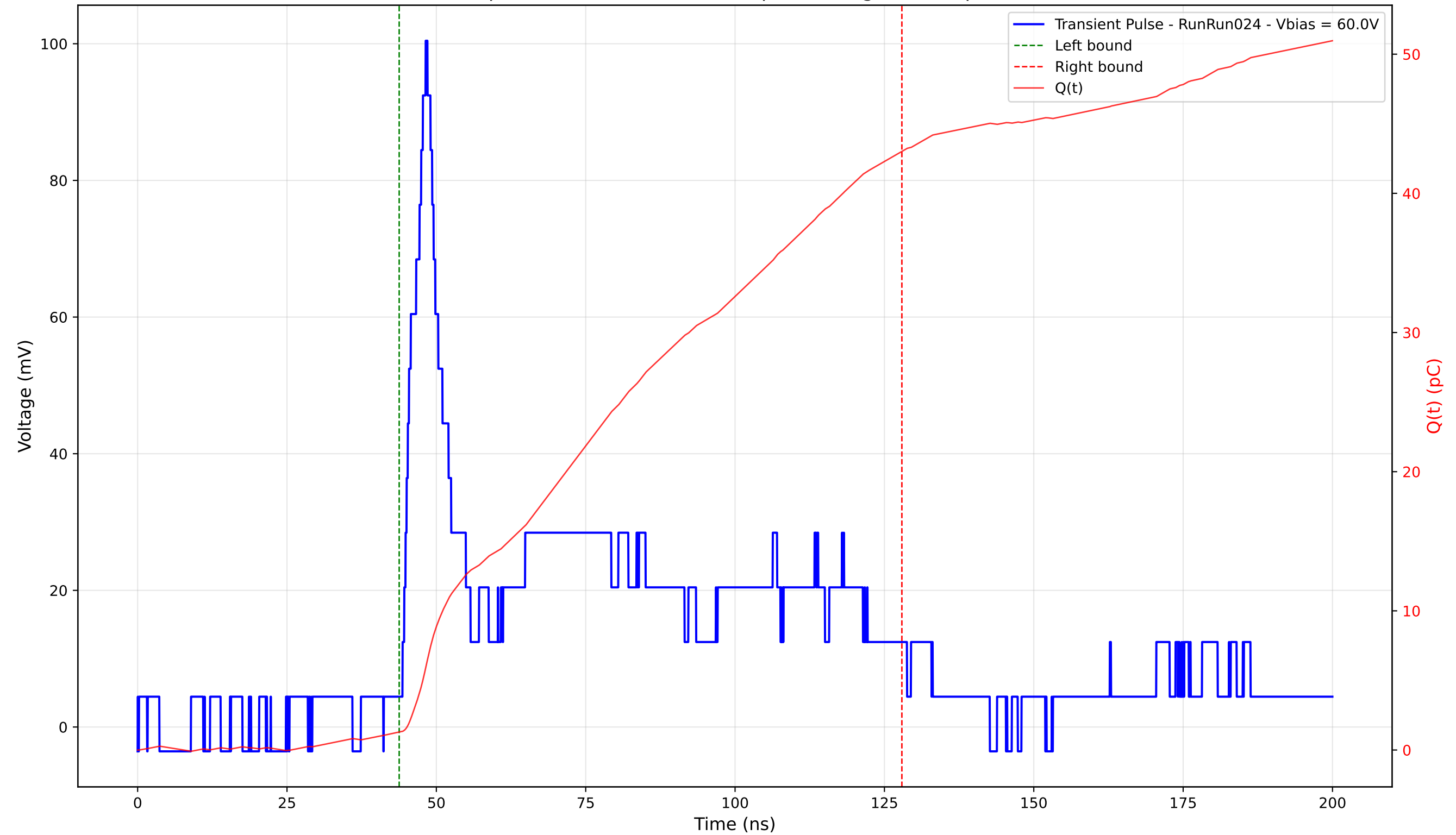
Transient Pulse - Sample: 4003 - Position: 215.0 \mu\text{m} - Charge: 41.74 pC - Rise Time: 3.41 ns
