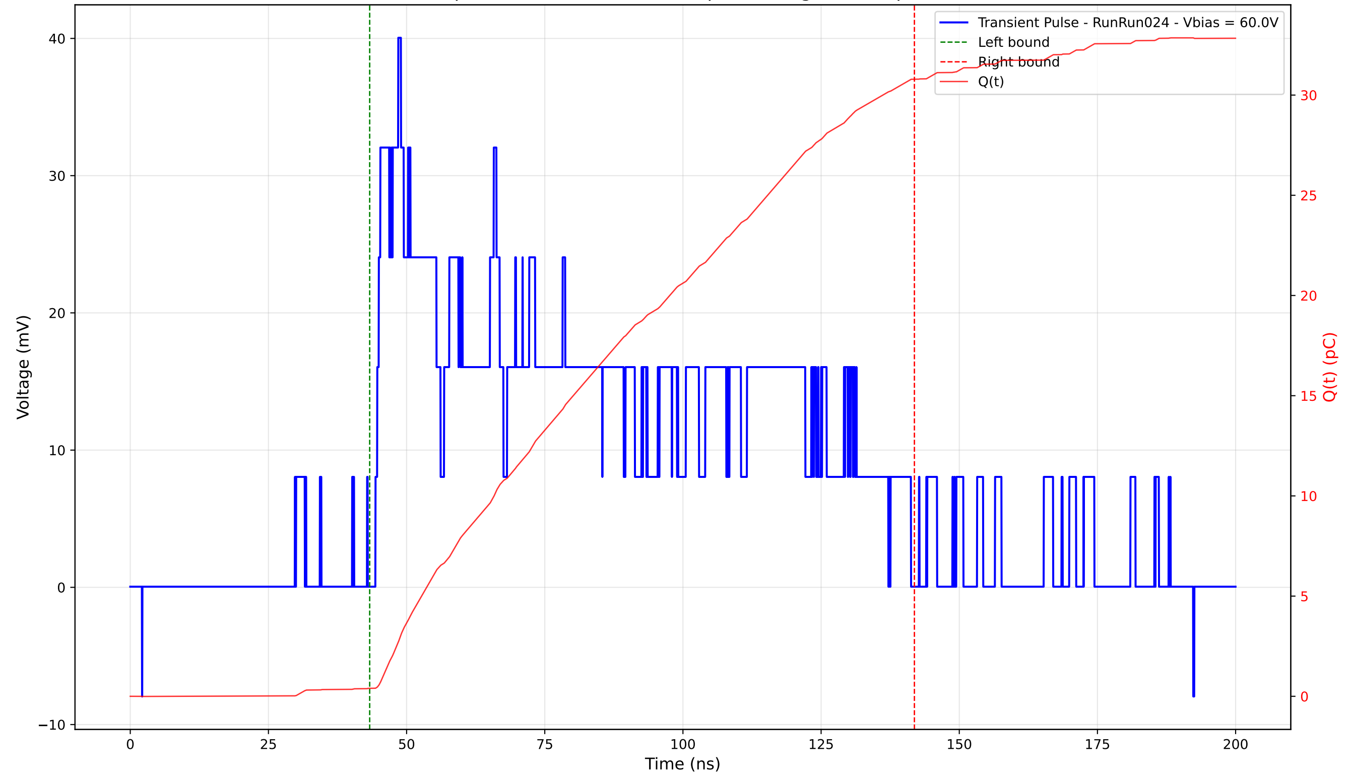
Transient Pulse - Sample: 4003 - Position: 225.0 \mu\text{m} - Charge: 30.39 pC - Rise Time: 4.13 ns
