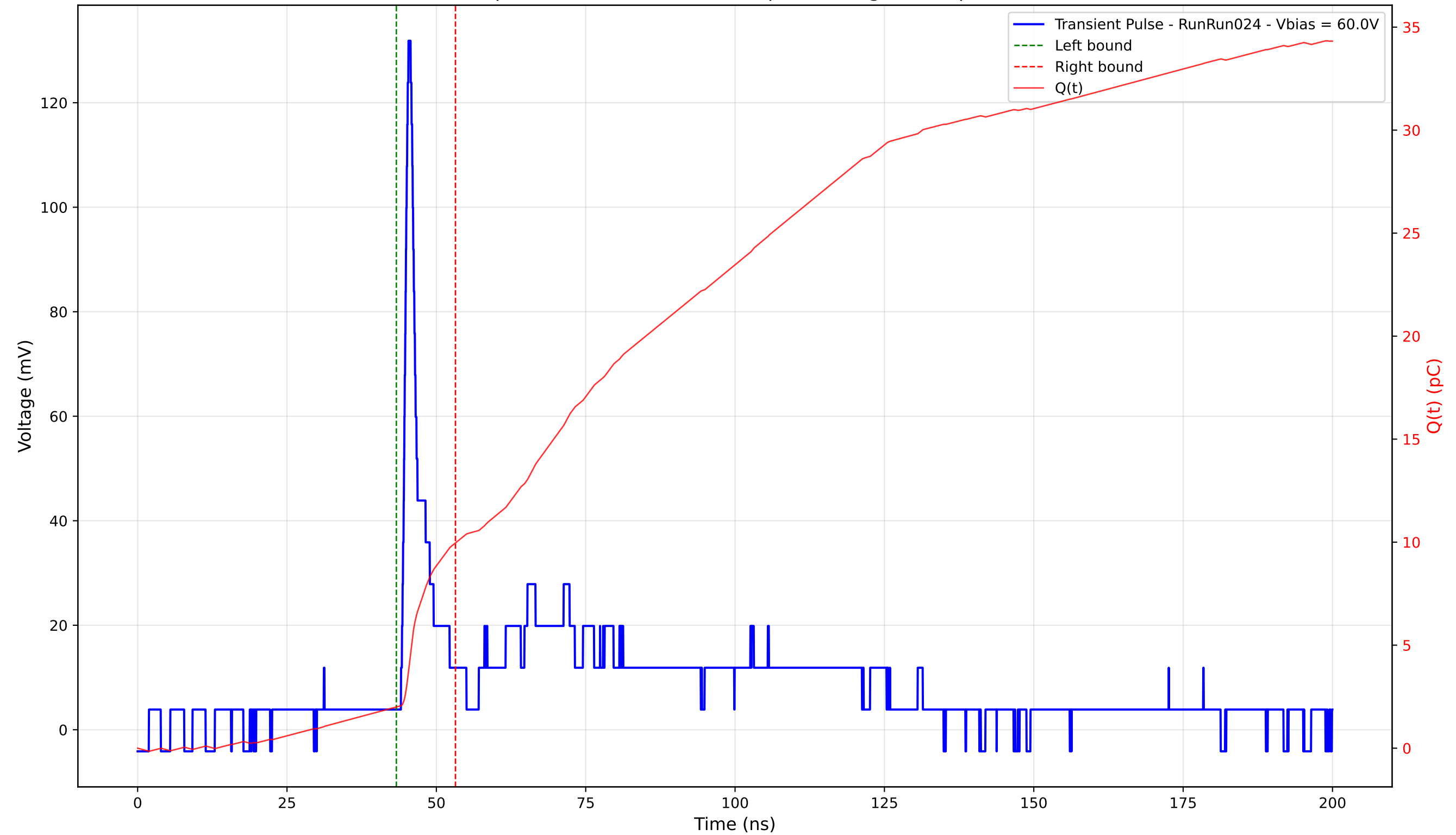
Transient Pulse - Sample: 4003 - Position: 100.0 \mu\text{m} - Charge: 7.97 pC - Rise Time: 0.98 ns
