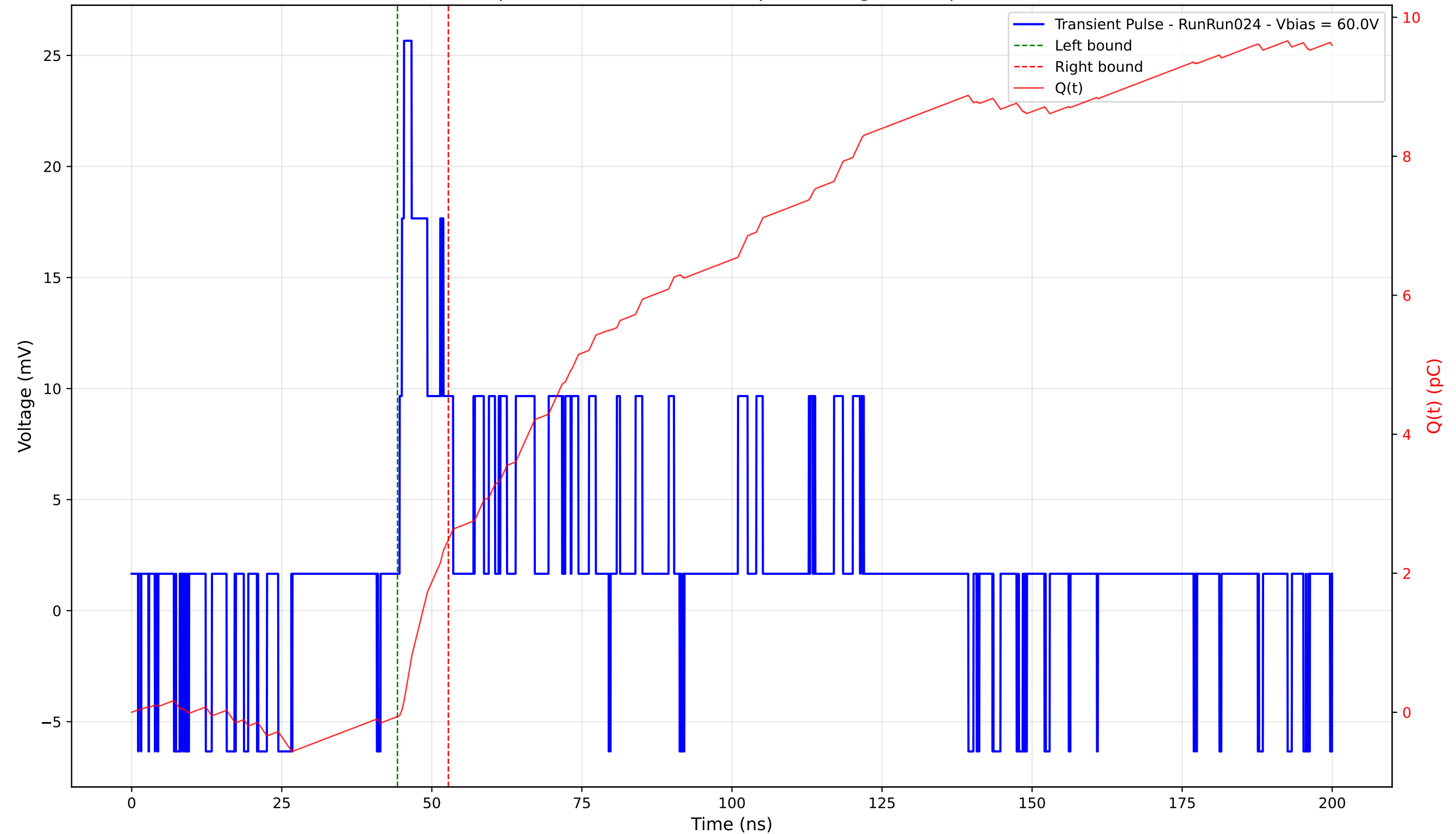
Transient Pulse - Sample: 4003 - Position: 55.0 \mu\text{m} - Charge: 2.55 pC - Rise Time: 0.74 ns
