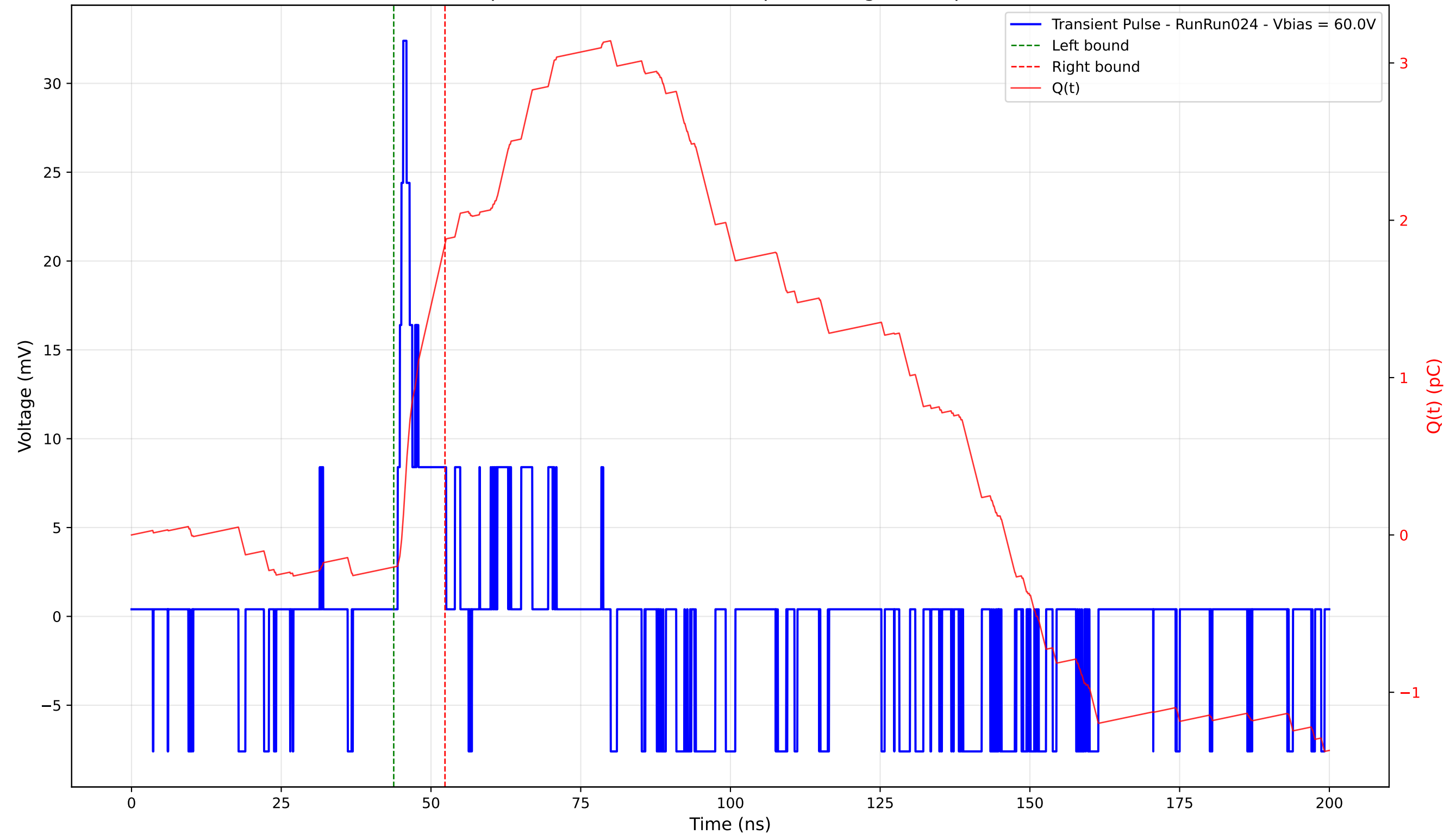
Transient Pulse - Sample: 4003 - Position: 400.0 \mu\text{m} - Charge: 2.05 pC - Rise Time: 0.93 ns
