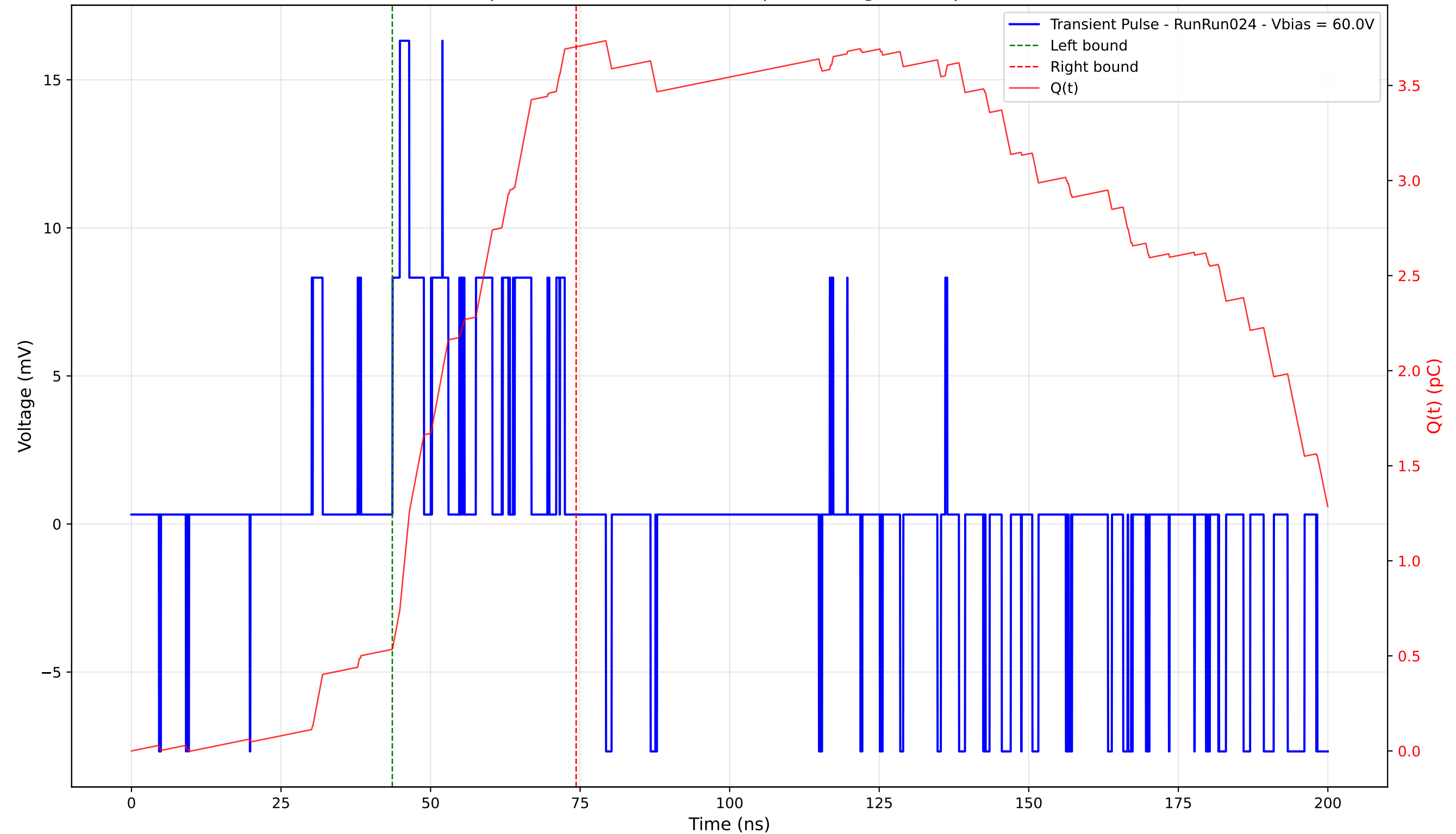
Transient Pulse - Sample: 4003 - Position: 360.0 \mu\text{m} - Charge: 3.17 pC - Rise Time: 1.24 ns
