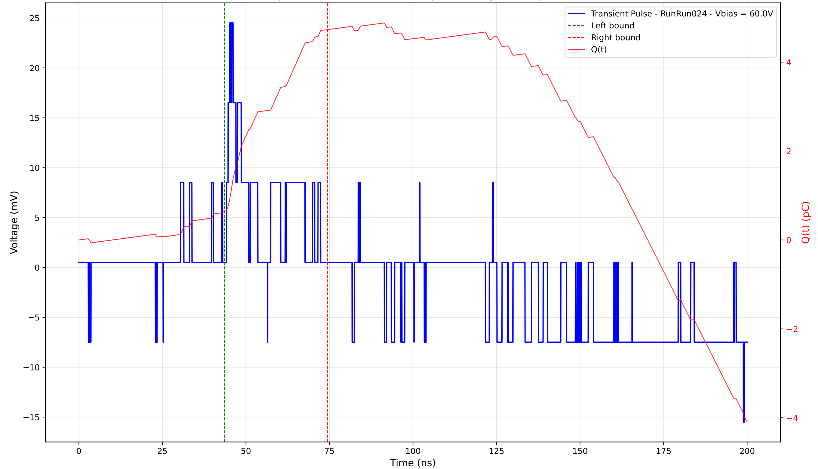
Transient Pulse - Sample: 4003 - Position: 320.0 \mu\text{m} - Charge: 4.08 pC - Rise Time: 1.04 ns
