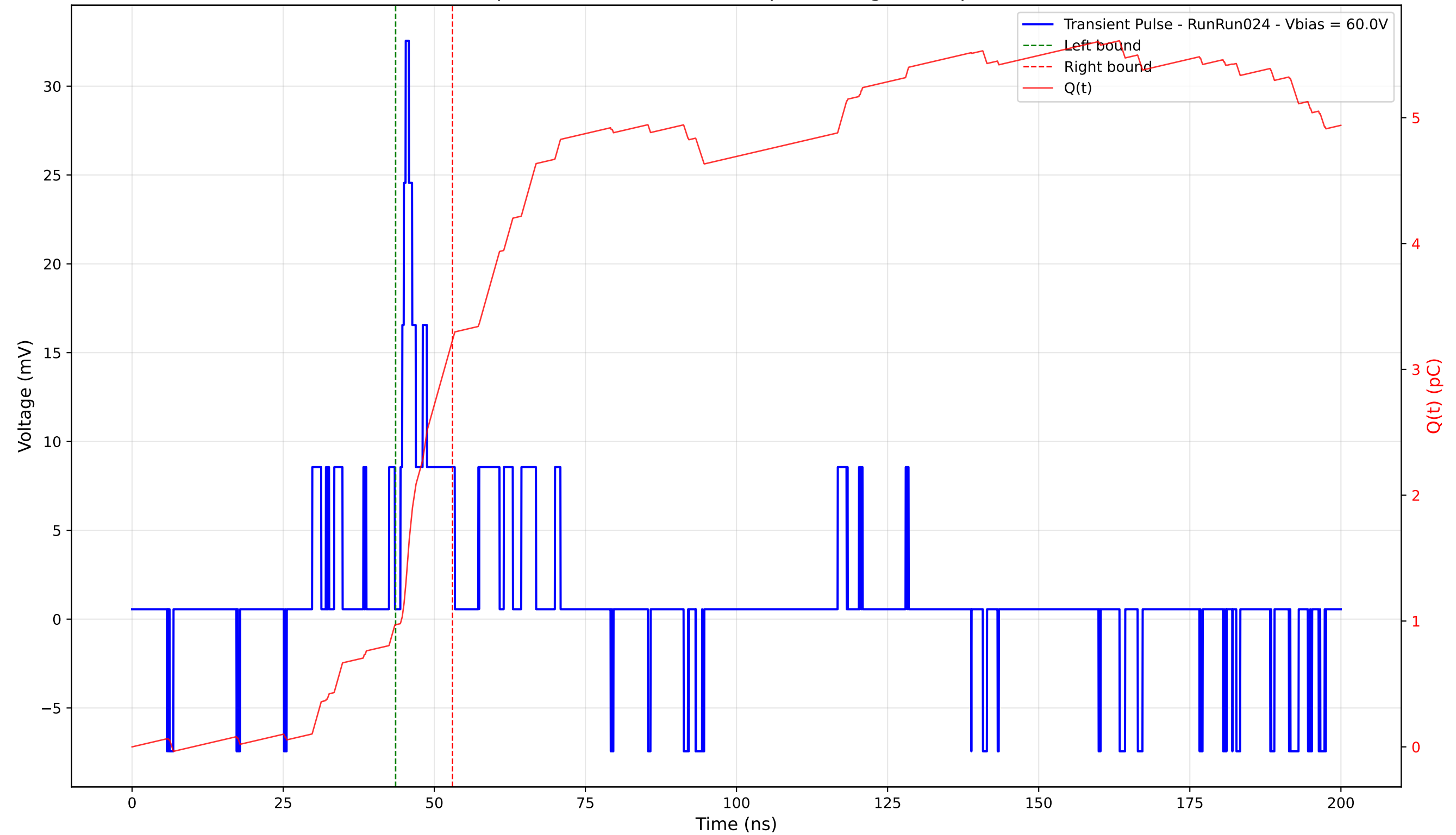
Transient Pulse - Sample: 4003 - Position: 305.0 \mu\text{m} - Charge: 2.26 pC - Rise Time: 0.87 ns
