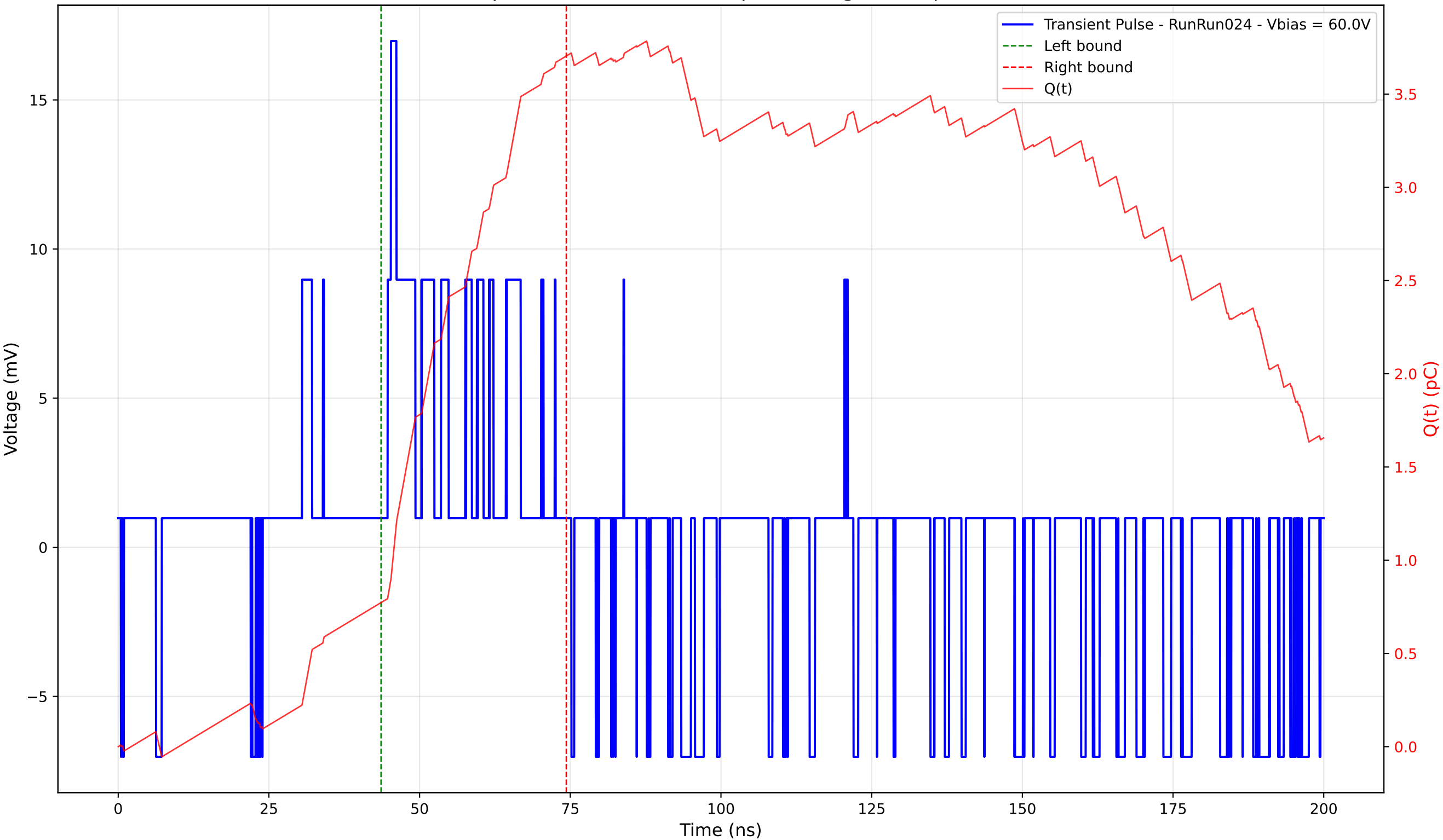
Transient Pulse - Sample: 4003 - Position: 0.0 \mu\text{m} - Charge: 2.93 pC - Rise Time: 0.56 ns
