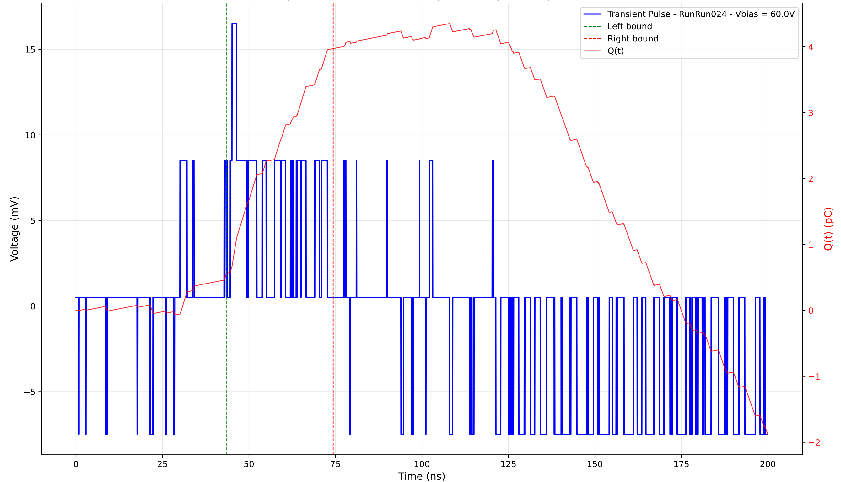
Transient Pulse - Sample: 4003 - Position: 25.0 \mu\text{m} - Charge: 3.41 pC - Rise Time: 0.54 ns
