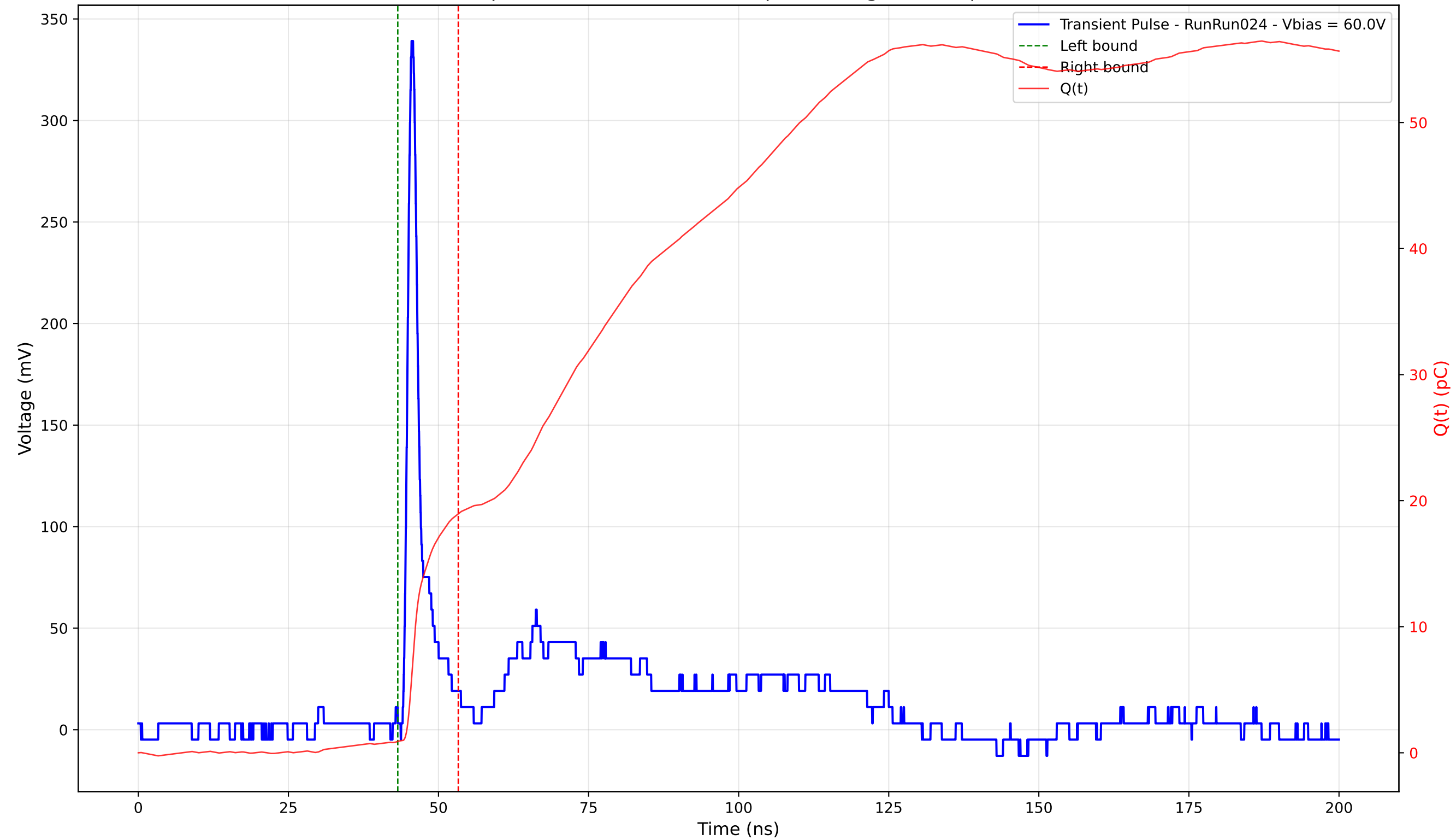
Transient Pulse - Sample: 4003 - Position: 140.0 \mu\text{m} - Charge: 18.05 pC - Rise Time: 1.04 ns
