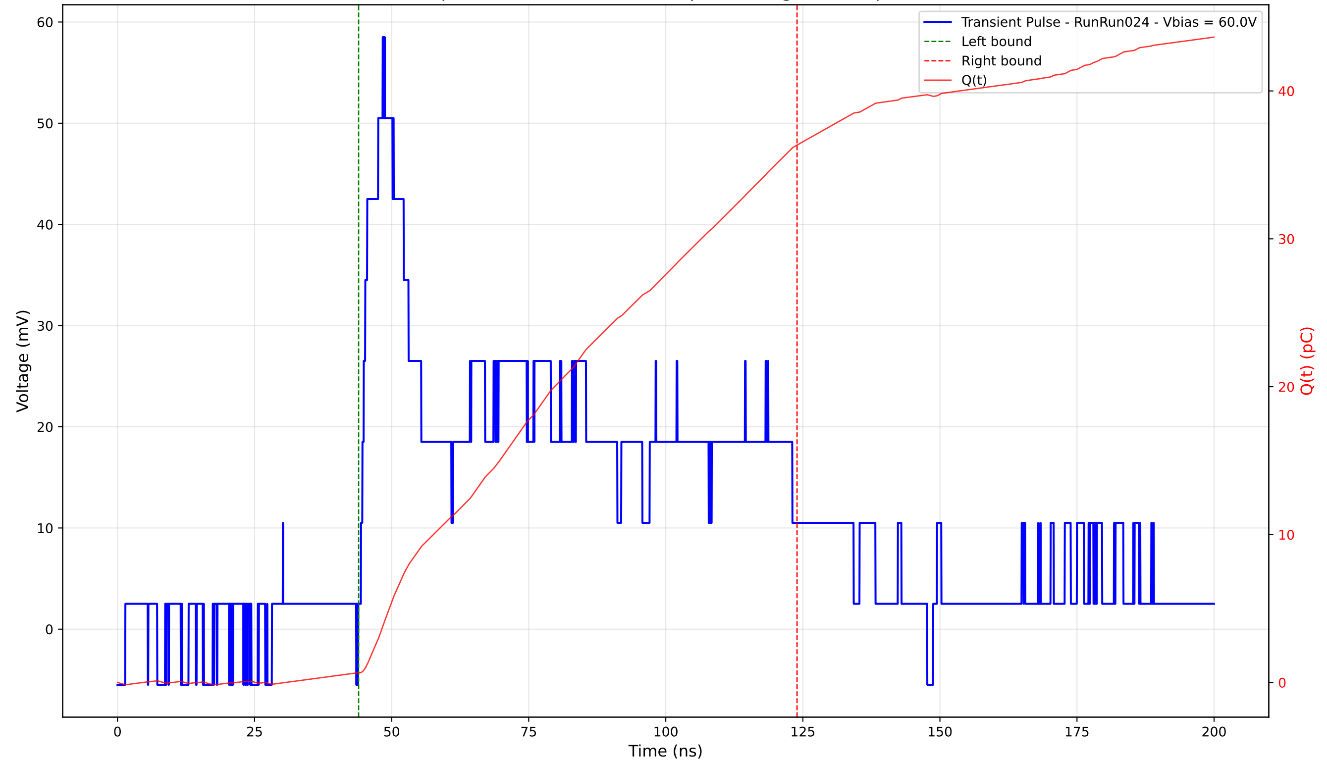
Transient Pulse - Sample: 4003 - Position: 220.0 \mu\text{m} - Charge: 35.69 pC - Rise Time: 3.97 ns
