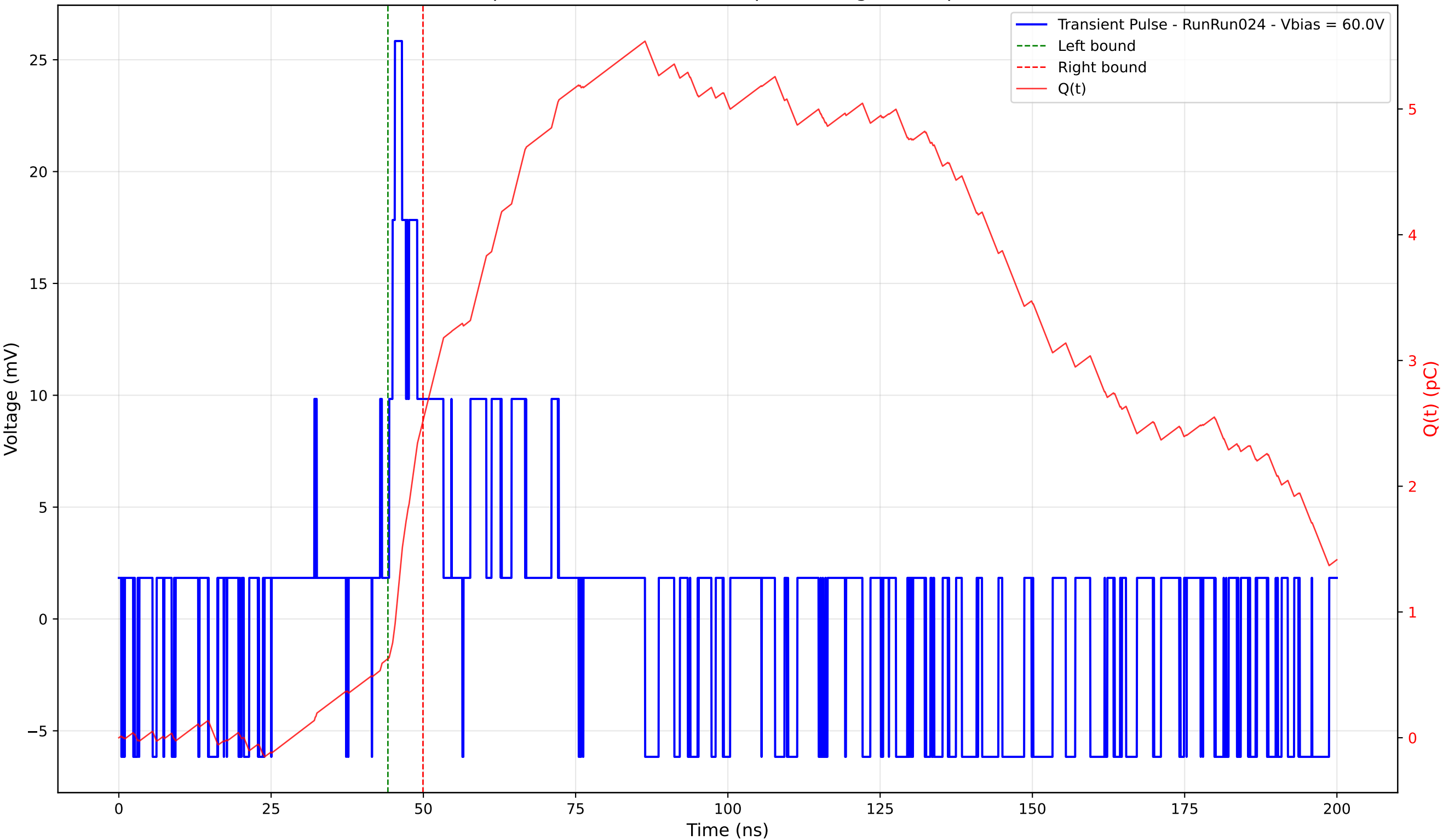
Transient Pulse - Sample: 4003 - Position: 50.0 \mu\text{m} - Charge: 1.89 pC - Rise Time: 0.96 ns
