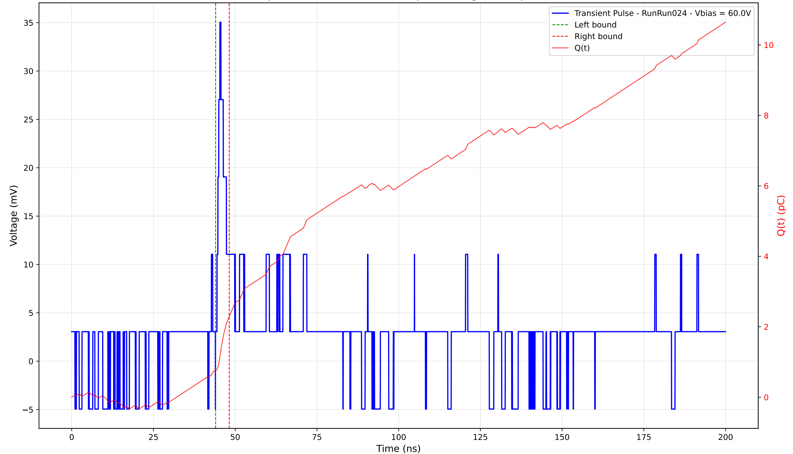
Transient Pulse - Sample: 4003 - Position: 280.0 \mu\text{m} - Charge: 1.53 pC - Rise Time: 0.90 ns
