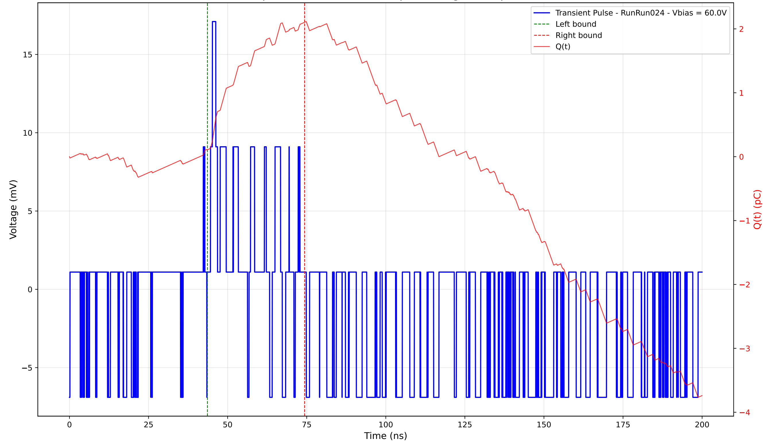
Transient Pulse - Sample: 4003 - Position: 15.0 \mu\text{m} - Charge: 1.99 pC - Rise Time: 0.62 ns
