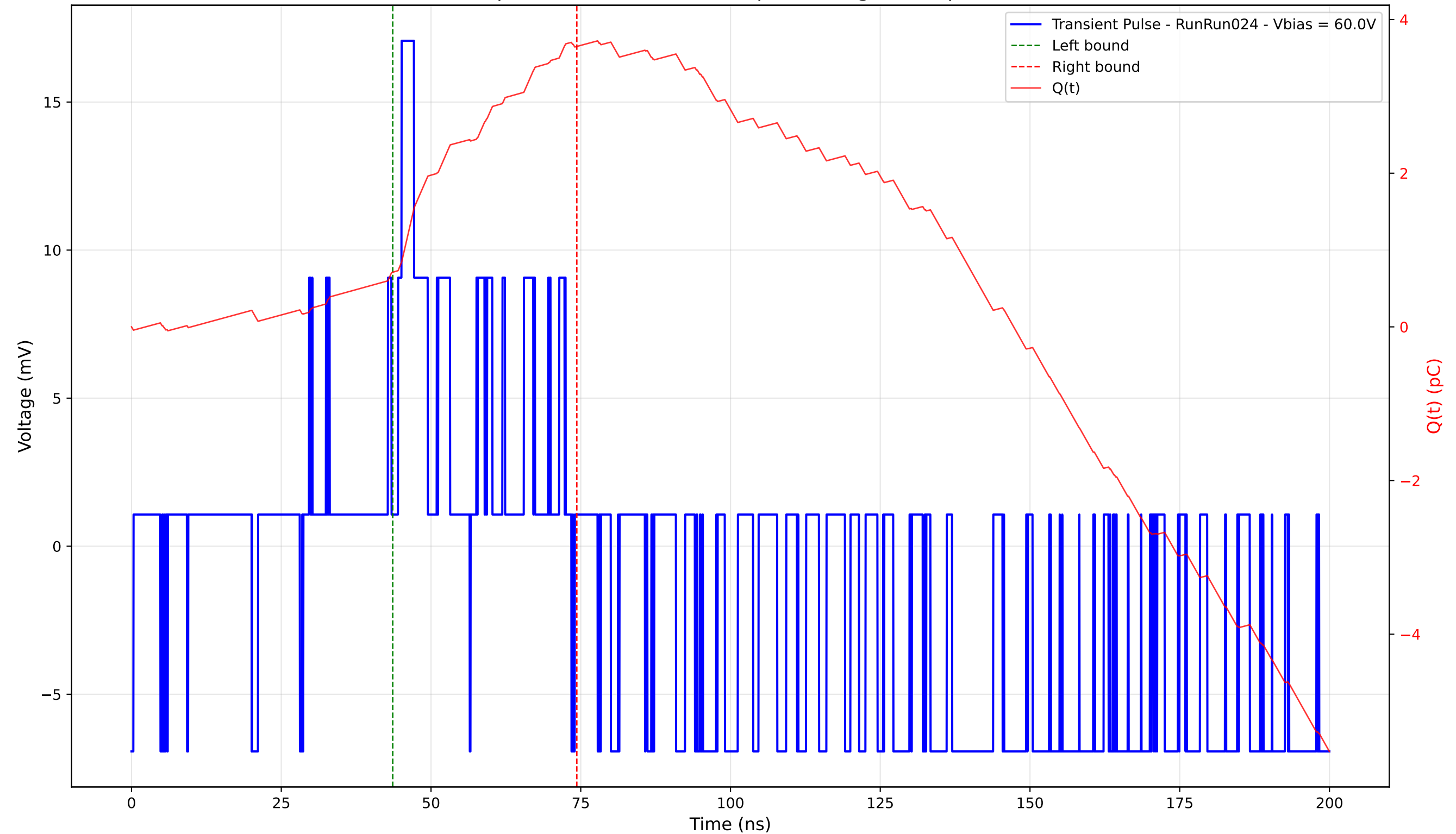
Transient Pulse - Sample: 4003 - Position: 40.0 \mu\text{m} - Charge: 2.94 pC - Rise Time: 0.60 ns
