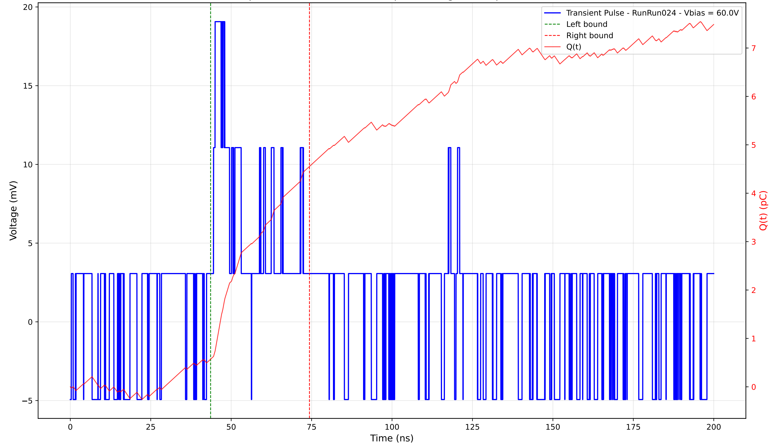
Transient Pulse - Sample: 4003 - Position: 325.0 \mu\text{m} - Charge: 3.98 pC - Rise Time: 0.00 ns (N/A)
