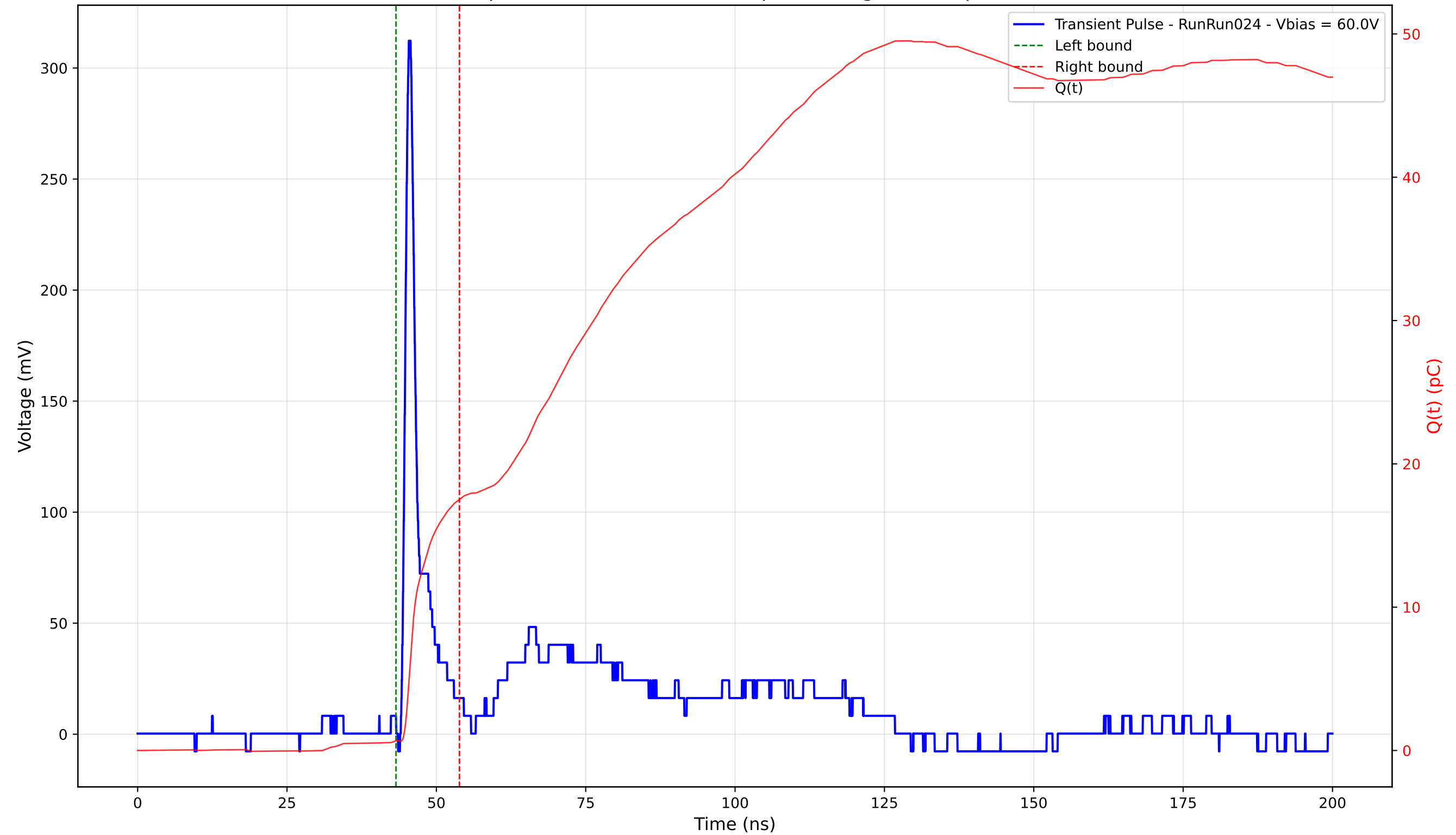
Transient Pulse - Sample: 4003 - Position: 120.0 \mu\text{m} - Charge: 16.83 pC - Rise Time: 0.96 ns
