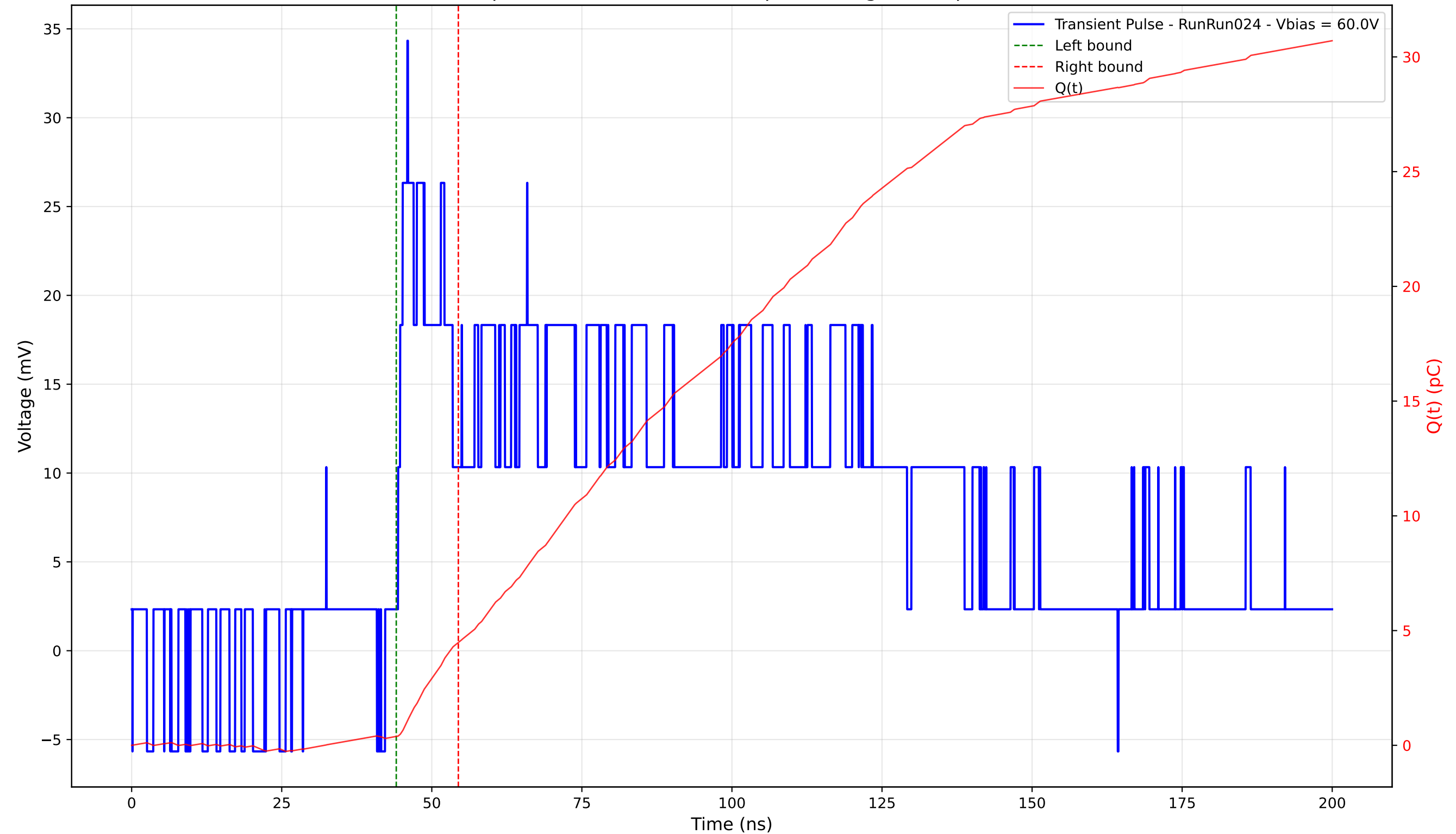
Transient Pulse - Sample: 4003 - Position: 230.0 \mu\text{m} - Charge: 4.09 pC - Rise Time: 1.56 ns
