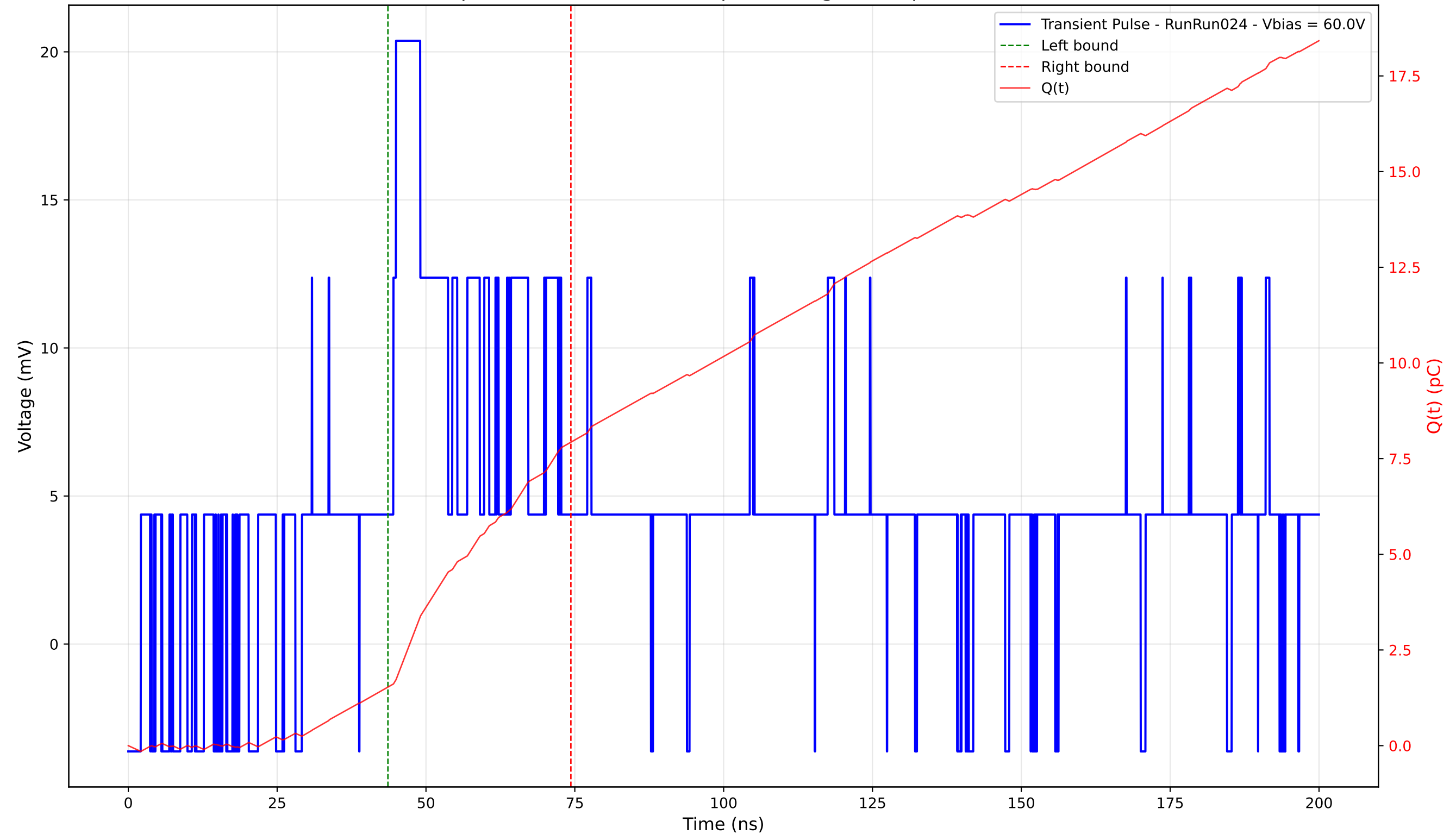
Transient Pulse - Sample: 4003 - Position: 65.0 \mu\text{m} - Charge: 6.40 pC - Rise Time: 0.00 ns (N/A)
