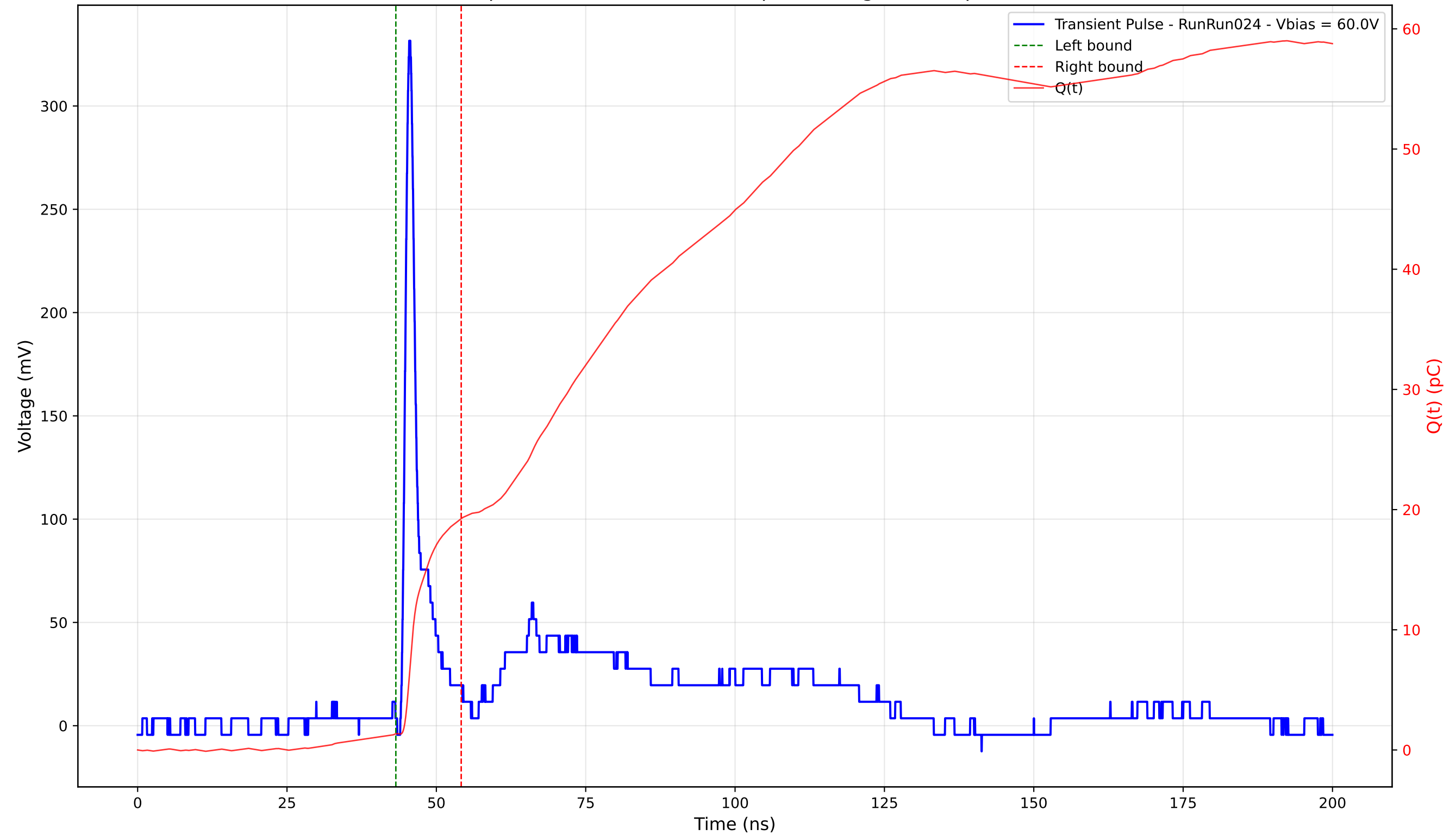
Transient Pulse - Sample: 4003 - Position: 125.0 \mu\text{m} - Charge: 17.91 pC - Rise Time: 0.97 ns
