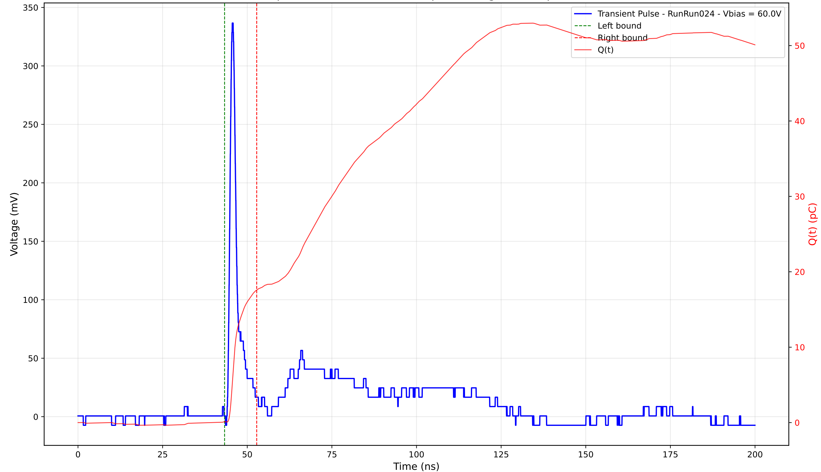
Transient Pulse - Sample: 4003 - Position: 145.0 \mu\text{m} - Charge: 17.47 pC - Rise Time: 1.00 ns
