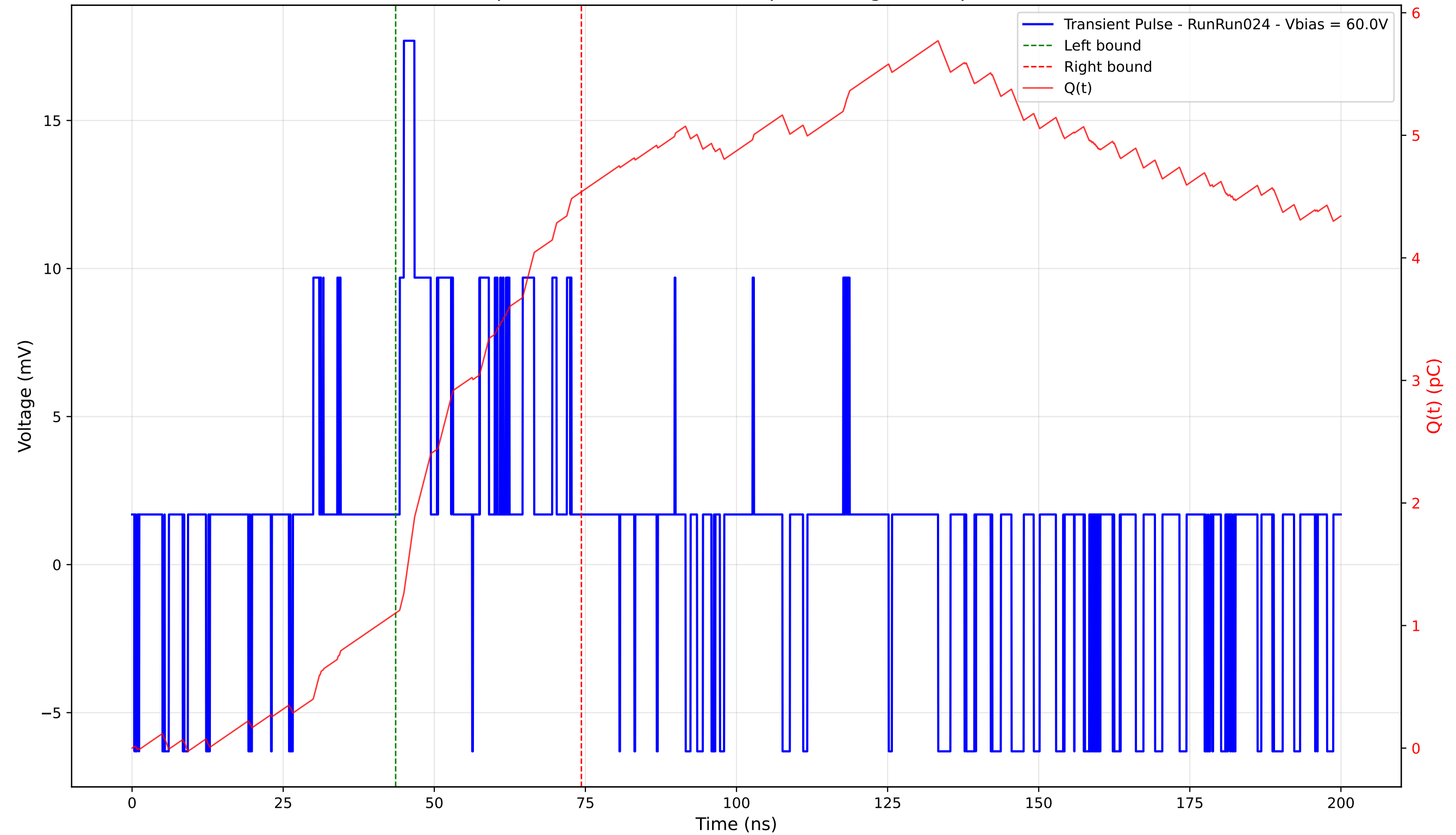
Transient Pulse - Sample: 4003 - Position: 355.0 \mu\text{m} - Charge: 3.44 pC - Rise Time: 0.70 ns
