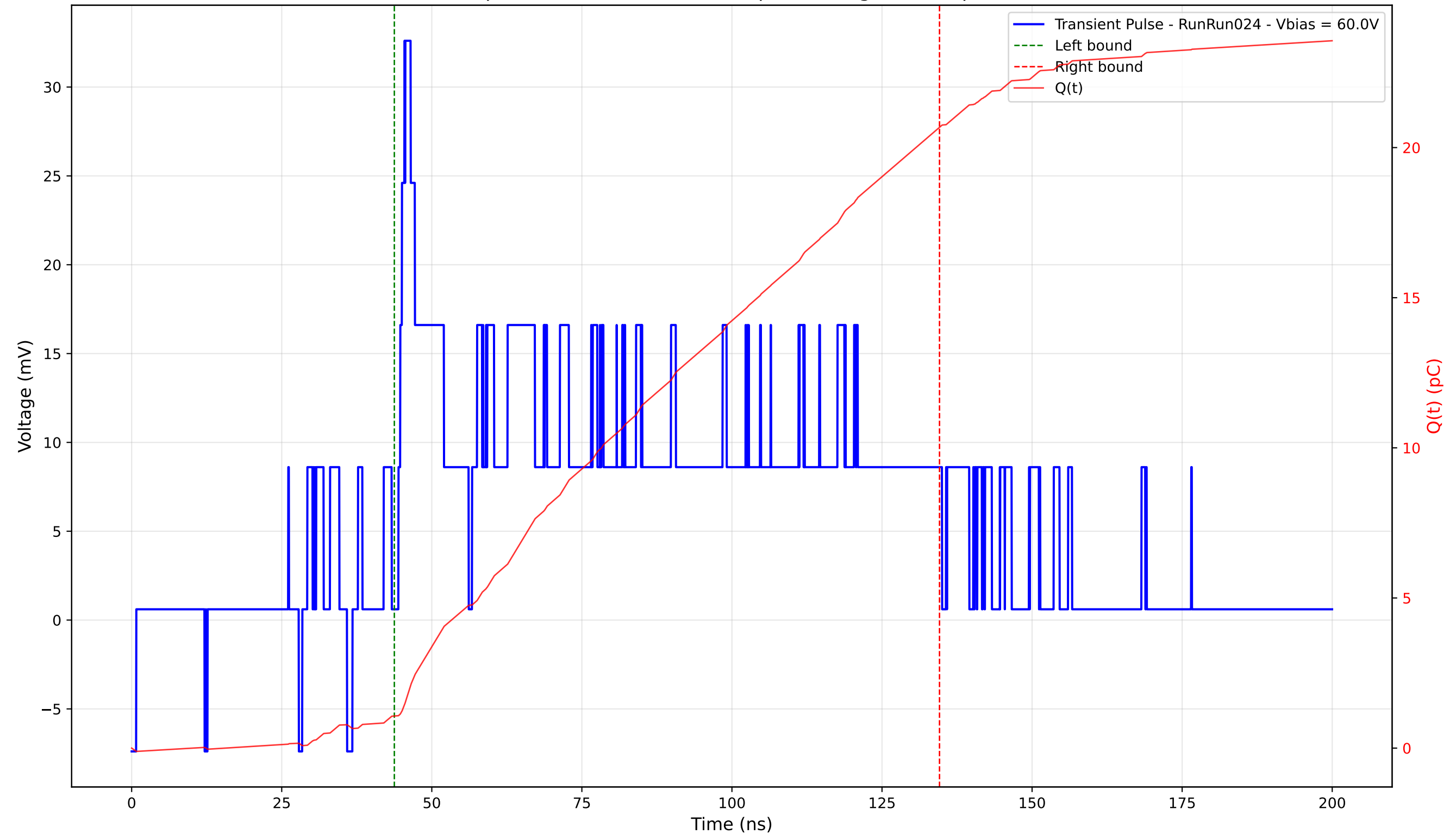
Transient Pulse - Sample: 4003 - Position: 235.0 \mu\text{m} - Charge: 19.61 pC - Rise Time: 1.01 ns
