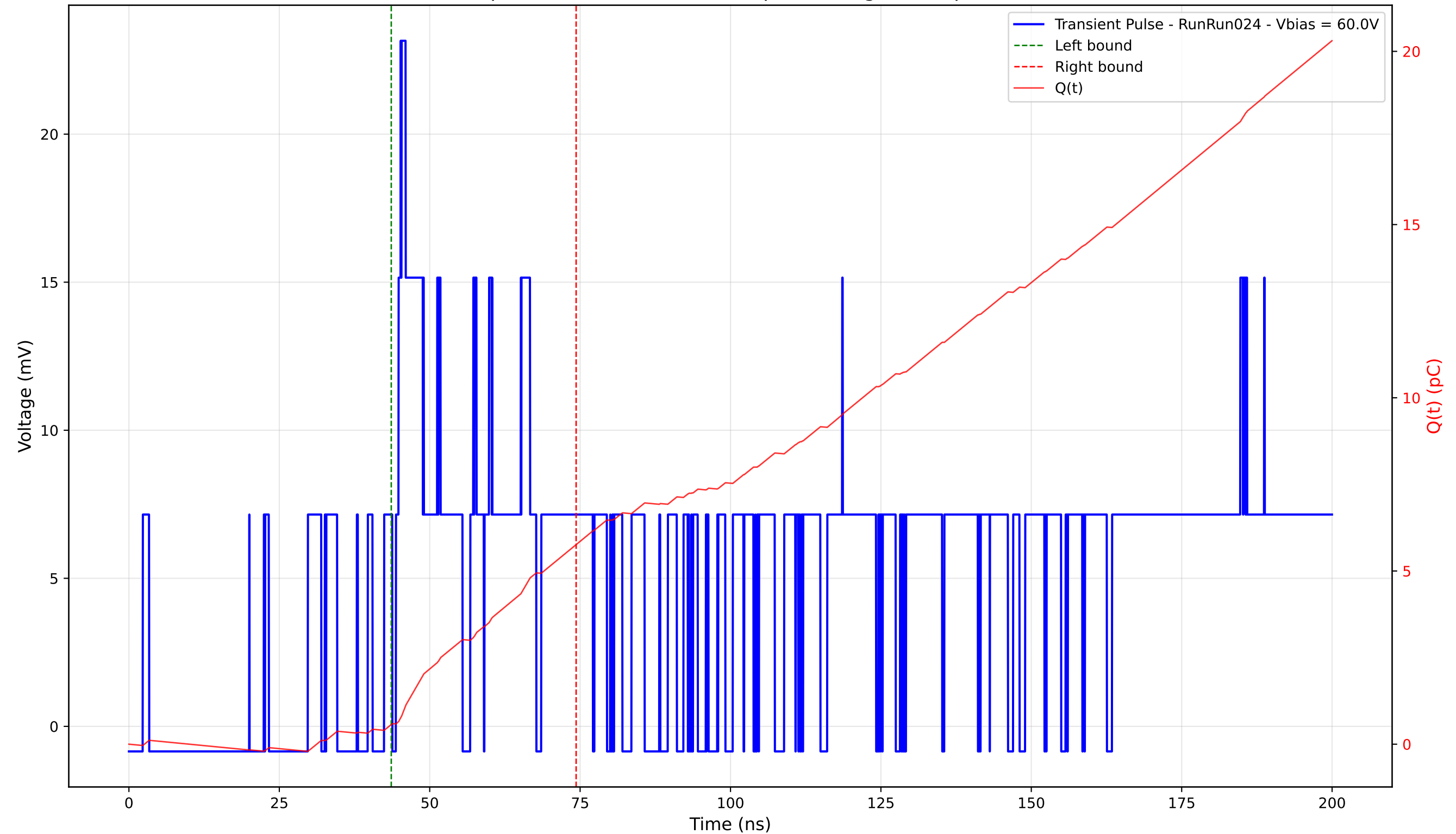
Transient Pulse - Sample: 4003 - Position: 340.0 \mu\text{m} - Charge: 5.19 pC - Rise Time: 0.82 ns
