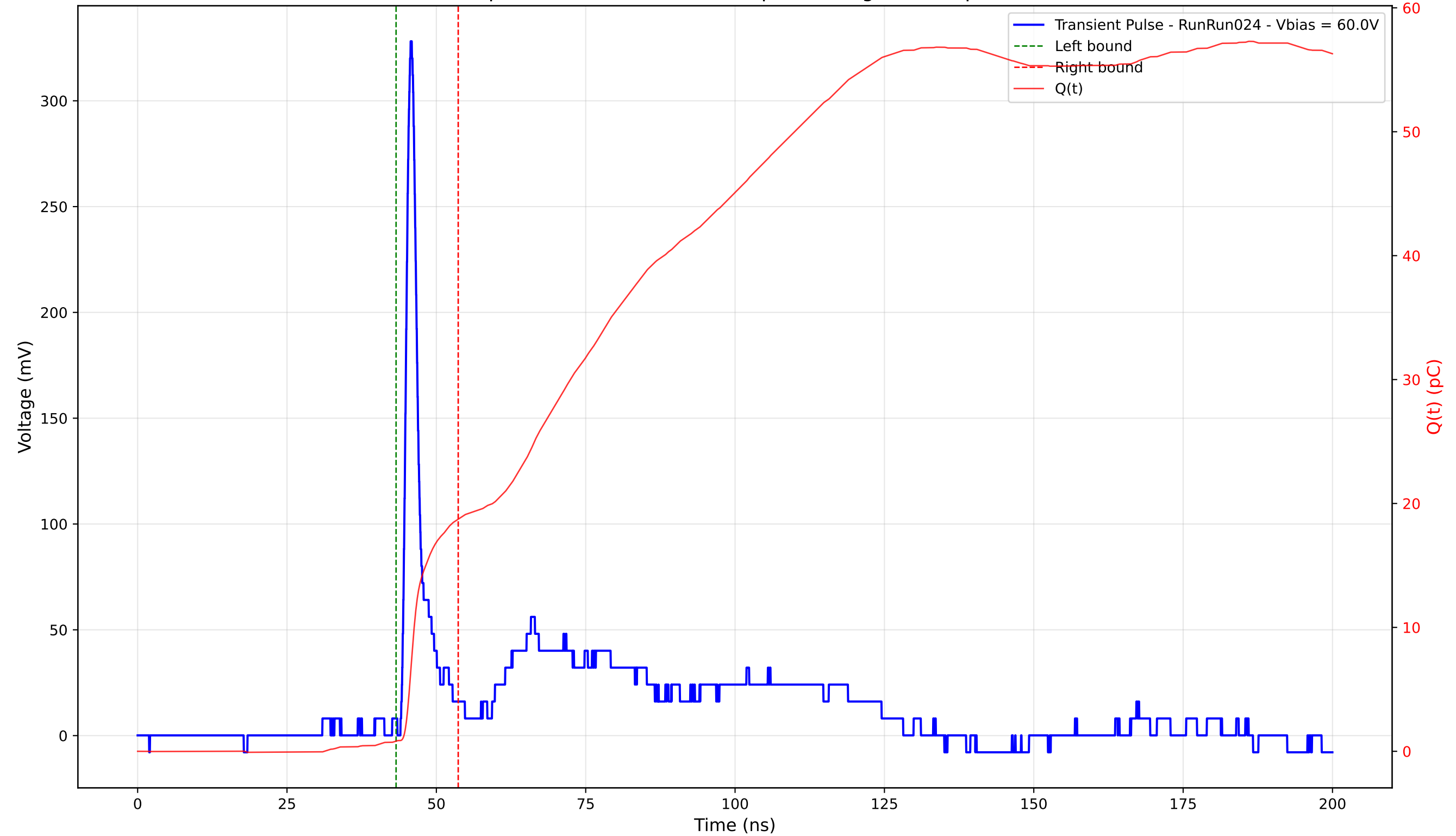
Transient Pulse - Sample: 4003 - Position: 155.0 \mu\text{m} - Charge: 17.91 pC - Rise Time: 1.08 ns
