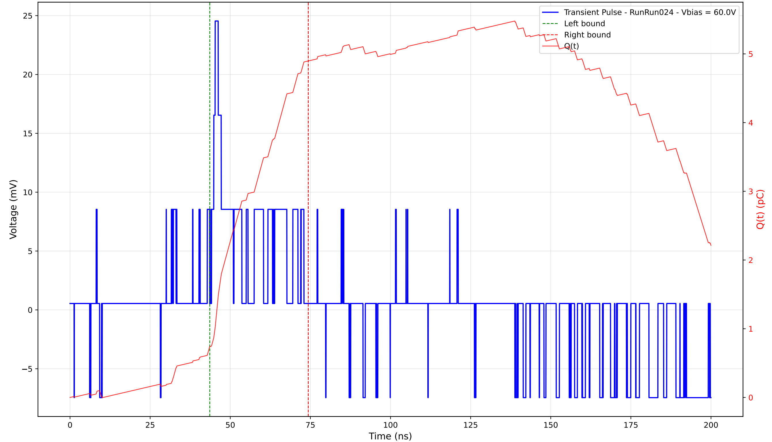
Transient Pulse - Sample: 4003 - Position: 380.0 \mu\text{m} - Charge: 4.16 pC - Rise Time: 1.14 ns
