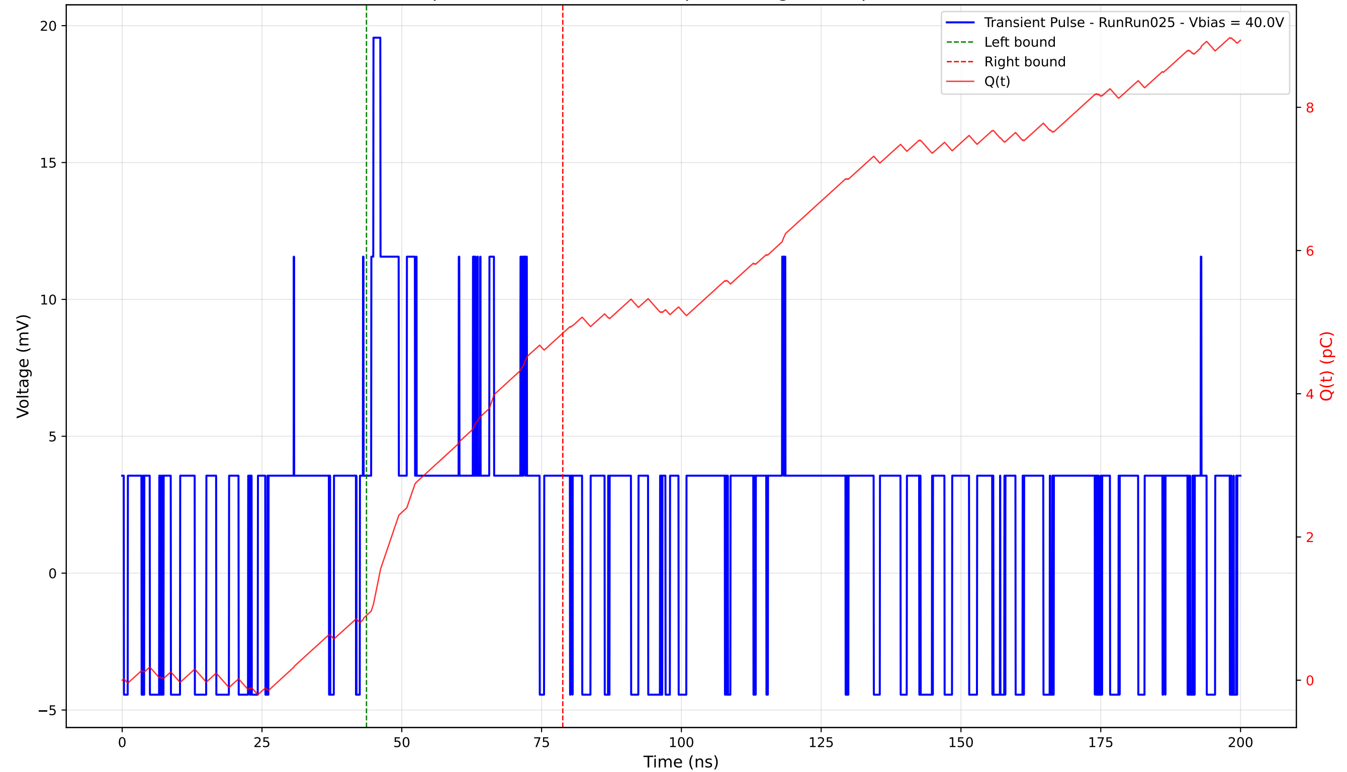
Transient Pulse - Sample: 4003 - Position: 405.0 \mu\text{m} - Charge: 3.94 pC - Rise Time: 0.00 ns (N/A)
