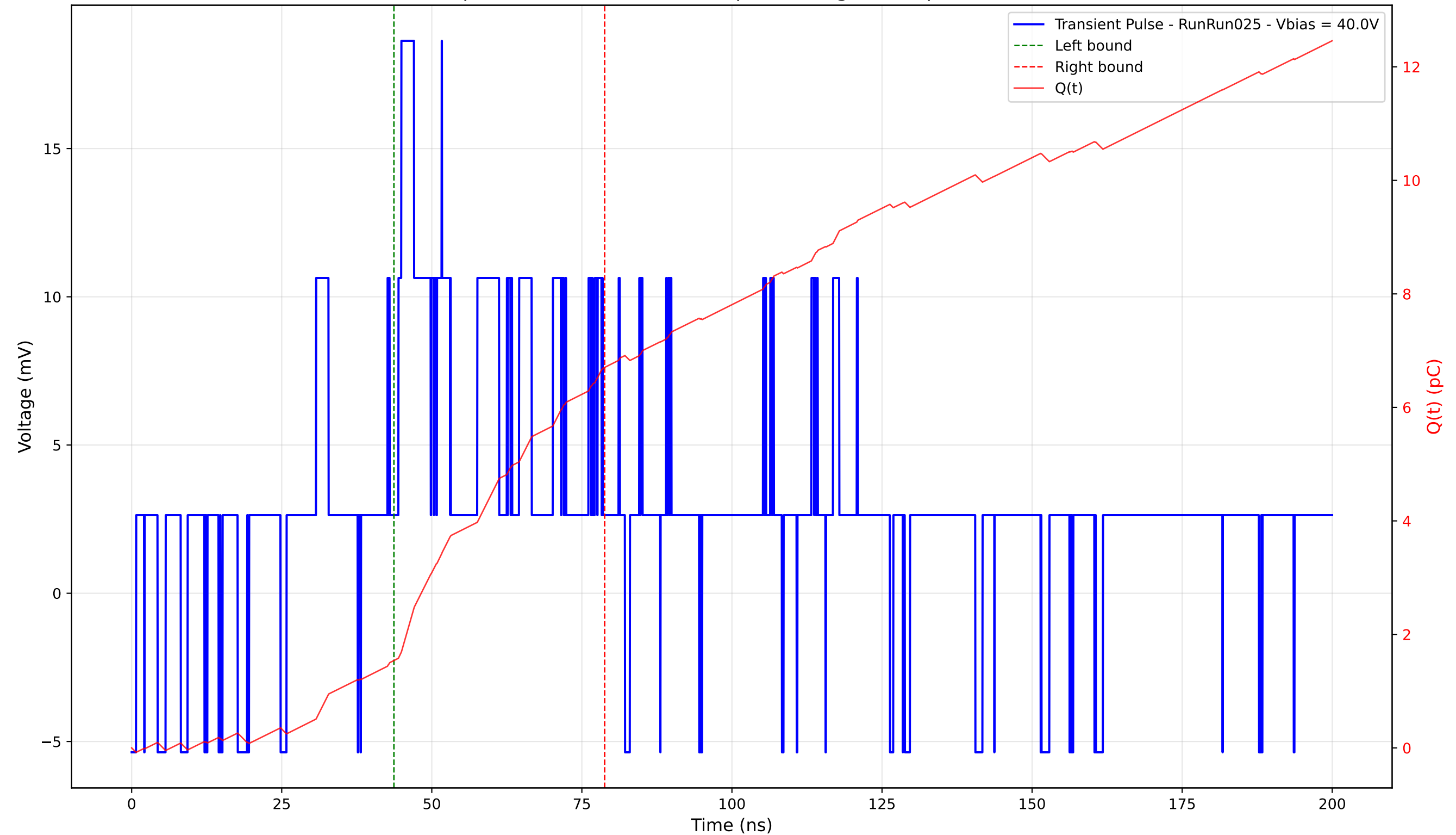
Transient Pulse - Sample: 4003 - Position: 385.0 \mu\text{m} - Charge: 5.16 pC - Rise Time: 0.00 ns (N/A)
