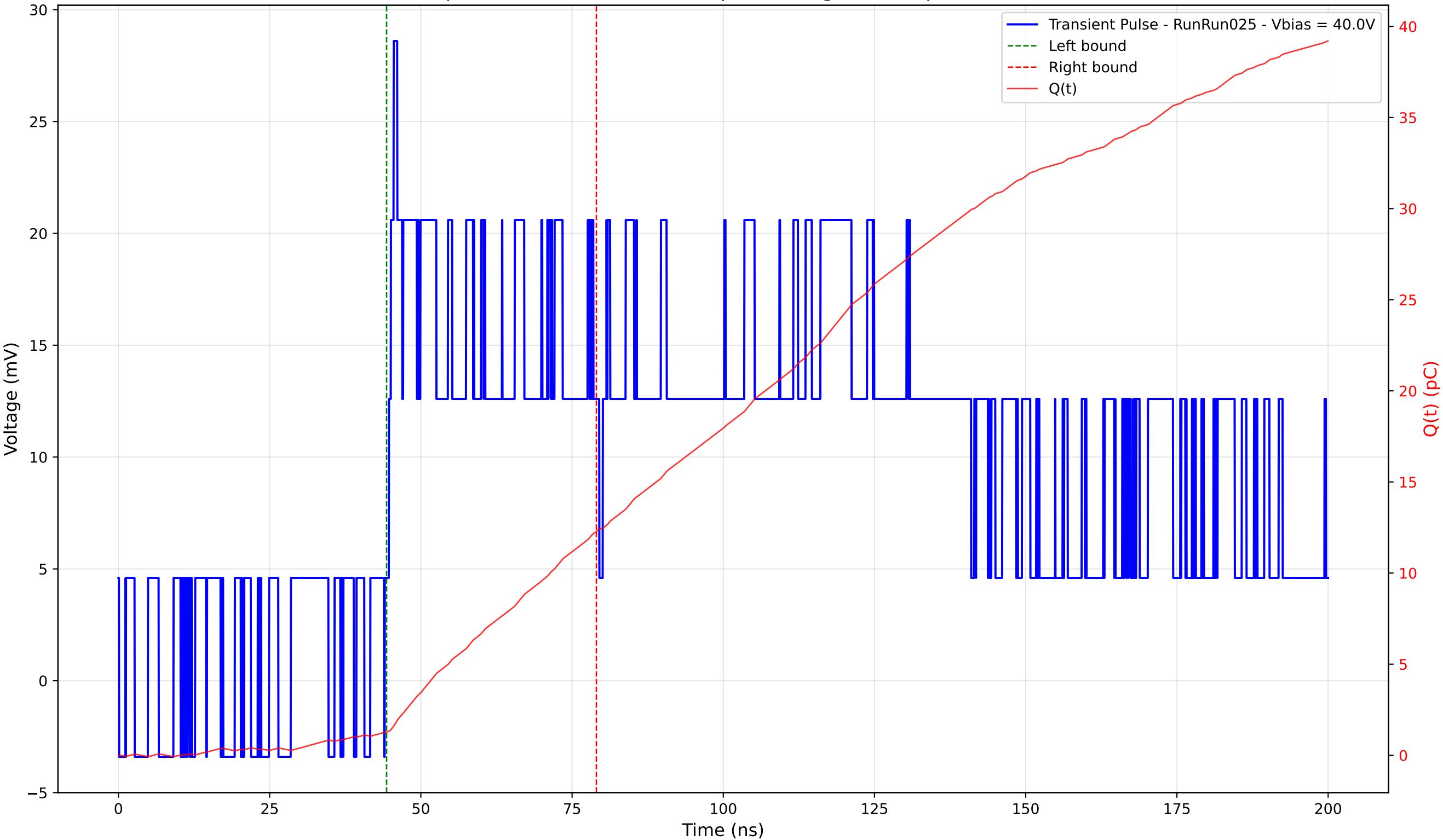
Transient Pulse - Sample: 4003 - Position: 205.0 \mu\text{m} - Charge: 11.01 pC - Rise Time: 0.00 ns (N/A)
