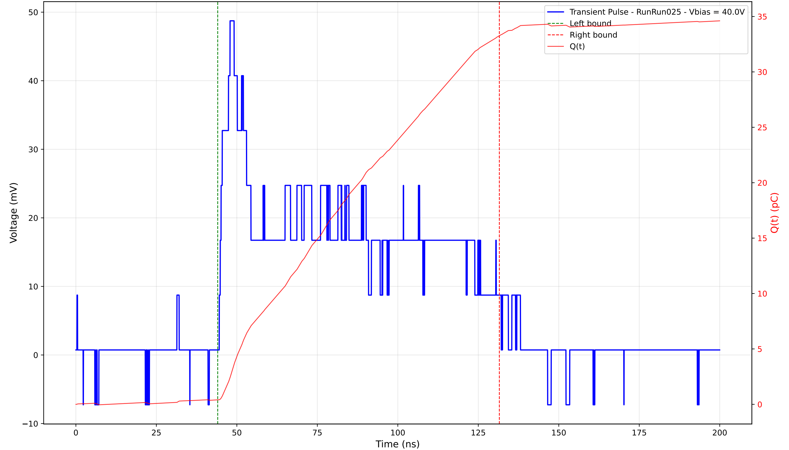
Transient Pulse - Sample: 4003 - Position: 195.0 \mu\text{m} - Charge: 32.87 pC - Rise Time: 3.35 ns
