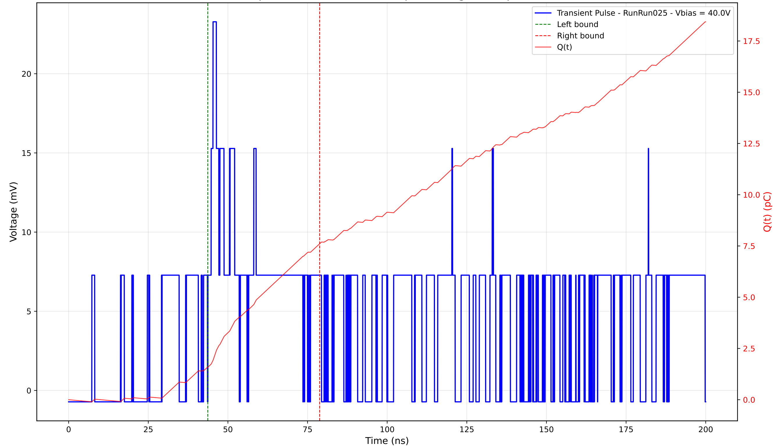
Transient Pulse - Sample: 4003 - Position: 365.0 \mu\text{m} - Charge: 6.03 pC - Rise Time: 1.62 ns
