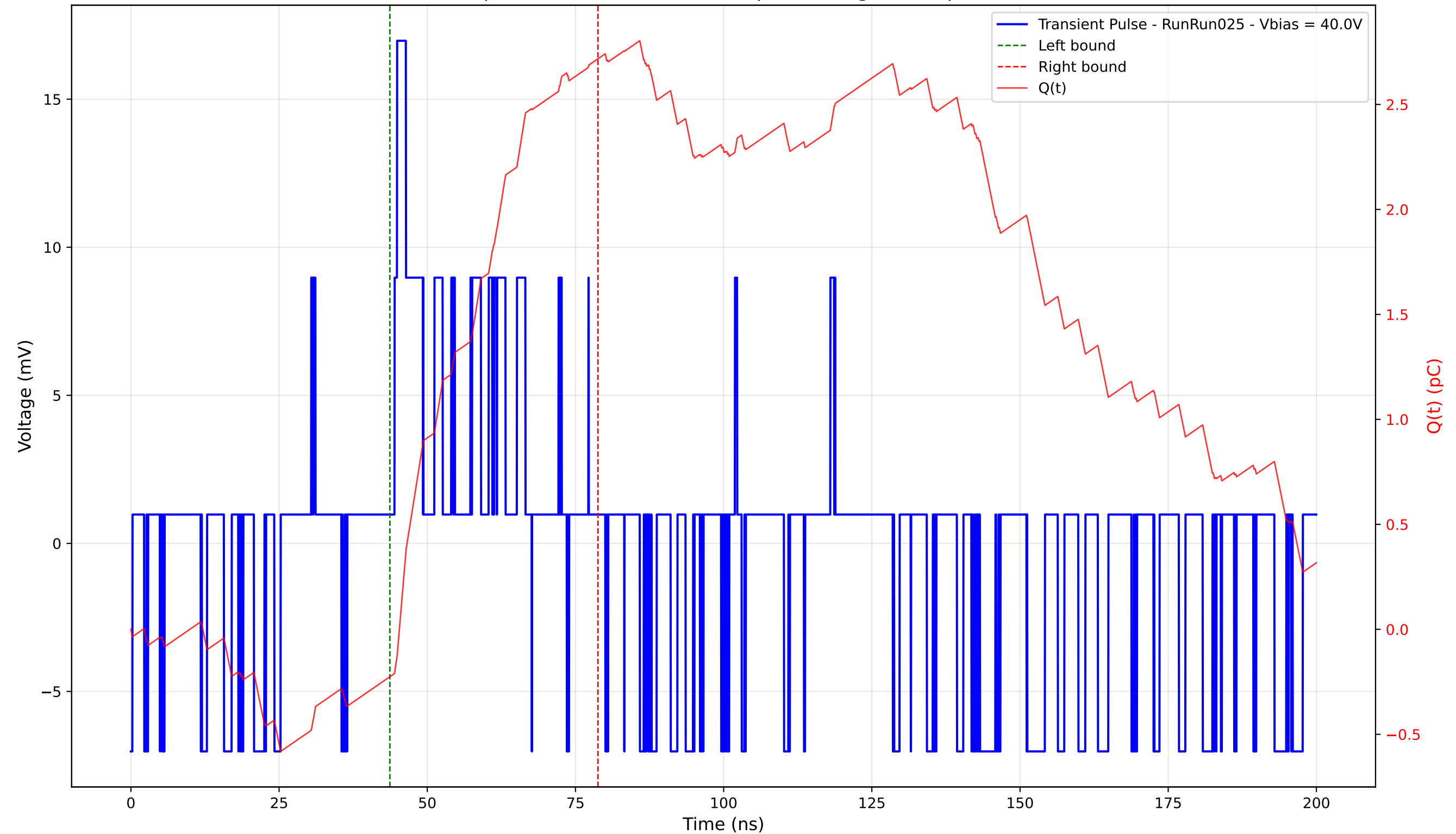
Transient Pulse - Sample: 4003 - Position: 380.0 \mu\text{m} - Charge: 2.94 pC - Rise Time: 0.44 ns
