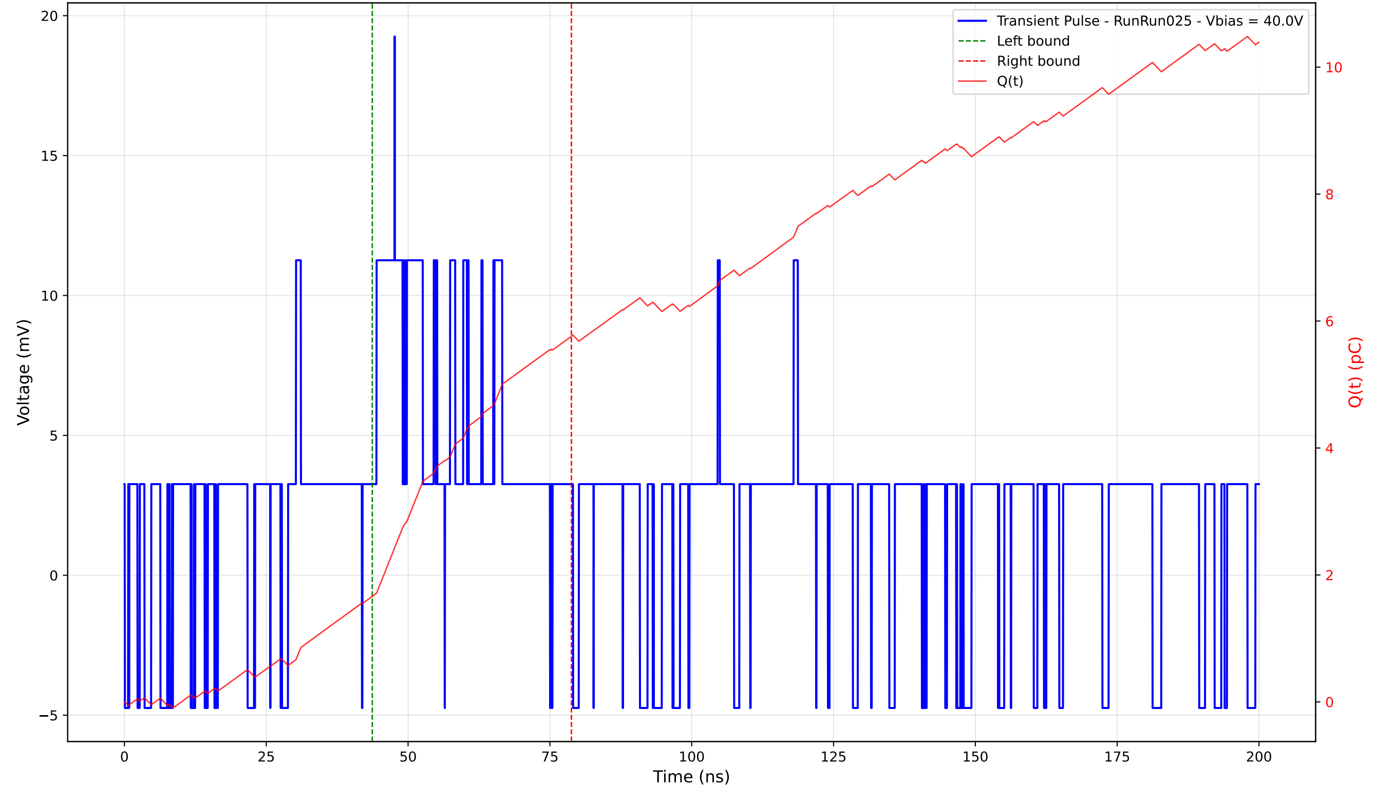
Transient Pulse - Sample: 4003 - Position: 70.0 \mu\text{m} - Charge: 4.10 pC - Rise Time: 0.00 ns (N/A)
