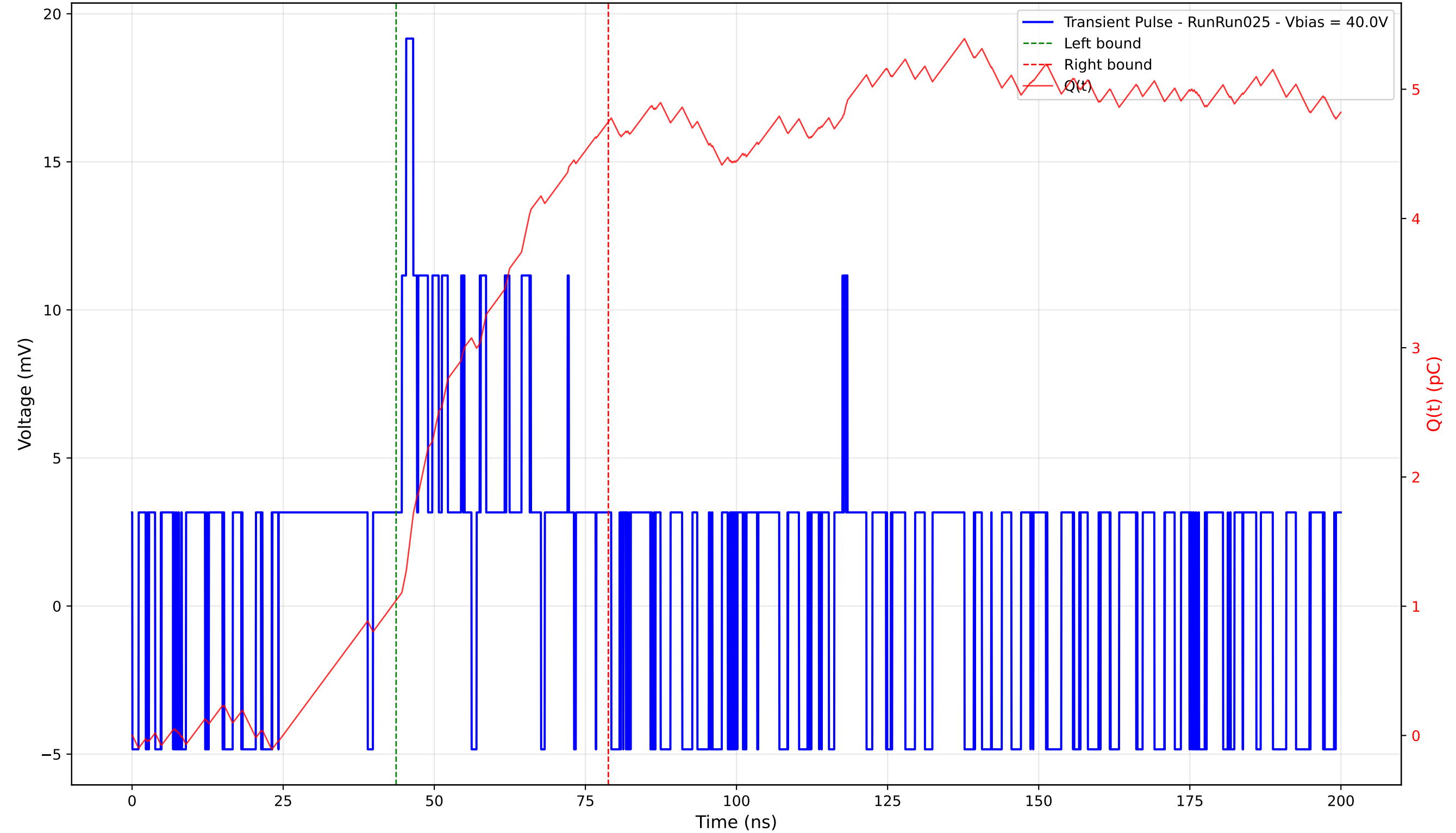
Transient Pulse - Sample: 4003 - Position: 415.0 \mu\text{m} - Charge: 3.70 pC - Rise Time: 0.00 ns (N/A)
