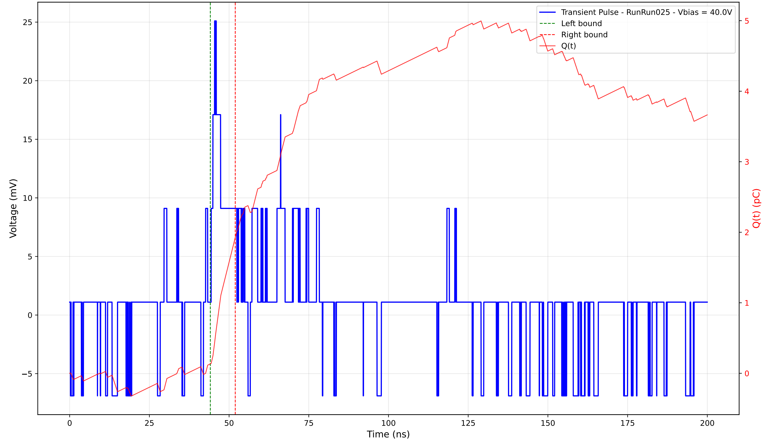
Transient Pulse - Sample: 4003 - Position: 285.0 \mu\text{m} - Charge: 1.80 pC - Rise Time: 1.10 ns
