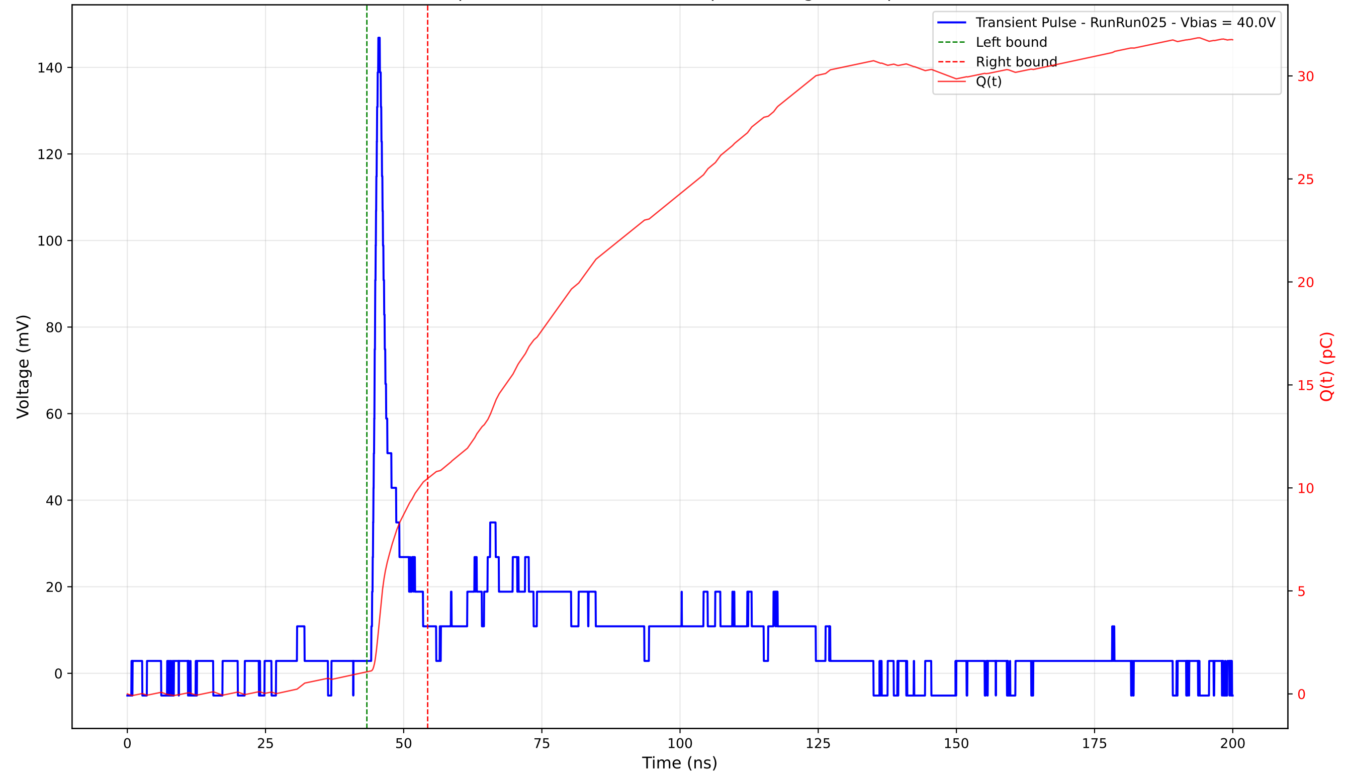
Transient Pulse - Sample: 4003 - Position: 105.0 \mu\text{m} - Charge: 9.40 pC - Rise Time: 1.01 ns
