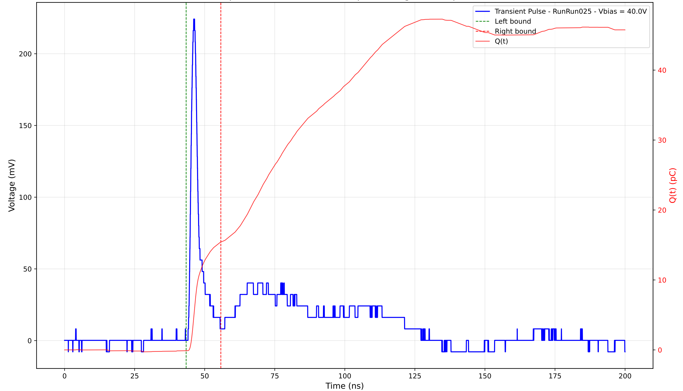
Transient Pulse - Sample: 4003 - Position: 160.0 \mu\text{m} - Charge: 15.53 pC - Rise Time: 1.40 ns
