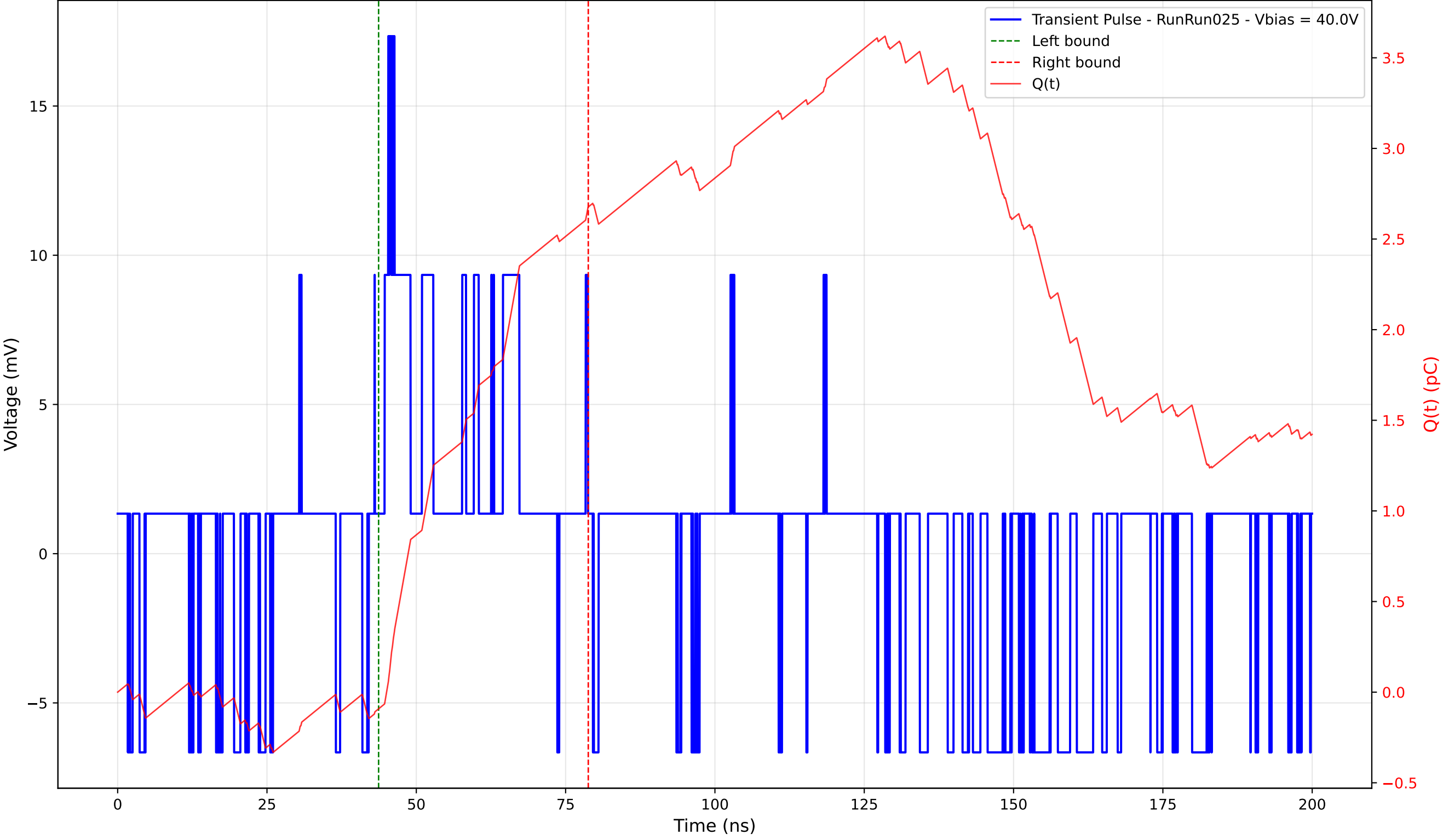
Transient Pulse - Sample: 4003 - Position: 35.0 \mu\text{m} - Charge: 2.77 pC - Rise Time: 0.62 ns
