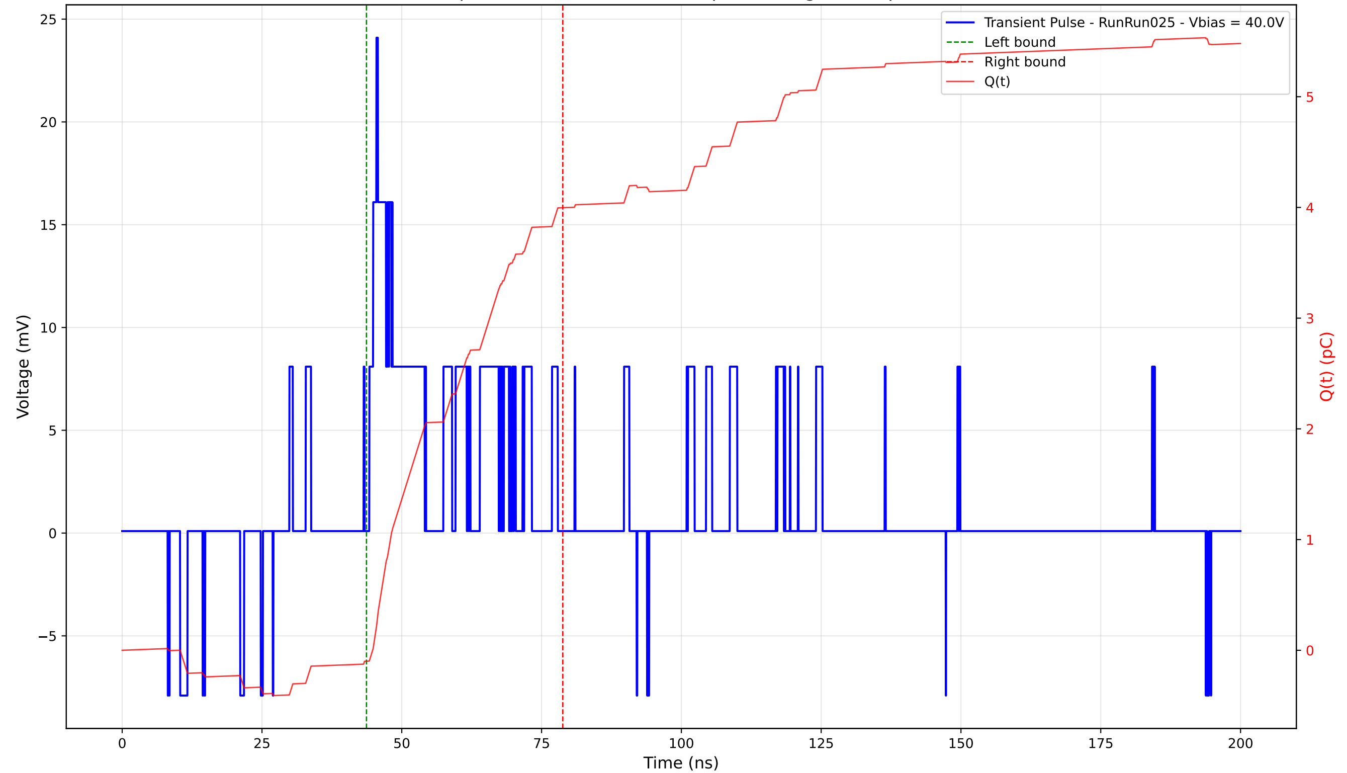
Transient Pulse - Sample: 4003 - Position: 250.0 \mu\text{m} - Charge: 4.10 pC - Rise Time: 1.27 ns
