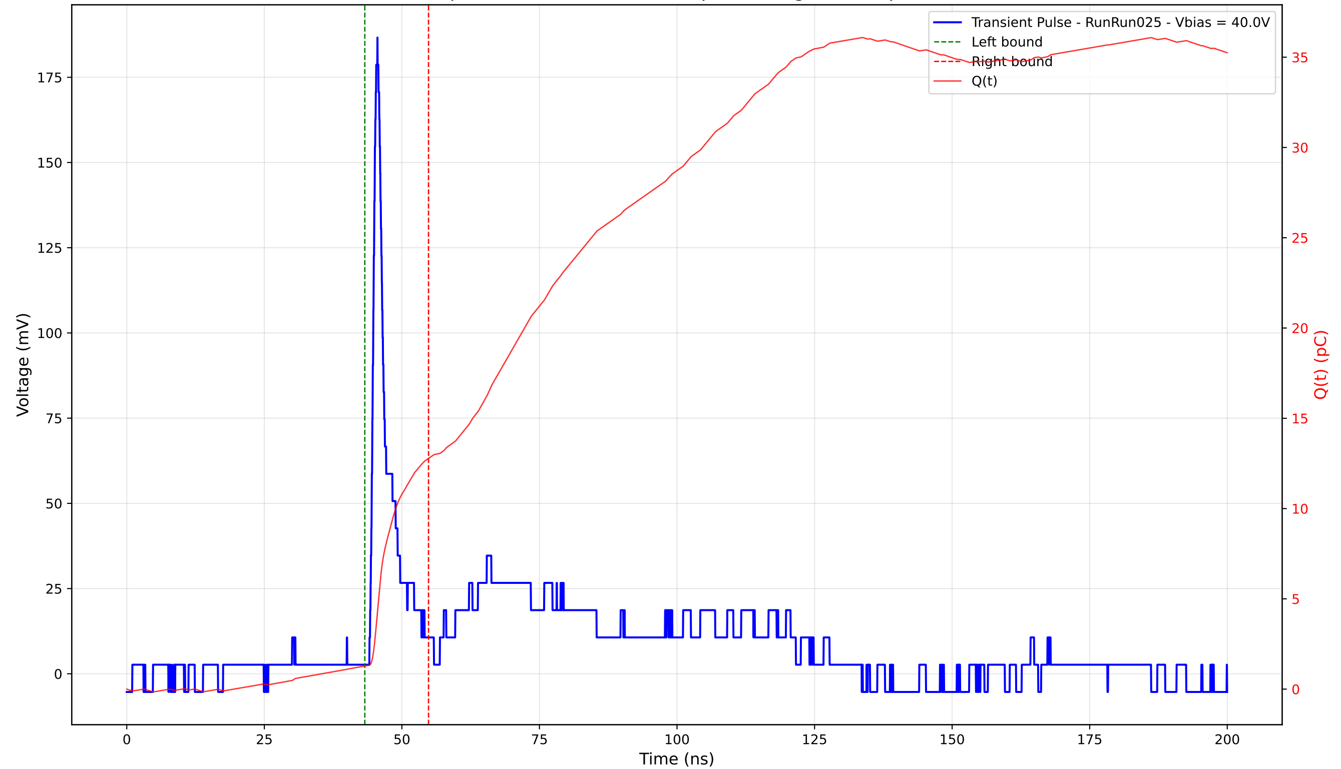
Transient Pulse - Sample: 4003 - Position: 110.0 \mu\text{m} - Charge: 11.51 pC - Rise Time: 0.96 ns
