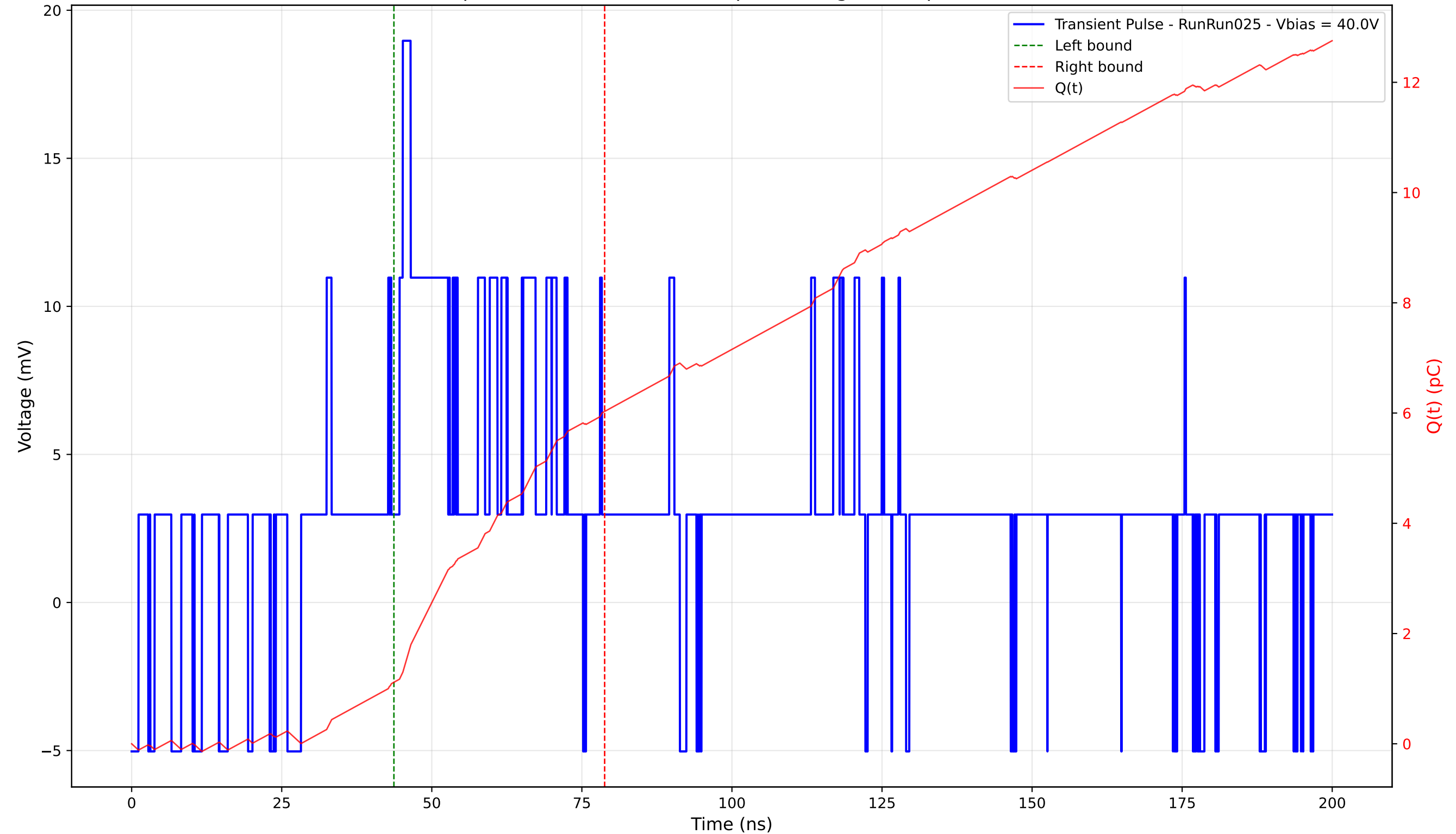
Transient Pulse - Sample: 4003 - Position: 360.0 \mu\text{m} - Charge: 4.91 pC - Rise Time: 0.00 ns (N/A)
