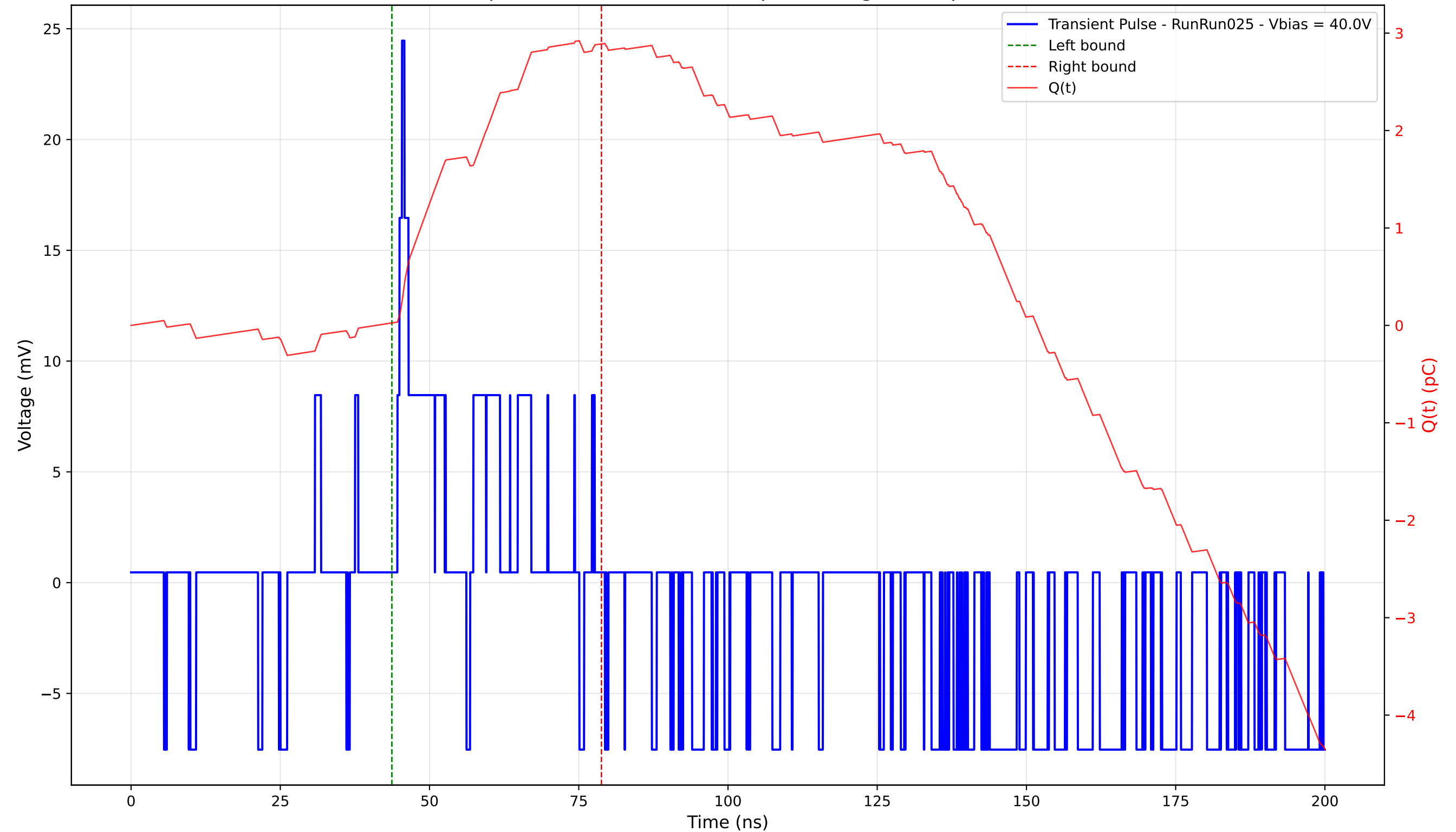
Transient Pulse - Sample: 4003 - Position: 305.0 \mu\text{m} - Charge: 2.87 pC - Rise Time: 0.78 ns
