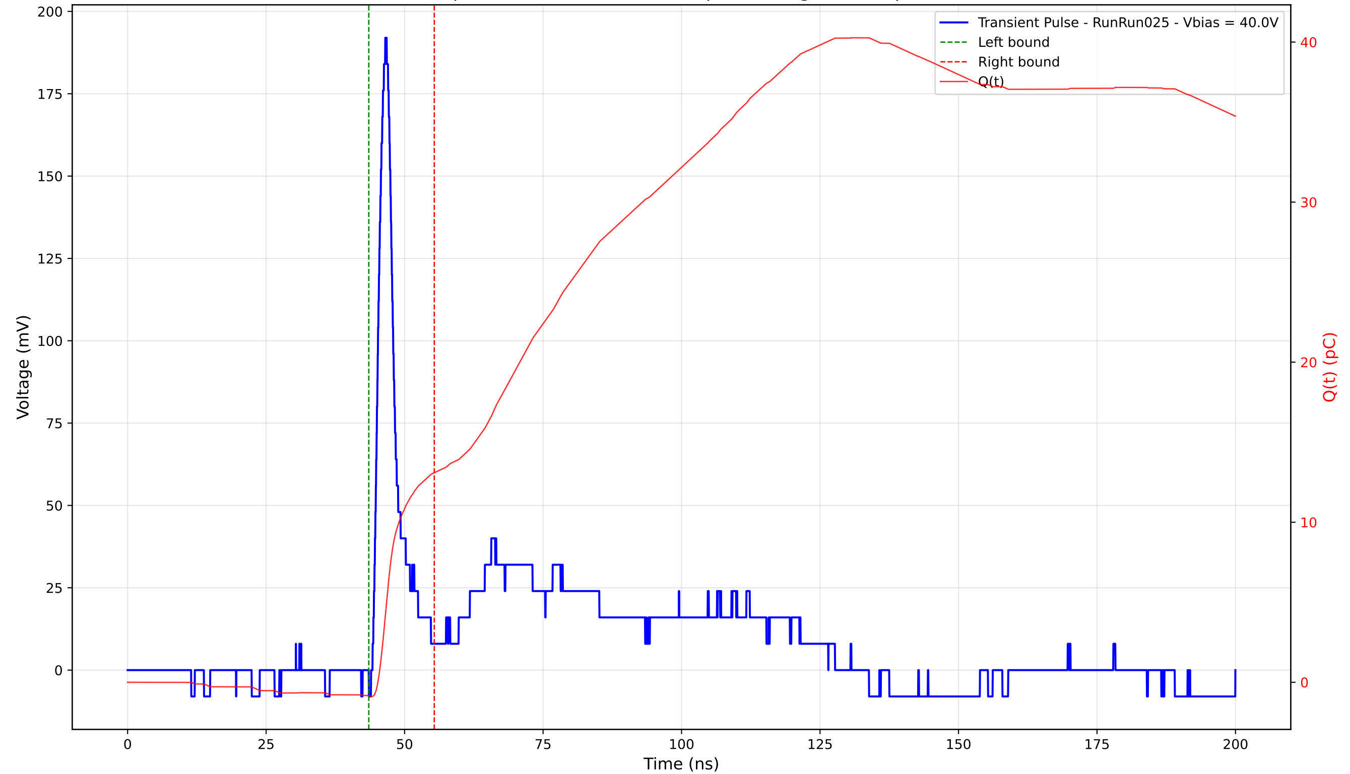
Transient Pulse - Sample: 4003 - Position: 170.0 \mu\text{m} - Charge: 13.91 pC - Rise Time: 1.63 ns
