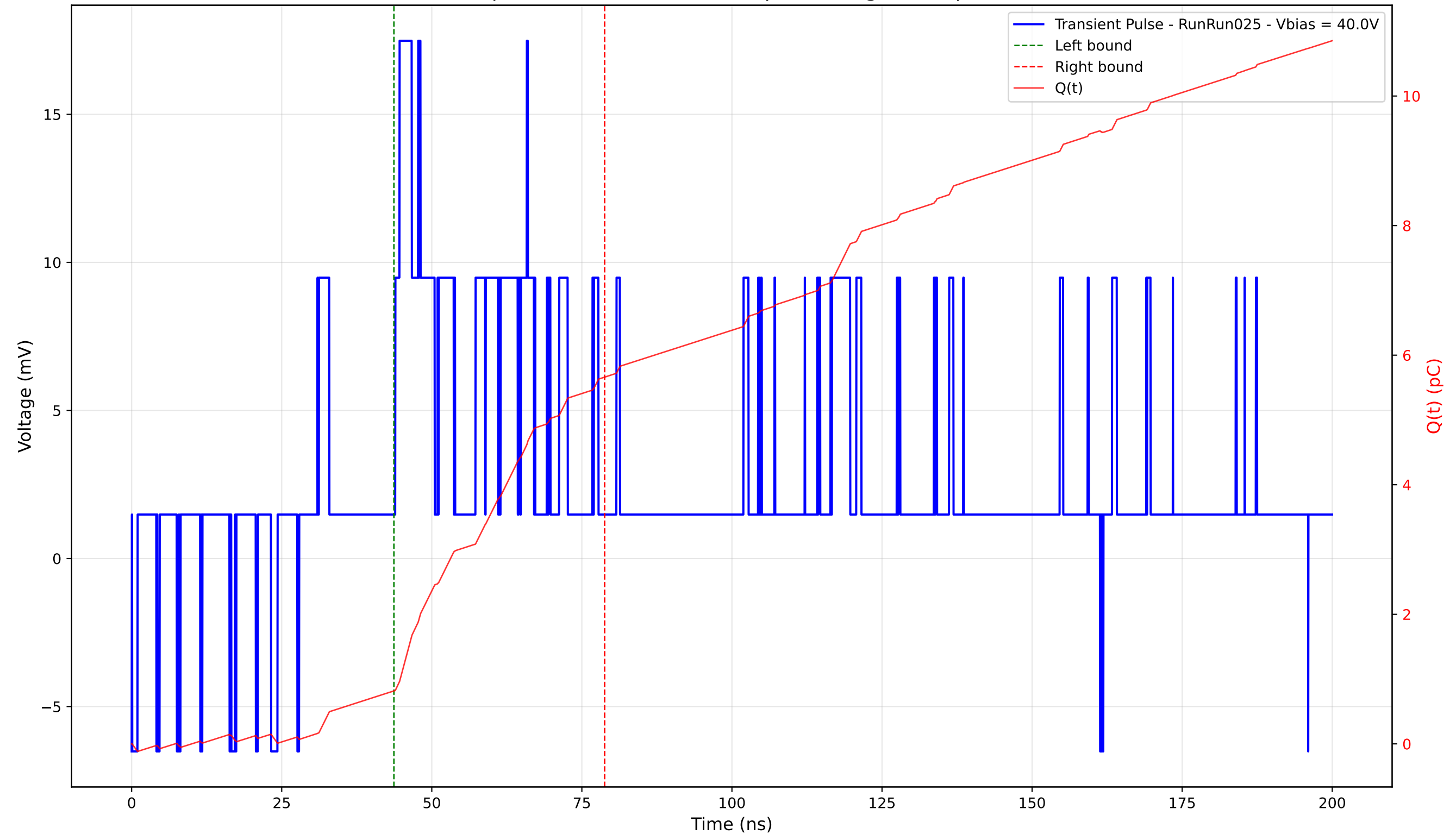
Transient Pulse - Sample: 4003 - Position: 310.0 \mu\text{m} - Charge: 4.84 pC - Rise Time: 0.72 ns
