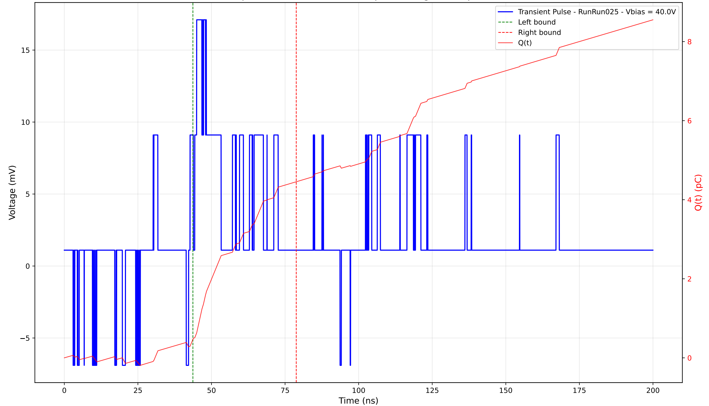
Transient Pulse - Sample: 4003 - Position: 235.0 \mu\text{m} - Charge: 3.98 pC - Rise Time: 0.66 ns
