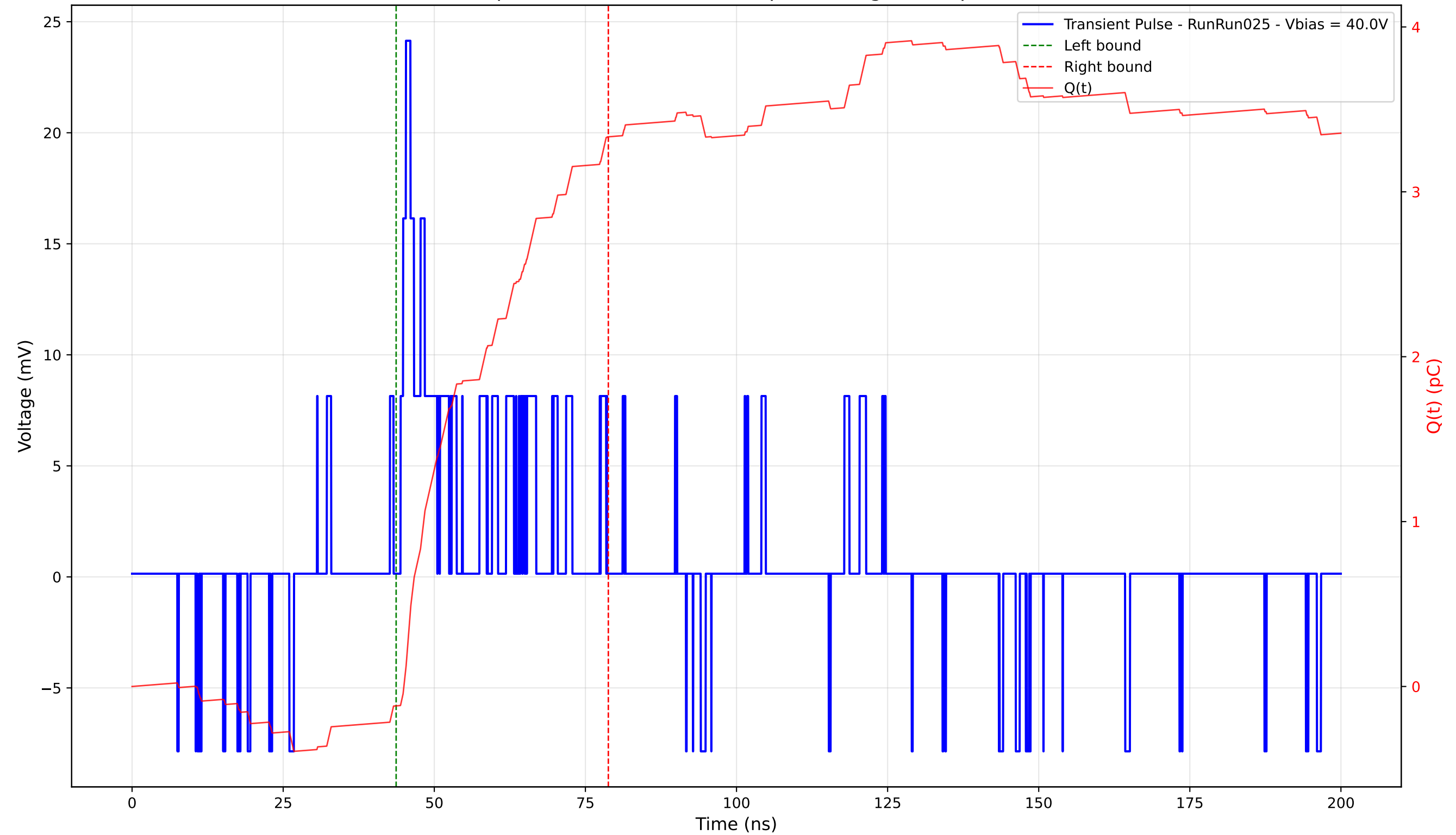
Transient Pulse - Sample: 4003 - Position: 290.0 \mu\text{m} - Charge: 3.45 pC - Rise Time: 0.89 ns
