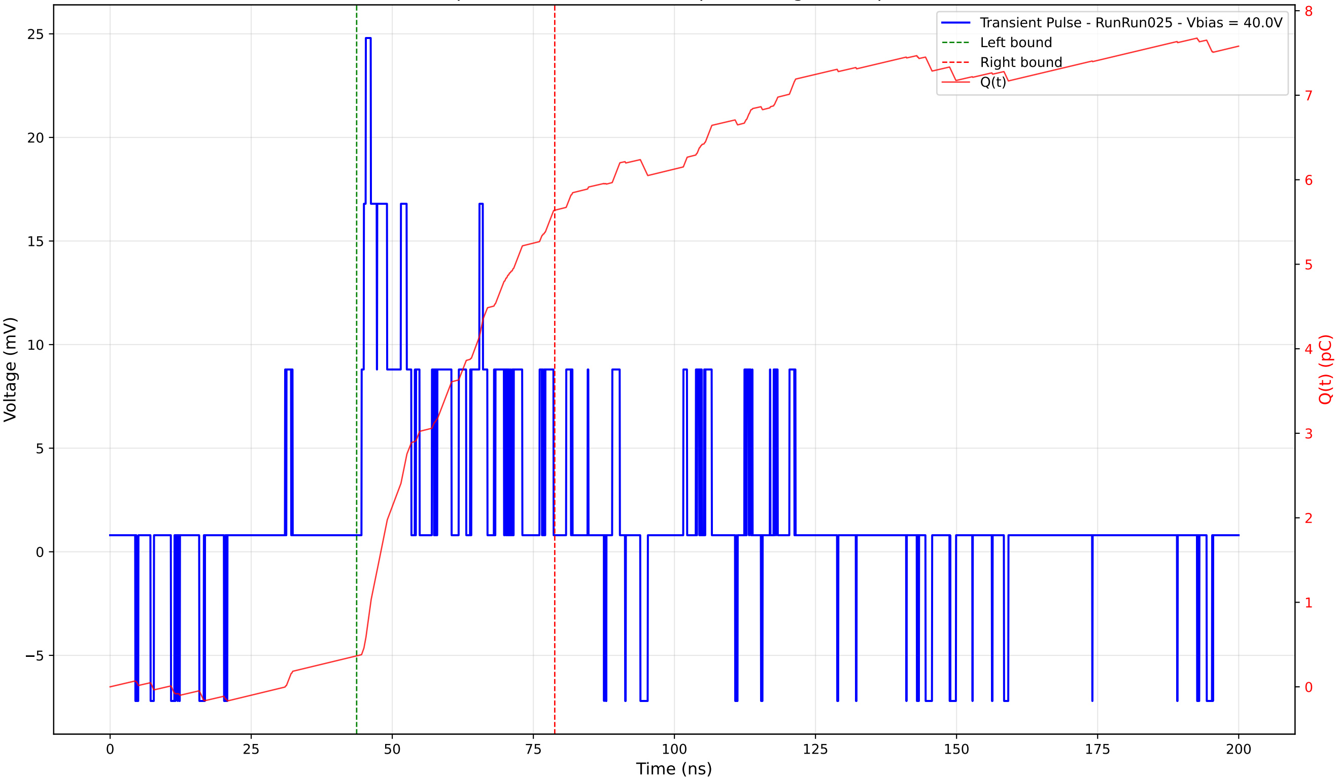
Transient Pulse - Sample: 4003 - Position: 50.0 \mu\text{m} - Charge: 5.27 pC - Rise Time: 0.76 ns
