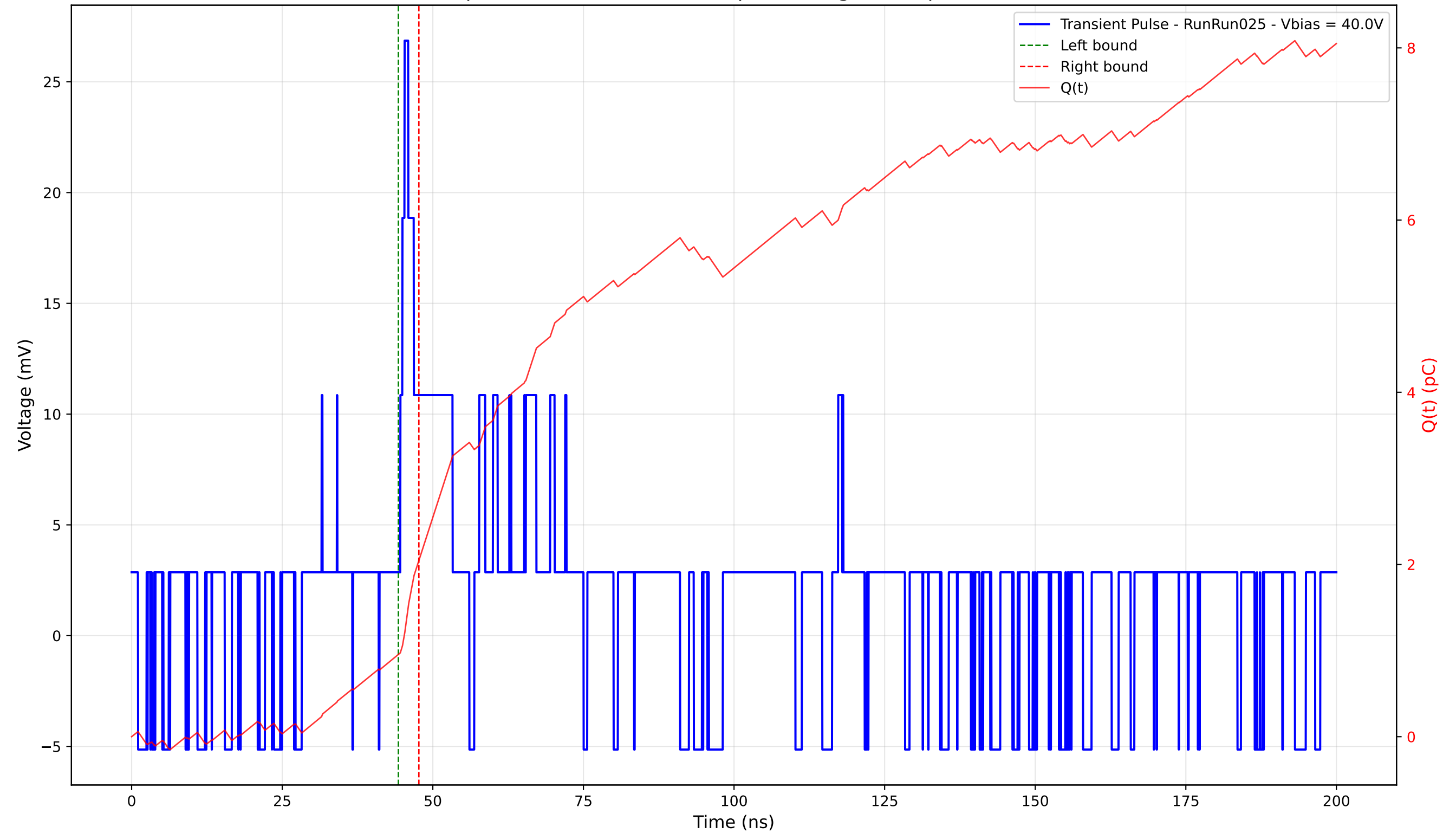
Transient Pulse - Sample: 4003 - Position: 260.0 \mu\text{m} - Charge: 1.09 pC - Rise Time: 0.00 ns (N/A)
