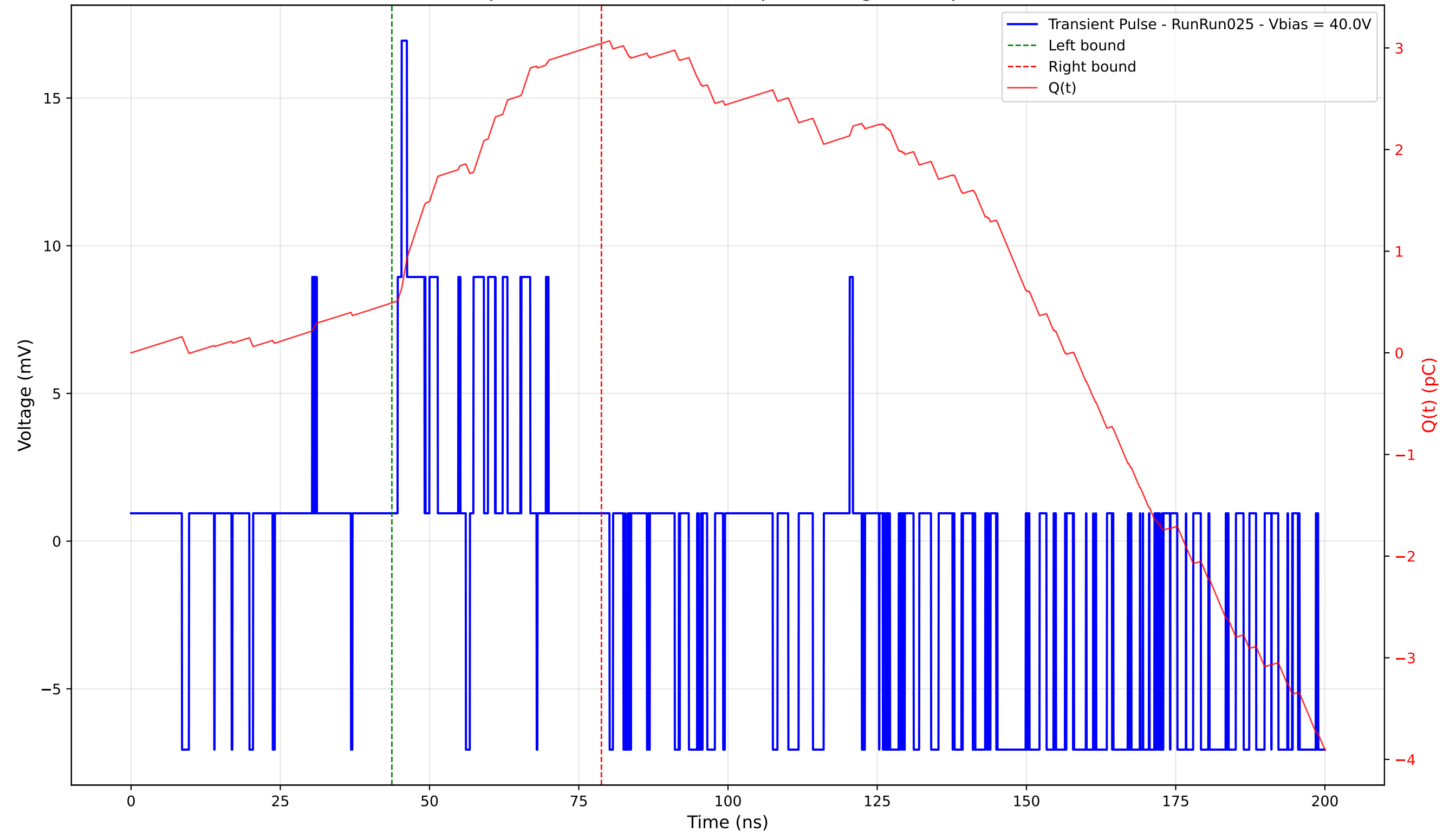
Transient Pulse - Sample: 4003 - Position: 420.0 \mu\text{m} - Charge: 2.56 pC - Rise Time: 0.68 ns
