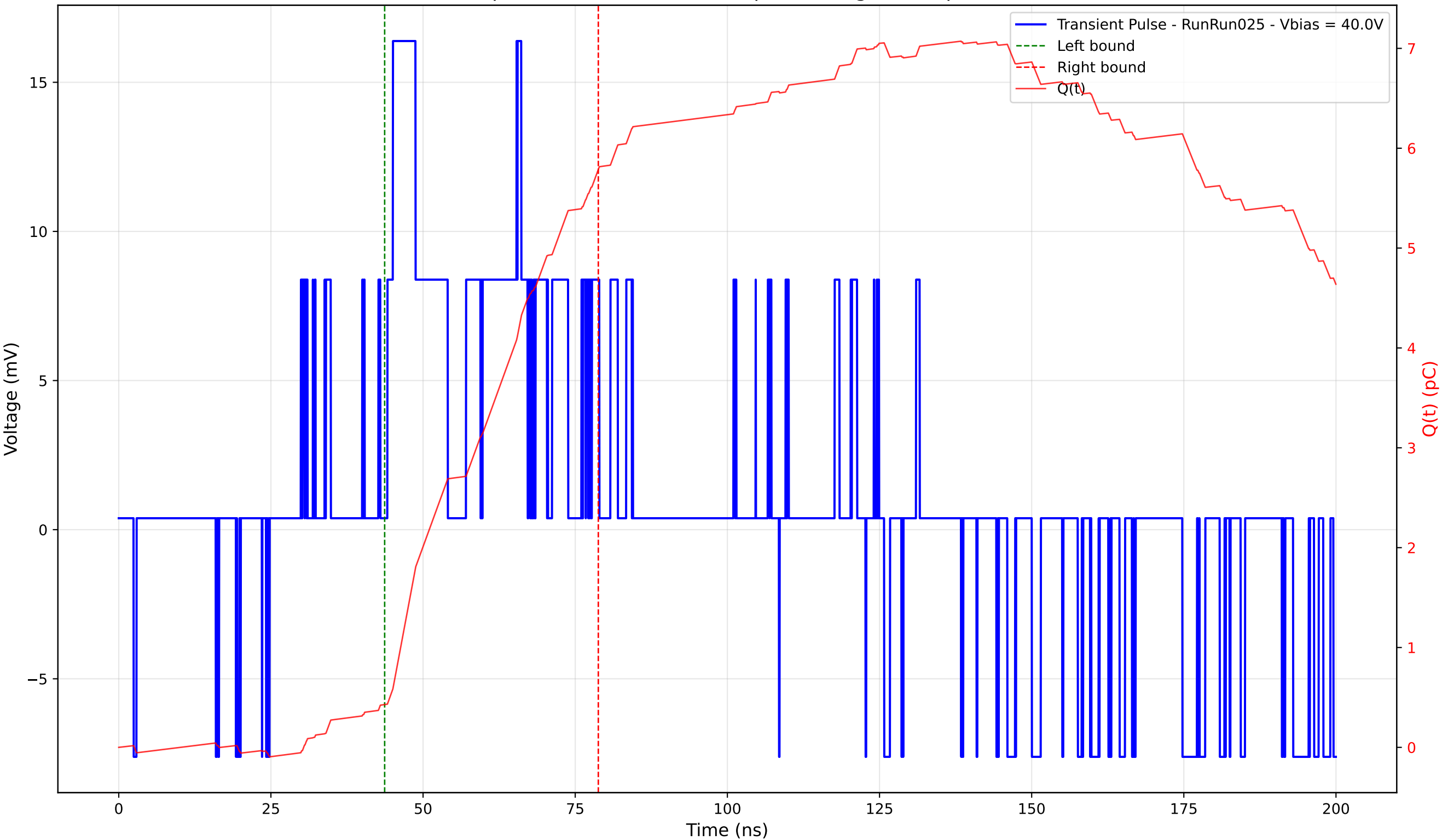
Transient Pulse - Sample: 4003 - Position: 45.0 \mu\text{m} - Charge: 5.36 pC - Rise Time: 0.92 ns
