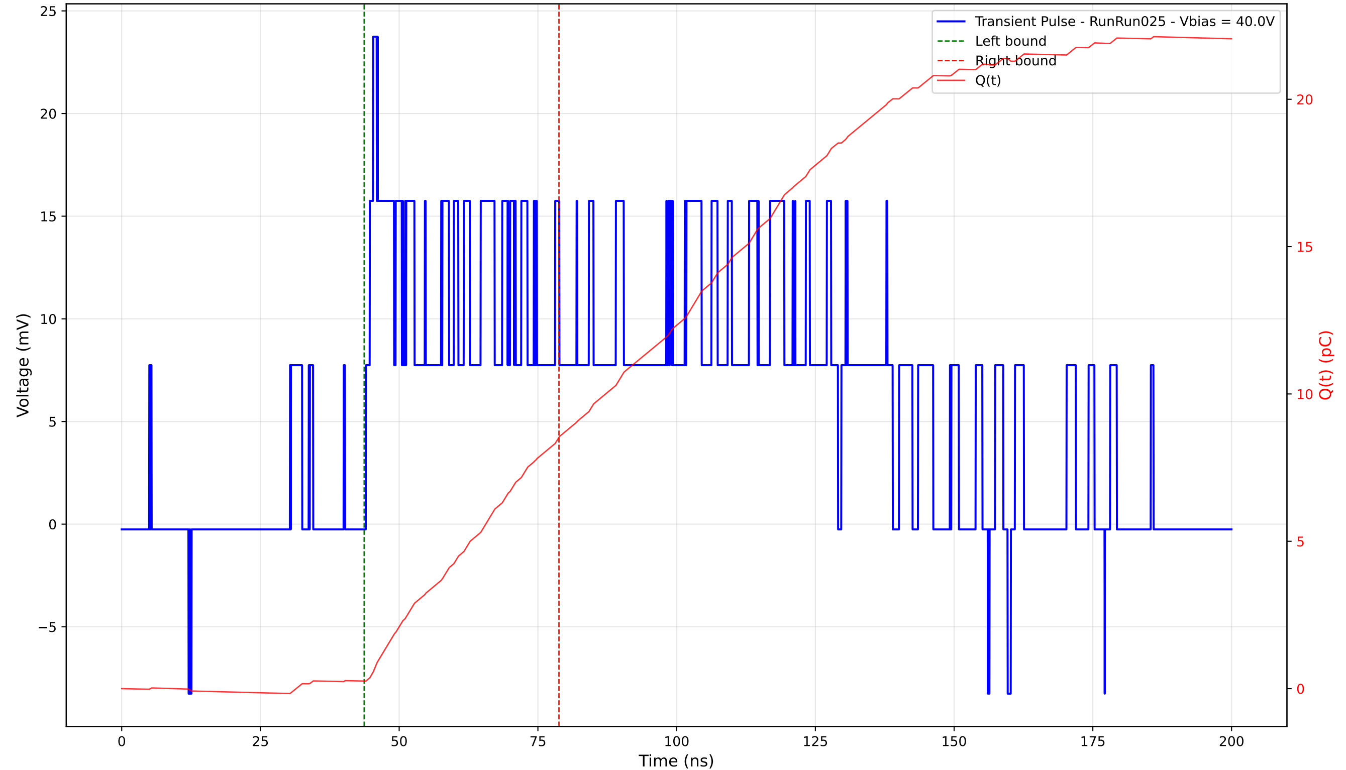
Transient Pulse - Sample: 4003 - Position: 210.0 \mu\text{m} - Charge: 8.28 pC - Rise Time: 1.31 ns
