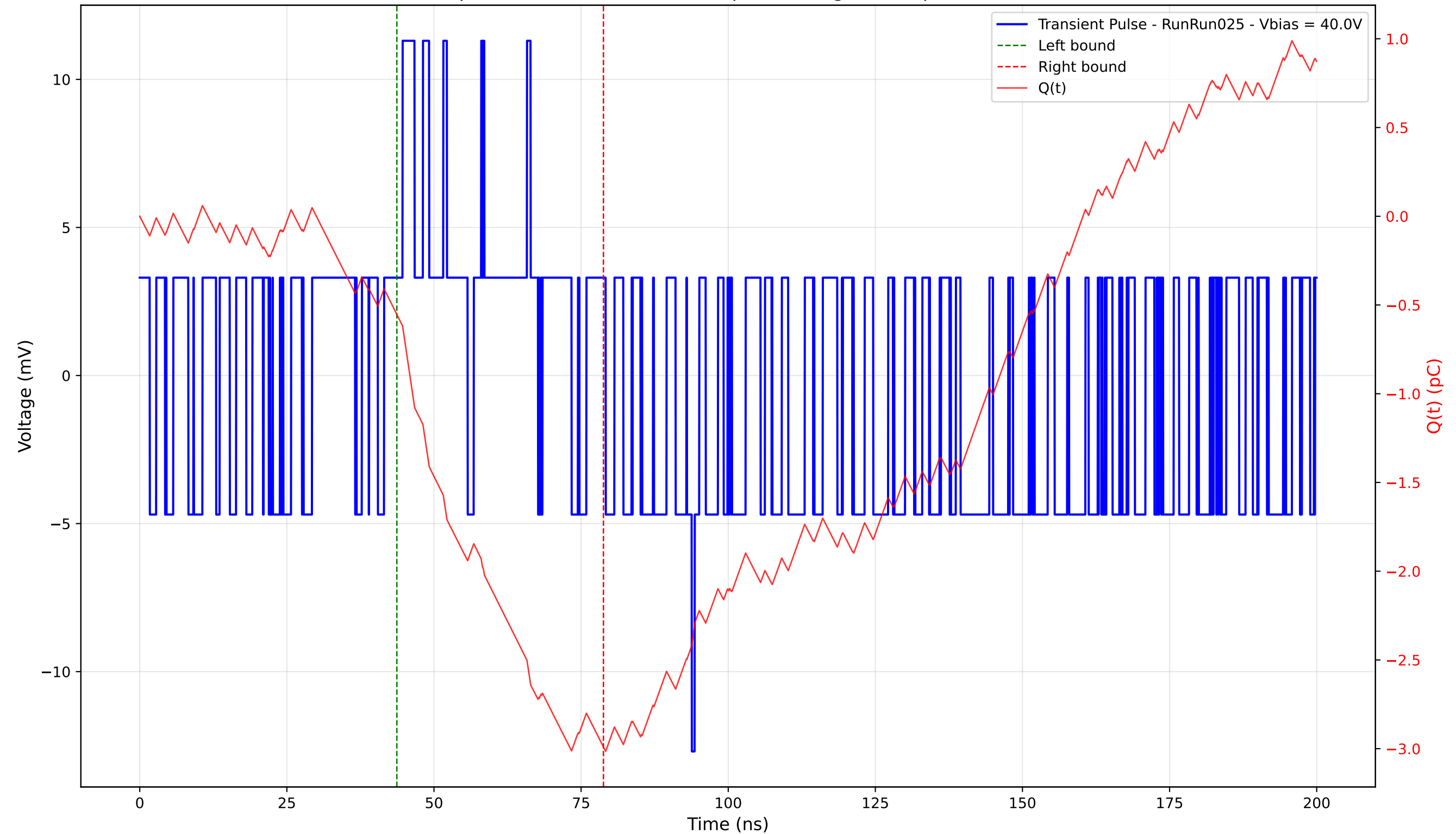
Transient Pulse - Sample: 4003 - Position: 425.0 \mu\text{m} - Charge: 2.44 pC - Rise Time: 0.00 ns (N/A)
