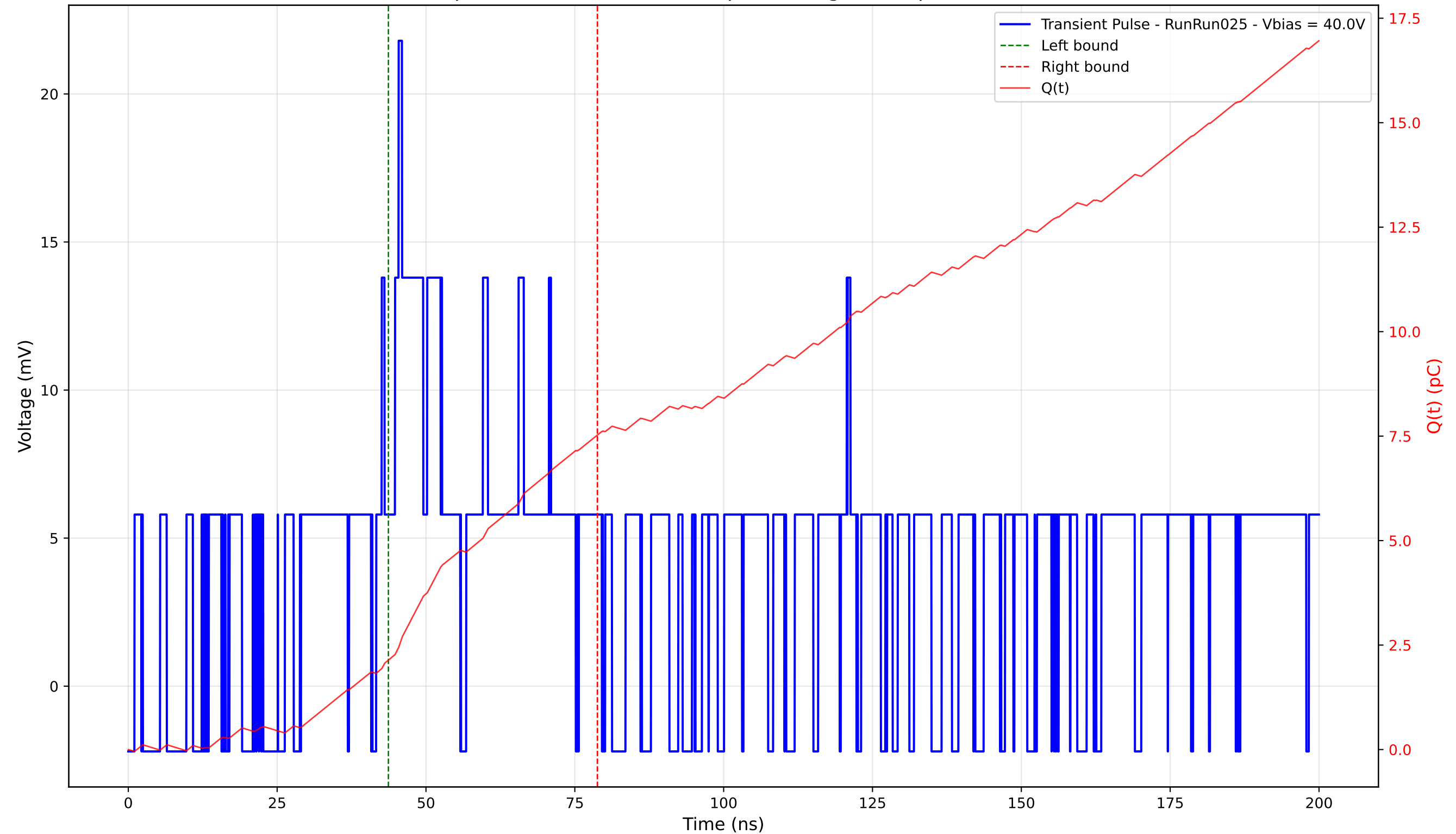
Transient Pulse - Sample: 4003 - Position: 335.0 \mu\text{m} - Charge: 5.39 pC - Rise Time: 0.00 ns (N/A)
