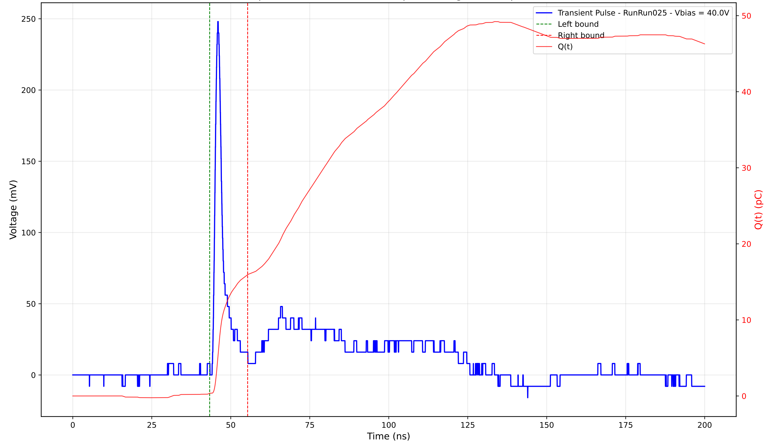
Transient Pulse - Sample: 4003 - Position: 150.0 \mu\text{m} - Charge: 15.60 pC - Rise Time: 1.16 ns
