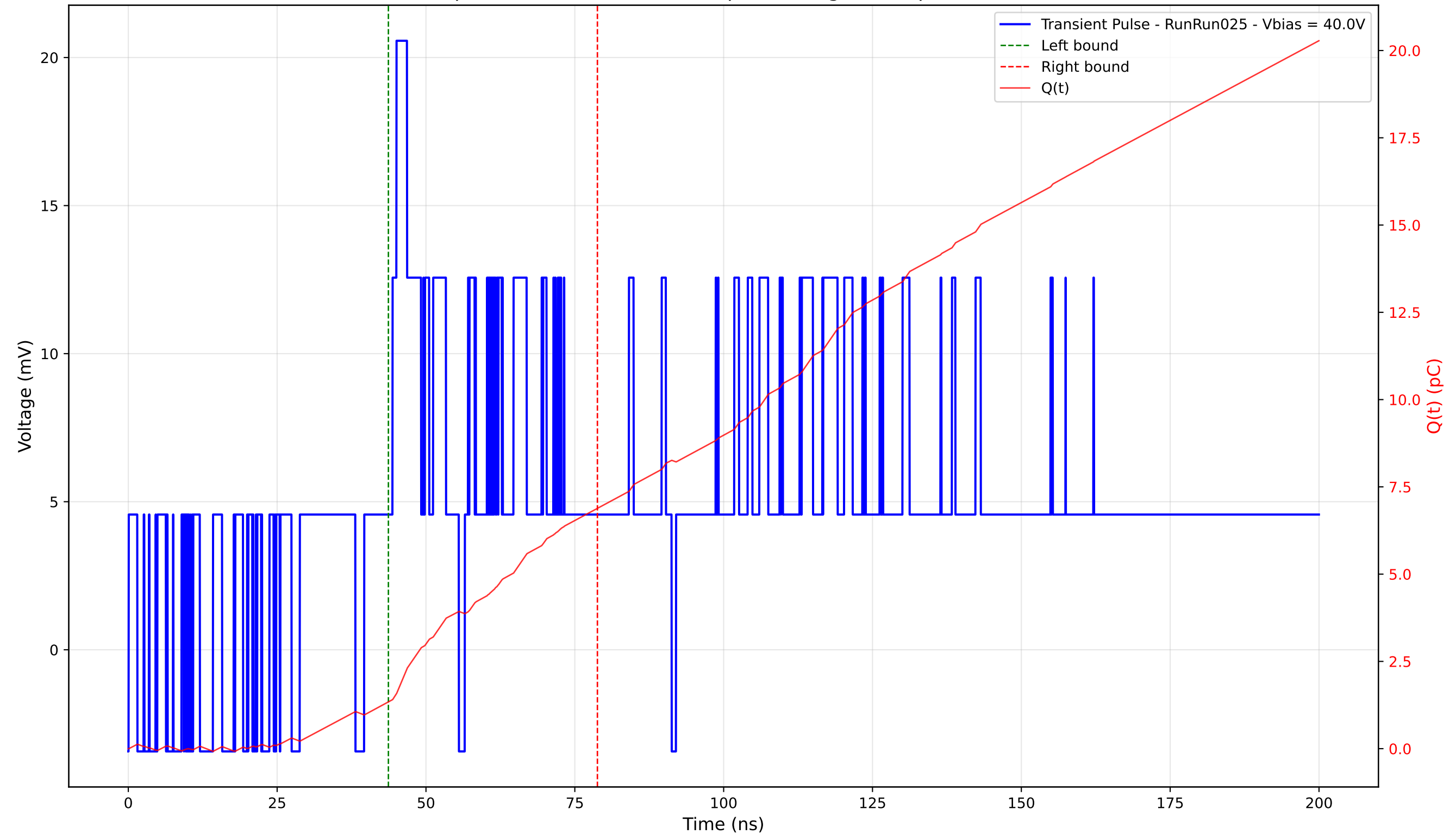
Transient Pulse - Sample: 4003 - Position: 220.0 \mu\text{m} - Charge: 5.54 pC - Rise Time: 0.00 ns (N/A)
