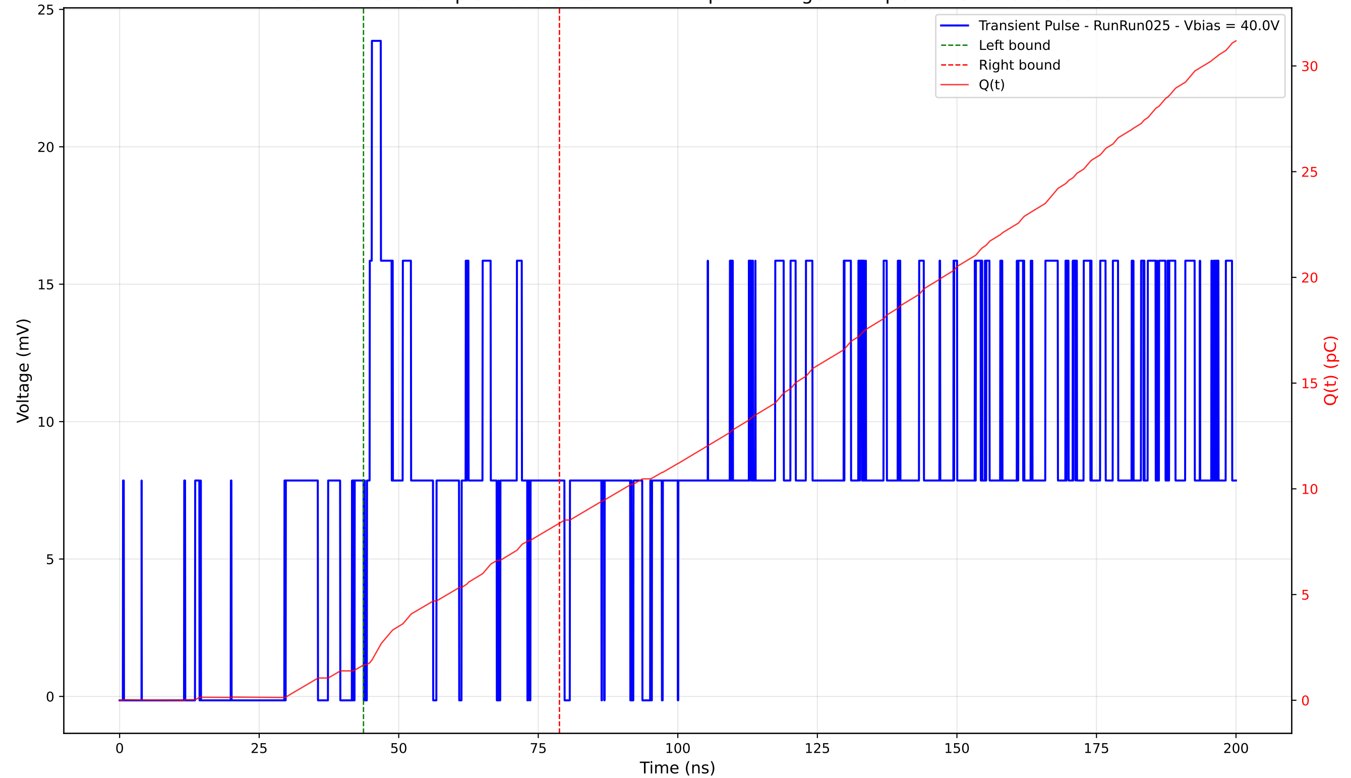
Transient Pulse - Sample: 4003 - Position: 240.0 \mu\text{m} - Charge: 6.71 pC - Rise Time: 0.89 ns
