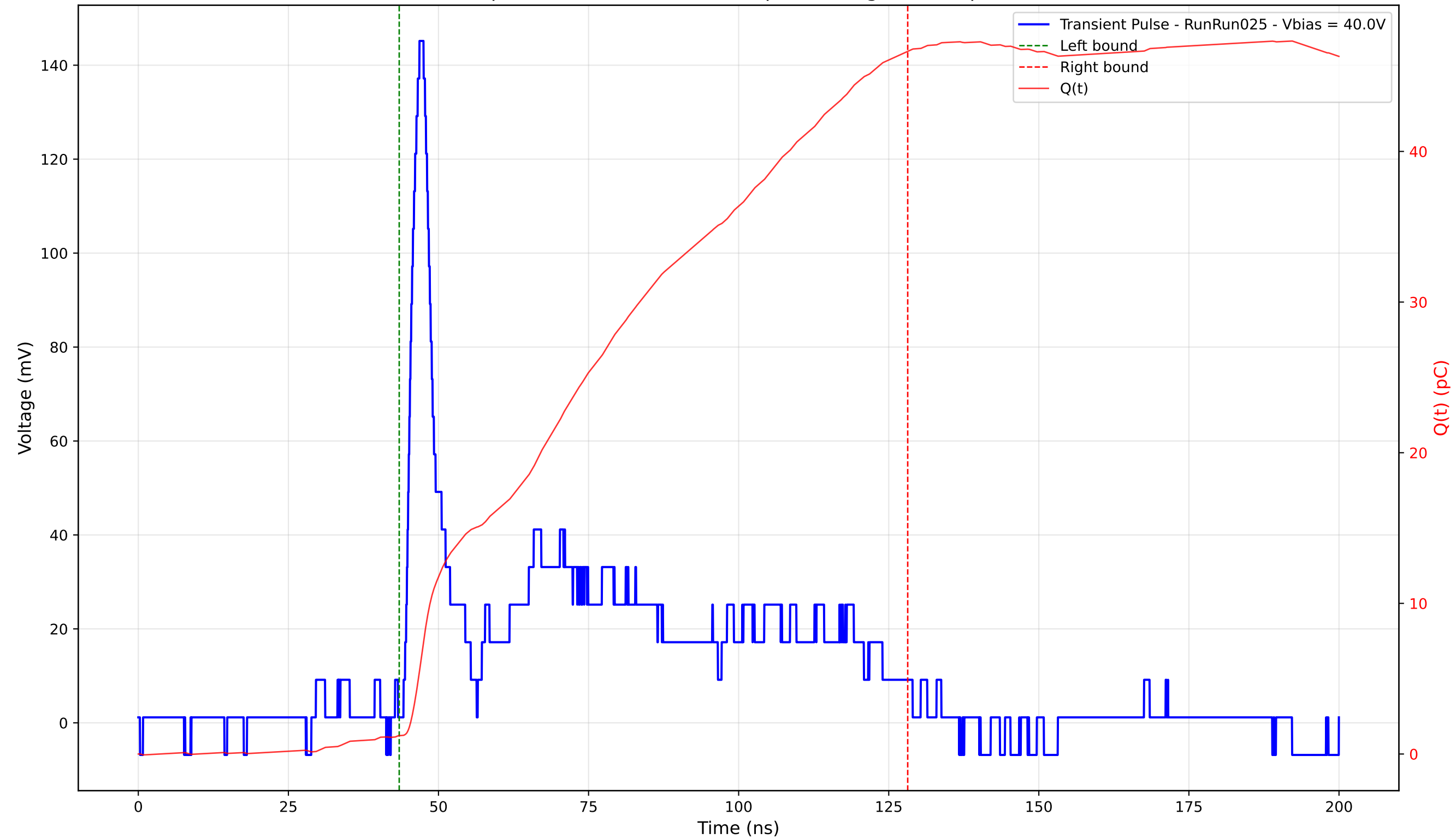
Transient Pulse - Sample: 4003 - Position: 180.0 \mu\text{m} - Charge: 45.43 pC - Rise Time: 2.11 ns
