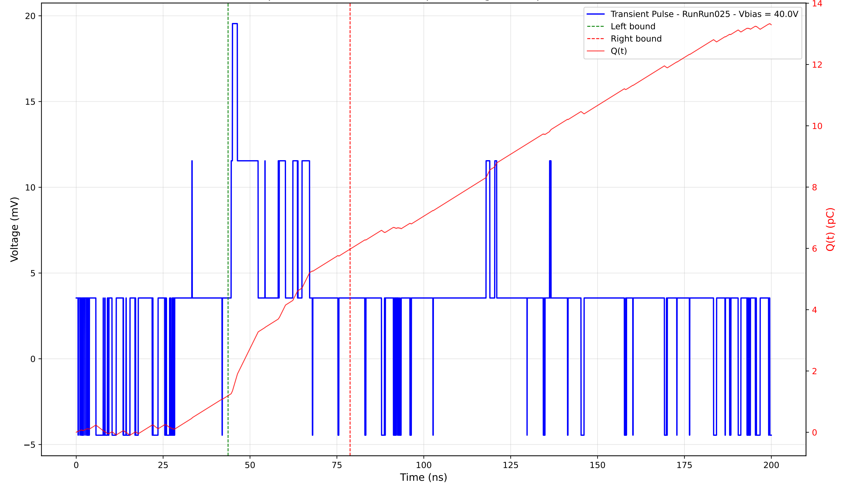
Transient Pulse - Sample: 4003 - Position: 370.0 \mu\text{m} - Charge: 4.78 pC - Rise Time: 0.00 ns (N/A)
