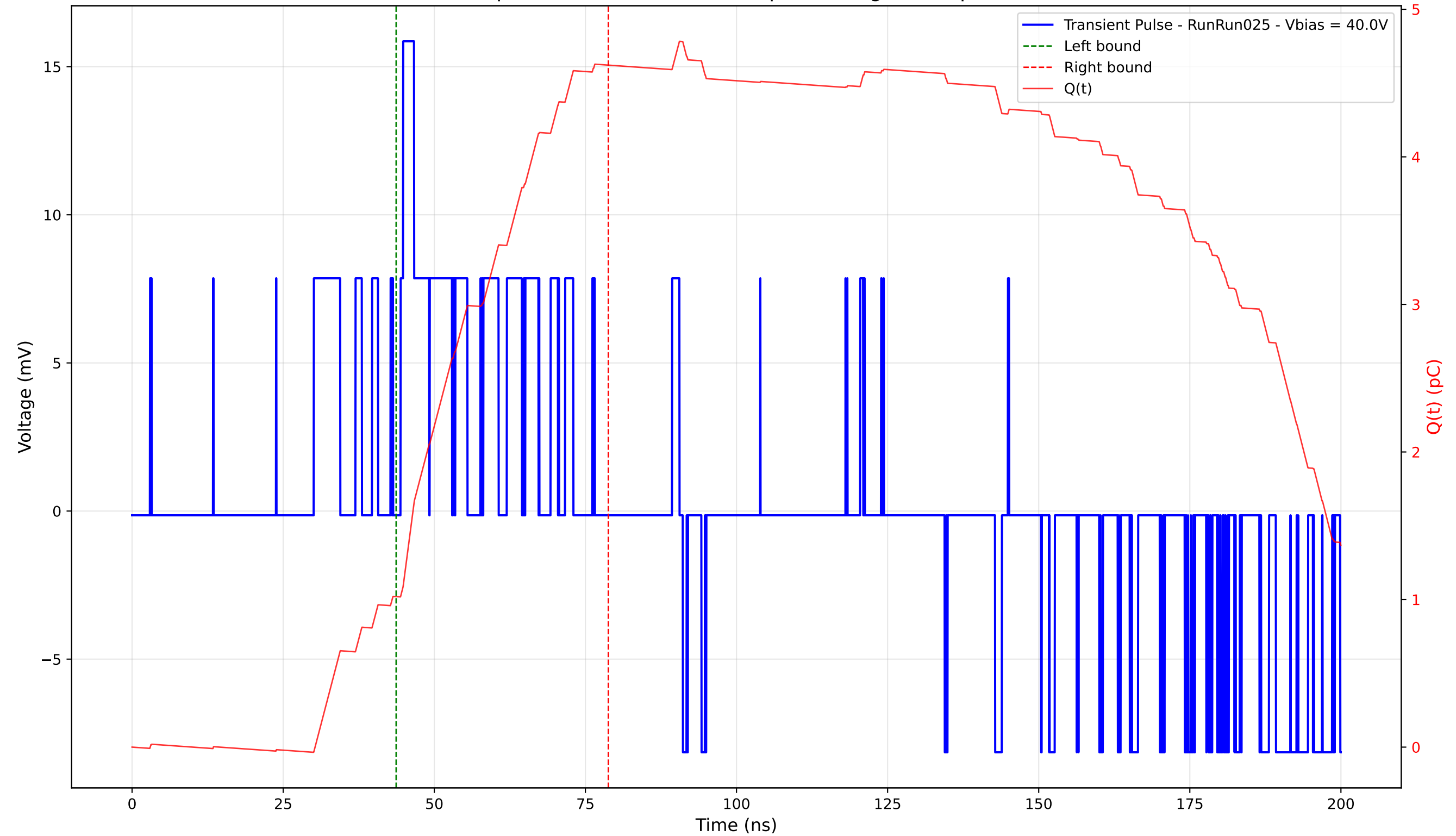
Transient Pulse - Sample: 4003 - Position: 330.0 \mu\text{m} - Charge: 3.60 pC - Rise Time: 0.44 ns
