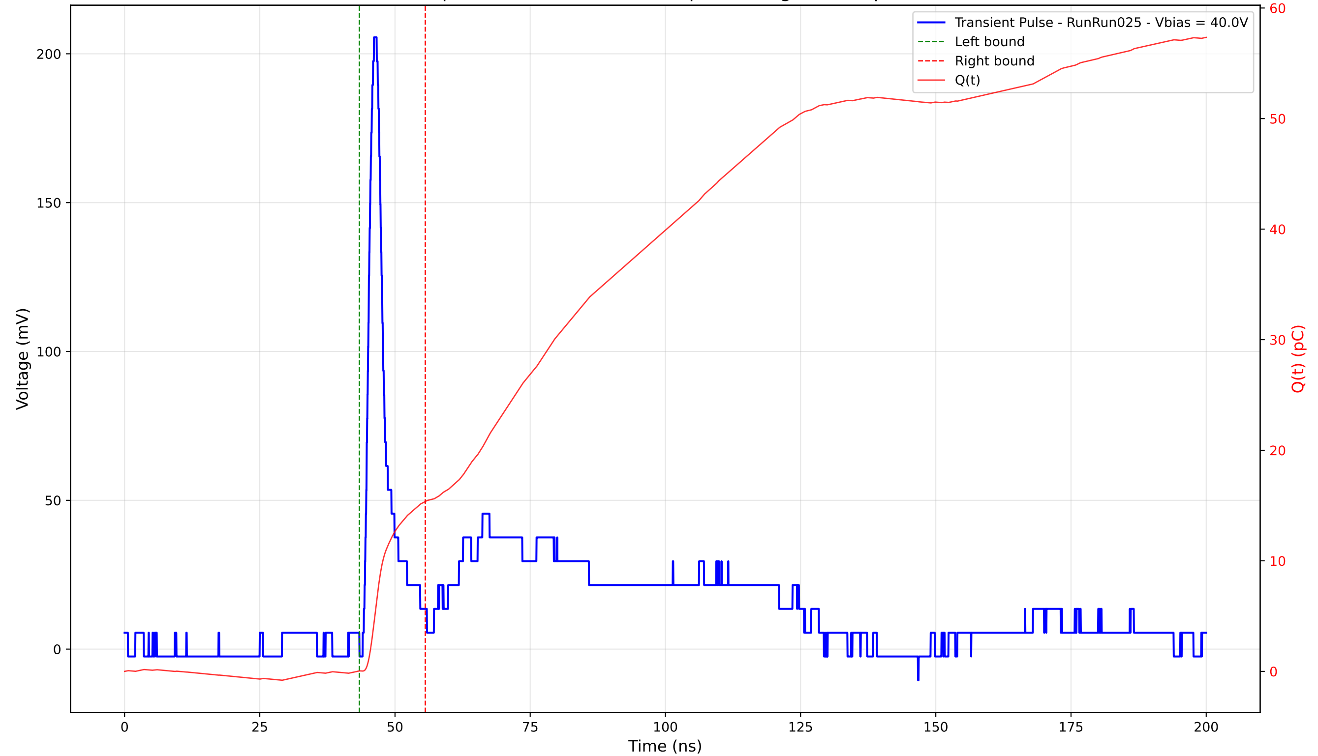
Transient Pulse - Sample: 4003 - Position: 165.0 \mu\text{m} - Charge: 15.32 pC - Rise Time: 1.44 ns
