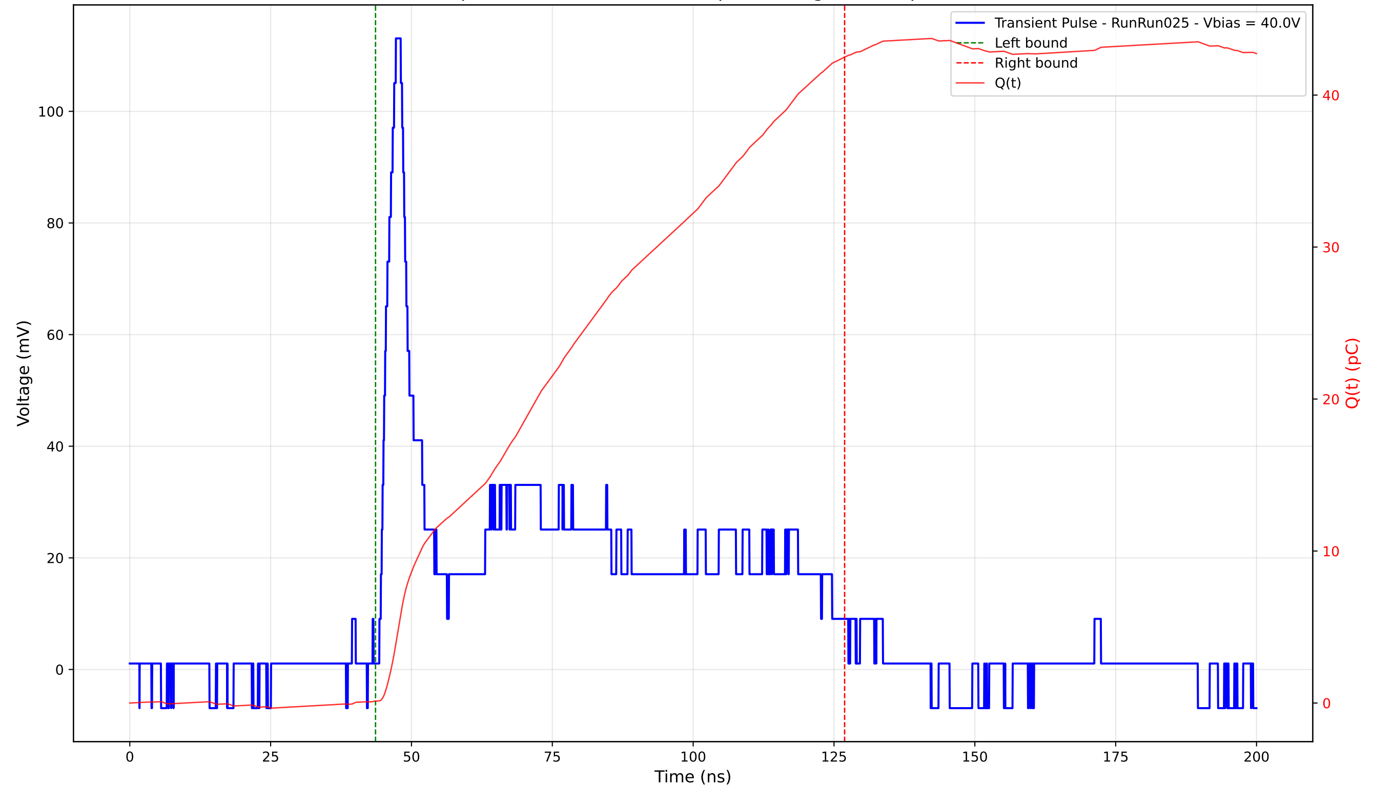
Transient Pulse - Sample: 4003 - Position: 185.0 \mu\text{m} - Charge: 42.38 pC - Rise Time: 2.37 ns
