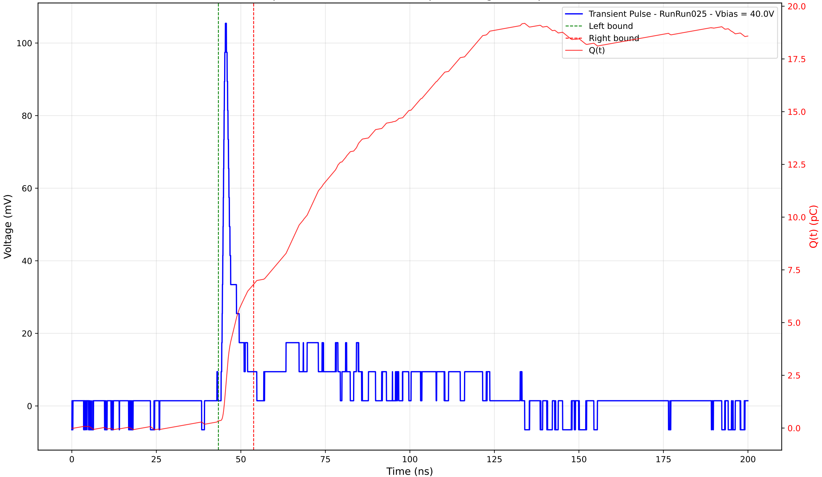
Transient Pulse - Sample: 4003 - Position: 100.0 \mu\text{m} - Charge: 6.48 pC - Rise Time: 0.92 ns
