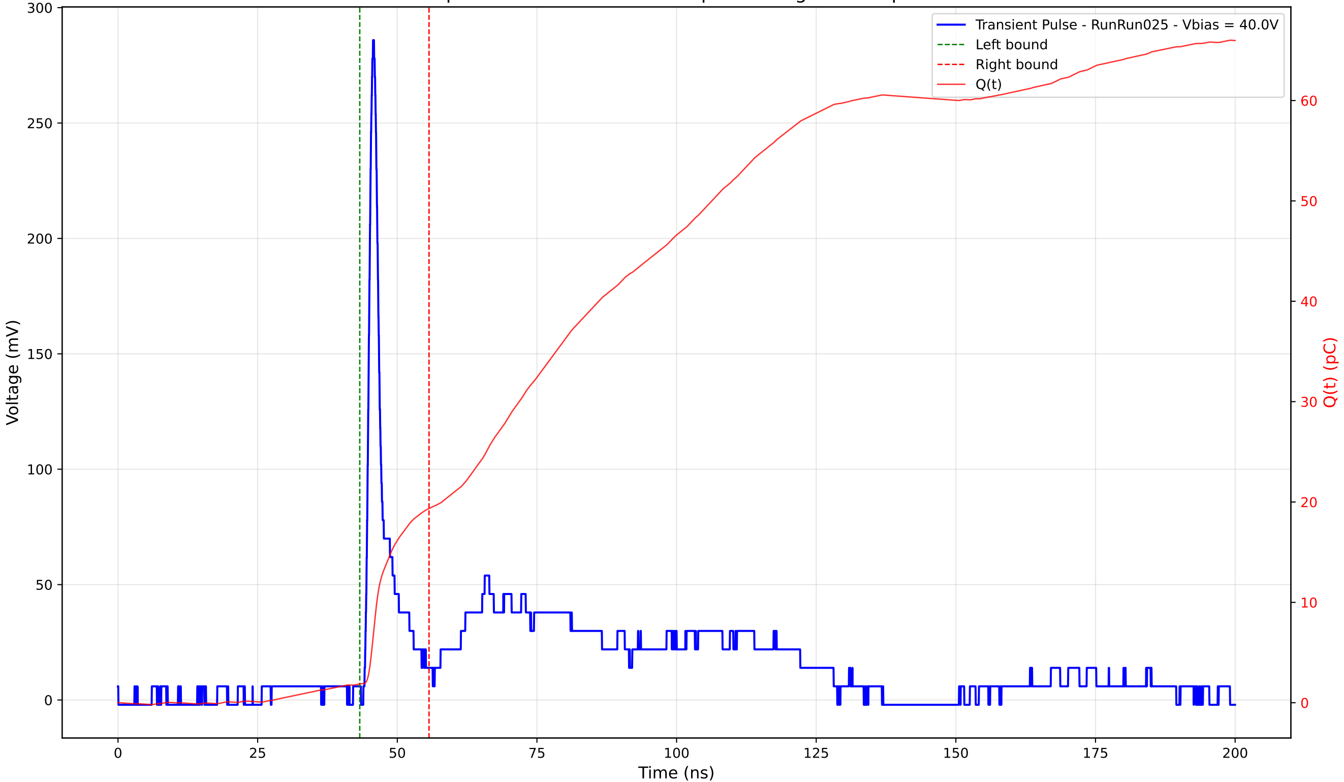
Transient Pulse - Sample: 4003 - Position: 135.0 \mu\text{m} - Charge: 17.47 pC - Rise Time: 1.10 ns
