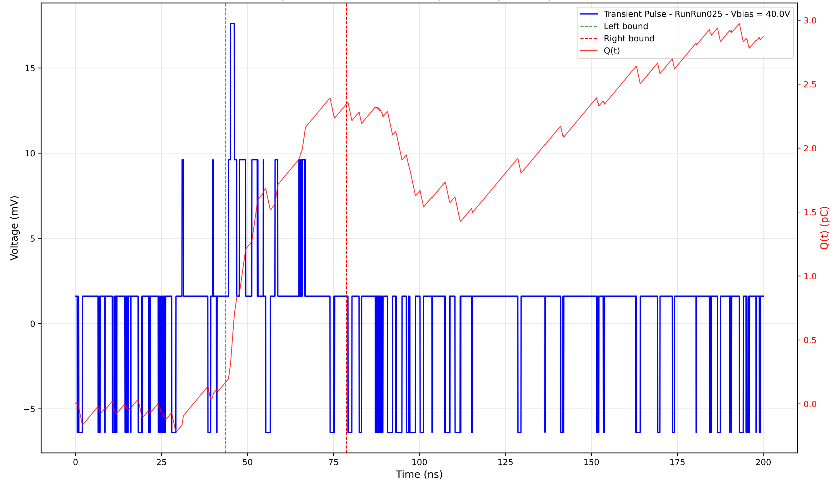
Transient Pulse - Sample: 4003 - Position: 340.0 \mu\text{m} - Charge: 2.17 pC - Rise Time: 0.58 ns
