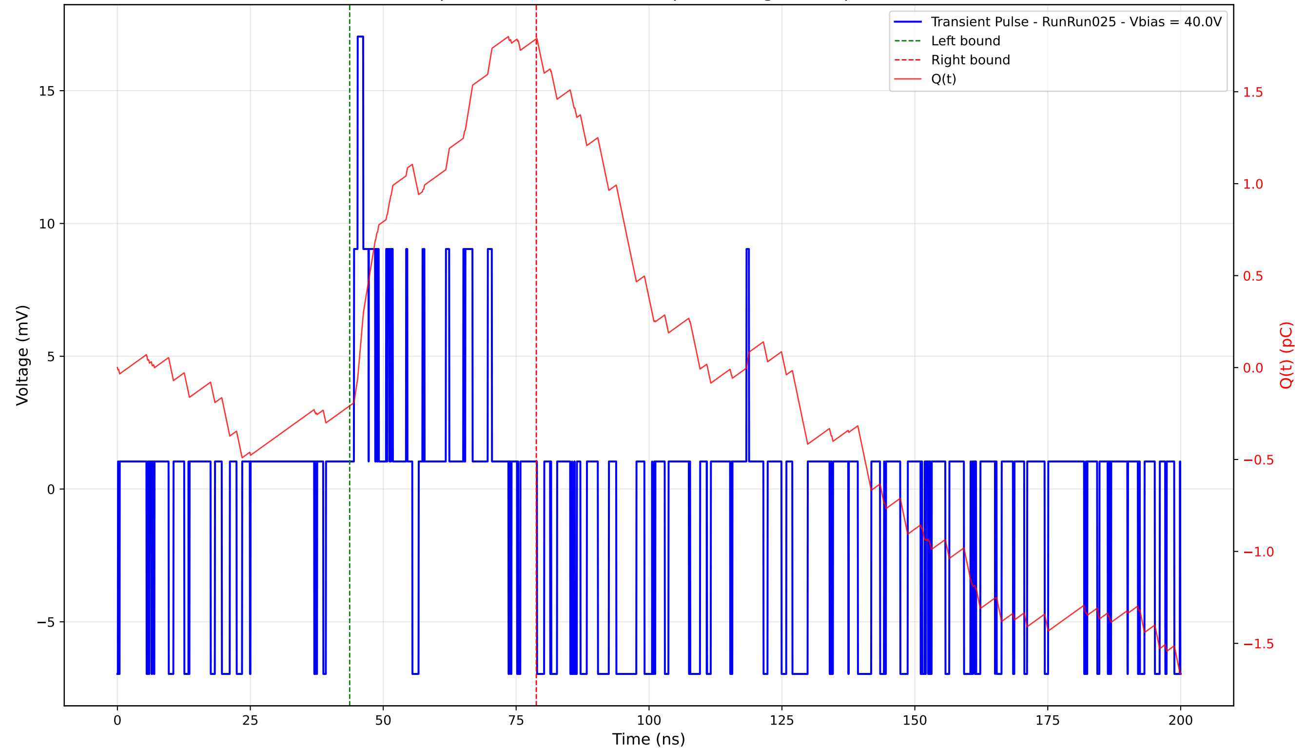
Transient Pulse - Sample: 4003 - Position: 25.0 \mu\text{m} - Charge: 2.00 pC - Rise Time: 0.70 ns
