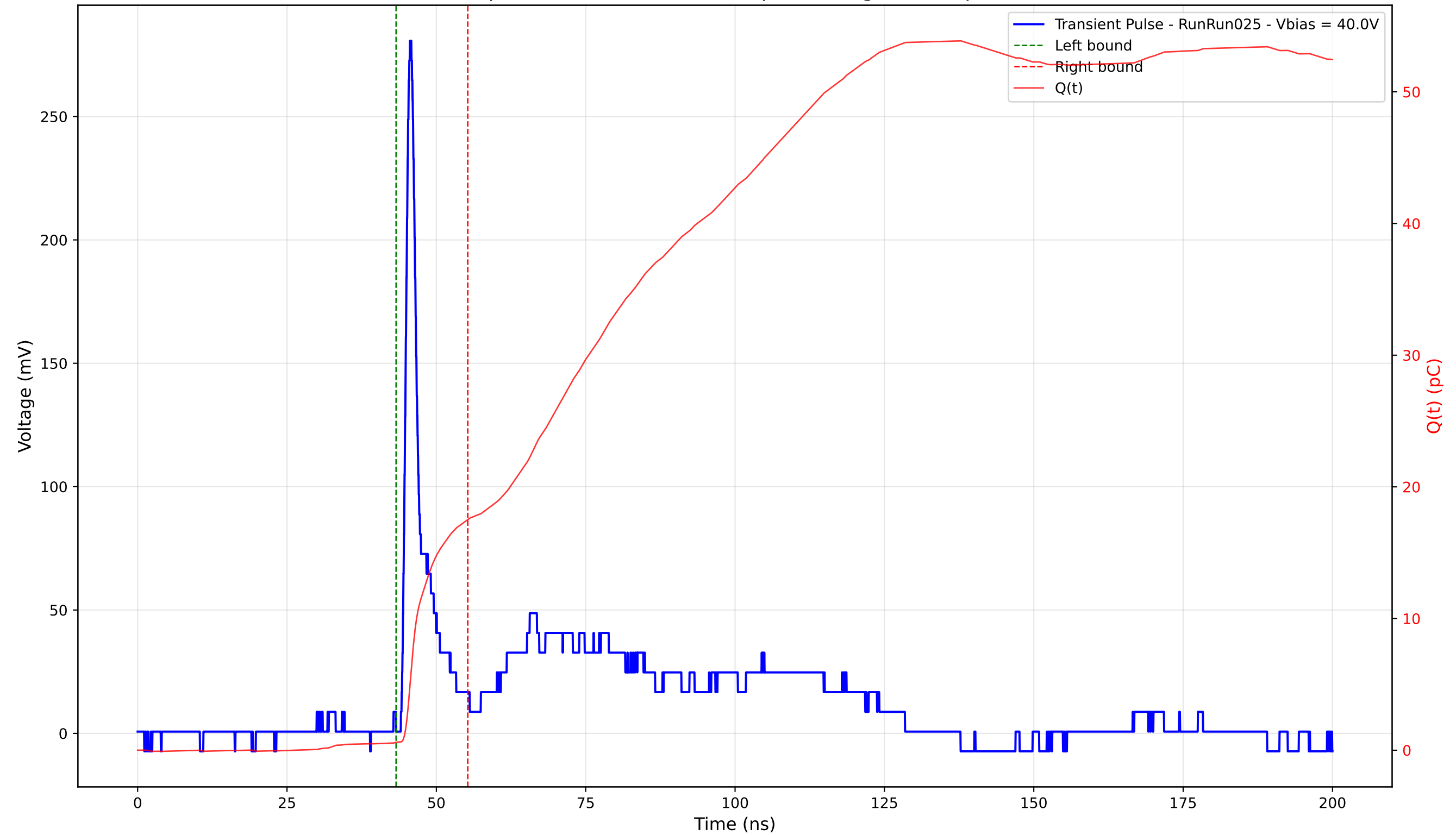
Transient Pulse - Sample: 4003 - Position: 130.0 \mu\text{m} - Charge: 16.91 pC - Rise Time: 1.03 ns
