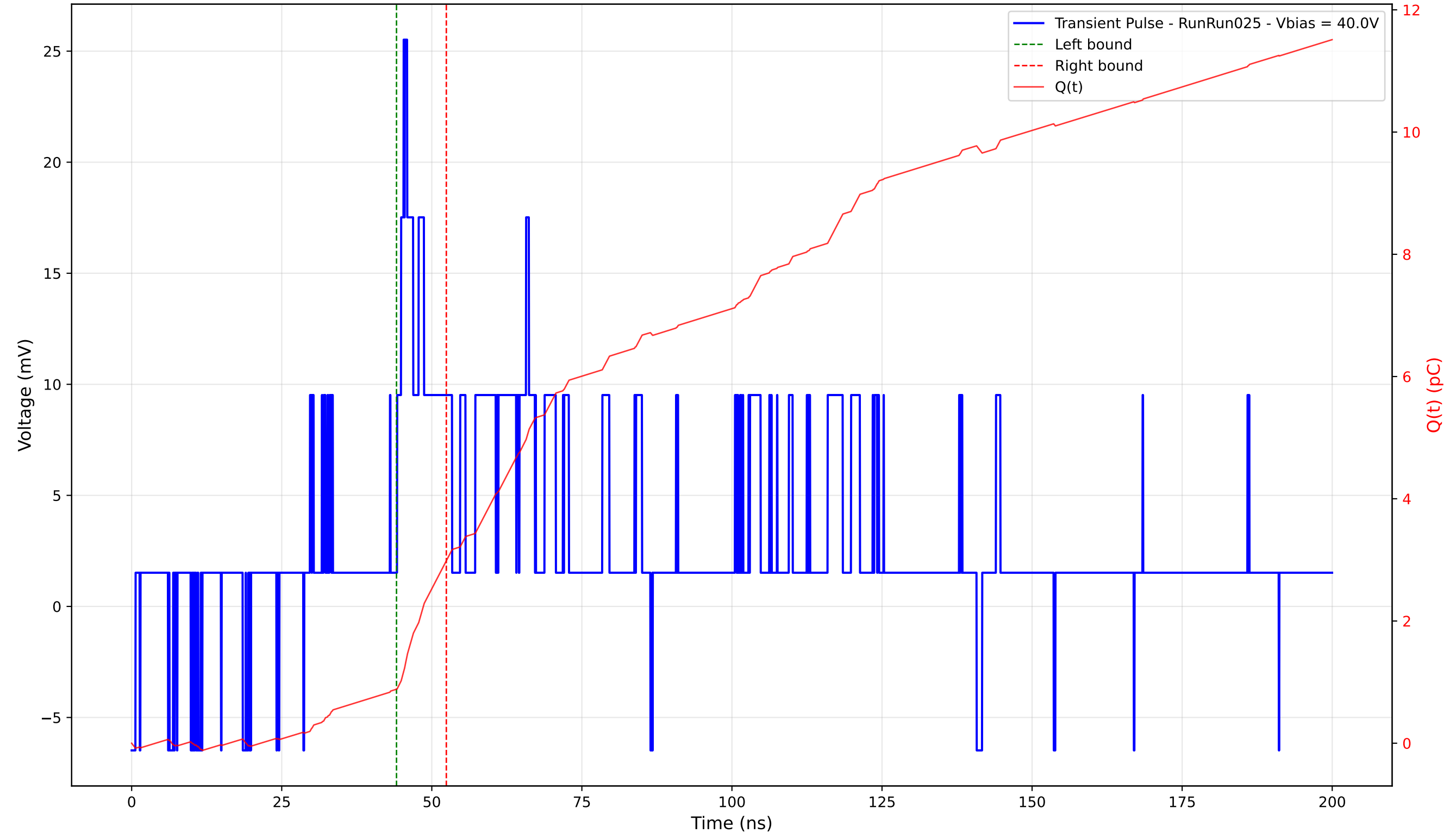
Transient Pulse - Sample: 4003 - Position: 85.0 \mu\text{m} - Charge: 2.11 pC - Rise Time: 1.10 ns
