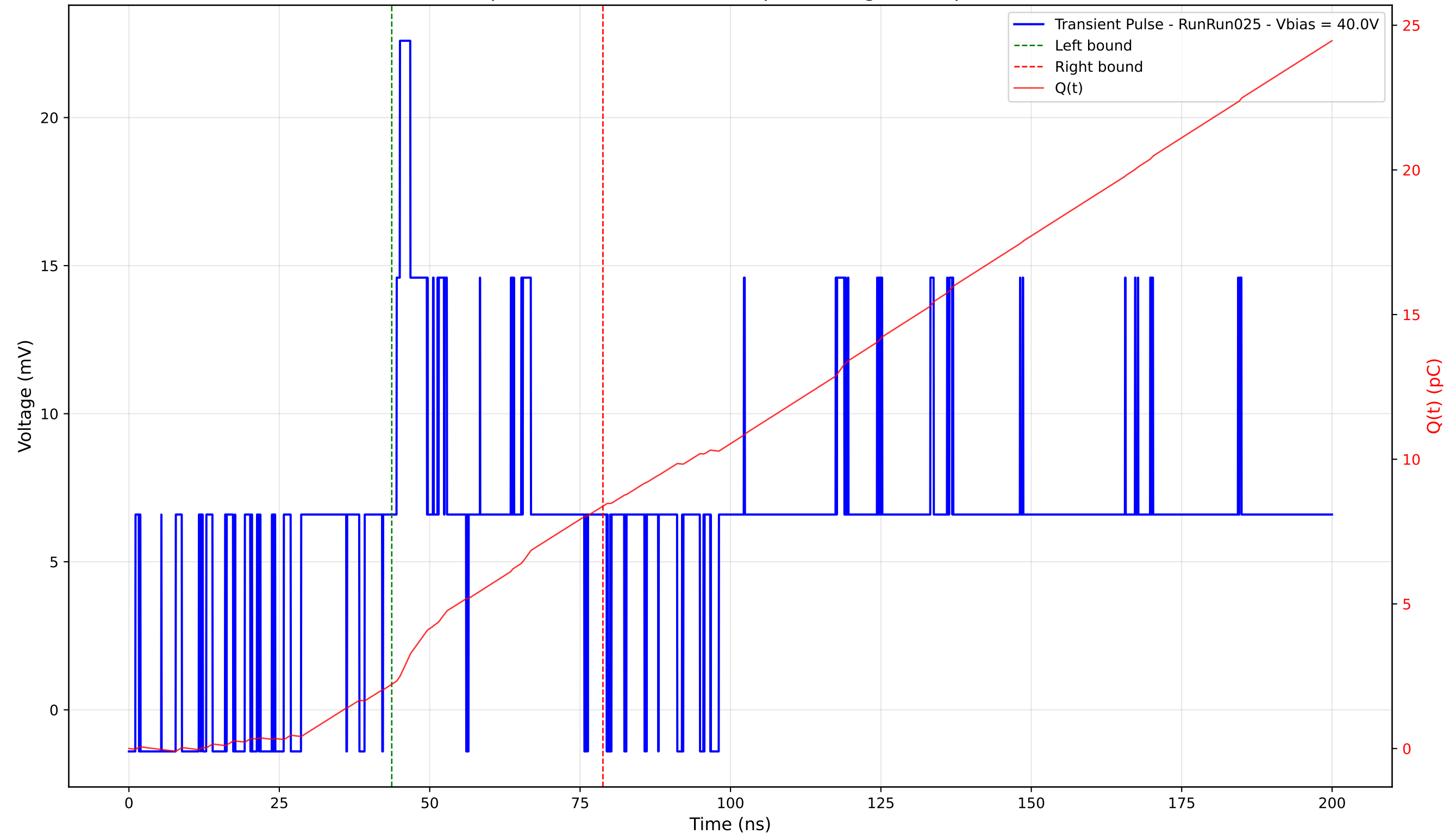
Transient Pulse - Sample: 4003 - Position: 245.0 \mu\text{m} - Charge: 6.16 pC - Rise Time: 2.82 ns
