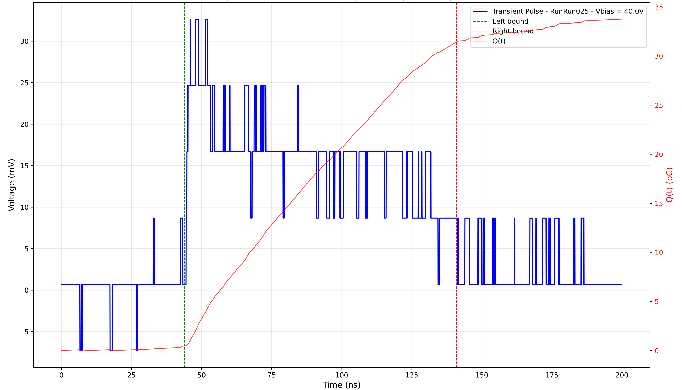
Transient Pulse - Sample: 4003 - Position: 200.0 \mu\text{m} - Charge: 30.97 pC - Rise Time: 1.49 ns
