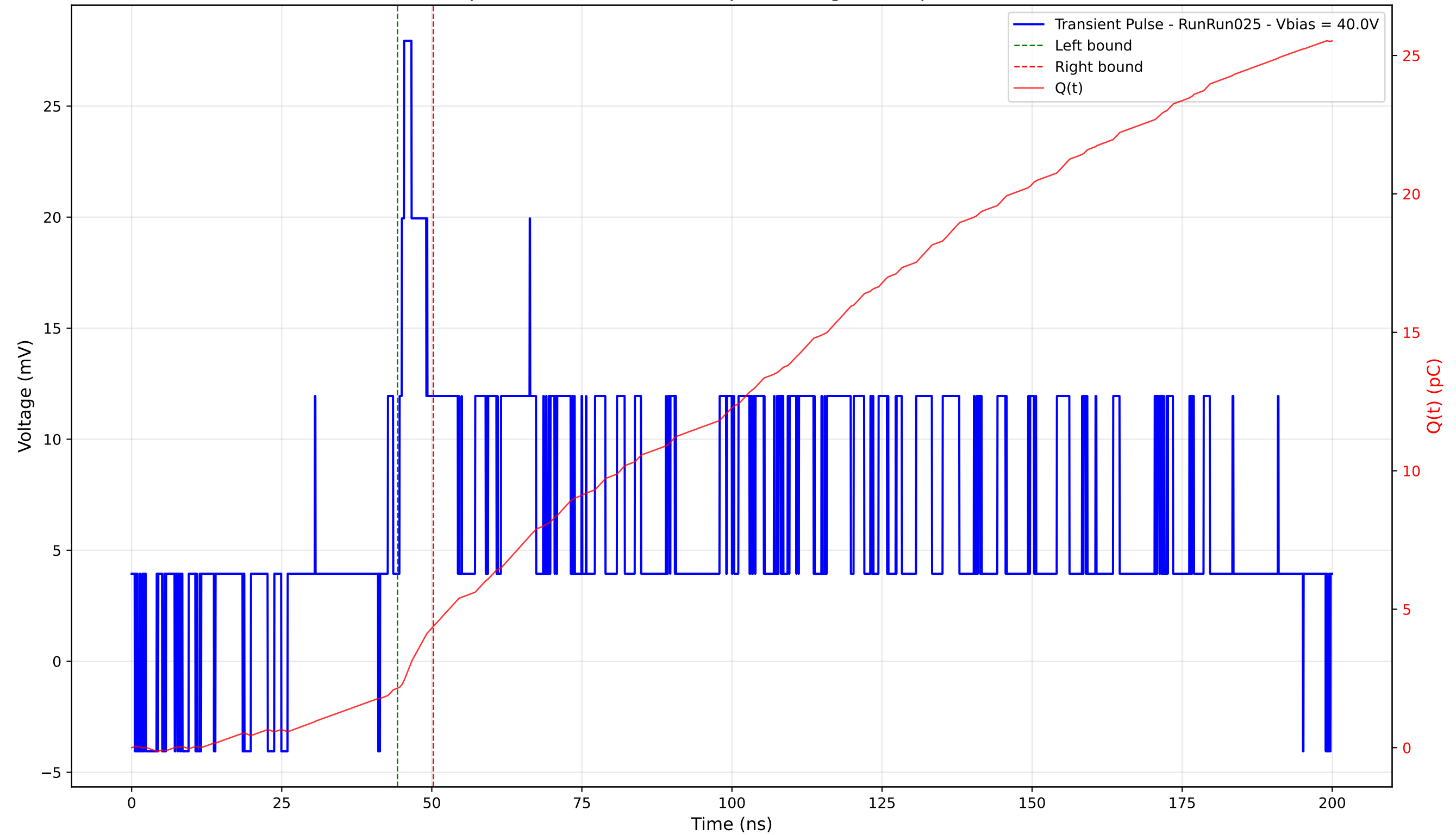
Transient Pulse - Sample: 4003 - Position: 55.0 \mu\text{m} - Charge: 2.24 pC - Rise Time: 0.00 ns (N/A)
