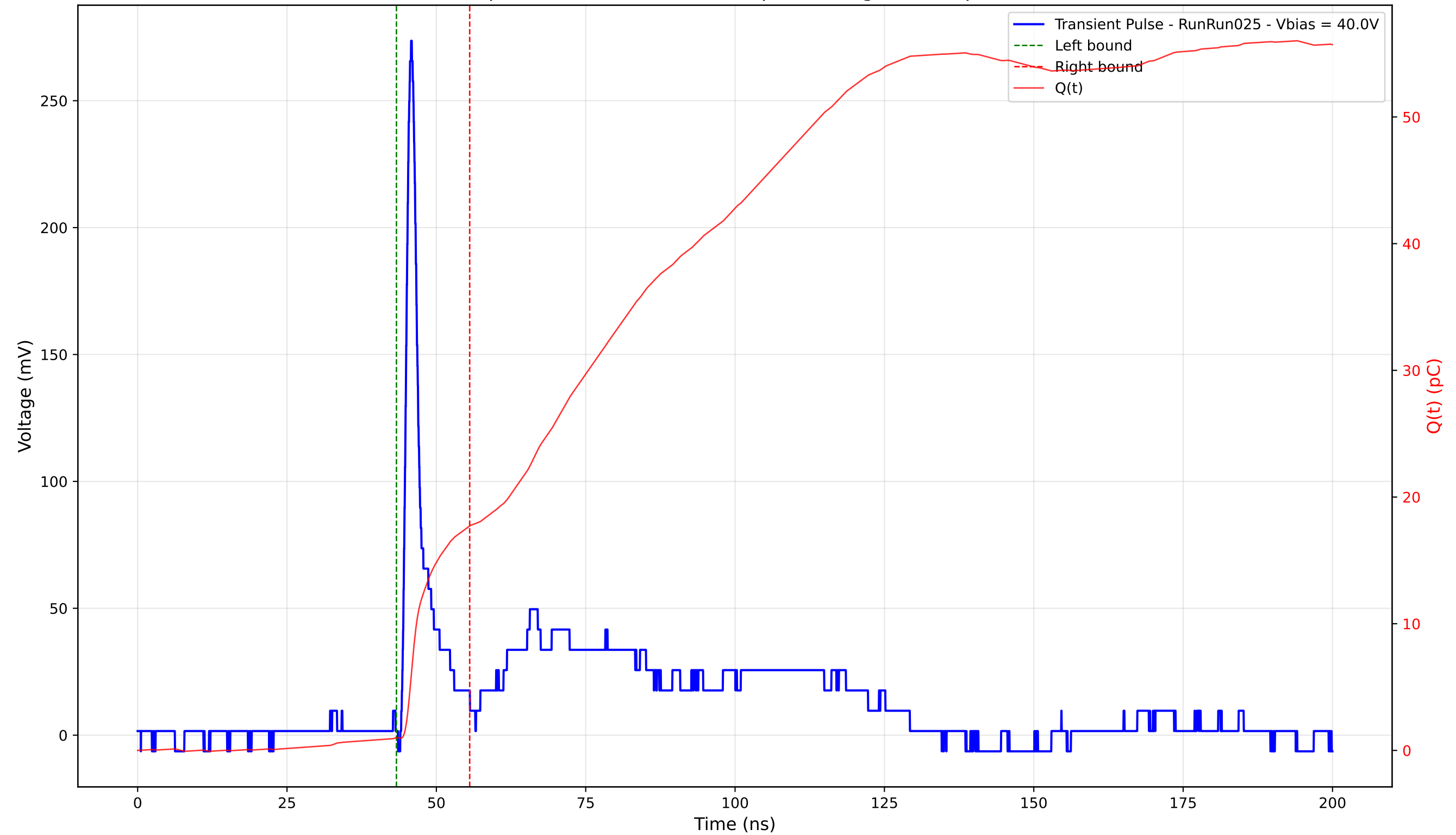
Transient Pulse - Sample: 4003 - Position: 140.0 \mu\text{m} - Charge: 16.73 pC - Rise Time: 1.10 ns
