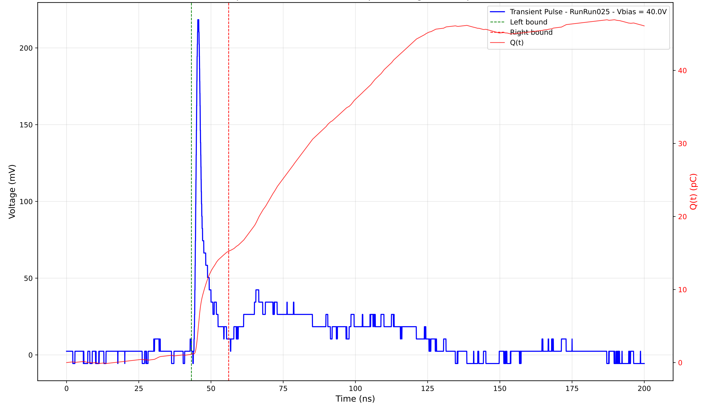
Transient Pulse - Sample: 4003 - Position: 115.0 \mu\text{m} - Charge: 14.07 pC - Rise Time: 0.97 ns
