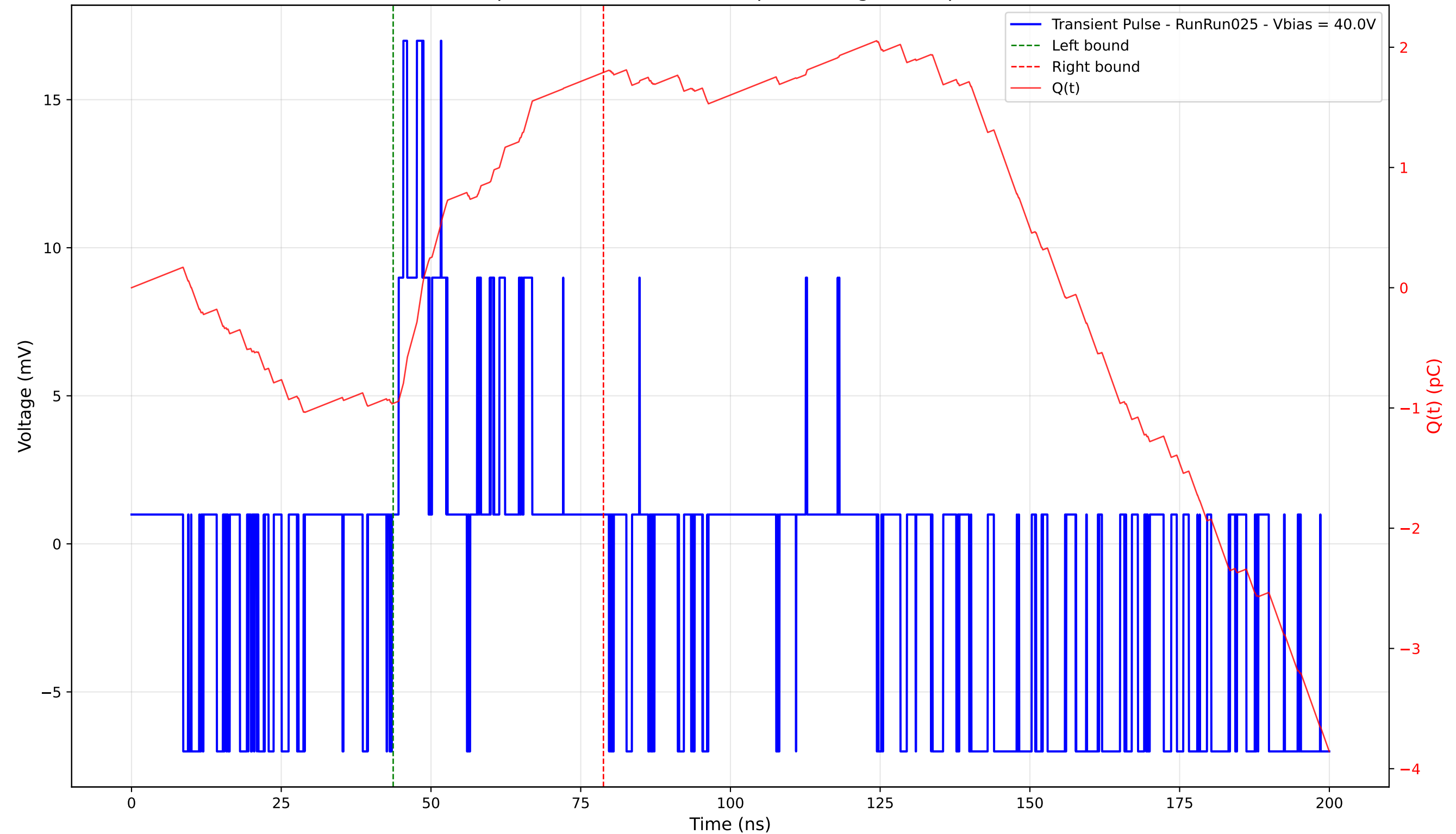
Transient Pulse - Sample: 4003 - Position: 65.0 \mu\text{m} - Charge: 2.75 pC - Rise Time: 0.80 ns
