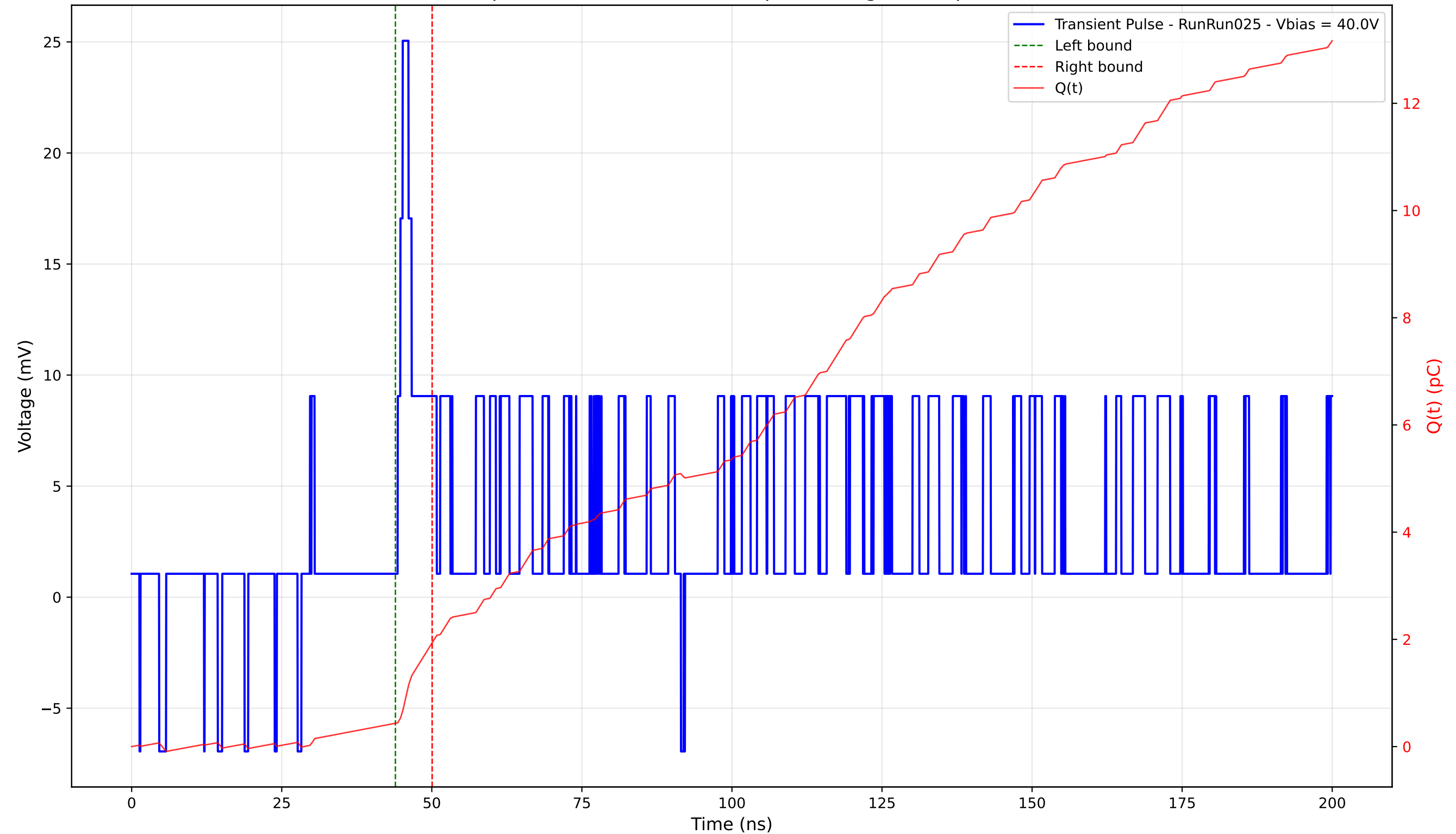
Transient Pulse - Sample: 4003 - Position: 225.0 \mu\text{m} - Charge: 1.51 pC - Rise Time: 0.84 ns
