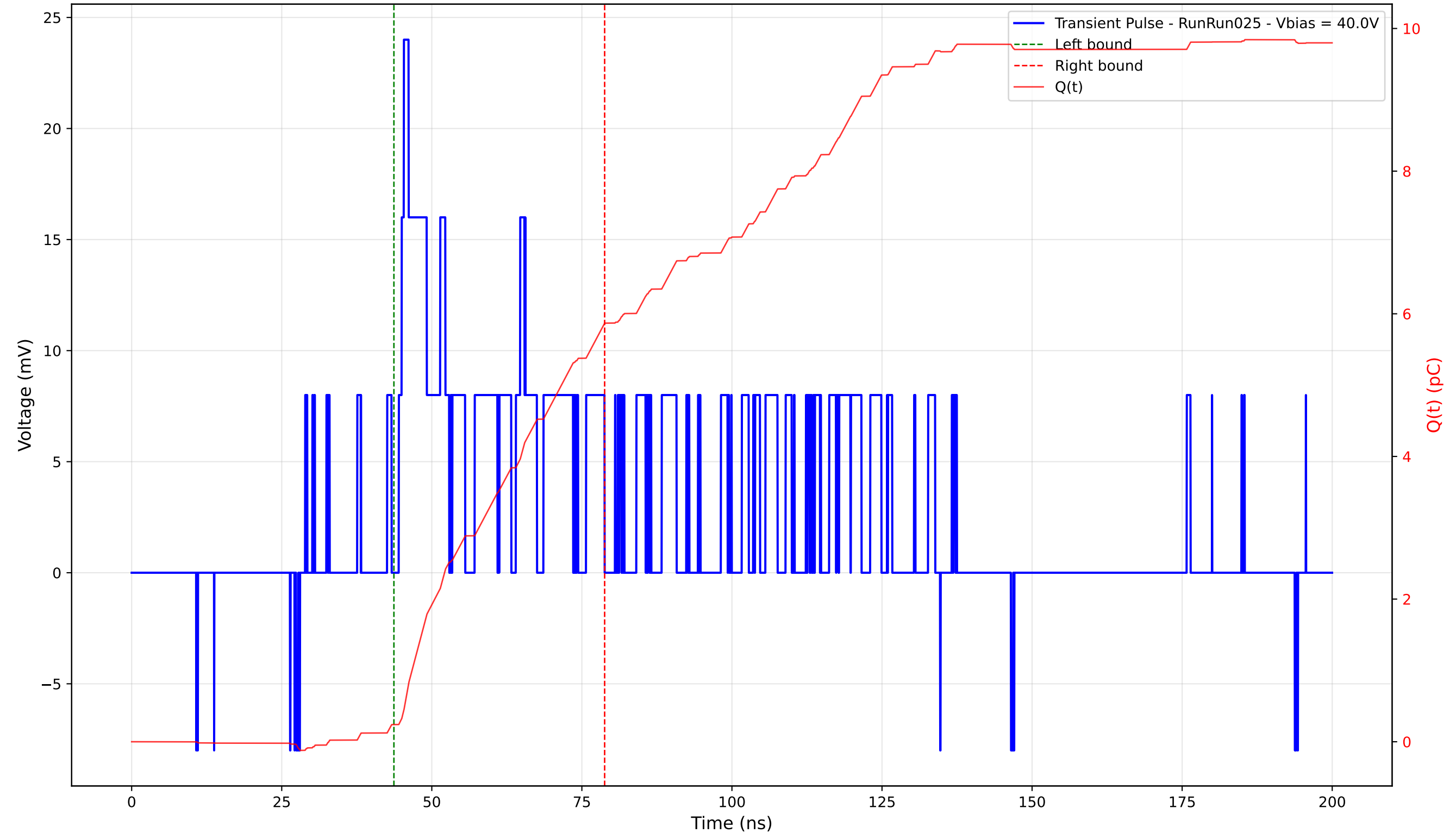
Transient Pulse - Sample: 4003 - Position: 60.0 \mu\text{m} - Charge: 5.63 pC - Rise Time: 0.85 ns
