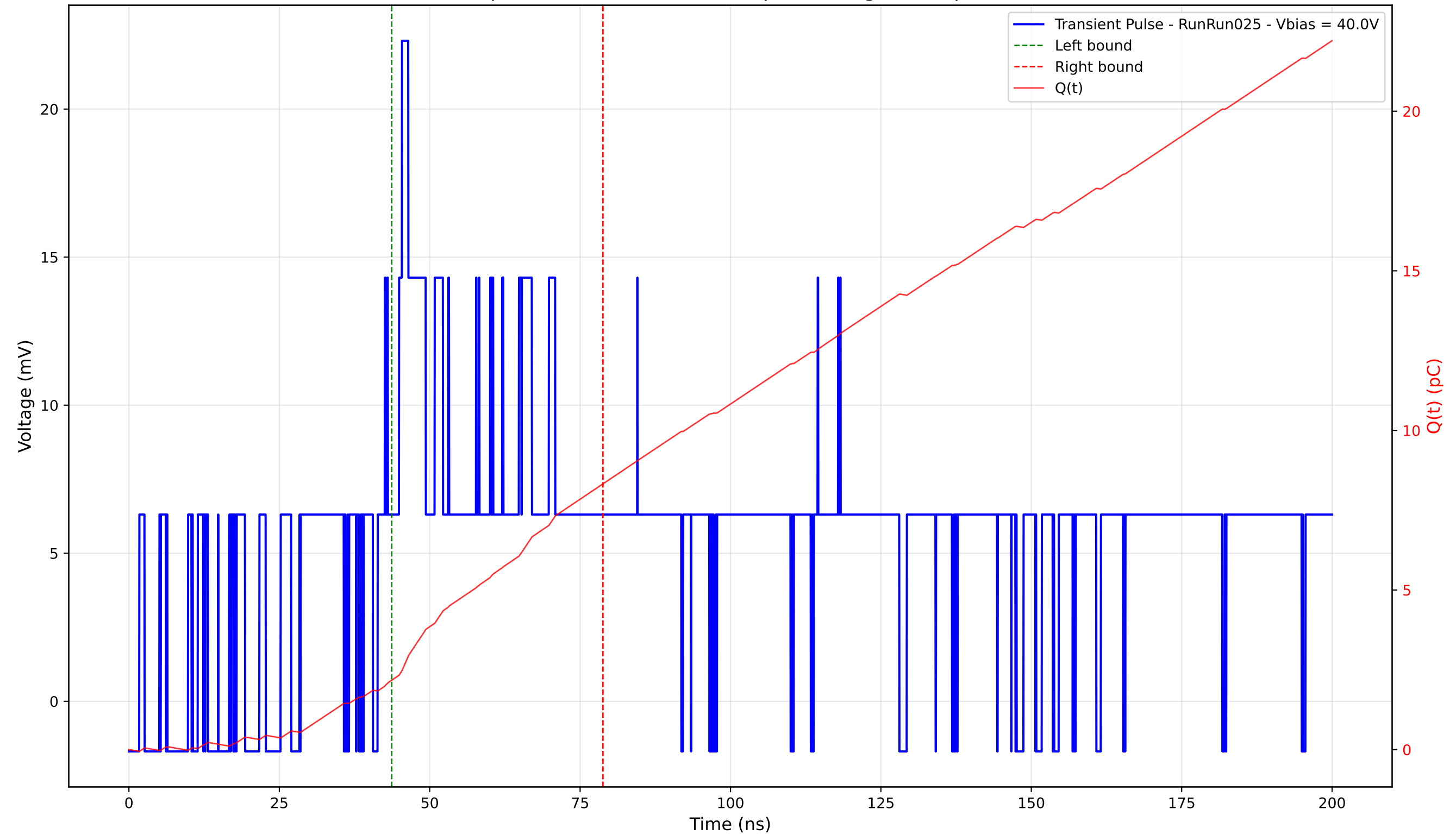
Transient Pulse - Sample: 4003 - Position: 345.0 \mu\text{m} - Charge: 6.15 pC - Rise Time: 4.06 ns
