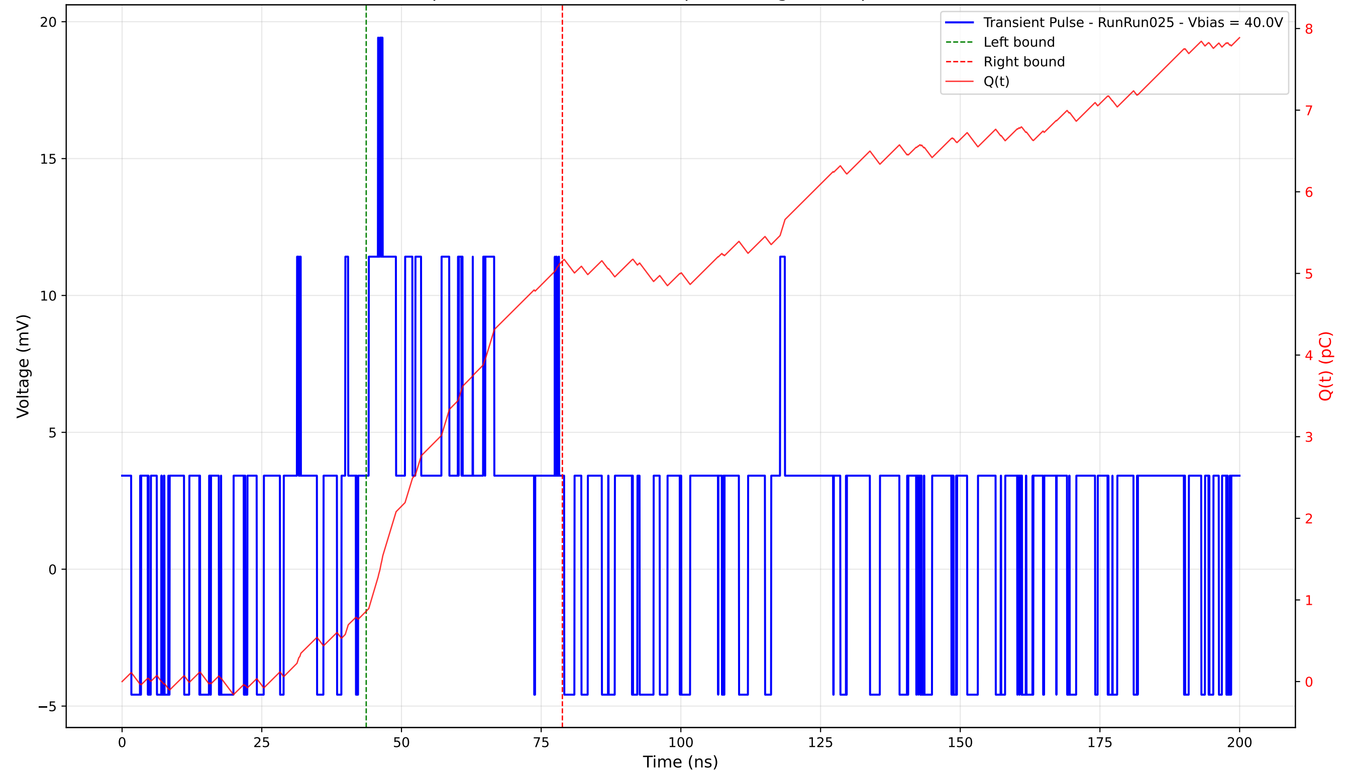
Transient Pulse - Sample: 4003 - Position: 325.0 \mu\text{m} - Charge: 4.29 pC - Rise Time: 0.00 ns (N/A)
