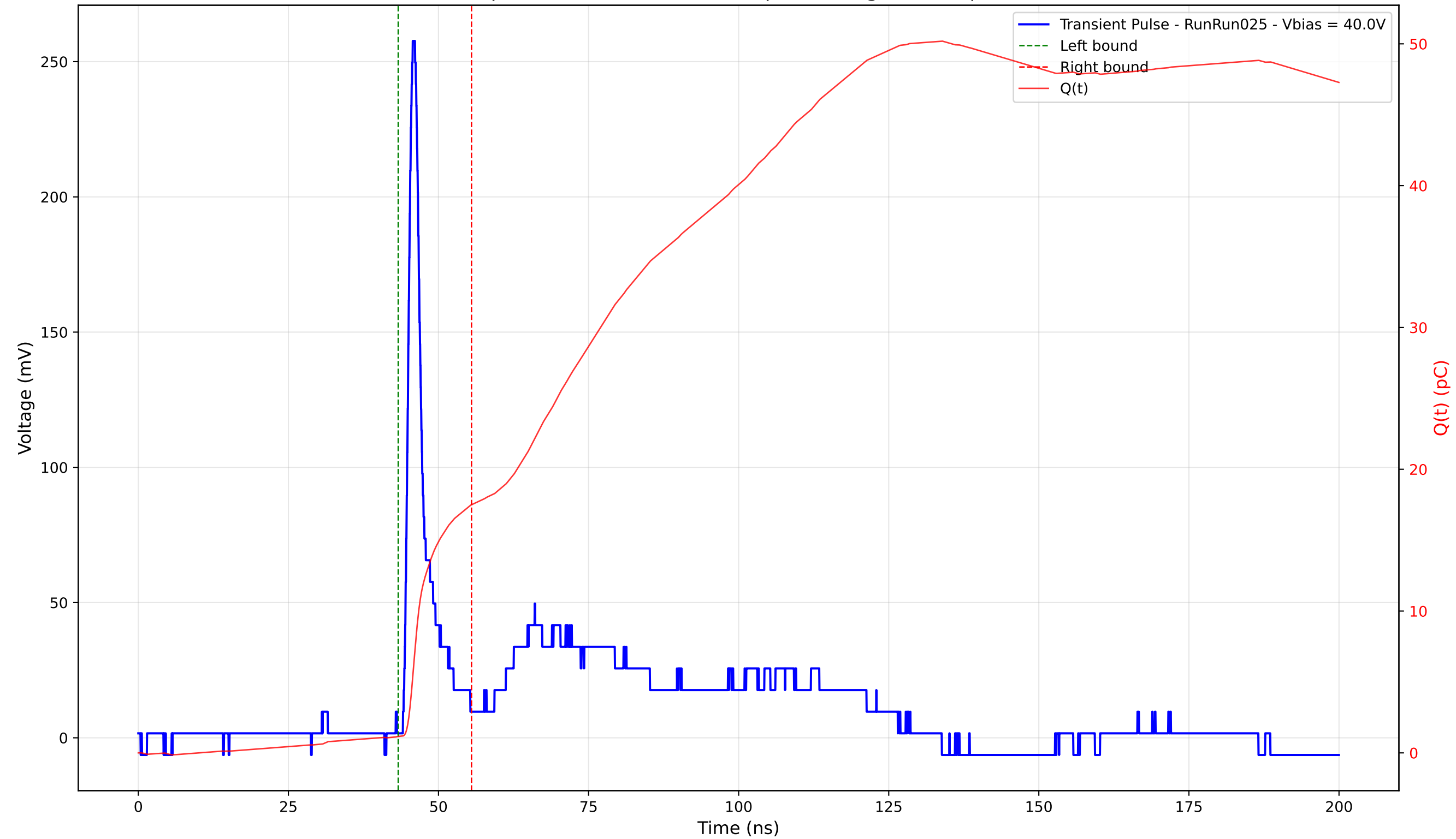
Transient Pulse - Sample: 4003 - Position: 145.0 \mu\text{m} - Charge: 16.34 pC - Rise Time: 1.10 ns
