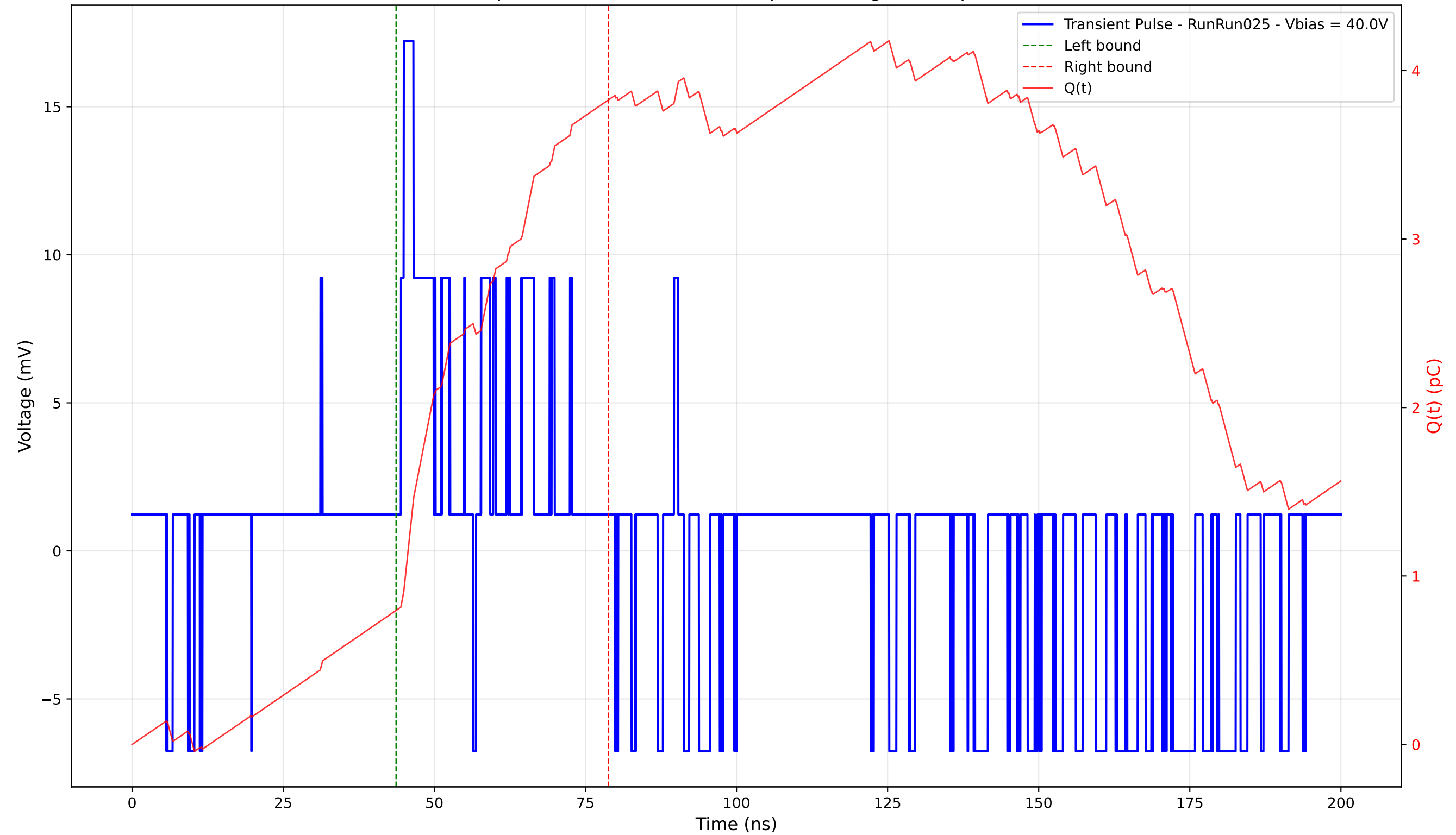
Transient Pulse - Sample: 4003 - Position: 375.0 \mu\text{m} - Charge: 3.03 pC - Rise Time: 0.48 ns
