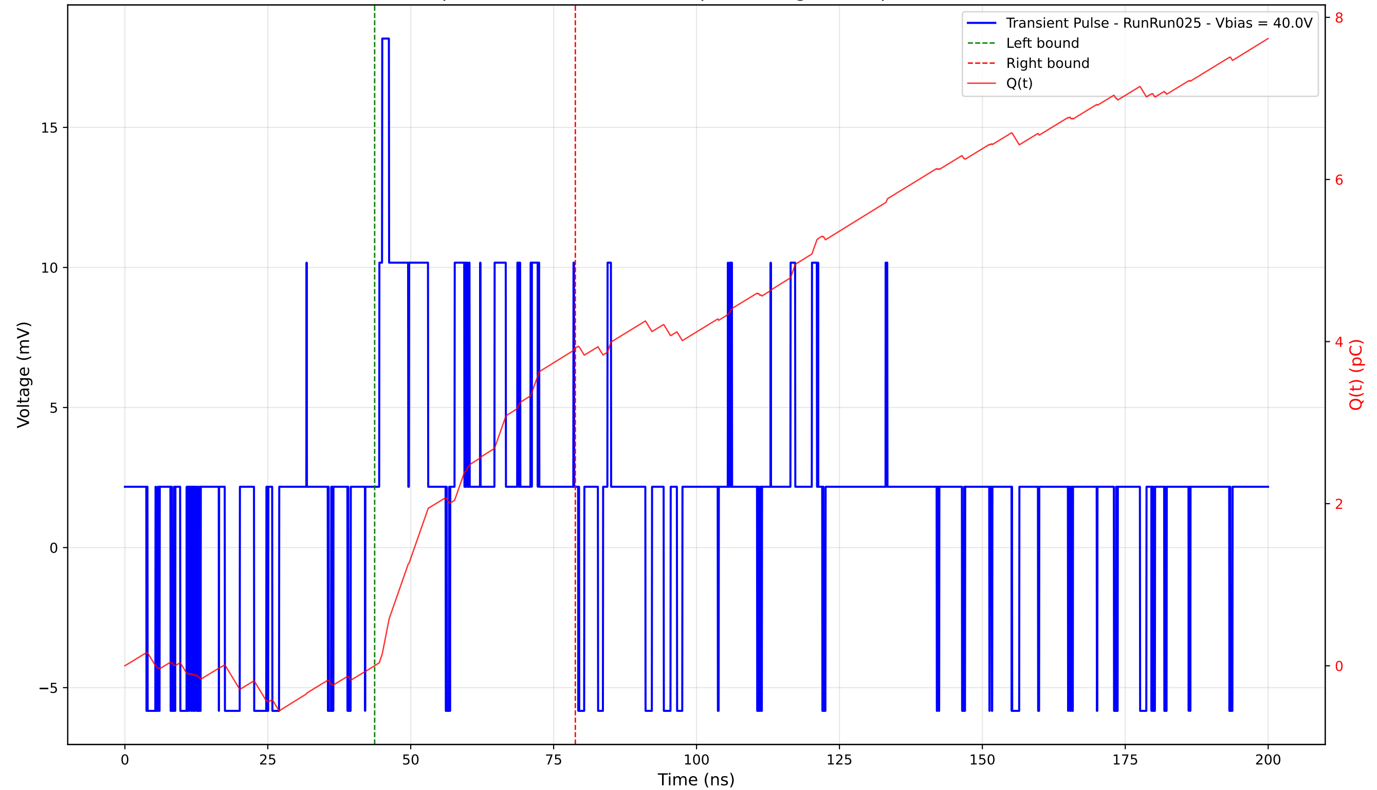
Transient Pulse - Sample: 4003 - Position: 350.0 \mu\text{m} - Charge: 3.92 pC - Rise Time: 0.00 ns (N/A)
