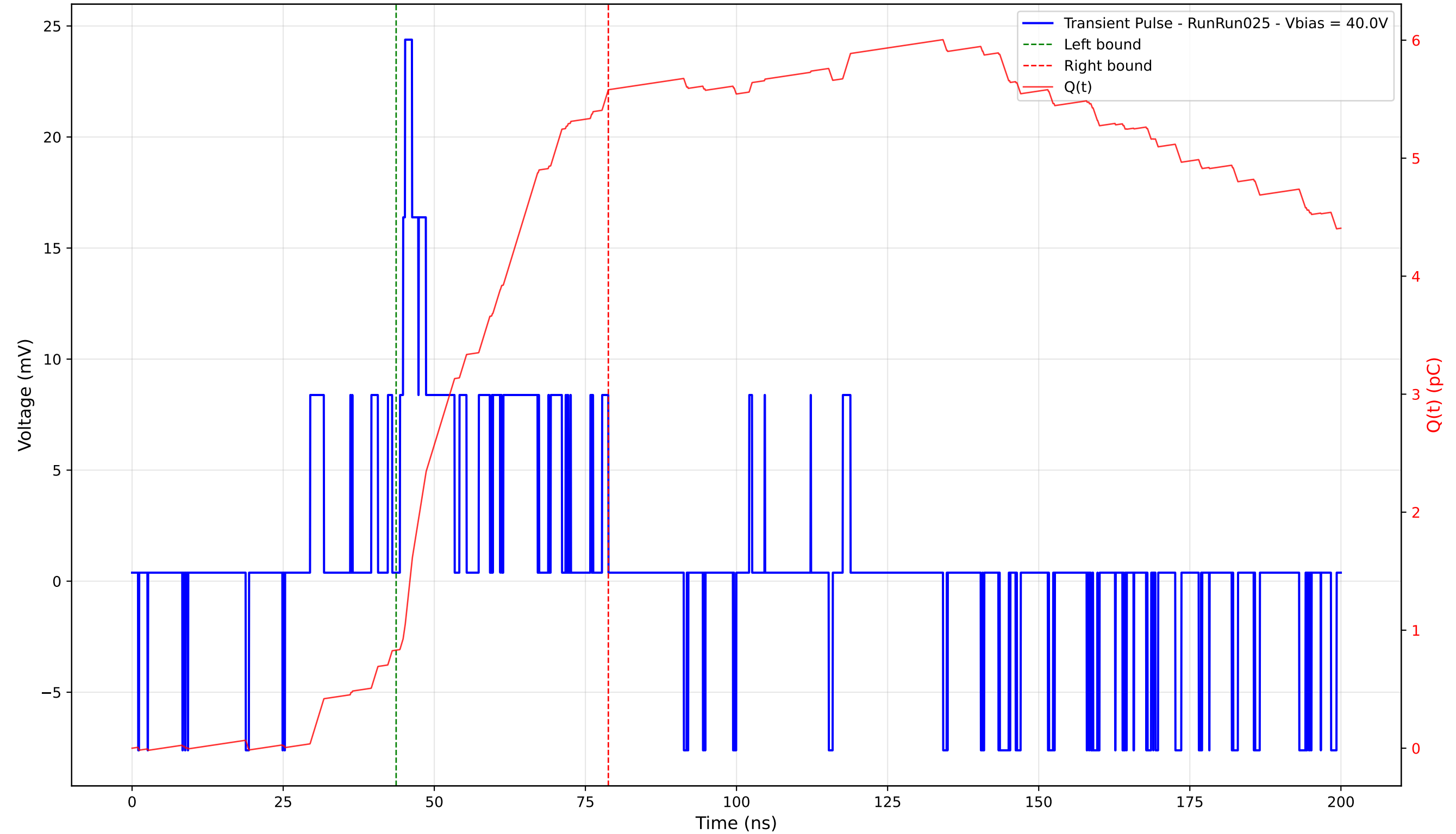
Transient Pulse - Sample: 4003 - Position: 280.0 \mu\text{m} - Charge: 4.75 pC - Rise Time: 0.85 ns
