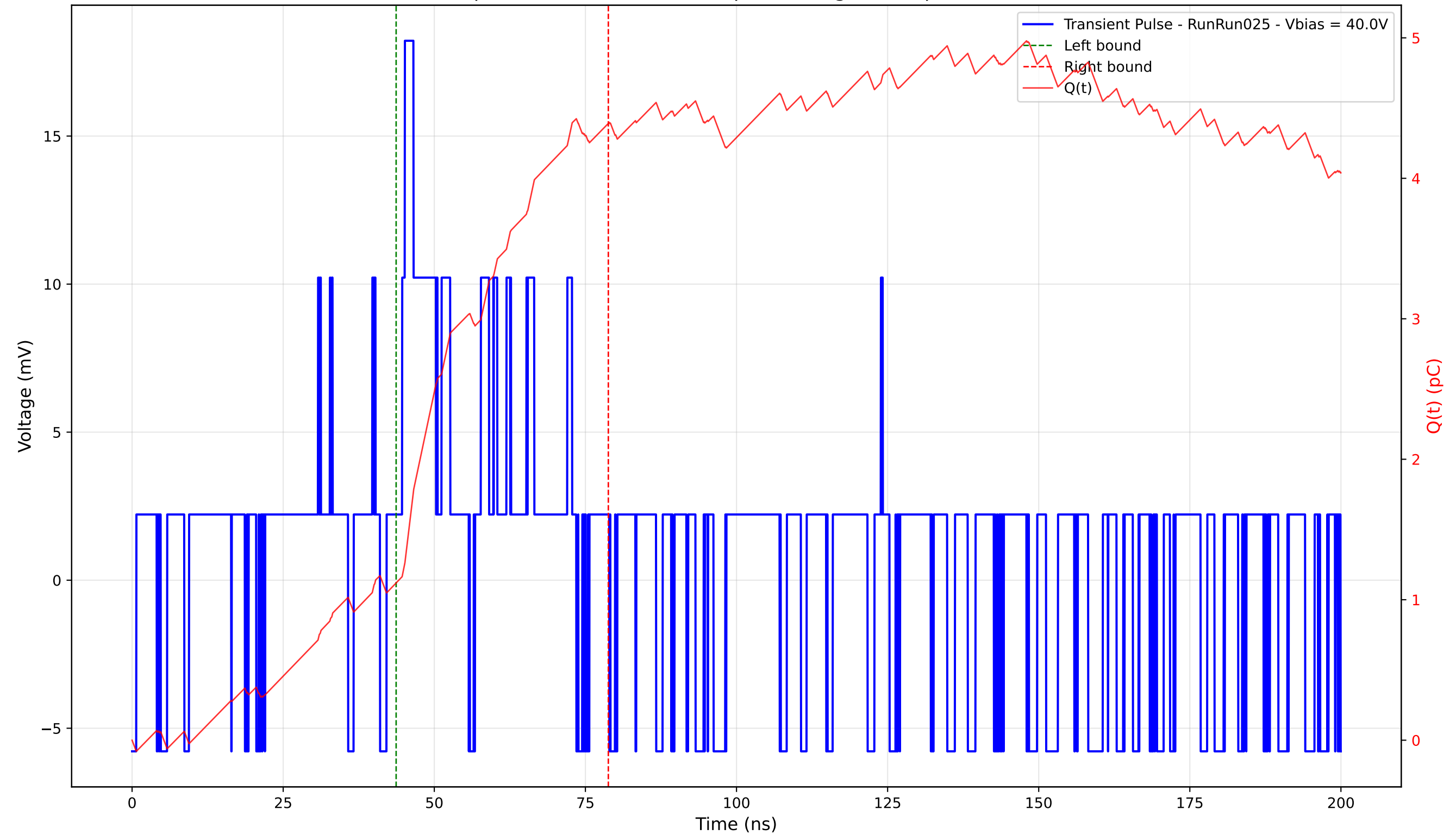
Transient Pulse - Sample: 4003 - Position: 80.0 \mu\text{m} - Charge: 3.27 pC - Rise Time: 0.00 ns (N/A)
