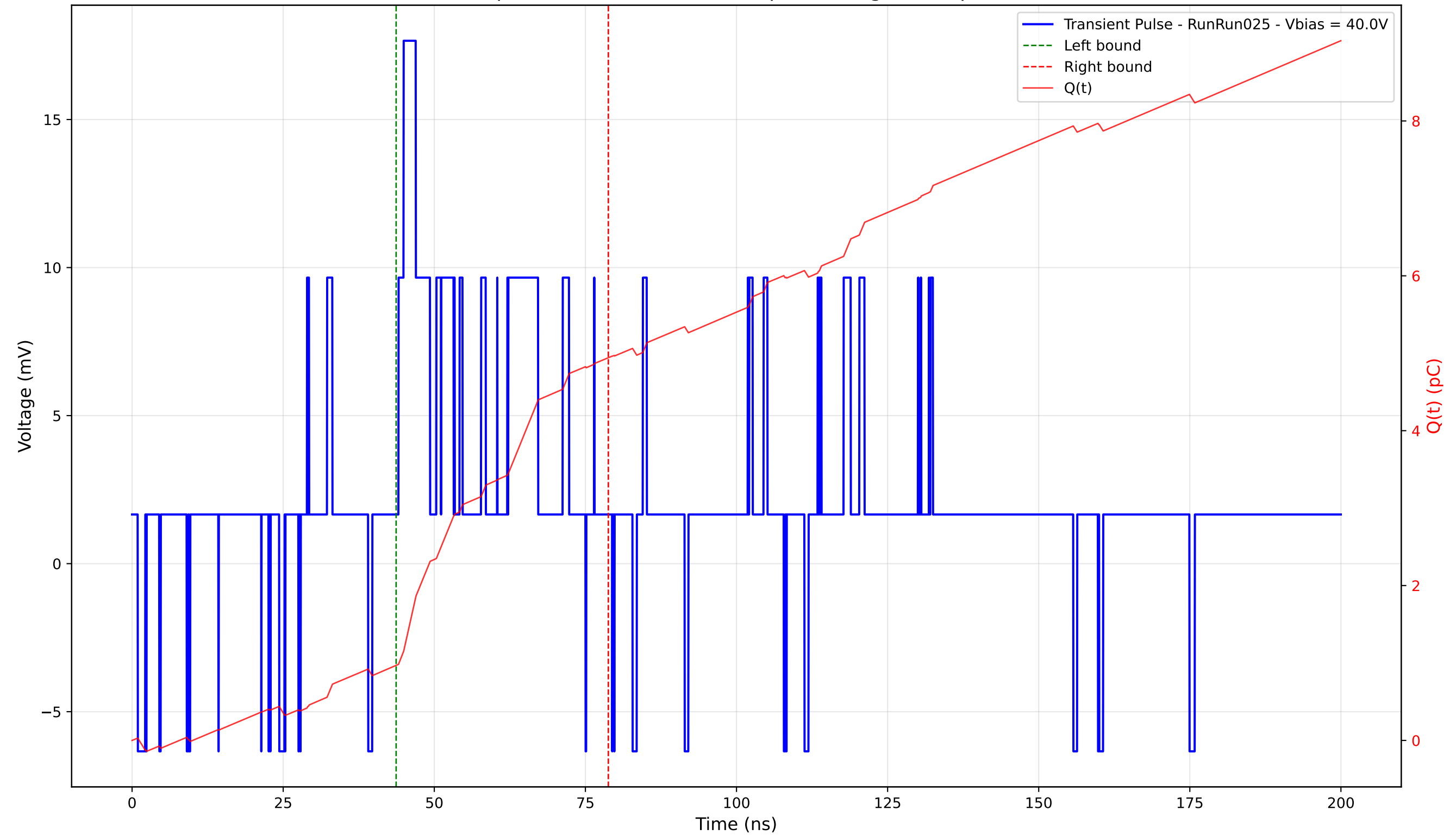
Transient Pulse - Sample: 4003 - Position: 355.0 \mu\text{m} - Charge: 3.97 pC - Rise Time: 0.86 ns
