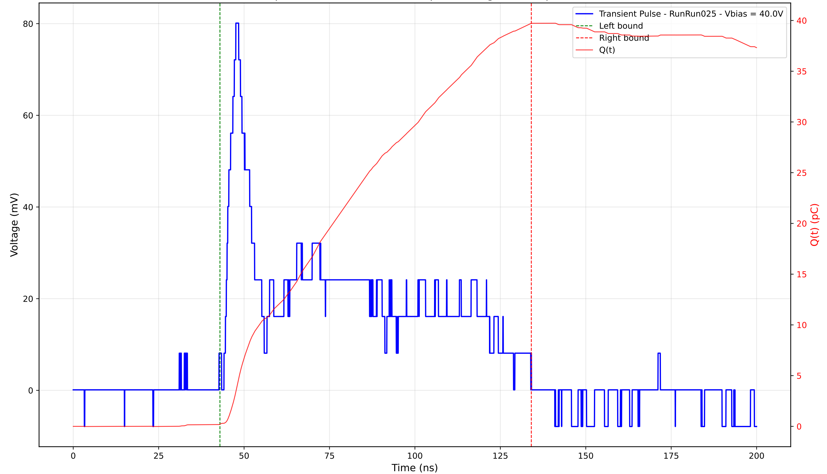
Transient Pulse - Sample: 4003 - Position: 190.0 \mu\text{m} - Charge: 39.50 pC - Rise Time: 3.02 ns
