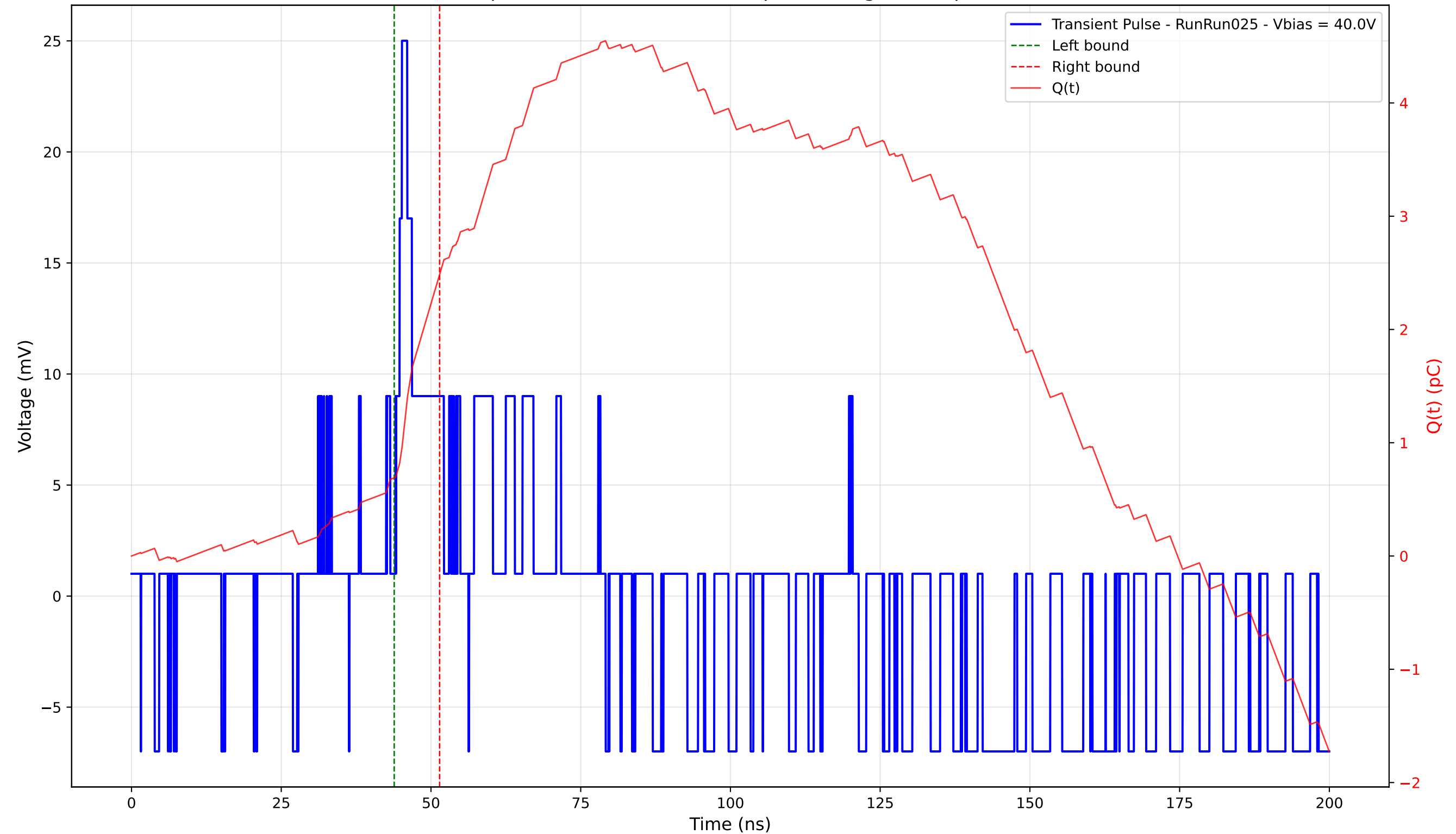
Transient Pulse - Sample: 4003 - Position: 275.0 \mu\text{m} - Charge: 1.80 pC - Rise Time: 0.98 ns
