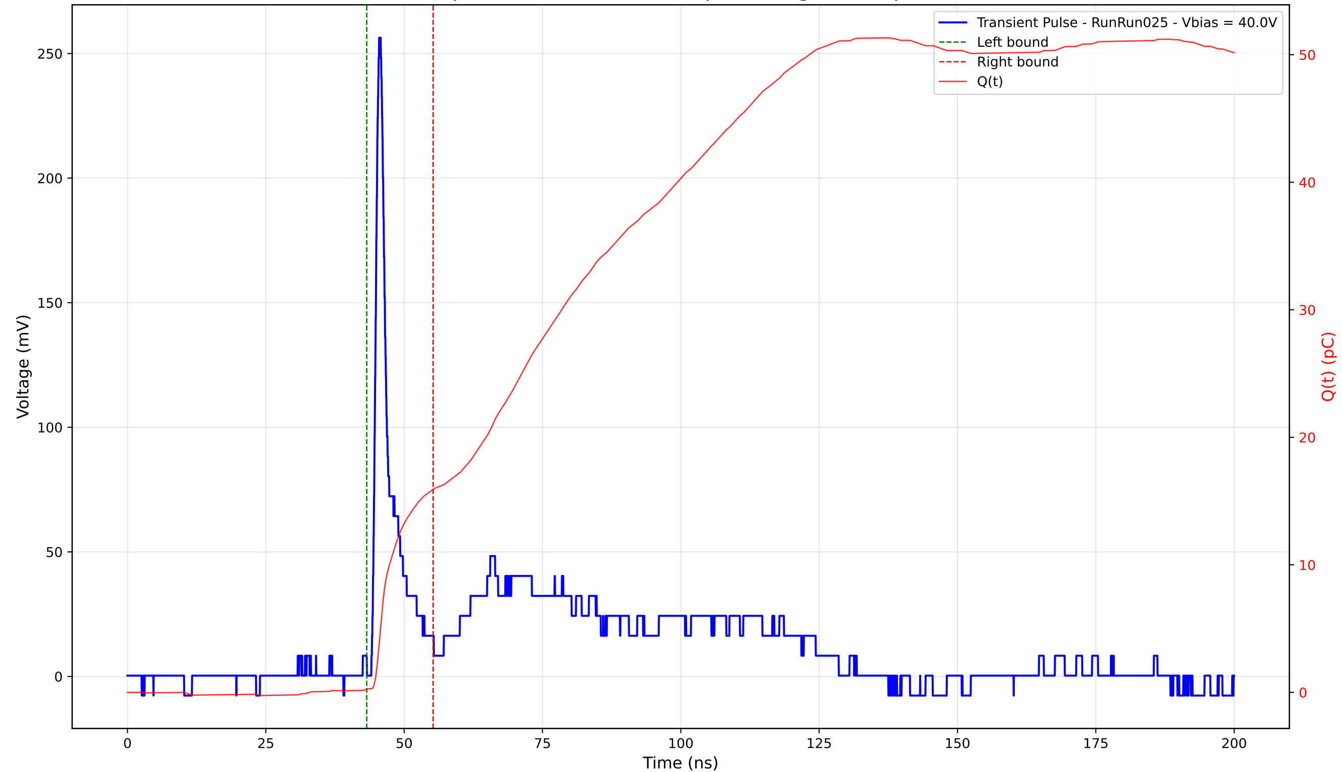
Transient Pulse - Sample: 4003 - Position: 120.0 \mu\text{m} - Charge: 15.67 pC - Rise Time: 0.94 ns
