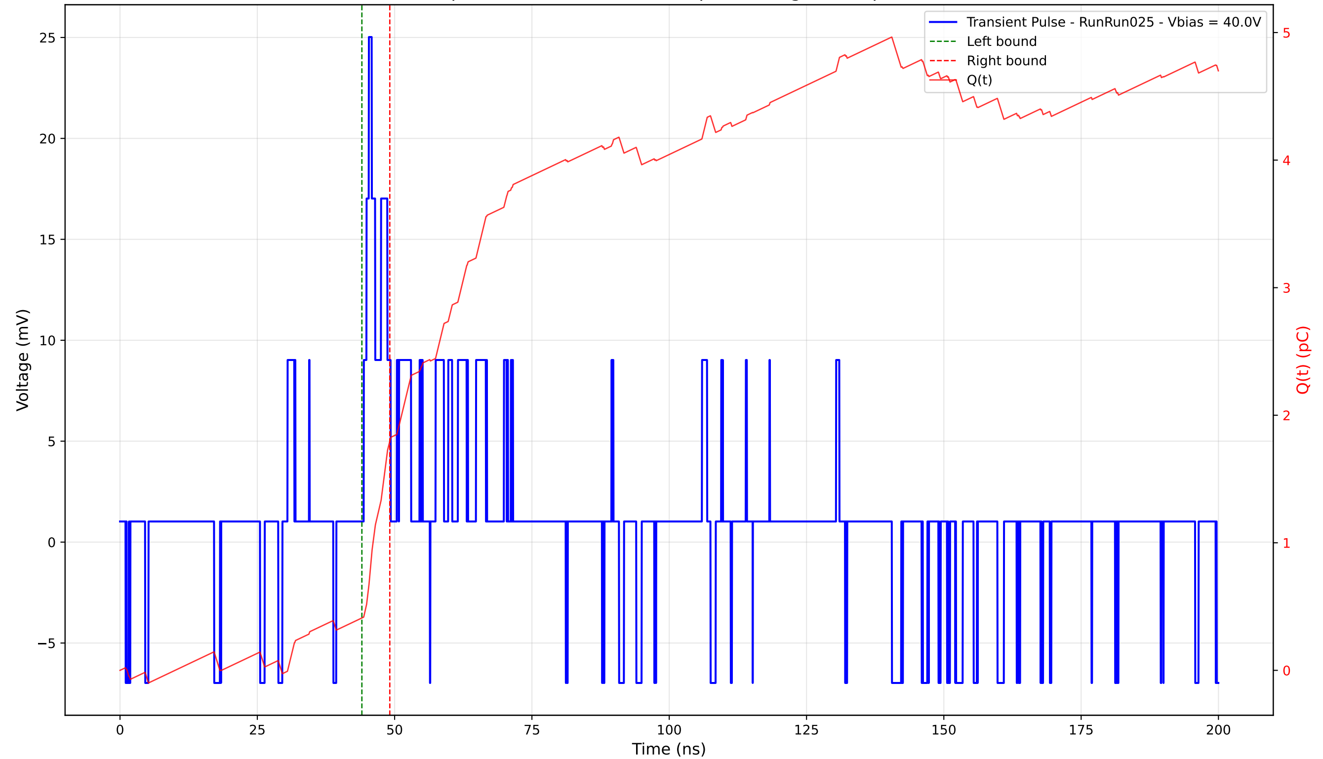
Transient Pulse - Sample: 4003 - Position: 300.0 \mu\text{m} - Charge: 1.39 pC - Rise Time: 0.94 ns
