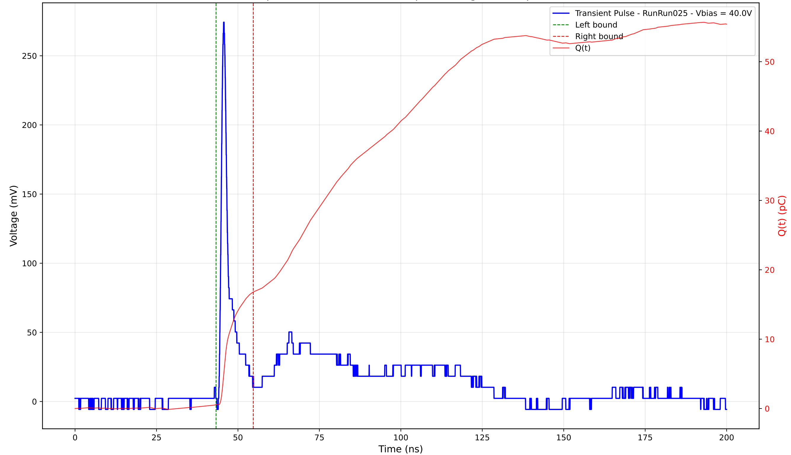
Transient Pulse - Sample: 4003 - Position: 125.0 \mu\text{m} - Charge: 16.22 pC - Rise Time: 1.00 ns
