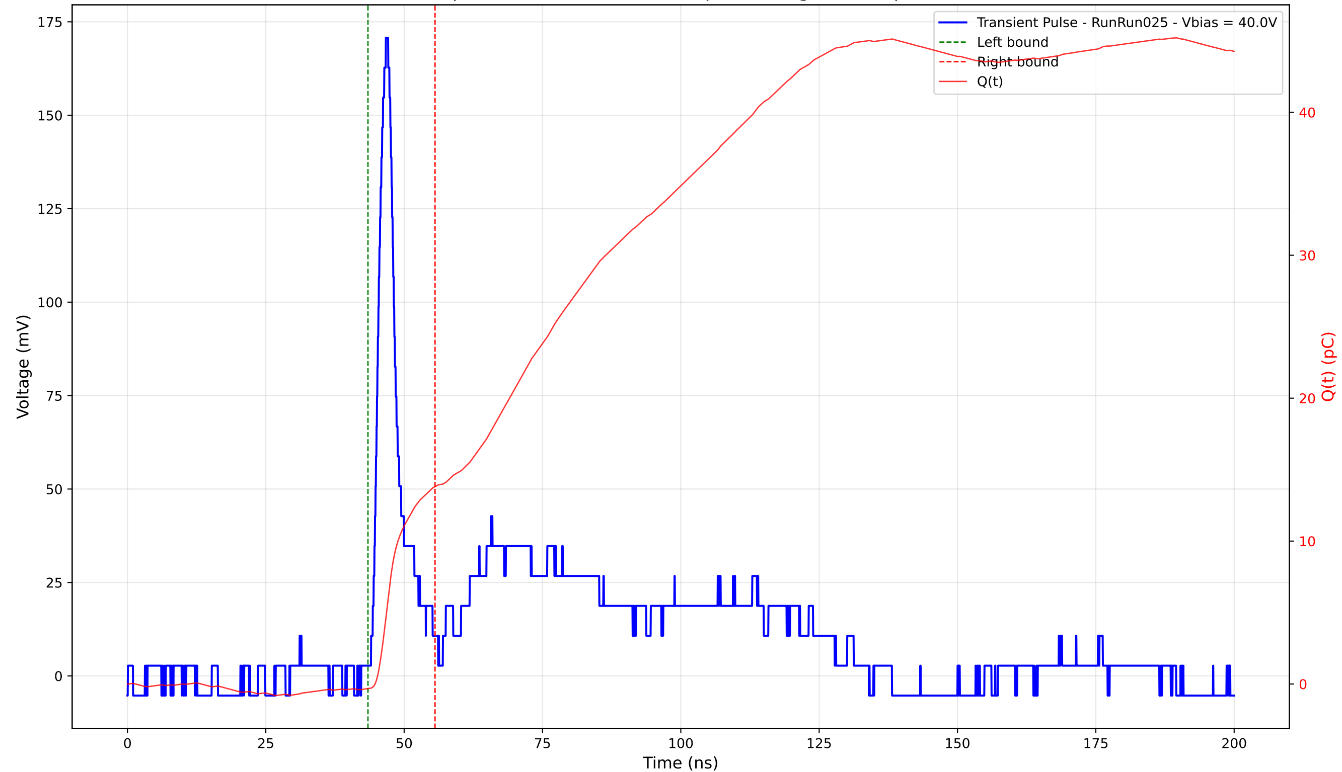
Transient Pulse - Sample: 4003 - Position: 175.0 \mu\text{m} - Charge: 14.14 pC - Rise Time: 1.86 ns
