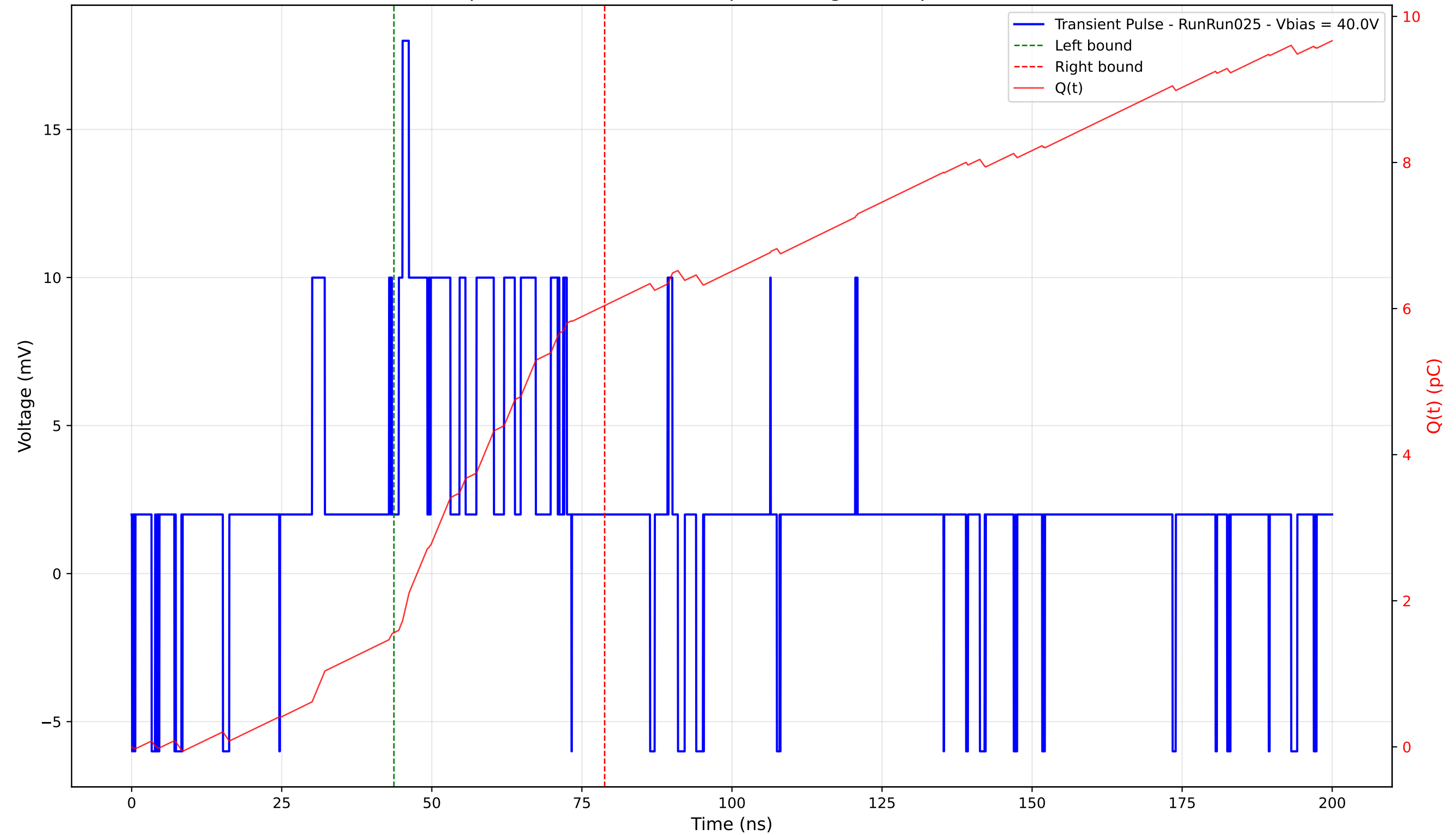
Transient Pulse - Sample: 4003 - Position: 75.0 \mu\text{m} - Charge: 4.48 pC - Rise Time: 0.00 ns (N/A)
