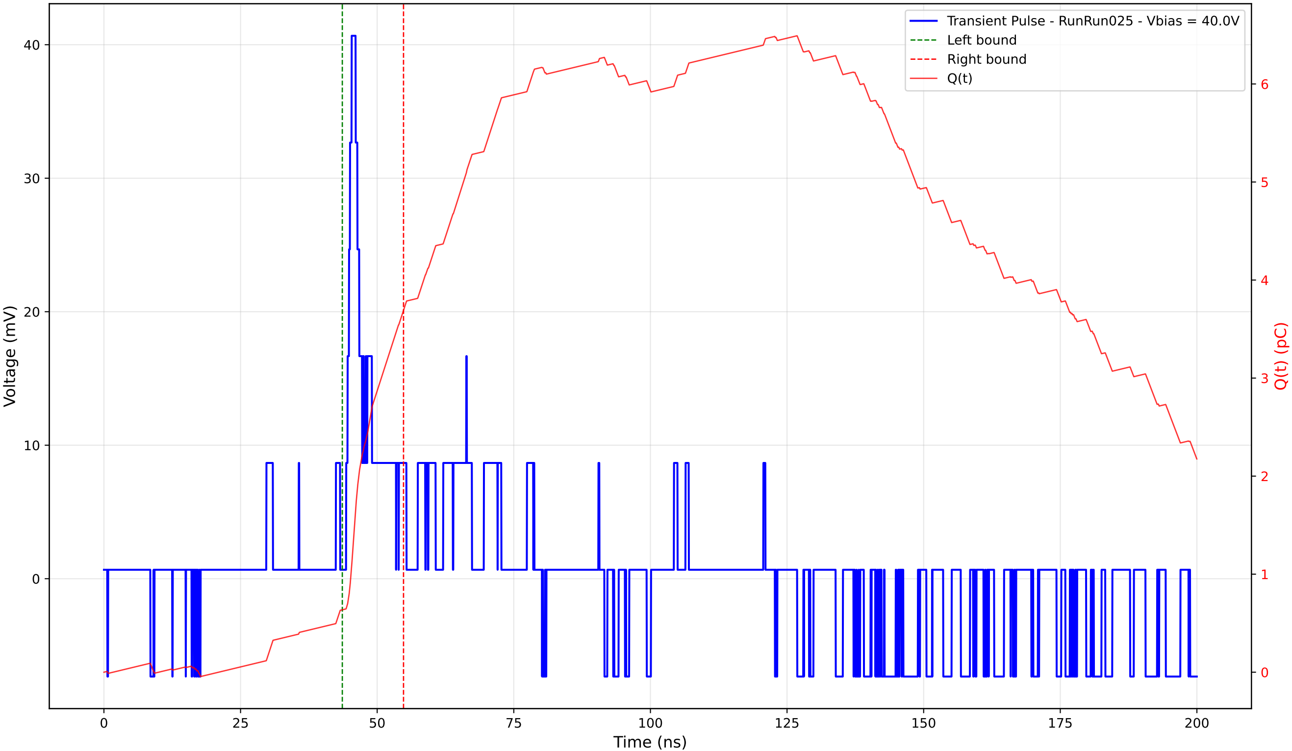
Transient Pulse - Sample: 4003 - Position: 90.0 \mu\text{m} - Charge: 3.06 pC - Rise Time: 1.01 ns
