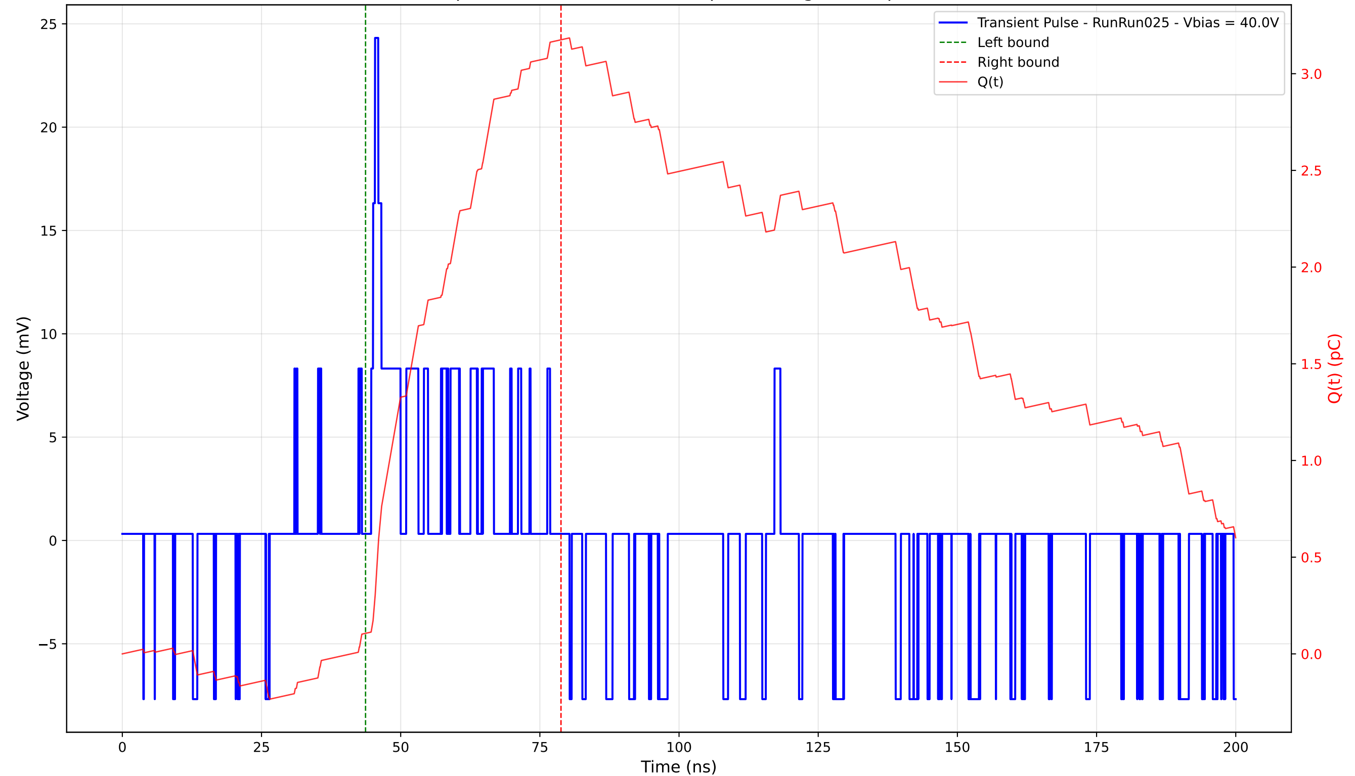
Transient Pulse - Sample: 4003 - Position: 320.0 \mu\text{m} - Charge: 3.07 pC - Rise Time: 0.69 ns
