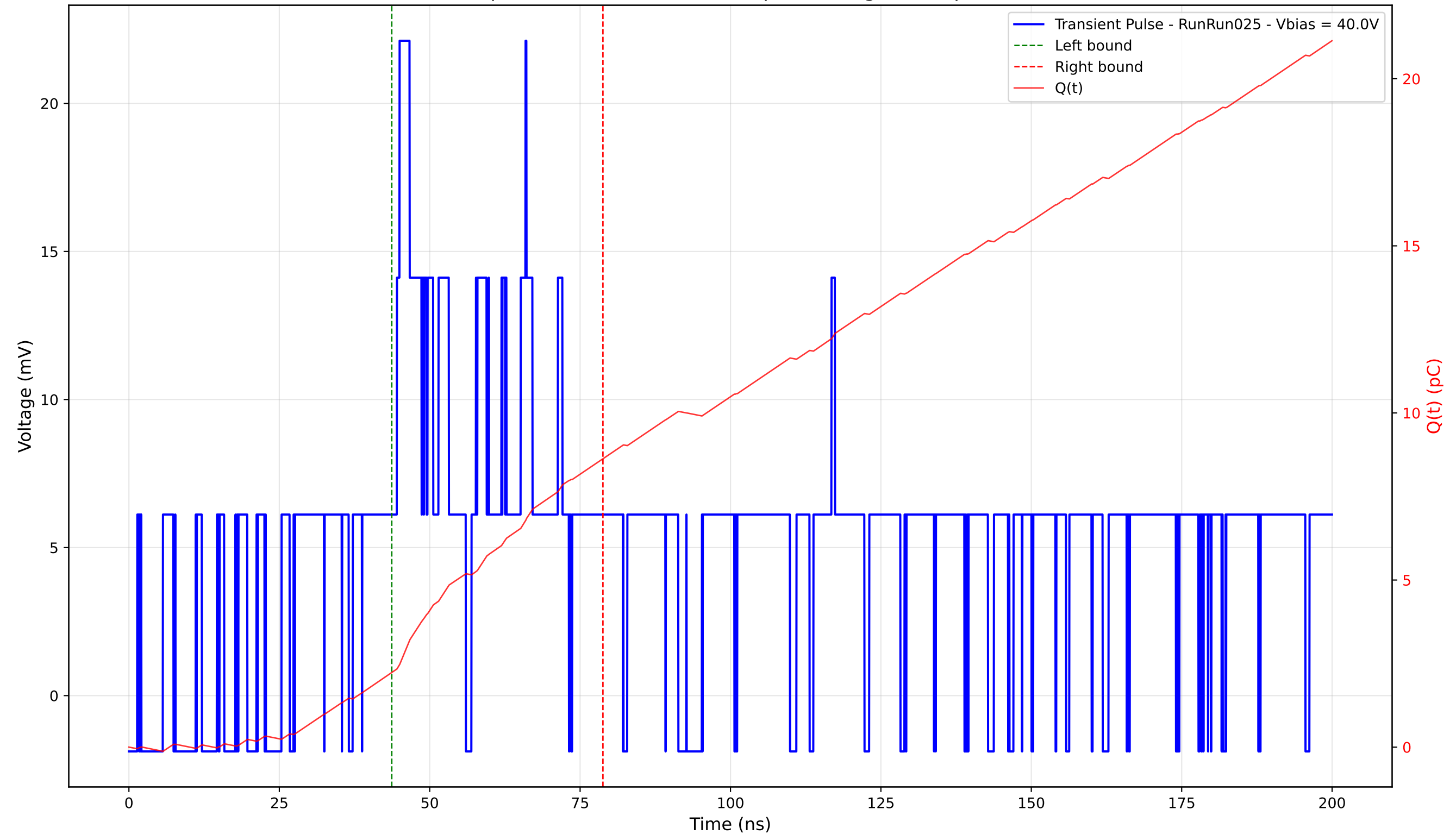
Transient Pulse - Sample: 4003 - Position: 315.0 \mu\text{m} - Charge: 6.40 pC - Rise Time: 6.22 ns
