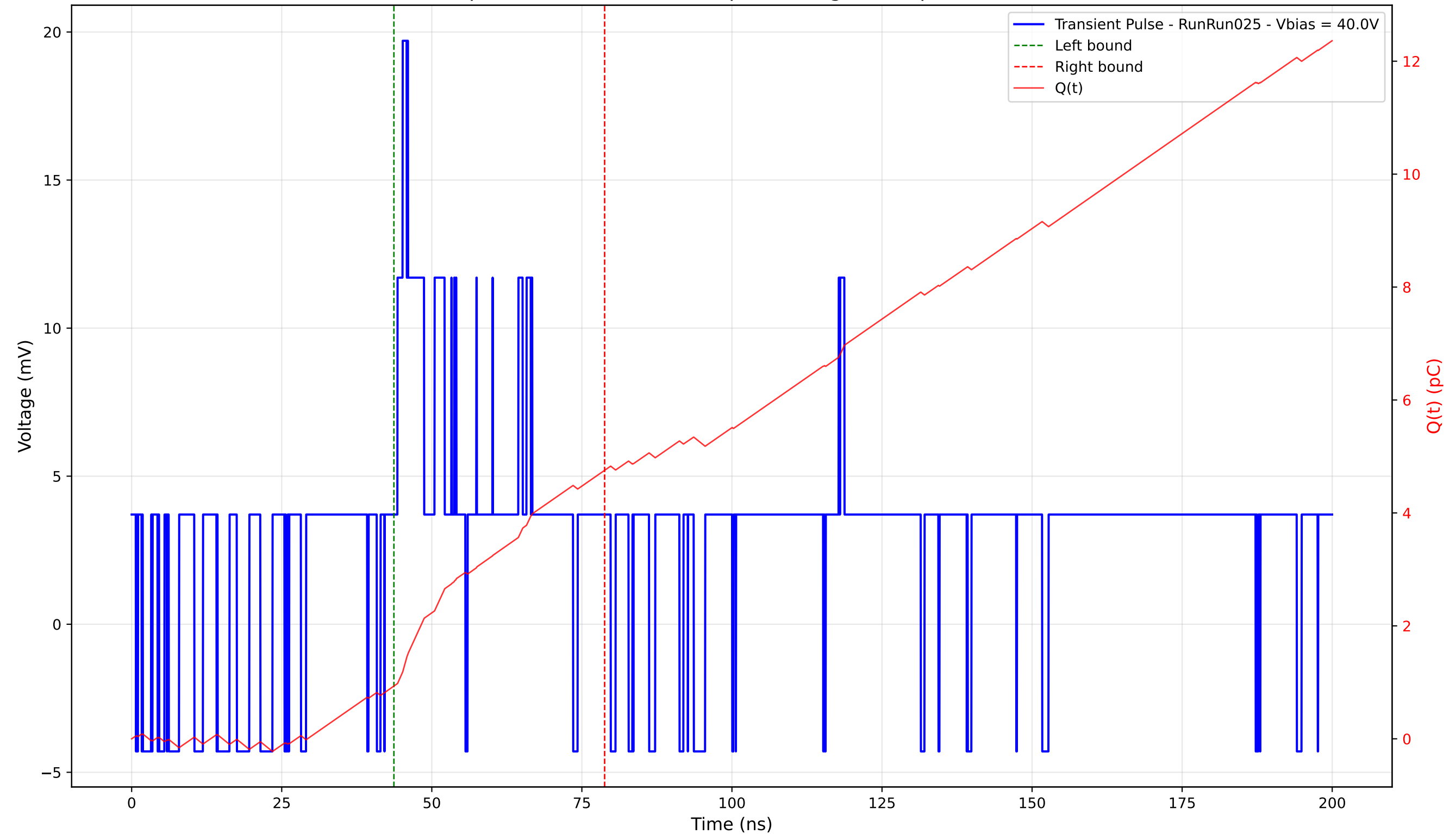
Transient Pulse - Sample: 4003 - Position: 30.0 \mu\text{m} - Charge: 3.82 pC - Rise Time: 0.00 ns (N/A)
