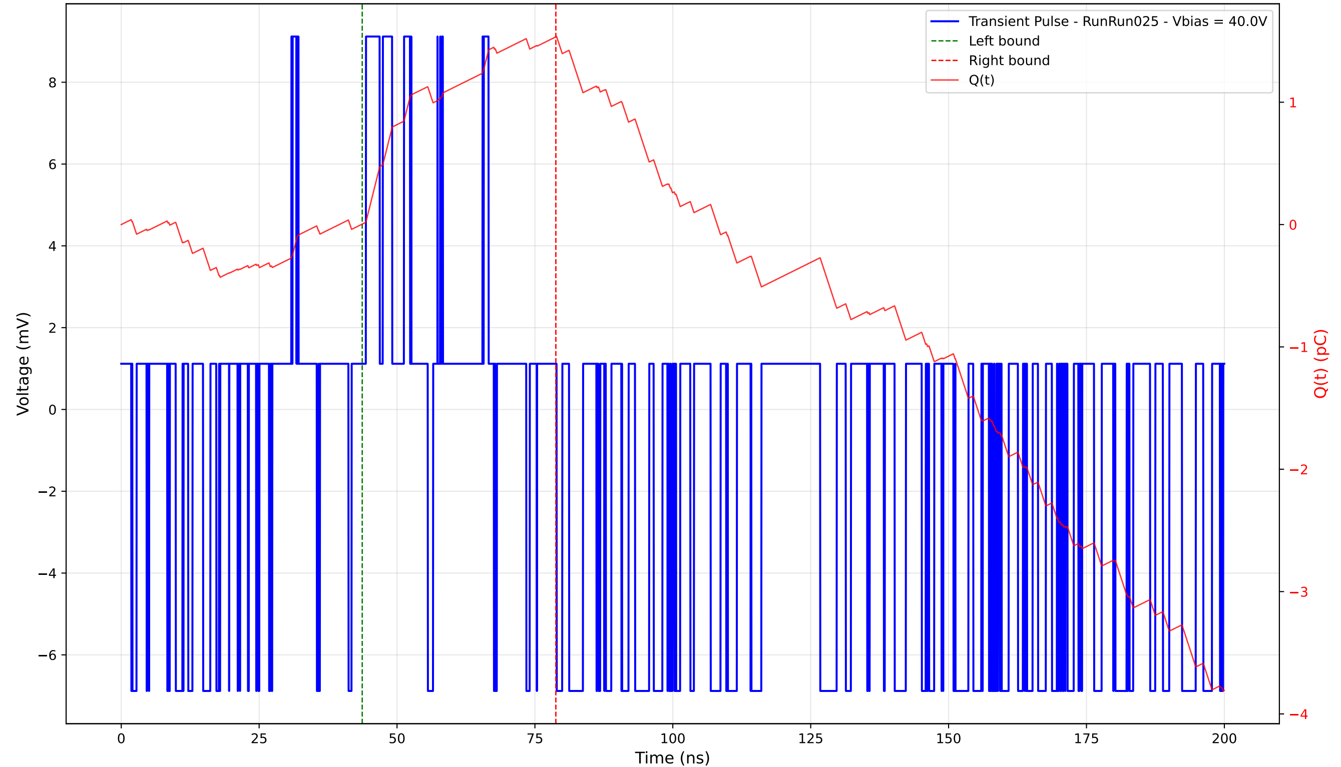
Transient Pulse - Sample: 4003 - Position: 15.0 \mu\text{m} - Charge: 1.53 pC - Rise Time: 0.00 ns (N/A)
