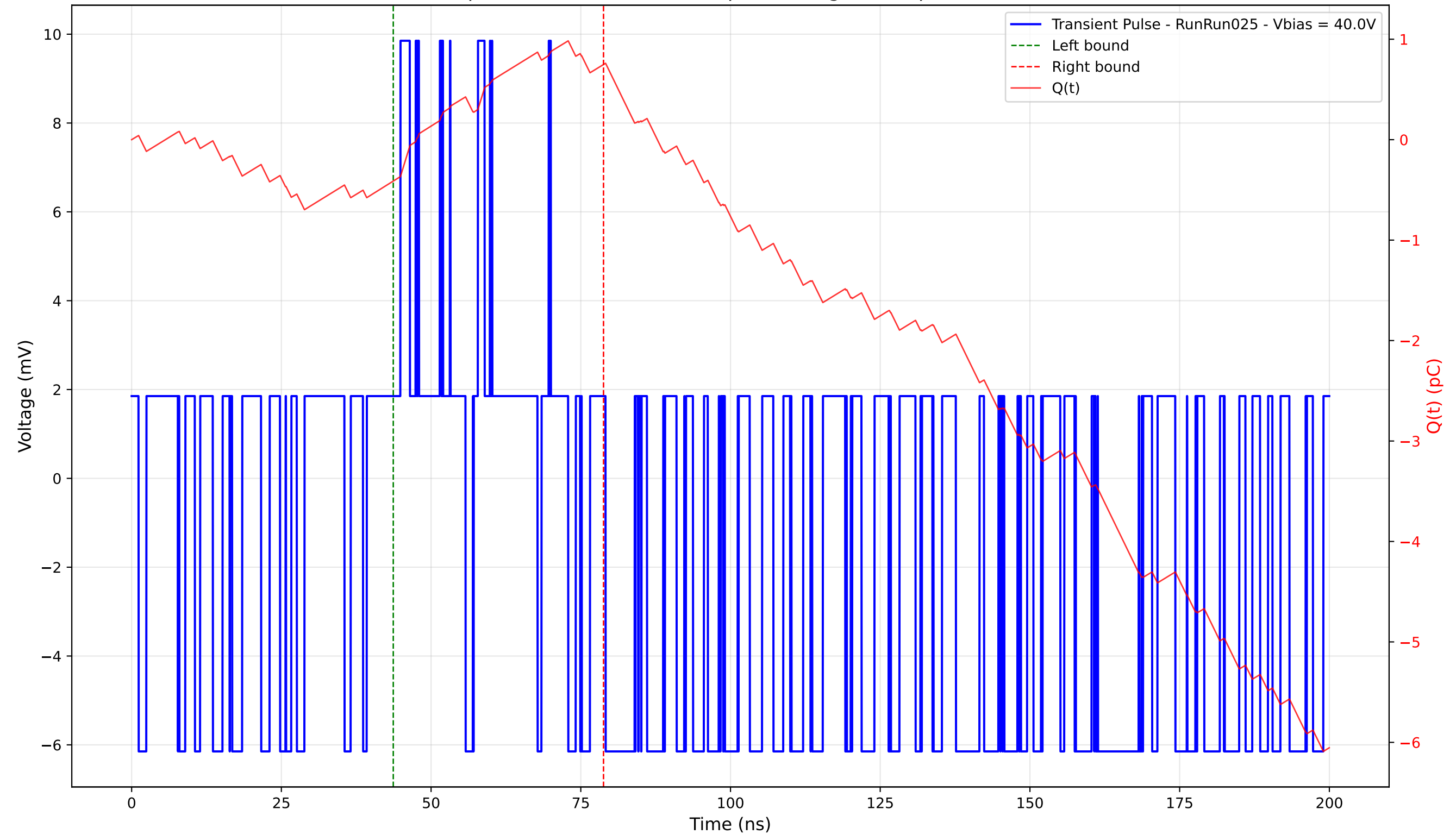
Transient Pulse - Sample: 4003 - Position: 10.0 \mu\text{m} - Charge: 1.16 pC - Rise Time: 0.00 ns (N/A)
