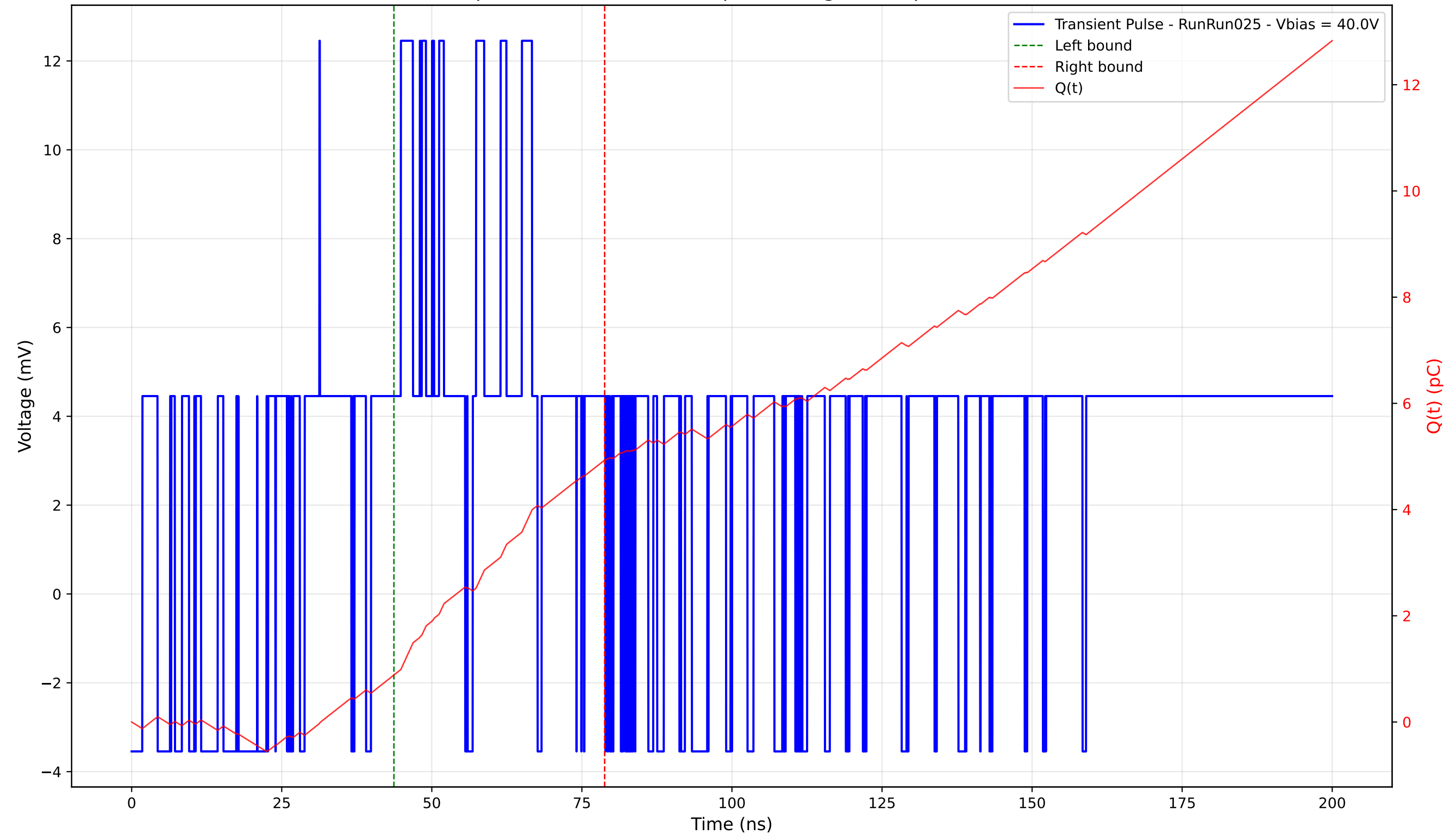
Transient Pulse - Sample: 4003 - Position: 5.0 \mu\text{m} - Charge: 4.05 pC - Rise Time: 0.00 ns (N/A)
