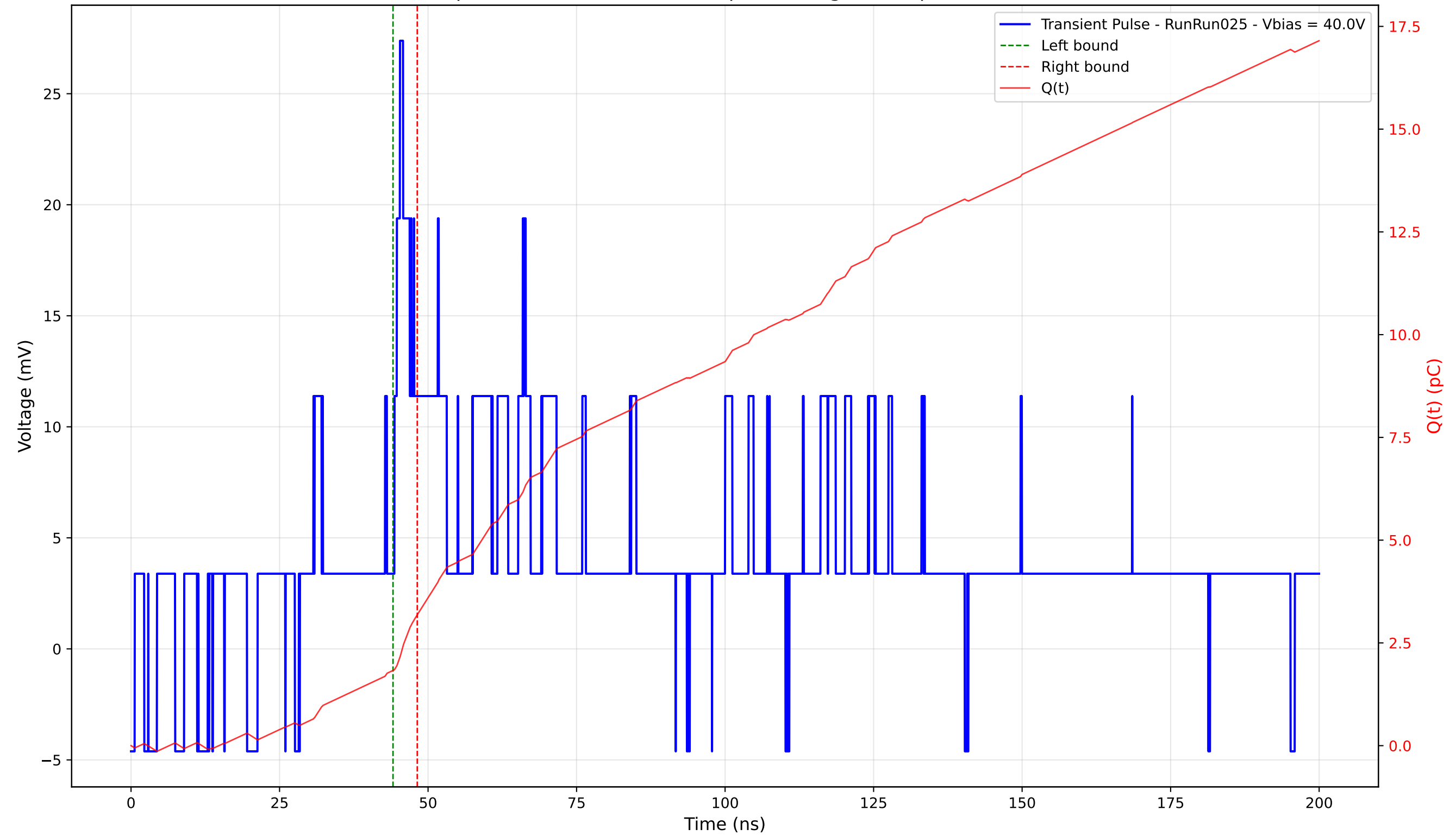
Transient Pulse - Sample: 4003 - Position: 295.0 \mu\text{m} - Charge: 1.35 pC - Rise Time: 0.00 ns (N/A)
