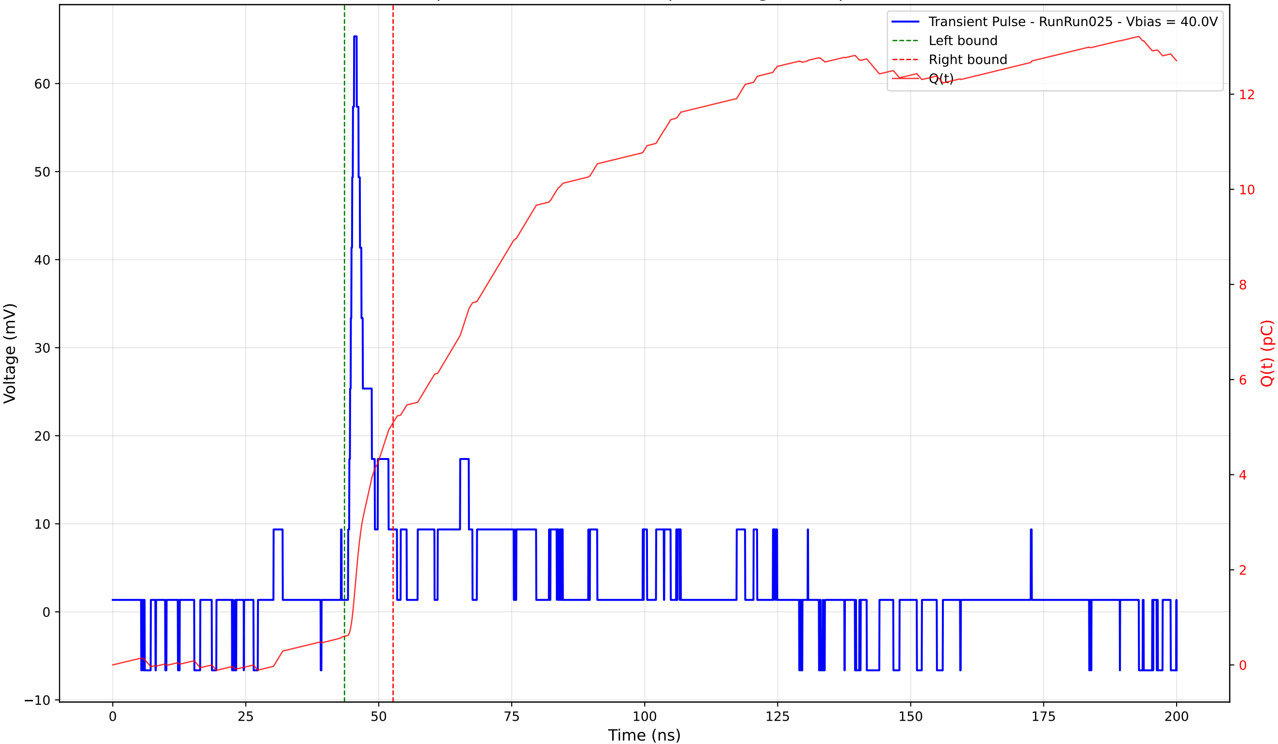
Transient Pulse - Sample: 4003 - Position: 95.0 \mu\text{m} - Charge: 4.50 pC - Rise Time: 1.13 ns
