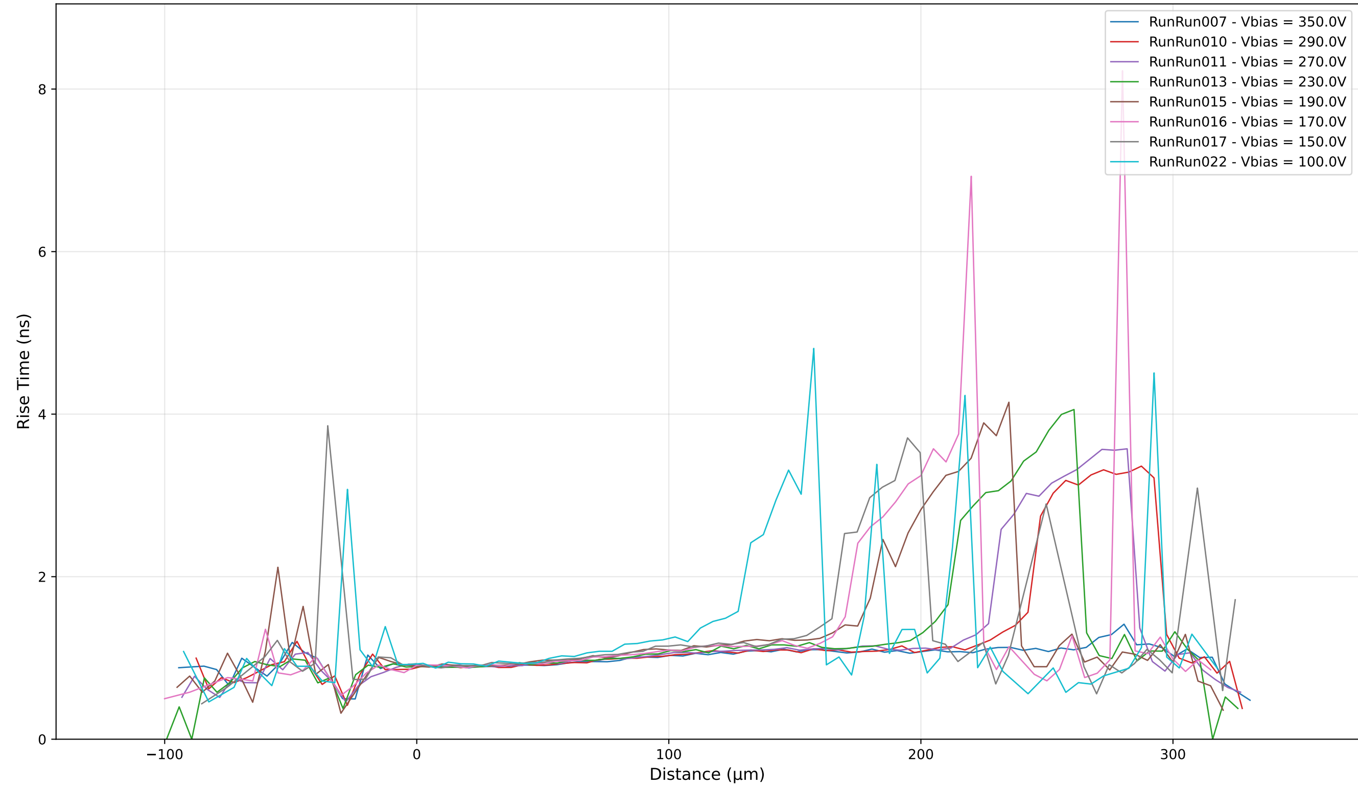
Rise Time
