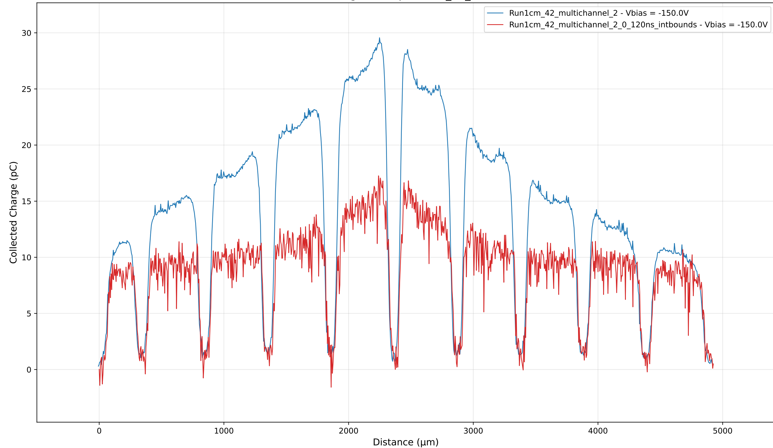
Collected Charge - Sample: 1cm_42_multichannel
