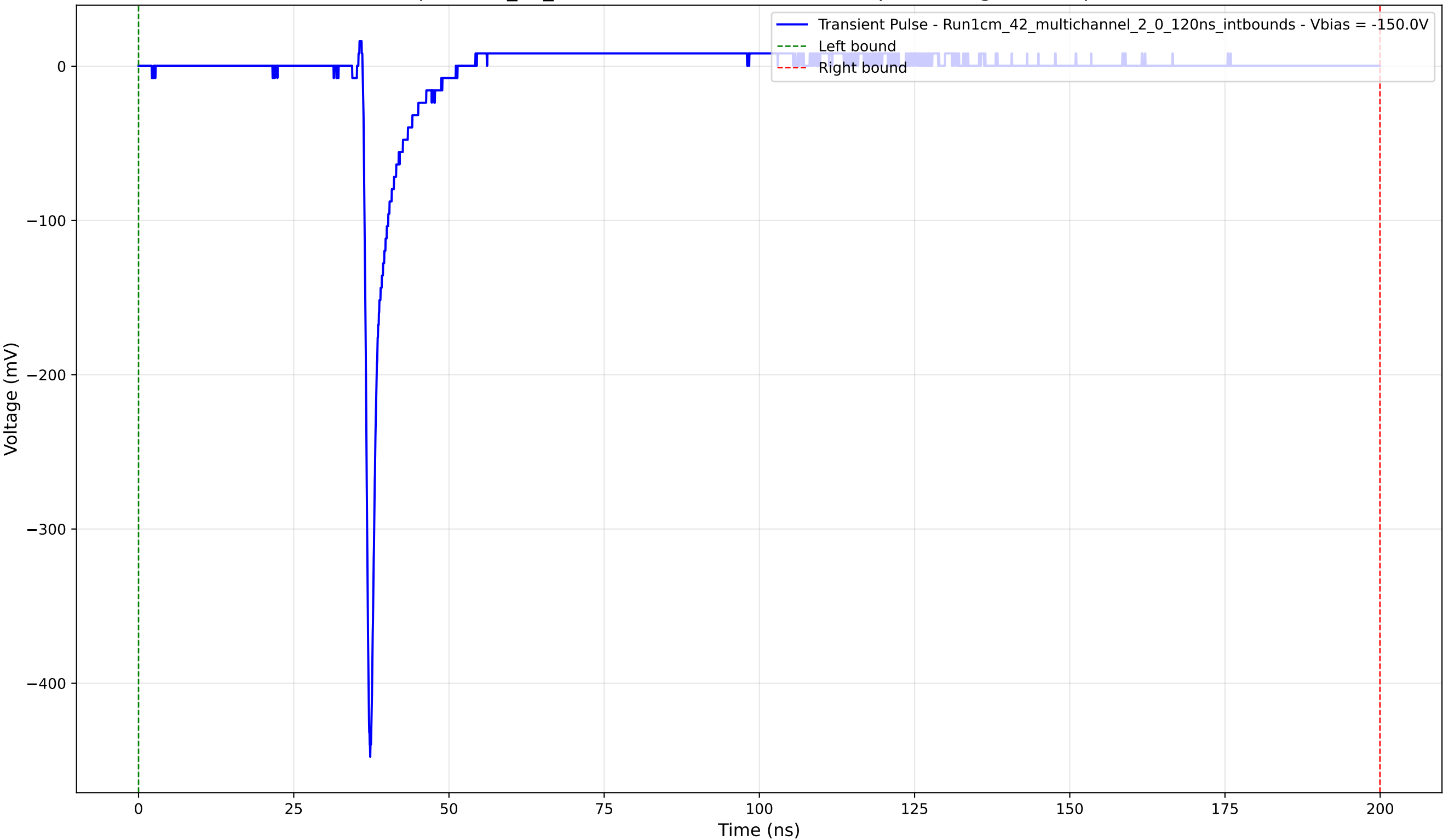
Transient Pulse - Sample: 1cm_42_multichannel - Position: 2665.0 \mu\text{m} - Charge: 12.75 pC - Rise Time: 0.80 ns
