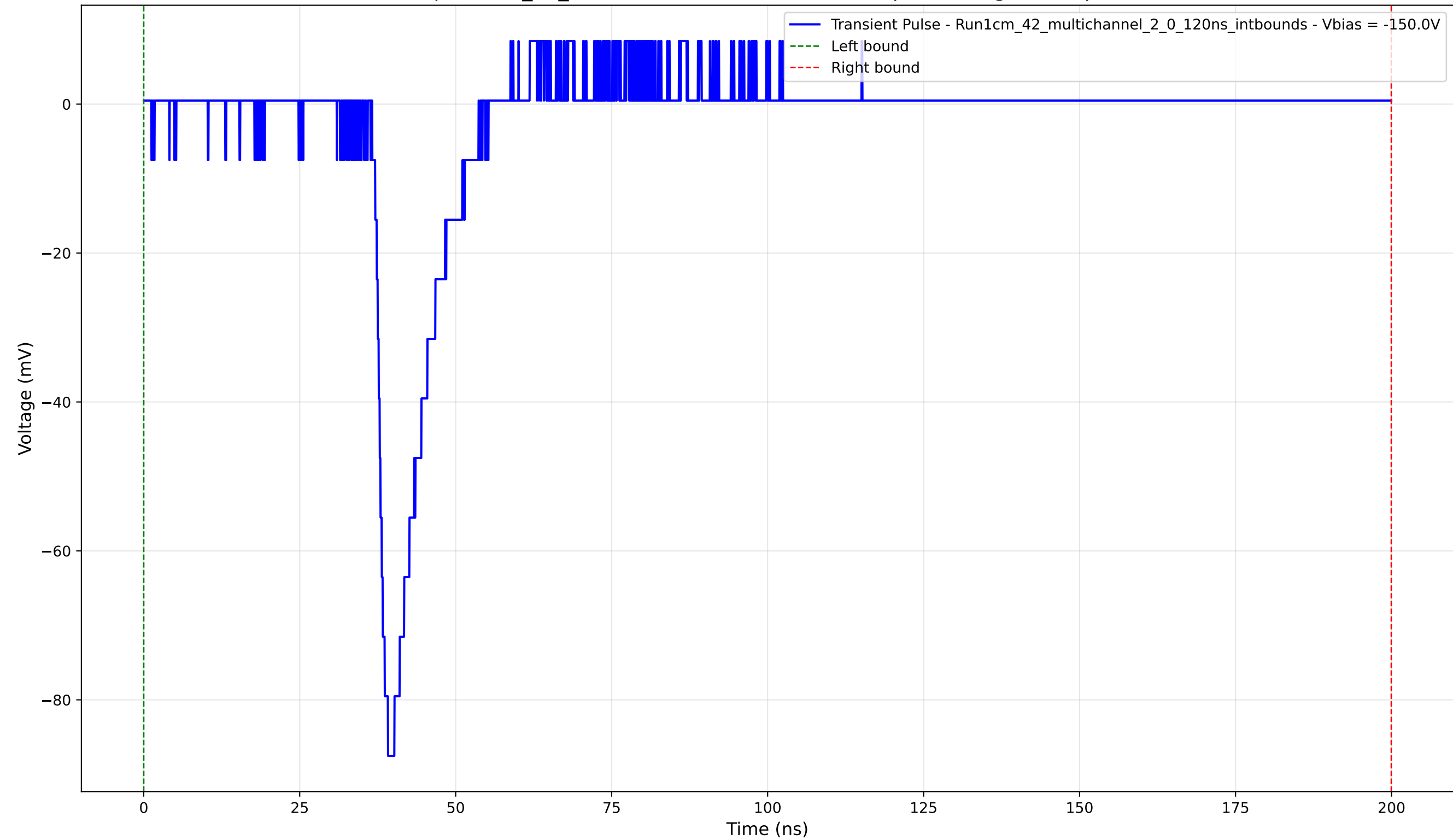
Transient Pulse - Sample: 1cm_42_multichannel - Position: 4115.0 \mu\text{m} - Charge: 9.76 pC - Rise Time: 1.55 ns
