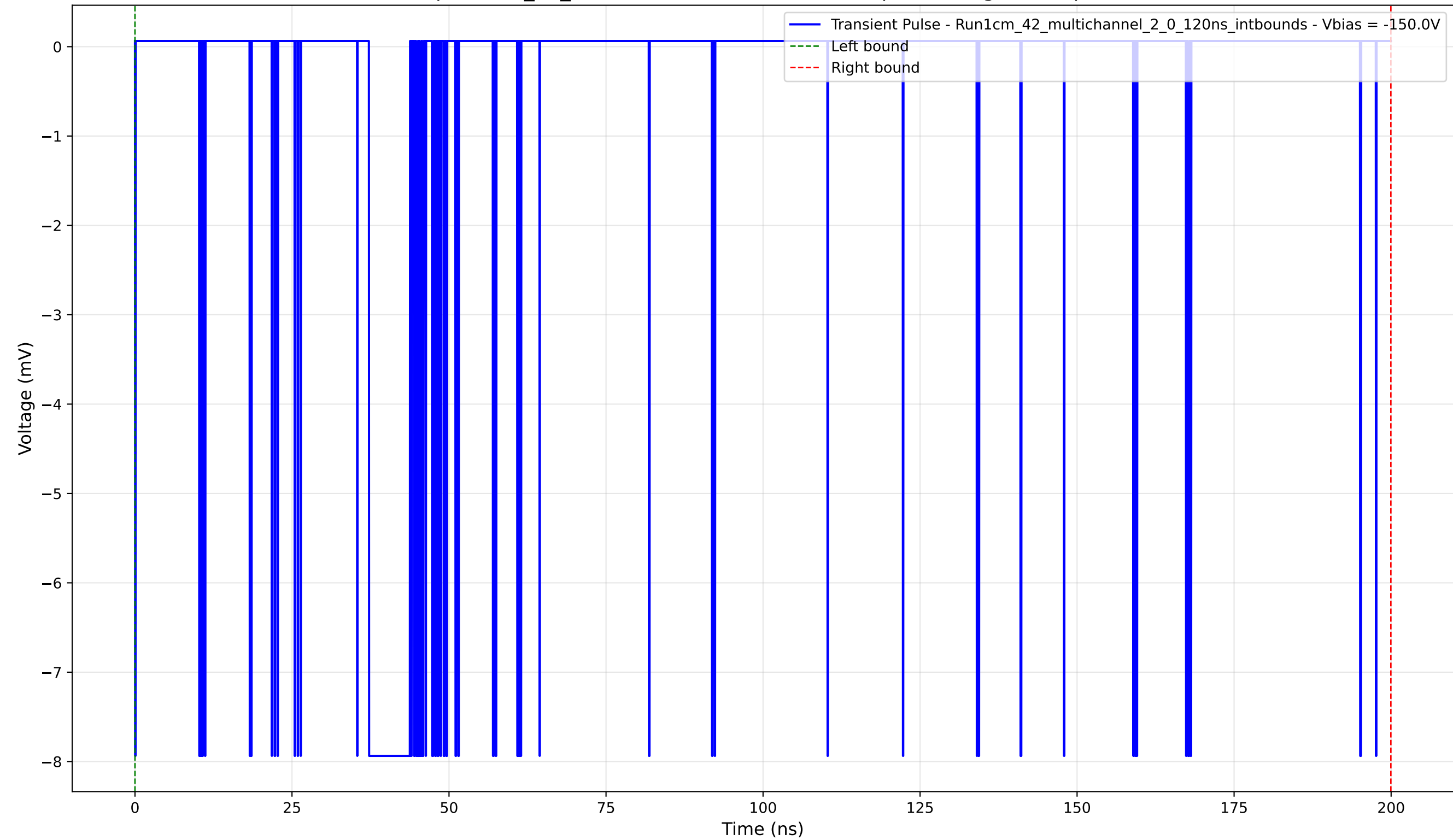
Transient Pulse - Sample: 1cm_42_multichannel - Position: 855.0 \mu\text{m} - Charge: 1.75 pC - Rise Time: 0.04 ns
