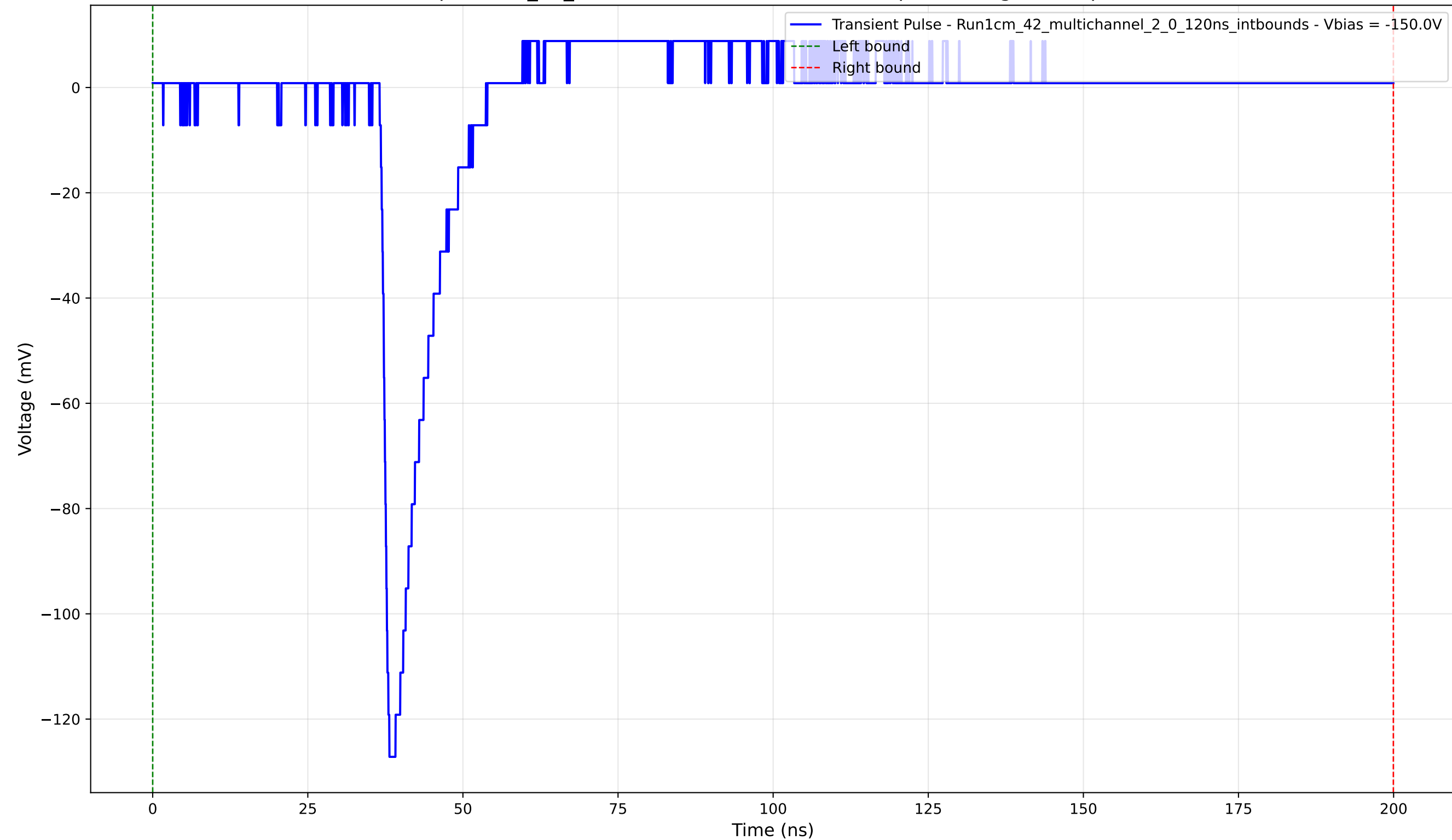
Transient Pulse - Sample: 1cm_42_multichannel - Position: 1065.0 \mu\text{m} - Charge: 7.28 pC - Rise Time: 1.21 ns
