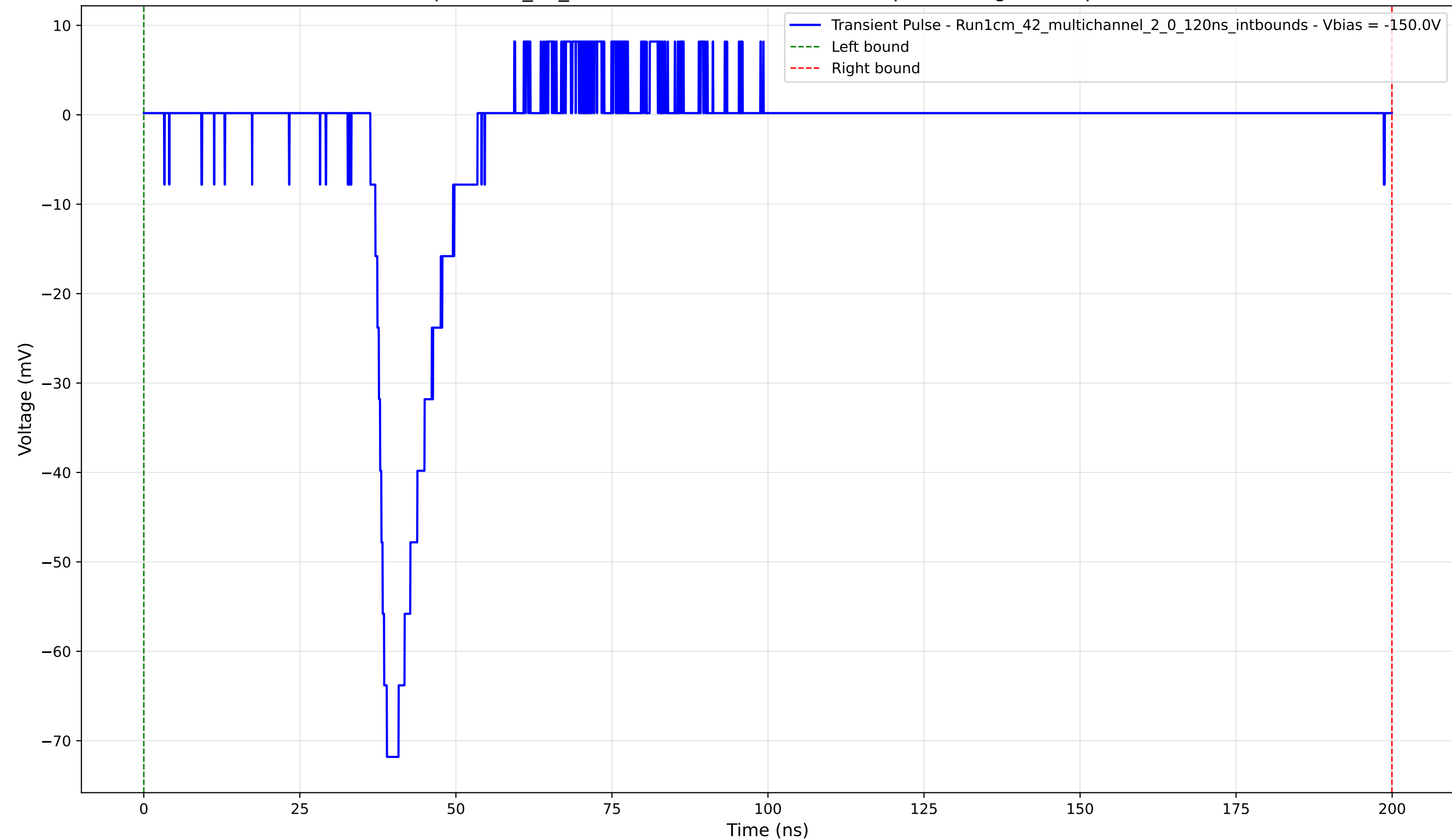
Transient Pulse - Sample: 1cm_42_multichannel - Position: 4550.0 \mu\text{m} - Charge: 8.62 pC - Rise Time: 2.64 ns
