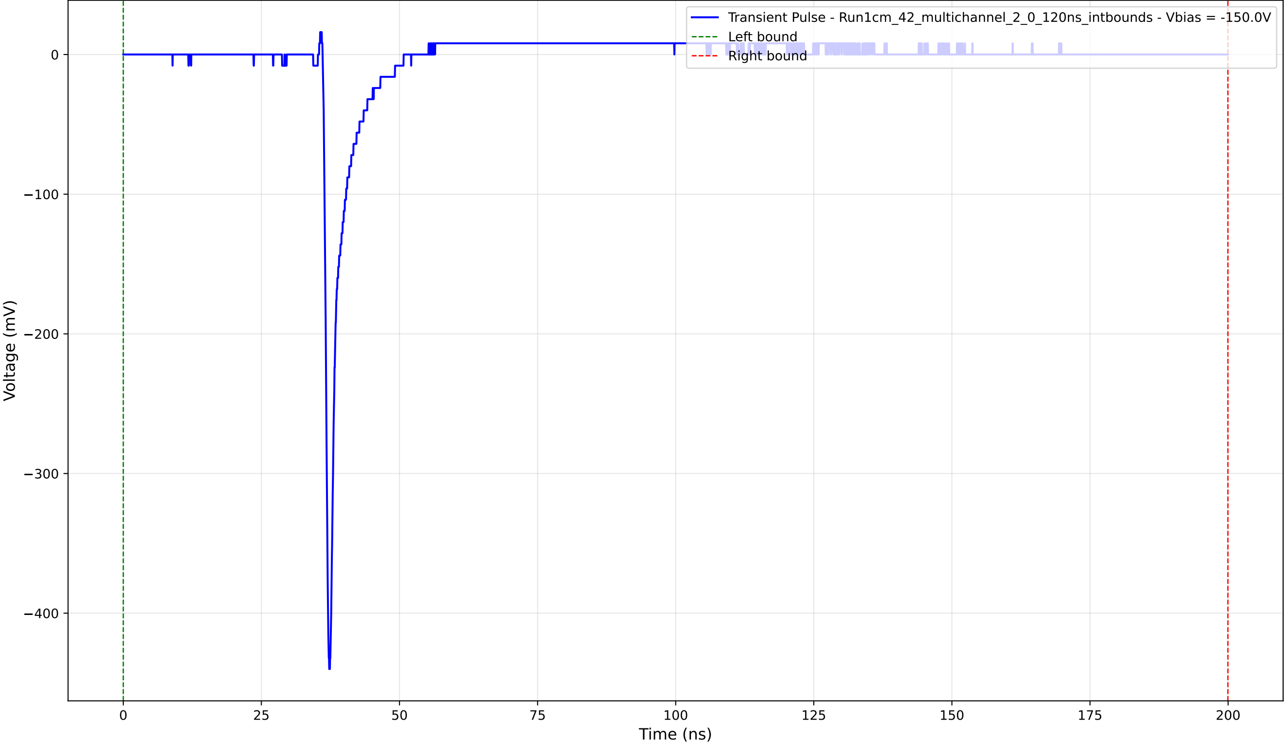
Transient Pulse - Sample: 1cm_42_multichannel - Position: 2685.0 \mu\text{m} - Charge: 13.83 pC - Rise Time: 0.78 ns
