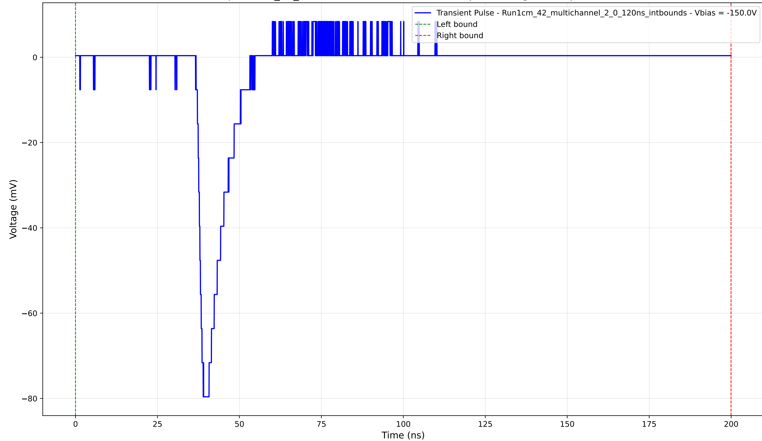
Transient Pulse - Sample: 1cm_42_multichannel - Position: 4250.0 \mu\text{m} - Charge: 9.04 pC - Rise Time: 1.80 ns
