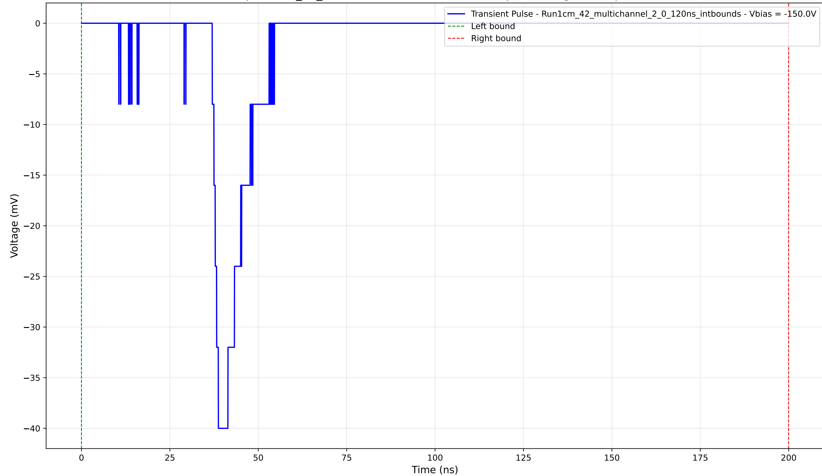
Transient Pulse - Sample: 1cm_42_multichannel - Position: 4335.0 \mu\text{m} - Charge: 6.88 pC - Rise Time: 1.74 ns
