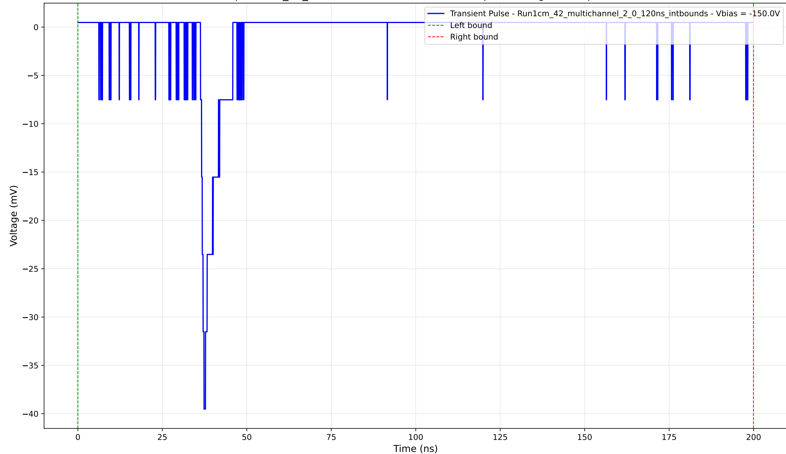
Transient Pulse - Sample: 1cm_42_multichannel - Position: 2905.0 \mu\text{m} - Charge: 1.97 pC - Rise Time: 1.06 ns
