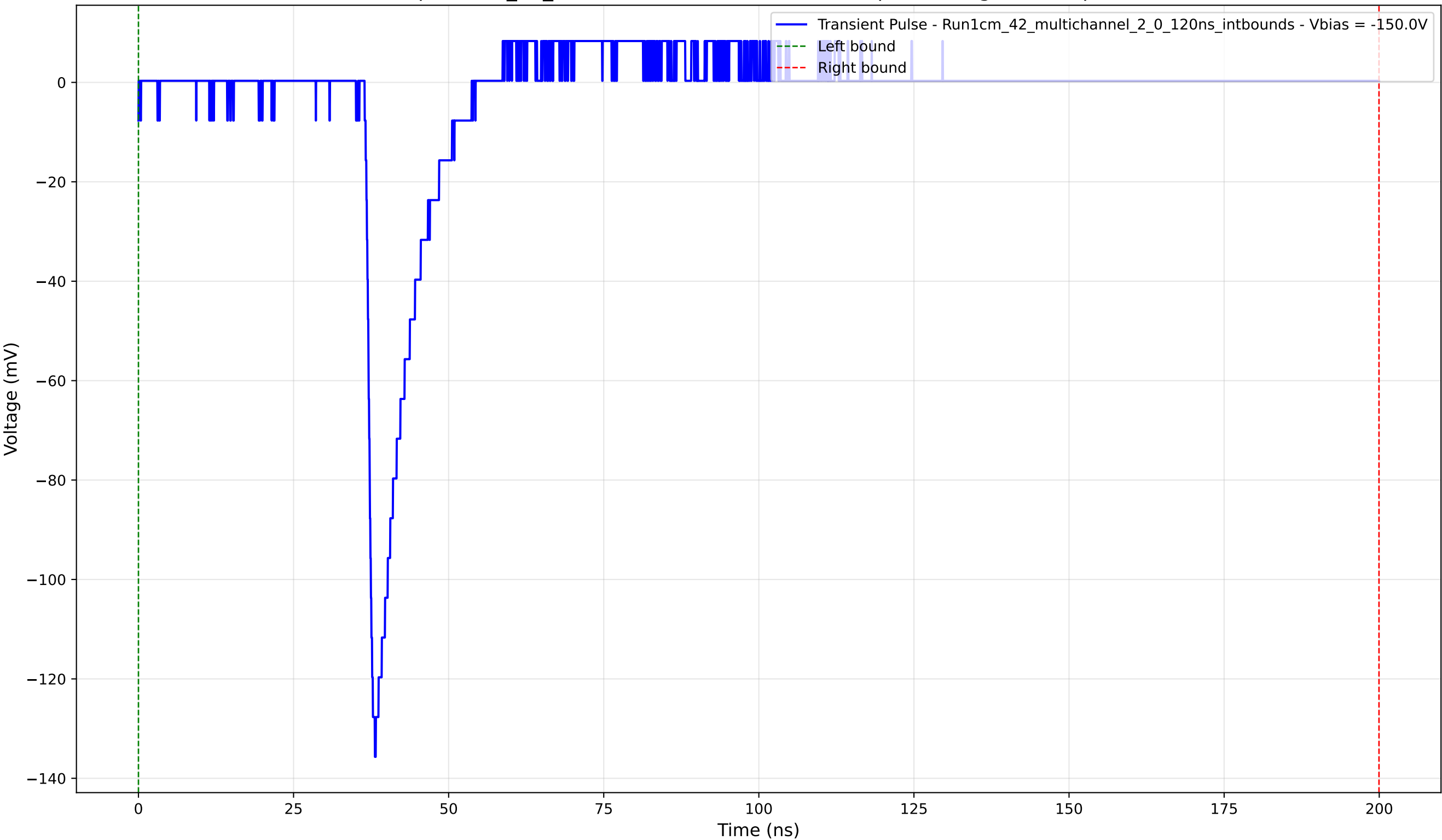
Transient Pulse - Sample: 1cm_42_multichannel - Position: 3465.0 \mu\text{m} - Charge: 10.56 pC - Rise Time: 1.17 ns
