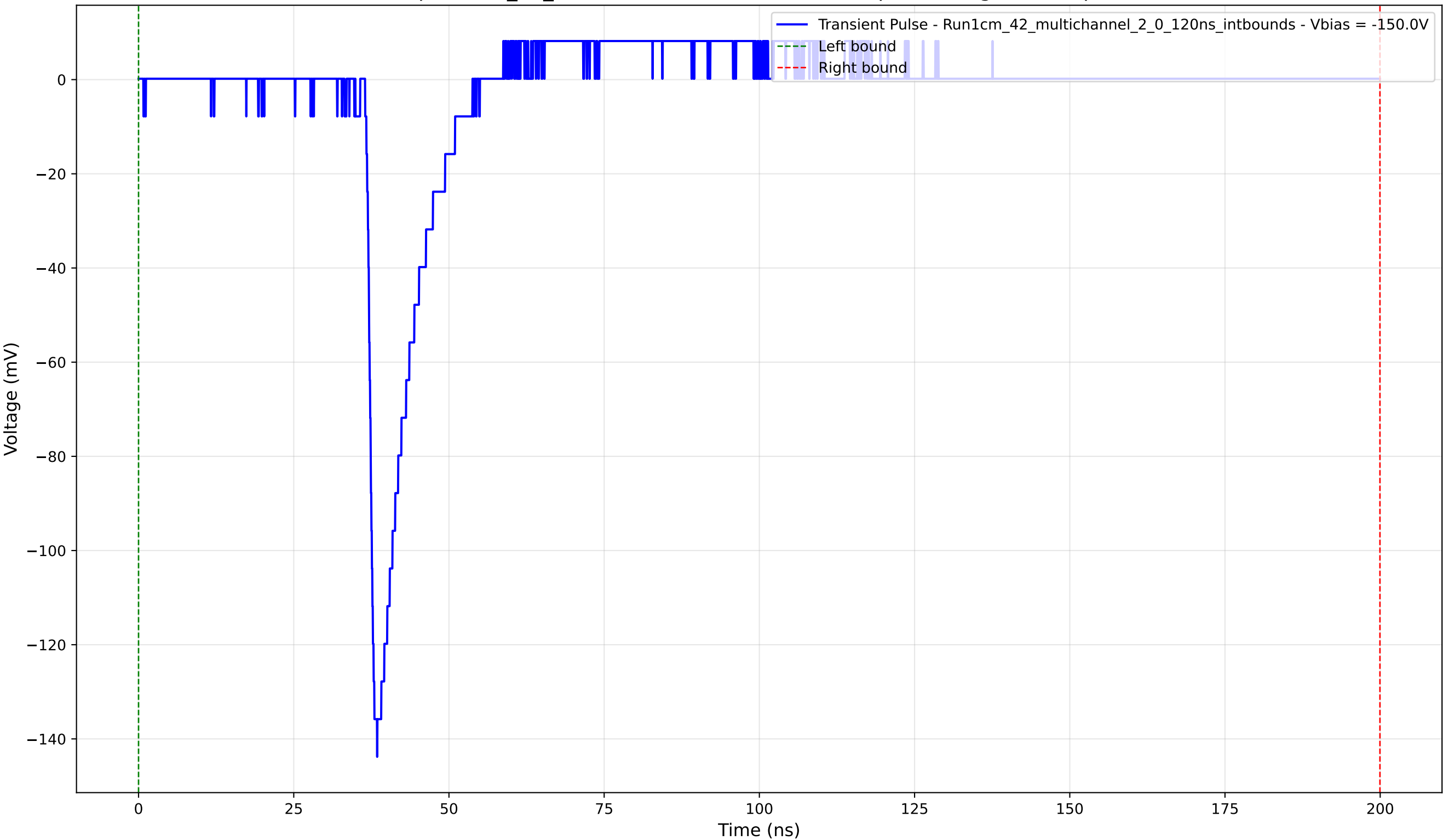
Transient Pulse - Sample: 1cm_42_multichannel - Position: 1145.0 \mu\text{m} - Charge: 10.76 pC - Rise Time: 1.29 ns
