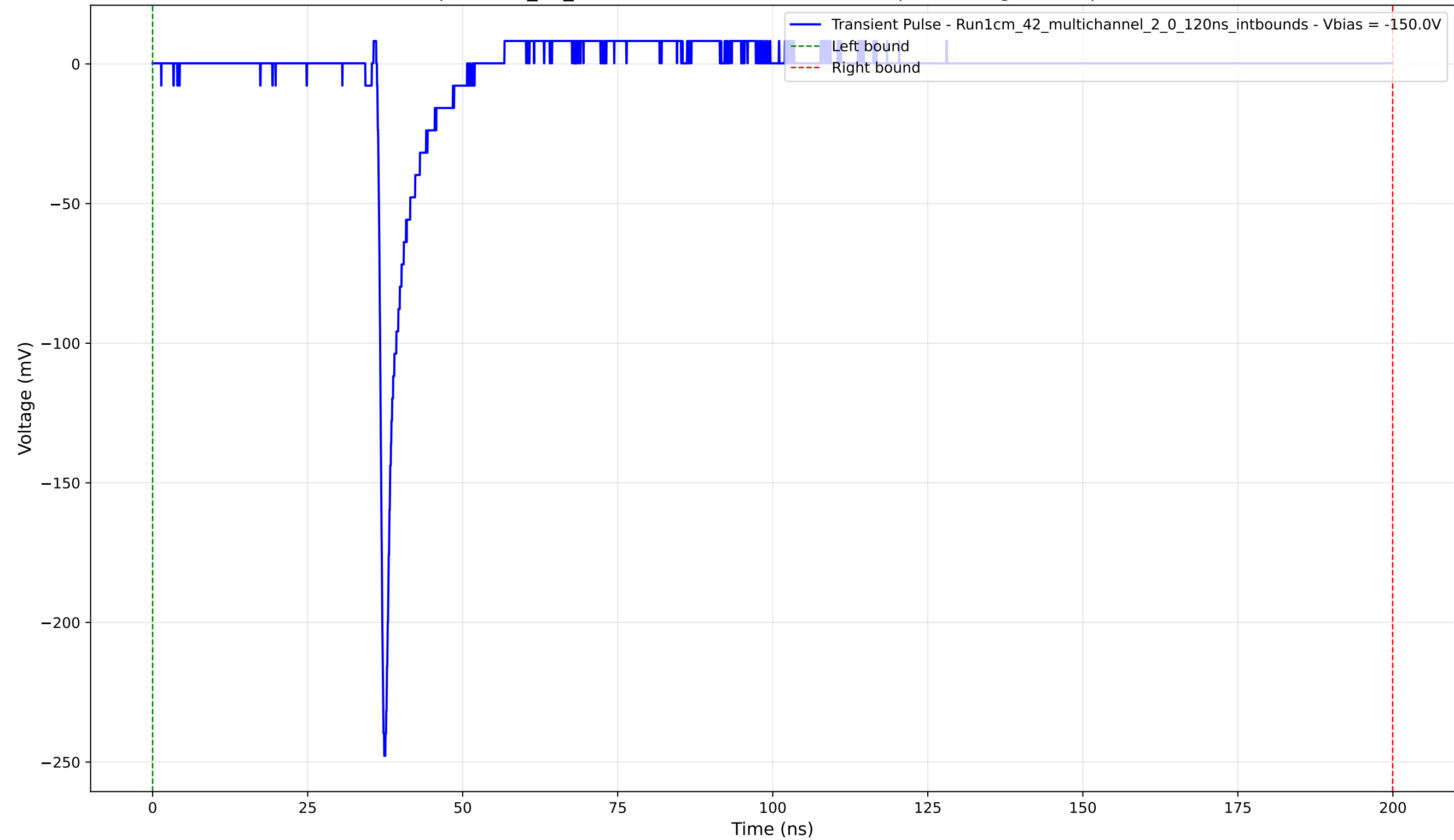
Transient Pulse - Sample: 1cm_42_multichannel - Position: 2815.0 \mu\text{m} - Charge: 9.58 pC - Rise Time: 0.79 ns
