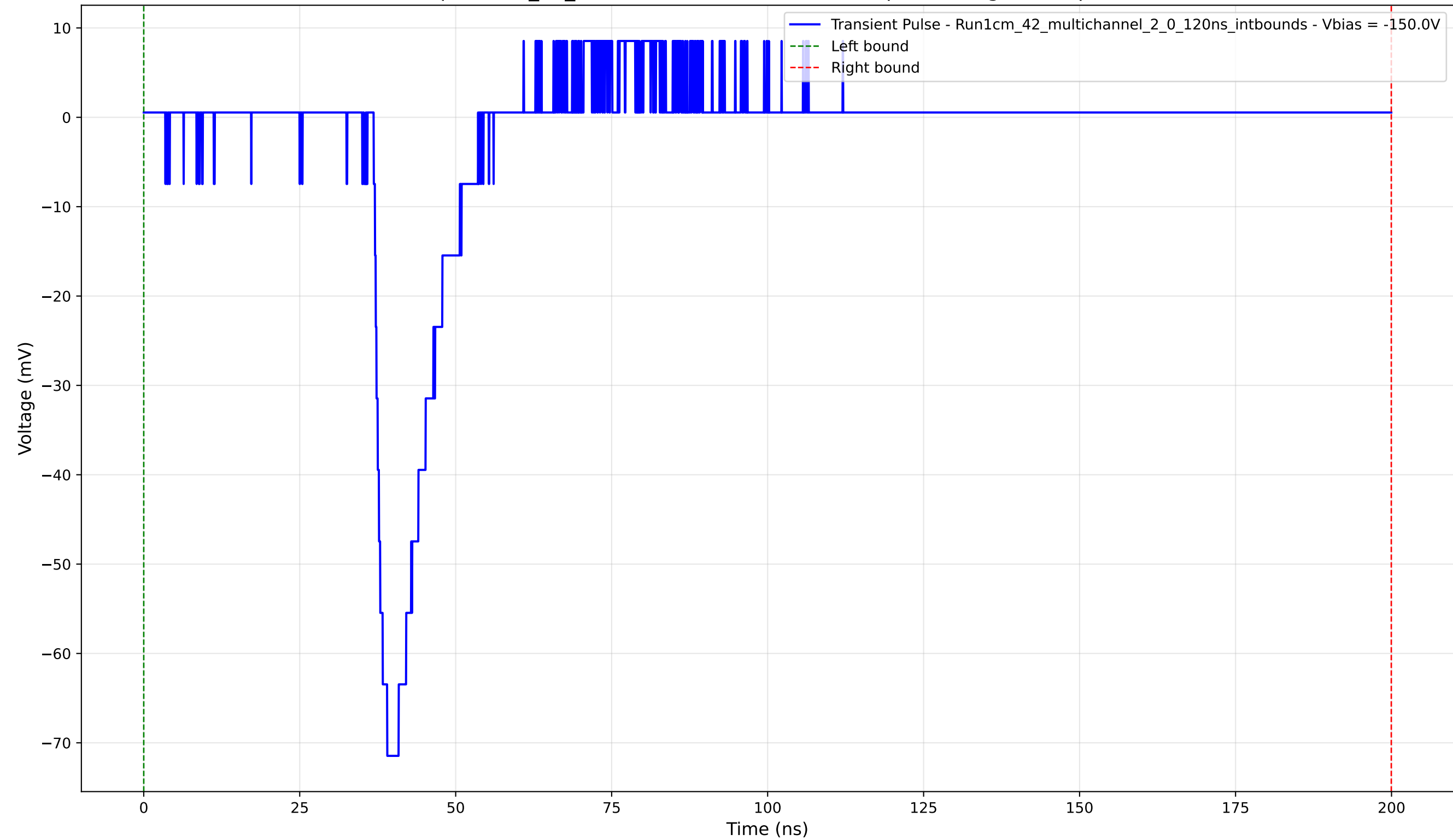
Transient Pulse - Sample: 1cm_42_multichannel - Position: 205.0 \mu\text{m} - Charge: 7.61 pC - Rise Time: 2.16 ns
