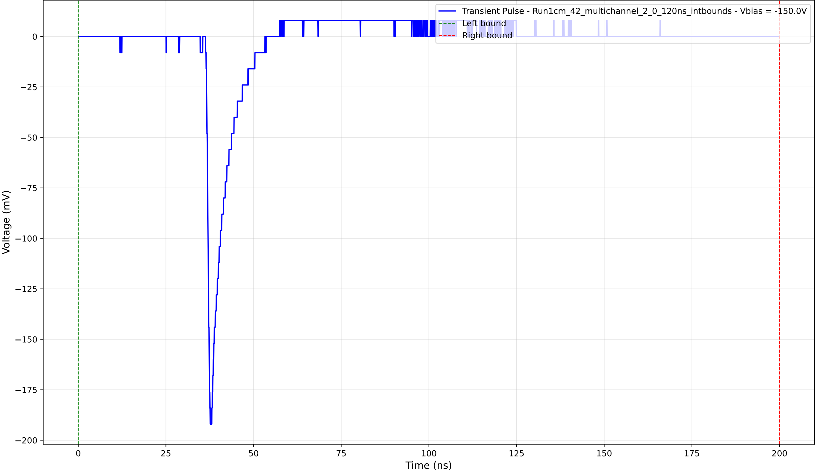
Transient Pulse - Sample: 1cm_42_multichannel - Position: 3215.0 \mu\text{m} - Charge: 11.37 pC - Rise Time: 0.94 ns
