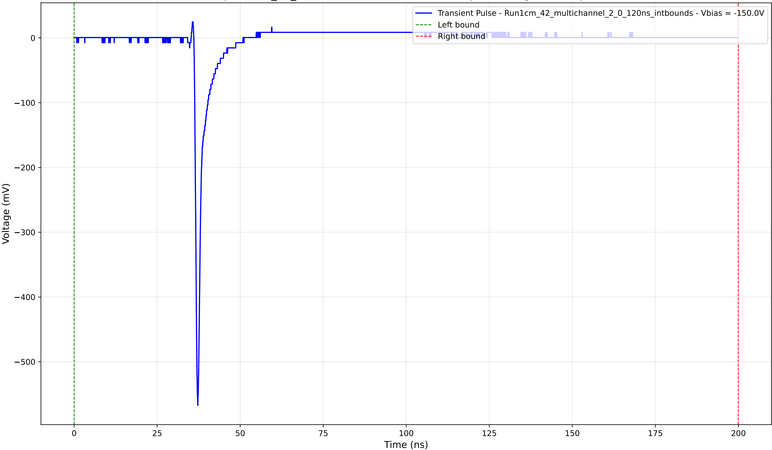
Transient Pulse - Sample: 1cm_42_multichannel - Position: 2185.0 \mu\text{m} - Charge: 15.05 pC - Rise Time: 0.75 ns
