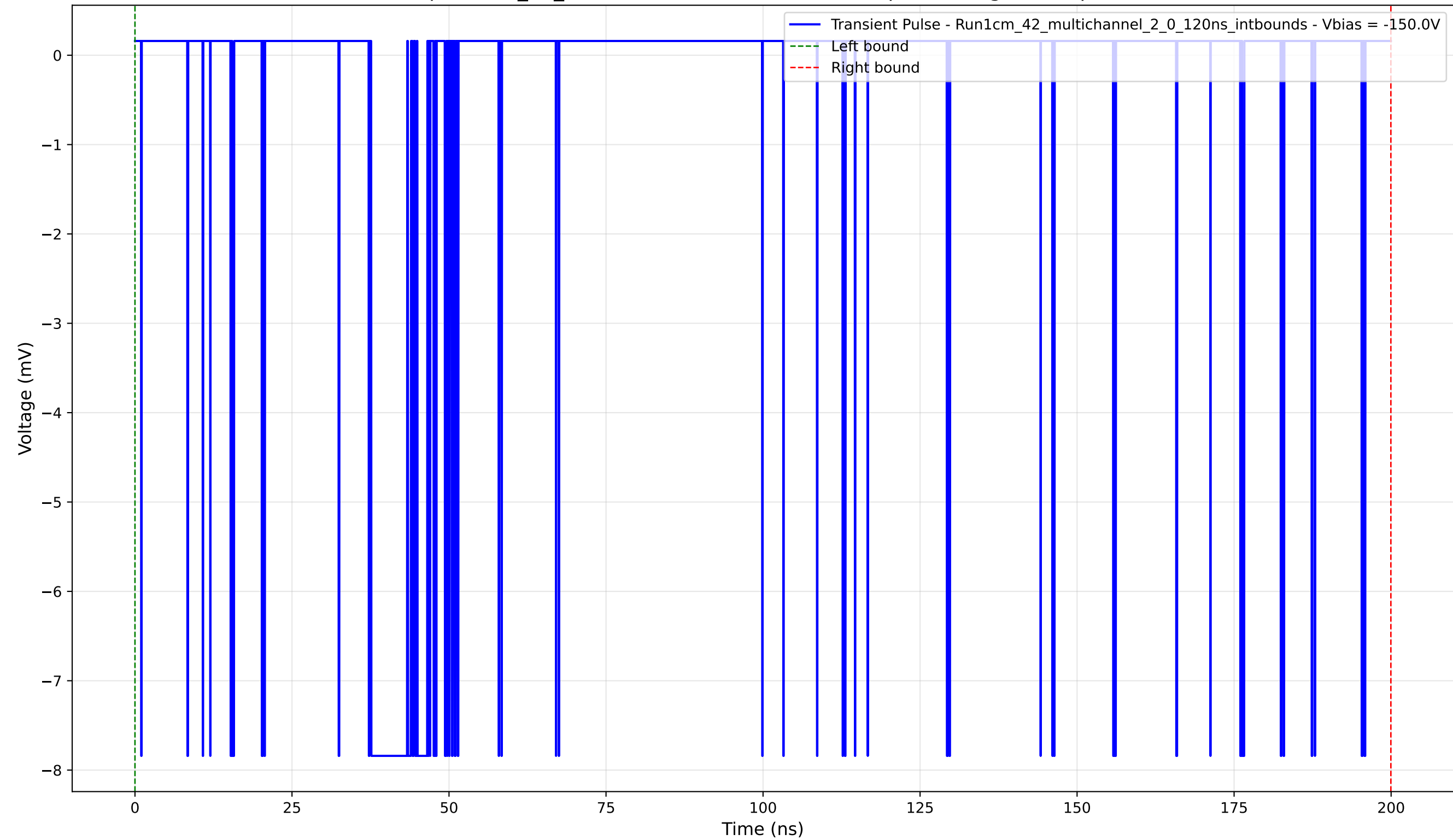
Transient Pulse - Sample: 1cm_42_multichannel - Position: 4375.0 \mu\text{m} - Charge: 1.55 pC - Rise Time: 0.04 ns
