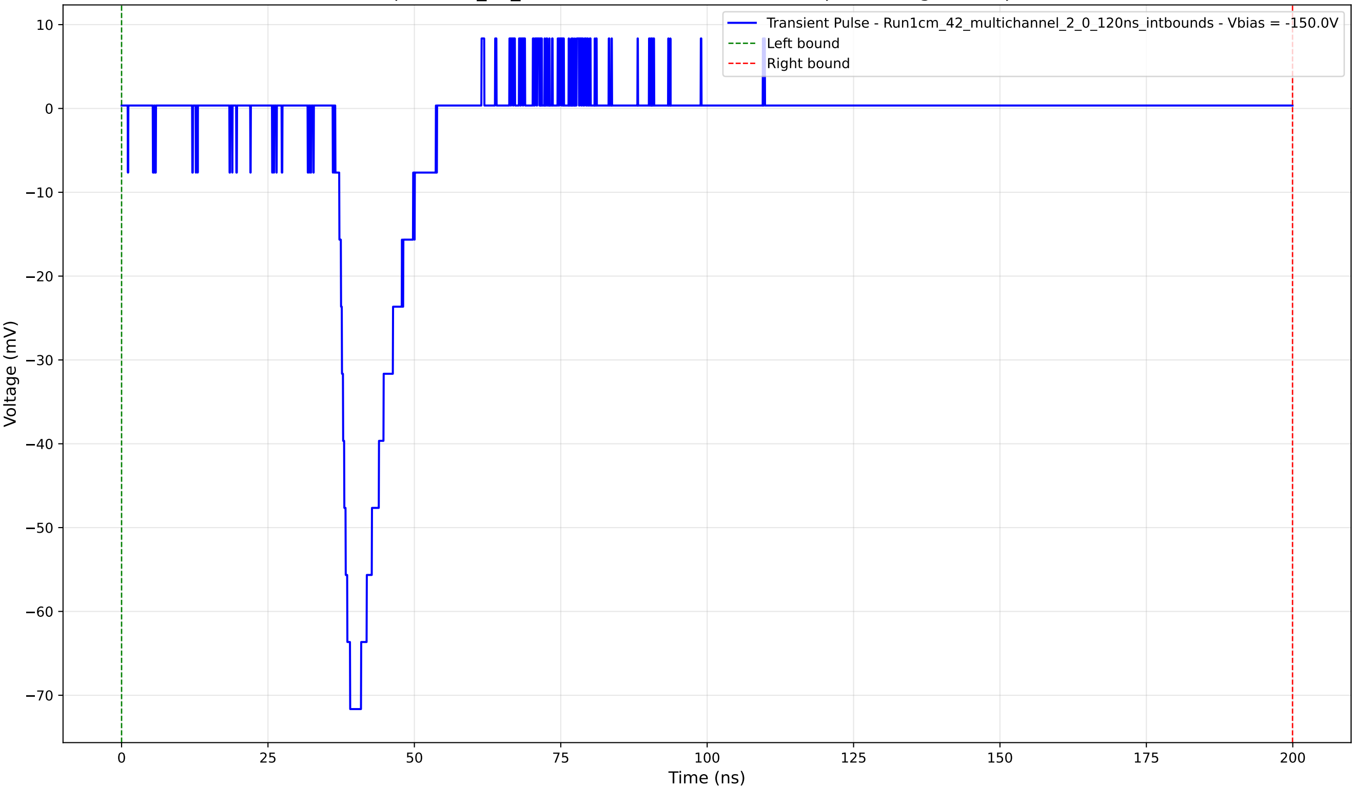
Transient Pulse - Sample: 1cm_42_multichannel - Position: 4505.0 \mu\text{m} - Charge: 9.21 pC - Rise Time: 2.52 ns
