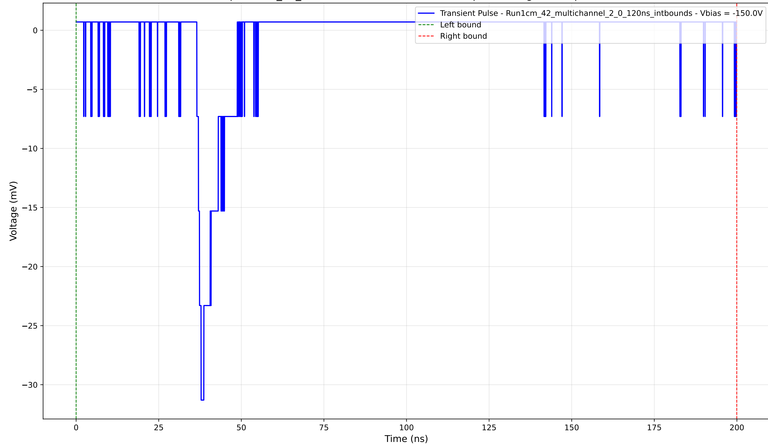
Transient Pulse - Sample: 1cm_42_multichannel - Position: 1325.0 \mu\text{m} - Charge: 1.61 pC - Rise Time: 1.31 ns
