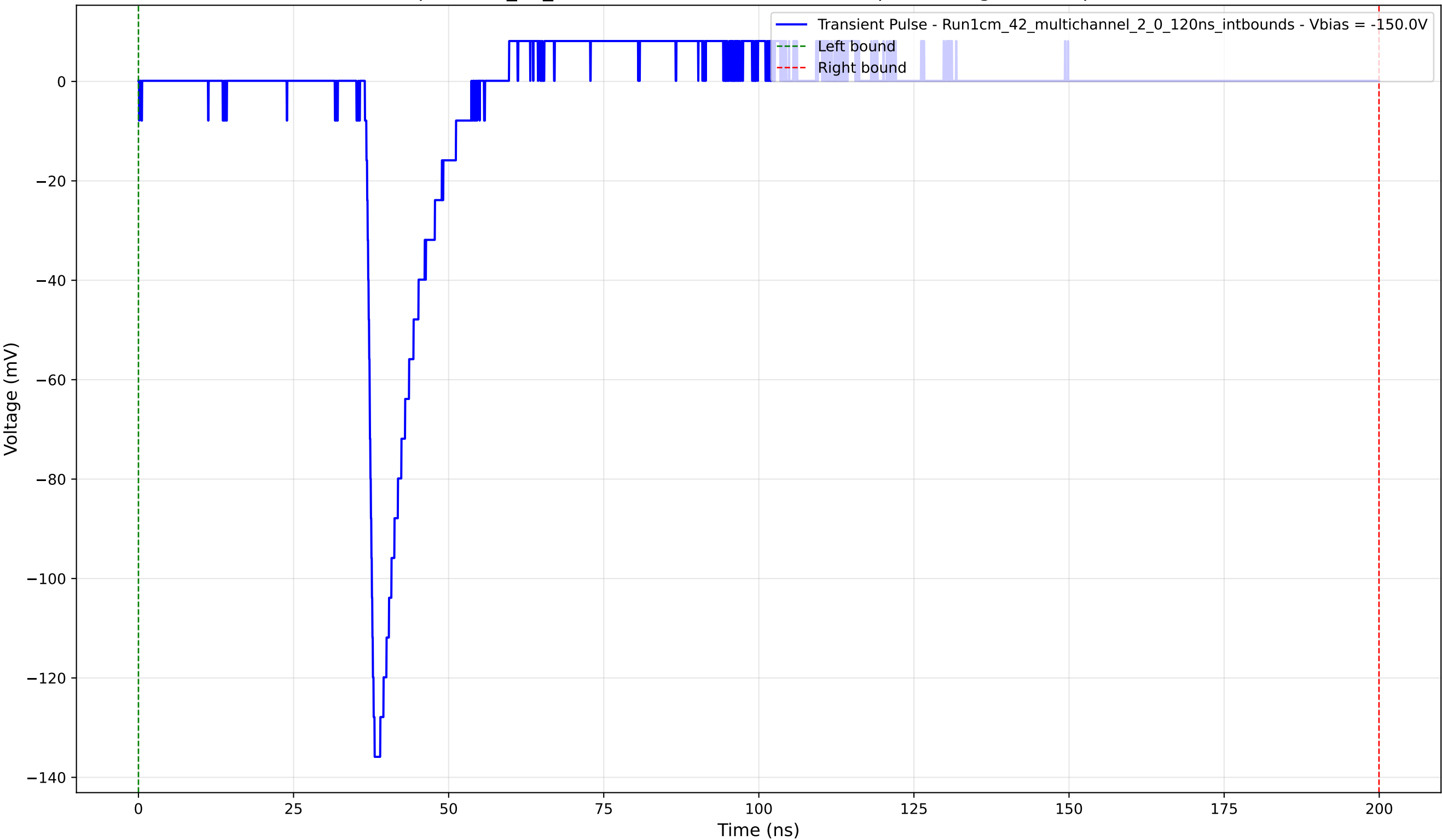
Transient Pulse - Sample: 1cm_42_multichannel - Position: 1135.0 \mu\text{m} - Charge: 10.81 pC - Rise Time: 1.17 ns
