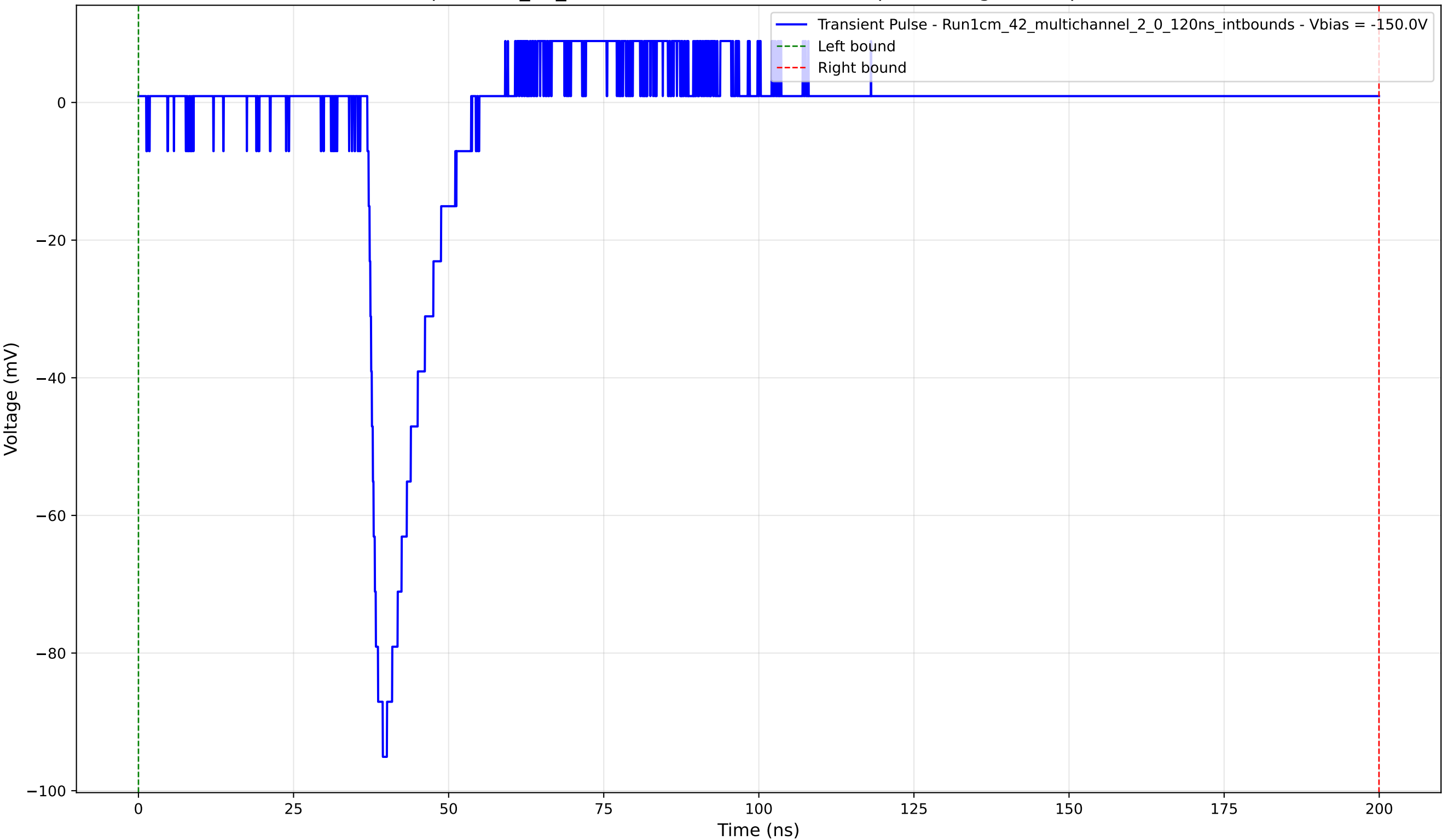
Transient Pulse - Sample: 1cm_42_multichannel - Position: 470.0 \mu\text{m} - Charge: 7.07 pC - Rise Time: 1.55 ns
