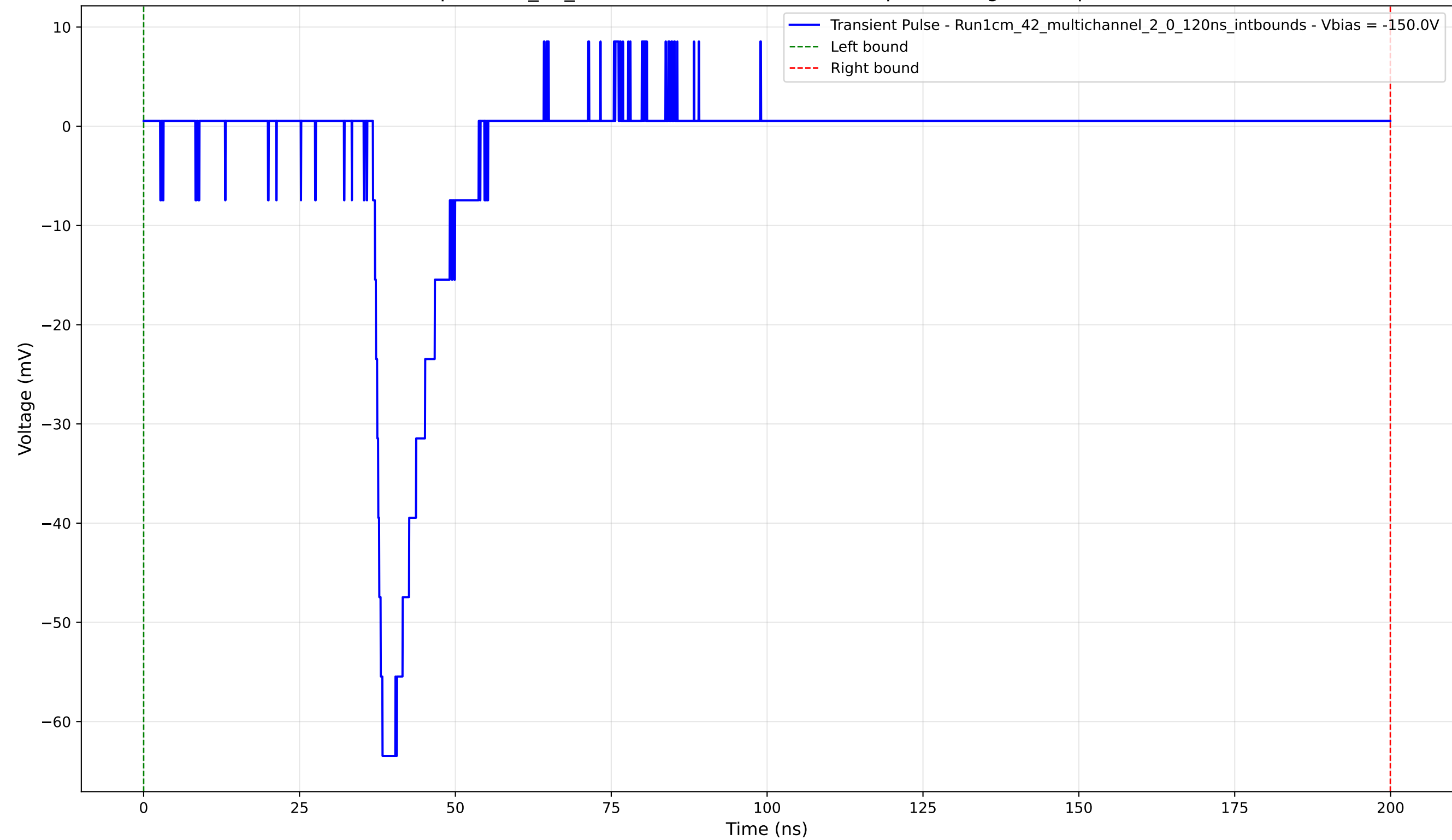
Transient Pulse - Sample: 1cm_42_multichannel - Position: 795.0 \mu\text{m} - Charge: 7.72 pC - Rise Time: 1.53 ns
