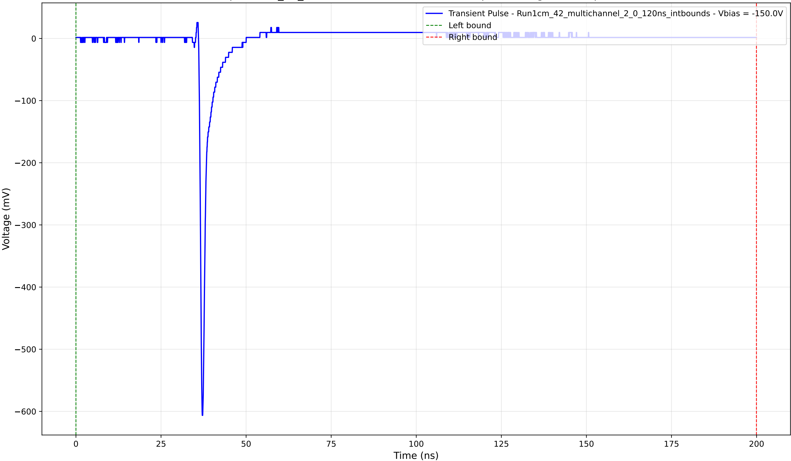
Transient Pulse - Sample: 1cm_42_multichannel - Position: 2230.0 \mu\text{m} - Charge: 11.22 pC - Rise Time: 0.73 ns
