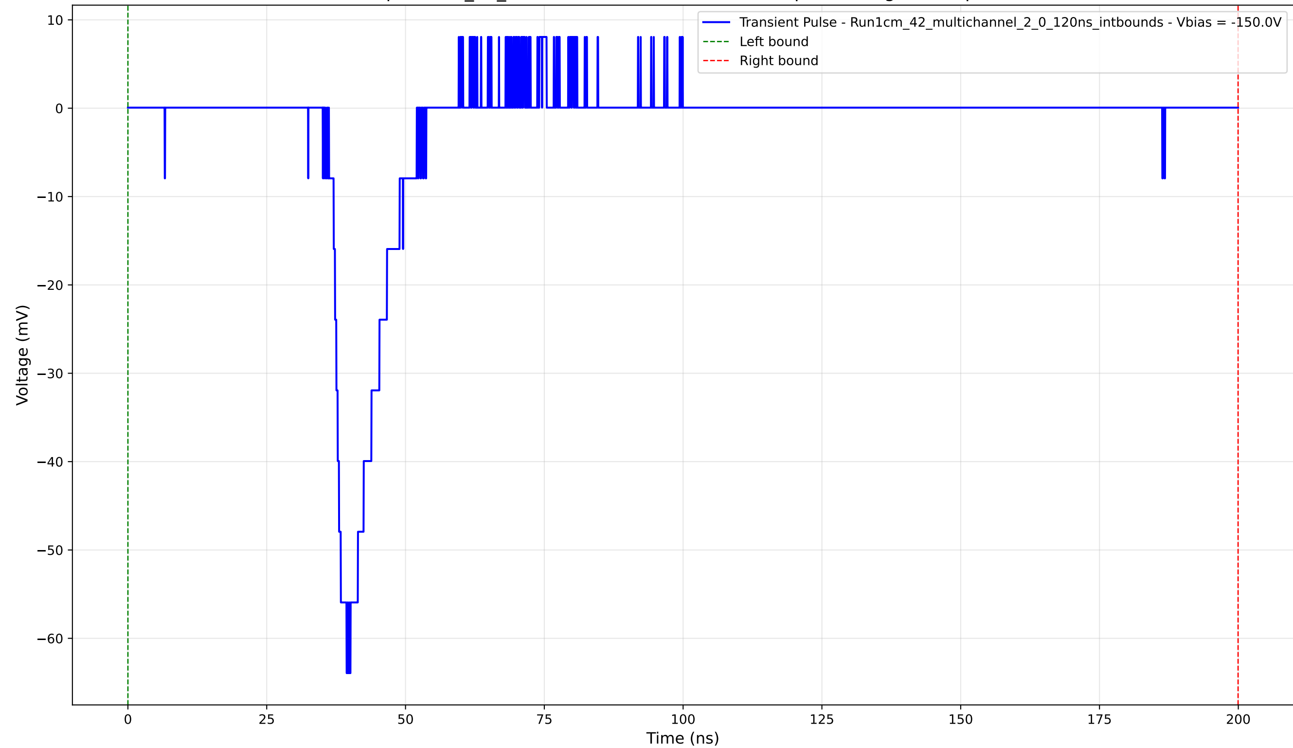
Transient Pulse - Sample: 1cm_42_multichannel - Position: 4795.0 \mu\text{m} - Charge: 8.21 pC - Rise Time: 3.17 ns
