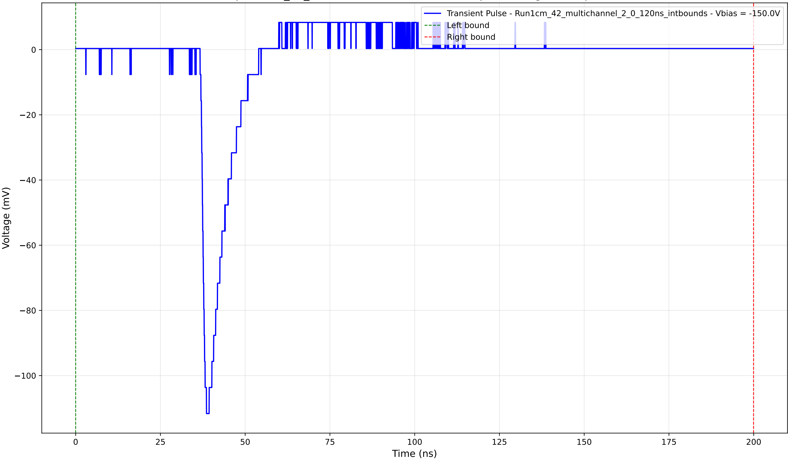
Transient Pulse - Sample: 1cm_42_multichannel - Position: 925.0 \mu\text{m} - Charge: 9.04 pC - Rise Time: 1.26 ns
