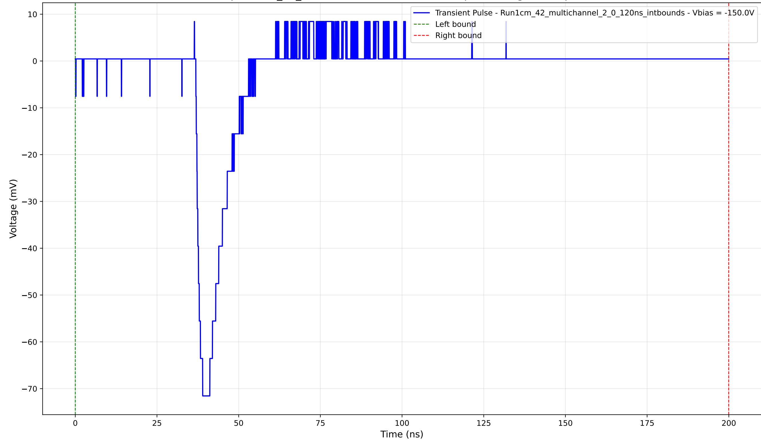
Transient Pulse - Sample: 1cm_42_multichannel - Position: 200.0 \mu\text{m} - Charge: 7.80 pC - Rise Time: 2.08 ns
