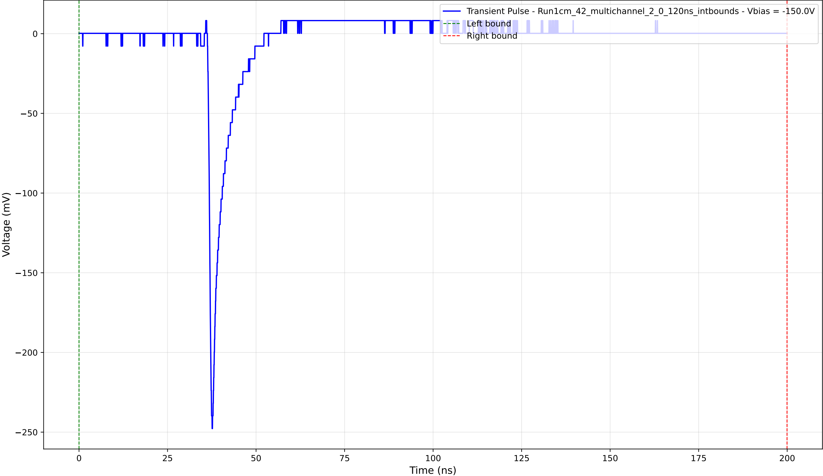
Transient Pulse - Sample: 1cm_42_multichannel - Position: 3030.0 \mu\text{m} - Charge: 11.79 pC - Rise Time: 0.87 ns
