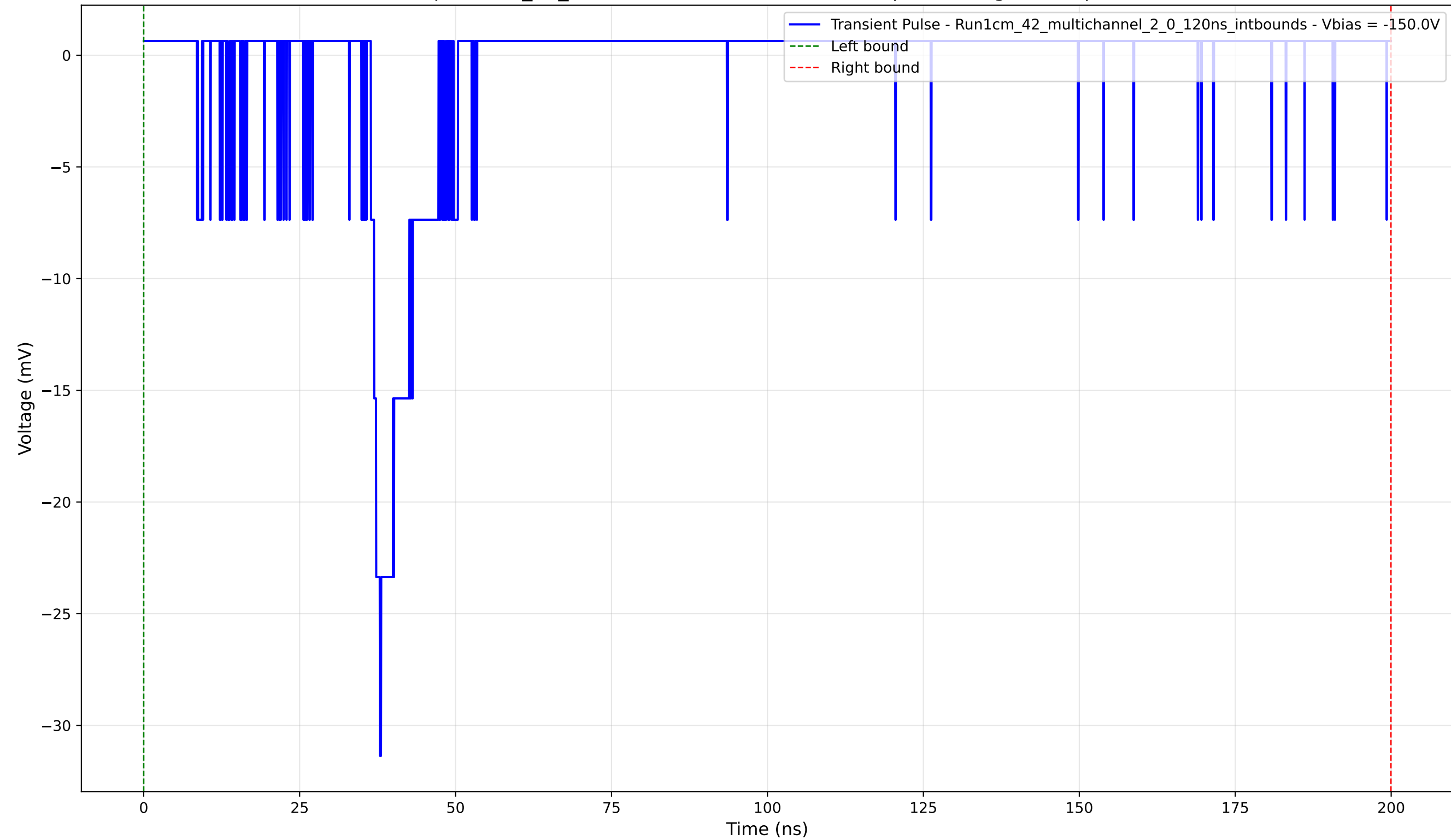
Transient Pulse - Sample: 1cm_42_multichannel - Position: 3350.0 \mu\text{m} - Charge: 1.83 pC - Rise Time: 1.47 ns
