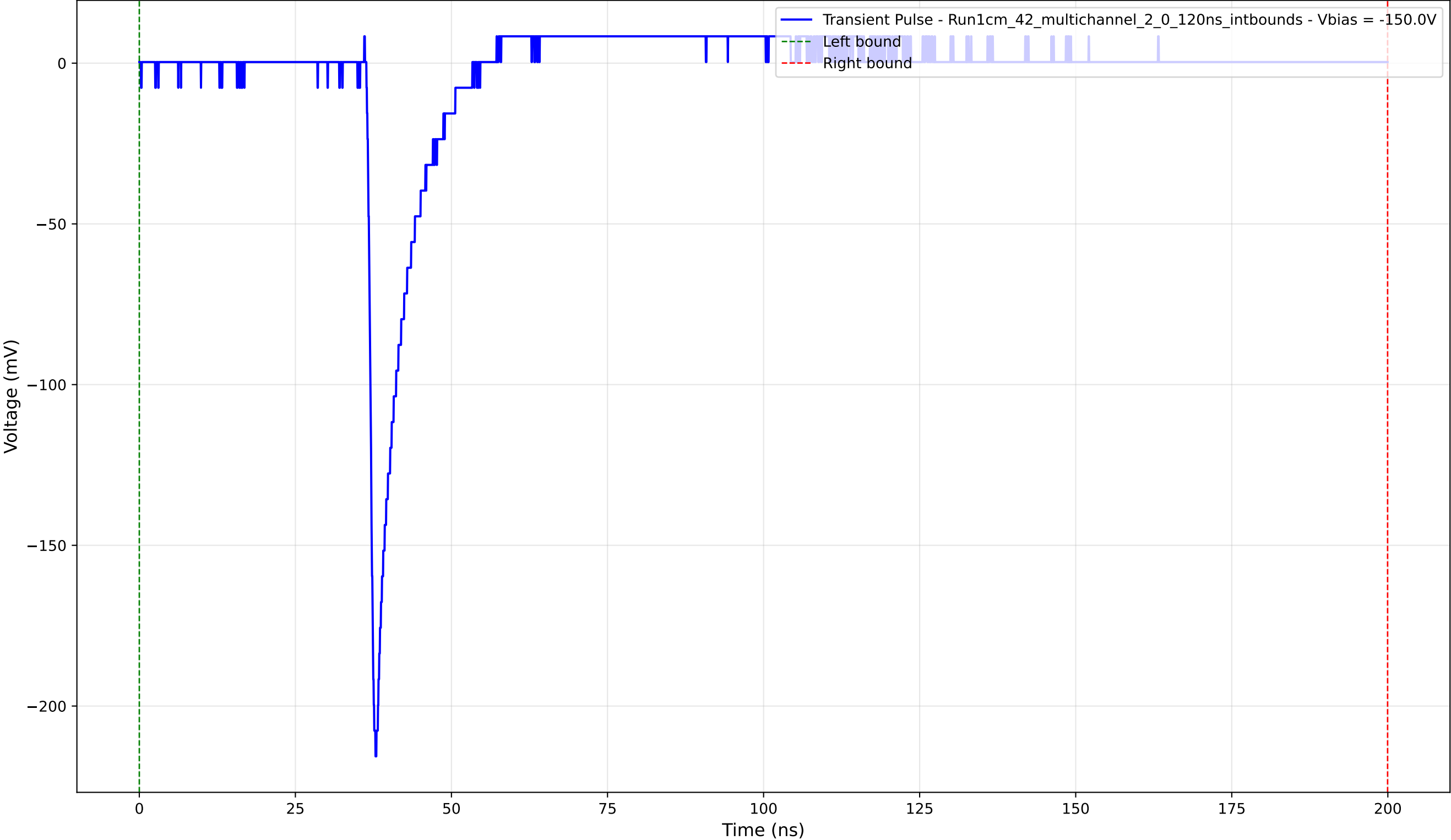
Transient Pulse - Sample: 1cm_42_multichannel - Position: 1505.0 \mu\text{m} - Charge: 11.24 pC - Rise Time: 1.01 ns
