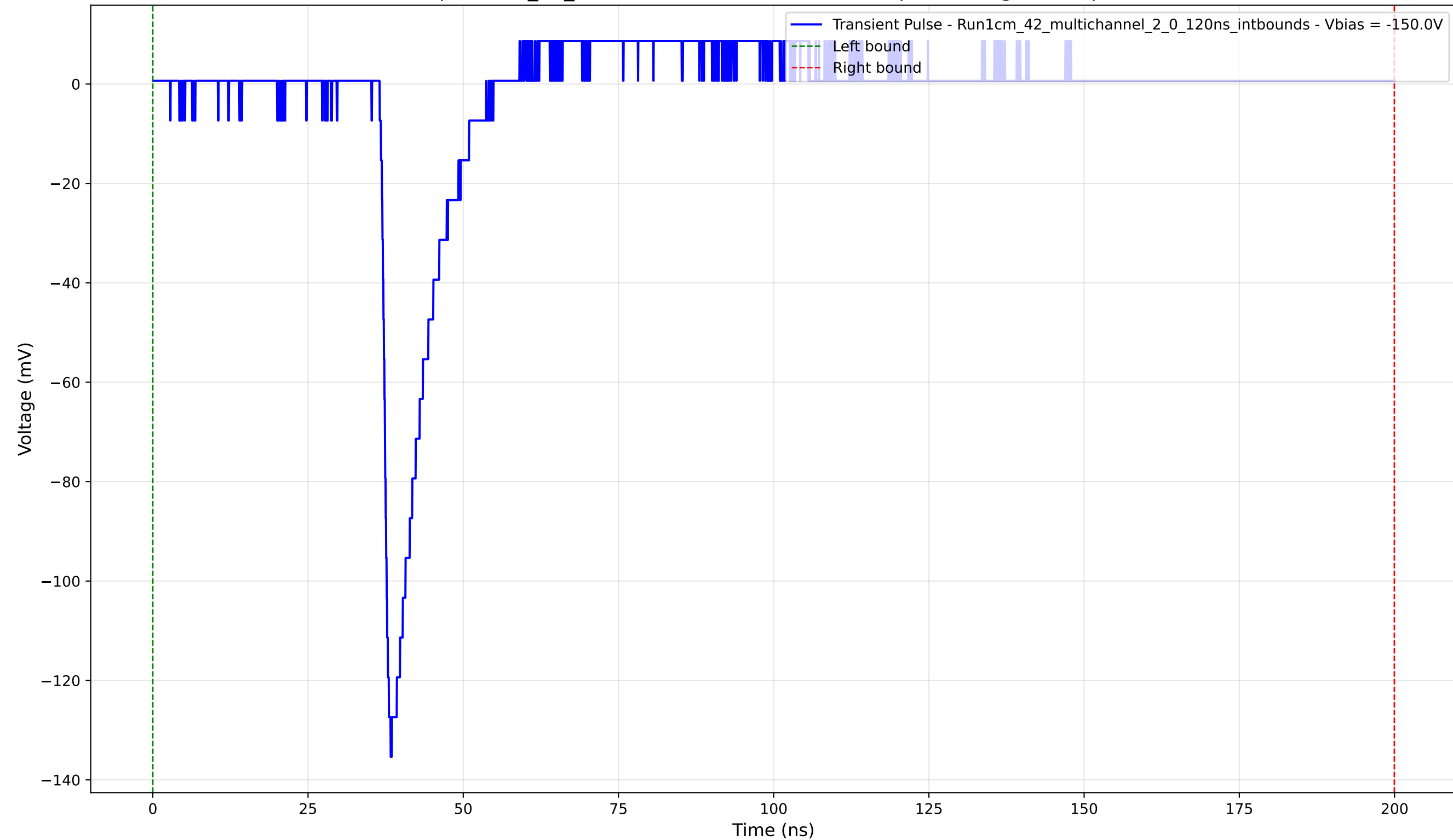
Transient Pulse - Sample: 1cm_42_multichannel - Position: 1105.0 \mu\text{m} - Charge: 8.82 pC - Rise Time: 1.29 ns
