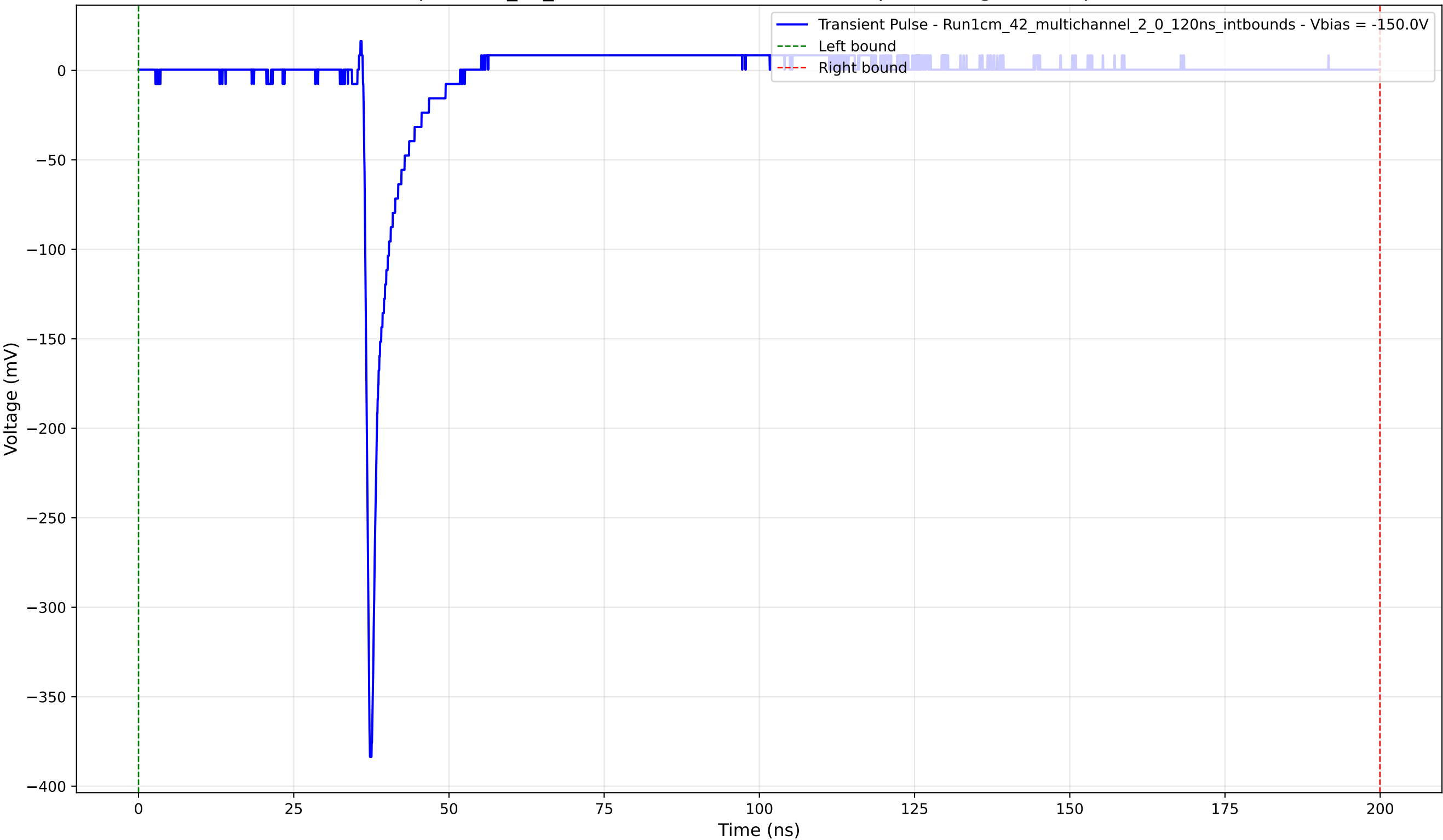
Transient Pulse - Sample: 1cm_42_multichannel - Position: 2765.0 \mu\text{m} - Charge: 12.15 pC - Rise Time: 0.83 ns
