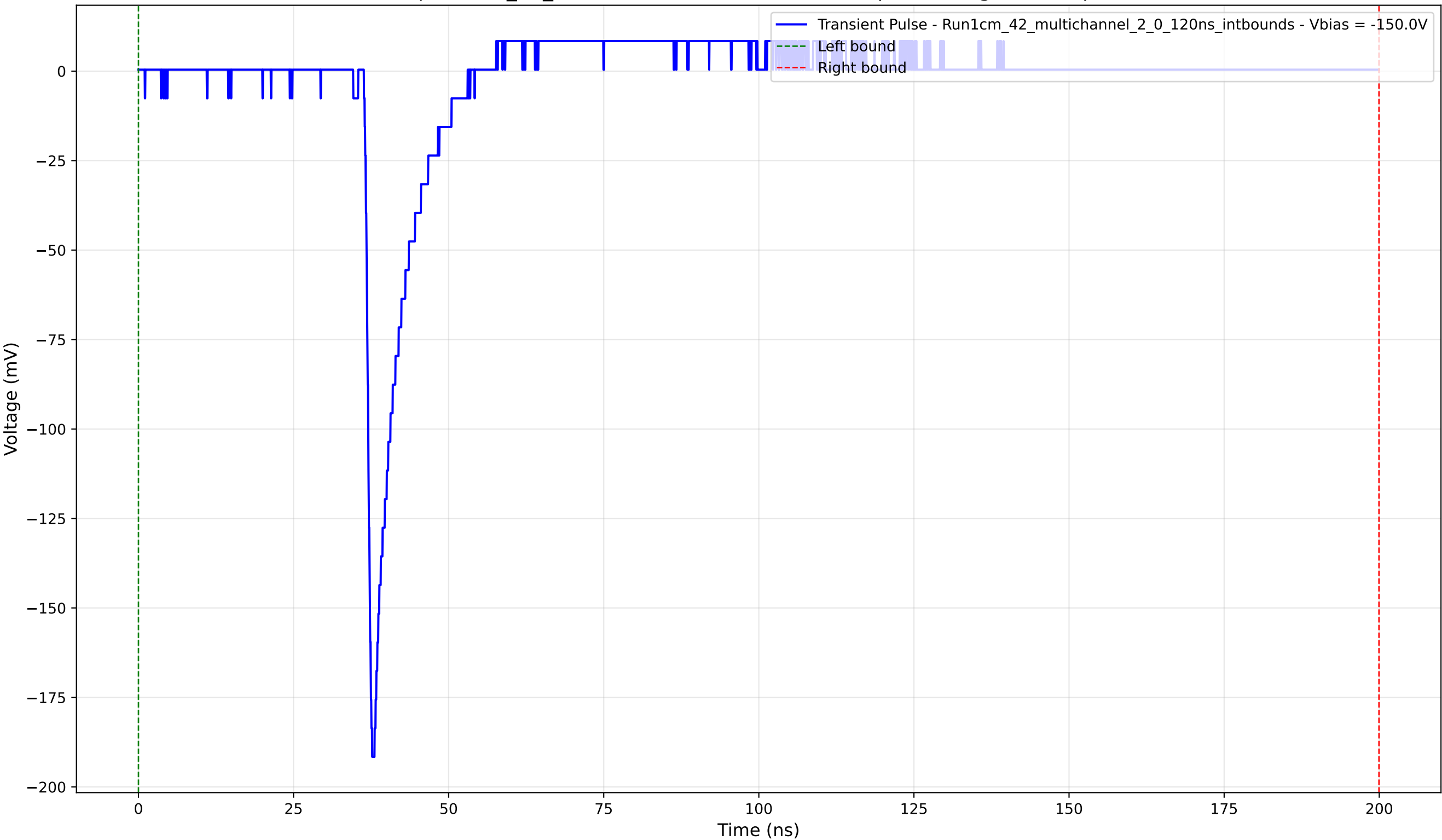
Transient Pulse - Sample: 1cm_42_multichannel - Position: 3225.0 \mu\text{m} - Charge: 10.04 pC - Rise Time: 0.94 ns
