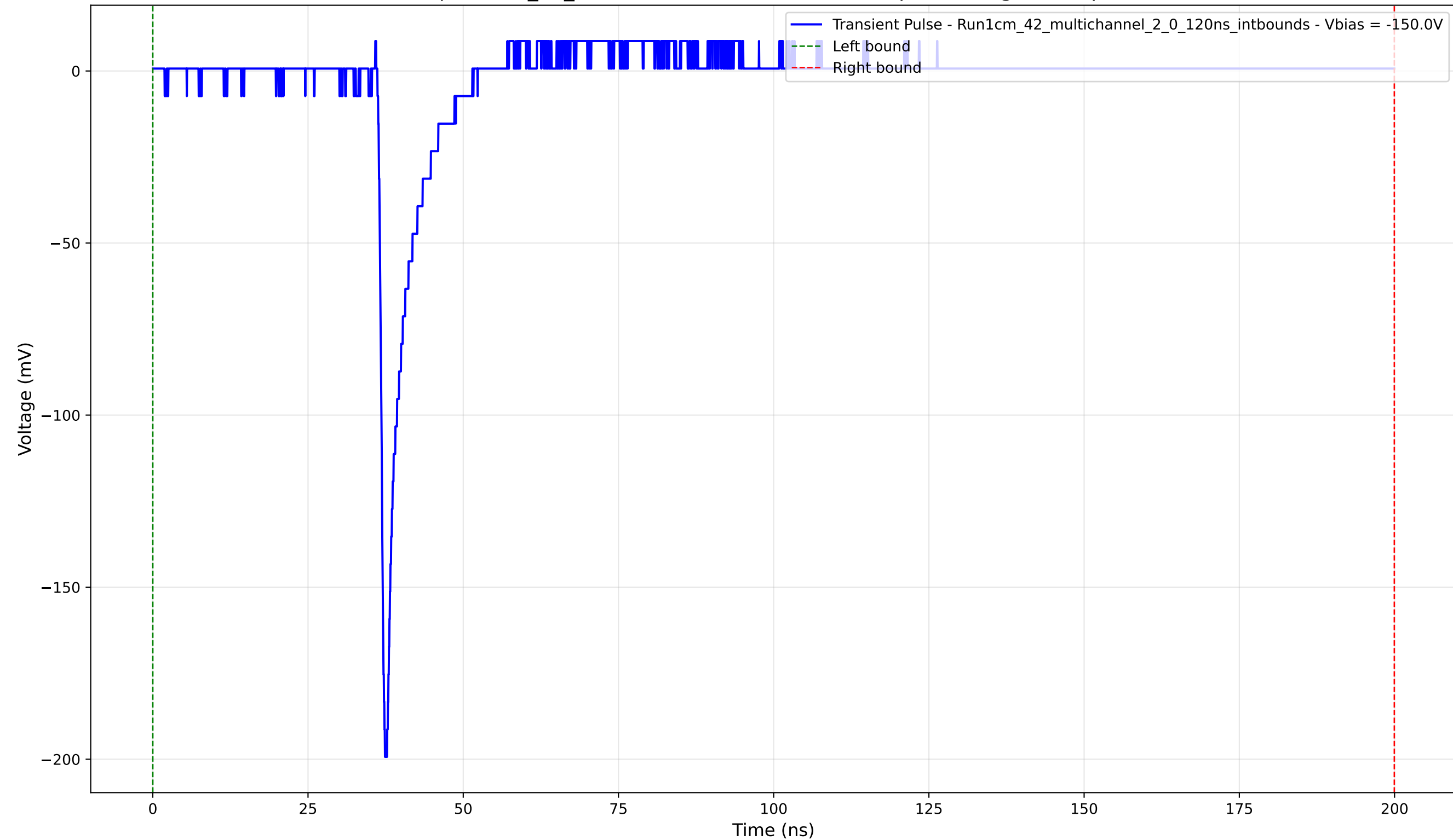
Transient Pulse - Sample: 1cm_42_multichannel - Position: 1805.0 \mu\text{m} - Charge: 9.23 pC - Rise Time: 0.86 ns
