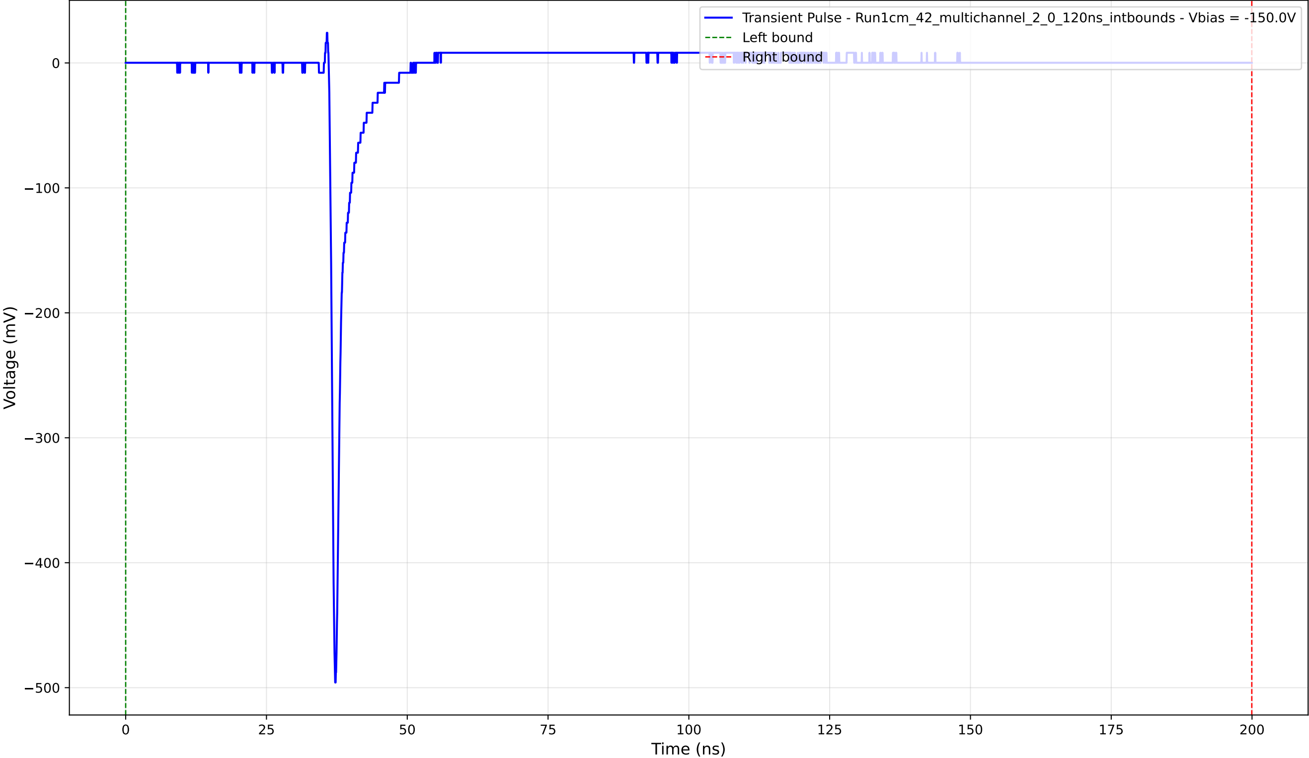
Transient Pulse - Sample: 1cm_42_multichannel - Position: 2575.0 \mu\text{m} - Charge: 14.65 pC - Rise Time: 0.75 ns
