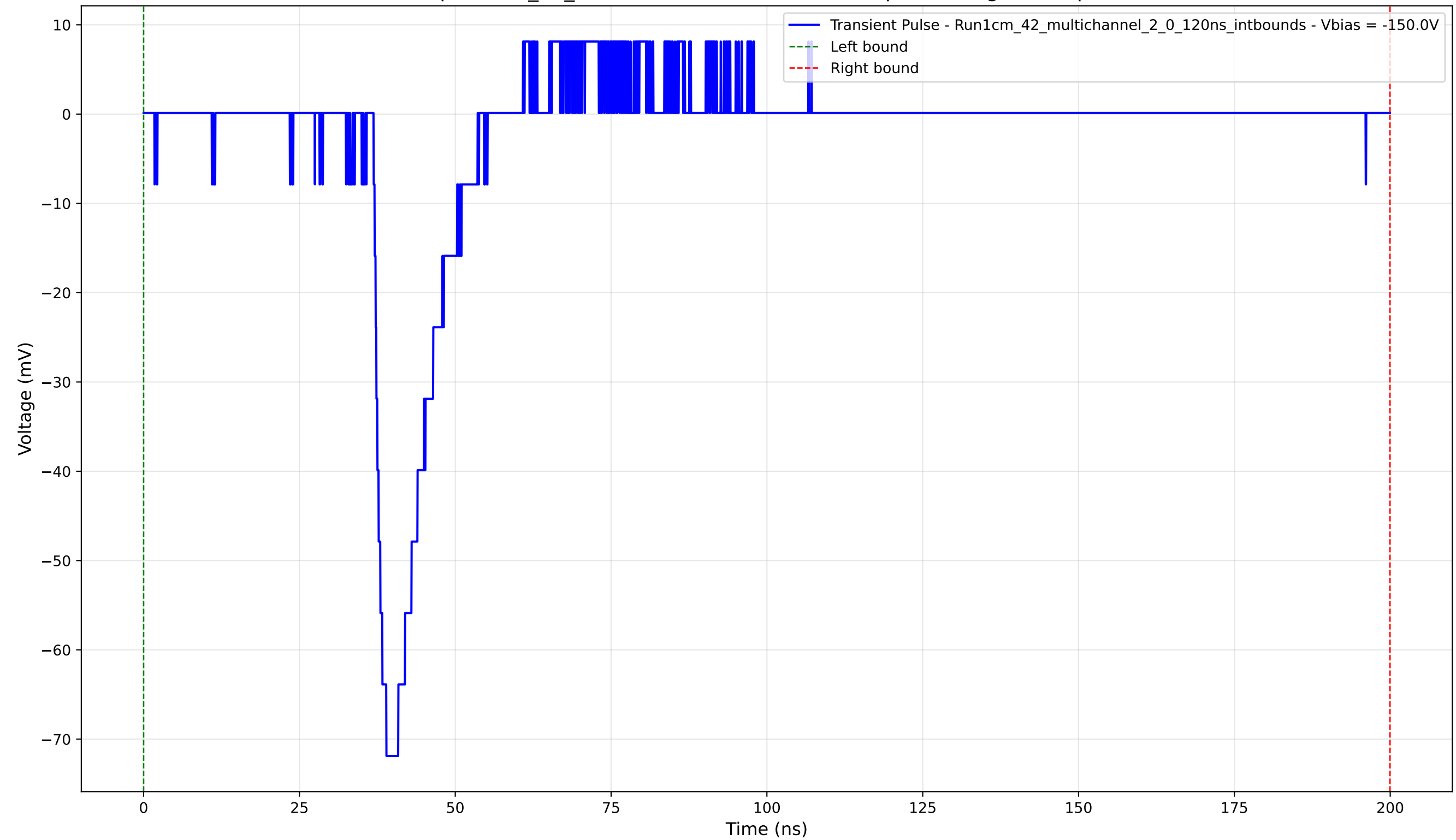
Transient Pulse - Sample: 1cm_42_multichannel - Position: 215.0 \mu\text{m} - Charge: 9.13 pC - Rise Time: 2.04 ns
