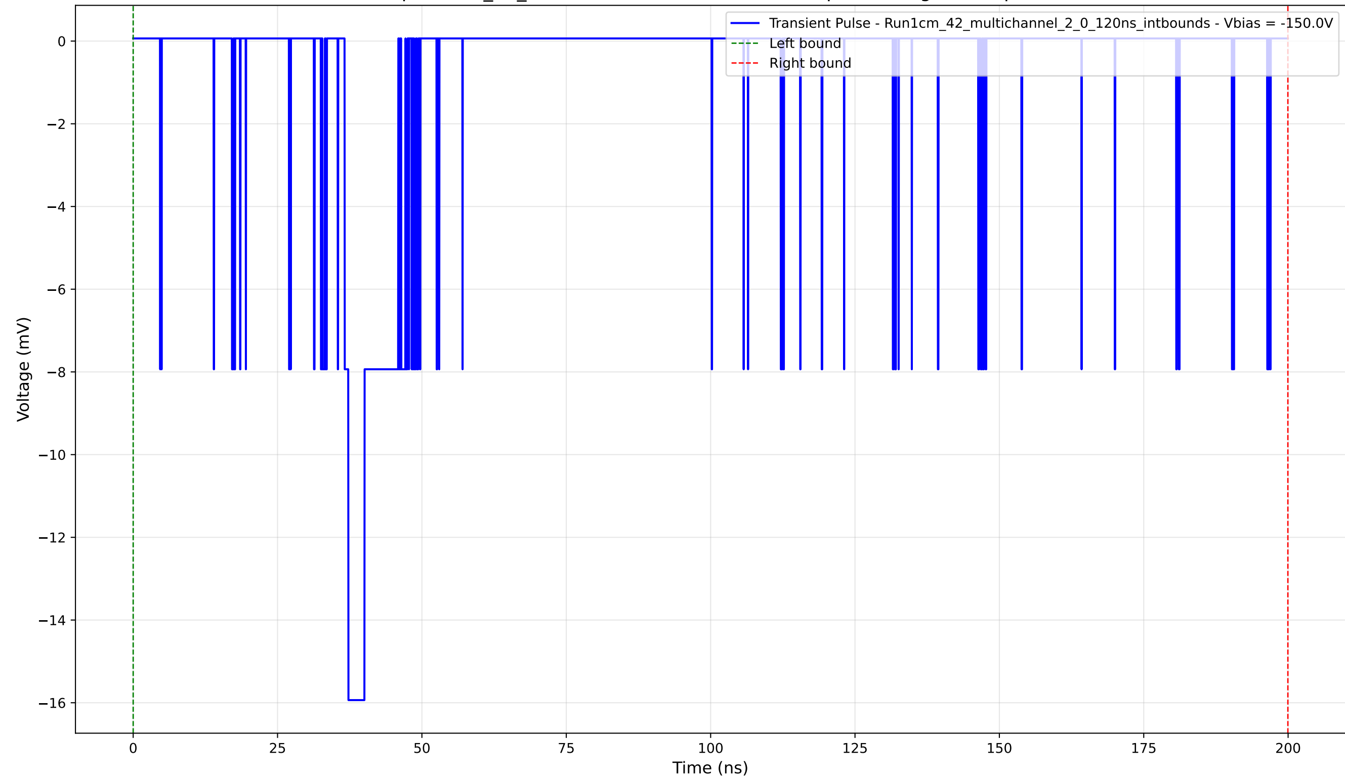
Transient Pulse - Sample: 1cm_42_multichannel - Position: 3360.0 \mu\text{m} - Charge: 2.78 pC - Rise Time: 0.67 ns
