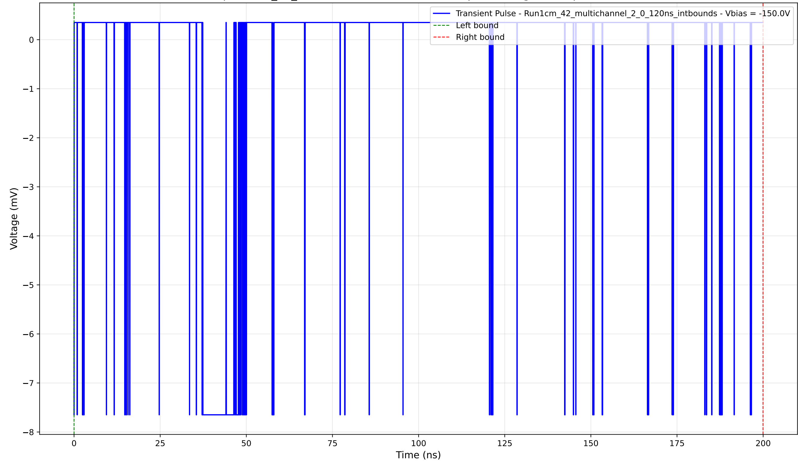
Transient Pulse - Sample: 1cm_42_multichannel - Position: 860.0 \mu\text{m} - Charge: 1.01 pC - Rise Time: 0.00 ns (N/A)
