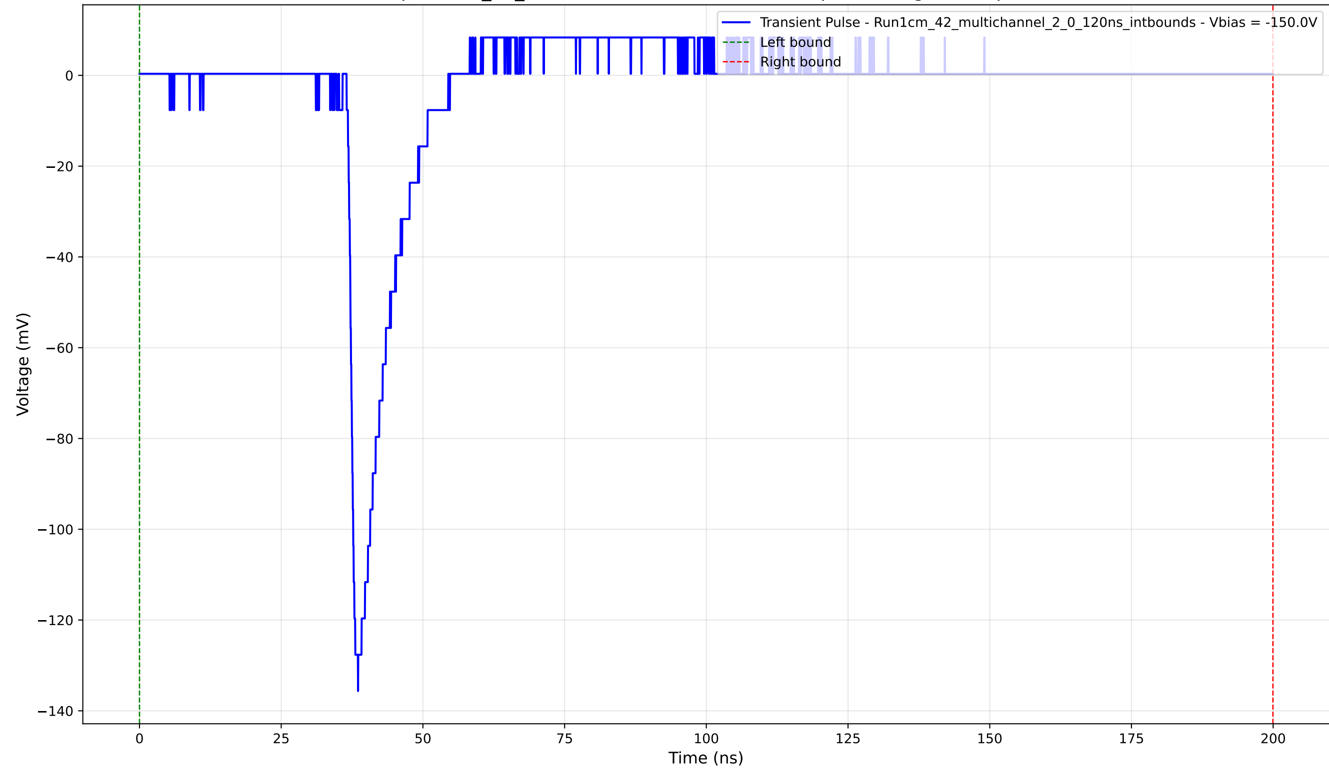
Transient Pulse - Sample: 1cm_42_multichannel - Position: 1095.0 \mu\text{m} - Charge: 9.77 pC - Rise Time: 1.29 ns
