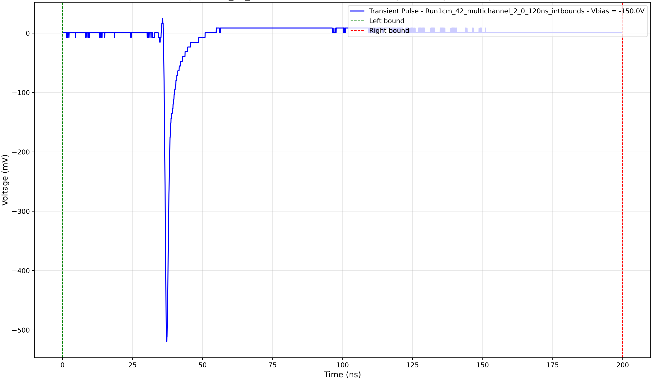
Transient Pulse - Sample: 1cm_42_multichannel - Position: 2550.0 \mu\text{m} - Charge: 12.65 pC - Rise Time: 0.73 ns
