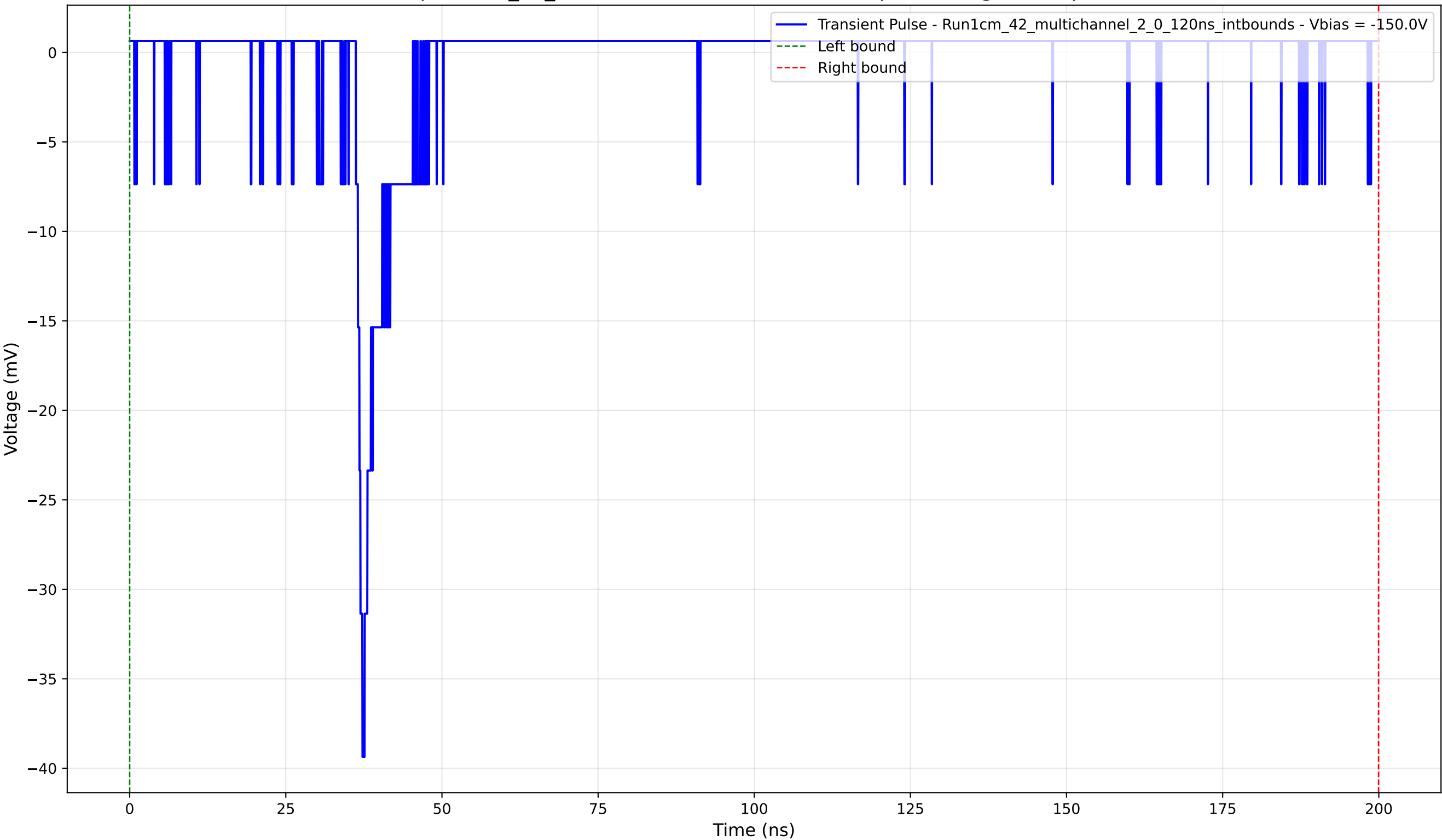
Transient Pulse - Sample: 1cm_42_multichannel - Position: 2850.0 \mu\text{m} - Charge: 1.30 pC - Rise Time: 1.06 ns
