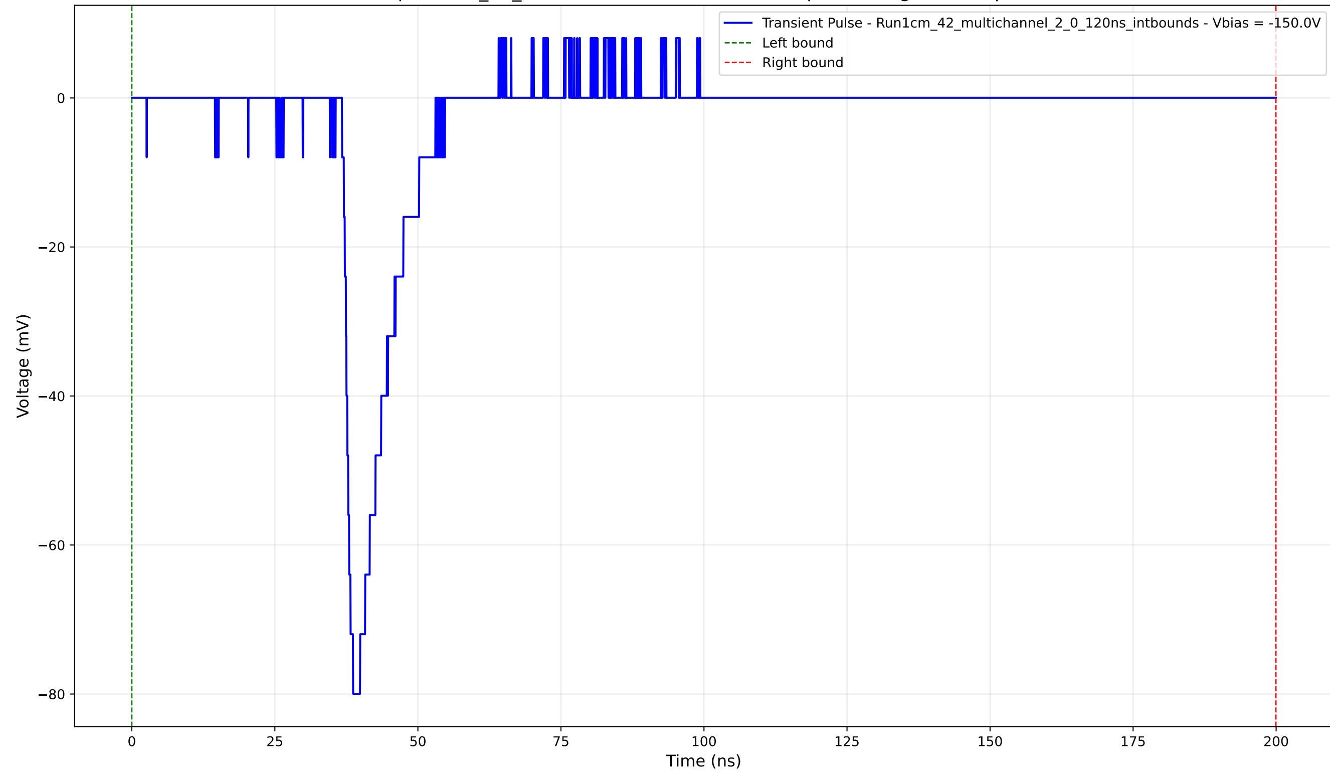
Transient Pulse - Sample: 1cm_42_multichannel - Position: 790.0 \mu\text{m} - Charge: 10.91 pC - Rise Time: 1.64 ns
