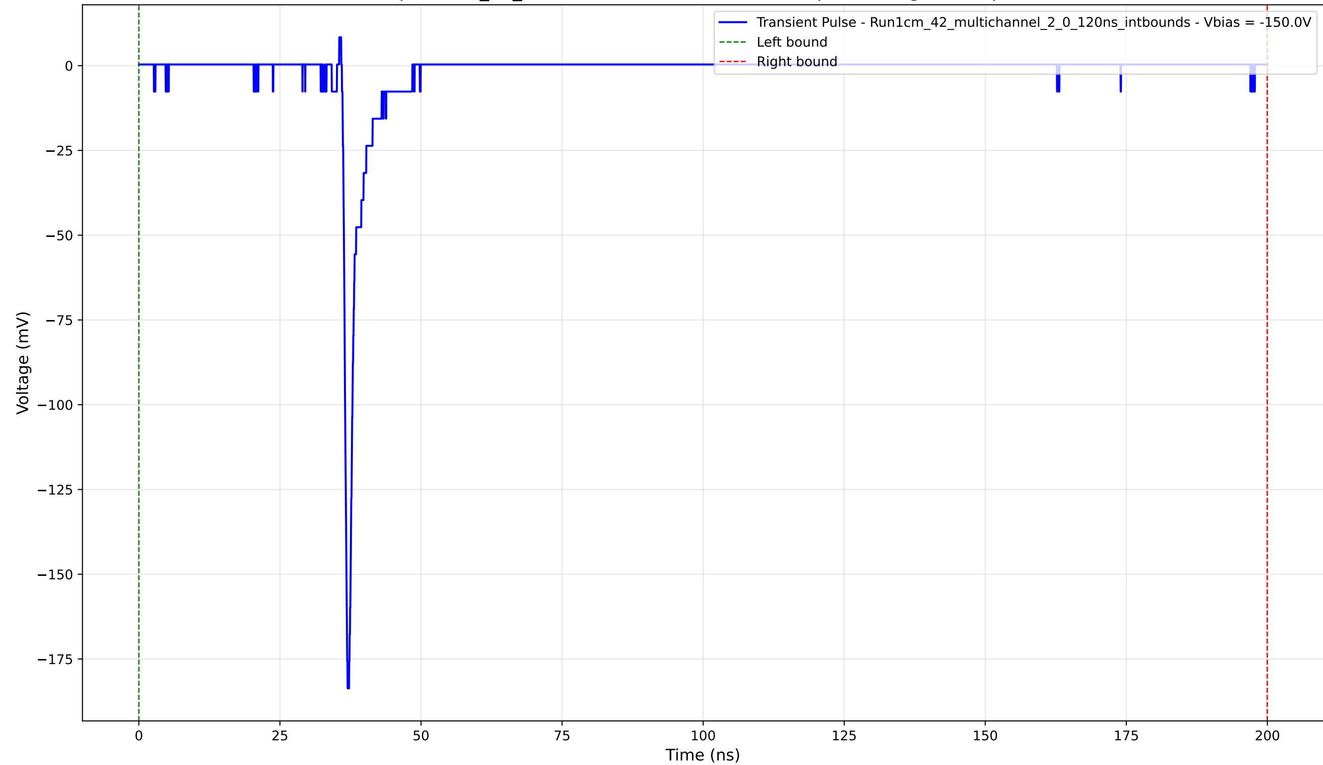
Transient Pulse - Sample: 1cm_42_multichannel - Position: 2410.0 \mu\text{m} - Charge: 7.89 pC - Rise Time: 0.73 ns
