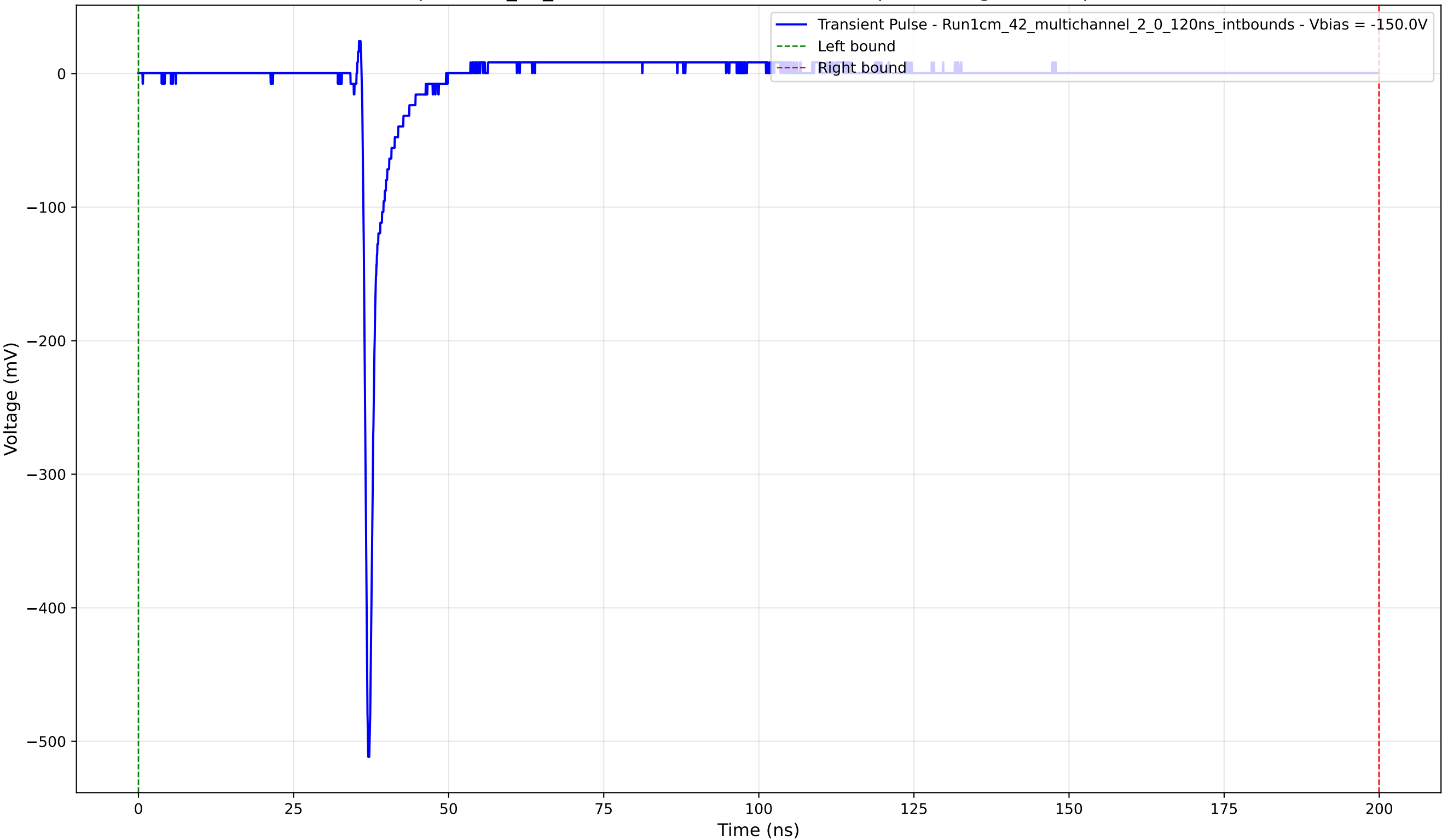
Transient Pulse - Sample: 1cm_42_multichannel - Position: 2305.0 \mu\text{m} - Charge: 12.98 pC - Rise Time: 0.72 ns
