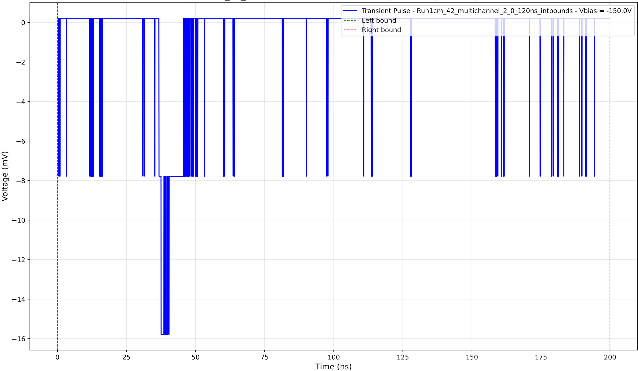
Transient Pulse - Sample: 1cm_42_multichannel - Position: 1340.0 \mu\text{m} - Charge: 1.89 pC - Rise Time: 0.79 ns
