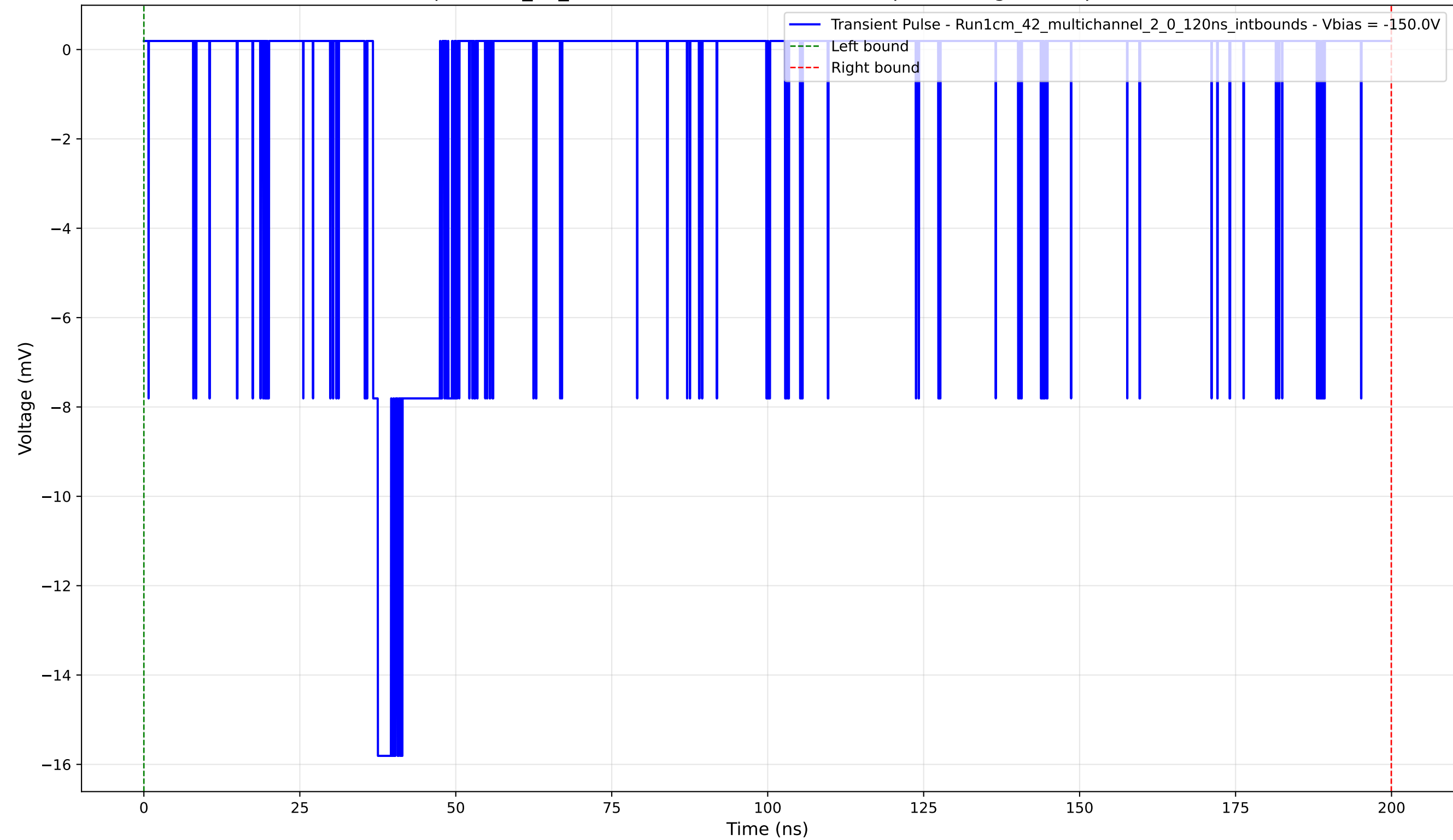
Transient Pulse - Sample: 1cm_42_multichannel - Position: 3405.0 \mu\text{m} - Charge: 3.01 pC - Rise Time: 0.79 ns
