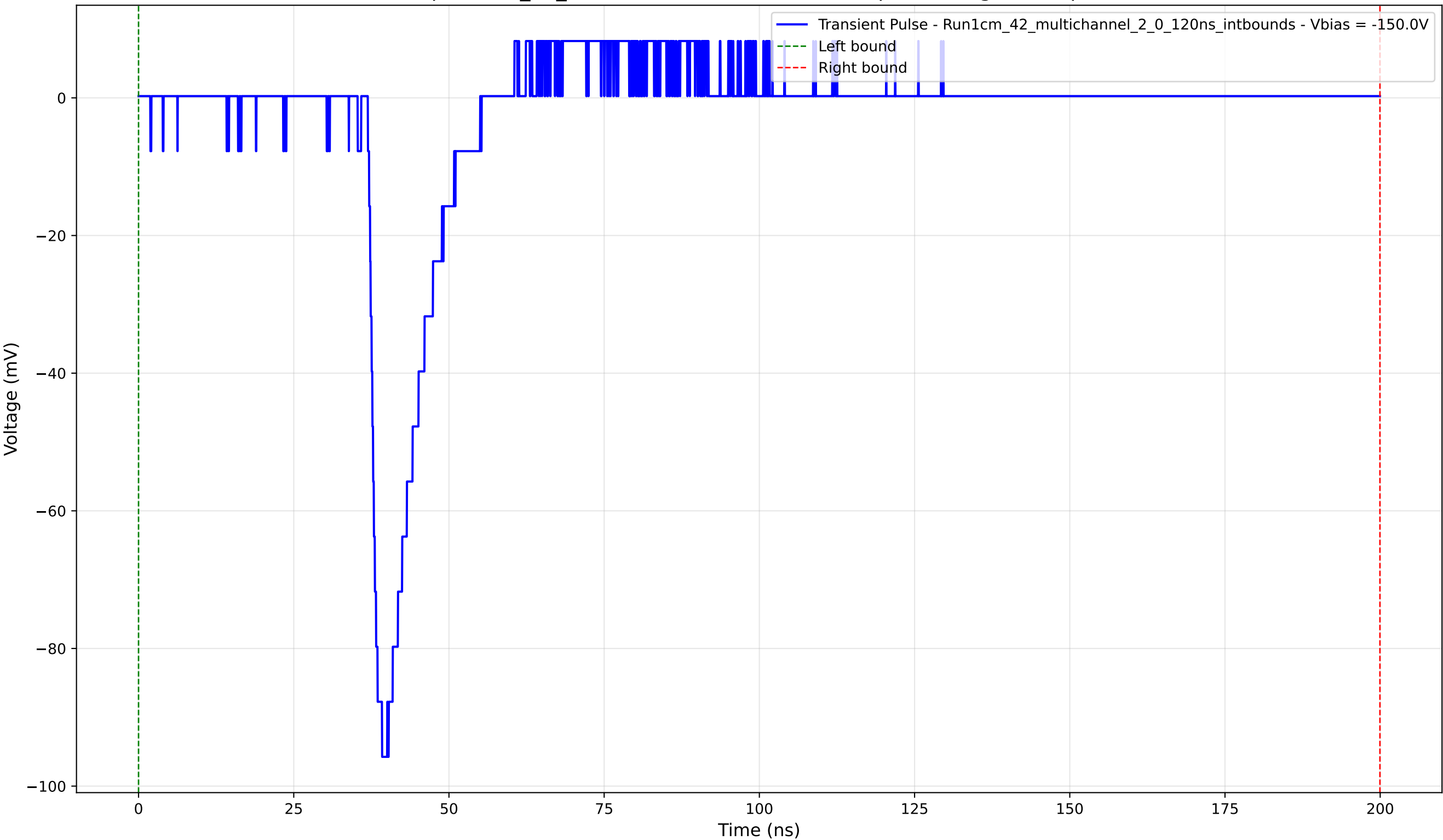
Transient Pulse - Sample: 1cm_42_multichannel - Position: 520.0 \mu\text{m} - Charge: 9.94 pC - Rise Time: 1.39 ns
