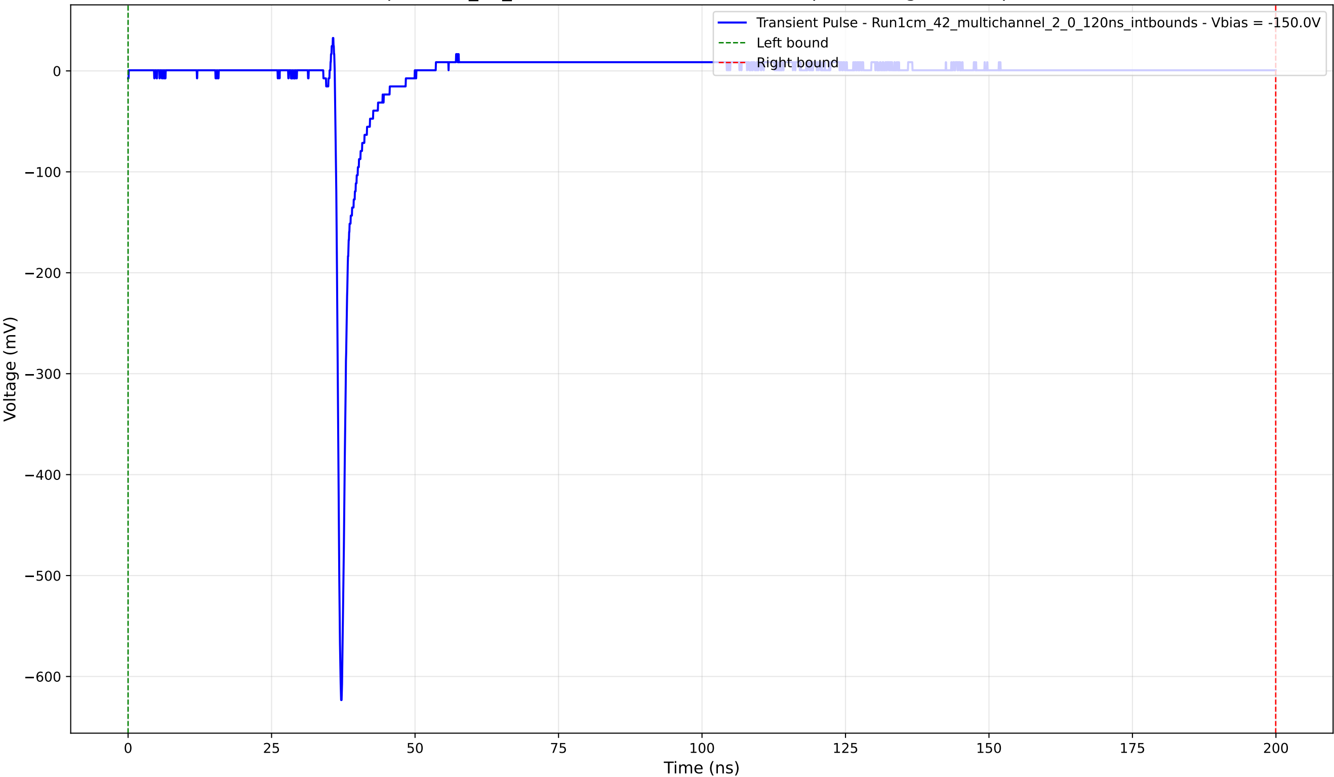
Transient Pulse - Sample: 1cm_42_multichannel - Position: 2285.0 \mu\text{m} - Charge: 14.65 pC - Rise Time: 0.73 ns
