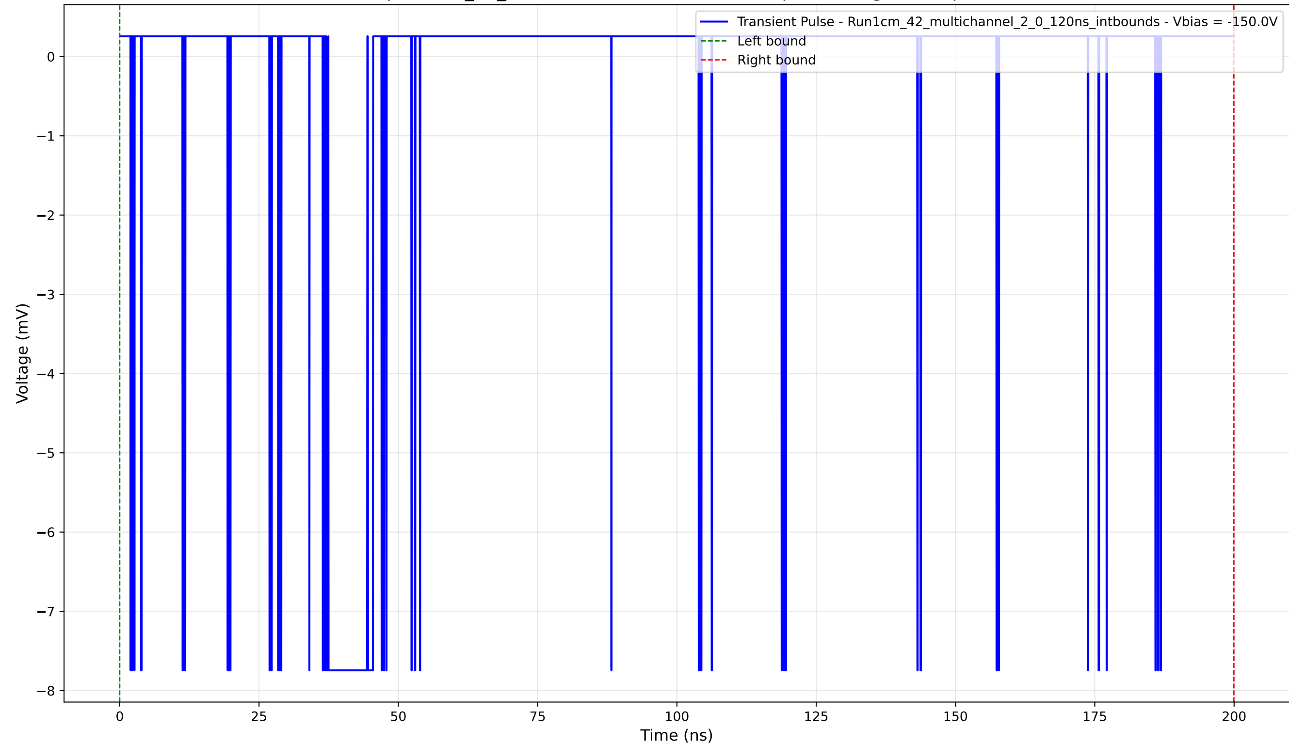
Transient Pulse - Sample: 1cm_42_multichannel - Position: 850.0 \mu\text{m} - Charge: 0.90 pC - Rise Time: 0.04 ns
