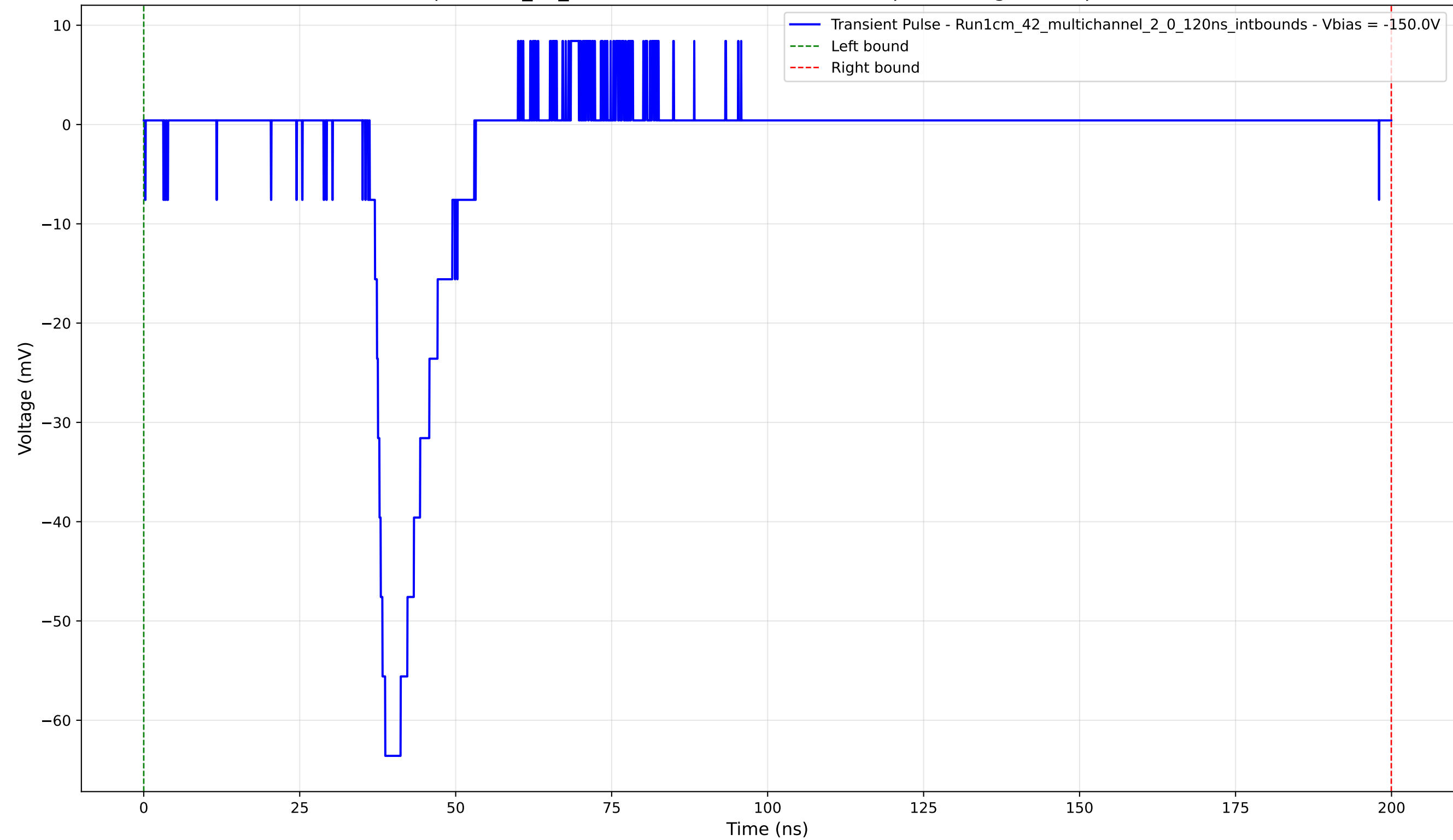
Transient Pulse - Sample: 1cm_42_multichannel - Position: 4730.0 \mu\text{m} - Charge: 7.74 pC - Rise Time: 2.49 ns
