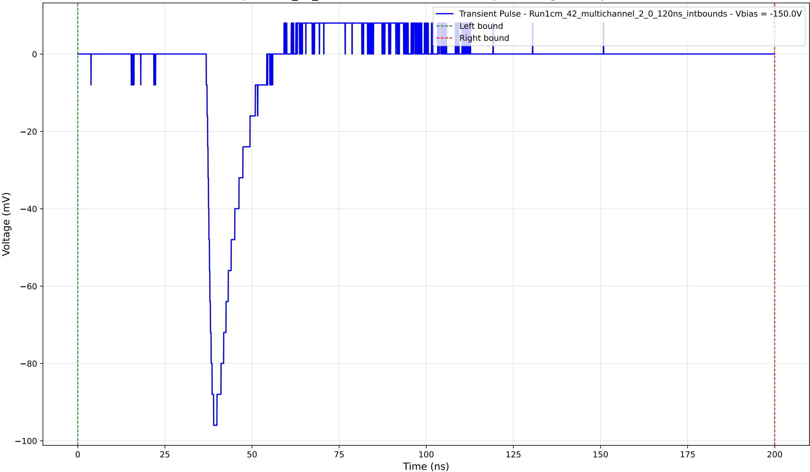
Transient Pulse - Sample: 1cm_42_multichannel - Position: 530.0 \mu\text{m} - Charge: 9.38 pC - Rise Time: 1.47 ns
