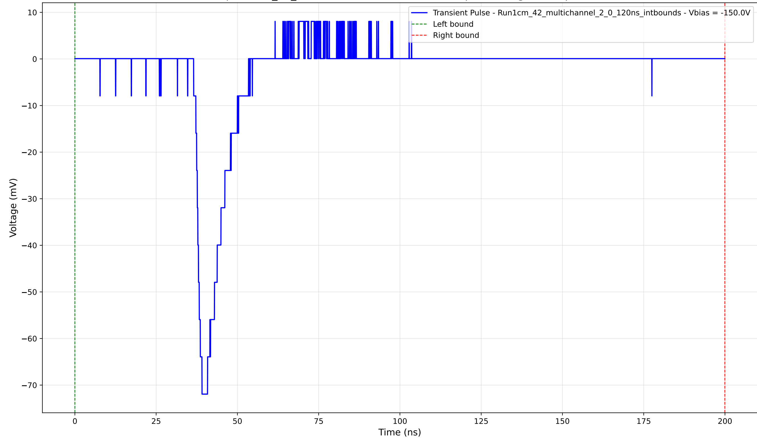
Transient Pulse - Sample: 1cm_42_multichannel - Position: 4530.0 \mu\text{m} - Charge: 9.66 pC - Rise Time: 2.56 ns
