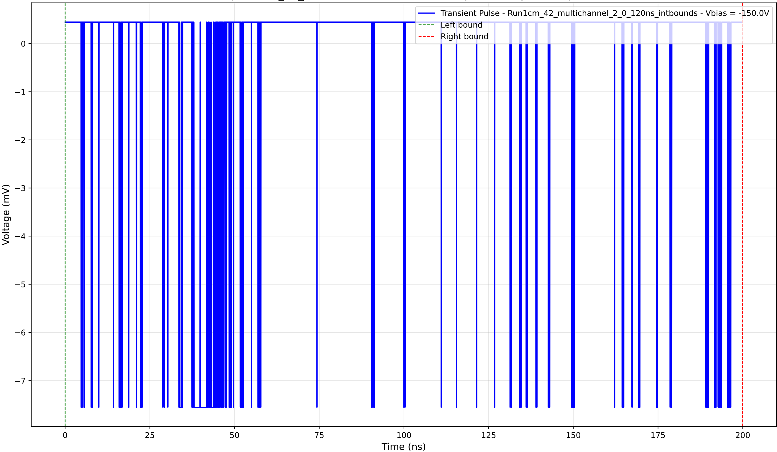
Transient Pulse - Sample: 1cm_42_multichannel - Position: 35.0 \mu\text{m} - Charge: 0.83 pC - Rise Time: 0.04 ns
