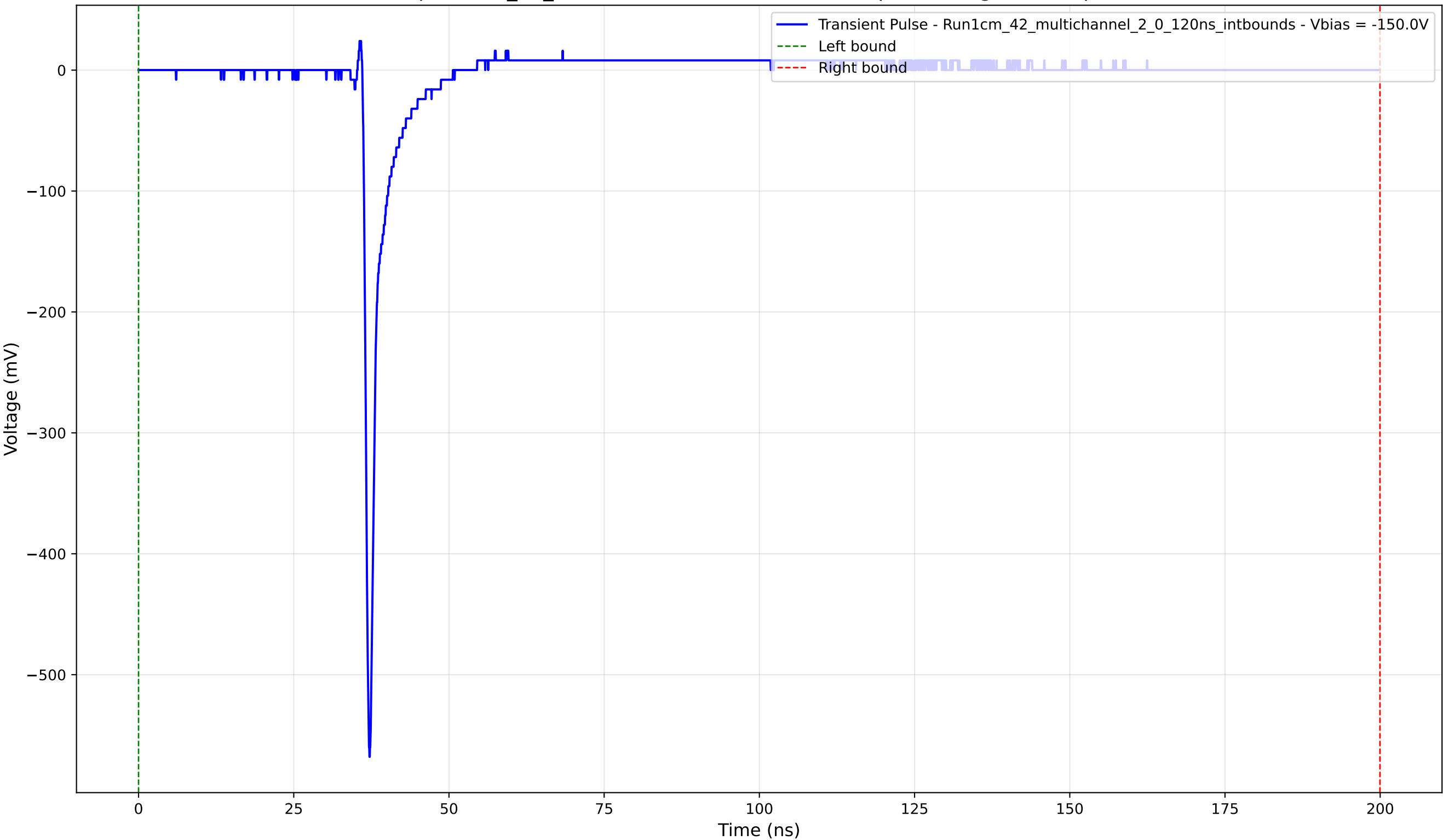
Transient Pulse - Sample: 1cm_42_multichannel - Position: 2190.0 \mu\text{m} - Charge: 15.64 pC - Rise Time: 0.76 ns
