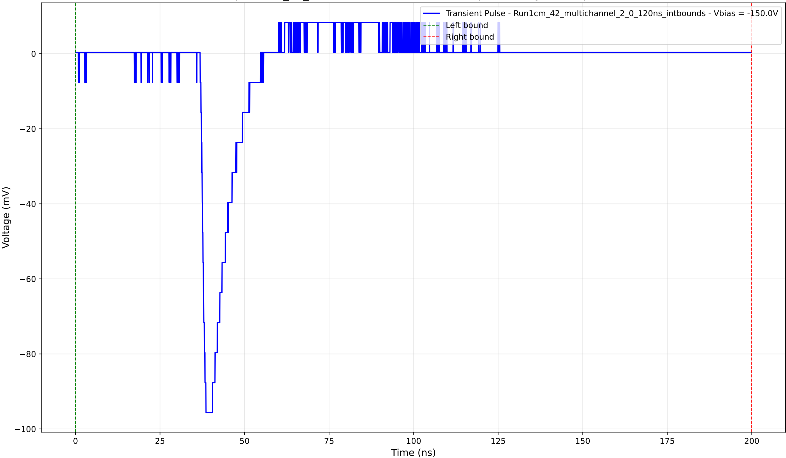
Transient Pulse - Sample: 1cm_42_multichannel - Position: 625.0 \mu\text{m} - Charge: 9.36 pC - Rise Time: 1.23 ns
