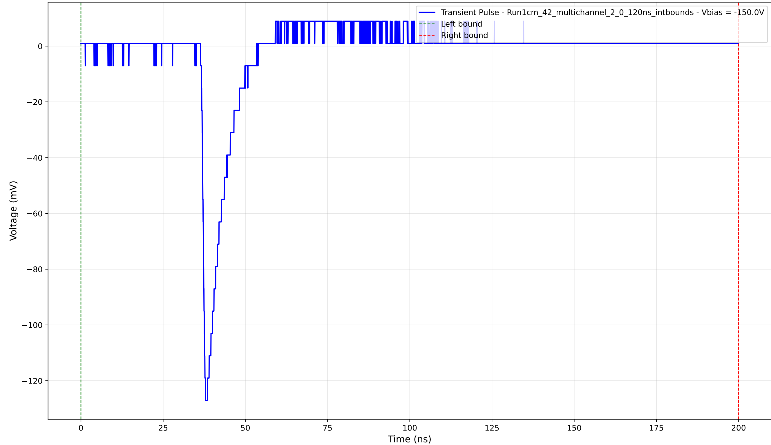
Transient Pulse - Sample: 1cm_42_multichannel - Position: 3460.0 \mu\text{m} - Charge: 7.41 pC - Rise Time: 1.09 ns
