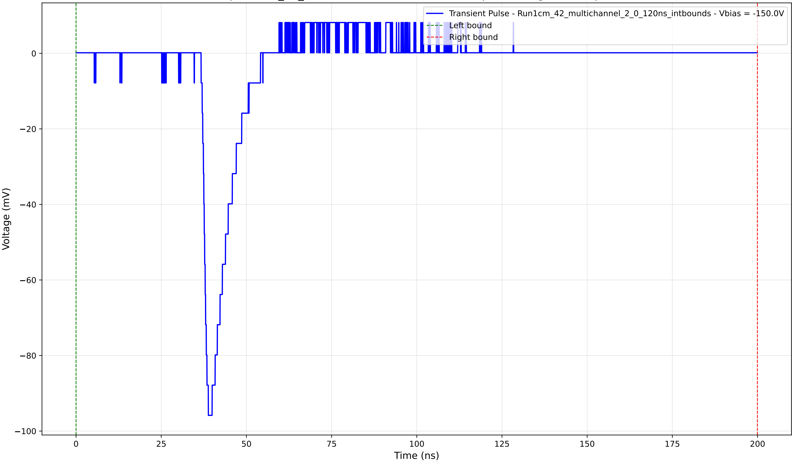
Transient Pulse - Sample: 1cm_42_multichannel - Position: 4005.0 \mu\text{m} - Charge: 10.03 pC - Rise Time: 1.43 ns
