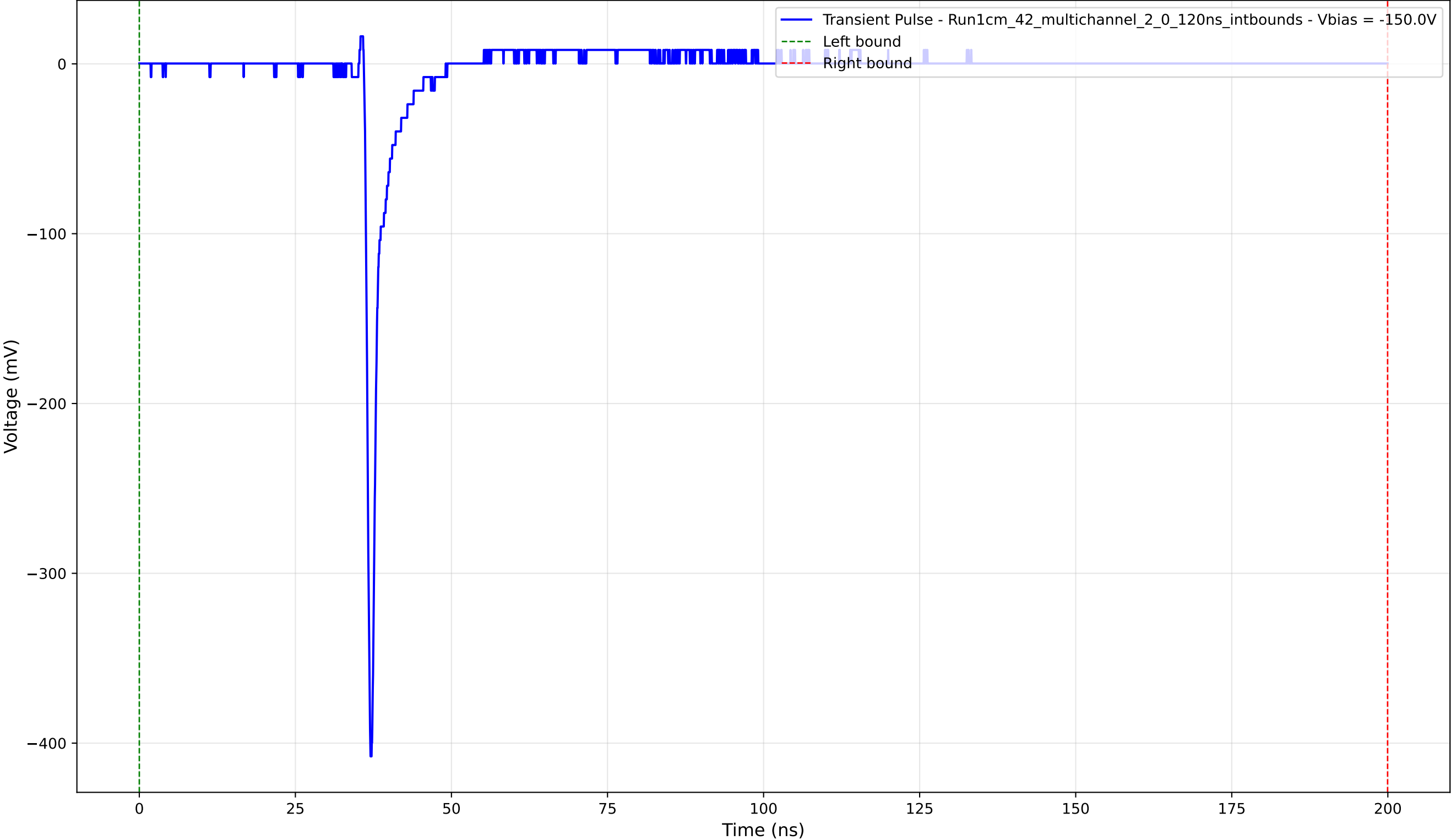
Transient Pulse - Sample: 1cm_42_multichannel - Position: 2425.0 \mu\text{m} - Charge: 12.03 pC - Rise Time: 0.72 ns
