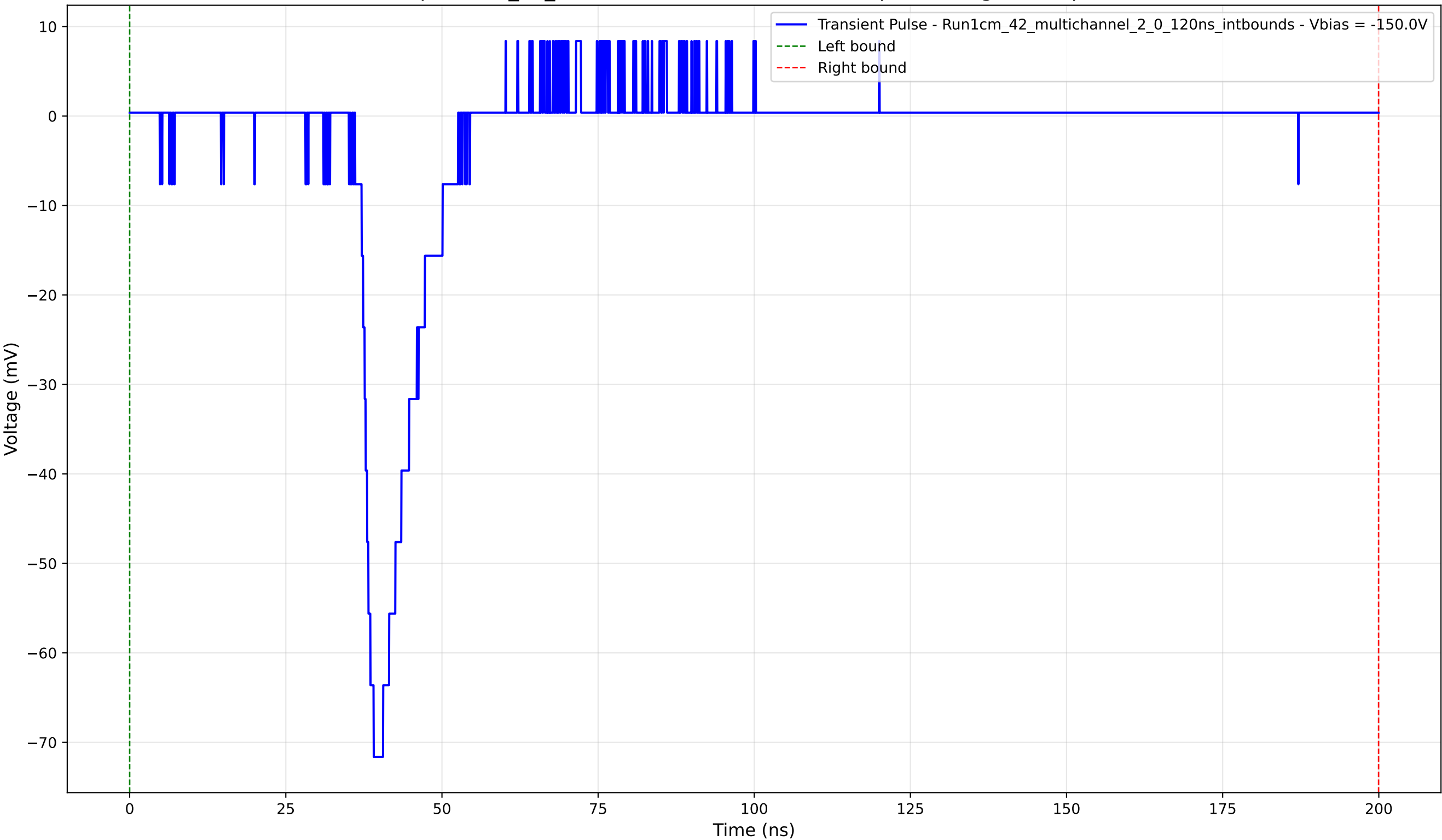
Transient Pulse - Sample: 1cm_42_multichannel - Position: 4655.0 \mu\text{m} - Charge: 8.51 pC - Rise Time: 2.96 ns
