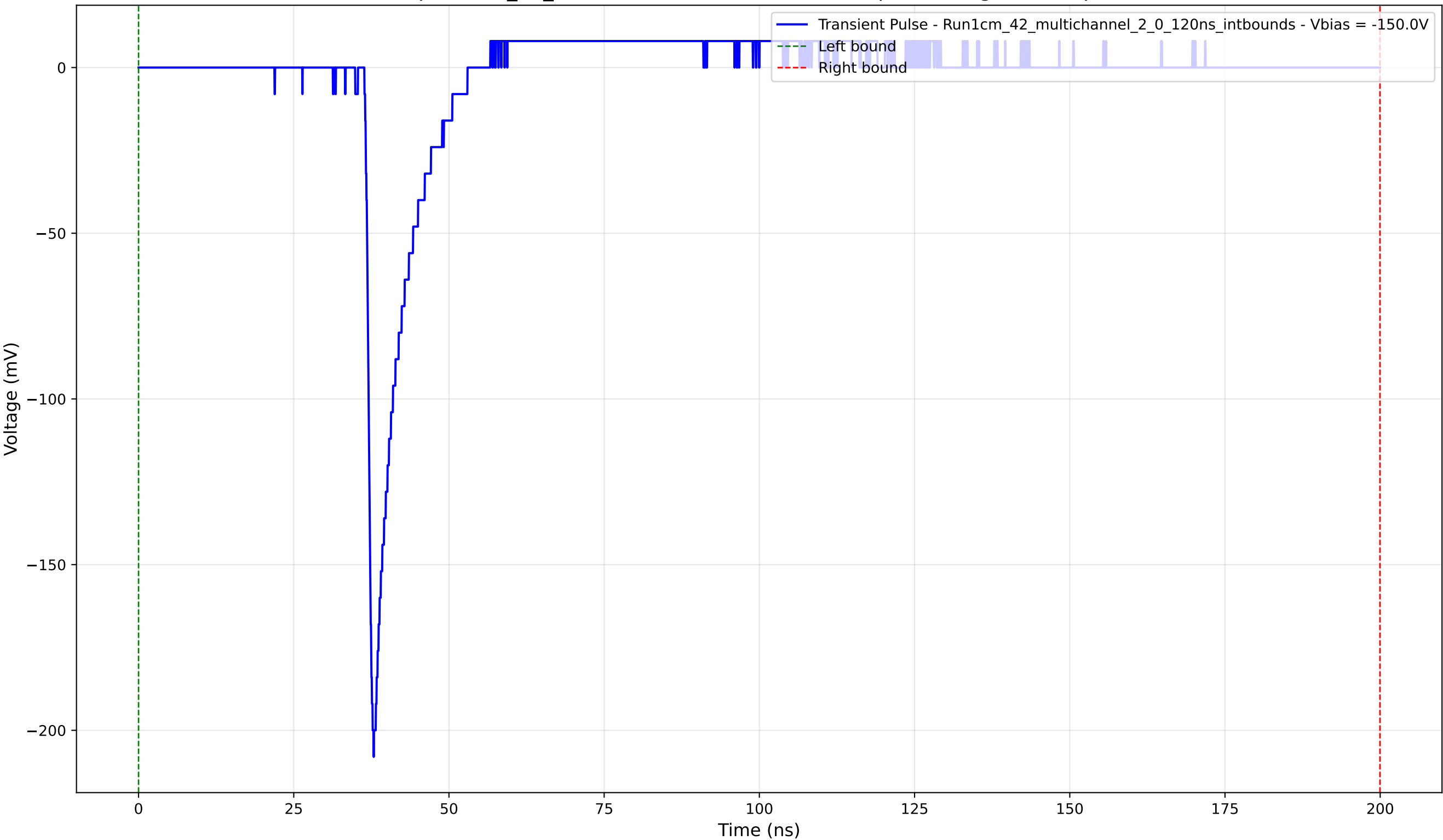
Transient Pulse - Sample: 1cm_42_multichannel - Position: 1475.0 \mu\text{m} - Charge: 11.17 pC - Rise Time: 1.02 ns
