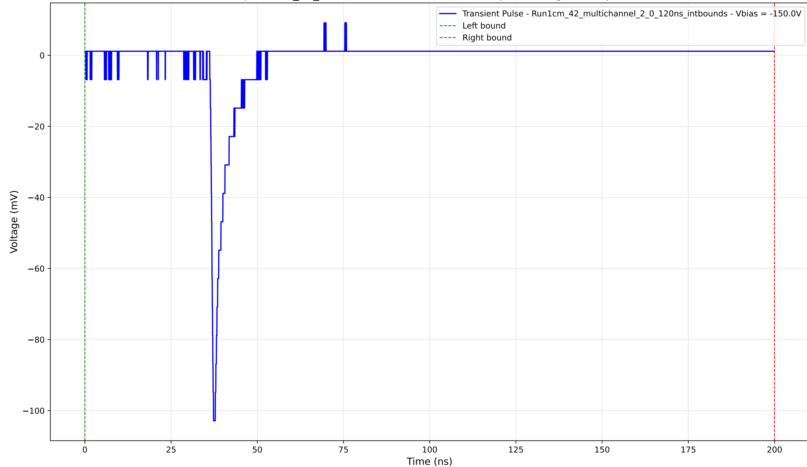
Transient Pulse - Sample: 1cm_42_multichannel - Position: 1820.0 \mu\text{m} - Charge: 4.36 pC - Rise Time: 0.82 ns
