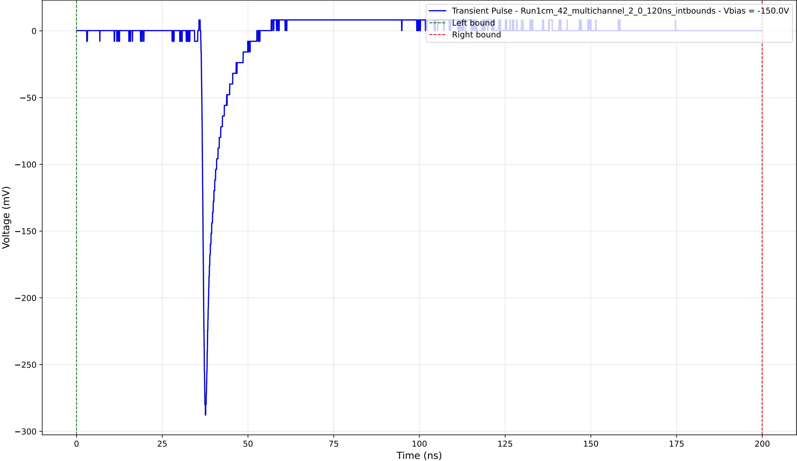
Transient Pulse - Sample: 1cm_42_multichannel - Position: 1725.0 \mu\text{m} - Charge: 13.59 pC - Rise Time: 0.91 ns
