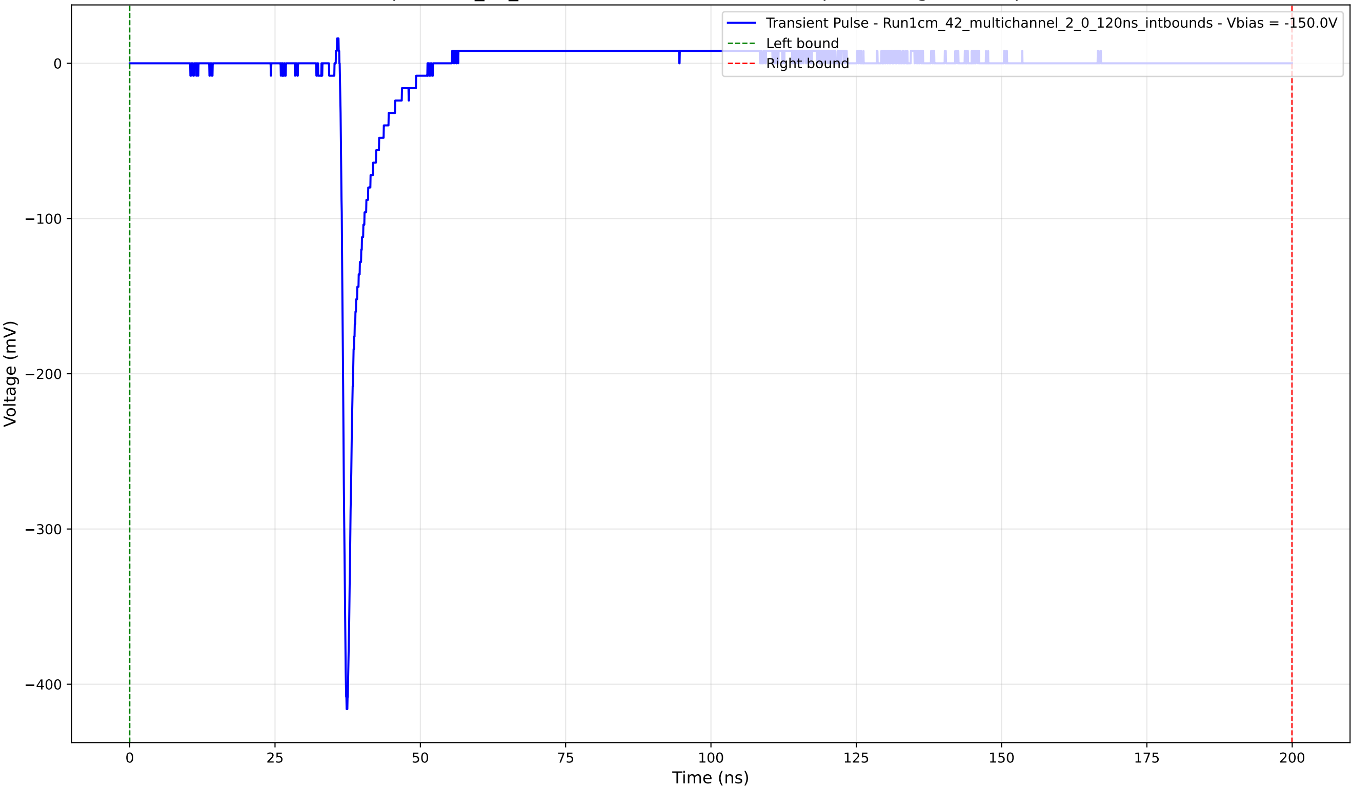
Transient Pulse - Sample: 1cm_42_multichannel - Position: 2735.0 \mu\text{m} - Charge: 14.54 pC - Rise Time: 0.81 ns
