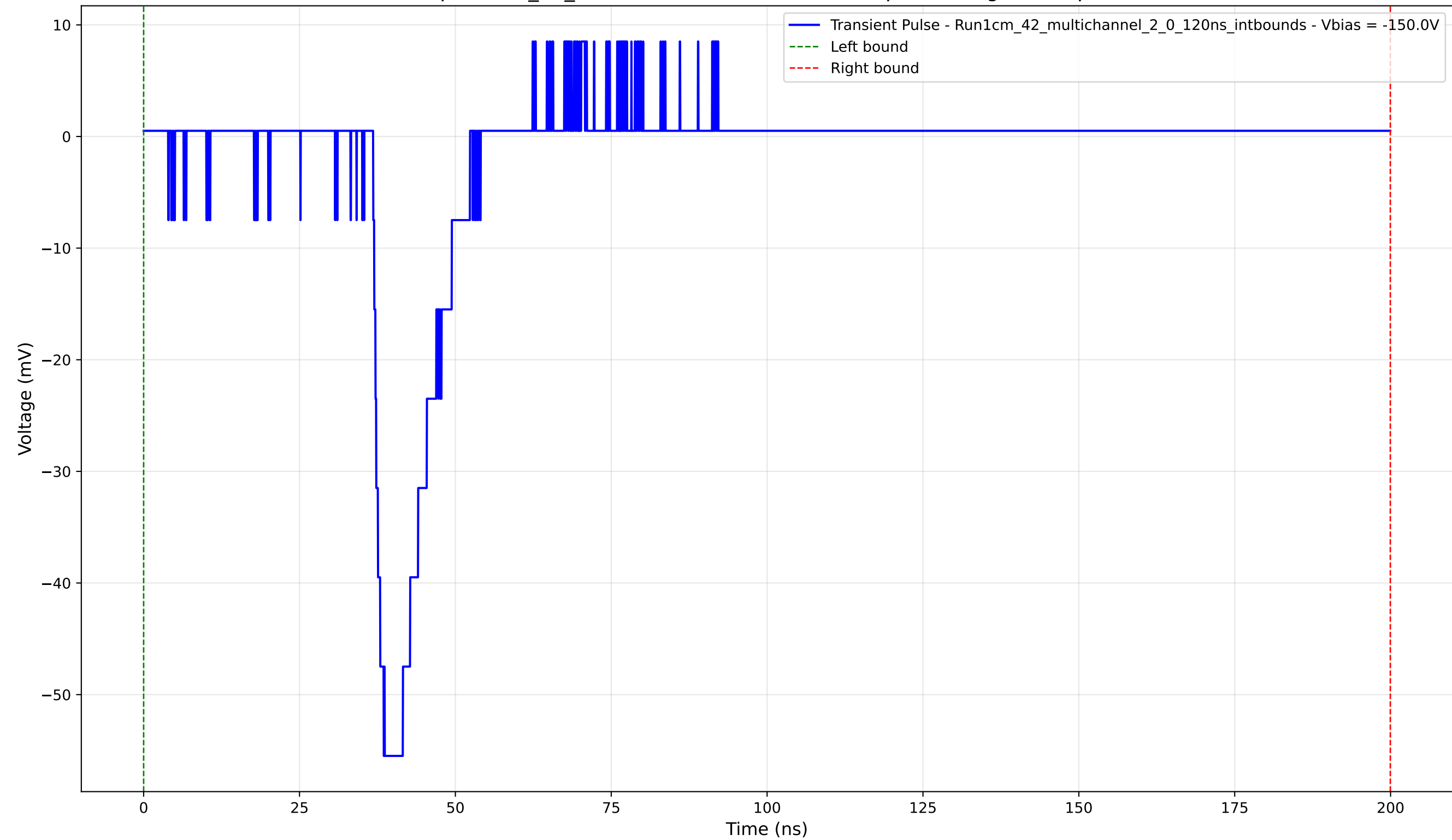
Transient Pulse - Sample: 1cm_42_multichannel - Position: 100.0 \mu\text{m} - Charge: 7.12 pC - Rise Time: 1.69 ns
