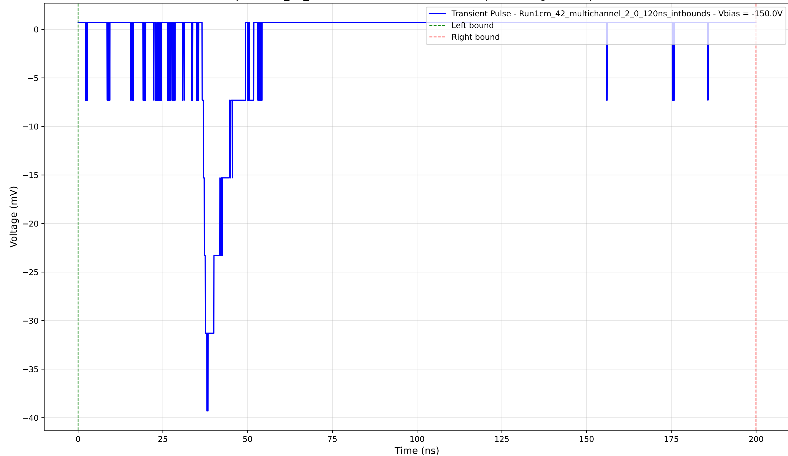
Transient Pulse - Sample: 1cm_42_multichannel - Position: 3420.0 \mu\text{m} - Charge: 2.85 pC - Rise Time: 1.42 ns
