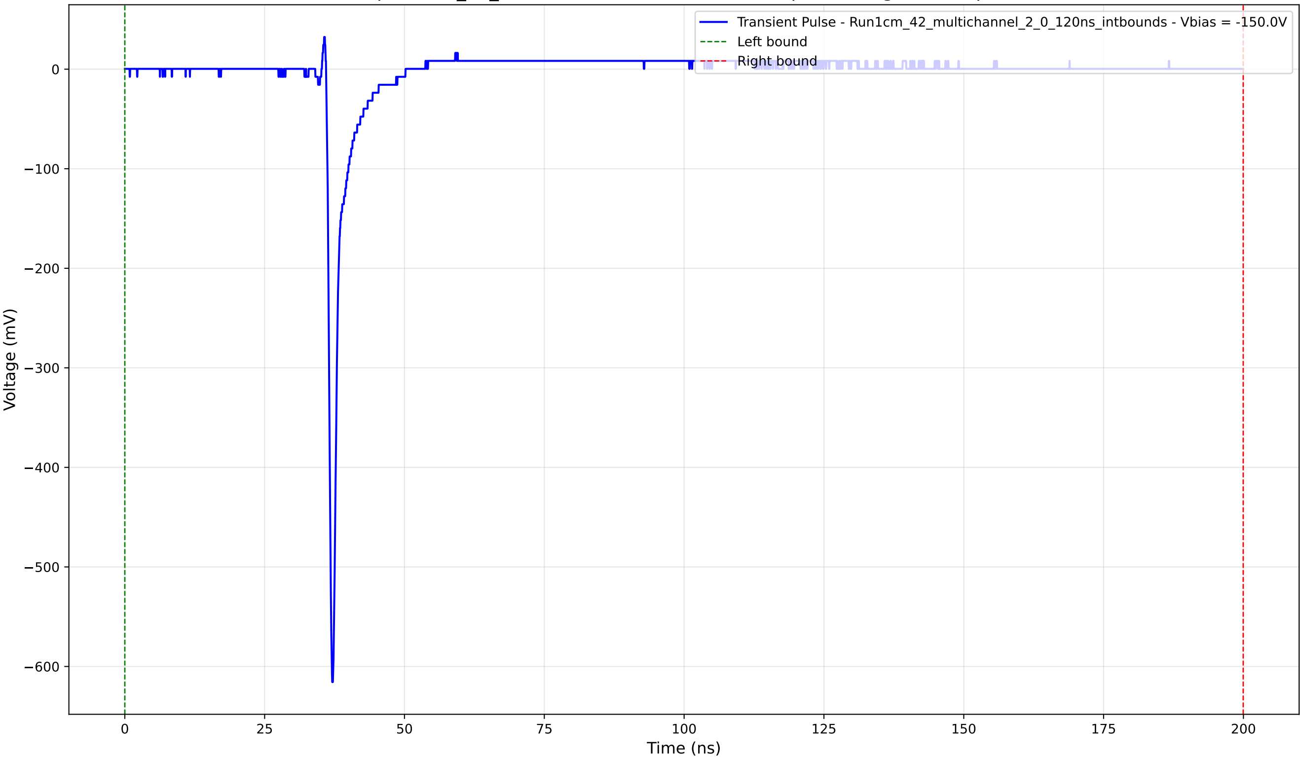
Transient Pulse - Sample: 1cm_42_multichannel - Position: 2450.0 \mu\text{m} - Charge: 14.67 pC - Rise Time: 0.73 ns
