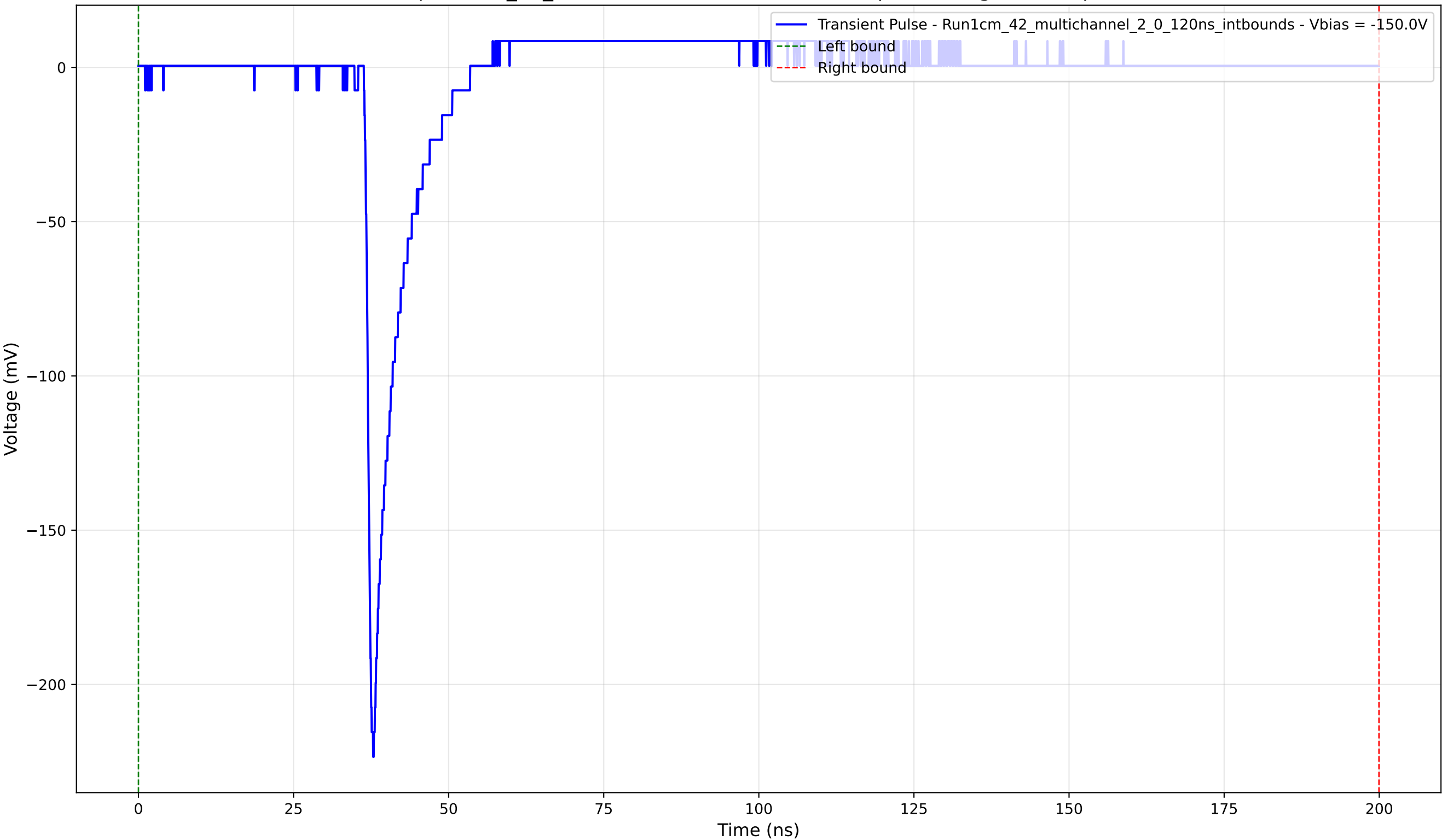
Transient Pulse - Sample: 1cm_42_multichannel - Position: 1540.0 \mu\text{m} - Charge: 10.24 pC - Rise Time: 1.01 ns
