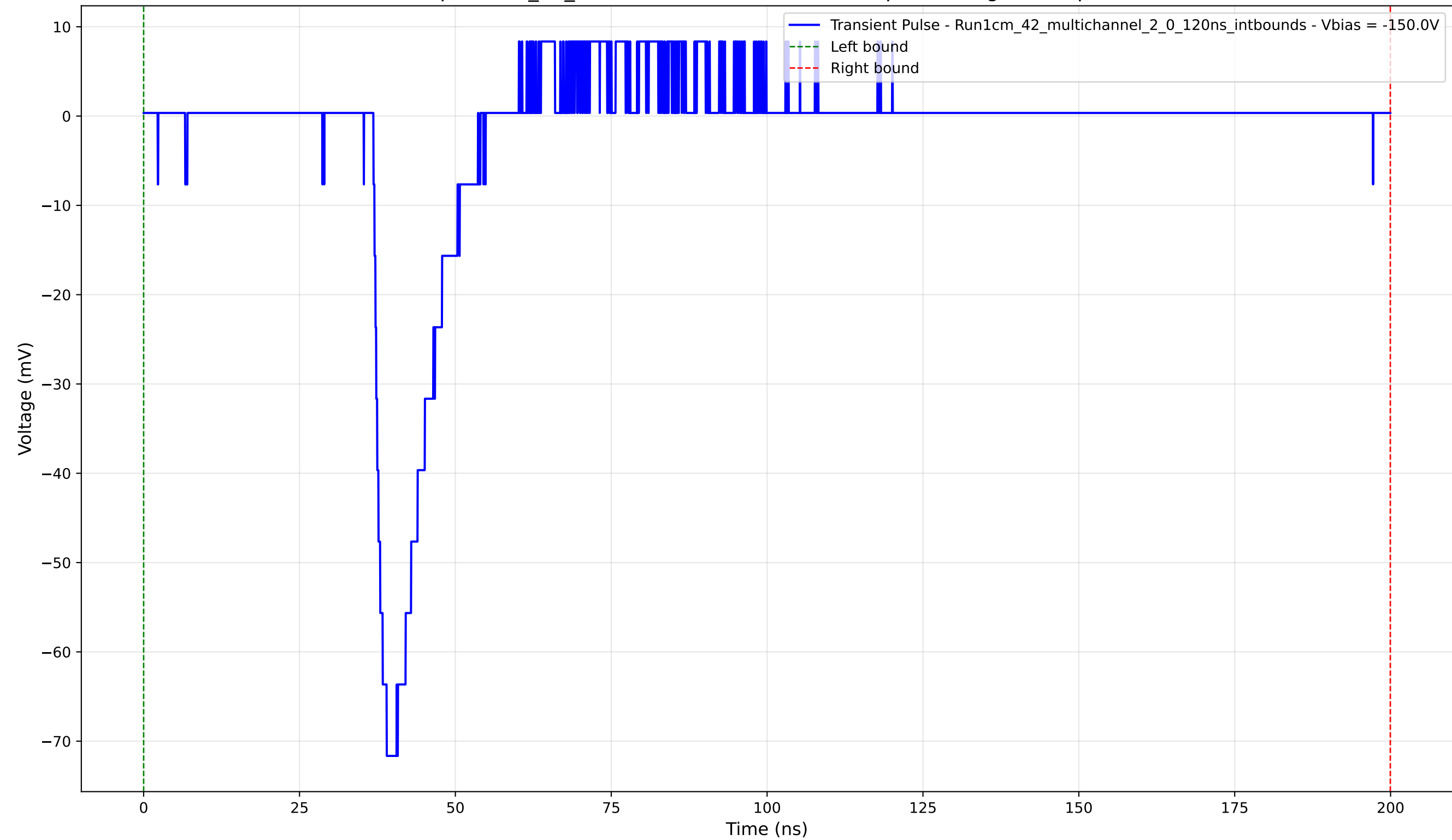
Transient Pulse - Sample: 1cm_42_multichannel - Position: 185.0 \mu\text{m} - Charge: 7.28 pC - Rise Time: 2.12 ns
