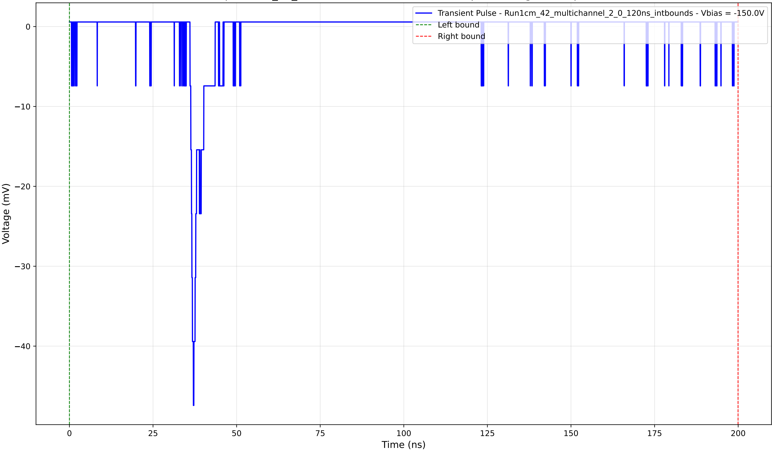
Transient Pulse - Sample: 1cm_42_multichannel - Position: 2390.0 \mu\text{m} - Charge: 1.10 pC - Rise Time: 1.02 ns
