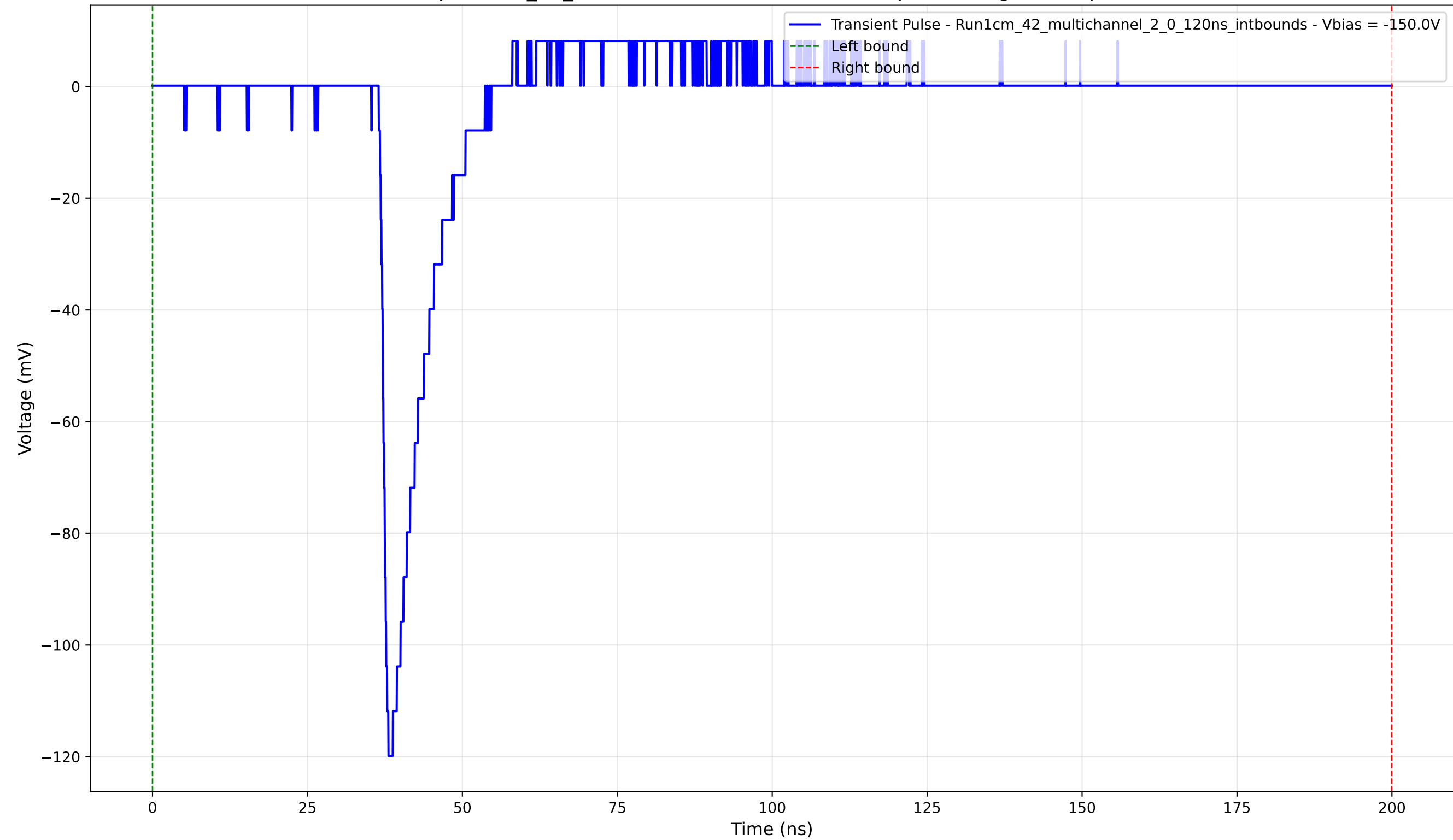
Transient Pulse - Sample: 1cm_42_multichannel - Position: 3565.0 \mu\text{m} - Charge: 9.92 pC - Rise Time: 1.18 ns
