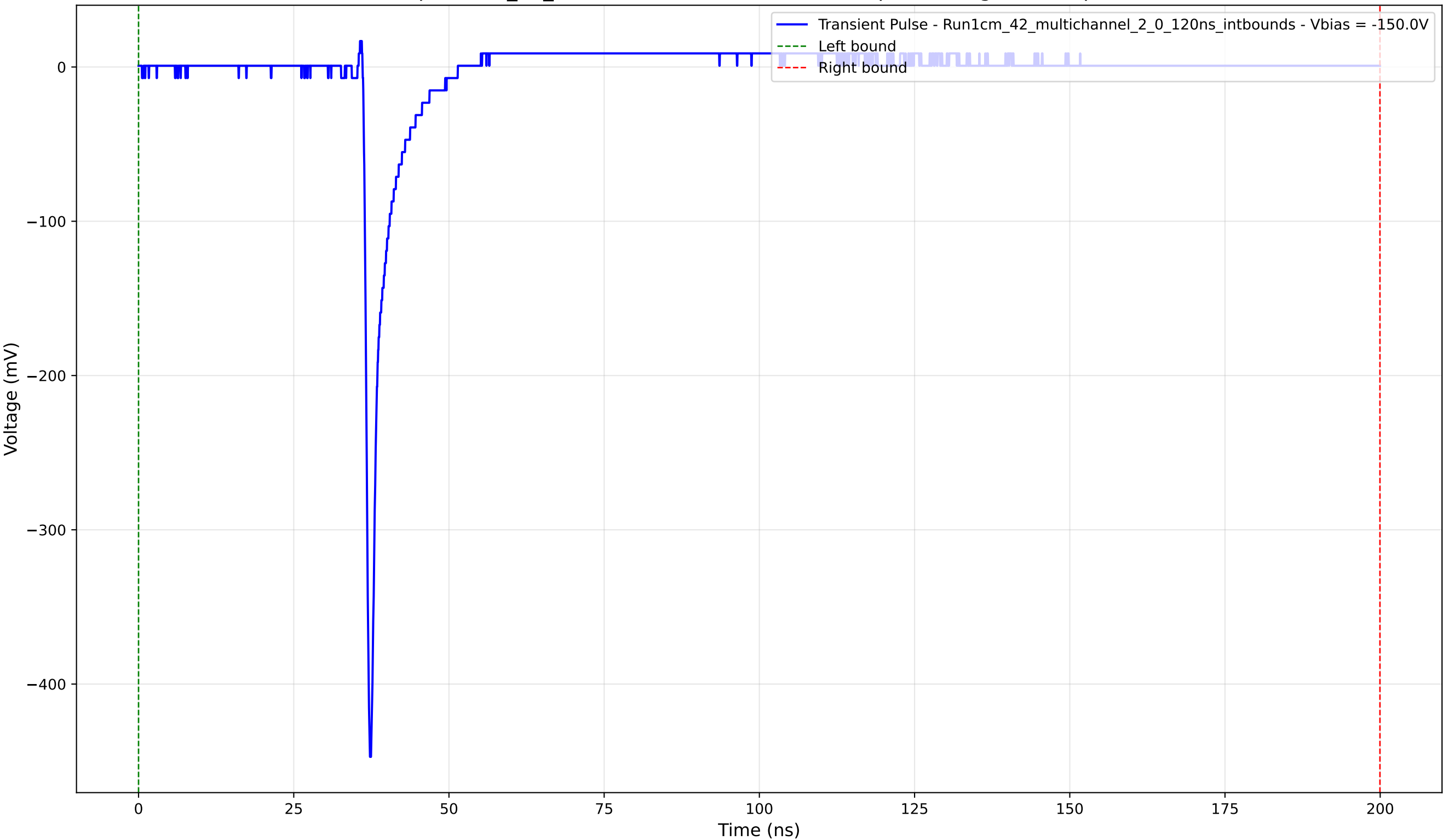
Transient Pulse - Sample: 1cm_42_multichannel - Position: 2035.0 \mu\text{m} - Charge: 12.47 pC - Rise Time: 0.76 ns
