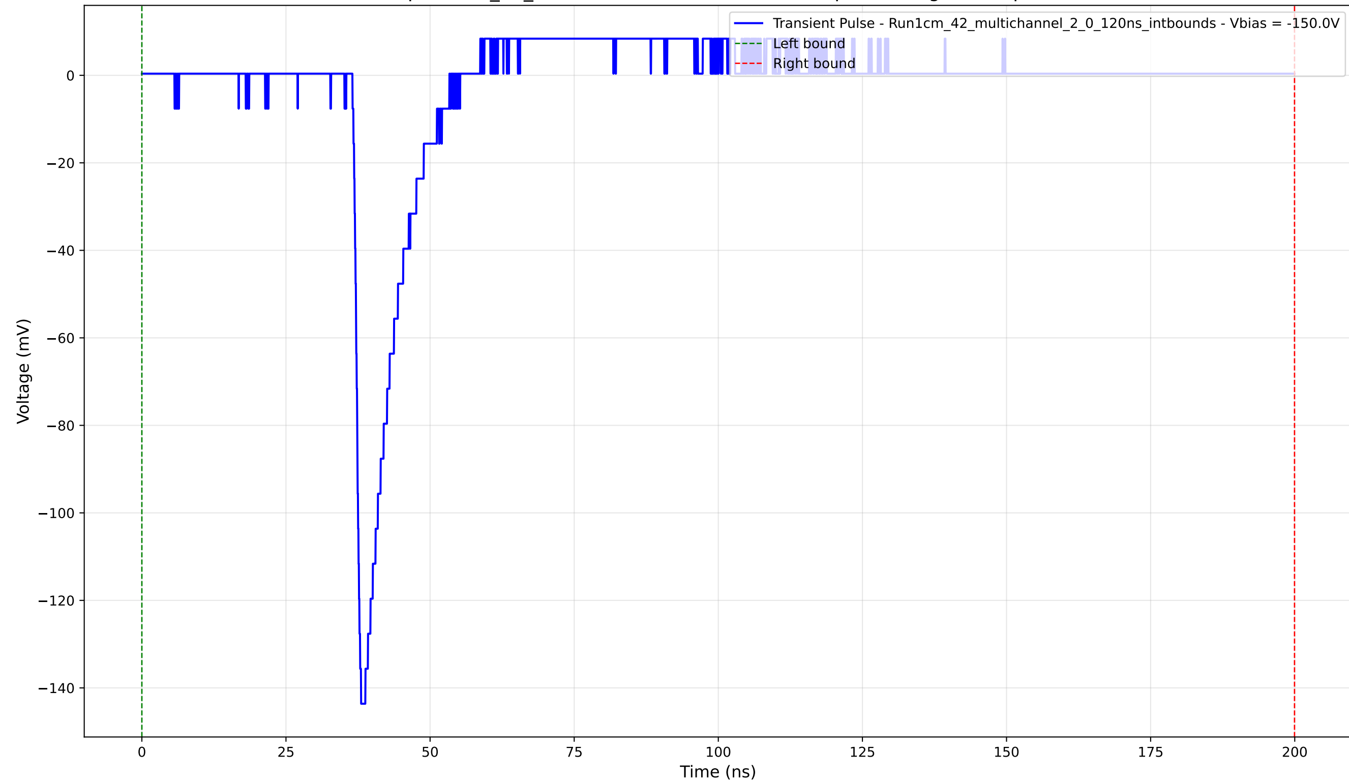
Transient Pulse - Sample: 1cm_42_multichannel - Position: 1175.0 \mu\text{m} - Charge: 9.87 pC - Rise Time: 1.17 ns
