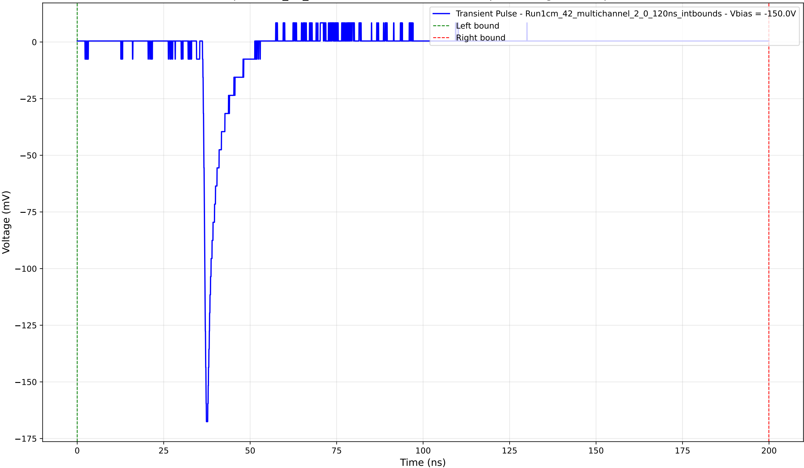
Transient Pulse - Sample: 1cm_42_multichannel - Position: 1810.0 \mu\text{m} - Charge: 10.50 pC - Rise Time: 0.83 ns
