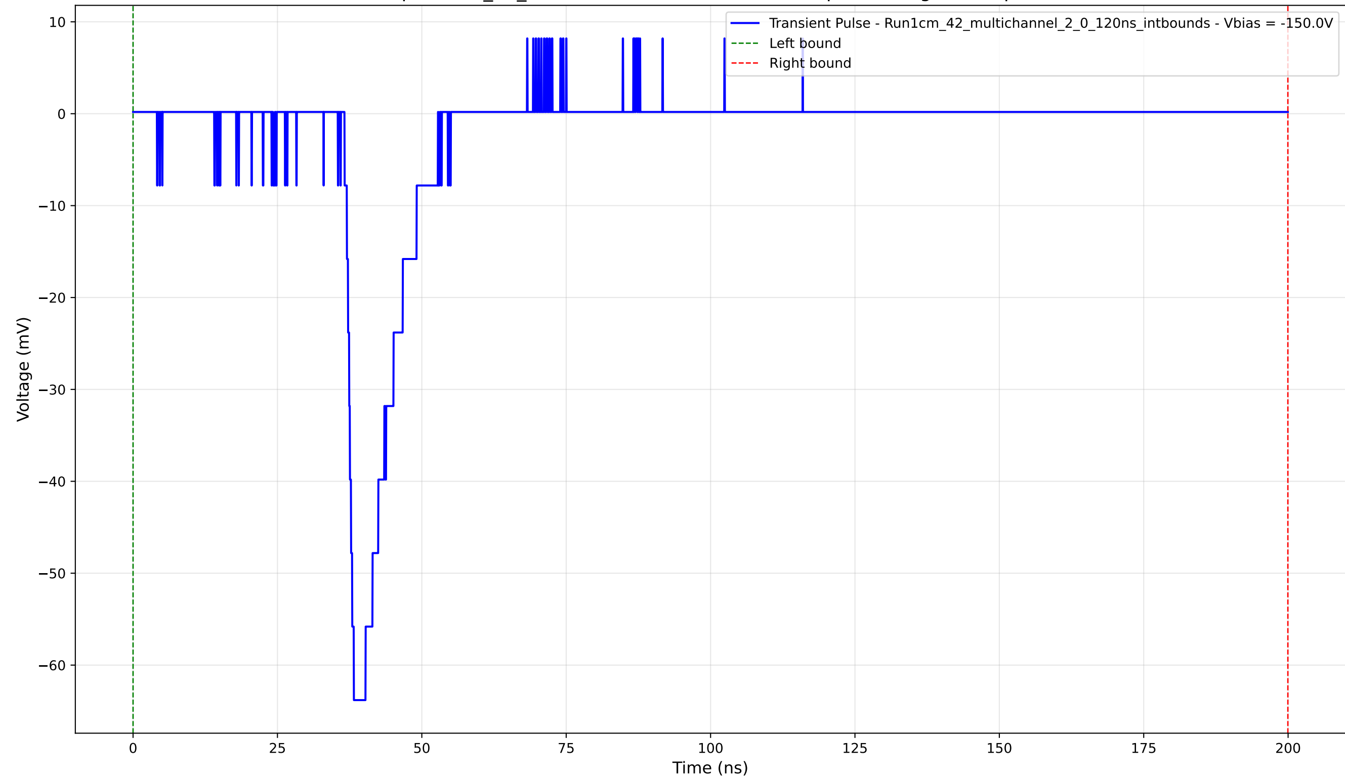
Transient Pulse - Sample: 1cm_42_multichannel - Position: 3830.0 \mu\text{m} - Charge: 9.17 pC - Rise Time: 1.61 ns
