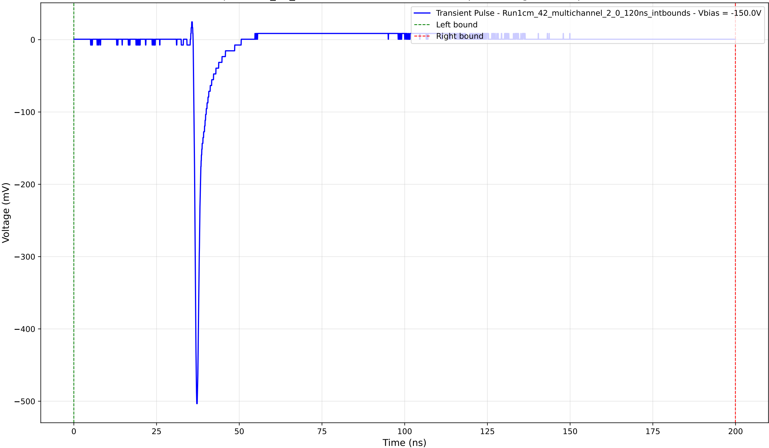
Transient Pulse - Sample: 1cm_42_multichannel - Position: 2565.0 \mu\text{m} - Charge: 13.16 pC - Rise Time: 0.77 ns
