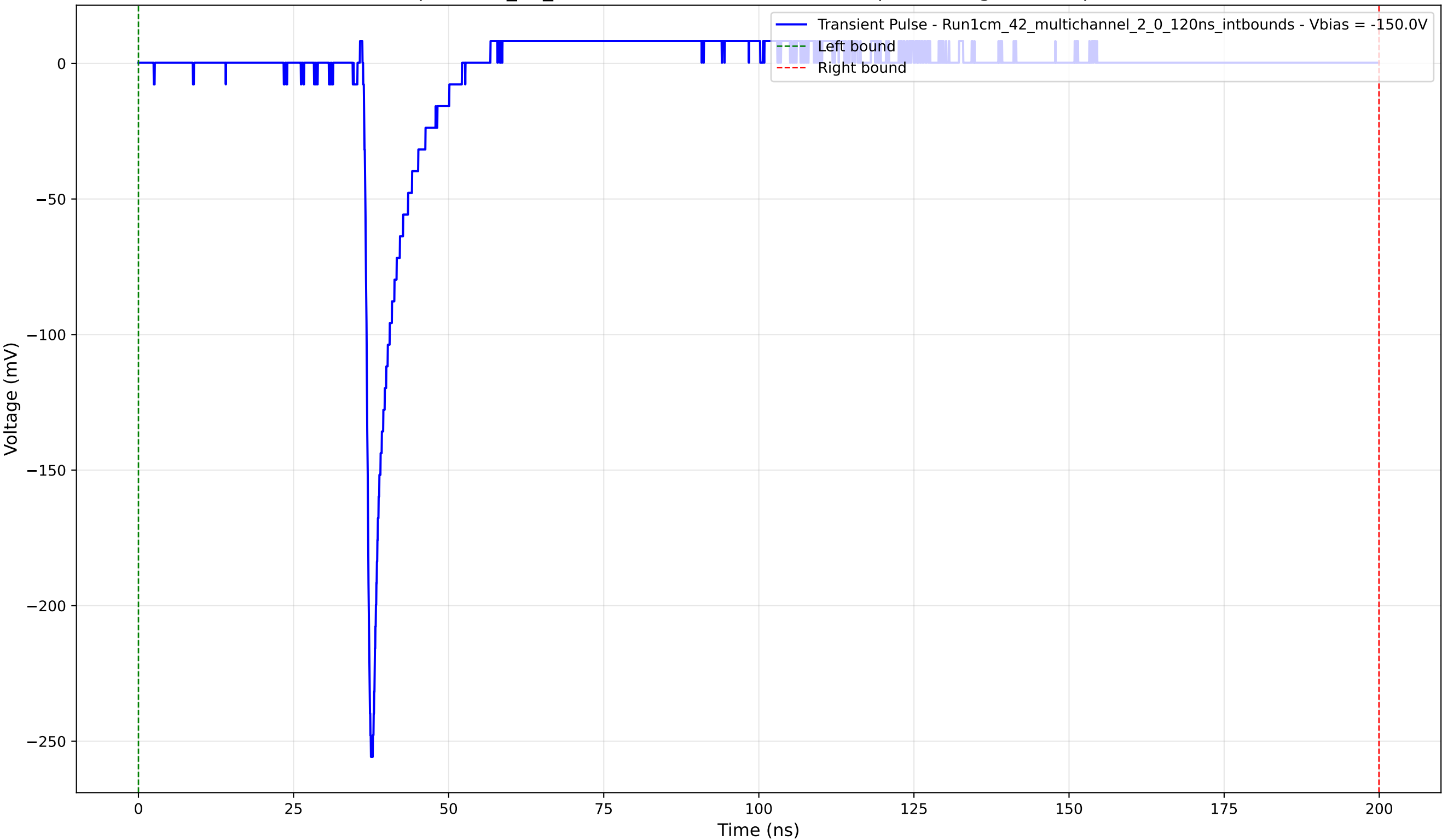
Transient Pulse - Sample: 1cm_42_multichannel - Position: 3010.0 \mu\text{m} - Charge: 10.87 pC - Rise Time: 0.86 ns
