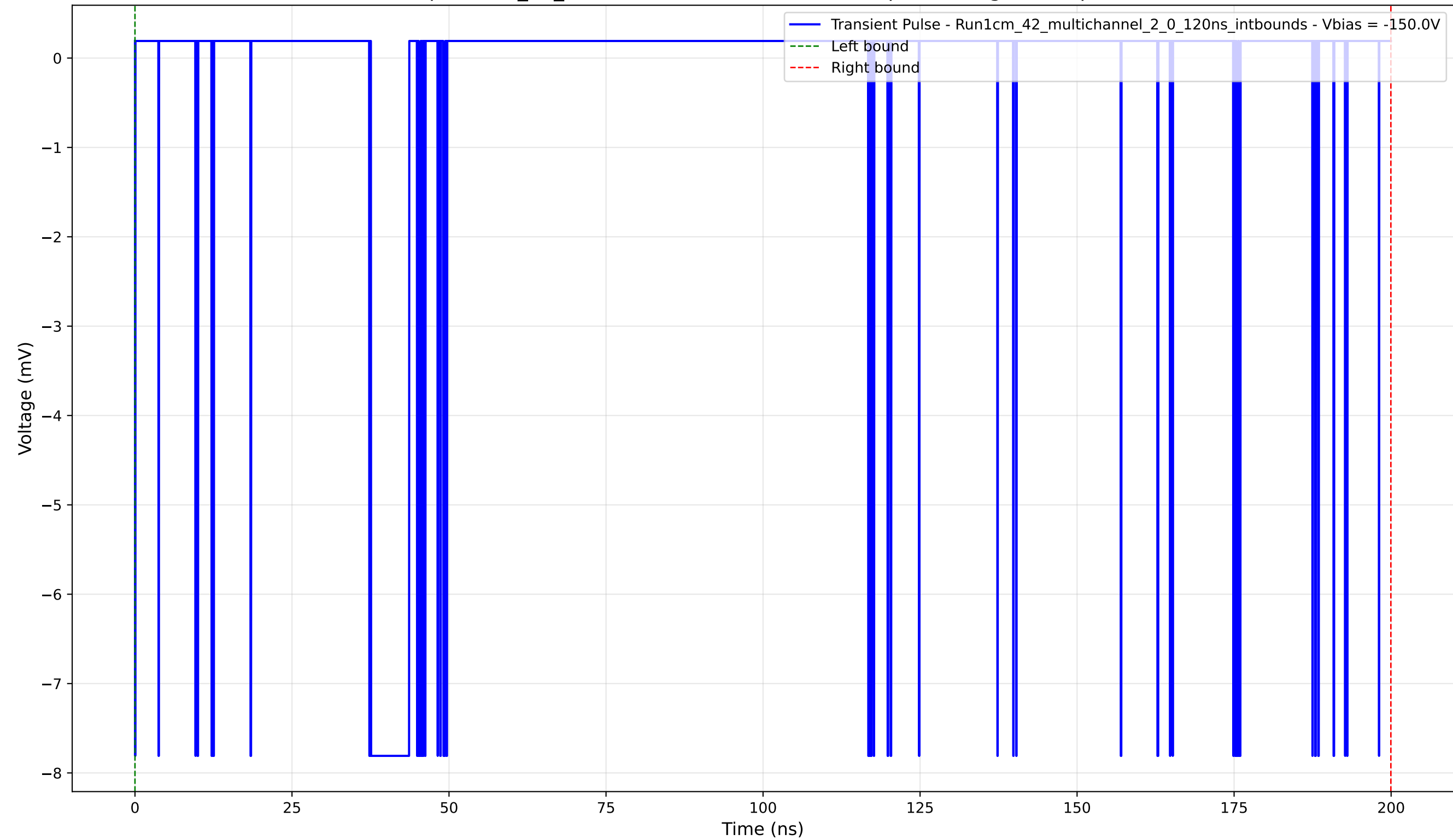
Transient Pulse - Sample: 1cm_42_multichannel - Position: 4370.0 \mu\text{m} - Charge: 0.99 pC - Rise Time: 0.04 ns
