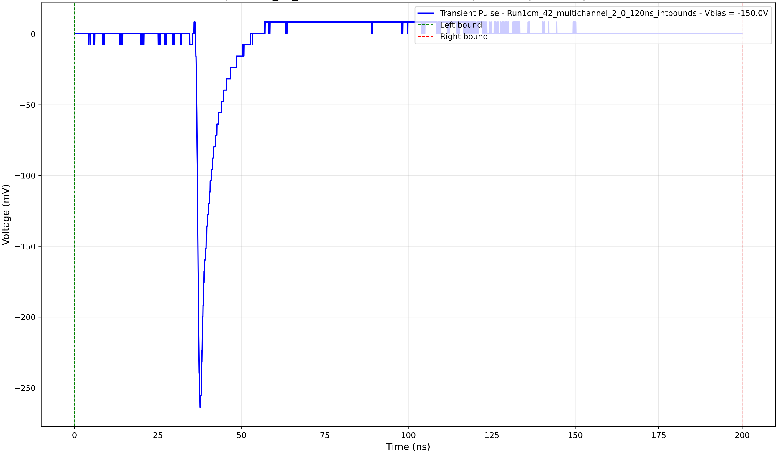
Transient Pulse - Sample: 1cm_42_multichannel - Position: 1665.0 \mu\text{m} - Charge: 11.60 pC - Rise Time: 0.91 ns
