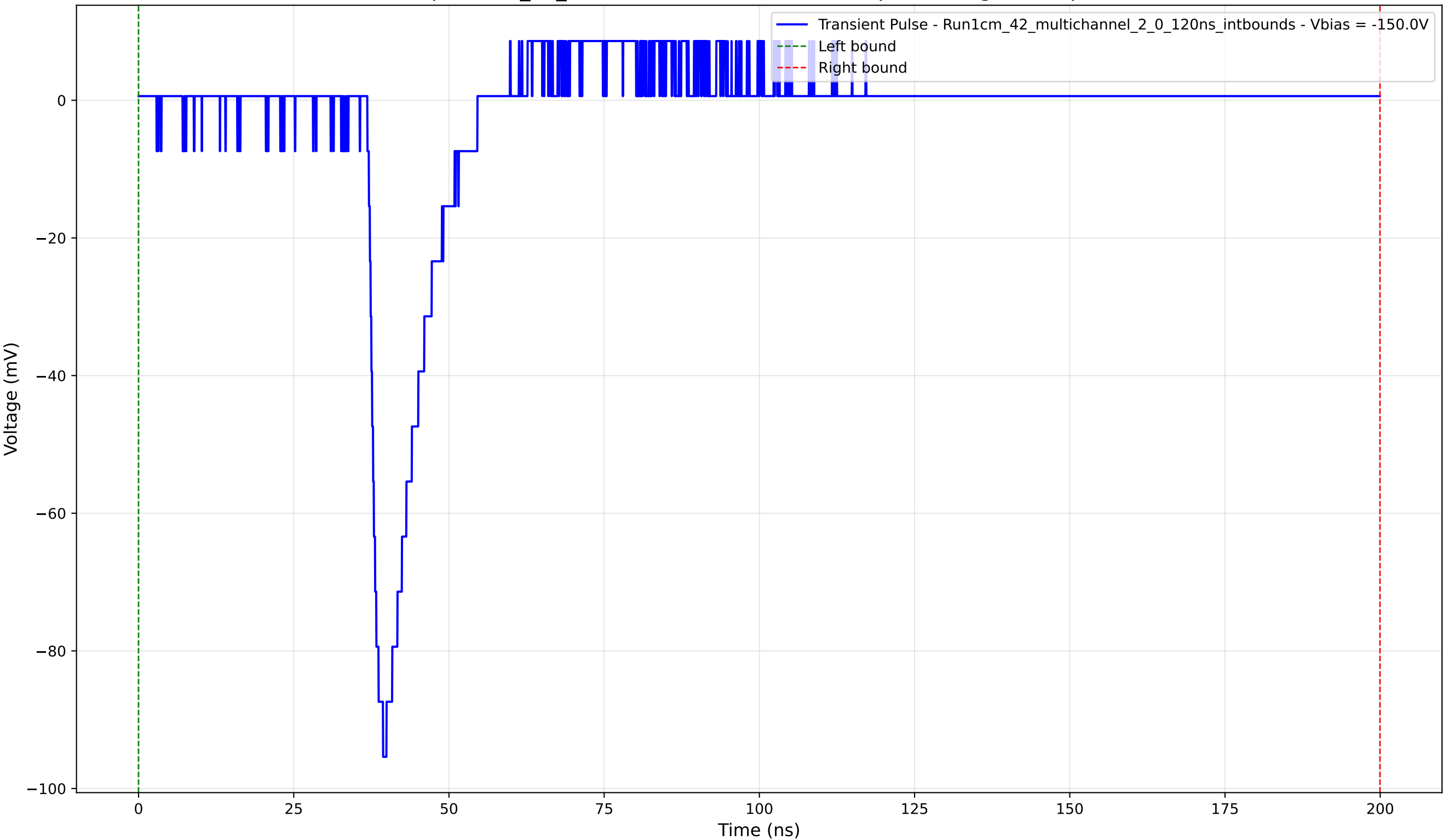
Transient Pulse - Sample: 1cm_42_multichannel - Position: 465.0 \mu\text{m} - Charge: 8.53 pC - Rise Time: 1.59 ns
