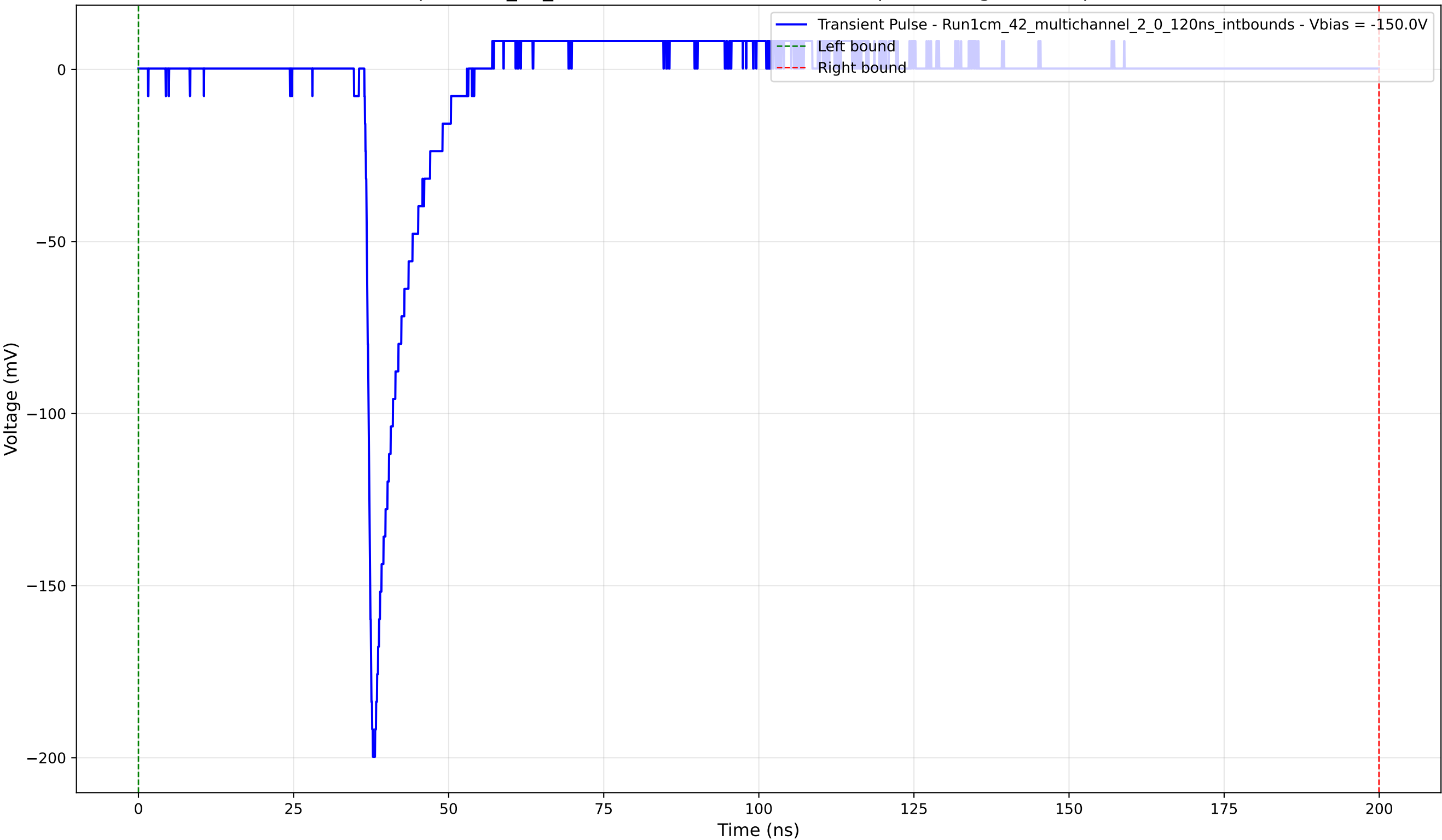
Transient Pulse - Sample: 1cm_42_multichannel - Position: 1460.0 \mu\text{m} - Charge: 11.13 pC - Rise Time: 0.98 ns
