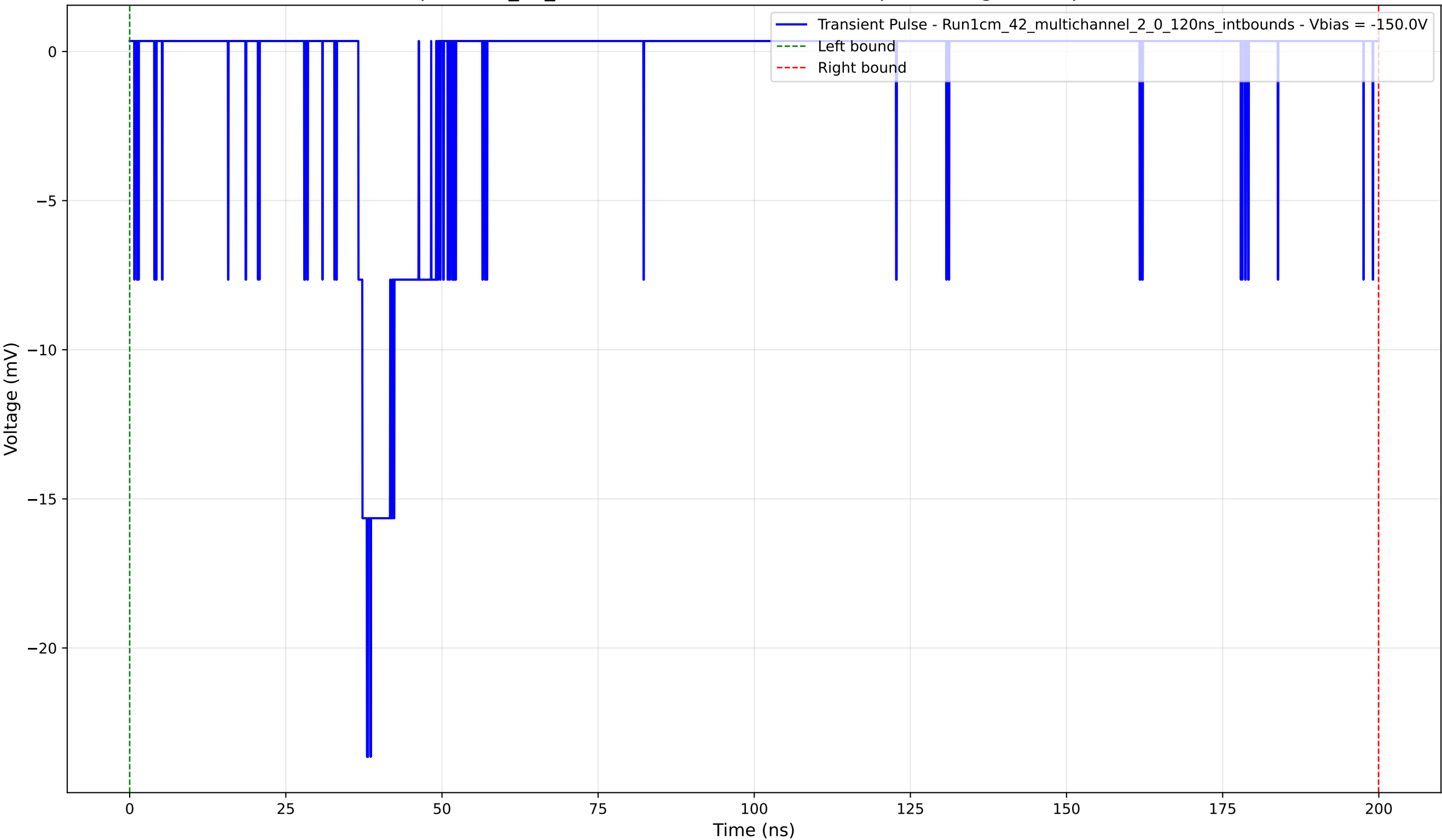
Transient Pulse - Sample: 1cm_42_multichannel - Position: 1330.0 \mu\text{m} - Charge: 1.98 pC - Rise Time: 1.39 ns
