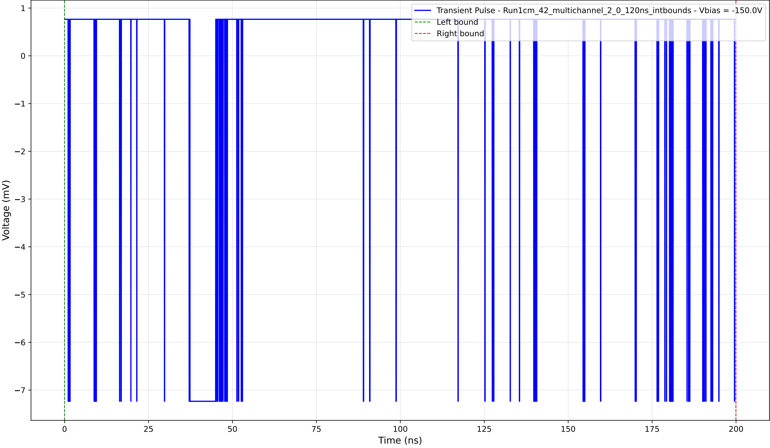
Transient Pulse - Sample: 1cm_42_multichannel - Position: 835.0 \mu\text{m} - Charge: -0.76 pC - Rise Time: 0.00 ns (N/A)
