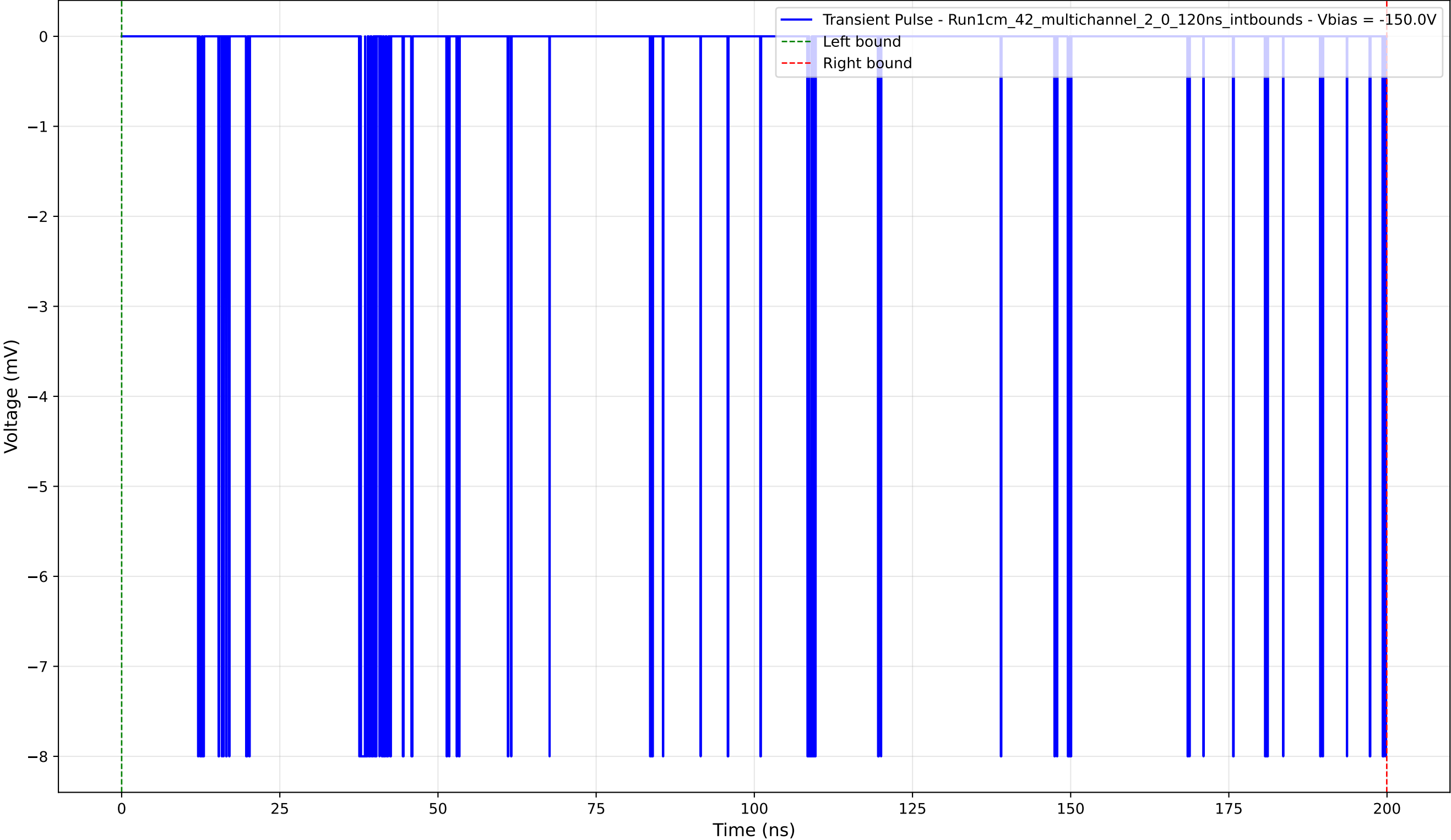
Transient Pulse - Sample: 1cm_42_multichannel - Position: 4900.0 \mu\text{m} - Charge: 1.42 pC - Rise Time: 0.04 ns
