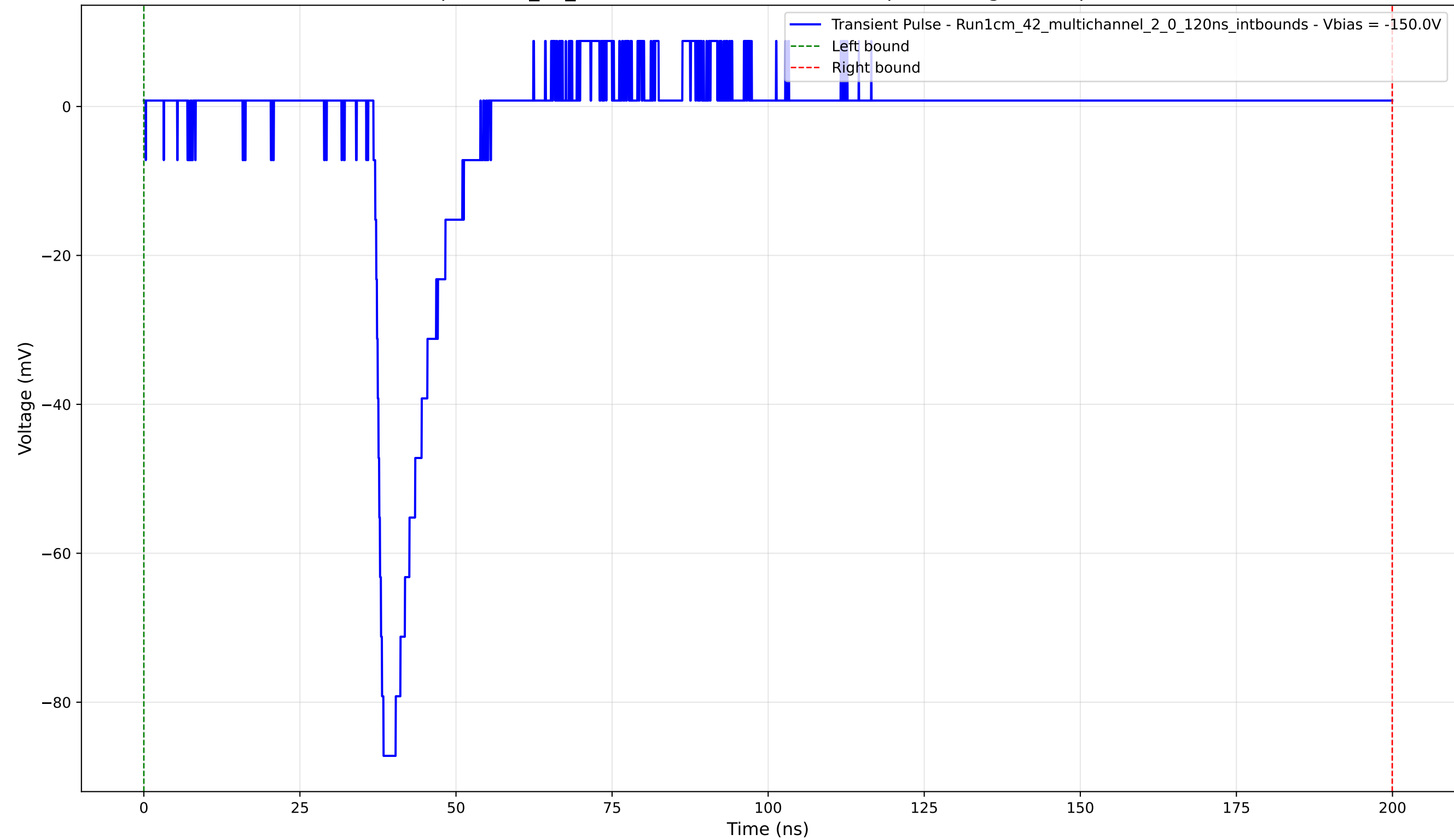
Transient Pulse - Sample: 1cm_42_multichannel - Position: 780.0 \mu\text{m} - Charge: 8.54 pC - Rise Time: 1.11 ns
