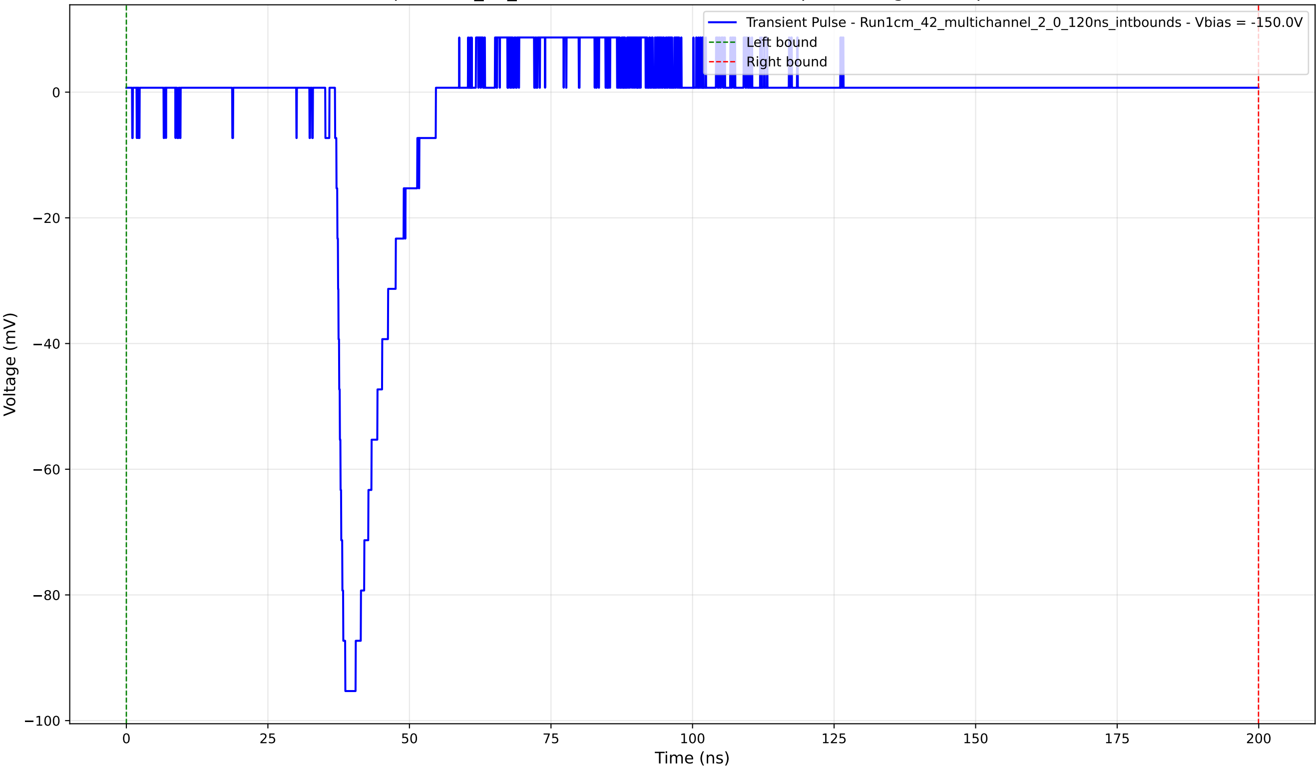
Transient Pulse - Sample: 1cm_42_multichannel - Position: 595.0 \mu\text{m} - Charge: 8.15 pC - Rise Time: 1.23 ns
