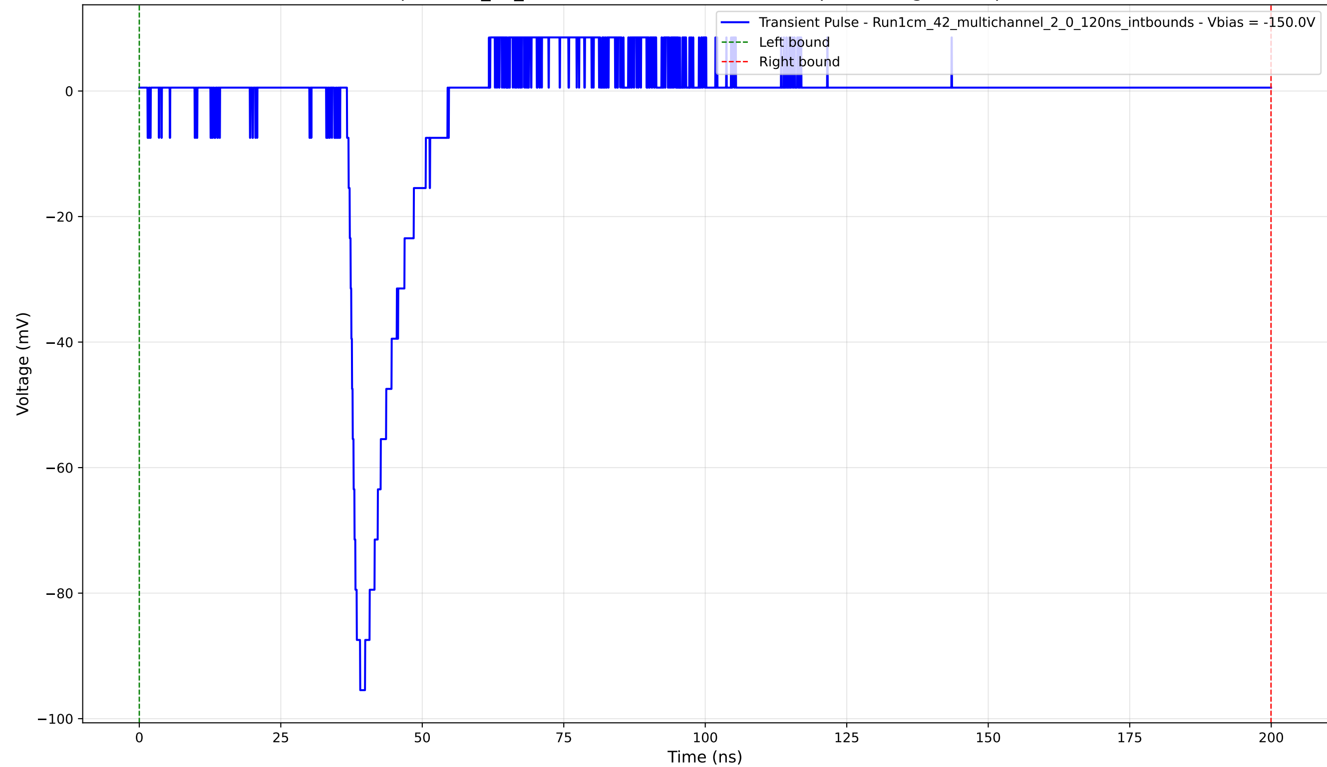
Transient Pulse - Sample: 1cm_42_multichannel - Position: 3975.0 \mu\text{m} - Charge: 8.10 pC - Rise Time: 1.47 ns
