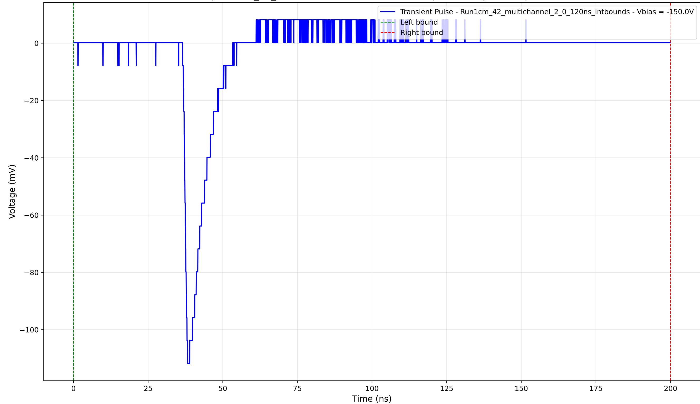
Transient Pulse - Sample: 1cm_42_multichannel - Position: 3680.0 \mu\text{m} - Charge: 9.64 pC - Rise Time: 1.26 ns
