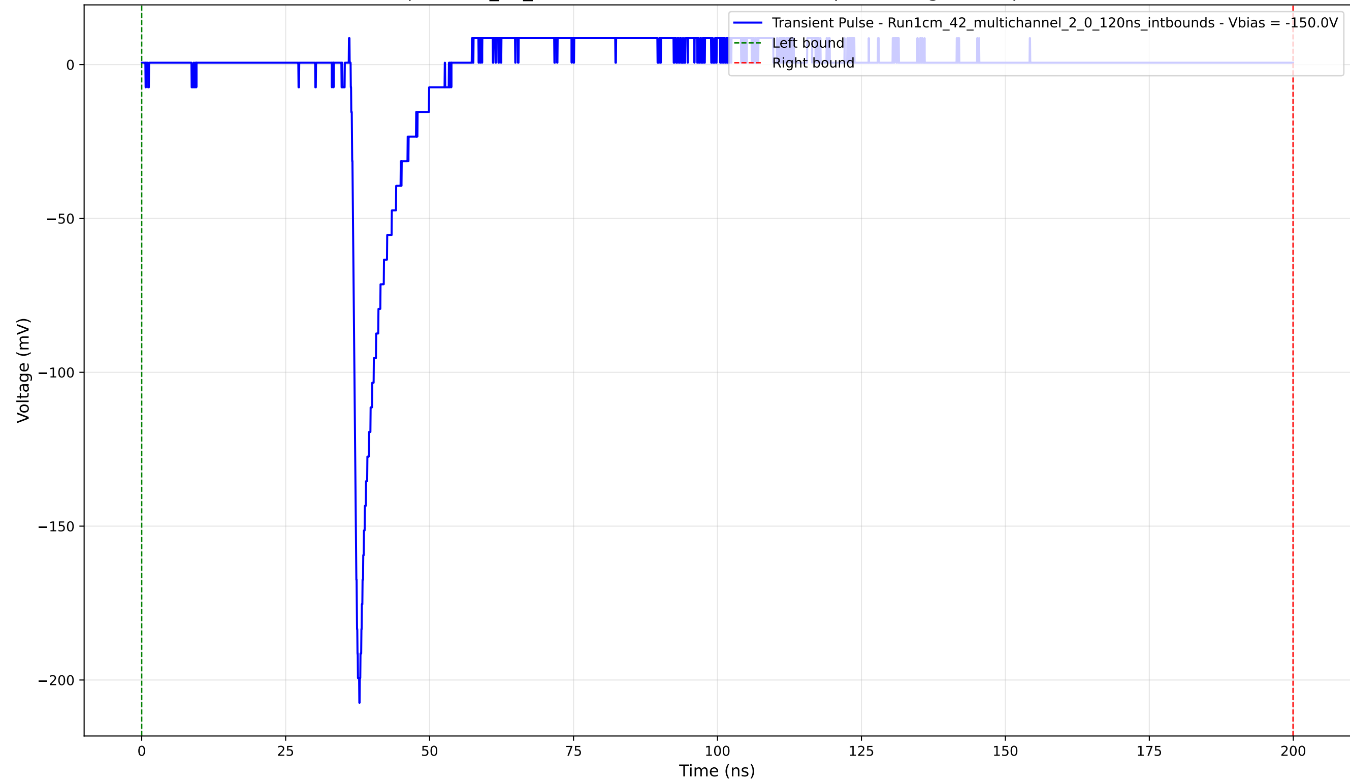
Transient Pulse - Sample: 1cm_42_multichannel - Position: 3140.0 \mu\text{m} - Charge: 8.73 pC - Rise Time: 0.97 ns
