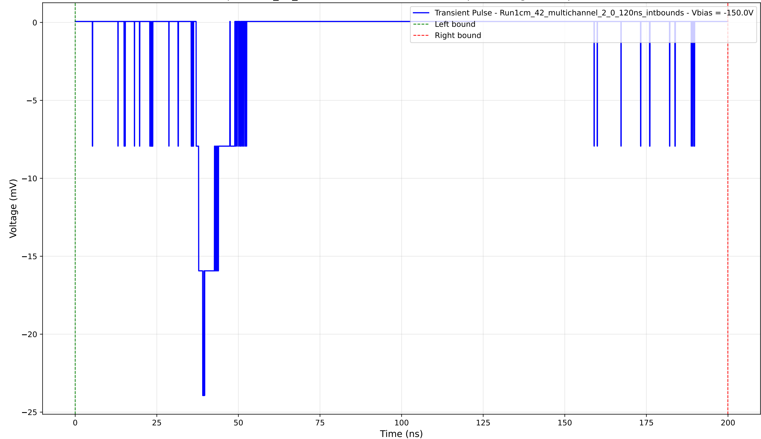
Transient Pulse - Sample: 1cm_42_multichannel - Position: 3920.0 \mu\text{m} - Charge: 3.10 pC - Rise Time: 2.03 ns
