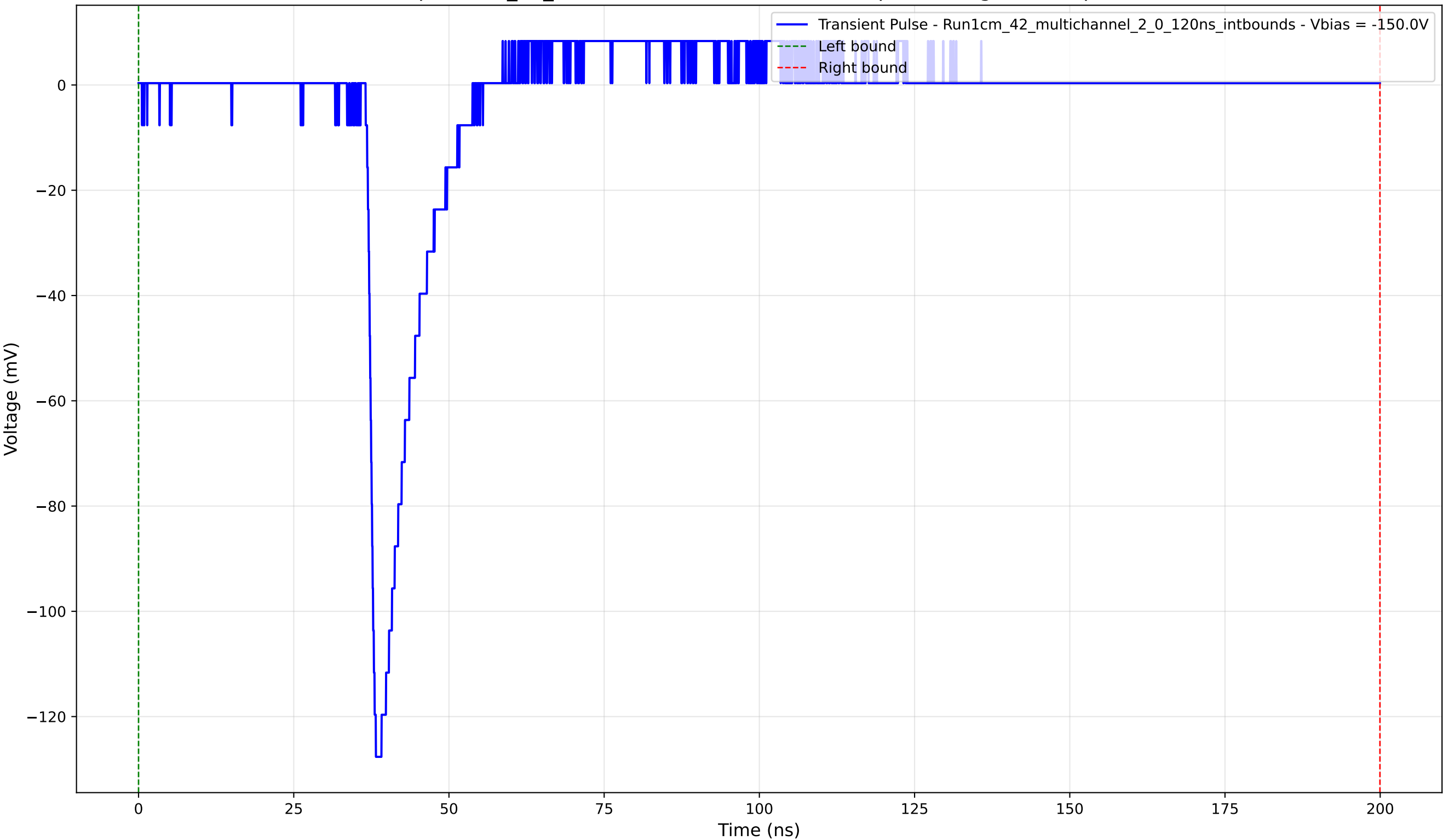
Transient Pulse - Sample: 1cm_42_multichannel - Position: 1045.0 \mu\text{m} - Charge: 10.11 pC - Rise Time: 1.21 ns
