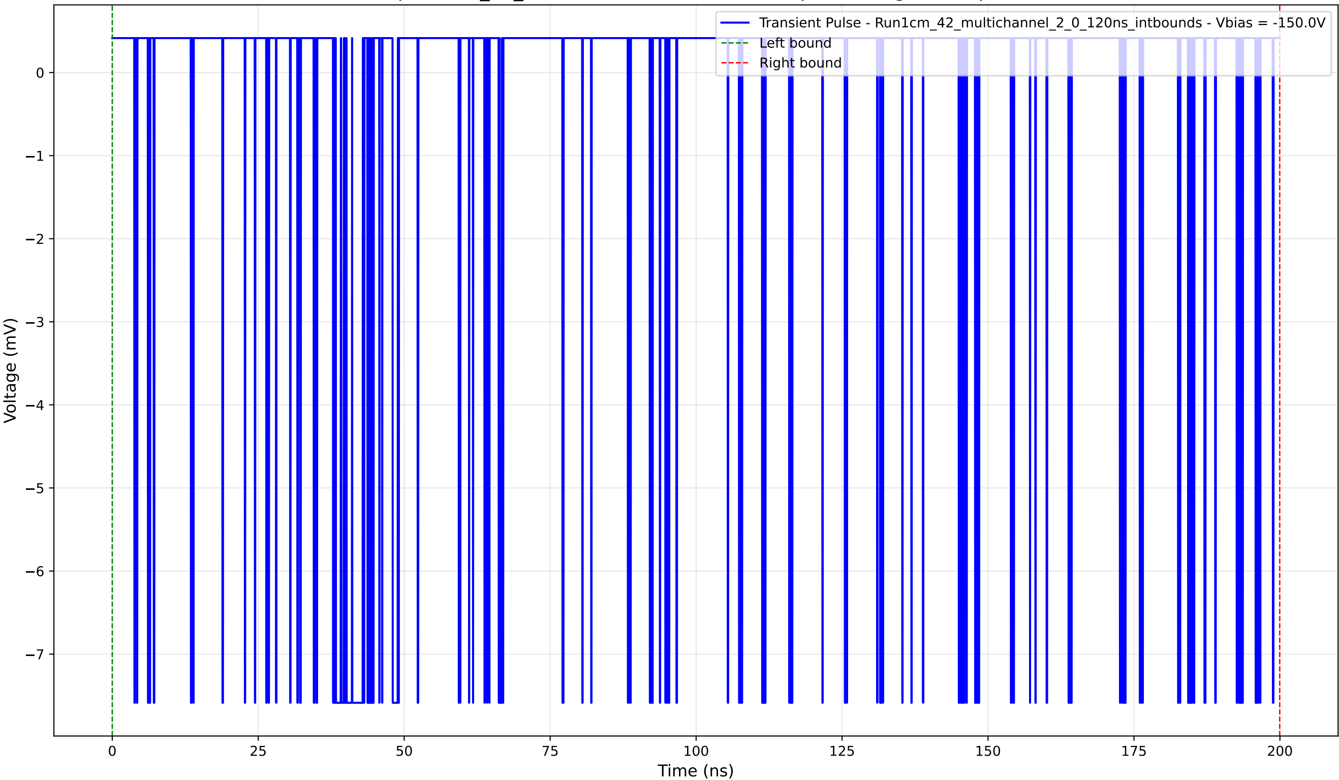
Transient Pulse - Sample: 1cm_42_multichannel - Position: 20.0 \mu\text{m} - Charge: 1.11 pC - Rise Time: 0.04 ns
