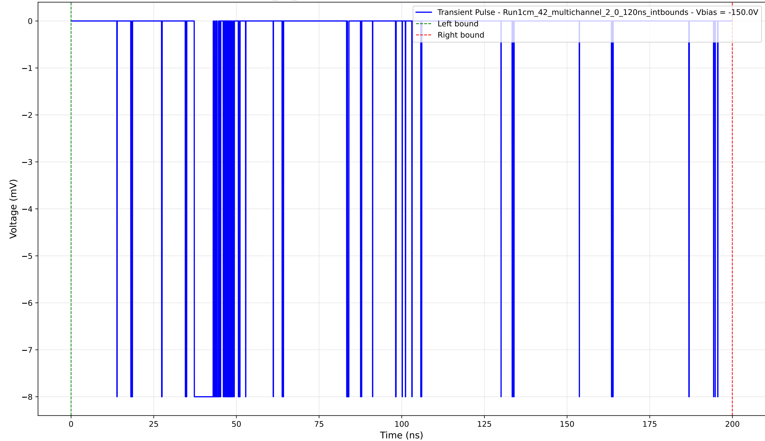
Transient Pulse - Sample: 1cm_42_multichannel - Position: 3885.0 \mu\text{m} - Charge: 2.00 pC - Rise Time: 0.04 ns
