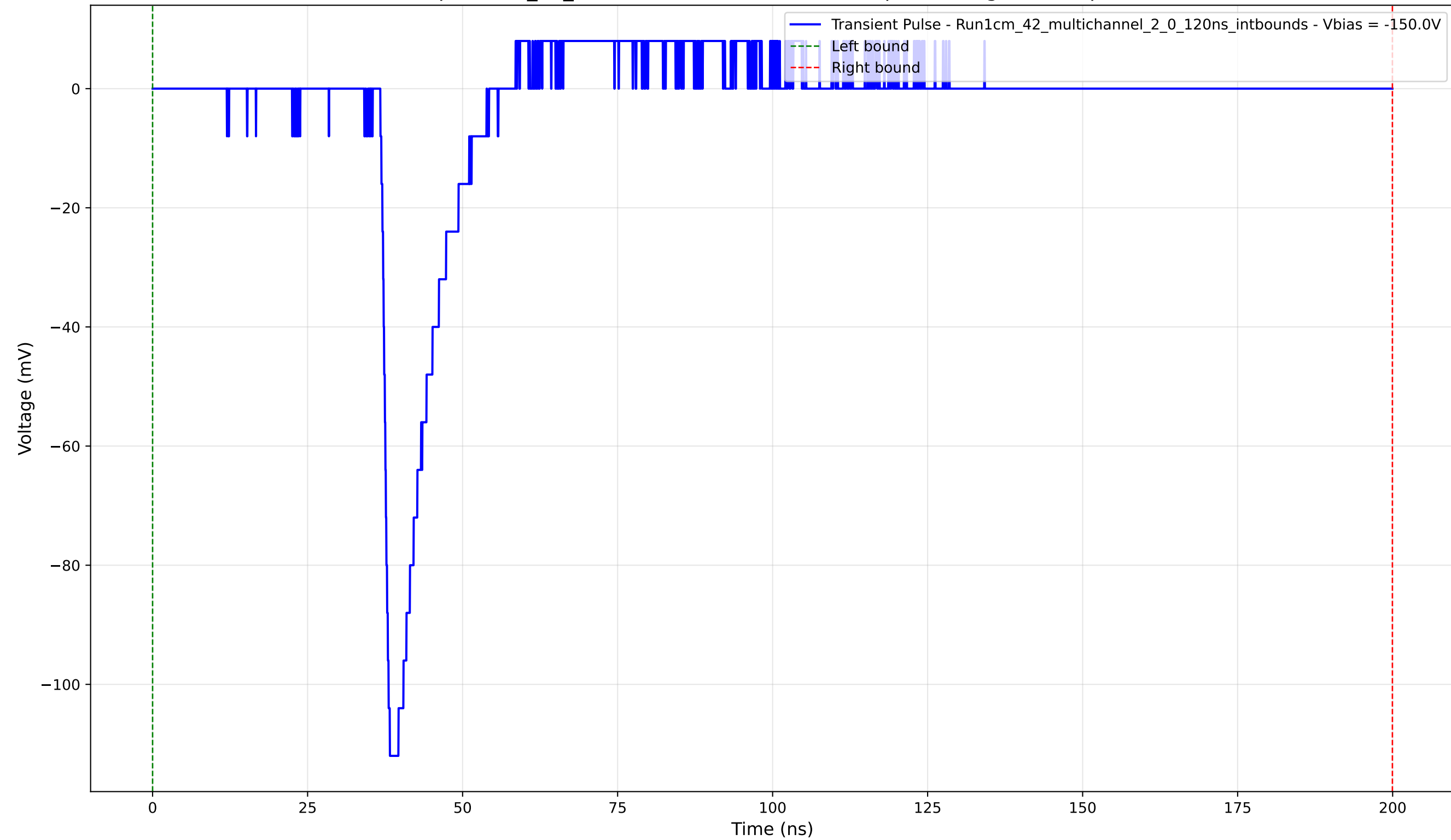
Transient Pulse - Sample: 1cm_42_multichannel - Position: 930.0 \mu\text{m} - Charge: 10.41 pC - Rise Time: 1.18 ns
