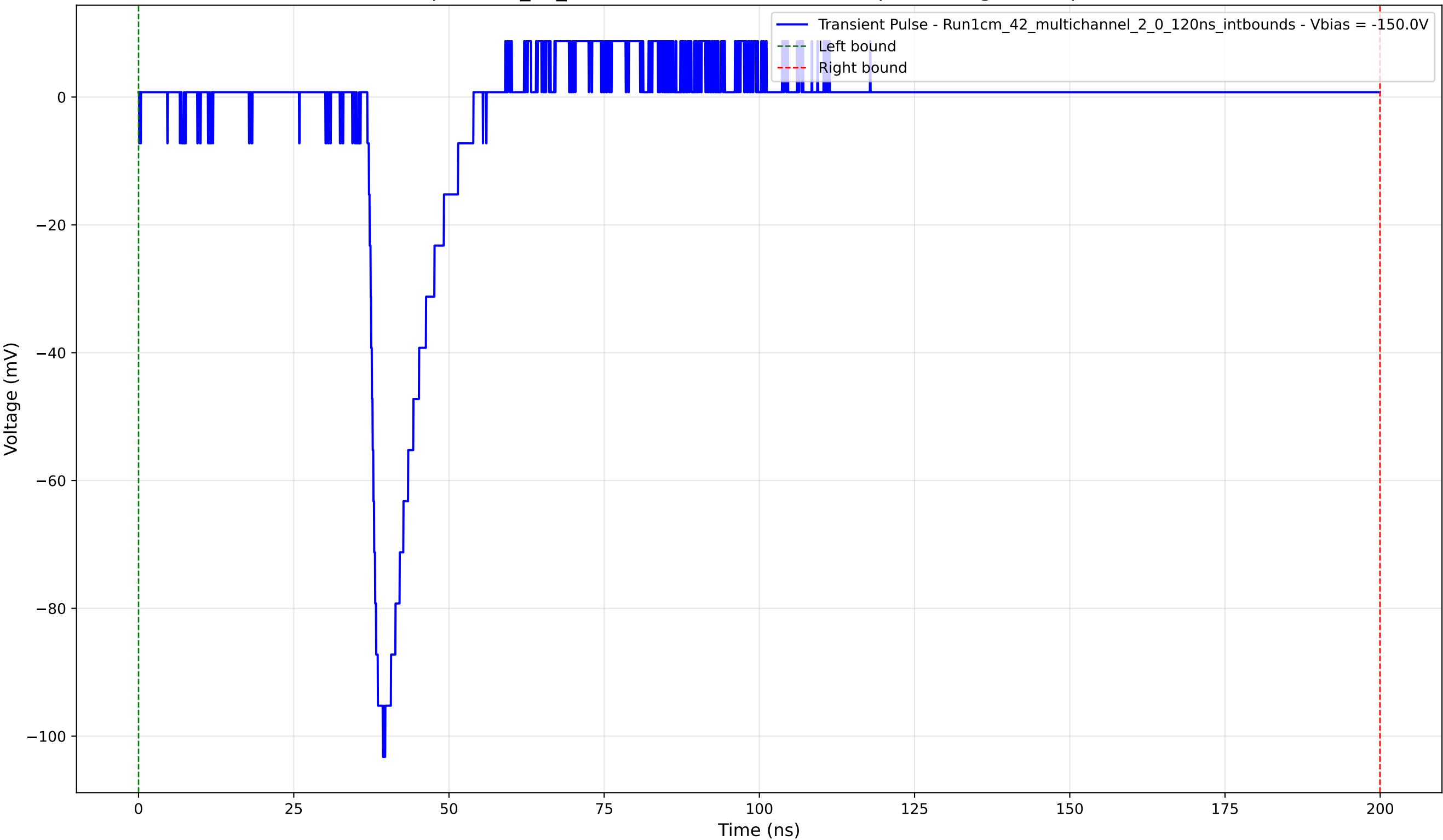
Transient Pulse - Sample: 1cm_42_multichannel - Position: 645.0 \mu\text{m} - Charge: 8.66 pC - Rise Time: 1.46 ns
