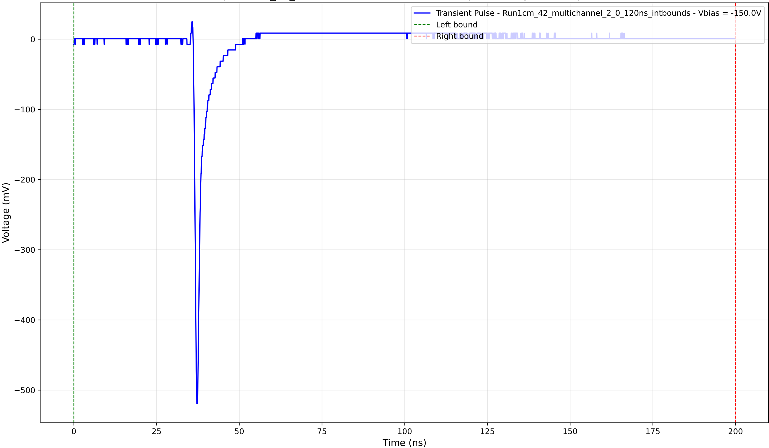
Transient Pulse - Sample: 1cm_42_multichannel - Position: 2140.0 \mu\text{m} - Charge: 13.54 pC - Rise Time: 0.73 ns
