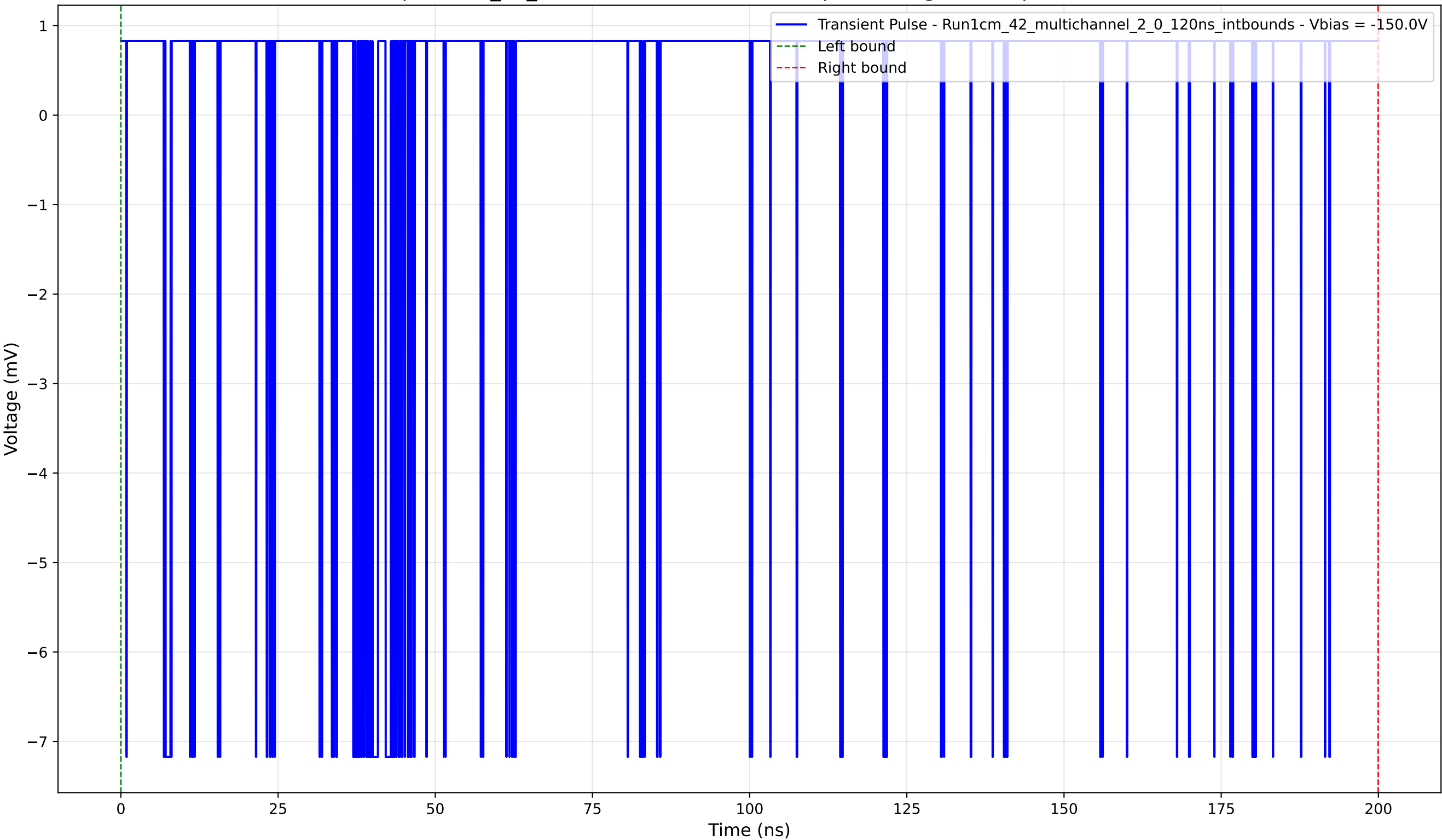
Transient Pulse - Sample: 1cm_42_multichannel - Position: 5.0 \mu\text{m} - Charge: -1.41 pC - Rise Time: 0.00 ns (N/A)
