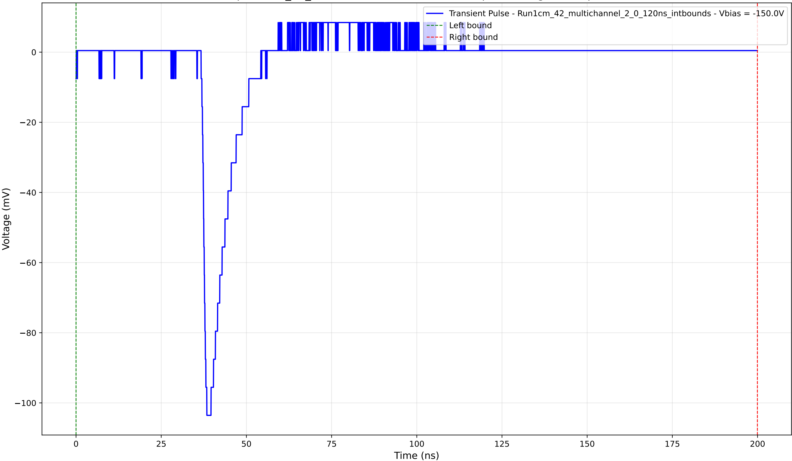
Transient Pulse - Sample: 1cm_42_multichannel - Position: 920.0 \mu\text{m} - Charge: 9.14 pC - Rise Time: 1.19 ns
