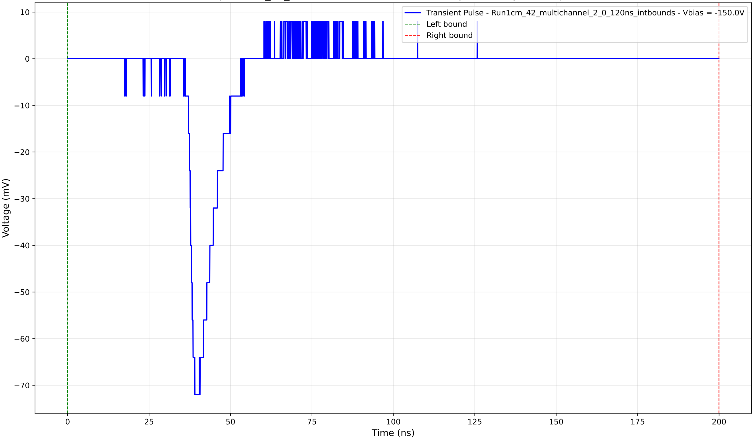
Transient Pulse - Sample: 1cm_42_multichannel - Position: 4620.0 \mu\text{m} - Charge: 9.61 pC - Rise Time: 2.88 ns
