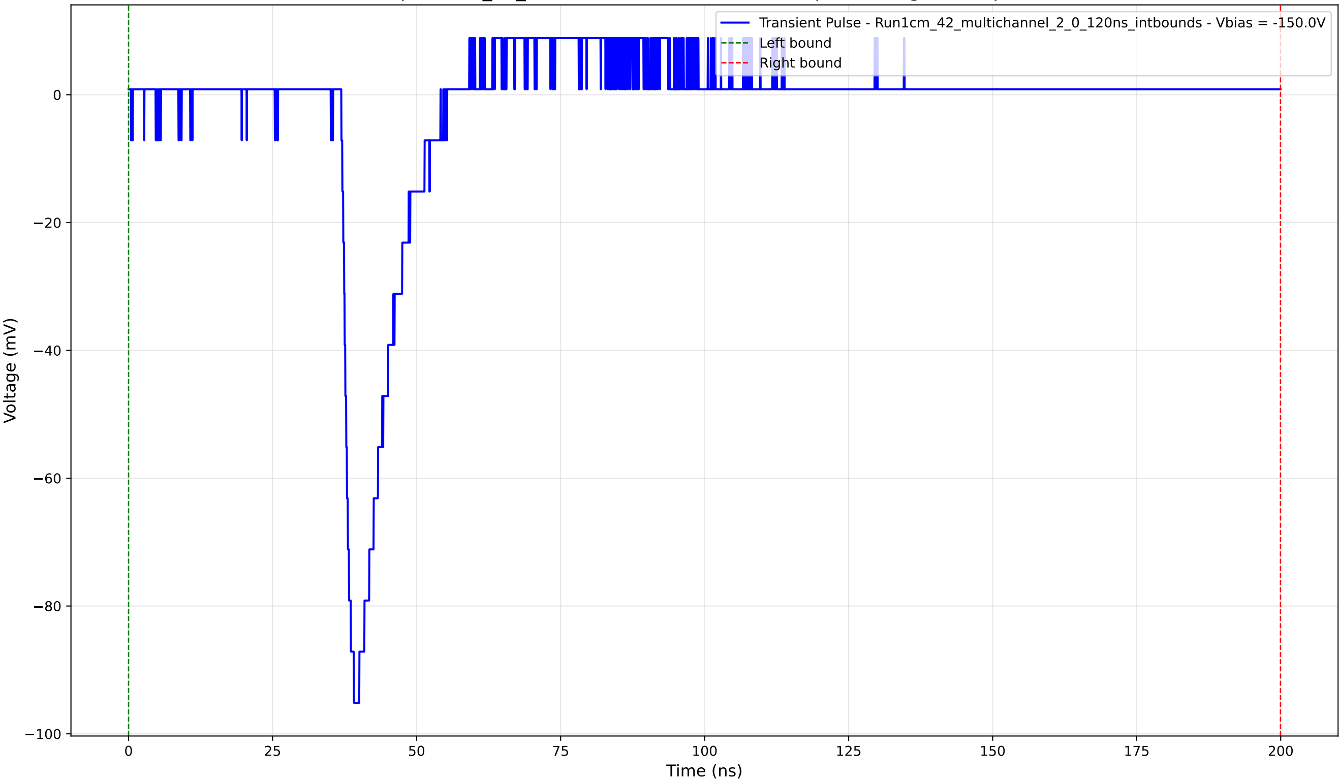
Transient Pulse - Sample: 1cm_42_multichannel - Position: 525.0 \mu\text{m} - Charge: 6.80 pC - Rise Time: 1.51 ns
