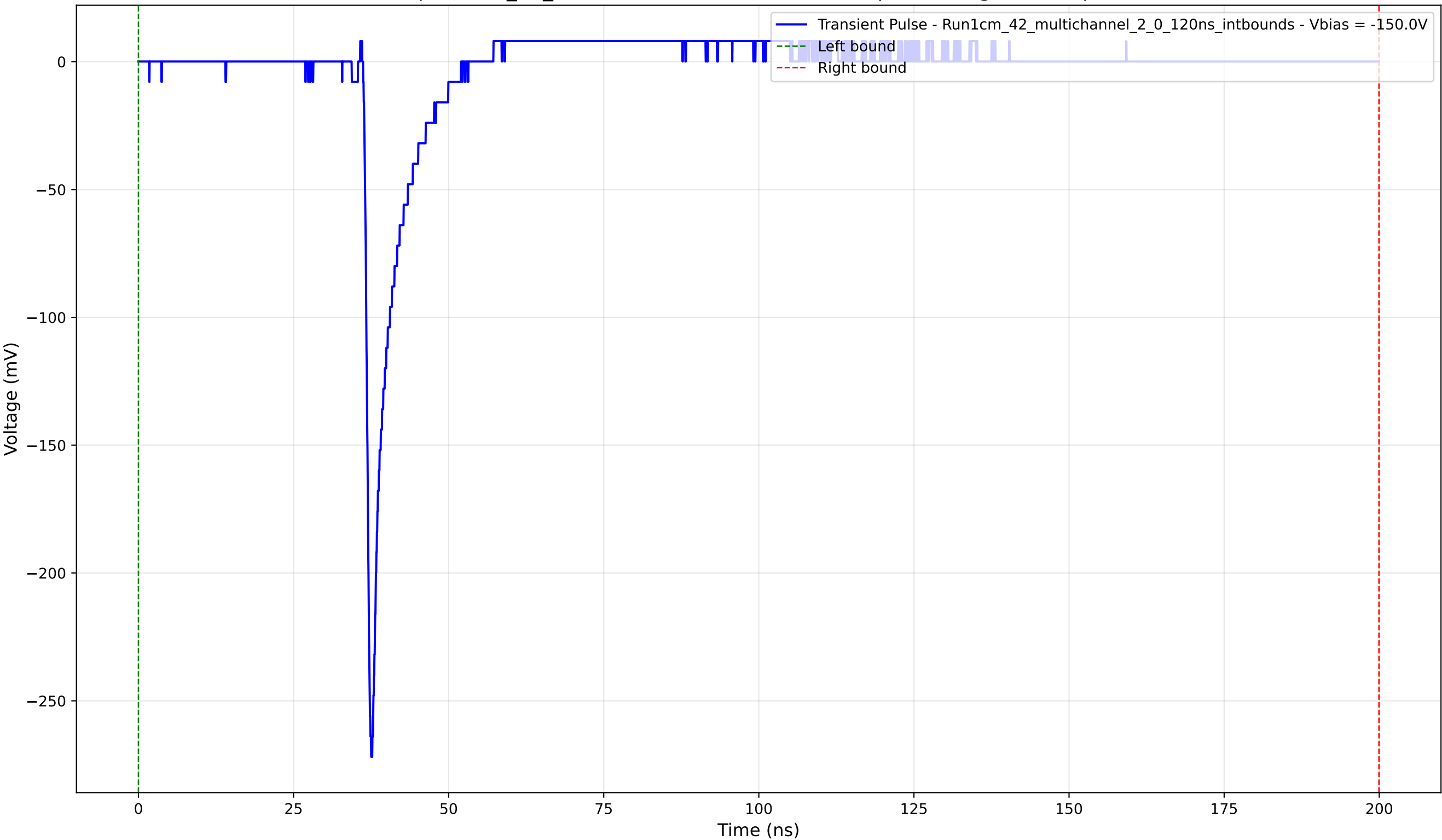
Transient Pulse - Sample: 1cm_42_multichannel - Position: 2985.0 \mu\text{m} - Charge: 12.40 pC - Rise Time: 0.85 ns
