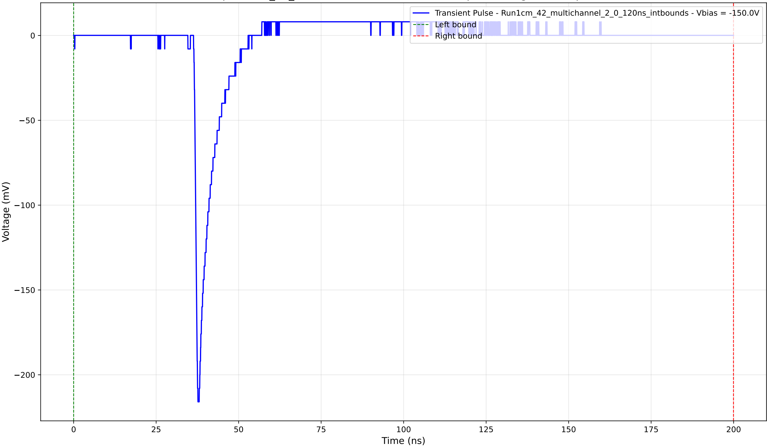
Transient Pulse - Sample: 1cm_42_multichannel - Position: 1530.0 \mu\text{m} - Charge: 11.71 pC - Rise Time: 0.94 ns
