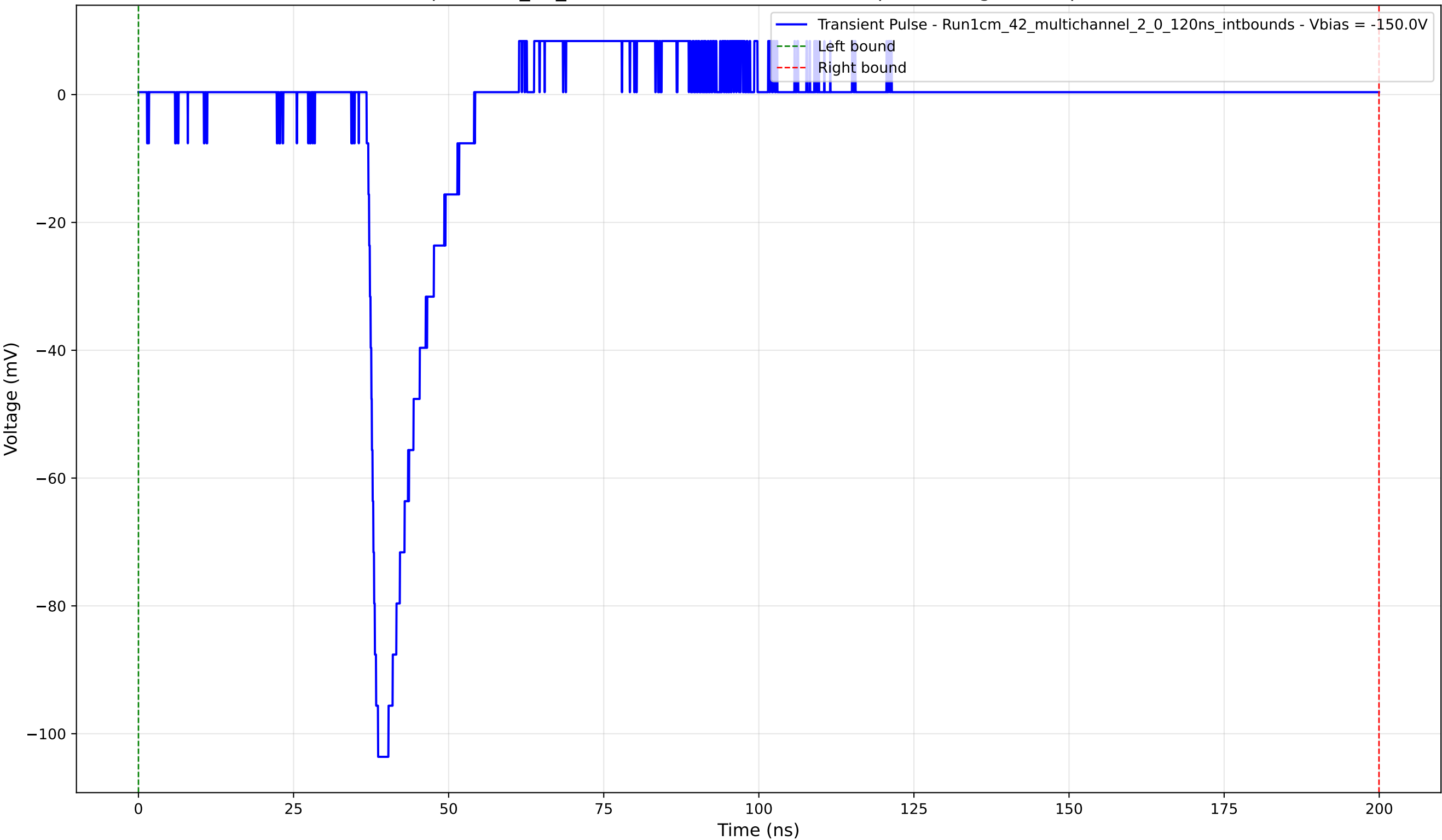
Transient Pulse - Sample: 1cm_42_multichannel - Position: 705.0 \mu\text{m} - Charge: 9.65 pC - Rise Time: 1.27 ns
