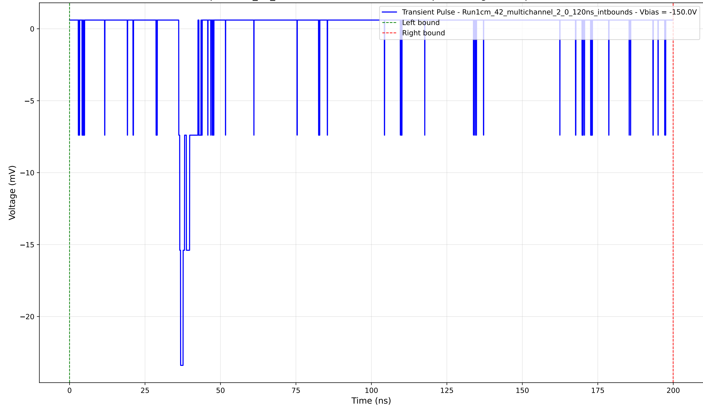
Transient Pulse - Sample: 1cm_42_multichannel - Position: 2375.0 \mu\text{m} - Charge: 0.01 pC - Rise Time: 0.63 ns
