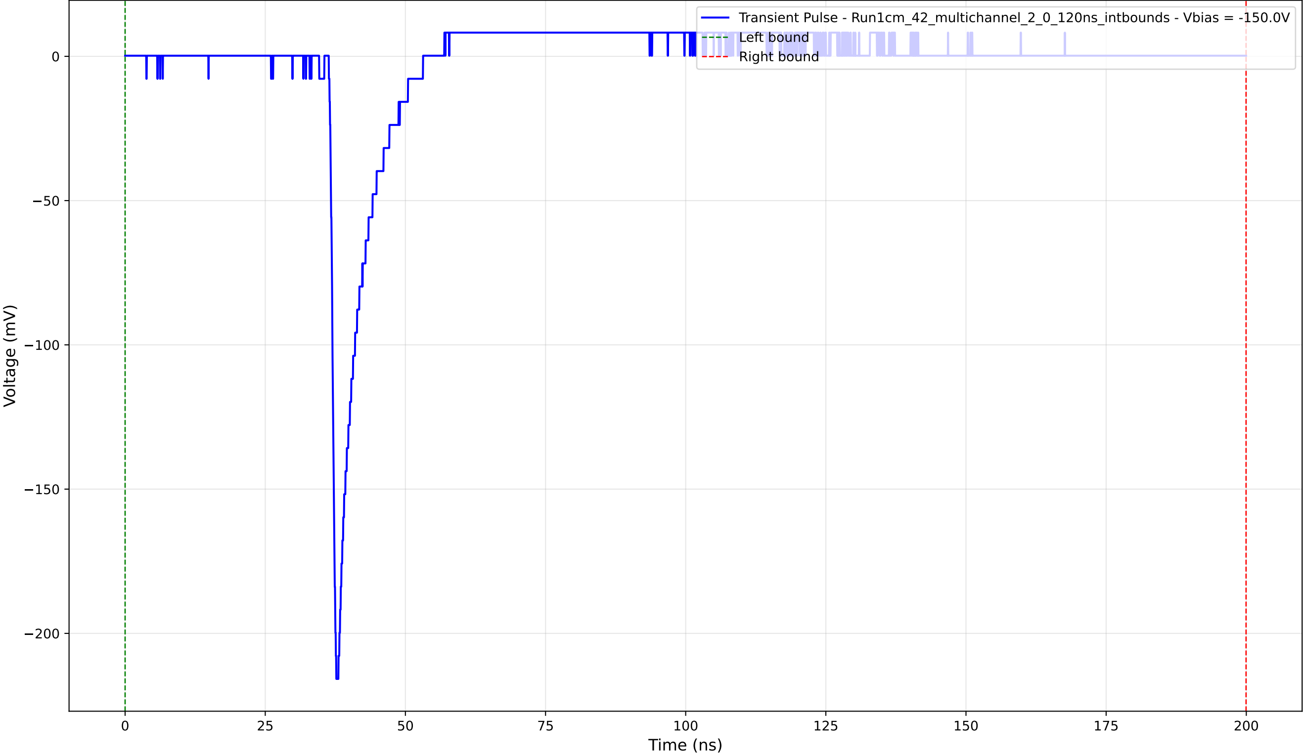
Transient Pulse - Sample: 1cm_42_multichannel - Position: 1520.0 \mu\text{m} - Charge: 10.40 pC - Rise Time: 0.97 ns
