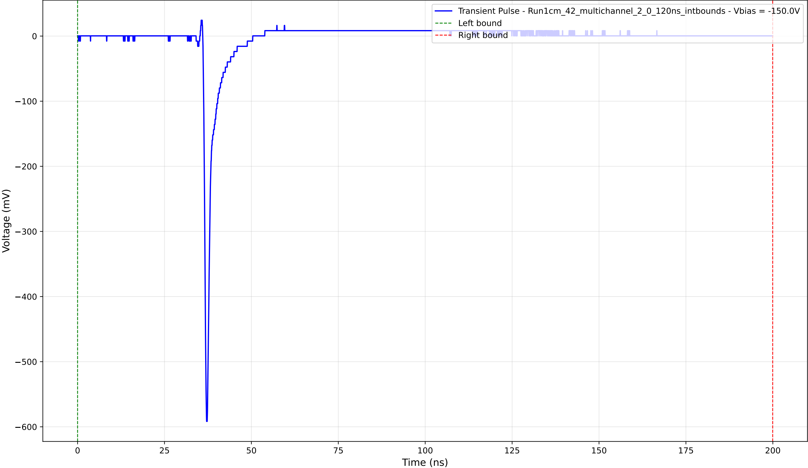
Transient Pulse - Sample: 1cm_42_multichannel - Position: 2215.0 \mu\text{m} - Charge: 15.28 pC - Rise Time: 0.73 ns
