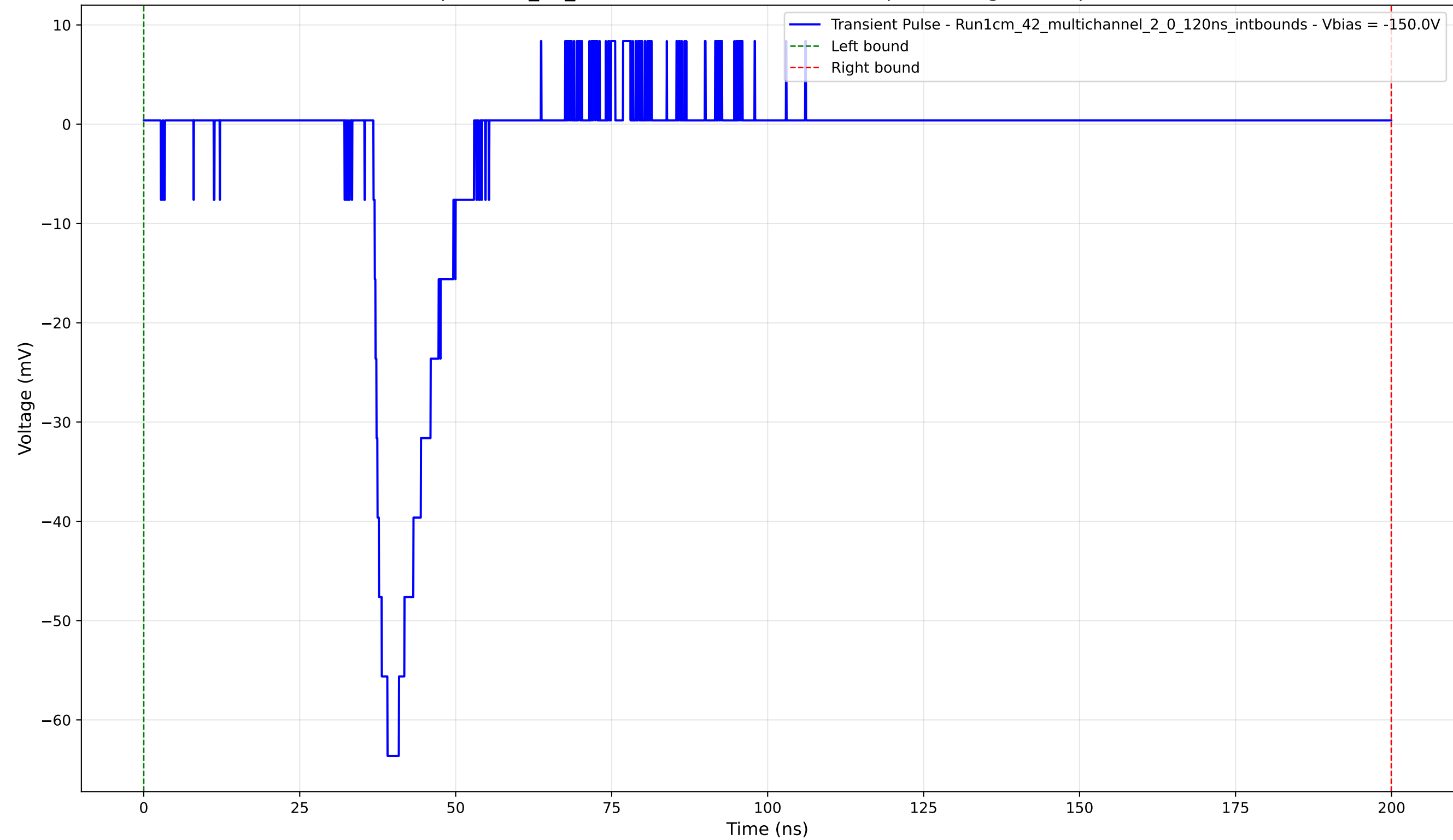
Transient Pulse - Sample: 1cm_42_multichannel - Position: 115.0 \mu\text{m} - Charge: 8.00 pC - Rise Time: 2.25 ns
