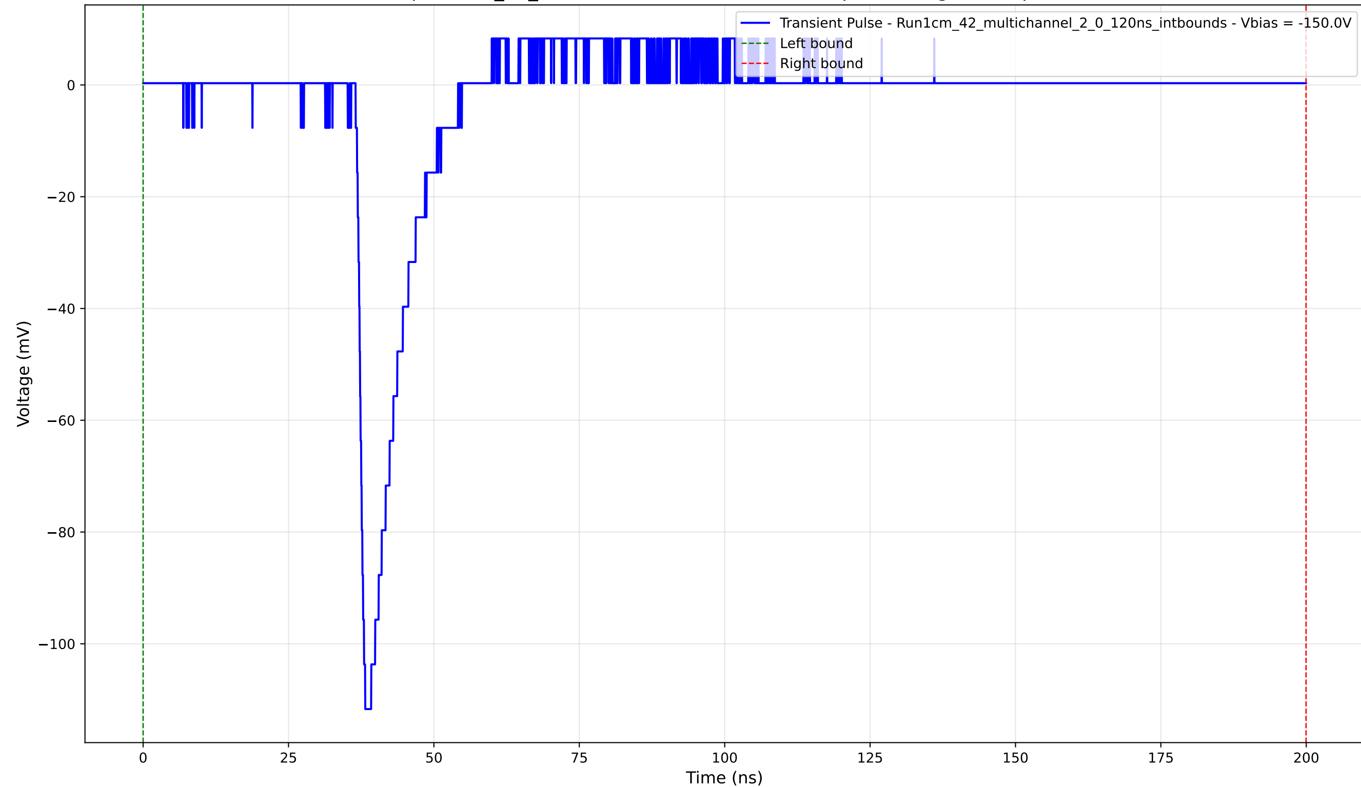
Transient Pulse - Sample: 1cm_42_multichannel - Position: 3660.0 \mu\text{m} - Charge: 9.78 pC - Rise Time: 1.22 ns
