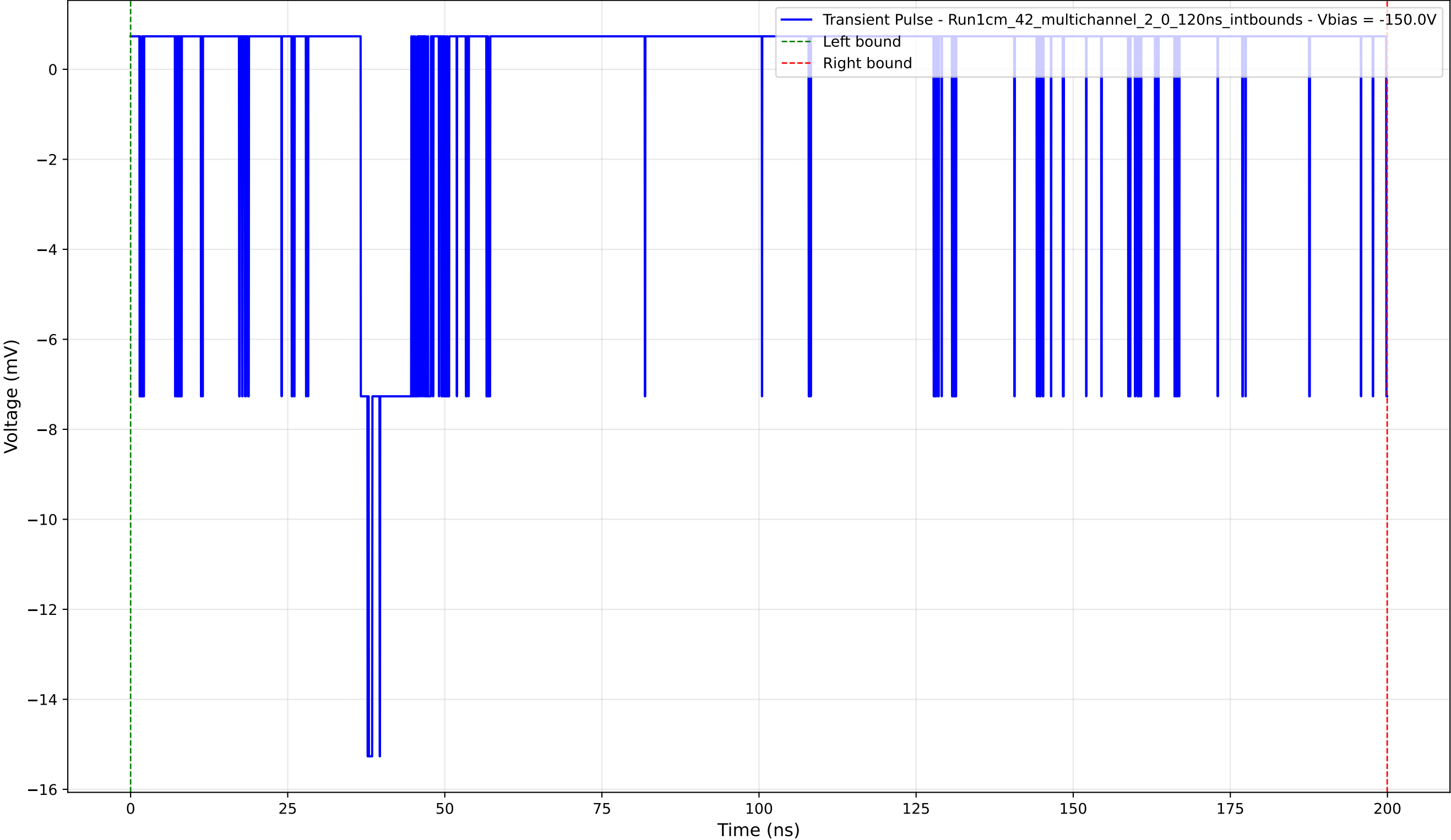
Transient Pulse - Sample: 1cm_42_multichannel - Position: 3400.0 \mu\text{m} - Charge: -0.04 pC - Rise Time: 1.12 ns
