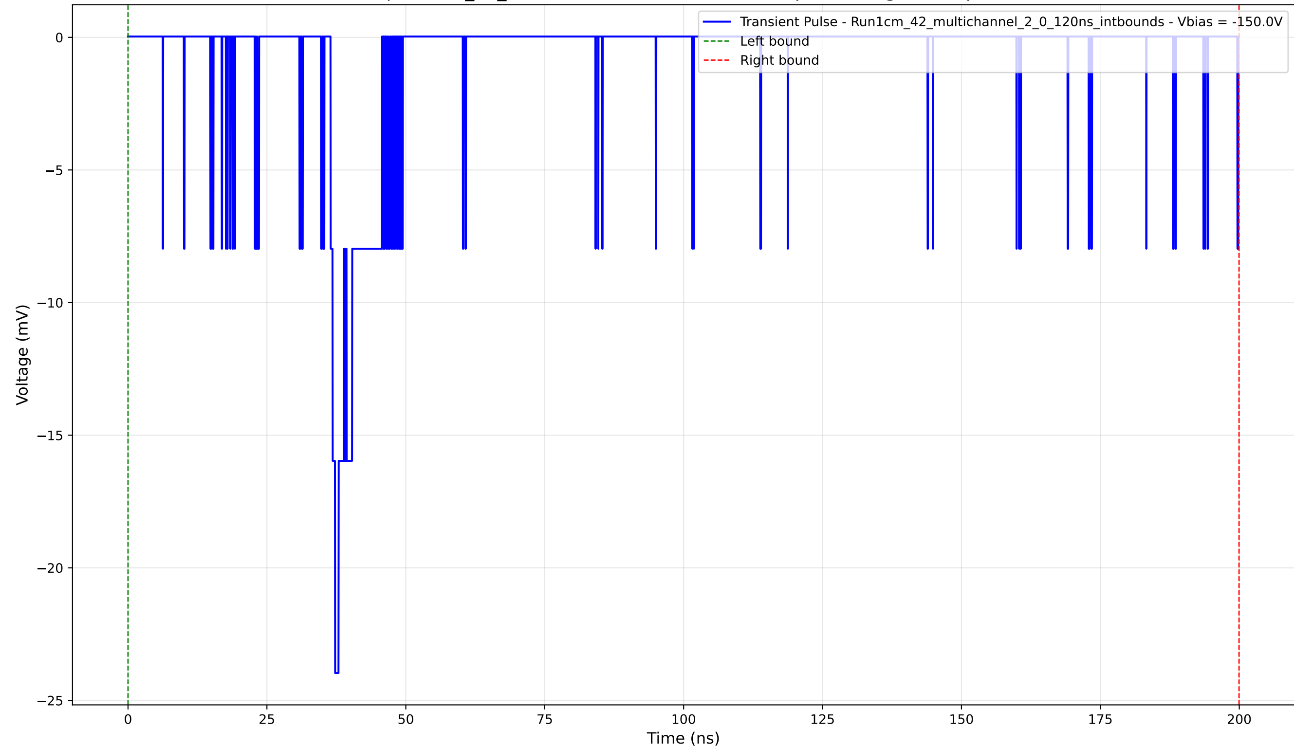
Transient Pulse - Sample: 1cm_42_multichannel - Position: 2895.0 \mu\text{m} - Charge: 2.93 pC - Rise Time: 0.83 ns
