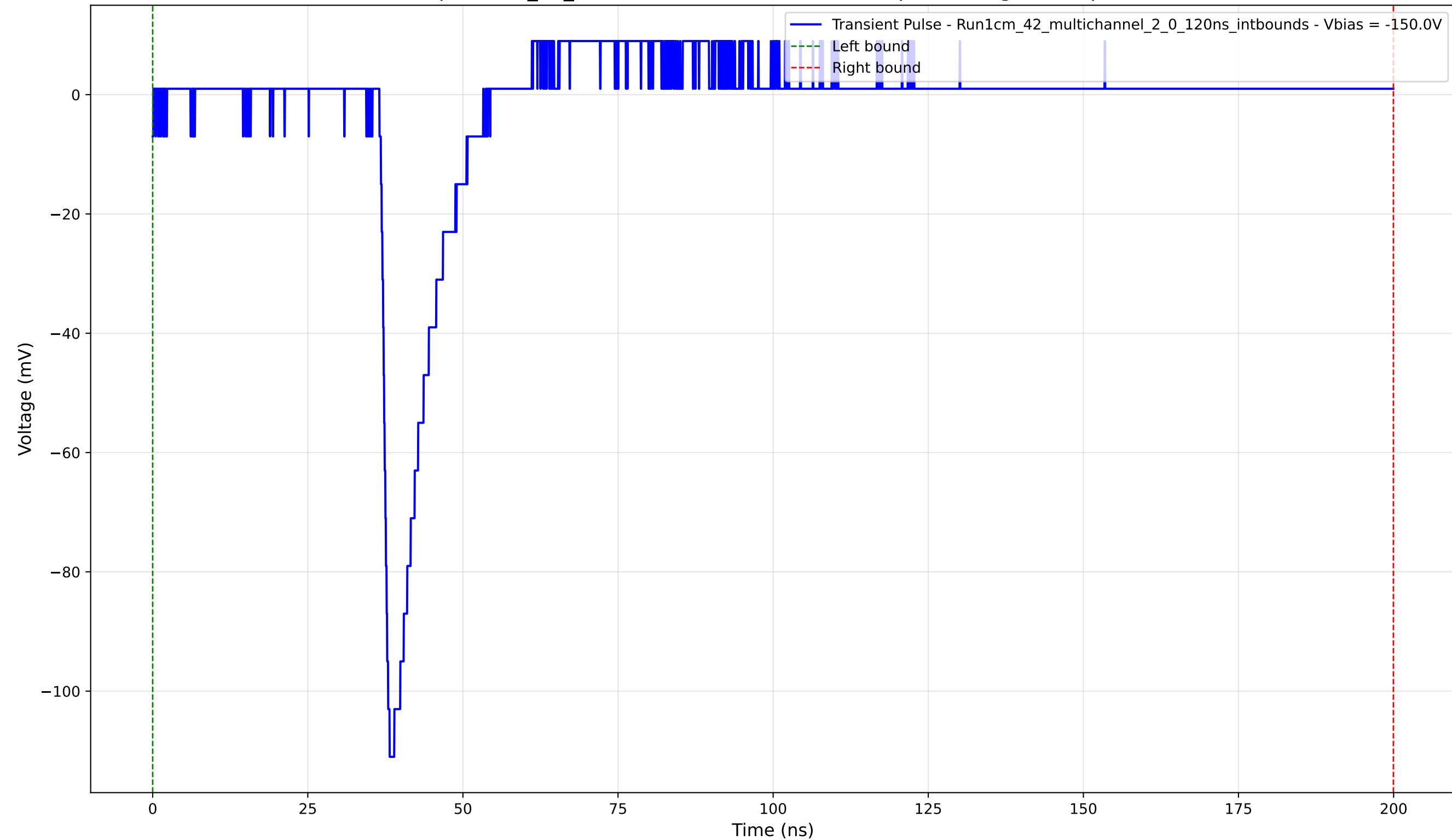
Transient Pulse - Sample: 1cm_42_multichannel - Position: 3645.0 \mu\text{m} - Charge: 7.21 pC - Rise Time: 1.18 ns
