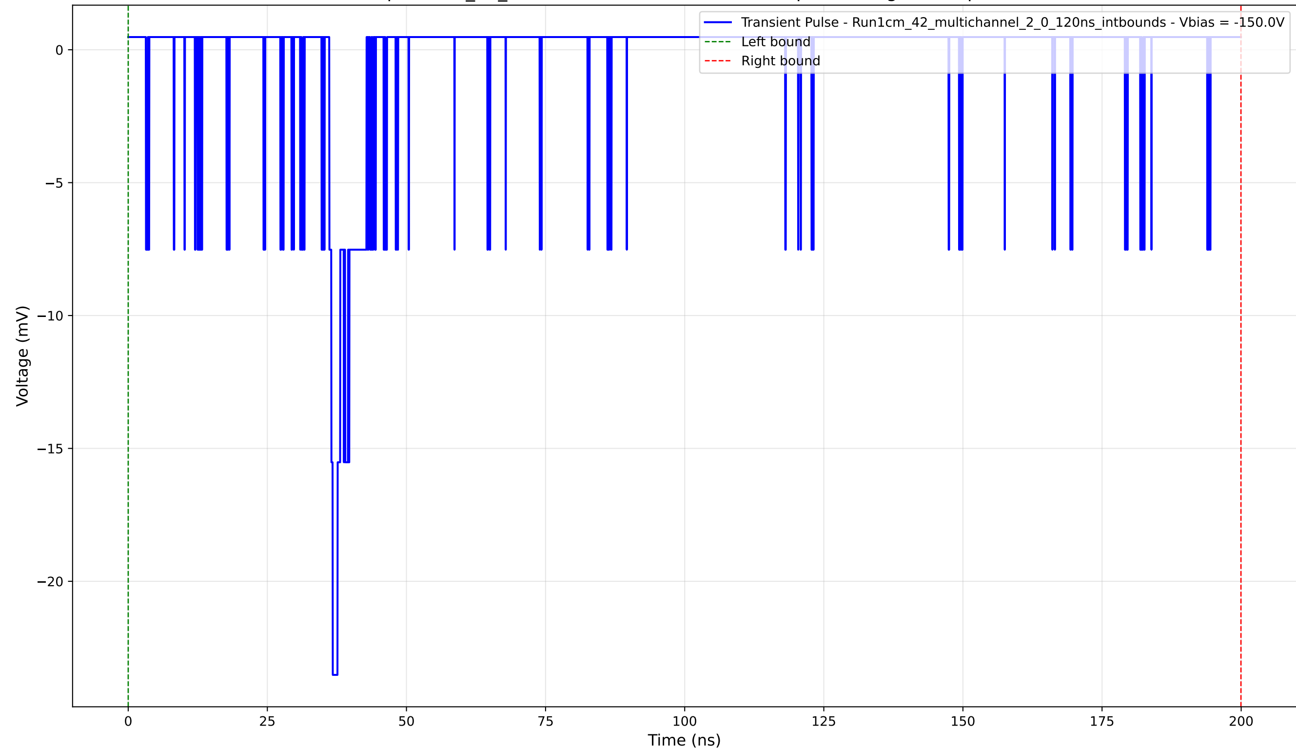
Transient Pulse - Sample: 1cm_42_multichannel - Position: 2365.0 \mu\text{m} - Charge: 0.88 pC - Rise Time: 0.63 ns
