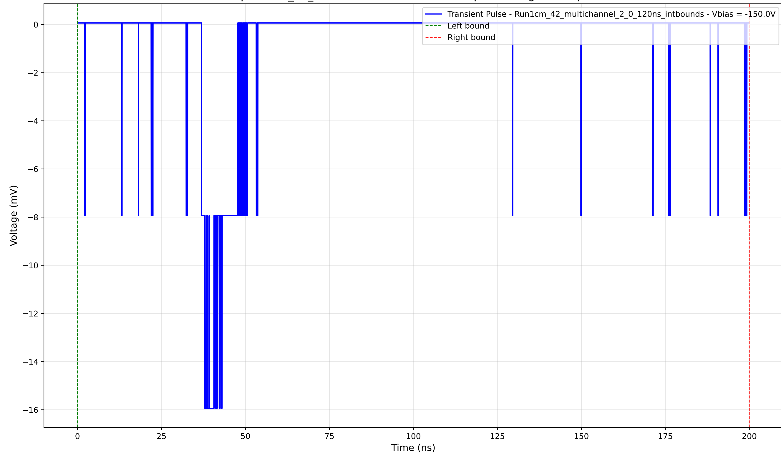
Transient Pulse - Sample: 1cm_42_multichannel - Position: 55.0 \mu\text{m} - Charge: 2.47 pC - Rise Time: 0.95 ns
