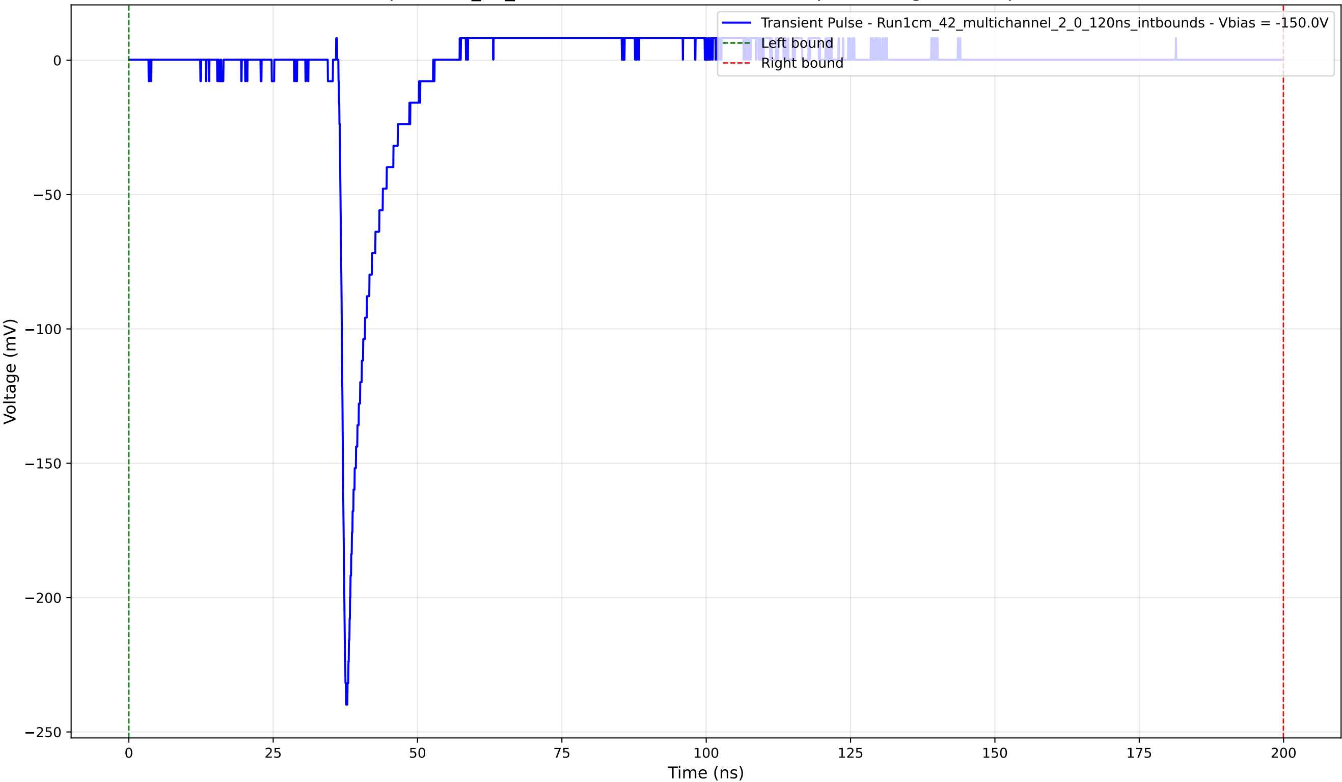
Transient Pulse - Sample: 1cm_42_multichannel - Position: 1615.0 \mu\text{m} - Charge: 12.66 pC - Rise Time: 0.92 ns
