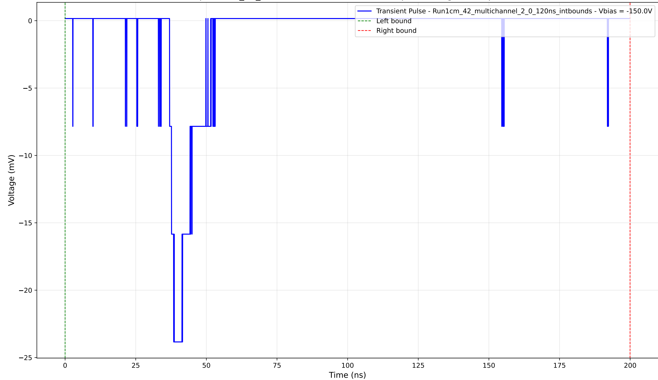
Transient Pulse - Sample: 1cm_42_multichannel - Position: 305.0 \mu\text{m} - Charge: 3.50 pC - Rise Time: 1.47 ns
