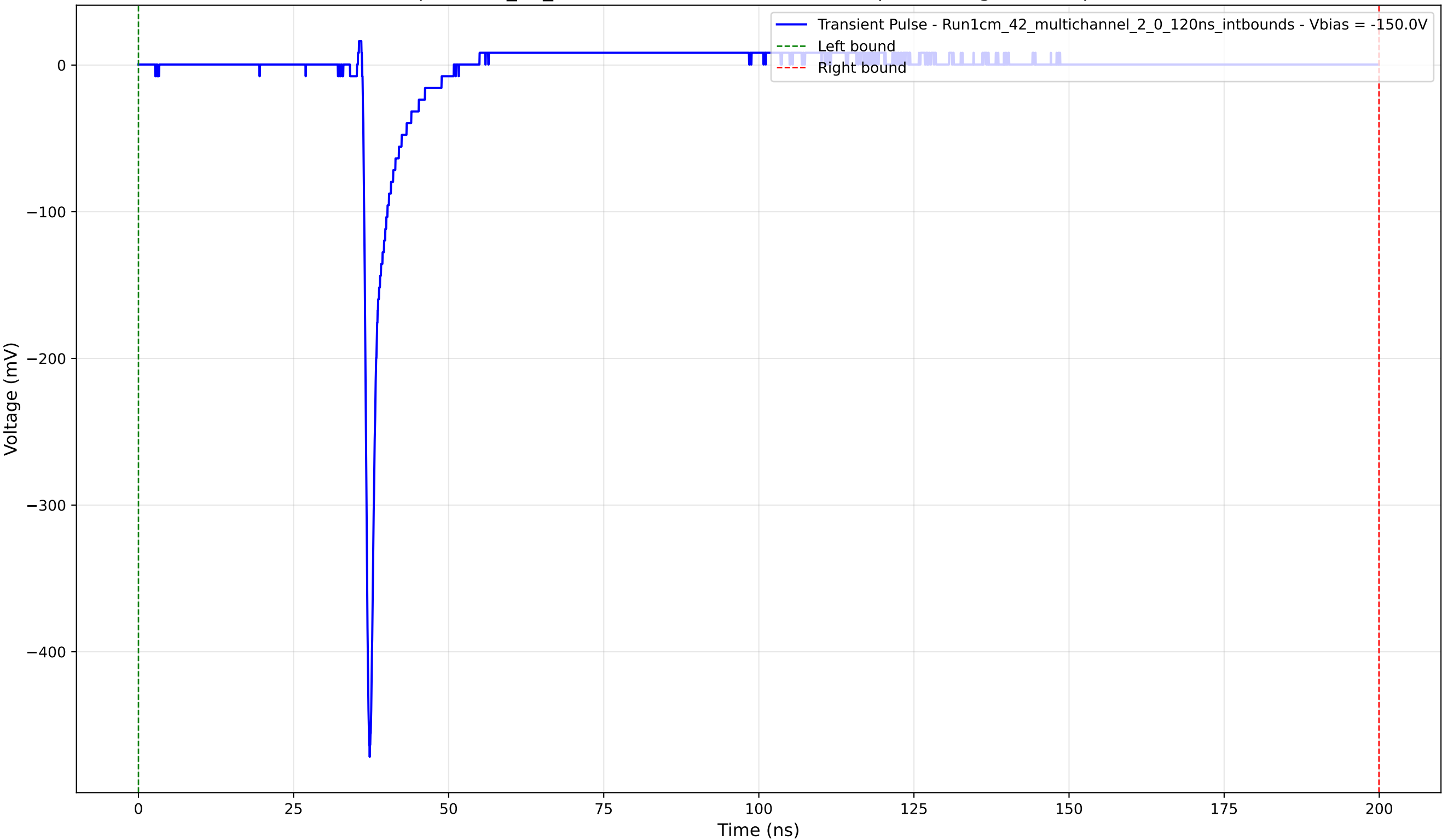
Transient Pulse - Sample: 1cm_42_multichannel - Position: 2630.0 \mu\text{m} - Charge: 13.18 pC - Rise Time: 0.75 ns
