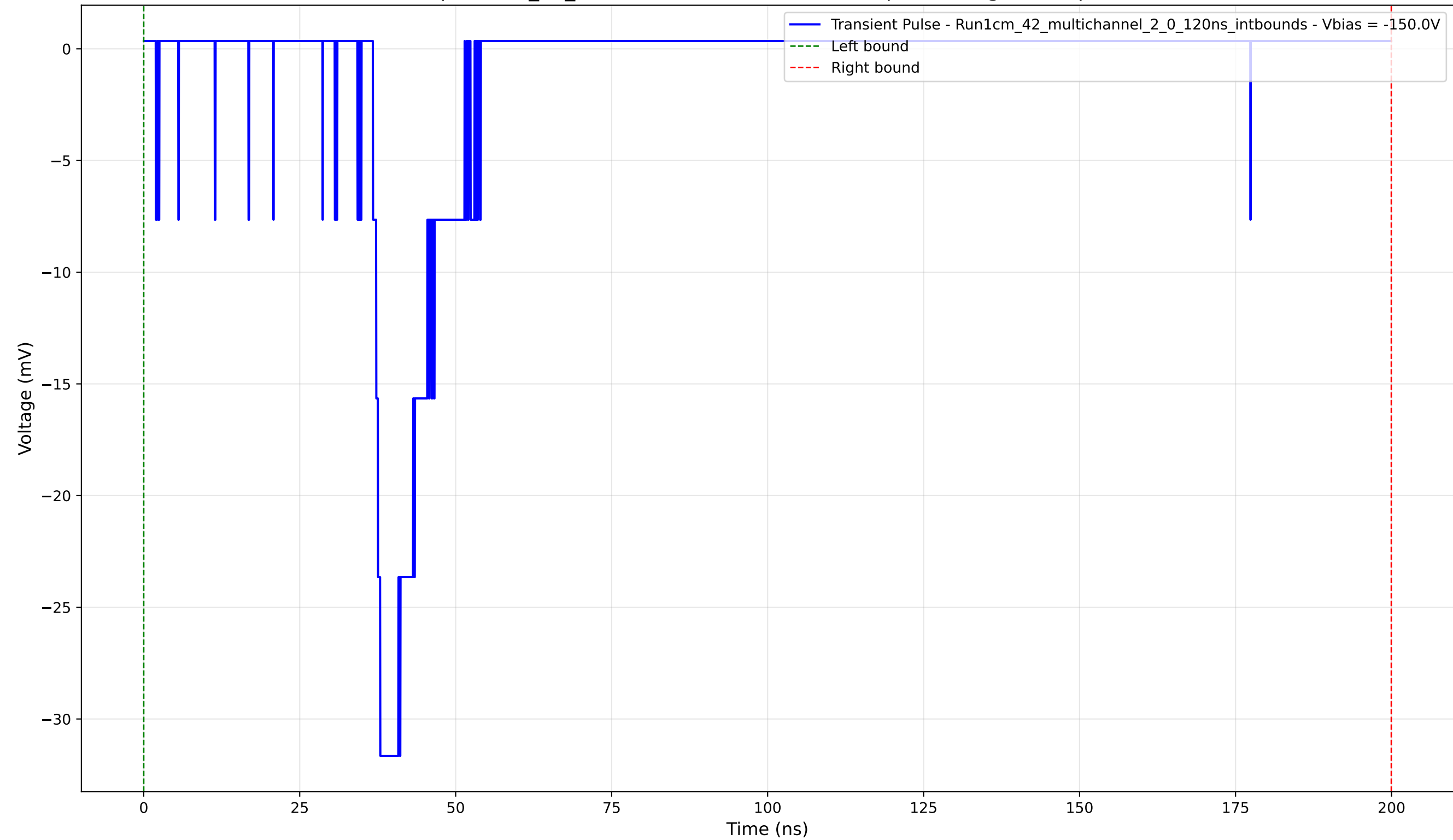
Transient Pulse - Sample: 1cm_42_multichannel - Position: 890.0 \mu\text{m} - Charge: 4.19 pC - Rise Time: 1.18 ns
