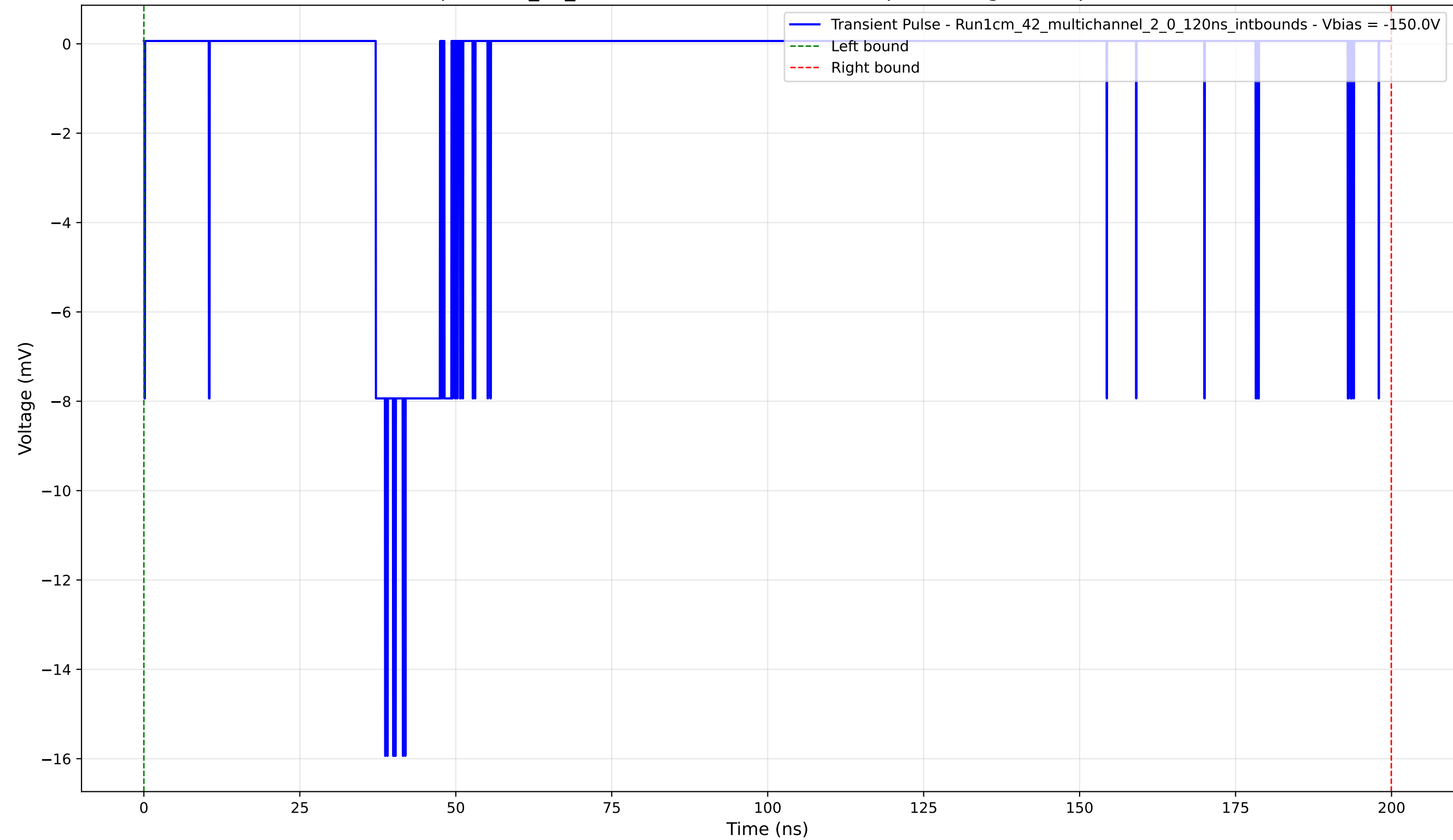
Transient Pulse - Sample: 1cm_42_multichannel - Position: 315.0 \mu\text{m} - Charge: 2.01 pC - Rise Time: 1.51 ns
