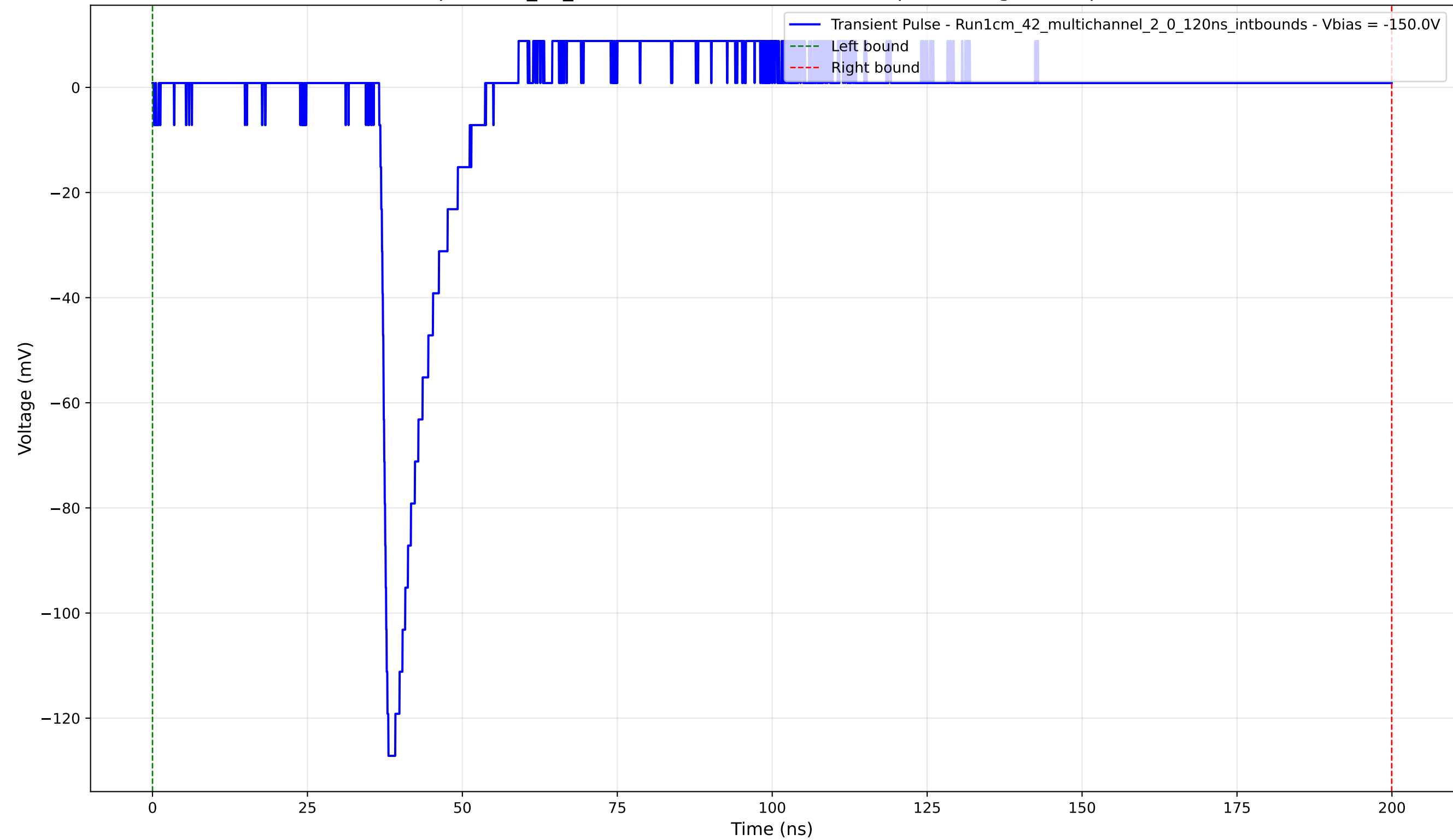
Transient Pulse - Sample: 1cm_42_multichannel - Position: 1075.0 \mu\text{m} - Charge: 7.97 pC - Rise Time: 1.13 ns
