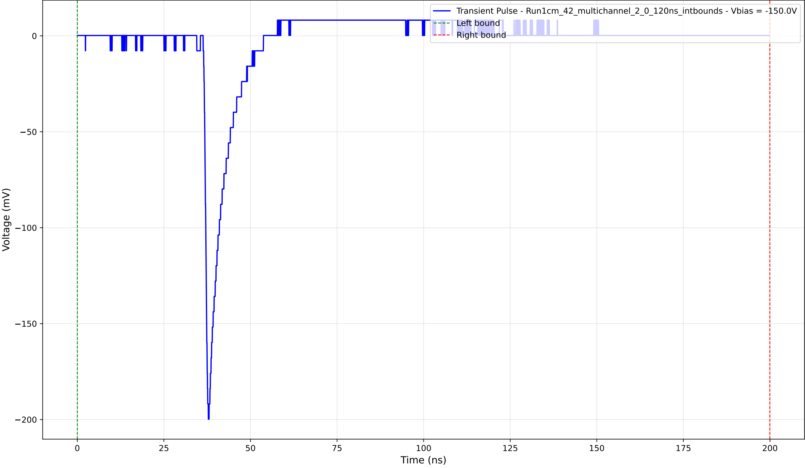
Transient Pulse - Sample: 1cm_42_multichannel - Position: 1455.0 \mu\text{m} - Charge: 11.41 pC - Rise Time: 1.02 ns
