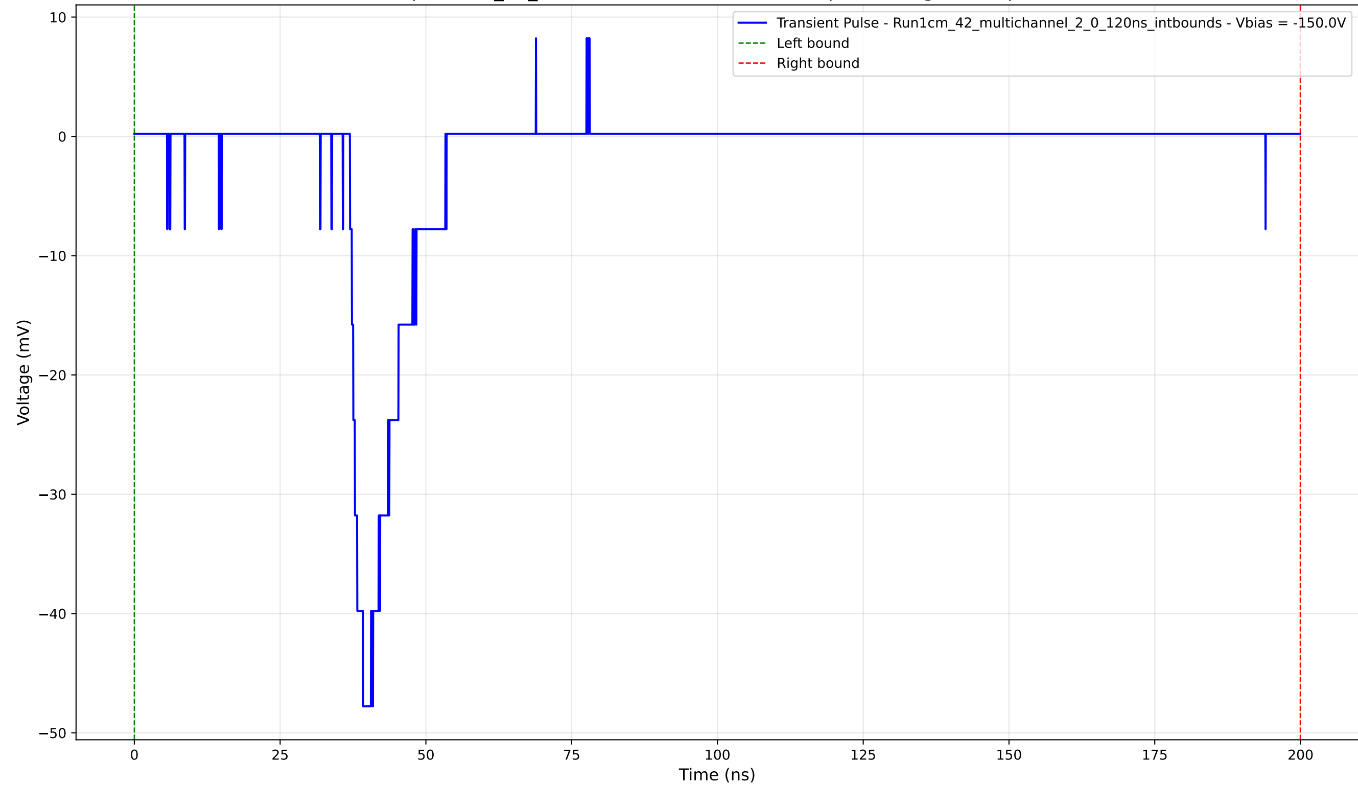
Transient Pulse - Sample: 1cm_42_multichannel - Position: 395.0 \mu\text{m} - Charge: 6.51 pC - Rise Time: 2.26 ns
