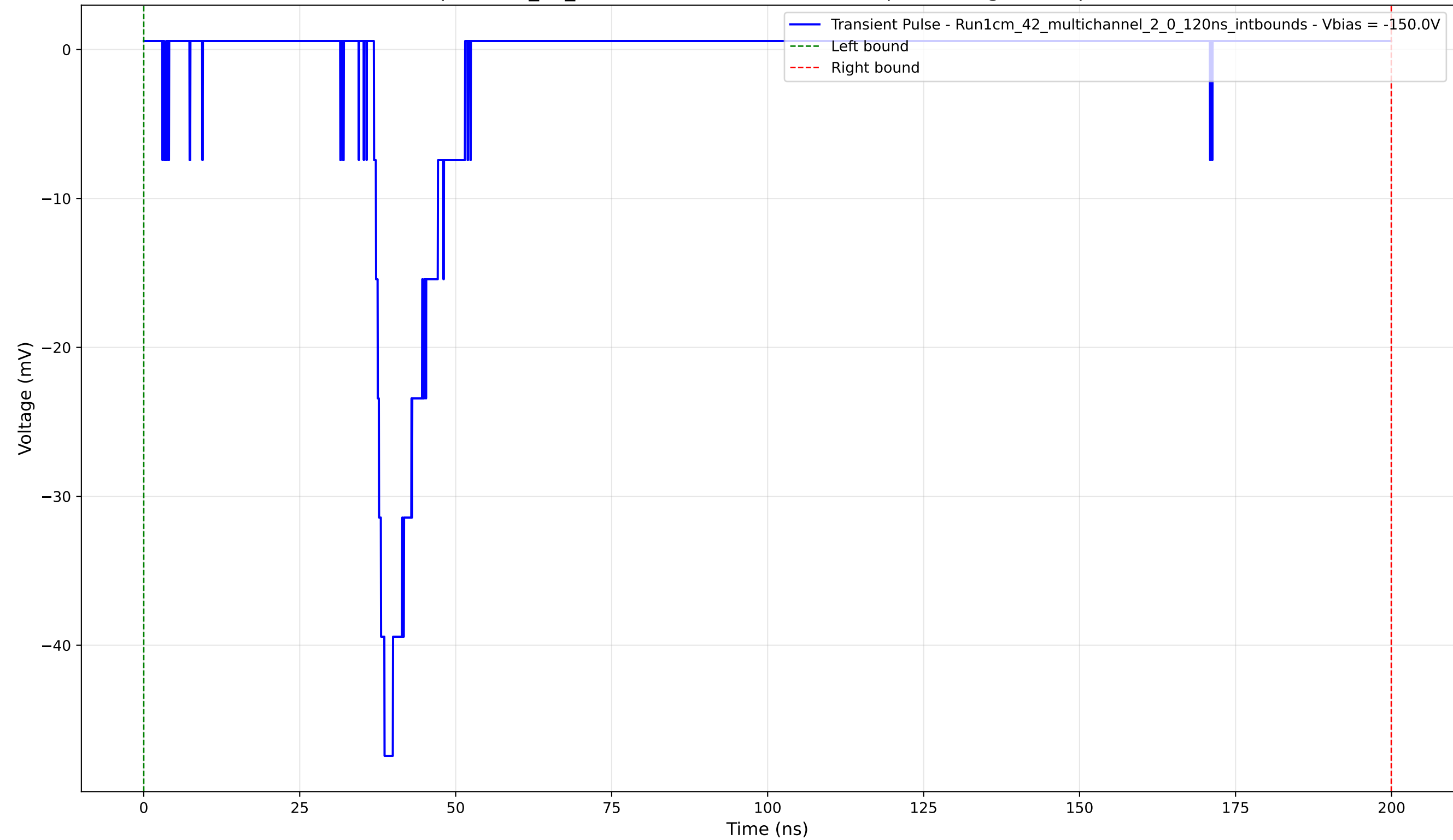
Transient Pulse - Sample: 1cm_42_multichannel - Position: 805.0 \mu\text{m} - Charge: 4.68 pC - Rise Time: 1.70 ns
