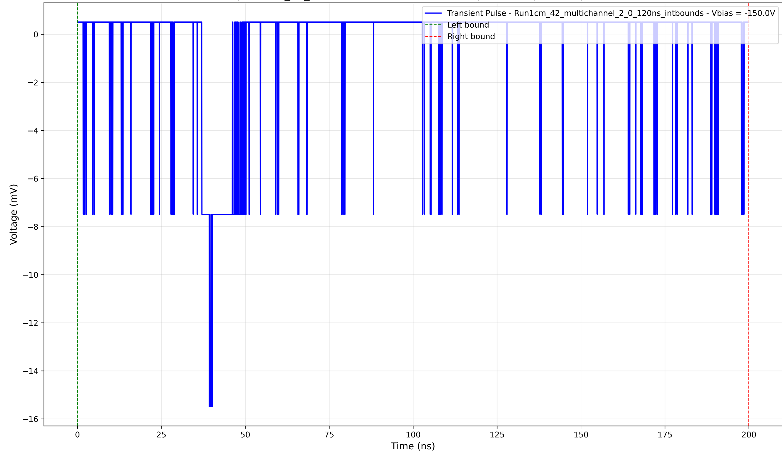
Transient Pulse - Sample: 1cm_42_multichannel - Position: 830.0 \mu\text{m} - Charge: 1.15 pC - Rise Time: 2.23 ns
