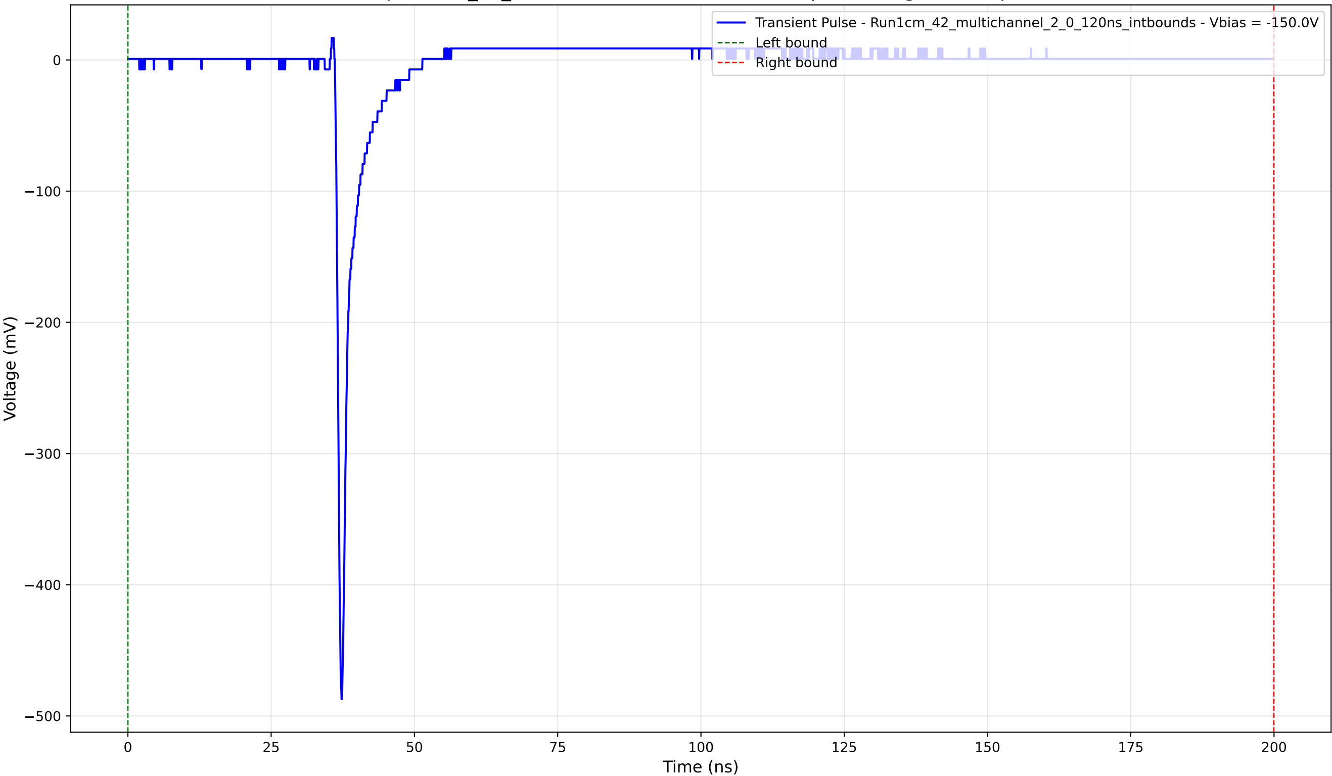
Transient Pulse - Sample: 1cm_42_multichannel - Position: 2095.0 \mu\text{m} - Charge: 13.34 pC - Rise Time: 0.77 ns
