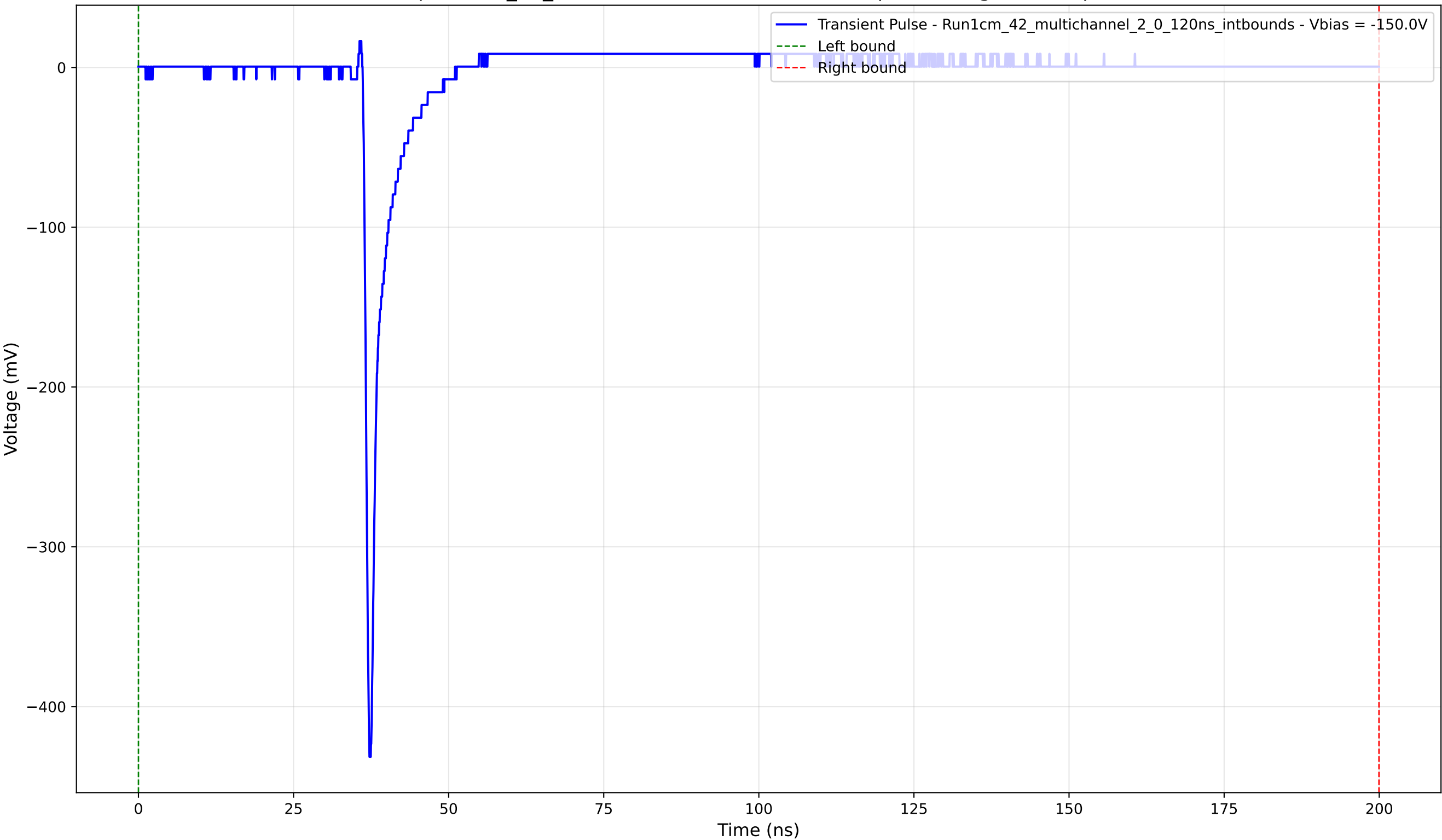
Transient Pulse - Sample: 1cm_42_multichannel - Position: 2700.0 \mu\text{m} - Charge: 12.42 pC - Rise Time: 0.77 ns
