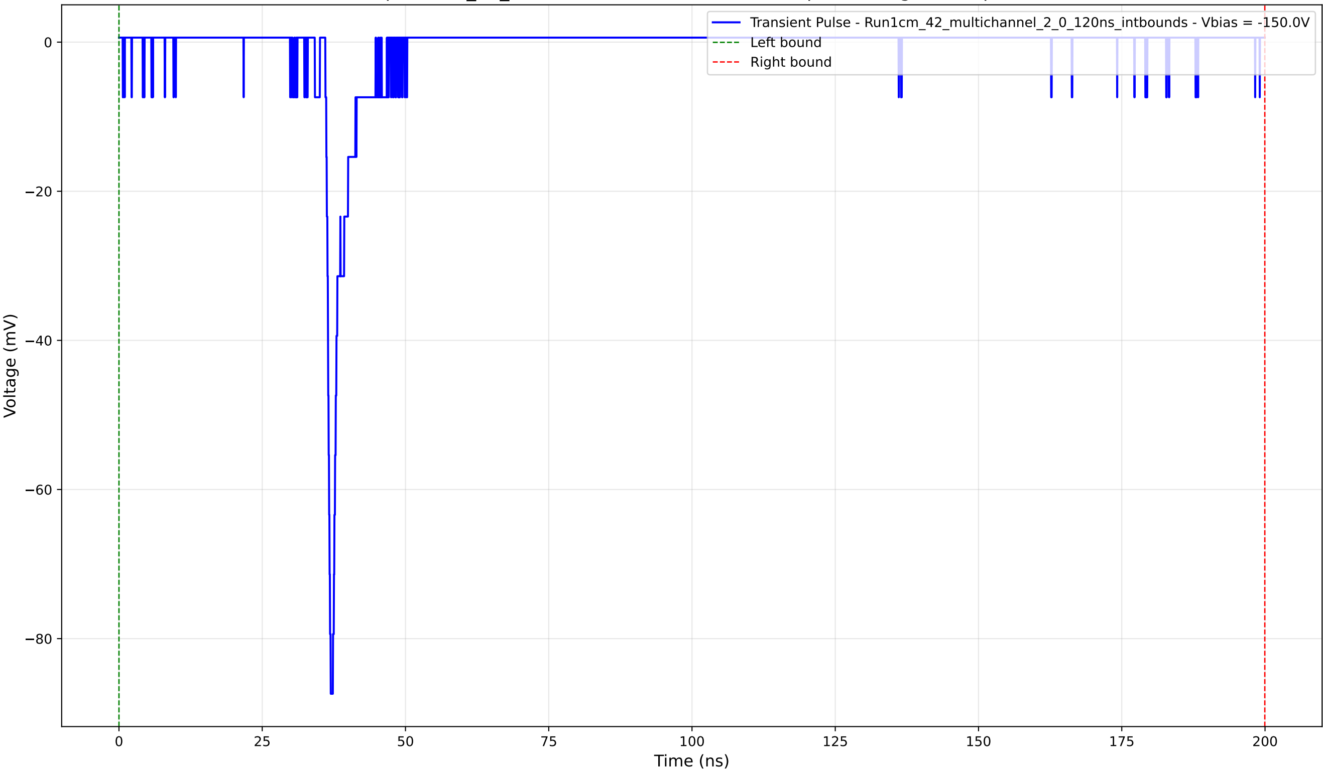
Transient Pulse - Sample: 1cm_42_multichannel - Position: 2400.0 \mu\text{m} - Charge: 3.14 pC - Rise Time: 0.67 ns
