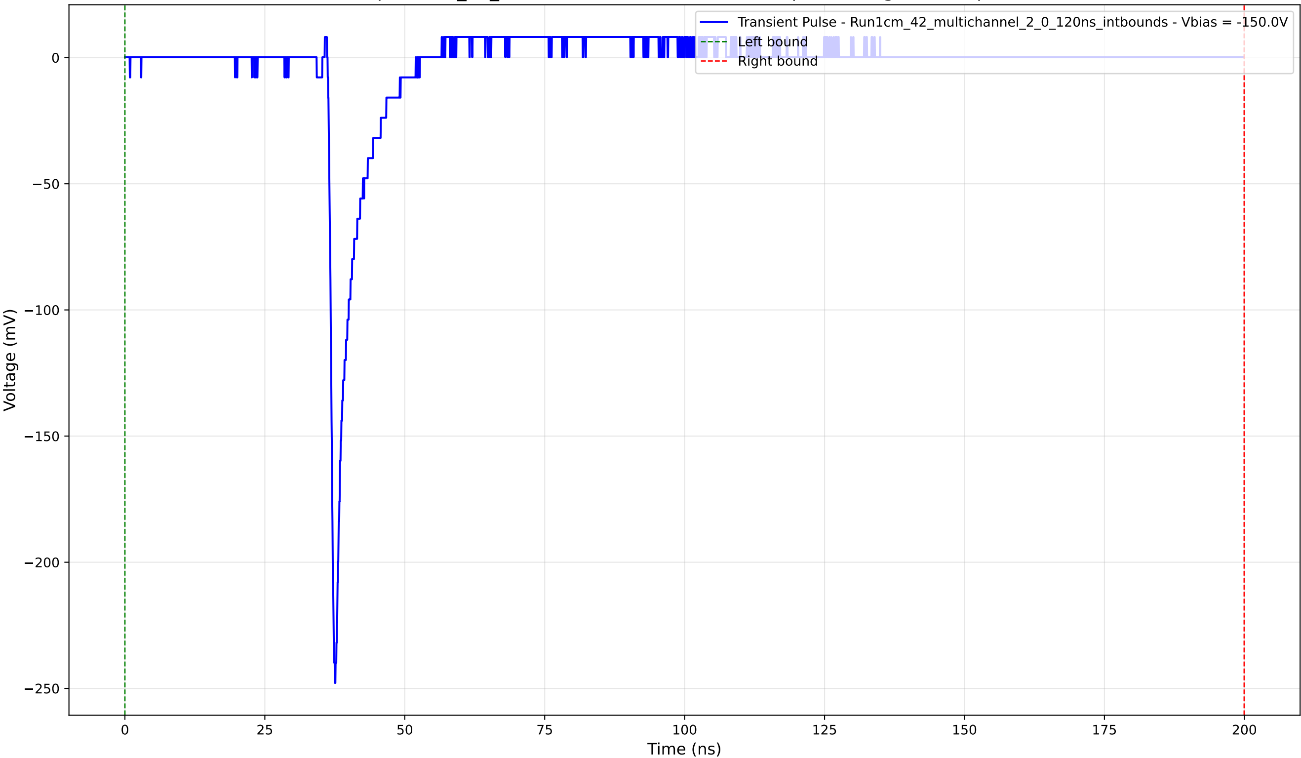
Transient Pulse - Sample: 1cm_42_multichannel - Position: 1795.0 \mu\text{m} - Charge: 11.13 pC - Rise Time: 0.87 ns
