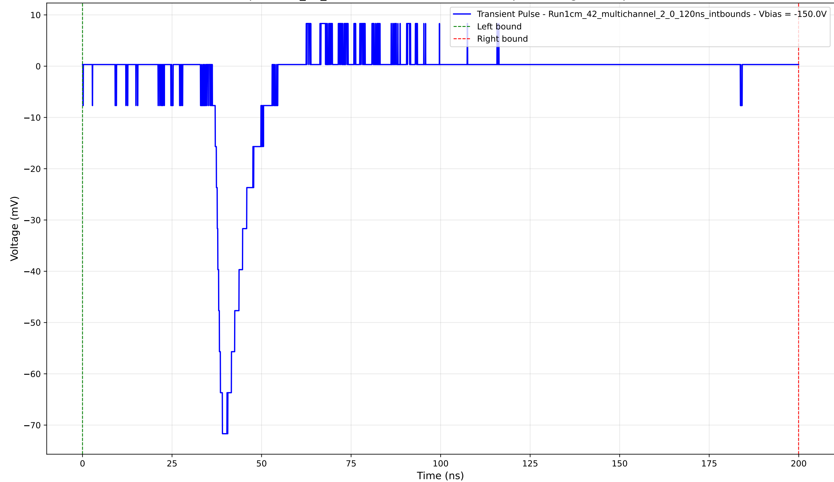
Transient Pulse - Sample: 1cm_42_multichannel - Position: 4640.0 \mu\text{m} - Charge: 9.12 pC - Rise Time: 2.80 ns
