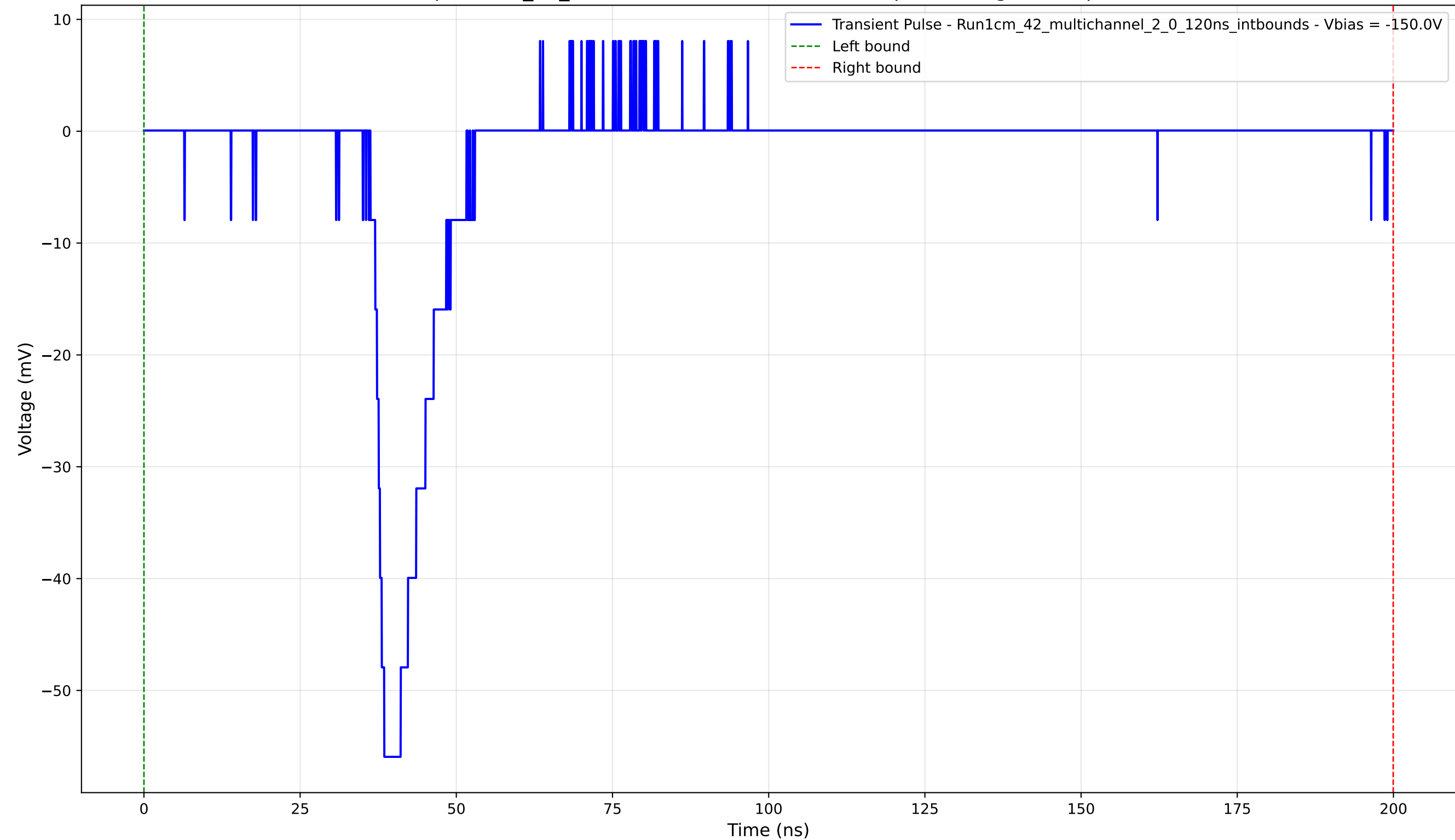
Transient Pulse - Sample: 1cm_42_multichannel - Position: 4810.0 \mu\text{m} - Charge: 8.50 pC - Rise Time: 2.21 ns
