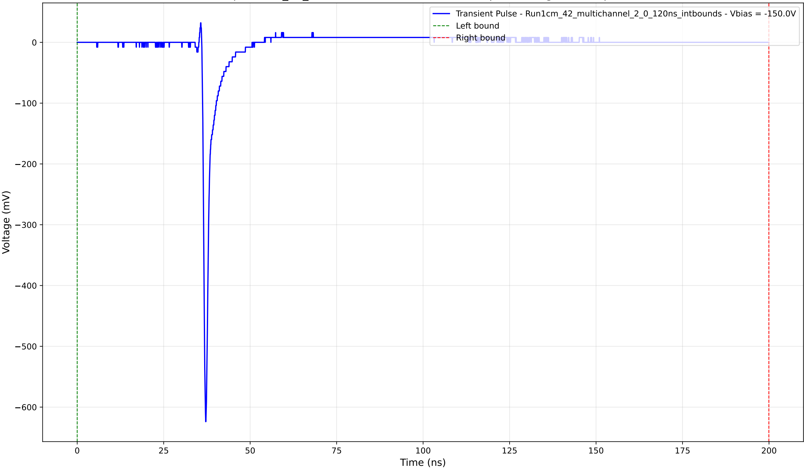
Transient Pulse - Sample: 1cm_42_multichannel - Position: 2240.0 \mu\text{m} - Charge: 17.26 pC - Rise Time: 0.73 ns
