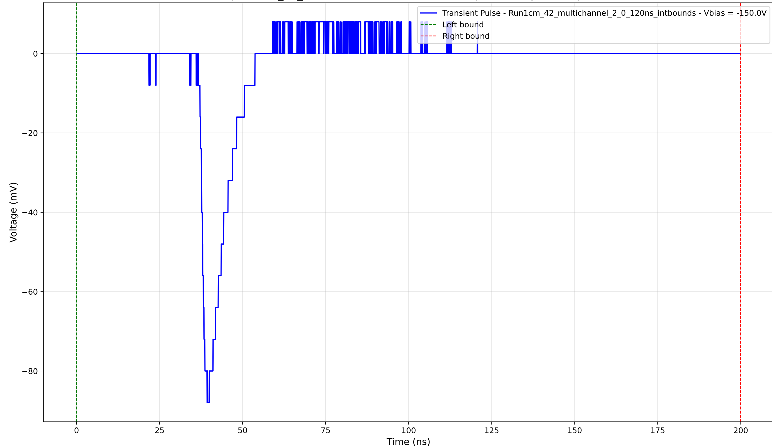
Transient Pulse - Sample: 1cm_42_multichannel - Position: 4210.0 \mu\text{m} - Charge: 9.57 pC - Rise Time: 1.52 ns
