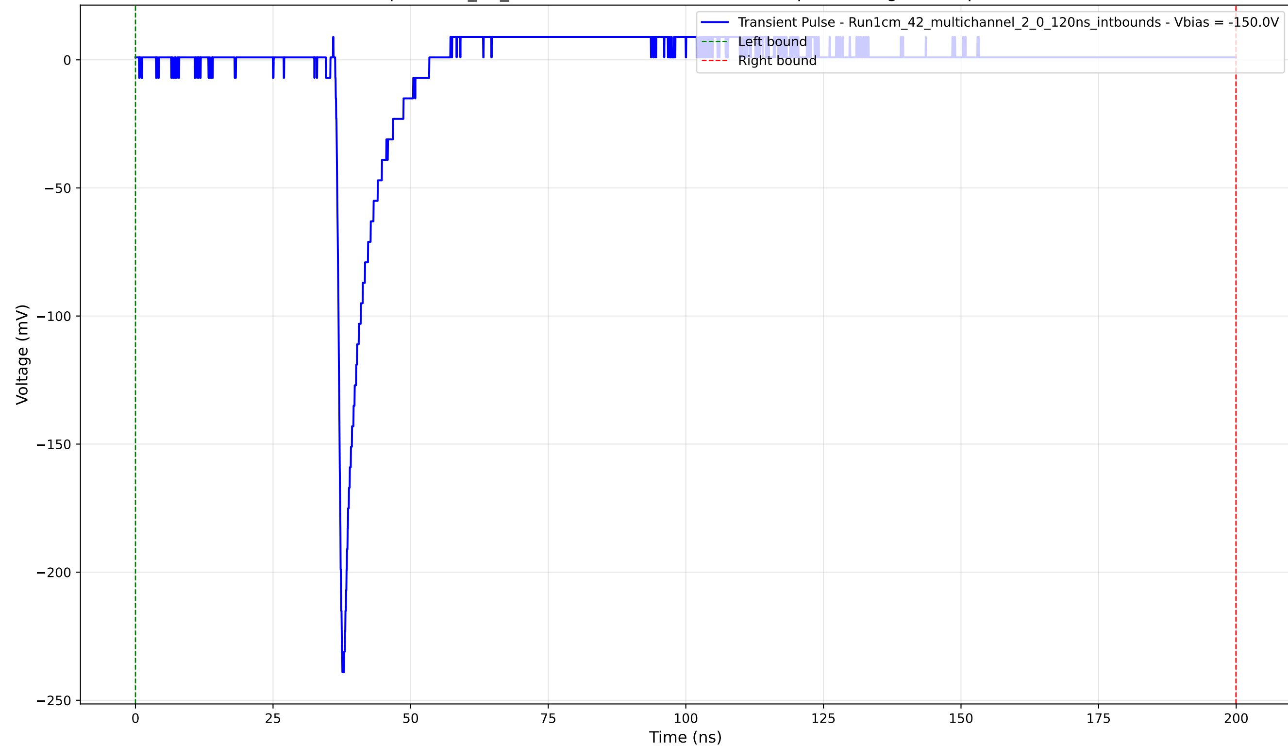
Transient Pulse - Sample: 1cm_42_multichannel - Position: 1610.0 \mu\text{m} - Charge: 9.81 pC - Rise Time: 0.92 ns
