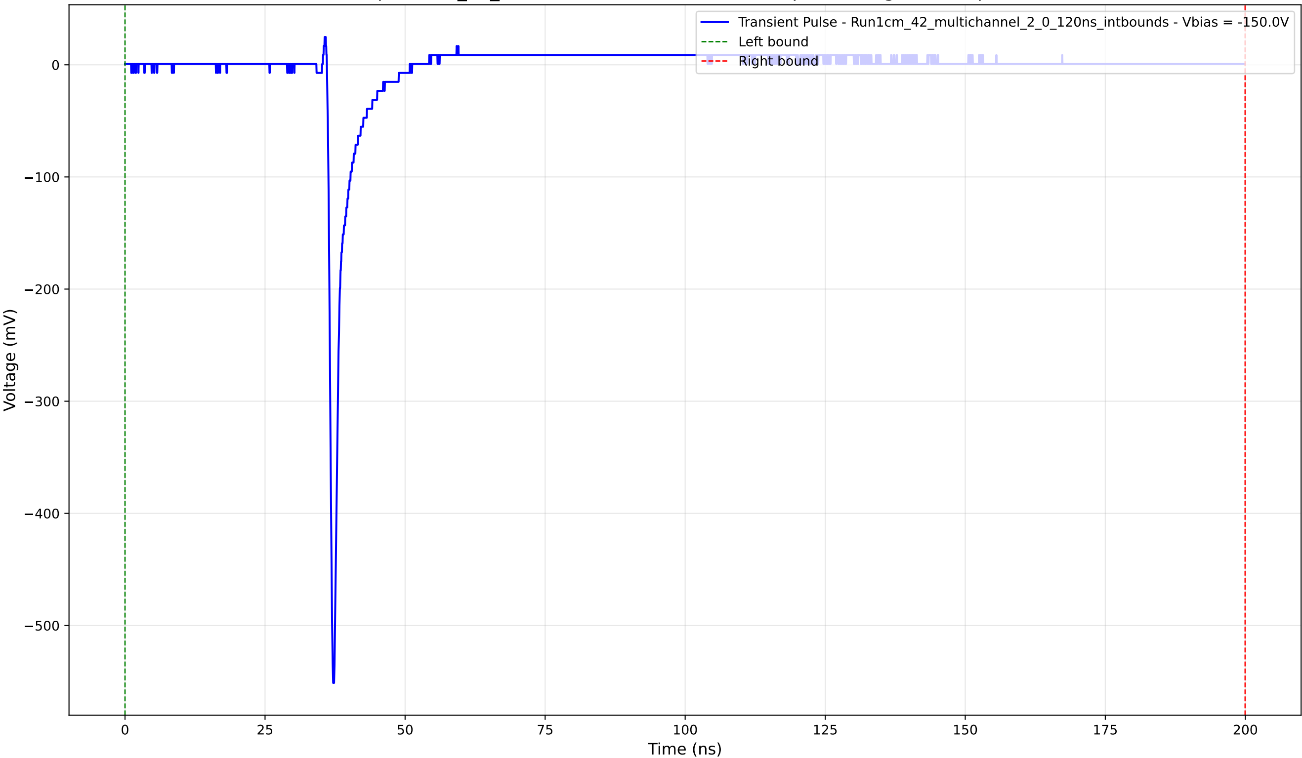
Transient Pulse - Sample: 1cm_42_multichannel - Position: 2175.0 \mu\text{m} - Charge: 13.18 pC - Rise Time: 0.74 ns
