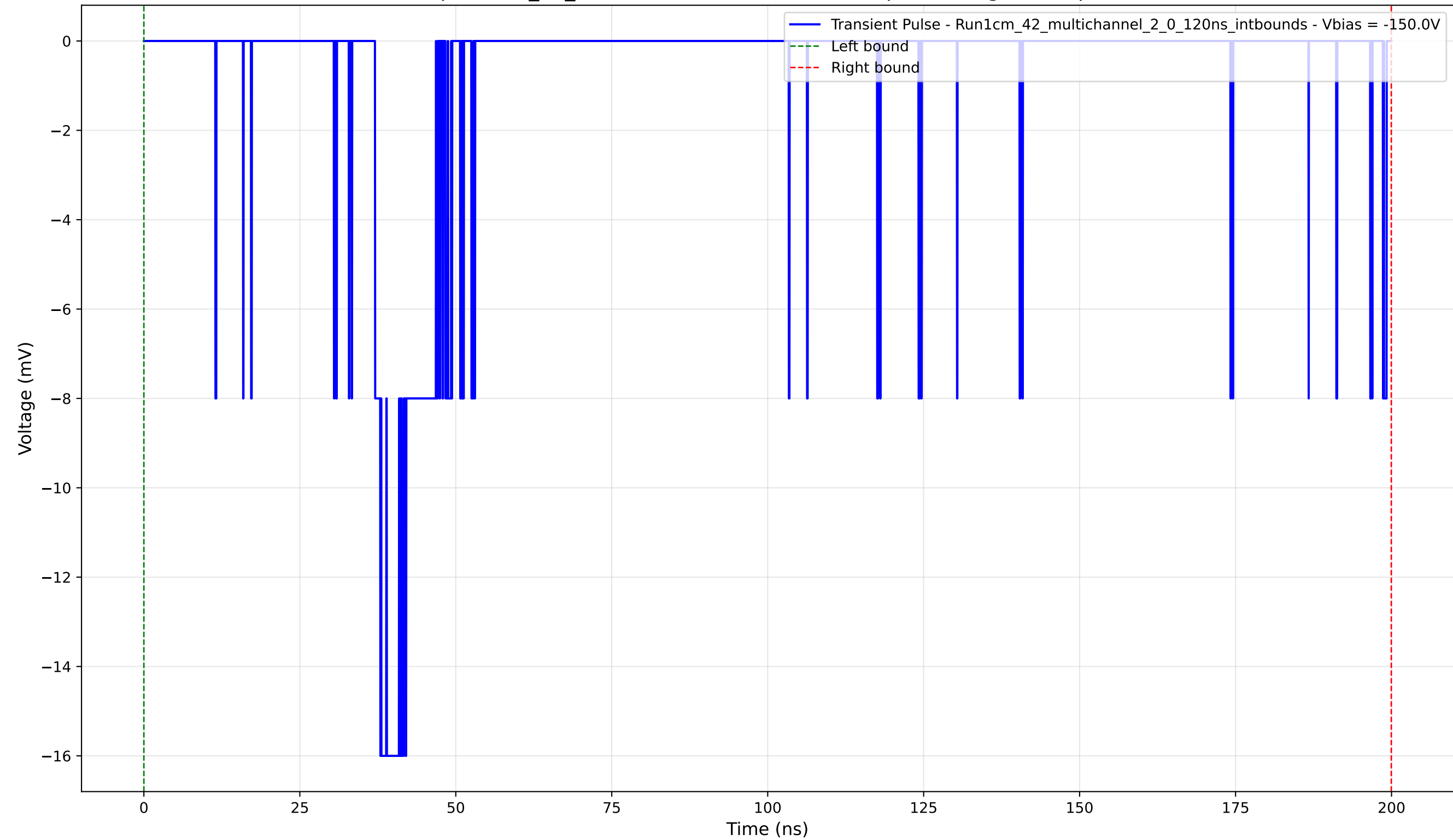
Transient Pulse - Sample: 1cm_42_multichannel - Position: 825.0 \mu\text{m} - Charge: 2.94 pC - Rise Time: 0.87 ns
