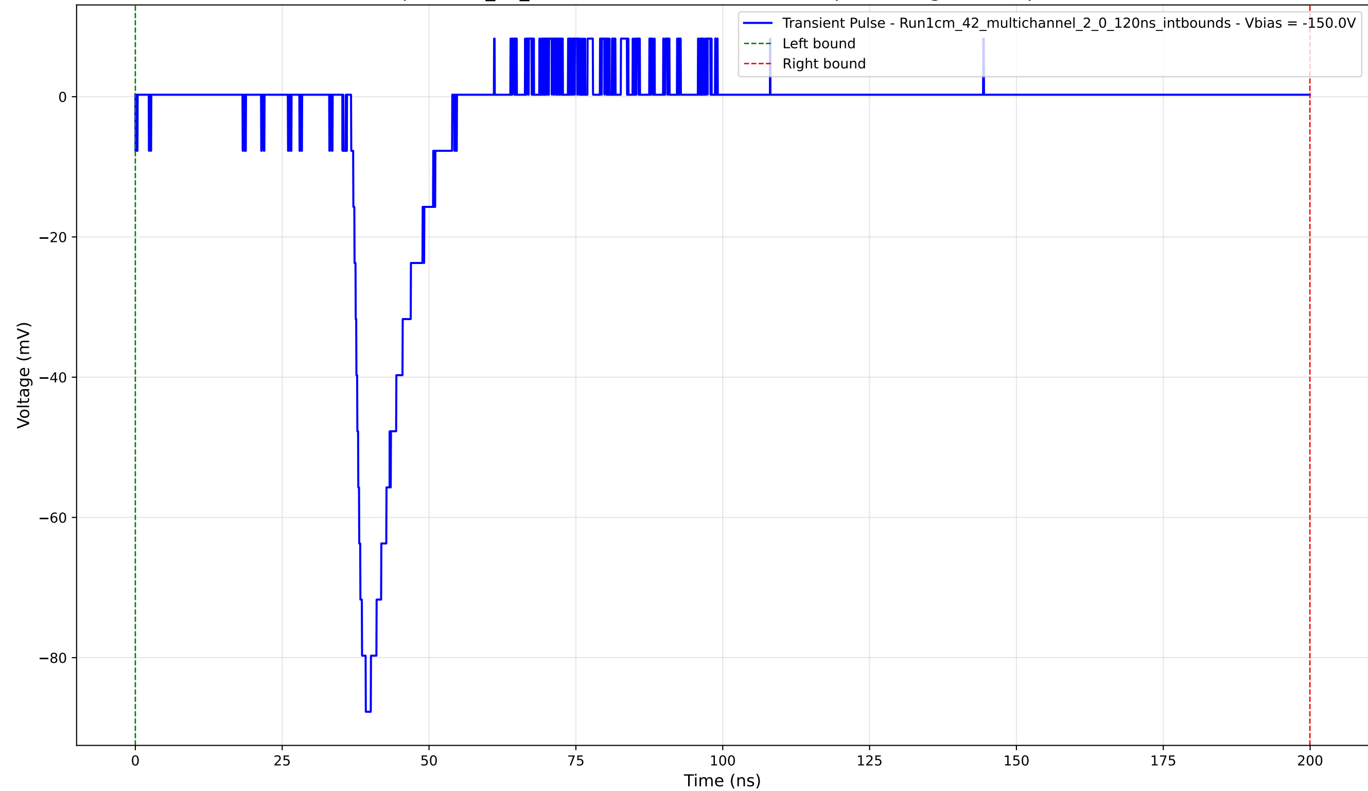
Transient Pulse - Sample: 1cm_42_multichannel - Position: 4100.0 \mu\text{m} - Charge: 10.49 pC - Rise Time: 1.51 ns
