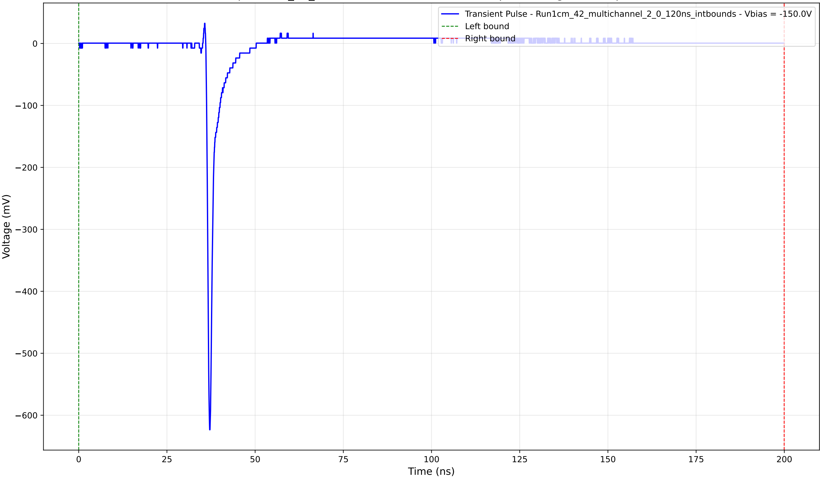
Transient Pulse - Sample: 1cm_42_multichannel - Position: 2465.0 \mu\text{m} - Charge: 14.32 pC - Rise Time: 0.73 ns
