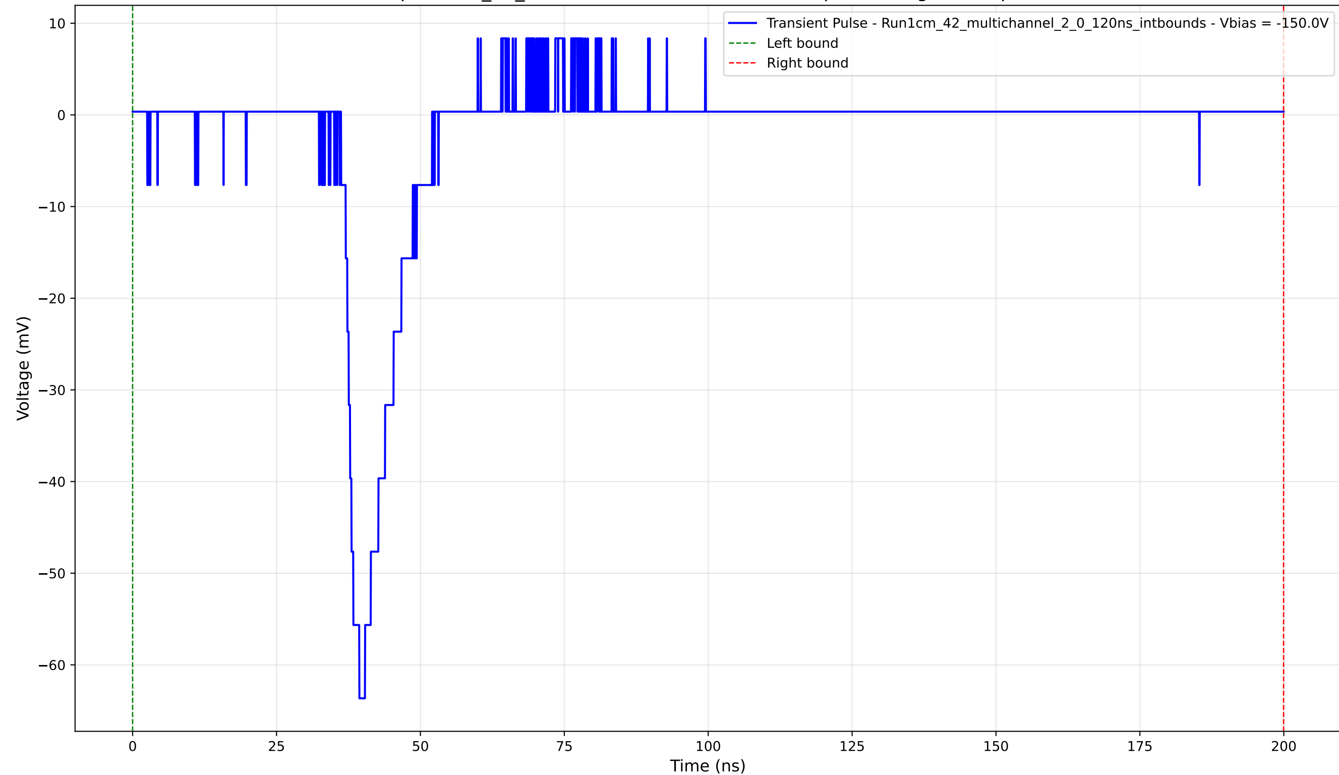
Transient Pulse - Sample: 1cm_42_multichannel - Position: 4800.0 \mu\text{m} - Charge: 7.37 pC - Rise Time: 3.17 ns
