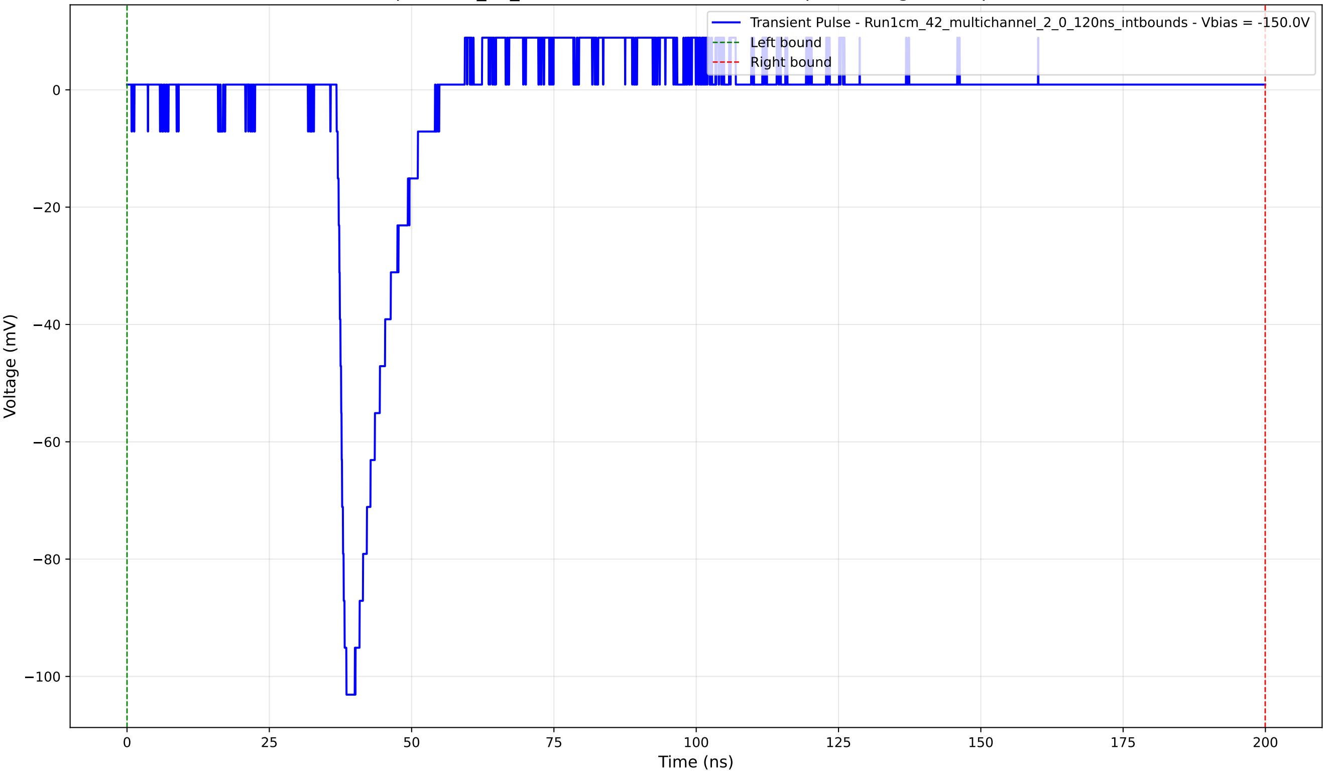
Transient Pulse - Sample: 1cm_42_multichannel - Position: 730.0 \mu\text{m} - Charge: 6.66 pC - Rise Time: 1.22 ns
