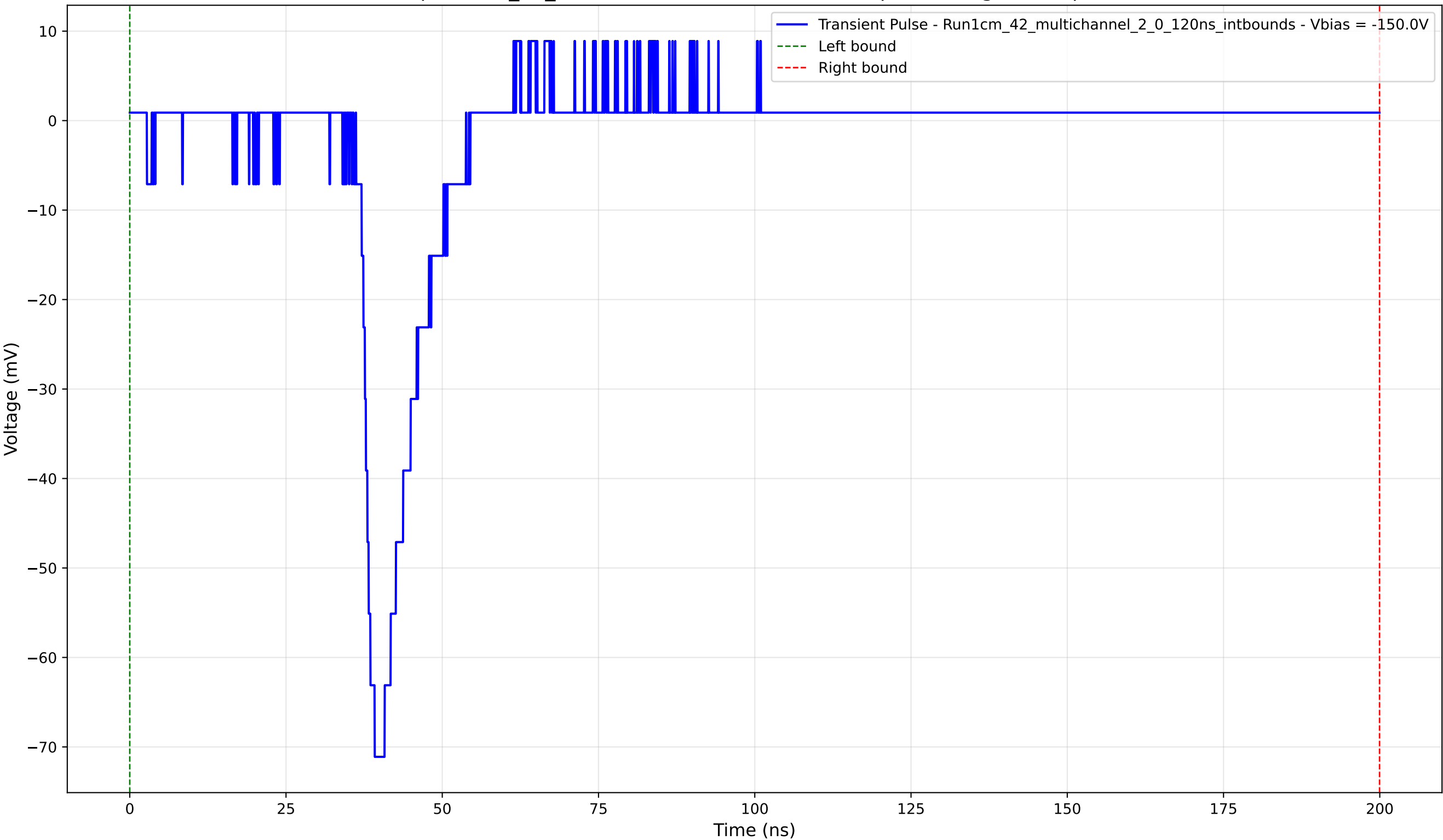
Transient Pulse - Sample: 1cm_42_multichannel - Position: 4590.0 \mu\text{m} - Charge: 7.46 pC - Rise Time: 2.12 ns
