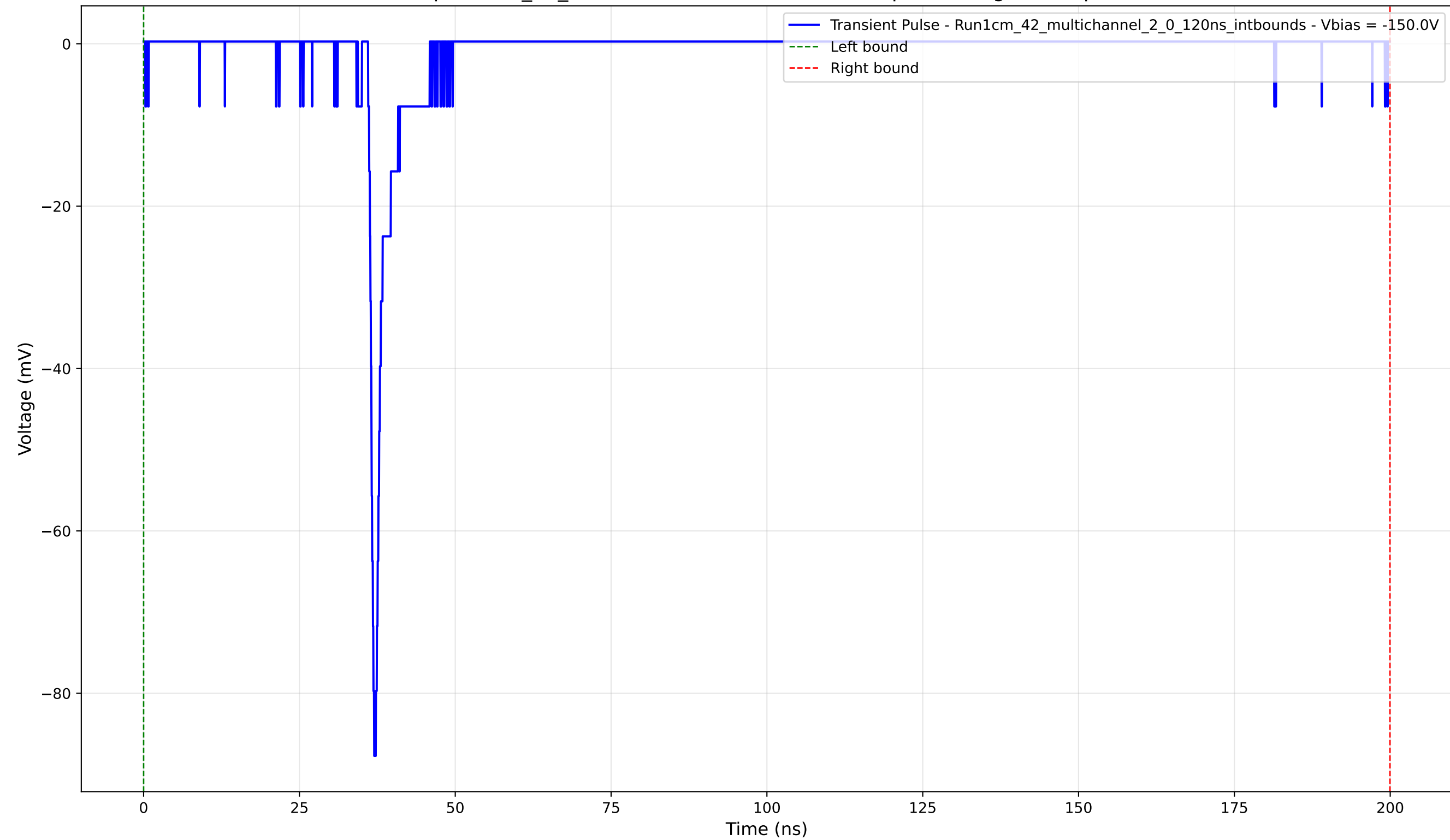
Transient Pulse - Sample: 1cm_42_multichannel - Position: 2340.0 \mu\text{m} - Charge: 3.69 pC - Rise Time: 0.71 ns
