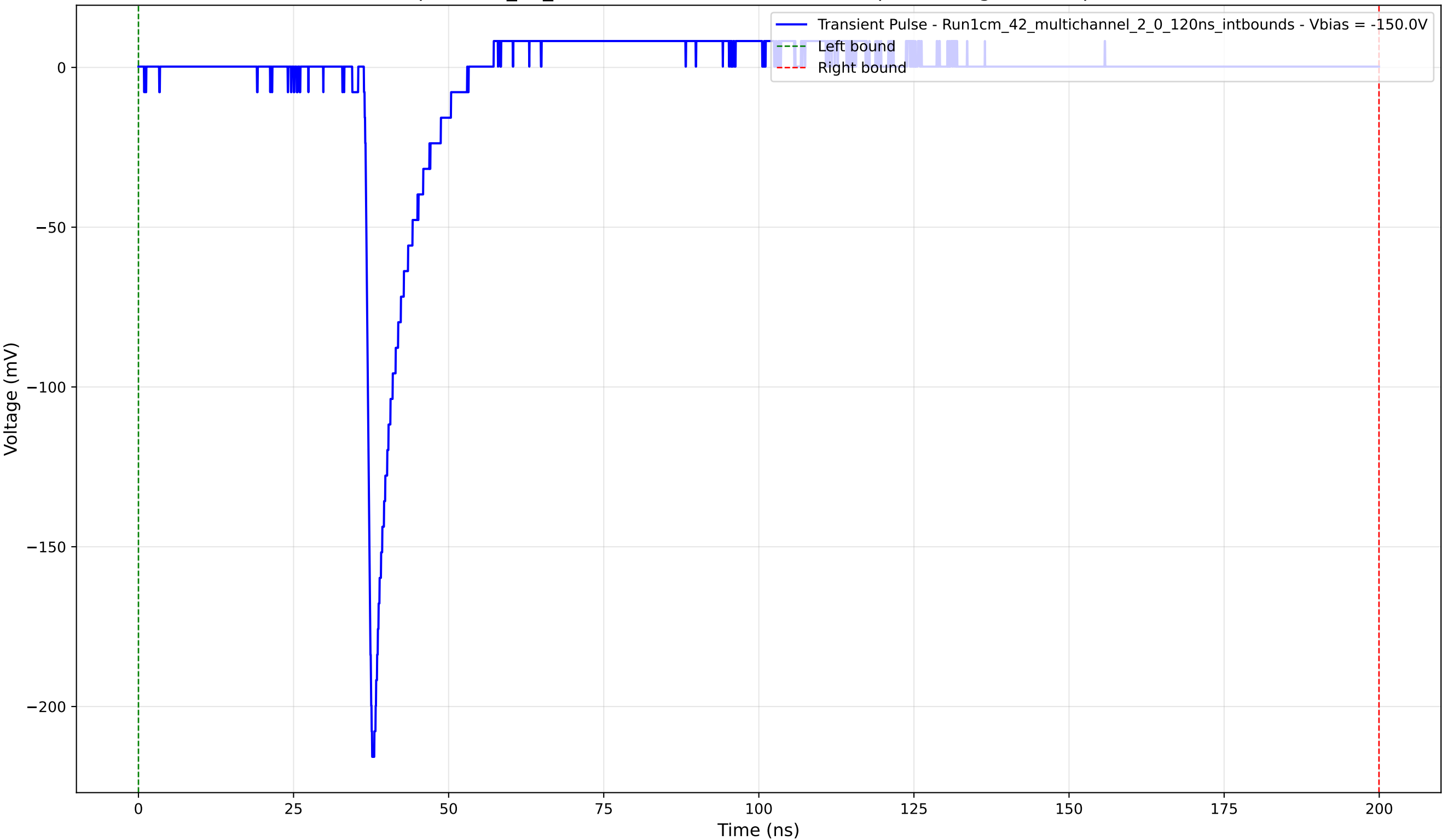
Transient Pulse - Sample: 1cm_42_multichannel - Position: 1525.0 \mu\text{m} - Charge: 11.71 pC - Rise Time: 0.97 ns
