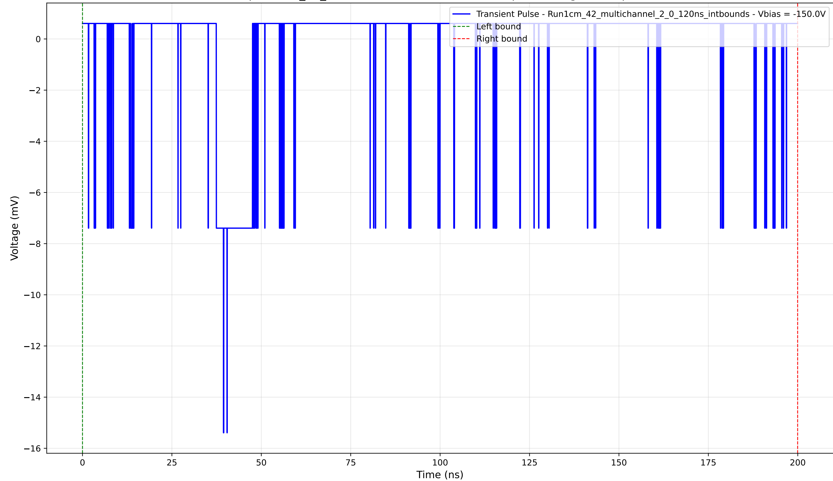
Transient Pulse - Sample: 1cm_42_multichannel - Position: 4415.0 \mu\text{m} - Charge: 0.51 pC - Rise Time: 2.03 ns
