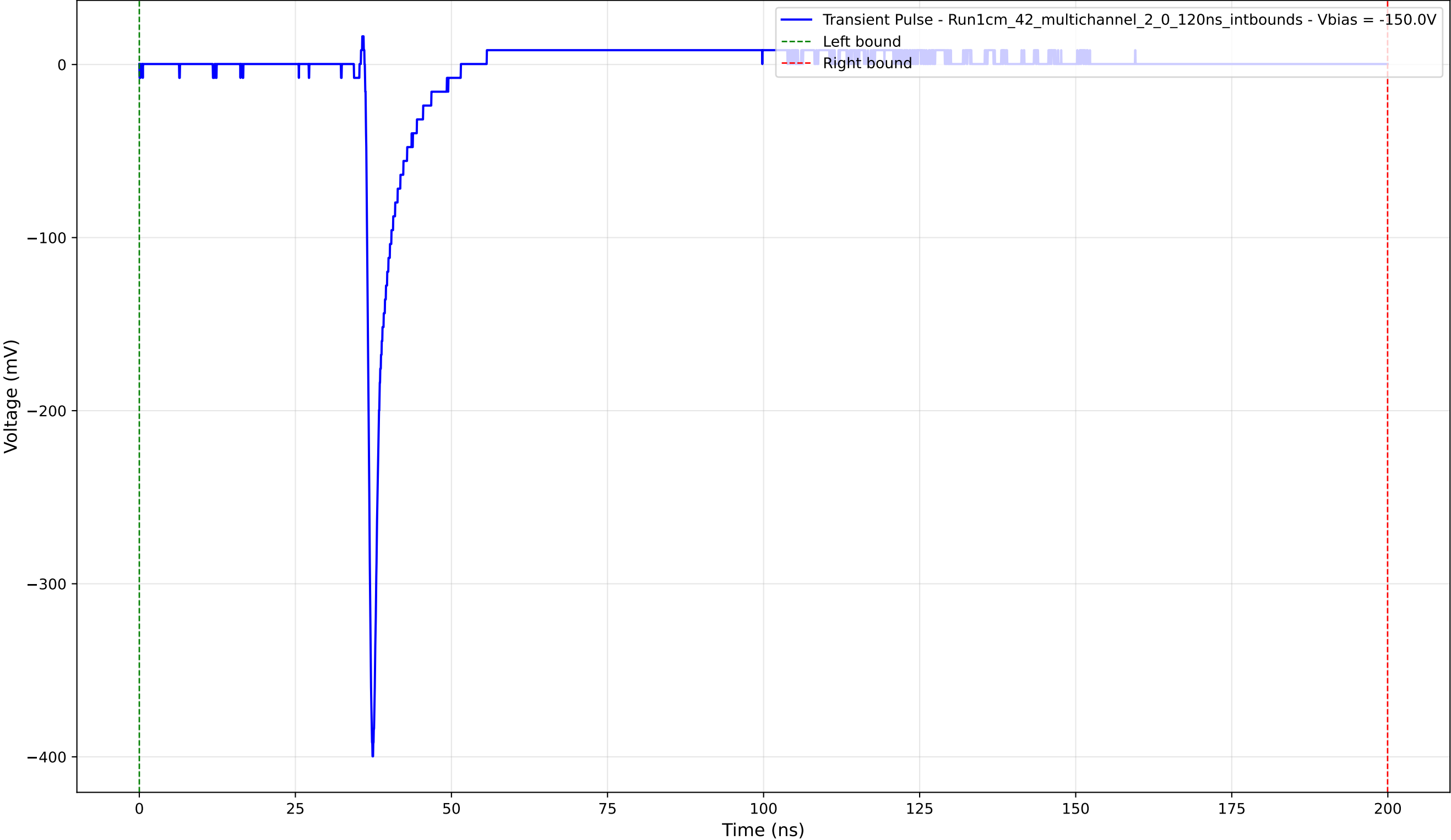
Transient Pulse - Sample: 1cm_42_multichannel - Position: 2755.0 \mu\text{m} - Charge: 12.23 pC - Rise Time: 0.80 ns
