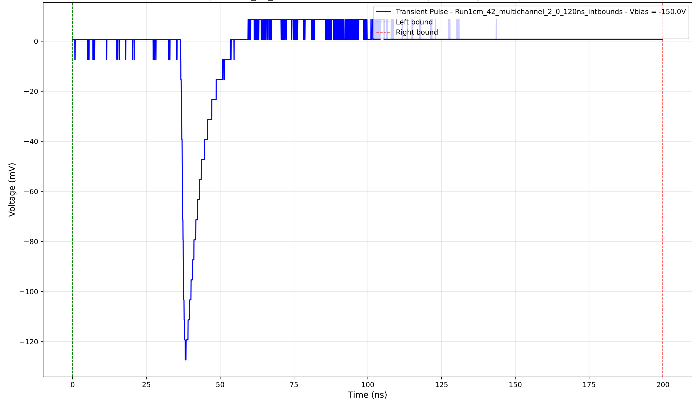
Transient Pulse - Sample: 1cm_42_multichannel - Position: 3540.0 \mu\text{m} - Charge: 8.99 pC - Rise Time: 1.25 ns
