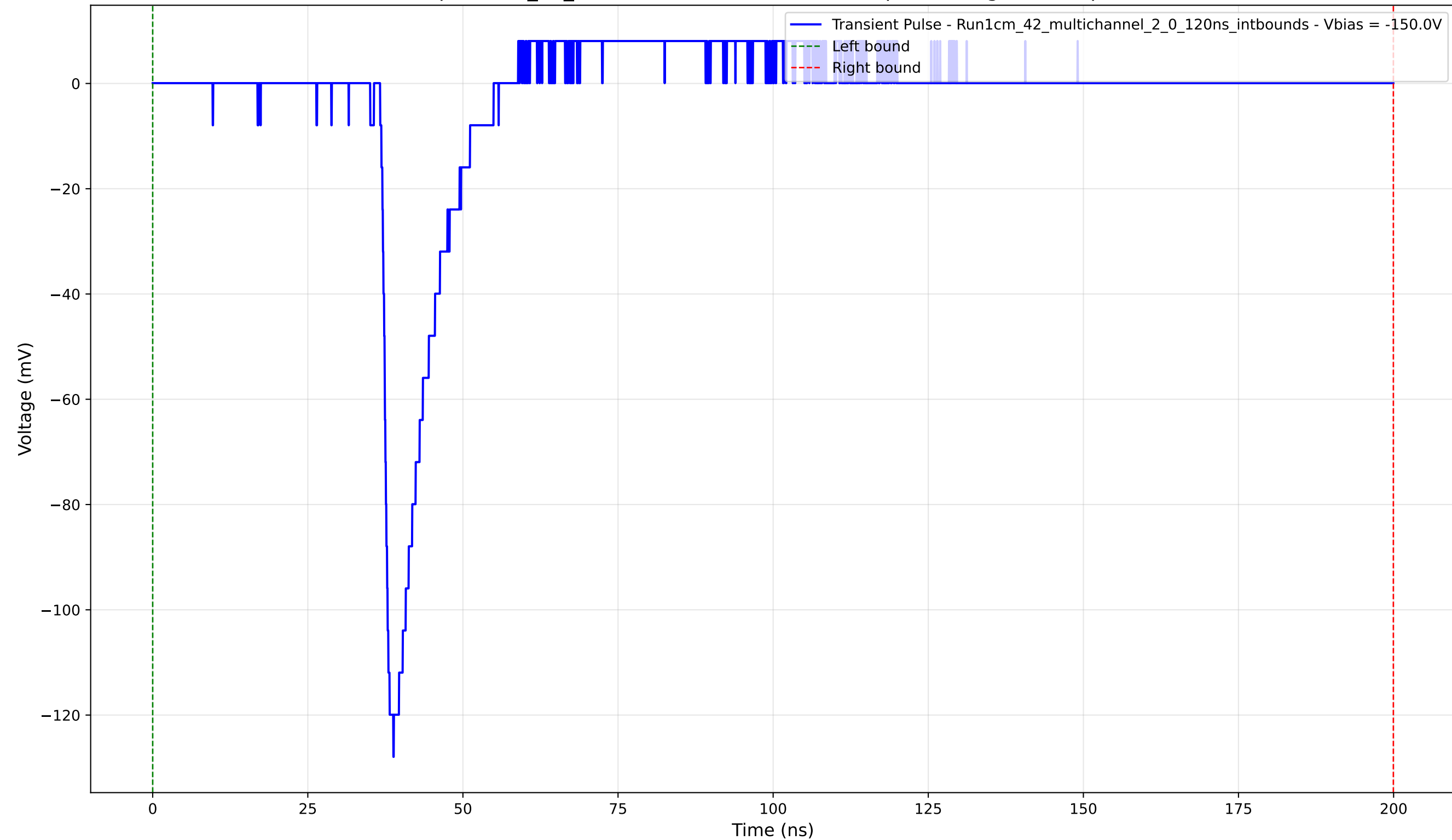
Transient Pulse - Sample: 1cm_42_multichannel - Position: 995.0 \mu\text{m} - Charge: 10.01 pC - Rise Time: 1.34 ns
