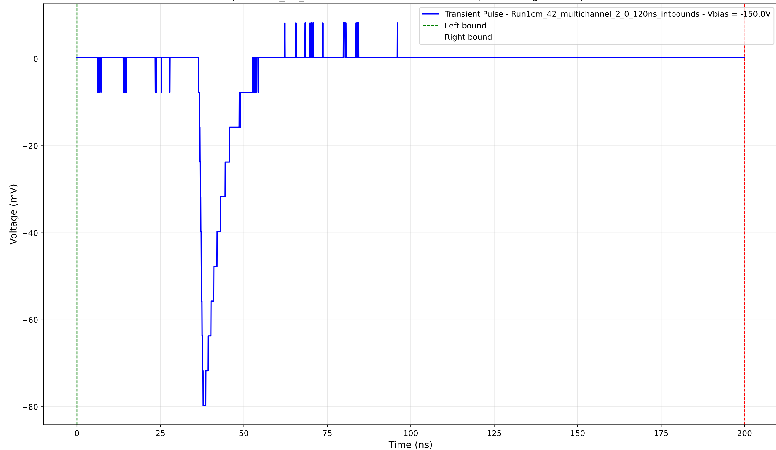
Transient Pulse - Sample: 1cm_42_multichannel - Position: 3435.0 \mu\text{m} - Charge: 9.04 pC - Rise Time: 1.12 ns
