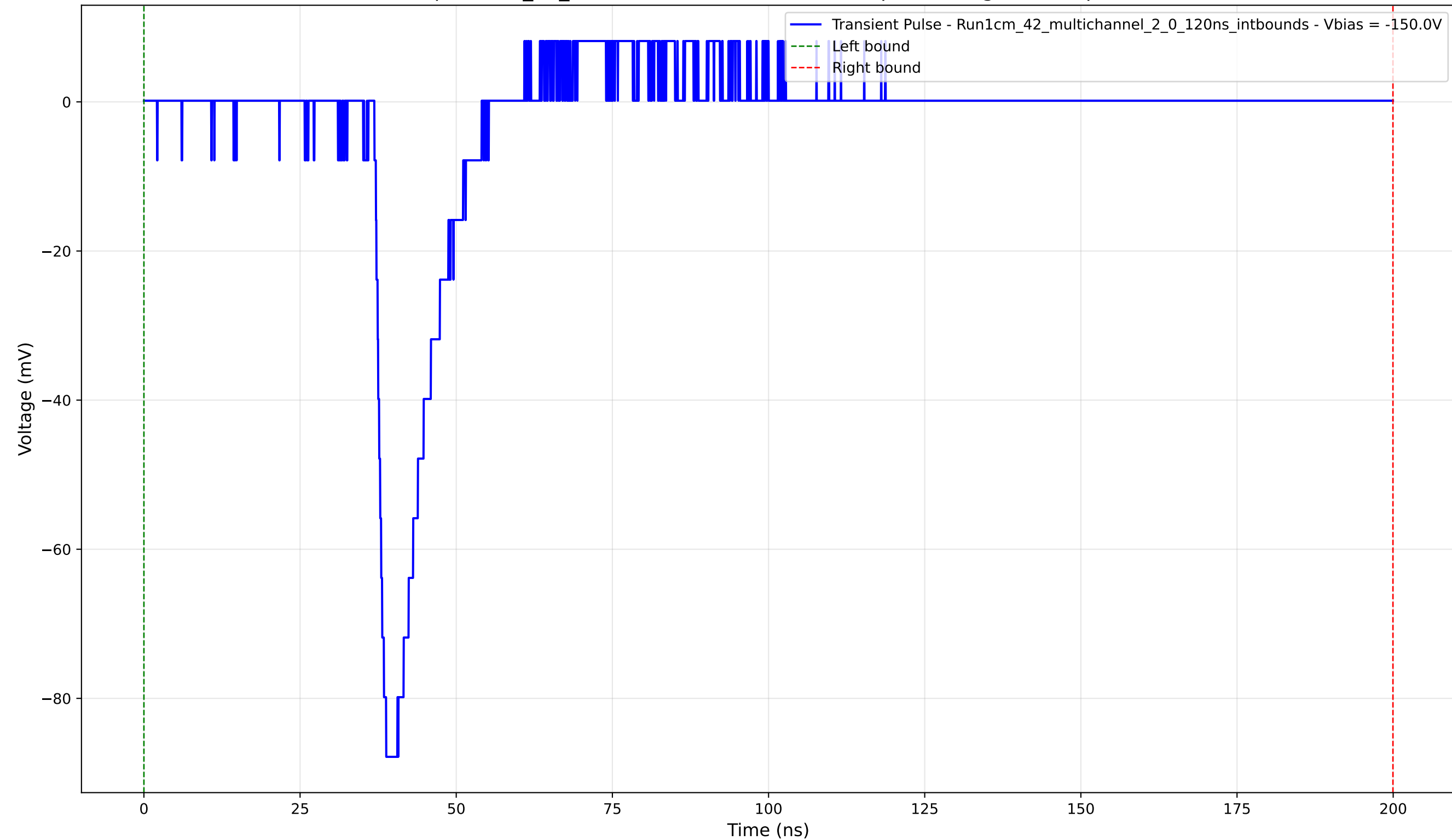
Transient Pulse - Sample: 1cm_42_multichannel - Position: 445.0 \mu\text{m} - Charge: 10.16 pC - Rise Time: 1.32 ns
