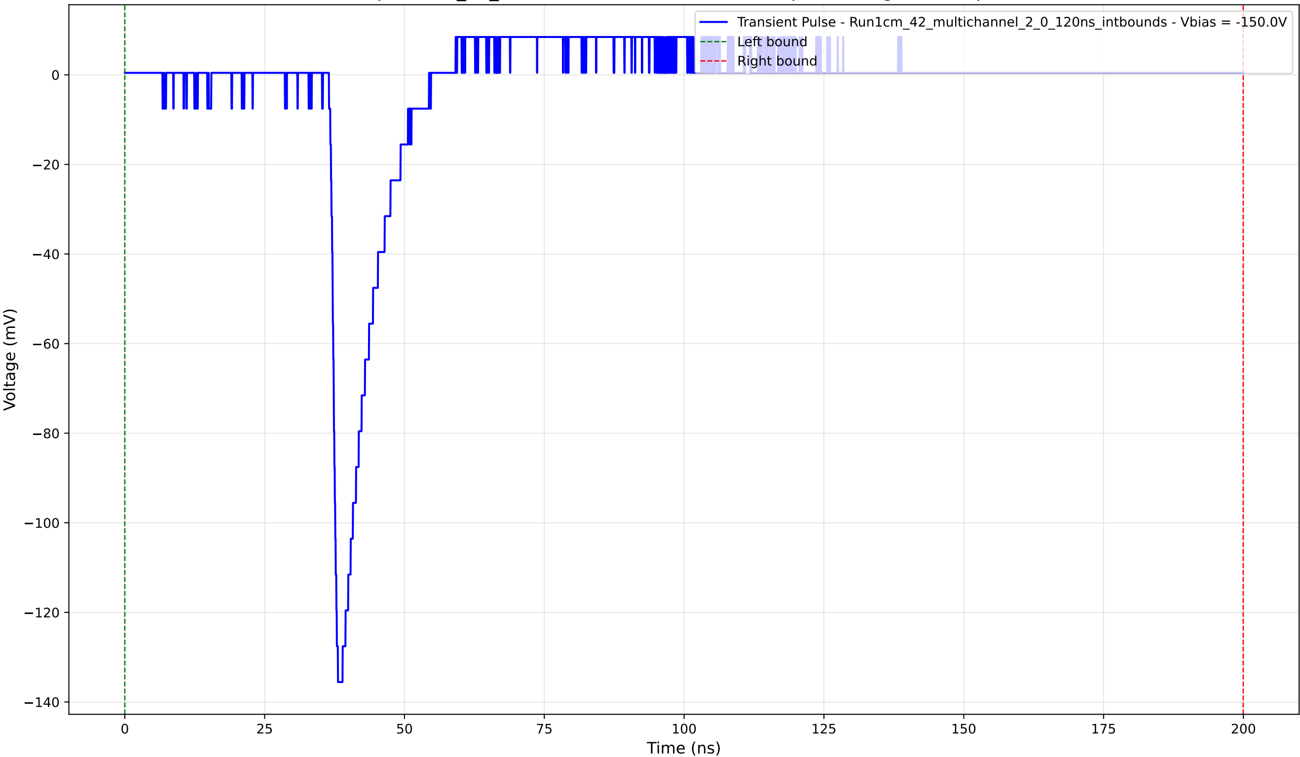
Transient Pulse - Sample: 1cm_42_multichannel - Position: 1130.0 \mu\text{m} - Charge: 10.01 pC - Rise Time: 1.17 ns
