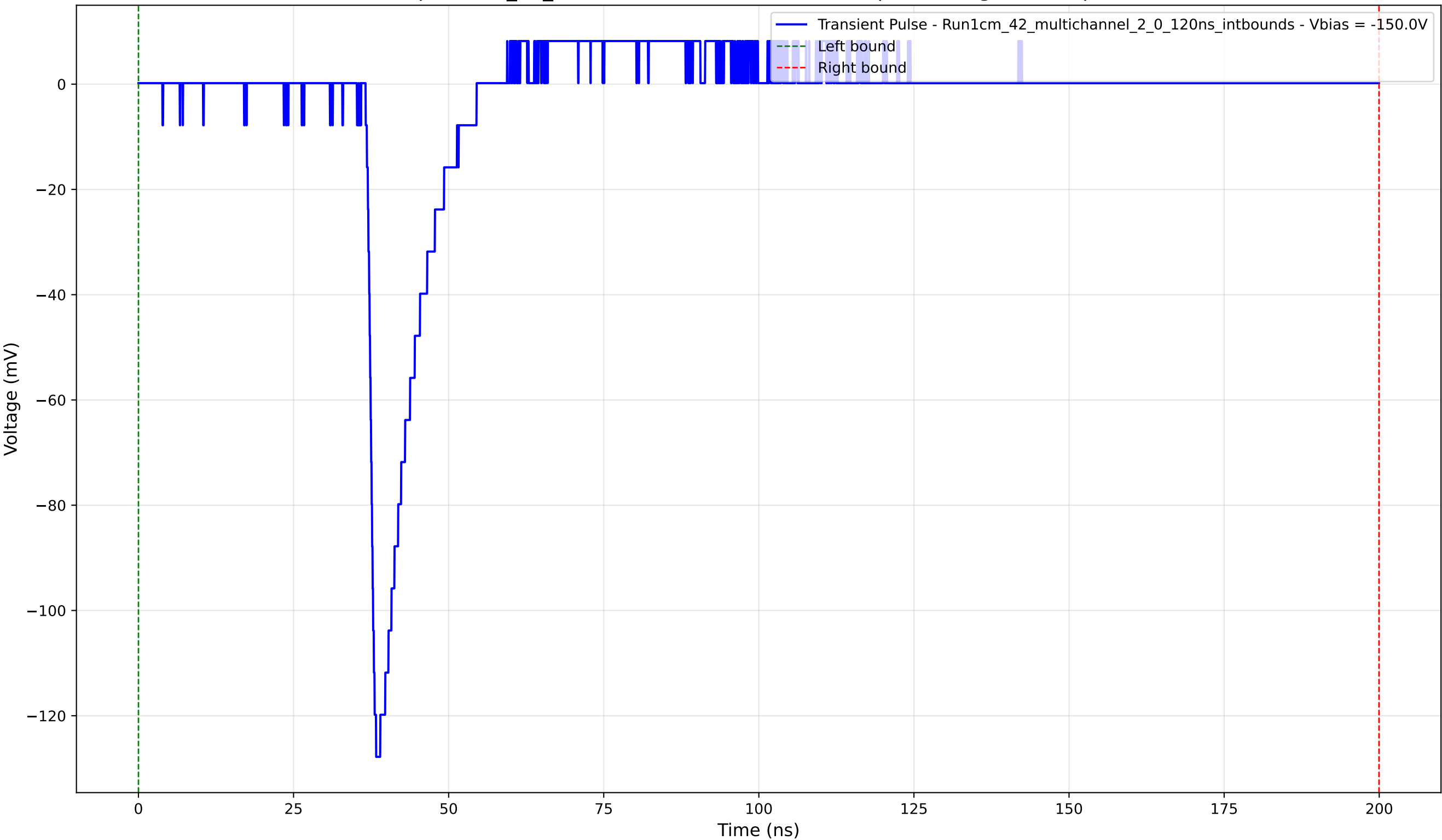
Transient Pulse - Sample: 1cm_42_multichannel - Position: 1010.0 \mu\text{m} - Charge: 11.18 pC - Rise Time: 1.26 ns
