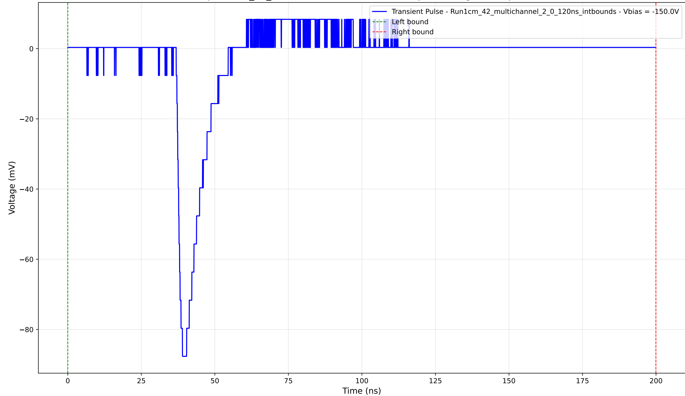
Transient Pulse - Sample: 1cm_42_multichannel - Position: 435.0 \mu\text{m} - Charge: 8.86 pC - Rise Time: 1.43 ns
