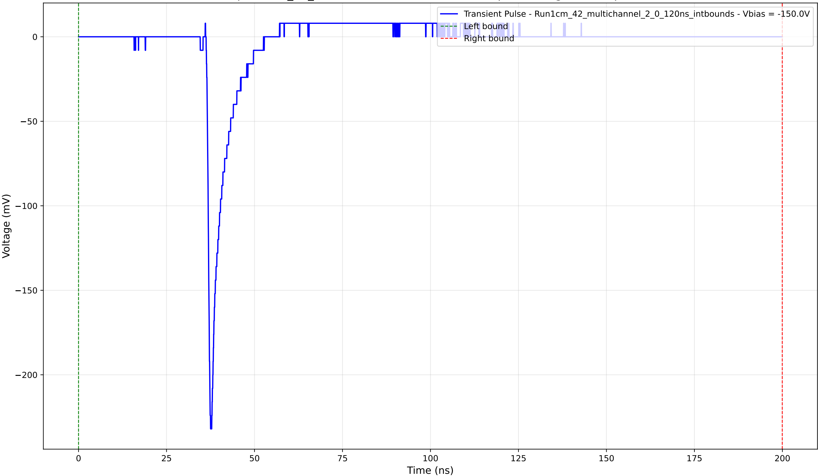
Transient Pulse - Sample: 1cm_42_multichannel - Position: 3050.0 \mu\text{m} - Charge: 12.18 pC - Rise Time: 0.89 ns
