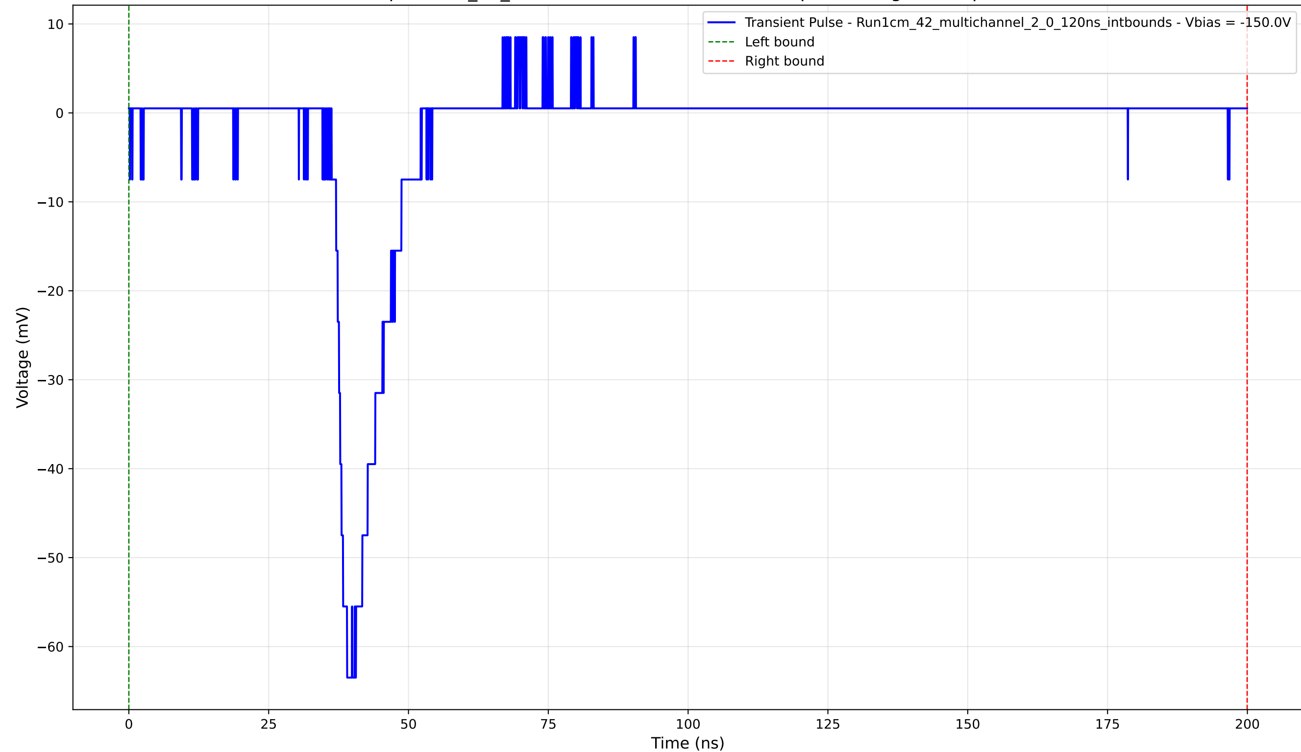
Transient Pulse - Sample: 1cm_42_multichannel - Position: 4790.0 \mu\text{m} - Charge: 7.68 pC - Rise Time: 2.77 ns
