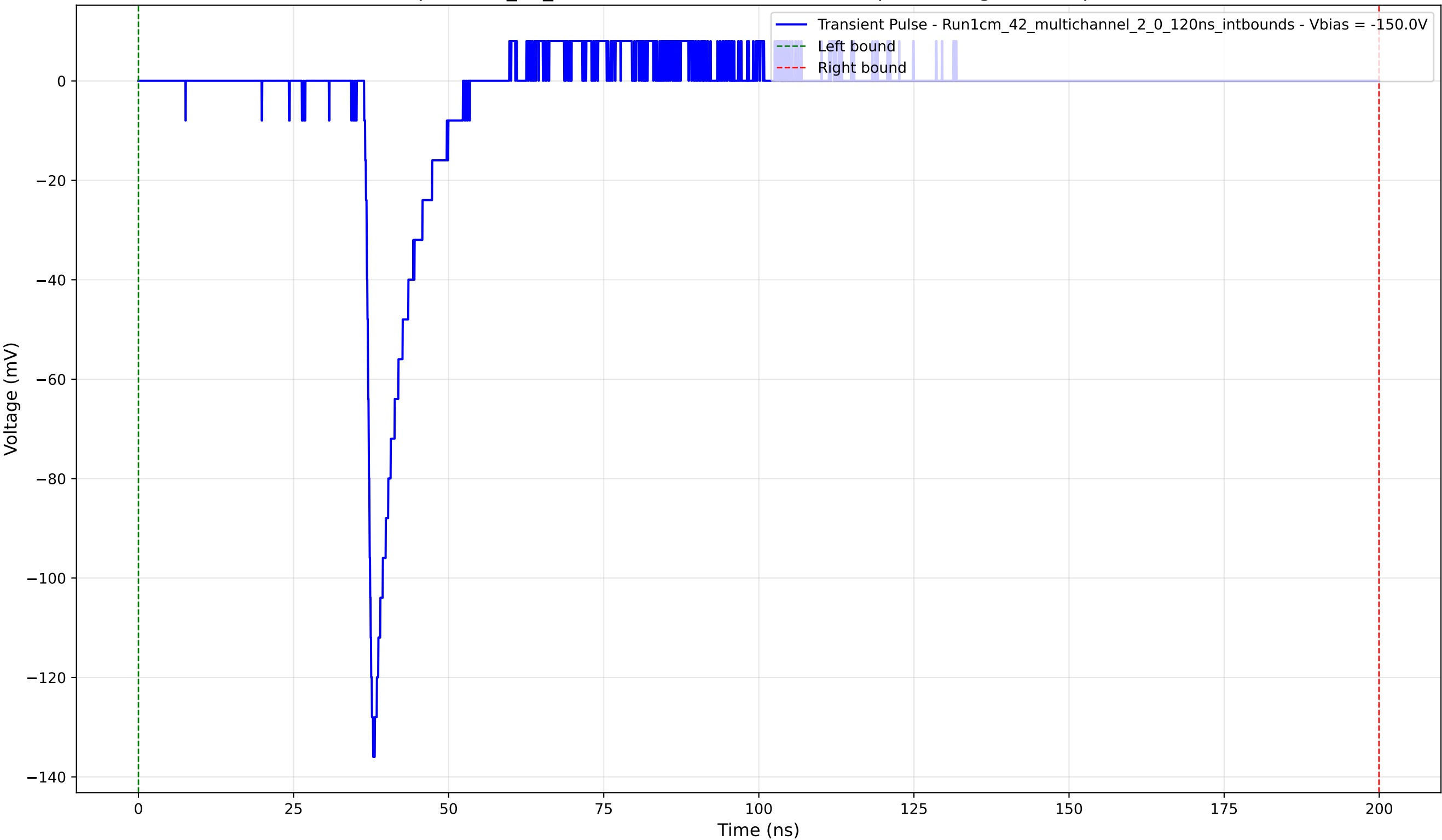
Transient Pulse - Sample: 1cm_42_multichannel - Position: 3315.0 \mu\text{m} - Charge: 10.35 pC - Rise Time: 1.09 ns
