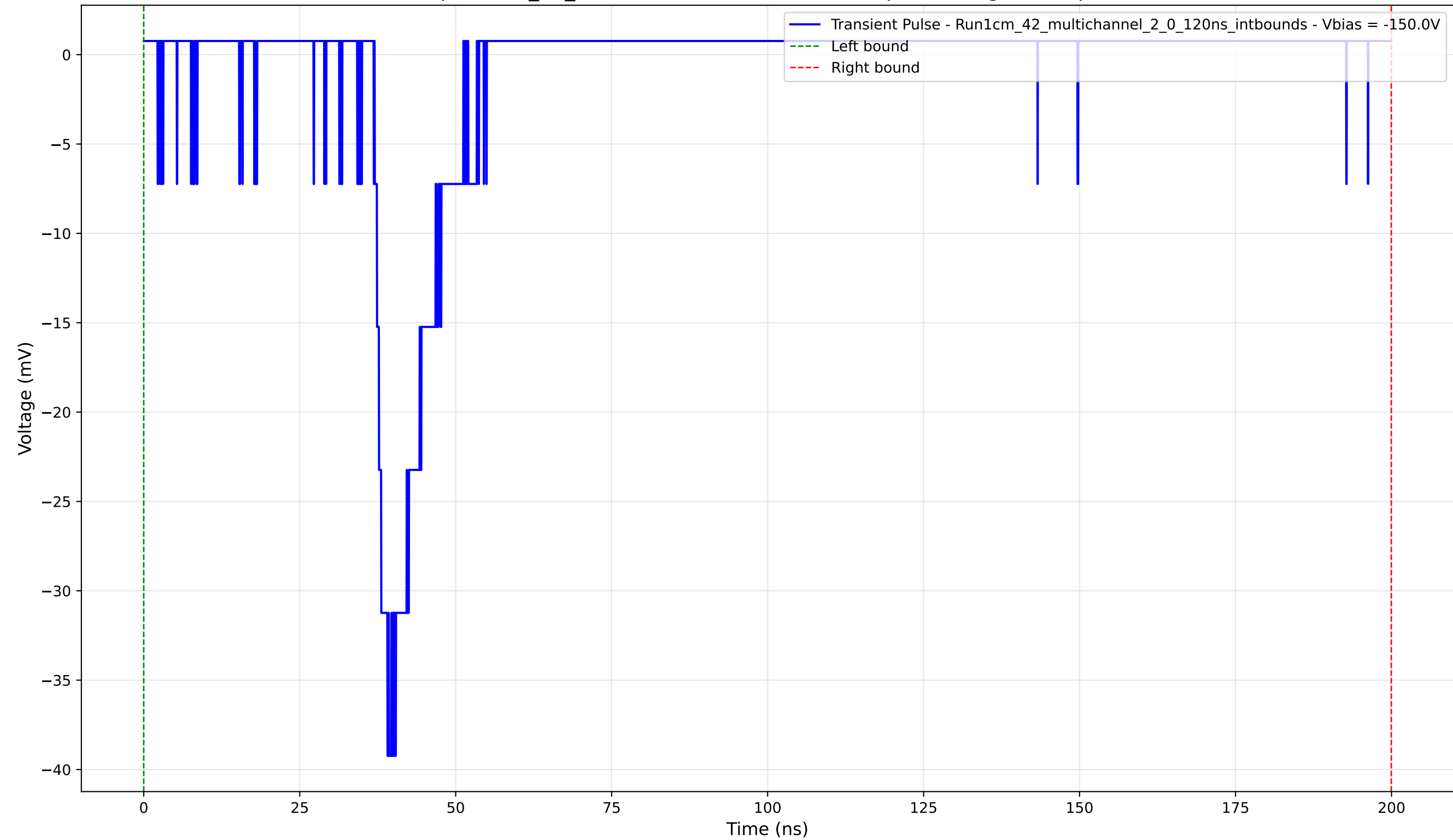
Transient Pulse - Sample: 1cm_42_multichannel - Position: 390.0 \mu\text{m} - Charge: 3.46 pC - Rise Time: 2.06 ns
