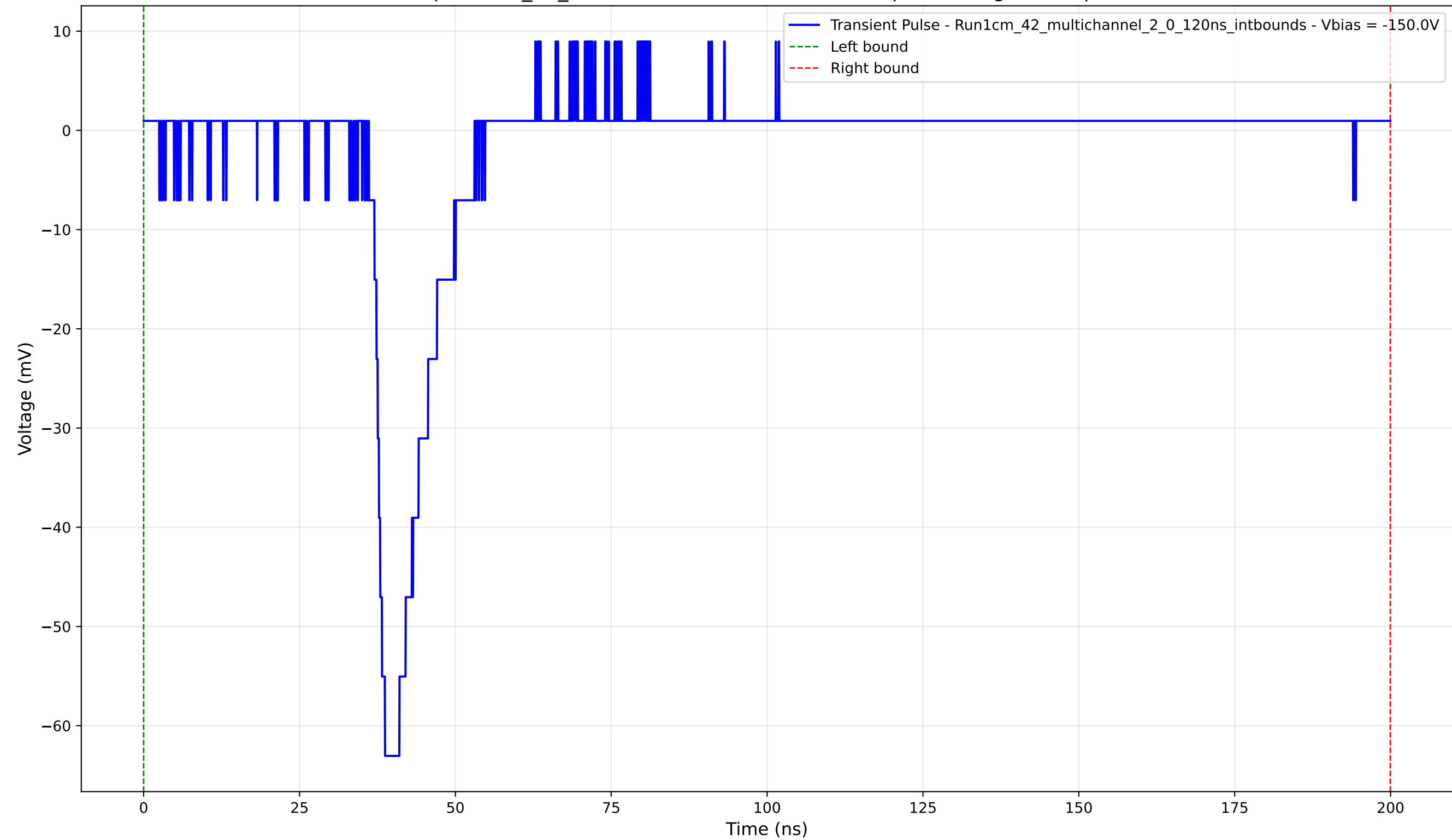
Transient Pulse - Sample: 1cm_42_multichannel - Position: 4765.0 \mu\text{m} - Charge: 6.57 pC - Rise Time: 2.56 ns
