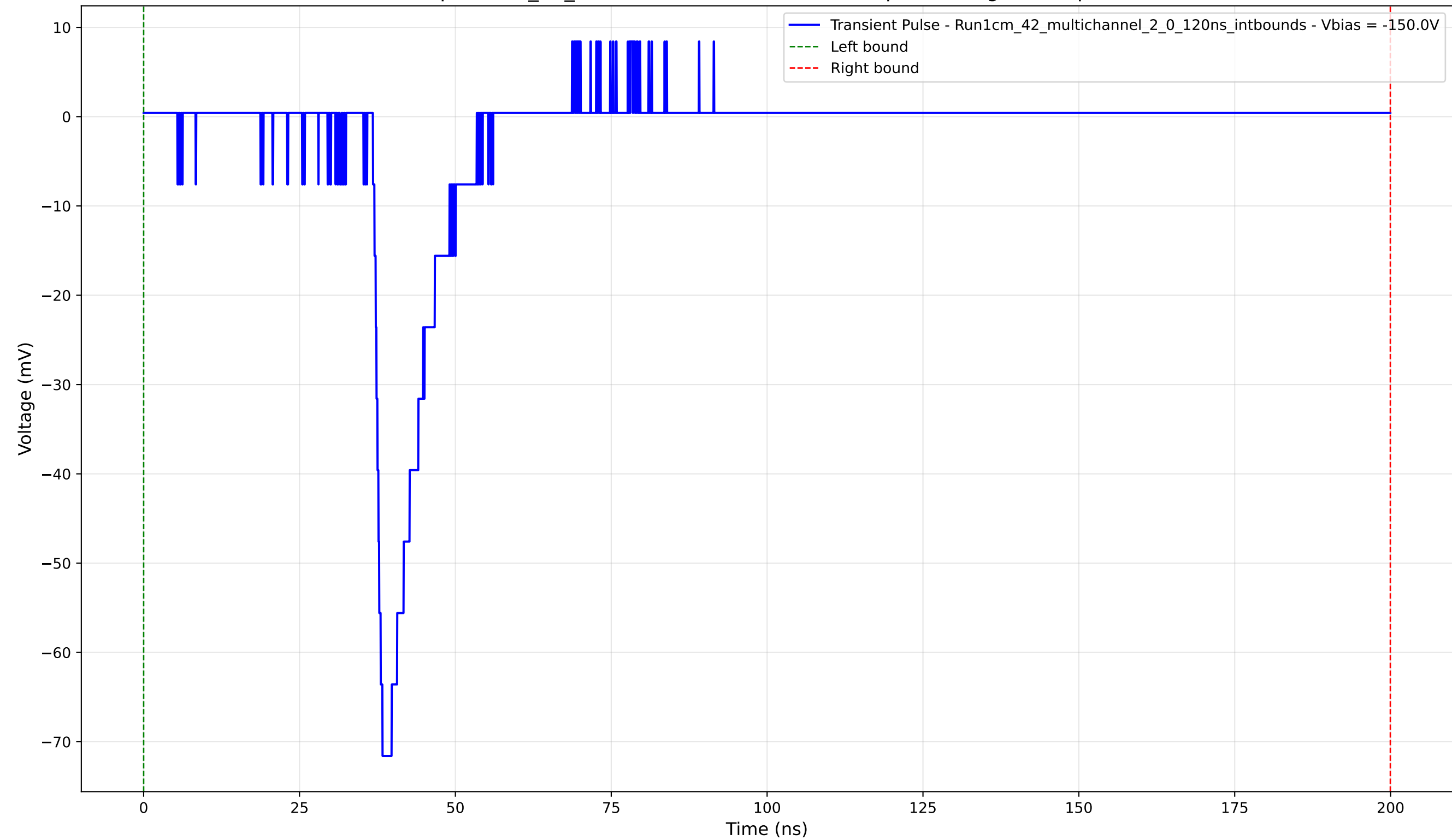
Transient Pulse - Sample: 1cm_42_multichannel - Position: 905.0 \mu\text{m} - Charge: 8.89 pC - Rise Time: 1.52 ns
