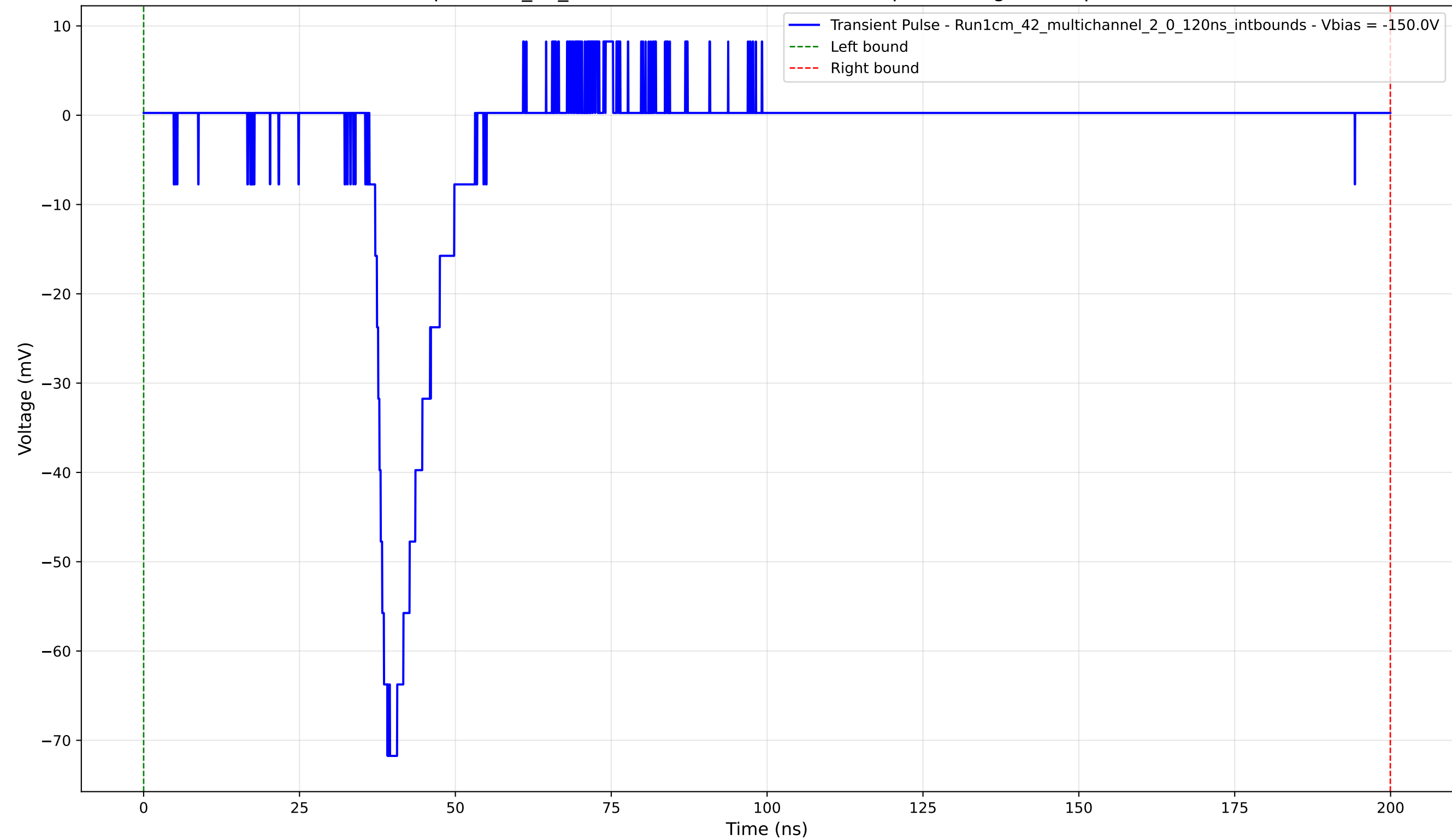
Transient Pulse - Sample: 1cm_42_multichannel - Position: 4630.0 \mu\text{m} - Charge: 9.31 pC - Rise Time: 2.88 ns
