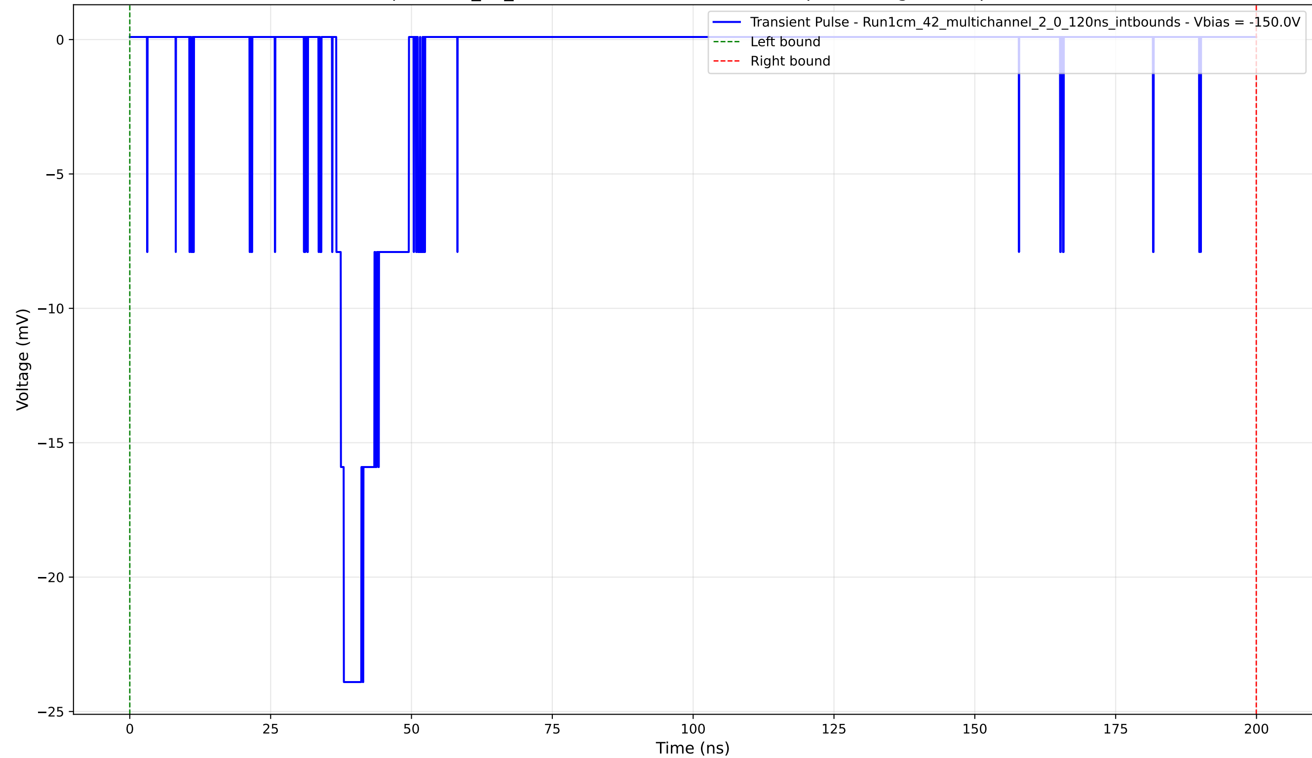
Transient Pulse - Sample: 1cm_42_multichannel - Position: 3850.0 \mu\text{m} - Charge: 3.74 pC - Rise Time: 1.35 ns
