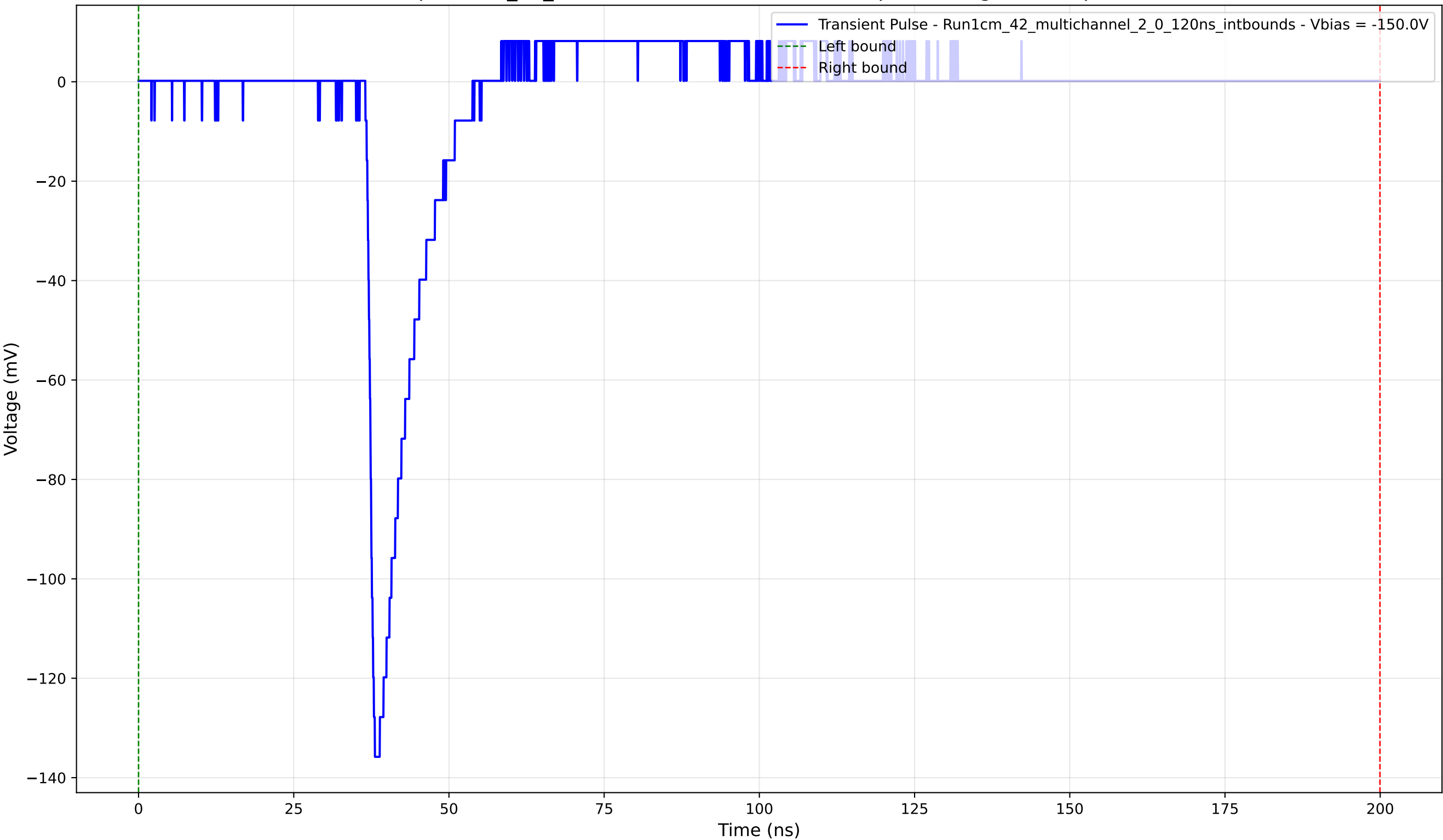
Transient Pulse - Sample: 1cm_42_multichannel - Position: 1140.0 \mu\text{m} - Charge: 10.70 pC - Rise Time: 1.17 ns
