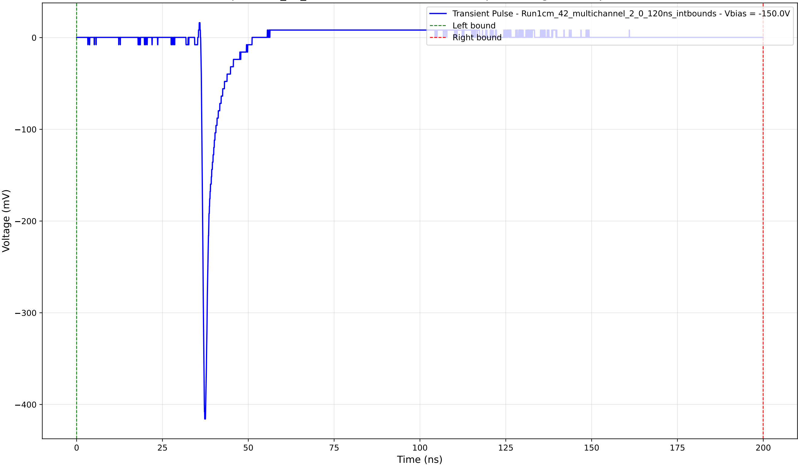
Transient Pulse - Sample: 1cm_42_multichannel - Position: 1980.0 \mu\text{m} - Charge: 14.79 pC - Rise Time: 0.79 ns
