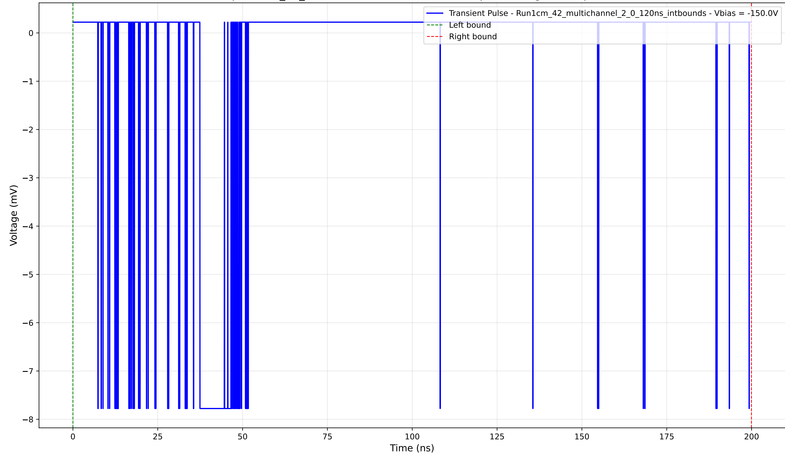
Transient Pulse - Sample: 1cm_42_multichannel - Position: 4360.0 \mu\text{m} - Charge: 1.45 pC - Rise Time: 0.04 ns
