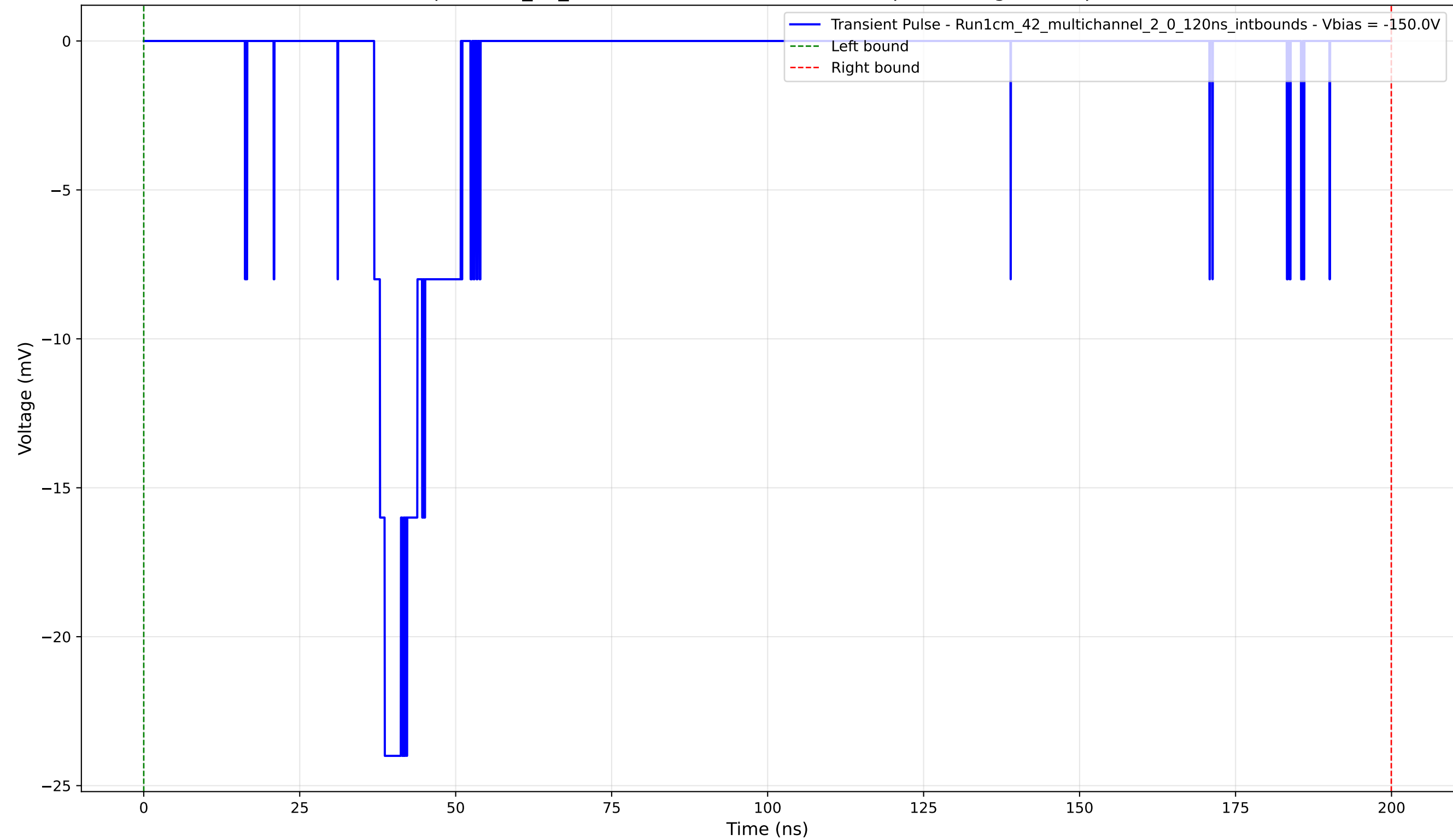
Transient Pulse - Sample: 1cm_42_multichannel - Position: 4430.0 \mu\text{m} - Charge: 4.07 pC - Rise Time: 1.71 ns
