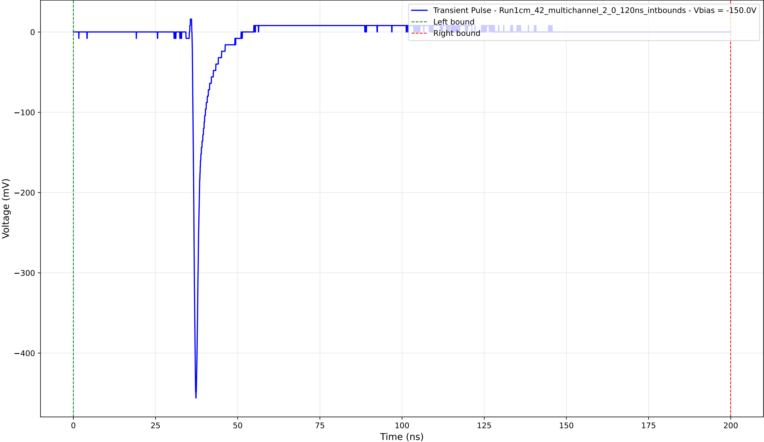
Transient Pulse - Sample: 1cm_42_multichannel - Position: 2650.0 \mu\text{m} - Charge: 14.37 pC - Rise Time: 0.74 ns
