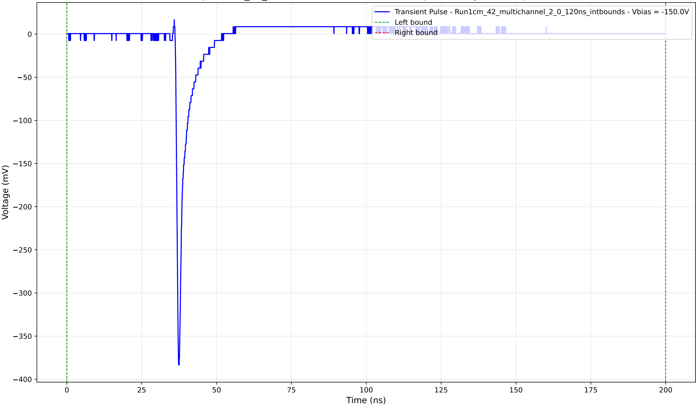
Transient Pulse - Sample: 1cm_42_multichannel - Position: 1960.0 \mu\text{m} - Charge: 12.28 pC - Rise Time: 0.77 ns
