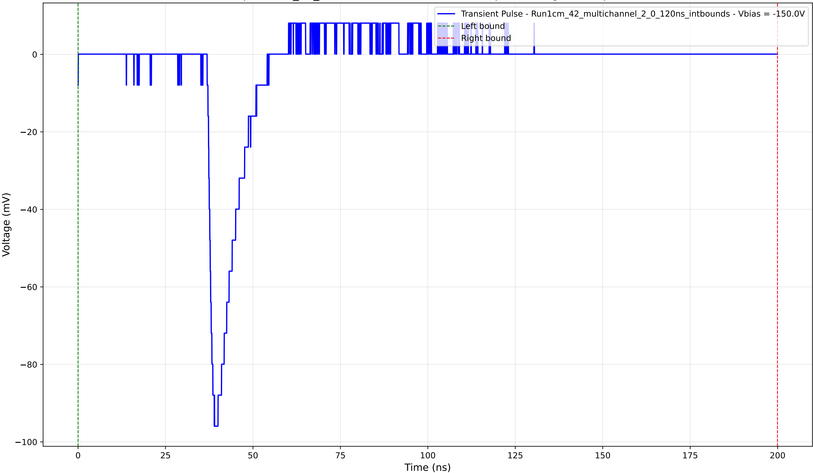
Transient Pulse - Sample: 1cm_42_multichannel - Position: 535.0 \mu\text{m} - Charge: 9.59 pC - Rise Time: 1.43 ns
