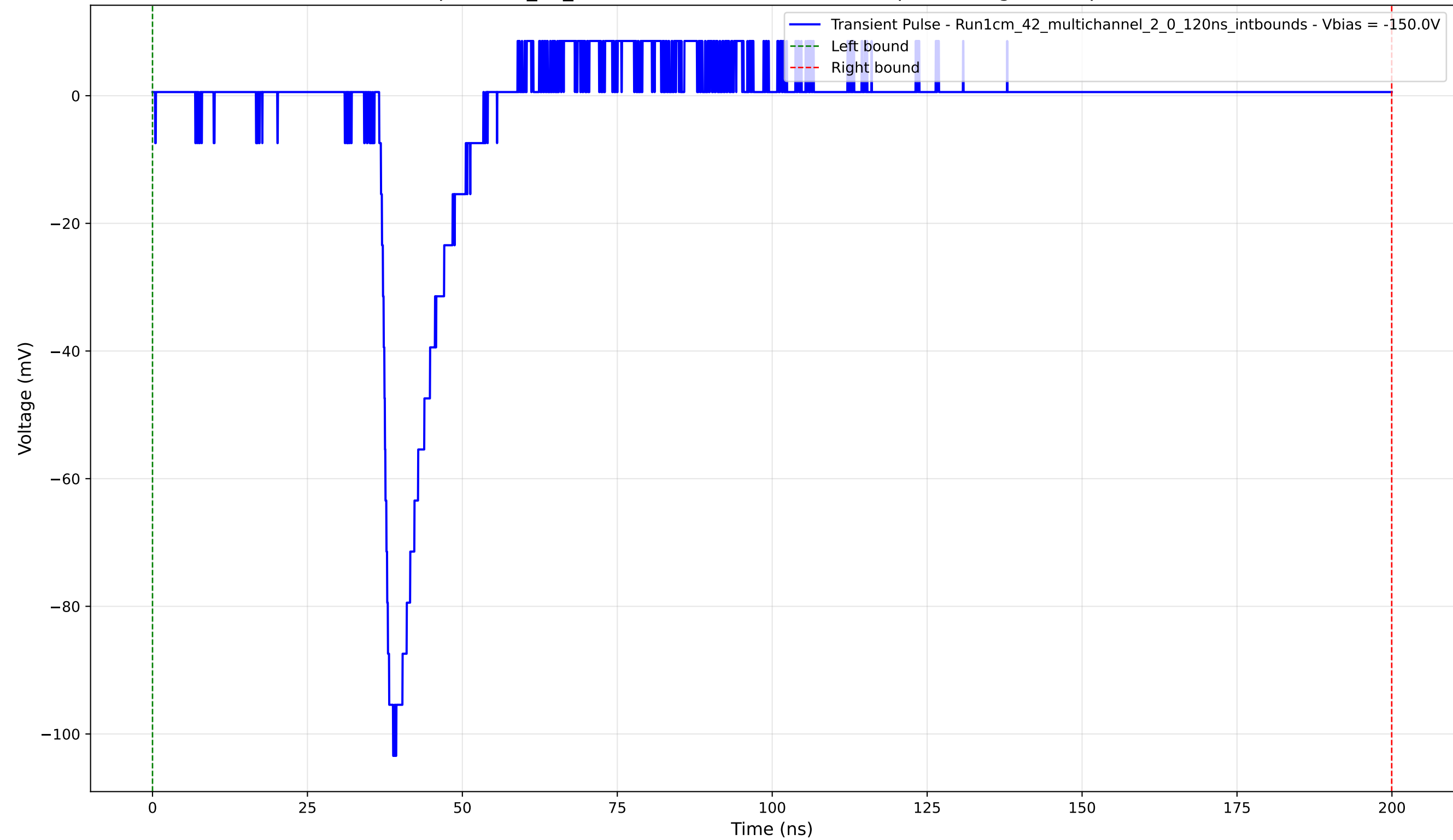
Transient Pulse - Sample: 1cm_42_multichannel - Position: 3790.0 \mu\text{m} - Charge: 8.57 pC - Rise Time: 1.35 ns
