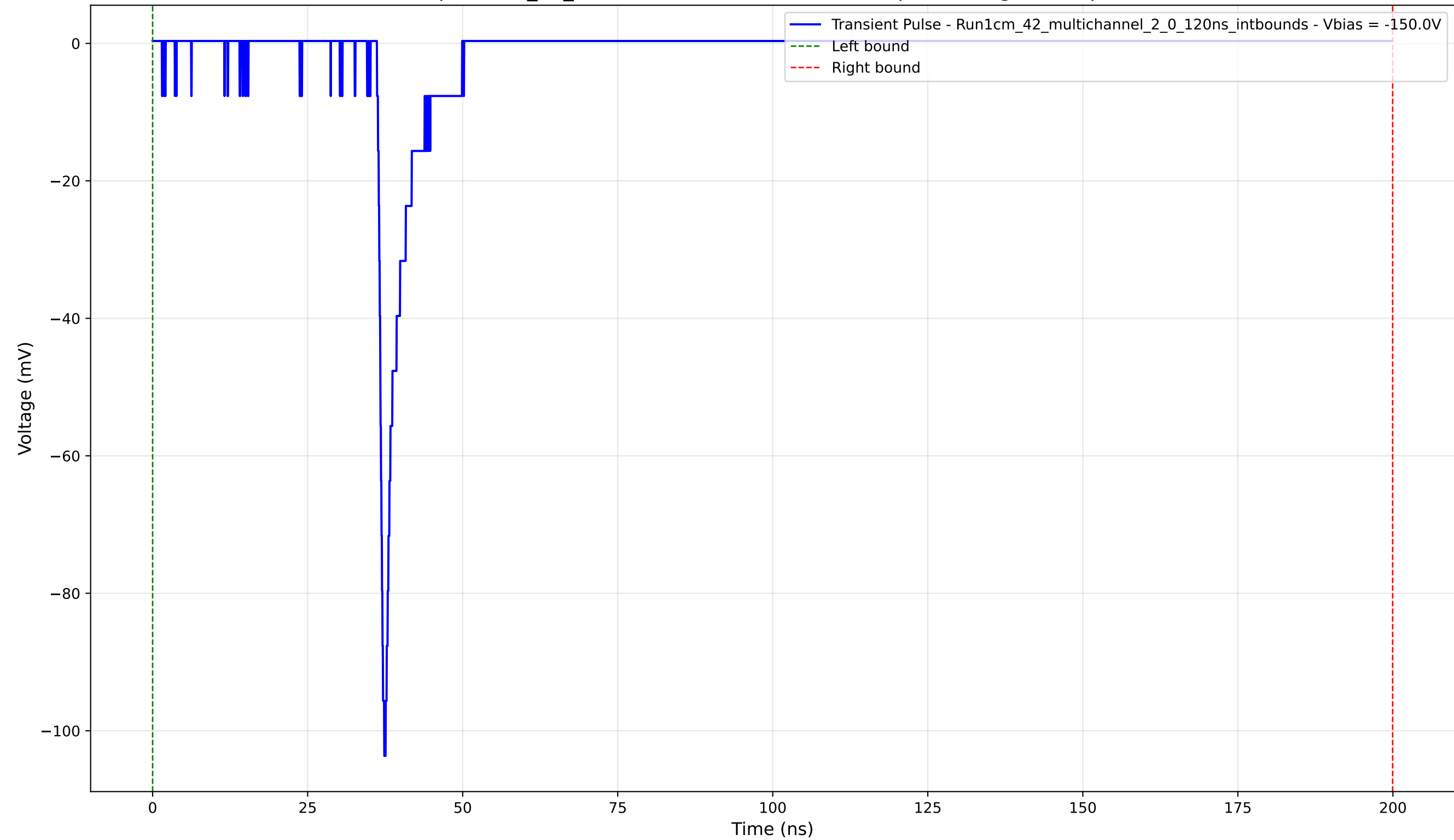
Transient Pulse - Sample: 1cm_42_multichannel - Position: 2835.0 \mu\text{m} - Charge: 6.11 pC - Rise Time: 0.83 ns
