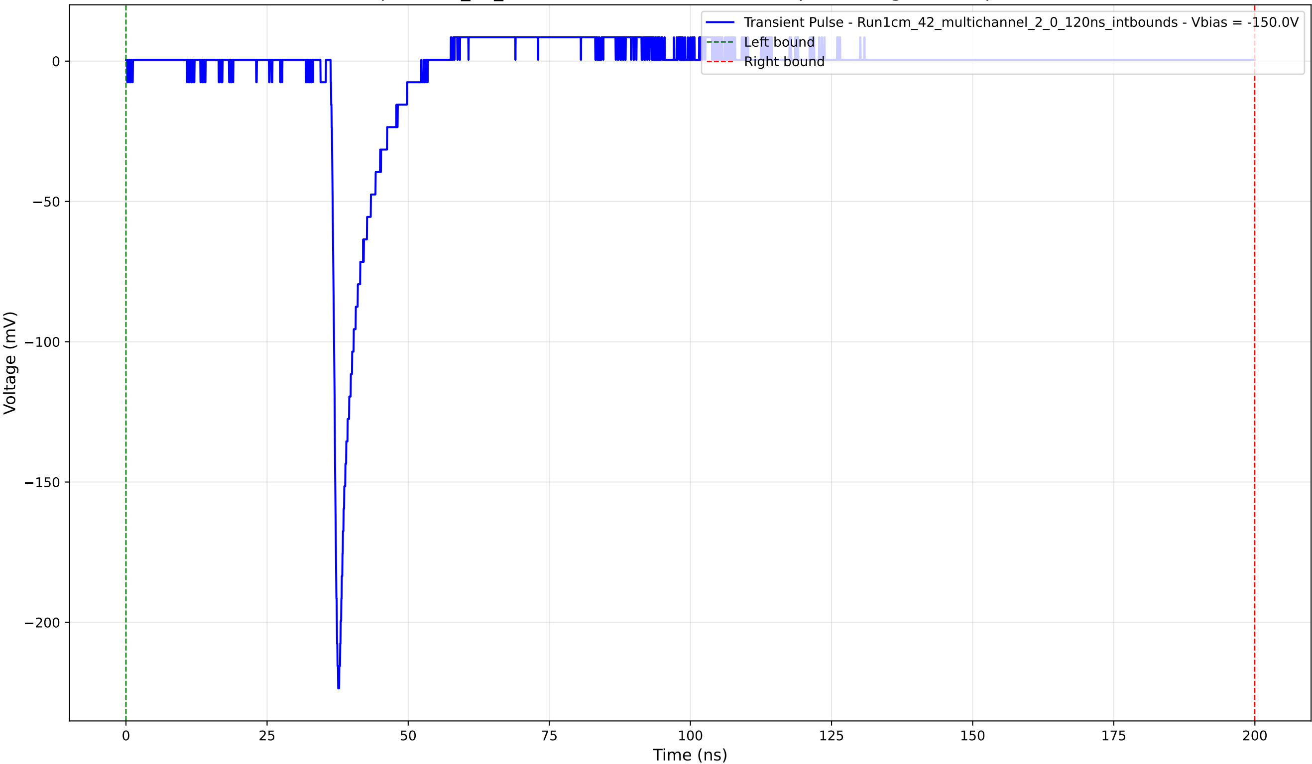
Transient Pulse - Sample: 1cm_42_multichannel - Position: 3080.0 \mu\text{m} - Charge: 12.14 pC - Rise Time: 0.97 ns
