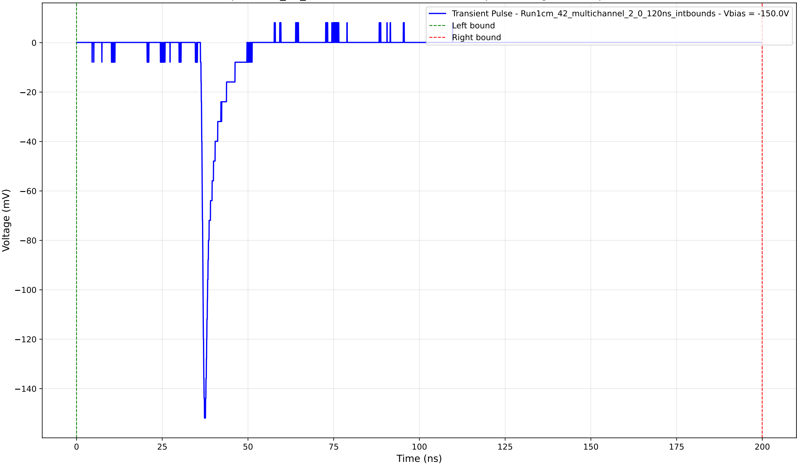
Transient Pulse - Sample: 1cm_42_multichannel - Position: 1910.0 \mu\text{m} - Charge: 10.04 pC - Rise Time: 0.88 ns
