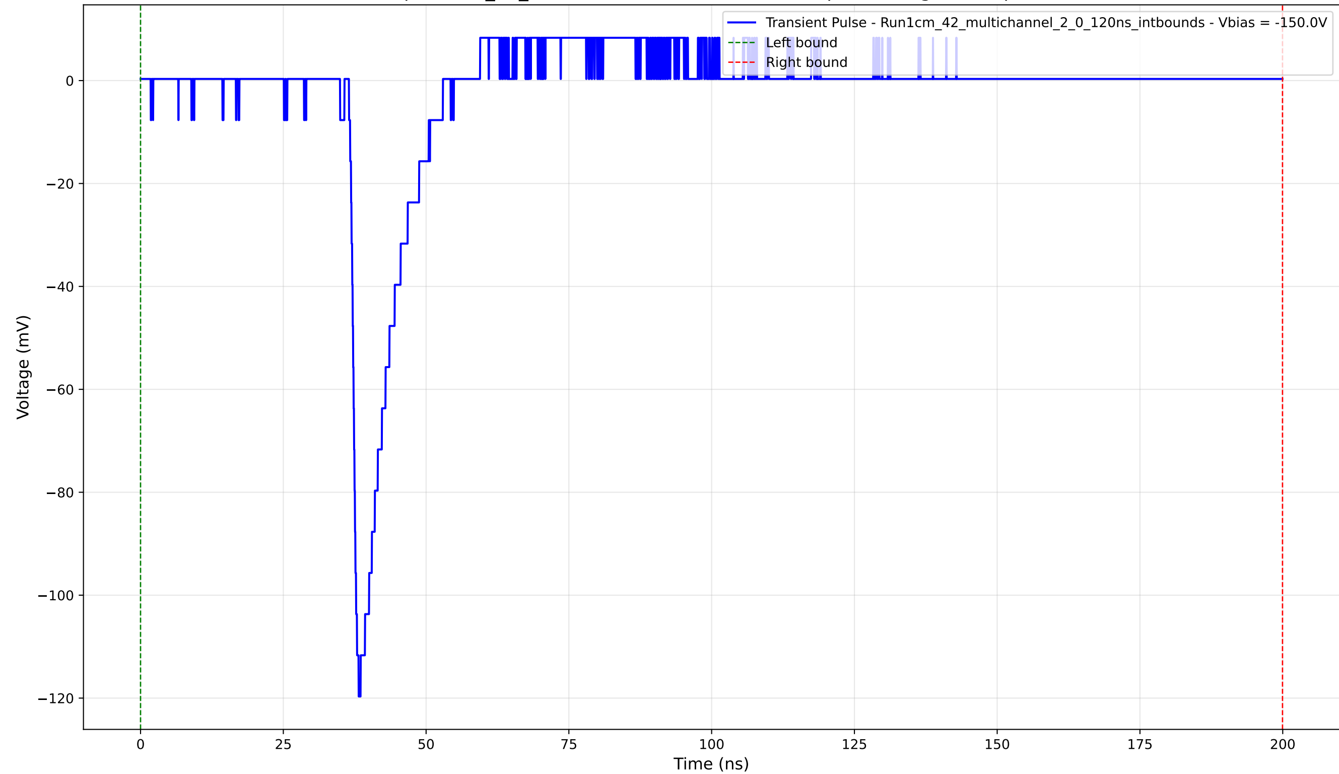
Transient Pulse - Sample: 1cm_42_multichannel - Position: 3575.0 \mu\text{m} - Charge: 9.39 pC - Rise Time: 1.22 ns
