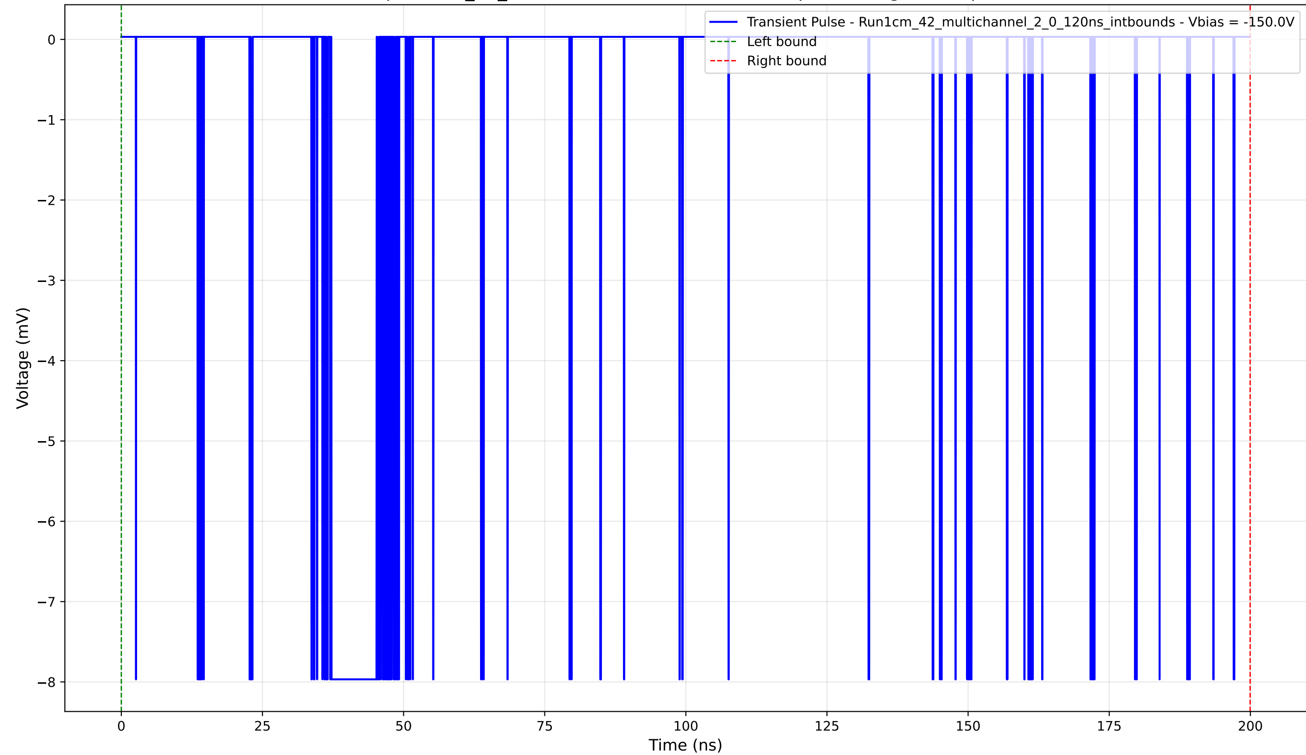
Transient Pulse - Sample: 1cm_42_multichannel - Position: 3900.0 \mu\text{m} - Charge: 2.40 pC - Rise Time: 0.04 ns
