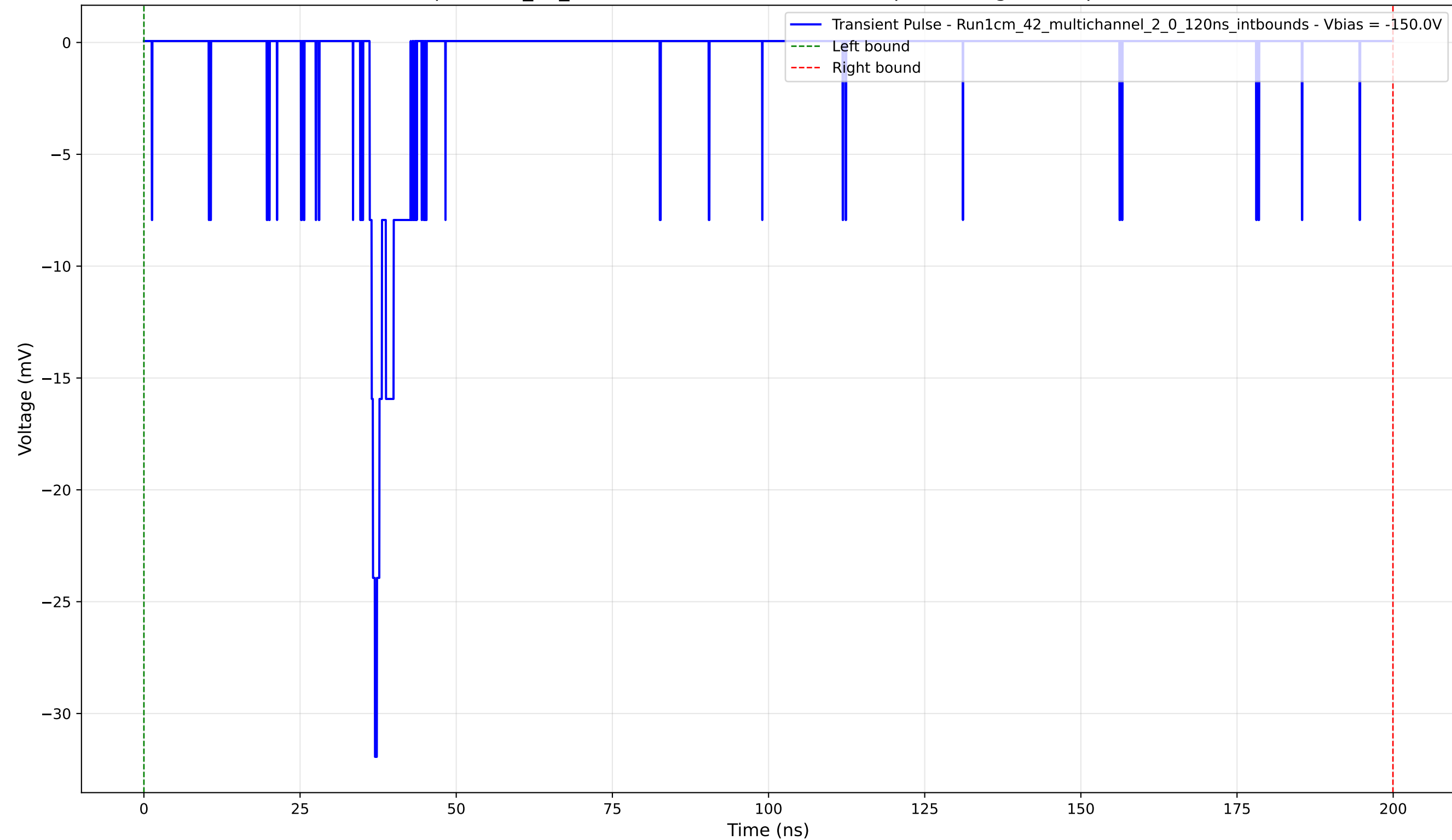
Transient Pulse - Sample: 1cm_42_multichannel - Position: 2380.0 \mu\text{m} - Charge: 2.03 pC - Rise Time: 0.86 ns
