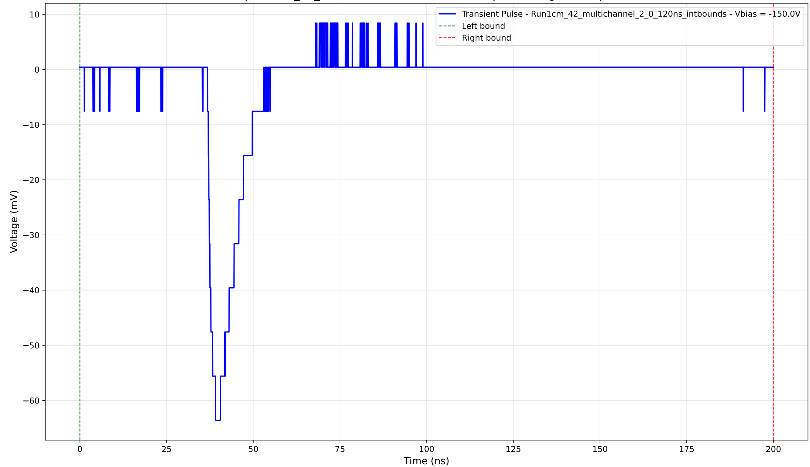
Transient Pulse - Sample: 1cm_42_multichannel - Position: 110.0 \mu\text{m} - Charge: 8.06 pC - Rise Time: 2.33 ns
