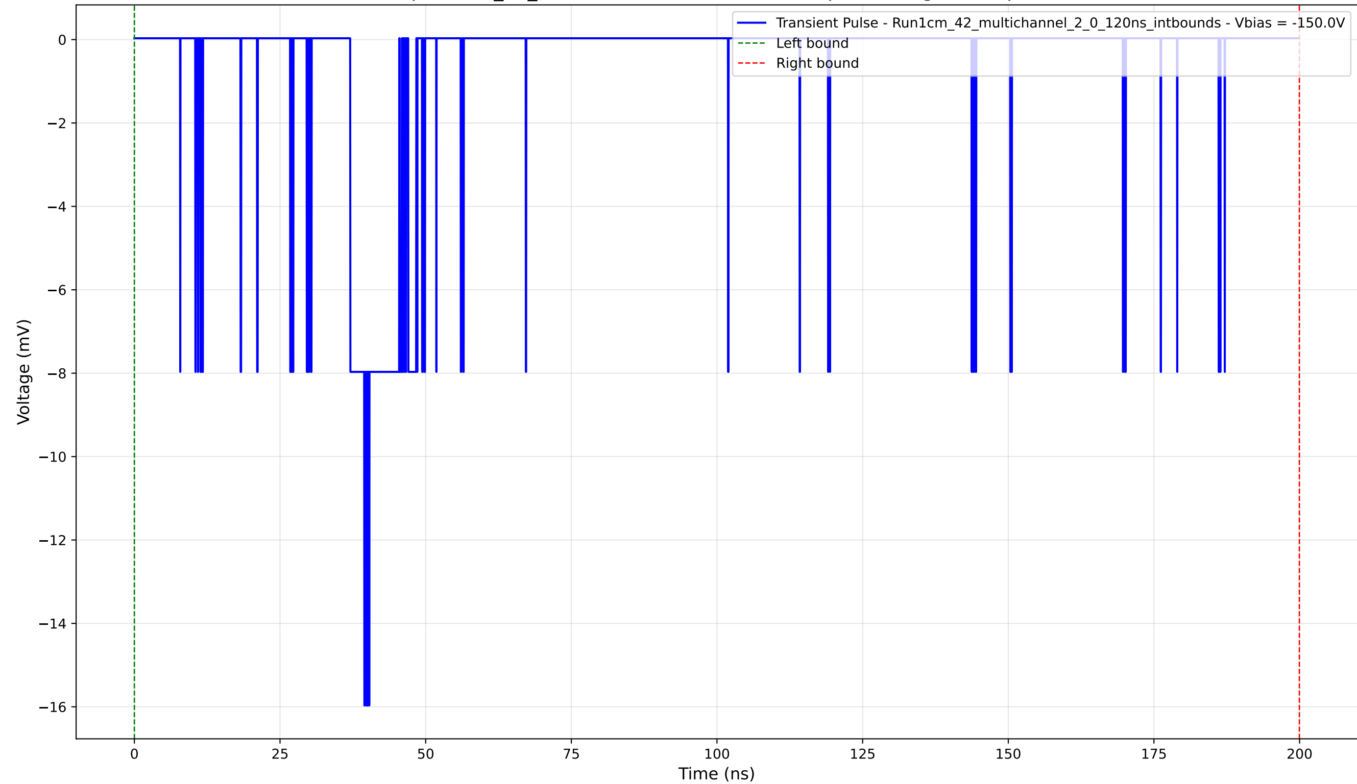
Transient Pulse - Sample: 1cm_42_multichannel - Position: 870.0 \mu\text{m} - Charge: 2.11 pC - Rise Time: 2.43 ns
