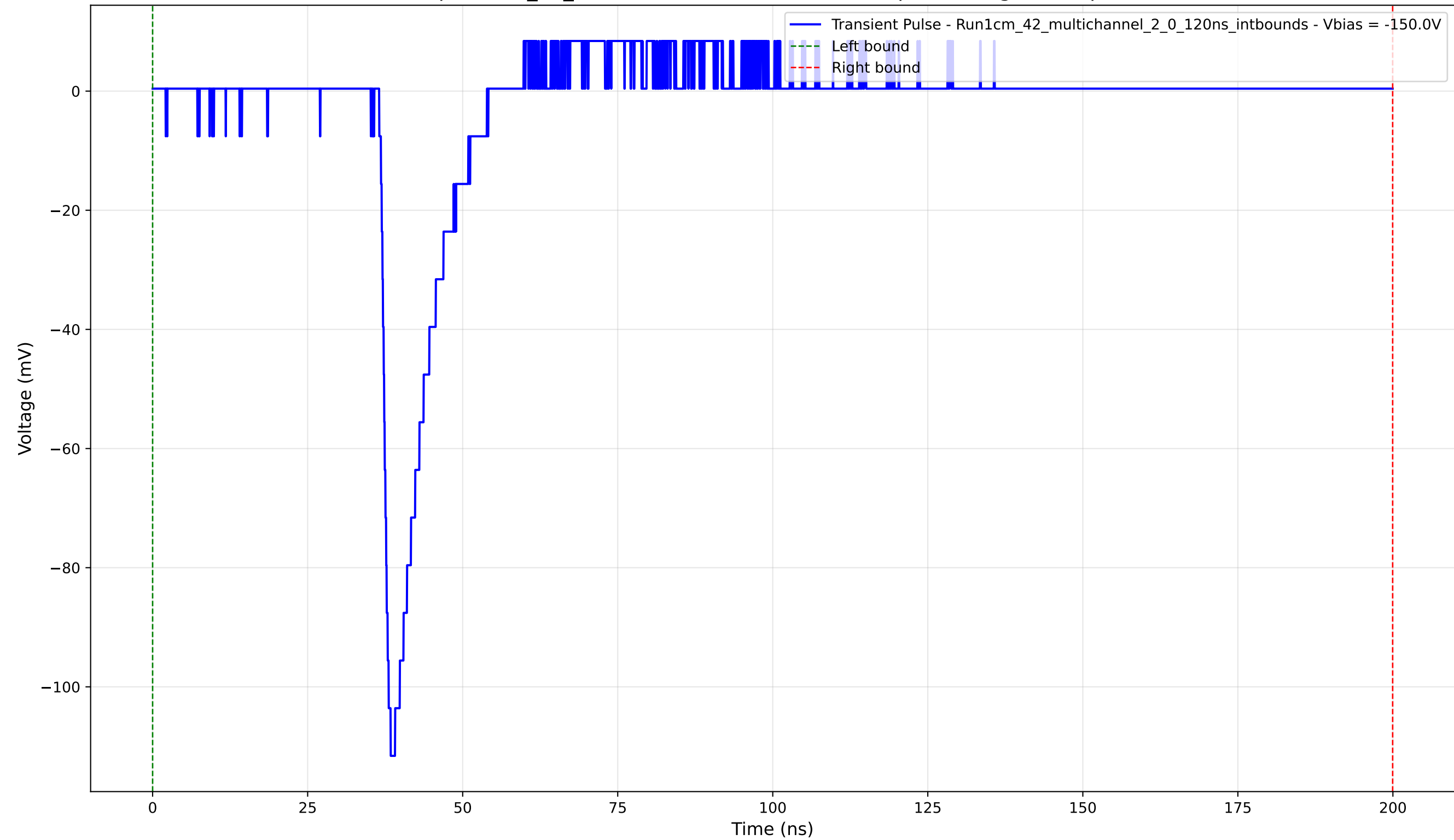
Transient Pulse - Sample: 1cm_42_multichannel - Position: 3690.0 \mu\text{m} - Charge: 9.61 pC - Rise Time: 1.26 ns
