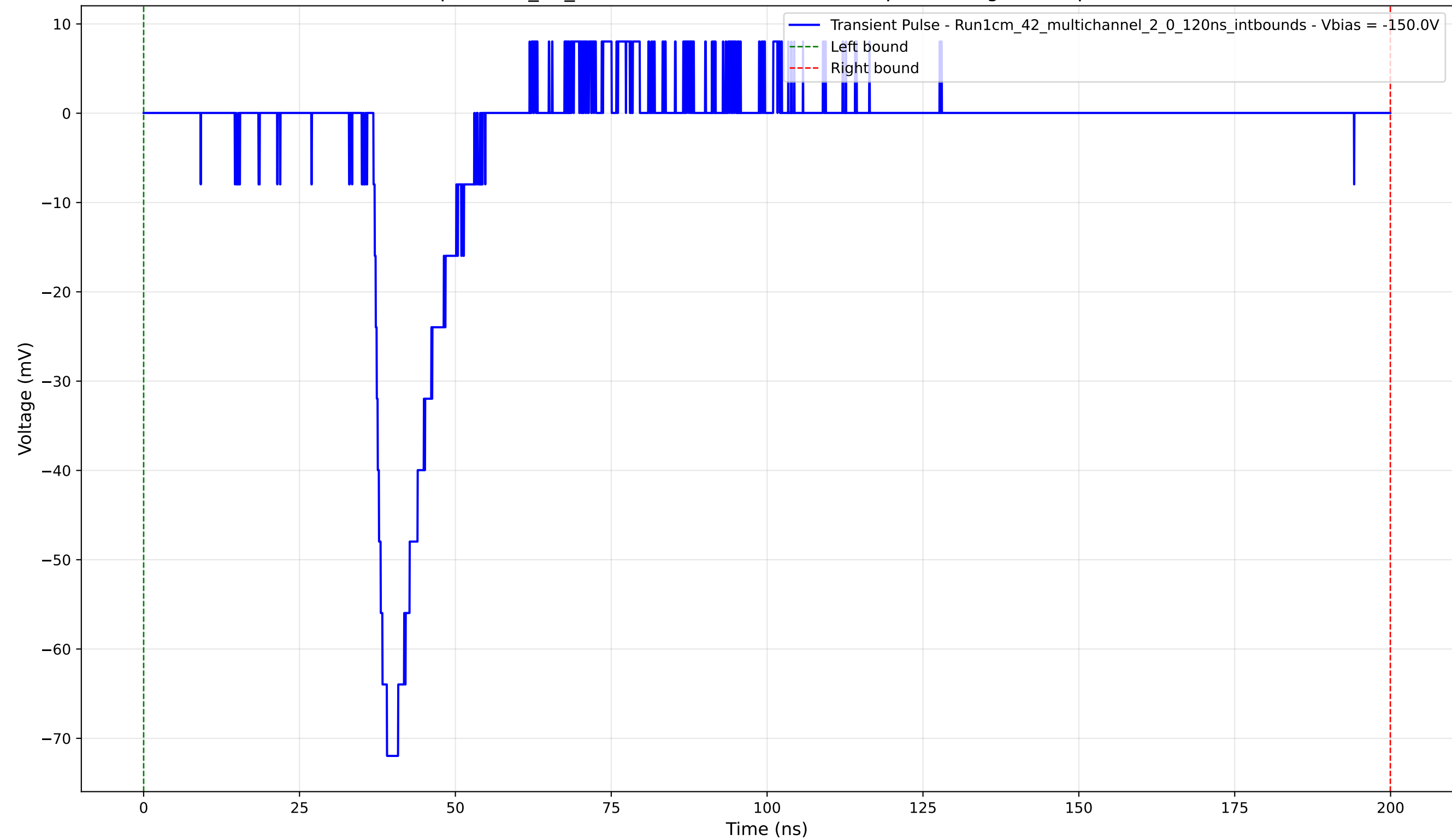
Transient Pulse - Sample: 1cm_42_multichannel - Position: 250.0 \mu\text{m} - Charge: 9.54 pC - Rise Time: 2.16 ns
