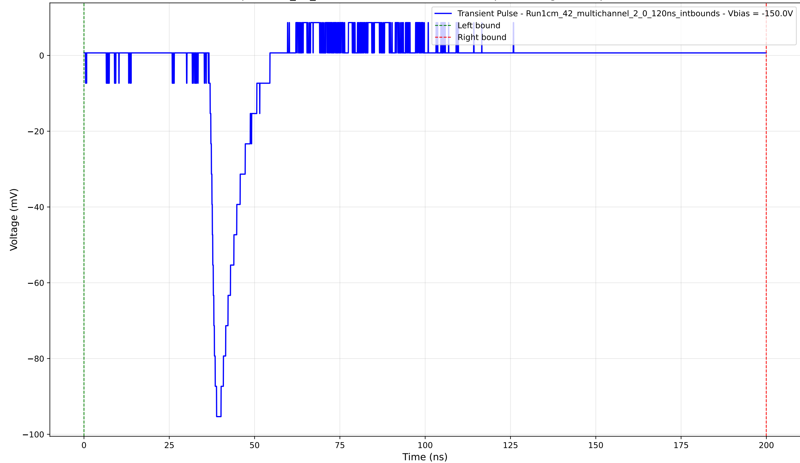
Transient Pulse - Sample: 1cm_42_multichannel - Position: 4000.0 \mu\text{m} - Charge: 8.71 pC - Rise Time: 1.51 ns
