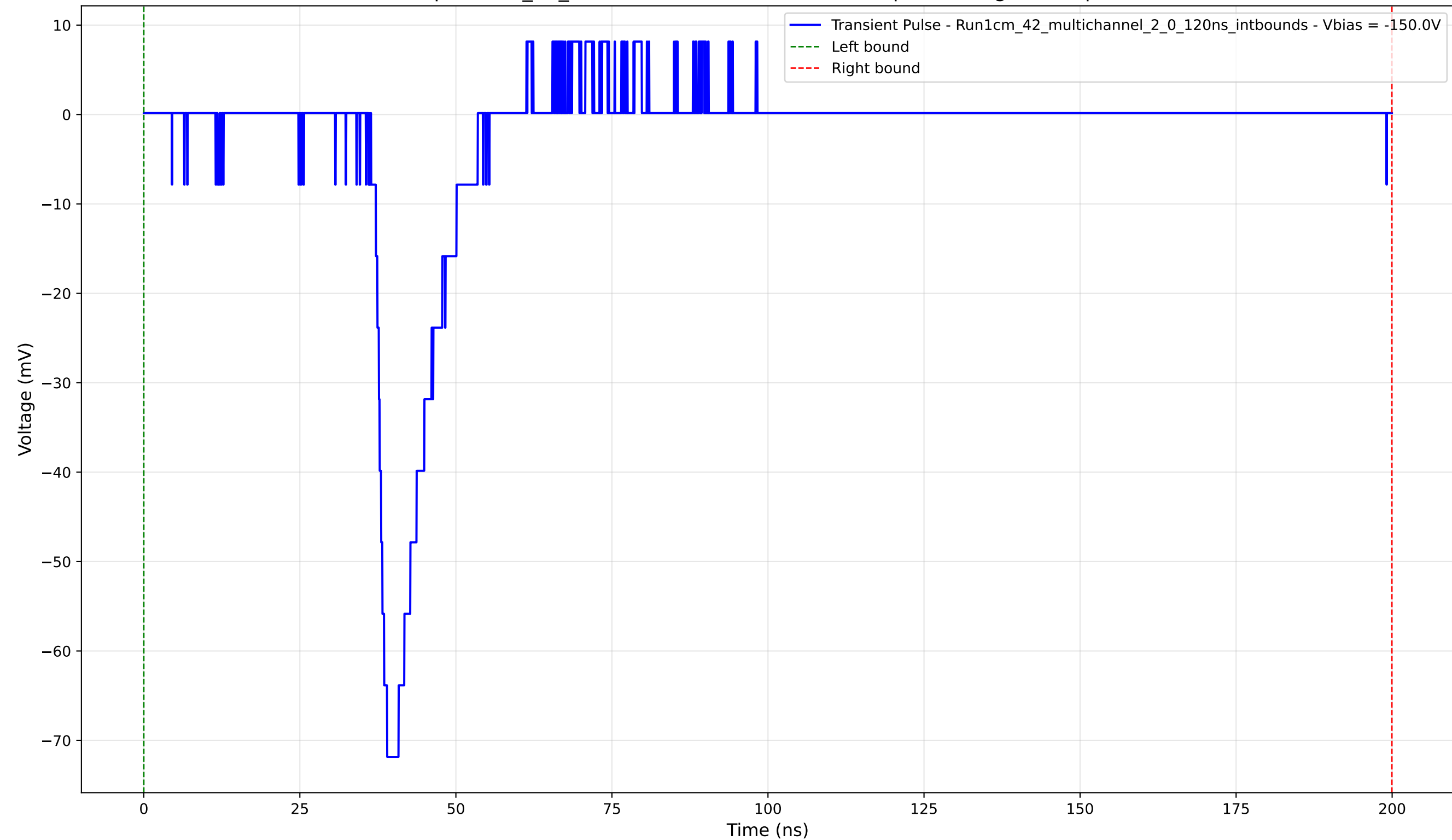
Transient Pulse - Sample: 1cm_42_multichannel - Position: 4540.0 \mu\text{m} - Charge: 9.57 pC - Rise Time: 2.56 ns
