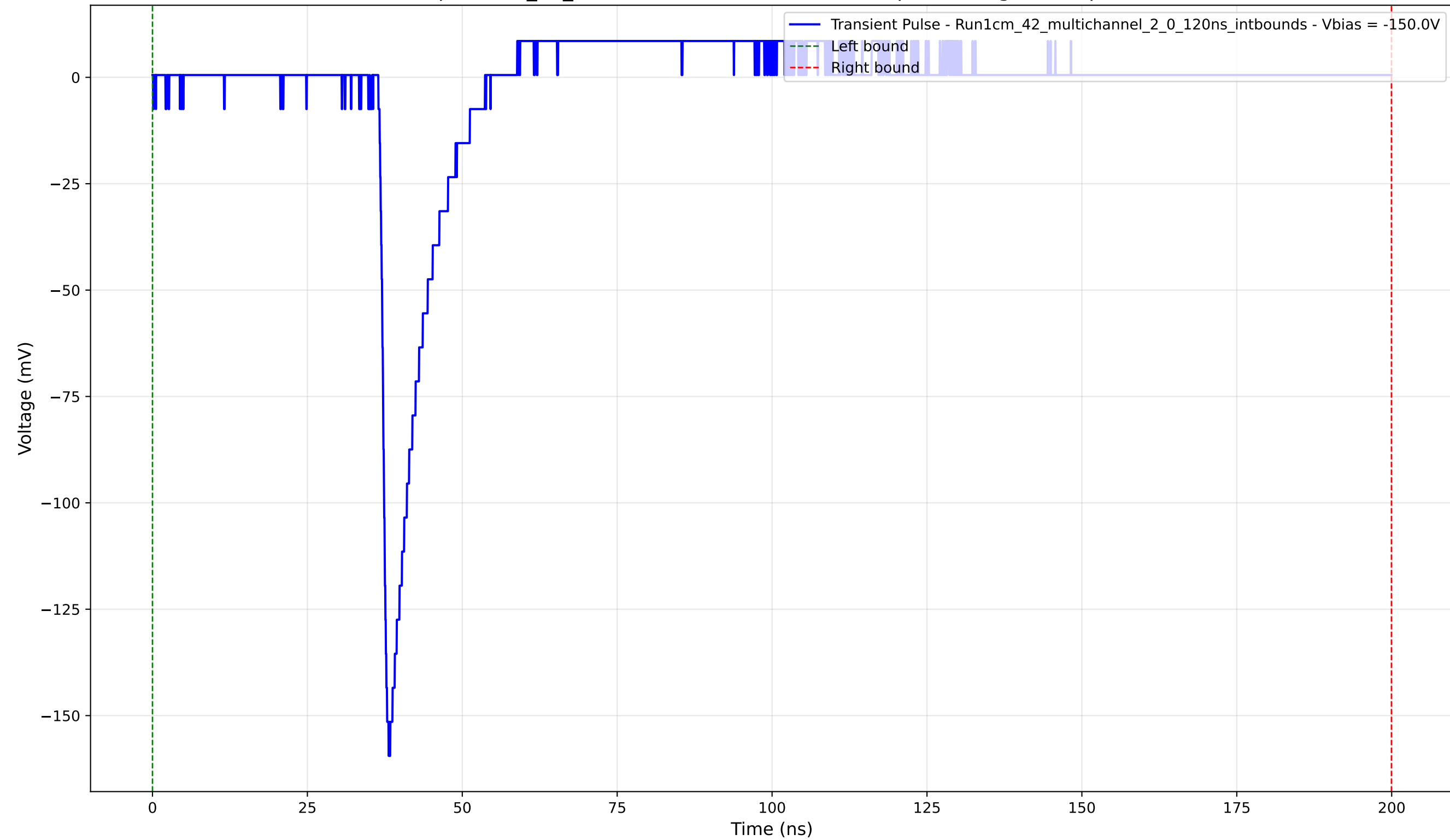
Transient Pulse - Sample: 1cm_42_multichannel - Position: 1245.0 \mu\text{m} - Charge: 9.14 pC - Rise Time: 1.16 ns
