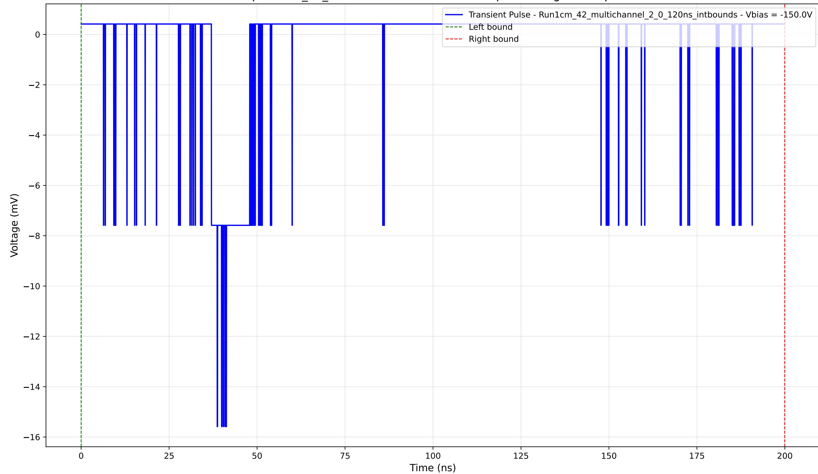
Transient Pulse - Sample: 1cm_42_multichannel - Position: 50.0 \mu\text{m} - Charge: 1.04 pC - Rise Time: 1.67 ns
