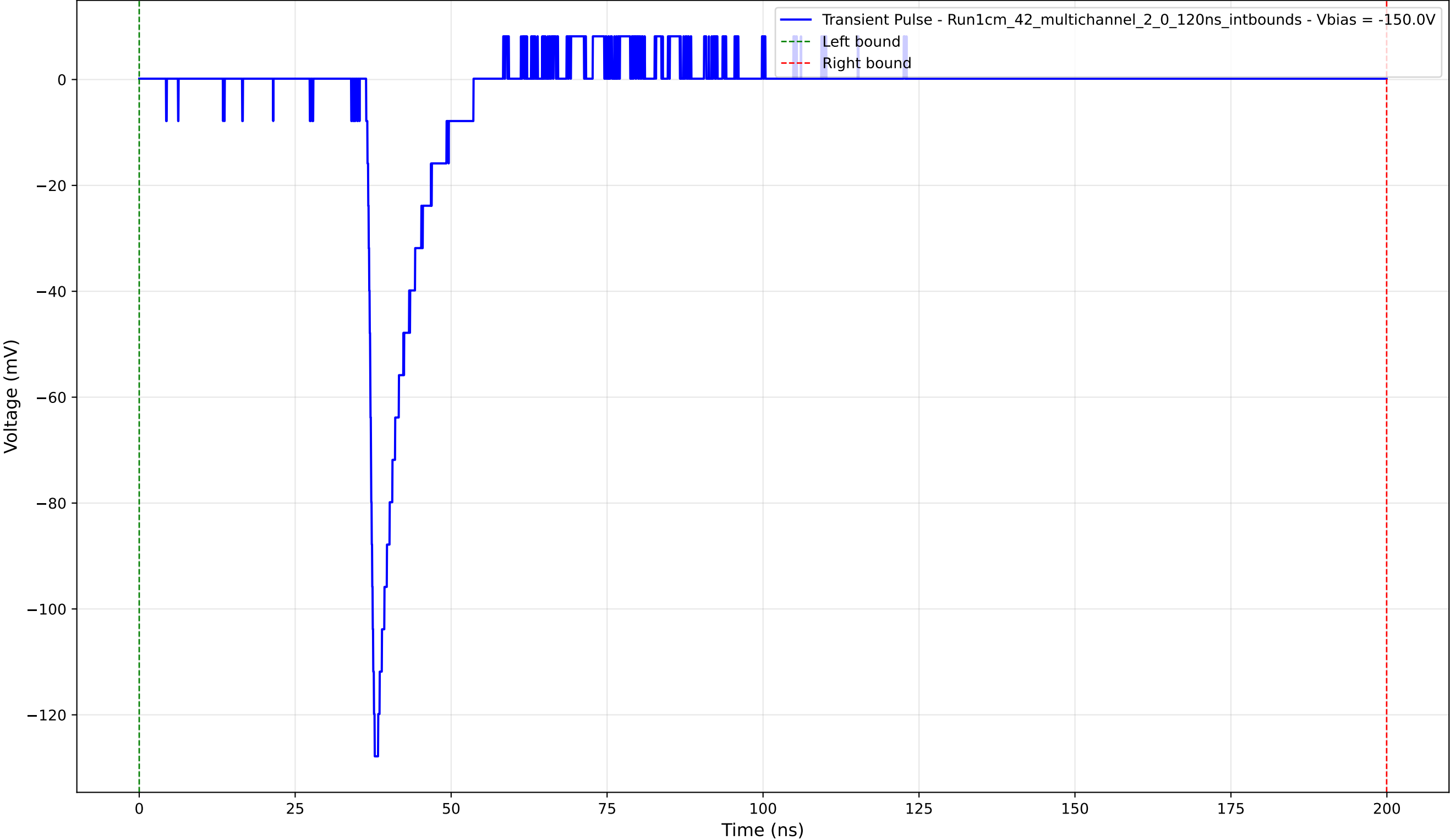
Transient Pulse - Sample: 1cm_42_multichannel - Position: 1415.0 \mu\text{m} - Charge: 11.05 pC - Rise Time: 1.06 ns
