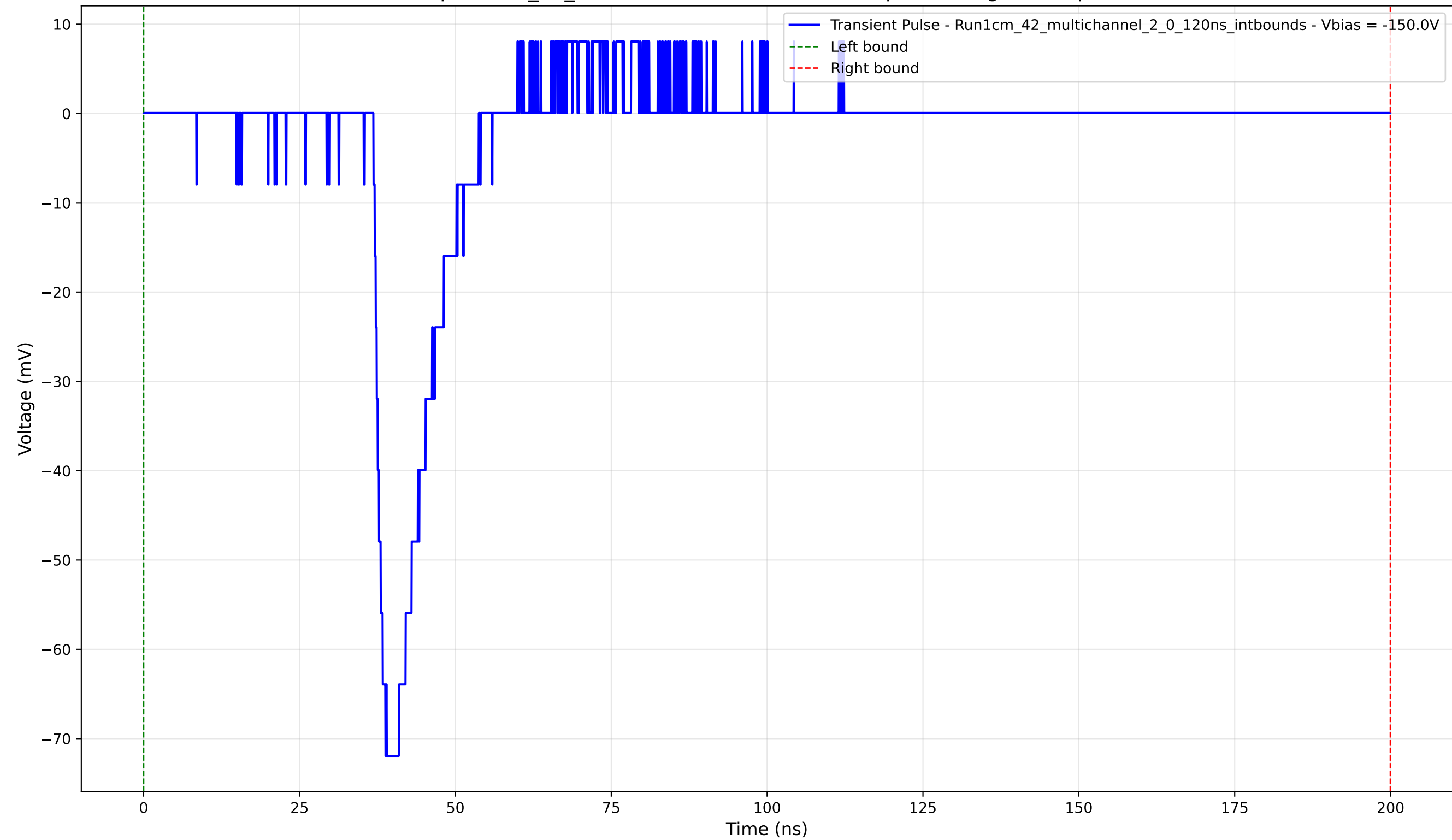
Transient Pulse - Sample: 1cm_42_multichannel - Position: 235.0 \mu\text{m} - Charge: 9.54 pC - Rise Time: 1.92 ns
