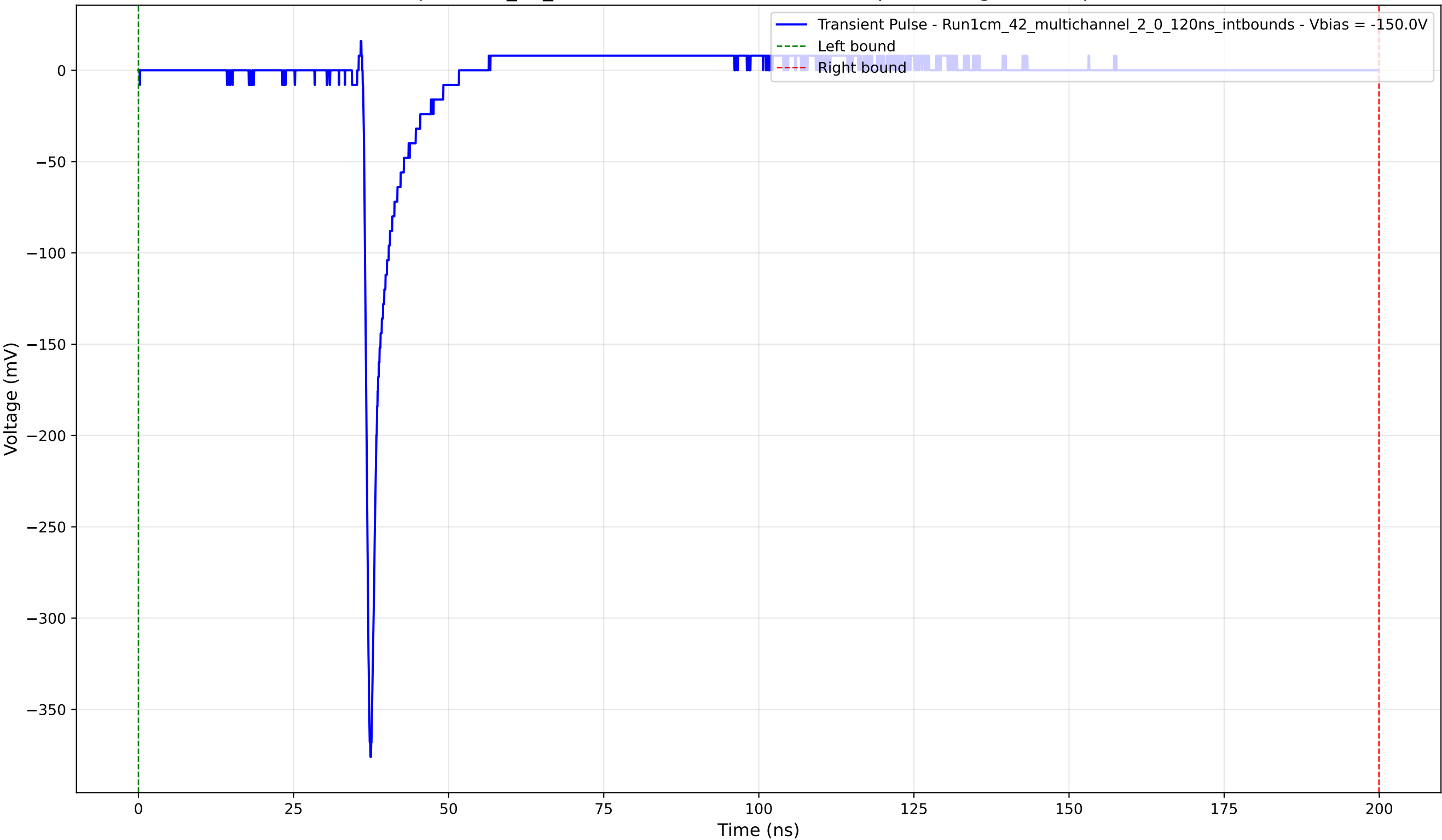
Transient Pulse - Sample: 1cm_42_multichannel - Position: 2775.0 \mu\text{m} - Charge: 13.54 pC - Rise Time: 0.78 ns
