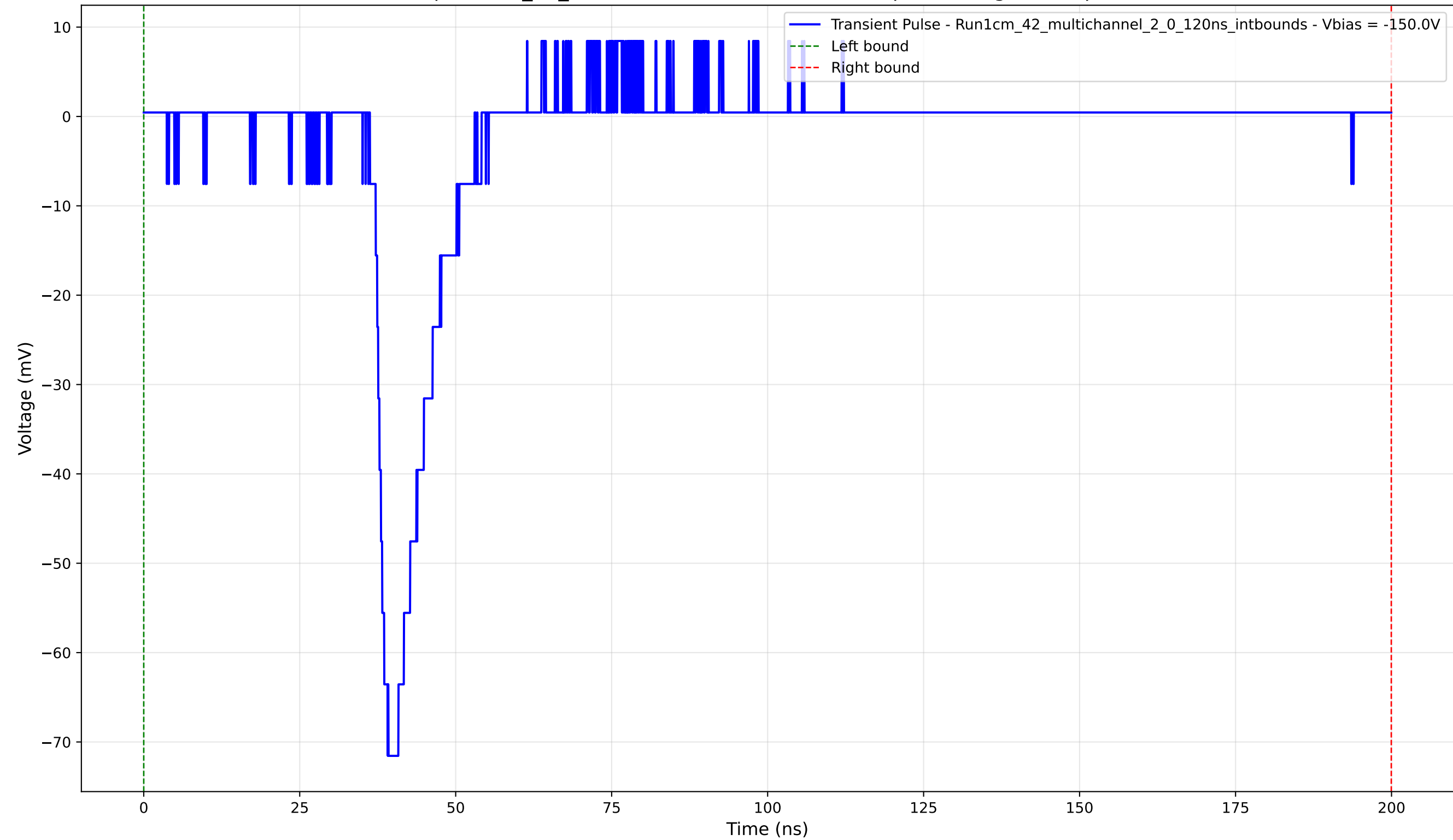
Transient Pulse - Sample: 1cm_42_multichannel - Position: 4595.0 \mu\text{m} - Charge: 8.65 pC - Rise Time: 2.84 ns
