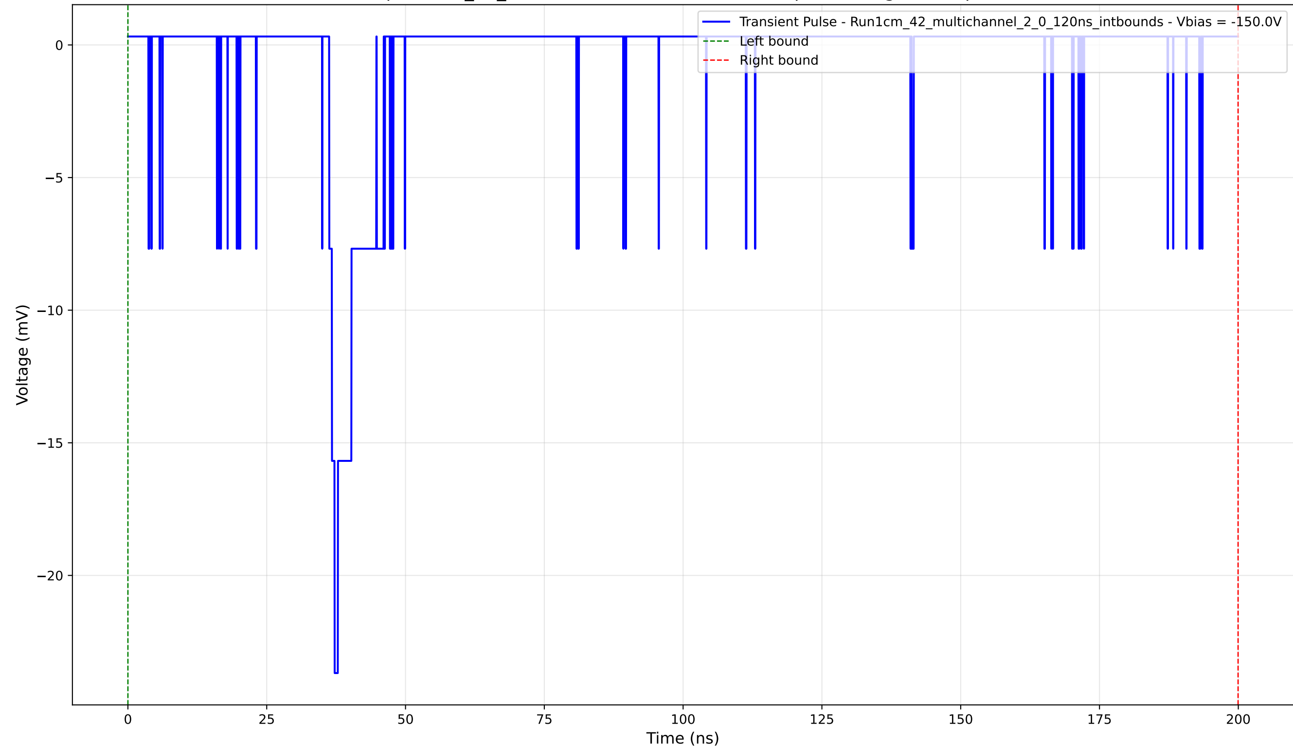
Transient Pulse - Sample: 1cm_42_multichannel - Position: 1880.0 \mu\text{m} - Charge: 1.58 pC - Rise Time: 0.99 ns
