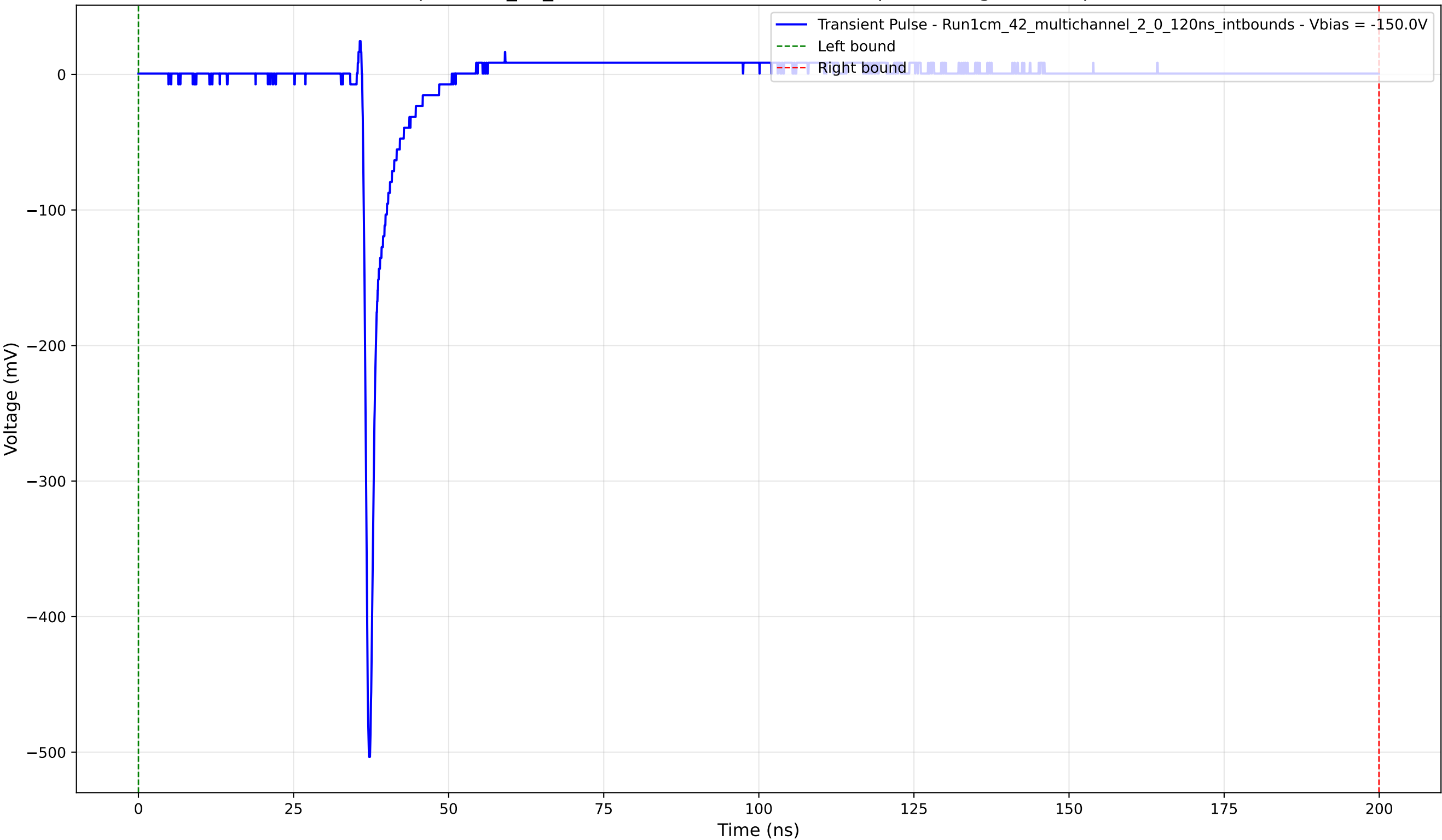
Transient Pulse - Sample: 1cm_42_multichannel - Position: 2560.0 \mu\text{m} - Charge: 12.54 pC - Rise Time: 0.74 ns
