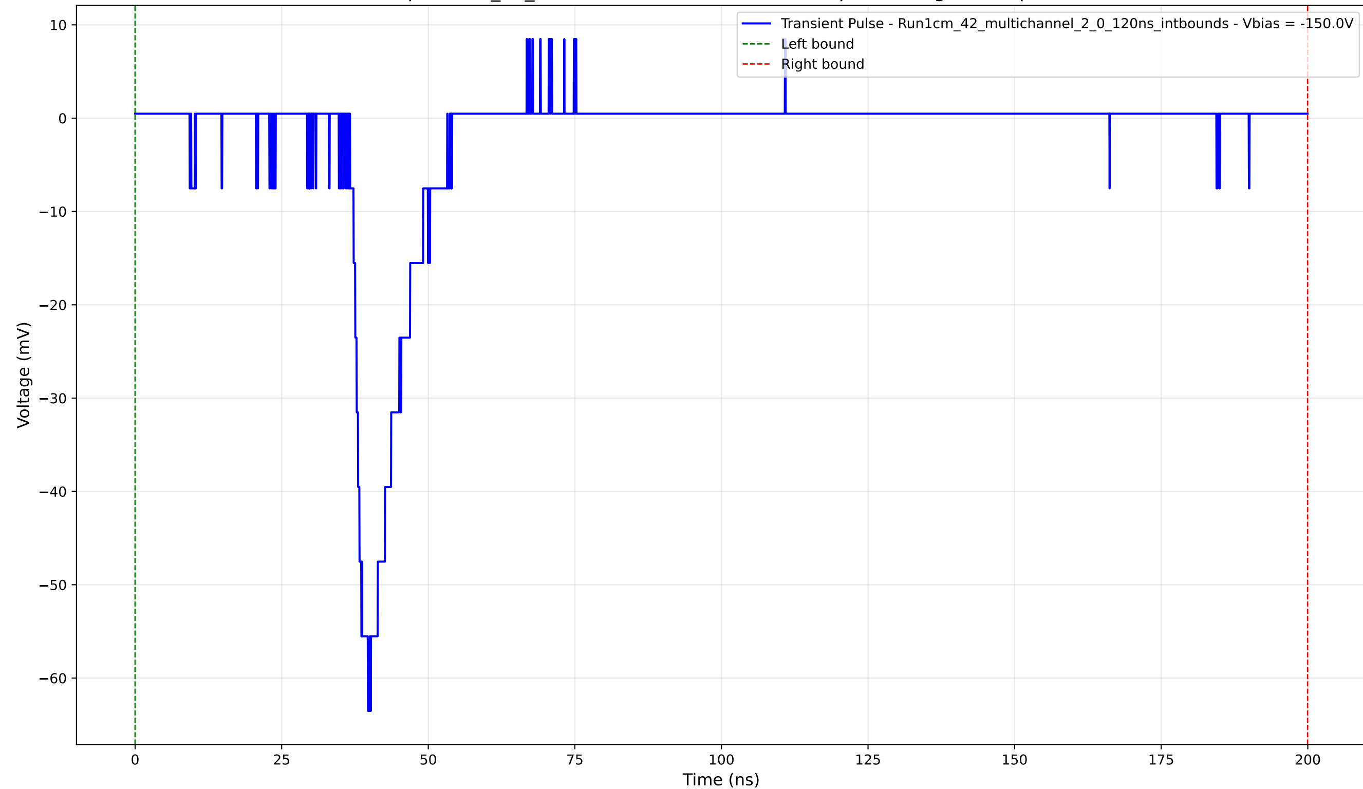
Transient Pulse - Sample: 1cm_42_multichannel - Position: 4320.0 \mu\text{m} - Charge: 7.89 pC - Rise Time: 3.05 ns
