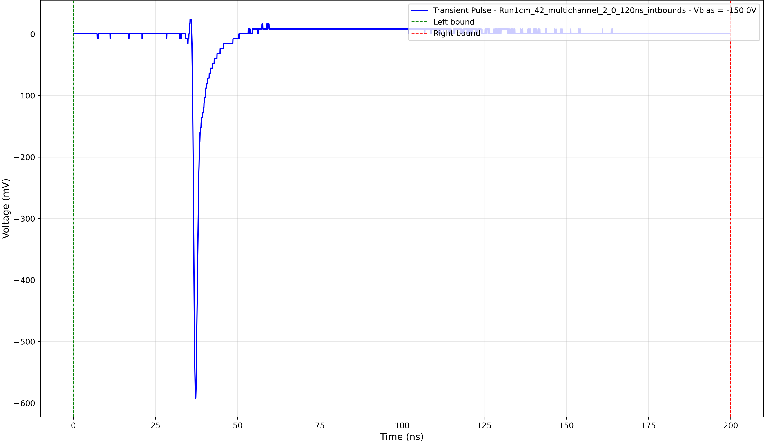
Transient Pulse - Sample: 1cm_42_multichannel - Position: 2495.0 \mu\text{m} - Charge: 14.78 pC - Rise Time: 0.74 ns
