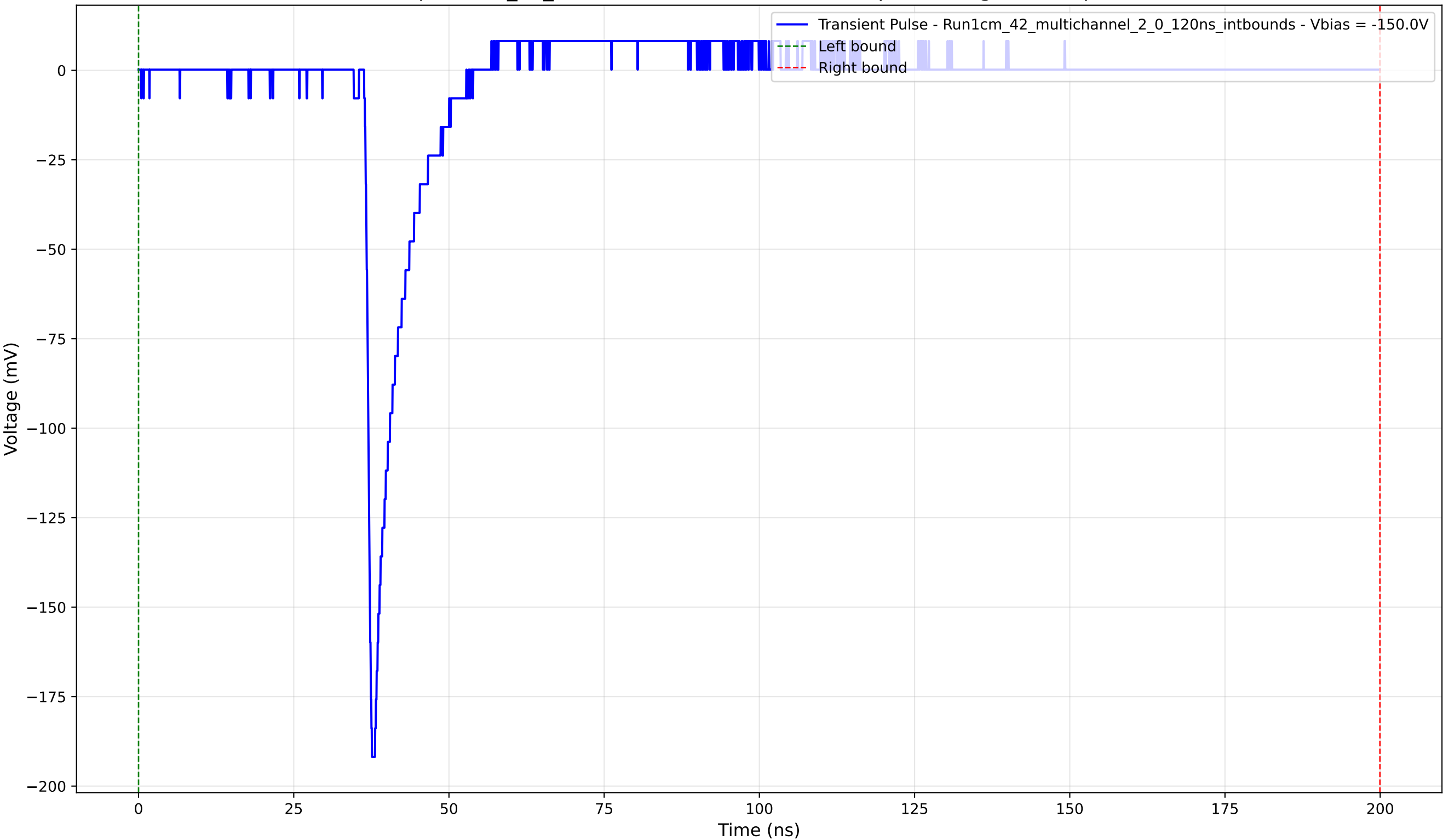
Transient Pulse - Sample: 1cm_42_multichannel - Position: 3195.0 \mu\text{m} - Charge: 11.47 pC - Rise Time: 0.90 ns
