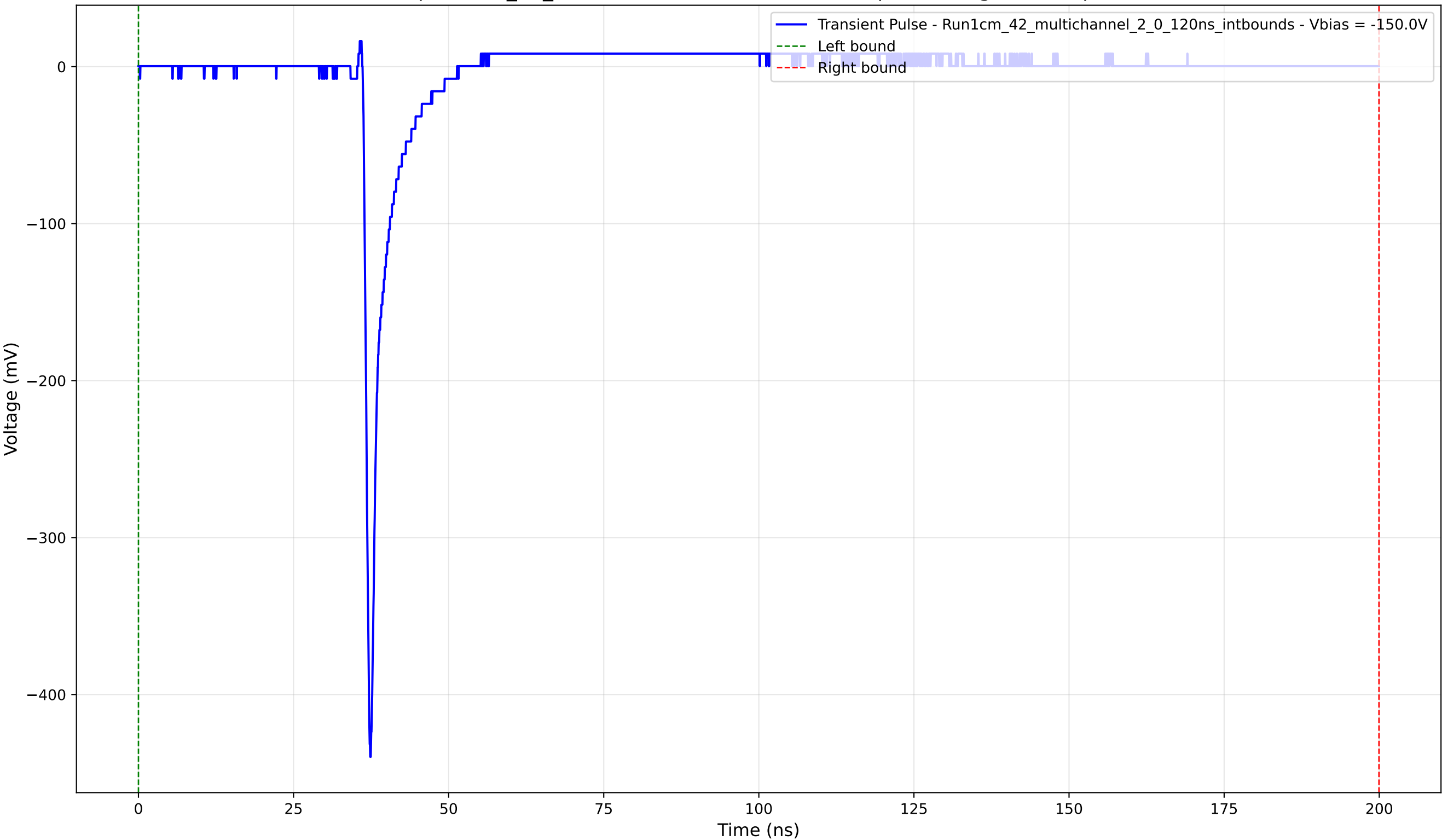
Transient Pulse - Sample: 1cm_42_multichannel - Position: 2010.0 \mu\text{m} - Charge: 13.85 pC - Rise Time: 0.79 ns
