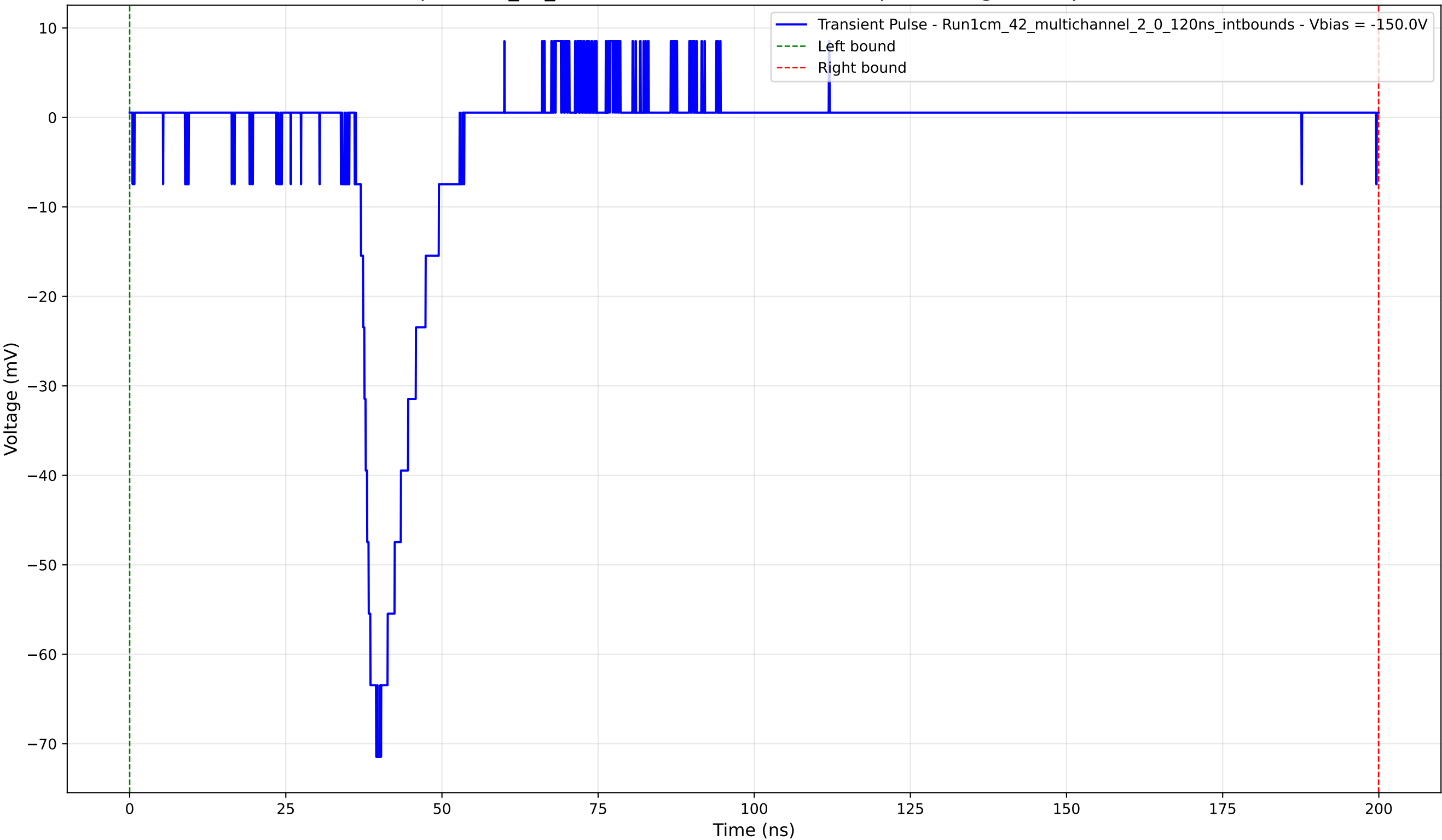
Transient Pulse - Sample: 1cm_42_multichannel - Position: 4710.0 \mu\text{m} - Charge: 7.80 pC - Rise Time: 3.24 ns
