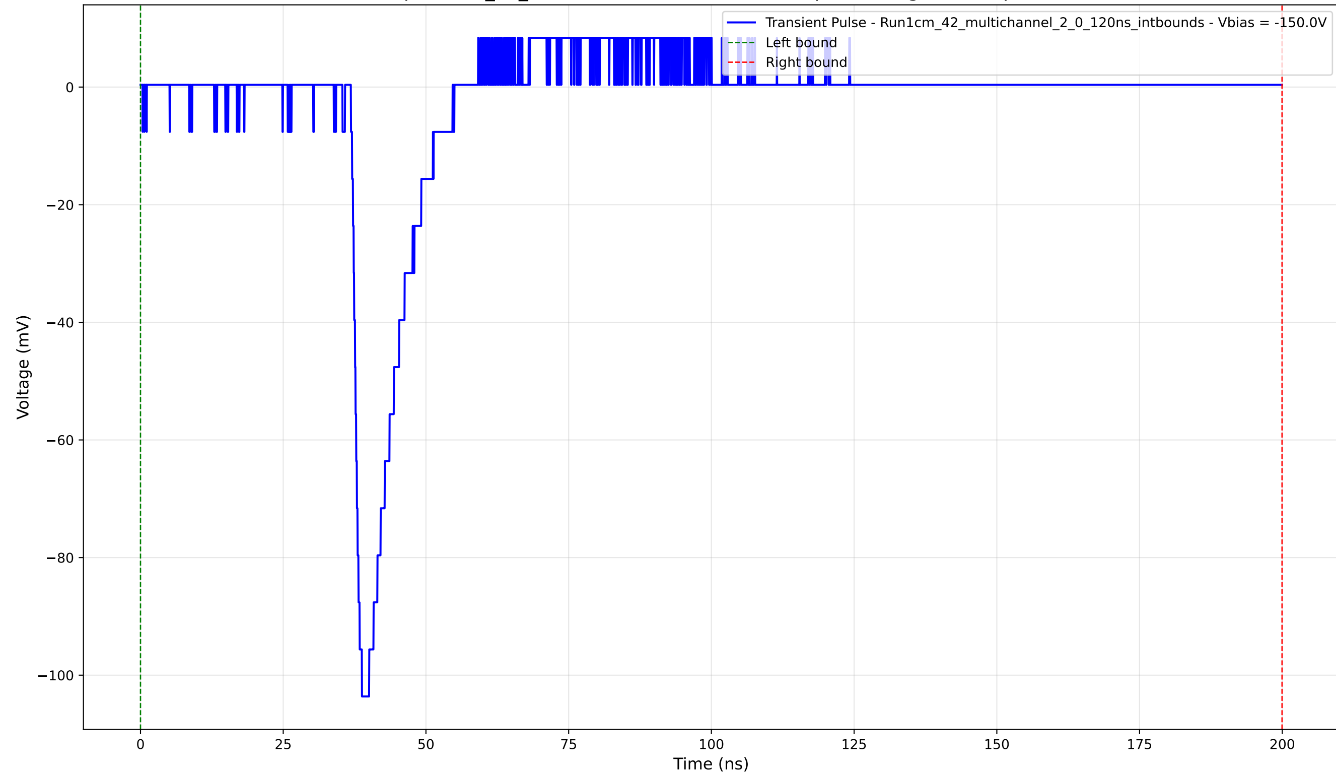
Transient Pulse - Sample: 1cm_42_multichannel - Position: 675.0 \mu\text{m} - Charge: 10.13 pC - Rise Time: 1.35 ns
