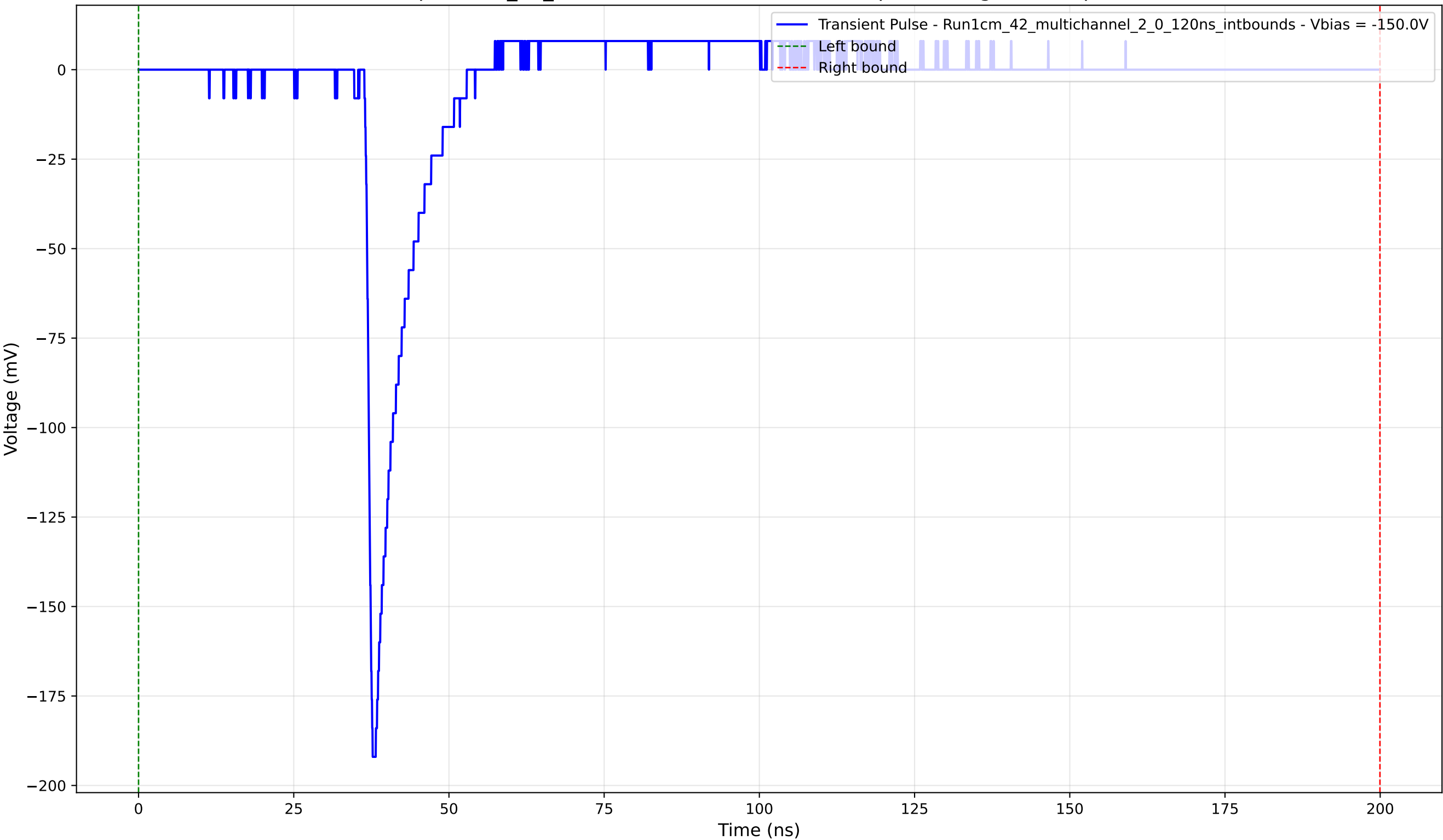
Transient Pulse - Sample: 1cm_42_multichannel - Position: 1450.0 \mu\text{m} - Charge: 12.56 pC - Rise Time: 0.98 ns
