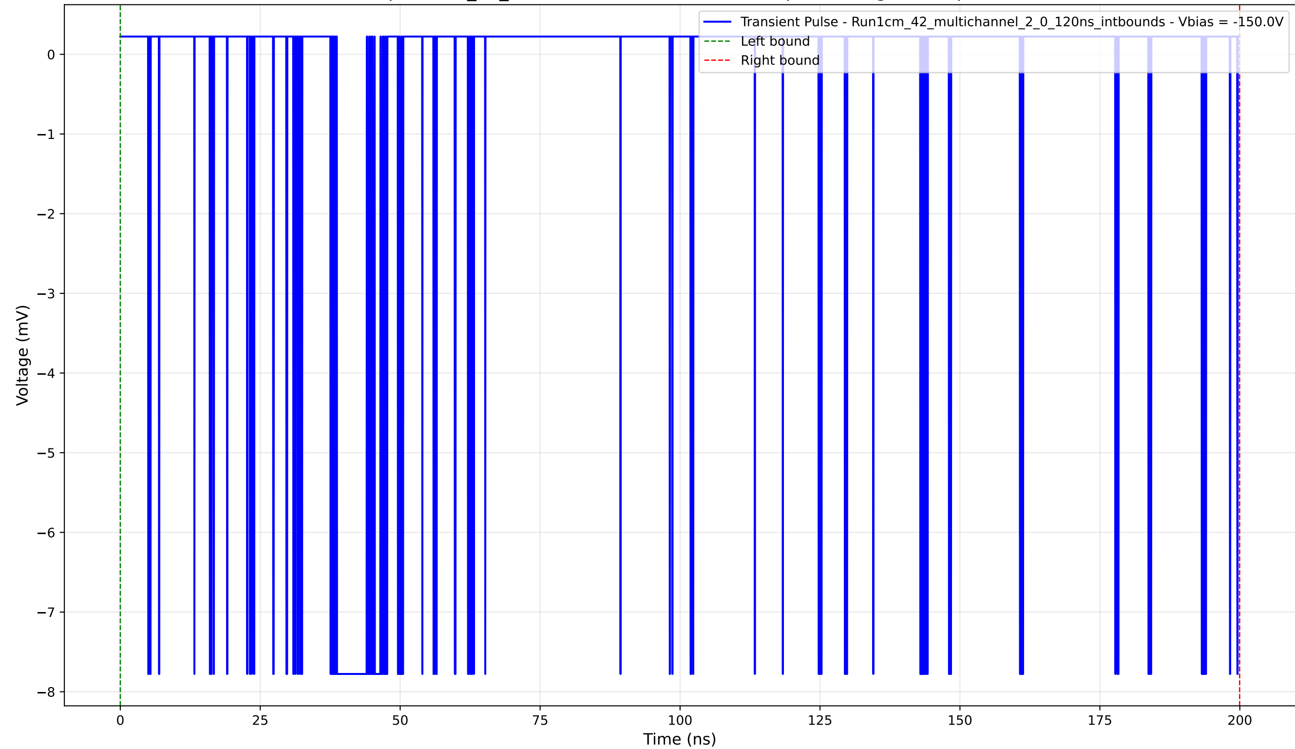
Transient Pulse - Sample: 1cm_42_multichannel - Position: 345.0 \mu\text{m} - Charge: 1.55 pC - Rise Time: 0.04 ns
