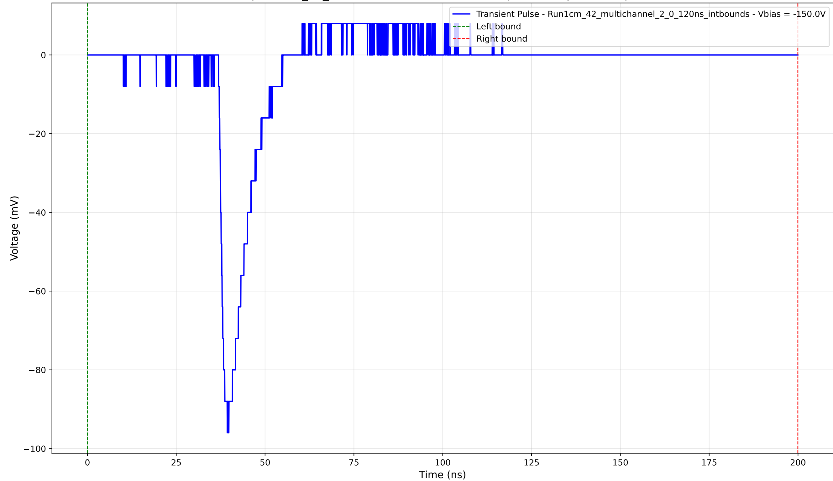
Transient Pulse - Sample: 1cm_42_multichannel - Position: 455.0 \mu\text{m} - Charge: 10.81 pC - Rise Time: 1.59 ns
