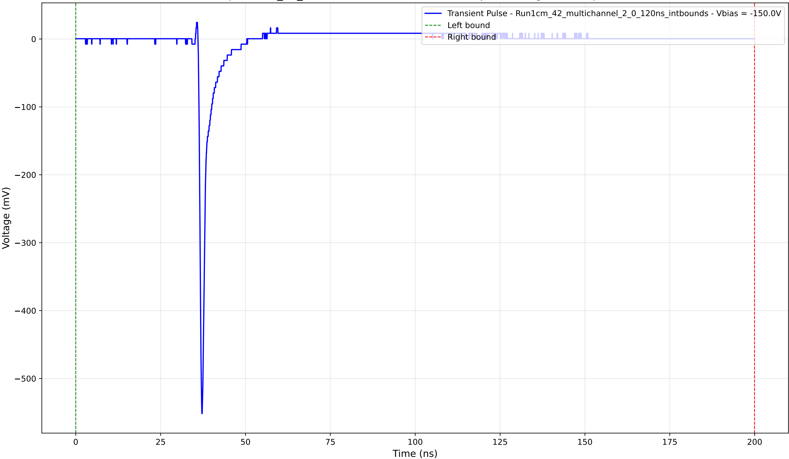
Transient Pulse - Sample: 1cm_42_multichannel - Position: 2525.0 \mu\text{m} - Charge: 14.30 pC - Rise Time: 0.76 ns
