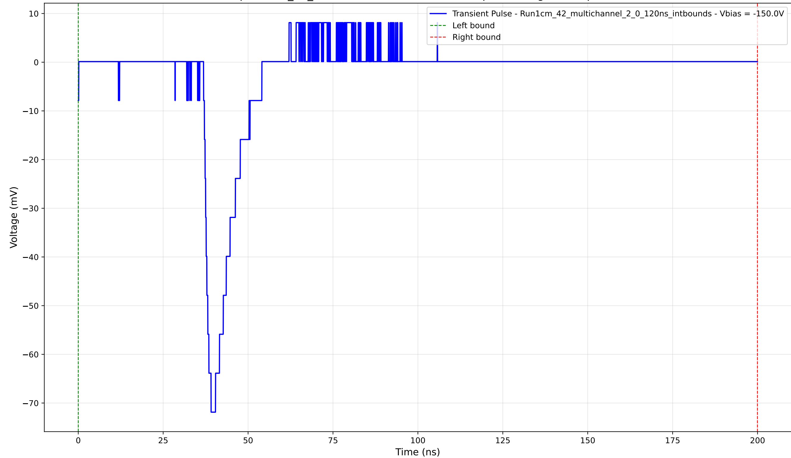
Transient Pulse - Sample: 1cm_42_multichannel - Position: 410.0 \mu\text{m} - Charge: 8.89 pC - Rise Time: 2.20 ns
