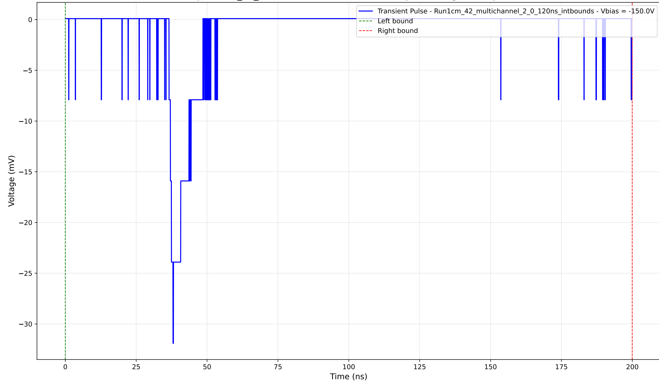
Transient Pulse - Sample: 1cm_42_multichannel - Position: 3415.0 \mu\text{m} - Charge: 3.76 pC - Rise Time: 1.42 ns
