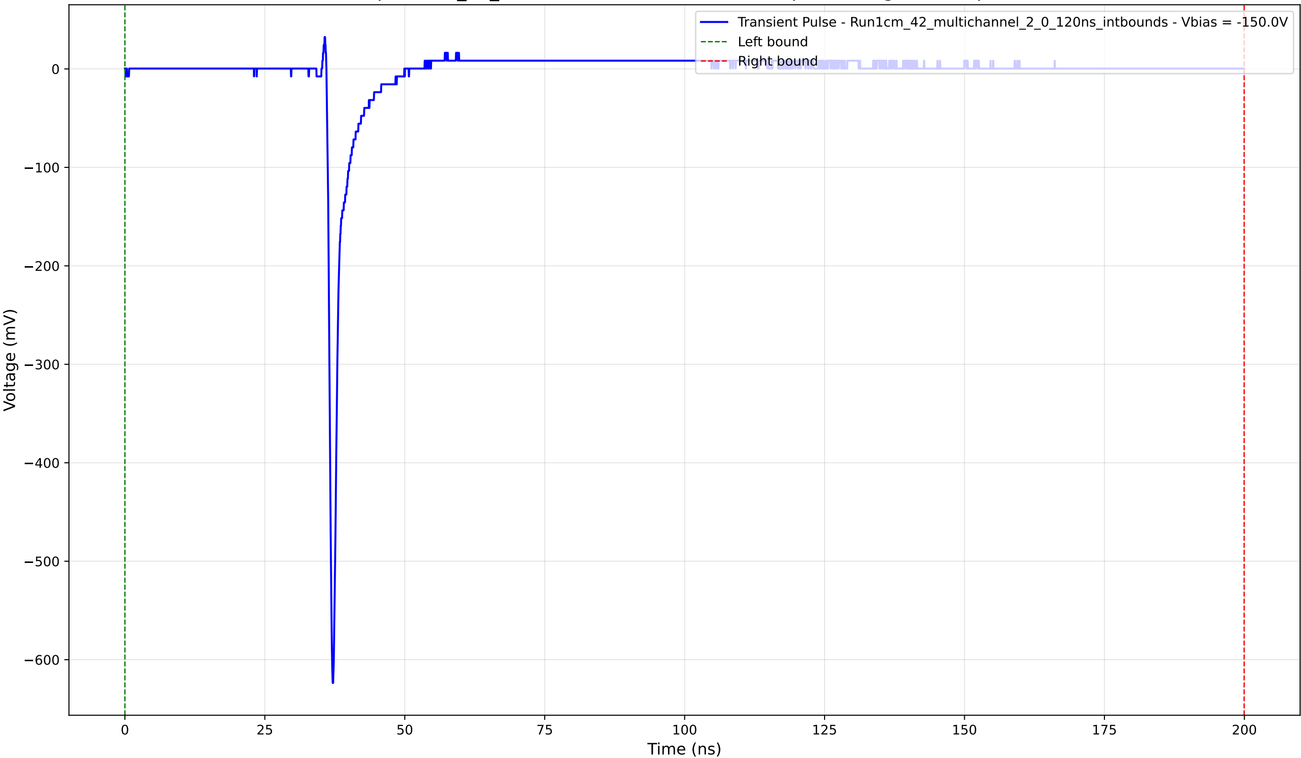
Transient Pulse - Sample: 1cm_42_multichannel - Position: 2470.0 \mu\text{m} - Charge: 14.77 pC - Rise Time: 0.73 ns
