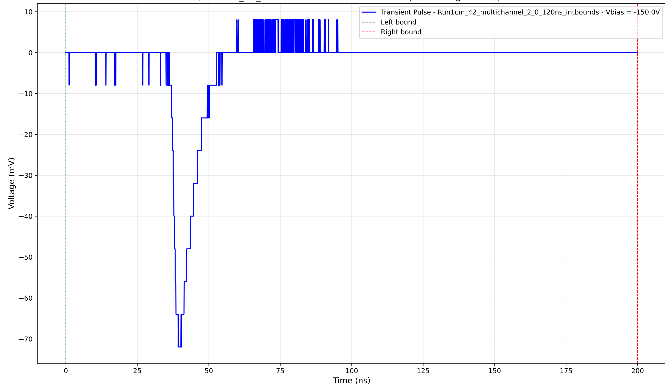
Transient Pulse - Sample: 1cm_42_multichannel - Position: 4705.0 \mu\text{m} - Charge: 9.34 pC - Rise Time: 3.08 ns
