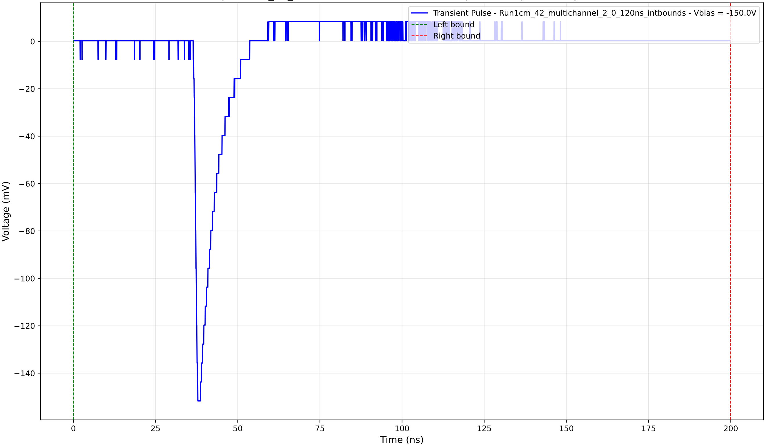
Transient Pulse - Sample: 1cm_42_multichannel - Position: 1265.0 \mu\text{m} - Charge: 10.53 pC - Rise Time: 1.12 ns
