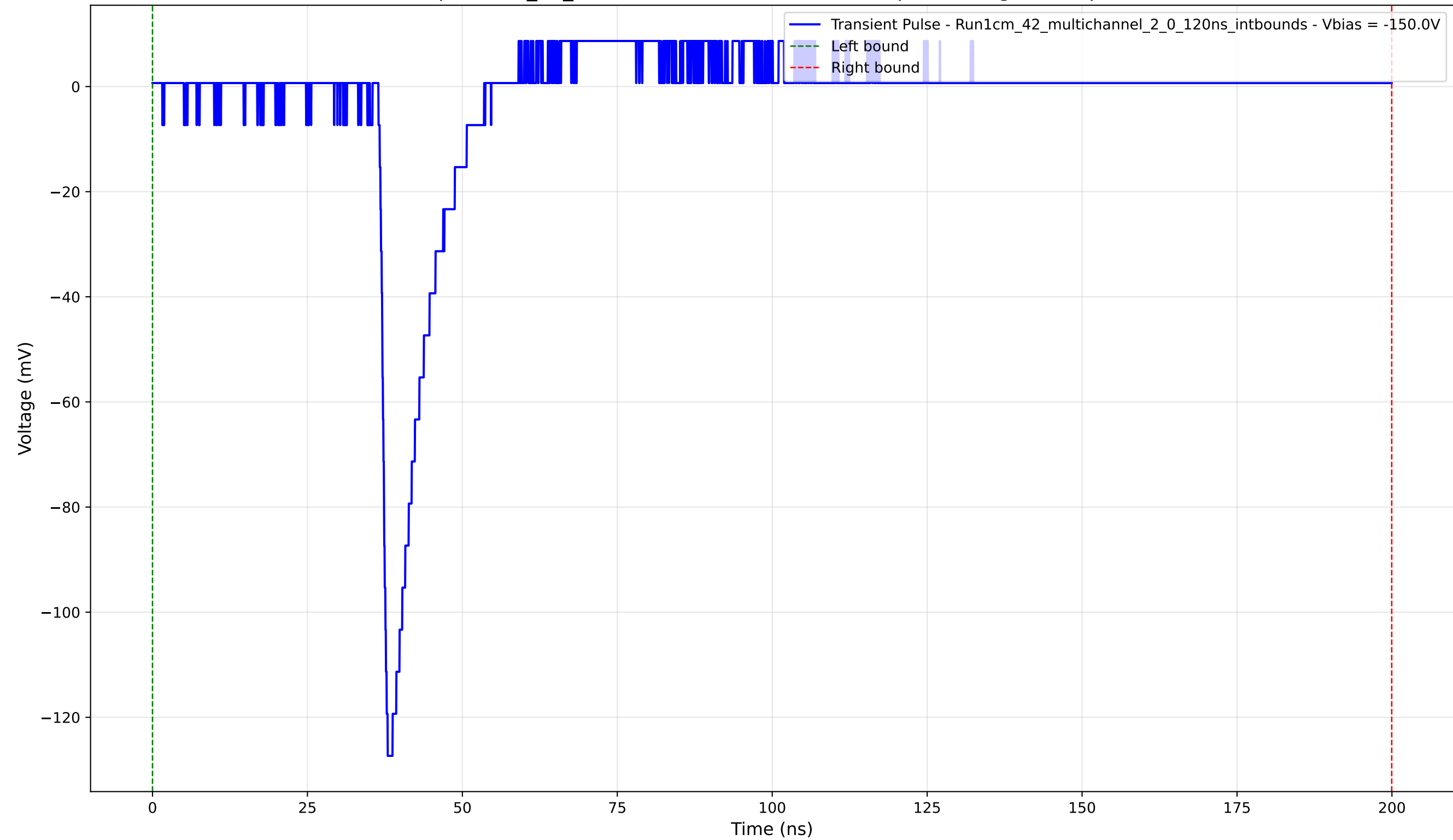
Transient Pulse - Sample: 1cm_42_multichannel - Position: 3520.0 \mu\text{m} - Charge: 9.54 pC - Rise Time: 1.13 ns
