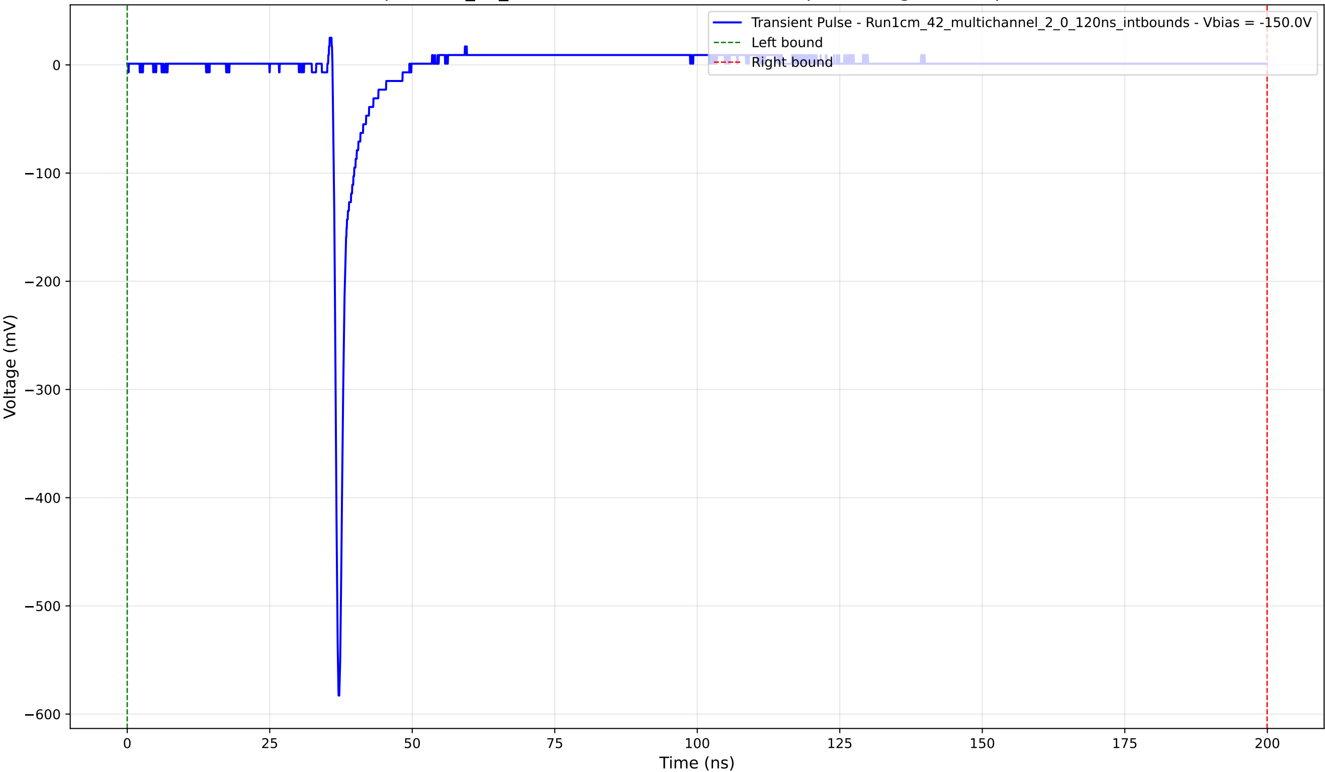
Transient Pulse - Sample: 1cm_42_multichannel - Position: 2295.0 \mu\text{m} - Charge: 12.51 pC - Rise Time: 0.73 ns
