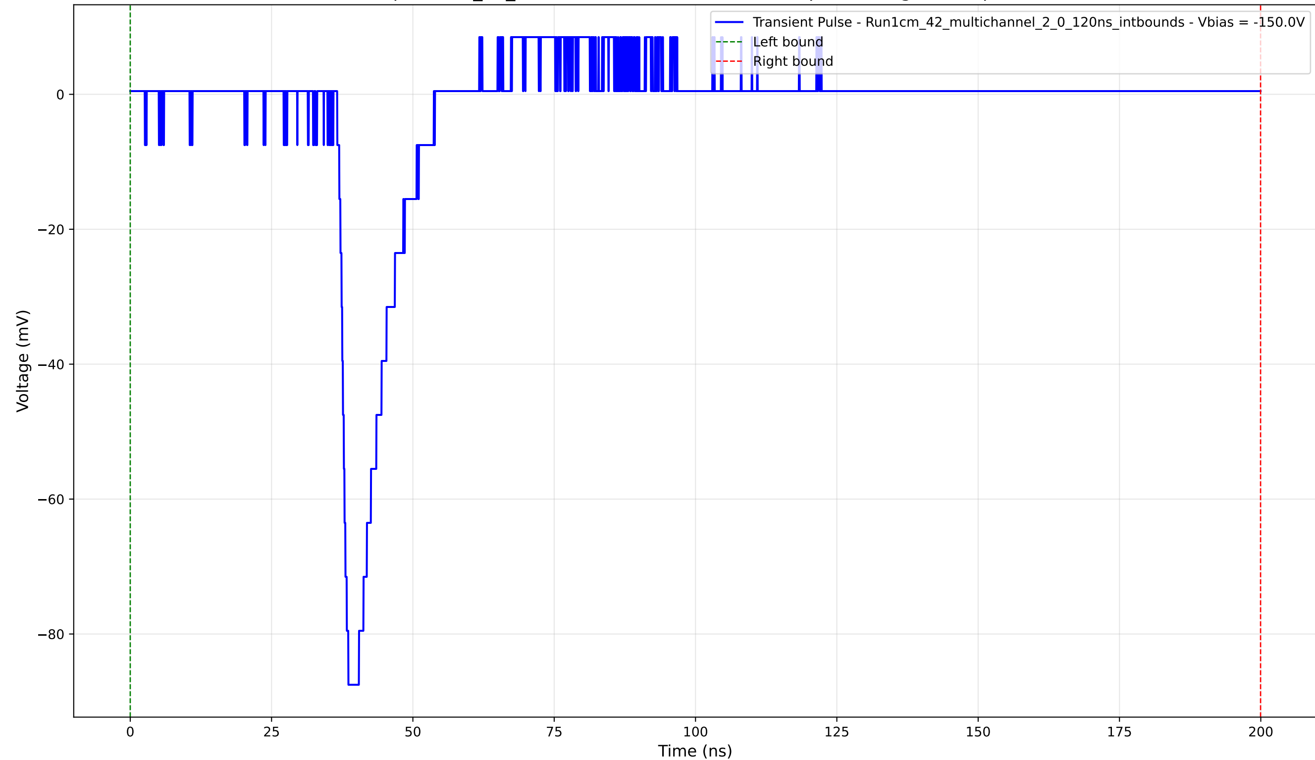
Transient Pulse - Sample: 1cm_42_multichannel - Position: 3965.0 \mu\text{m} - Charge: 8.76 pC - Rise Time: 1.35 ns
