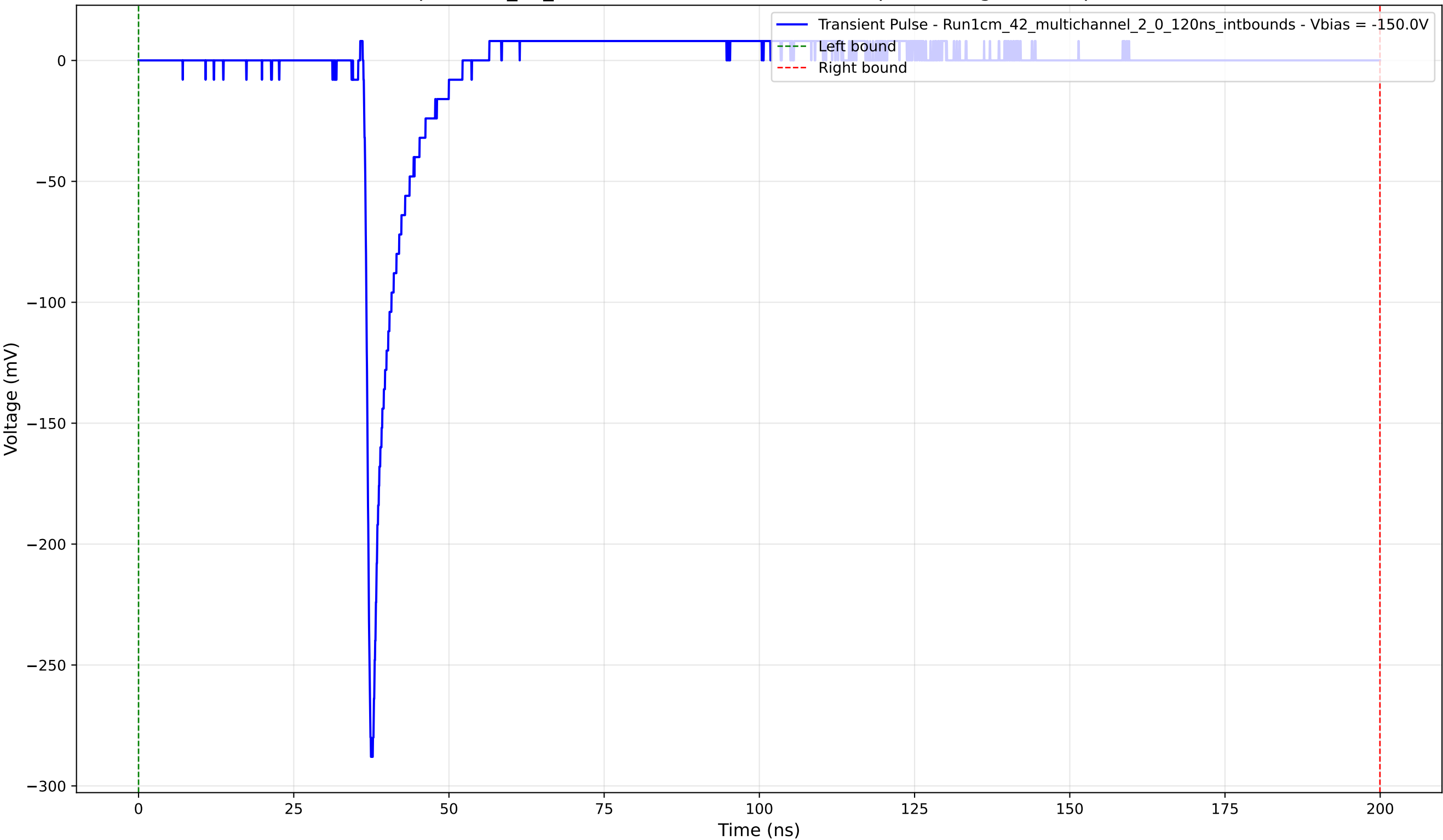
Transient Pulse - Sample: 1cm_42_multichannel - Position: 1765.0 \mu\text{m} - Charge: 12.65 pC - Rise Time: 0.87 ns
