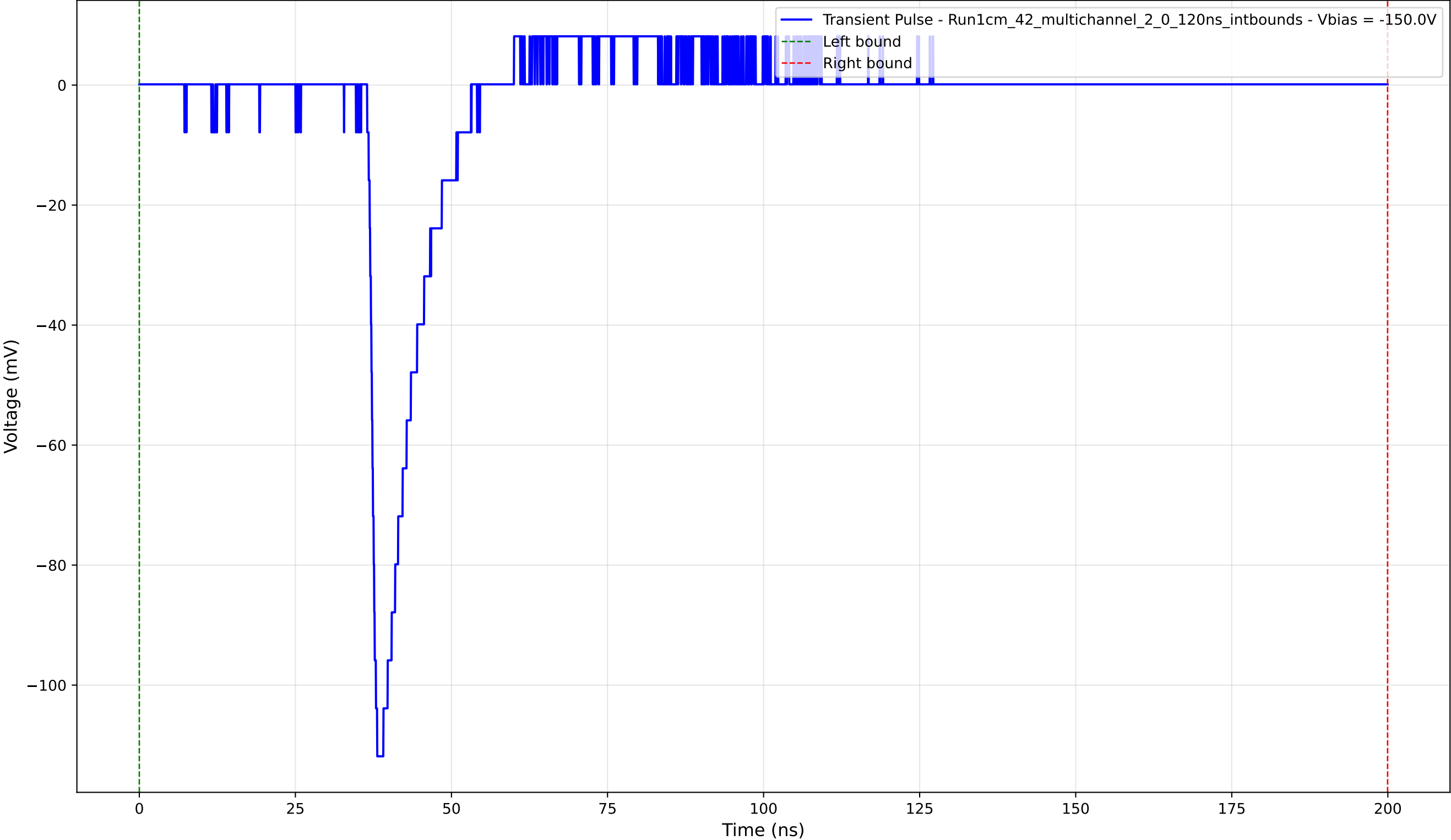
Transient Pulse - Sample: 1cm_42_multichannel - Position: 3610.0 \mu\text{m} - Charge: 10.41 pC - Rise Time: 1.18 ns
