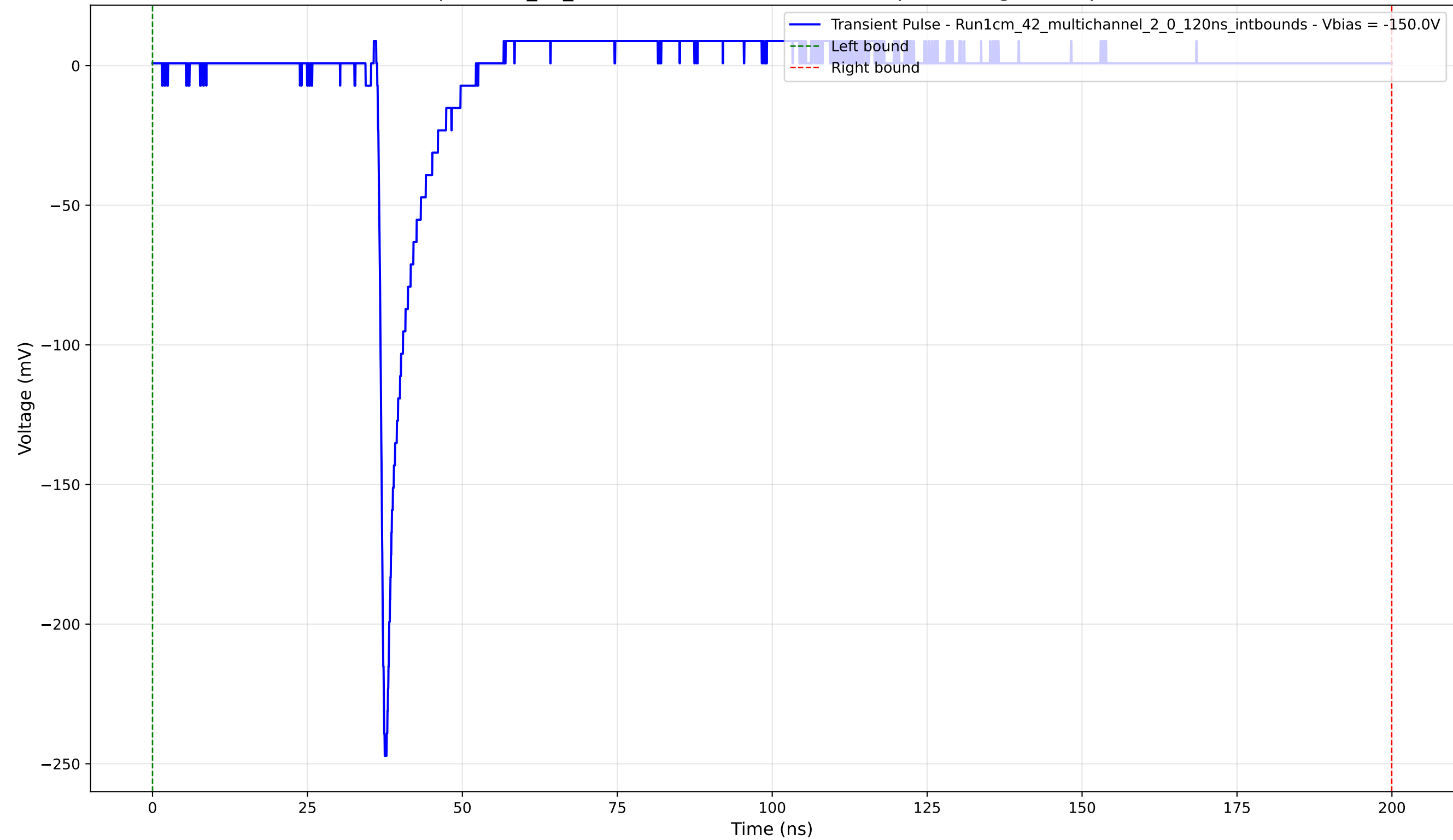
Transient Pulse - Sample: 1cm_42_multichannel - Position: 3025.0 \mu\text{m} - Charge: 8.83 pC - Rise Time: 0.87 ns
