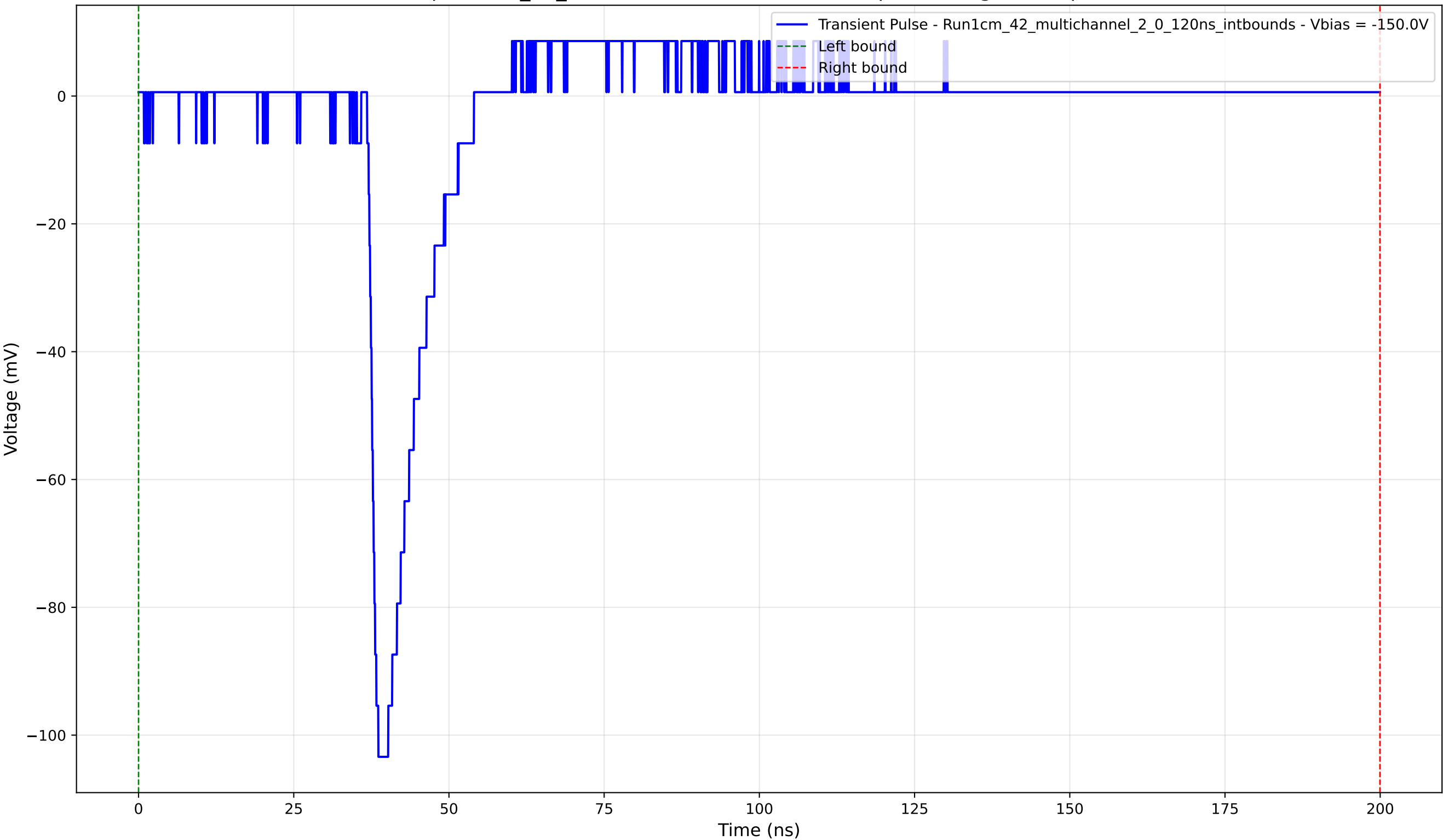
Transient Pulse - Sample: 1cm_42_multichannel - Position: 695.0 \mu\text{m} - Charge: 8.21 pC - Rise Time: 1.27 ns
