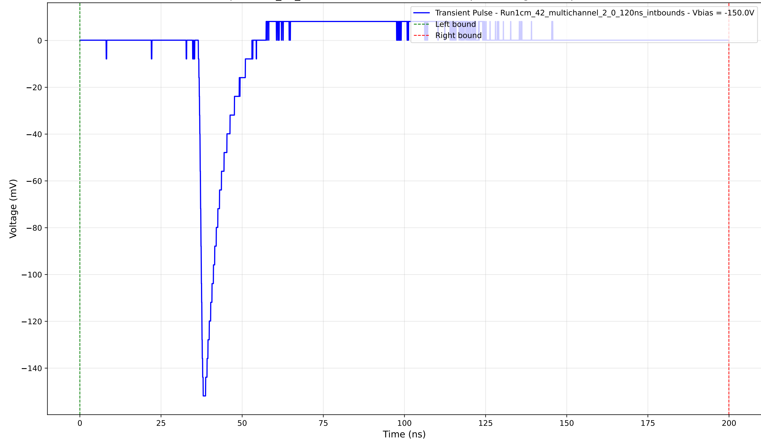
Transient Pulse - Sample: 1cm_42_multichannel - Position: 1215.0 \mu\text{m} - Charge: 9.28 pC - Rise Time: 1.16 ns
