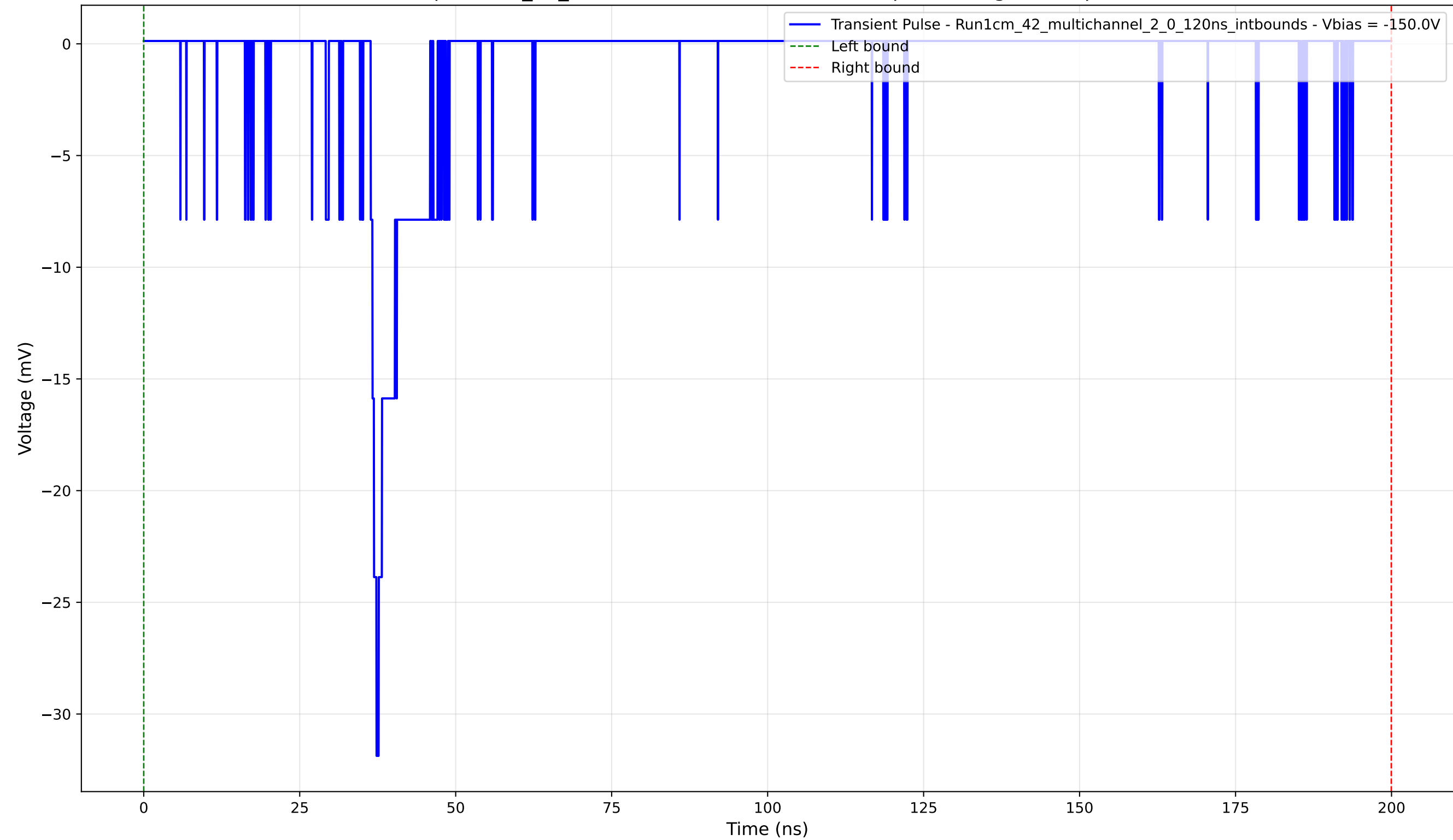
Transient Pulse - Sample: 1cm_42_multichannel - Position: 2855.0 \mu\text{m} - Charge: 2.97 pC - Rise Time: 0.94 ns
