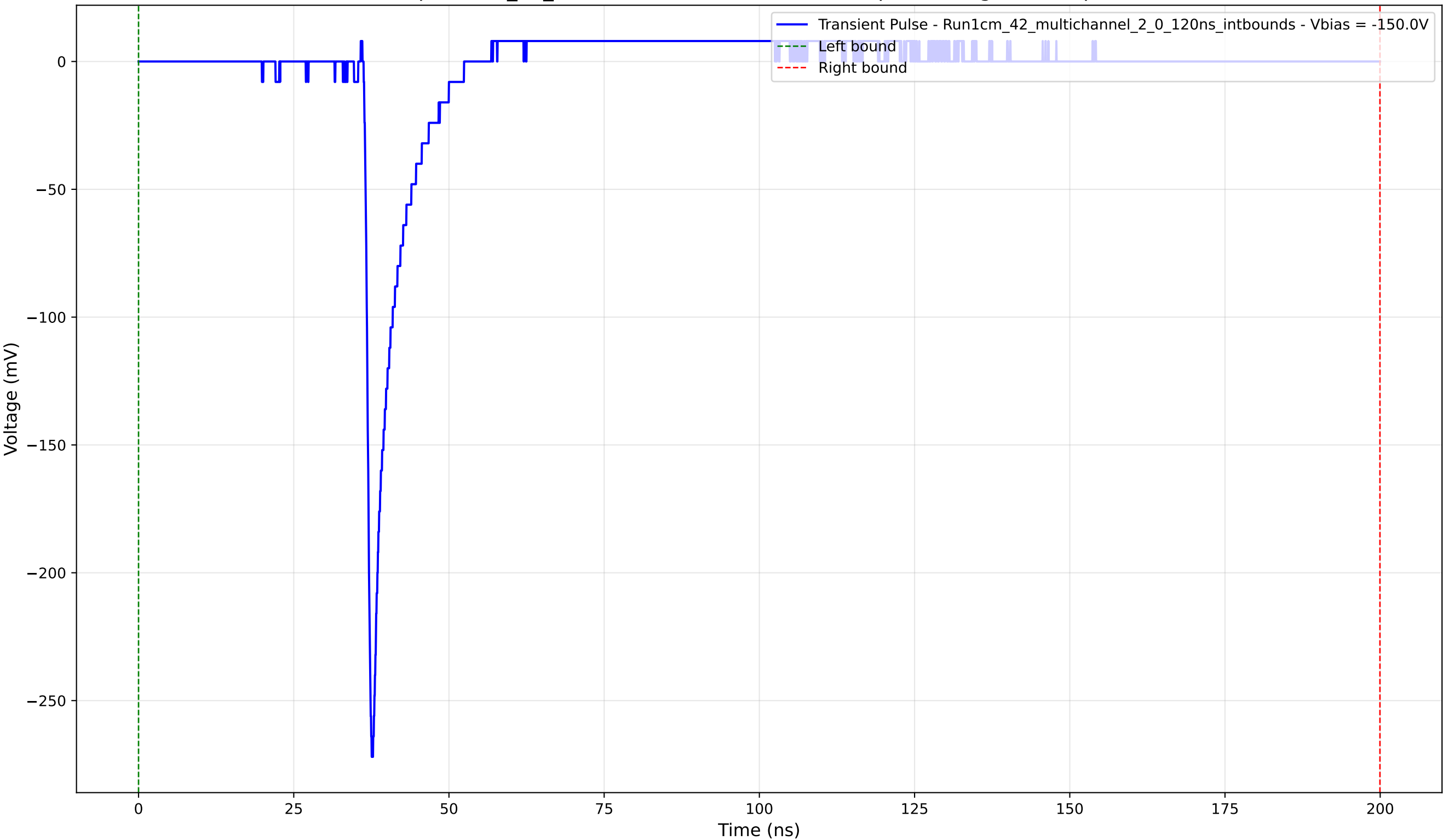
Transient Pulse - Sample: 1cm_42_multichannel - Position: 1685.0 \mu\text{m} - Charge: 12.93 pC - Rise Time: 0.89 ns
