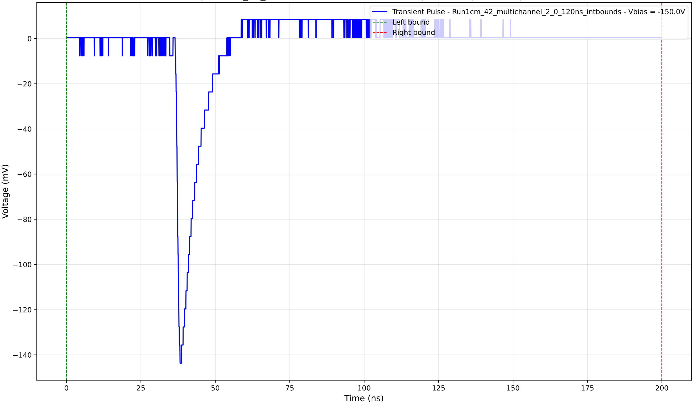
Transient Pulse - Sample: 1cm_42_multichannel - Position: 1160.0 \mu\text{m} - Charge: 10.47 pC - Rise Time: 1.21 ns
