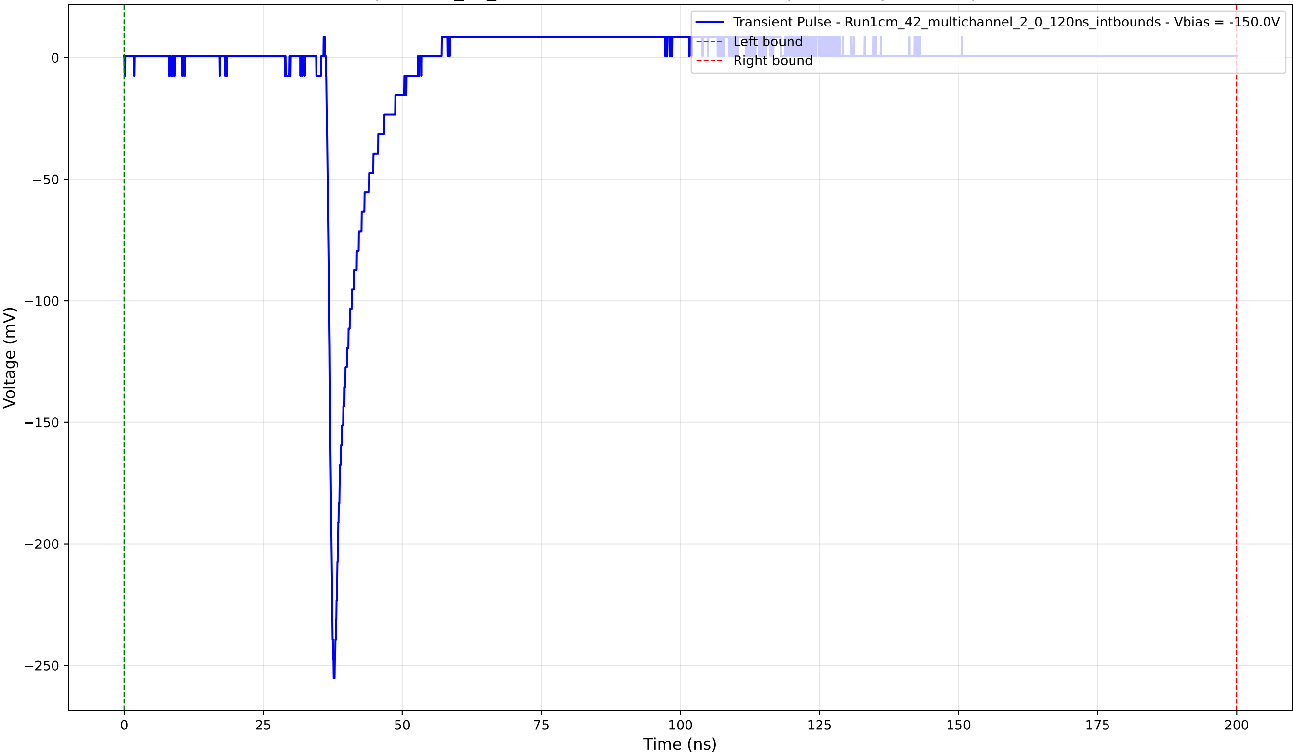
Transient Pulse - Sample: 1cm_42_multichannel - Position: 1650.0 \mu\text{m} - Charge: 10.59 pC - Rise Time: 0.90 ns
