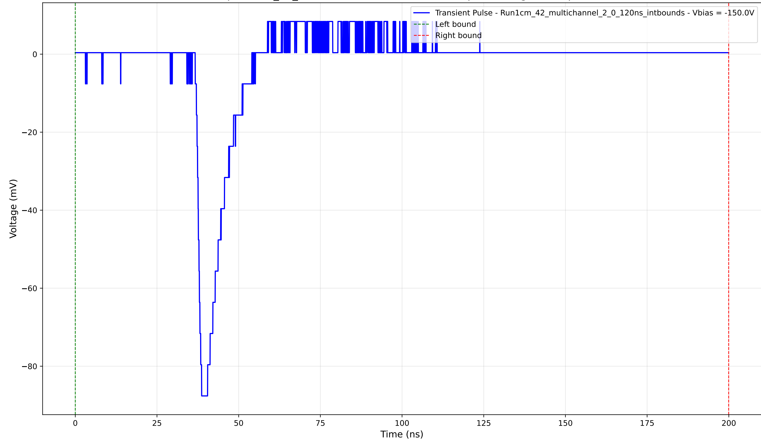
Transient Pulse - Sample: 1cm_42_multichannel - Position: 4030.0 \mu\text{m} - Charge: 8.67 pC - Rise Time: 1.35 ns
