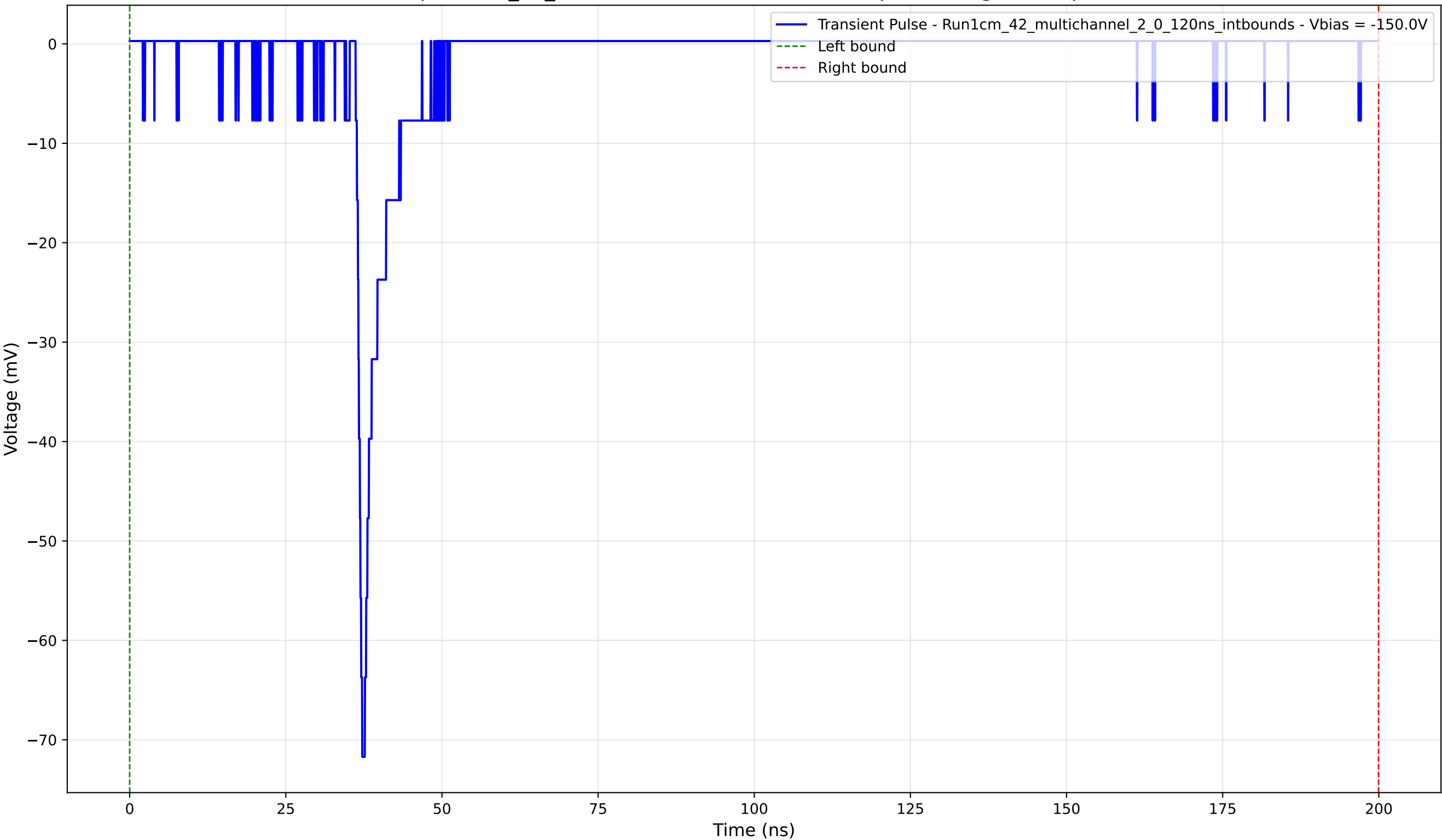
Transient Pulse - Sample: 1cm_42_multichannel - Position: 2840.0 \mu\text{m} - Charge: 4.99 pC - Rise Time: 1.04 ns
