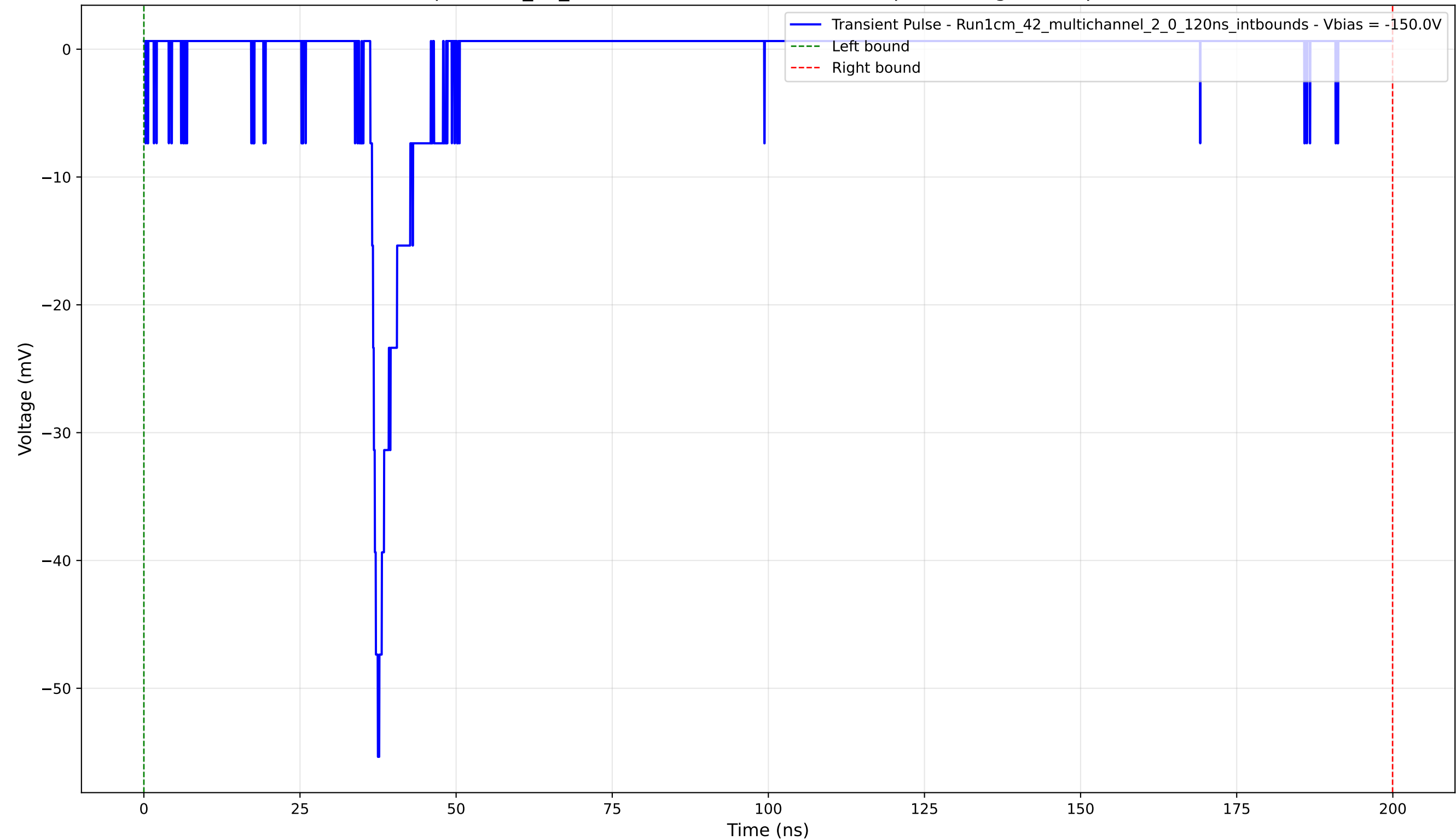
Transient Pulse - Sample: 1cm_42_multichannel - Position: 1830.0 \mu\text{m} - Charge: 2.31 pC - Rise Time: 1.21 ns
