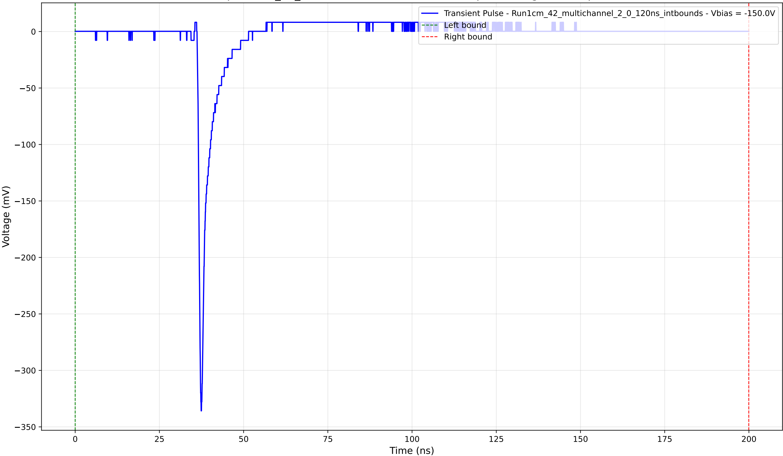
Transient Pulse - Sample: 1cm_42_multichannel - Position: 1935.0 \mu\text{m} - Charge: 11.83 pC - Rise Time: 0.82 ns
