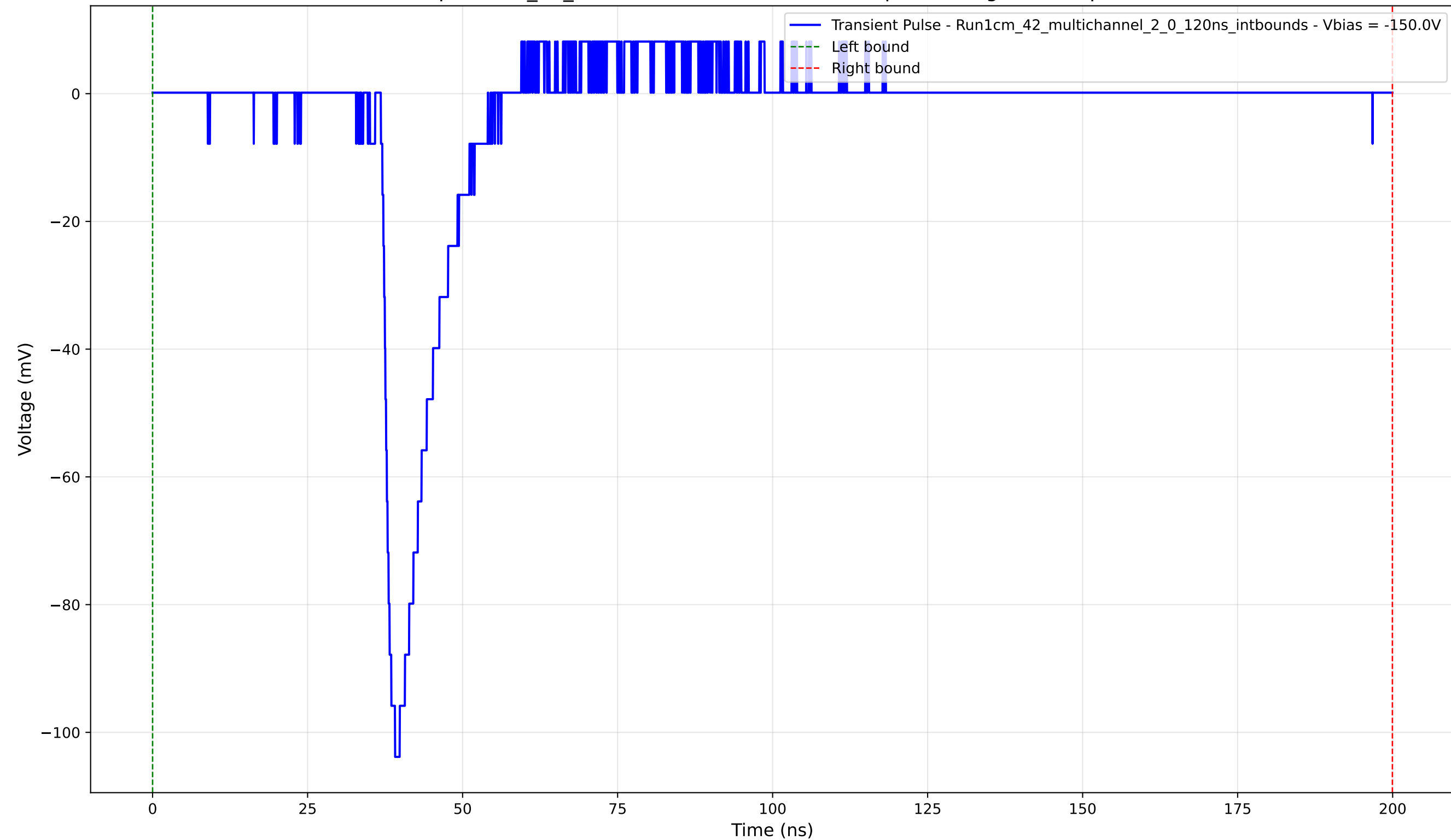
Transient Pulse - Sample: 1cm_42_multichannel - Position: 640.0 \mu\text{m} - Charge: 11.39 pC - Rise Time: 1.47 ns
