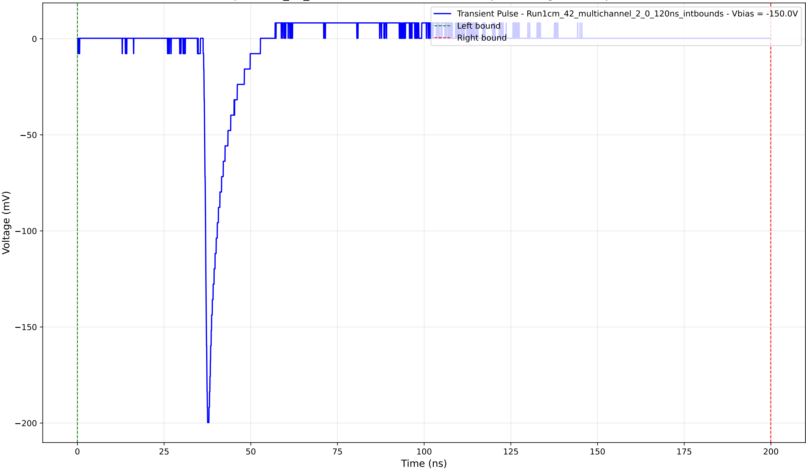
Transient Pulse - Sample: 1cm_42_multichannel - Position: 3145.0 \mu\text{m} - Charge: 10.30 pC - Rise Time: 0.90 ns
