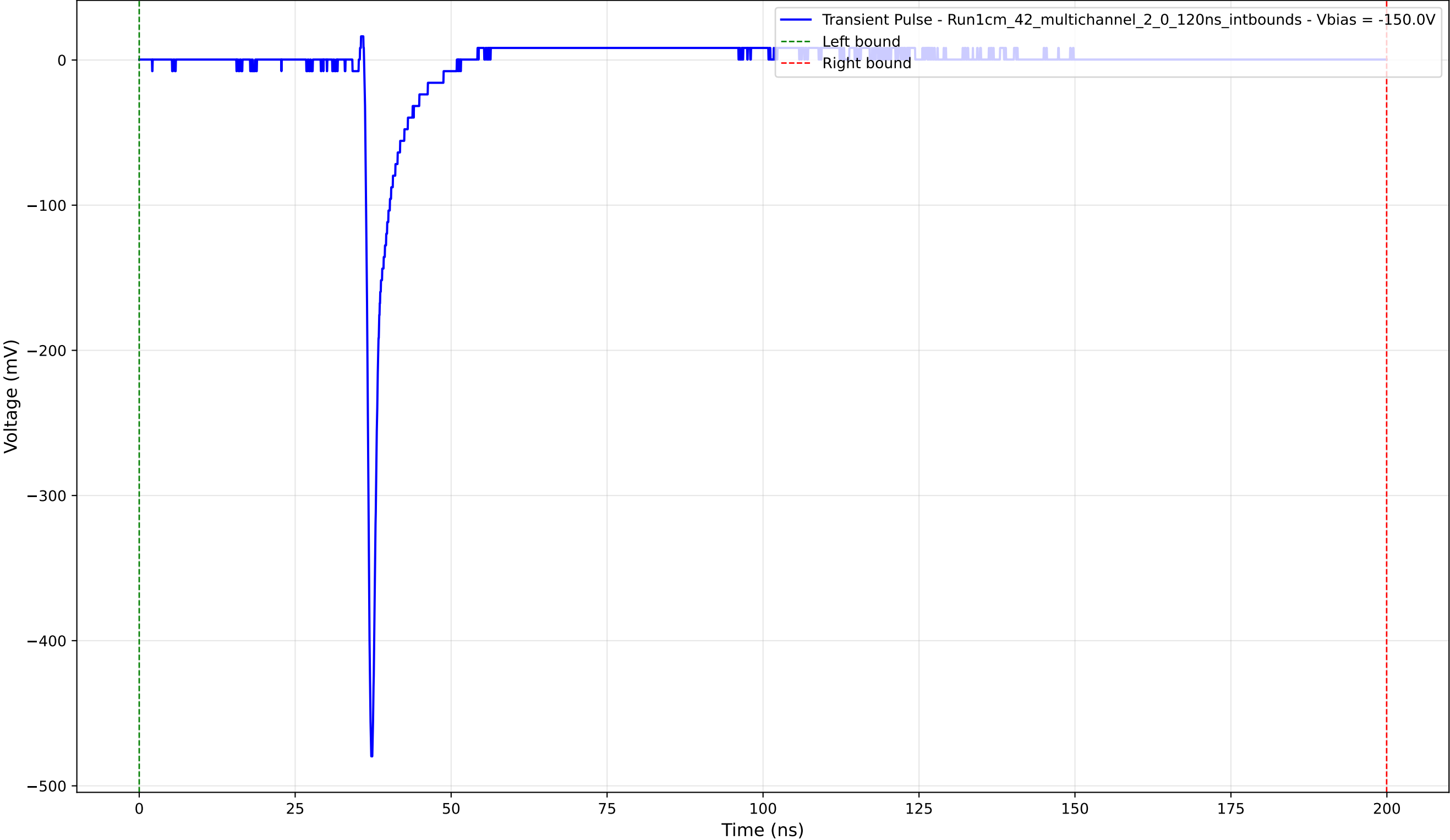
Transient Pulse - Sample: 1cm_42_multichannel - Position: 2610.0 \mu\text{m} - Charge: 14.11 pC - Rise Time: 0.78 ns
