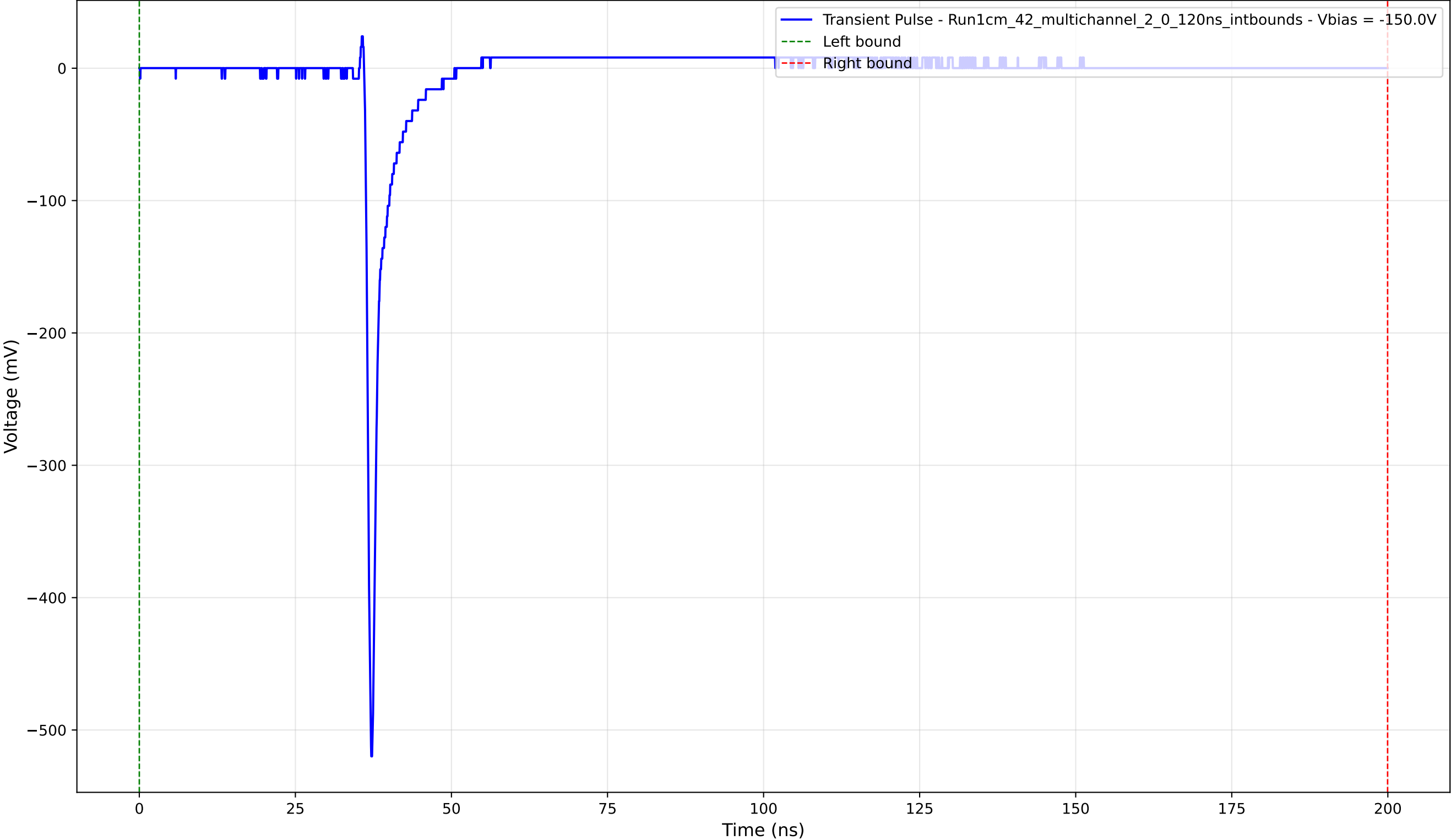
Transient Pulse - Sample: 1cm_42_multichannel - Position: 2545.0 \mu\text{m} - Charge: 14.47 pC - Rise Time: 0.76 ns
