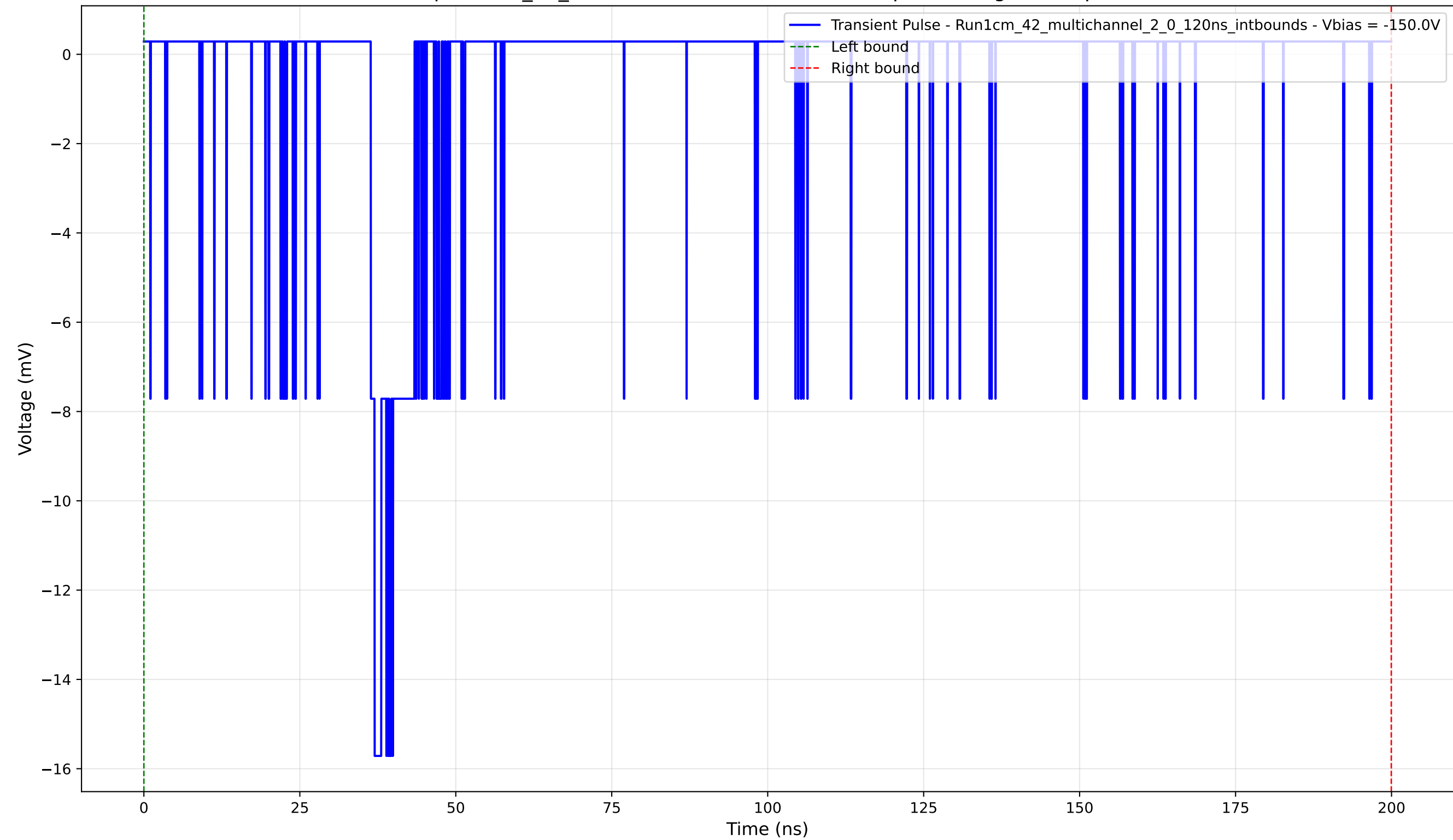
Transient Pulse - Sample: 1cm_42_multichannel - Position: 2885.0 \mu\text{m} - Charge: 1.50 pC - Rise Time: 0.63 ns
