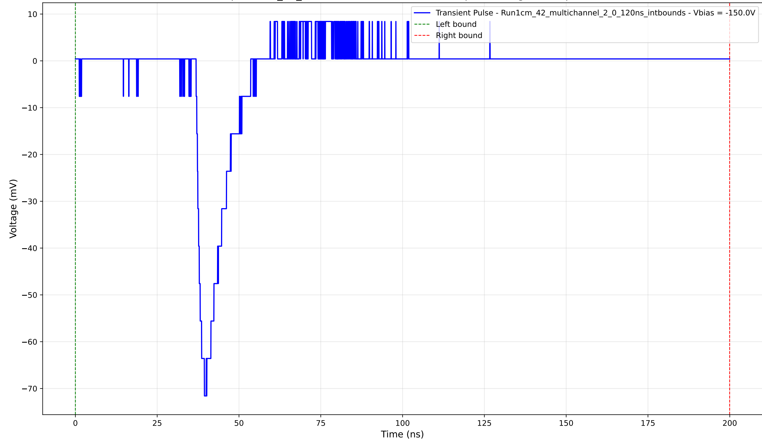
Transient Pulse - Sample: 1cm_42_multichannel - Position: 265.0 \mu\text{m} - Charge: 7.51 pC - Rise Time: 2.52 ns
