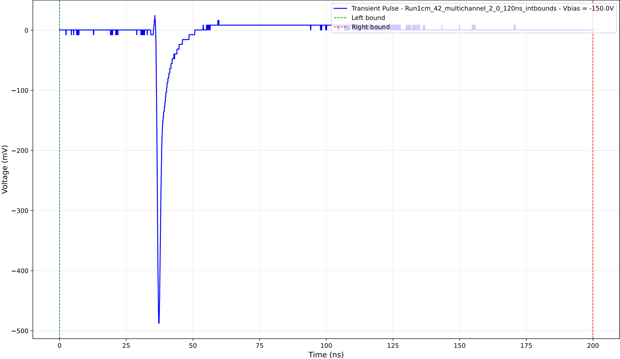
Transient Pulse - Sample: 1cm_42_multichannel - Position: 2590.0 \mu\text{m} - Charge: 13.06 pC - Rise Time: 0.75 ns
