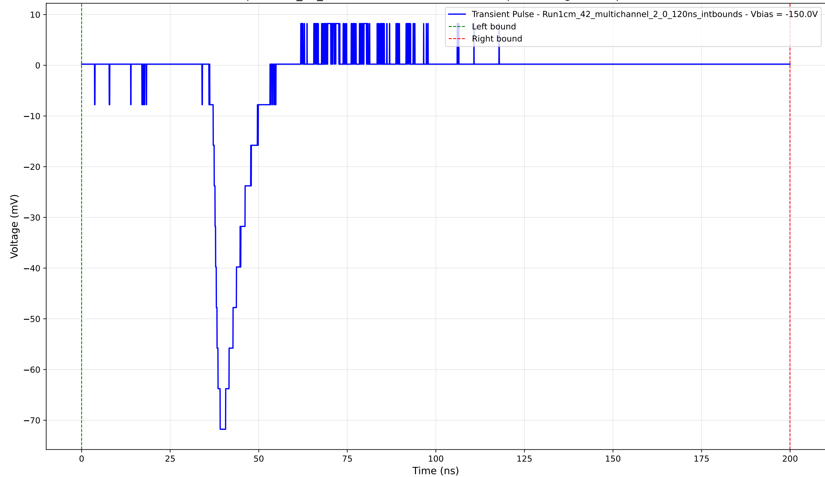
Transient Pulse - Sample: 1cm_42_multichannel - Position: 4570.0 \mu\text{m} - Charge: 8.84 pC - Rise Time: 2.92 ns
