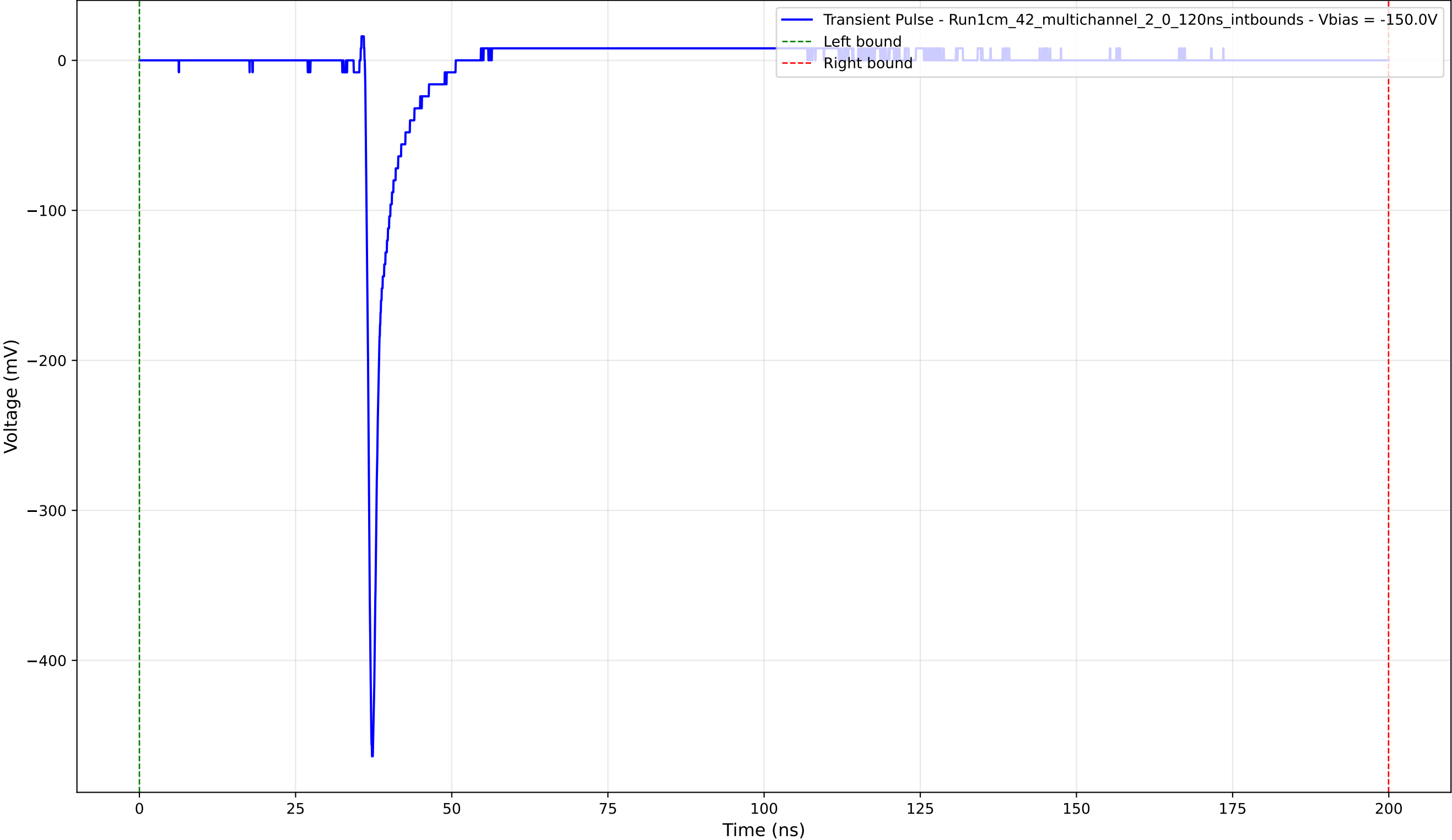
Transient Pulse - Sample: 1cm_42_multichannel - Position: 2640.0 \mu\text{m} - Charge: 14.43 pC - Rise Time: 0.75 ns
