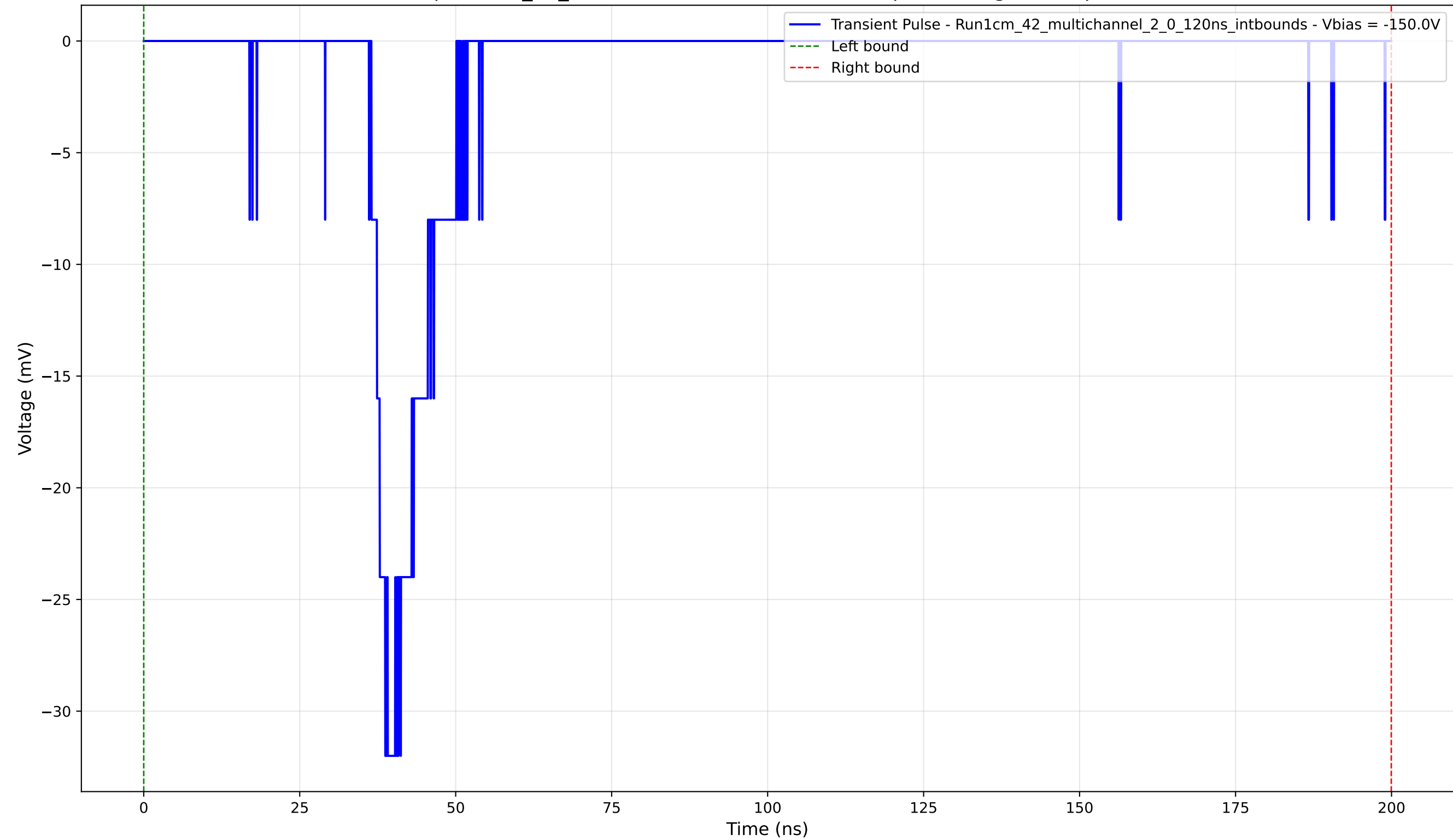
Transient Pulse - Sample: 1cm_42_multichannel - Position: 4850.0 \mu\text{m} - Charge: 4.97 pC - Rise Time: 2.22 ns
