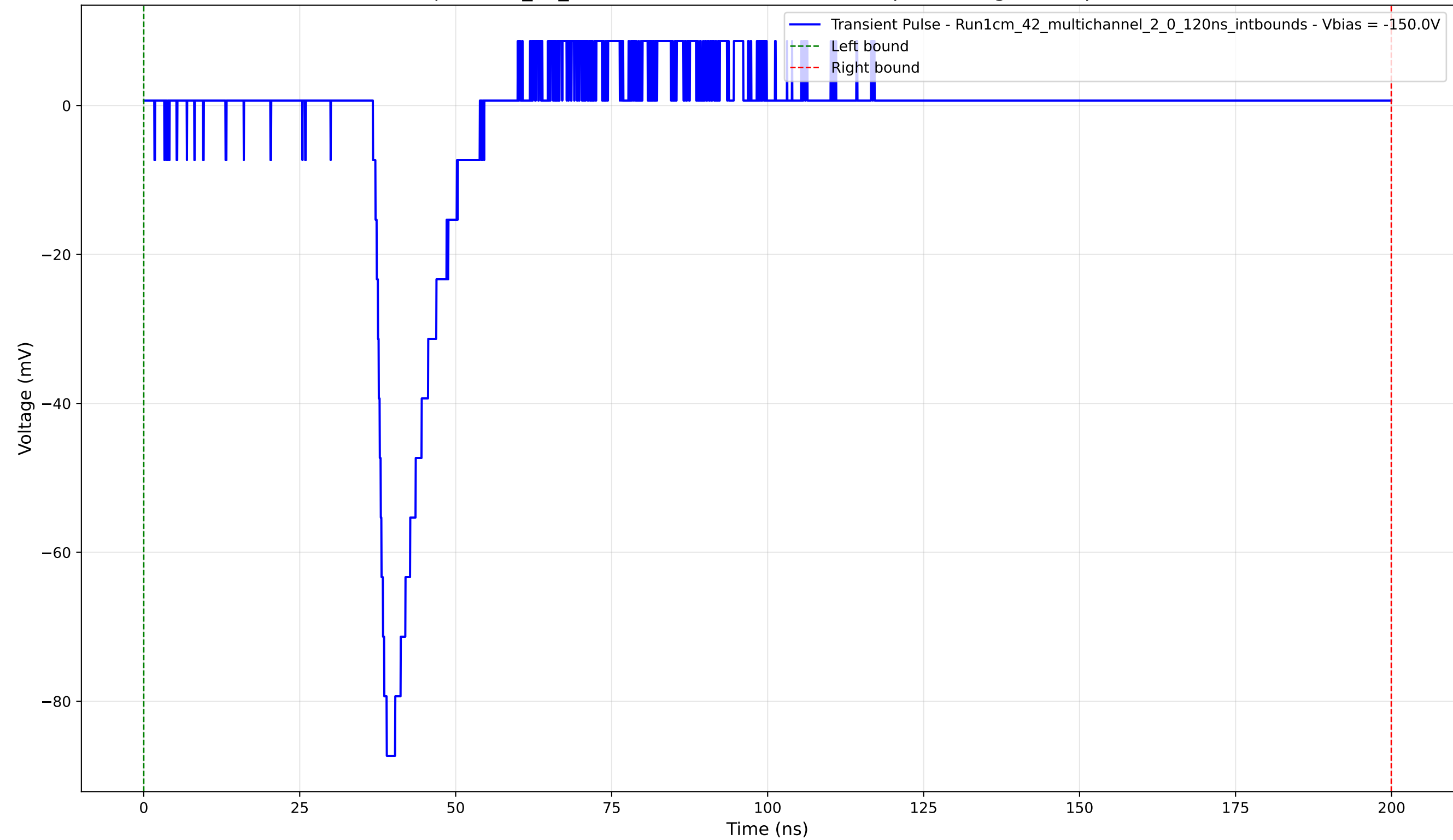
Transient Pulse - Sample: 1cm_42_multichannel - Position: 4150.0 \mu\text{m} - Charge: 6.85 pC - Rise Time: 1.43 ns
