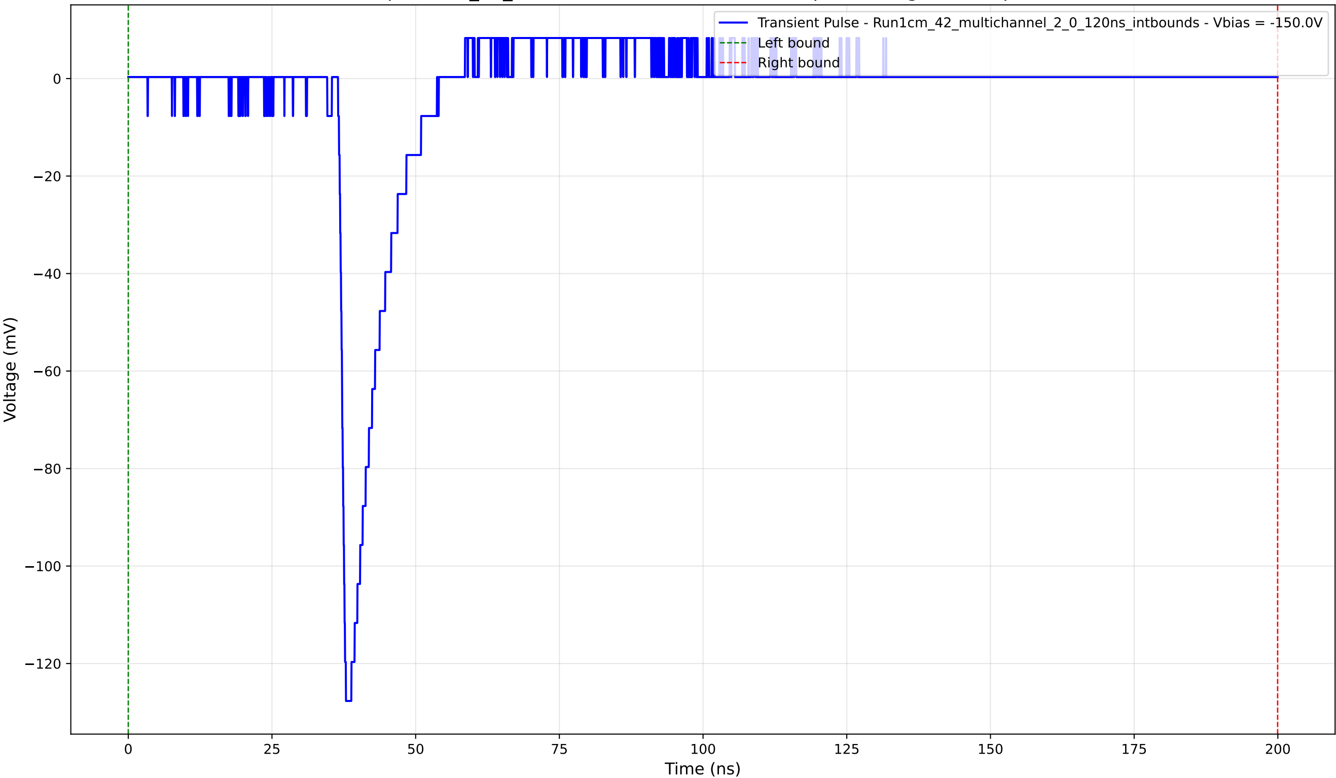
Transient Pulse - Sample: 1cm_42_multichannel - Position: 3505.0 \mu\text{m} - Charge: 10.32 pC - Rise Time: 1.05 ns
