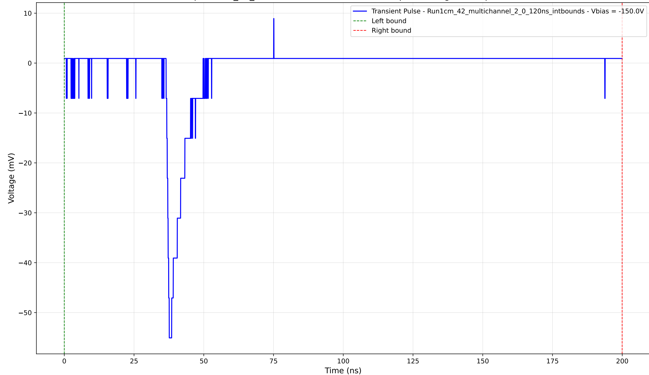
Transient Pulse - Sample: 1cm_42_multichannel - Position: 3340.0 \mu\text{m} - Charge: 3.00 pC - Rise Time: 1.13 ns
