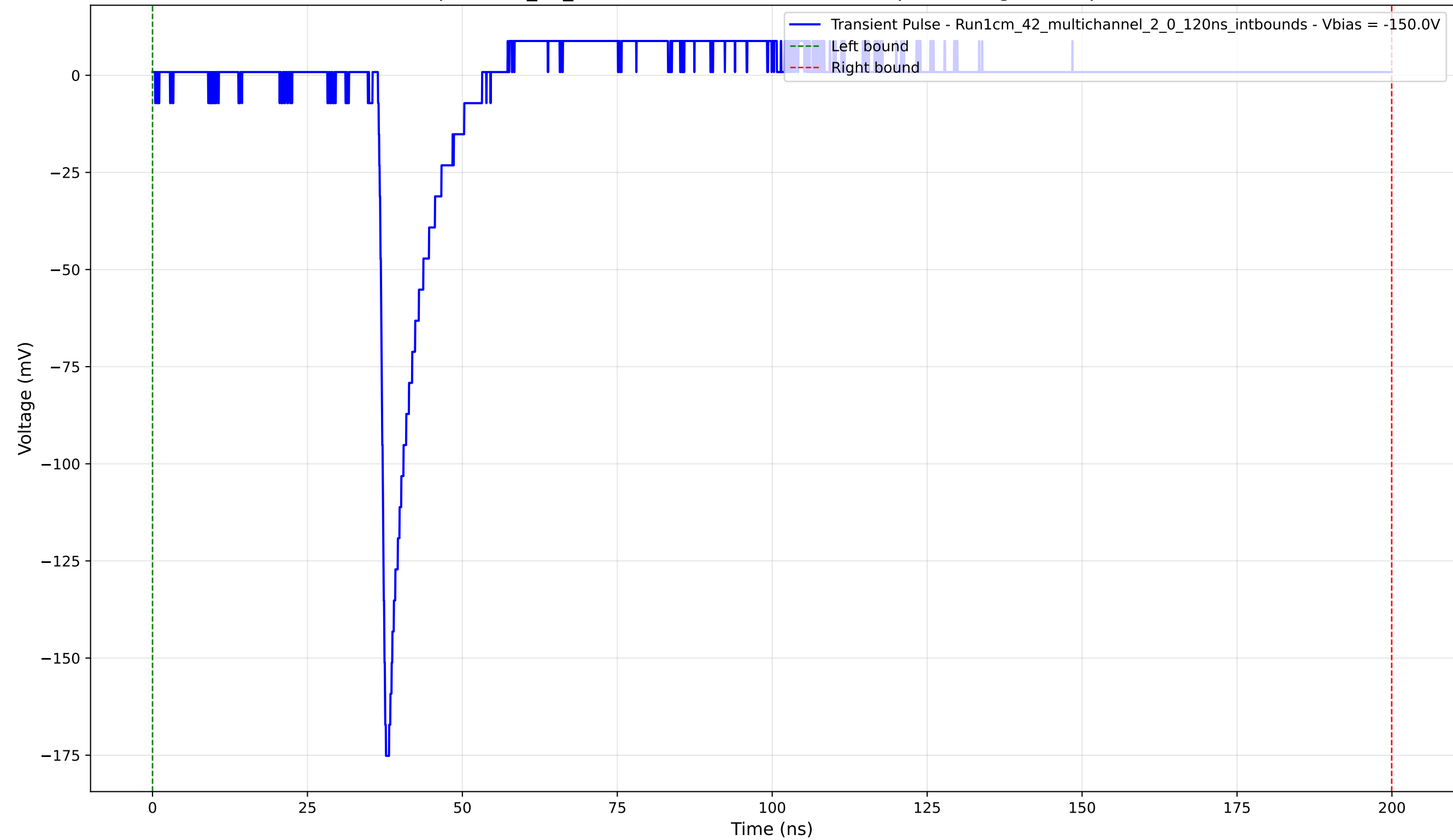
Transient Pulse - Sample: 1cm_42_multichannel - Position: 3270.0 \mu\text{m} - Charge: 8.83 pC - Rise Time: 0.94 ns
