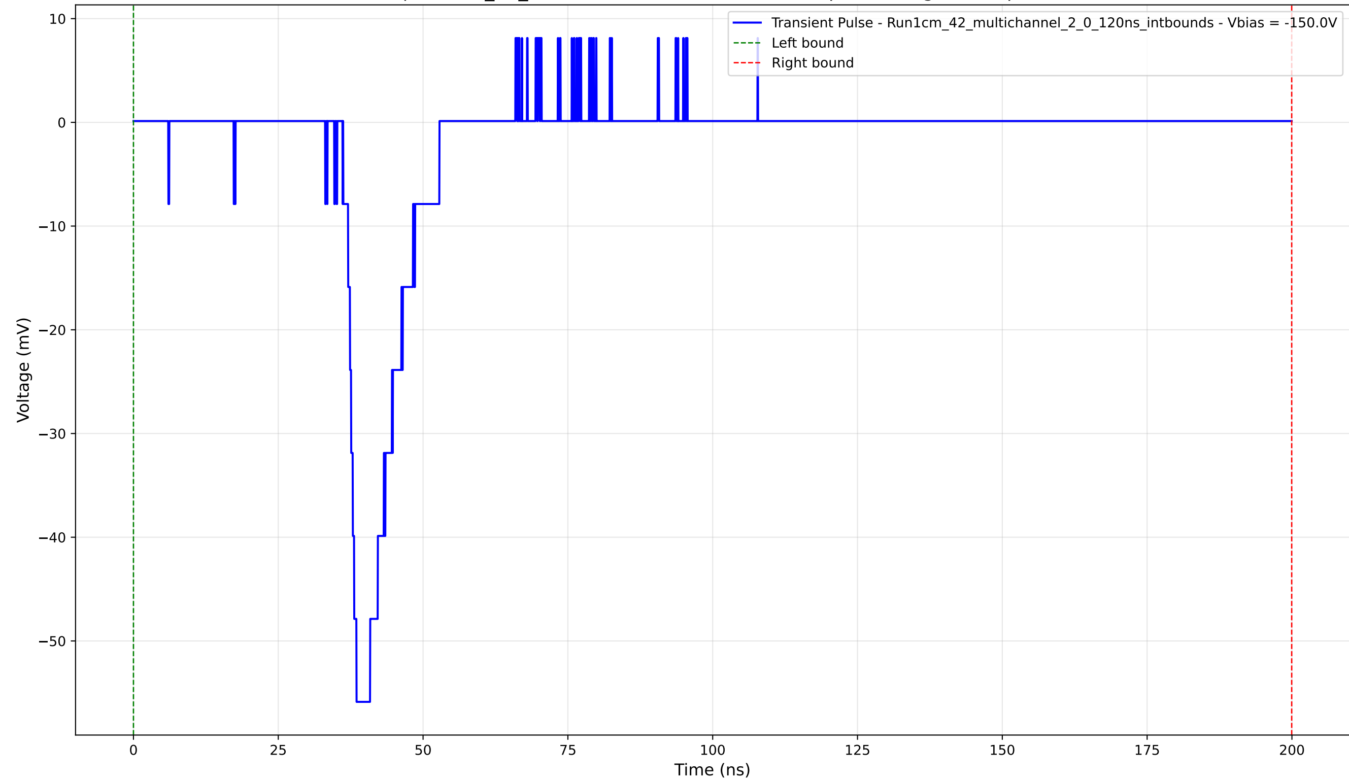
Transient Pulse - Sample: 1cm_42_multichannel - Position: 4815.0 \mu\text{m} - Charge: 7.98 pC - Rise Time: 2.29 ns
