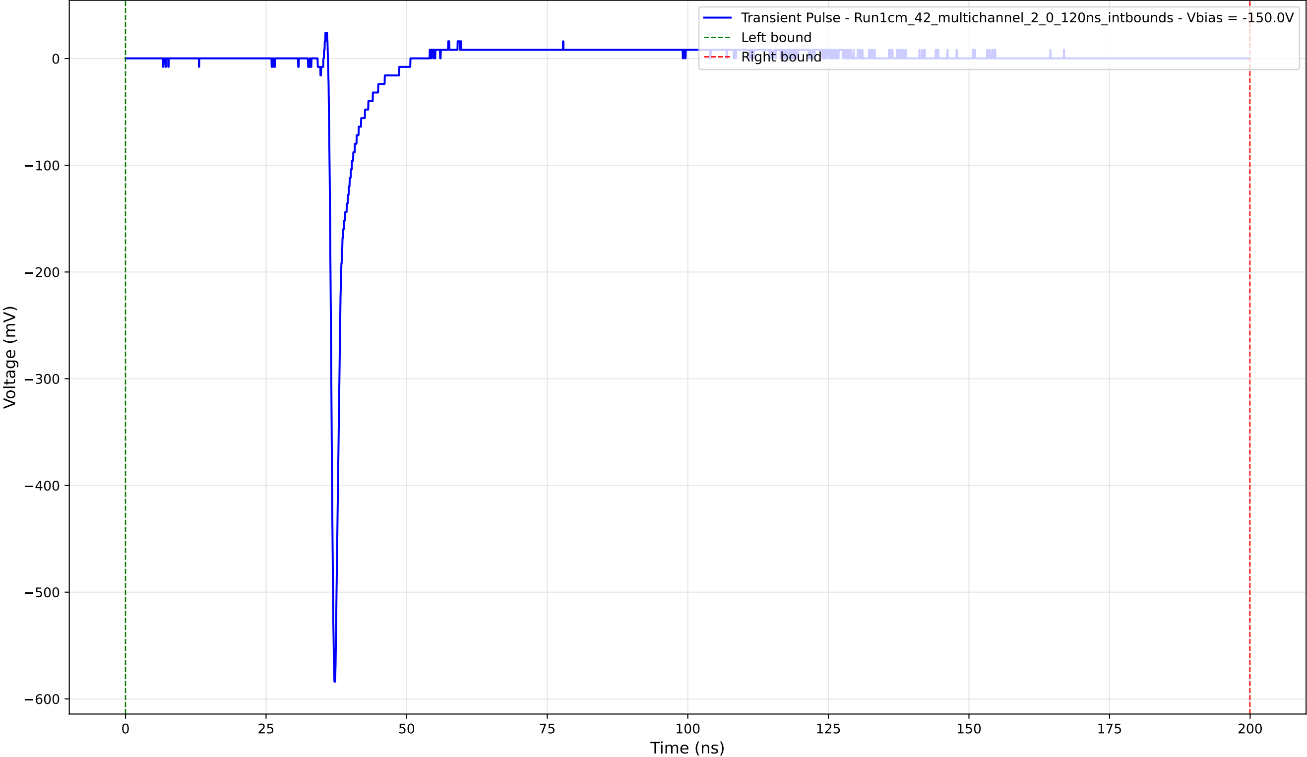
Transient Pulse - Sample: 1cm_42_multichannel - Position: 2205.0 \mu\text{m} - Charge: 16.34 pC - Rise Time: 0.75 ns
