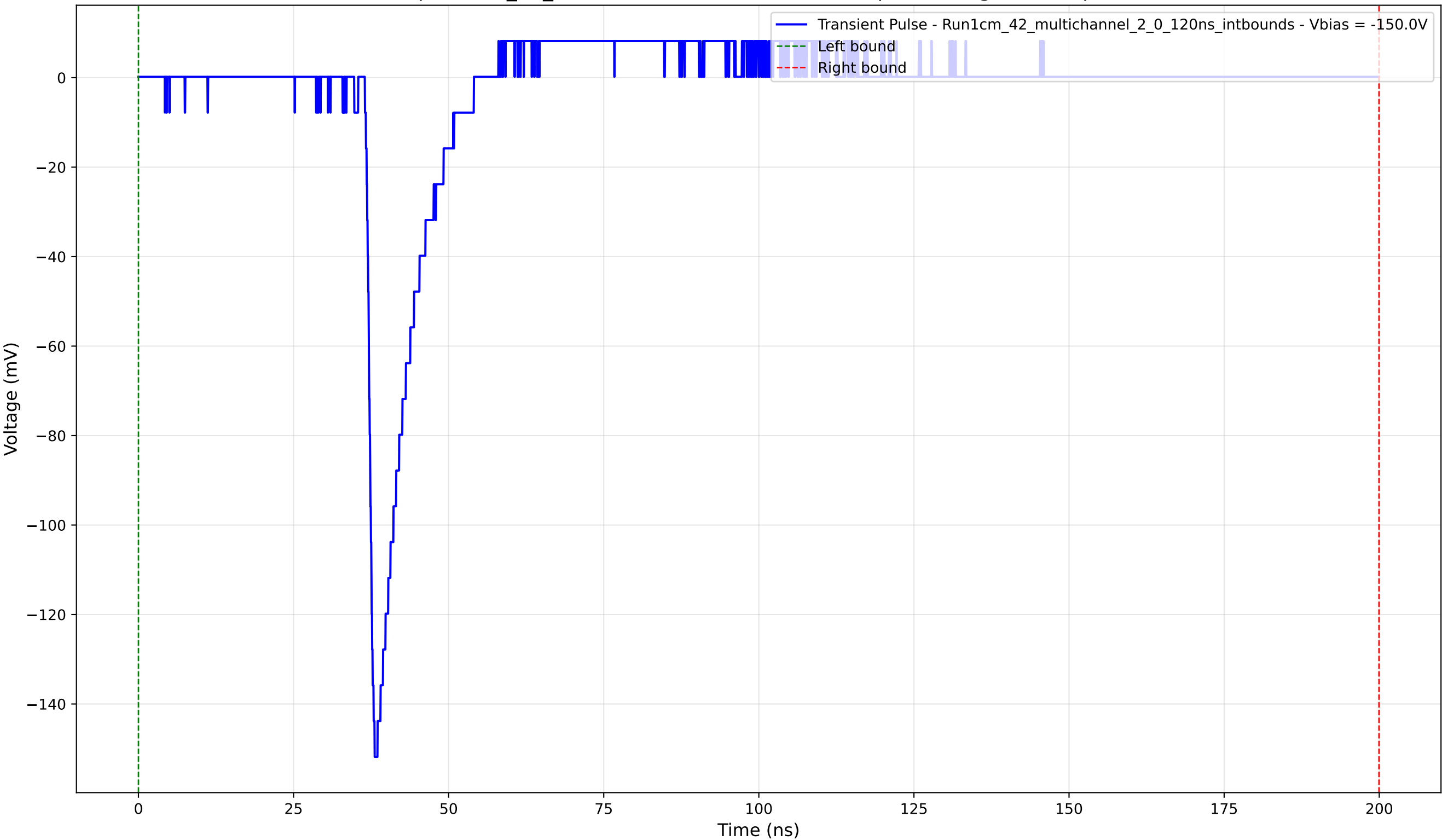
Transient Pulse - Sample: 1cm_42_multichannel - Position: 1200.0 \mu\text{m} - Charge: 11.06 pC - Rise Time: 1.24 ns
