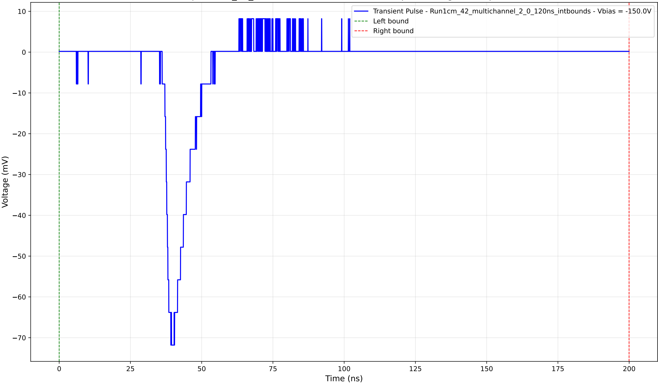
Transient Pulse - Sample: 1cm_42_multichannel - Position: 4695.0 \mu\text{m} - Charge: 9.11 pC - Rise Time: 3.04 ns
