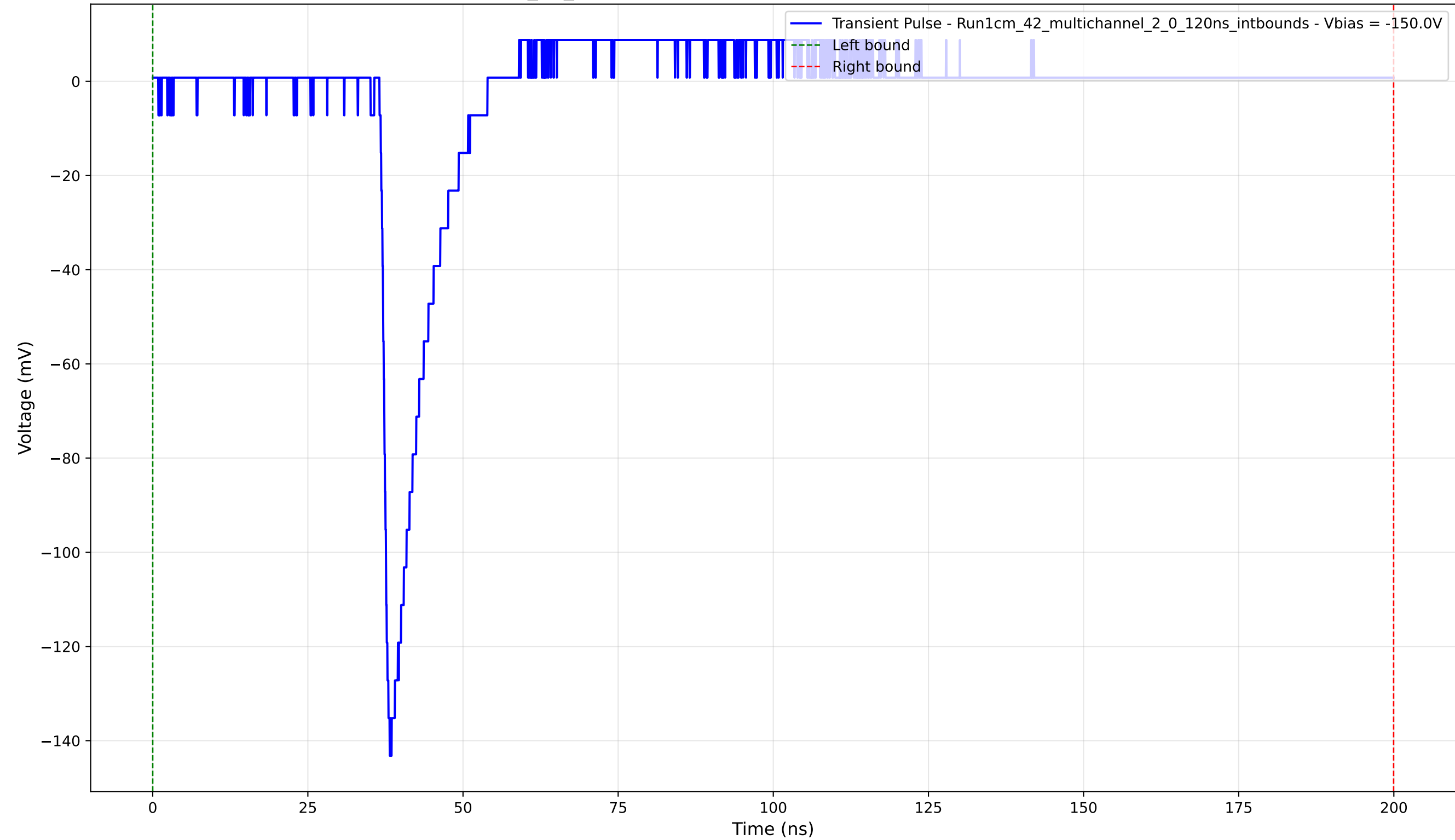
Transient Pulse - Sample: 1cm_42_multichannel - Position: 1155.0 \mu\text{m} - Charge: 8.26 pC - Rise Time: 1.24 ns
