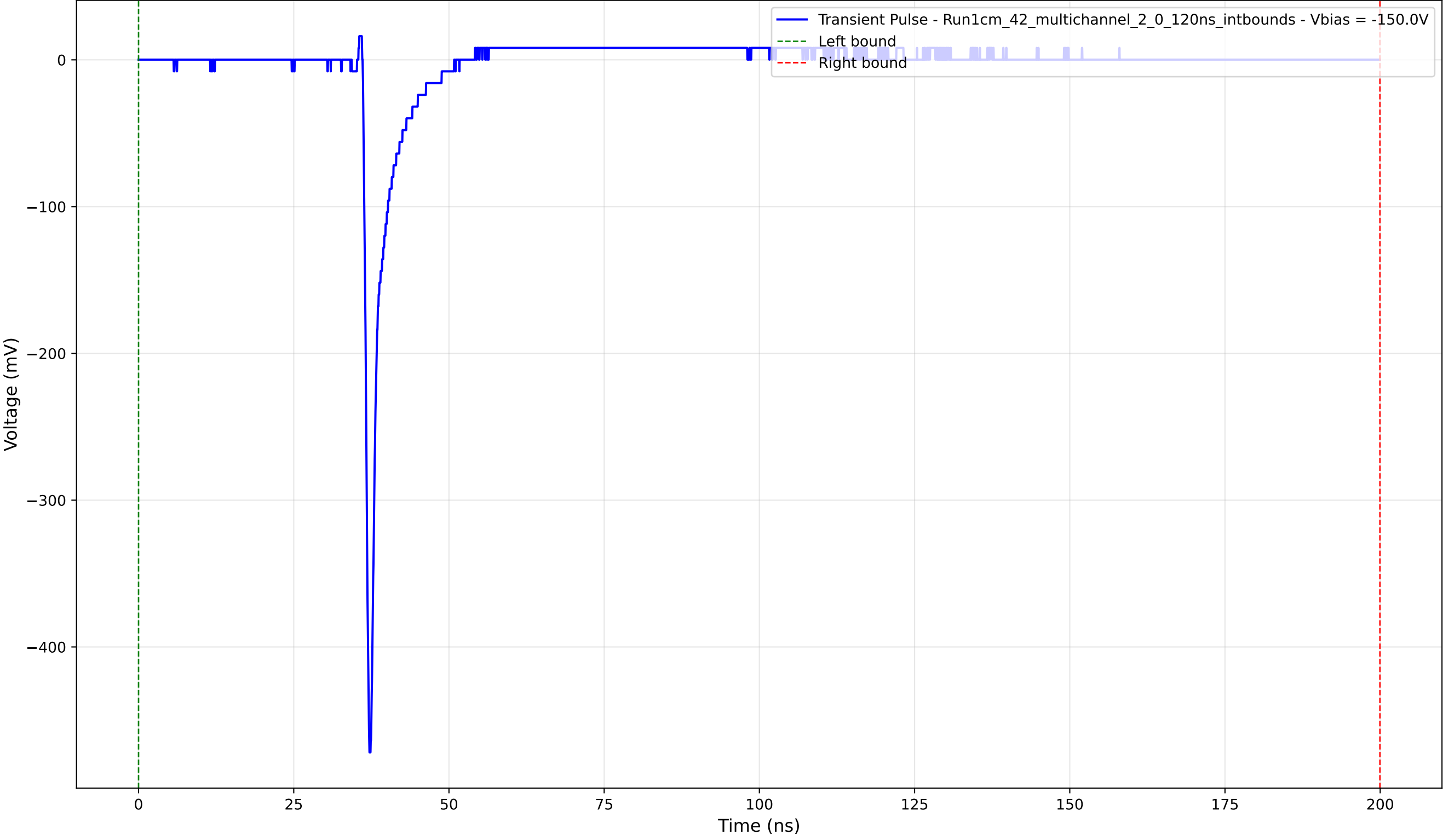
Transient Pulse - Sample: 1cm_42_multichannel - Position: 2625.0 \mu\text{m} - Charge: 14.88 pC - Rise Time: 0.76 ns
