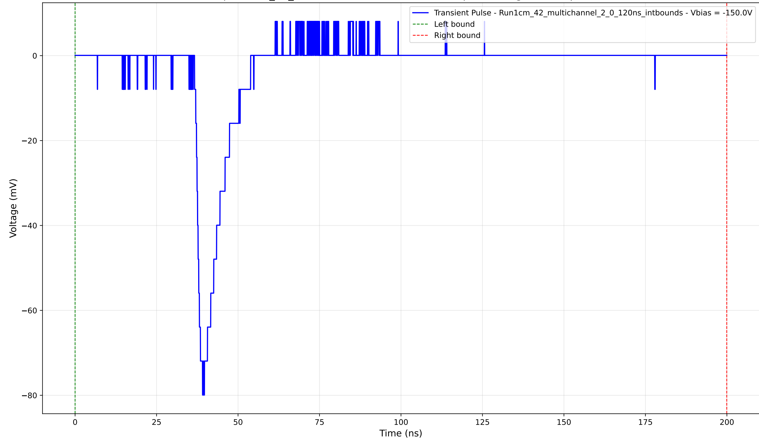
Transient Pulse - Sample: 1cm_42_multichannel - Position: 3950.0 \mu\text{m} - Charge: 10.18 pC - Rise Time: 2.12 ns
