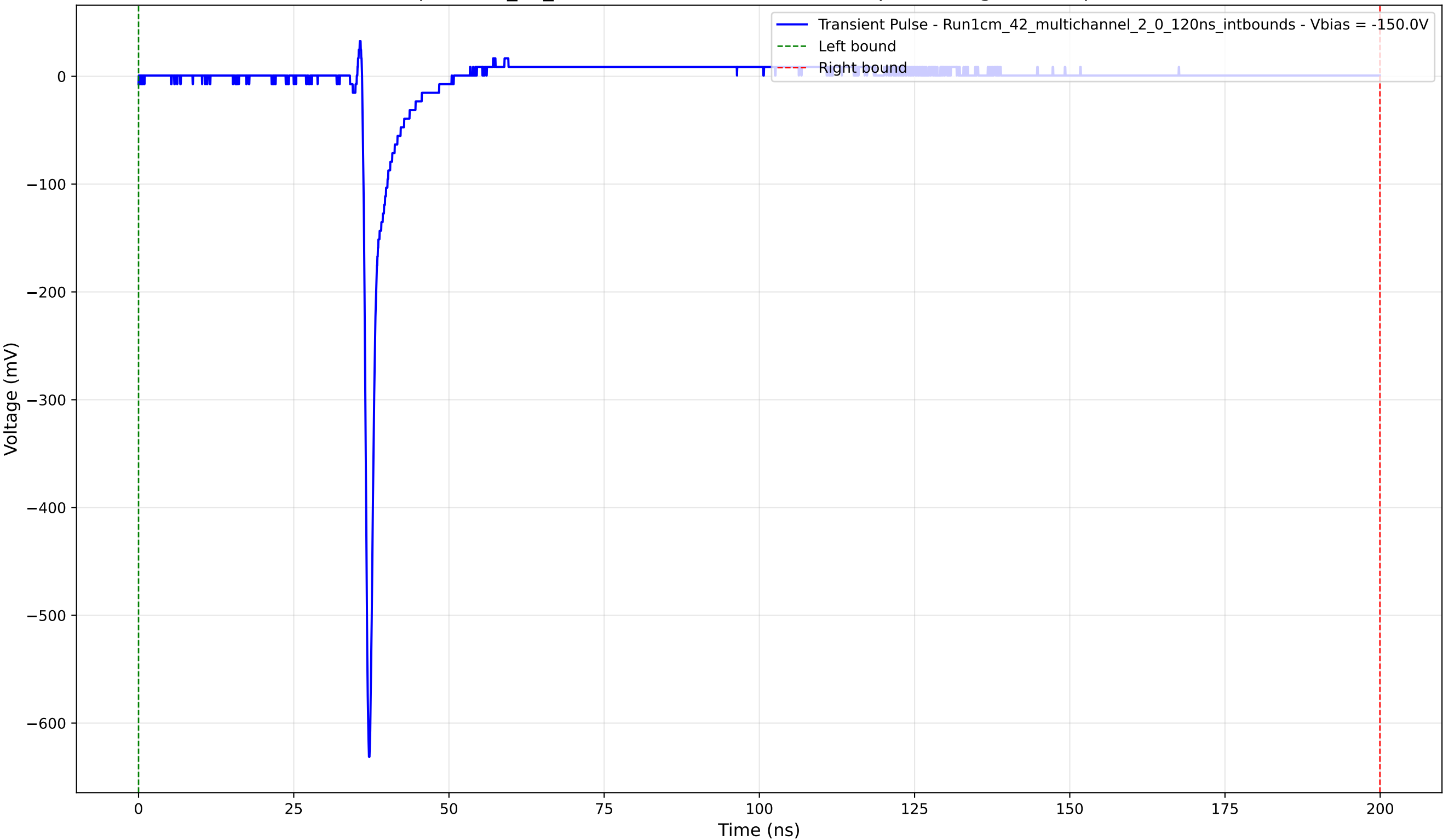
Transient Pulse - Sample: 1cm_42_multichannel - Position: 2280.0 \mu\text{m} - Charge: 14.81 pC - Rise Time: 0.73 ns
