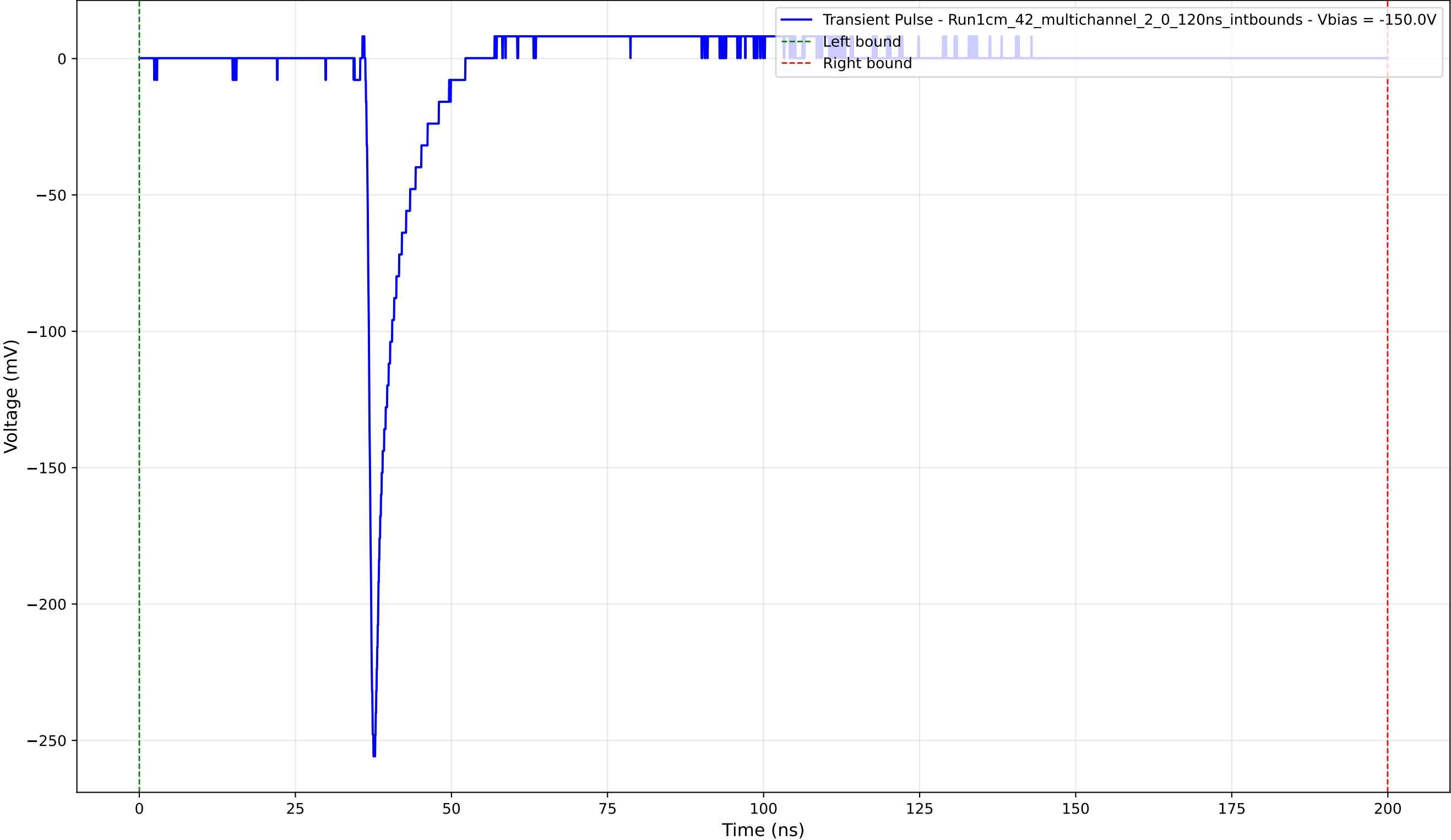
Transient Pulse - Sample: 1cm_42_multichannel - Position: 3015.0 \mu\text{m} - Charge: 12.32 pC - Rise Time: 0.87 ns
