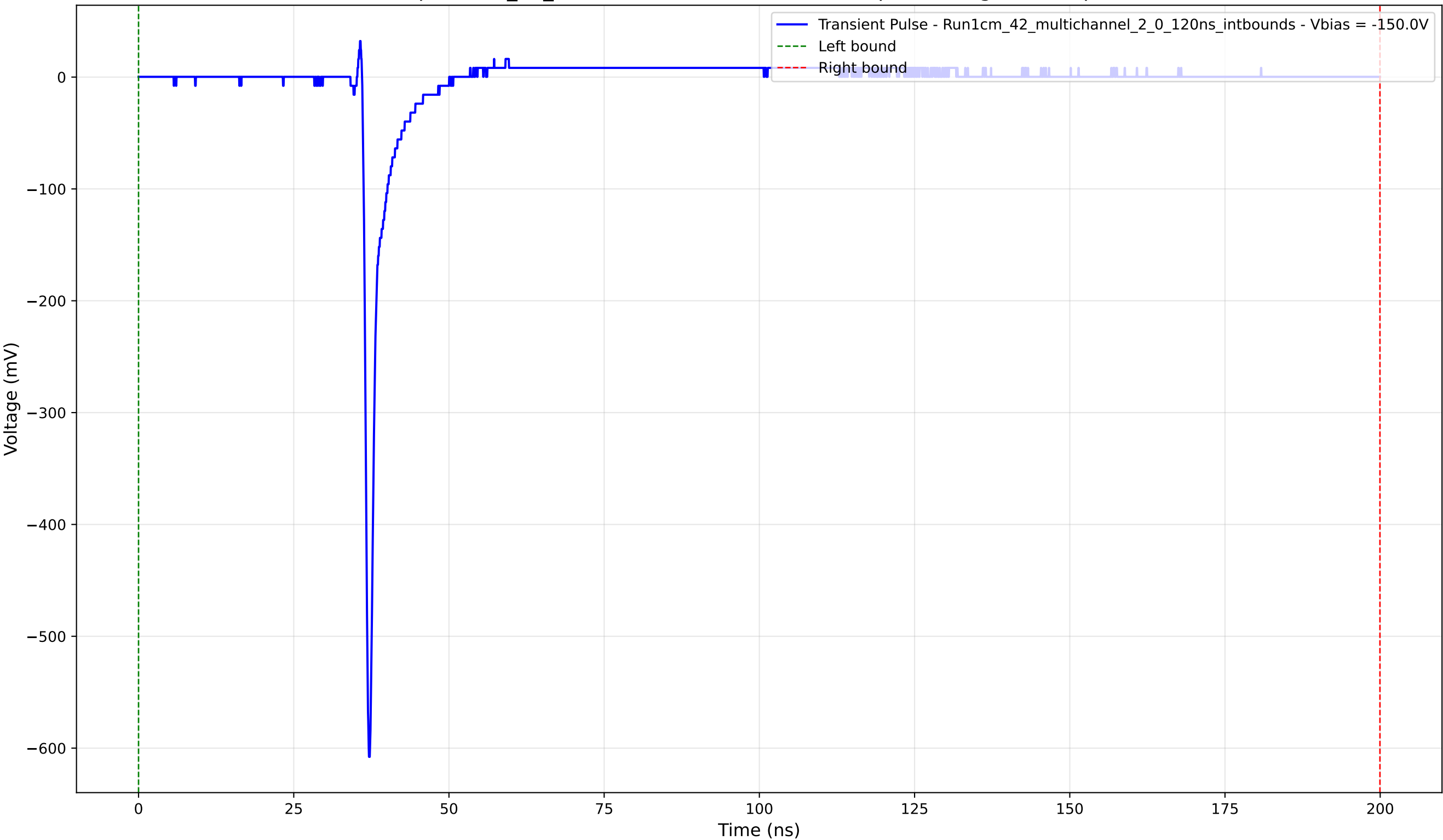
Transient Pulse - Sample: 1cm_42_multichannel - Position: 2485.0 \mu\text{m} - Charge: 15.89 pC - Rise Time: 0.66 ns
