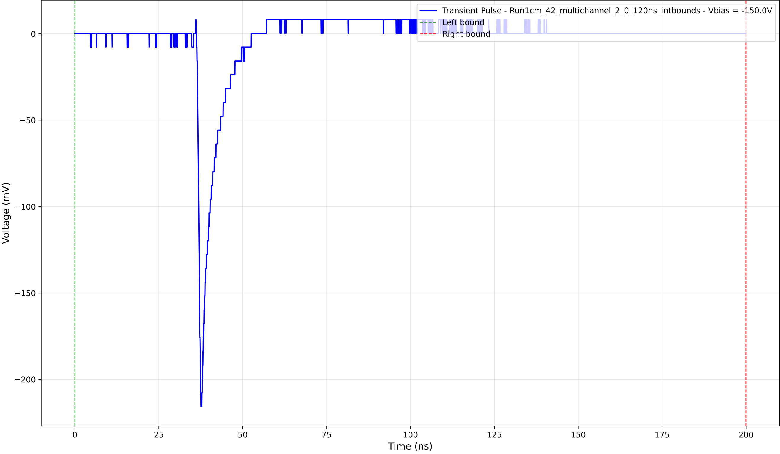
Transient Pulse - Sample: 1cm_42_multichannel - Position: 3105.0 \mu\text{m} - Charge: 10.42 pC - Rise Time: 0.93 ns
