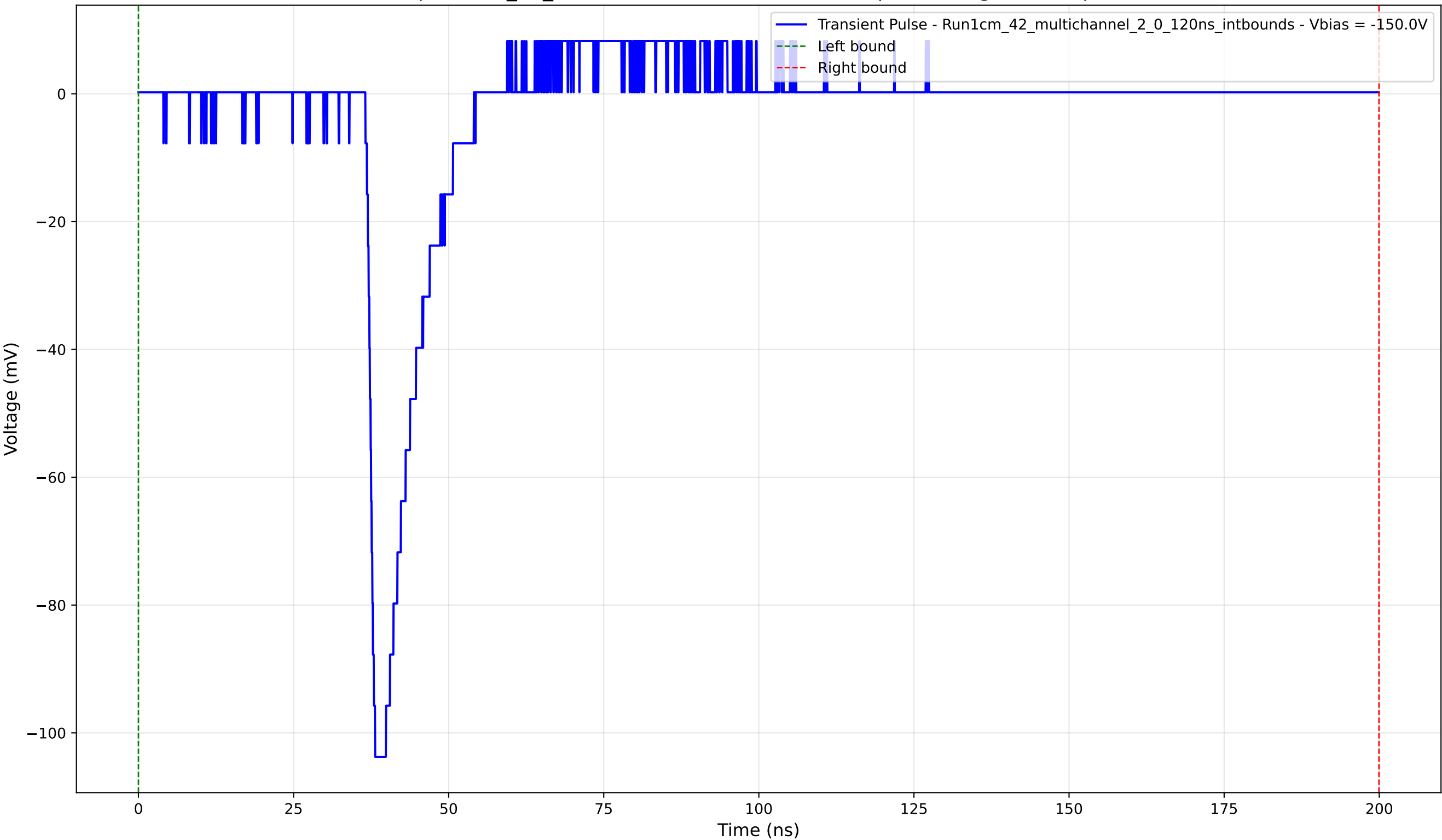
Transient Pulse - Sample: 1cm_42_multichannel - Position: 3725.0 \mu\text{m} - Charge: 10.49 pC - Rise Time: 1.15 ns
