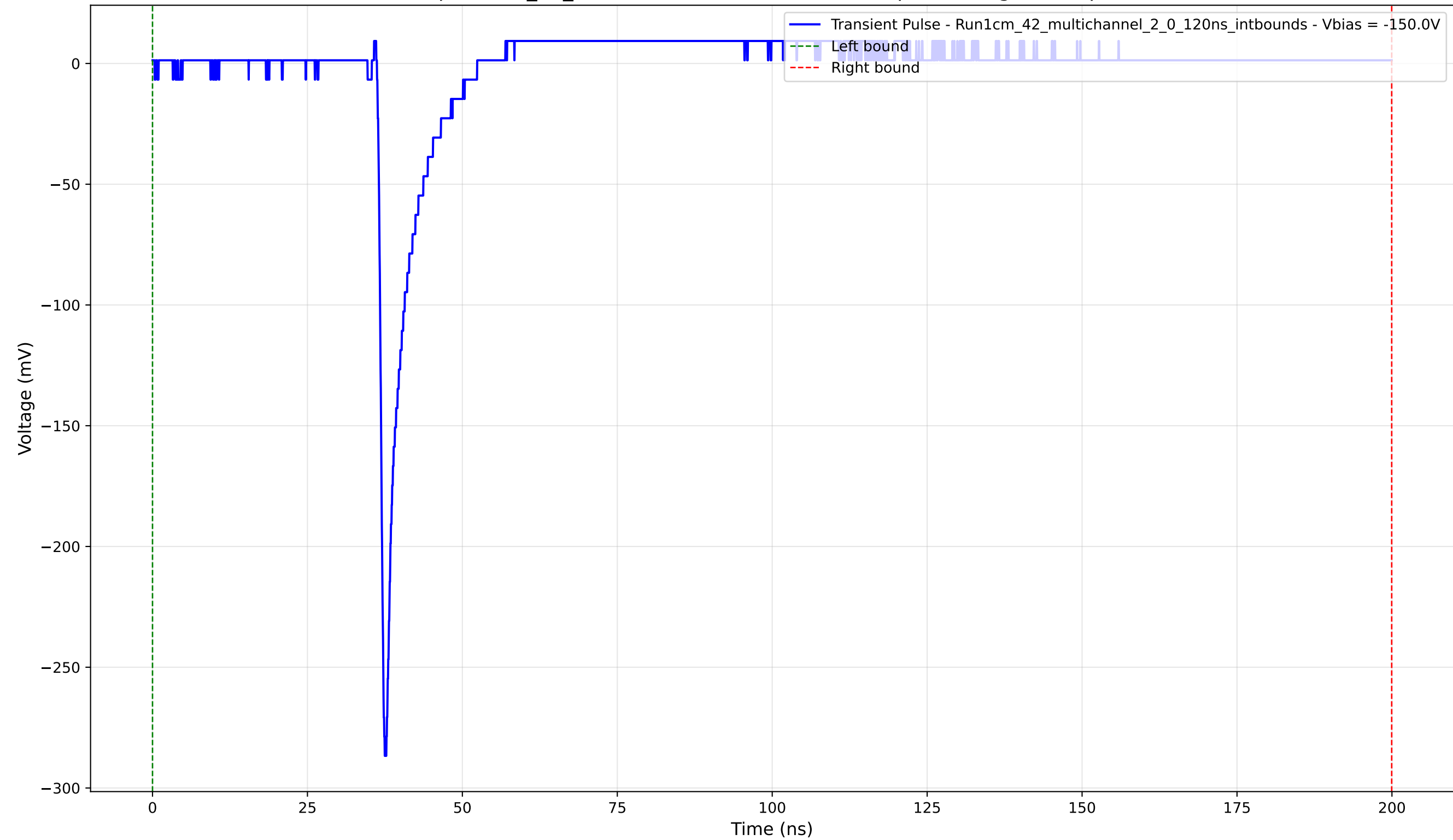
Transient Pulse - Sample: 1cm_42_multichannel - Position: 1760.0 \mu\text{m} - Charge: 8.32 pC - Rise Time: 0.83 ns
