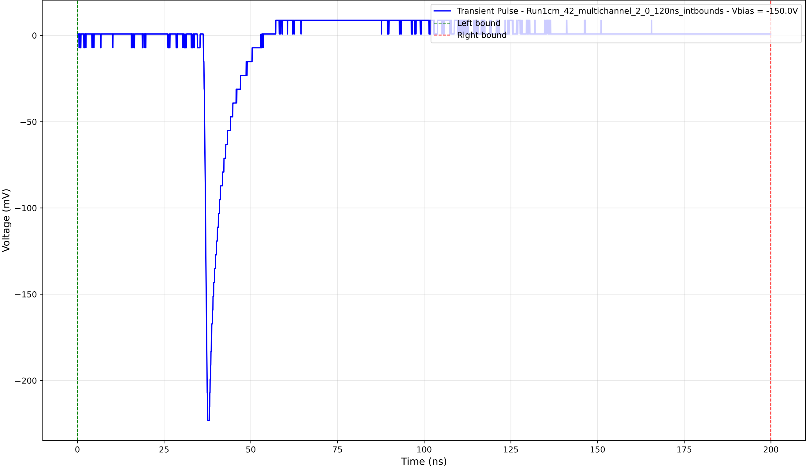
Transient Pulse - Sample: 1cm_42_multichannel - Position: 1565.0 \mu\text{m} - Charge: 10.51 pC - Rise Time: 0.92 ns
