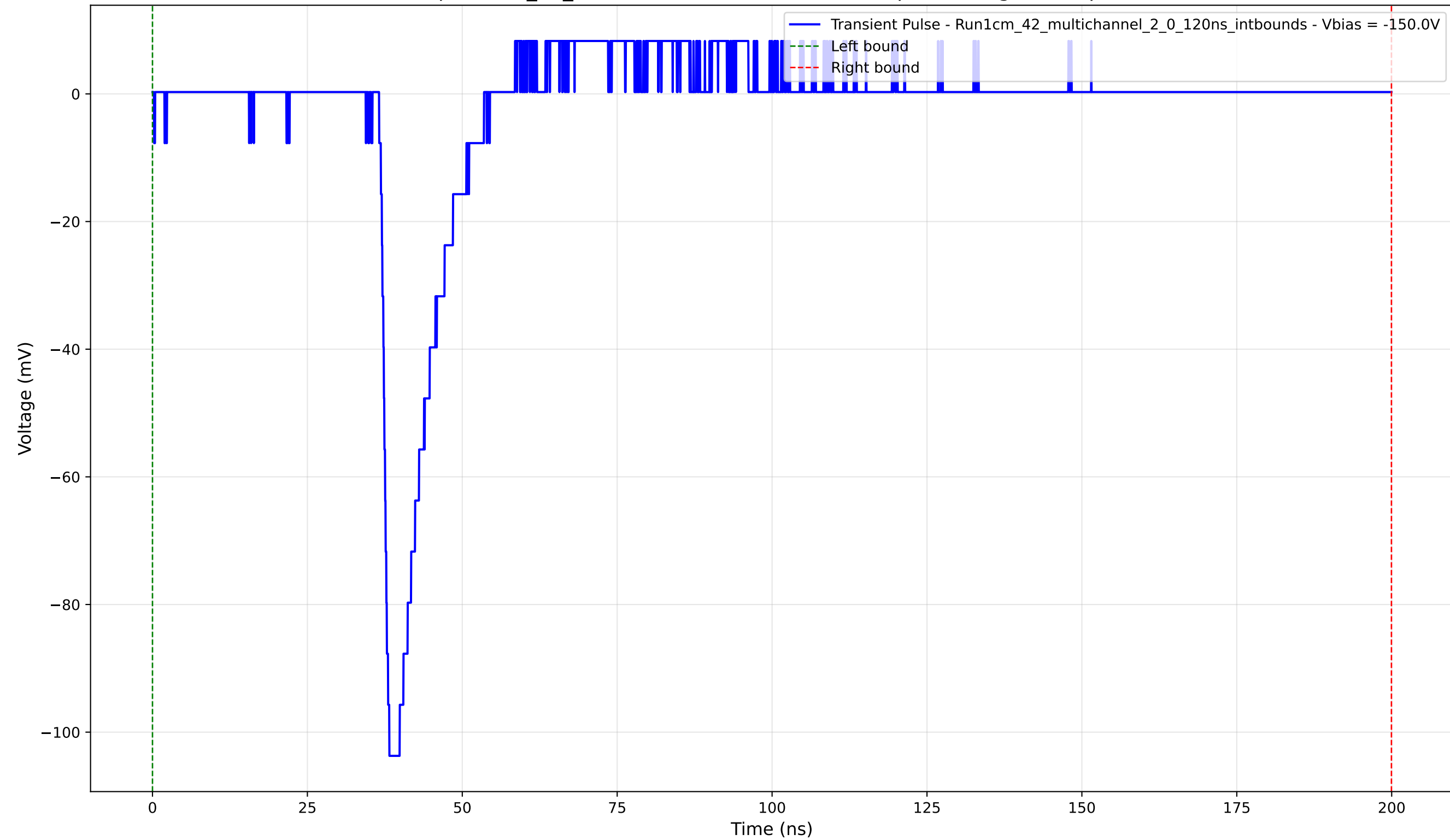
Transient Pulse - Sample: 1cm_42_multichannel - Position: 3745.0 \mu\text{m} - Charge: 9.12 pC - Rise Time: 1.19 ns
