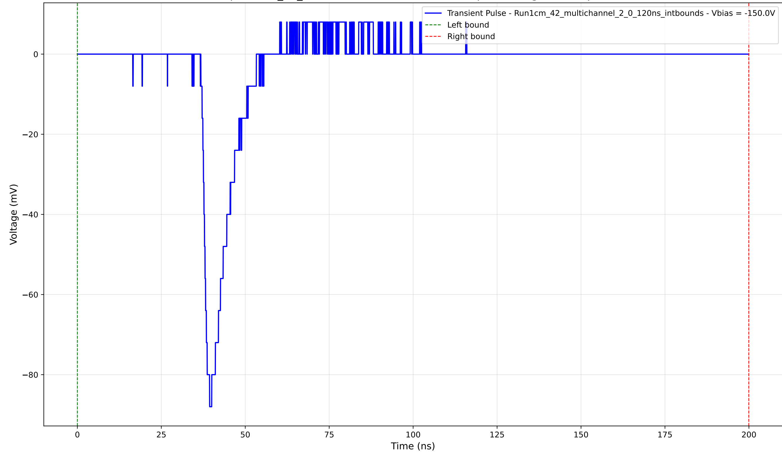
Transient Pulse - Sample: 1cm_42_multichannel - Position: 4200.0 \mu\text{m} - Charge: 10.16 pC - Rise Time: 1.56 ns
