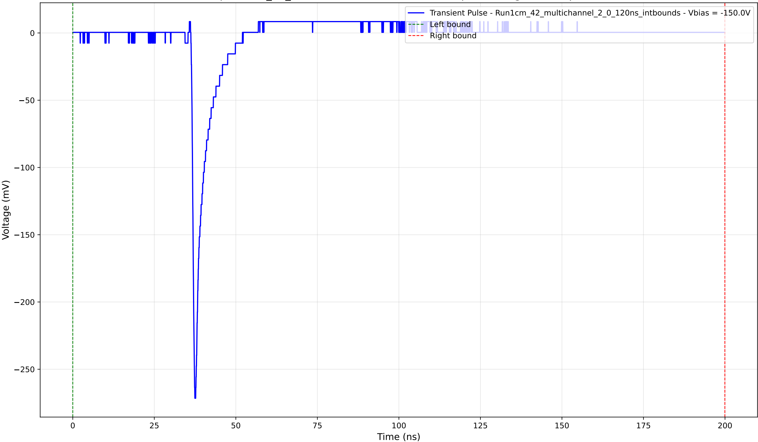
Transient Pulse - Sample: 1cm_42_multichannel - Position: 2960.0 \mu\text{m} - Charge: 11.30 pC - Rise Time: 0.85 ns
