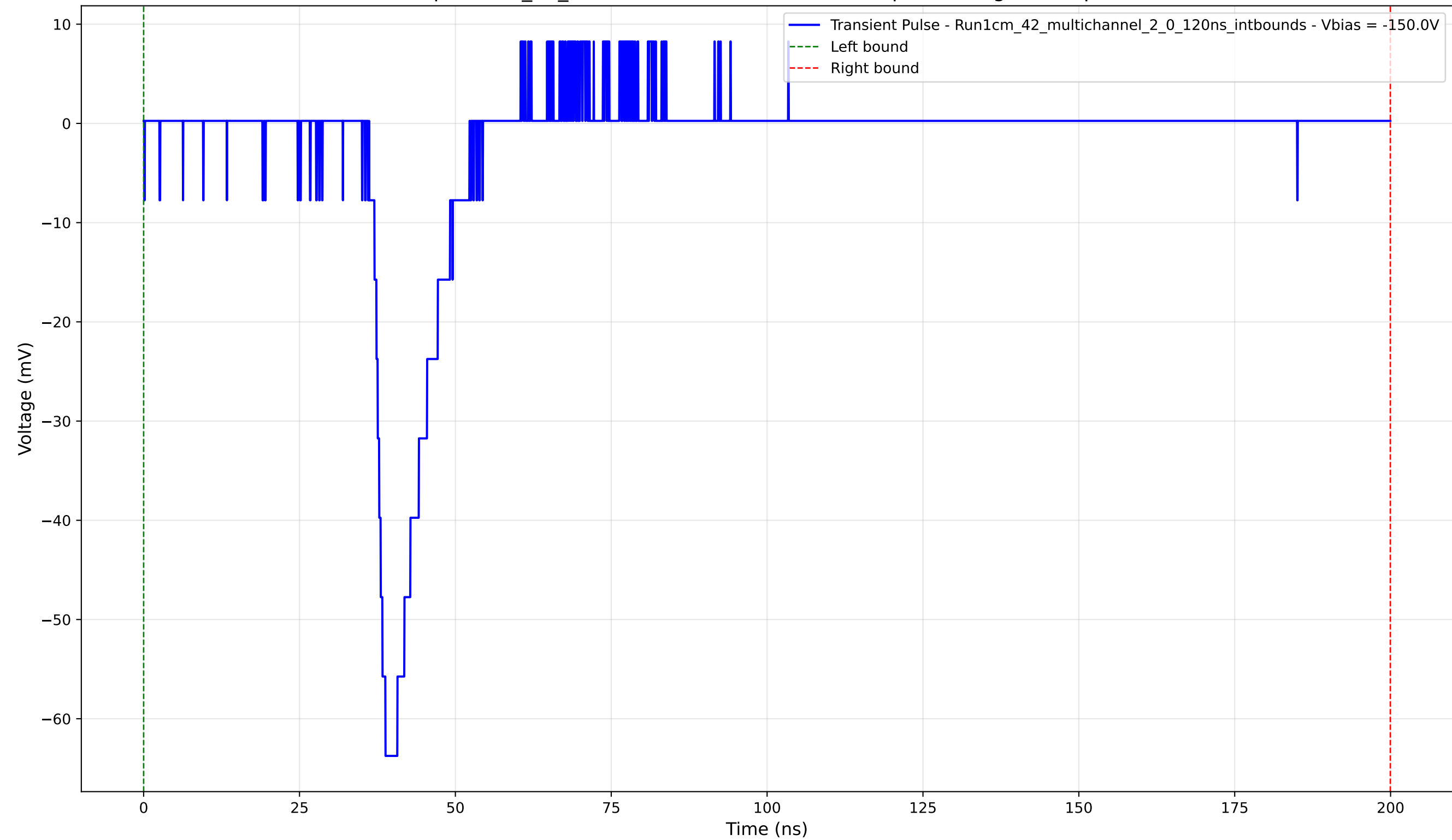
Transient Pulse - Sample: 1cm_42_multichannel - Position: 4780.0 \mu\text{m} - Charge: 8.04 pC - Rise Time: 2.61 ns
