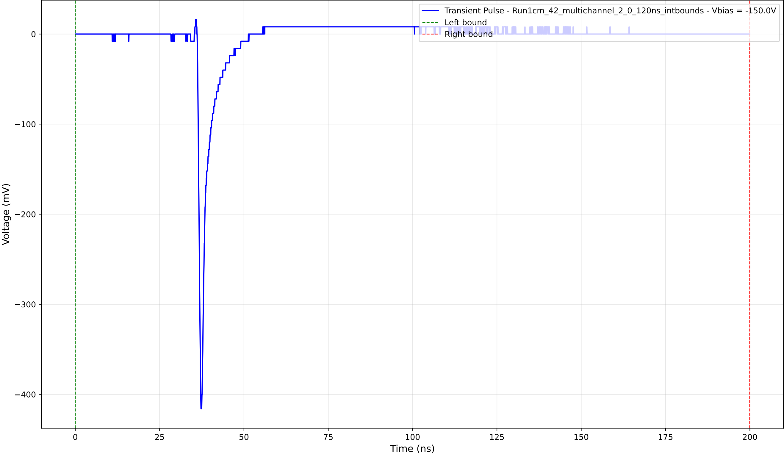
Transient Pulse - Sample: 1cm_42_multichannel - Position: 2730.0 \mu\text{m} - Charge: 14.56 pC - Rise Time: 0.77 ns
