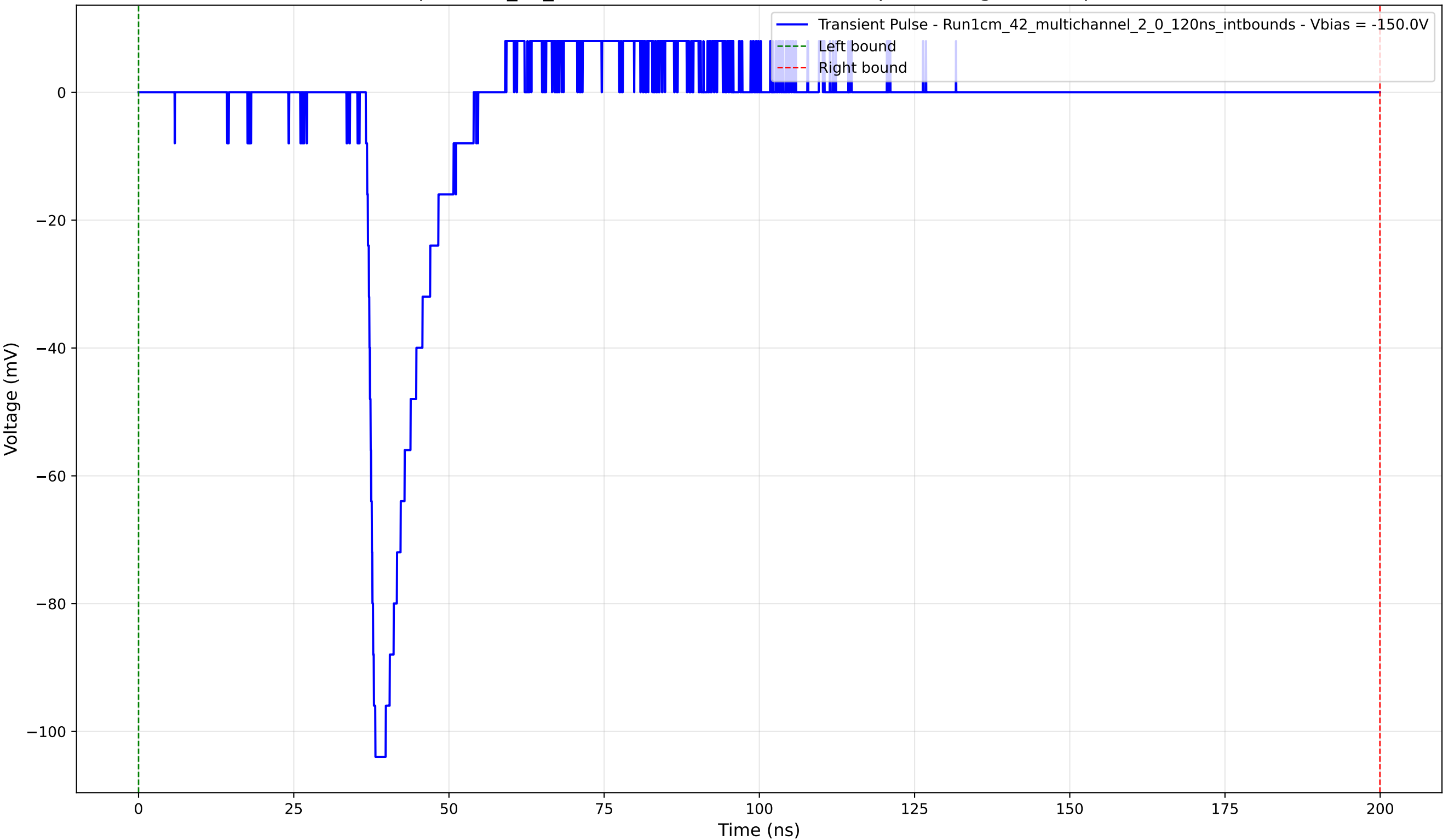
Transient Pulse - Sample: 1cm_42_multichannel - Position: 3705.0 \mu\text{m} - Charge: 10.36 pC - Rise Time: 1.11 ns
