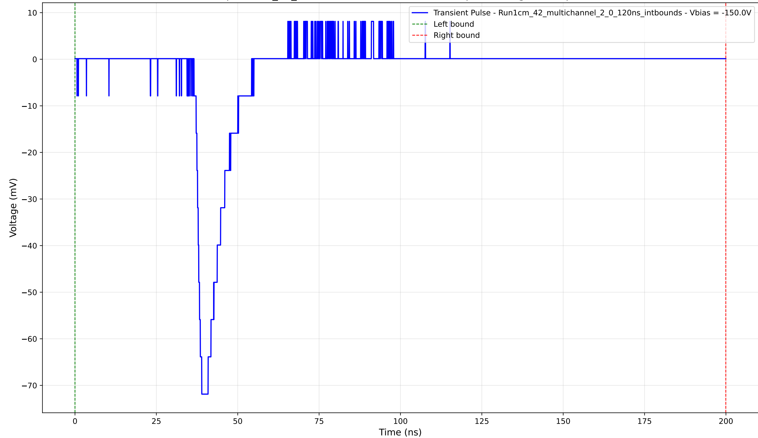
Transient Pulse - Sample: 1cm_42_multichannel - Position: 4290.0 \mu\text{m} - Charge: 9.86 pC - Rise Time: 2.36 ns
