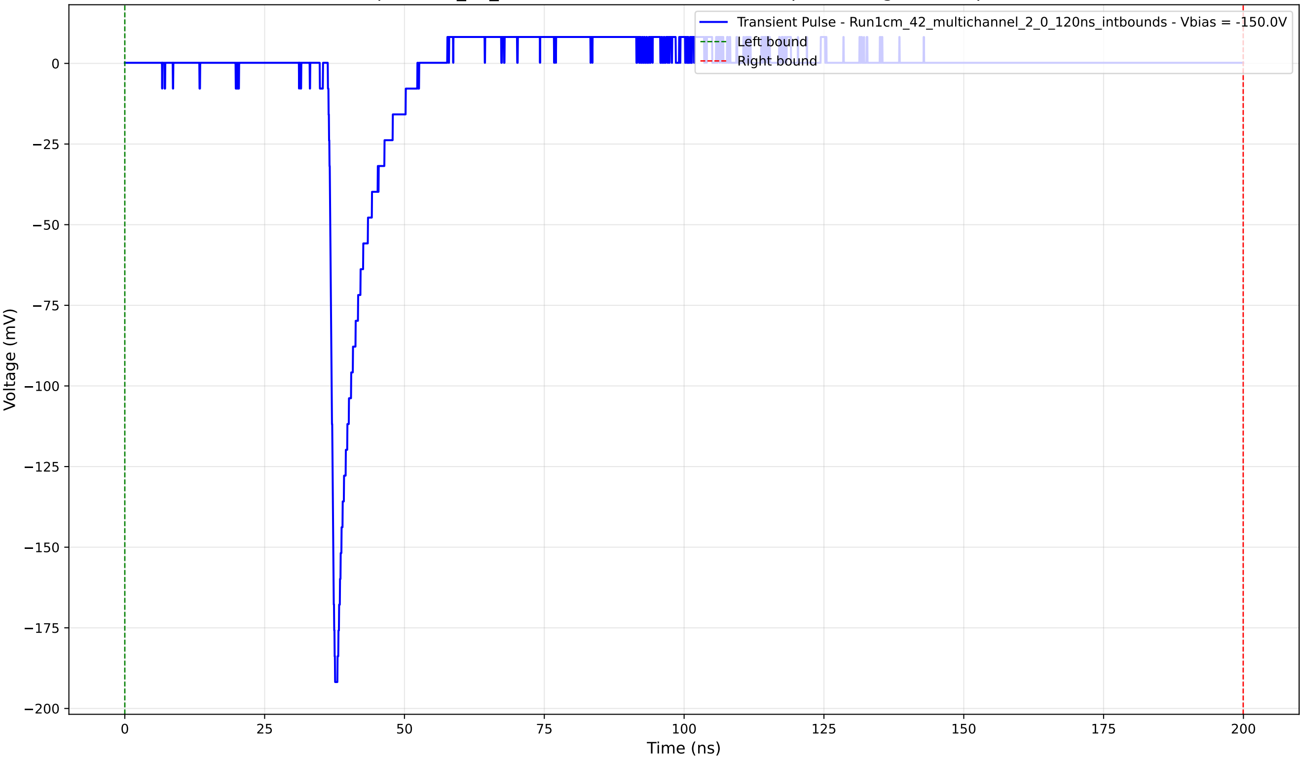
Transient Pulse - Sample: 1cm_42_multichannel - Position: 3180.0 \mu\text{m} - Charge: 10.75 pC - Rise Time: 0.94 ns
