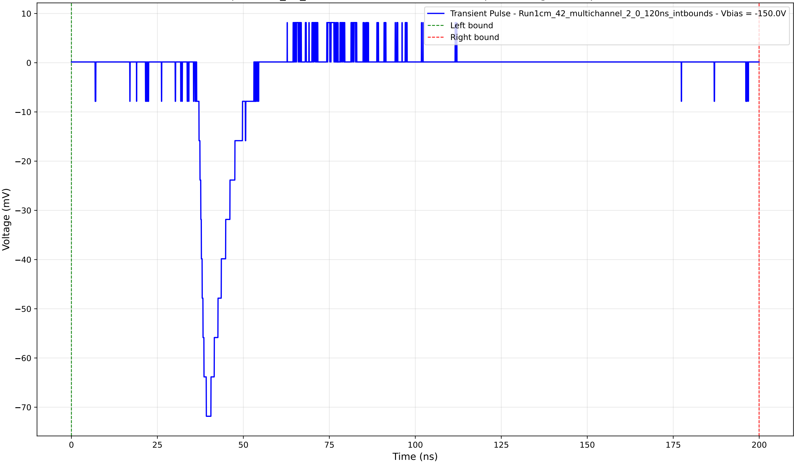
Transient Pulse - Sample: 1cm_42_multichannel - Position: 4650.0 \mu\text{m} - Charge: 9.37 pC - Rise Time: 2.80 ns
