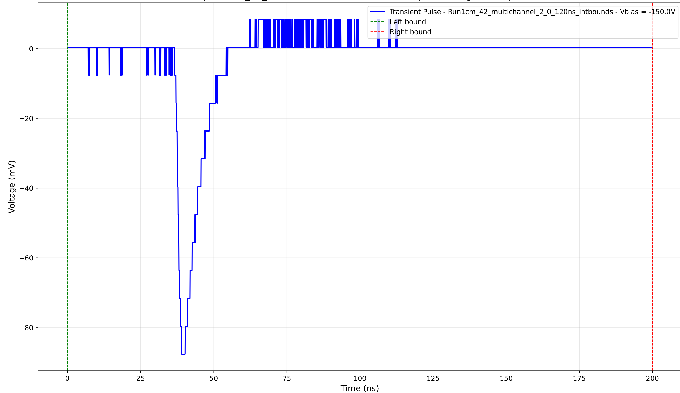
Transient Pulse - Sample: 1cm_42_multichannel - Position: 4165.0 \mu\text{m} - Charge: 9.69 pC - Rise Time: 1.51 ns
