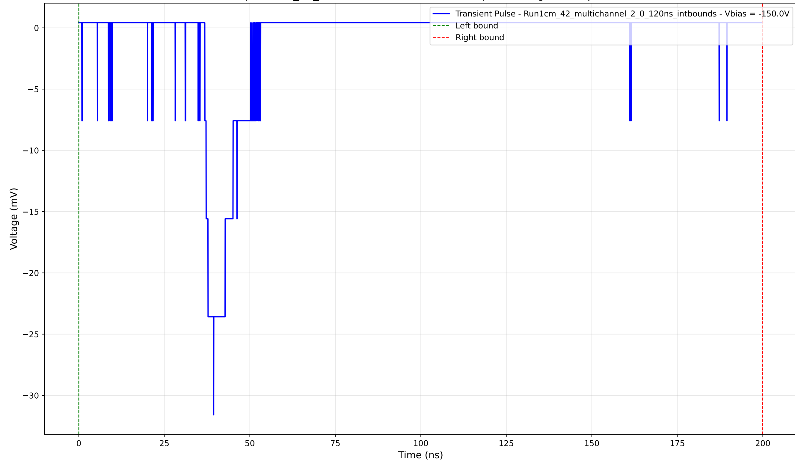
Transient Pulse - Sample: 1cm_42_multichannel - Position: 65.0 \mu\text{m} - Charge: 3.02 pC - Rise Time: 2.58 ns
