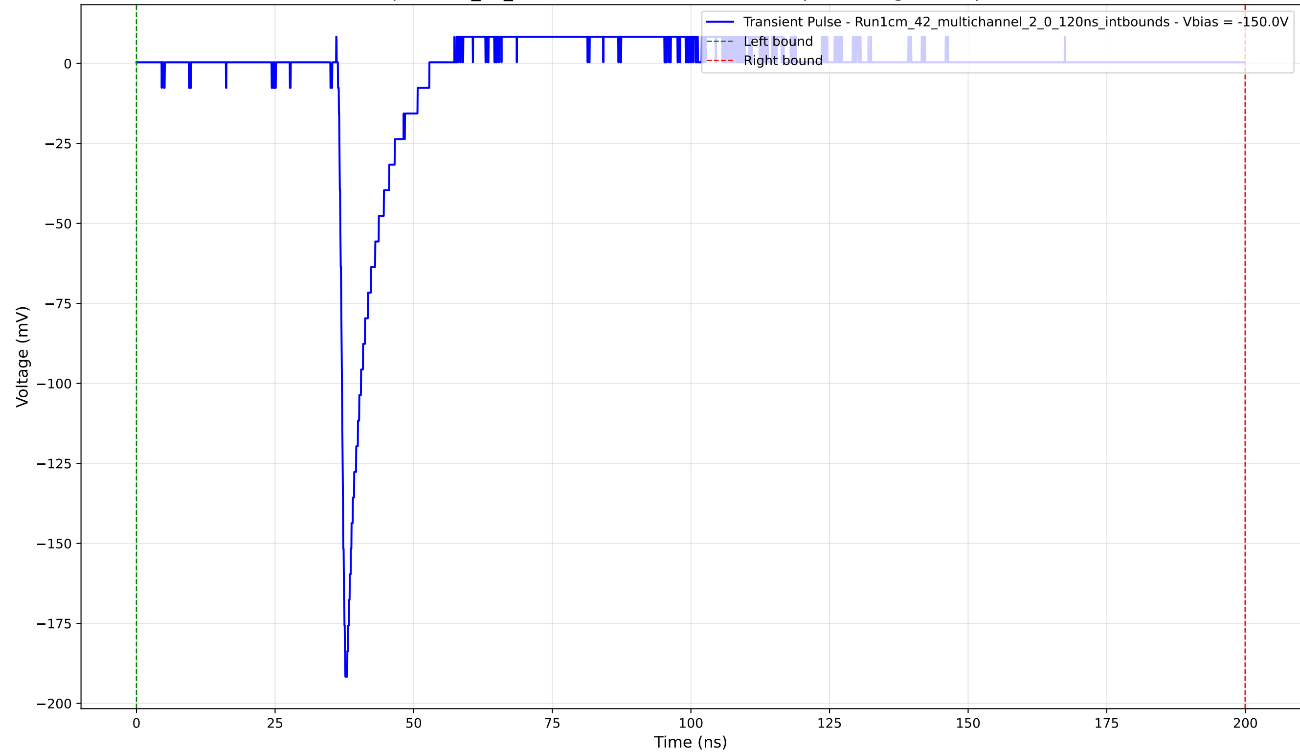
Transient Pulse - Sample: 1cm_42_multichannel - Position: 3220.0 \mu\text{m} - Charge: 9.71 pC - Rise Time: 0.94 ns
