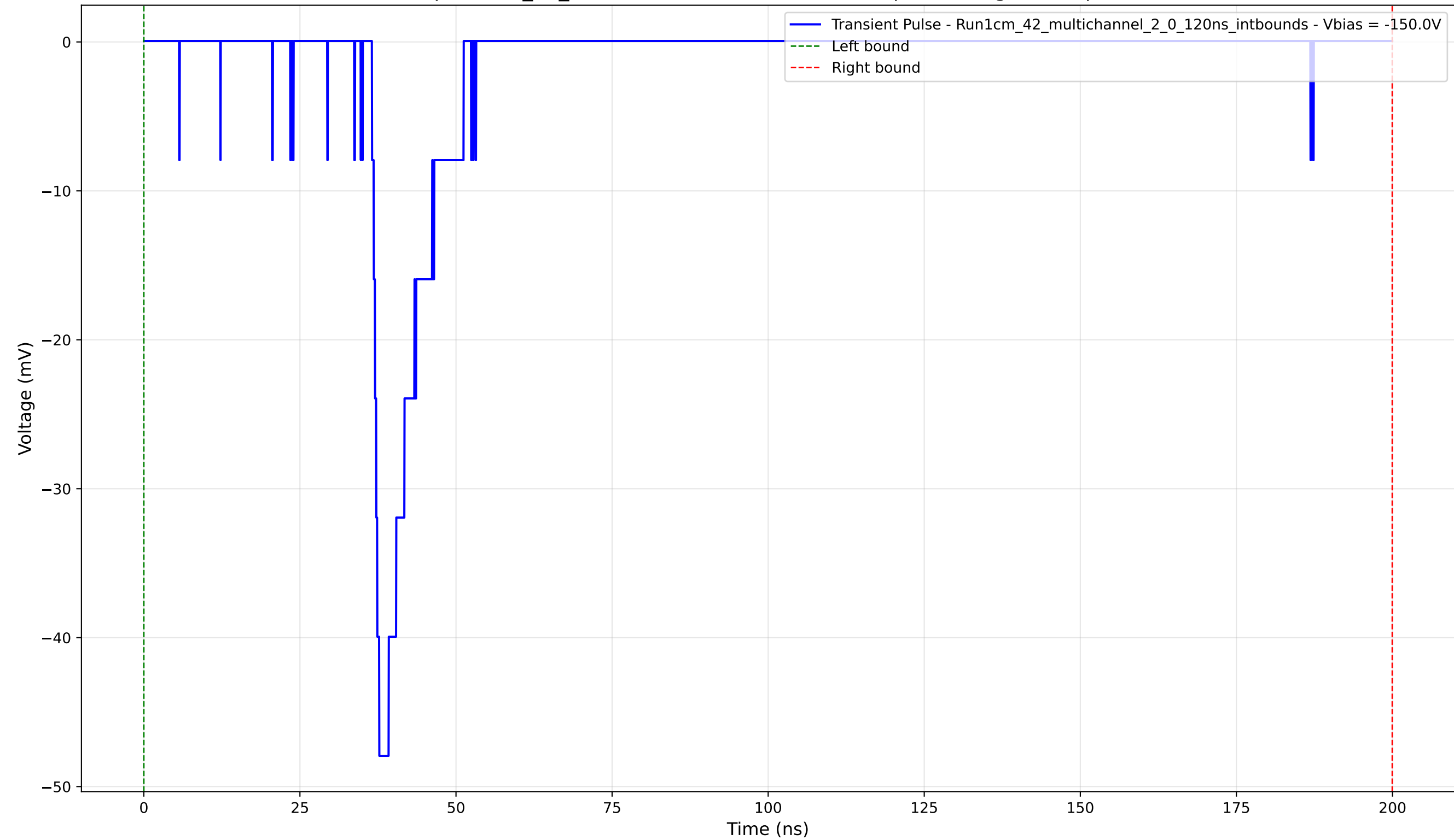
Transient Pulse - Sample: 1cm_42_multichannel - Position: 3425.0 \mu\text{m} - Charge: 6.34 pC - Rise Time: 1.18 ns
