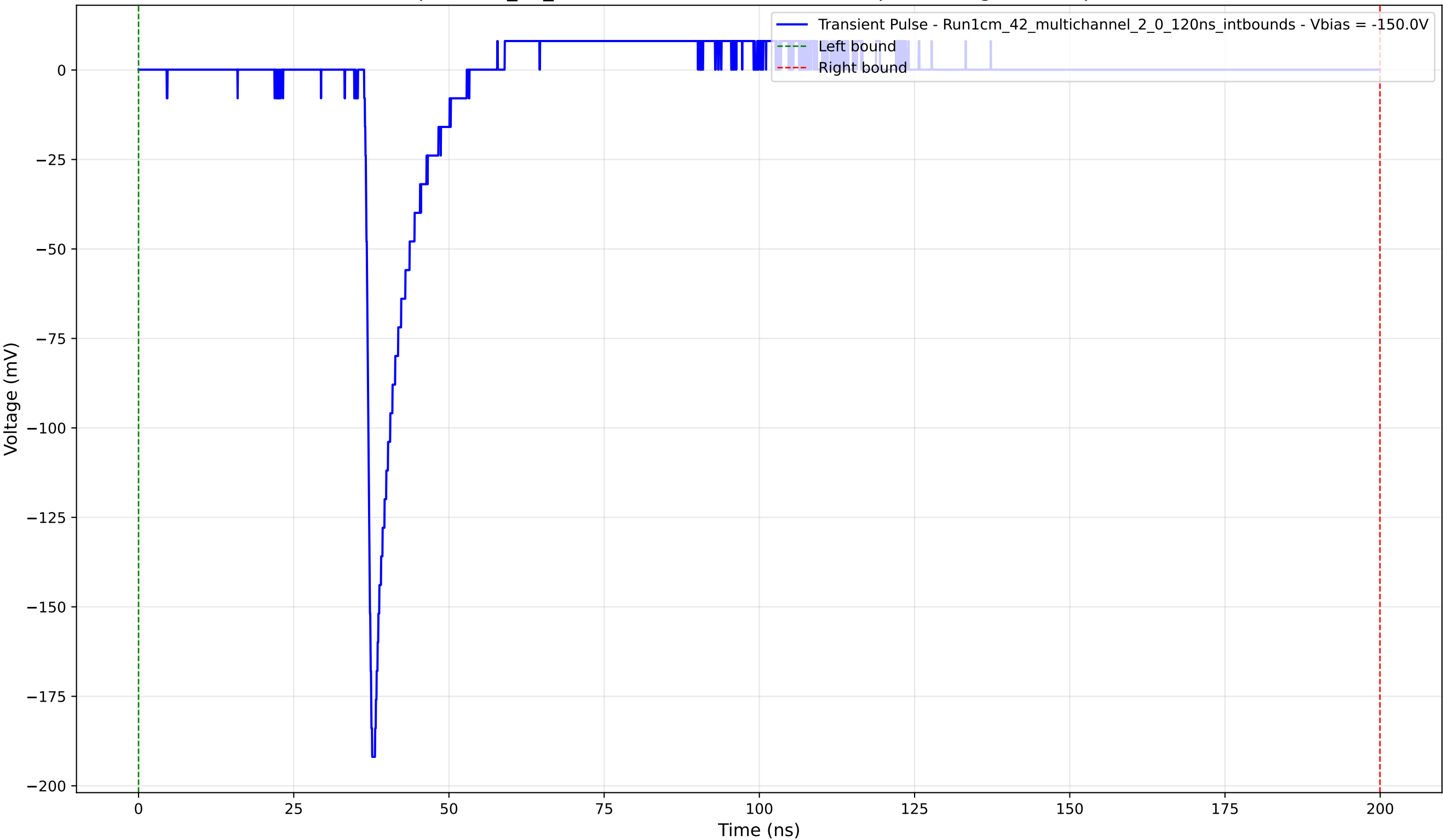
Transient Pulse - Sample: 1cm_42_multichannel - Position: 3205.0 \mu\text{m} - Charge: 11.28 pC - Rise Time: 0.93 ns
