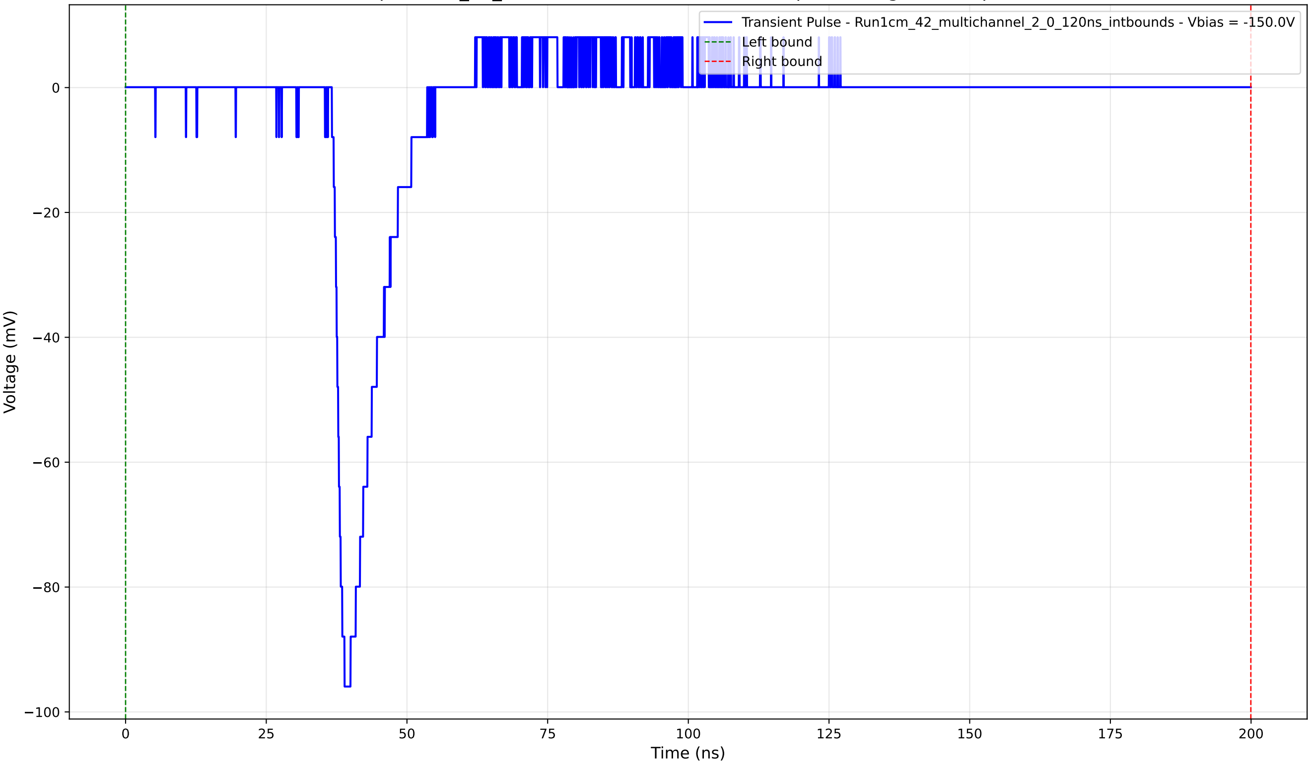
Transient Pulse - Sample: 1cm_42_multichannel - Position: 4010.0 \mu\text{m} - Charge: 10.24 pC - Rise Time: 1.55 ns
