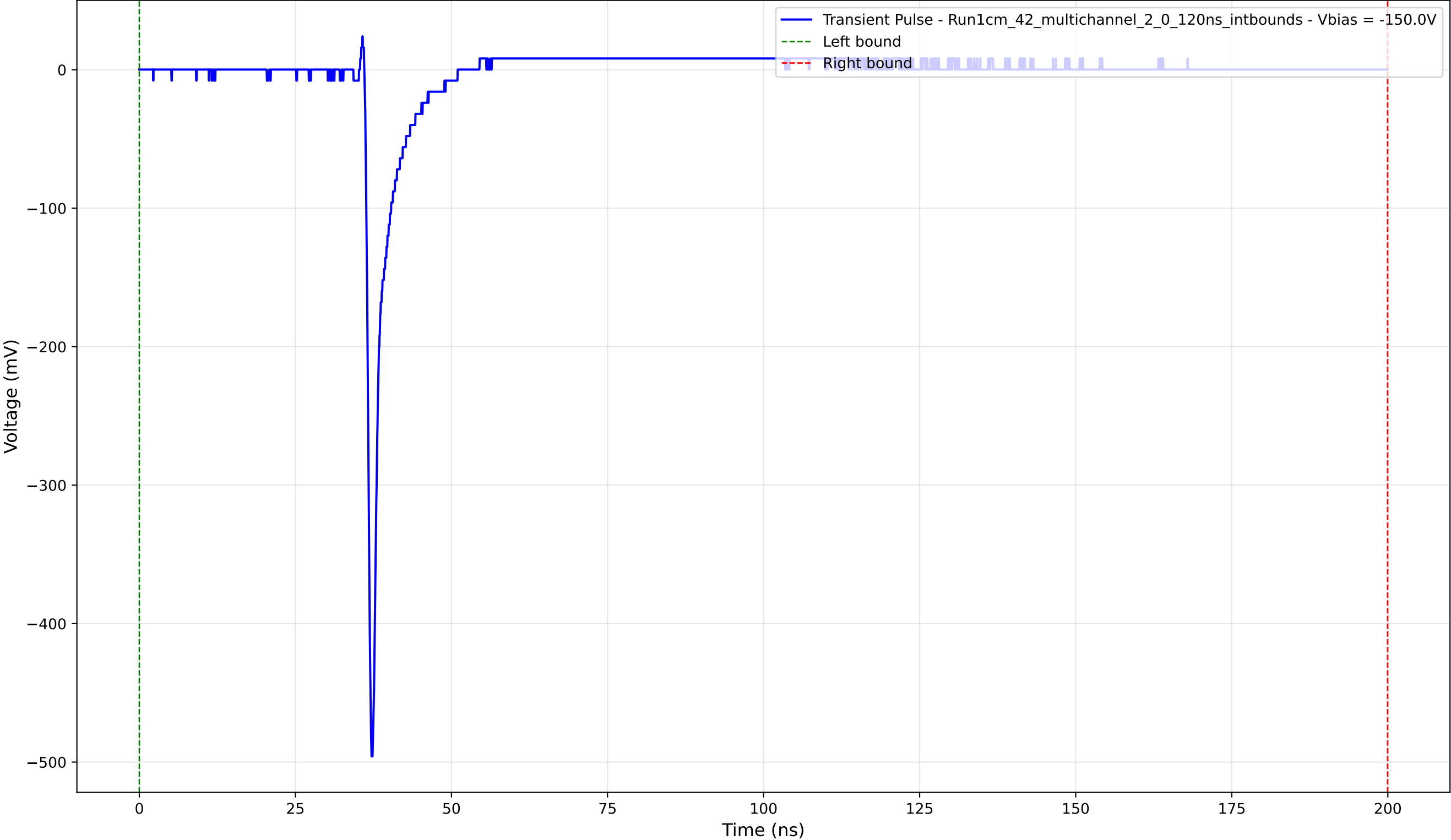
Transient Pulse - Sample: 1cm_42_multichannel - Position: 2110.0 \mu\text{m} - Charge: 15.52 pC - Rise Time: 0.77 ns
