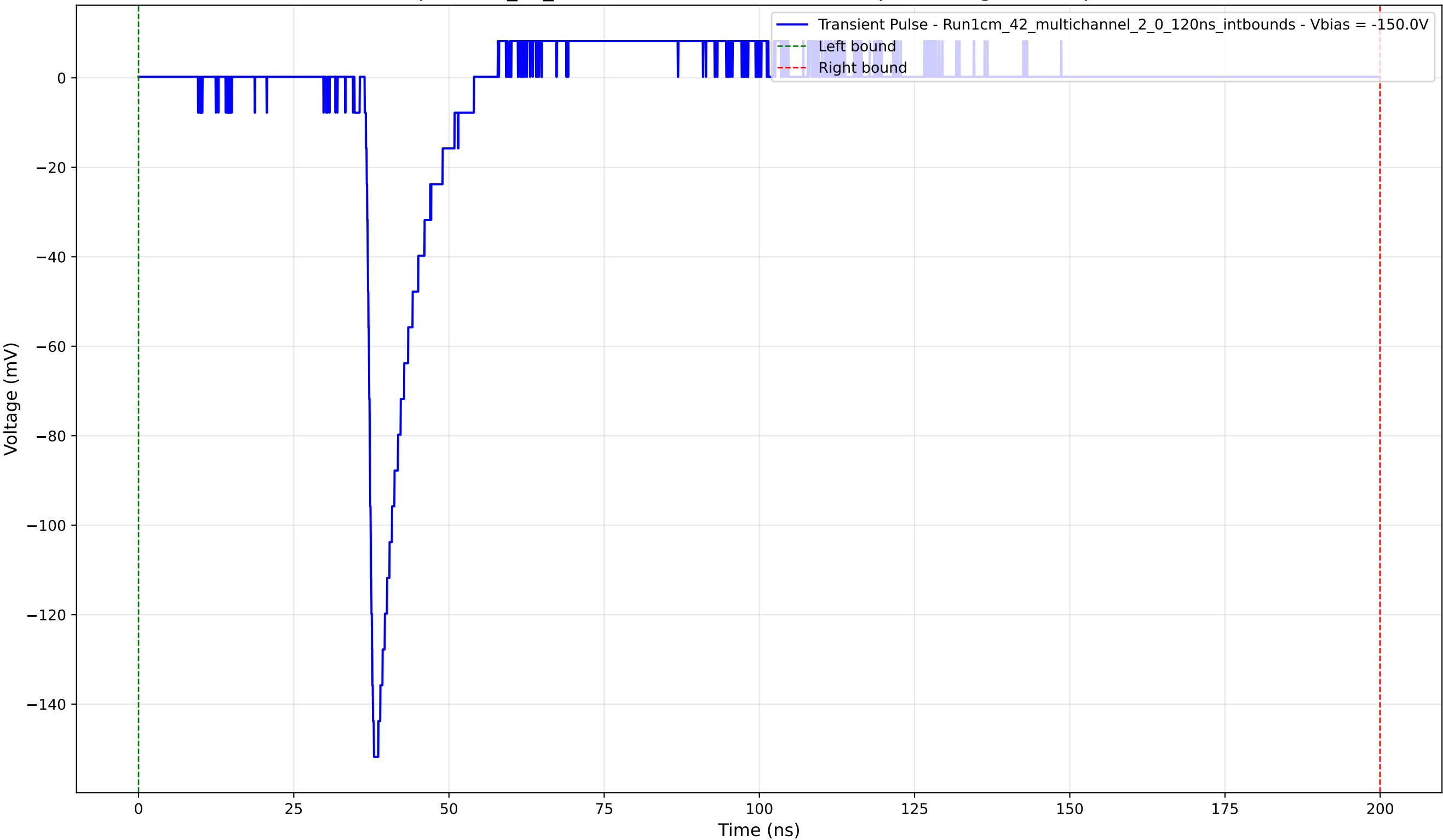
Transient Pulse - Sample: 1cm_42_multichannel - Position: 1270.0 \mu\text{m} - Charge: 10.97 pC - Rise Time: 1.12 ns
