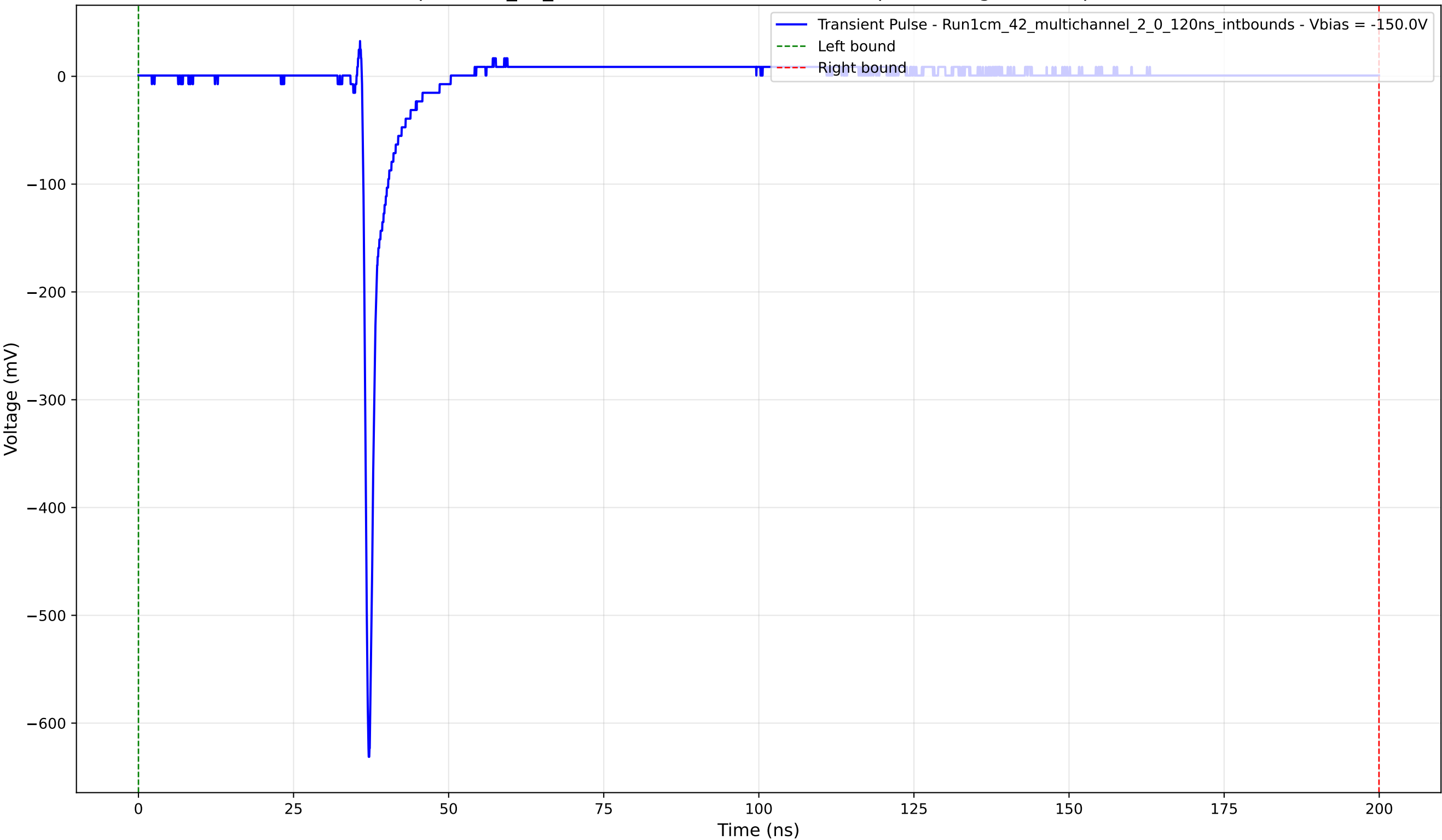
Transient Pulse - Sample: 1cm_42_multichannel - Position: 2250.0 \mu\text{m} - Charge: 14.65 pC - Rise Time: 0.74 ns
