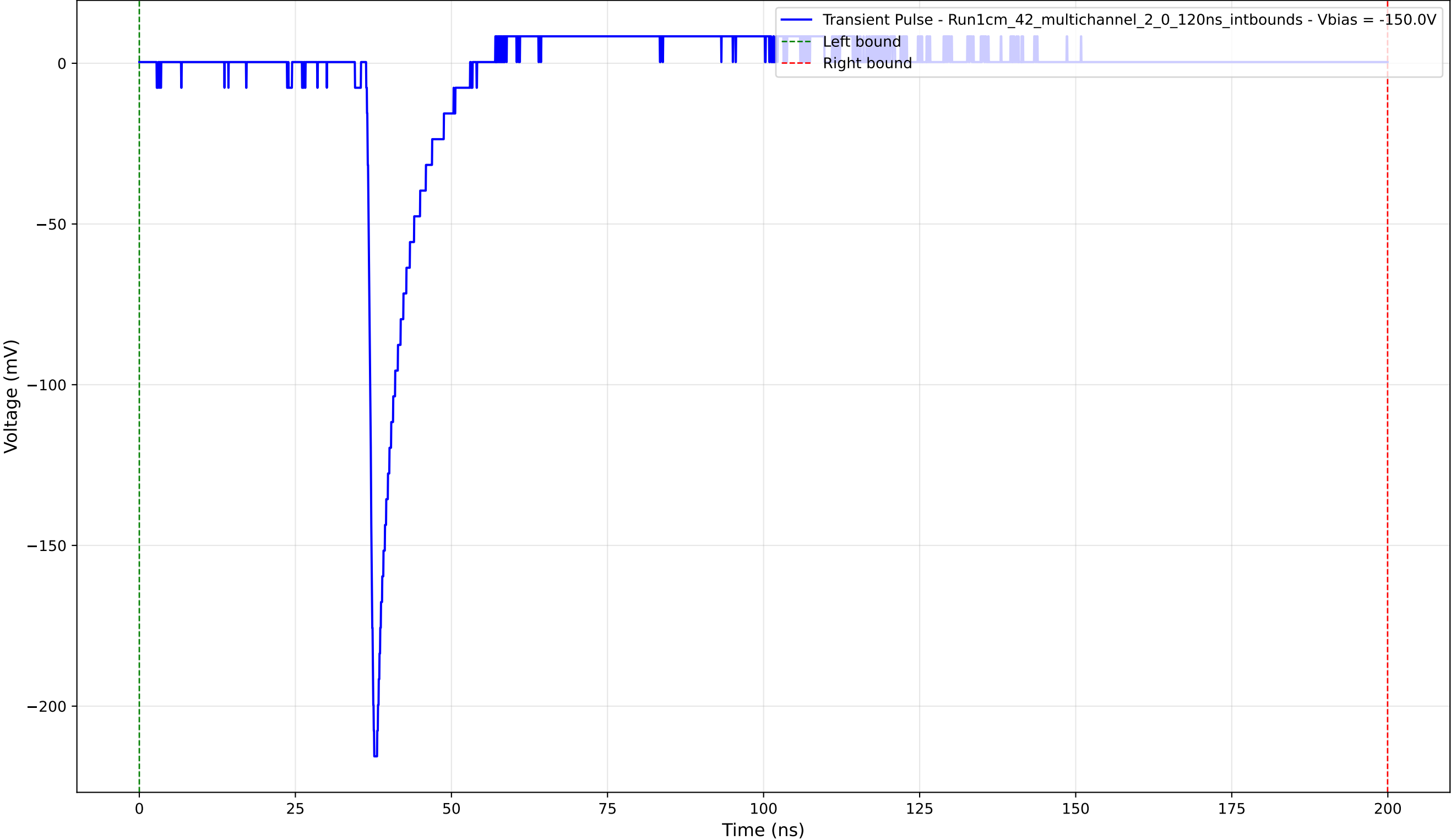
Transient Pulse - Sample: 1cm_42_multichannel - Position: 1535.0 \mu\text{m} - Charge: 11.10 pC - Rise Time: 0.93 ns
