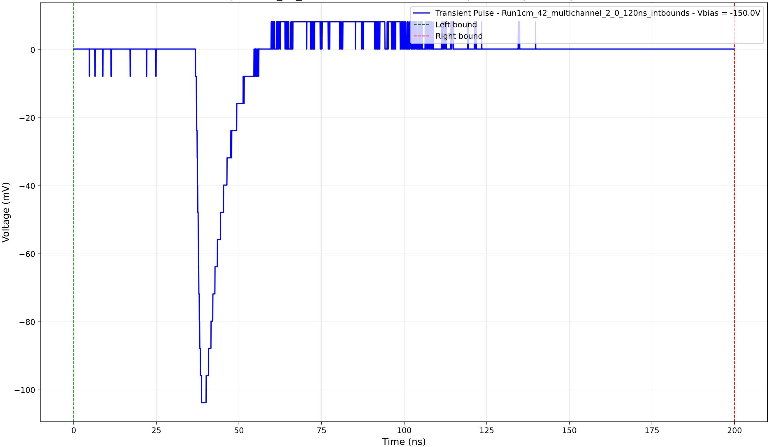
Transient Pulse - Sample: 1cm_42_multichannel - Position: 690.0 \mu\text{m} - Charge: 9.15 pC - Rise Time: 1.23 ns
