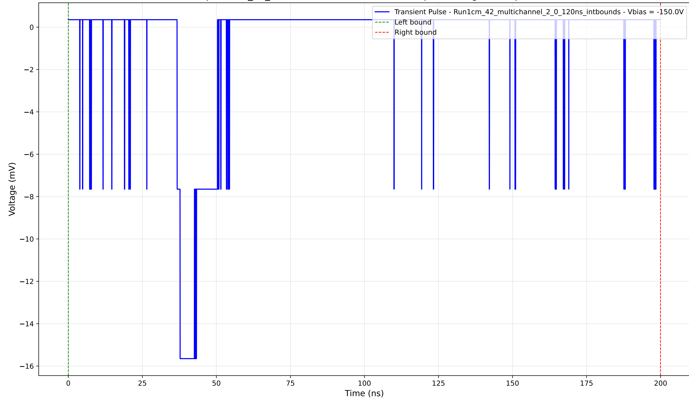
Transient Pulse - Sample: 1cm_42_multichannel - Position: 3855.0 \mu\text{m} - Charge: 2.18 pC - Rise Time: 1.03 ns
