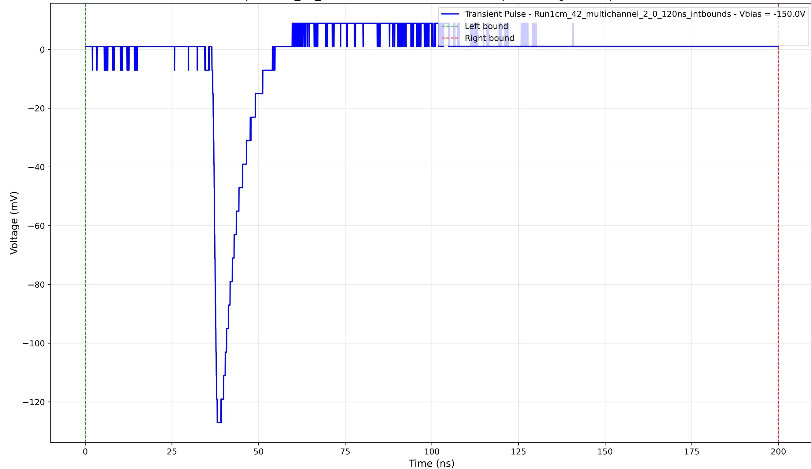
Transient Pulse - Sample: 1cm_42_multichannel - Position: 1080.0 \mu\text{m} - Charge: 8.28 pC - Rise Time: 1.13 ns
