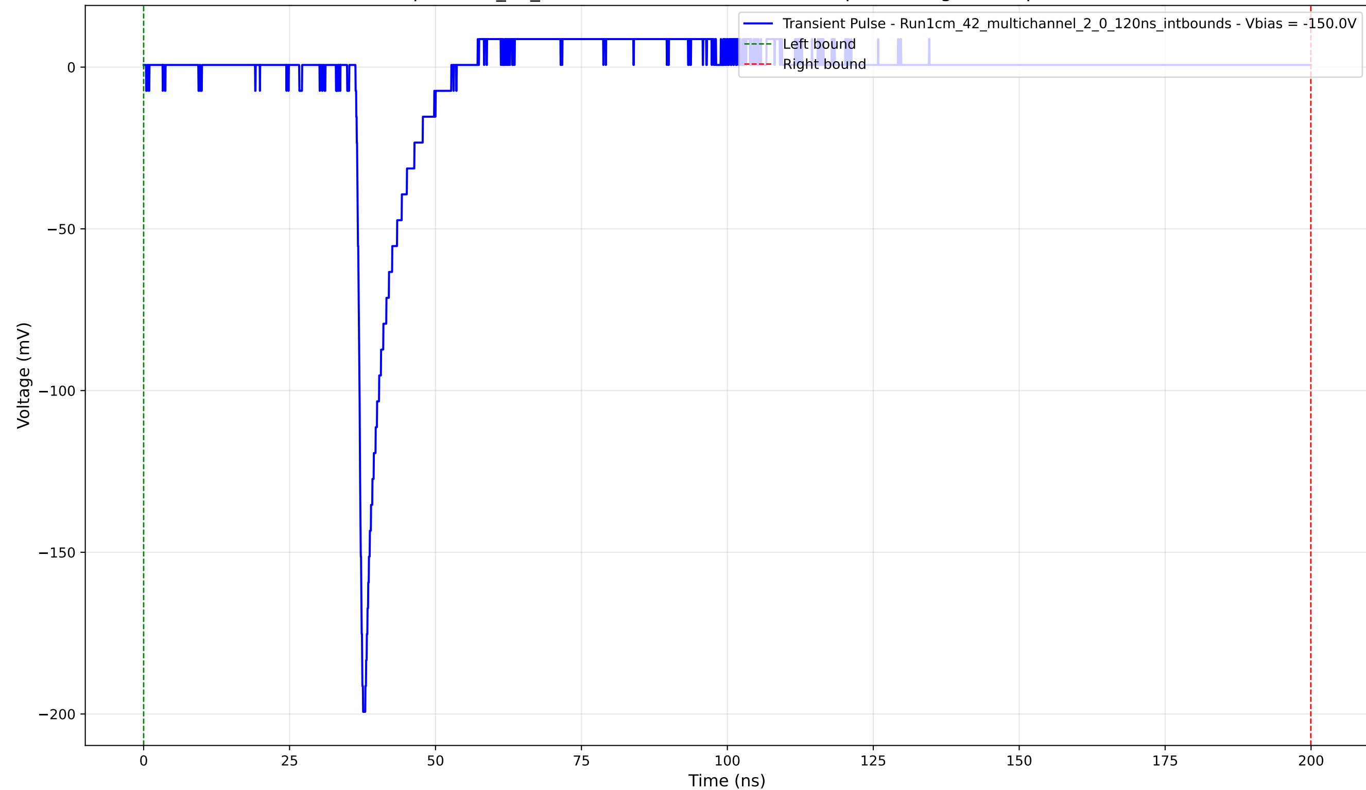
Transient Pulse - Sample: 1cm_42_multichannel - Position: 3150.0 \mu\text{m} - Charge: 9.43 pC - Rise Time: 0.92 ns
