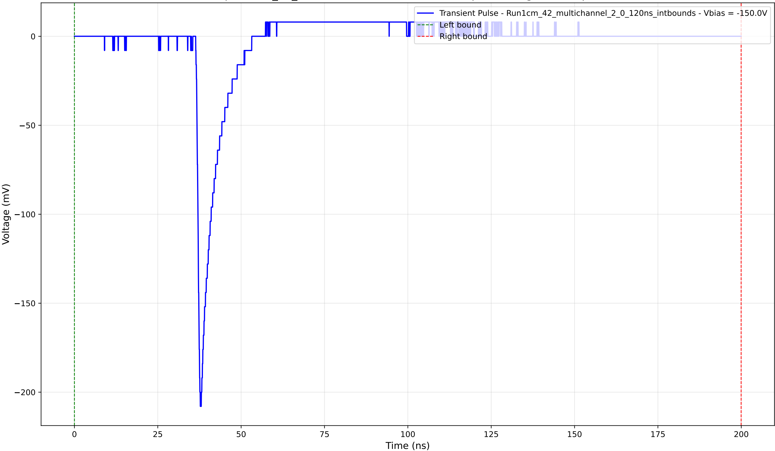
Transient Pulse - Sample: 1cm_42_multichannel - Position: 1480.0 \mu\text{m} - Charge: 12.08 pC - Rise Time: 0.98 ns
