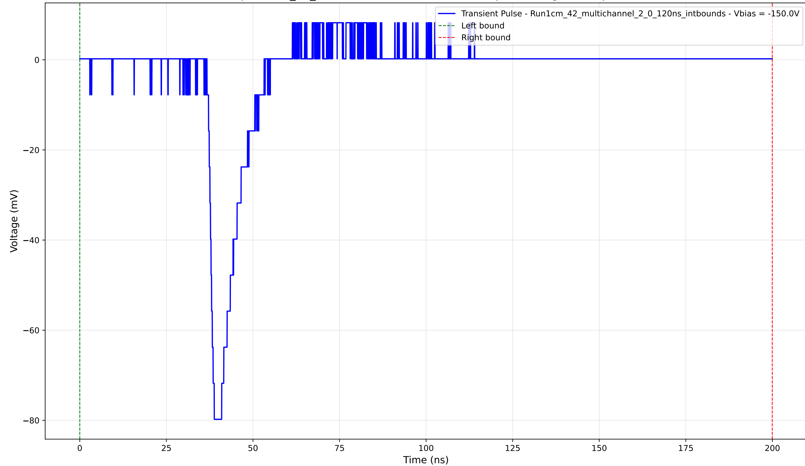
Transient Pulse - Sample: 1cm_42_multichannel - Position: 4235.0 \mu\text{m} - Charge: 9.67 pC - Rise Time: 1.68 ns
