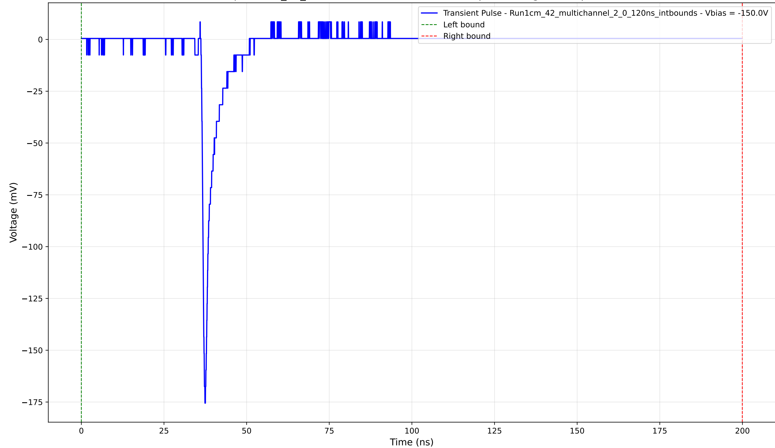
Transient Pulse - Sample: 1cm_42_multichannel - Position: 2825.0 \mu\text{m} - Charge: 9.28 pC - Rise Time: 0.86 ns
