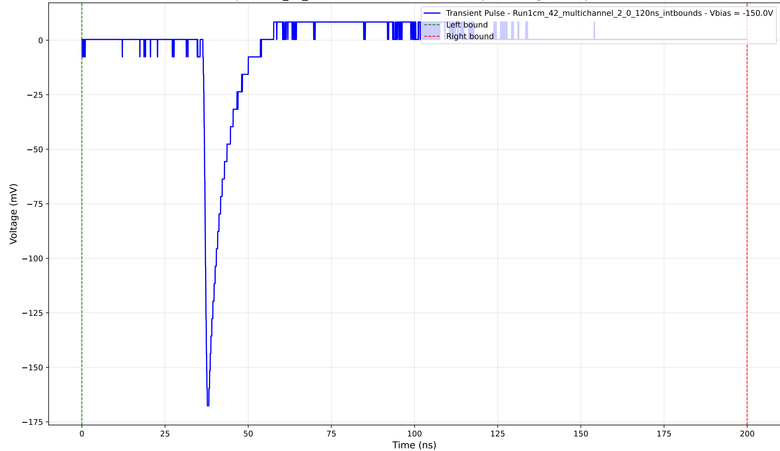
Transient Pulse - Sample: 1cm_42_multichannel - Position: 3290.0 \mu\text{m} - Charge: 9.40 pC - Rise Time: 0.91 ns
