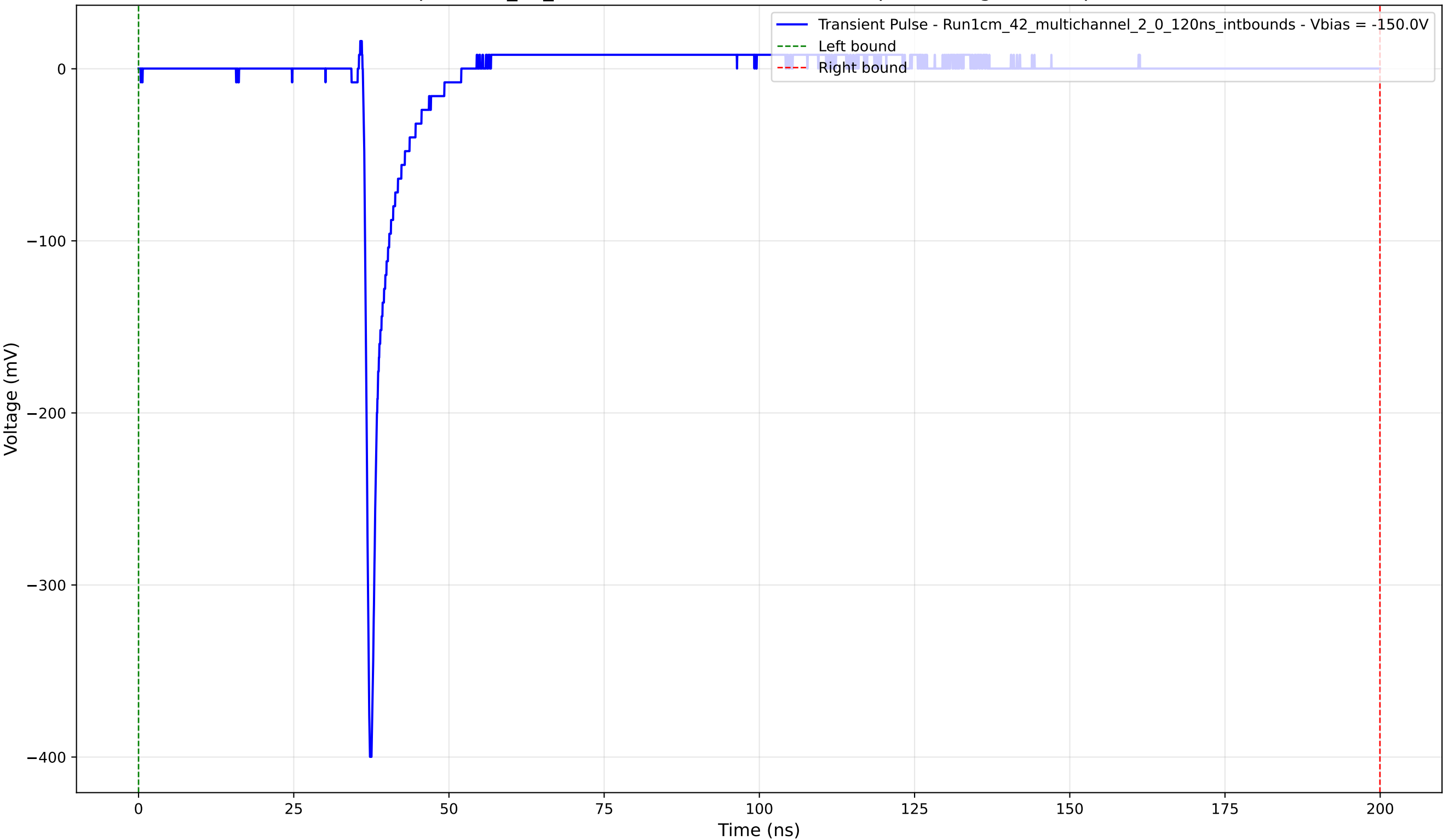
Transient Pulse - Sample: 1cm_42_multichannel - Position: 2750.0 \mu\text{m} - Charge: 13.19 pC - Rise Time: 0.76 ns
