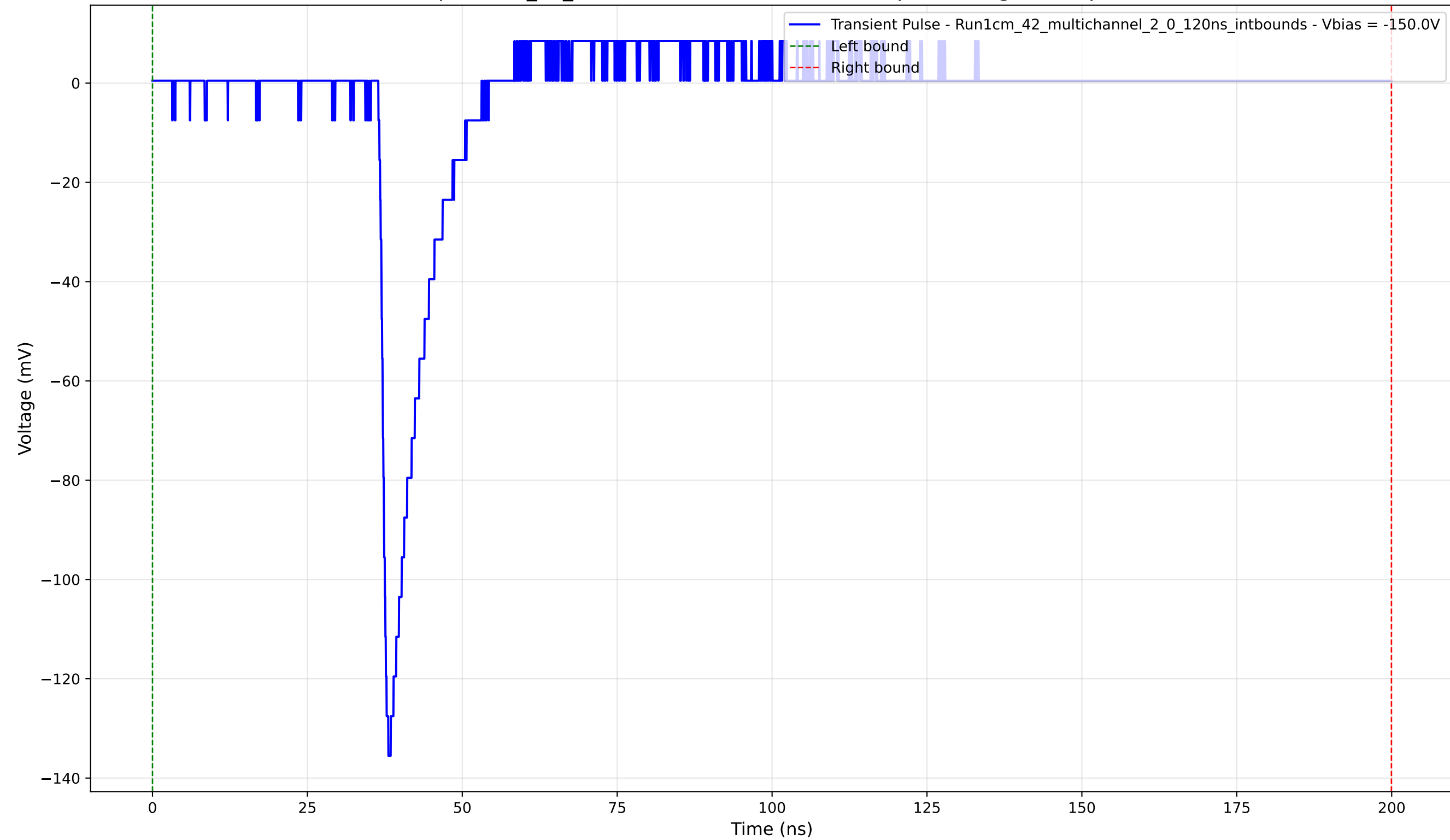
Transient Pulse - Sample: 1cm_42_multichannel - Position: 3470.0 \mu\text{m} - Charge: 9.62 pC - Rise Time: 1.17 ns
