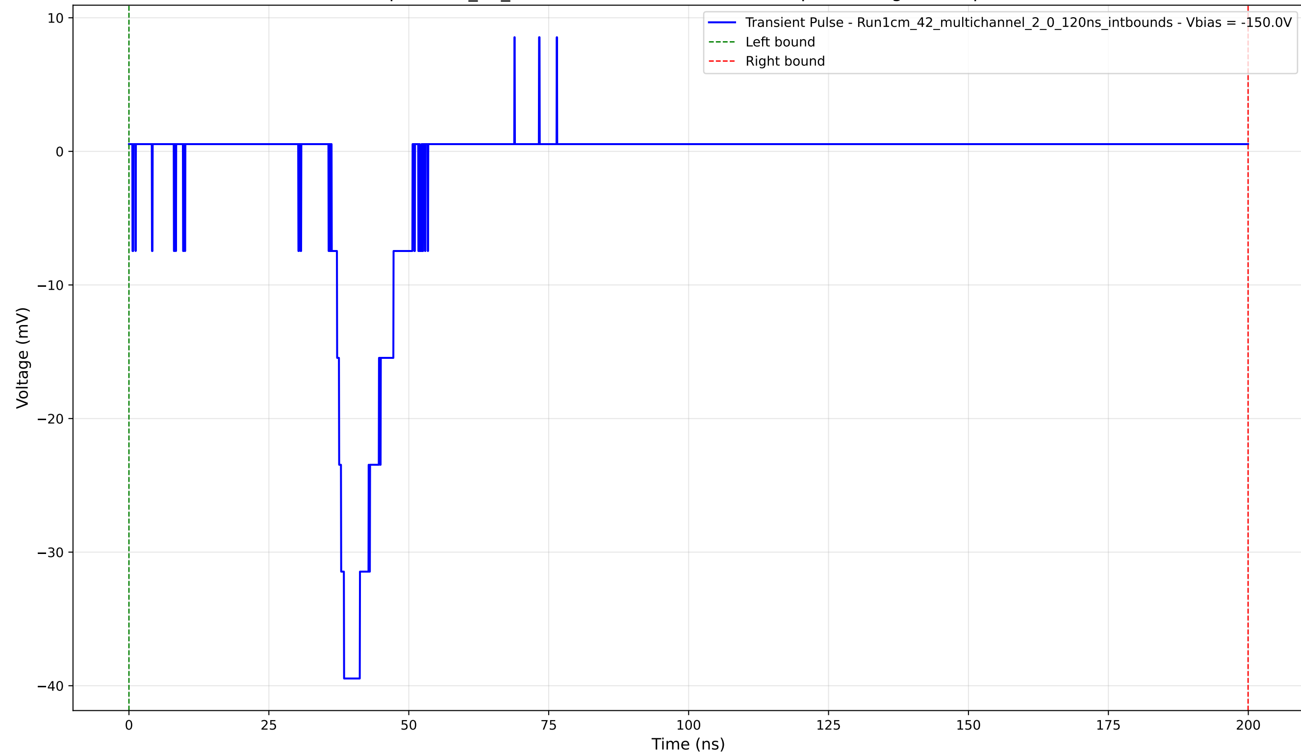
Transient Pulse - Sample: 1cm_42_multichannel - Position: 4840.0 \mu\text{m} - Charge: 4.48 pC - Rise Time: 2.22 ns
