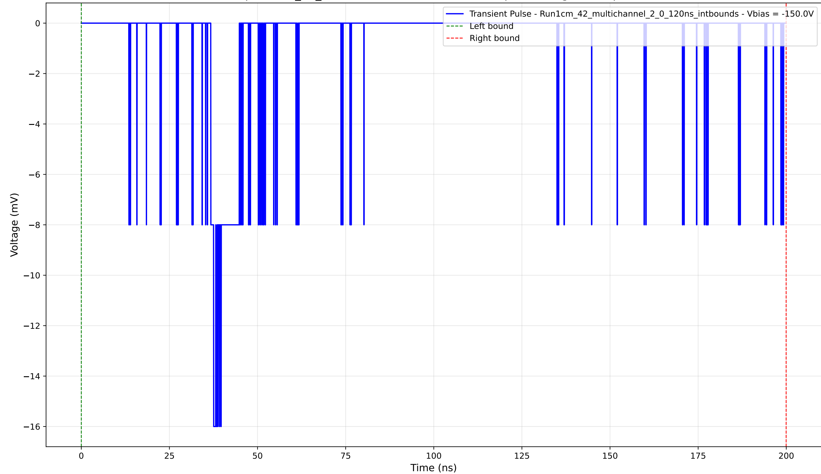
Transient Pulse - Sample: 1cm_42_multichannel - Position: 3365.0 \mu\text{m} - Charge: 2.51 pC - Rise Time: 0.83 ns
