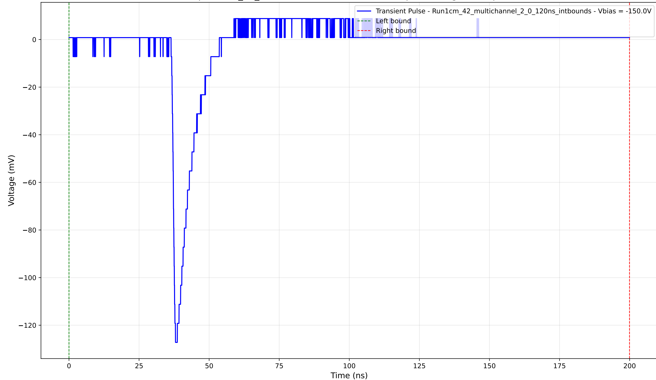
Transient Pulse - Sample: 1cm_42_multichannel - Position: 3525.0 \mu\text{m} - Charge: 7.80 pC - Rise Time: 1.13 ns
