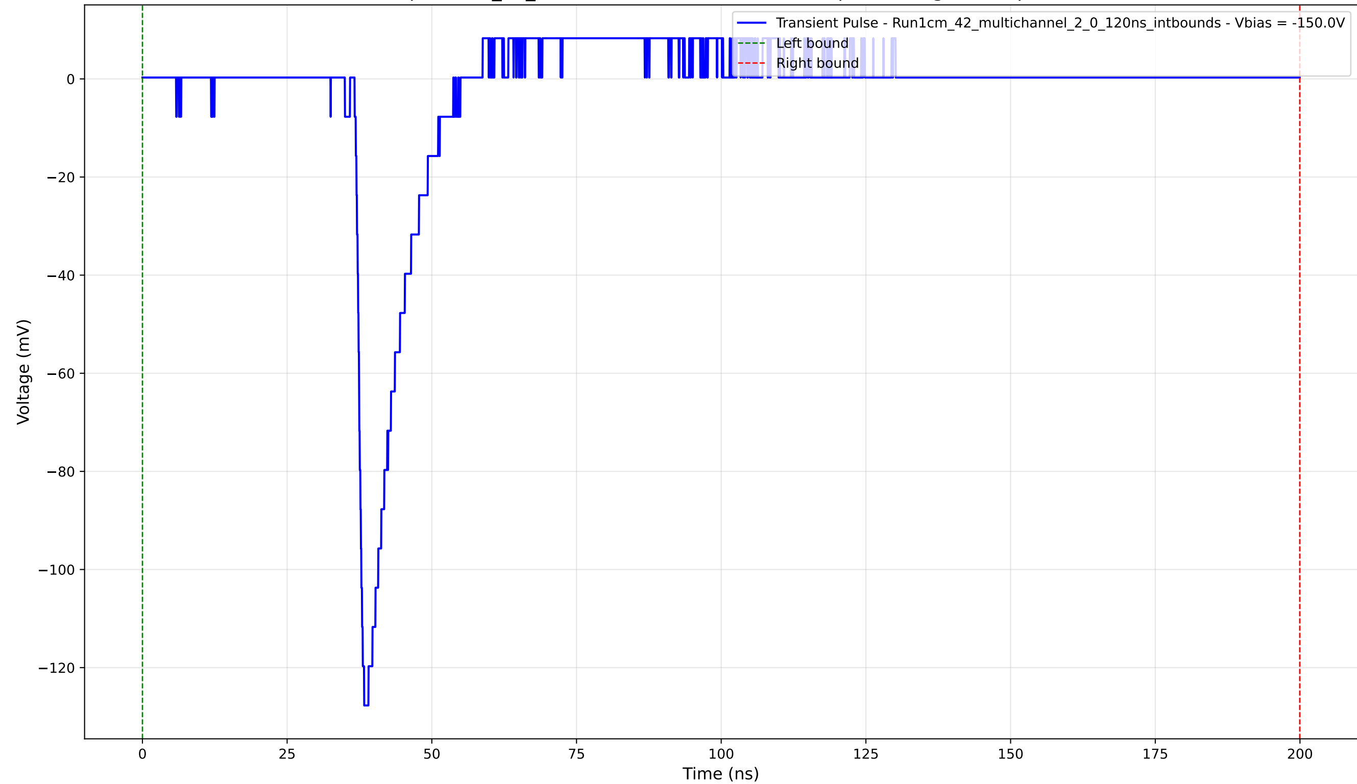
Transient Pulse - Sample: 1cm_42_multichannel - Position: 1015.0 \mu\text{m} - Charge: 9.75 pC - Rise Time: 1.21 ns
