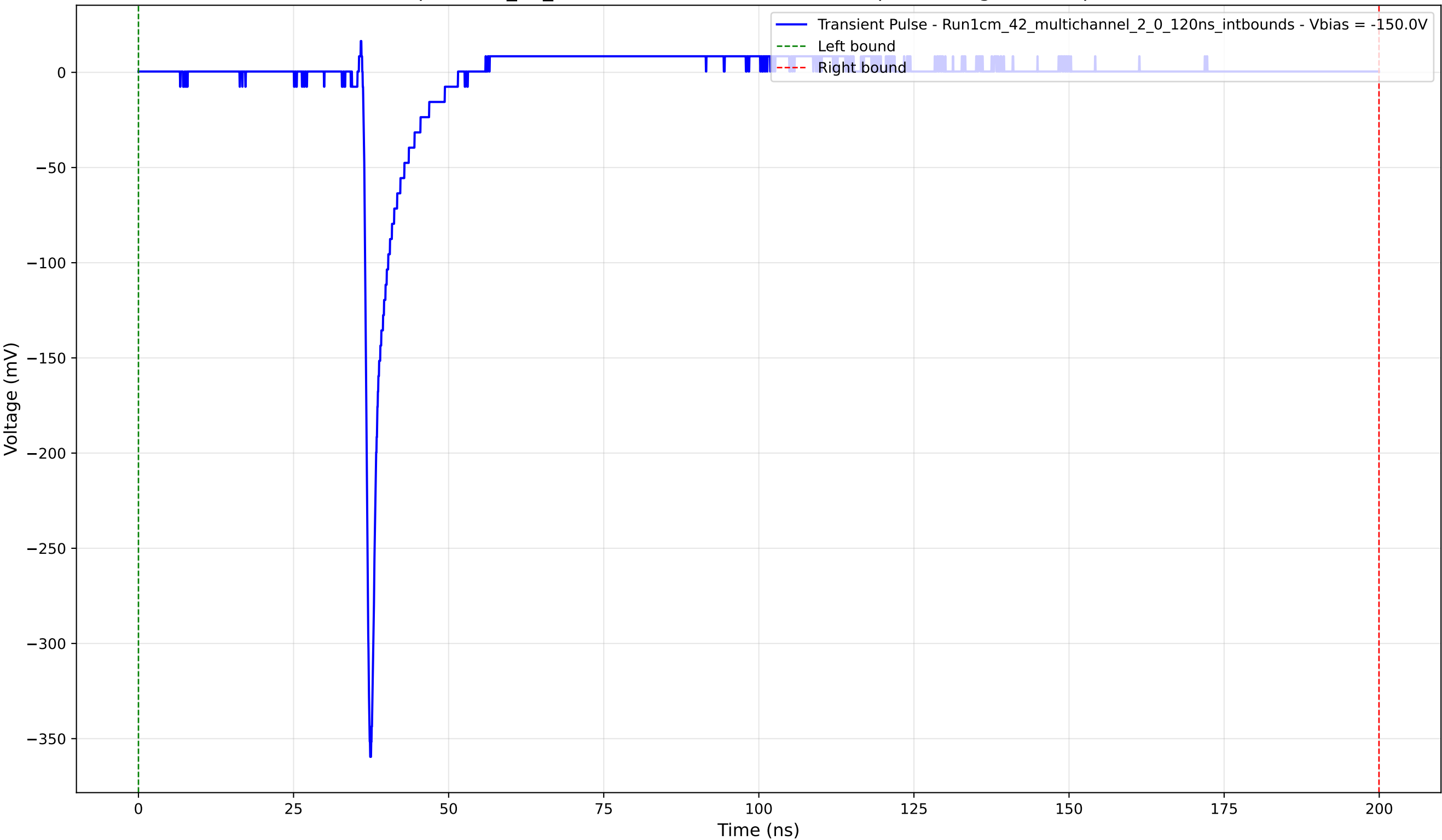
Transient Pulse - Sample: 1cm_42_multichannel - Position: 2785.0 \mu\text{m} - Charge: 11.51 pC - Rise Time: 0.80 ns
