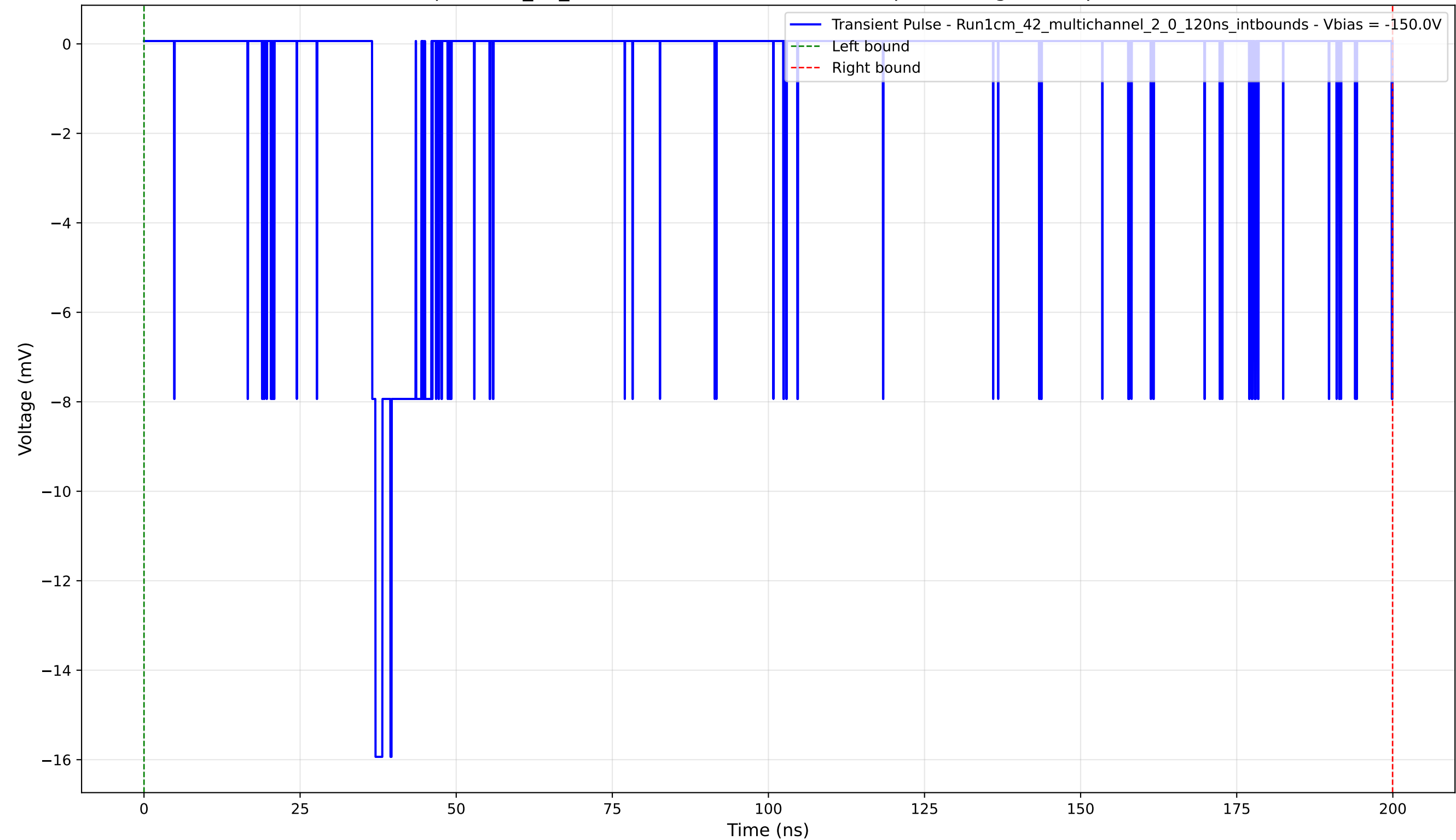
Transient Pulse - Sample: 1cm_42_multichannel - Position: 1865.0 \mu\text{m} - Charge: 2.20 pC - Rise Time: 0.55 ns
