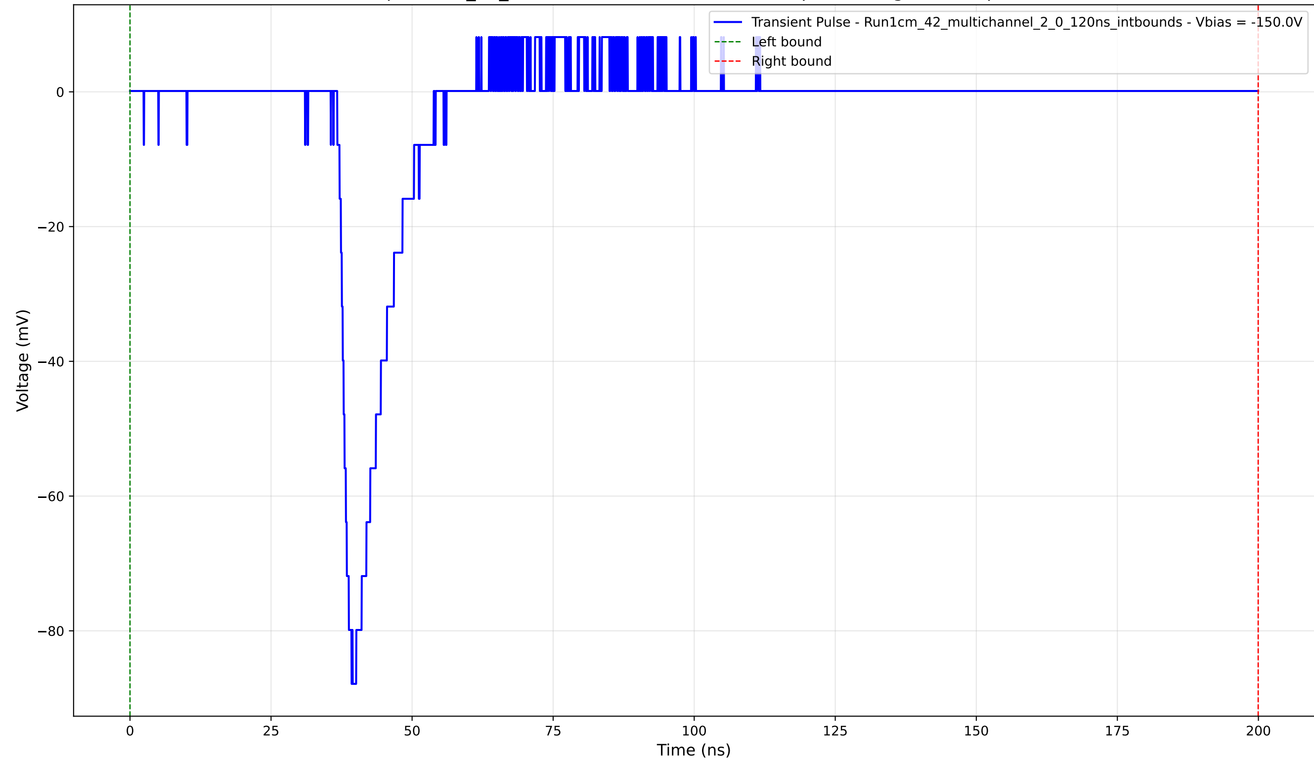
Transient Pulse - Sample: 1cm_42_multichannel - Position: 4215.0 \mu\text{m} - Charge: 10.06 pC - Rise Time: 1.68 ns
