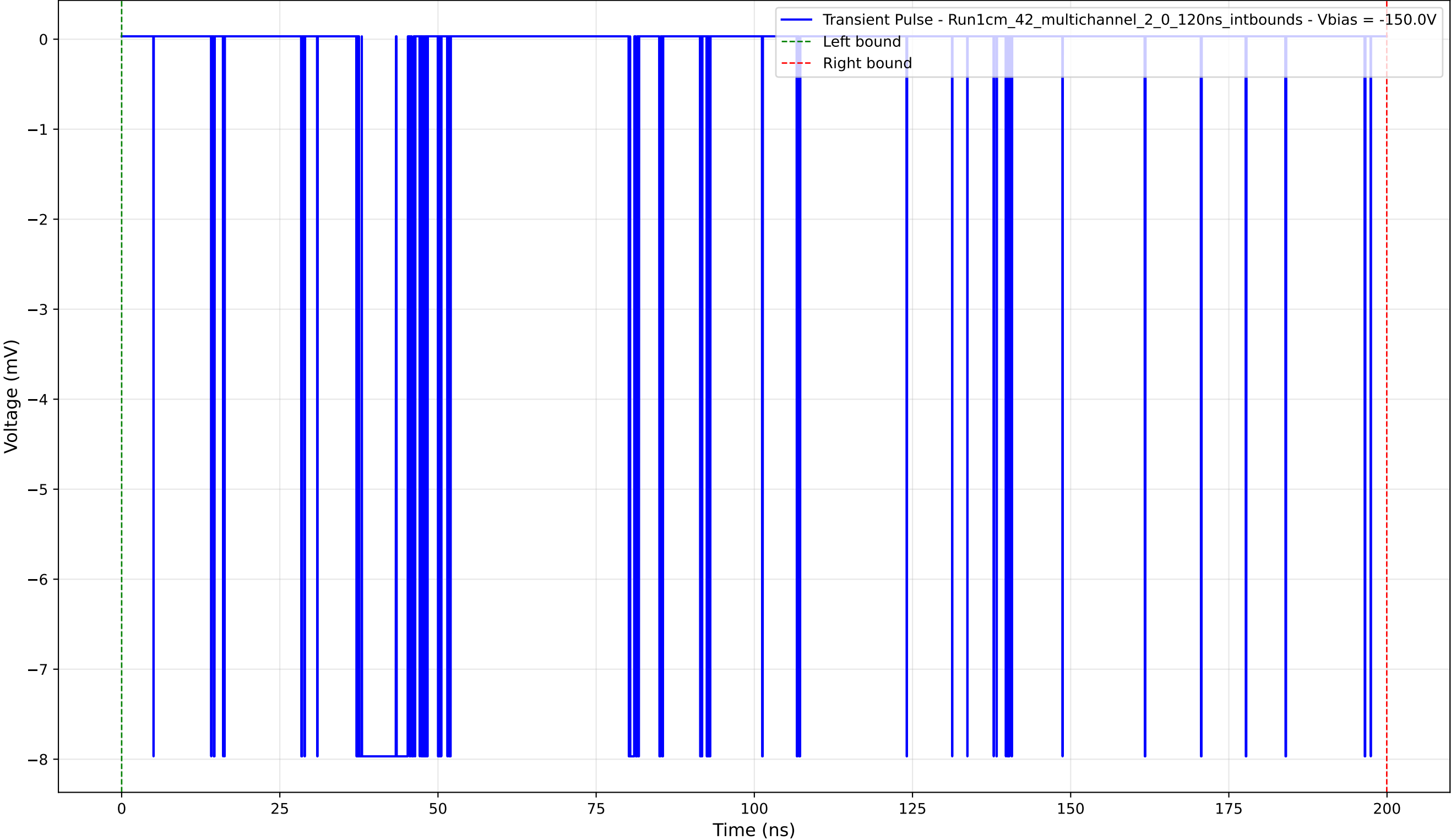
Transient Pulse - Sample: 1cm_42_multichannel - Position: 3880.0 \mu\text{m} - Charge: 2.07 pC - Rise Time: 0.04 ns
