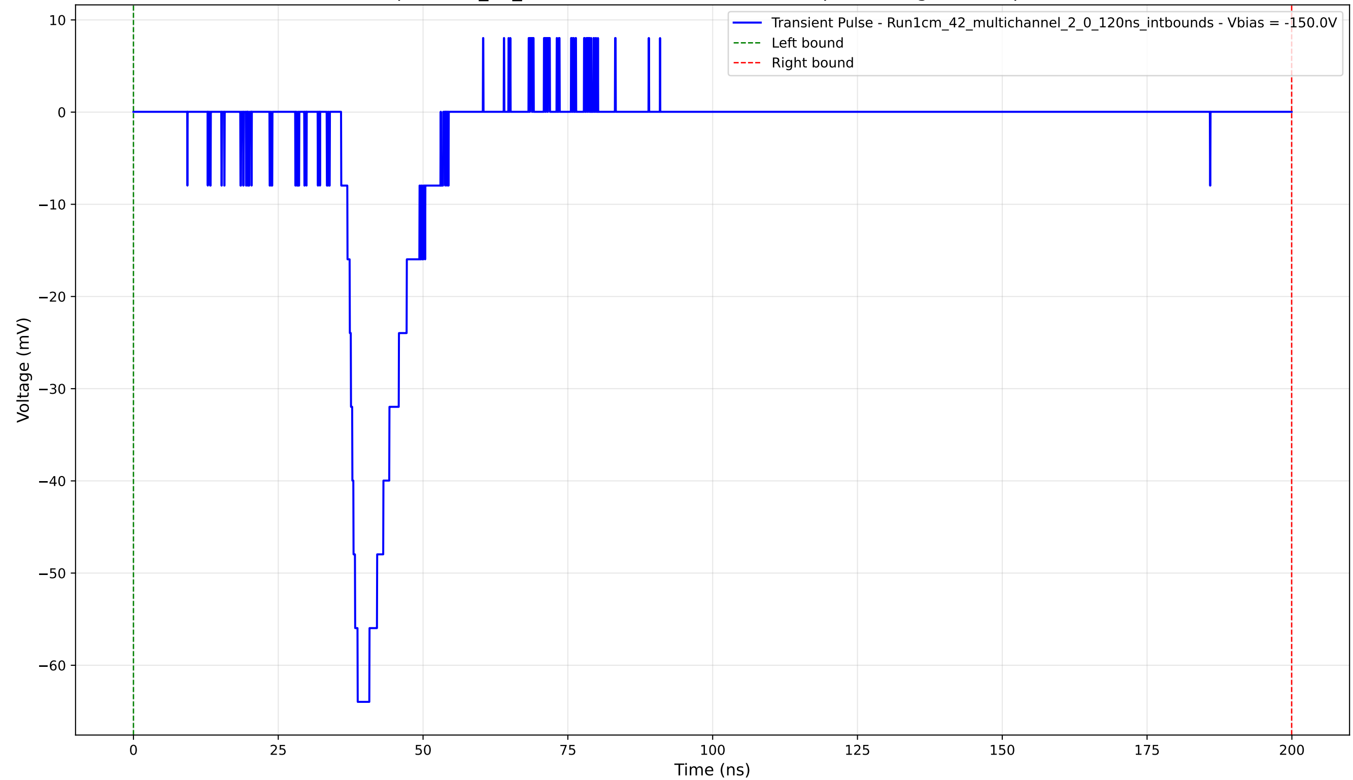
Transient Pulse - Sample: 1cm_42_multichannel - Position: 4755.0 \mu\text{m} - Charge: 10.23 pC - Rise Time: 2.85 ns
