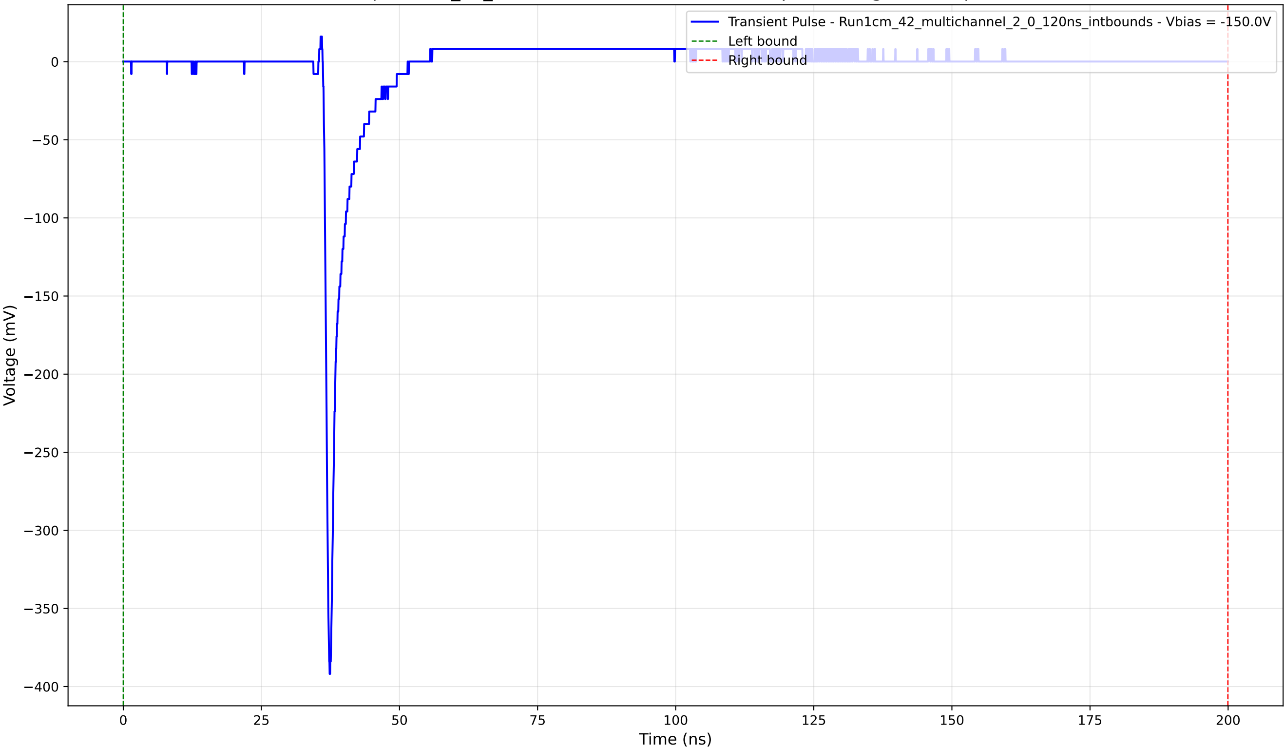
Transient Pulse - Sample: 1cm_42_multichannel - Position: 2760.0 \mu\text{m} - Charge: 12.76 pC - Rise Time: 0.81 ns
