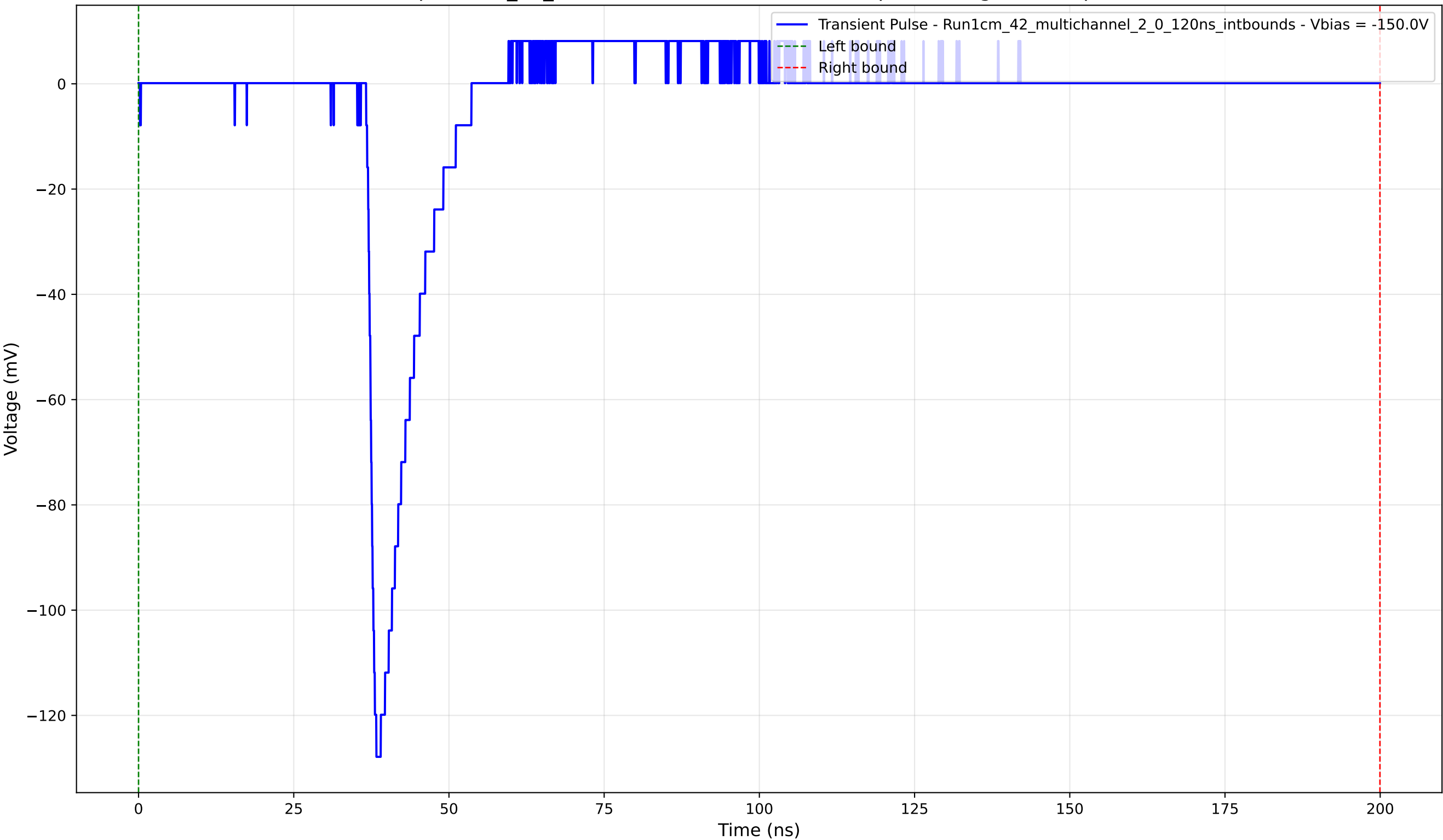
Transient Pulse - Sample: 1cm_42_multichannel - Position: 1020.0 \mu\text{m} - Charge: 10.77 pC - Rise Time: 1.26 ns
