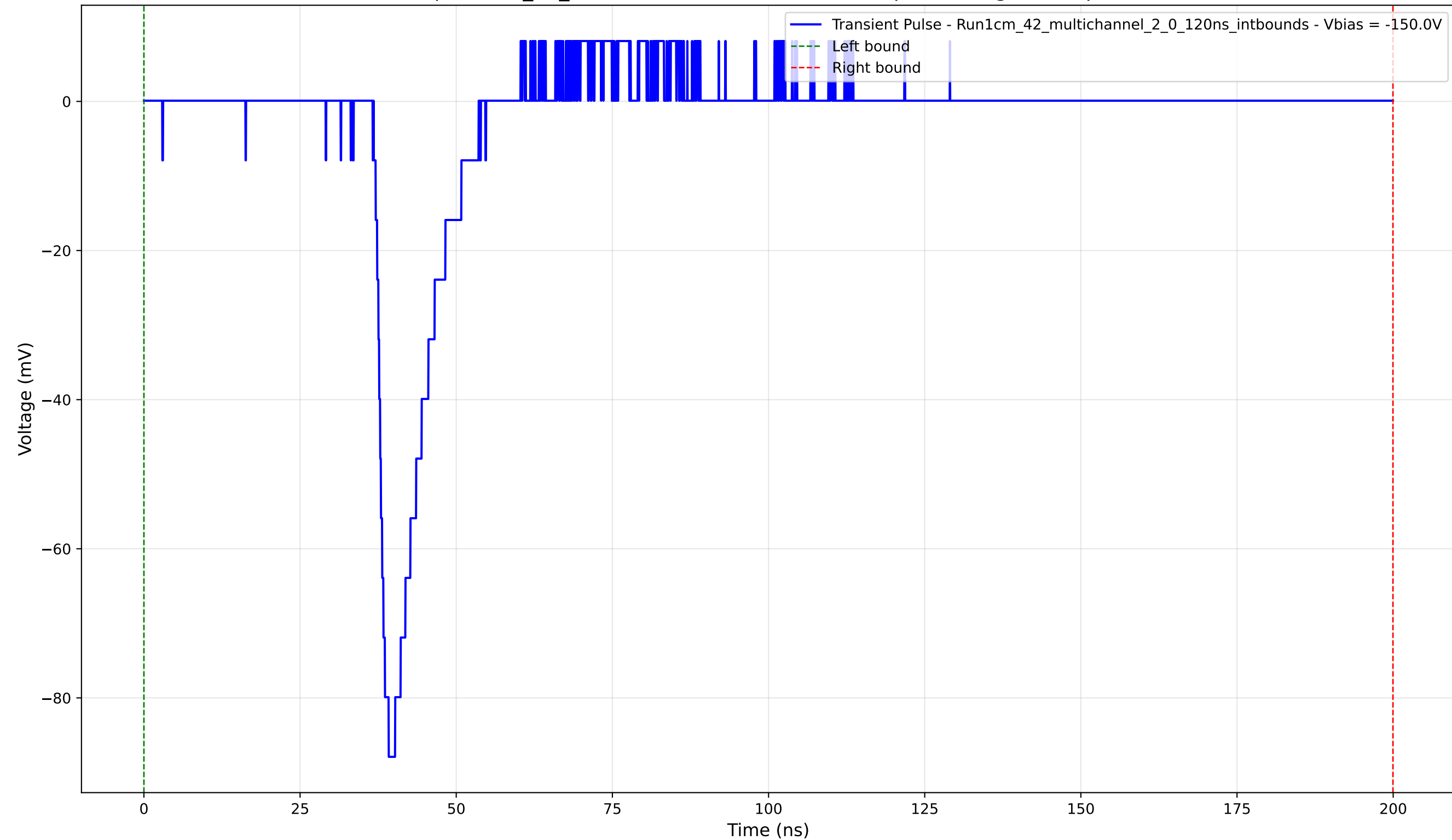
Transient Pulse - Sample: 1cm_42_multichannel - Position: 4130.0 \mu\text{m} - Charge: 9.79 pC - Rise Time: 1.52 ns
