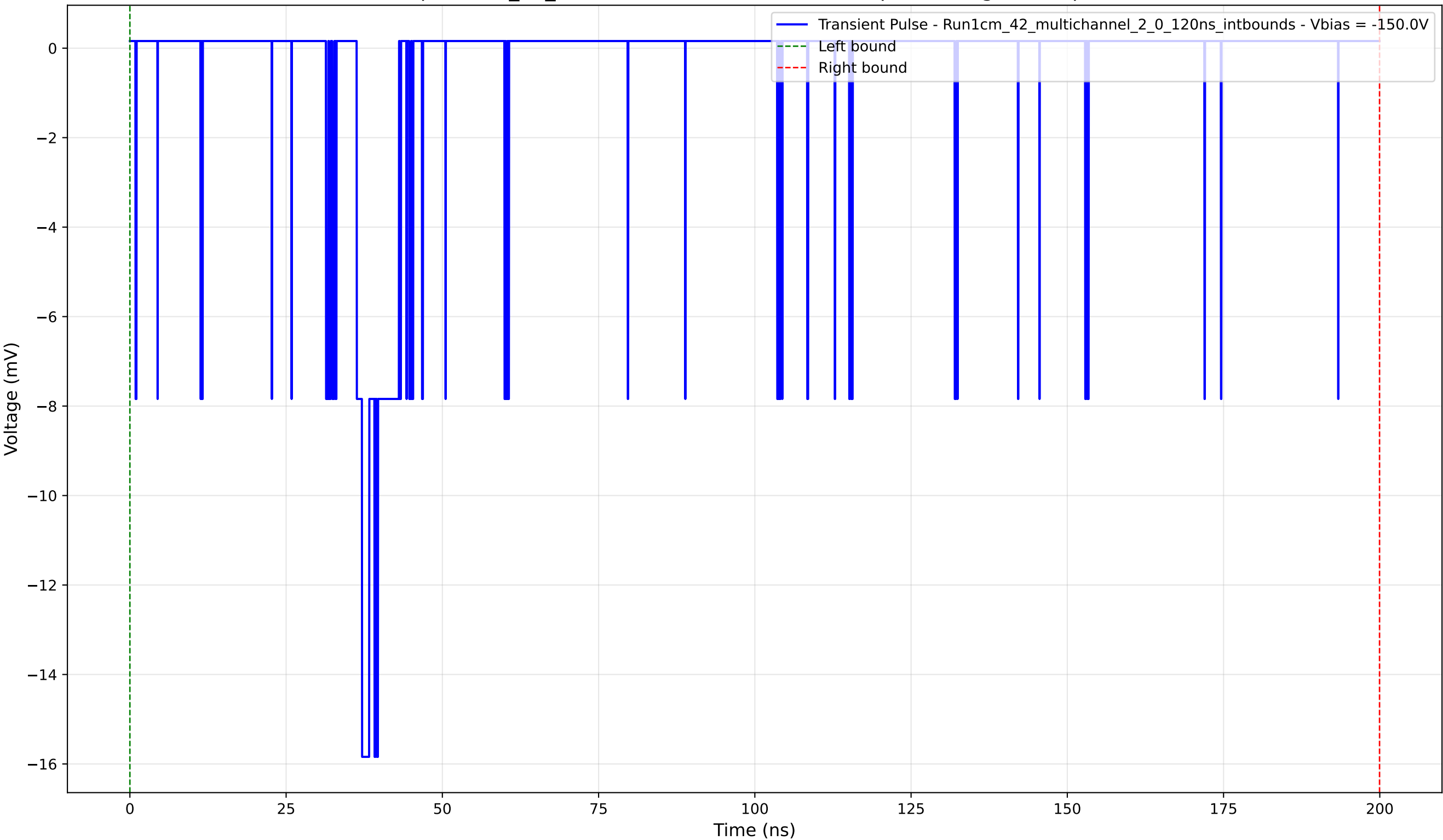
Transient Pulse - Sample: 1cm_42_multichannel - Position: 2875.0 \mu\text{m} - Charge: 1.52 pC - Rise Time: 0.87 ns
