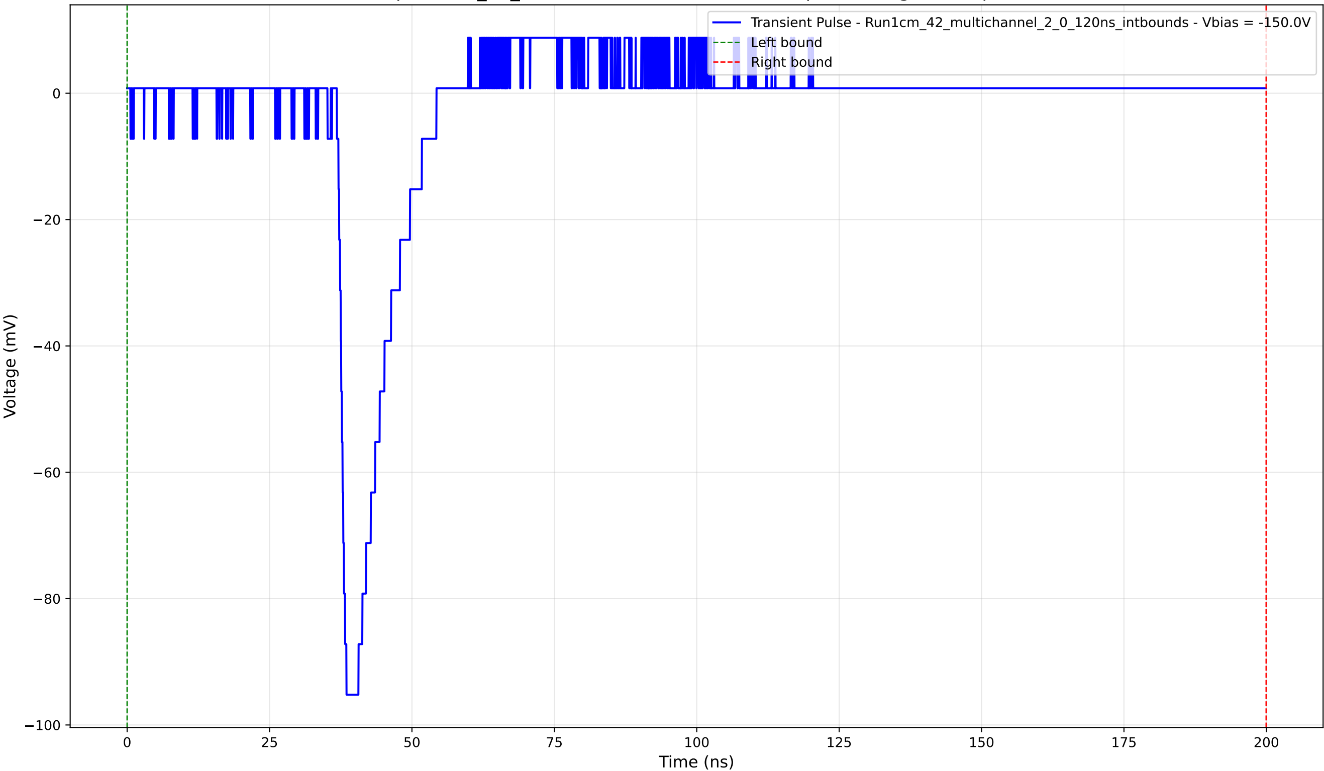
Transient Pulse - Sample: 1cm_42_multichannel - Position: 630.0 \mu\text{m} - Charge: 8.77 pC - Rise Time: 1.19 ns
