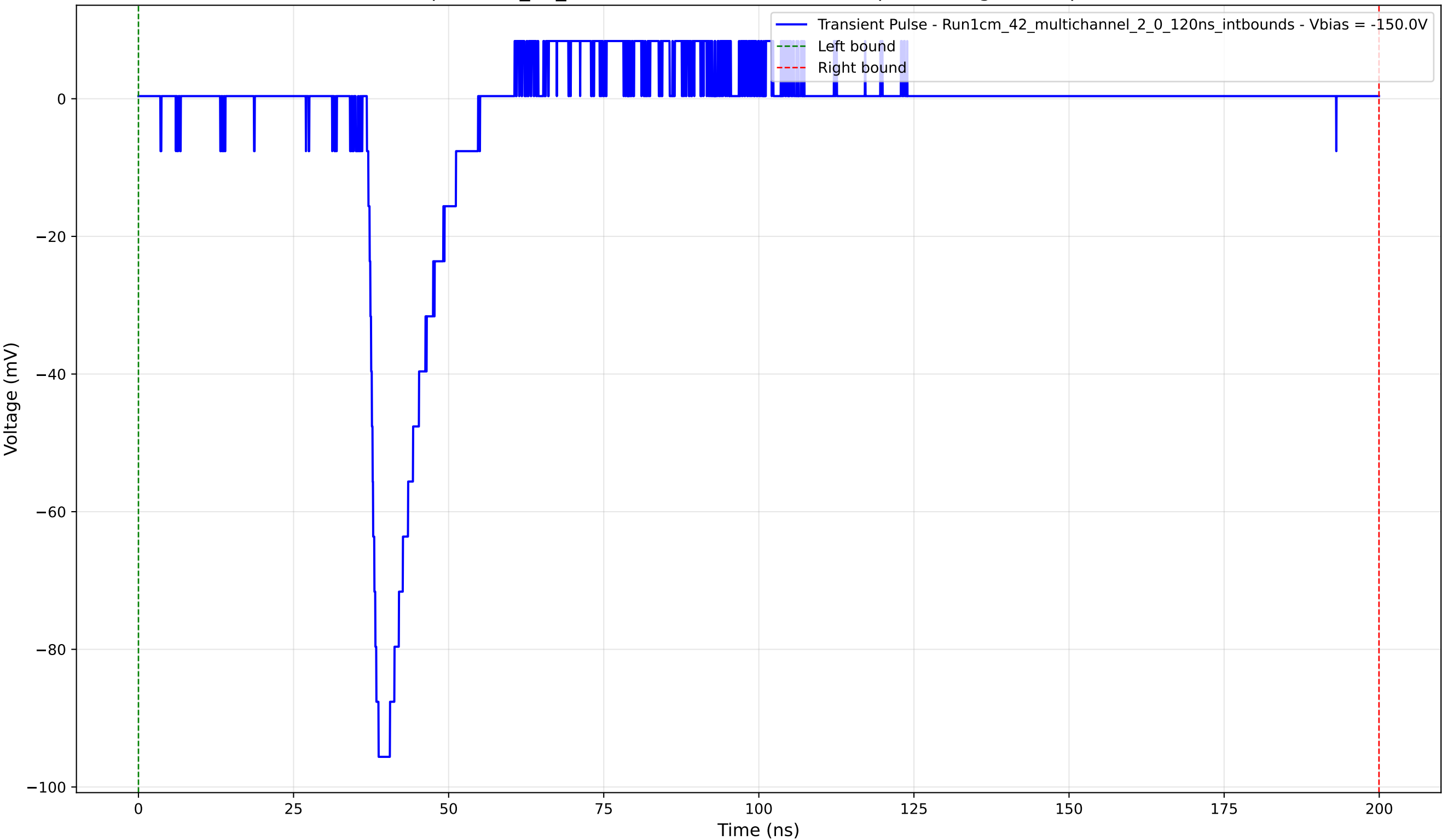
Transient Pulse - Sample: 1cm_42_multichannel - Position: 580.0 \mu\text{m} - Charge: 9.32 pC - Rise Time: 1.31 ns
