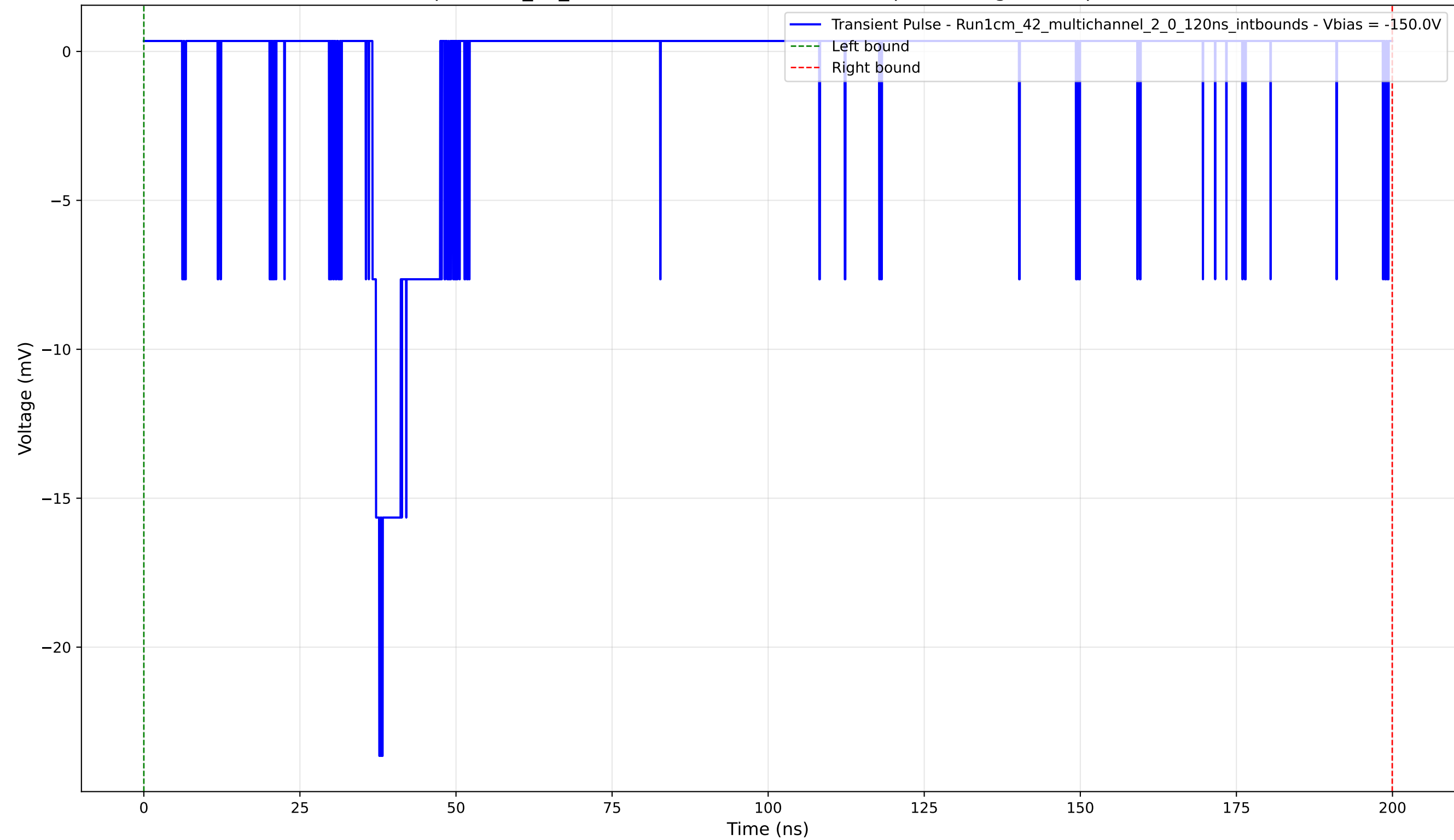
Transient Pulse - Sample: 1cm_42_multichannel - Position: 3355.0 \mu\text{m} - Charge: 2.04 pC - Rise Time: 1.11 ns
