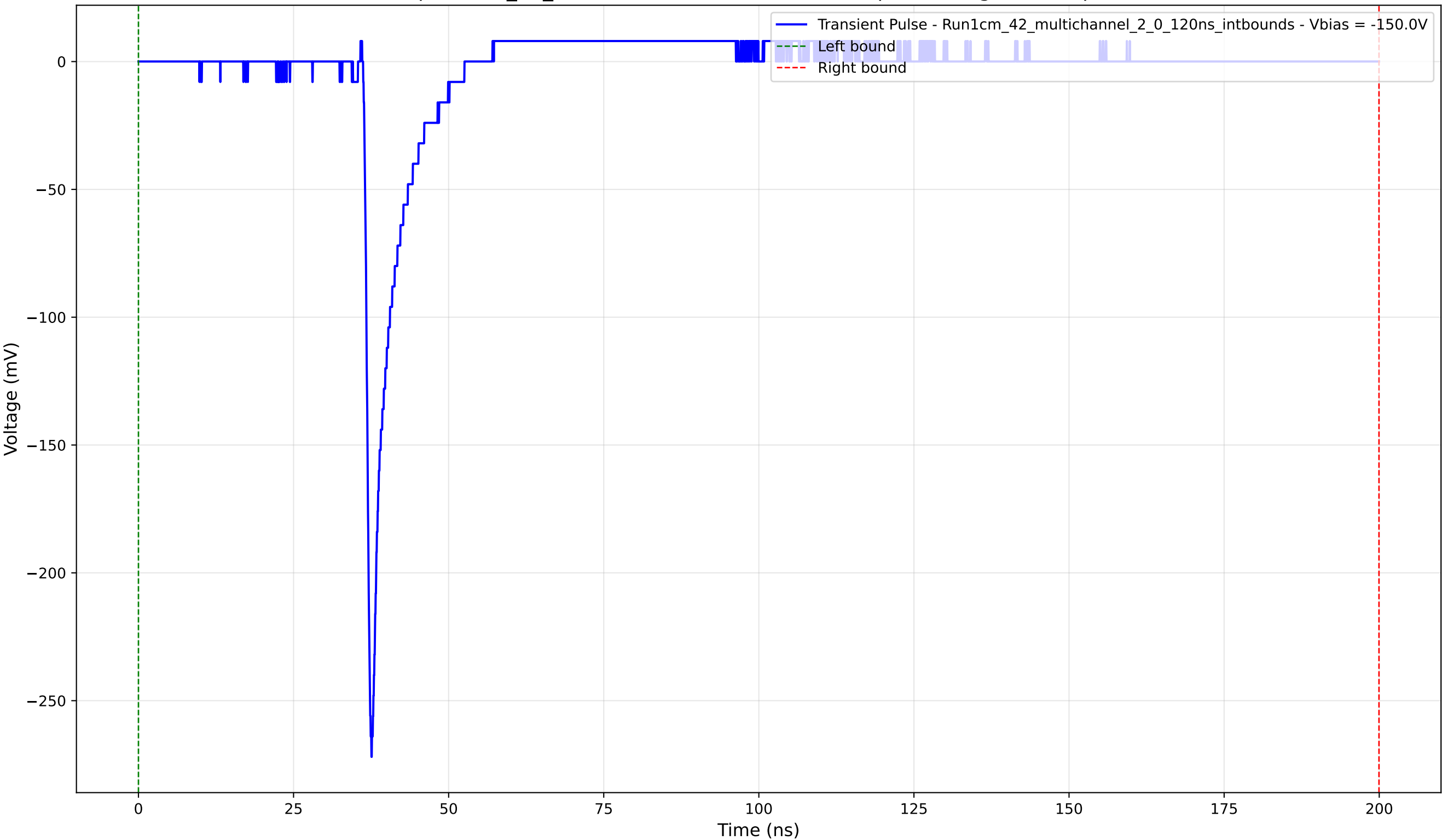
Transient Pulse - Sample: 1cm_42_multichannel - Position: 2995.0 \mu\text{m} - Charge: 13.05 pC - Rise Time: 0.89 ns
