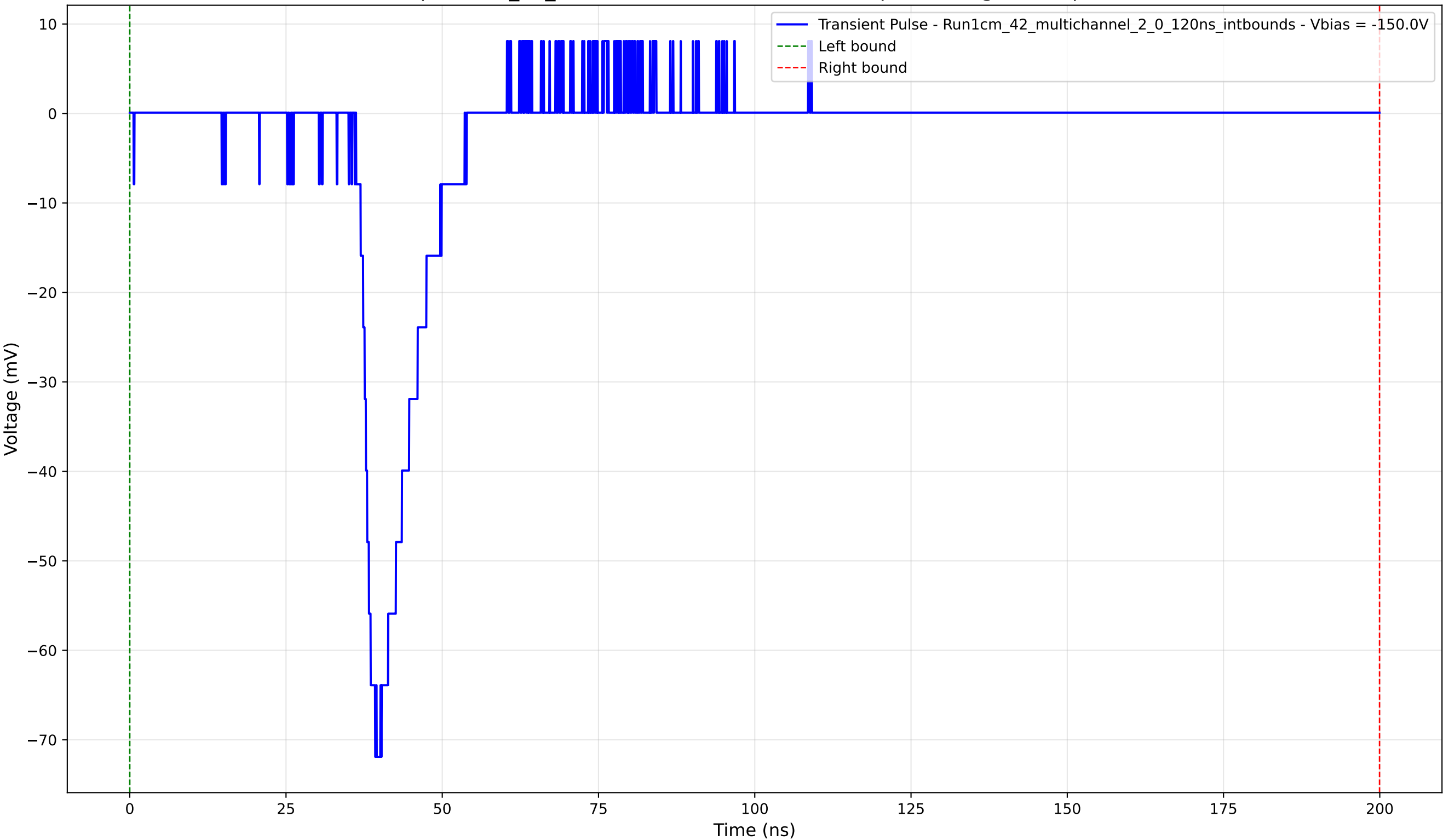
Transient Pulse - Sample: 1cm_42_multichannel - Position: 4685.0 \mu\text{m} - Charge: 9.79 pC - Rise Time: 3.04 ns
