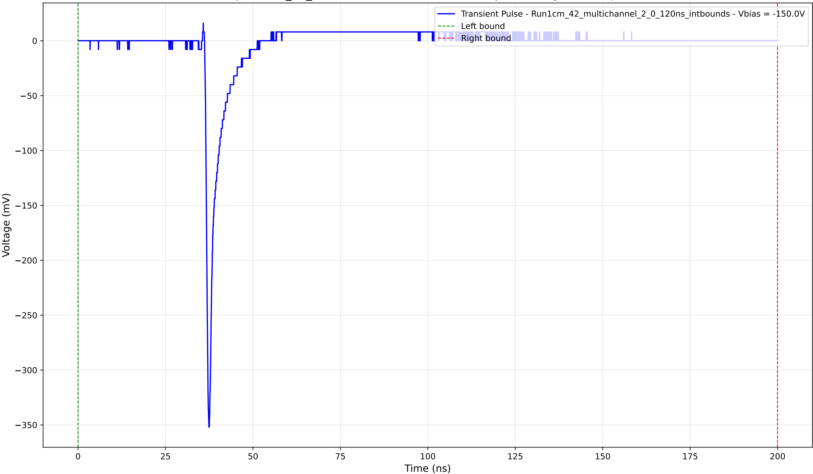
Transient Pulse - Sample: 1cm_42_multichannel - Position: 1940.0 \mu\text{m} - Charge: 12.65 pC - Rise Time: 0.81 ns
