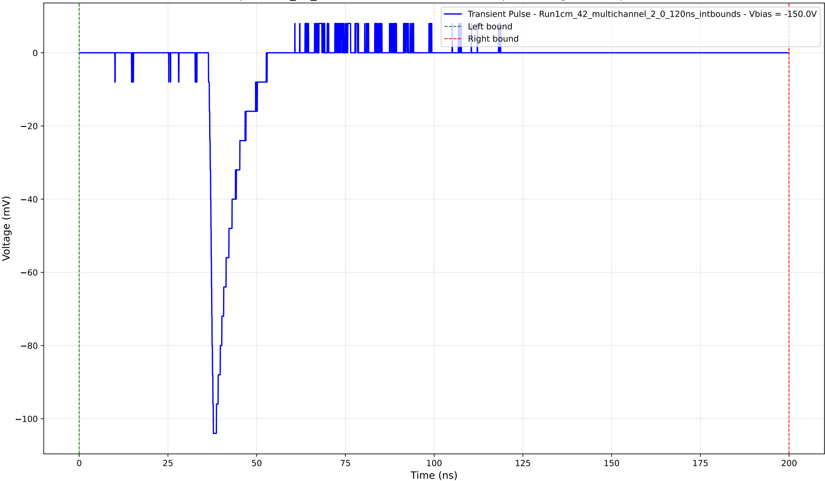
Transient Pulse - Sample: 1cm_42_multichannel - Position: 1300.0 \mu\text{m} - Charge: 11.26 pC - Rise Time: 1.03 ns
