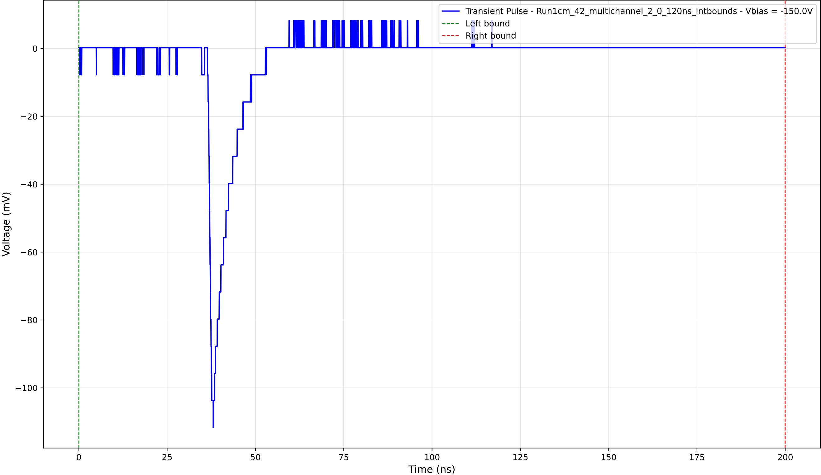
Transient Pulse - Sample: 1cm_42_multichannel - Position: 3325.0 \mu\text{m} - Charge: 10.50 pC - Rise Time: 1.06 ns
