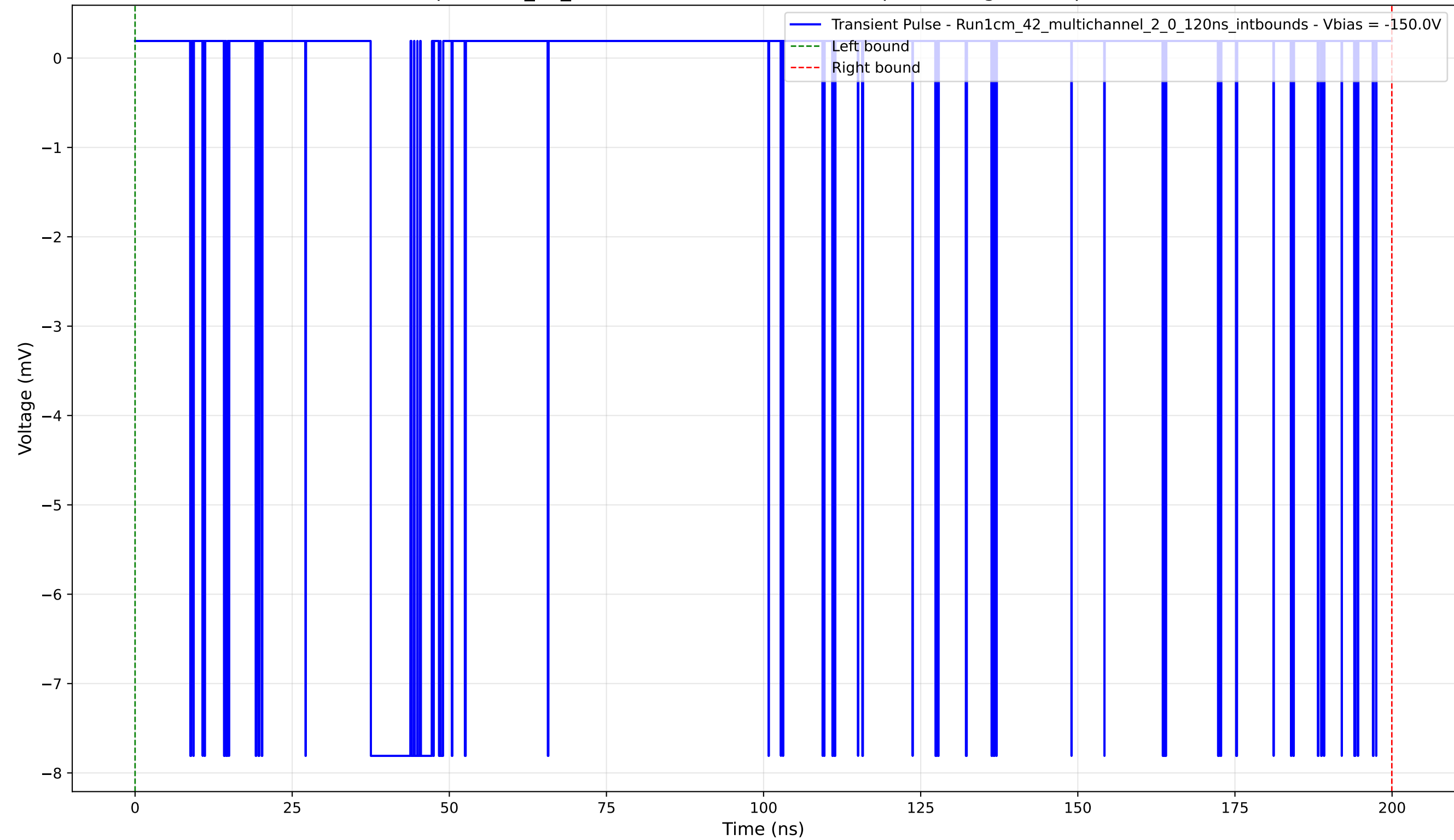
Transient Pulse - Sample: 1cm_42_multichannel - Position: 845.0 \mu\text{m} - Charge: 1.71 pC - Rise Time: 0.04 ns
