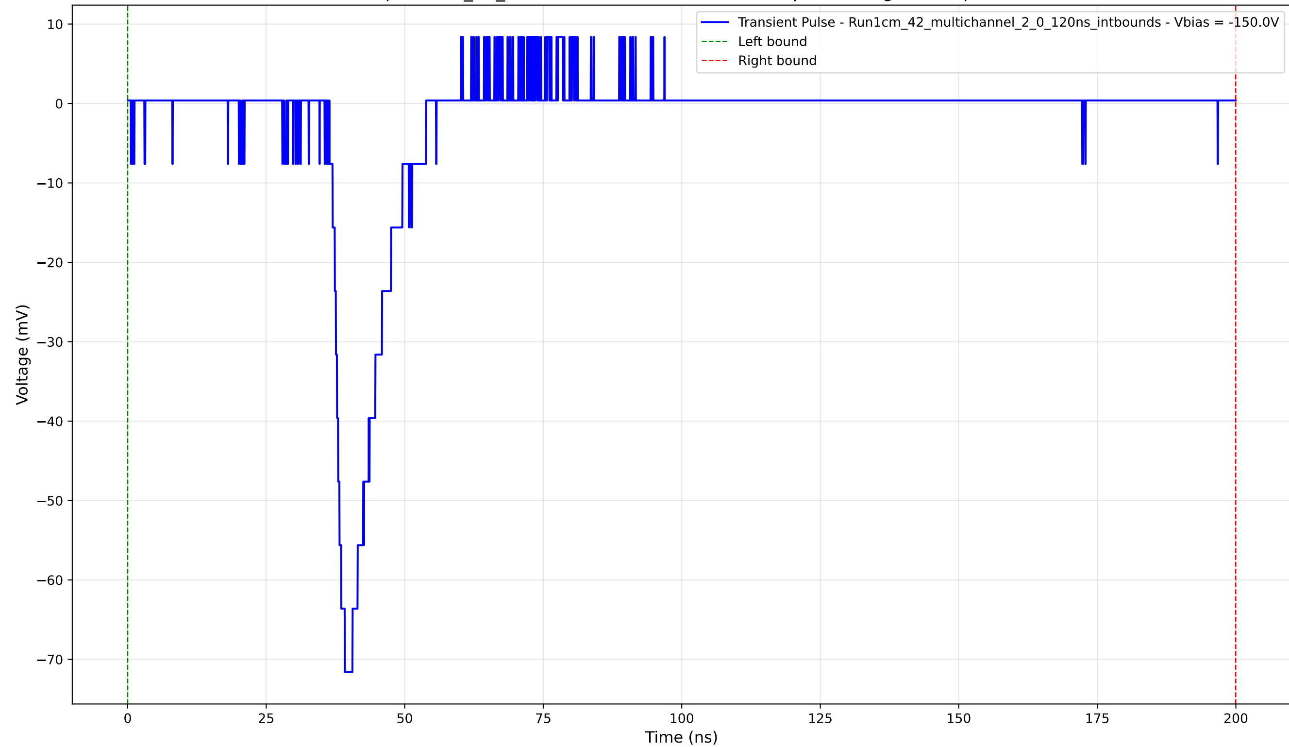
Transient Pulse - Sample: 1cm_42_multichannel - Position: 4660.0 \mu\text{m} - Charge: 8.86 pC - Rise Time: 2.76 ns
