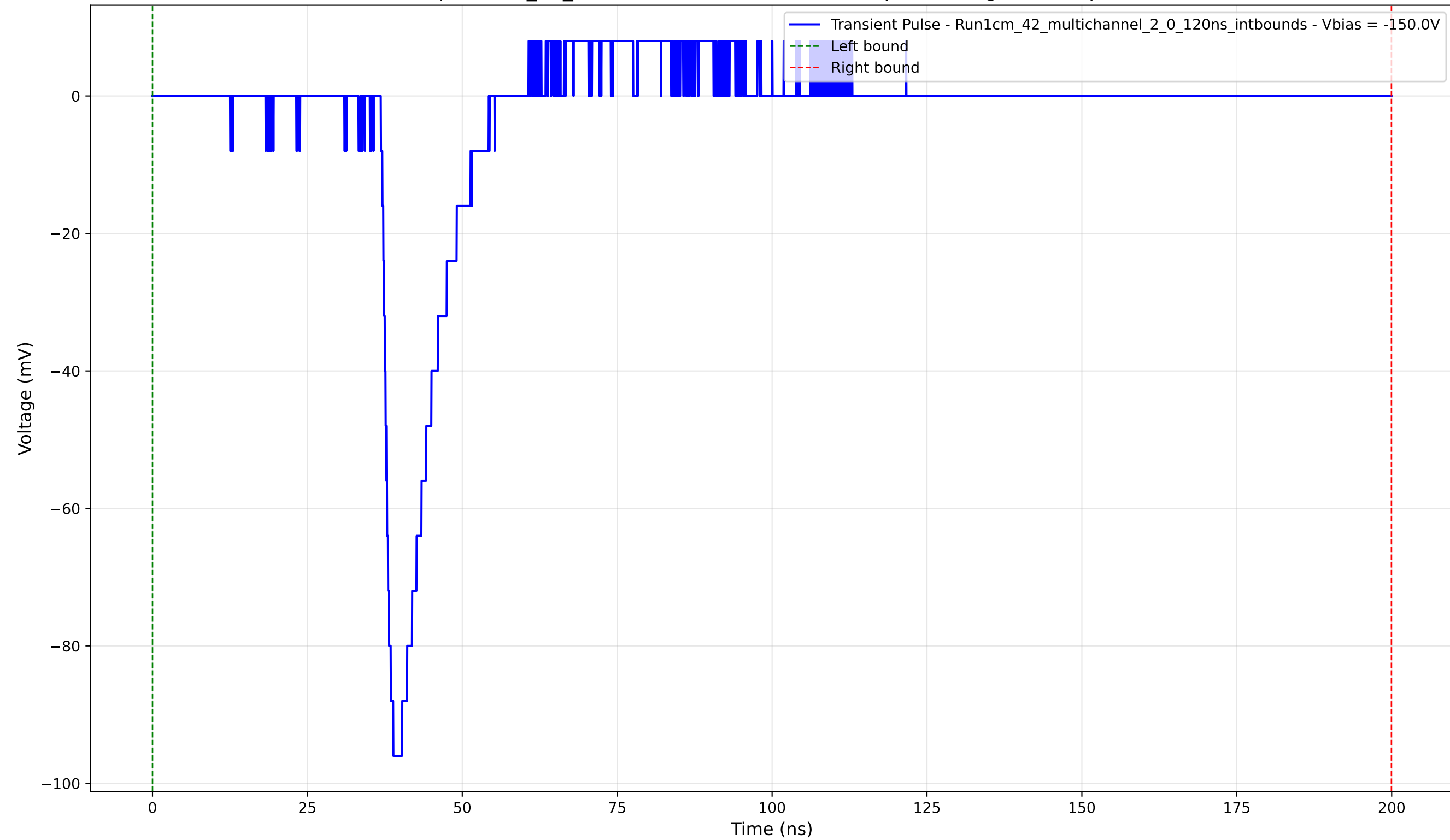
Transient Pulse - Sample: 1cm_42_multichannel - Position: 560.0 \mu\text{m} - Charge: 10.37 pC - Rise Time: 1.39 ns
