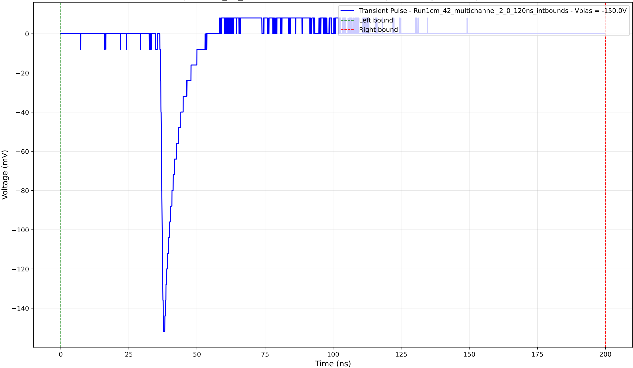
Transient Pulse - Sample: 1cm_42_multichannel - Position: 3305.0 \mu\text{m} - Charge: 10.60 pC - Rise Time: 1.04 ns
