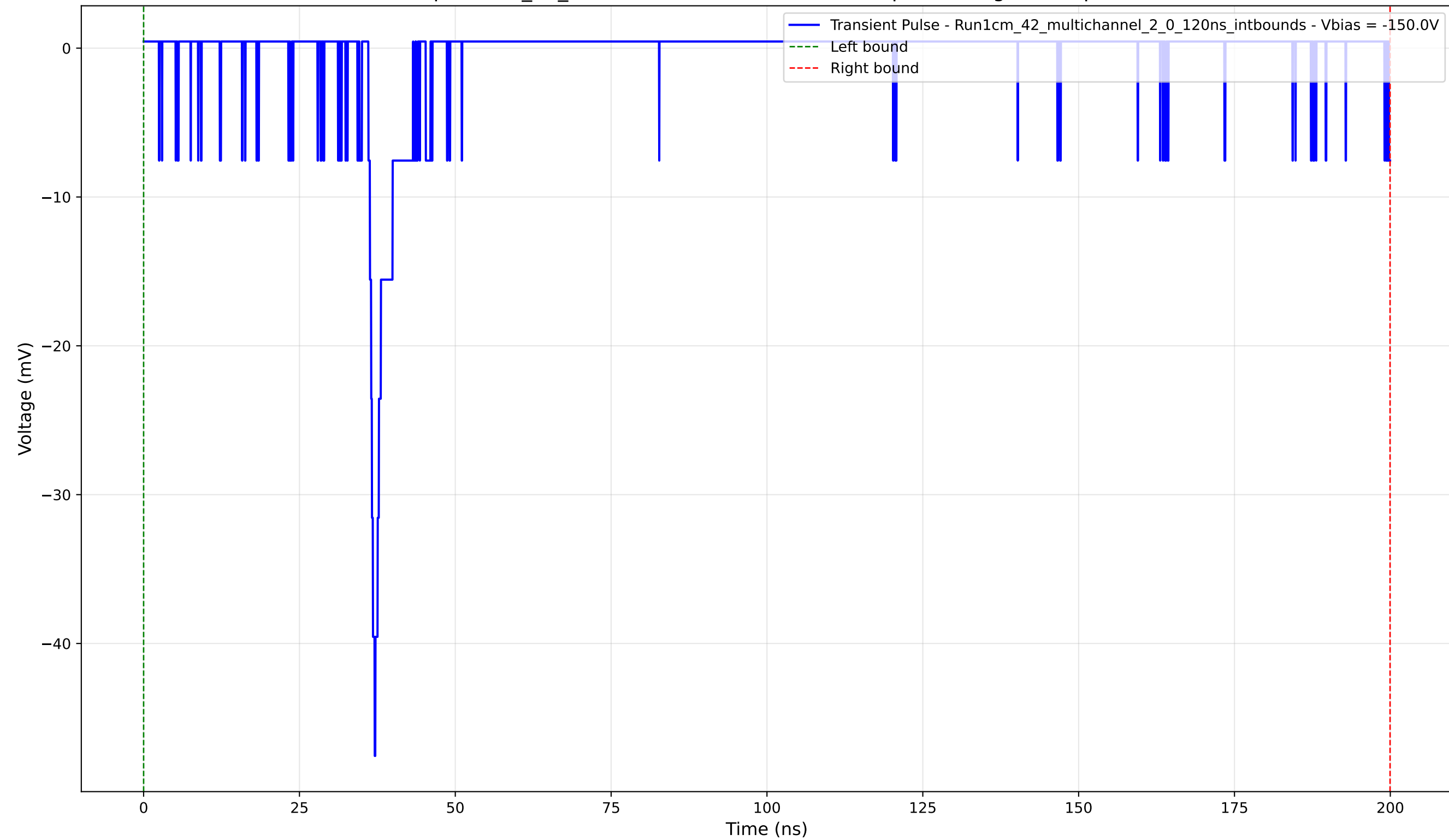
Transient Pulse - Sample: 1cm_42_multichannel - Position: 2350.0 \mu\text{m} - Charge: 1.67 pC - Rise Time: 1.02 ns
