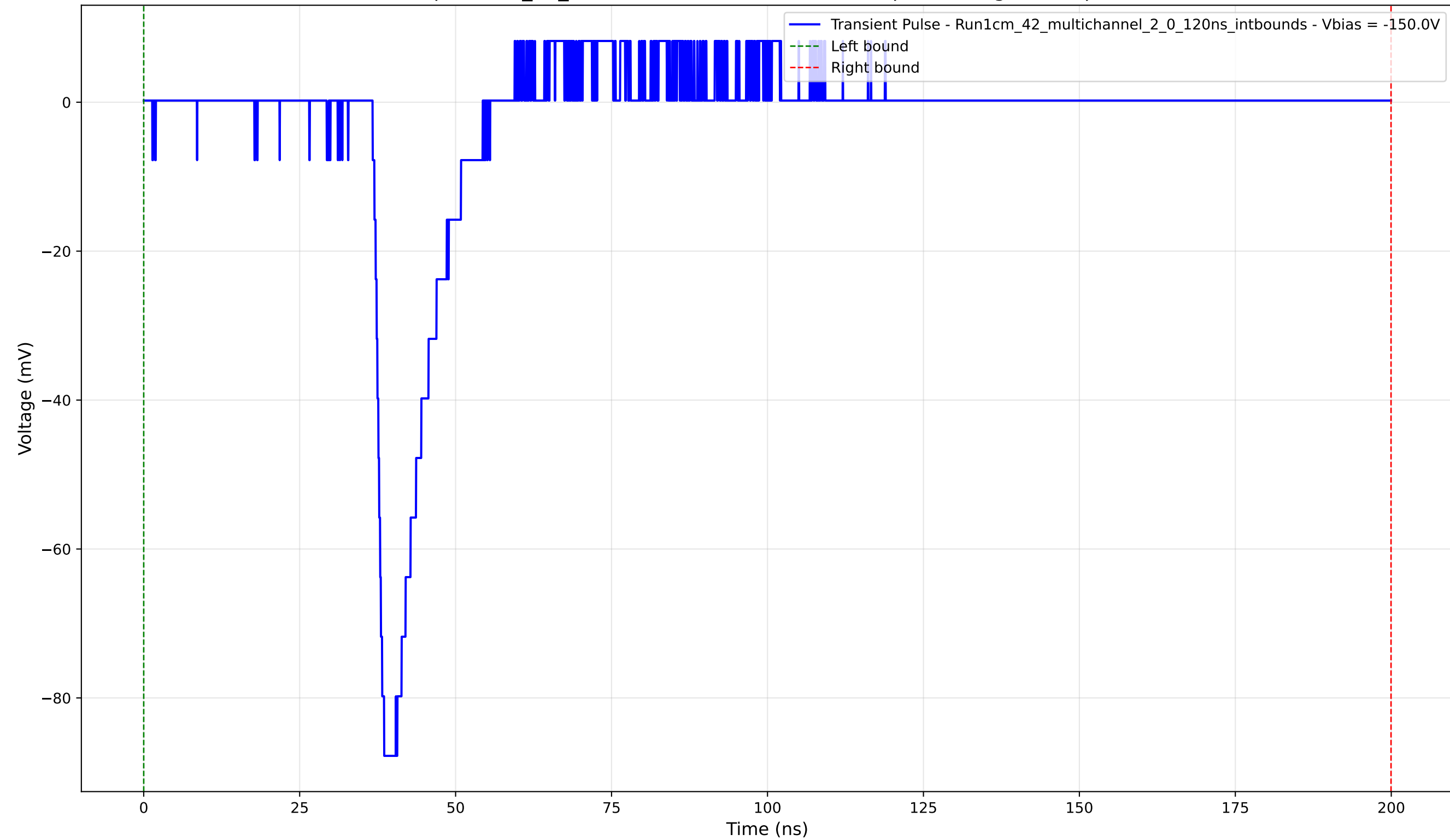
Transient Pulse - Sample: 1cm_42_multichannel - Position: 3970.0 \mu\text{m} - Charge: 9.65 pC - Rise Time: 1.27 ns
