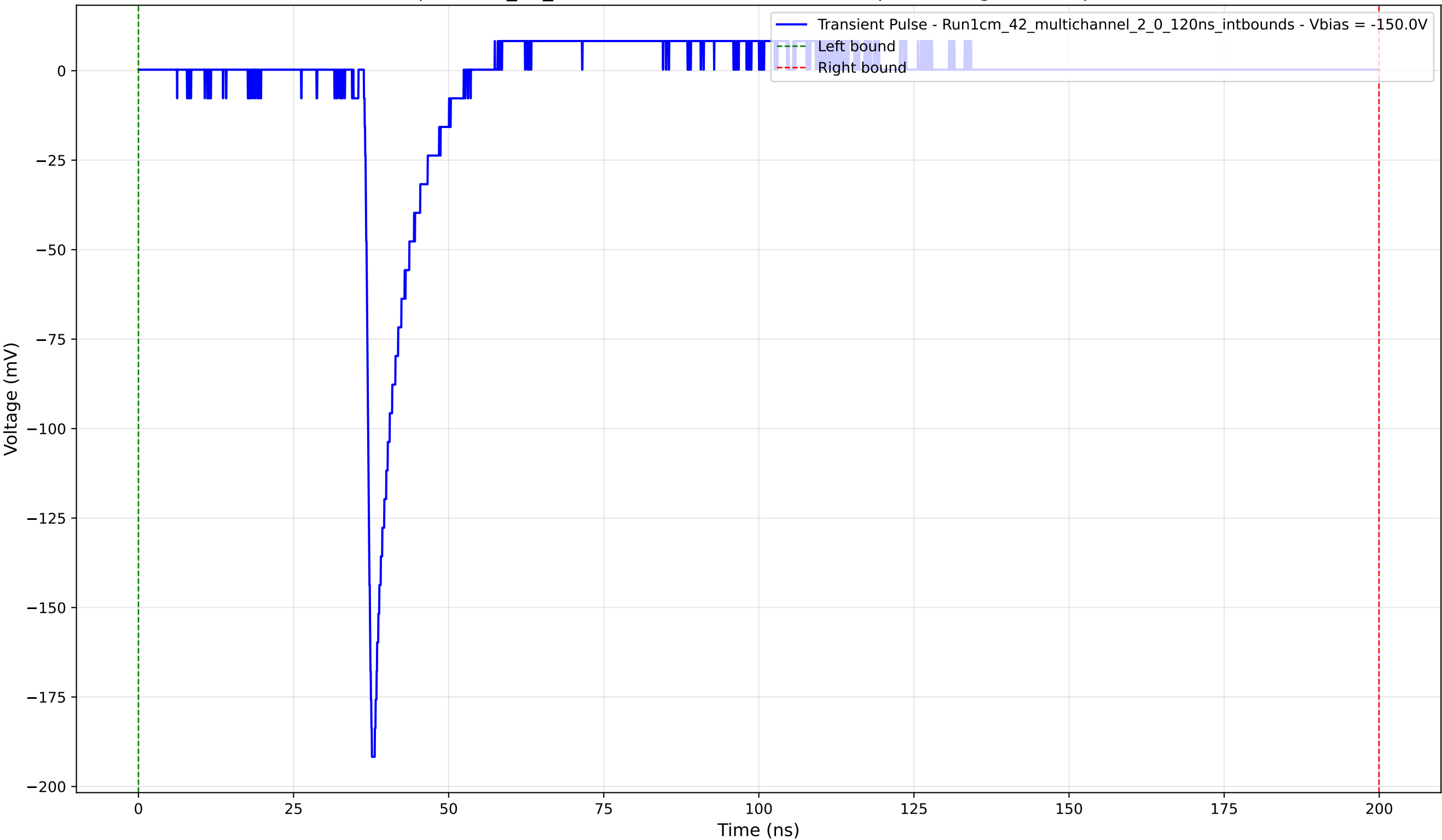
Transient Pulse - Sample: 1cm_42_multichannel - Position: 3210.0 \mu\text{m} - Charge: 10.37 pC - Rise Time: 0.94 ns
