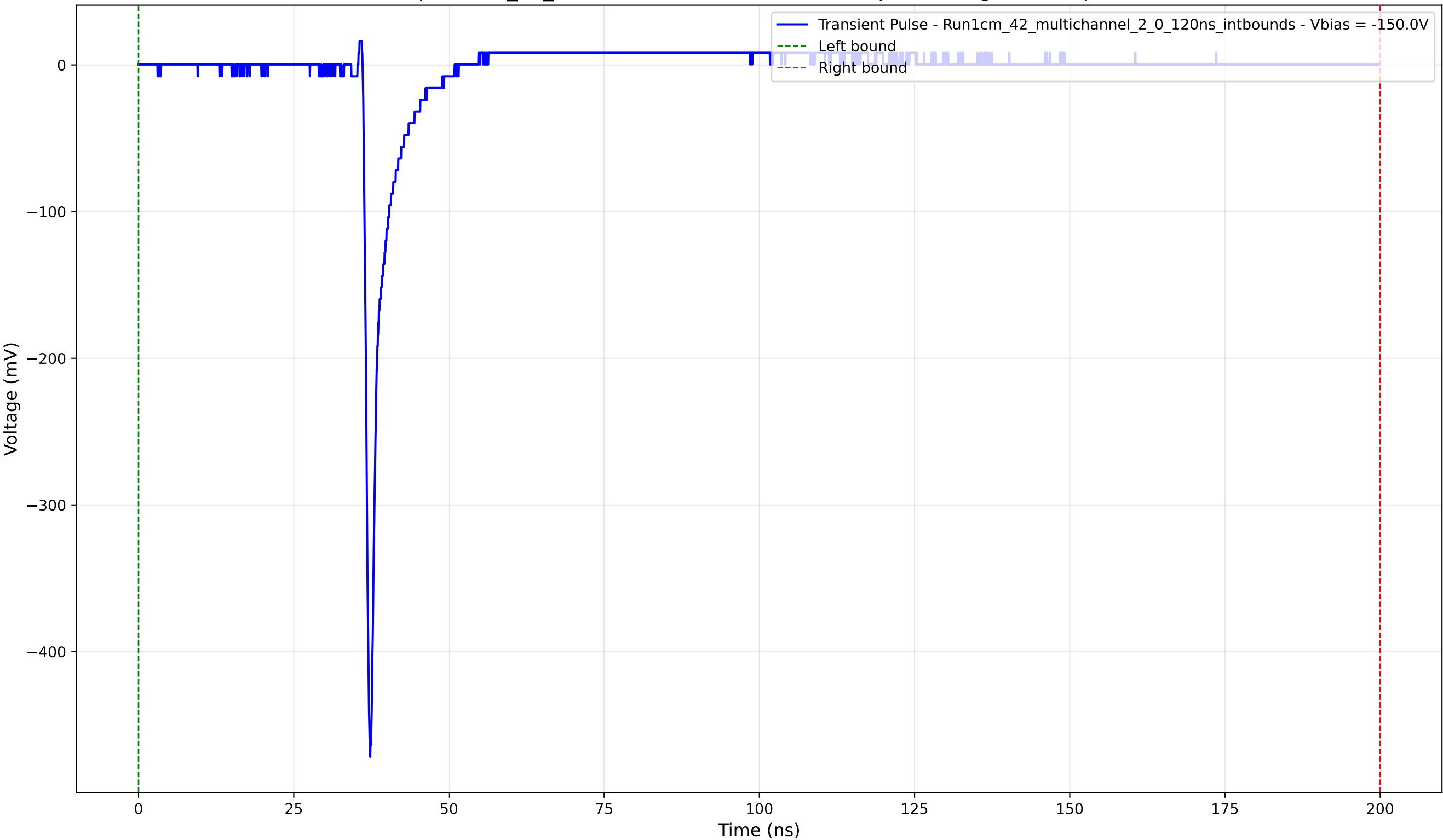
Transient Pulse - Sample: 1cm_42_multichannel - Position: 2070.0 \mu\text{m} - Charge: 15.15 pC - Rise Time: 0.77 ns
