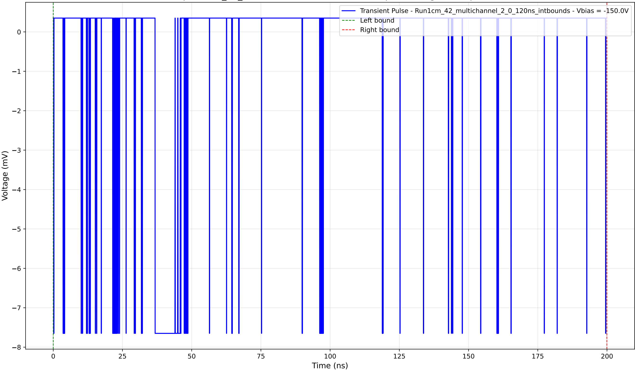
Transient Pulse - Sample: 1cm_42_multichannel - Position: 3385.0 \mu\text{m} - Charge: 1.02 pC - Rise Time: 0.04 ns
