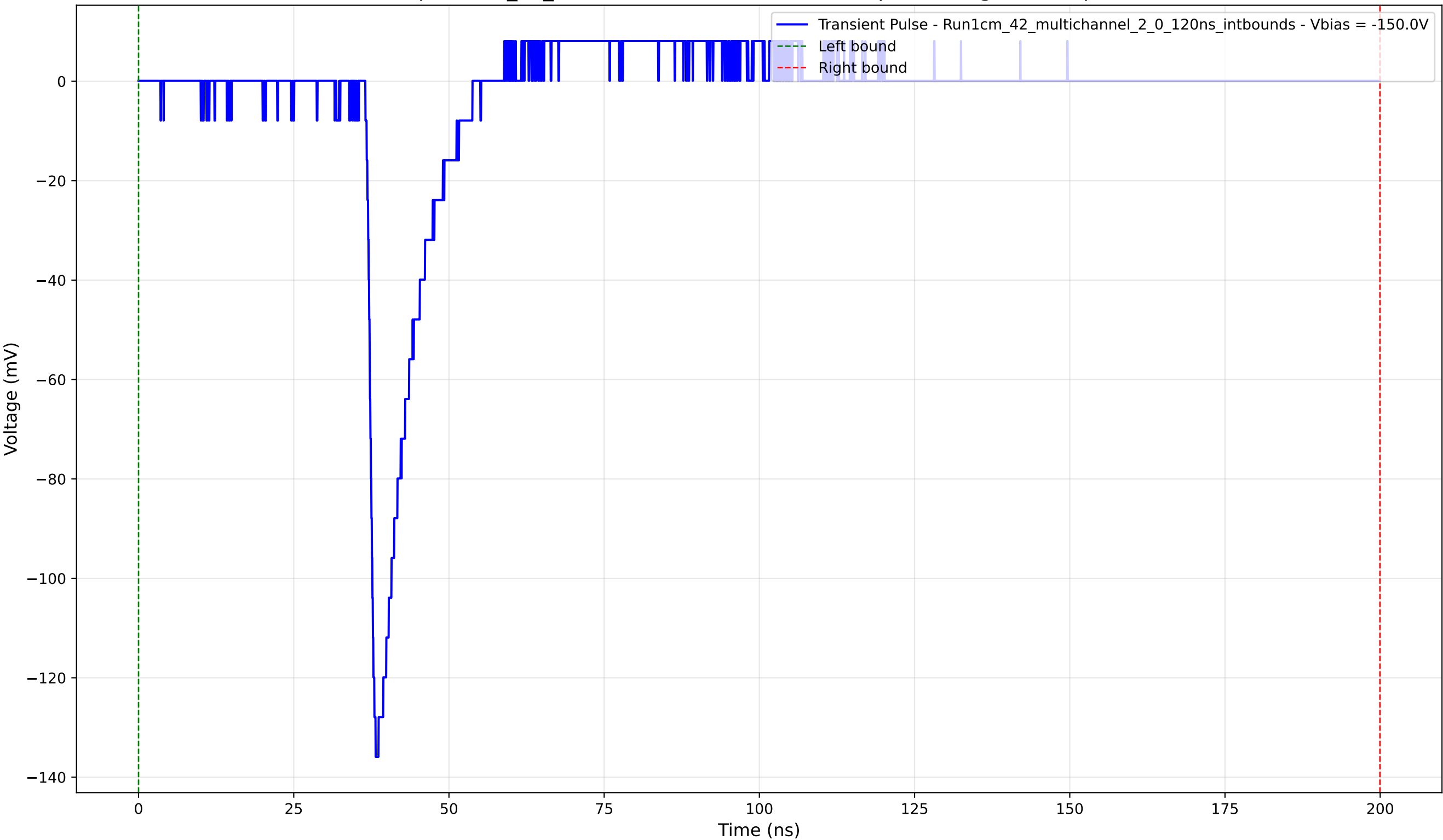
Transient Pulse - Sample: 1cm_42_multichannel - Position: 1120.0 \mu\text{m} - Charge: 11.62 pC - Rise Time: 1.25 ns
