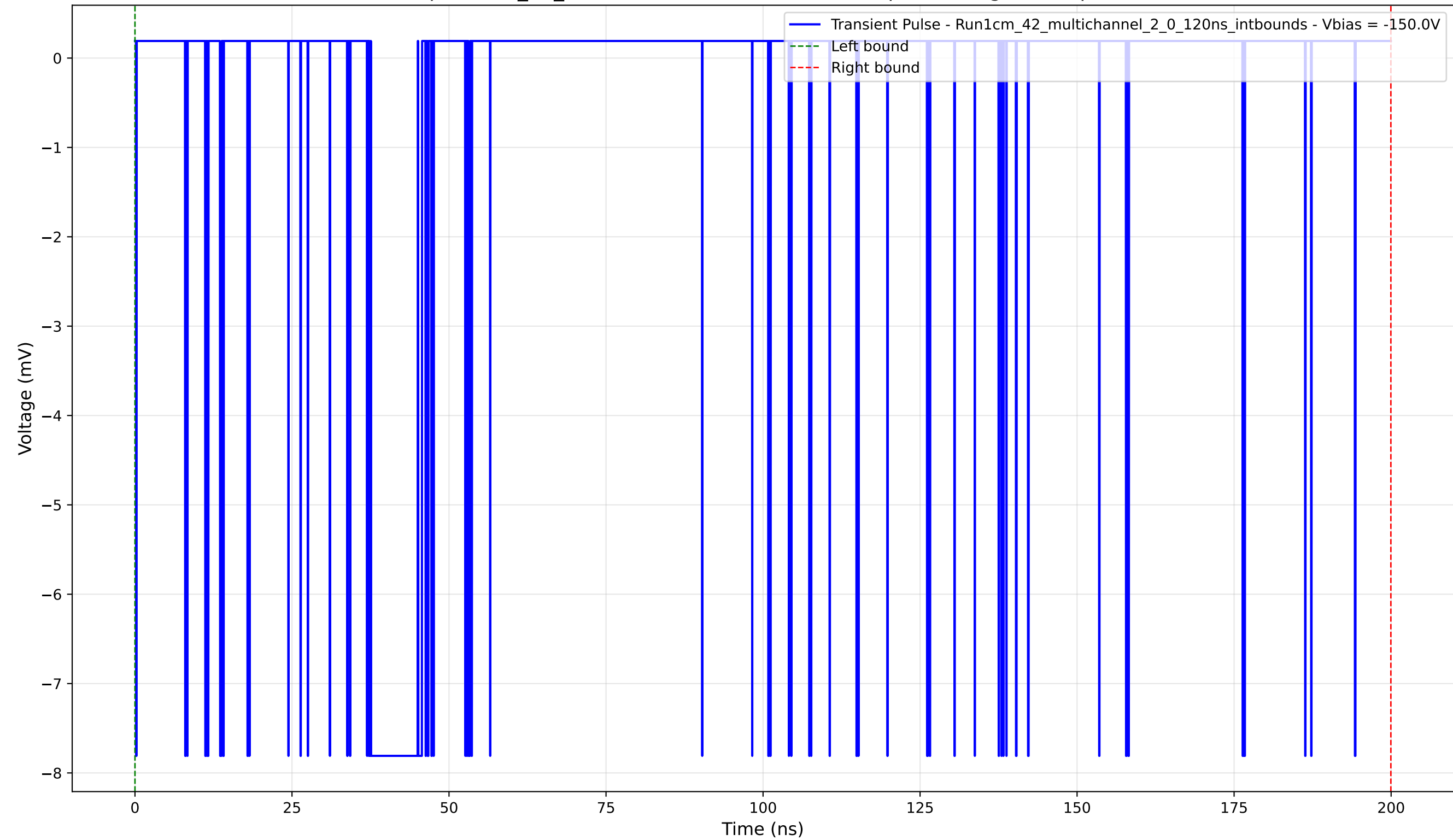
Transient Pulse - Sample: 1cm_42_multichannel - Position: 4410.0 \mu\text{m} - Charge: 1.35 pC - Rise Time: 0.04 ns
