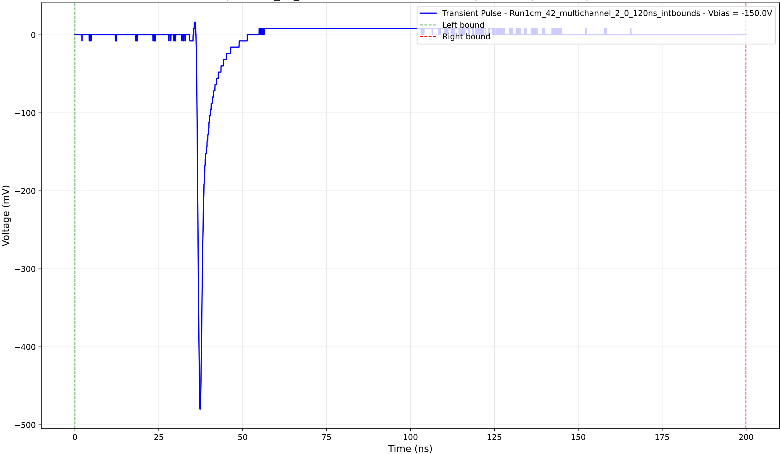
Transient Pulse - Sample: 1cm_42_multichannel - Position: 2090.0 \mu\text{m} - Charge: 14.88 pC - Rise Time: 0.74 ns
