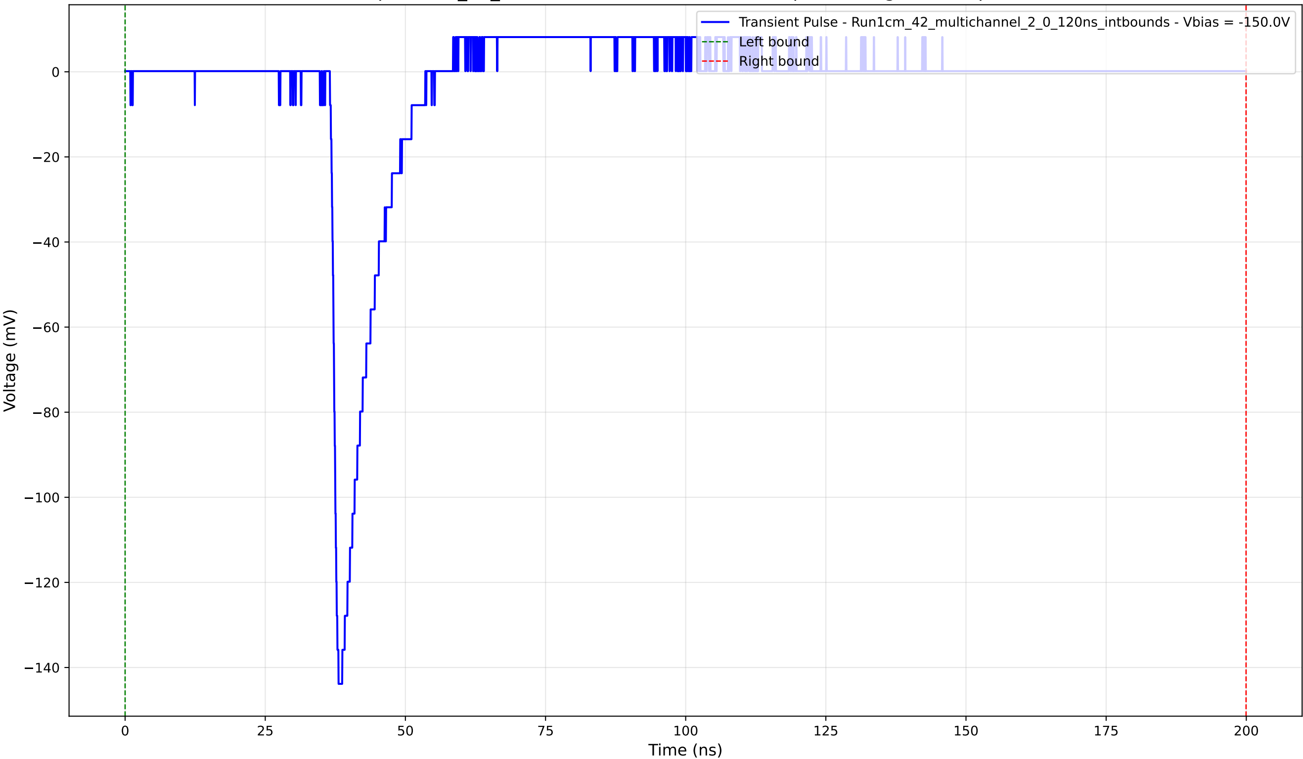
Transient Pulse - Sample: 1cm_42_multichannel - Position: 1180.0 \mu\text{m} - Charge: 10.82 pC - Rise Time: 1.17 ns
