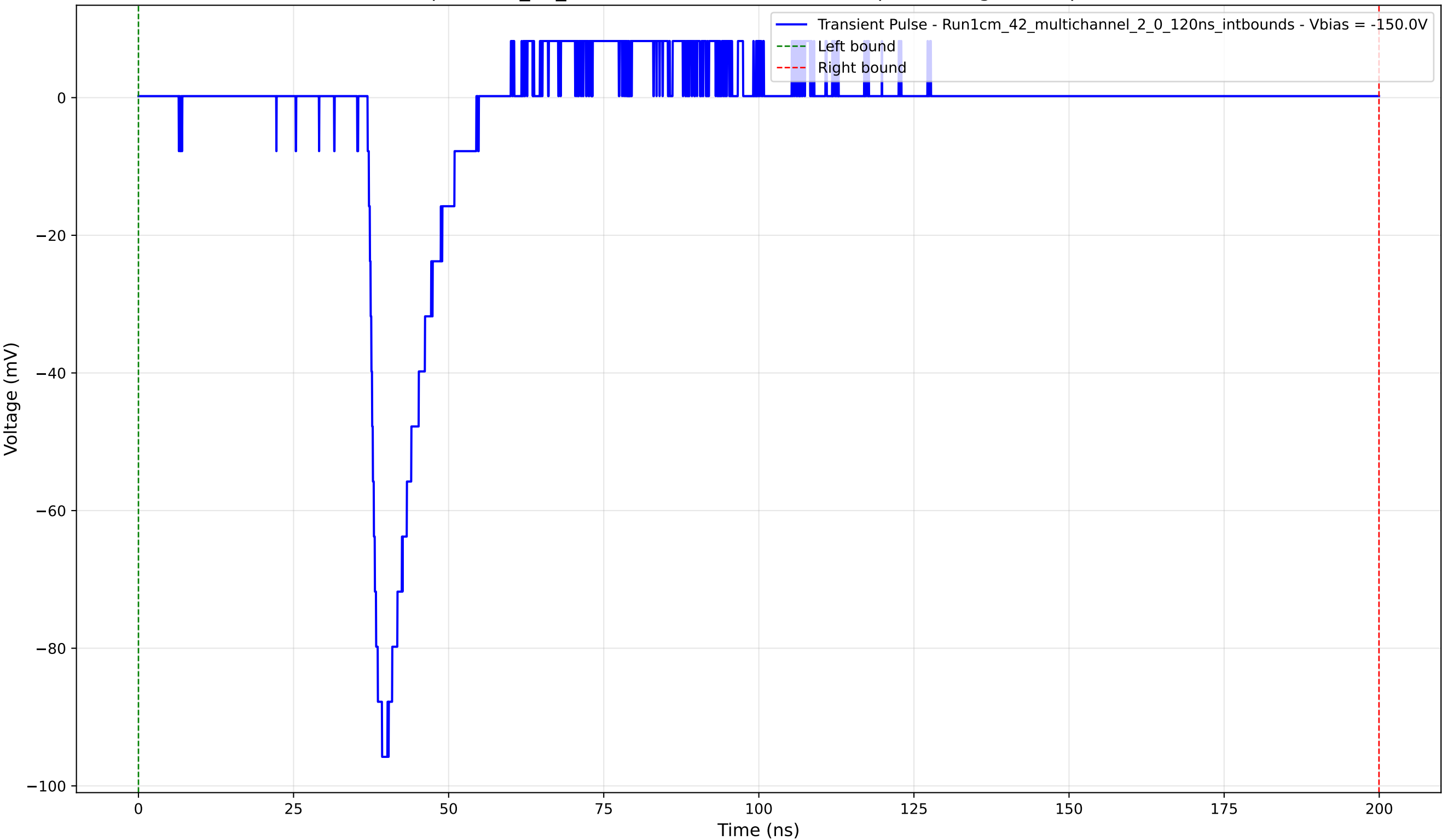
Transient Pulse - Sample: 1cm_42_multichannel - Position: 480.0 \mu\text{m} - Charge: 8.73 pC - Rise Time: 1.47 ns
