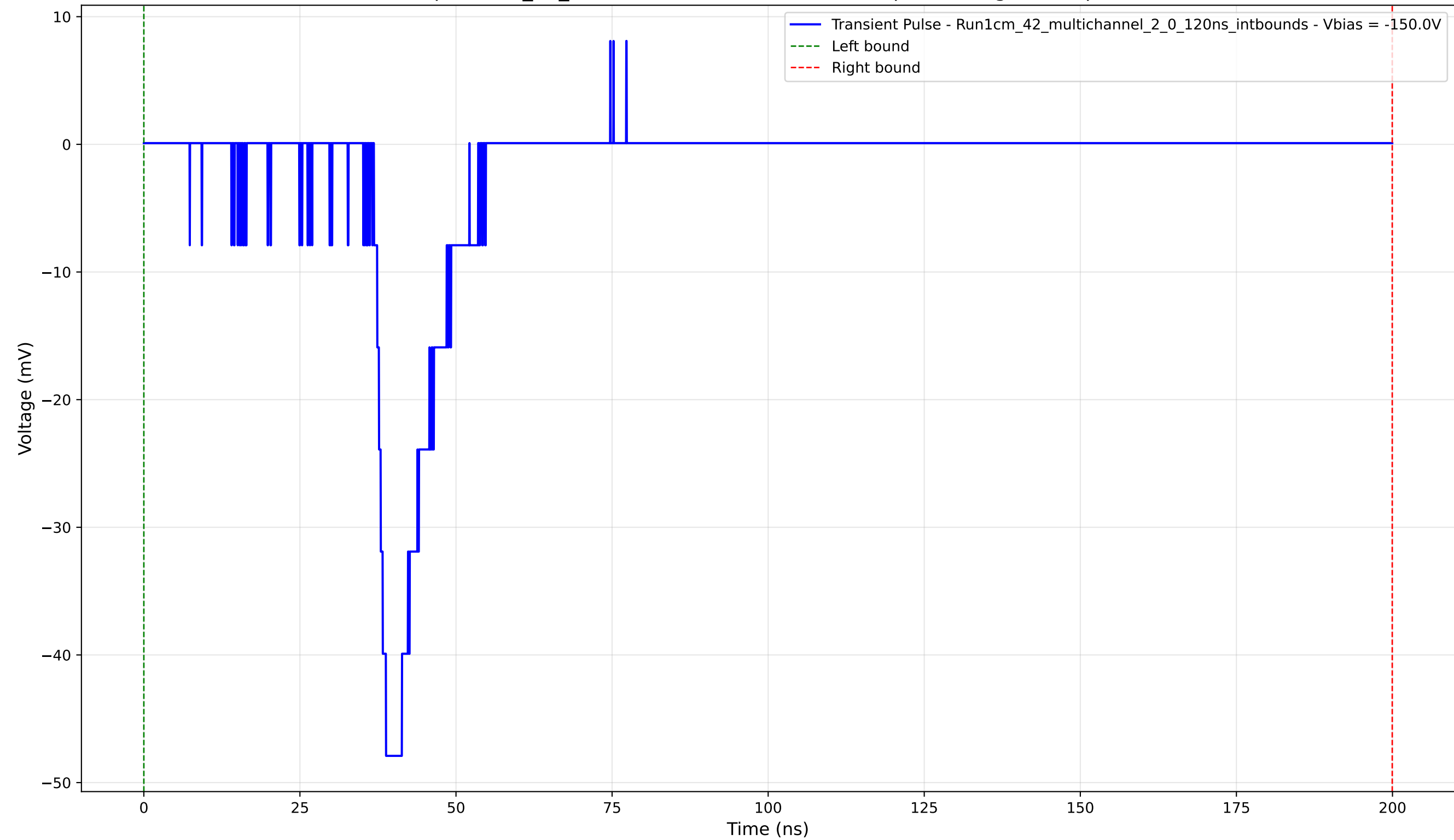
Transient Pulse - Sample: 1cm_42_multichannel - Position: 4330.0 \mu\text{m} - Charge: 7.98 pC - Rise Time: 1.94 ns
