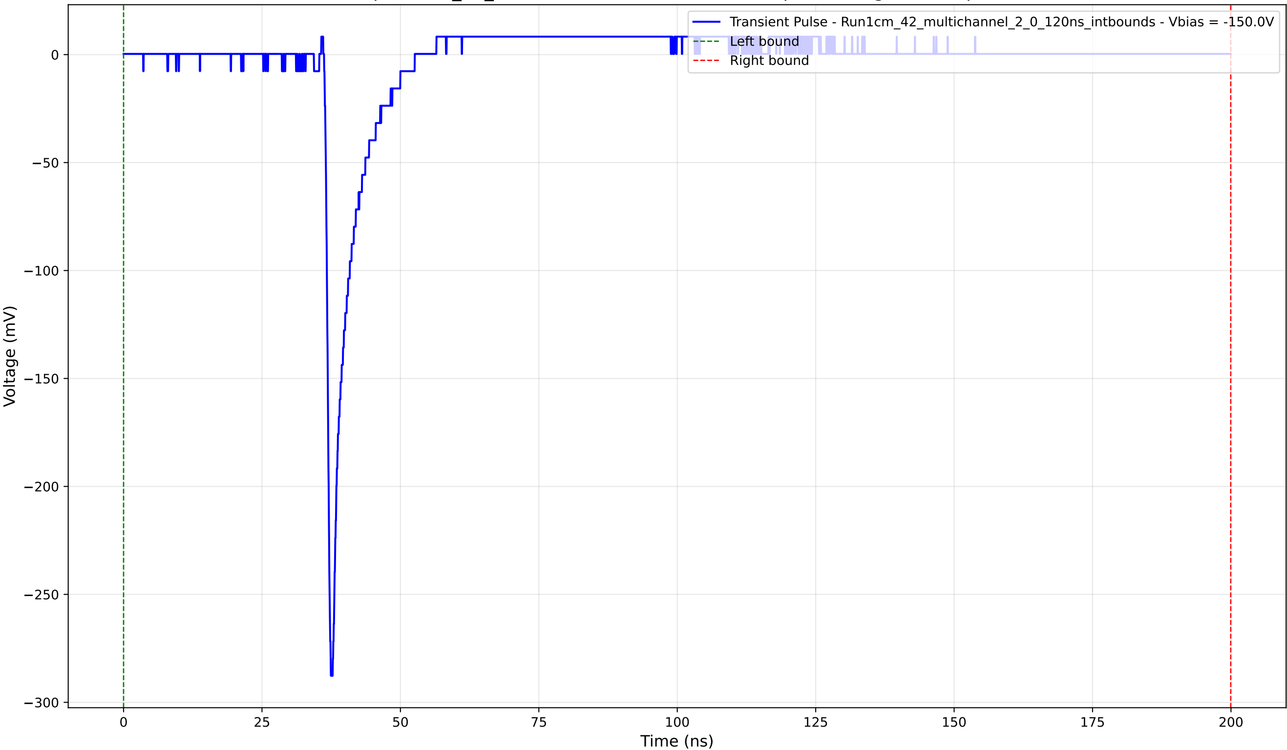
Transient Pulse - Sample: 1cm_42_multichannel - Position: 1750.0 \mu\text{m} - Charge: 12.63 pC - Rise Time: 0.83 ns
