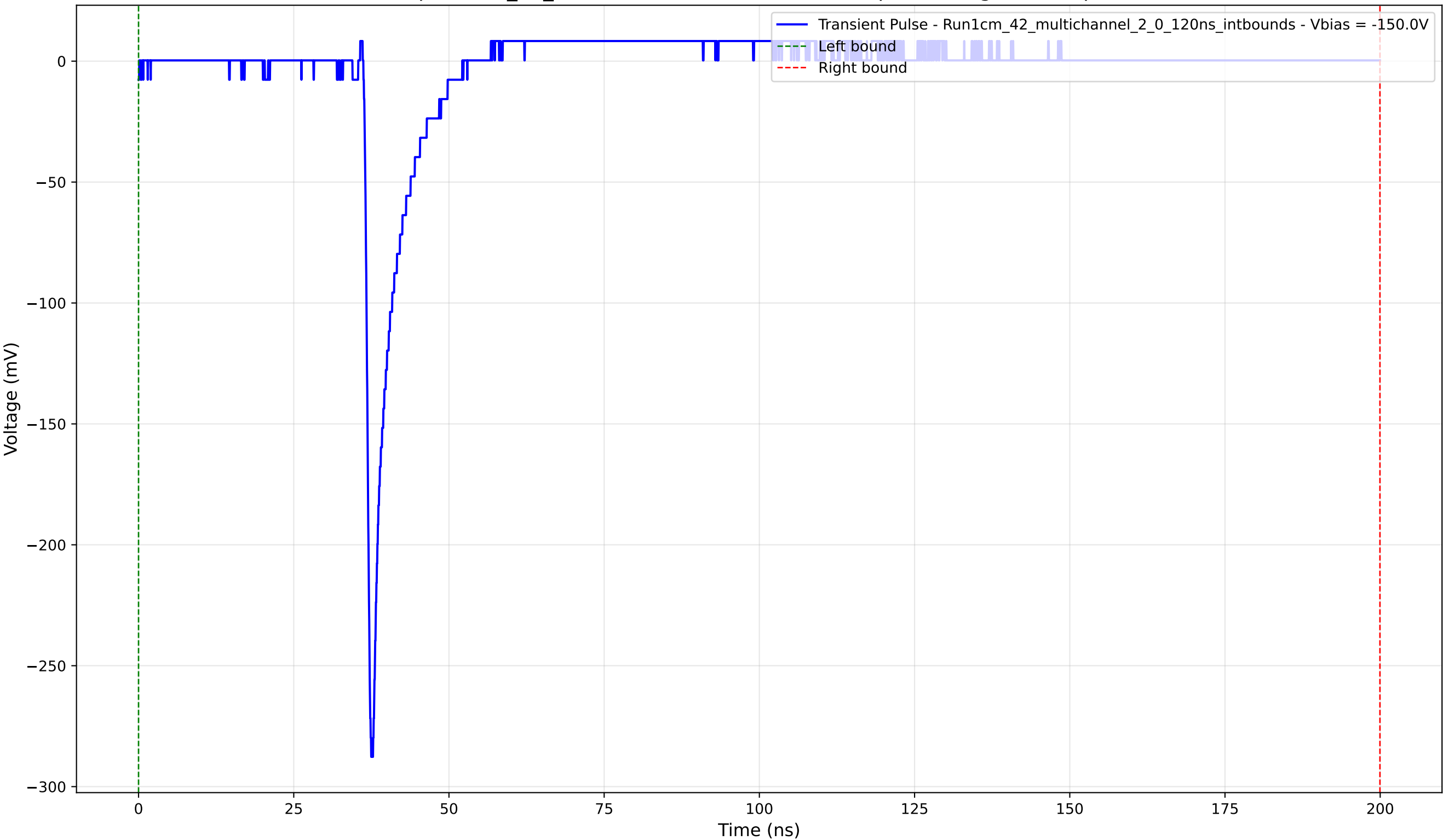
Transient Pulse - Sample: 1cm_42_multichannel - Position: 1745.0 \mu\text{m} - Charge: 12.84 pC - Rise Time: 0.83 ns
