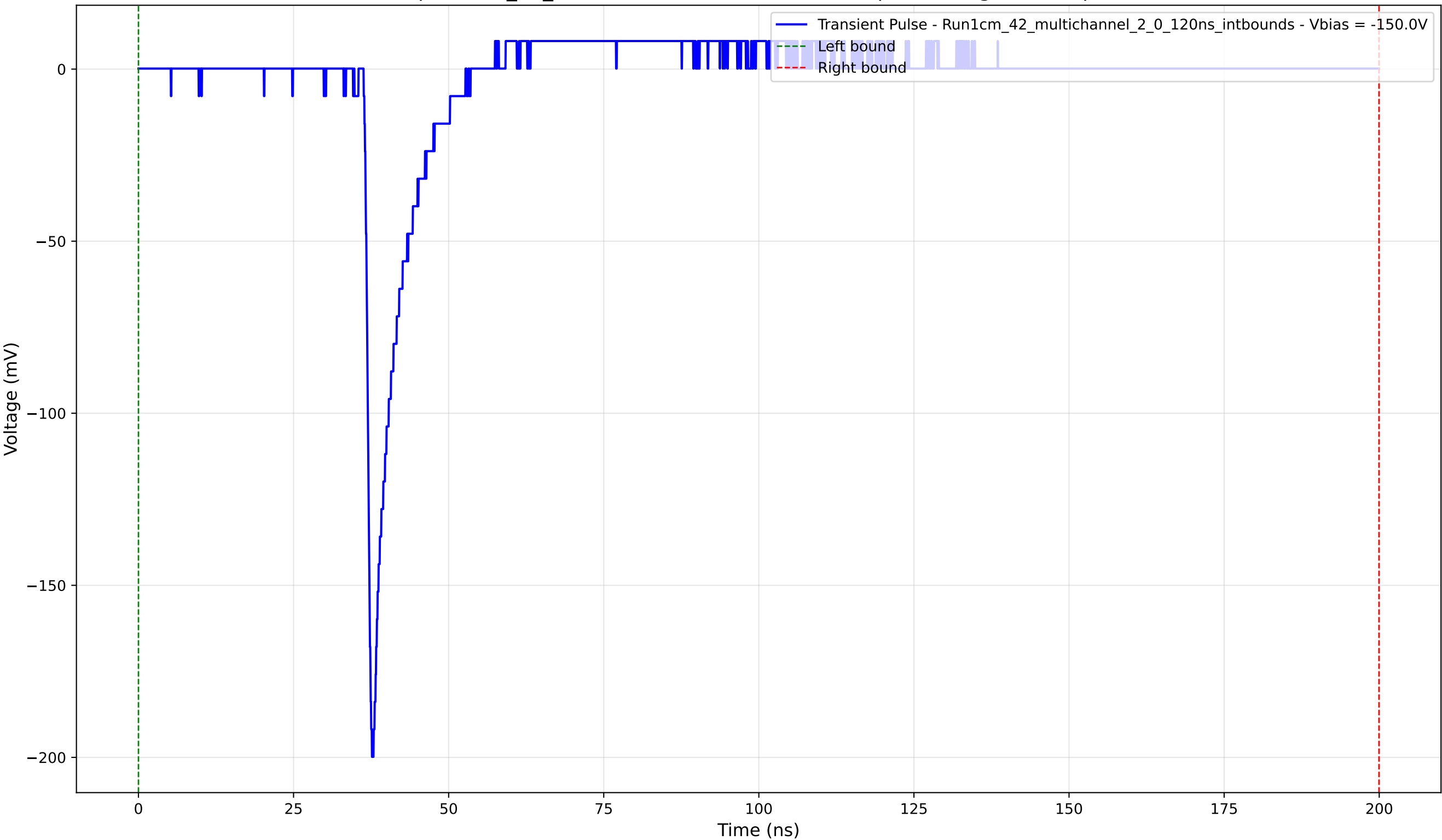
Transient Pulse - Sample: 1cm_42_multichannel - Position: 3155.0 \mu\text{m} - Charge: 10.44 pC - Rise Time: 0.94 ns
