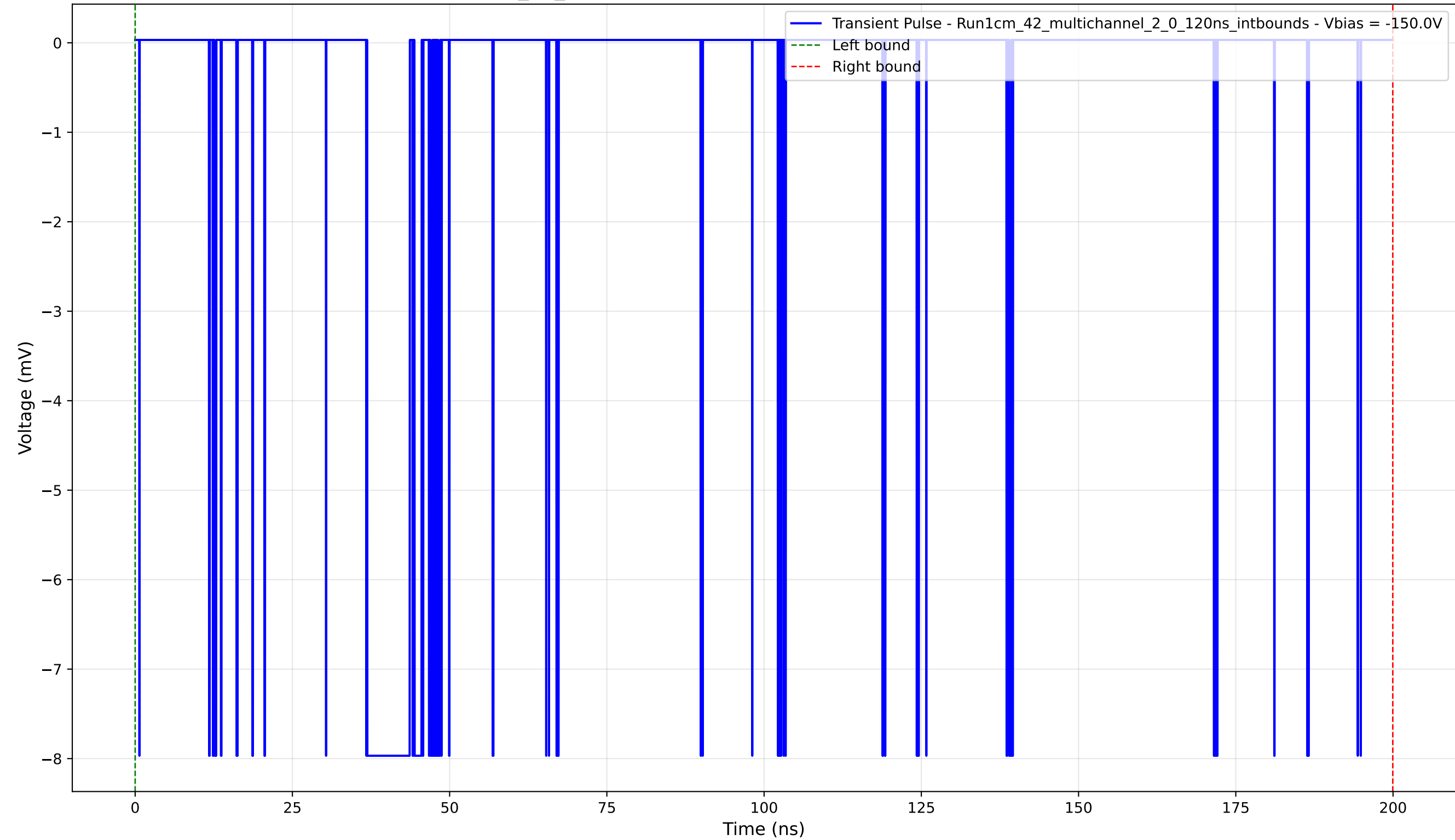
Transient Pulse - Sample: 1cm_42_multichannel - Position: 1355.0 \mu\text{m} - Charge: 1.98 pC - Rise Time: 0.04 ns
