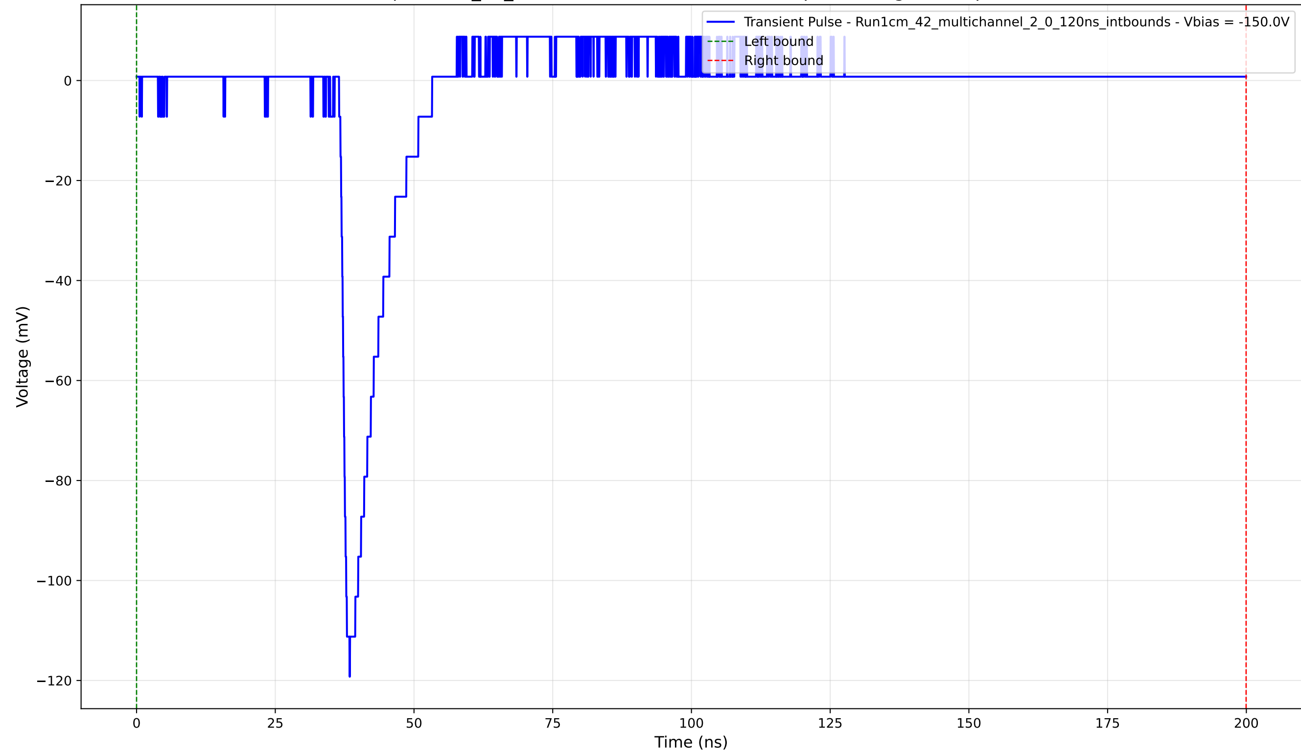
Transient Pulse - Sample: 1cm_42_multichannel - Position: 3590.0 \mu\text{m} - Charge: 7.19 pC - Rise Time: 1.18 ns
