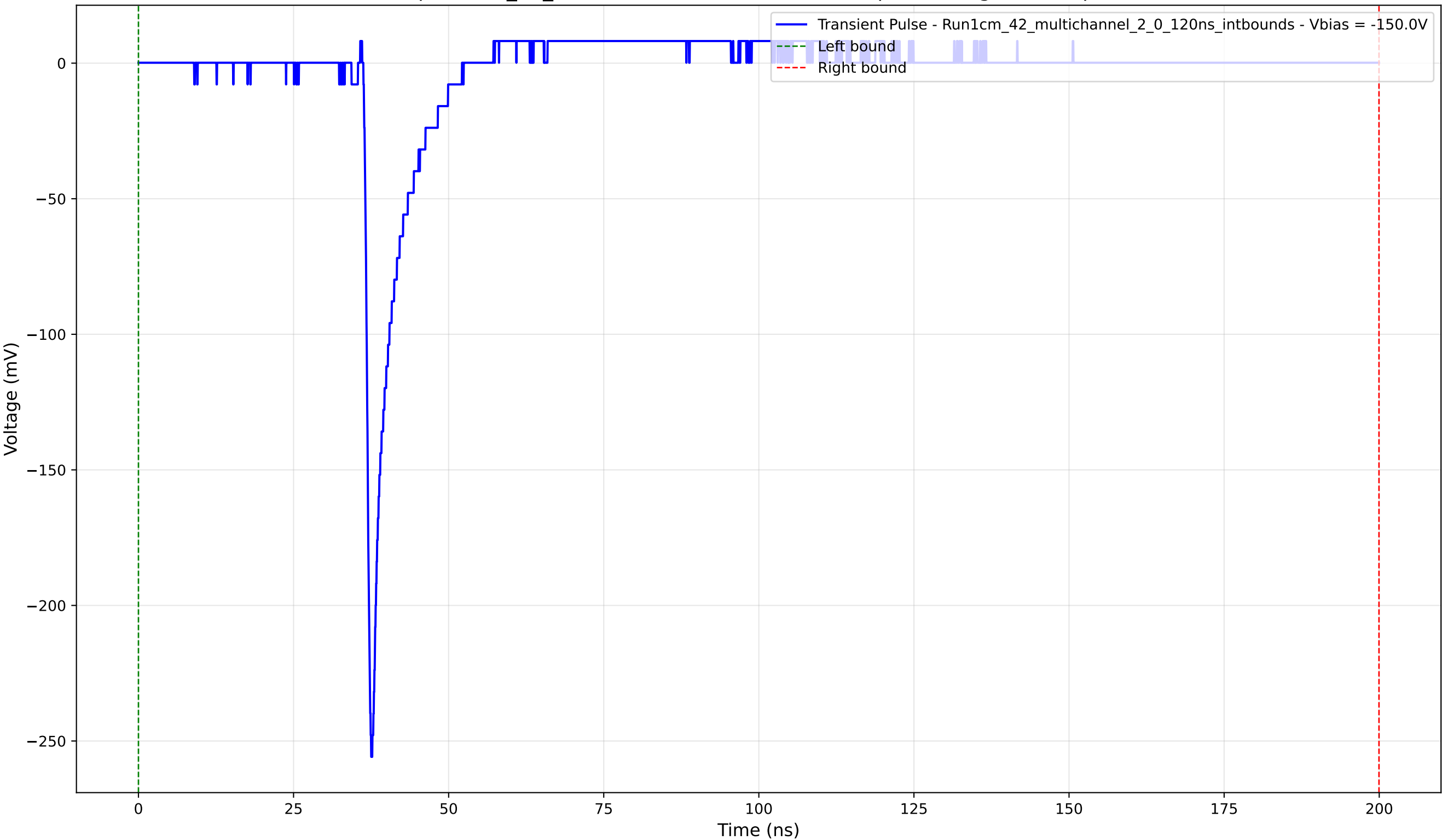
Transient Pulse - Sample: 1cm_42_multichannel - Position: 3020.0 \mu\text{m} - Charge: 12.27 pC - Rise Time: 0.86 ns
