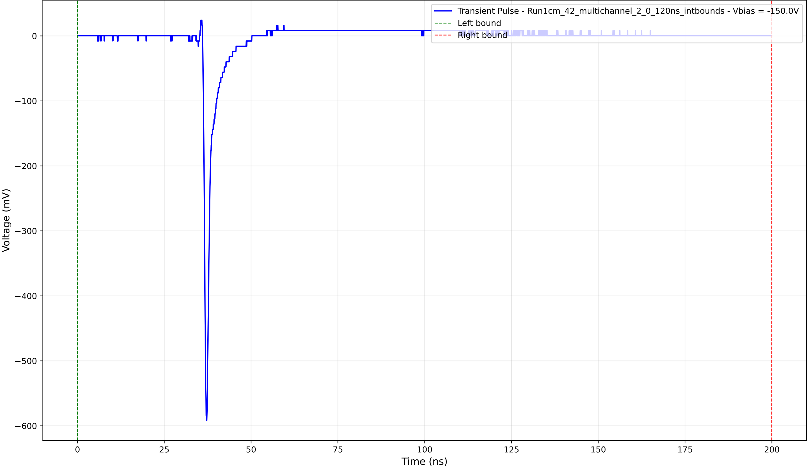
Transient Pulse - Sample: 1cm_42_multichannel - Position: 2500.0 \mu\text{m} - Charge: 16.03 pC - Rise Time: 0.74 ns
