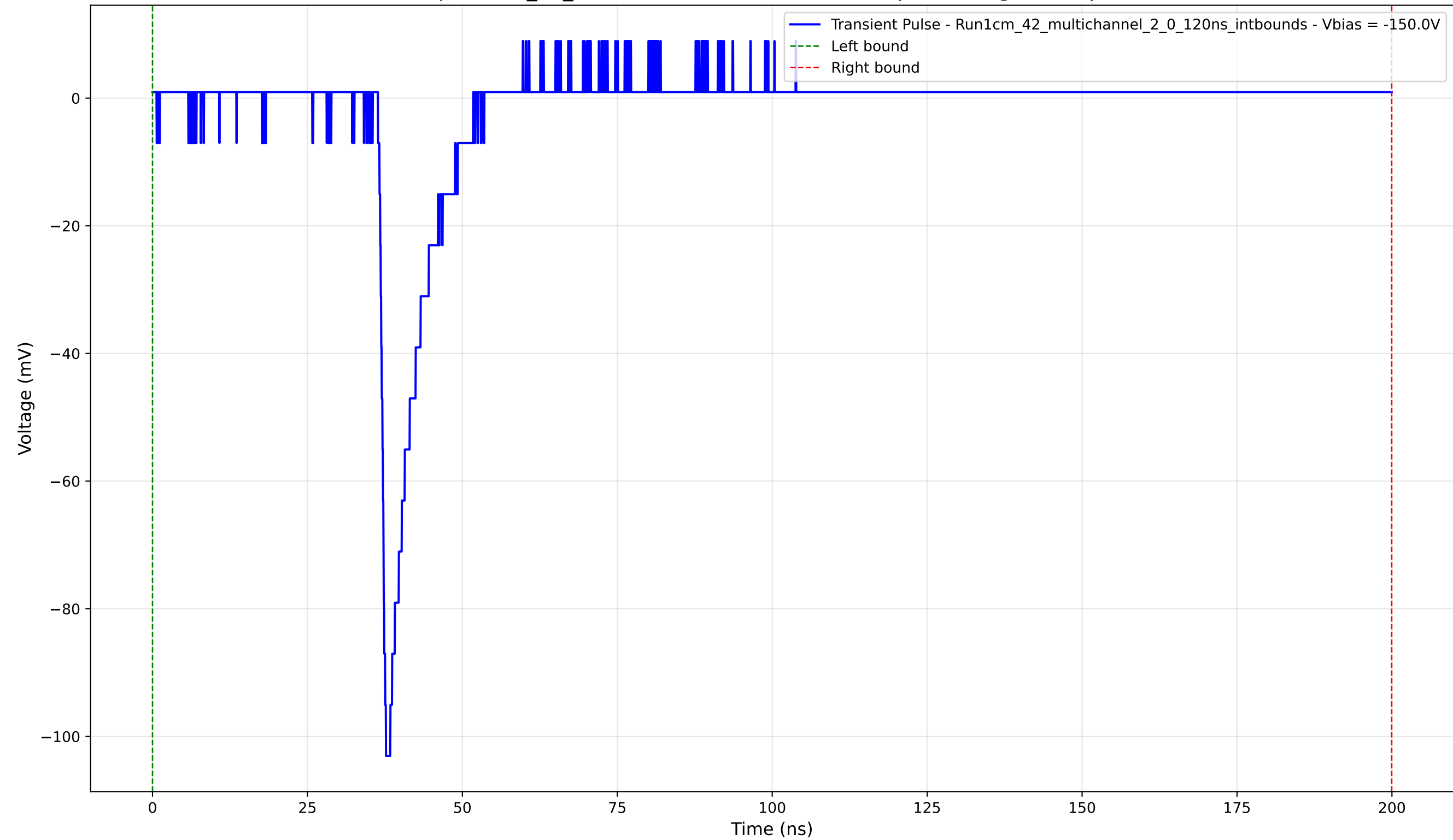
Transient Pulse - Sample: 1cm_42_multichannel - Position: 1410.0 \mu\text{m} - Charge: 7.57 pC - Rise Time: 0.94 ns
