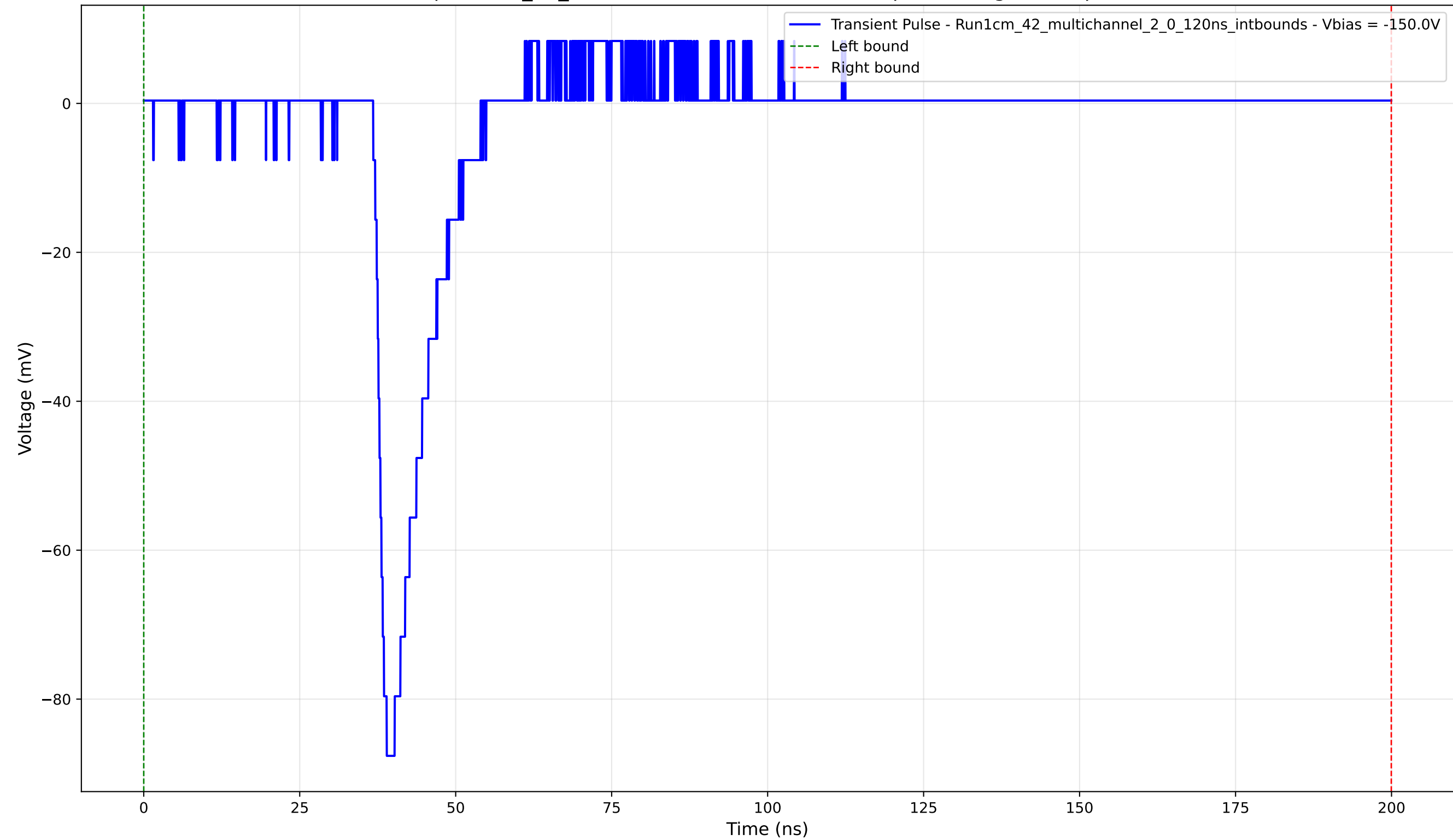
Transient Pulse - Sample: 1cm_42_multichannel - Position: 4140.0 \mu\text{m} - Charge: 9.30 pC - Rise Time: 1.43 ns
