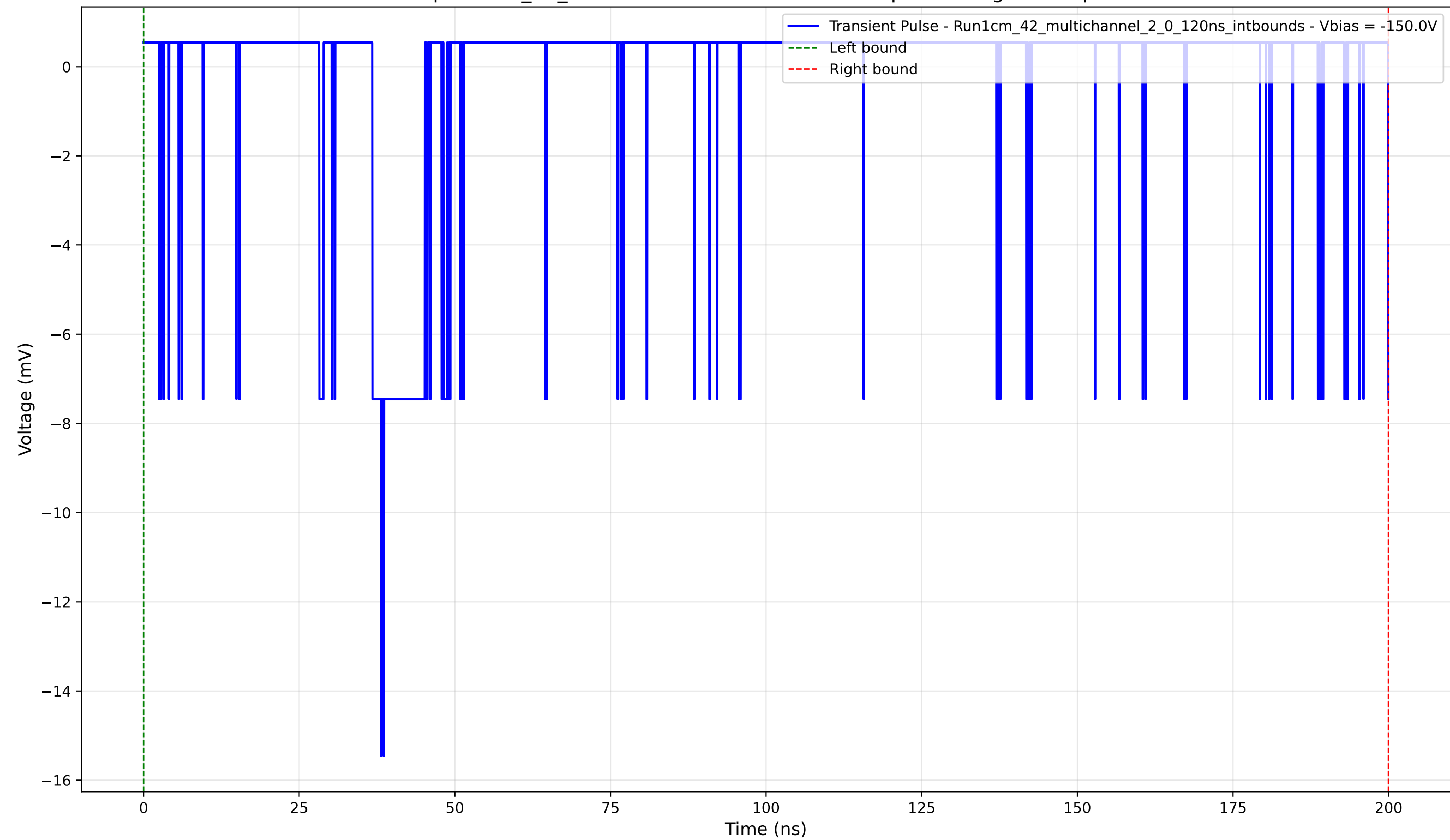
Transient Pulse - Sample: 1cm_42_multichannel - Position: 3370.0 \mu\text{m} - Charge: 0.35 pC - Rise Time: 1.43 ns
