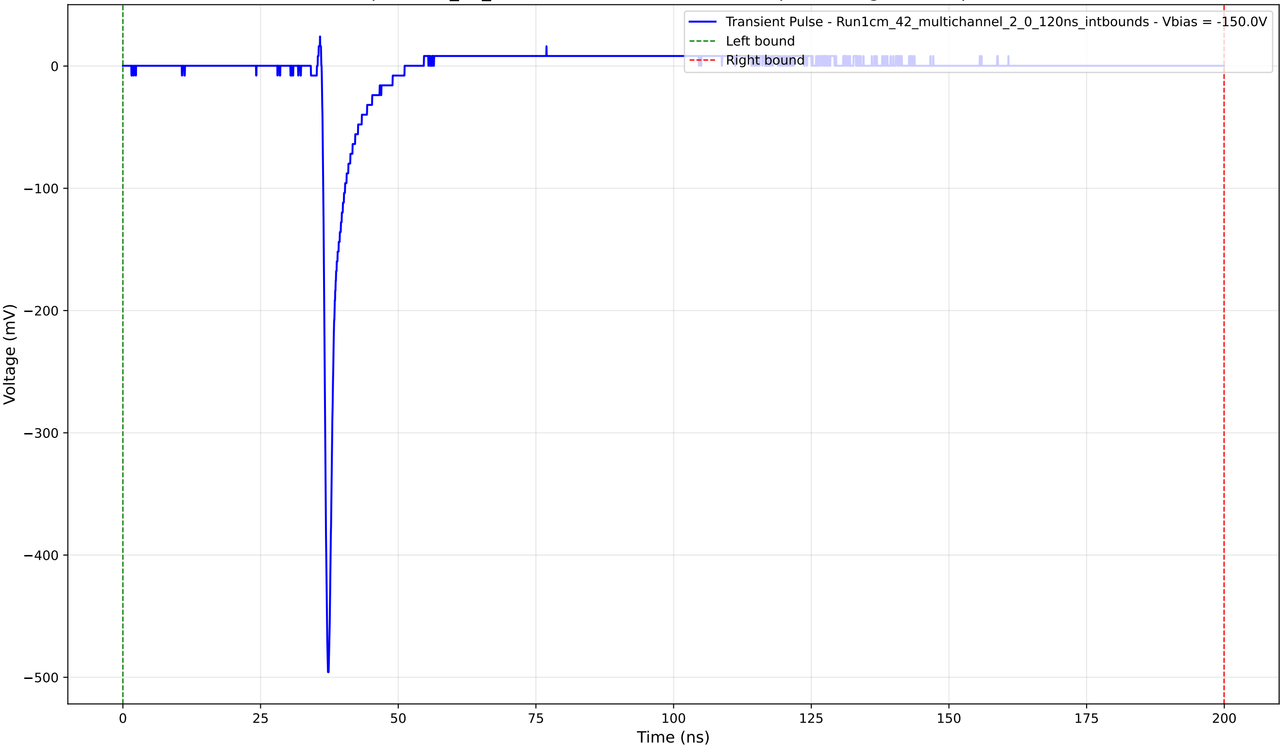
Transient Pulse - Sample: 1cm_42_multichannel - Position: 2105.0 \mu\text{m} - Charge: 14.83 pC - Rise Time: 0.77 ns
