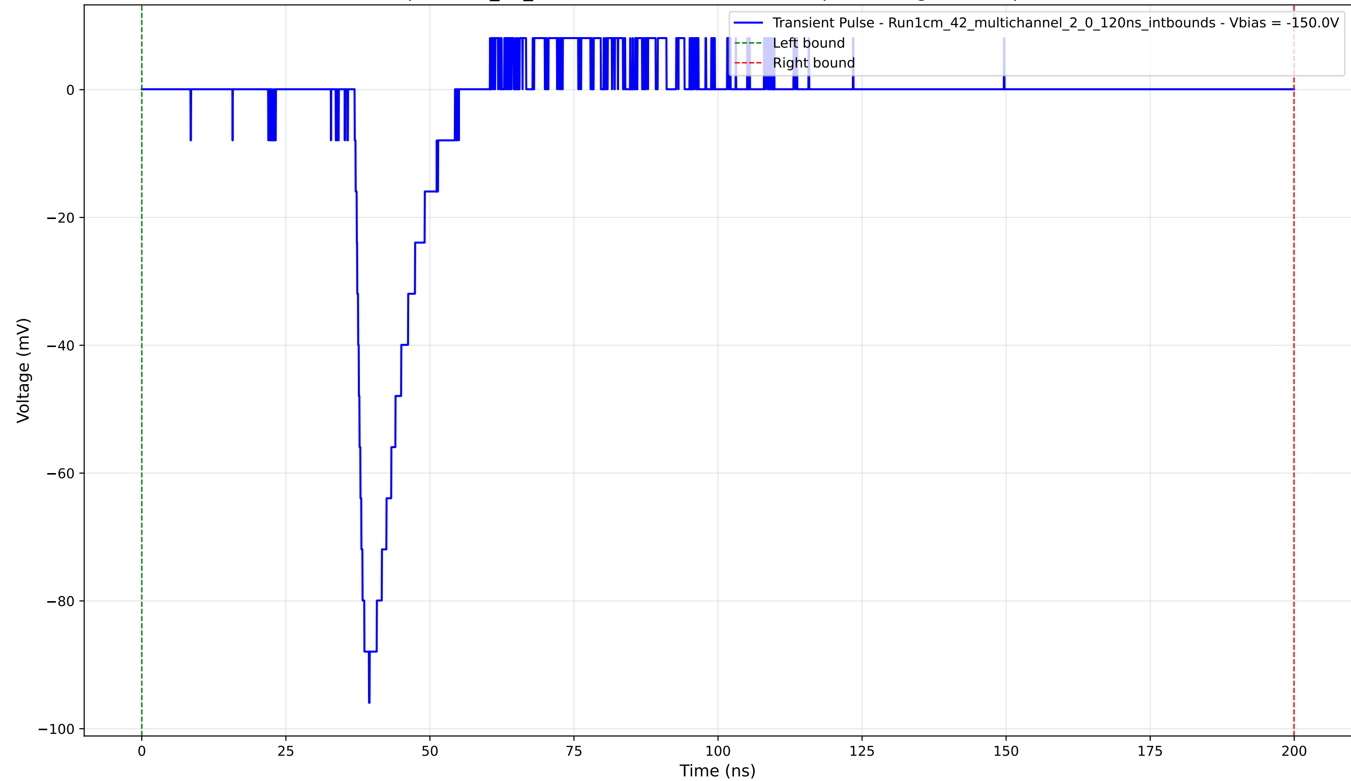
Transient Pulse - Sample: 1cm_42_multichannel - Position: 475.0 \mu\text{m} - Charge: 10.35 pC - Rise Time: 1.55 ns
