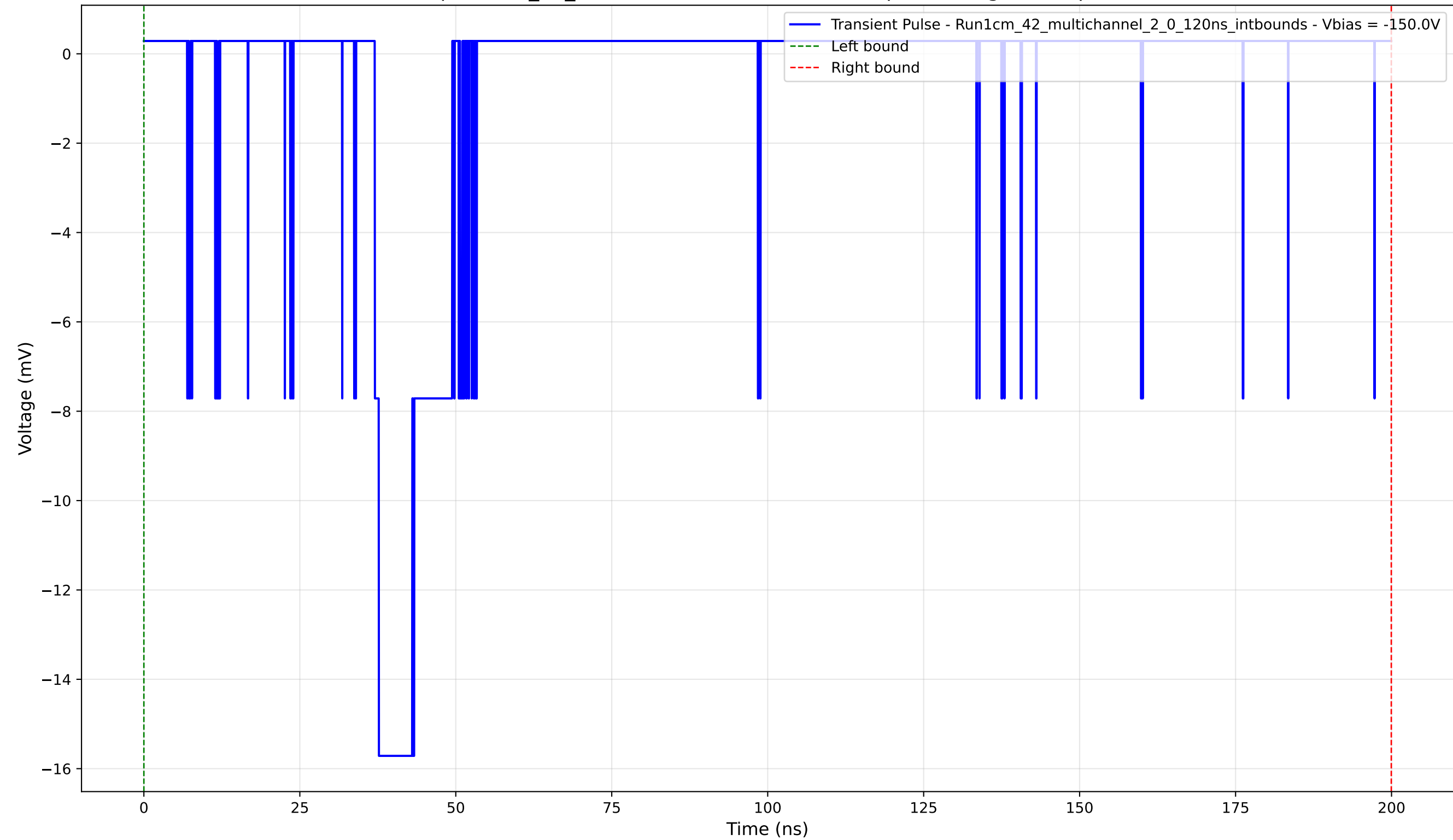
Transient Pulse - Sample: 1cm_42_multichannel - Position: 820.0 \mu\text{m} - Charge: 2.35 pC - Rise Time: 0.67 ns
