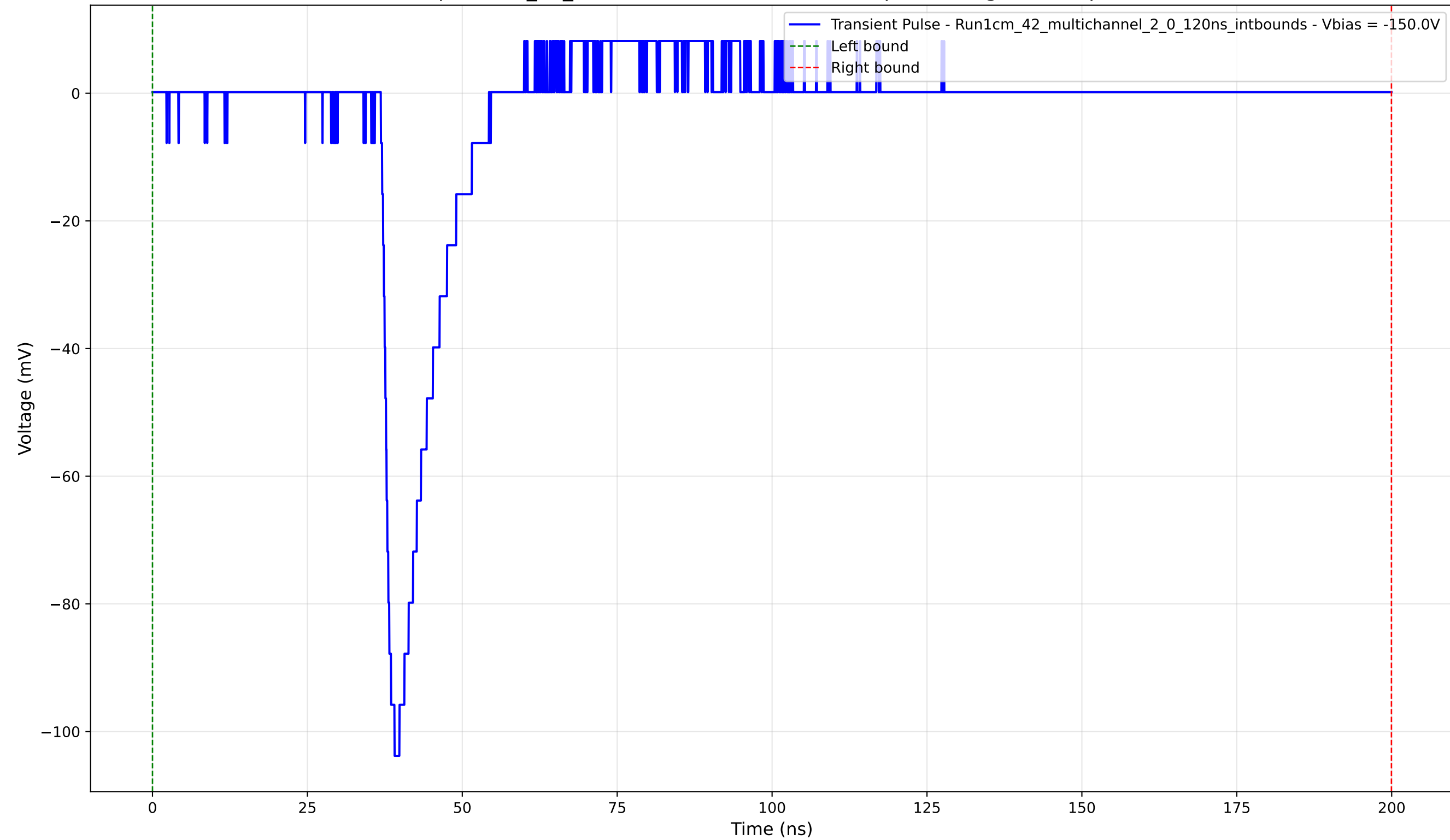
Transient Pulse - Sample: 1cm_42_multichannel - Position: 650.0 \mu\text{m} - Charge: 10.43 pC - Rise Time: 1.47 ns
