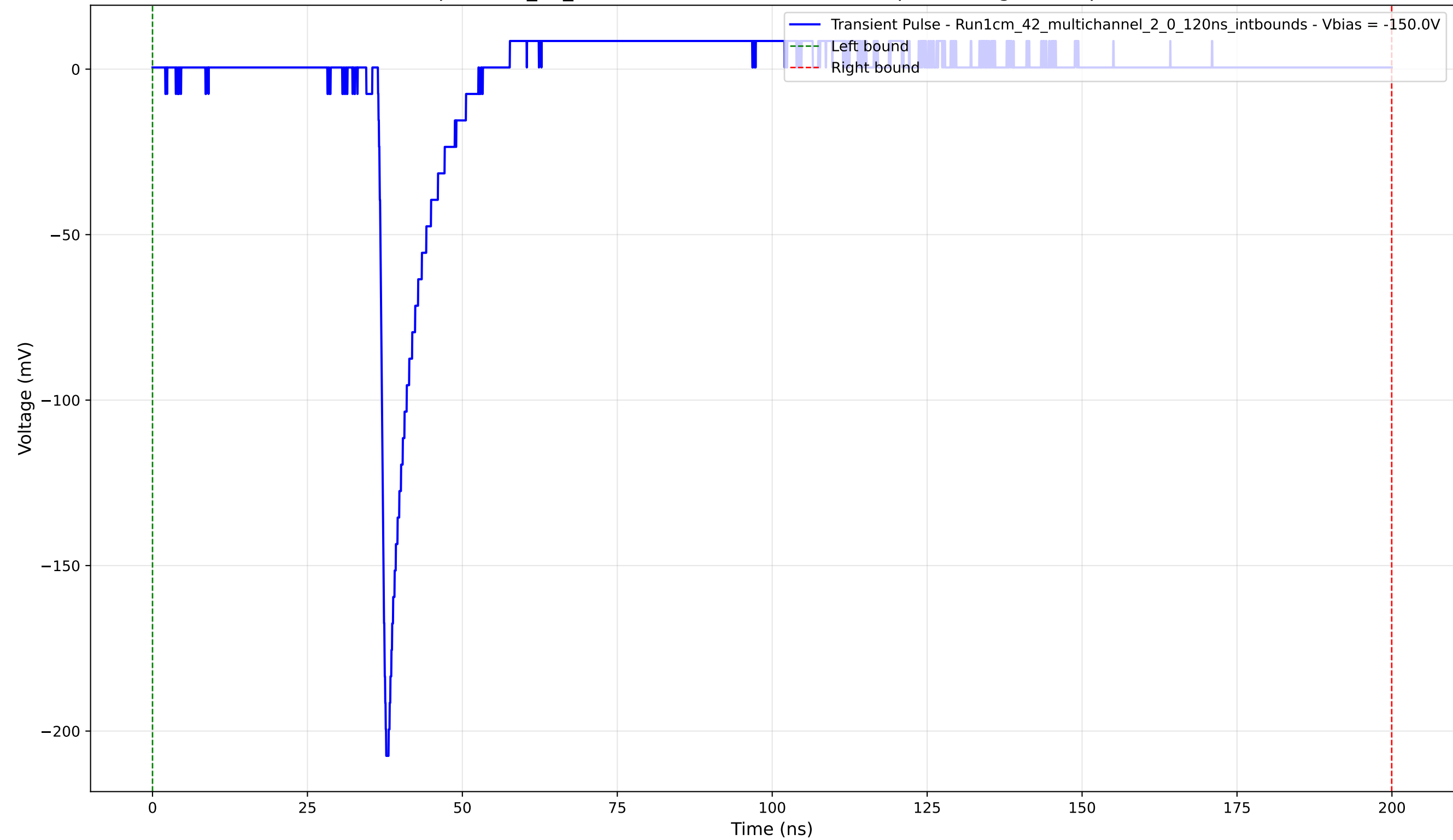
Transient Pulse - Sample: 1cm_42_multichannel - Position: 1490.0 \mu\text{m} - Charge: 9.74 pC - Rise Time: 1.01 ns
