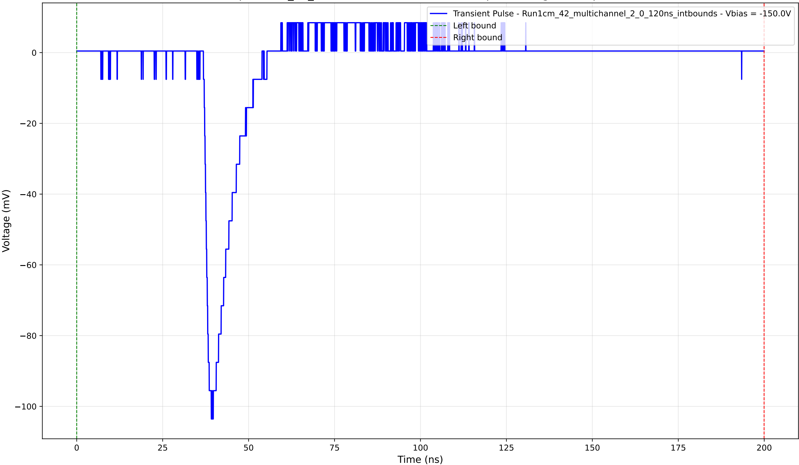
Transient Pulse - Sample: 1cm_42_multichannel - Position: 600.0 \mu\text{m} - Charge: 9.31 pC - Rise Time: 1.47 ns
