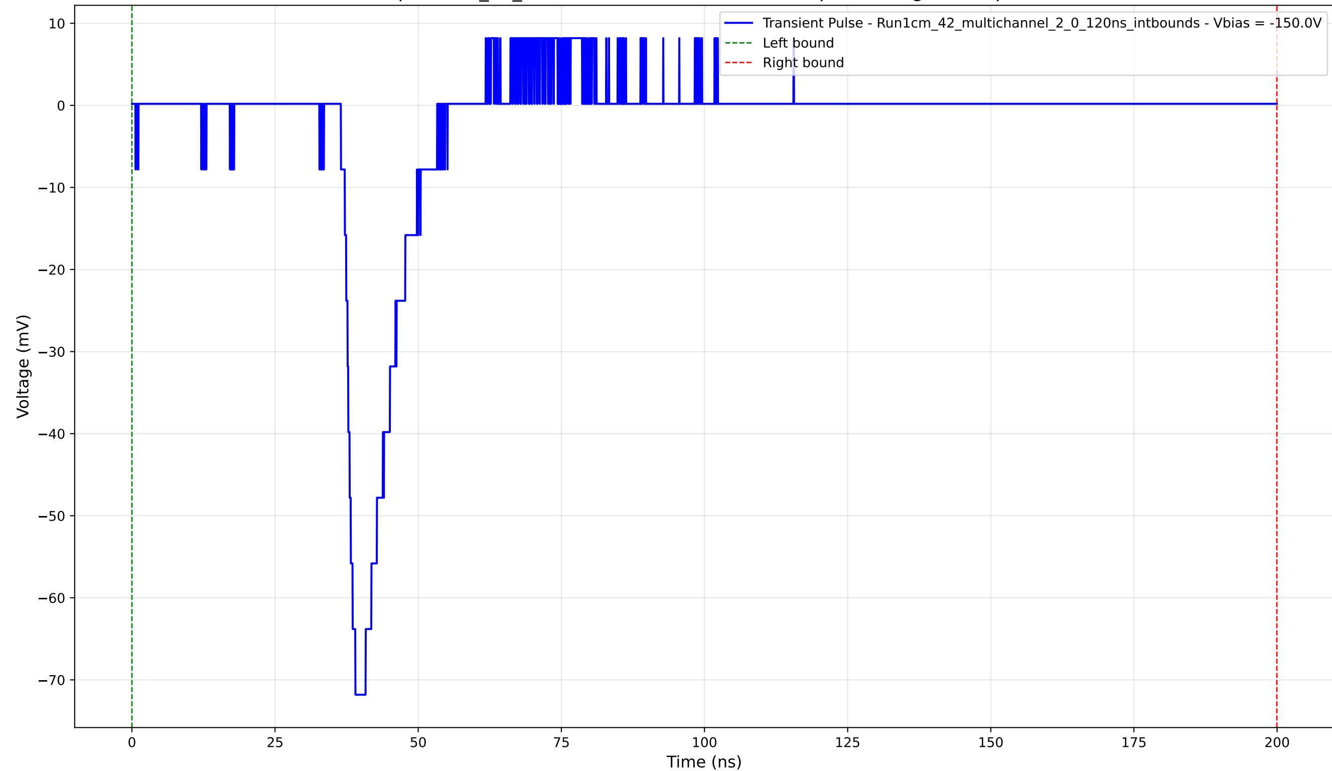
Transient Pulse - Sample: 1cm_42_multichannel - Position: 4565.0 \mu\text{m} - Charge: 8.77 pC - Rise Time: 2.52 ns
