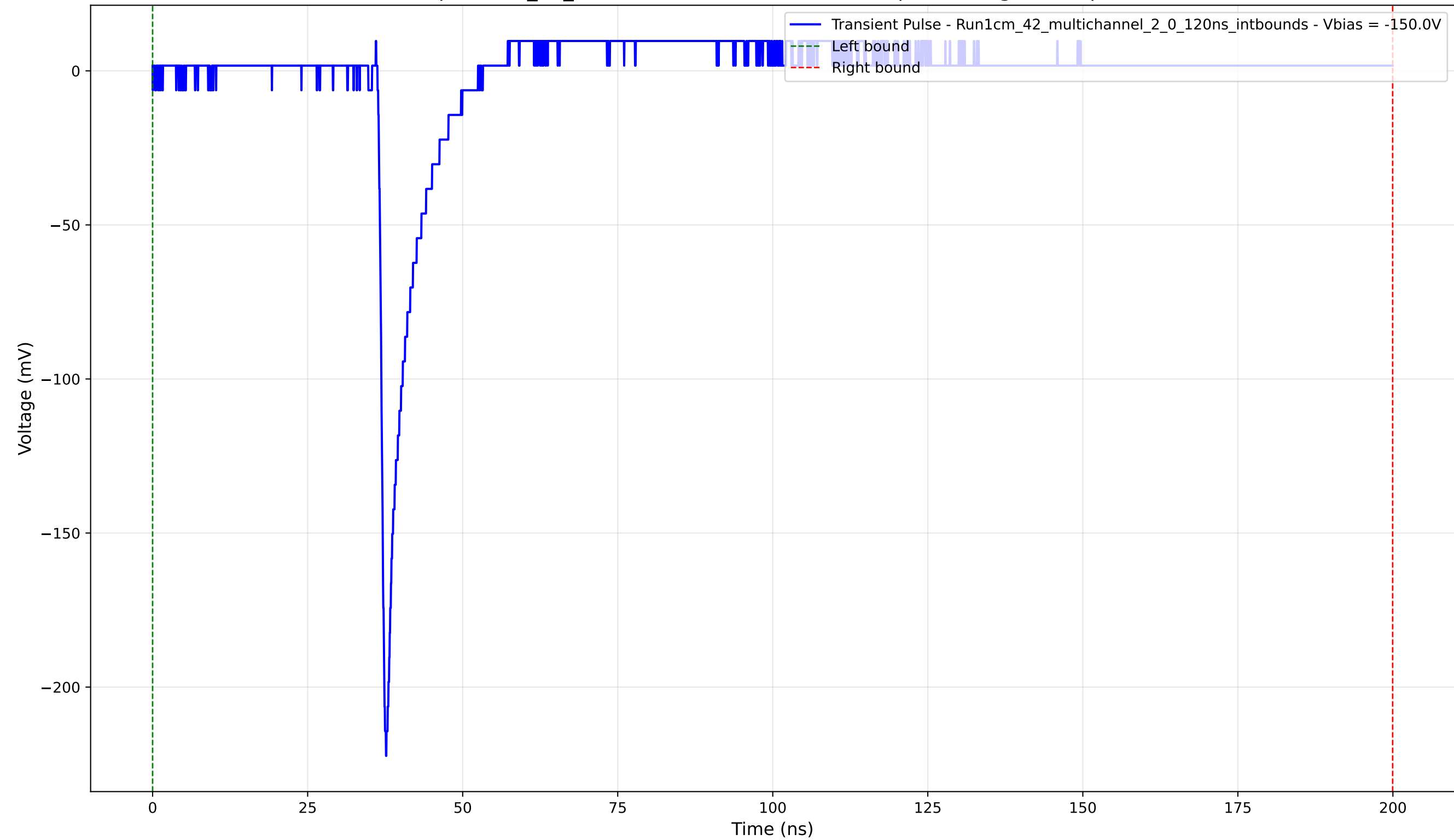
Transient Pulse - Sample: 1cm_42_multichannel - Position: 3085.0 \mu\text{m} - Charge: 5.13 pC - Rise Time: 0.92 ns
