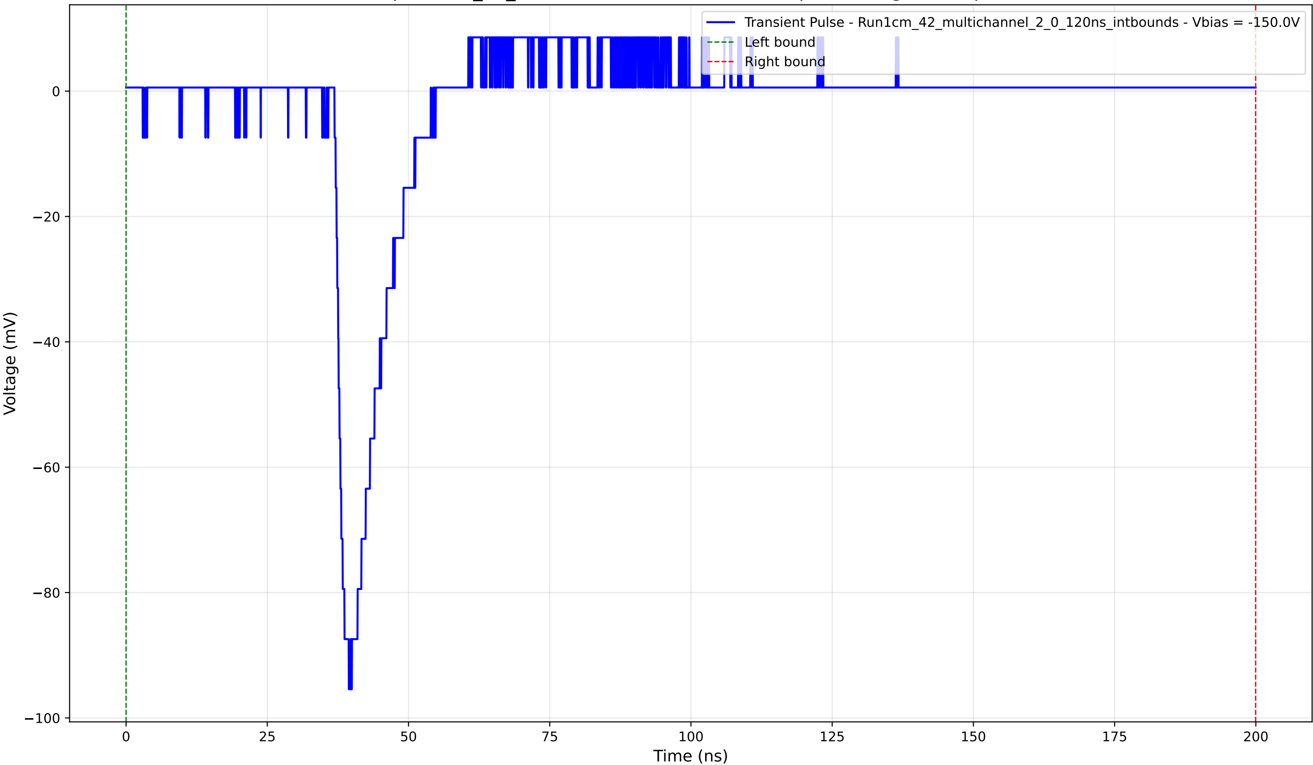
Transient Pulse - Sample: 1cm_42_multichannel - Position: 460.0 \mu\text{m} - Charge: 8.01 pC - Rise Time: 1.59 ns
