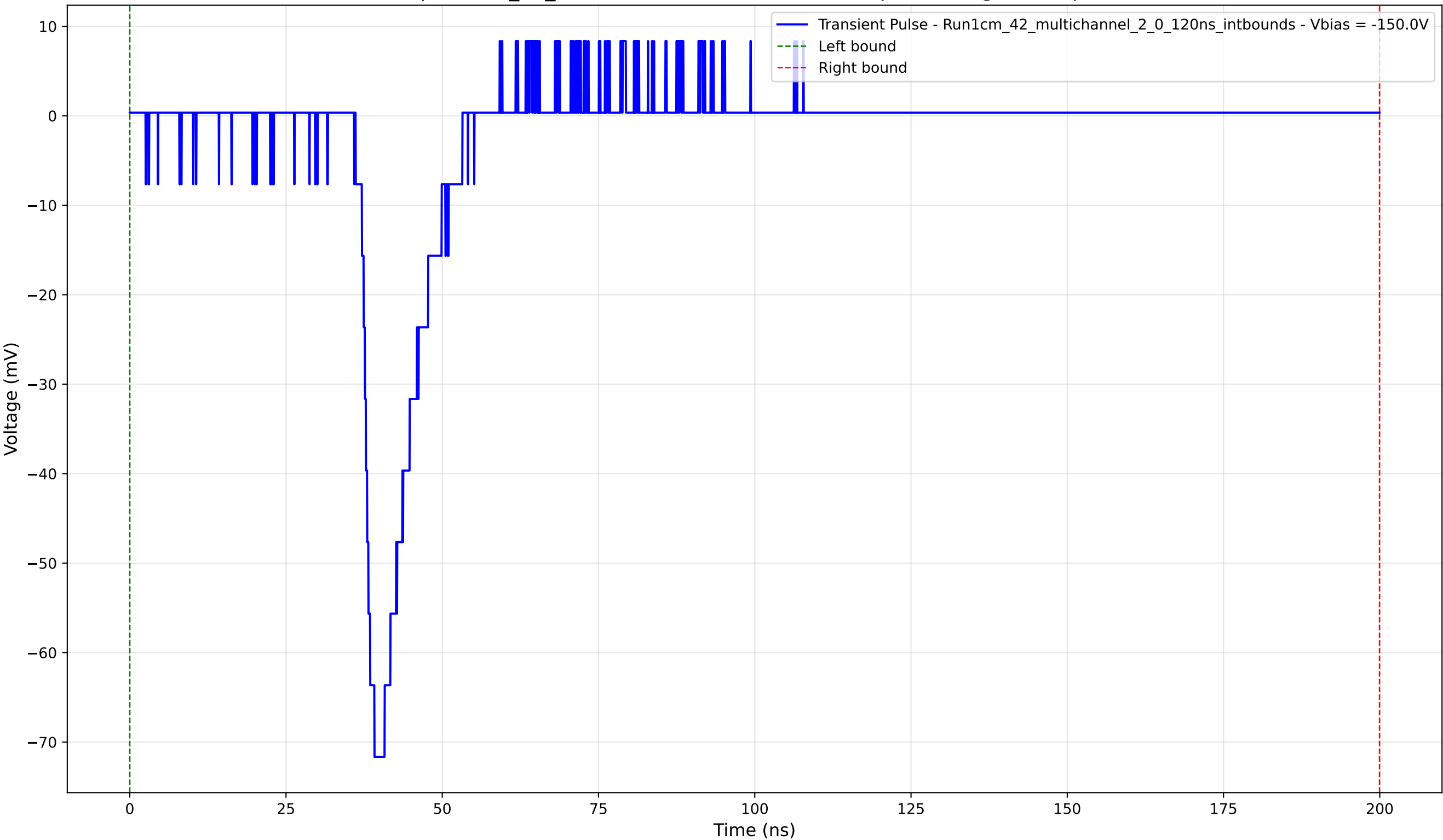
Transient Pulse - Sample: 1cm_42_multichannel - Position: 4585.0 \mu\text{m} - Charge: 8.97 pC - Rise Time: 3.00 ns
