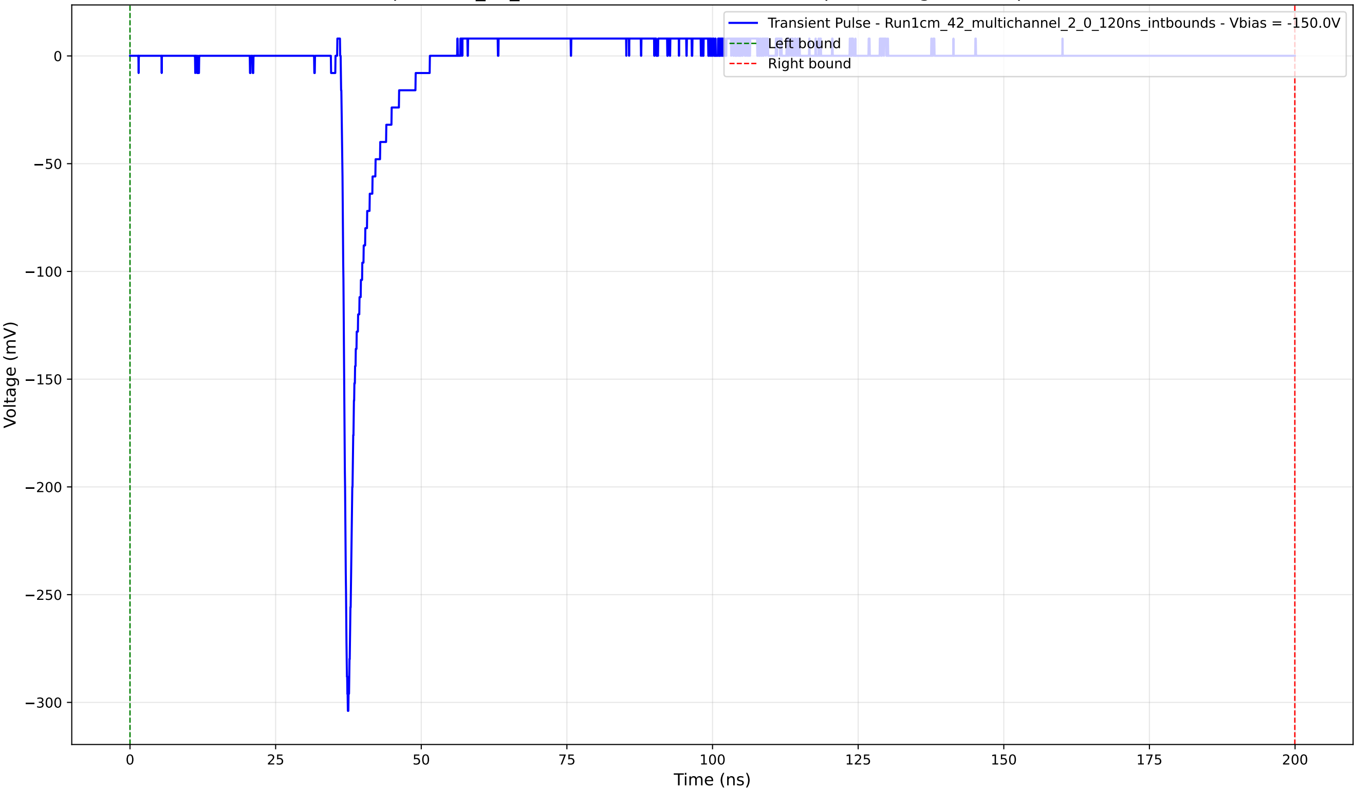
Transient Pulse - Sample: 1cm_42_multichannel - Position: 2805.0 \mu\text{m} - Charge: 11.41 pC - Rise Time: 0.82 ns
