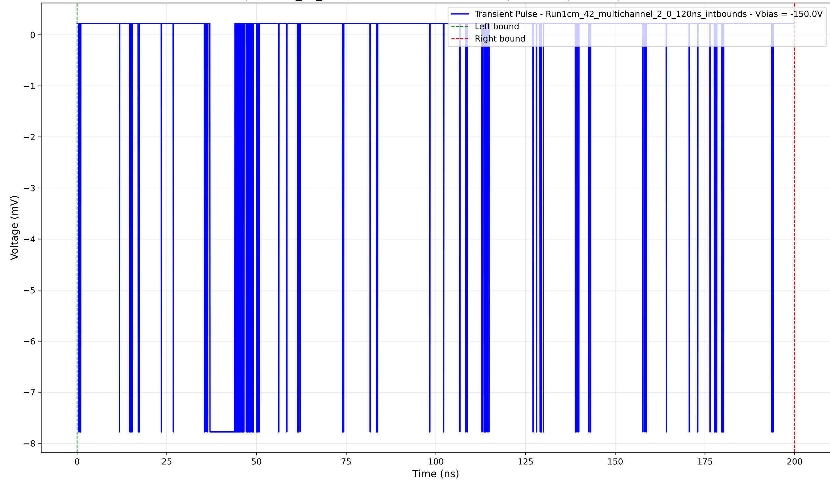
Transient Pulse - Sample: 1cm_42_multichannel - Position: 3375.0 \mu\text{m} - Charge: 1.52 pC - Rise Time: 0.04 ns
