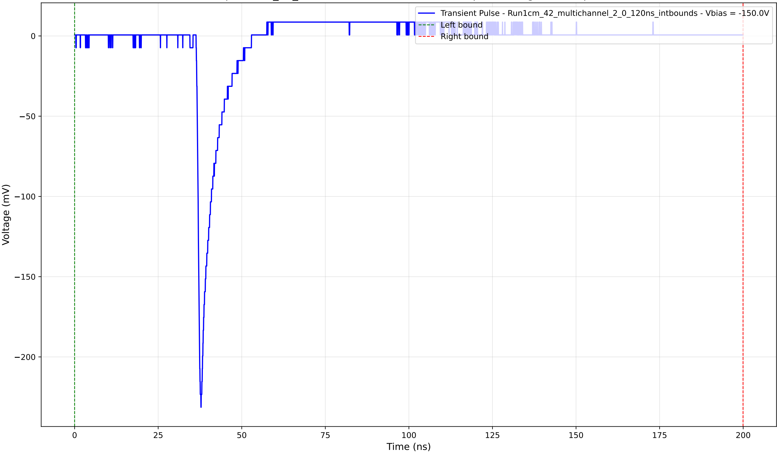
Transient Pulse - Sample: 1cm_42_multichannel - Position: 1570.0 \mu\text{m} - Charge: 10.63 pC - Rise Time: 1.00 ns
