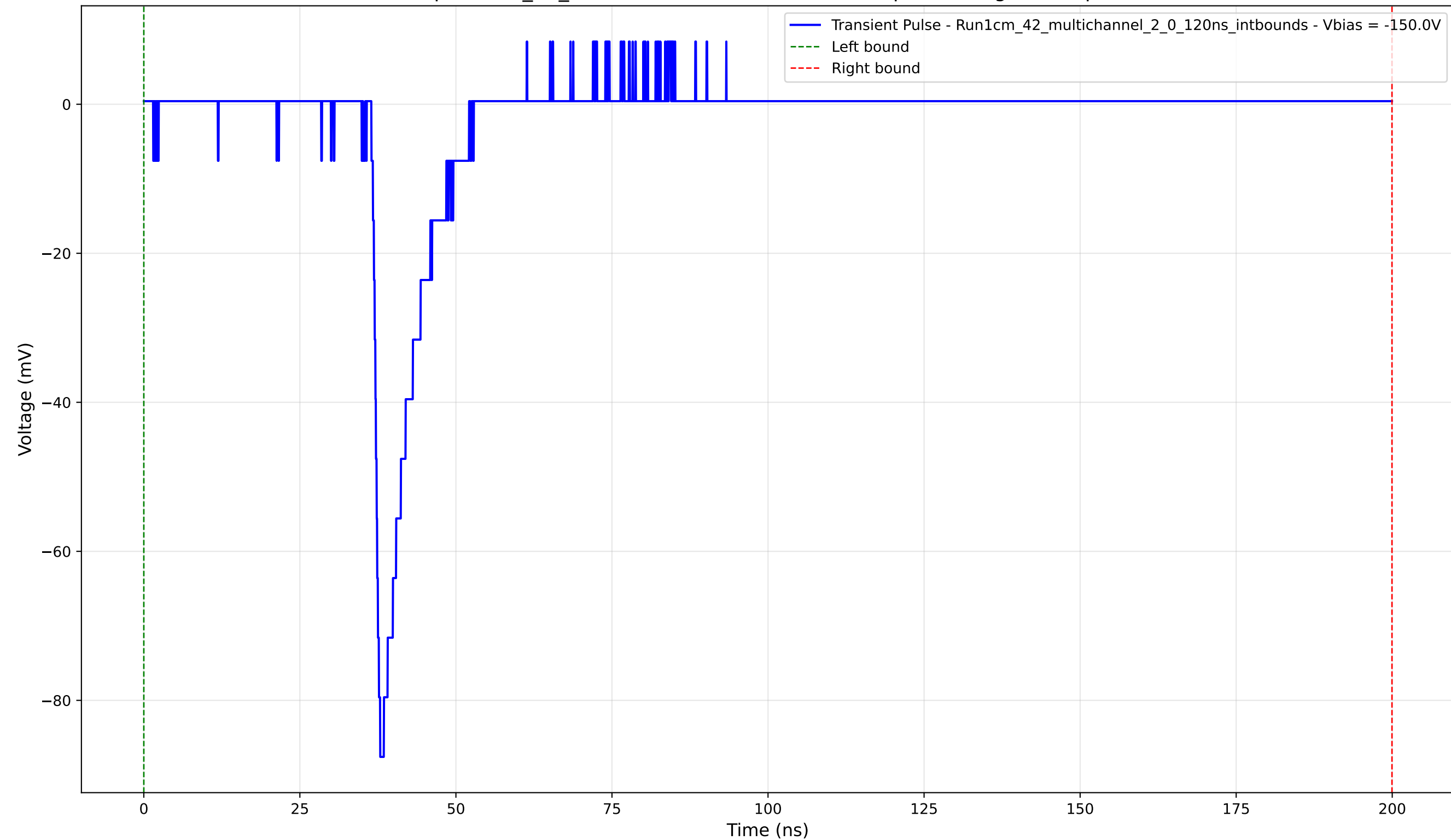
Transient Pulse - Sample: 1cm_42_multichannel - Position: 1305.0 \mu\text{m} - Charge: 8.67 pC - Rise Time: 0.99 ns
