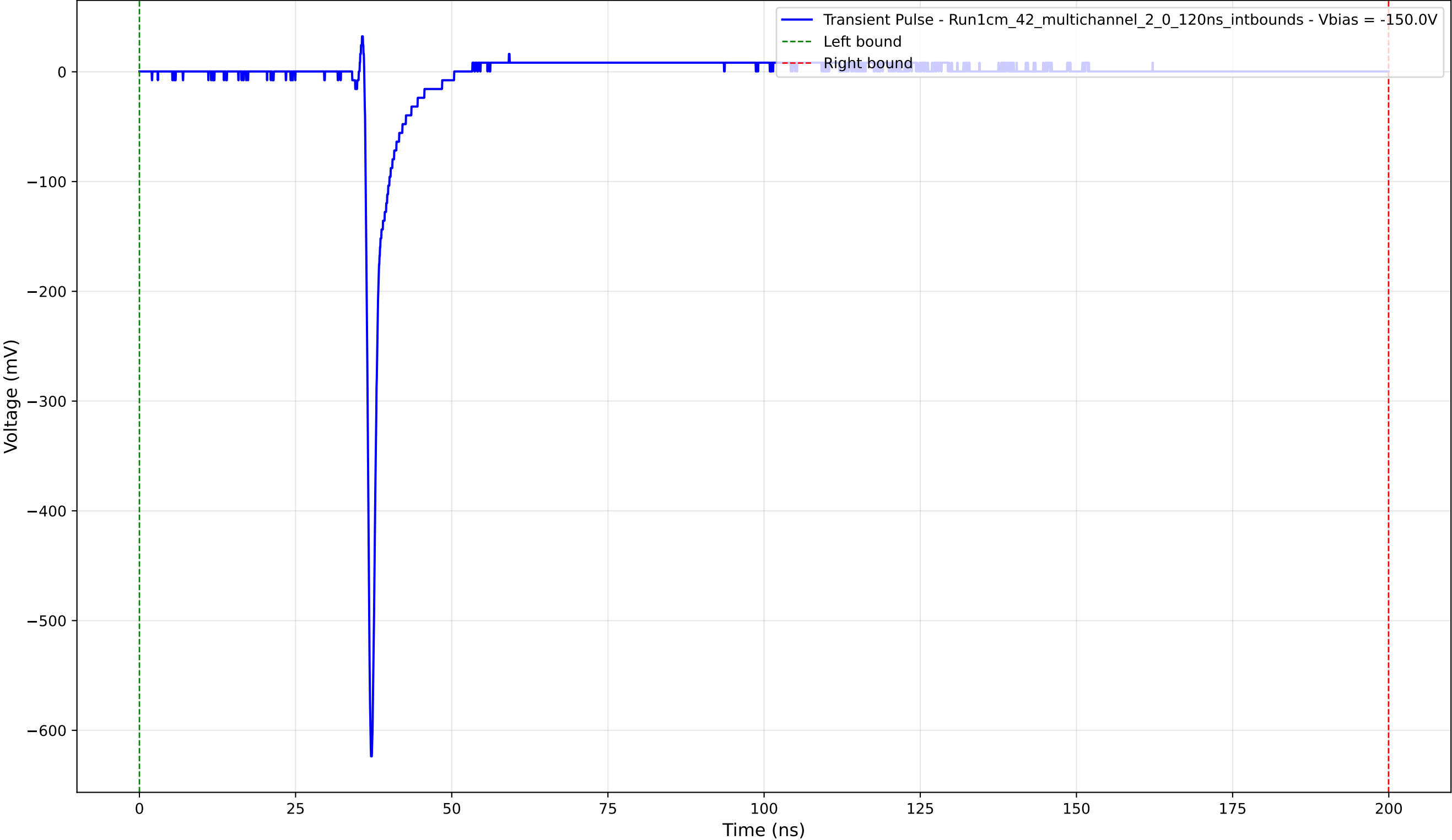
Transient Pulse - Sample: 1cm_42_multichannel - Position: 2455.0 \mu\text{m} - Charge: 15.99 pC - Rise Time: 0.73 ns
