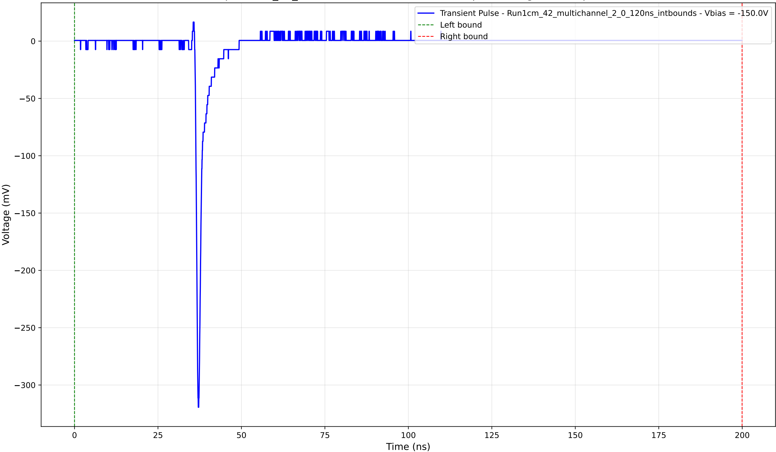
Transient Pulse - Sample: 1cm_42_multichannel - Position: 2420.0 \mu\text{m} - Charge: 10.54 pC - Rise Time: 0.72 ns
