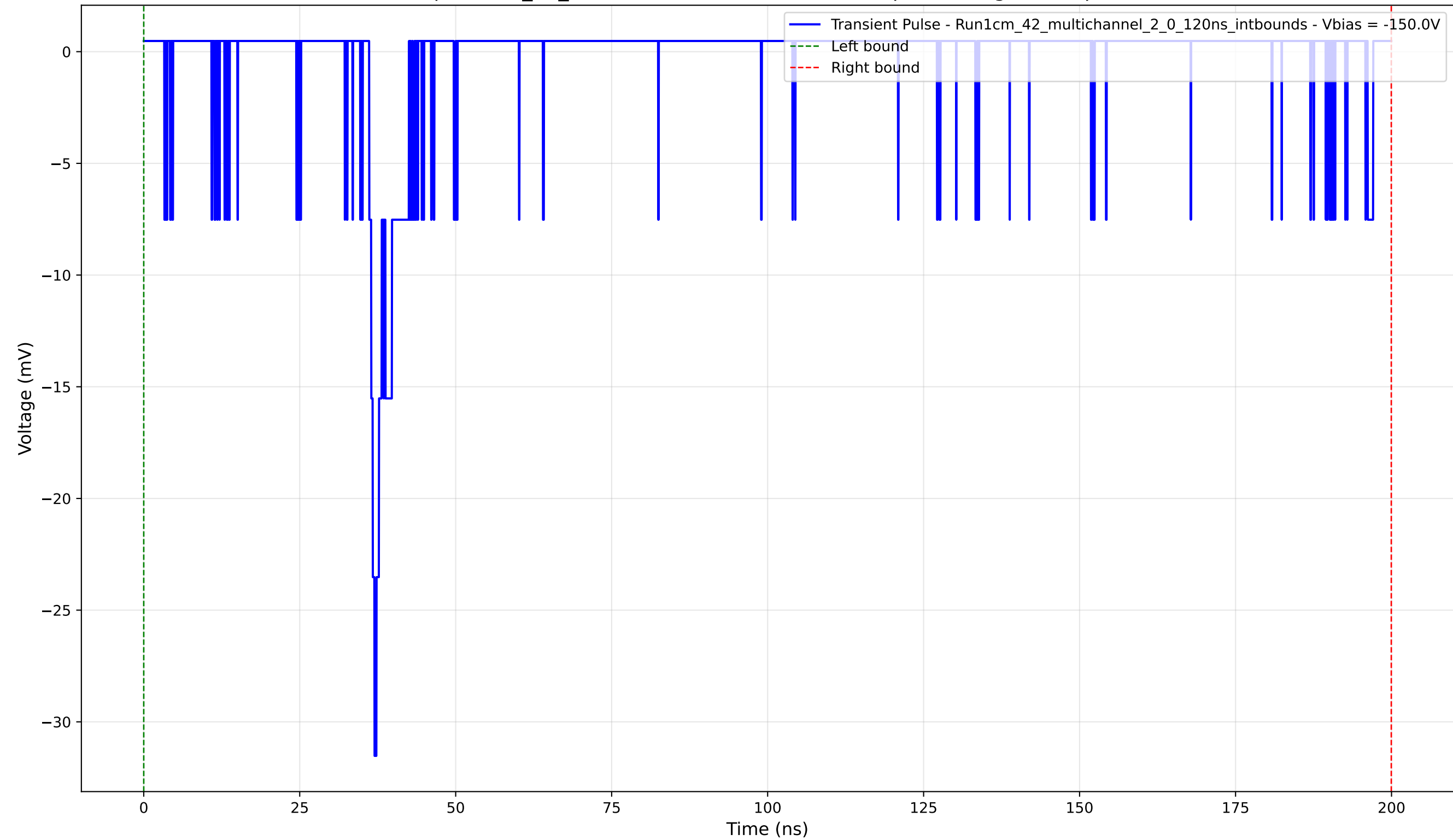
Transient Pulse - Sample: 1cm_42_multichannel - Position: 2360.0 \mu\text{m} - Charge: 1.06 pC - Rise Time: 0.86 ns
