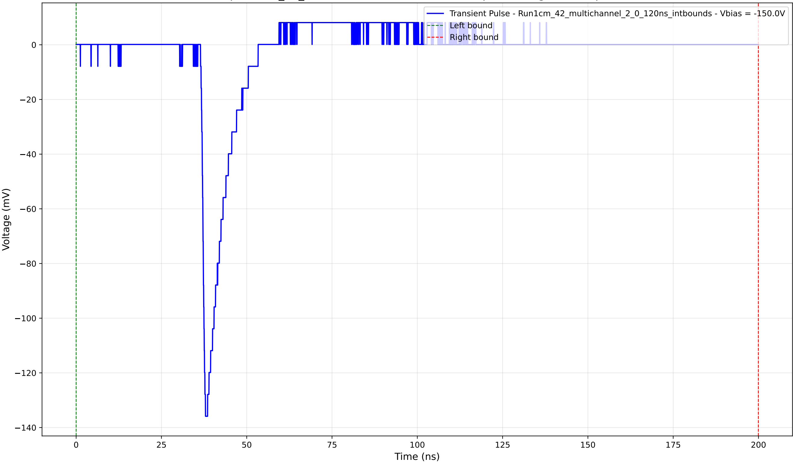
Transient Pulse - Sample: 1cm_42_multichannel - Position: 3485.0 \mu\text{m} - Charge: 10.24 pC - Rise Time: 1.13 ns
