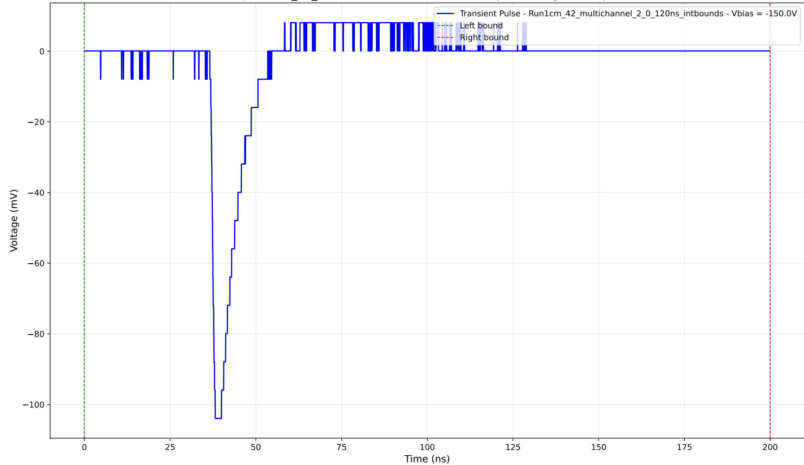
Transient Pulse - Sample: 1cm_42_multichannel - Position: 3720.0 \mu\text{m} - Charge: 9.76 pC - Rise Time: 1.11 ns
