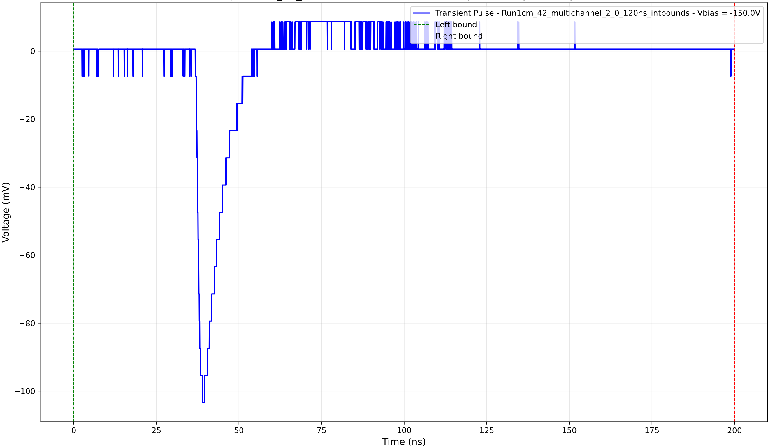
Transient Pulse - Sample: 1cm_42_multichannel - Position: 760.0 \mu\text{m} - Charge: 8.50 pC - Rise Time: 1.31 ns
