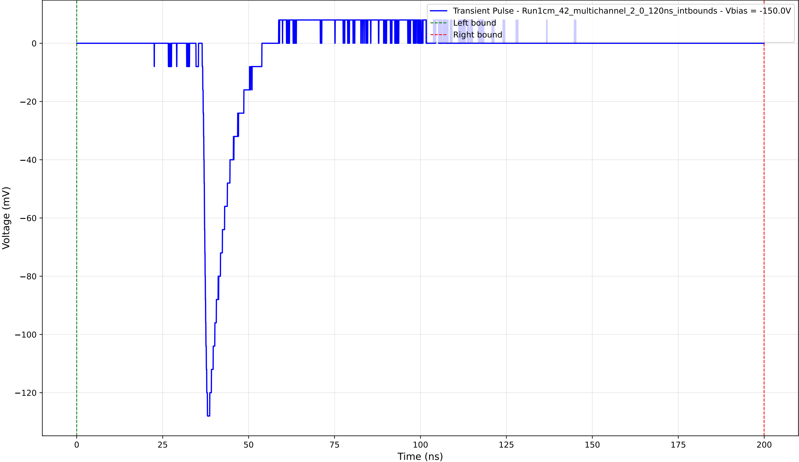
Transient Pulse - Sample: 1cm_42_multichannel - Position: 3530.0 \mu\text{m} - Charge: 10.31 pC - Rise Time: 1.18 ns
