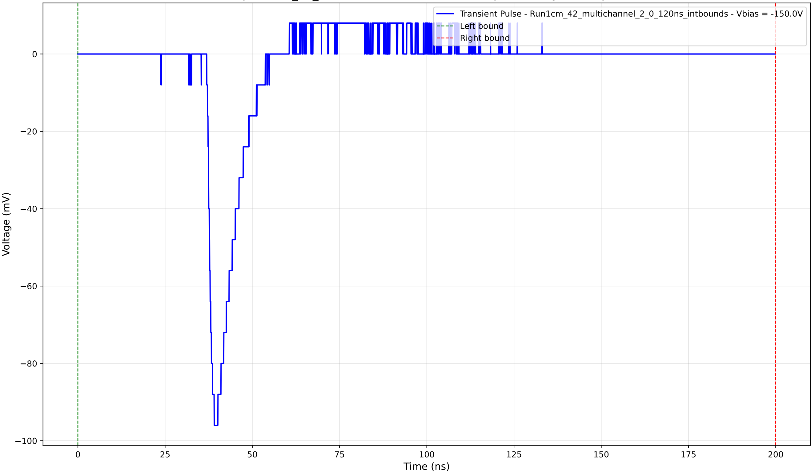
Transient Pulse - Sample: 1cm_42_multichannel - Position: 500.0 \mu\text{m} - Charge: 9.47 pC - Rise Time: 1.47 ns
