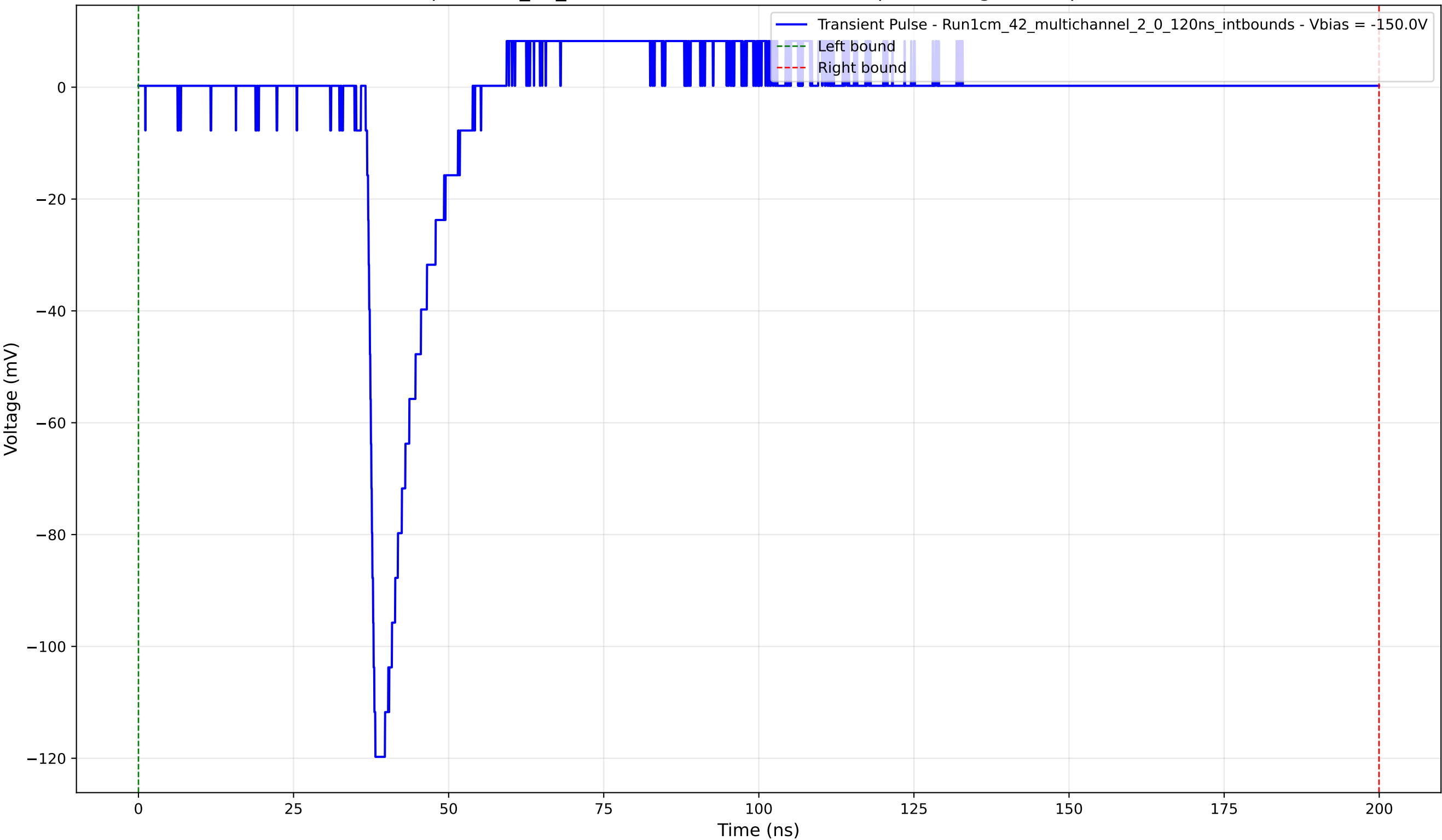
Transient Pulse - Sample: 1cm_42_multichannel - Position: 970.0 \mu\text{m} - Charge: 9.85 pC - Rise Time: 1.18 ns
