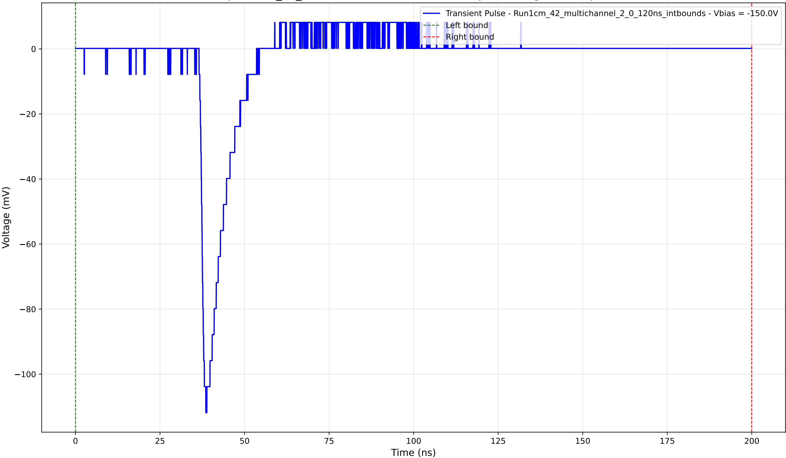
Transient Pulse - Sample: 1cm_42_multichannel - Position: 3695.0 \mu\text{m} - Charge: 10.03 pC - Rise Time: 1.34 ns
