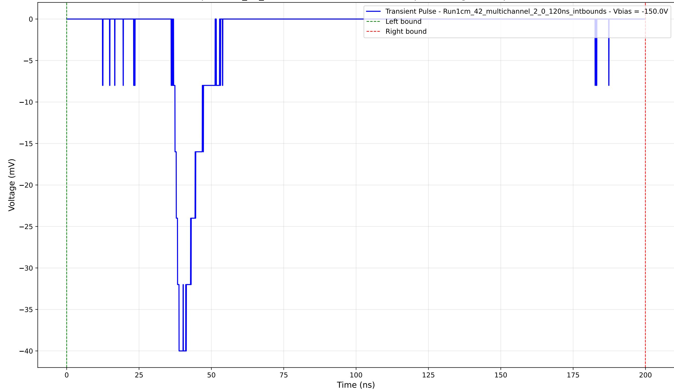
Transient Pulse - Sample: 1cm_42_multichannel - Position: 4440.0 \mu\text{m} - Charge: 6.50 pC - Rise Time: 1.90 ns
