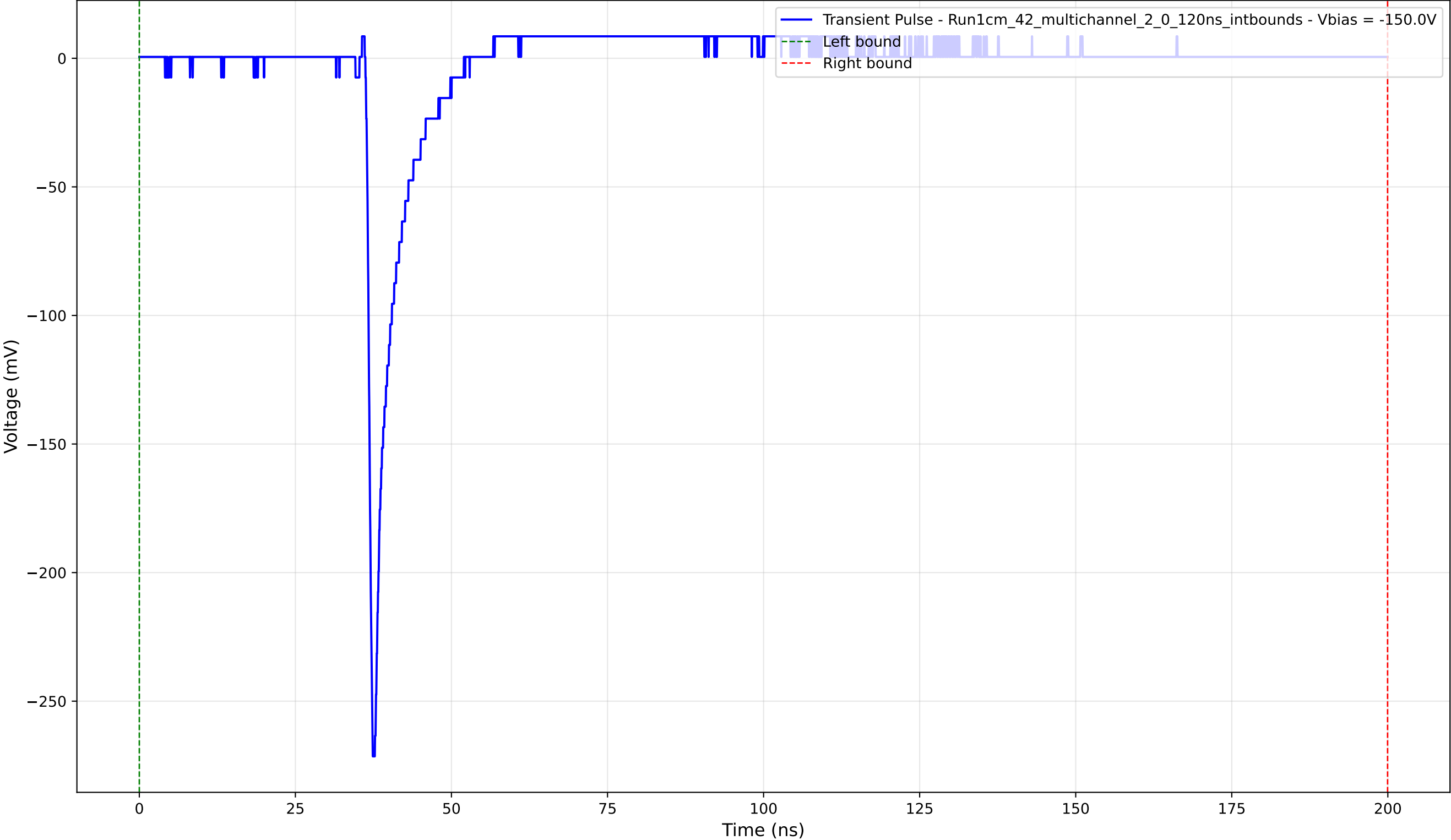
Transient Pulse - Sample: 1cm_42_multichannel - Position: 1780.0 \mu\text{m} - Charge: 10.47 pC - Rise Time: 0.85 ns
