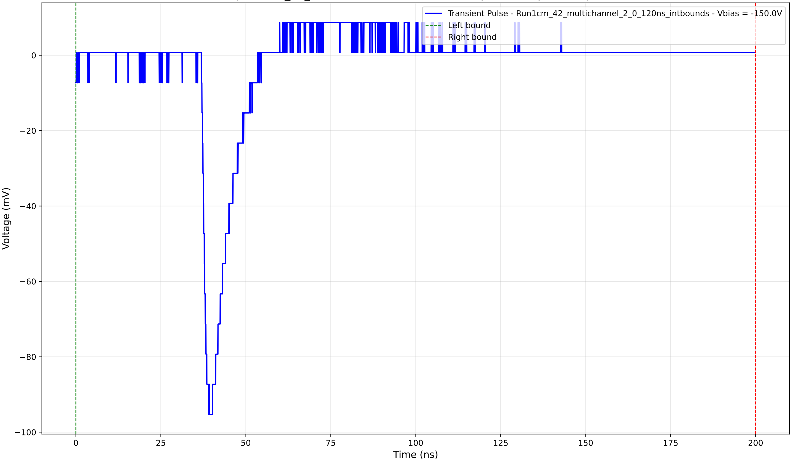
Transient Pulse - Sample: 1cm_42_multichannel - Position: 510.0 \mu\text{m} - Charge: 7.43 pC - Rise Time: 1.47 ns
