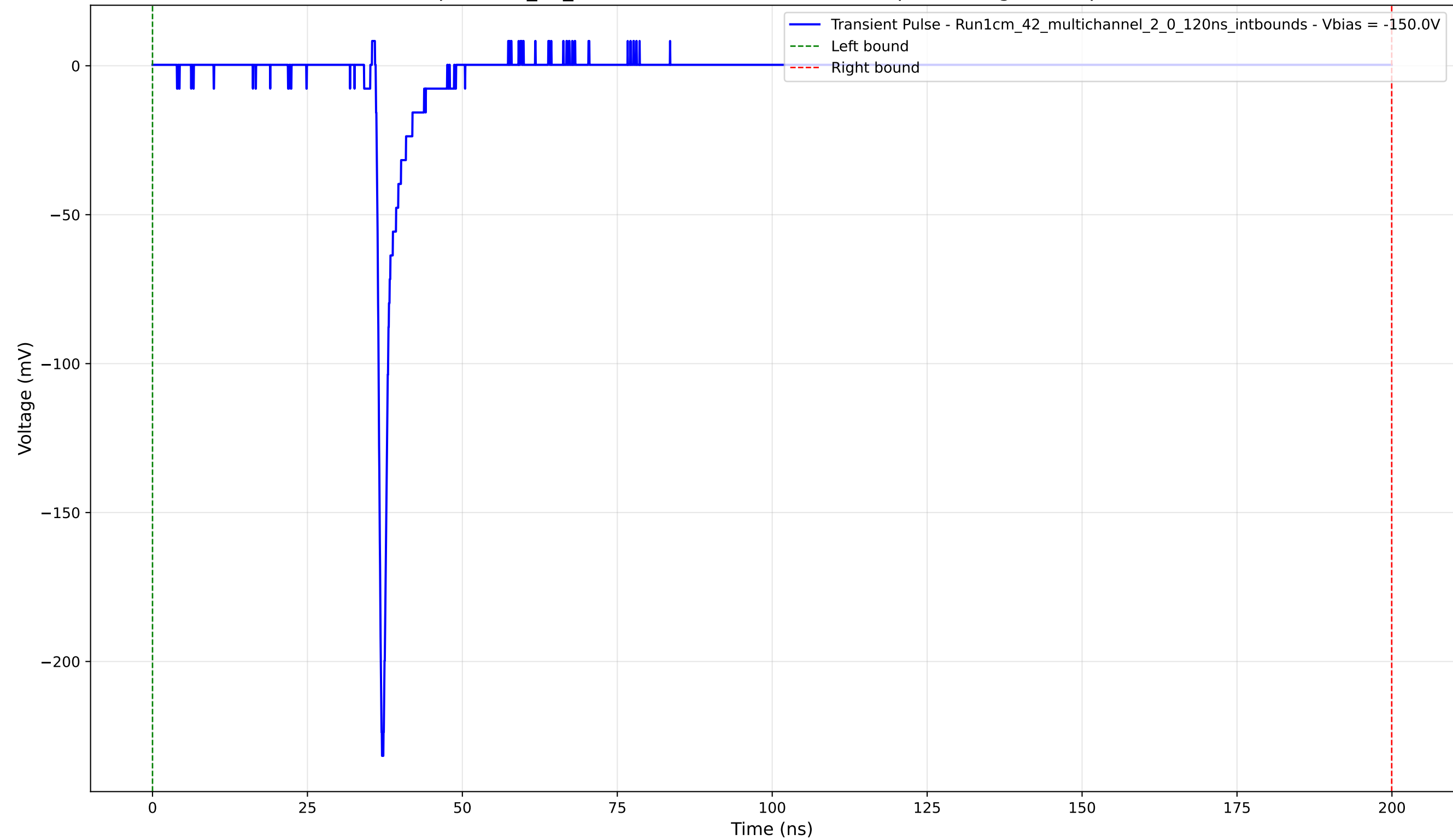
Transient Pulse - Sample: 1cm_42_multichannel - Position: 2325.0 \mu\text{m} - Charge: 9.34 pC - Rise Time: 0.73 ns
