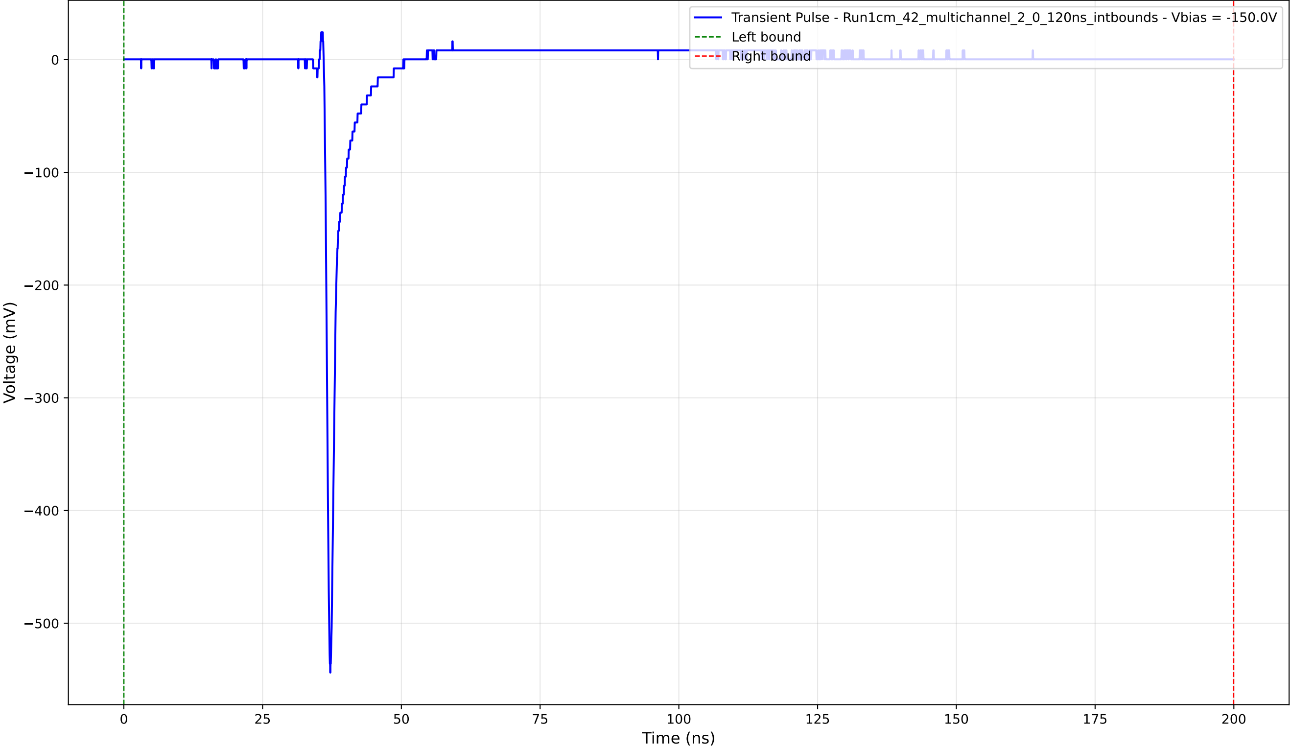
Transient Pulse - Sample: 1cm_42_multichannel - Position: 2530.0 \mu\text{m} - Charge: 14.88 pC - Rise Time: 0.75 ns
