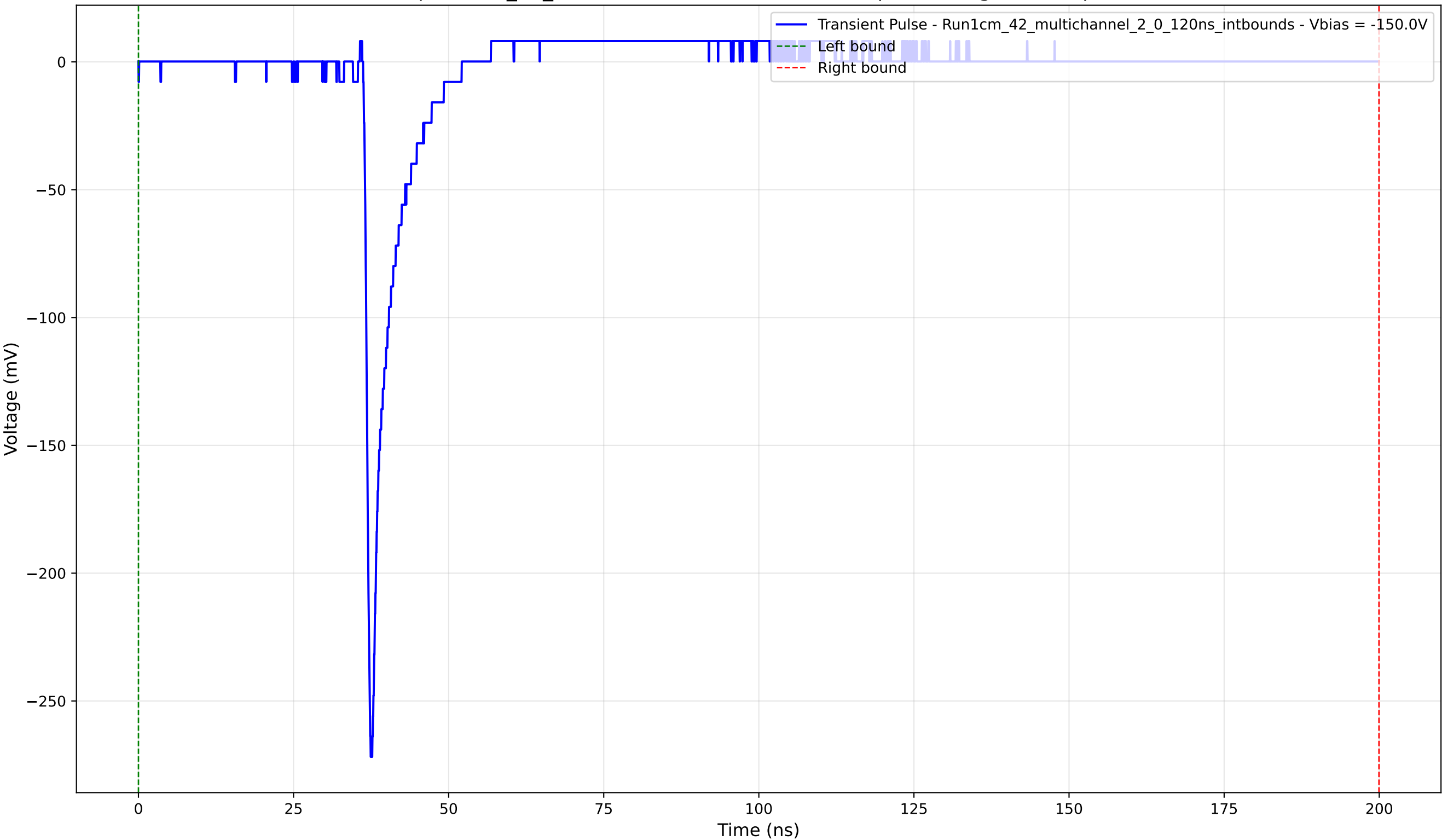
Transient Pulse - Sample: 1cm_42_multichannel - Position: 1785.0 \mu\text{m} - Charge: 12.07 pC - Rise Time: 0.85 ns
