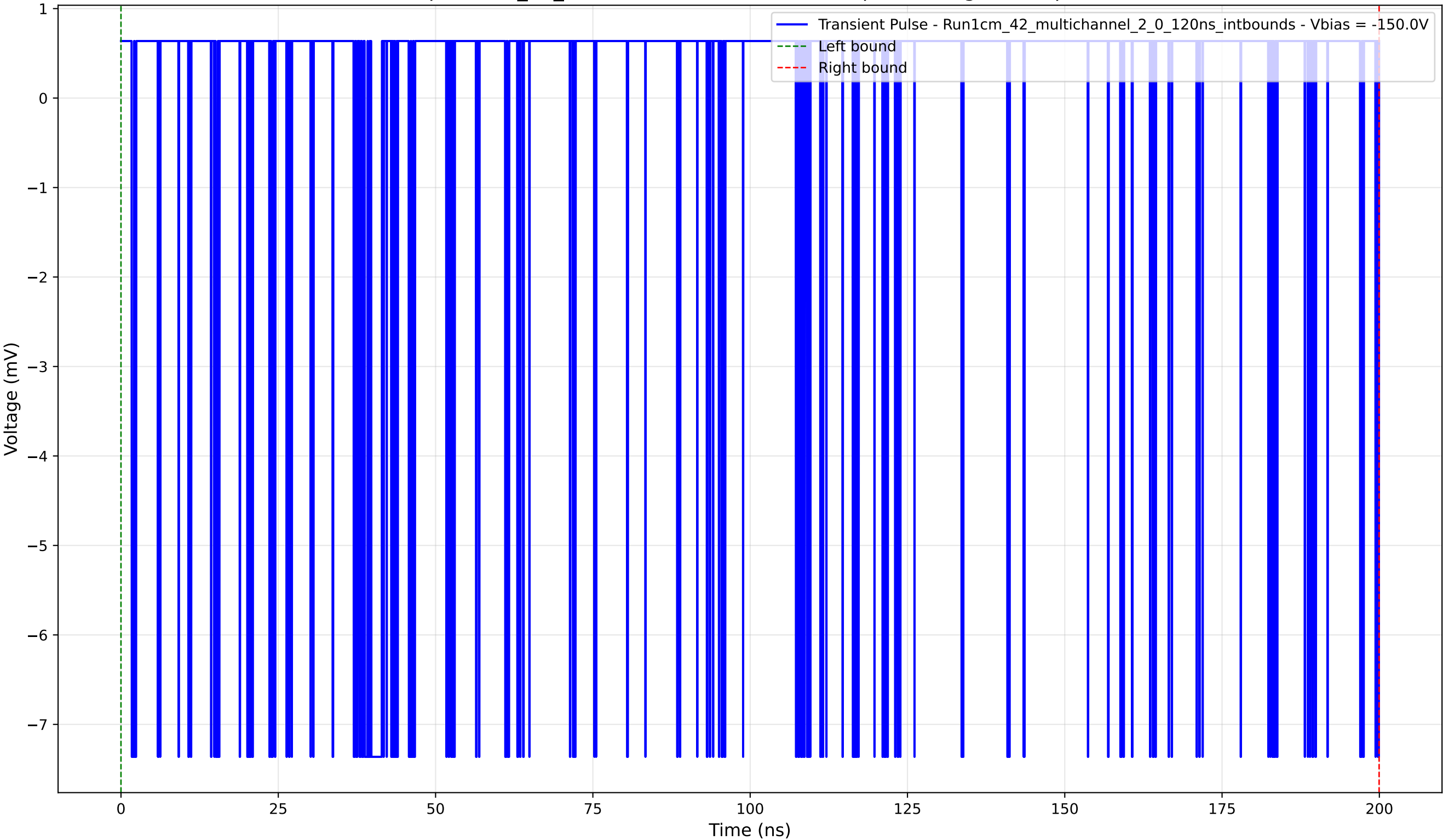
Transient Pulse - Sample: 1cm_42_multichannel - Position: 10.0 \mu\text{m} - Charge: 0.25 pC - Rise Time: 0.04 ns
