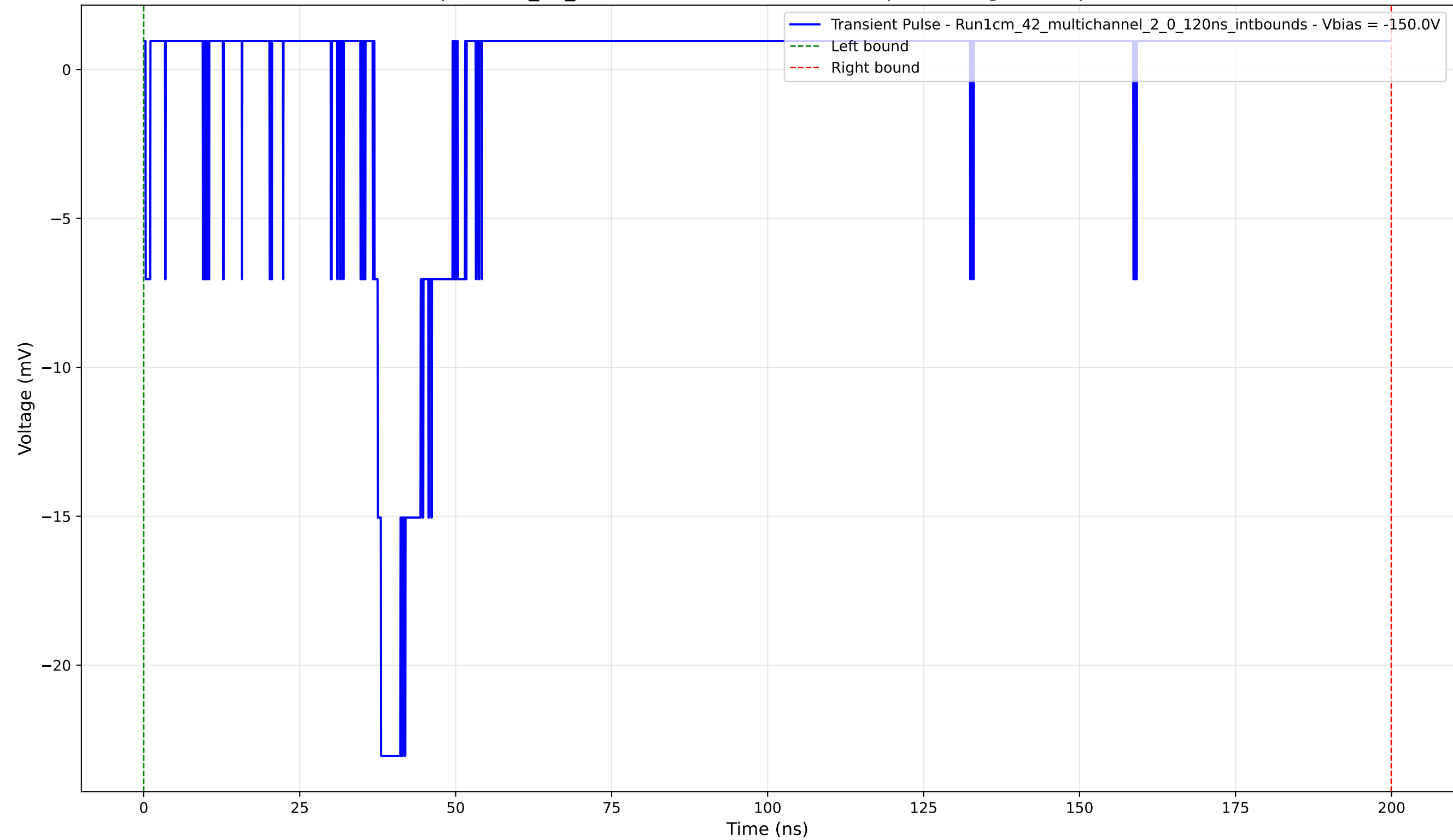
Transient Pulse - Sample: 1cm_42_multichannel - Position: 815.0 \mu\text{m} - Charge: 0.79 pC - Rise Time: 1.07 ns
