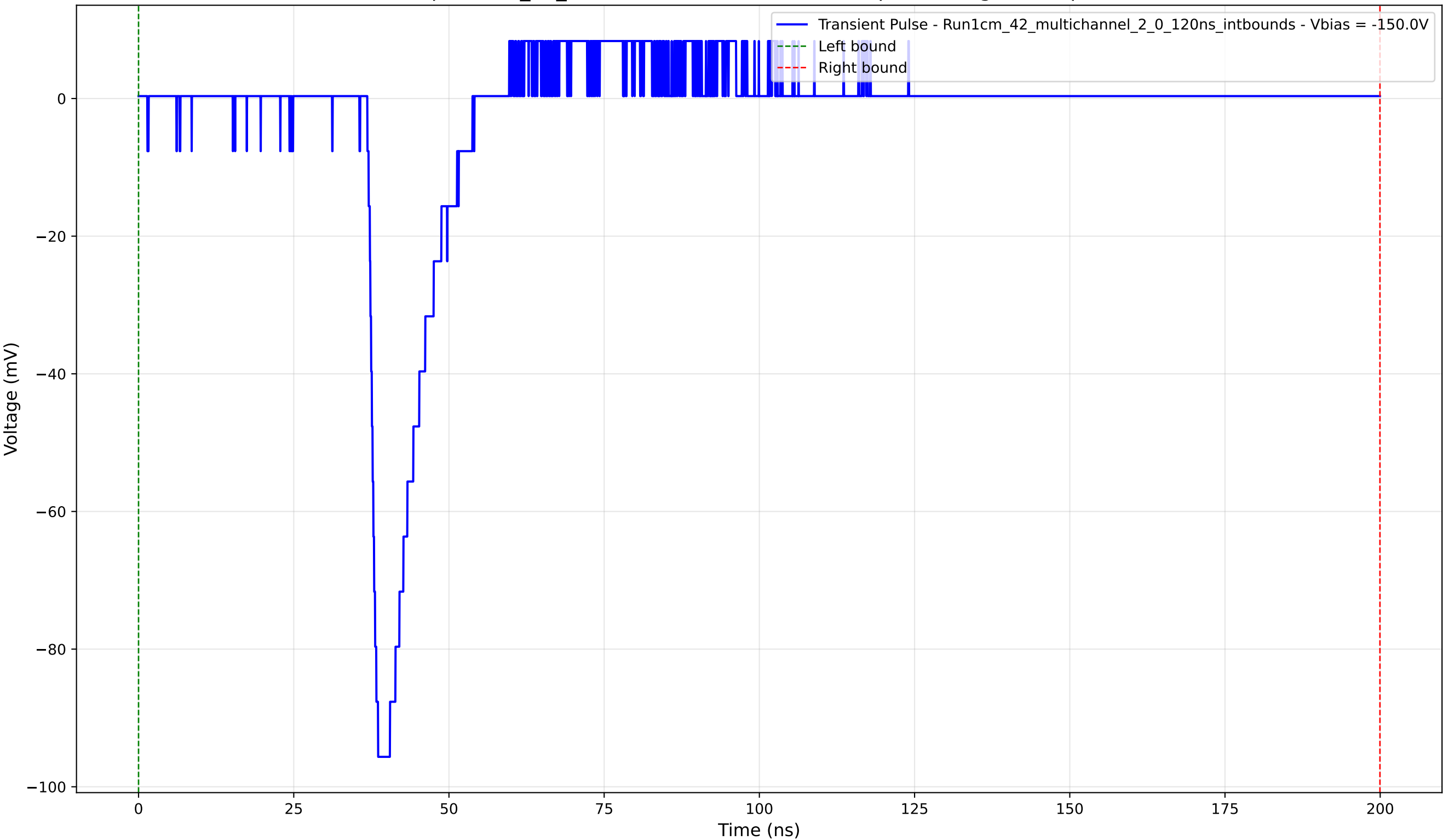
Transient Pulse - Sample: 1cm_42_multichannel - Position: 610.0 \mu\text{m} - Charge: 9.48 pC - Rise Time: 1.27 ns
