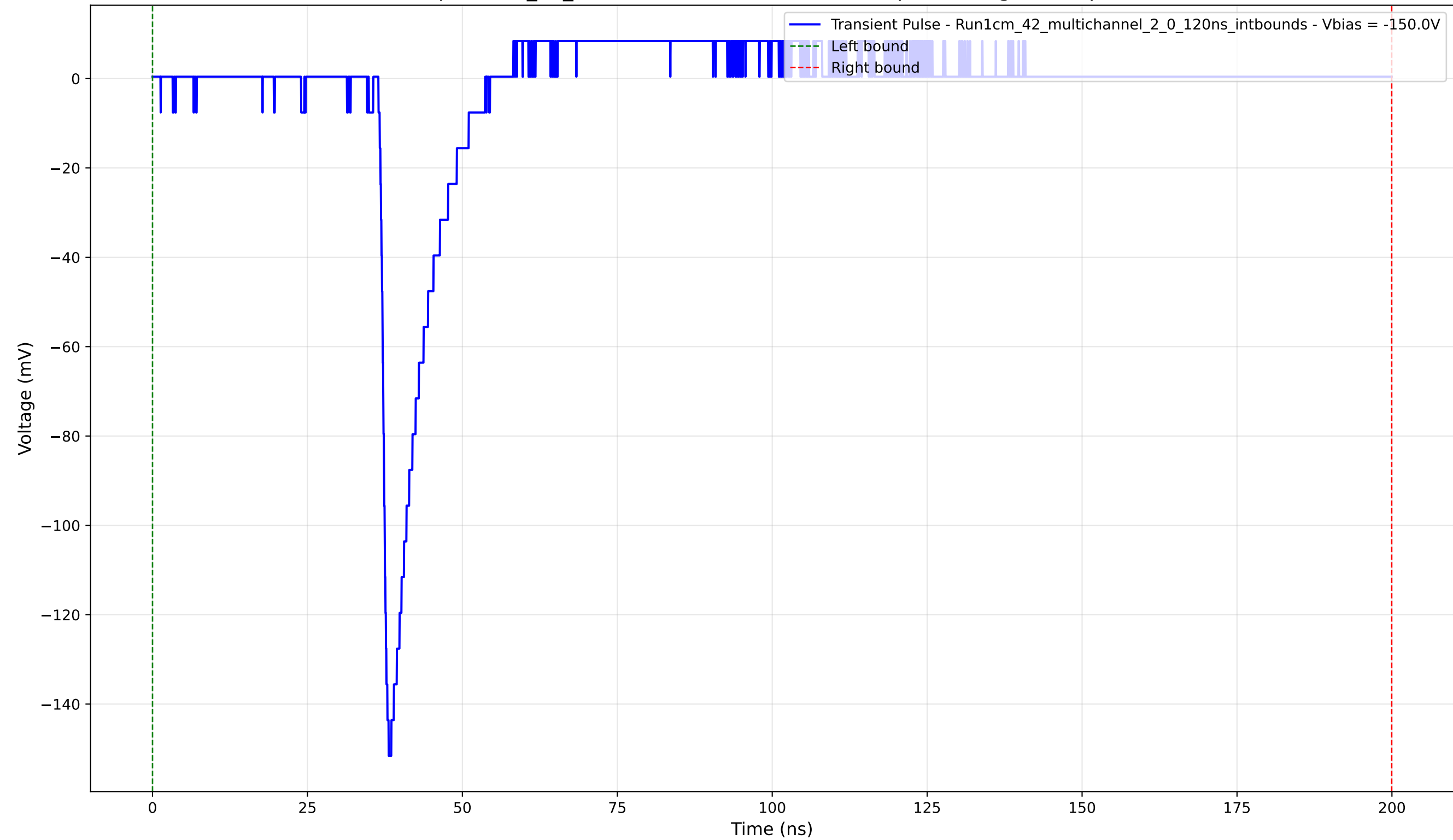
Transient Pulse - Sample: 1cm_42_multichannel - Position: 1205.0 \mu\text{m} - Charge: 9.77 pC - Rise Time: 1.24 ns
