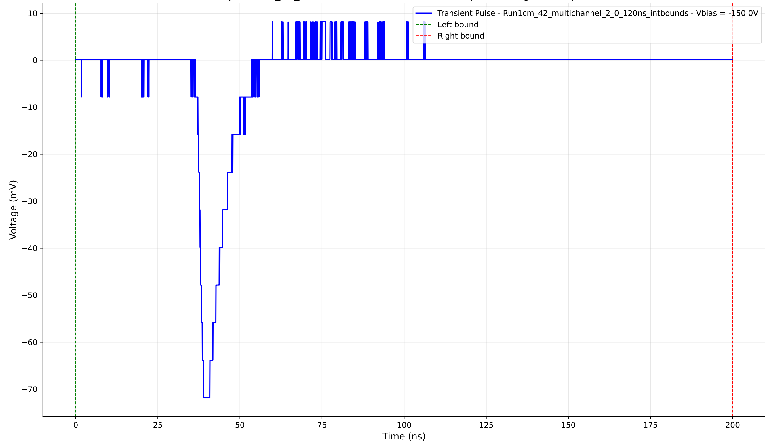
Transient Pulse - Sample: 1cm_42_multichannel - Position: 4520.0 \mu\text{m} - Charge: 9.73 pC - Rise Time: 2.40 ns
