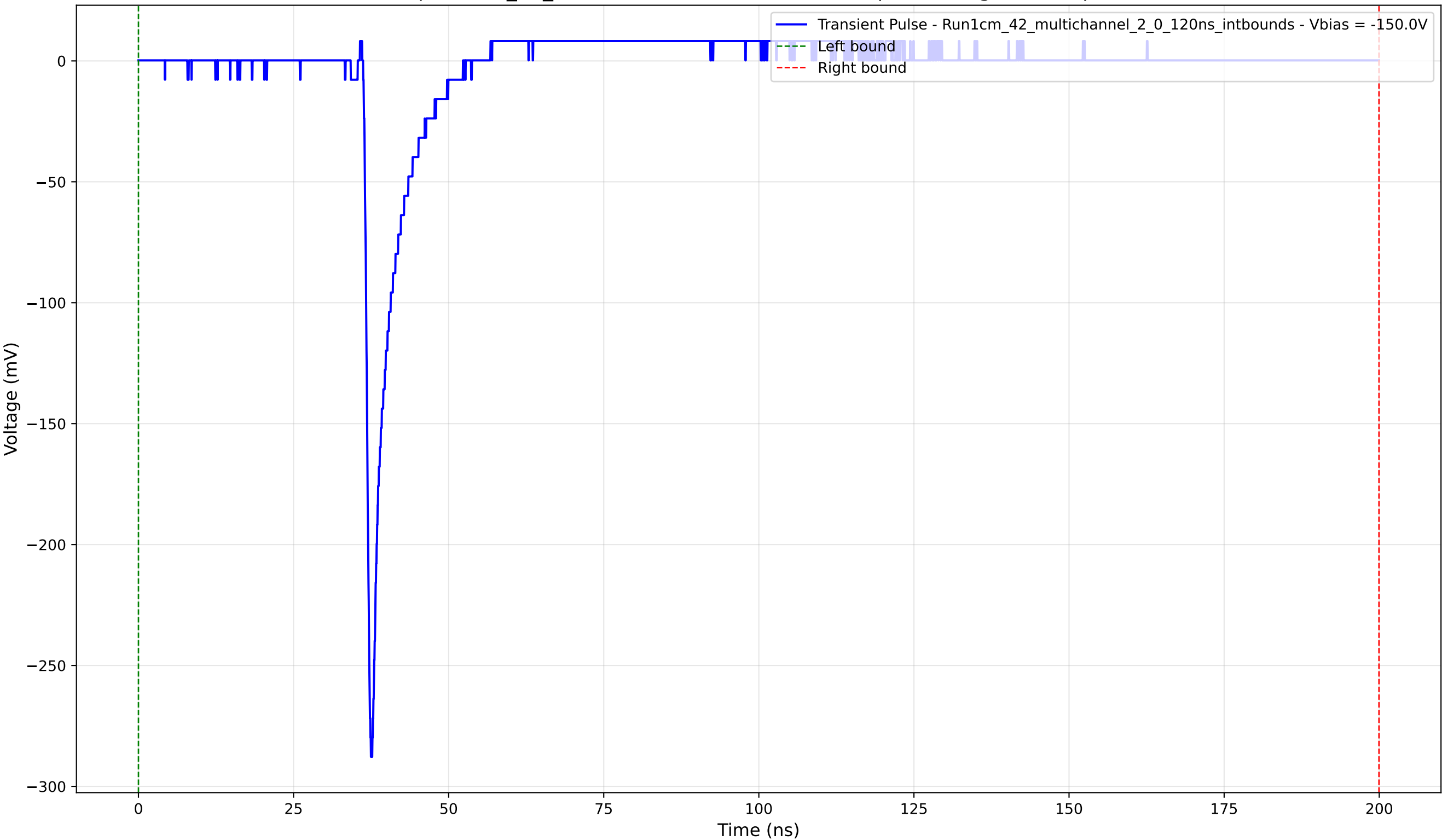
Transient Pulse - Sample: 1cm_42_multichannel - Position: 1770.0 \mu\text{m} - Charge: 12.27 pC - Rise Time: 0.83 ns
