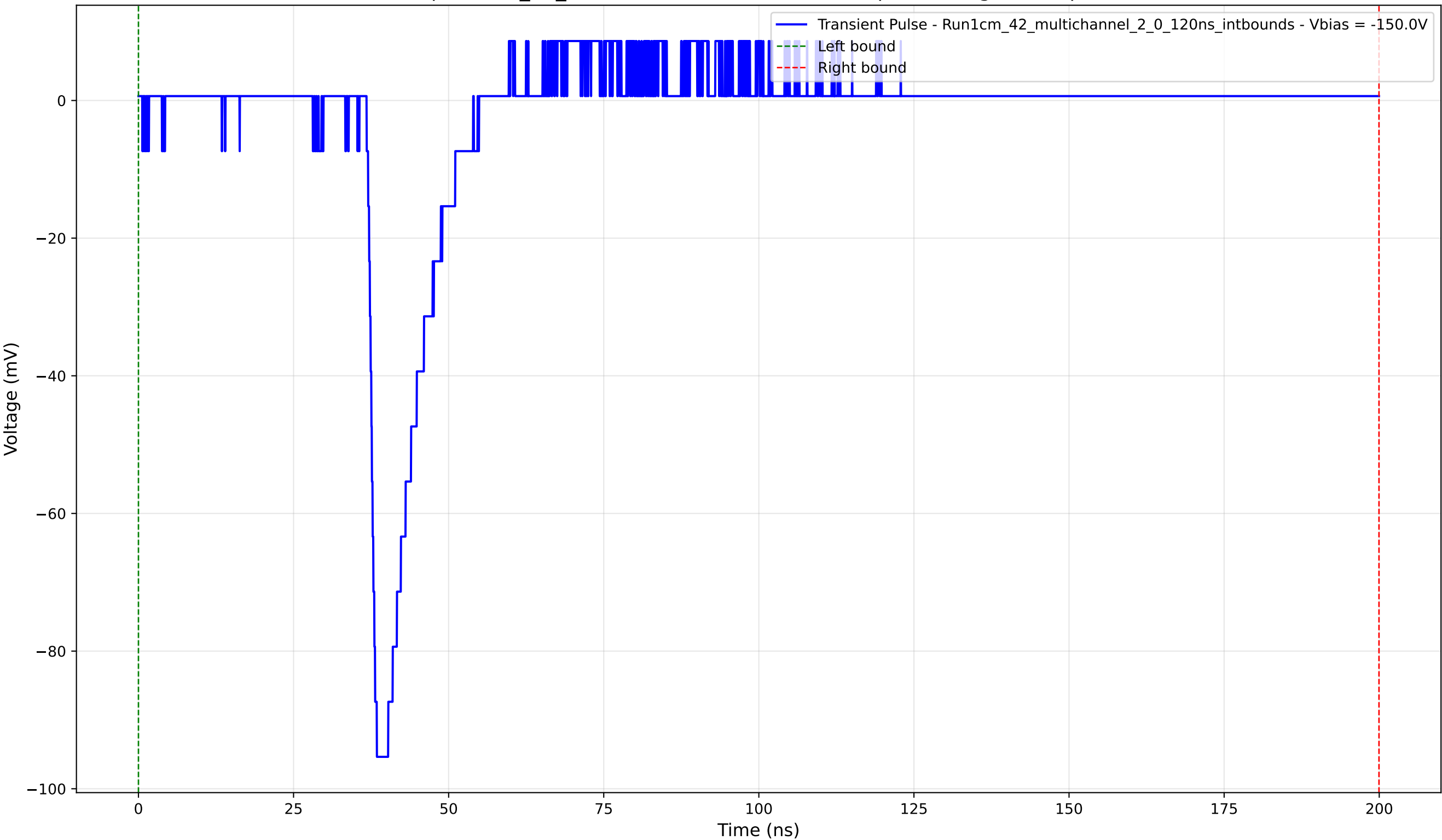
Transient Pulse - Sample: 1cm_42_multichannel - Position: 765.0 \mu\text{m} - Charge: 9.25 pC - Rise Time: 1.15 ns
