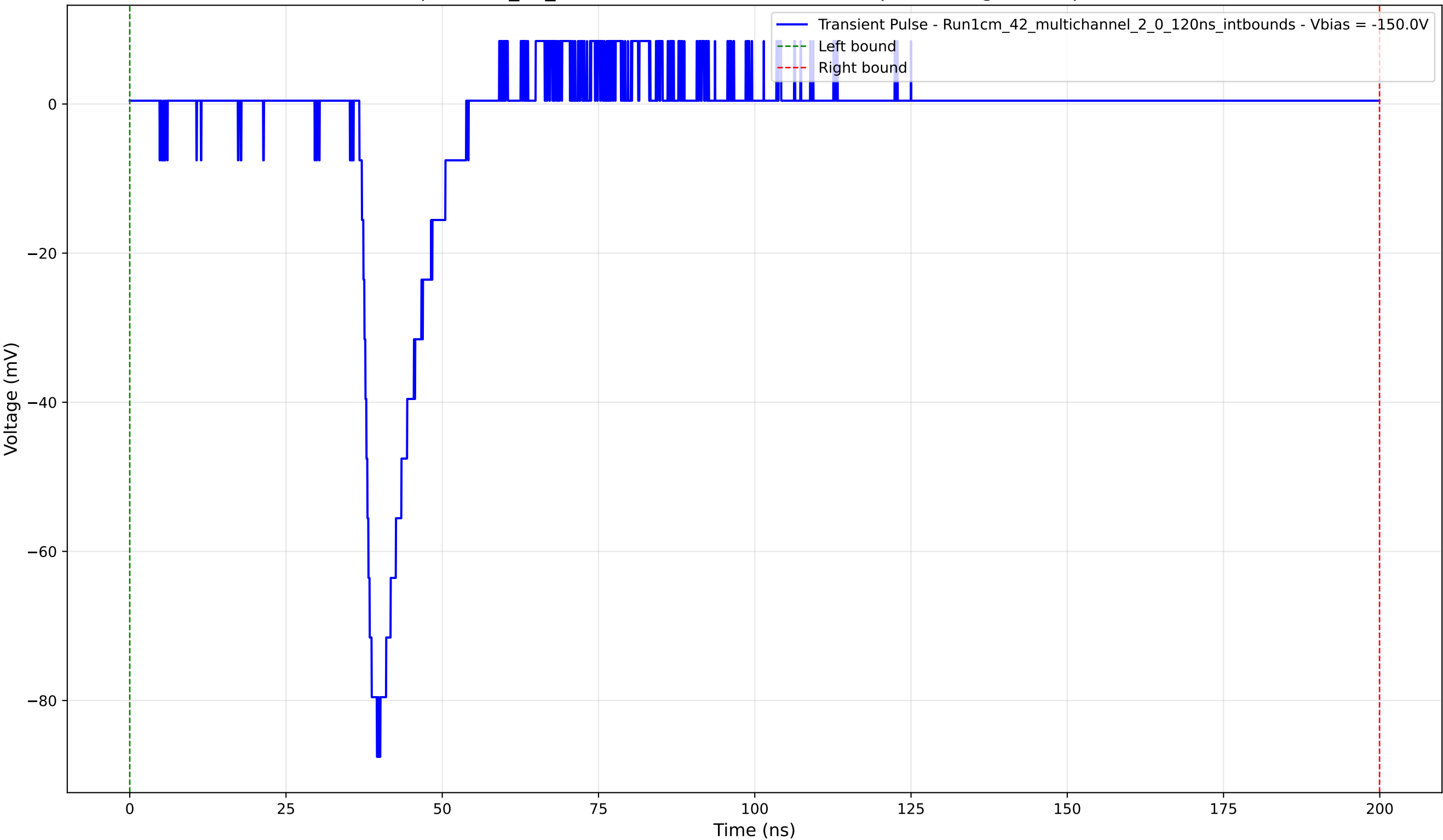
Transient Pulse - Sample: 1cm_42_multichannel - Position: 4190.0 \mu\text{m} - Charge: 8.37 pC - Rise Time: 1.59 ns
