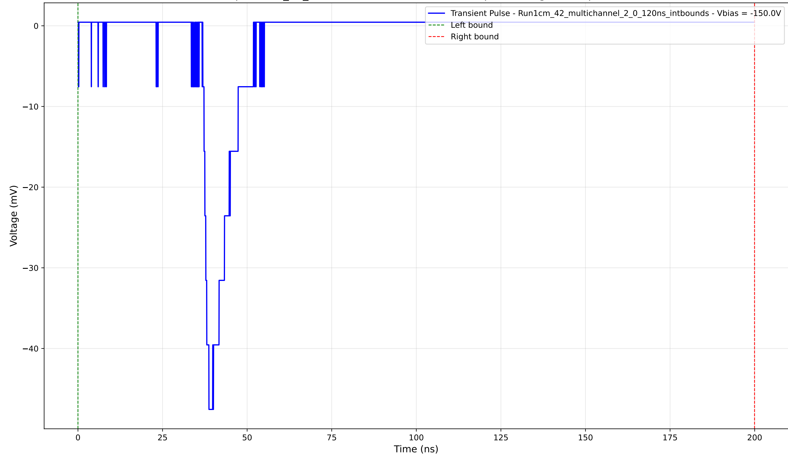
Transient Pulse - Sample: 1cm_42_multichannel - Position: 3935.0 \mu\text{m} - Charge: 5.59 pC - Rise Time: 1.82 ns
