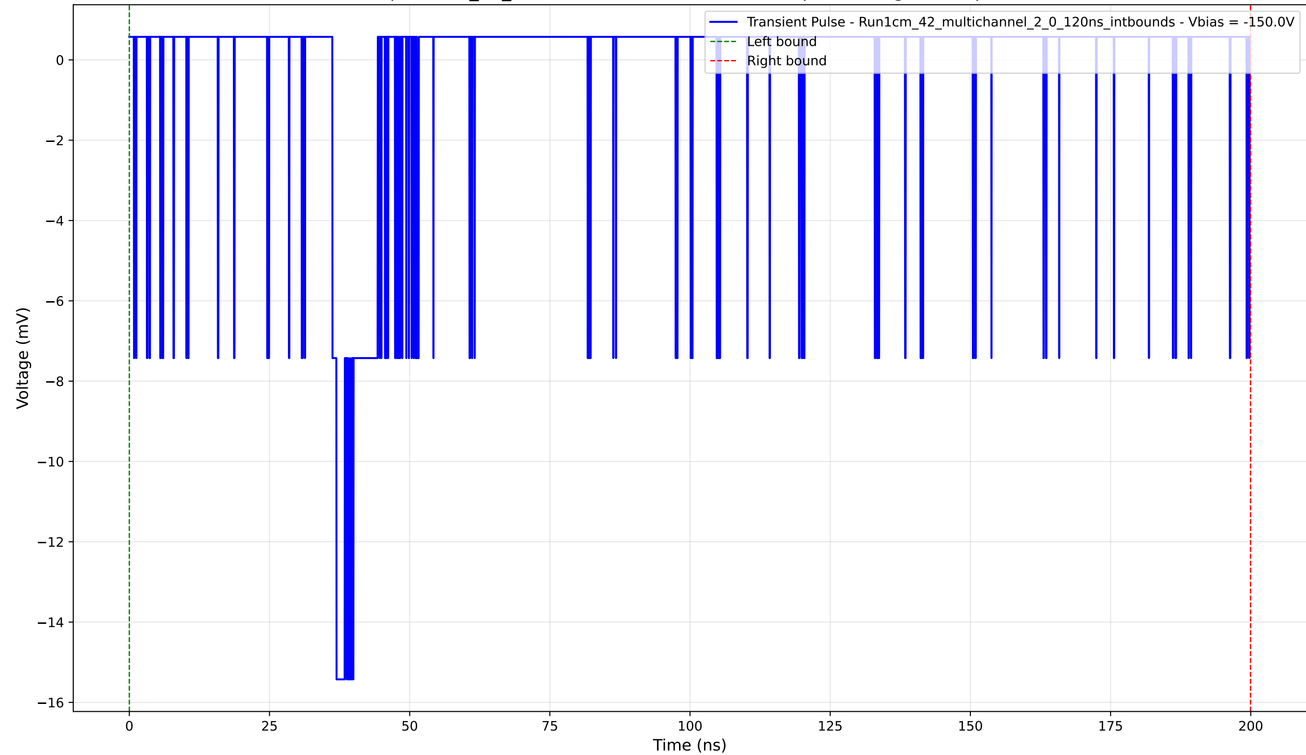
Transient Pulse - Sample: 1cm_42_multichannel - Position: 2865.0 \mu\text{m} - Charge: 0.58 pC - Rise Time: 0.75 ns
