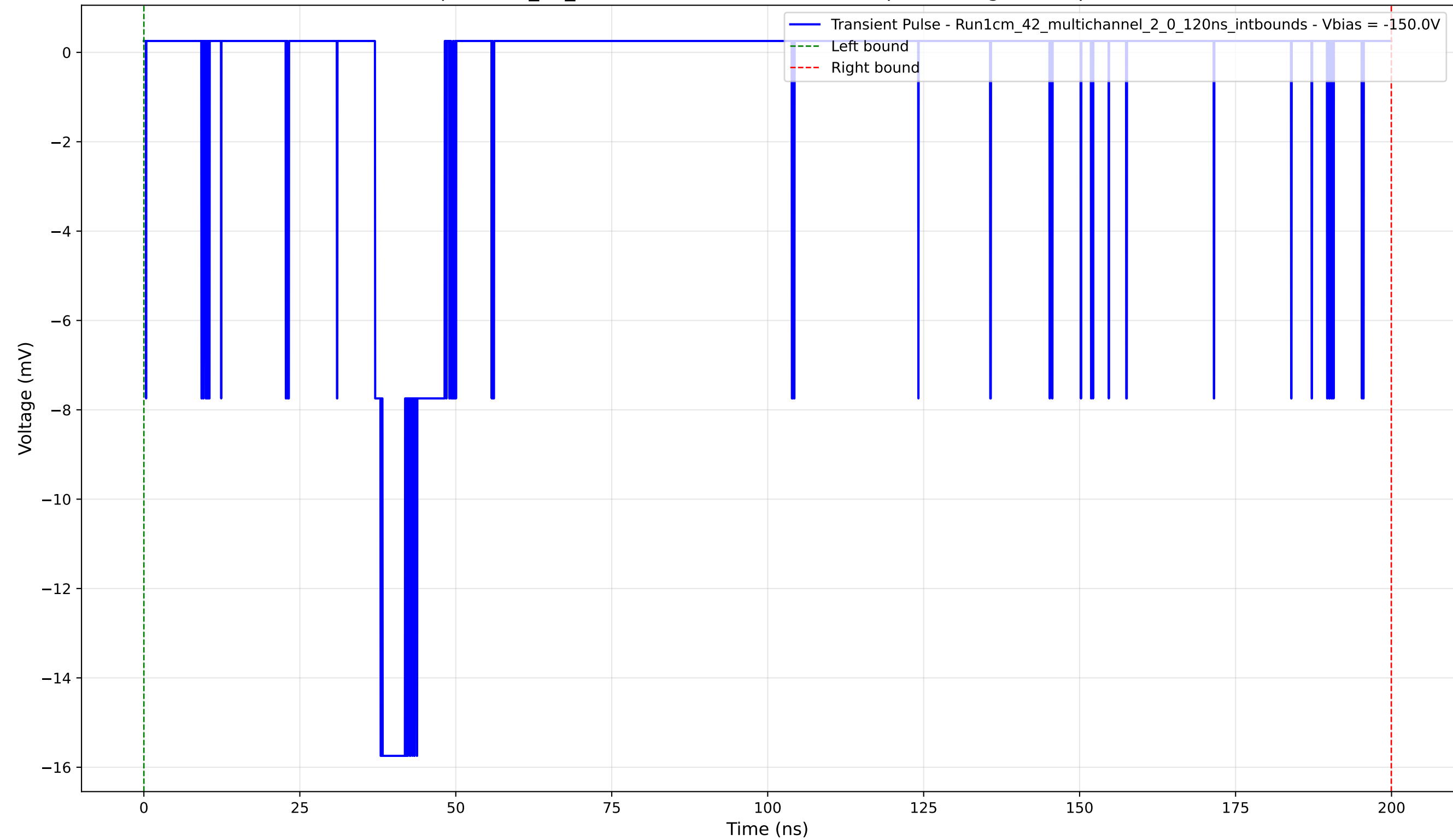
Transient Pulse - Sample: 1cm_42_multichannel - Position: 375.0 \mu\text{m} - Charge: 2.03 pC - Rise Time: 0.91 ns
