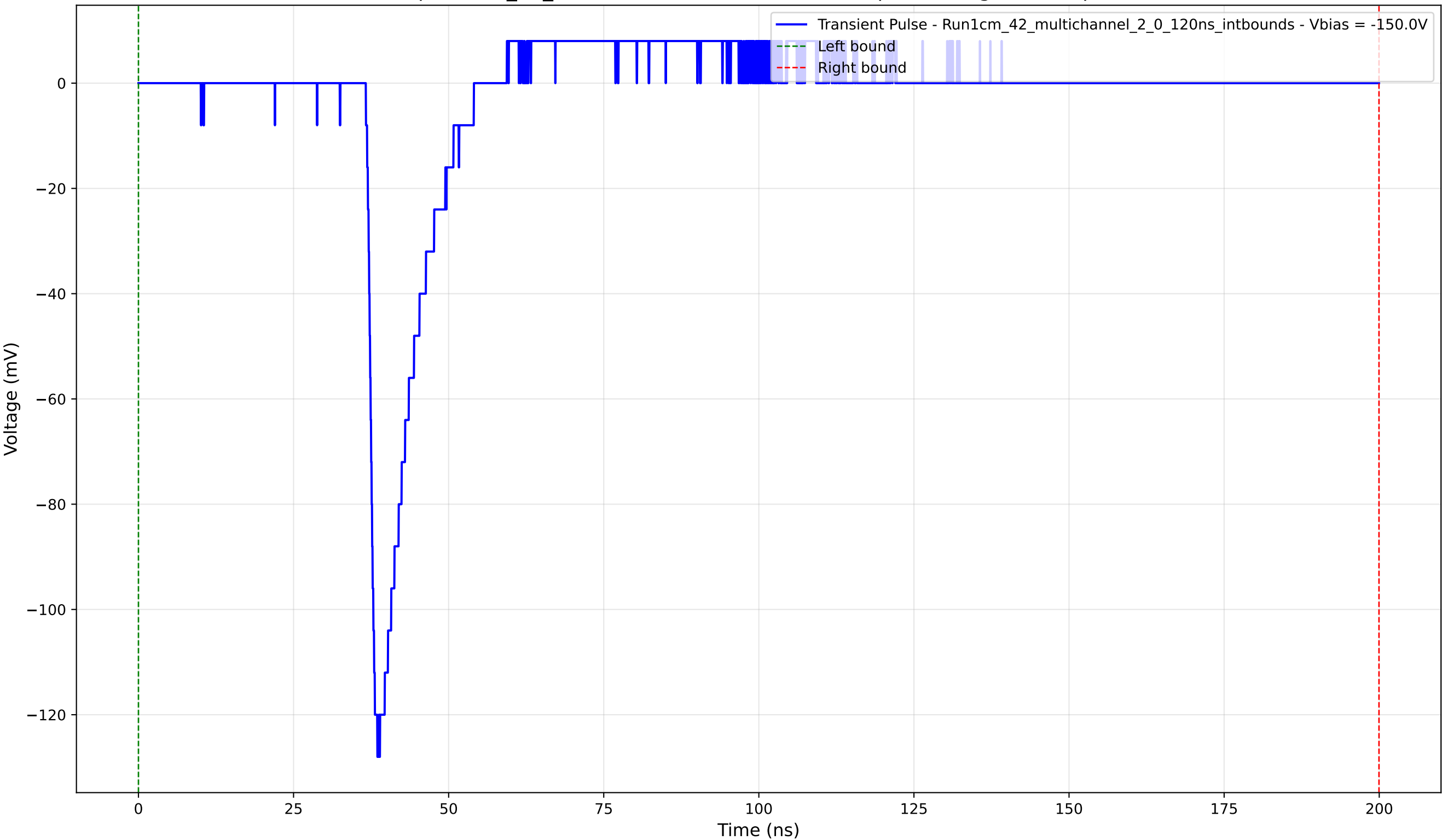
Transient Pulse - Sample: 1cm_42_multichannel - Position: 1005.0 \mu\text{m} - Charge: 10.00 pC - Rise Time: 1.26 ns
