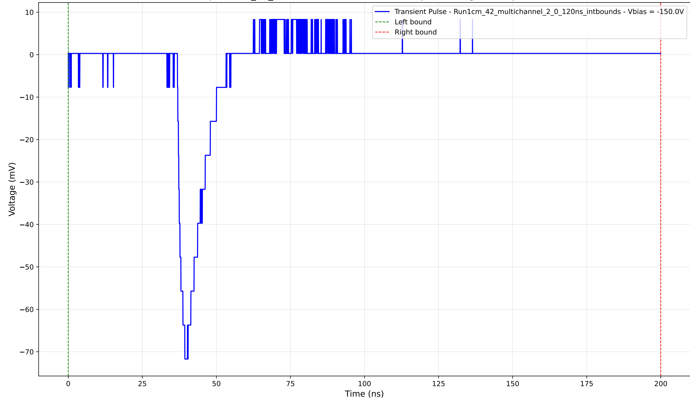
Transient Pulse - Sample: 1cm_42_multichannel - Position: 145.0 \mu\text{m} - Charge: 8.36 pC - Rise Time: 2.48 ns
