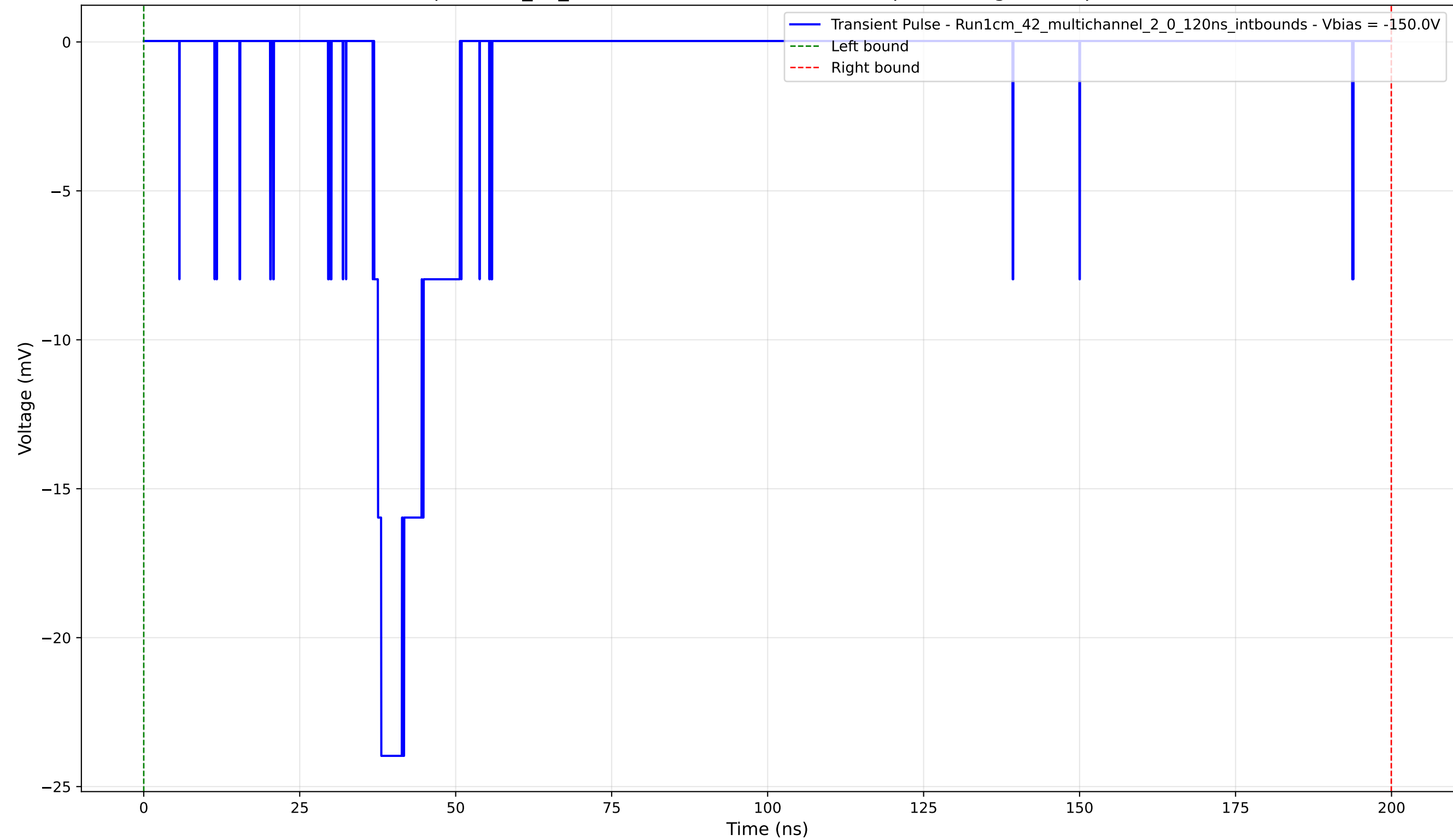
Transient Pulse - Sample: 1cm_42_multichannel - Position: 3925.0 \mu\text{m} - Charge: 4.05 pC - Rise Time: 1.15 ns
