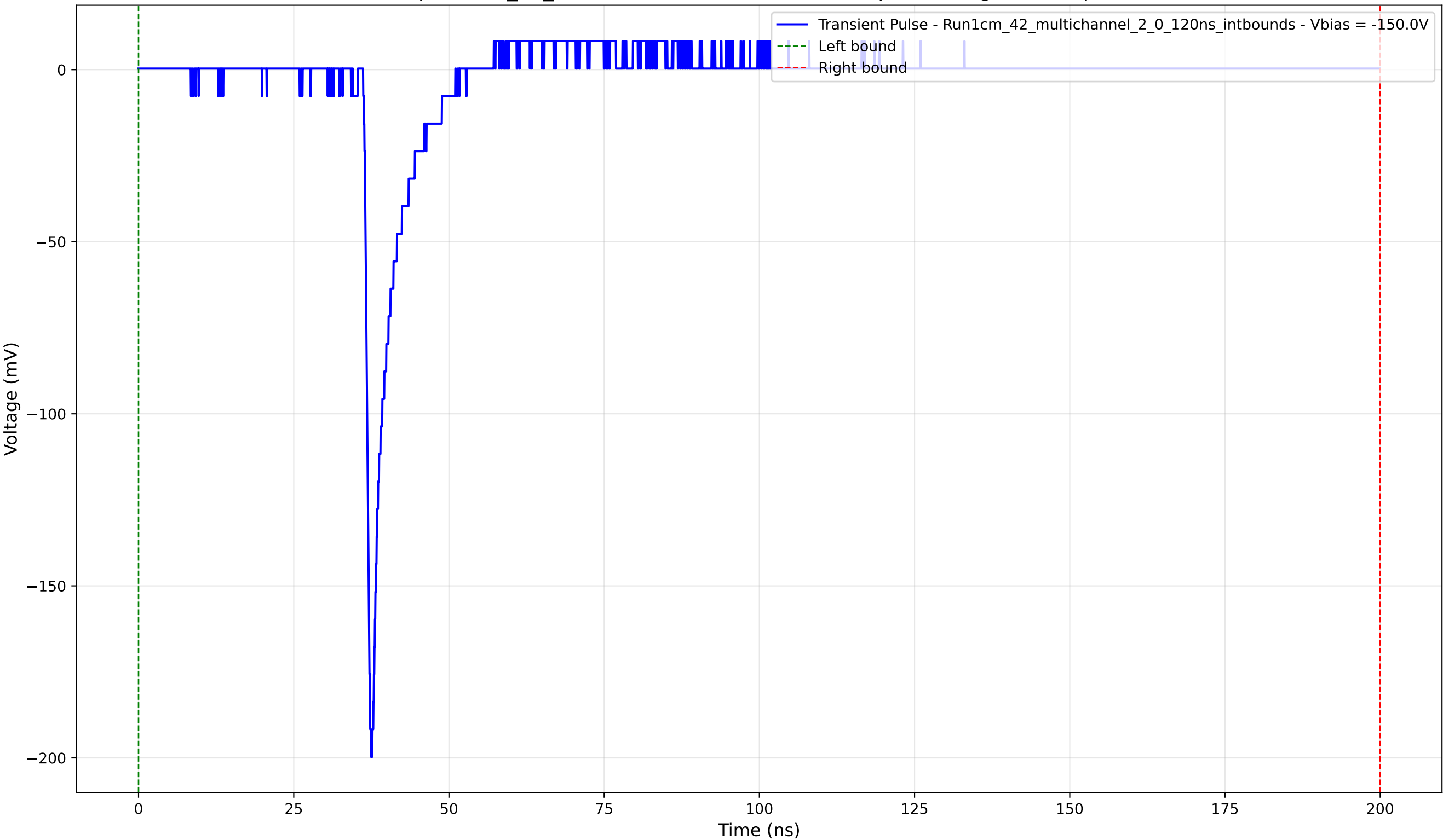
Transient Pulse - Sample: 1cm_42_multichannel - Position: 2935.0 \mu\text{m} - Charge: 10.54 pC - Rise Time: 0.88 ns
