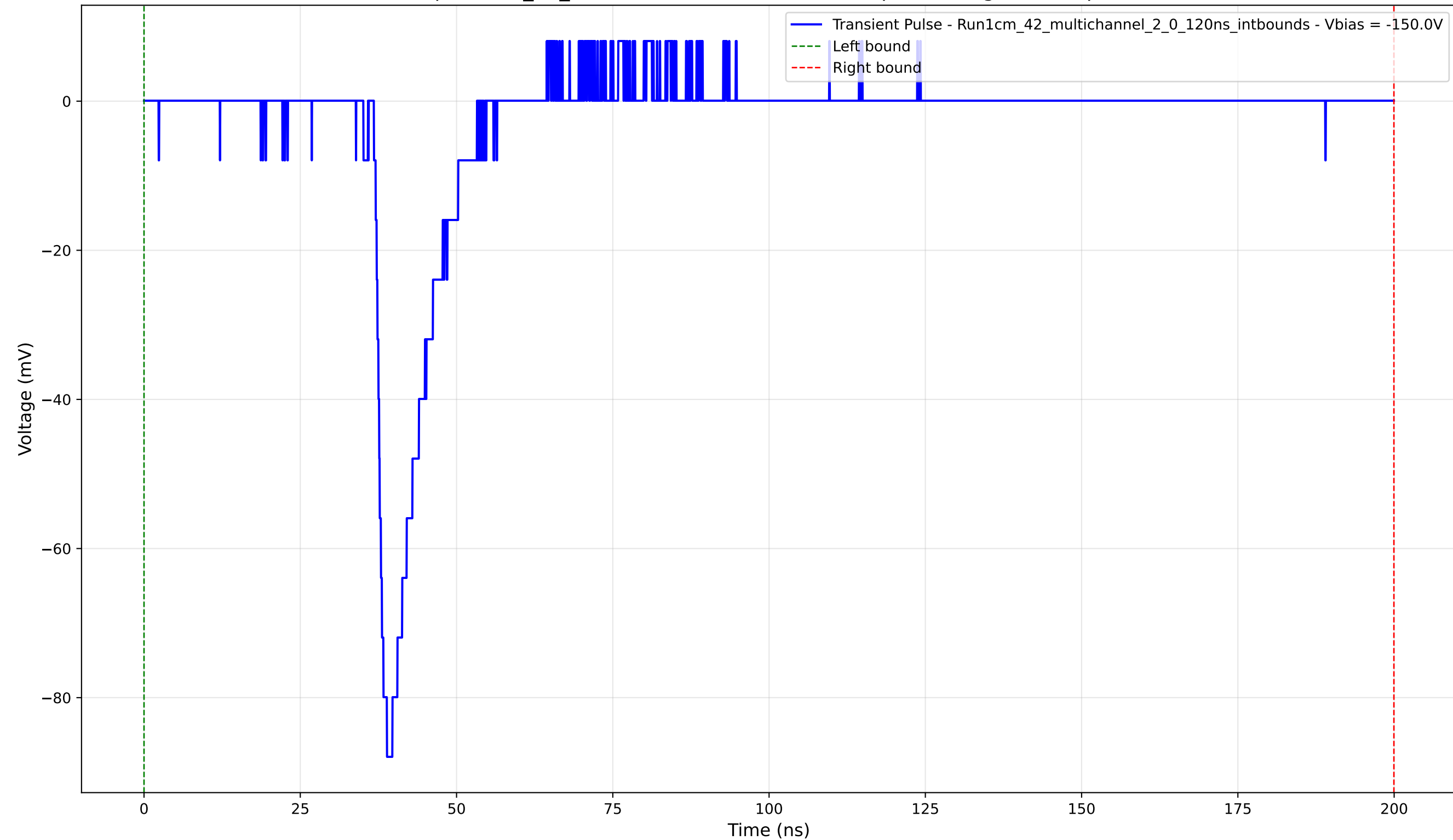
Transient Pulse - Sample: 1cm_42_multichannel - Position: 785.0 \mu\text{m} - Charge: 11.20 pC - Rise Time: 1.28 ns
