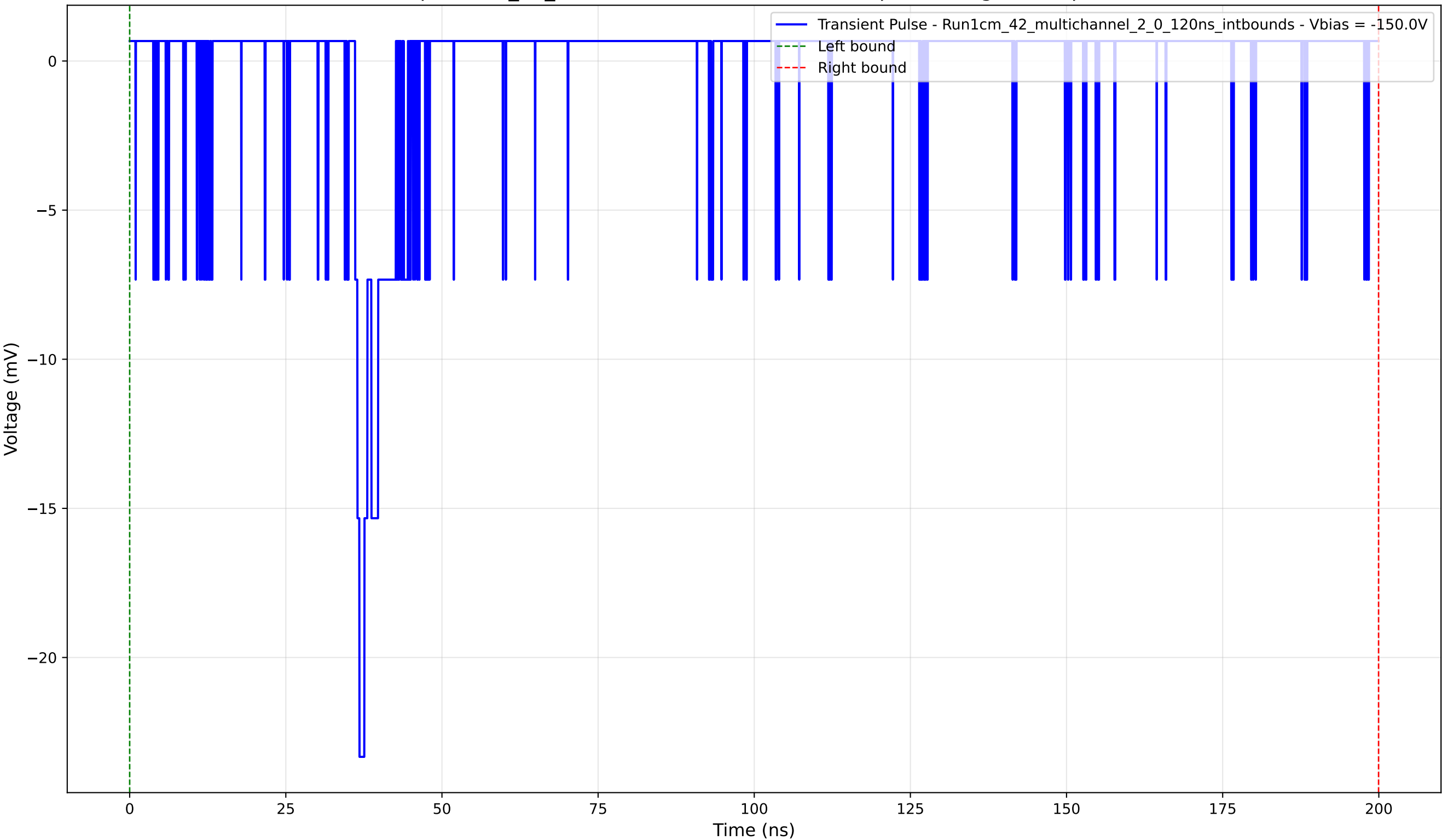
Transient Pulse - Sample: 1cm_42_multichannel - Position: 2370.0 \mu\text{m} - Charge: 0.56 pC - Rise Time: 0.71 ns
