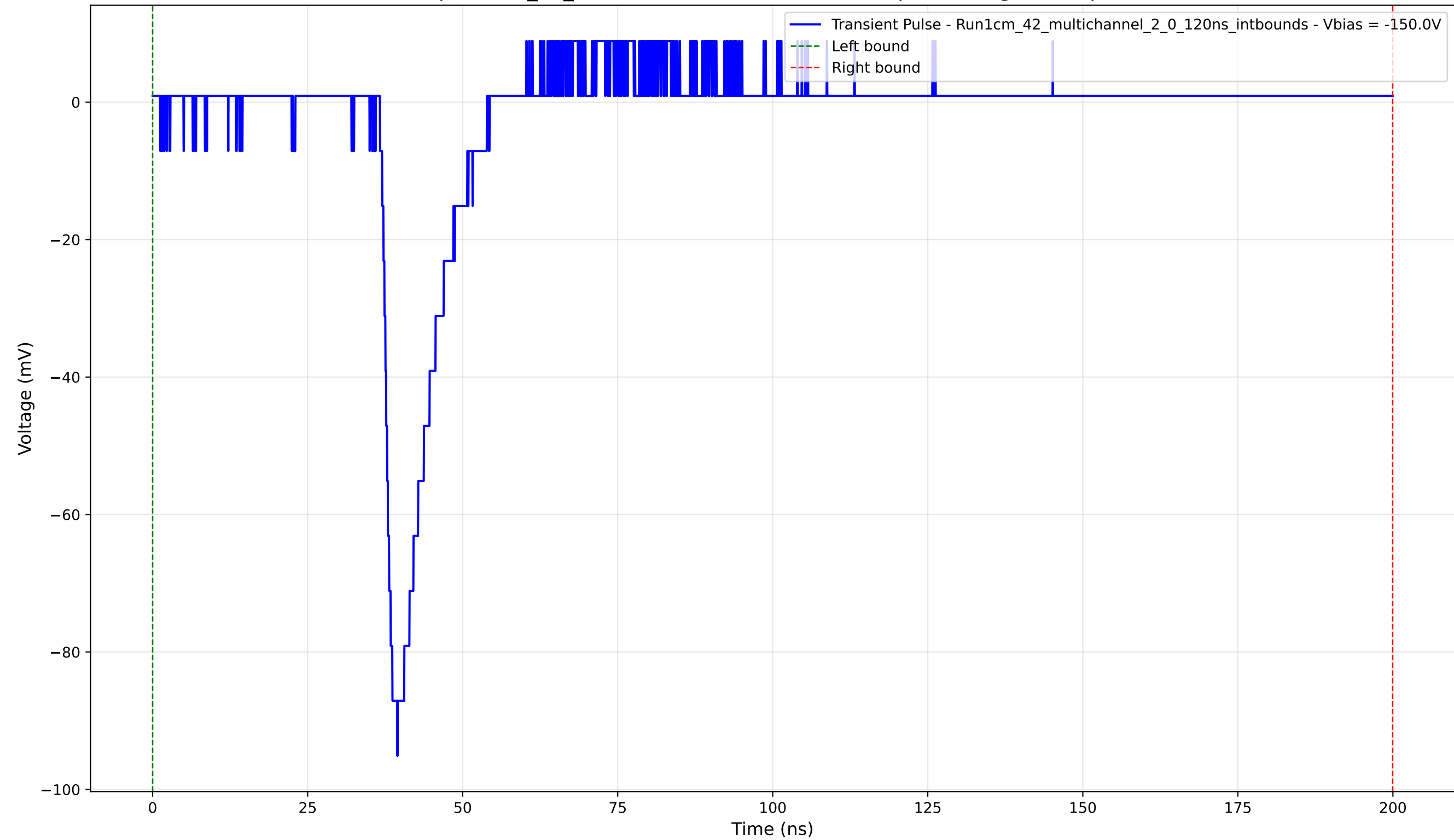
Transient Pulse - Sample: 1cm_42_multichannel - Position: 4035.0 \mu\text{m} - Charge: 7.91 pC - Rise Time: 1.67 ns
