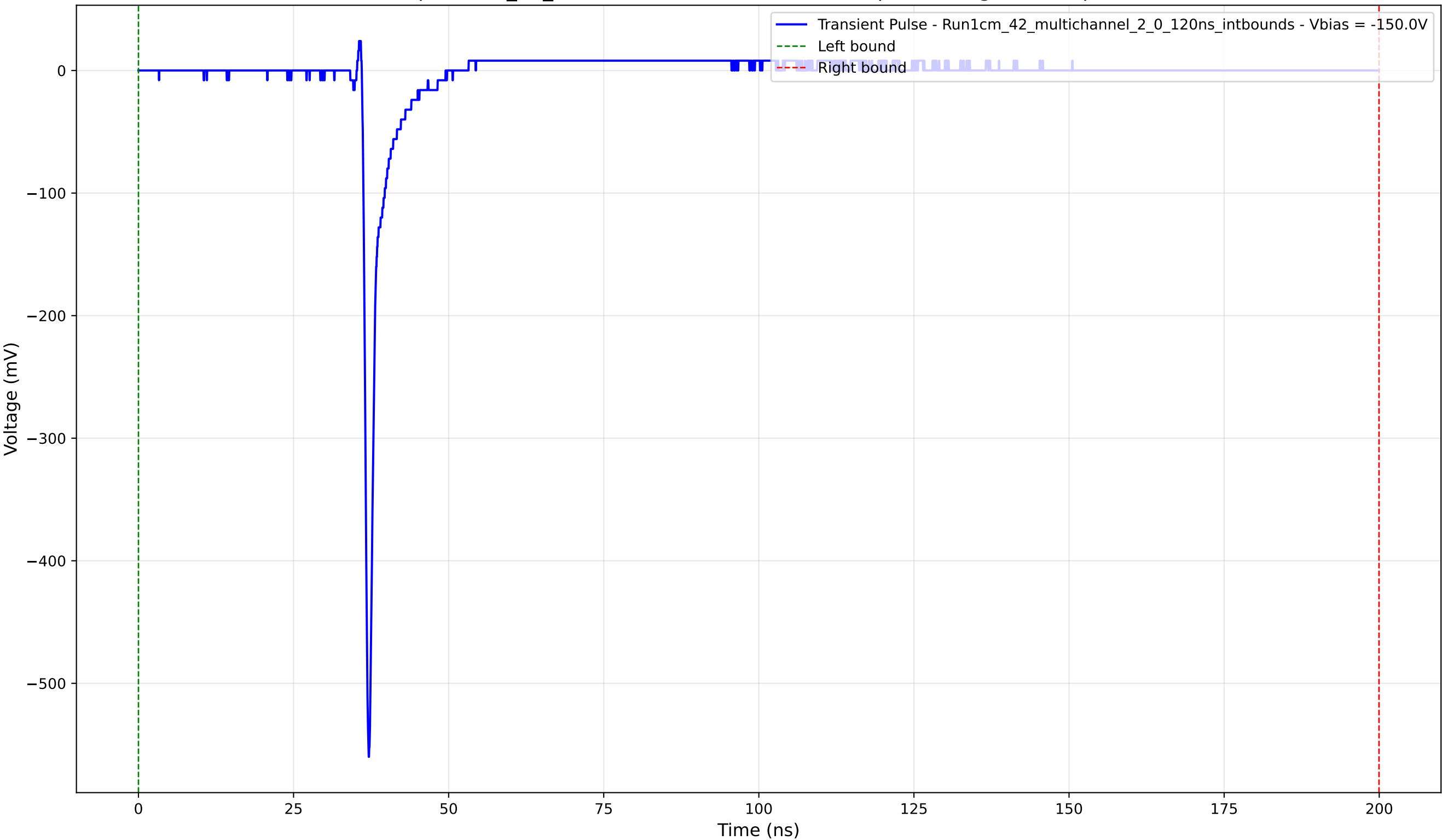
Transient Pulse - Sample: 1cm_42_multichannel - Position: 2300.0 \mu\text{m} - Charge: 15.01 pC - Rise Time: 0.73 ns
