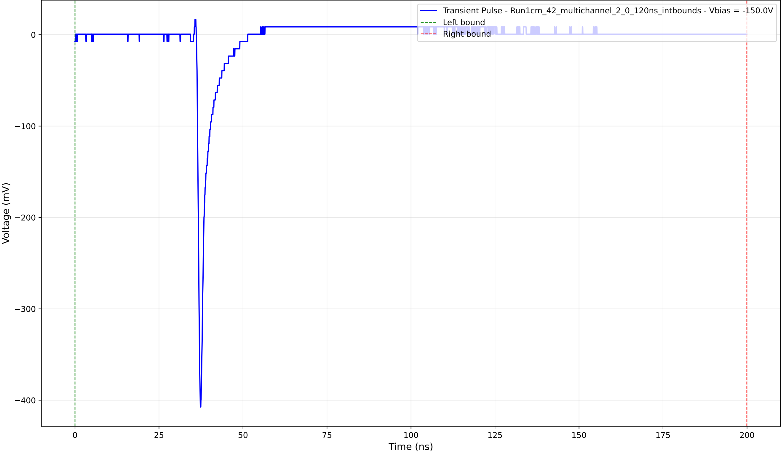
Transient Pulse - Sample: 1cm_42_multichannel - Position: 2745.0 \mu\text{m} - Charge: 11.95 pC - Rise Time: 0.79 ns
