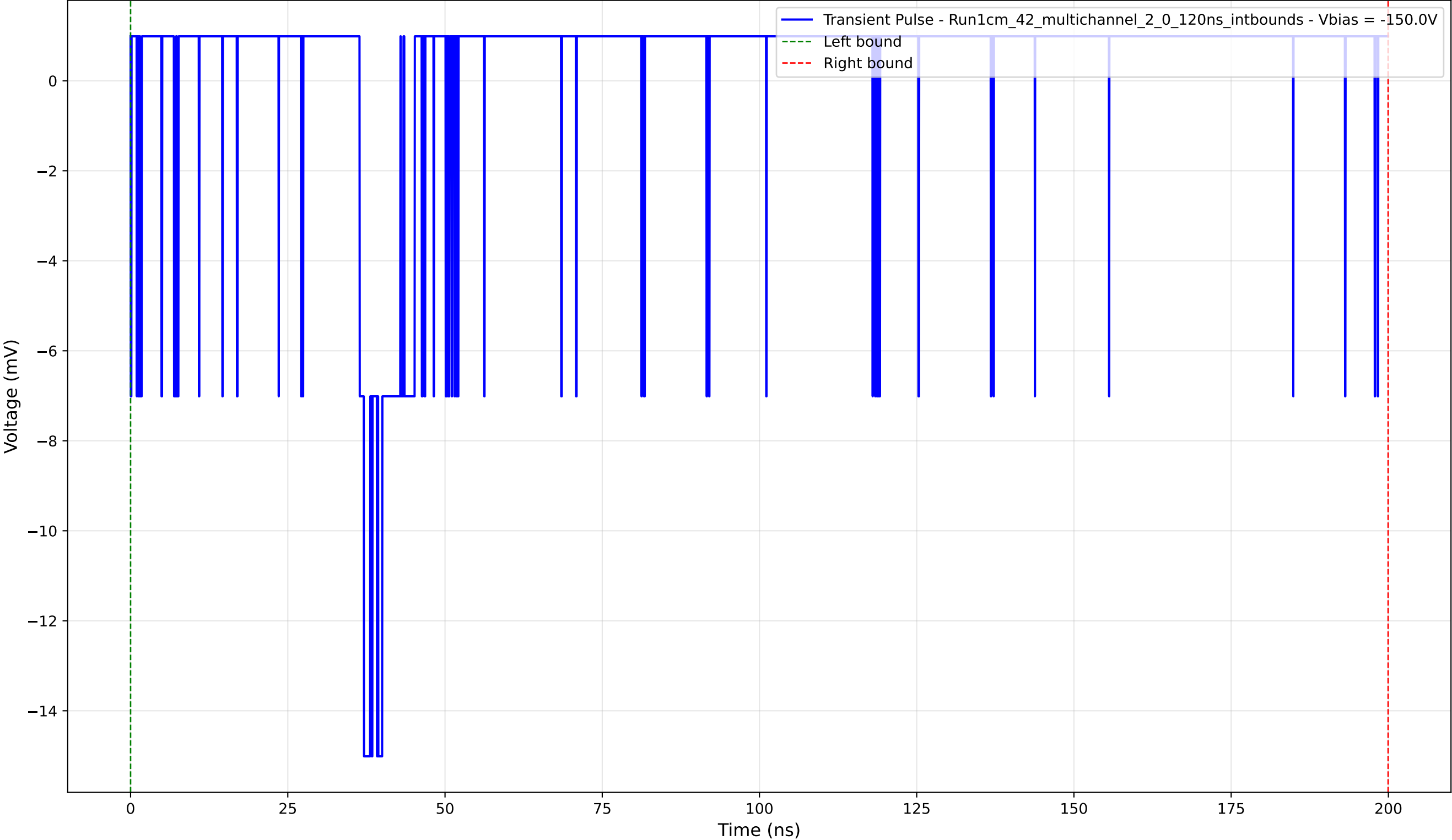
Transient Pulse - Sample: 1cm_42_multichannel - Position: 1860.0 \mu\text{m} - Charge: -1.58 pC - Rise Time: 0.72 ns
