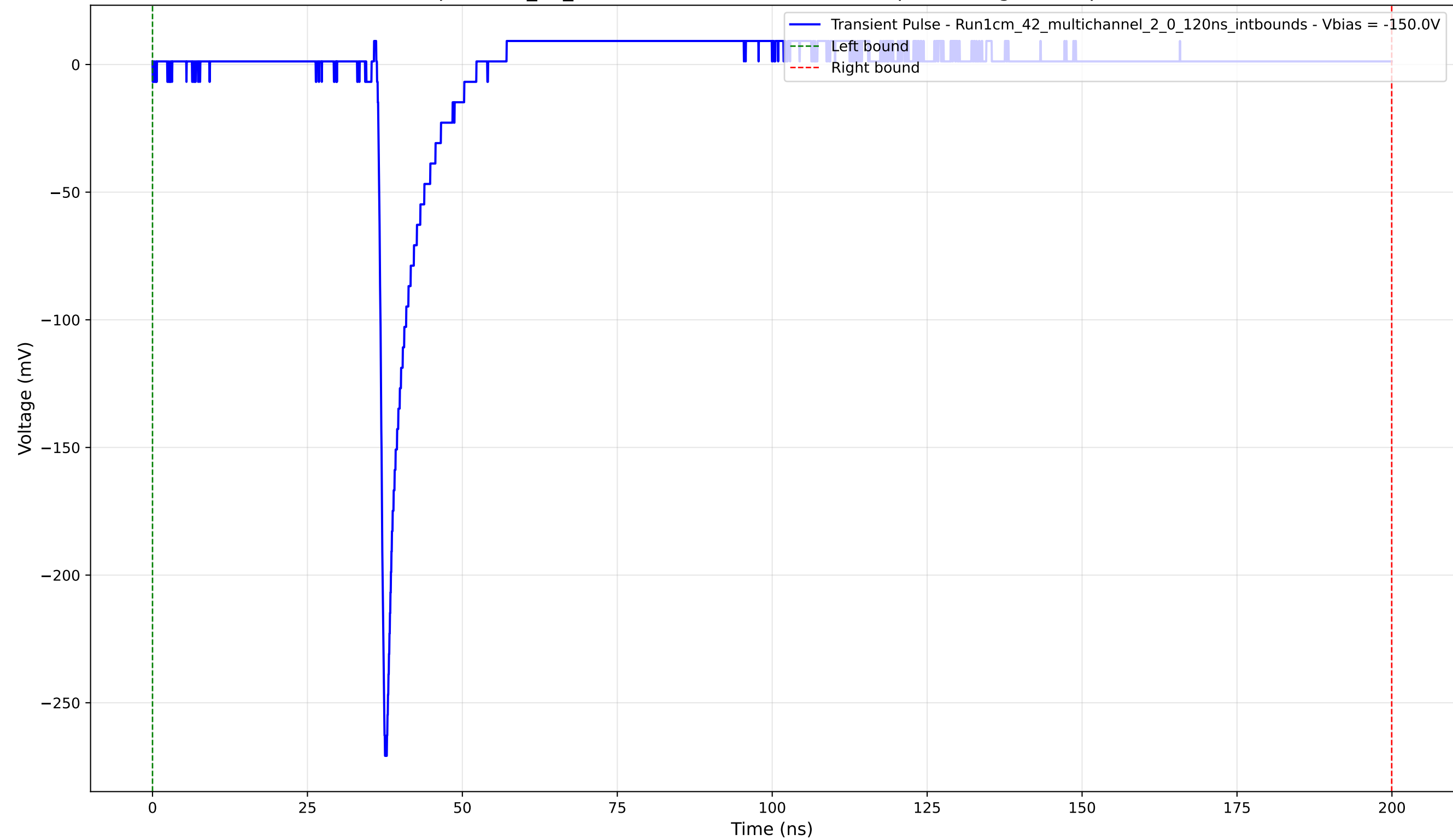
Transient Pulse - Sample: 1cm_42_multichannel - Position: 1690.0 \mu\text{m} - Charge: 9.03 pC - Rise Time: 0.88 ns
