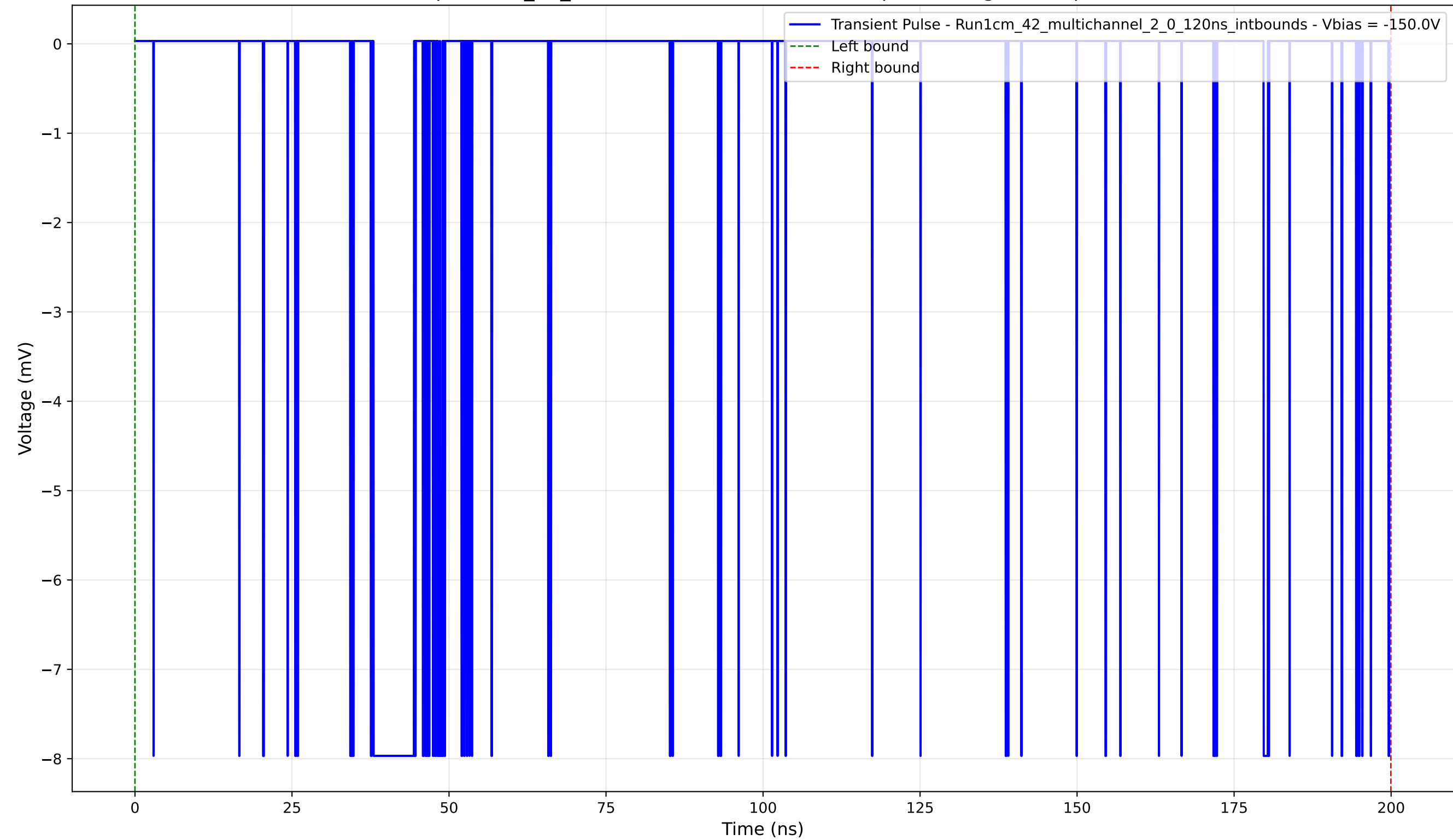
Transient Pulse - Sample: 1cm_42_multichannel - Position: 335.0 \mu\text{m} - Charge: 2.05 pC - Rise Time: 0.04 ns
