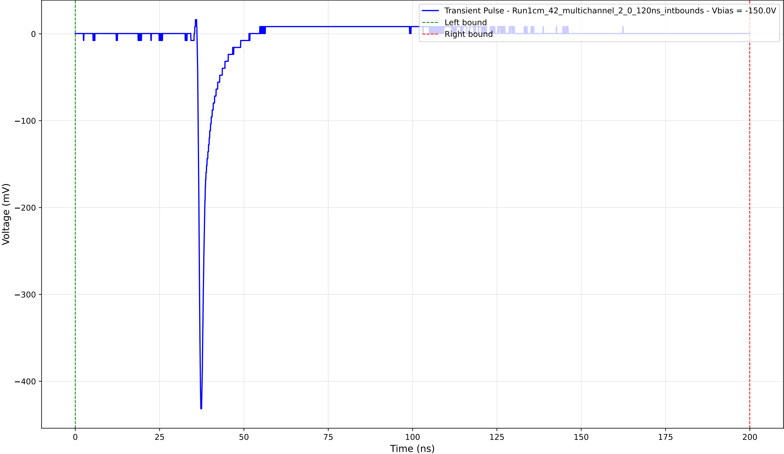
Transient Pulse - Sample: 1cm_42_multichannel - Position: 2695.0 \mu\text{m} - Charge: 13.84 pC - Rise Time: 0.78 ns
