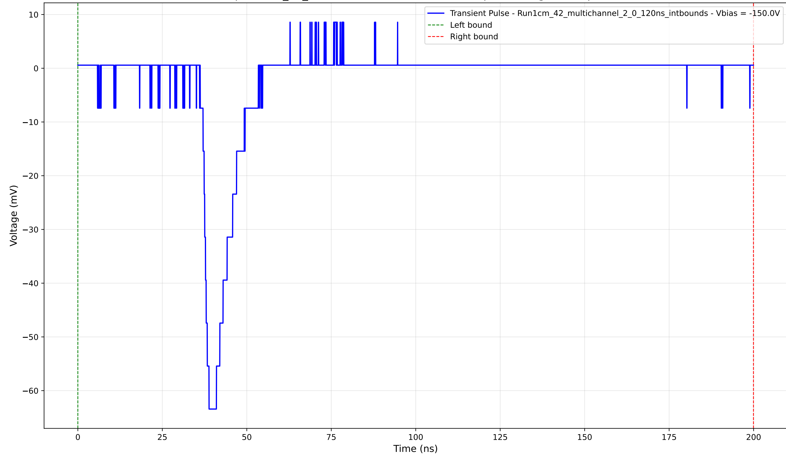
Transient Pulse - Sample: 1cm_42_multichannel - Position: 4760.0 \mu\text{m} - Charge: 8.25 pC - Rise Time: 2.61 ns
