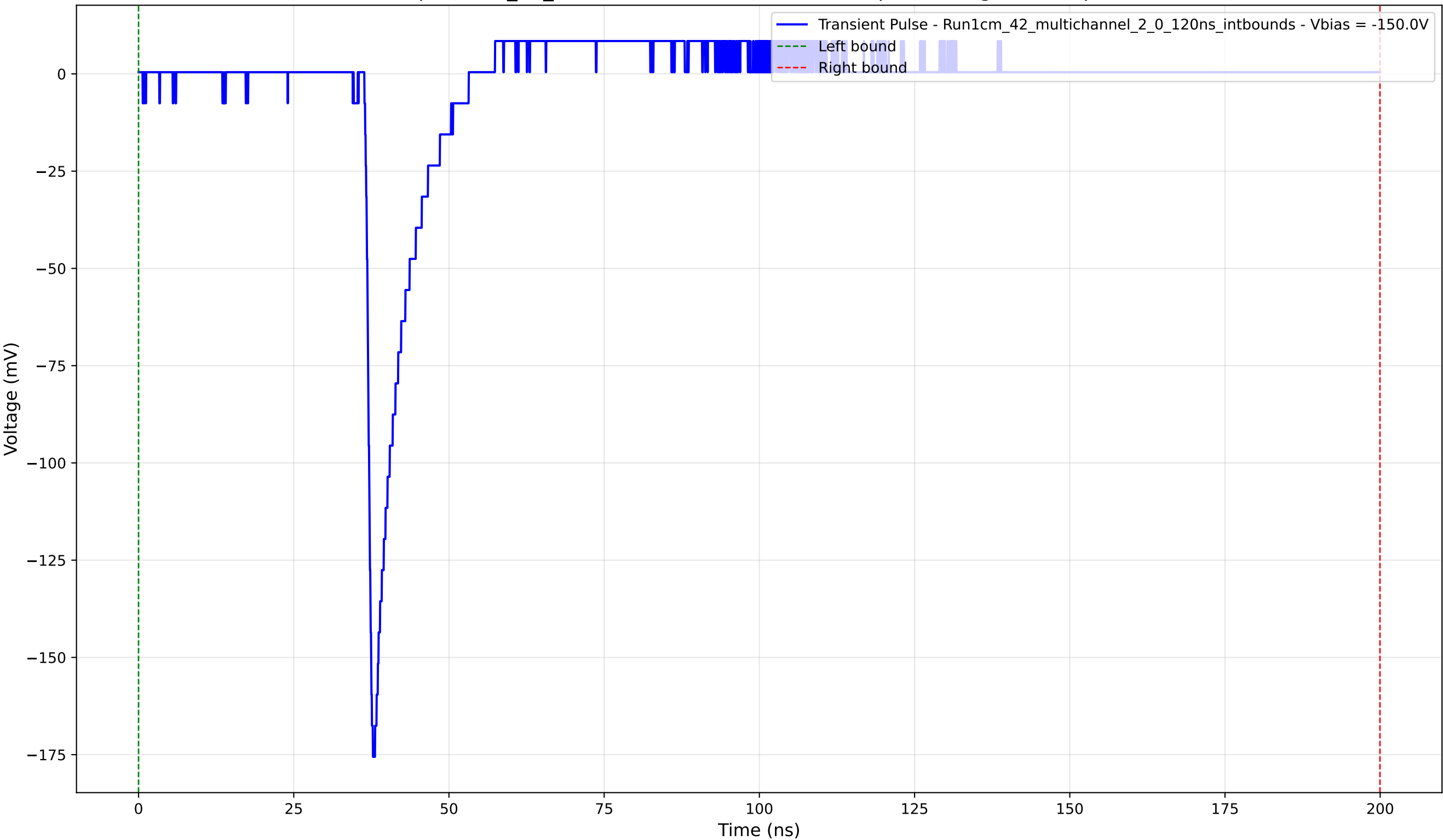
Transient Pulse - Sample: 1cm_42_multichannel - Position: 3280.0 \mu\text{m} - Charge: 10.01 pC - Rise Time: 0.95 ns
