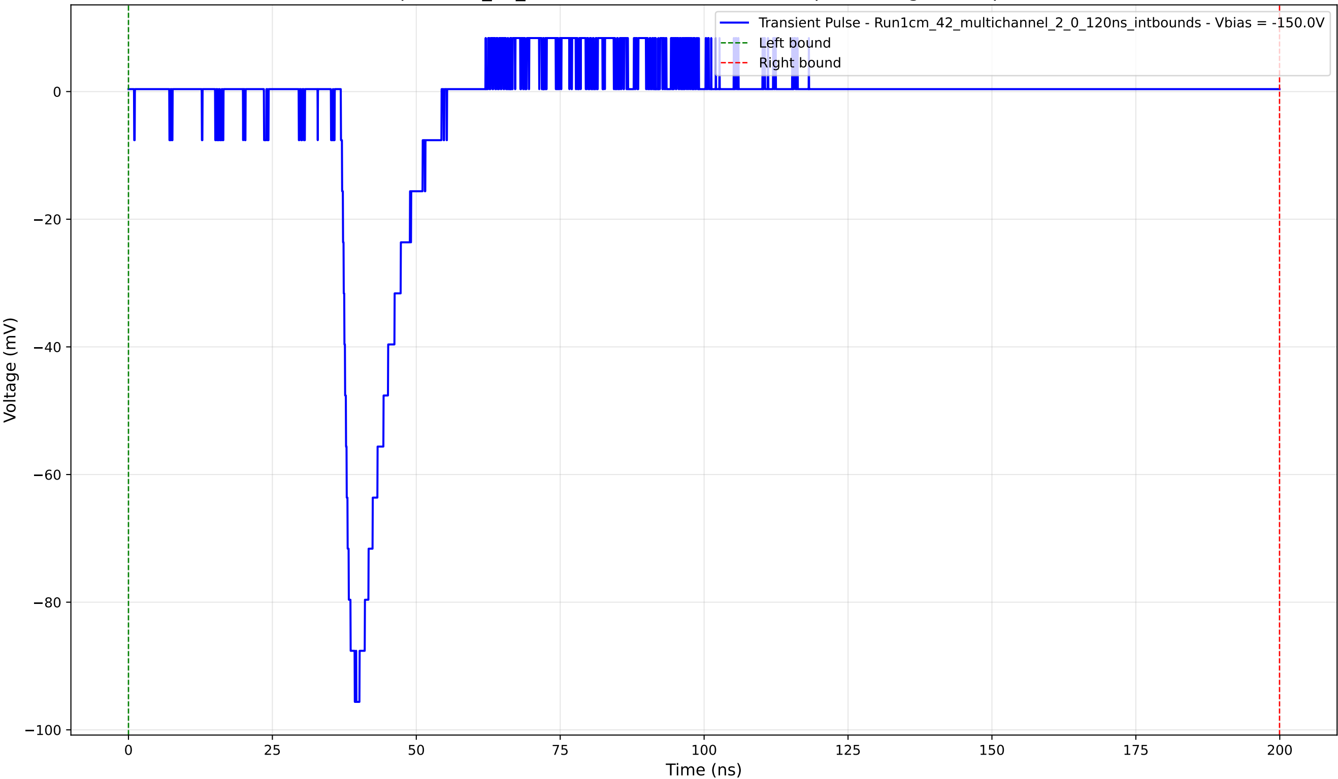
Transient Pulse - Sample: 1cm_42_multichannel - Position: 490.0 \mu\text{m} - Charge: 9.86 pC - Rise Time: 1.51 ns
