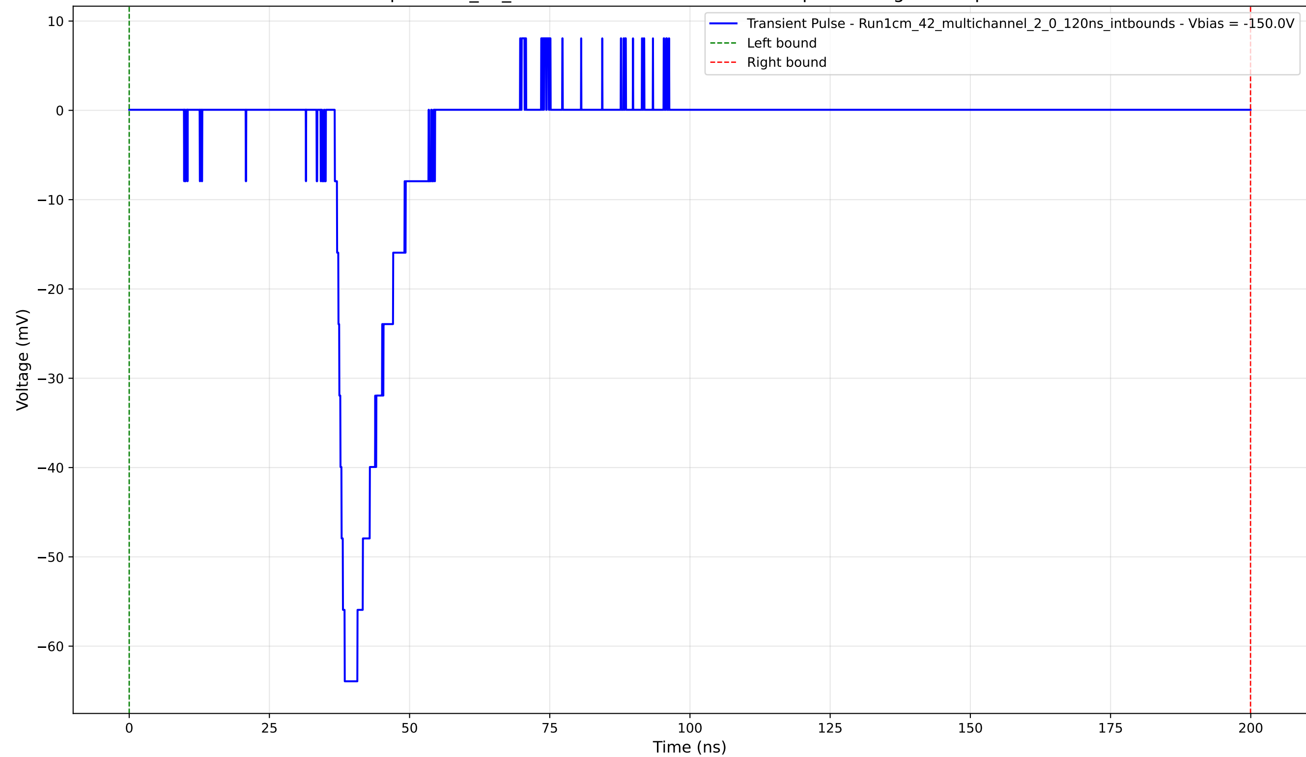
Transient Pulse - Sample: 1cm_42_multichannel - Position: 3945.0 \mu\text{m} - Charge: 9.75 pC - Rise Time: 1.77 ns
