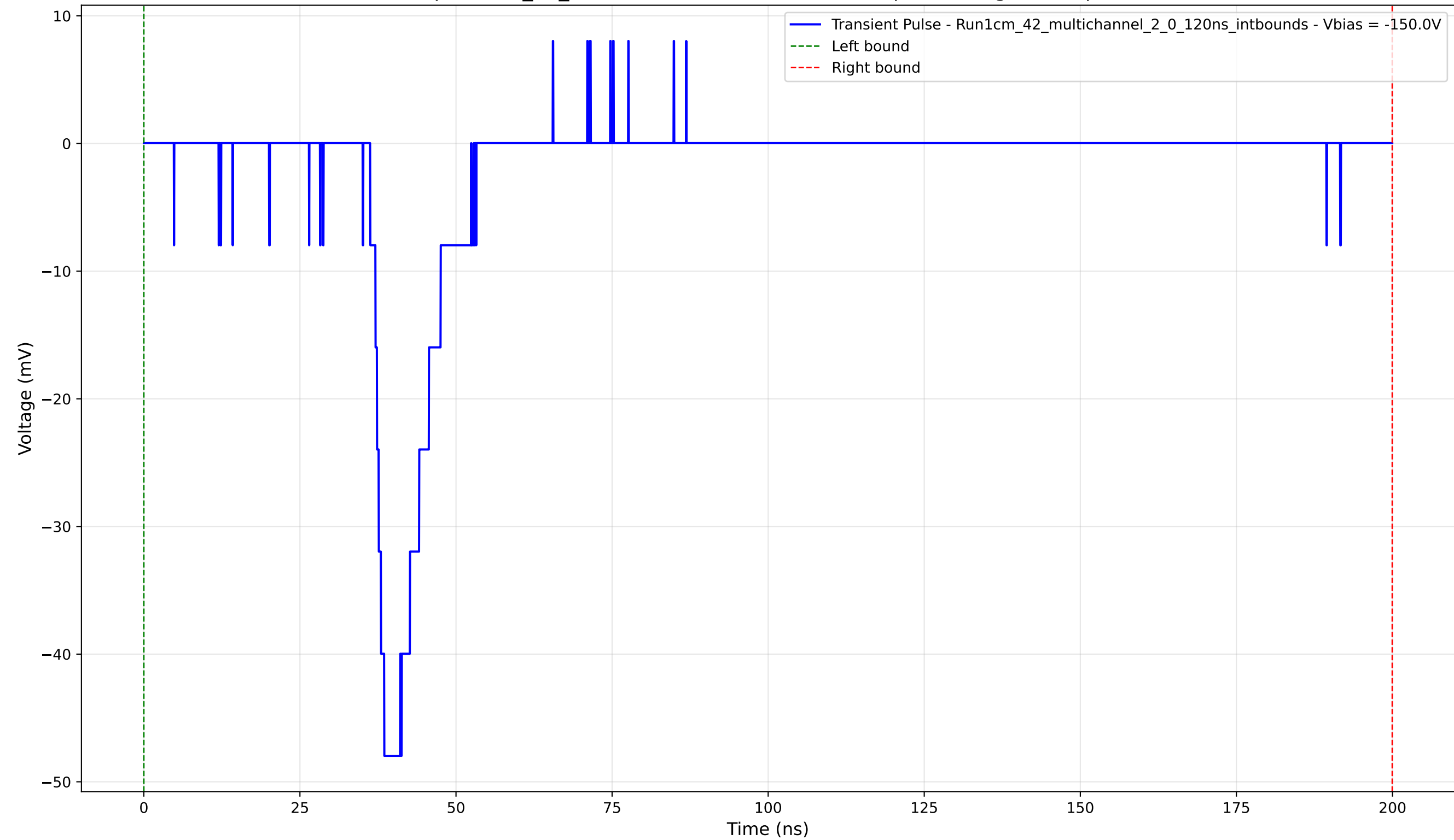
Transient Pulse - Sample: 1cm_42_multichannel - Position: 4830.0 \mu\text{m} - Charge: 7.78 pC - Rise Time: 2.26 ns
