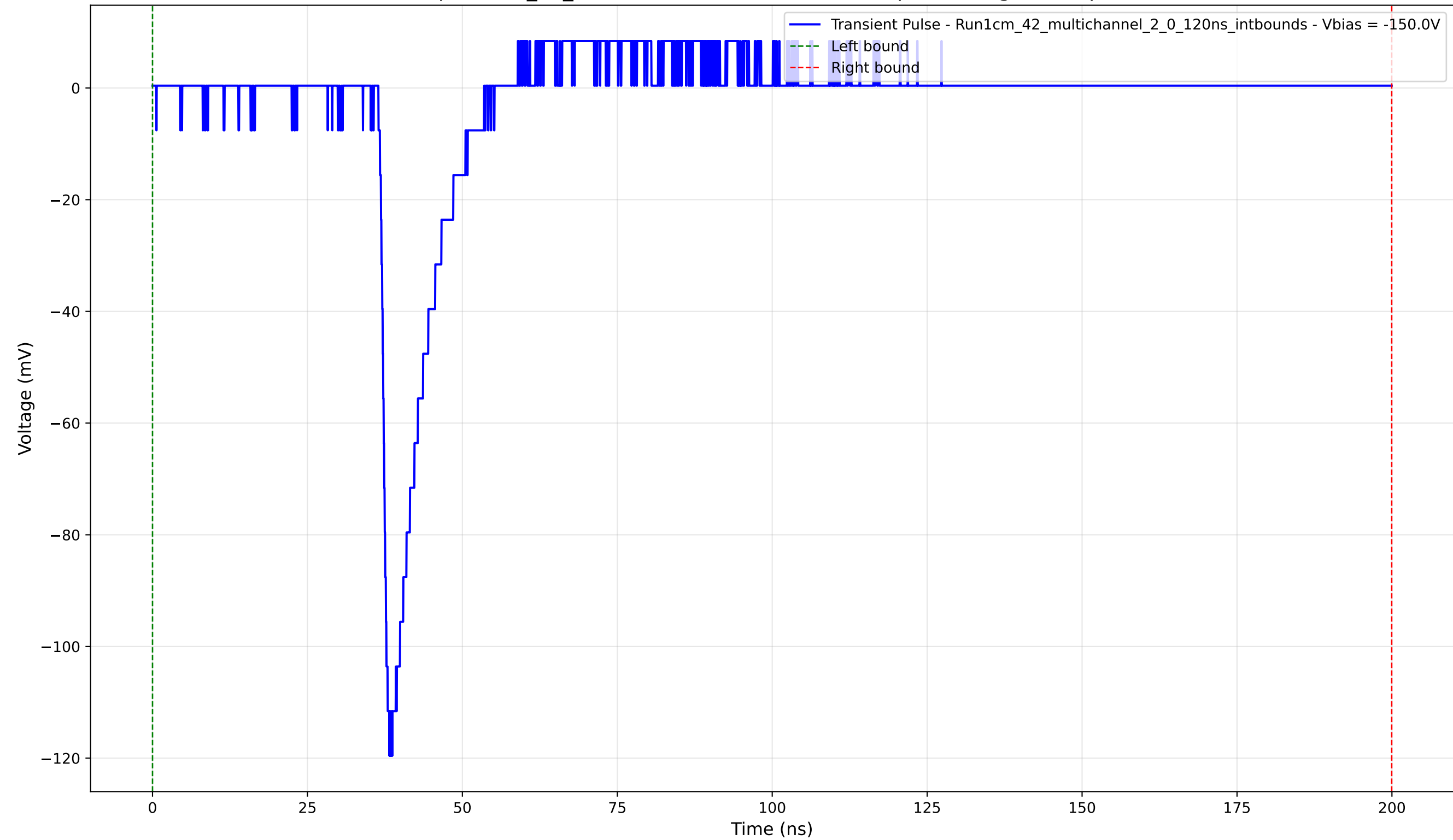
Transient Pulse - Sample: 1cm_42_multichannel - Position: 3585.0 \mu\text{m} - Charge: 9.75 pC - Rise Time: 1.26 ns
