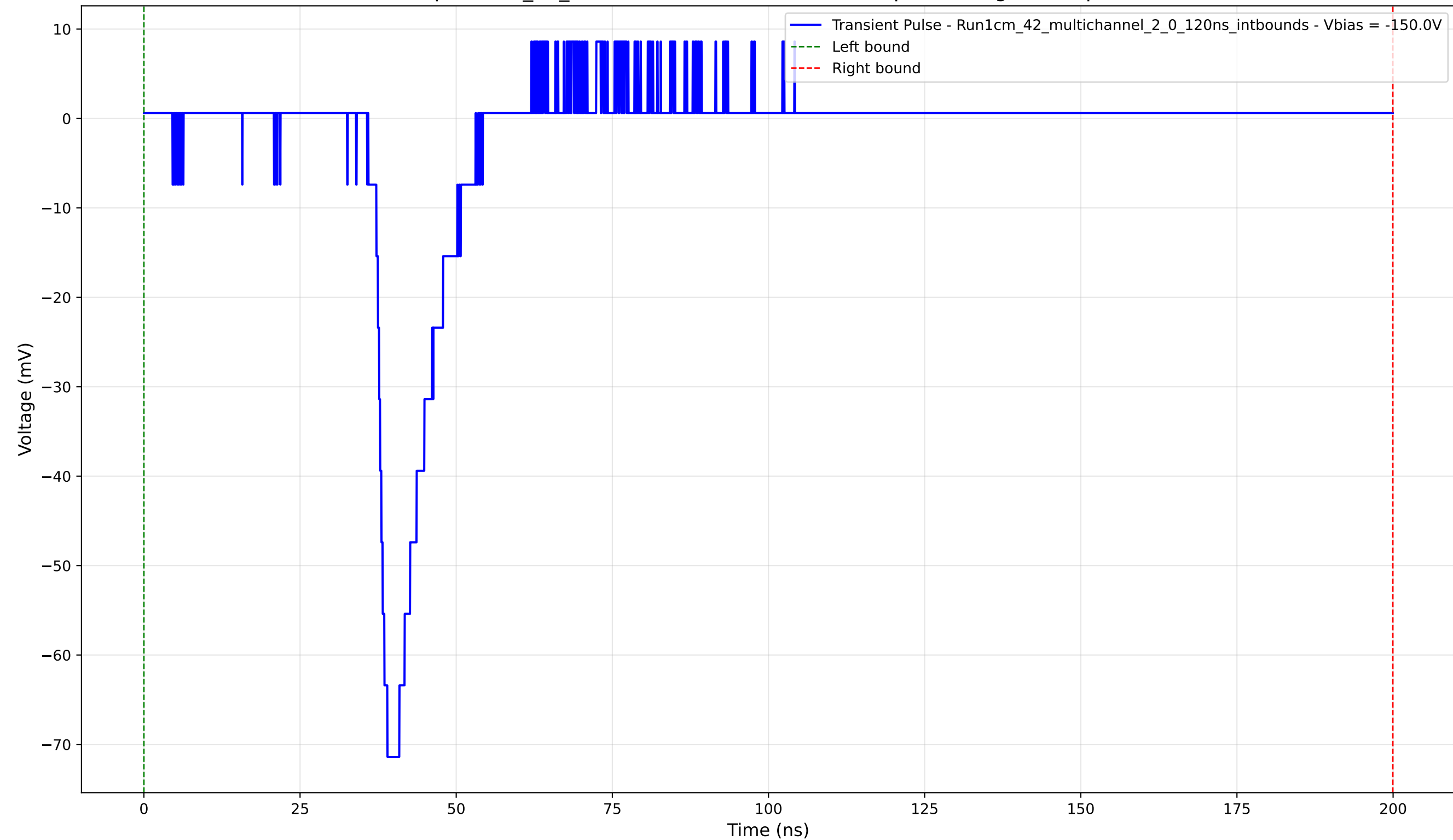
Transient Pulse - Sample: 1cm_42_multichannel - Position: 4560.0 \mu\text{m} - Charge: 7.79 pC - Rise Time: 3.04 ns
