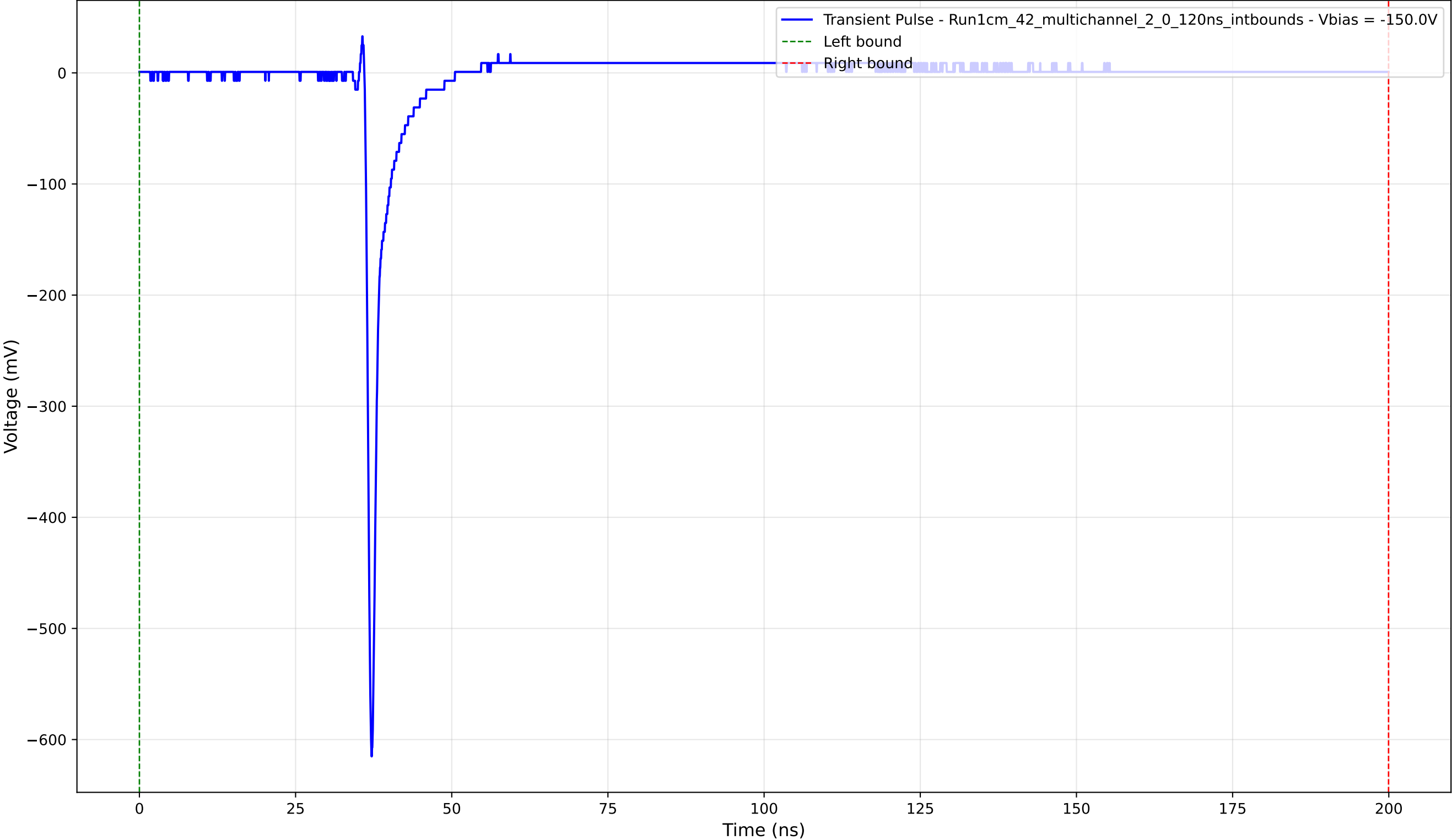
Transient Pulse - Sample: 1cm_42_multichannel - Position: 2235.0 \mu\text{m} - Charge: 14.66 pC - Rise Time: 0.75 ns
