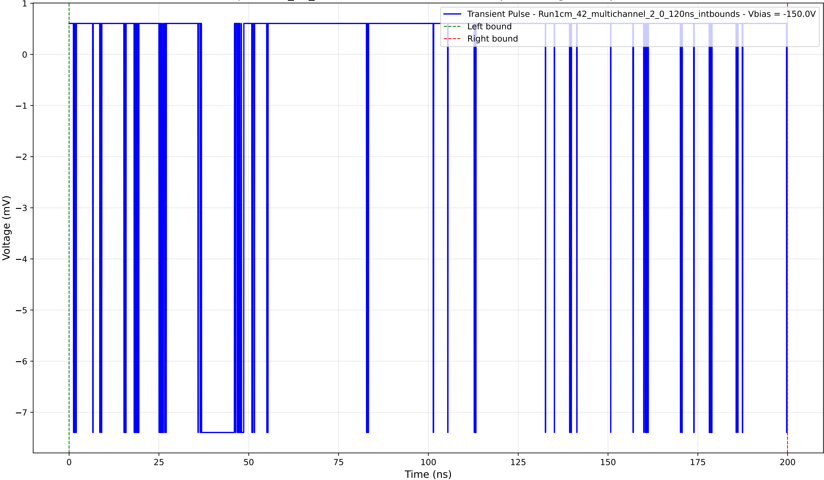
Transient Pulse - Sample: 1cm_42_multichannel - Position: 3395.0 \mu\text{m} - Charge: 0.30 pC - Rise Time: 0.04 ns
