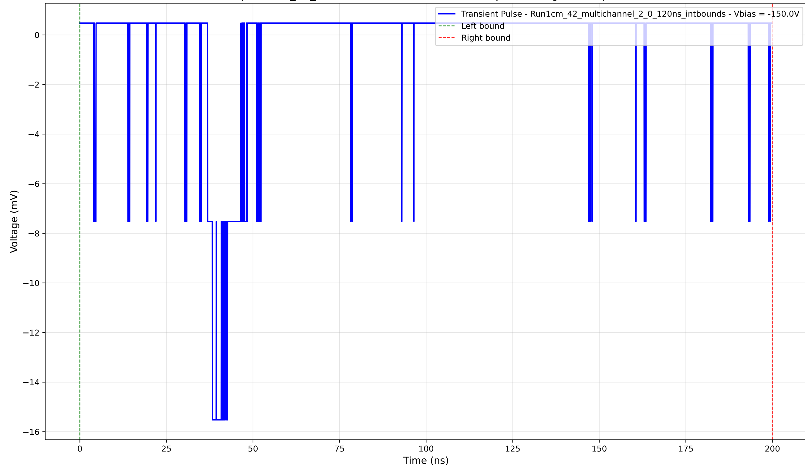
Transient Pulse - Sample: 1cm_42_multichannel - Position: 4865.0 \mu\text{m} - Charge: 1.09 pC - Rise Time: 1.39 ns
