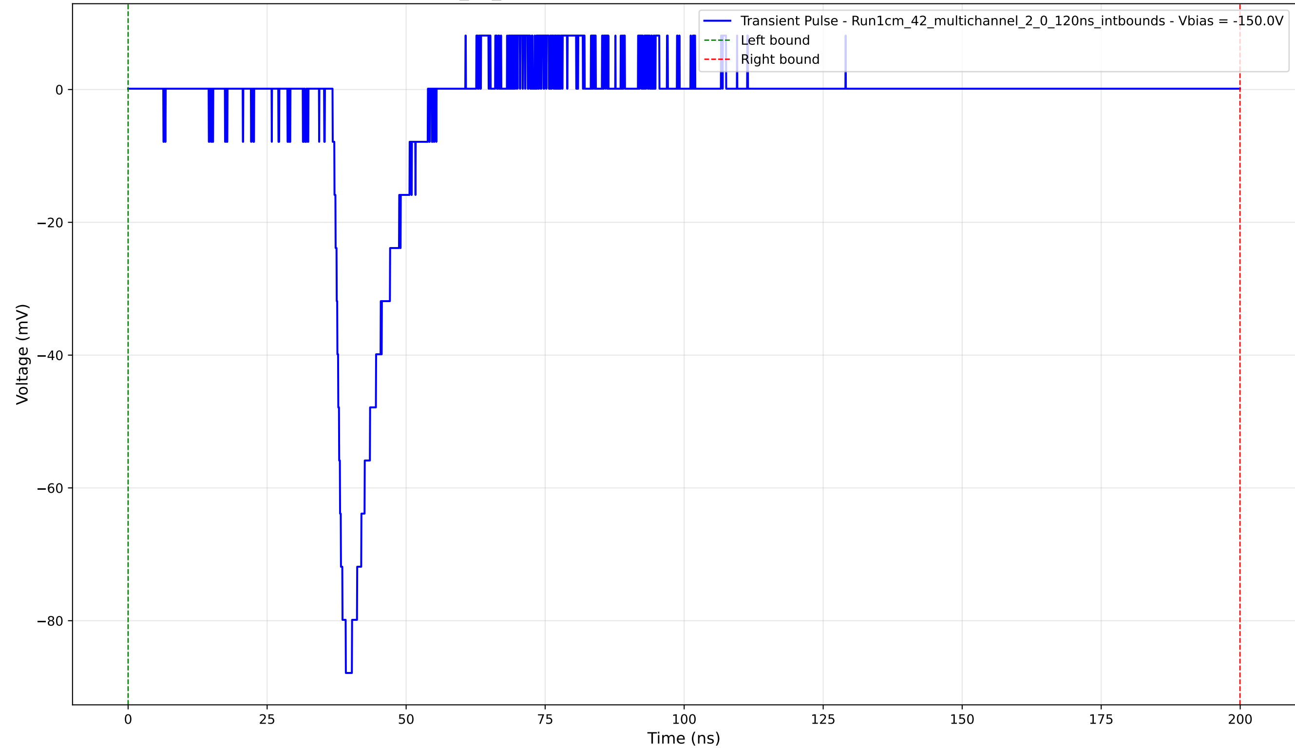
Transient Pulse - Sample: 1cm_42_multichannel - Position: 4110.0 \mu\text{m} - Charge: 10.49 pC - Rise Time: 1.48 ns
