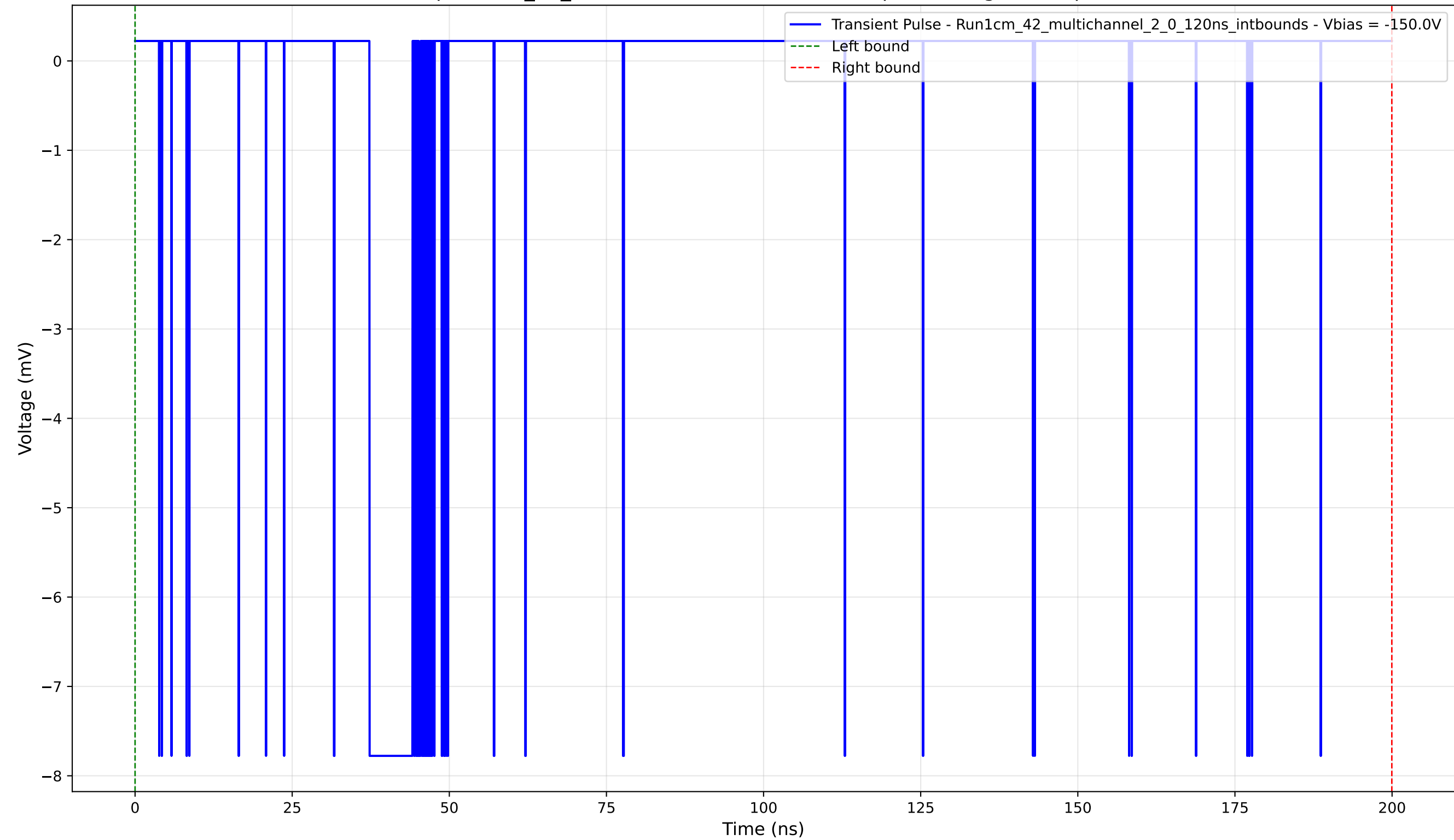
Transient Pulse - Sample: 1cm_42_multichannel - Position: 325.0 \mu\text{m} - Charge: 0.78 pC - Rise Time: 0.04 ns
