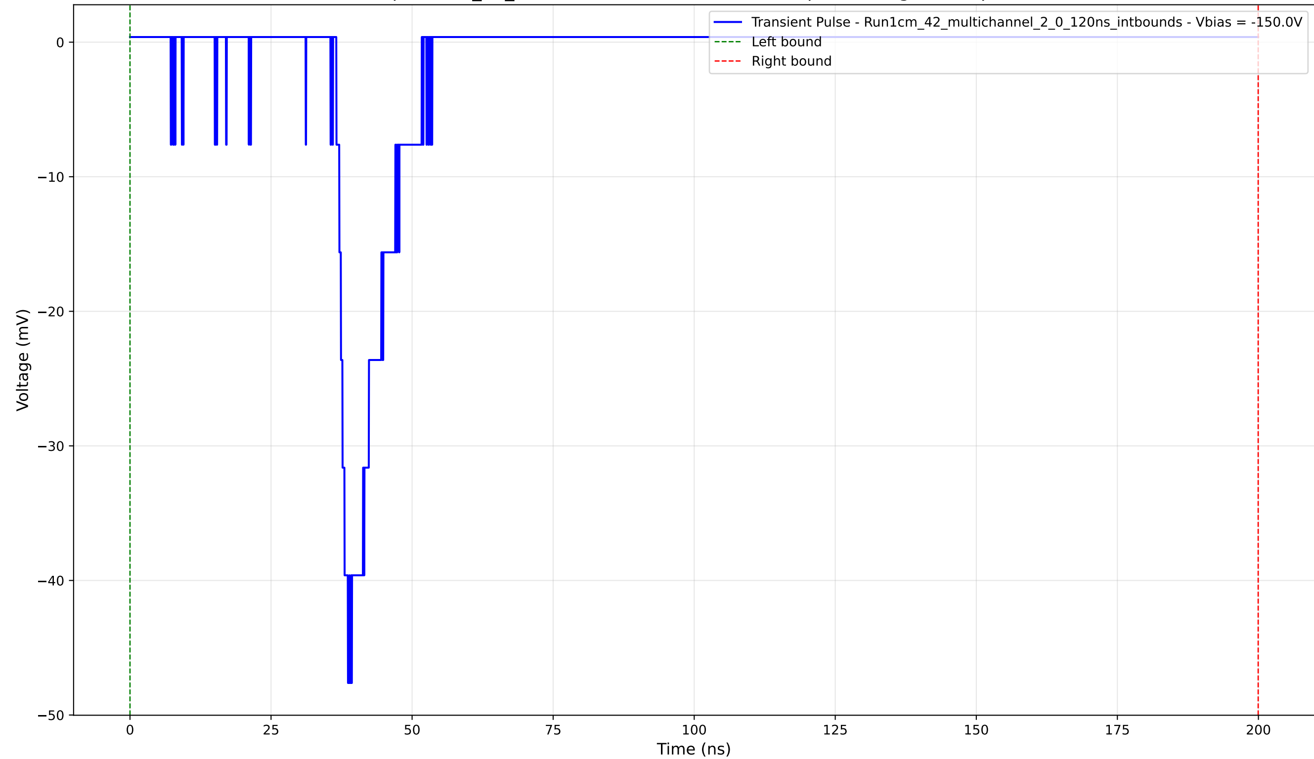
Transient Pulse - Sample: 1cm_42_multichannel - Position: 3840.0 \mu\text{m} - Charge: 5.36 pC - Rise Time: 2.06 ns
