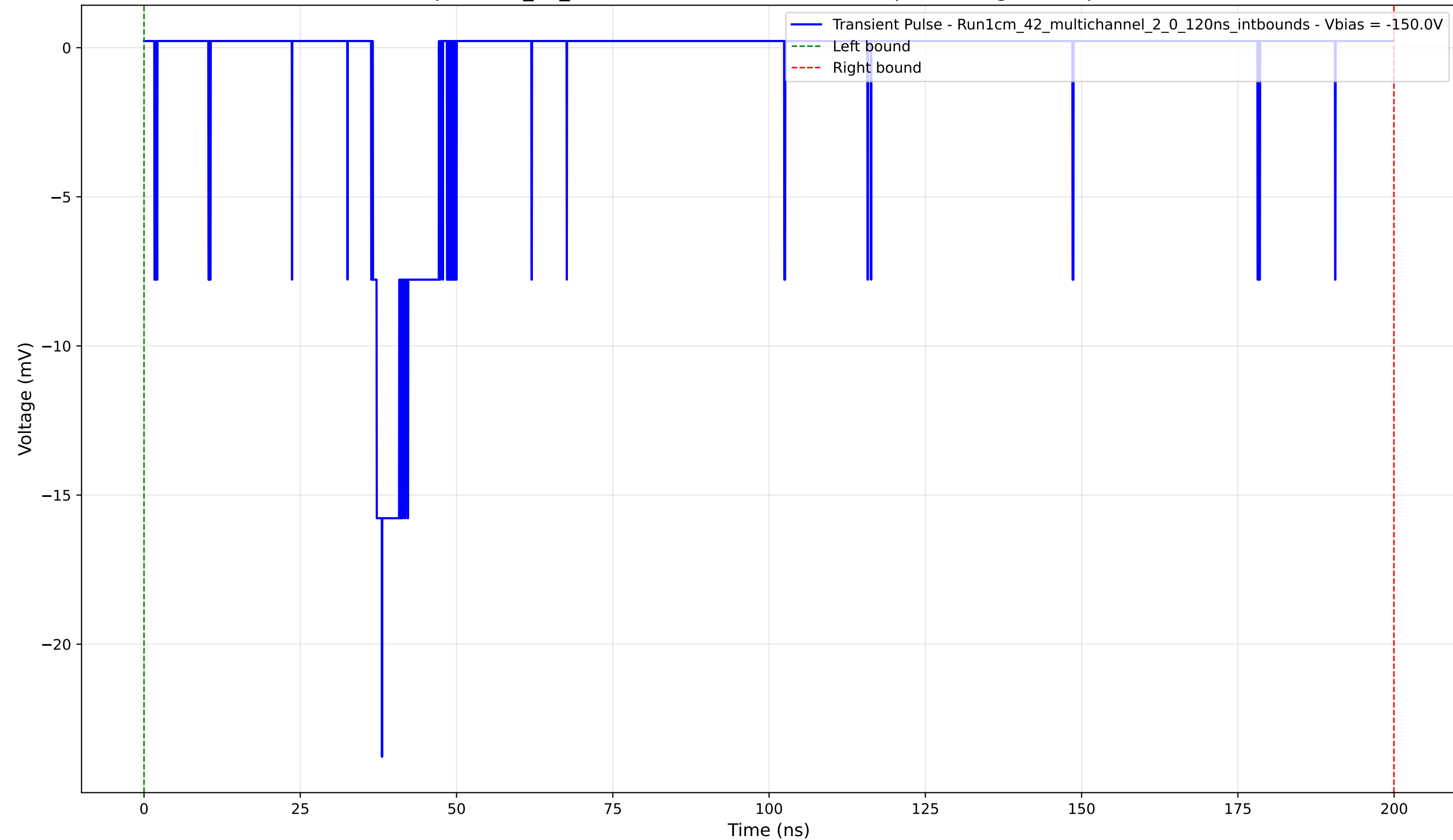
Transient Pulse - Sample: 1cm_42_multichannel - Position: 1380.0 \mu\text{m} - Charge: 1.89 pC - Rise Time: 1.47 ns
