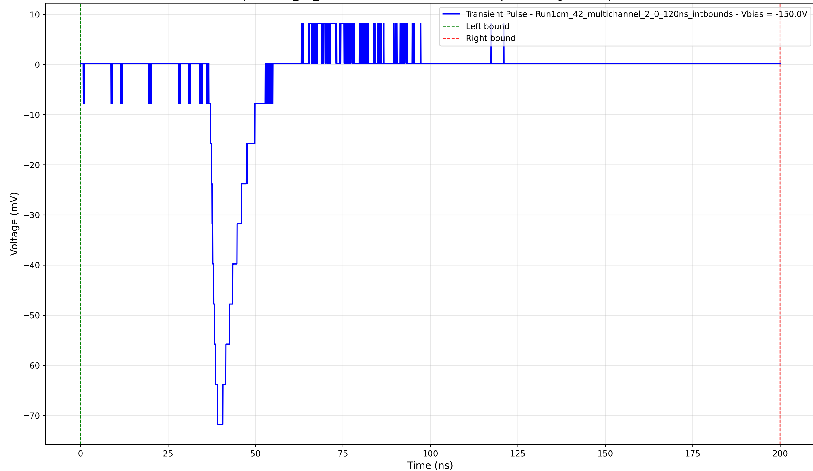
Transient Pulse - Sample: 1cm_42_multichannel - Position: 4635.0 \mu\text{m} - Charge: 8.52 pC - Rise Time: 2.56 ns
