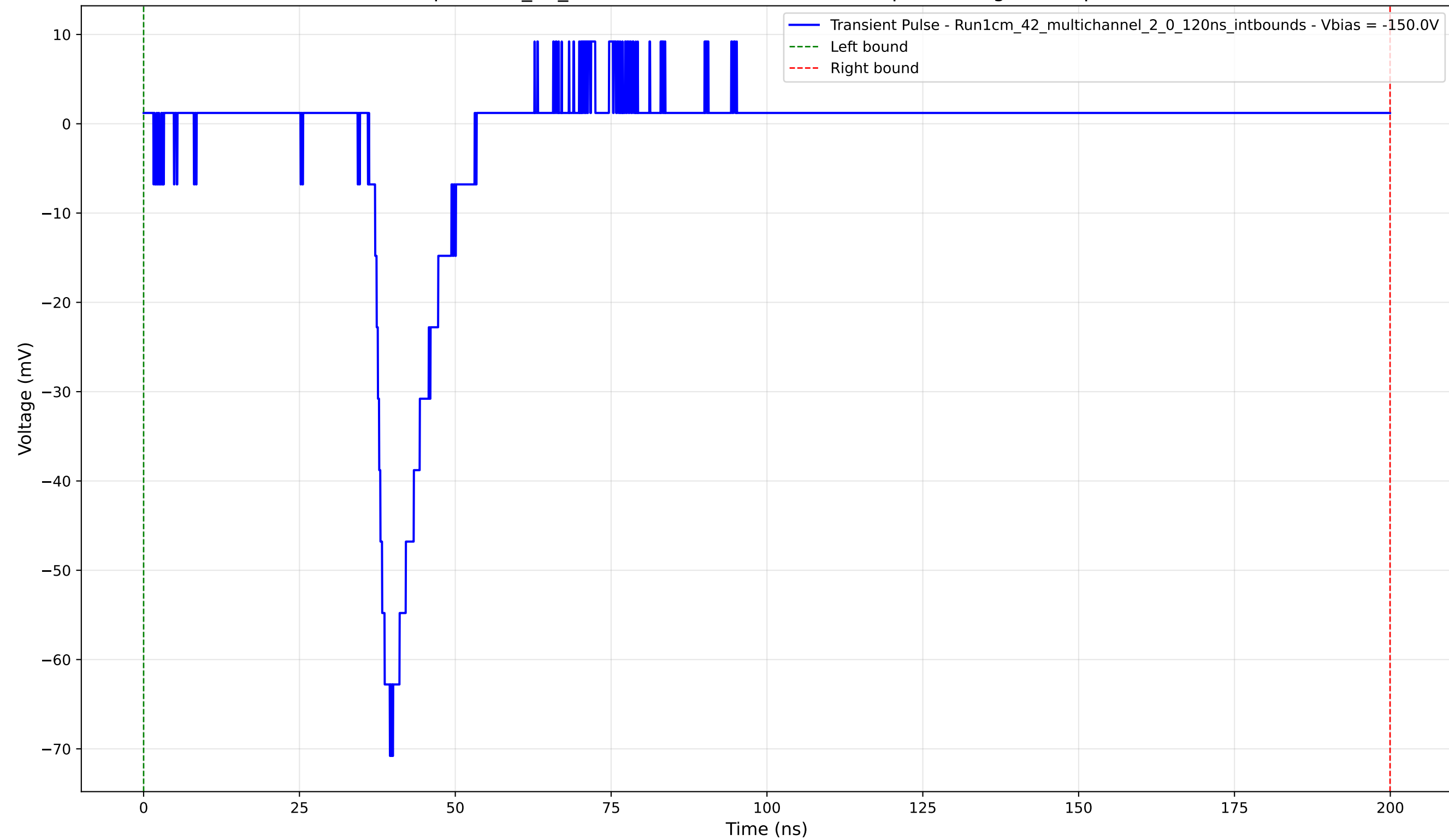
Transient Pulse - Sample: 1cm_42_multichannel - Position: 4735.0 \mu\text{m} - Charge: 5.10 pC - Rise Time: 2.40 ns
