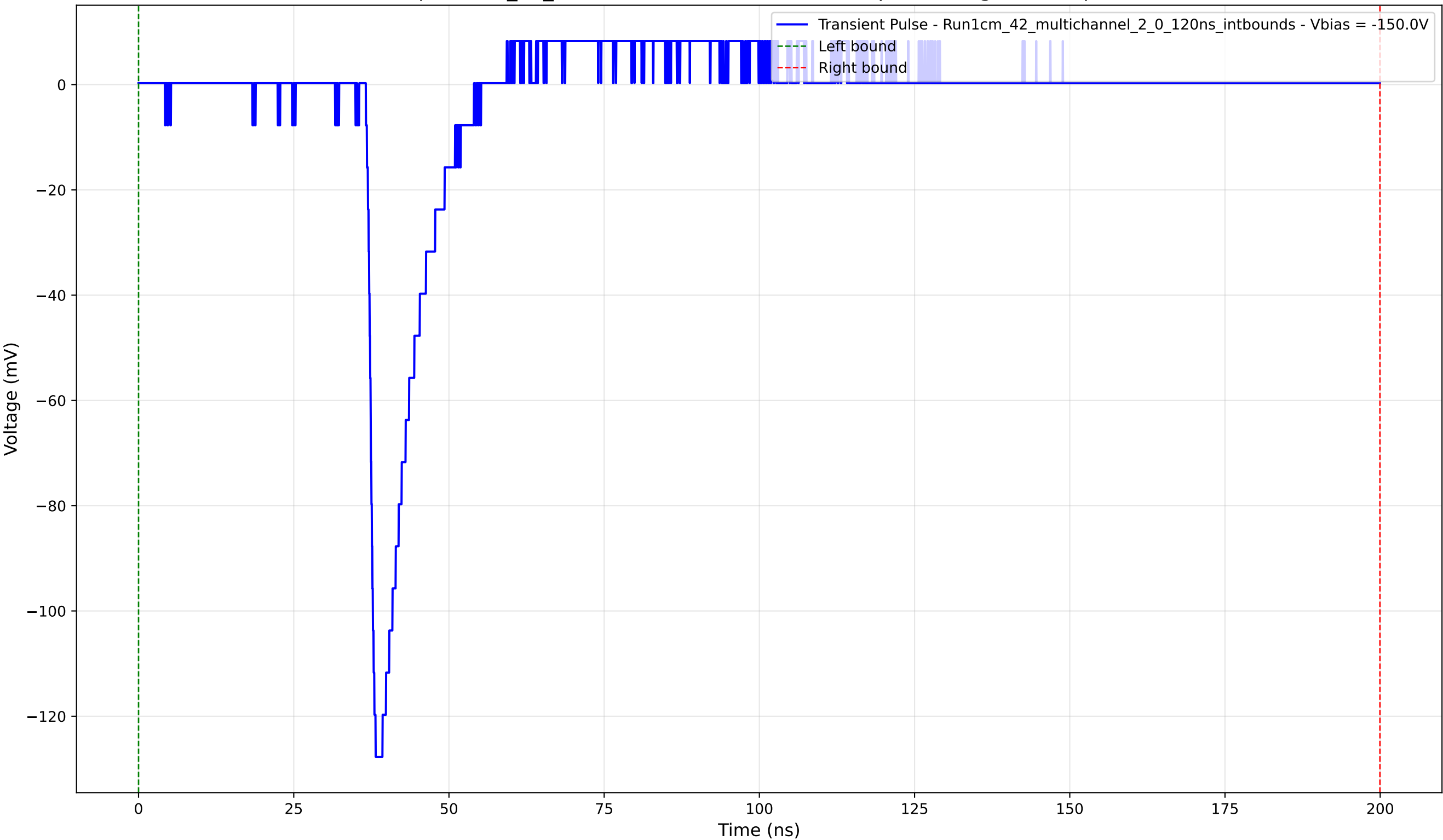
Transient Pulse - Sample: 1cm_42_multichannel - Position: 1050.0 \mu\text{m} - Charge: 10.25 pC - Rise Time: 1.21 ns
