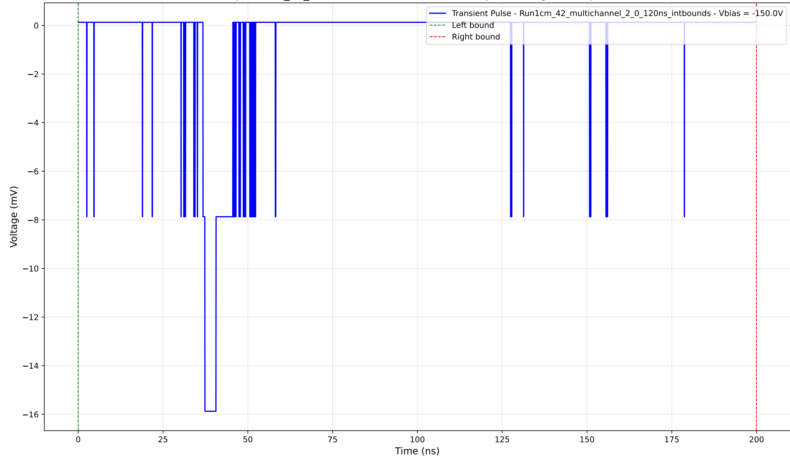
Transient Pulse - Sample: 1cm_42_multichannel - Position: 1335.0 \mu\text{m} - Charge: 2.00 pC - Rise Time: 0.59 ns
