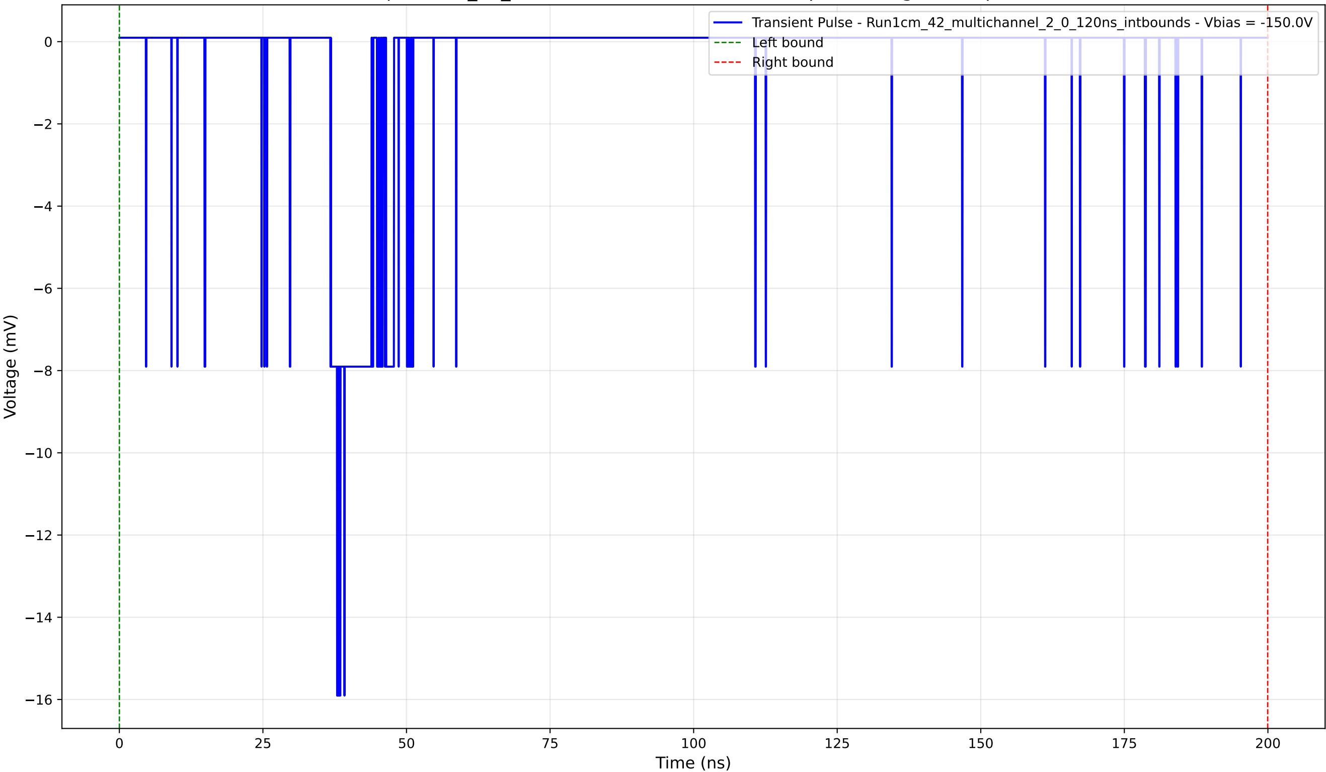
Transient Pulse - Sample: 1cm_42_multichannel - Position: 1345.0 \mu\text{m} - Charge: 1.65 pC - Rise Time: 1.07 ns
