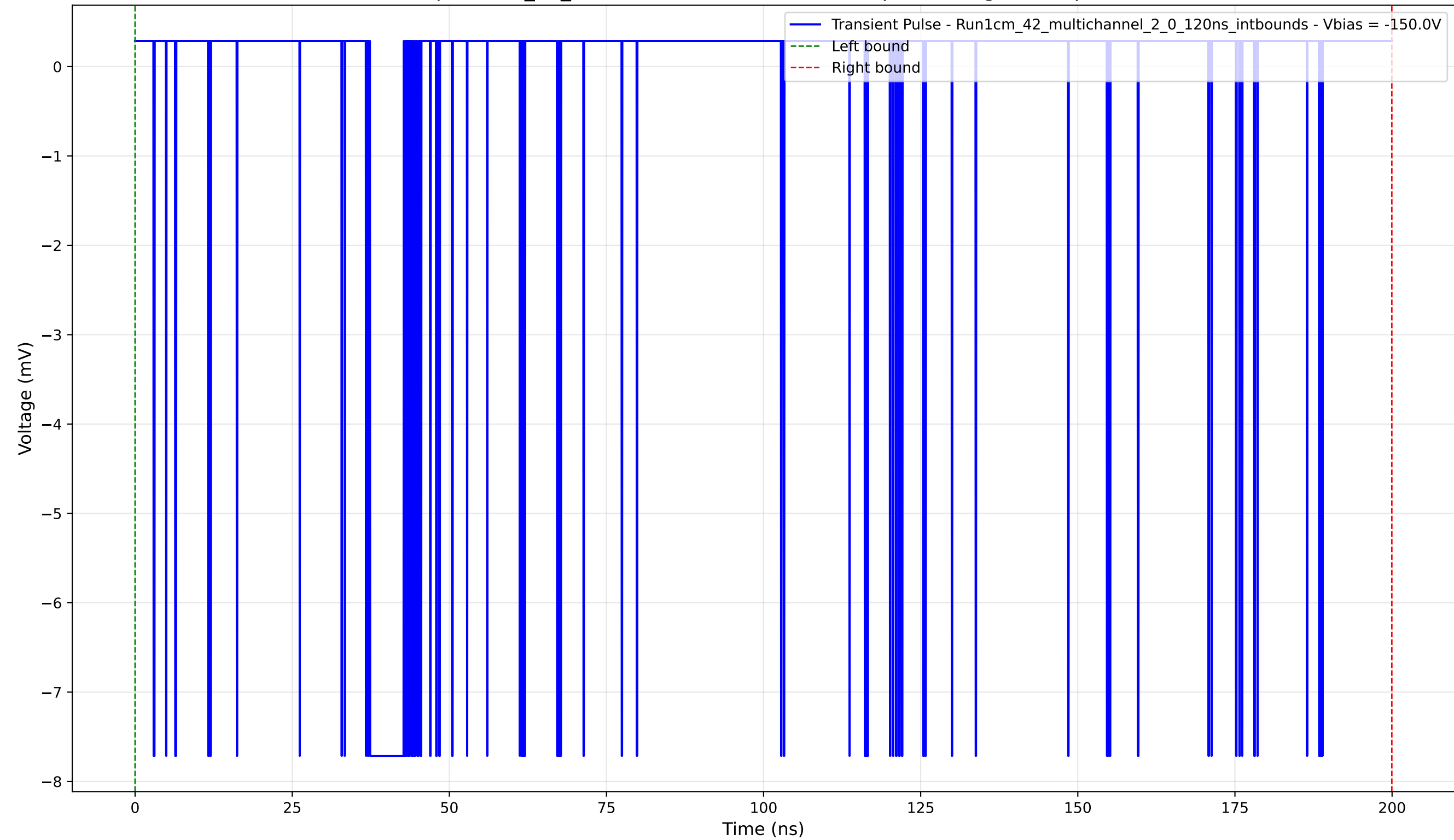
Transient Pulse - Sample: 1cm_42_multichannel - Position: 340.0 \mu\text{m} - Charge: 0.79 pC - Rise Time: 0.04 ns
