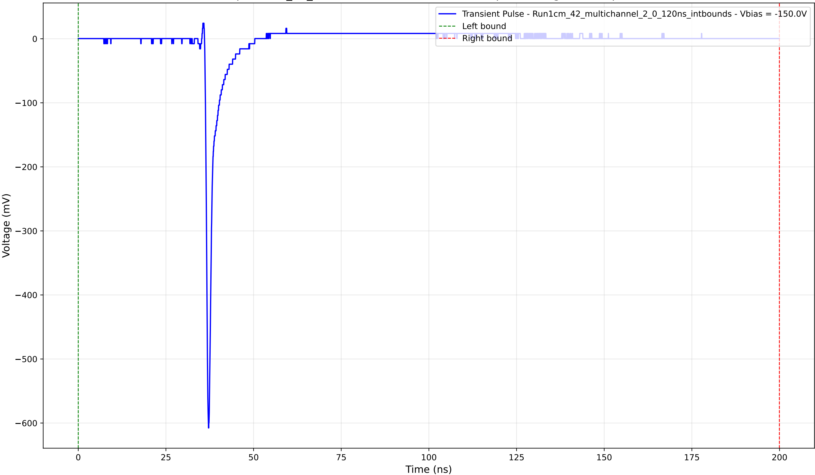
Transient Pulse - Sample: 1cm_42_multichannel - Position: 2225.0 \mu\text{m} - Charge: 15.88 pC - Rise Time: 0.74 ns
