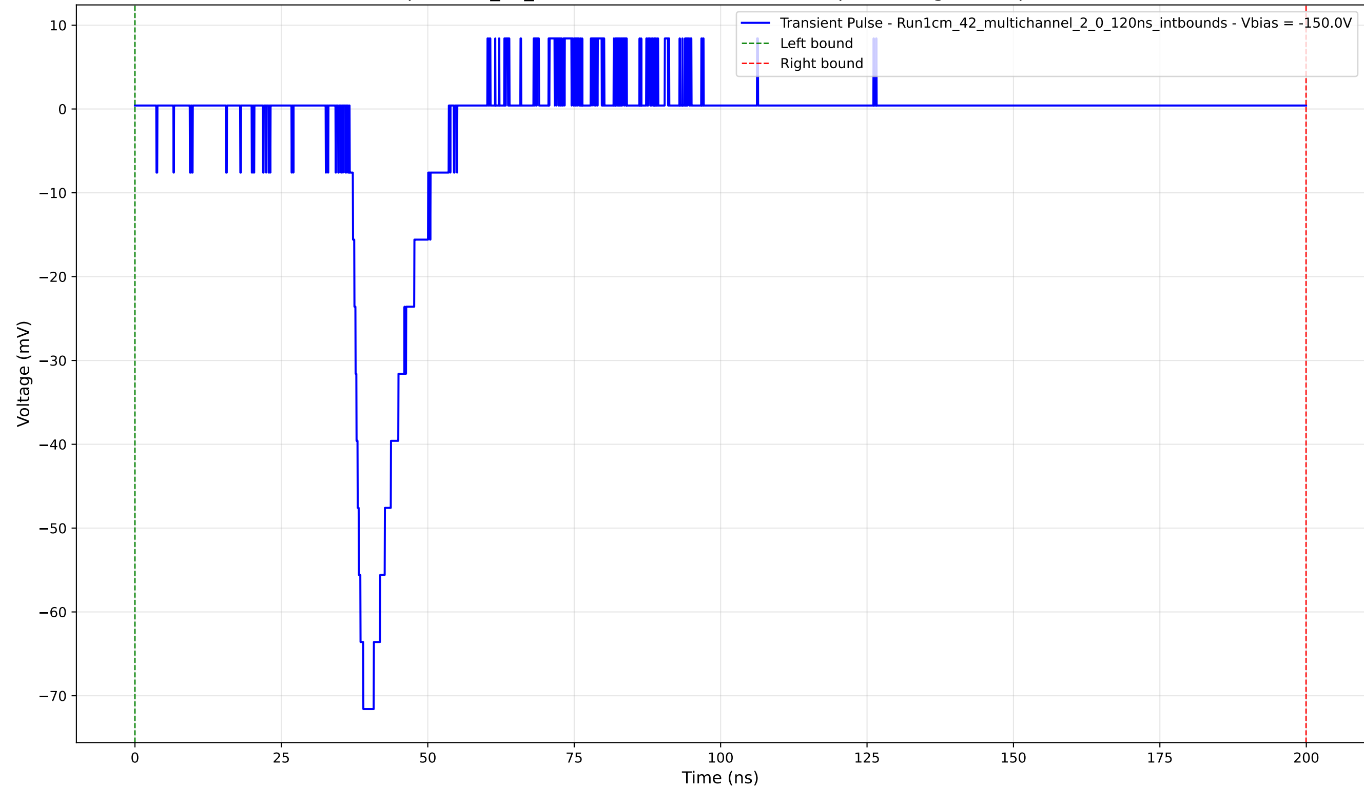
Transient Pulse - Sample: 1cm_42_multichannel - Position: 4510.0 \mu\text{m} - Charge: 8.16 pC - Rise Time: 2.32 ns
