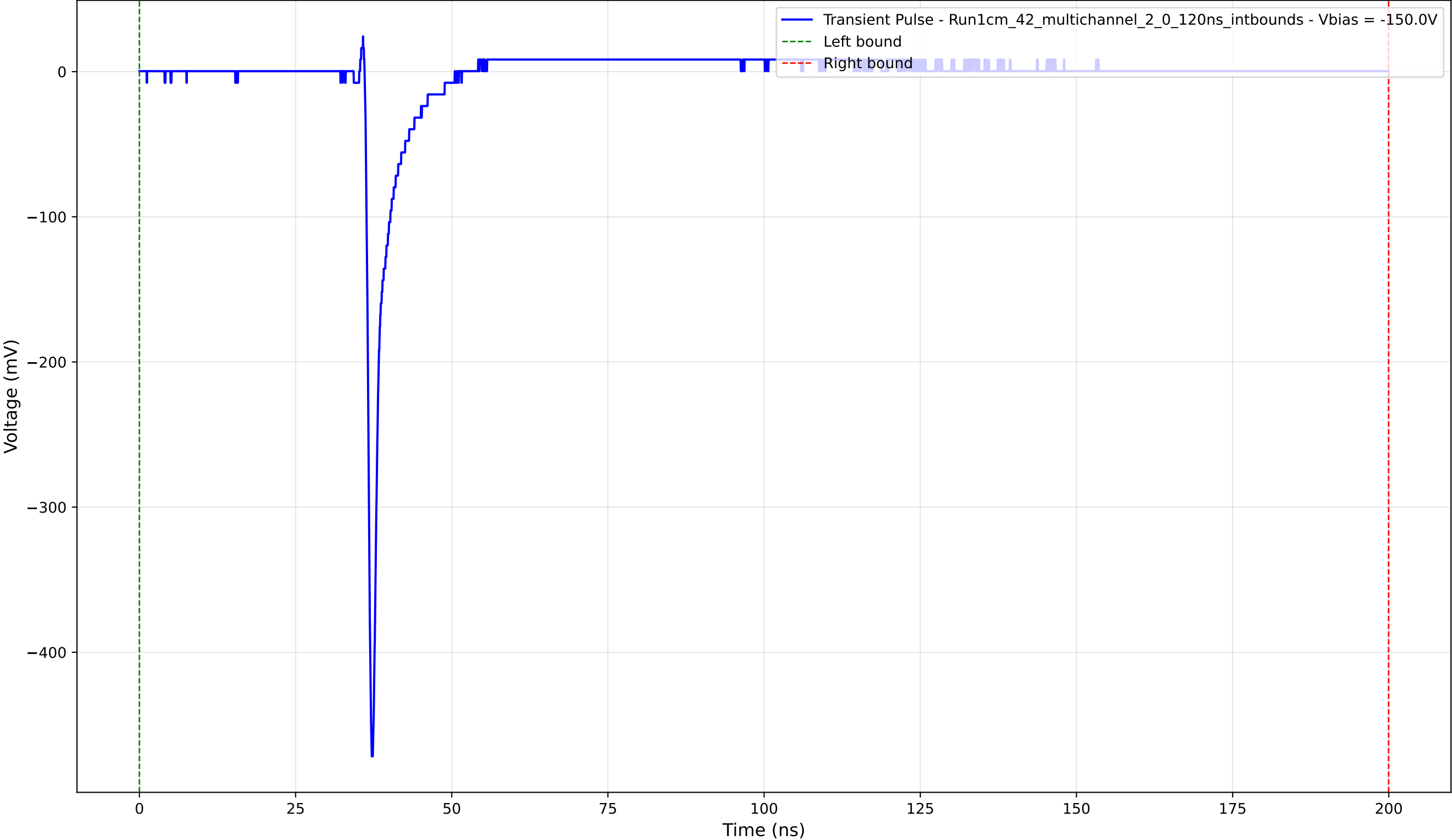
Transient Pulse - Sample: 1cm_42_multichannel - Position: 2620.0 \mu\text{m} - Charge: 13.25 pC - Rise Time: 0.73 ns
