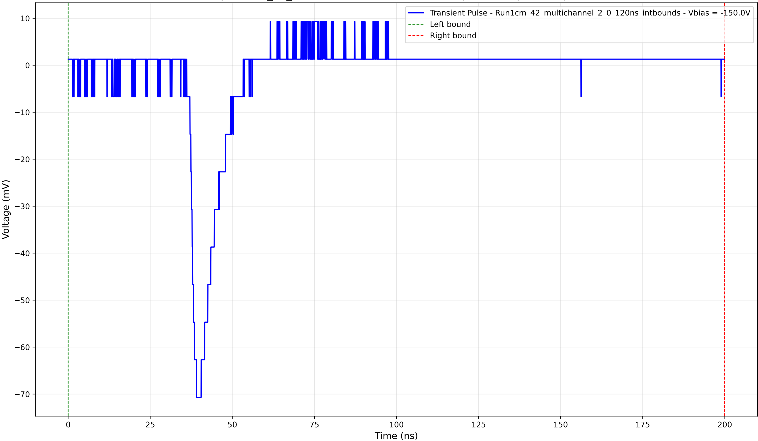
Transient Pulse - Sample: 1cm_42_multichannel - Position: 4700.0 \mu\text{m} - Charge: 5.46 pC - Rise Time: 2.08 ns
