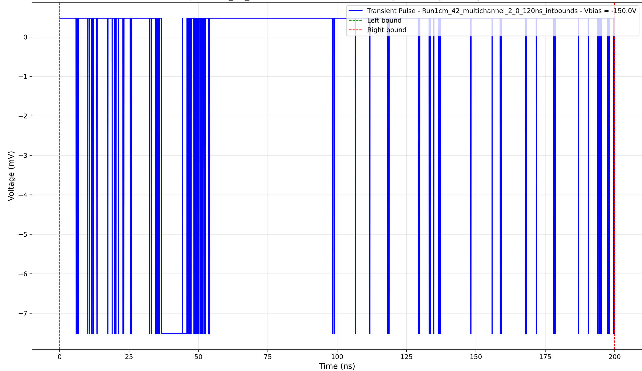
Transient Pulse - Sample: 1cm_42_multichannel - Position: 1350.0 \mu\text{m} - Charge: 0.89 pC - Rise Time: 0.04 ns
