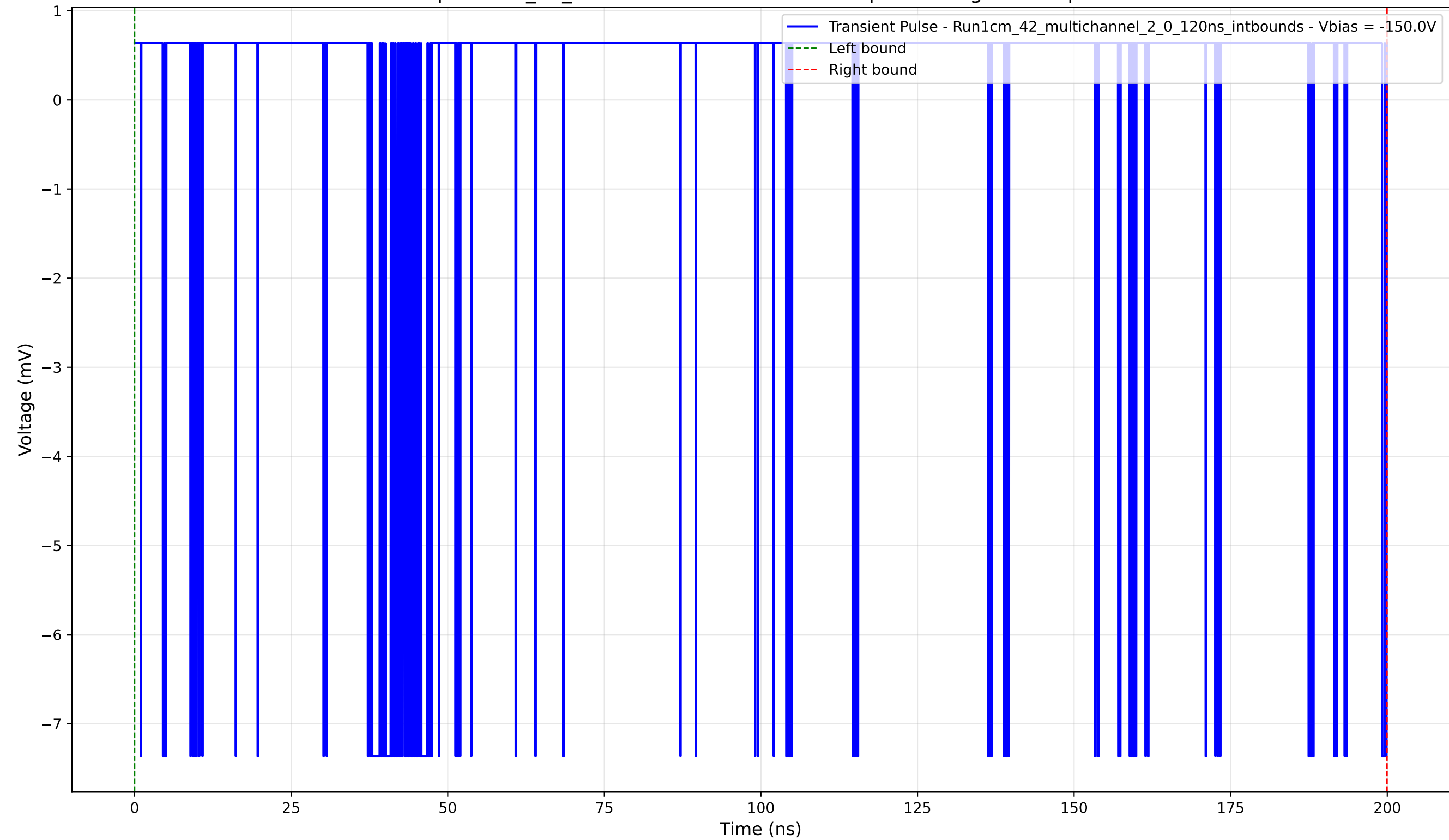
Transient Pulse - Sample: 1cm_42_multichannel - Position: 30.0 \mu\text{m} - Charge: -0.44 pC - Rise Time: 0.04 ns
