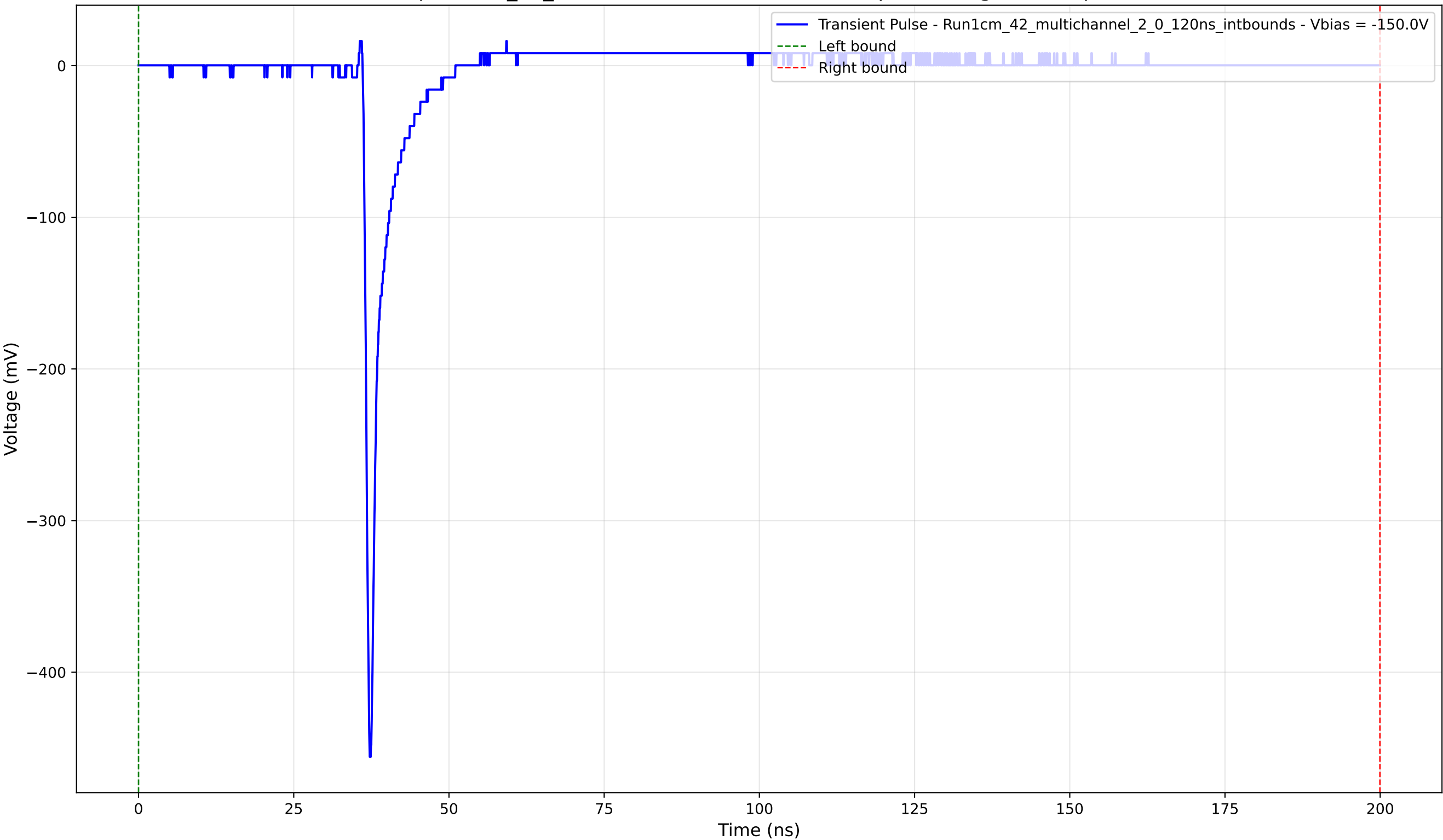
Transient Pulse - Sample: 1cm_42_multichannel - Position: 2060.0 \mu\text{m} - Charge: 14.51 pC - Rise Time: 0.74 ns
