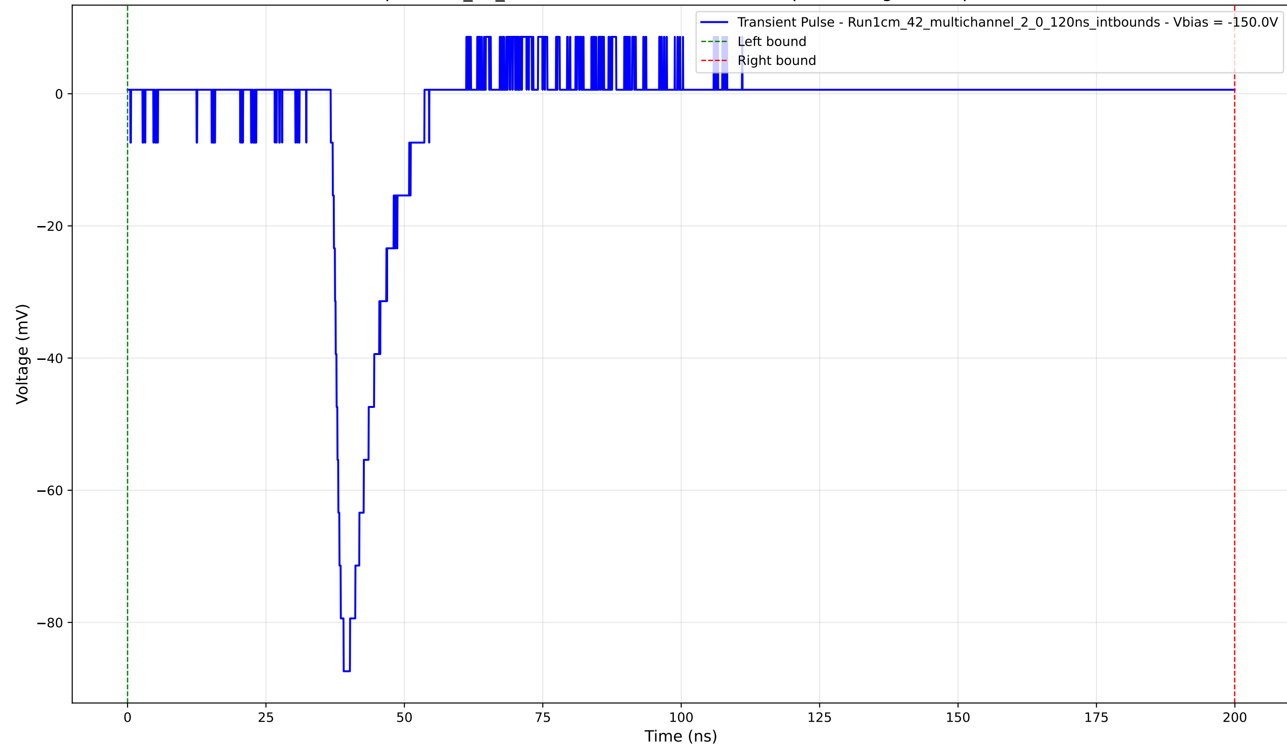
Transient Pulse - Sample: 1cm_42_multichannel - Position: 4085.0 \mu\text{m} - Charge: 9.10 pC - Rise Time: 1.47 ns
