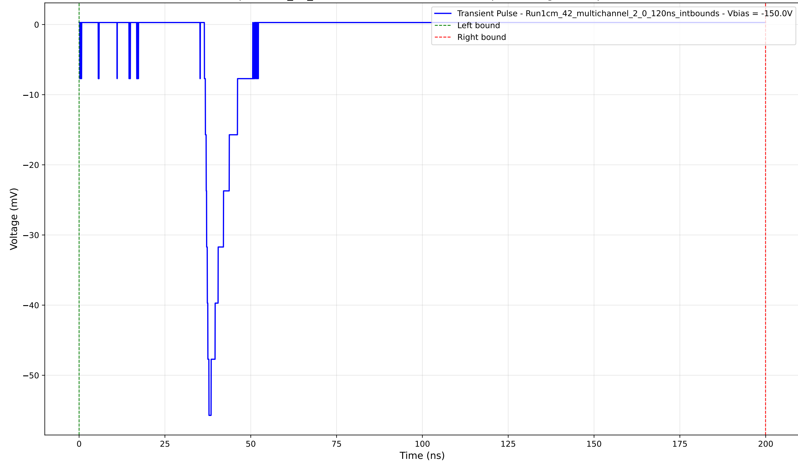
Transient Pulse - Sample: 1cm_42_multichannel - Position: 1315.0 \mu\text{m} - Charge: 5.65 pC - Rise Time: 1.33 ns
