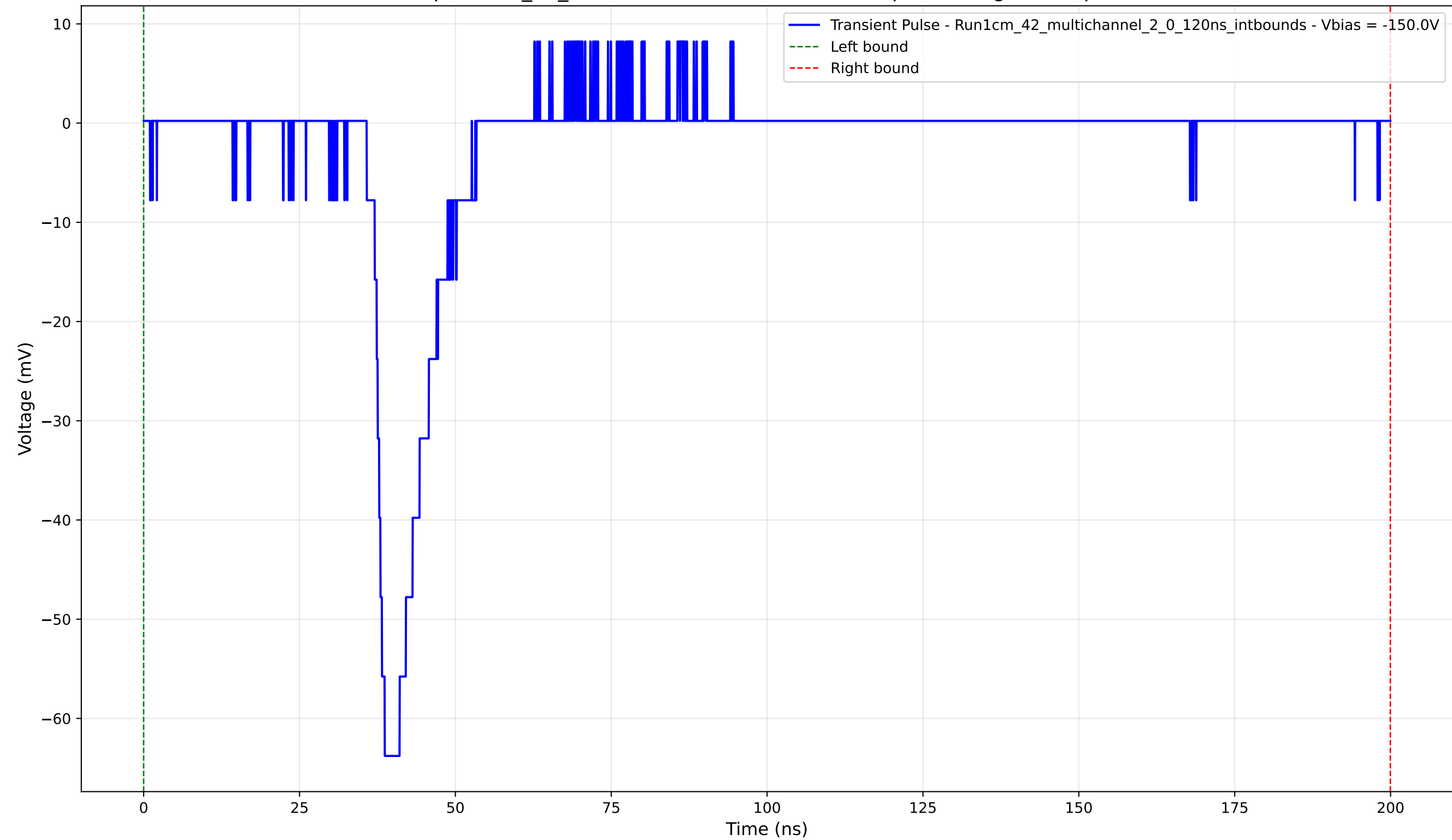
Transient Pulse - Sample: 1cm_42_multichannel - Position: 4750.0 \mu\text{m} - Charge: 8.98 pC - Rise Time: 2.89 ns
