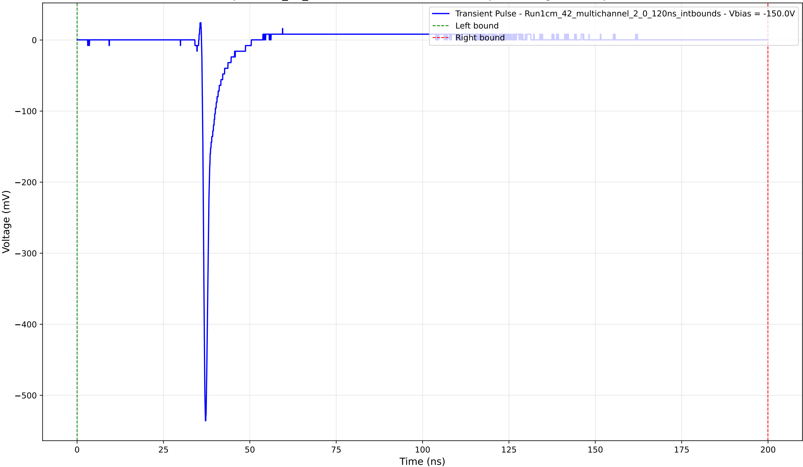
Transient Pulse - Sample: 1cm_42_multichannel - Position: 2535.0 \mu\text{m} - Charge: 13.99 pC - Rise Time: 0.73 ns
