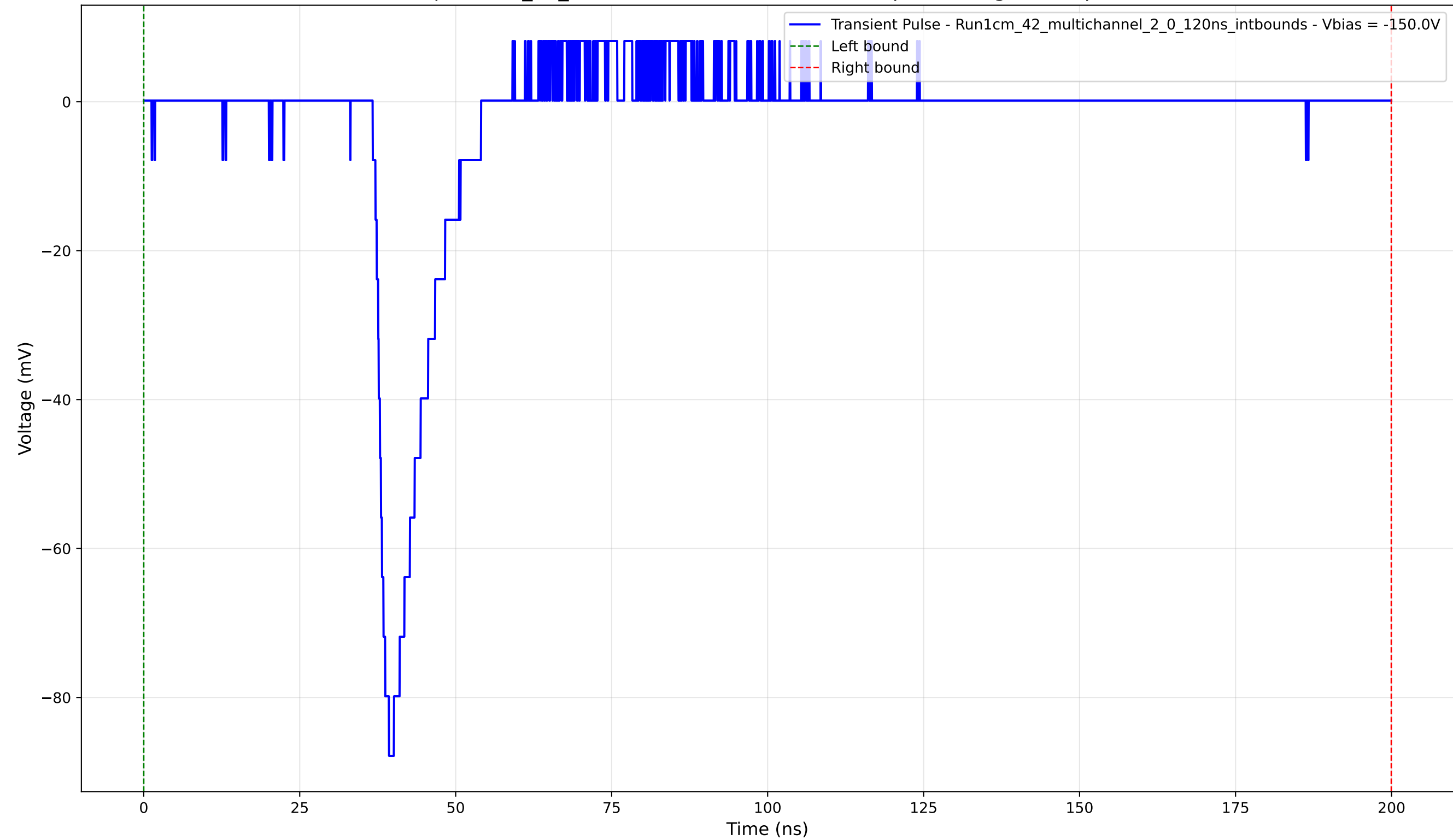
Transient Pulse - Sample: 1cm_42_multichannel - Position: 4205.0 \mu\text{m} - Charge: 9.16 pC - Rise Time: 1.60 ns
