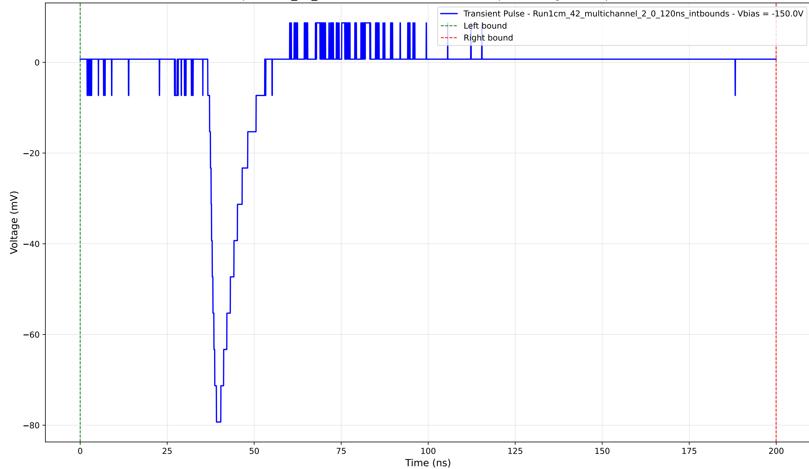
Transient Pulse - Sample: 1cm_42_multichannel - Position: 4260.0 \mu\text{m} - Charge: 7.99 pC - Rise Time: 2.00 ns
