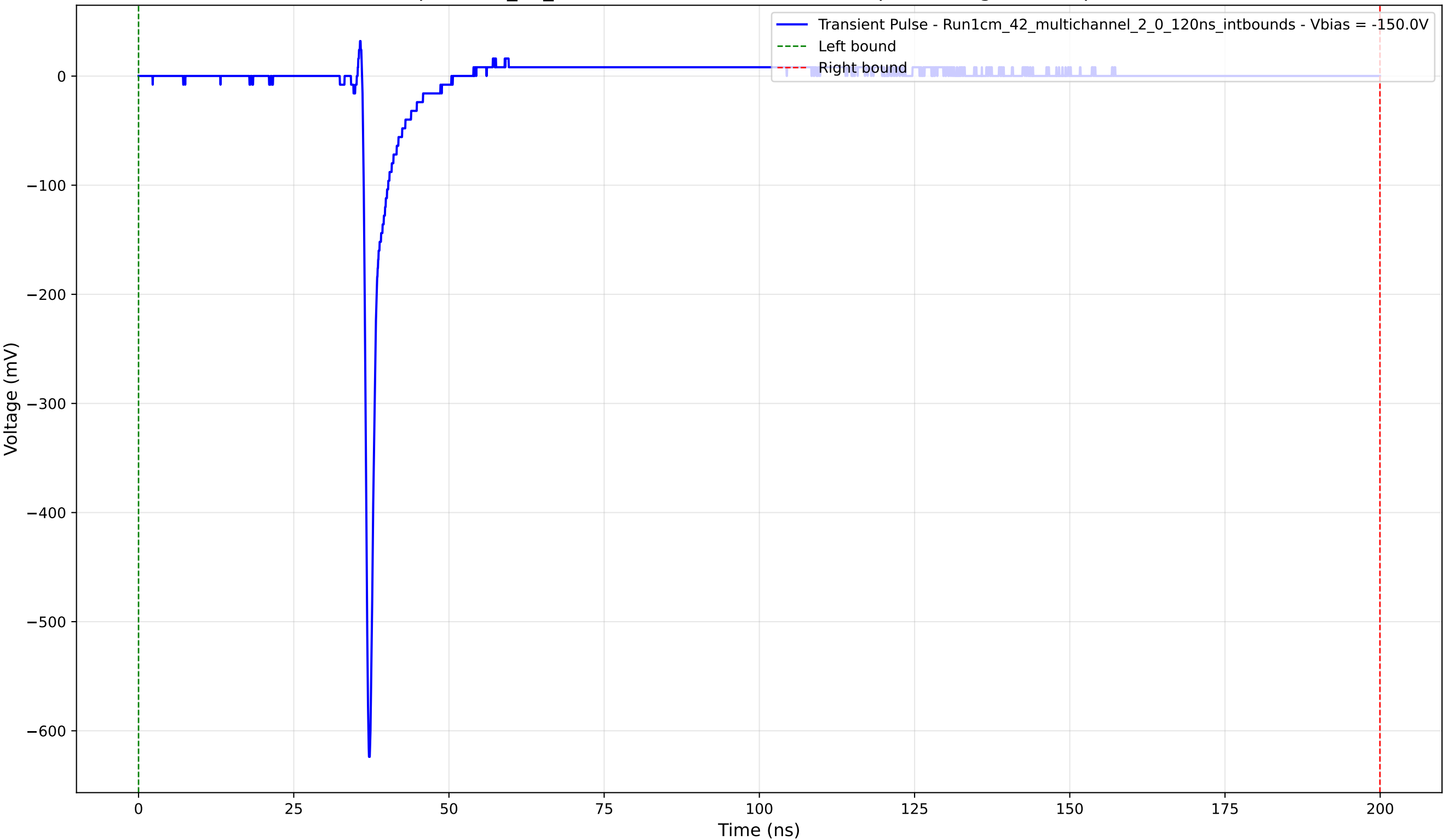
Transient Pulse - Sample: 1cm_42_multichannel - Position: 2245.0 \mu\text{m} - Charge: 16.79 pC - Rise Time: 0.73 ns
