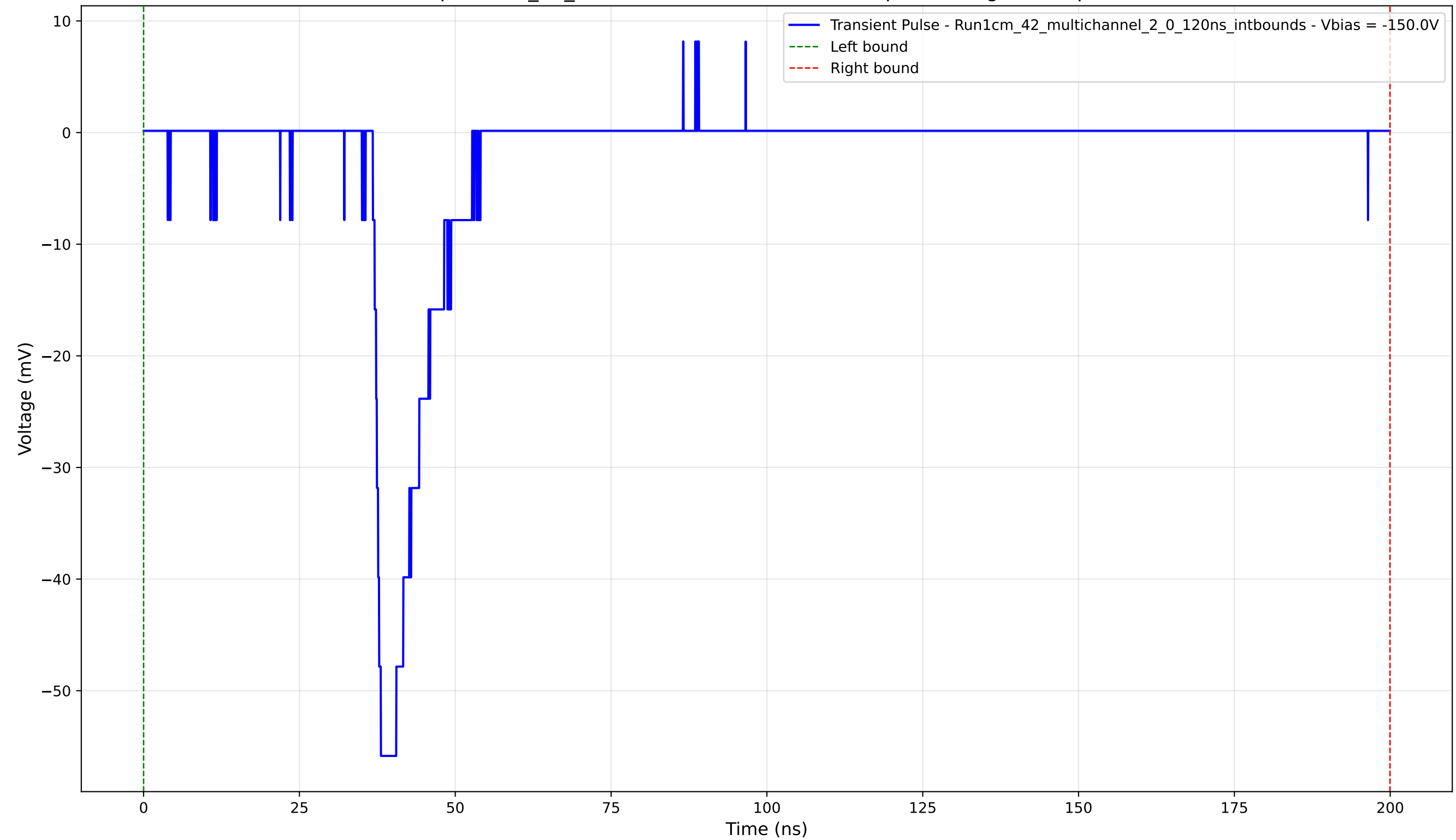
Transient Pulse - Sample: 1cm_42_multichannel - Position: 900.0 \mu\text{m} - Charge: 8.32 pC - Rise Time: 1.29 ns
