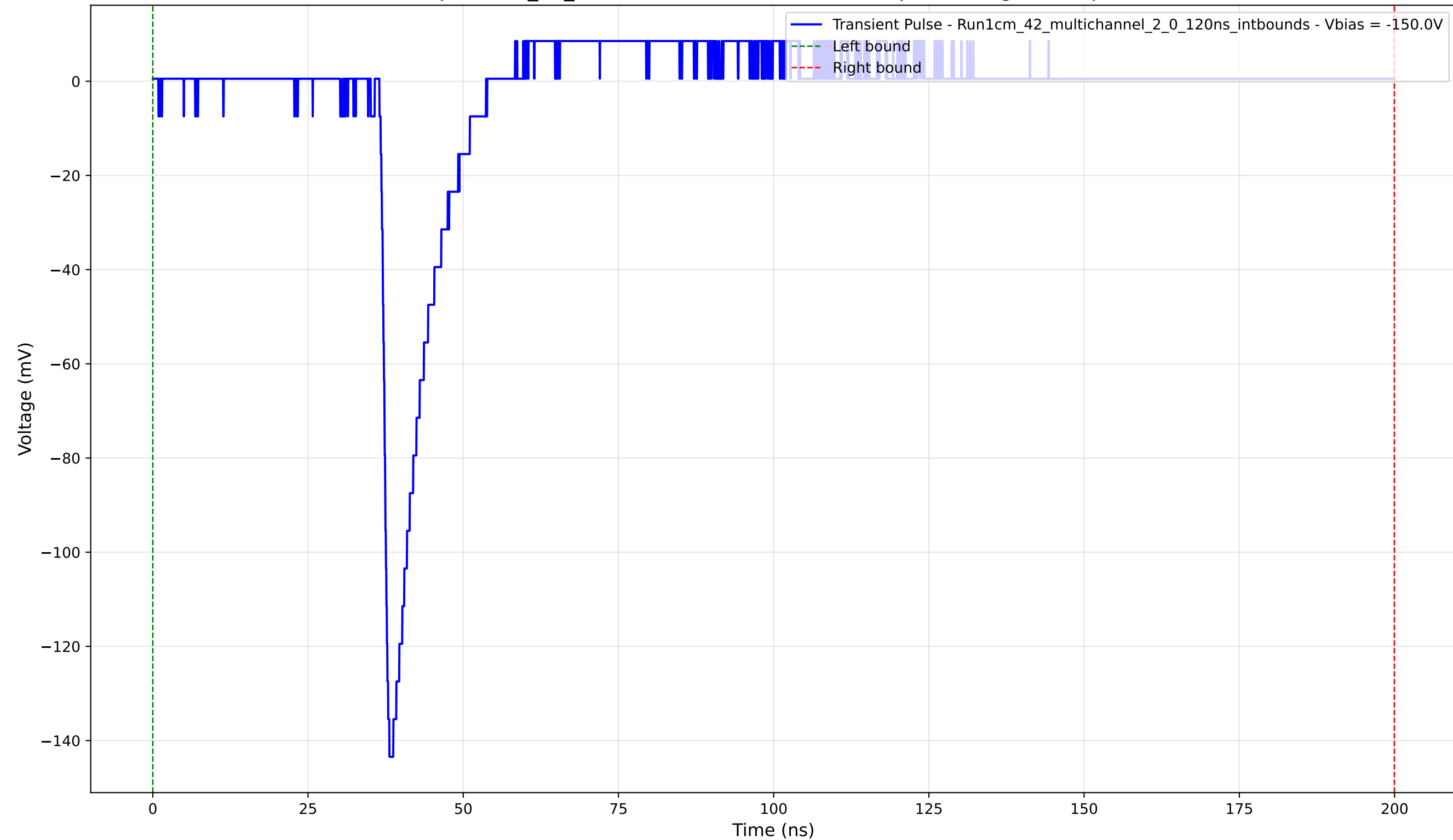
Transient Pulse - Sample: 1cm_42_multichannel - Position: 1165.0 \mu\text{m} - Charge: 9.60 pC - Rise Time: 1.21 ns
