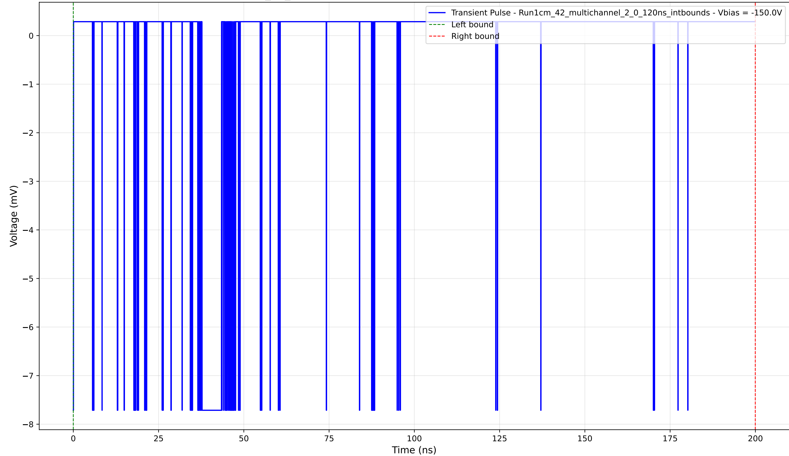
Transient Pulse - Sample: 1cm_42_multichannel - Position: 3890.0 \mu\text{m} - Charge: 0.83 pC - Rise Time: 0.00 ns (N/A)
