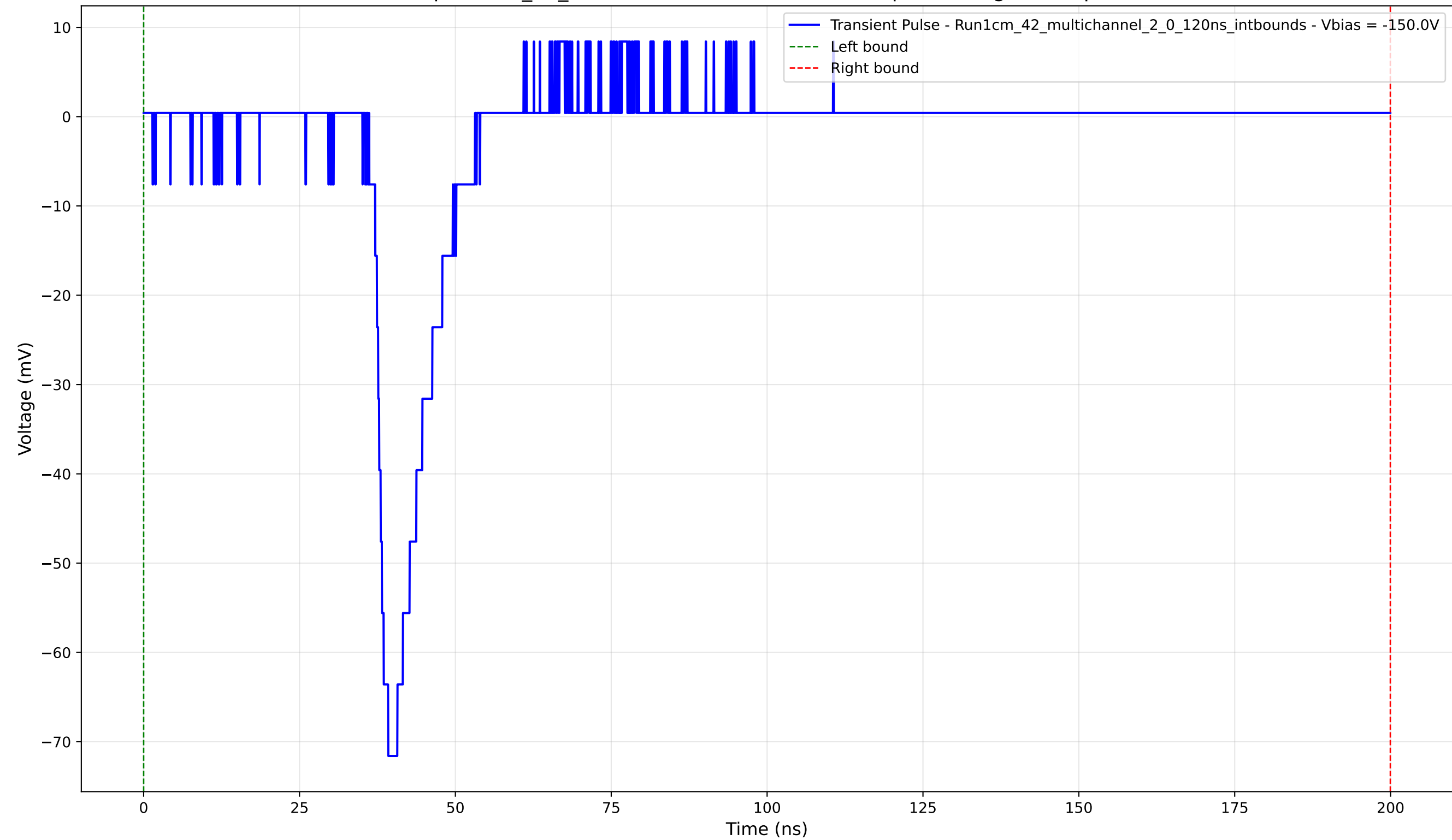
Transient Pulse - Sample: 1cm_42_multichannel - Position: 4600.0 \mu\text{m} - Charge: 8.80 pC - Rise Time: 3.04 ns
