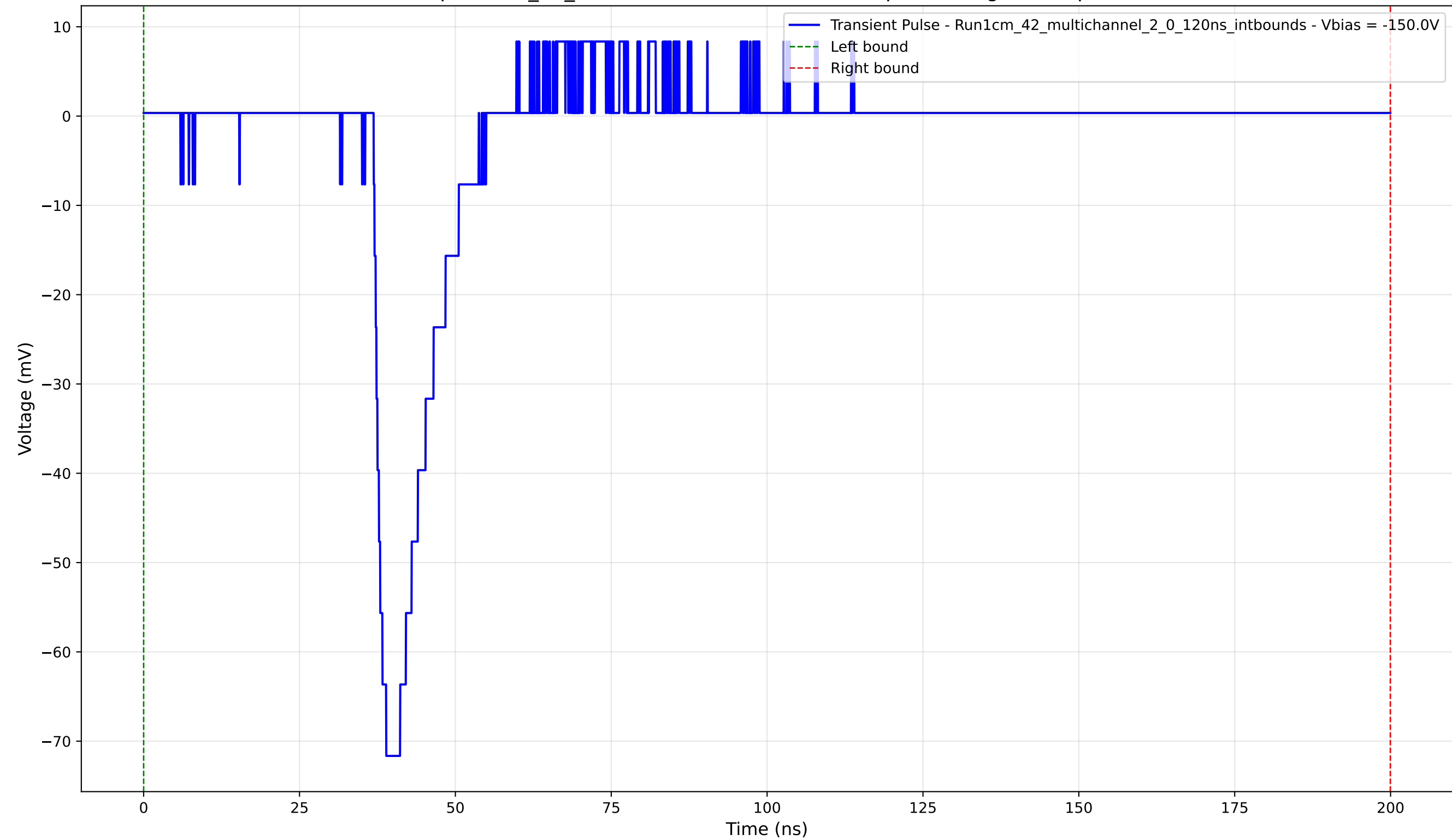
Transient Pulse - Sample: 1cm_42_multichannel - Position: 230.0 \mu\text{m} - Charge: 8.68 pC - Rise Time: 2.00 ns
