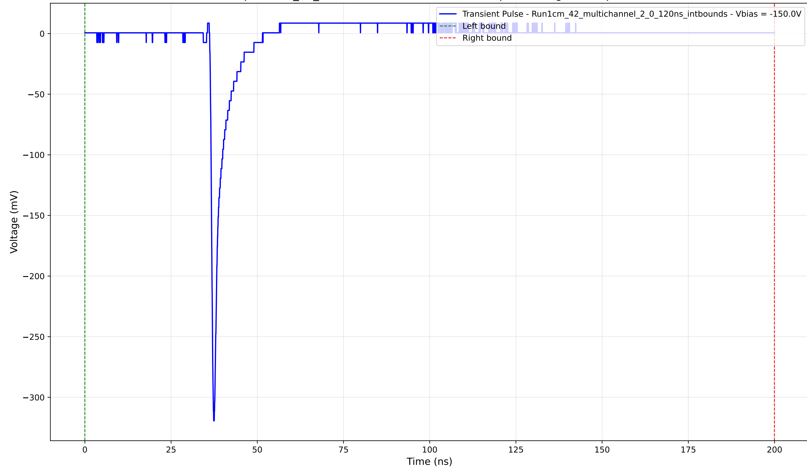
Transient Pulse - Sample: 1cm_42_multichannel - Position: 2800.0 \mu\text{m} - Charge: 9.89 pC - Rise Time: 0.80 ns
