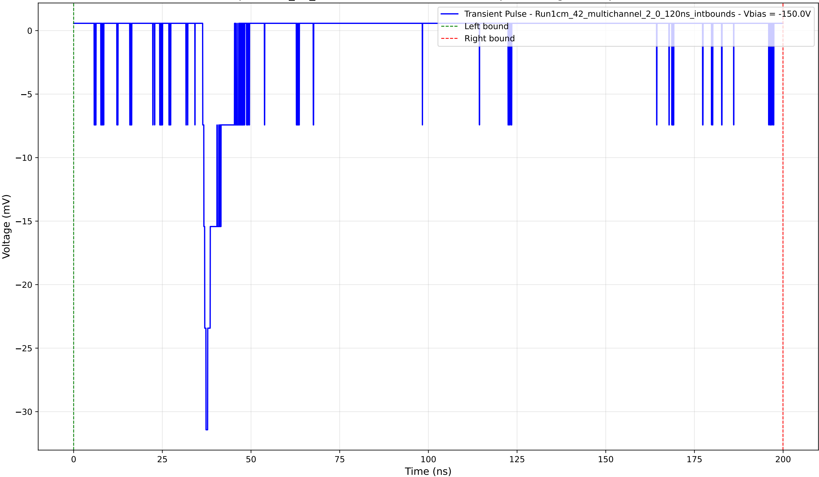
Transient Pulse - Sample: 1cm_42_multichannel - Position: 1840.0 \mu\text{m} - Charge: 1.28 pC - Rise Time: 0.95 ns
