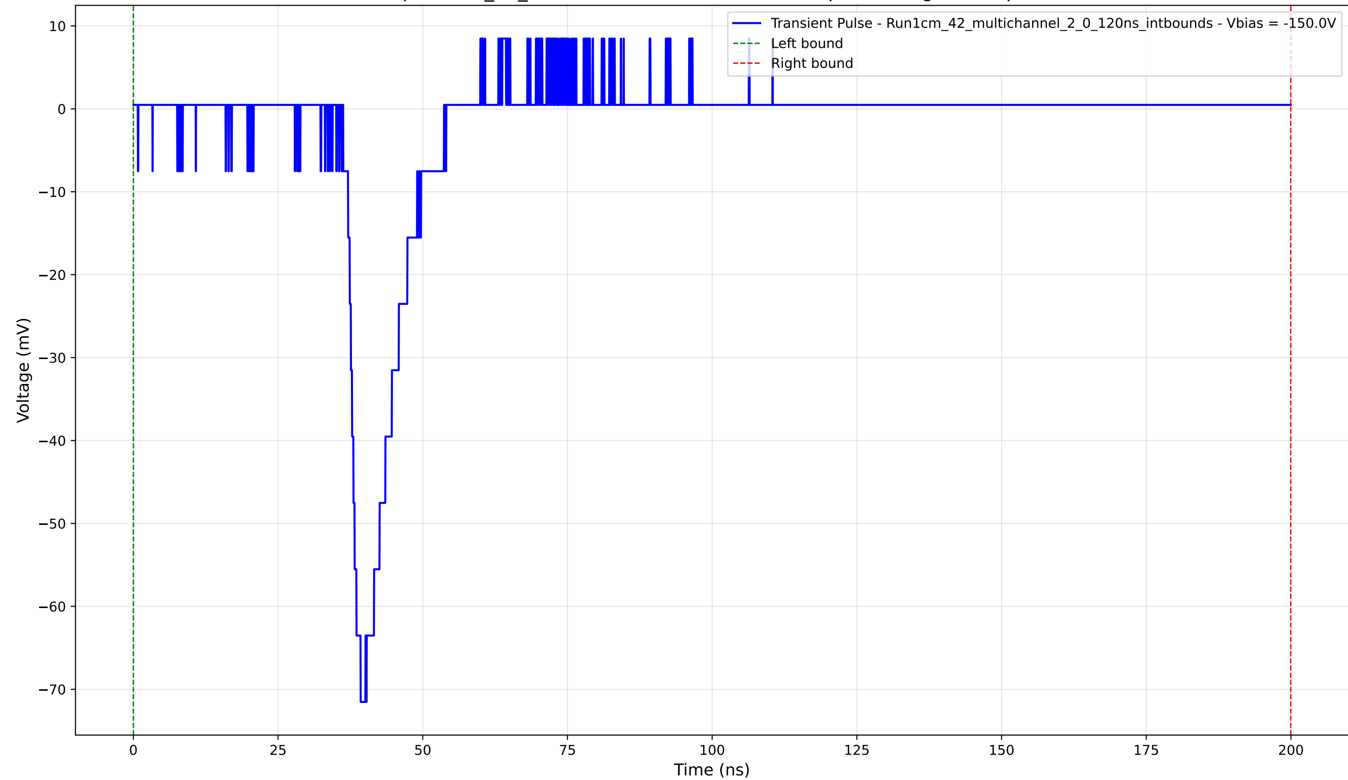
Transient Pulse - Sample: 1cm_42_multichannel - Position: 4690.0 \mu\text{m} - Charge: 8.24 pC - Rise Time: 3.00 ns
