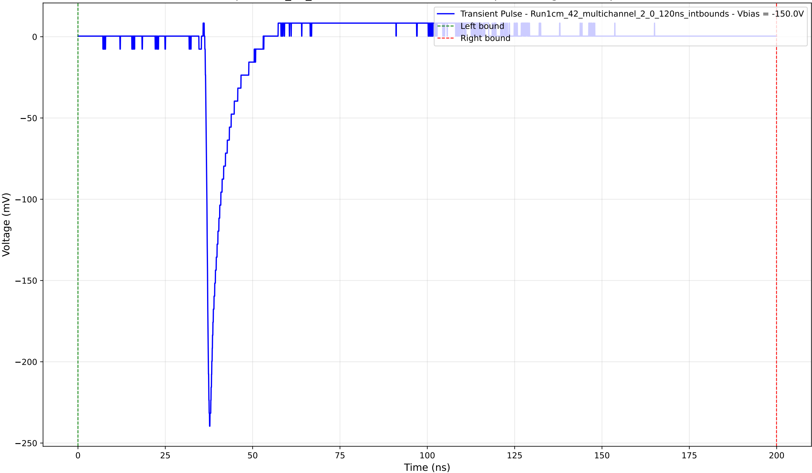
Transient Pulse - Sample: 1cm_42_multichannel - Position: 1600.0 \mu\text{m} - Charge: 11.65 pC - Rise Time: 0.96 ns
