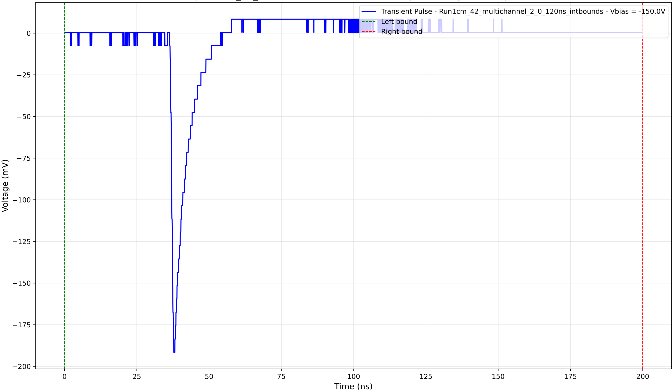
Transient Pulse - Sample: 1cm_42_multichannel - Position: 1445.0 \mu\text{m} - Charge: 11.30 pC - Rise Time: 0.98 ns
