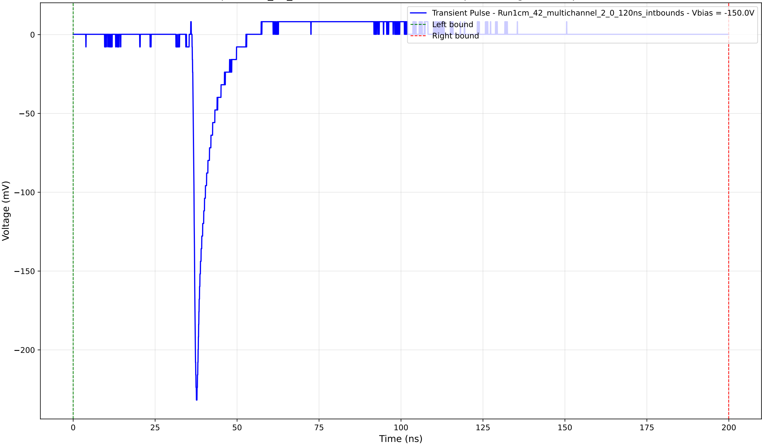
Transient Pulse - Sample: 1cm_42_multichannel - Position: 3060.0 \mu\text{m} - Charge: 12.50 pC - Rise Time: 0.96 ns
