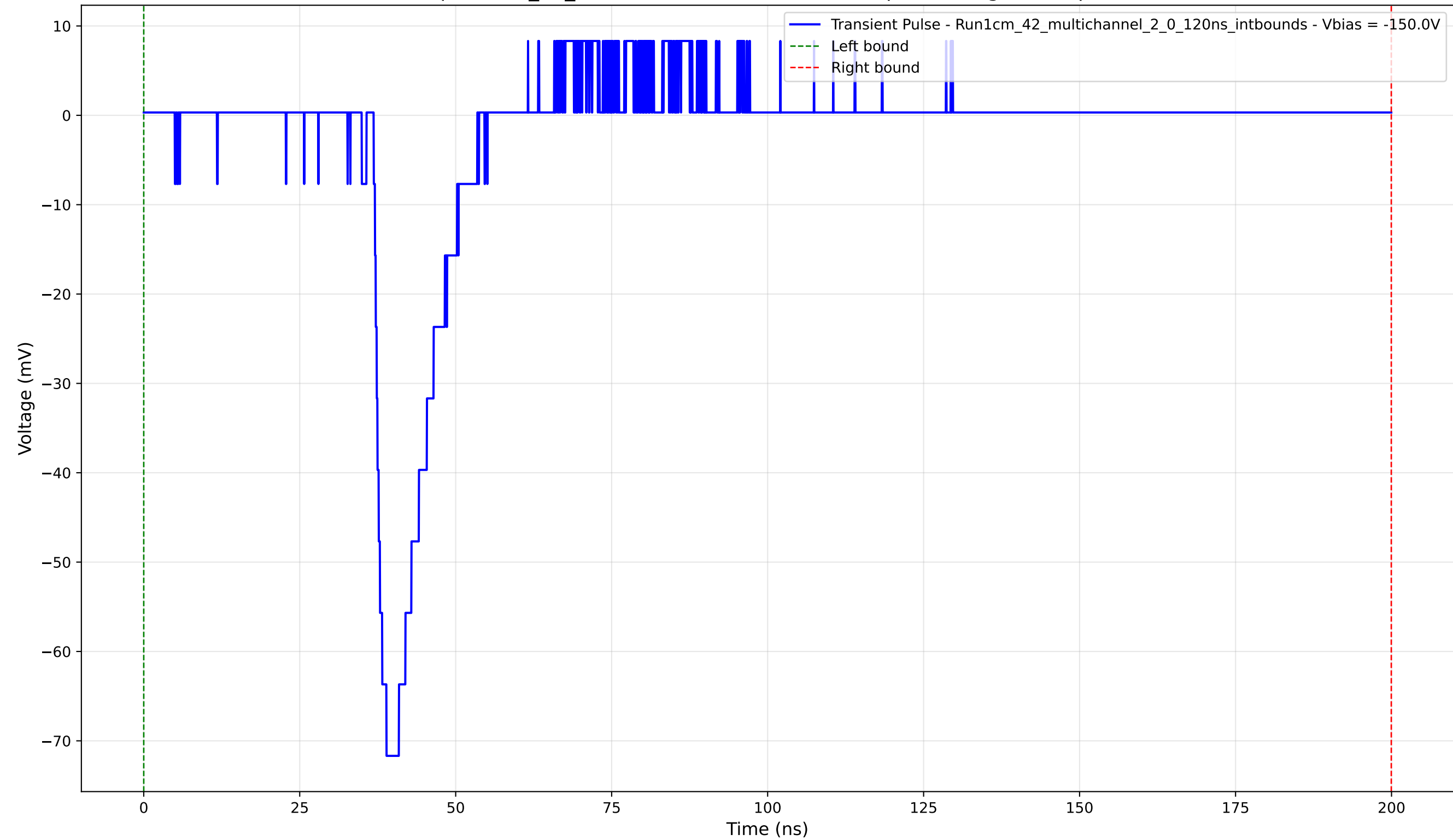
Transient Pulse - Sample: 1cm_42_multichannel - Position: 195.0 \mu\text{m} - Charge: 8.39 pC - Rise Time: 2.04 ns
