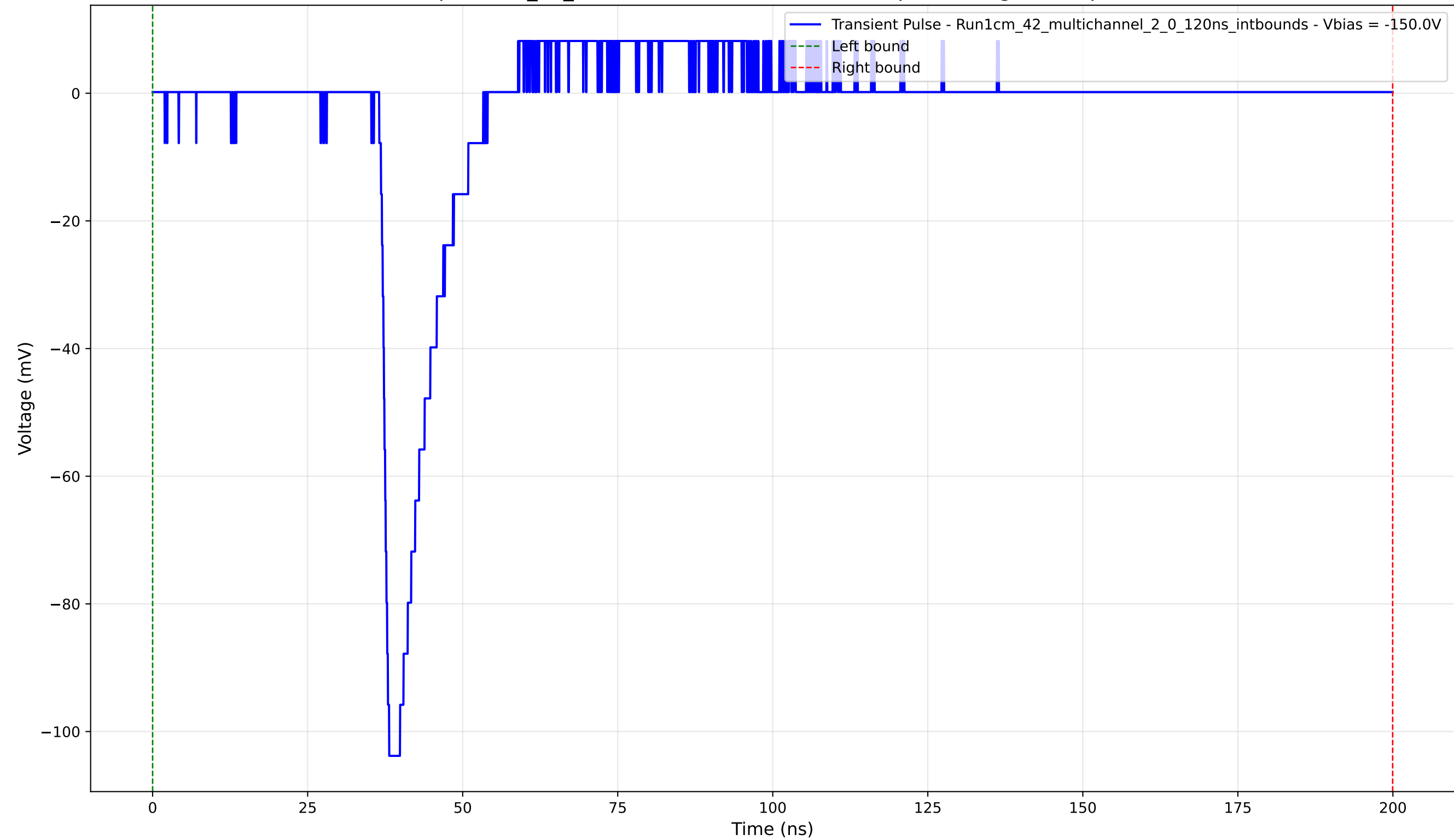
Transient Pulse - Sample: 1cm_42_multichannel - Position: 3730.0 \mu\text{m} - Charge: 9.04 pC - Rise Time: 1.15 ns
