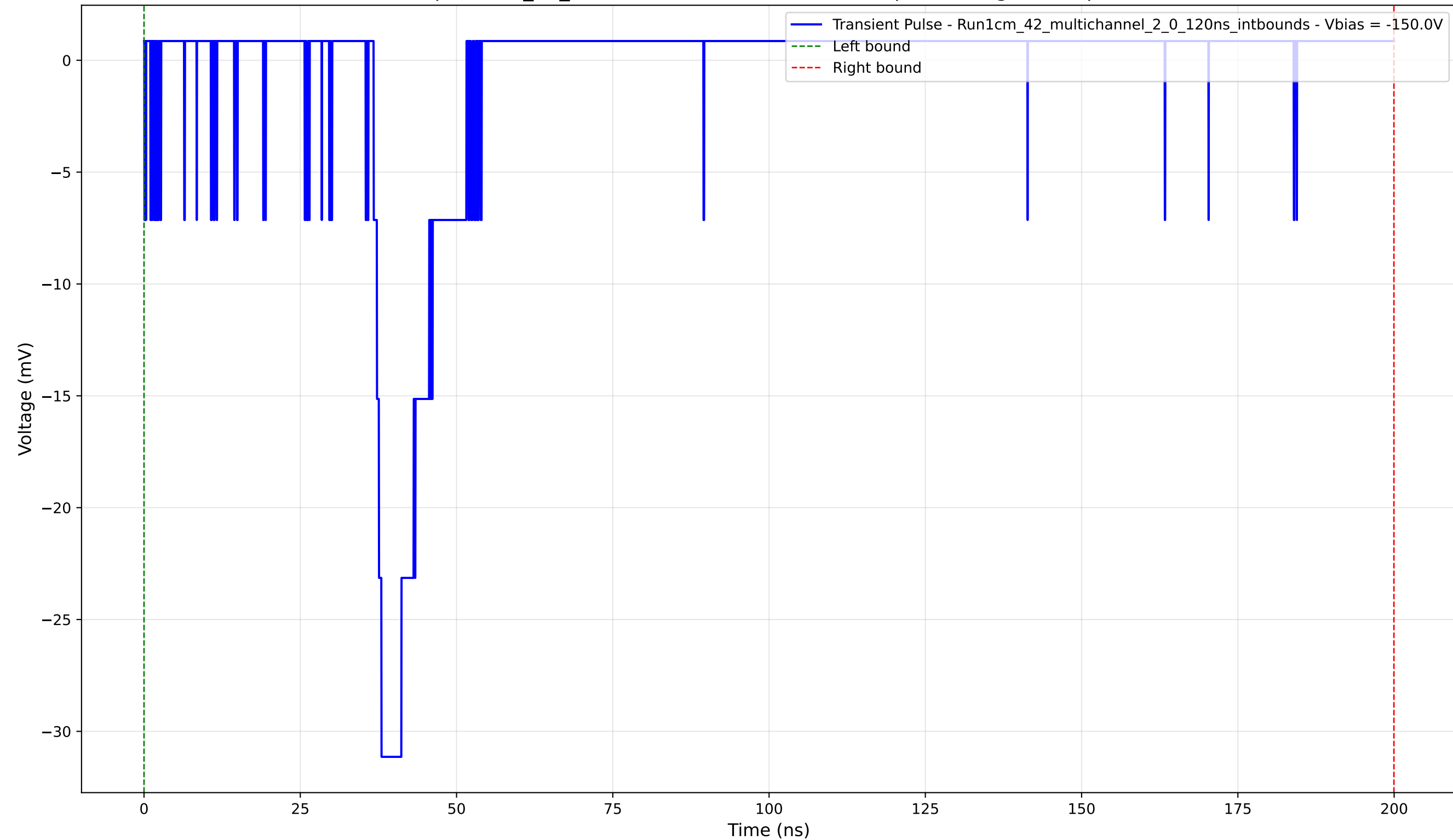
Transient Pulse - Sample: 1cm_42_multichannel - Position: 3845.0 \mu\text{m} - Charge: 2.42 pC - Rise Time: 1.27 ns
