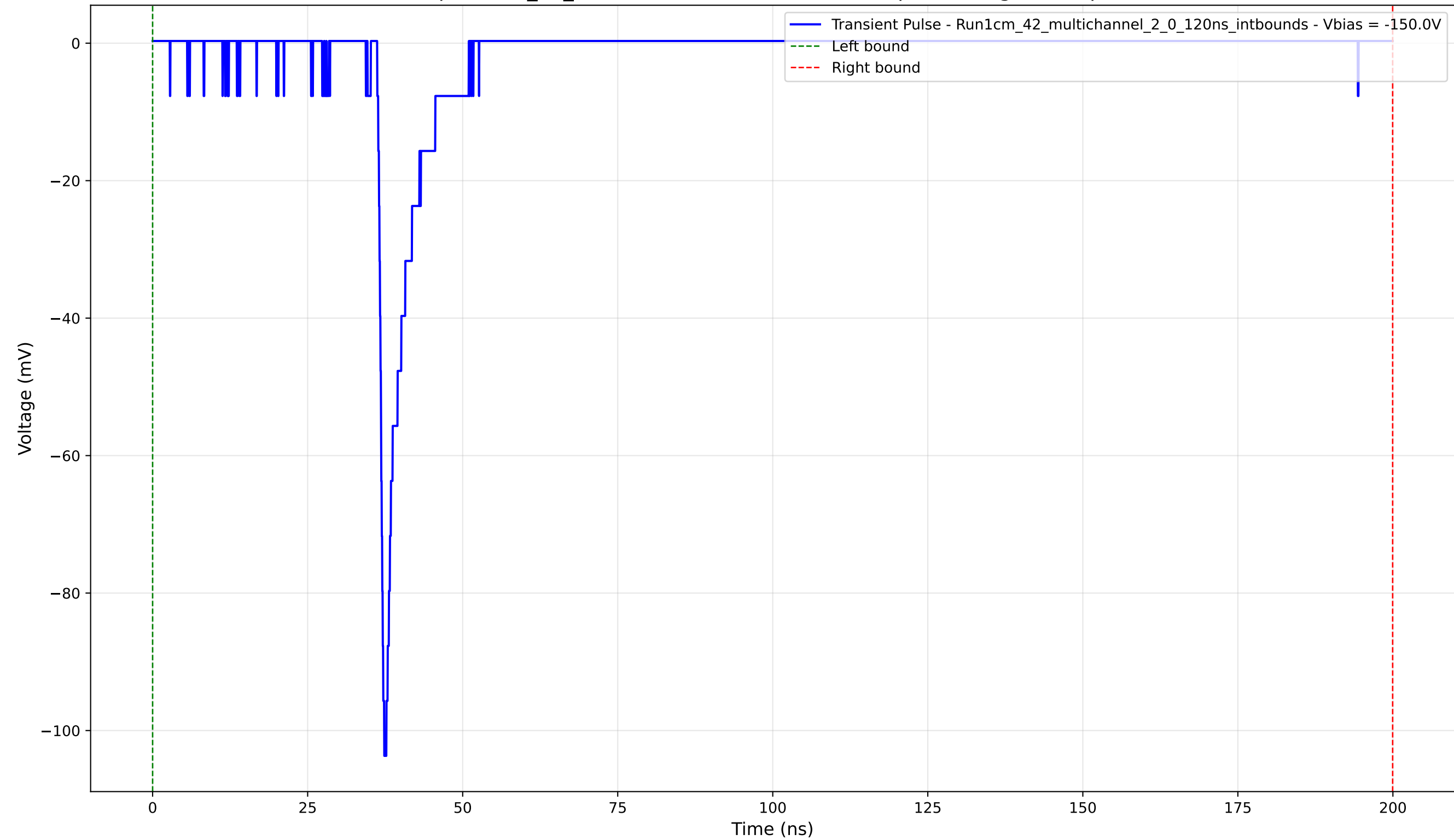
Transient Pulse - Sample: 1cm_42_multichannel - Position: 2920.0 \mu\text{m} - Charge: 7.71 pC - Rise Time: 0.83 ns
