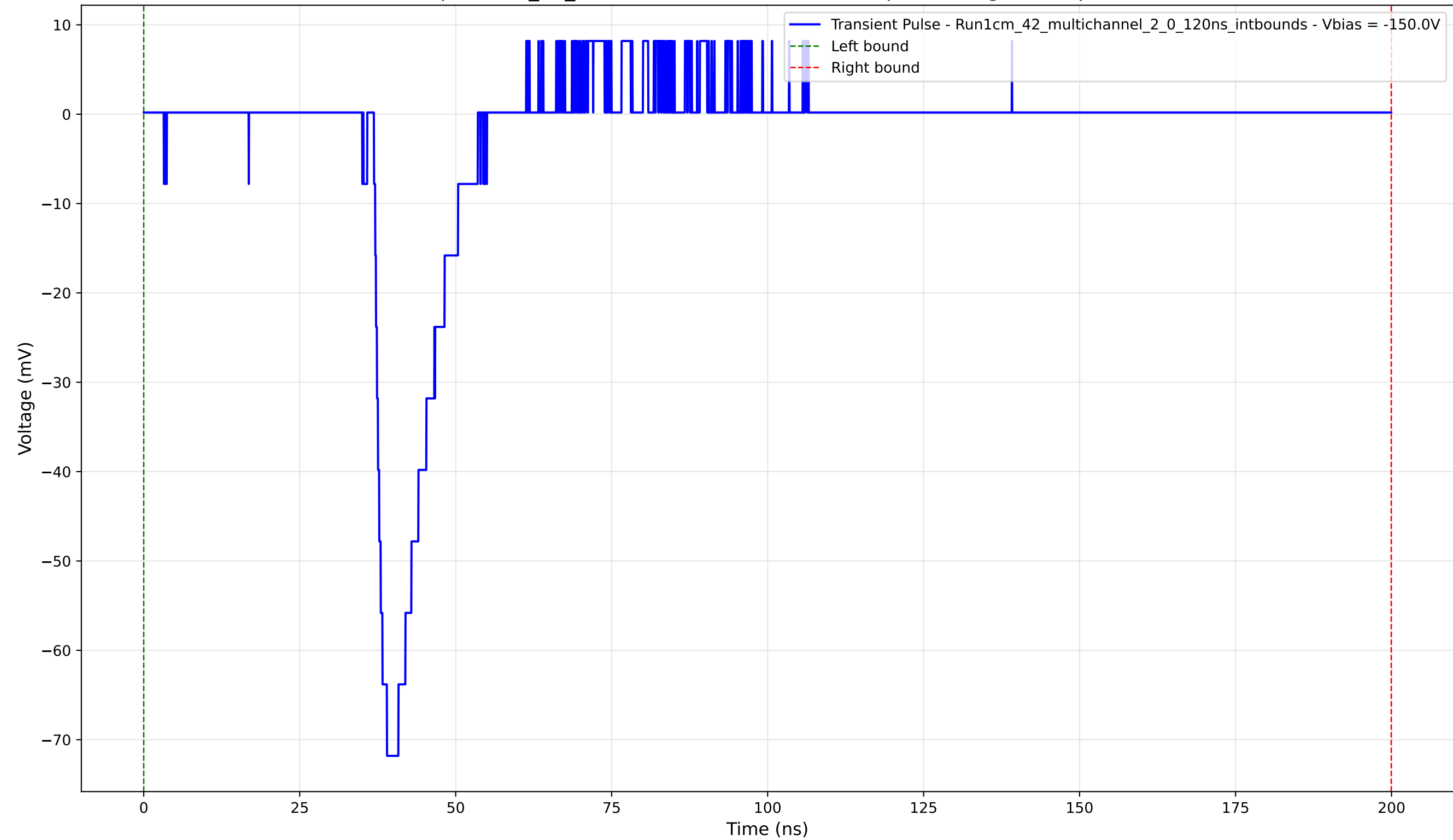
Transient Pulse - Sample: 1cm_42_multichannel - Position: 240.0 \mu\text{m} - Charge: 8.93 pC - Rise Time: 2.08 ns
