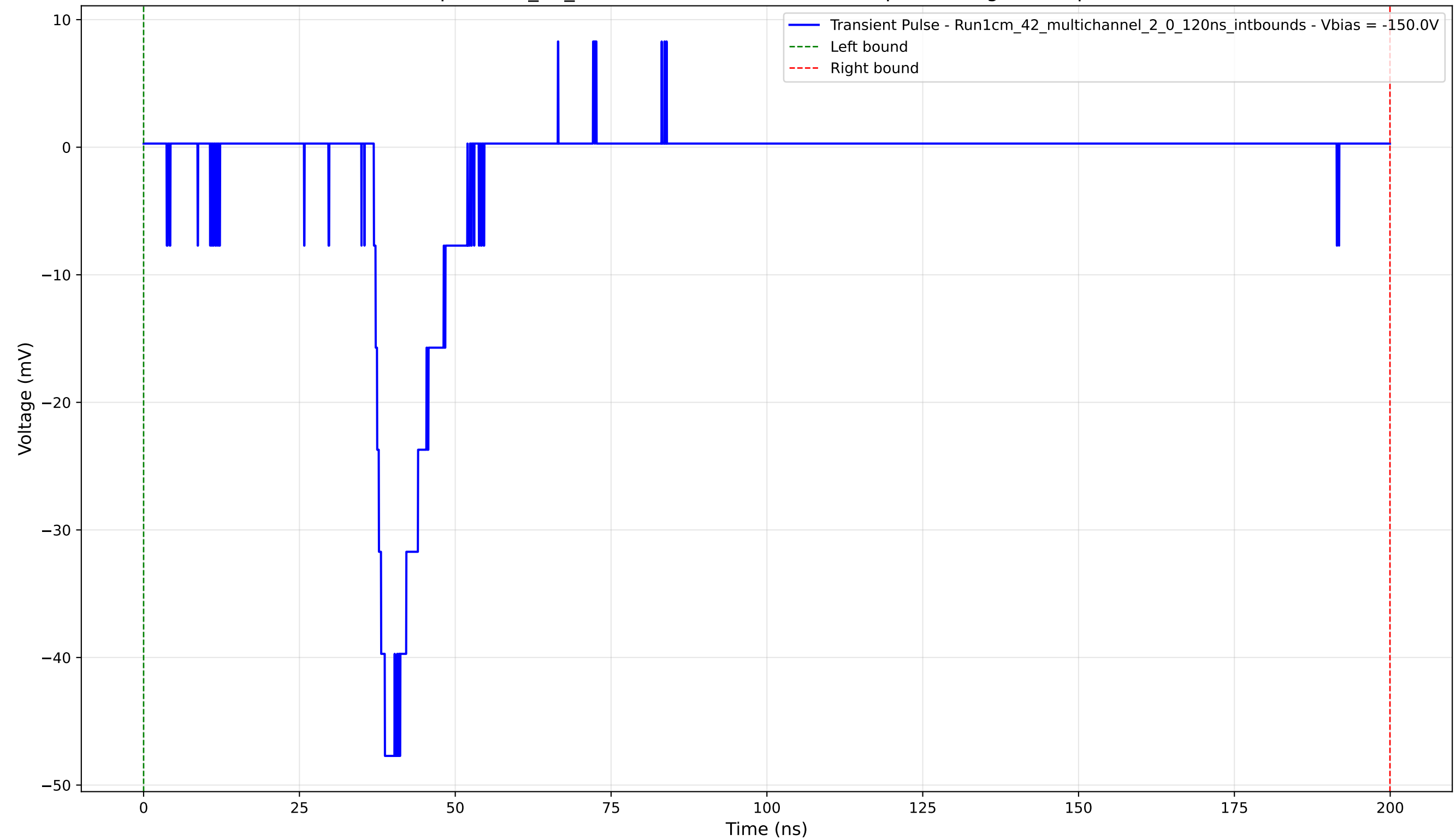
Transient Pulse - Sample: 1cm_42_multichannel - Position: 290.0 \mu\text{m} - Charge: 6.59 pC - Rise Time: 1.78 ns
