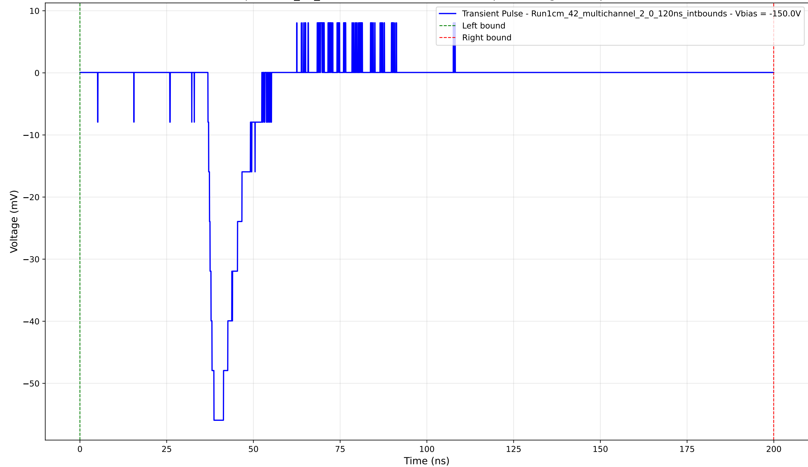
Transient Pulse - Sample: 1cm_42_multichannel - Position: 280.0 \mu\text{m} - Charge: 8.36 pC - Rise Time: 1.73 ns
