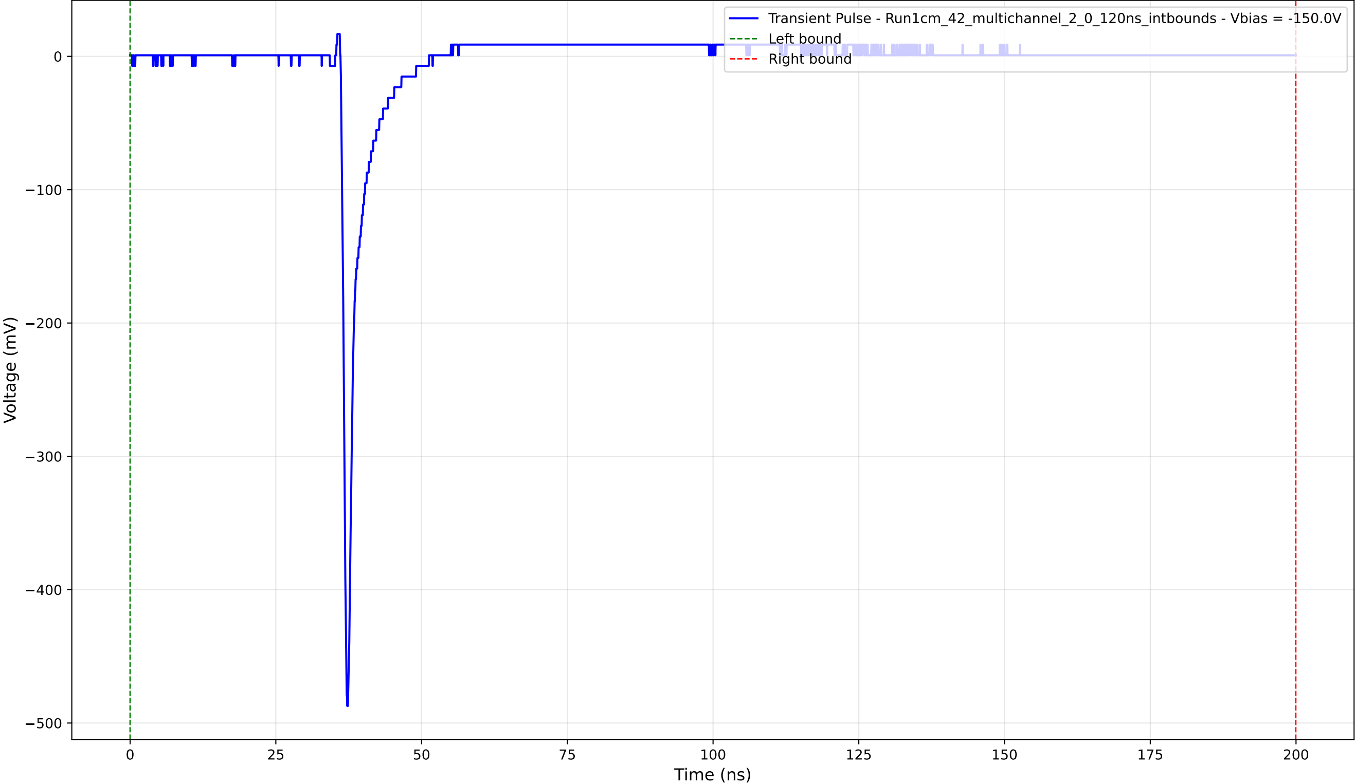
Transient Pulse - Sample: 1cm_42_multichannel - Position: 2100.0 \mu\text{m} - Charge: 12.92 pC - Rise Time: 0.77 ns
