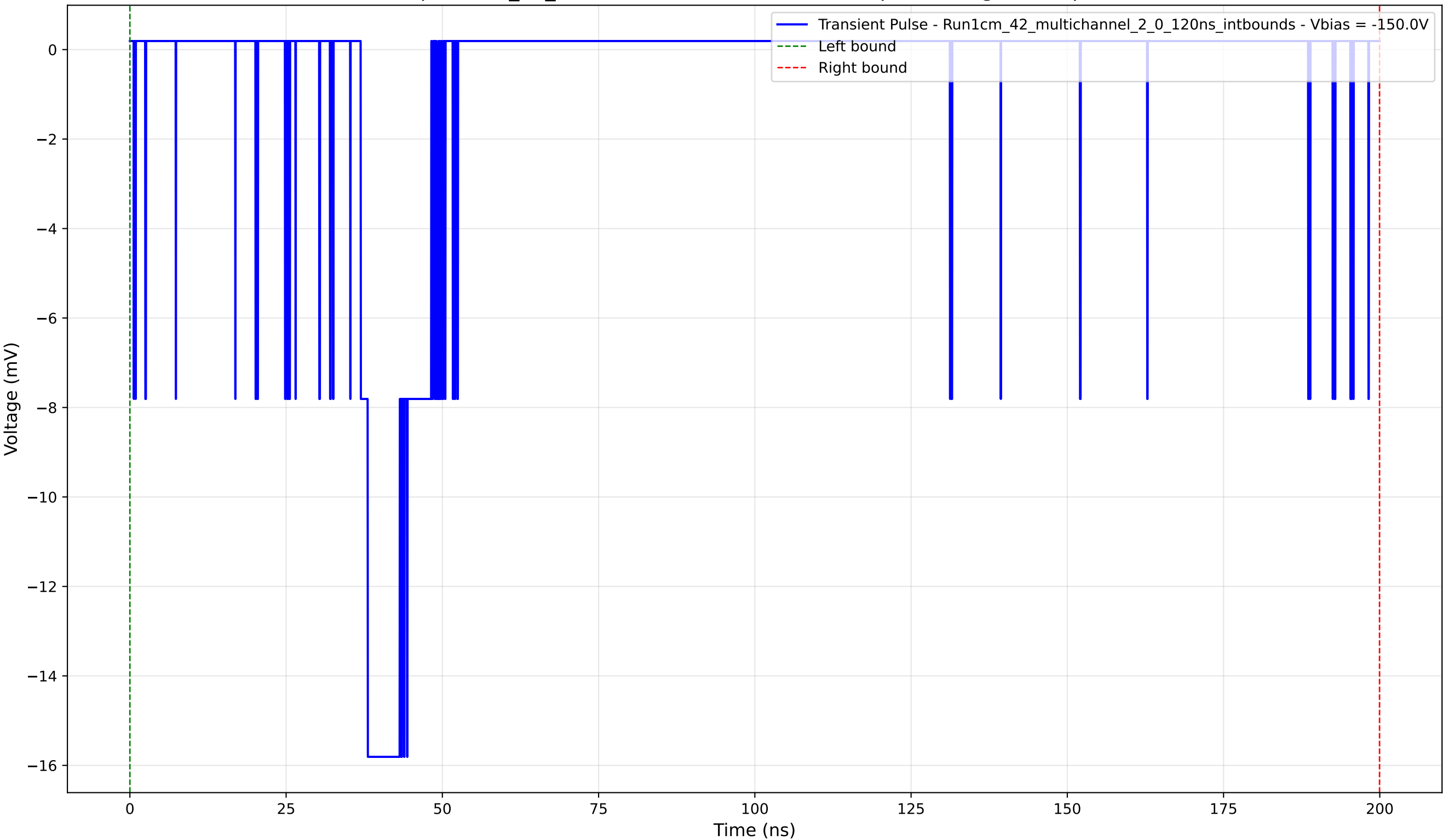
Transient Pulse - Sample: 1cm_42_multichannel - Position: 4425.0 \mu\text{m} - Charge: 2.50 pC - Rise Time: 1.15 ns
