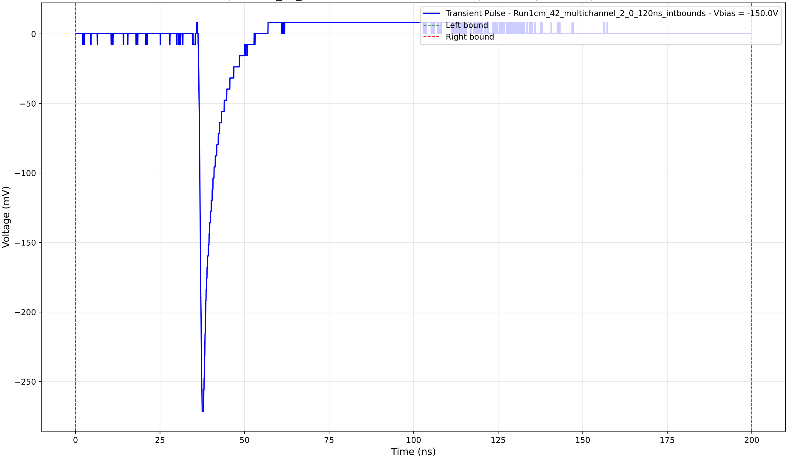
Transient Pulse - Sample: 1cm_42_multichannel - Position: 1695.0 \mu\text{m} - Charge: 12.37 pC - Rise Time: 0.85 ns
