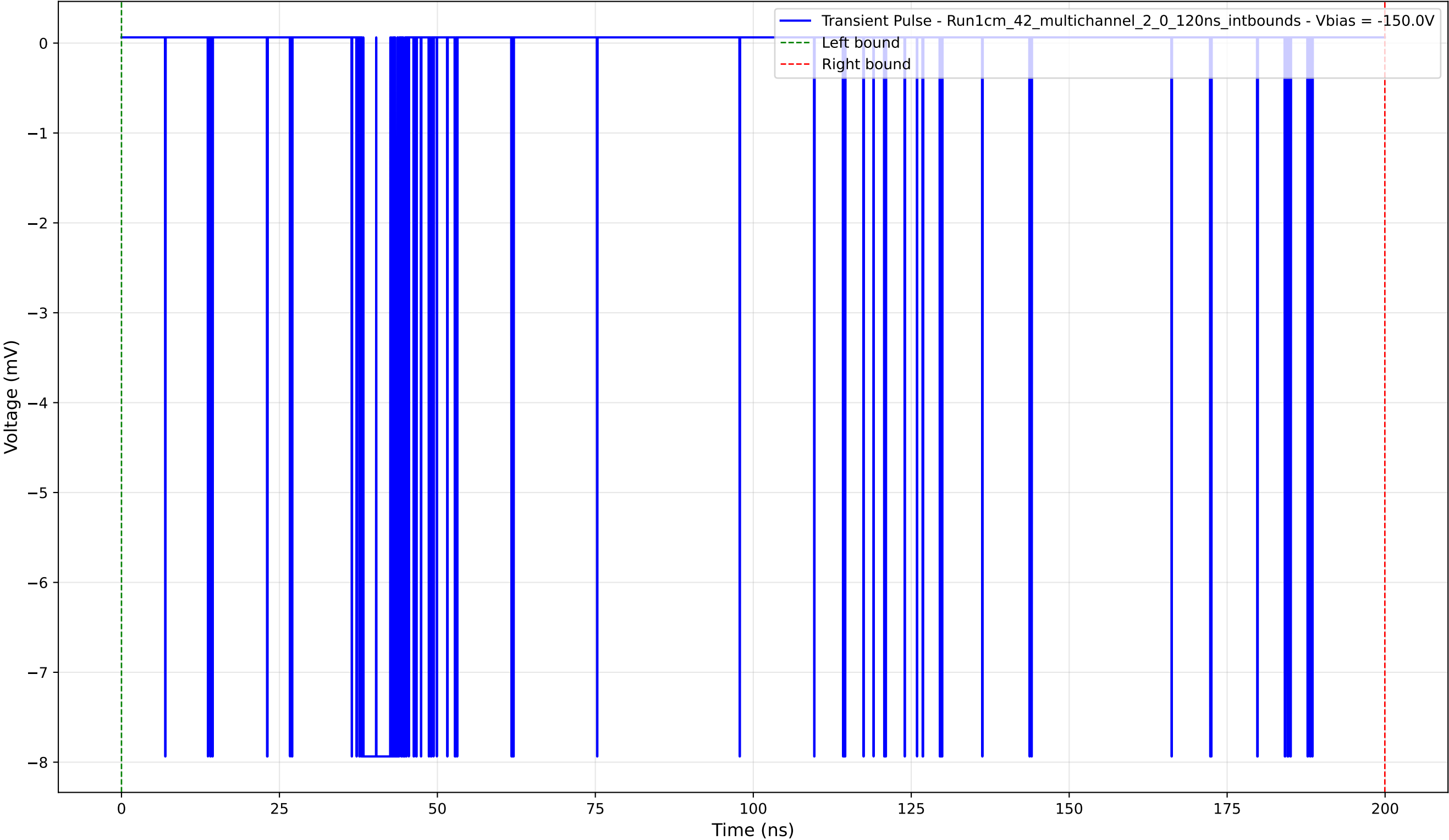
Transient Pulse - Sample: 1cm_42_multichannel - Position: 4385.0 \mu\text{m} - Charge: 1.47 pC - Rise Time: 0.04 ns
