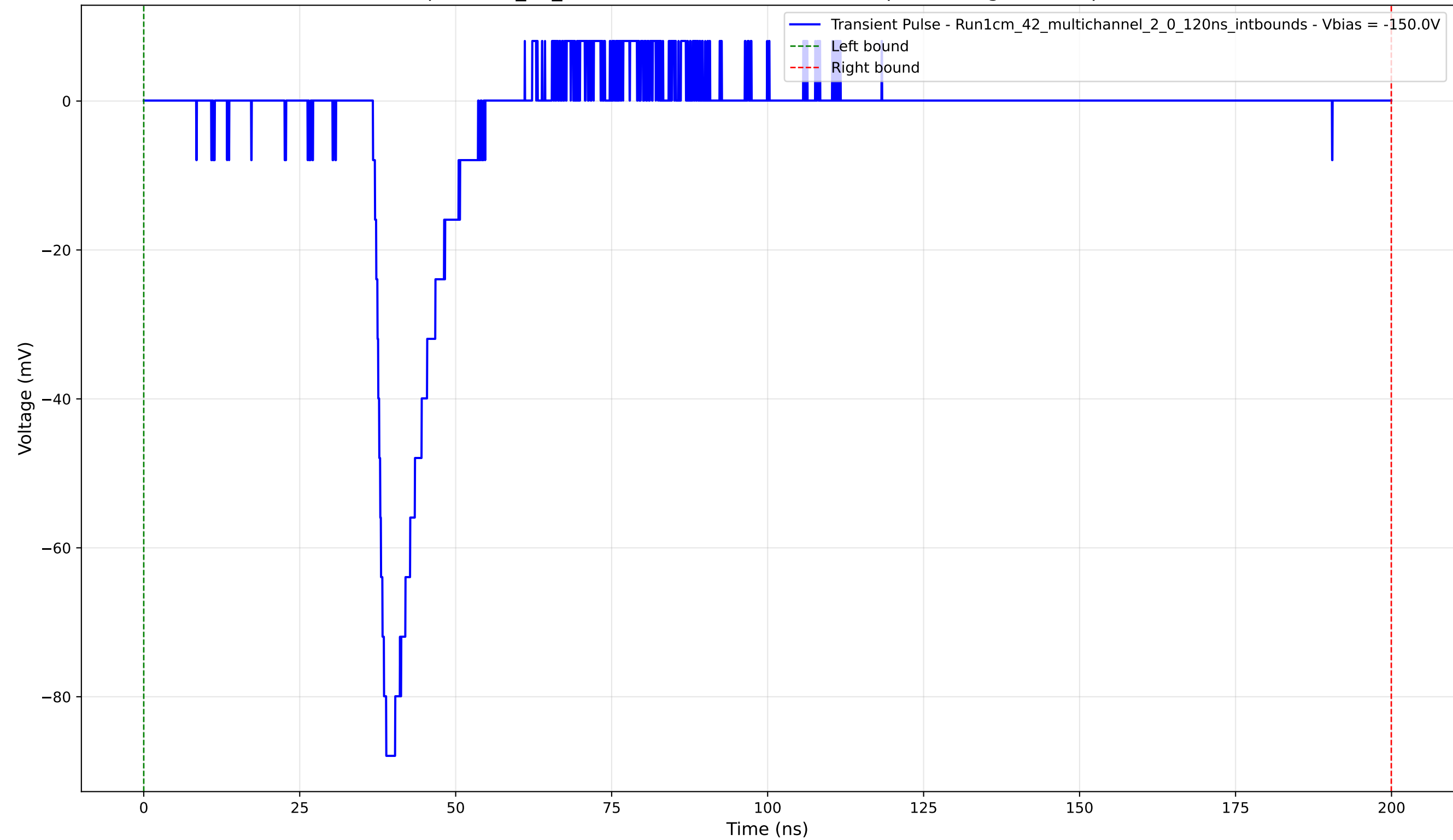
Transient Pulse - Sample: 1cm_42_multichannel - Position: 4070.0 \mu\text{m} - Charge: 10.52 pC - Rise Time: 1.48 ns
