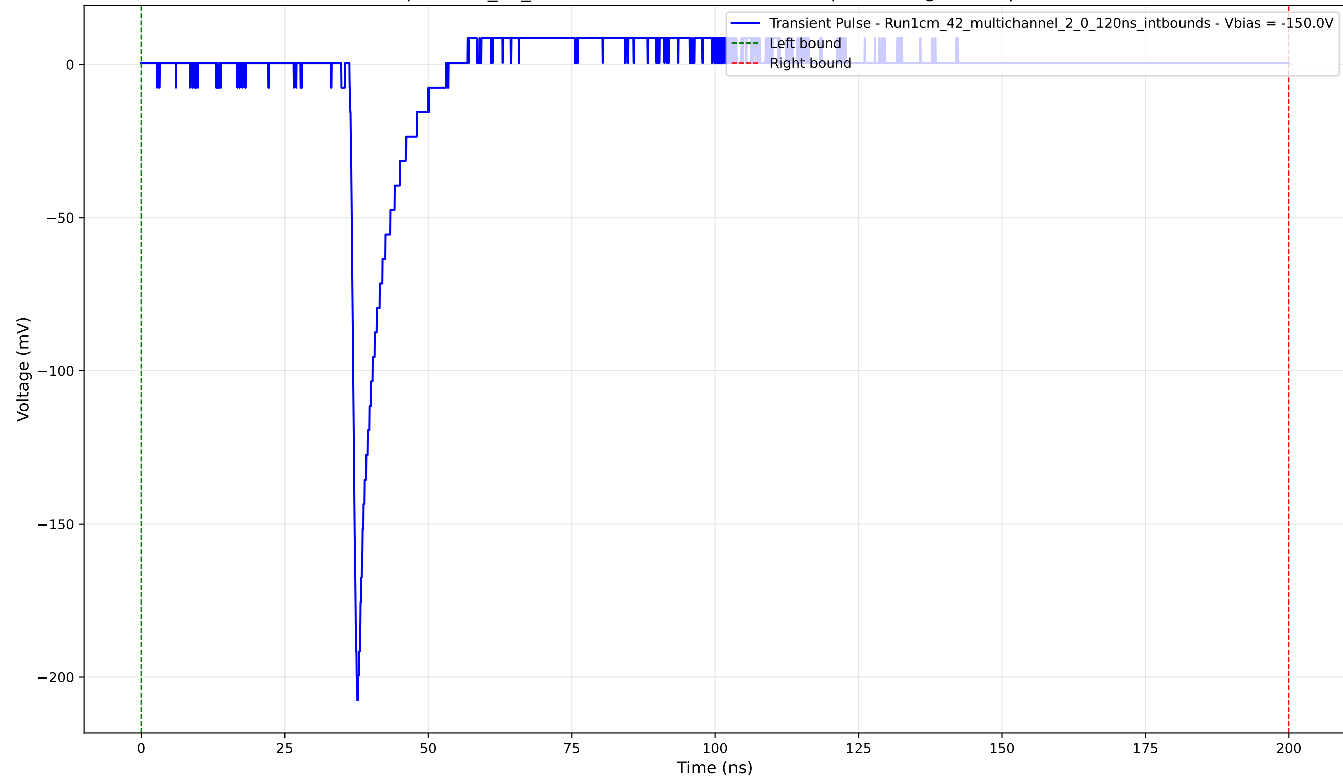
Transient Pulse - Sample: 1cm_42_multichannel - Position: 3135.0 \mu\text{m} - Charge: 9.71 pC - Rise Time: 0.97 ns
