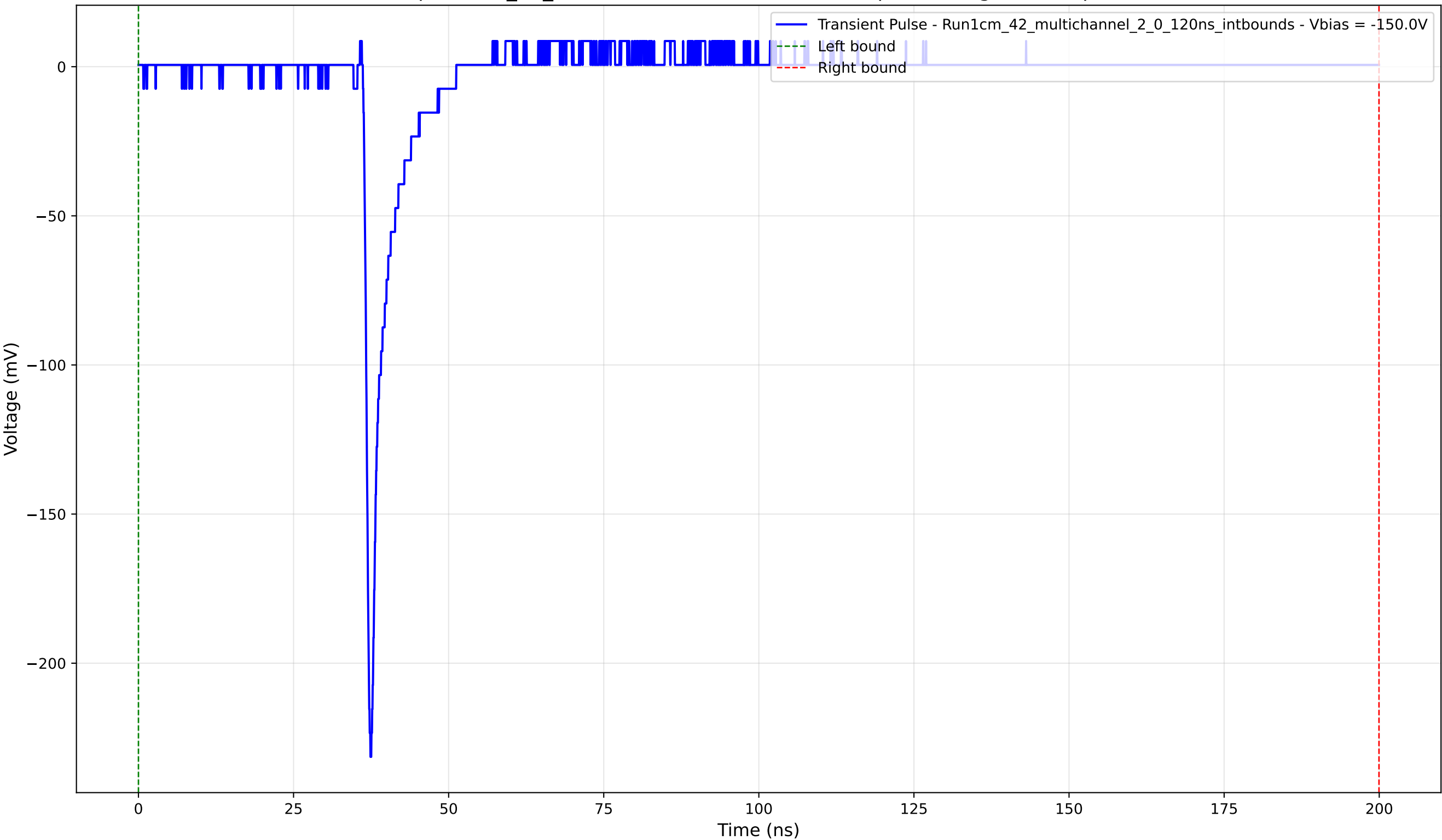
Transient Pulse - Sample: 1cm_42_multichannel - Position: 1920.0 \mu\text{m} - Charge: 10.13 pC - Rise Time: 0.84 ns
