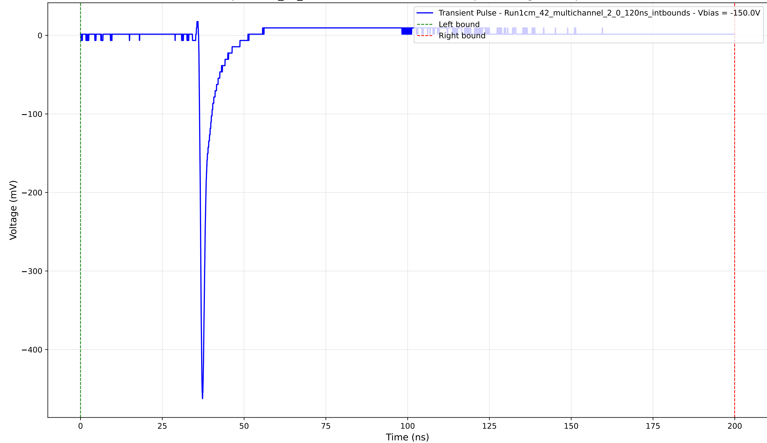
Transient Pulse - Sample: 1cm_42_multichannel - Position: 2645.0 \mu\text{m} - Charge: 9.43 pC - Rise Time: 0.73 ns
