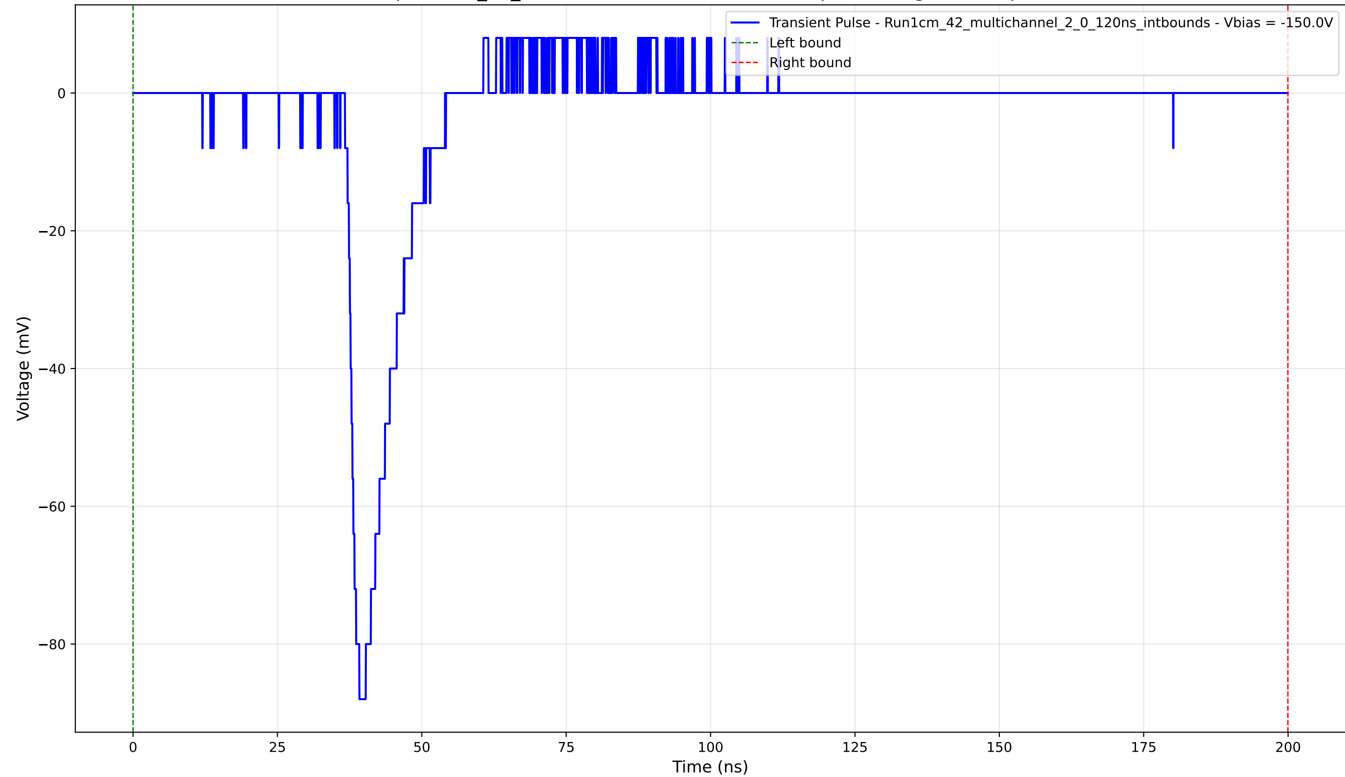
Transient Pulse - Sample: 1cm_42_multichannel - Position: 4175.0 \mu\text{m} - Charge: 10.40 pC - Rise Time: 1.52 ns
