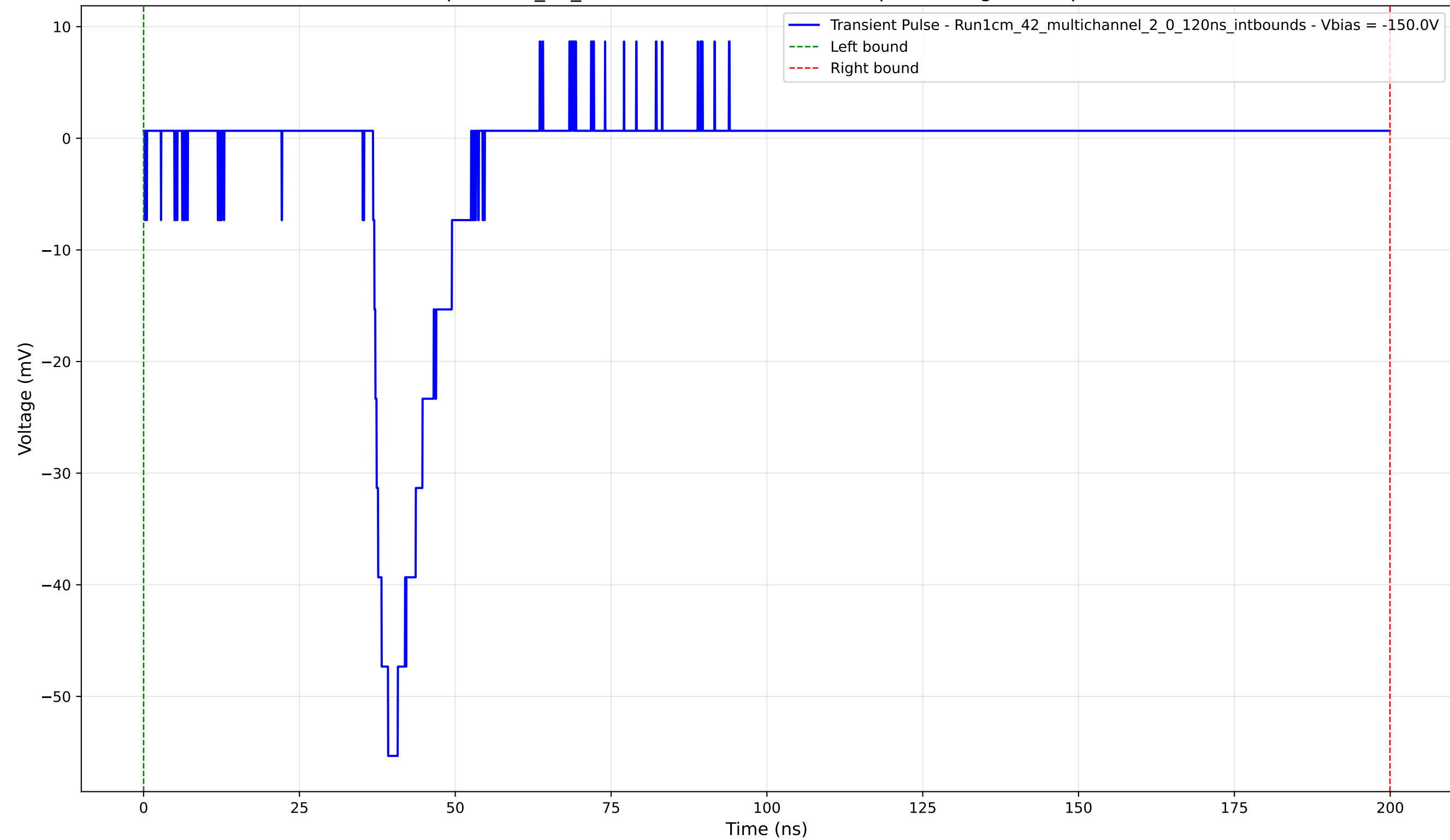
Transient Pulse - Sample: 1cm_42_multichannel - Position: 90.0 \mu\text{m} - Charge: 6.40 pC - Rise Time: 2.41 ns
