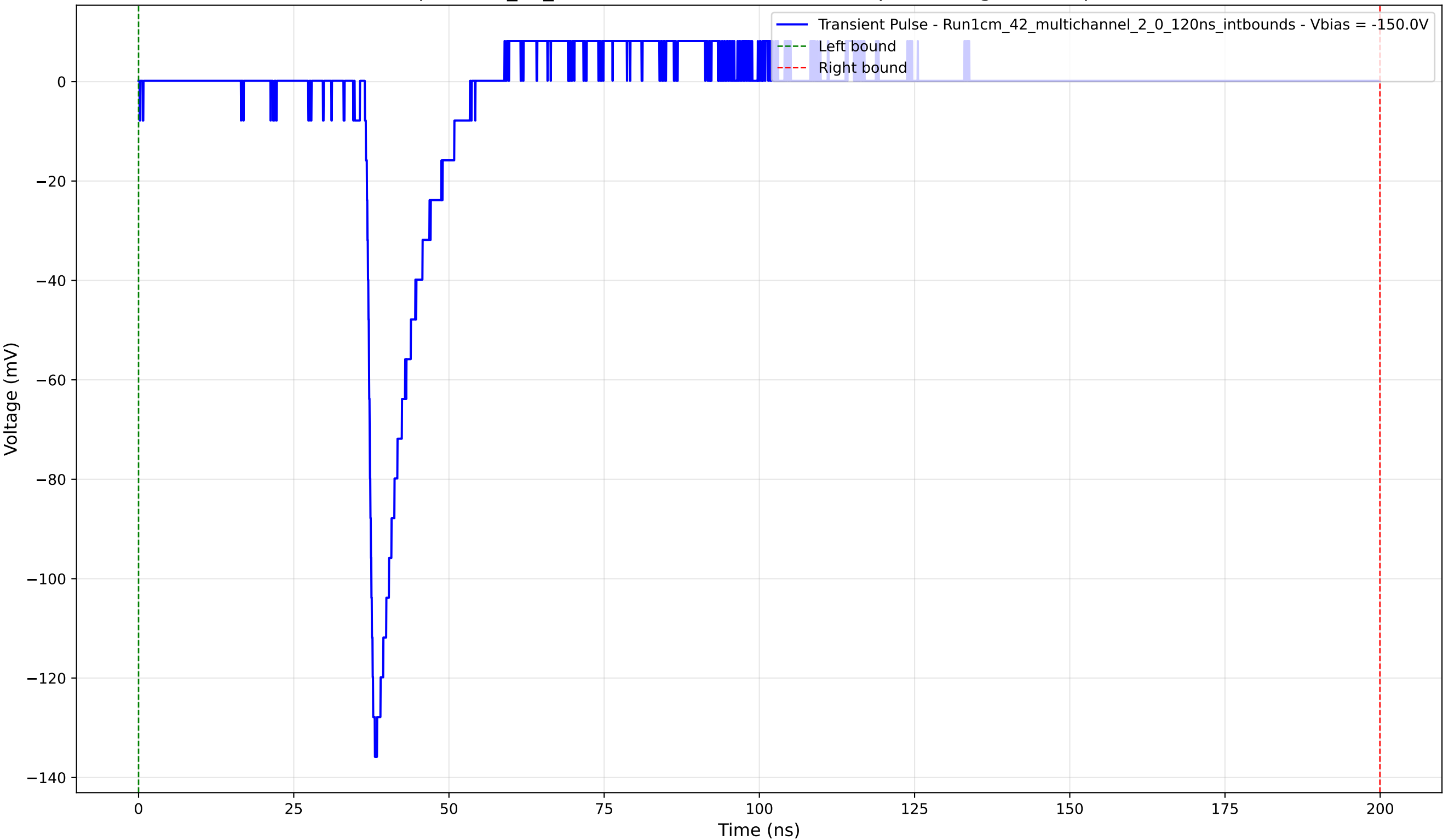
Transient Pulse - Sample: 1cm_42_multichannel - Position: 3490.0 \mu\text{m} - Charge: 10.75 pC - Rise Time: 1.17 ns
