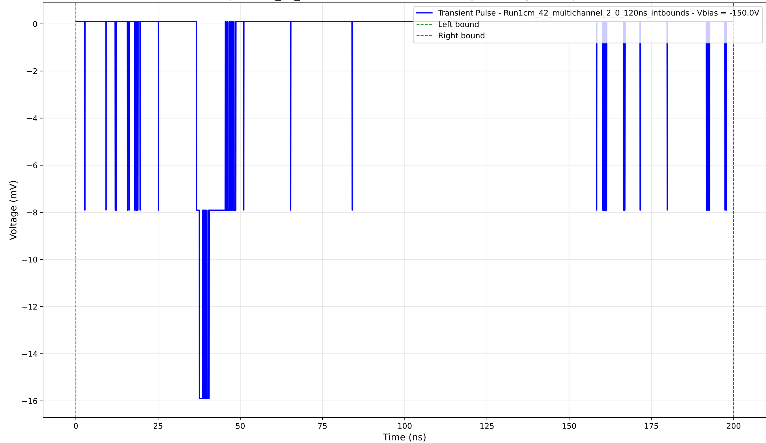
Transient Pulse - Sample: 1cm_42_multichannel - Position: 1375.0 \mu\text{m} - Charge: 2.18 pC - Rise Time: 0.87 ns
