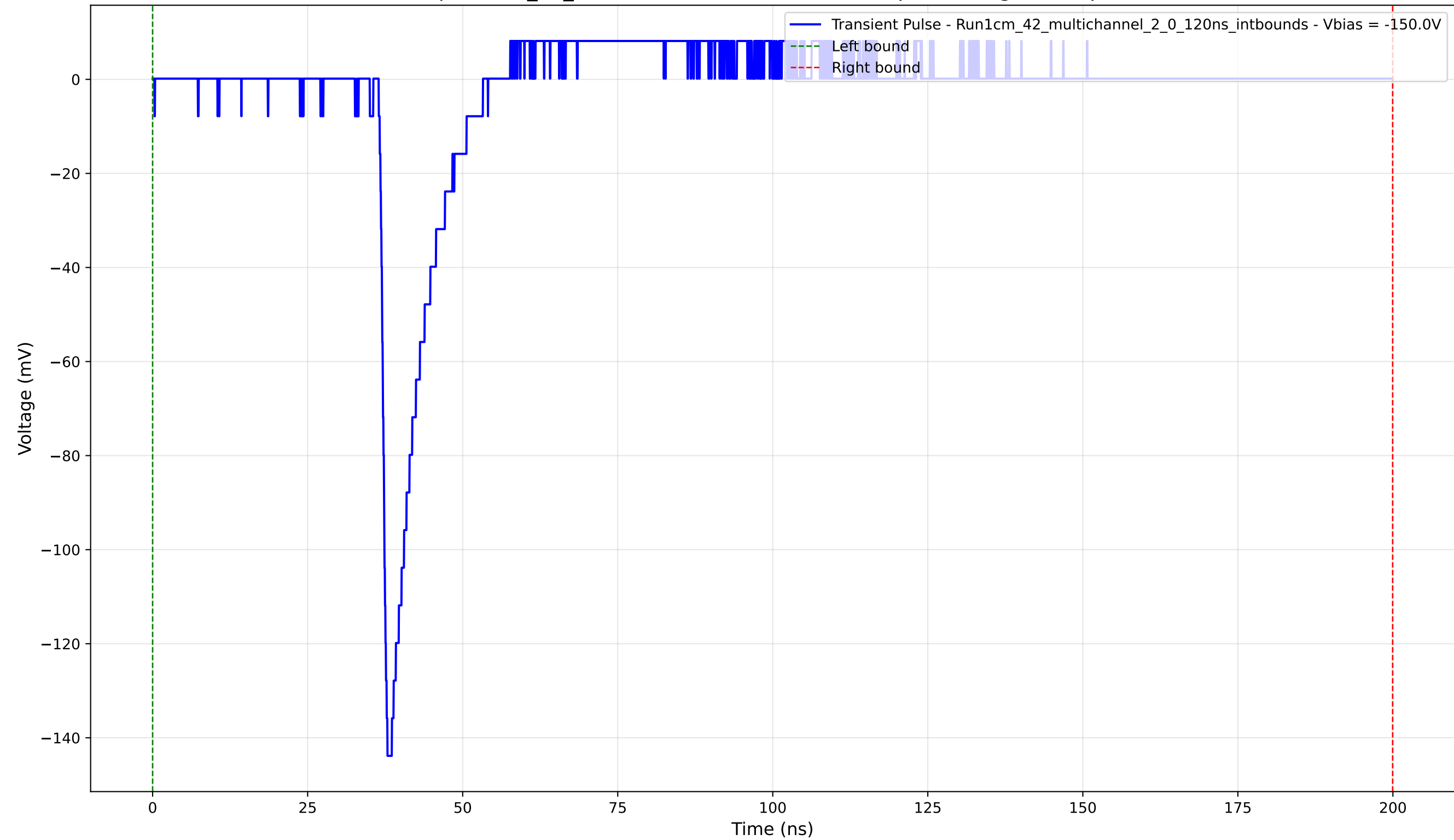
Transient Pulse - Sample: 1cm_42_multichannel - Position: 1280.0 \mu\text{m} - Charge: 9.94 pC - Rise Time: 1.13 ns
