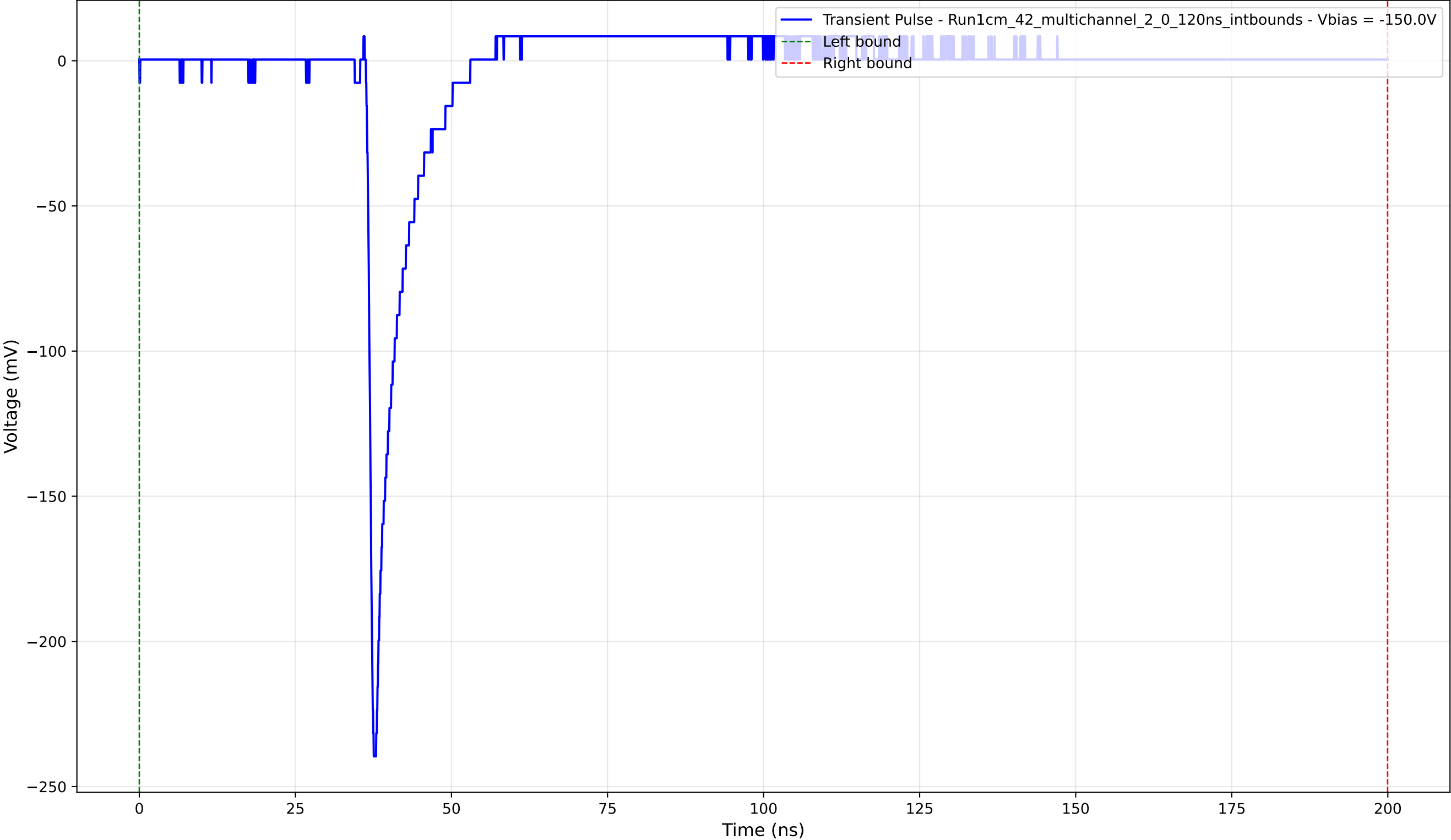
Transient Pulse - Sample: 1cm_42_multichannel - Position: 1620.0 \mu\text{m} - Charge: 11.69 pC - Rise Time: 0.92 ns
