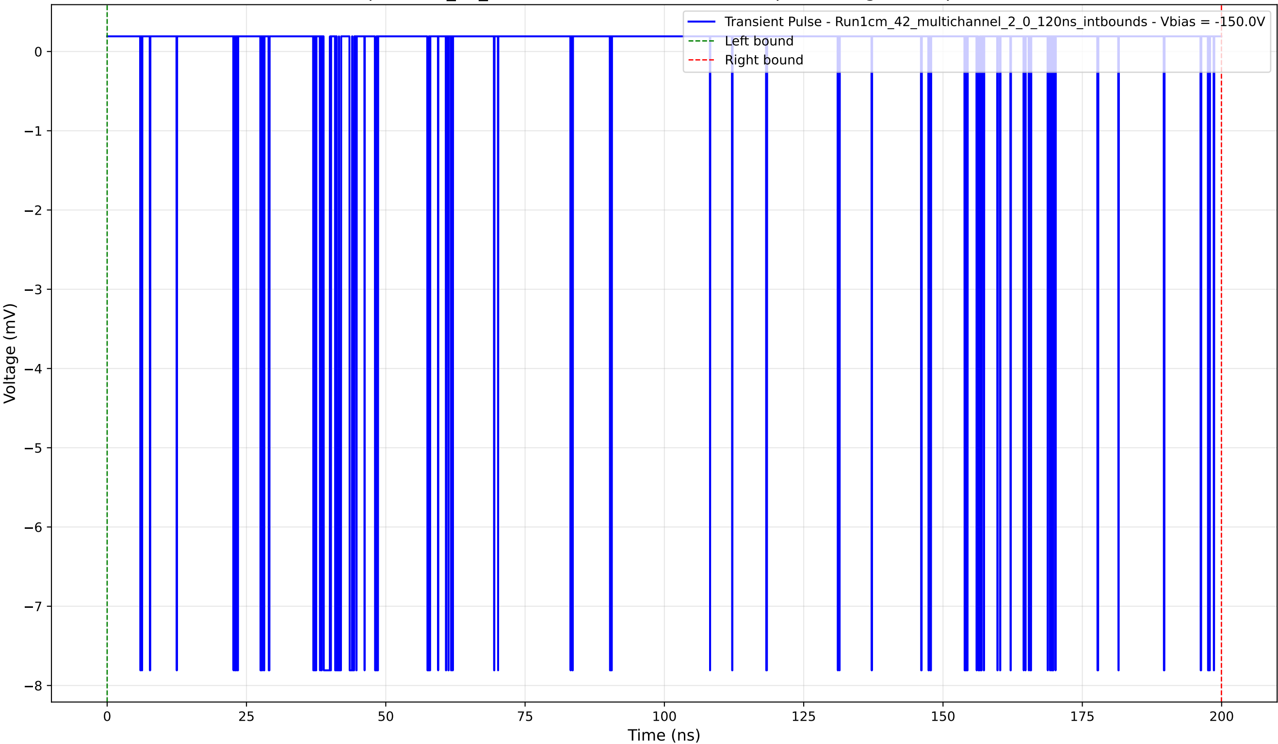
Transient Pulse - Sample: 1cm_42_multichannel - Position: 4895.0 \mu\text{m} - Charge: 0.77 pC - Rise Time: 0.04 ns
