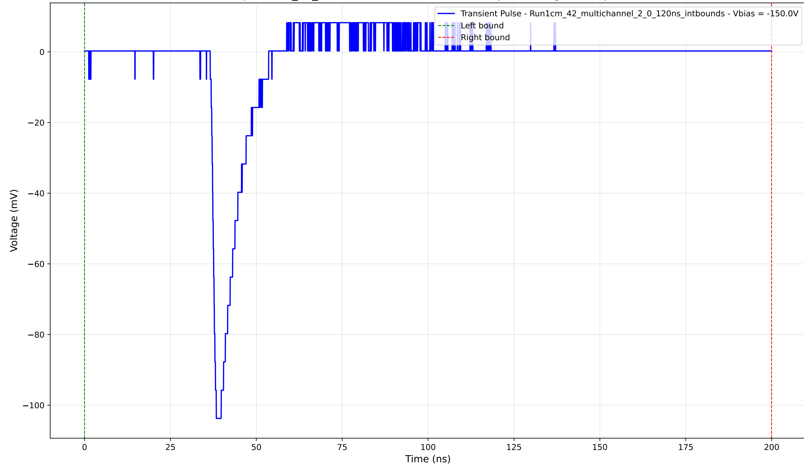
Transient Pulse - Sample: 1cm_42_multichannel - Position: 3775.0 \mu\text{m} - Charge: 9.52 pC - Rise Time: 1.27 ns
