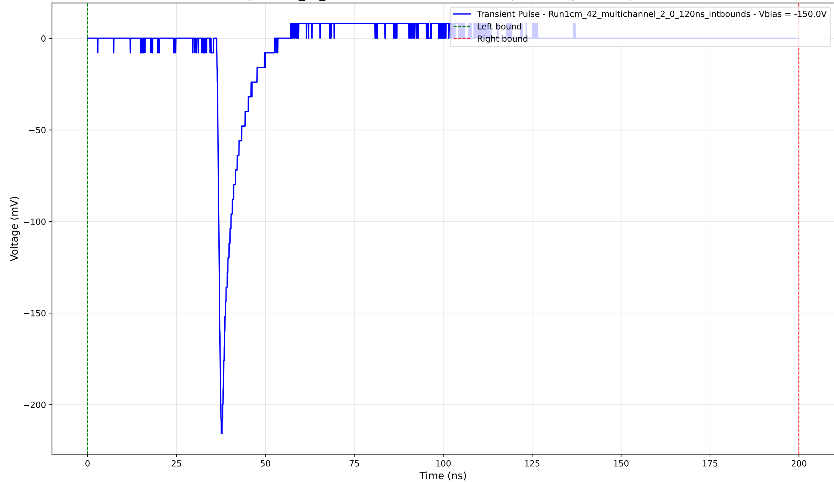
Transient Pulse - Sample: 1cm_42_multichannel - Position: 3100.0 \mu\text{m} - Charge: 12.16 pC - Rise Time: 0.97 ns
