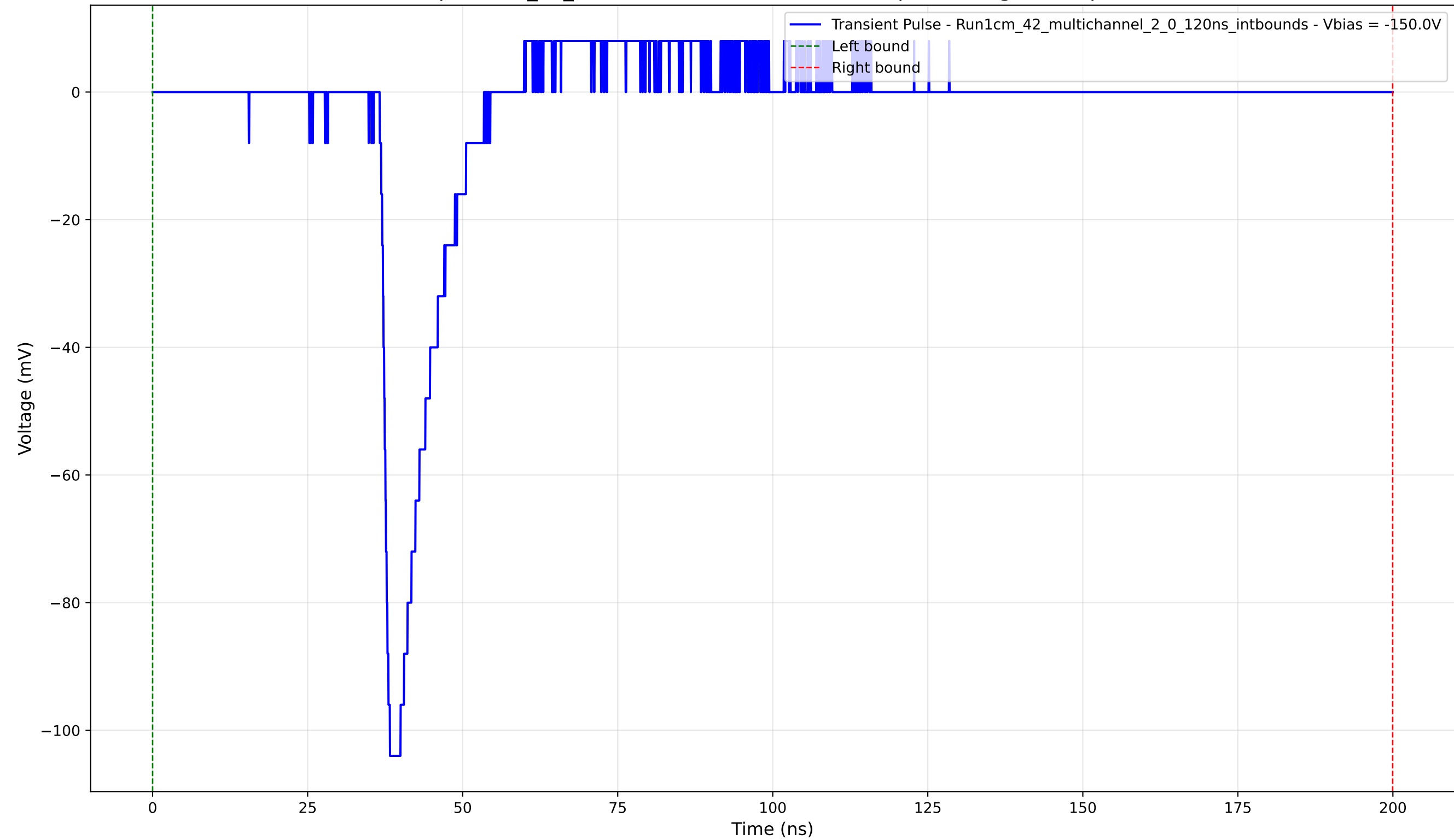
Transient Pulse - Sample: 1cm_42_multichannel - Position: 3755.0 \mu\text{m} - Charge: 9.99 pC - Rise Time: 1.19 ns
