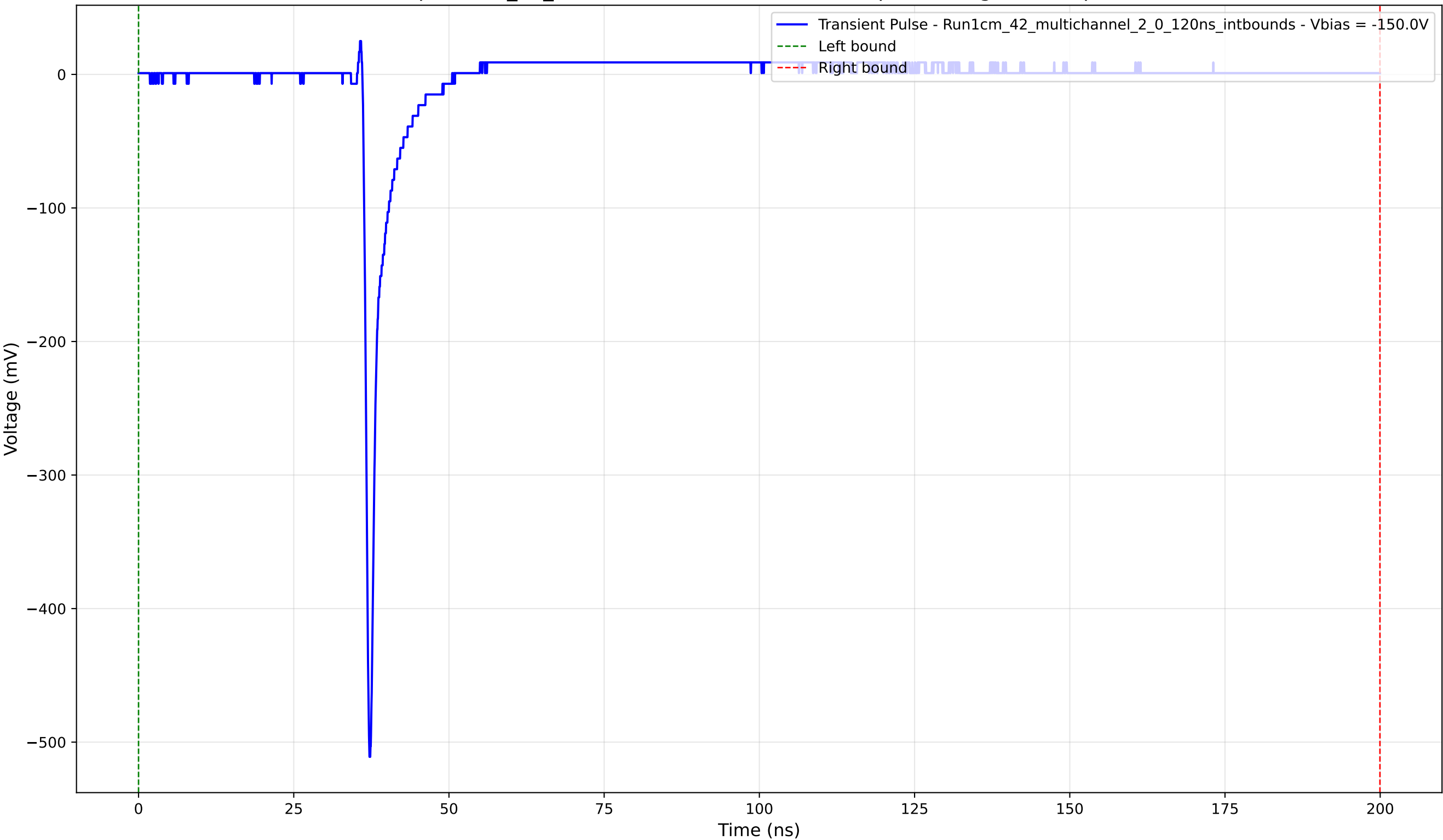
Transient Pulse - Sample: 1cm_42_multichannel - Position: 2130.0 \mu\text{m} - Charge: 12.11 pC - Rise Time: 0.76 ns
