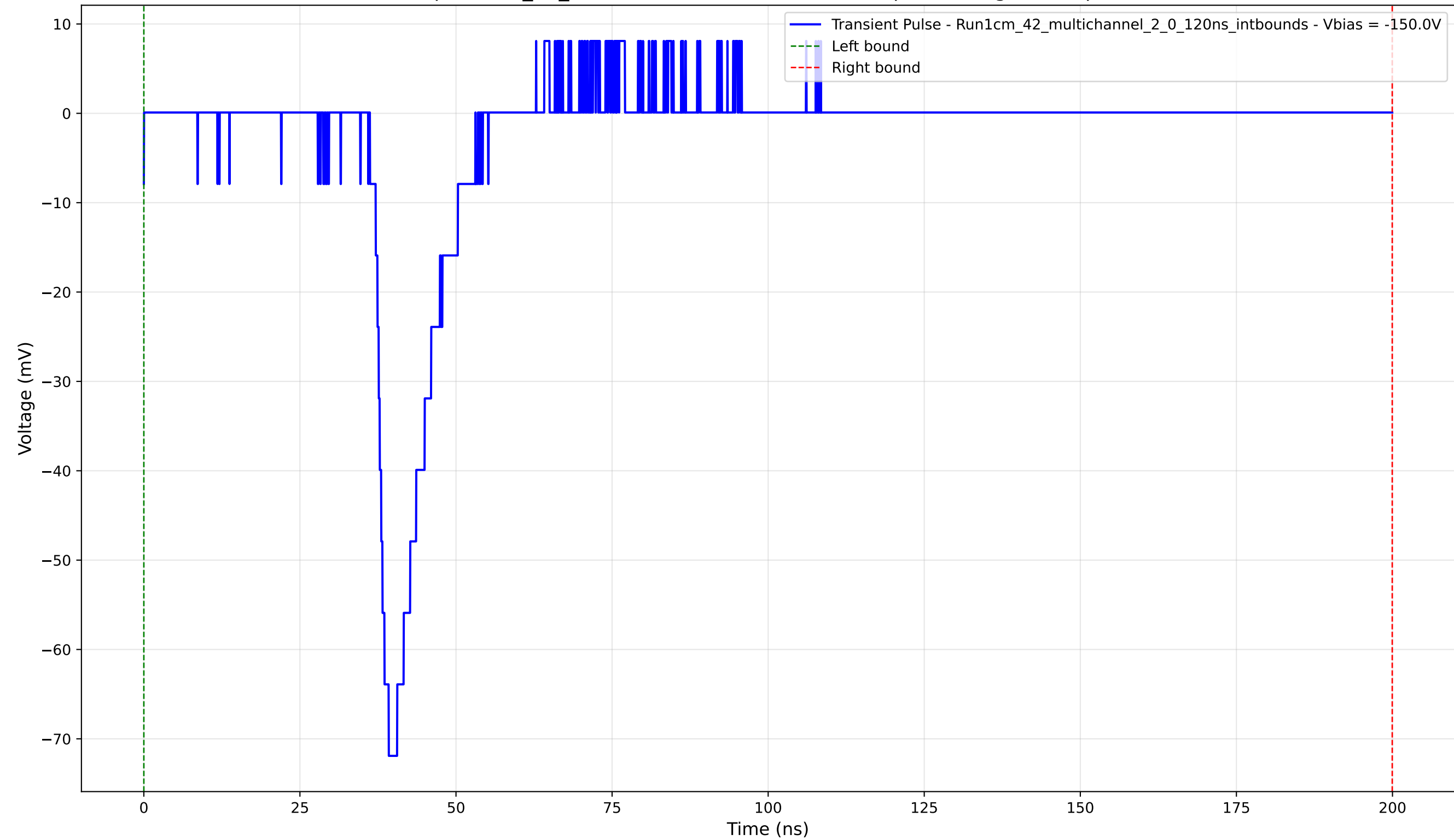
Transient Pulse - Sample: 1cm_42_multichannel - Position: 4625.0 \mu\text{m} - Charge: 9.71 pC - Rise Time: 3.00 ns
