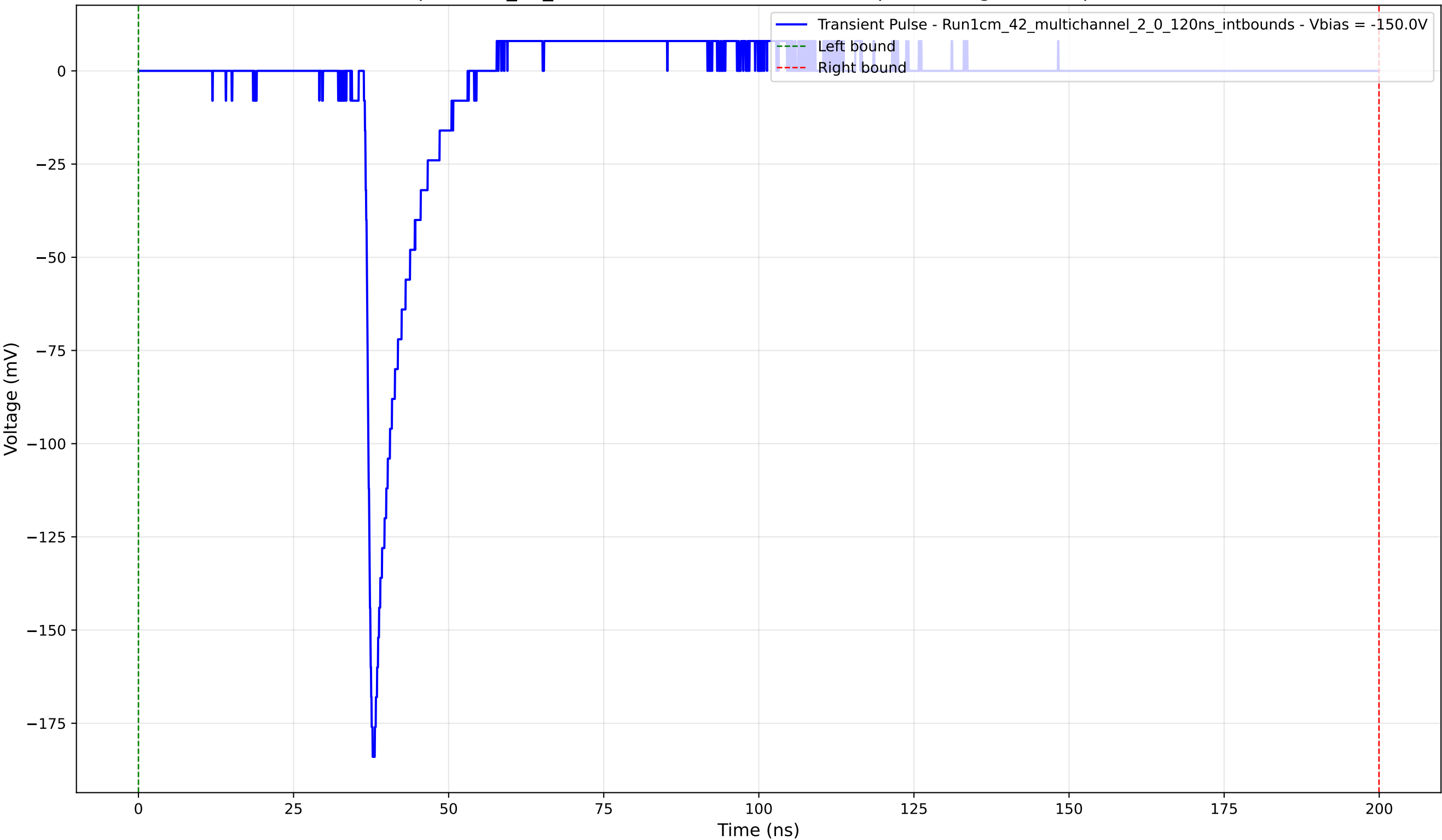
Transient Pulse - Sample: 1cm_42_multichannel - Position: 3250.0 \mu\text{m} - Charge: 11.97 pC - Rise Time: 0.95 ns
