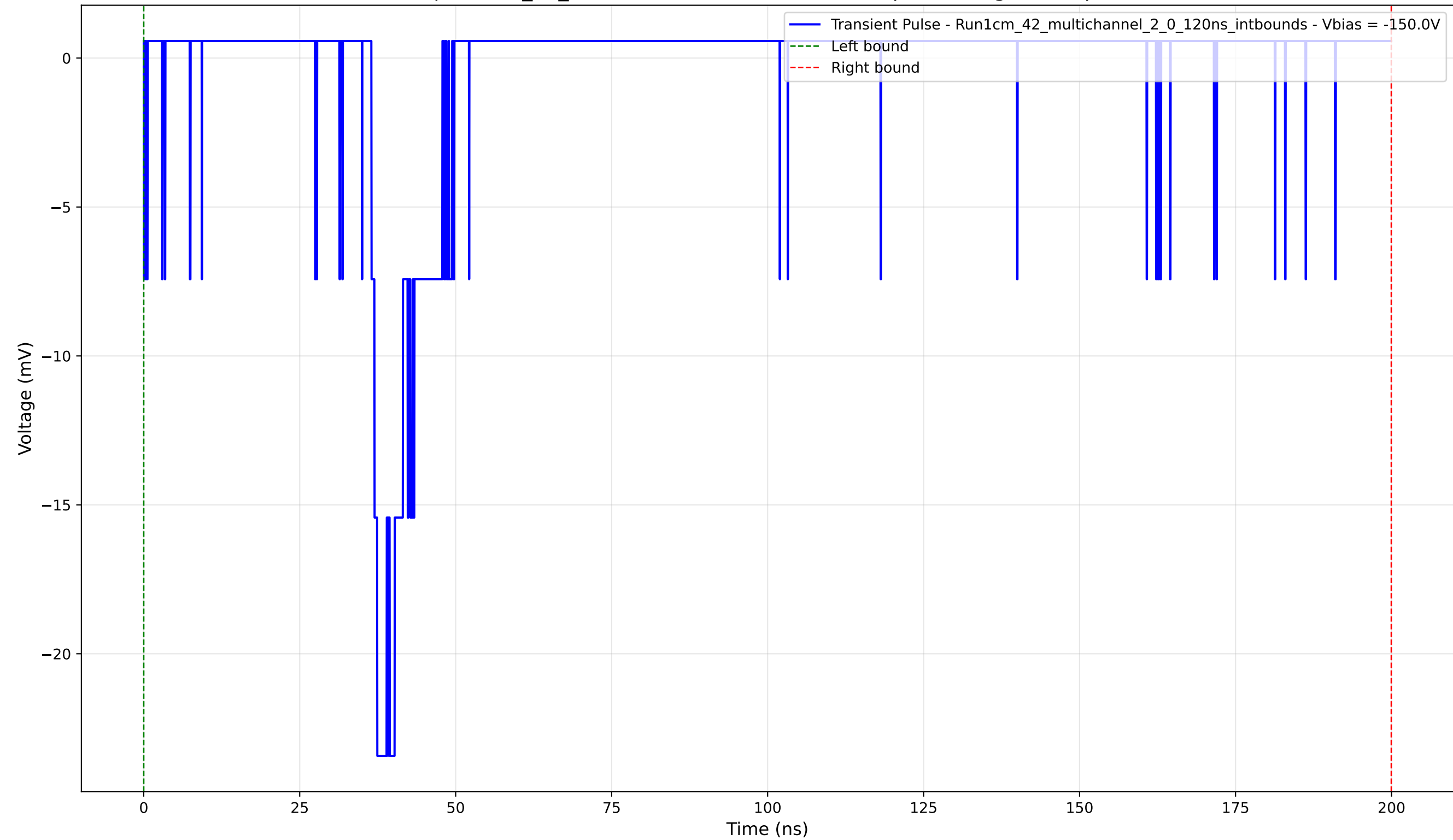
Transient Pulse - Sample: 1cm_42_multichannel - Position: 1385.0 \mu\text{m} - Charge: 1.30 pC - Rise Time: 0.95 ns
