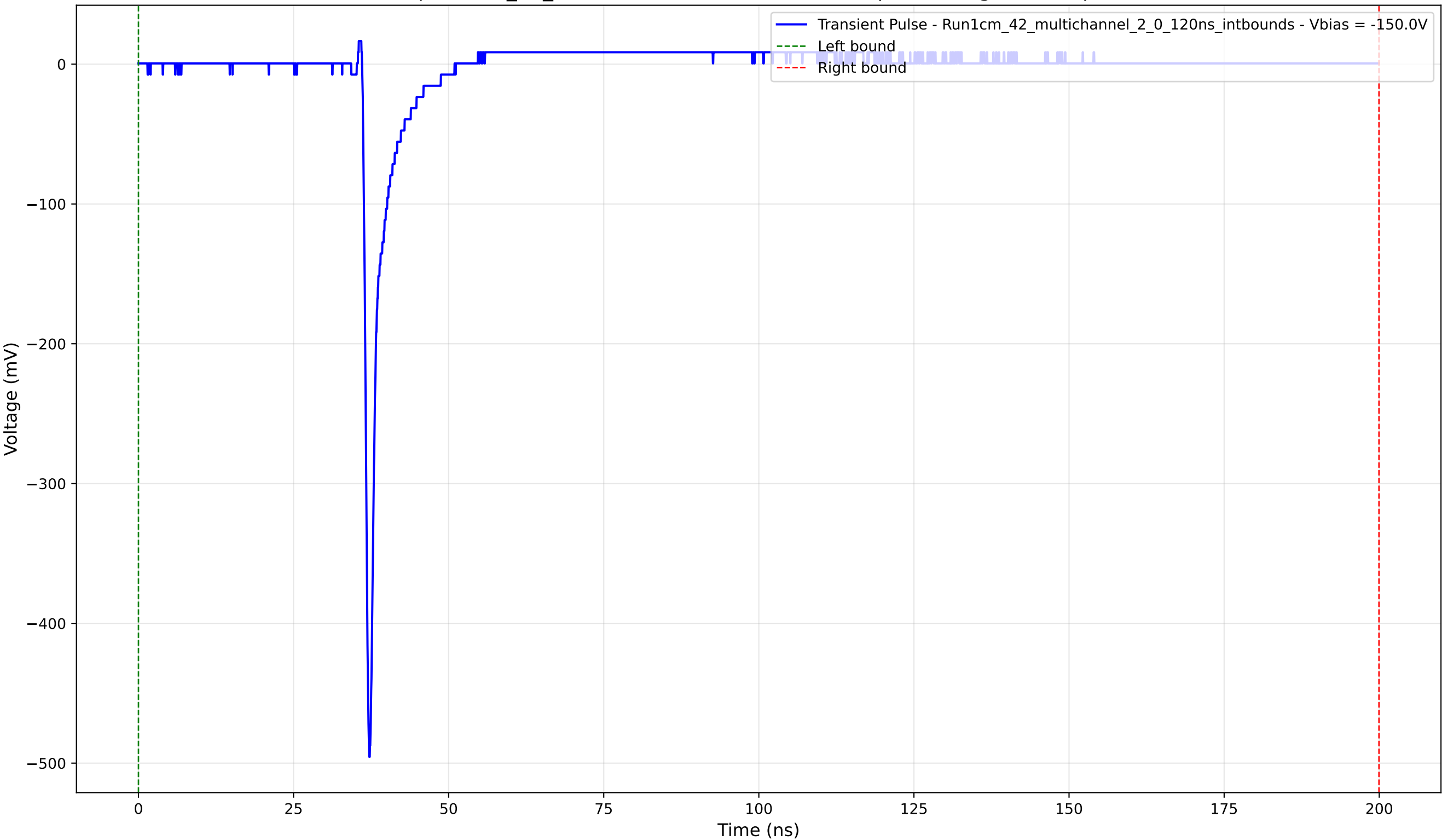
Transient Pulse - Sample: 1cm_42_multichannel - Position: 2580.0 \mu\text{m} - Charge: 13.13 pC - Rise Time: 0.77 ns
