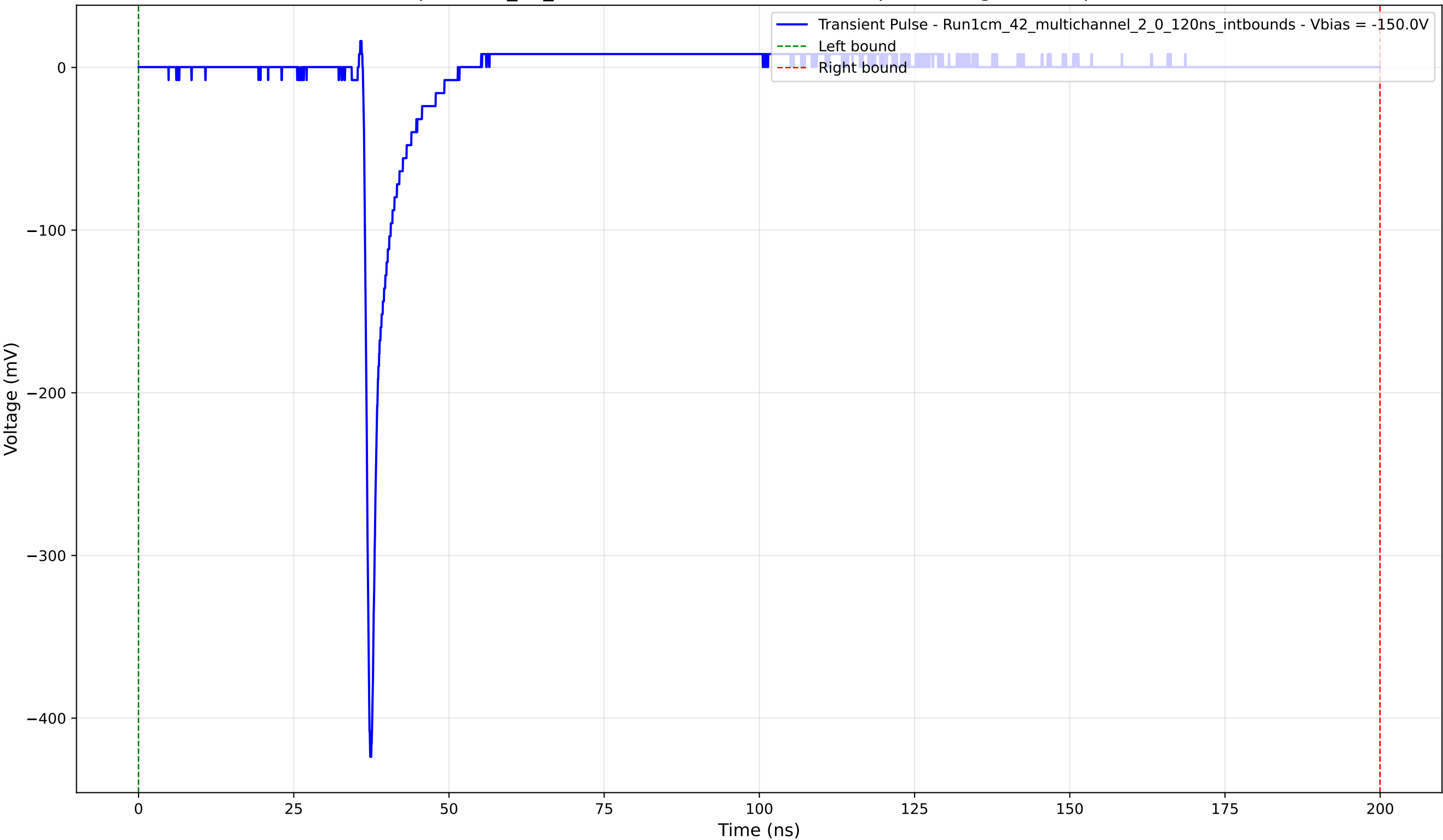
Transient Pulse - Sample: 1cm_42_multichannel - Position: 1990.0 \mu\text{m} - Charge: 14.32 pC - Rise Time: 0.78 ns
