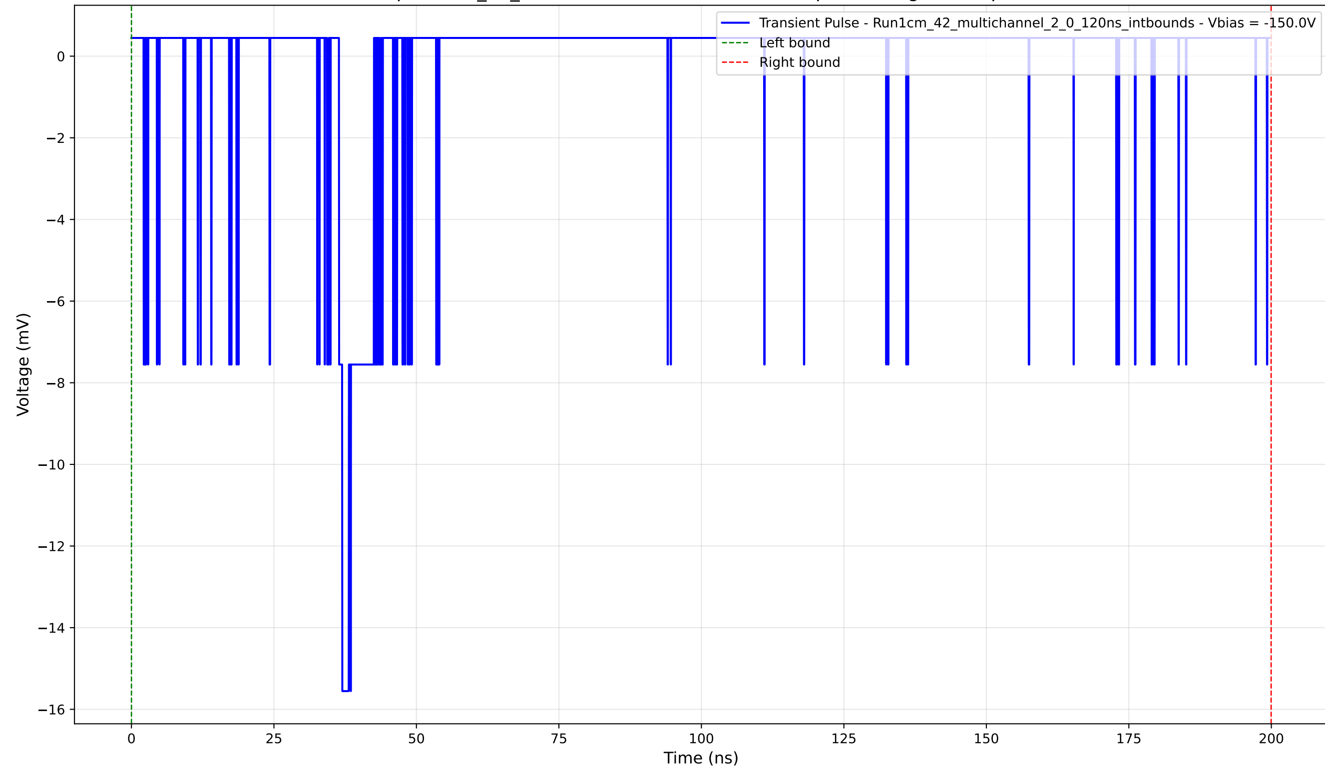
Transient Pulse - Sample: 1cm_42_multichannel - Position: 2870.0 \mu\text{m} - Charge: 0.24 pC - Rise Time: 0.59 ns
