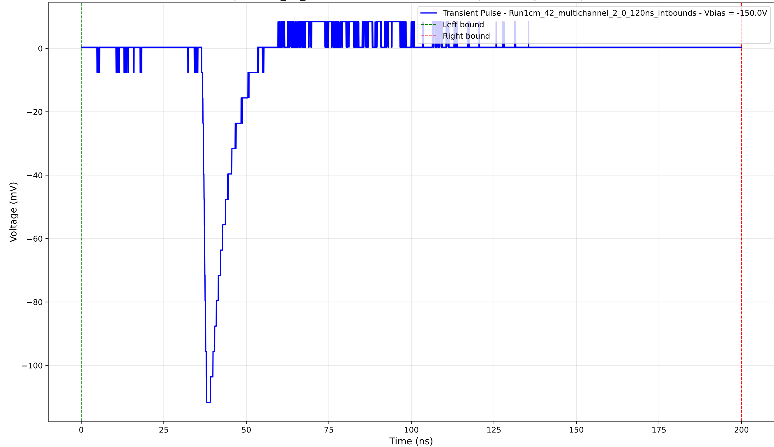
Transient Pulse - Sample: 1cm_42_multichannel - Position: 3600.0 \mu\text{m} - Charge: 9.85 pC - Rise Time: 1.14 ns
