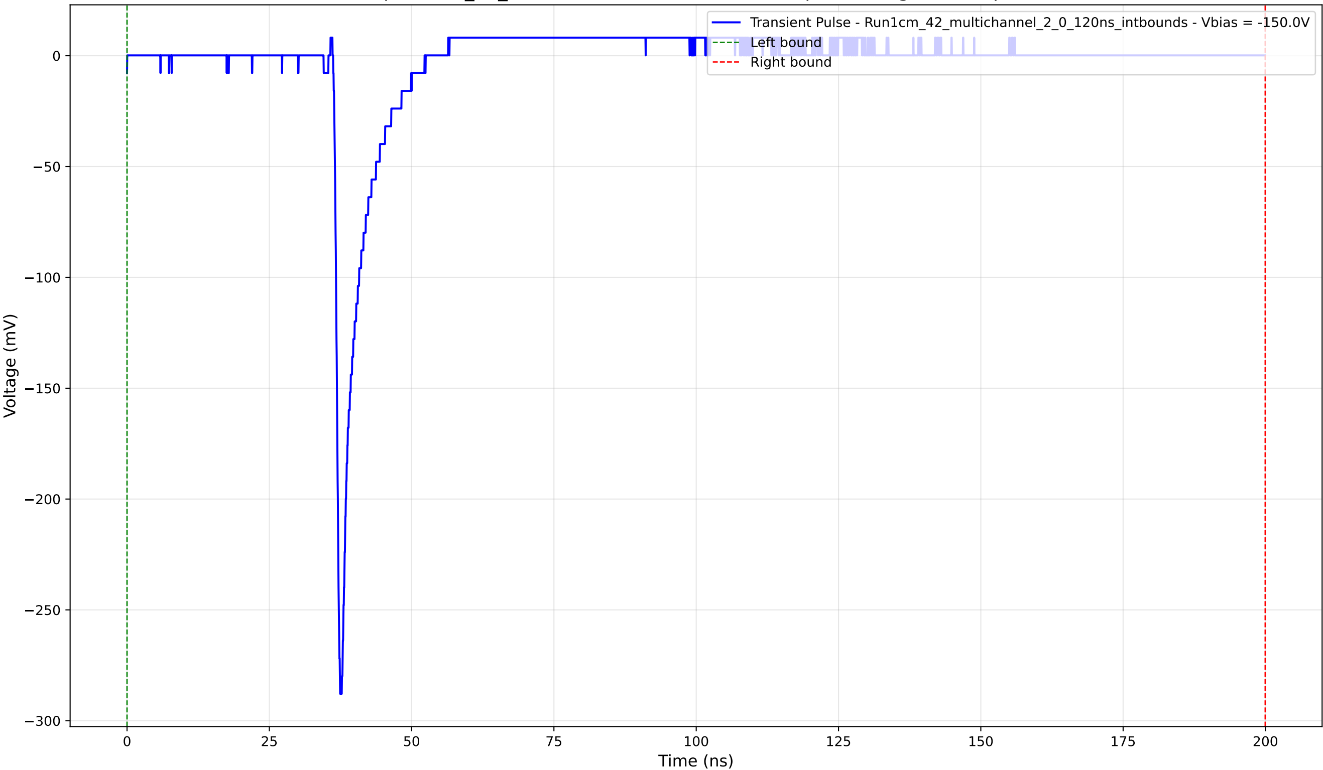
Transient Pulse - Sample: 1cm_42_multichannel - Position: 1755.0 \mu\text{m} - Charge: 12.71 pC - Rise Time: 0.83 ns
