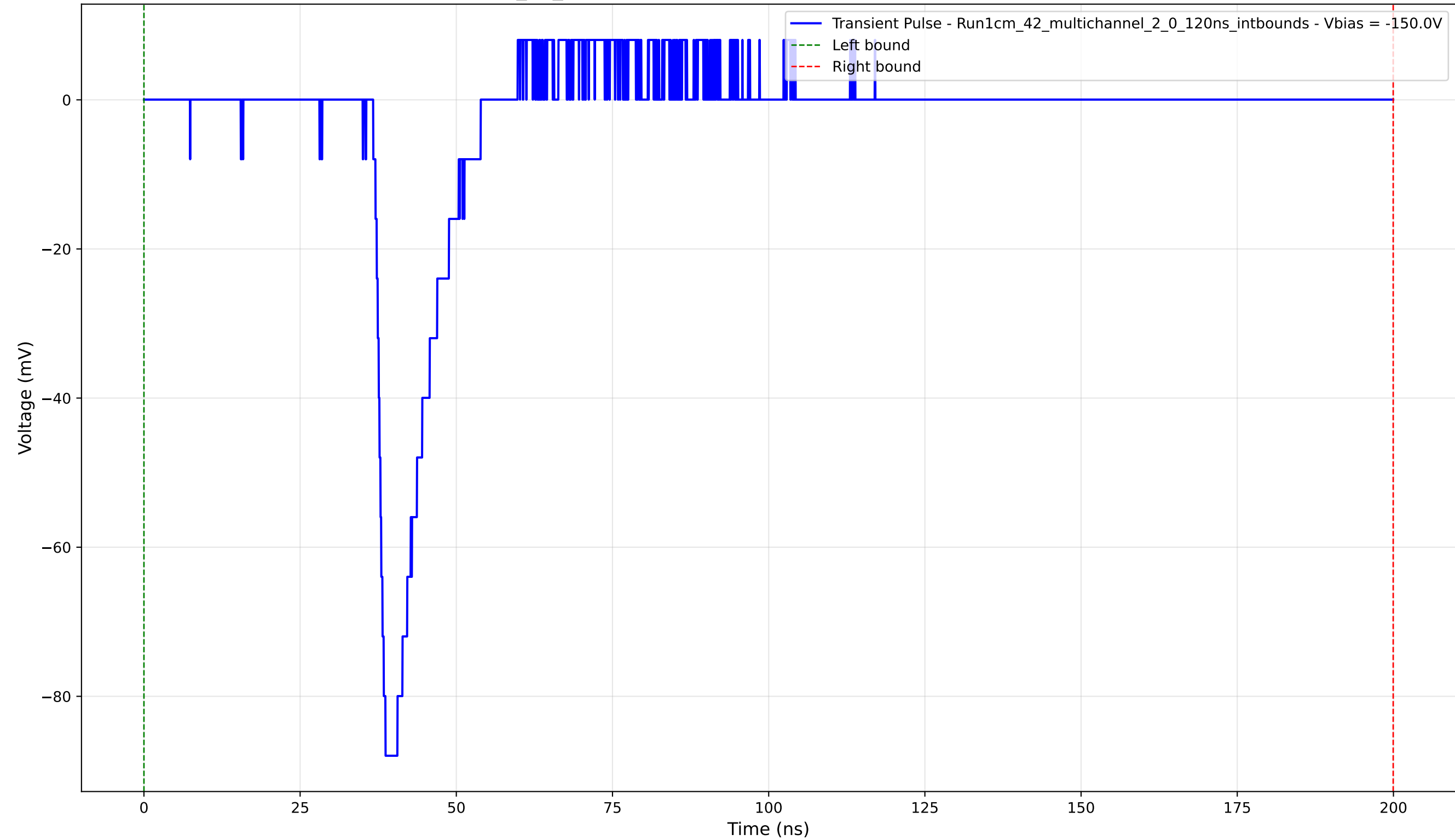
Transient Pulse - Sample: 1cm_42_multichannel - Position: 4050.0 \mu\text{m} - Charge: 10.00 pC - Rise Time: 1.36 ns
