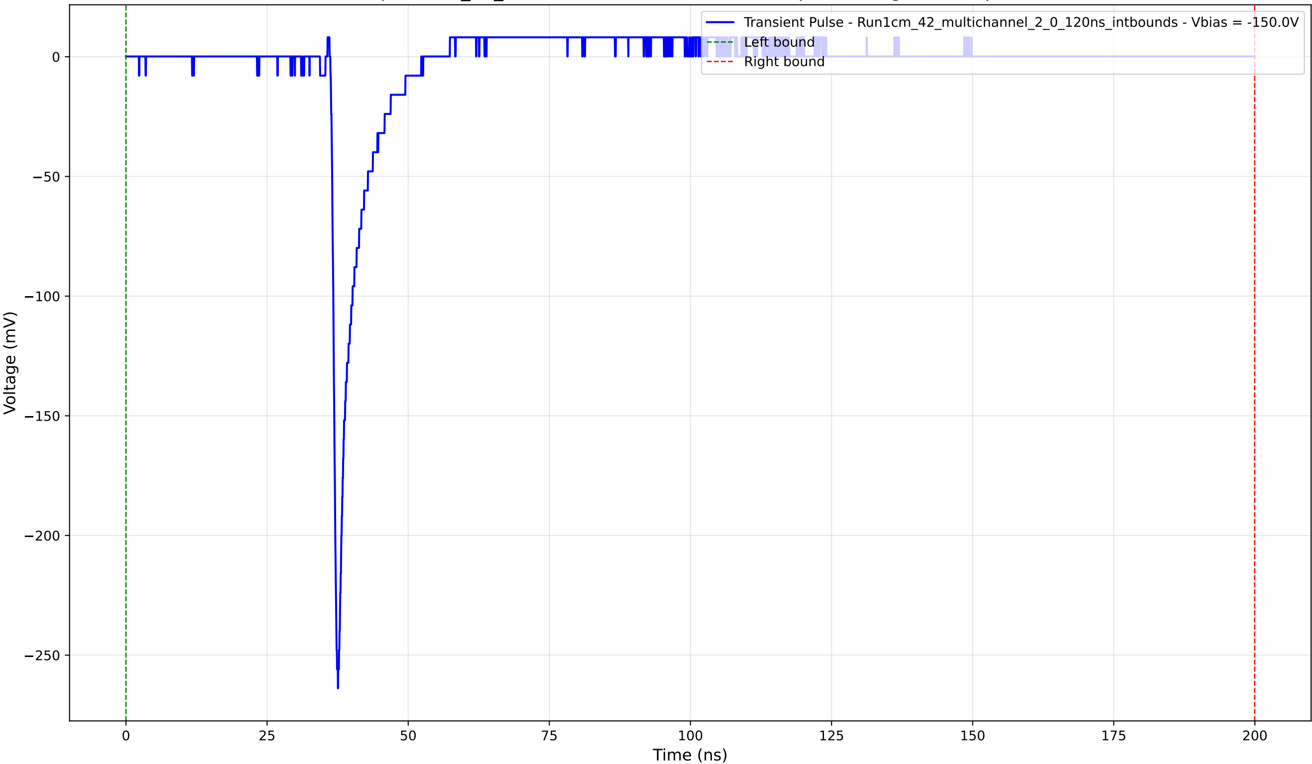
Transient Pulse - Sample: 1cm_42_multichannel - Position: 2950.0 \mu\text{m} - Charge: 11.68 pC - Rise Time: 0.86 ns
