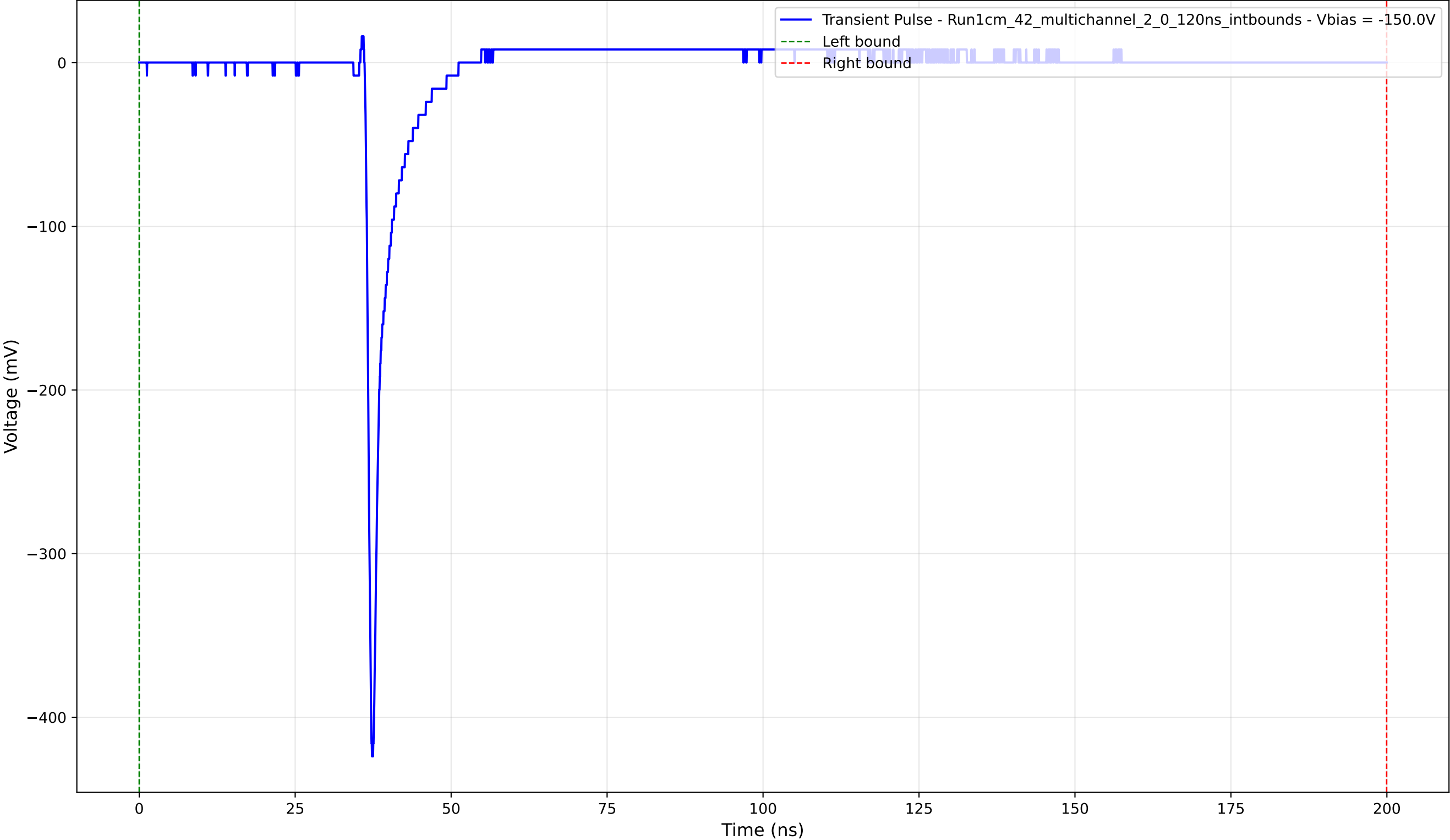
Transient Pulse - Sample: 1cm_42_multichannel - Position: 1995.0 \mu\text{m} - Charge: 14.14 pC - Rise Time: 0.81 ns
