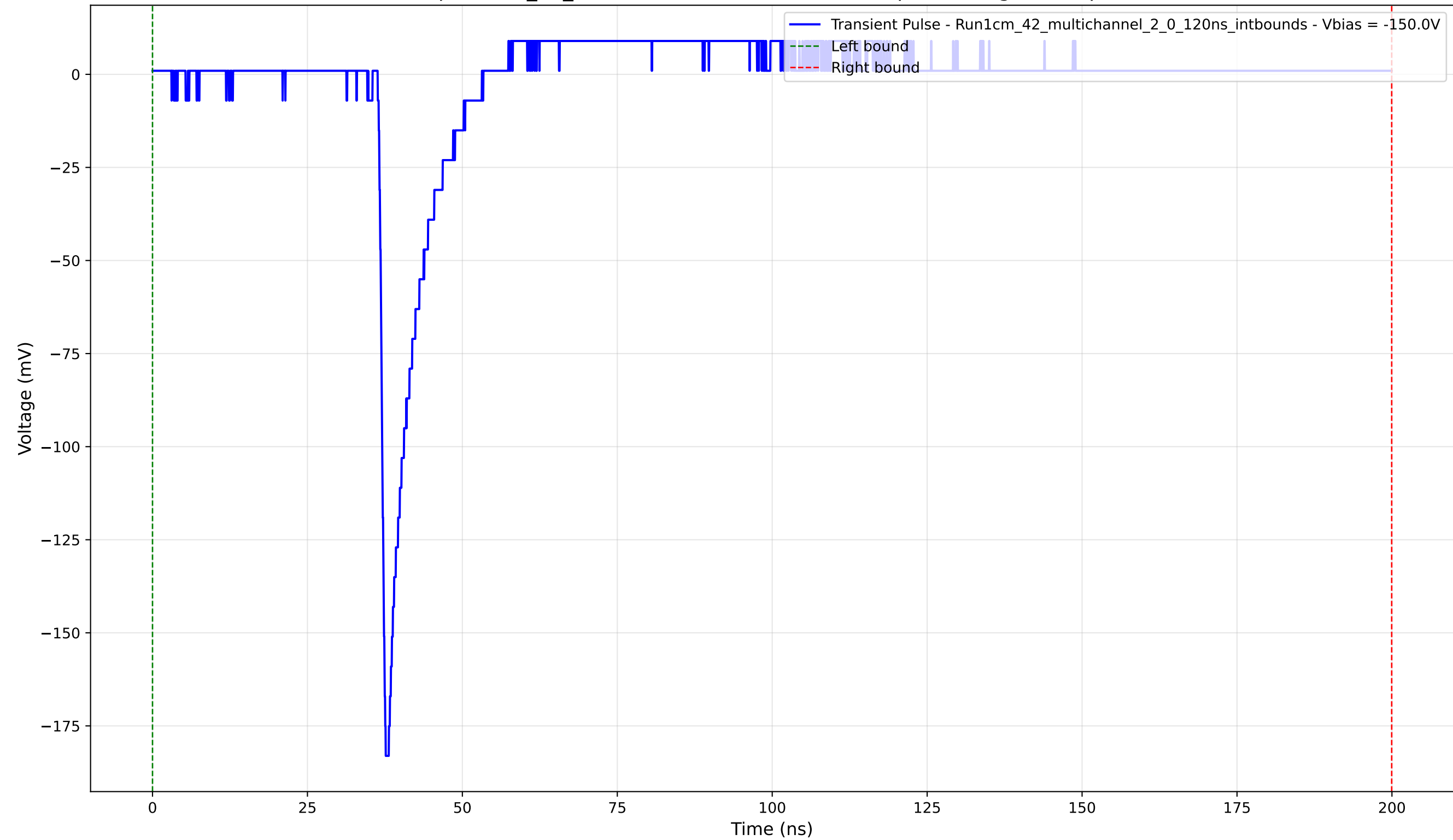
Transient Pulse - Sample: 1cm_42_multichannel - Position: 3245.0 \mu\text{m} - Charge: 7.77 pC - Rise Time: 0.90 ns
