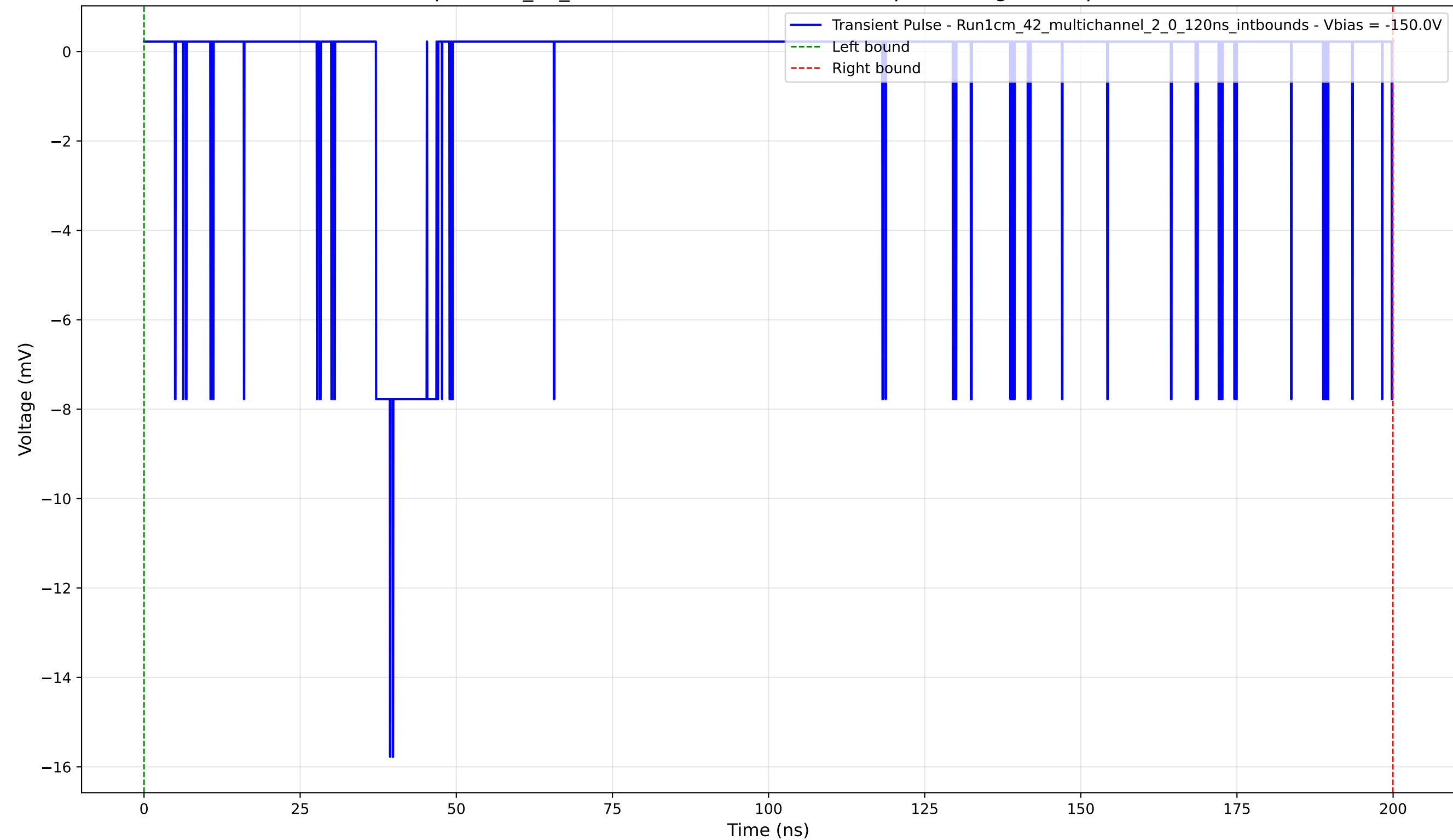
Transient Pulse - Sample: 1cm_42_multichannel - Position: 3865.0 \mu\text{m} - Charge: 1.43 pC - Rise Time: 2.27 ns
