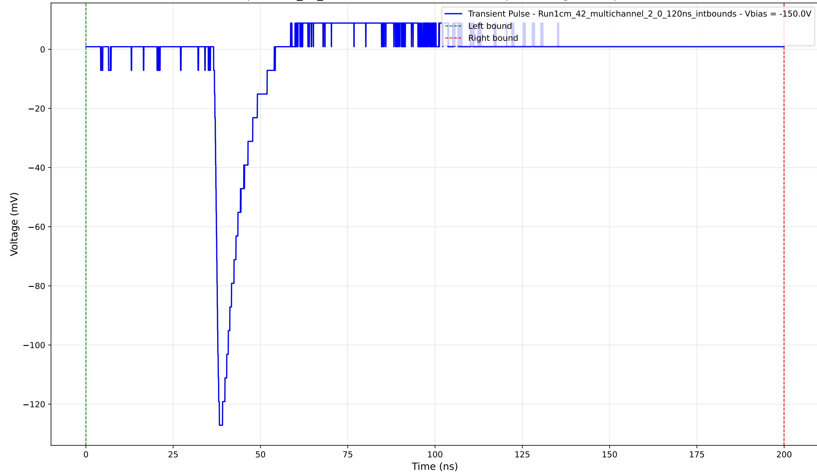
Transient Pulse - Sample: 1cm_42_multichannel - Position: 1035.0 \mu\text{m} - Charge: 8.14 pC - Rise Time: 1.21 ns
