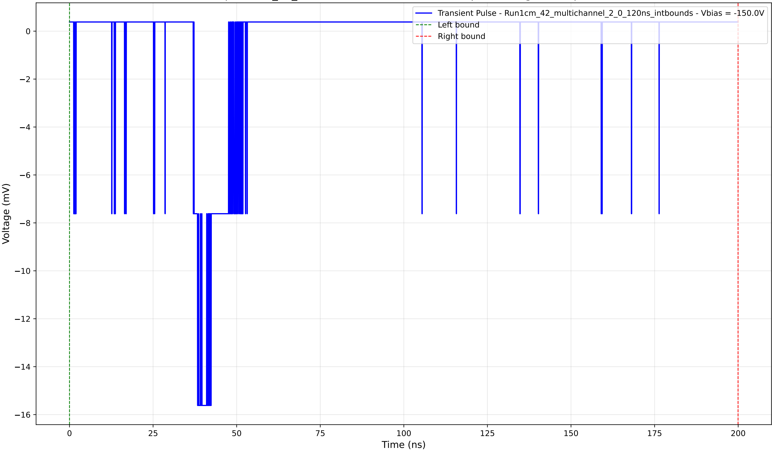
Transient Pulse - Sample: 1cm_42_multichannel - Position: 4355.0 \mu\text{m} - Charge: 1.32 pC - Rise Time: 1.07 ns
