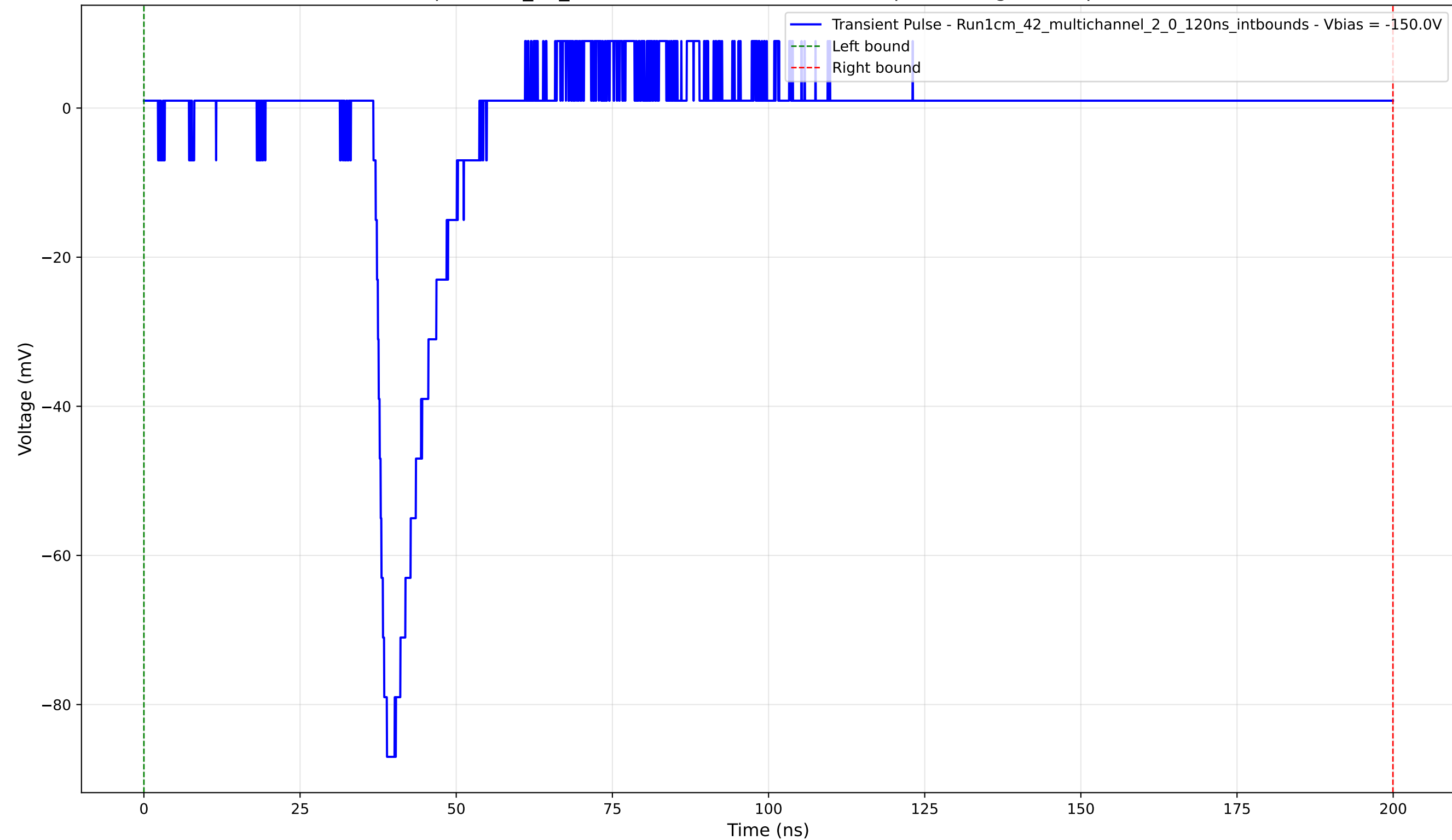
Transient Pulse - Sample: 1cm_42_multichannel - Position: 4080.0 \mu\text{m} - Charge: 6.77 pC - Rise Time: 1.39 ns
