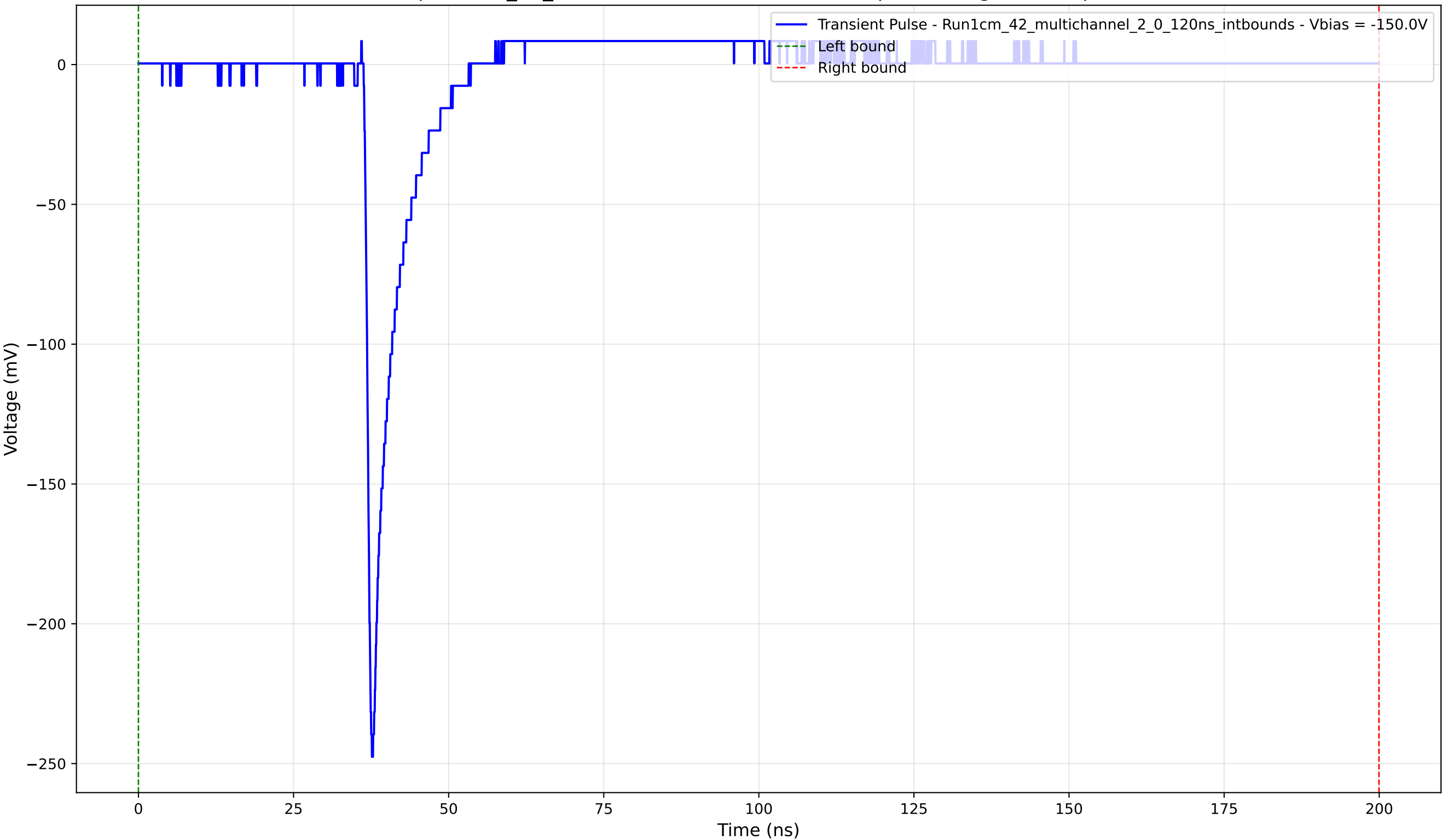
Transient Pulse - Sample: 1cm_42_multichannel - Position: 1635.0 \mu\text{m} - Charge: 12.06 pC - Rise Time: 0.91 ns
