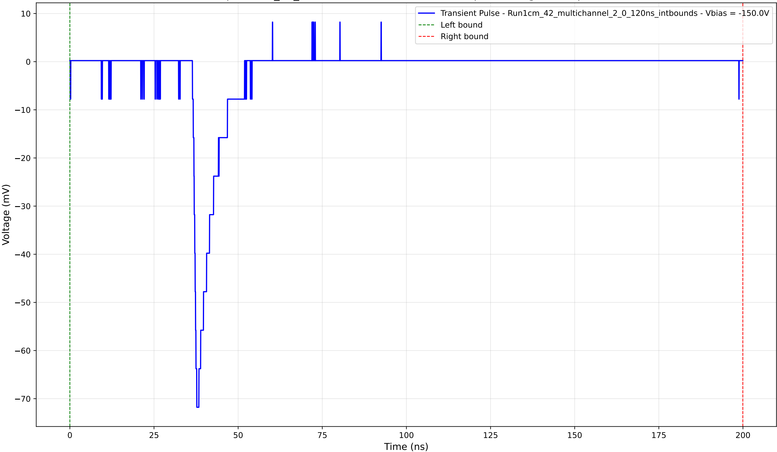
Transient Pulse - Sample: 1cm_42_multichannel - Position: 3335.0 \mu\text{m} - Charge: 7.51 pC - Rise Time: 1.28 ns
