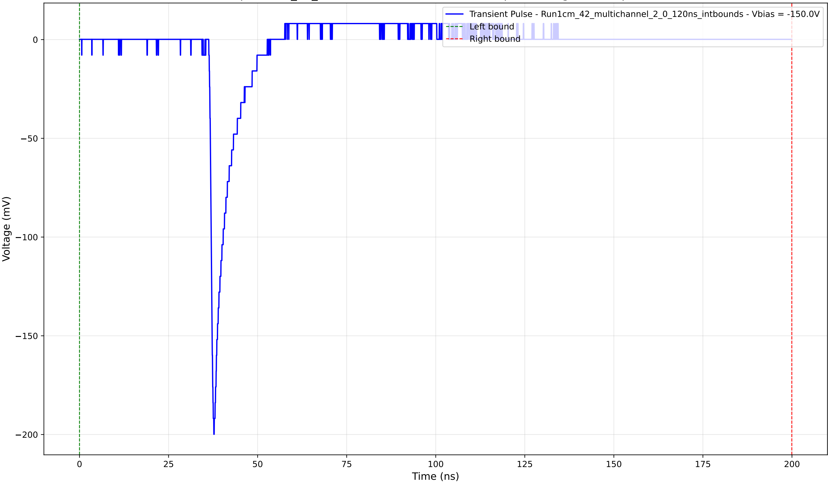
Transient Pulse - Sample: 1cm_42_multichannel - Position: 3160.0 \mu\text{m} - Charge: 10.90 pC - Rise Time: 0.98 ns
