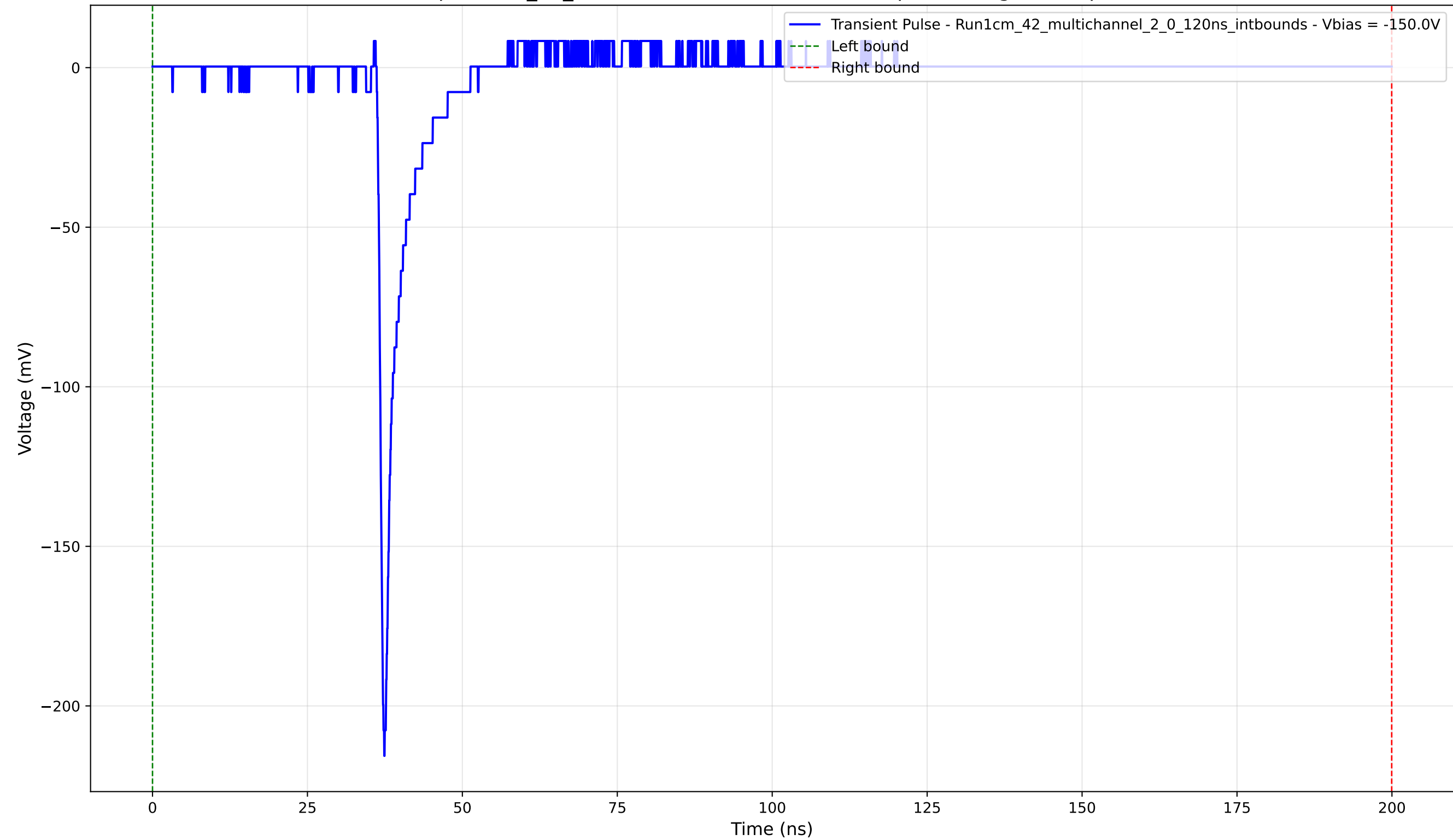
Transient Pulse - Sample: 1cm_42_multichannel - Position: 2820.0 \mu\text{m} - Charge: 9.96 pC - Rise Time: 0.85 ns
