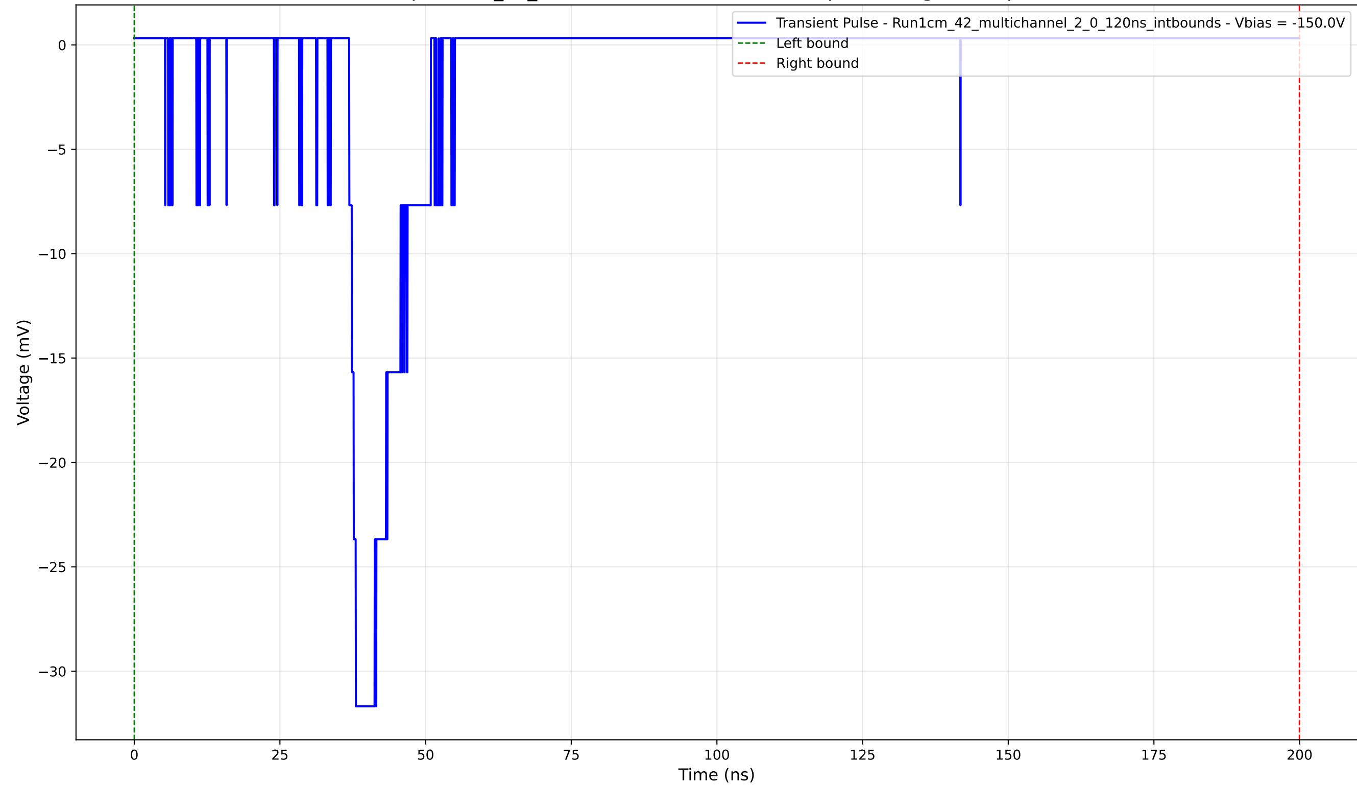
Transient Pulse - Sample: 1cm_42_multichannel - Position: 810.0 \mu\text{m} - Charge: 4.31 pC - Rise Time: 1.14 ns
