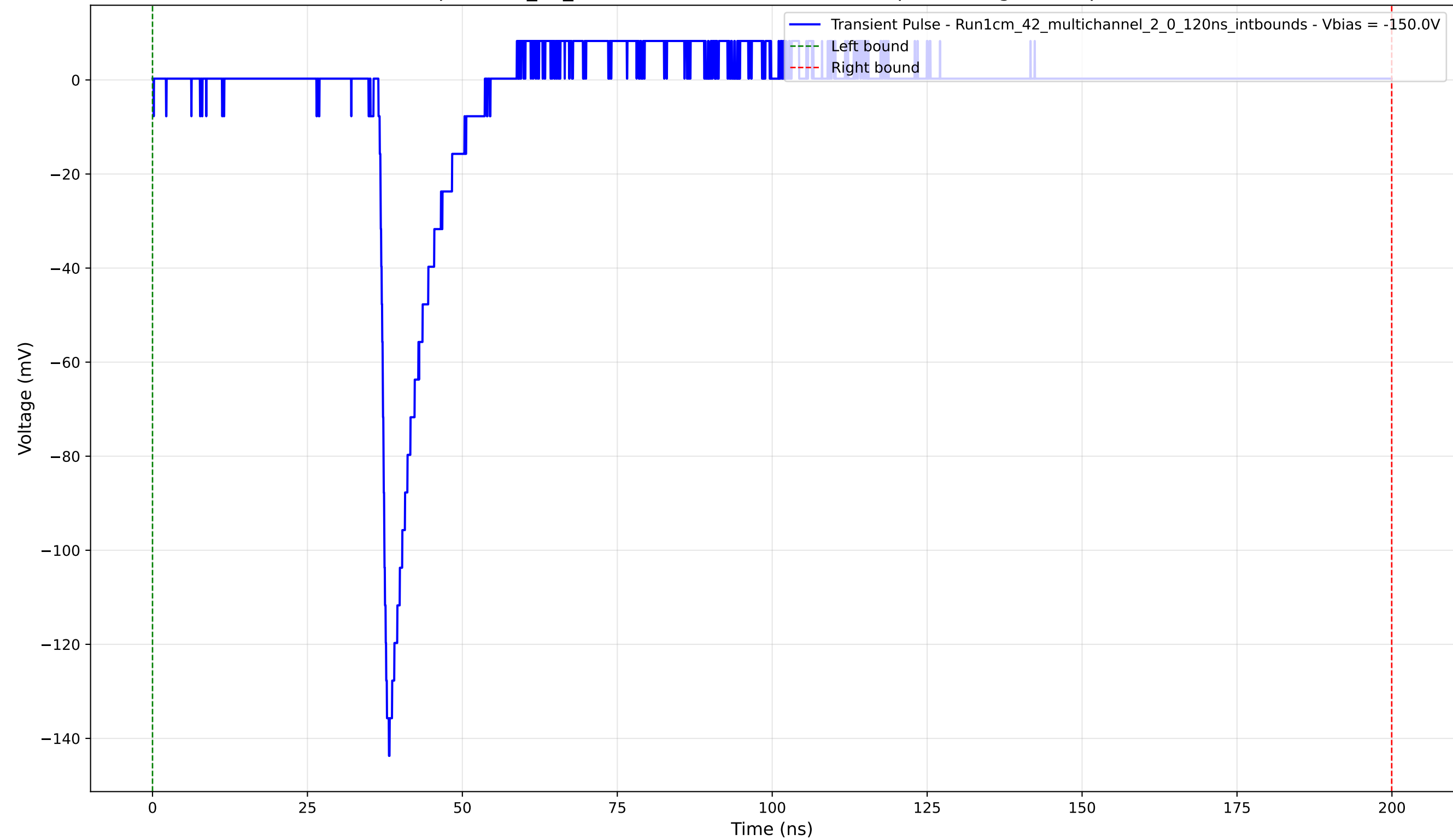
Transient Pulse - Sample: 1cm_42_multichannel - Position: 1285.0 \mu\text{m} - Charge: 9.82 pC - Rise Time: 1.17 ns
