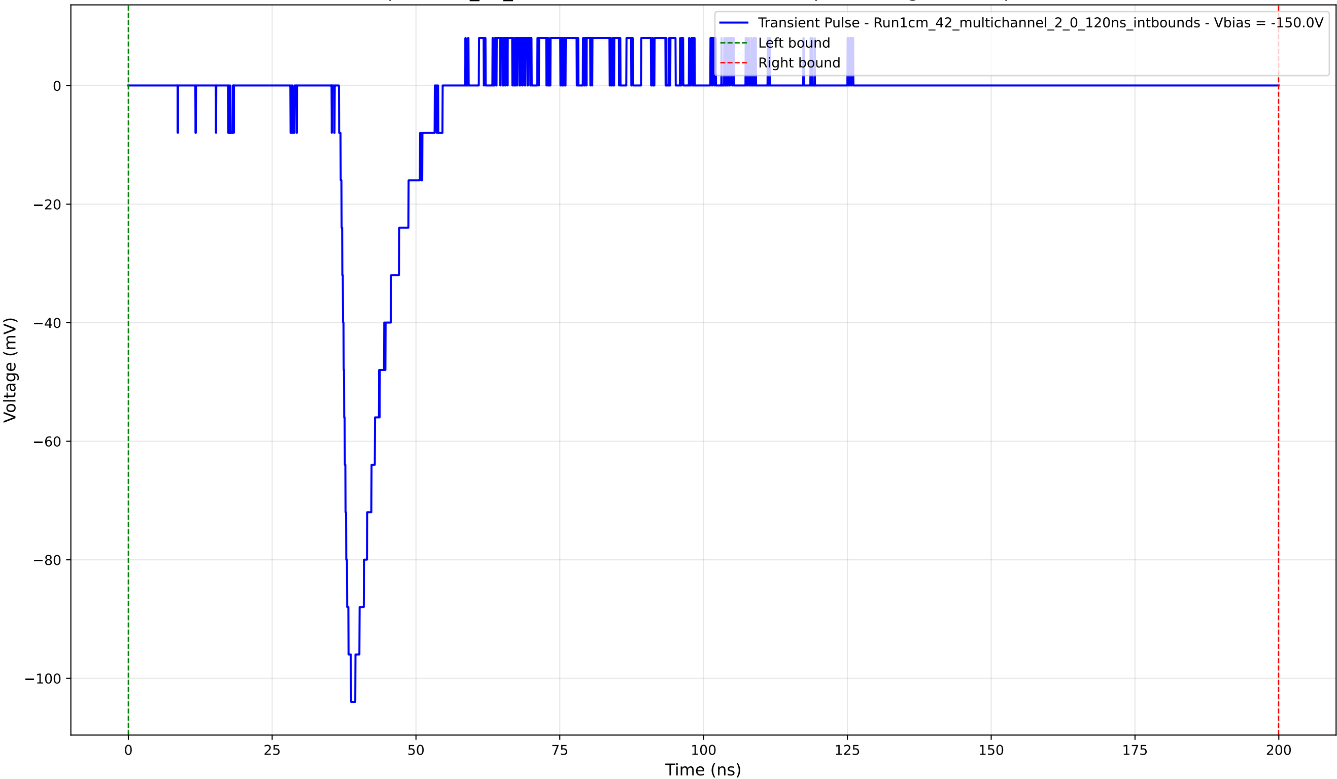
Transient Pulse - Sample: 1cm_42_multichannel - Position: 3795.0 \mu\text{m} - Charge: 10.71 pC - Rise Time: 1.39 ns
