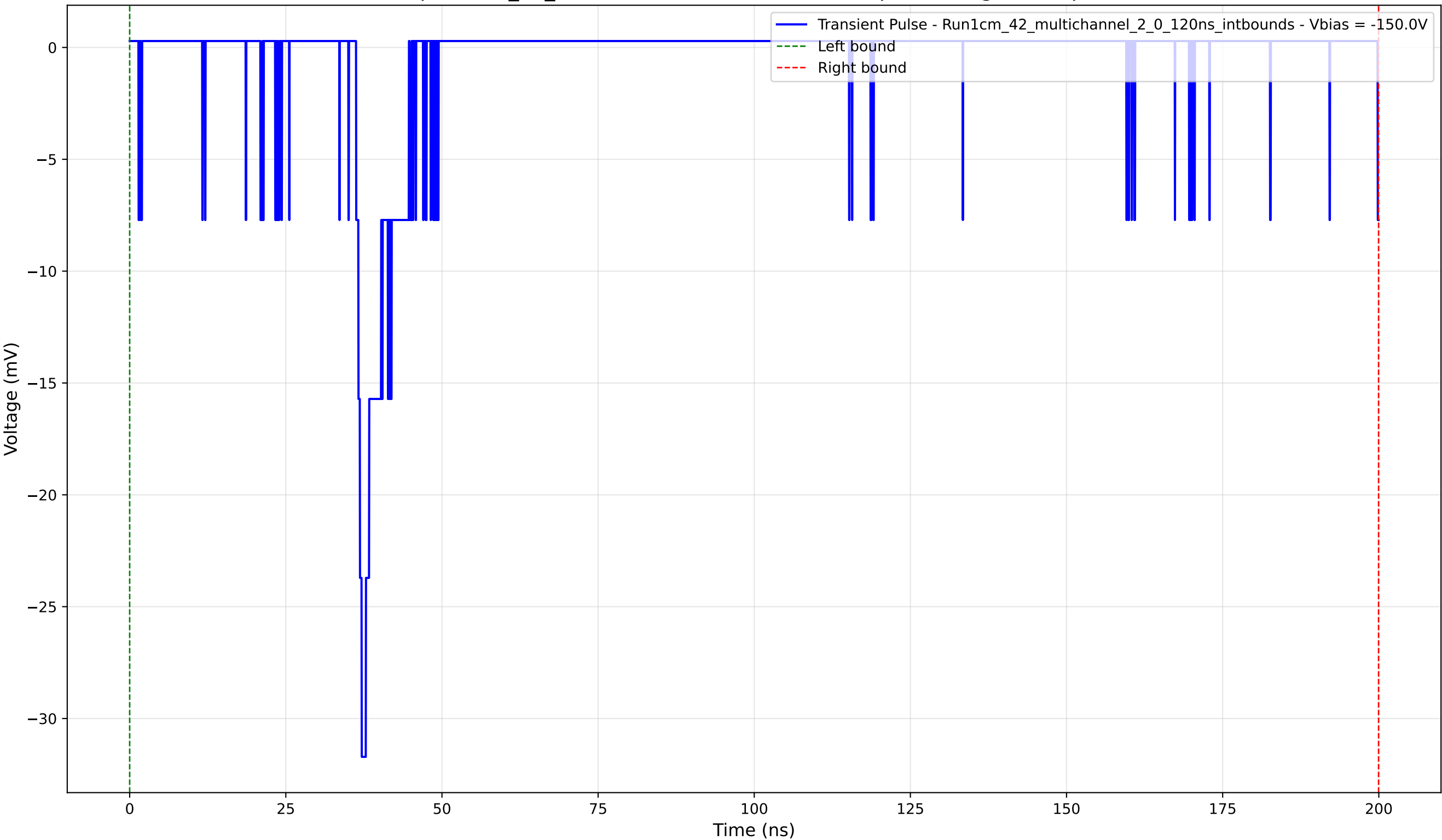
Transient Pulse - Sample: 1cm_42_multichannel - Position: 1885.0 \mu\text{m} - Charge: 1.97 pC - Rise Time: 0.90 ns
