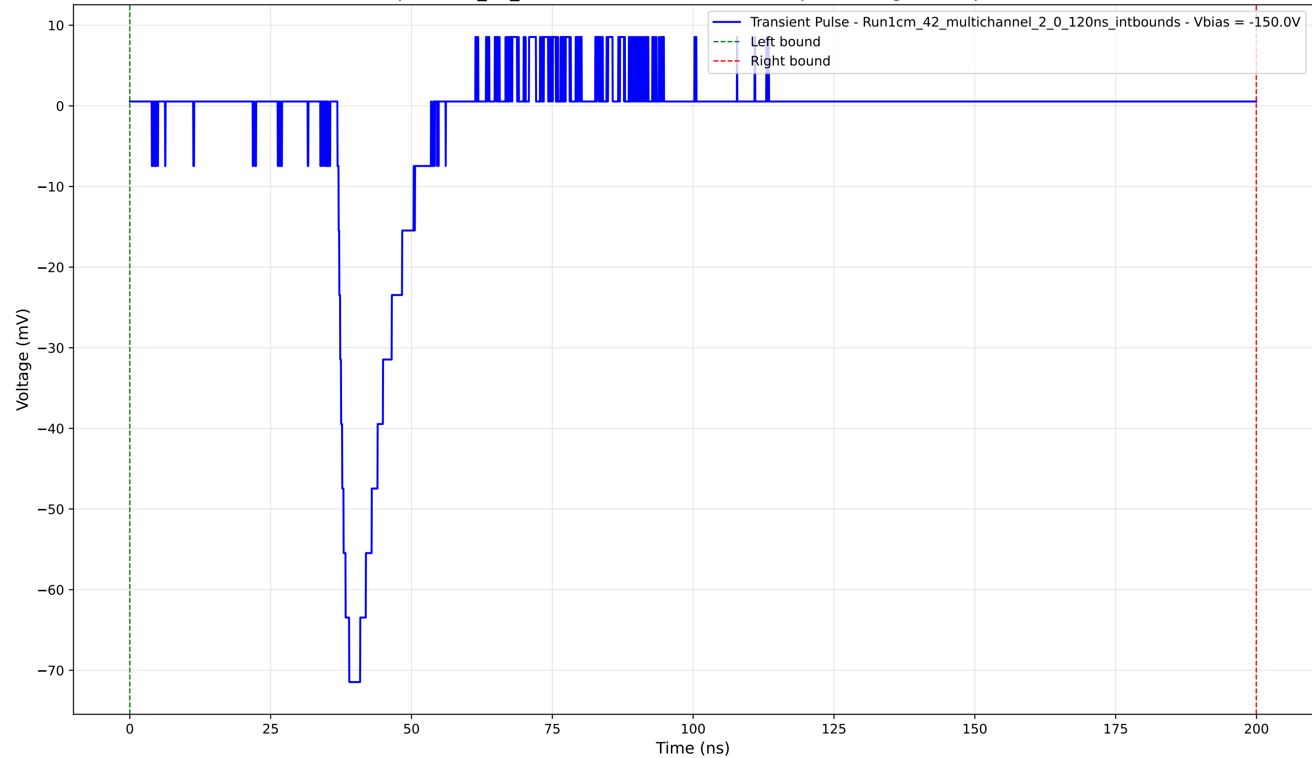
Transient Pulse - Sample: 1cm_42_multichannel - Position: 180.0 \mu\text{m} - Charge: 8.02 pC - Rise Time: 2.08 ns
