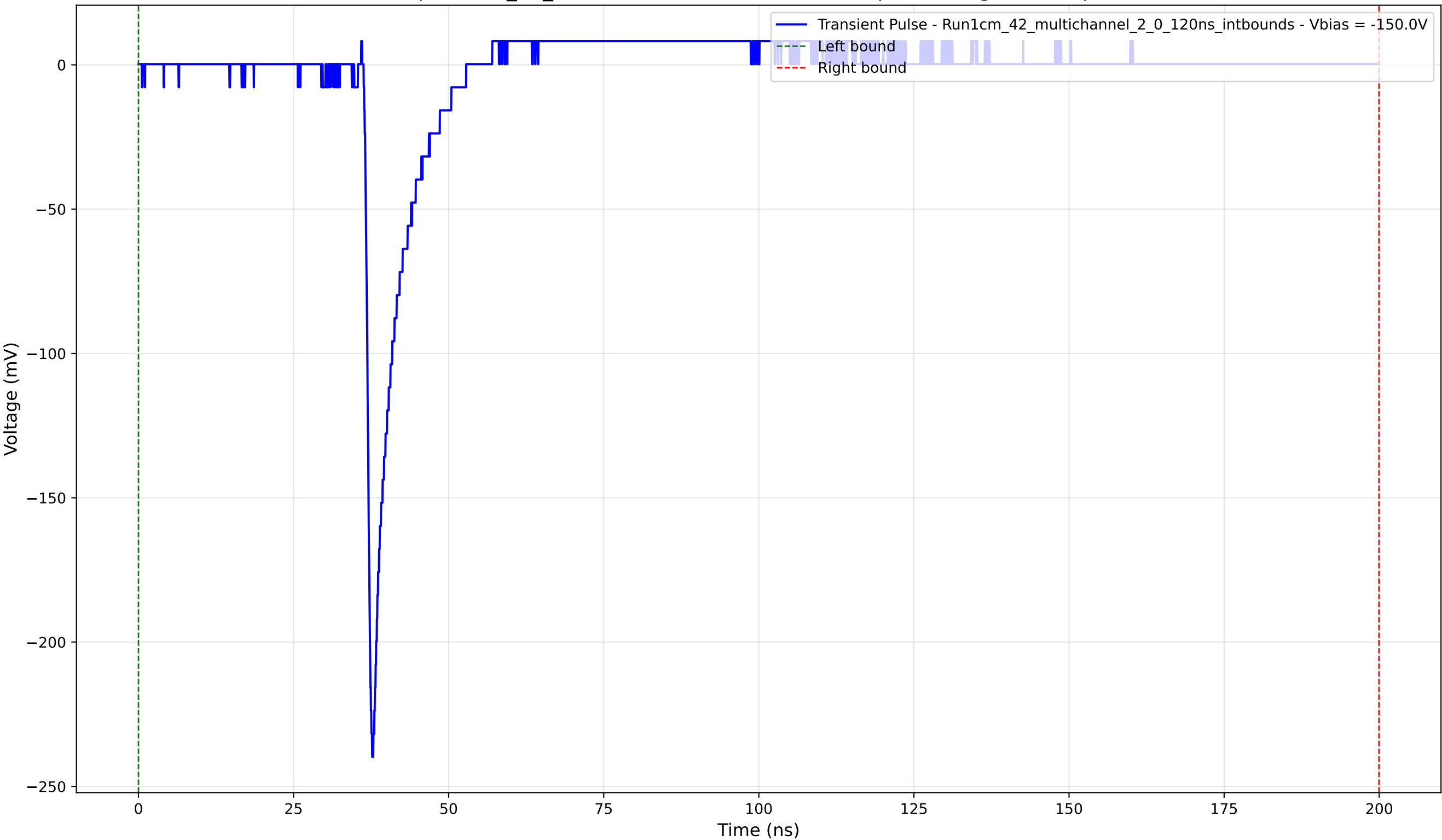
Transient Pulse - Sample: 1cm_42_multichannel - Position: 1605.0 \mu\text{m} - Charge: 11.96 pC - Rise Time: 0.96 ns
