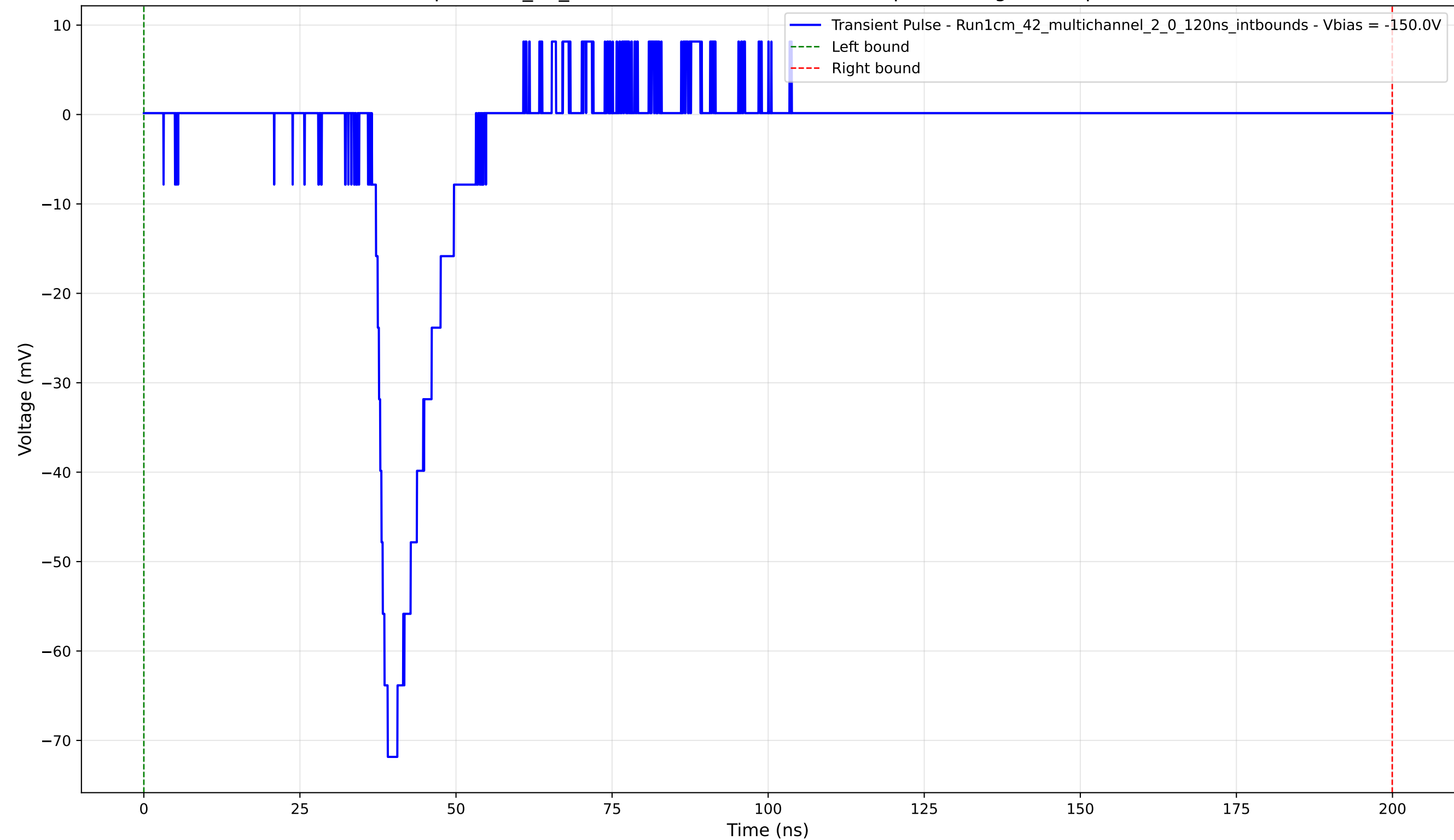
Transient Pulse - Sample: 1cm_42_multichannel - Position: 4500.0 \mu\text{m} - Charge: 8.98 pC - Rise Time: 2.52 ns
