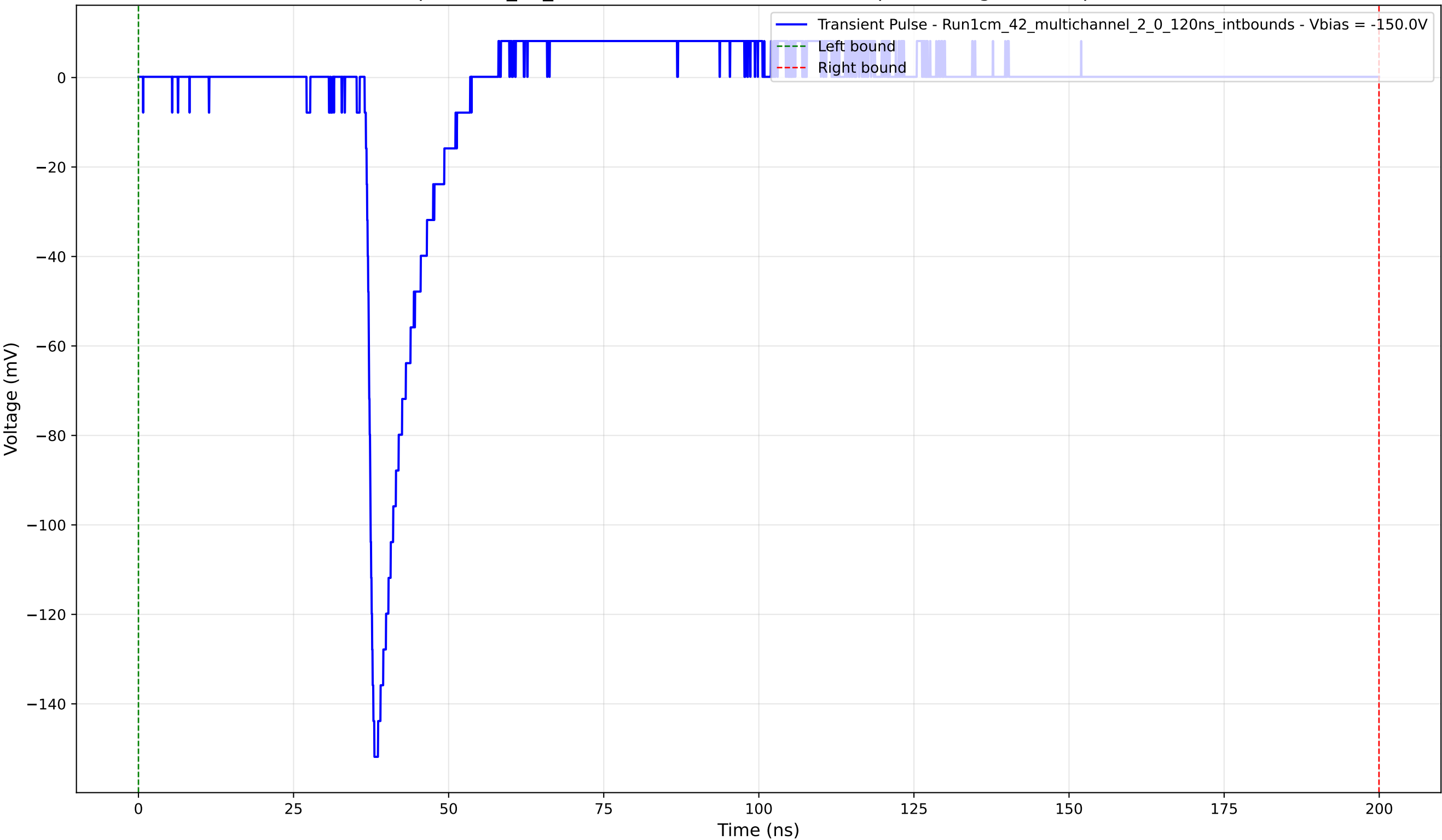
Transient Pulse - Sample: 1cm_42_multichannel - Position: 1210.0 \mu\text{m} - Charge: 10.37 pC - Rise Time: 1.20 ns
