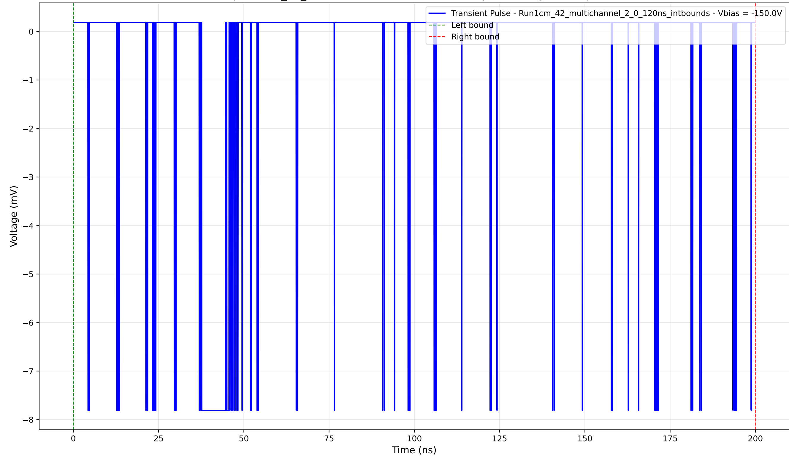
Transient Pulse - Sample: 1cm_42_multichannel - Position: 3875.0 \mu\text{m} - Charge: 1.63 pC - Rise Time: 0.04 ns
