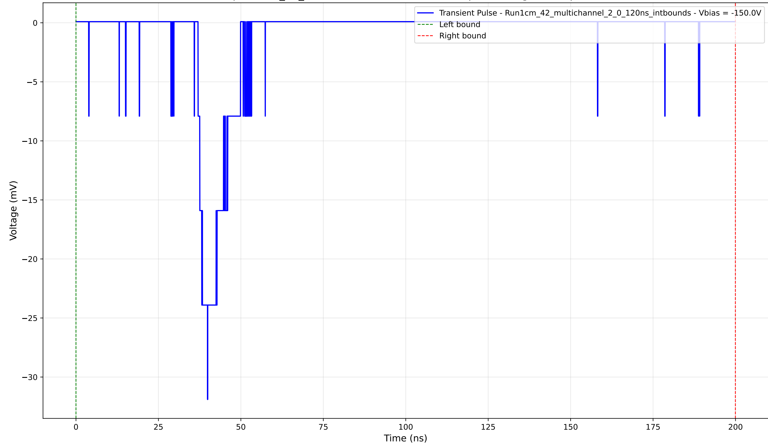
Transient Pulse - Sample: 1cm_42_multichannel - Position: 385.0 \mu\text{m} - Charge: 4.11 pC - Rise Time: 2.90 ns
