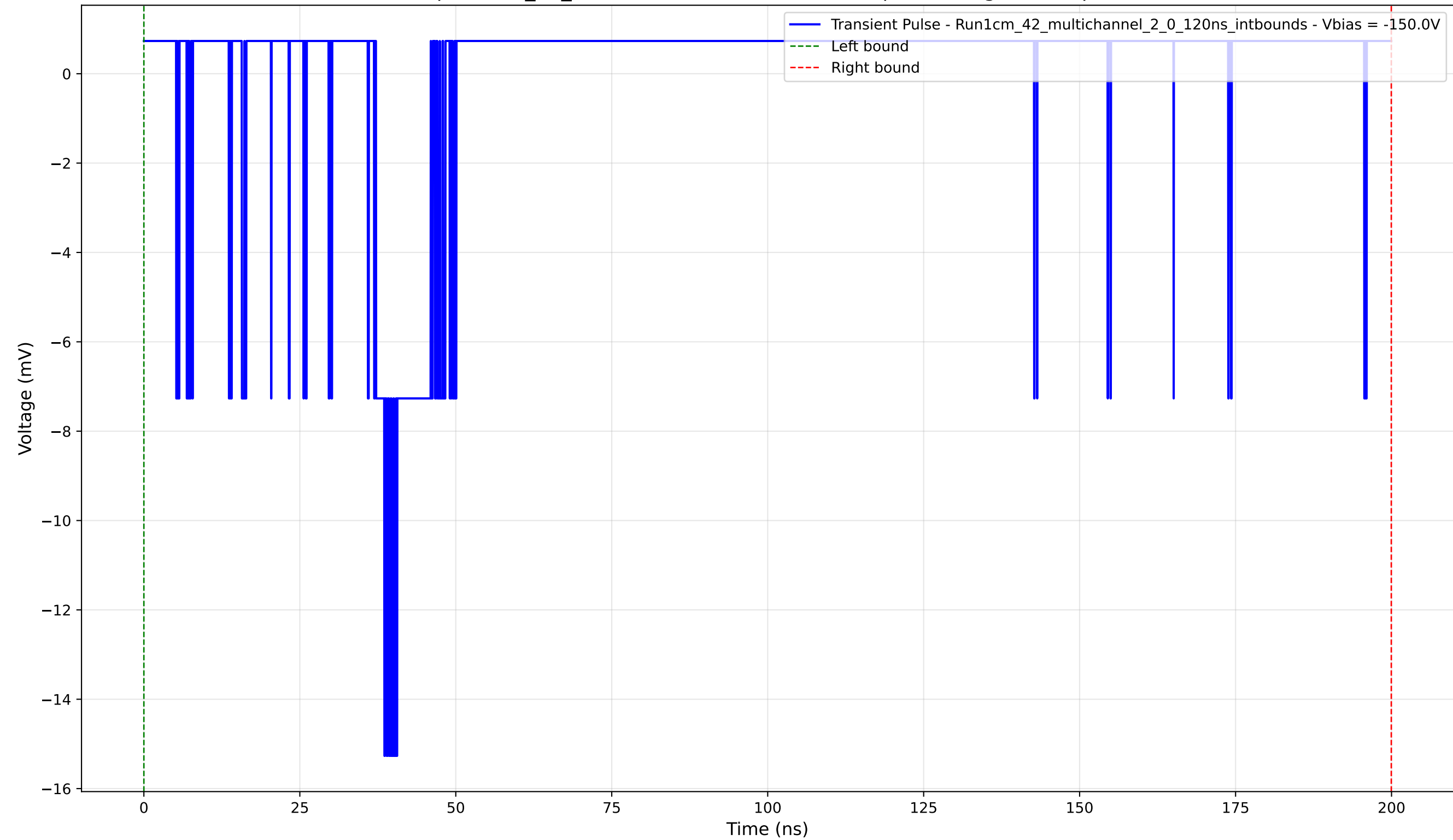
Transient Pulse - Sample: 1cm_42_multichannel - Position: 370.0 \mu\text{m} - Charge: -0.40 pC - Rise Time: 1.36 ns
