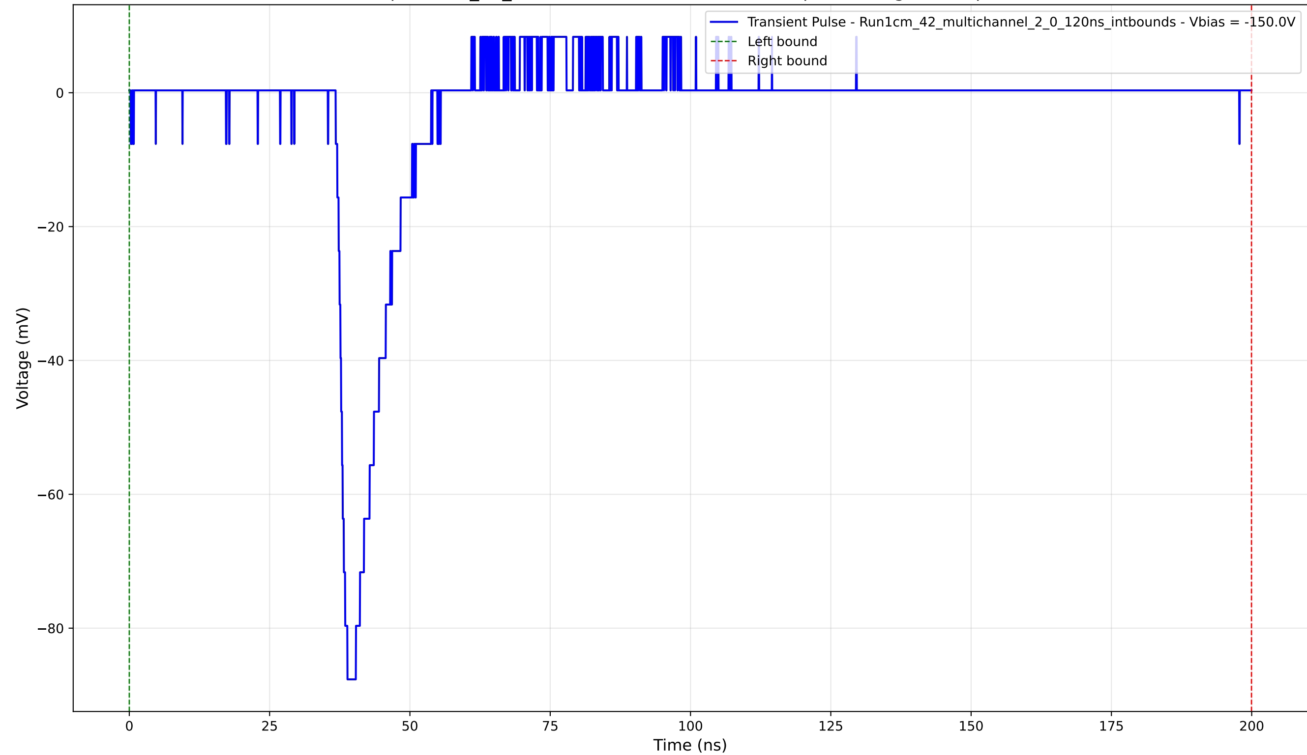
Transient Pulse - Sample: 1cm_42_multichannel - Position: 4075.0 \mu\text{m} - Charge: 9.26 pC - Rise Time: 1.43 ns
