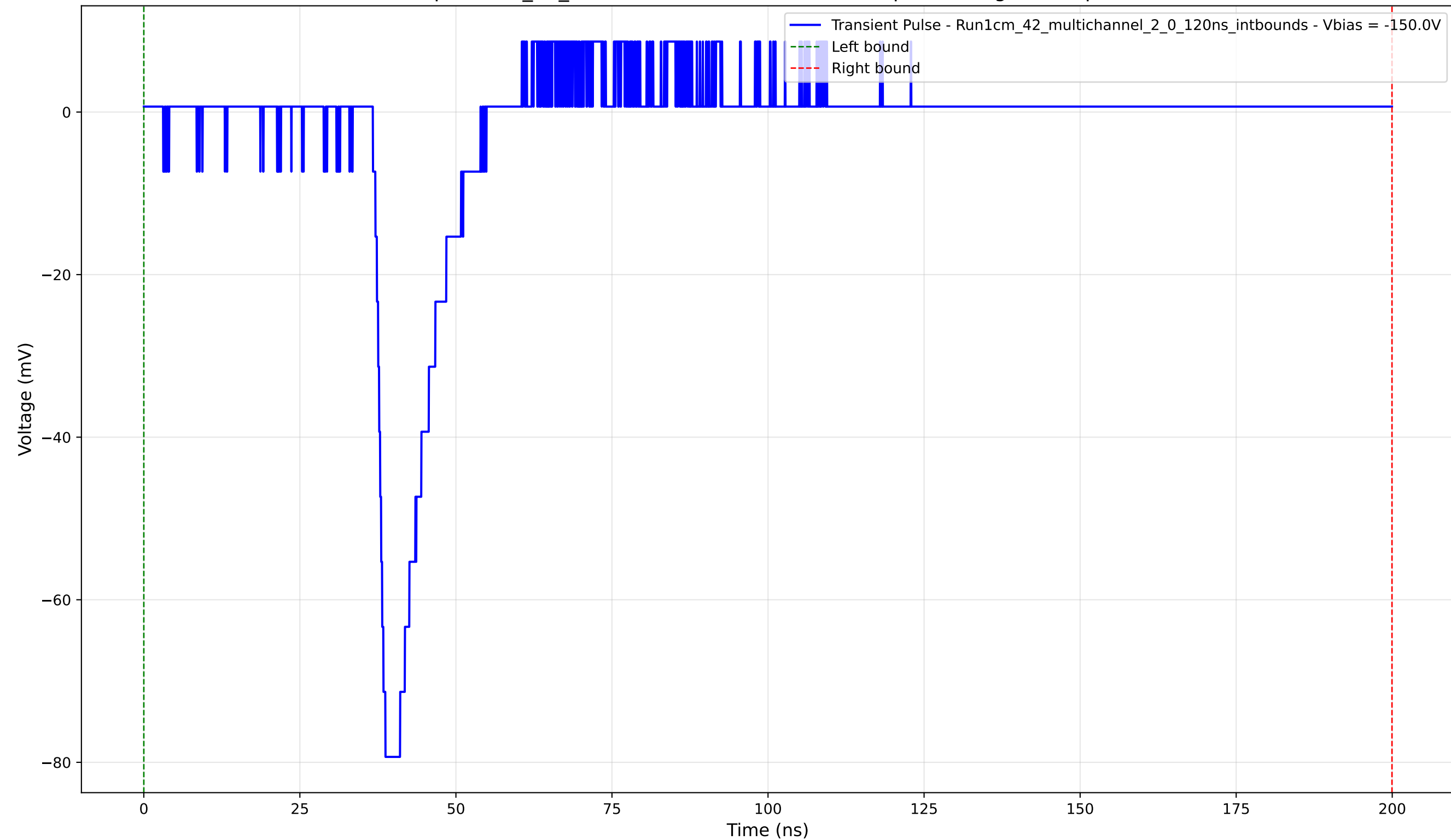
Transient Pulse - Sample: 1cm_42_multichannel - Position: 4185.0 \mu\text{m} - Charge: 7.84 pC - Rise Time: 1.64 ns
