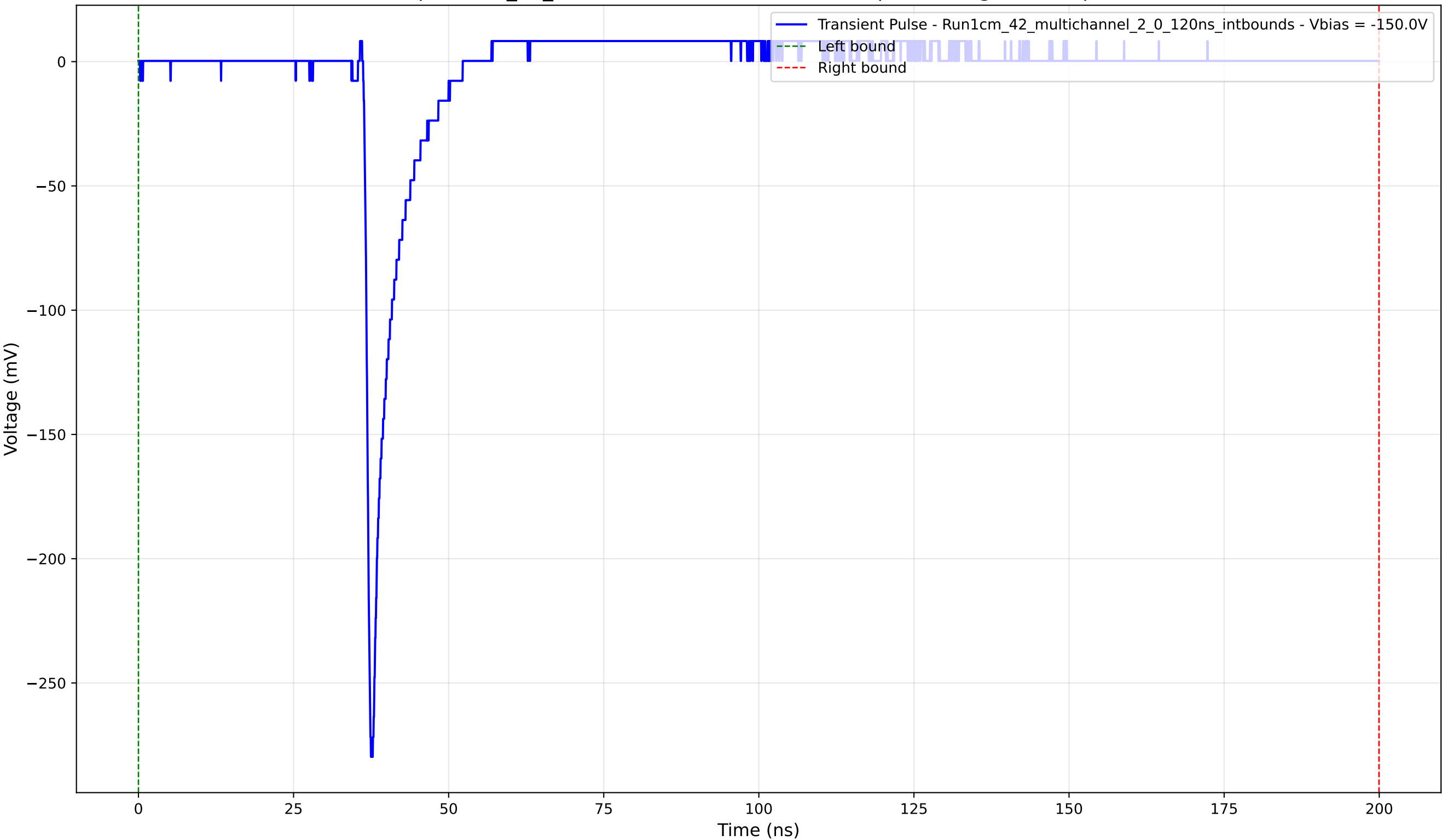
Transient Pulse - Sample: 1cm_42_multichannel - Position: 1720.0 \mu\text{m} - Charge: 11.86 pC - Rise Time: 0.88 ns
