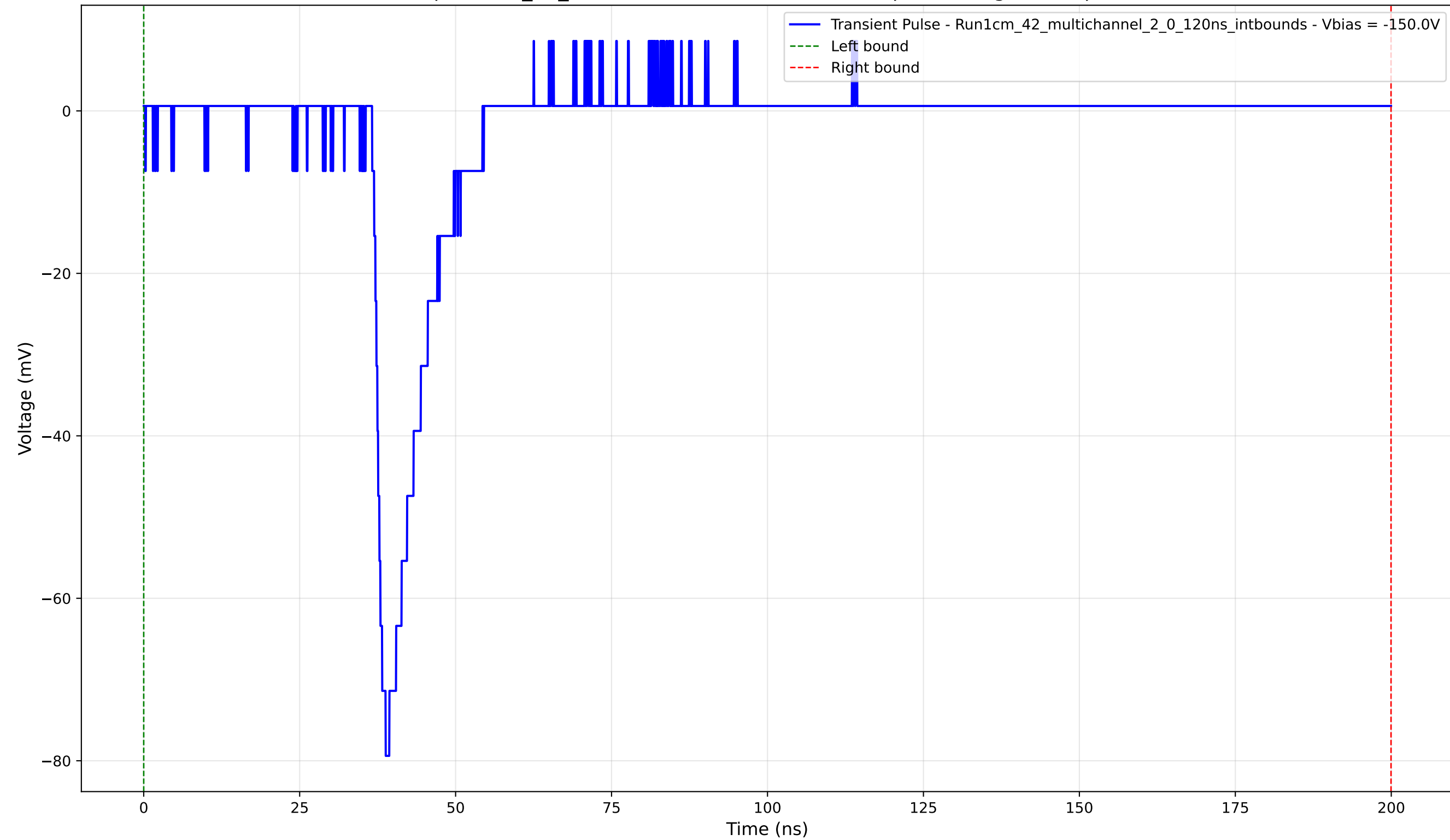
Transient Pulse - Sample: 1cm_42_multichannel - Position: 3825.0 \mu\text{m} - Charge: 8.77 pC - Rise Time: 1.88 ns
