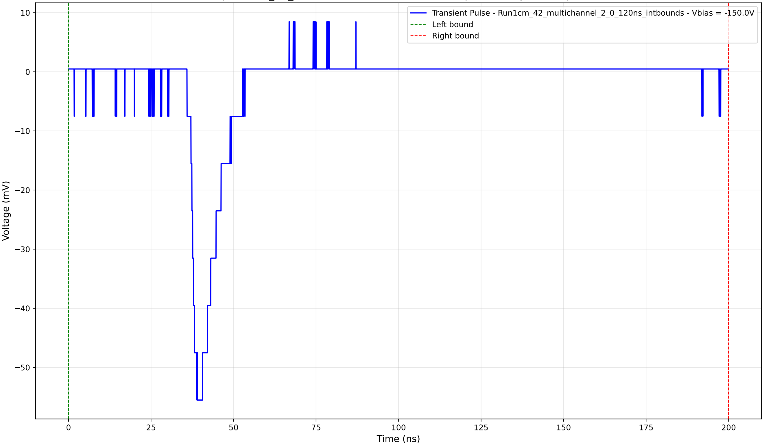
Transient Pulse - Sample: 1cm_42_multichannel - Position: 4820.0 \mu\text{m} - Charge: 7.12 pC - Rise Time: 3.01 ns
