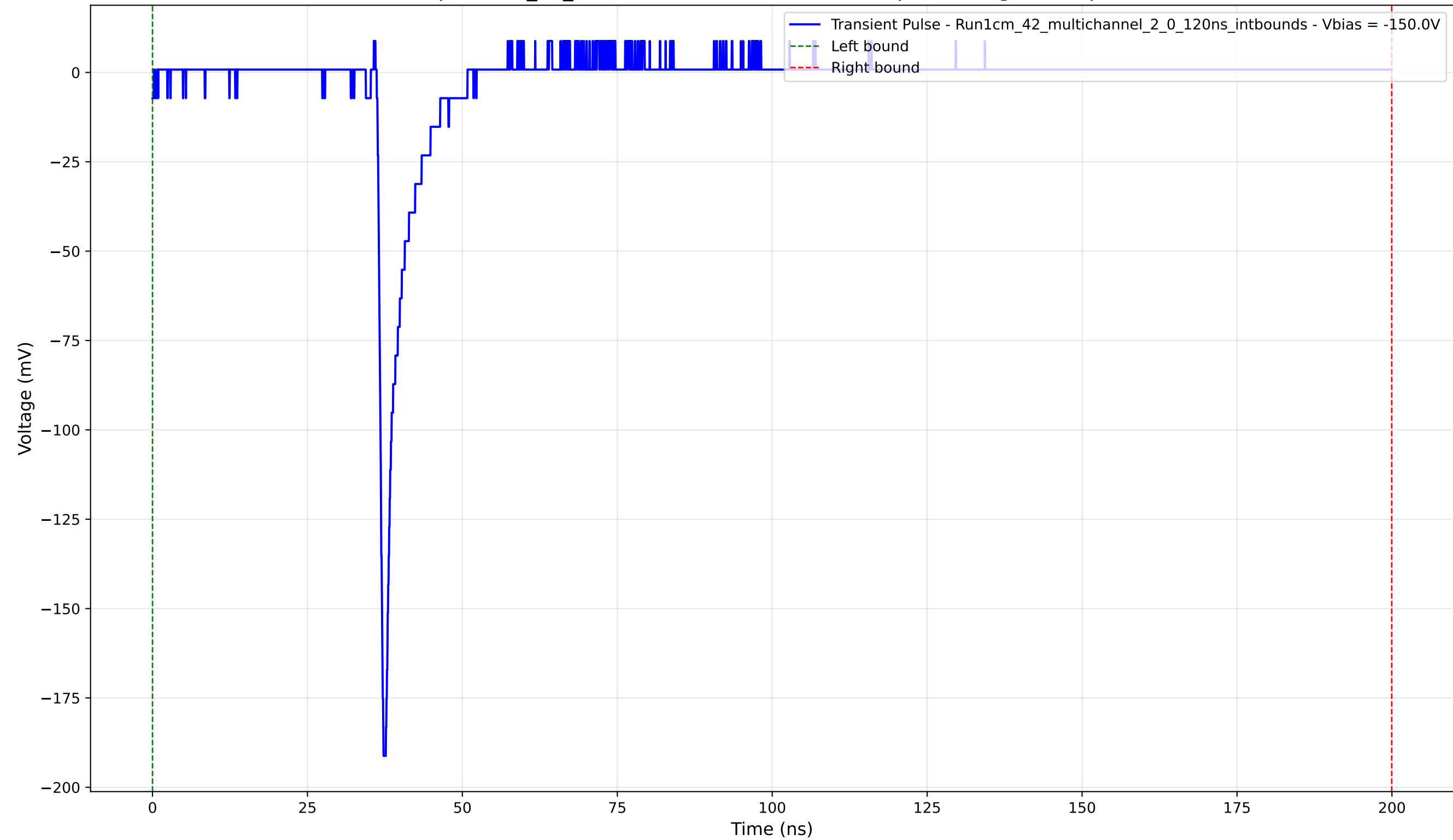
Transient Pulse - Sample: 1cm_42_multichannel - Position: 1915.0 \mu\text{m} - Charge: 8.81 pC - Rise Time: 0.82 ns
