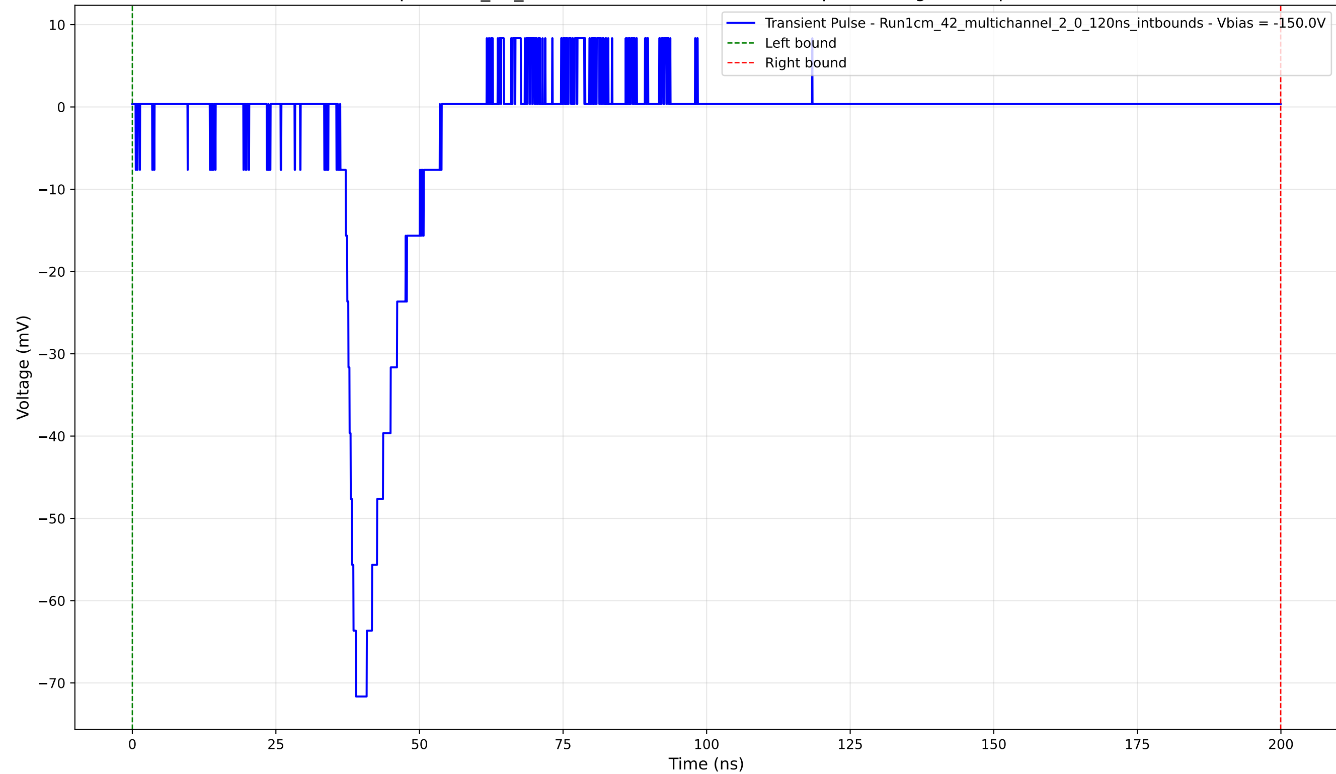
Transient Pulse - Sample: 1cm_42_multichannel - Position: 4555.0 \mu\text{m} - Charge: 8.67 pC - Rise Time: 2.72 ns
