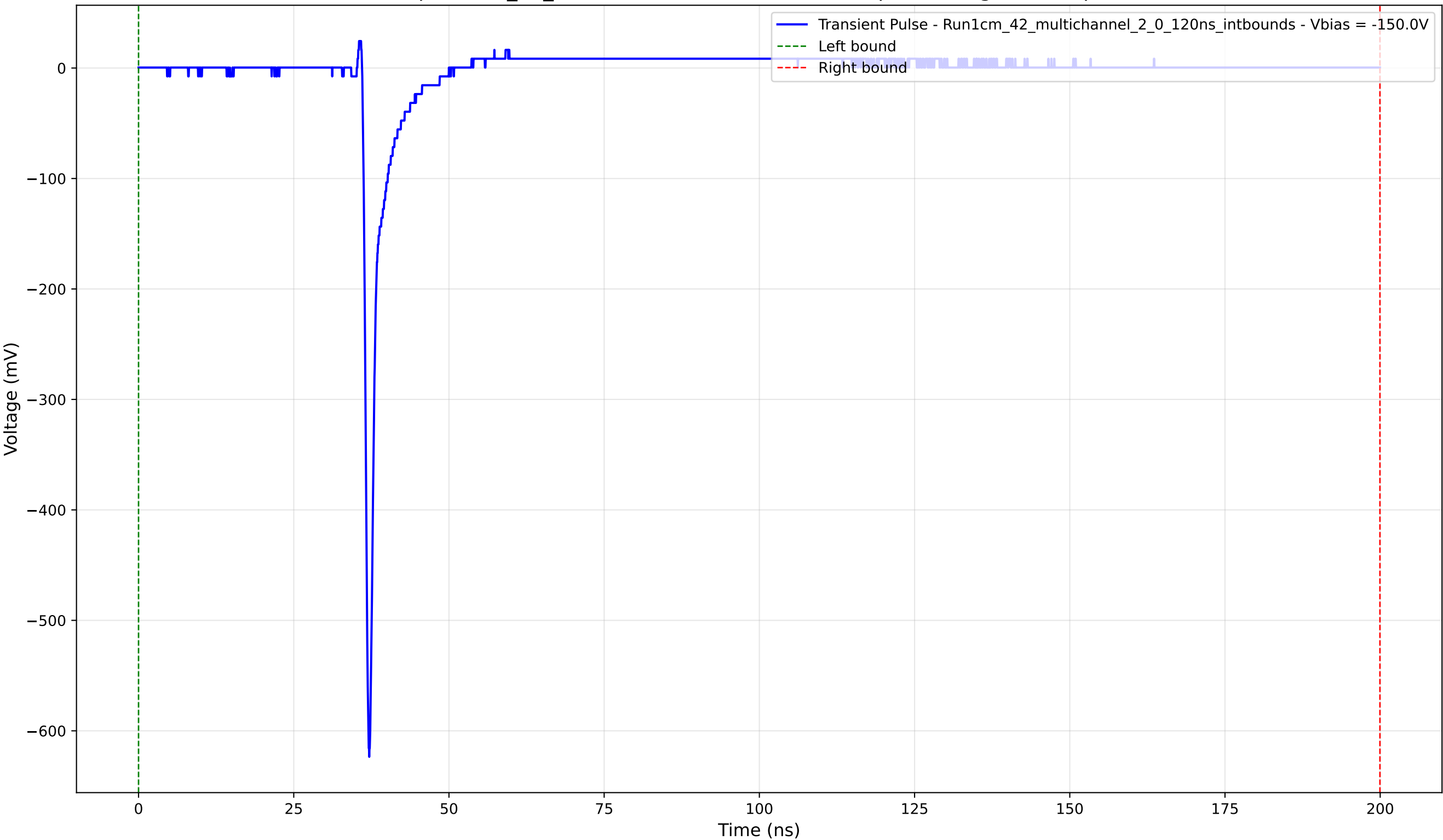
Transient Pulse - Sample: 1cm_42_multichannel - Position: 2475.0 \mu\text{m} - Charge: 15.11 pC - Rise Time: 0.75 ns
