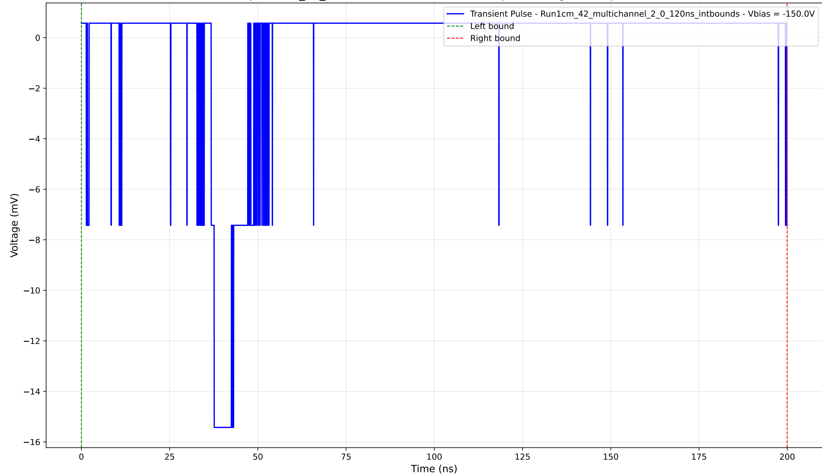
Transient Pulse - Sample: 1cm_42_multichannel - Position: 880.0 \mu\text{m} - Charge: 1.08 pC - Rise Time: 0.87 ns
