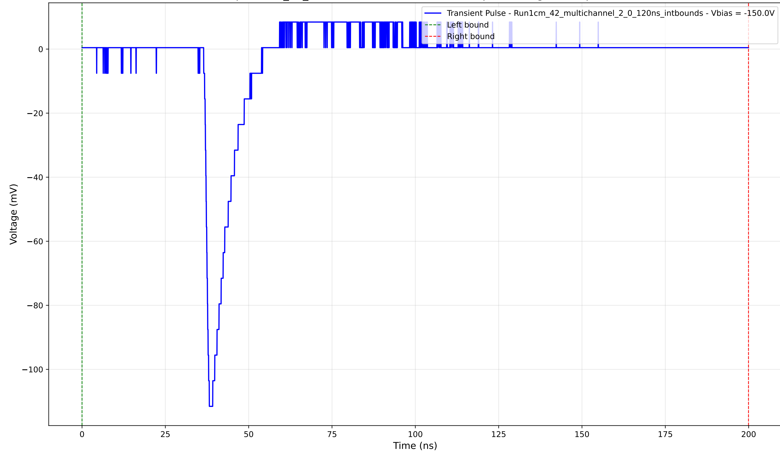
Transient Pulse - Sample: 1cm_42_multichannel - Position: 3670.0 \mu\text{m} - Charge: 8.61 pC - Rise Time: 1.22 ns
