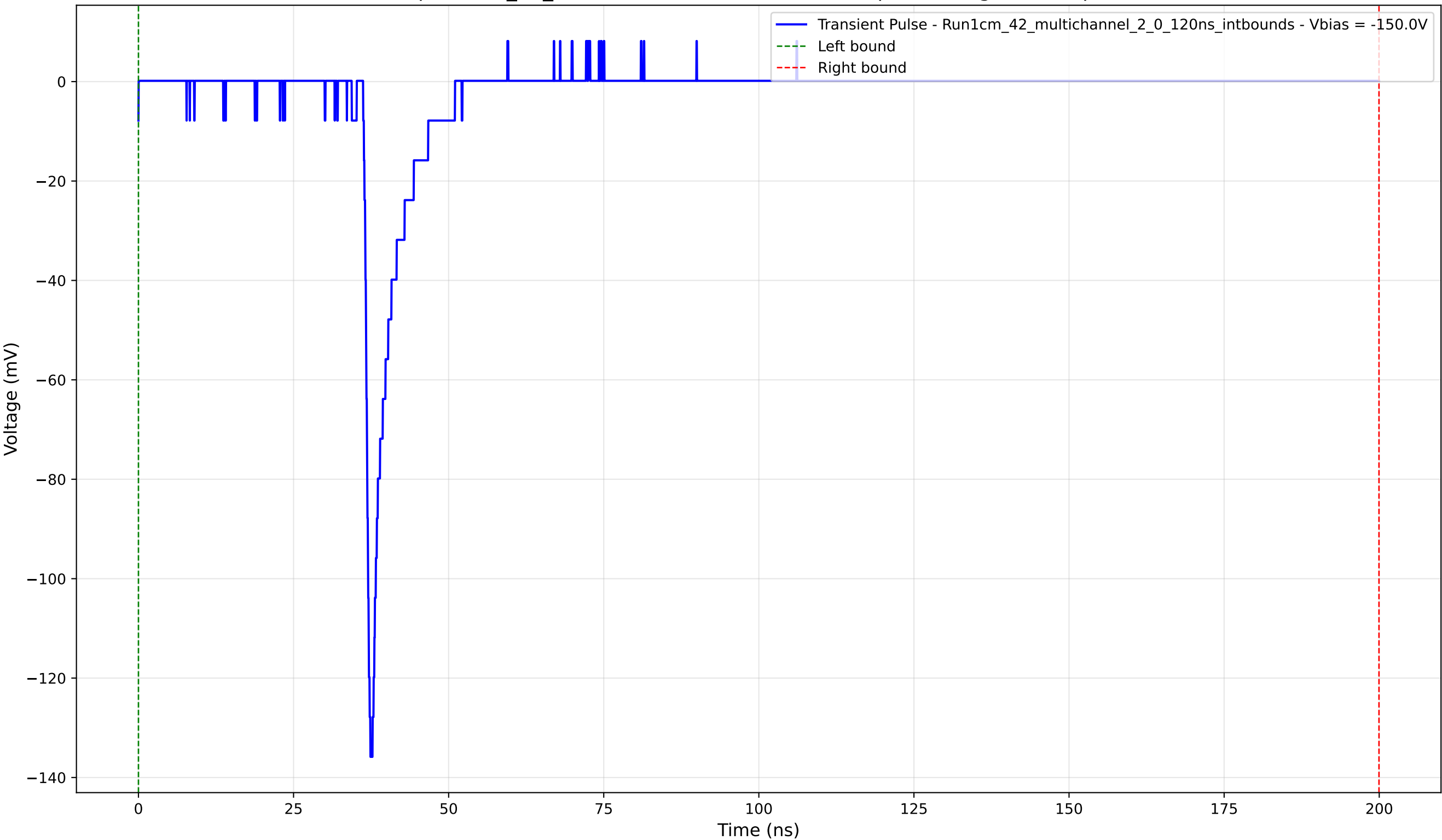
Transient Pulse - Sample: 1cm_42_multichannel - Position: 1815.0 \mu\text{m} - Charge: 10.16 pC - Rise Time: 0.93 ns
