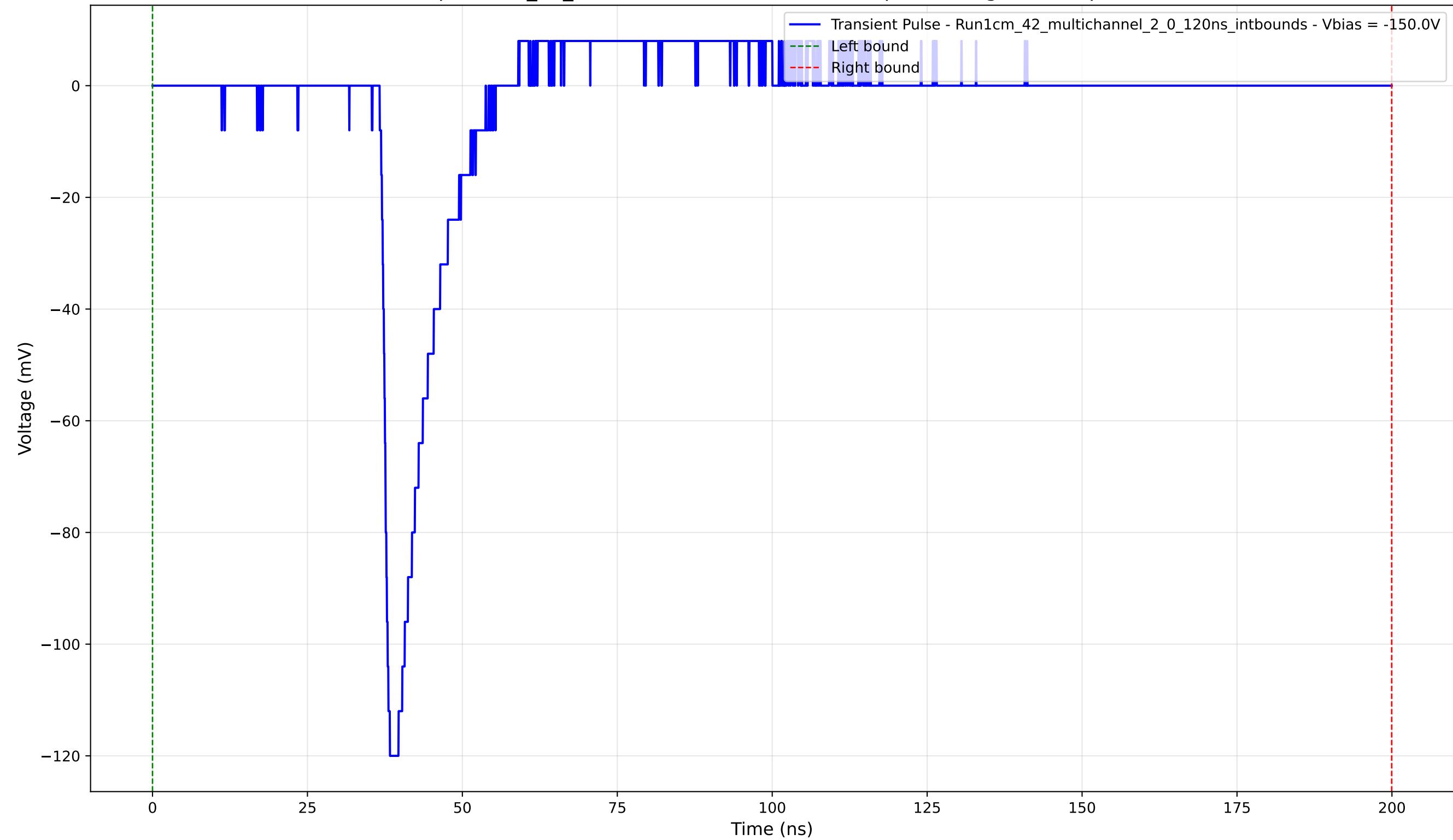
Transient Pulse - Sample: 1cm_42_multichannel - Position: 955.0 \mu\text{m} - Charge: 10.50 pC - Rise Time: 1.18 ns
