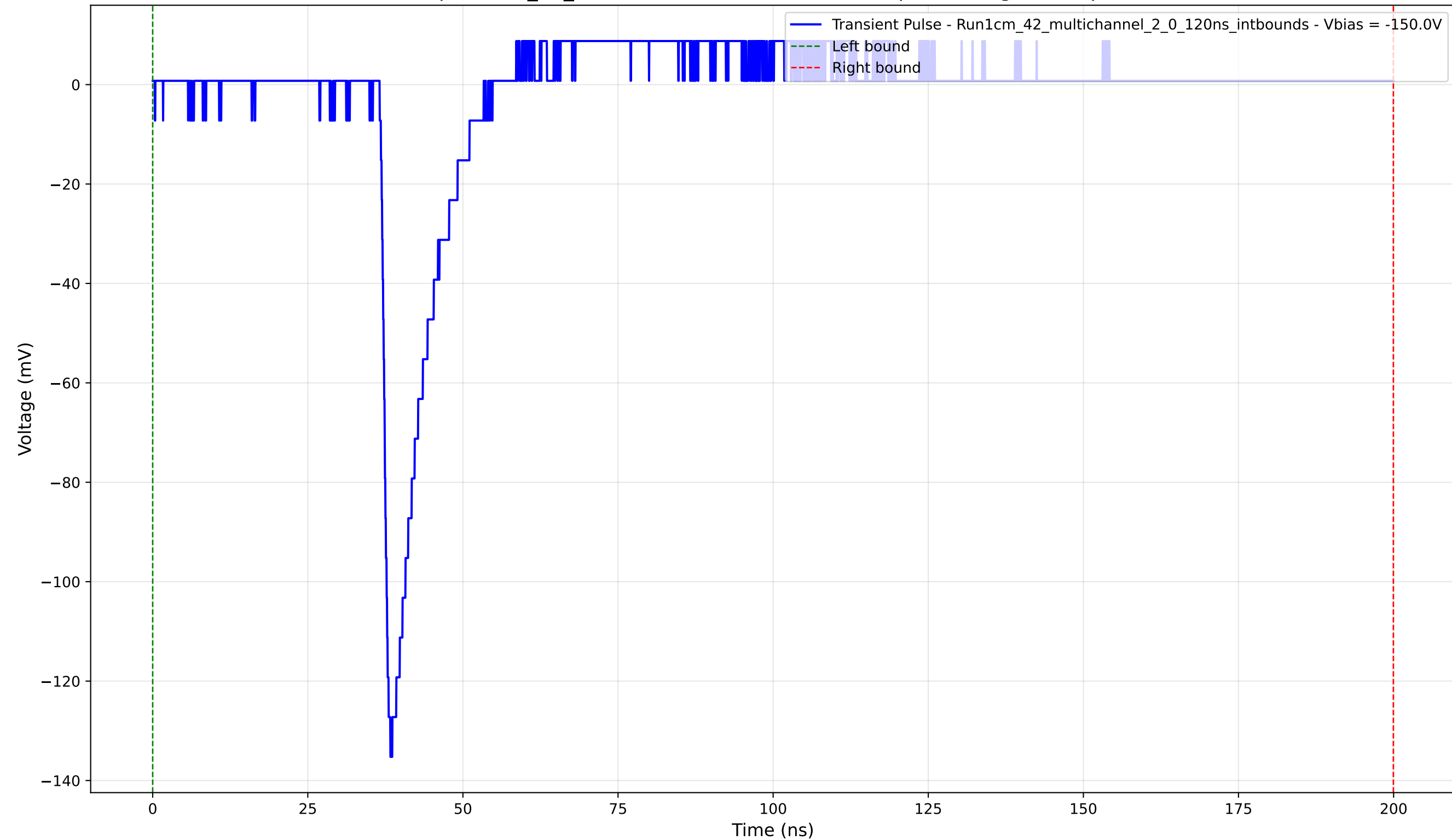
Transient Pulse - Sample: 1cm_42_multichannel - Position: 1100.0 \mu\text{m} - Charge: 7.83 pC - Rise Time: 1.25 ns
