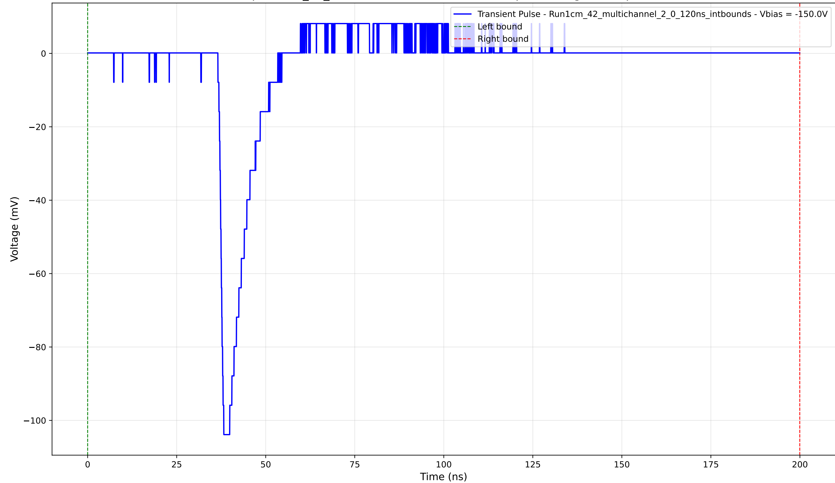
Transient Pulse - Sample: 1cm_42_multichannel - Position: 3760.0 \mu\text{m} - Charge: 9.26 pC - Rise Time: 1.19 ns
