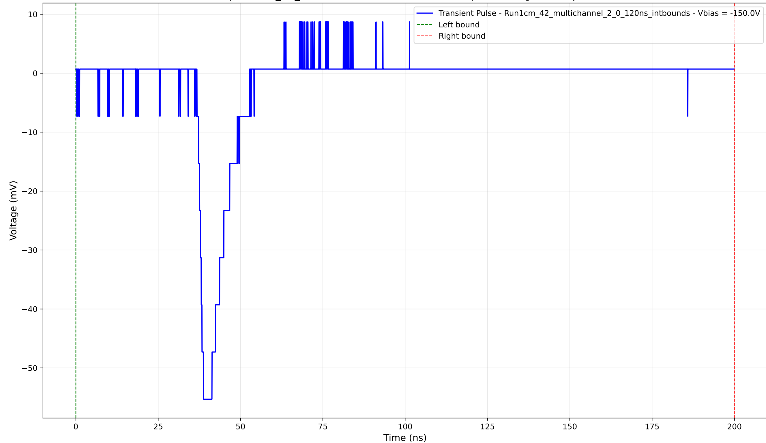
Transient Pulse - Sample: 1cm_42_multichannel - Position: 4455.0 \mu\text{m} - Charge: 6.16 pC - Rise Time: 1.97 ns
