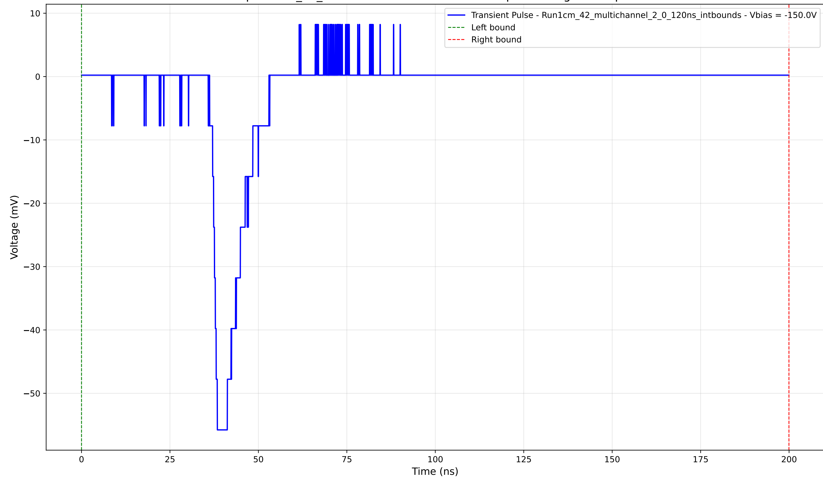
Transient Pulse - Sample: 1cm_42_multichannel - Position: 4805.0 \mu\text{m} - Charge: 7.81 pC - Rise Time: 2.17 ns
