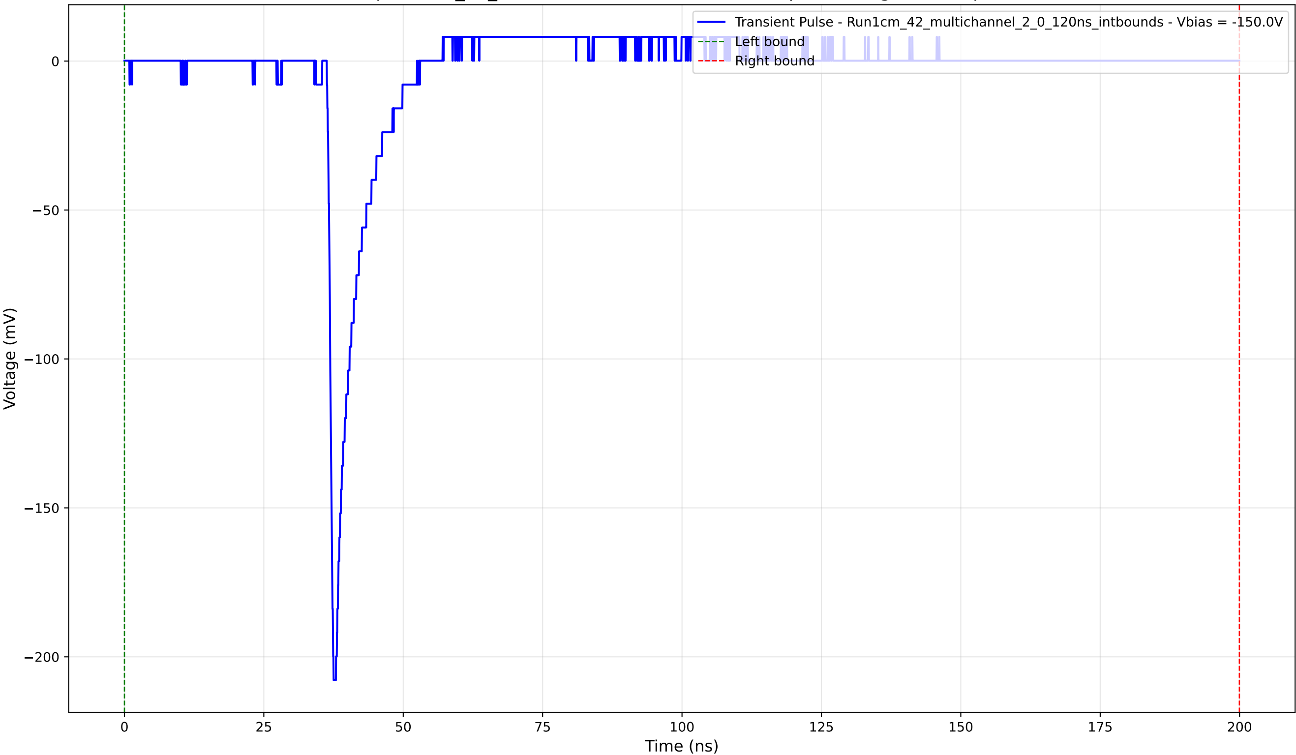
Transient Pulse - Sample: 1cm_42_multichannel - Position: 3115.0 \mu\text{m} - Charge: 11.45 pC - Rise Time: 0.91 ns
