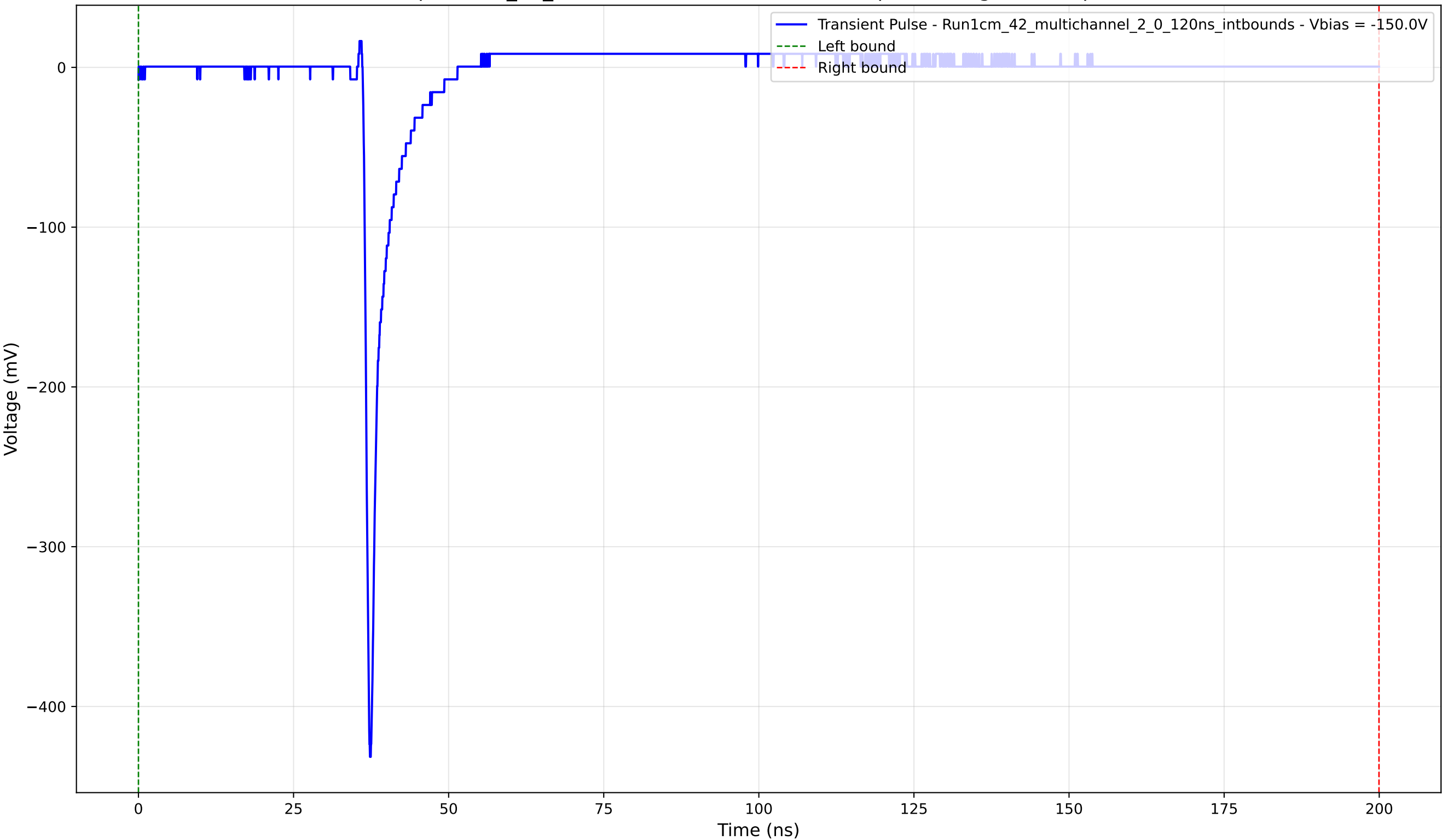
Transient Pulse - Sample: 1cm_42_multichannel - Position: 2005.0 \mu\text{m} - Charge: 13.44 pC - Rise Time: 0.81 ns
