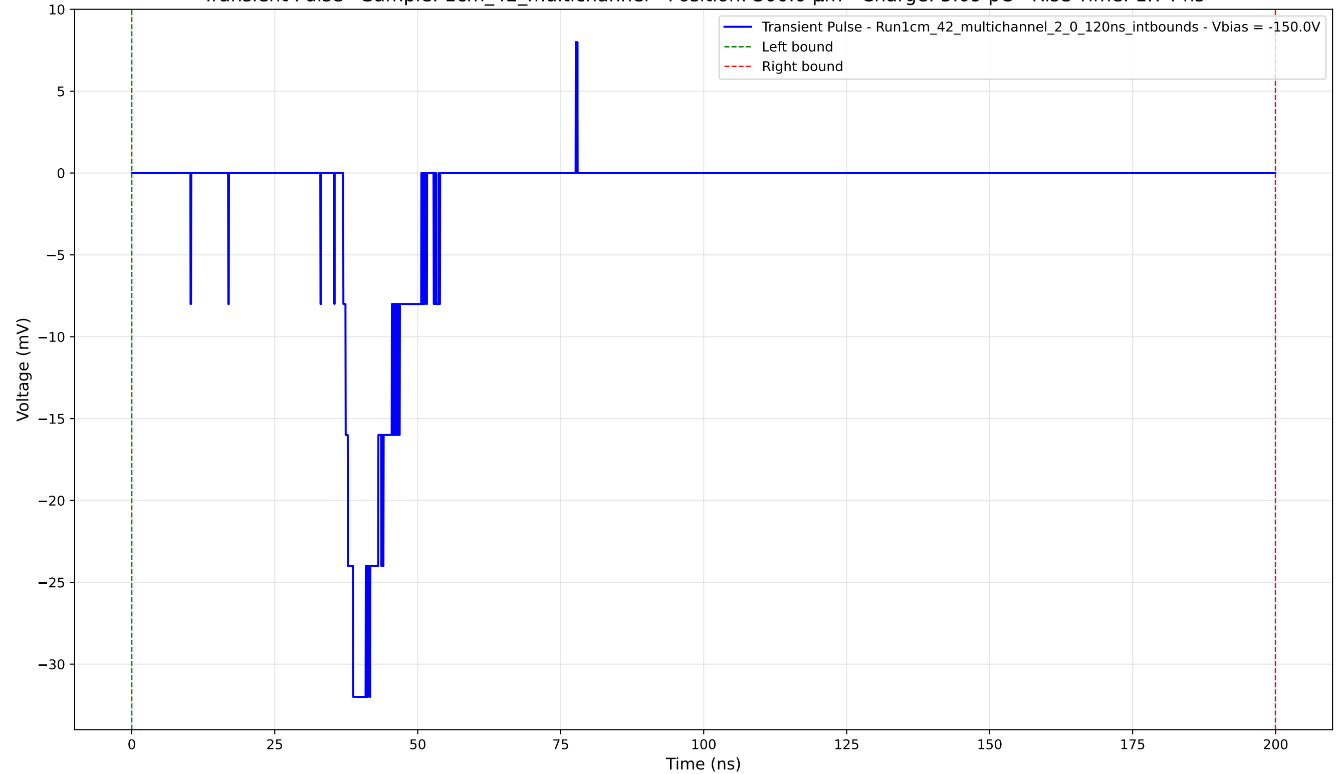
Transient Pulse - Sample: 1cm_42_multichannel - Position: 300.0 \mu\text{m} - Charge: 5.09 pC - Rise Time: 1.74 ns
