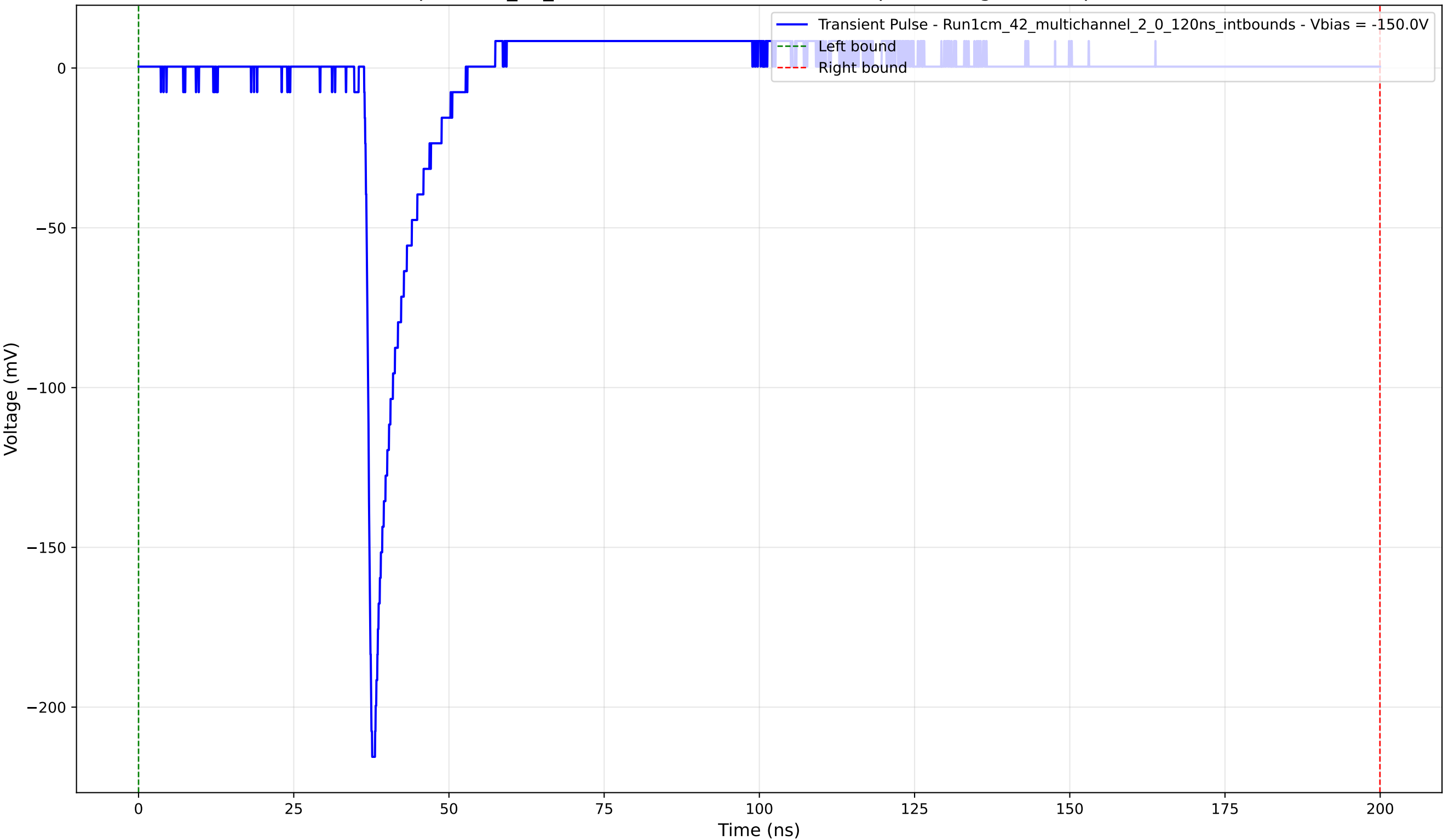
Transient Pulse - Sample: 1cm_42_multichannel - Position: 1545.0 \mu\text{m} - Charge: 10.65 pC - Rise Time: 0.94 ns
