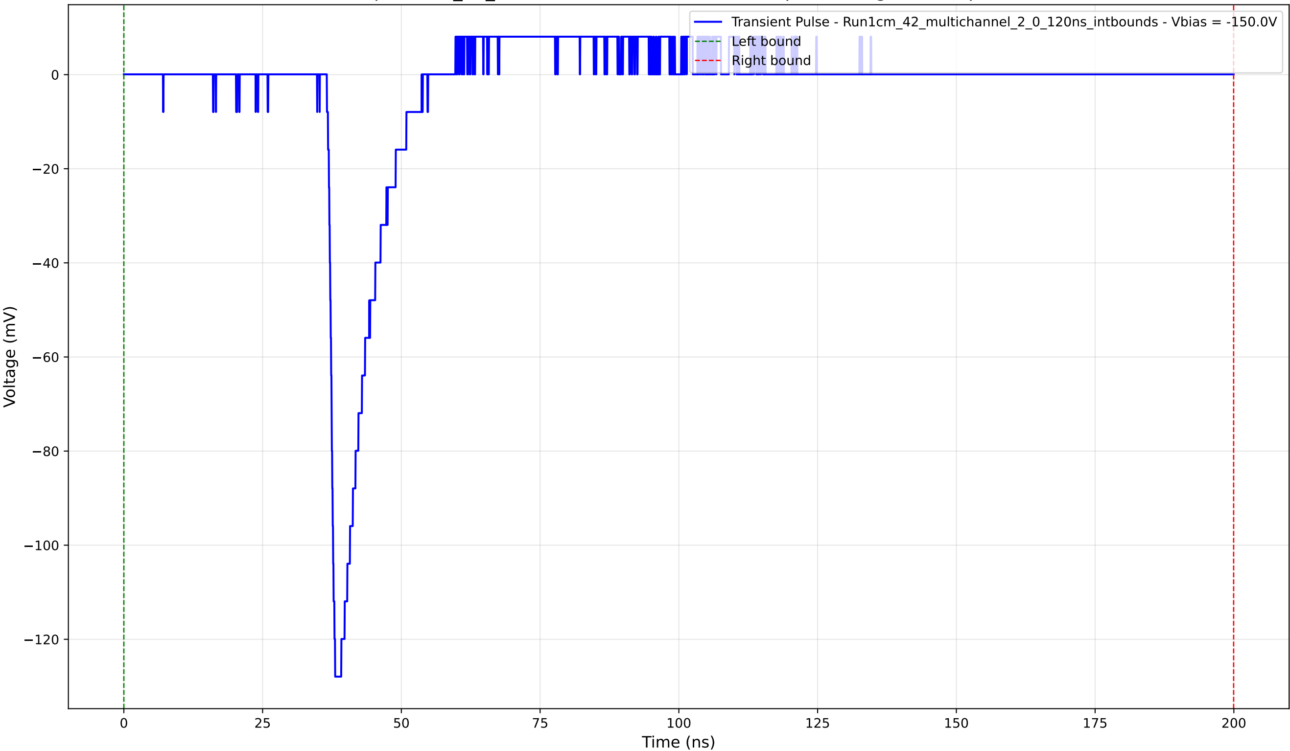
Transient Pulse - Sample: 1cm_42_multichannel - Position: 1085.0 \mu\text{m} - Charge: 10.80 pC - Rise Time: 1.18 ns
