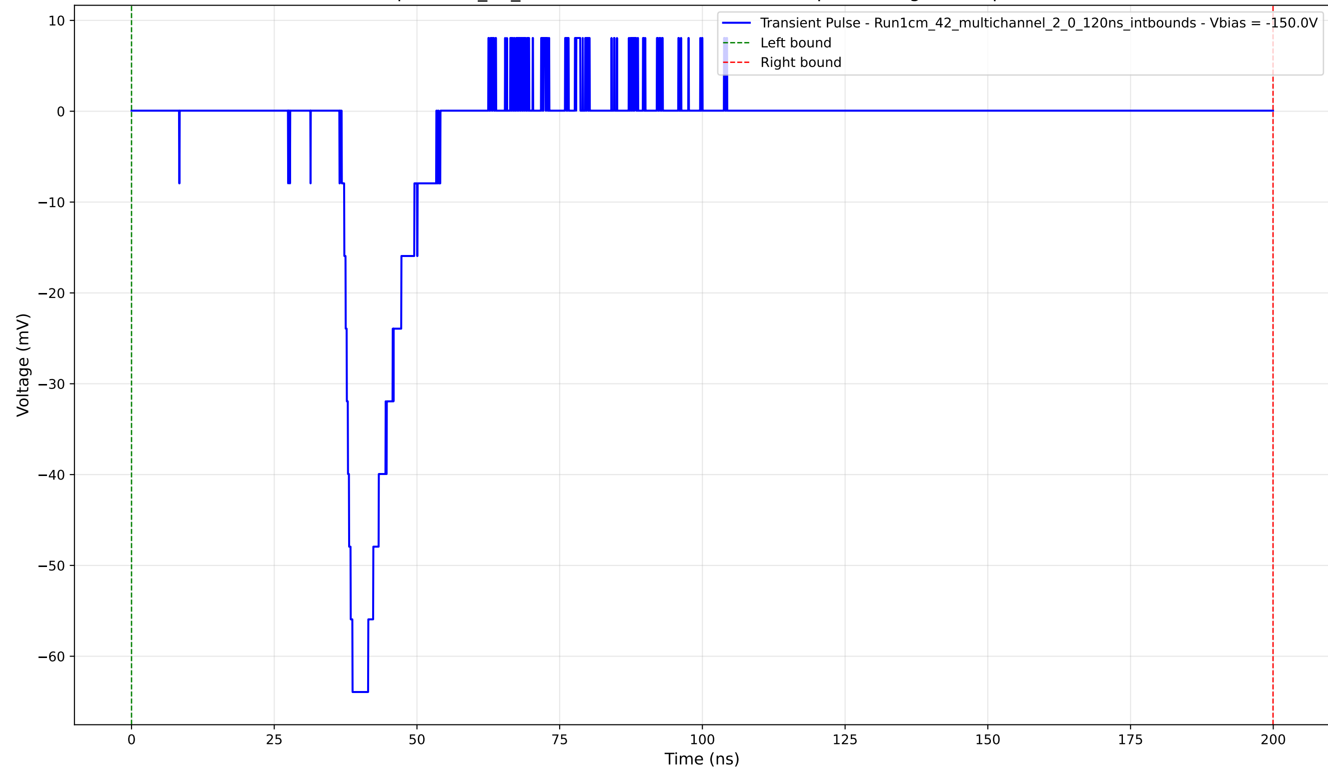
Transient Pulse - Sample: 1cm_42_multichannel - Position: 4475.0 \mu\text{m} - Charge: 9.03 pC - Rise Time: 1.89 ns
