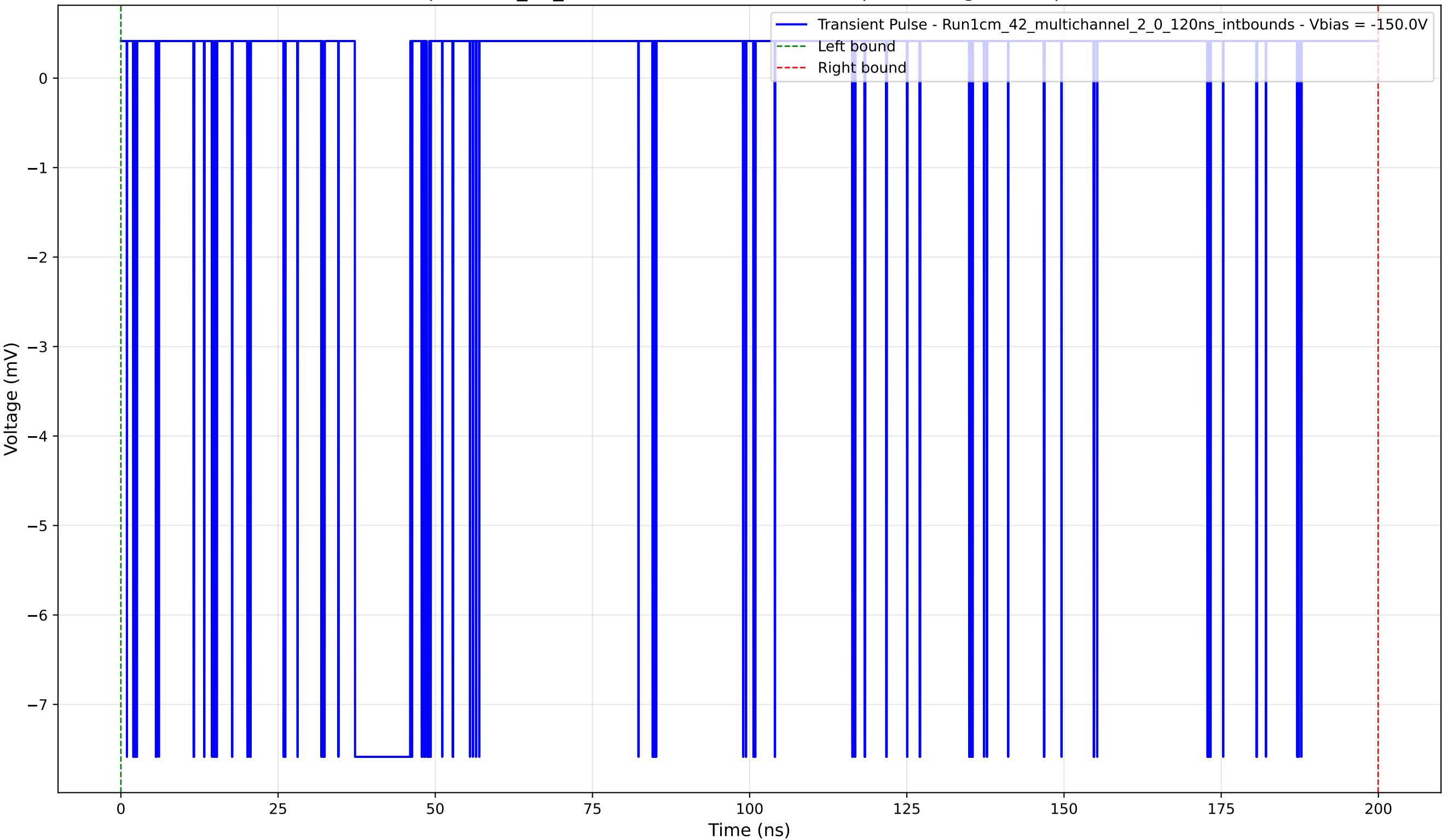
Transient Pulse - Sample: 1cm_42_multichannel - Position: 45.0 \mu\text{m} - Charge: 0.83 pC - Rise Time: 0.04 ns
