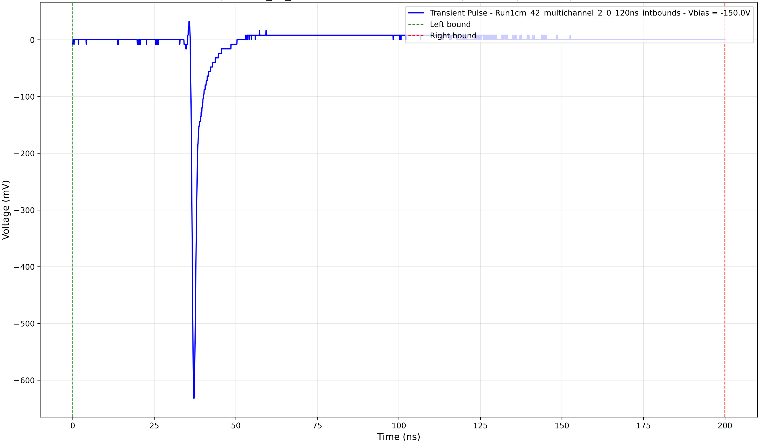
Transient Pulse - Sample: 1cm_42_multichannel - Position: 2275.0 \mu\text{m} - Charge: 16.80 pC - Rise Time: 0.72 ns
