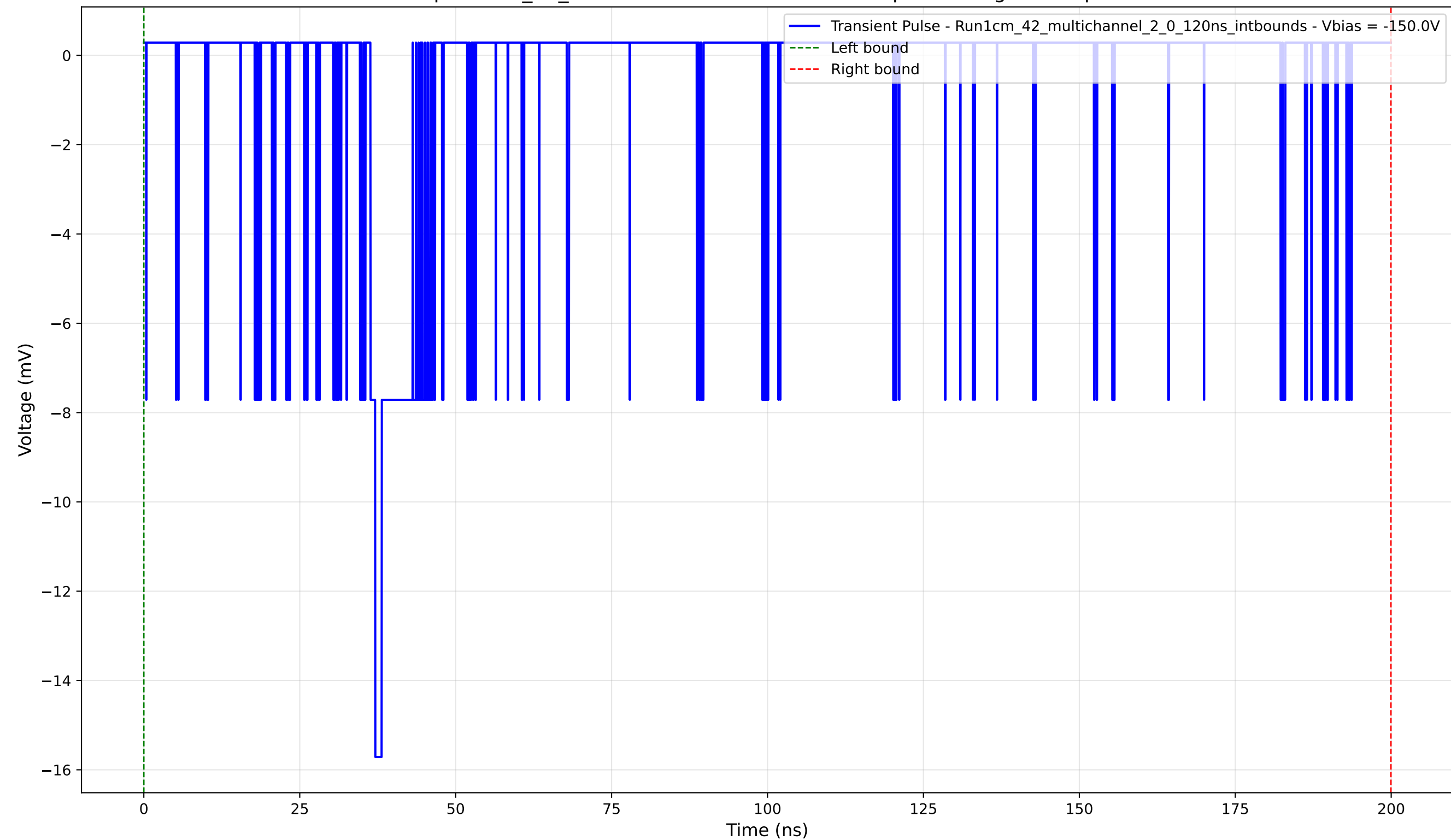
Transient Pulse - Sample: 1cm_42_multichannel - Position: 2880.0 \mu\text{m} - Charge: 2.21 pC - Rise Time: 0.79 ns
