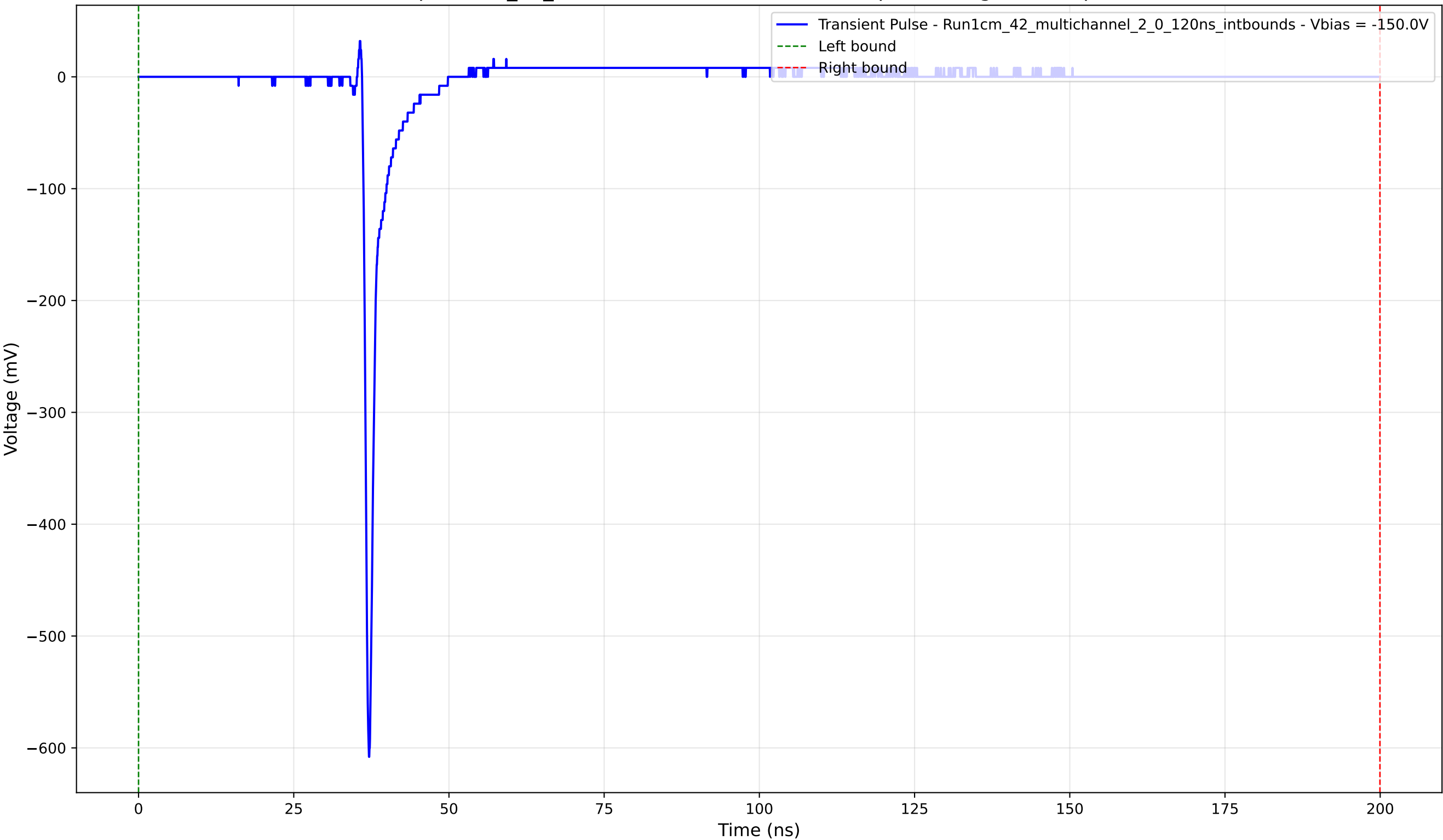
Transient Pulse - Sample: 1cm_42_multichannel - Position: 2445.0 \mu\text{m} - Charge: 16.65 pC - Rise Time: 0.72 ns
