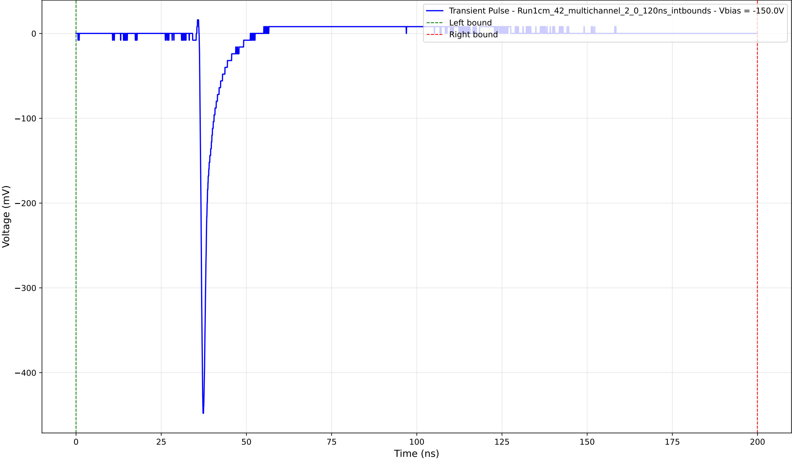
Transient Pulse - Sample: 1cm_42_multichannel - Position: 2030.0 \mu\text{m} - Charge: 15.44 pC - Rise Time: 0.75 ns
