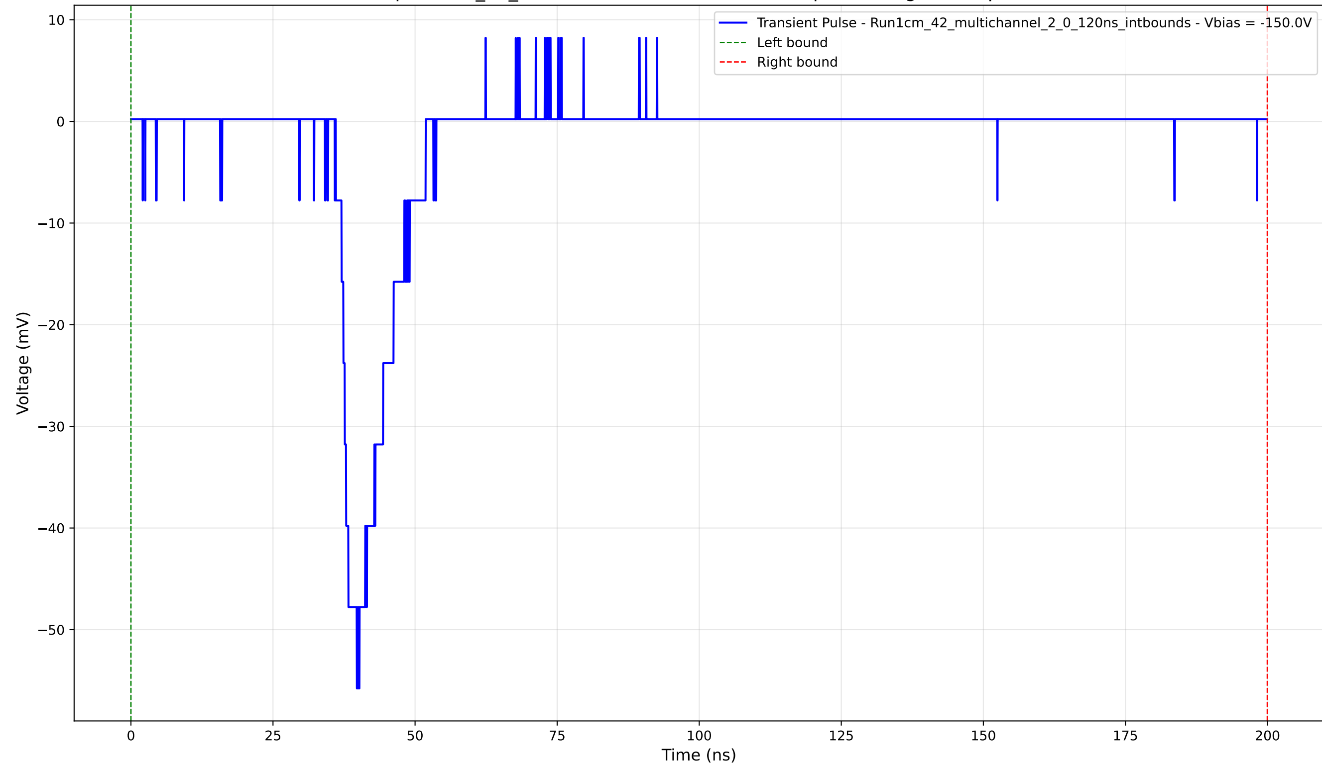
Transient Pulse - Sample: 1cm_42_multichannel - Position: 4825.0 \mu\text{m} - Charge: 7.36 pC - Rise Time: 3.69 ns
