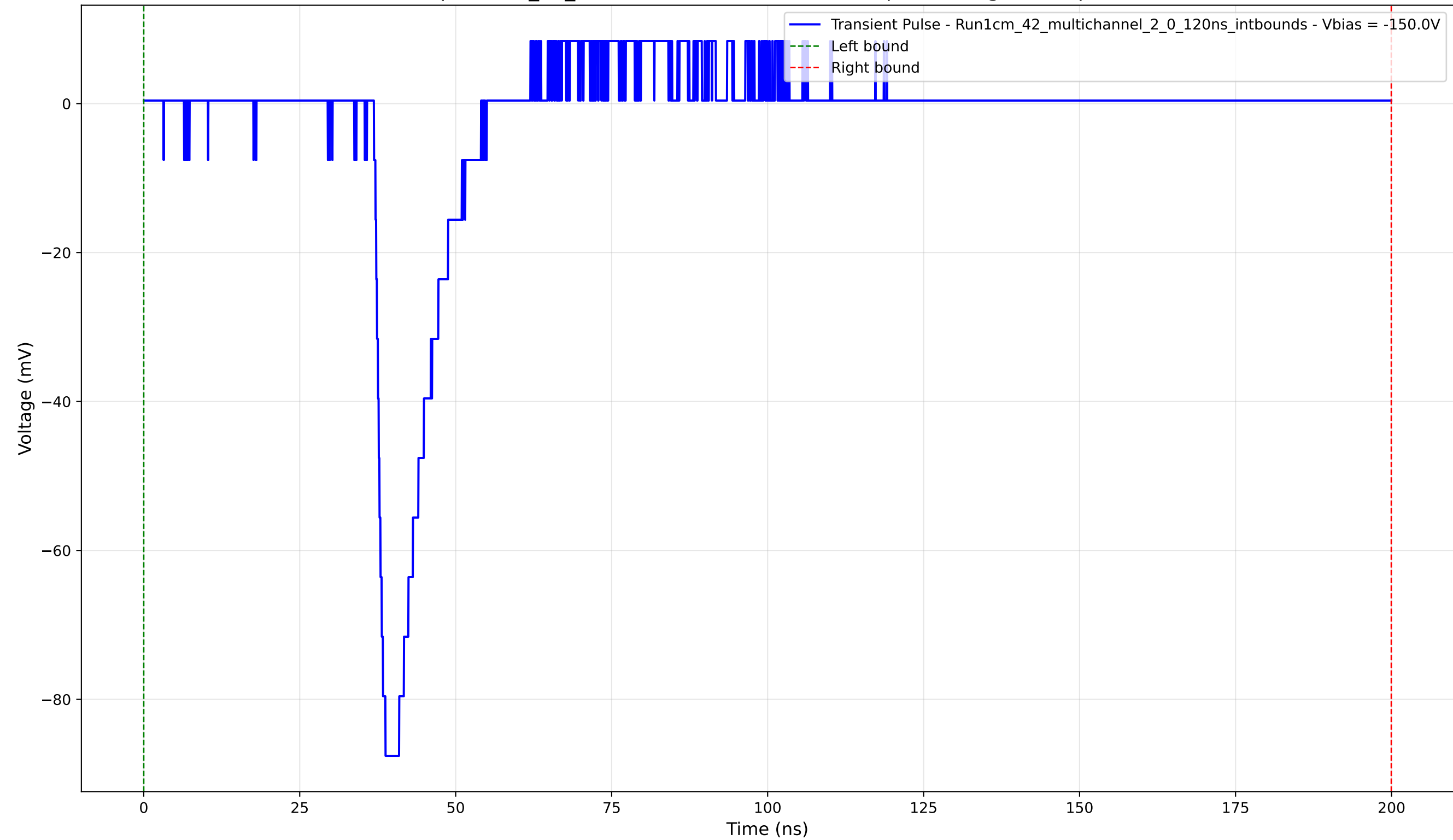
Transient Pulse - Sample: 1cm_42_multichannel - Position: 450.0 \mu\text{m} - Charge: 8.95 pC - Rise Time: 1.23 ns
