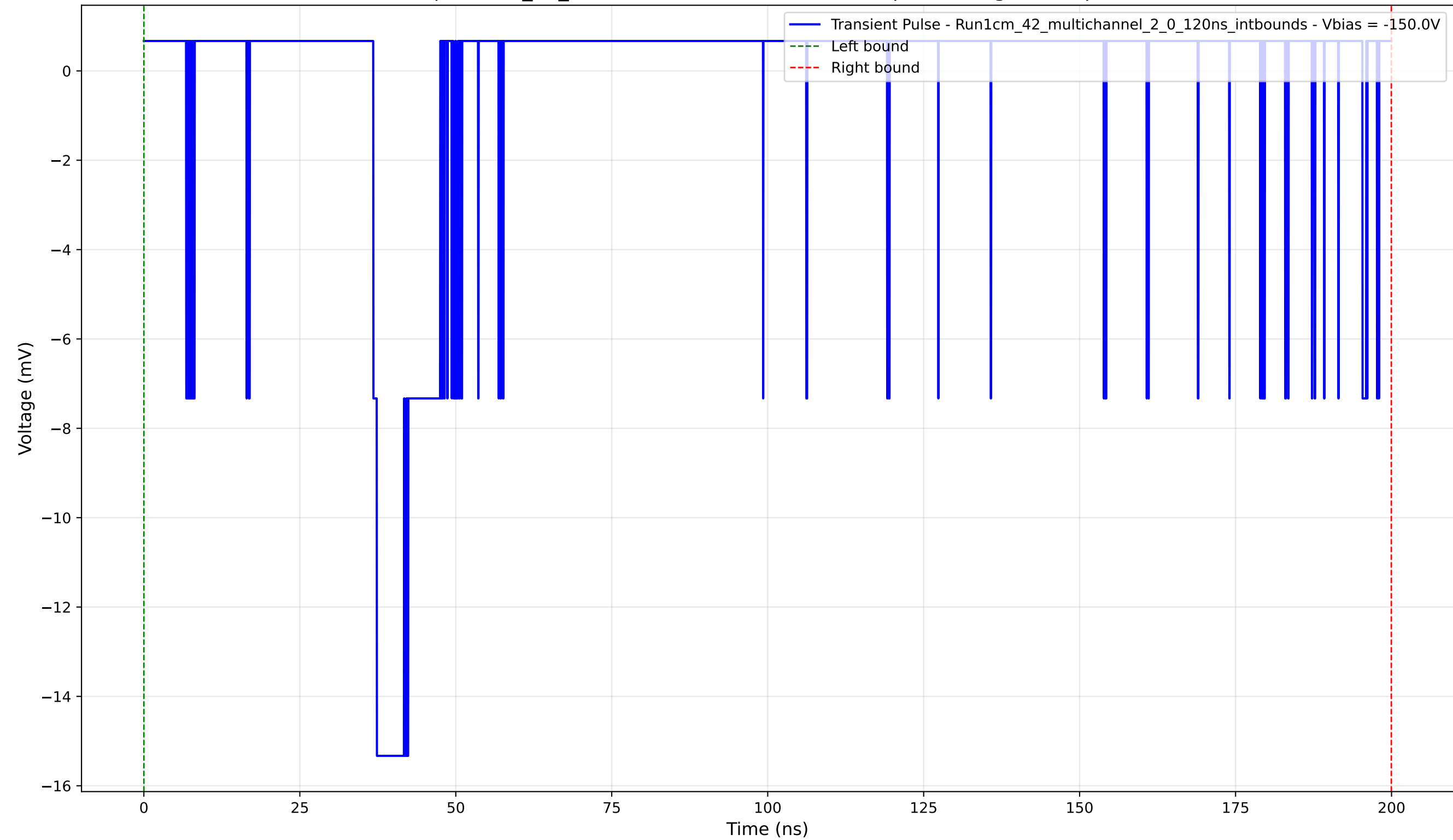
Transient Pulse - Sample: 1cm_42_multichannel - Position: 3410.0 \mu\text{m} - Charge: 0.68 pC - Rise Time: 0.59 ns
