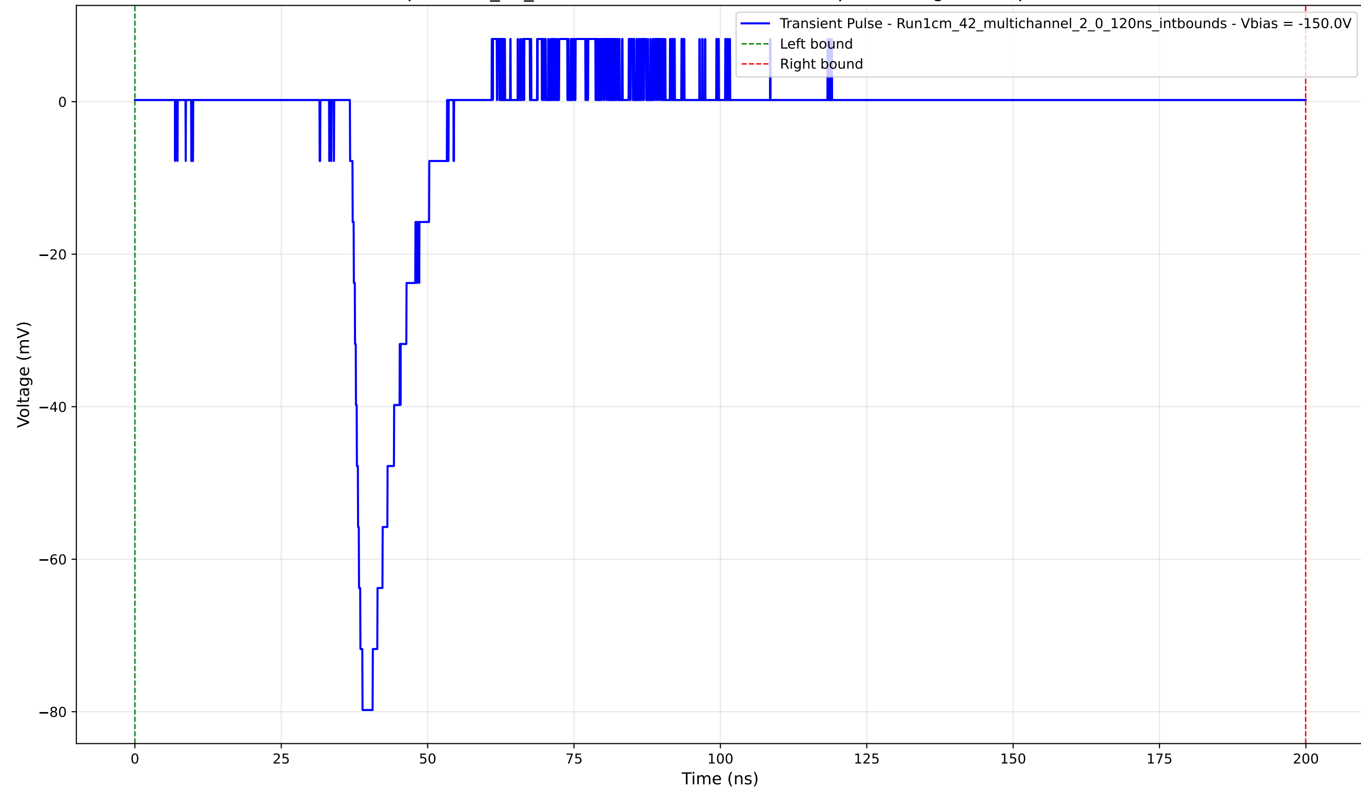
Transient Pulse - Sample: 1cm_42_multichannel - Position: 4245.0 \mu\text{m} - Charge: 8.73 pC - Rise Time: 1.72 ns
