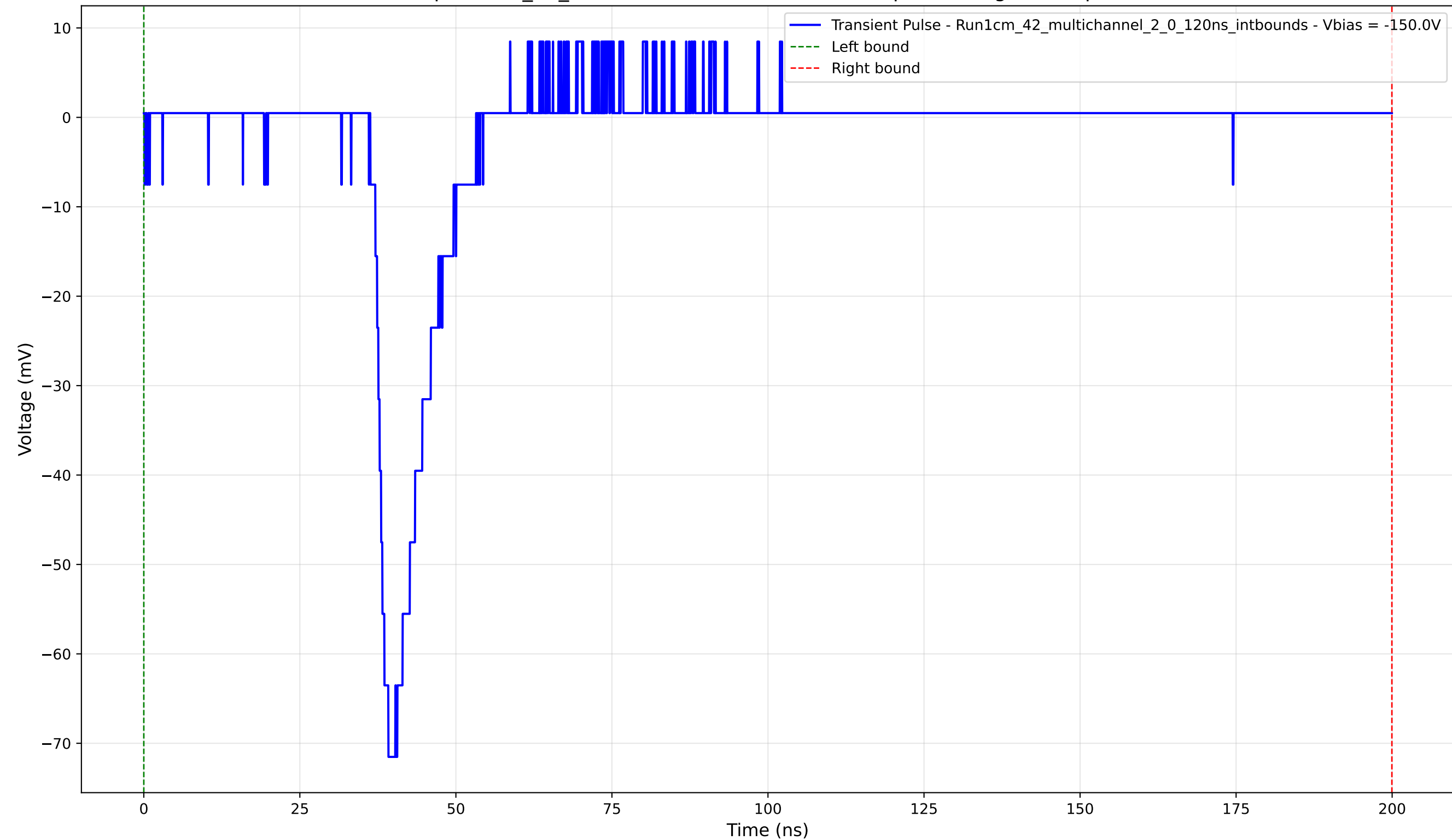
Transient Pulse - Sample: 1cm_42_multichannel - Position: 4665.0 \mu\text{m} - Charge: 8.10 pC - Rise Time: 2.88 ns
