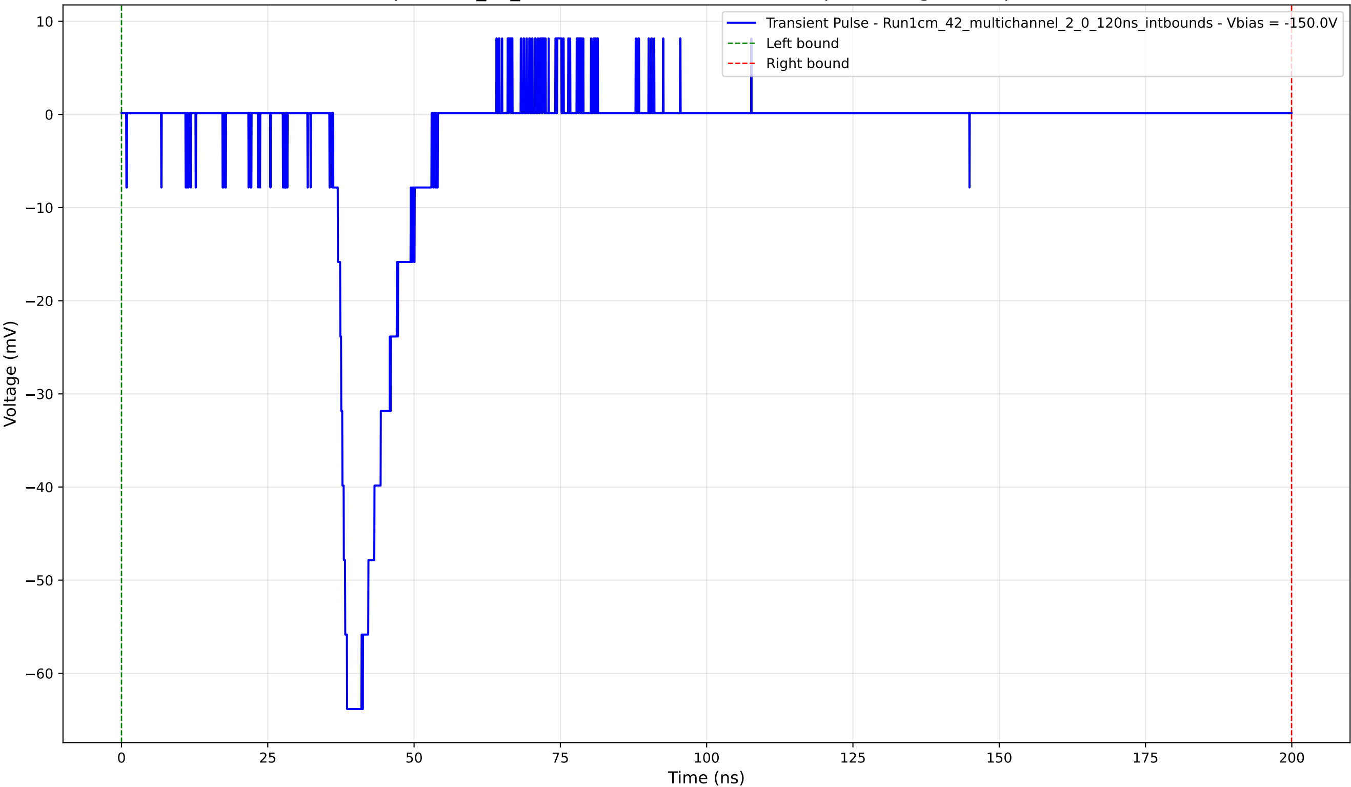
Transient Pulse - Sample: 1cm_42_multichannel - Position: 4745.0 \mu\text{m} - Charge: 9.45 pC - Rise Time: 2.37 ns
