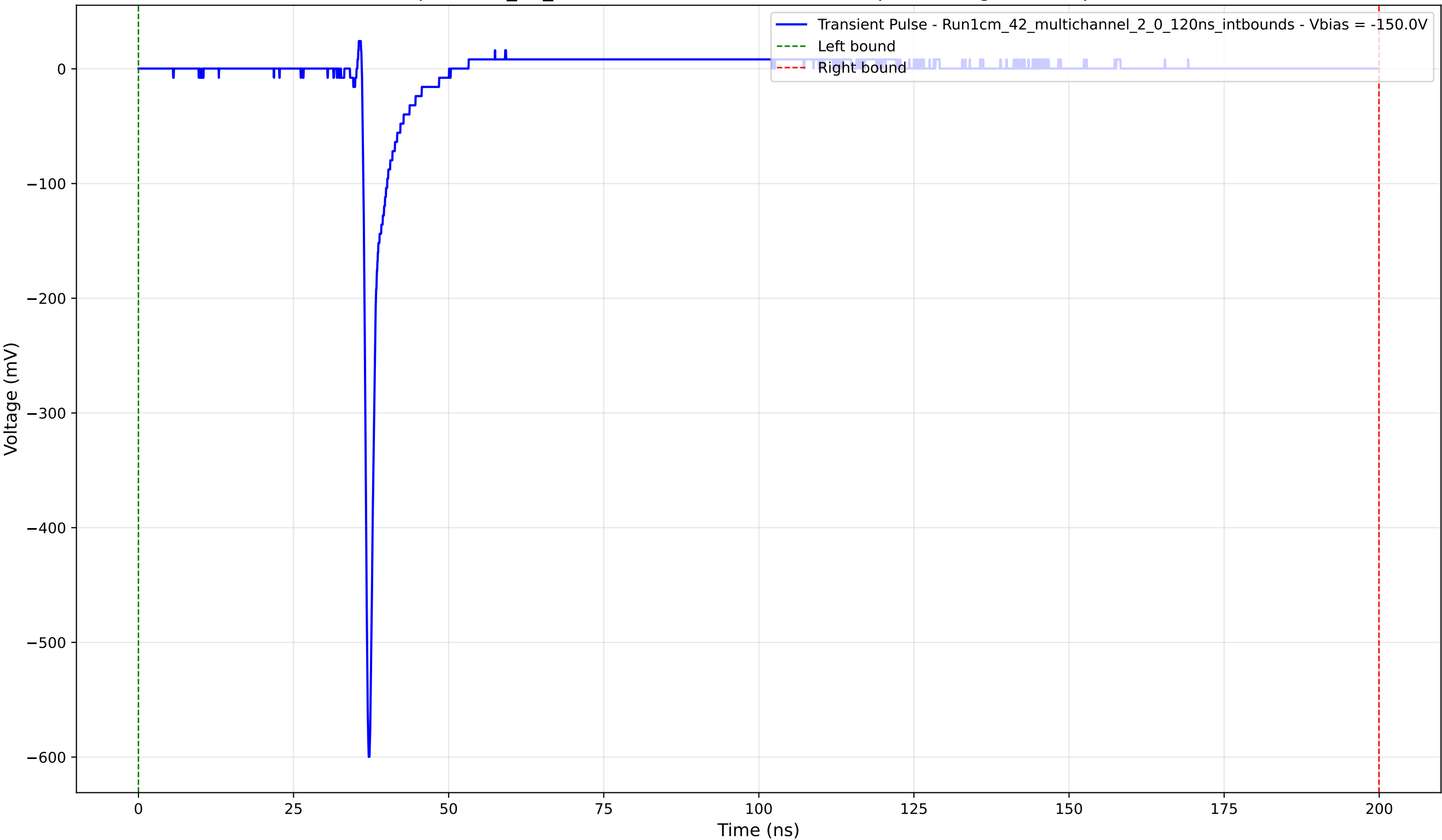
Transient Pulse - Sample: 1cm_42_multichannel - Position: 2490.0 \mu\text{m} - Charge: 16.15 pC - Rise Time: 0.72 ns
