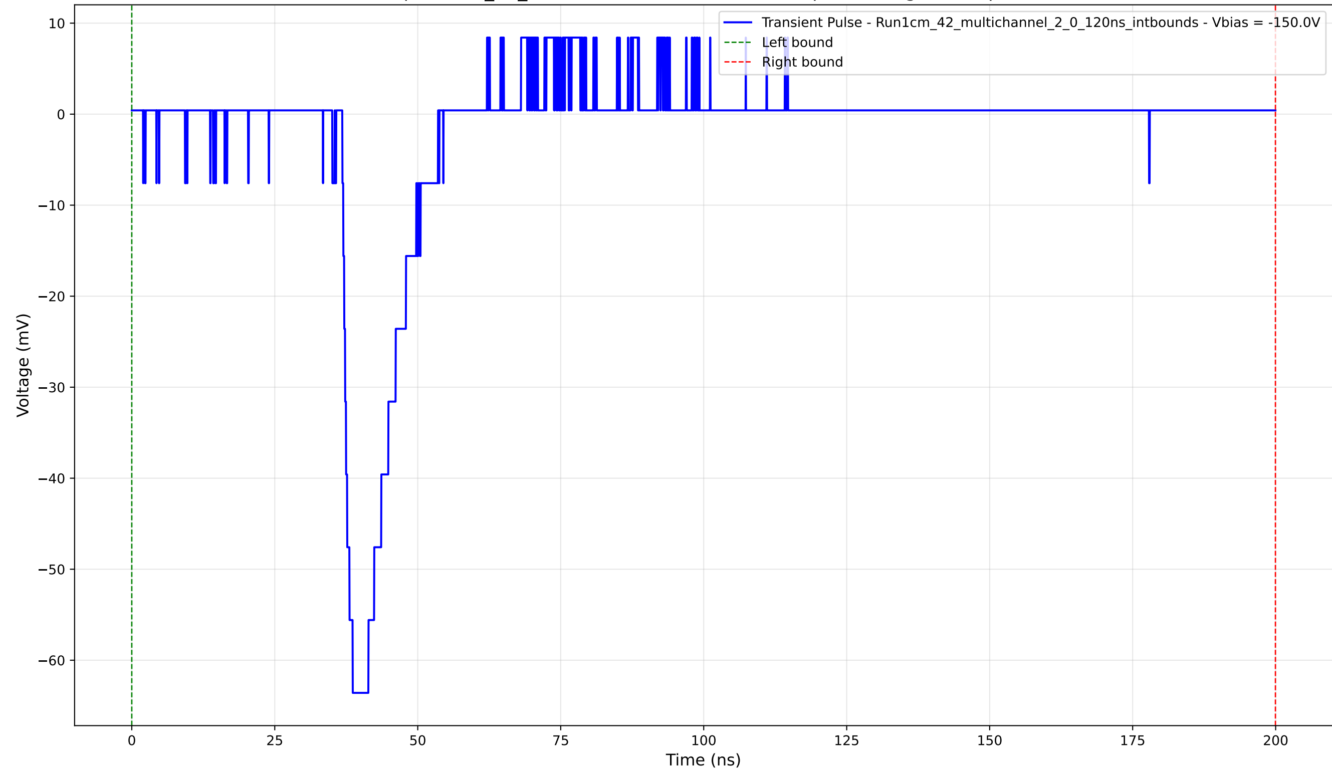
Transient Pulse - Sample: 1cm_42_multichannel - Position: 135.0 \mu\text{m} - Charge: 7.84 pC - Rise Time: 1.81 ns
