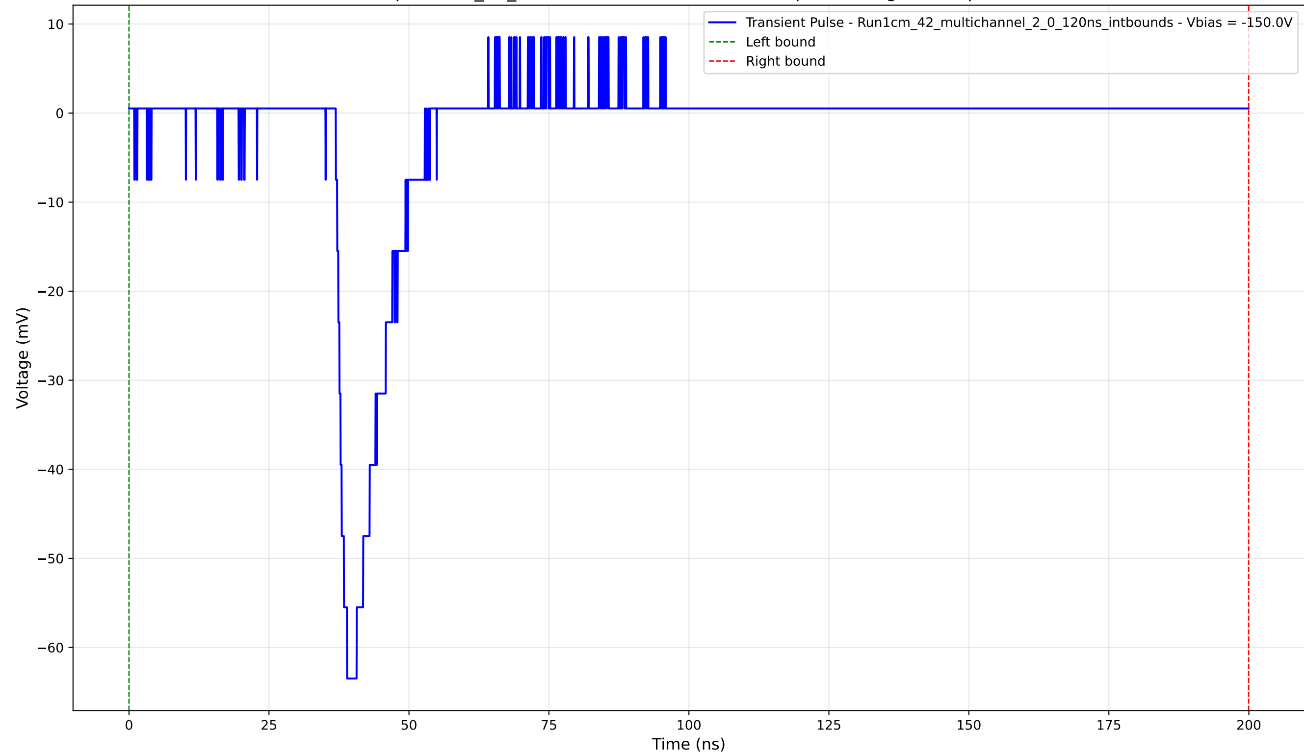
Transient Pulse - Sample: 1cm_42_multichannel - Position: 405.0 \mu\text{m} - Charge: 7.33 pC - Rise Time: 2.01 ns
