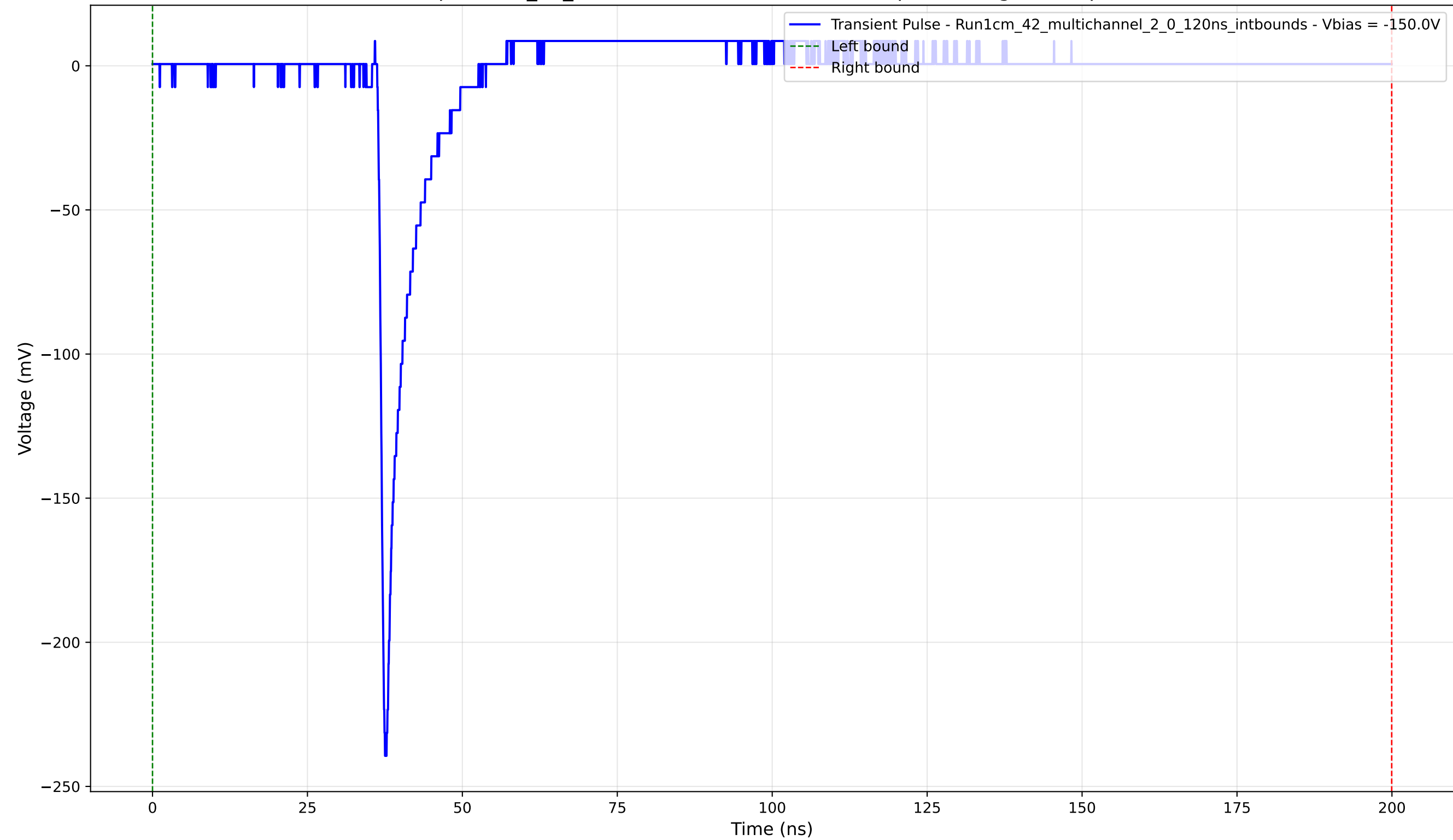
Transient Pulse - Sample: 1cm_42_multichannel - Position: 3040.0 \mu\text{m} - Charge: 9.90 pC - Rise Time: 0.92 ns
