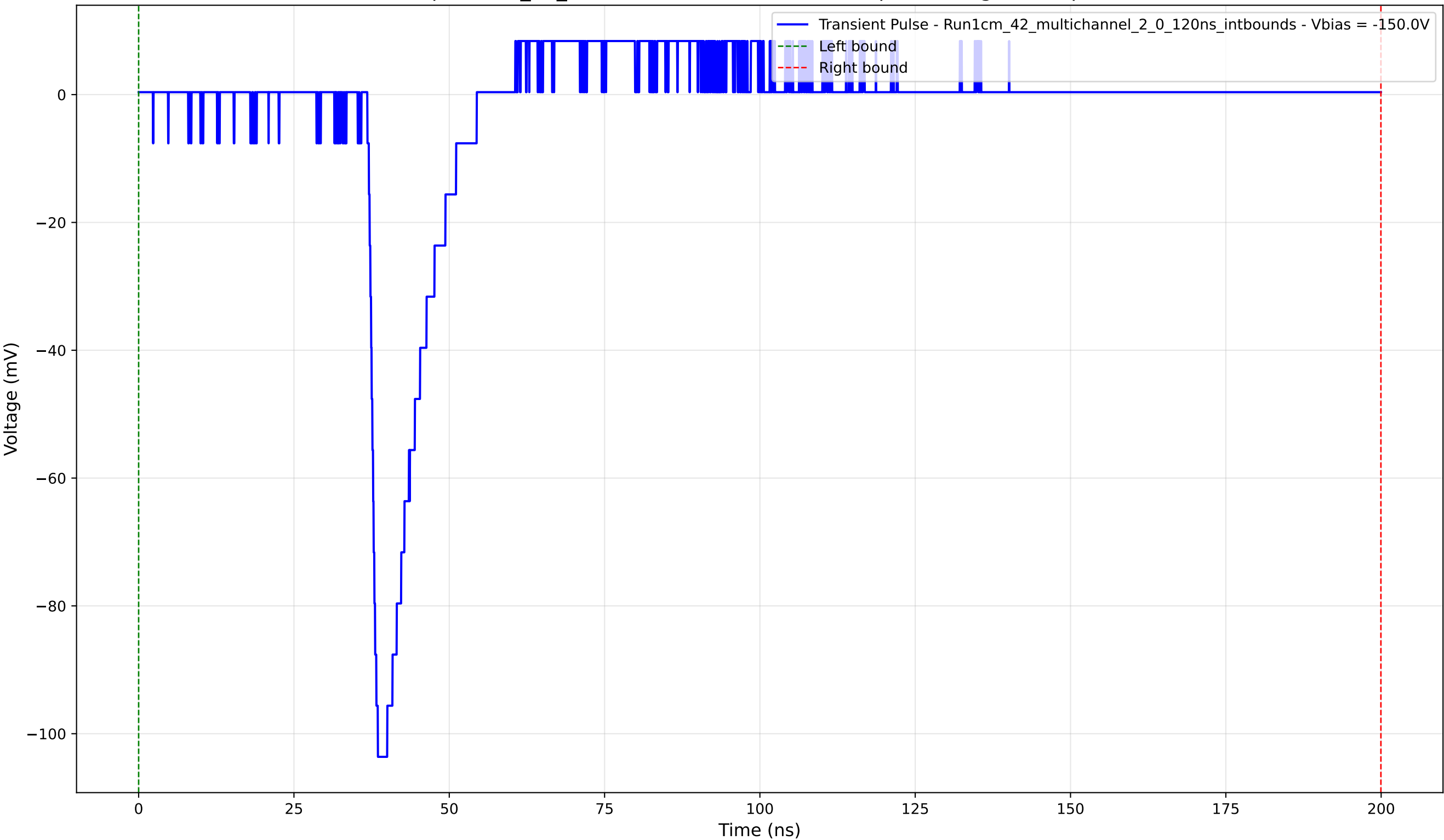
Transient Pulse - Sample: 1cm_42_multichannel - Position: 725.0 \mu\text{m} - Charge: 9.34 pC - Rise Time: 1.23 ns
