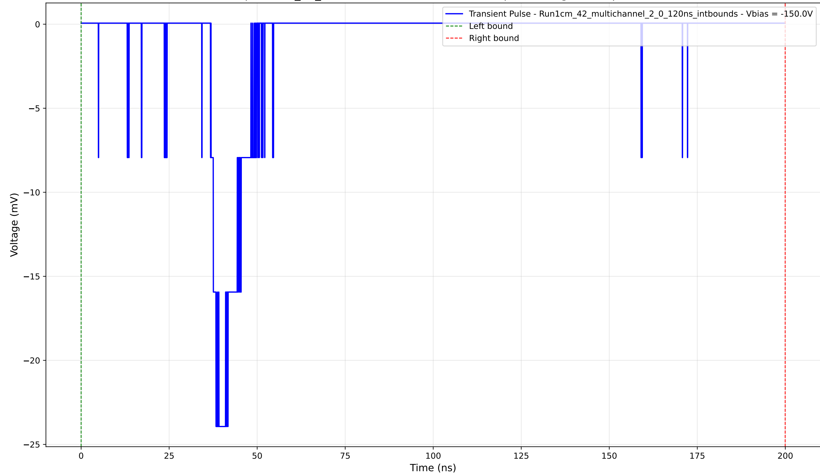
Transient Pulse - Sample: 1cm_42_multichannel - Position: 4855.0 \mu\text{m} - Charge: 3.73 pC - Rise Time: 1.43 ns
