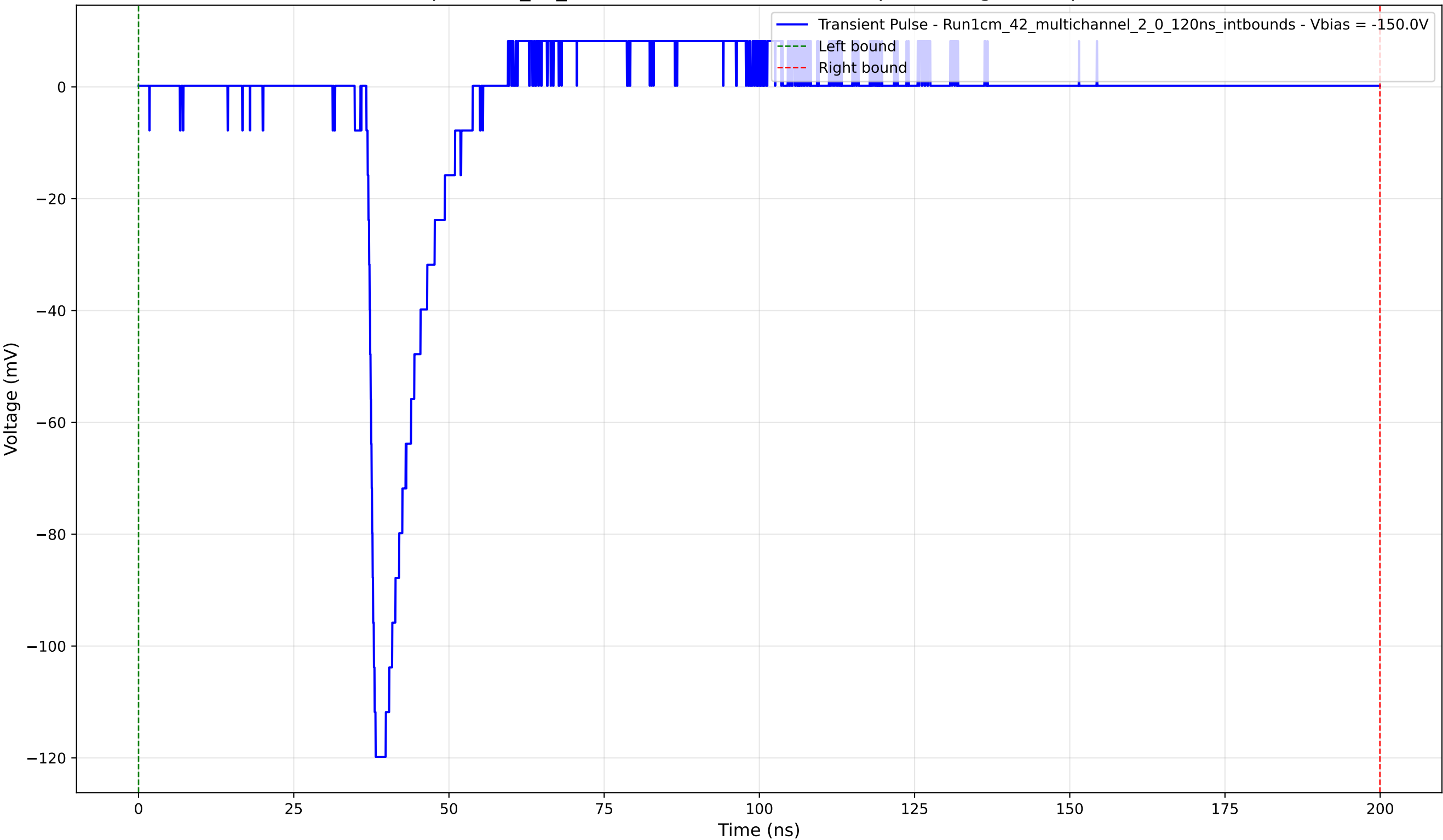
Transient Pulse - Sample: 1cm_42_multichannel - Position: 960.0 \mu\text{m} - Charge: 9.67 pC - Rise Time: 1.14 ns
