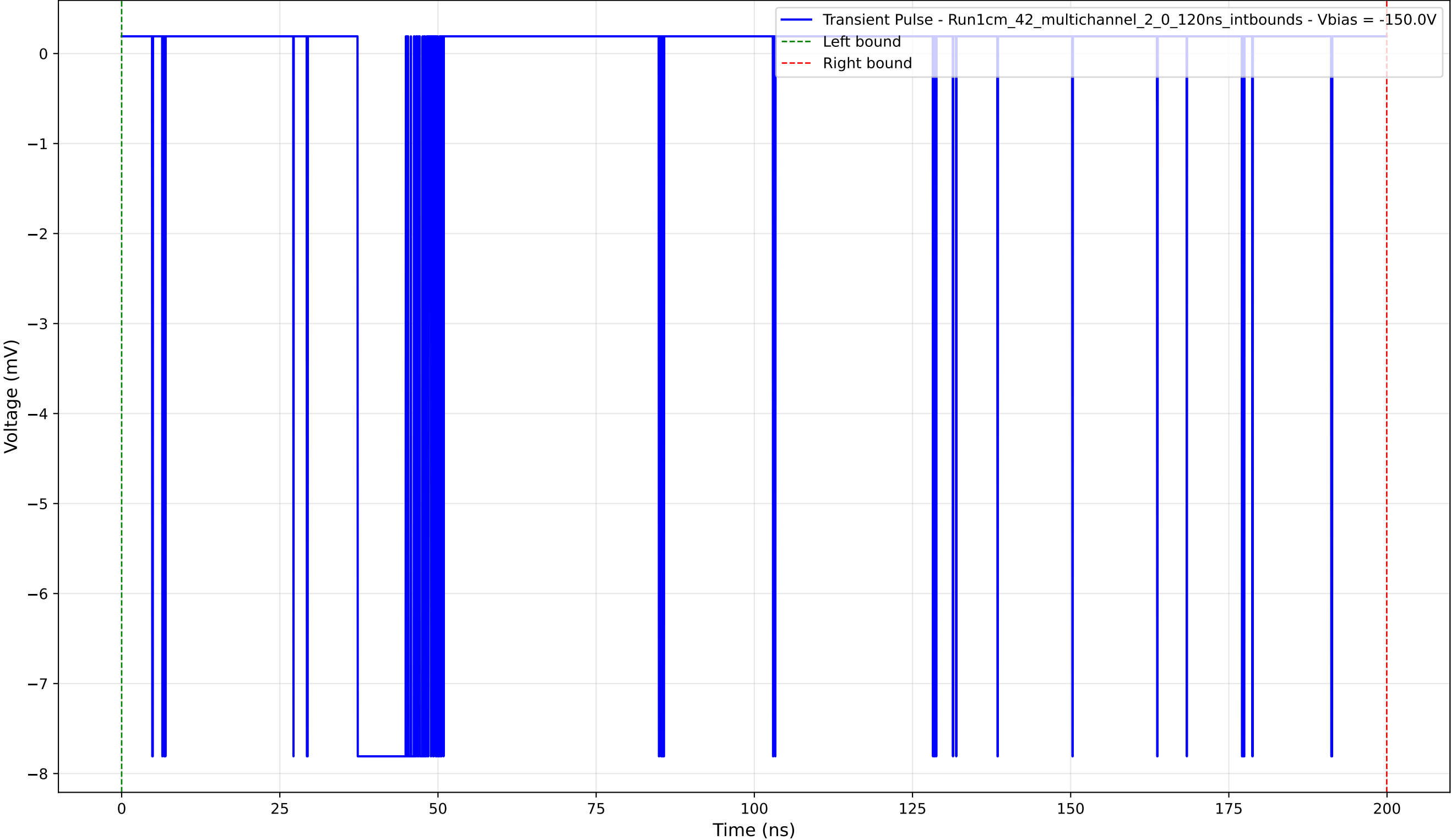
Transient Pulse - Sample: 1cm_42_multichannel - Position: 40.0 \mu\text{m} - Charge: 1.28 pC - Rise Time: 0.04 ns
