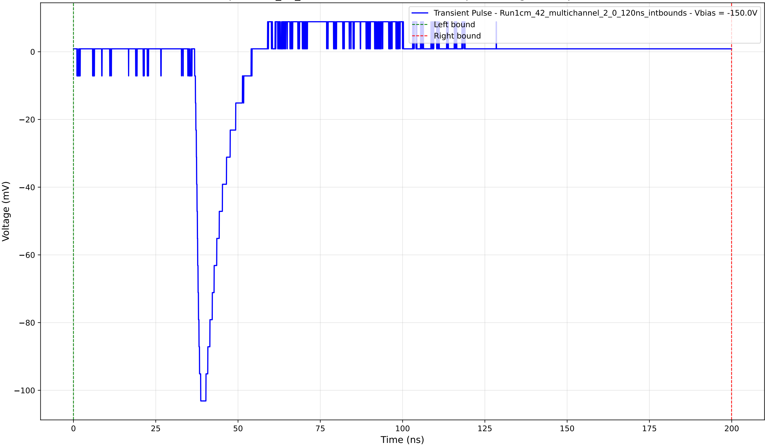
Transient Pulse - Sample: 1cm_42_multichannel - Position: 685.0 \mu\text{m} - Charge: 7.09 pC - Rise Time: 1.26 ns
