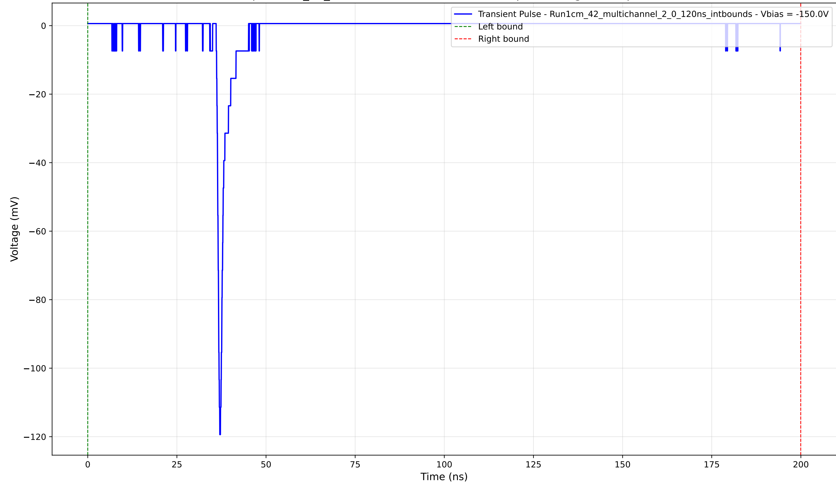
Transient Pulse - Sample: 1cm_42_multichannel - Position: 2335.0 \mu\text{m} - Charge: 3.54 pC - Rise Time: 0.78 ns
