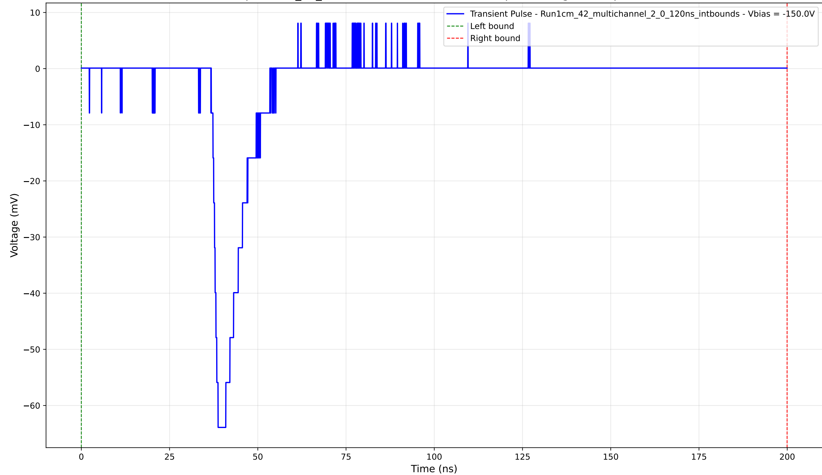
Transient Pulse - Sample: 1cm_42_multichannel - Position: 4310.0 \mu\text{m} - Charge: 9.44 pC - Rise Time: 1.93 ns
