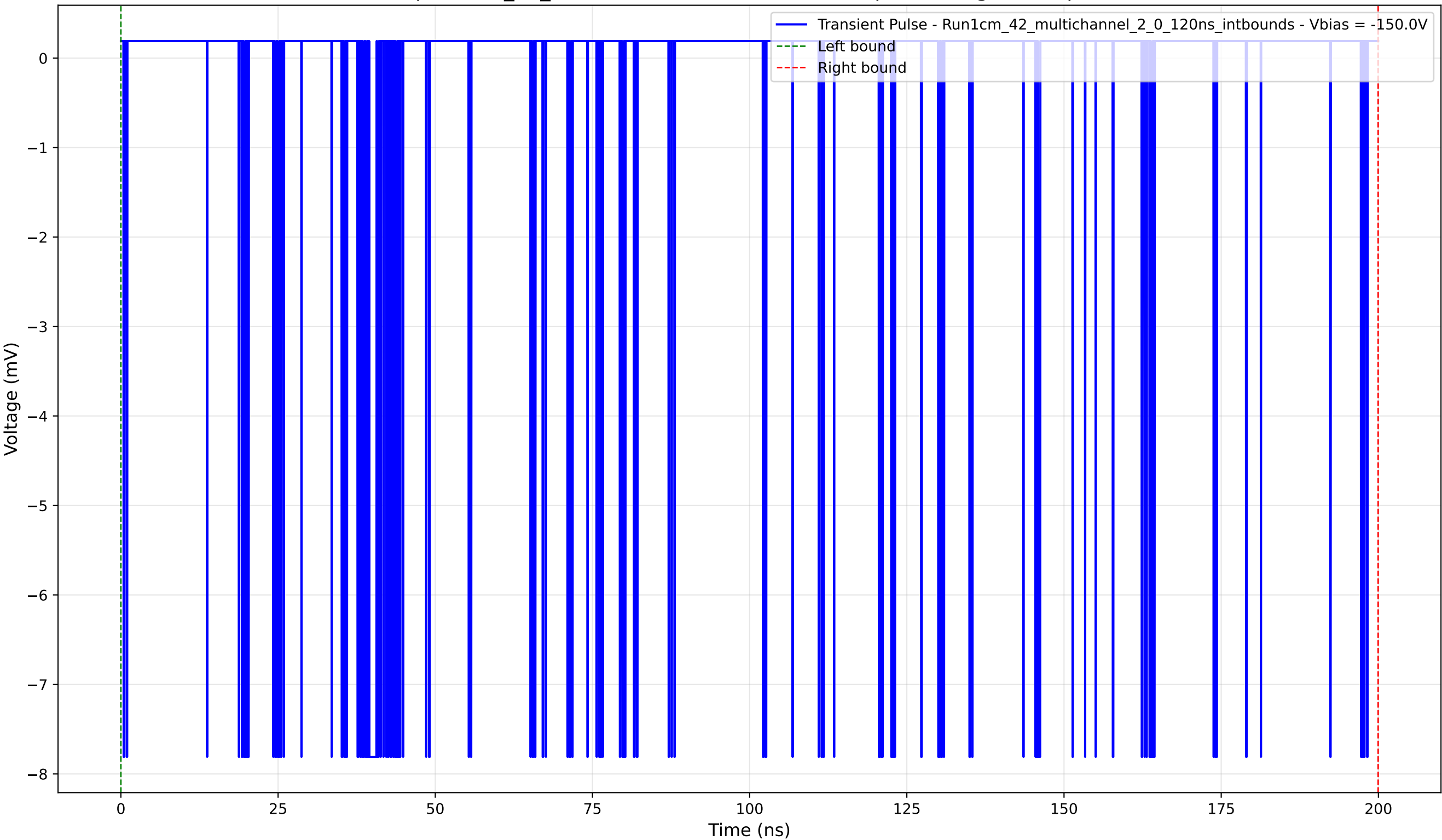
Transient Pulse - Sample: 1cm_42_multichannel - Position: 4905.0 \mu\text{m} - Charge: 1.40 pC - Rise Time: 0.04 ns
