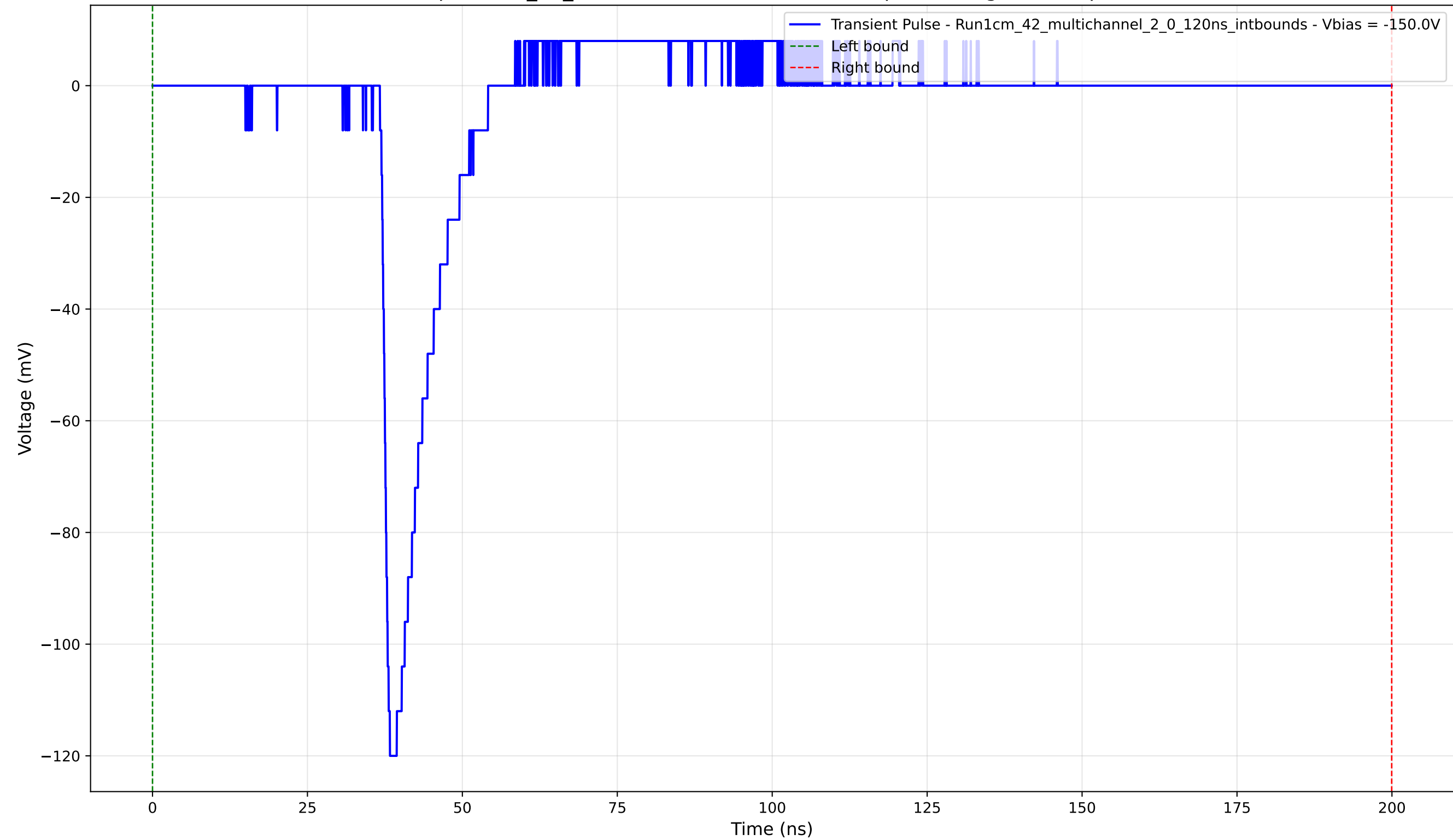
Transient Pulse - Sample: 1cm_42_multichannel - Position: 950.0 \mu\text{m} - Charge: 10.46 pC - Rise Time: 1.18 ns
