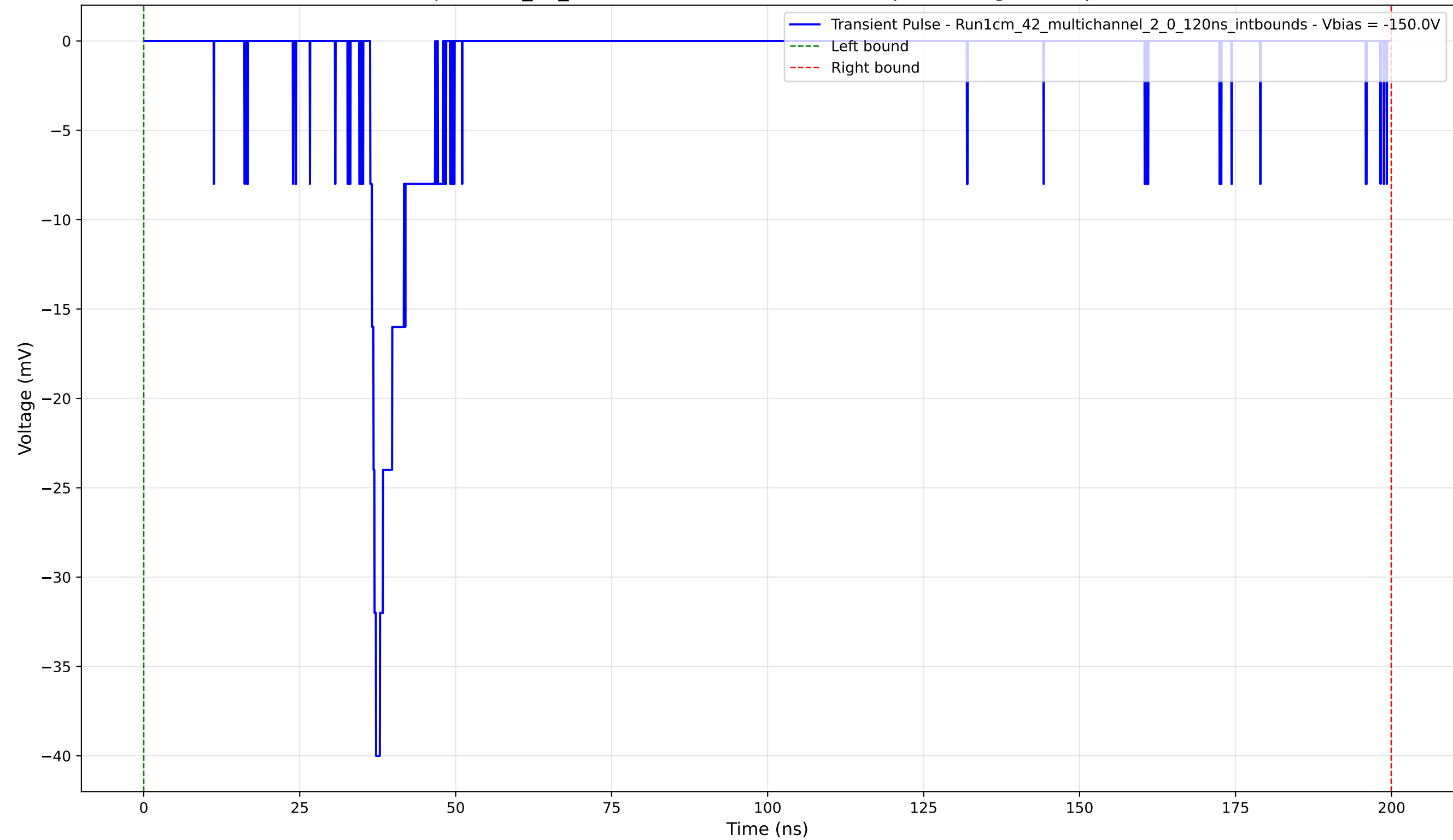
Transient Pulse - Sample: 1cm_42_multichannel - Position: 1835.0 \mu\text{m} - Charge: 3.90 pC - Rise Time: 0.94 ns
