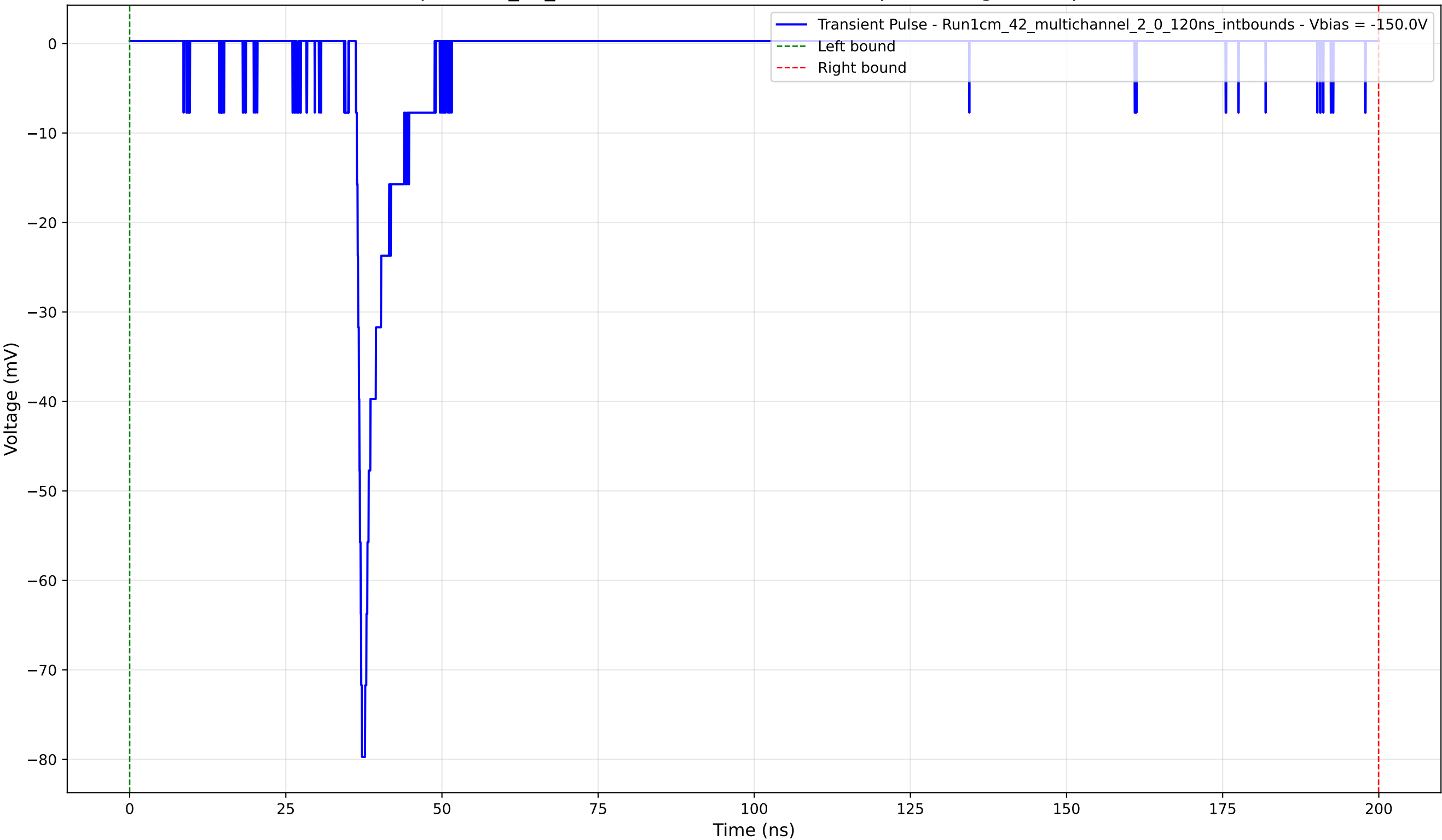
Transient Pulse - Sample: 1cm_42_multichannel - Position: 1900.0 \mu\text{m} - Charge: 5.61 pC - Rise Time: 0.84 ns
