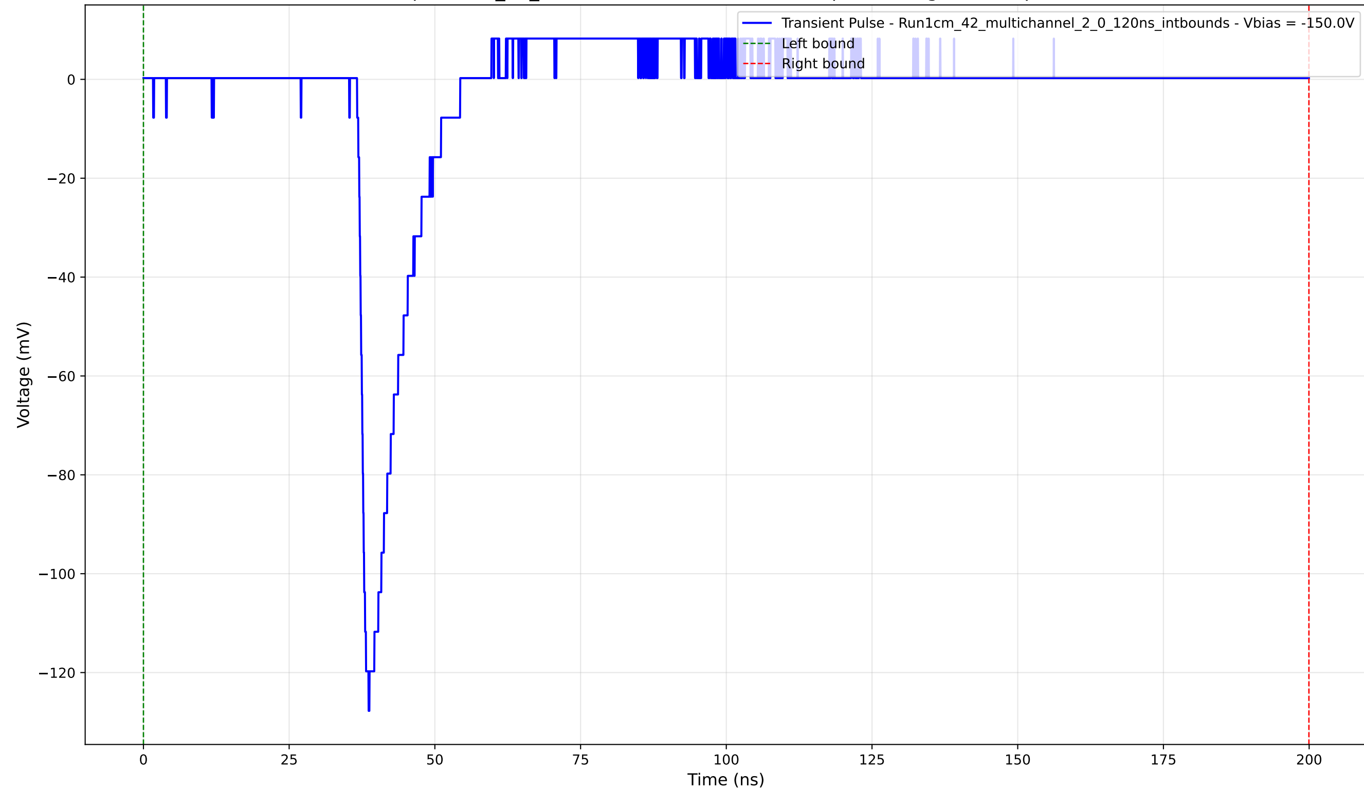
Transient Pulse - Sample: 1cm_42_multichannel - Position: 990.0 \mu\text{m} - Charge: 10.09 pC - Rise Time: 1.33 ns
