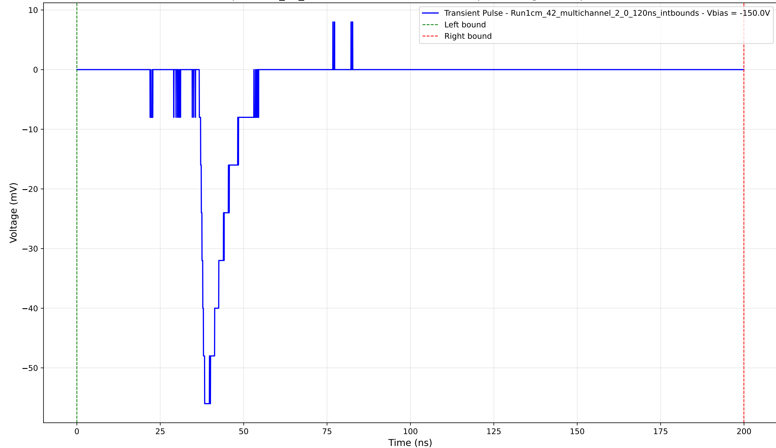
Transient Pulse - Sample: 1cm_42_multichannel - Position: 3835.0 \mu\text{m} - Charge: 8.62 pC - Rise Time: 1.61 ns
