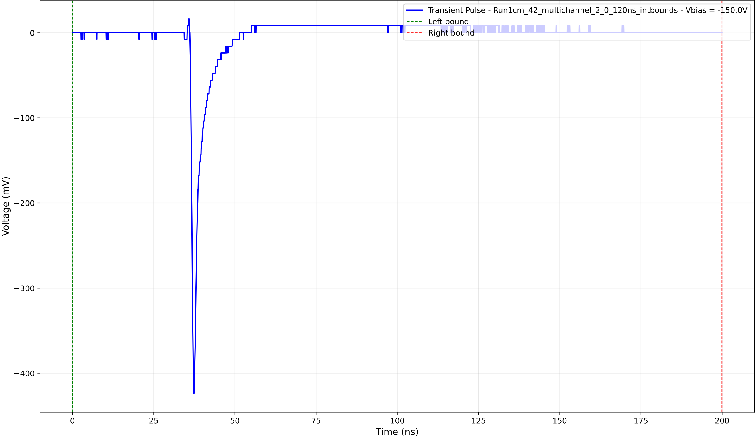
Transient Pulse - Sample: 1cm_42_multichannel - Position: 1985.0 \mu\text{m} - Charge: 13.09 pC - Rise Time: 0.78 ns
