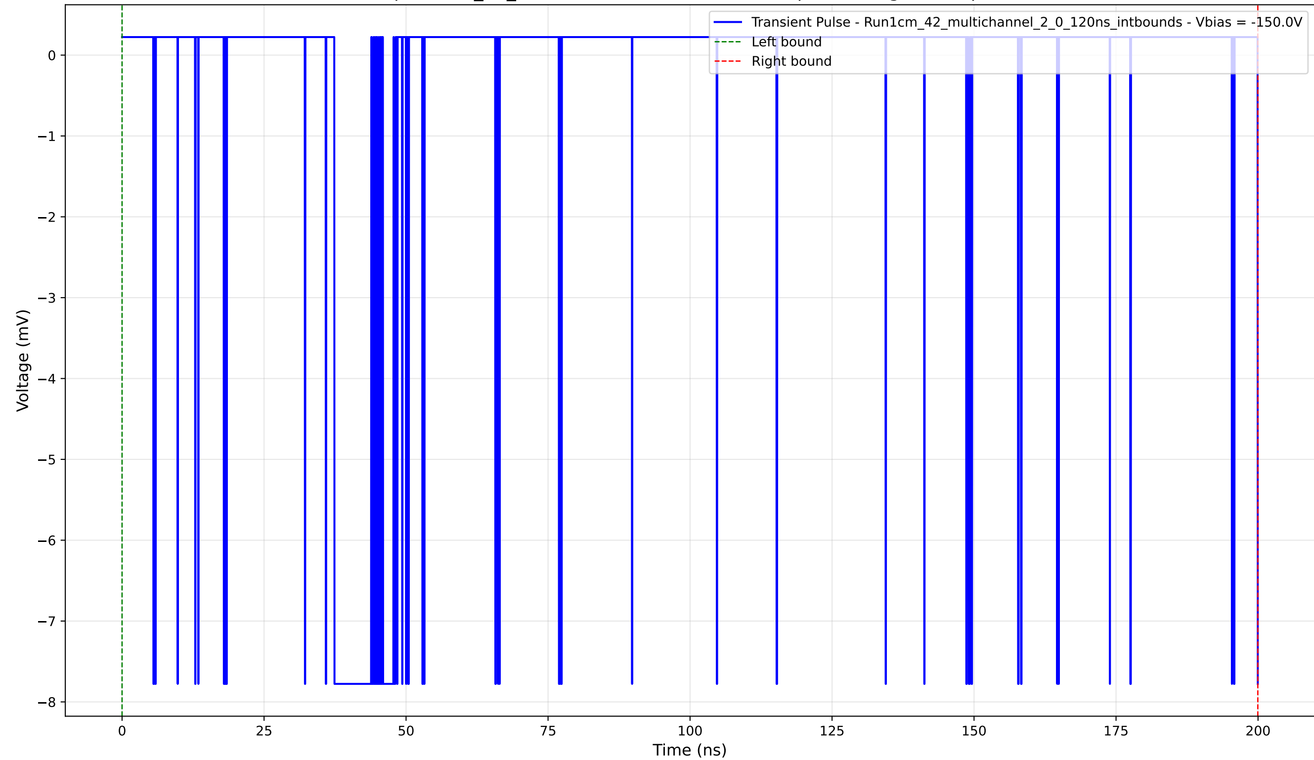
Transient Pulse - Sample: 1cm_42_multichannel - Position: 865.0 \mu\text{m} - Charge: 1.28 pC - Rise Time: 0.04 ns
