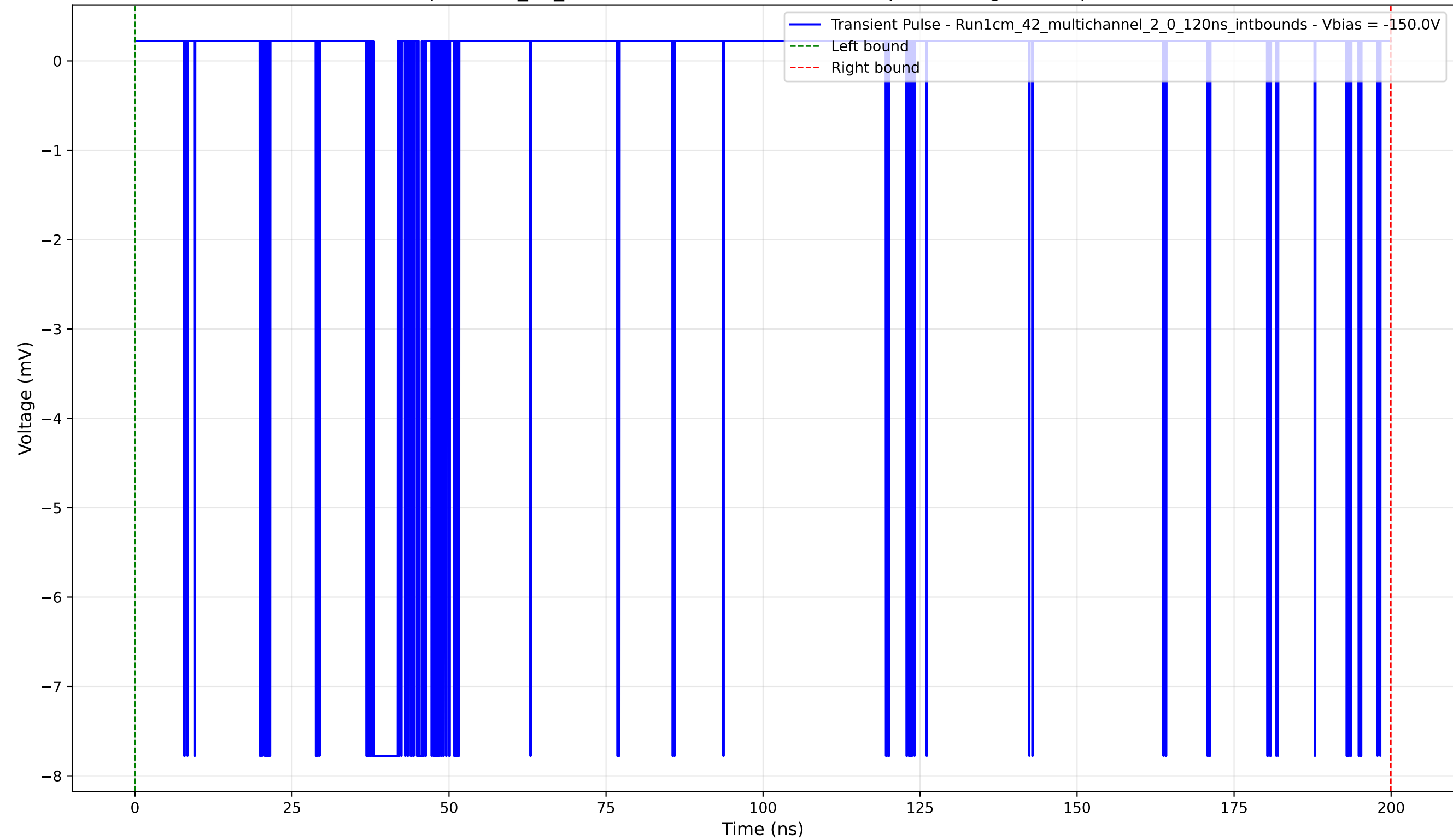
Transient Pulse - Sample: 1cm_42_multichannel - Position: 4400.0 \mu\text{m} - Charge: 1.17 pC - Rise Time: 0.04 ns
