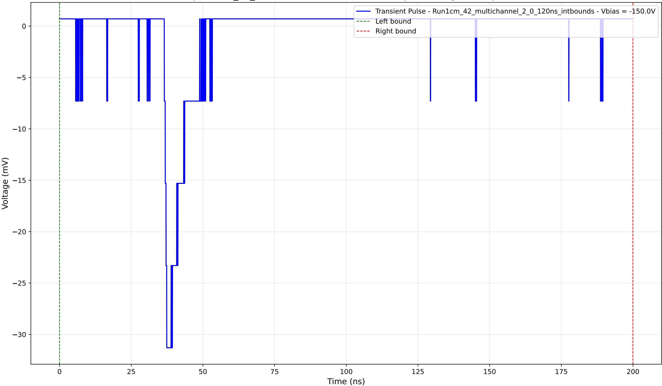
Transient Pulse - Sample: 1cm_42_multichannel - Position: 1390.0 \mu\text{m} - Charge: 1.81 pC - Rise Time: 0.87 ns
