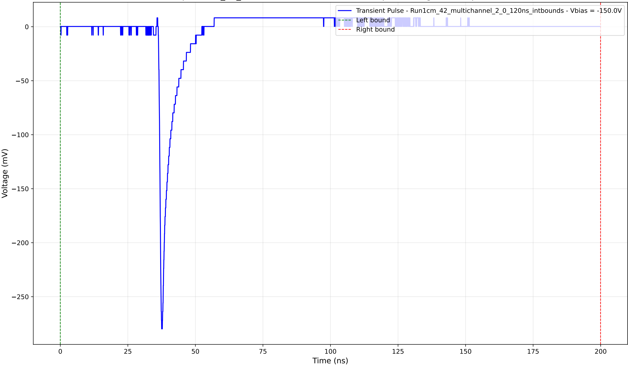
Transient Pulse - Sample: 1cm_42_multichannel - Position: 1715.0 \mu\text{m} - Charge: 12.96 pC - Rise Time: 0.88 ns
