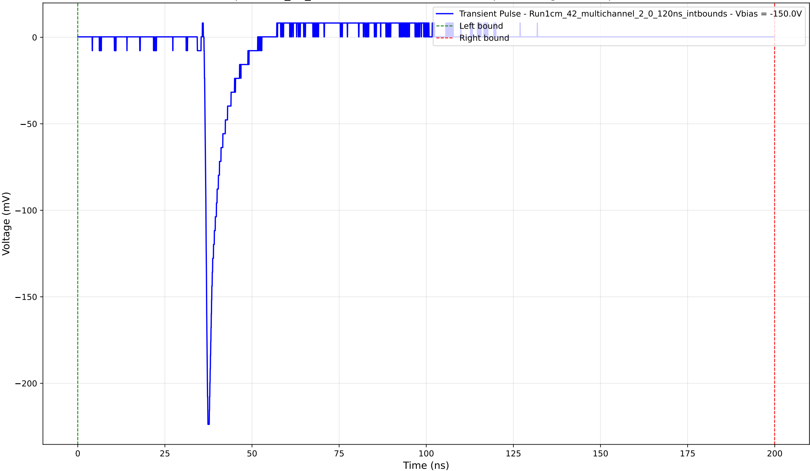
Transient Pulse - Sample: 1cm_42_multichannel - Position: 1800.0 \mu\text{m} - Charge: 10.69 pC - Rise Time: 0.89 ns
