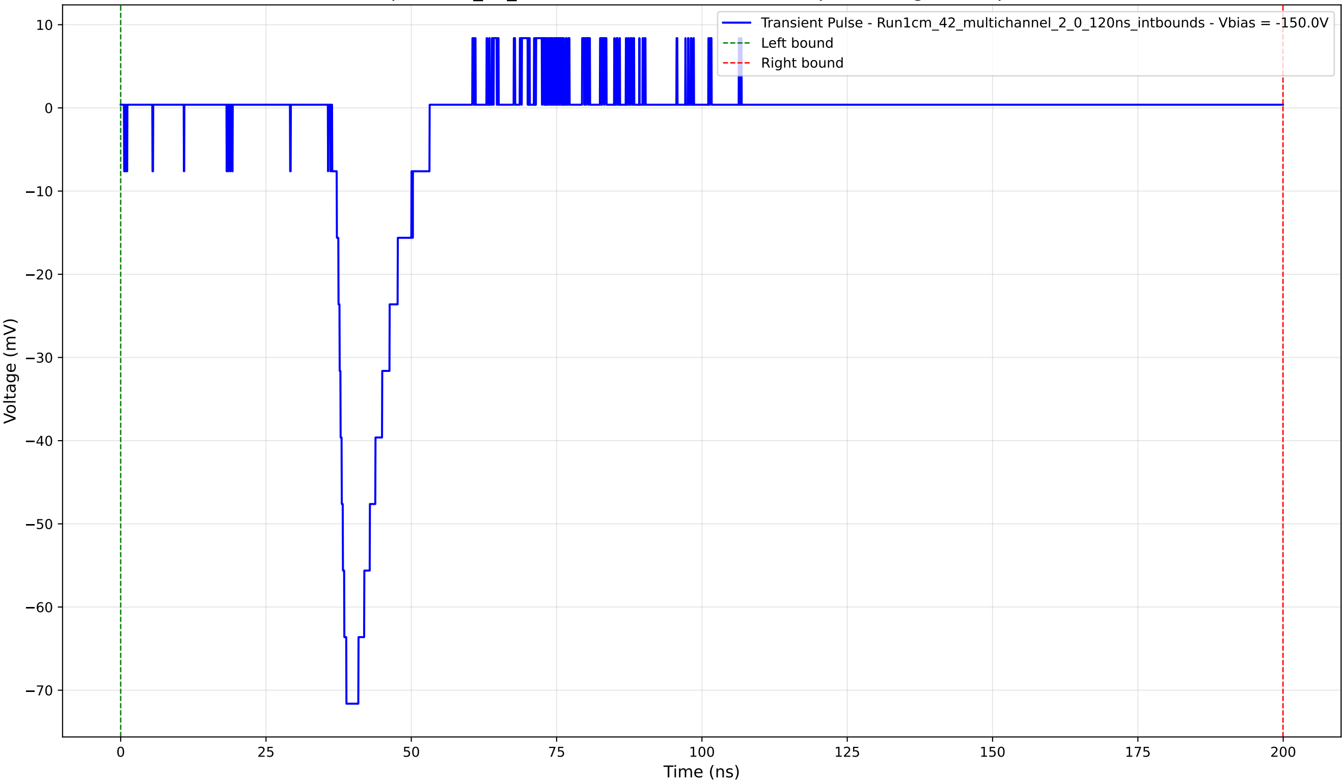
Transient Pulse - Sample: 1cm_42_multichannel - Position: 4545.0 \mu\text{m} - Charge: 8.31 pC - Rise Time: 2.44 ns
