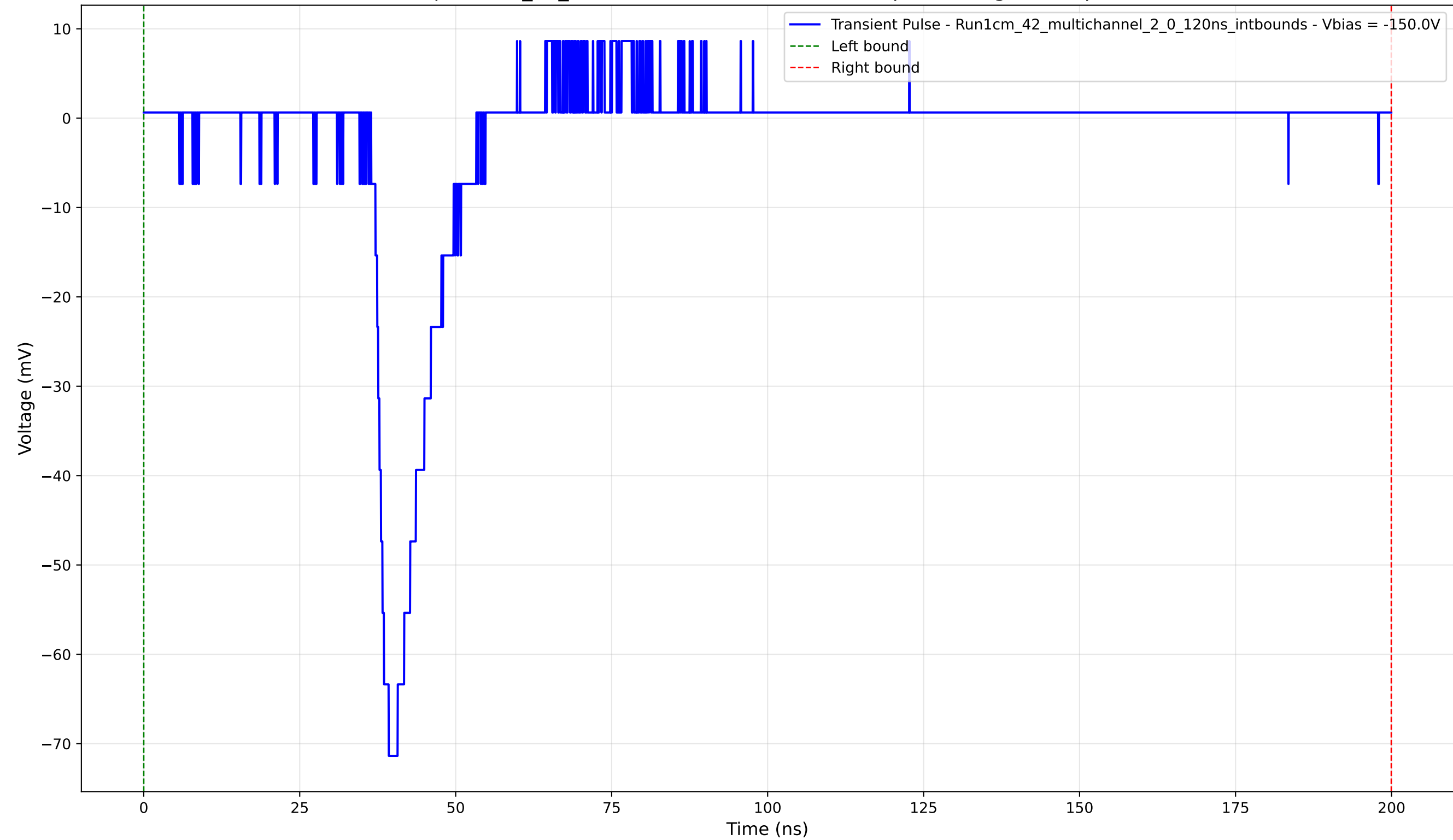
Transient Pulse - Sample: 1cm_42_multichannel - Position: 4615.0 \mu\text{m} - Charge: 7.61 pC - Rise Time: 2.80 ns
