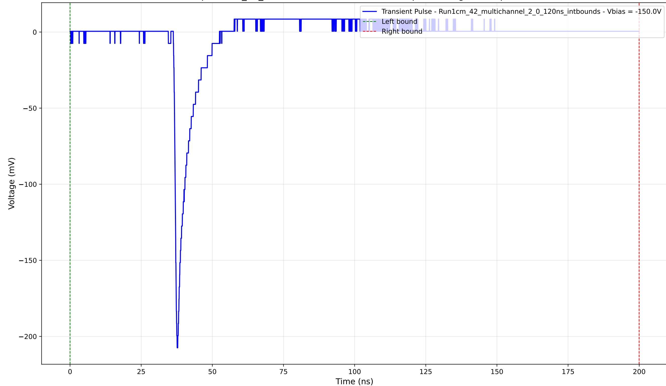
Transient Pulse - Sample: 1cm_42_multichannel - Position: 3130.0 \mu\text{m} - Charge: 9.06 pC - Rise Time: 0.97 ns
