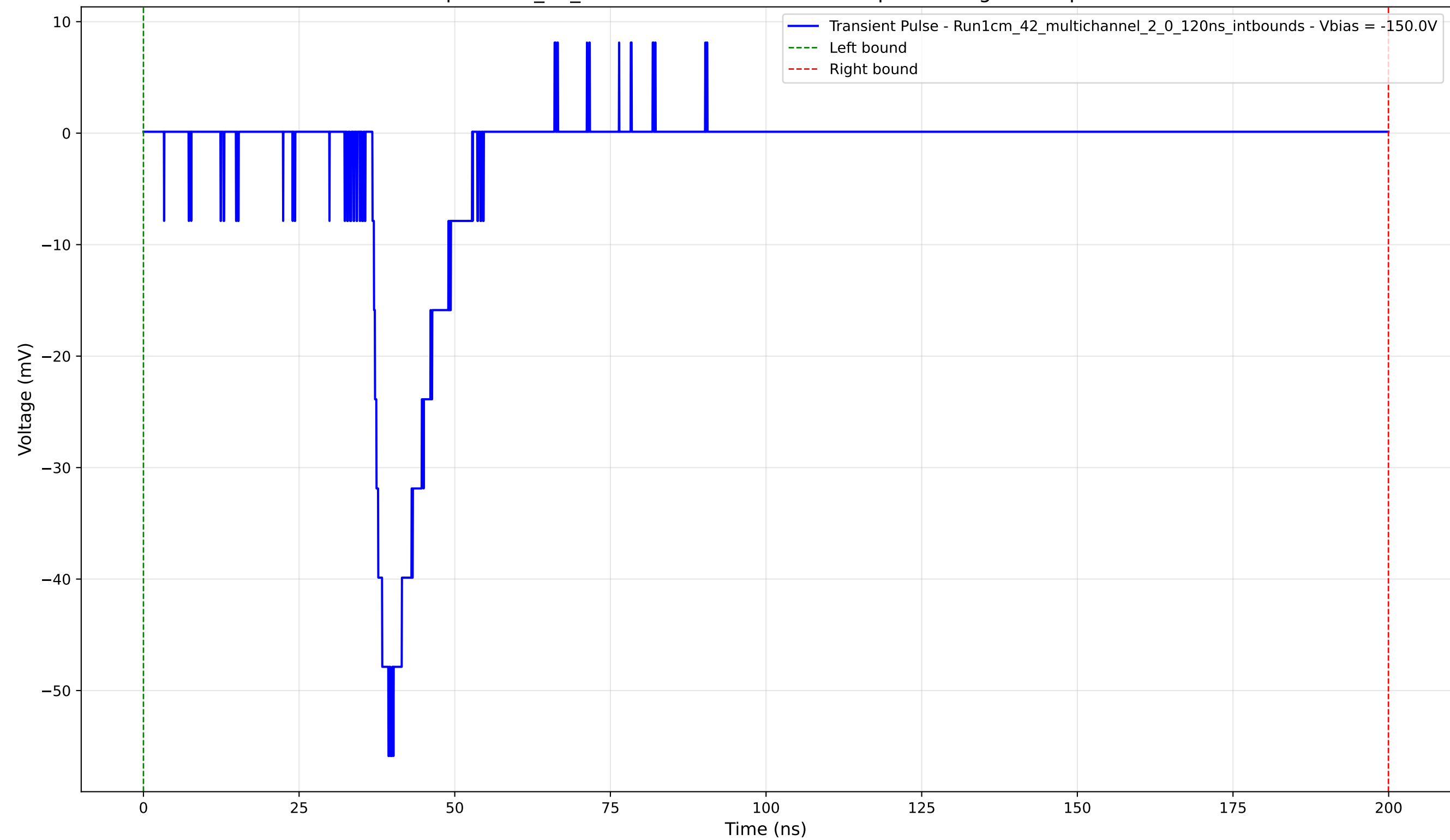
Transient Pulse - Sample: 1cm_42_multichannel - Position: 85.0 \mu\text{m} - Charge: 8.29 pC - Rise Time: 2.57 ns
