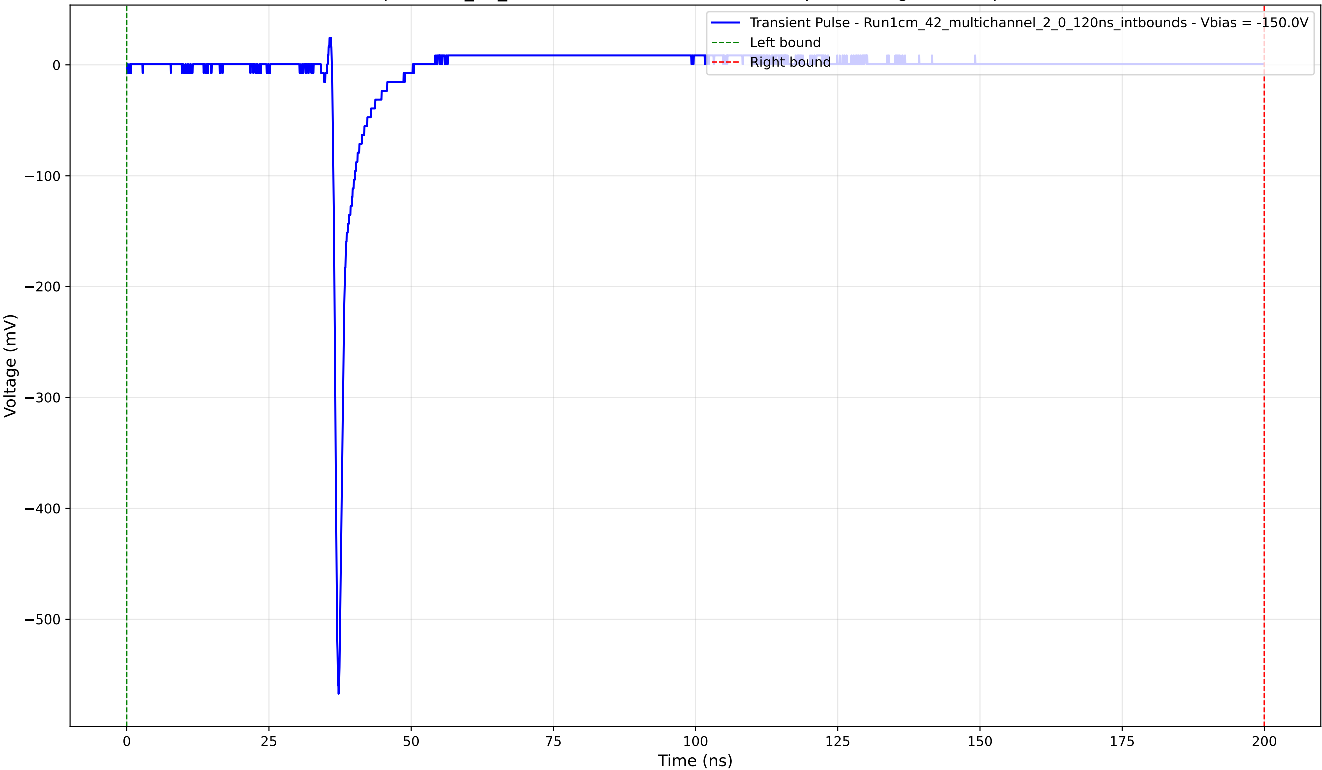
Transient Pulse - Sample: 1cm_42_multichannel - Position: 2515.0 \mu\text{m} - Charge: 15.51 pC - Rise Time: 0.71 ns
