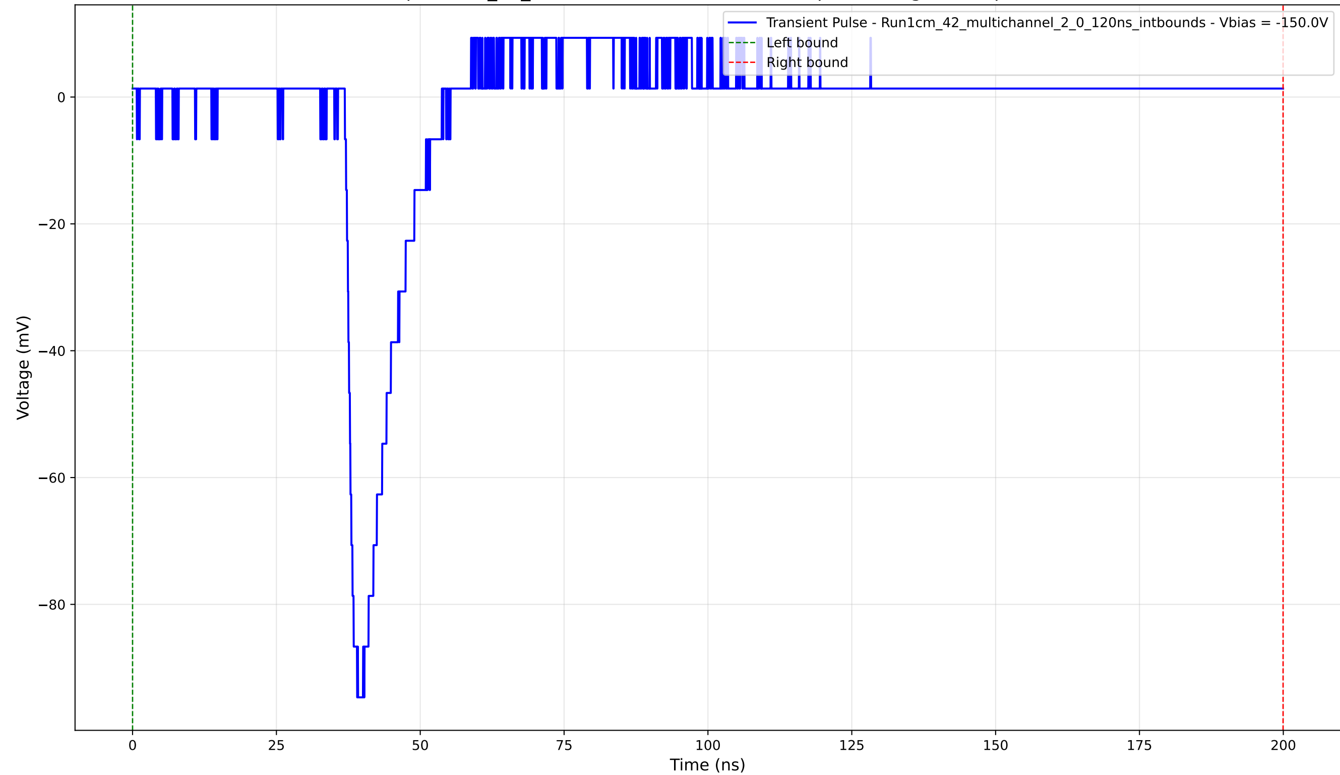
Transient Pulse - Sample: 1cm_42_multichannel - Position: 550.0 \mu\text{m} - Charge: 5.23 pC - Rise Time: 1.35 ns
