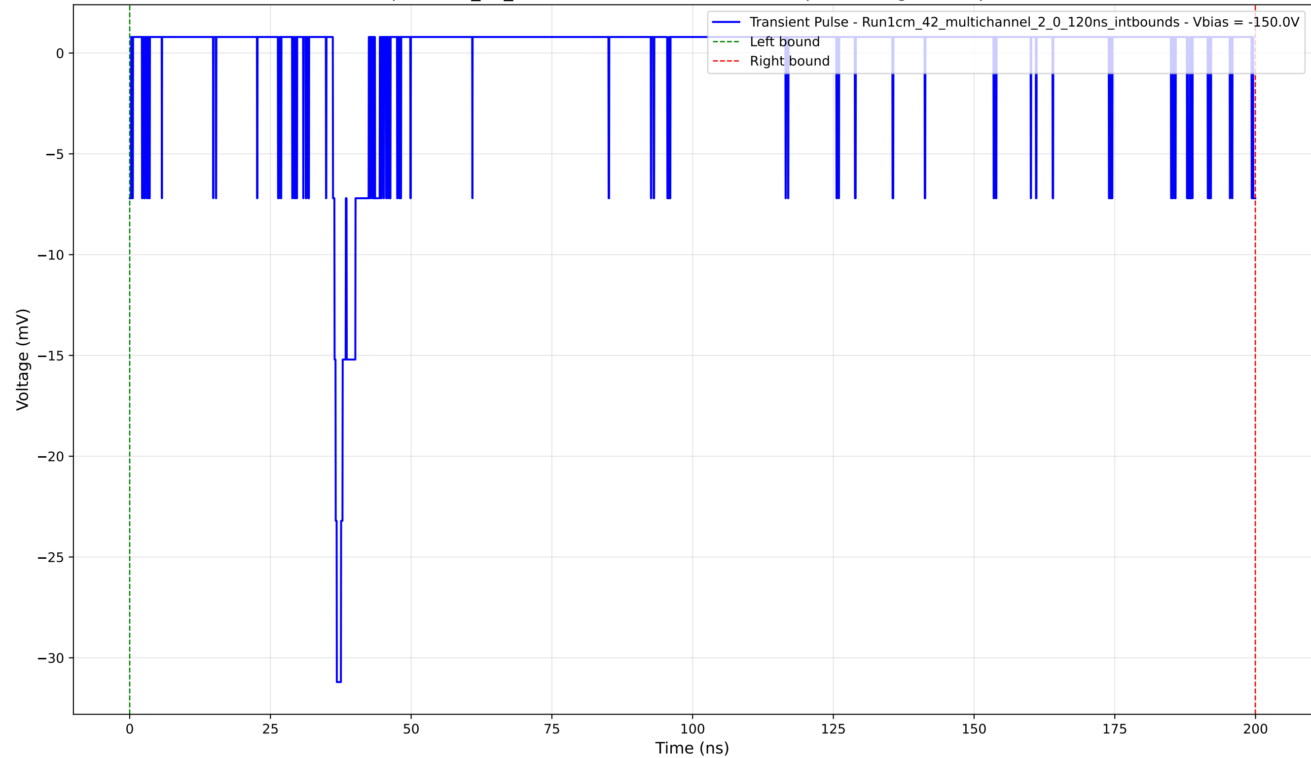
Transient Pulse - Sample: 1cm_42_multichannel - Position: 2385.0 \mu\text{m} - Charge: 0.17 pC - Rise Time: 0.71 ns
