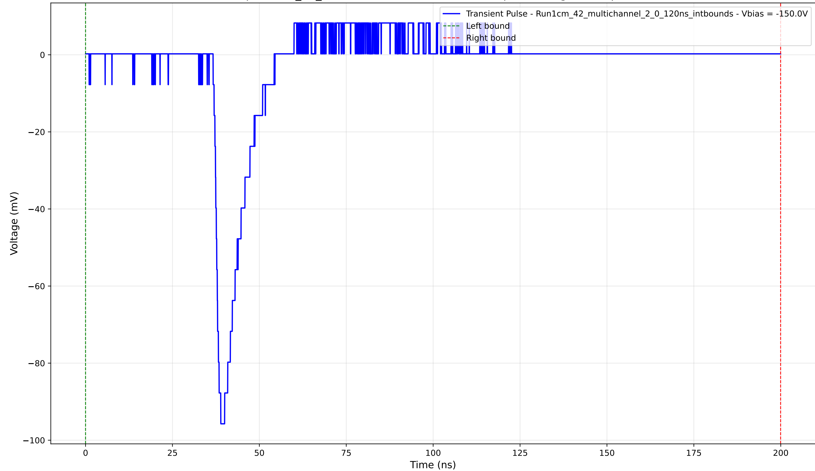
Transient Pulse - Sample: 1cm_42_multichannel - Position: 3985.0 \mu\text{m} - Charge: 9.07 pC - Rise Time: 1.47 ns
