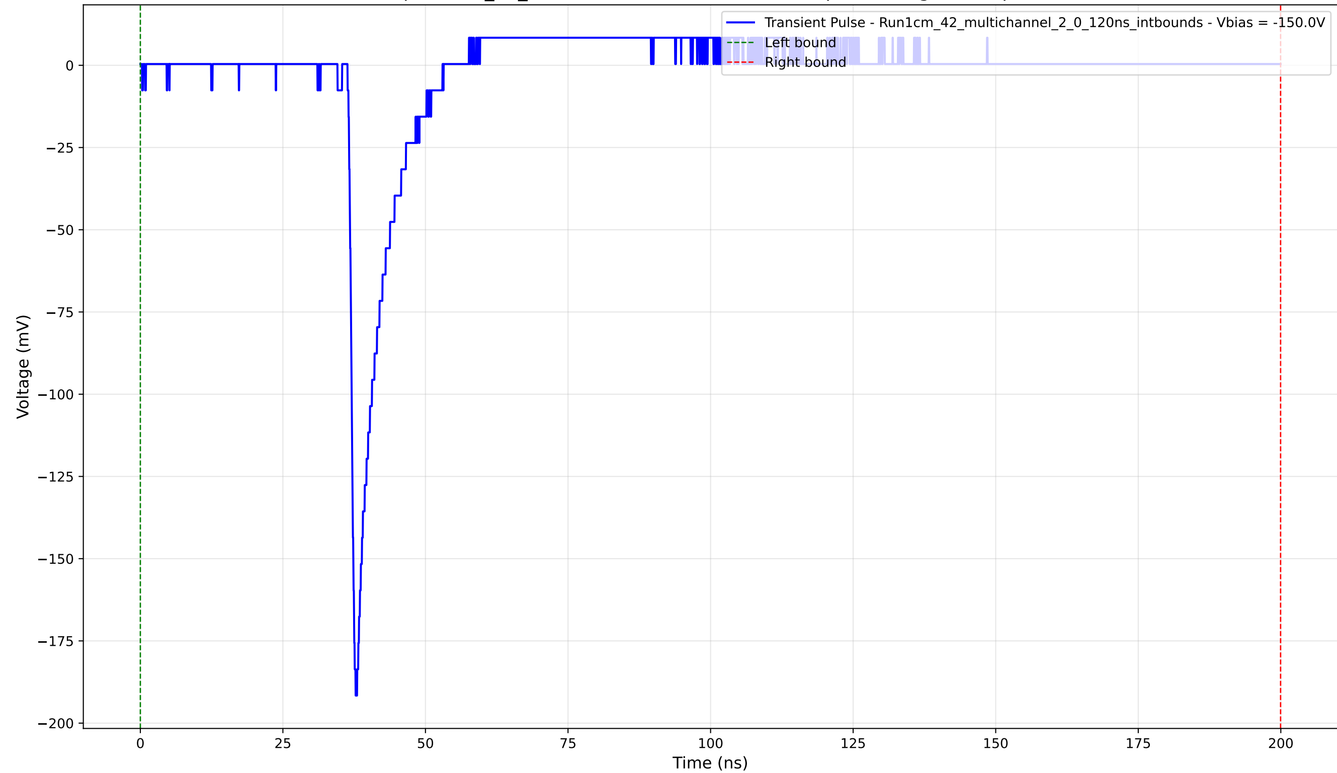
Transient Pulse - Sample: 1cm_42_multichannel - Position: 3235.0 \mu\text{m} - Charge: 9.91 pC - Rise Time: 0.94 ns
