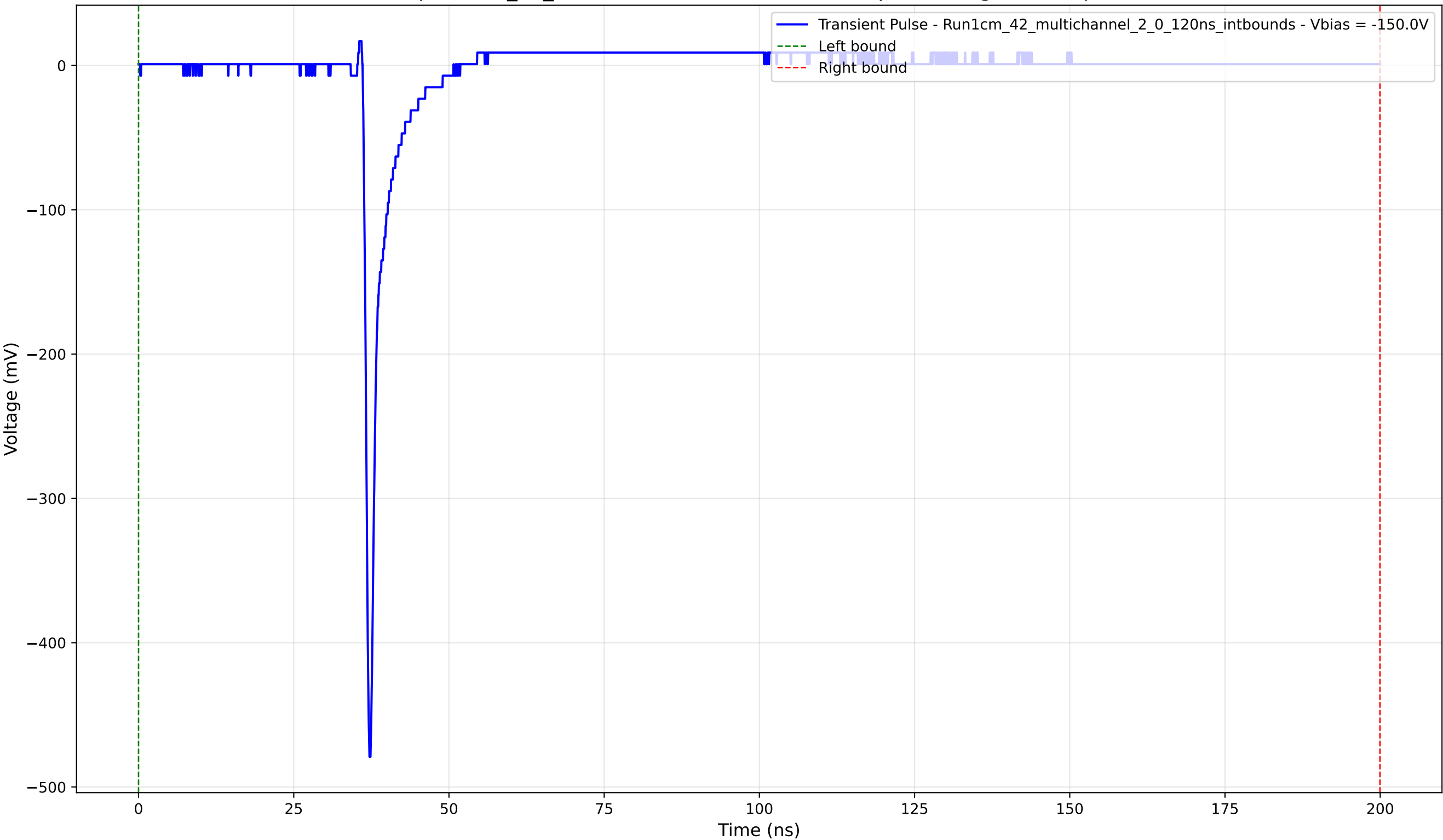
Transient Pulse - Sample: 1cm_42_multichannel - Position: 2605.0 \mu\text{m} - Charge: 11.57 pC - Rise Time: 0.78 ns
