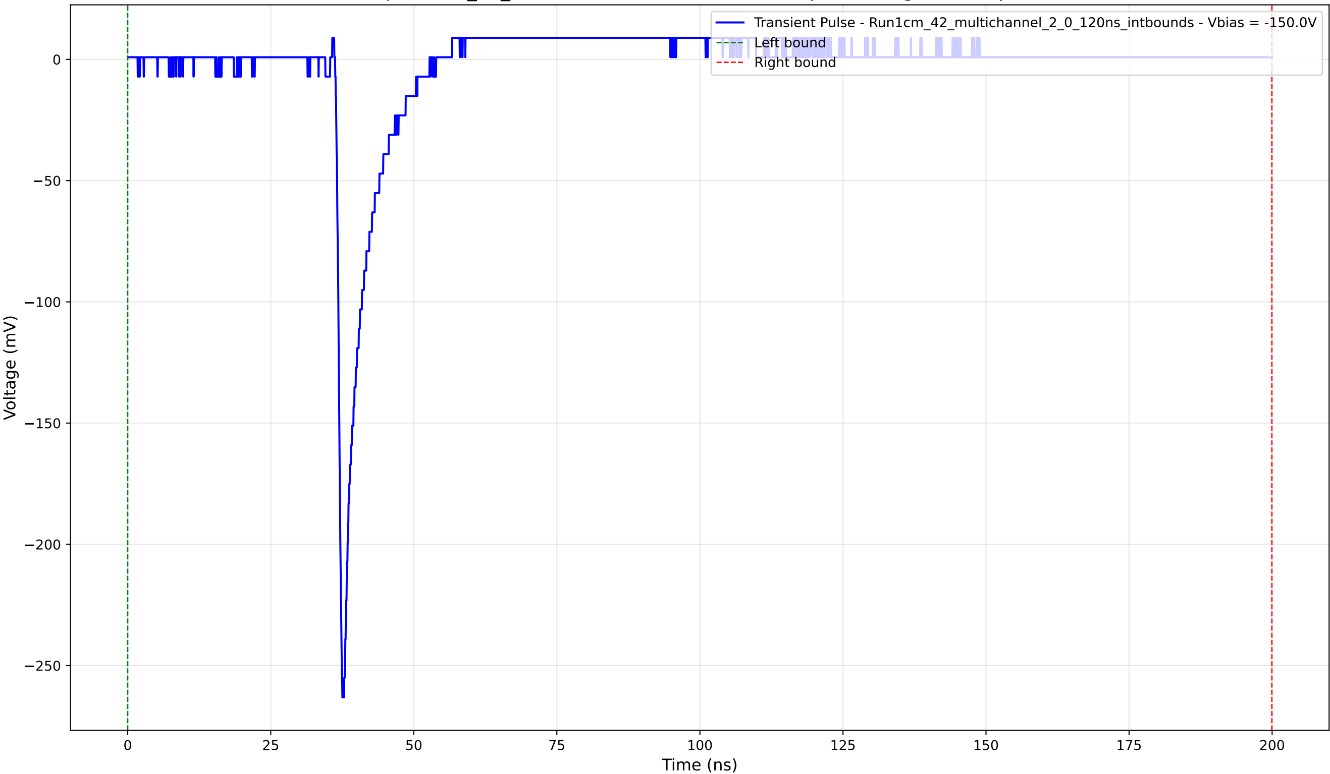
Transient Pulse - Sample: 1cm_42_multichannel - Position: 1675.0 \mu\text{m} - Charge: 10.77 pC - Rise Time: 0.89 ns
