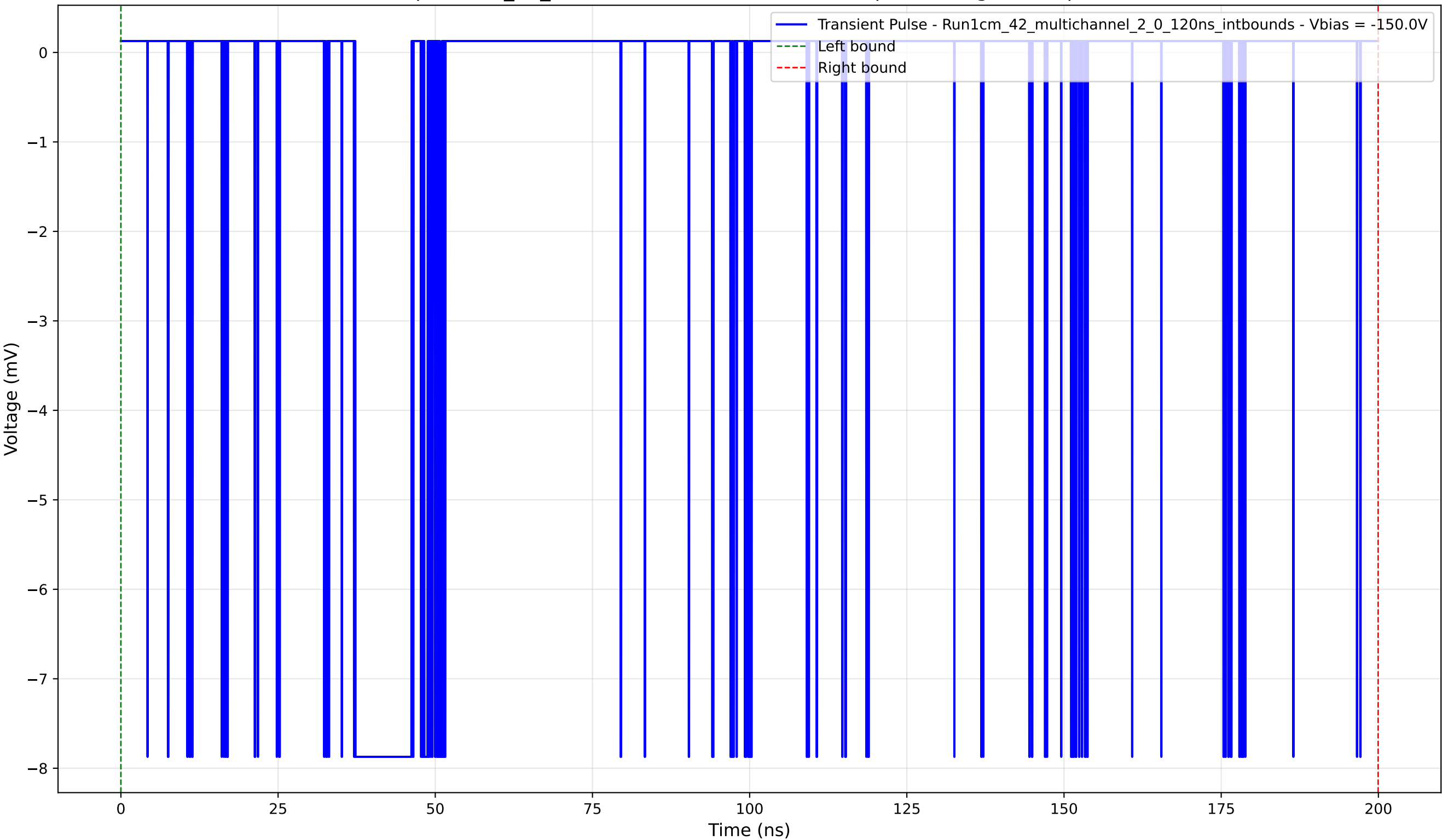
Transient Pulse - Sample: 1cm_42_multichannel - Position: 4875.0 \mu\text{m} - Charge: 2.33 pC - Rise Time: 0.04 ns
