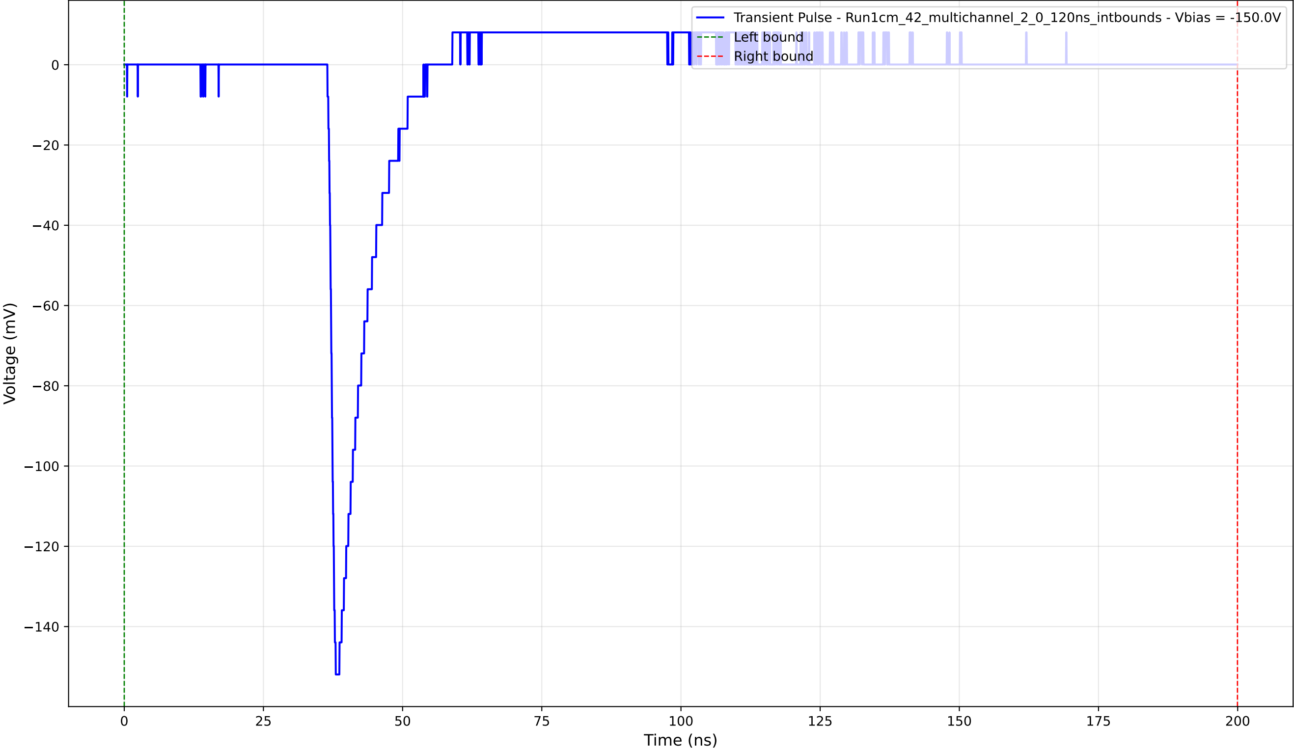
Transient Pulse - Sample: 1cm_42_multichannel - Position: 1220.0 \mu\text{m} - Charge: 10.51 pC - Rise Time: 1.16 ns
