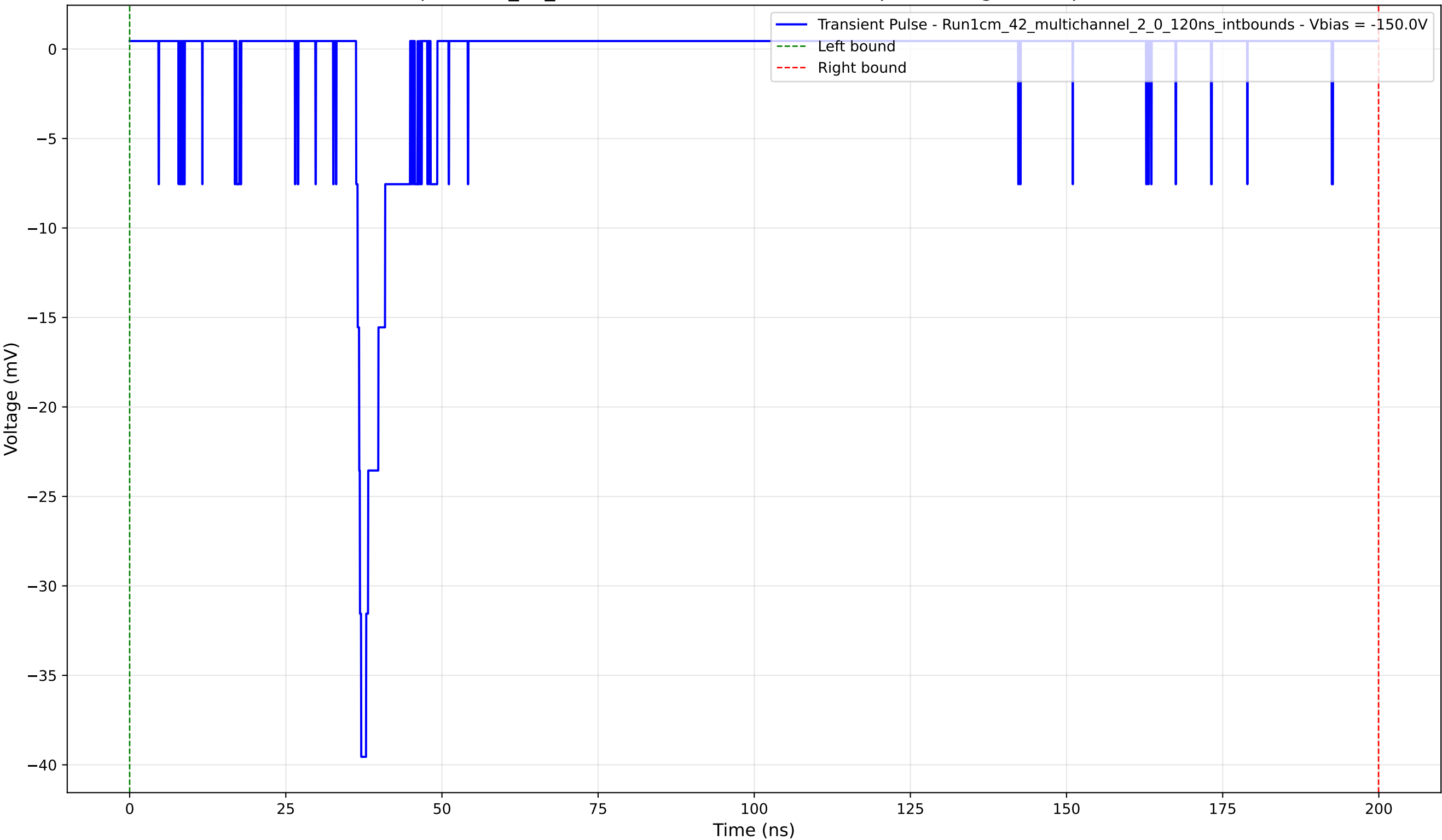
Transient Pulse - Sample: 1cm_42_multichannel - Position: 1890.0 \mu\text{m} - Charge: 1.94 pC - Rise Time: 0.82 ns
