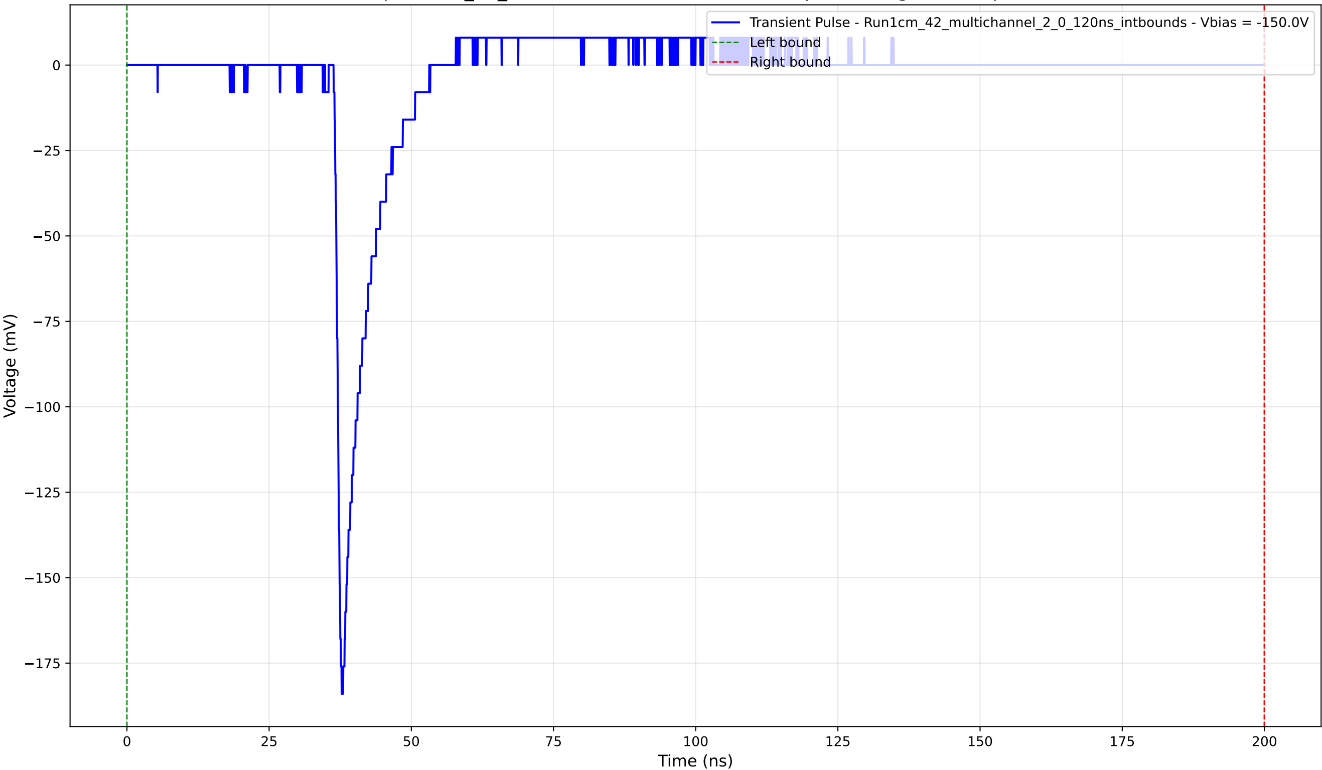
Transient Pulse - Sample: 1cm_42_multichannel - Position: 3260.0 \mu\text{m} - Charge: 11.97 pC - Rise Time: 0.95 ns
