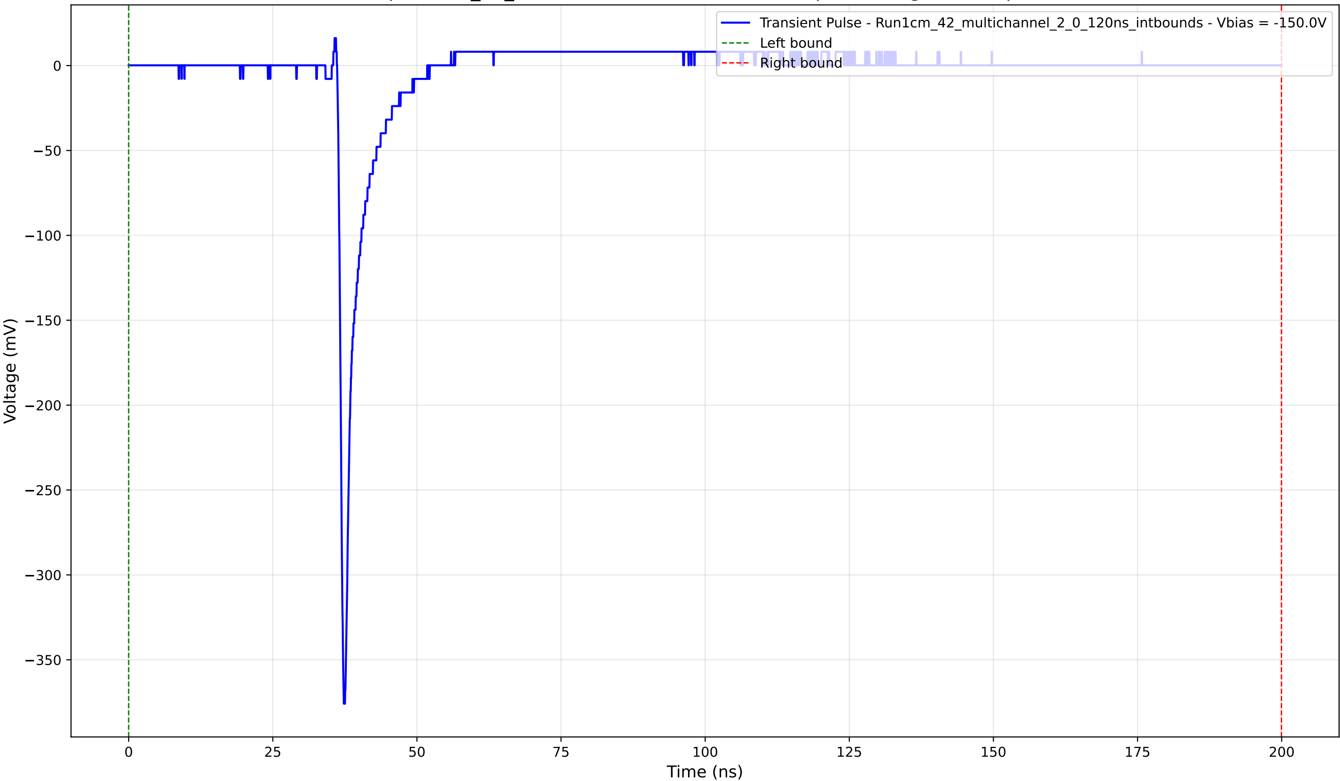
Transient Pulse - Sample: 1cm_42_multichannel - Position: 1955.0 \mu\text{m} - Charge: 13.74 pC - Rise Time: 0.78 ns
