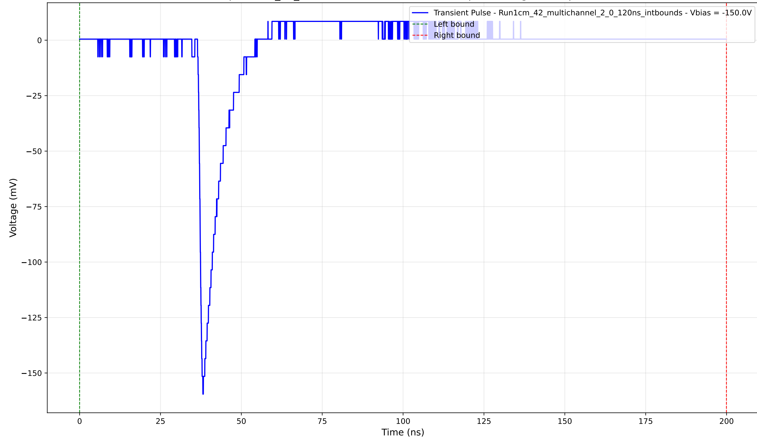
Transient Pulse - Sample: 1cm_42_multichannel - Position: 1255.0 \mu\text{m} - Charge: 9.94 pC - Rise Time: 1.16 ns
