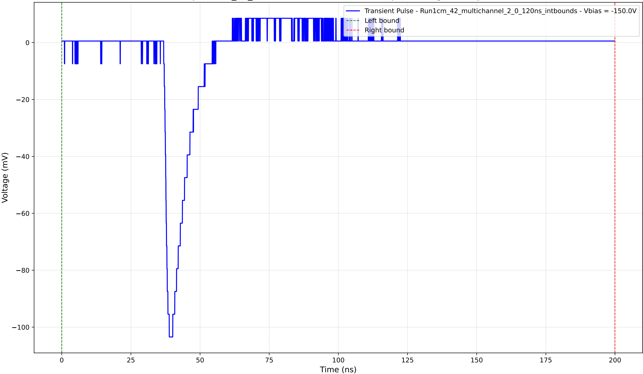
Transient Pulse - Sample: 1cm_42_multichannel - Position: 670.0 \mu\text{m} - Charge: 9.47 pC - Rise Time: 1.35 ns
