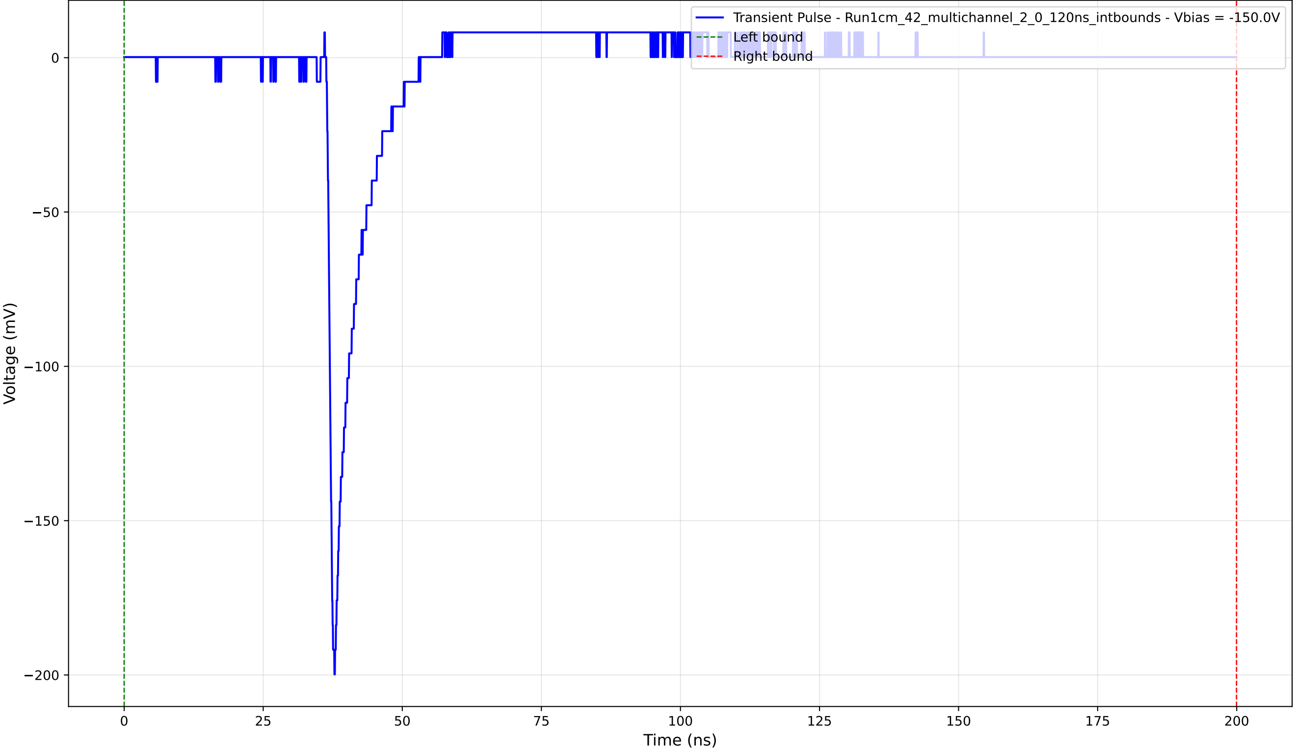
Transient Pulse - Sample: 1cm_42_multichannel - Position: 3185.0 \mu\text{m} - Charge: 10.84 pC - Rise Time: 0.98 ns
