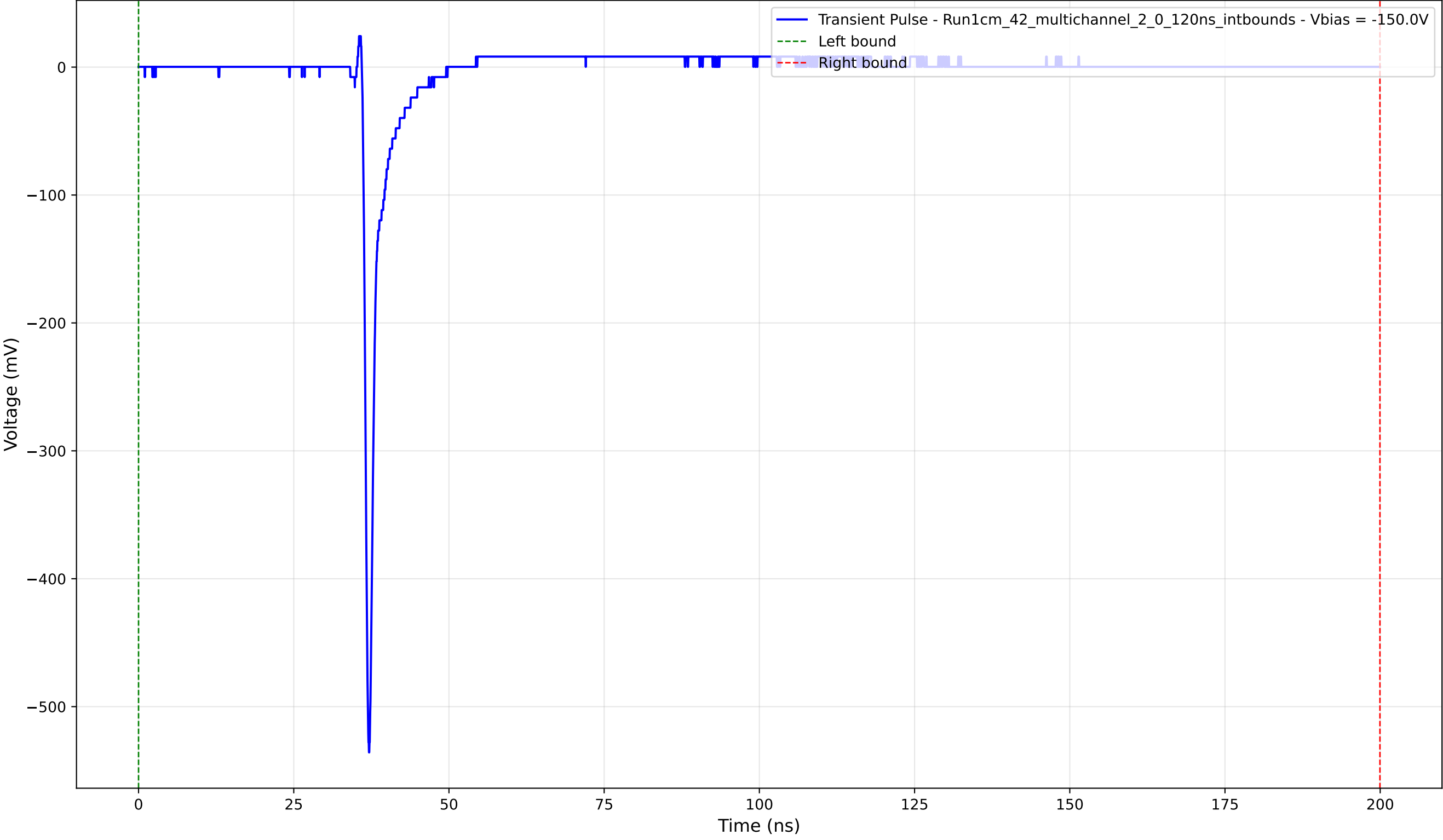
Transient Pulse - Sample: 1cm_42_multichannel - Position: 2435.0 \mu\text{m} - Charge: 13.05 pC - Rise Time: 0.70 ns
