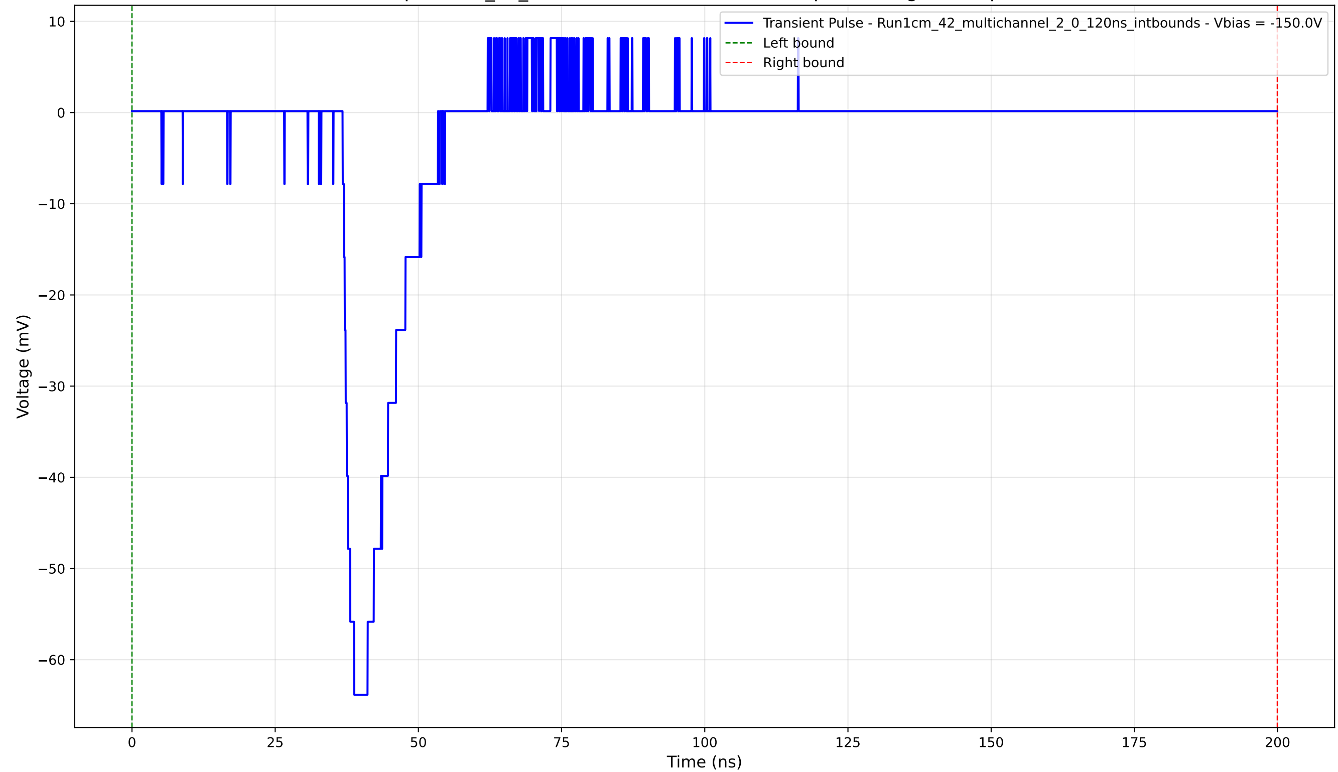
Transient Pulse - Sample: 1cm_42_multichannel - Position: 130.0 \mu\text{m} - Charge: 8.92 pC - Rise Time: 2.01 ns
