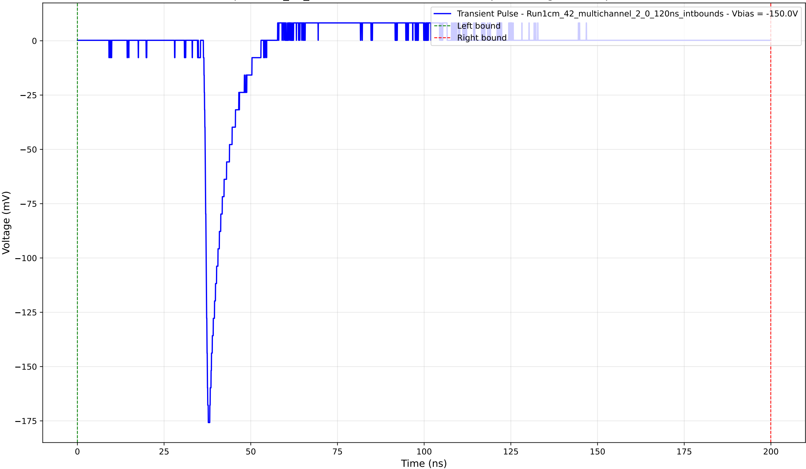
Transient Pulse - Sample: 1cm_42_multichannel - Position: 3275.0 \mu\text{m} - Charge: 10.81 pC - Rise Time: 0.95 ns
