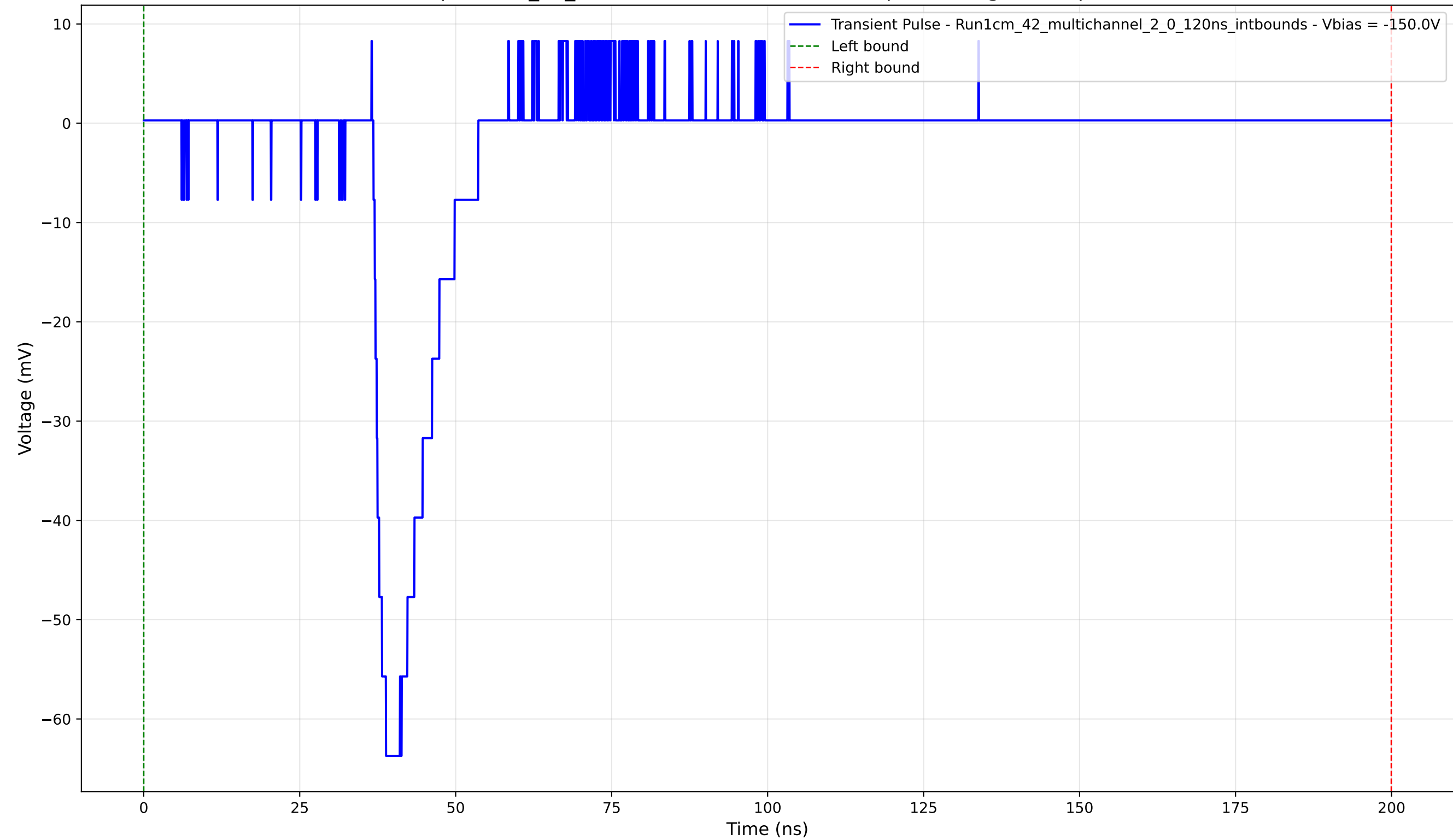
Transient Pulse - Sample: 1cm_42_multichannel - Position: 125.0 \mu\text{m} - Charge: 8.38 pC - Rise Time: 2.01 ns
