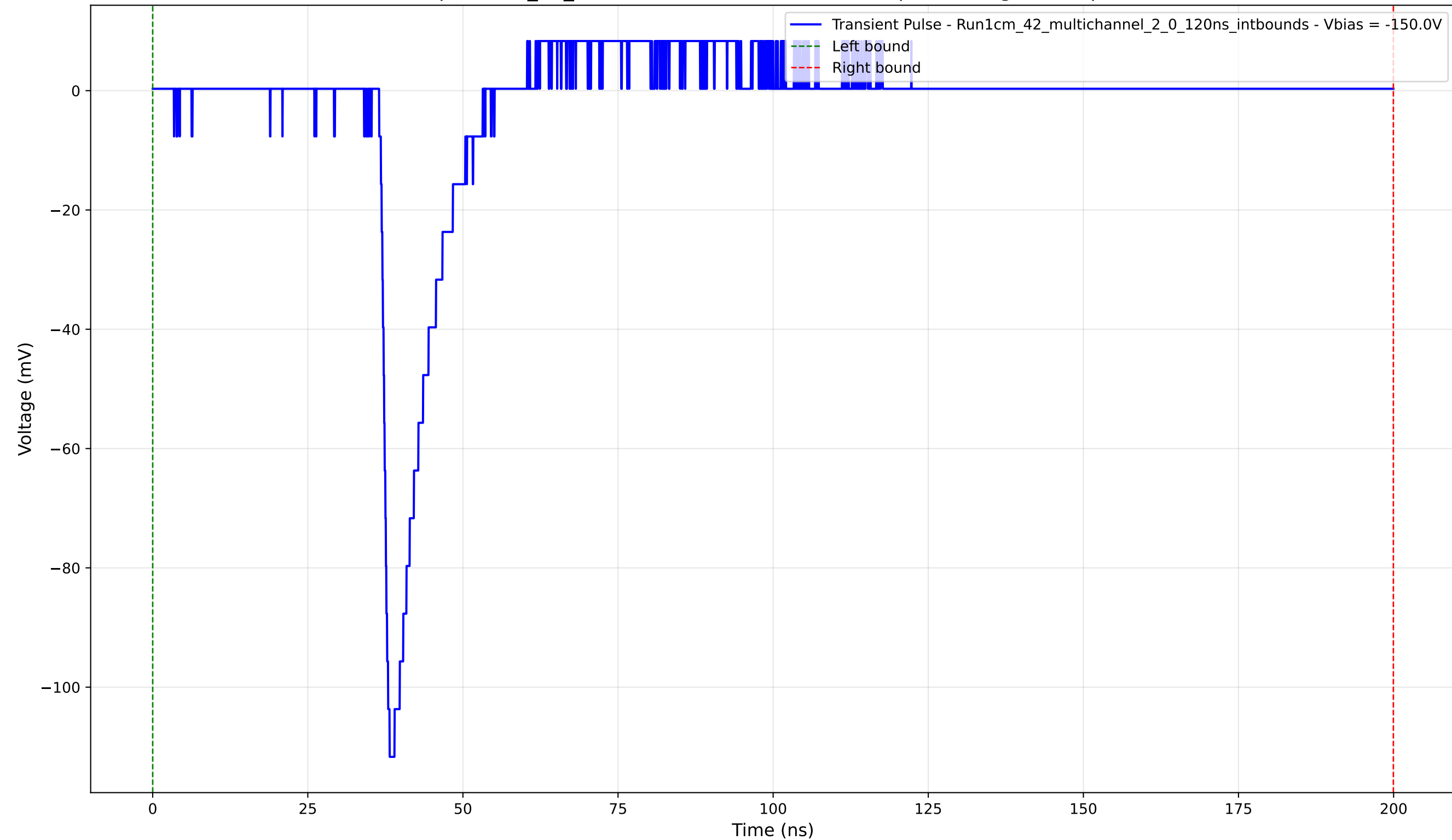
Transient Pulse - Sample: 1cm_42_multichannel - Position: 3640.0 \mu\text{m} - Charge: 8.63 pC - Rise Time: 1.18 ns
