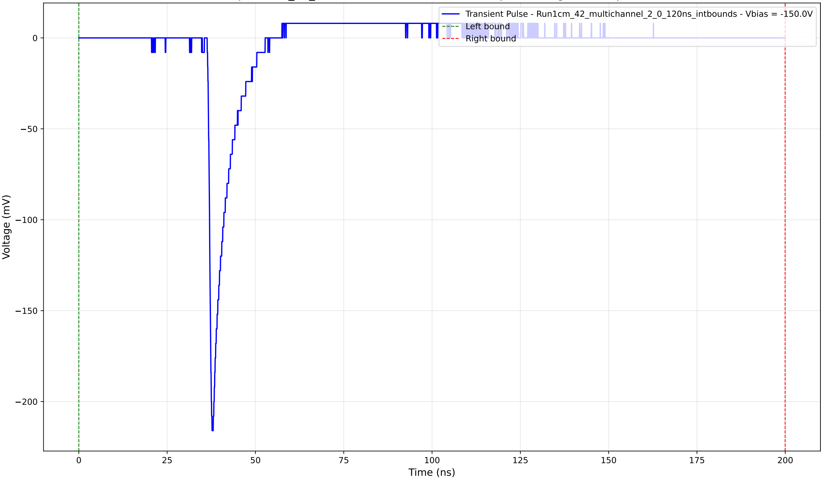
Transient Pulse - Sample: 1cm_42_multichannel - Position: 1510.0 \mu\text{m} - Charge: 12.28 pC - Rise Time: 0.97 ns
