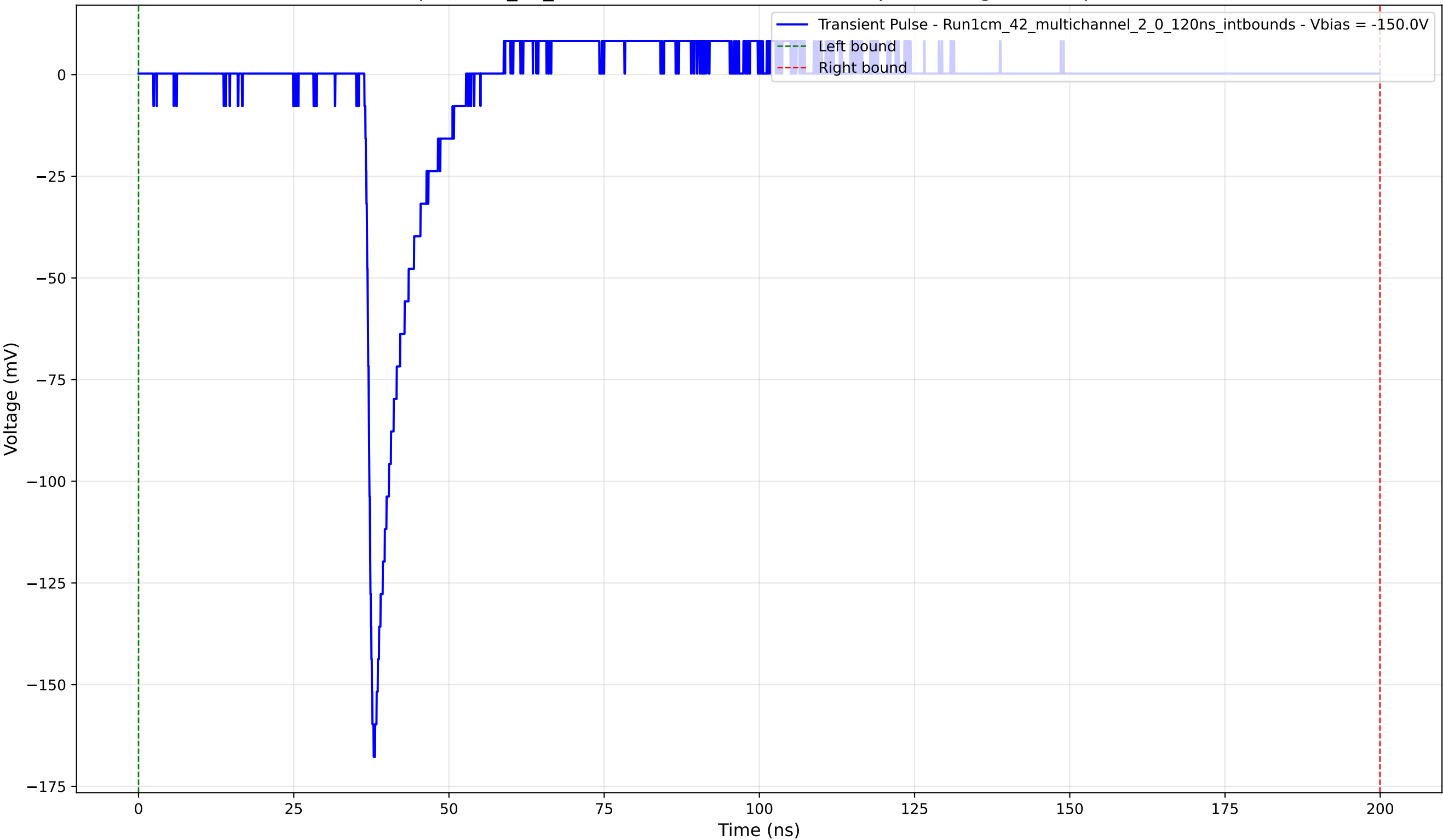
Transient Pulse - Sample: 1cm_42_multichannel - Position: 3295.0 \mu\text{m} - Charge: 10.33 pC - Rise Time: 0.99 ns
