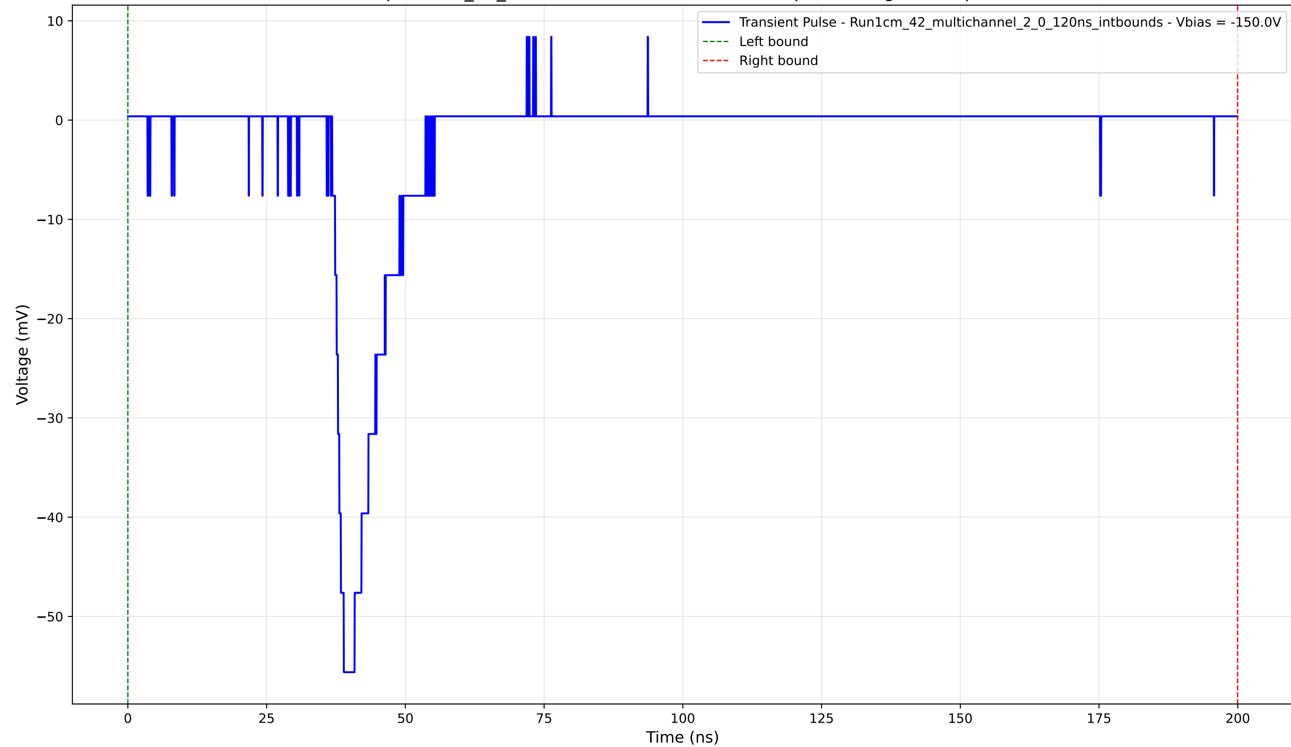
Transient Pulse - Sample: 1cm_42_multichannel - Position: 4325.0 \mu\text{m} - Charge: 7.65 pC - Rise Time: 2.09 ns
