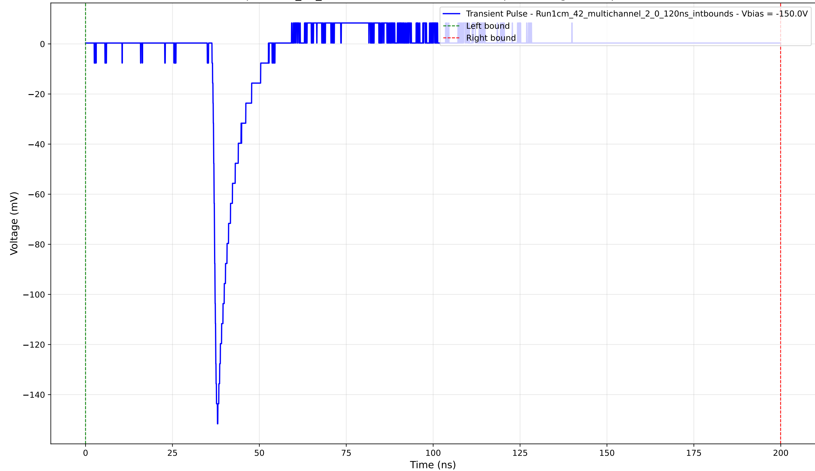
Transient Pulse - Sample: 1cm_42_multichannel - Position: 1420.0 \mu\text{m} - Charge: 9.83 pC - Rise Time: 1.12 ns
