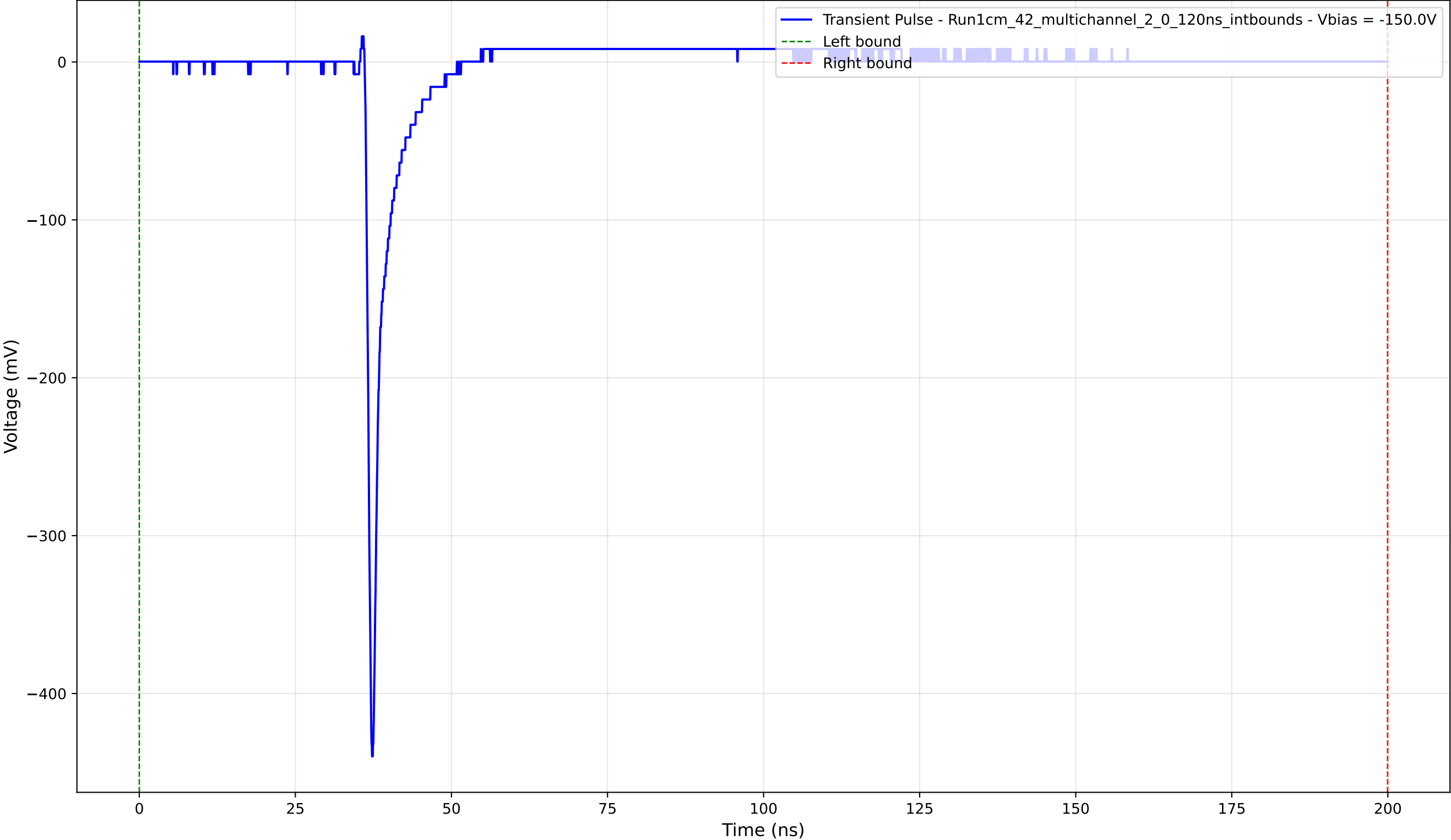
Transient Pulse - Sample: 1cm_42_multichannel - Position: 2680.0 \mu\text{m} - Charge: 13.28 pC - Rise Time: 0.80 ns
