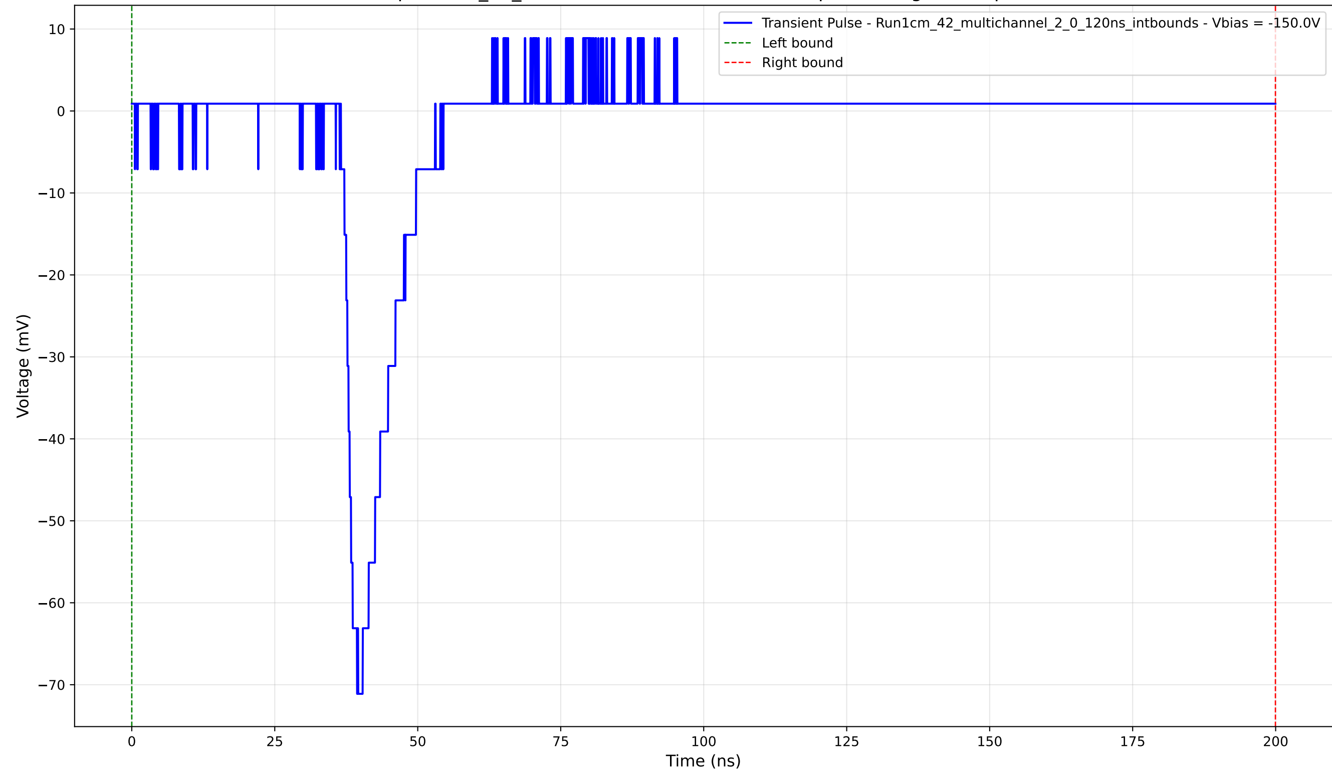
Transient Pulse - Sample: 1cm_42_multichannel - Position: 4480.0 \mu\text{m} - Charge: 6.77 pC - Rise Time: 2.24 ns
