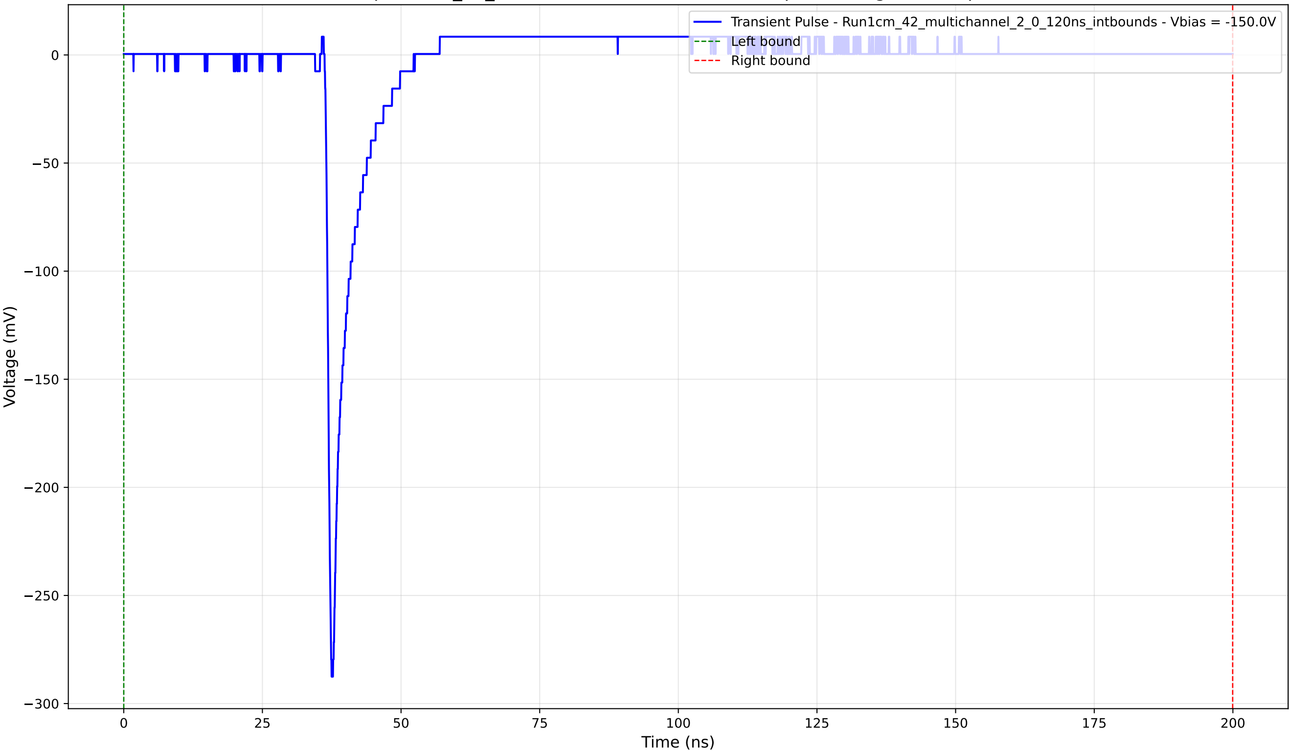
Transient Pulse - Sample: 1cm_42_multichannel - Position: 1735.0 \mu\text{m} - Charge: 11.69 pC - Rise Time: 0.87 ns
