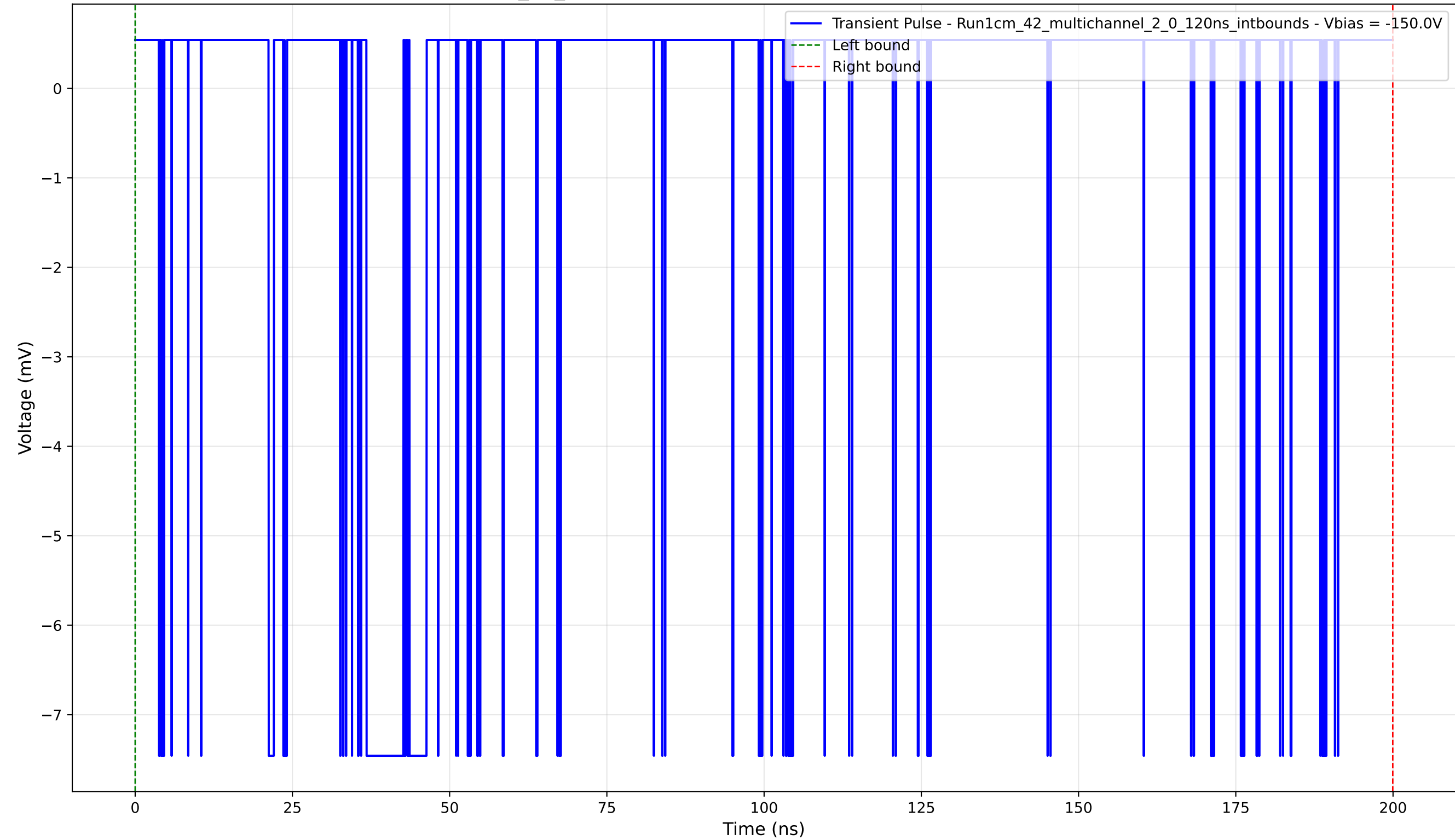
Transient Pulse - Sample: 1cm_42_multichannel - Position: 3390.0 \mu\text{m} - Charge: 0.69 pC - Rise Time: 0.04 ns
