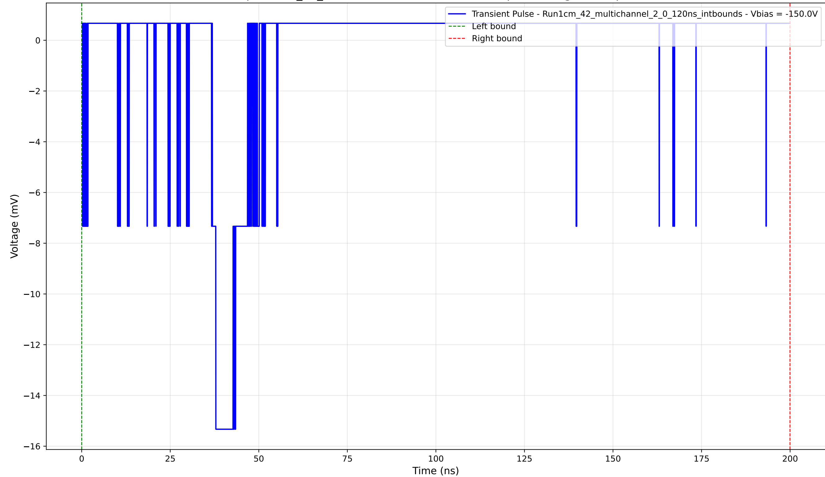
Transient Pulse - Sample: 1cm_42_multichannel - Position: 4860.0 \mu\text{m} - Charge: 0.70 pC - Rise Time: 0.99 ns
