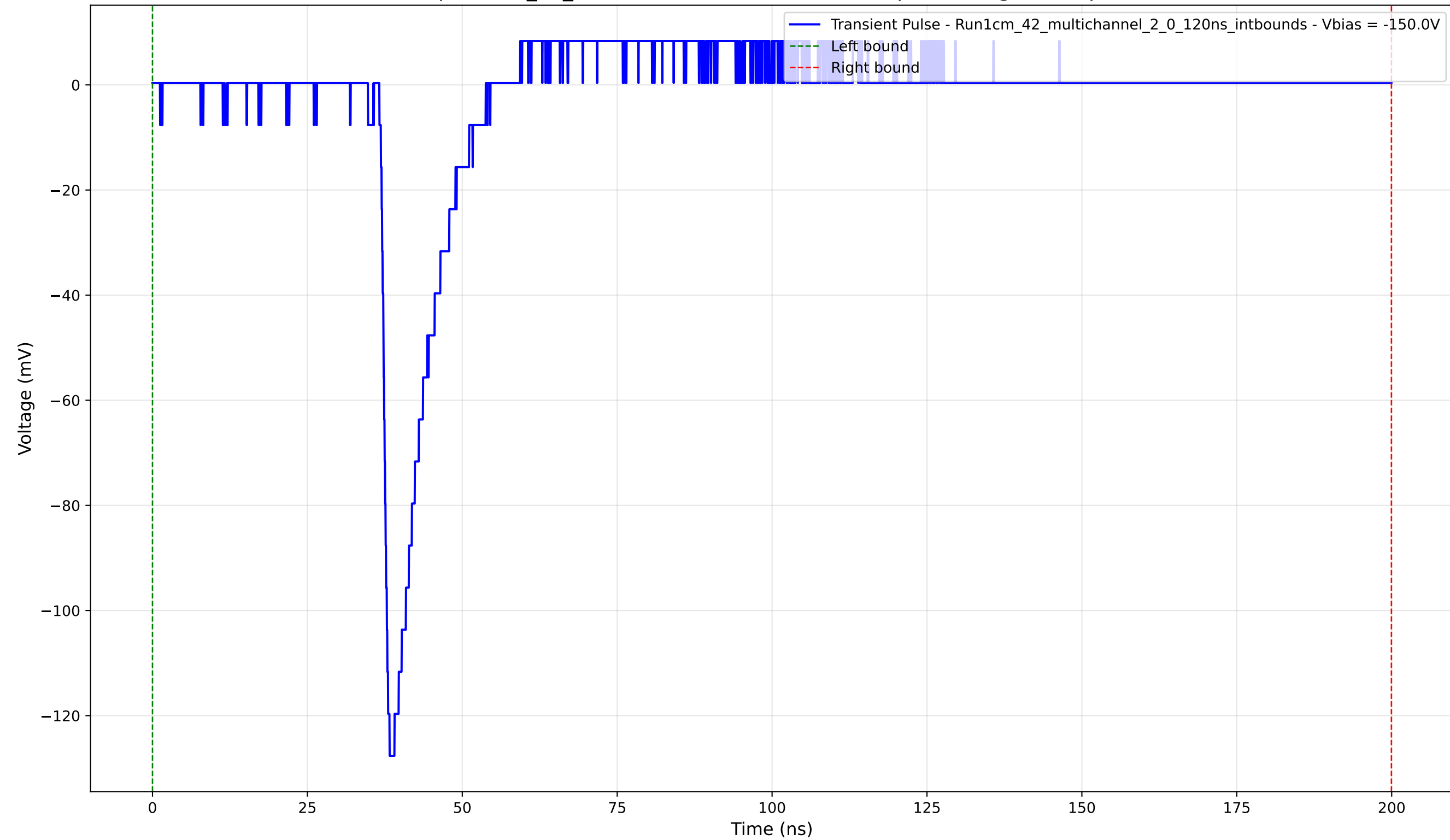
Transient Pulse - Sample: 1cm_42_multichannel - Position: 1025.0 \mu\text{m} - Charge: 9.52 pC - Rise Time: 1.17 ns
