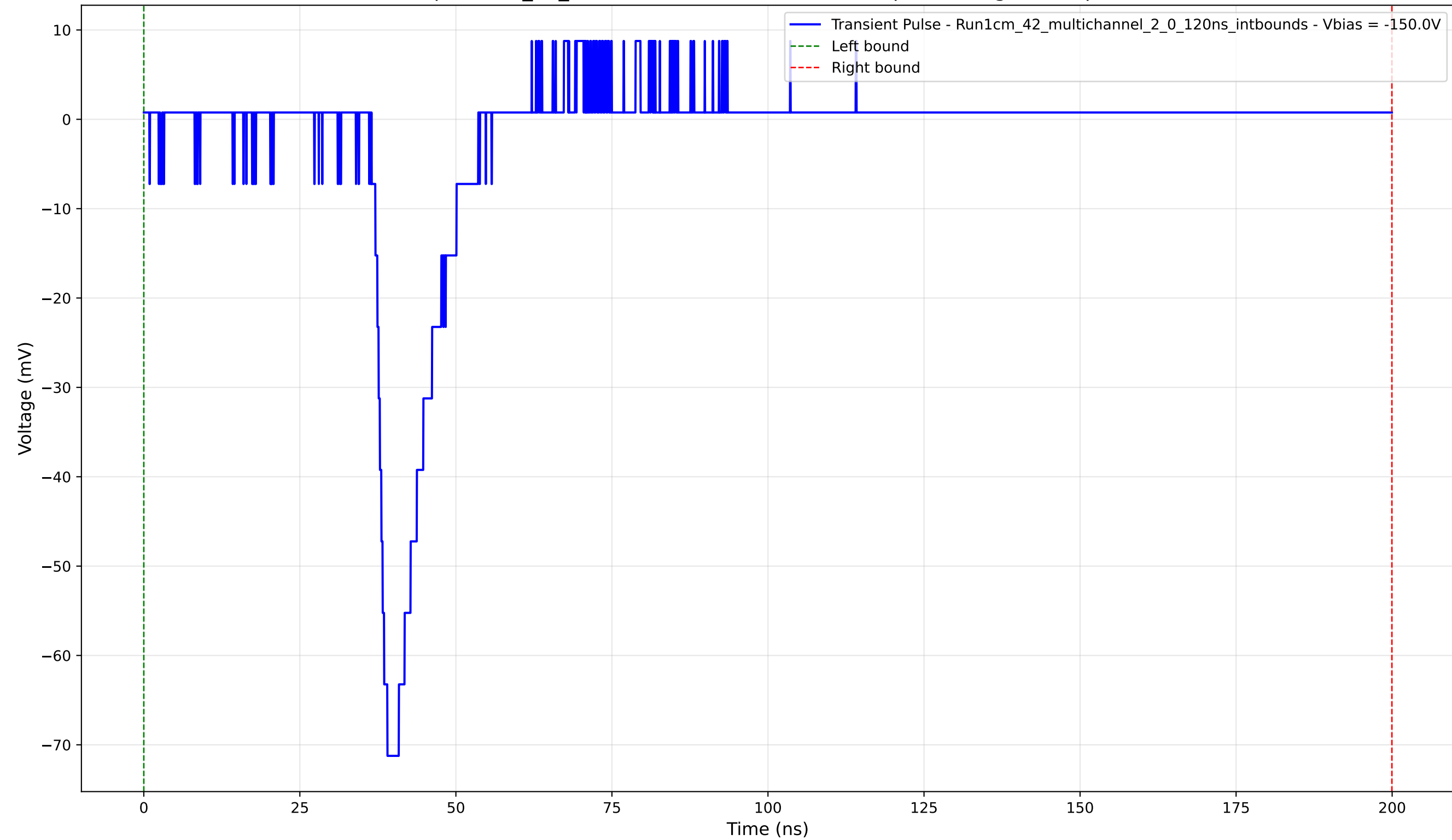
Transient Pulse - Sample: 1cm_42_multichannel - Position: 4575.0 \mu\text{m} - Charge: 7.53 pC - Rise Time: 2.52 ns
