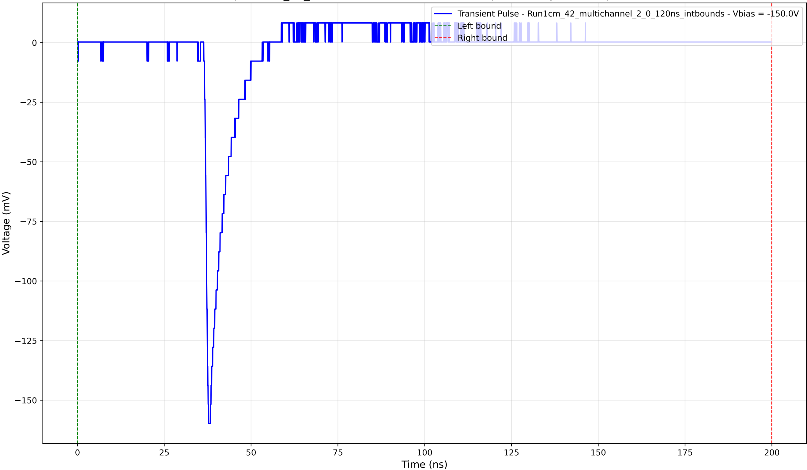
Transient Pulse - Sample: 1cm_42_multichannel - Position: 1425.0 \mu\text{m} - Charge: 10.54 pC - Rise Time: 1.04 ns
