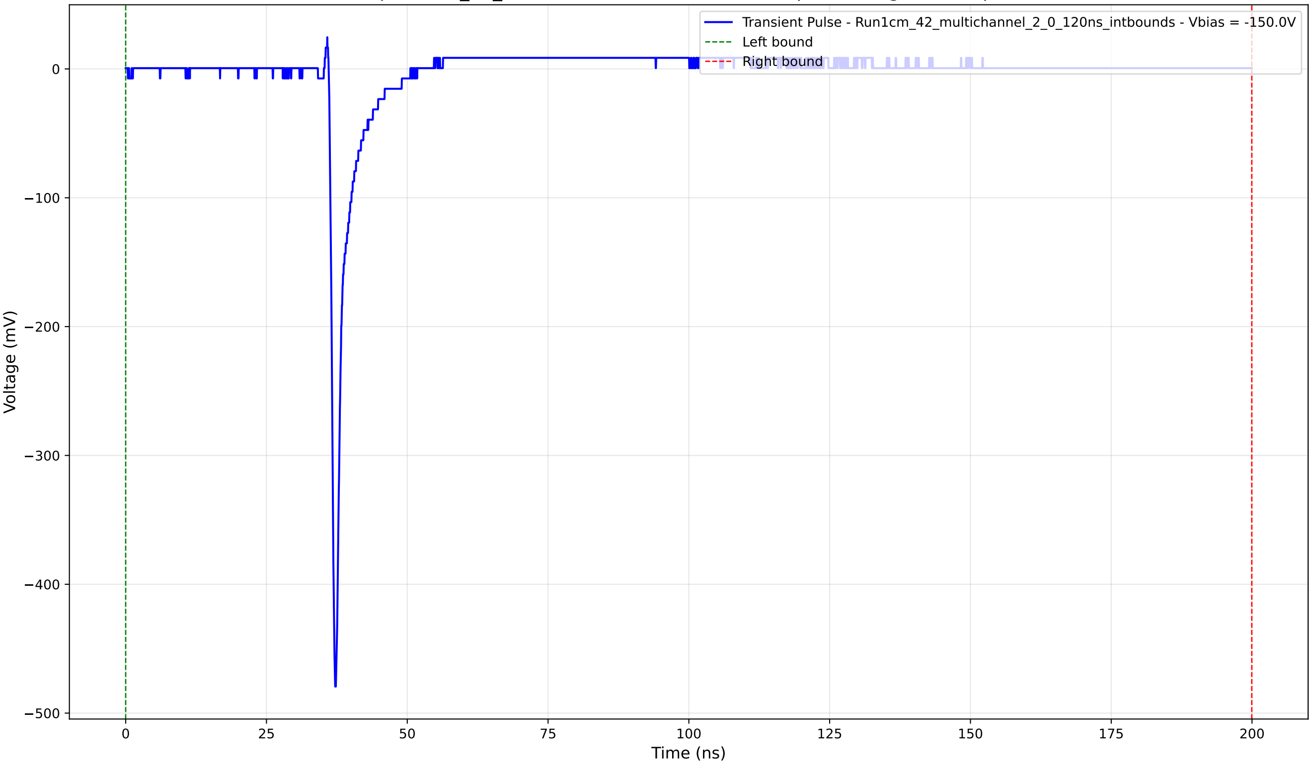
Transient Pulse - Sample: 1cm_42_multichannel - Position: 2600.0 \mu\text{m} - Charge: 12.37 pC - Rise Time: 0.72 ns
