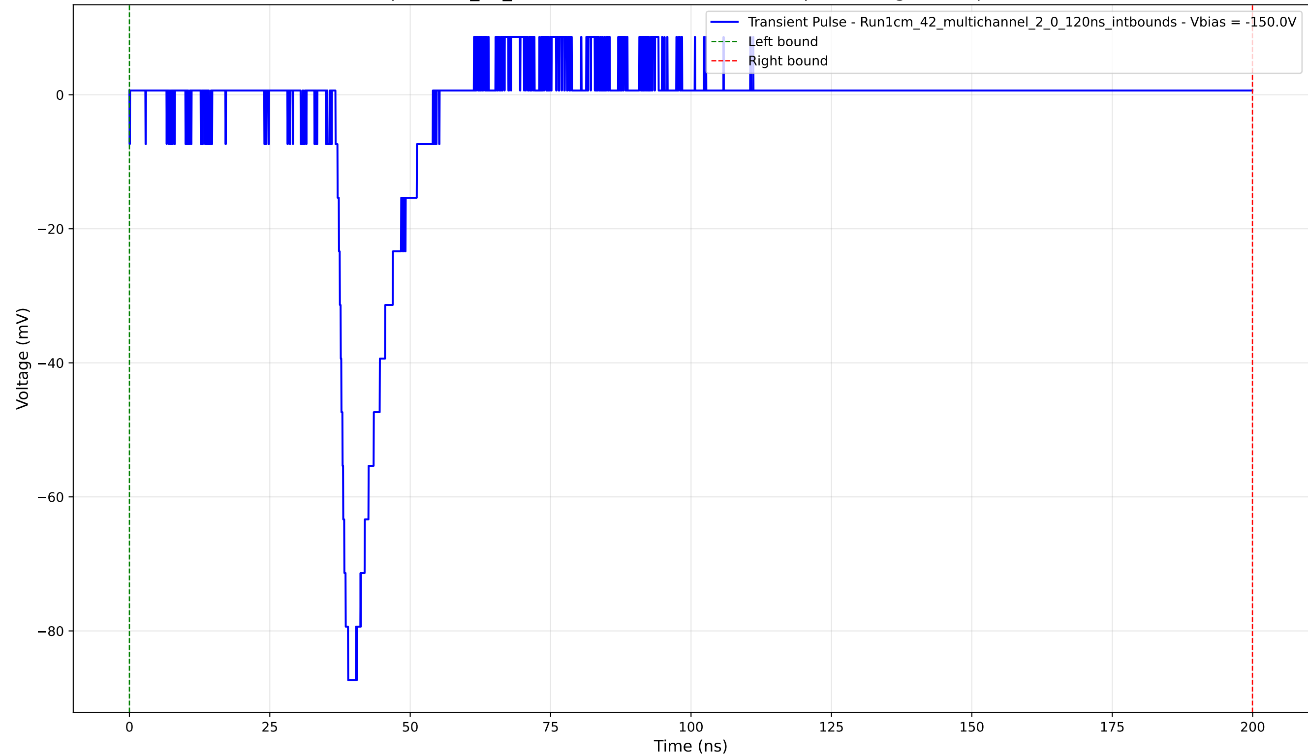
Transient Pulse - Sample: 1cm_42_multichannel - Position: 4095.0 \mu\text{m} - Charge: 8.87 pC - Rise Time: 1.47 ns
