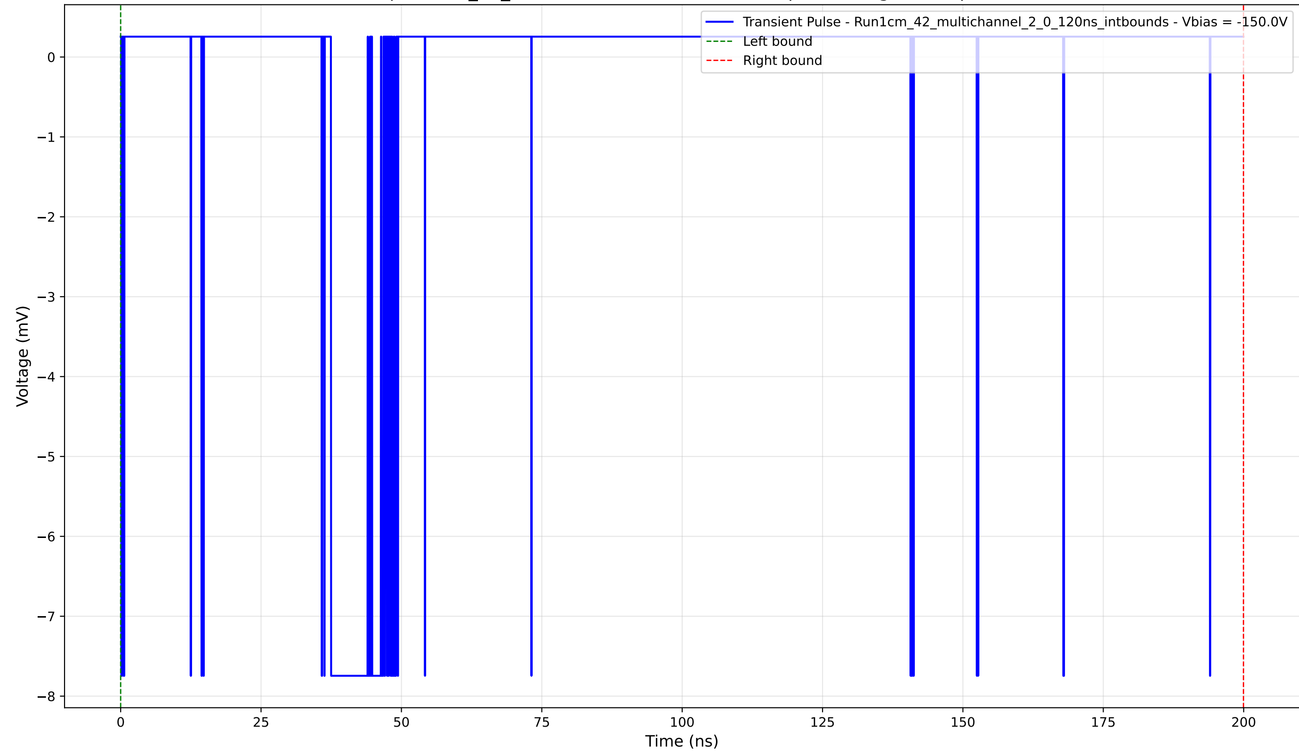
Transient Pulse - Sample: 1cm_42_multichannel - Position: 365.0 \mu\text{m} - Charge: 0.80 pC - Rise Time: 0.04 ns
