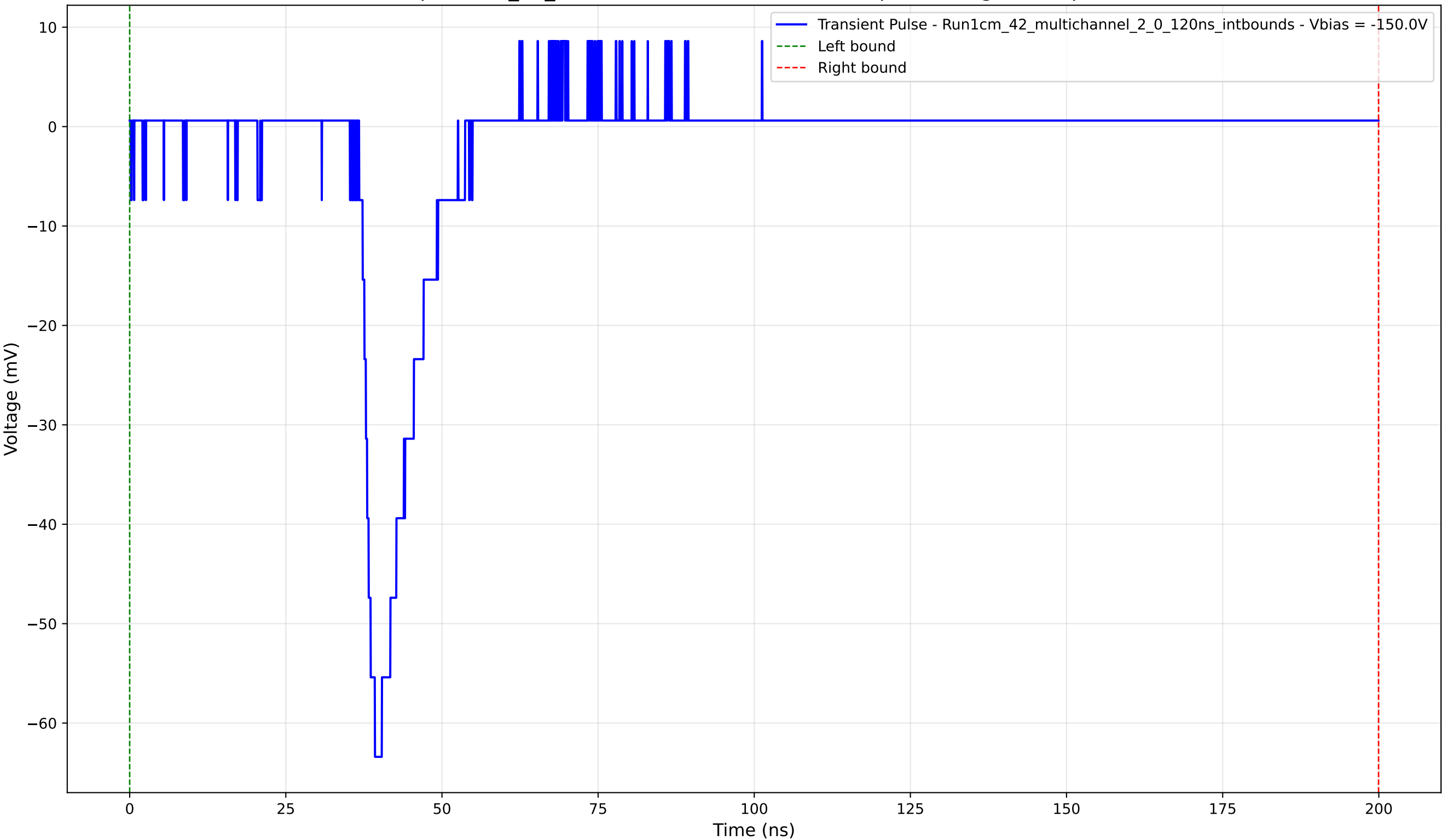
Transient Pulse - Sample: 1cm_42_multichannel - Position: 4460.0 \mu\text{m} - Charge: 7.04 pC - Rise Time: 2.53 ns
