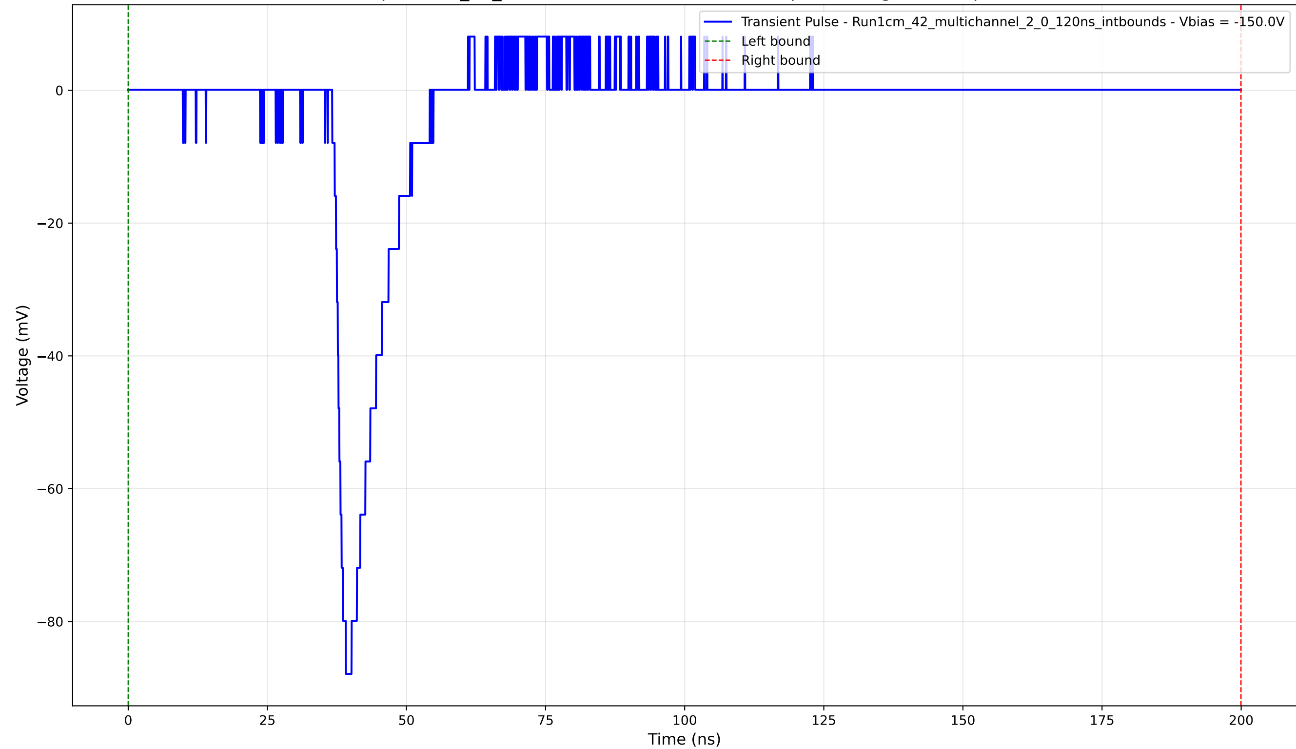
Transient Pulse - Sample: 1cm_42_multichannel - Position: 4135.0 \mu\text{m} - Charge: 10.61 pC - Rise Time: 1.52 ns
