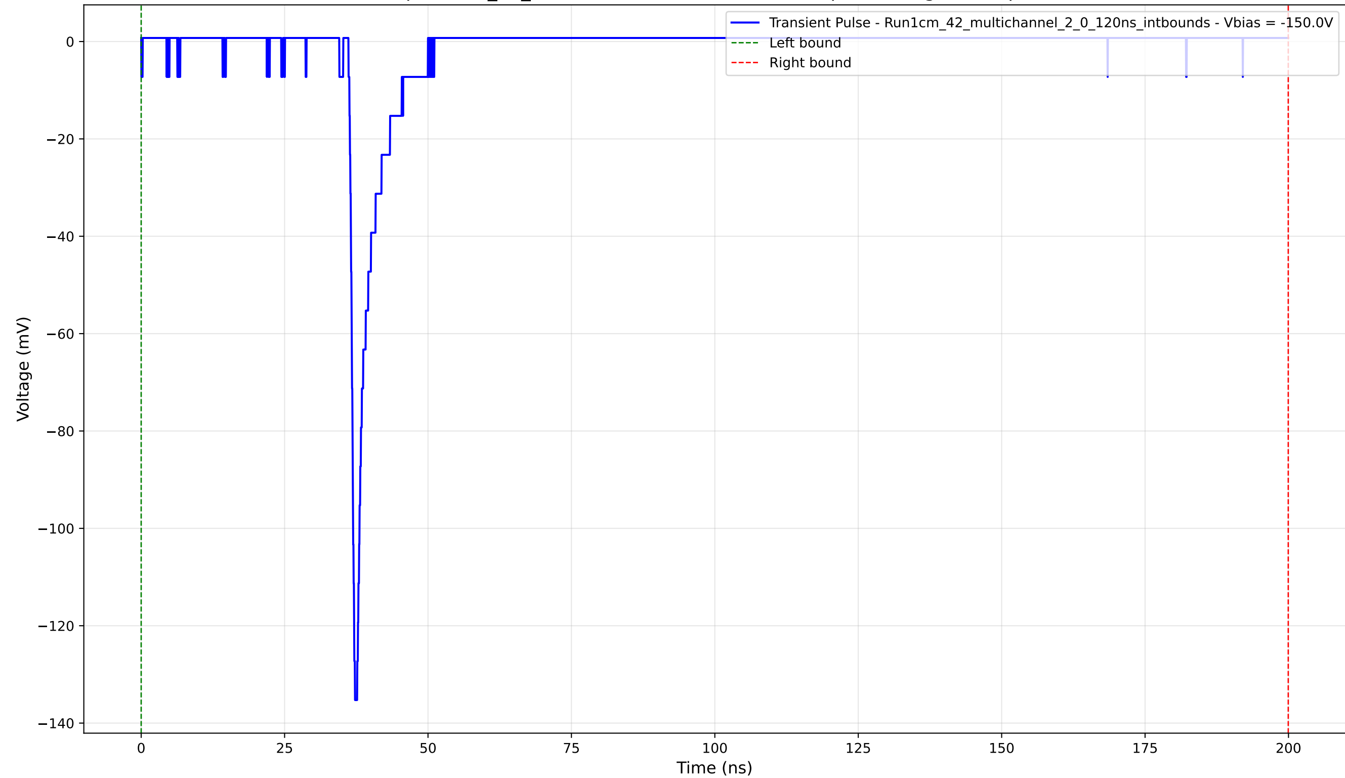
Transient Pulse - Sample: 1cm_42_multichannel - Position: 2830.0 \mu\text{m} - Charge: 7.02 pC - Rise Time: 0.85 ns
