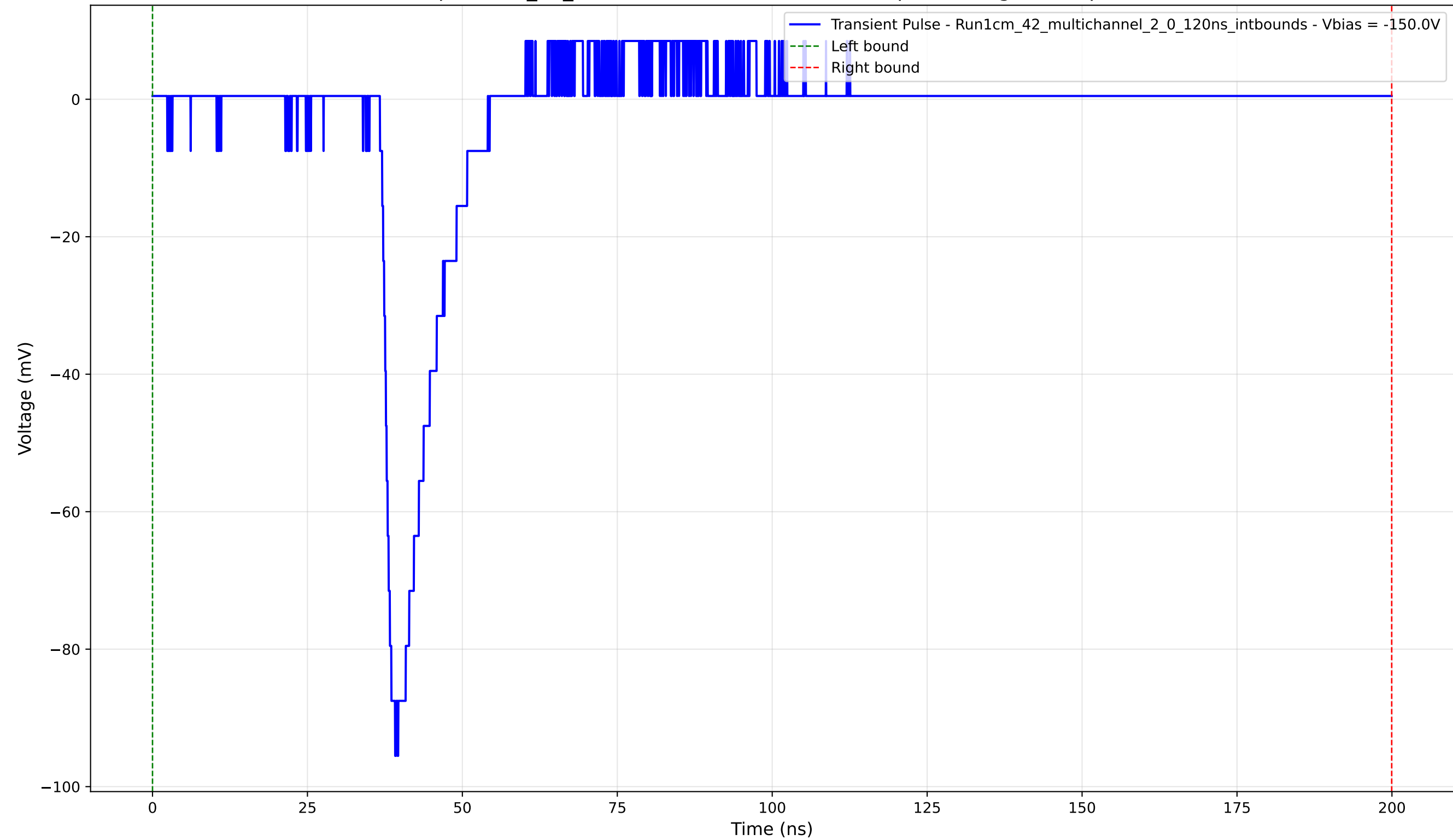
Transient Pulse - Sample: 1cm_42_multichannel - Position: 4020.0 \mu\text{m} - Charge: 9.09 pC - Rise Time: 1.51 ns
