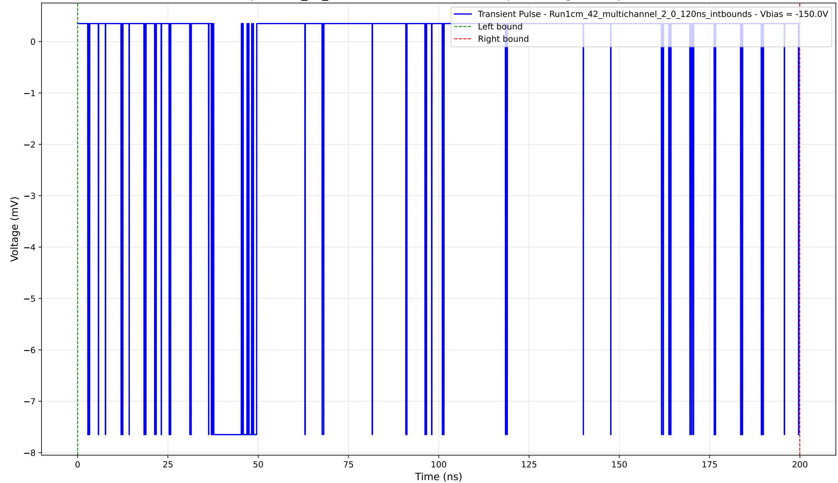
Transient Pulse - Sample: 1cm_42_multichannel - Position: 360.0 \mu\text{m} - Charge: 1.14 pC - Rise Time: 0.04 ns
