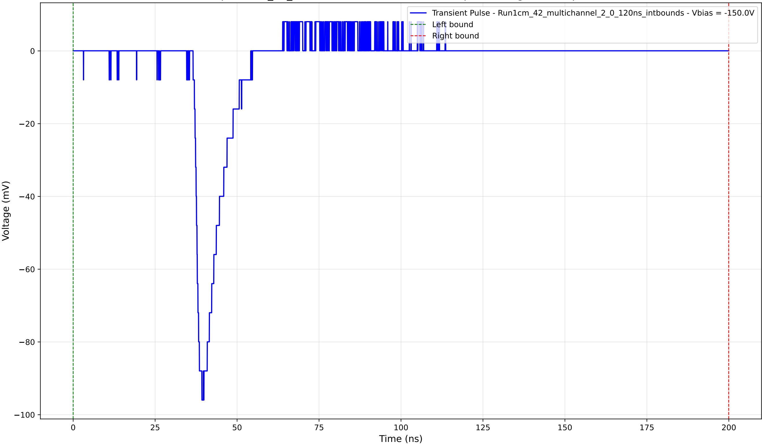
Transient Pulse - Sample: 1cm_42_multichannel - Position: 3980.0 \mu\text{m} - Charge: 11.42 pC - Rise Time: 1.55 ns
