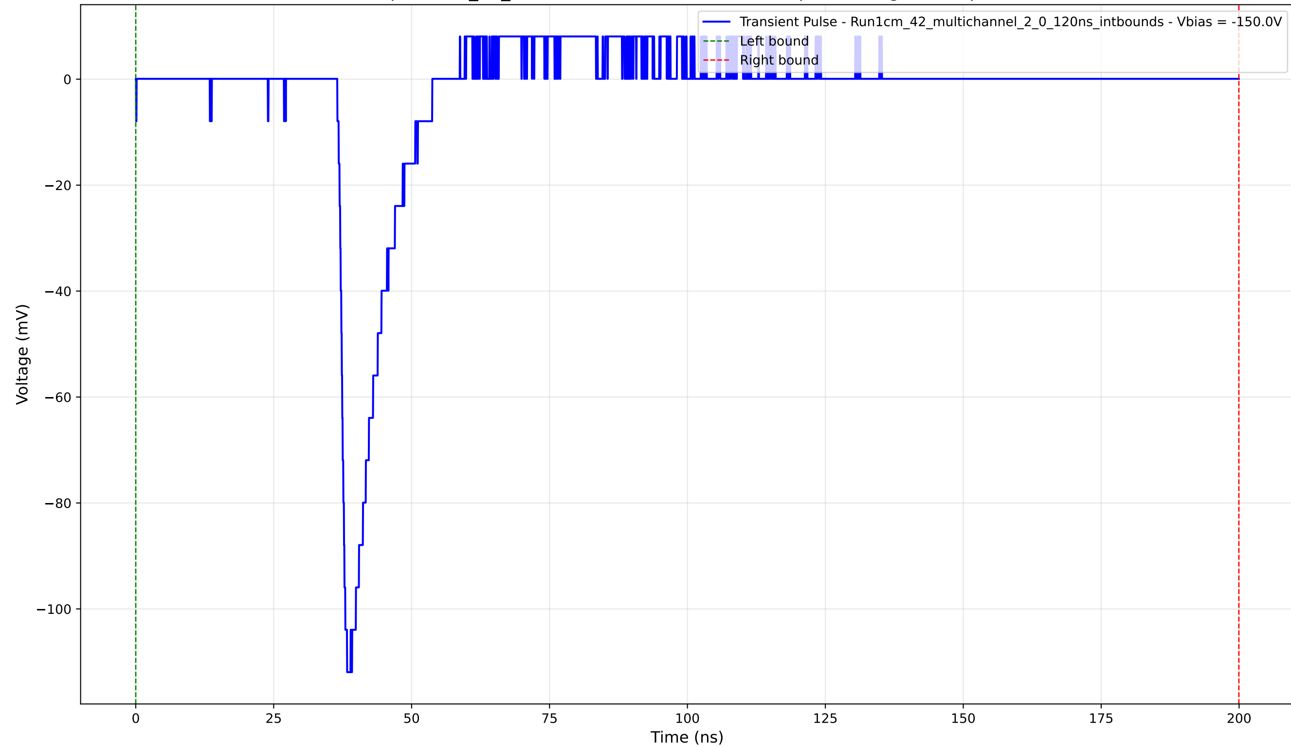
Transient Pulse - Sample: 1cm_42_multichannel - Position: 3675.0 \mu\text{m} - Charge: 9.71 pC - Rise Time: 1.22 ns
