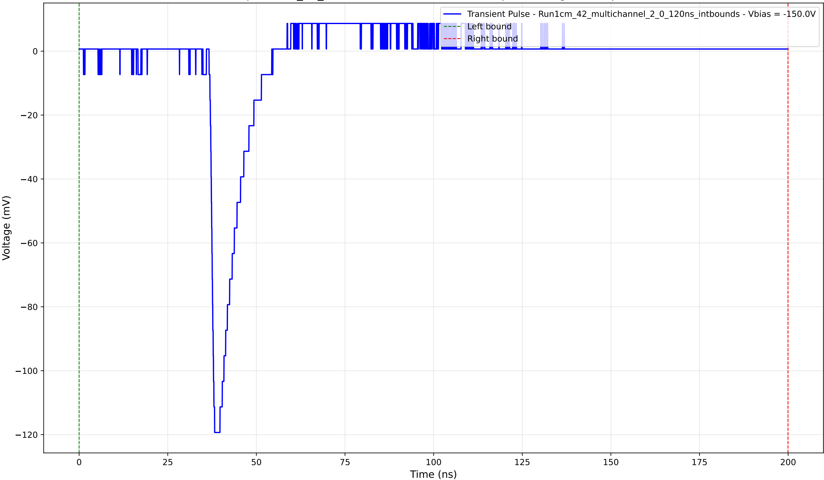
Transient Pulse - Sample: 1cm_42_multichannel - Position: 965.0 \mu\text{m} - Charge: 8.94 pC - Rise Time: 1.14 ns
