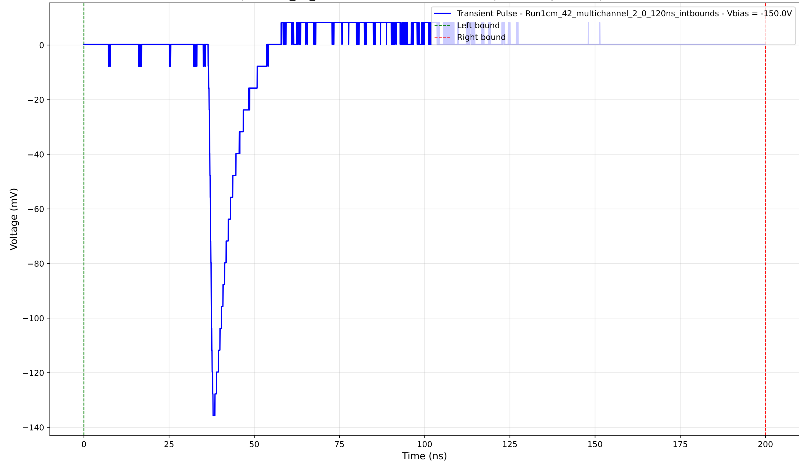
Transient Pulse - Sample: 1cm_42_multichannel - Position: 3480.0 \mu\text{m} - Charge: 9.98 pC - Rise Time: 1.17 ns
