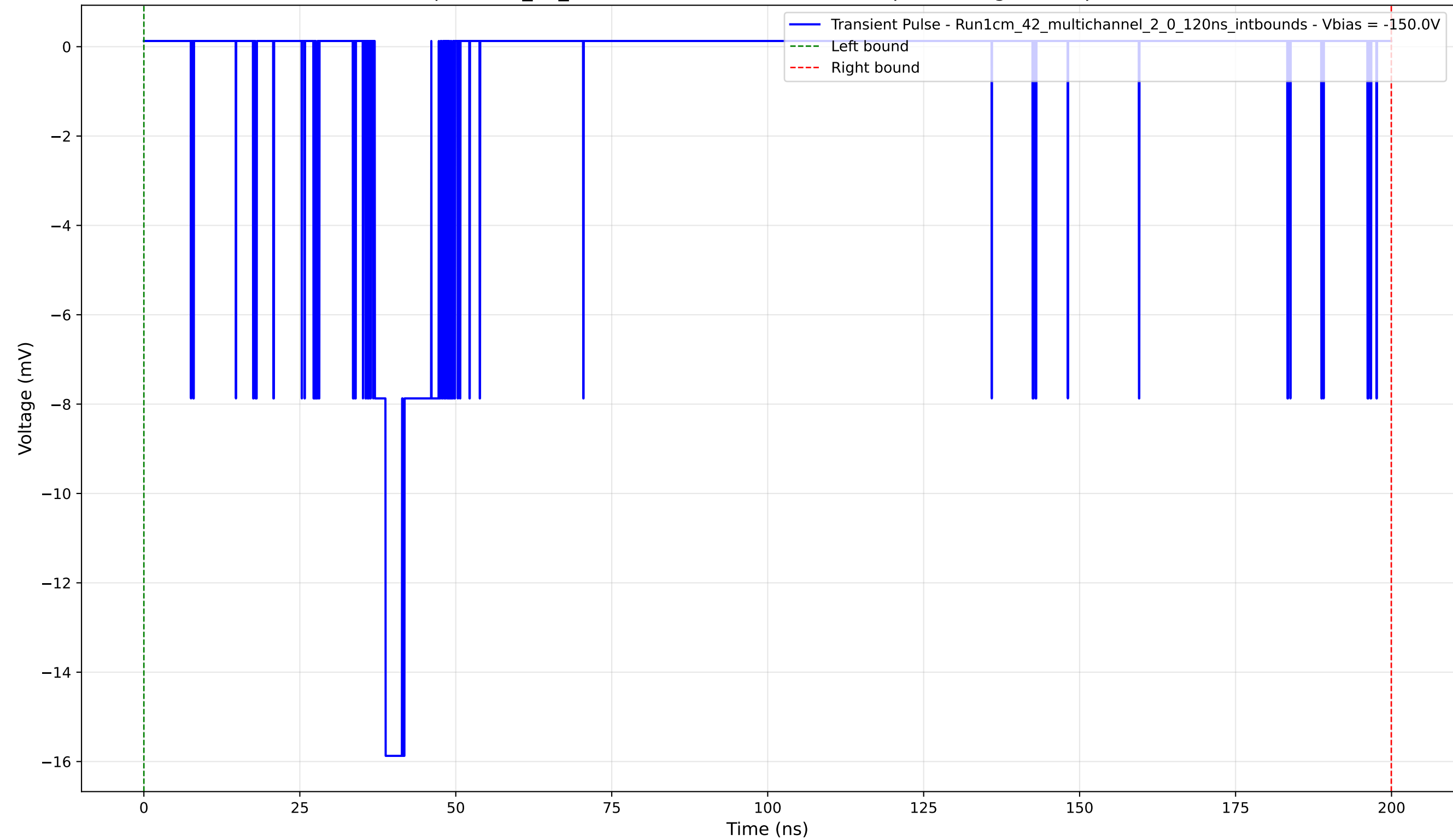
Transient Pulse - Sample: 1cm_42_multichannel - Position: 4420.0 \mu\text{m} - Charge: 2.40 pC - Rise Time: 1.75 ns
