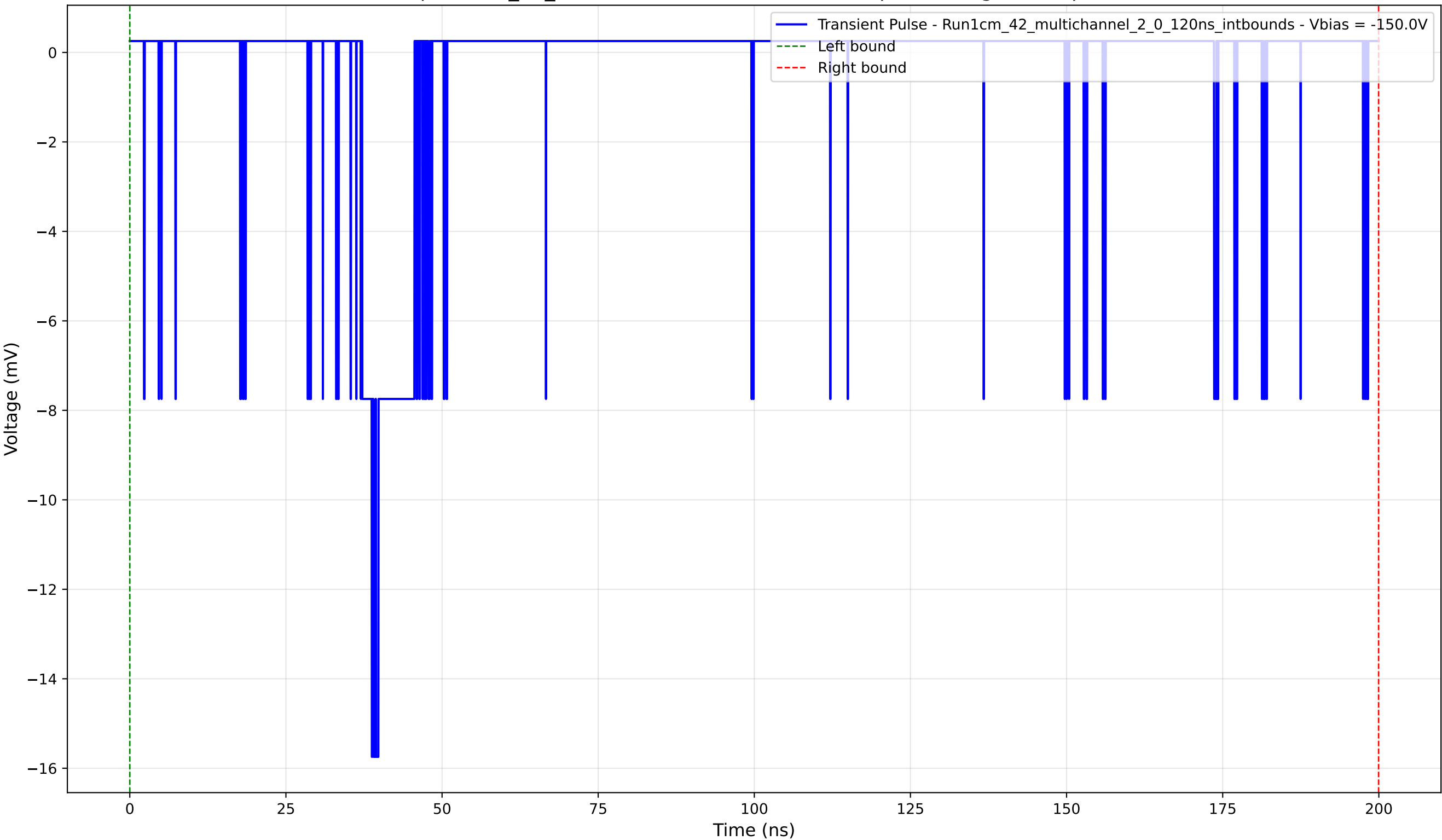
Transient Pulse - Sample: 1cm_42_multichannel - Position: 3910.0 \mu\text{m} - Charge: 1.30 pC - Rise Time: 1.55 ns
