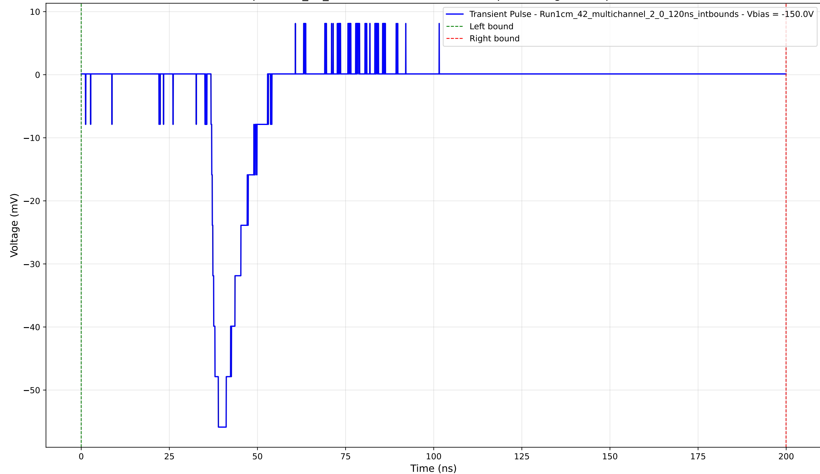
Transient Pulse - Sample: 1cm_42_multichannel - Position: 95.0 \mu\text{m} - Charge: 8.53 pC - Rise Time: 2.09 ns
