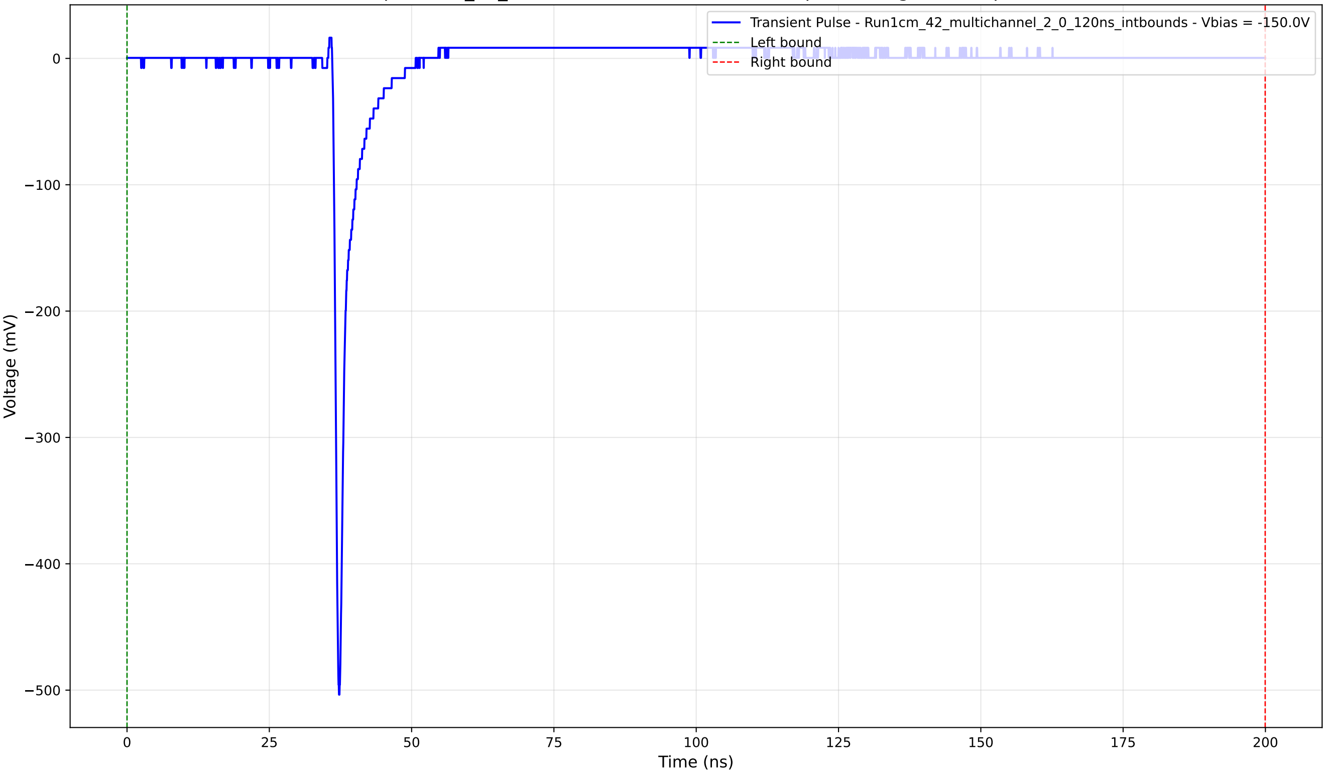
Transient Pulse - Sample: 1cm_42_multichannel - Position: 2115.0 \mu\text{m} - Charge: 14.26 pC - Rise Time: 0.74 ns
