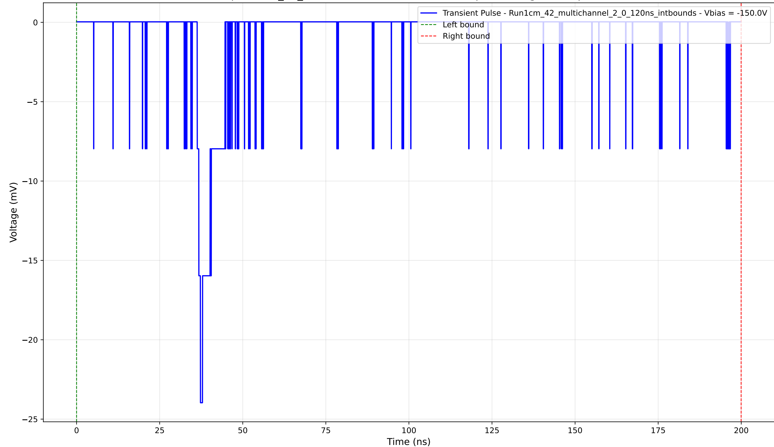
Transient Pulse - Sample: 1cm_42_multichannel - Position: 1845.0 \mu\text{m} - Charge: 2.88 pC - Rise Time: 0.99 ns
