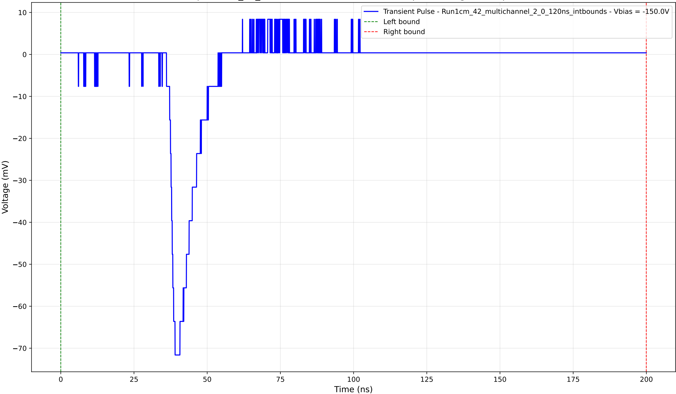
Transient Pulse - Sample: 1cm_42_multichannel - Position: 4525.0 \mu\text{m} - Charge: 8.79 pC - Rise Time: 2.92 ns
