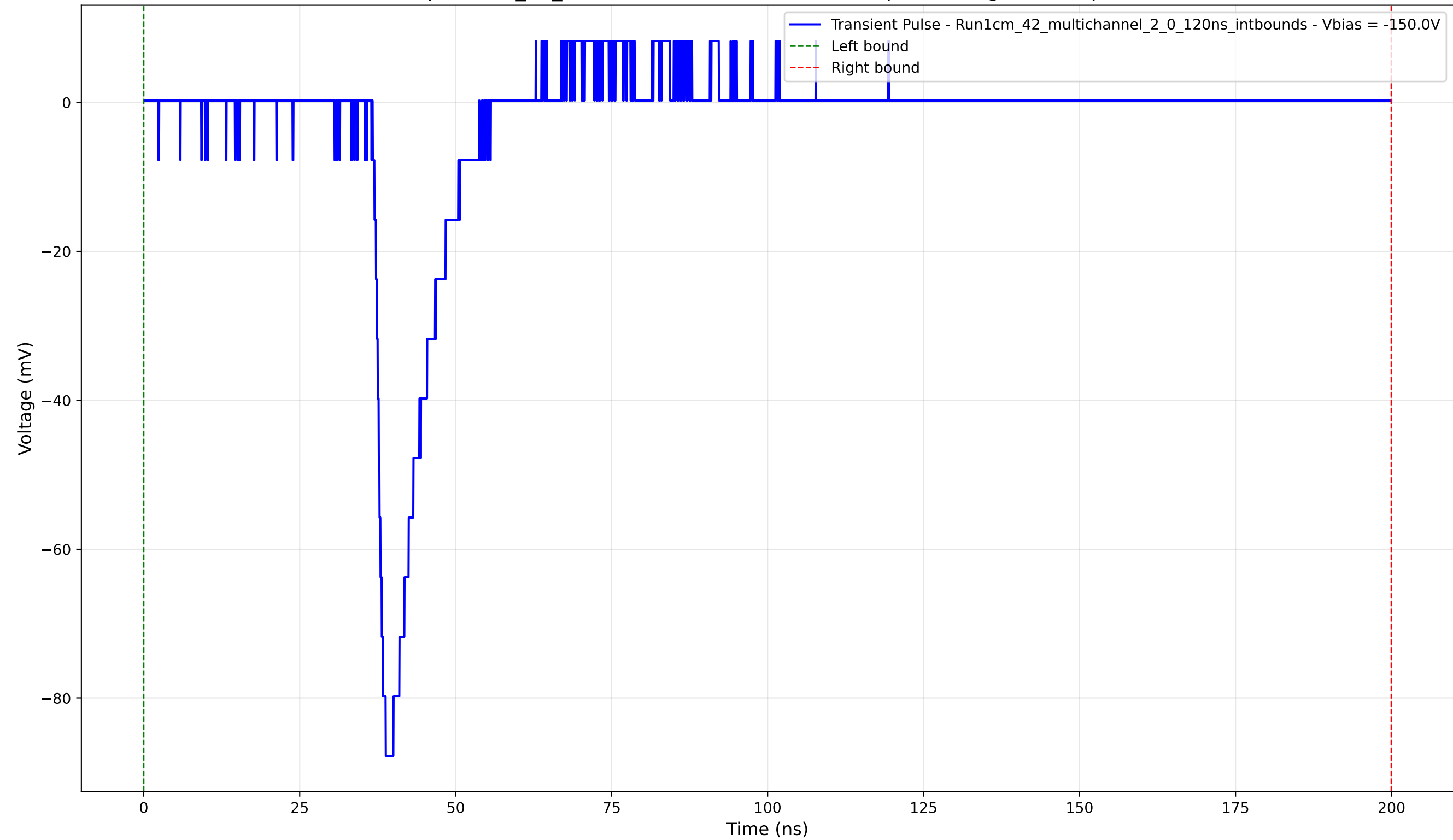
Transient Pulse - Sample: 1cm_42_multichannel - Position: 3960.0 \mu\text{m} - Charge: 10.10 pC - Rise Time: 1.39 ns
