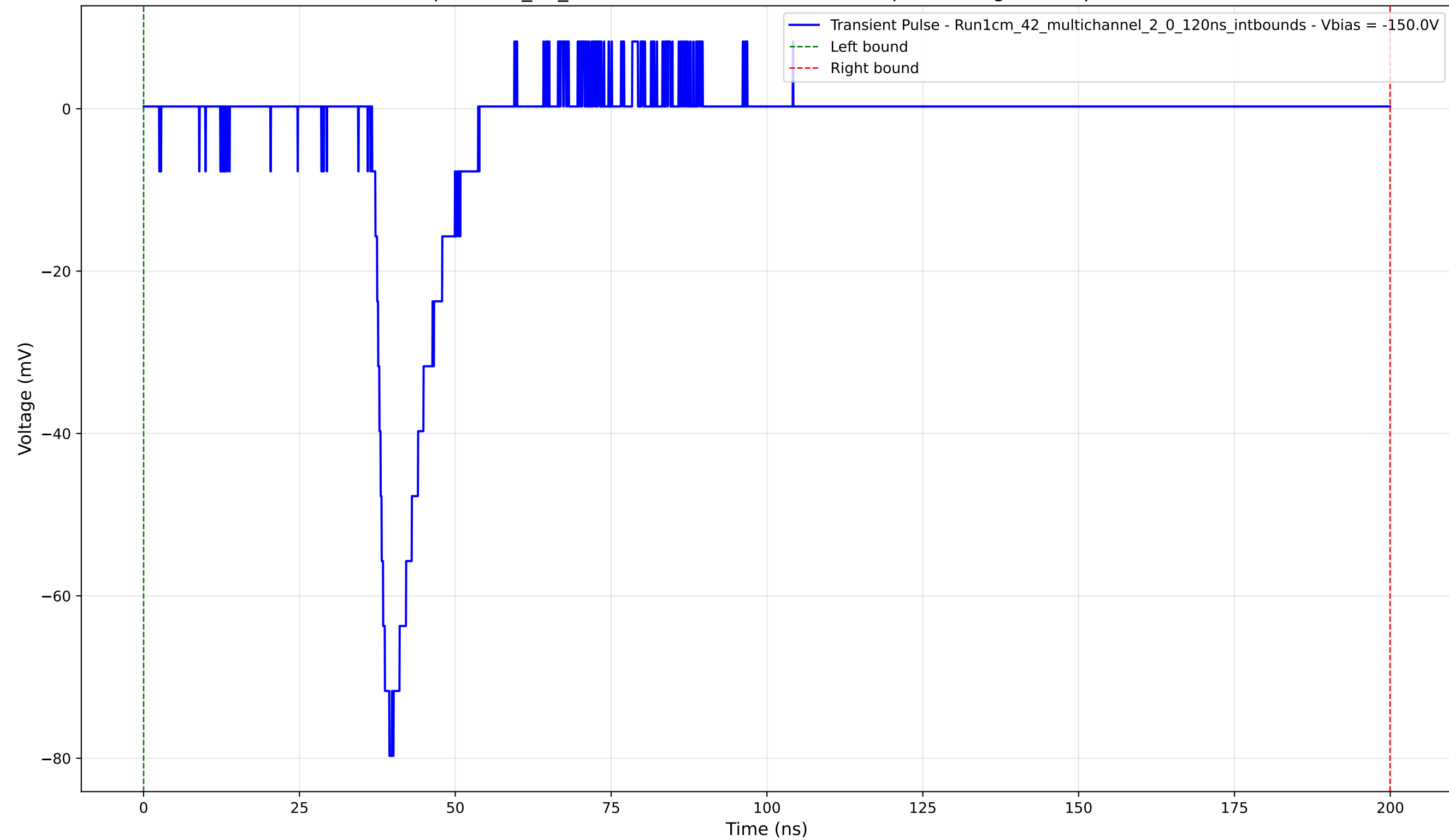
Transient Pulse - Sample: 1cm_42_multichannel - Position: 4270.0 \mu\text{m} - Charge: 9.38 pC - Rise Time: 2.28 ns
