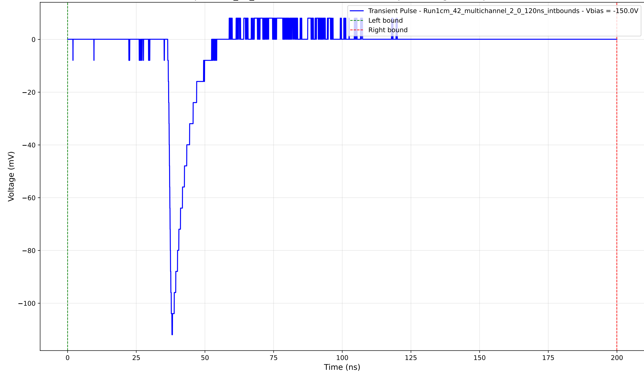
Transient Pulse - Sample: 1cm_42_multichannel - Position: 3445.0 \mu\text{m} - Charge: 9.93 pC - Rise Time: 1.10 ns
