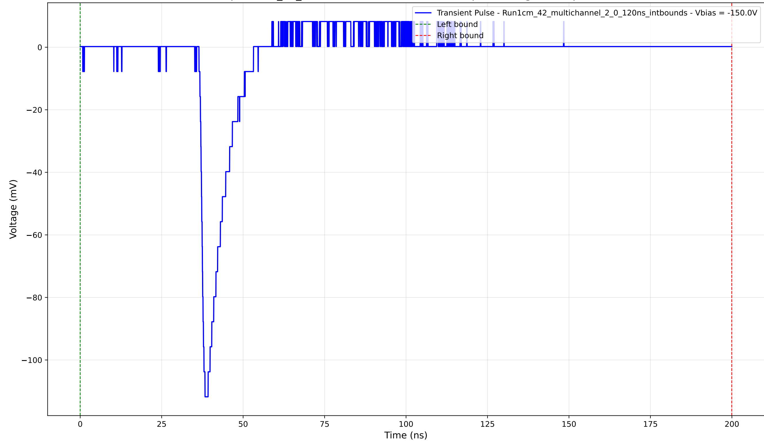
Transient Pulse - Sample: 1cm_42_multichannel - Position: 3655.0 \mu\text{m} - Charge: 9.64 pC - Rise Time: 1.26 ns
