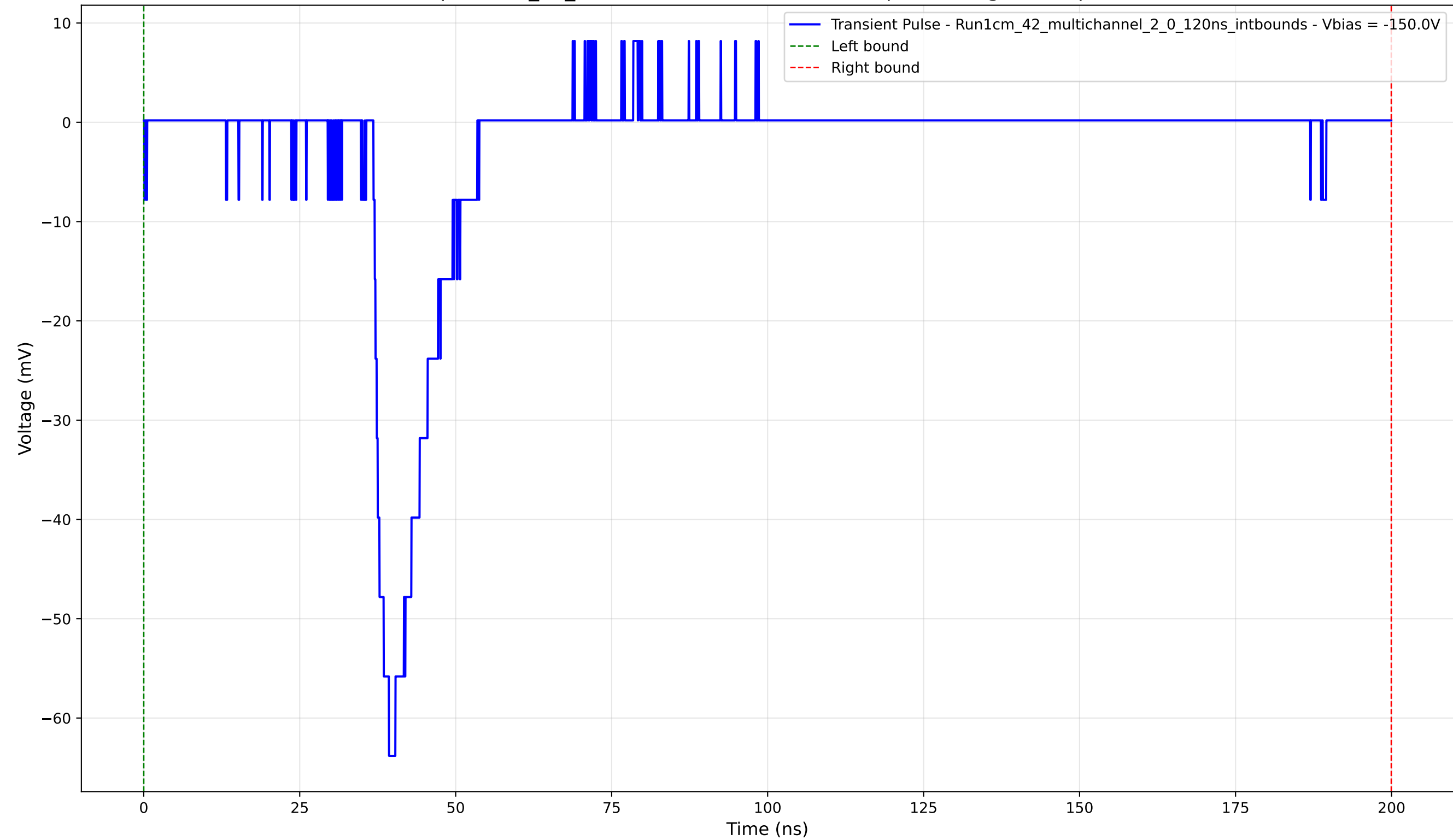
Transient Pulse - Sample: 1cm_42_multichannel - Position: 105.0 \mu\text{m} - Charge: 9.47 pC - Rise Time: 2.49 ns
