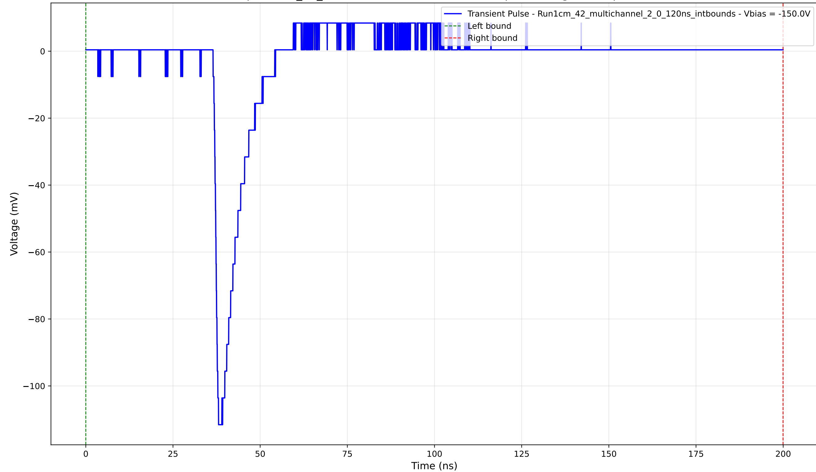
Transient Pulse - Sample: 1cm_42_multichannel - Position: 3605.0 \mu\text{m} - Charge: 8.87 pC - Rise Time: 1.14 ns
