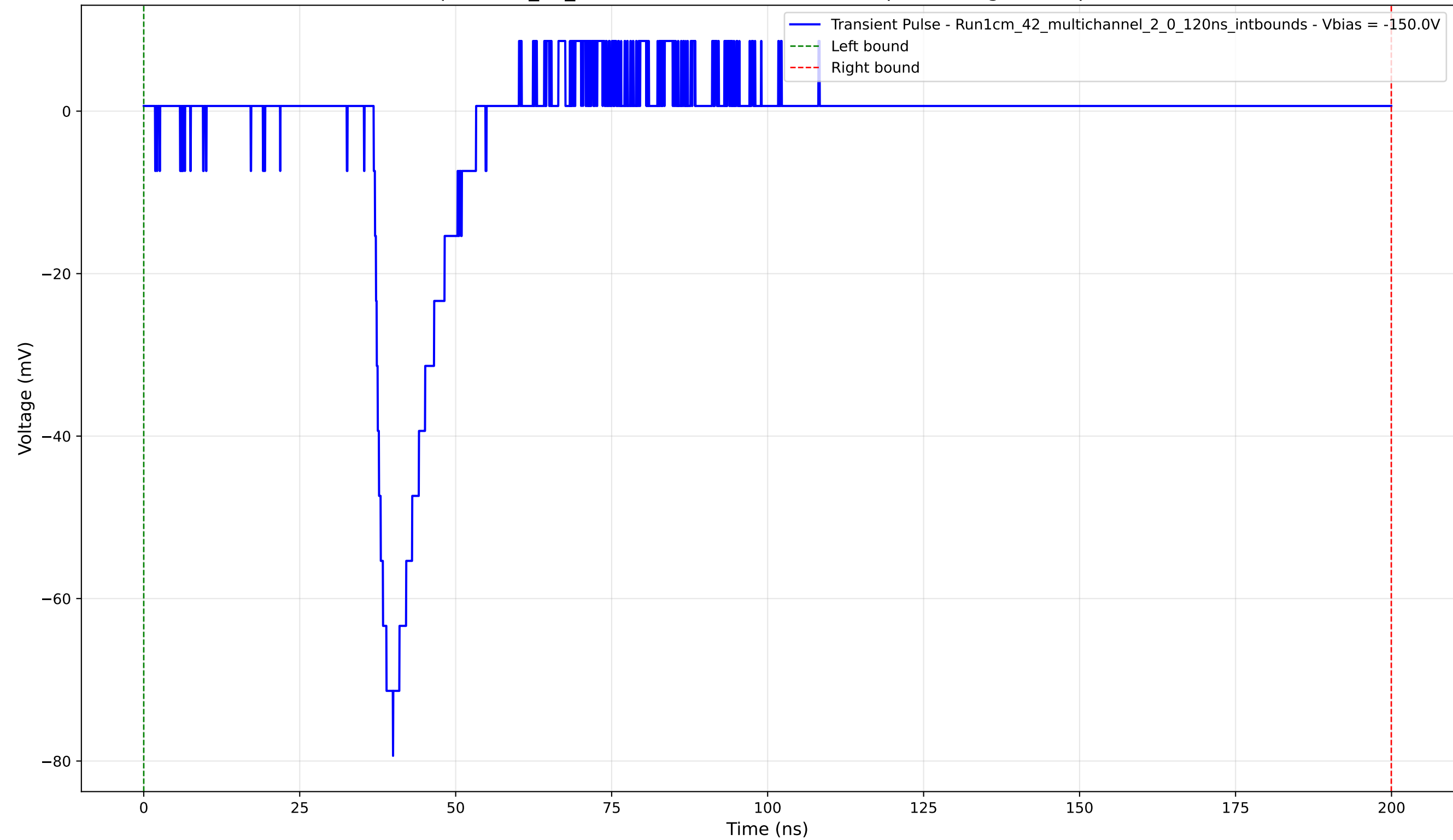
Transient Pulse - Sample: 1cm_42_multichannel - Position: 210.0 \mu\text{m} - Charge: 7.11 pC - Rise Time: 2.92 ns
