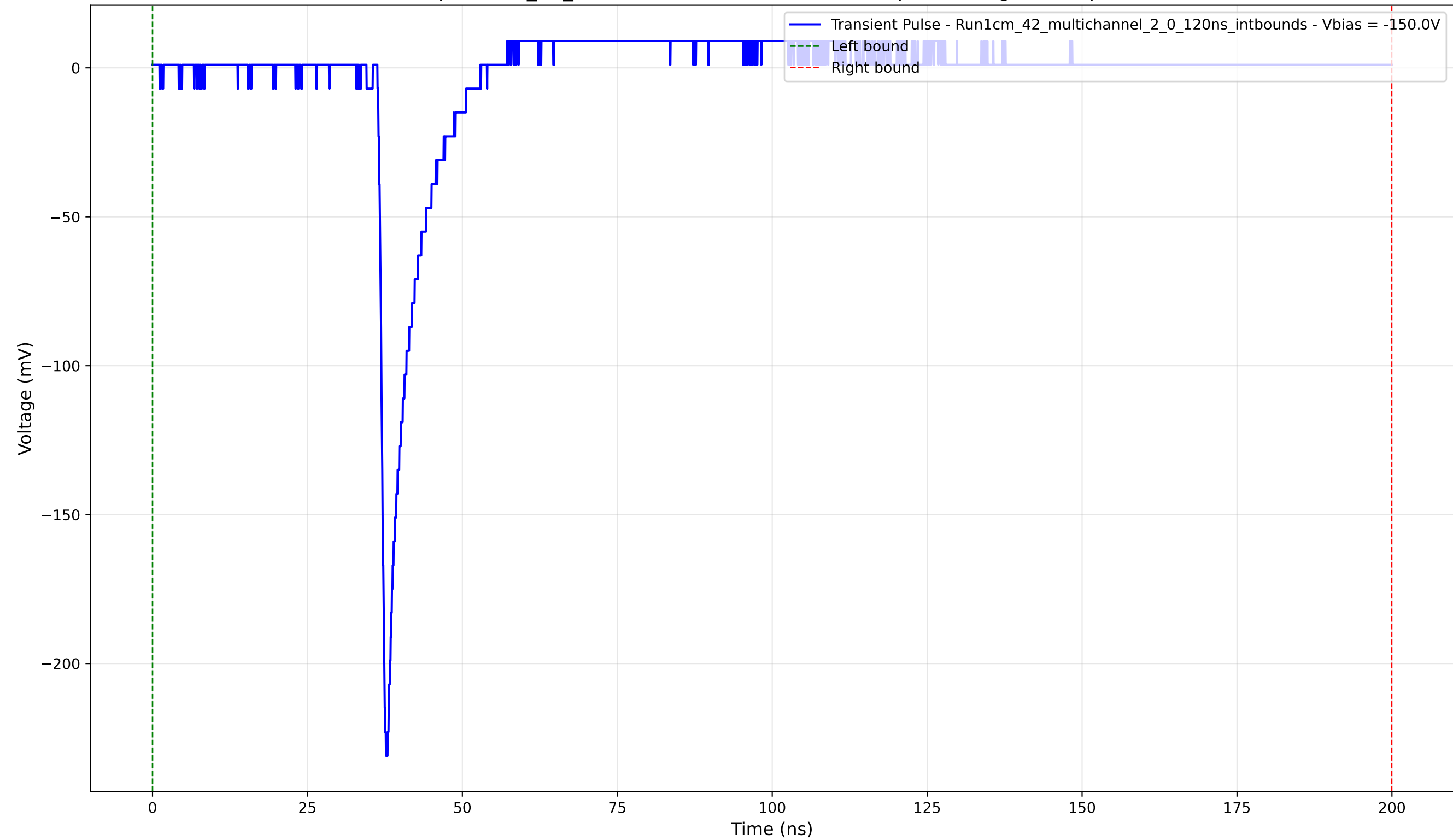
Transient Pulse - Sample: 1cm_42_multichannel - Position: 1575.0 \mu\text{m} - Charge: 9.83 pC - Rise Time: 0.96 ns
