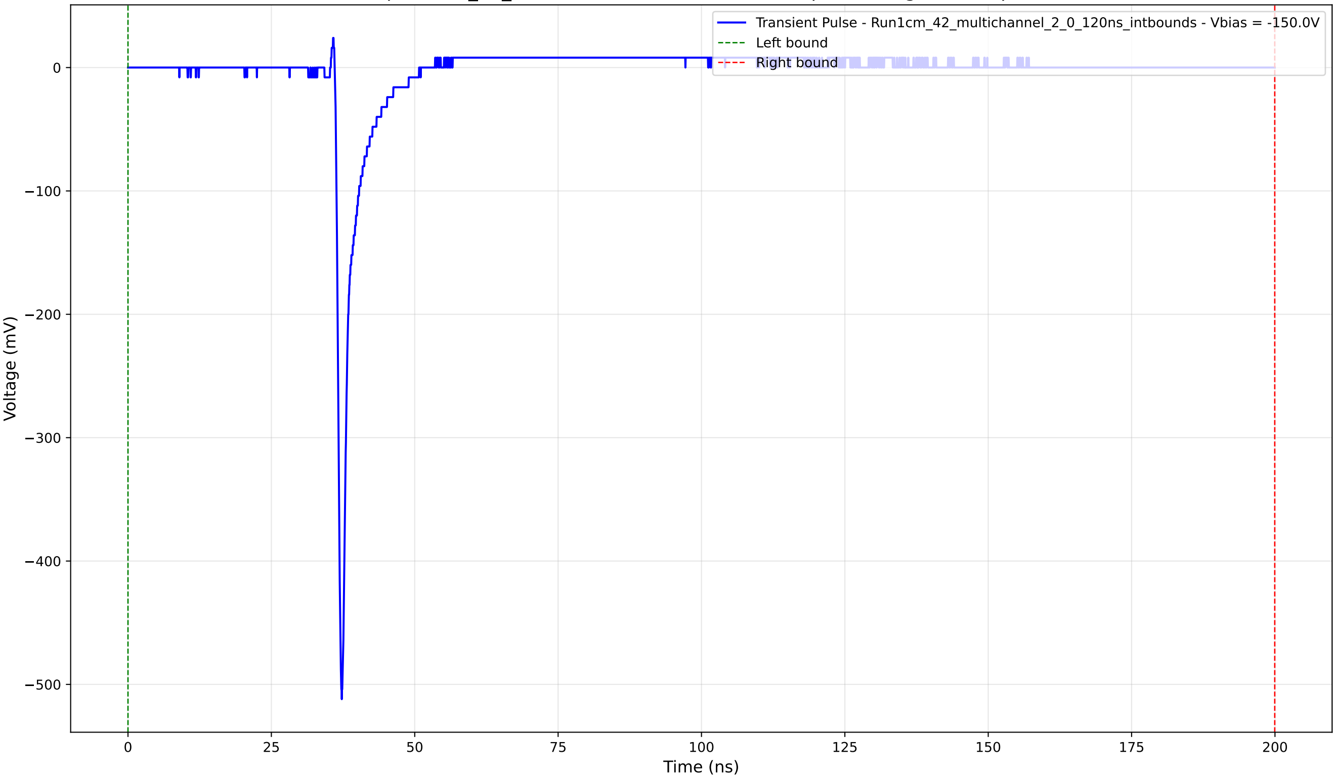
Transient Pulse - Sample: 1cm_42_multichannel - Position: 2120.0 \mu\text{m} - Charge: 15.35 pC - Rise Time: 0.78 ns
