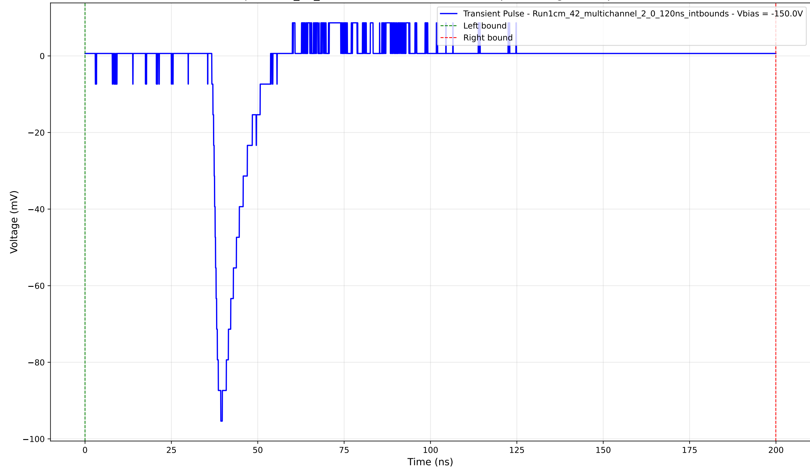
Transient Pulse - Sample: 1cm_42_multichannel - Position: 4015.0 \mu\text{m} - Charge: 8.77 pC - Rise Time: 1.59 ns
