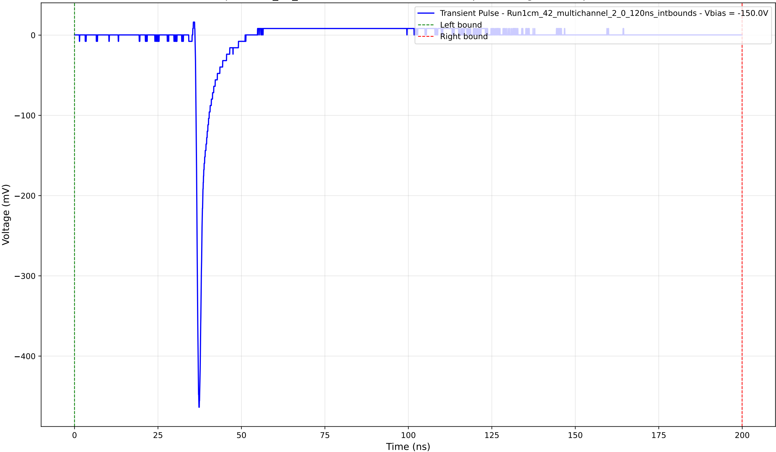
Transient Pulse - Sample: 1cm_42_multichannel - Position: 2065.0 \mu\text{m} - Charge: 14.79 pC - Rise Time: 0.77 ns
