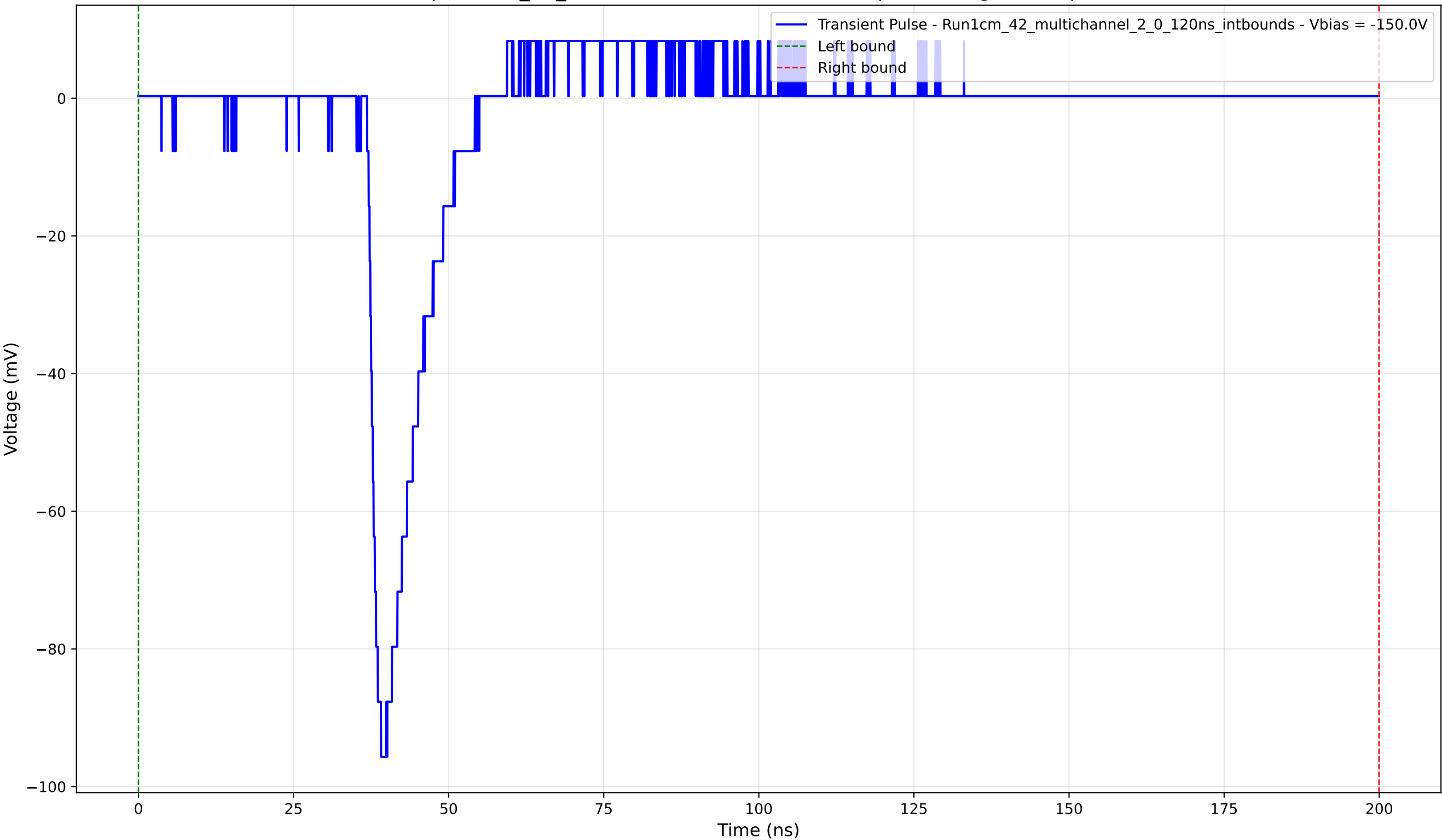
Transient Pulse - Sample: 1cm_42_multichannel - Position: 495.0 \mu\text{m} - Charge: 8.35 pC - Rise Time: 1.51 ns
