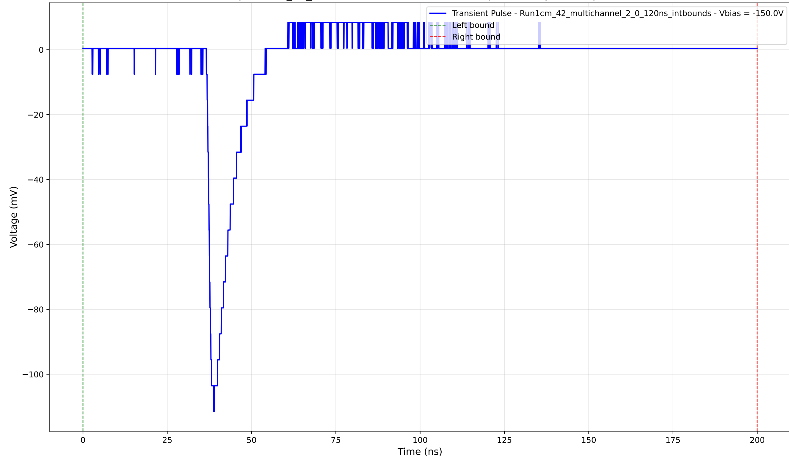
Transient Pulse - Sample: 1cm_42_multichannel - Position: 3700.0 \mu\text{m} - Charge: 8.95 pC - Rise Time: 1.34 ns
