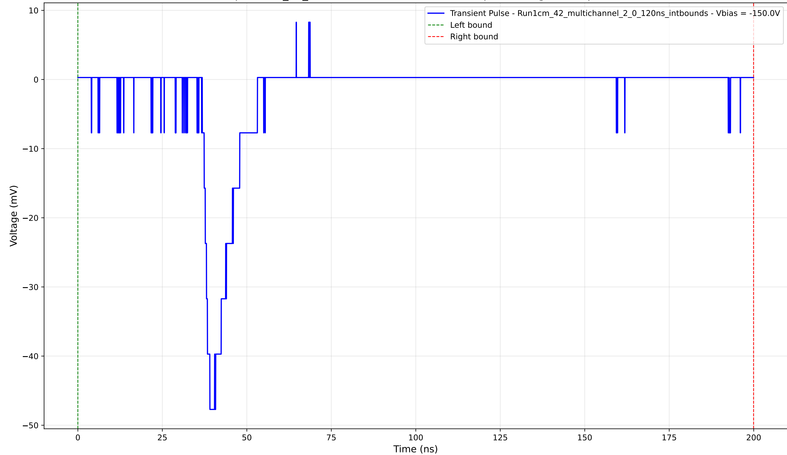
Transient Pulse - Sample: 1cm_42_multichannel - Position: 4445.0 \mu\text{m} - Charge: 6.80 pC - Rise Time: 2.26 ns
