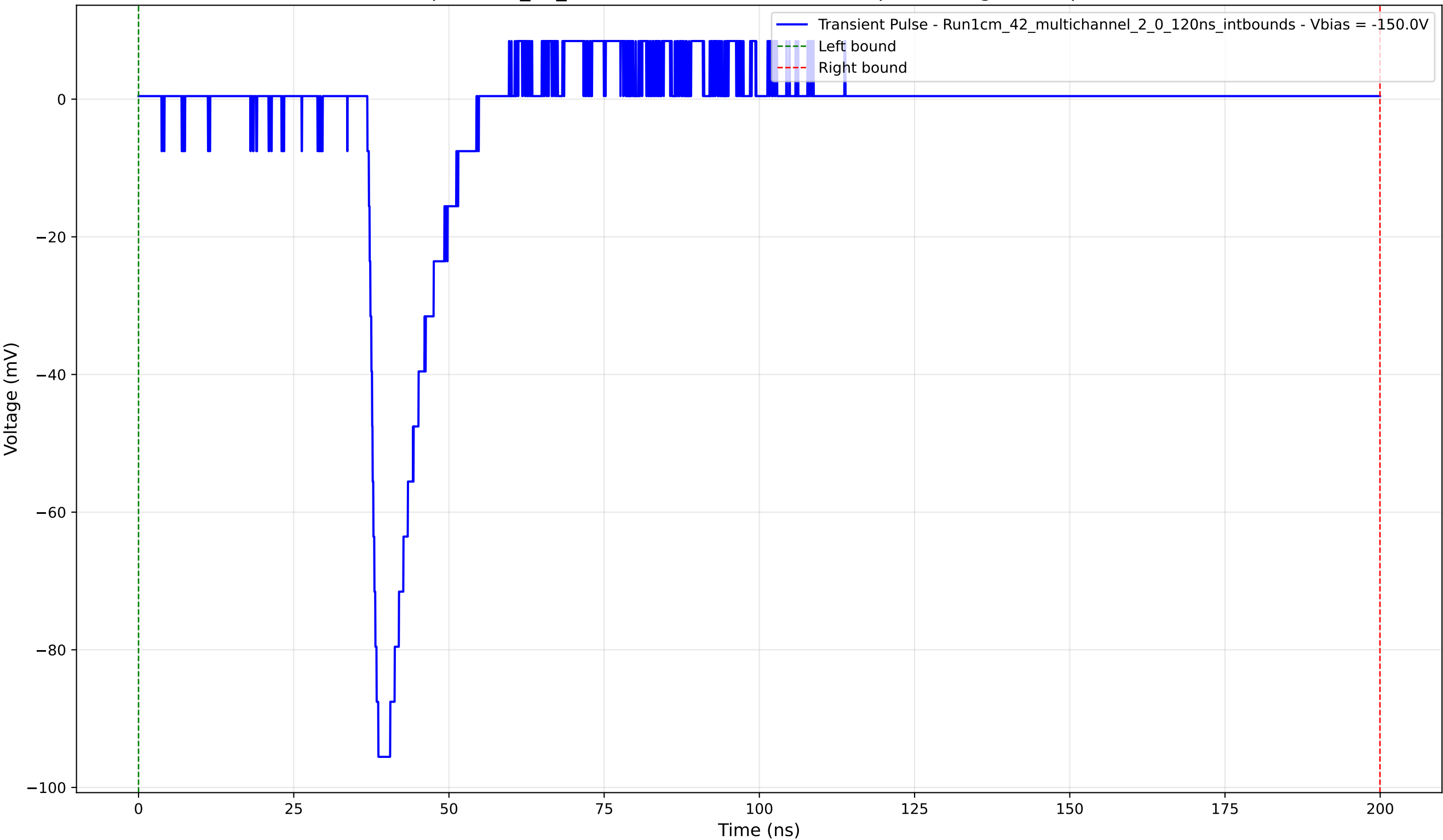
Transient Pulse - Sample: 1cm_42_multichannel - Position: 590.0 \mu\text{m} - Charge: 9.77 pC - Rise Time: 1.27 ns
