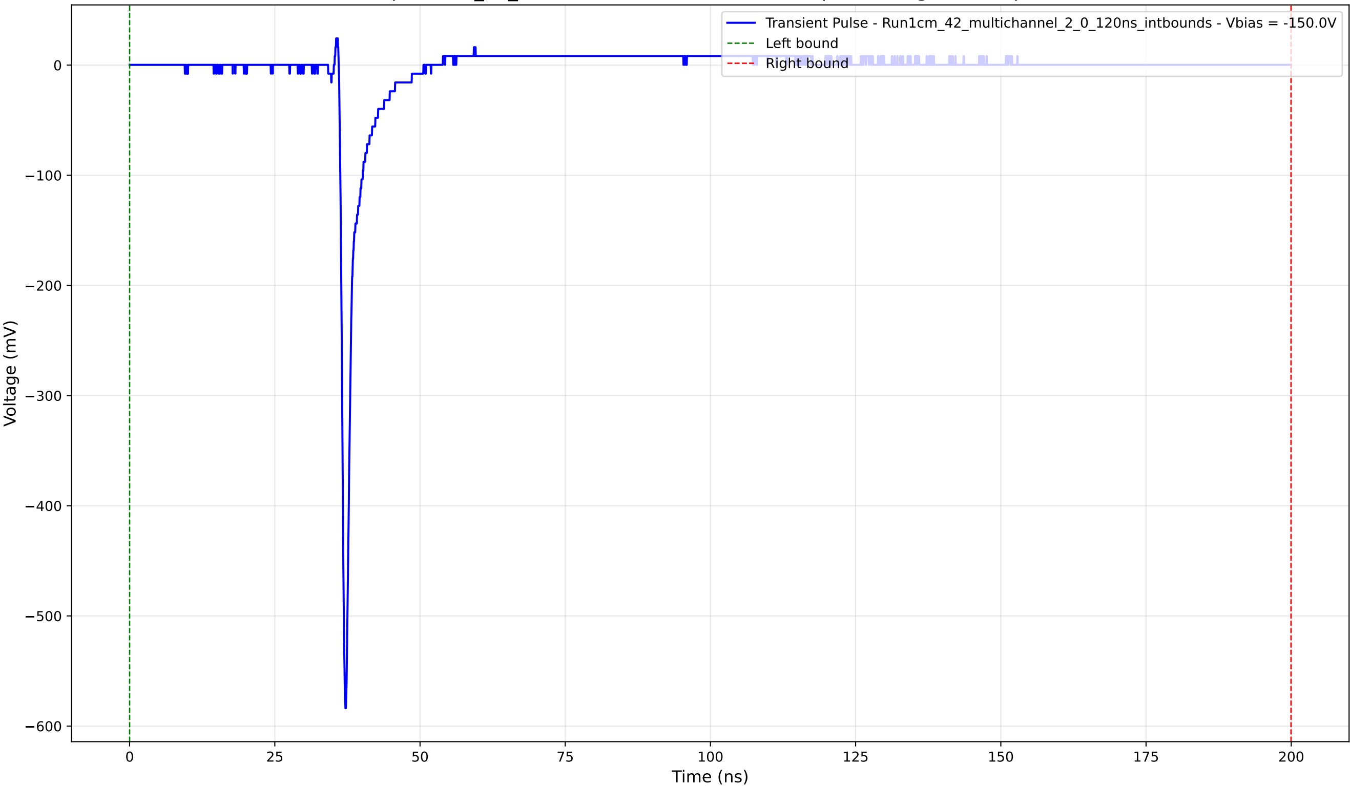
Transient Pulse - Sample: 1cm_42_multichannel - Position: 2505.0 \mu\text{m} - Charge: 16.07 pC - Rise Time: 0.75 ns
