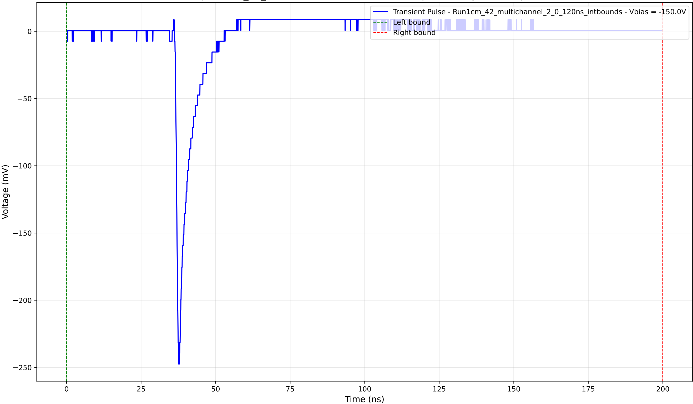
Transient Pulse - Sample: 1cm_42_multichannel - Position: 1630.0 \mu\text{m} - Charge: 10.68 pC - Rise Time: 0.91 ns
