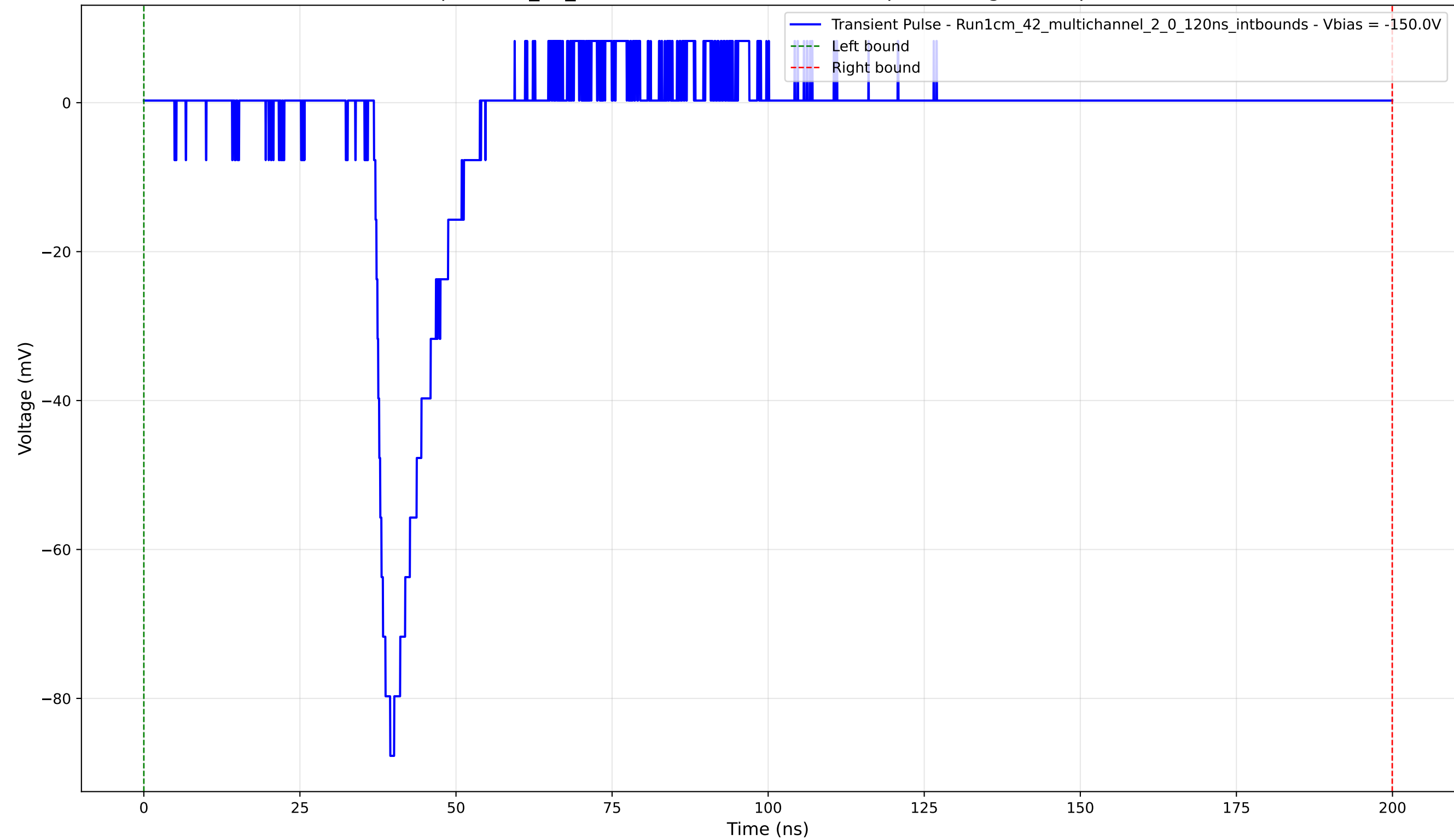
Transient Pulse - Sample: 1cm_42_multichannel - Position: 425.0 \mu\text{m} - Charge: 9.64 pC - Rise Time: 1.63 ns
