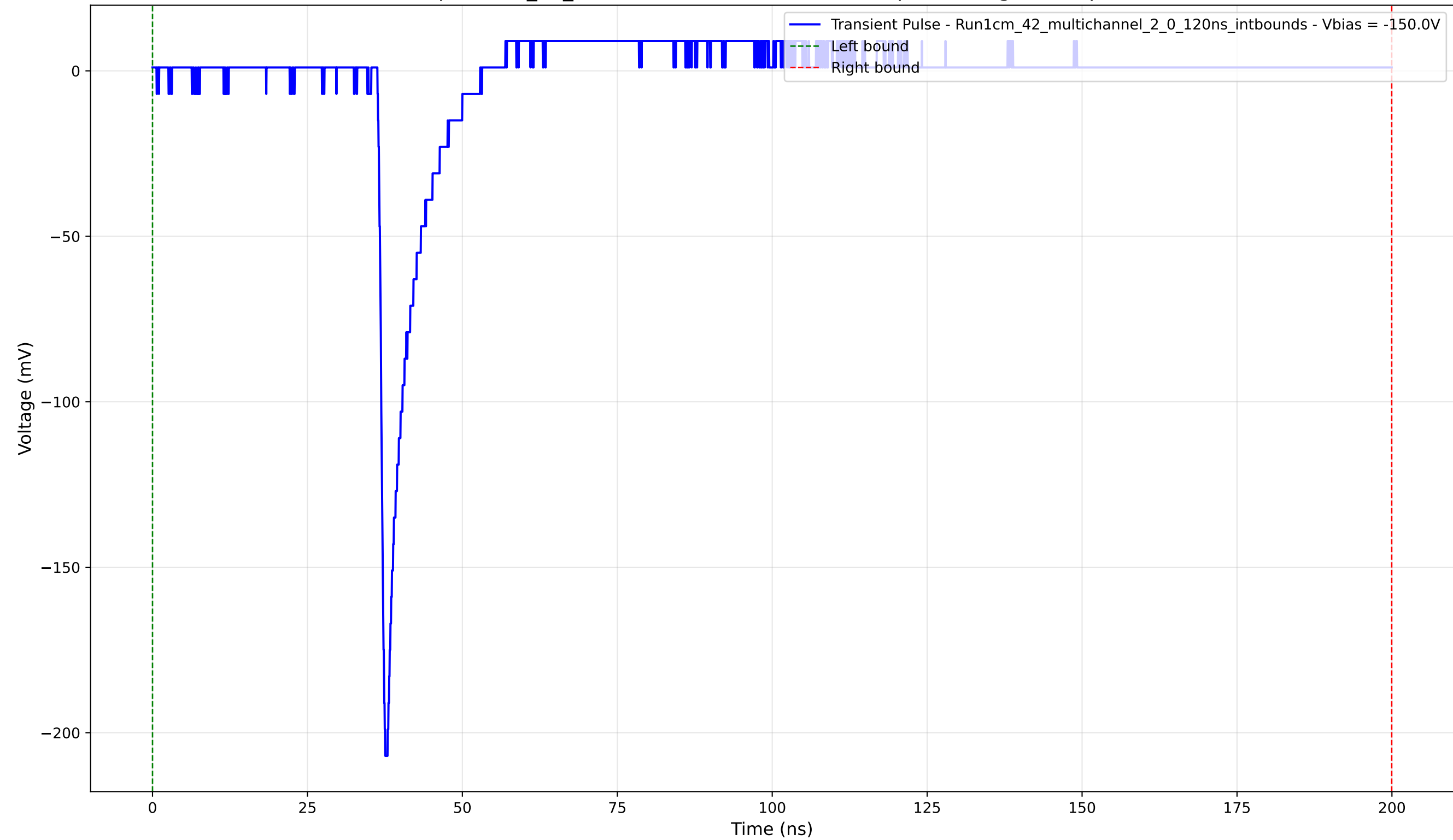
Transient Pulse - Sample: 1cm_42_multichannel - Position: 3120.0 \mu\text{m} - Charge: 7.98 pC - Rise Time: 0.93 ns
