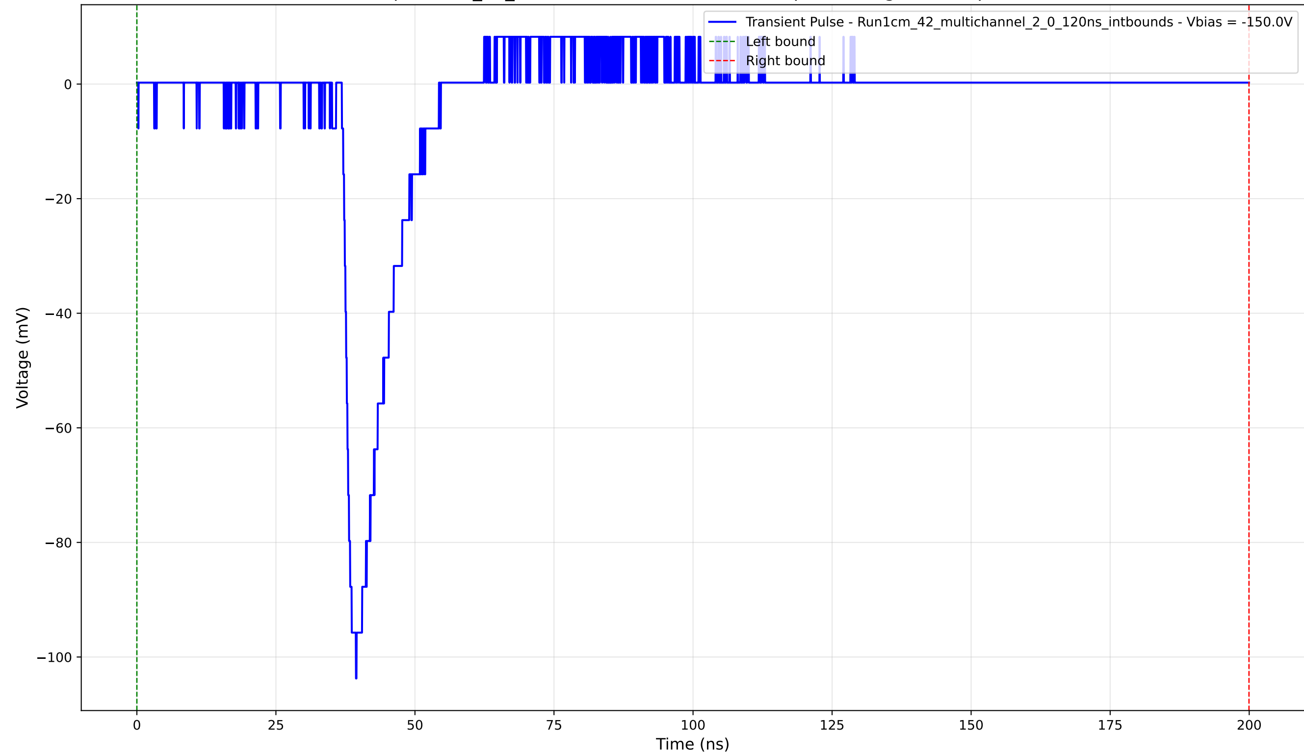
Transient Pulse - Sample: 1cm_42_multichannel - Position: 585.0 \mu\text{m} - Charge: 10.20 pC - Rise Time: 1.55 ns
