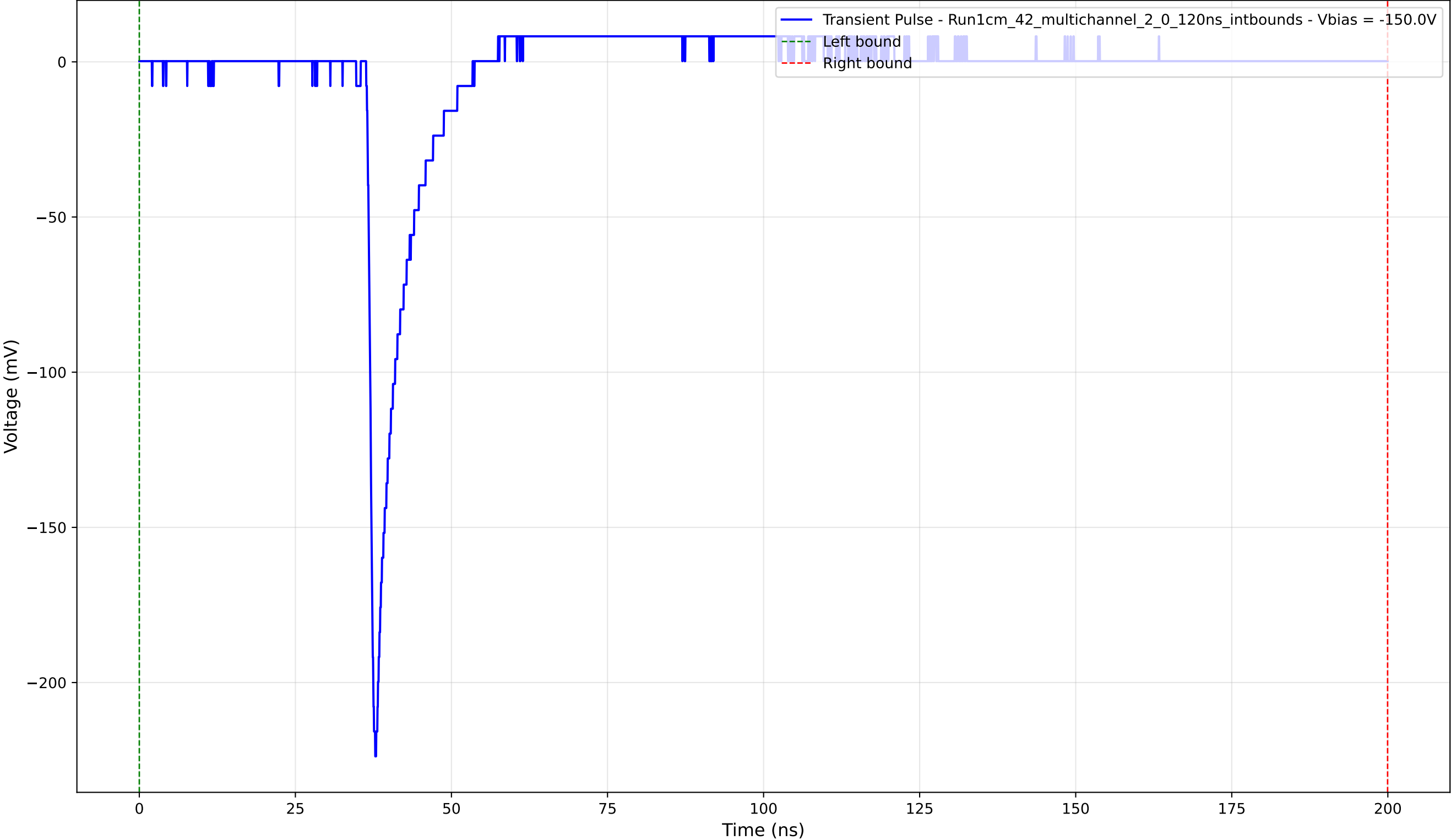
Transient Pulse - Sample: 1cm_42_multichannel - Position: 1550.0 \mu\text{m} - Charge: 12.21 pC - Rise Time: 0.97 ns
