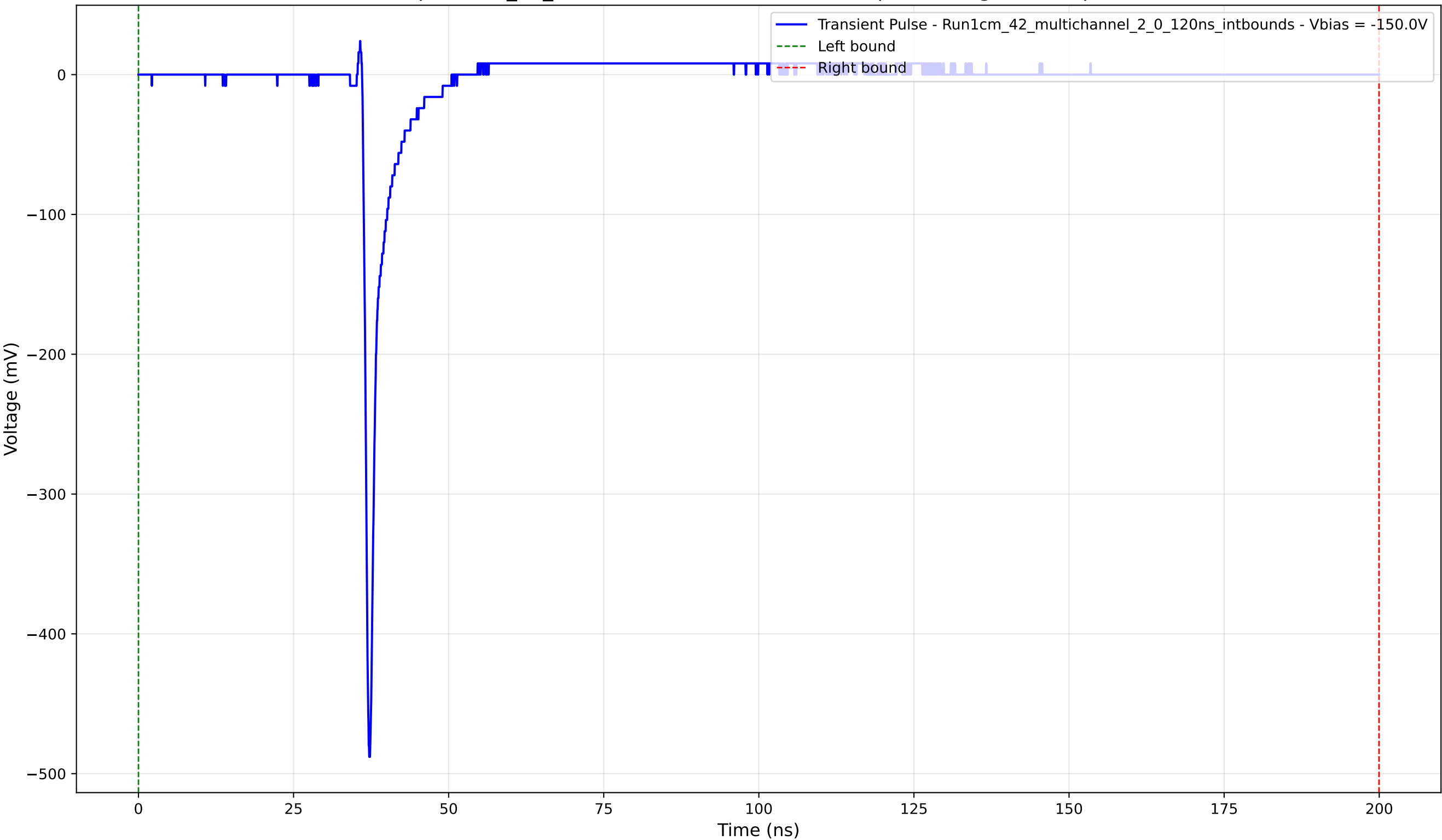
Transient Pulse - Sample: 1cm_42_multichannel - Position: 2595.0 \mu\text{m} - Charge: 15.09 pC - Rise Time: 0.78 ns
