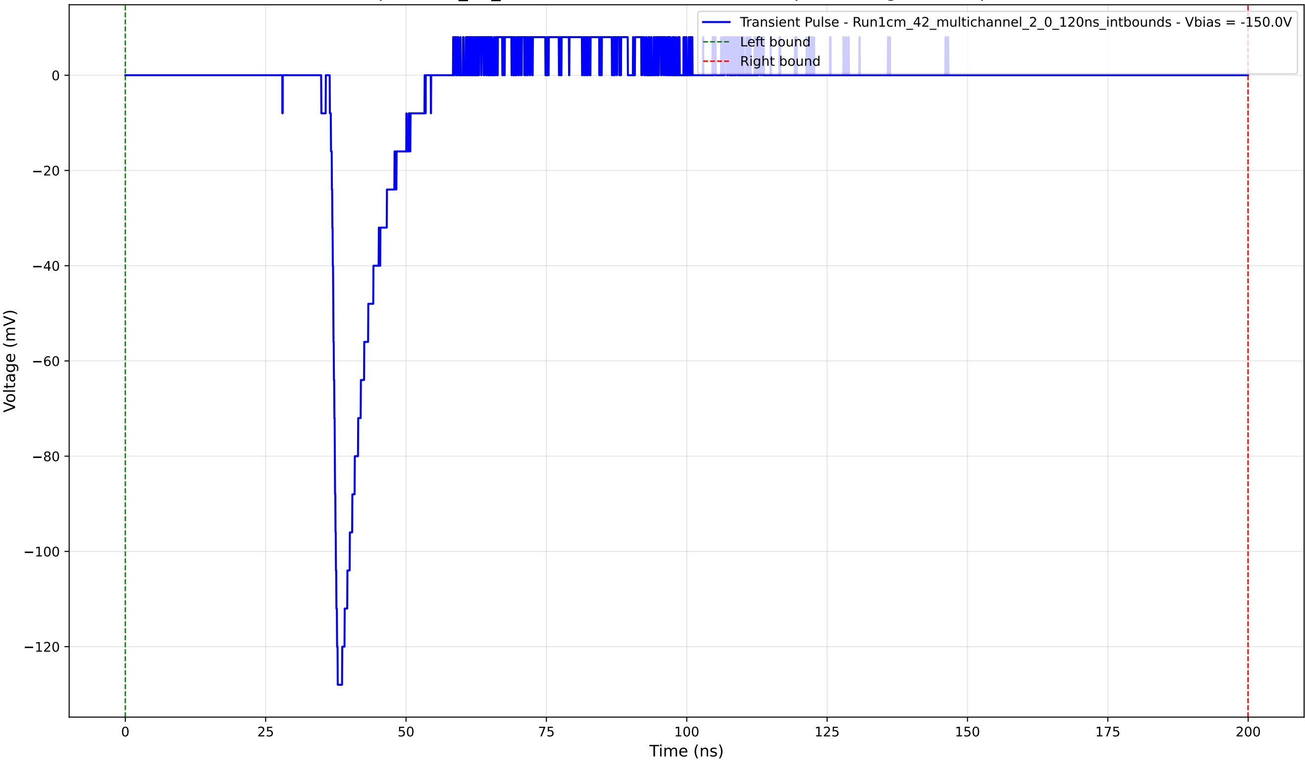
Transient Pulse - Sample: 1cm_42_multichannel - Position: 1290.0 \mu\text{m} - Charge: 11.05 pC - Rise Time: 1.10 ns
