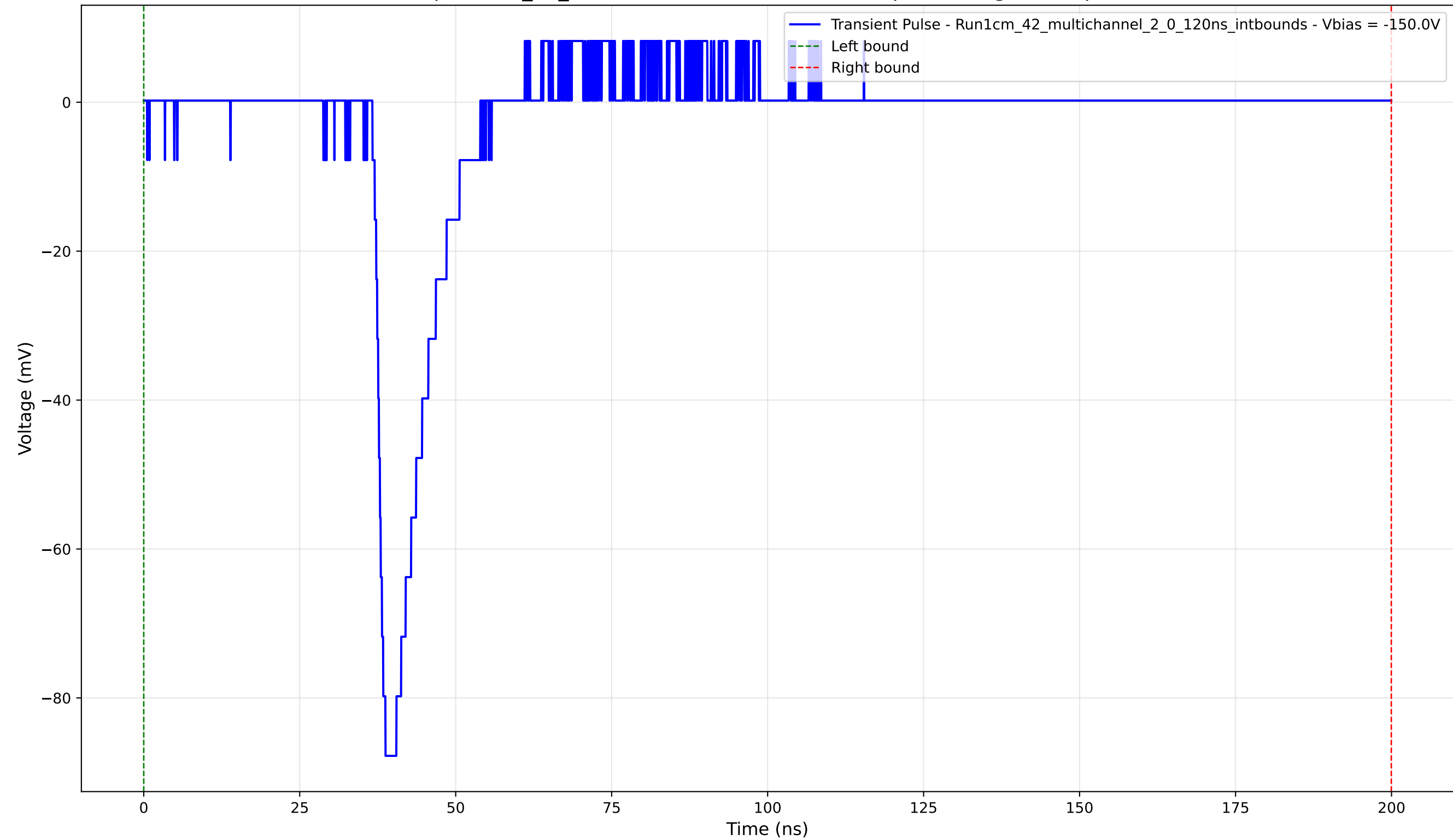
Transient Pulse - Sample: 1cm_42_multichannel - Position: 4055.0 \mu\text{m} - Charge: 9.94 pC - Rise Time: 1.39 ns
