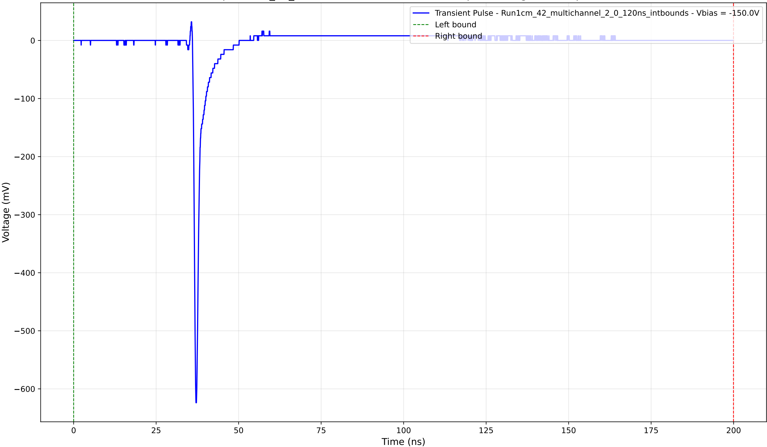
Transient Pulse - Sample: 1cm_42_multichannel - Position: 2460.0 \mu\text{m} - Charge: 15.13 pC - Rise Time: 0.71 ns
