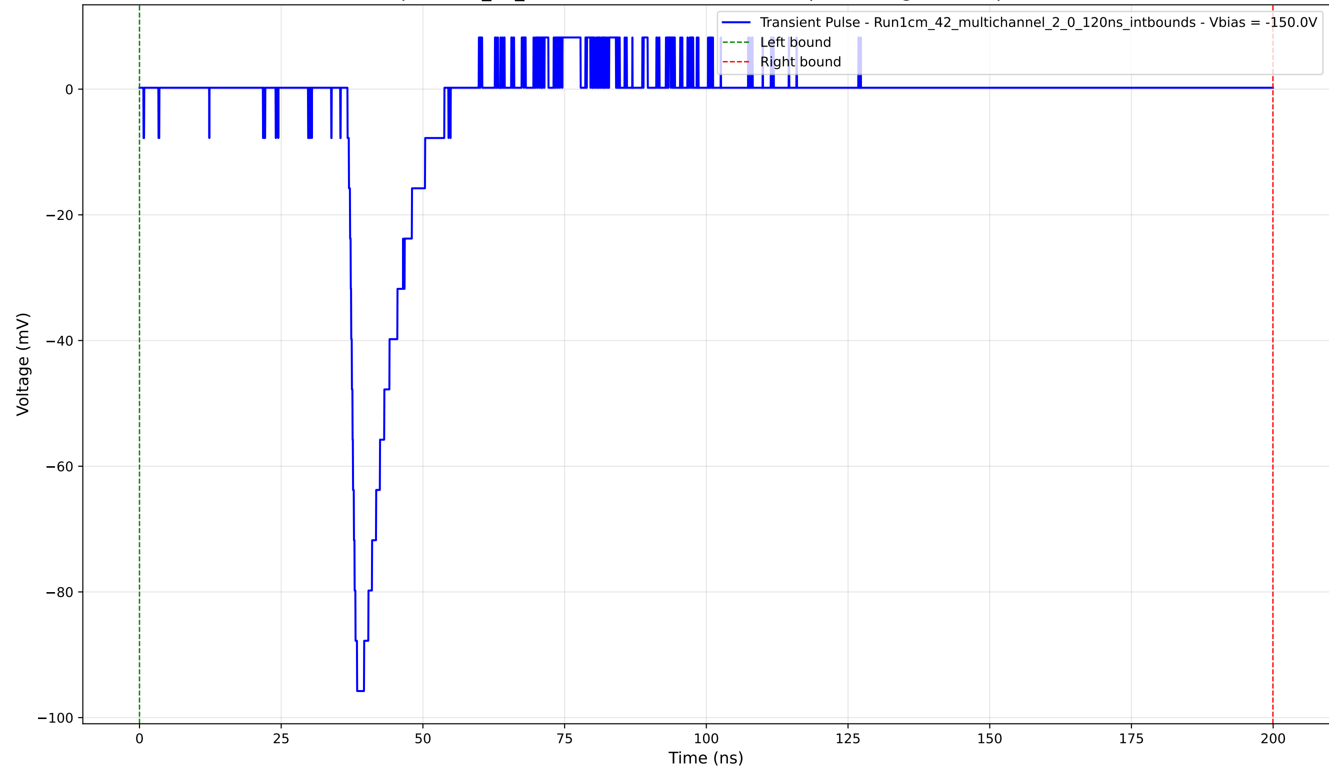
Transient Pulse - Sample: 1cm_42_multichannel - Position: 915.0 \mu\text{m} - Charge: 10.58 pC - Rise Time: 1.19 ns
