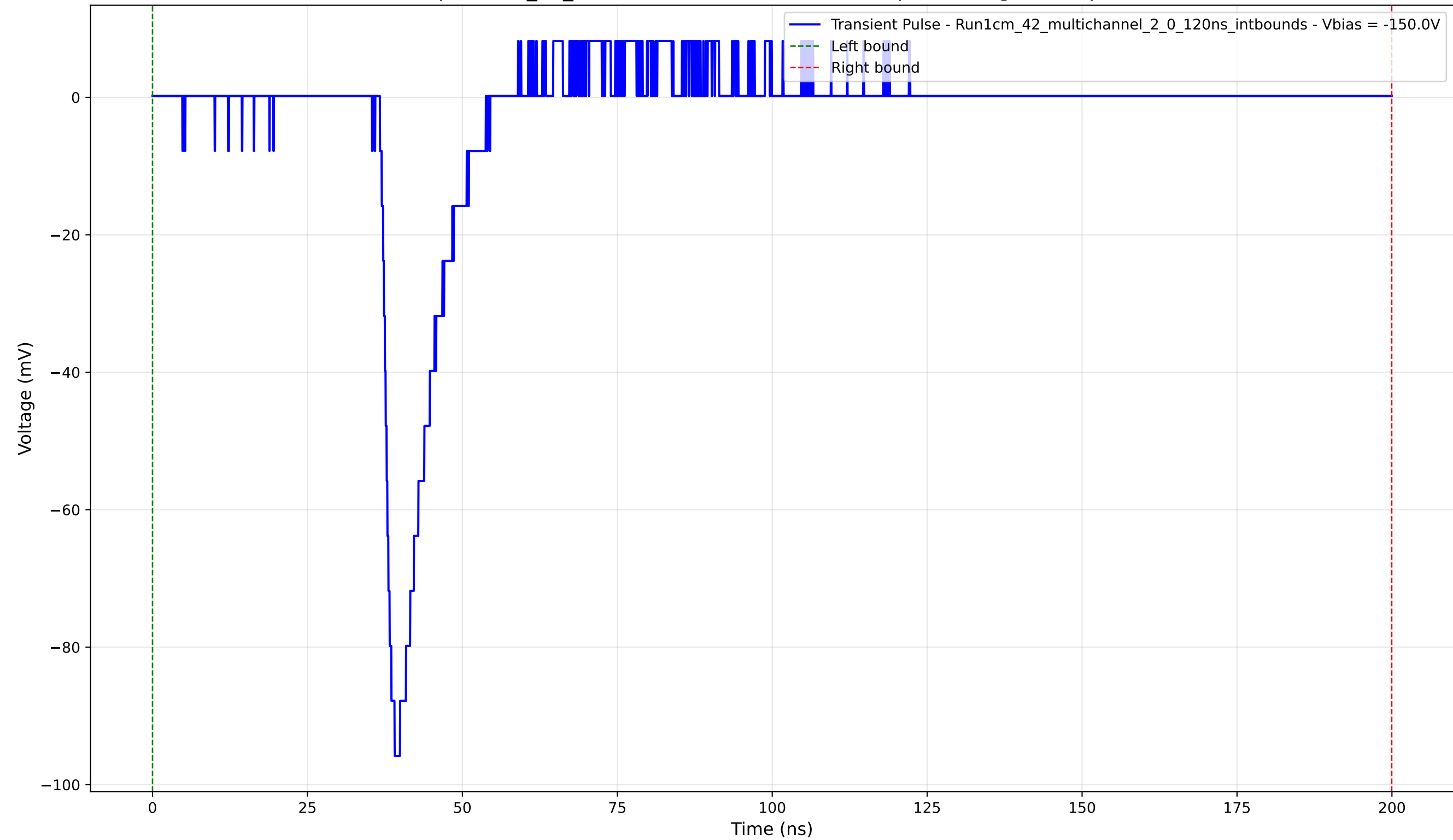
Transient Pulse - Sample: 1cm_42_multichannel - Position: 3990.0 \mu\text{m} - Charge: 9.98 pC - Rise Time: 1.59 ns
