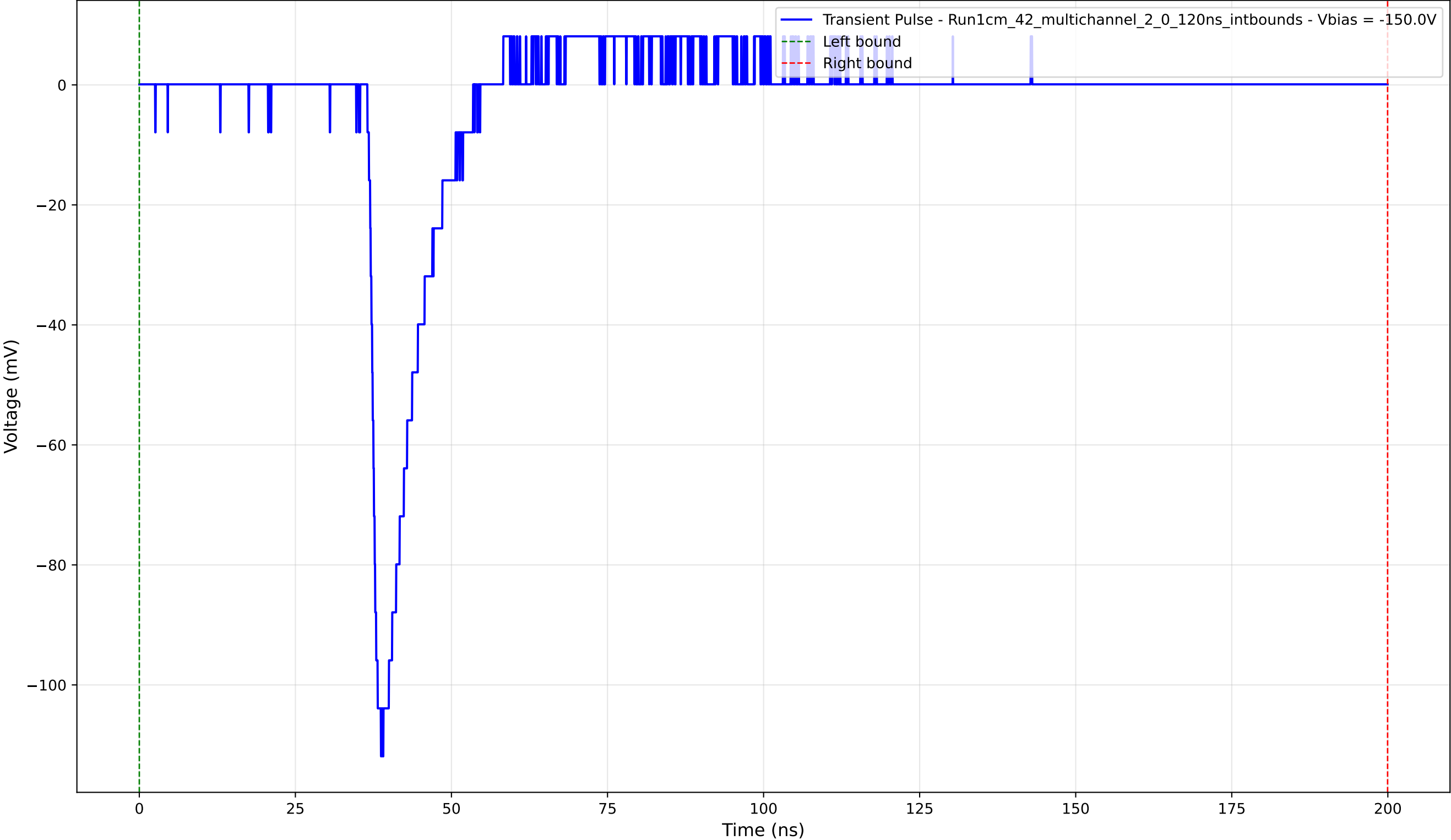
Transient Pulse - Sample: 1cm_42_multichannel - Position: 3715.0 \mu\text{m} - Charge: 10.29 pC - Rise Time: 1.42 ns
