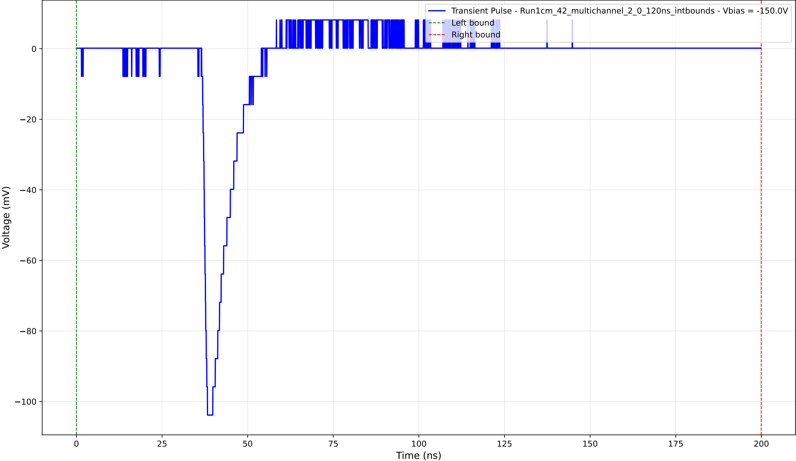
Transient Pulse - Sample: 1cm_42_multichannel - Position: 3765.0 \mu\text{m} - Charge: 10.89 pC - Rise Time: 1.23 ns
