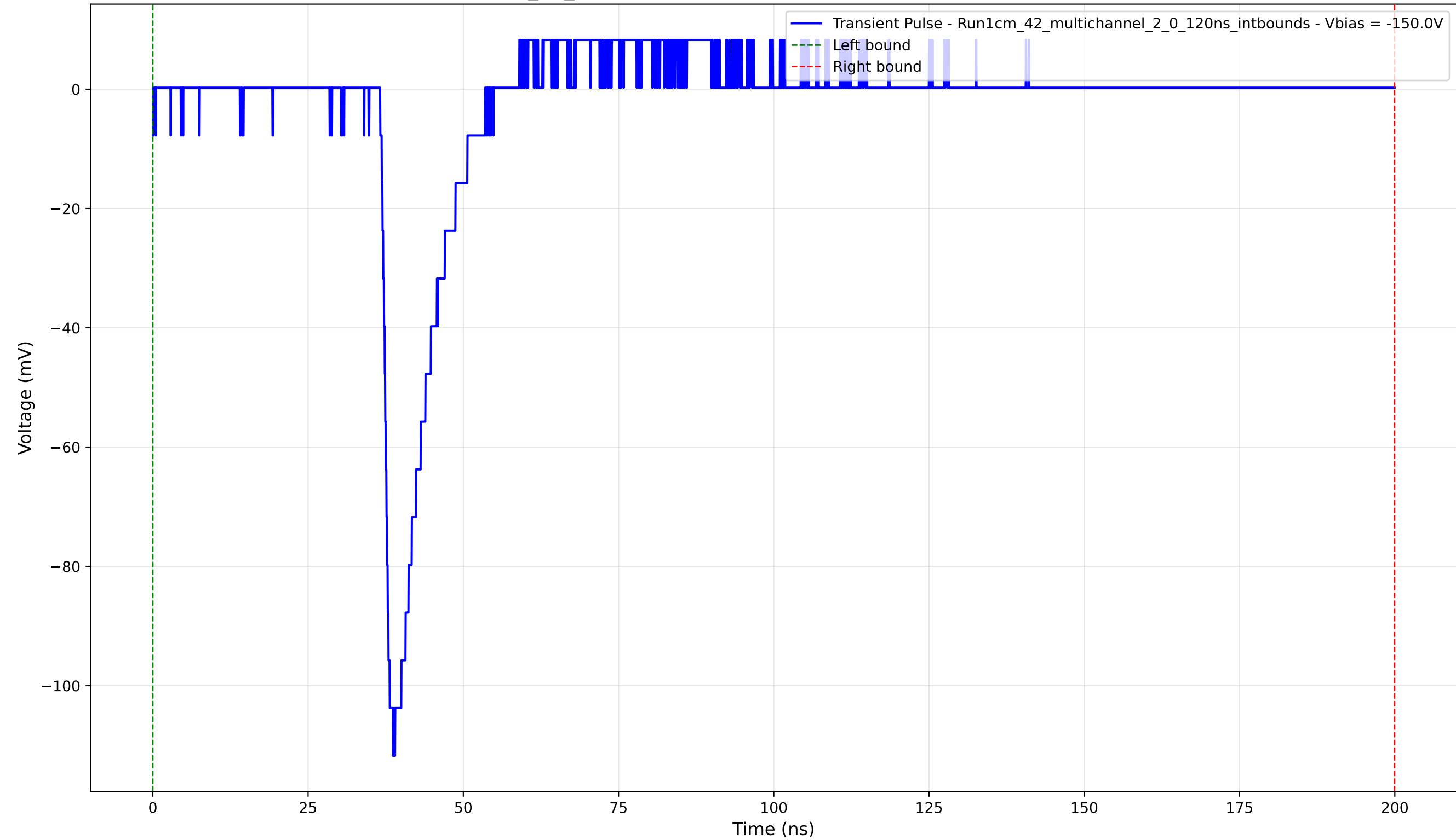
Transient Pulse - Sample: 1cm_42_multichannel - Position: 3735.0 \mu\text{m} - Charge: 9.90 pC - Rise Time: 1.30 ns
