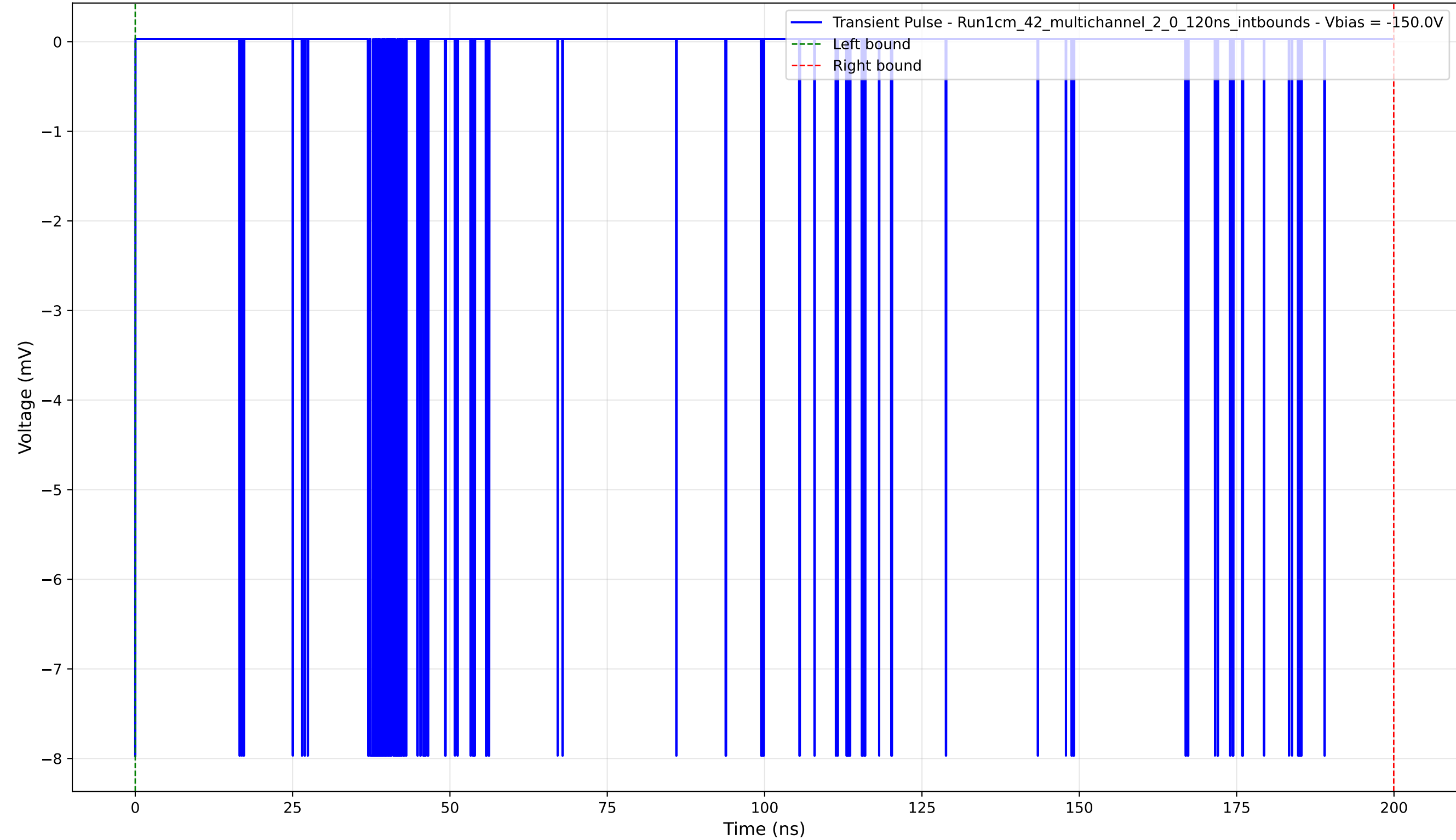
Transient Pulse - Sample: 1cm_42_multichannel - Position: 4890.0 \mu\text{m} - Charge: 1.40 pC - Rise Time: 0.00 ns (N/A)
