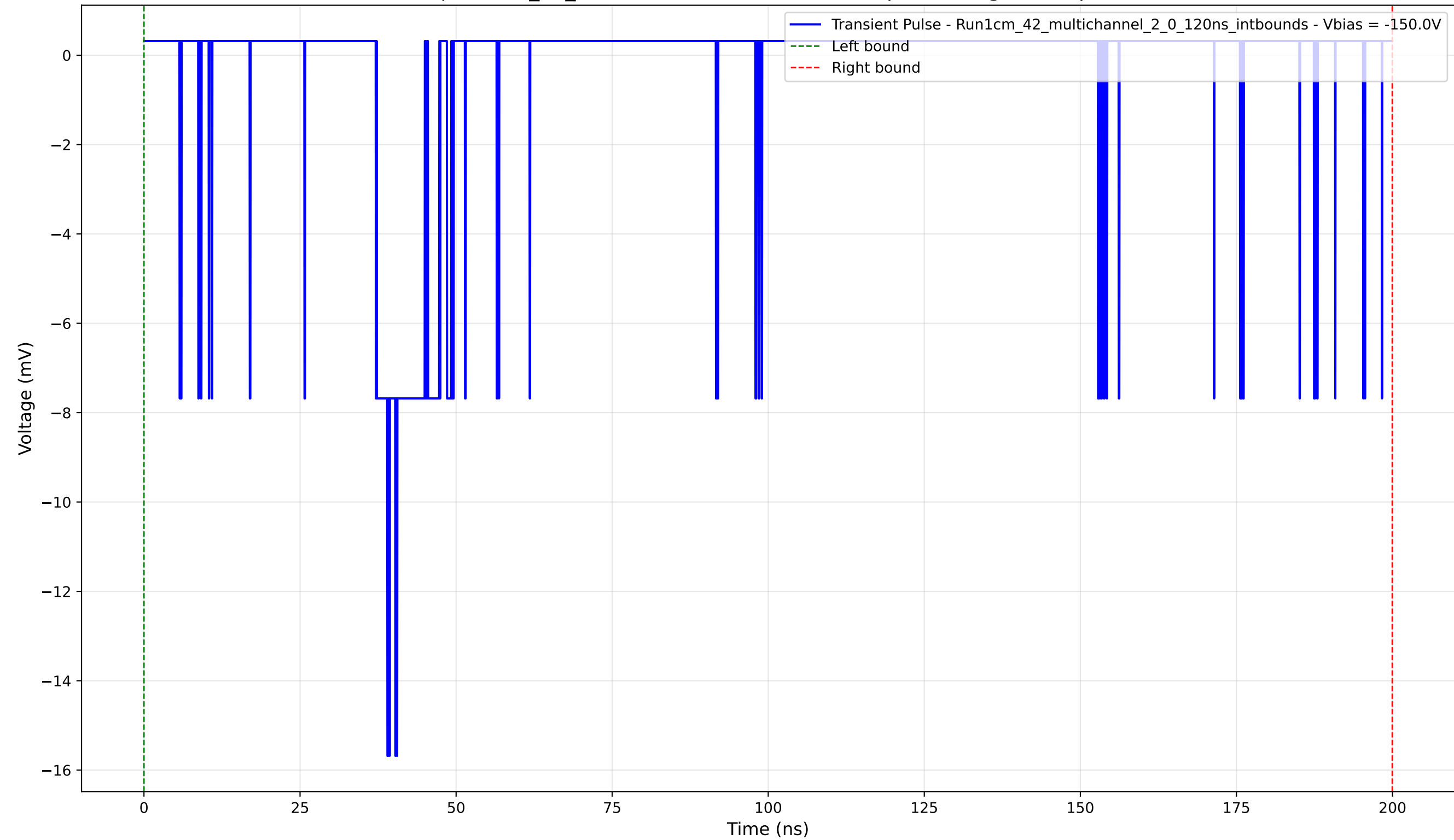
Transient Pulse - Sample: 1cm_42_multichannel - Position: 320.0 \mu\text{m} - Charge: 1.07 pC - Rise Time: 1.71 ns
