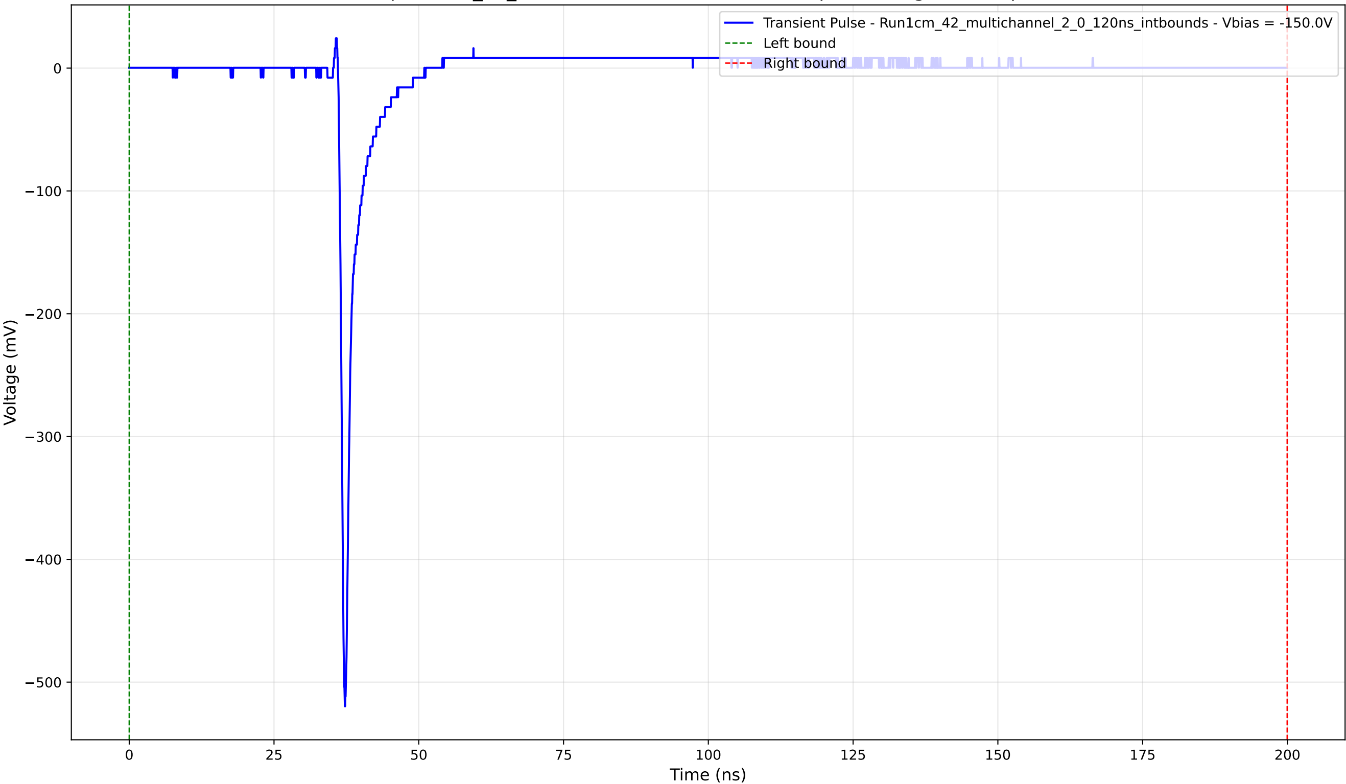
Transient Pulse - Sample: 1cm_42_multichannel - Position: 2135.0 \mu\text{m} - Charge: 14.81 pC - Rise Time: 0.73 ns
