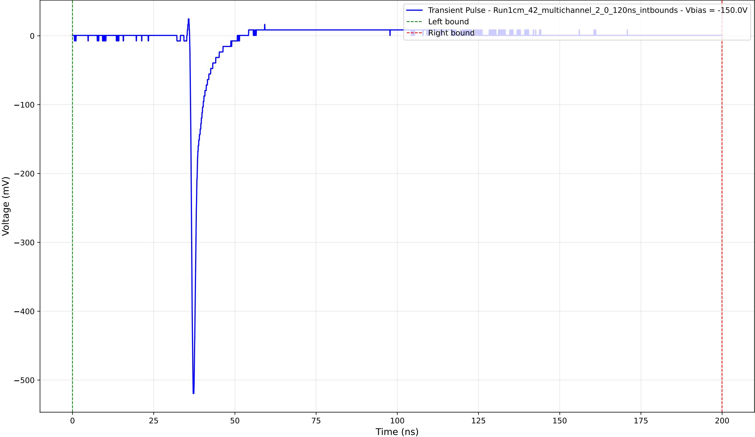
Transient Pulse - Sample: 1cm_42_multichannel - Position: 2150.0 \mu\text{m} - Charge: 14.33 pC - Rise Time: 0.76 ns
