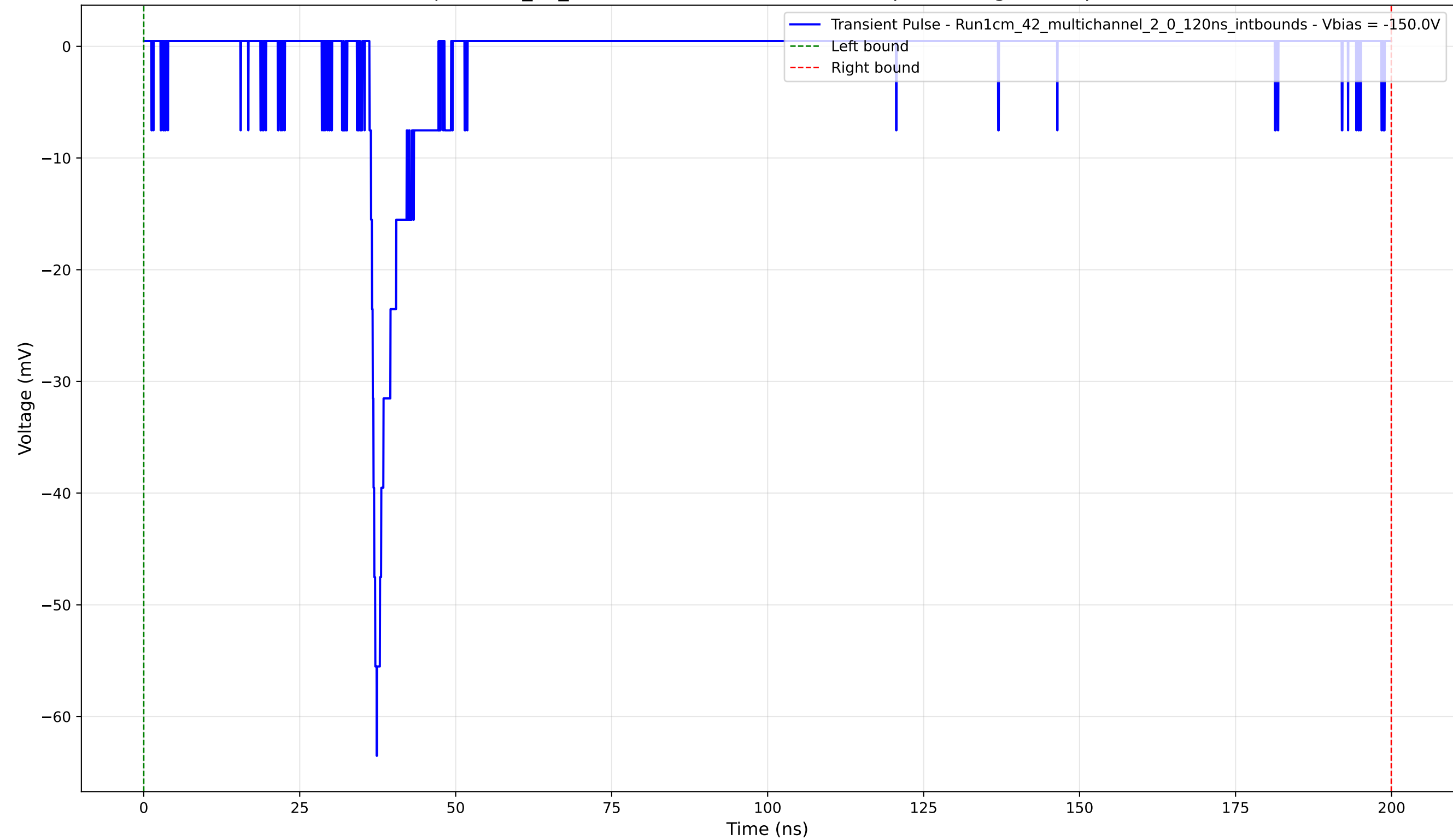
Transient Pulse - Sample: 1cm_42_multichannel - Position: 1895.0 \mu\text{m} - Charge: 3.51 pC - Rise Time: 1.17 ns
