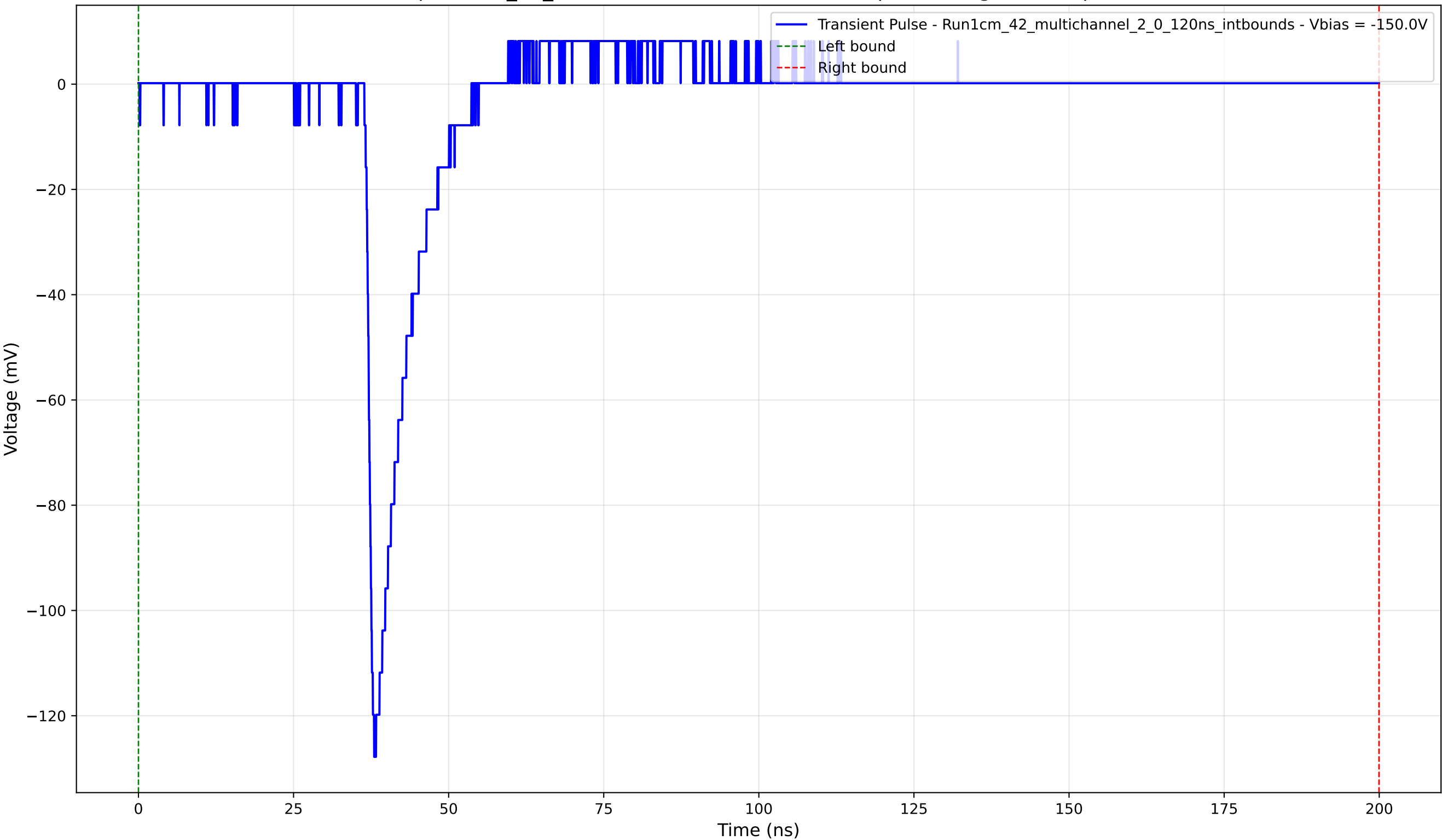
Transient Pulse - Sample: 1cm_42_multichannel - Position: 3455.0 \mu\text{m} - Charge: 10.82 pC - Rise Time: 1.18 ns
