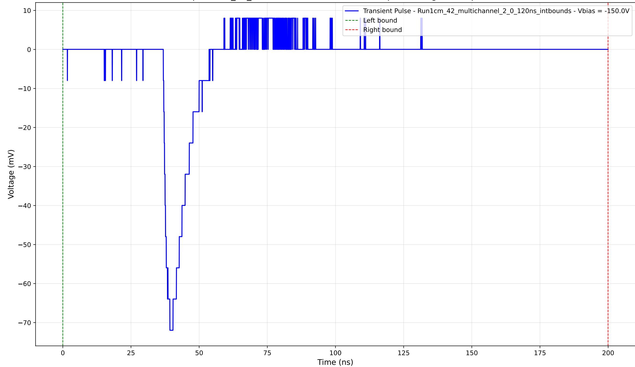
Transient Pulse - Sample: 1cm_42_multichannel - Position: 155.0 \mu\text{m} - Charge: 8.88 pC - Rise Time: 2.40 ns
