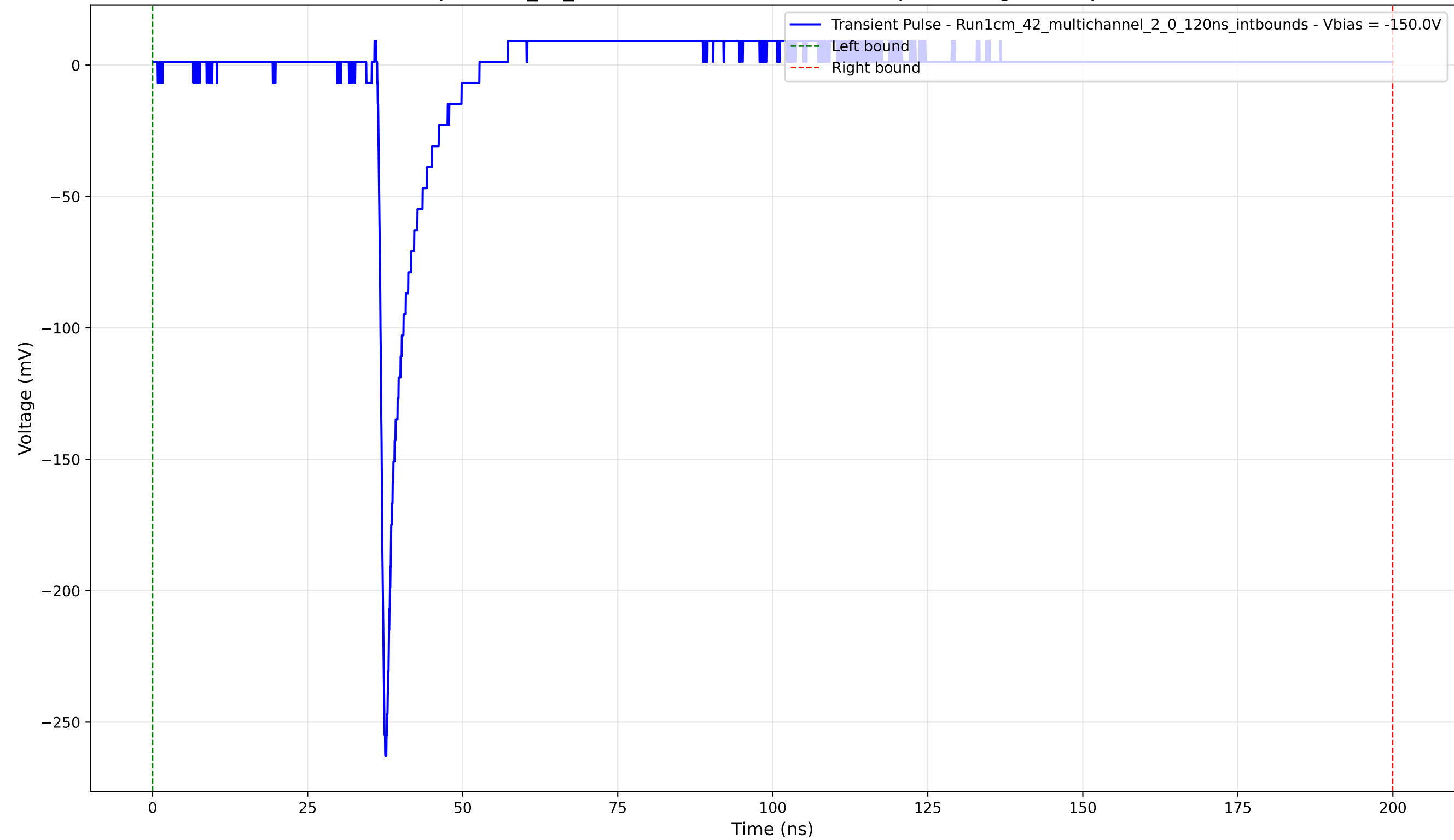
Transient Pulse - Sample: 1cm_42_multichannel - Position: 3005.0 \mu\text{m} - Charge: 8.40 pC - Rise Time: 0.89 ns
