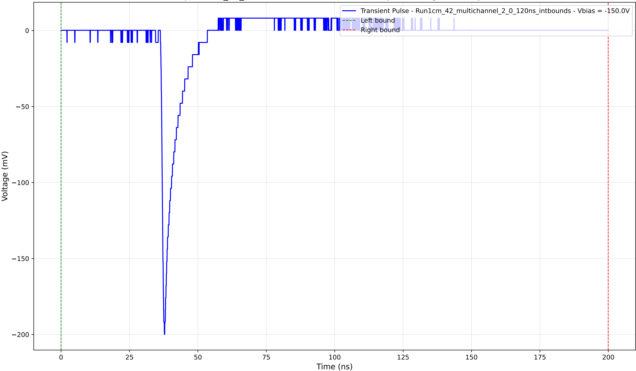
Transient Pulse - Sample: 1cm_42_multichannel - Position: 3170.0 \mu\text{m} - Charge: 11.49 pC - Rise Time: 0.98 ns
