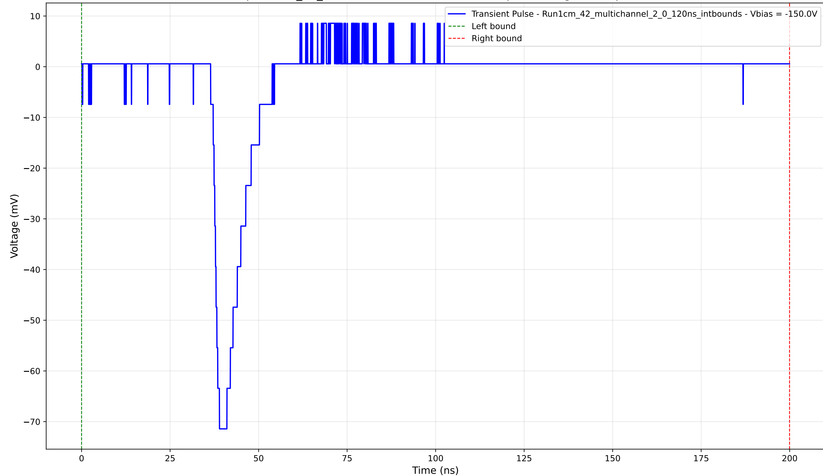
Transient Pulse - Sample: 1cm_42_multichannel - Position: 4535.0 \mu\text{m} - Charge: 8.33 pC - Rise Time: 2.48 ns
