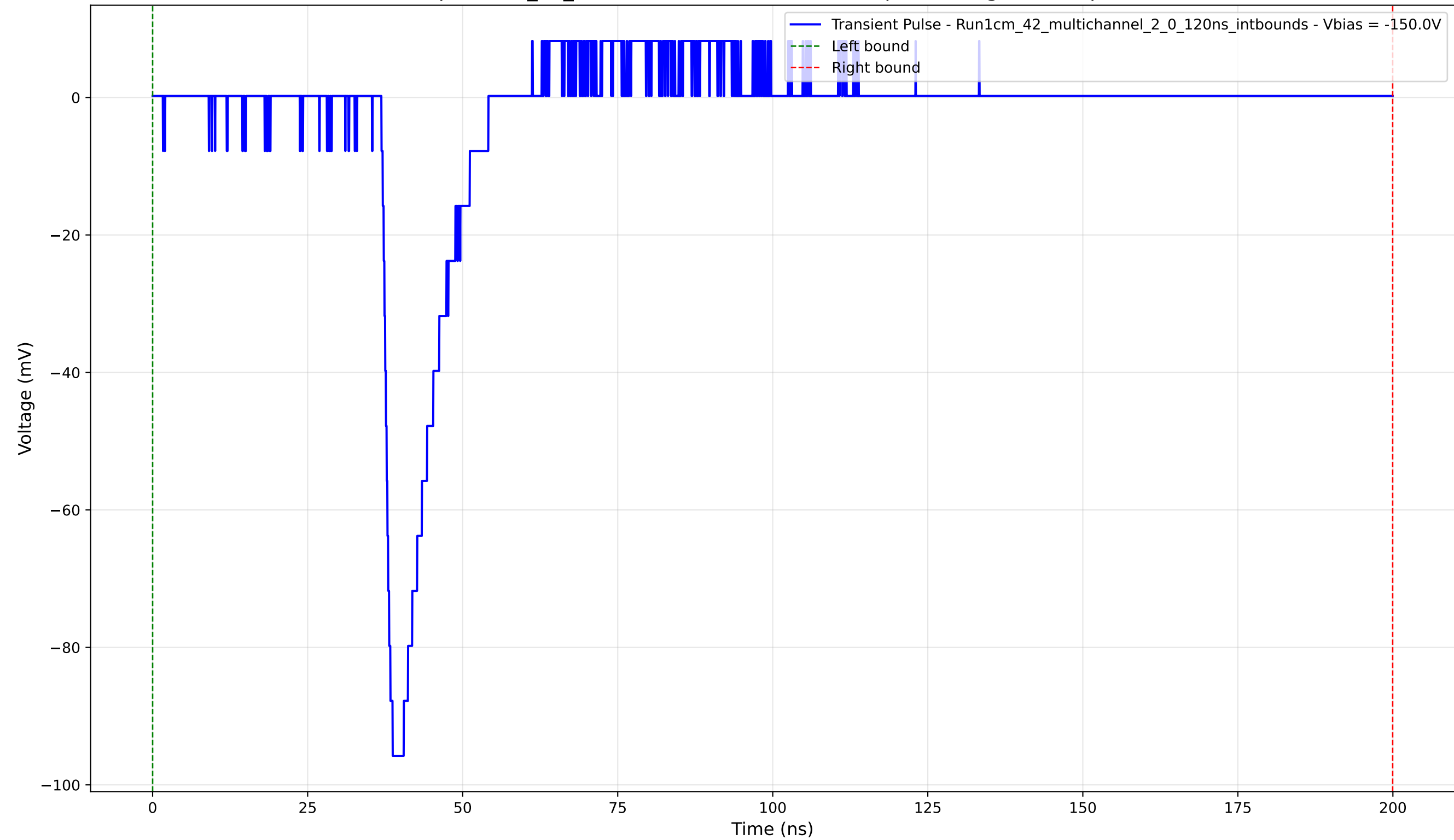
Transient Pulse - Sample: 1cm_42_multichannel - Position: 575.0 \mu\text{m} - Charge: 10.15 pC - Rise Time: 1.27 ns
