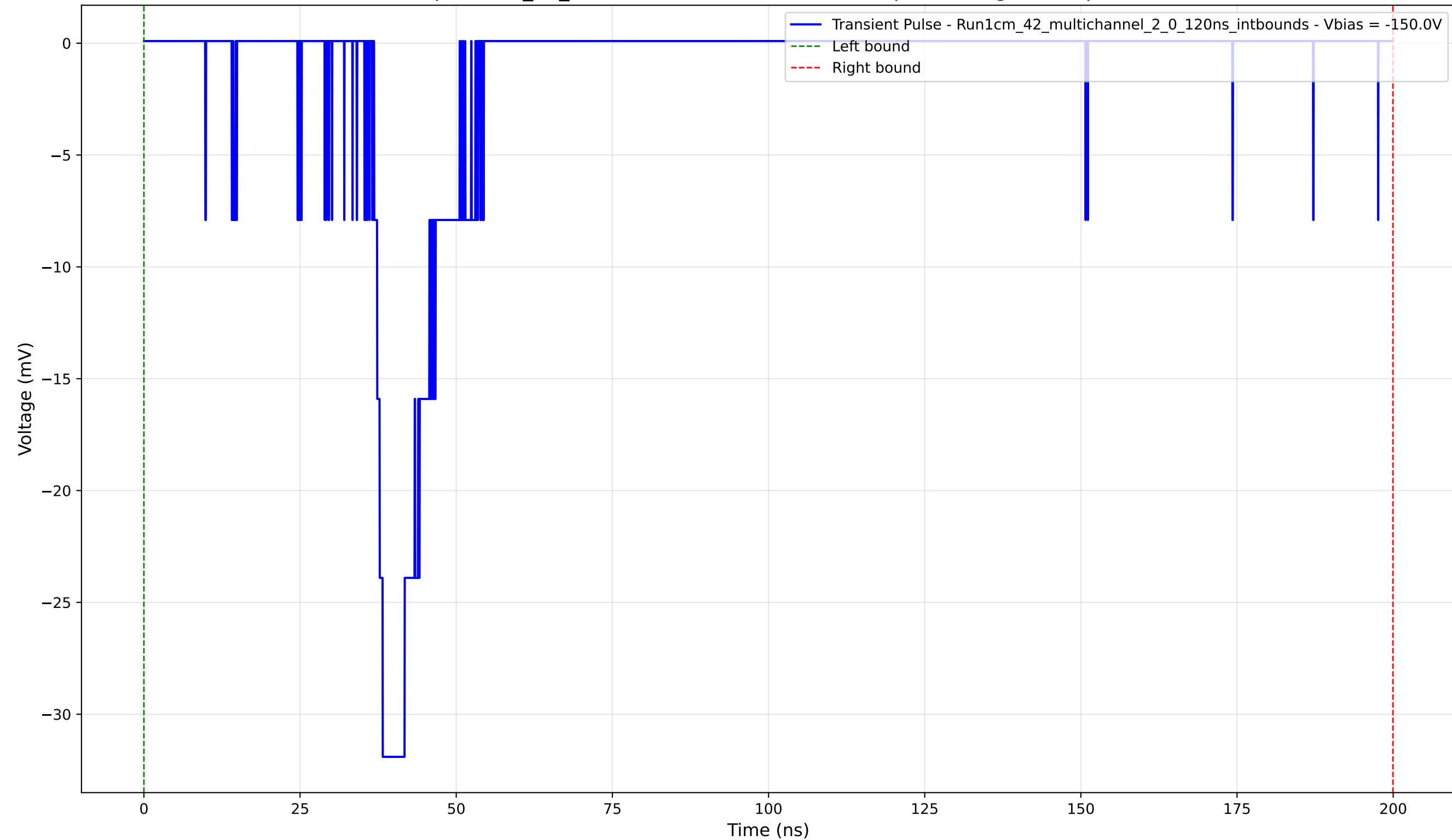
Transient Pulse - Sample: 1cm_42_multichannel - Position: 3930.0 \mu\text{m} - Charge: 5.56 pC - Rise Time: 1.38 ns
