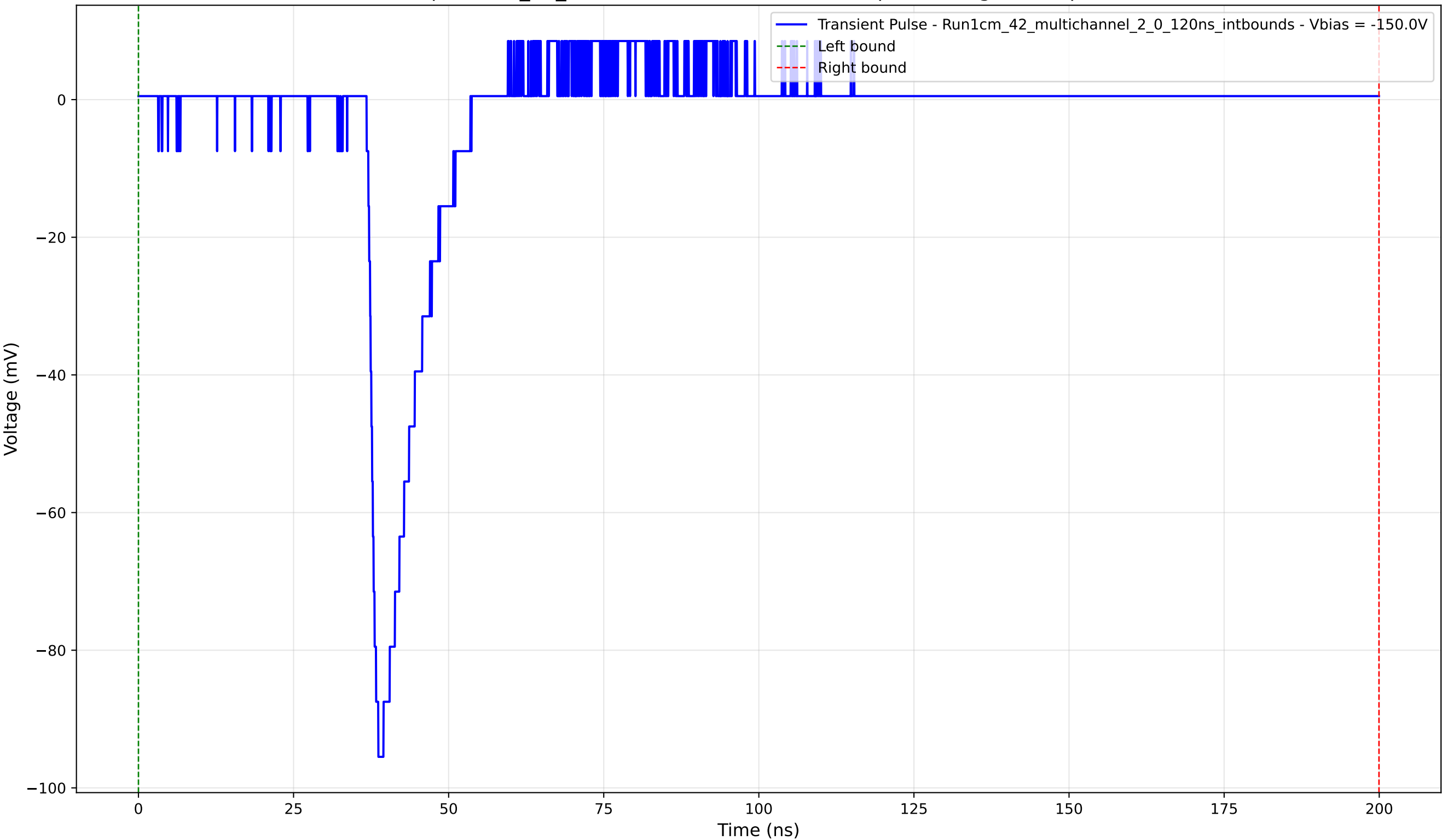
Transient Pulse - Sample: 1cm_42_multichannel - Position: 775.0 \mu\text{m} - Charge: 8.78 pC - Rise Time: 1.27 ns
