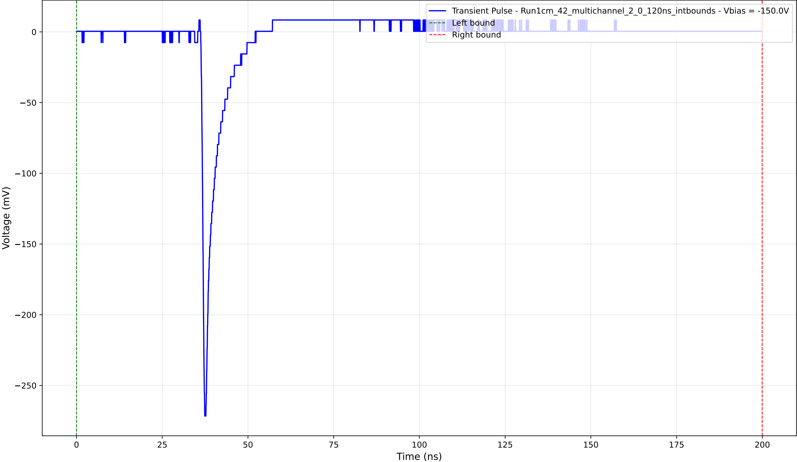
Transient Pulse - Sample: 1cm_42_multichannel - Position: 2965.0 \mu\text{m} - Charge: 11.46 pC - Rise Time: 0.85 ns
