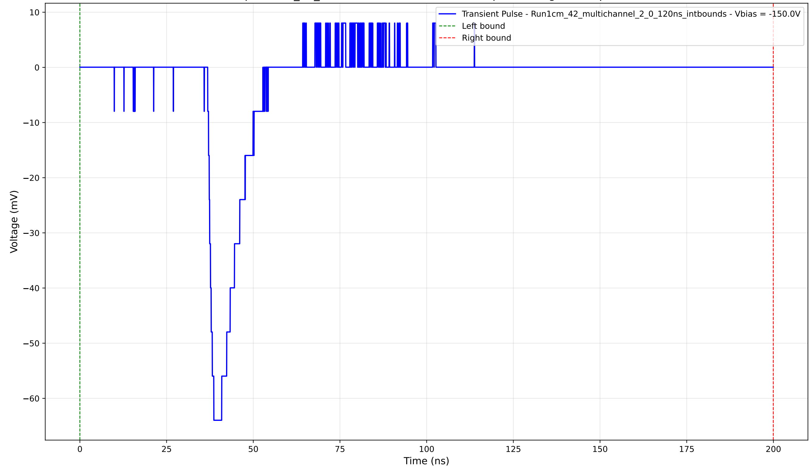
Transient Pulse - Sample: 1cm_42_multichannel - Position: 270.0 \mu\text{m} - Charge: 9.15 pC - Rise Time: 1.77 ns
