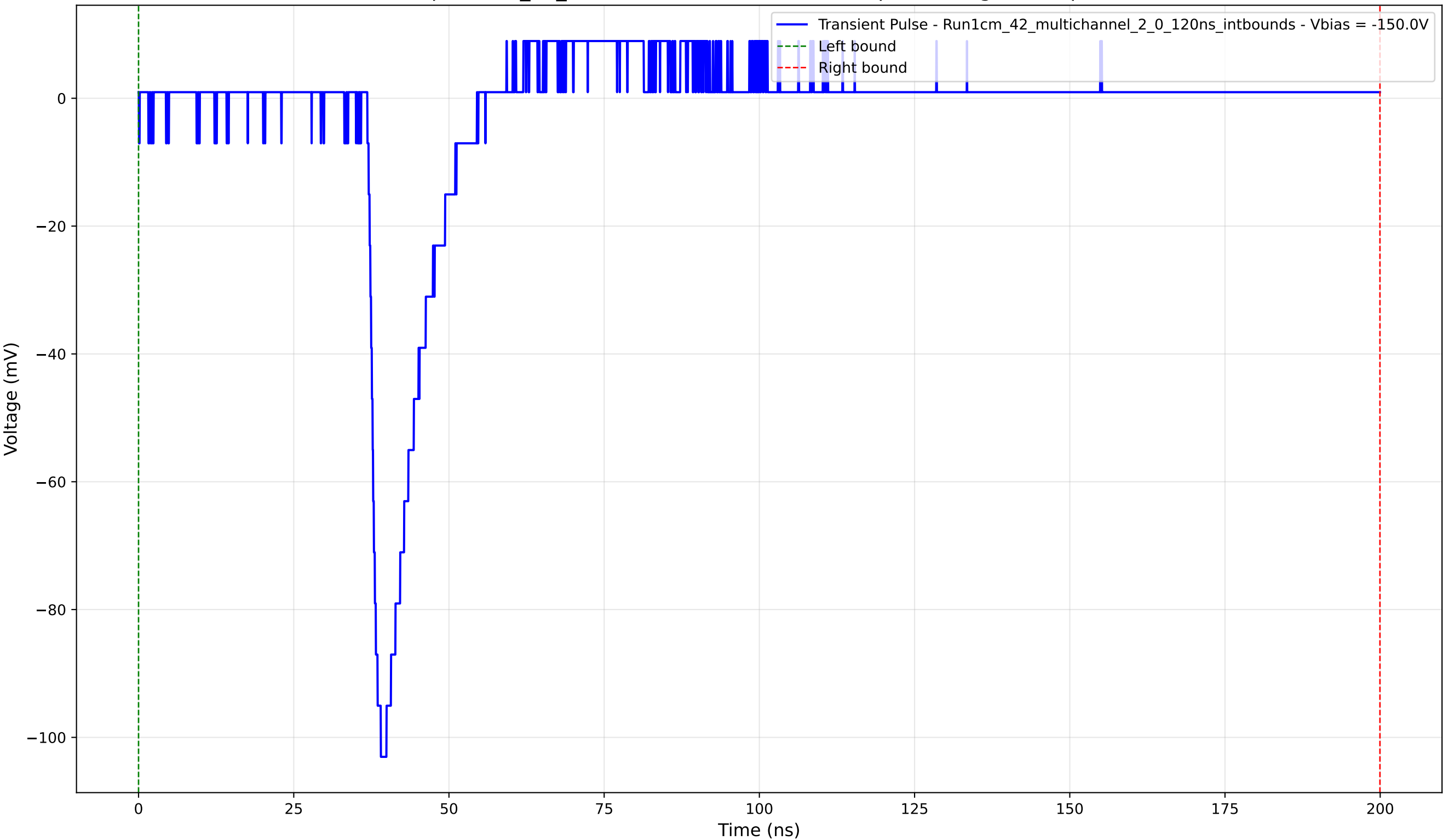
Transient Pulse - Sample: 1cm_42_multichannel - Position: 655.0 \mu\text{m} - Charge: 7.87 pC - Rise Time: 1.46 ns
