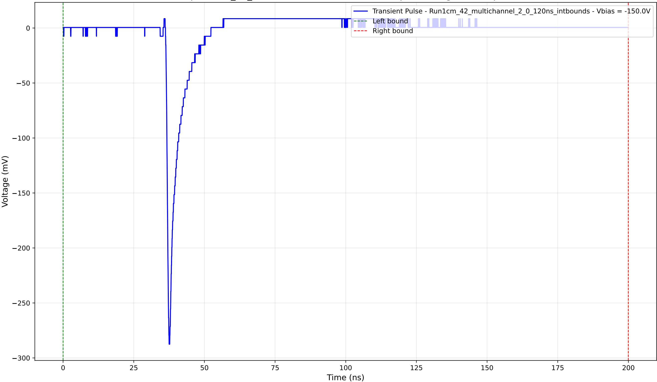
Transient Pulse - Sample: 1cm_42_multichannel - Position: 1730.0 \mu\text{m} - Charge: 12.09 pC - Rise Time: 0.89 ns
