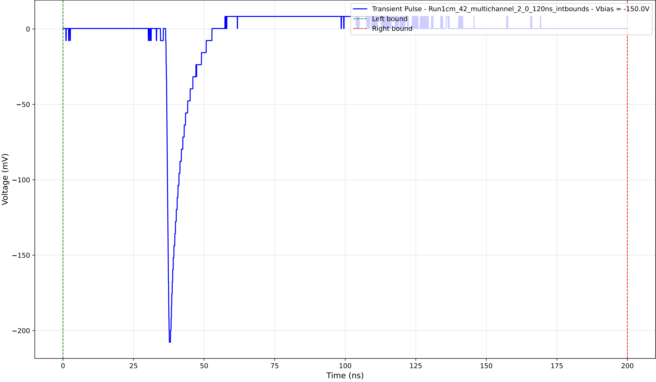
Transient Pulse - Sample: 1cm_42_multichannel - Position: 1495.0 \mu\text{m} - Charge: 10.40 pC - Rise Time: 0.97 ns
