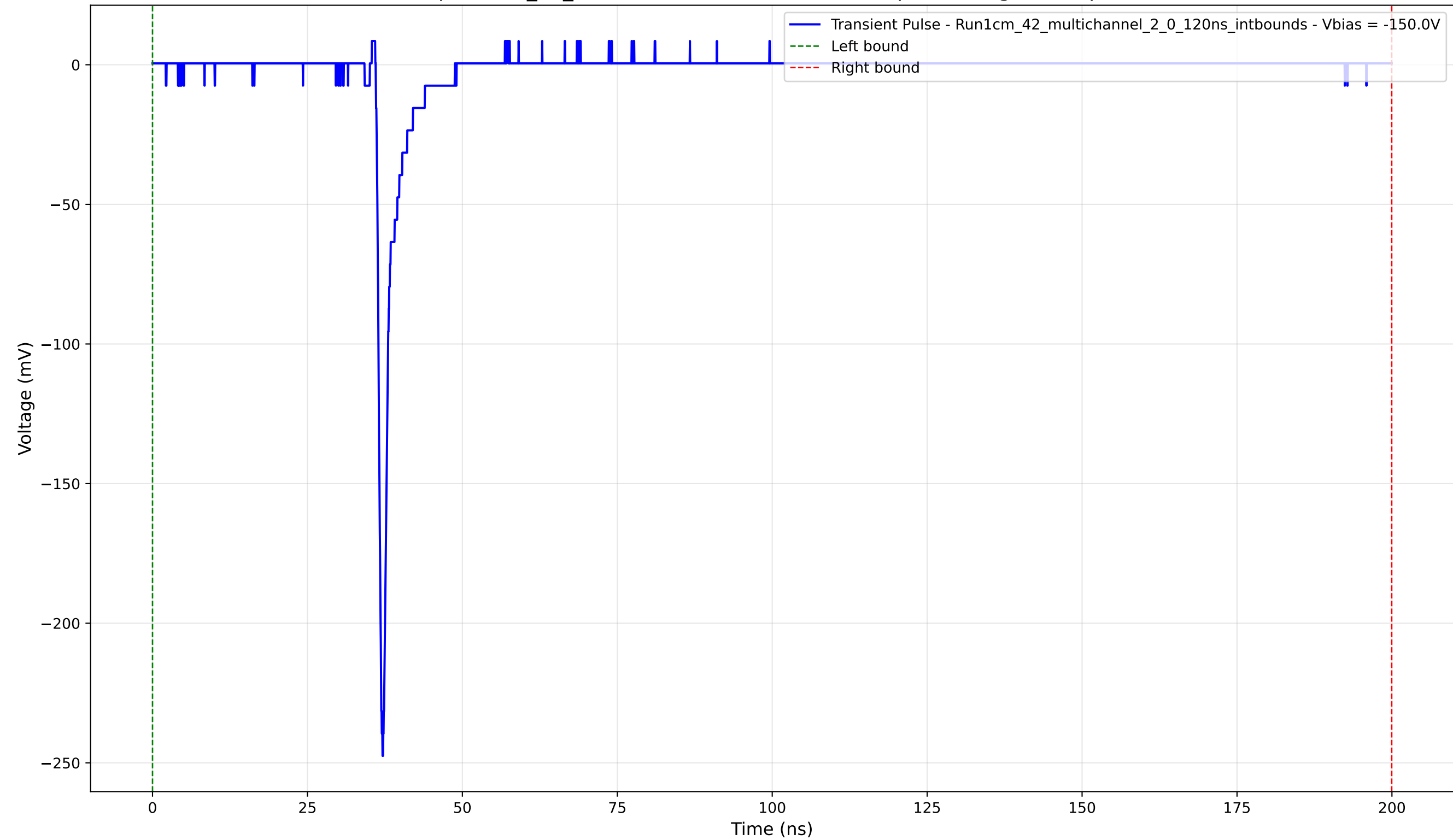
Transient Pulse - Sample: 1cm_42_multichannel - Position: 2415.0 \mu\text{m} - Charge: 9.26 pC - Rise Time: 0.71 ns
