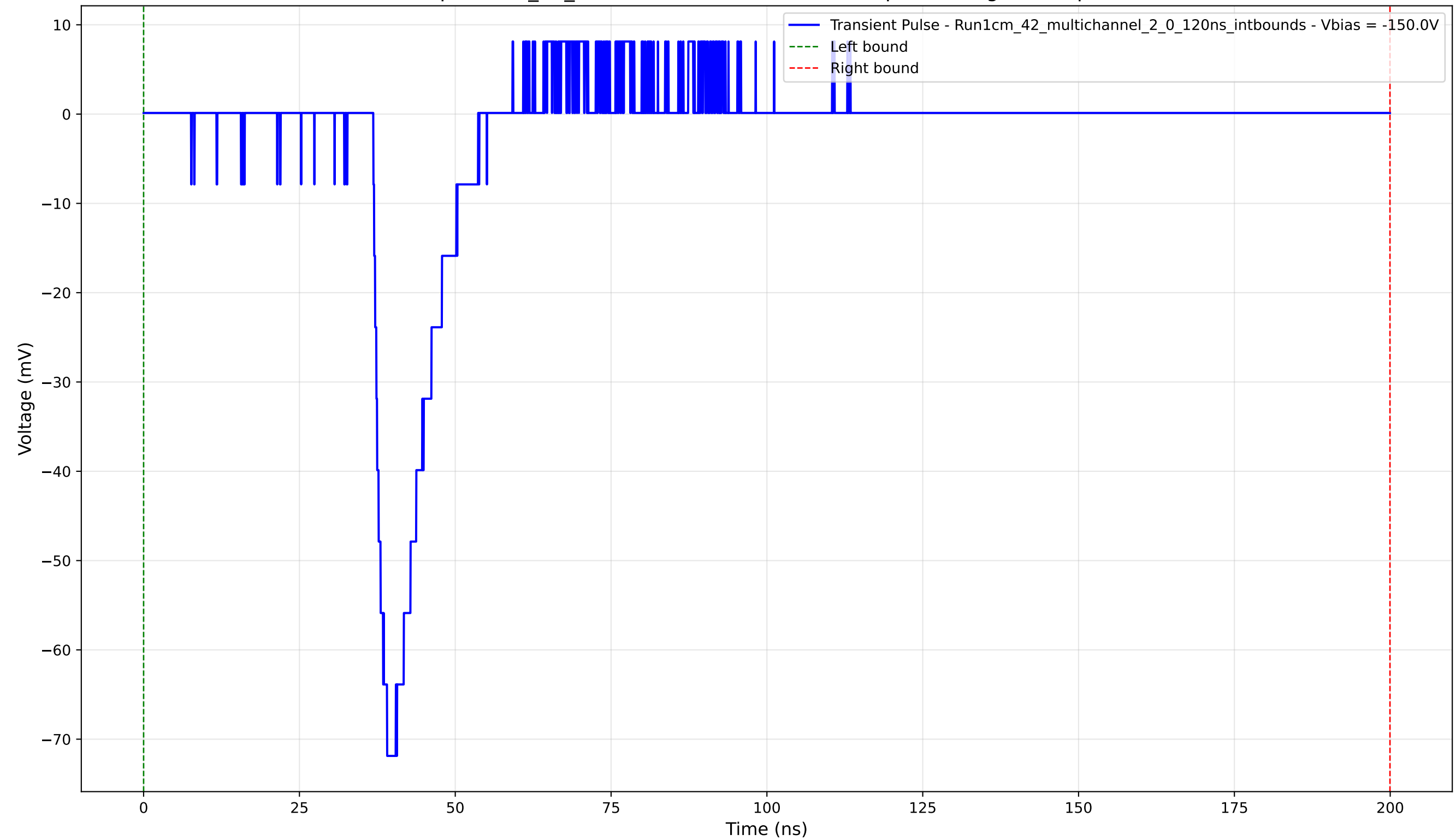
Transient Pulse - Sample: 1cm_42_multichannel - Position: 160.0 \mu\text{m} - Charge: 8.97 pC - Rise Time: 2.20 ns
