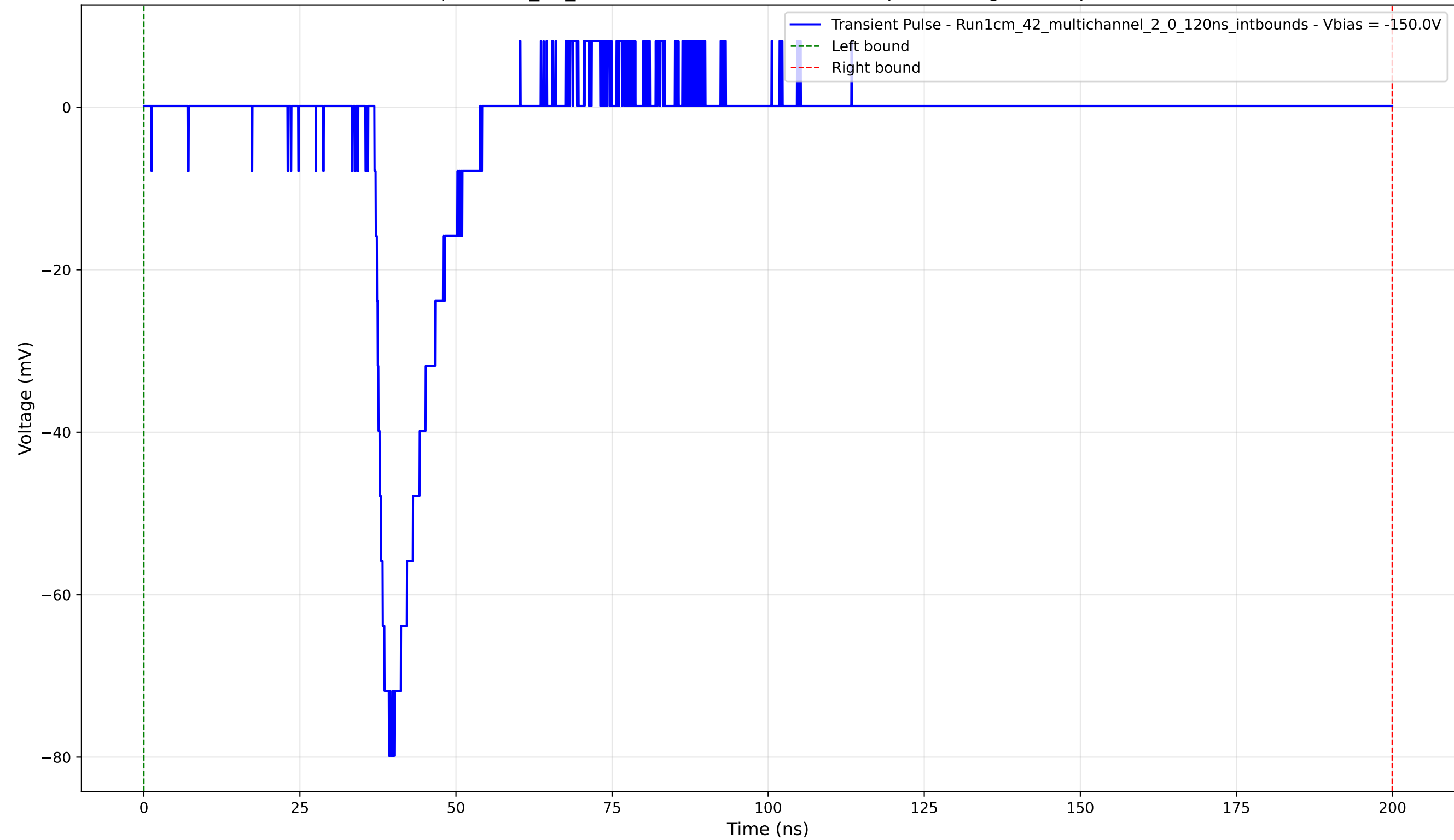
Transient Pulse - Sample: 1cm_42_multichannel - Position: 415.0 \mu\text{m} - Charge: 9.90 pC - Rise Time: 2.16 ns
