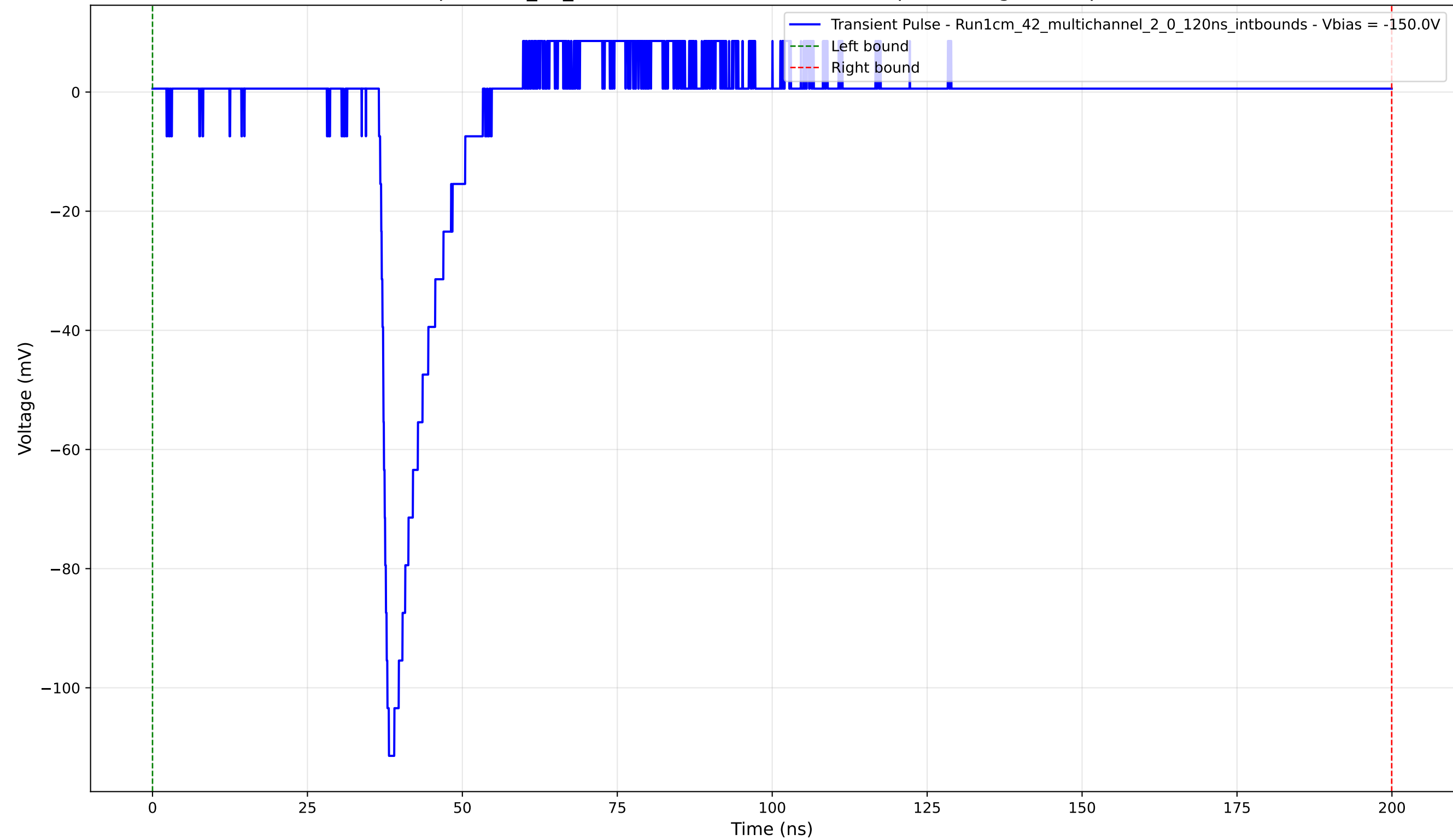
Transient Pulse - Sample: 1cm_42_multichannel - Position: 3625.0 \mu\text{m} - Charge: 8.98 pC - Rise Time: 1.18 ns
