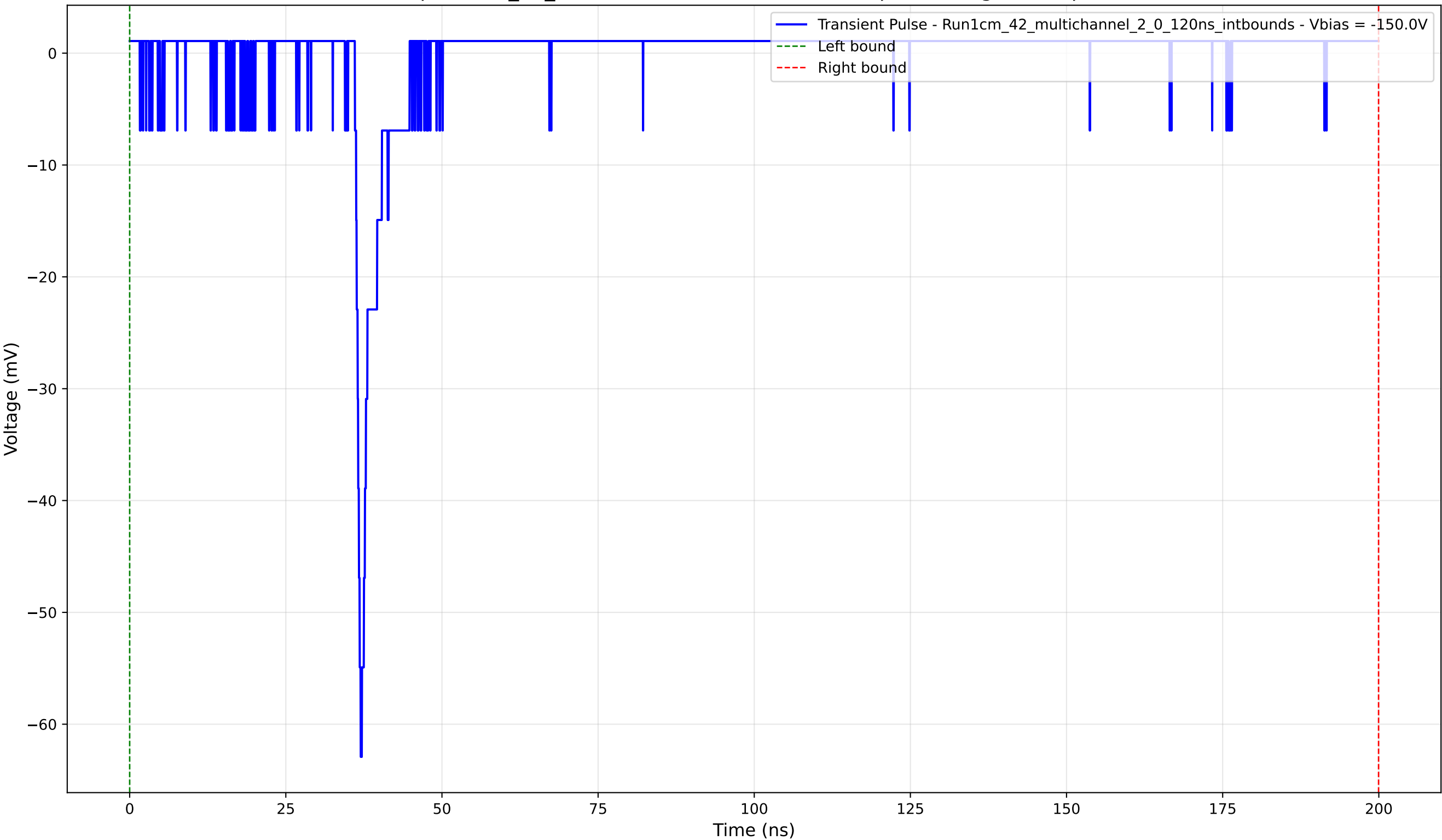
Transient Pulse - Sample: 1cm_42_multichannel - Position: 2395.0 \mu\text{m} - Charge: 0.22 pC - Rise Time: 0.92 ns
