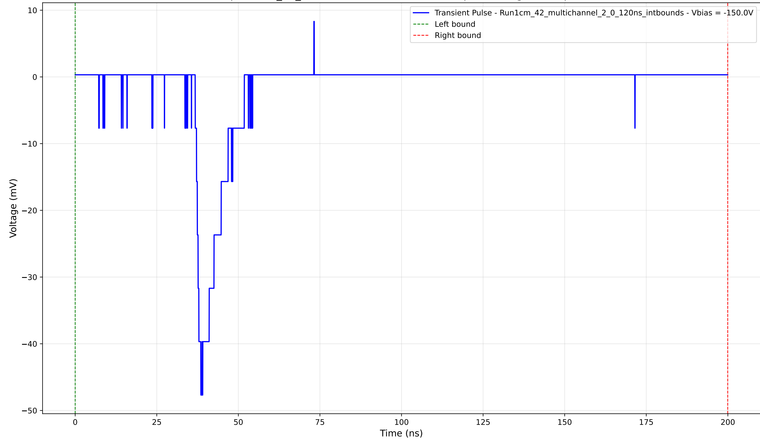
Transient Pulse - Sample: 1cm_42_multichannel - Position: 895.0 \mu\text{m} - Charge: 5.52 pC - Rise Time: 1.74 ns
