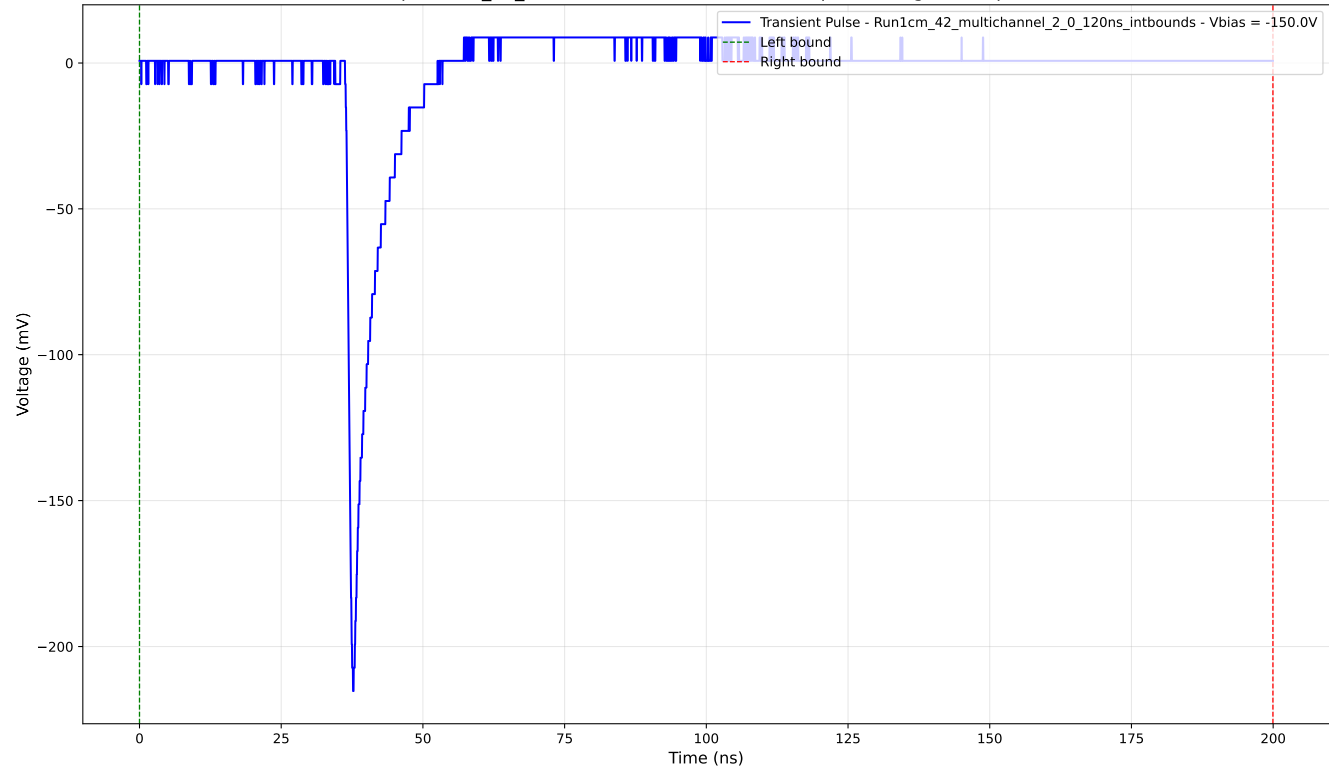
Transient Pulse - Sample: 1cm_42_multichannel - Position: 3110.0 \mu\text{m} - Charge: 9.77 pC - Rise Time: 0.97 ns
