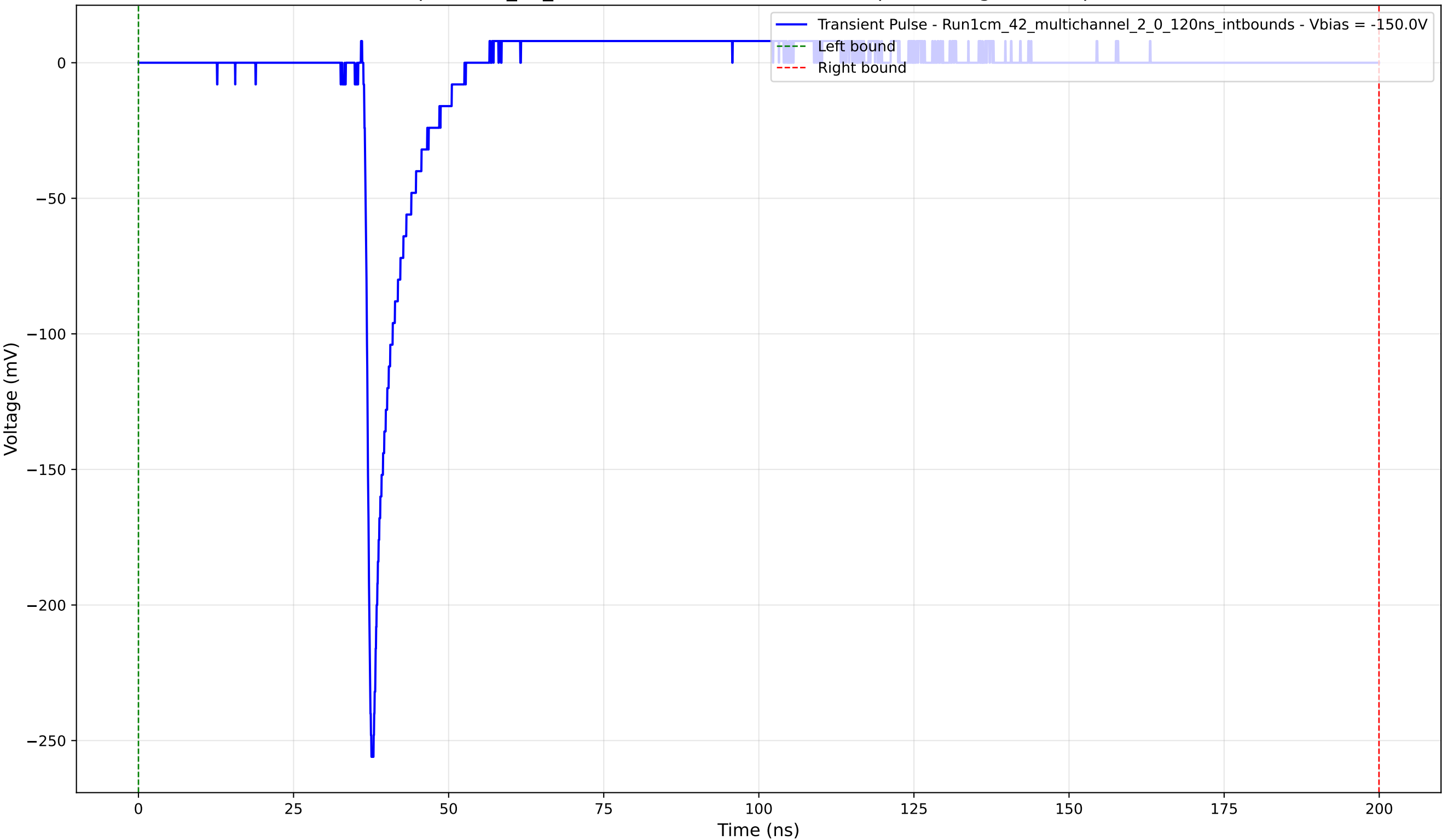
Transient Pulse - Sample: 1cm_42_multichannel - Position: 1655.0 \mu\text{m} - Charge: 12.73 pC - Rise Time: 0.86 ns
