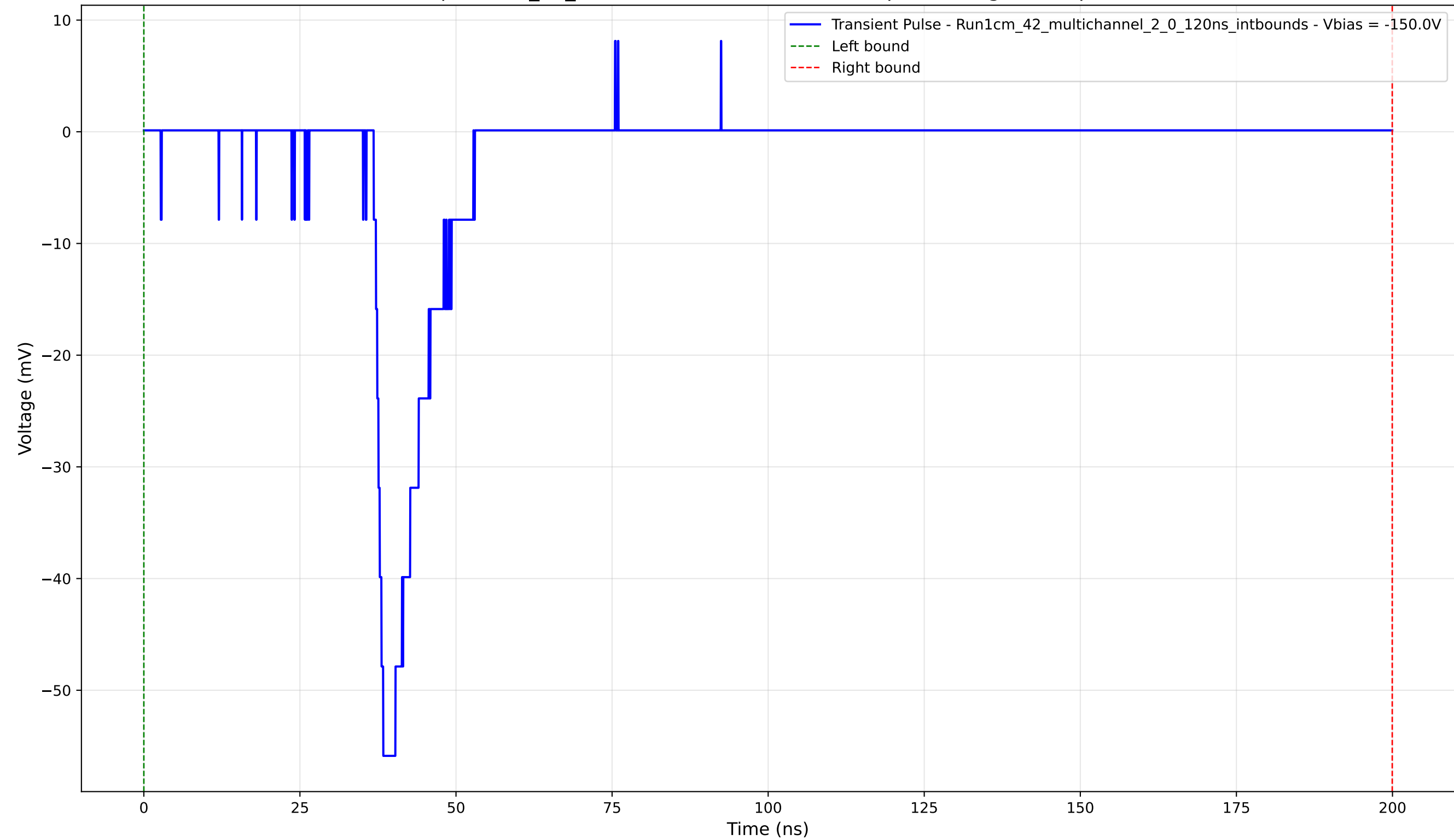
Transient Pulse - Sample: 1cm_42_multichannel - Position: 800.0 \mu\text{m} - Charge: 8.06 pC - Rise Time: 1.53 ns
