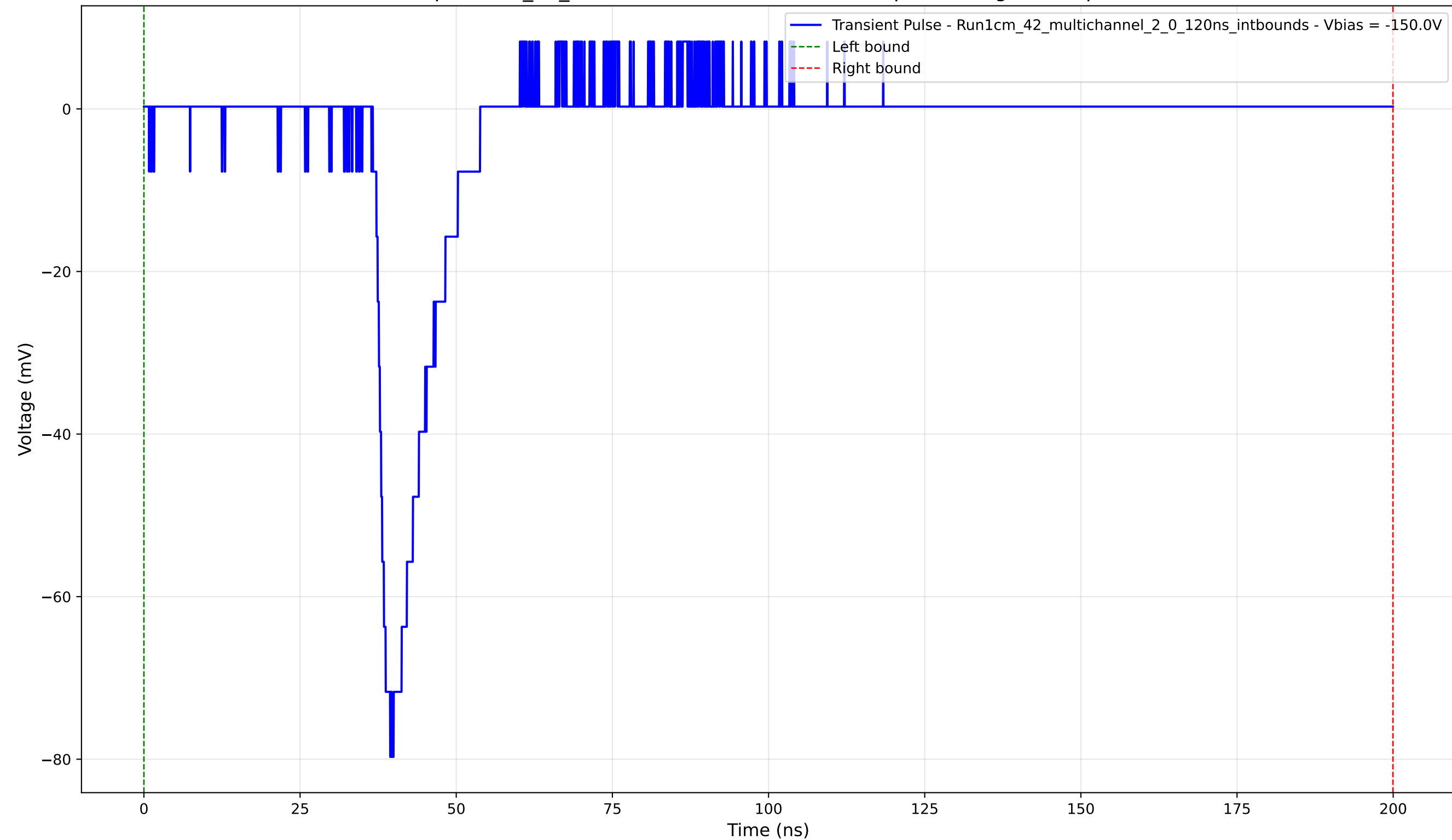
Transient Pulse - Sample: 1cm_42_multichannel - Position: 4265.0 \mu\text{m} - Charge: 9.35 pC - Rise Time: 2.24 ns
