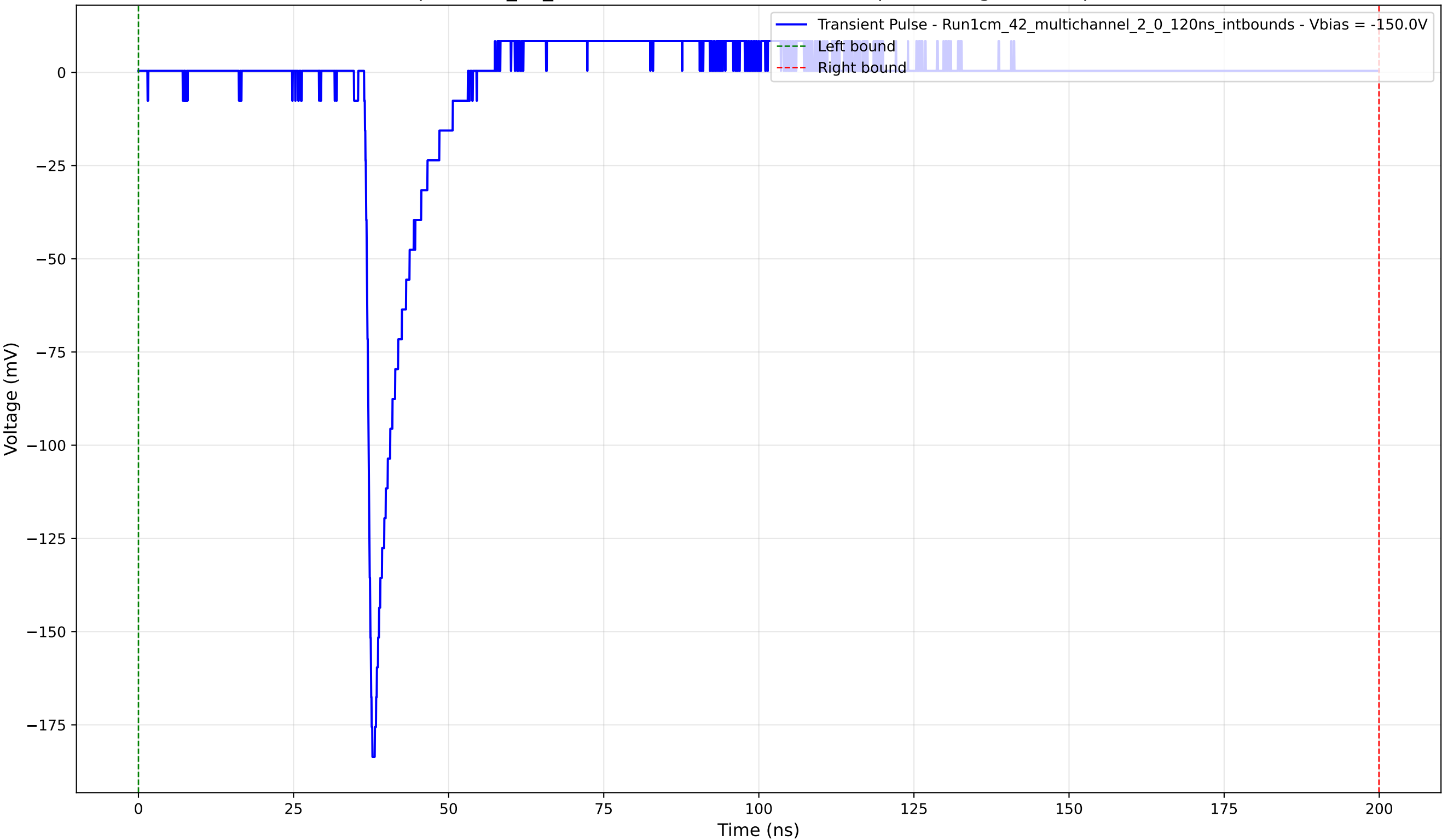
Transient Pulse - Sample: 1cm_42_multichannel - Position: 3255.0 \mu\text{m} - Charge: 10.08 pC - Rise Time: 0.95 ns
