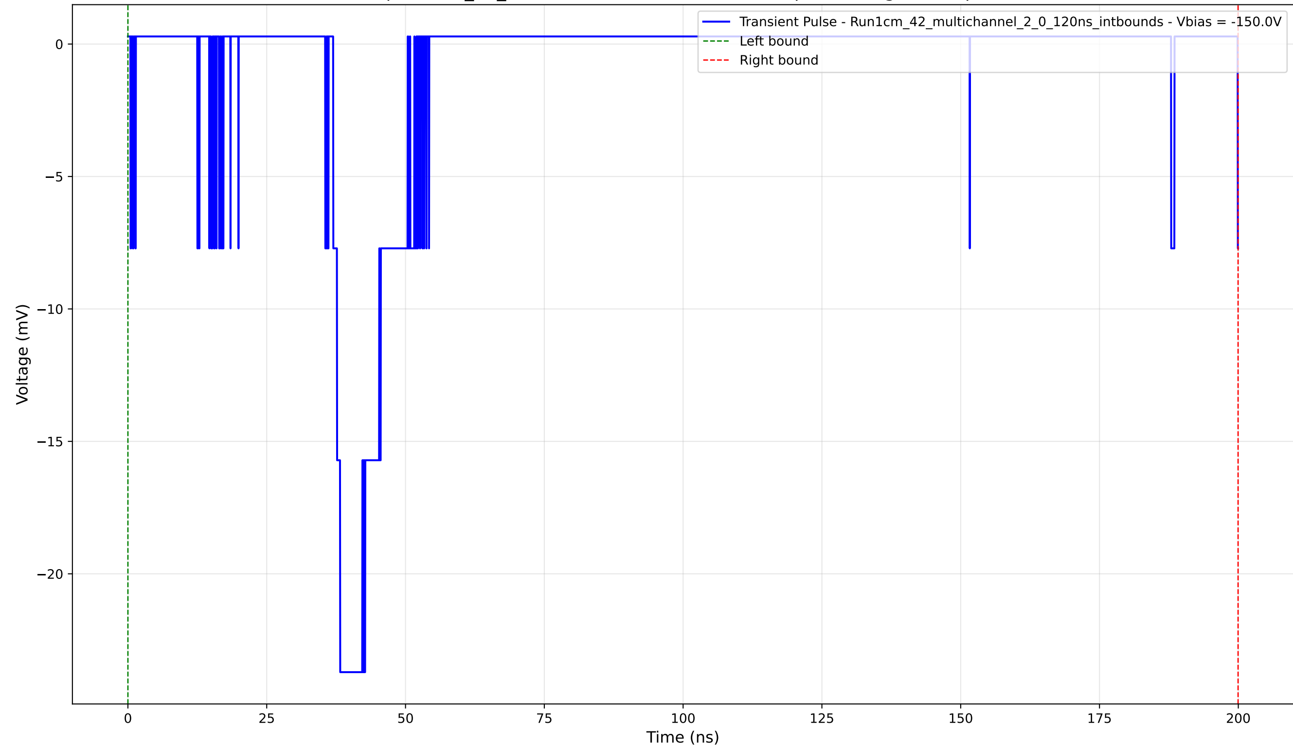
Transient Pulse - Sample: 1cm_42_multichannel - Position: 4345.0 \mu\text{m} - Charge: 3.66 pC - Rise Time: 1.27 ns
