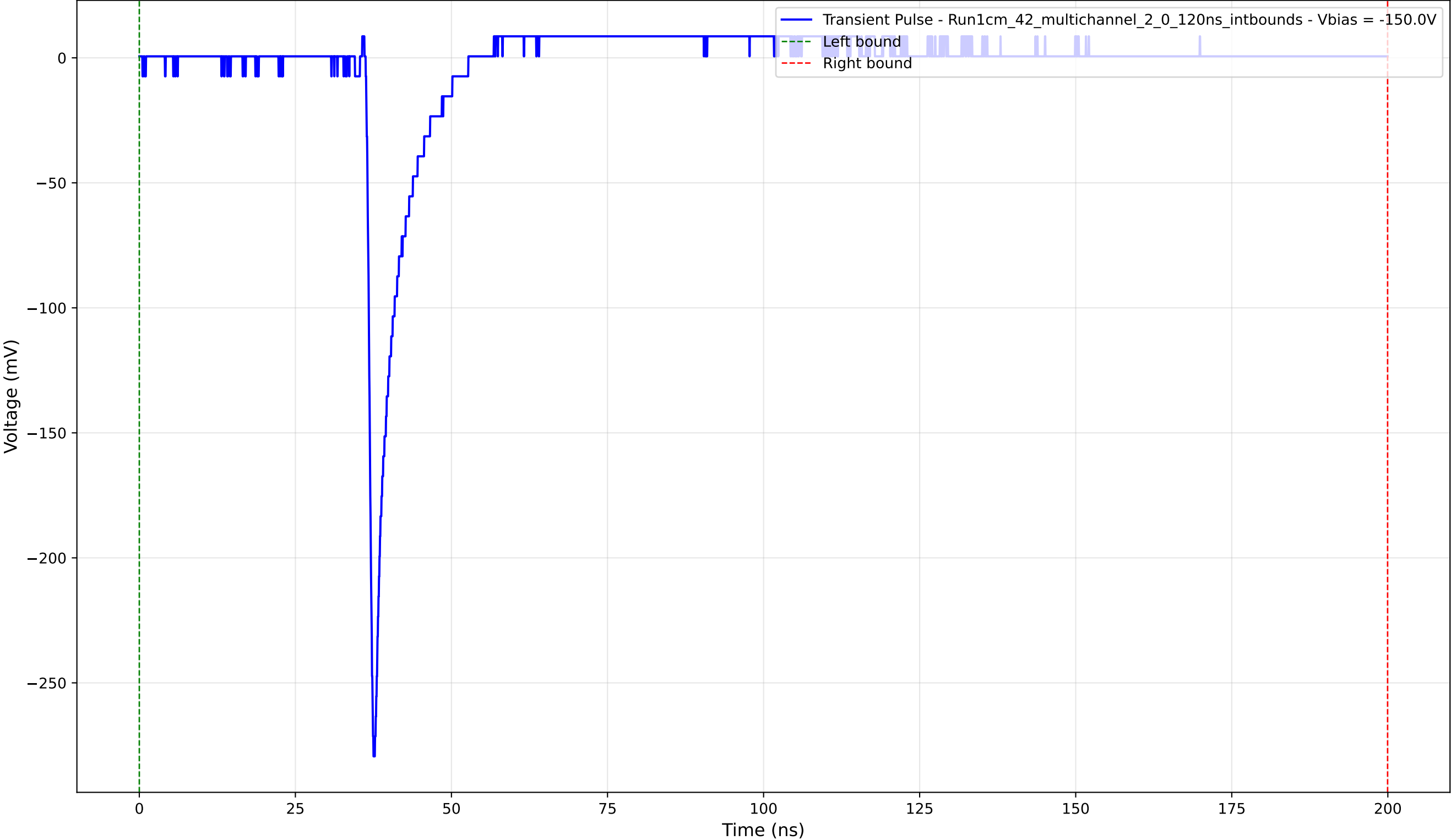
Transient Pulse - Sample: 1cm_42_multichannel - Position: 1710.0 \mu\text{m} - Charge: 11.65 pC - Rise Time: 0.92 ns
