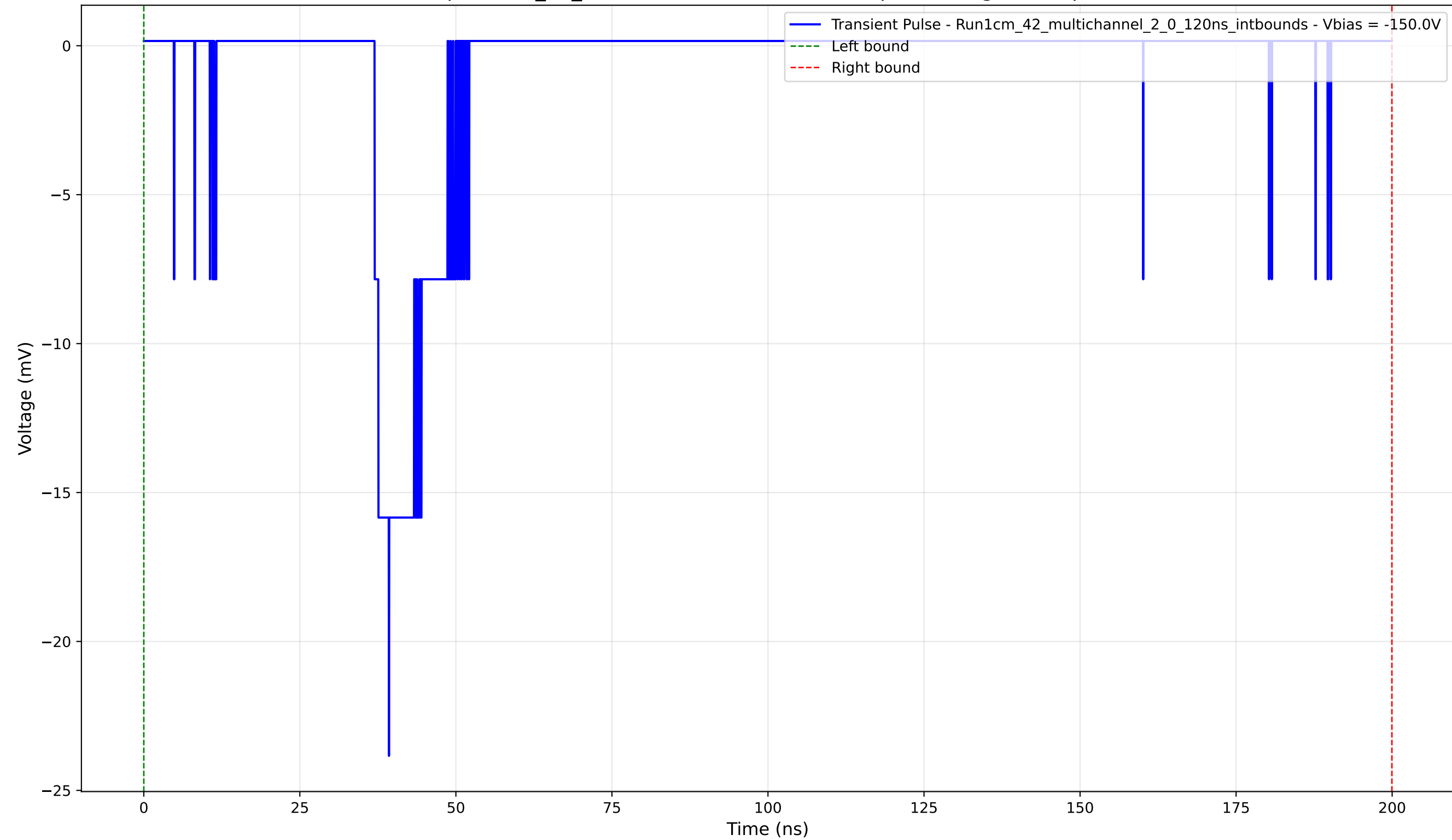
Transient Pulse - Sample: 1cm_42_multichannel - Position: 60.0 \mu\text{m} - Charge: 2.68 pC - Rise Time: 2.31 ns
