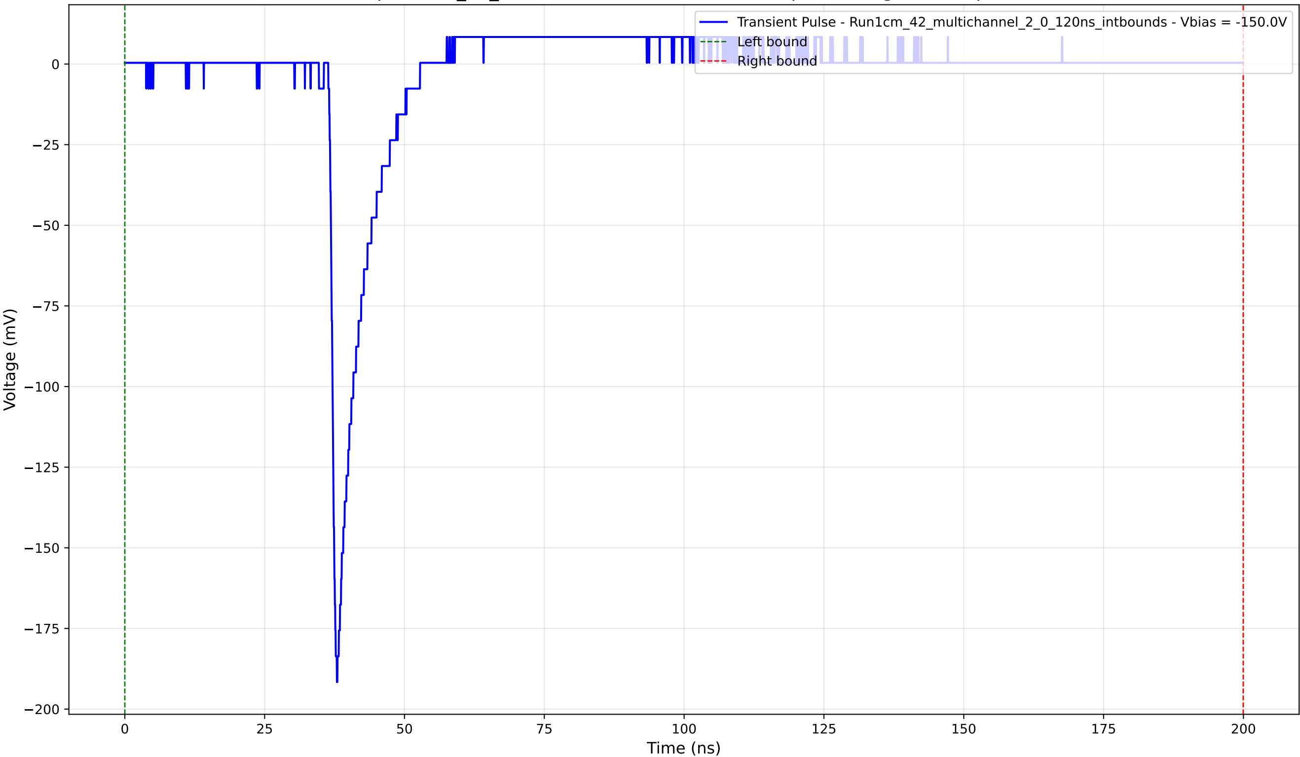
Transient Pulse - Sample: 1cm_42_multichannel - Position: 1440.0 \mu\text{m} - Charge: 10.12 pC - Rise Time: 1.02 ns
