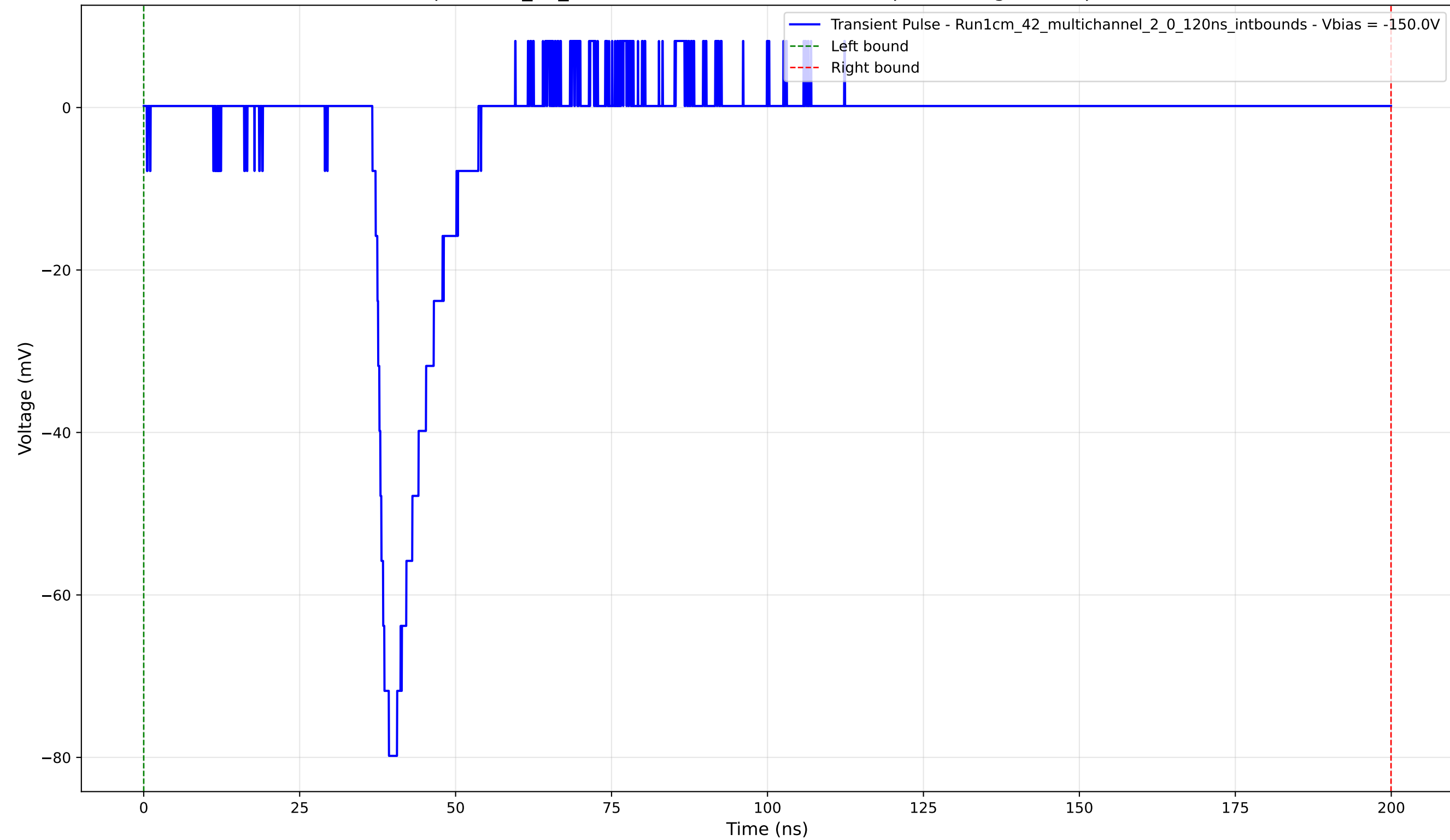
Transient Pulse - Sample: 1cm_42_multichannel - Position: 4255.0 \mu\text{m} - Charge: 9.83 pC - Rise Time: 2.16 ns
