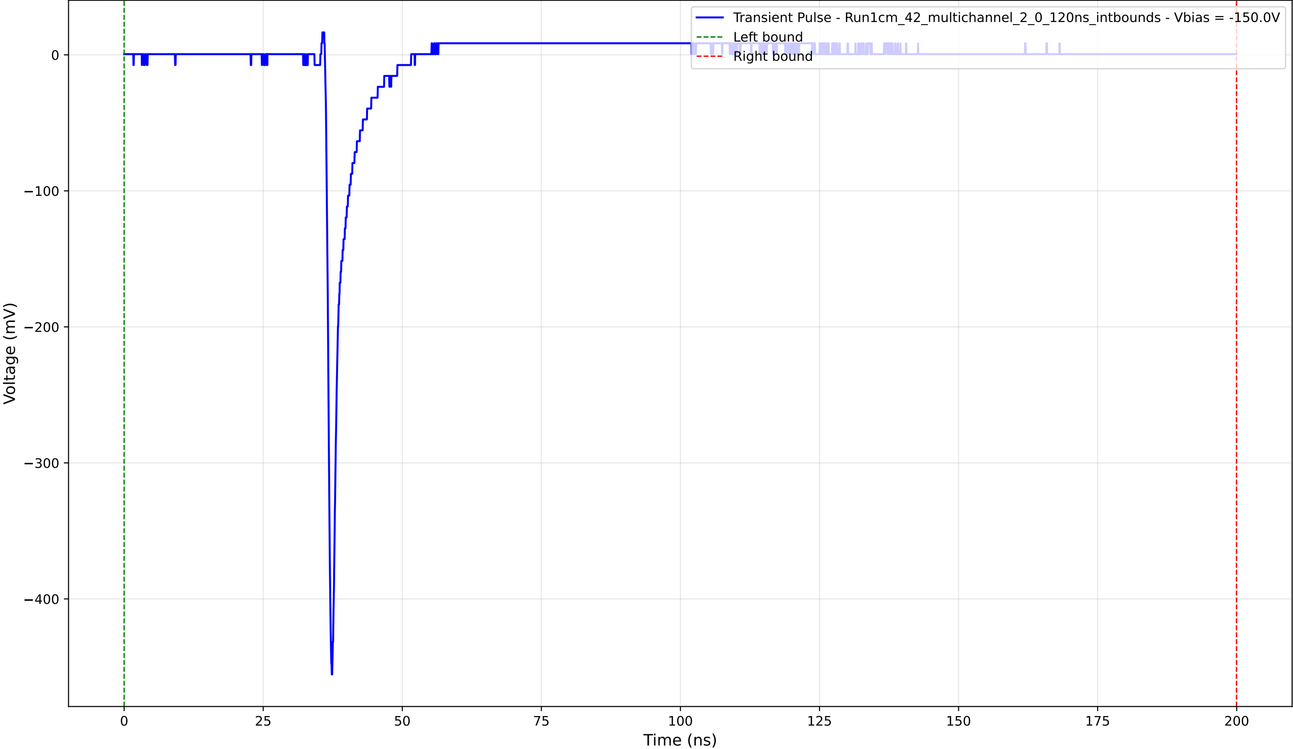
Transient Pulse - Sample: 1cm_42_multichannel - Position: 2045.0 \mu\text{m} - Charge: 13.76 pC - Rise Time: 0.76 ns
