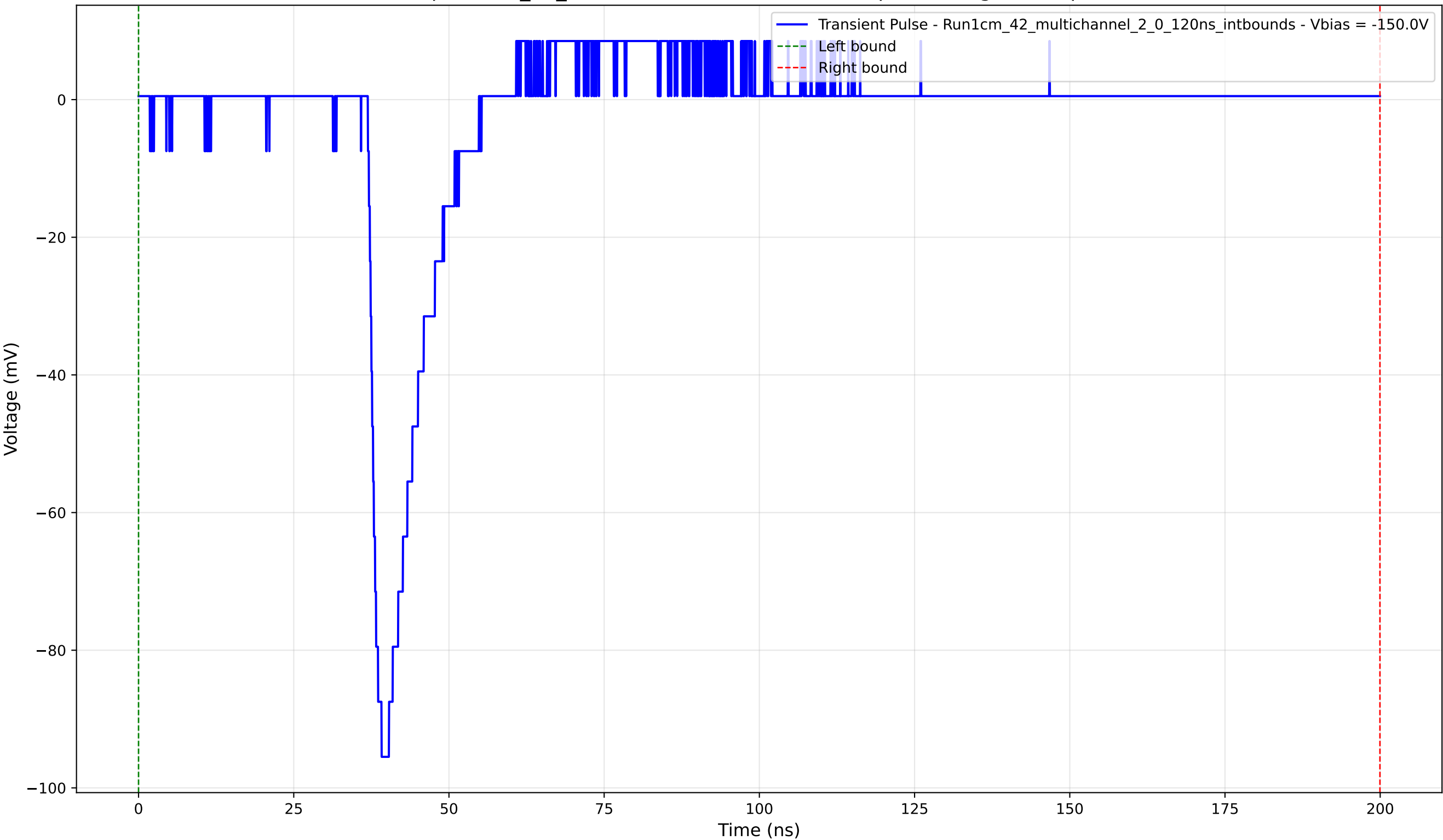
Transient Pulse - Sample: 1cm_42_multichannel - Position: 505.0 \mu\text{m} - Charge: 8.30 pC - Rise Time: 1.51 ns
