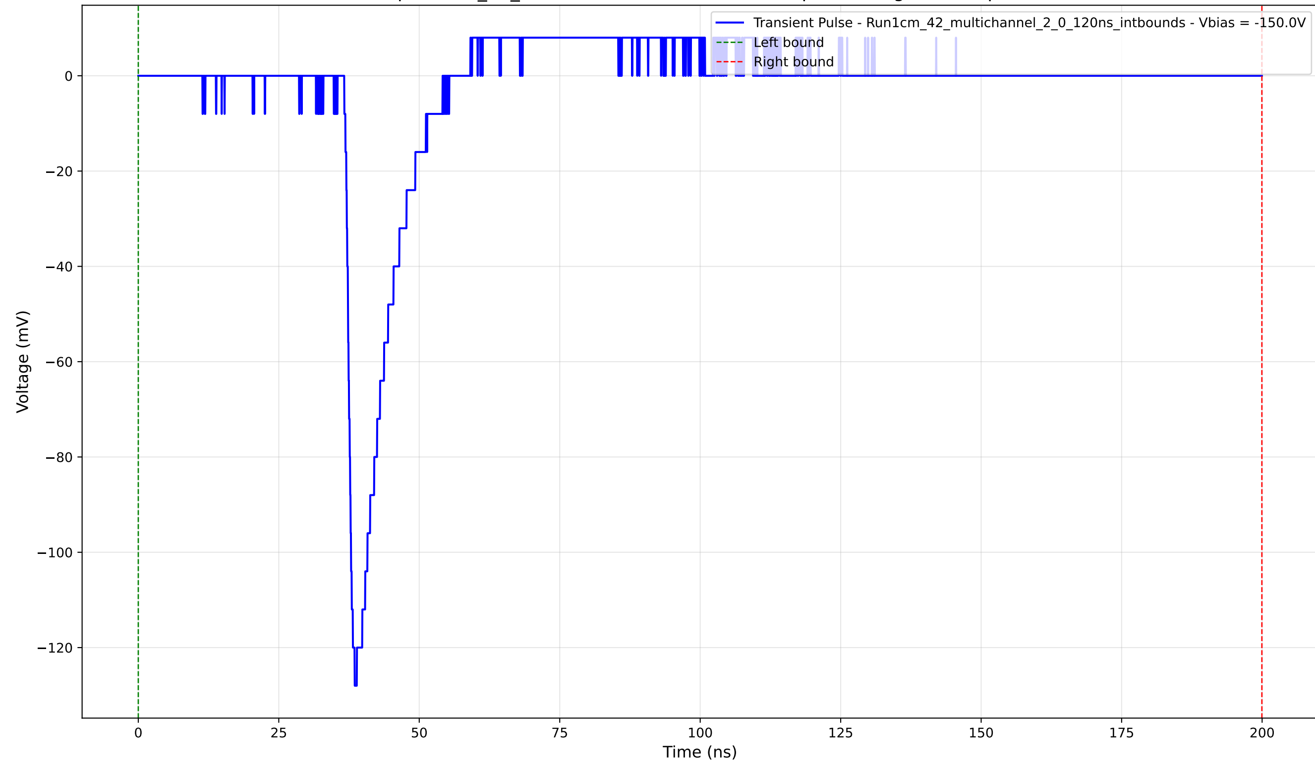
Transient Pulse - Sample: 1cm_42_multichannel - Position: 985.0 \mu\text{m} - Charge: 10.44 pC - Rise Time: 1.34 ns
