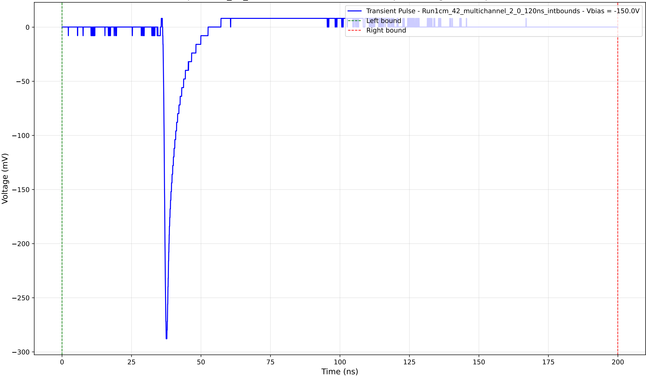
Transient Pulse - Sample: 1cm_42_multichannel - Position: 1740.0 \mu\text{m} - Charge: 13.80 pC - Rise Time: 0.87 ns
