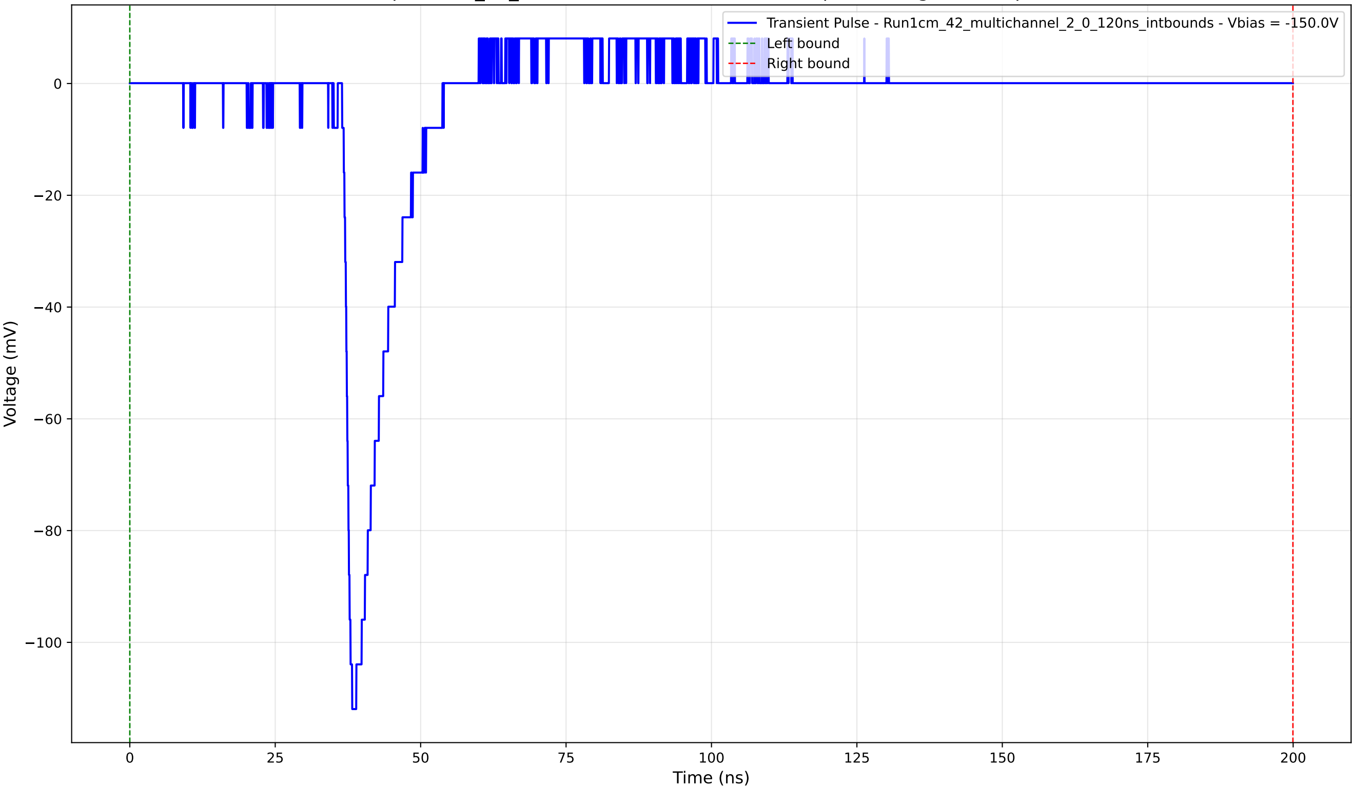
Transient Pulse - Sample: 1cm_42_multichannel - Position: 3635.0 \mu\text{m} - Charge: 10.52 pC - Rise Time: 1.18 ns
