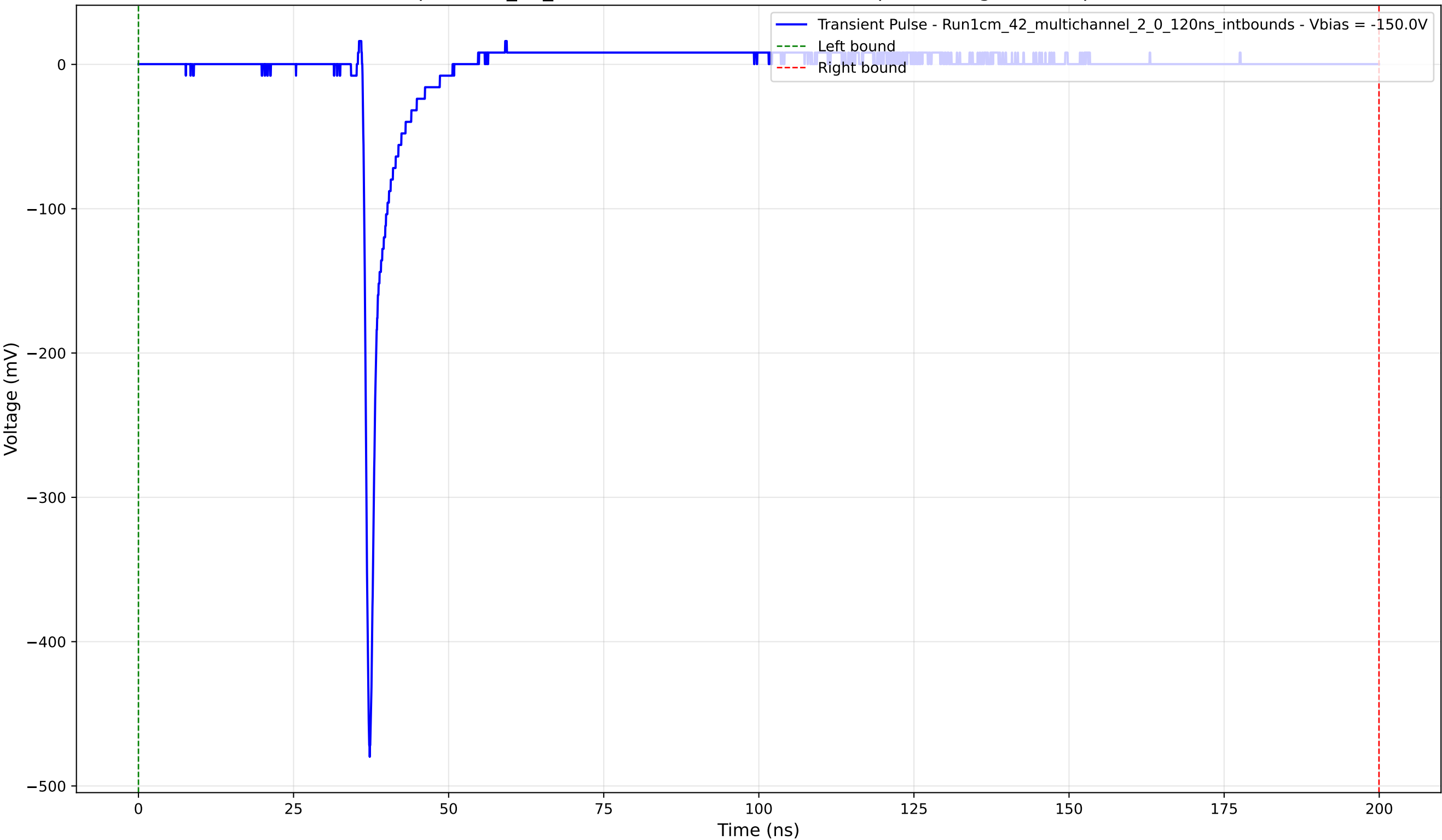
Transient Pulse - Sample: 1cm_42_multichannel - Position: 2615.0 \mu\text{m} - Charge: 13.04 pC - Rise Time: 0.76 ns
