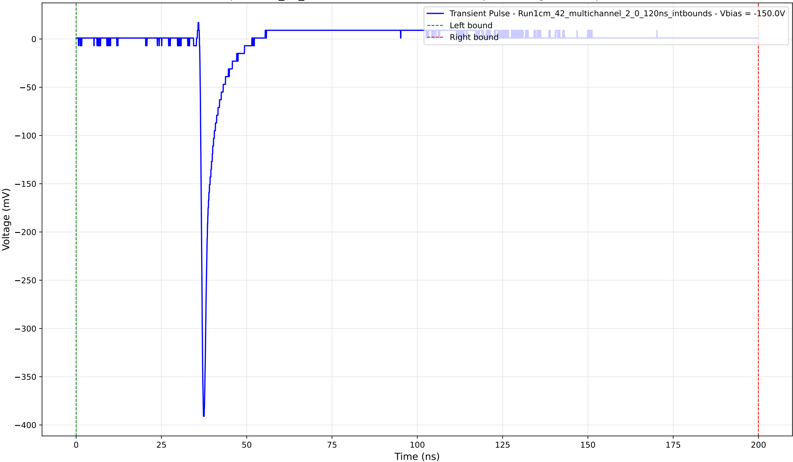
Transient Pulse - Sample: 1cm_42_multichannel - Position: 1965.0 \mu\text{m} - Charge: 10.50 pC - Rise Time: 0.80 ns
