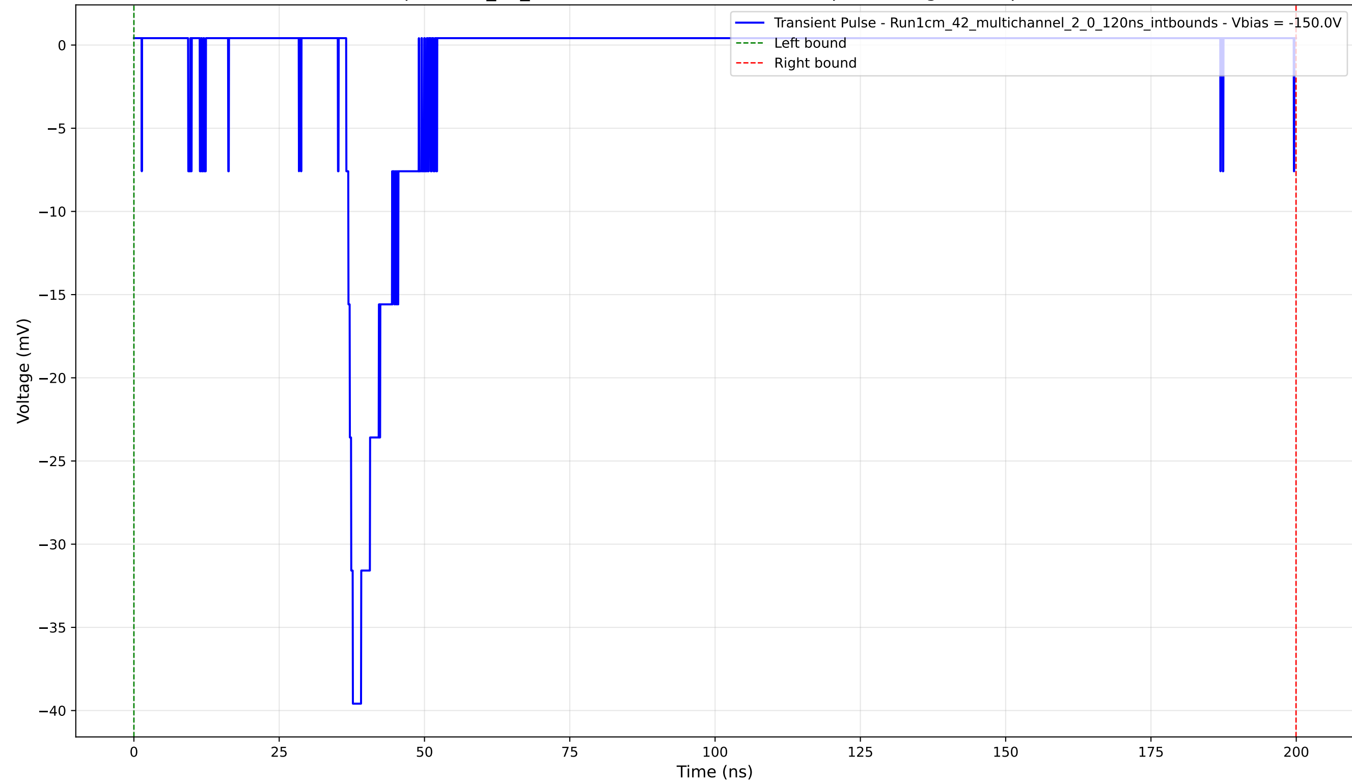
Transient Pulse - Sample: 1cm_42_multichannel - Position: 1320.0 \mu\text{m} - Charge: 3.78 pC - Rise Time: 1.14 ns
