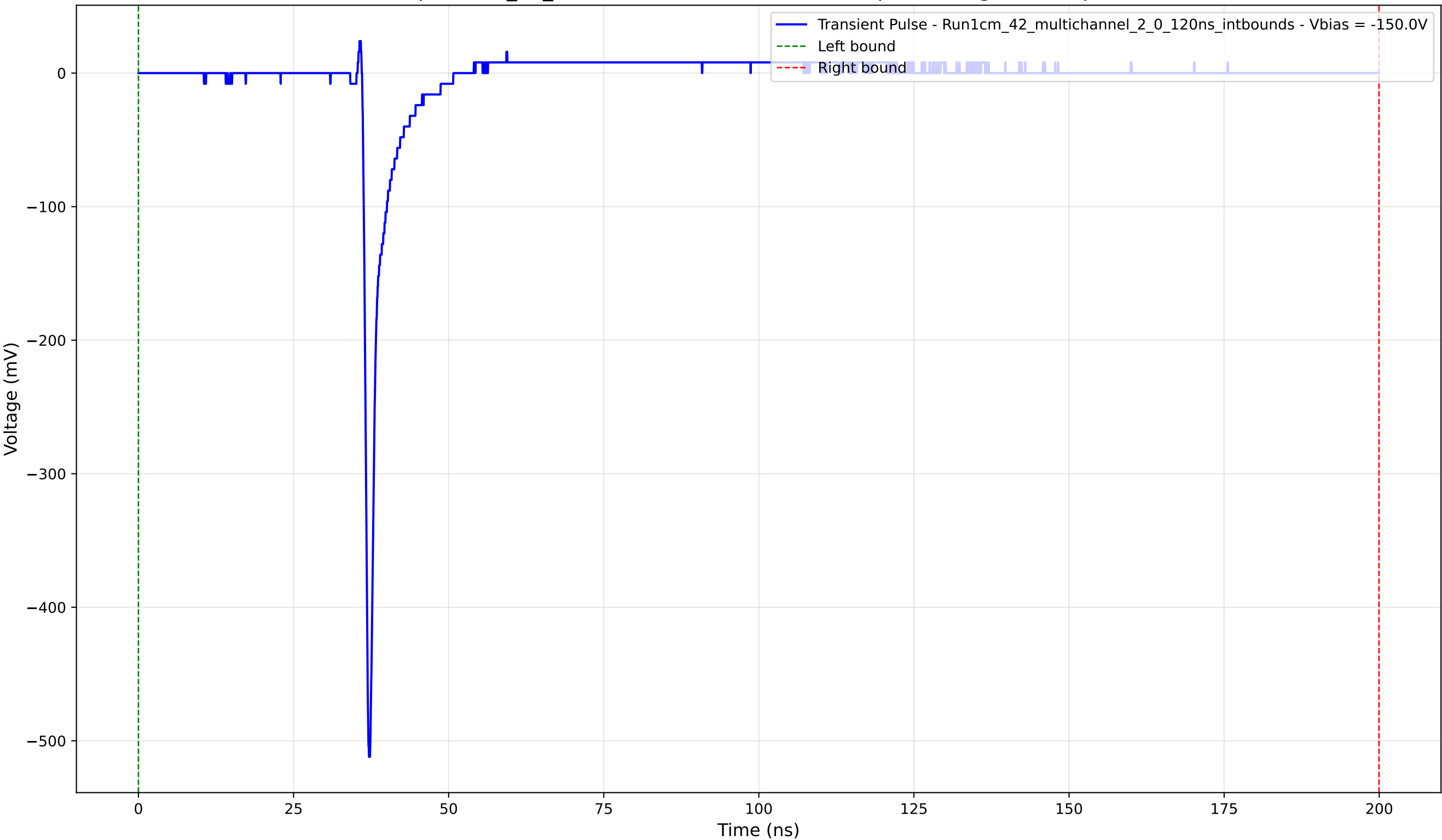
Transient Pulse - Sample: 1cm_42_multichannel - Position: 2555.0 \mu\text{m} - Charge: 14.93 pC - Rise Time: 0.74 ns
