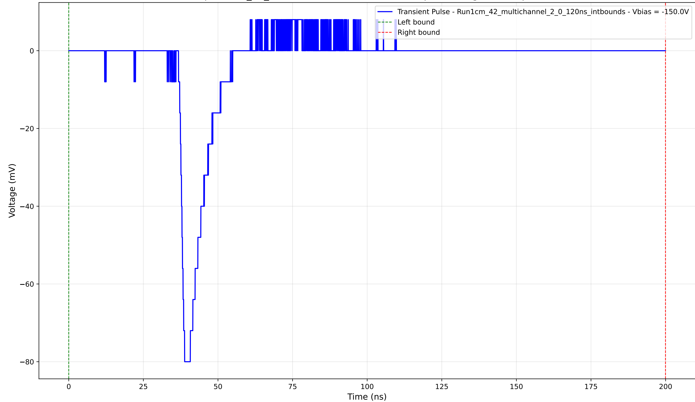
Transient Pulse - Sample: 1cm_42_multichannel - Position: 4240.0 \mu\text{m} - Charge: 10.32 pC - Rise Time: 1.36 ns
