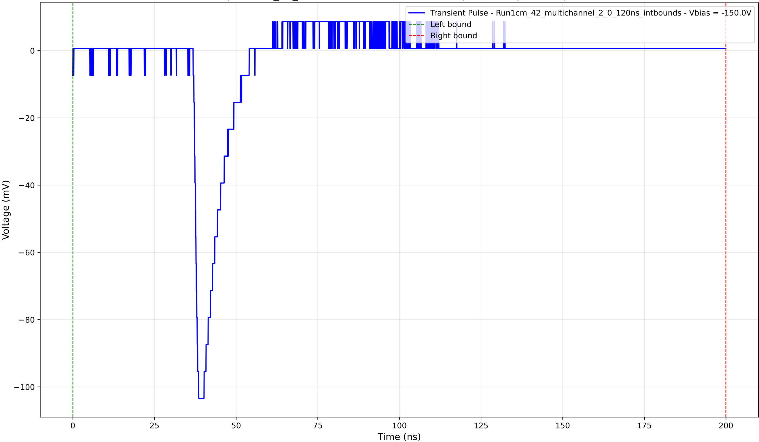
Transient Pulse - Sample: 1cm_42_multichannel - Position: 735.0 \mu\text{m} - Charge: 8.51 pC - Rise Time: 1.19 ns
