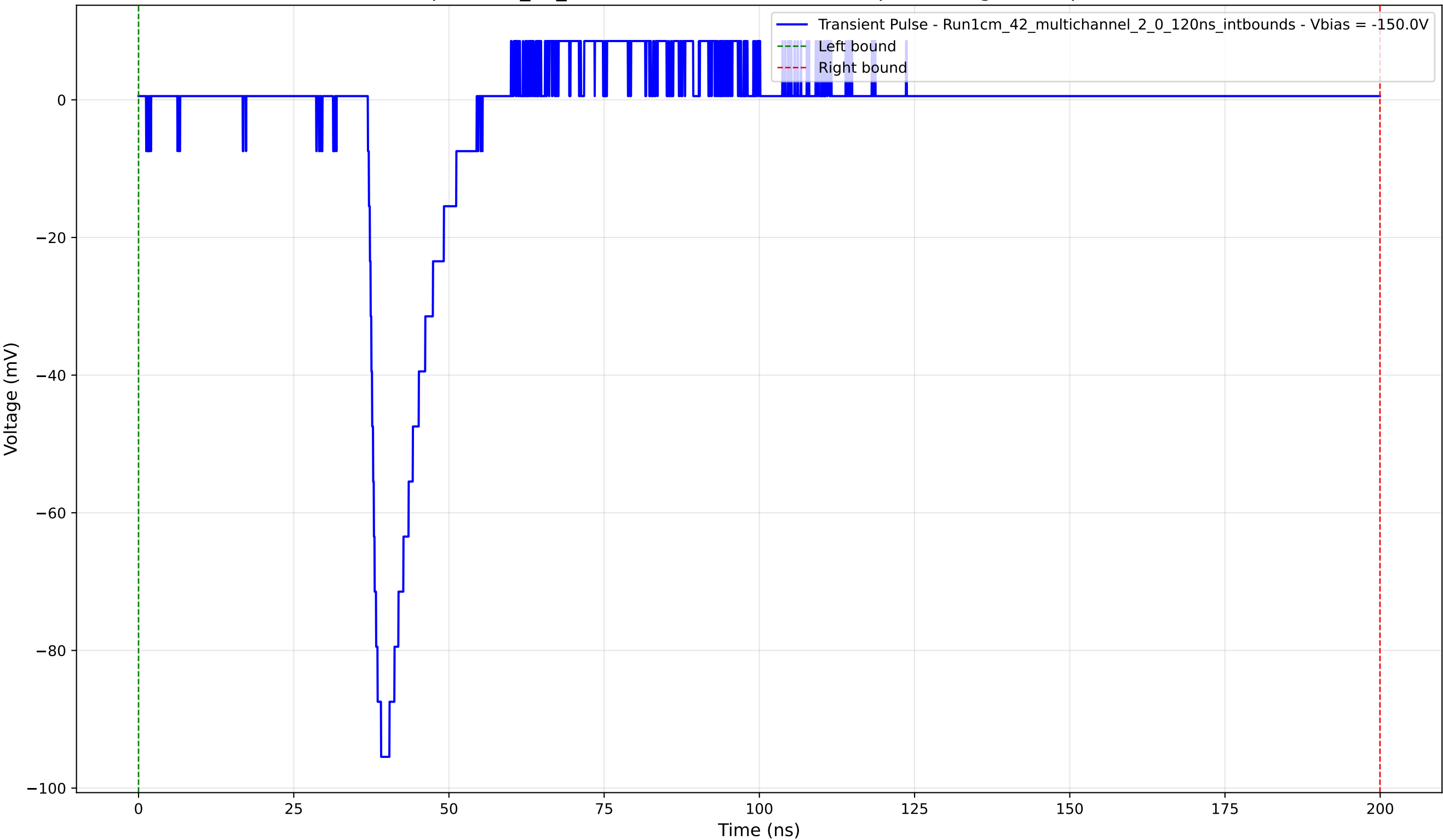
Transient Pulse - Sample: 1cm_42_multichannel - Position: 515.0 \mu\text{m} - Charge: 8.41 pC - Rise Time: 1.43 ns
