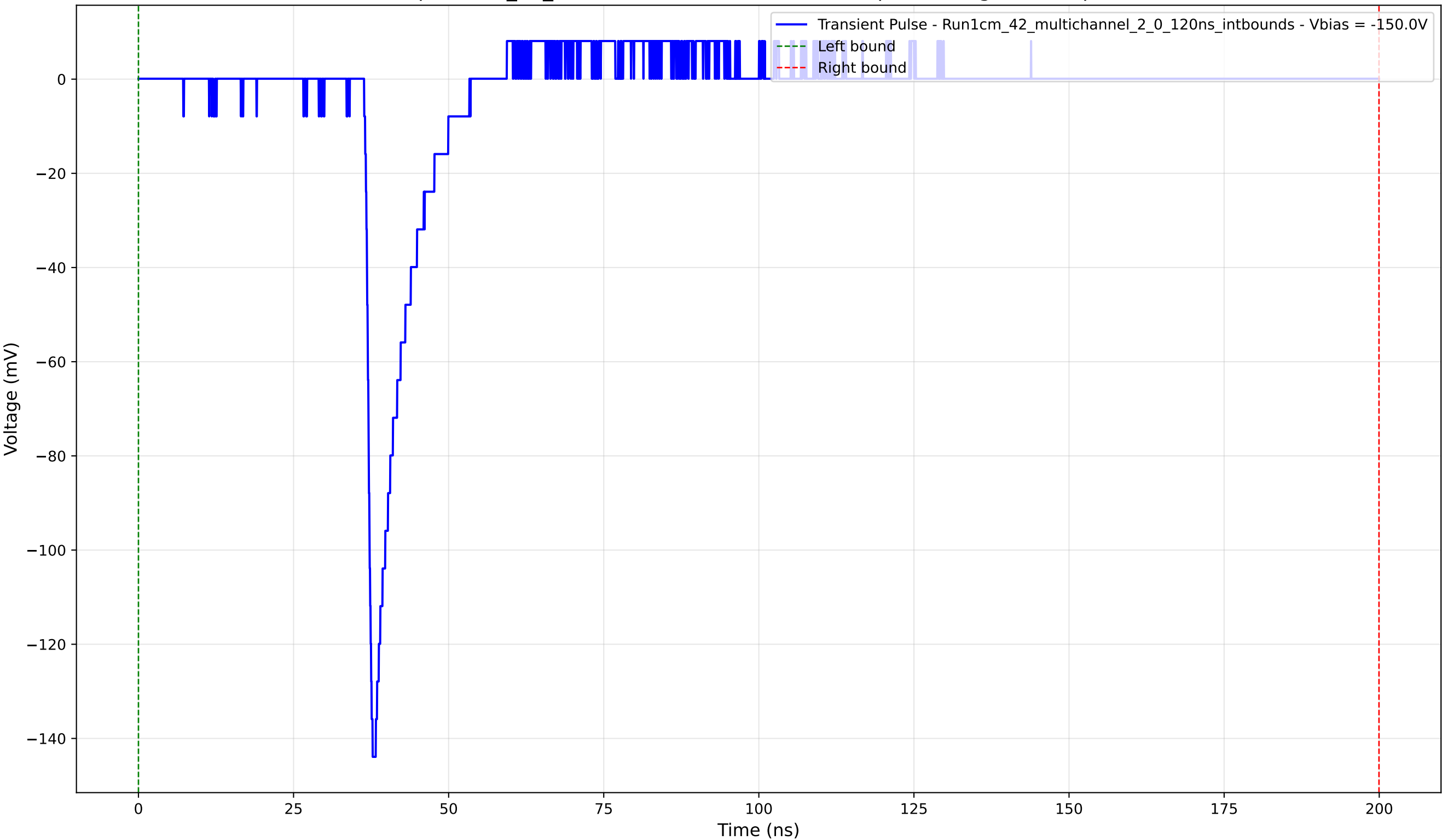
Transient Pulse - Sample: 1cm_42_multichannel - Position: 3310.0 \mu\text{m} - Charge: 10.64 pC - Rise Time: 1.05 ns
