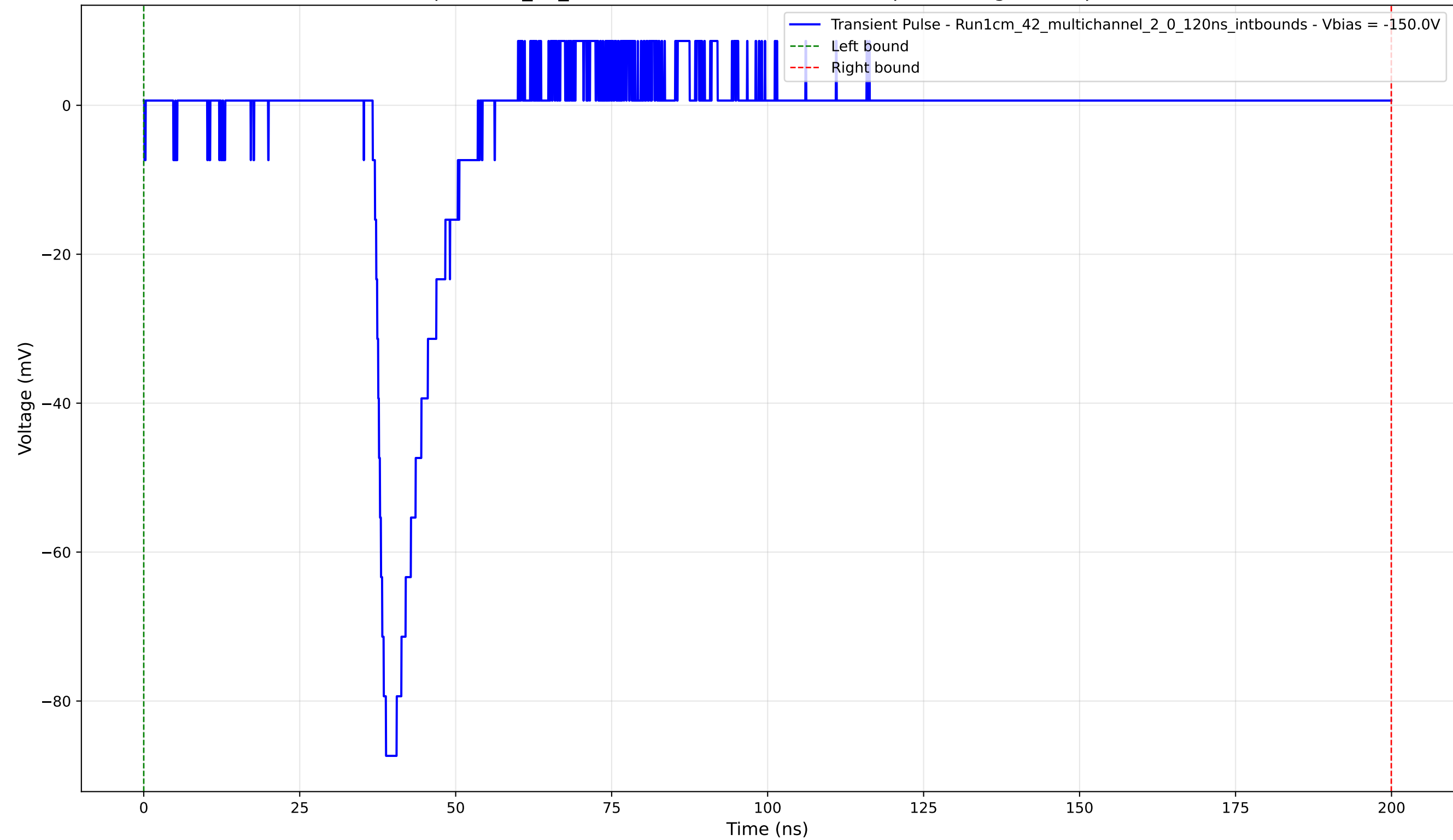
Transient Pulse - Sample: 1cm_42_multichannel - Position: 4065.0 \mu\text{m} - Charge: 8.38 pC - Rise Time: 1.43 ns
