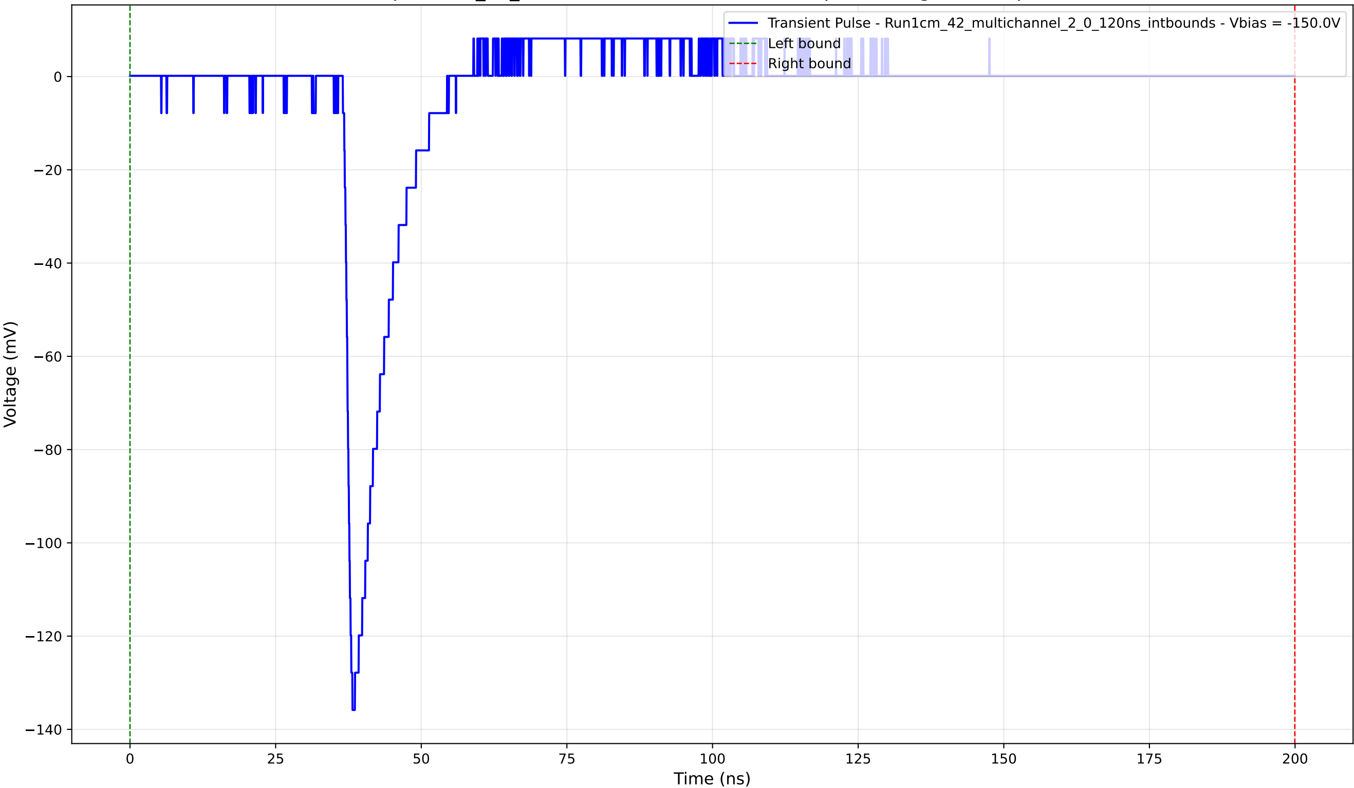
Transient Pulse - Sample: 1cm_42_multichannel - Position: 1110.0 \mu\text{m} - Charge: 11.37 pC - Rise Time: 1.21 ns
