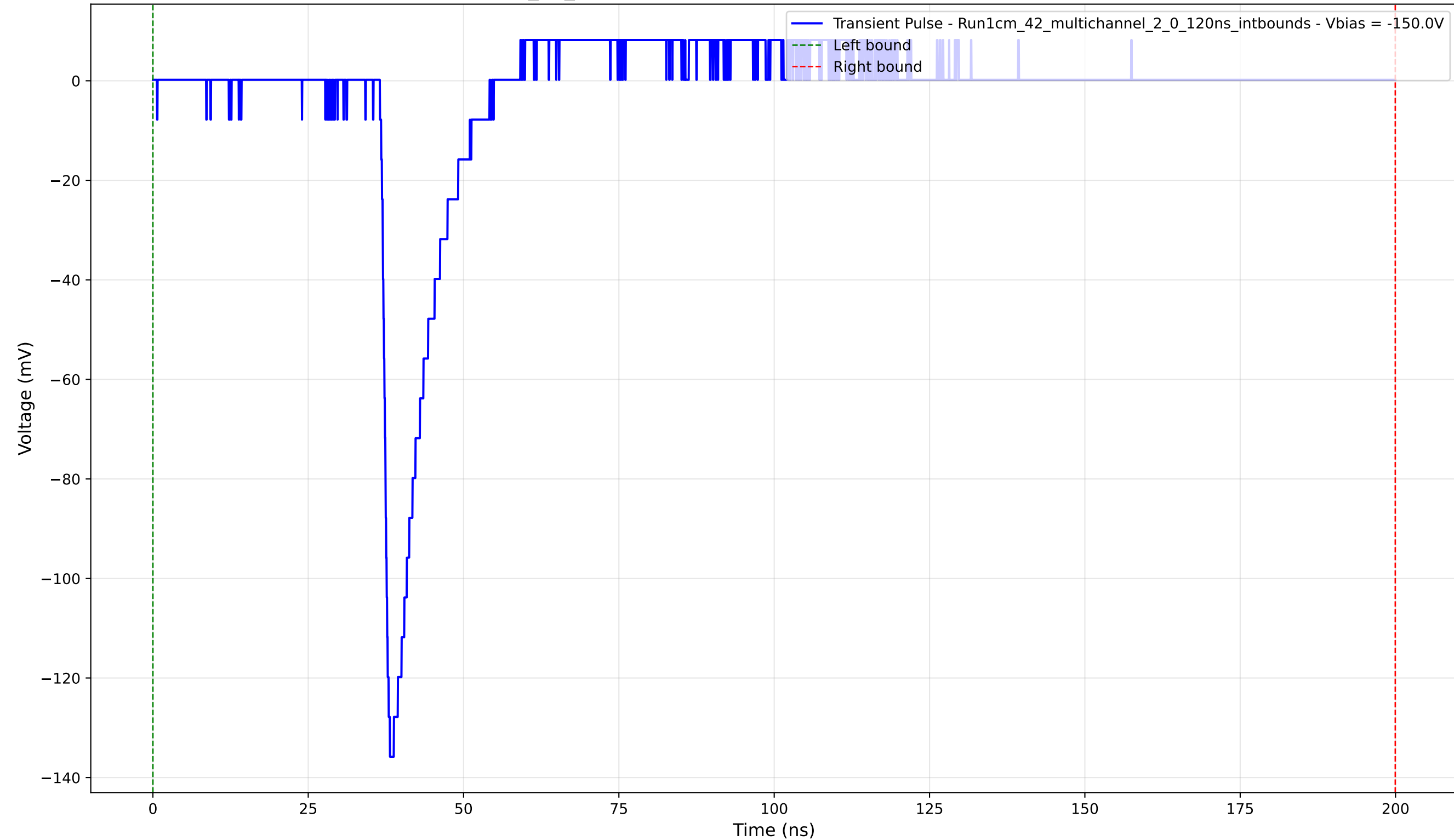
Transient Pulse - Sample: 1cm_42_multichannel - Position: 1125.0 \mu\text{m} - Charge: 9.88 pC - Rise Time: 1.21 ns
