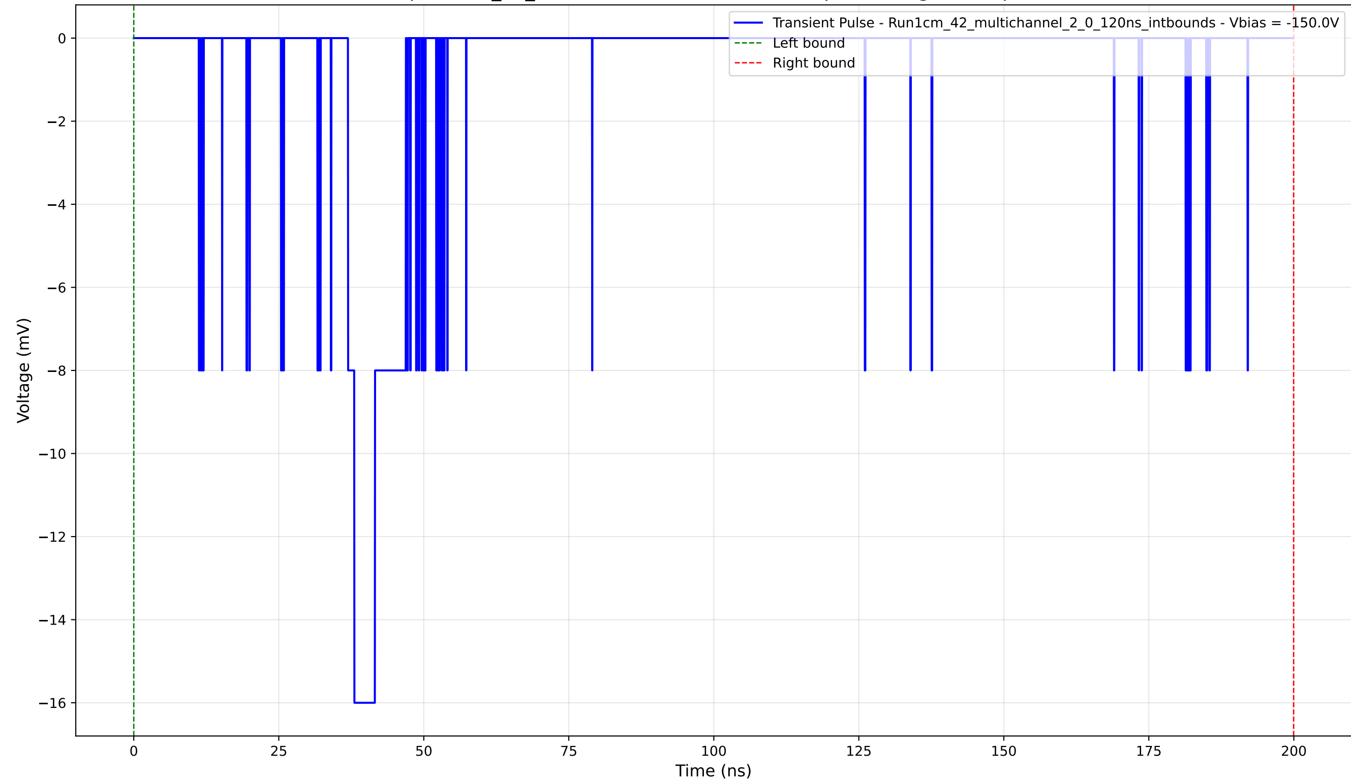
Transient Pulse - Sample: 1cm_42_multichannel - Position: 875.0 \mu\text{m} - Charge: 2.87 pC - Rise Time: 1.11 ns
