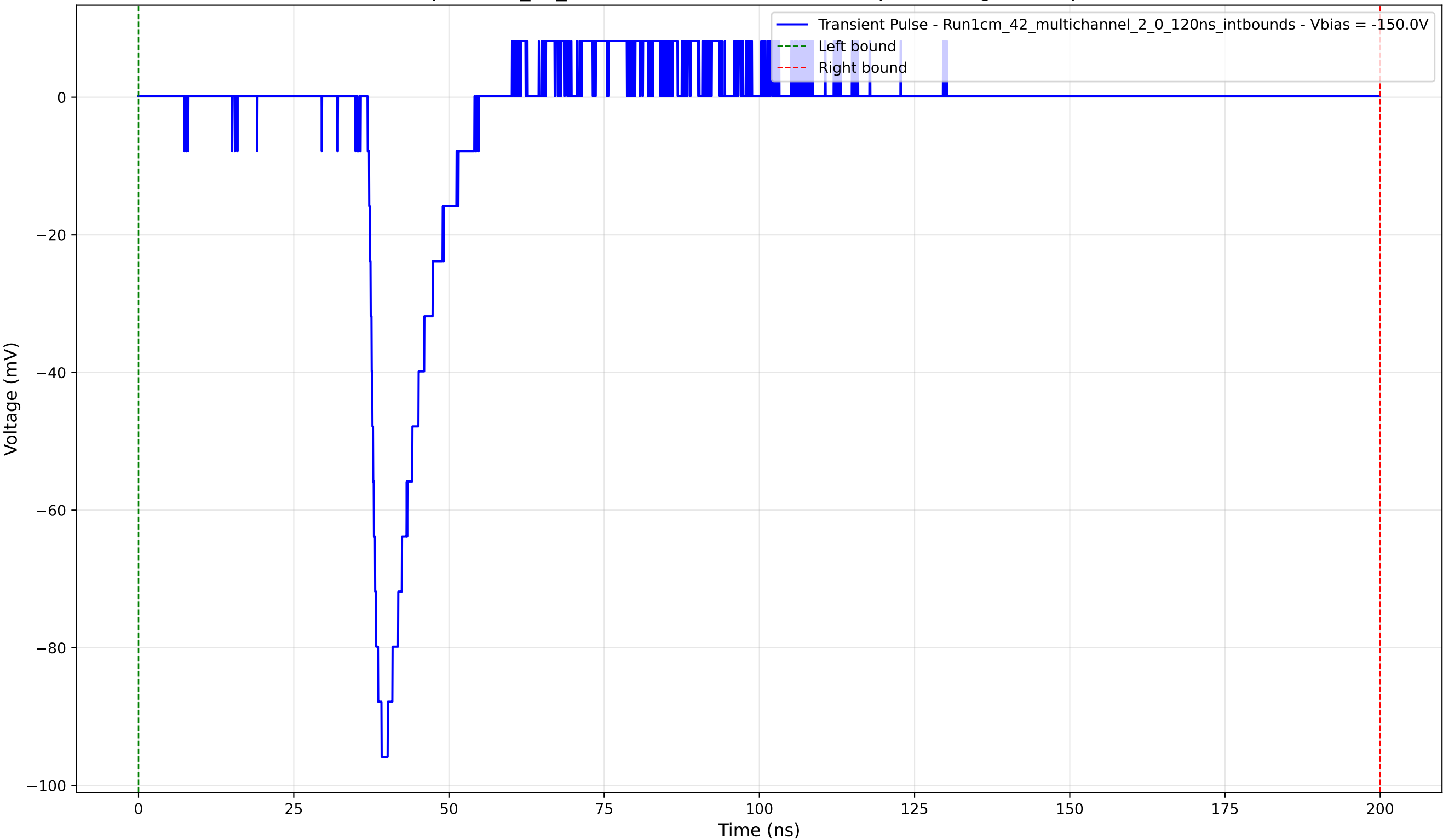
Transient Pulse - Sample: 1cm_42_multichannel - Position: 485.0 \mu\text{m} - Charge: 9.87 pC - Rise Time: 1.47 ns
