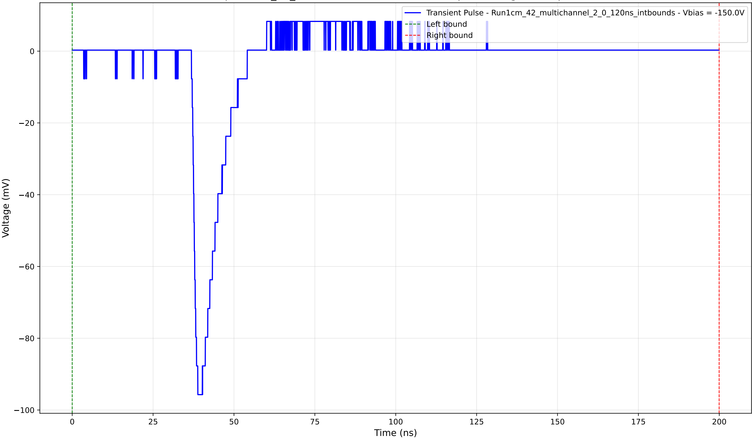
Transient Pulse - Sample: 1cm_42_multichannel - Position: 565.0 \mu\text{m} - Charge: 9.75 pC - Rise Time: 1.35 ns
