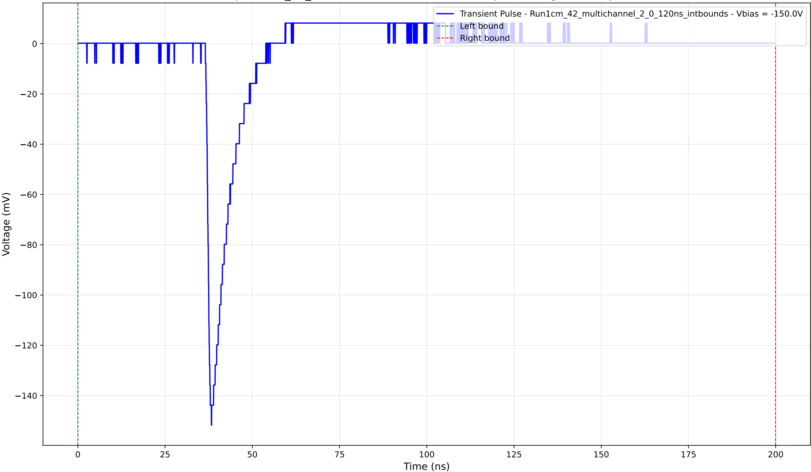
Transient Pulse - Sample: 1cm_42_multichannel - Position: 1185.0 \mu\text{m} - Charge: 10.42 pC - Rise Time: 1.24 ns
