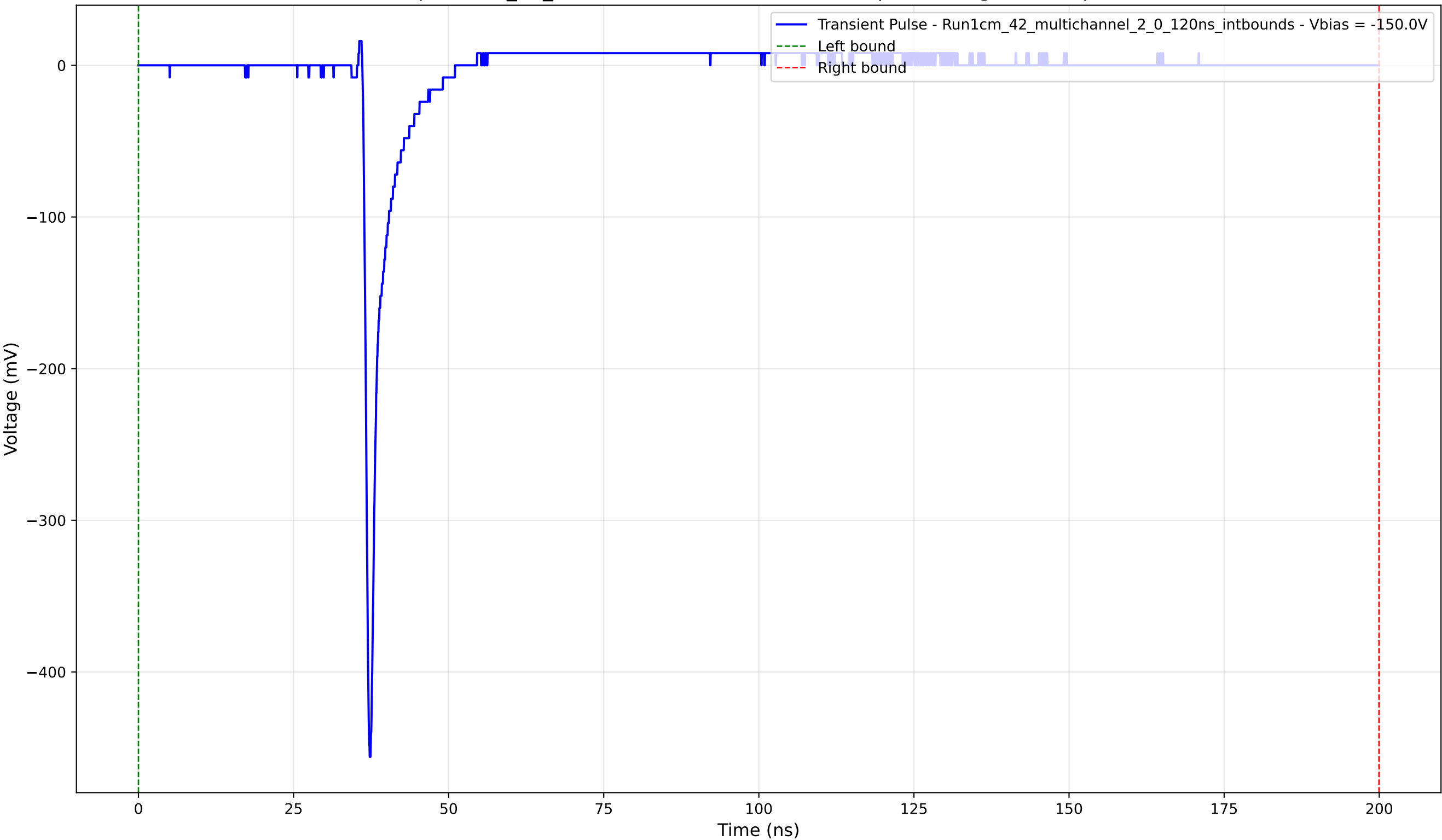
Transient Pulse - Sample: 1cm_42_multichannel - Position: 2055.0 \mu\text{m} - Charge: 14.78 pC - Rise Time: 0.79 ns
