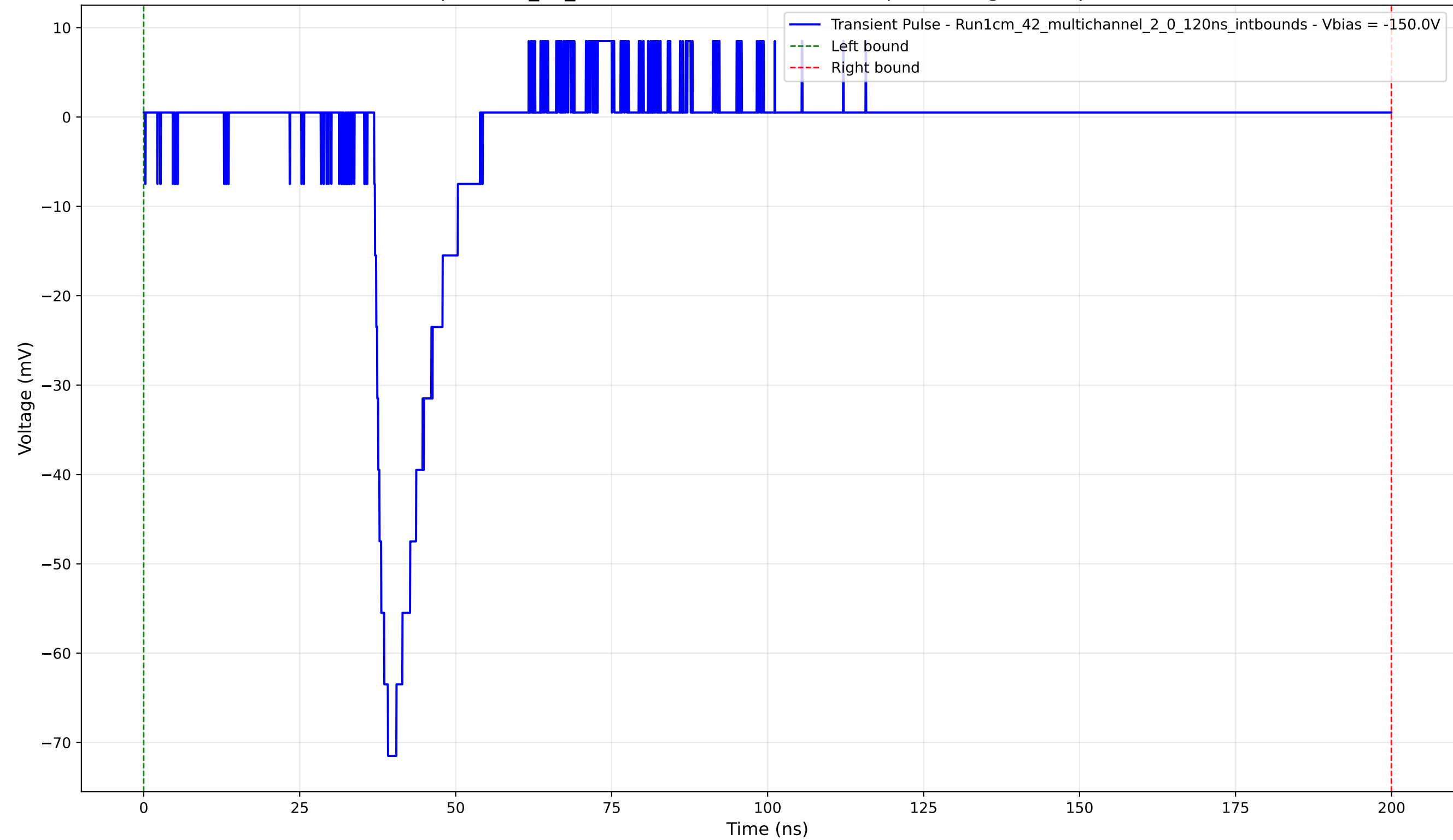
Transient Pulse - Sample: 1cm_42_multichannel - Position: 260.0 \mu\text{m} - Charge: 8.07 pC - Rise Time: 2.20 ns
