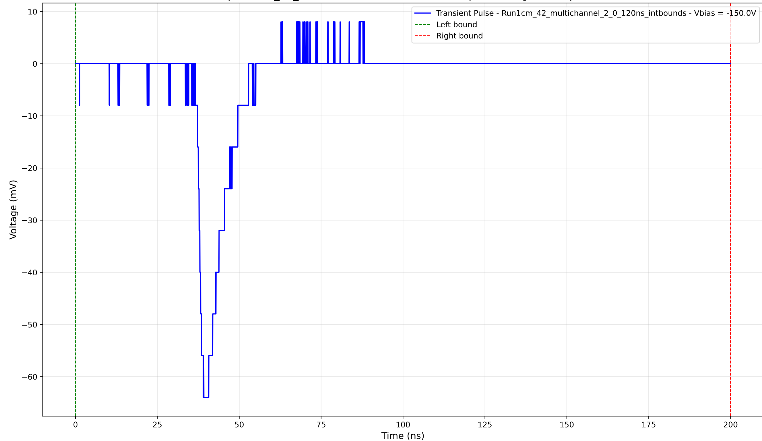
Transient Pulse - Sample: 1cm_42_multichannel - Position: 4315.0 \mu\text{m} - Charge: 9.58 pC - Rise Time: 2.33 ns
