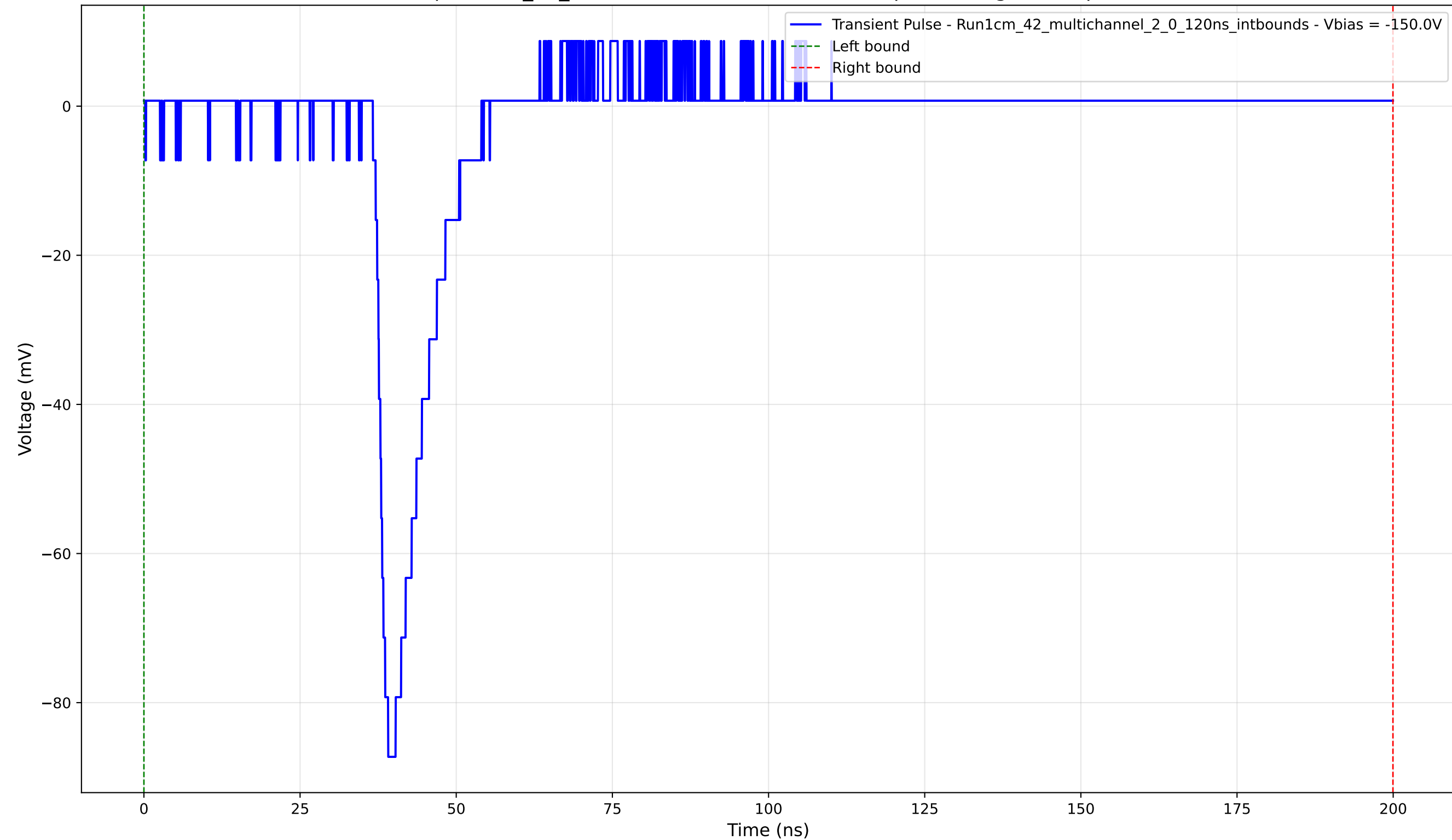
Transient Pulse - Sample: 1cm_42_multichannel - Position: 4155.0 \mu\text{m} - Charge: 8.58 pC - Rise Time: 1.55 ns
