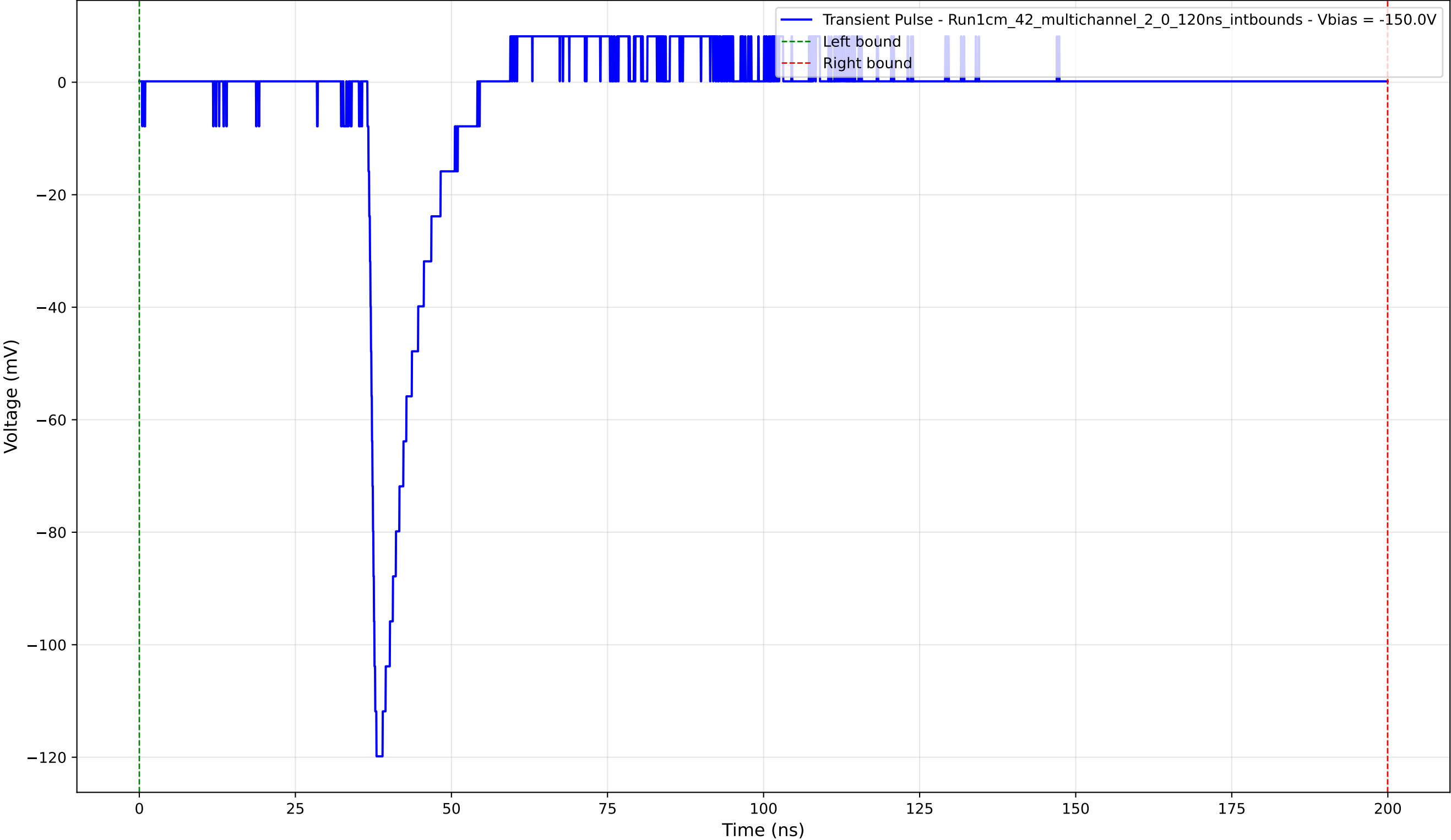
Transient Pulse - Sample: 1cm_42_multichannel - Position: 3555.0 \mu\text{m} - Charge: 10.29 pC - Rise Time: 1.10 ns
