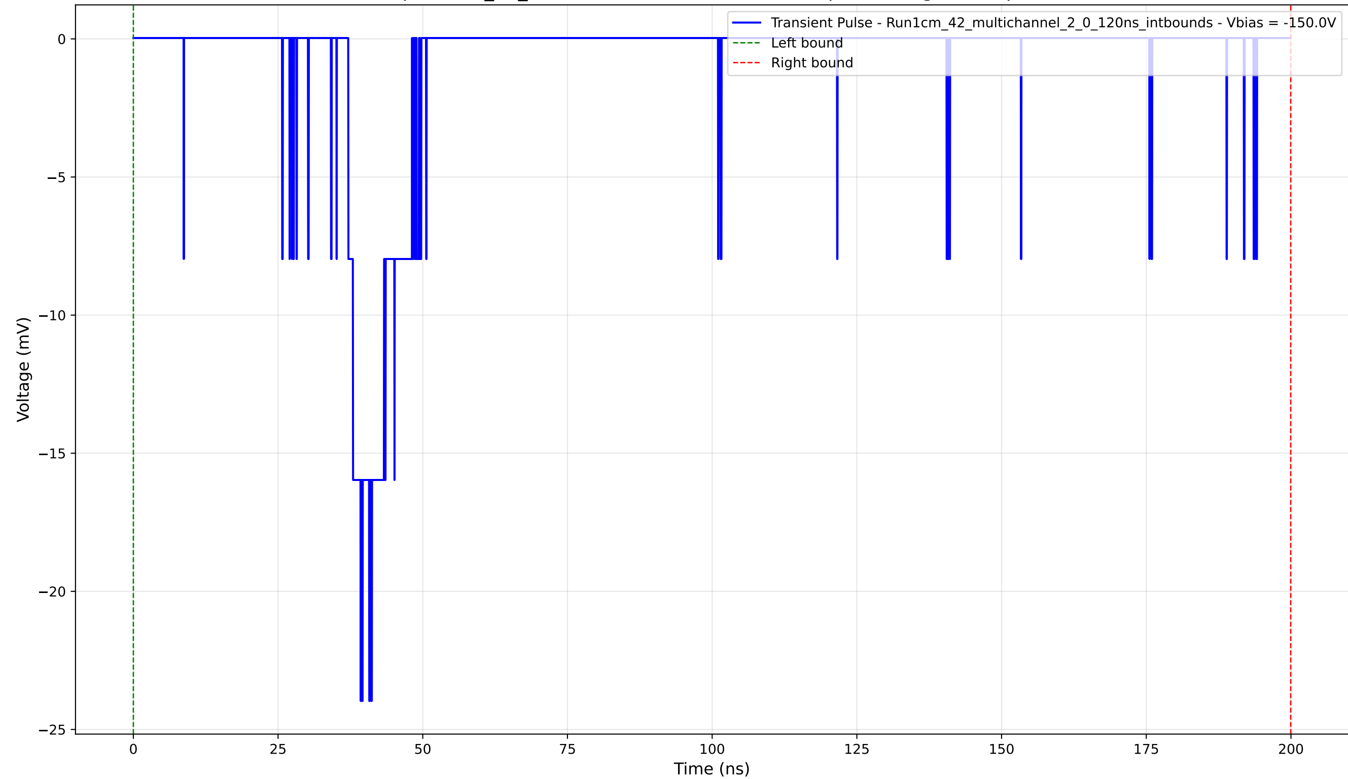
Transient Pulse - Sample: 1cm_42_multichannel - Position: 4350.0 \mu\text{m} - Charge: 3.08 pC - Rise Time: 2.15 ns
