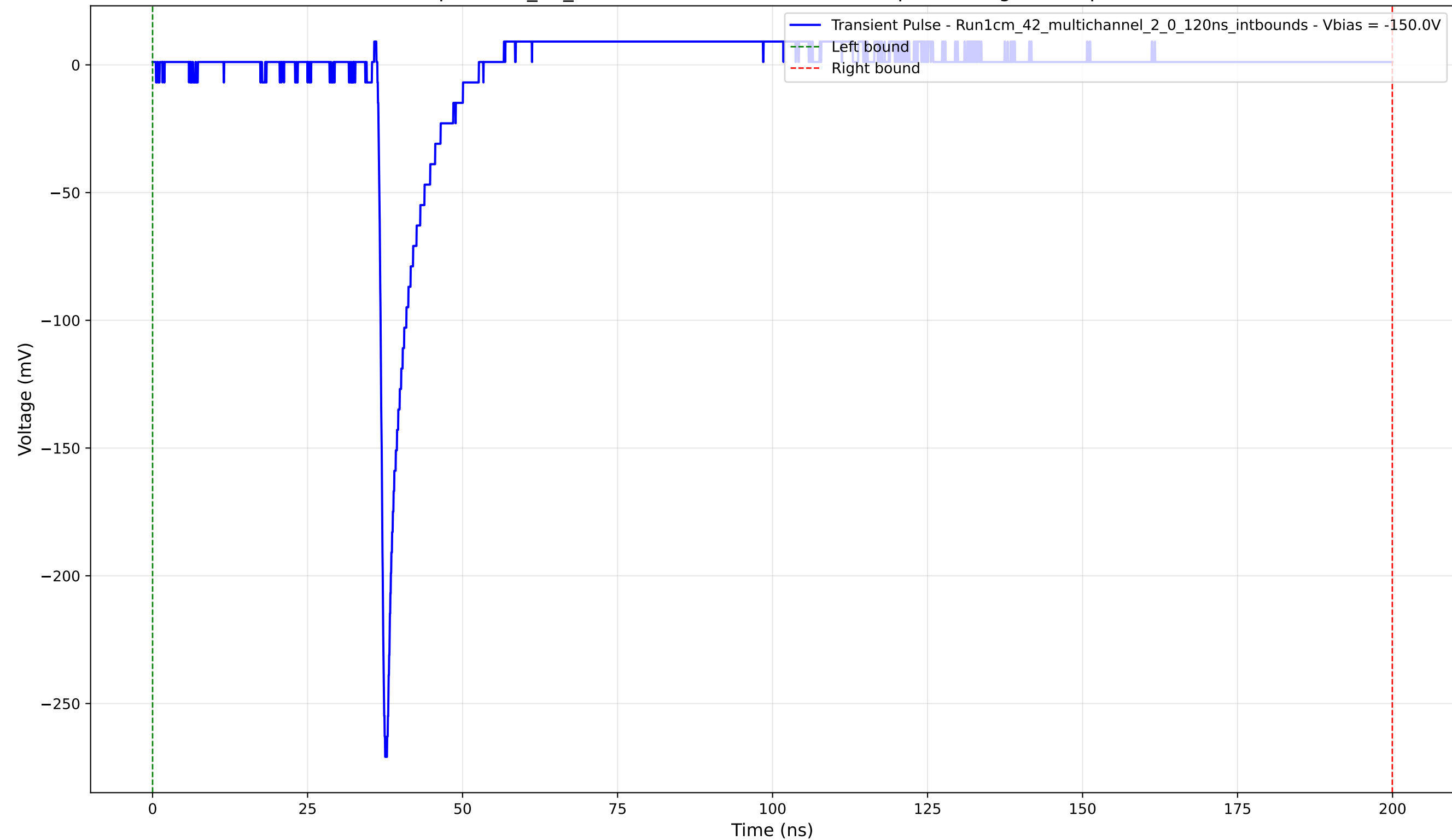
Transient Pulse - Sample: 1cm_42_multichannel - Position: 1700.0 \mu\text{m} - Charge: 9.36 pC - Rise Time: 0.84 ns
