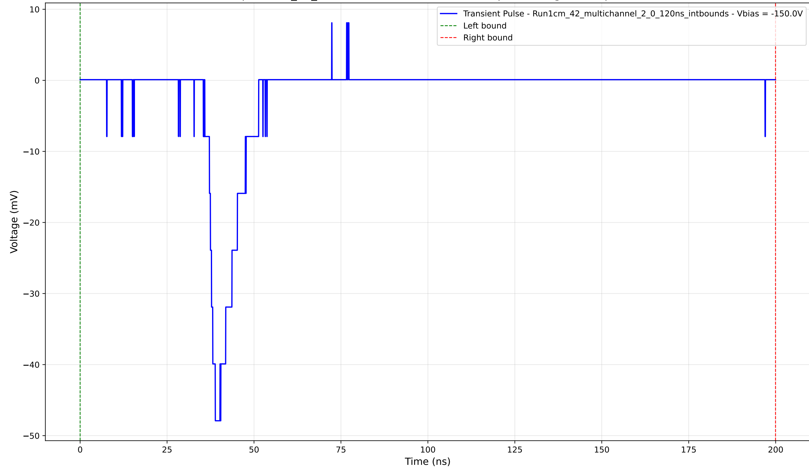
Transient Pulse - Sample: 1cm_42_multichannel - Position: 4835.0 \mu\text{m} - Charge: 6.94 pC - Rise Time: 3.02 ns
