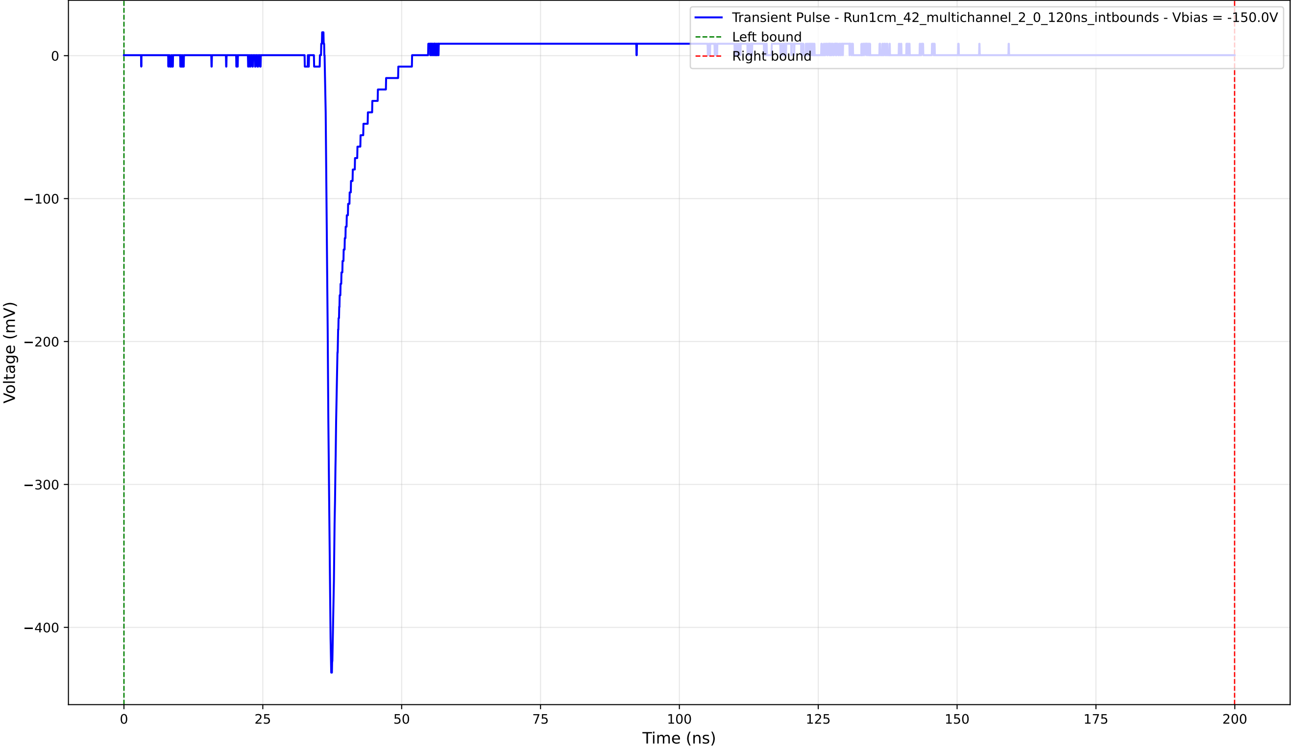
Transient Pulse - Sample: 1cm_42_multichannel - Position: 2000.0 \mu\text{m} - Charge: 13.96 pC - Rise Time: 0.78 ns
