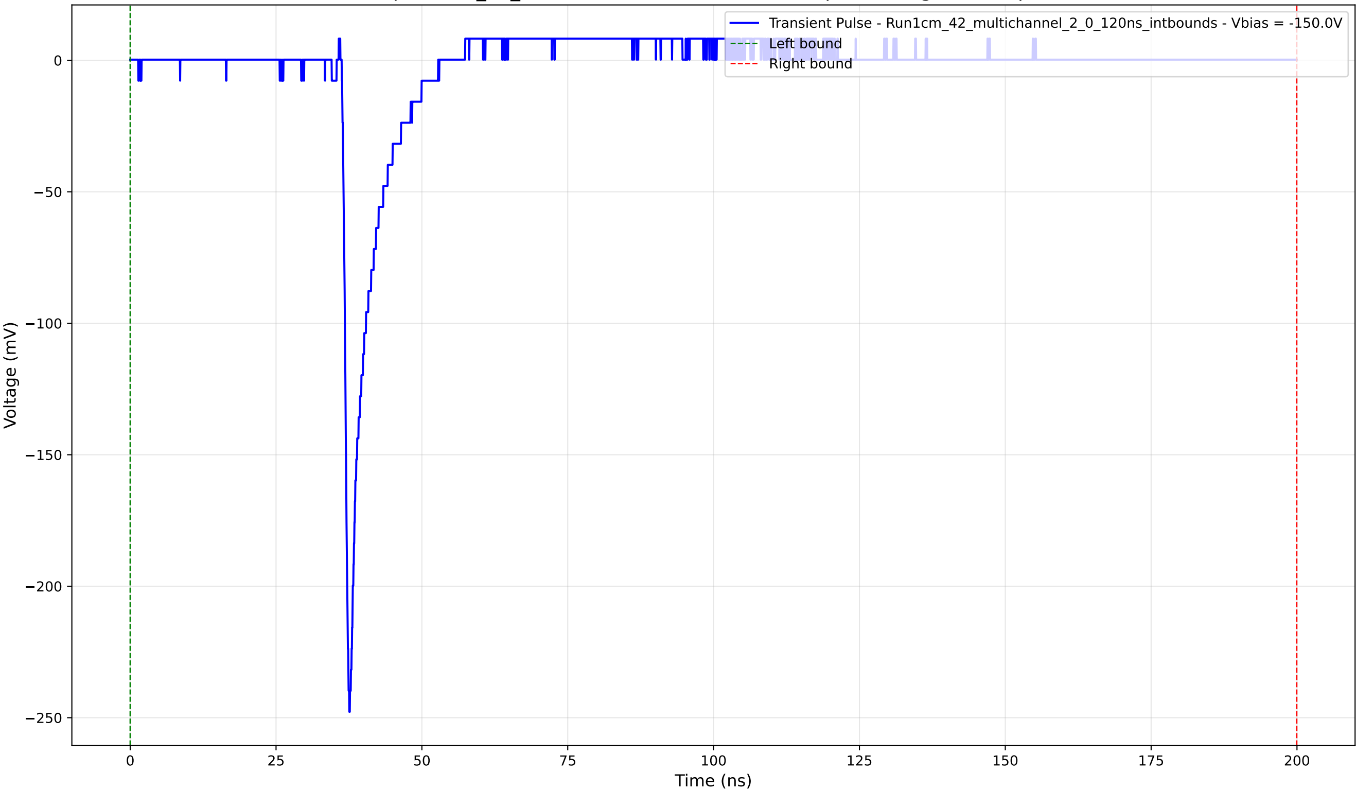
Transient Pulse - Sample: 1cm_42_multichannel - Position: 3035.0 \mu\text{m} - Charge: 11.84 pC - Rise Time: 0.87 ns
