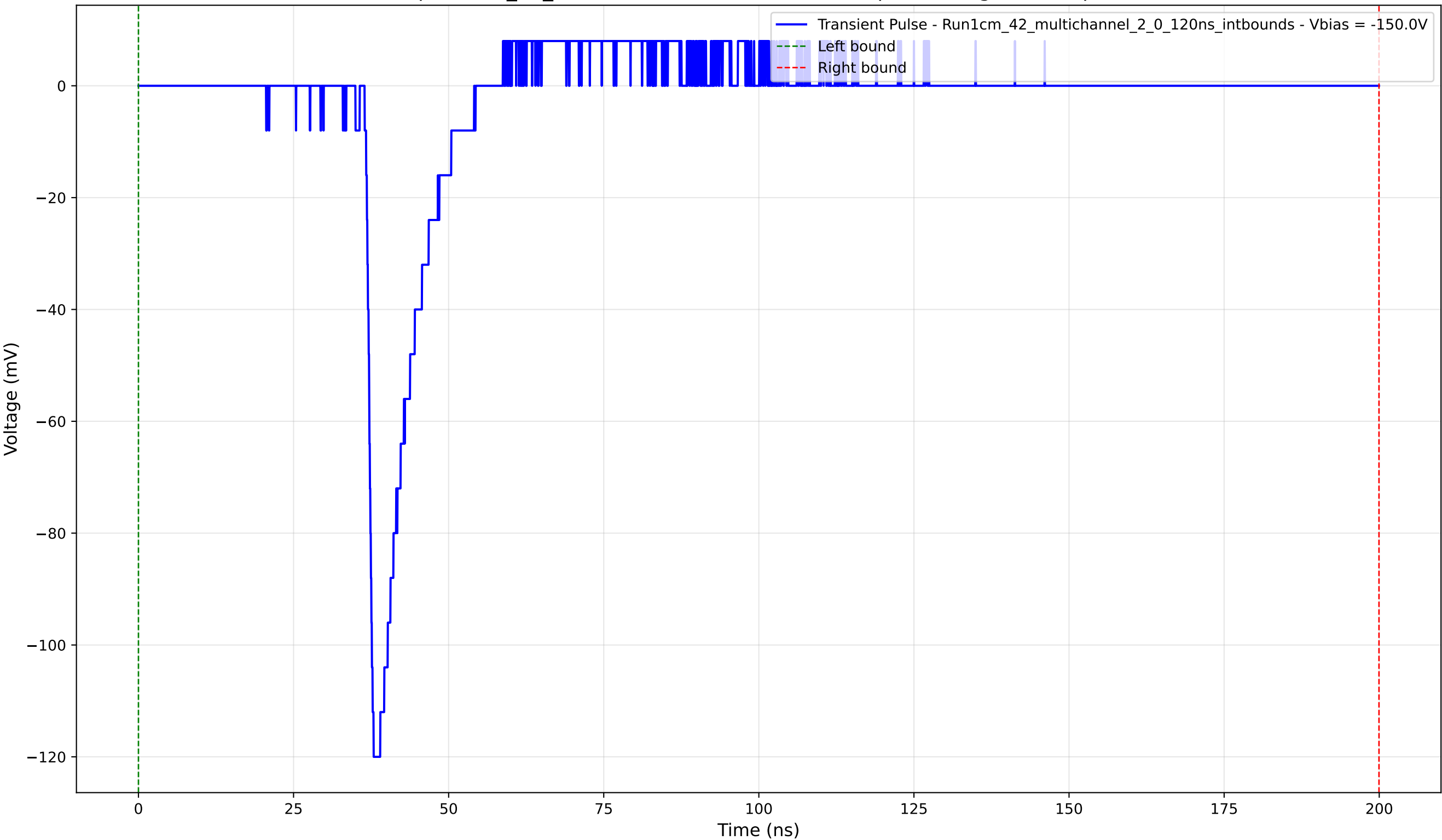
Transient Pulse - Sample: 1cm_42_multichannel - Position: 3545.0 \mu\text{m} - Charge: 10.60 pC - Rise Time: 1.06 ns
