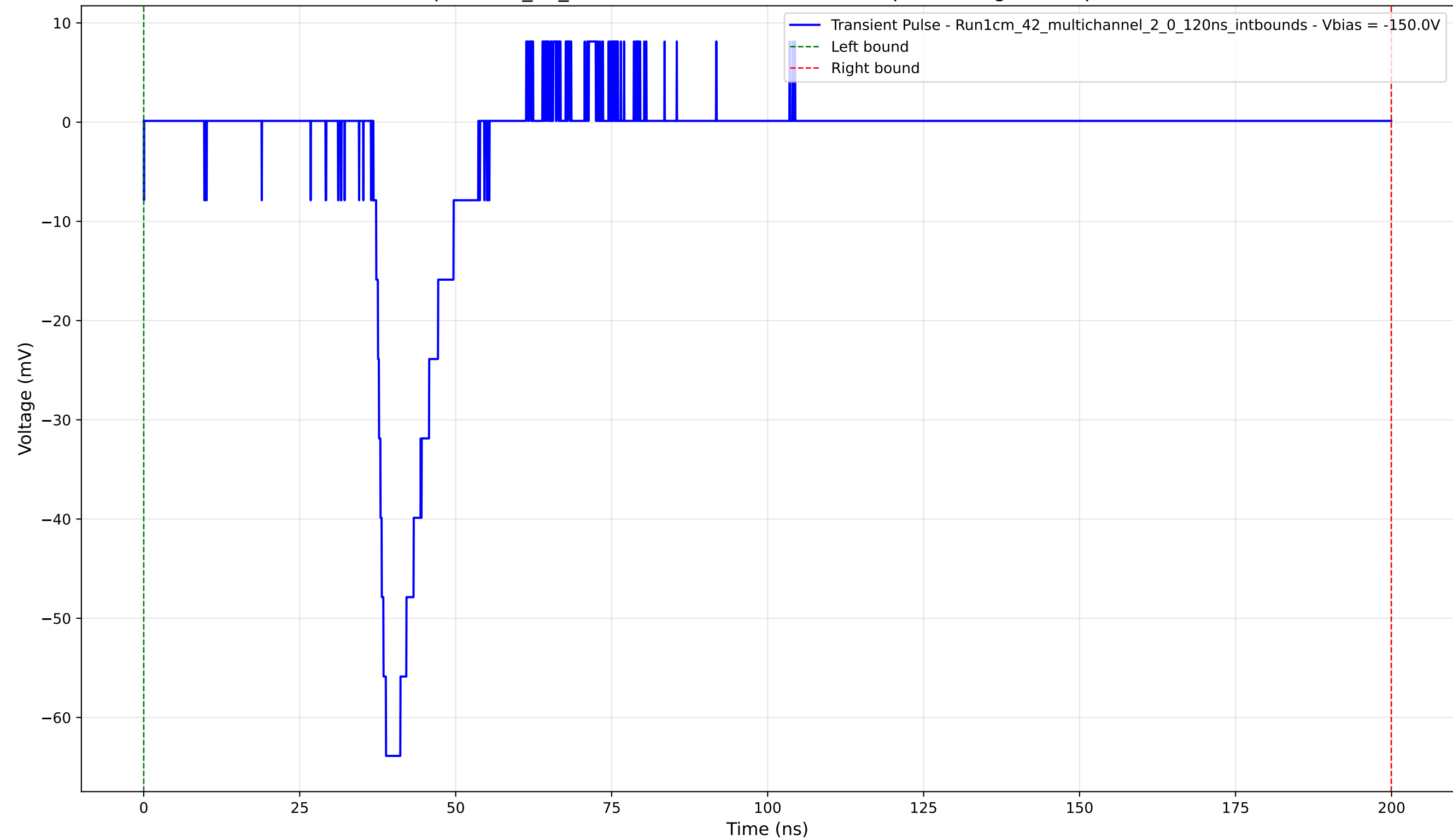
Transient Pulse - Sample: 1cm_42_multichannel - Position: 4470.0 \mu\text{m} - Charge: 8.95 pC - Rise Time: 2.01 ns
