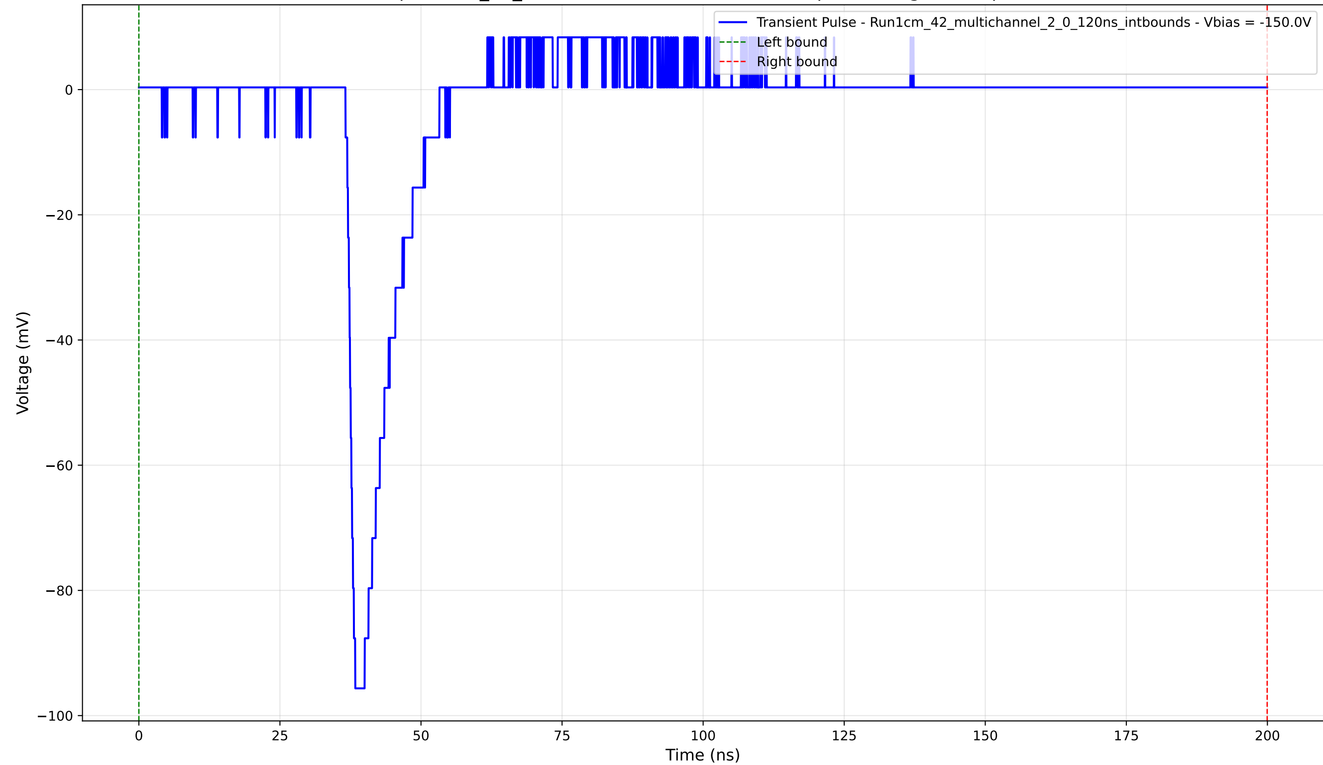
Transient Pulse - Sample: 1cm_42_multichannel - Position: 3805.0 \mu\text{m} - Charge: 8.96 pC - Rise Time: 1.19 ns
