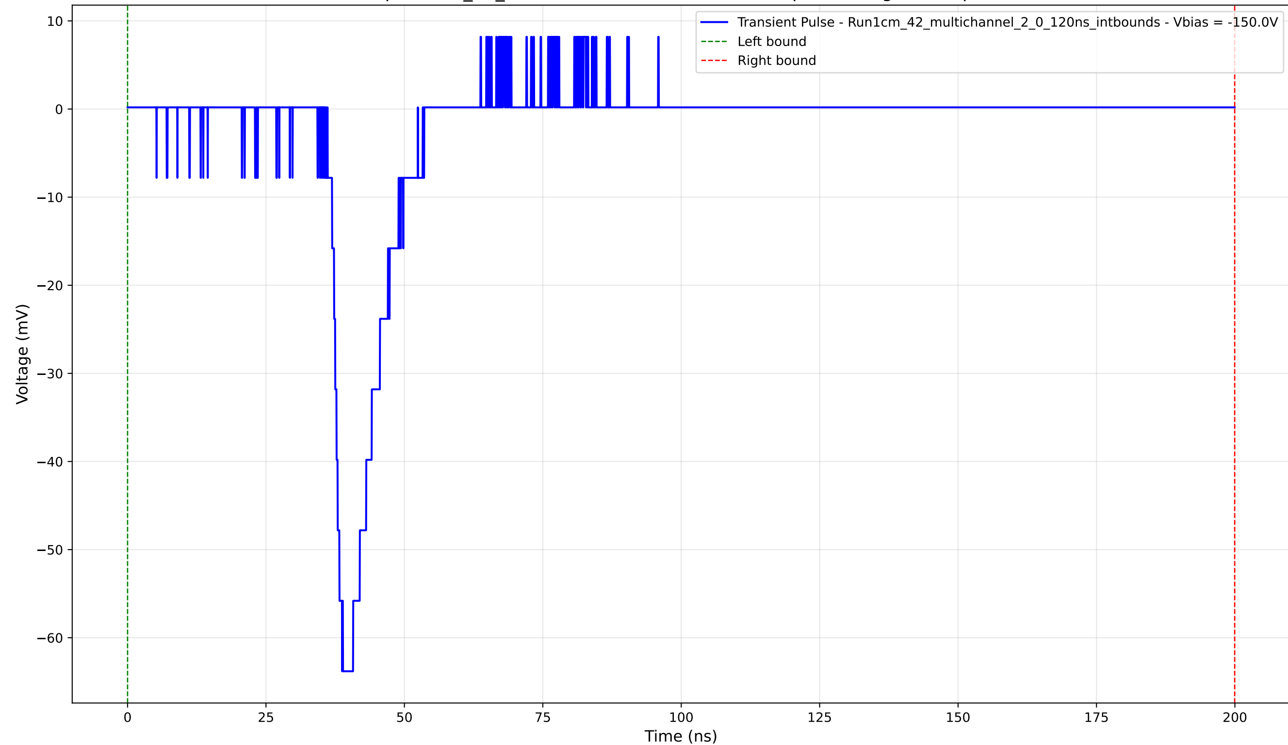
Transient Pulse - Sample: 1cm_42_multichannel - Position: 4770.0 \mu\text{m} - Charge: 8.79 pC - Rise Time: 2.61 ns
