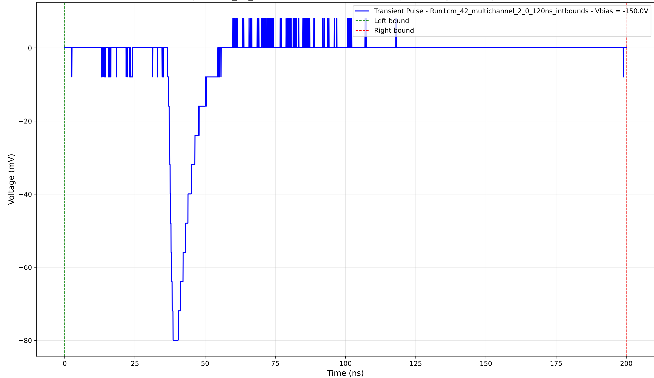
Transient Pulse - Sample: 1cm_42_multichannel - Position: 3955.0 \mu\text{m} - Charge: 11.39 pC - Rise Time: 1.60 ns
