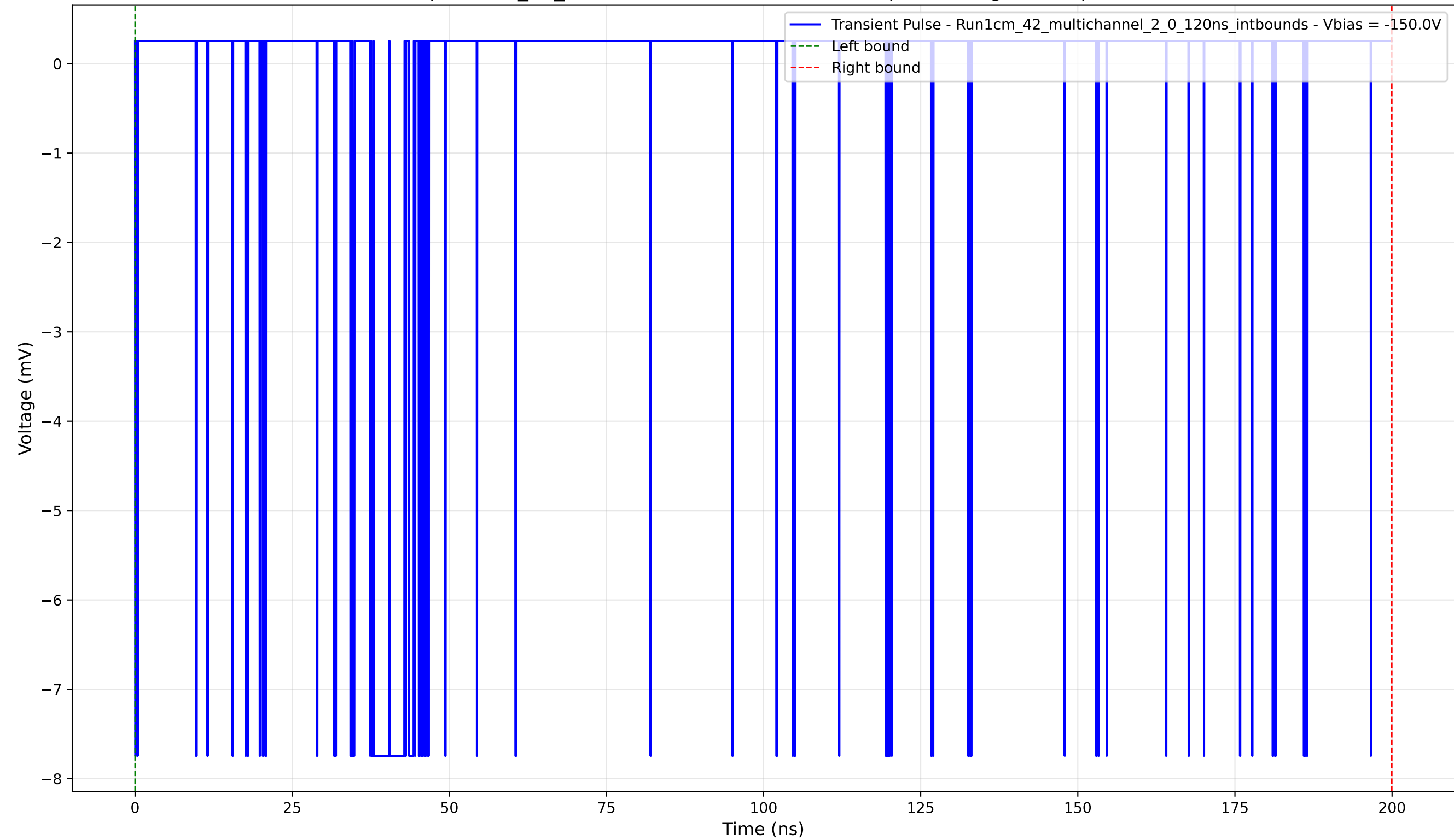
Transient Pulse - Sample: 1cm_42_multichannel - Position: 4390.0 \mu\text{m} - Charge: 0.86 pC - Rise Time: 0.04 ns
