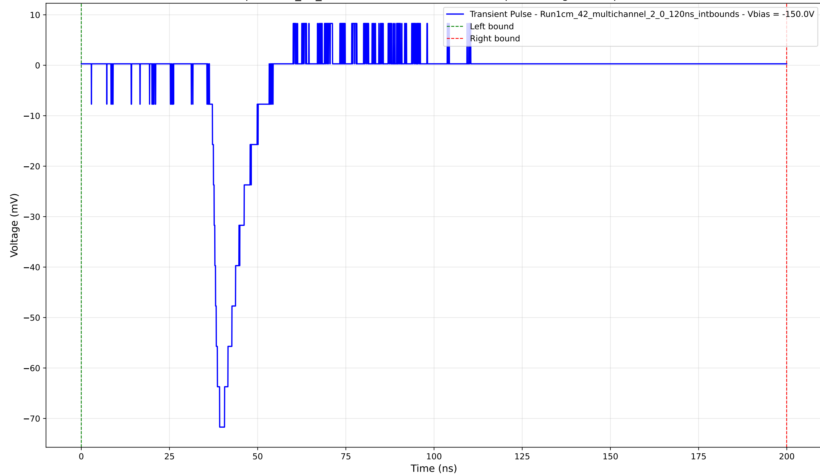
Transient Pulse - Sample: 1cm_42_multichannel - Position: 4490.0 \mu\text{m} - Charge: 8.52 pC - Rise Time: 2.88 ns
