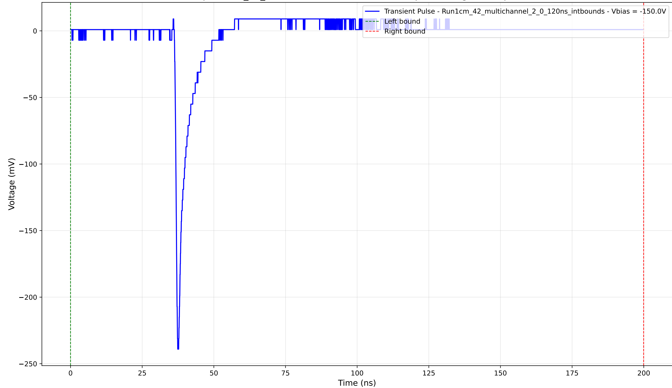
Transient Pulse - Sample: 1cm_42_multichannel - Position: 2945.0 \mu\text{m} - Charge: 8.25 pC - Rise Time: 0.84 ns
