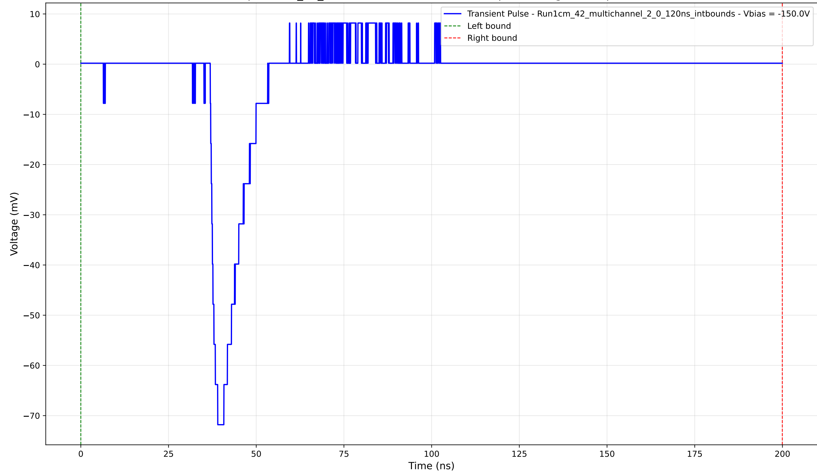
Transient Pulse - Sample: 1cm_42_multichannel - Position: 175.0 \mu\text{m} - Charge: 8.46 pC - Rise Time: 2.12 ns
