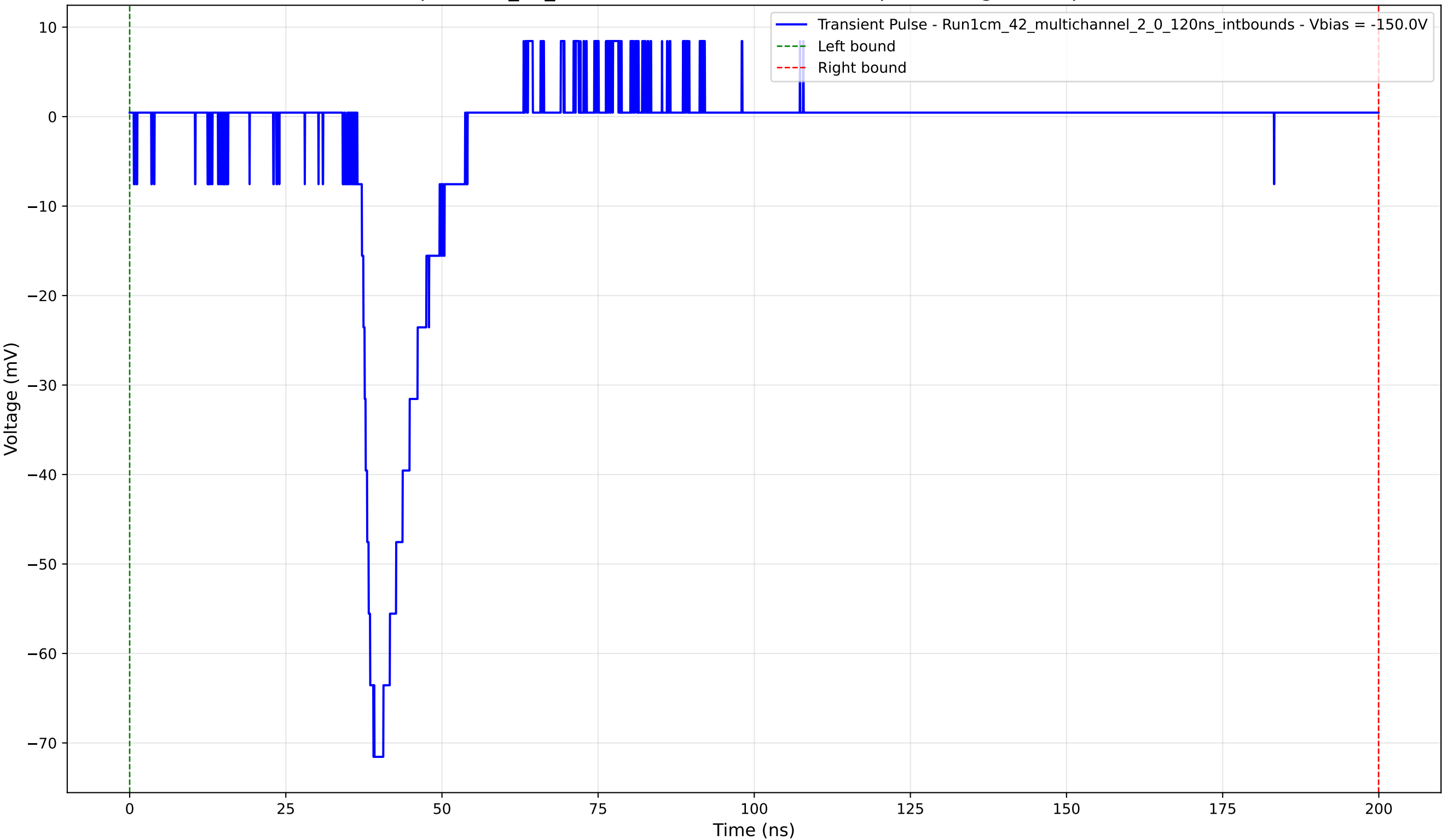
Transient Pulse - Sample: 1cm_42_multichannel - Position: 4605.0 \mu\text{m} - Charge: 8.74 pC - Rise Time: 2.56 ns
