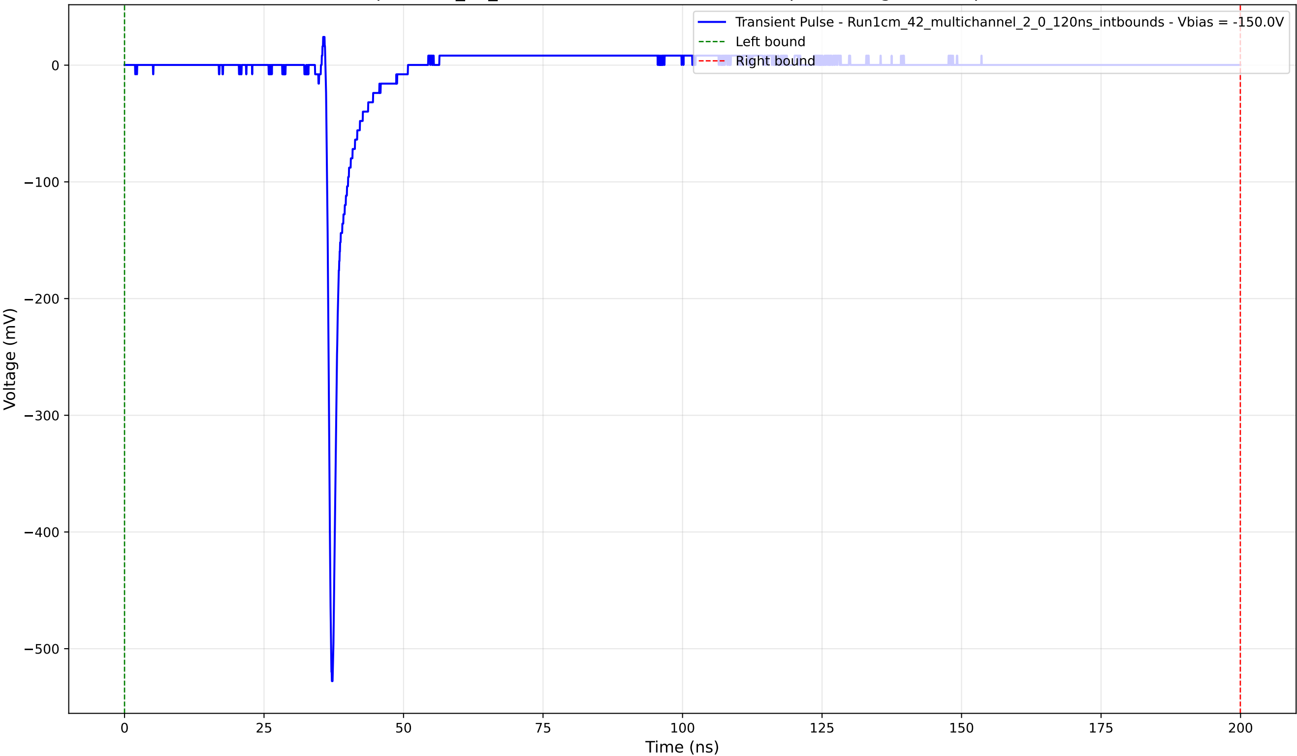
Transient Pulse - Sample: 1cm_42_multichannel - Position: 2540.0 \mu\text{m} - Charge: 15.70 pC - Rise Time: 0.74 ns
