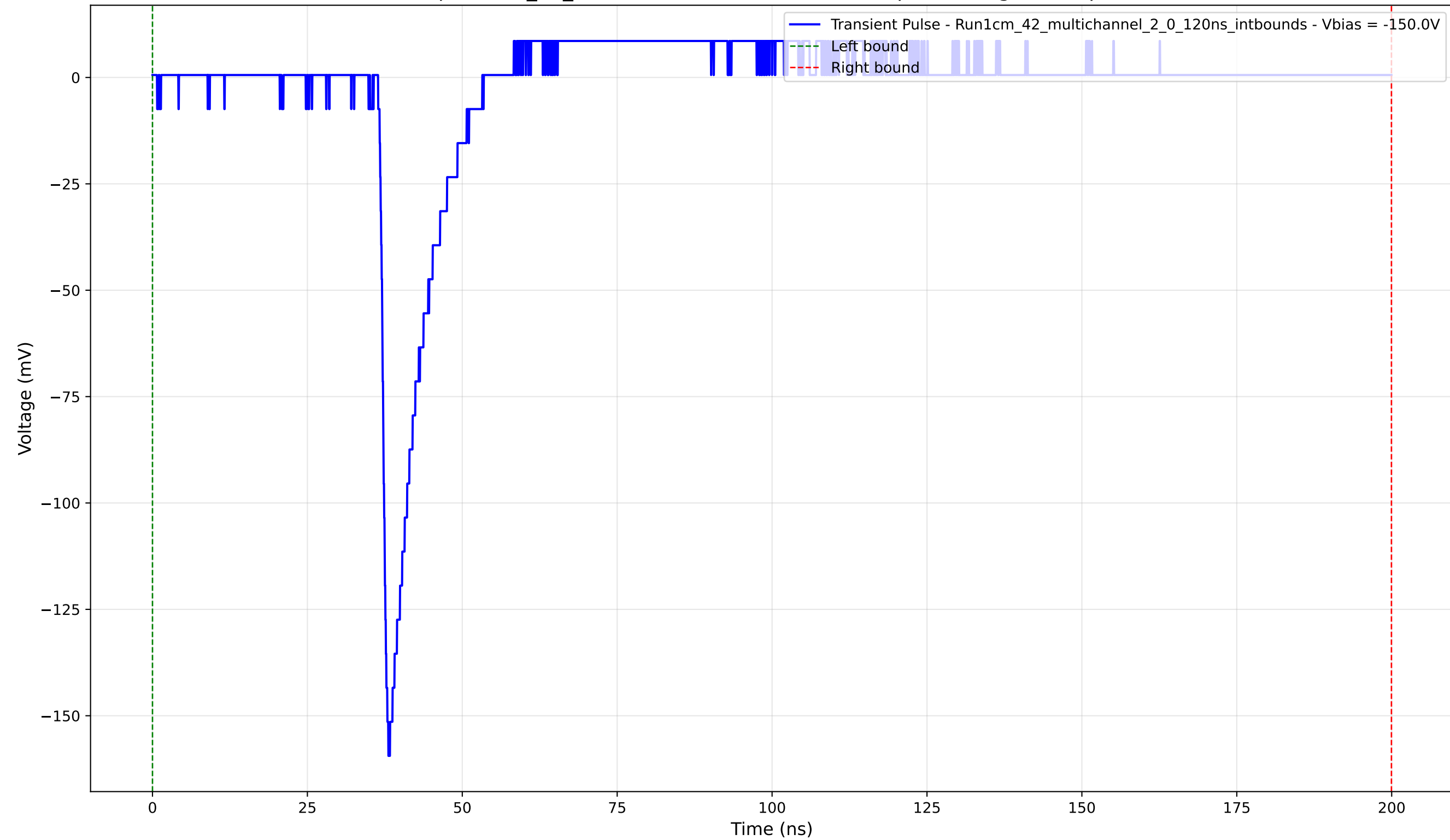
Transient Pulse - Sample: 1cm_42_multichannel - Position: 1240.0 \mu\text{m} - Charge: 8.98 pC - Rise Time: 1.20 ns
