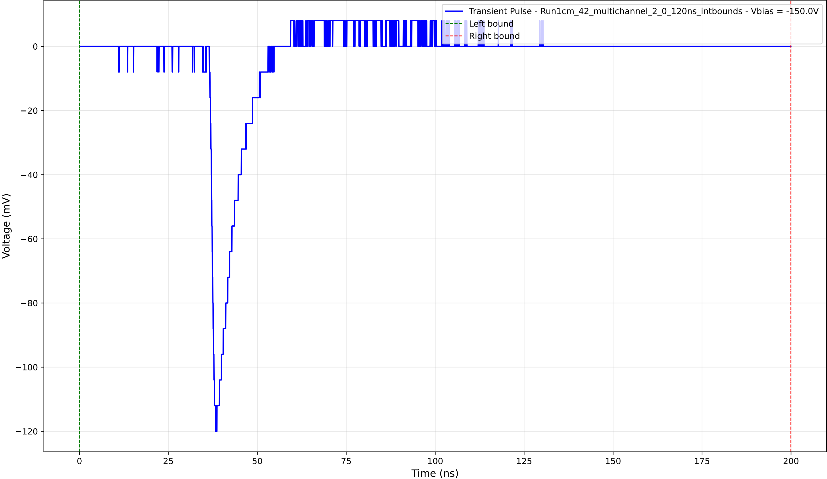
Transient Pulse - Sample: 1cm_42_multichannel - Position: 3595.0 \mu\text{m} - Charge: 11.31 pC - Rise Time: 1.26 ns
