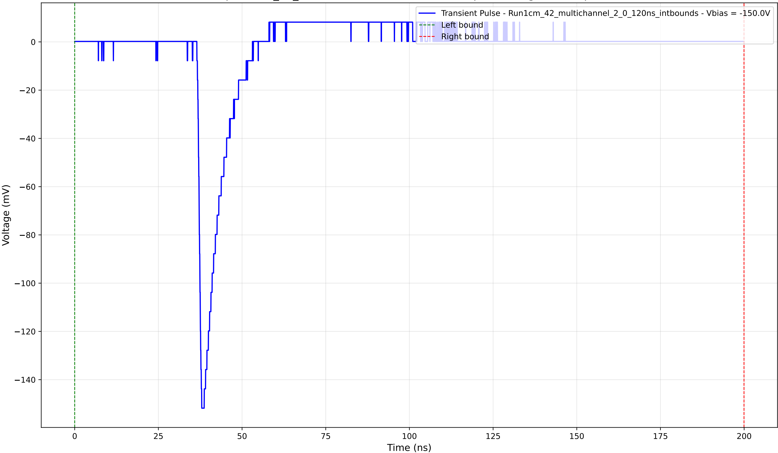
Transient Pulse - Sample: 1cm_42_multichannel - Position: 1225.0 \mu\text{m} - Charge: 10.79 pC - Rise Time: 1.16 ns
