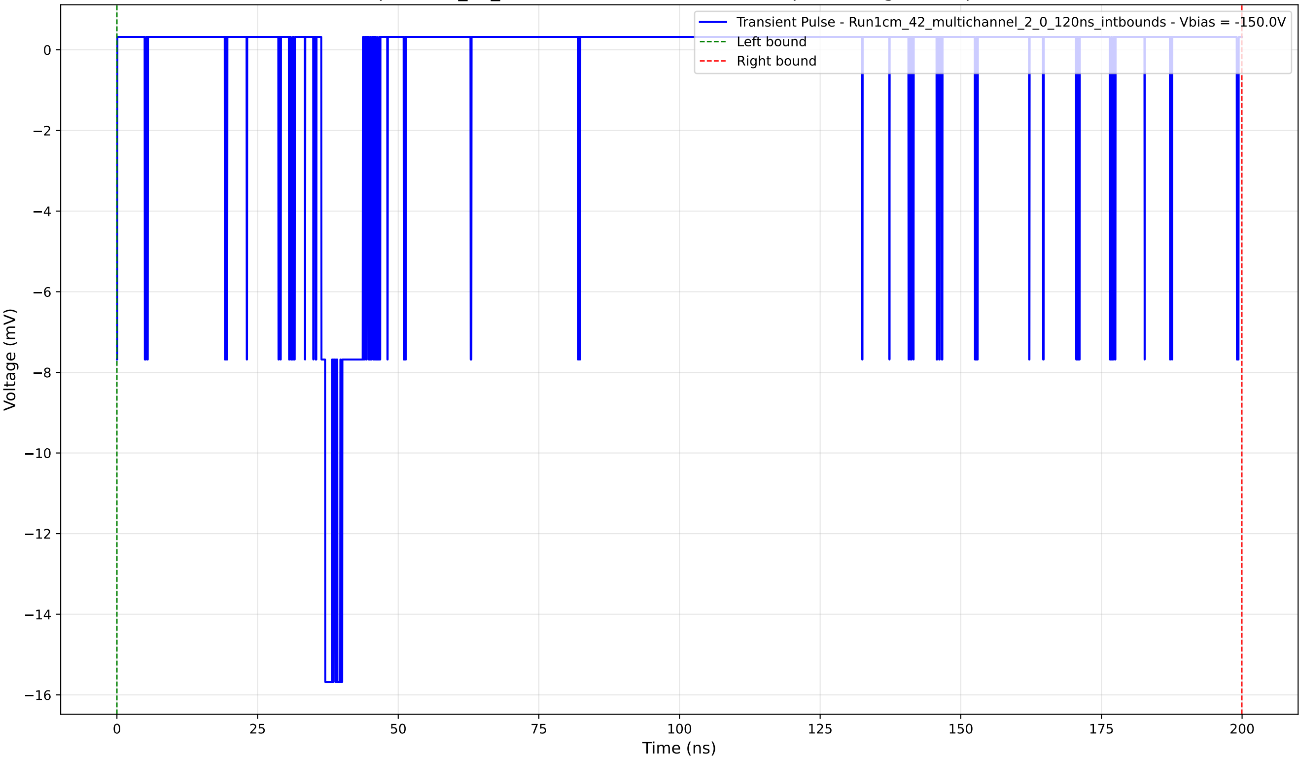
Transient Pulse - Sample: 1cm_42_multichannel - Position: 2890.0 \mu\text{m} - Charge: 1.33 pC - Rise Time: 0.71 ns
