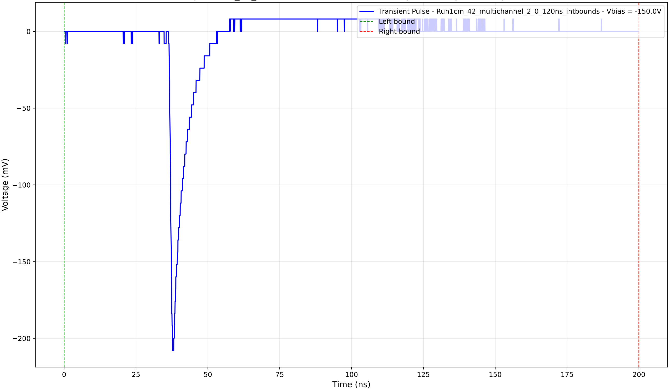
Transient Pulse - Sample: 1cm_42_multichannel - Position: 1485.0 \mu\text{m} - Charge: 11.13 pC - Rise Time: 0.98 ns
