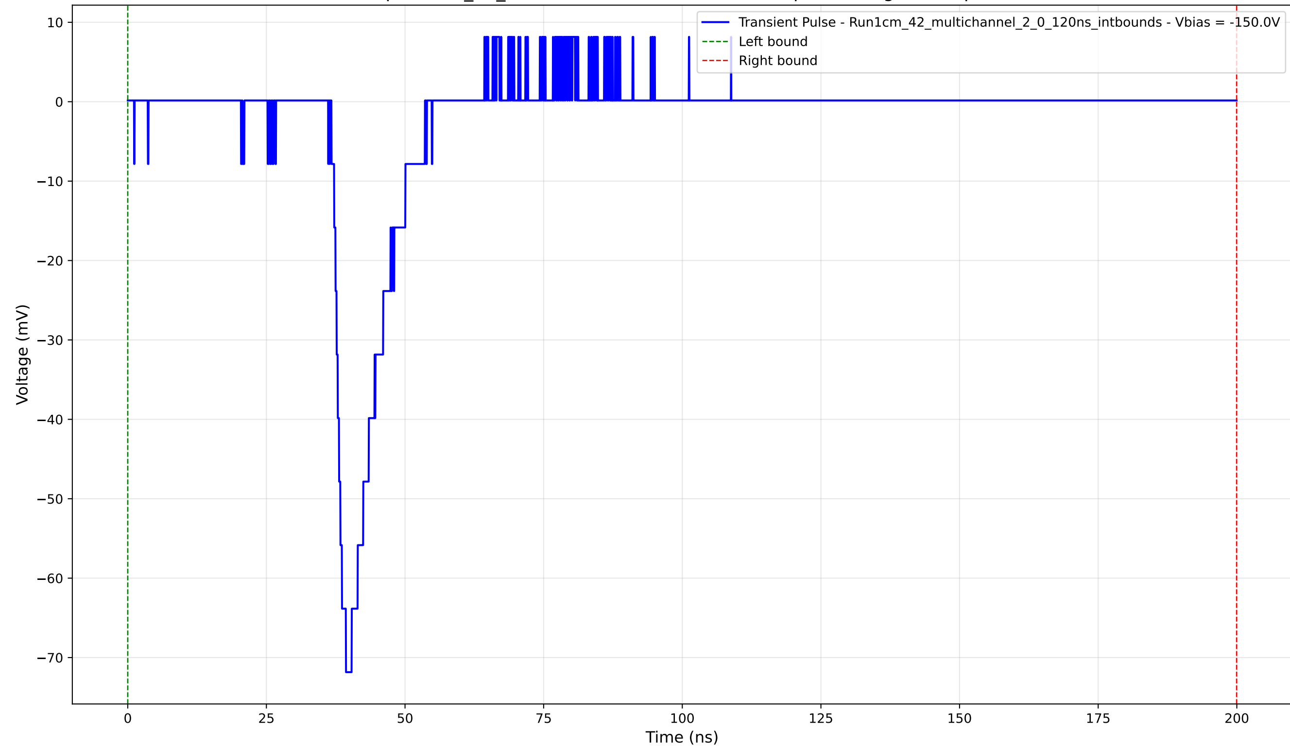
Transient Pulse - Sample: 1cm_42_multichannel - Position: 4300.0 \mu\text{m} - Charge: 9.24 pC - Rise Time: 2.60 ns
