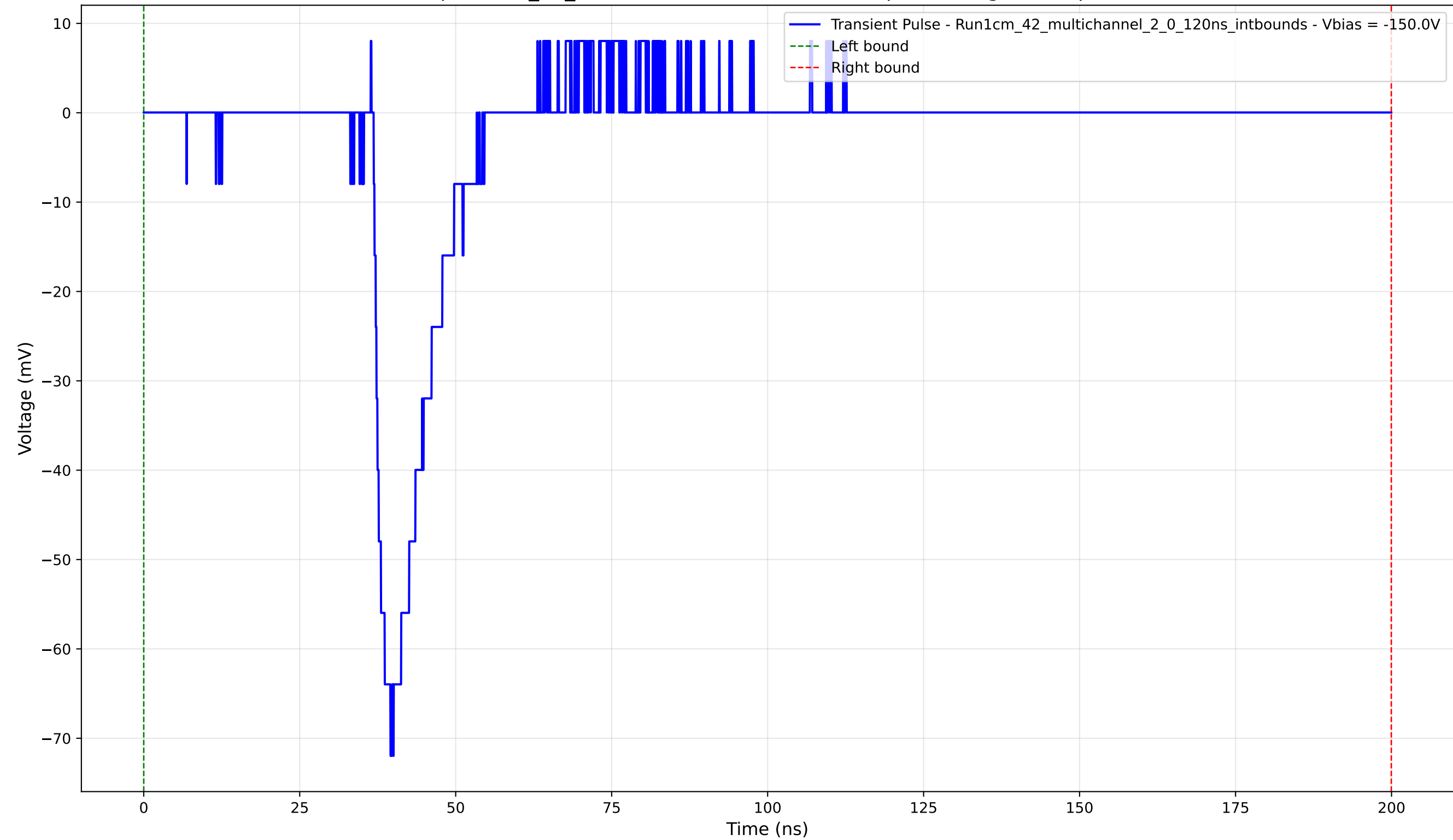
Transient Pulse - Sample: 1cm_42_multichannel - Position: 140.0 \mu\text{m} - Charge: 9.38 pC - Rise Time: 2.68 ns
