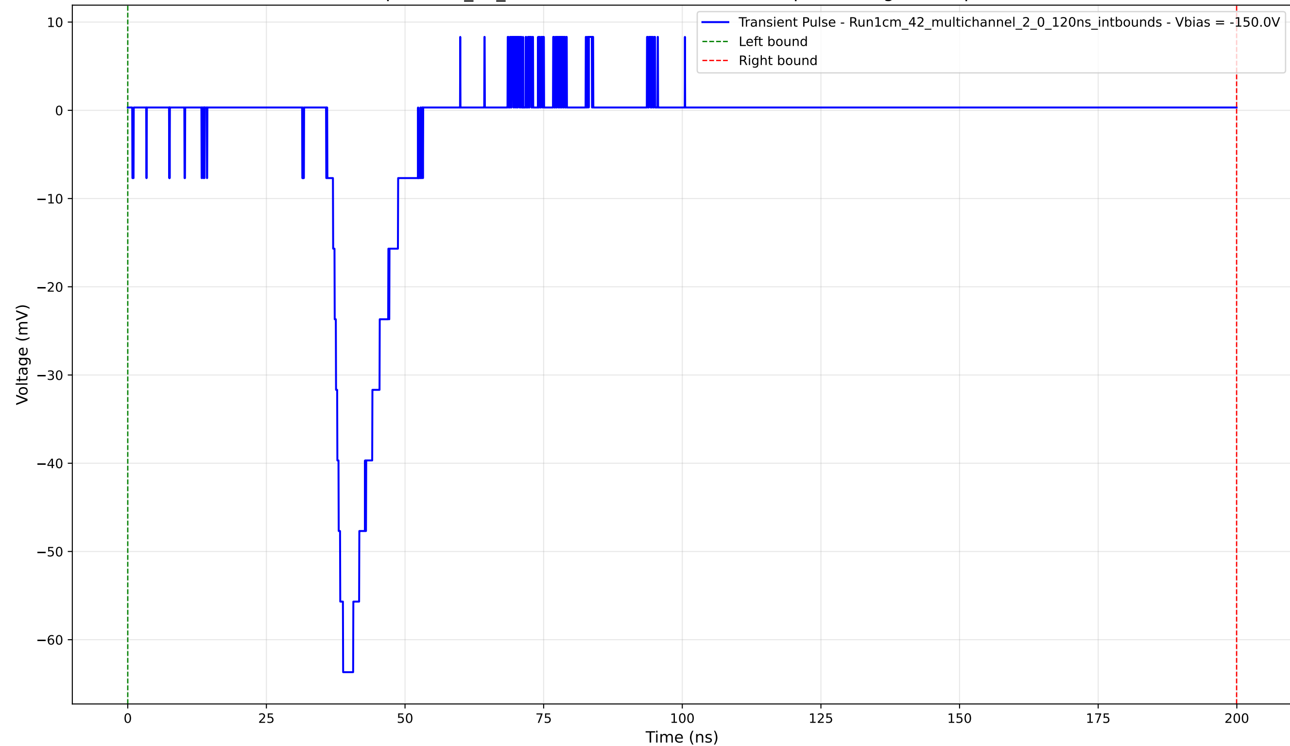
Transient Pulse - Sample: 1cm_42_multichannel - Position: 4785.0 \mu\text{m} - Charge: 7.93 pC - Rise Time: 2.85 ns
