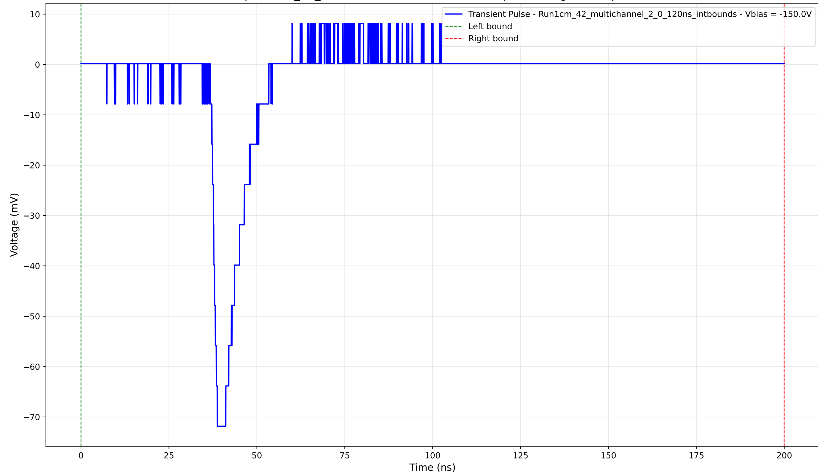
Transient Pulse - Sample: 1cm_42_multichannel - Position: 4275.0 \mu\text{m} - Charge: 9.76 pC - Rise Time: 2.00 ns
