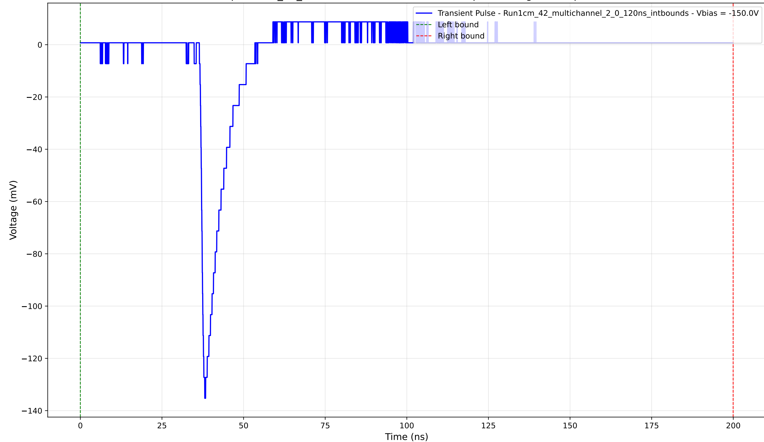
Transient Pulse - Sample: 1cm_42_multichannel - Position: 3495.0 \mu\text{m} - Charge: 8.43 pC - Rise Time: 1.17 ns
