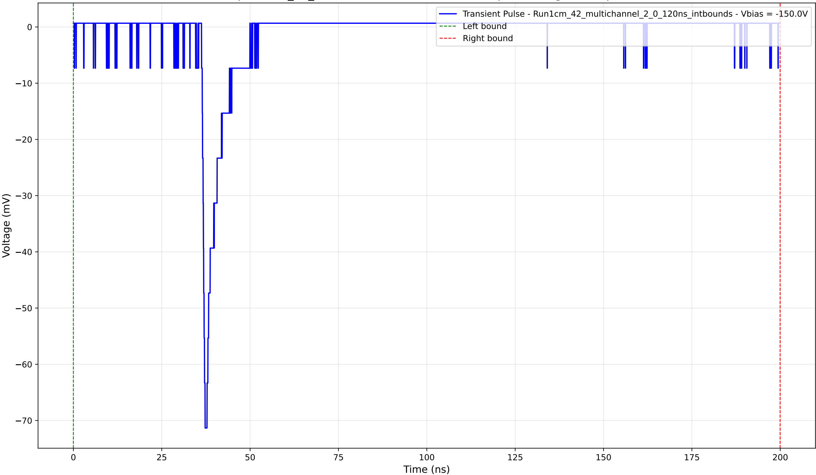
Transient Pulse - Sample: 1cm_42_multichannel - Position: 2915.0 \mu\text{m} - Charge: 4.52 pC - Rise Time: 1.00 ns
