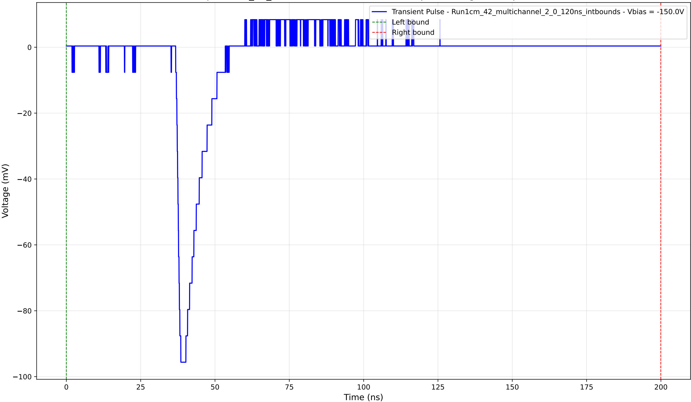
Transient Pulse - Sample: 1cm_42_multichannel - Position: 770.0 \mu\text{m} - Charge: 9.26 pC - Rise Time: 1.19 ns
