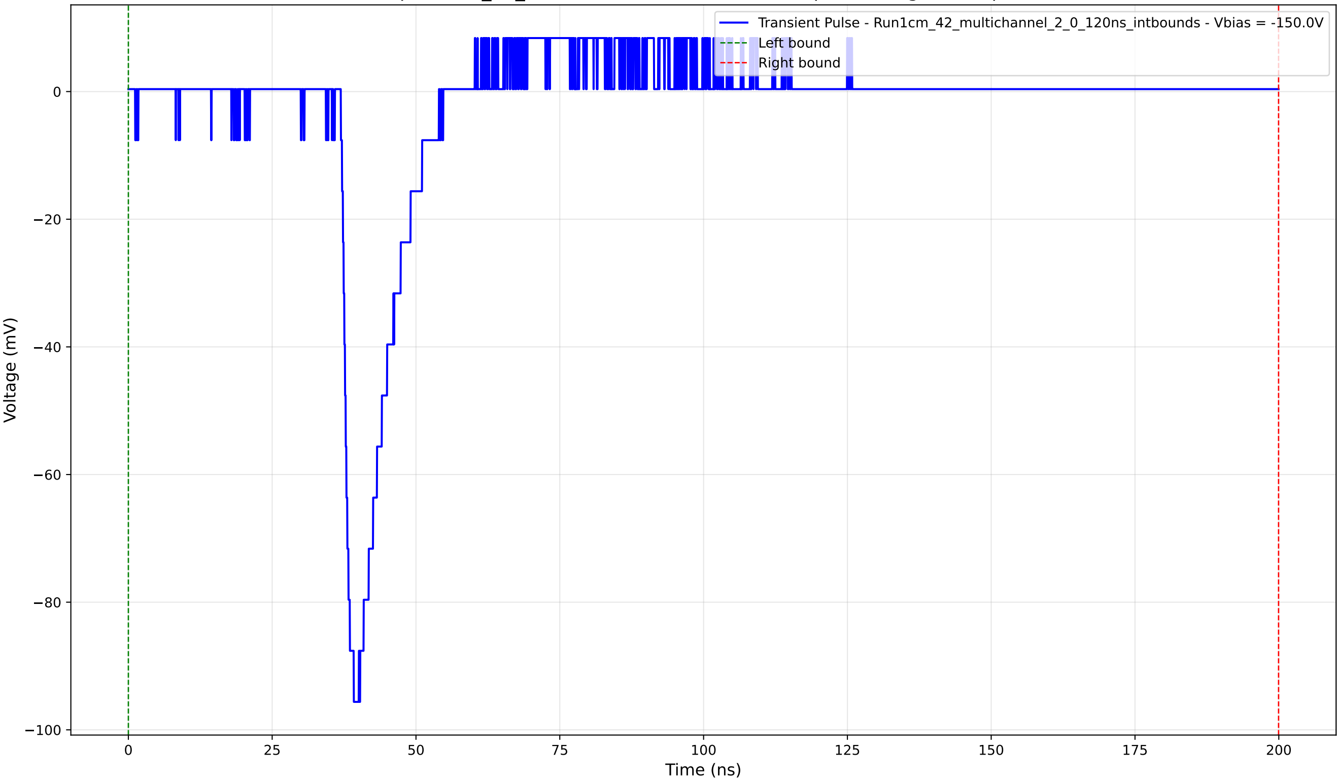
Transient Pulse - Sample: 1cm_42_multichannel - Position: 545.0 \mu\text{m} - Charge: 8.74 pC - Rise Time: 1.39 ns
