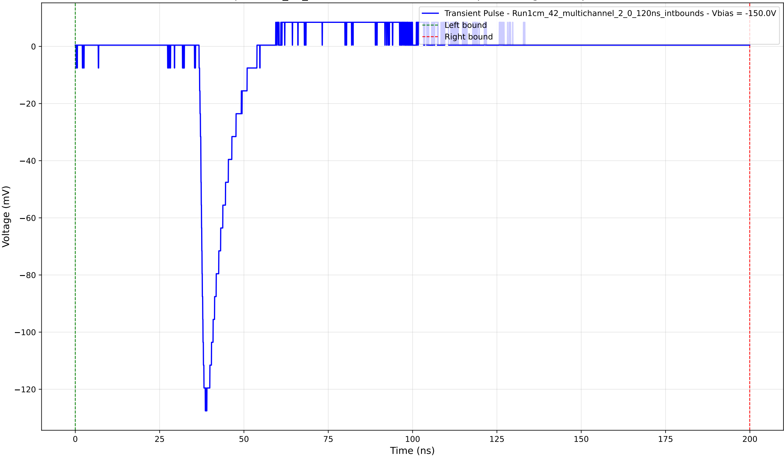
Transient Pulse - Sample: 1cm_42_multichannel - Position: 980.0 \mu\text{m} - Charge: 8.79 pC - Rise Time: 1.29 ns
