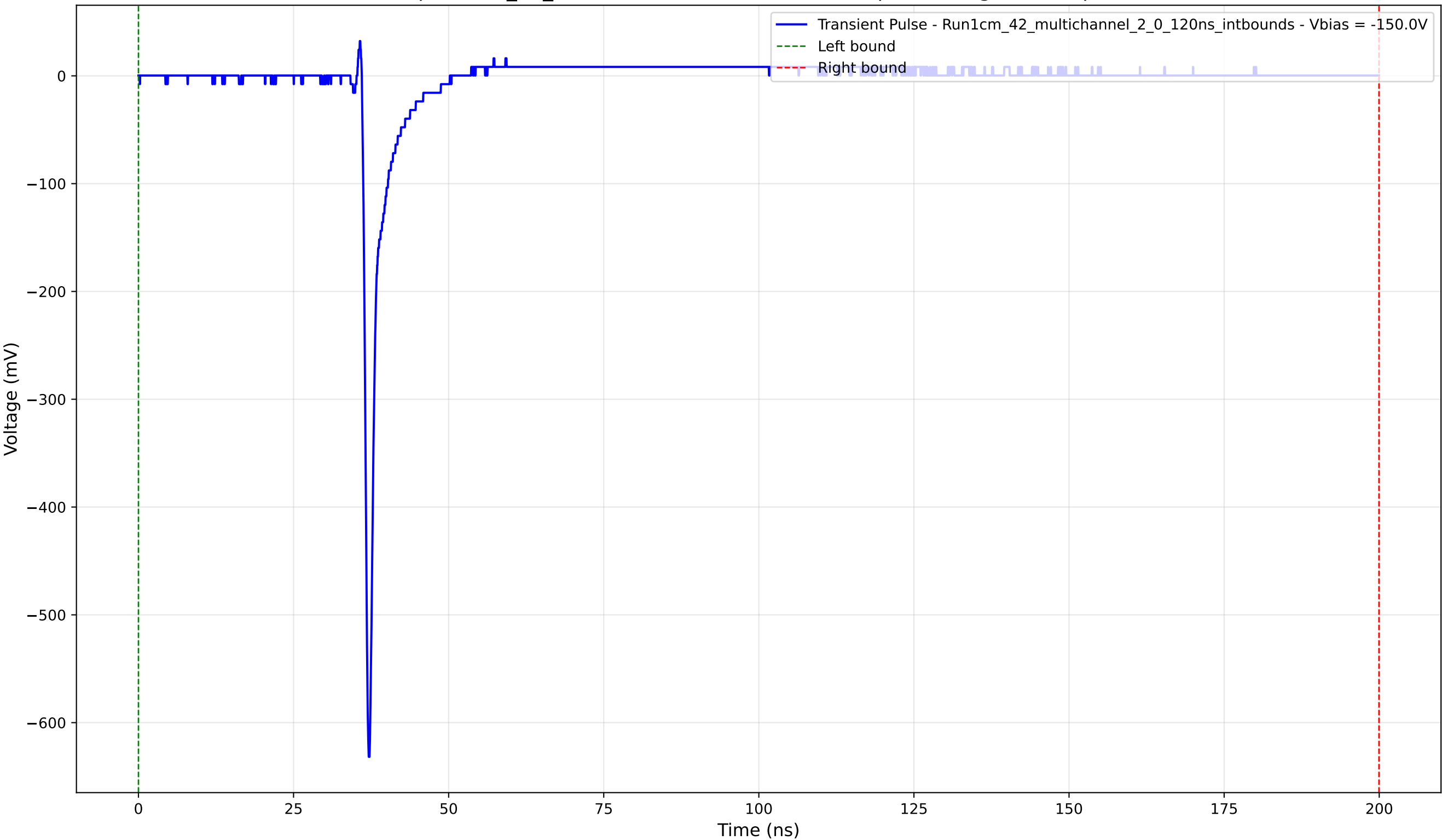
Transient Pulse - Sample: 1cm_42_multichannel - Position: 2260.0 \mu\text{m} - Charge: 16.63 pC - Rise Time: 0.72 ns
