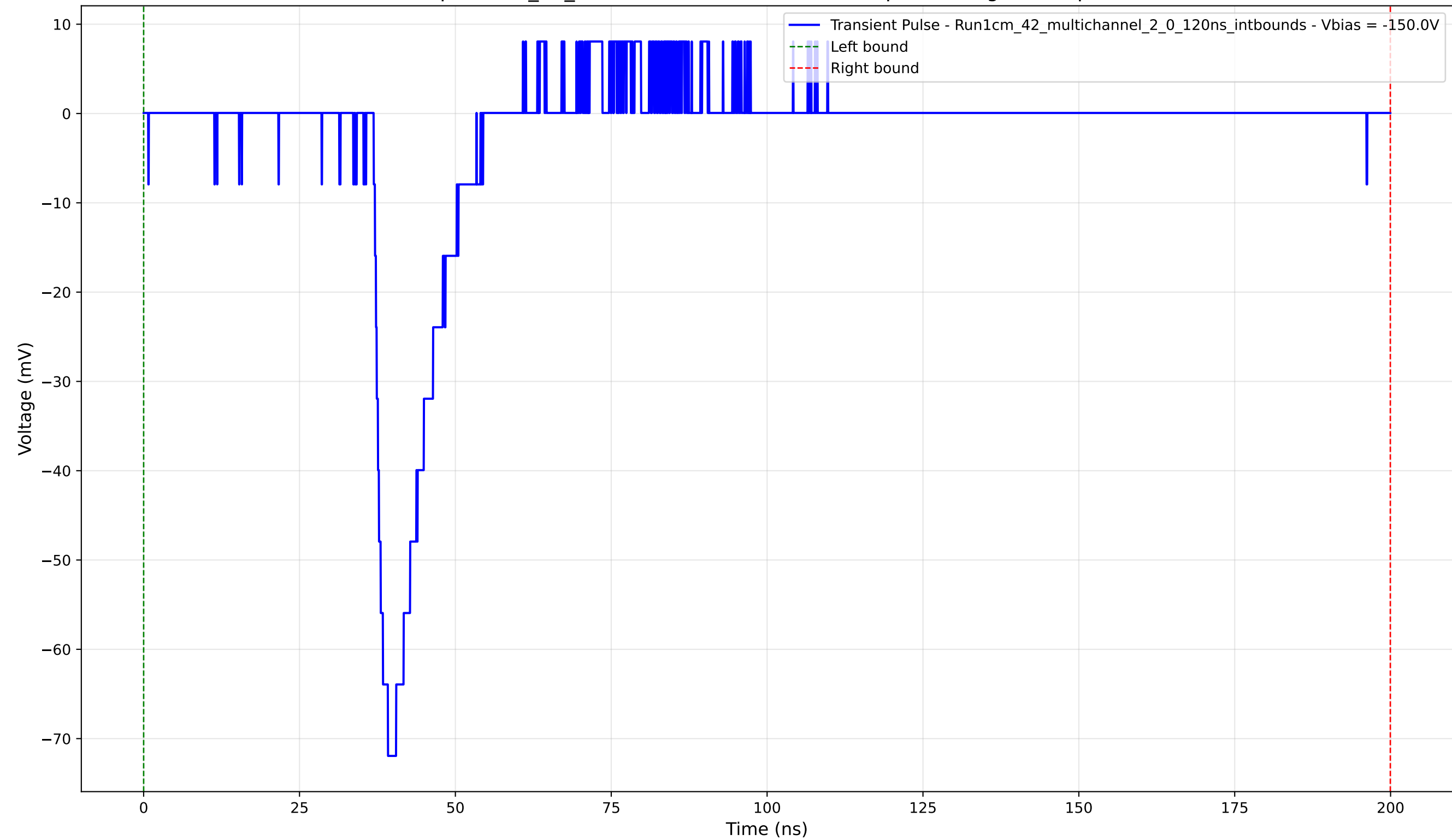
Transient Pulse - Sample: 1cm_42_multichannel - Position: 255.0 \mu\text{m} - Charge: 9.40 pC - Rise Time: 2.28 ns
