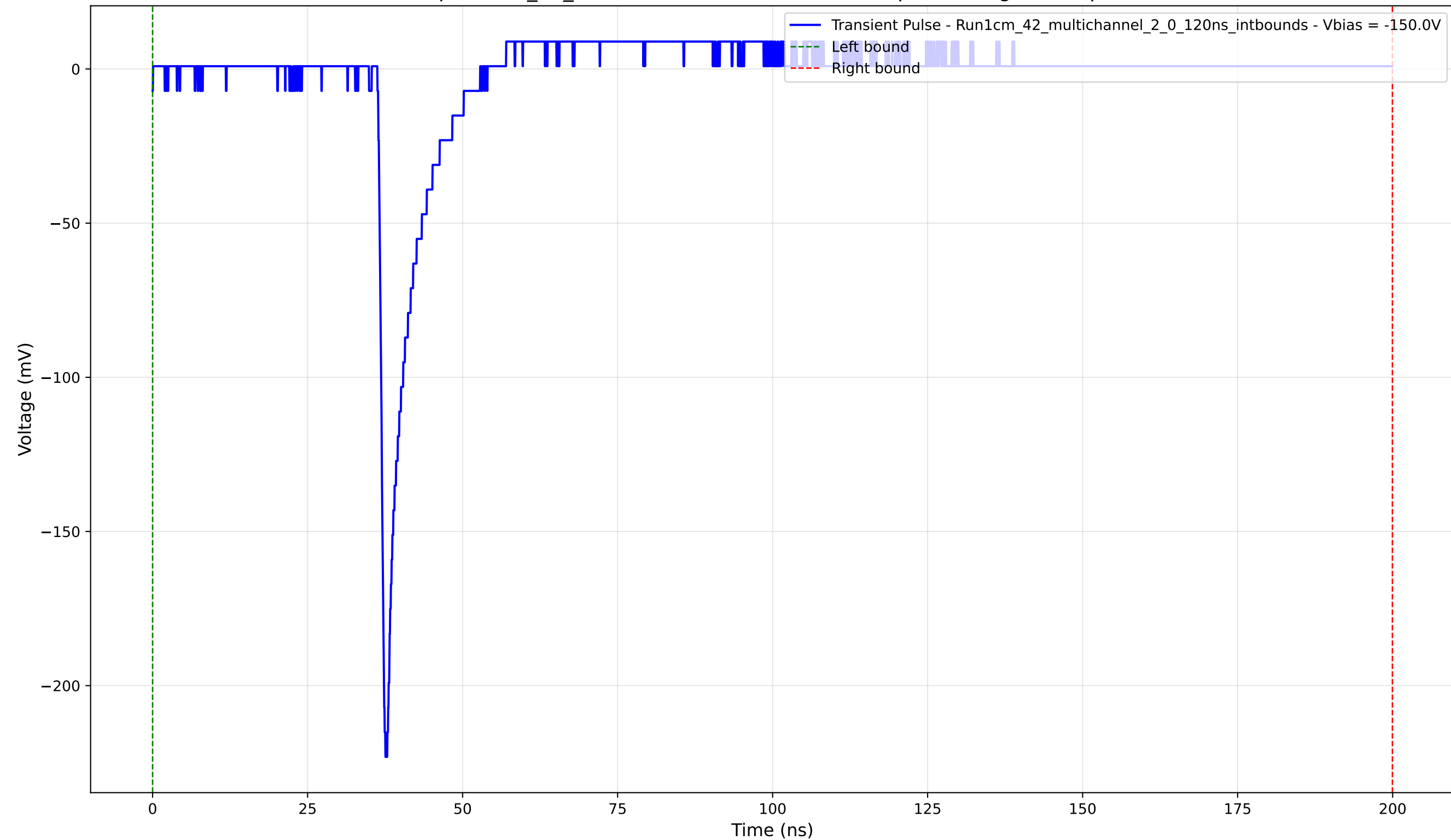
Transient Pulse - Sample: 1cm_42_multichannel - Position: 3075.0 \mu\text{m} - Charge: 9.29 pC - Rise Time: 0.92 ns
