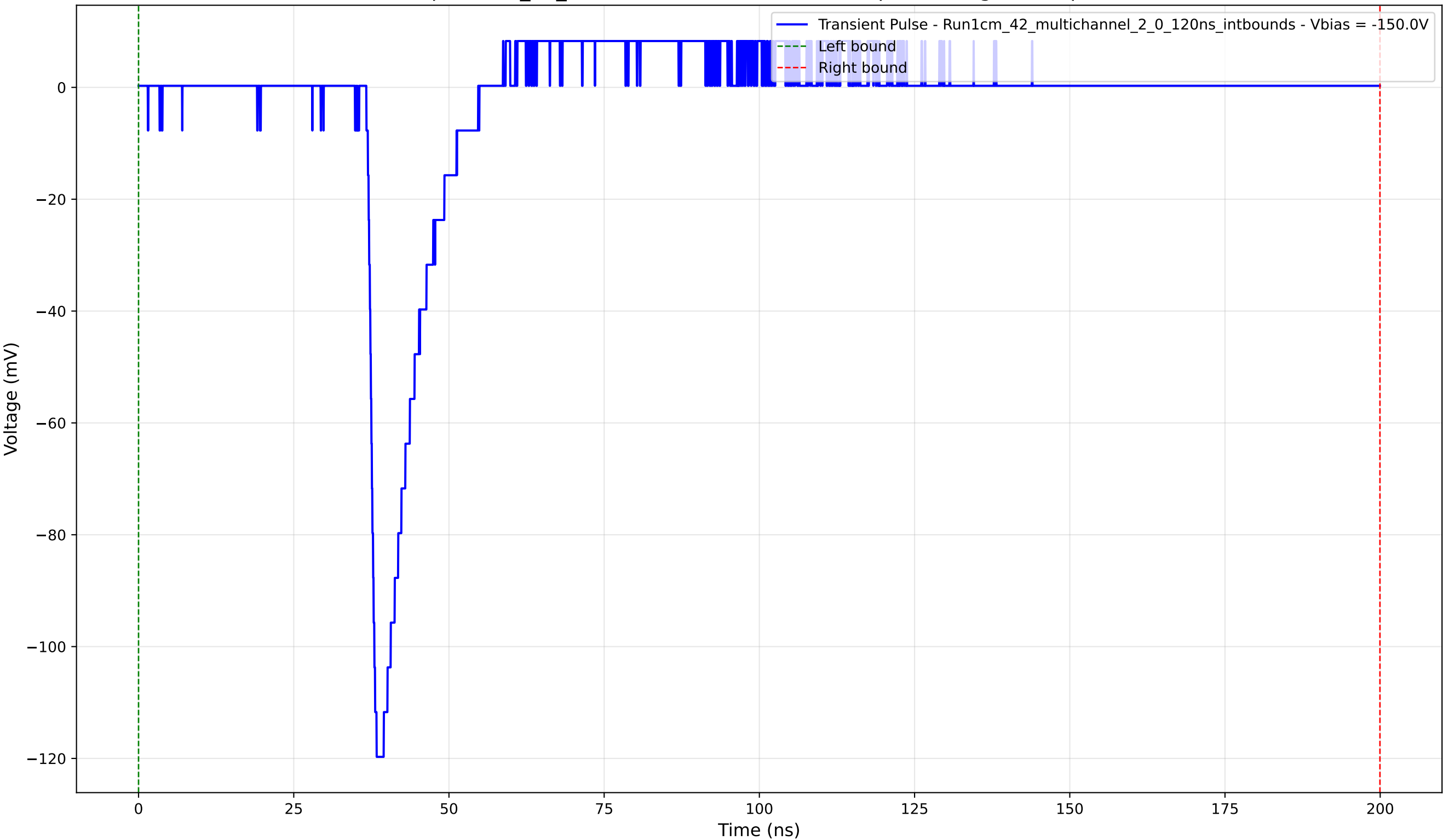
Transient Pulse - Sample: 1cm_42_multichannel - Position: 940.0 \mu\text{m} - Charge: 8.91 pC - Rise Time: 1.18 ns
