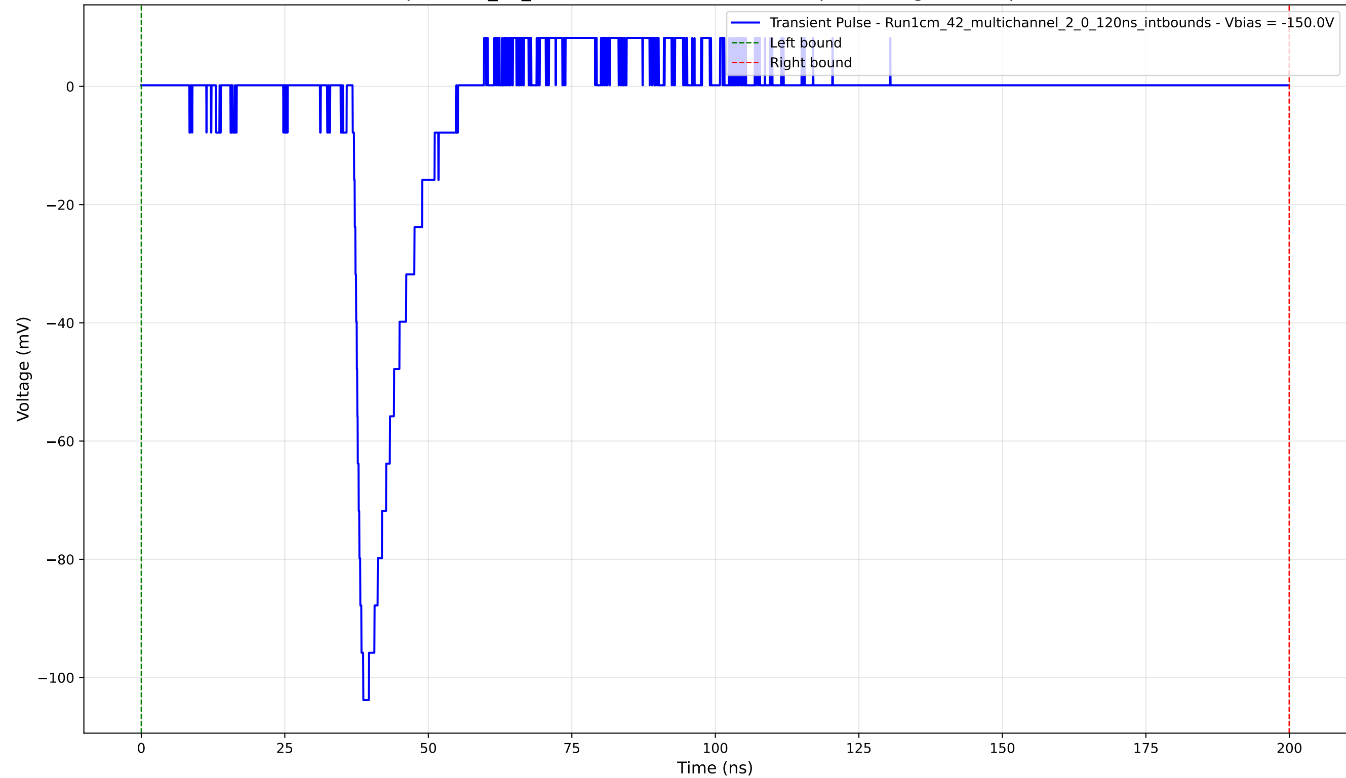
Transient Pulse - Sample: 1cm_42_multichannel - Position: 755.0 \mu\text{m} - Charge: 10.49 pC - Rise Time: 1.31 ns
