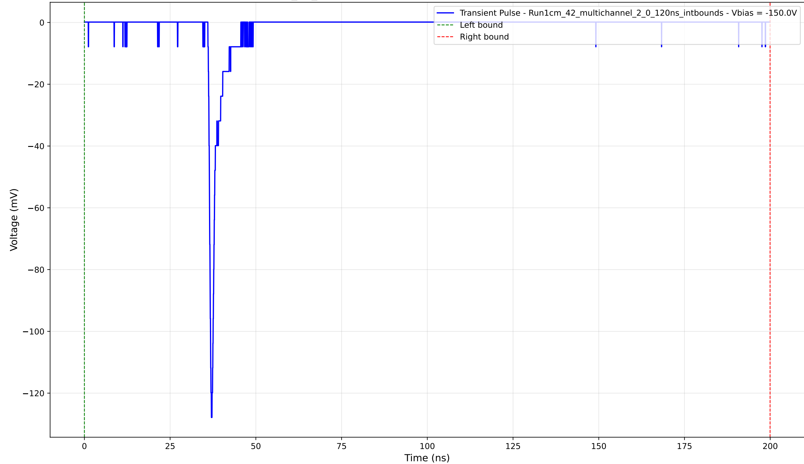
Transient Pulse - Sample: 1cm_42_multichannel - Position: 2405.0 \mu\text{m} - Charge: 5.97 pC - Rise Time: 0.78 ns
