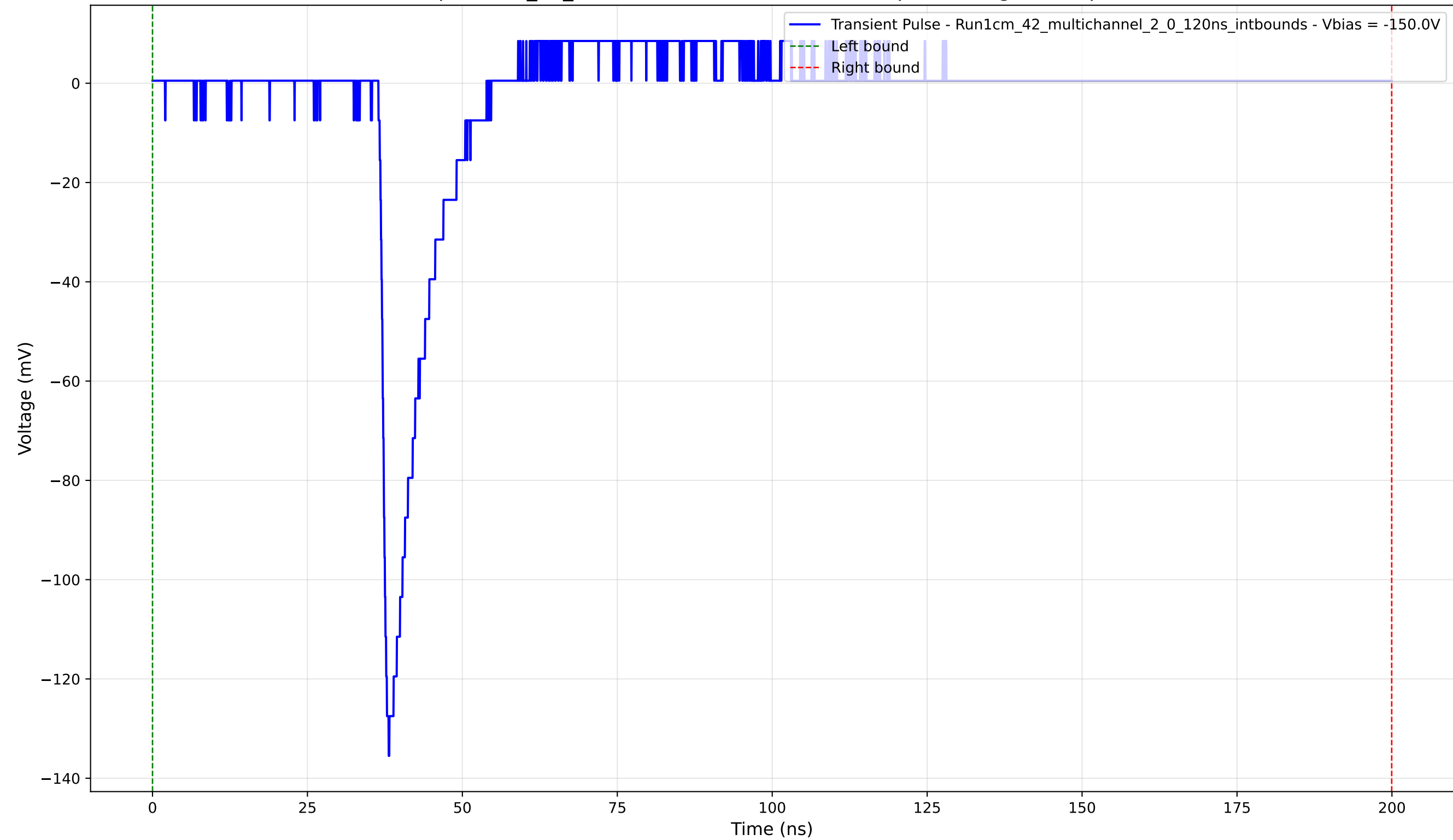
Transient Pulse - Sample: 1cm_42_multichannel - Position: 3500.0 \mu\text{m} - Charge: 9.88 pC - Rise Time: 1.17 ns
