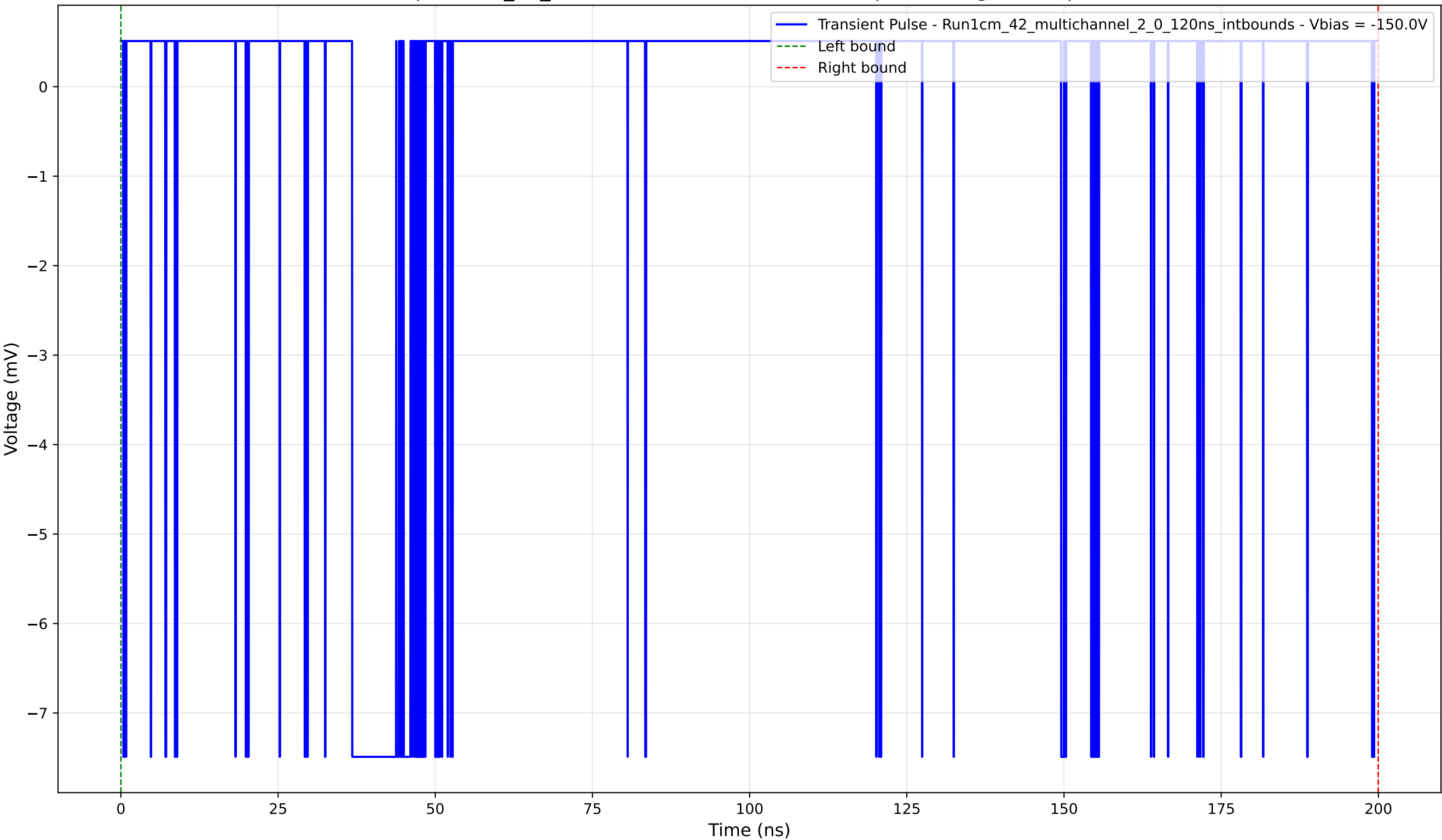
Transient Pulse - Sample: 1cm_42_multichannel - Position: 1365.0 \mu\text{m} - Charge: 0.33 pC - Rise Time: 0.04 ns
