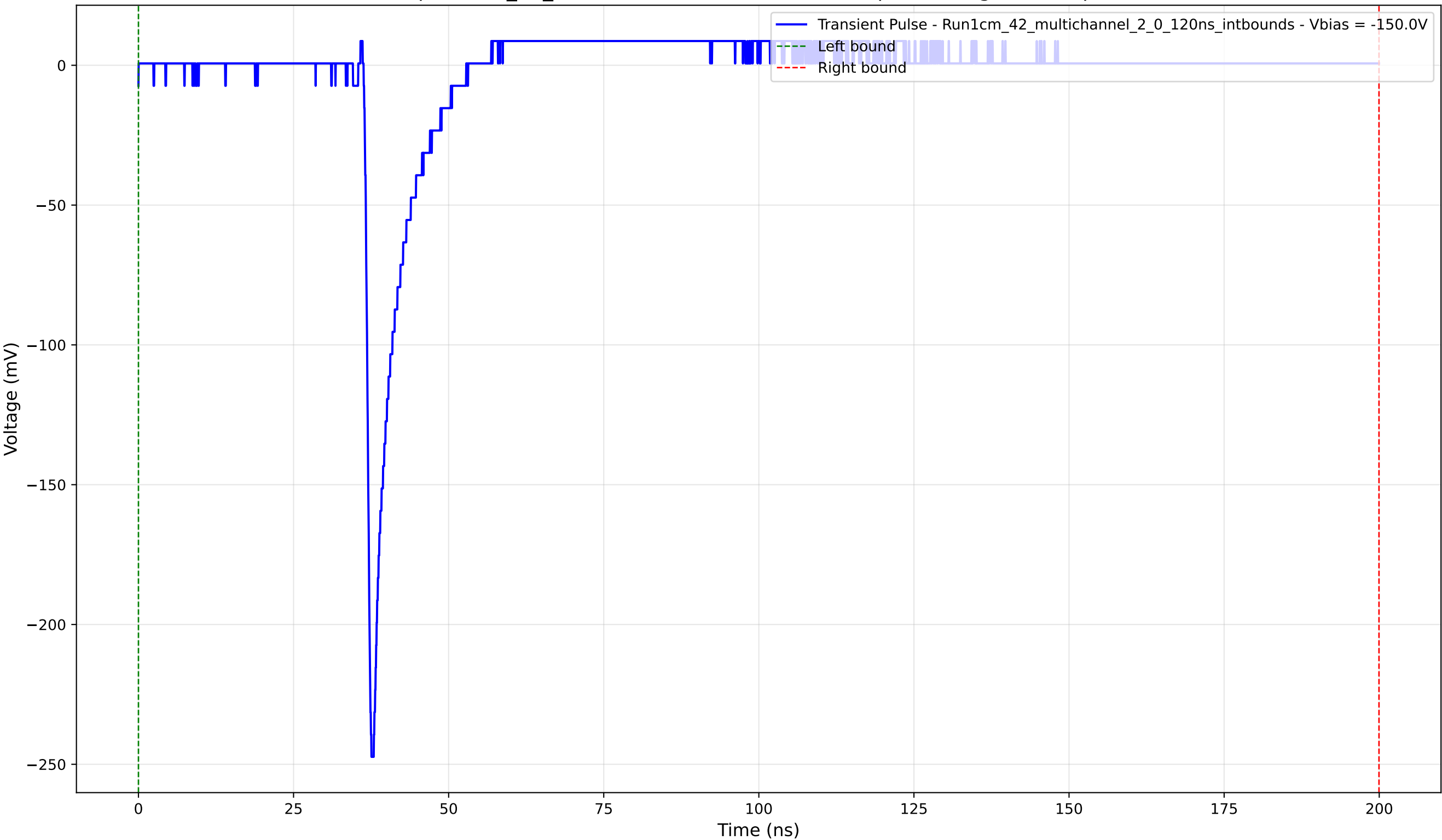
Transient Pulse - Sample: 1cm_42_multichannel - Position: 1640.0 \mu\text{m} - Charge: 10.80 pC - Rise Time: 0.87 ns
