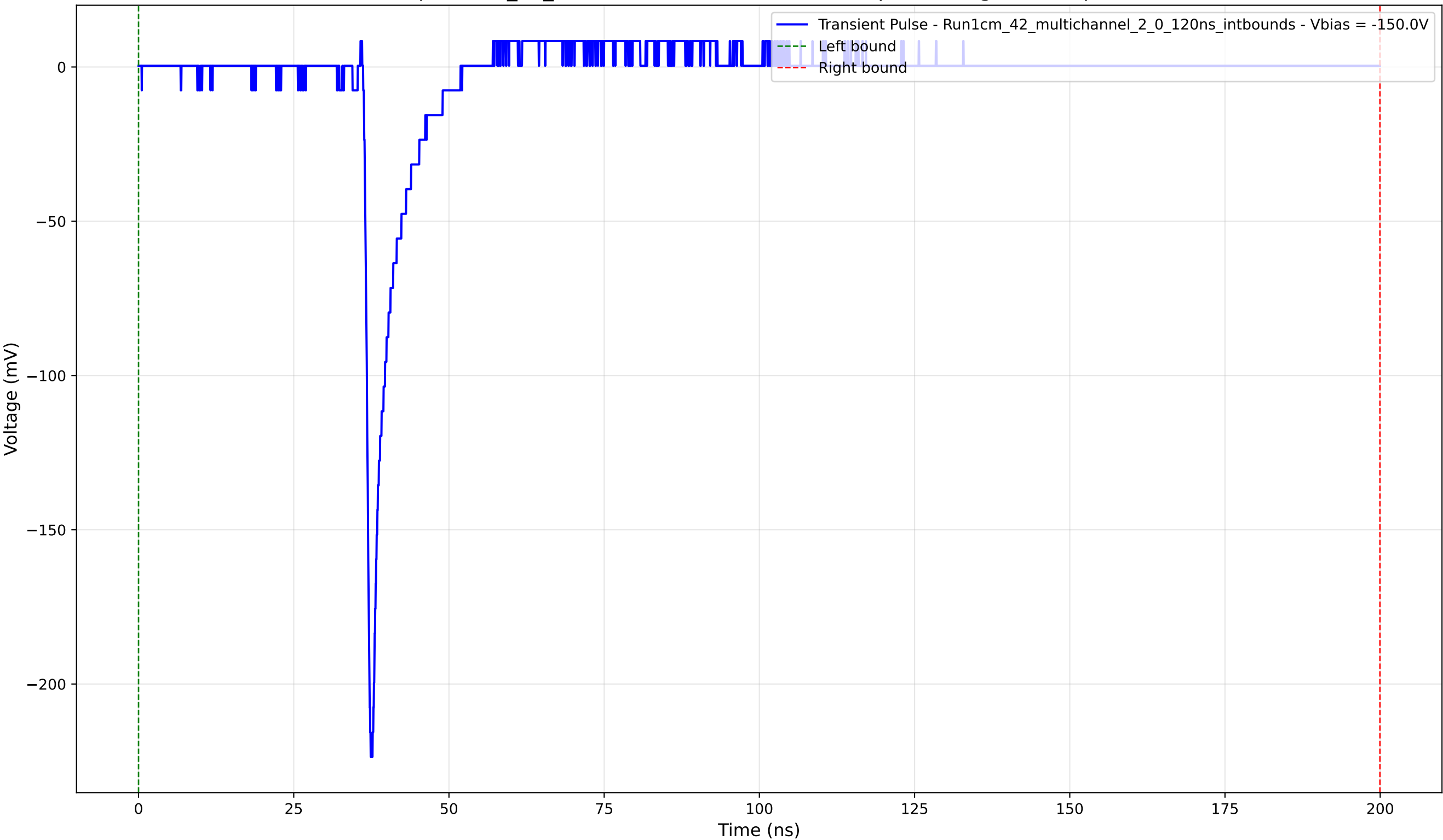
Transient Pulse - Sample: 1cm_42_multichannel - Position: 2940.0 \mu\text{m} - Charge: 10.91 pC - Rise Time: 0.89 ns
