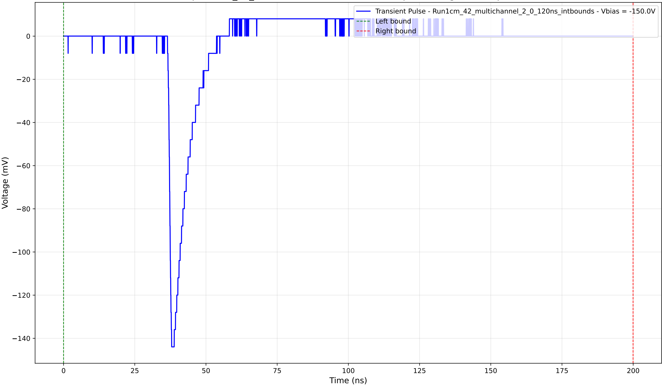
Transient Pulse - Sample: 1cm_42_multichannel - Position: 1190.0 \mu\text{m} - Charge: 10.66 pC - Rise Time: 1.17 ns
