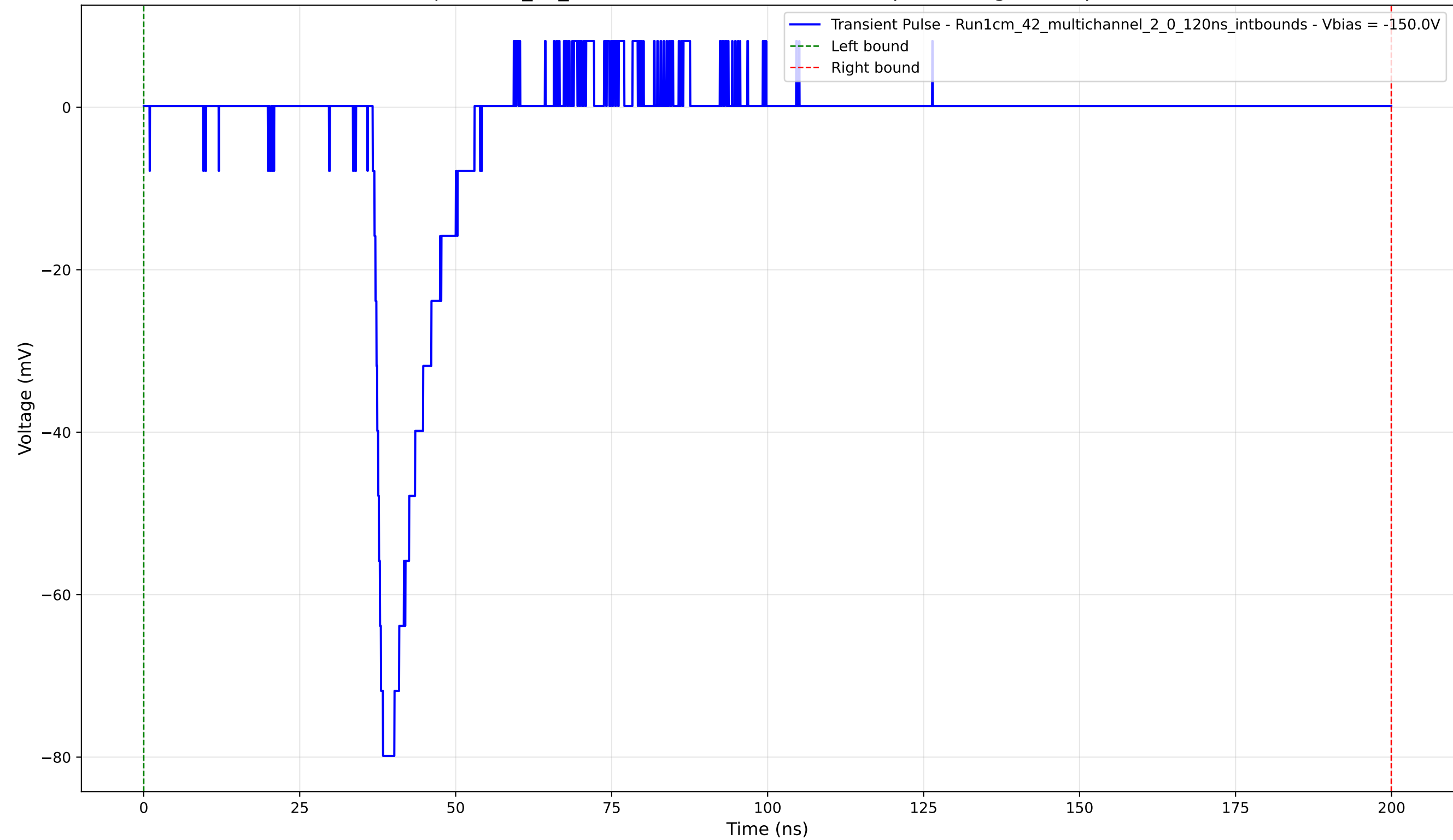
Transient Pulse - Sample: 1cm_42_multichannel - Position: 3820.0 \mu\text{m} - Charge: 9.70 pC - Rise Time: 1.40 ns
