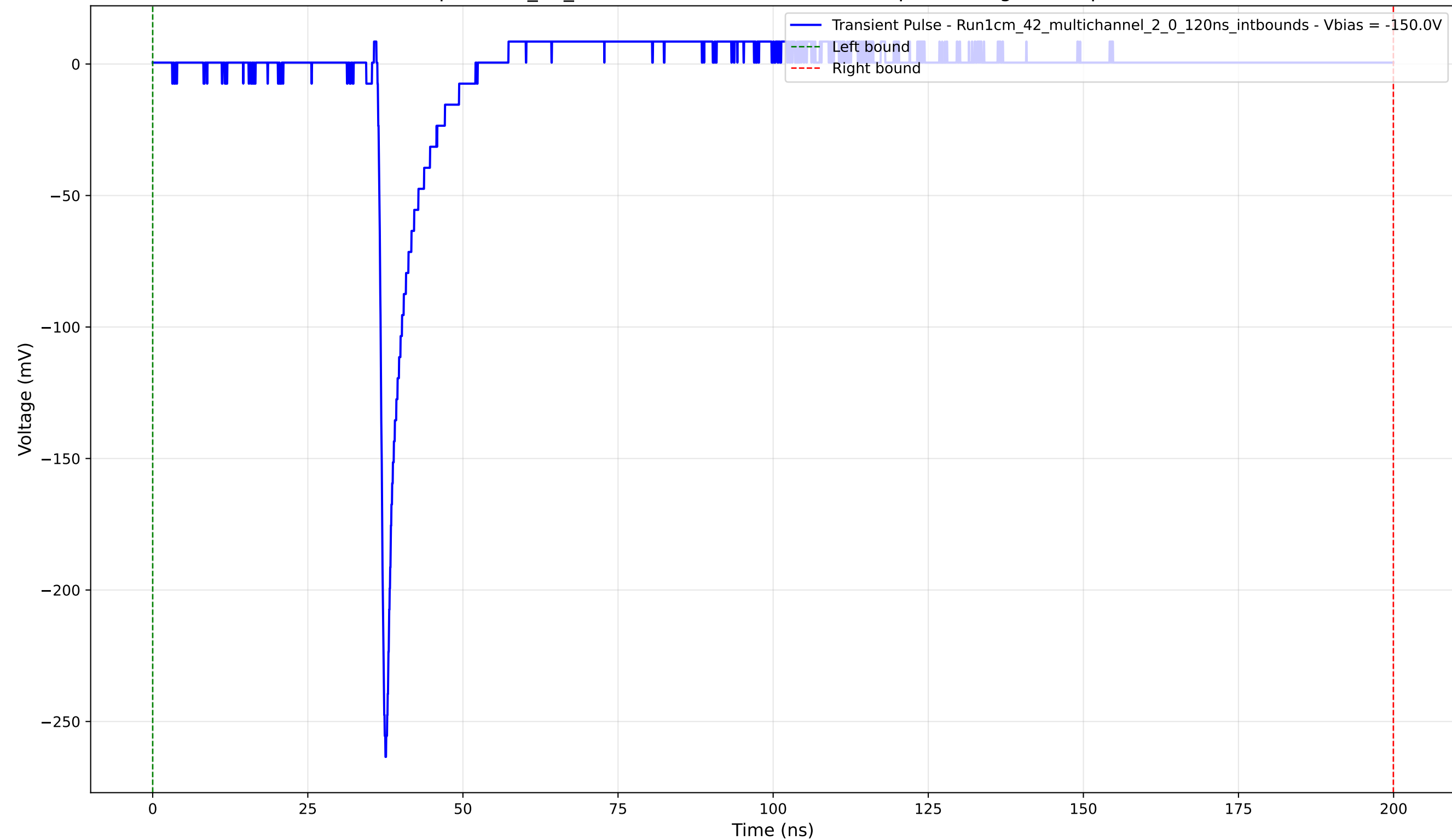
Transient Pulse - Sample: 1cm_42_multichannel - Position: 1790.0 \mu\text{m} - Charge: 9.86 pC - Rise Time: 0.85 ns
