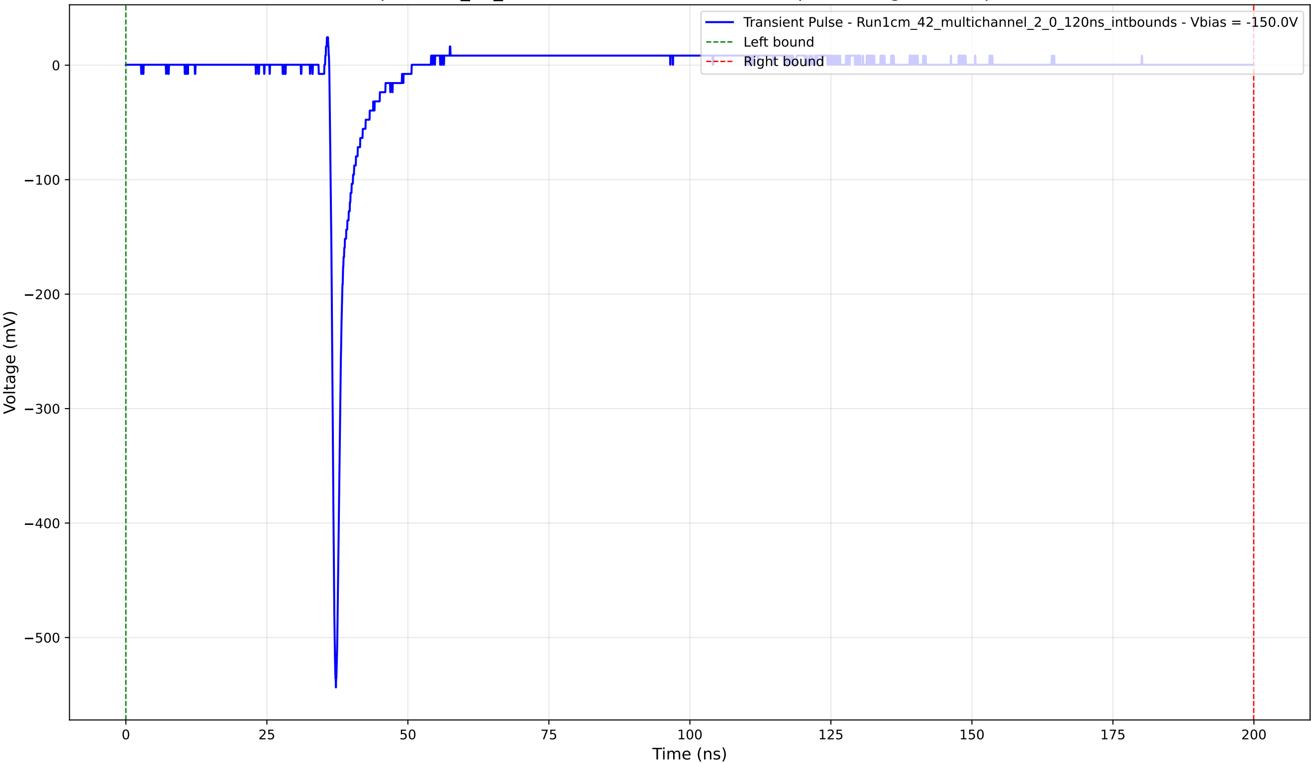
Transient Pulse - Sample: 1cm_42_multichannel - Position: 2170.0 \mu\text{m} - Charge: 14.52 pC - Rise Time: 0.77 ns
