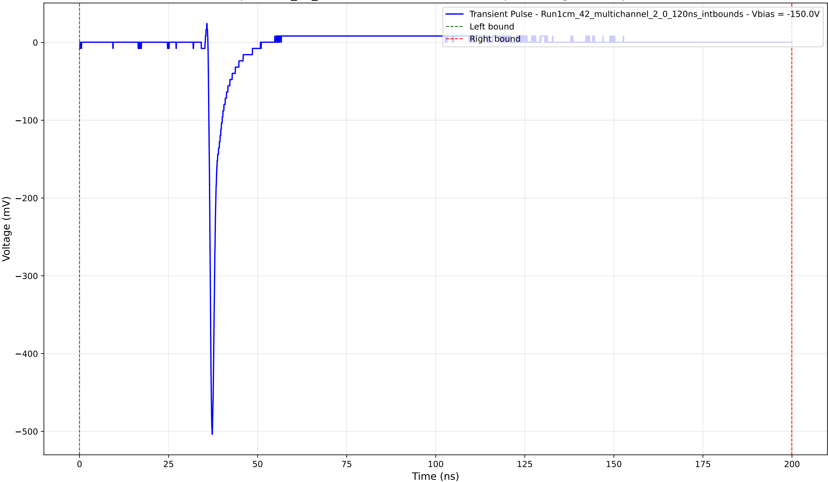
Transient Pulse - Sample: 1cm_42_multichannel - Position: 2570.0 \mu\text{m} - Charge: 13.77 pC - Rise Time: 0.77 ns
