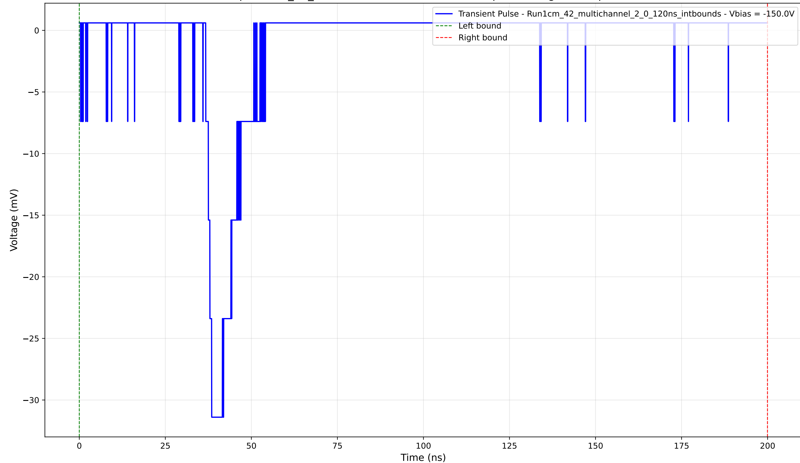
Transient Pulse - Sample: 1cm_42_multichannel - Position: 4340.0 \mu\text{m} - Charge: 3.45 pC - Rise Time: 1.75 ns
