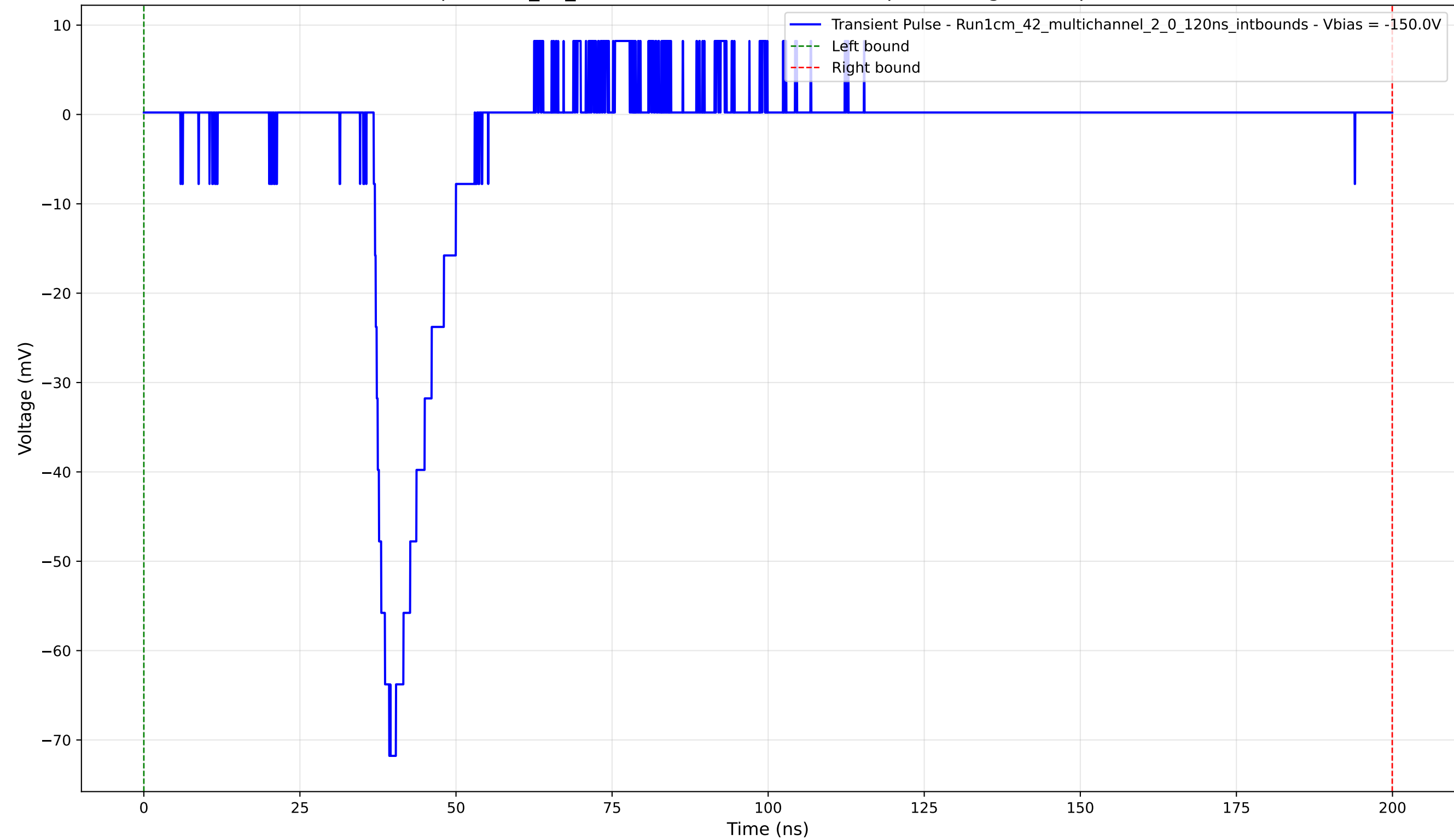
Transient Pulse - Sample: 1cm_42_multichannel - Position: 150.0 \mu\text{m} - Charge: 8.75 pC - Rise Time: 2.48 ns
