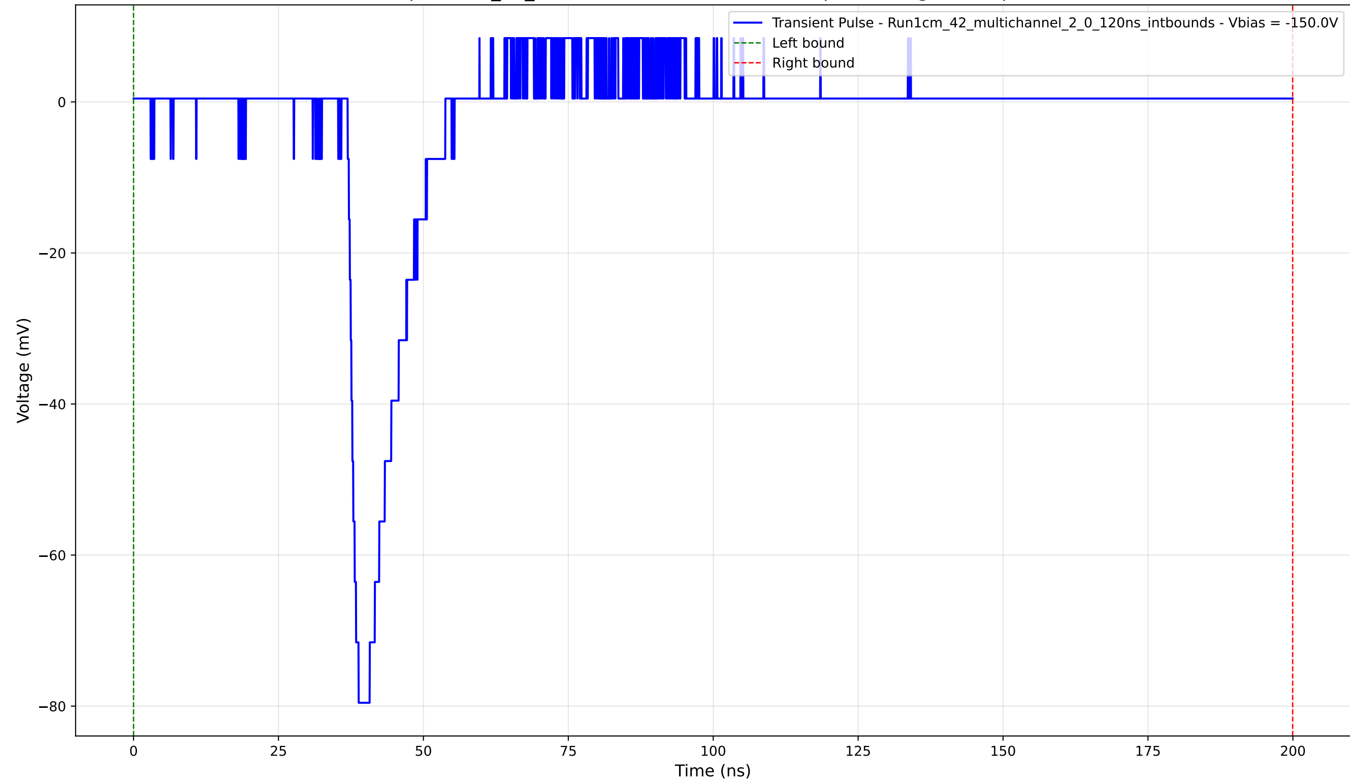
Transient Pulse - Sample: 1cm_42_multichannel - Position: 420.0 \mu\text{m} - Charge: 8.38 pC - Rise Time: 1.72 ns
