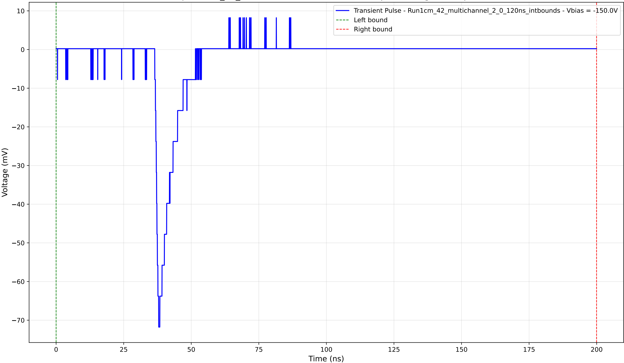
Transient Pulse - Sample: 1cm_42_multichannel - Position: 1310.0 \mu\text{m} - Charge: 7.63 pC - Rise Time: 1.44 ns
