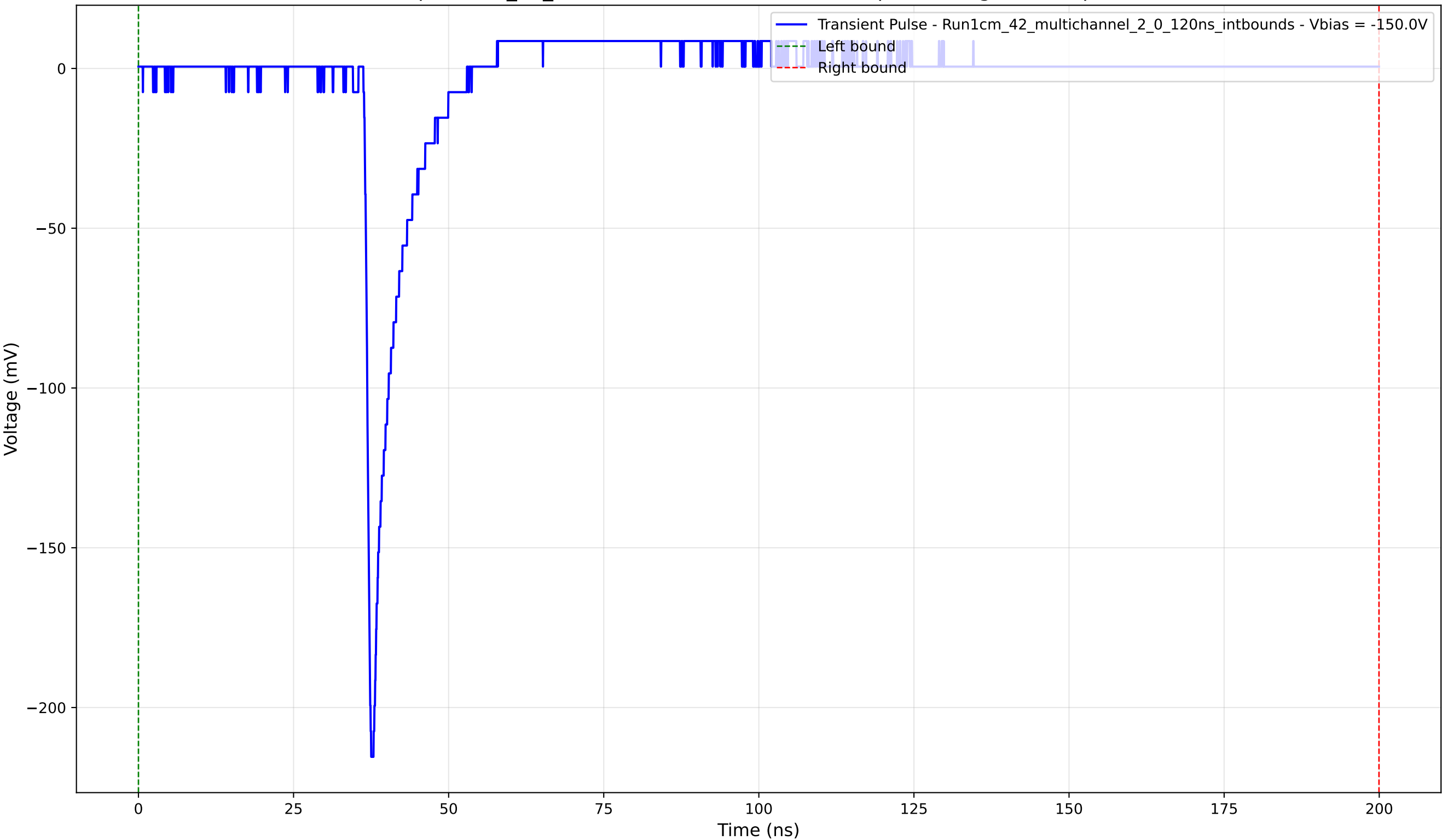
Transient Pulse - Sample: 1cm_42_multichannel - Position: 3090.0 \mu\text{m} - Charge: 10.31 pC - Rise Time: 0.89 ns
