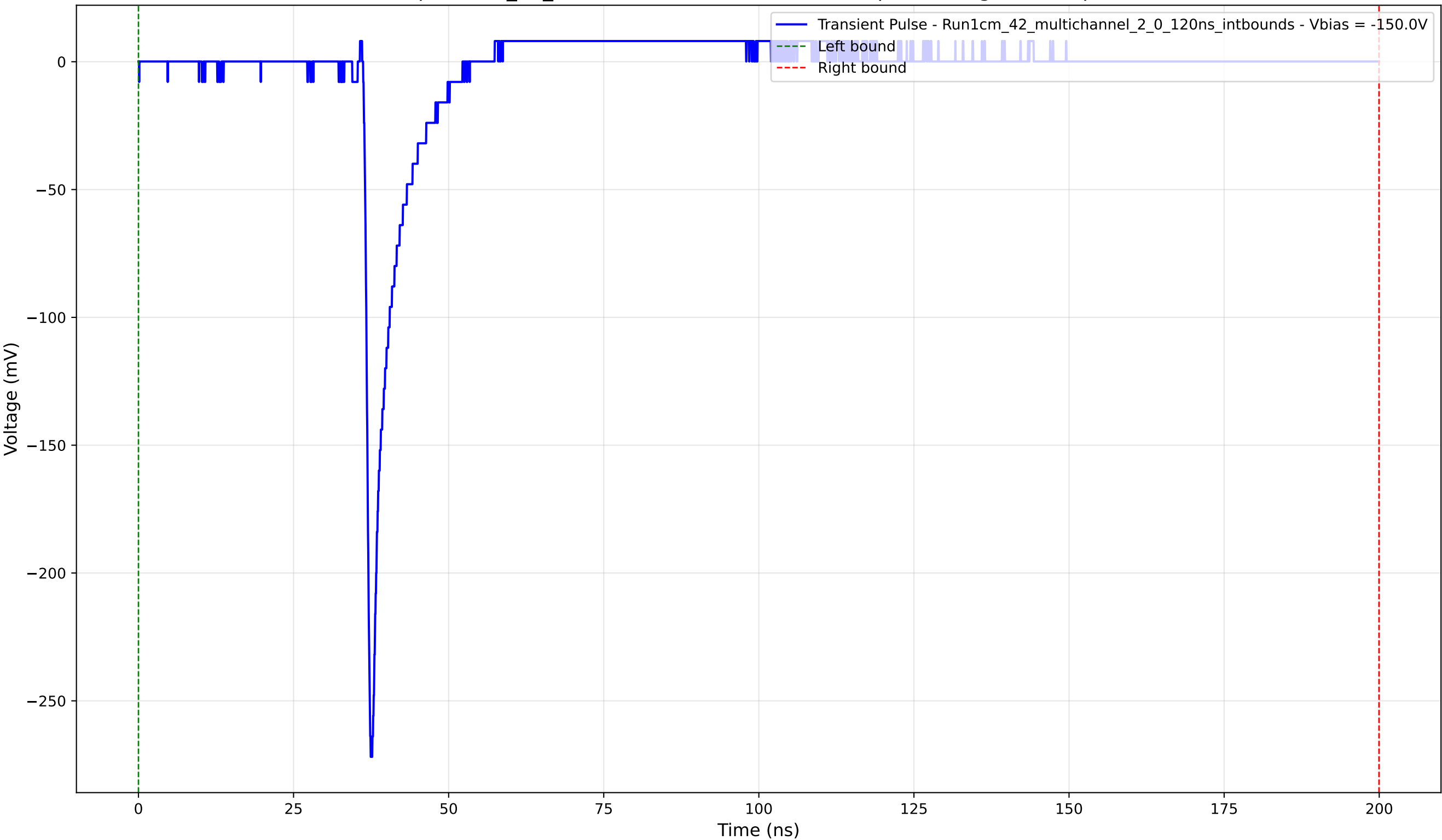
Transient Pulse - Sample: 1cm_42_multichannel - Position: 2980.0 \mu\text{m} - Charge: 12.96 pC - Rise Time: 0.85 ns
