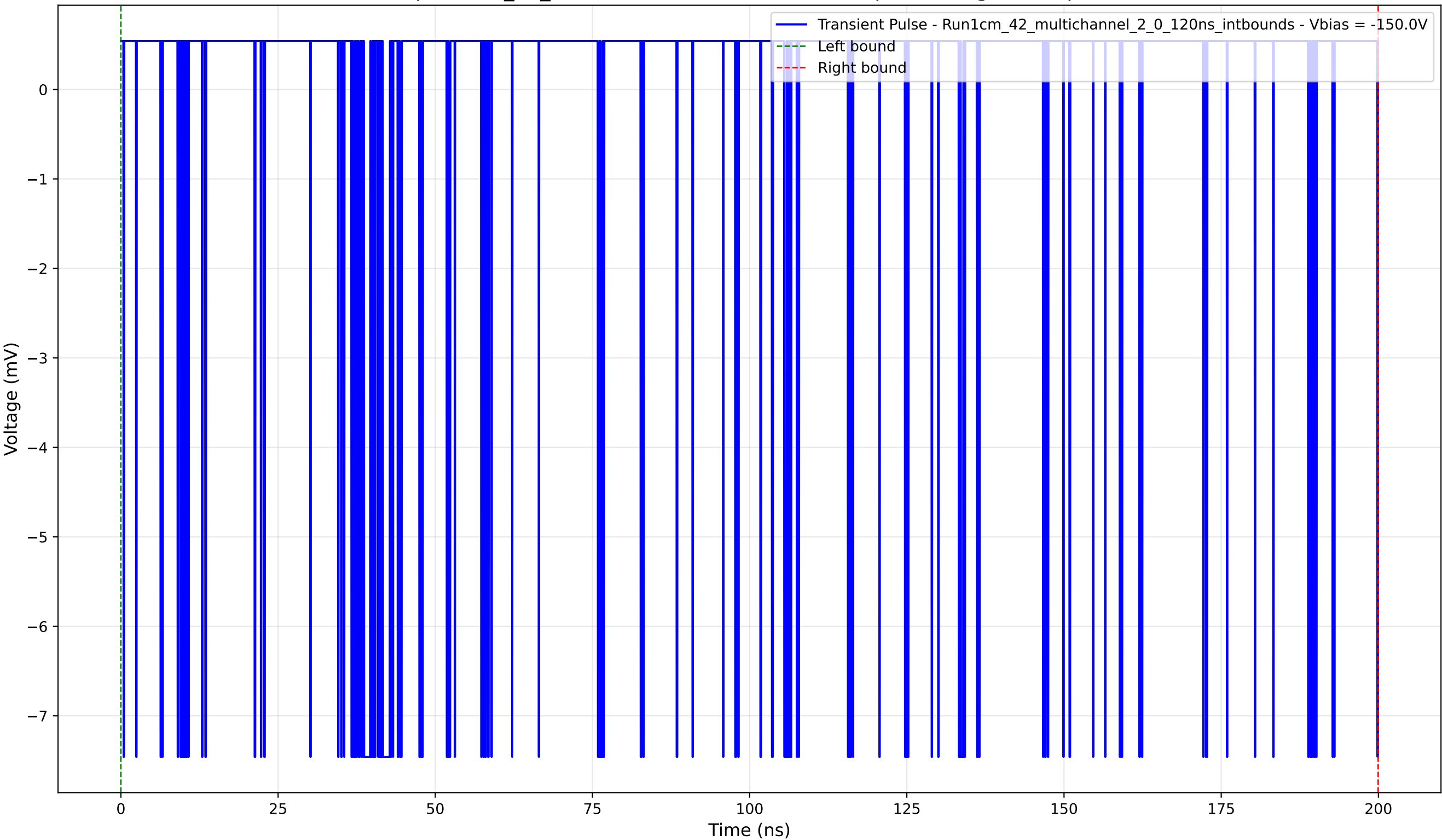
Transient Pulse - Sample: 1cm_42_multichannel - Position: 4920.0 \mu\text{m} - Charge: 0.11 pC - Rise Time: 0.04 ns
