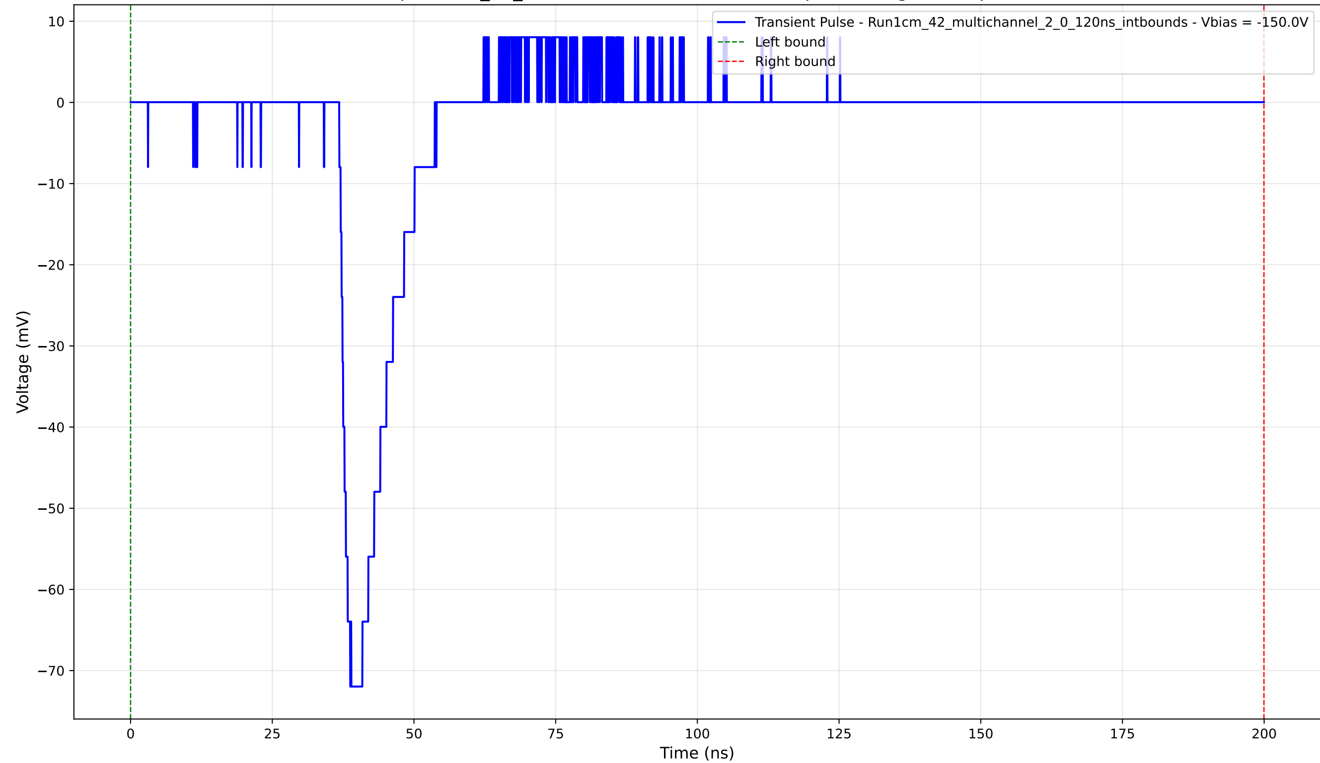
Transient Pulse - Sample: 1cm_42_multichannel - Position: 245.0 \mu\text{m} - Charge: 9.34 pC - Rise Time: 1.92 ns
