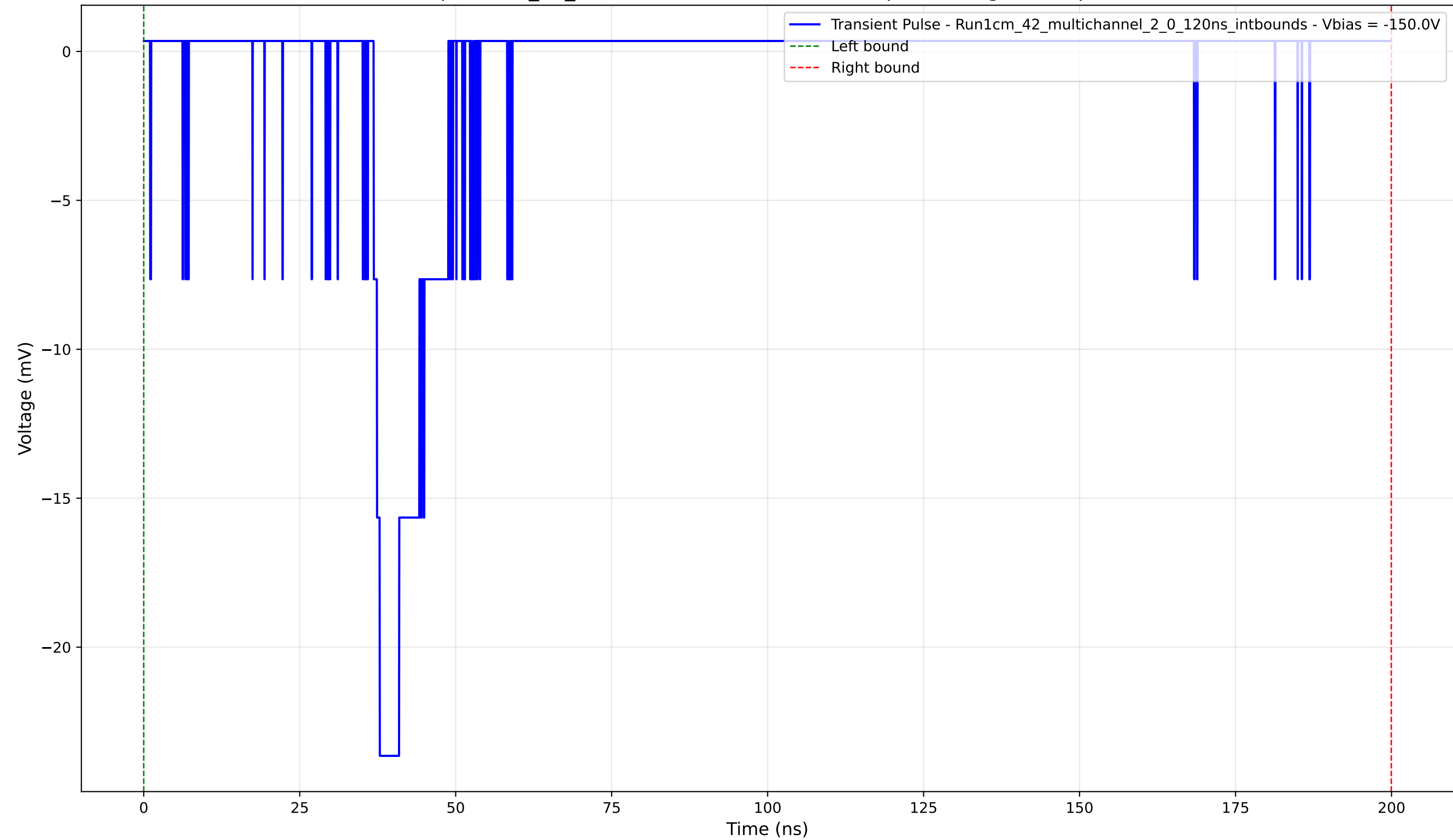
Transient Pulse - Sample: 1cm_42_multichannel - Position: 885.0 \mu\text{m} - Charge: 2.74 pC - Rise Time: 0.99 ns
