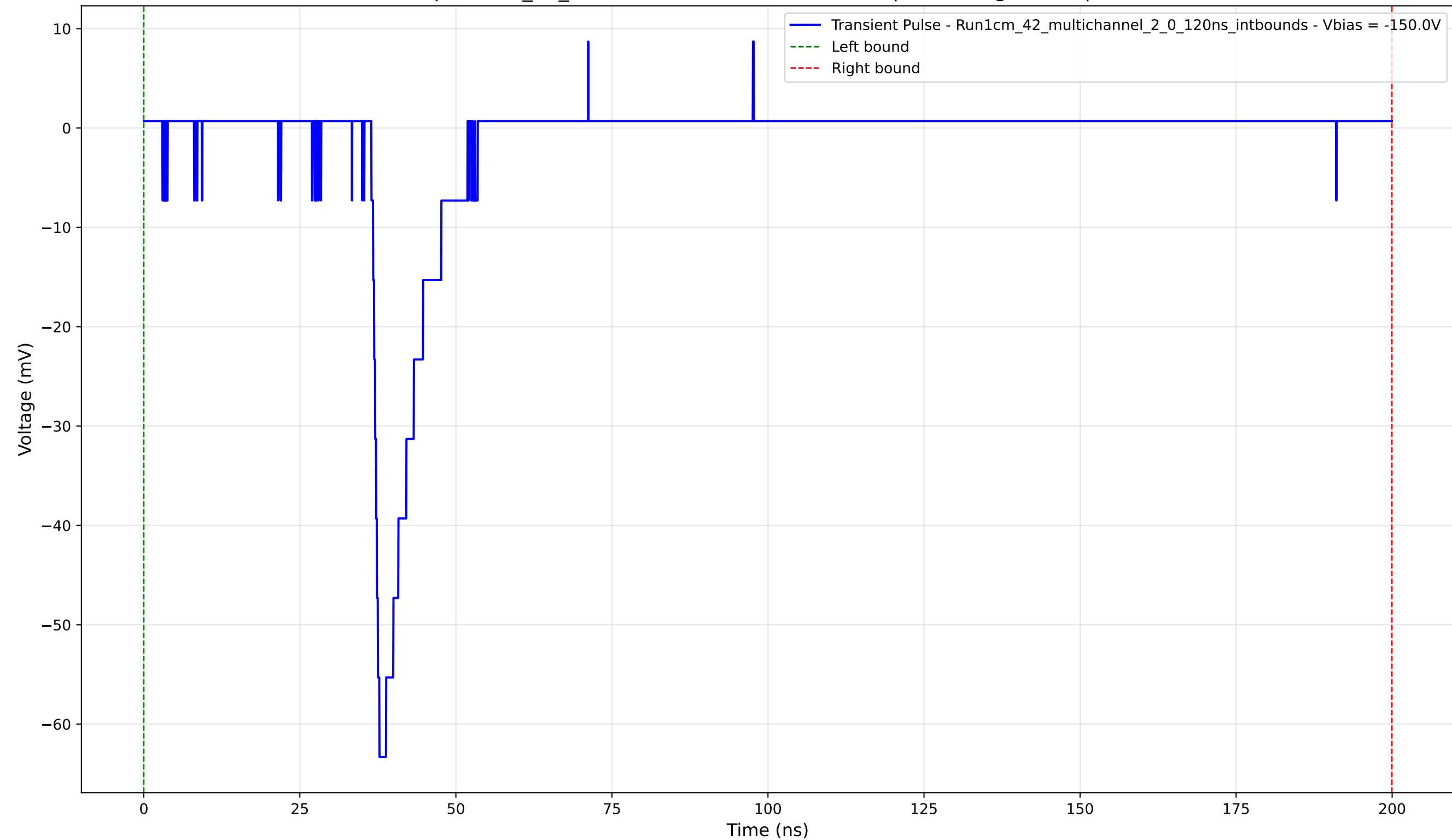
Transient Pulse - Sample: 1cm_42_multichannel - Position: 3430.0 \mu\text{m} - Charge: 5.95 pC - Rise Time: 1.29 ns
