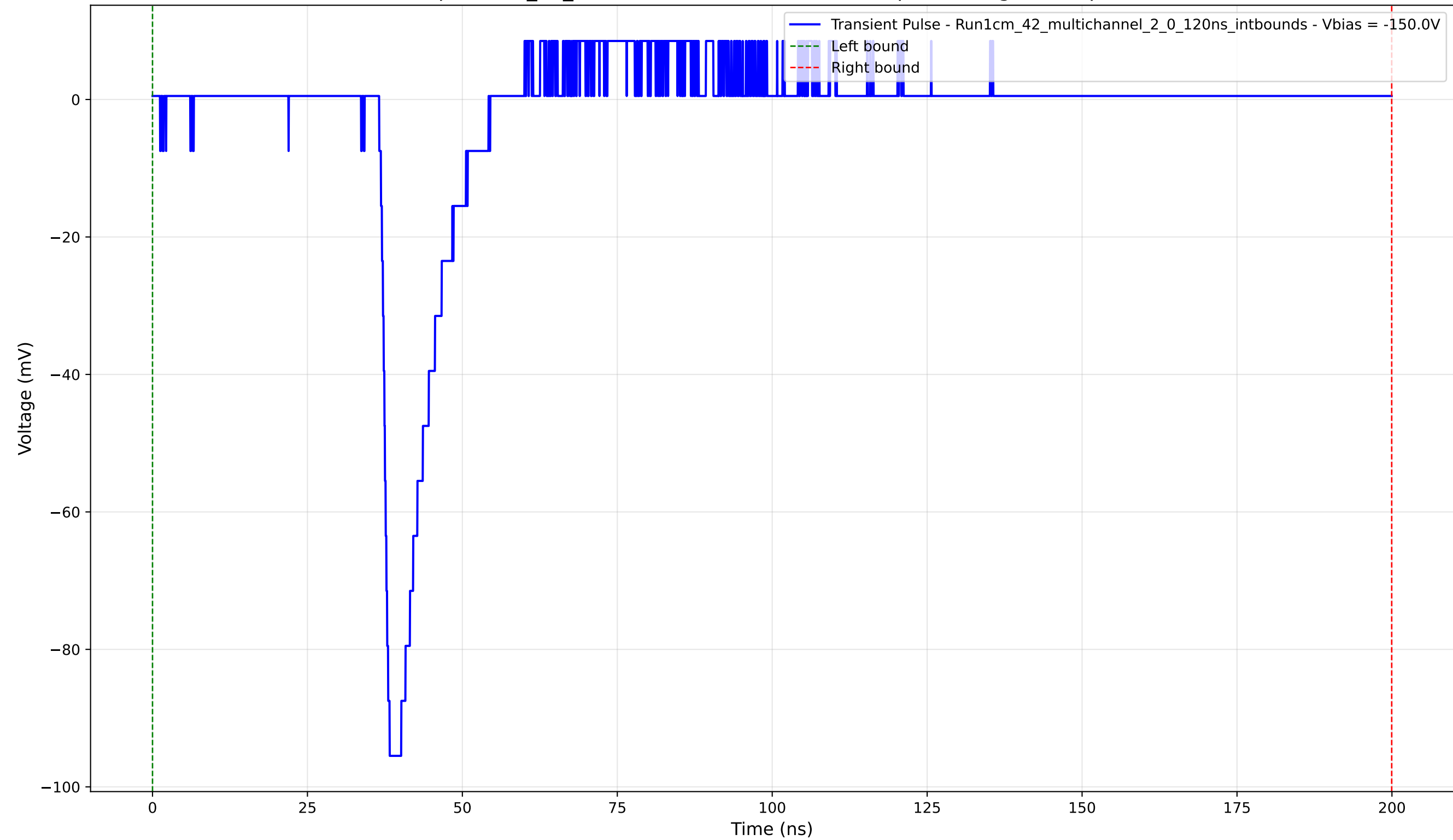
Transient Pulse - Sample: 1cm_42_multichannel - Position: 3800.0 \mu\text{m} - Charge: 8.21 pC - Rise Time: 1.19 ns
