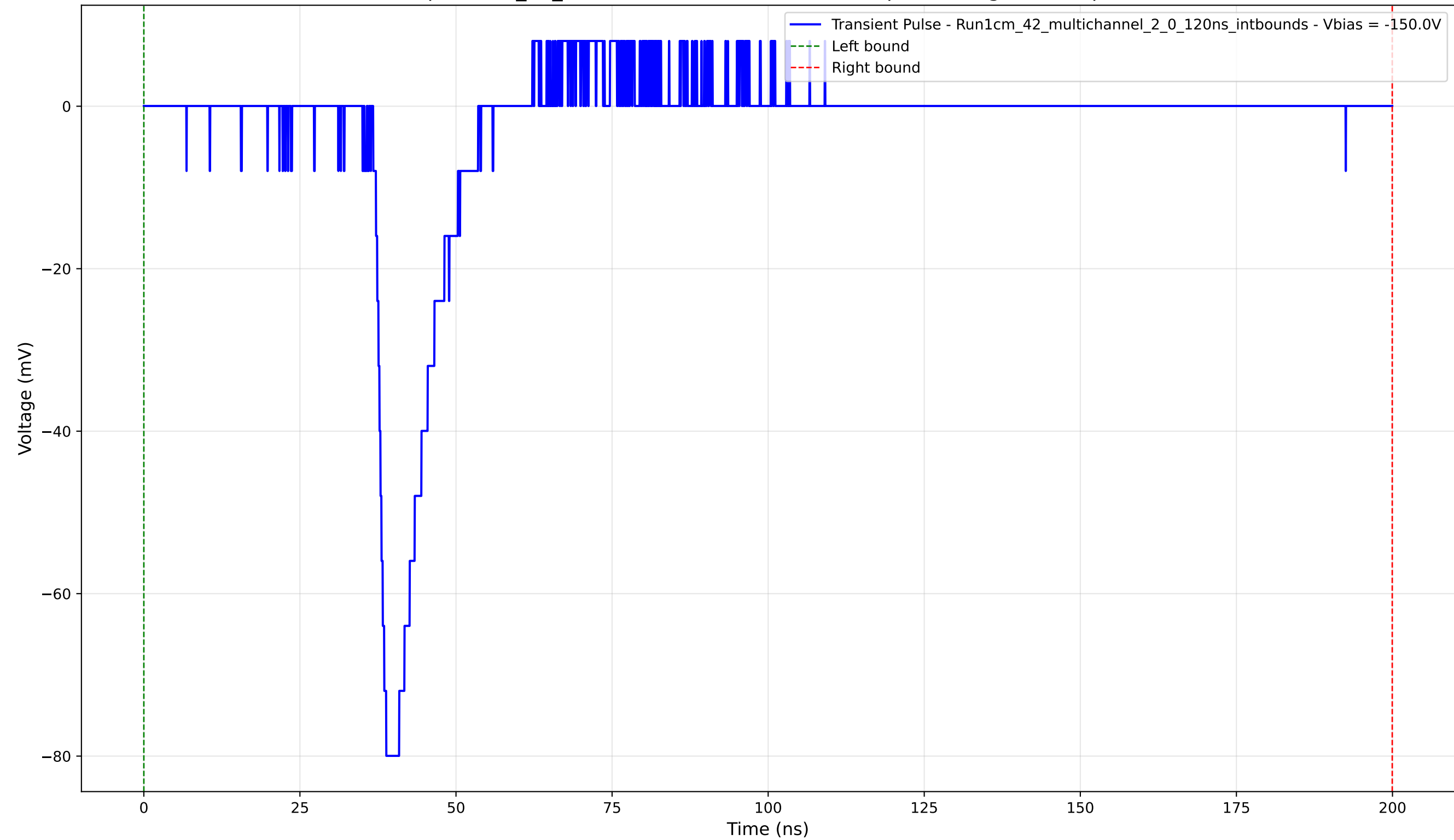
Transient Pulse - Sample: 1cm_42_multichannel - Position: 4230.0 \mu\text{m} - Charge: 10.18 pC - Rise Time: 1.68 ns
