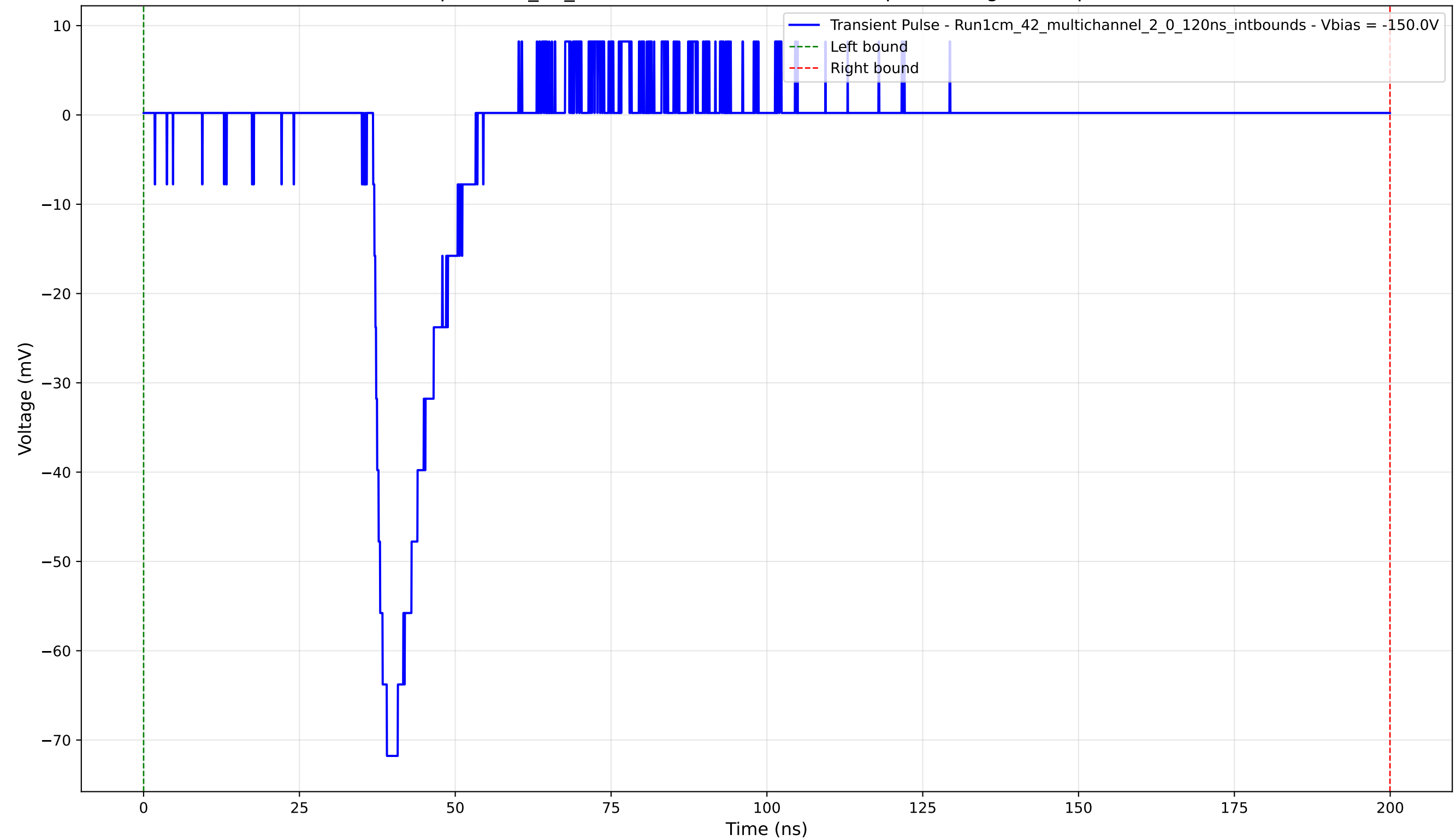
Transient Pulse - Sample: 1cm_42_multichannel - Position: 170.0 \mu\text{m} - Charge: 8.98 pC - Rise Time: 2.20 ns
