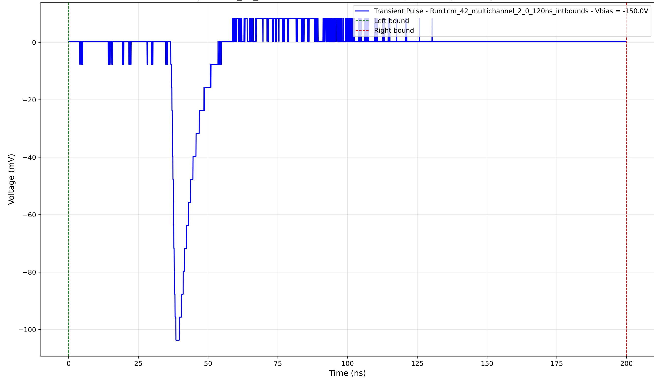
Transient Pulse - Sample: 1cm_42_multichannel - Position: 3785.0 \mu\text{m} - Charge: 9.30 pC - Rise Time: 1.27 ns
