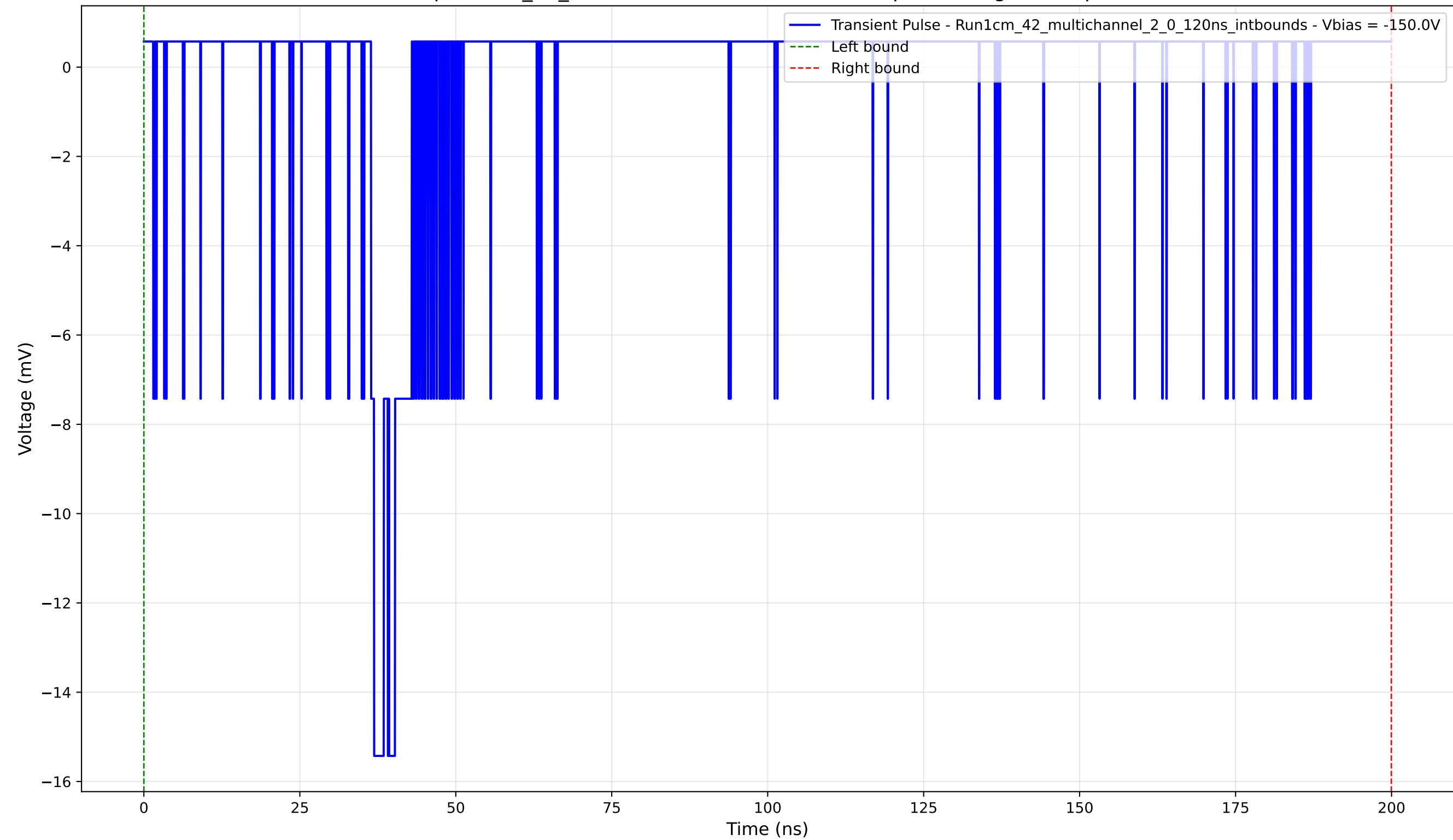
Transient Pulse - Sample: 1cm_42_multichannel - Position: 1875.0 \mu\text{m} - Charge: 0.46 pC - Rise Time: 0.51 ns
