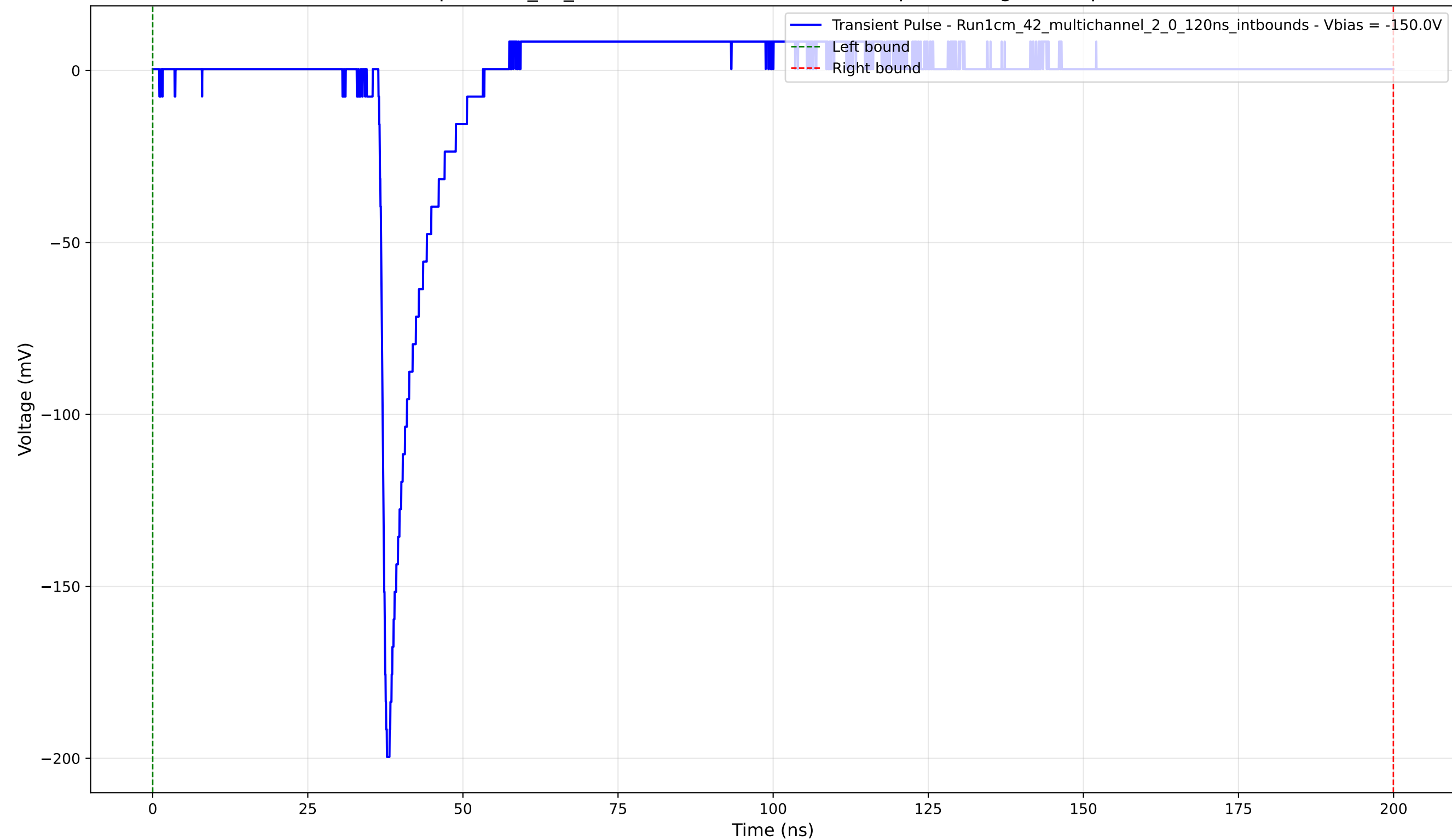
Transient Pulse - Sample: 1cm_42_multichannel - Position: 1465.0 \mu\text{m} - Charge: 9.91 pC - Rise Time: 0.98 ns
