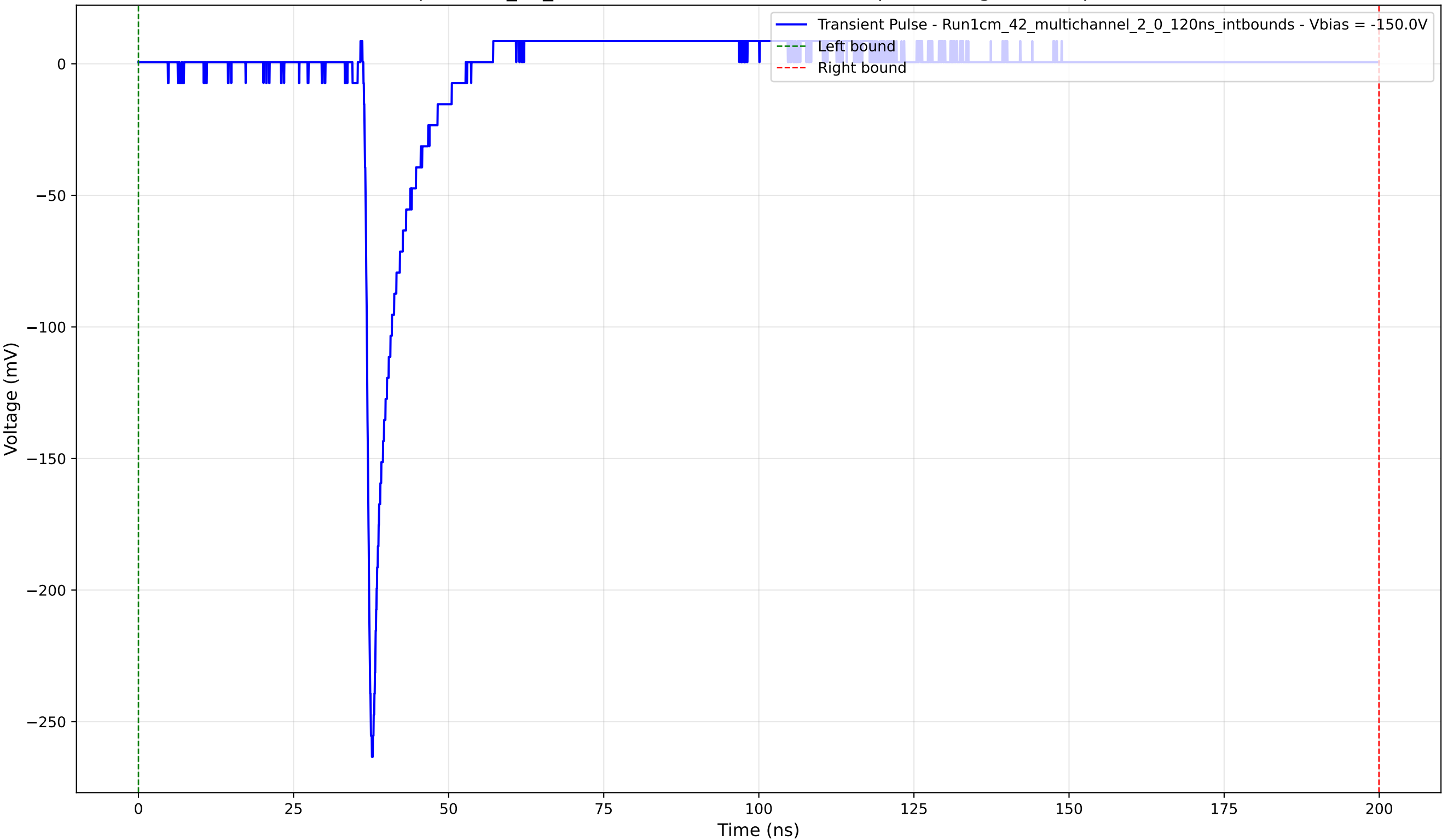
Transient Pulse - Sample: 1cm_42_multichannel - Position: 1670.0 \mu\text{m} - Charge: 10.95 pC - Rise Time: 0.91 ns
