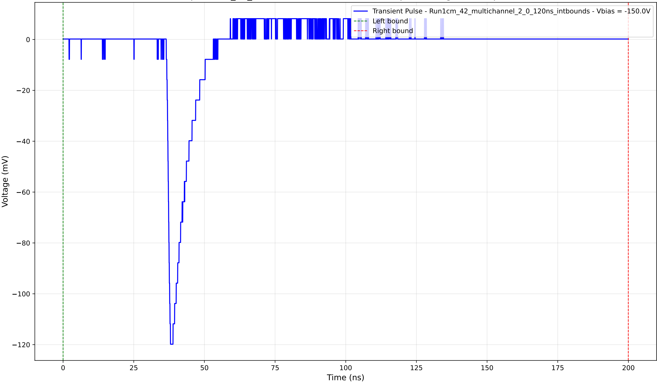
Transient Pulse - Sample: 1cm_42_multichannel - Position: 3560.0 \mu\text{m} - Charge: 10.28 pC - Rise Time: 1.14 ns
