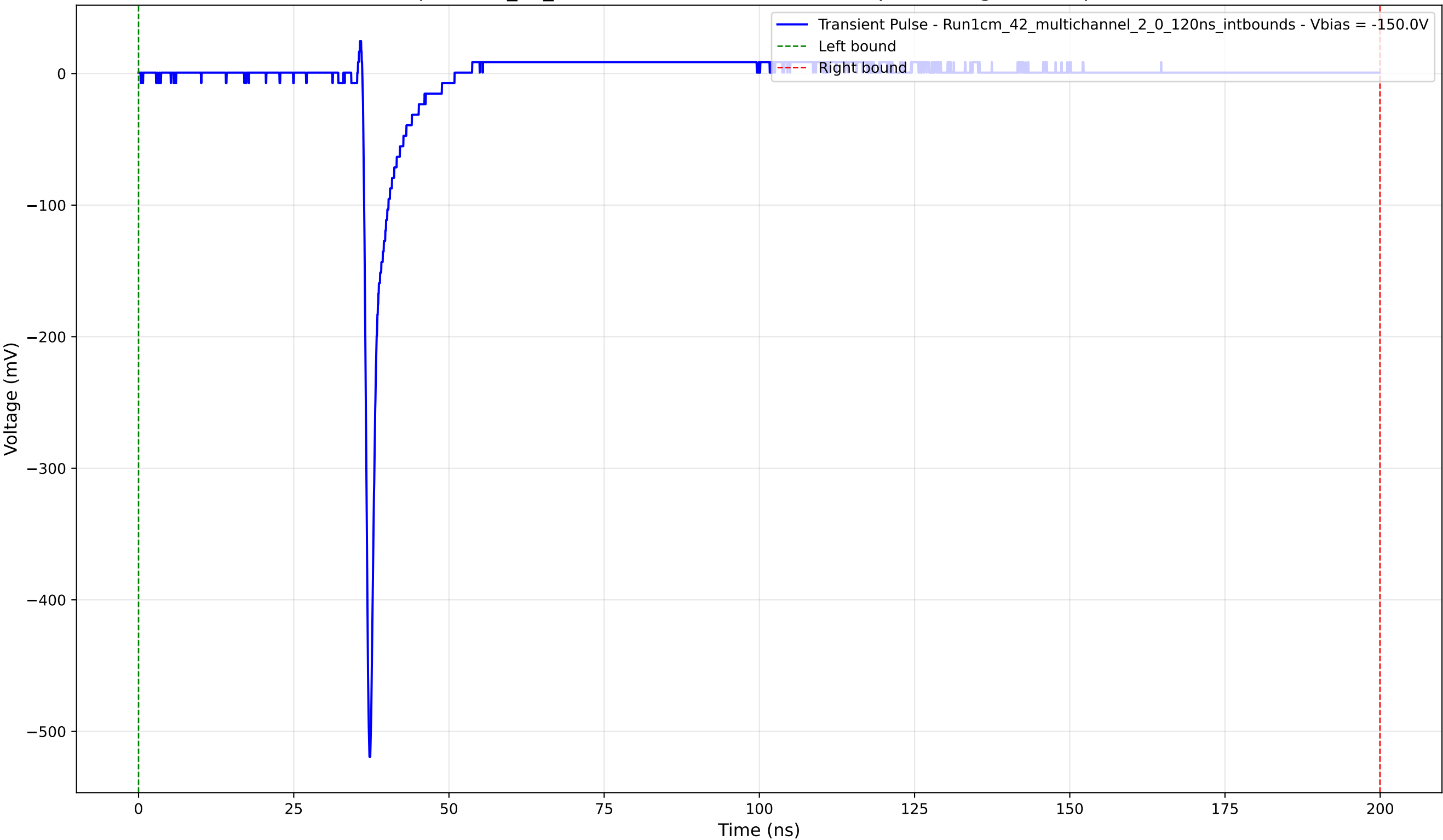
Transient Pulse - Sample: 1cm_42_multichannel - Position: 2145.0 \mu\text{m} - Charge: 13.45 pC - Rise Time: 0.76 ns
