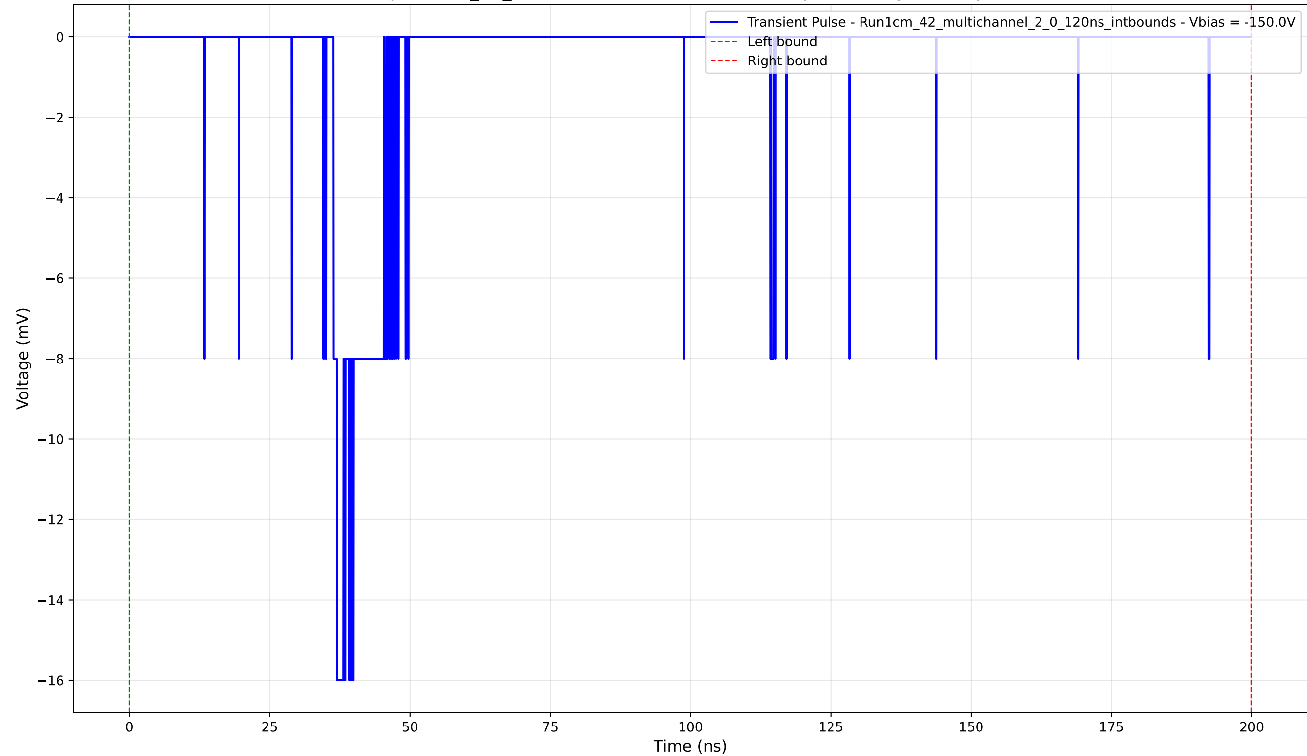
Transient Pulse - Sample: 1cm_42_multichannel - Position: 1855.0 \mu\text{m} - Charge: 2.16 pC - Rise Time: 0.63 ns
