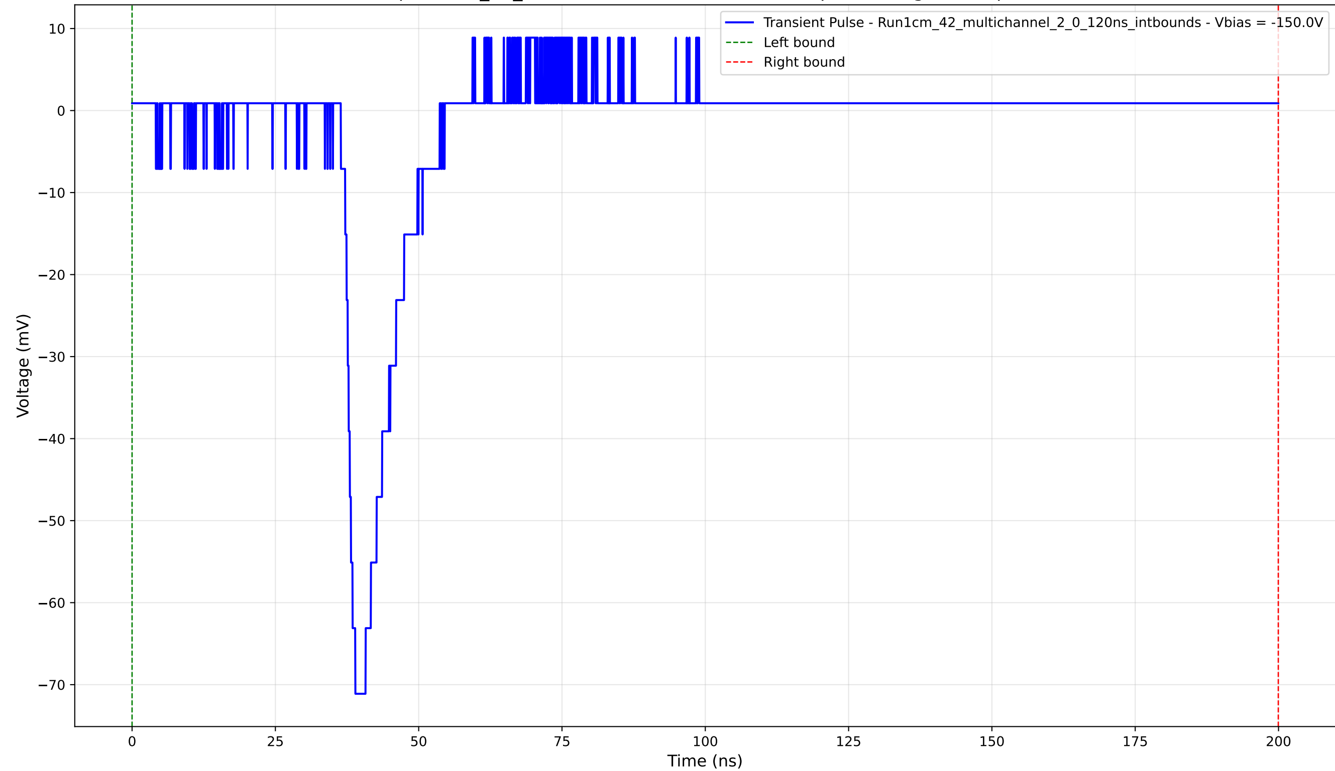
Transient Pulse - Sample: 1cm_42_multichannel - Position: 4610.0 \mu\text{m} - Charge: 6.79 pC - Rise Time: 1.80 ns
