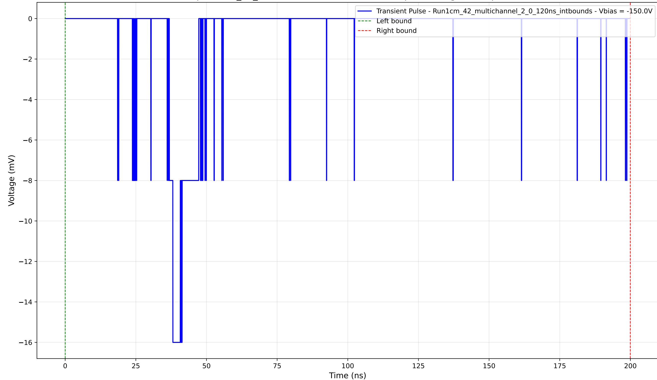
Transient Pulse - Sample: 1cm_42_multichannel - Position: 3860.0 \mu\text{m} - Charge: 2.64 pC - Rise Time: 1.27 ns
