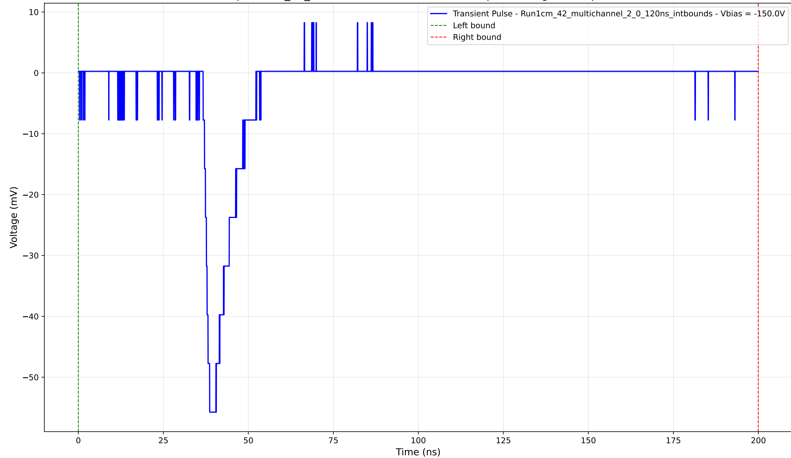
Transient Pulse - Sample: 1cm_42_multichannel - Position: 3940.0 \mu\text{m} - Charge: 7.81 pC - Rise Time: 1.93 ns
