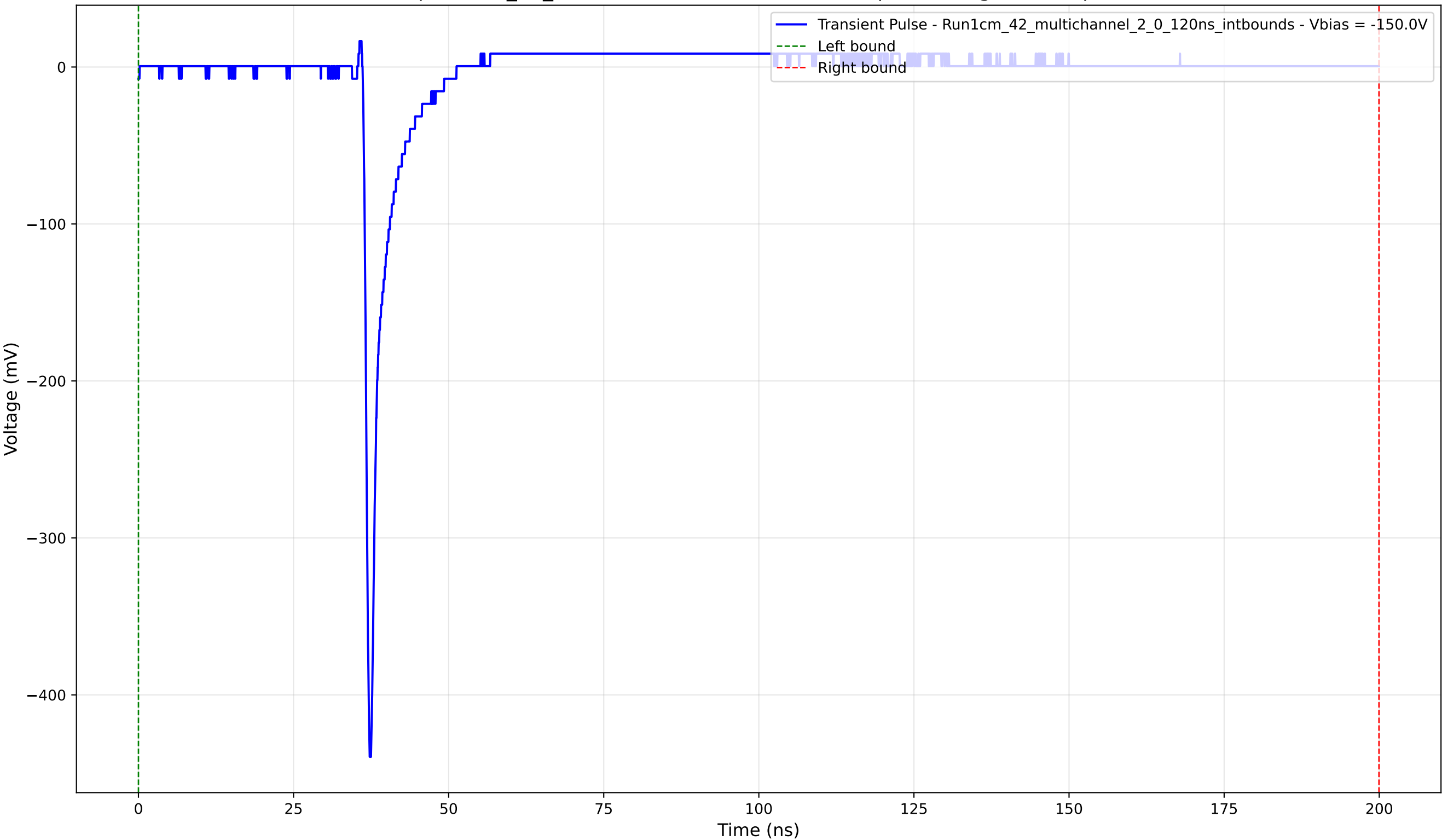
Transient Pulse - Sample: 1cm_42_multichannel - Position: 2020.0 \mu\text{m} - Charge: 13.60 pC - Rise Time: 0.76 ns
