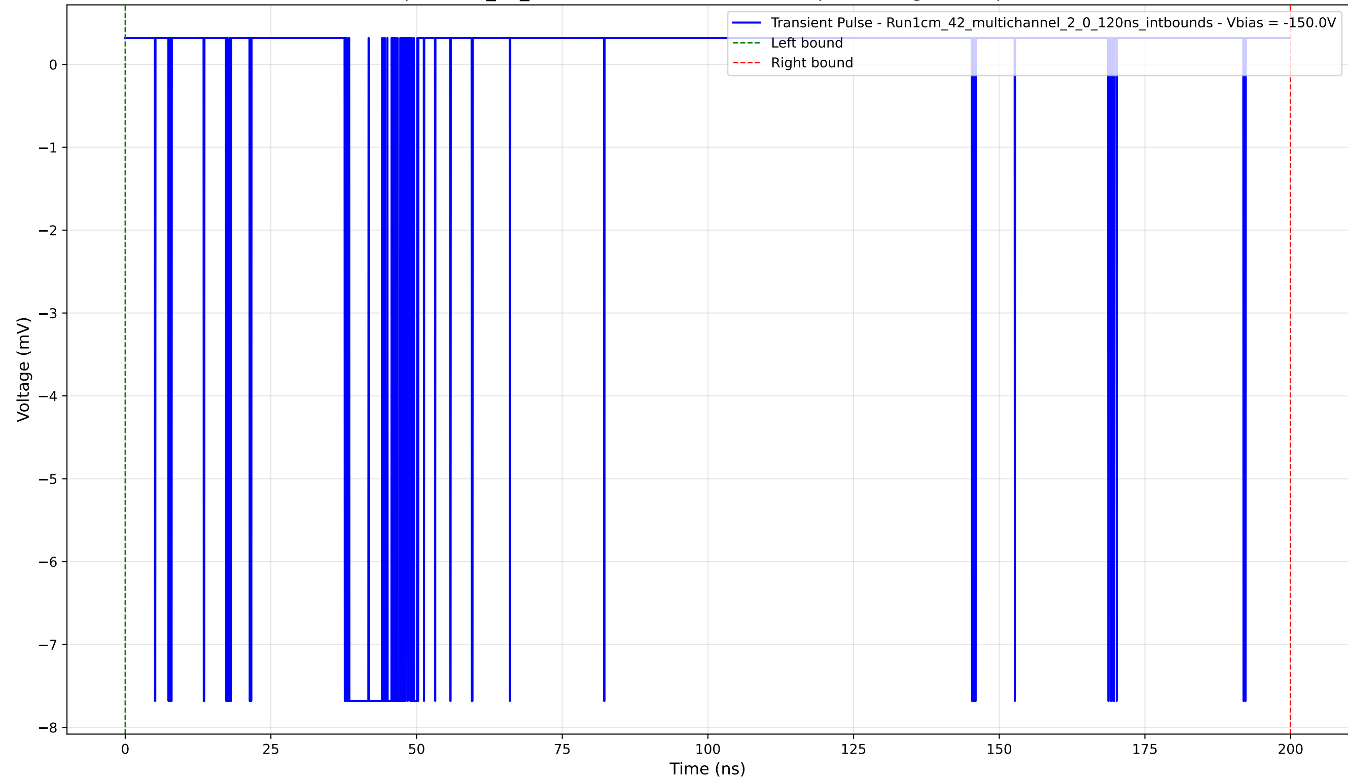
Transient Pulse - Sample: 1cm_42_multichannel - Position: 355.0 \mu\text{m} - Charge: 0.73 pC - Rise Time: 0.04 ns
