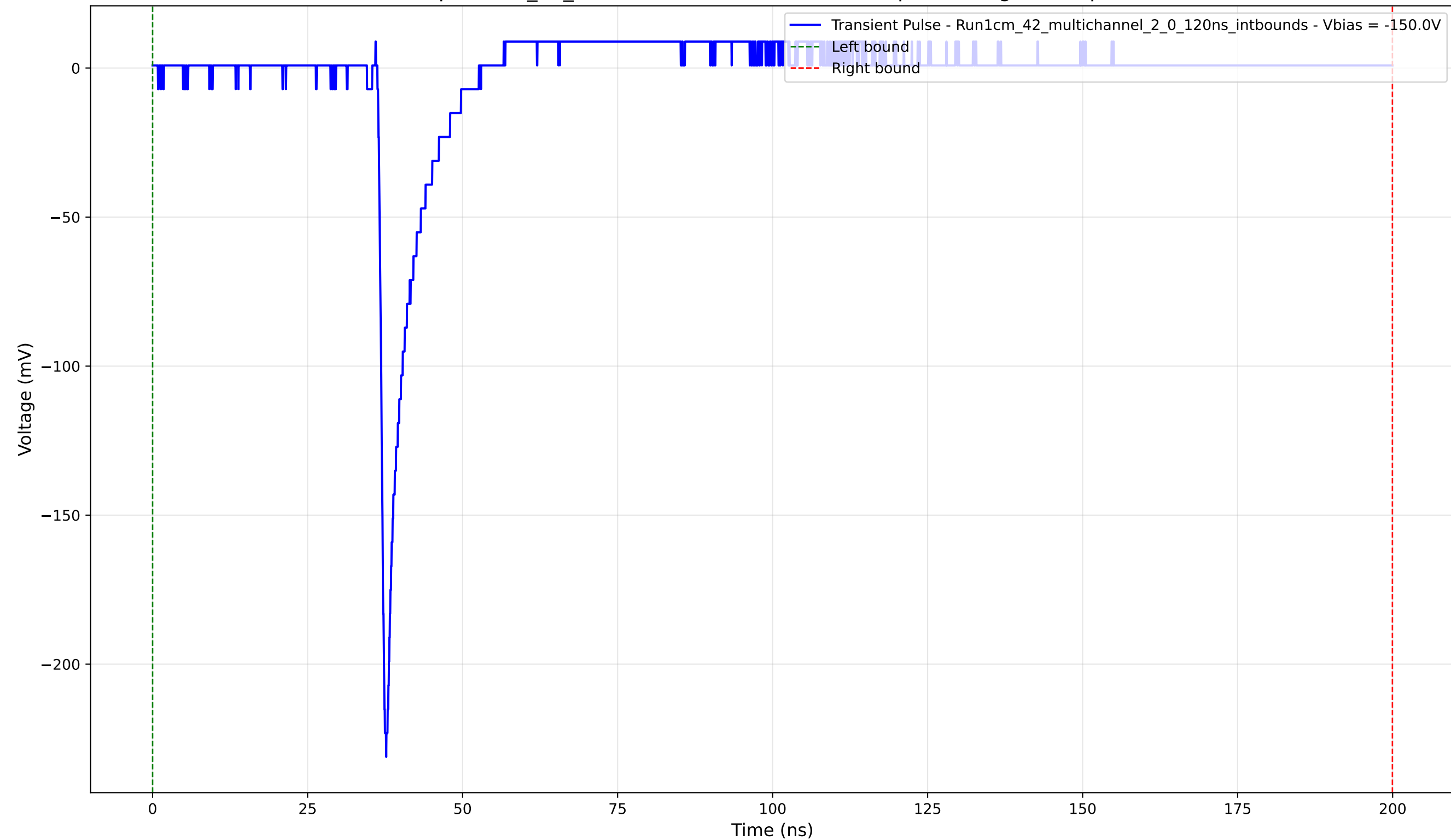
Transient Pulse - Sample: 1cm_42_multichannel - Position: 3065.0 \mu\text{m} - Charge: 8.55 pC - Rise Time: 0.92 ns
