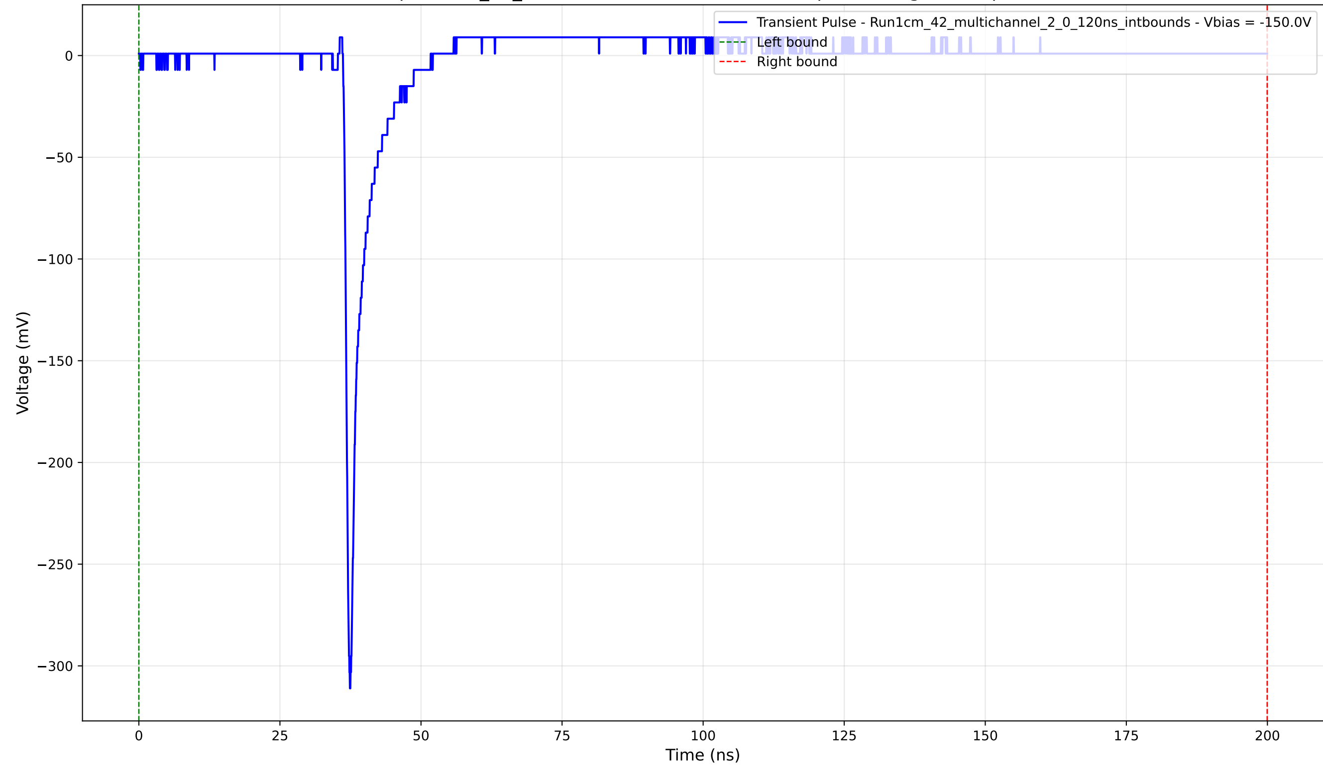
Transient Pulse - Sample: 1cm_42_multichannel - Position: 1930.0 \mu\text{m} - Charge: 7.55 pC - Rise Time: 0.80 ns
