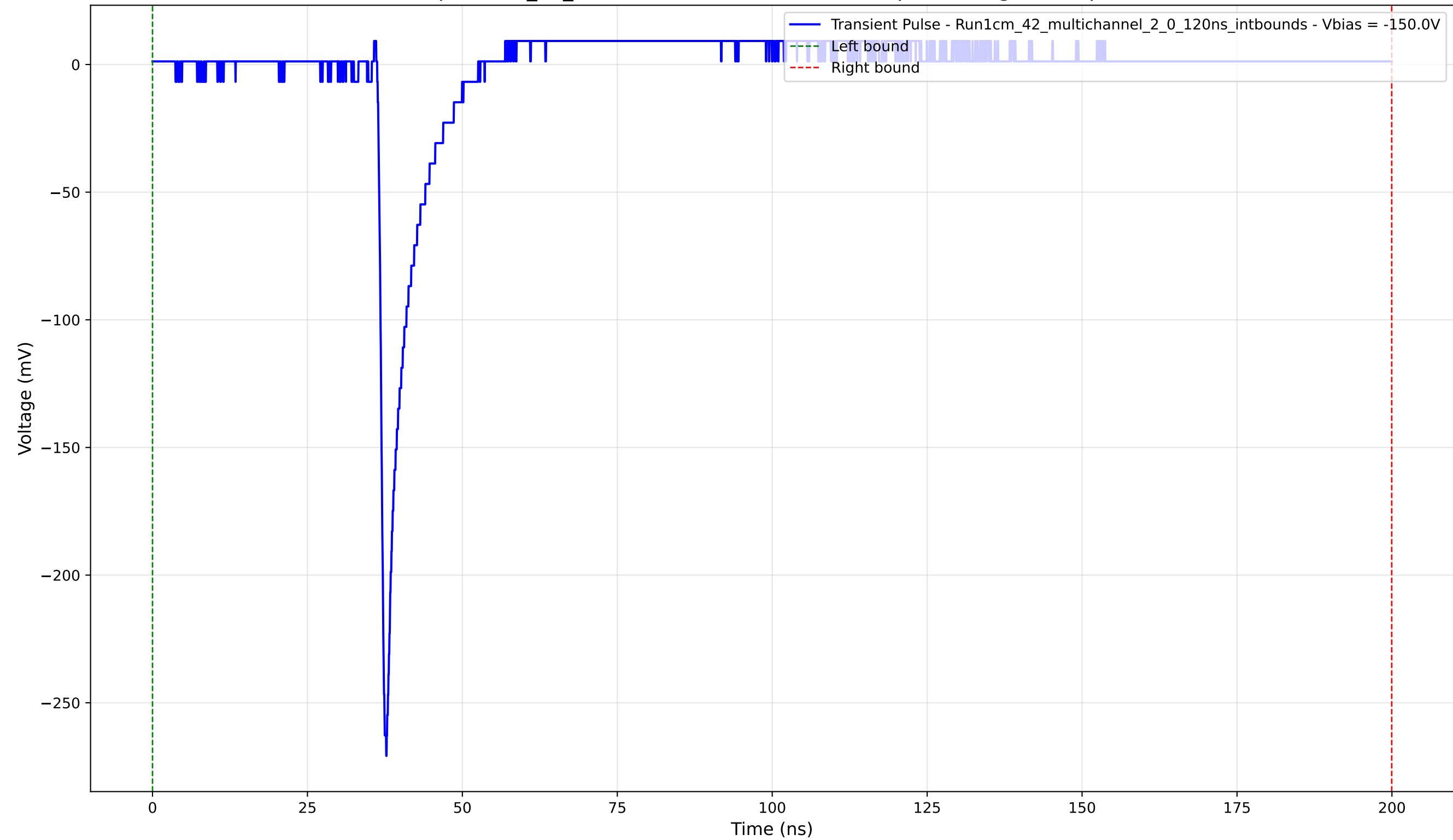
Transient Pulse - Sample: 1cm_42_multichannel - Position: 1680.0 \mu\text{m} - Charge: 8.69 pC - Rise Time: 0.90 ns
