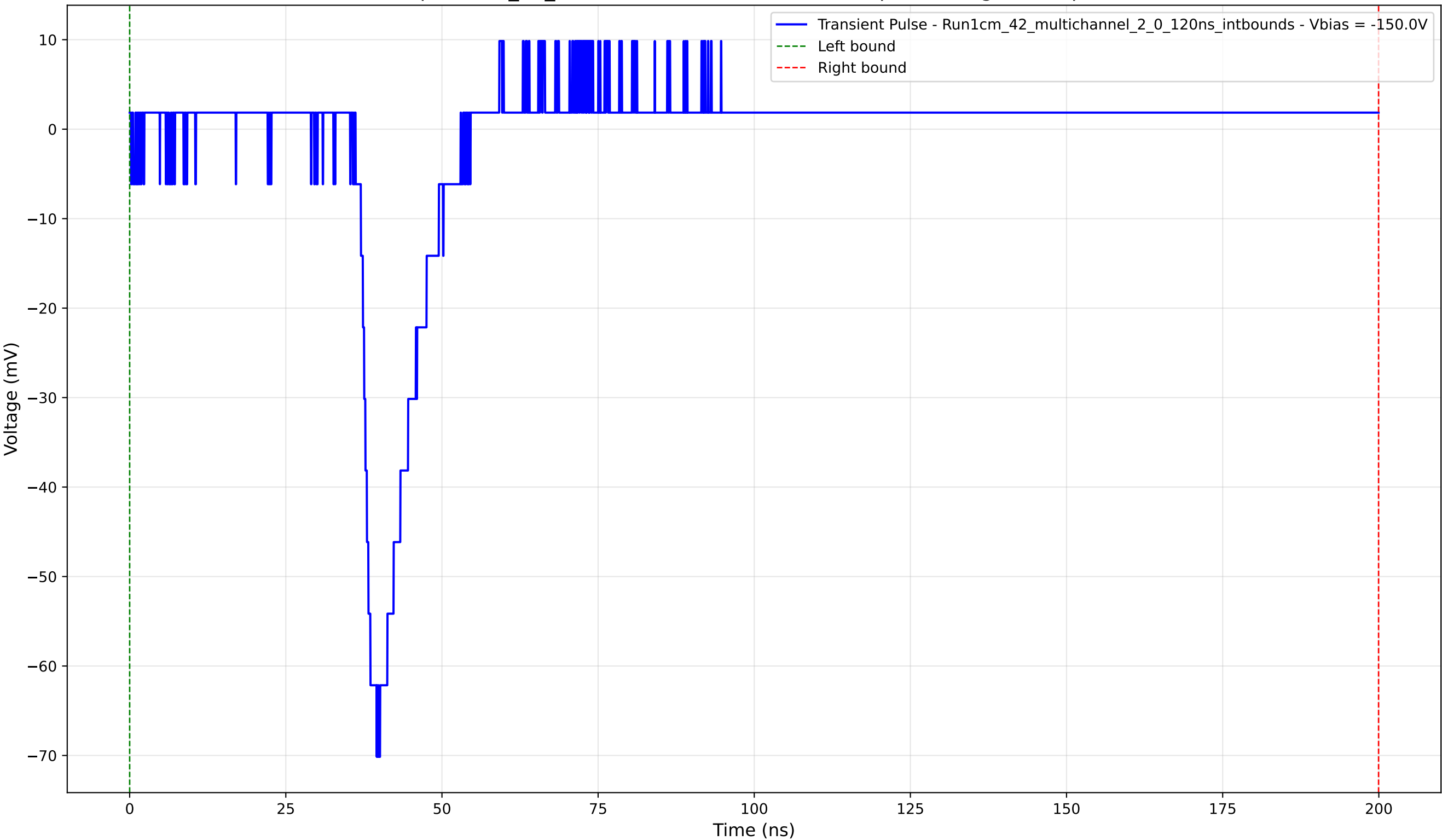
Transient Pulse - Sample: 1cm_42_multichannel - Position: 4725.0 \mu\text{m} - Charge: 3.03 pC - Rise Time: 2.56 ns
