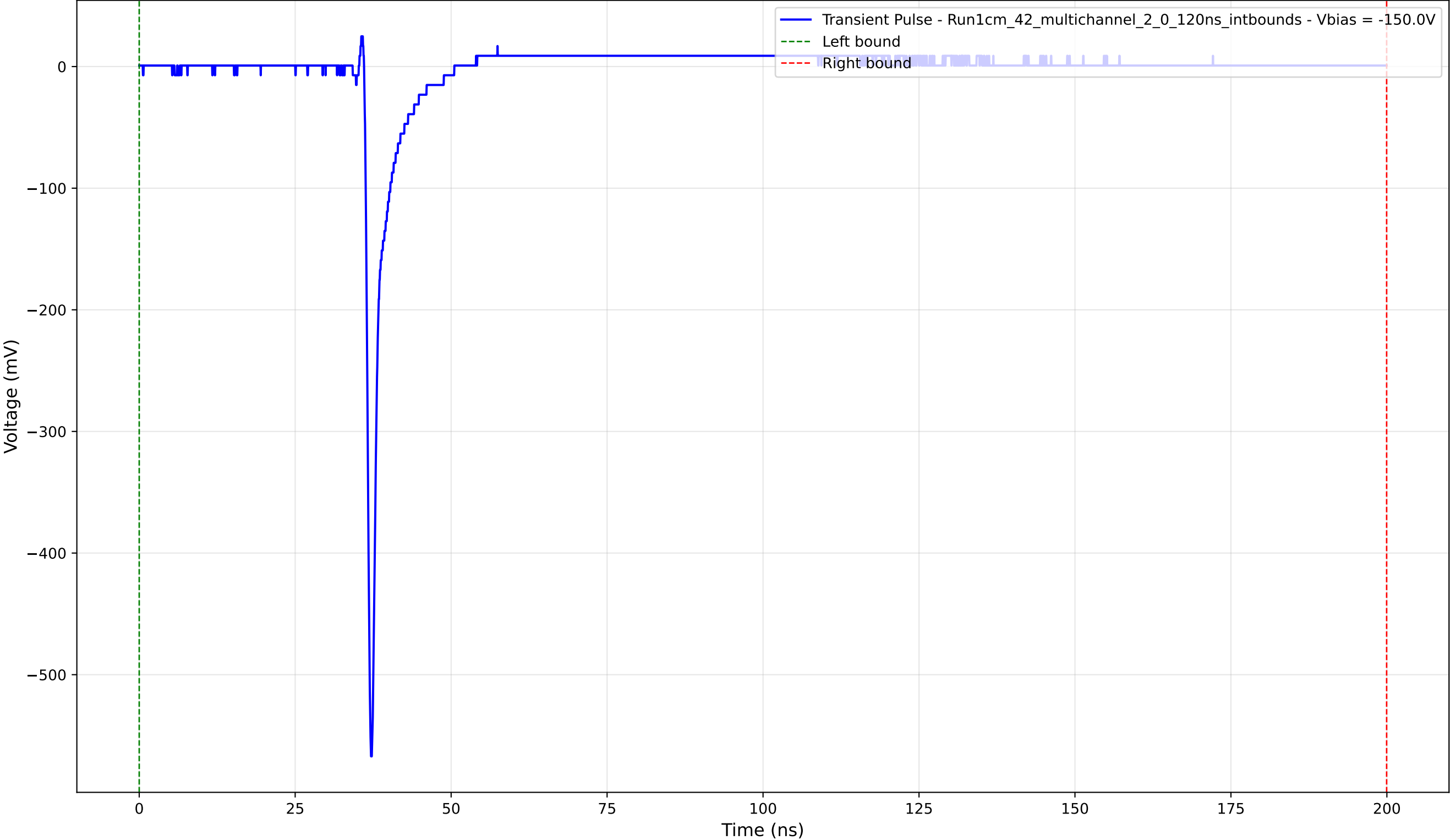
Transient Pulse - Sample: 1cm_42_multichannel - Position: 2195.0 \mu\text{m} - Charge: 13.24 pC - Rise Time: 0.74 ns
