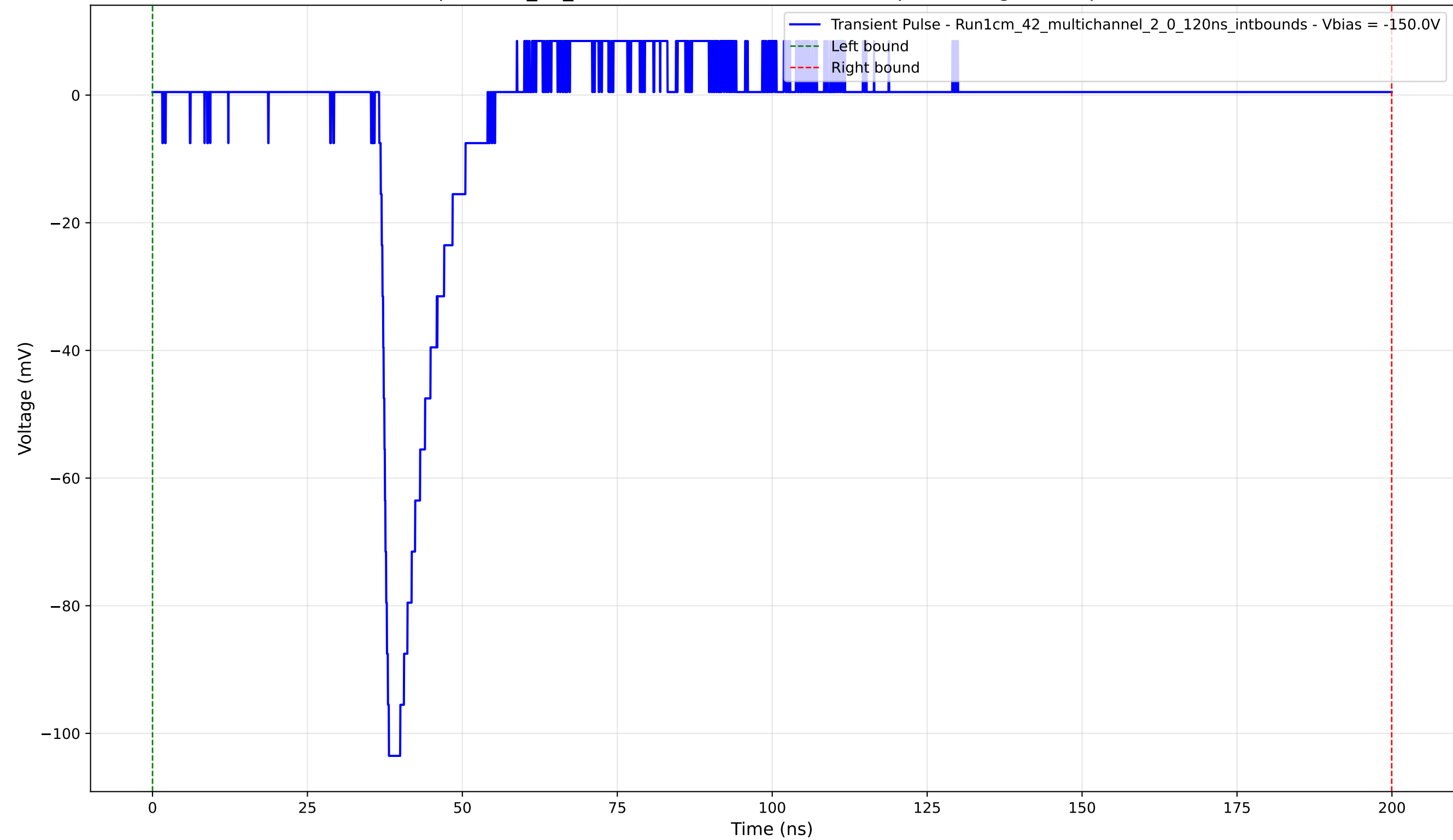
Transient Pulse - Sample: 1cm_42_multichannel - Position: 3740.0 \mu\text{m} - Charge: 9.03 pC - Rise Time: 1.19 ns
