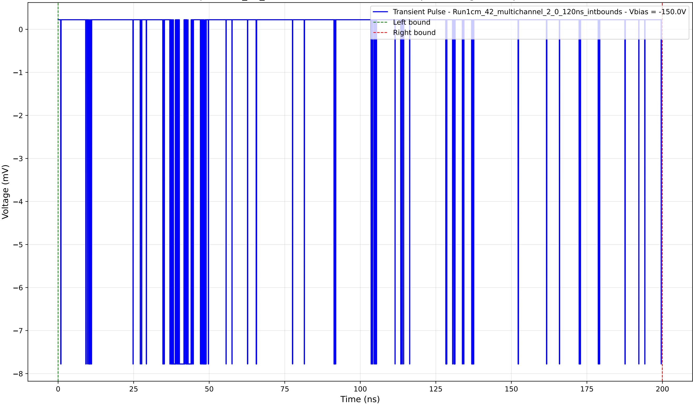
Transient Pulse - Sample: 1cm_42_multichannel - Position: 4915.0 \mu\text{m} - Charge: 0.96 pC - Rise Time: 0.04 ns
