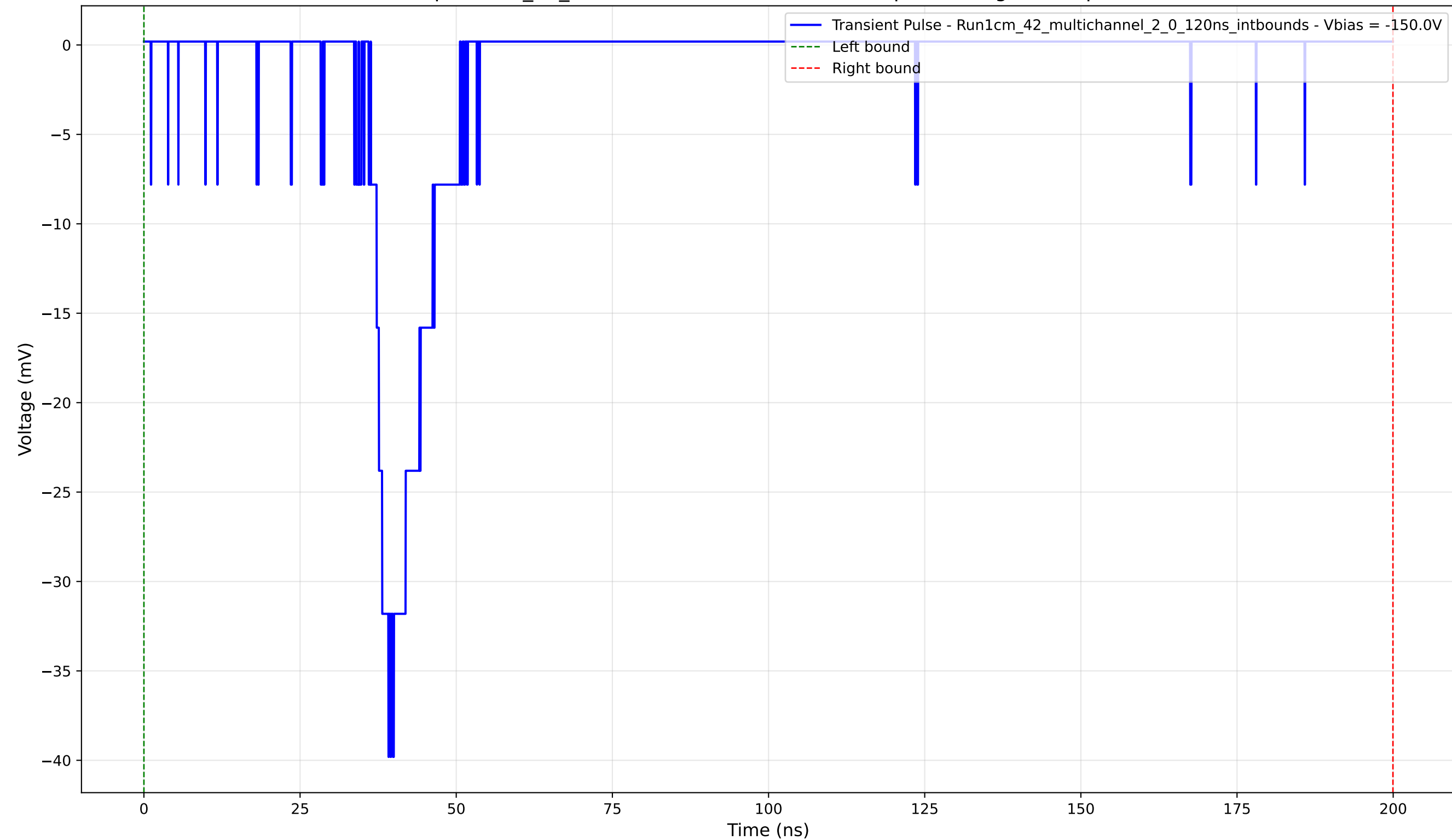
Transient Pulse - Sample: 1cm_42_multichannel - Position: 4845.0 \mu\text{m} - Charge: 5.31 pC - Rise Time: 2.82 ns
