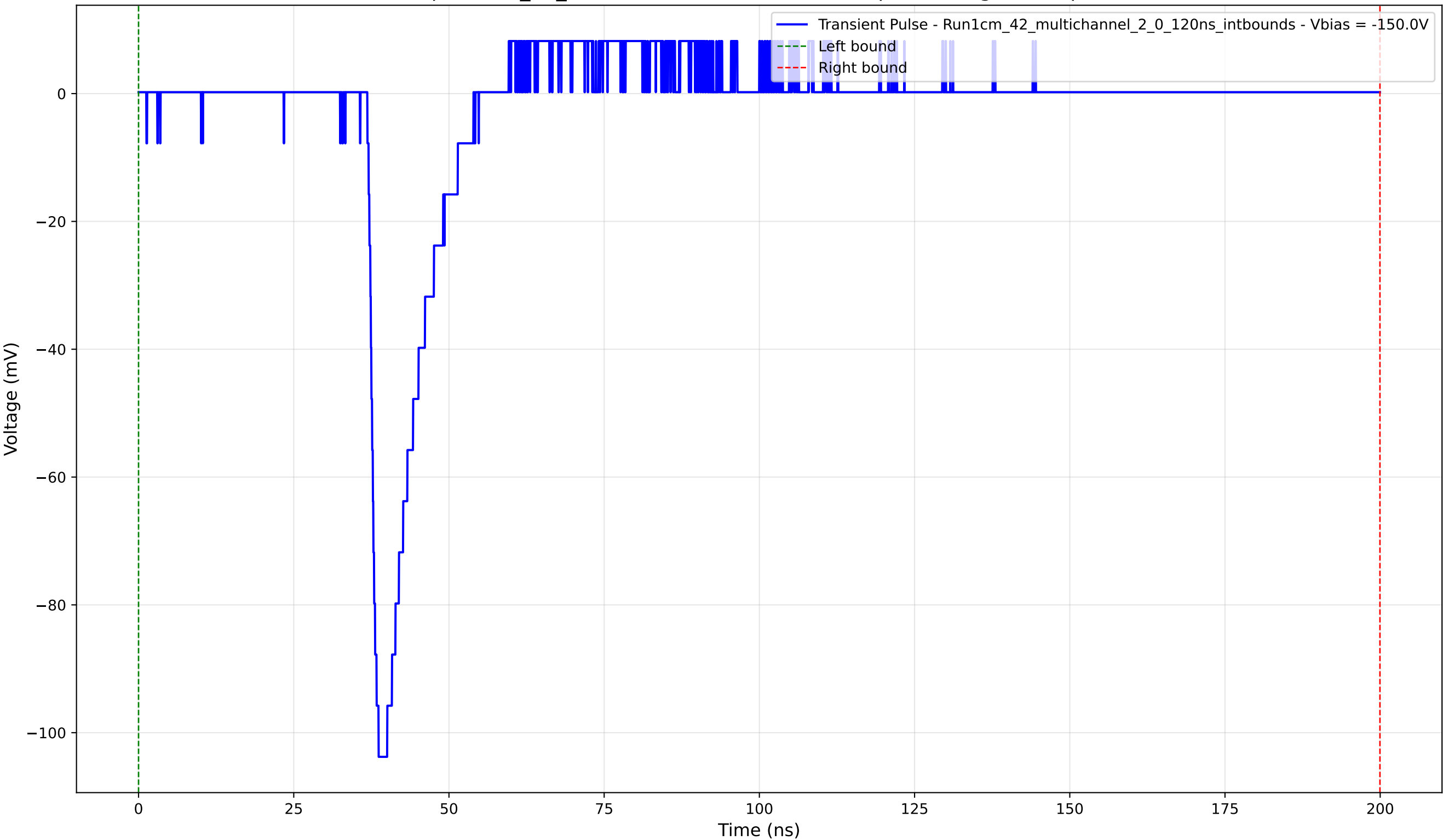
Transient Pulse - Sample: 1cm_42_multichannel - Position: 740.0 \mu\text{m} - Charge: 9.89 pC - Rise Time: 1.31 ns
