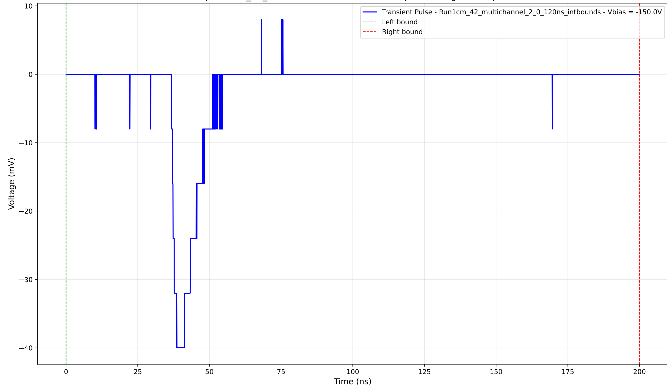
Transient Pulse - Sample: 1cm_42_multichannel - Position: 75.0 \mu\text{m} - Charge: 6.88 pC - Rise Time: 1.66 ns
