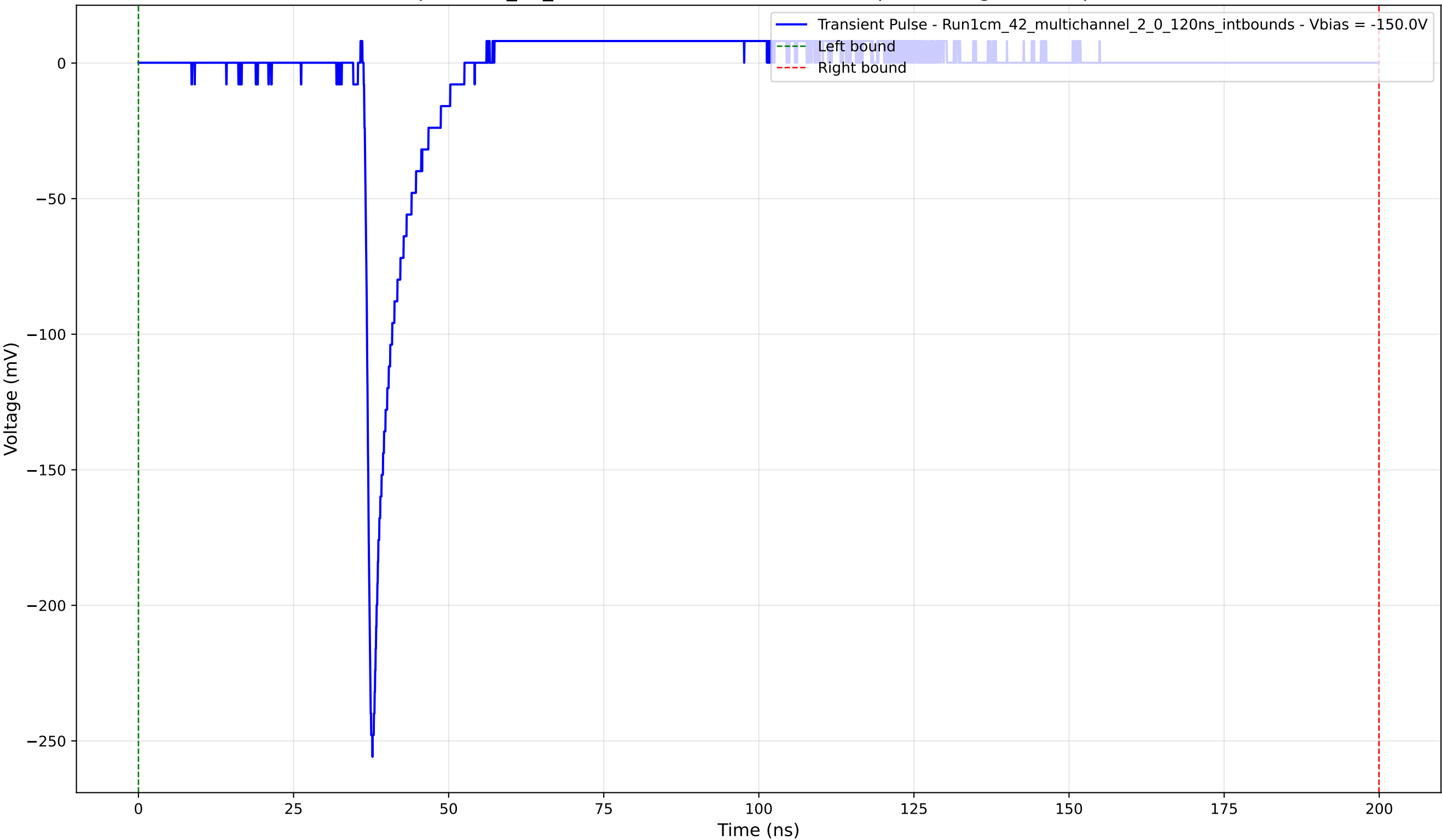
Transient Pulse - Sample: 1cm_42_multichannel - Position: 1645.0 \mu\text{m} - Charge: 11.73 pC - Rise Time: 0.90 ns
