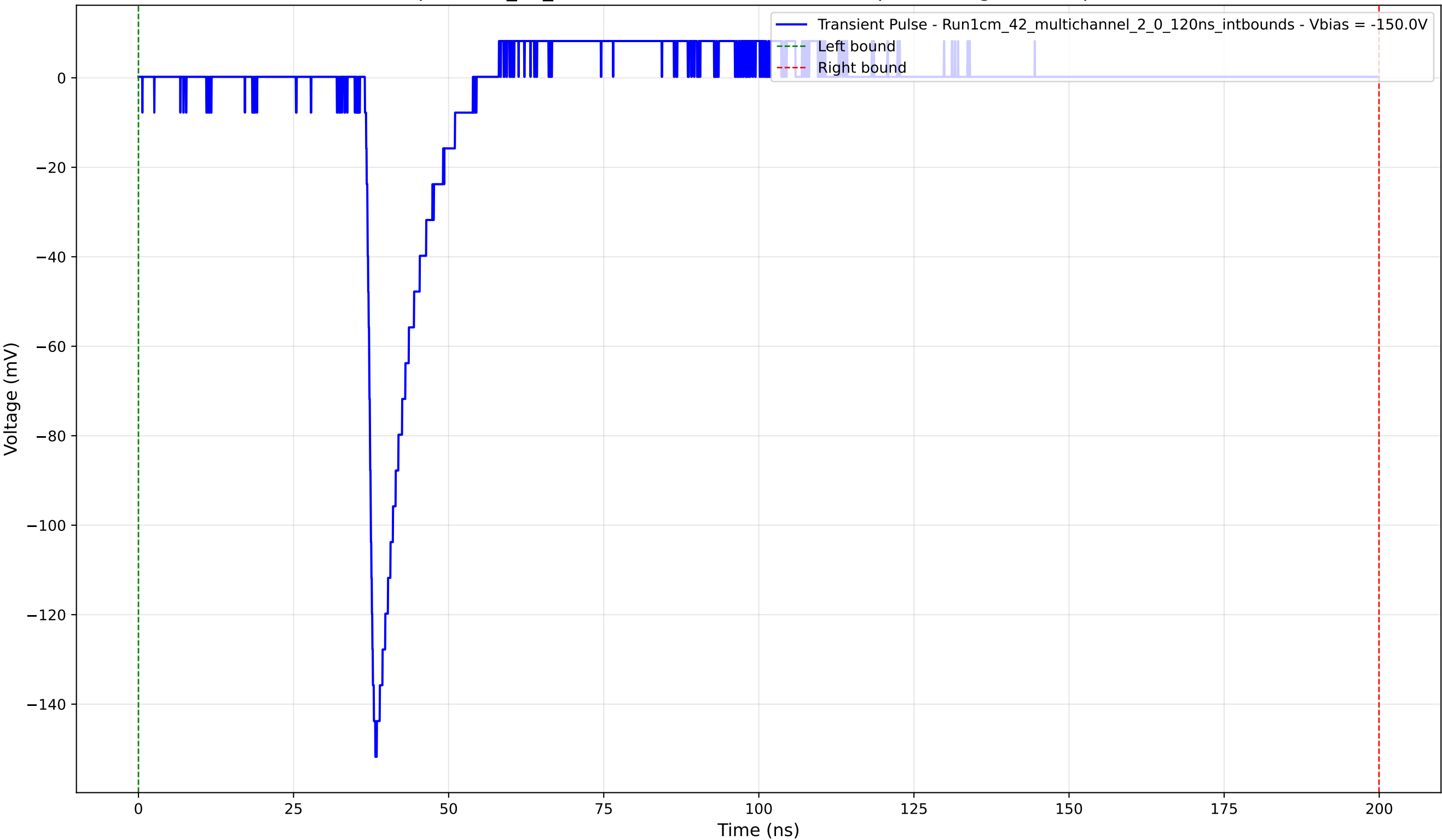
Transient Pulse - Sample: 1cm_42_multichannel - Position: 1195.0 \mu\text{m} - Charge: 11.39 pC - Rise Time: 1.24 ns
