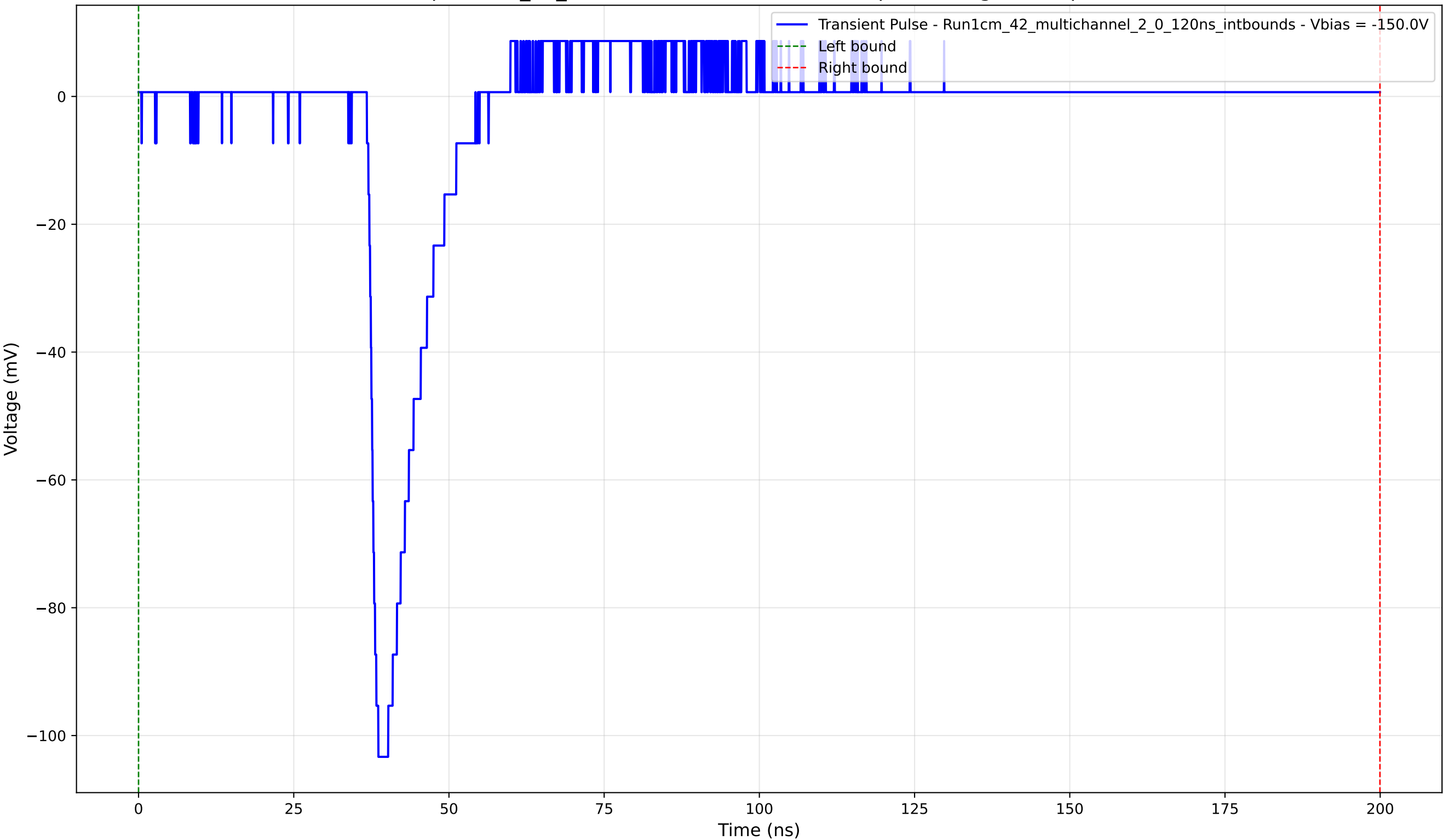
Transient Pulse - Sample: 1cm_42_multichannel - Position: 715.0 \mu\text{m} - Charge: 9.02 pC - Rise Time: 1.30 ns
