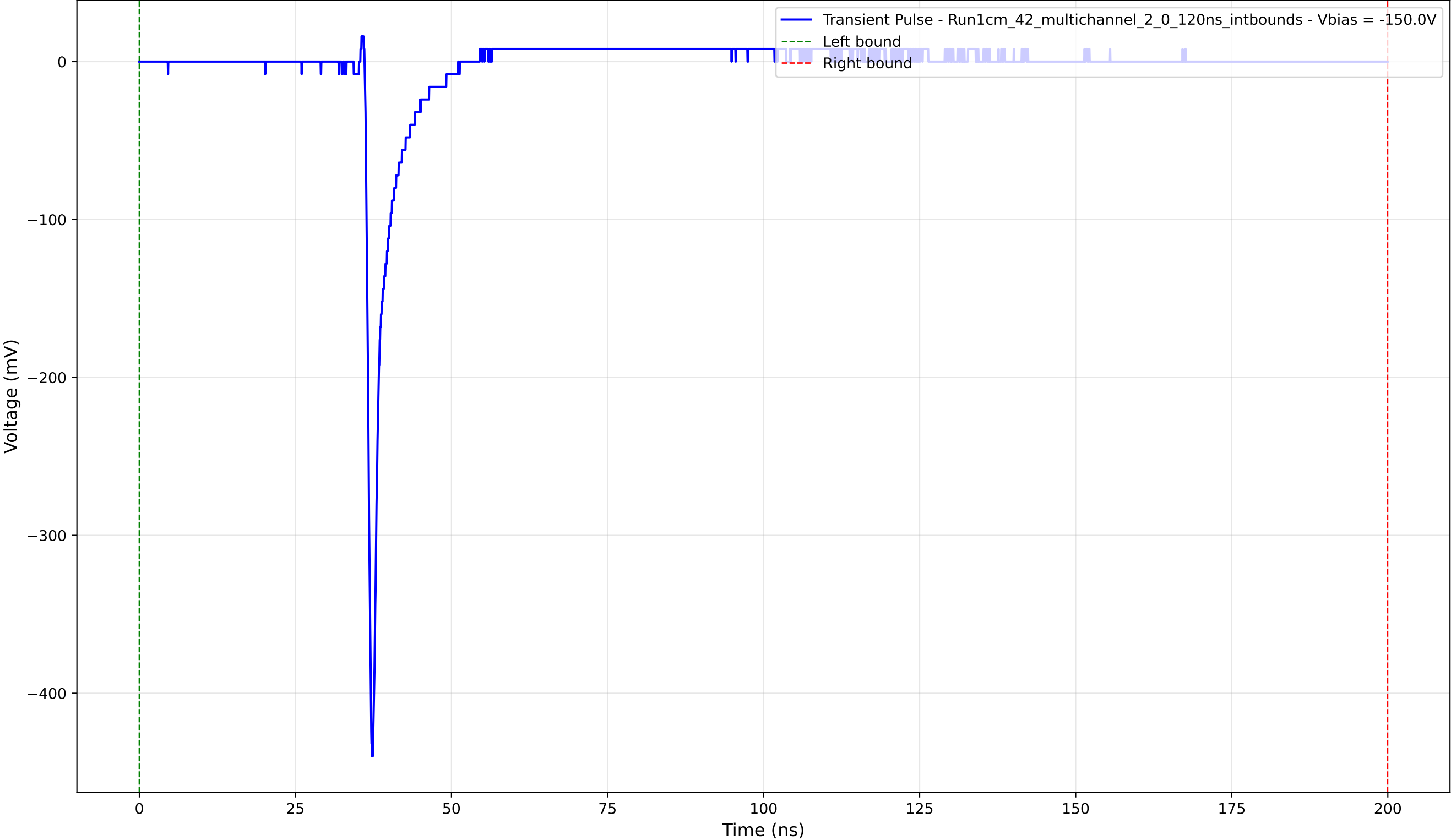
Transient Pulse - Sample: 1cm_42_multichannel - Position: 2675.0 \mu\text{m} - Charge: 14.00 pC - Rise Time: 0.80 ns
