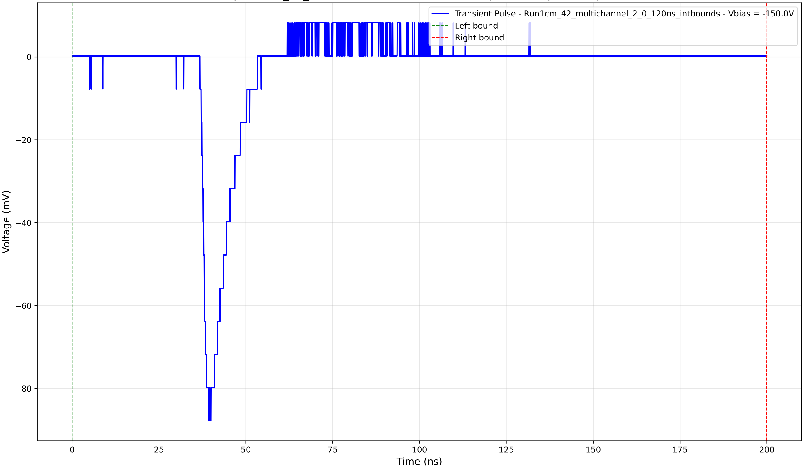
Transient Pulse - Sample: 1cm_42_multichannel - Position: 4195.0 \mu\text{m} - Charge: 8.33 pC - Rise Time: 1.55 ns
