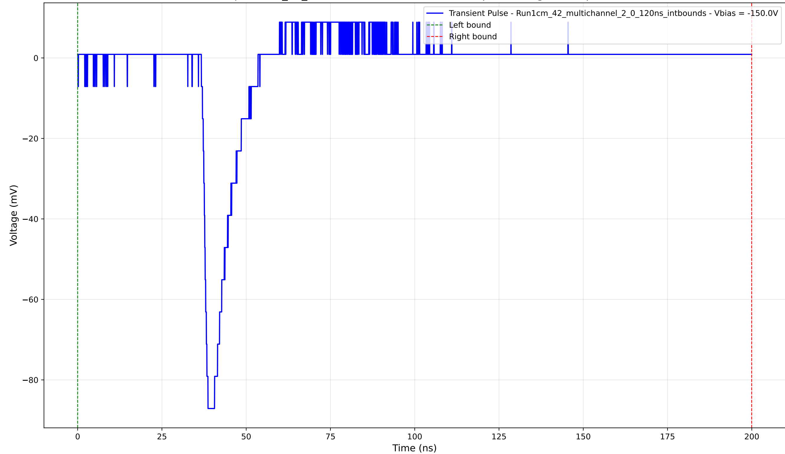
Transient Pulse - Sample: 1cm_42_multichannel - Position: 4045.0 \mu\text{m} - Charge: 6.68 pC - Rise Time: 1.35 ns
