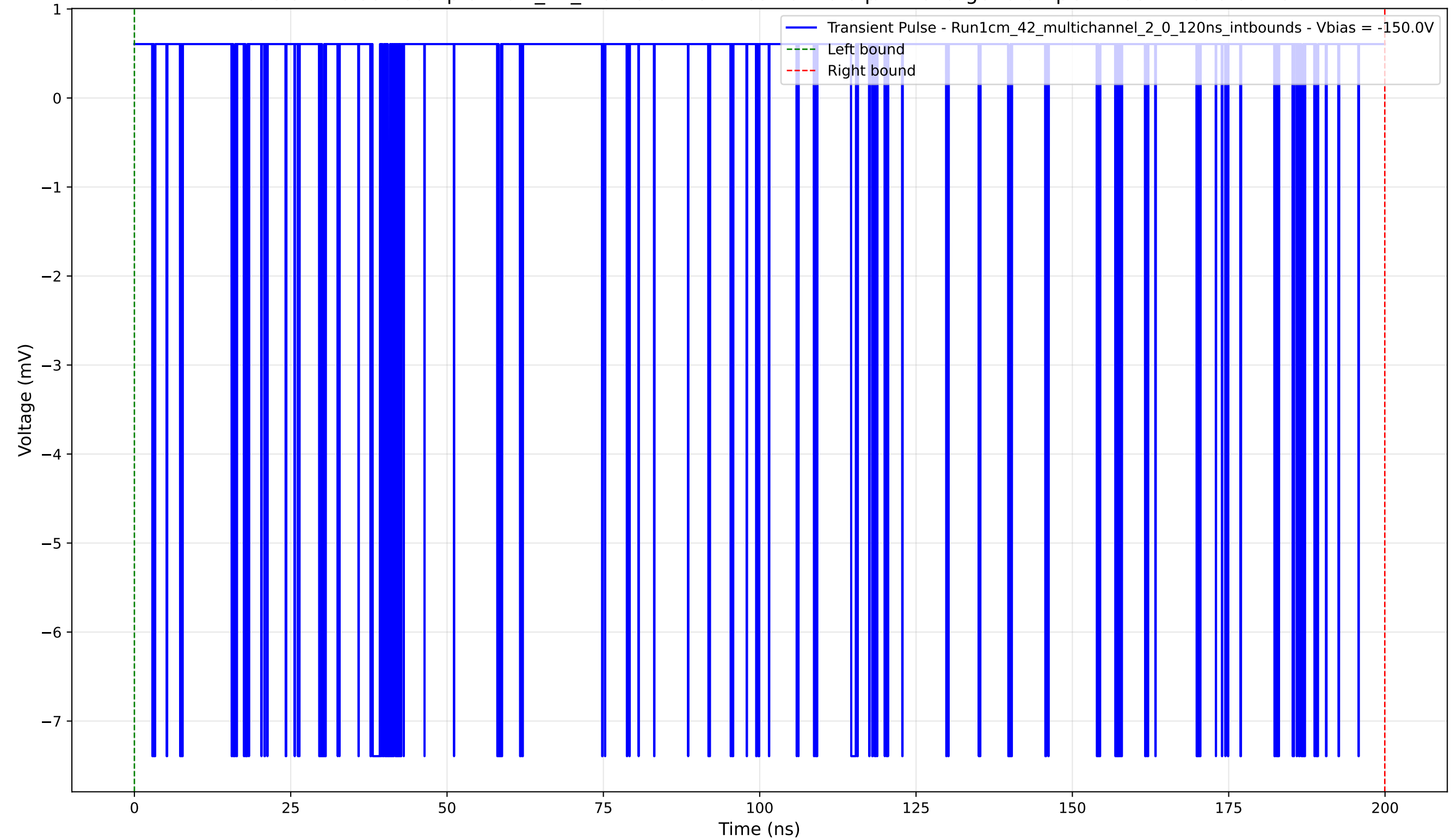
Transient Pulse - Sample: 1cm_42_multichannel - Position: 0.0 \mu\text{m} - Charge: 0.02 pC - Rise Time: 0.04 ns
