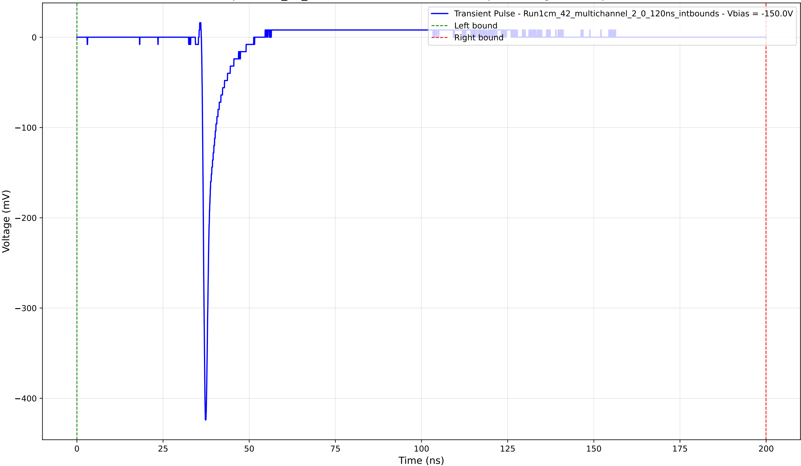
Transient Pulse - Sample: 1cm_42_multichannel - Position: 2720.0 \mu\text{m} - Charge: 13.58 pC - Rise Time: 0.78 ns
