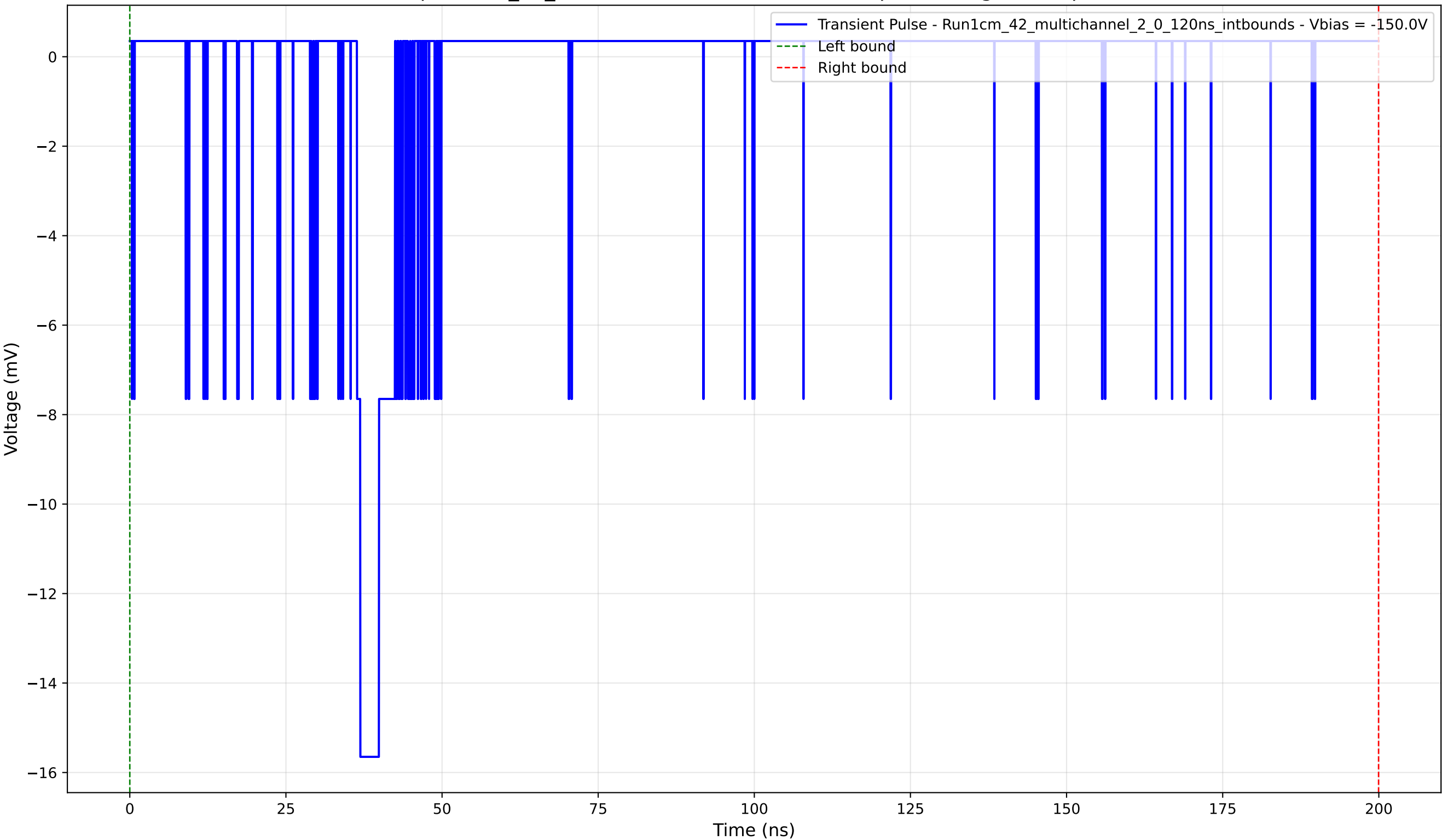
Transient Pulse - Sample: 1cm_42_multichannel - Position: 1850.0 \mu\text{m} - Charge: 1.13 pC - Rise Time: 0.55 ns
