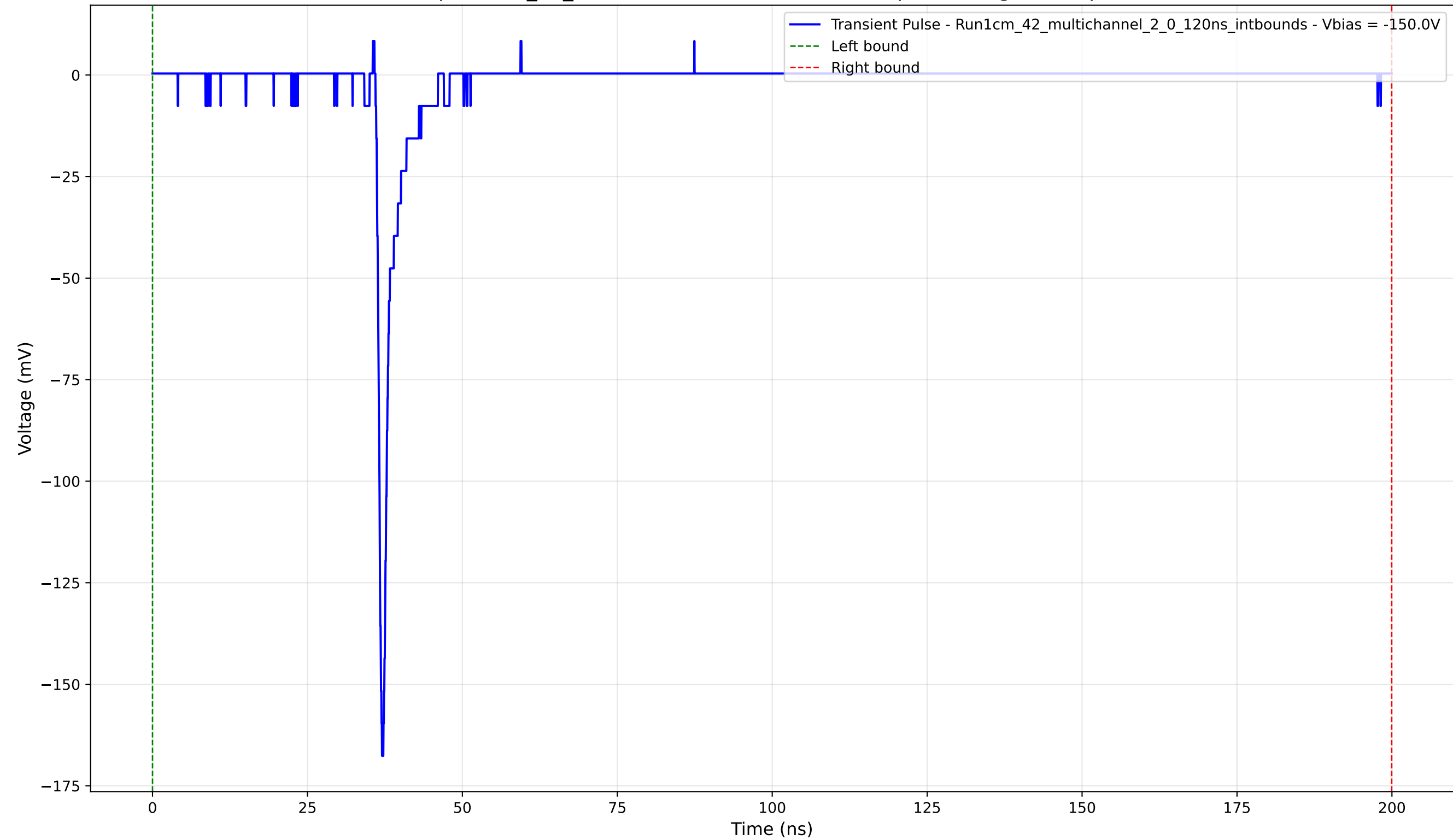
Transient Pulse - Sample: 1cm_42_multichannel - Position: 2330.0 \mu\text{m} - Charge: 6.62 pC - Rise Time: 0.71 ns
