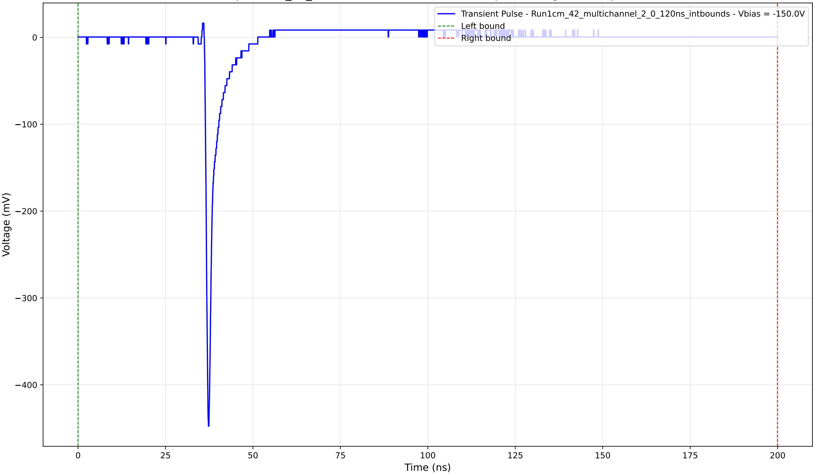
Transient Pulse - Sample: 1cm_42_multichannel - Position: 2660.0 \mu\text{m} - Charge: 13.57 pC - Rise Time: 0.74 ns
