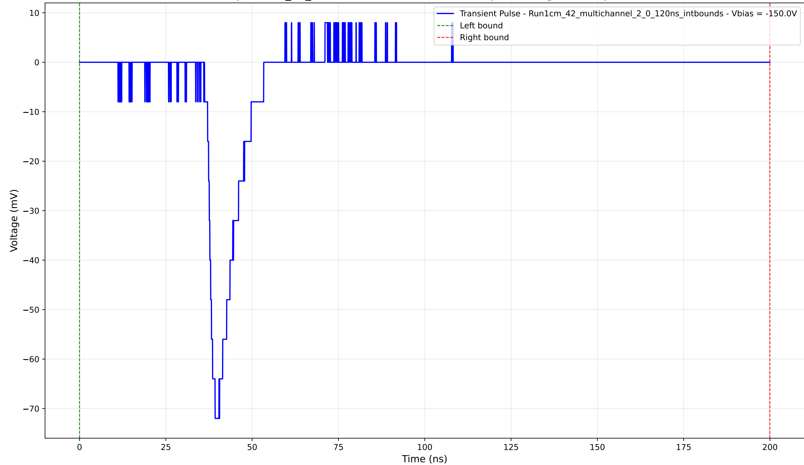
Transient Pulse - Sample: 1cm_42_multichannel - Position: 4680.0 \mu\text{m} - Charge: 10.68 pC - Rise Time: 3.04 ns
