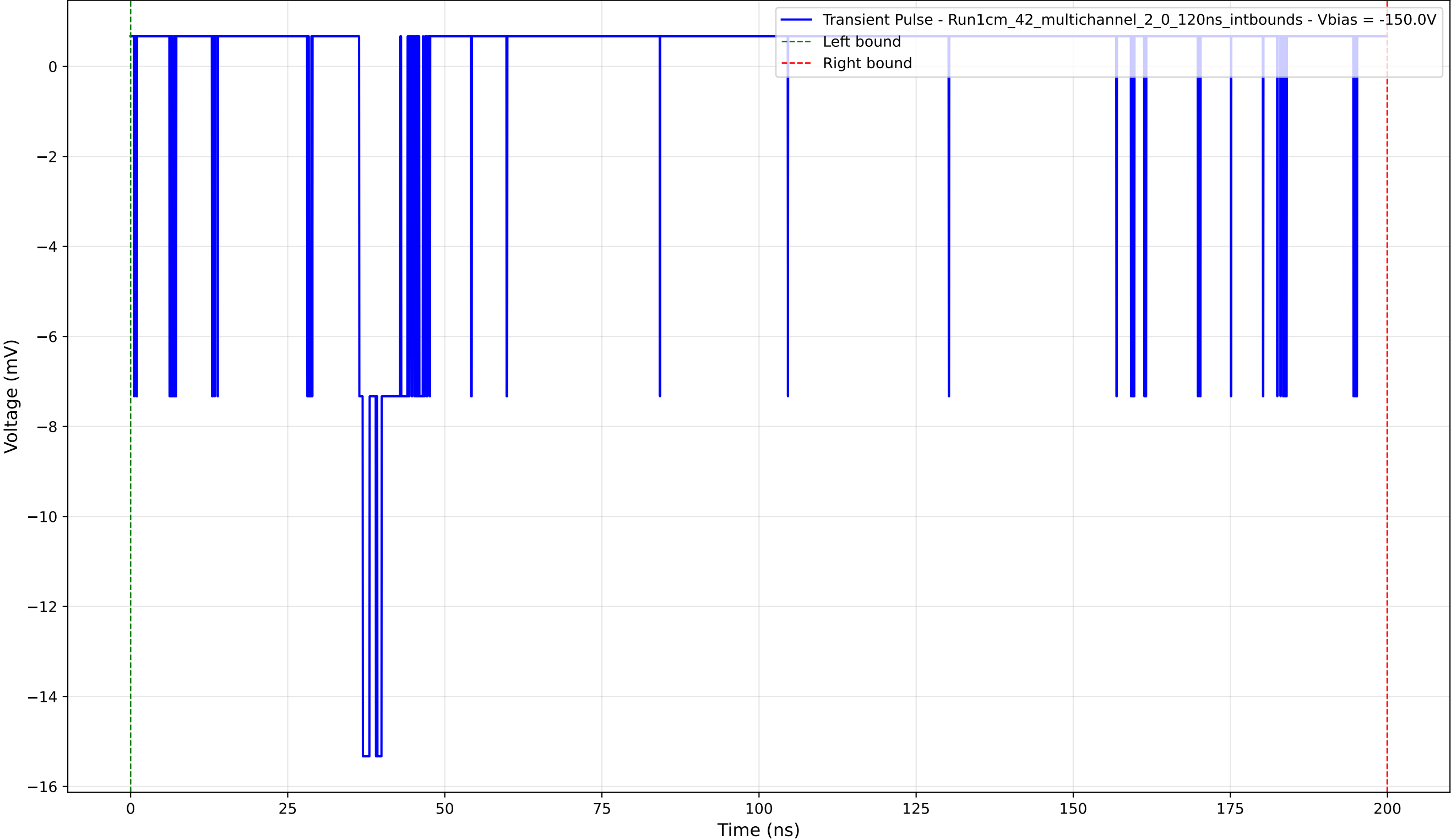
Transient Pulse - Sample: 1cm_42_multichannel - Position: 1870.0 \mu\text{m} - Charge: -0.33 pC - Rise Time: 0.59 ns
