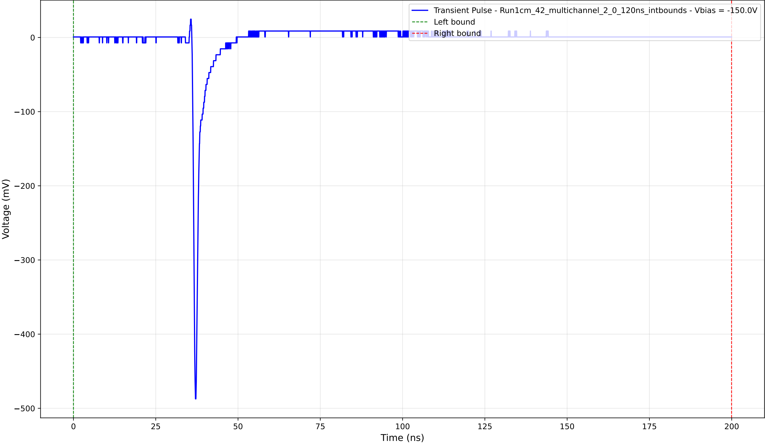
Transient Pulse - Sample: 1cm_42_multichannel - Position: 2430.0 \mu\text{m} - Charge: 11.26 pC - Rise Time: 0.71 ns
