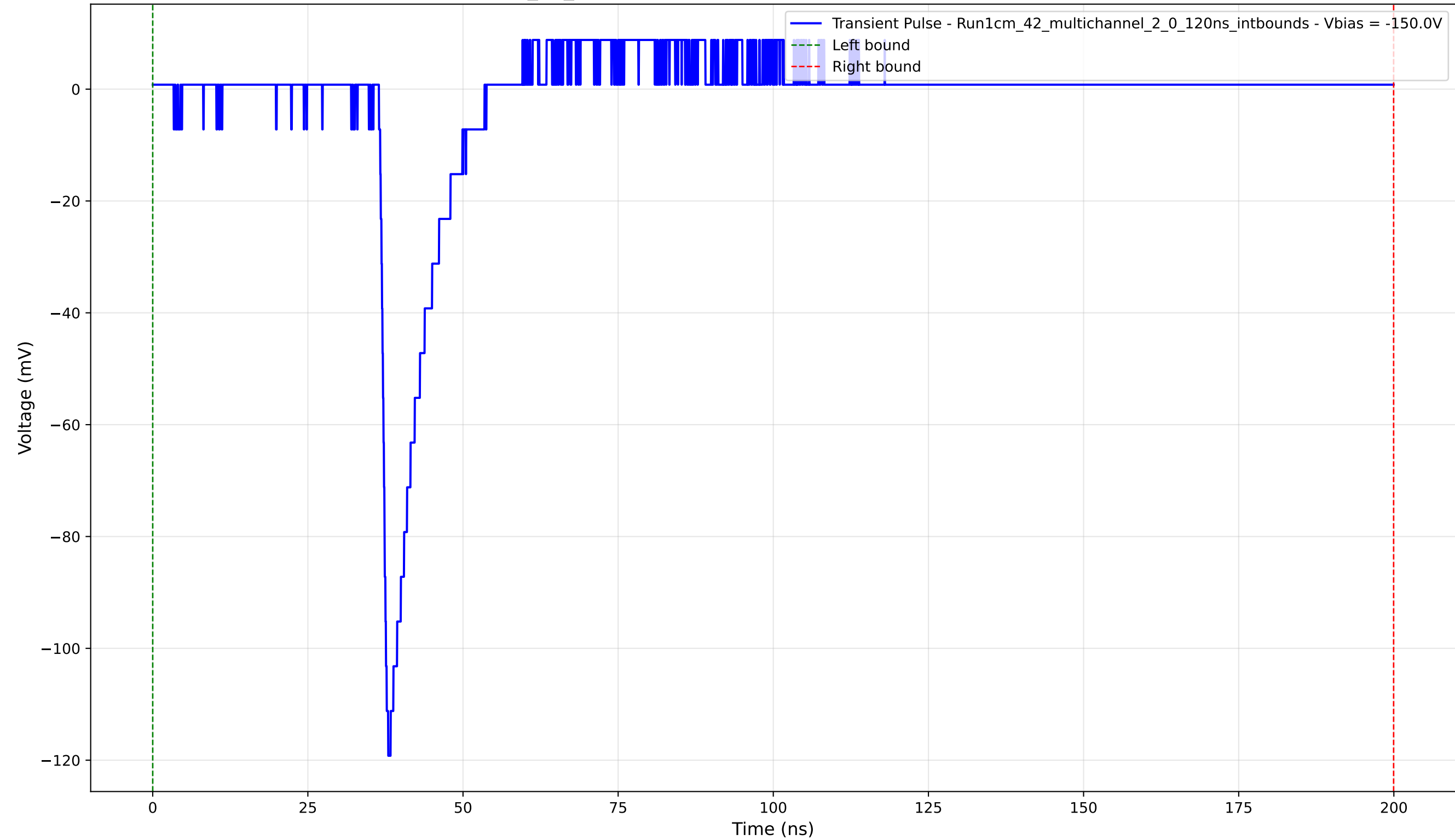
Transient Pulse - Sample: 1cm_42_multichannel - Position: 3450.0 \mu\text{m} - Charge: 7.57 pC - Rise Time: 1.06 ns
