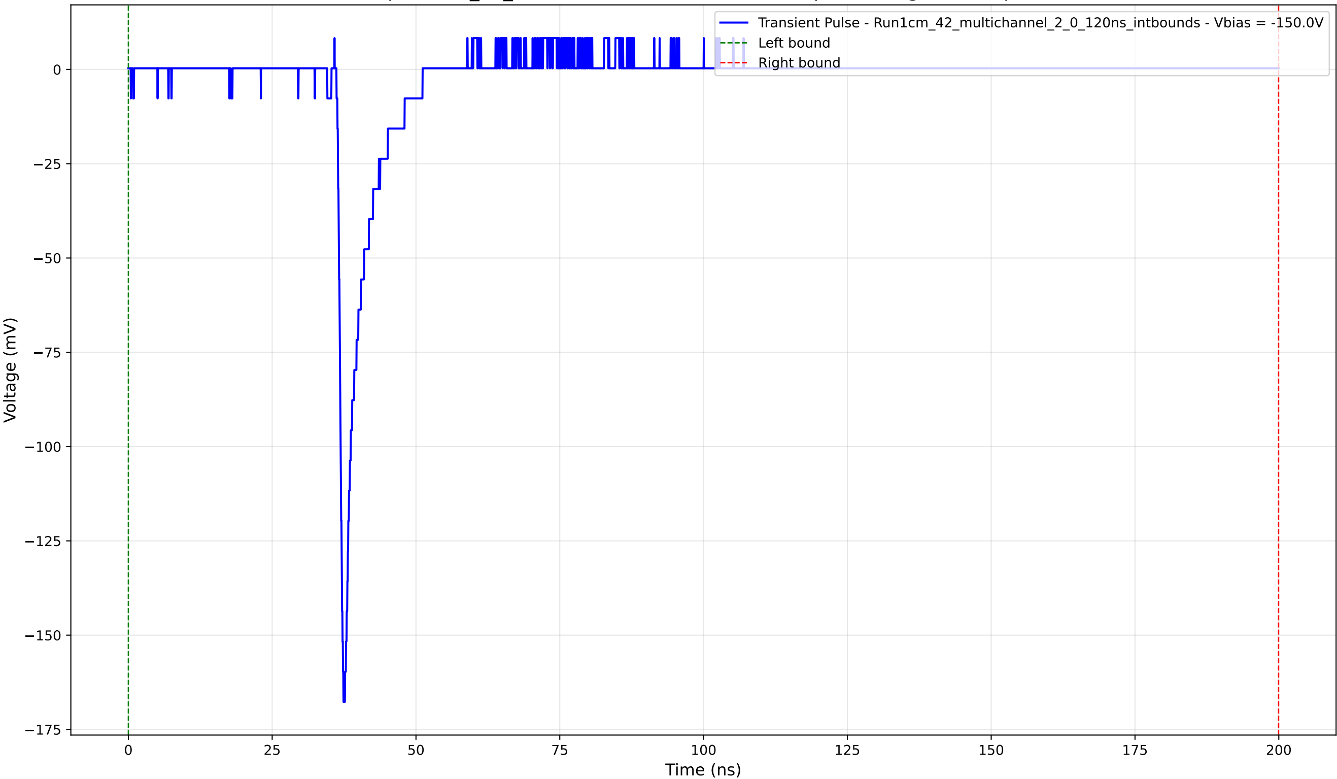
Transient Pulse - Sample: 1cm_42_multichannel - Position: 2930.0 \mu\text{m} - Charge: 10.10 pC - Rise Time: 0.83 ns
