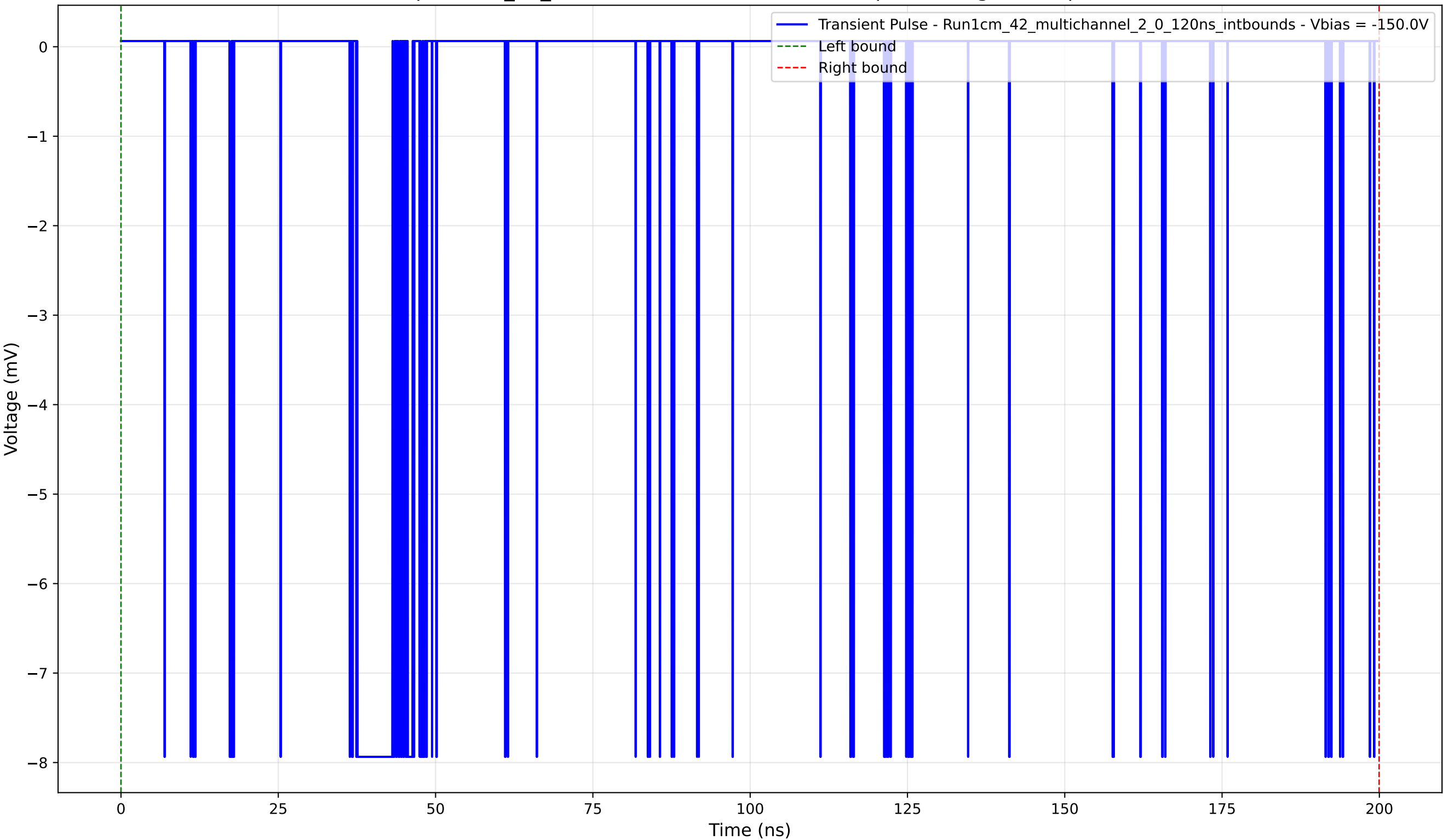
Transient Pulse - Sample: 1cm_42_multichannel - Position: 3895.0 \mu\text{m} - Charge: 1.91 pC - Rise Time: 0.04 ns
