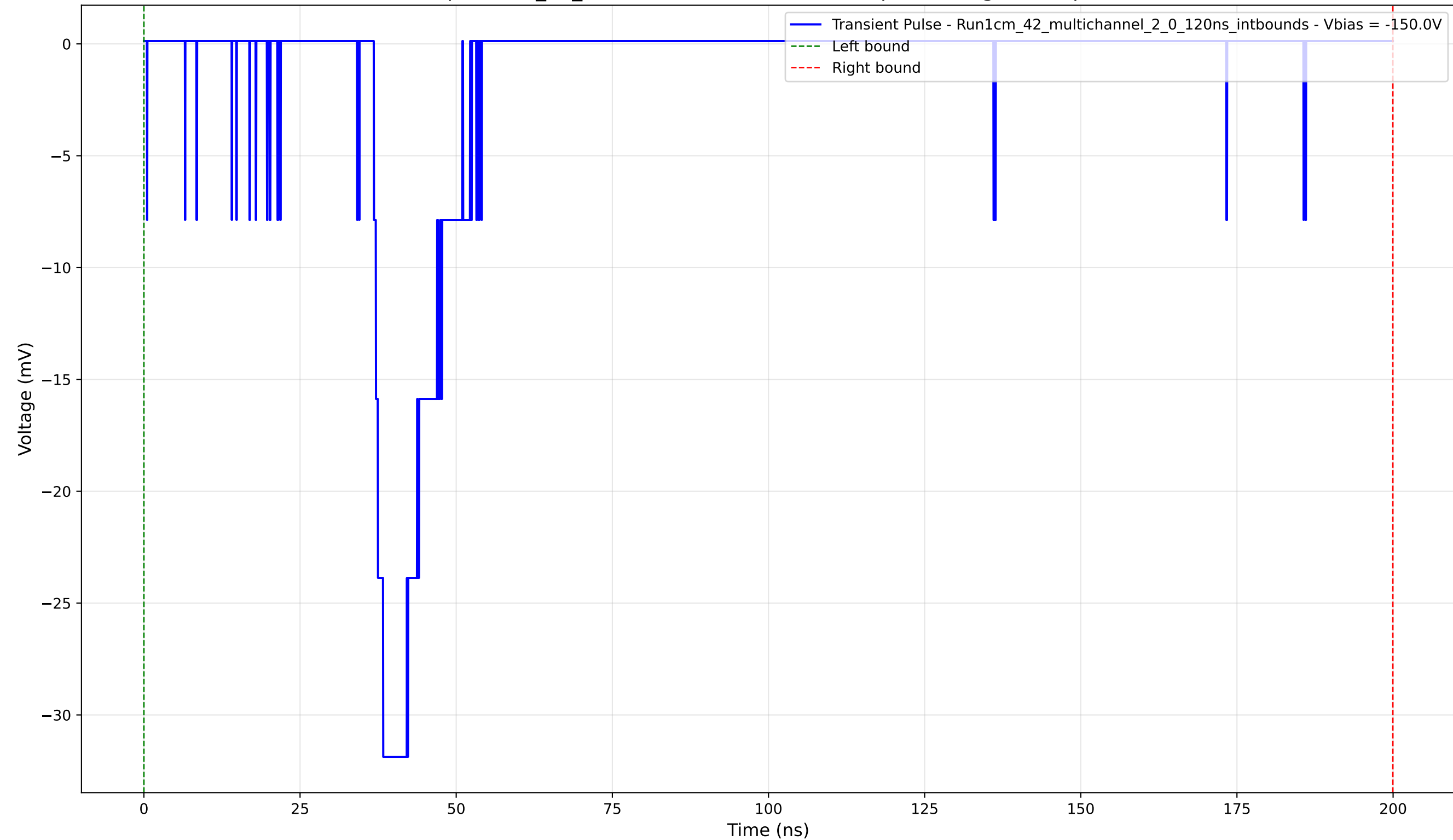
Transient Pulse - Sample: 1cm_42_multichannel - Position: 70.0 \mu\text{m} - Charge: 5.54 pC - Rise Time: 1.50 ns
