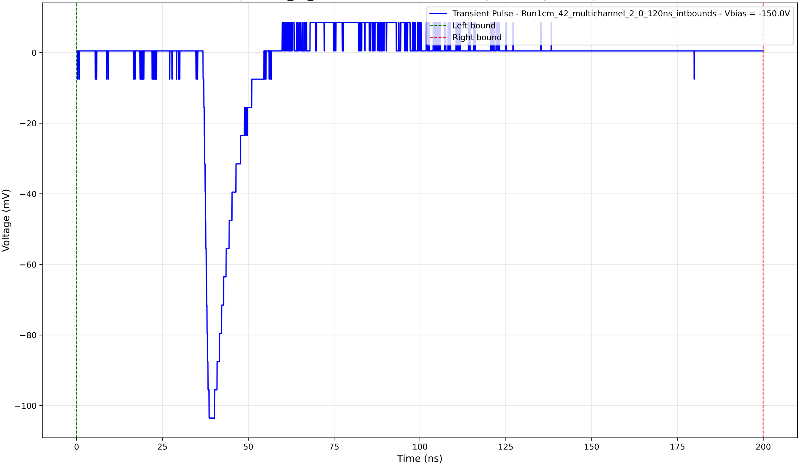
Transient Pulse - Sample: 1cm_42_multichannel - Position: 700.0 \mu\text{m} - Charge: 9.36 pC - Rise Time: 1.23 ns
