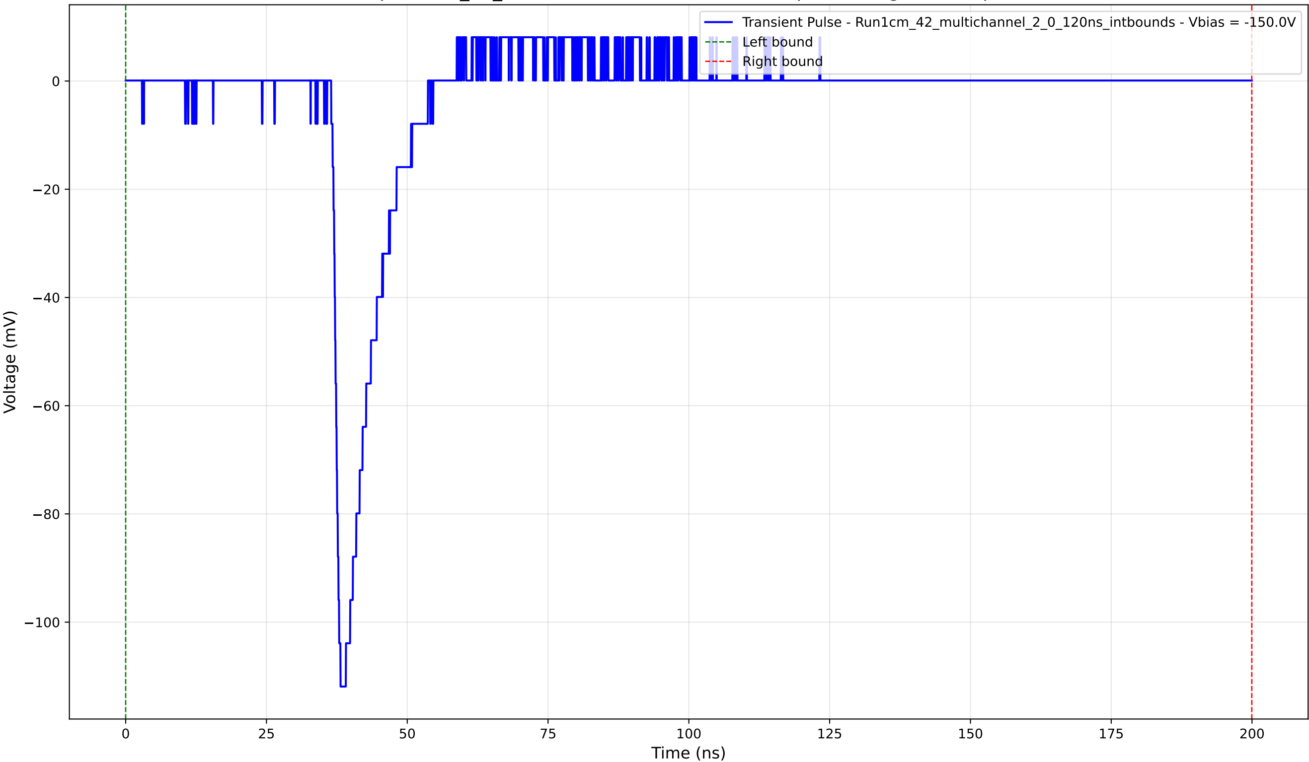
Transient Pulse - Sample: 1cm_42_multichannel - Position: 3620.0 \mu\text{m} - Charge: 11.25 pC - Rise Time: 1.18 ns
