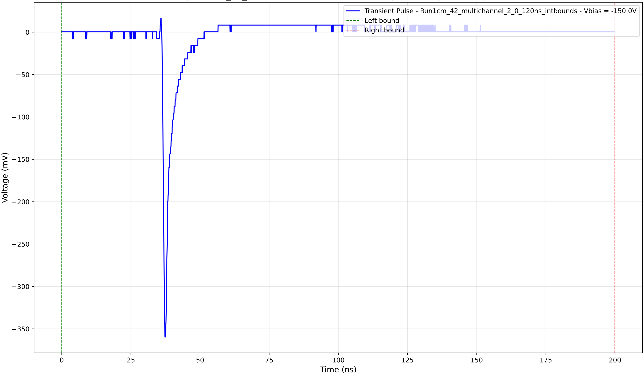
Transient Pulse - Sample: 1cm_42_multichannel - Position: 1945.0 \mu\text{m} - Charge: 11.94 pC - Rise Time: 0.80 ns
