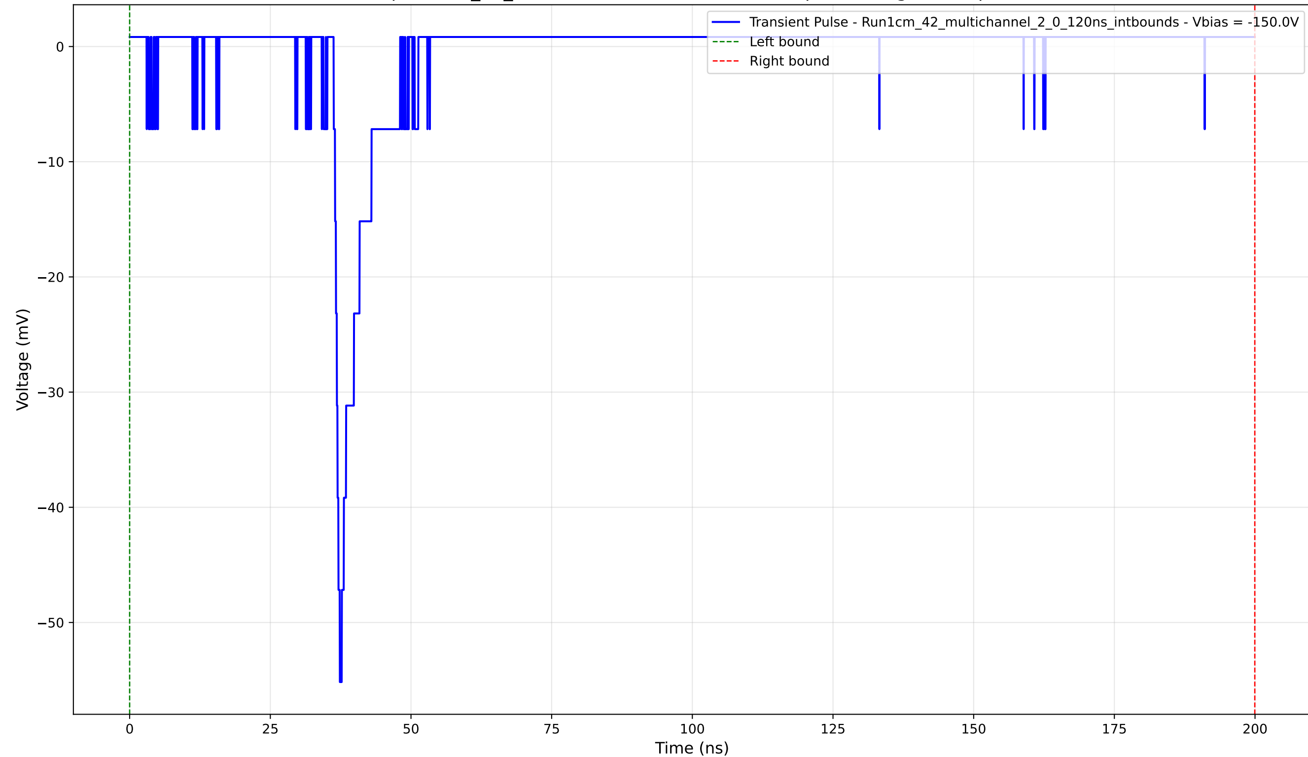
Transient Pulse - Sample: 1cm_42_multichannel - Position: 2910.0 \mu\text{m} - Charge: 2.13 pC - Rise Time: 1.09 ns
