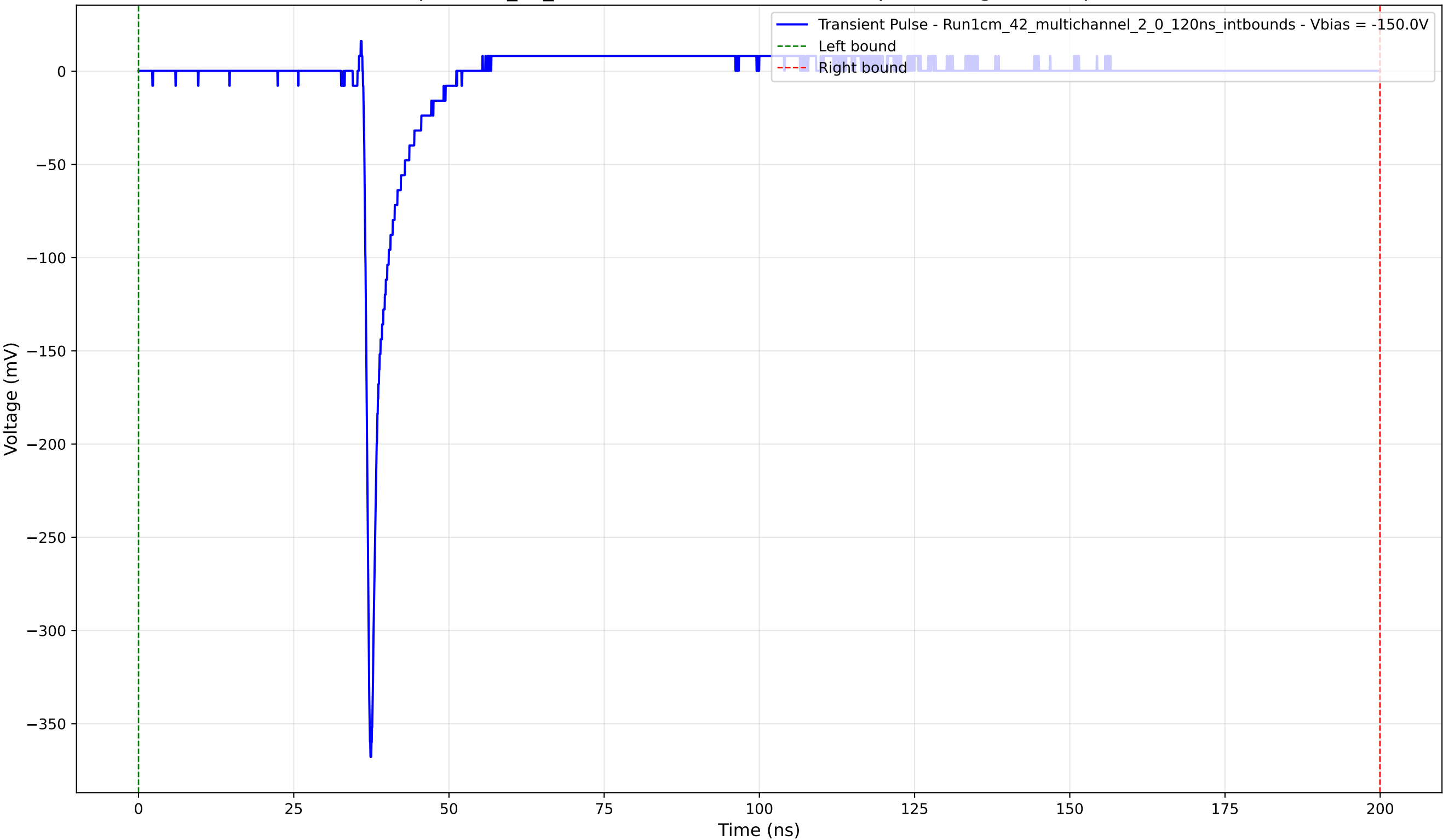
Transient Pulse - Sample: 1cm_42_multichannel - Position: 2780.0 \mu\text{m} - Charge: 12.36 pC - Rise Time: 0.79 ns
