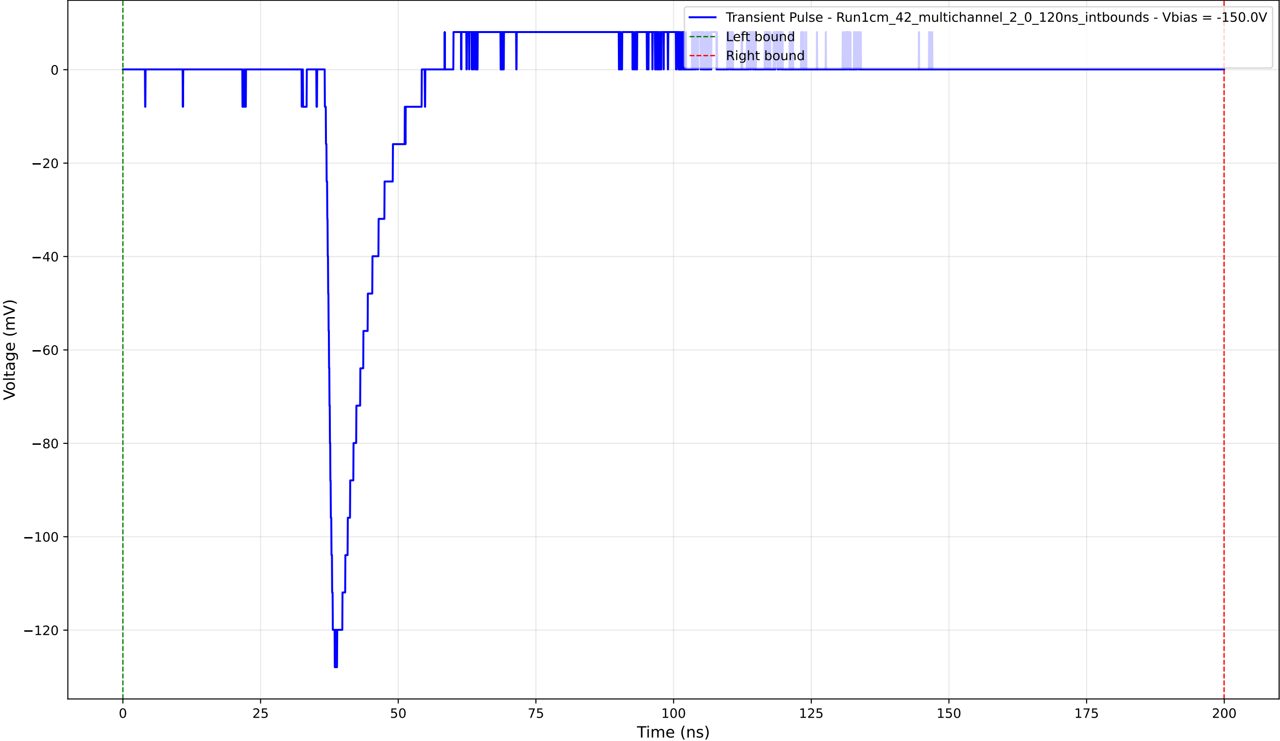
Transient Pulse - Sample: 1cm_42_multichannel - Position: 1000.0 \mu\text{m} - Charge: 10.31 pC - Rise Time: 1.26 ns
