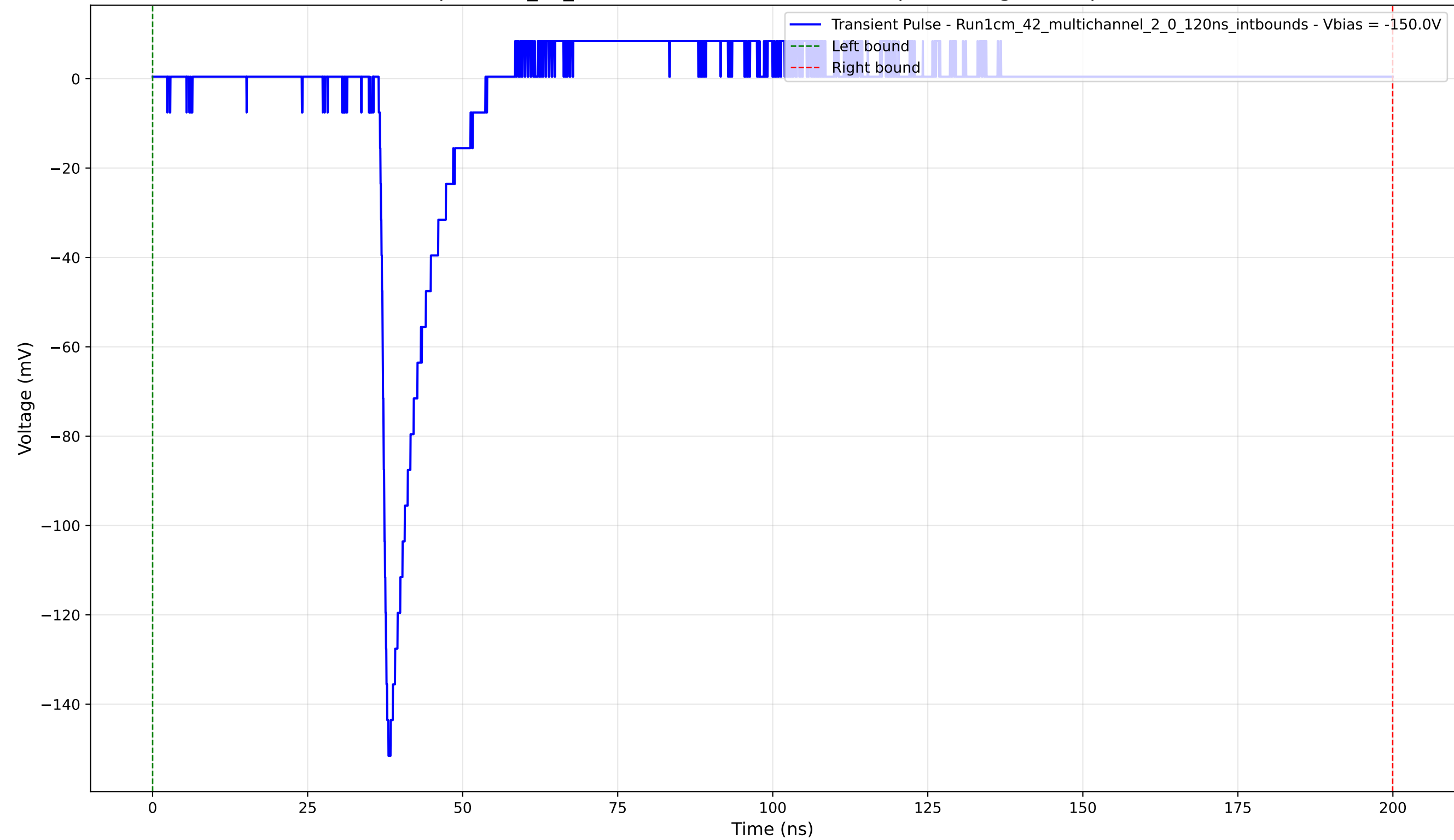
Transient Pulse - Sample: 1cm_42_multichannel - Position: 1275.0 \mu\text{m} - Charge: 9.44 pC - Rise Time: 1.16 ns
