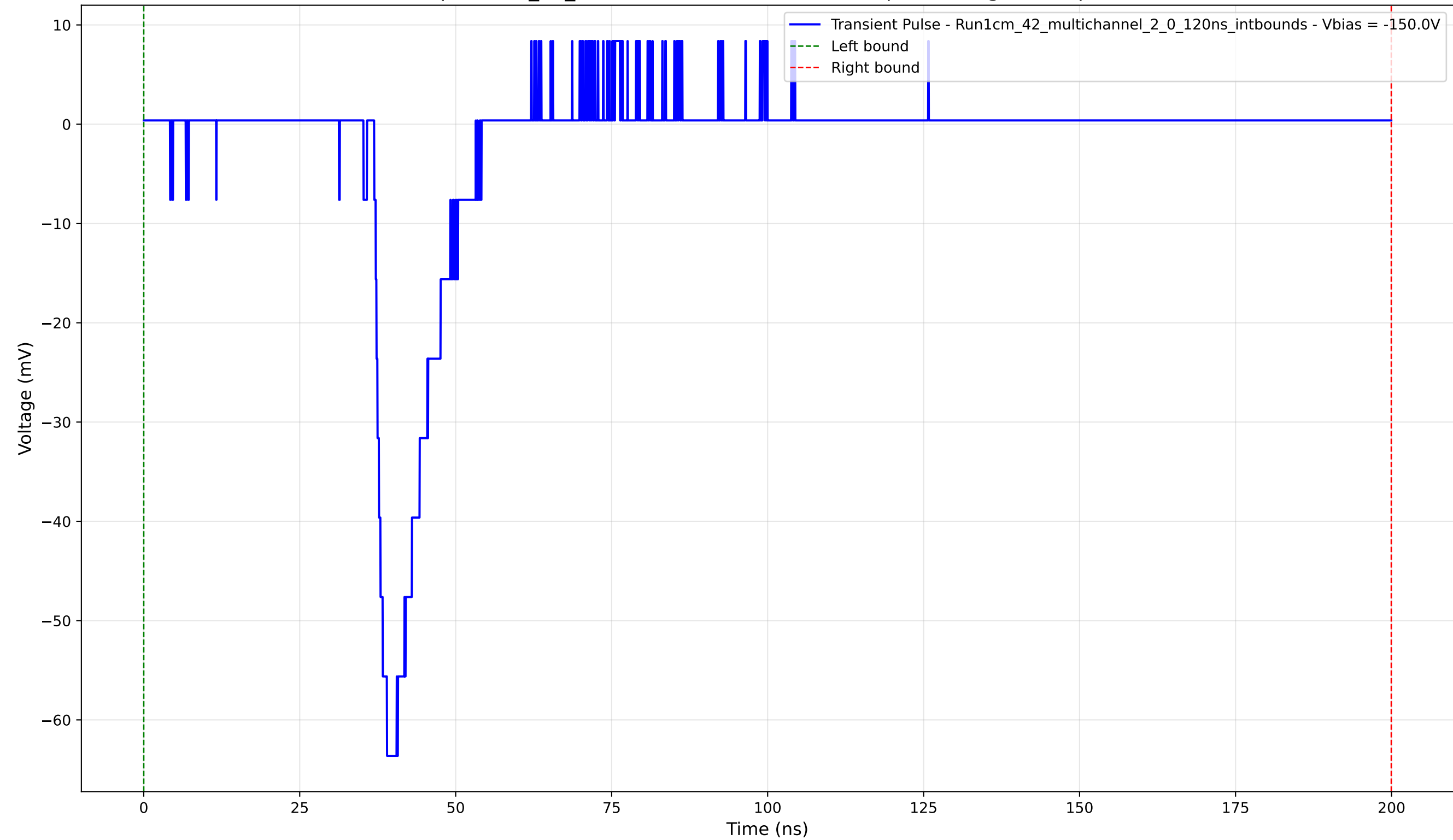
Transient Pulse - Sample: 1cm_42_multichannel - Position: 275.0 \mu\text{m} - Charge: 7.98 pC - Rise Time: 2.05 ns
