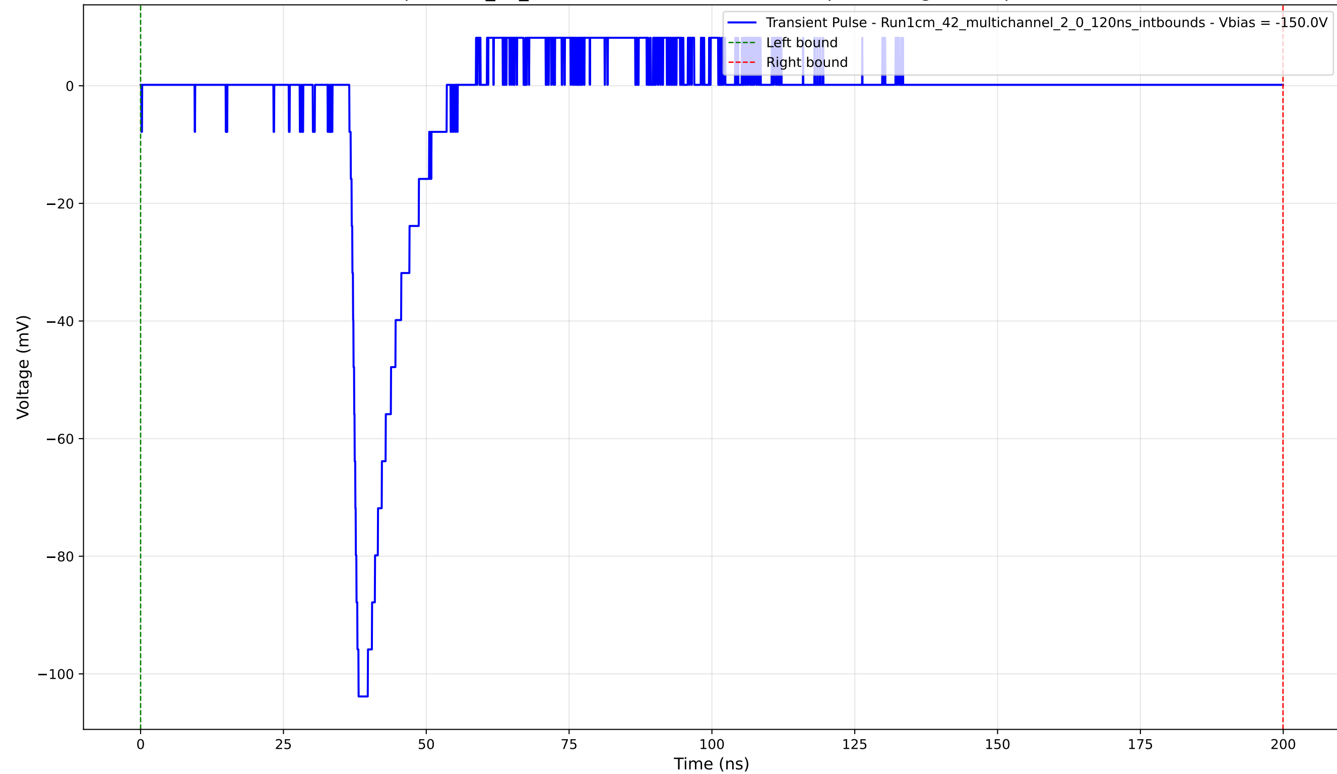
Transient Pulse - Sample: 1cm_42_multichannel - Position: 3710.0 \mu\text{m} - Charge: 9.35 pC - Rise Time: 1.19 ns
