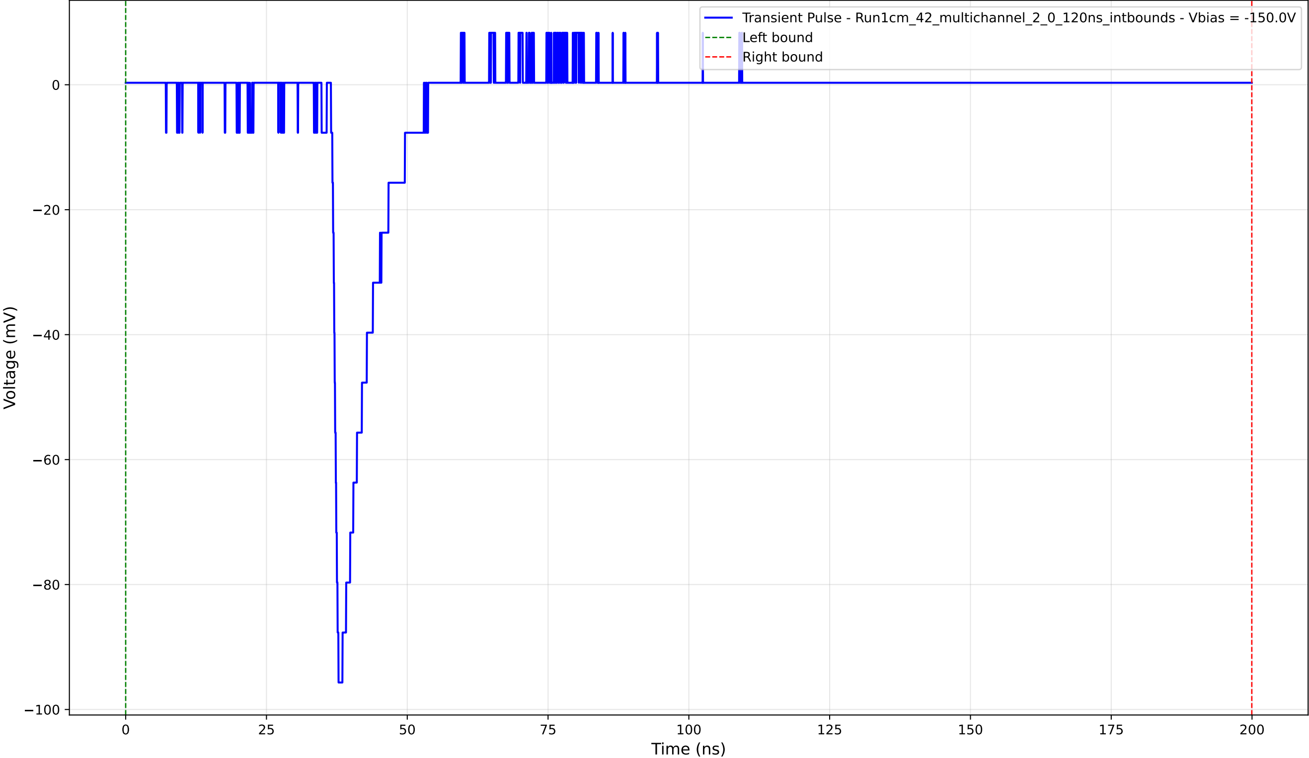
Transient Pulse - Sample: 1cm_42_multichannel - Position: 3440.0 \mu\text{m} - Charge: 10.51 pC - Rise Time: 0.95 ns
