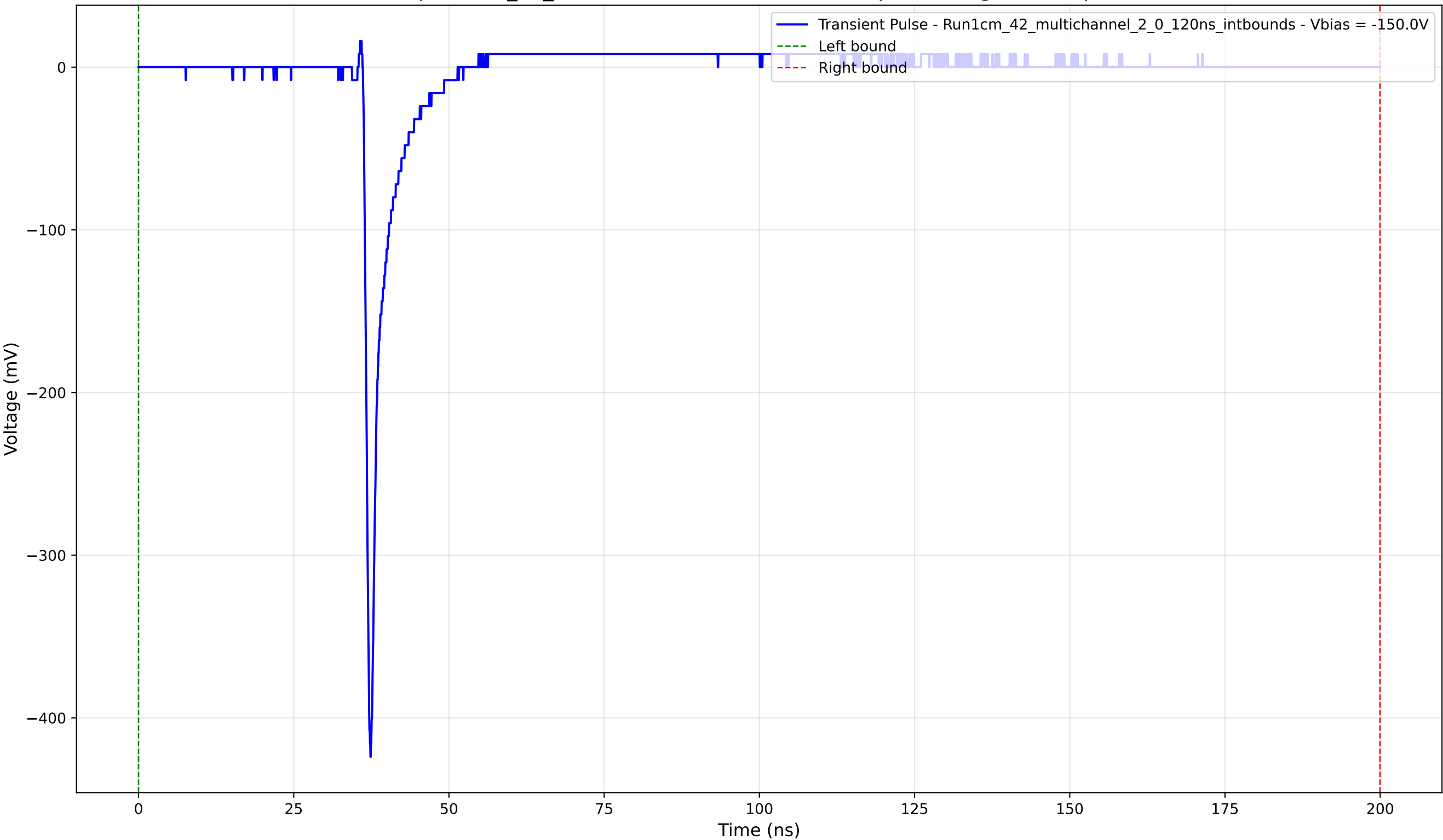
Transient Pulse - Sample: 1cm_42_multichannel - Position: 2725.0 \mu\text{m} - Charge: 13.33 pC - Rise Time: 0.81 ns
