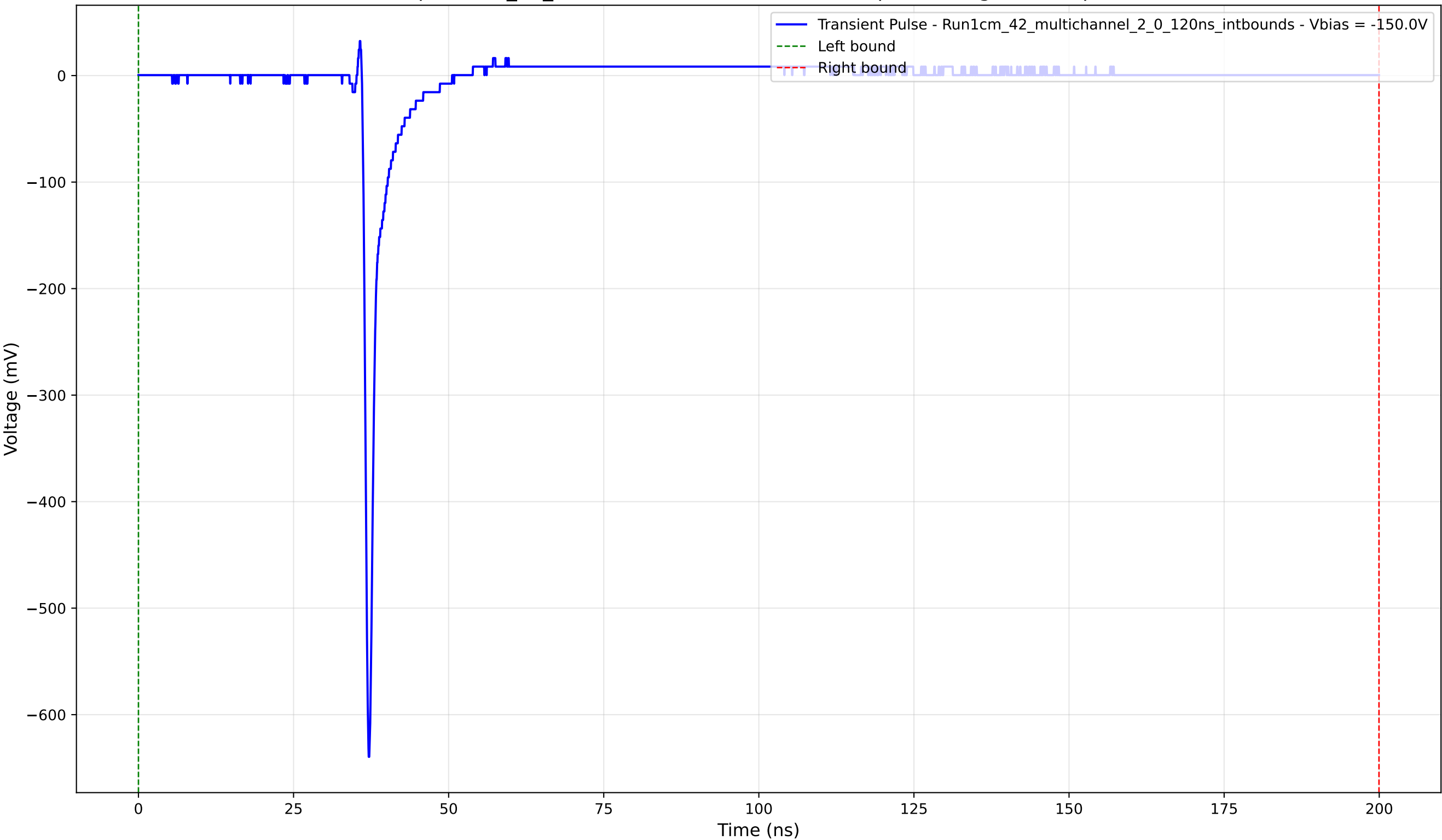
Transient Pulse - Sample: 1cm_42_multichannel - Position: 2265.0 \mu\text{m} - Charge: 16.29 pC - Rise Time: 0.74 ns
