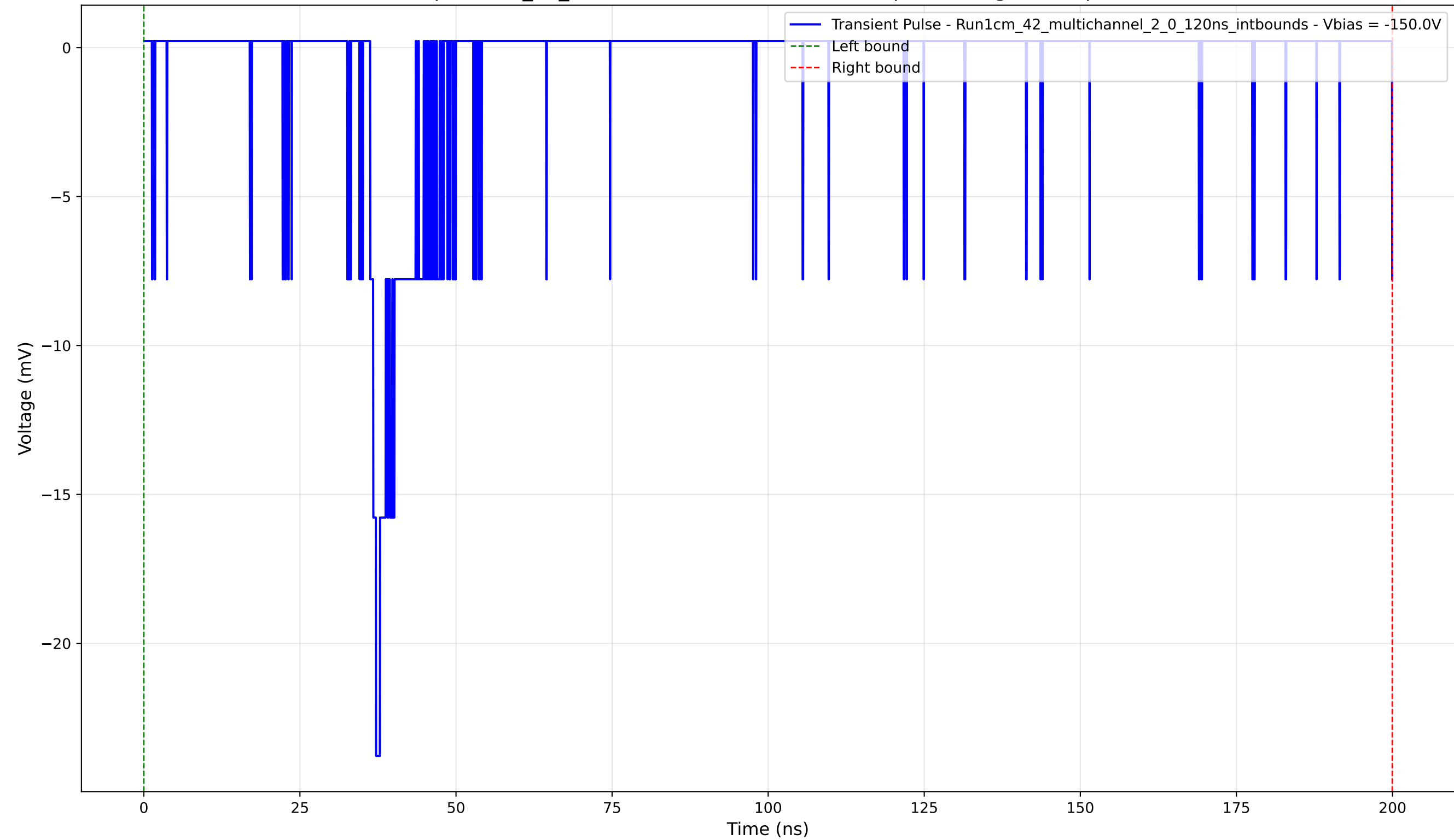
Transient Pulse - Sample: 1cm_42_multichannel - Position: 2860.0 \mu\text{m} - Charge: 1.96 pC - Rise Time: 0.95 ns
