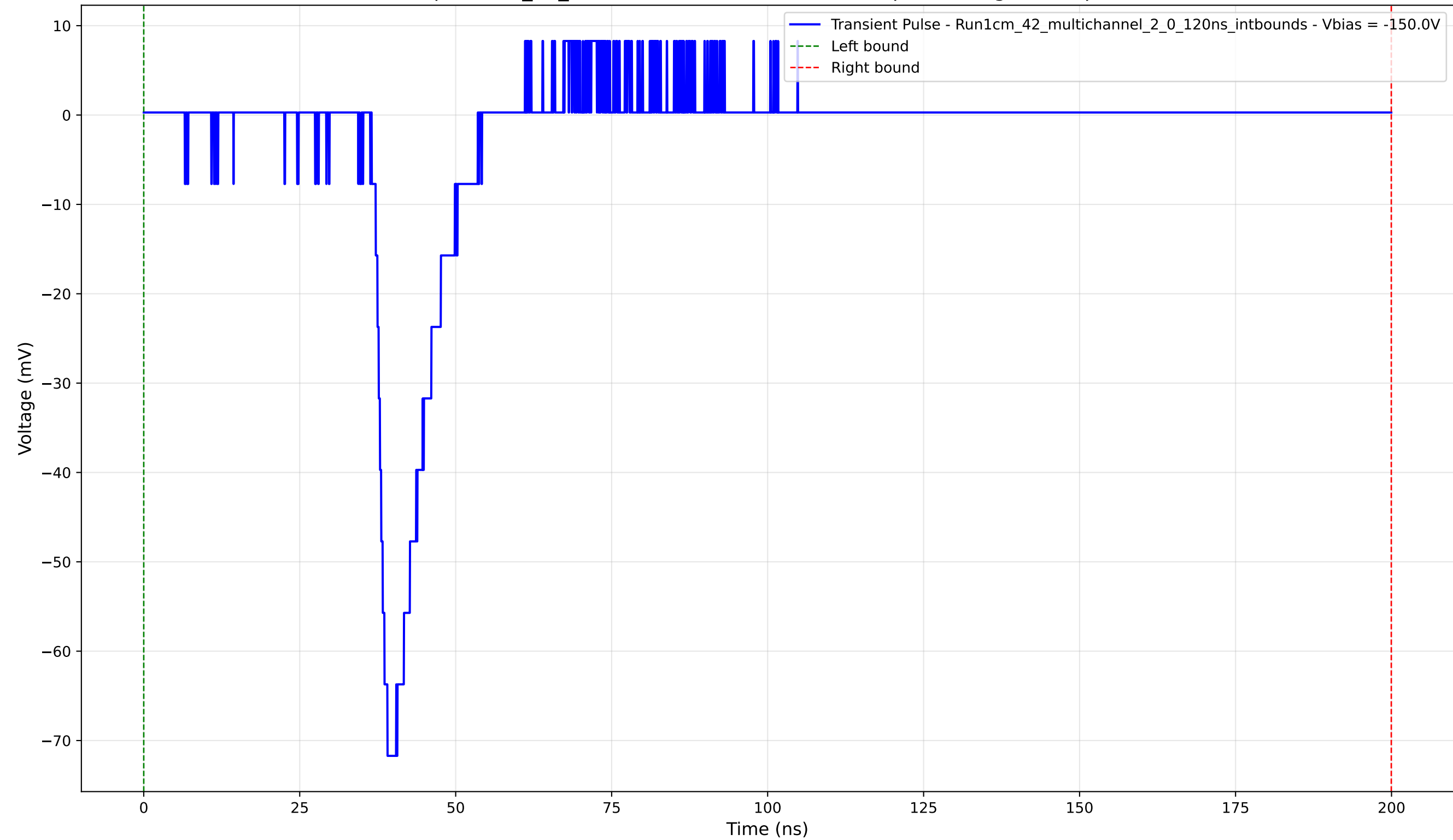
Transient Pulse - Sample: 1cm_42_multichannel - Position: 4495.0 \mu\text{m} - Charge: 8.59 pC - Rise Time: 2.52 ns
