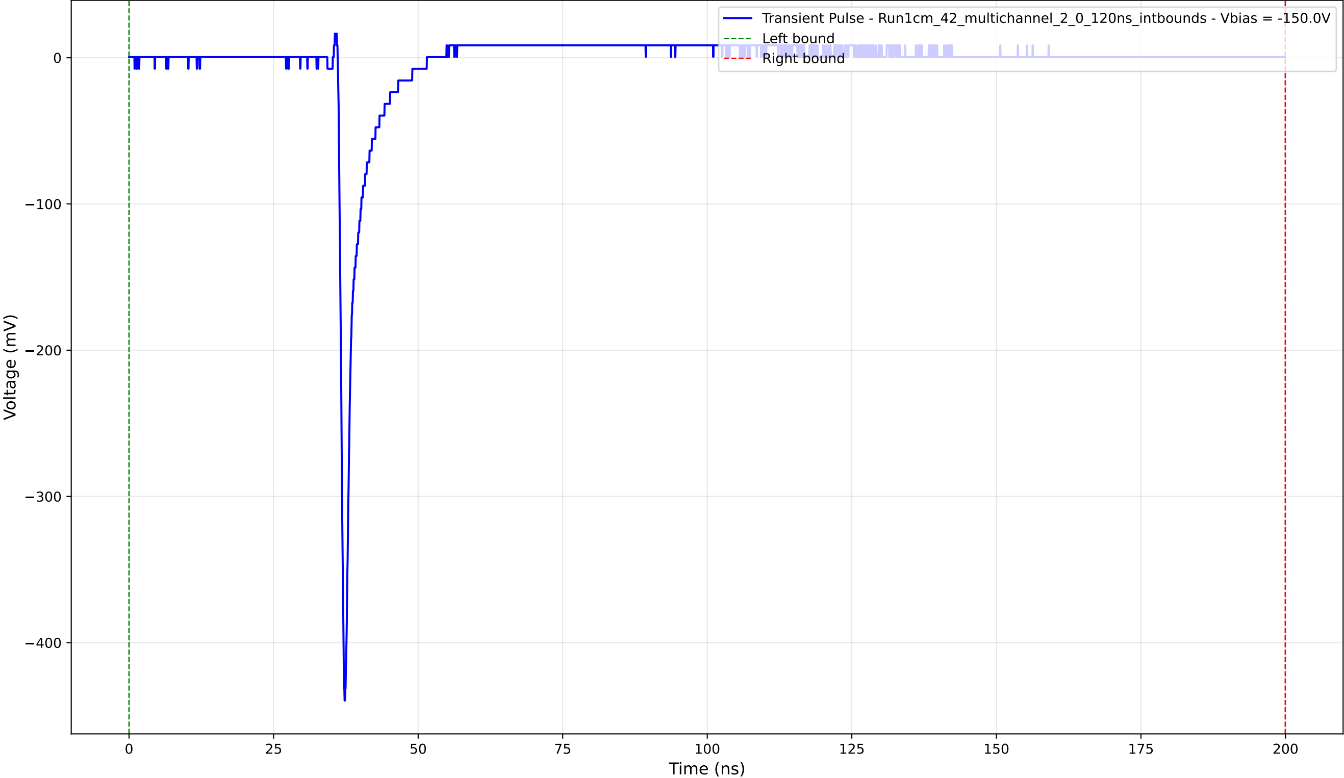
Transient Pulse - Sample: 1cm_42_multichannel - Position: 2670.0 \mu\text{m} - Charge: 12.53 pC - Rise Time: 0.80 ns
