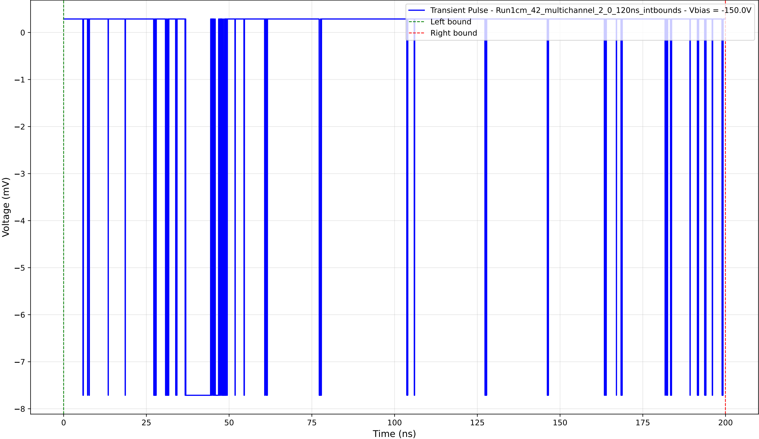
Transient Pulse - Sample: 1cm_42_multichannel - Position: 1360.0 \mu\text{m} - Charge: 1.34 pC - Rise Time: 0.04 ns
