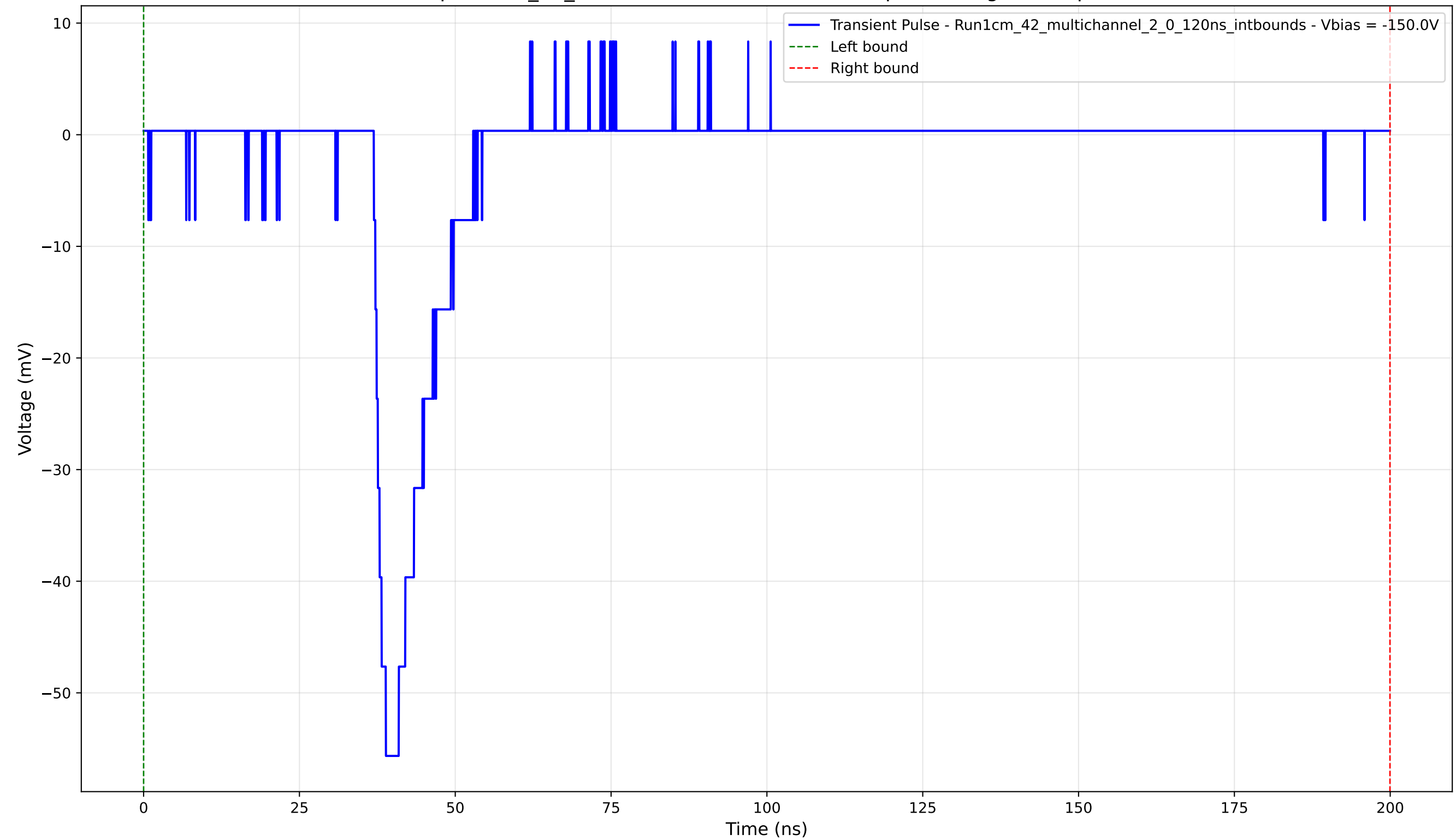
Transient Pulse - Sample: 1cm_42_multichannel - Position: 285.0 \mu\text{m} - Charge: 7.47 pC - Rise Time: 1.93 ns
