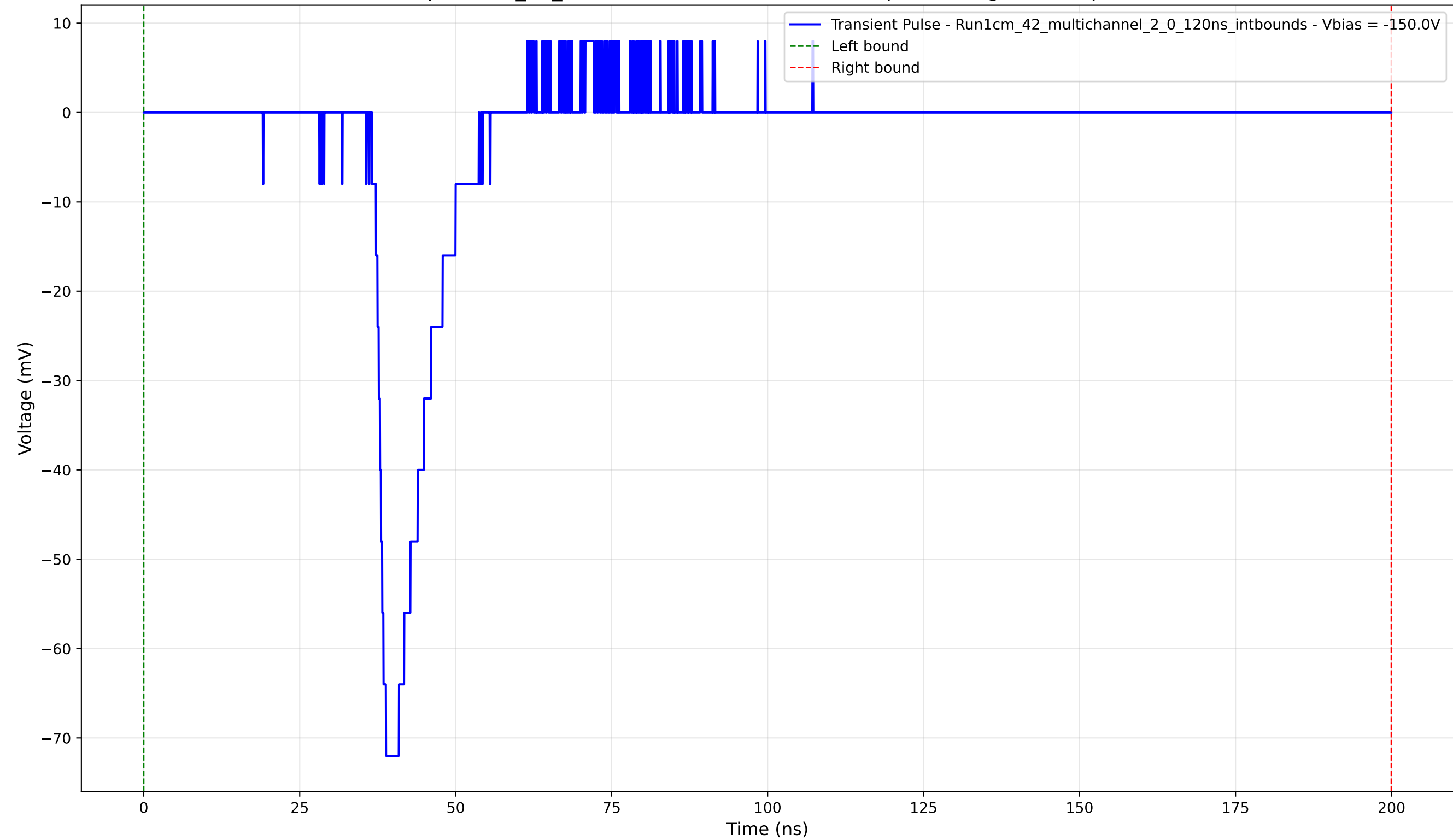
Transient Pulse - Sample: 1cm_42_multichannel - Position: 4285.0 \mu\text{m} - Charge: 10.18 pC - Rise Time: 2.24 ns
