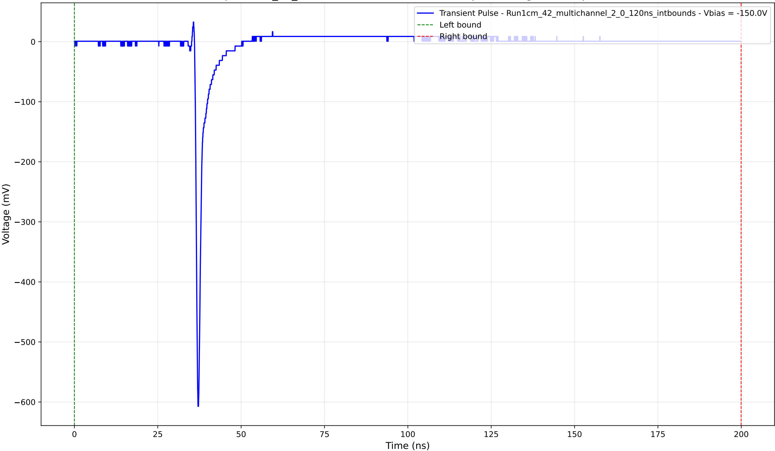
Transient Pulse - Sample: 1cm_42_multichannel - Position: 2290.0 \mu\text{m} - Charge: 14.49 pC - Rise Time: 0.71 ns
