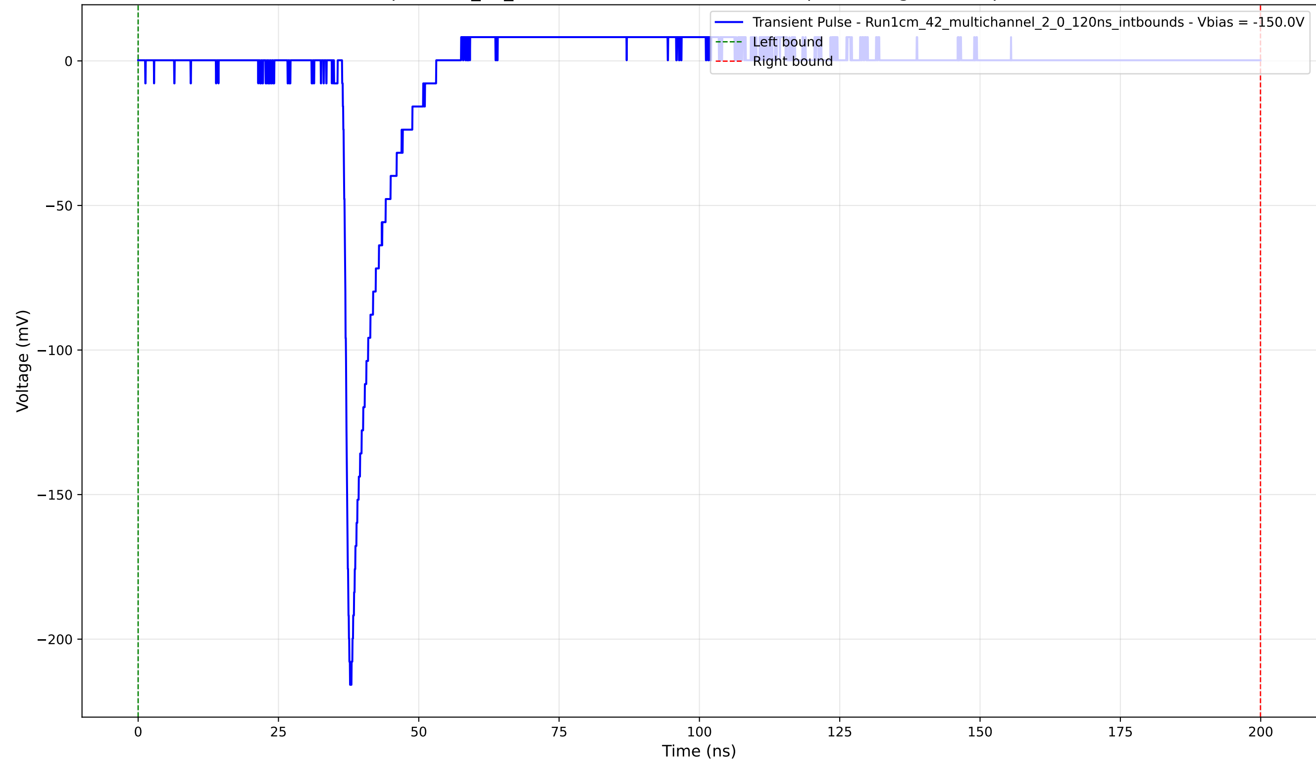
Transient Pulse - Sample: 1cm_42_multichannel - Position: 1515.0 \mu\text{m} - Charge: 12.37 pC - Rise Time: 1.01 ns
