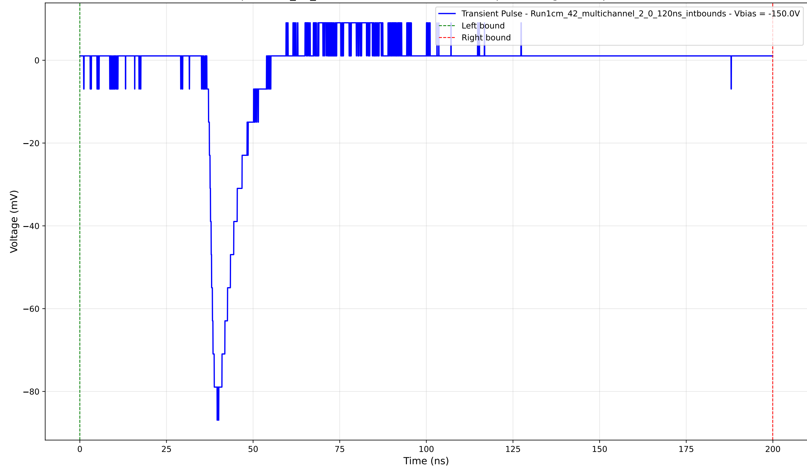
Transient Pulse - Sample: 1cm_42_multichannel - Position: 4220.0 \mu\text{m} - Charge: 6.24 pC - Rise Time: 1.67 ns
