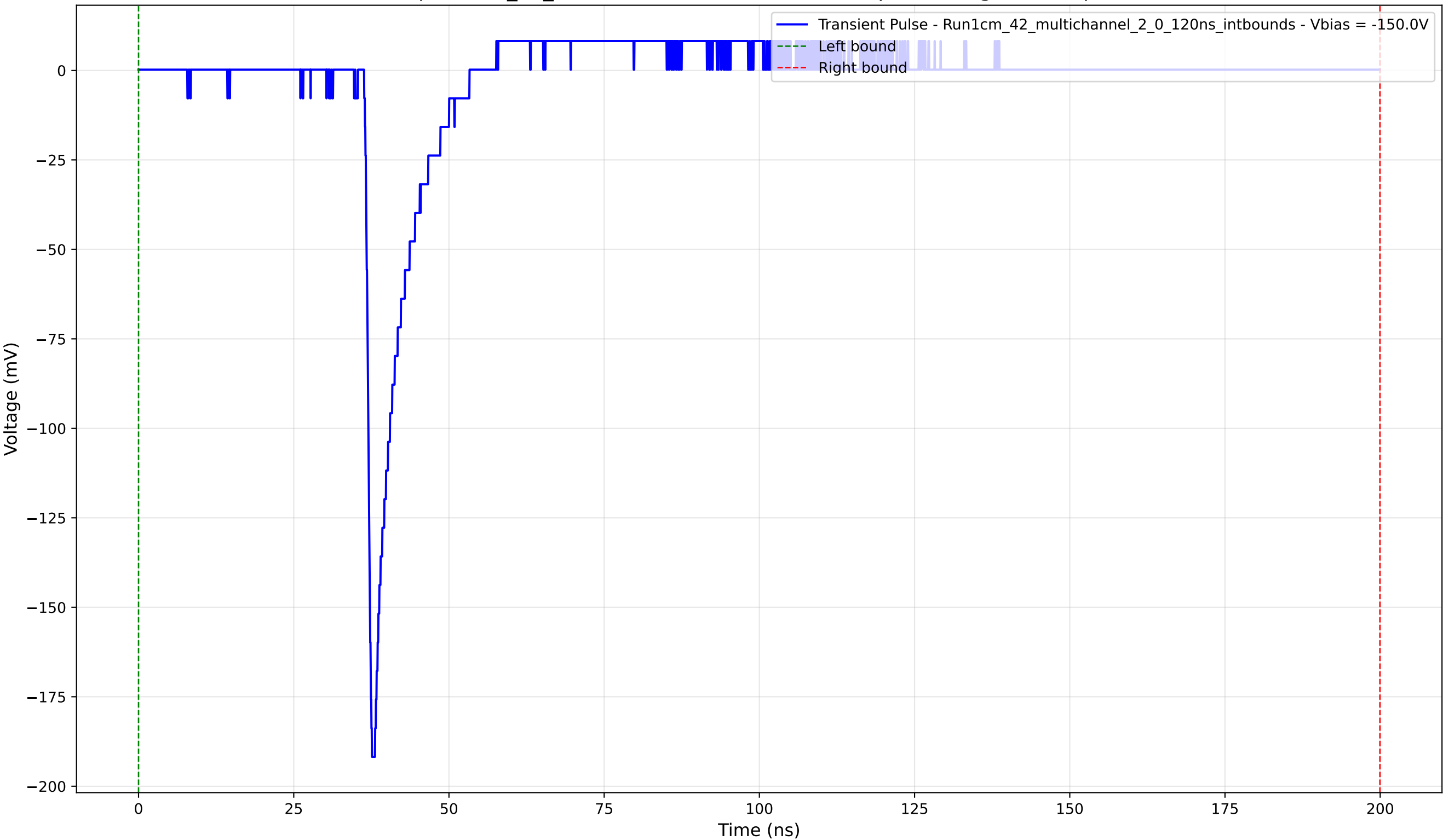
Transient Pulse - Sample: 1cm_42_multichannel - Position: 3200.0 \mu\text{m} - Charge: 10.99 pC - Rise Time: 0.90 ns
