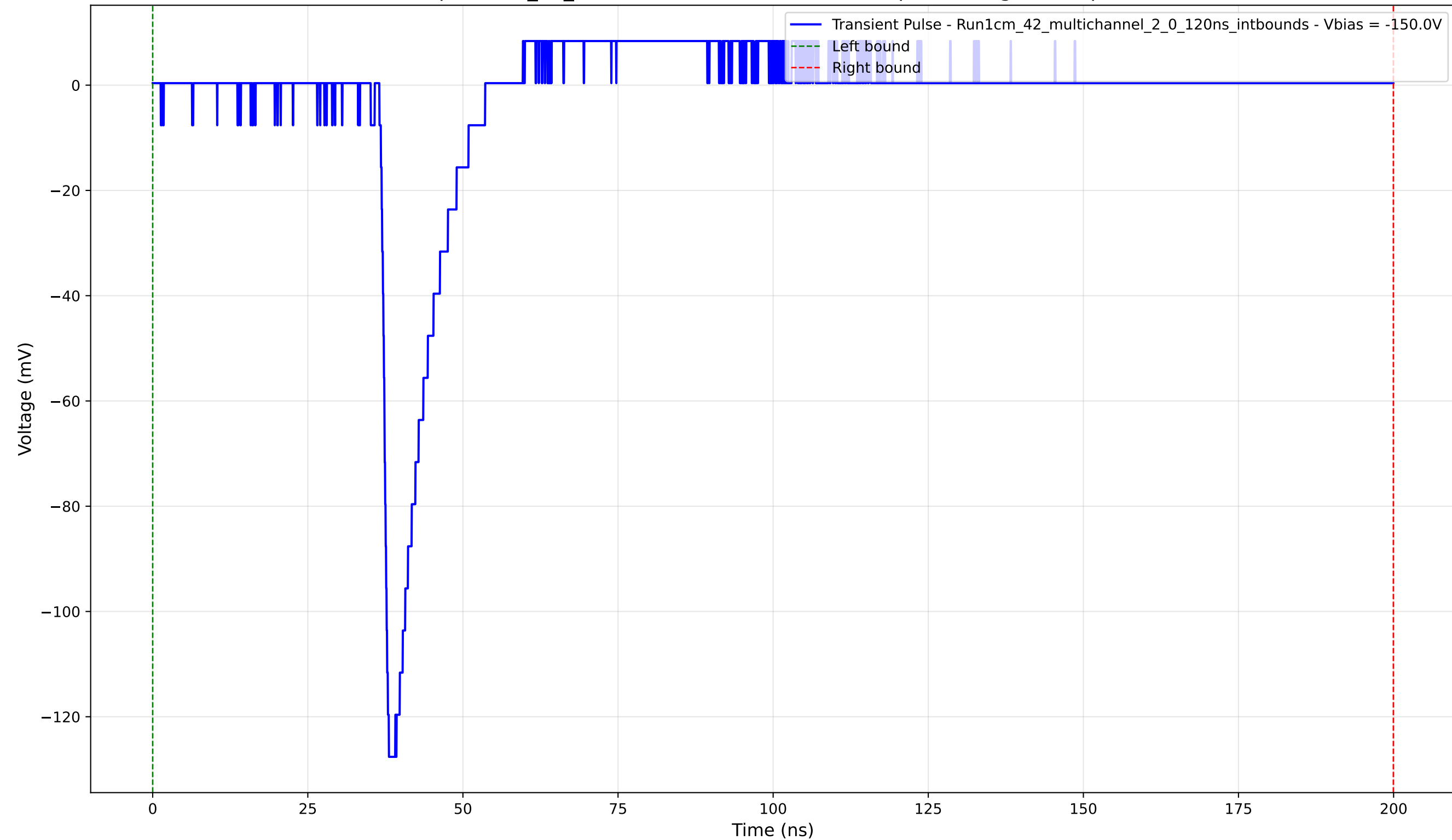
Transient Pulse - Sample: 1cm_42_multichannel - Position: 1090.0 \mu\text{m} - Charge: 9.48 pC - Rise Time: 1.13 ns
