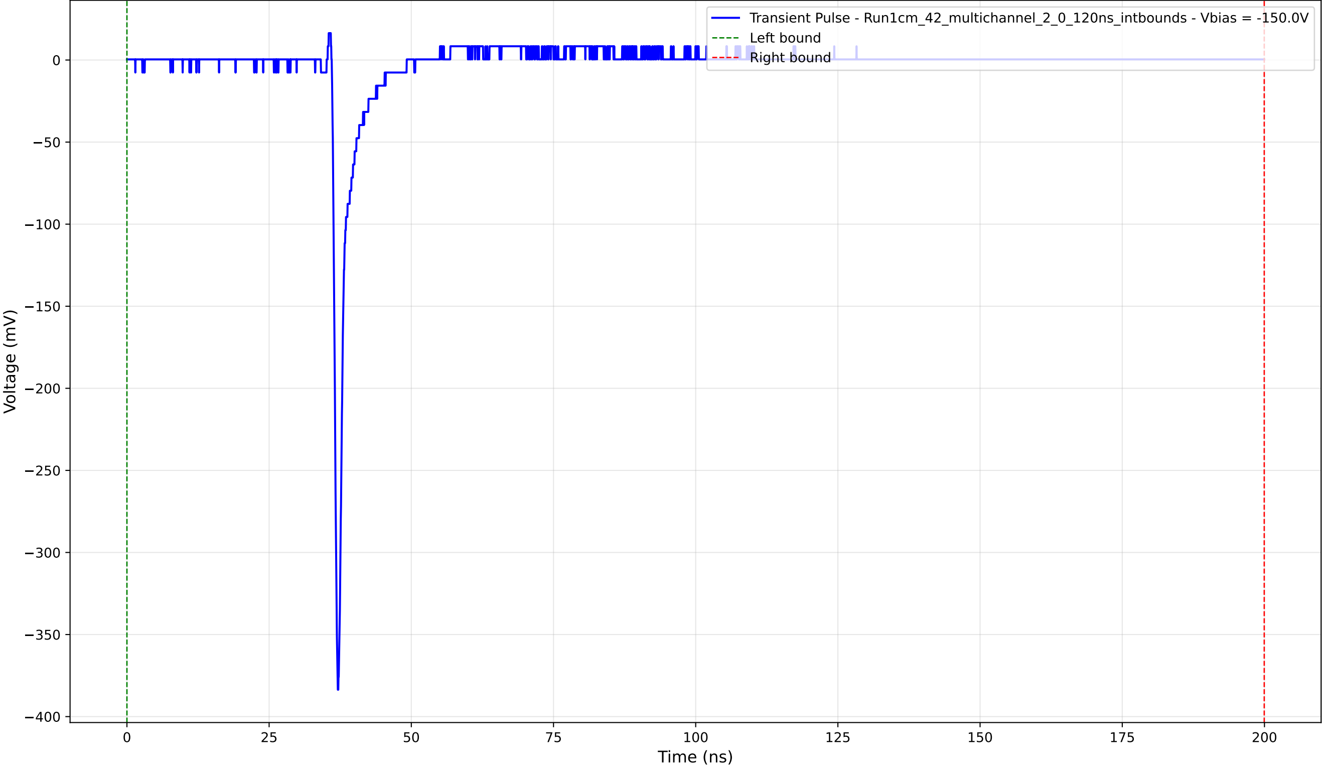
Transient Pulse - Sample: 1cm_42_multichannel - Position: 2315.0 \mu\text{m} - Charge: 11.30 pC - Rise Time: 0.73 ns
