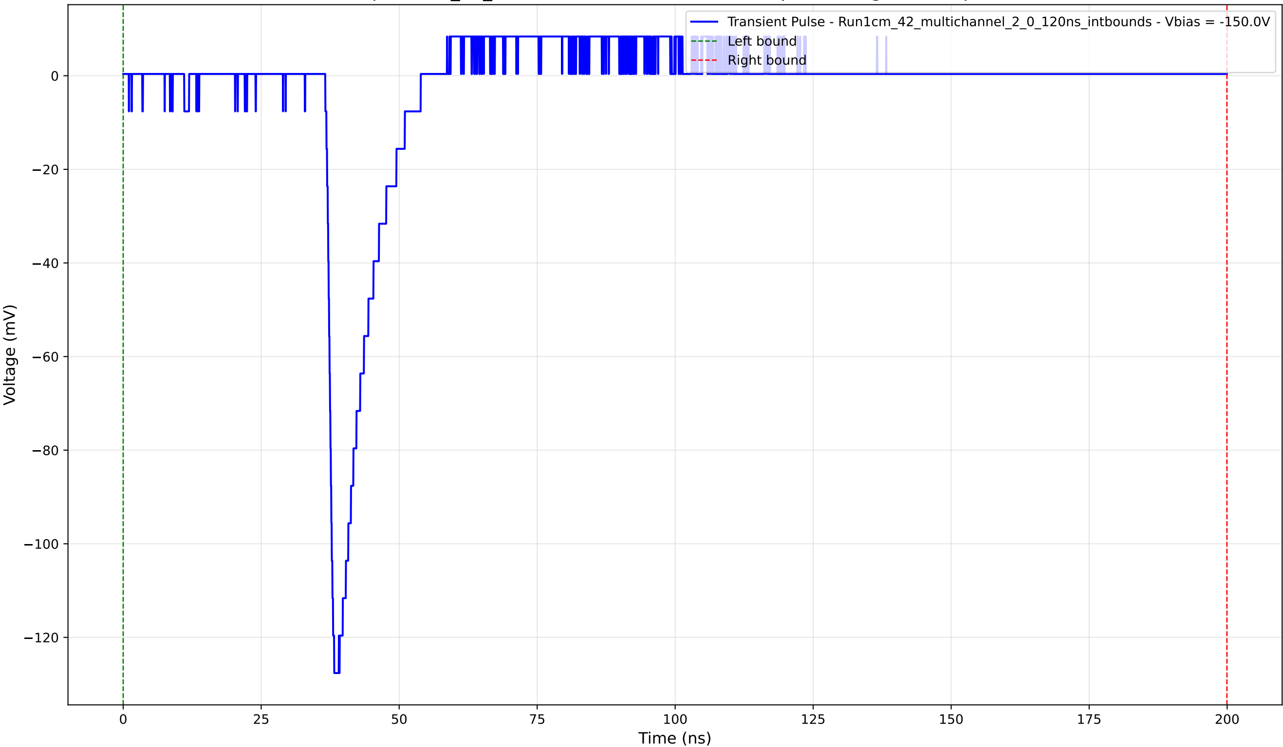
Transient Pulse - Sample: 1cm_42_multichannel - Position: 1040.0 \mu\text{m} - Charge: 10.11 pC - Rise Time: 1.21 ns
