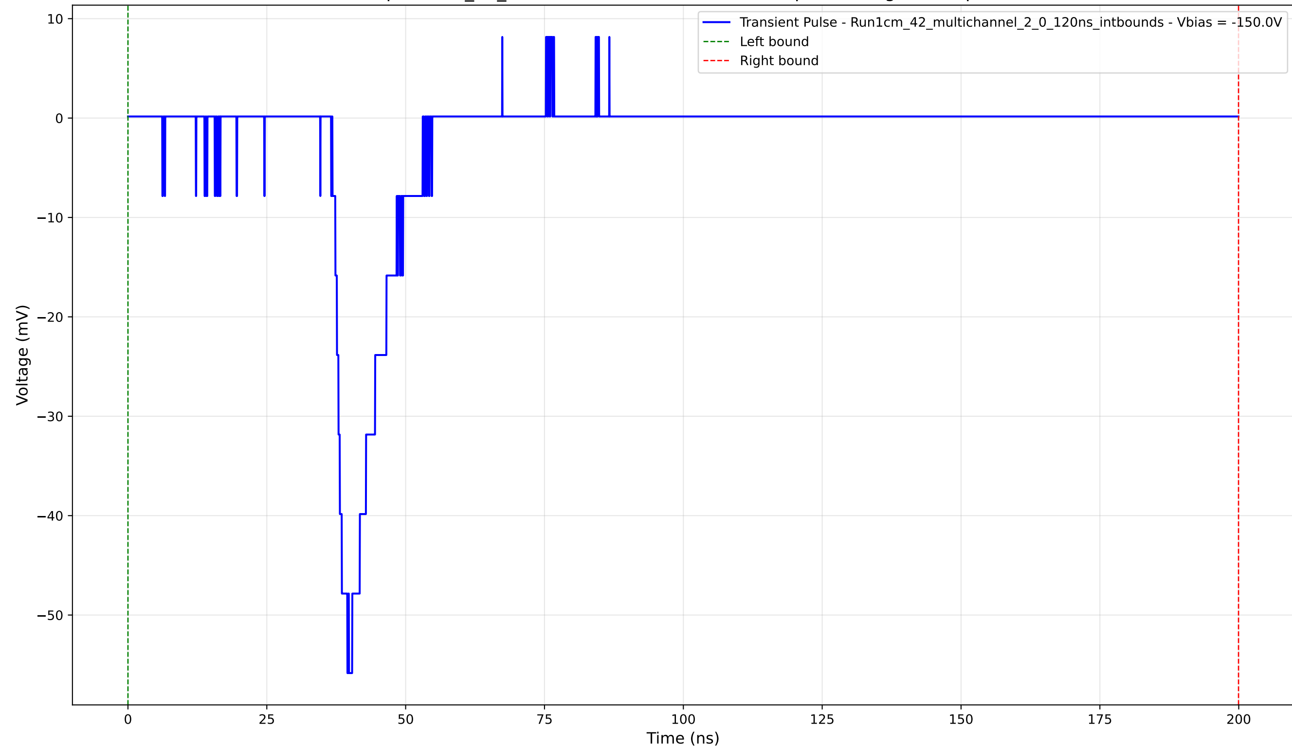
Transient Pulse - Sample: 1cm_42_multichannel - Position: 4450.0 \mu\text{m} - Charge: 7.78 pC - Rise Time: 2.69 ns
