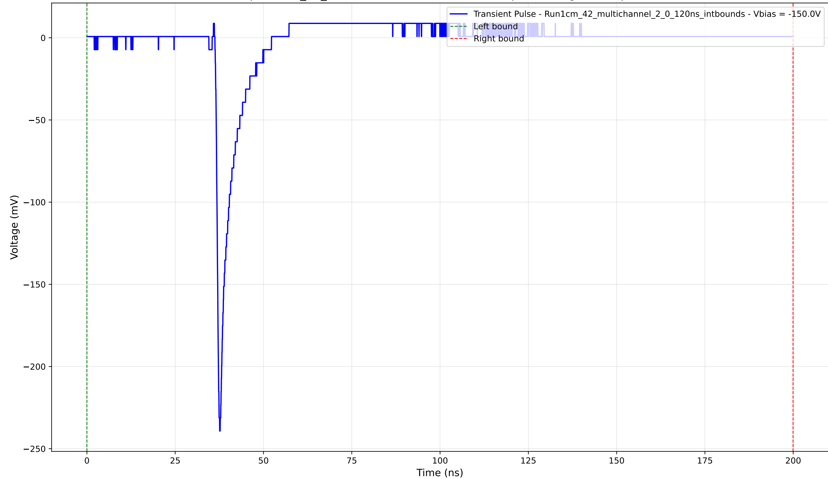
Transient Pulse - Sample: 1cm_42_multichannel - Position: 3045.0 \mu\text{m} - Charge: 8.70 pC - Rise Time: 0.92 ns
