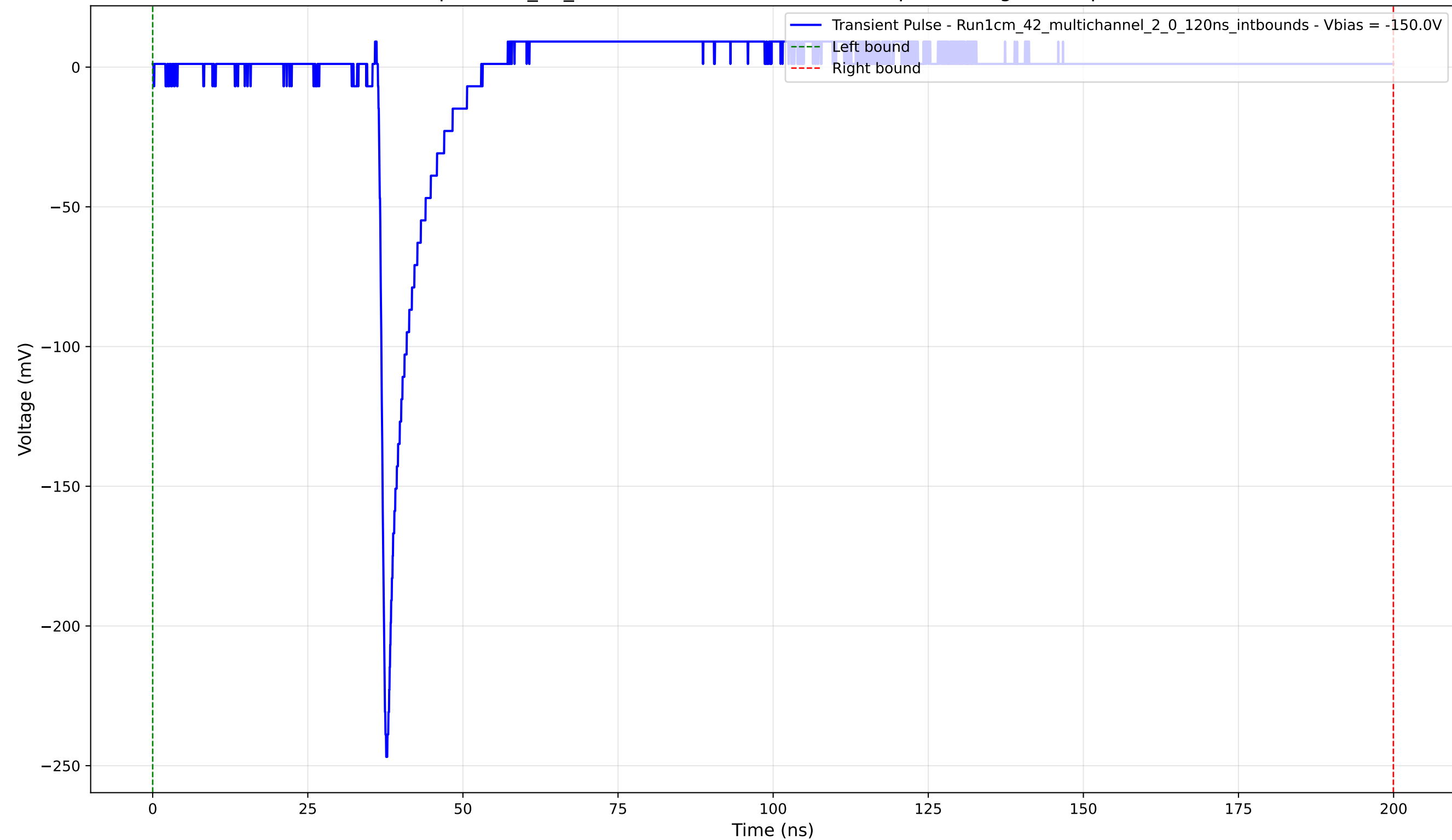
Transient Pulse - Sample: 1cm_42_multichannel - Position: 1625.0 \mu\text{m} - Charge: 9.04 pC - Rise Time: 0.91 ns
