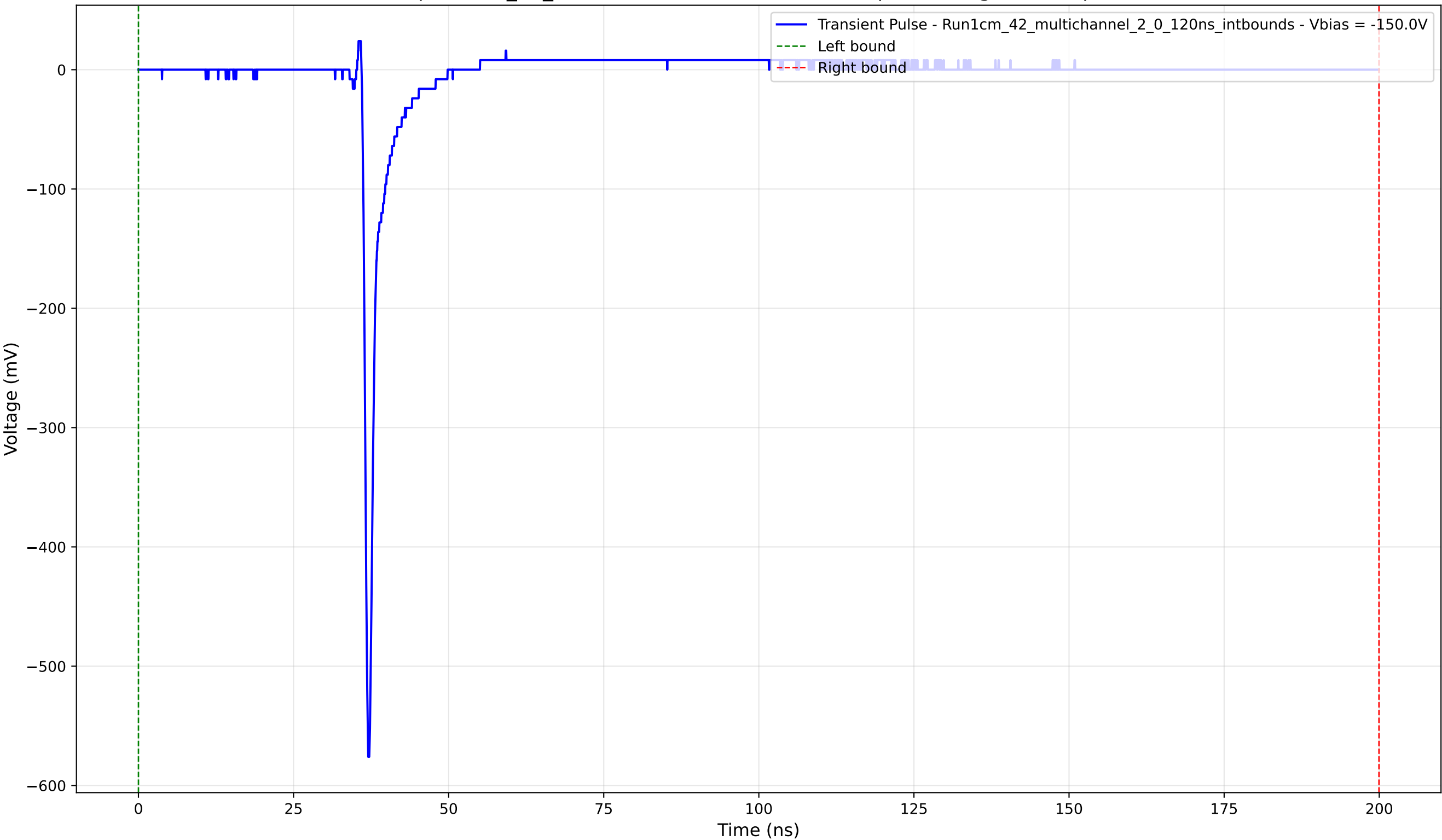
Transient Pulse - Sample: 1cm_42_multichannel - Position: 2440.0 \mu\text{m} - Charge: 15.69 pC - Rise Time: 0.73 ns
