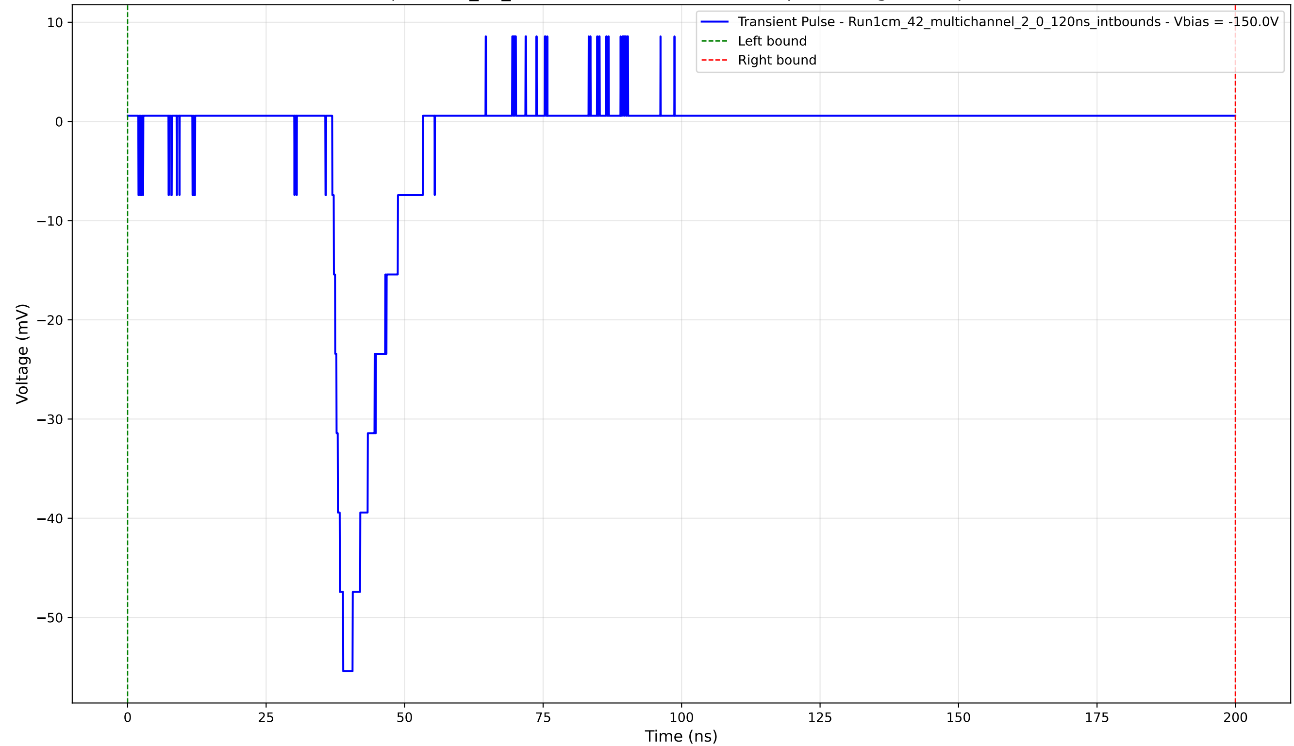
Transient Pulse - Sample: 1cm_42_multichannel - Position: 400.0 \mu\text{m} - Charge: 6.34 pC - Rise Time: 1.97 ns
