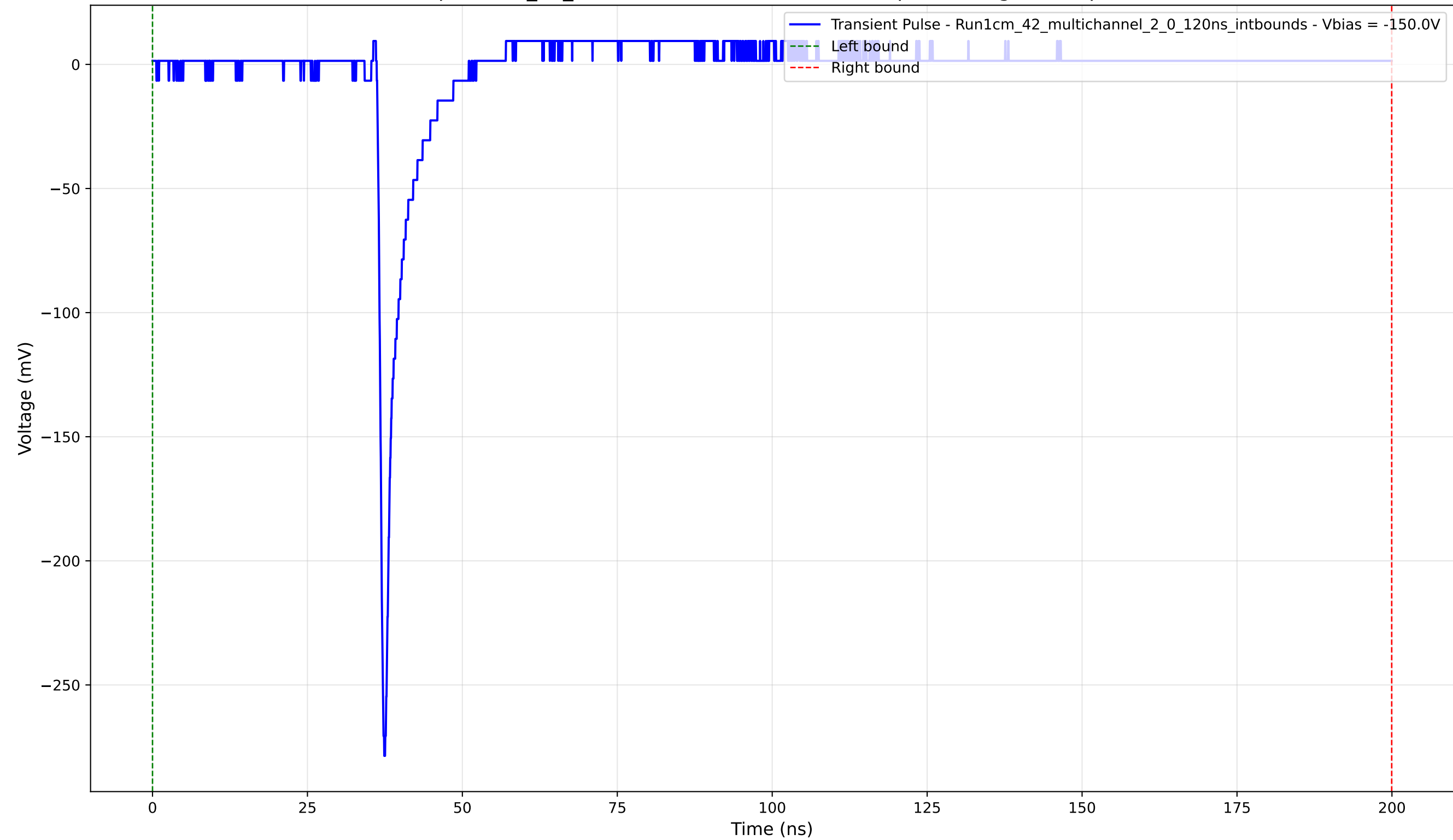
Transient Pulse - Sample: 1cm_42_multichannel - Position: 1925.0 \mu\text{m} - Charge: 6.74 pC - Rise Time: 0.83 ns
