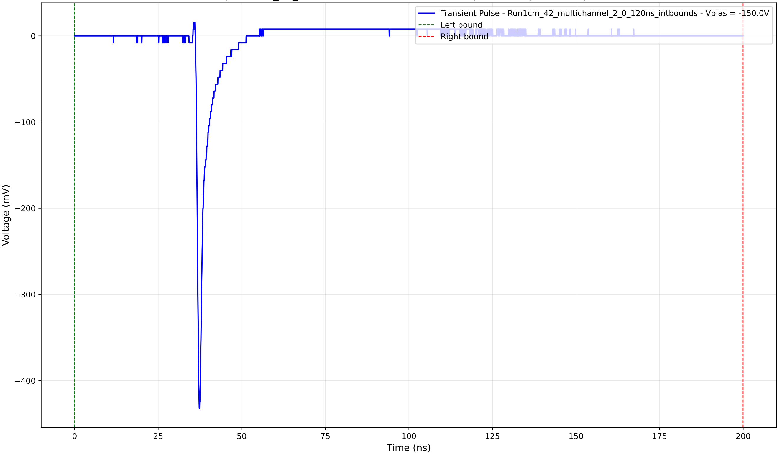
Transient Pulse - Sample: 1cm_42_multichannel - Position: 2705.0 \mu\text{m} - Charge: 14.53 pC - Rise Time: 0.77 ns
