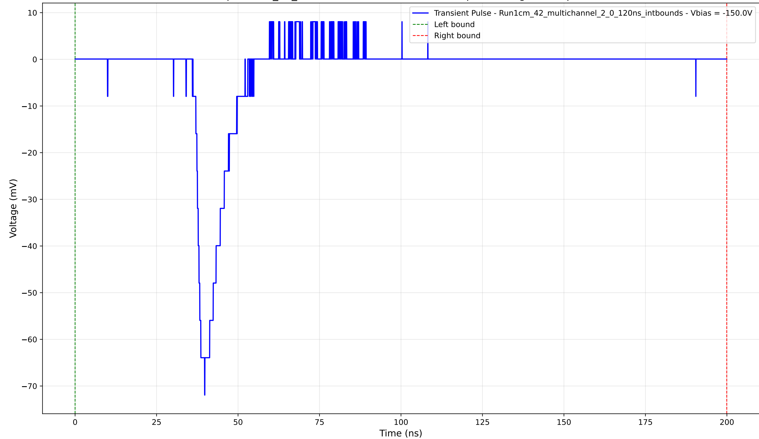
Transient Pulse - Sample: 1cm_42_multichannel - Position: 4720.0 \mu\text{m} - Charge: 9.11 pC - Rise Time: 3.56 ns
