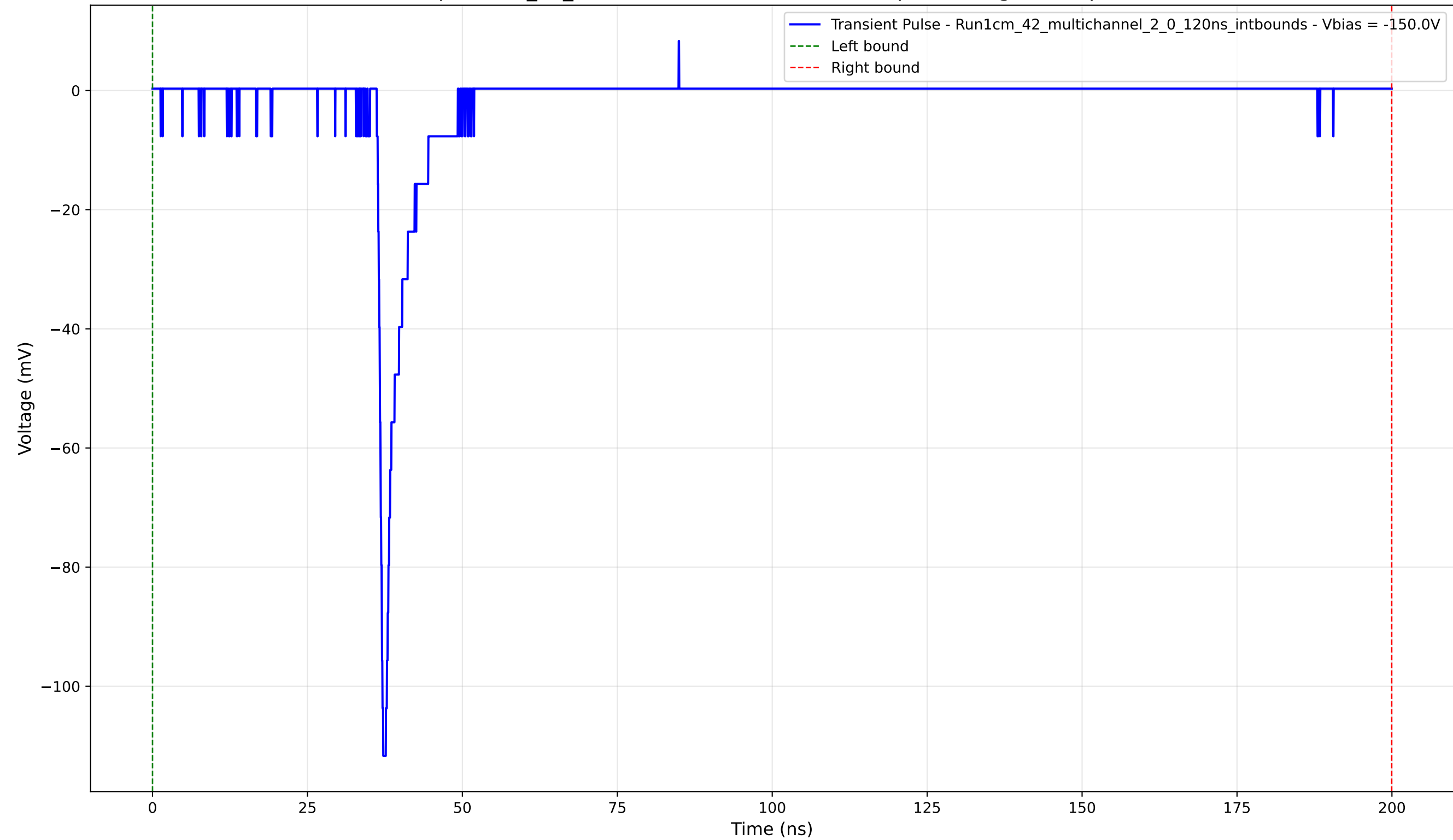
Transient Pulse - Sample: 1cm_42_multichannel - Position: 1905.0 \mu\text{m} - Charge: 7.14 pC - Rise Time: 0.78 ns
