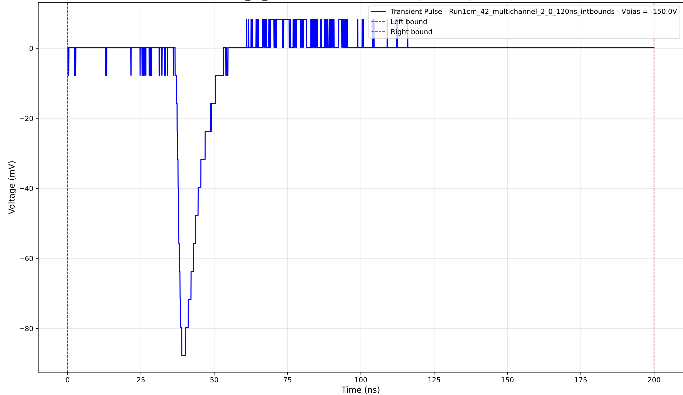
Transient Pulse - Sample: 1cm_42_multichannel - Position: 4160.0 \mu\text{m} - Charge: 9.98 pC - Rise Time: 1.47 ns
