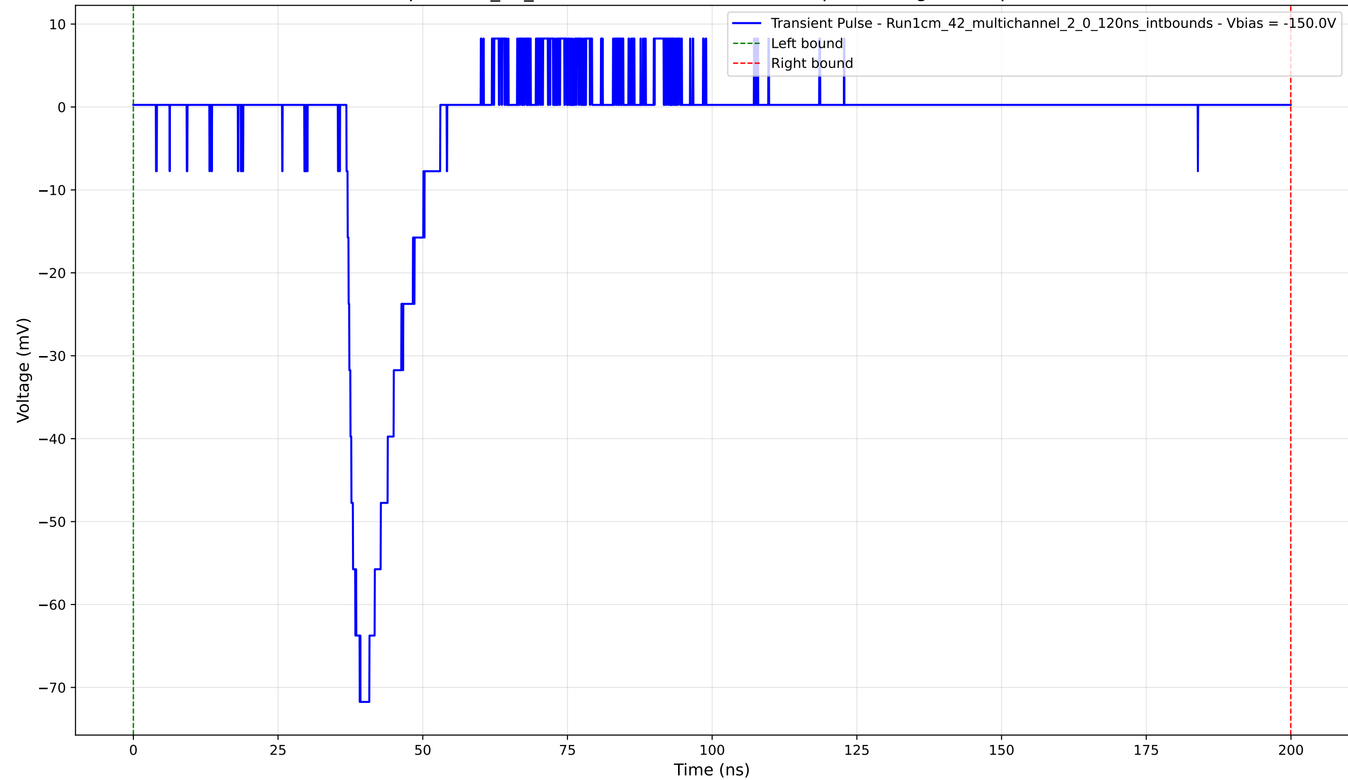
Transient Pulse - Sample: 1cm_42_multichannel - Position: 165.0 \mu\text{m} - Charge: 8.29 pC - Rise Time: 2.28 ns
