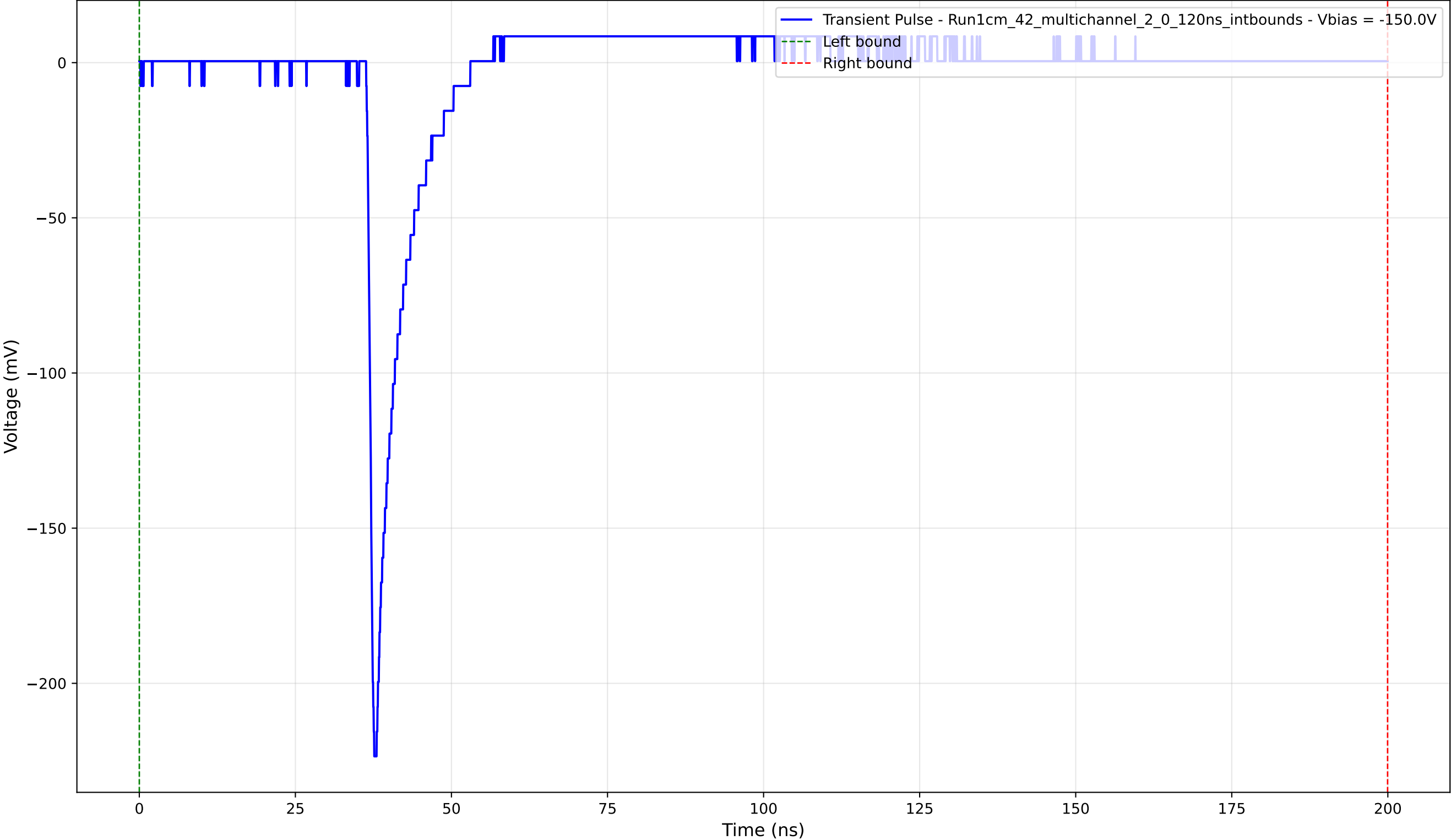
Transient Pulse - Sample: 1cm_42_multichannel - Position: 1560.0 \mu\text{m} - Charge: 10.06 pC - Rise Time: 0.97 ns
