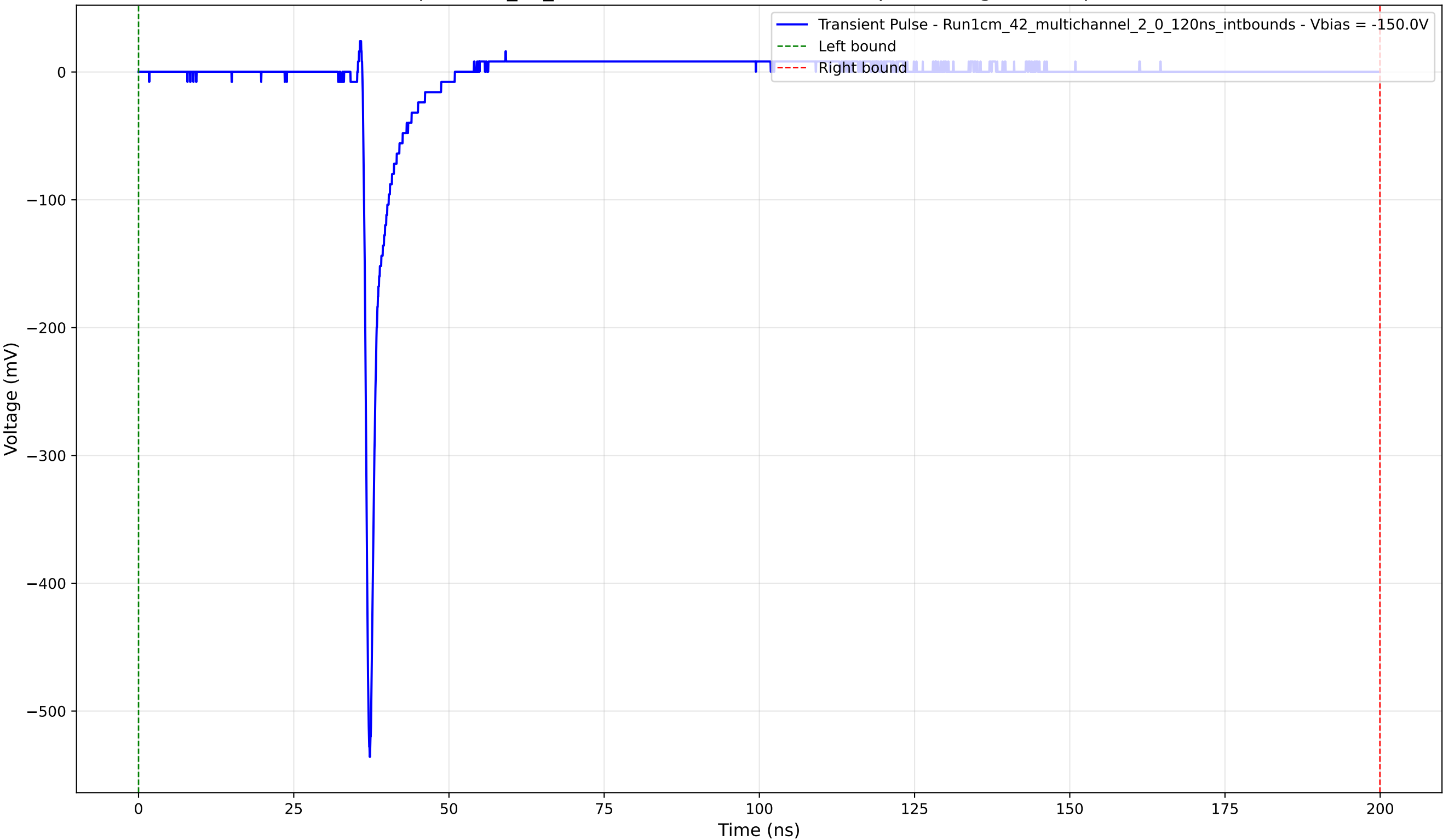
Transient Pulse - Sample: 1cm_42_multichannel - Position: 2155.0 \mu\text{m} - Charge: 15.42 pC - Rise Time: 0.74 ns
