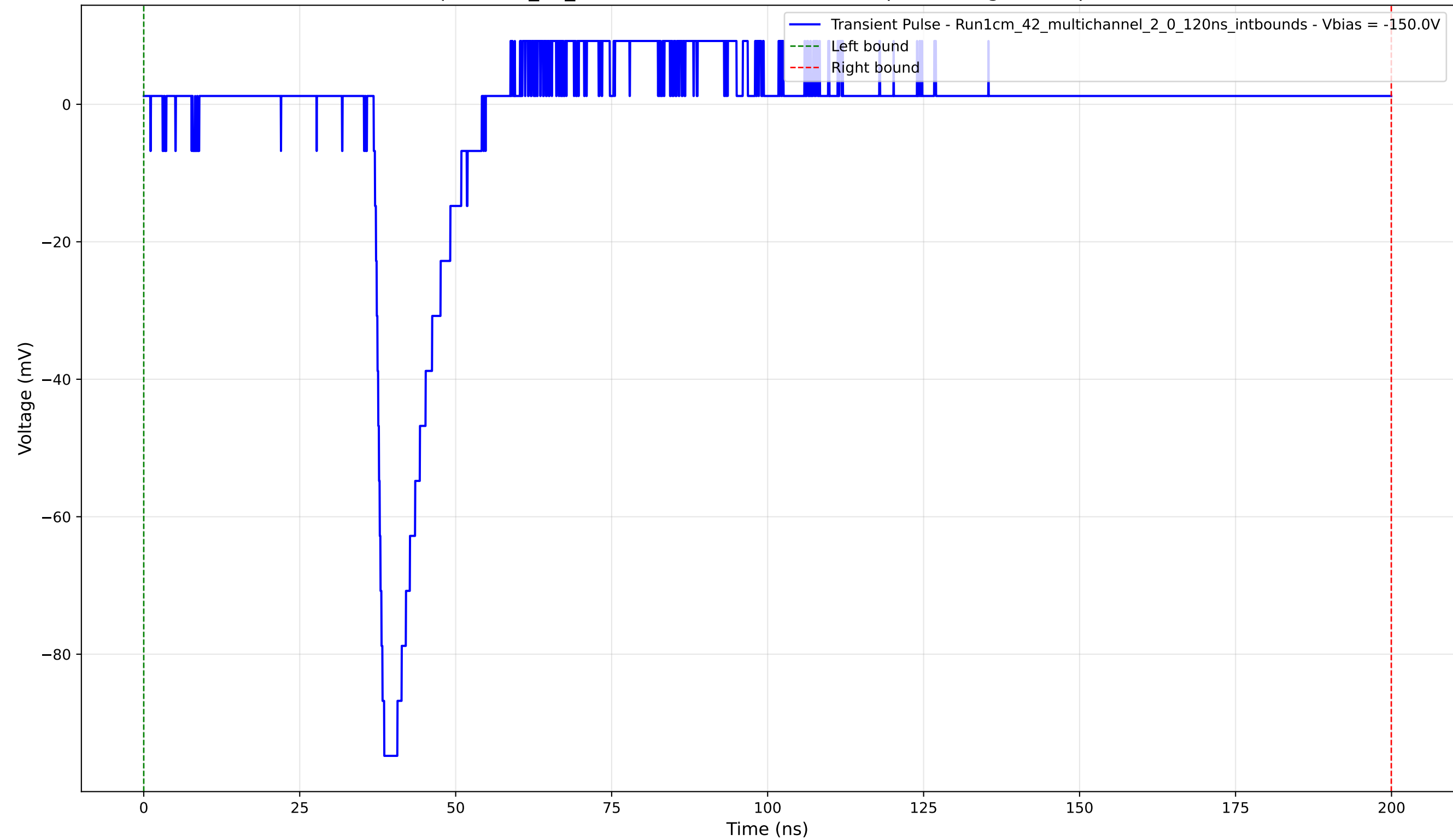
Transient Pulse - Sample: 1cm_42_multichannel - Position: 620.0 \mu\text{m} - Charge: 5.42 pC - Rise Time: 1.23 ns
