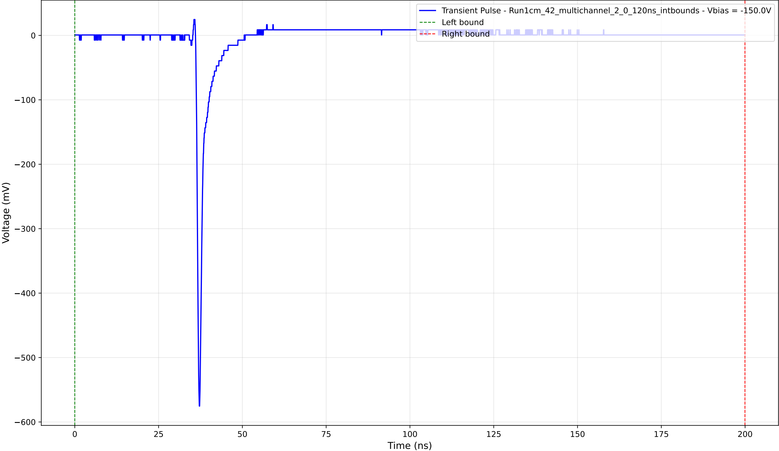
Transient Pulse - Sample: 1cm_42_multichannel - Position: 2510.0 \mu\text{m} - Charge: 14.40 pC - Rise Time: 0.73 ns
