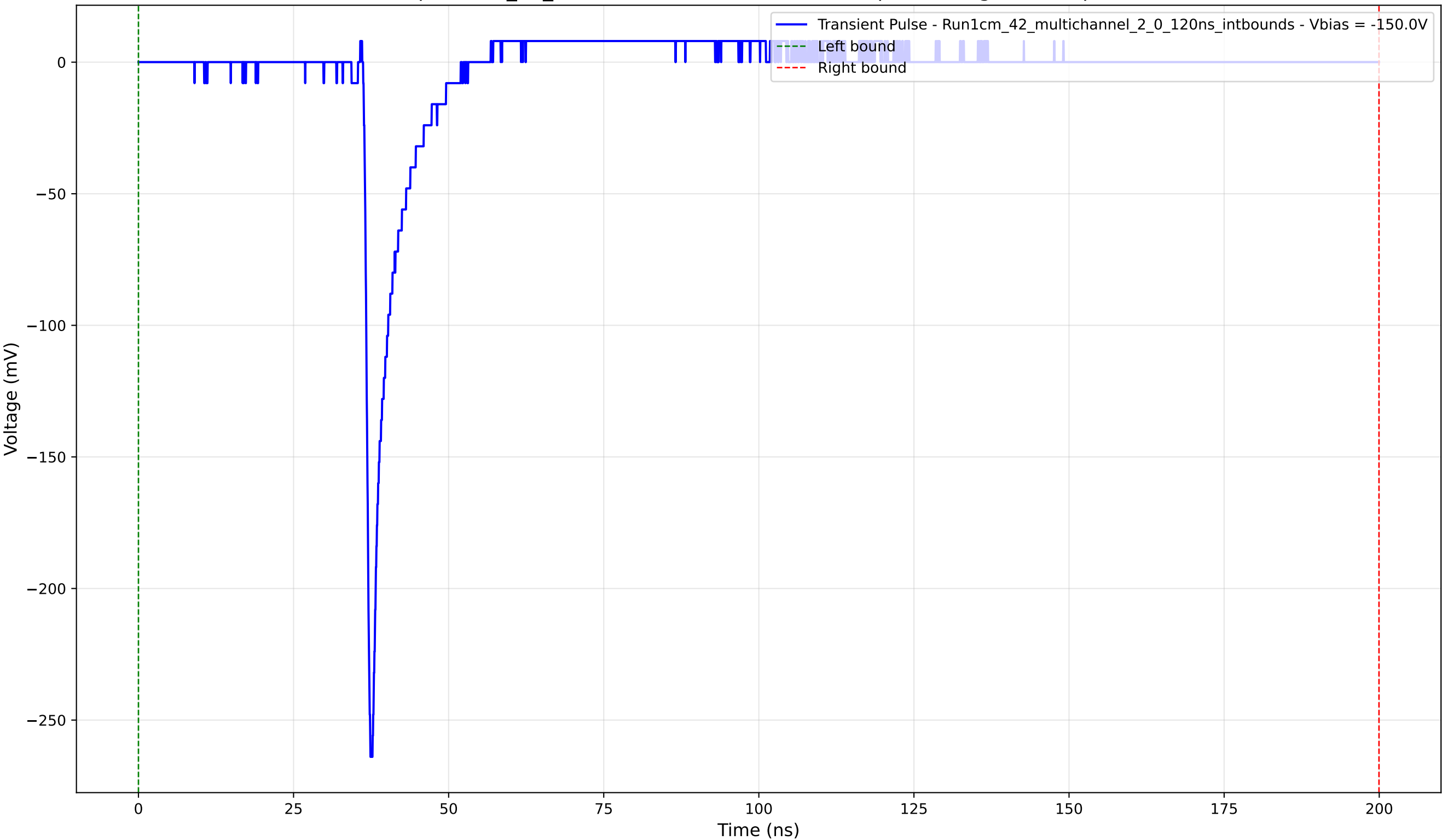
Transient Pulse - Sample: 1cm_42_multichannel - Position: 2955.0 \mu\text{m} - Charge: 12.36 pC - Rise Time: 0.82 ns
