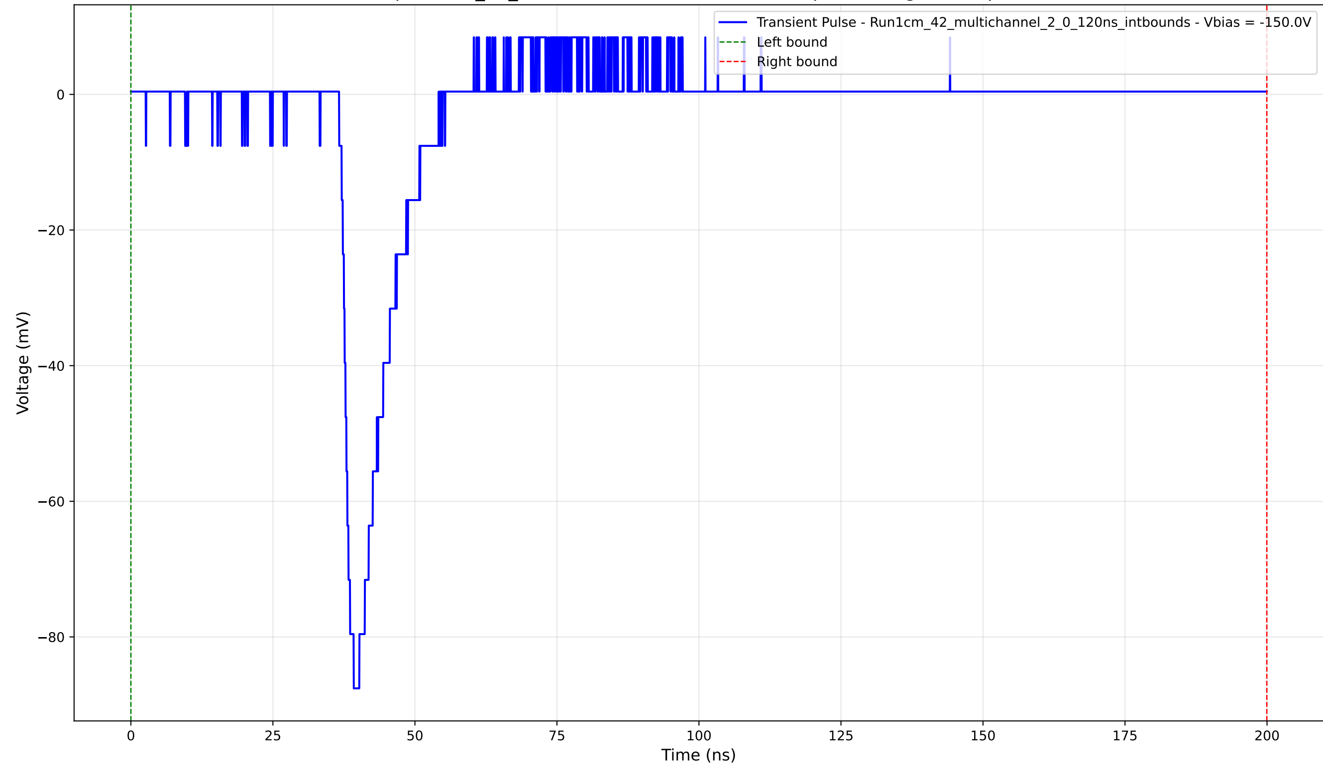
Transient Pulse - Sample: 1cm_42_multichannel - Position: 4120.0 \mu\text{m} - Charge: 9.41 pC - Rise Time: 1.51 ns
