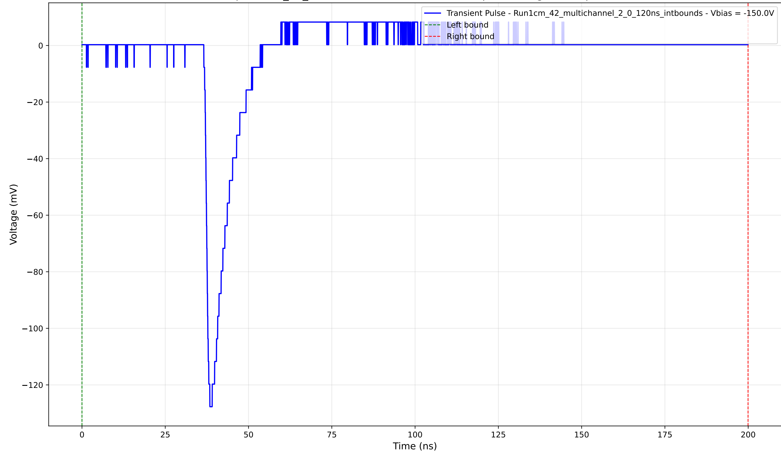
Transient Pulse - Sample: 1cm_42_multichannel - Position: 1030.0 \mu\text{m} - Charge: 9.65 pC - Rise Time: 1.25 ns
