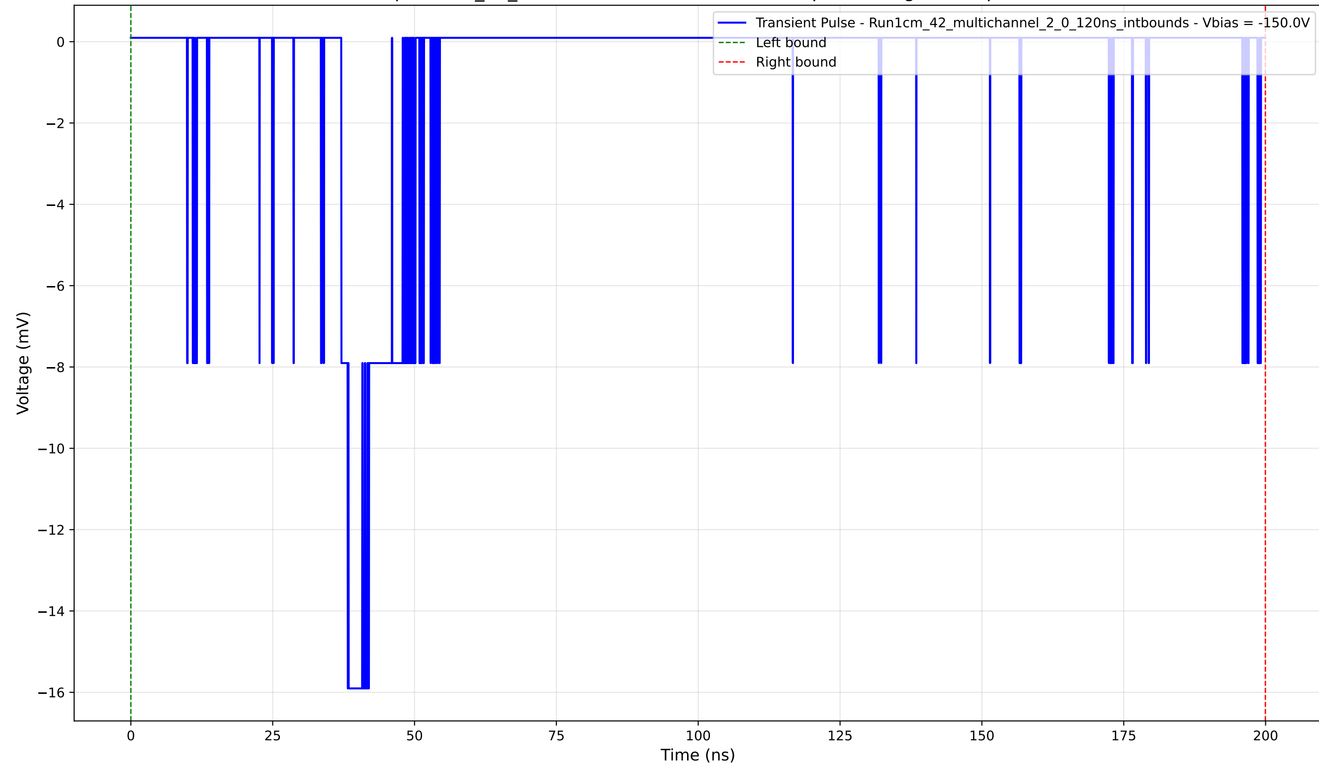
Transient Pulse - Sample: 1cm_42_multichannel - Position: 3915.0 \mu\text{m} - Charge: 2.80 pC - Rise Time: 1.15 ns
