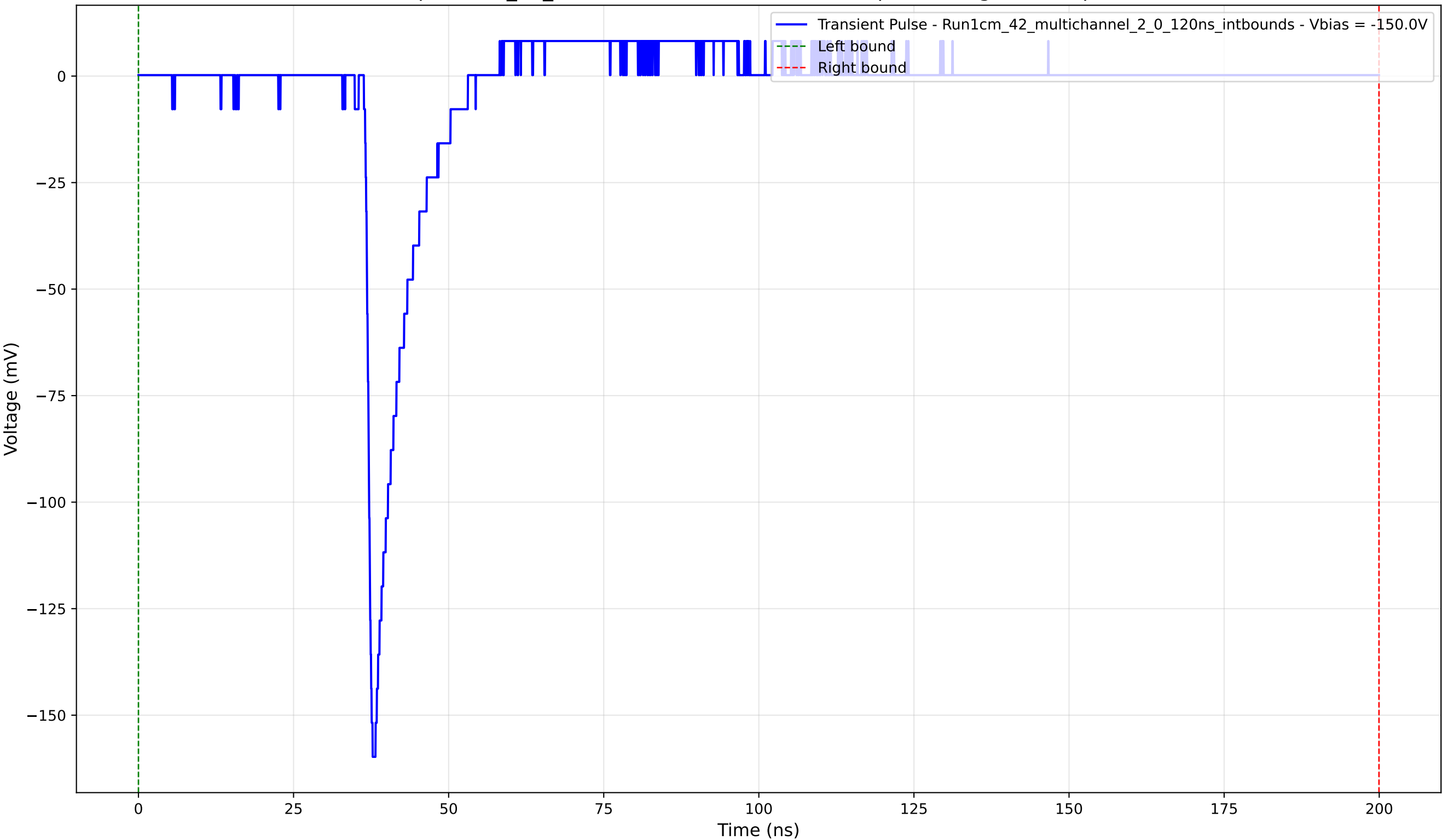
Transient Pulse - Sample: 1cm_42_multichannel - Position: 3300.0 \mu\text{m} - Charge: 10.29 pC - Rise Time: 1.00 ns
