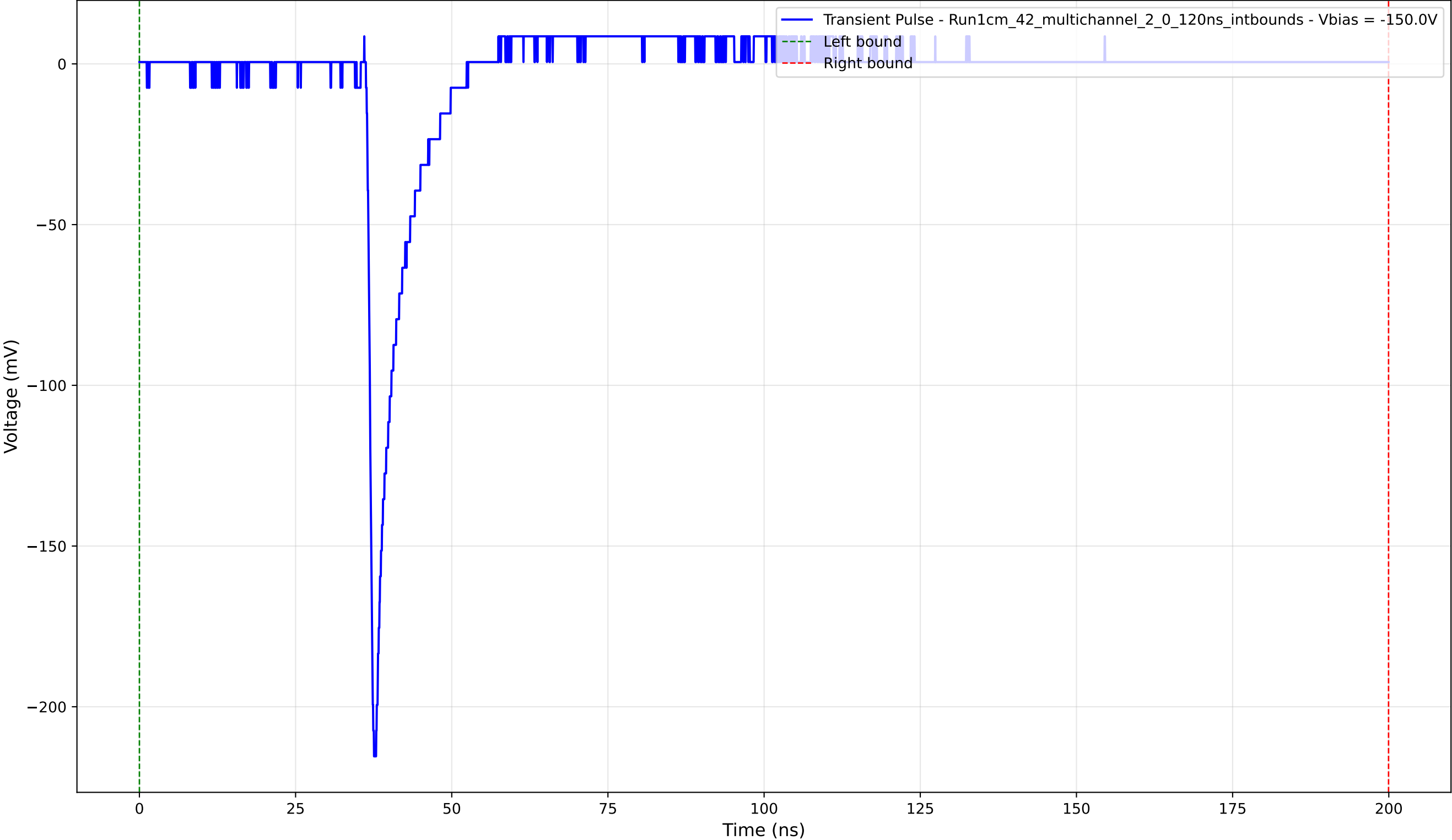
Transient Pulse - Sample: 1cm_42_multichannel - Position: 3095.0 \mu\text{m} - Charge: 10.87 pC - Rise Time: 0.89 ns
