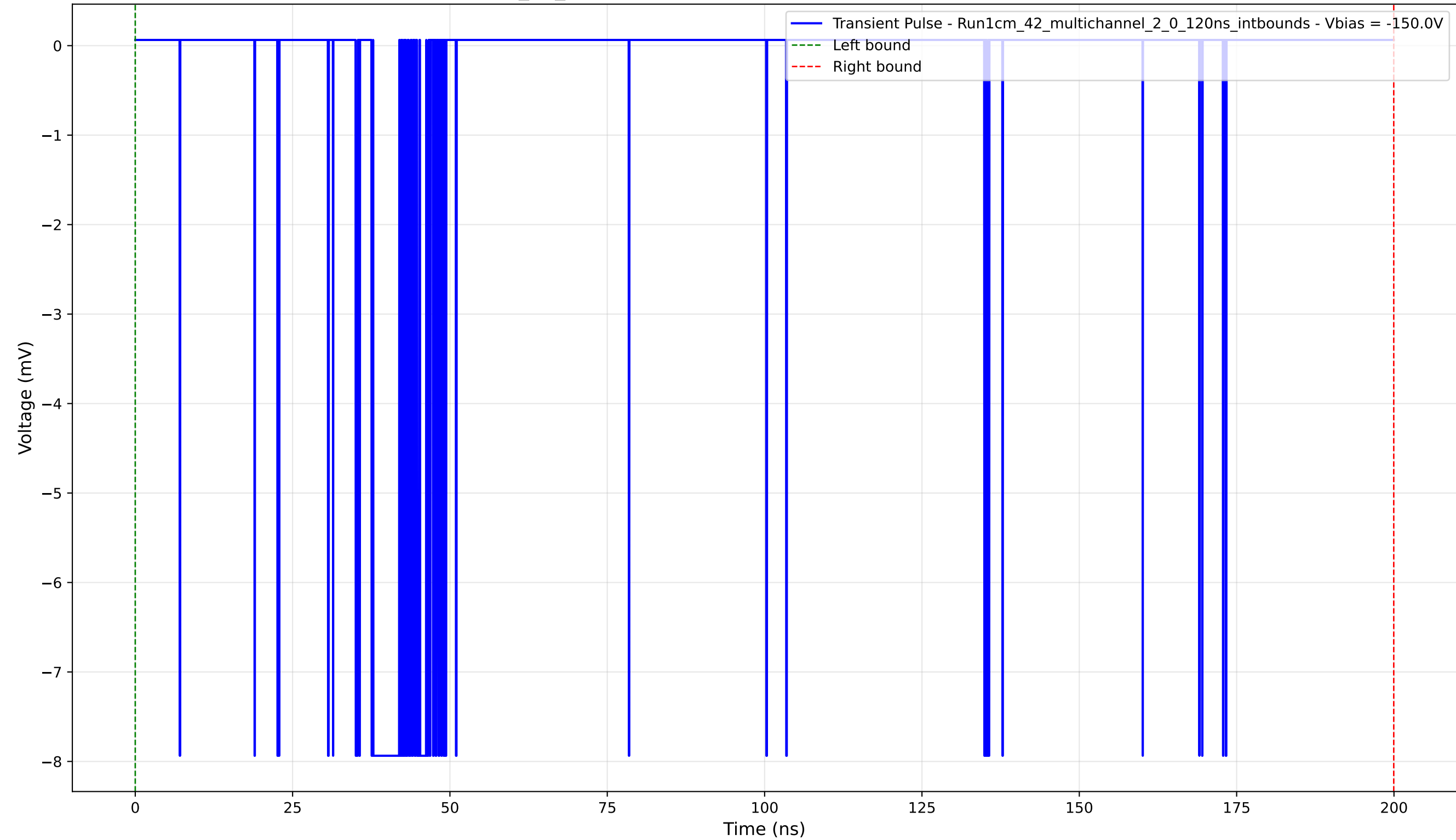
Transient Pulse - Sample: 1cm_42_multichannel - Position: 4405.0 \mu\text{m} - Charge: 1.48 pC - Rise Time: 0.04 ns
