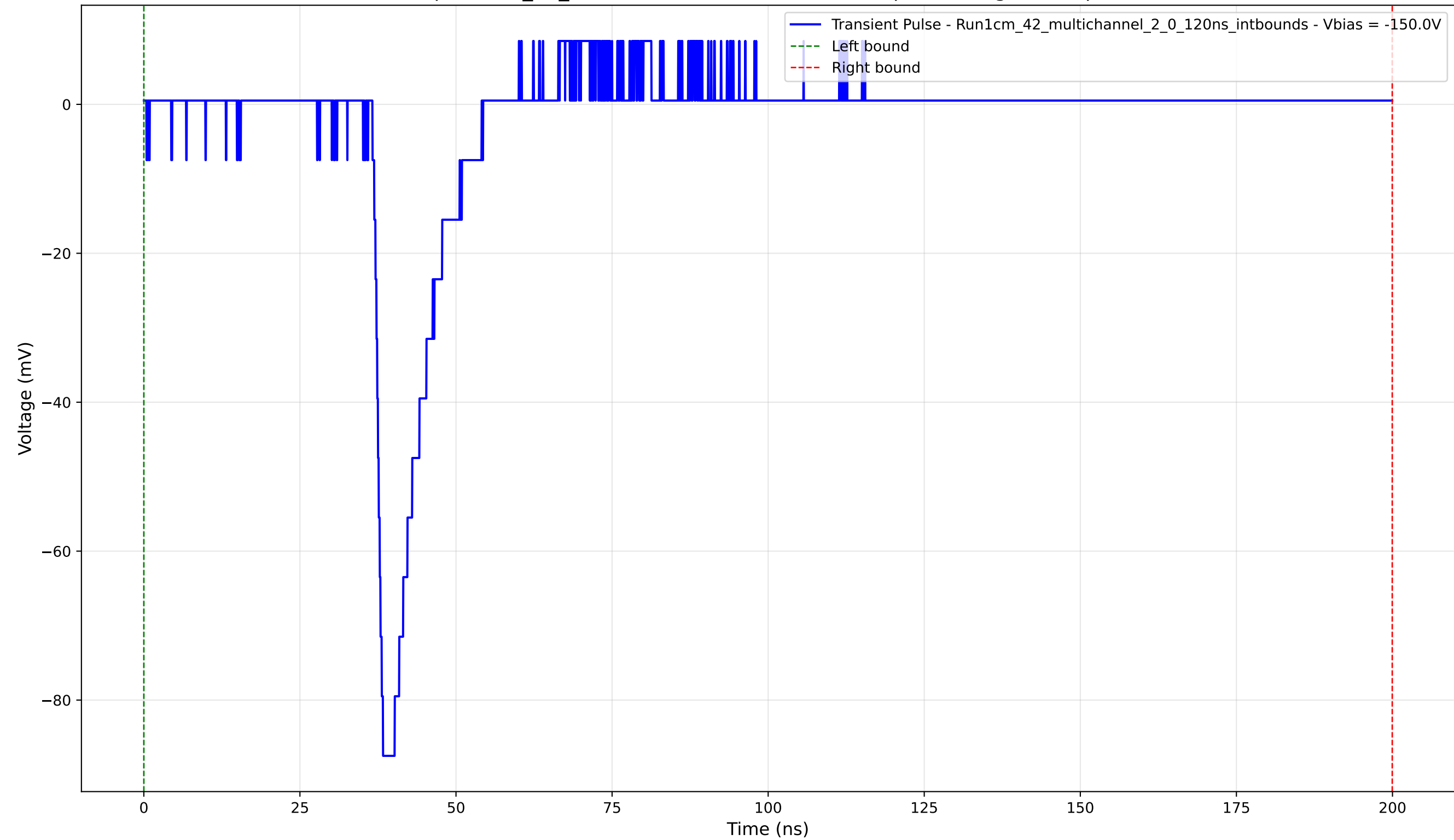
Transient Pulse - Sample: 1cm_42_multichannel - Position: 3815.0 \mu\text{m} - Charge: 9.53 pC - Rise Time: 1.23 ns
