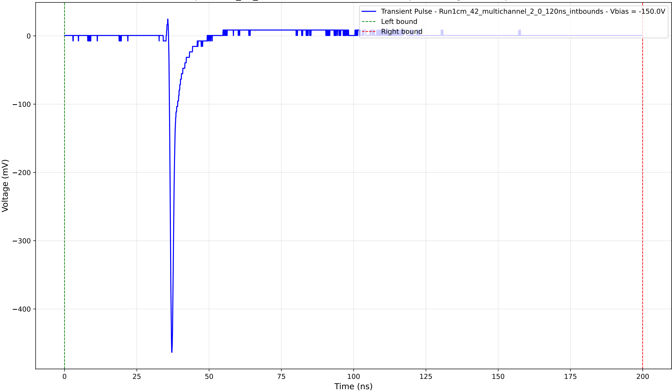
Transient Pulse - Sample: 1cm_42_multichannel - Position: 2310.0 \mu\text{m} - Charge: 10.68 pC - Rise Time: 0.75 ns
