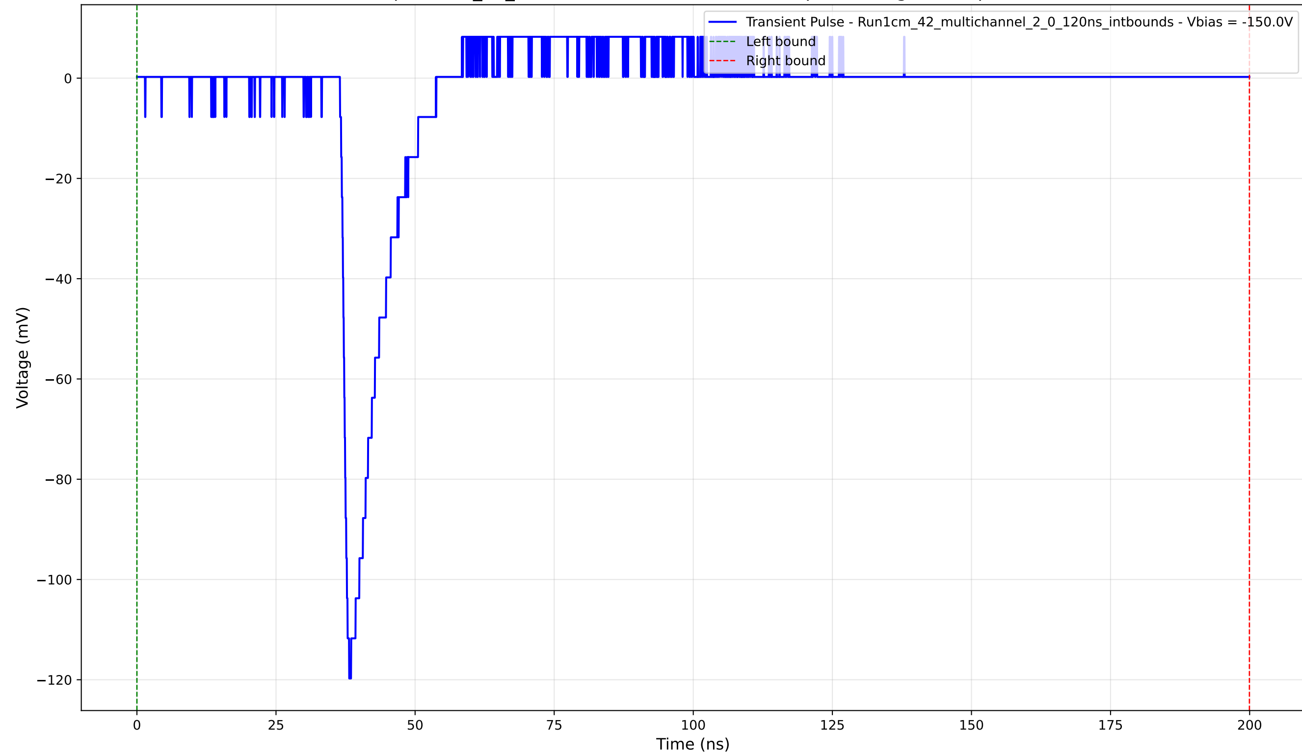
Transient Pulse - Sample: 1cm_42_multichannel - Position: 3570.0 \mu\text{m} - Charge: 9.00 pC - Rise Time: 1.18 ns
