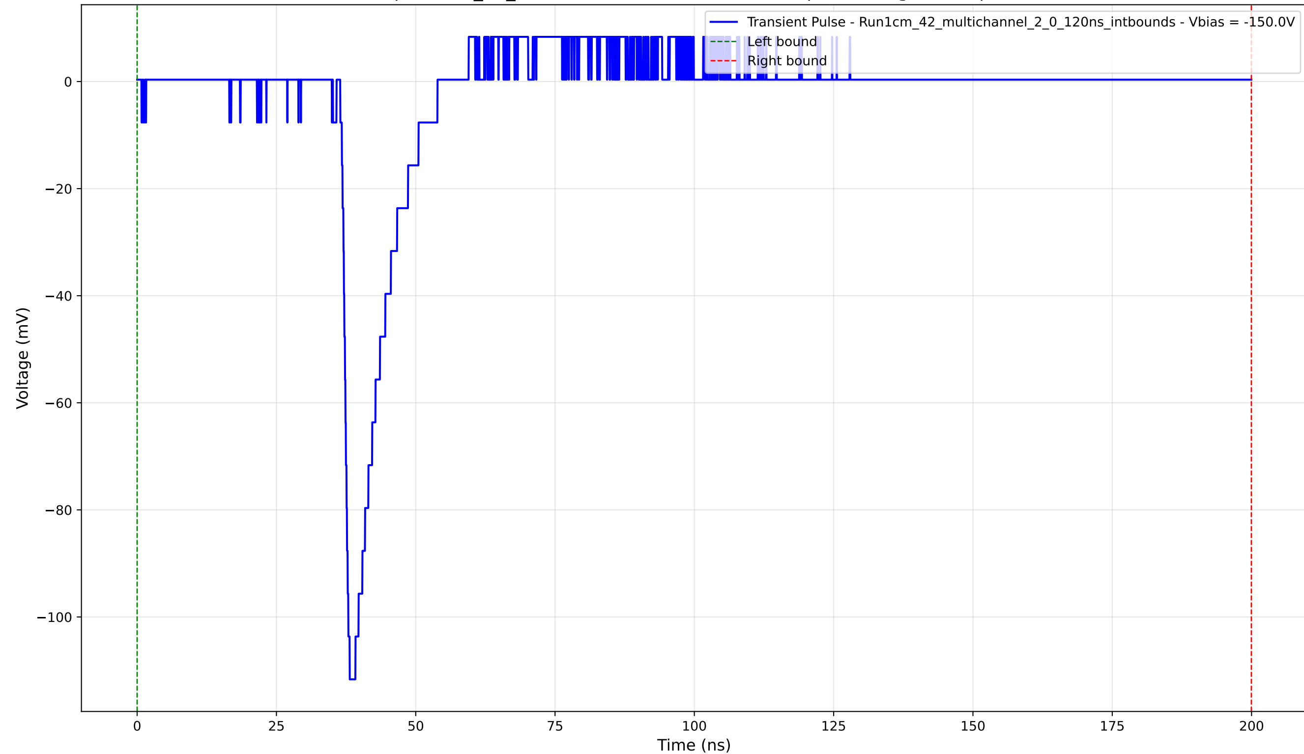
Transient Pulse - Sample: 1cm_42_multichannel - Position: 3630.0 \mu\text{m} - Charge: 9.26 pC - Rise Time: 1.18 ns
