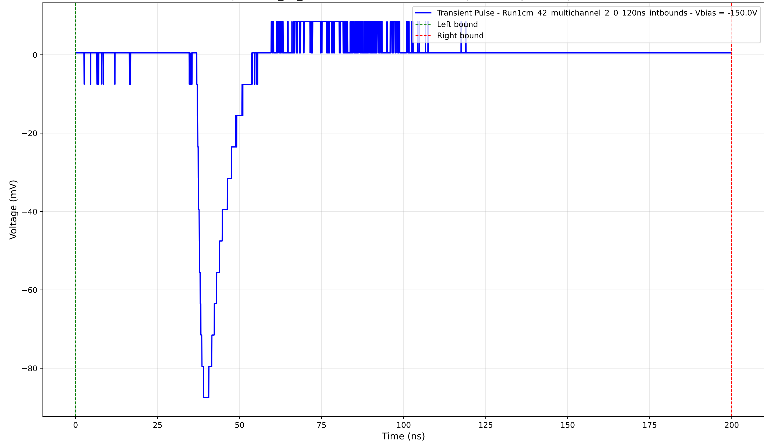
Transient Pulse - Sample: 1cm_42_multichannel - Position: 440.0 \mu\text{m} - Charge: 8.62 pC - Rise Time: 1.43 ns
