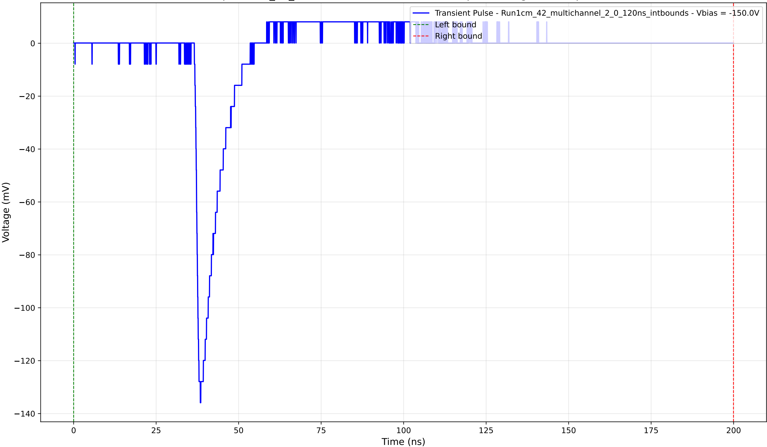
Transient Pulse - Sample: 1cm_42_multichannel - Position: 1115.0 \mu\text{m} - Charge: 10.56 pC - Rise Time: 1.25 ns
