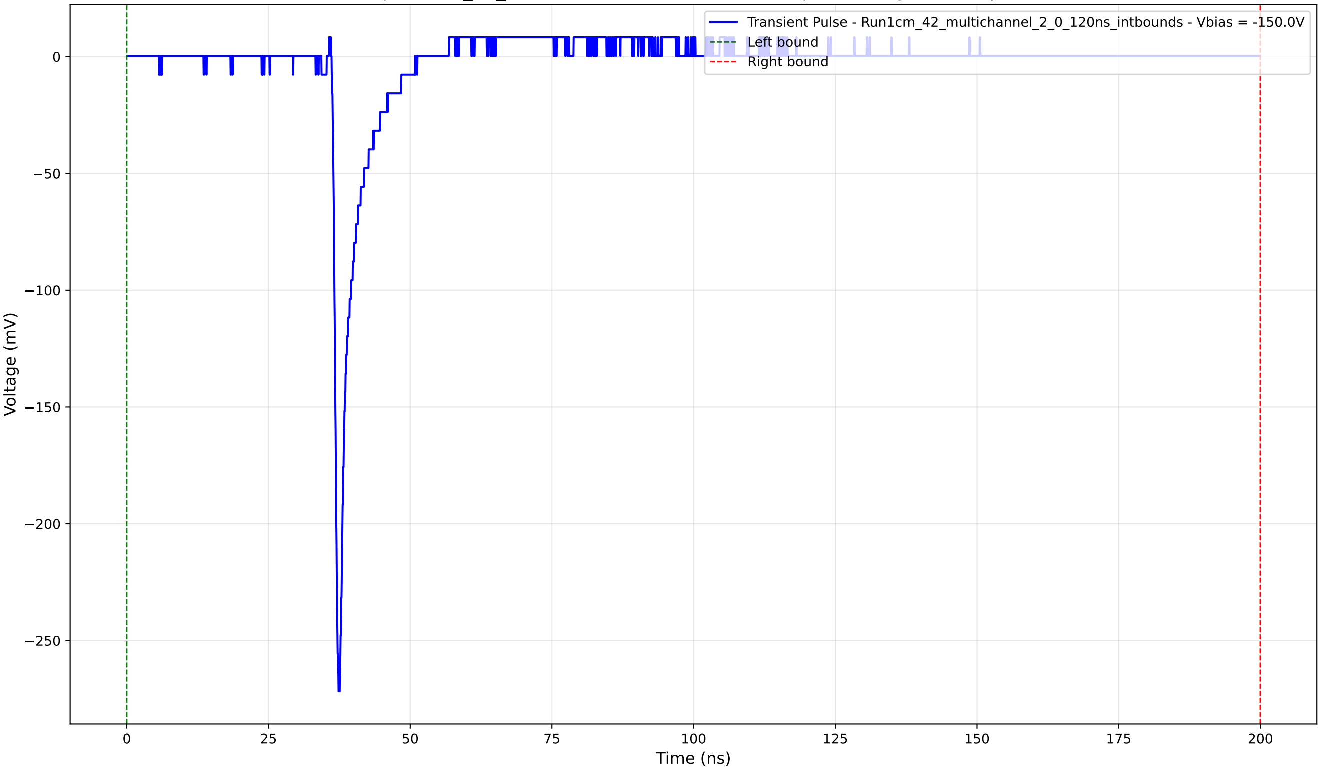
Transient Pulse - Sample: 1cm_42_multichannel - Position: 2810.0 \mu\text{m} - Charge: 10.85 pC - Rise Time: 0.81 ns
