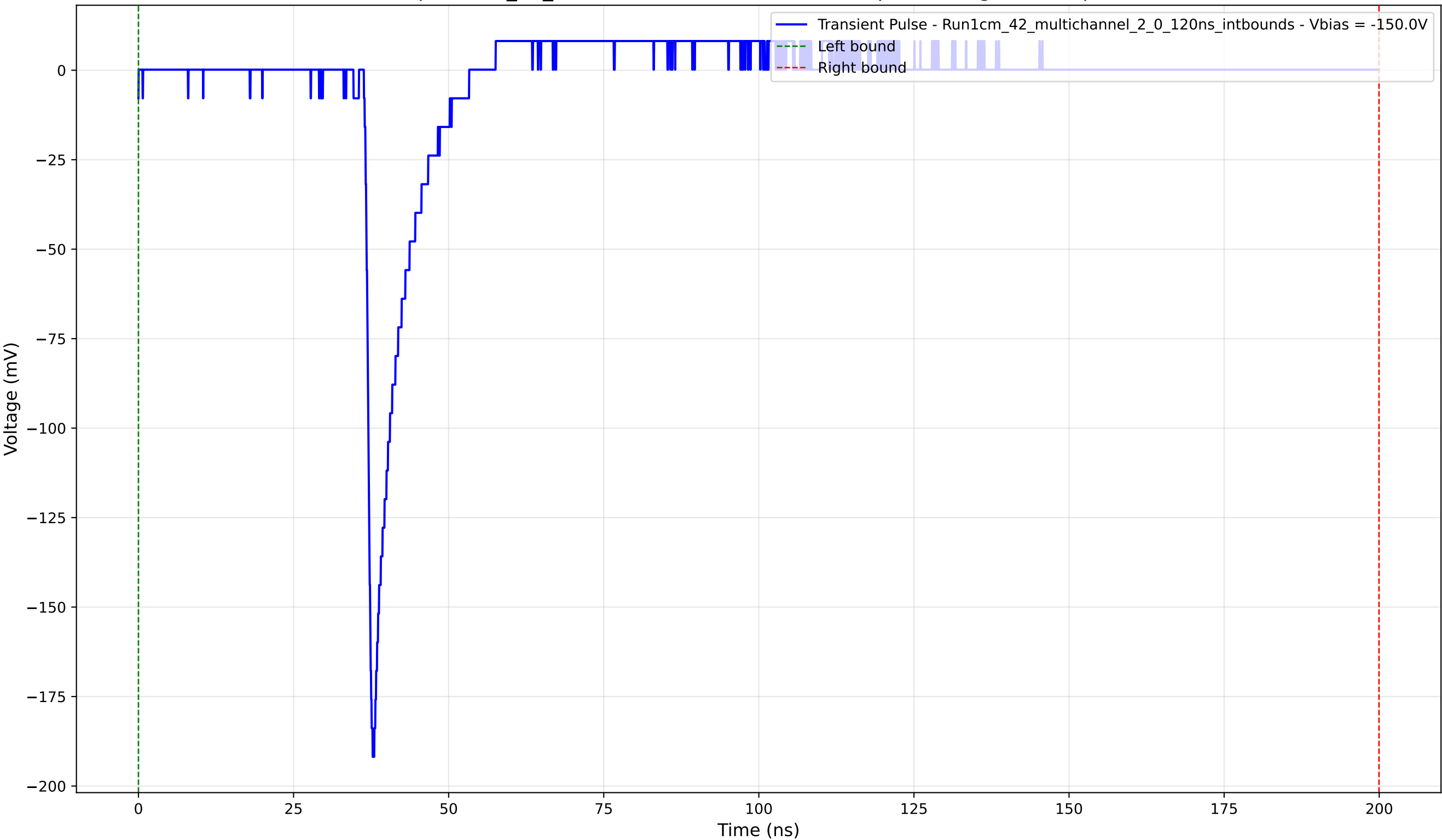
Transient Pulse - Sample: 1cm_42_multichannel - Position: 3230.0 \mu\text{m} - Charge: 10.73 pC - Rise Time: 0.94 ns
