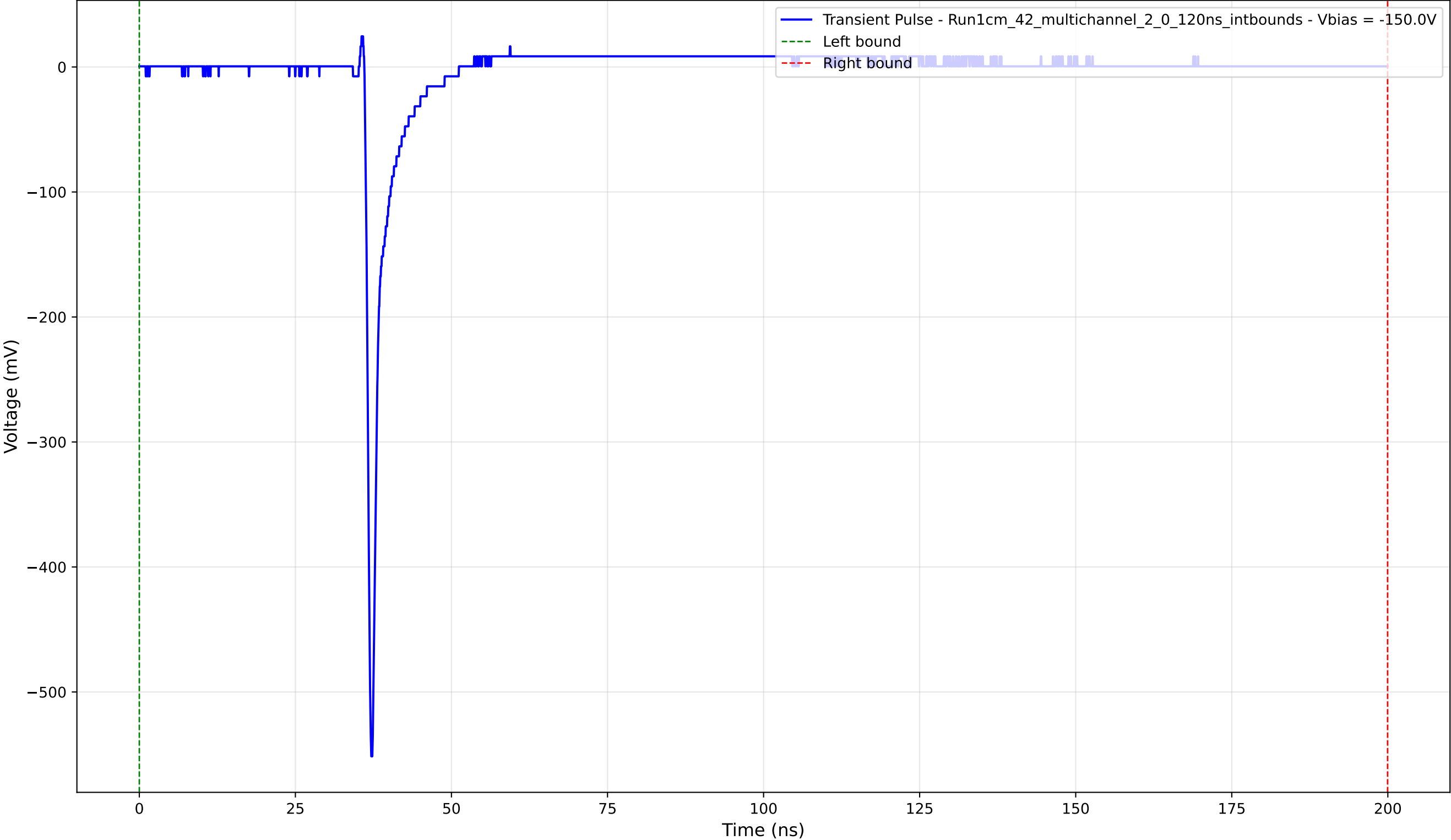
Transient Pulse - Sample: 1cm_42_multichannel - Position: 2180.0 \mu\text{m} - Charge: 14.59 pC - Rise Time: 0.74 ns
