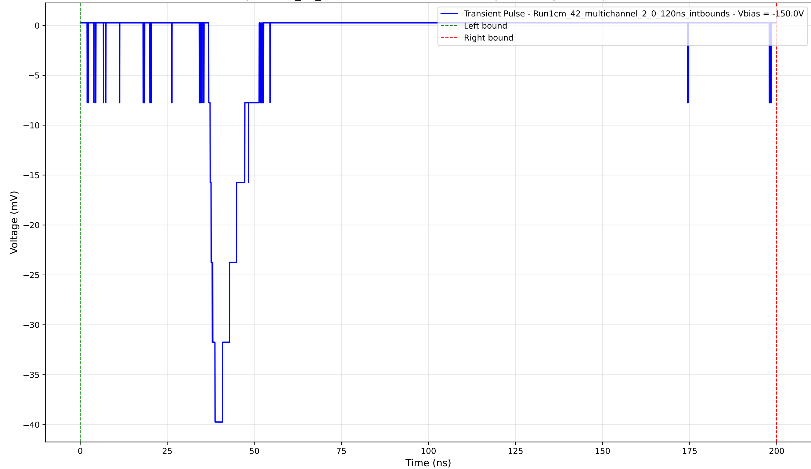
Transient Pulse - Sample: 1cm_42_multichannel - Position: 295.0 \mu\text{m} - Charge: 5.64 pC - Rise Time: 1.82 ns
