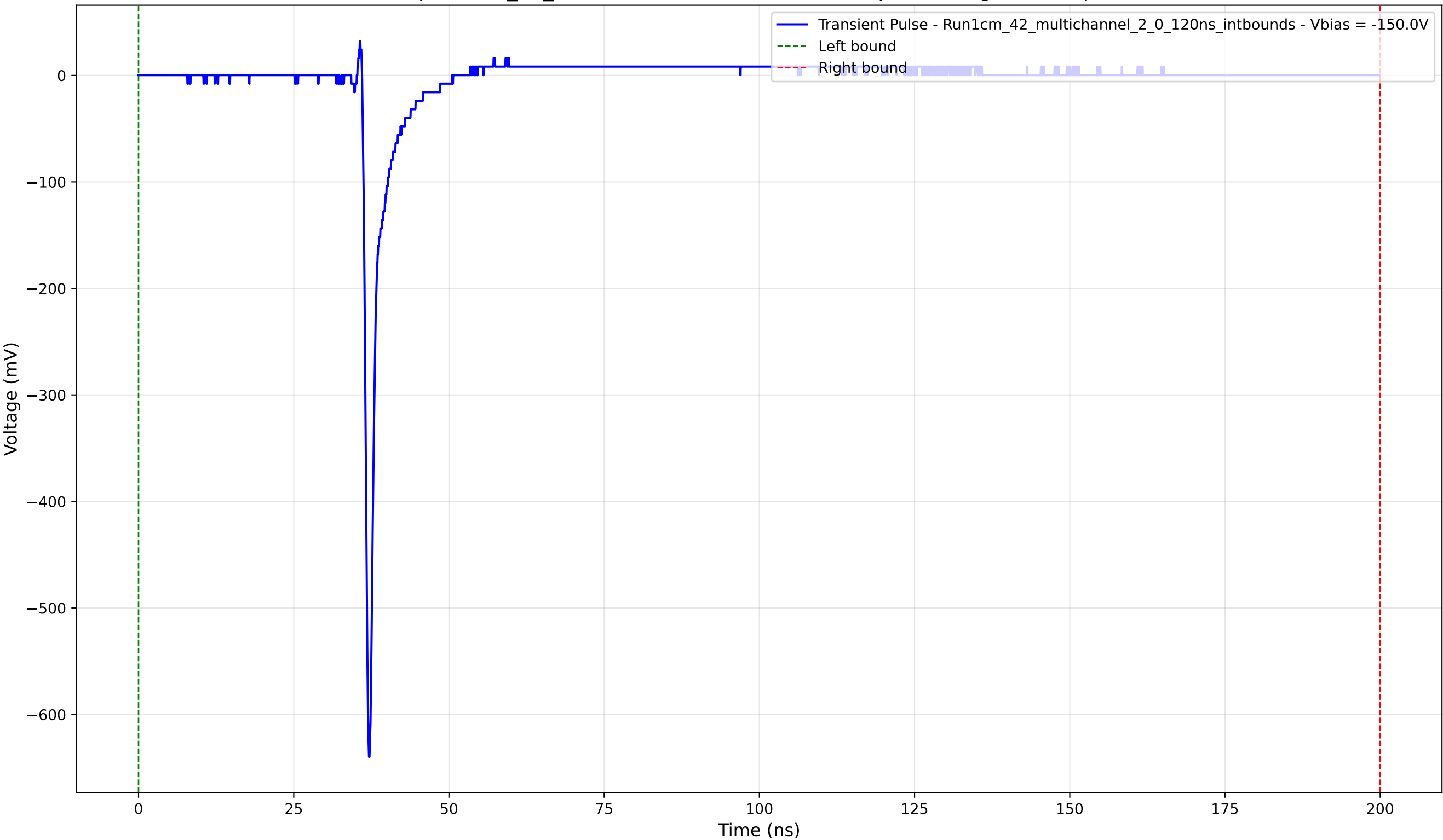
Transient Pulse - Sample: 1cm_42_multichannel - Position: 2270.0 \mu\text{m} - Charge: 16.17 pC - Rise Time: 0.72 ns
