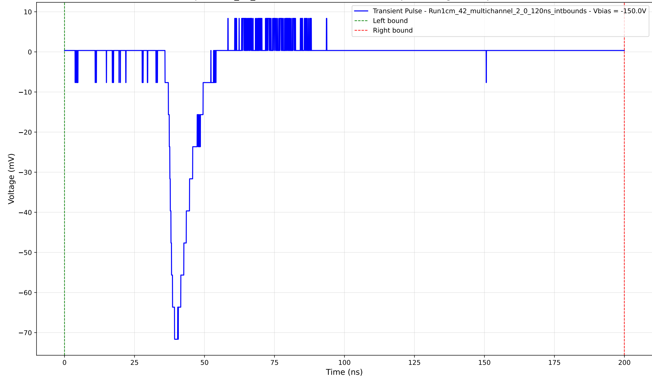
Transient Pulse - Sample: 1cm_42_multichannel - Position: 4670.0 \mu\text{m} - Charge: 8.27 pC - Rise Time: 3.40 ns
