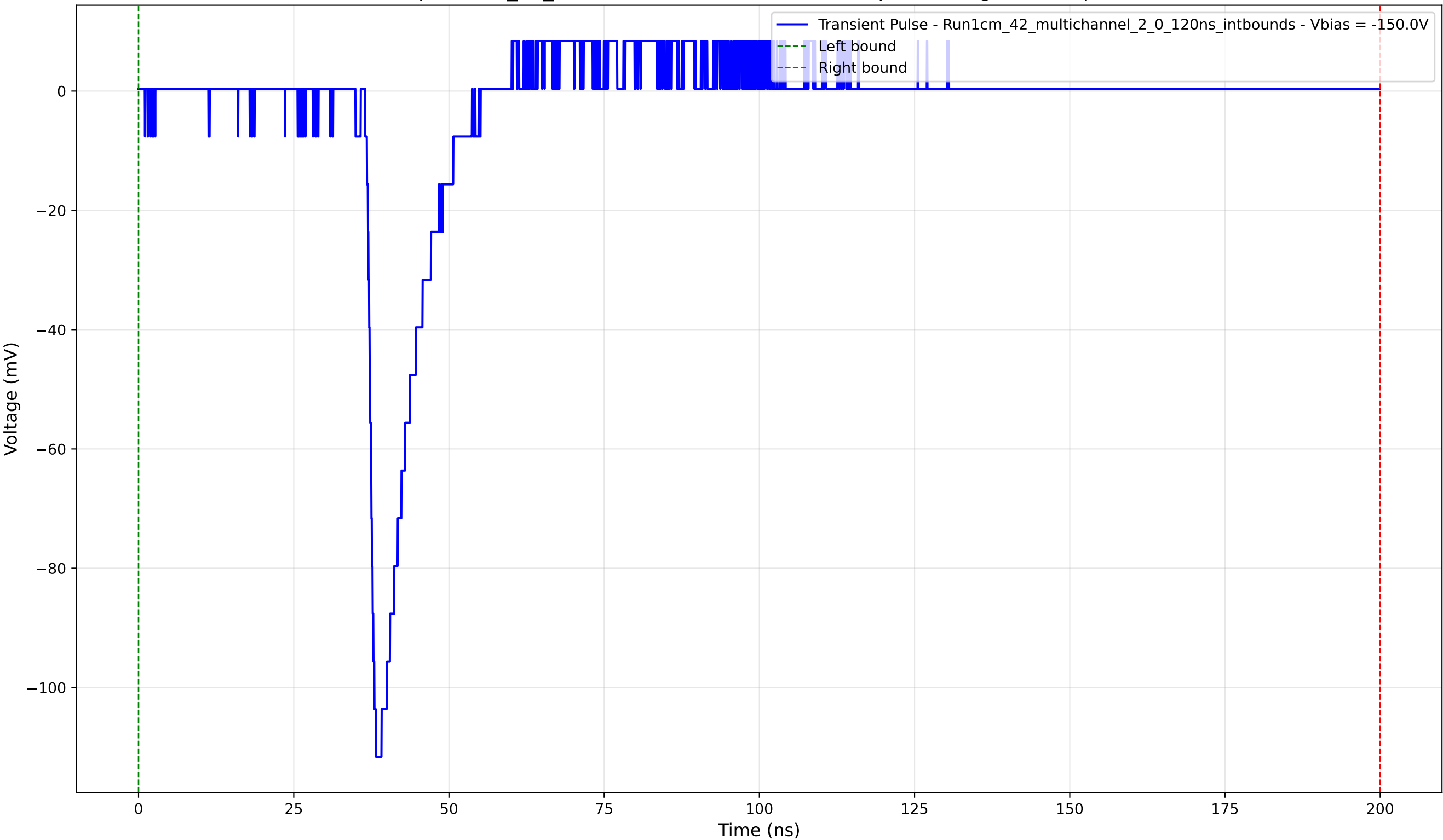
Transient Pulse - Sample: 1cm_42_multichannel - Position: 3665.0 \mu\text{m} - Charge: 10.11 pC - Rise Time: 1.22 ns
