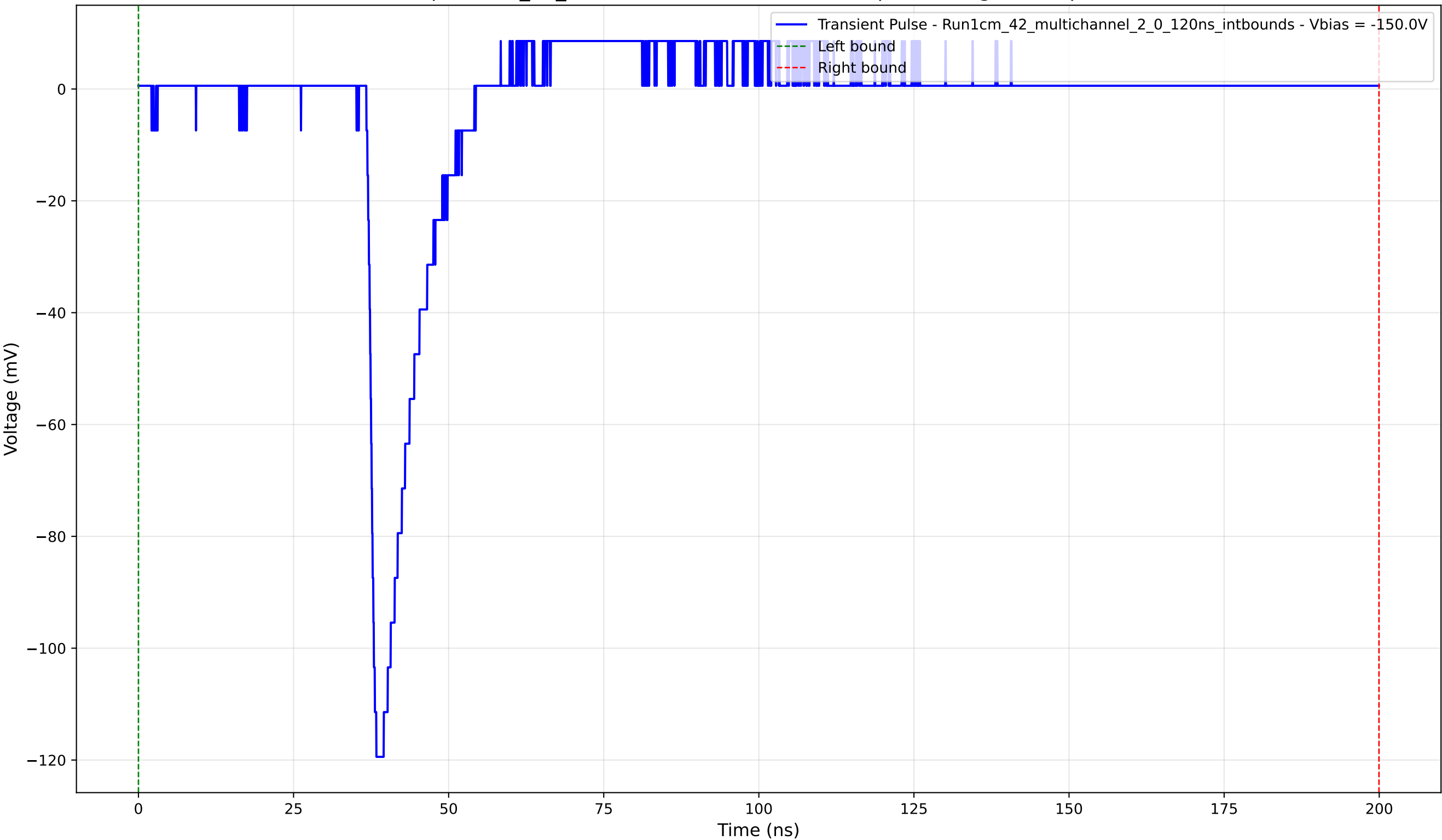
Transient Pulse - Sample: 1cm_42_multichannel - Position: 945.0 \mu\text{m} - Charge: 8.66 pC - Rise Time: 1.22 ns
