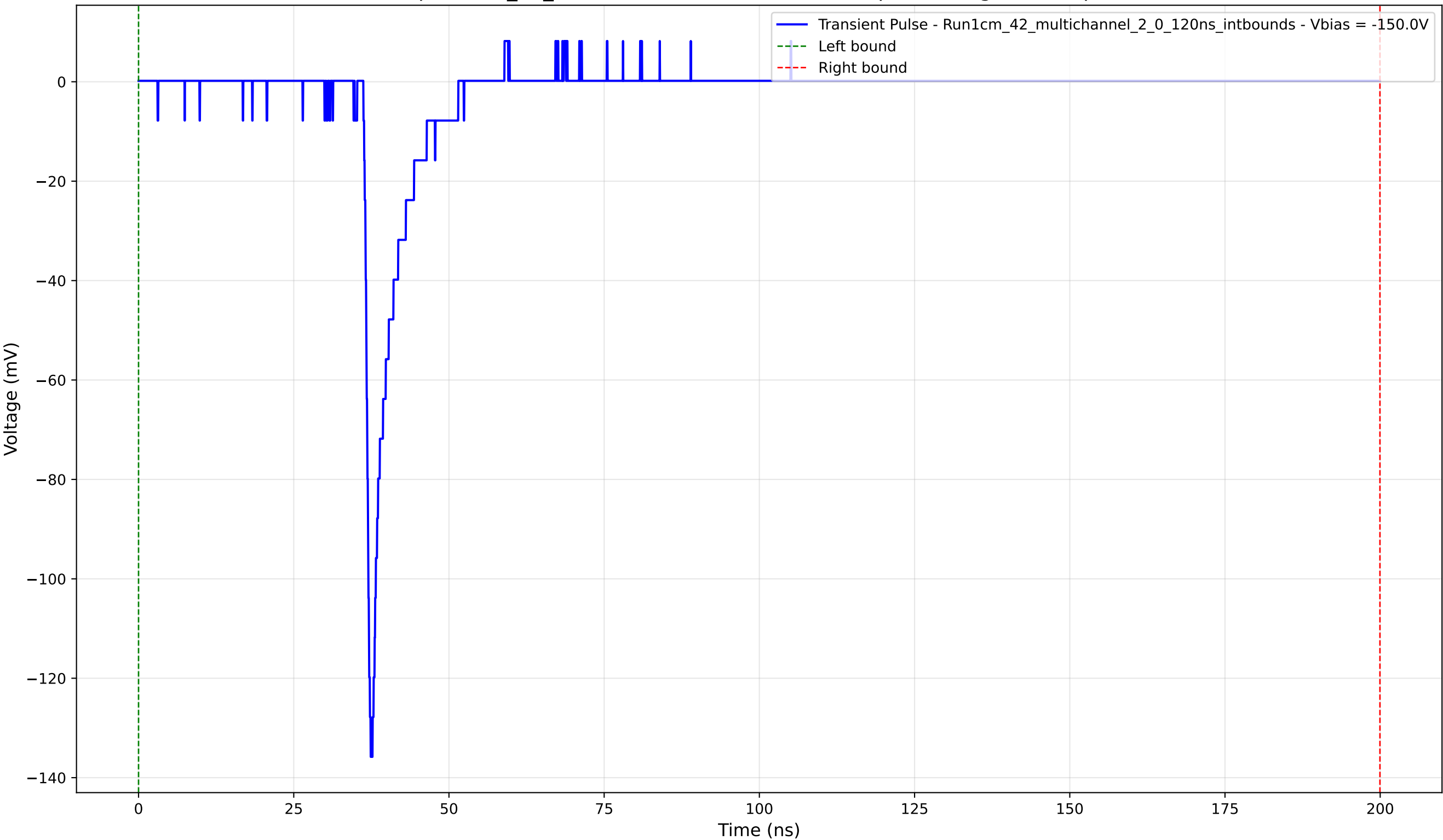
Transient Pulse - Sample: 1cm_42_multichannel - Position: 2925.0 \mu\text{m} - Charge: 10.02 pC - Rise Time: 0.93 ns
