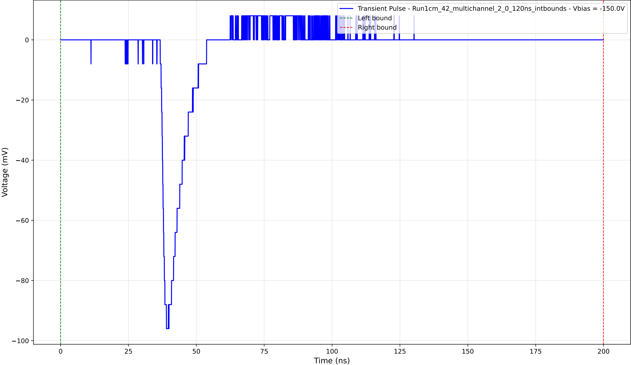
Transient Pulse - Sample: 1cm_42_multichannel - Position: 3995.0 \mu\text{m} - Charge: 10.61 pC - Rise Time: 1.43 ns
