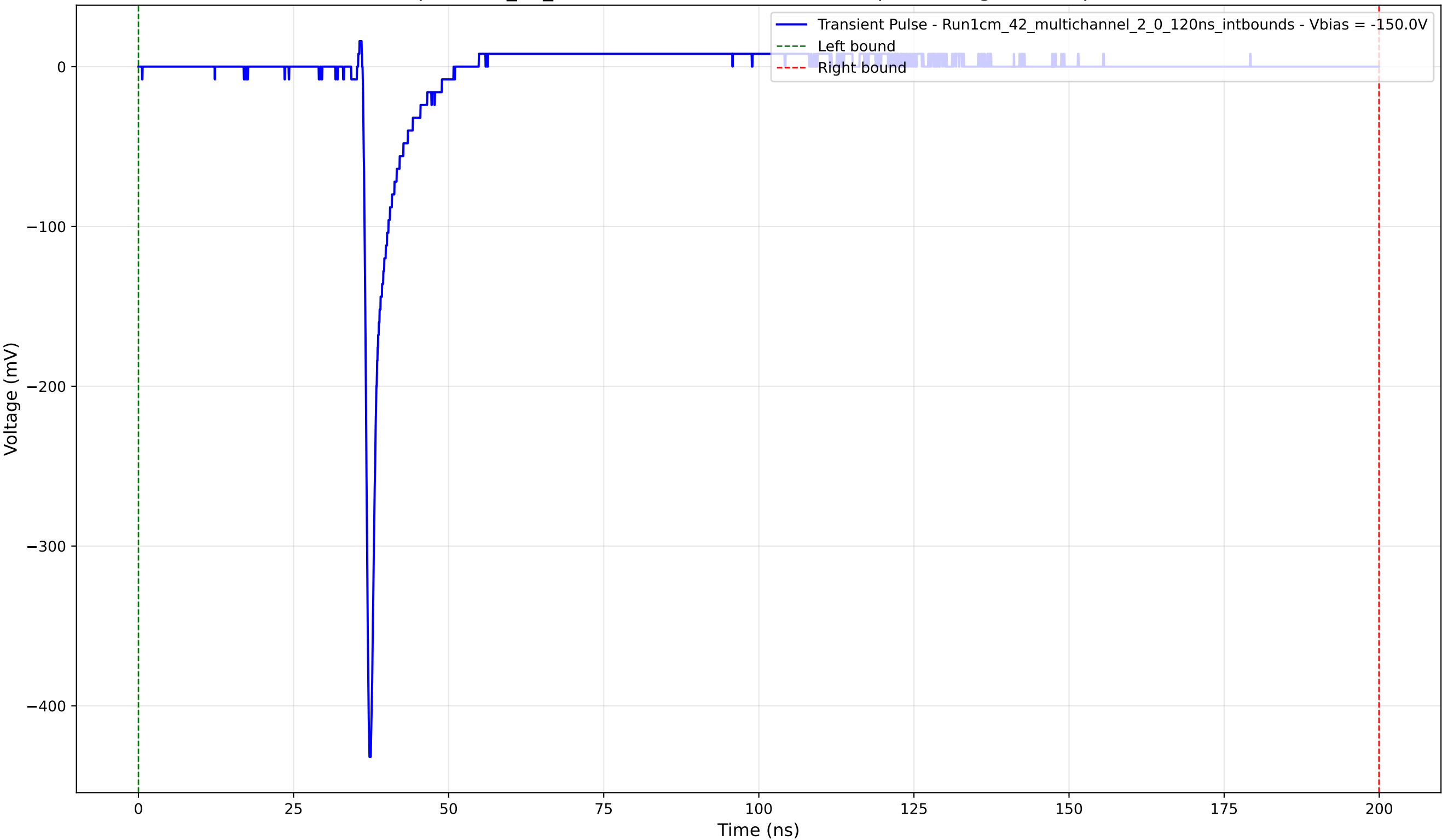
Transient Pulse - Sample: 1cm_42_multichannel - Position: 2690.0 \mu\text{m} - Charge: 13.80 pC - Rise Time: 0.78 ns
