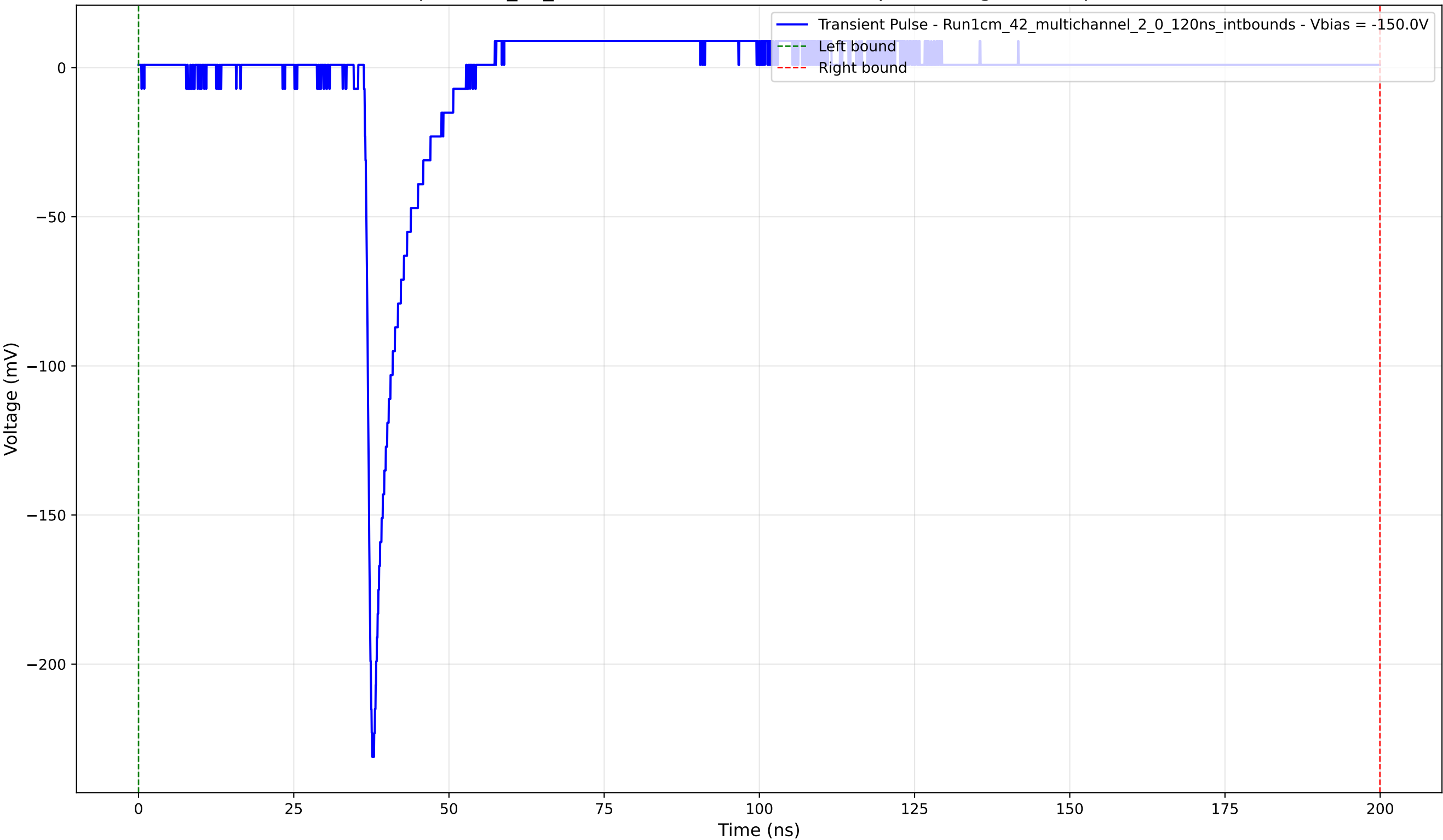
Transient Pulse - Sample: 1cm_42_multichannel - Position: 1580.0 \mu\text{m} - Charge: 10.09 pC - Rise Time: 0.96 ns
