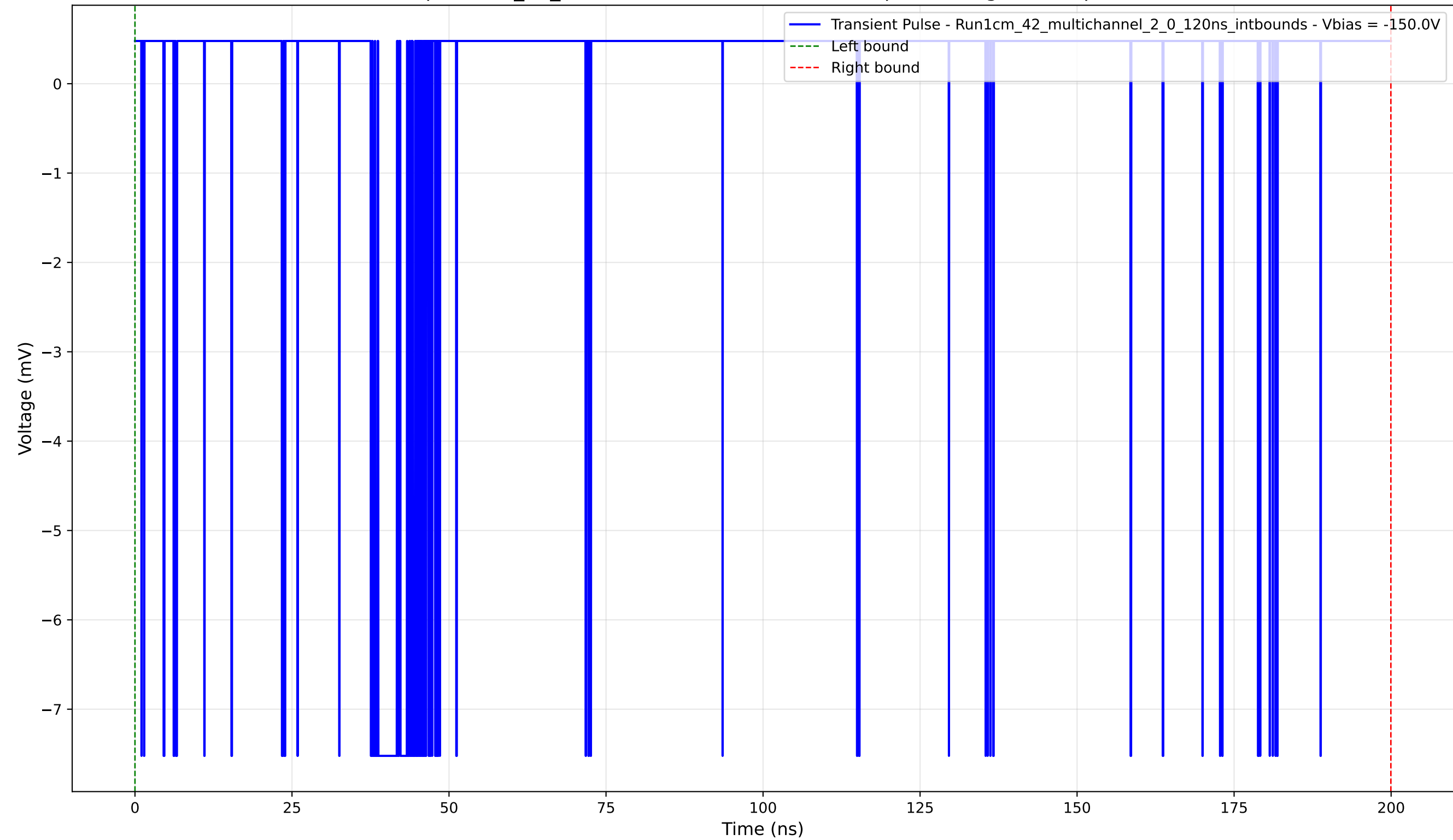
Transient Pulse - Sample: 1cm_42_multichannel - Position: 4395.0 \mu\text{m} - Charge: -0.22 pC - Rise Time: 0.04 ns
