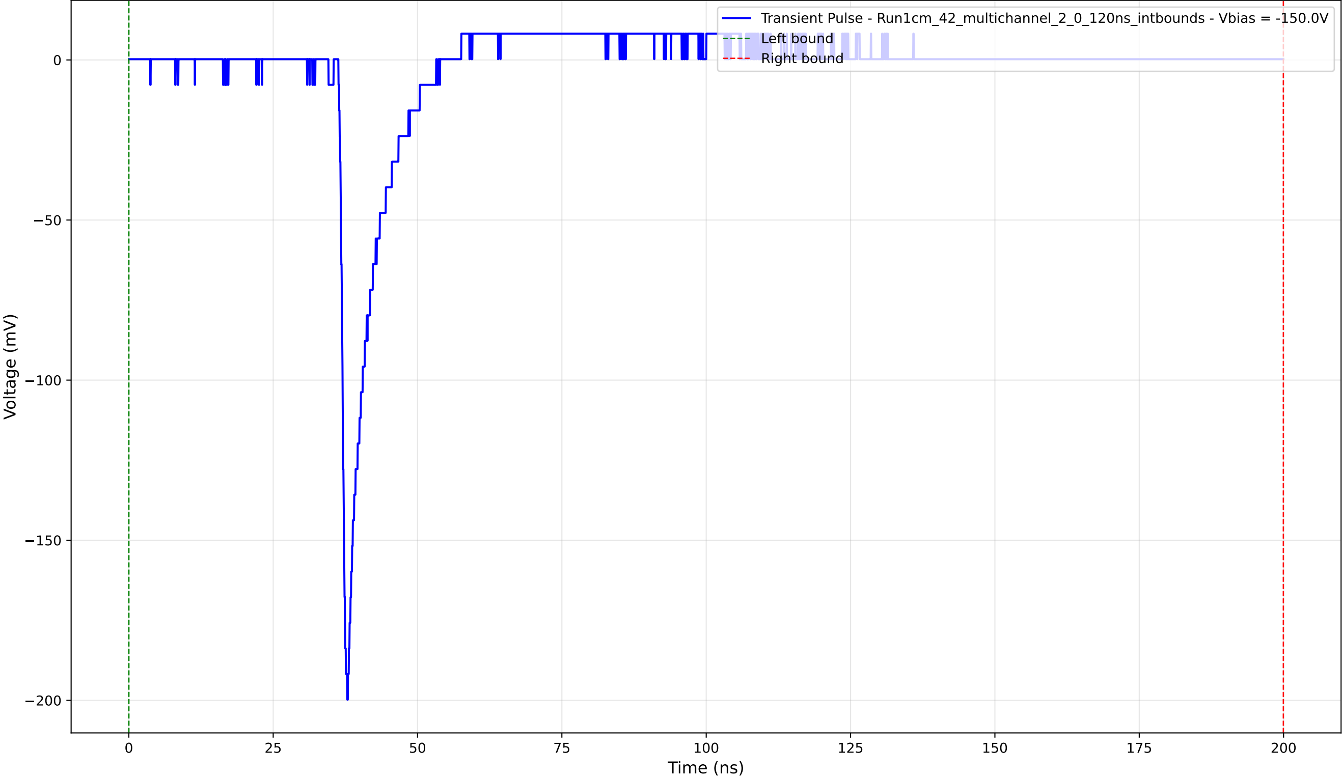
Transient Pulse - Sample: 1cm_42_multichannel - Position: 3190.0 \mu\text{m} - Charge: 11.11 pC - Rise Time: 0.98 ns
