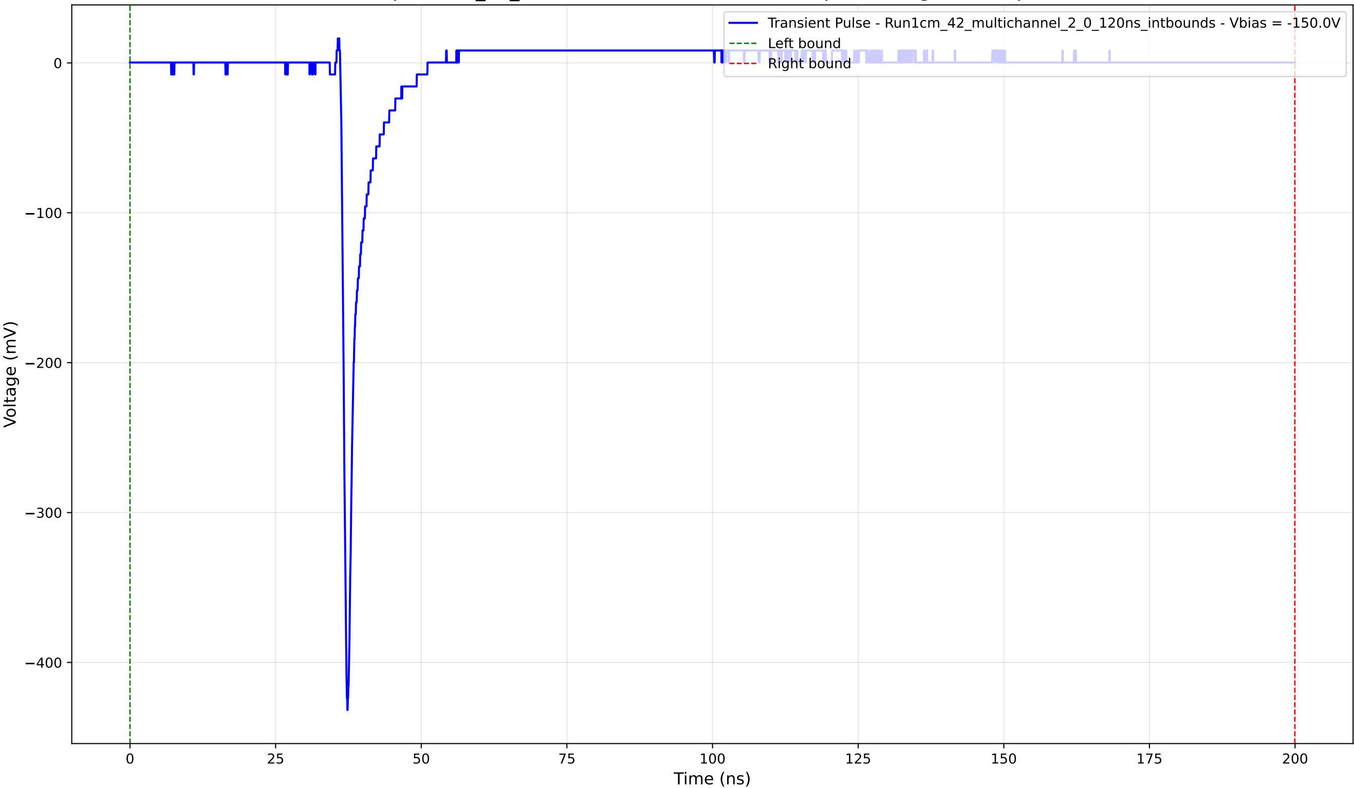
Transient Pulse - Sample: 1cm_42_multichannel - Position: 2710.0 \mu\text{m} - Charge: 13.32 pC - Rise Time: 0.78 ns
