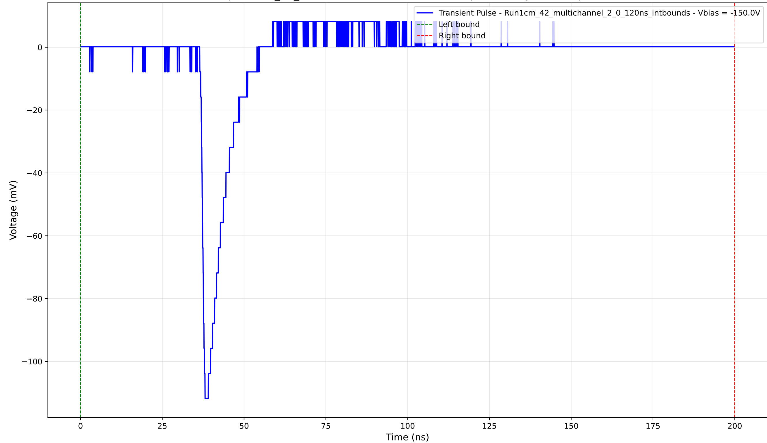
Transient Pulse - Sample: 1cm_42_multichannel - Position: 3615.0 \mu\text{m} - Charge: 10.33 pC - Rise Time: 1.18 ns
