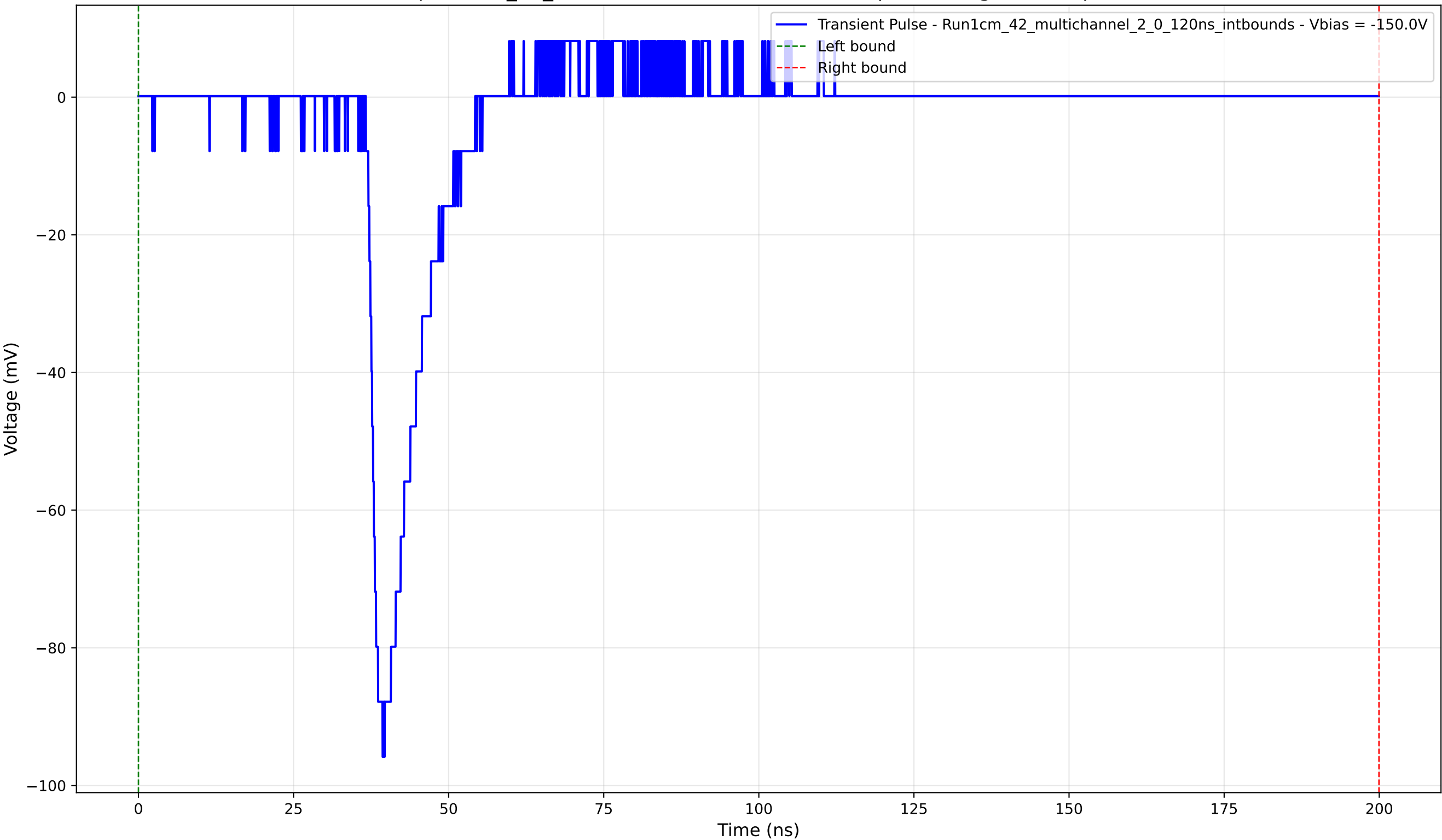
Transient Pulse - Sample: 1cm_42_multichannel - Position: 4025.0 \mu\text{m} - Charge: 10.81 pC - Rise Time: 1.59 ns
