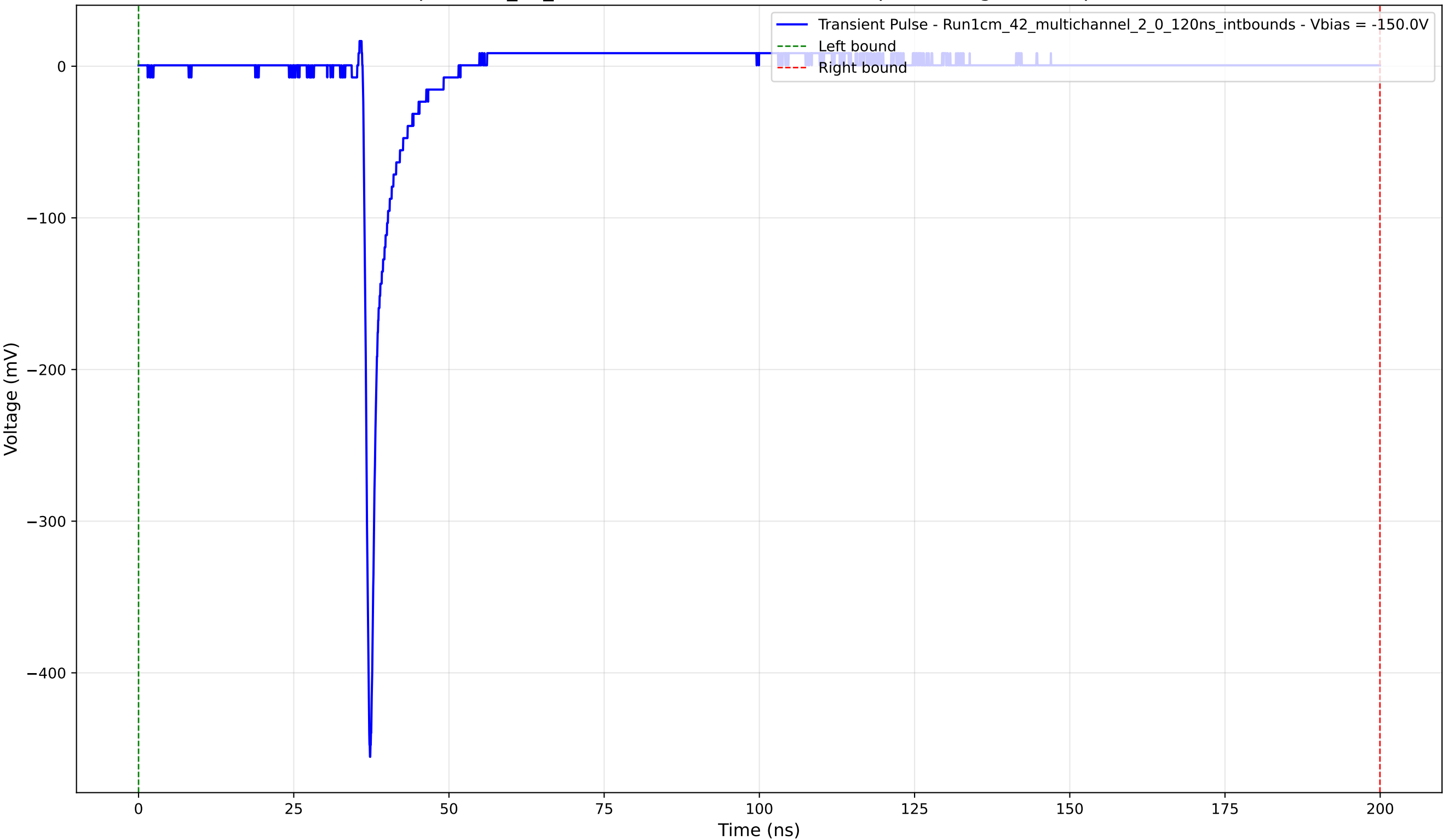
Transient Pulse - Sample: 1cm_42_multichannel - Position: 2655.0 \mu\text{m} - Charge: 13.23 pC - Rise Time: 0.74 ns
