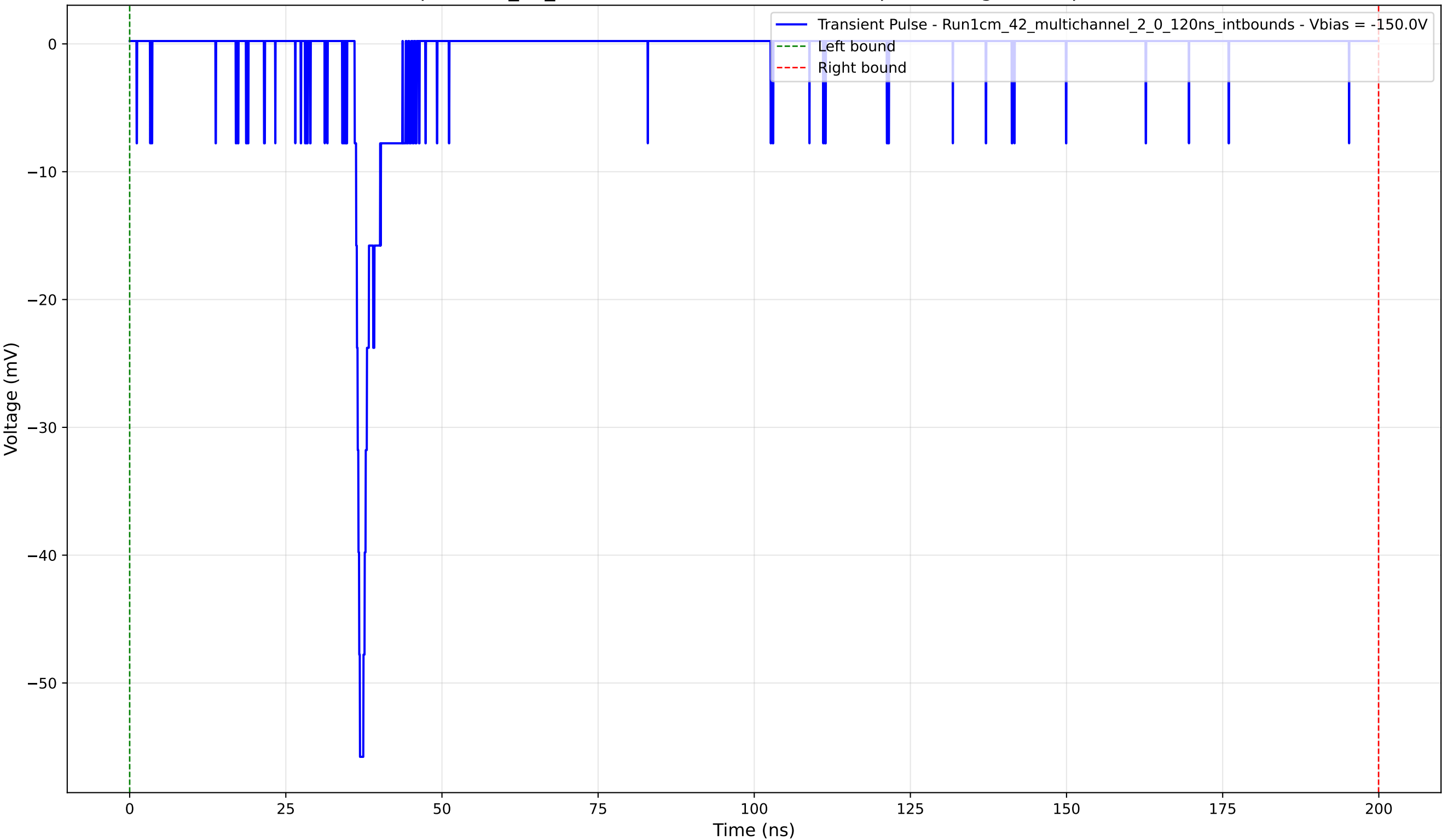
Transient Pulse - Sample: 1cm_42_multichannel - Position: 2345.0 \mu\text{m} - Charge: 2.76 pC - Rise Time: 0.85 ns
