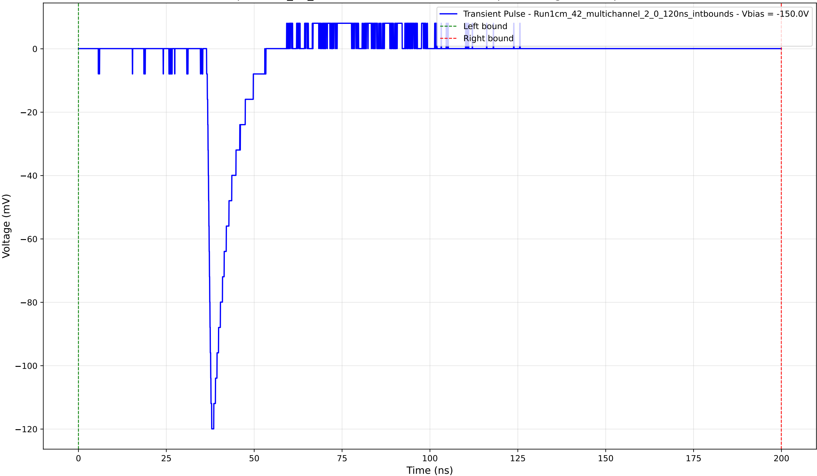
Transient Pulse - Sample: 1cm_42_multichannel - Position: 1295.0 \mu\text{m} - Charge: 10.61 pC - Rise Time: 1.06 ns
