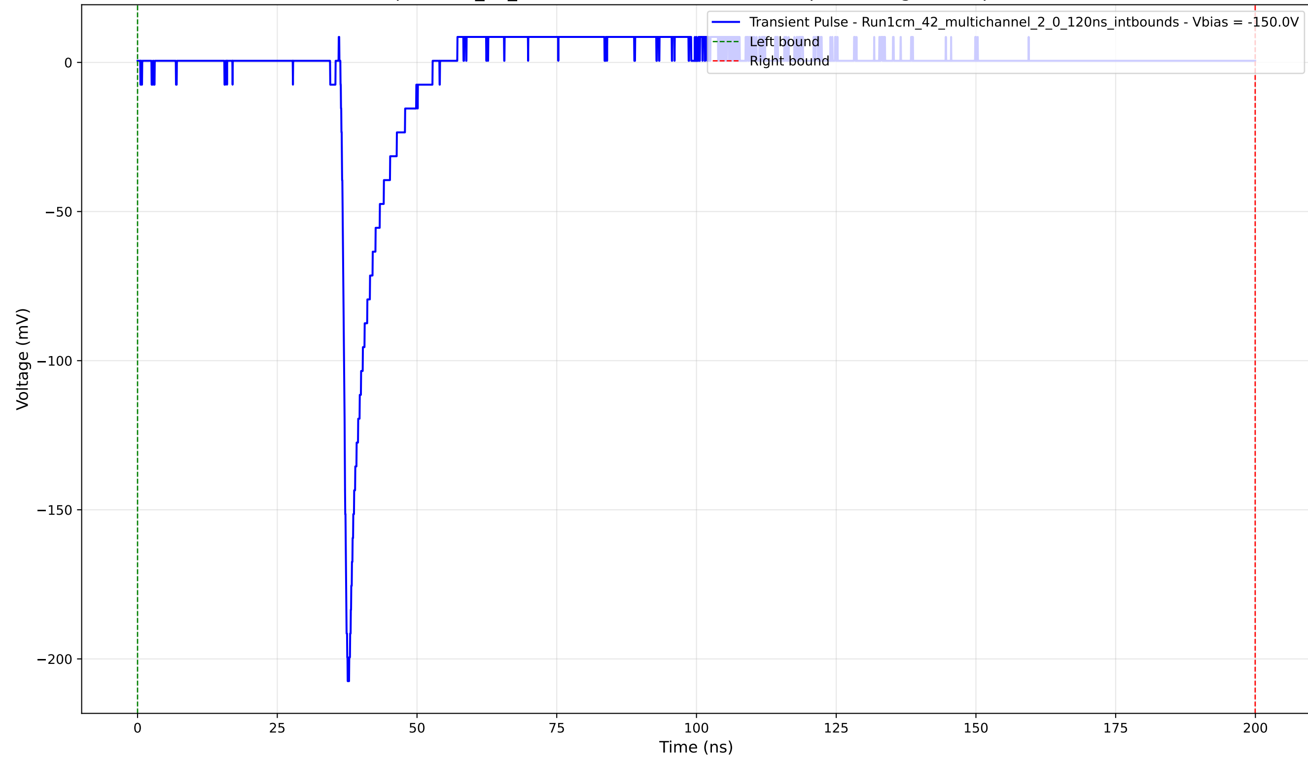
Transient Pulse - Sample: 1cm_42_multichannel - Position: 3125.0 \mu\text{m} - Charge: 9.15 pC - Rise Time: 0.93 ns
