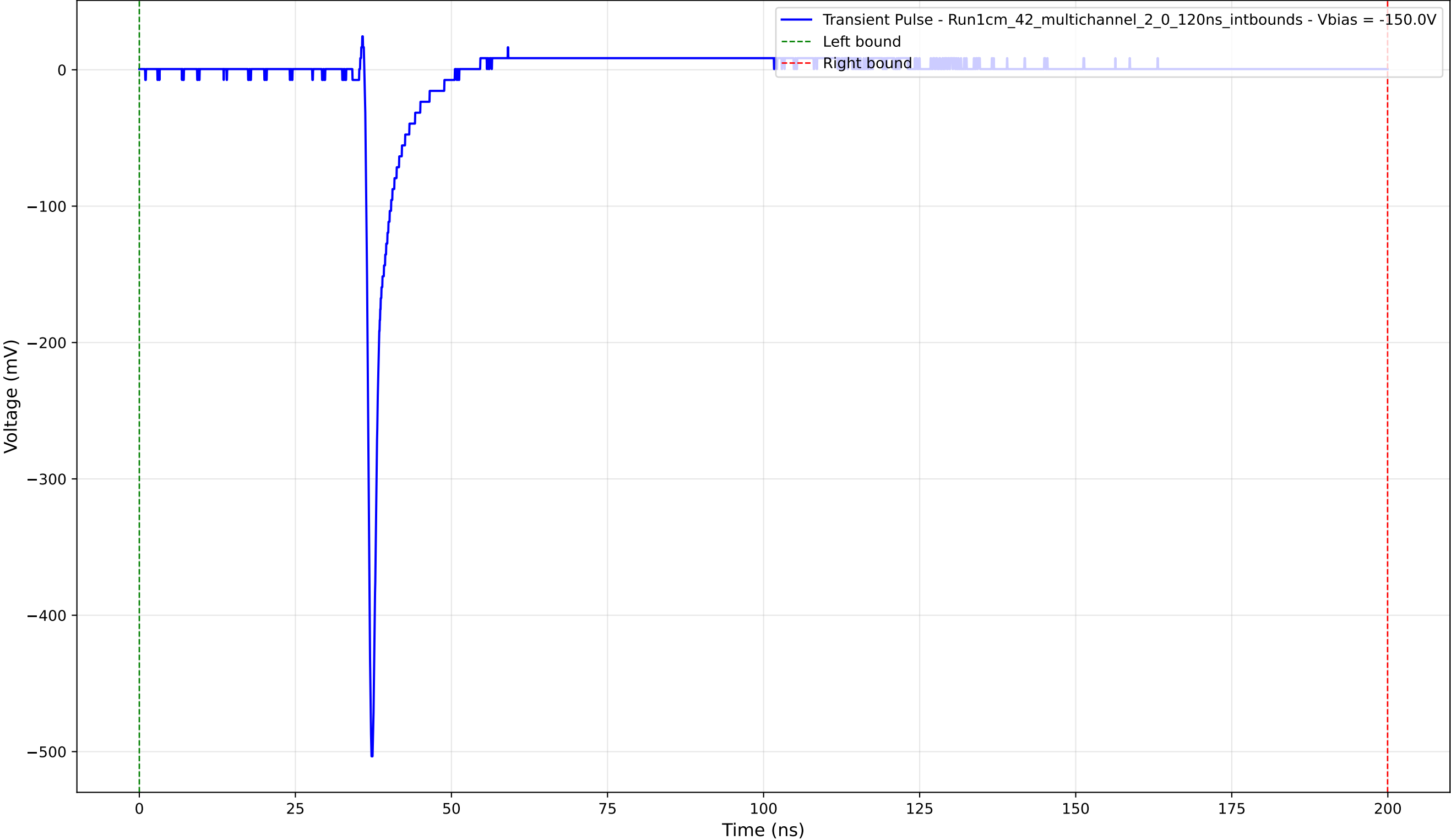
Transient Pulse - Sample: 1cm_42_multichannel - Position: 2125.0 \mu\text{m} - Charge: 14.26 pC - Rise Time: 0.77 ns
