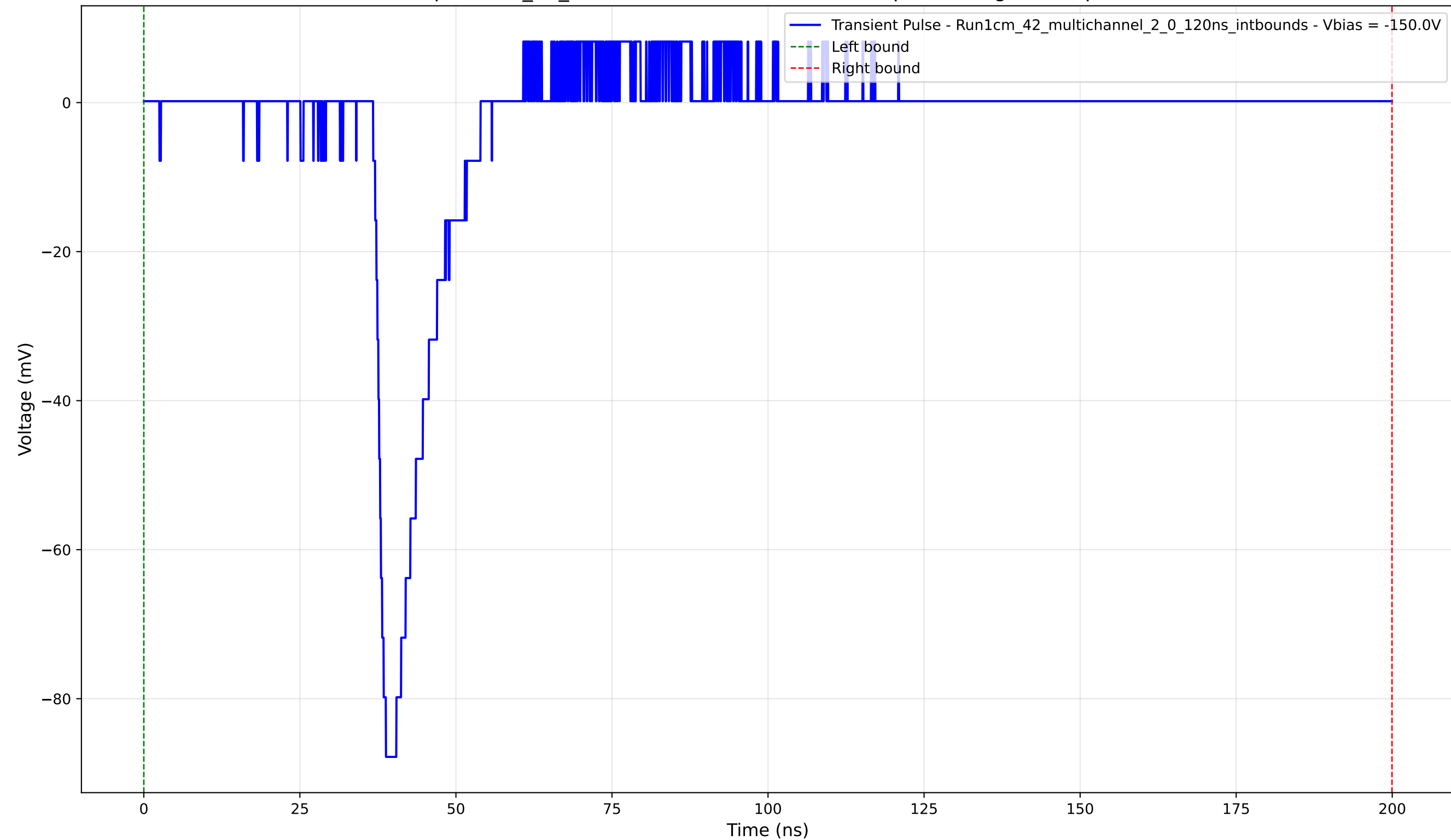
Transient Pulse - Sample: 1cm_42_multichannel - Position: 4060.0 \mu\text{m} - Charge: 9.92 pC - Rise Time: 1.40 ns
