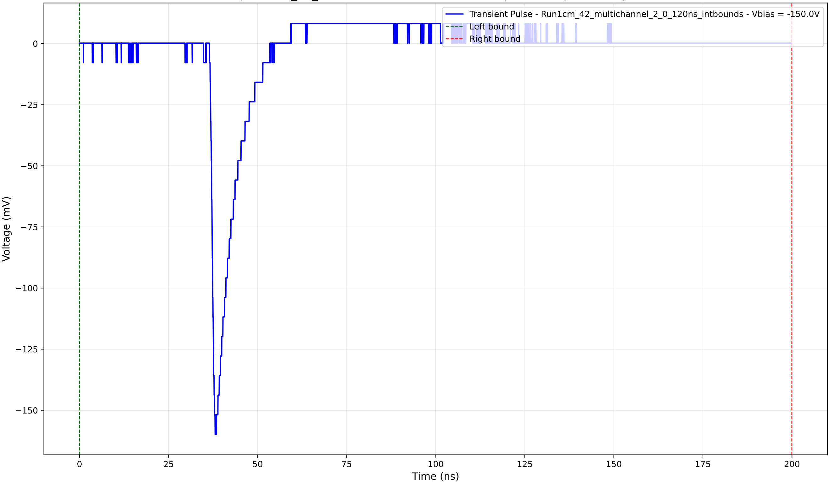
Transient Pulse - Sample: 1cm_42_multichannel - Position: 1235.0 \mu\text{m} - Charge: 11.08 pC - Rise Time: 1.20 ns
