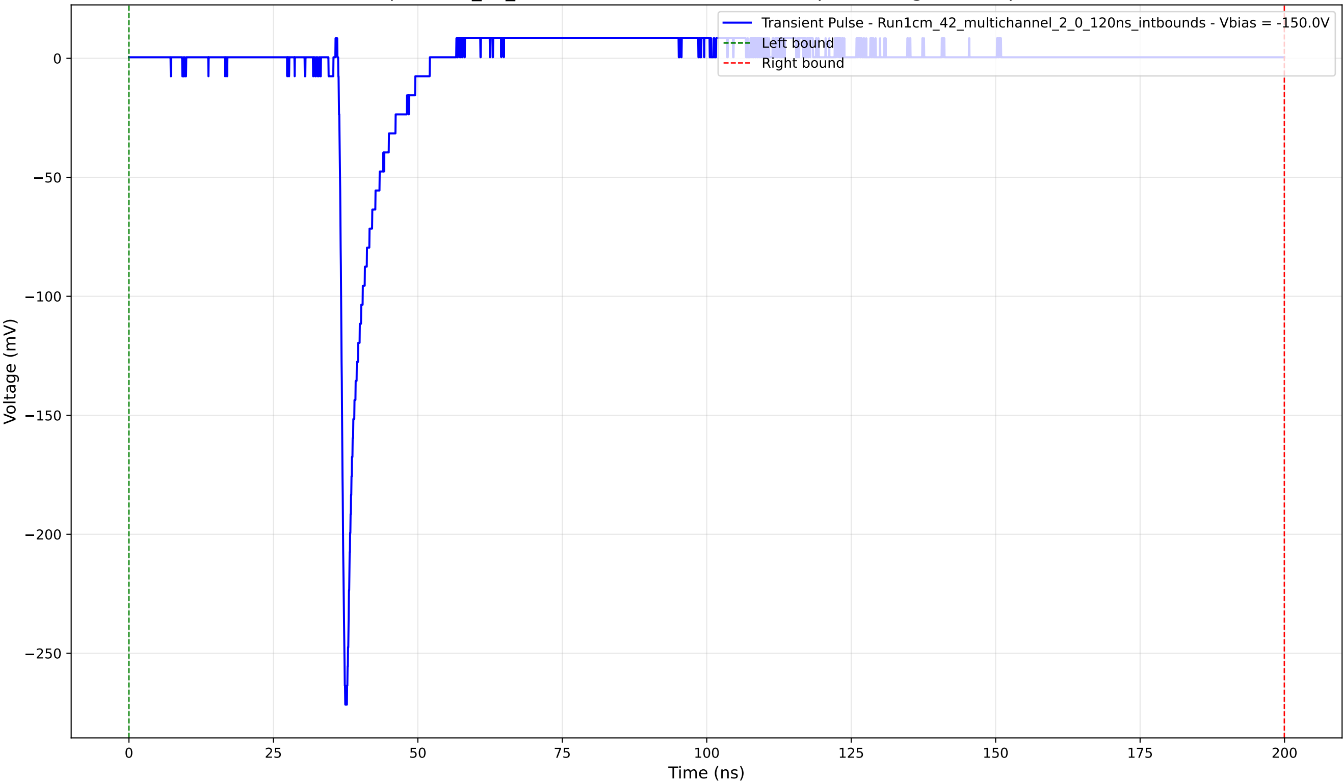
Transient Pulse - Sample: 1cm_42_multichannel - Position: 2970.0 \mu\text{m} - Charge: 10.85 pC - Rise Time: 0.85 ns
