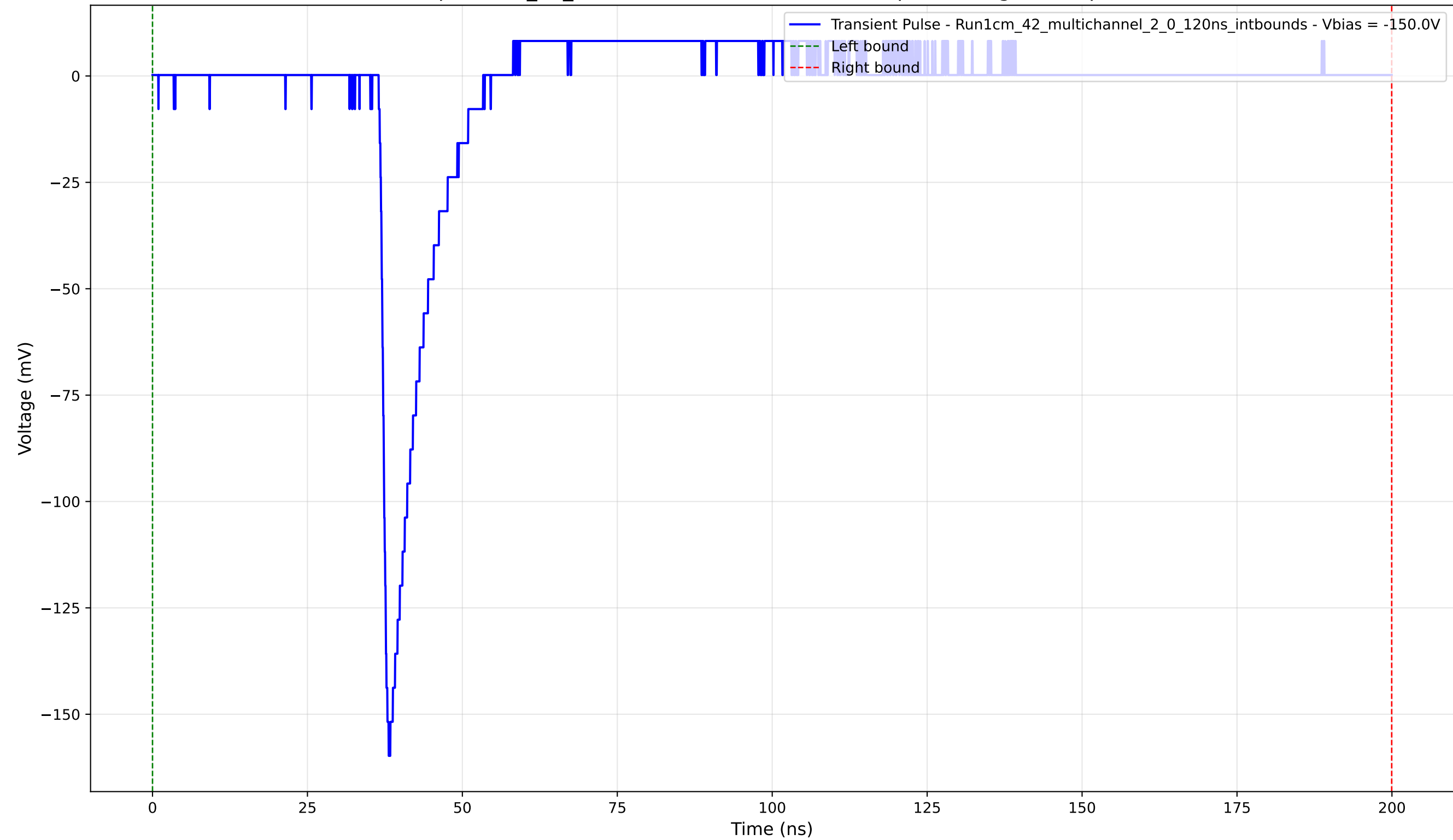
Transient Pulse - Sample: 1cm_42_multichannel - Position: 1230.0 \mu\text{m} - Charge: 9.97 pC - Rise Time: 1.16 ns
