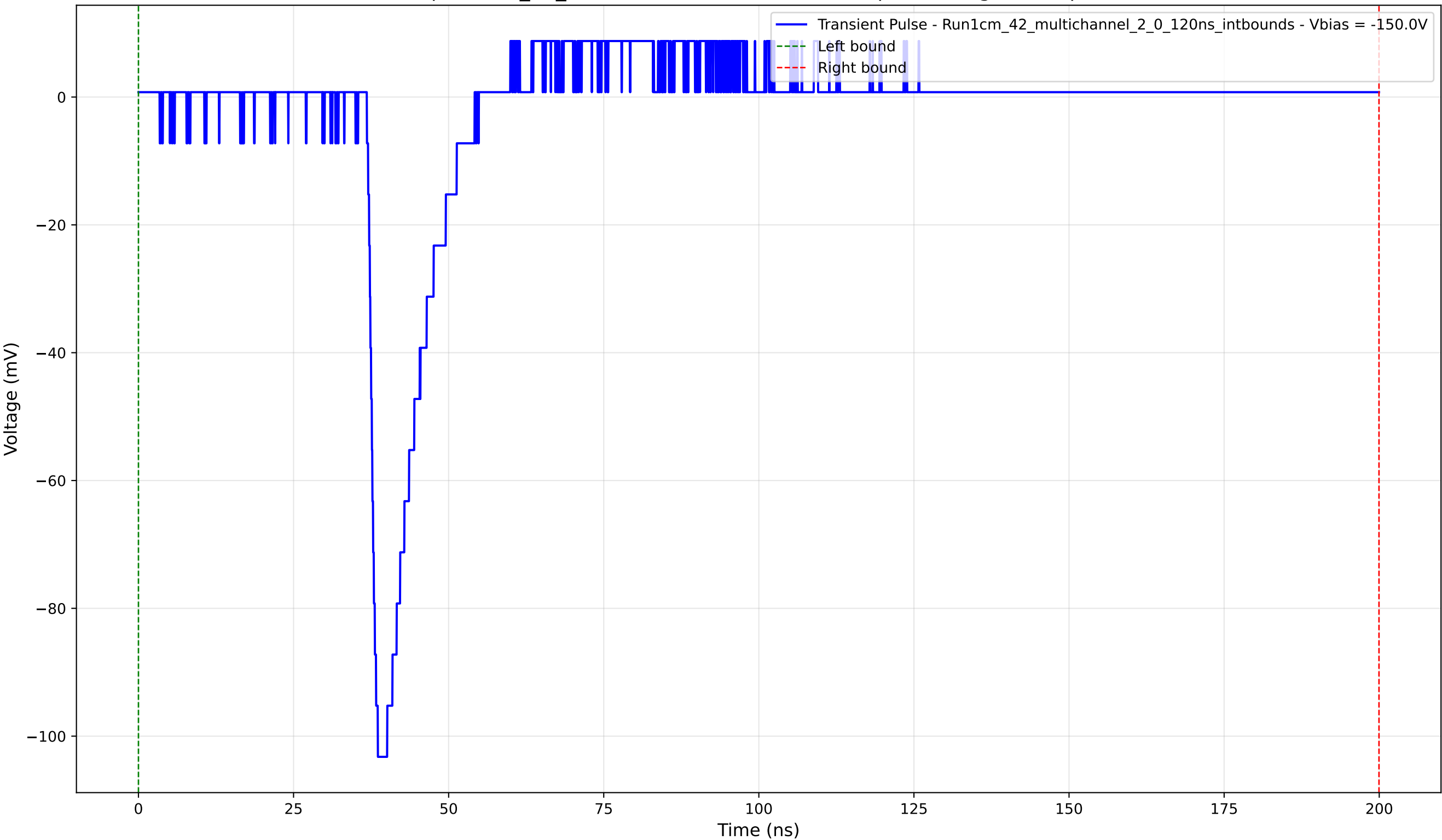
Transient Pulse - Sample: 1cm_42_multichannel - Position: 710.0 \mu\text{m} - Charge: 8.70 pC - Rise Time: 1.30 ns
