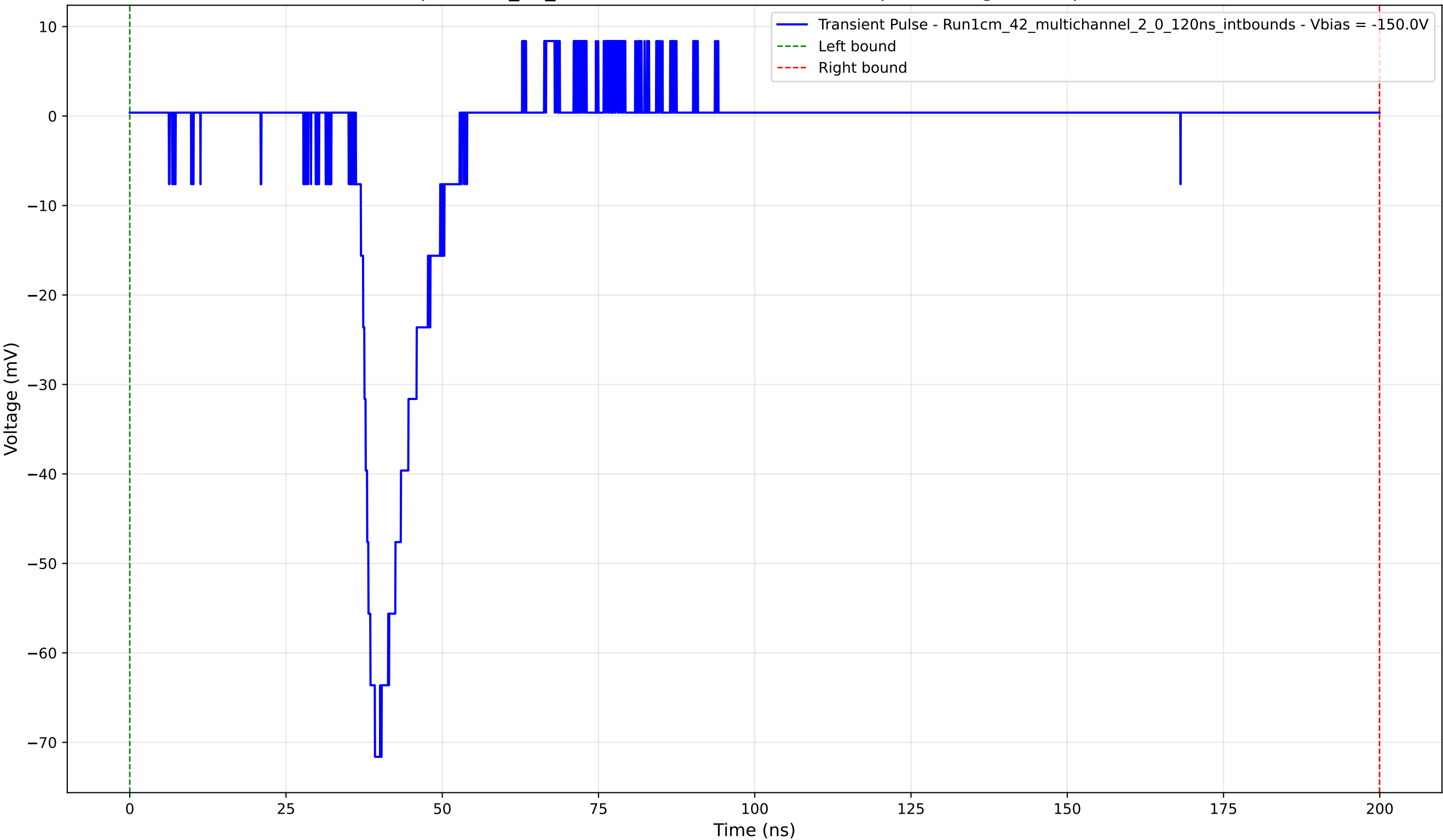
Transient Pulse - Sample: 1cm_42_multichannel - Position: 4715.0 \mu\text{m} - Charge: 8.64 pC - Rise Time: 3.04 ns
