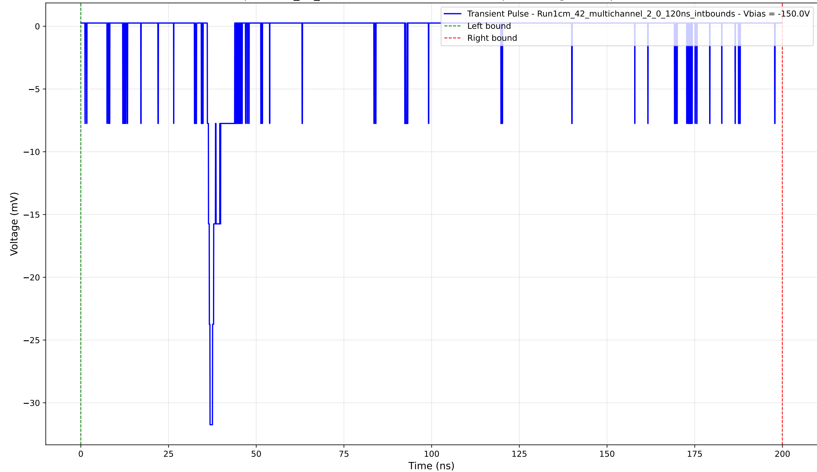
Transient Pulse - Sample: 1cm_42_multichannel - Position: 2355.0 \mu\text{m} - Charge: 2.11 pC - Rise Time: 0.78 ns
