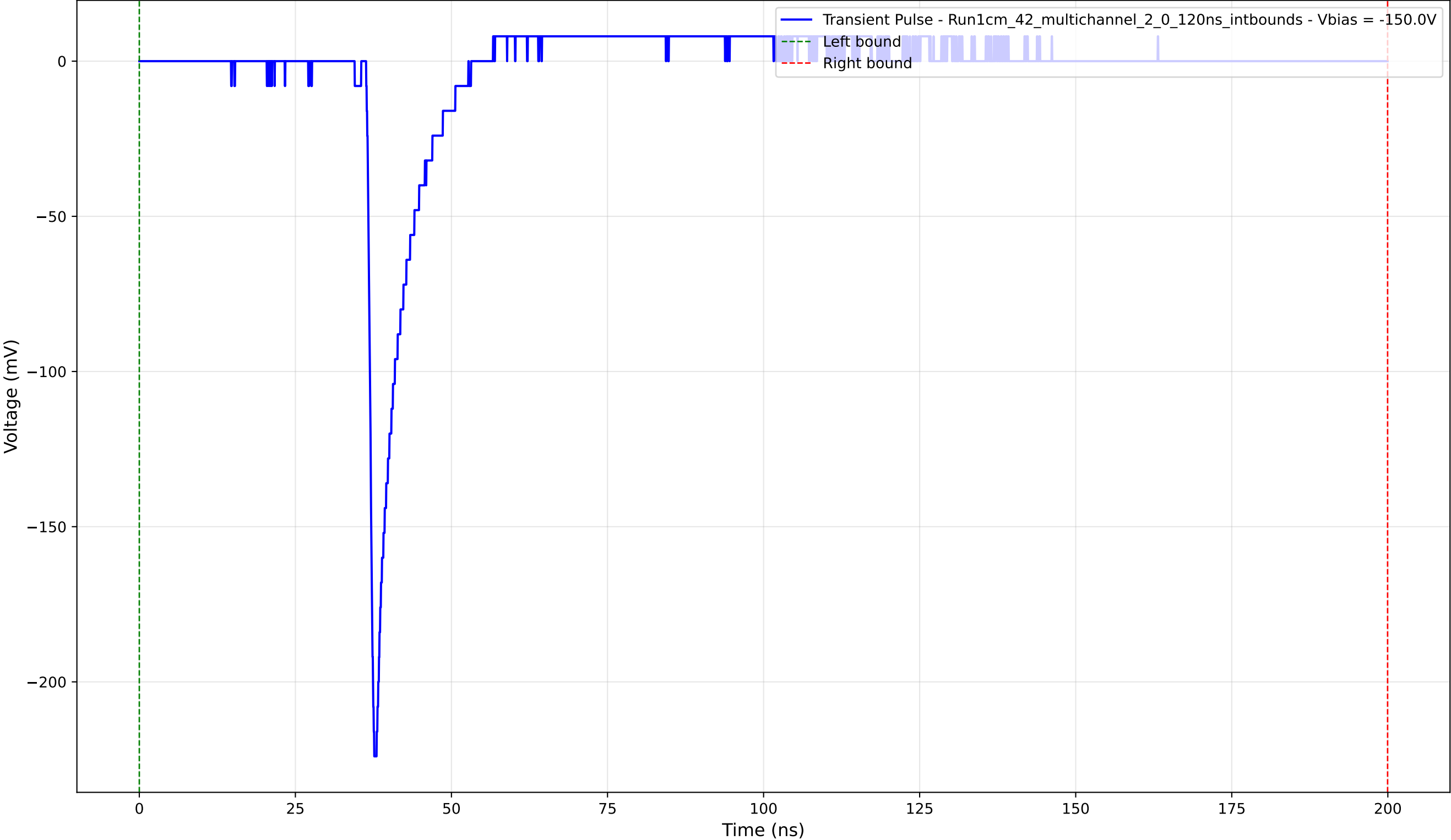
Transient Pulse - Sample: 1cm_42_multichannel - Position: 1555.0 \mu\text{m} - Charge: 12.07 pC - Rise Time: 0.97 ns
