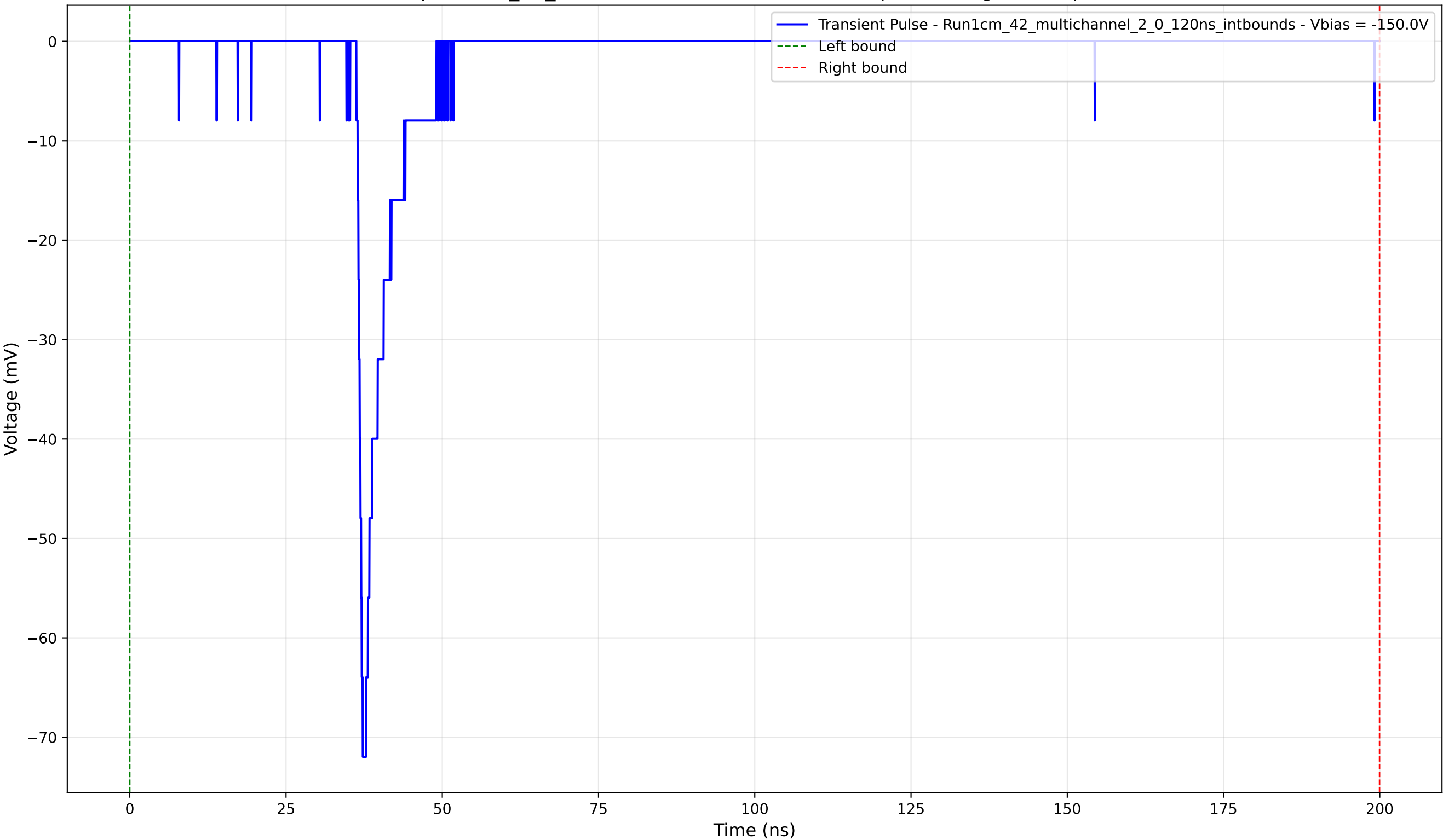
Transient Pulse - Sample: 1cm_42_multichannel - Position: 1825.0 \mu\text{m} - Charge: 6.10 pC - Rise Time: 1.00 ns
