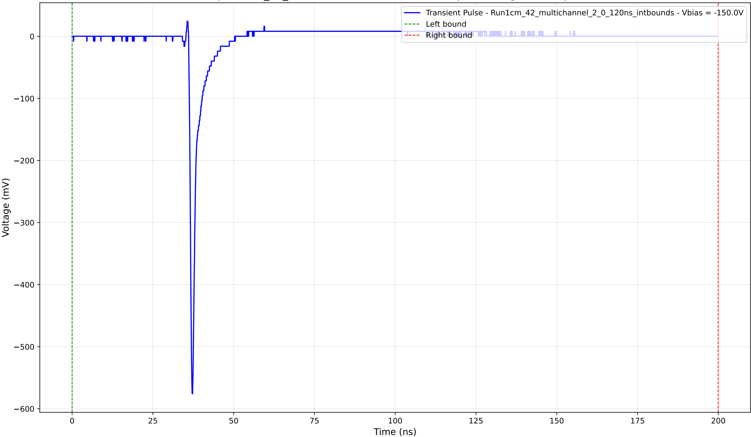
Transient Pulse - Sample: 1cm_42_multichannel - Position: 2200.0 \mu\text{m} - Charge: 15.77 pC - Rise Time: 0.75 ns
