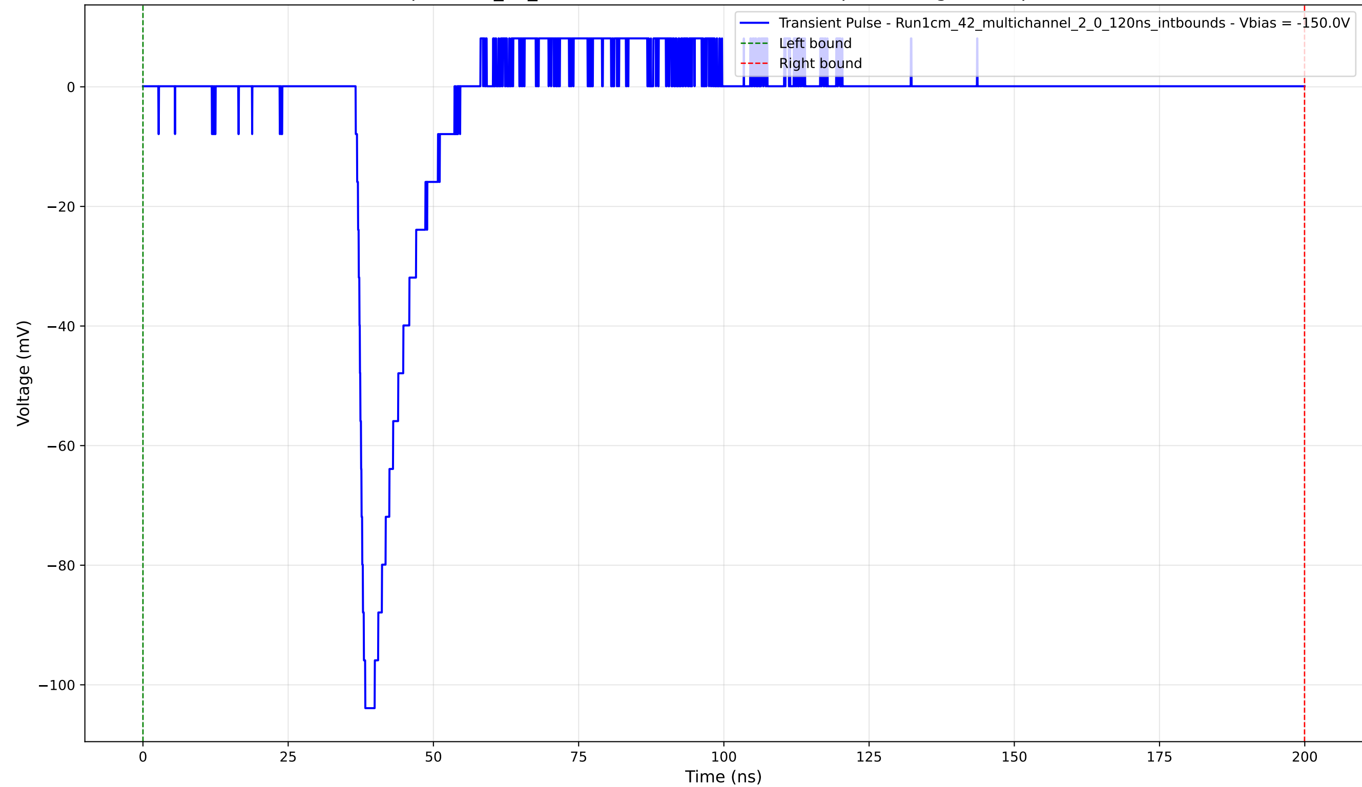
Transient Pulse - Sample: 1cm_42_multichannel - Position: 3750.0 \mu\text{m} - Charge: 9.76 pC - Rise Time: 1.19 ns
