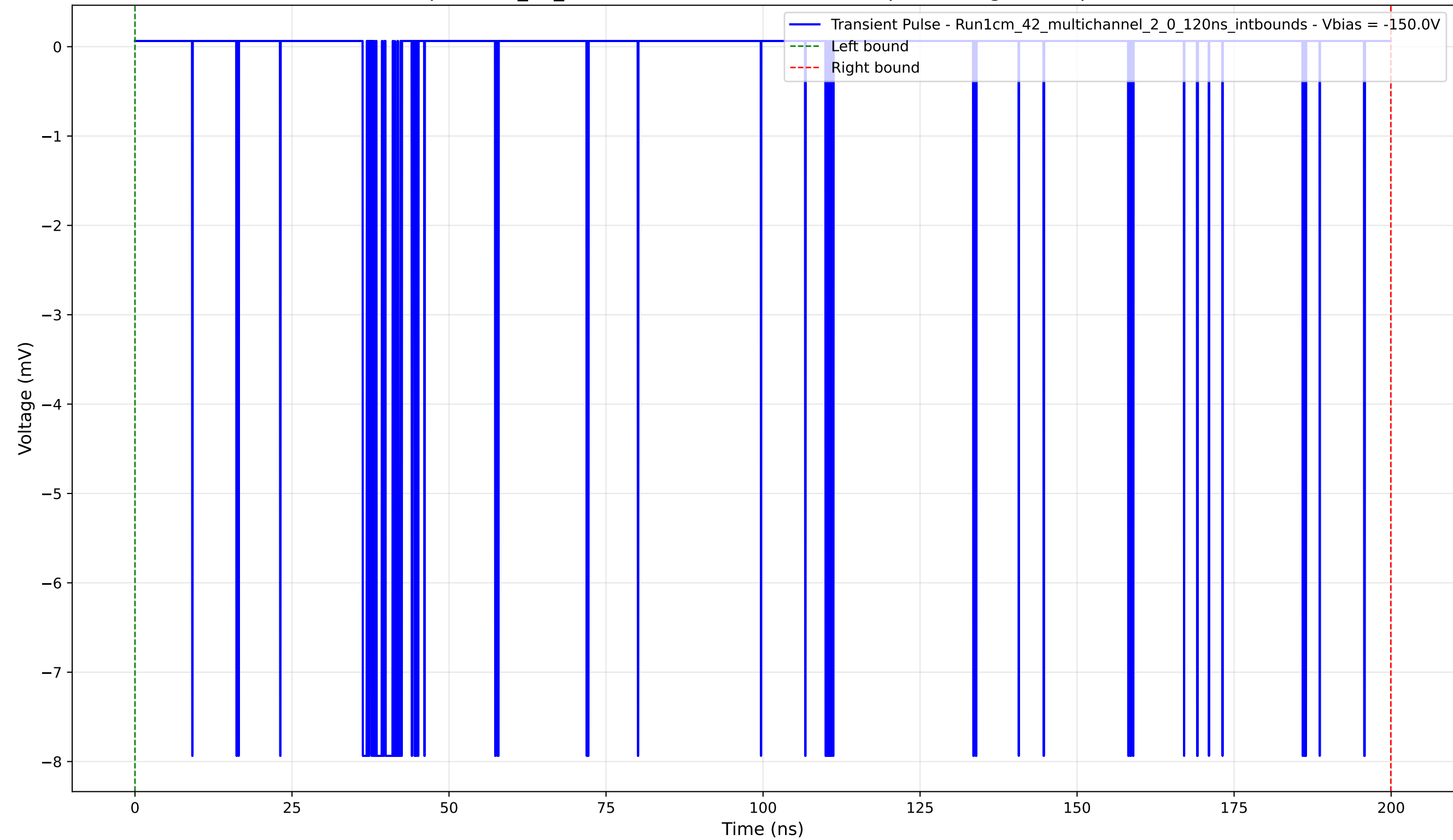
Transient Pulse - Sample: 1cm_42_multichannel - Position: 4910.0 \mu\text{m} - Charge: 1.03 pC - Rise Time: 0.04 ns
