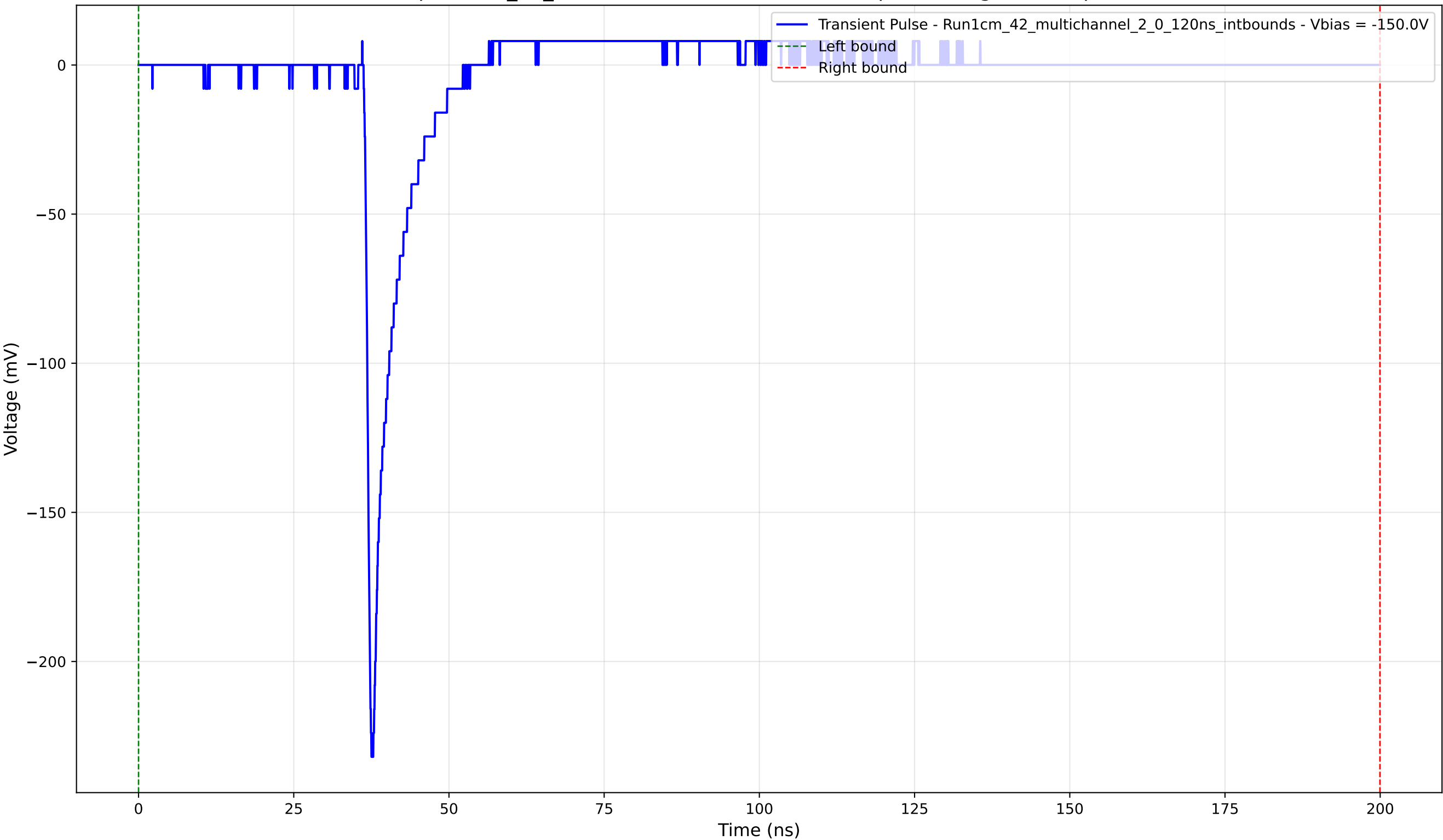
Transient Pulse - Sample: 1cm_42_multichannel - Position: 3055.0 \mu\text{m} - Charge: 11.26 pC - Rise Time: 0.92 ns
