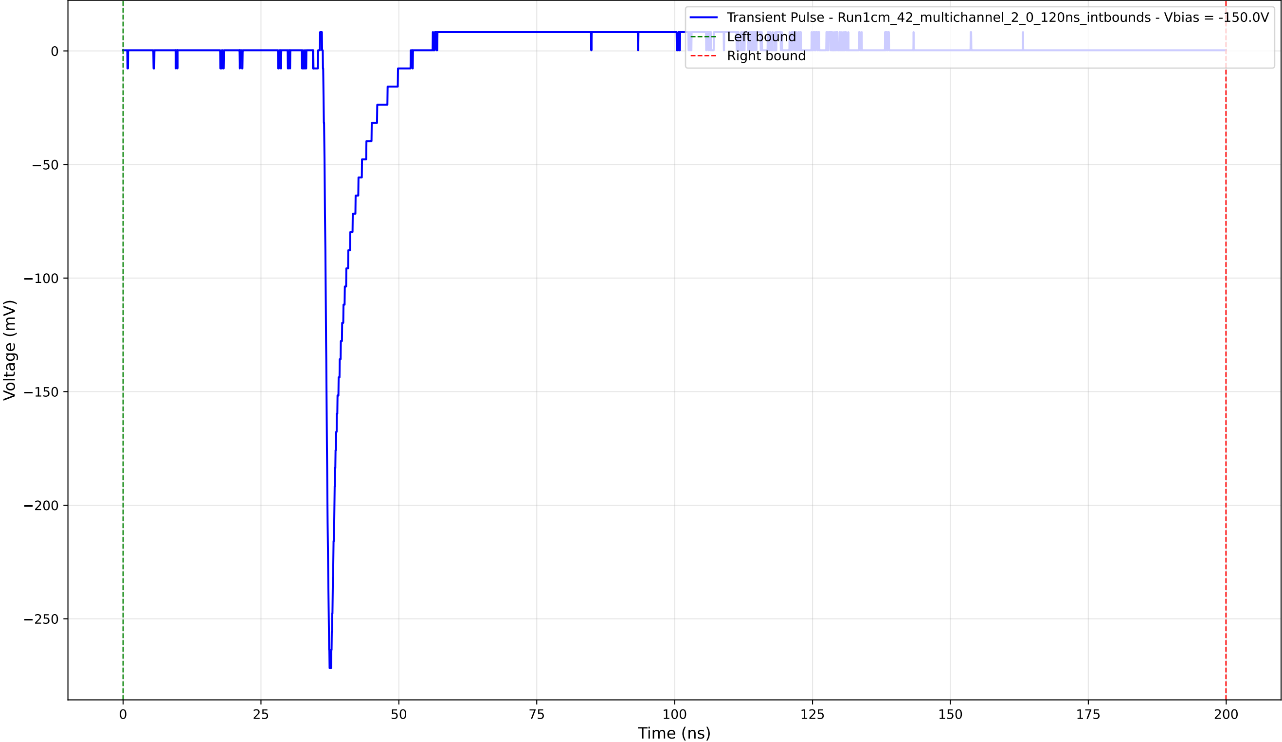
Transient Pulse - Sample: 1cm_42_multichannel - Position: 2975.0 \mu\text{m} - Charge: 11.31 pC - Rise Time: 0.89 ns
