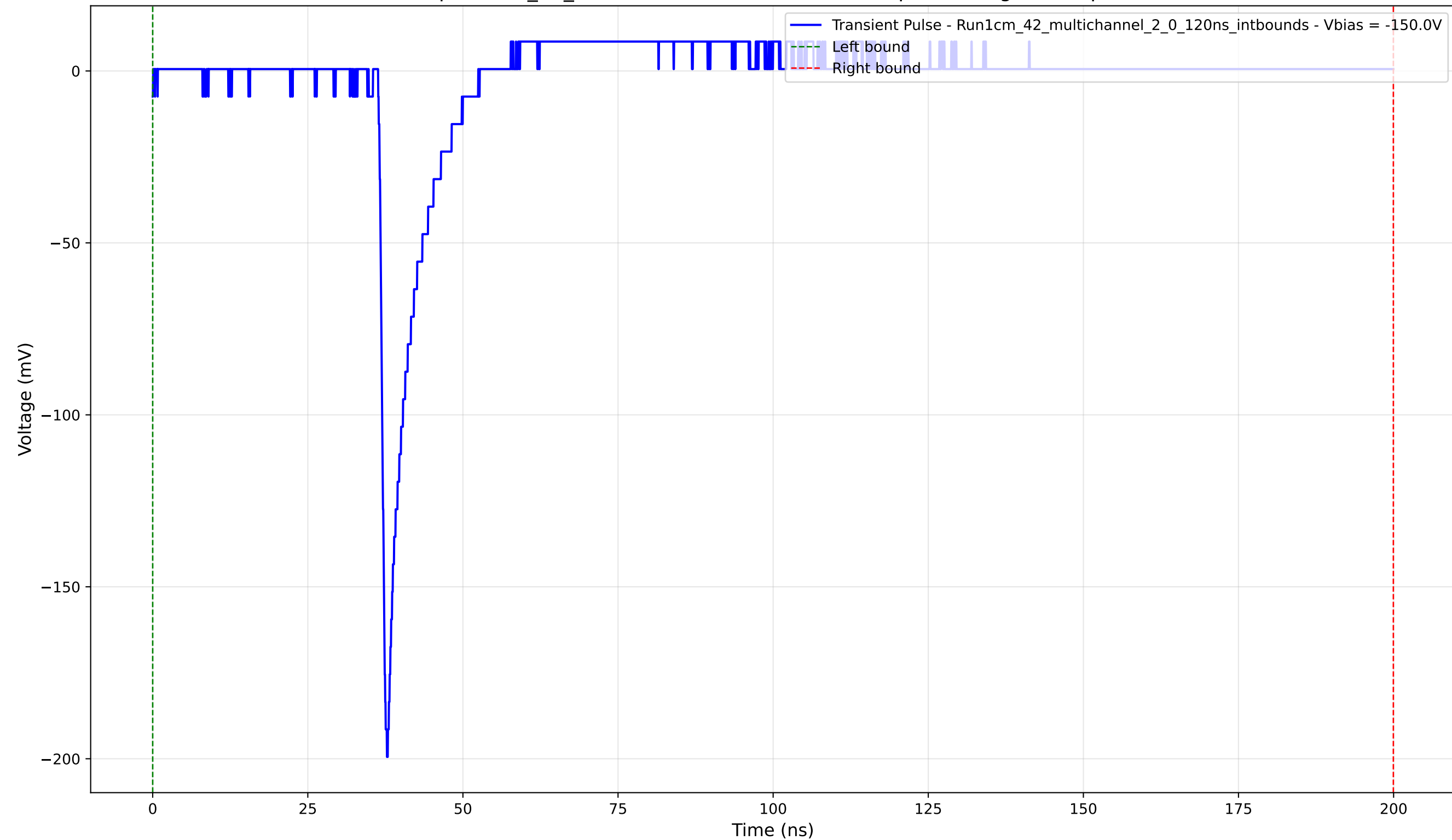
Transient Pulse - Sample: 1cm_42_multichannel - Position: 3175.0 \mu\text{m} - Charge: 9.86 pC - Rise Time: 0.94 ns
