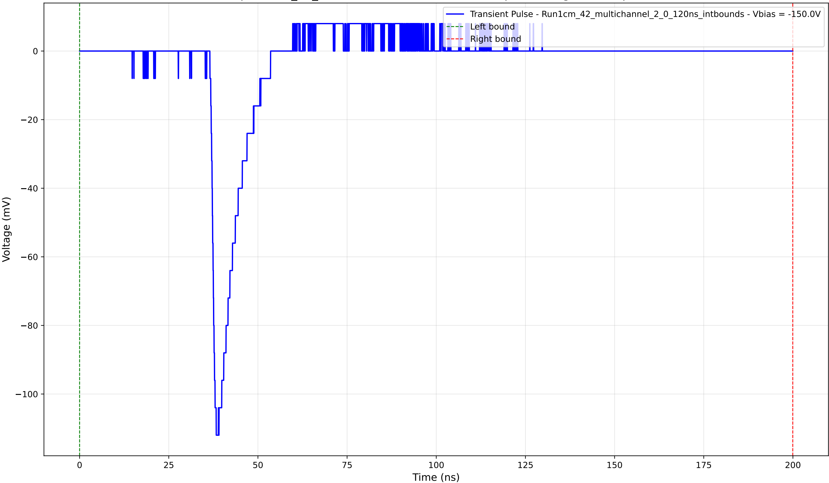
Transient Pulse - Sample: 1cm_42_multichannel - Position: 3650.0 \mu\text{m} - Charge: 10.57 pC - Rise Time: 1.22 ns
