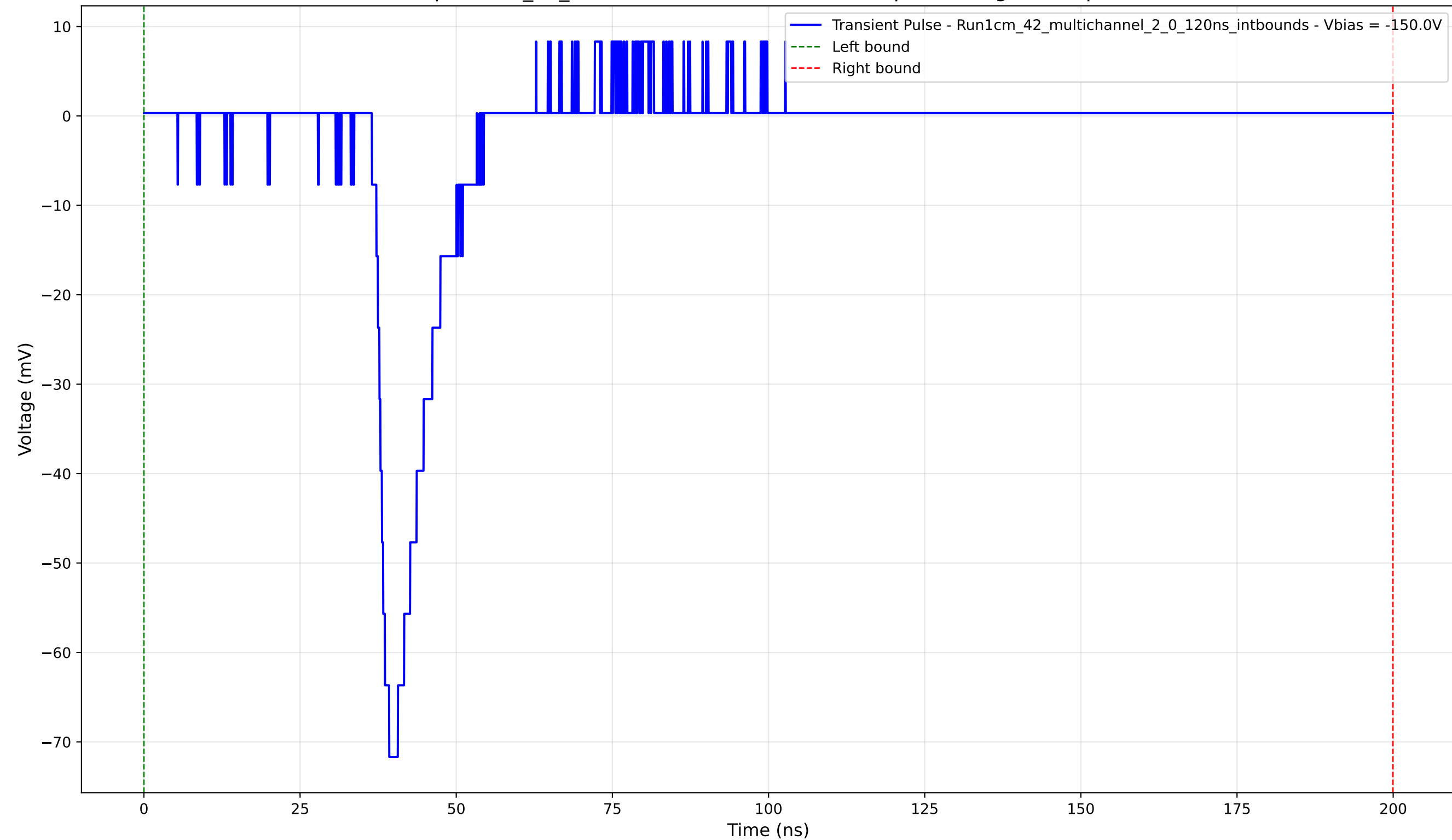
Transient Pulse - Sample: 1cm_42_multichannel - Position: 4485.0 \mu\text{m} - Charge: 8.99 pC - Rise Time: 2.76 ns
