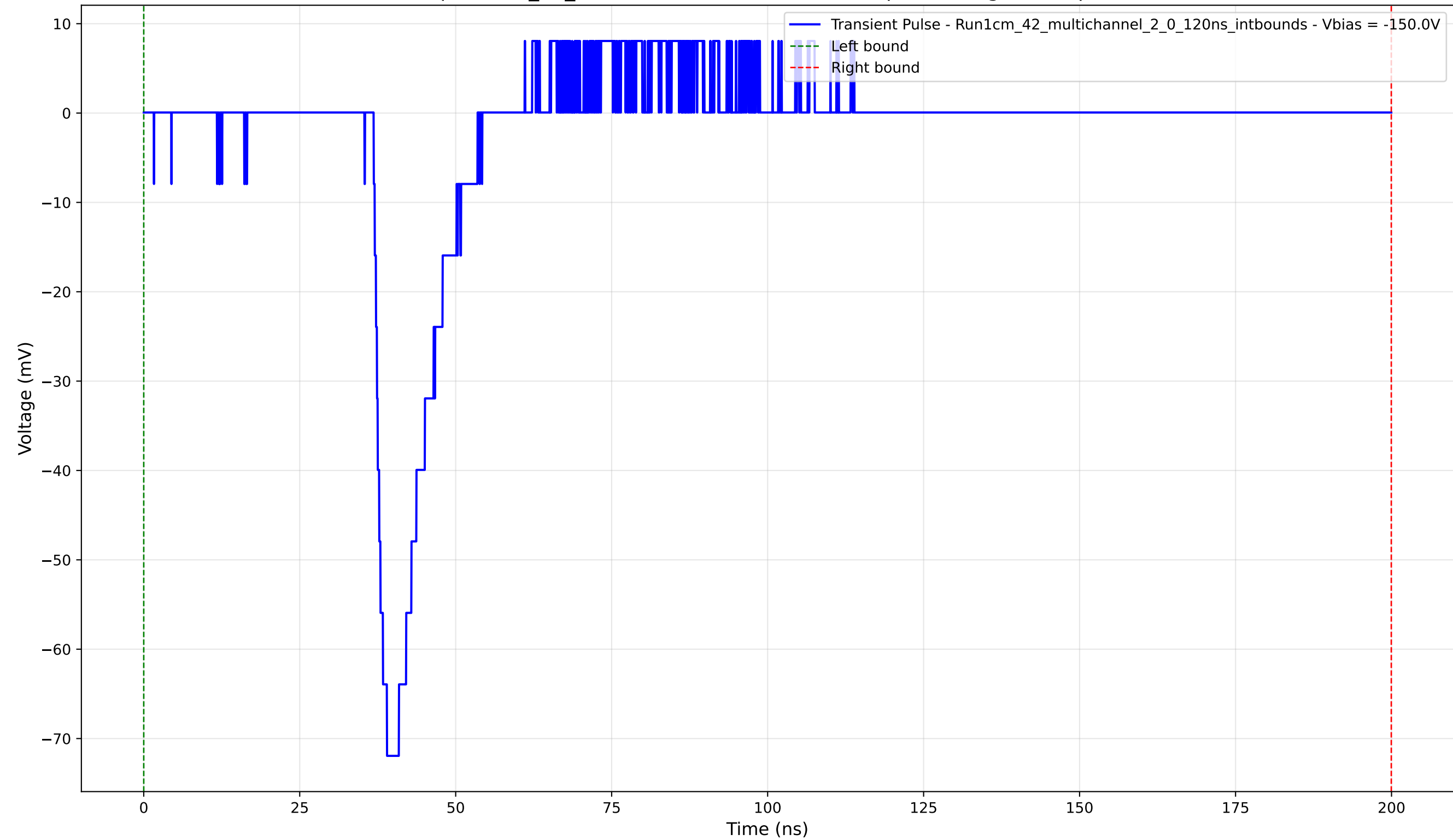
Transient Pulse - Sample: 1cm_42_multichannel - Position: 225.0 \mu\text{m} - Charge: 8.05 pC - Rise Time: 2.12 ns
