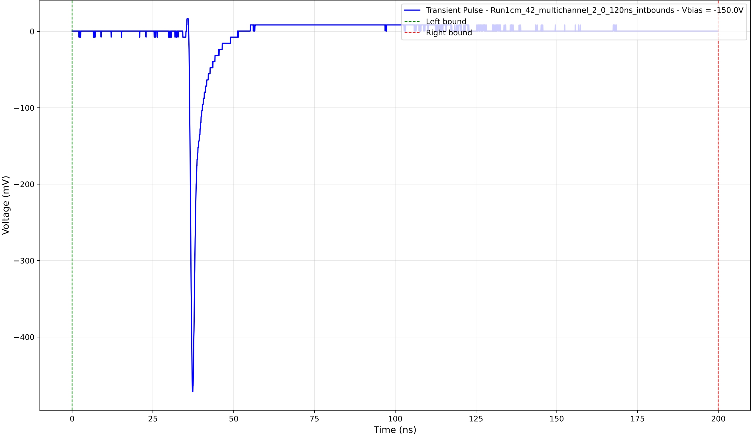
Transient Pulse - Sample: 1cm_42_multichannel - Position: 2080.0 \mu\text{m} - Charge: 14.25 pC - Rise Time: 0.78 ns
