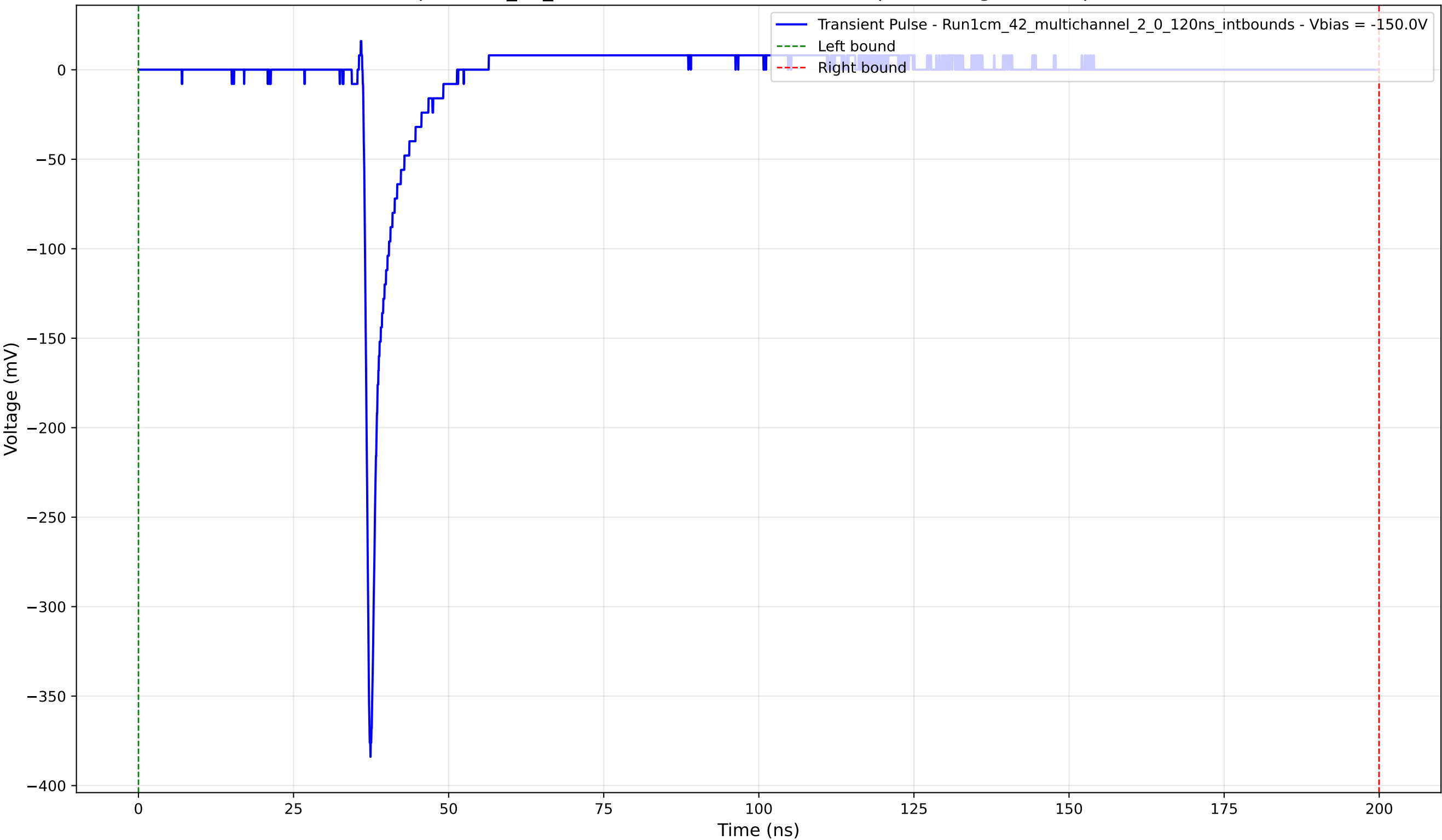
Transient Pulse - Sample: 1cm_42_multichannel - Position: 2770.0 \mu\text{m} - Charge: 12.88 pC - Rise Time: 0.82 ns
