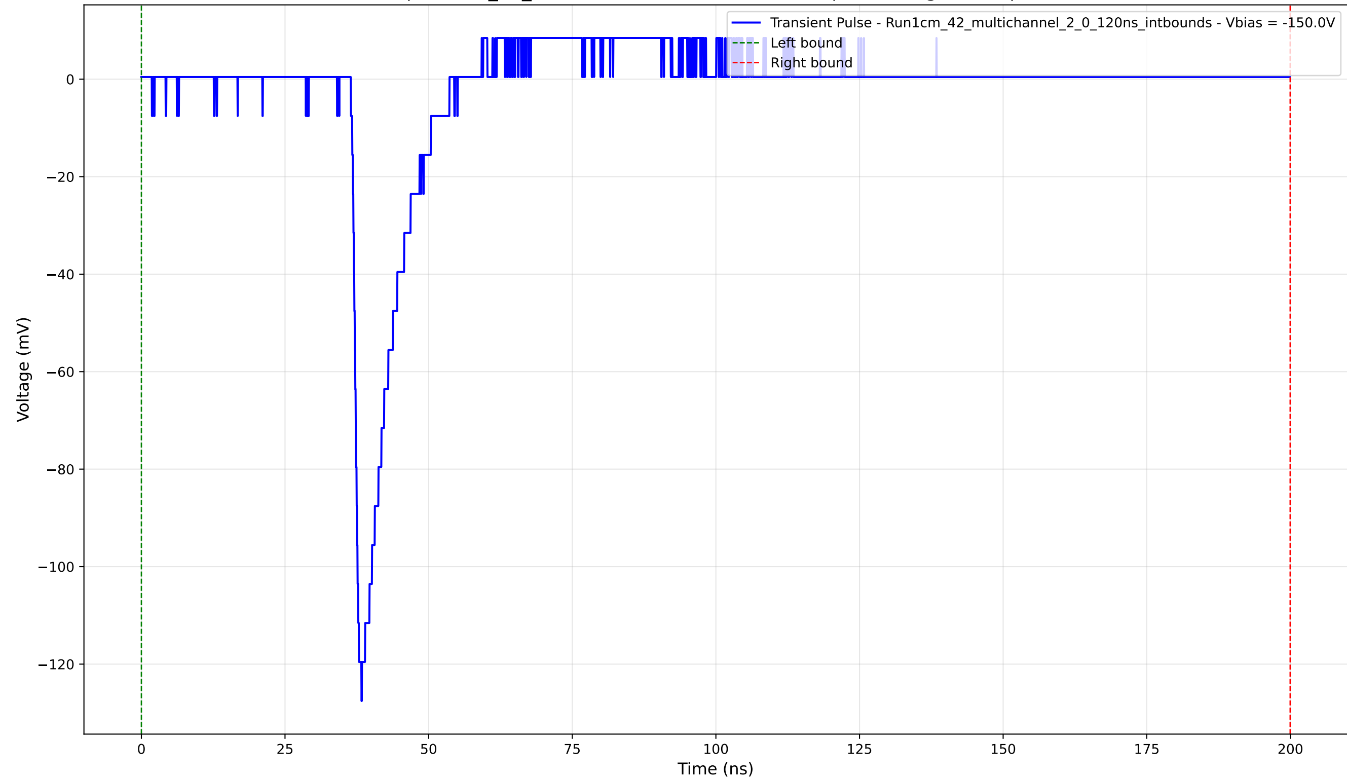
Transient Pulse - Sample: 1cm_42_multichannel - Position: 3535.0 \mu\text{m} - Charge: 9.05 pC - Rise Time: 1.17 ns
