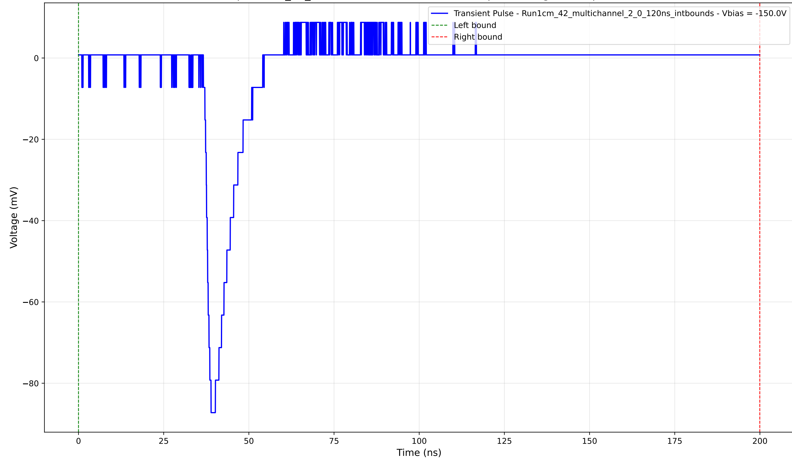
Transient Pulse - Sample: 1cm_42_multichannel - Position: 4105.0 \mu\text{m} - Charge: 8.18 pC - Rise Time: 1.47 ns
