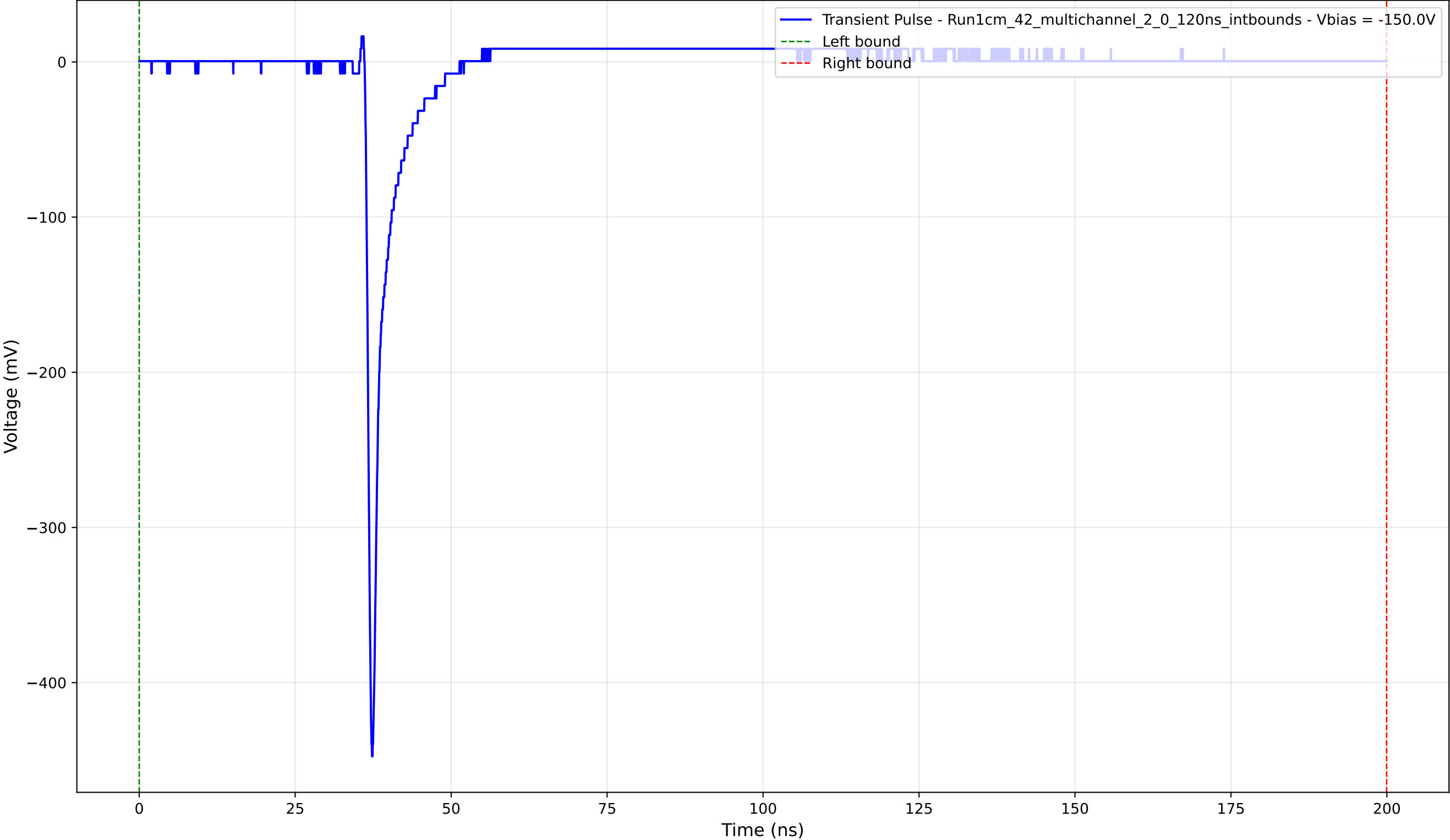
Transient Pulse - Sample: 1cm_42_multichannel - Position: 2025.0 \mu\text{m} - Charge: 13.32 pC - Rise Time: 0.75 ns
