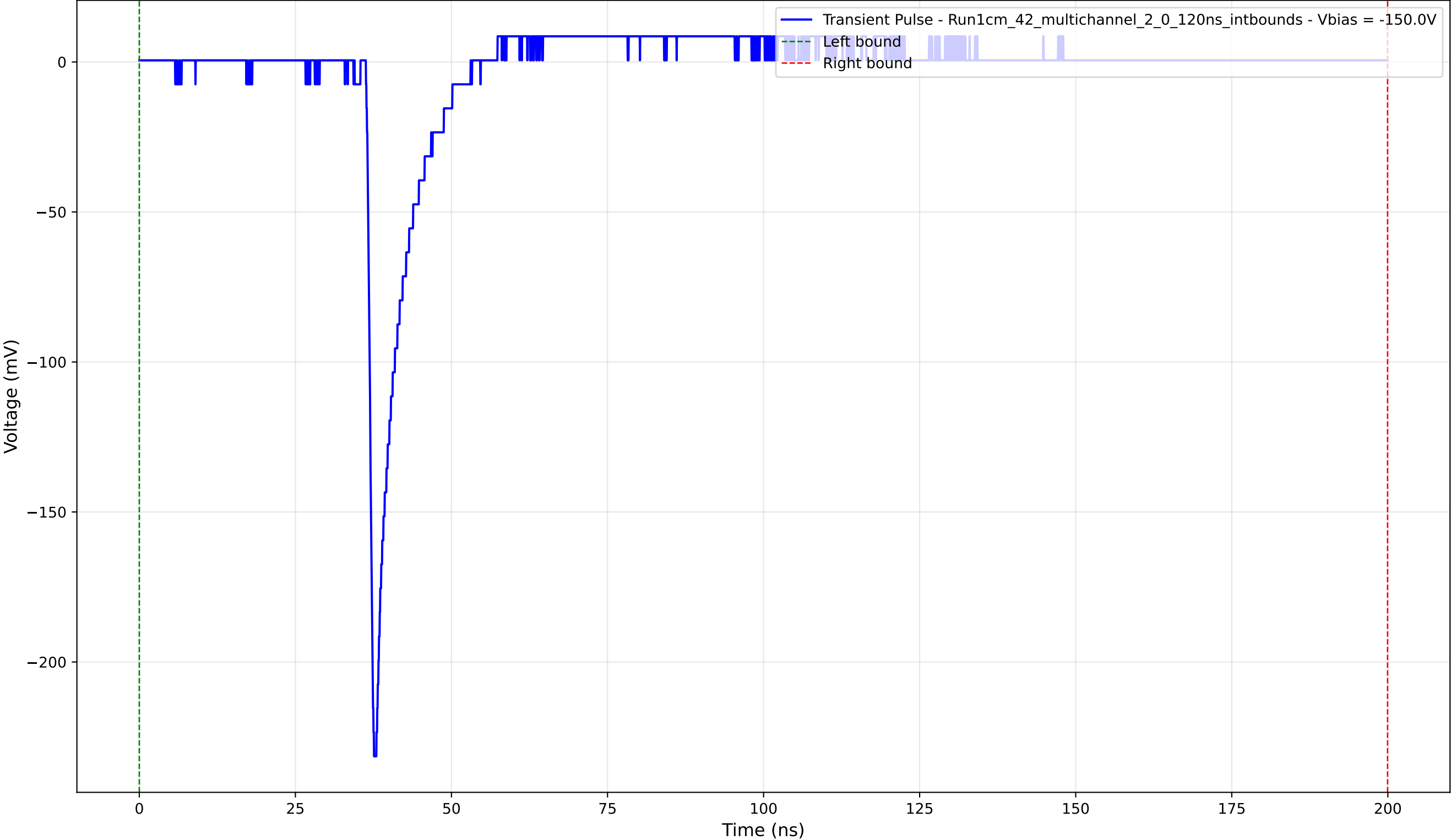
Transient Pulse - Sample: 1cm_42_multichannel - Position: 1595.0 \mu\text{m} - Charge: 11.55 pC - Rise Time: 0.96 ns
