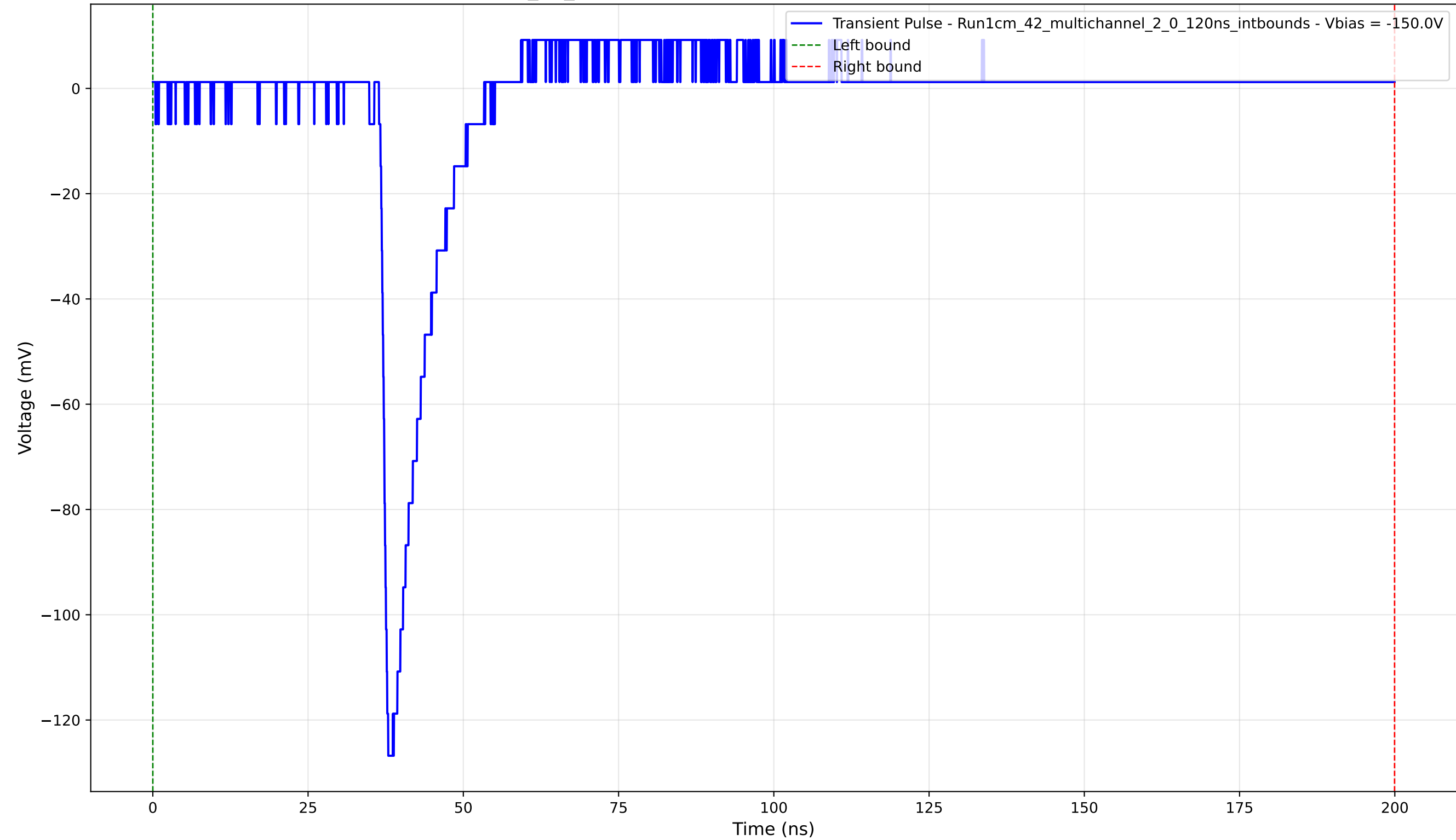
Transient Pulse - Sample: 1cm_42_multichannel - Position: 3515.0 \mu\text{m} - Charge: 7.77 pC - Rise Time: 1.09 ns
