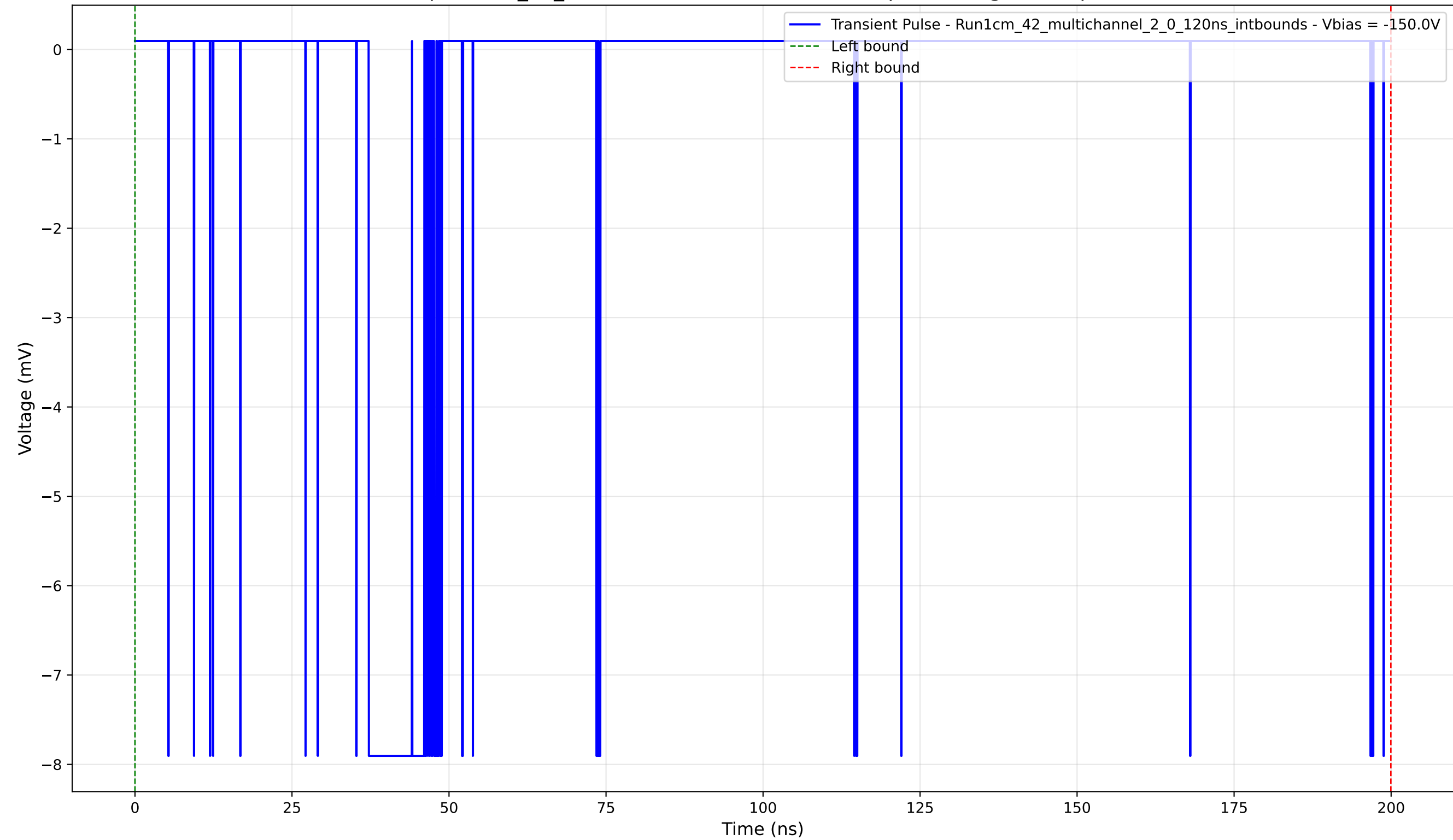
Transient Pulse - Sample: 1cm_42_multichannel - Position: 3870.0 \mu\text{m} - Charge: 1.54 pC - Rise Time: 0.04 ns
