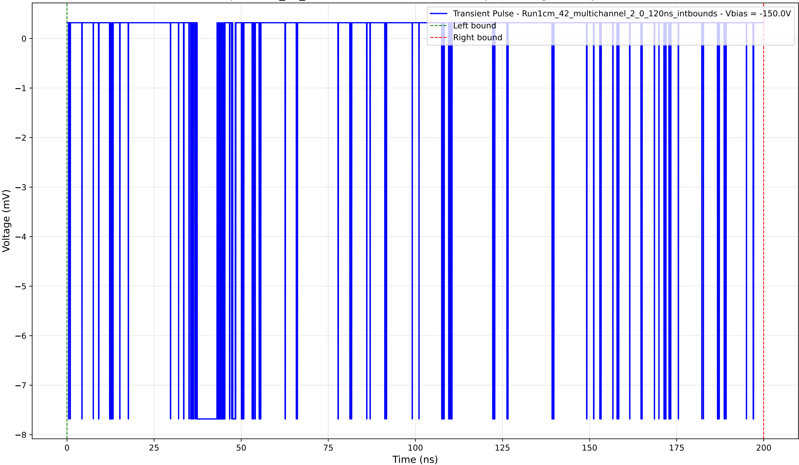
Transient Pulse - Sample: 1cm_42_multichannel - Position: 4880.0 \mu\text{m} - Charge: 1.45 pC - Rise Time: 0.04 ns
