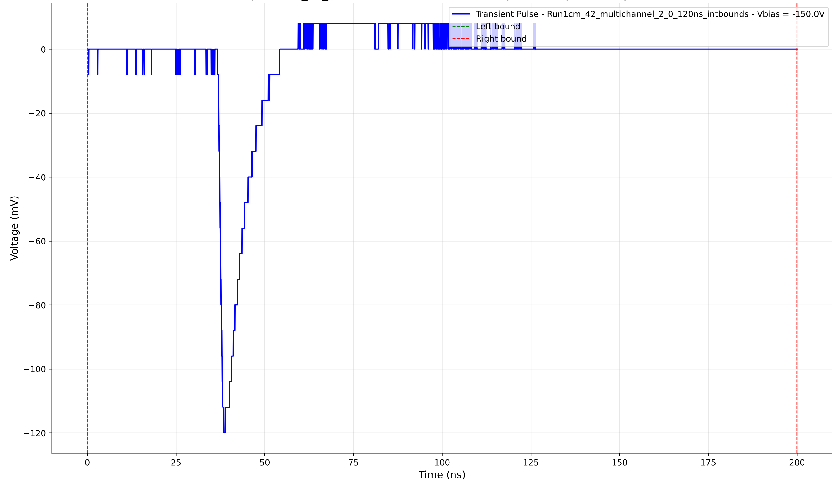
Transient Pulse - Sample: 1cm_42_multichannel - Position: 935.0 \mu\text{m} - Charge: 10.49 pC - Rise Time: 1.30 ns
