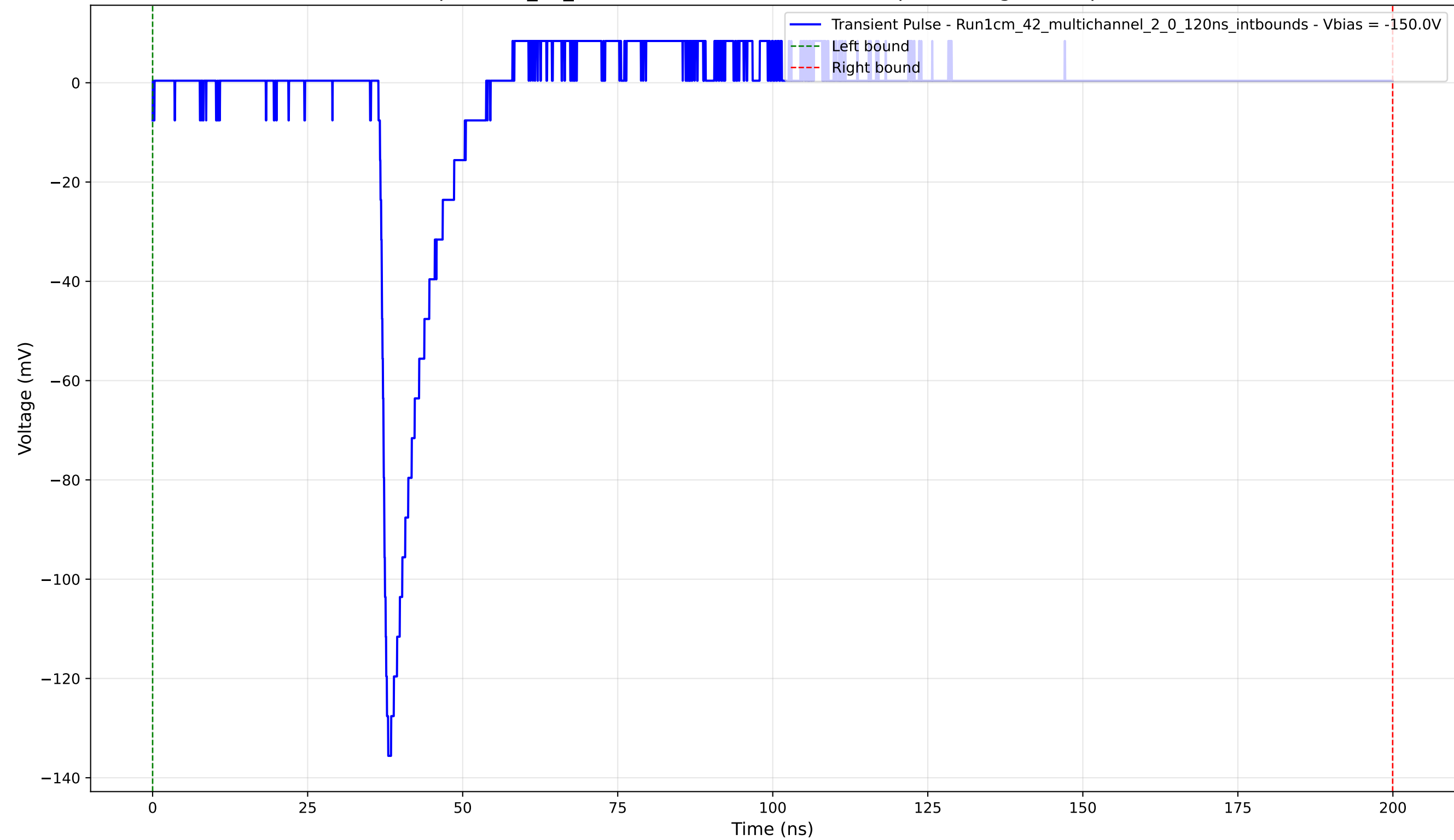
Transient Pulse - Sample: 1cm_42_multichannel - Position: 3475.0 \mu\text{m} - Charge: 9.39 pC - Rise Time: 1.13 ns
