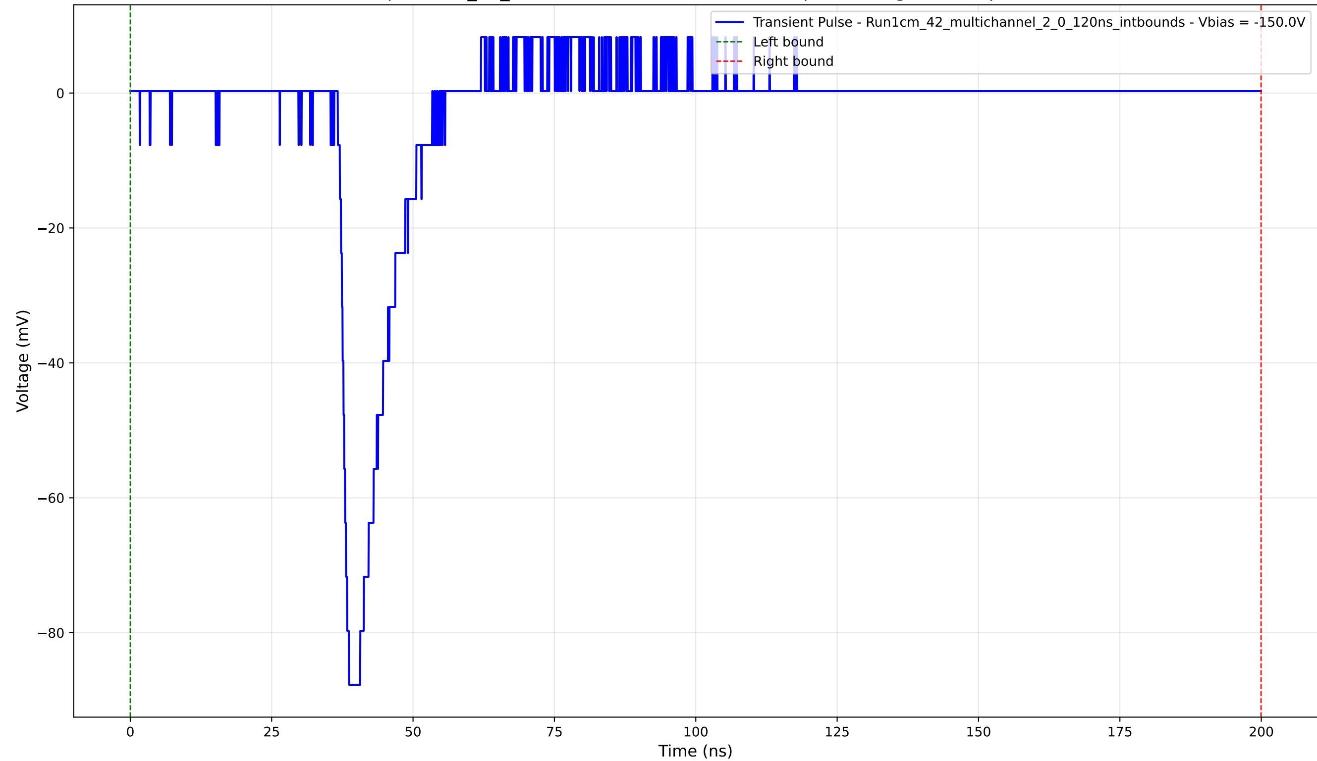
Transient Pulse - Sample: 1cm_42_multichannel - Position: 4040.0 \mu\text{m} - Charge: 10.05 pC - Rise Time: 1.31 ns
