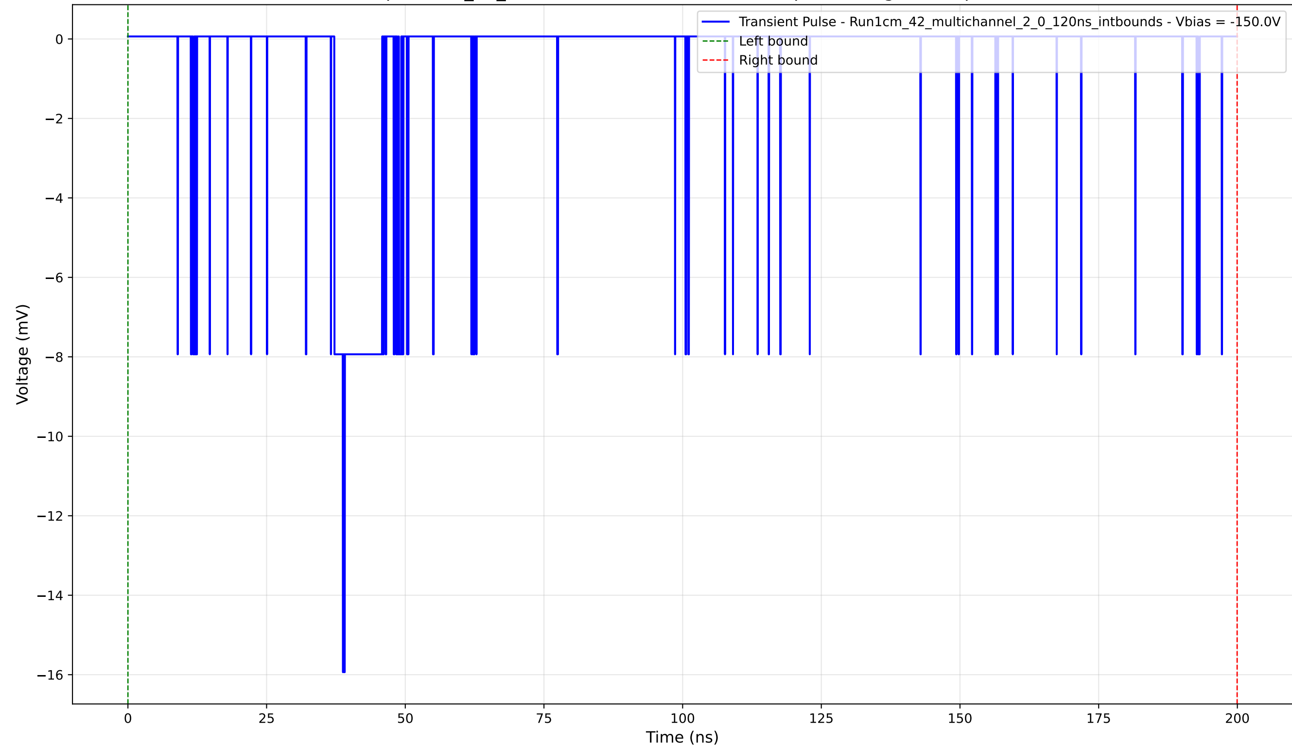
Transient Pulse - Sample: 1cm_42_multichannel - Position: 4870.0 \mu\text{m} - Charge: 1.96 pC - Rise Time: 1.55 ns
