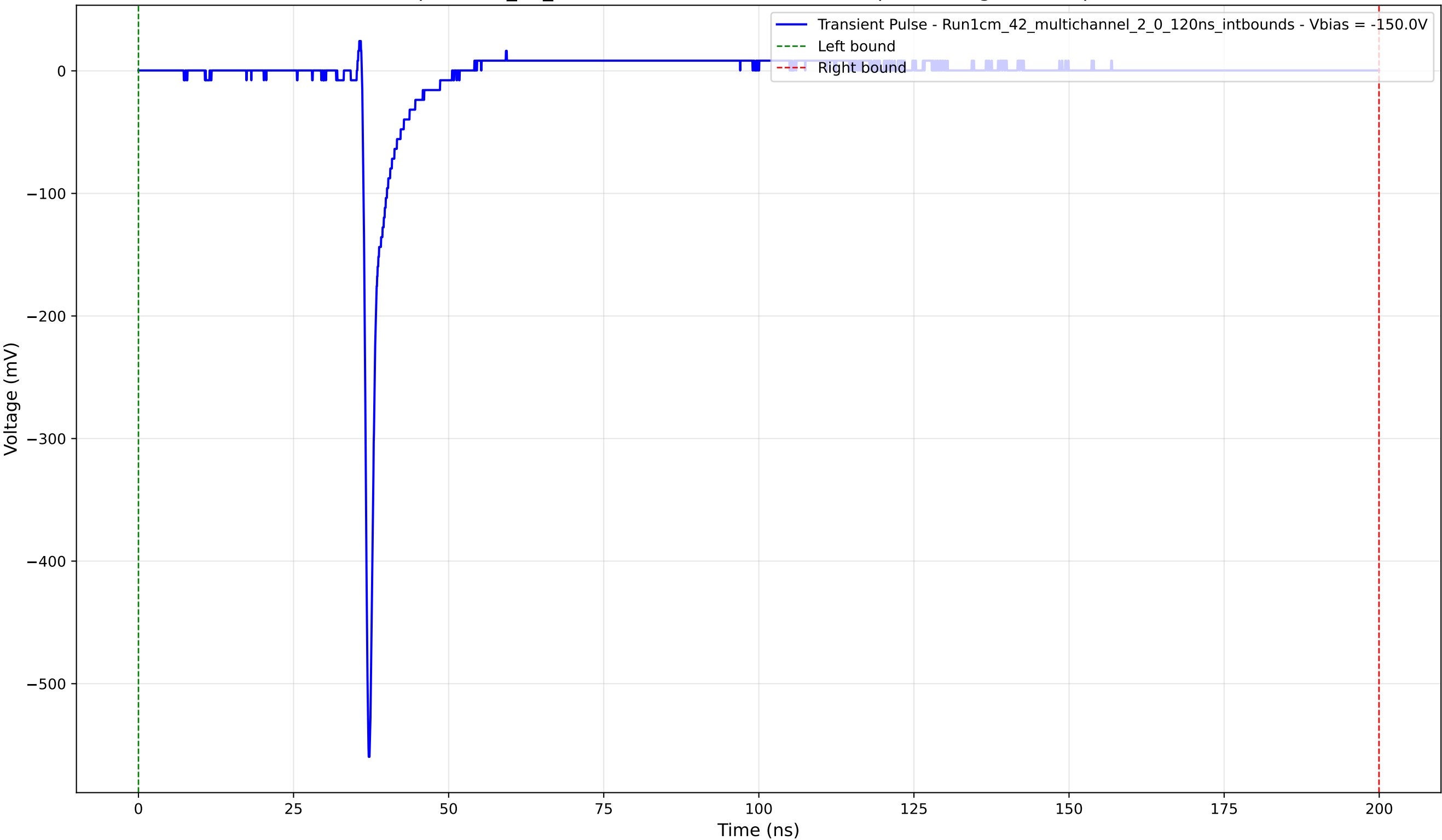
Transient Pulse - Sample: 1cm_42_multichannel - Position: 2520.0 \mu\text{m} - Charge: 15.21 pC - Rise Time: 0.74 ns
