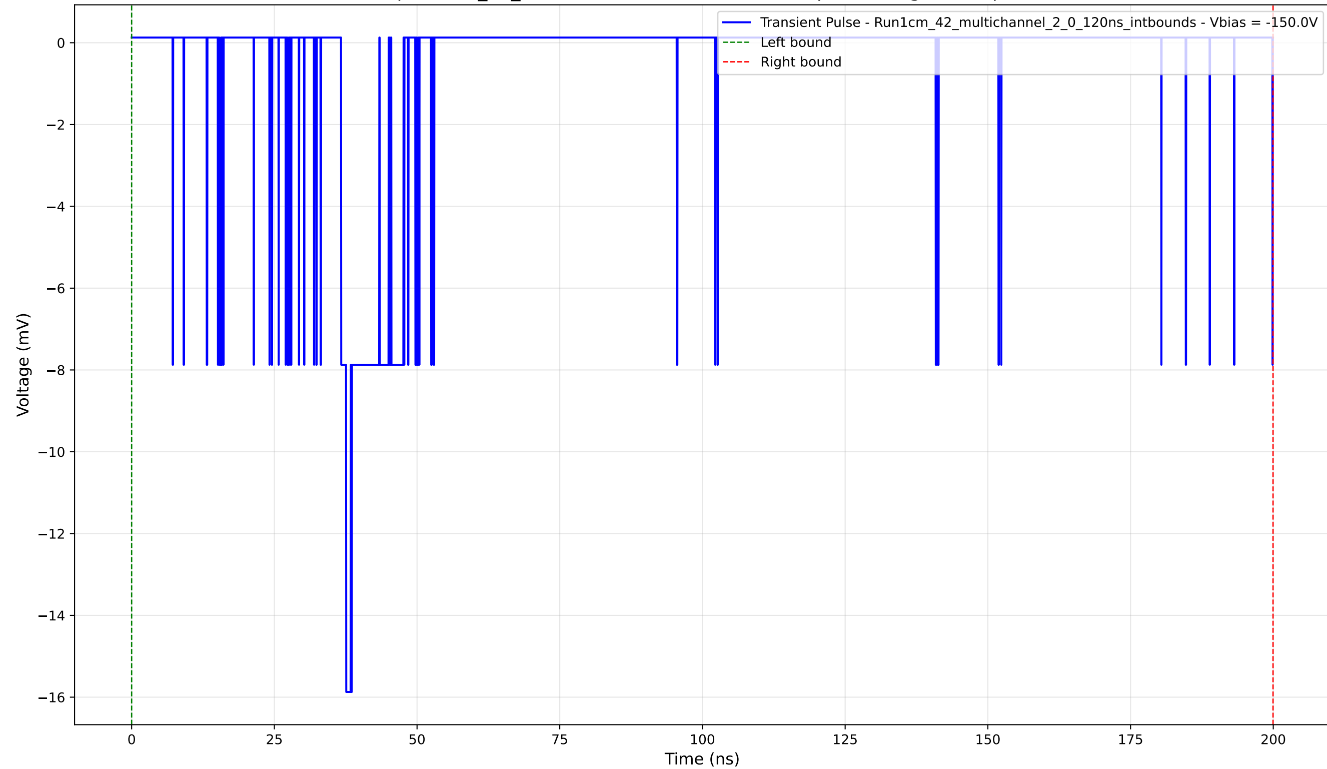
Transient Pulse - Sample: 1cm_42_multichannel - Position: 1370.0 \mu\text{m} - Charge: 1.83 pC - Rise Time: 0.91 ns
