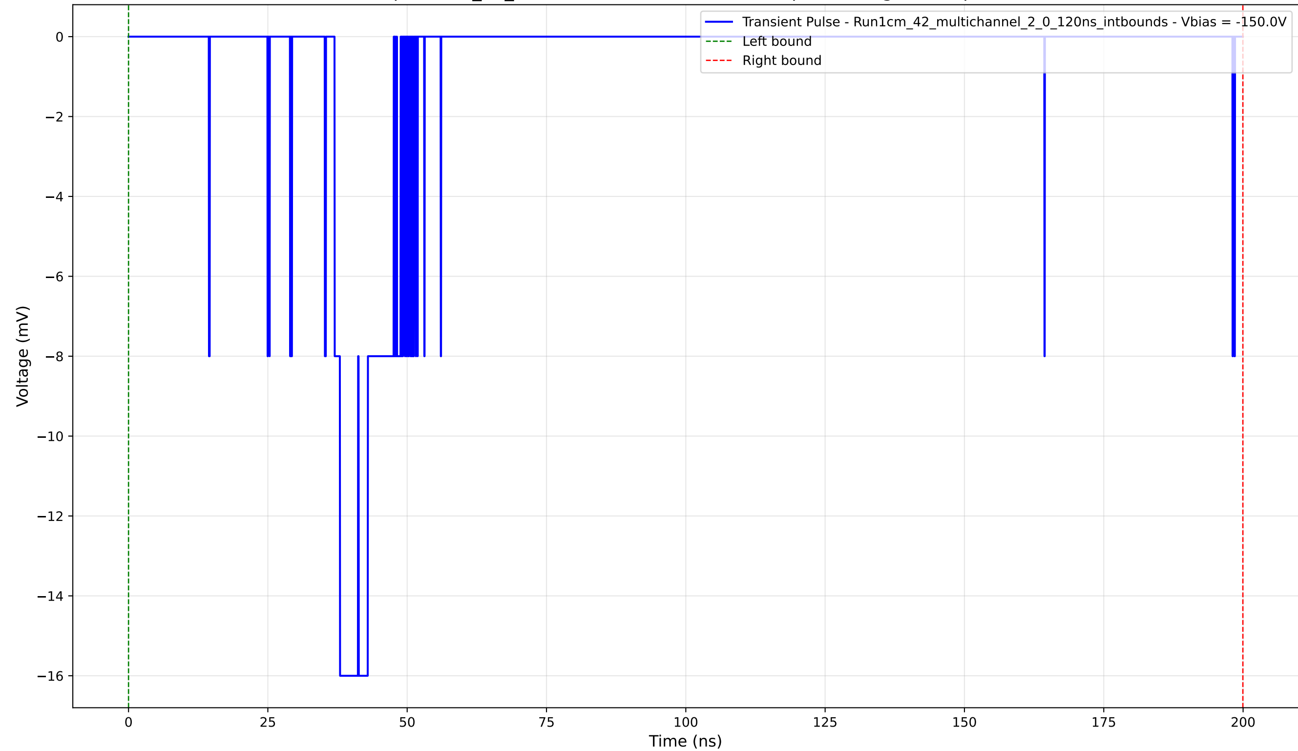
Transient Pulse - Sample: 1cm_42_multichannel - Position: 310.0 \mu\text{m} - Charge: 2.98 pC - Rise Time: 0.99 ns
