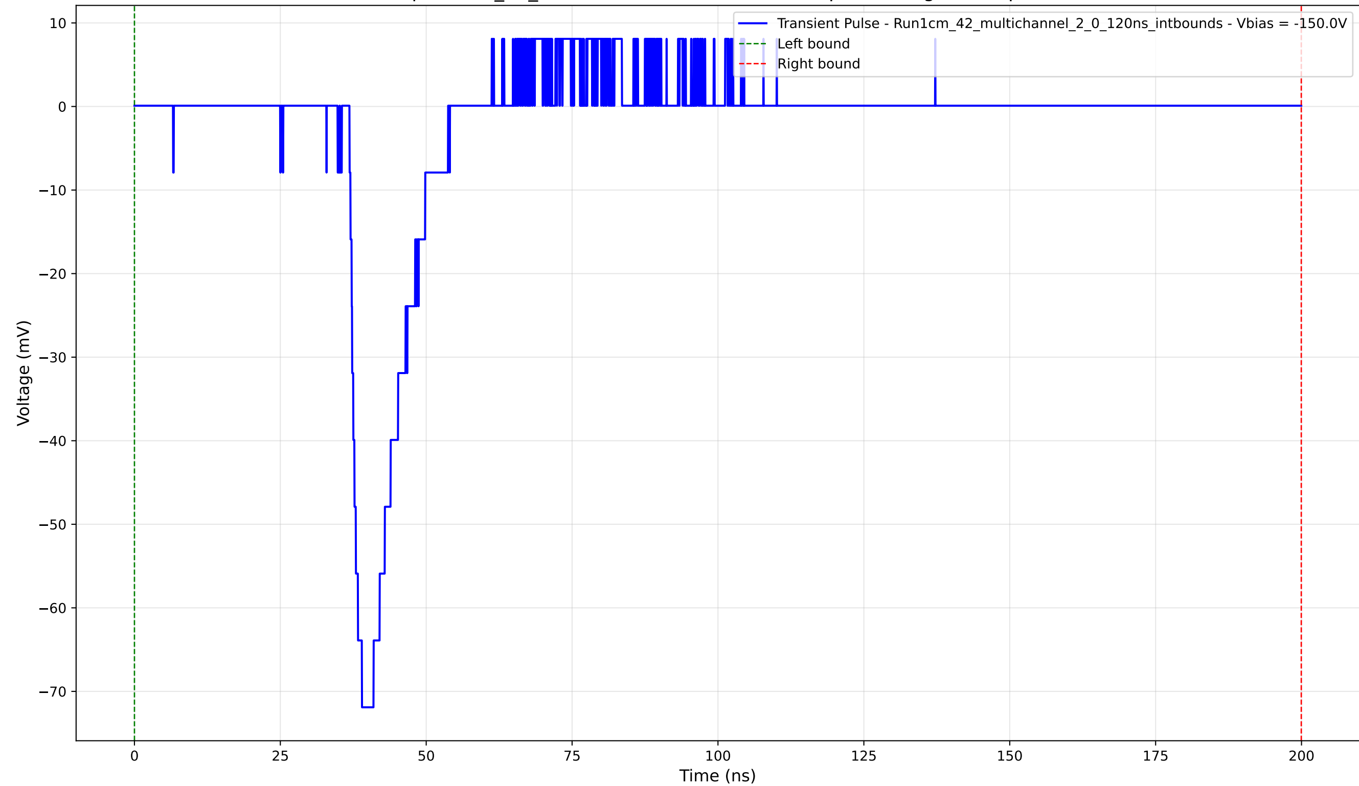
Transient Pulse - Sample: 1cm_42_multichannel - Position: 190.0 \mu\text{m} - Charge: 8.80 pC - Rise Time: 2.12 ns
