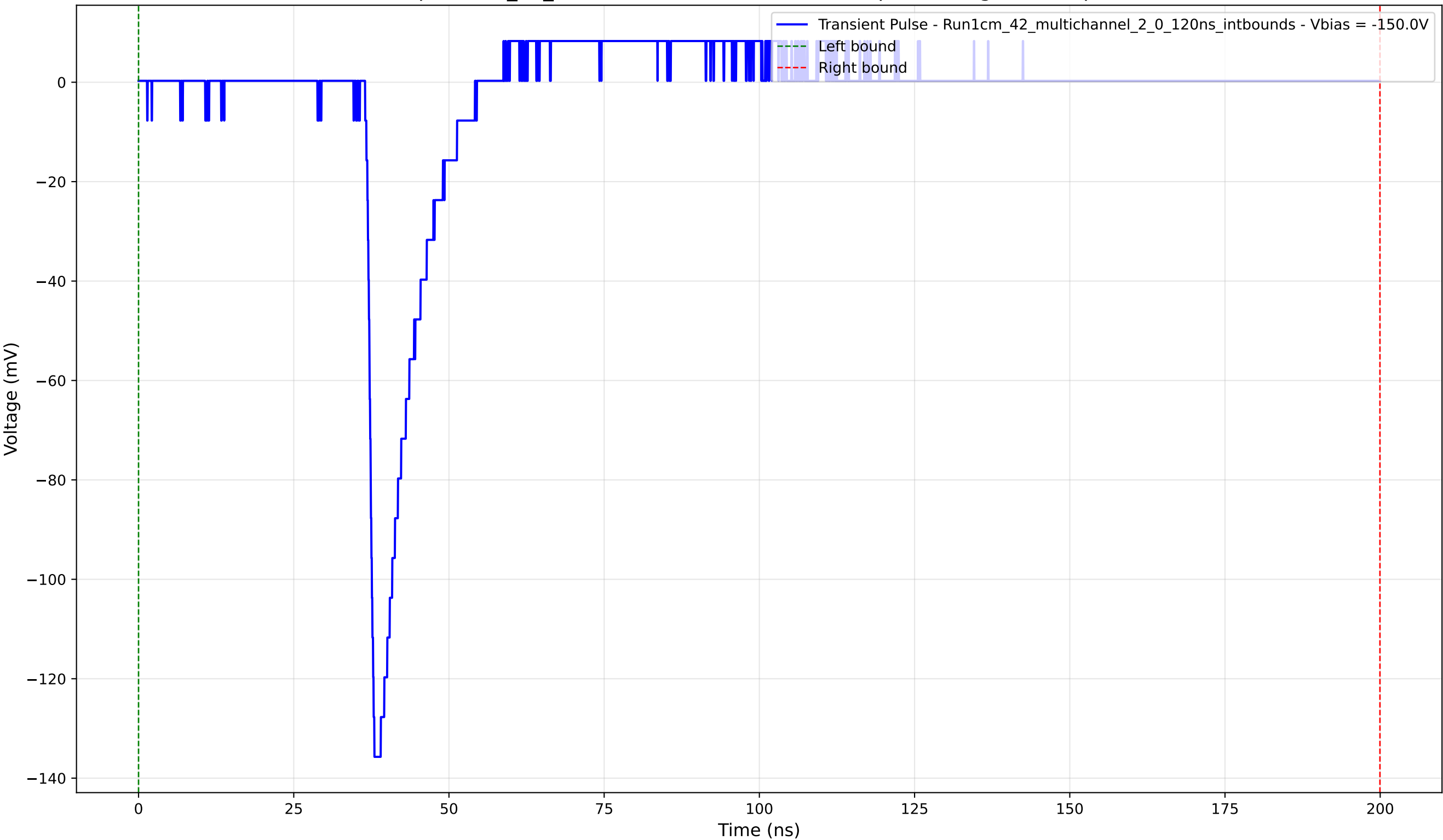
Transient Pulse - Sample: 1cm_42_multichannel - Position: 1150.0 \mu\text{m} - Charge: 10.51 pC - Rise Time: 1.17 ns
