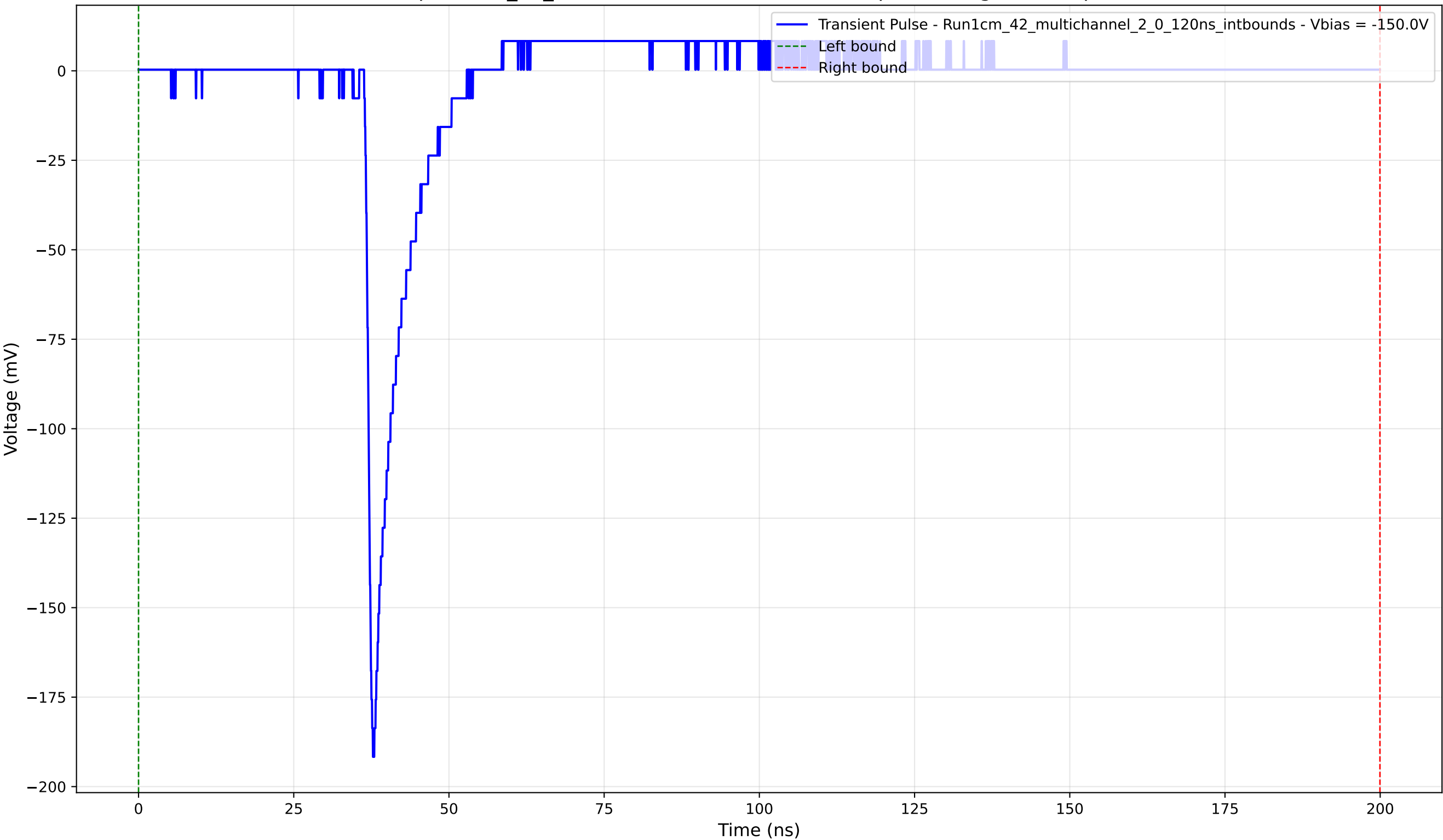
Transient Pulse - Sample: 1cm_42_multichannel - Position: 3240.0 \mu\text{m} - Charge: 10.37 pC - Rise Time: 0.98 ns
