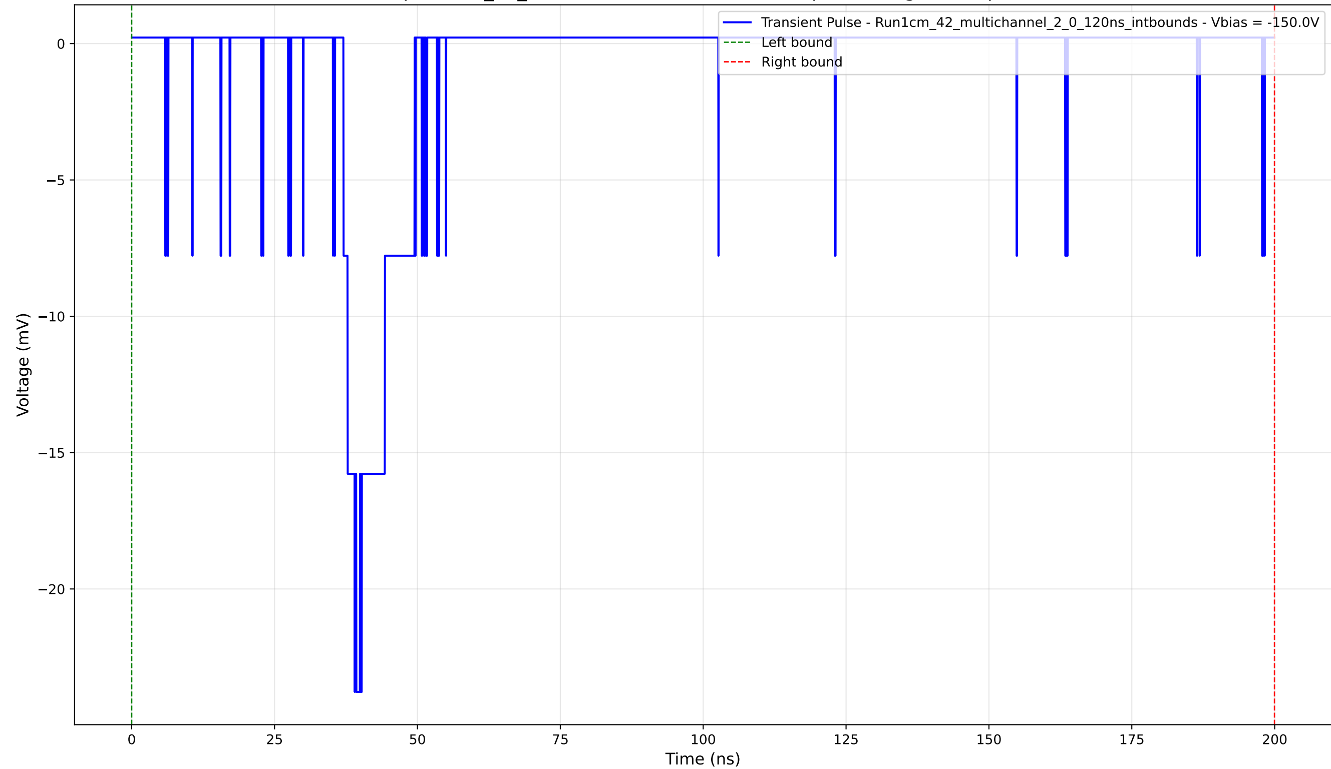
Transient Pulse - Sample: 1cm_42_multichannel - Position: 380.0 \mu\text{m} - Charge: 2.79 pC - Rise Time: 1.99 ns
