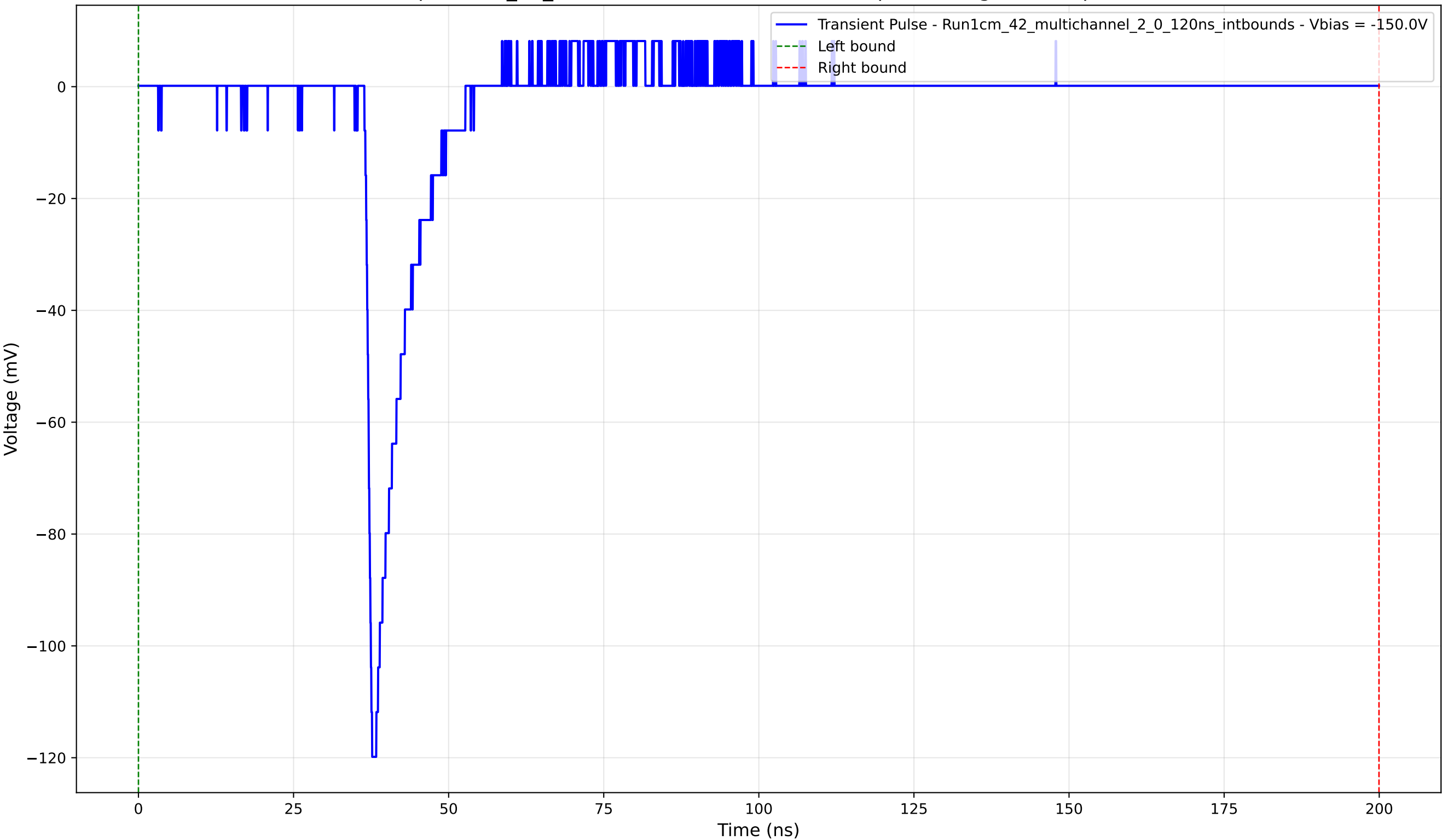
Transient Pulse - Sample: 1cm_42_multichannel - Position: 3320.0 \mu\text{m} - Charge: 10.25 pC - Rise Time: 0.98 ns
