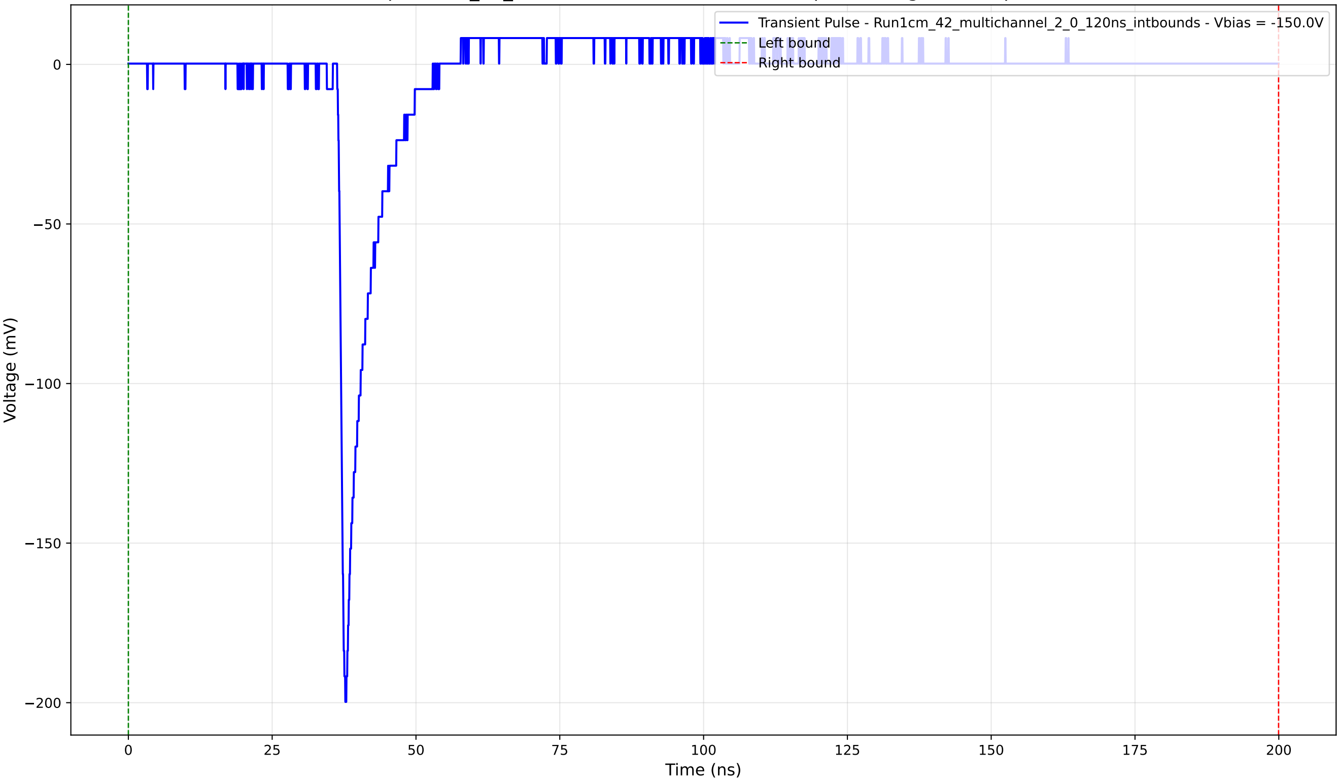
Transient Pulse - Sample: 1cm_42_multichannel - Position: 3165.0 \mu\text{m} - Charge: 10.99 pC - Rise Time: 0.94 ns
