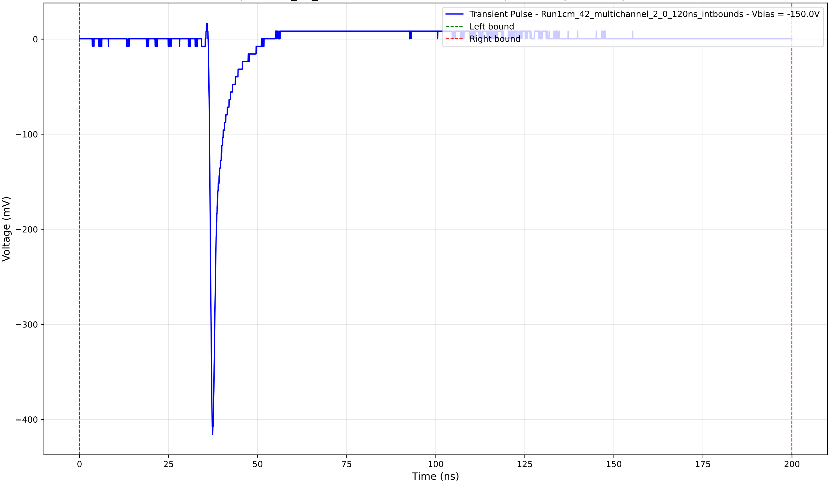
Transient Pulse - Sample: 1cm_42_multichannel - Position: 2740.0 \mu\text{m} - Charge: 13.31 pC - Rise Time: 0.81 ns
