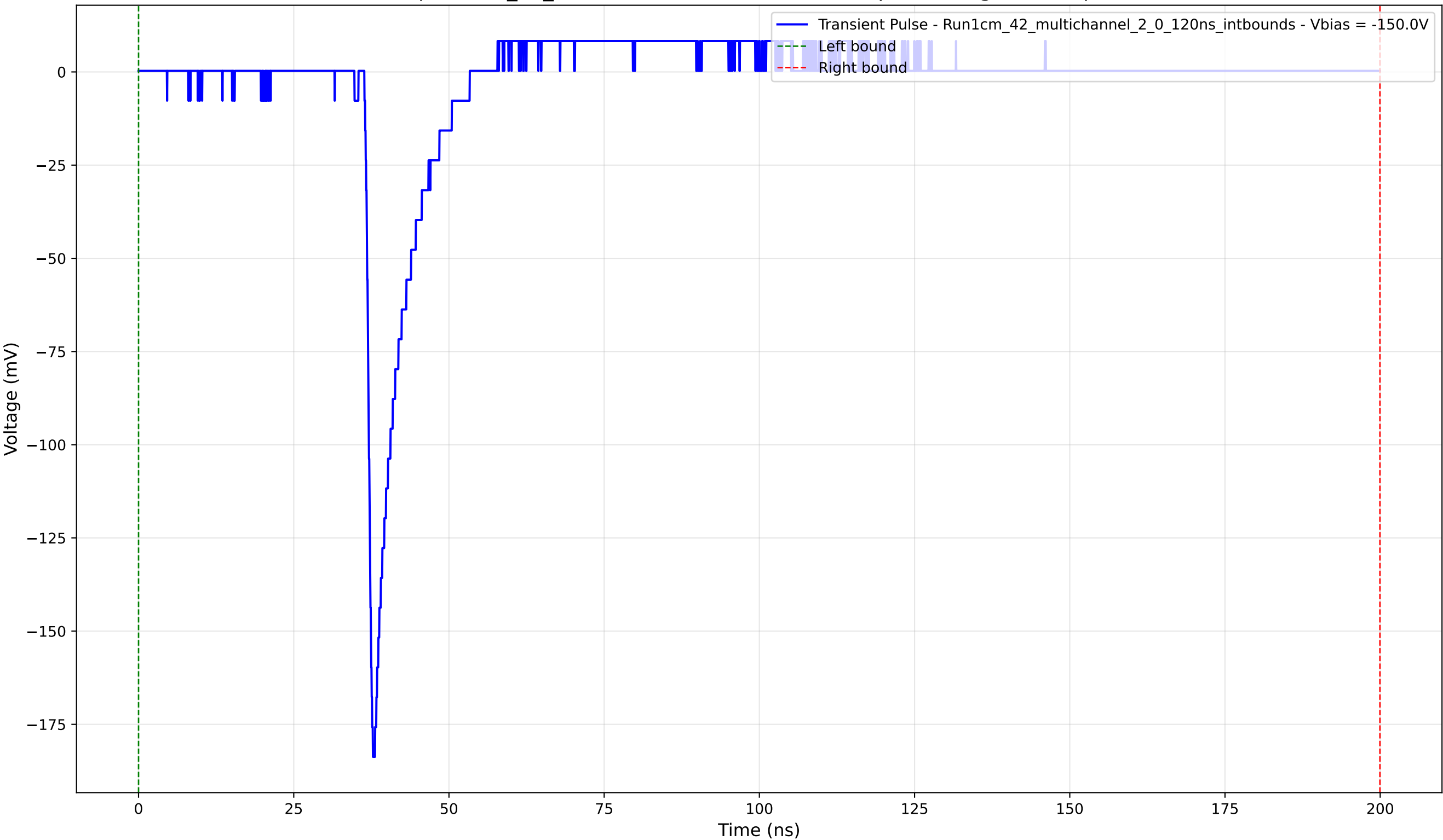
Transient Pulse - Sample: 1cm_42_multichannel - Position: 3265.0 \mu\text{m} - Charge: 10.42 pC - Rise Time: 0.99 ns
