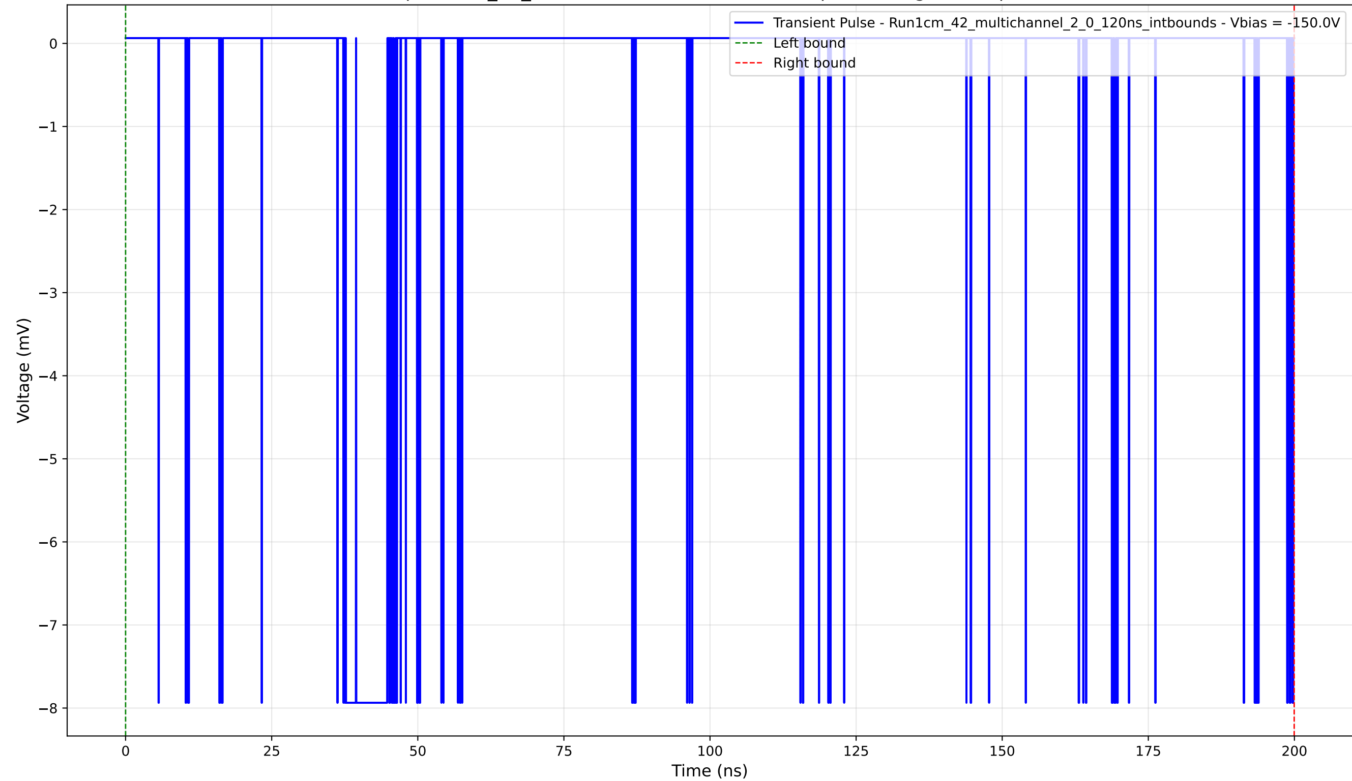
Transient Pulse - Sample: 1cm_42_multichannel - Position: 350.0 \mu\text{m} - Charge: 1.79 pC - Rise Time: 0.04 ns
