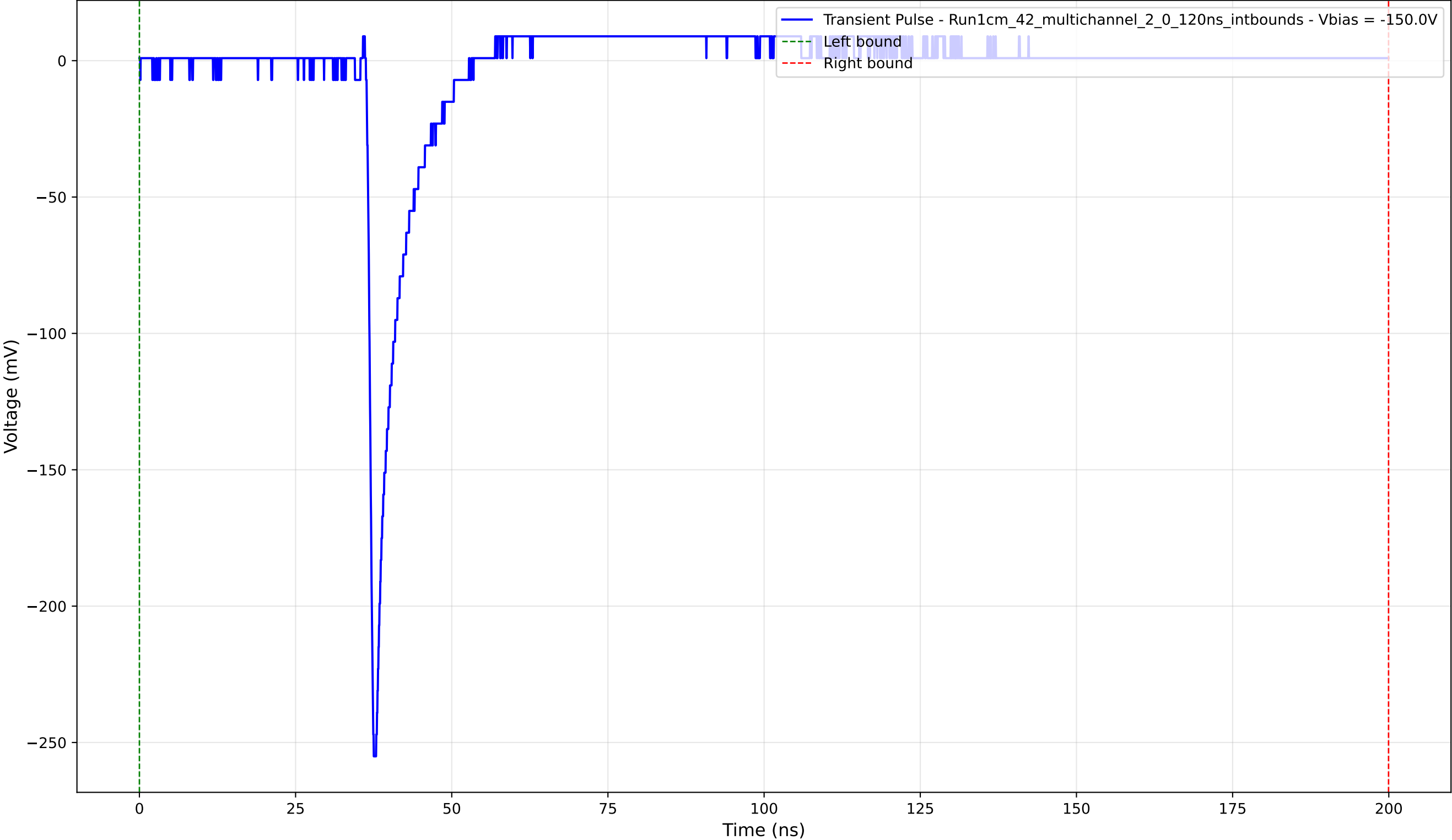
Transient Pulse - Sample: 1cm_42_multichannel - Position: 1660.0 \mu\text{m} - Charge: 10.35 pC - Rise Time: 0.90 ns
