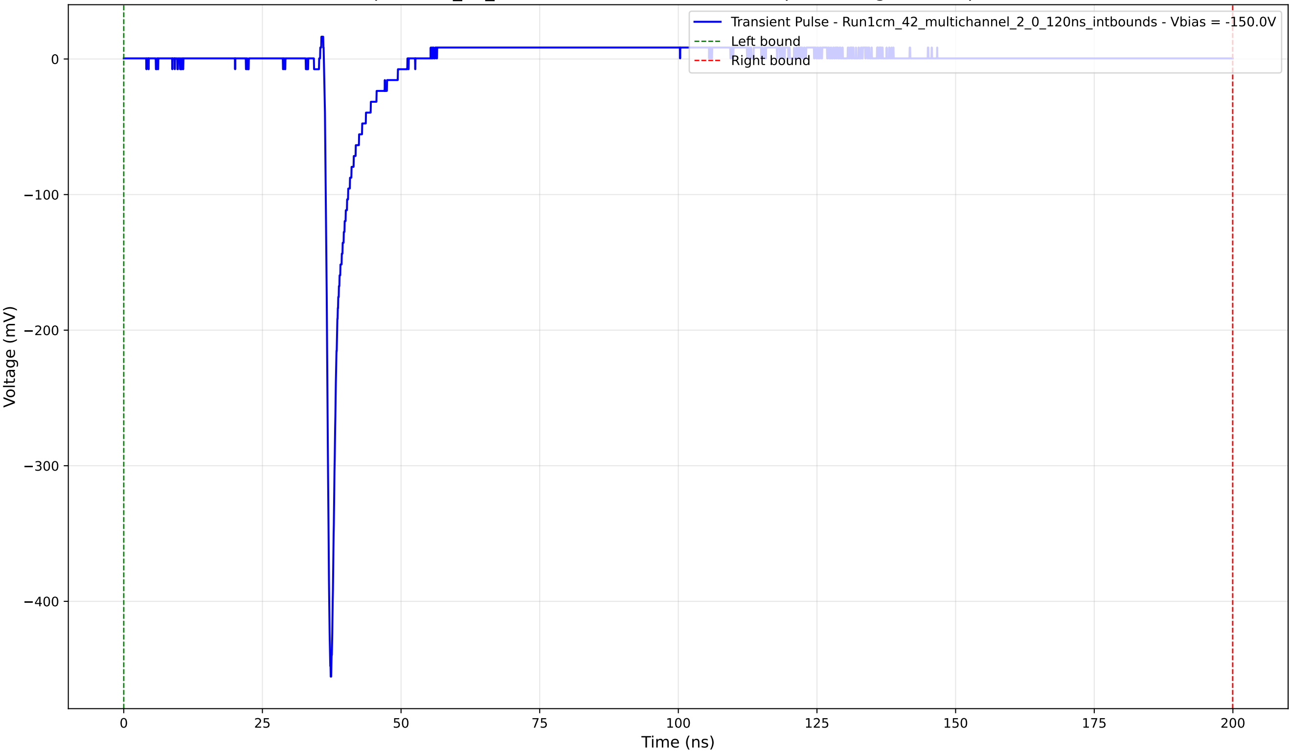
Transient Pulse - Sample: 1cm_42_multichannel - Position: 2040.0 \mu\text{m} - Charge: 13.86 pC - Rise Time: 0.76 ns
