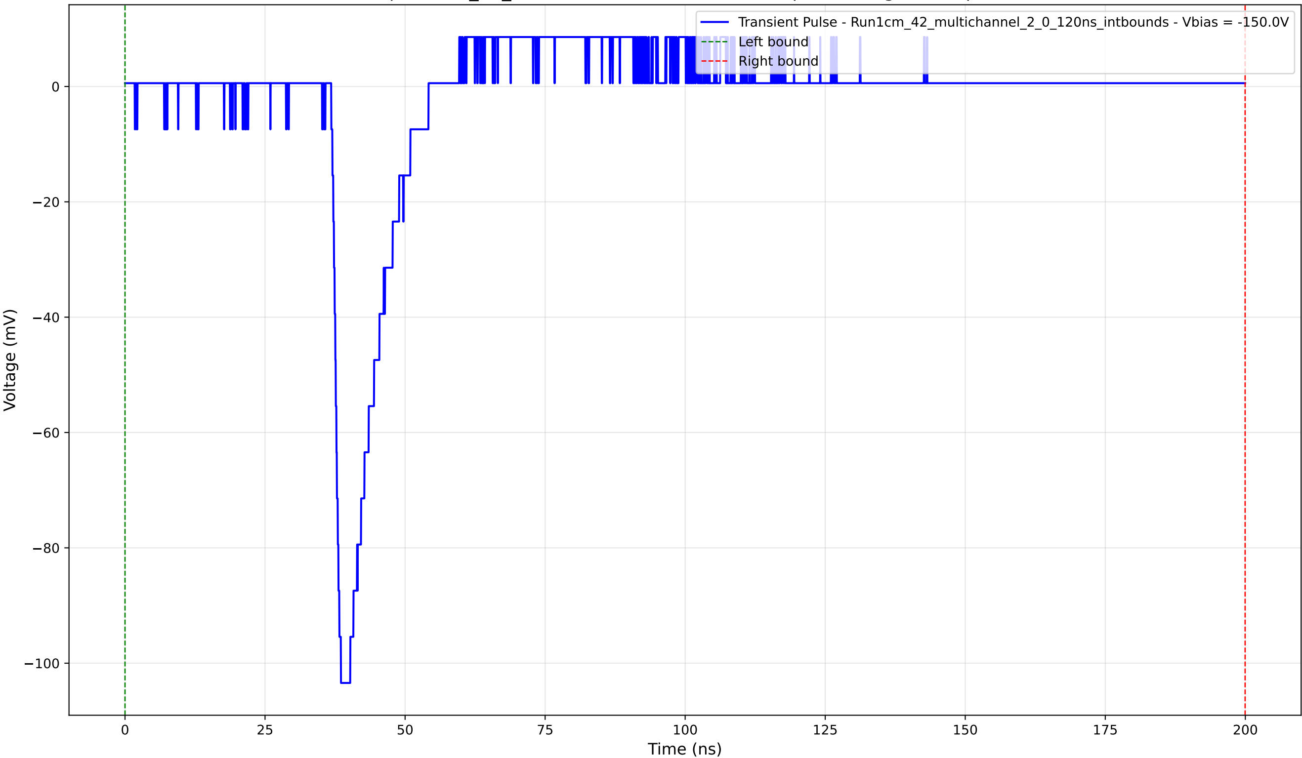
Transient Pulse - Sample: 1cm_42_multichannel - Position: 720.0 \mu\text{m} - Charge: 7.75 pC - Rise Time: 1.27 ns
