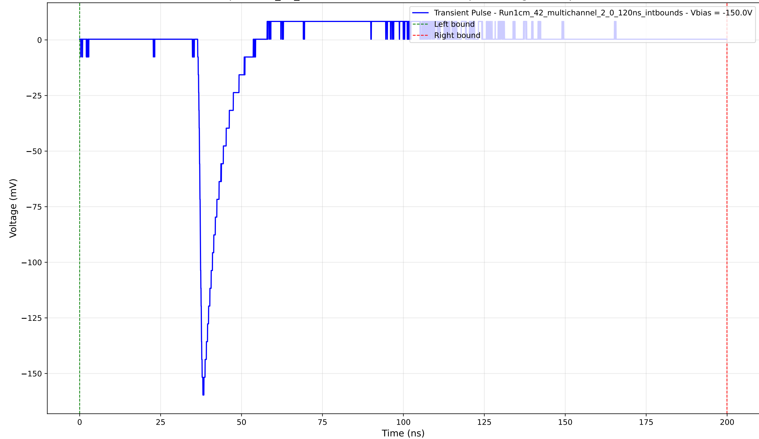
Transient Pulse - Sample: 1cm_42_multichannel - Position: 1250.0 \mu\text{m} - Charge: 9.09 pC - Rise Time: 1.12 ns
