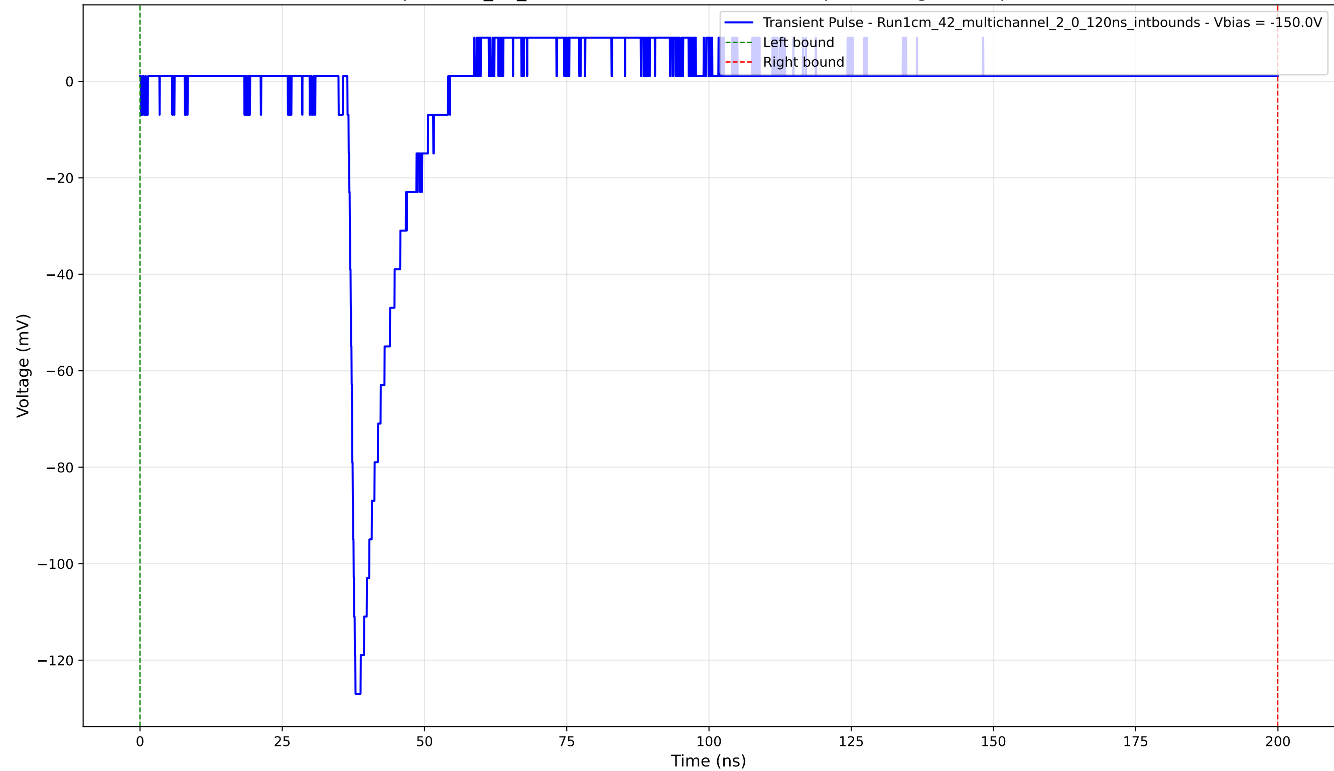
Transient Pulse - Sample: 1cm_42_multichannel - Position: 3510.0 \mu\text{m} - Charge: 7.38 pC - Rise Time: 1.09 ns
