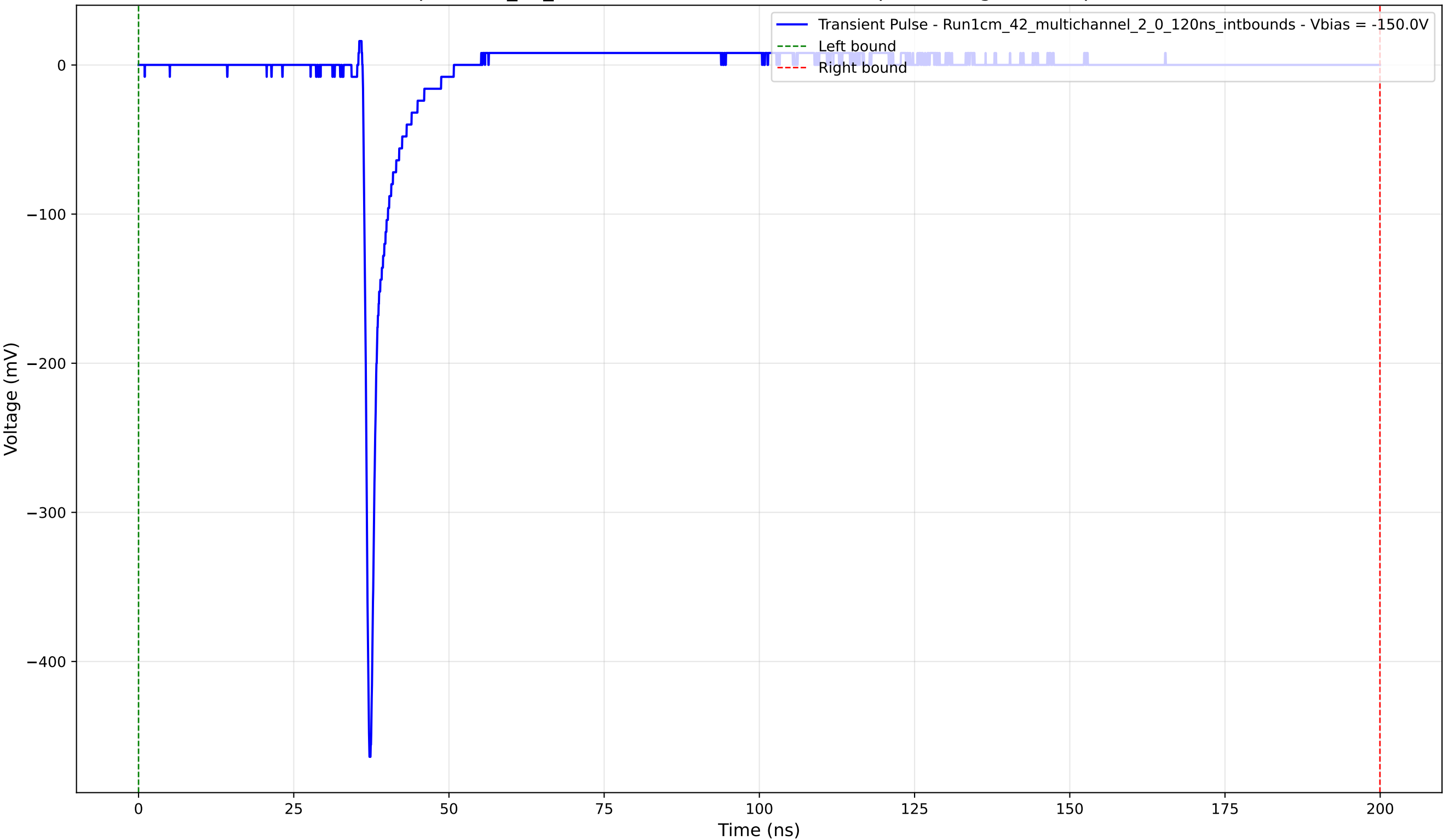
Transient Pulse - Sample: 1cm_42_multichannel - Position: 2635.0 \mu\text{m} - Charge: 14.33 pC - Rise Time: 0.77 ns
