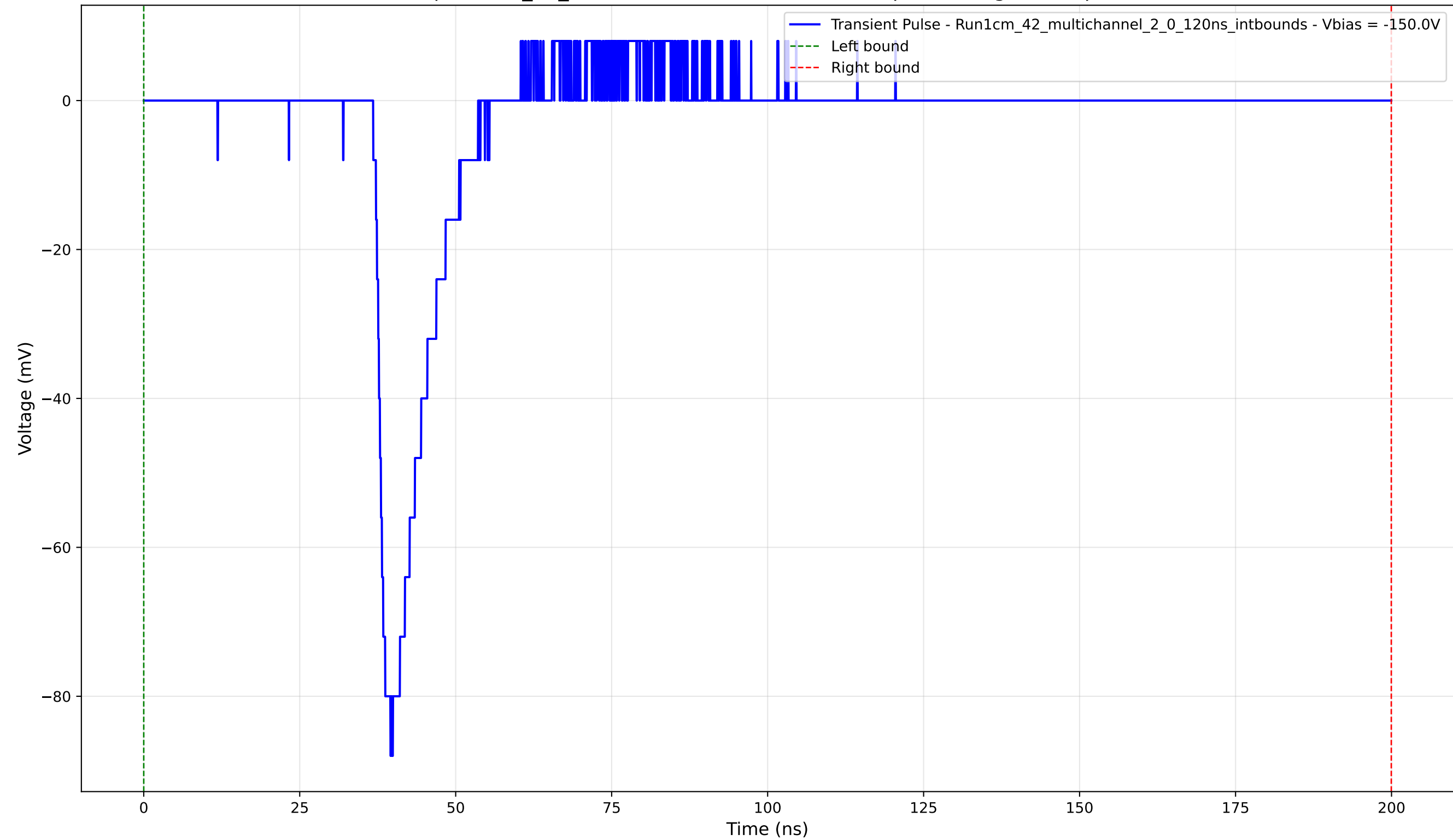
Transient Pulse - Sample: 1cm_42_multichannel - Position: 4180.0 \mu\text{m} - Charge: 9.97 pC - Rise Time: 1.52 ns
