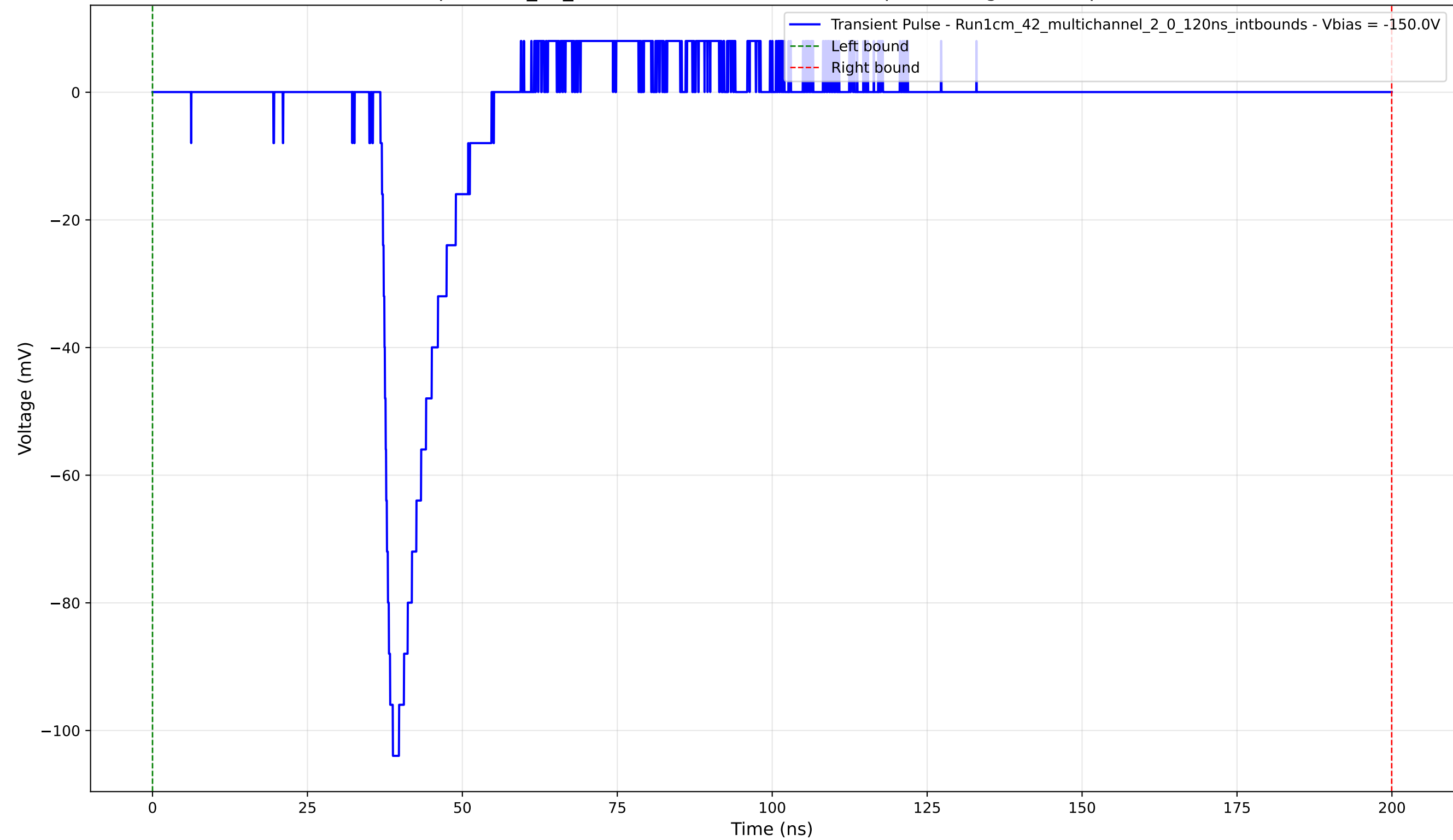
Transient Pulse - Sample: 1cm_42_multichannel - Position: 750.0 \mu\text{m} - Charge: 10.31 pC - Rise Time: 1.35 ns
