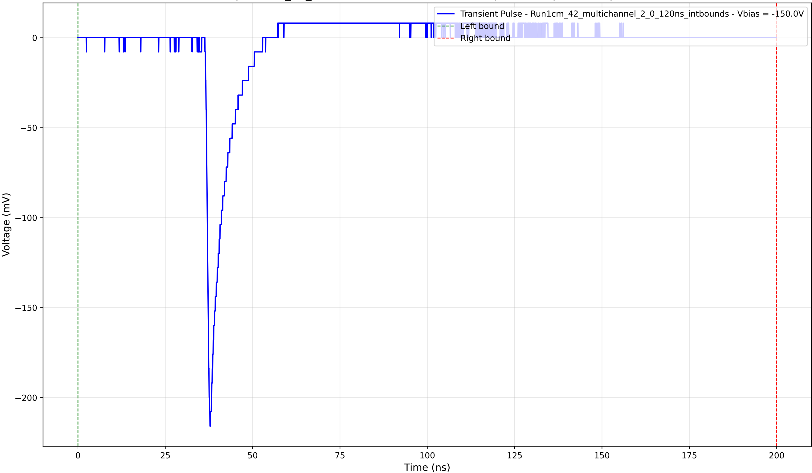
Transient Pulse - Sample: 1cm_42_multichannel - Position: 1500.0 \mu\text{m} - Charge: 11.16 pC - Rise Time: 1.01 ns
