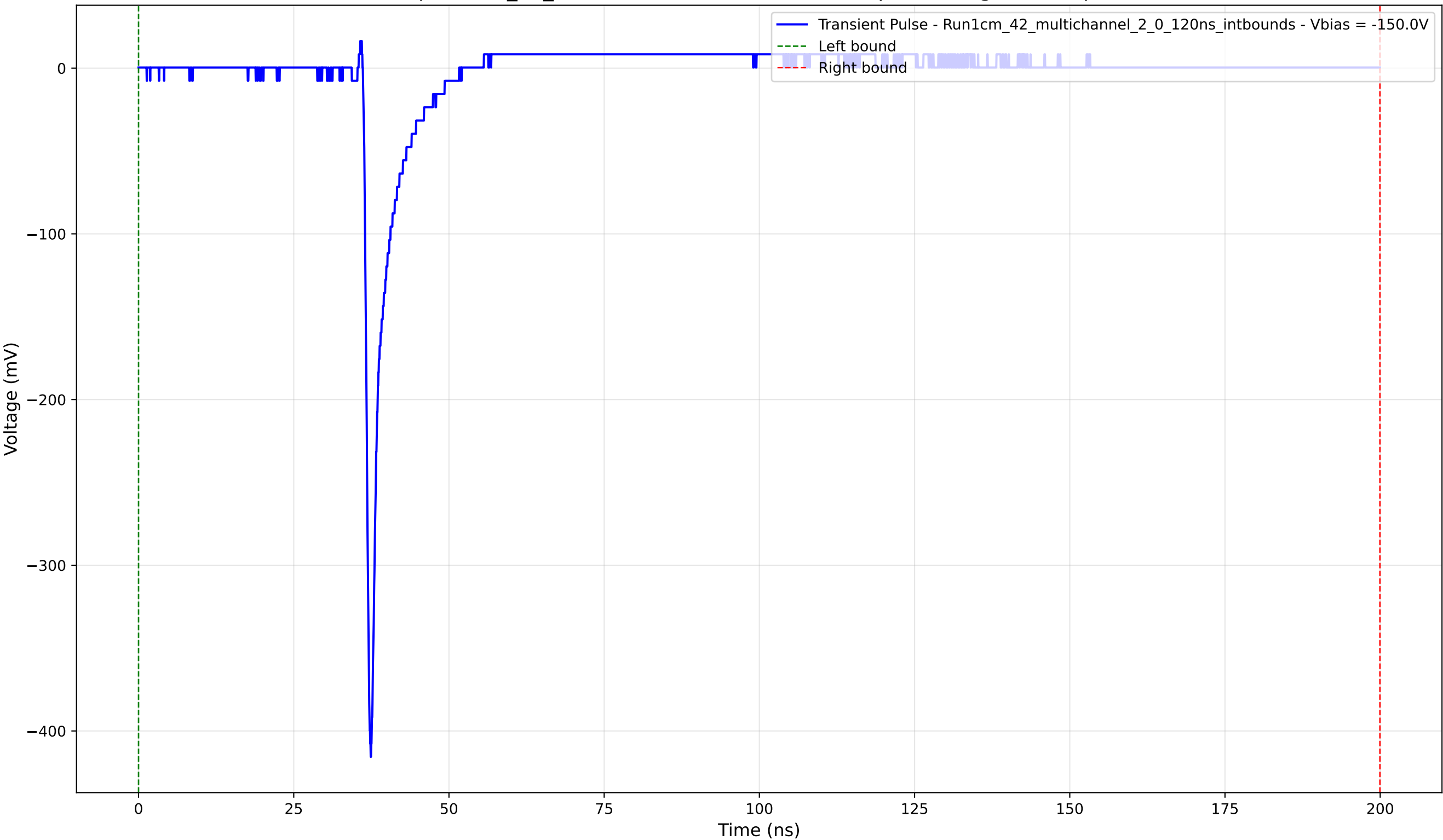
Transient Pulse - Sample: 1cm_42_multichannel - Position: 1975.0 \mu\text{m} - Charge: 13.38 pC - Rise Time: 0.78 ns
