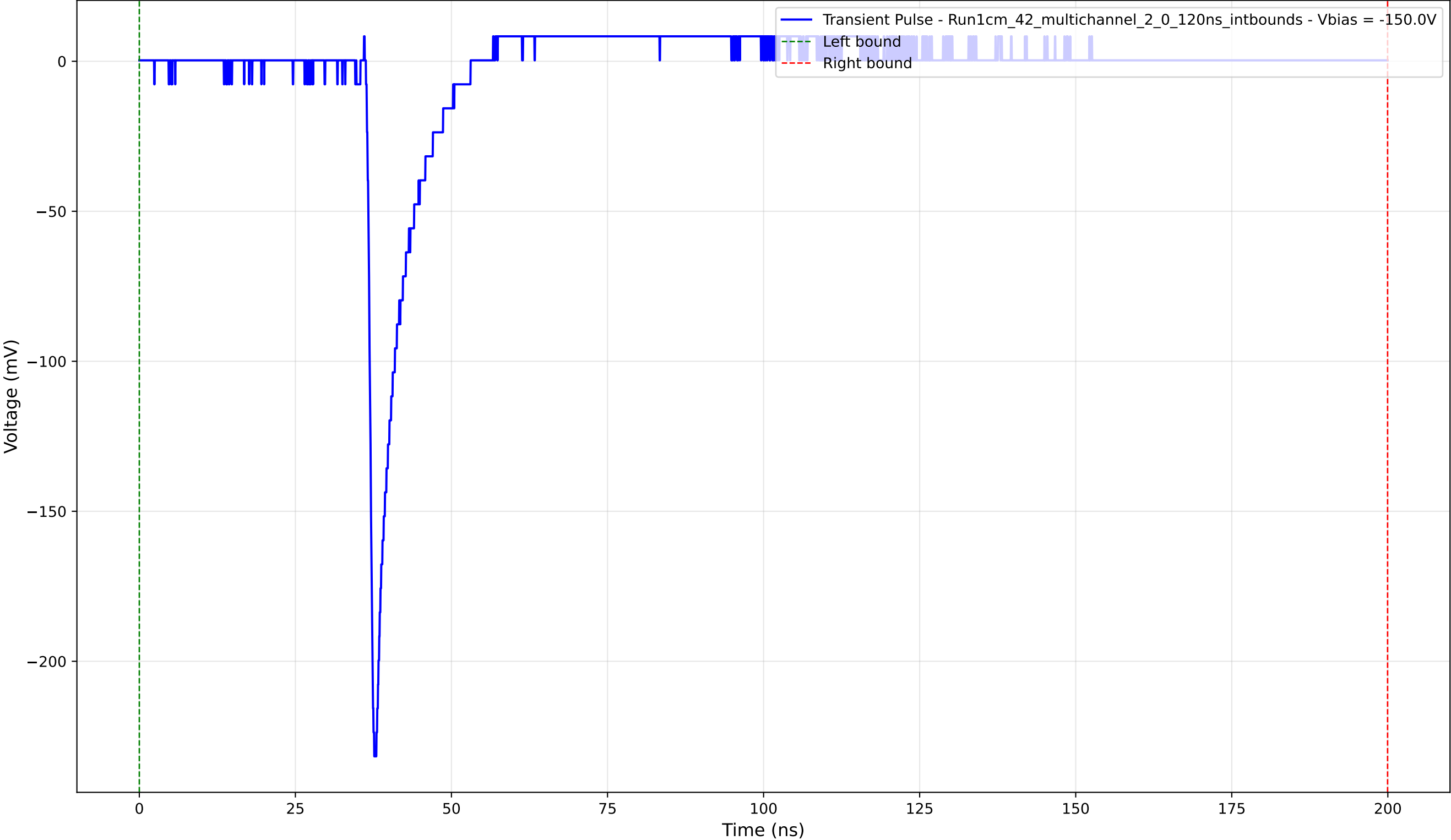
Transient Pulse - Sample: 1cm_42_multichannel - Position: 1590.0 \mu\text{m} - Charge: 11.73 pC - Rise Time: 0.96 ns
