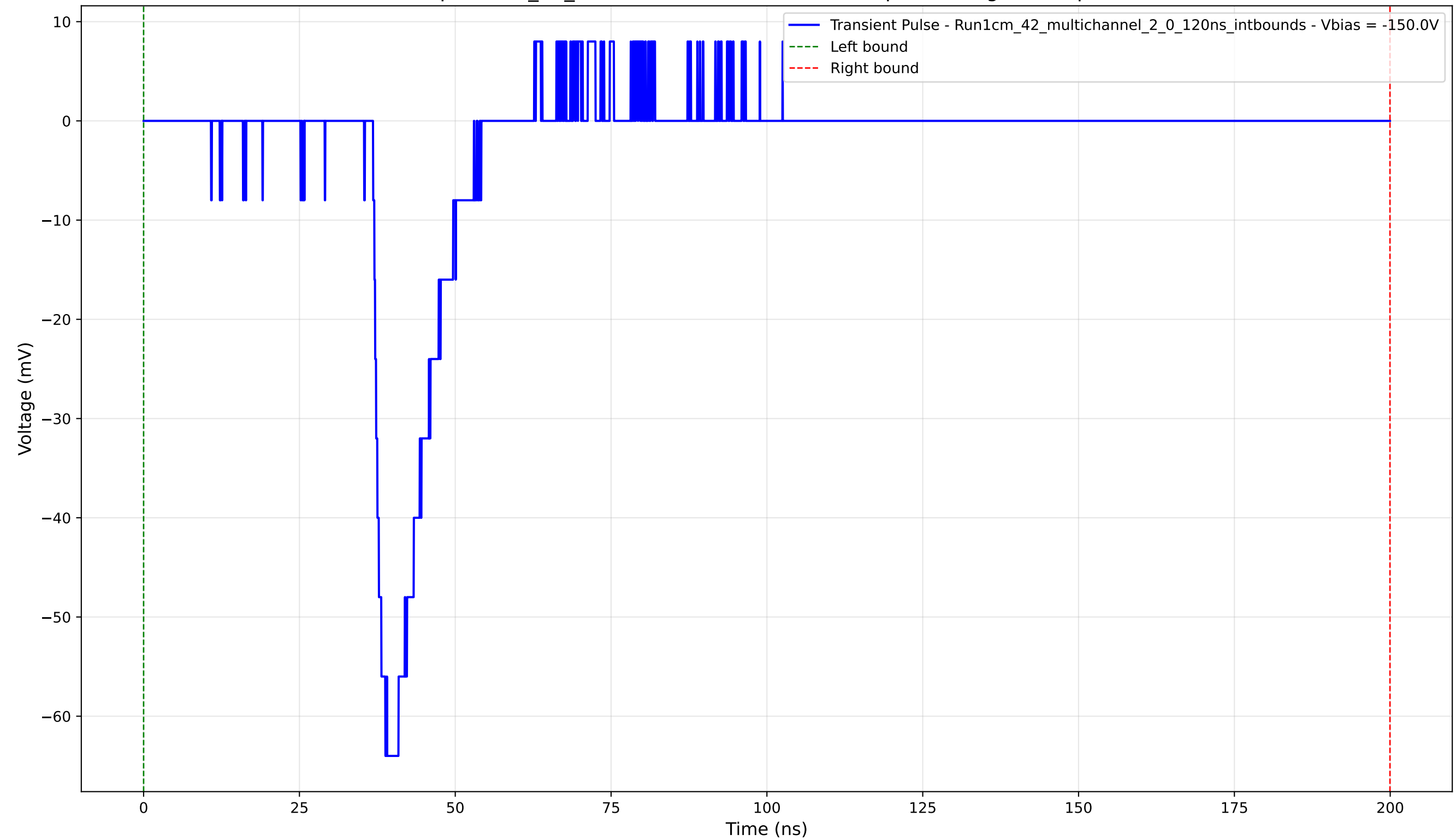
Transient Pulse - Sample: 1cm_42_multichannel - Position: 120.0 \mu\text{m} - Charge: 9.36 pC - Rise Time: 1.97 ns
