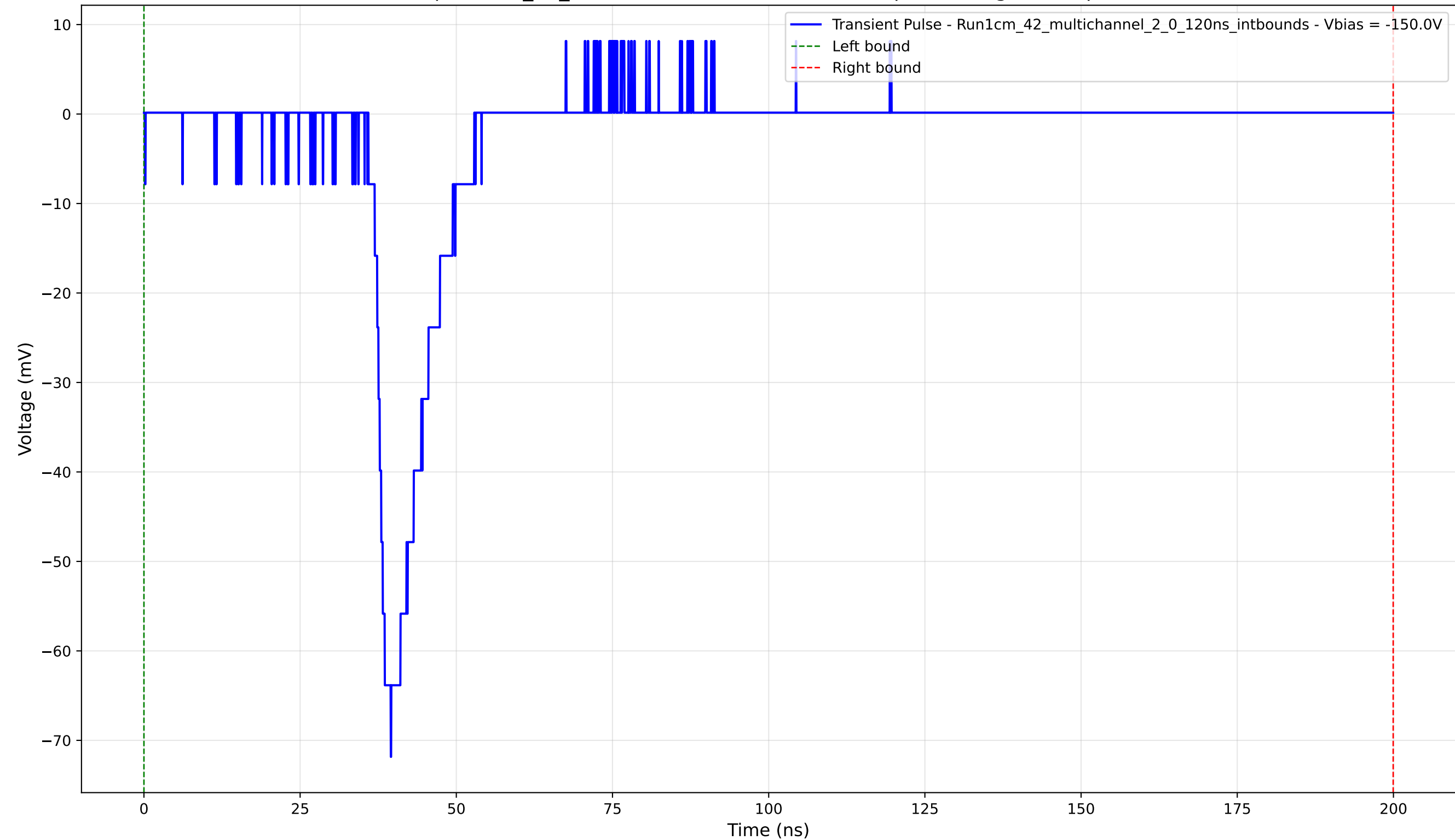
Transient Pulse - Sample: 1cm_42_multichannel - Position: 4740.0 \mu\text{m} - Charge: 9.66 pC - Rise Time: 3.56 ns
