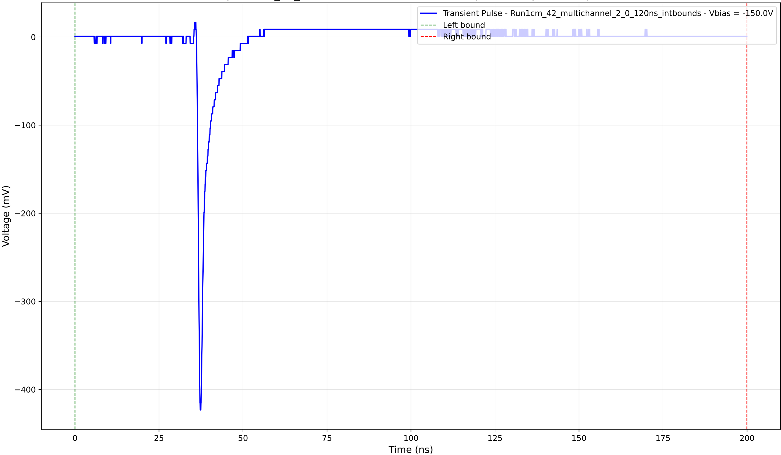
Transient Pulse - Sample: 1cm_42_multichannel - Position: 2715.0 \mu\text{m} - Charge: 11.52 pC - Rise Time: 0.77 ns
