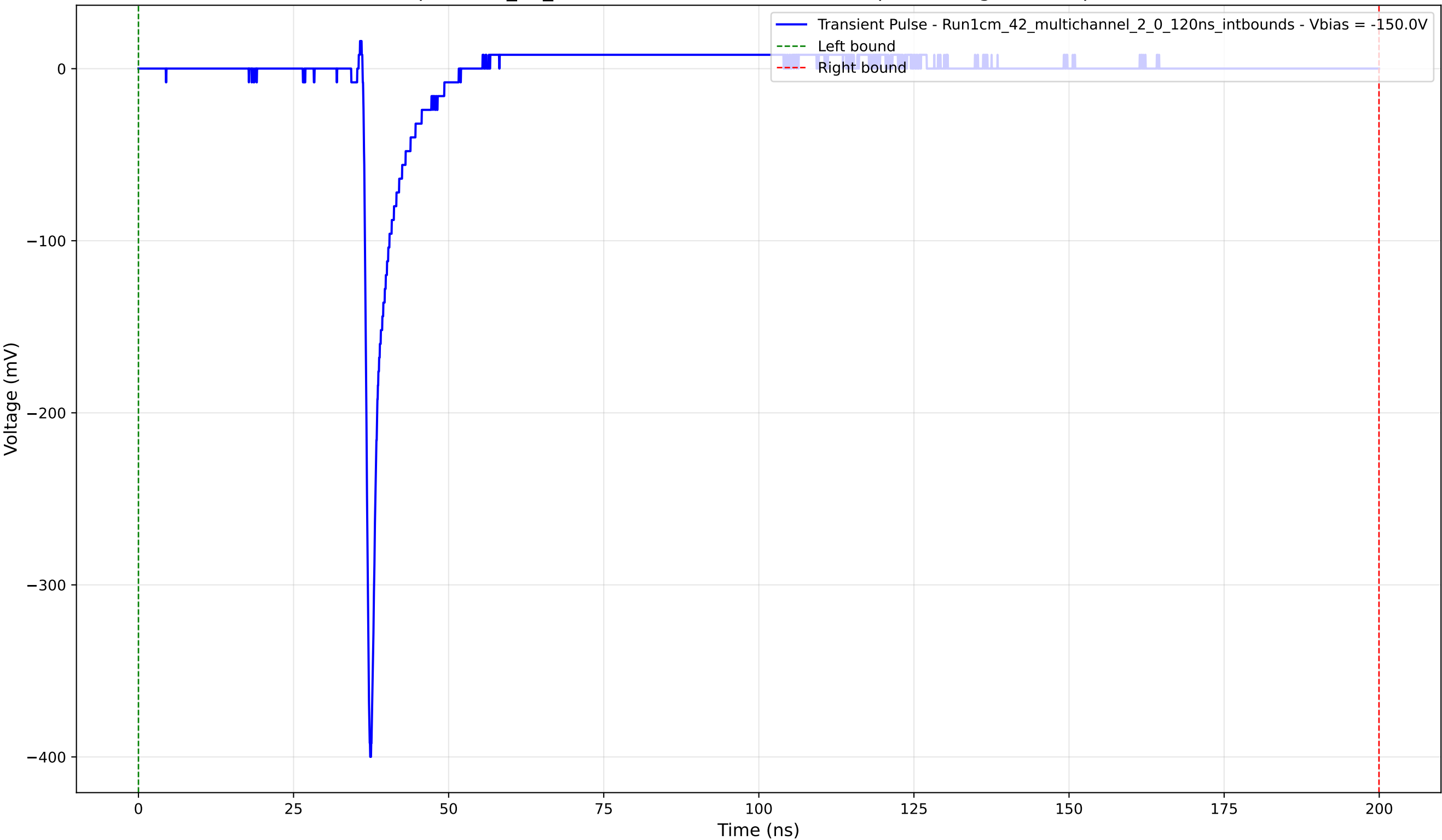
Transient Pulse - Sample: 1cm_42_multichannel - Position: 1970.0 \mu\text{m} - Charge: 14.39 pC - Rise Time: 0.80 ns
