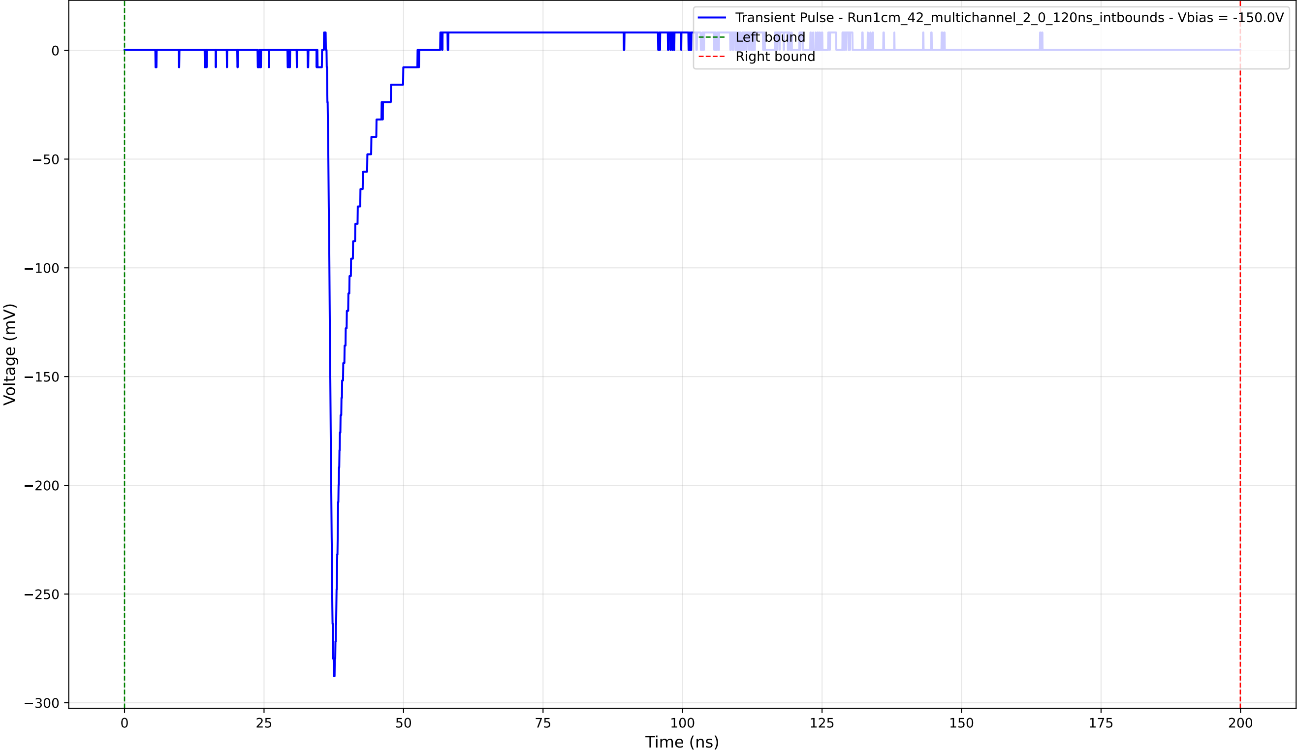
Transient Pulse - Sample: 1cm_42_multichannel - Position: 1775.0 \mu\text{m} - Charge: 12.25 pC - Rise Time: 0.85 ns
