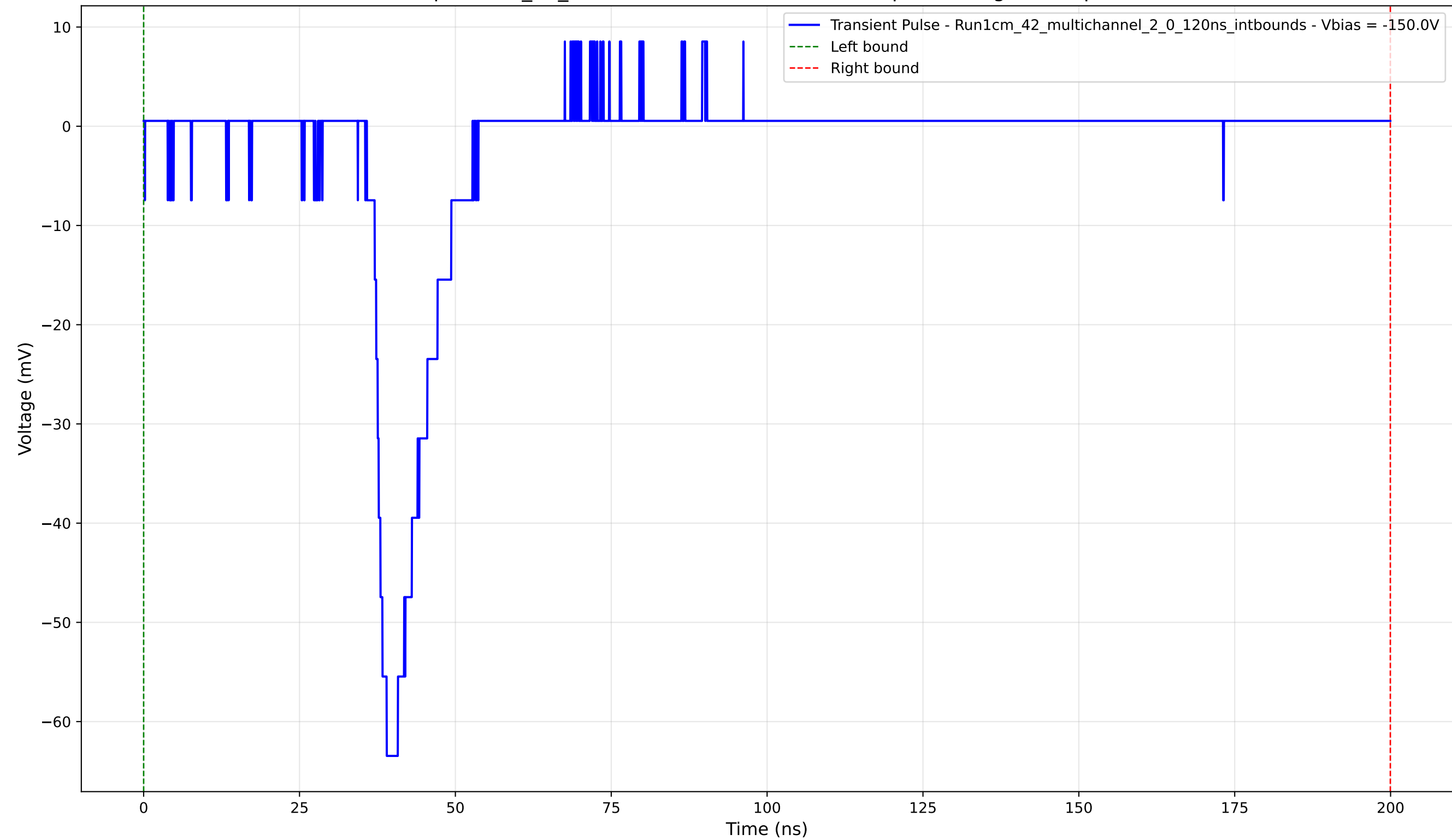
Transient Pulse - Sample: 1cm_42_multichannel - Position: 4775.0 \mu\text{m} - Charge: 7.87 pC - Rise Time: 3.17 ns
