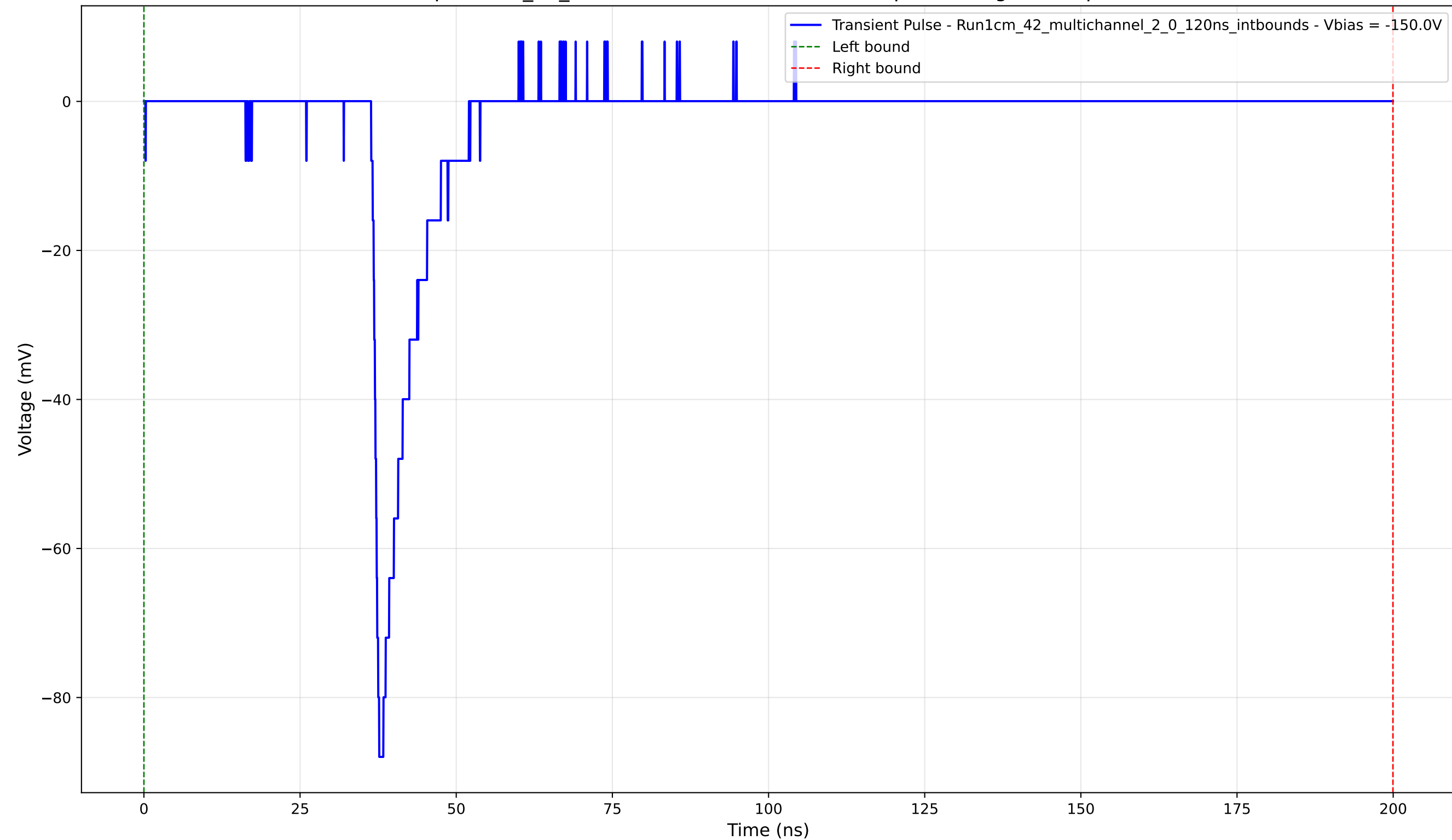
Transient Pulse - Sample: 1cm_42_multichannel - Position: 3330.0 \mu\text{m} - Charge: 9.68 pC - Rise Time: 0.92 ns
