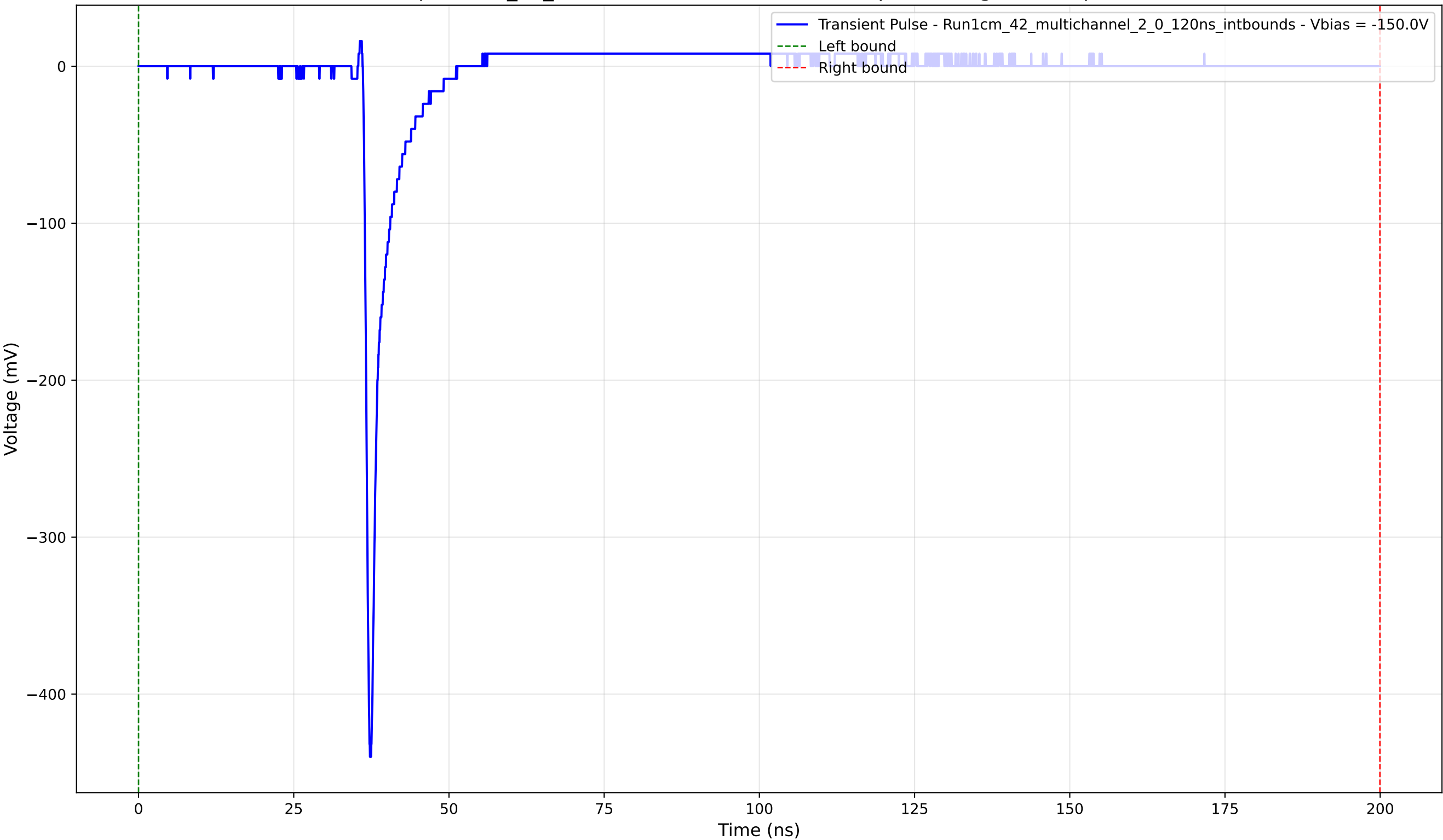
Transient Pulse - Sample: 1cm_42_multichannel - Position: 2015.0 \mu\text{m} - Charge: 15.17 pC - Rise Time: 0.76 ns
