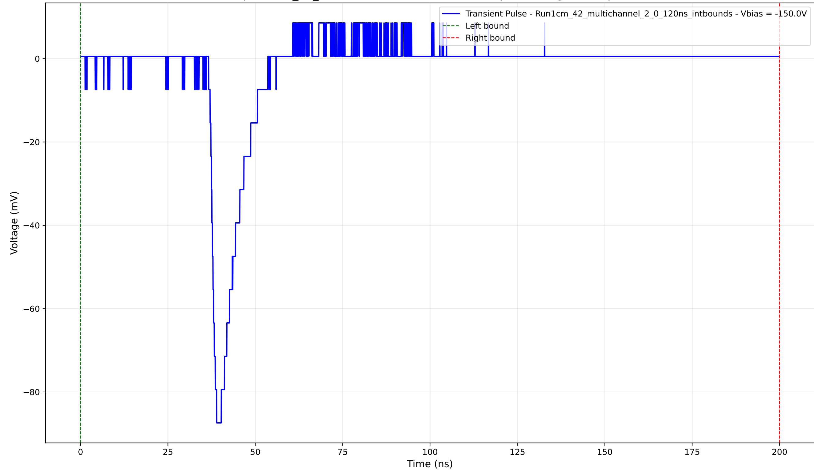
Transient Pulse - Sample: 1cm_42_multichannel - Position: 4090.0 \mu\text{m} - Charge: 8.86 pC - Rise Time: 1.51 ns
