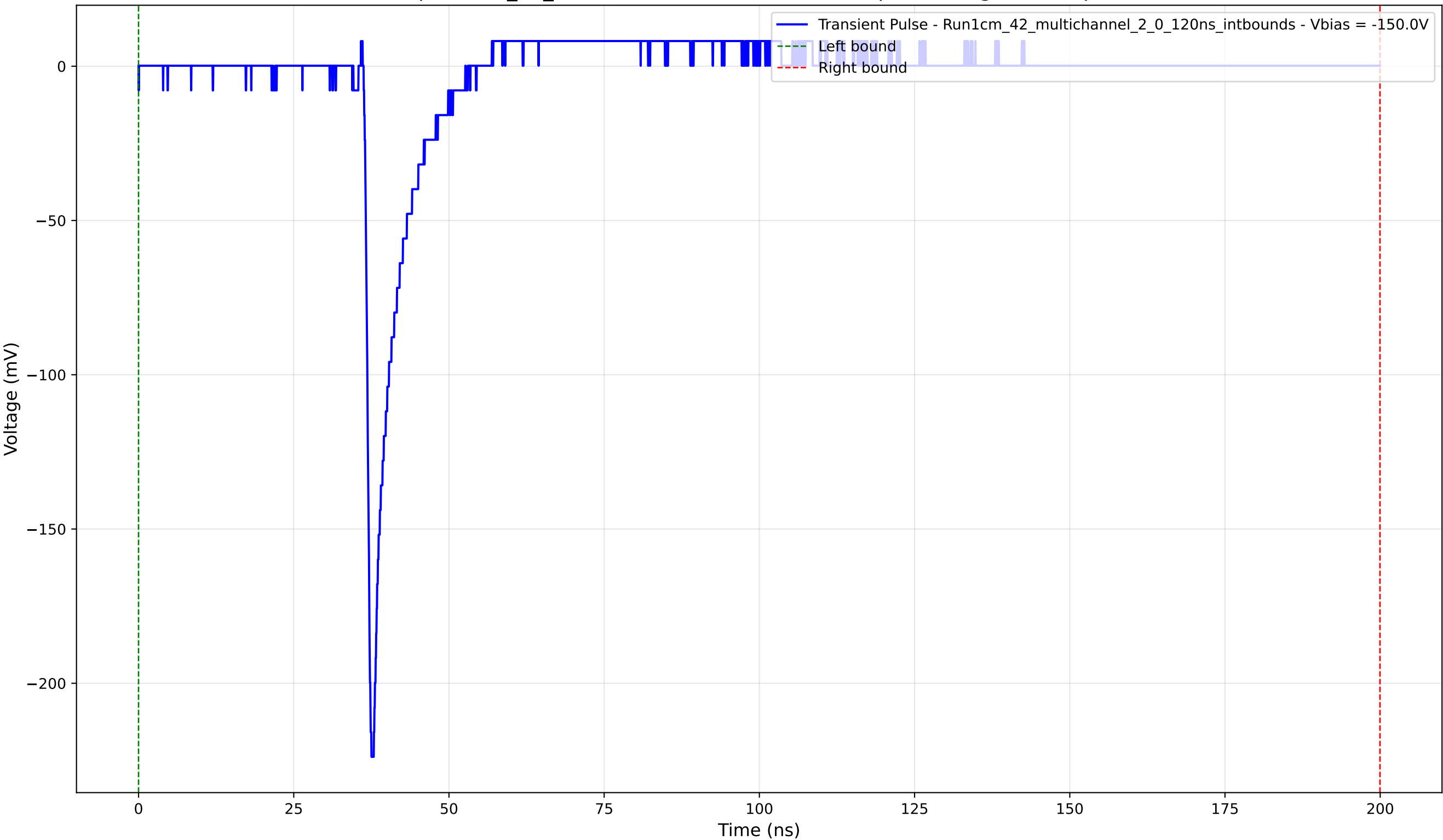
Transient Pulse - Sample: 1cm_42_multichannel - Position: 3070.0 \mu\text{m} - Charge: 11.73 pC - Rise Time: 0.90 ns
