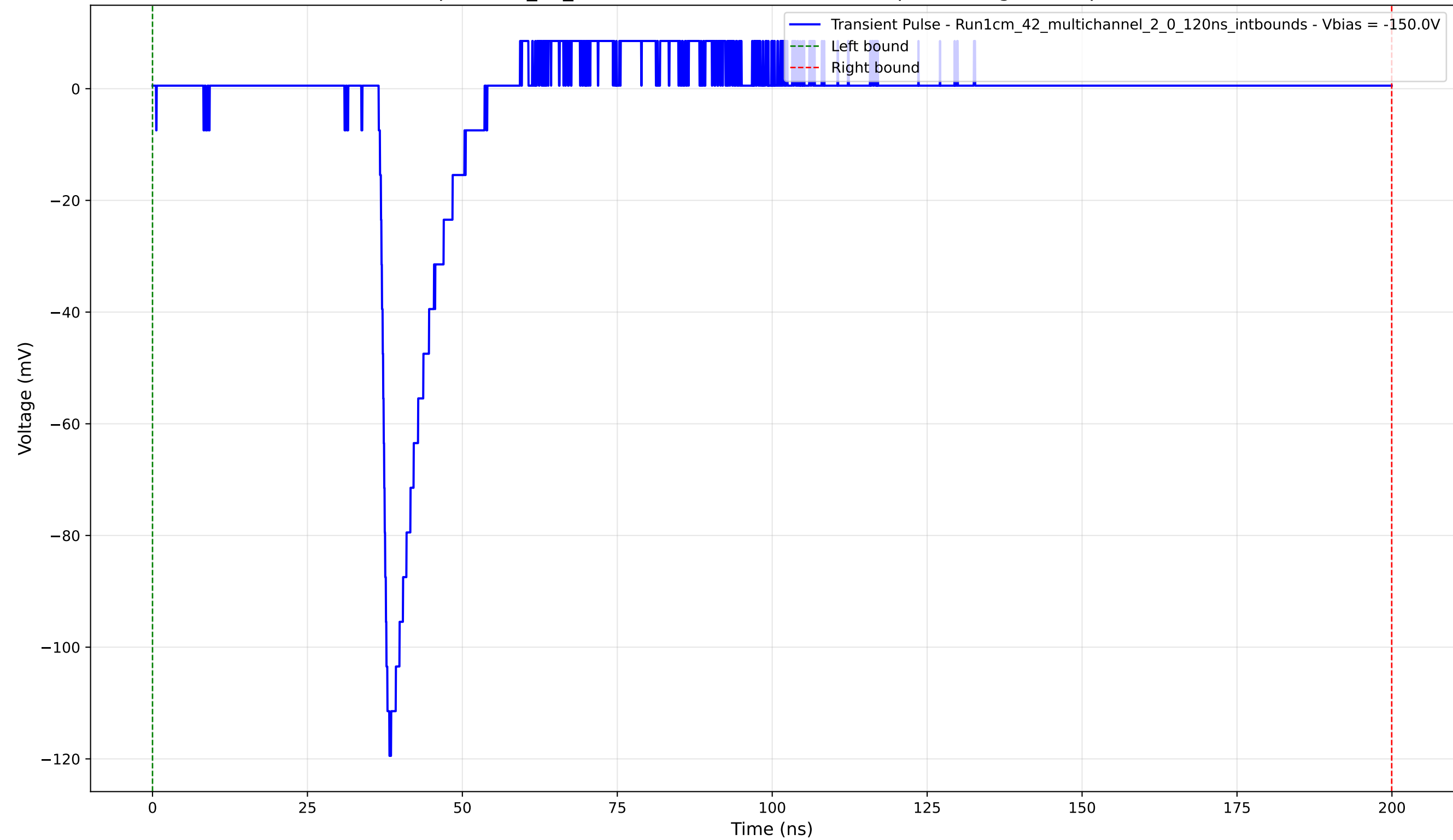
Transient Pulse - Sample: 1cm_42_multichannel - Position: 3580.0 \mu\text{m} - Charge: 8.79 pC - Rise Time: 1.22 ns
