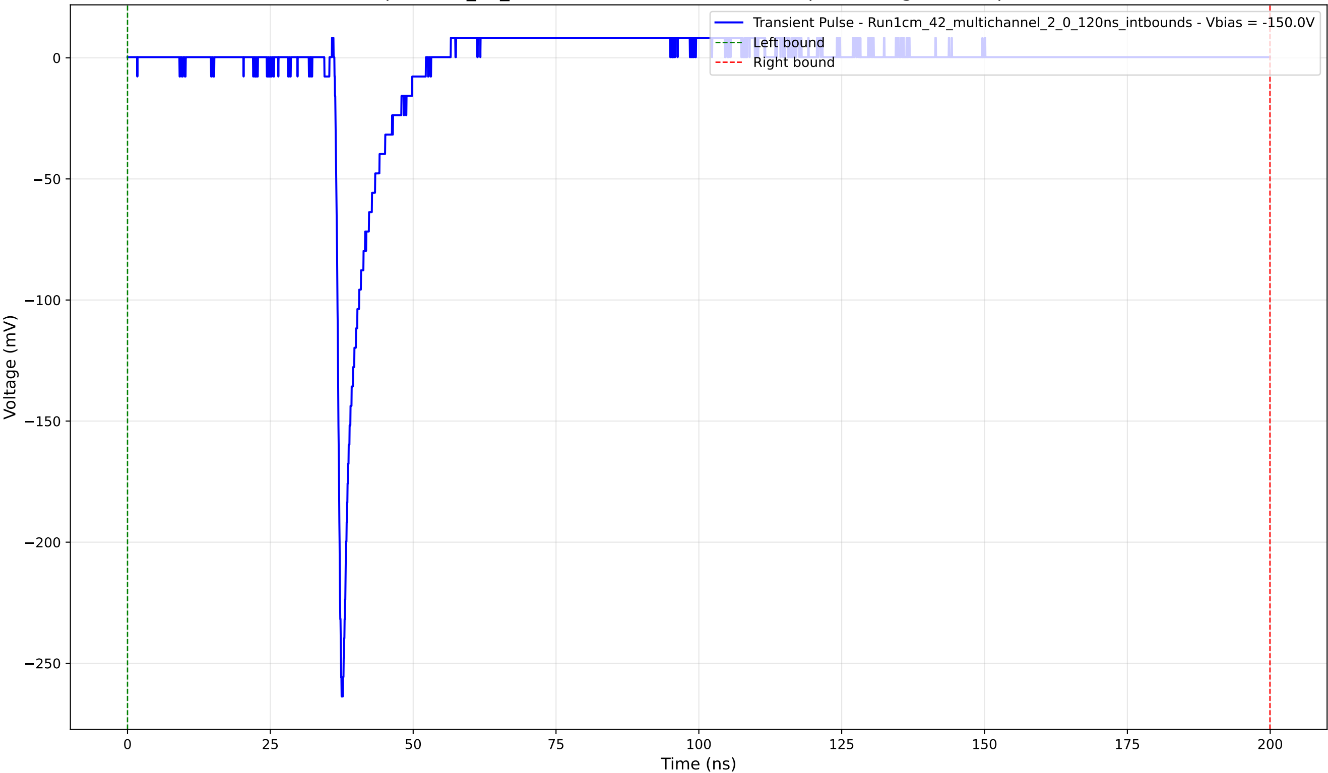
Transient Pulse - Sample: 1cm_42_multichannel - Position: 3000.0 \mu\text{m} - Charge: 11.64 pC - Rise Time: 0.89 ns
