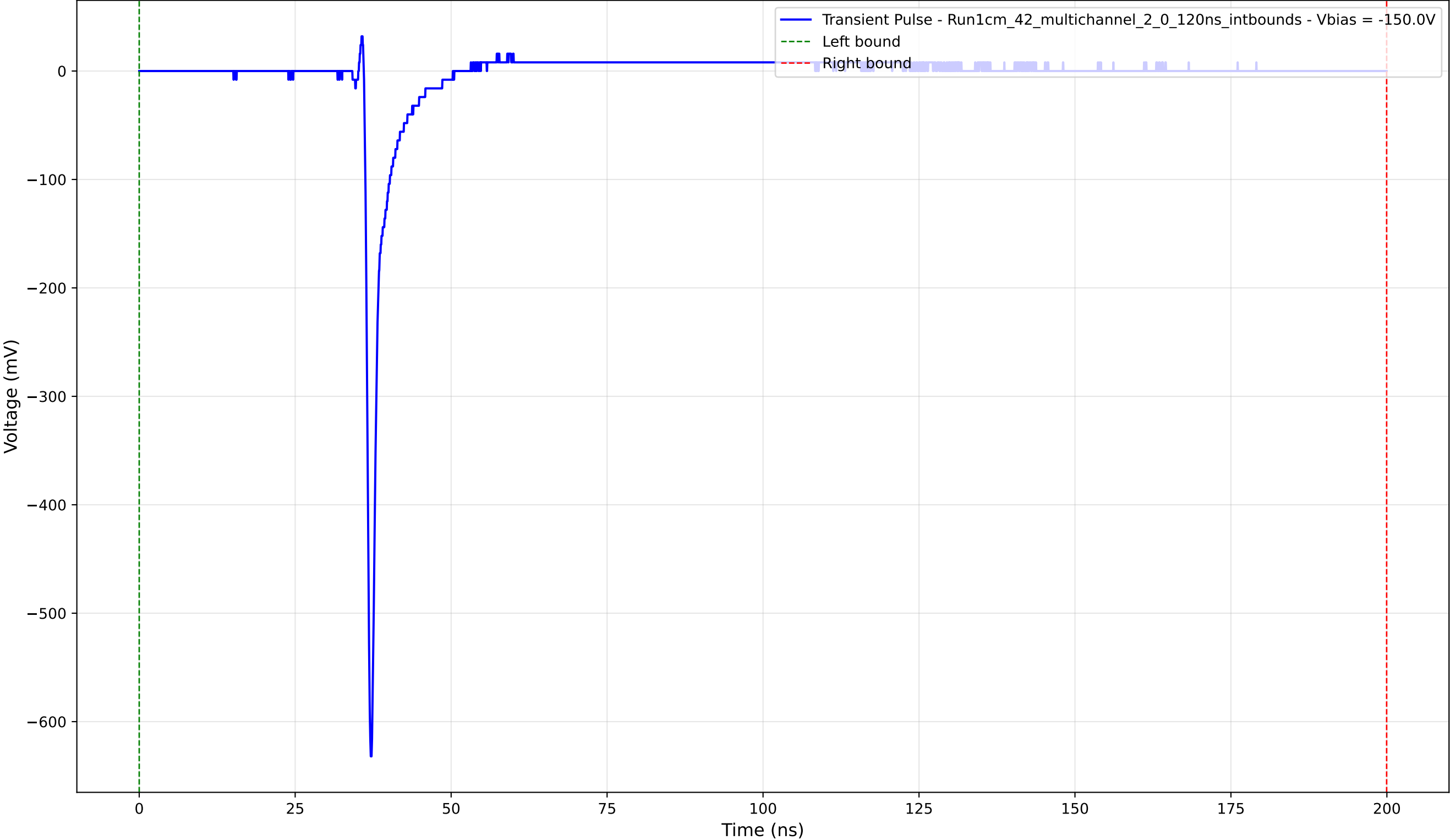
Transient Pulse - Sample: 1cm_42_multichannel - Position: 2255.0 \mu\text{m} - Charge: 17.06 pC - Rise Time: 0.72 ns
