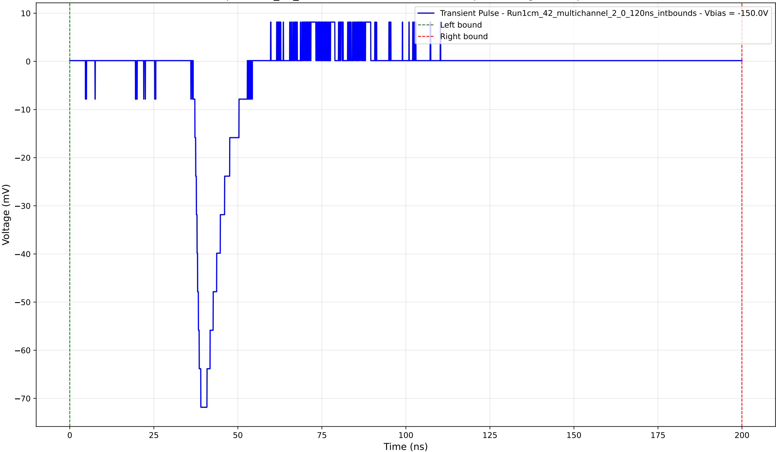
Transient Pulse - Sample: 1cm_42_multichannel - Position: 4515.0 \mu\text{m} - Charge: 8.46 pC - Rise Time: 2.28 ns
