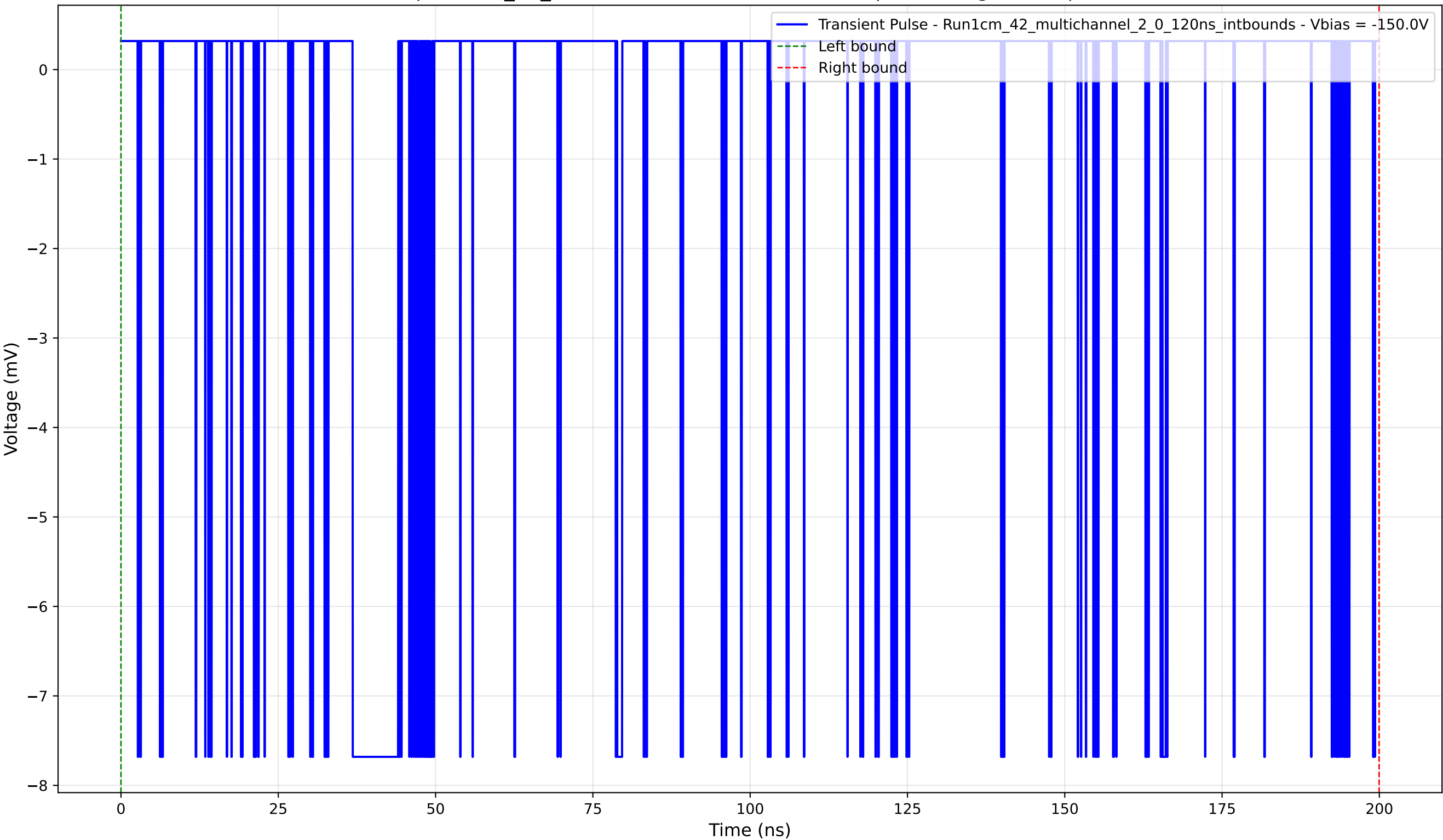
Transient Pulse - Sample: 1cm_42_multichannel - Position: 3380.0 \mu\text{m} - Charge: 1.85 pC - Rise Time: 0.04 ns
