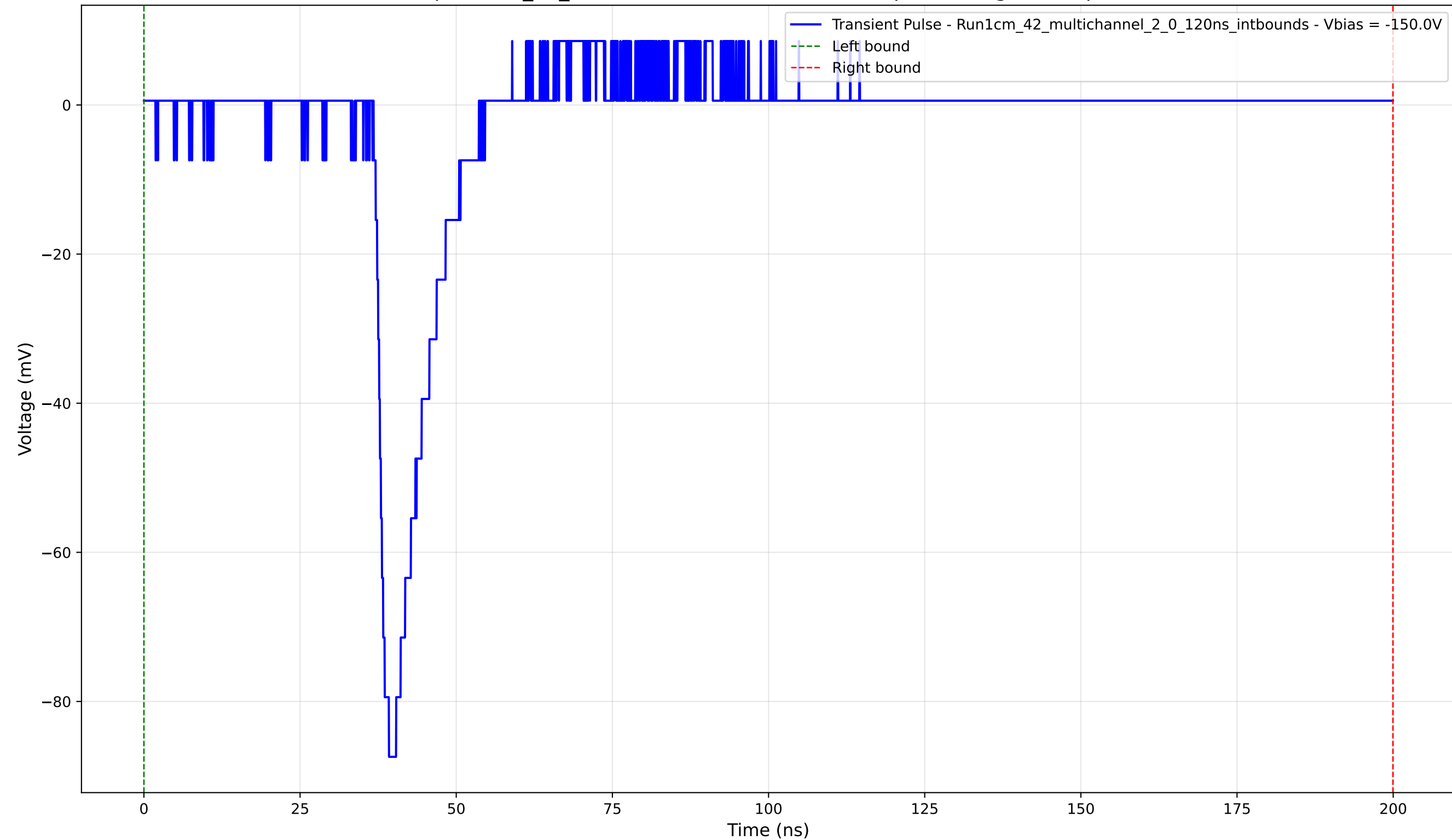
Transient Pulse - Sample: 1cm_42_multichannel - Position: 4145.0 \mu\text{m} - Charge: 8.57 pC - Rise Time: 1.47 ns
