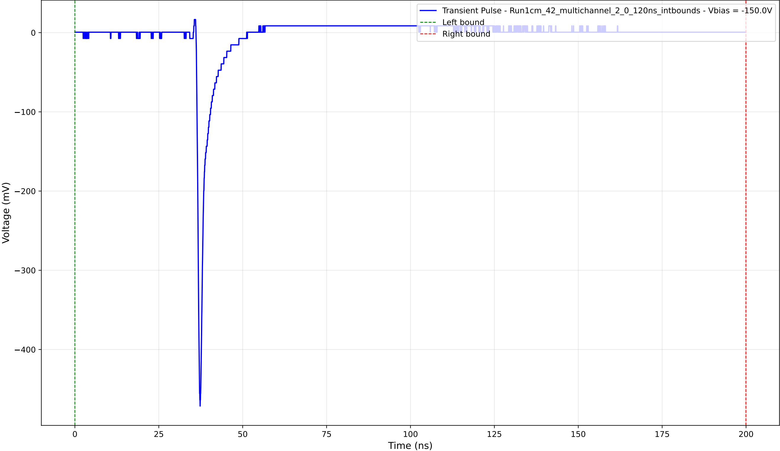
Transient Pulse - Sample: 1cm_42_multichannel - Position: 2075.0 \mu\text{m} - Charge: 13.07 pC - Rise Time: 0.77 ns
