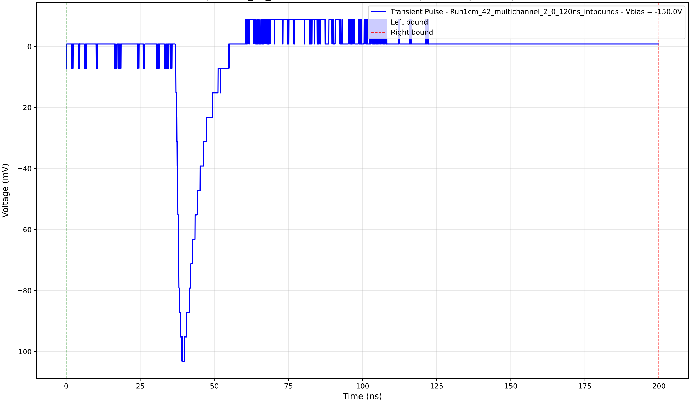
Transient Pulse - Sample: 1cm_42_multichannel - Position: 660.0 \mu\text{m} - Charge: 8.51 pC - Rise Time: 1.46 ns
