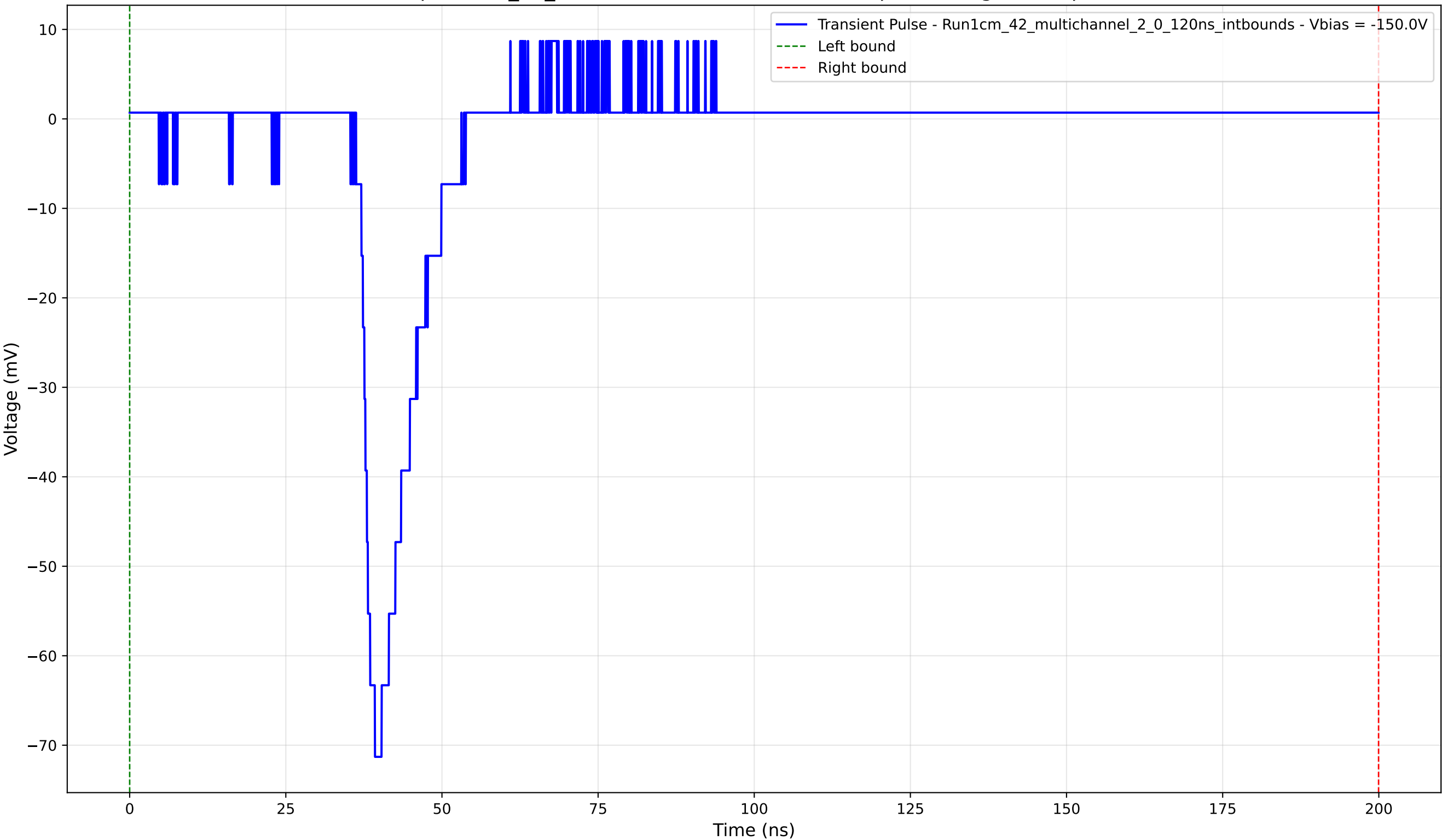
Transient Pulse - Sample: 1cm_42_multichannel - Position: 4675.0 \mu\text{m} - Charge: 7.40 pC - Rise Time: 3.00 ns
