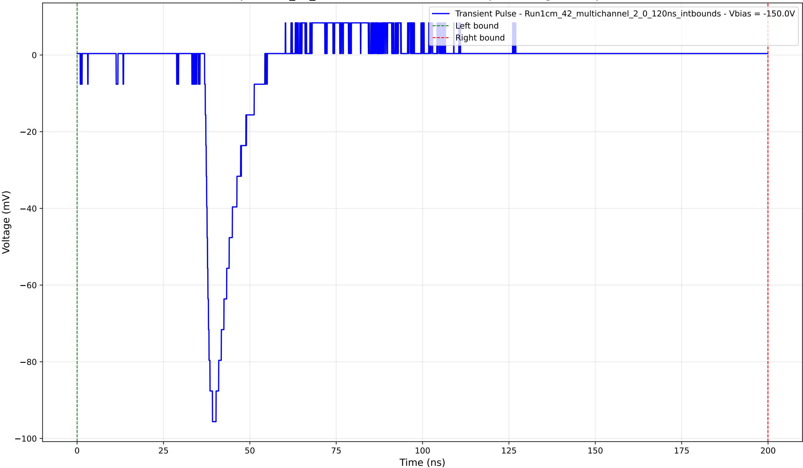
Transient Pulse - Sample: 1cm_42_multichannel - Position: 555.0 \mu\text{m} - Charge: 9.45 pC - Rise Time: 1.39 ns
