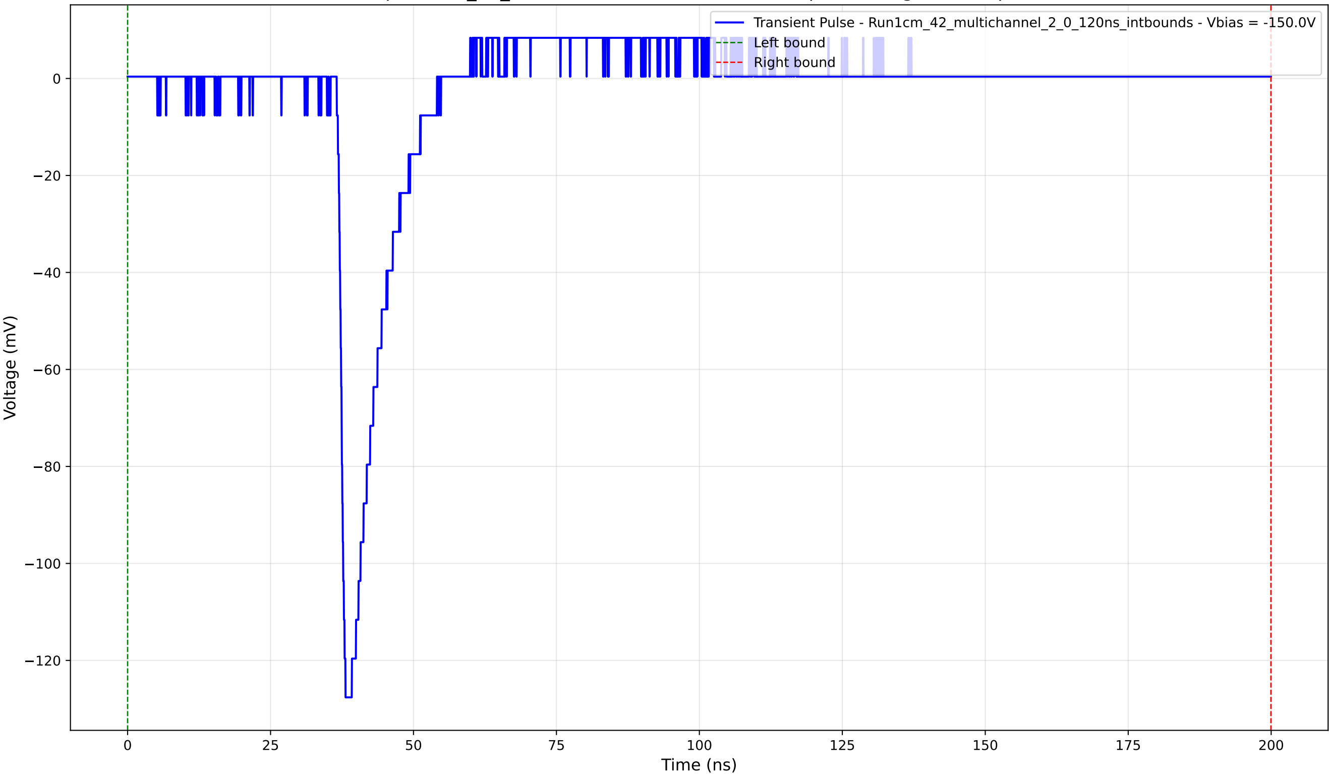
Transient Pulse - Sample: 1cm_42_multichannel - Position: 1070.0 \mu\text{m} - Charge: 10.34 pC - Rise Time: 1.17 ns
