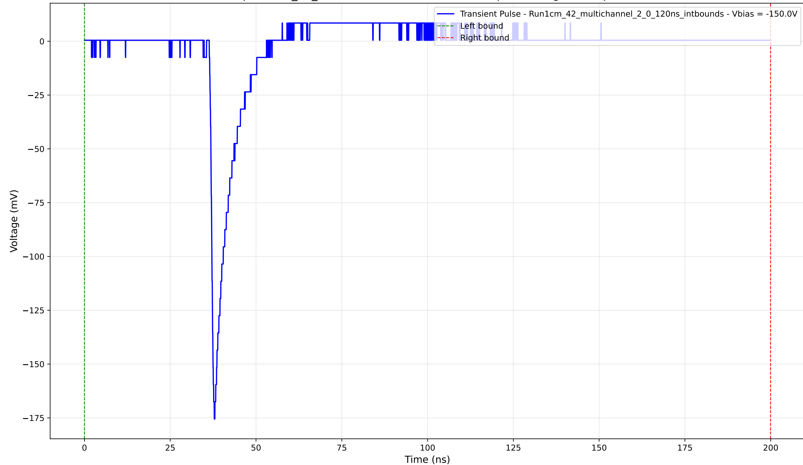
Transient Pulse - Sample: 1cm_42_multichannel - Position: 3285.0 \mu\text{m} - Charge: 9.81 pC - Rise Time: 0.99 ns
