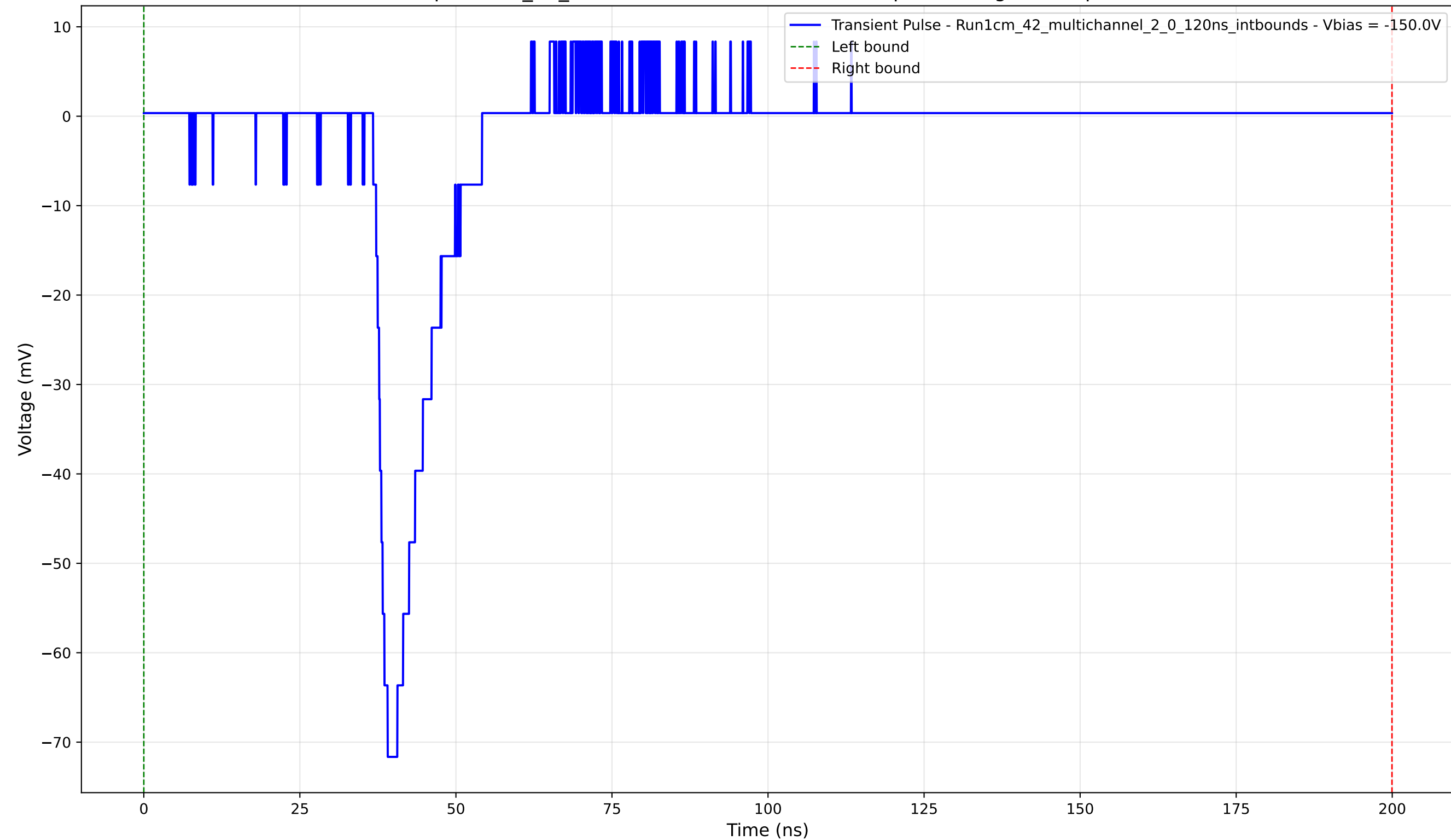
Transient Pulse - Sample: 1cm_42_multichannel - Position: 4295.0 \mu\text{m} - Charge: 8.55 pC - Rise Time: 2.32 ns
