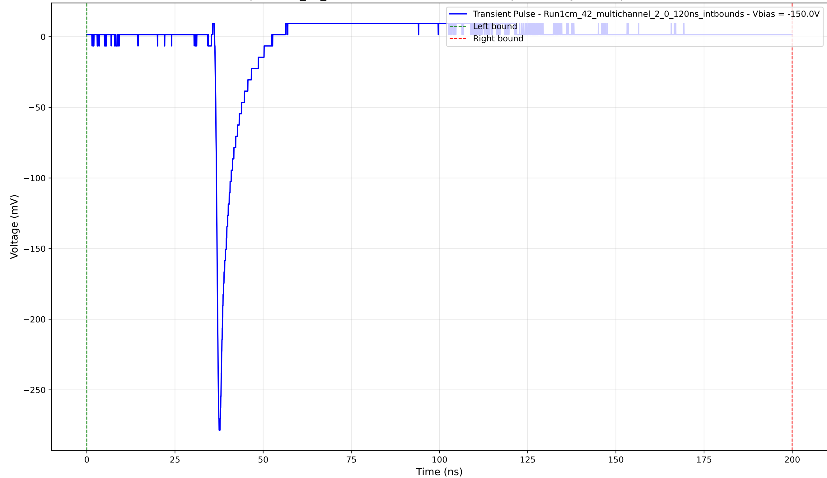
Transient Pulse - Sample: 1cm_42_multichannel - Position: 1705.0 \mu\text{m} - Charge: 7.78 pC - Rise Time: 0.89 ns
