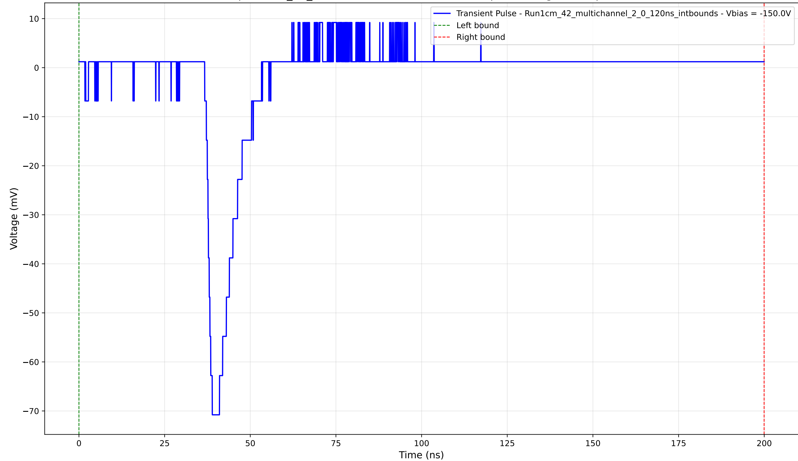
Transient Pulse - Sample: 1cm_42_multichannel - Position: 4280.0 \mu\text{m} - Charge: 5.58 pC - Rise Time: 1.76 ns
