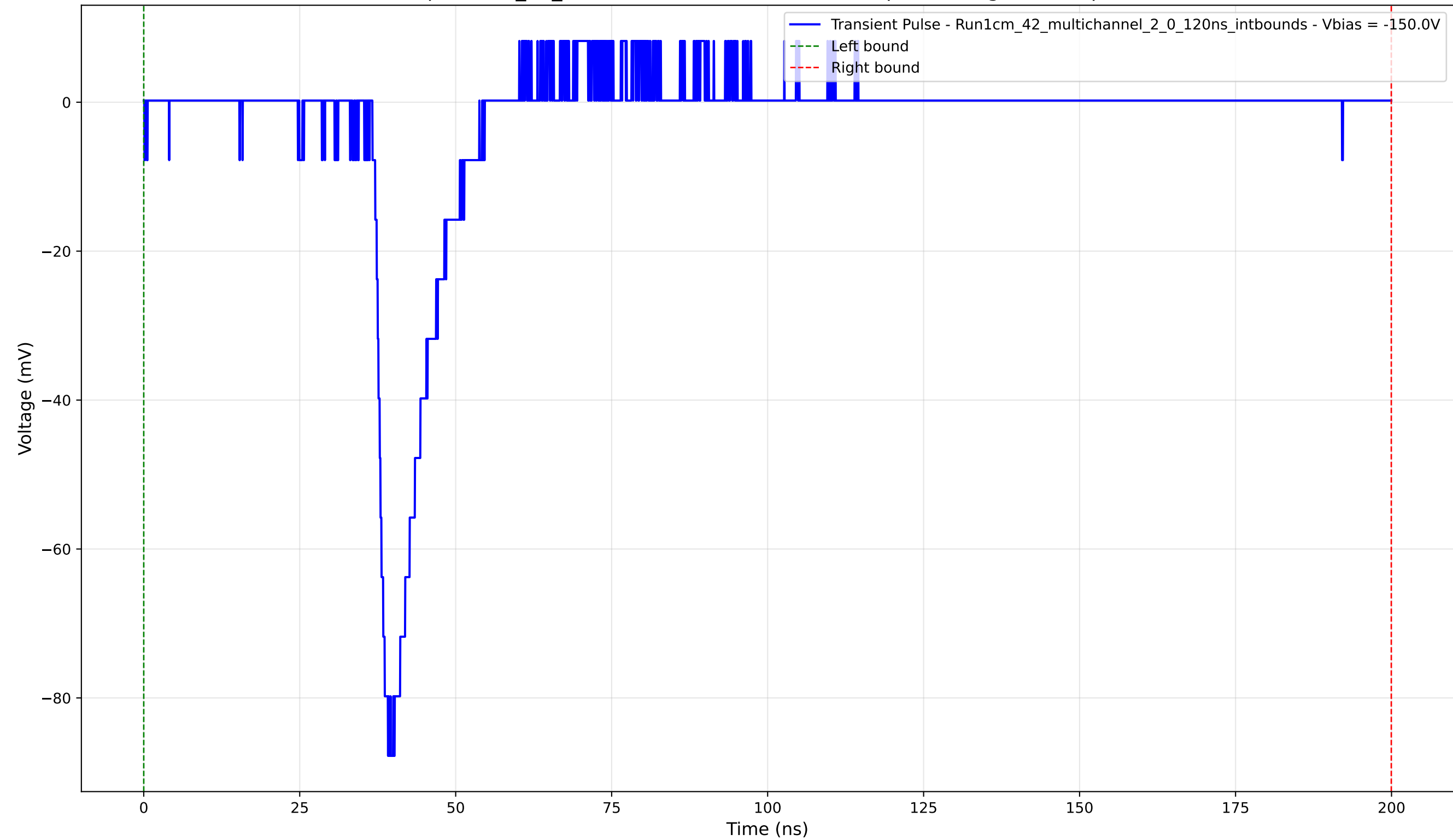
Transient Pulse - Sample: 1cm_42_multichannel - Position: 4125.0 \mu\text{m} - Charge: 10.30 pC - Rise Time: 1.55 ns
