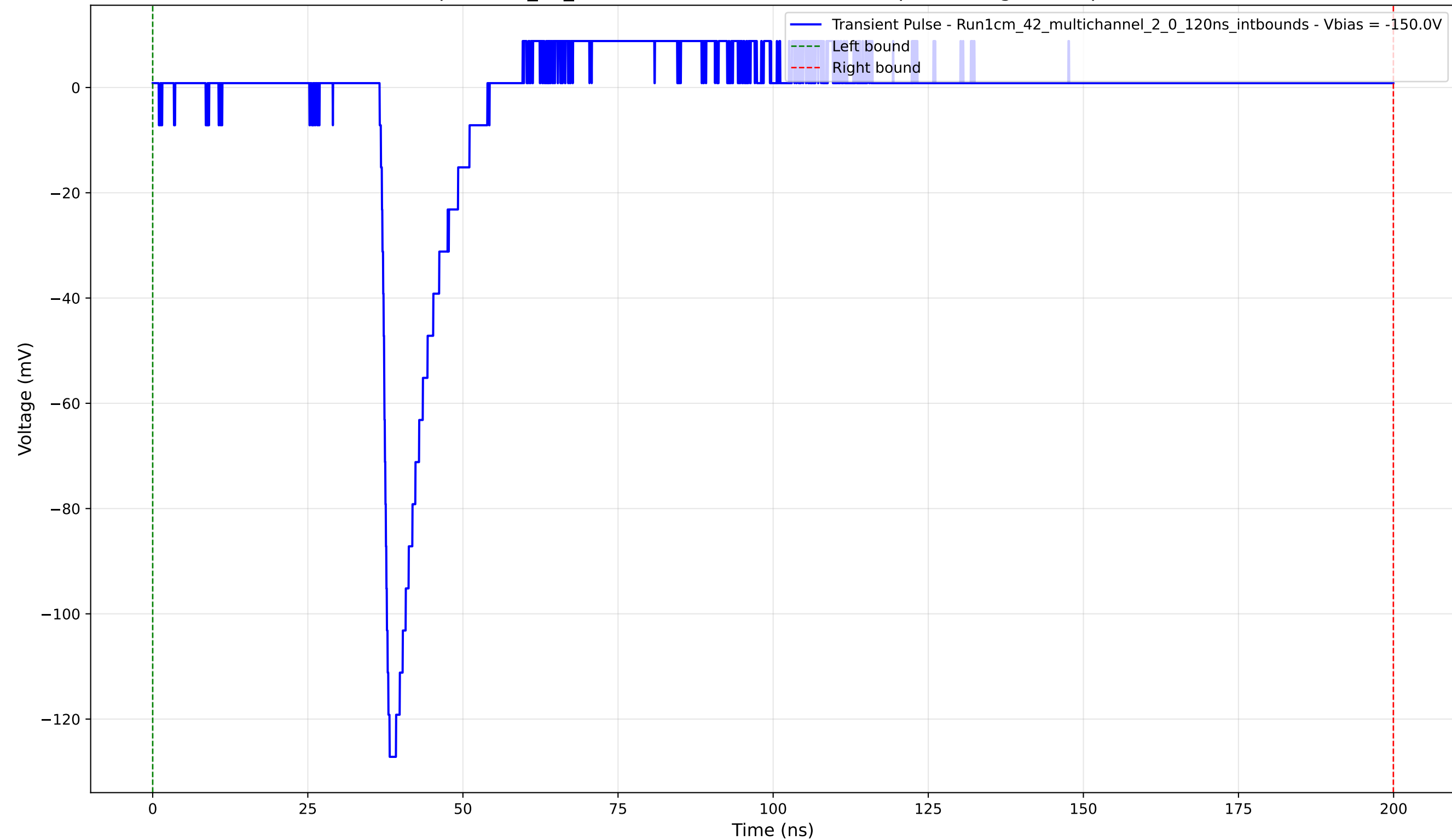
Transient Pulse - Sample: 1cm_42_multichannel - Position: 1055.0 \mu\text{m} - Charge: 8.14 pC - Rise Time: 1.21 ns
