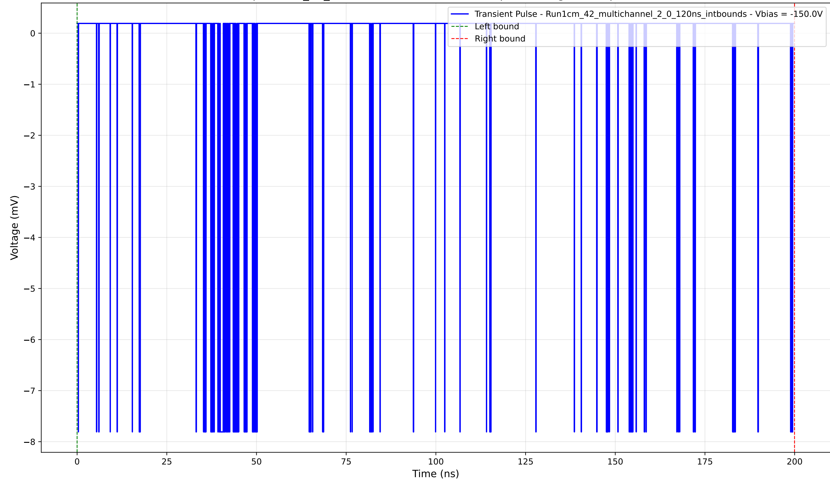
Transient Pulse - Sample: 1cm_42_multichannel - Position: 15.0 \mu\text{m} - Charge: 0.96 pC - Rise Time: 0.04 ns
