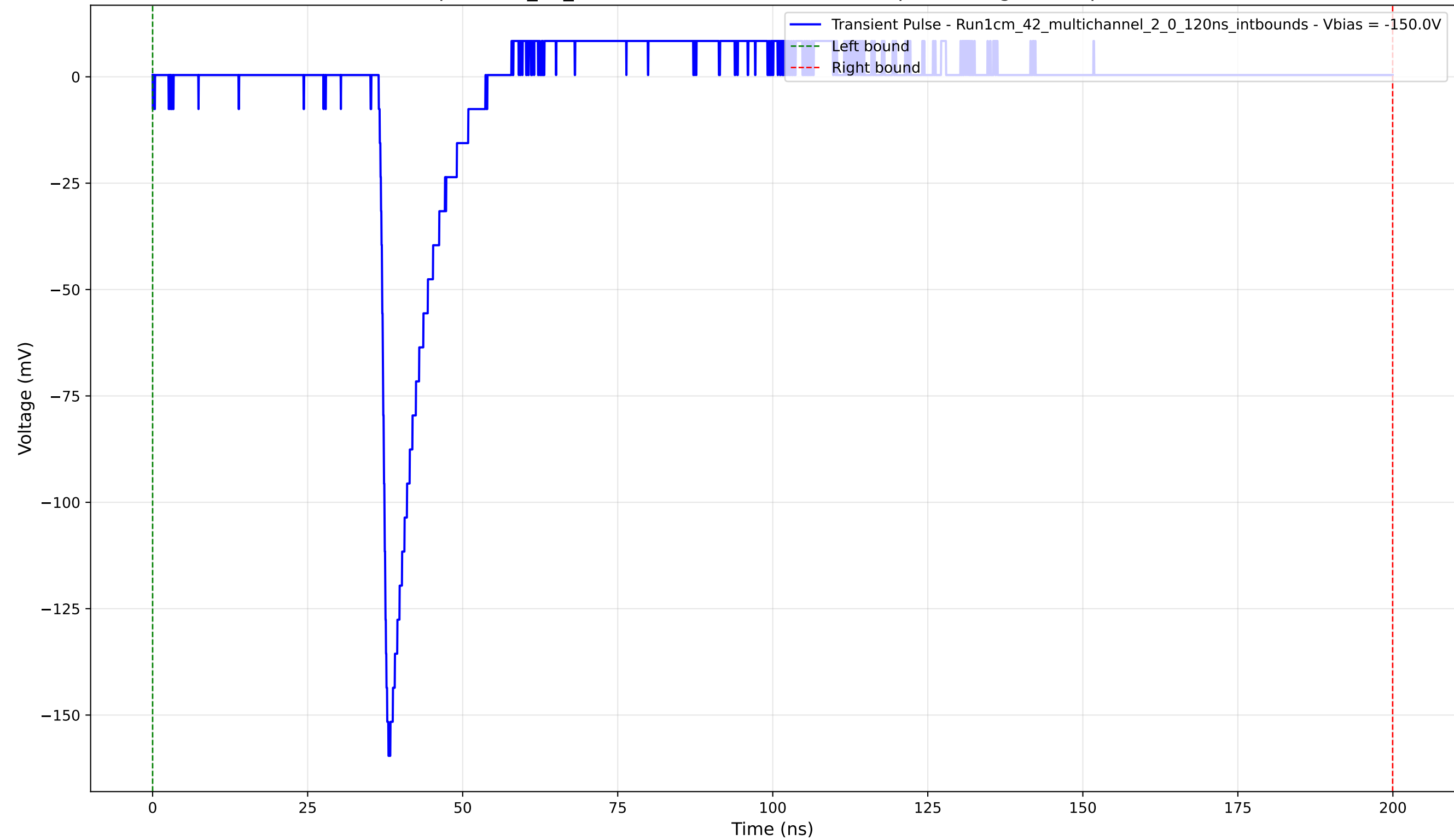
Transient Pulse - Sample: 1cm_42_multichannel - Position: 1260.0 \mu\text{m} - Charge: 9.48 pC - Rise Time: 1.12 ns
