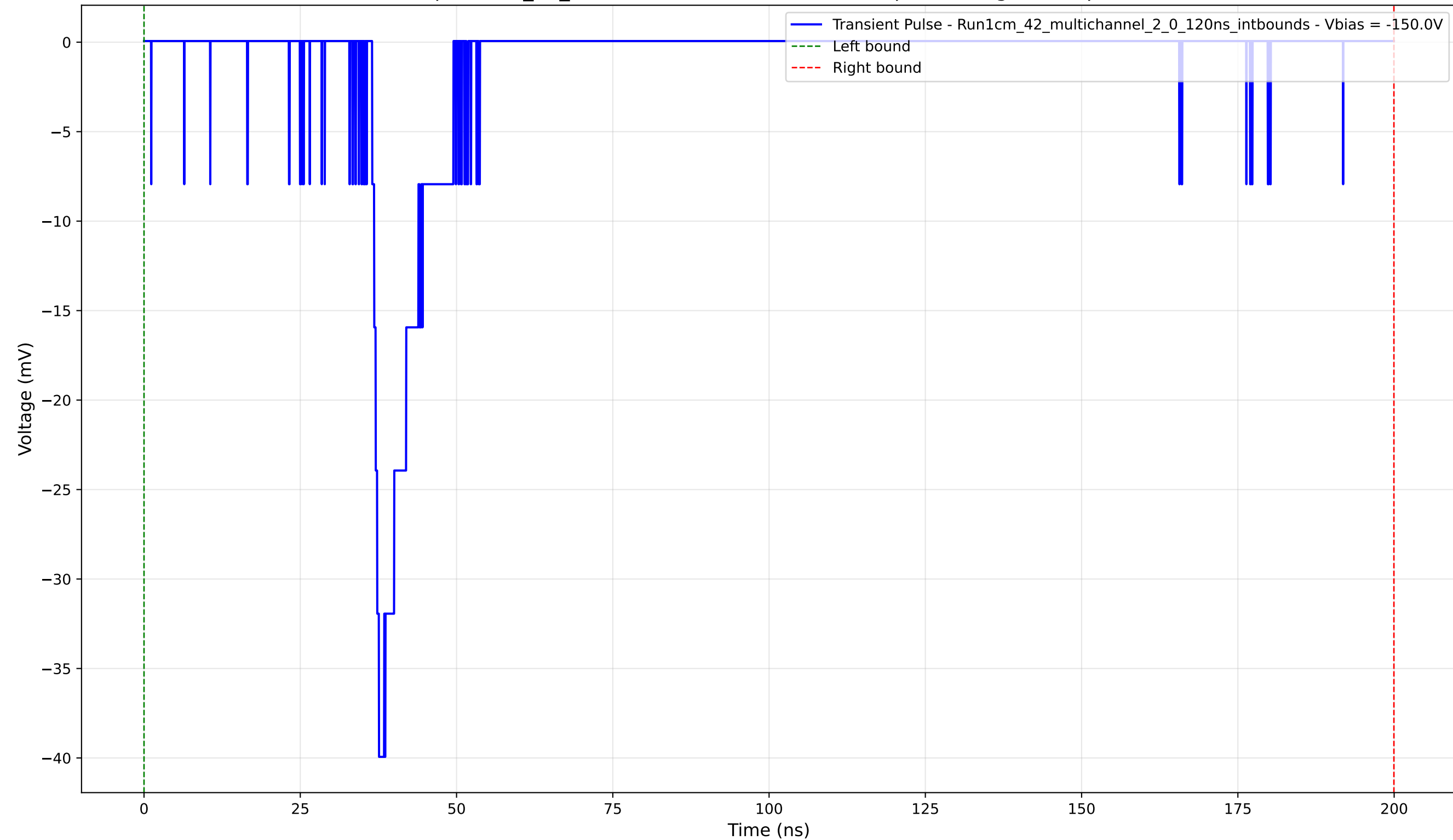
Transient Pulse - Sample: 1cm_42_multichannel - Position: 3345.0 \mu\text{m} - Charge: 4.92 pC - Rise Time: 1.10 ns
