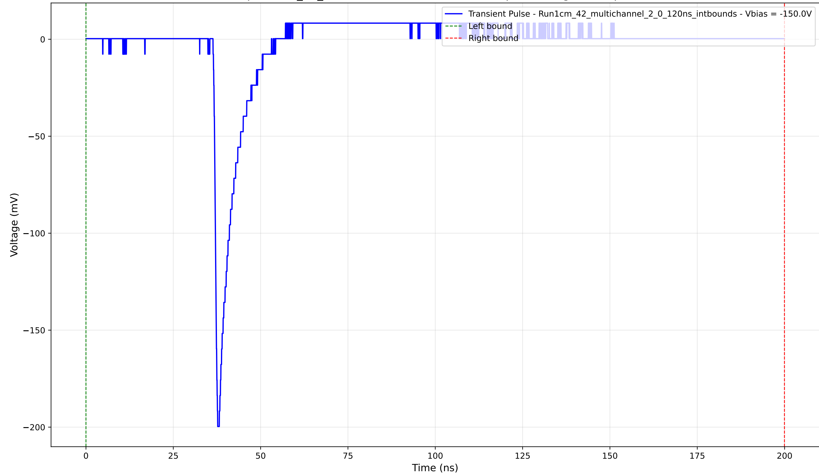
Transient Pulse - Sample: 1cm_42_multichannel - Position: 1470.0 \mu\text{m} - Charge: 9.93 pC - Rise Time: 0.98 ns
