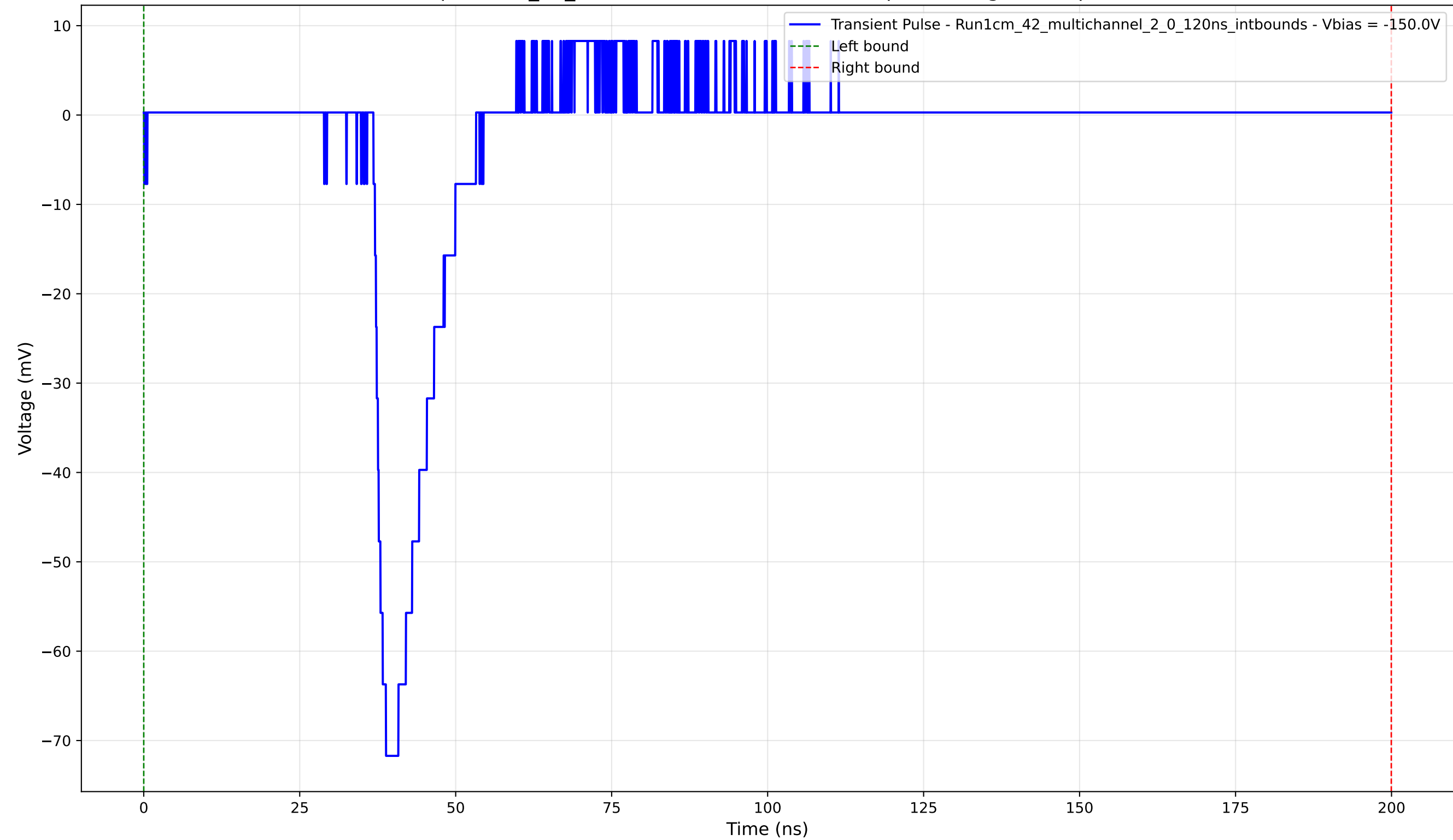
Transient Pulse - Sample: 1cm_42_multichannel - Position: 220.0 \mu\text{m} - Charge: 8.34 pC - Rise Time: 2.00 ns
