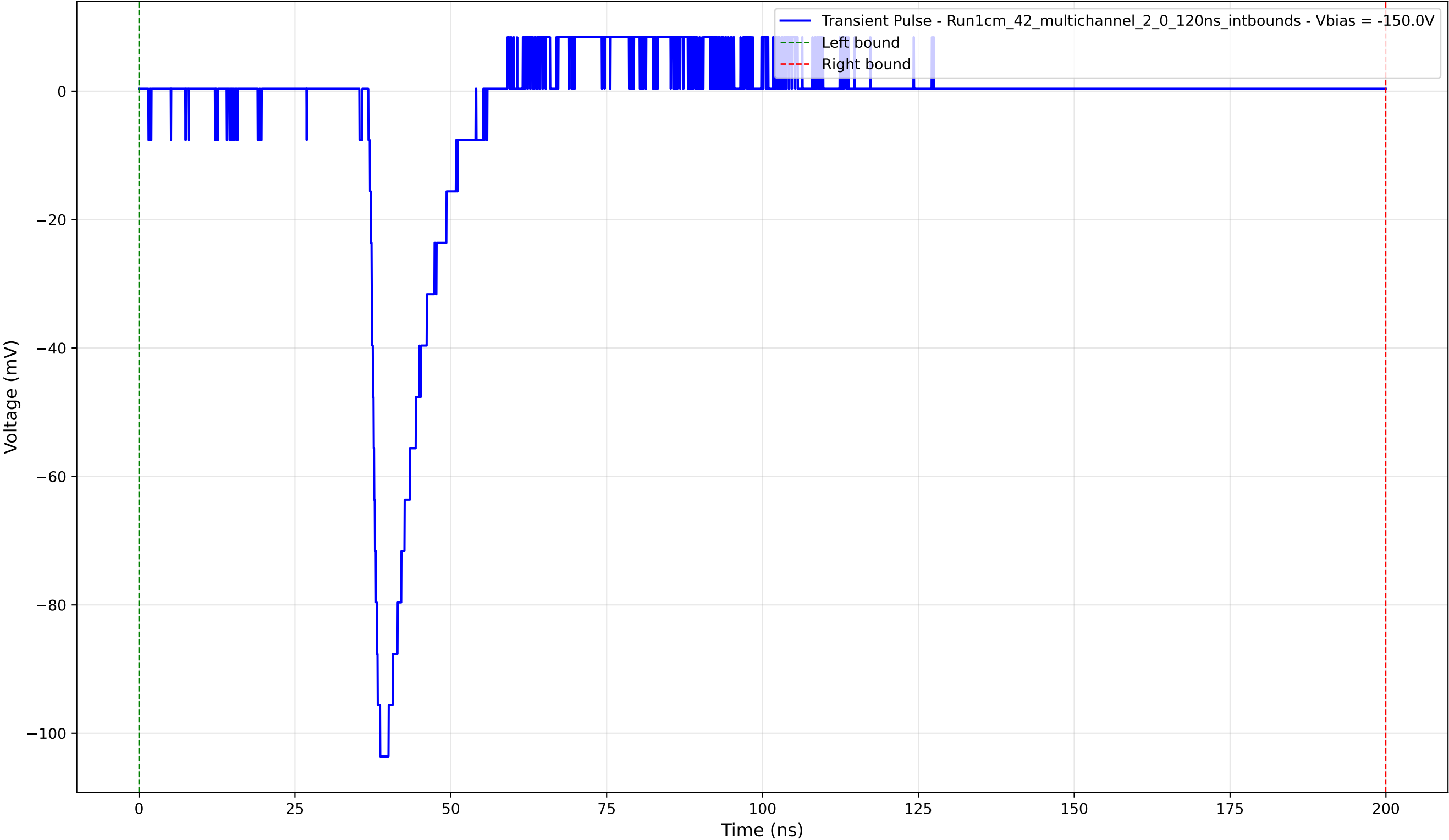
Transient Pulse - Sample: 1cm_42_multichannel - Position: 745.0 \mu\text{m} - Charge: 9.47 pC - Rise Time: 1.27 ns
