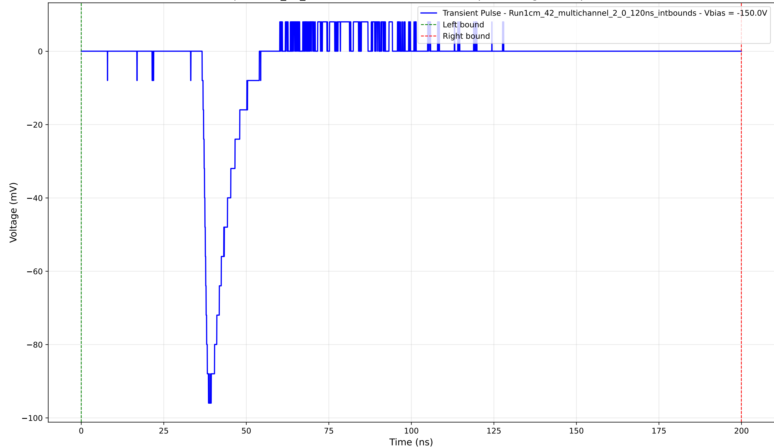
Transient Pulse - Sample: 1cm_42_multichannel - Position: 3810.0 \mu\text{m} - Charge: 9.87 pC - Rise Time: 1.31 ns
