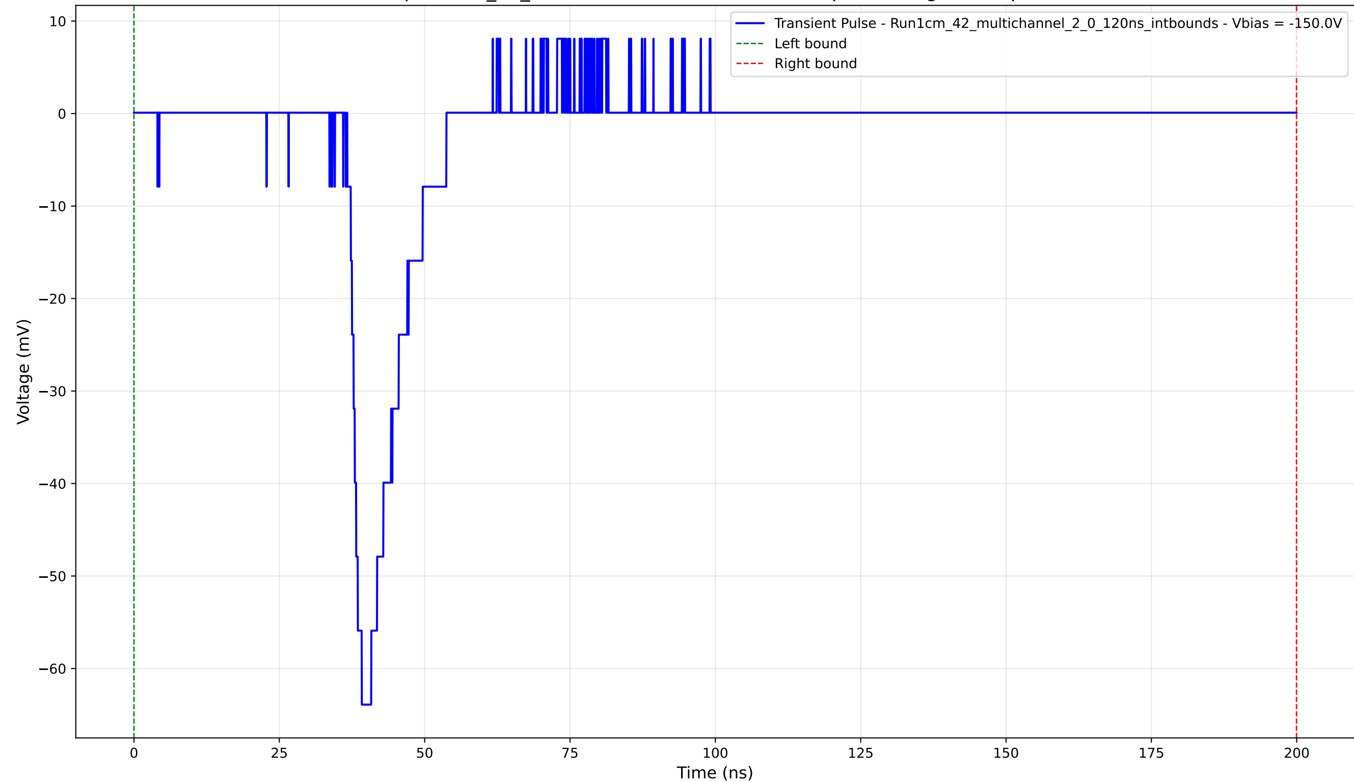
Transient Pulse - Sample: 1cm_42_multichannel - Position: 4465.0 \mu\text{m} - Charge: 8.74 pC - Rise Time: 2.49 ns
