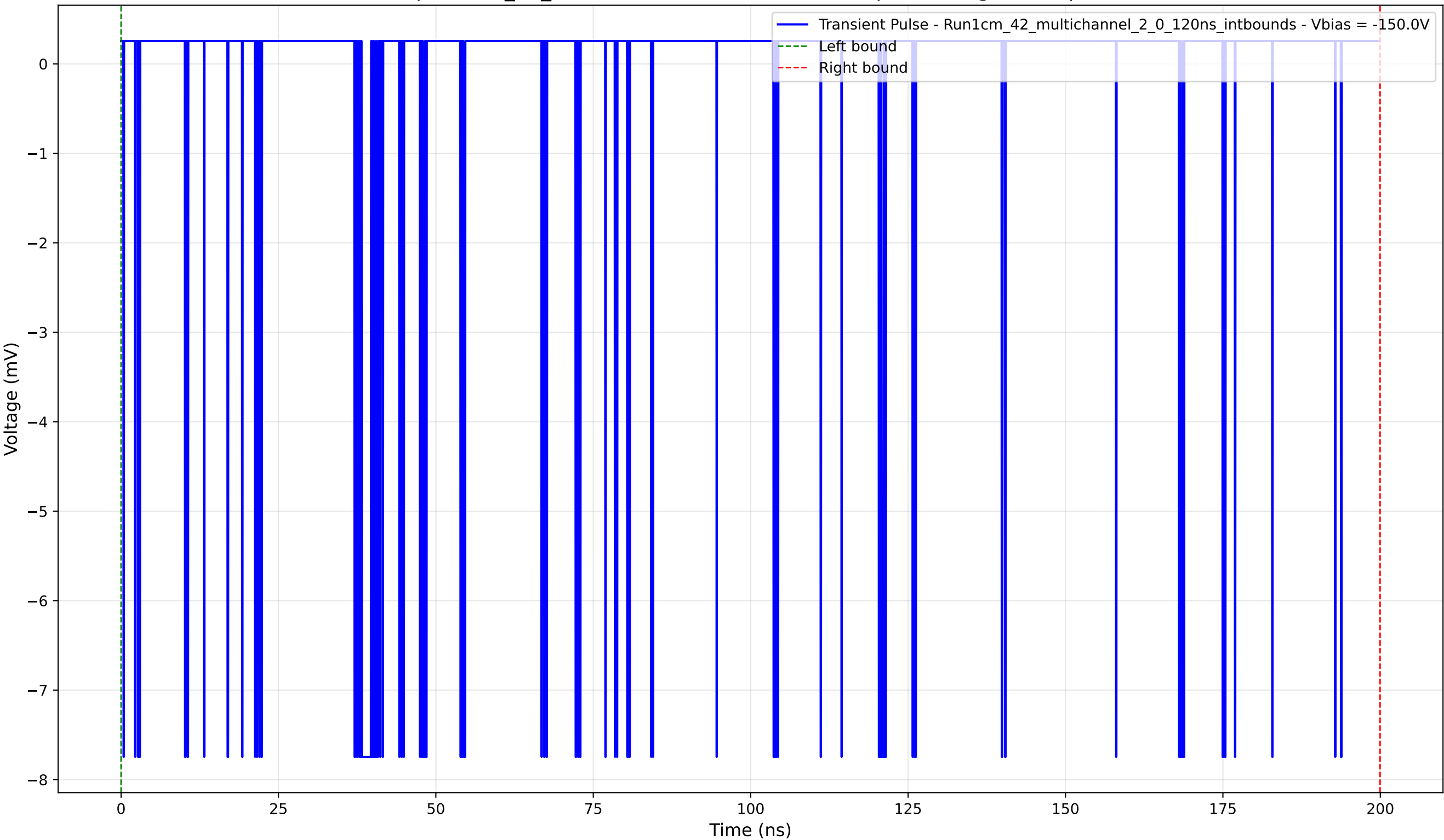
Transient Pulse - Sample: 1cm_42_multichannel - Position: 4925.0 \mu\text{m} - Charge: 0.50 pC - Rise Time: 0.04 ns
