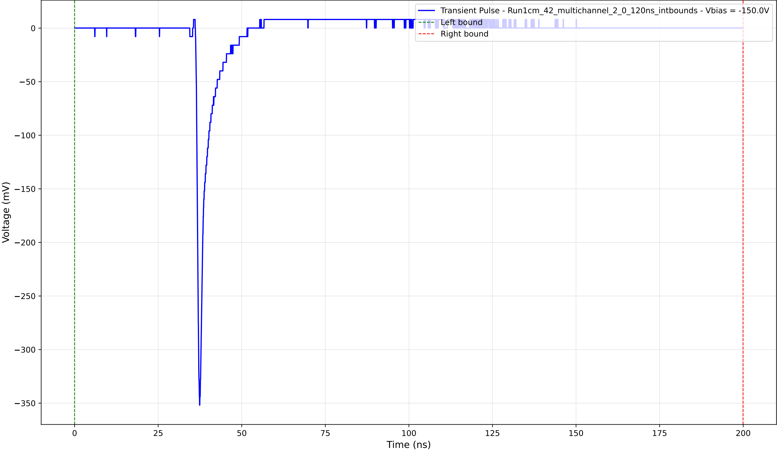
Transient Pulse - Sample: 1cm_42_multichannel - Position: 2790.0 \mu\text{m} - Charge: 12.50 pC - Rise Time: 0.81 ns
