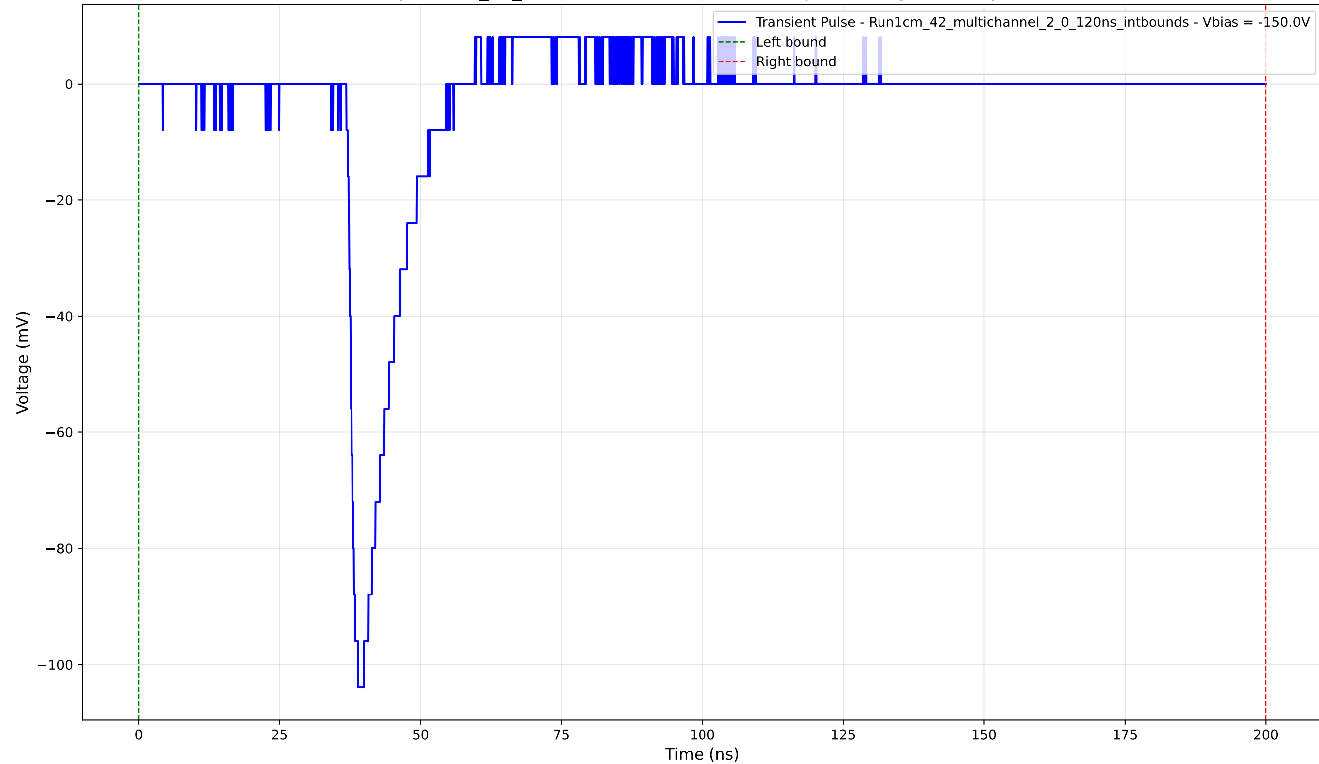
Transient Pulse - Sample: 1cm_42_multichannel - Position: 665.0 \mu\text{m} - Charge: 11.26 pC - Rise Time: 1.39 ns
