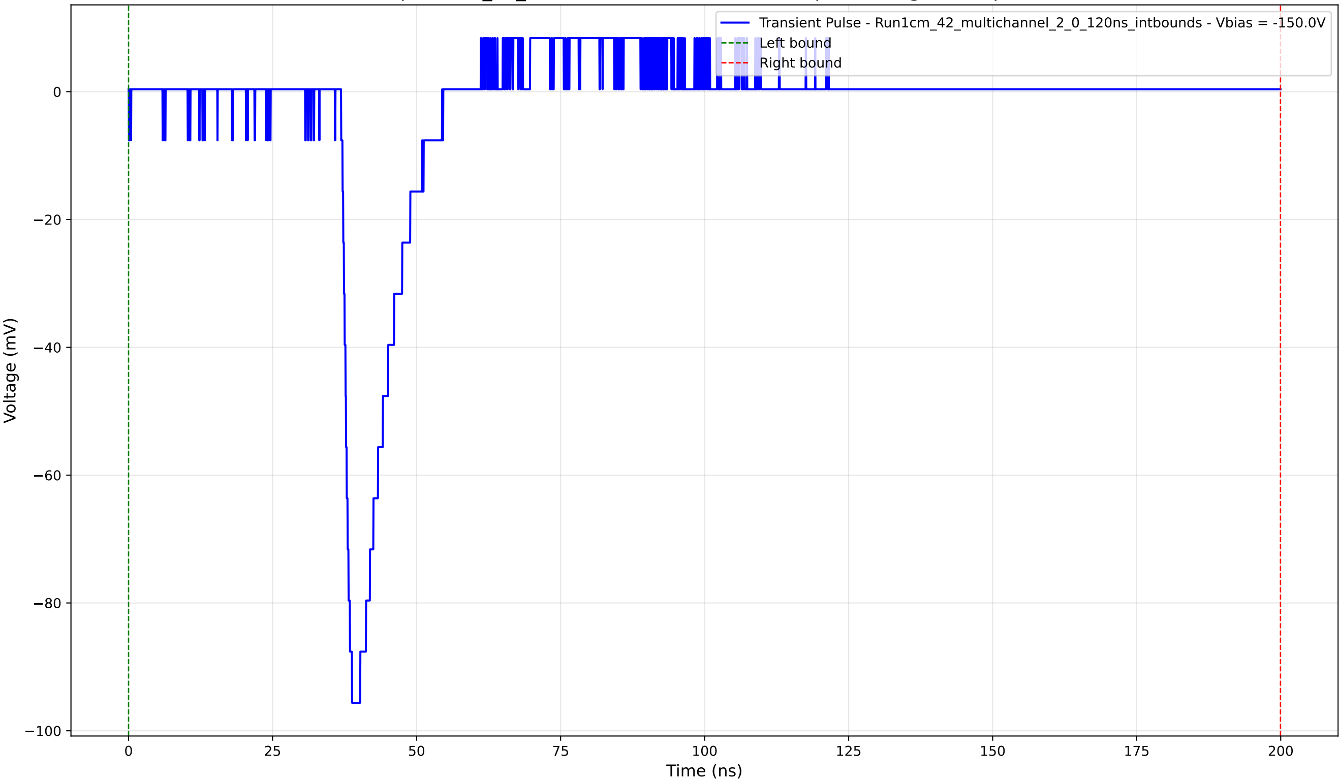
Transient Pulse - Sample: 1cm_42_multichannel - Position: 570.0 \mu\text{m} - Charge: 9.38 pC - Rise Time: 1.31 ns
