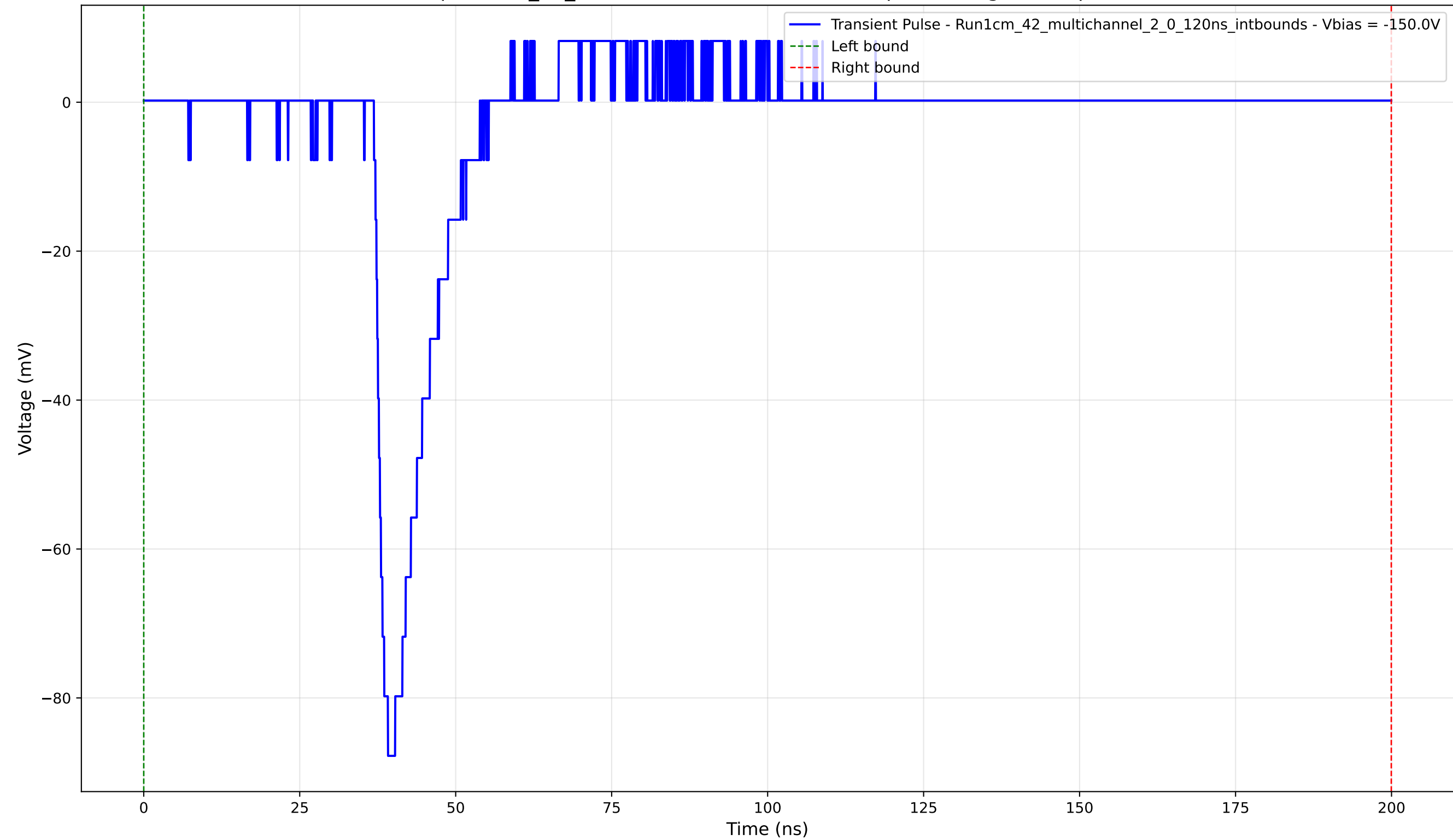
Transient Pulse - Sample: 1cm_42_multichannel - Position: 430.0 \mu\text{m} - Charge: 9.68 pC - Rise Time: 1.43 ns
