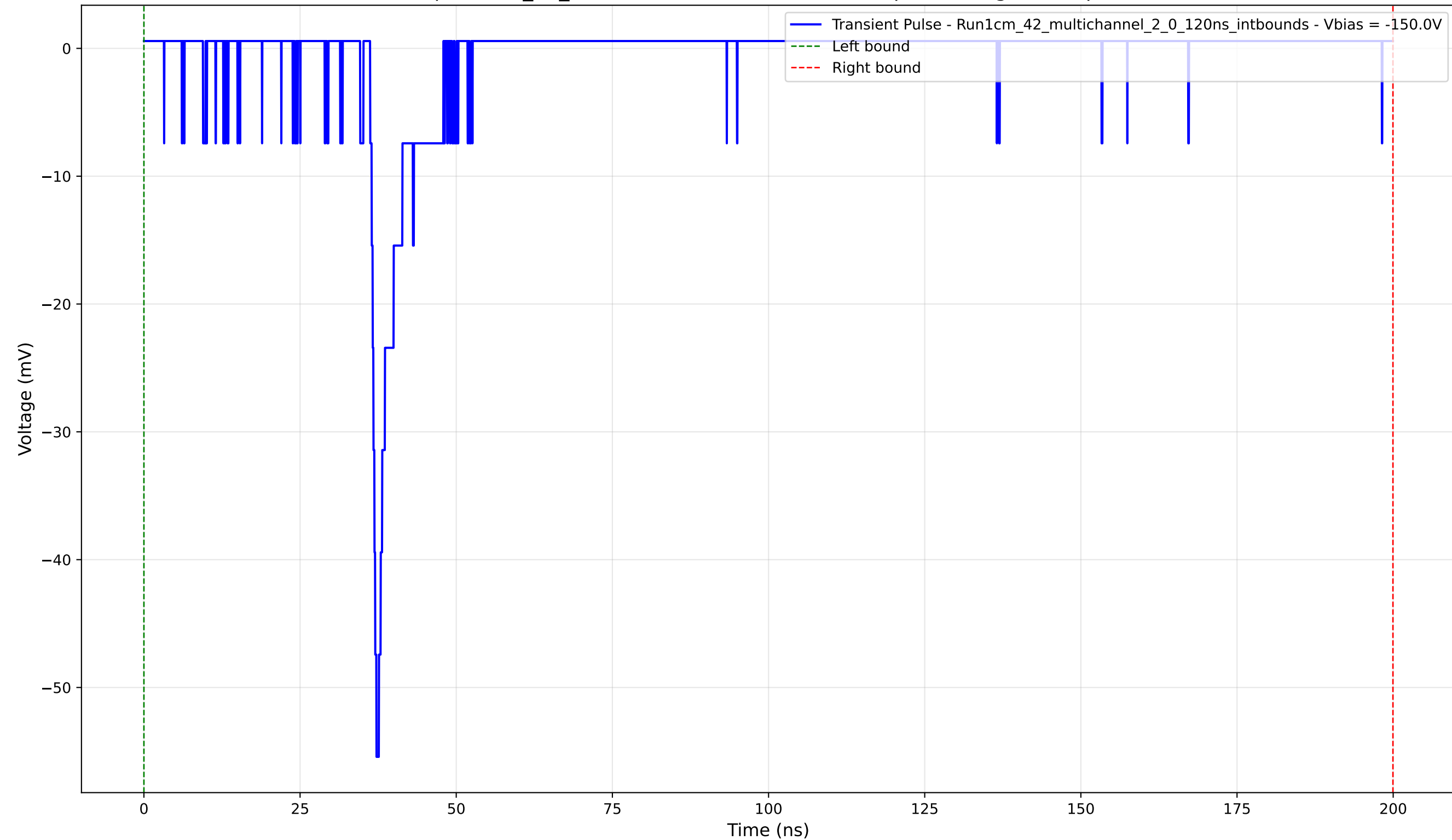
Transient Pulse - Sample: 1cm_42_multichannel - Position: 2845.0 \mu\text{m} - Charge: 2.46 pC - Rise Time: 1.01 ns
