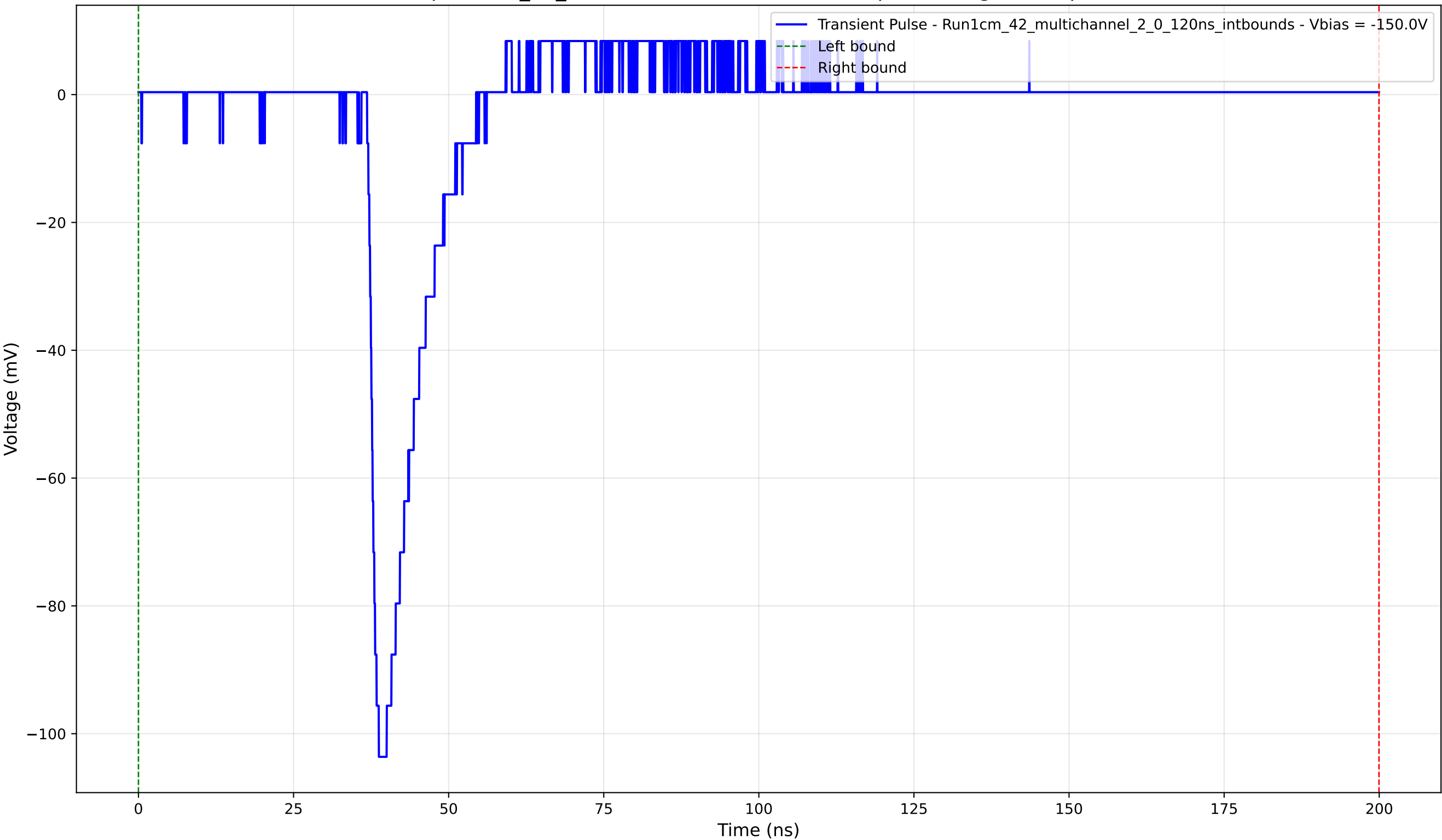
Transient Pulse - Sample: 1cm_42_multichannel - Position: 680.0 \mu\text{m} - Charge: 9.75 pC - Rise Time: 1.35 ns
