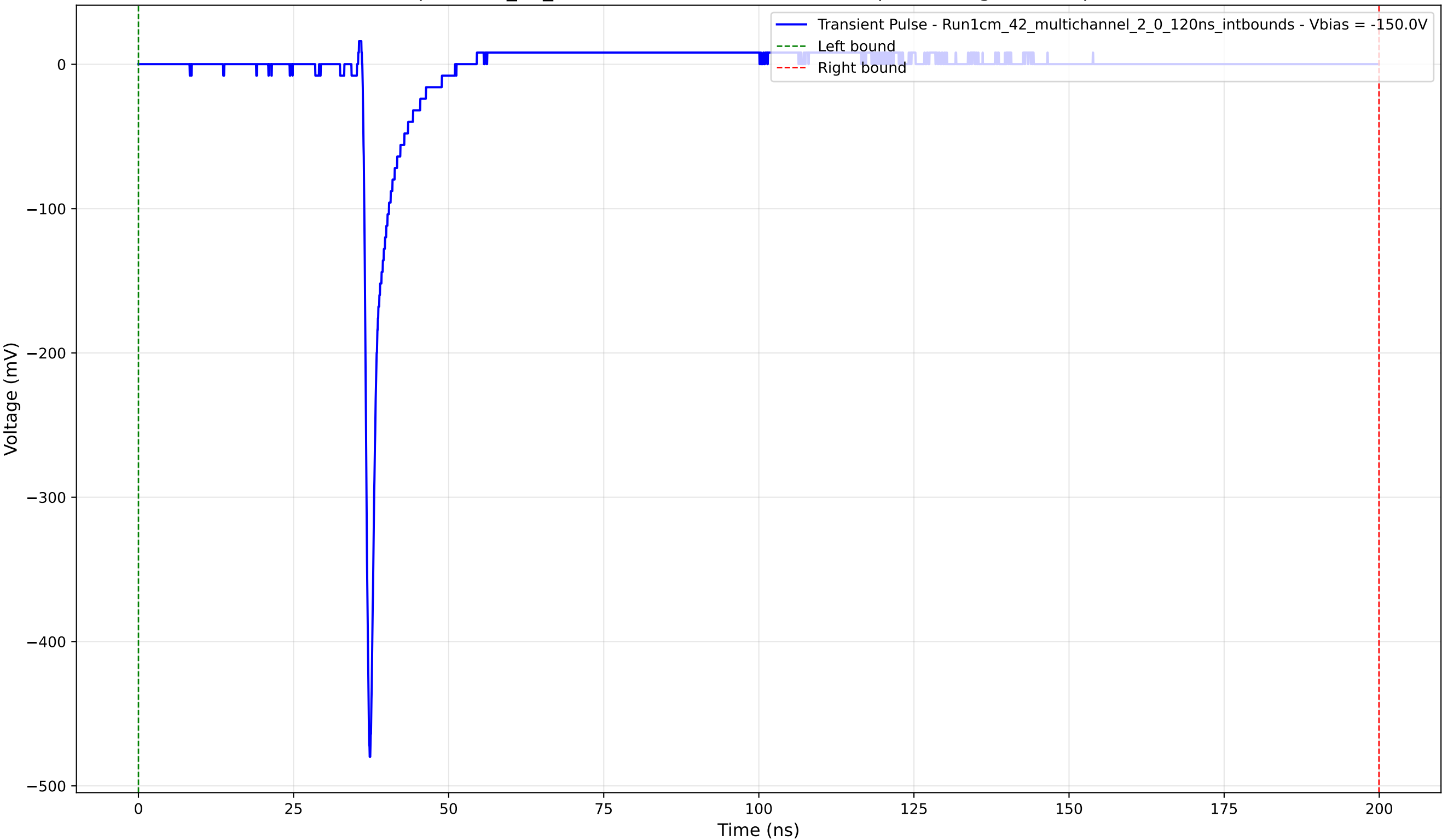
Transient Pulse - Sample: 1cm_42_multichannel - Position: 2085.0 \mu\text{m} - Charge: 14.98 pC - Rise Time: 0.74 ns
