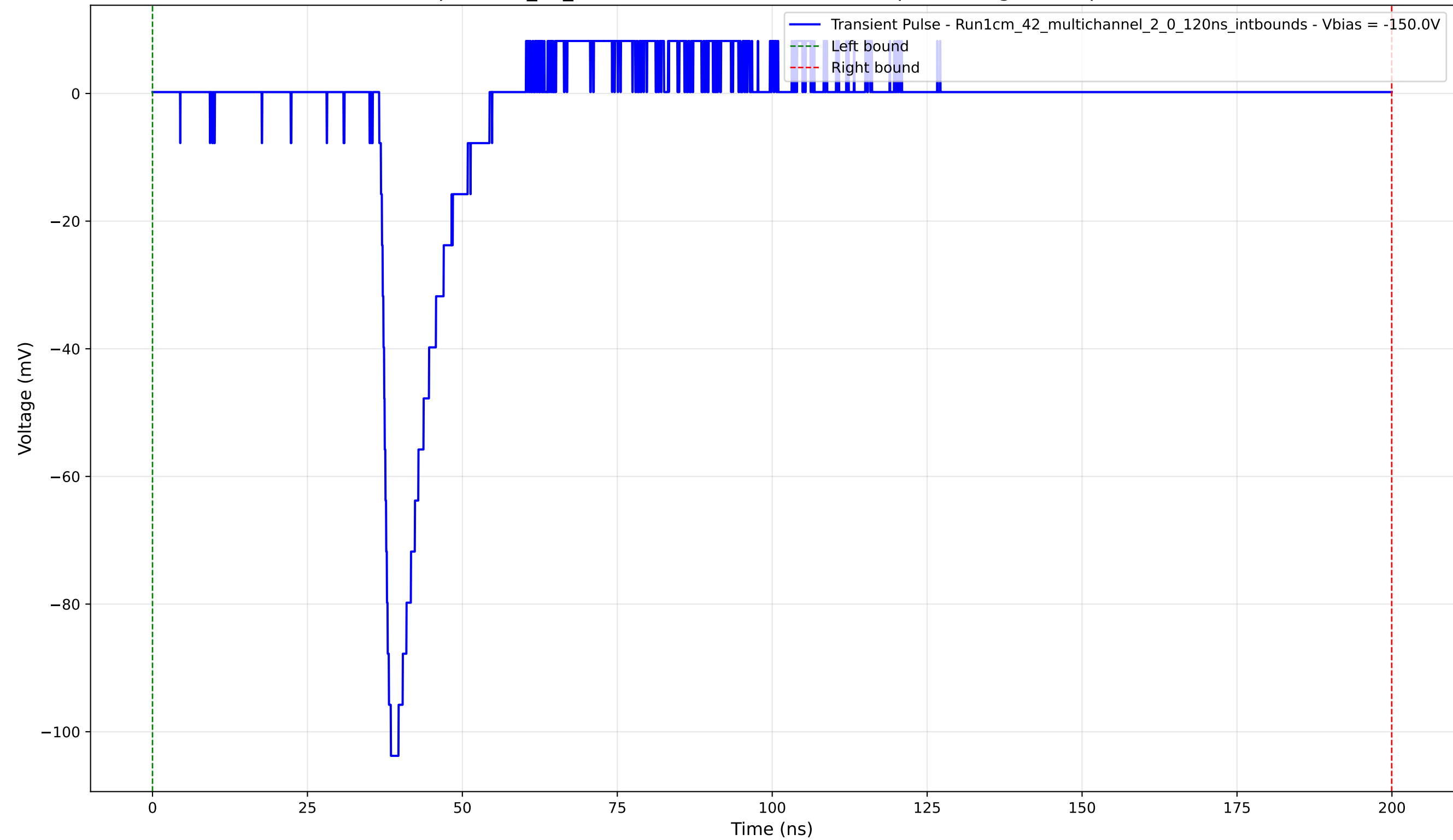
Transient Pulse - Sample: 1cm_42_multichannel - Position: 3780.0 \mu\text{m} - Charge: 9.32 pC - Rise Time: 1.31 ns
