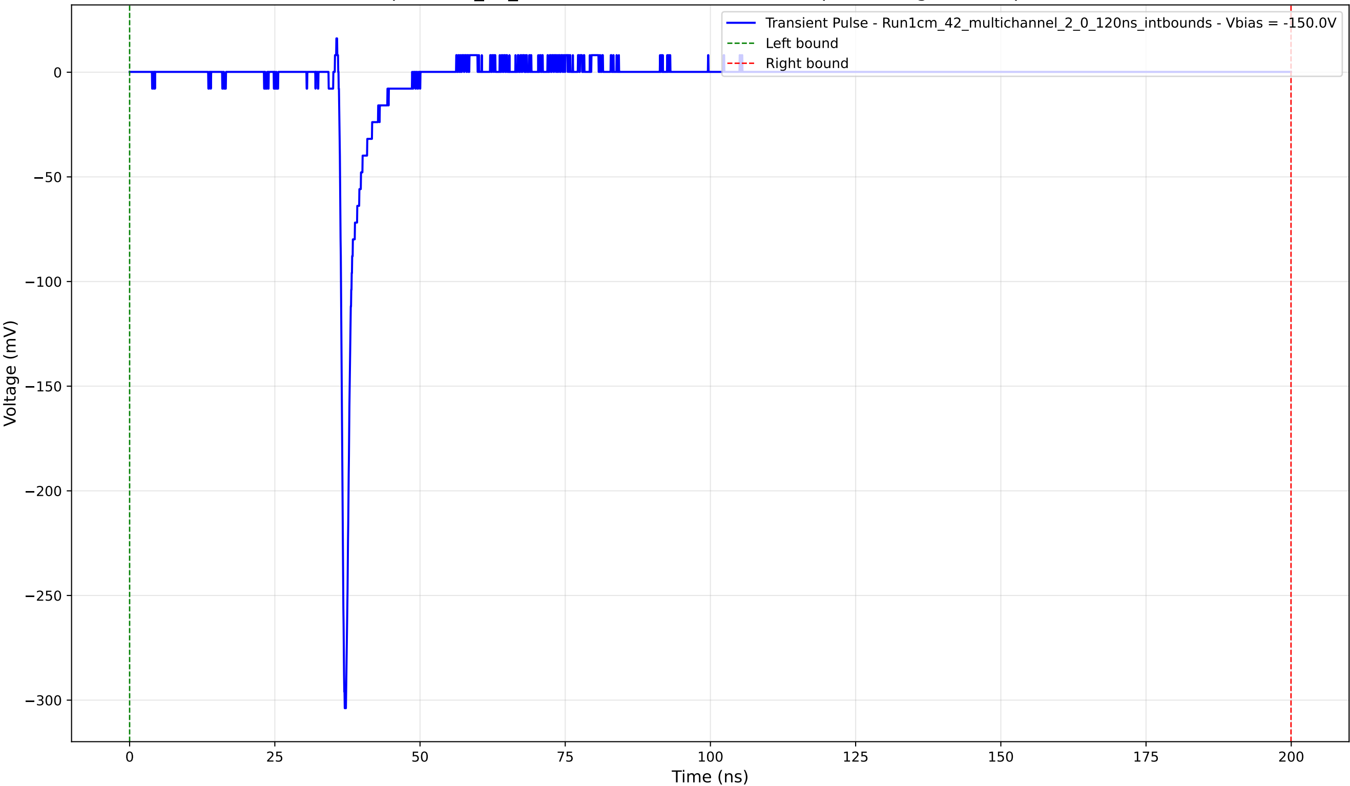
Transient Pulse - Sample: 1cm_42_multichannel - Position: 2320.0 \mu\text{m} - Charge: 11.60 pC - Rise Time: 0.70 ns
