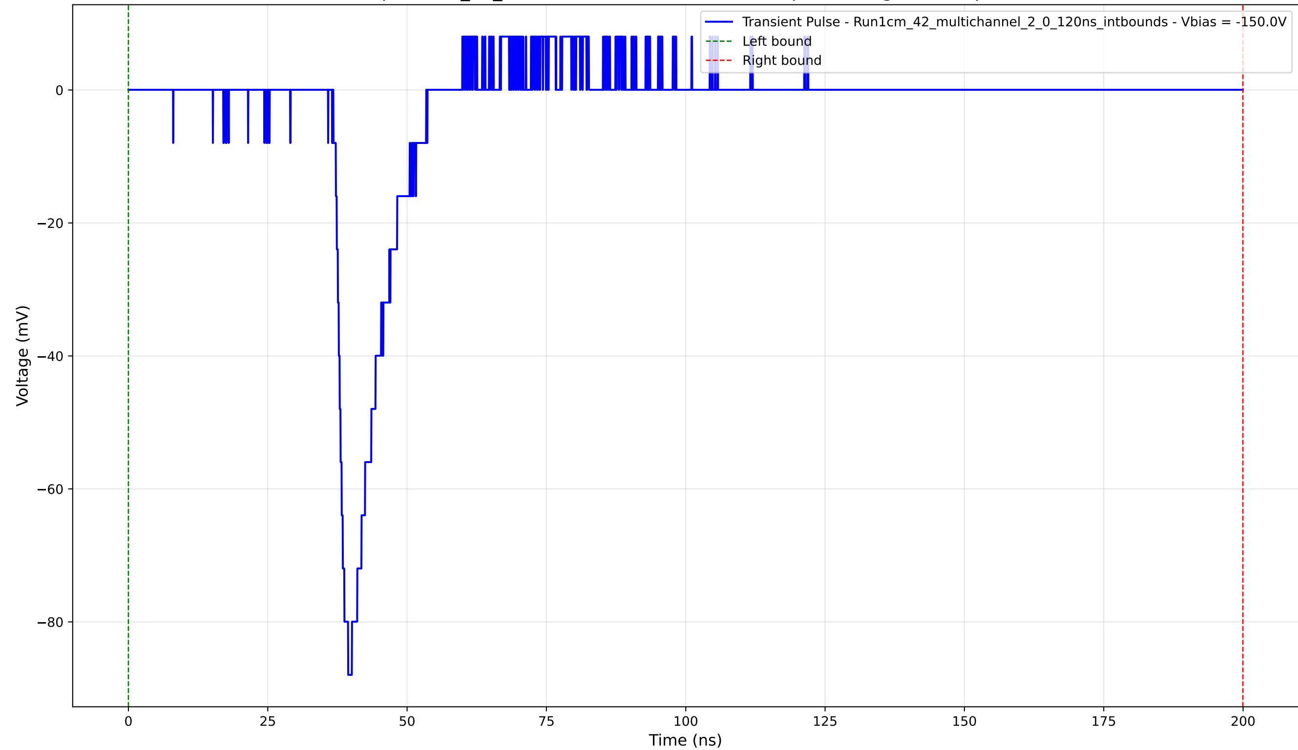
Transient Pulse - Sample: 1cm_42_multichannel - Position: 4225.0 \mu\text{m} - Charge: 10.21 pC - Rise Time: 1.56 ns
