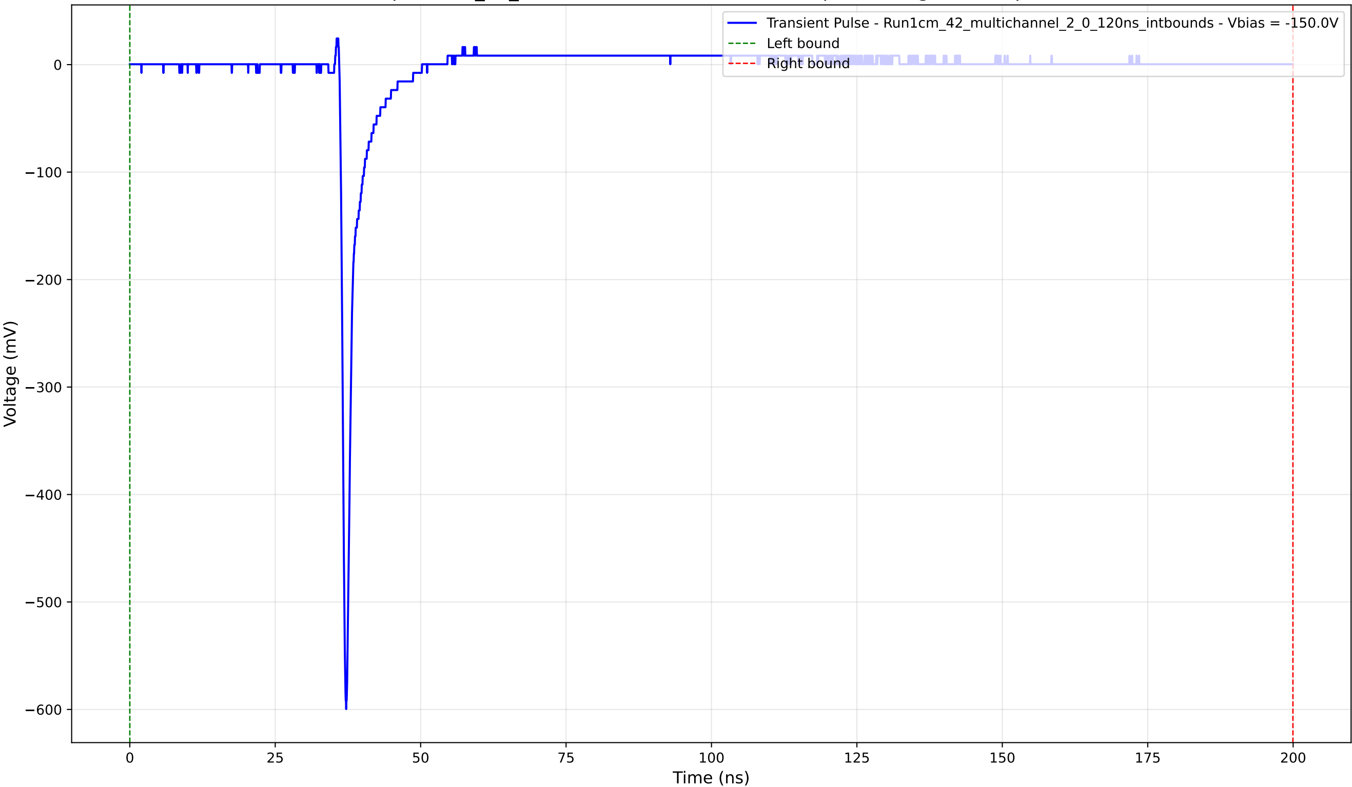
Transient Pulse - Sample: 1cm_42_multichannel - Position: 2220.0 \mu\text{m} - Charge: 15.72 pC - Rise Time: 0.74 ns
