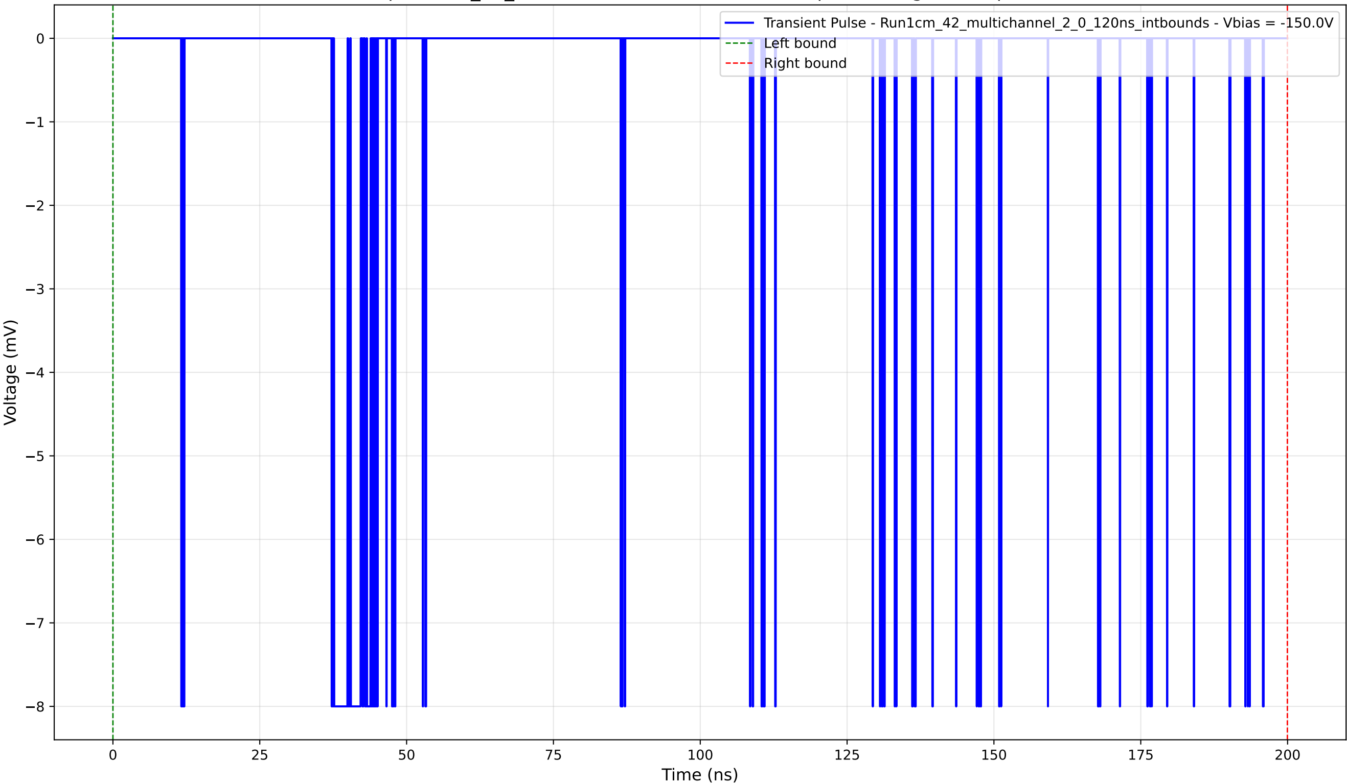
Transient Pulse - Sample: 1cm_42_multichannel - Position: 4885.0 \mu\text{m} - Charge: 1.73 pC - Rise Time: 0.04 ns
