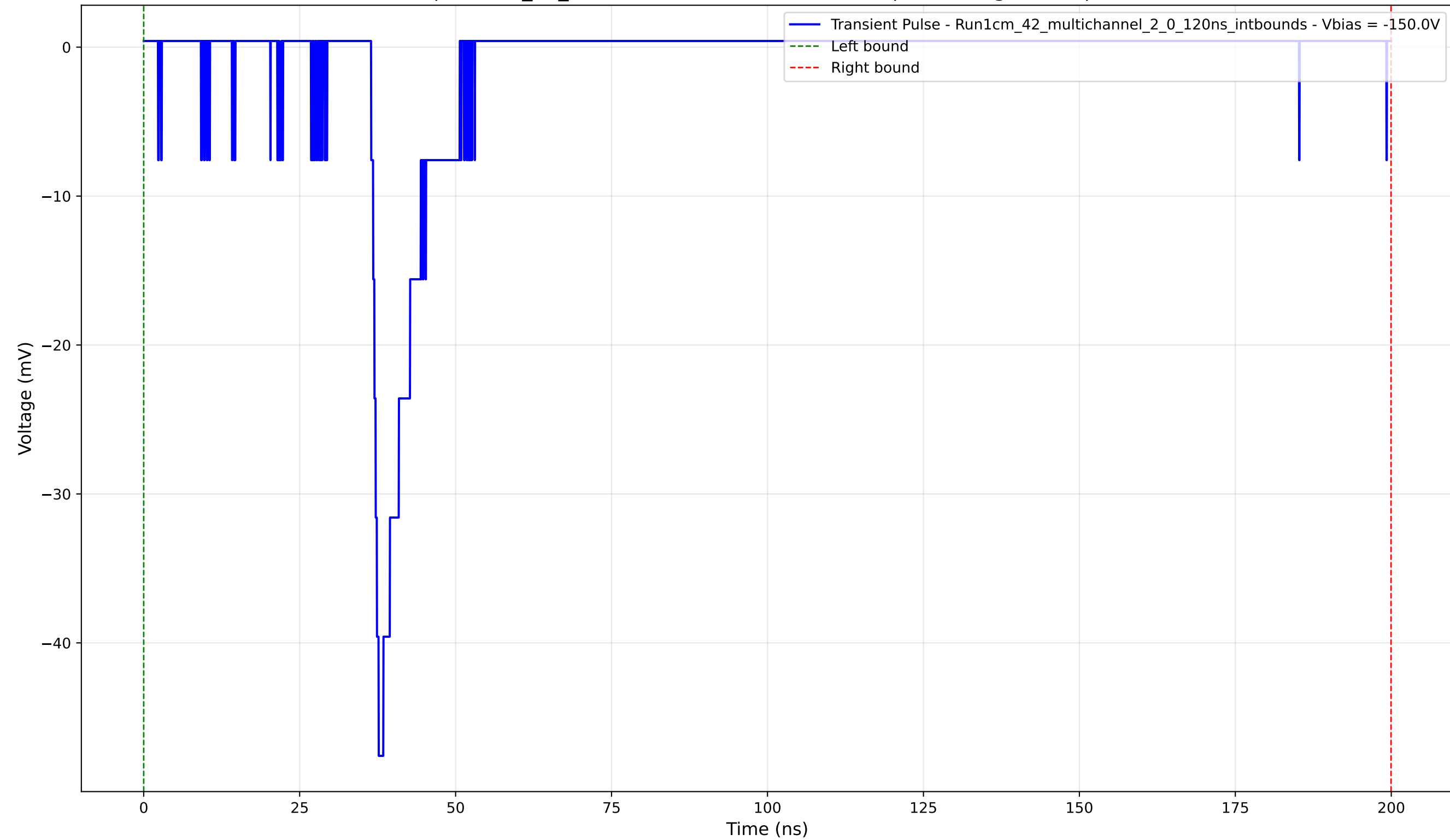
Transient Pulse - Sample: 1cm_42_multichannel - Position: 1395.0 \mu\text{m} - Charge: 4.44 pC - Rise Time: 1.22 ns
