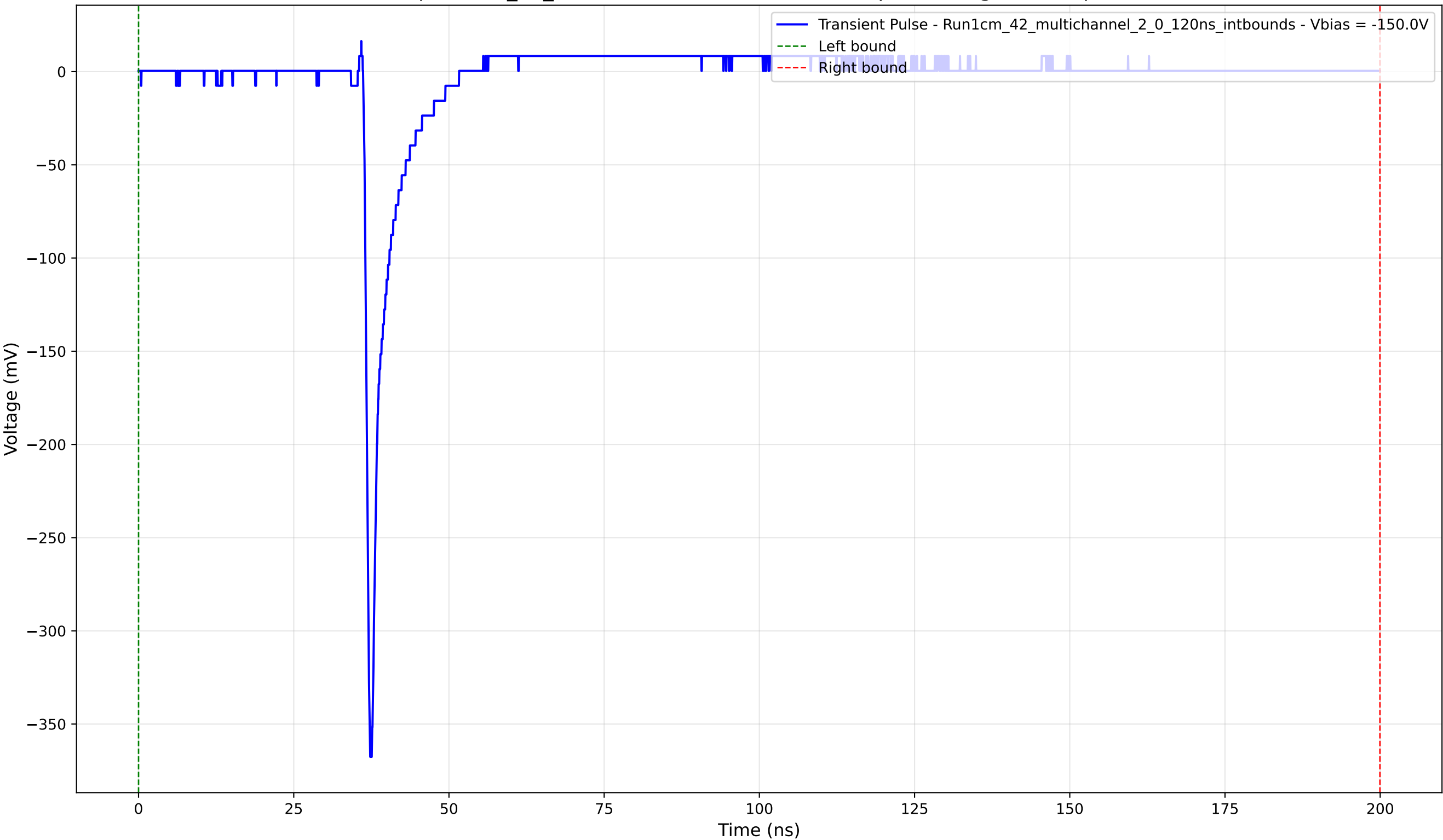
Transient Pulse - Sample: 1cm_42_multichannel - Position: 1950.0 \mu\text{m} - Charge: 12.36 pC - Rise Time: 0.79 ns
