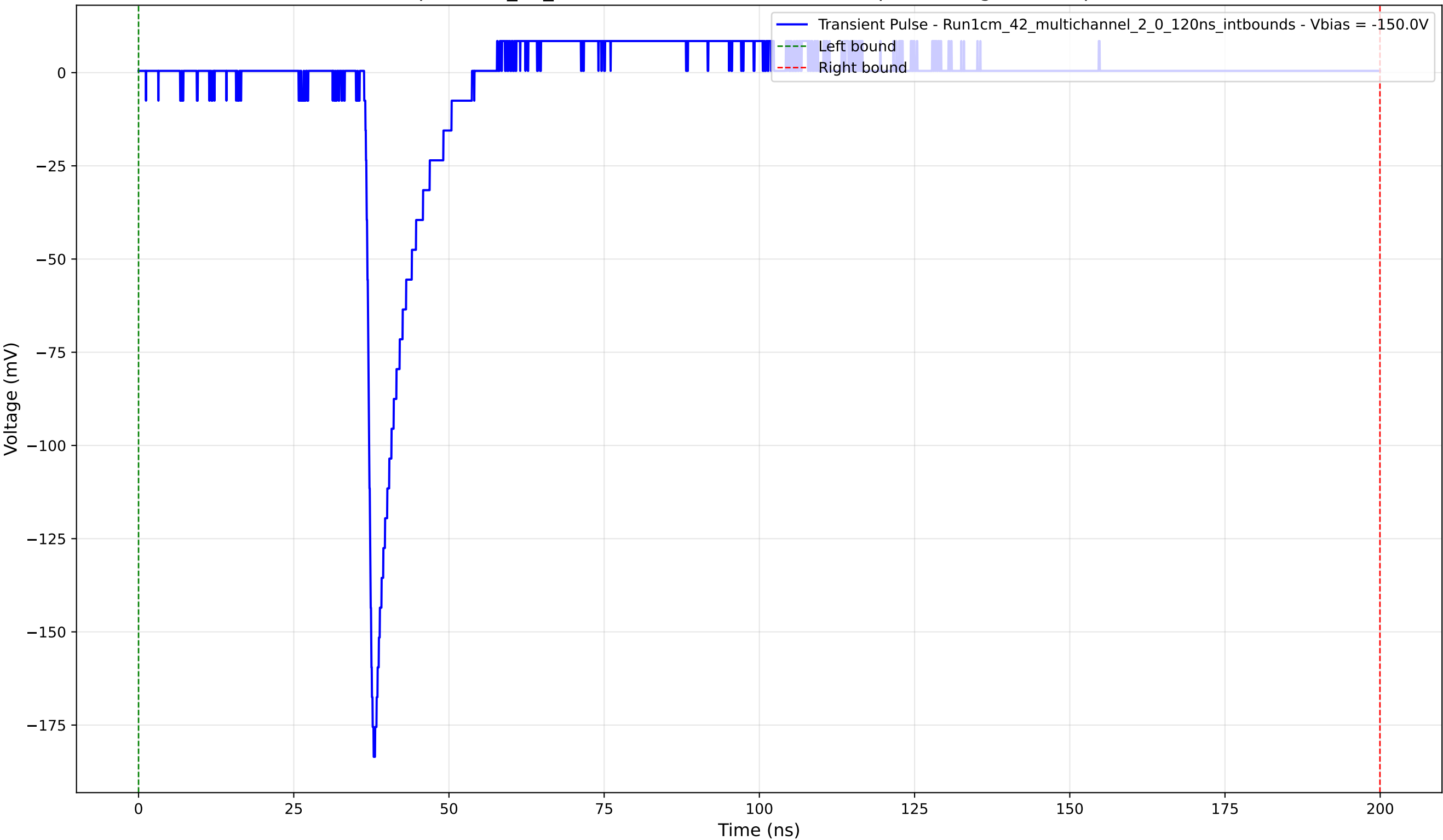
Transient Pulse - Sample: 1cm_42_multichannel - Position: 1435.0 \mu\text{m} - Charge: 10.72 pC - Rise Time: 0.99 ns
