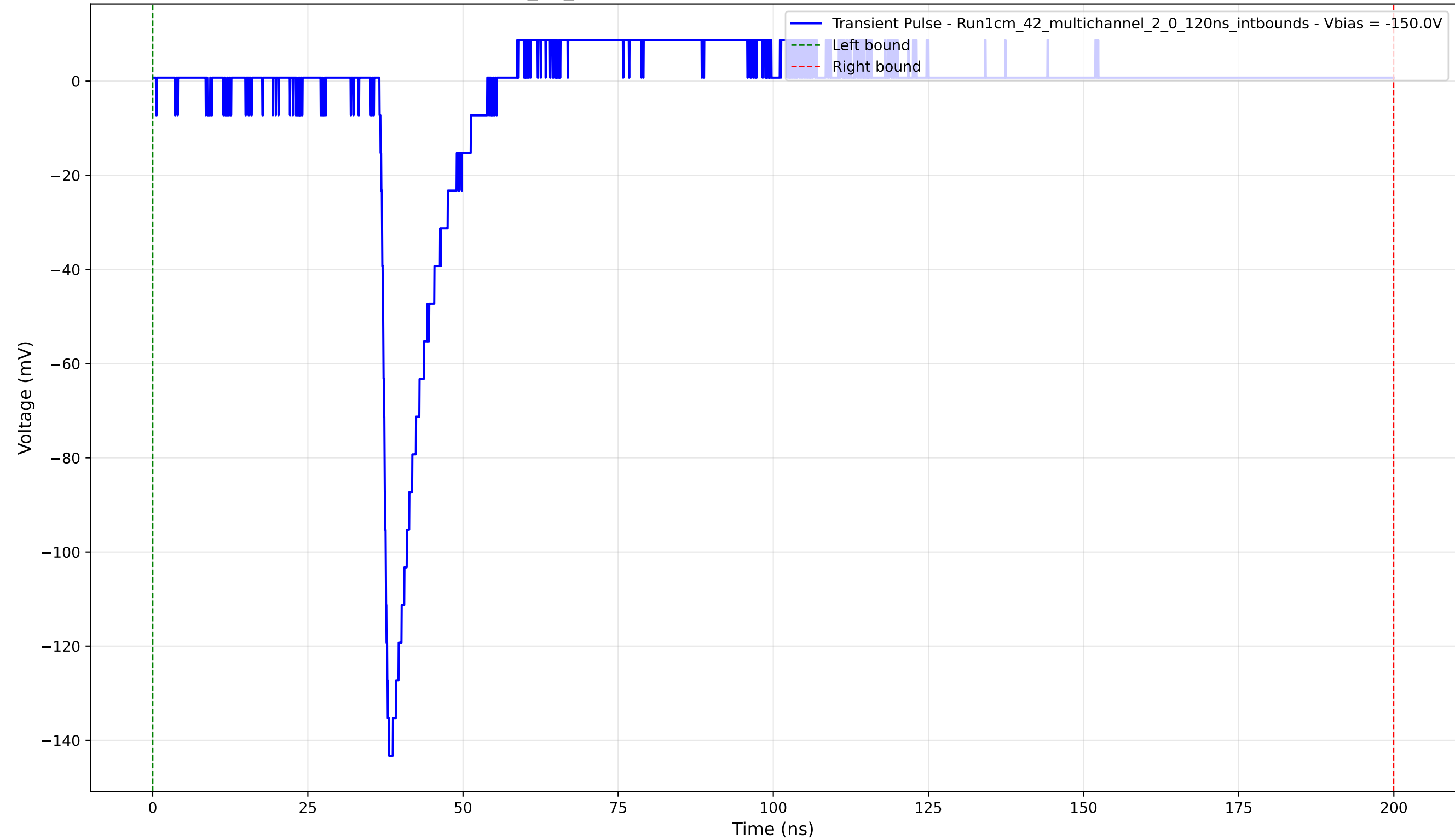
Transient Pulse - Sample: 1cm_42_multichannel - Position: 1170.0 \mu\text{m} - Charge: 9.39 pC - Rise Time: 1.16 ns
