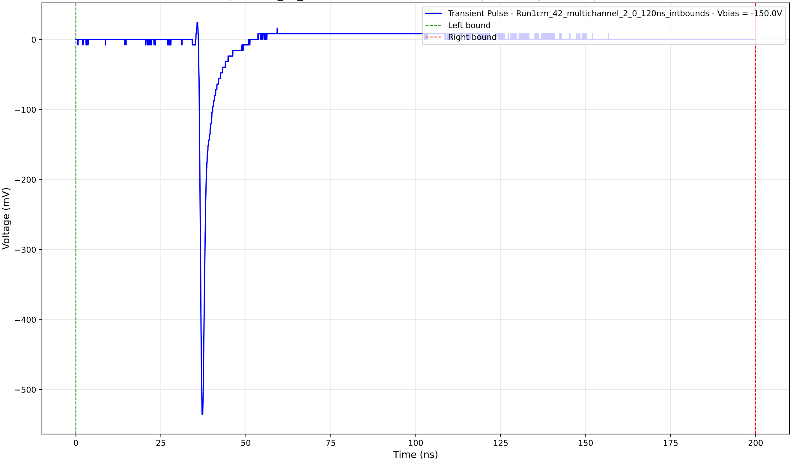
Transient Pulse - Sample: 1cm_42_multichannel - Position: 2165.0 \mu\text{m} - Charge: 14.42 pC - Rise Time: 0.76 ns
