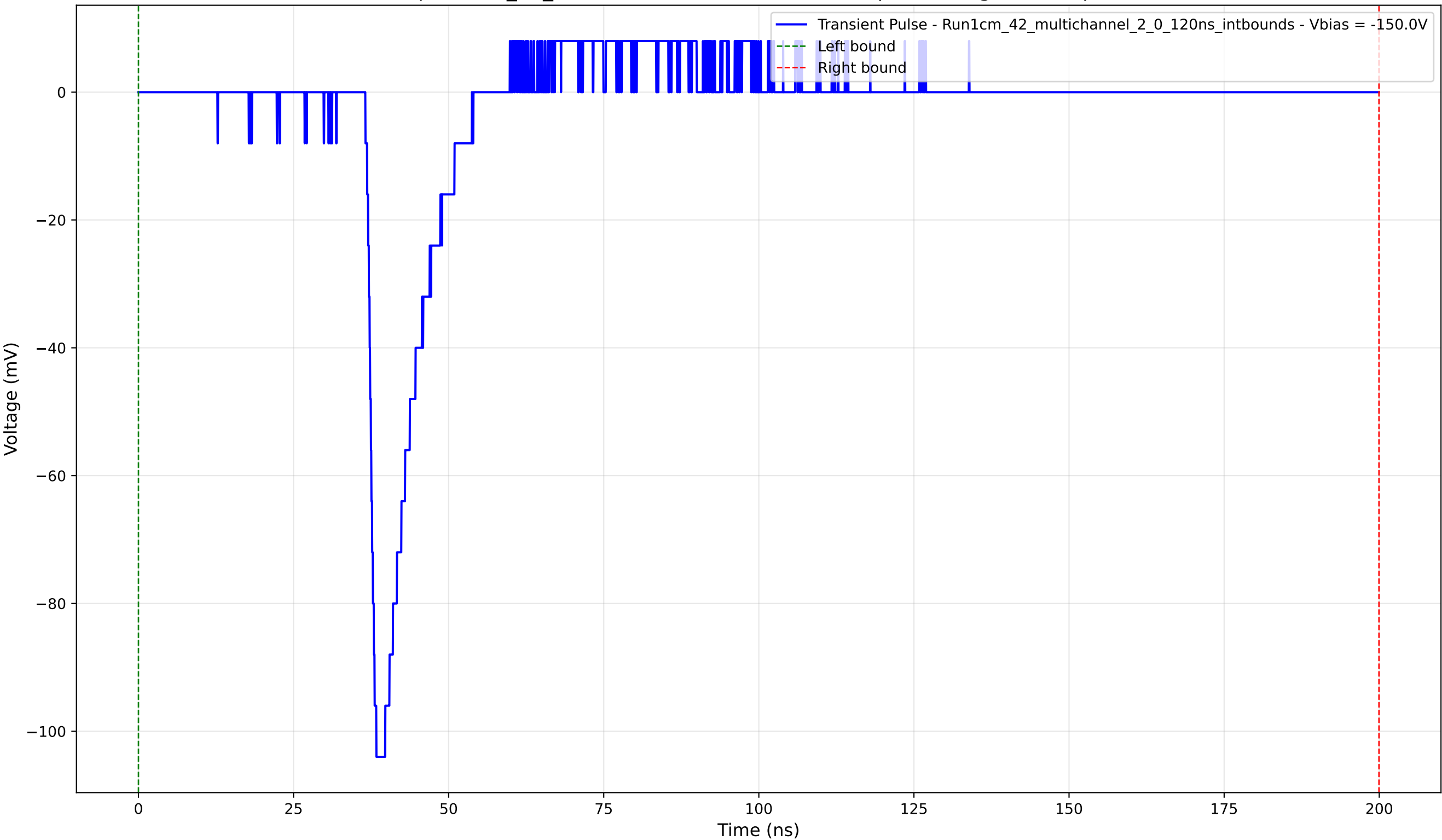
Transient Pulse - Sample: 1cm_42_multichannel - Position: 3770.0 \mu\text{m} - Charge: 10.63 pC - Rise Time: 1.23 ns
