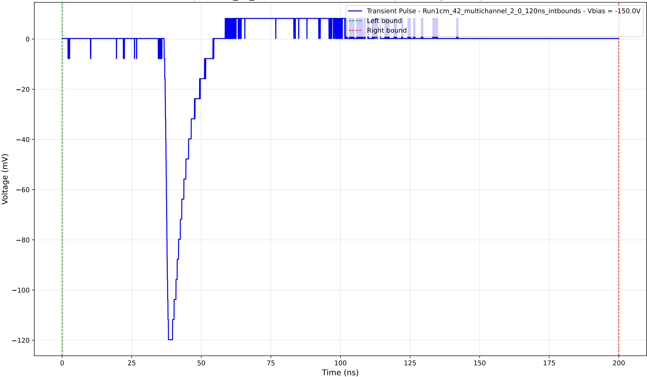
Transient Pulse - Sample: 1cm_42_multichannel - Position: 975.0 \mu\text{m} - Charge: 9.46 pC - Rise Time: 1.18 ns
