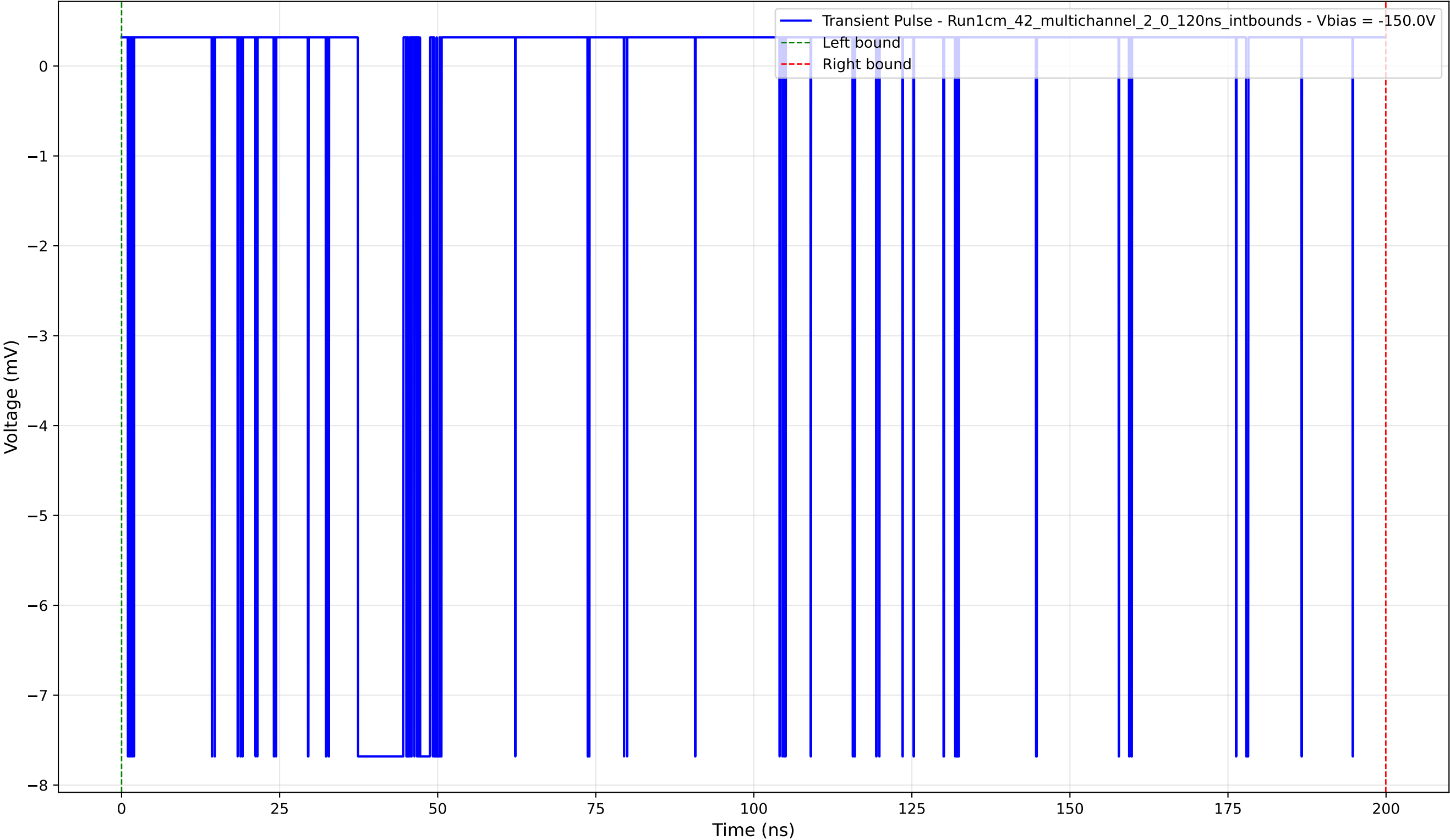
Transient Pulse - Sample: 1cm_42_multichannel - Position: 3905.0 \mu\text{m} - Charge: 1.07 pC - Rise Time: 0.04 ns
