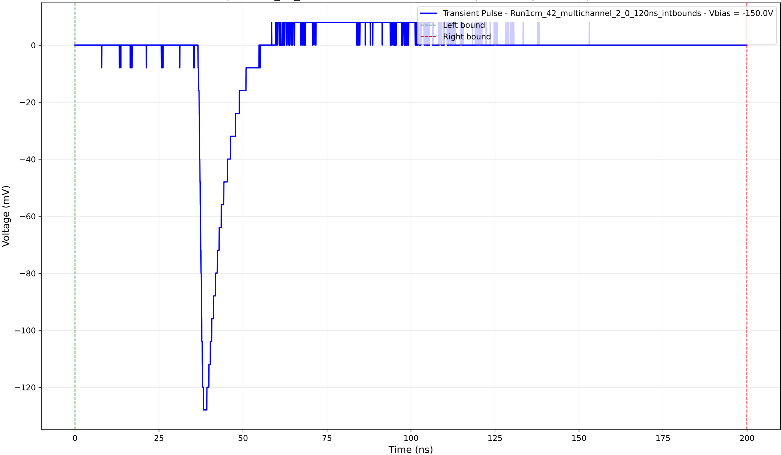
Transient Pulse - Sample: 1cm_42_multichannel - Position: 1060.0 \mu\text{m} - Charge: 10.70 pC - Rise Time: 1.22 ns
