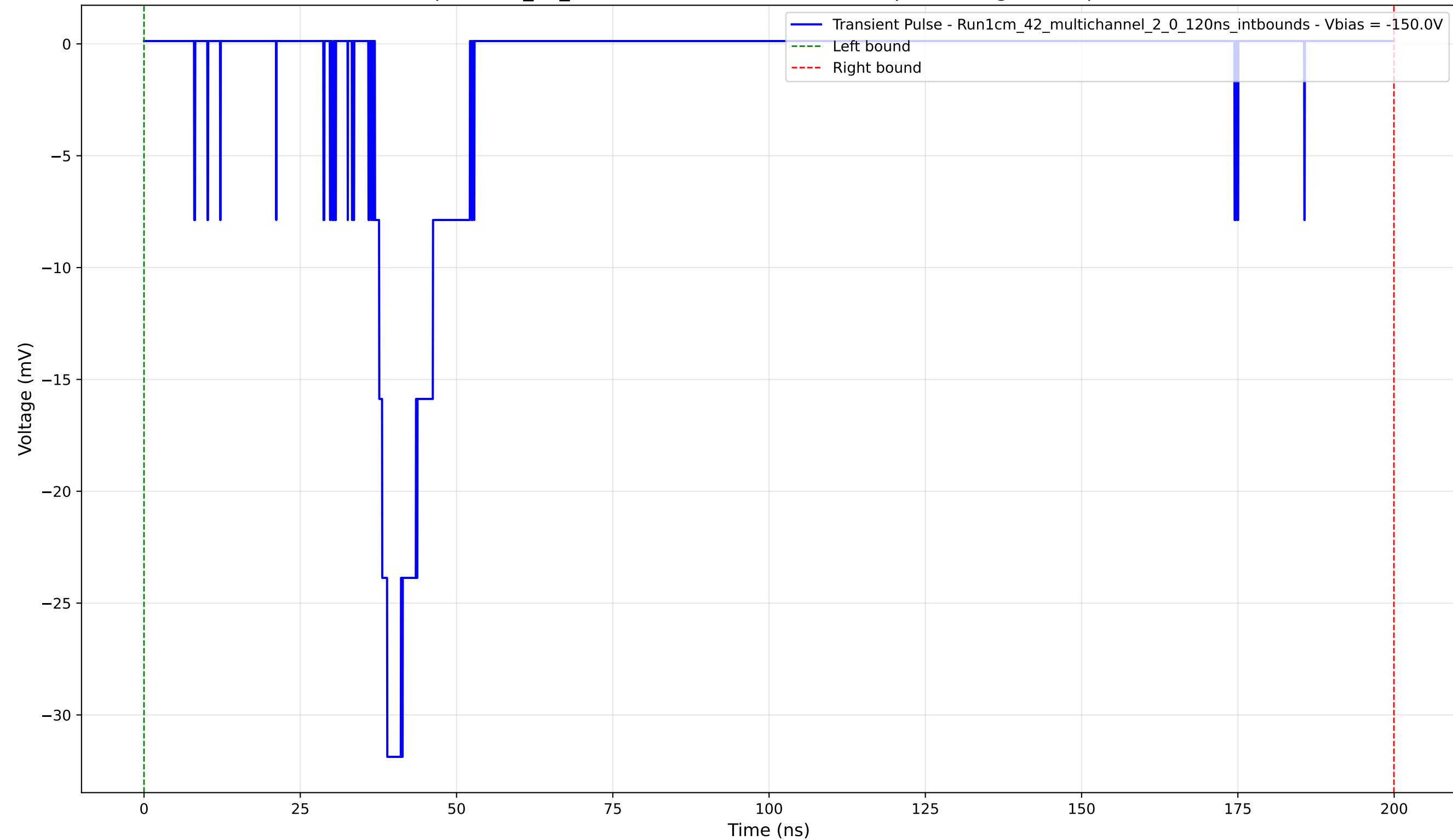
Transient Pulse - Sample: 1cm_42_multichannel - Position: 4435.0 \mu\text{m} - Charge: 4.92 pC - Rise Time: 1.98 ns
