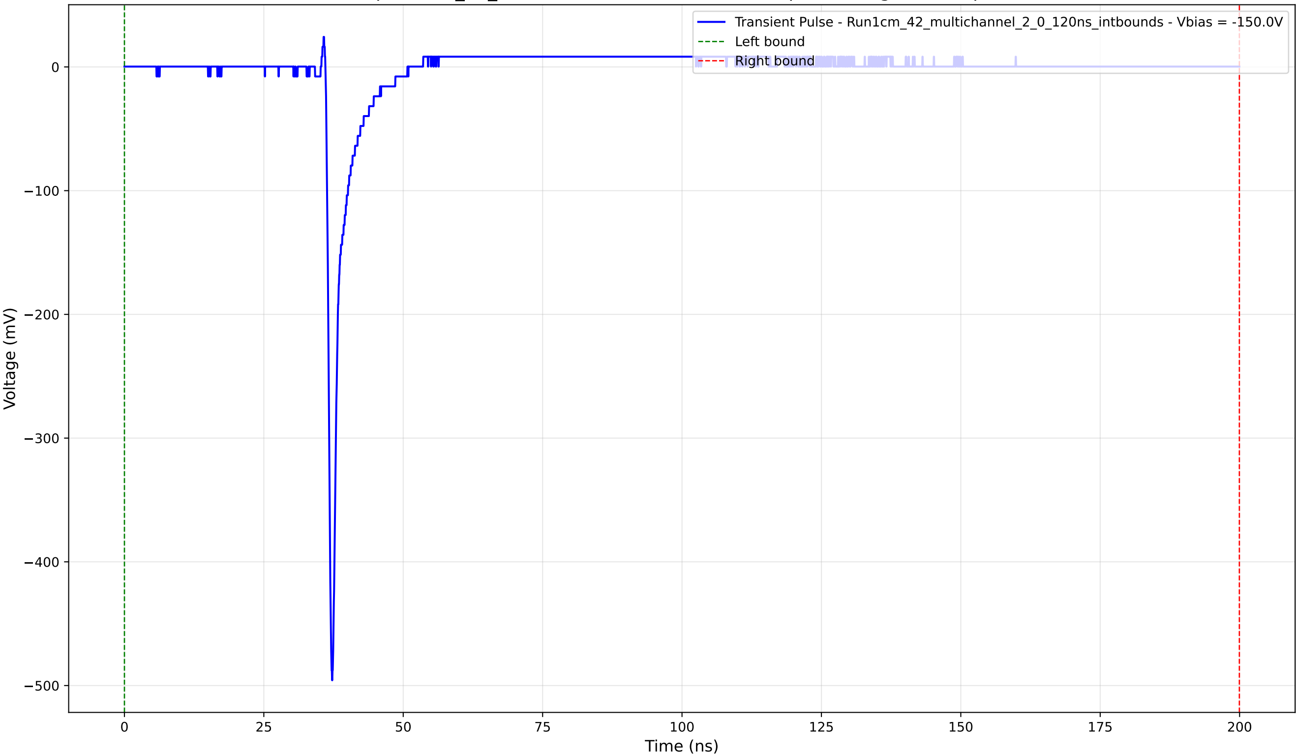
Transient Pulse - Sample: 1cm_42_multichannel - Position: 2585.0 \mu\text{m} - Charge: 13.19 pC - Rise Time: 0.77 ns
