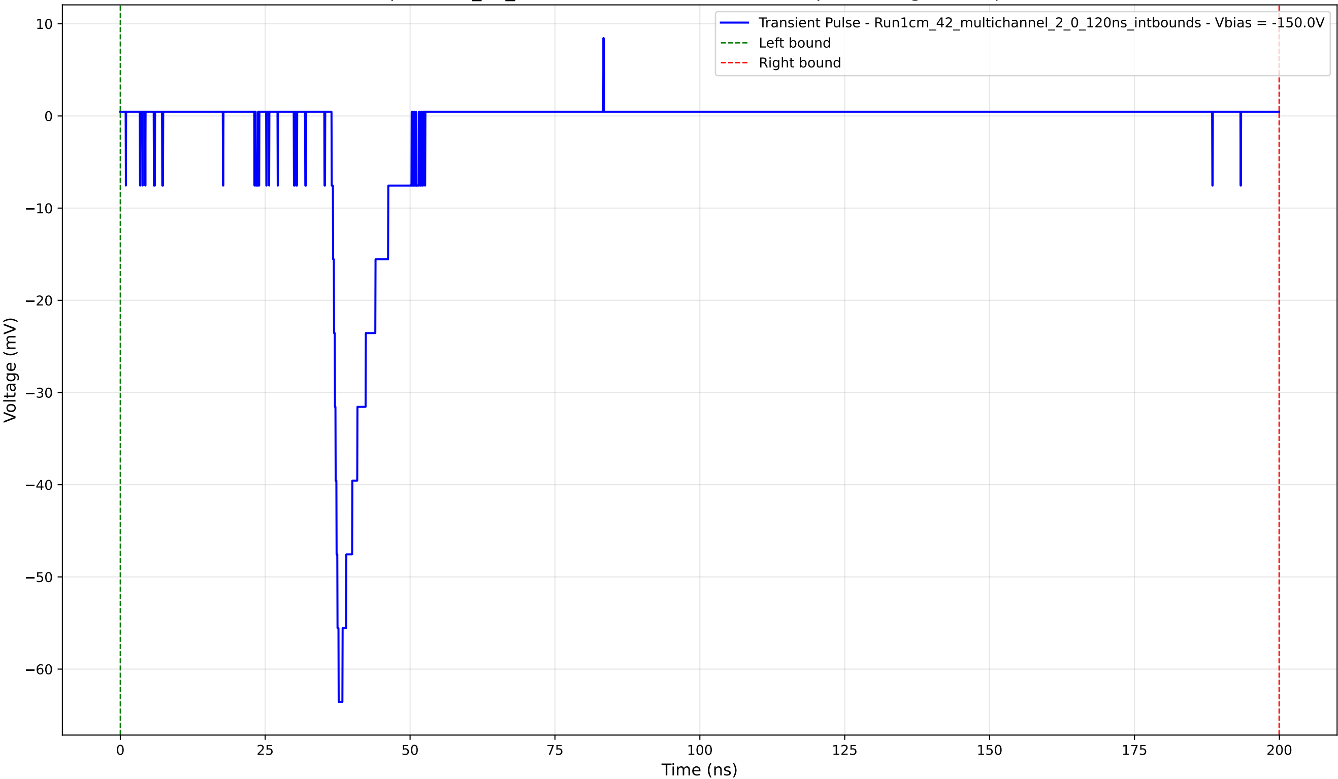
Transient Pulse - Sample: 1cm_42_multichannel - Position: 1400.0 \mu\text{m} - Charge: 5.90 pC - Rise Time: 1.21 ns
