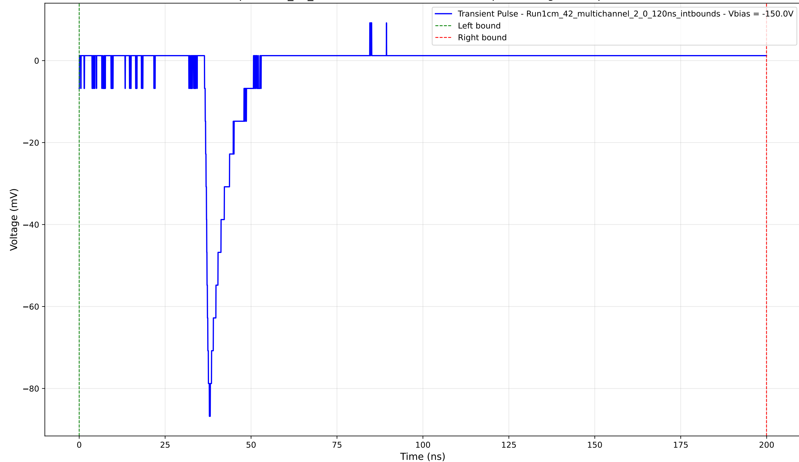
Transient Pulse - Sample: 1cm_42_multichannel - Position: 1405.0 \mu\text{m} - Charge: 5.22 pC - Rise Time: 0.95 ns
