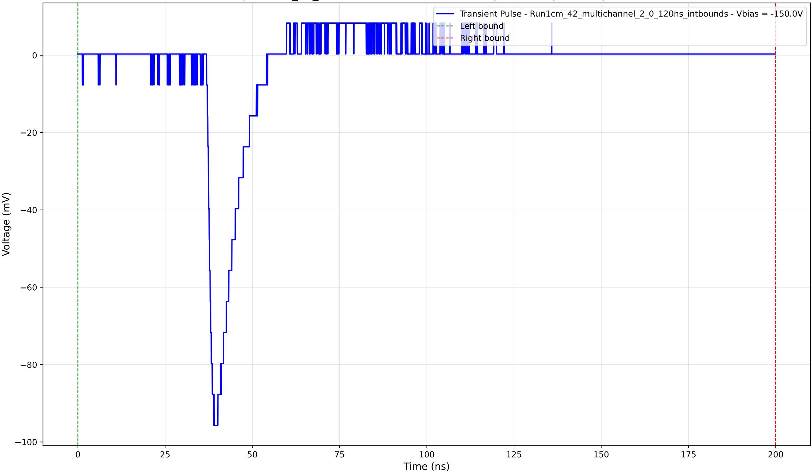
Transient Pulse - Sample: 1cm_42_multichannel - Position: 540.0 \mu\text{m} - Charge: 9.10 pC - Rise Time: 1.43 ns
