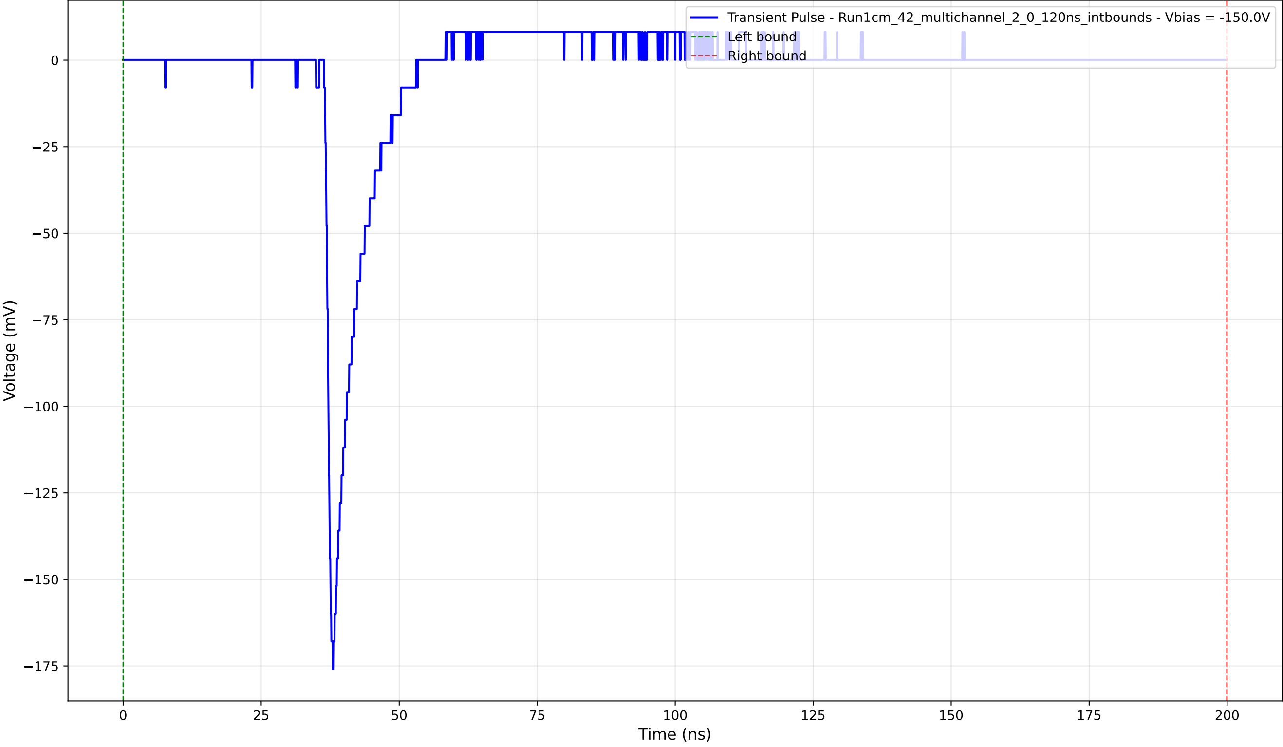
Transient Pulse - Sample: 1cm_42_multichannel - Position: 1430.0 \mu\text{m} - Charge: 11.16 pC - Rise Time: 0.99 ns
