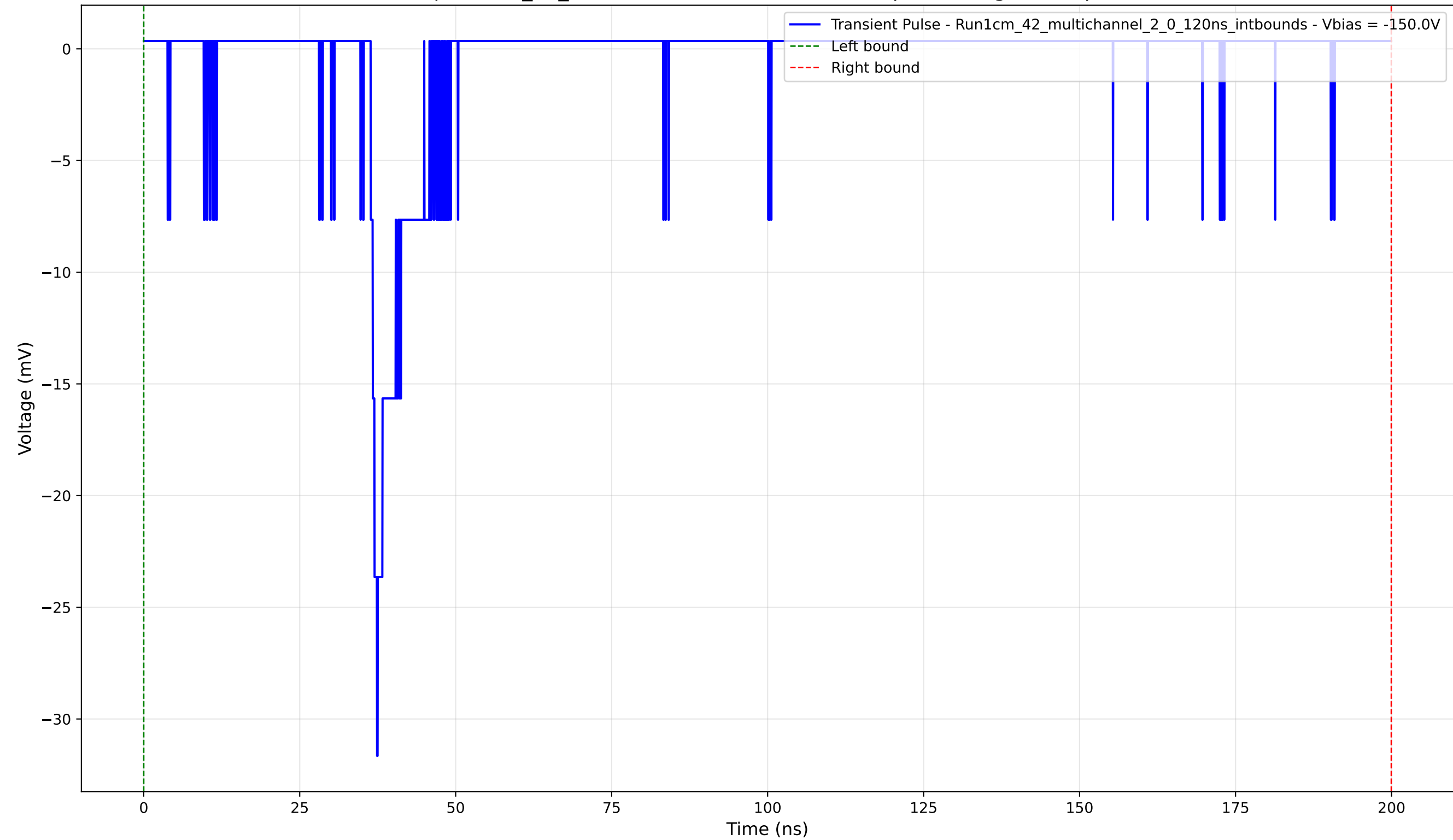
Transient Pulse - Sample: 1cm_42_multichannel - Position: 2900.0 \mu\text{m} - Charge: 1.79 pC - Rise Time: 1.02 ns
