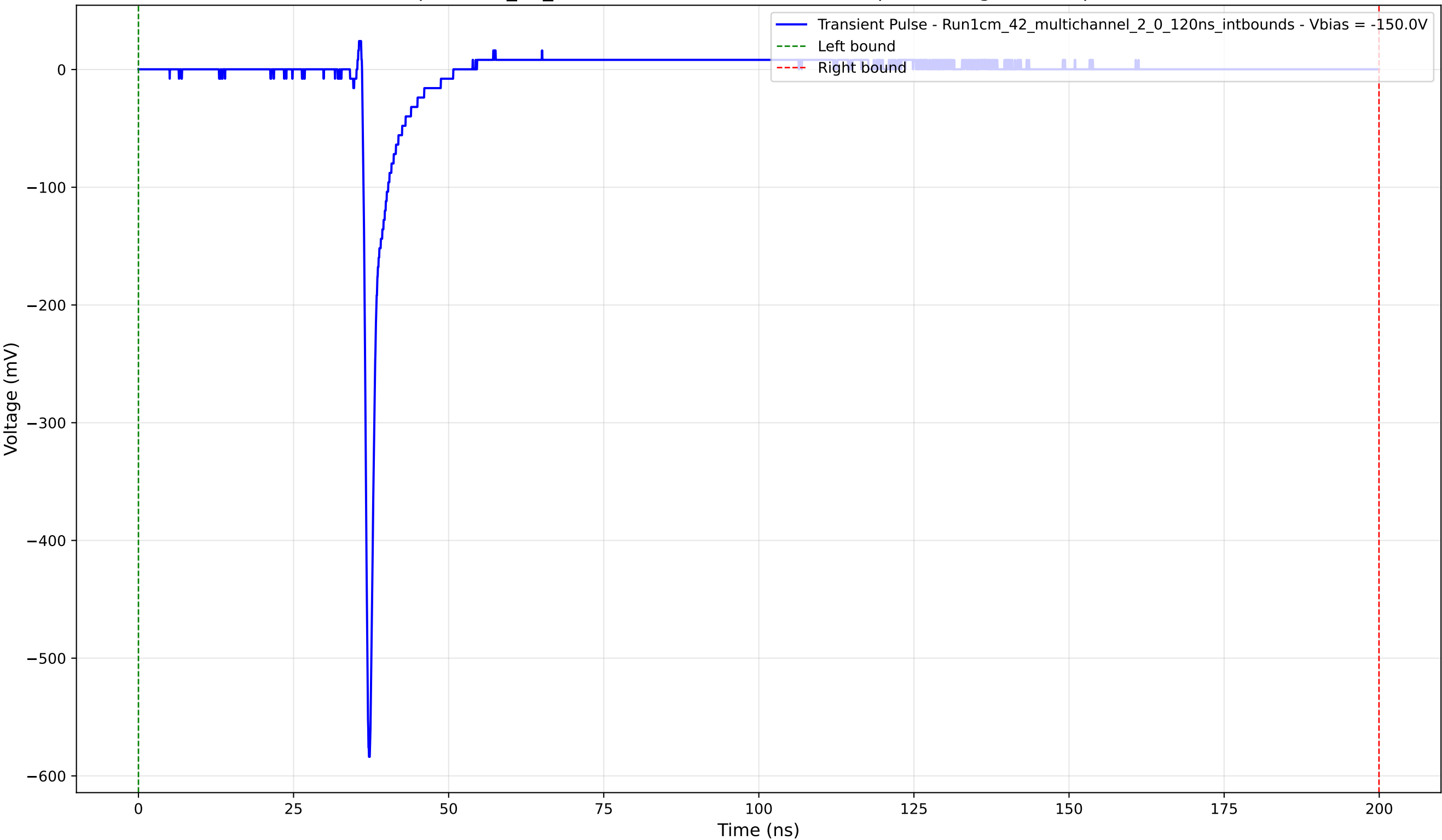
Transient Pulse - Sample: 1cm_42_multichannel - Position: 2210.0 \mu\text{m} - Charge: 16.18 pC - Rise Time: 0.73 ns
