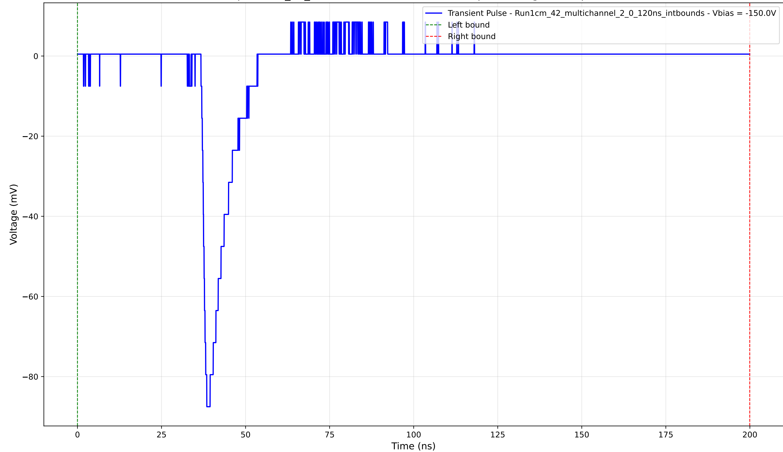
Transient Pulse - Sample: 1cm_42_multichannel - Position: 910.0 \mu\text{m} - Charge: 9.26 pC - Rise Time: 1.19 ns
