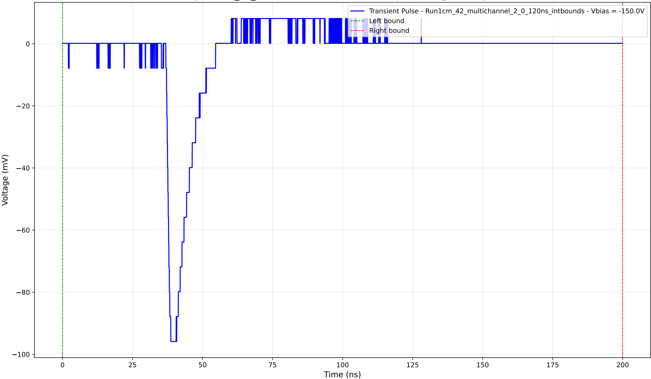
Transient Pulse - Sample: 1cm_42_multichannel - Position: 605.0 \mu\text{m} - Charge: 9.98 pC - Rise Time: 1.19 ns
