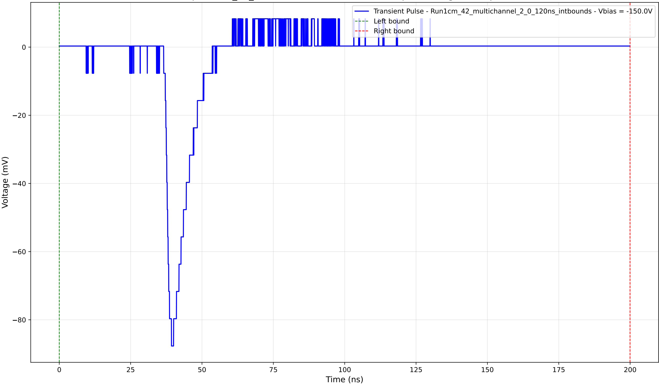
Transient Pulse - Sample: 1cm_42_multichannel - Position: 4170.0 \mu\text{m} - Charge: 9.39 pC - Rise Time: 1.51 ns
