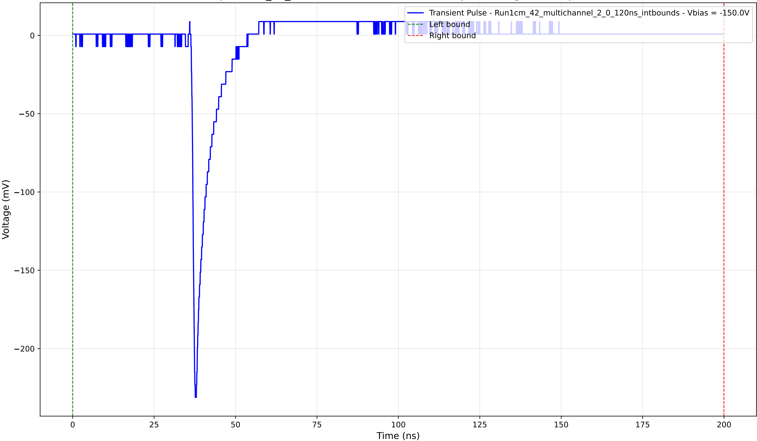
Transient Pulse - Sample: 1cm_42_multichannel - Position: 1585.0 \mu\text{m} - Charge: 10.33 pC - Rise Time: 0.96 ns
