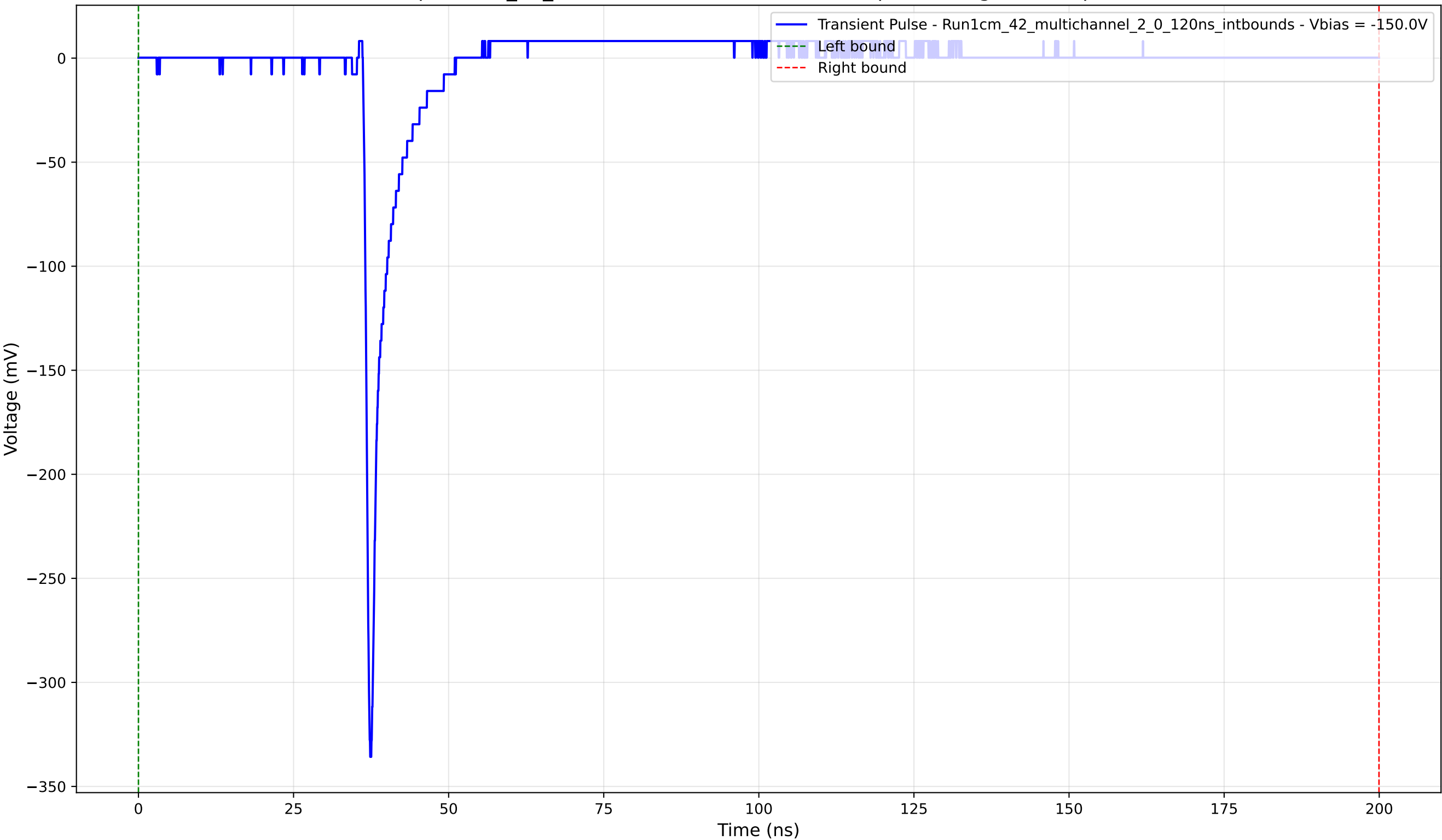
Transient Pulse - Sample: 1cm_42_multichannel - Position: 2795.0 \mu\text{m} - Charge: 11.02 pC - Rise Time: 0.82 ns
