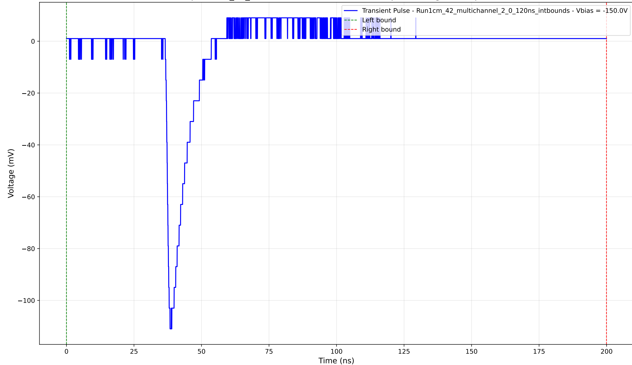
Transient Pulse - Sample: 1cm_42_multichannel - Position: 3685.0 \mu\text{m} - Charge: 6.69 pC - Rise Time: 1.26 ns
