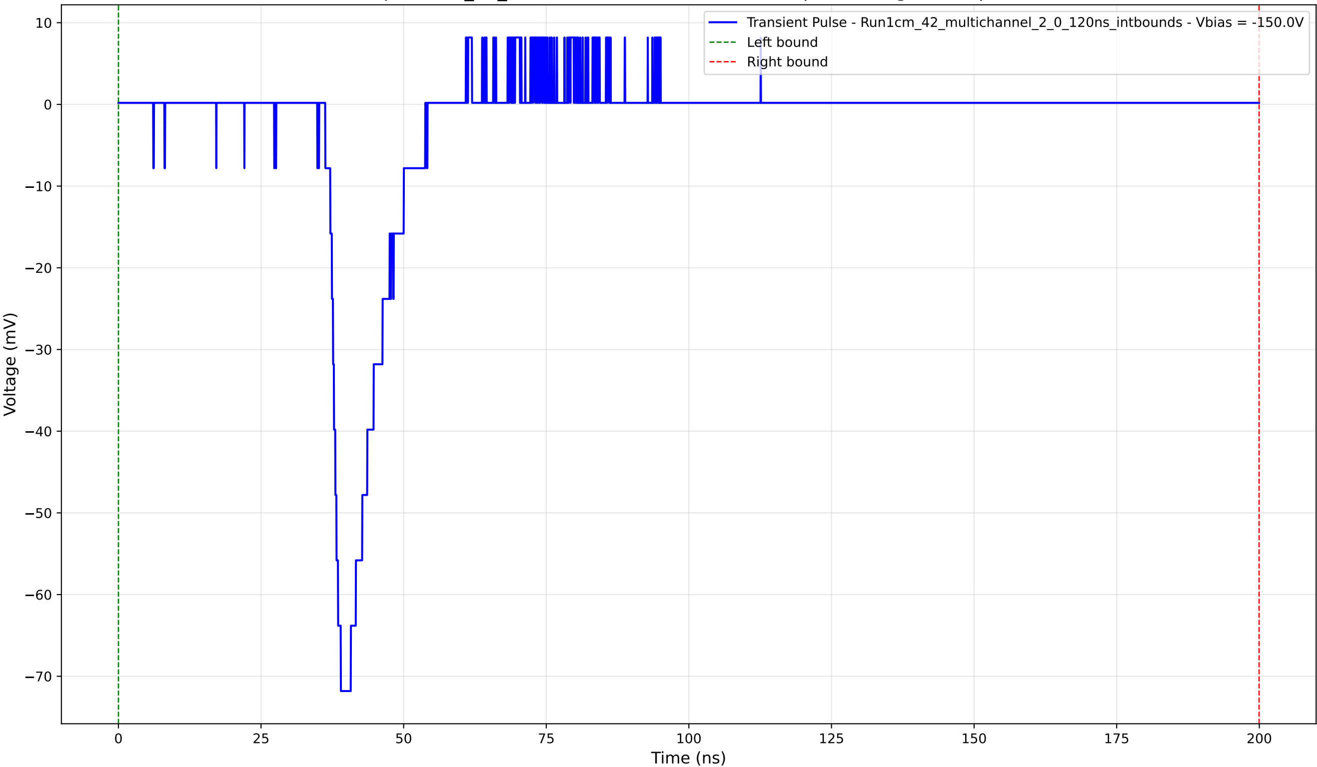
Transient Pulse - Sample: 1cm_42_multichannel - Position: 4580.0 \mu\text{m} - Charge: 9.35 pC - Rise Time: 2.72 ns
