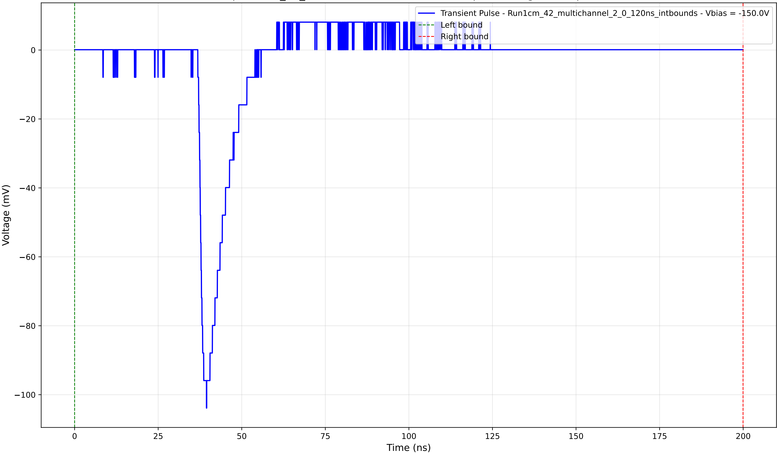
Transient Pulse - Sample: 1cm_42_multichannel - Position: 615.0 \mu\text{m} - Charge: 9.89 pC - Rise Time: 1.55 ns
