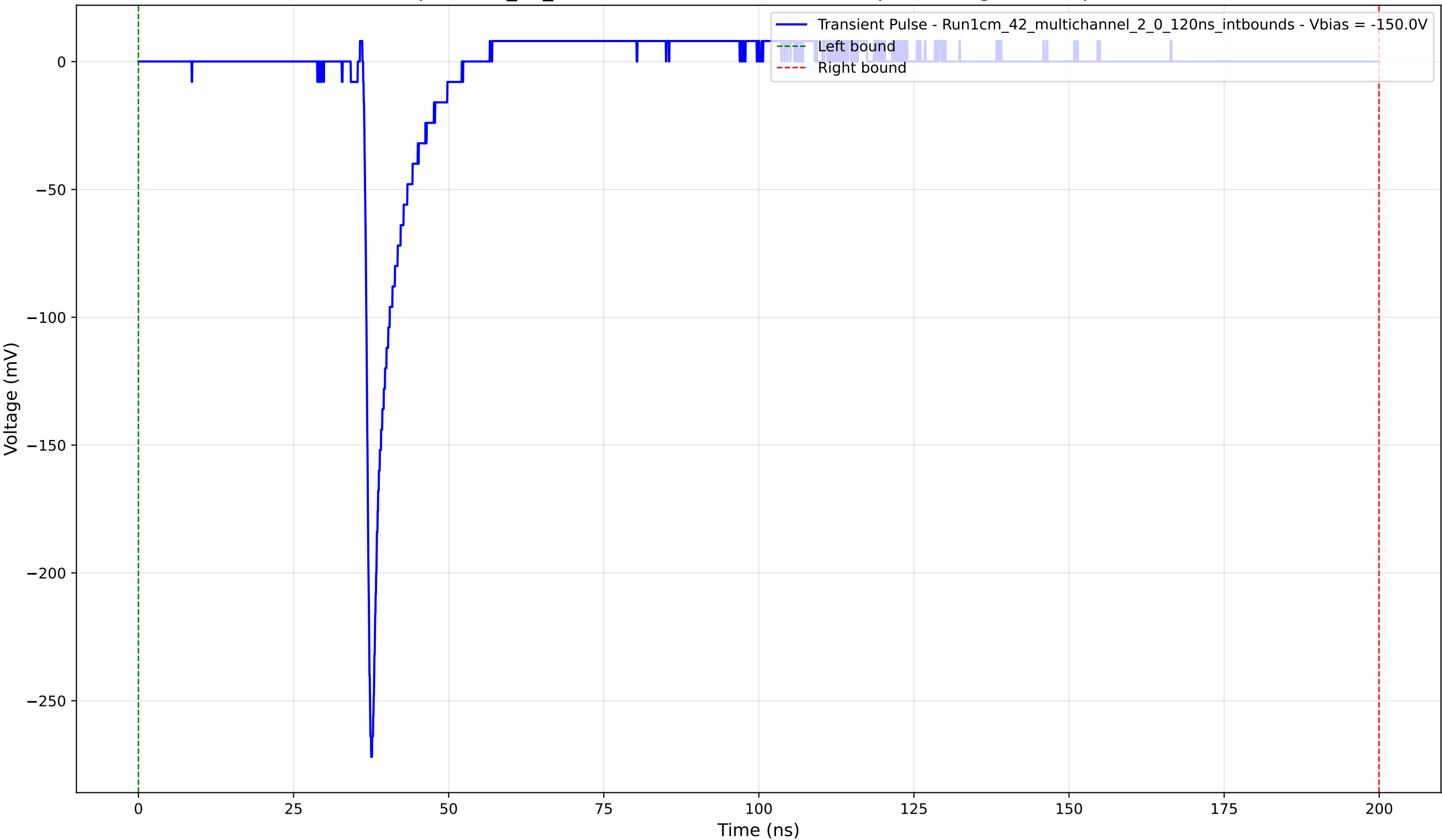
Transient Pulse - Sample: 1cm_42_multichannel - Position: 2990.0 \mu\text{m} - Charge: 12.34 pC - Rise Time: 0.89 ns
