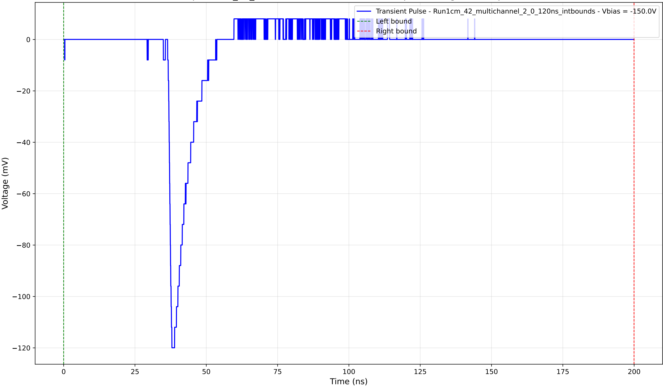
Transient Pulse - Sample: 1cm_42_multichannel - Position: 3550.0 \mu\text{m} - Charge: 10.62 pC - Rise Time: 1.14 ns
