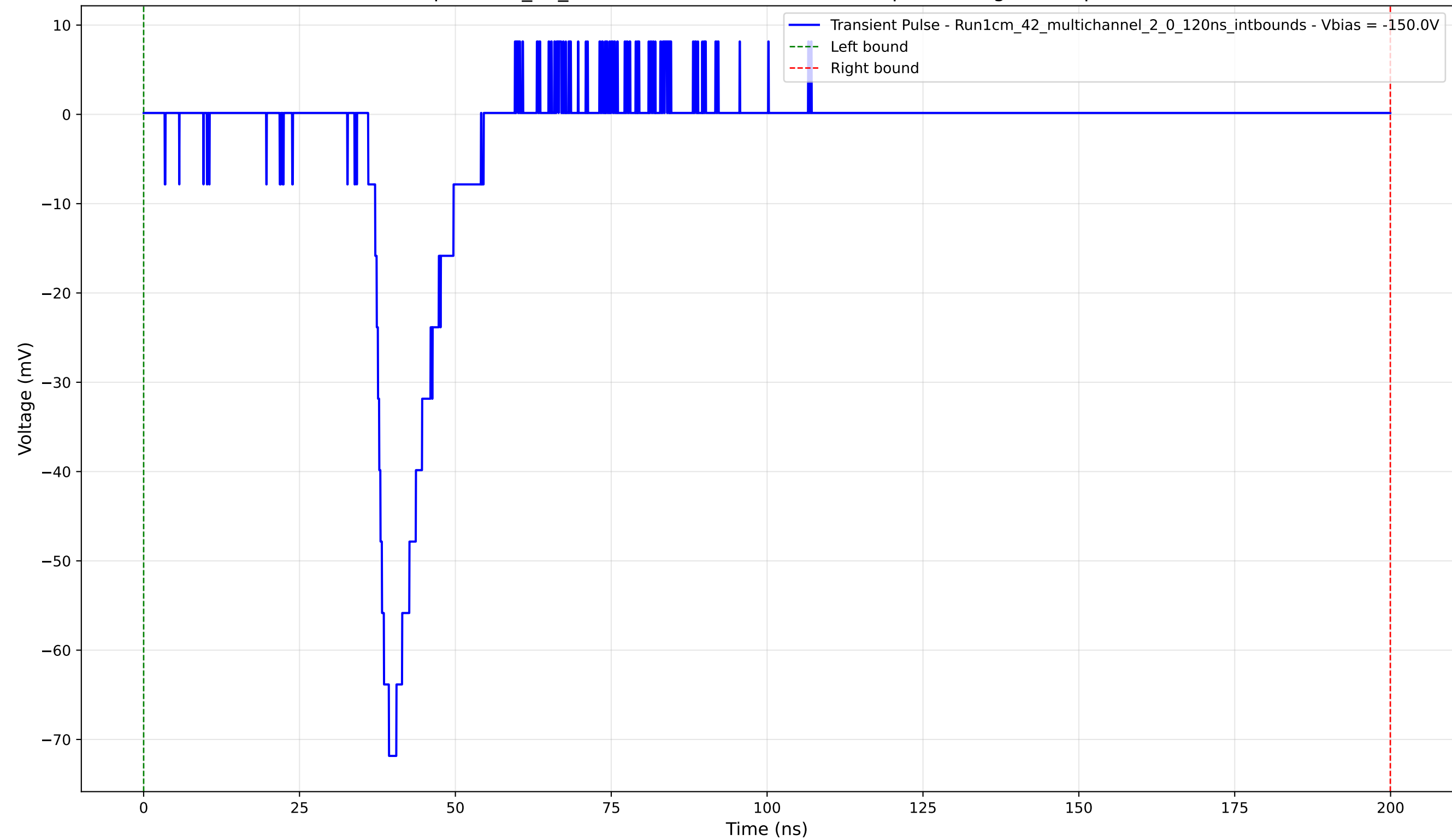
Transient Pulse - Sample: 1cm_42_multichannel - Position: 4645.0 \mu\text{m} - Charge: 9.62 pC - Rise Time: 3.32 ns
