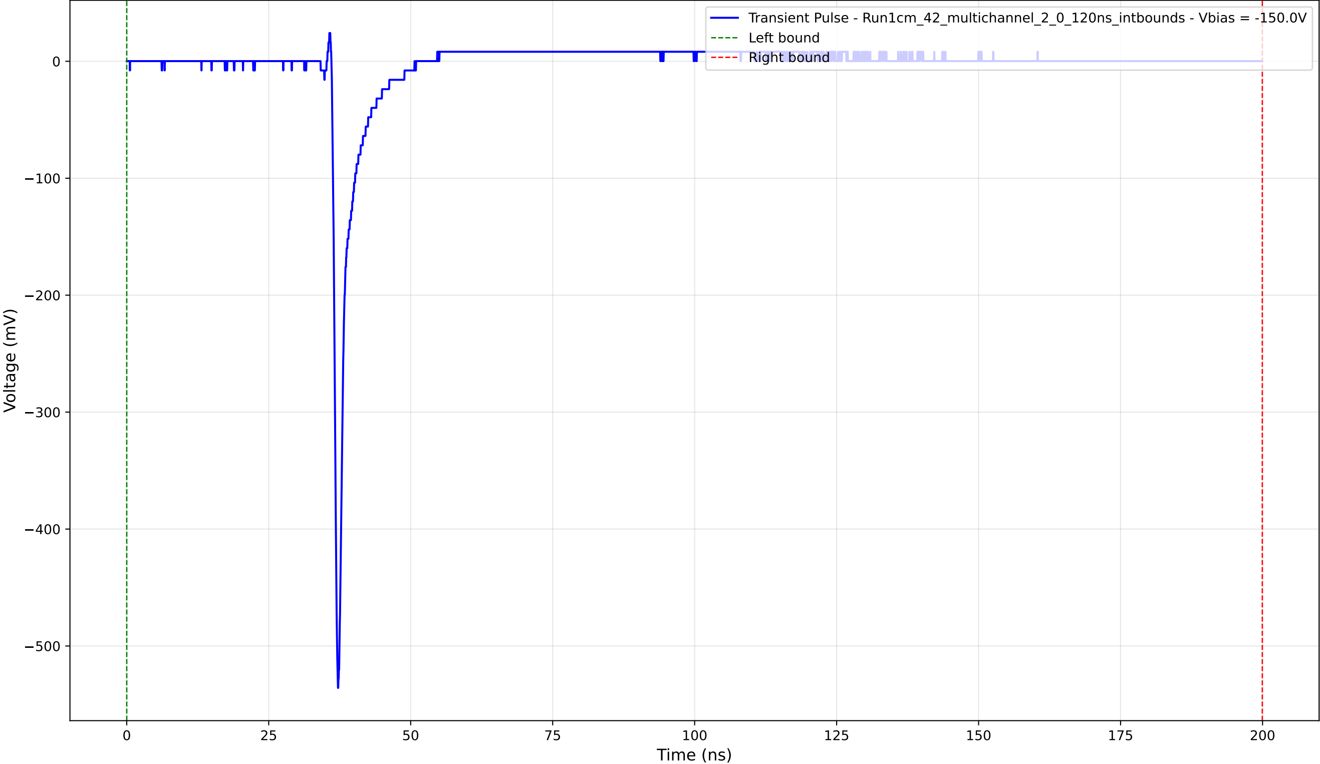
Transient Pulse - Sample: 1cm_42_multichannel - Position: 2160.0 \mu\text{m} - Charge: 15.89 pC - Rise Time: 0.75 ns
