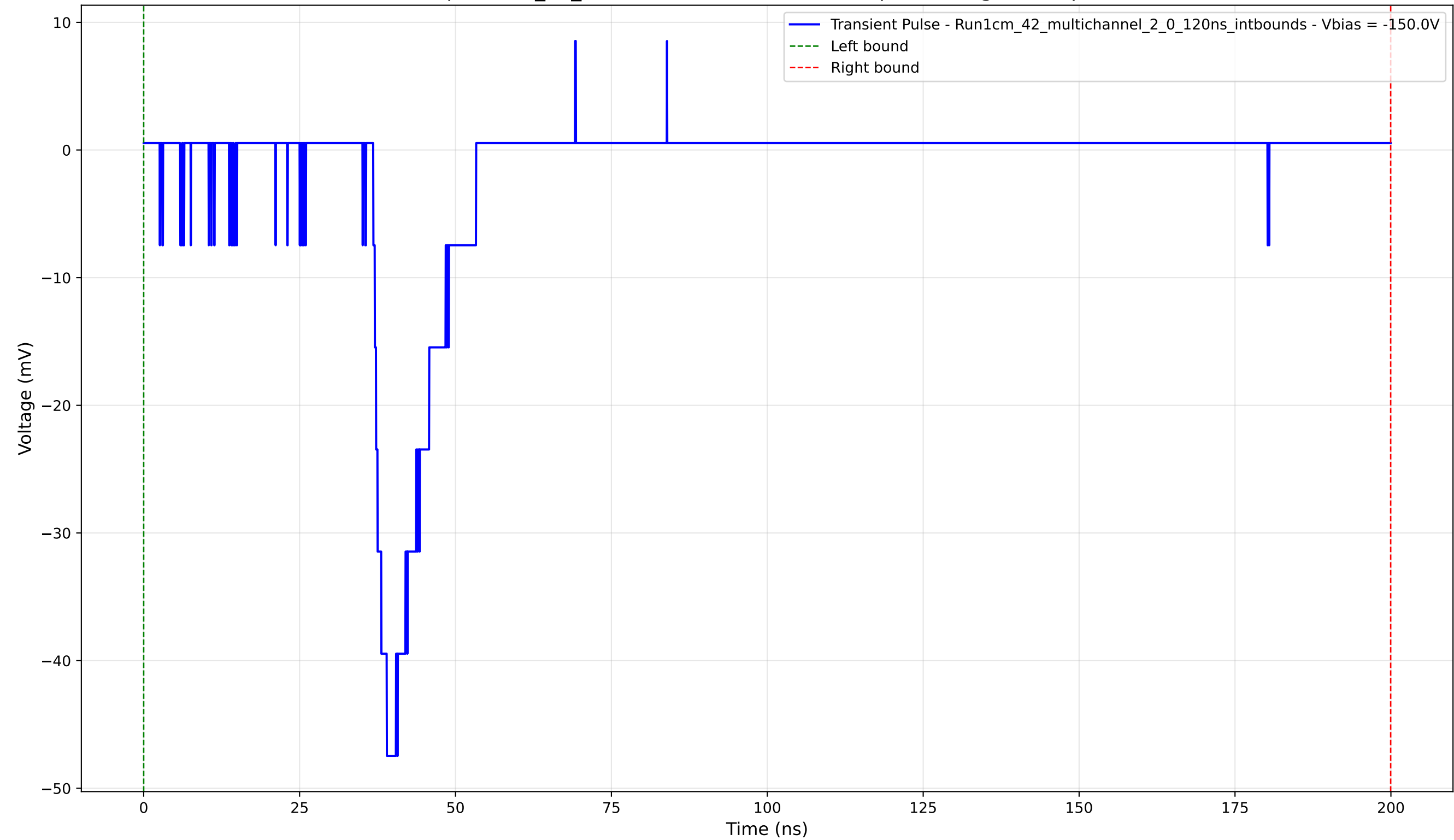
Transient Pulse - Sample: 1cm_42_multichannel - Position: 80.0 \mu\text{m} - Charge: 5.93 pC - Rise Time: 2.18 ns
