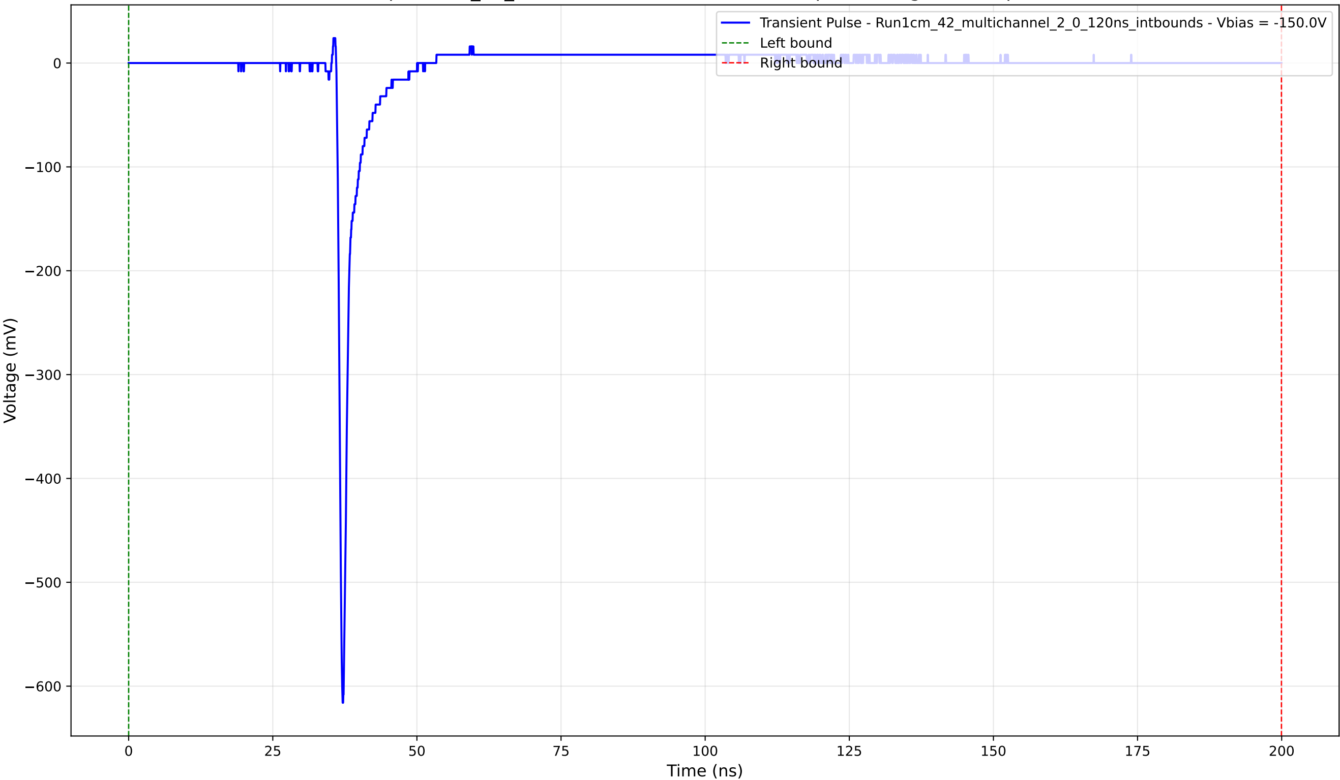
Transient Pulse - Sample: 1cm_42_multichannel - Position: 2480.0 \mu\text{m} - Charge: 16.82 pC - Rise Time: 0.73 ns
