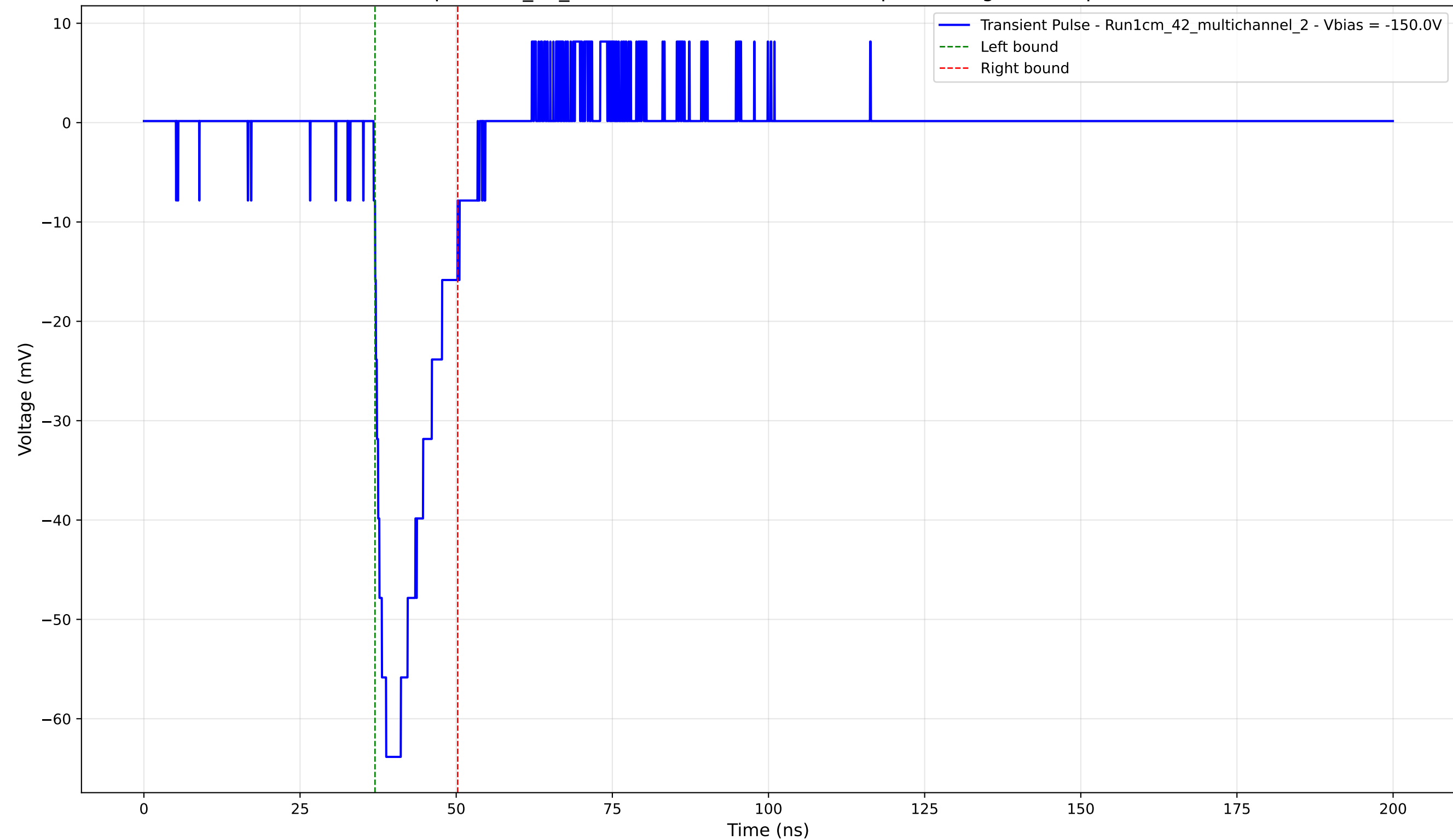
Transient Pulse - Sample: 1cm_42_multichannel - Position: 130.0 \mu\text{m} - Charge: 10.42 pC - Rise Time: 2.01 ns
