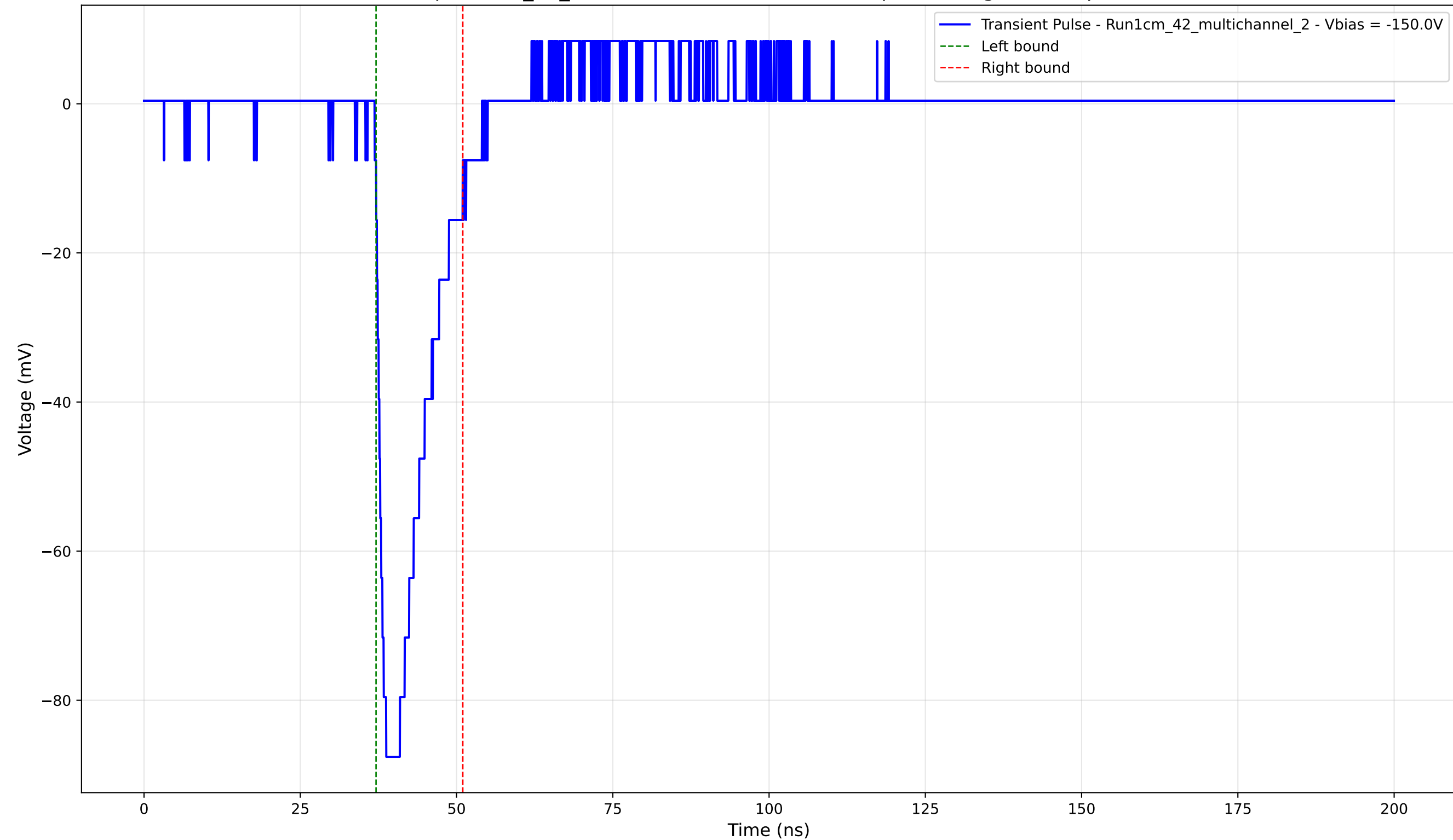
Transient Pulse - Sample: 1cm_42_multichannel - Position: 450.0 \mu\text{m} - Charge: 13.67 pC - Rise Time: 1.23 ns
