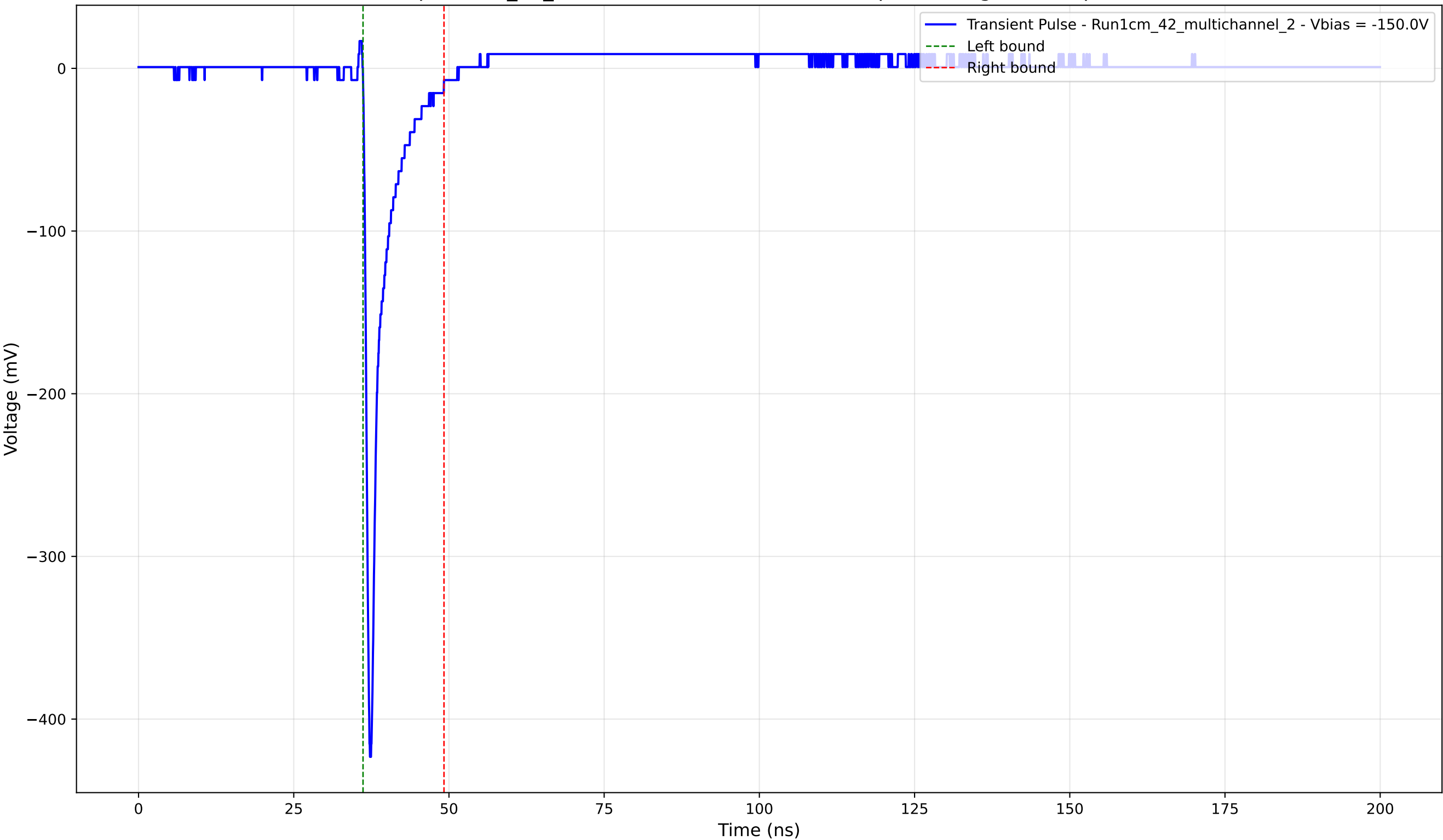
Transient Pulse - Sample: 1cm_42_multichannel - Position: 2715.0 \mu\text{m} - Charge: 24.89 pC - Rise Time: 0.77 ns
