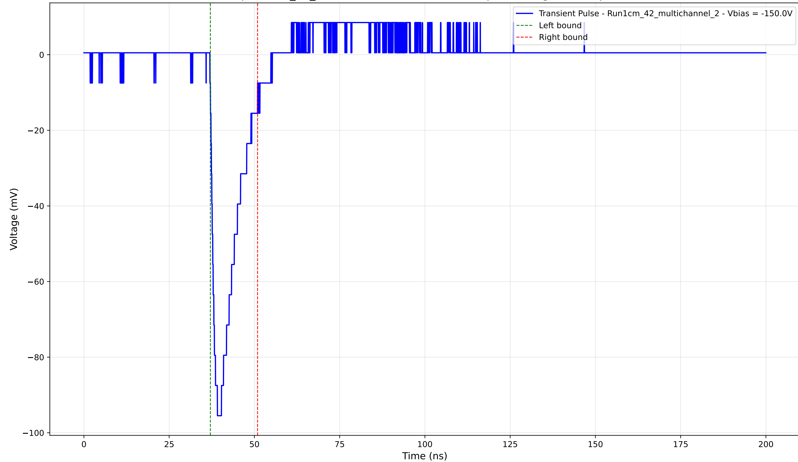
Transient Pulse - Sample: 1cm_42_multichannel - Position: 505.0 \mu\text{m} - Charge: 14.09 pC - Rise Time: 1.51 ns
