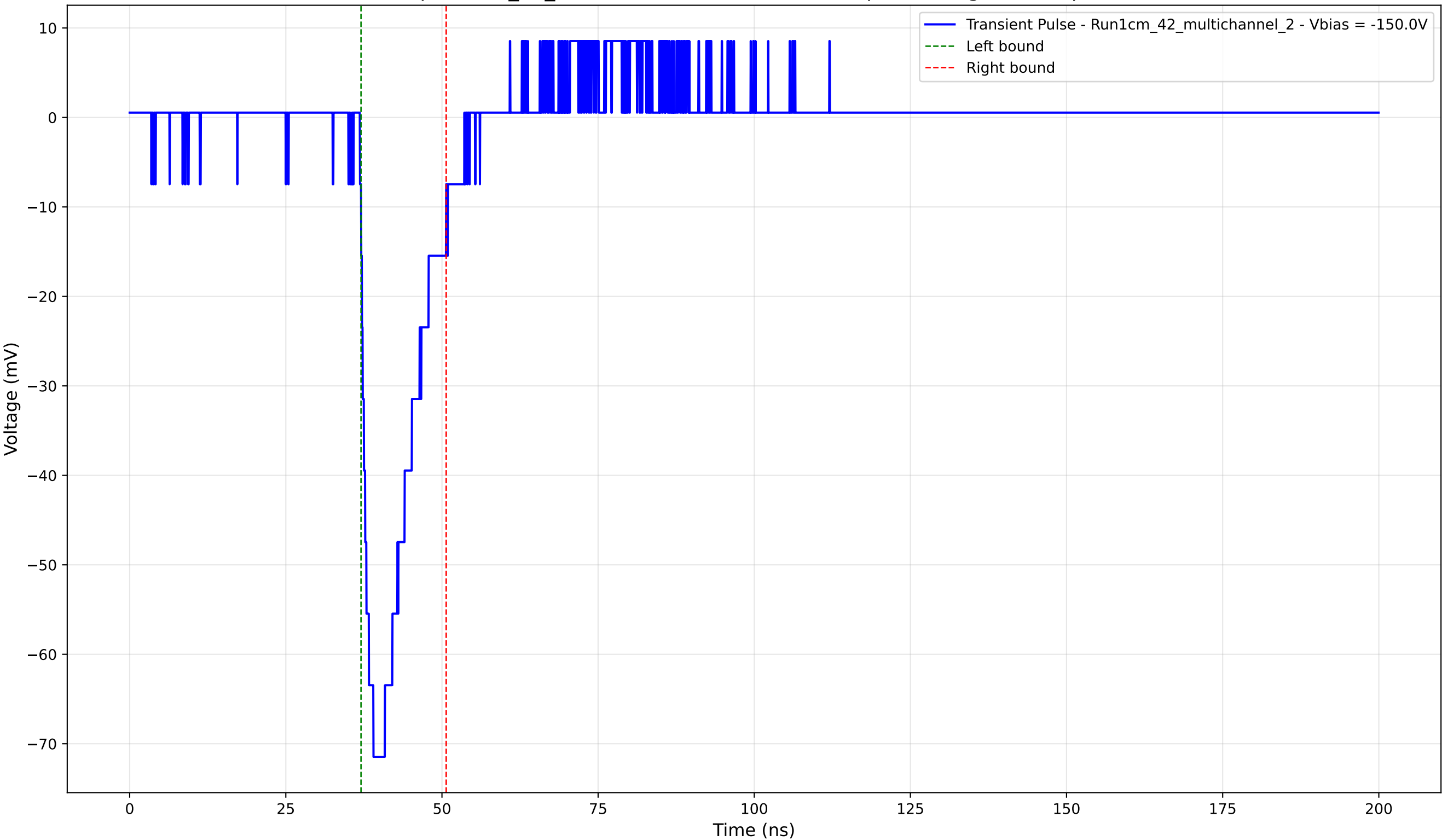
Transient Pulse - Sample: 1cm_42_multichannel - Position: 205.0 \mu\text{m} - Charge: 11.34 pC - Rise Time: 2.16 ns
