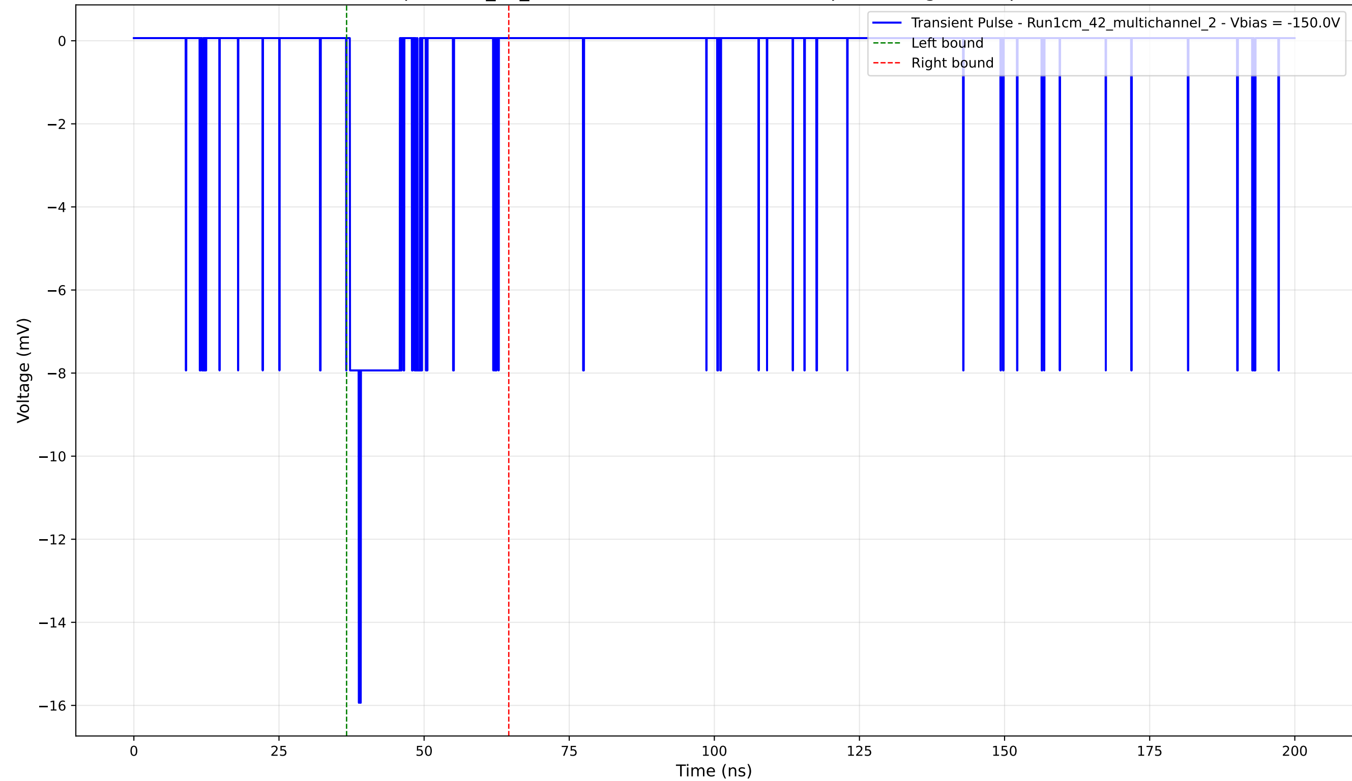
Transient Pulse - Sample: 1cm_42_multichannel - Position: 4870.0 \mu\text{m} - Charge: 1.68 pC - Rise Time: 1.55 ns
