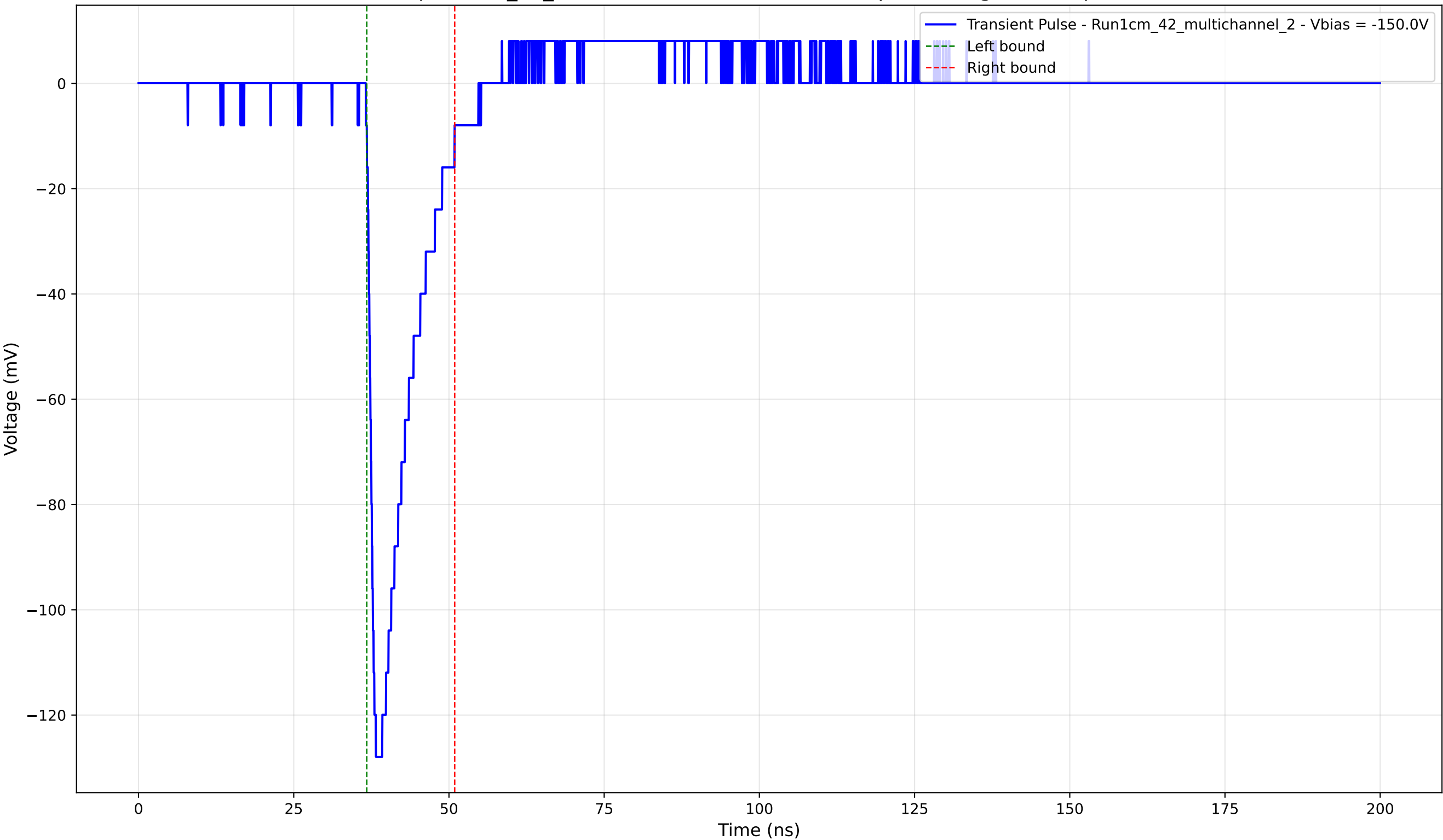
Transient Pulse - Sample: 1cm_42_multichannel - Position: 1060.0 \mu\text{m} - Charge: 17.26 pC - Rise Time: 1.22 ns
