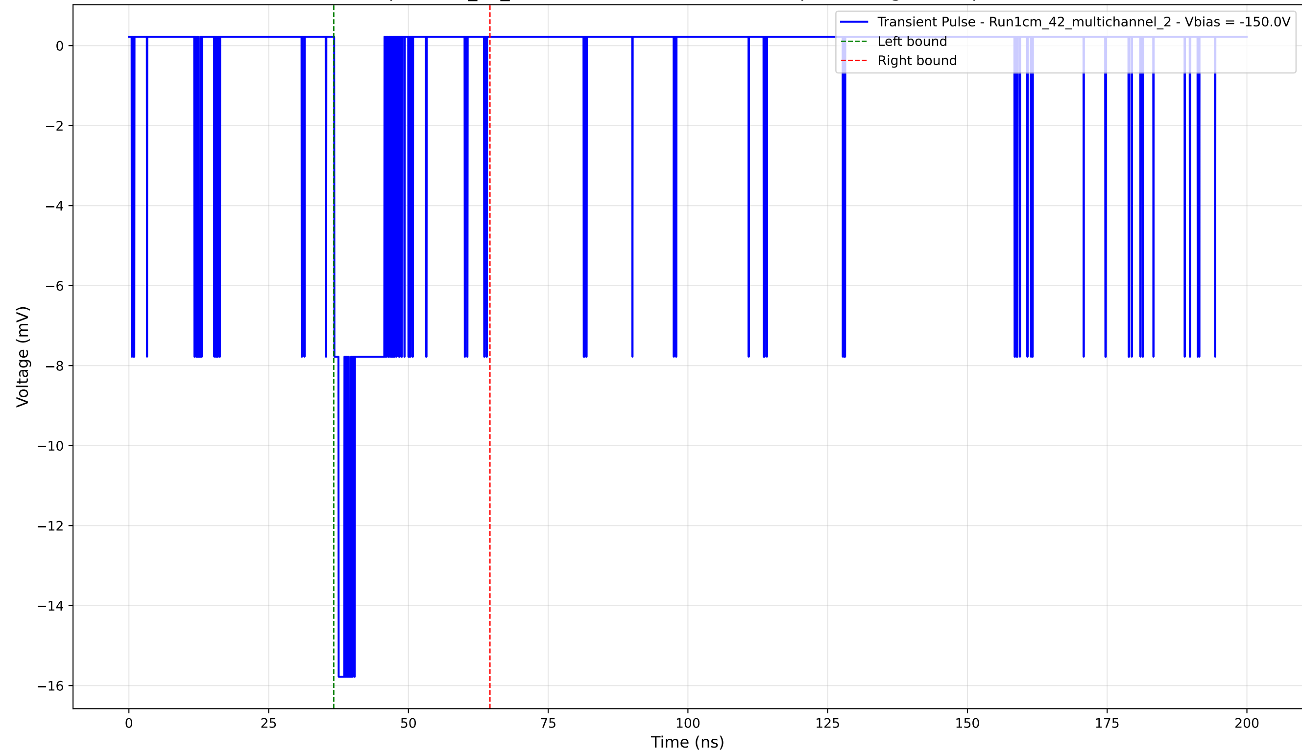
Transient Pulse - Sample: 1cm_42_multichannel - Position: 1340.0 \mu\text{m} - Charge: 2.01 pC - Rise Time: 0.79 ns
