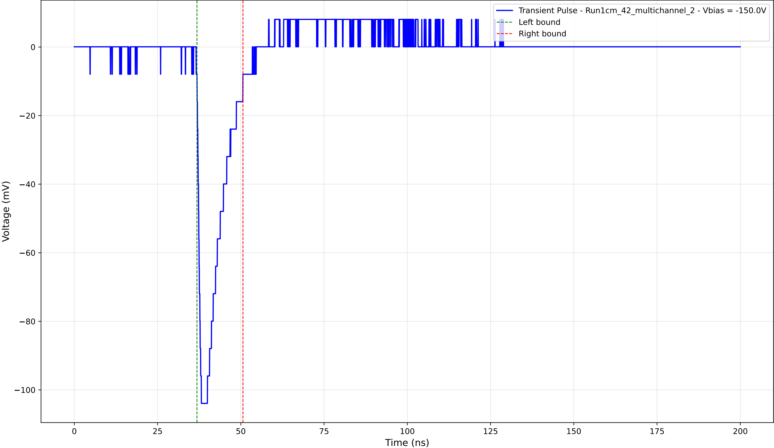
Transient Pulse - Sample: 1cm_42_multichannel - Position: 3720.0 \mu\text{m} - Charge: 14.99 pC - Rise Time: 1.11 ns
