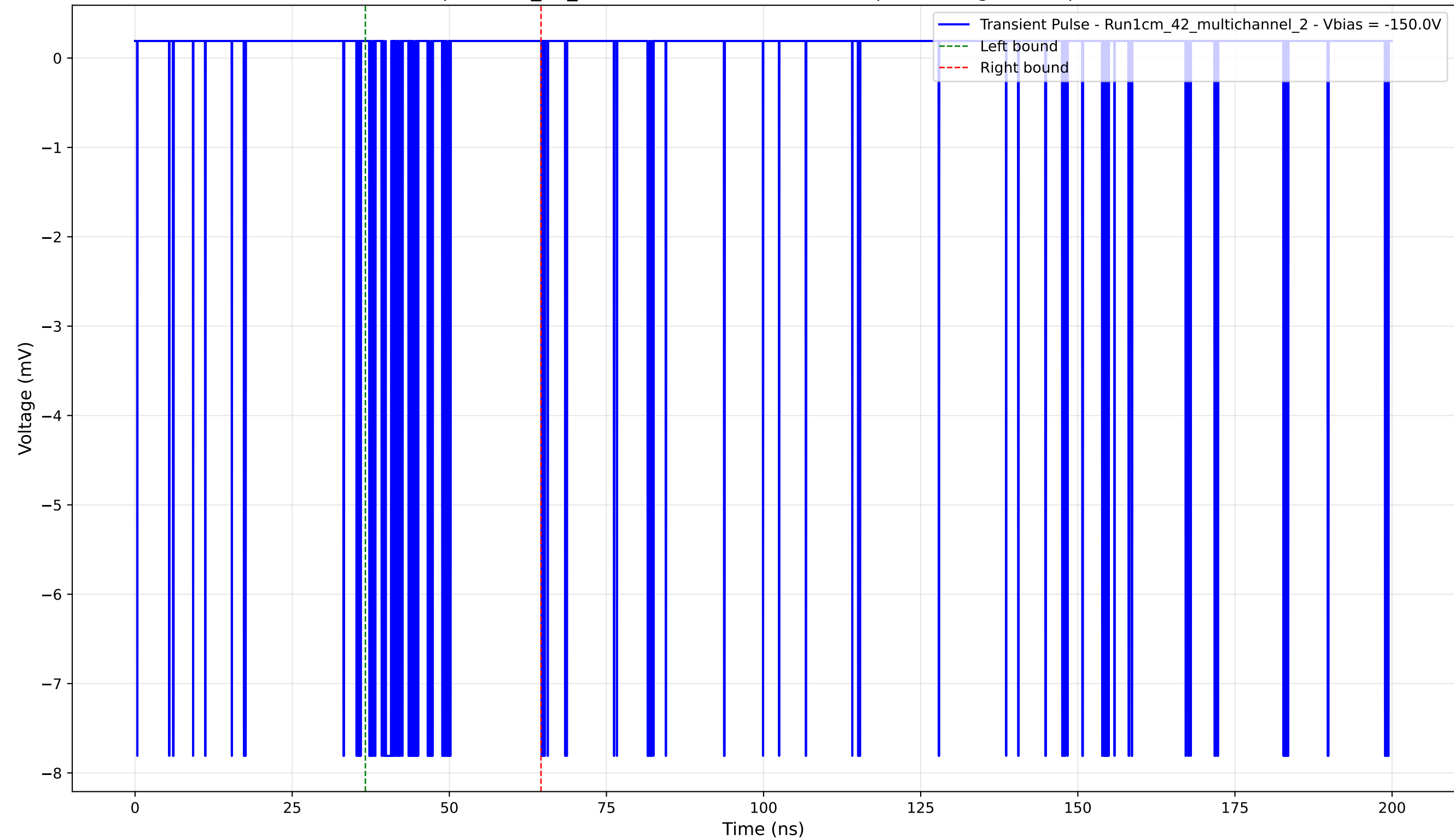
Transient Pulse - Sample: 1cm_42_multichannel - Position: 15.0 \mu\text{m} - Charge: 0.67 pC - Rise Time: 0.04 ns
