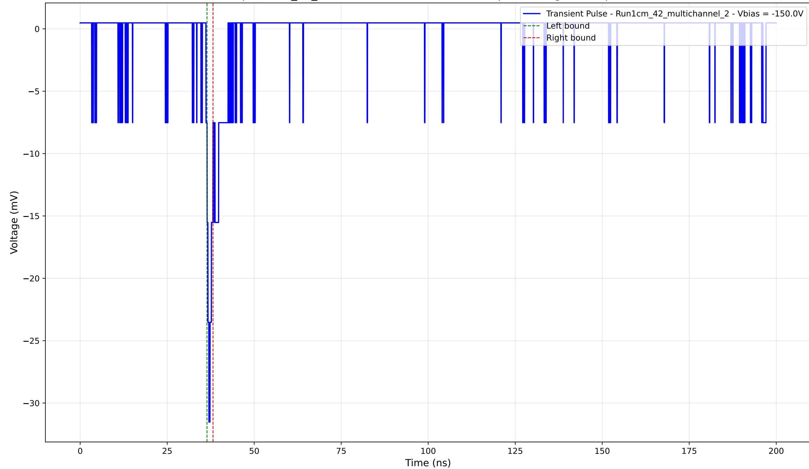
Transient Pulse - Sample: 1cm_42_multichannel - Position: 2360.0 \mu\text{m} - Charge: 0.74 pC - Rise Time: 0.86 ns
