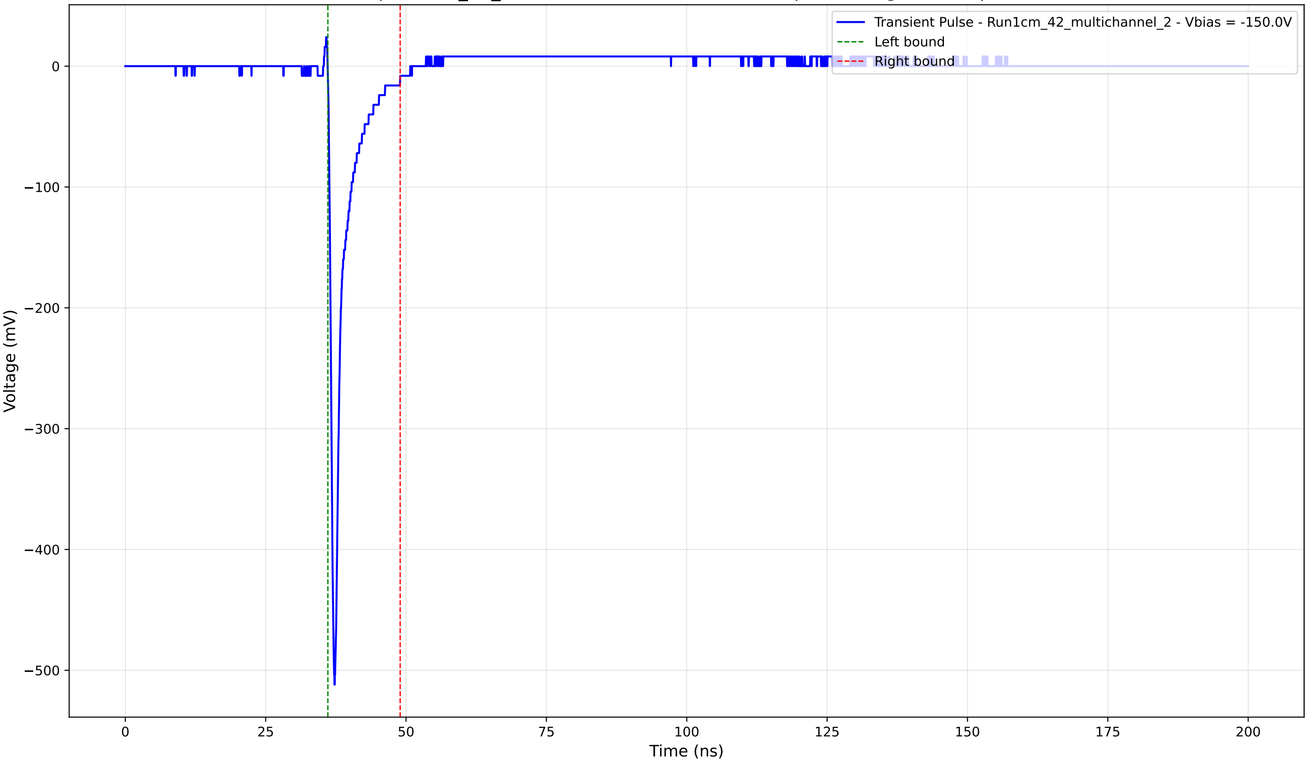
Transient Pulse - Sample: 1cm_42_multichannel - Position: 2120.0 \mu\text{m} - Charge: 26.75 pC - Rise Time: 0.78 ns
