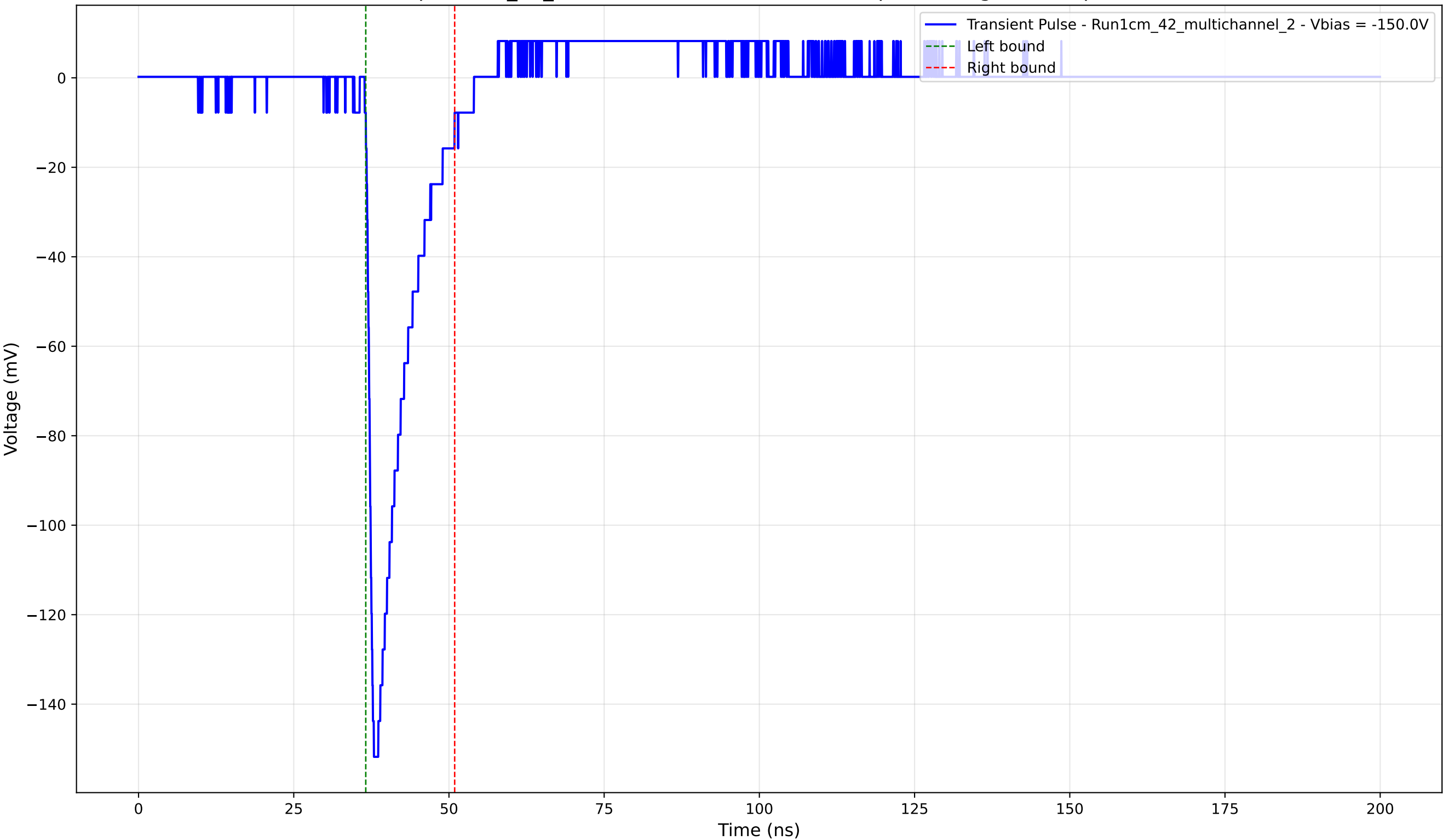
Transient Pulse - Sample: 1cm_42_multichannel - Position: 1270.0 \mu\text{m} - Charge: 18.41 pC - Rise Time: 1.12 ns
