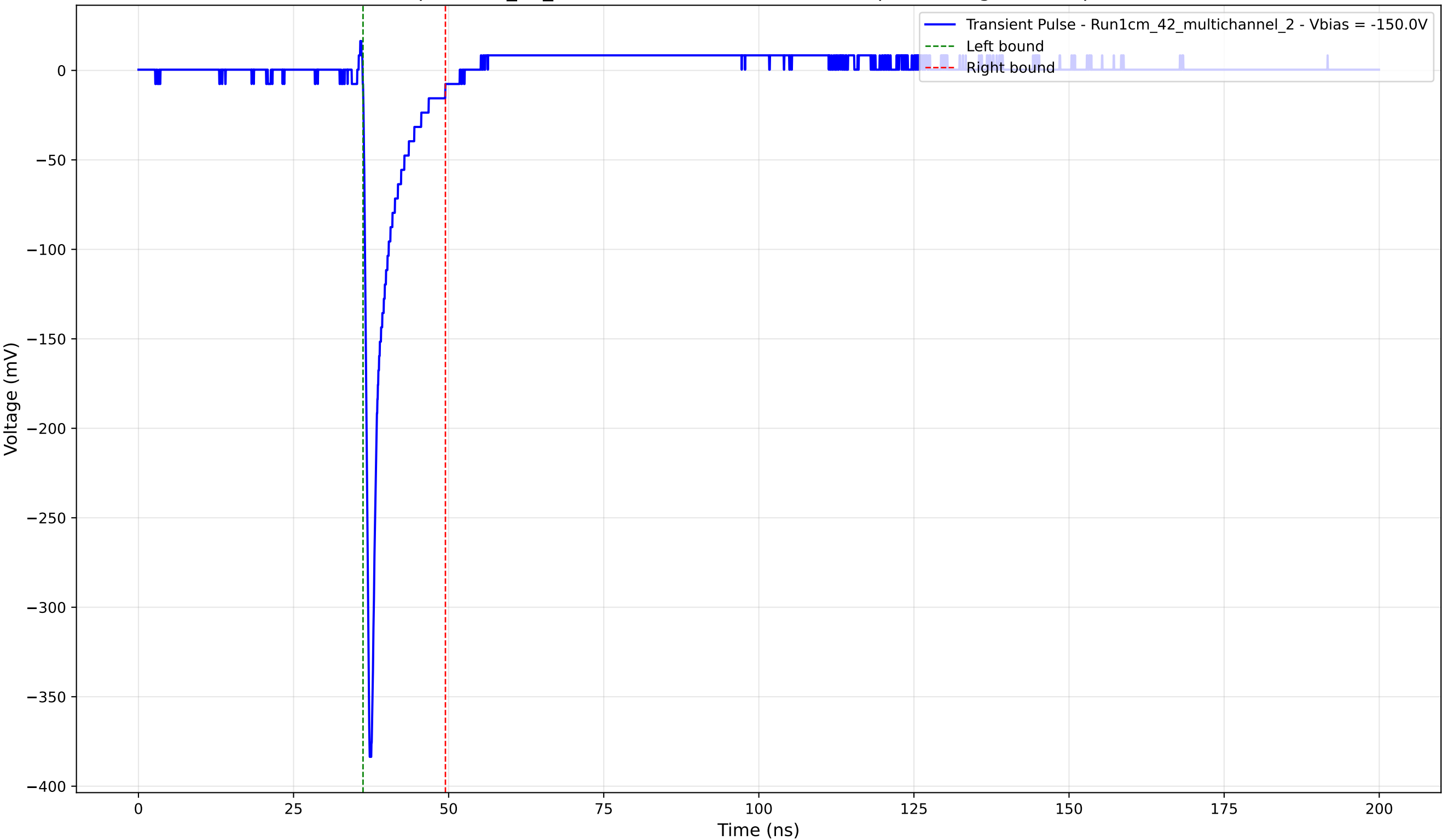
Transient Pulse - Sample: 1cm_42_multichannel - Position: 2765.0 \mu\text{m} - Charge: 23.77 pC - Rise Time: 0.83 ns
