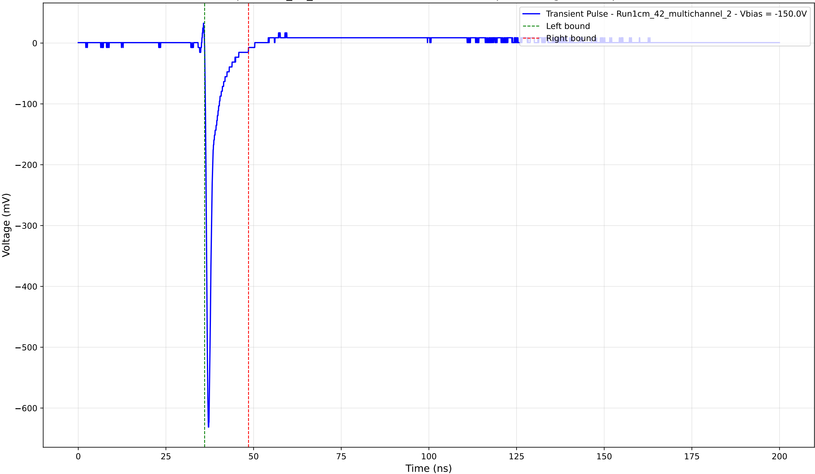
Transient Pulse - Sample: 1cm_42_multichannel - Position: 2250.0 \mu\text{m} - Charge: 29.00 pC - Rise Time: 0.74 ns
