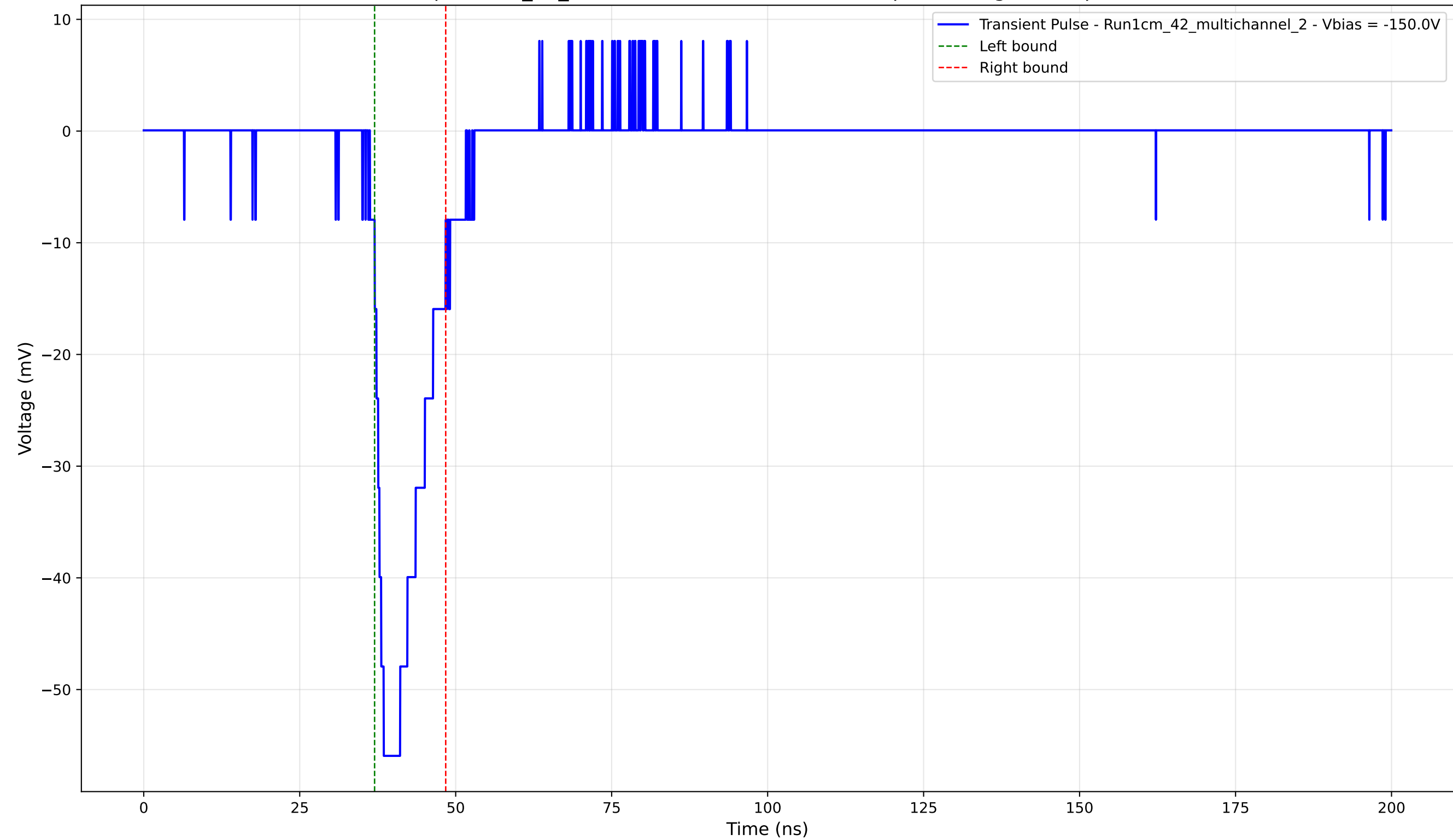
Transient Pulse - Sample: 1cm_42_multichannel - Position: 4810.0 \mu\text{m} - Charge: 8.30 pC - Rise Time: 2.21 ns
