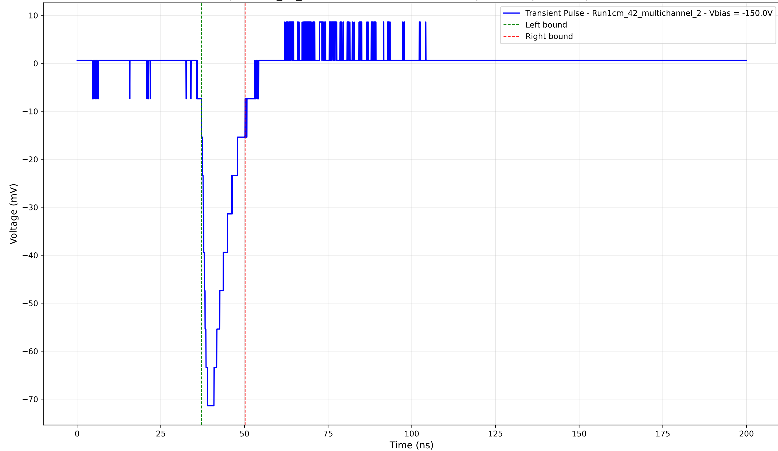
Transient Pulse - Sample: 1cm_42_multichannel - Position: 4560.0 \mu\text{m} - Charge: 10.59 pC - Rise Time: 3.04 ns
