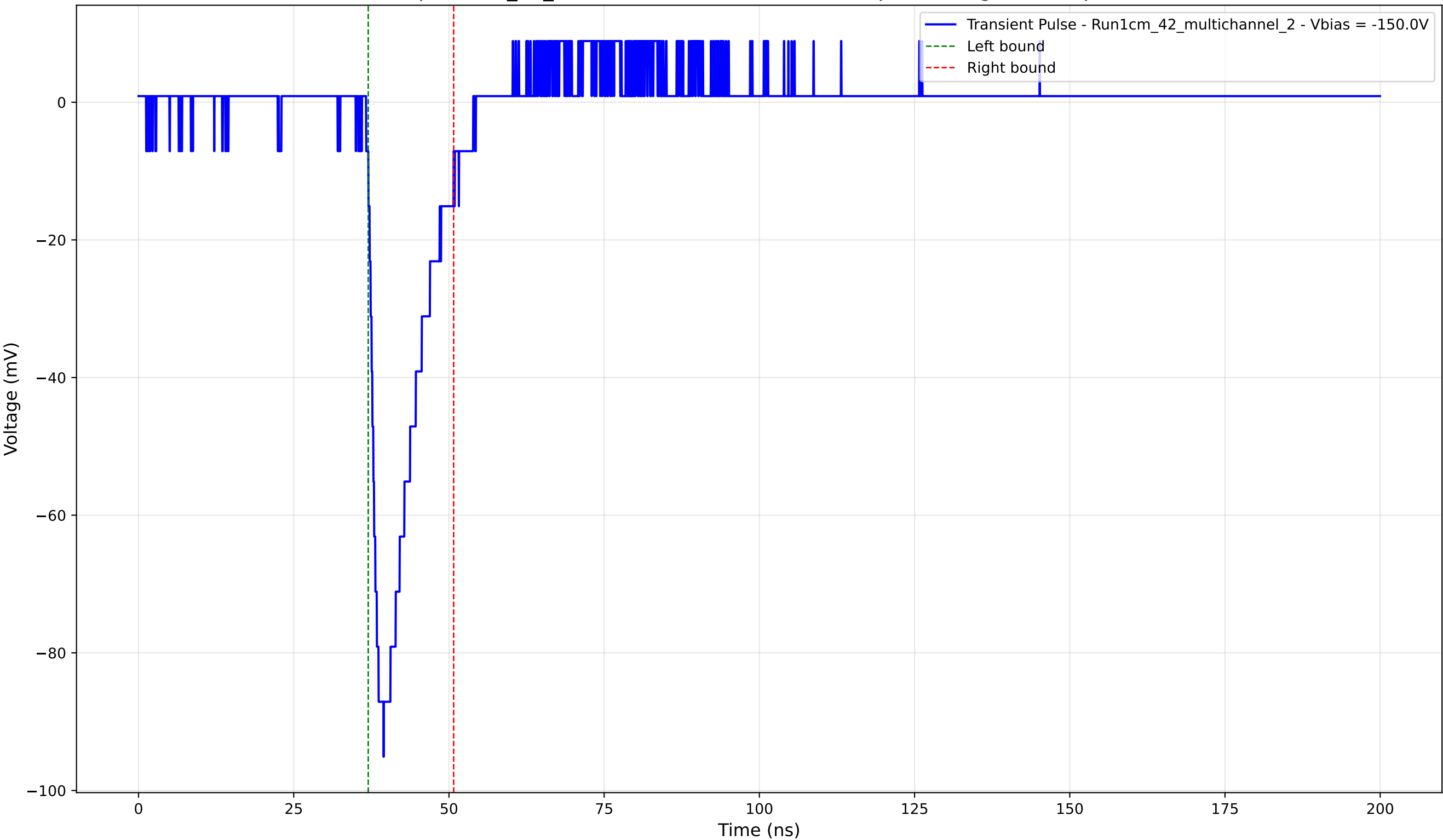
Transient Pulse - Sample: 1cm_42_multichannel - Position: 4035.0 \mu\text{m} - Charge: 13.08 pC - Rise Time: 1.67 ns
