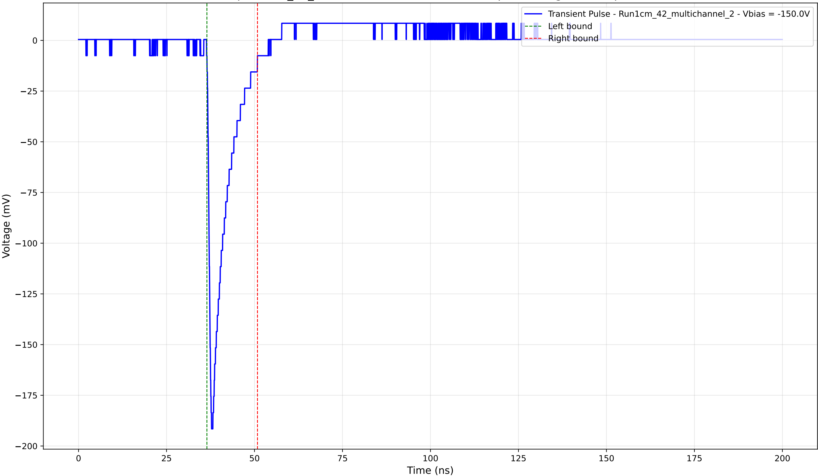
Transient Pulse - Sample: 1cm_42_multichannel - Position: 1445.0 \mu\text{m} - Charge: 20.20 pC - Rise Time: 0.98 ns
