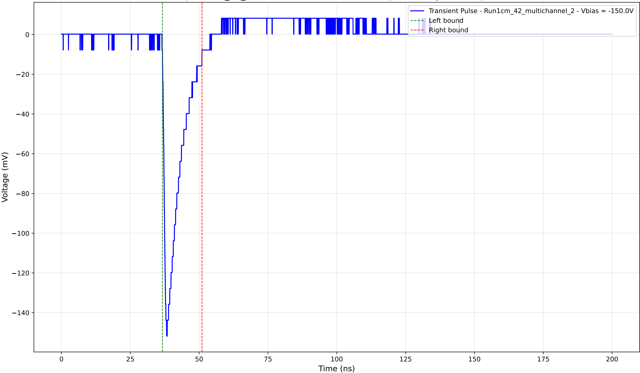
Transient Pulse - Sample: 1cm_42_multichannel - Position: 1195.0 \mu\text{m} - Charge: 18.63 pC - Rise Time: 1.24 ns
