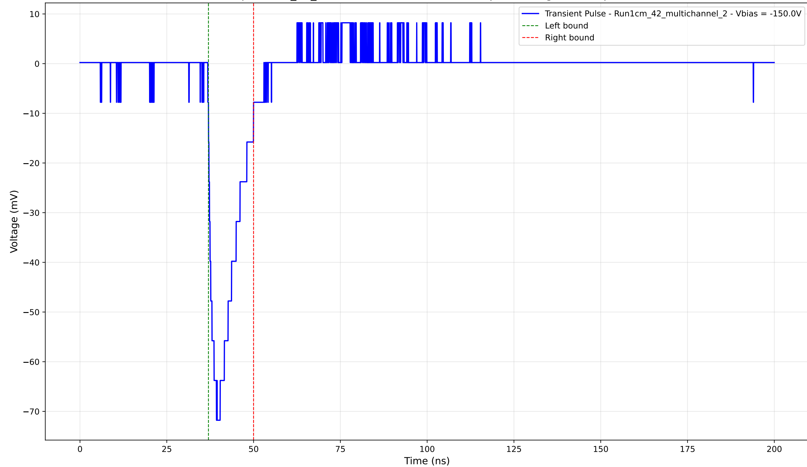
Transient Pulse - Sample: 1cm_42_multichannel - Position: 150.0 \mu\text{m} - Charge: 10.80 pC - Rise Time: 2.48 ns
