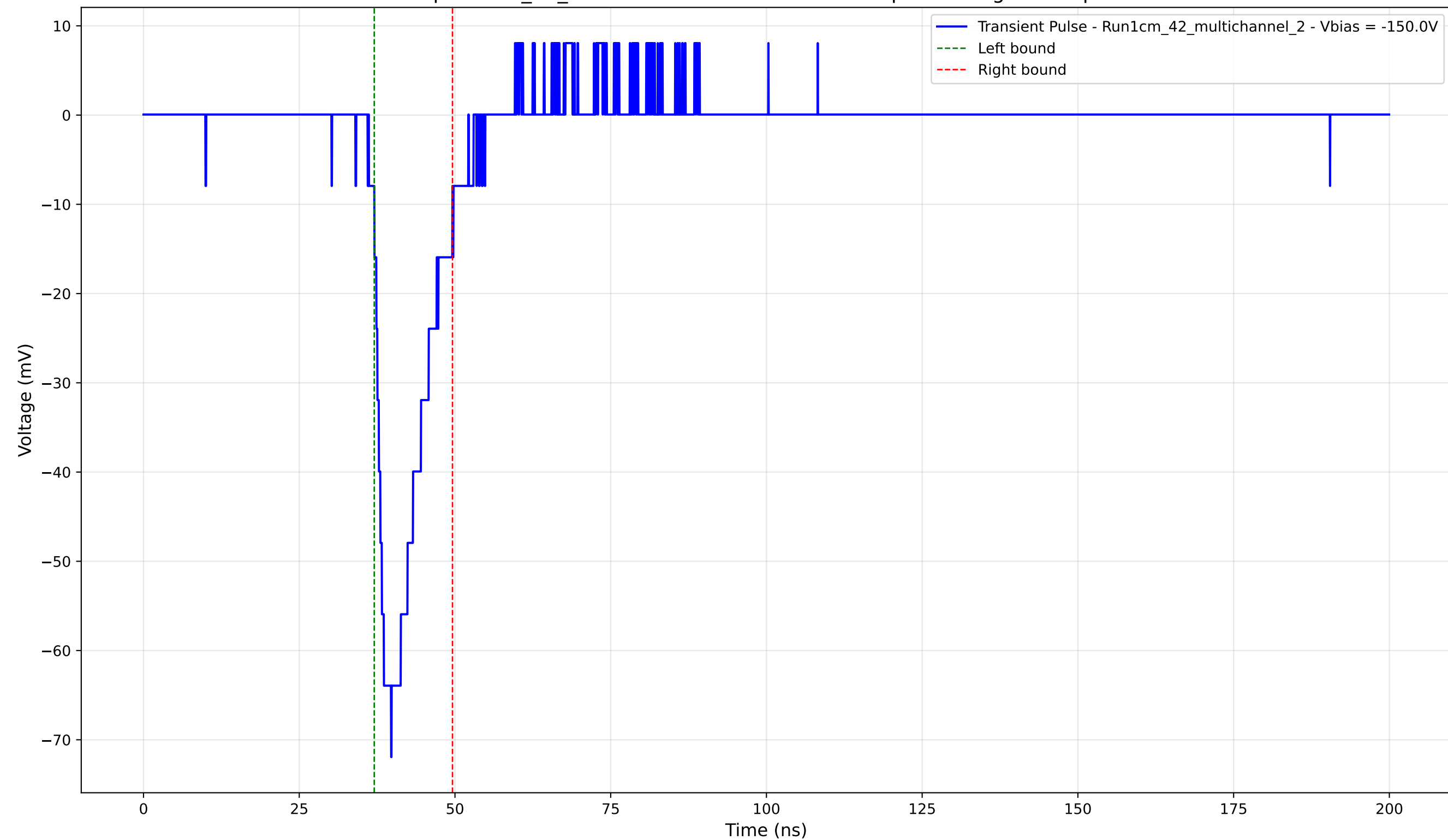
Transient Pulse - Sample: 1cm_42_multichannel - Position: 4720.0 \mu\text{m} - Charge: 9.91 pC - Rise Time: 3.56 ns
