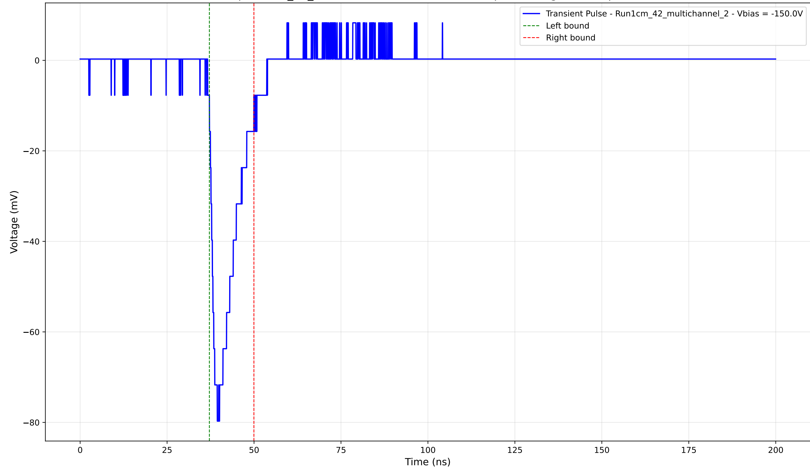
Transient Pulse - Sample: 1cm_42_multichannel - Position: 4270.0 \mu\text{m} - Charge: 11.04 pC - Rise Time: 2.28 ns
