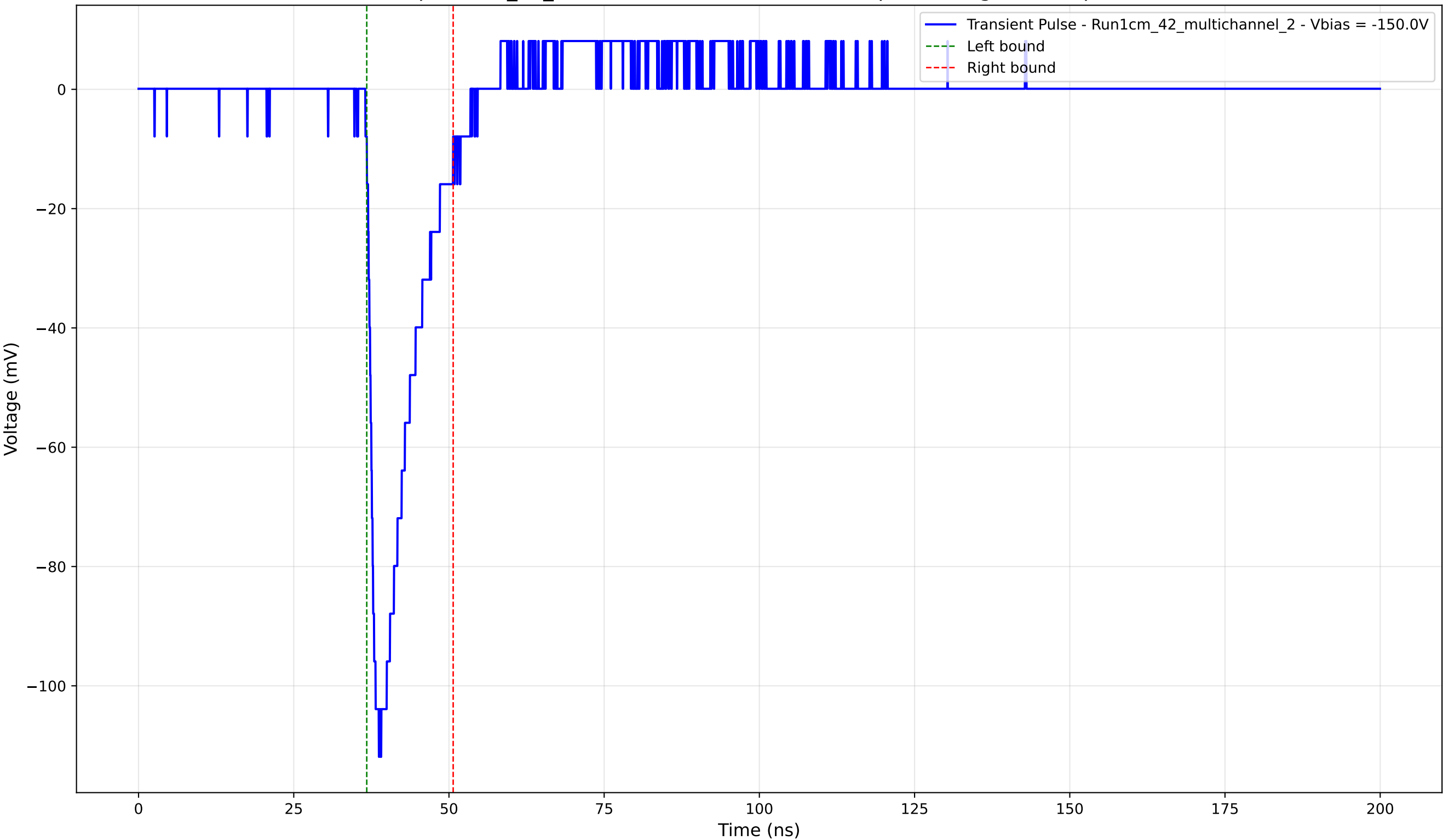
Transient Pulse - Sample: 1cm_42_multichannel - Position: 3715.0 \mu\text{m} - Charge: 14.94 pC - Rise Time: 1.42 ns
