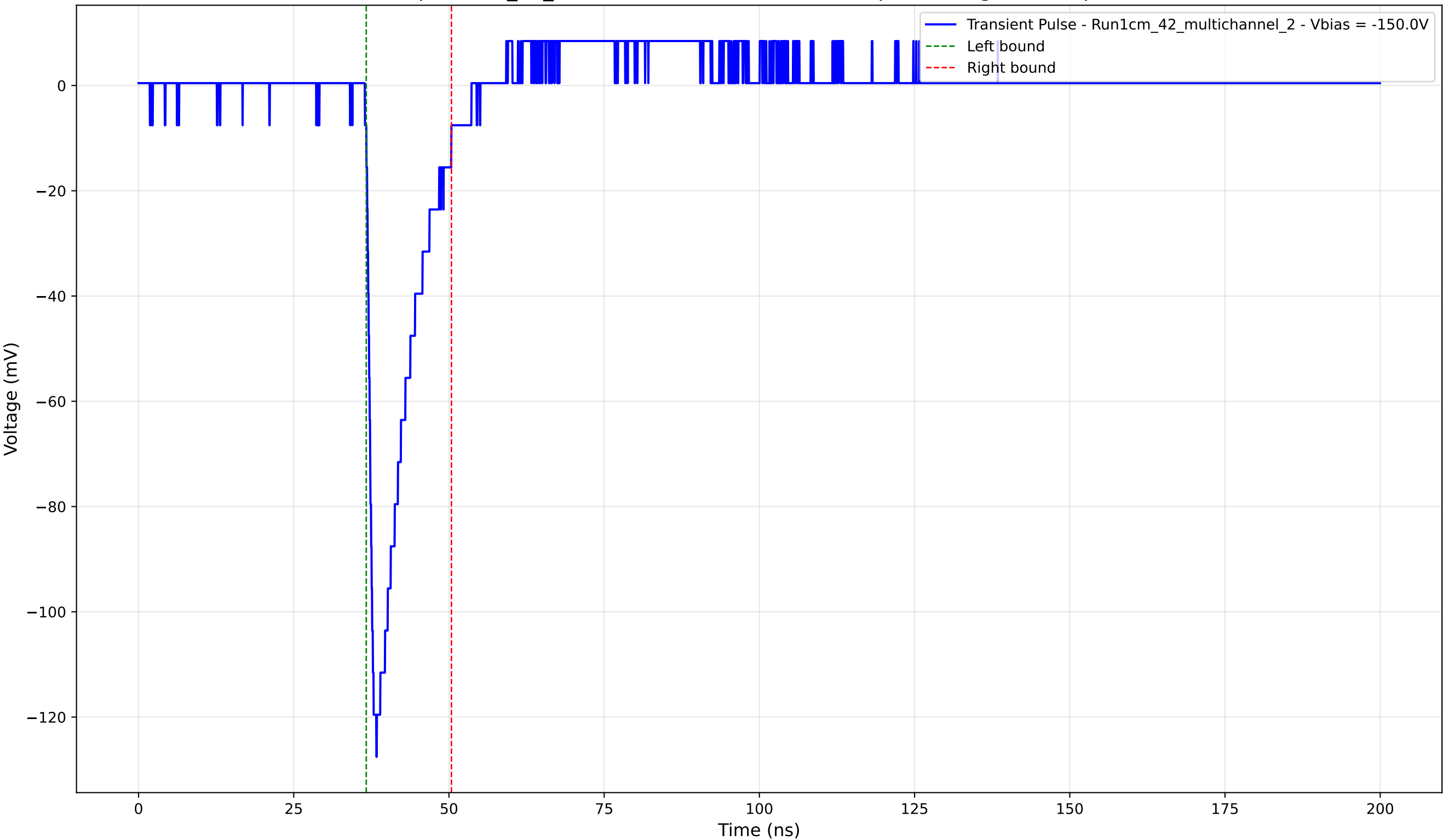
Transient Pulse - Sample: 1cm_42_multichannel - Position: 3535.0 \mu\text{m} - Charge: 15.83 pC - Rise Time: 1.17 ns
