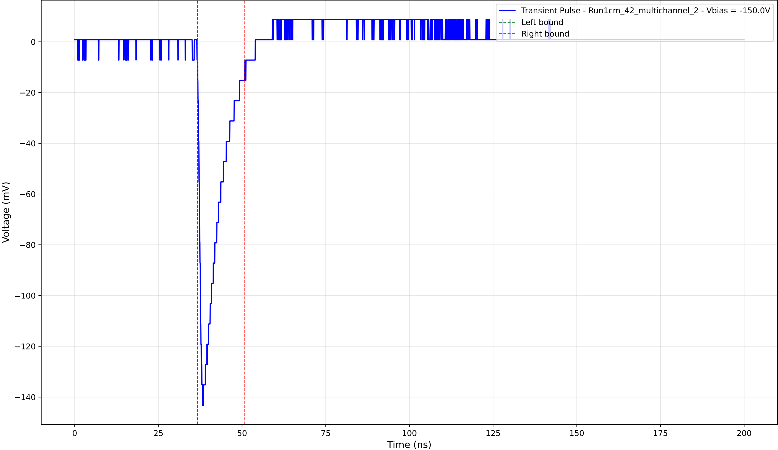
Transient Pulse - Sample: 1cm_42_multichannel - Position: 1155.0 \mu\text{m} - Charge: 17.87 pC - Rise Time: 1.24 ns
