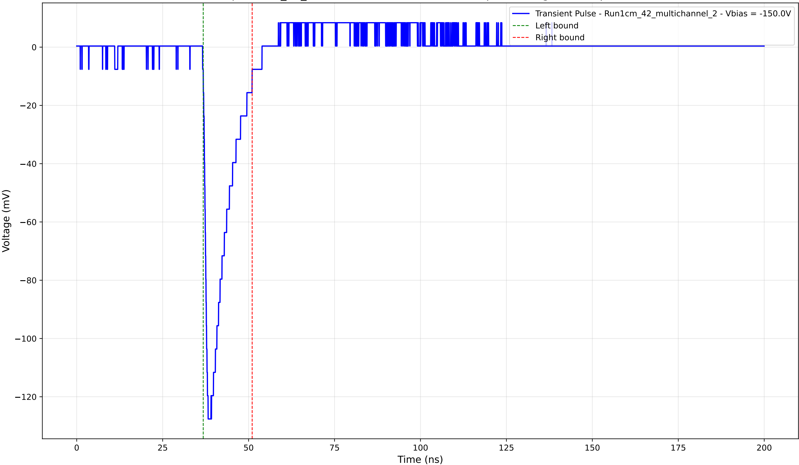
Transient Pulse - Sample: 1cm_42_multichannel - Position: 1040.0 \mu\text{m} - Charge: 17.22 pC - Rise Time: 1.21 ns
