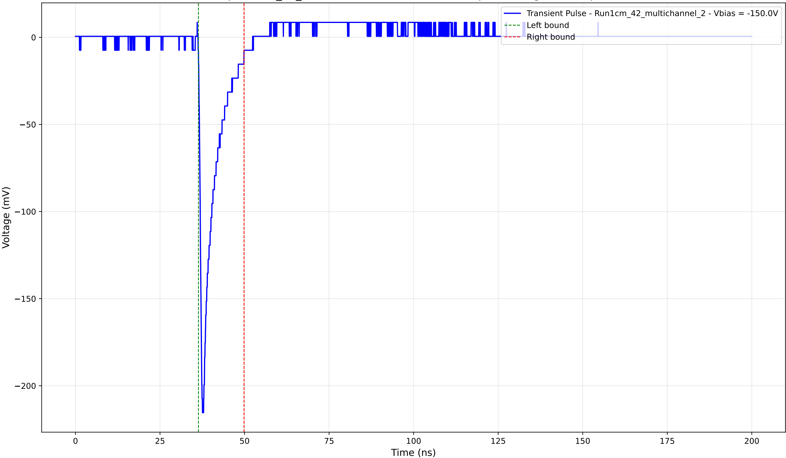
Transient Pulse - Sample: 1cm_42_multichannel - Position: 3095.0 \mu\text{m} - Charge: 19.15 pC - Rise Time: 0.89 ns
