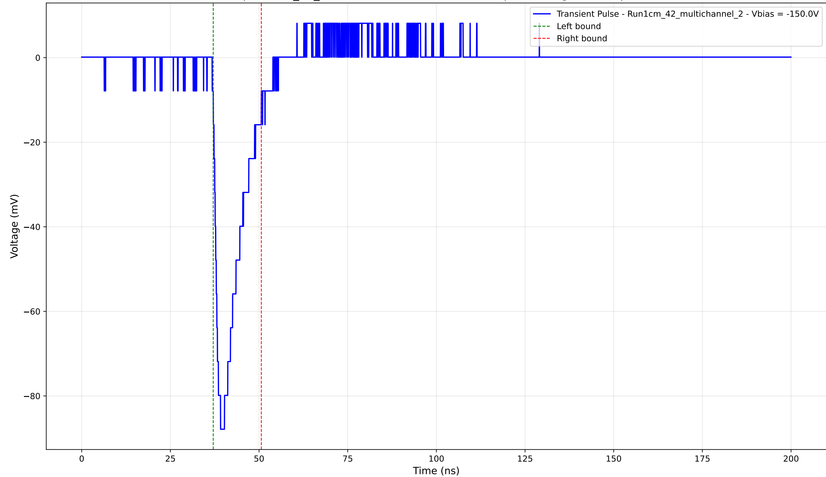
Transient Pulse - Sample: 1cm_42_multichannel - Position: 4110.0 \mu\text{m} - Charge: 12.82 pC - Rise Time: 1.48 ns
