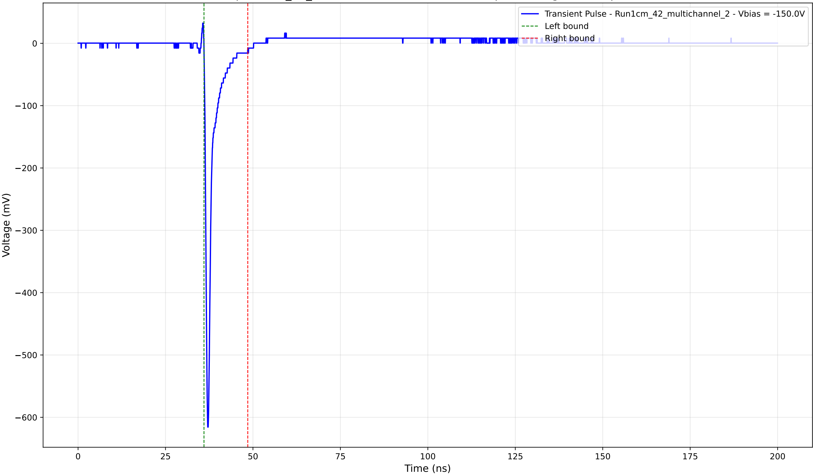
Transient Pulse - Sample: 1cm_42_multichannel - Position: 2450.0 \mu\text{m} - Charge: 27.52 pC - Rise Time: 0.73 ns
