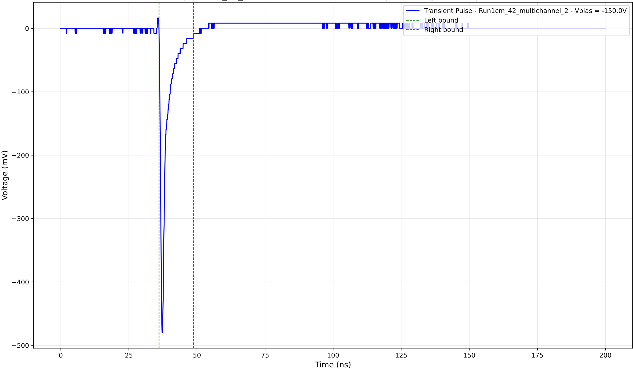
Transient Pulse - Sample: 1cm_42_multichannel - Position: 2610.0 \mu\text{m} - Charge: 25.17 pC - Rise Time: 0.78 ns
