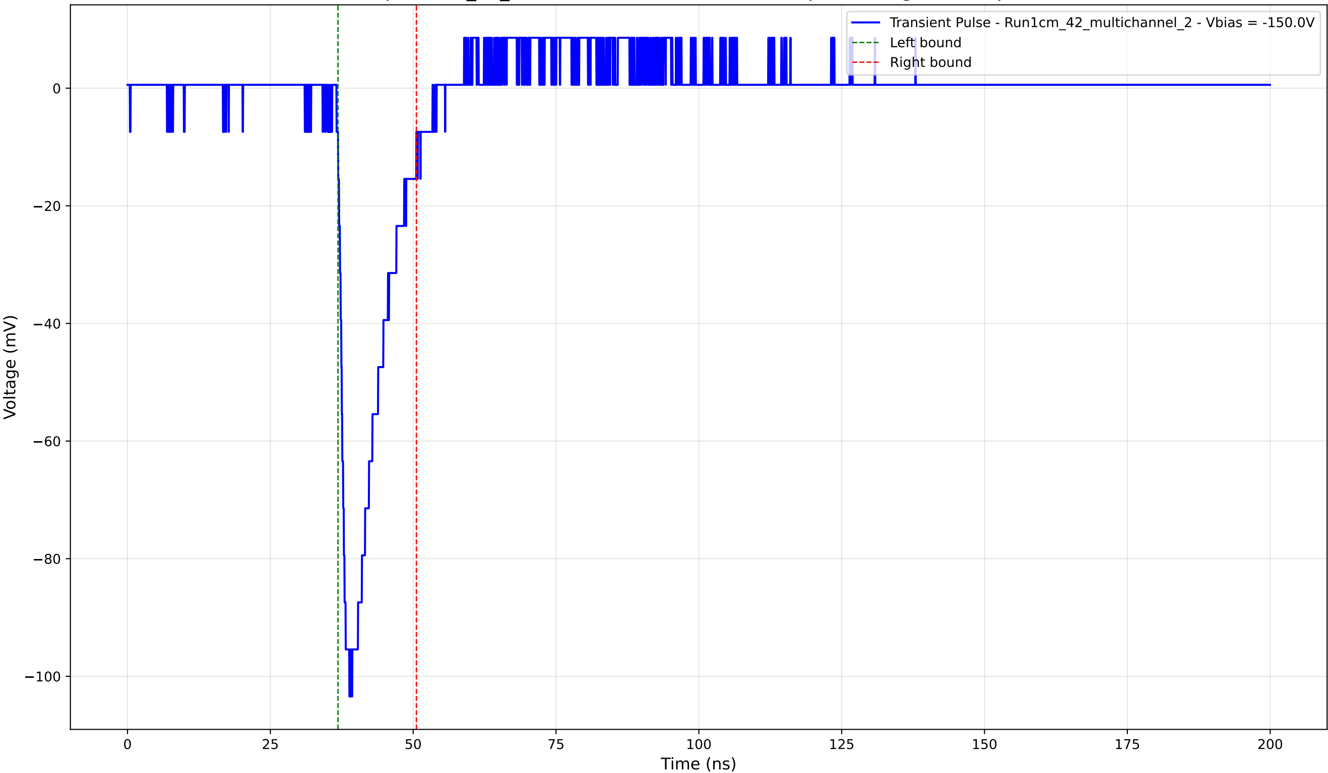
Transient Pulse - Sample: 1cm_42_multichannel - Position: 3790.0 \mu\text{m} - Charge: 14.24 pC - Rise Time: 1.35 ns
