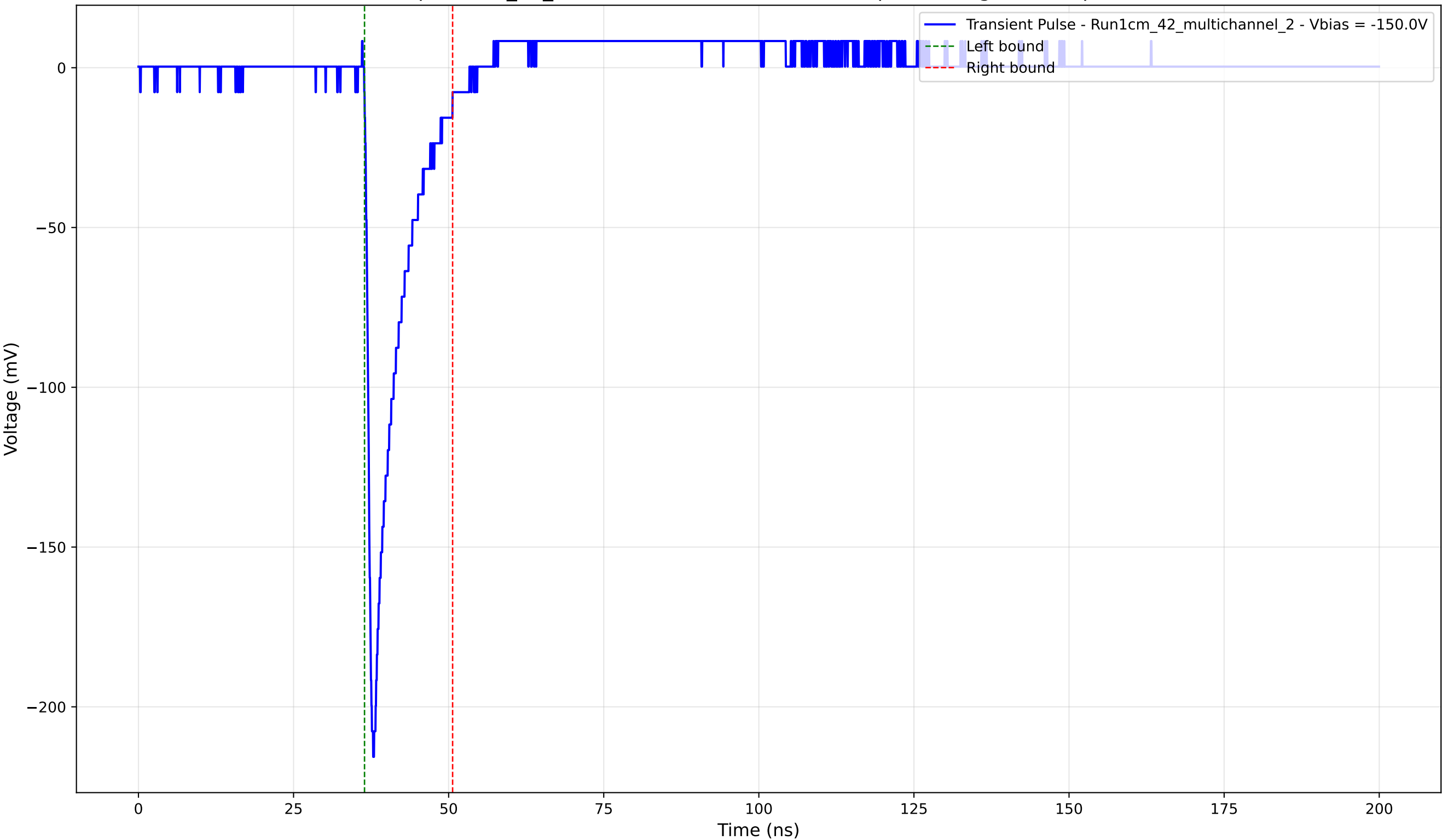
Transient Pulse - Sample: 1cm_42_multichannel - Position: 1505.0 \mu\text{m} - Charge: 21.26 pC - Rise Time: 1.01 ns
