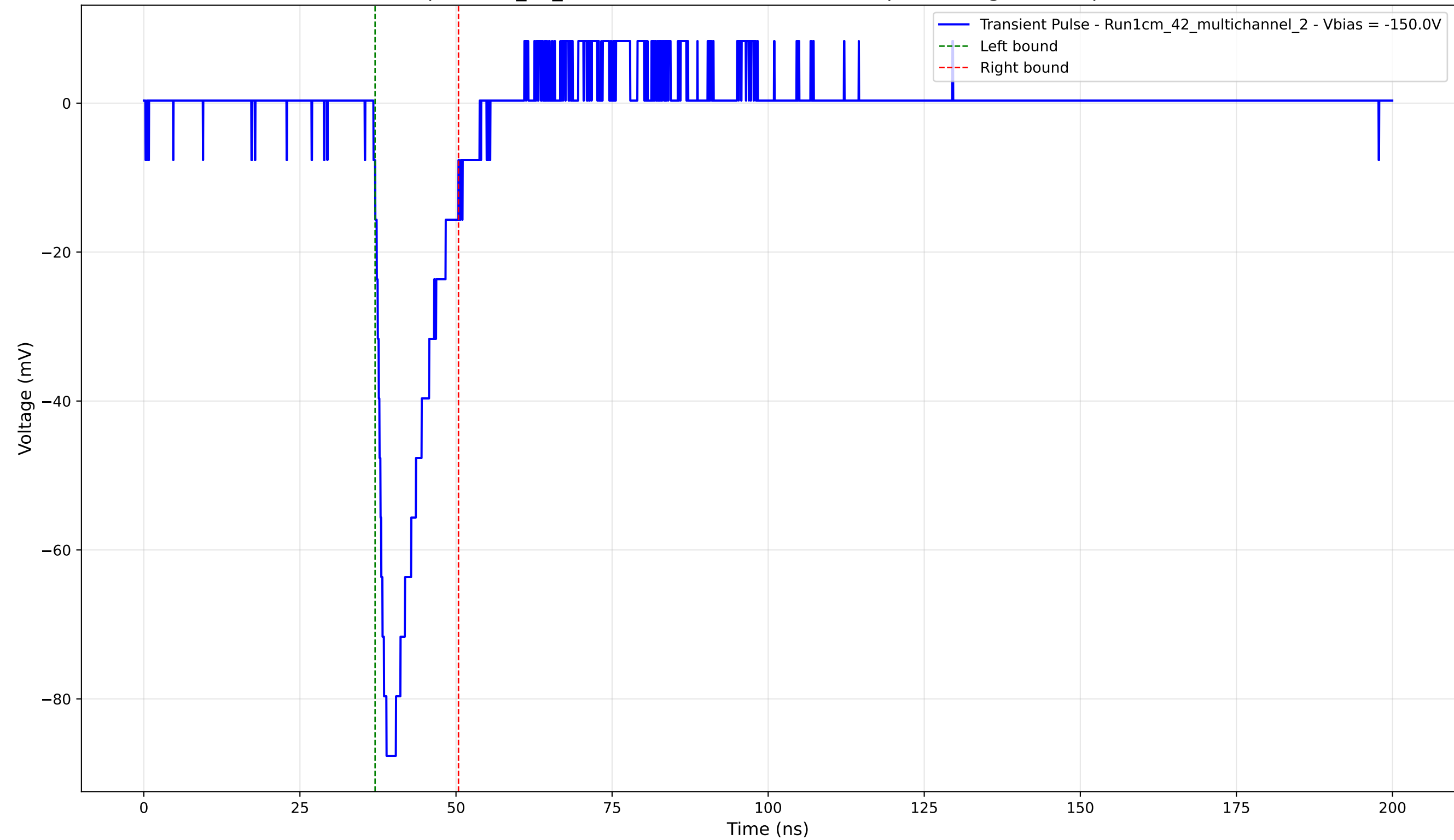
Transient Pulse - Sample: 1cm_42_multichannel - Position: 4075.0 \mu\text{m} - Charge: 12.71 pC - Rise Time: 1.43 ns
