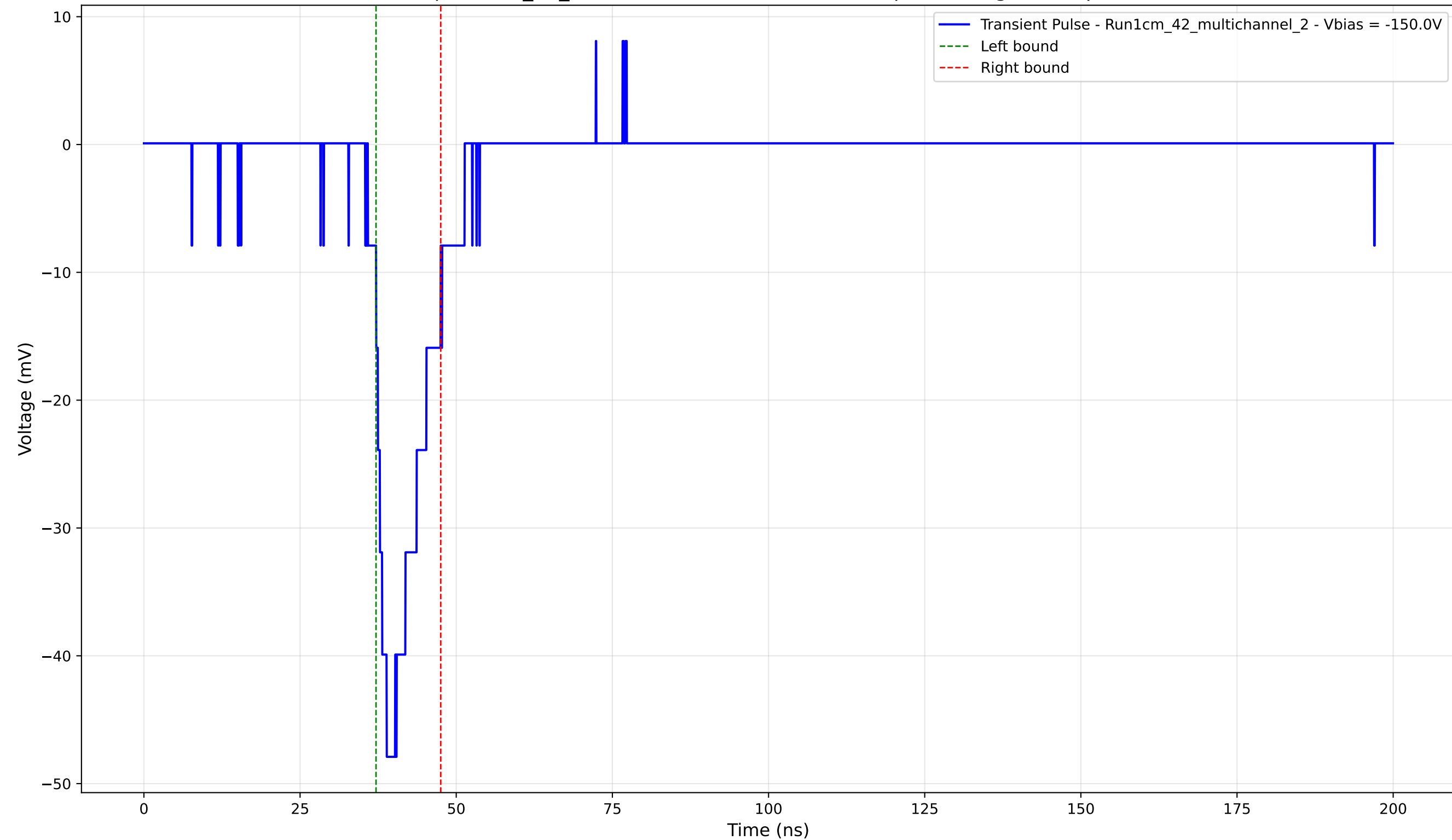
Transient Pulse - Sample: 1cm_42_multichannel - Position: 4835.0 \mu\text{m} - Charge: 6.30 pC - Rise Time: 3.02 ns
