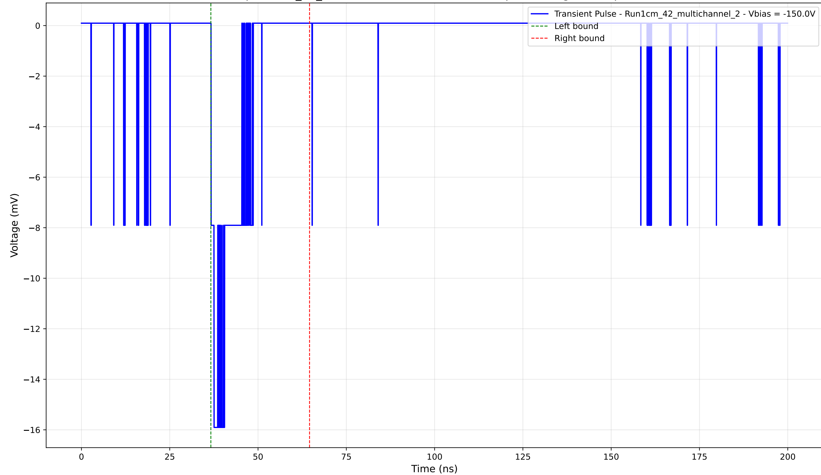
Transient Pulse - Sample: 1cm_42_multichannel - Position: 1375.0 \mu\text{m} - Charge: 2.04 pC - Rise Time: 0.87 ns
