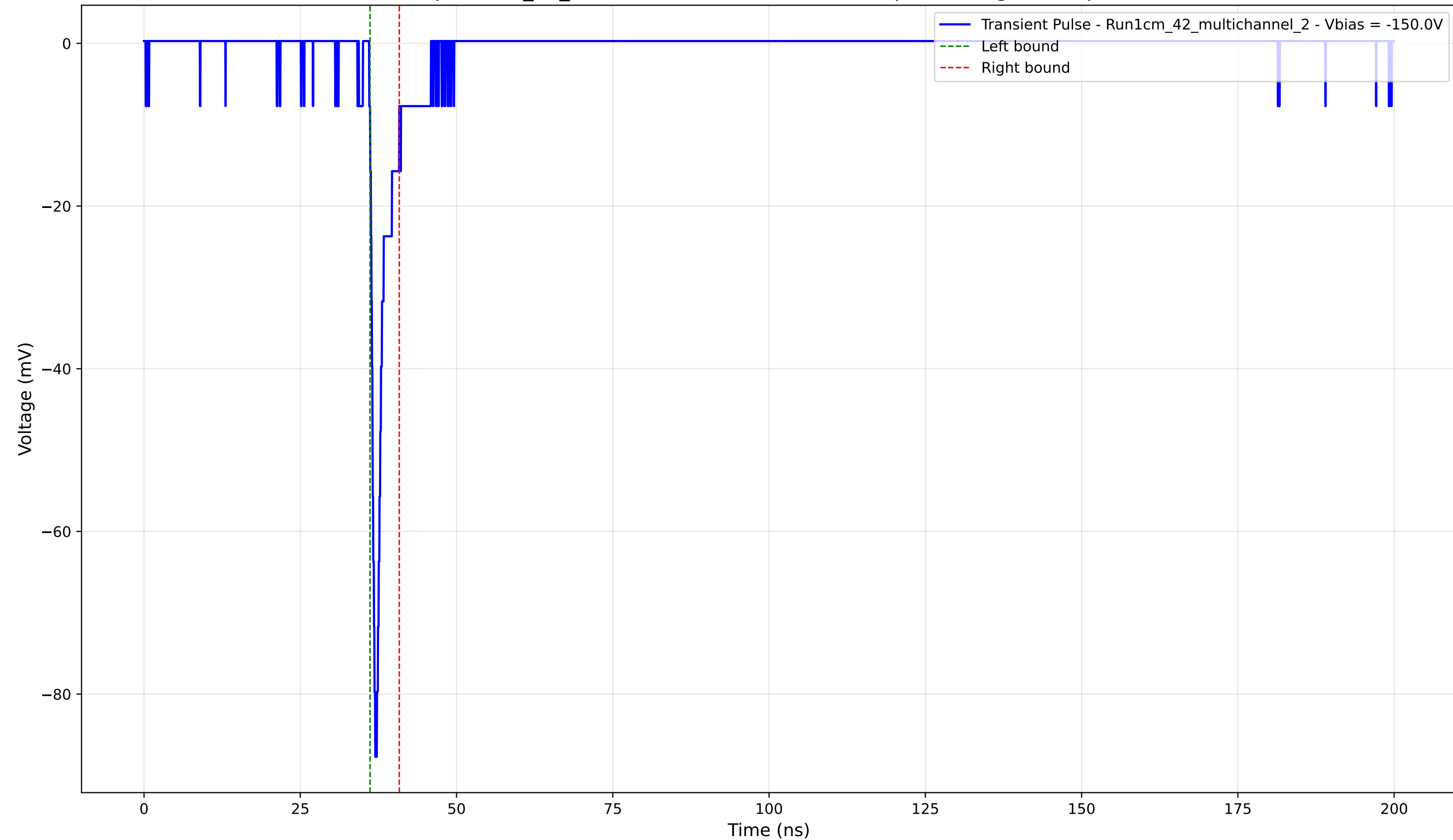
Transient Pulse - Sample: 1cm_42_multichannel - Position: 2340.0 \mu\text{m} - Charge: 3.40 pC - Rise Time: 0.71 ns
