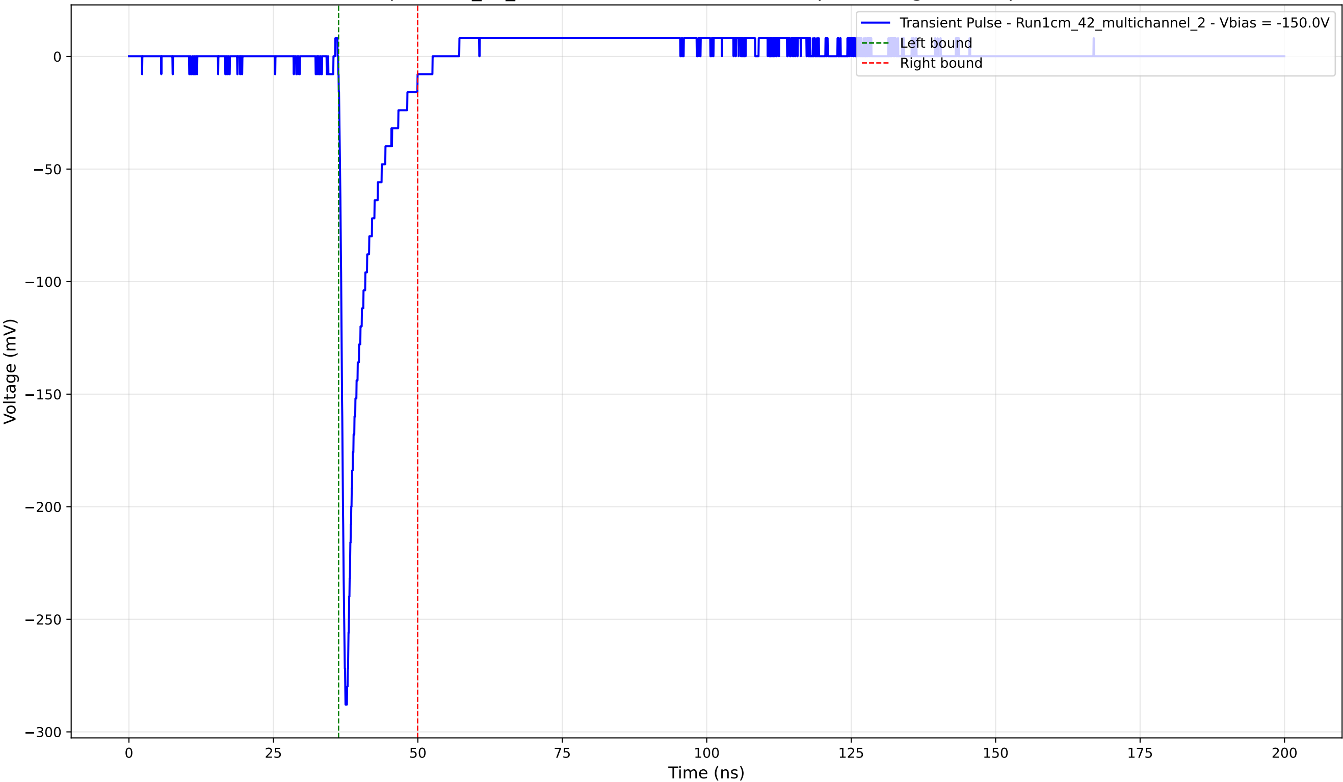
Transient Pulse - Sample: 1cm_42_multichannel - Position: 1740.0 \mu\text{m} - Charge: 23.09 pC - Rise Time: 0.87 ns
