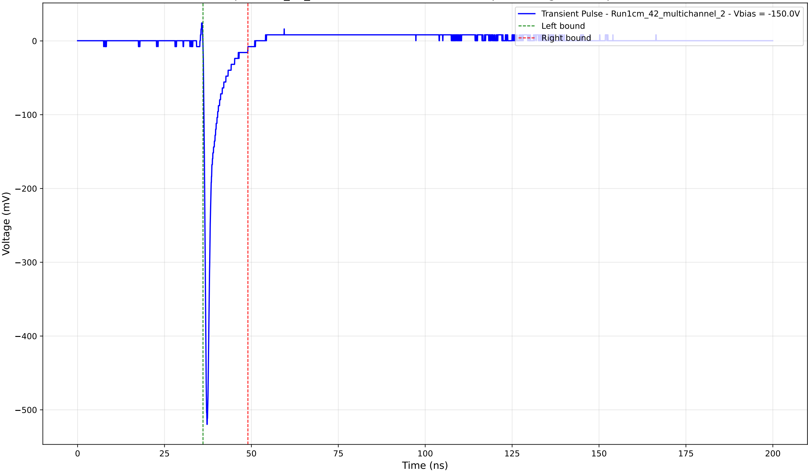
Transient Pulse - Sample: 1cm_42_multichannel - Position: 2135.0 \mu\text{m} - Charge: 26.84 pC - Rise Time: 0.73 ns
