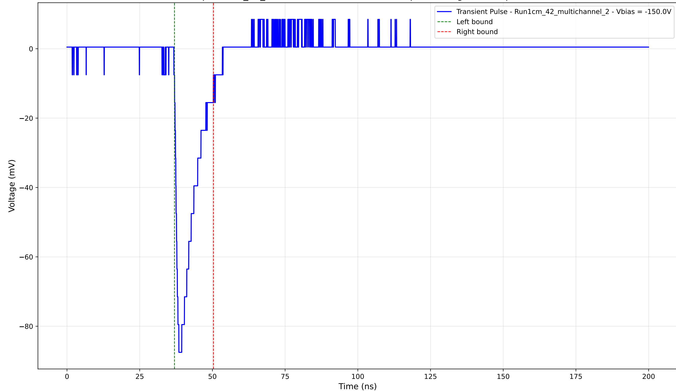
Transient Pulse - Sample: 1cm_42_multichannel - Position: 910.0 \mu\text{m} - Charge: 11.96 pC - Rise Time: 1.19 ns
