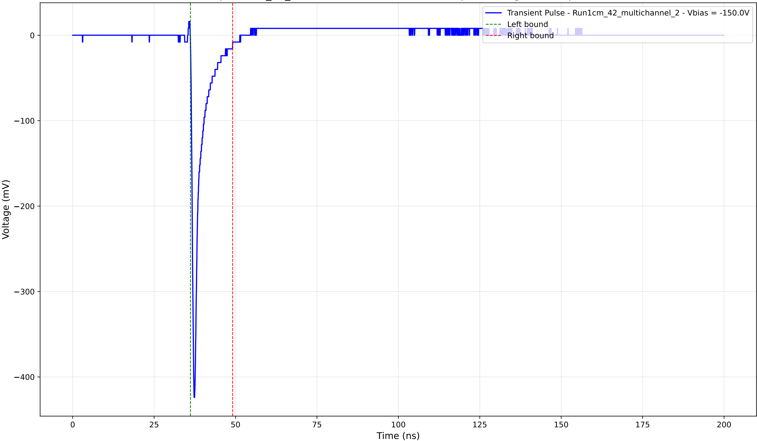
Transient Pulse - Sample: 1cm_42_multichannel - Position: 2720.0 \mu\text{m} - Charge: 24.97 pC - Rise Time: 0.78 ns
