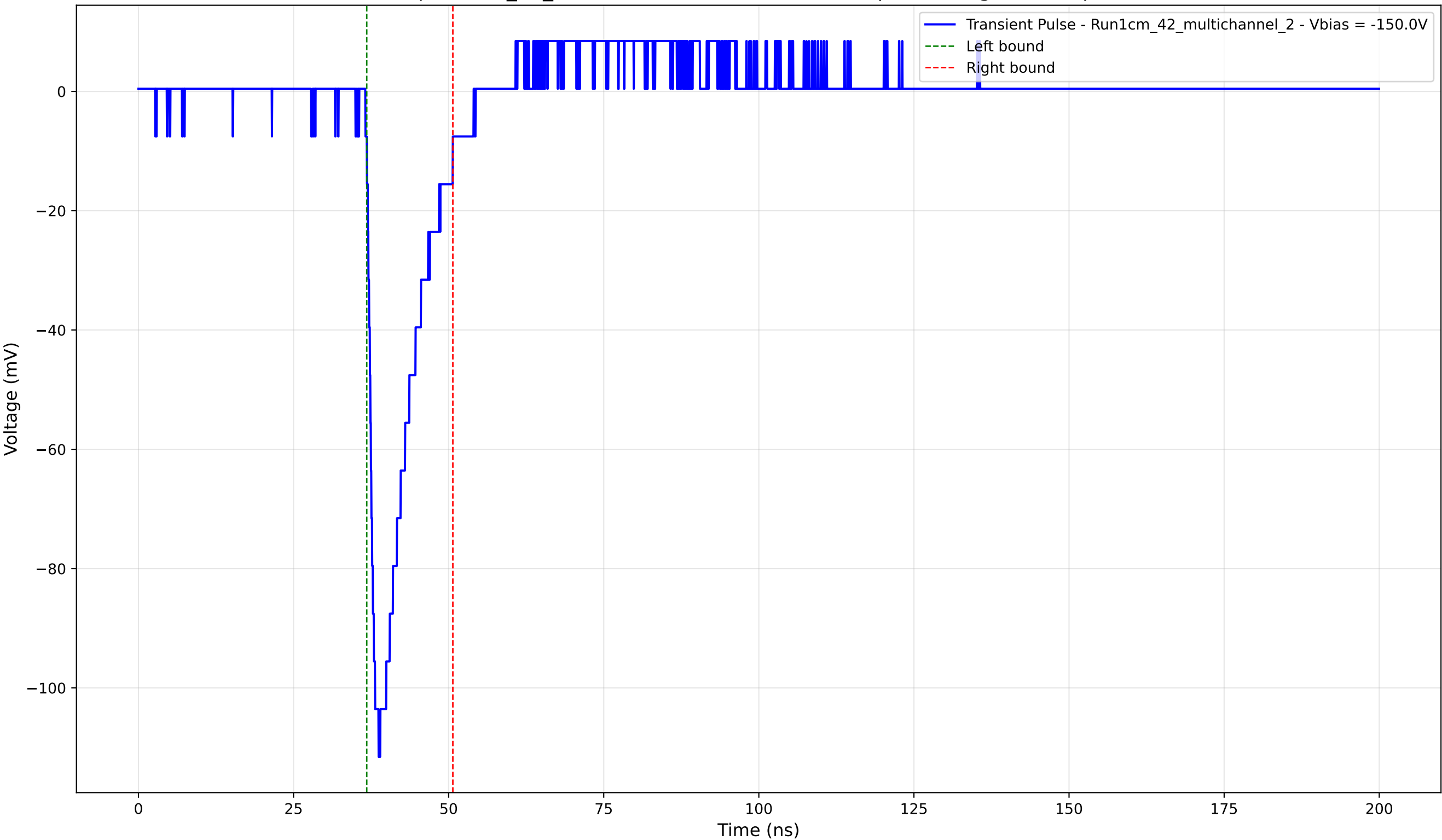
Transient Pulse - Sample: 1cm_42_multichannel - Position: 3700.0 \mu\text{m} - Charge: 14.78 pC - Rise Time: 1.34 ns
