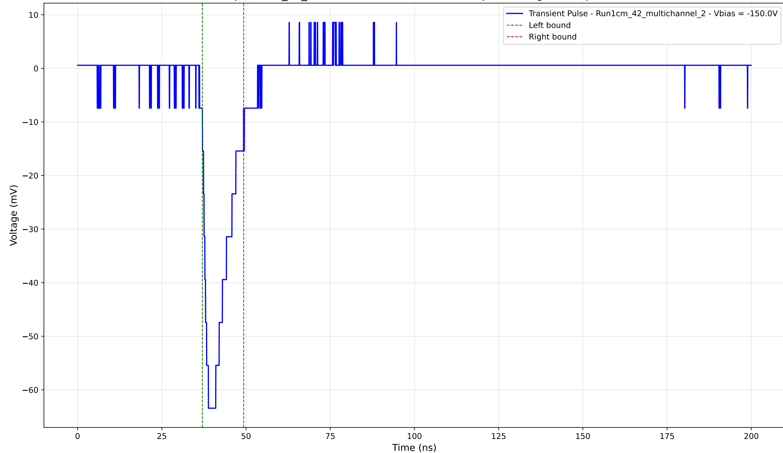
Transient Pulse - Sample: 1cm_42_multichannel - Position: 4760.0 \mu\text{m} - Charge: 9.40 pC - Rise Time: 2.61 ns
