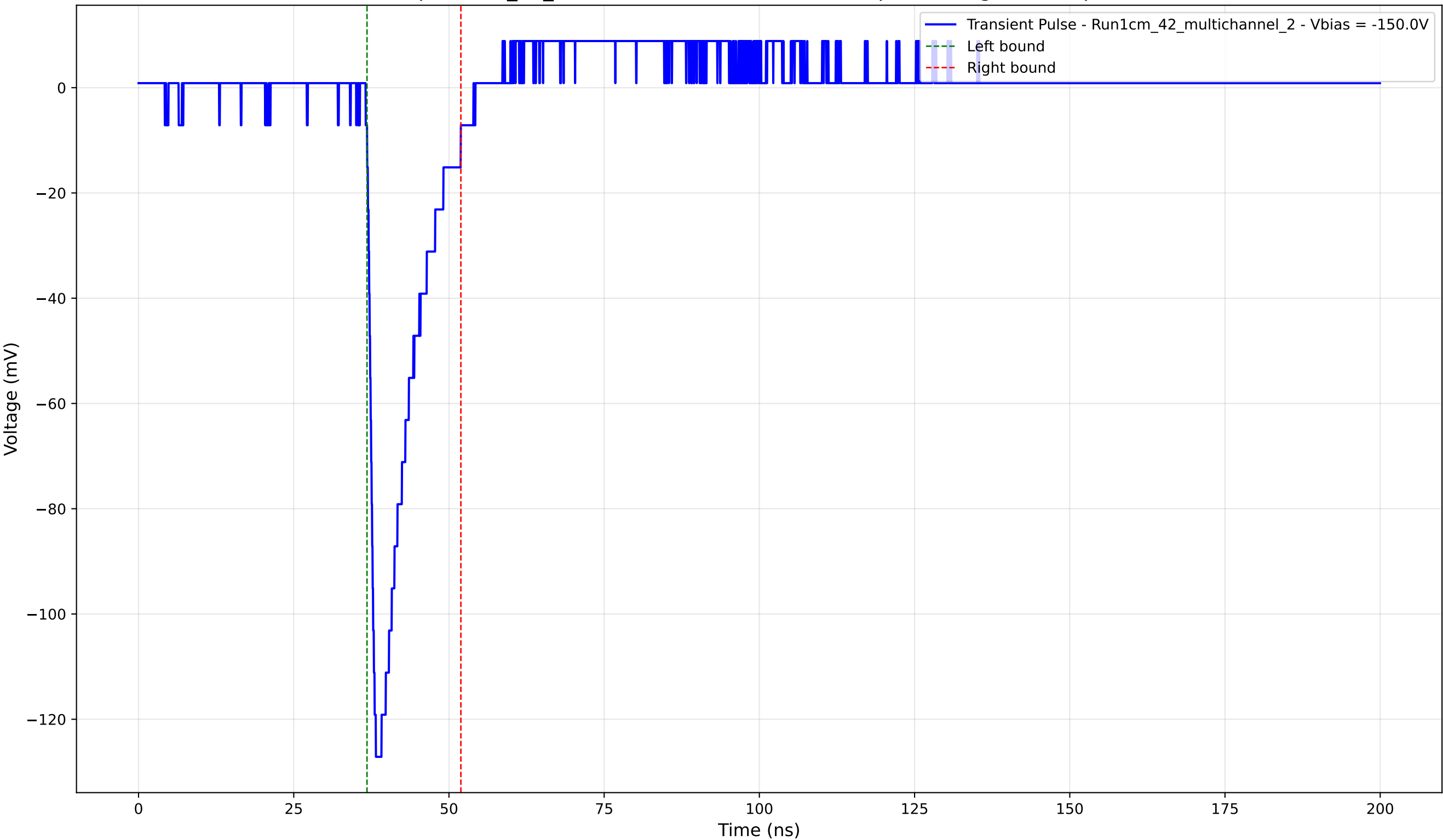
Transient Pulse - Sample: 1cm_42_multichannel - Position: 1035.0 \mu\text{m} - Charge: 17.31 pC - Rise Time: 1.21 ns
