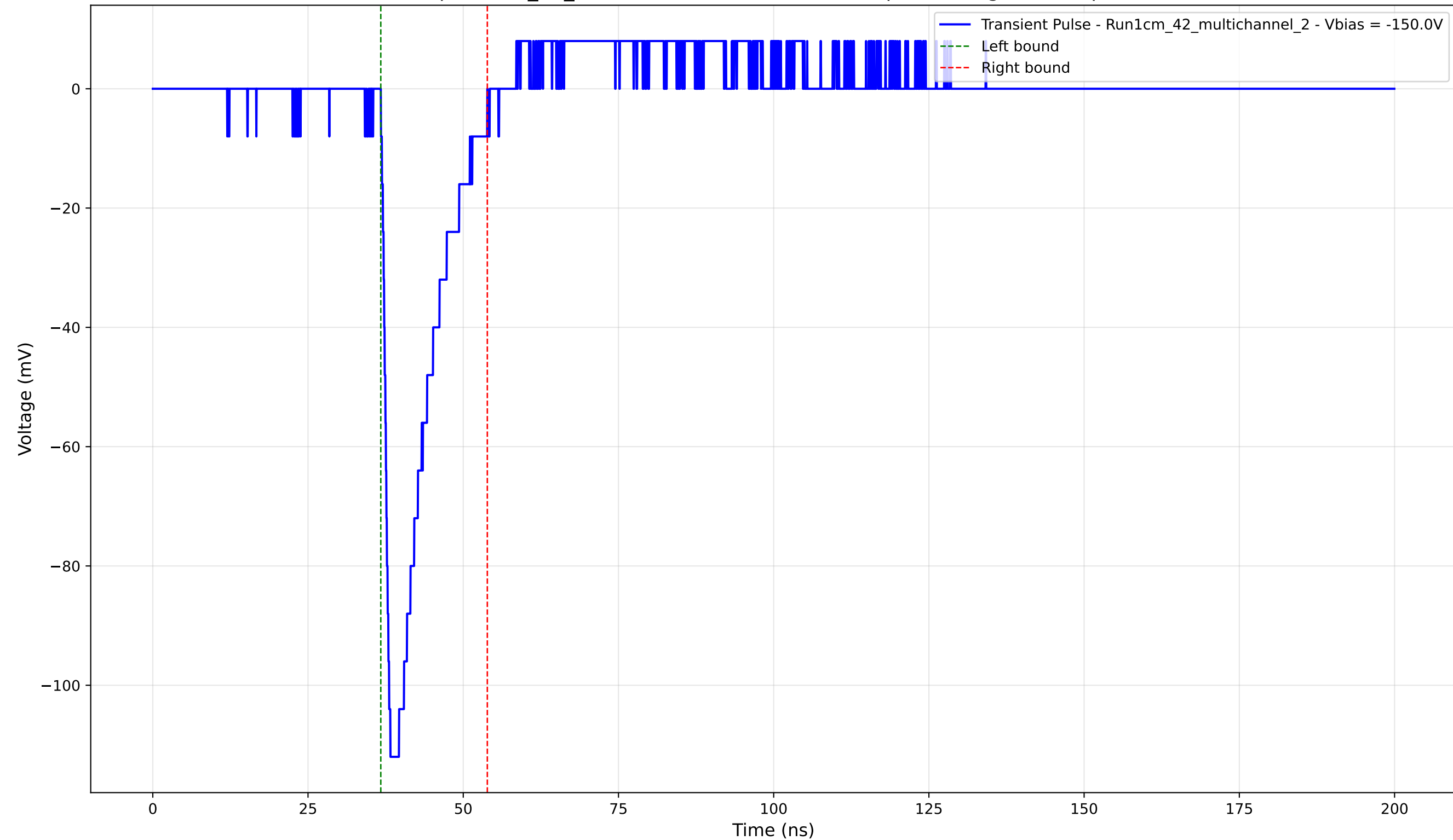
Transient Pulse - Sample: 1cm_42_multichannel - Position: 930.0 \mu\text{m} - Charge: 16.51 pC - Rise Time: 1.18 ns
