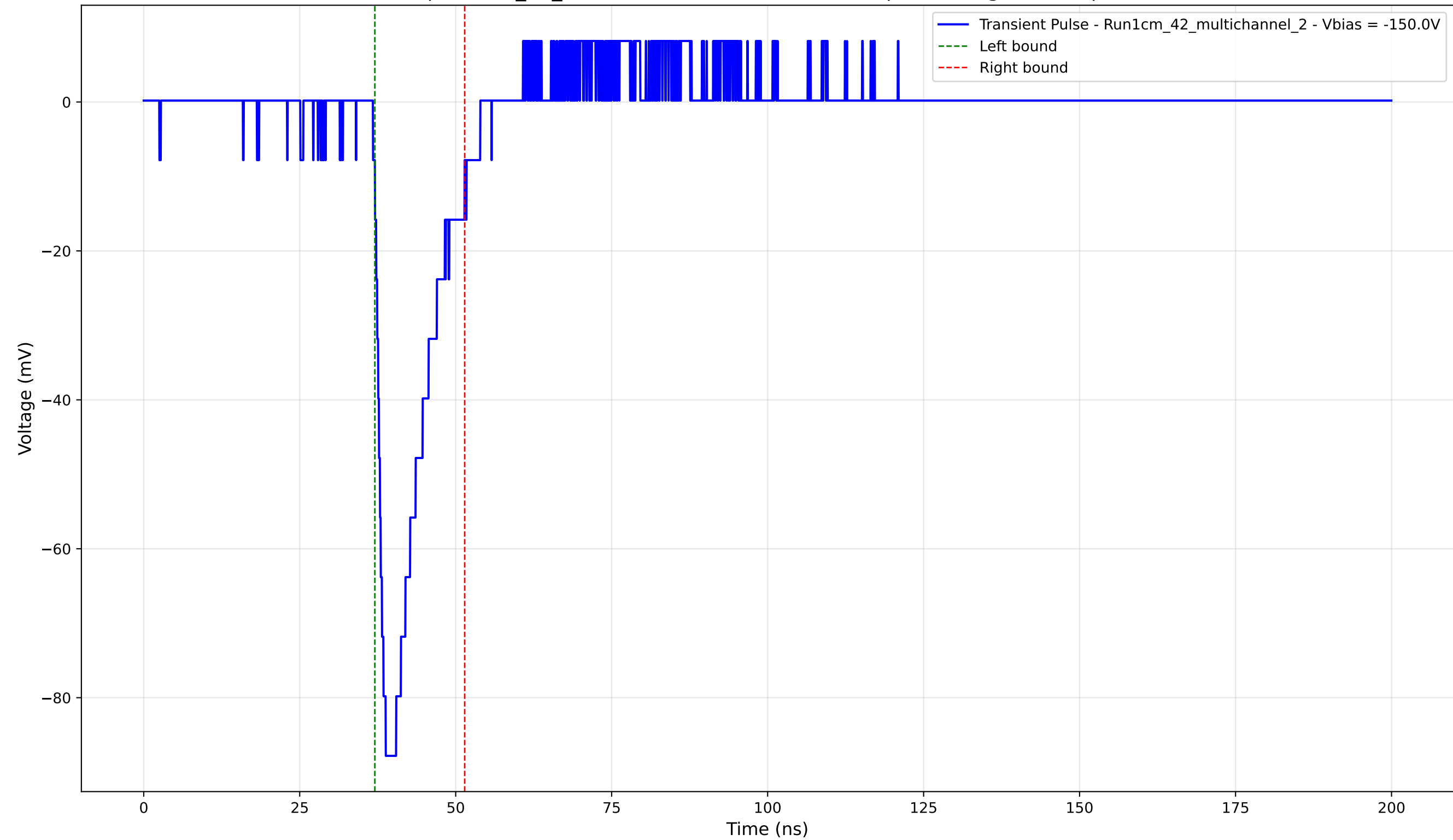
Transient Pulse - Sample: 1cm_42_multichannel - Position: 4060.0 \mu\text{m} - Charge: 13.27 pC - Rise Time: 1.40 ns
