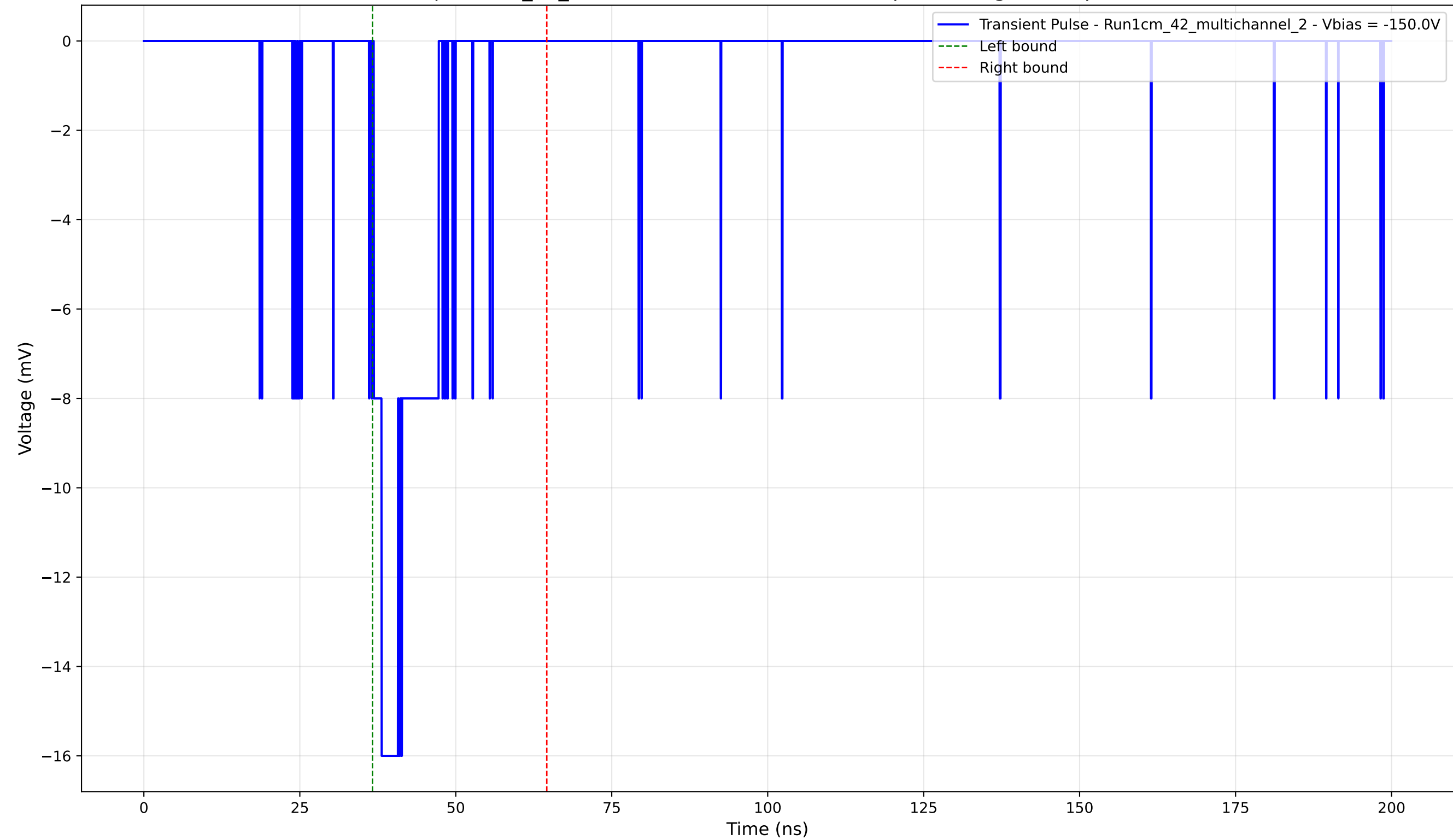
Transient Pulse - Sample: 1cm_42_multichannel - Position: 3860.0 \mu\text{m} - Charge: 2.28 pC - Rise Time: 1.27 ns
