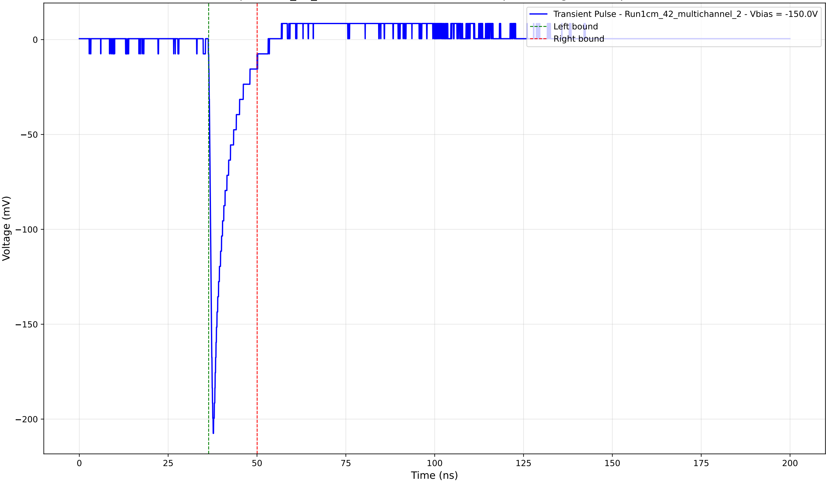
Transient Pulse - Sample: 1cm_42_multichannel - Position: 3135.0 \mu\text{m} - Charge: 18.64 pC - Rise Time: 0.97 ns
