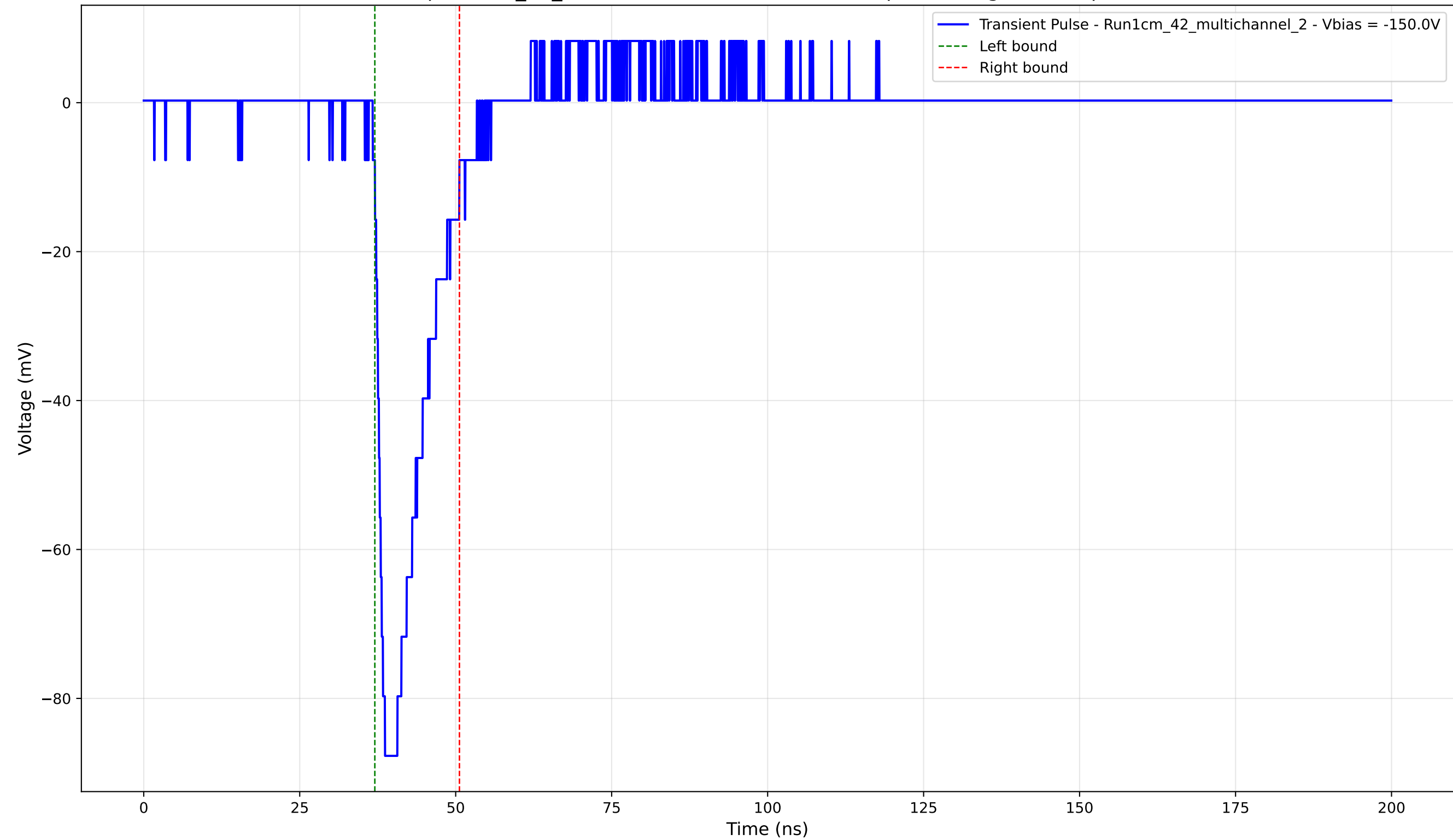
Transient Pulse - Sample: 1cm_42_multichannel - Position: 4040.0 \mu\text{m} - Charge: 13.20 pC - Rise Time: 1.31 ns
