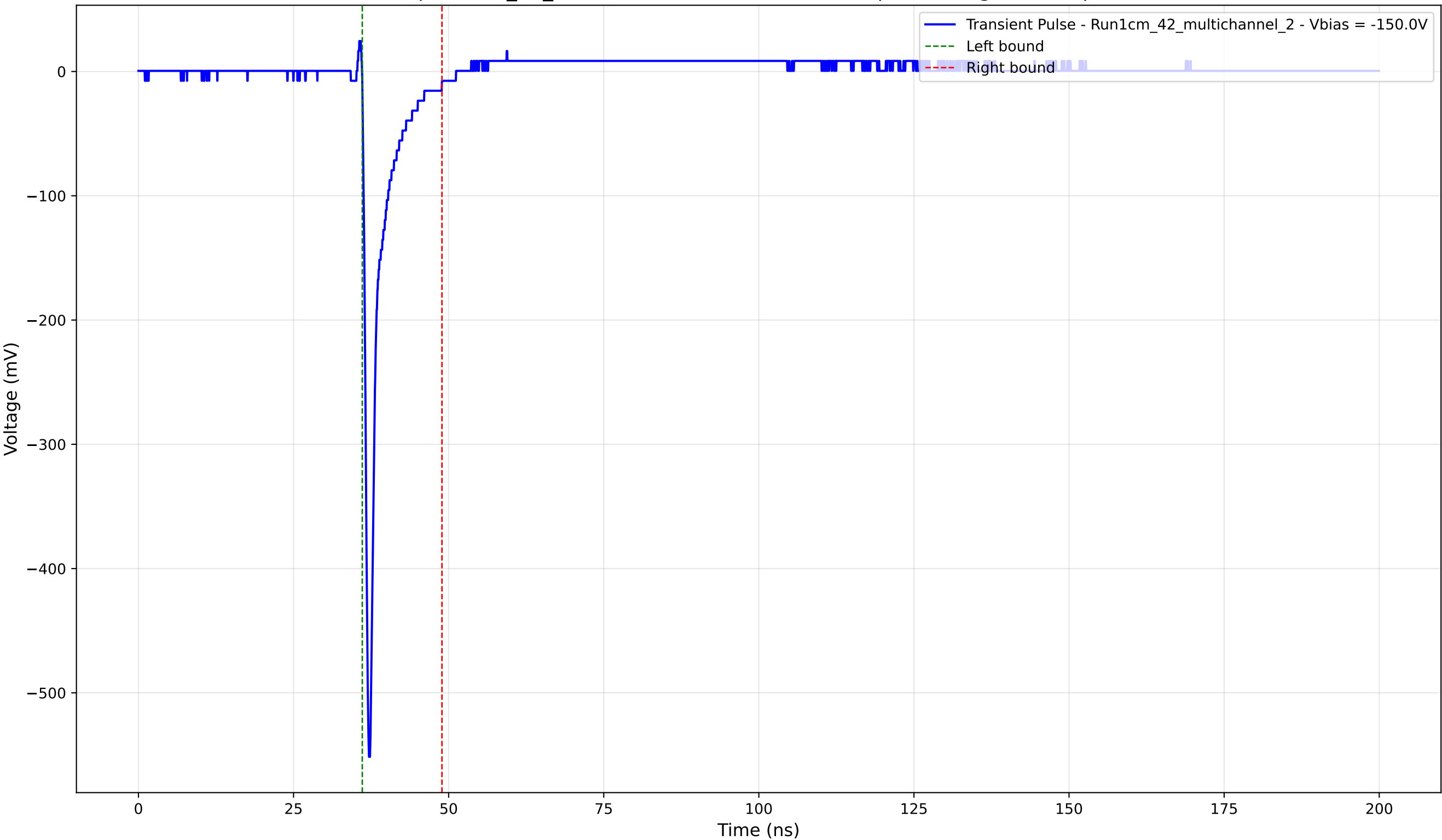
Transient Pulse - Sample: 1cm_42_multichannel - Position: 2180.0 \mu\text{m} - Charge: 27.49 pC - Rise Time: 0.74 ns
