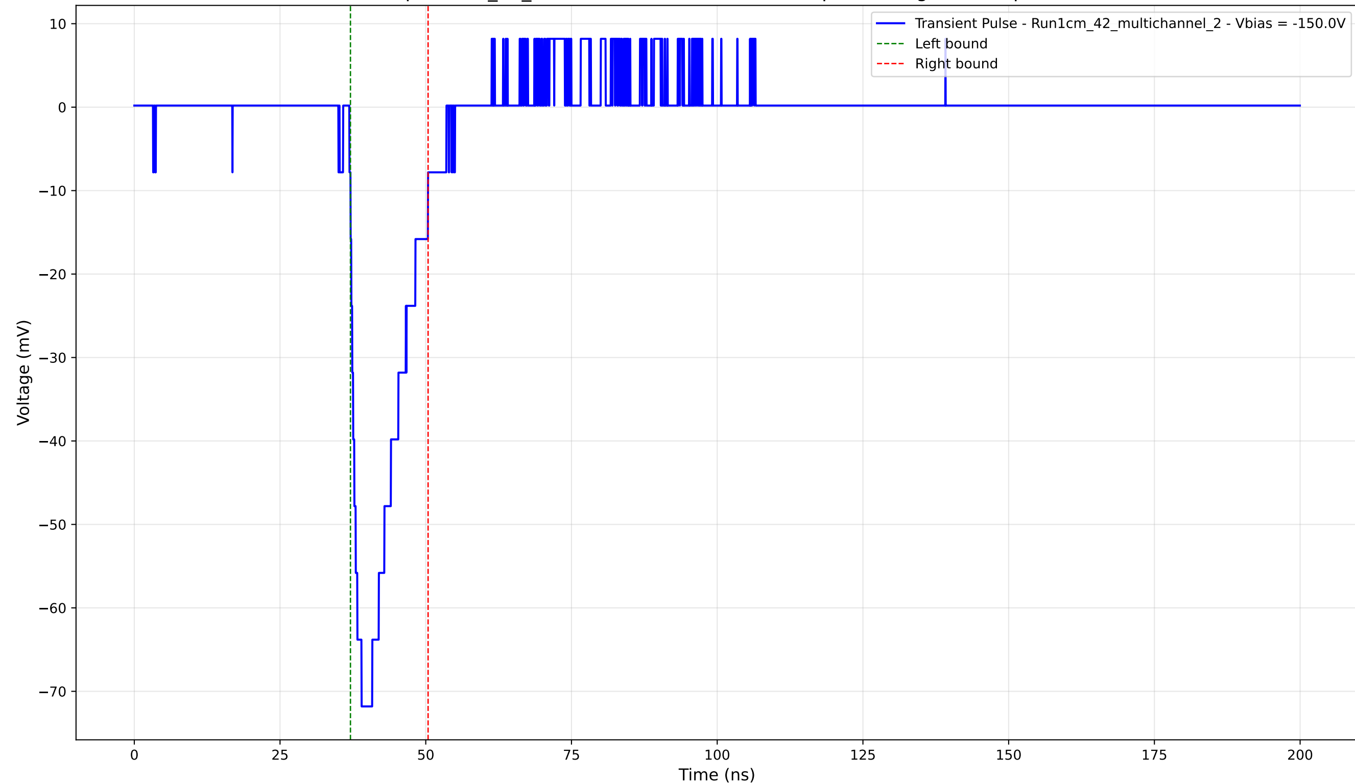
Transient Pulse - Sample: 1cm_42_multichannel - Position: 240.0 \mu\text{m} - Charge: 11.37 pC - Rise Time: 2.08 ns
