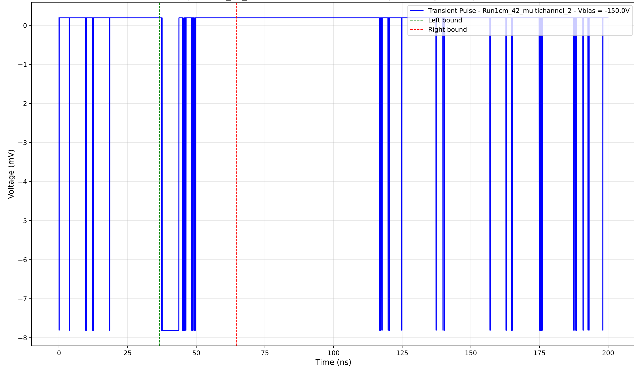
Transient Pulse - Sample: 1cm_42_multichannel - Position: 4370.0 \mu\text{m} - Charge: 1.10 pC - Rise Time: 0.04 ns
