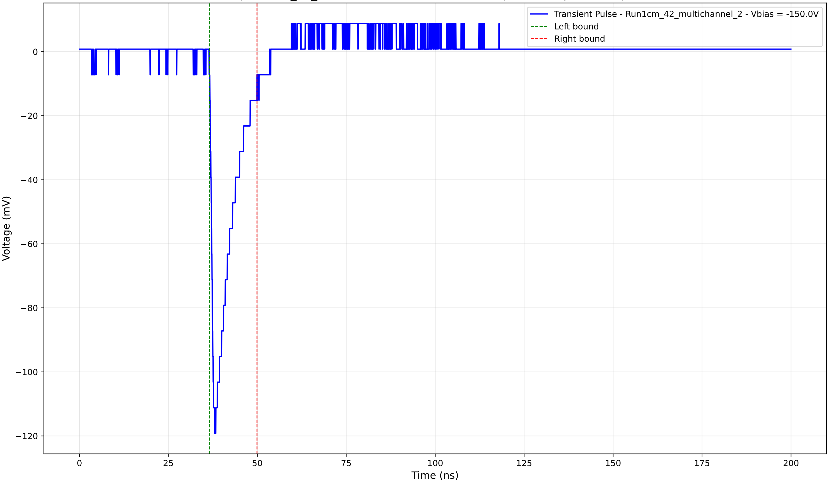
Transient Pulse - Sample: 1cm_42_multichannel - Position: 3450.0 \mu\text{m} - Charge: 14.14 pC - Rise Time: 1.06 ns
