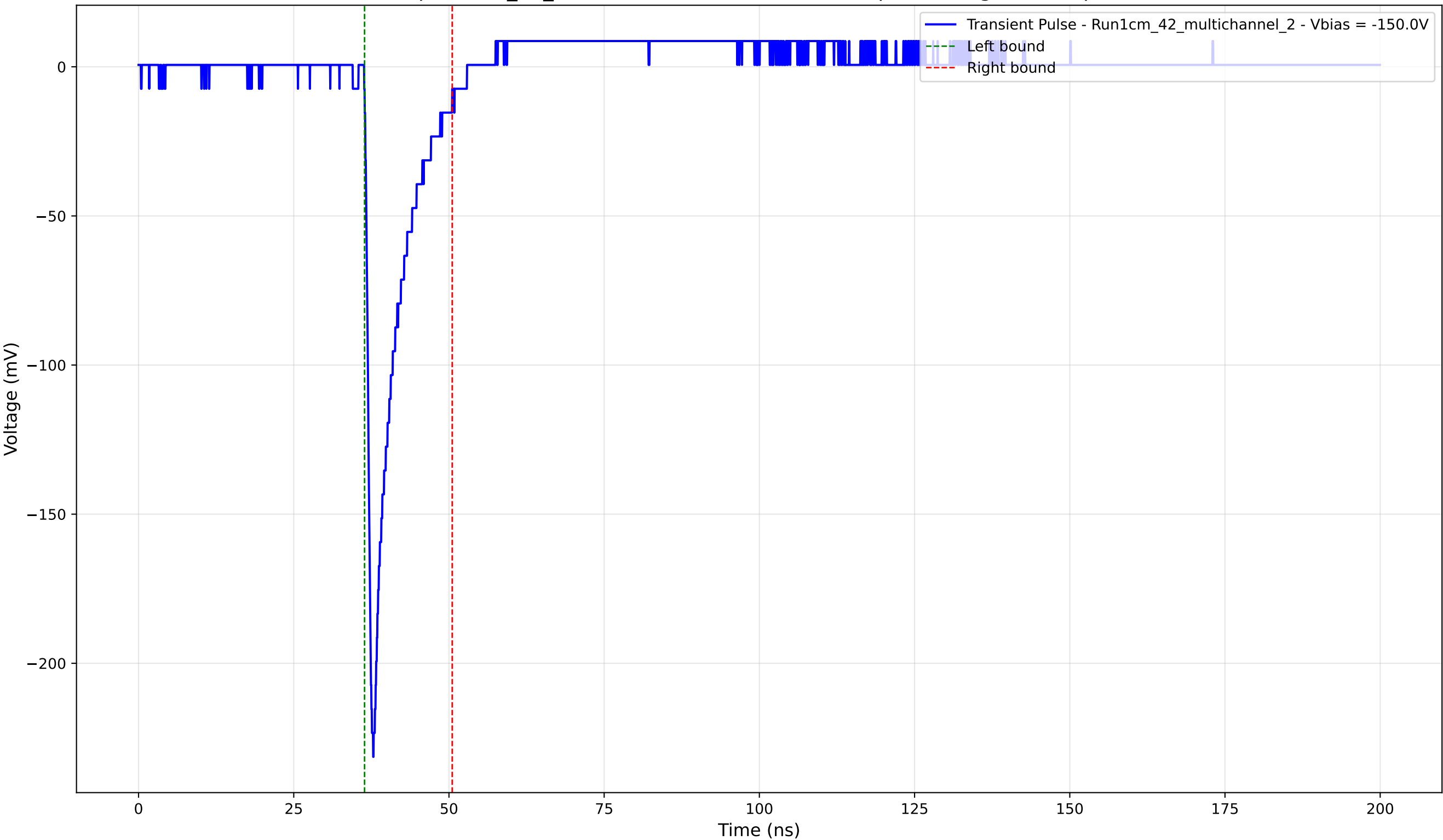
Transient Pulse - Sample: 1cm_42_multichannel - Position: 1570.0 \mu\text{m} - Charge: 21.39 pC - Rise Time: 1.00 ns
