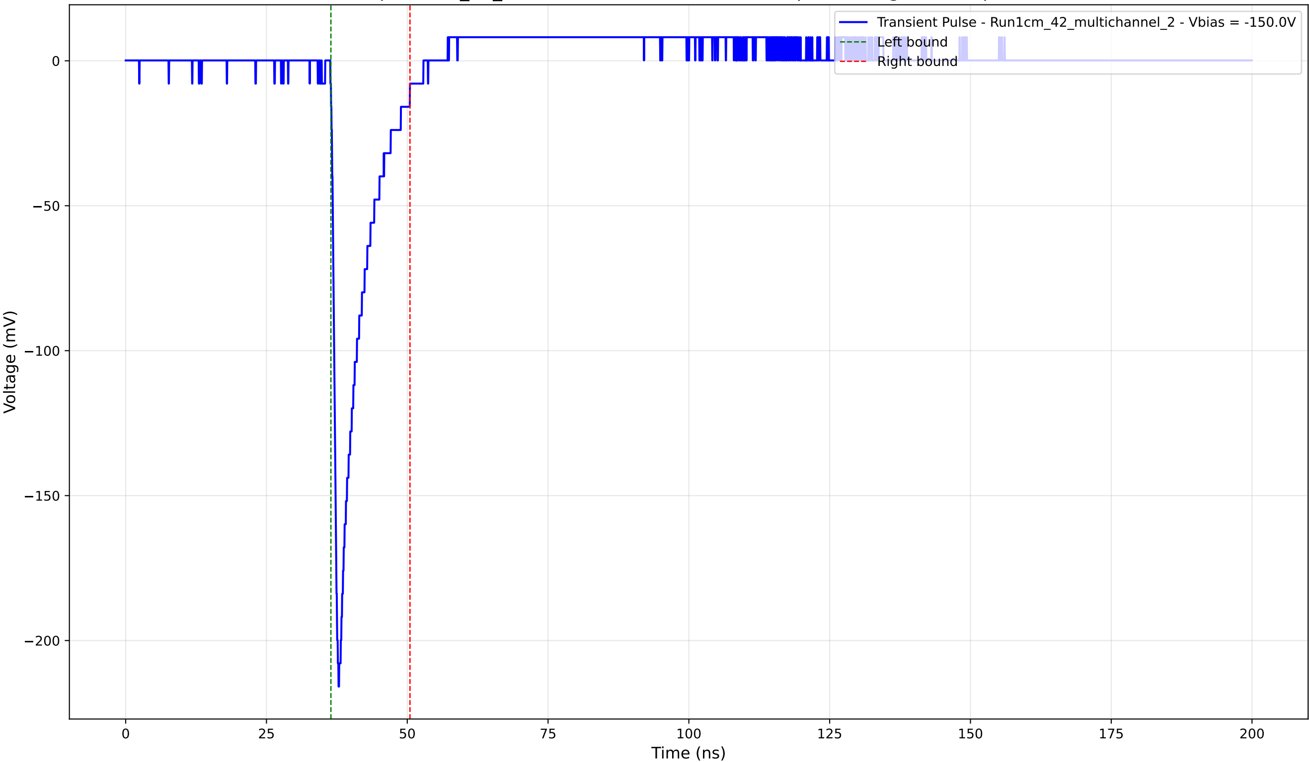
Transient Pulse - Sample: 1cm_42_multichannel - Position: 1500.0 \mu\text{m} - Charge: 21.17 pC - Rise Time: 1.01 ns
