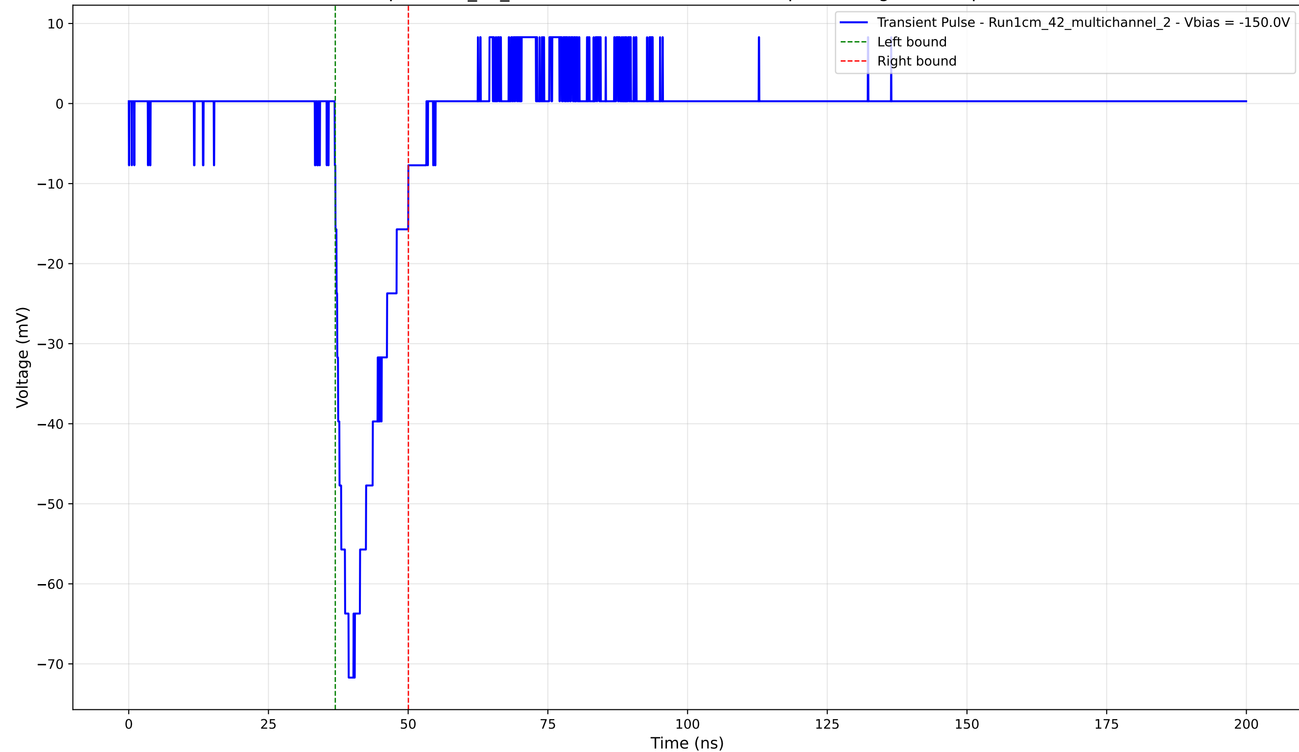
Transient Pulse - Sample: 1cm_42_multichannel - Position: 145.0 \mu\text{m} - Charge: 10.70 pC - Rise Time: 2.48 ns
