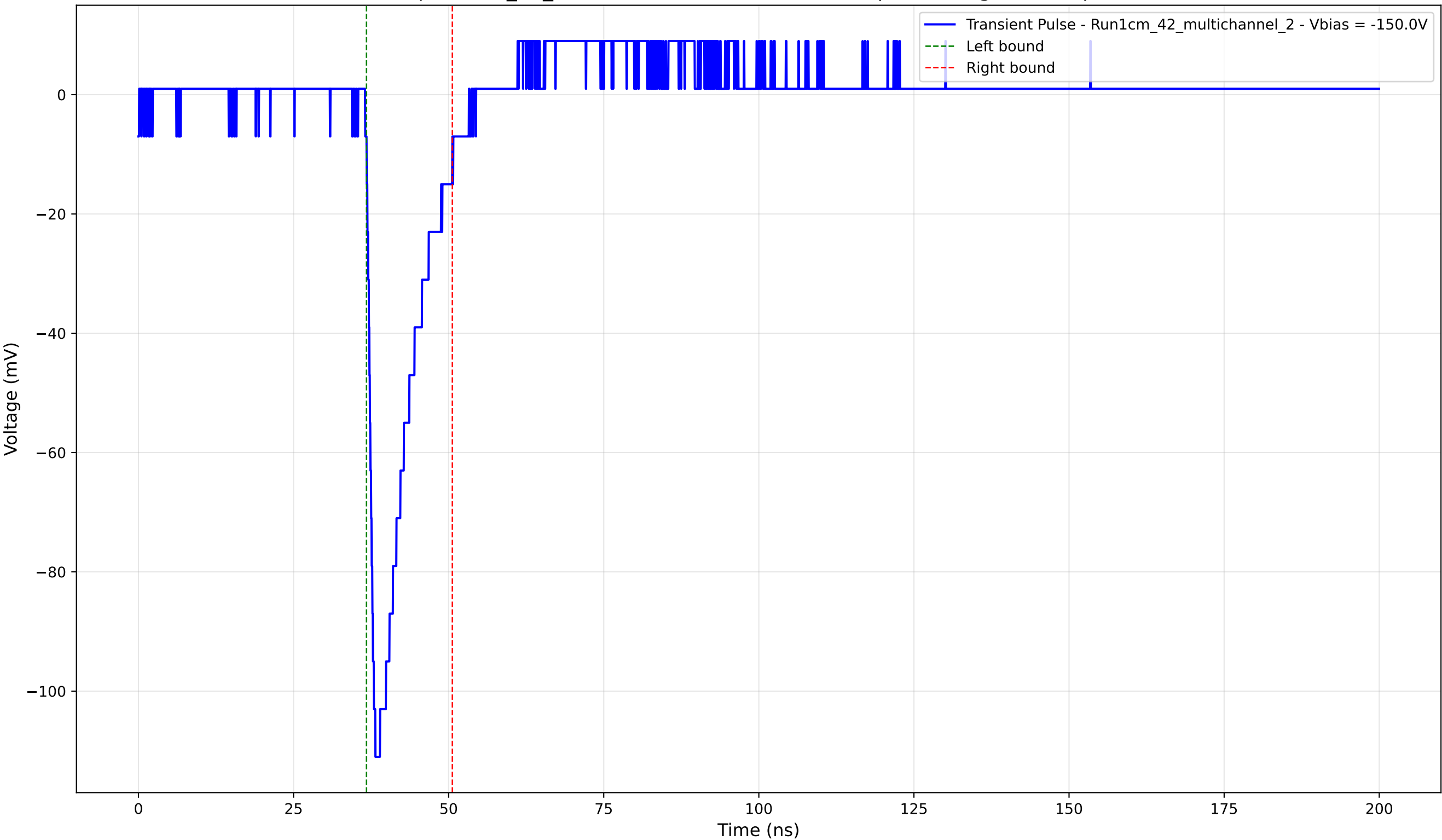
Transient Pulse - Sample: 1cm_42_multichannel - Position: 3645.0 \mu\text{m} - Charge: 14.83 pC - Rise Time: 1.18 ns
