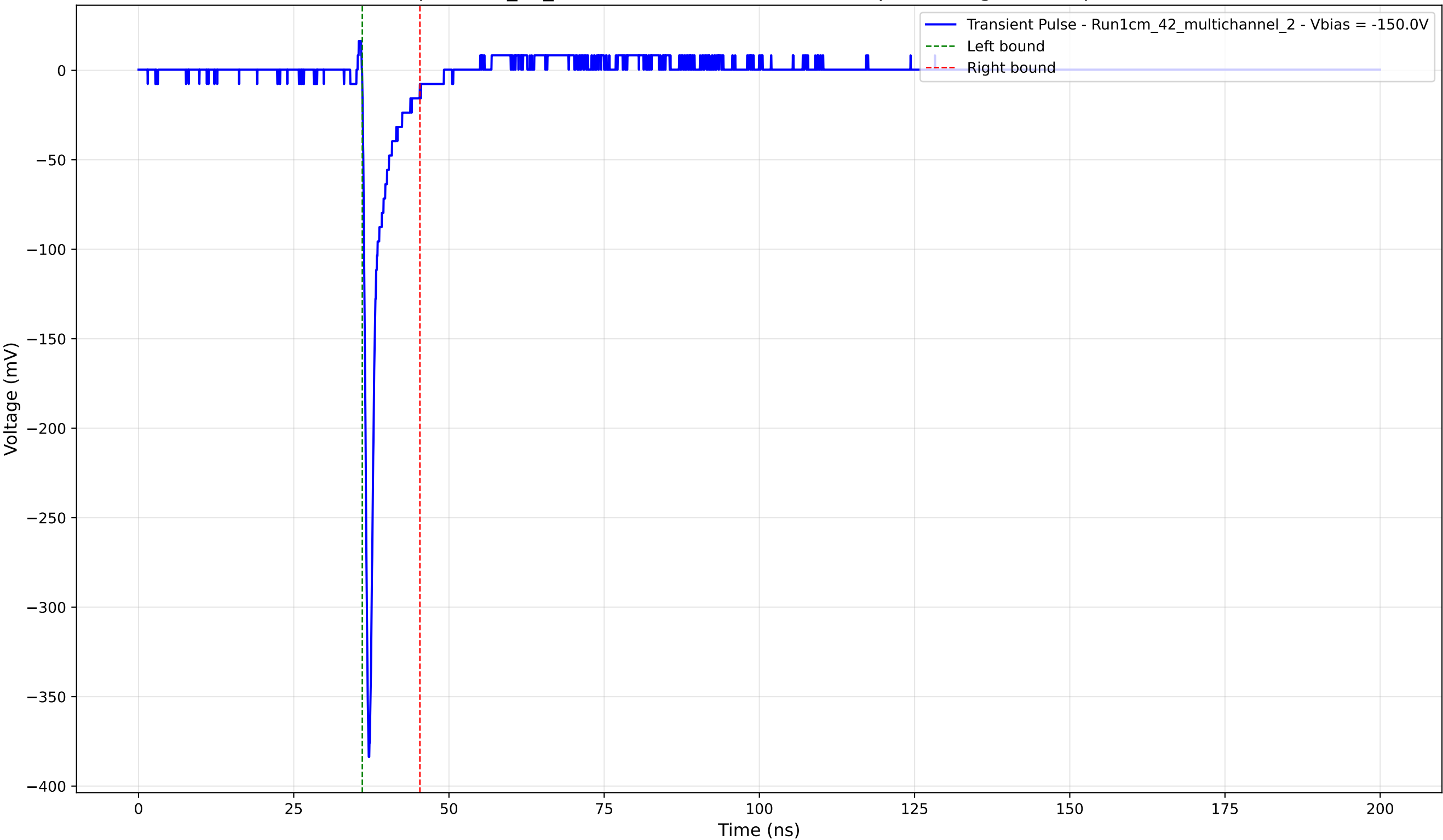
Transient Pulse - Sample: 1cm_42_multichannel - Position: 2315.0 \mu\text{m} - Charge: 16.31 pC - Rise Time: 0.73 ns
