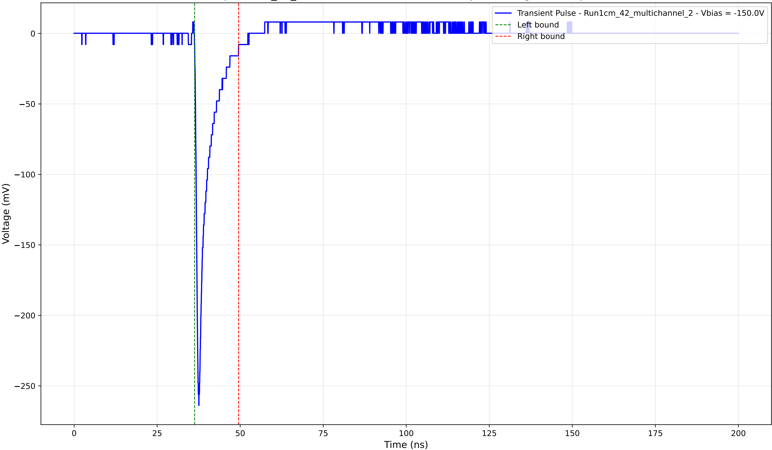
Transient Pulse - Sample: 1cm_42_multichannel - Position: 2950.0 \mu\text{m} - Charge: 19.75 pC - Rise Time: 0.86 ns
