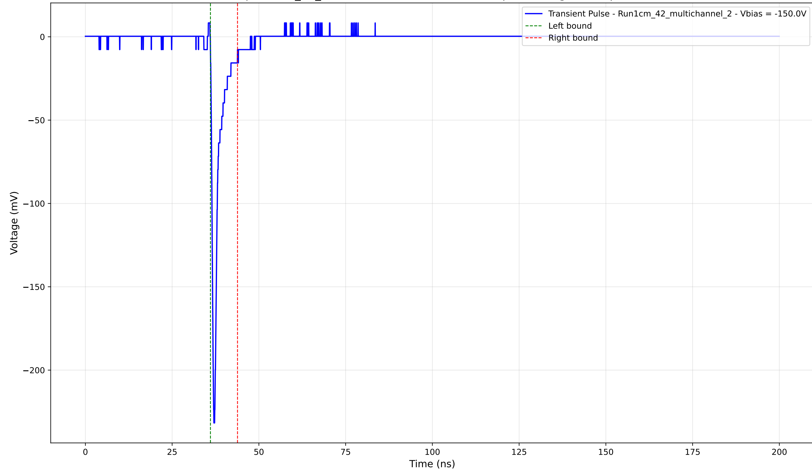
Transient Pulse - Sample: 1cm_42_multichannel - Position: 2325.0 \mu\text{m} - Charge: 9.88 pC - Rise Time: 0.73 ns
