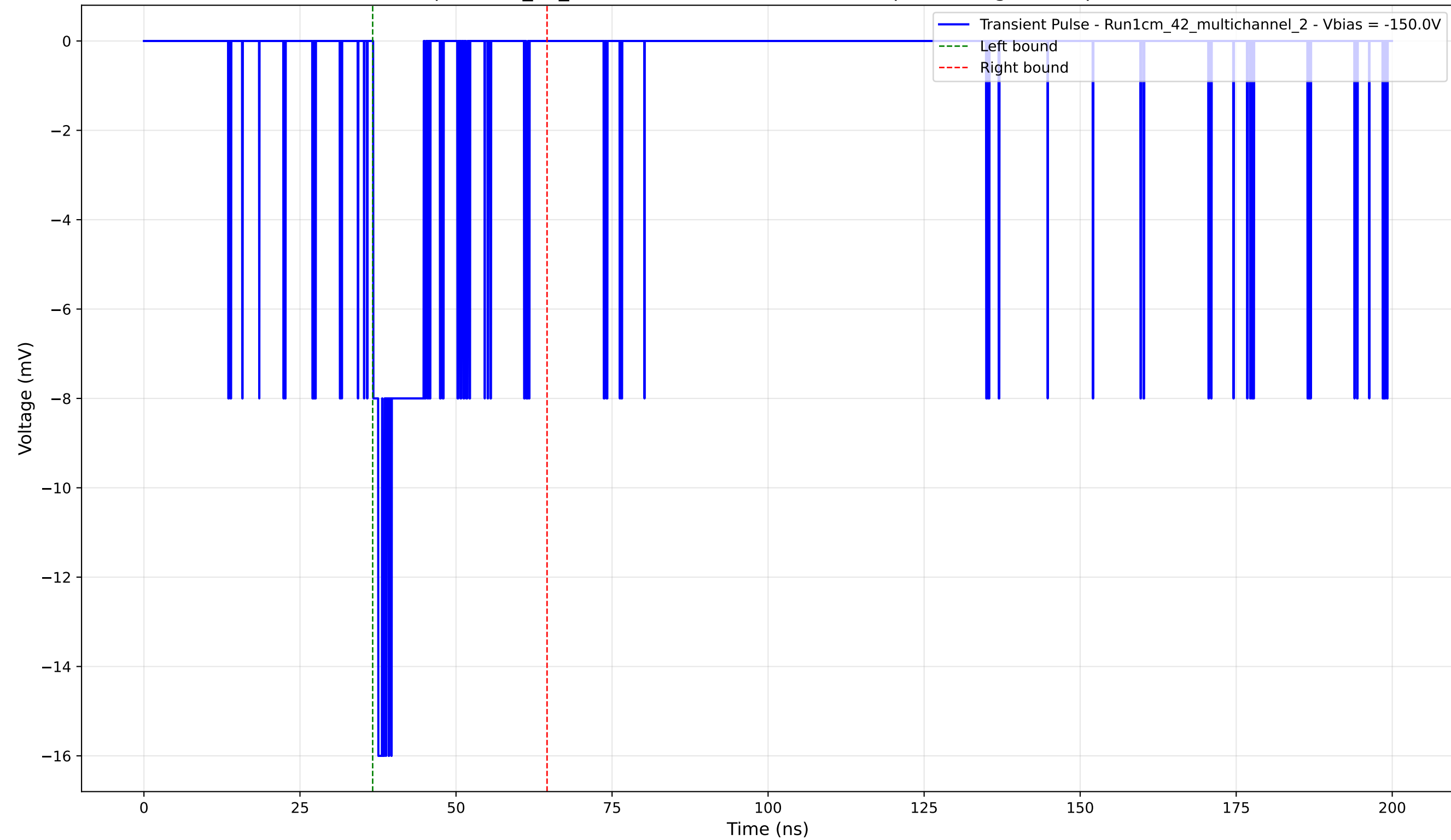
Transient Pulse - Sample: 1cm_42_multichannel - Position: 3365.0 \mu\text{m} - Charge: 1.85 pC - Rise Time: 0.83 ns
