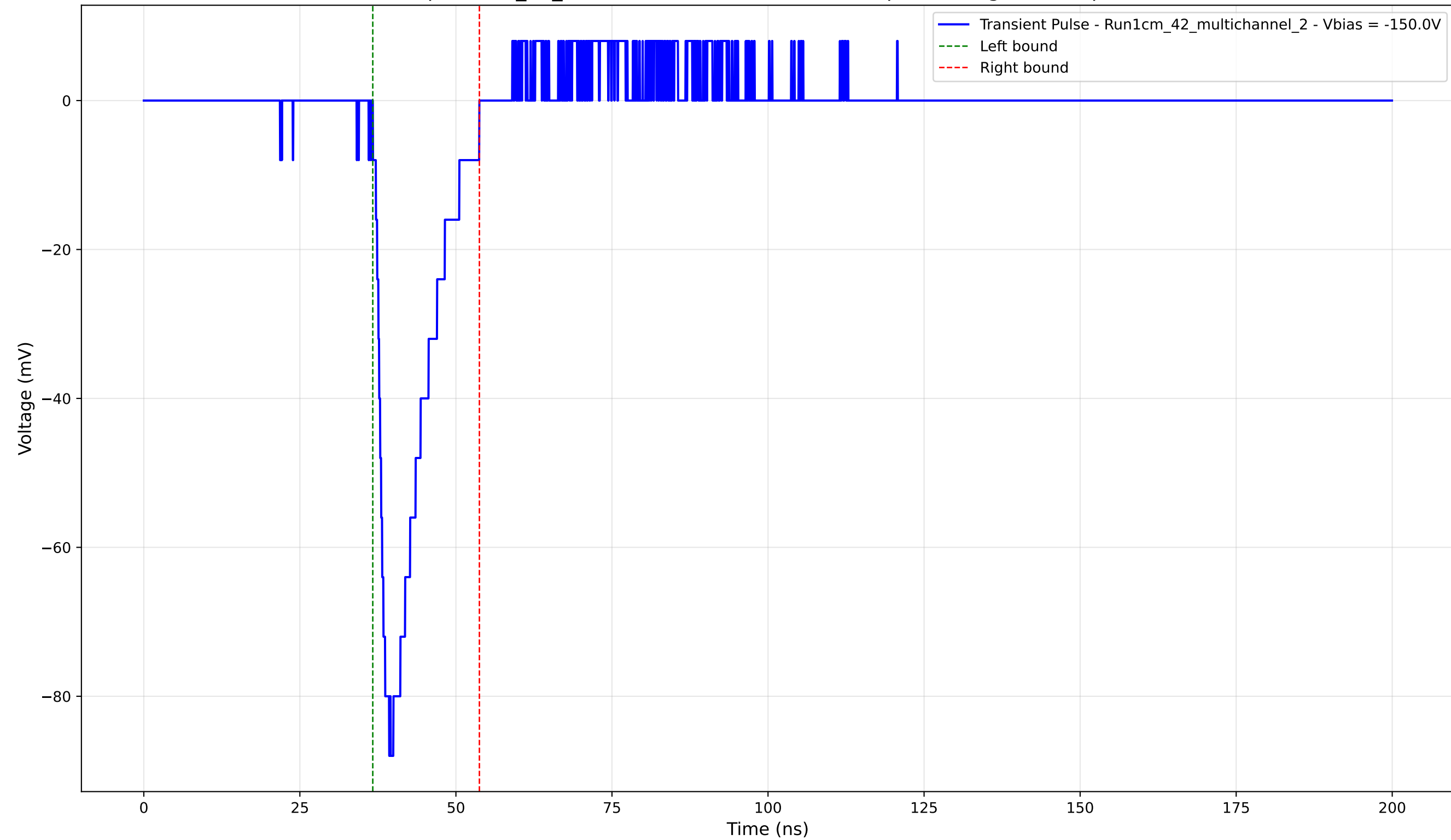
Transient Pulse - Sample: 1cm_42_multichannel - Position: 4210.0 \mu\text{m} - Charge: 13.04 pC - Rise Time: 1.52 ns
