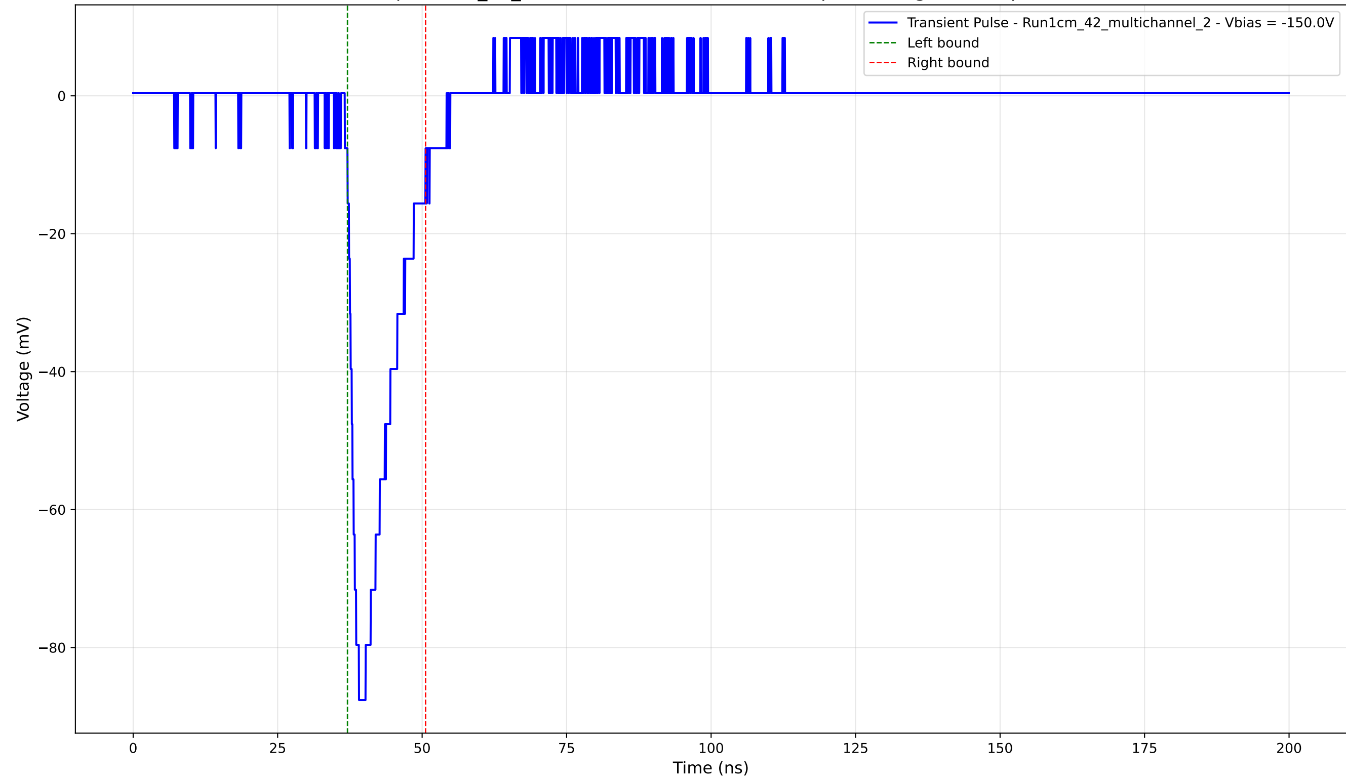
Transient Pulse - Sample: 1cm_42_multichannel - Position: 4165.0 \mu\text{m} - Charge: 12.68 pC - Rise Time: 1.51 ns
