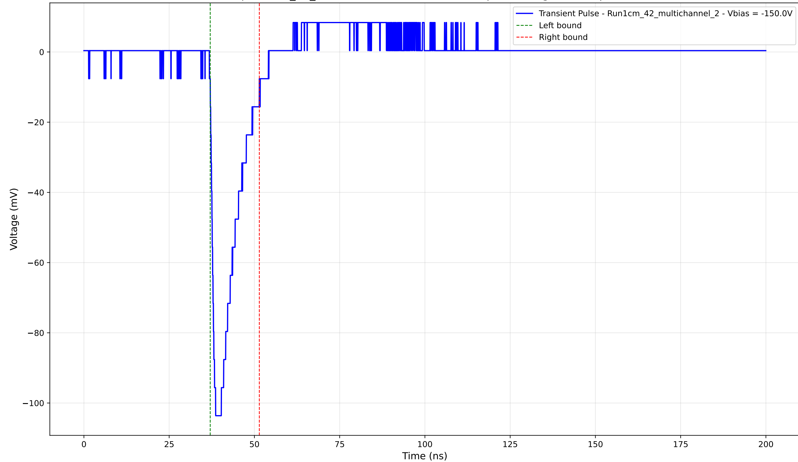
Transient Pulse - Sample: 1cm_42_multichannel - Position: 705.0 \mu\text{m} - Charge: 15.52 pC - Rise Time: 1.27 ns
