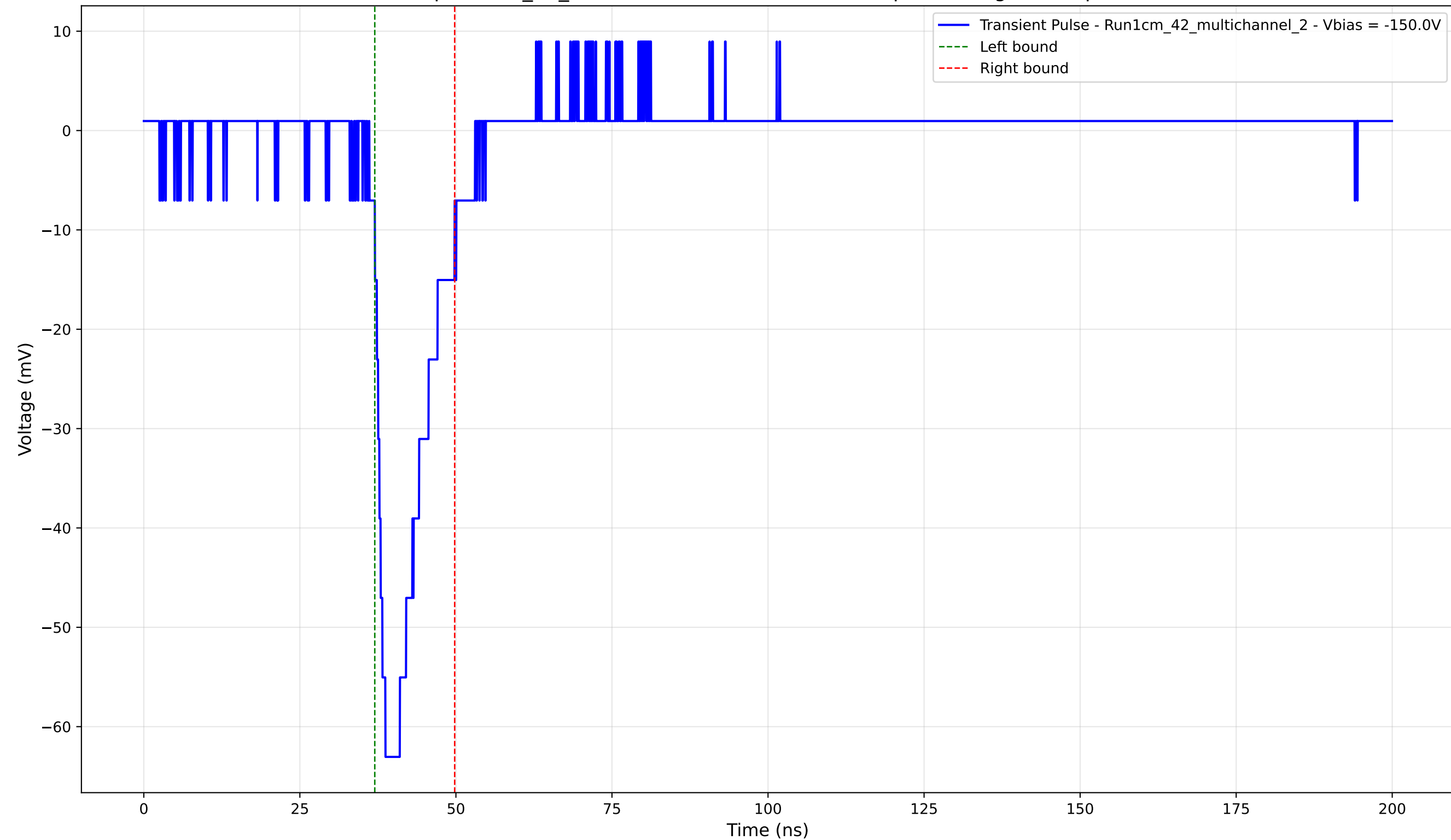
Transient Pulse - Sample: 1cm_42_multichannel - Position: 4765.0 \mu\text{m} - Charge: 9.52 pC - Rise Time: 2.56 ns
