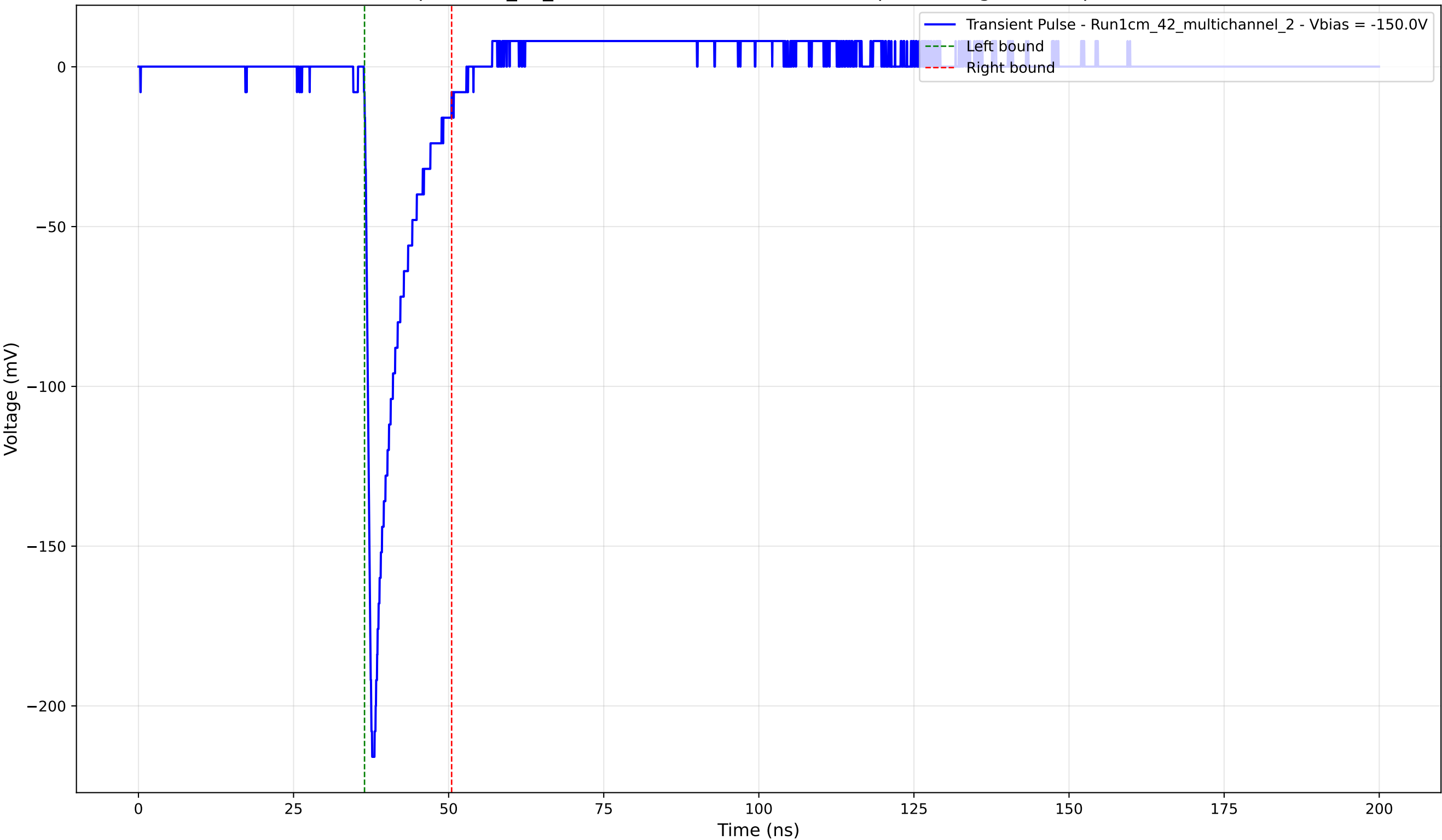
Transient Pulse - Sample: 1cm_42_multichannel - Position: 1530.0 \mu\text{m} - Charge: 21.26 pC - Rise Time: 0.94 ns
