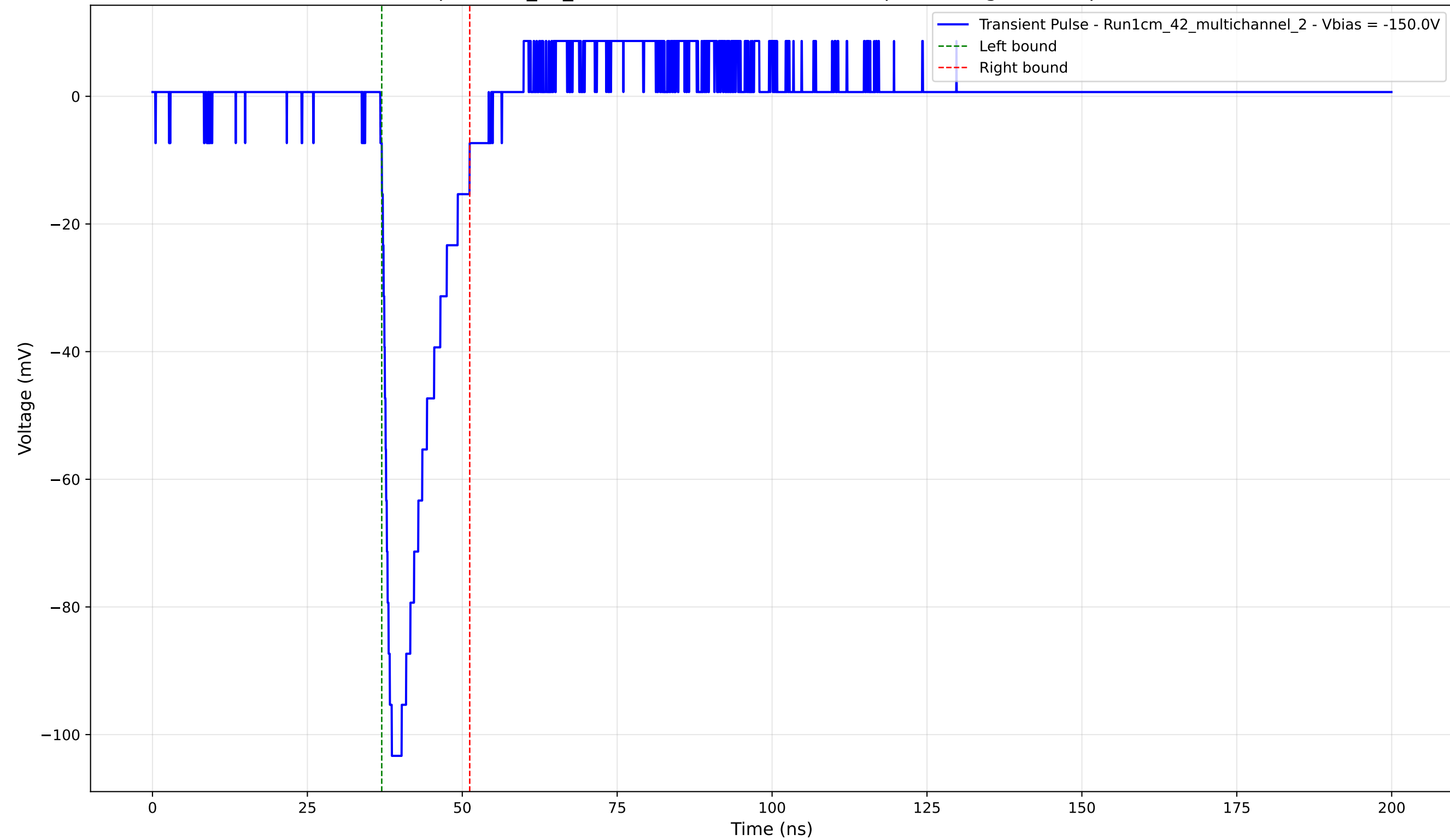
Transient Pulse - Sample: 1cm_42_multichannel - Position: 715.0 \mu\text{m} - Charge: 15.37 pC - Rise Time: 1.30 ns
