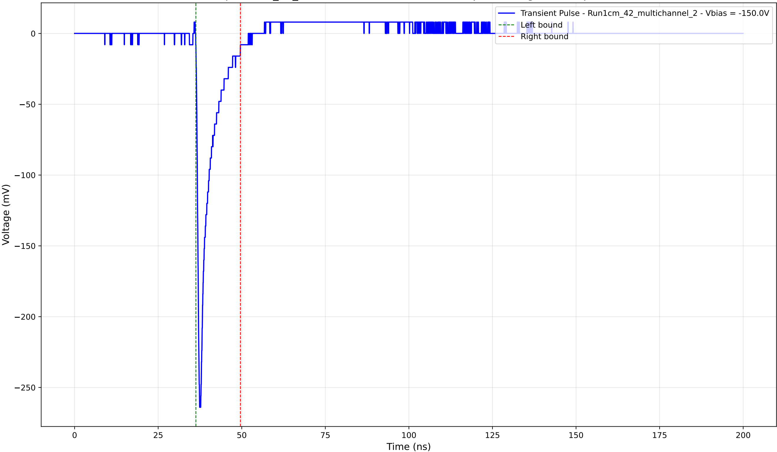
Transient Pulse - Sample: 1cm_42_multichannel - Position: 2955.0 \mu\text{m} - Charge: 20.46 pC - Rise Time: 0.82 ns
