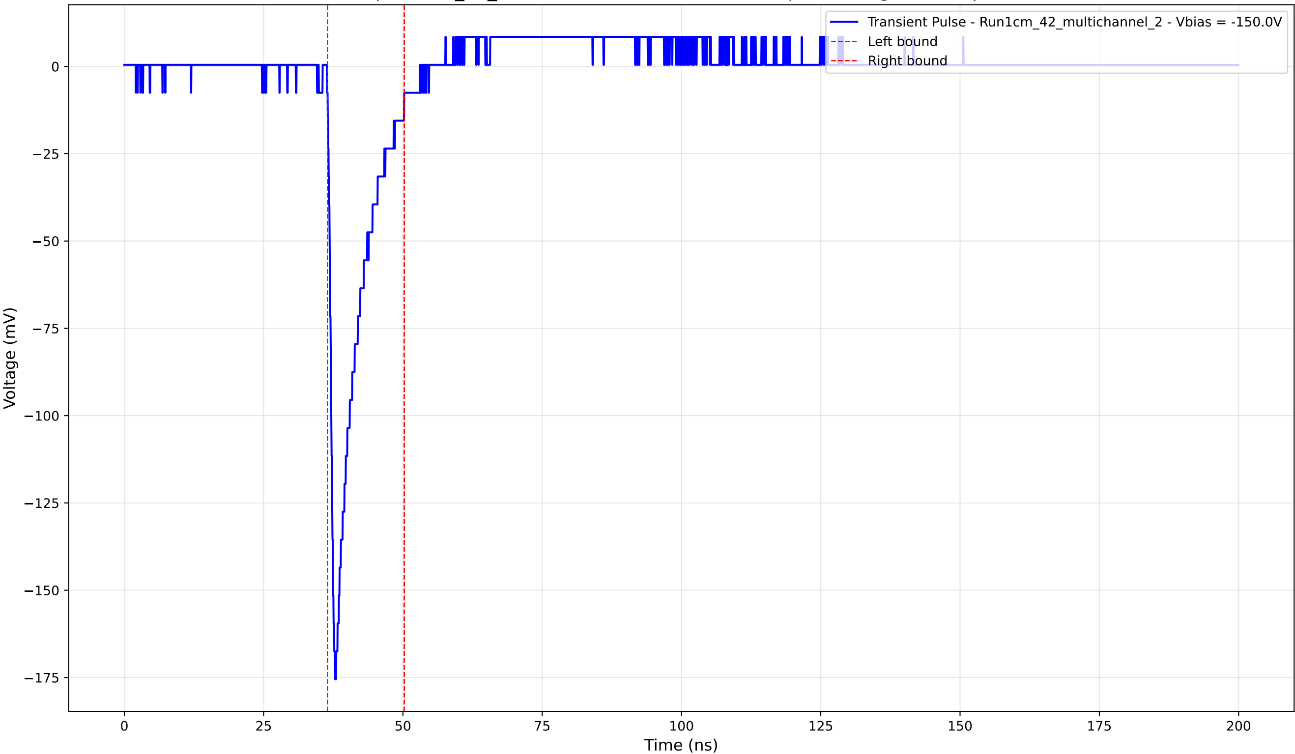
Transient Pulse - Sample: 1cm_42_multichannel - Position: 3285.0 \mu\text{m} - Charge: 18.14 pC - Rise Time: 0.99 ns
