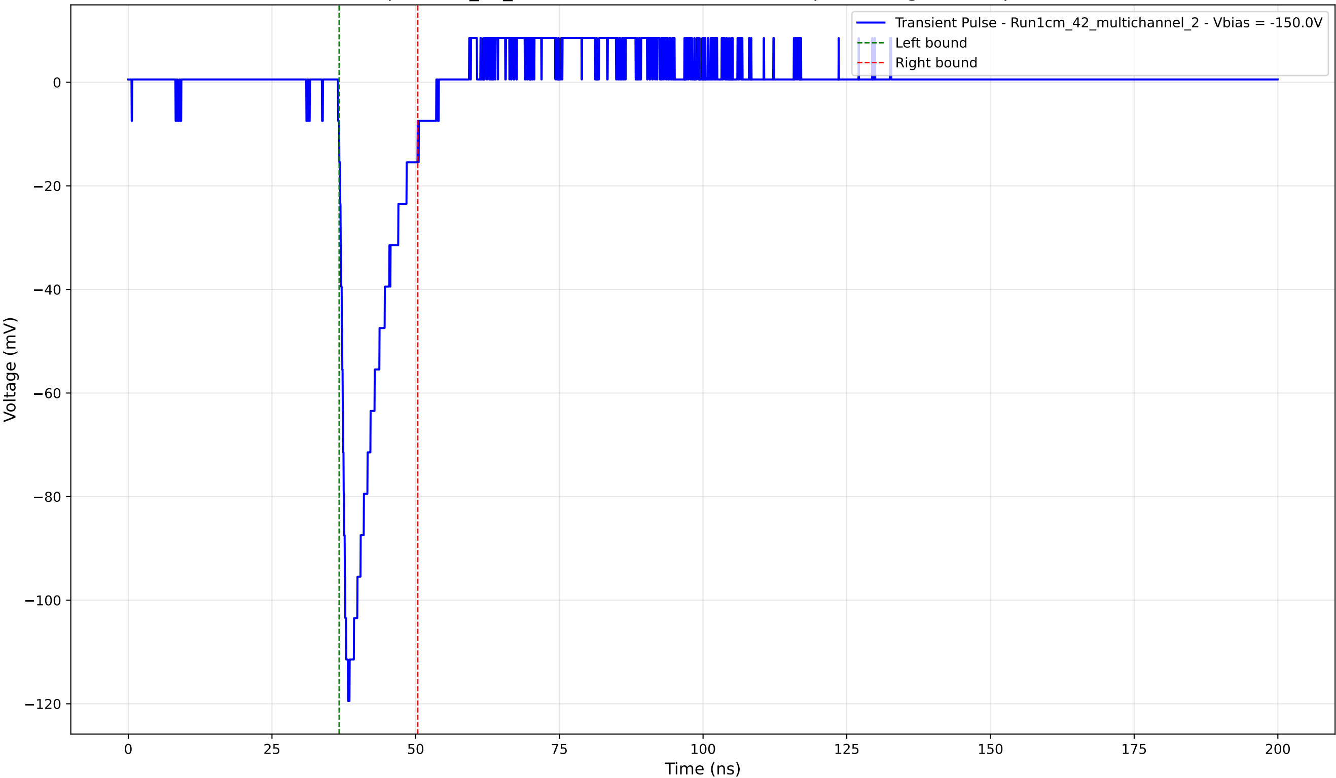
Transient Pulse - Sample: 1cm_42_multichannel - Position: 3580.0 \mu\text{m} - Charge: 15.17 pC - Rise Time: 1.22 ns
