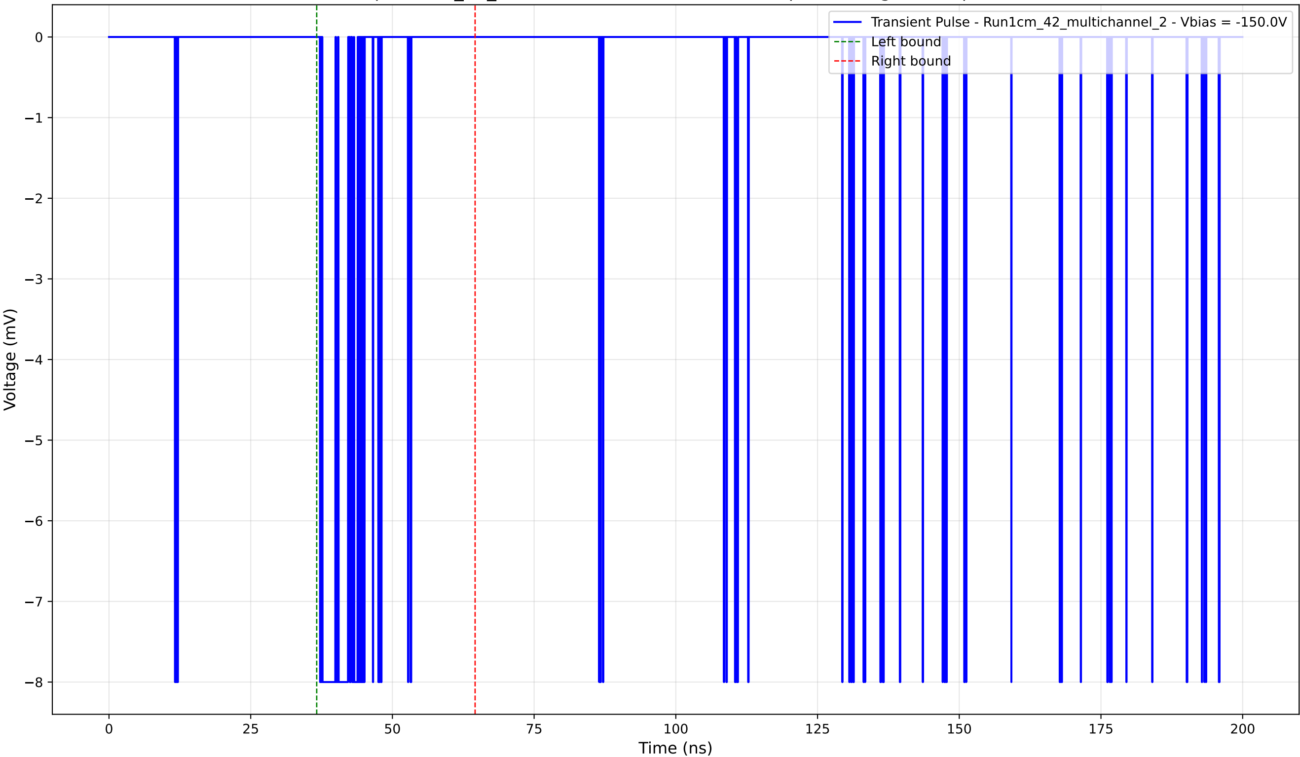
Transient Pulse - Sample: 1cm_42_multichannel - Position: 4885.0 \mu\text{m} - Charge: 1.08 pC - Rise Time: 0.04 ns
