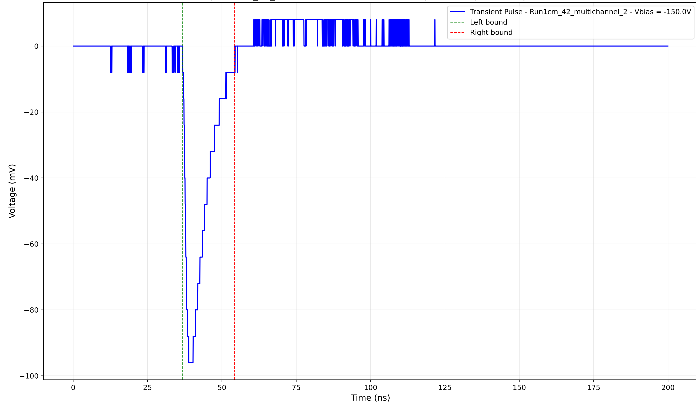
Transient Pulse - Sample: 1cm_42_multichannel - Position: 560.0 \mu\text{m} - Charge: 15.04 pC - Rise Time: 1.39 ns
