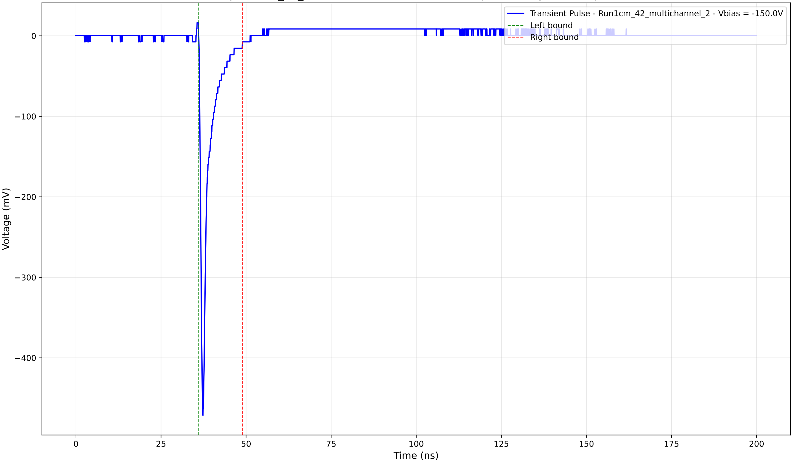
Transient Pulse - Sample: 1cm_42_multichannel - Position: 2075.0 \mu\text{m} - Charge: 25.72 pC - Rise Time: 0.77 ns
