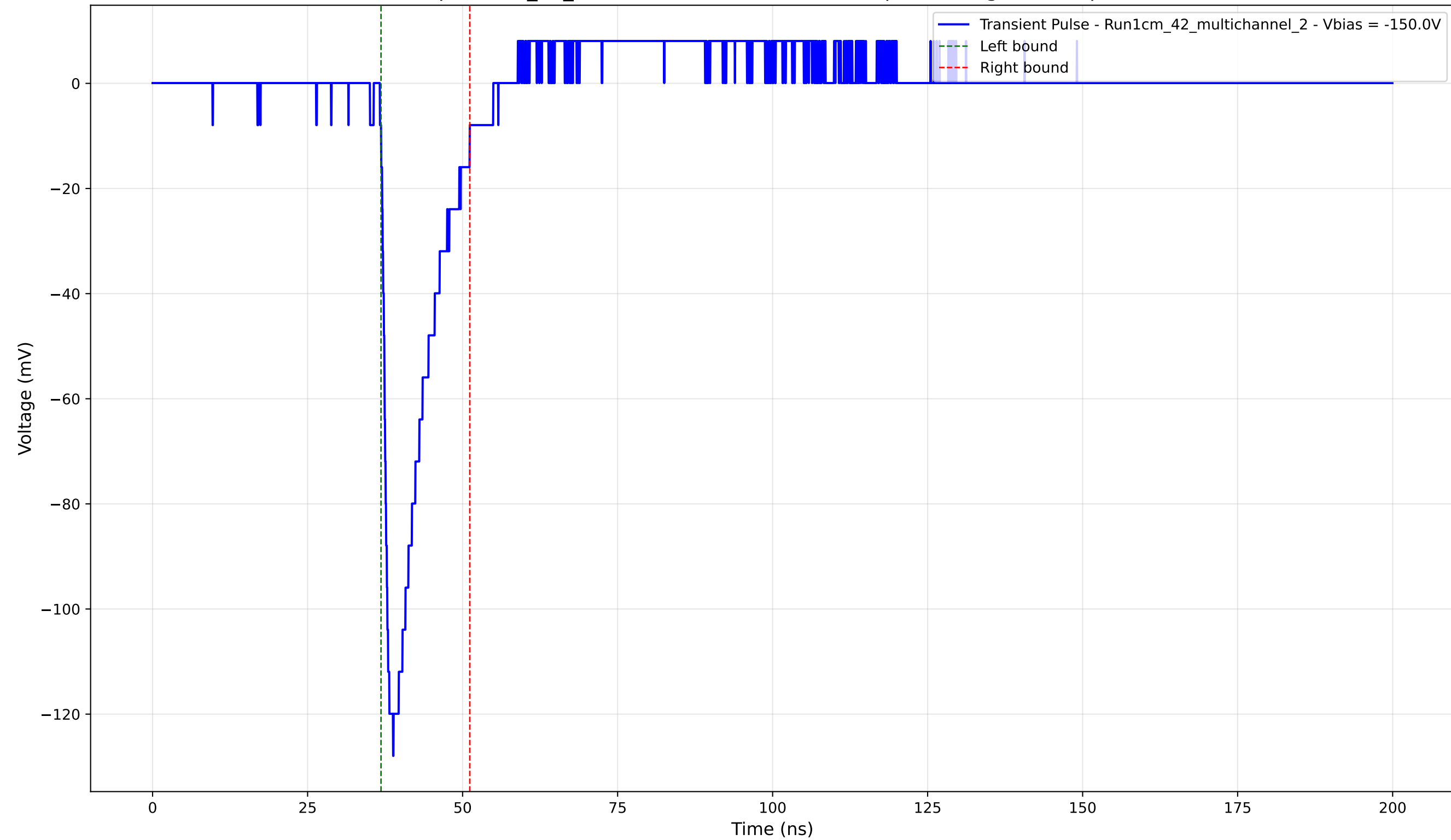
Transient Pulse - Sample: 1cm_42_multichannel - Position: 995.0 \mu\text{m} - Charge: 17.11 pC - Rise Time: 1.34 ns
