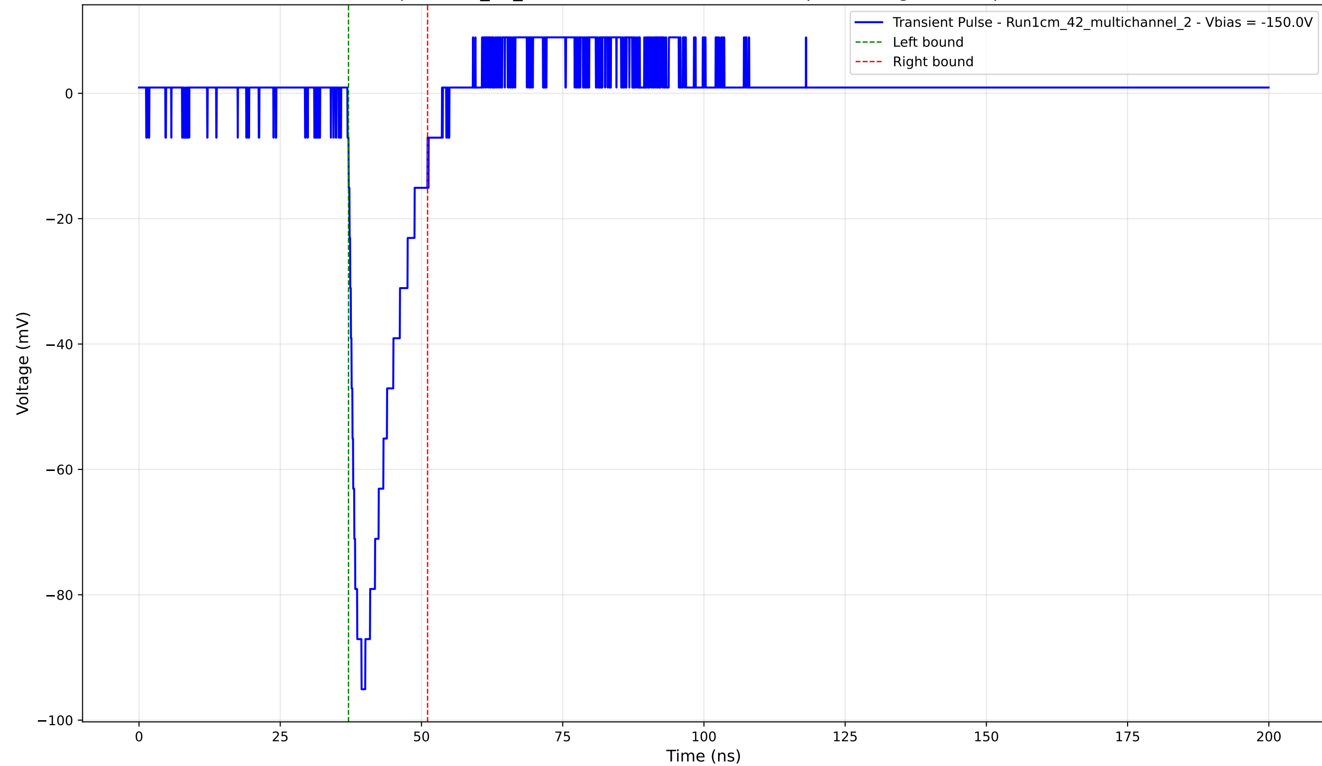
Transient Pulse - Sample: 1cm_42_multichannel - Position: 470.0 \mu\text{m} - Charge: 13.82 pC - Rise Time: 1.55 ns
