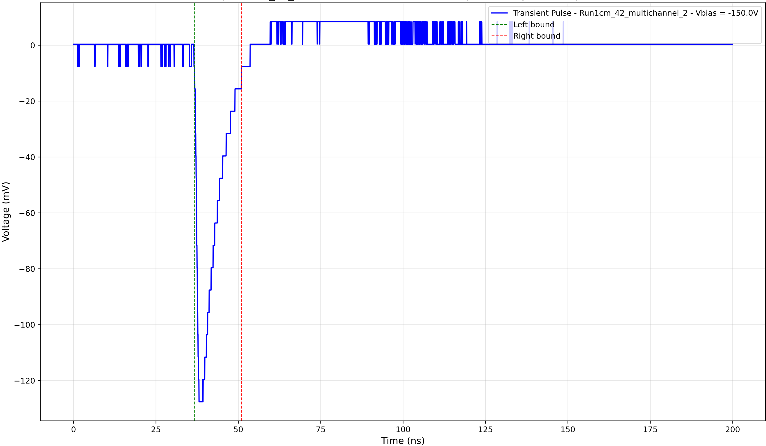
Transient Pulse - Sample: 1cm_42_multichannel - Position: 1090.0 \mu\text{m} - Charge: 17.21 pC - Rise Time: 1.13 ns
