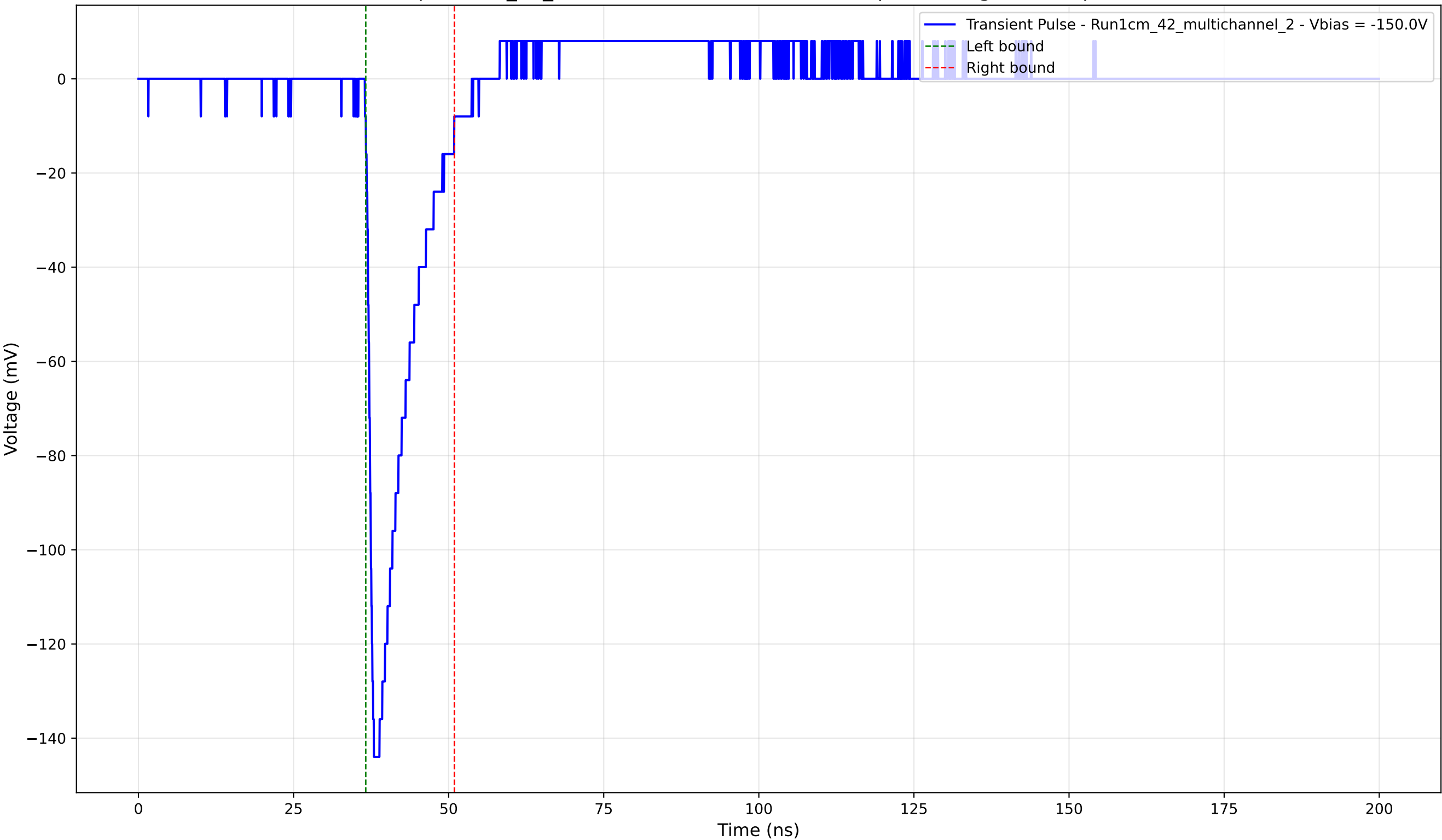
Transient Pulse - Sample: 1cm_42_multichannel - Position: 1190.0 \mu\text{m} - Charge: 18.54 pC - Rise Time: 1.17 ns
