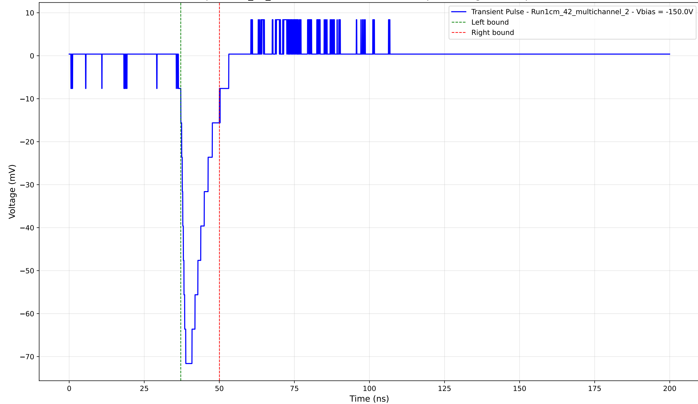
Transient Pulse - Sample: 1cm_42_multichannel - Position: 4545.0 \mu\text{m} - Charge: 10.72 pC - Rise Time: 2.44 ns
