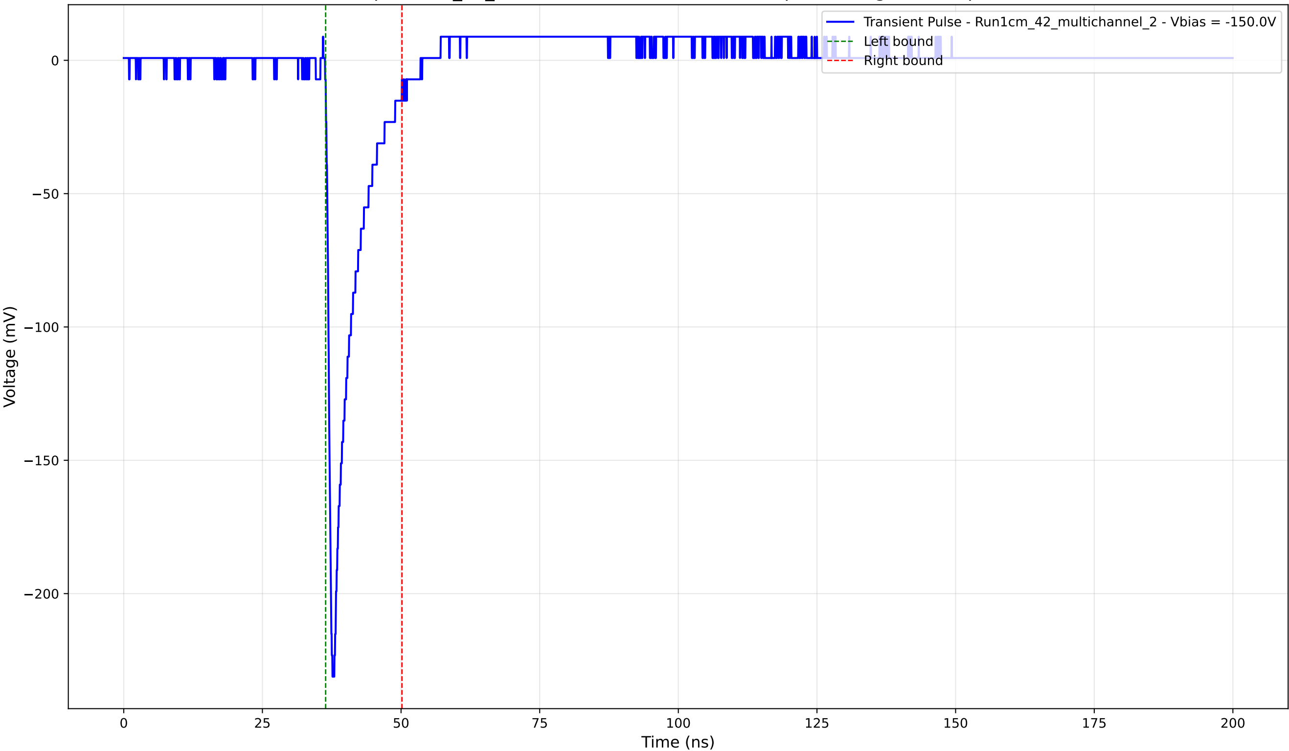
Transient Pulse - Sample: 1cm_42_multichannel - Position: 1585.0 \mu\text{m} - Charge: 21.49 pC - Rise Time: 0.96 ns
