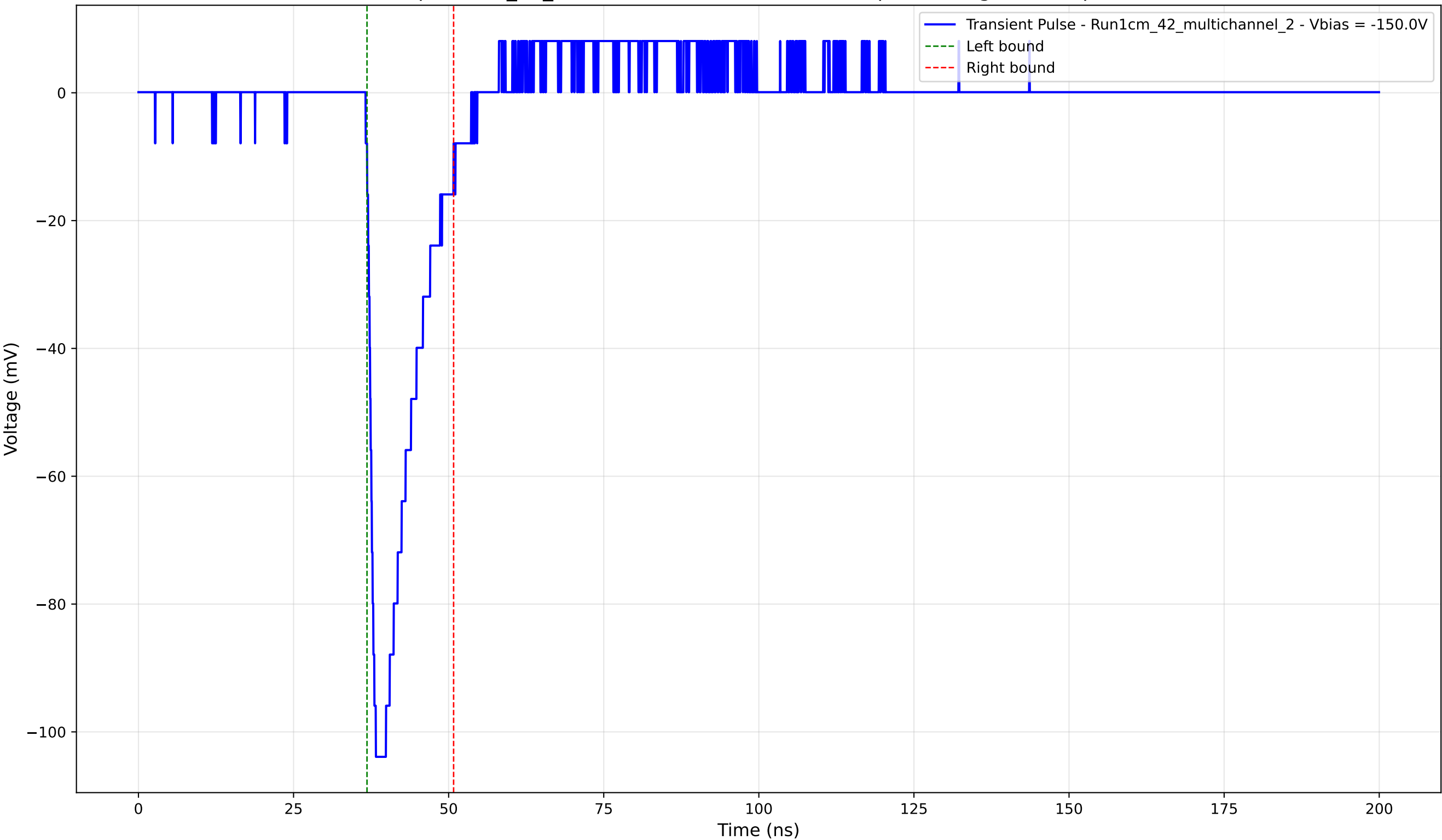
Transient Pulse - Sample: 1cm_42_multichannel - Position: 3750.0 \mu\text{m} - Charge: 14.98 pC - Rise Time: 1.19 ns
