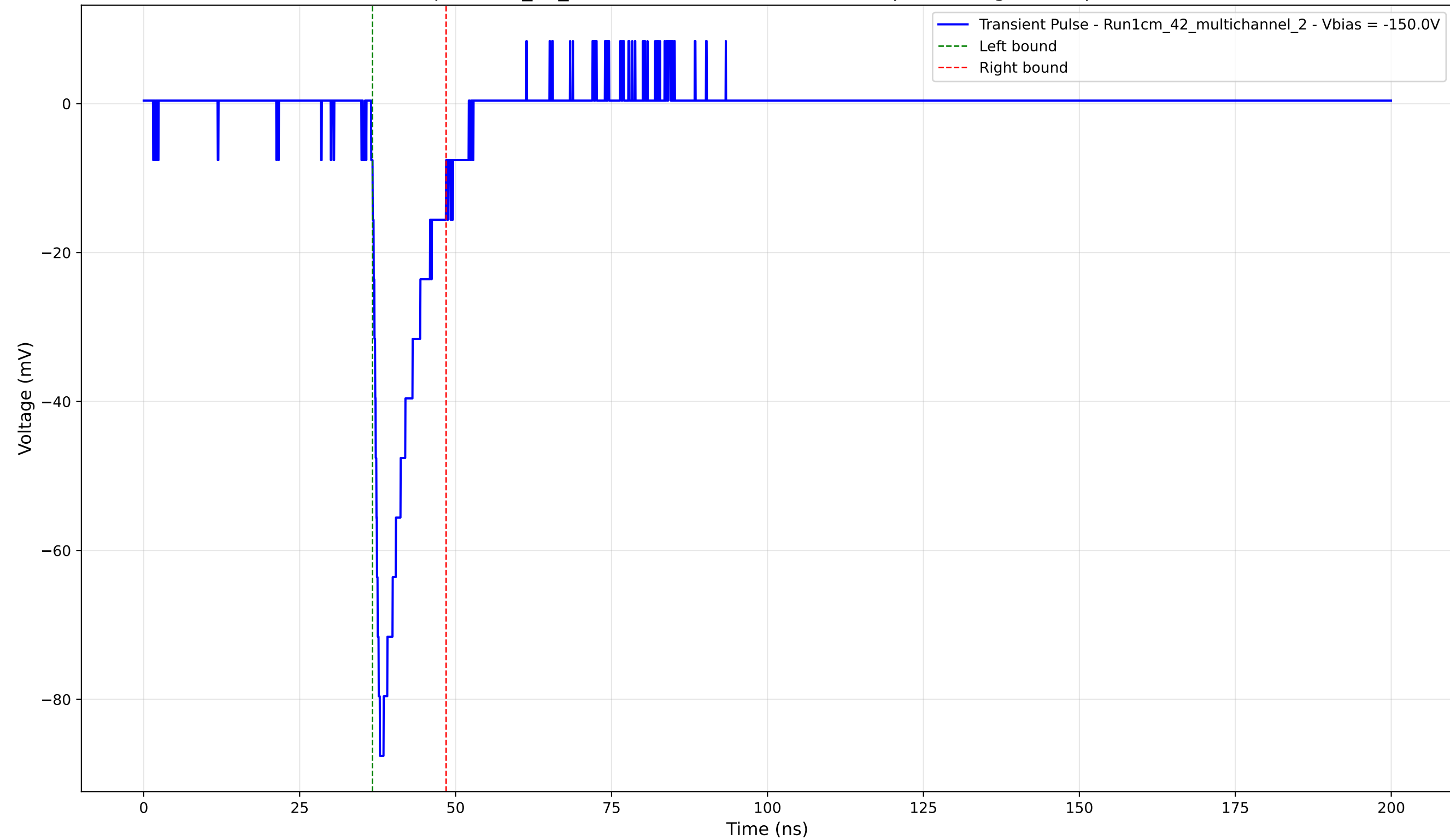
Transient Pulse - Sample: 1cm_42_multichannel - Position: 1305.0 \mu\text{m} - Charge: 9.84 pC - Rise Time: 0.99 ns
