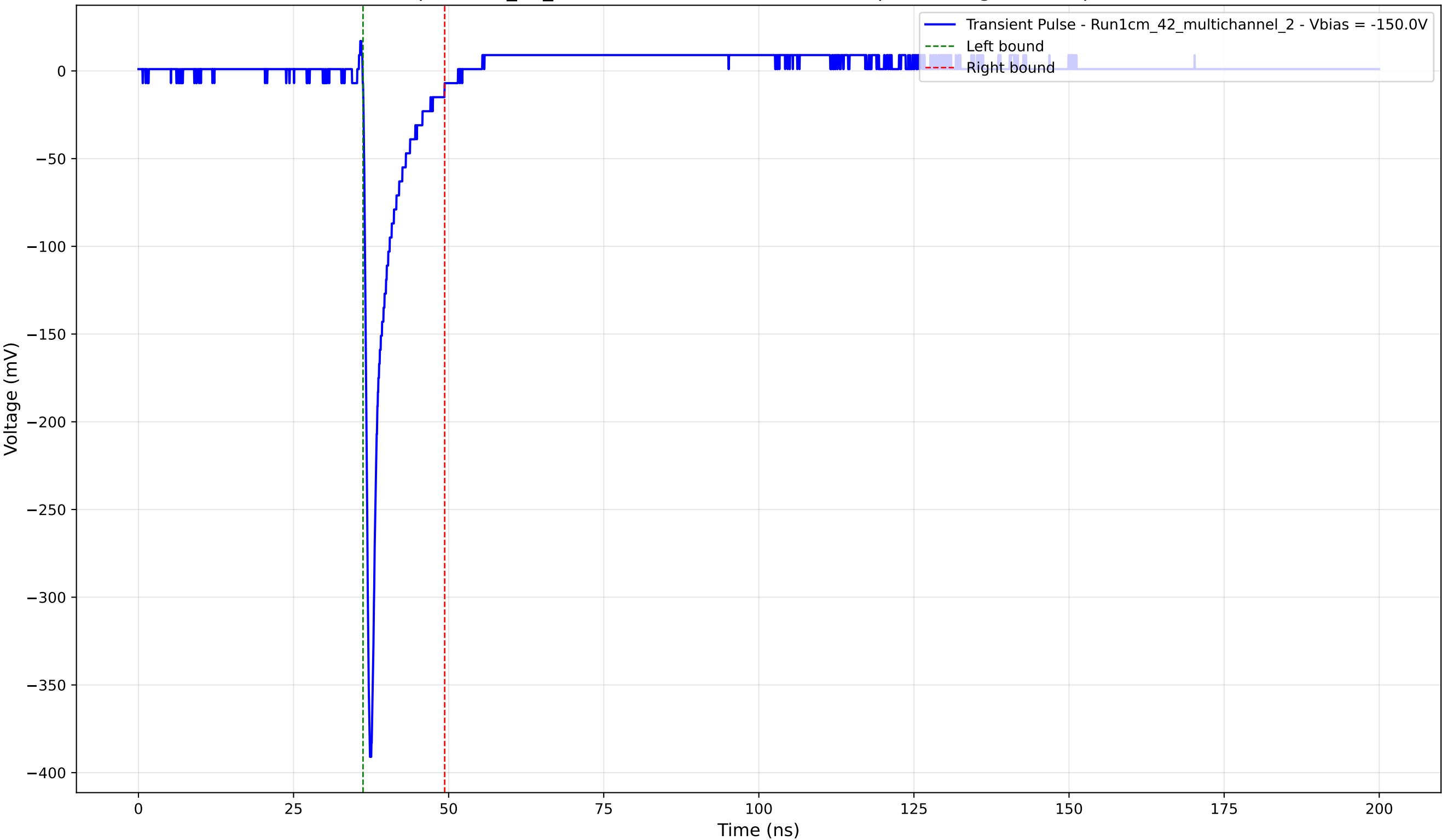
Transient Pulse - Sample: 1cm_42_multichannel - Position: 1965.0 \mu\text{m} - Charge: 24.49 pC - Rise Time: 0.80 ns
