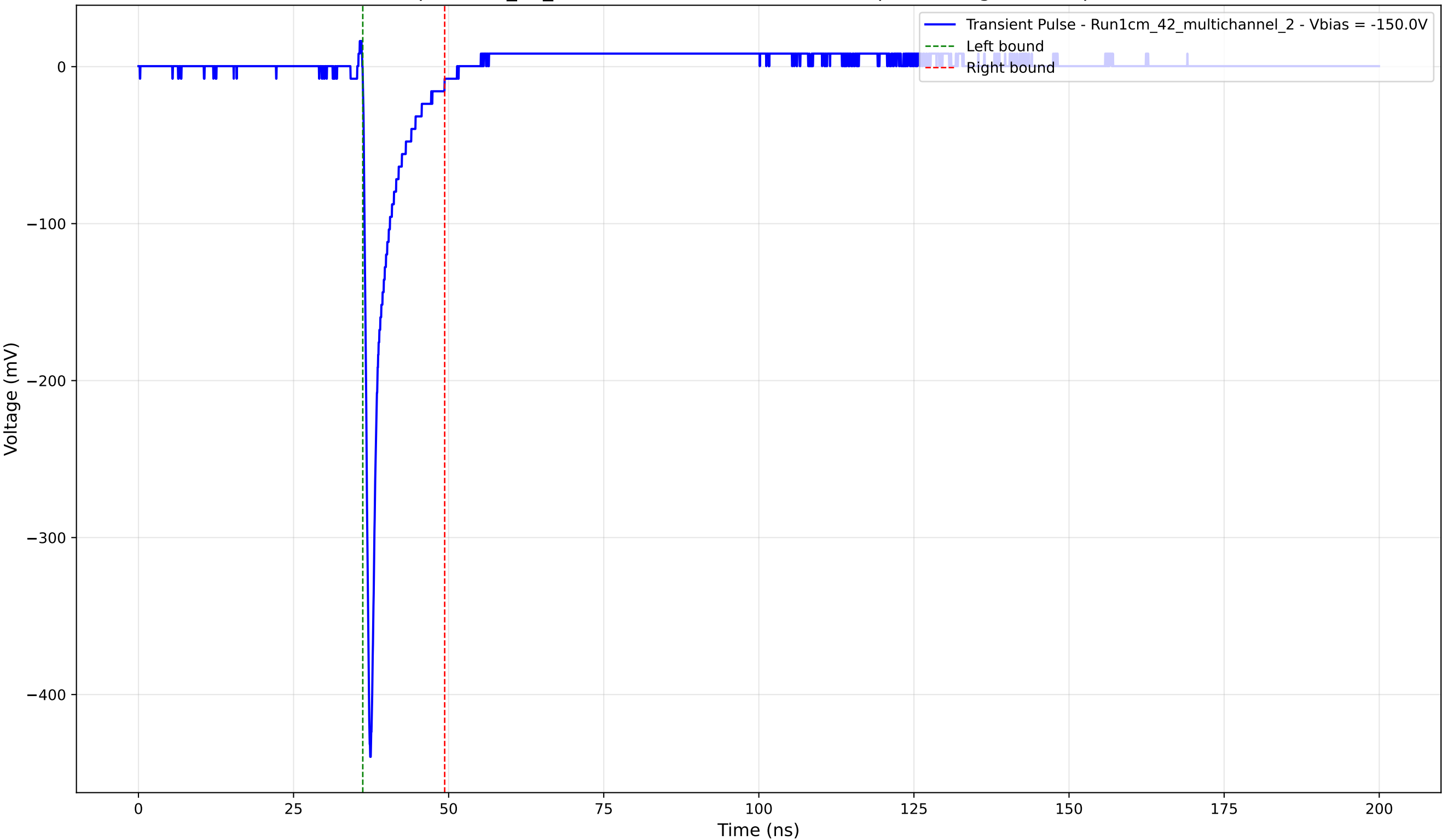
Transient Pulse - Sample: 1cm_42_multichannel - Position: 2010.0 \mu\text{m} - Charge: 25.98 pC - Rise Time: 0.79 ns
