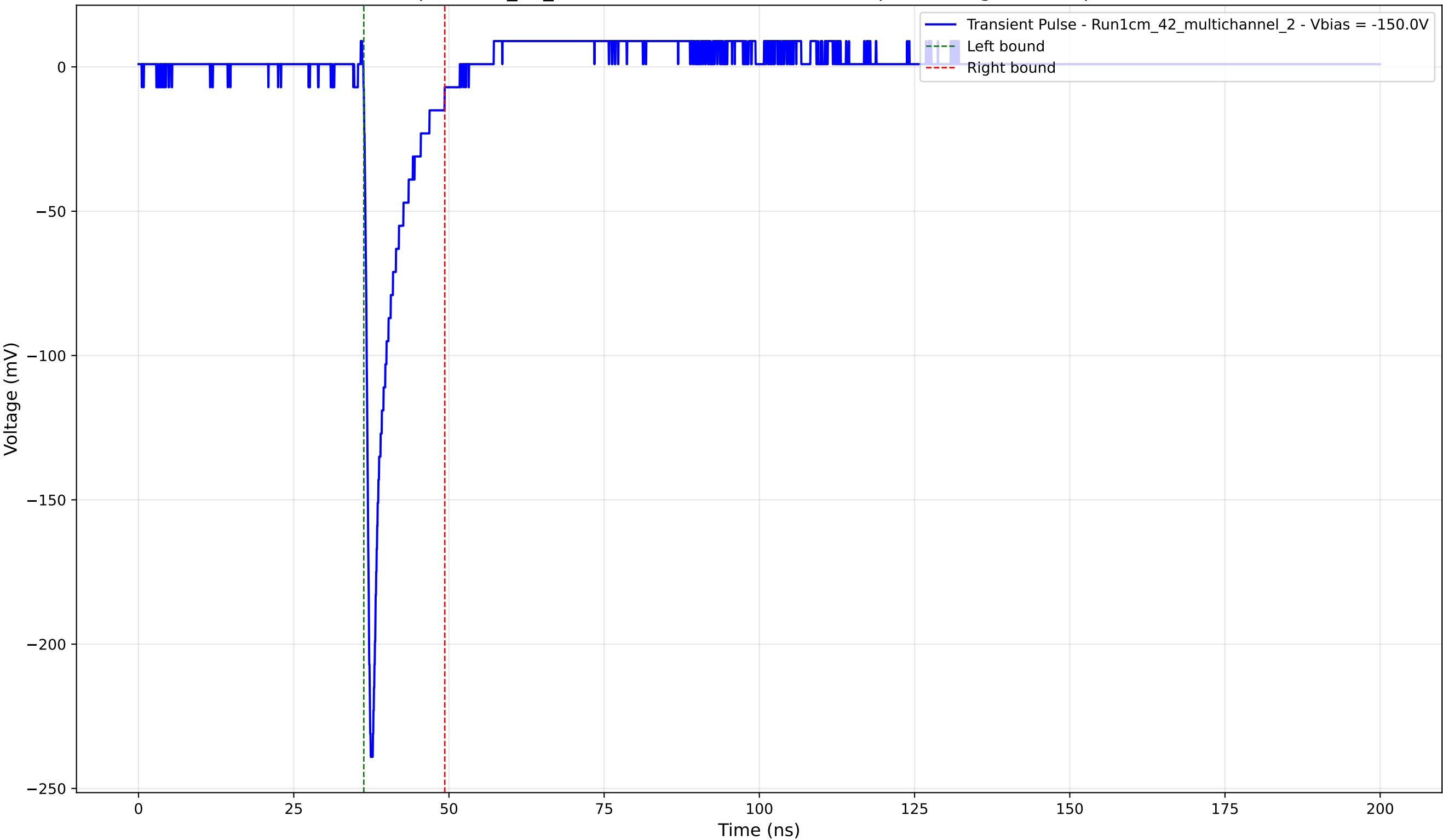
Transient Pulse - Sample: 1cm_42_multichannel - Position: 2945.0 \mu\text{m} - Charge: 18.36 pC - Rise Time: 0.84 ns
