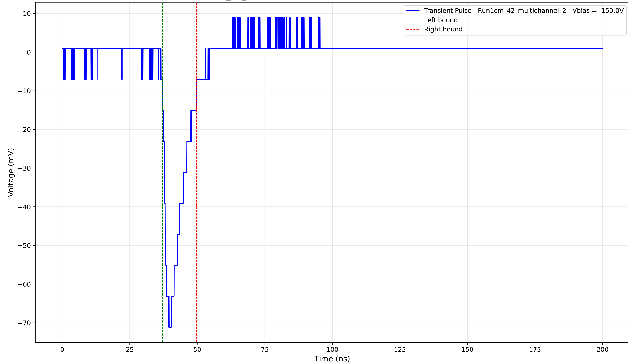
Transient Pulse - Sample: 1cm_42_multichannel - Position: 4480.0 \mu\text{m} - Charge: 9.98 pC - Rise Time: 2.24 ns
