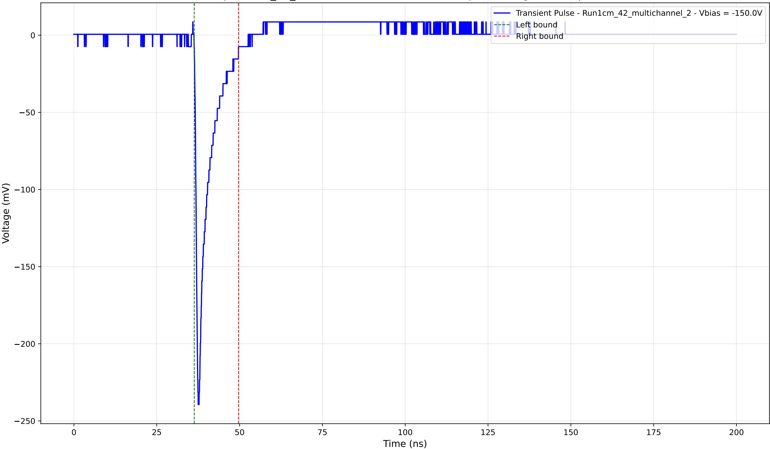
Transient Pulse - Sample: 1cm_42_multichannel - Position: 3040.0 \mu\text{m} - Charge: 19.84 pC - Rise Time: 0.92 ns
