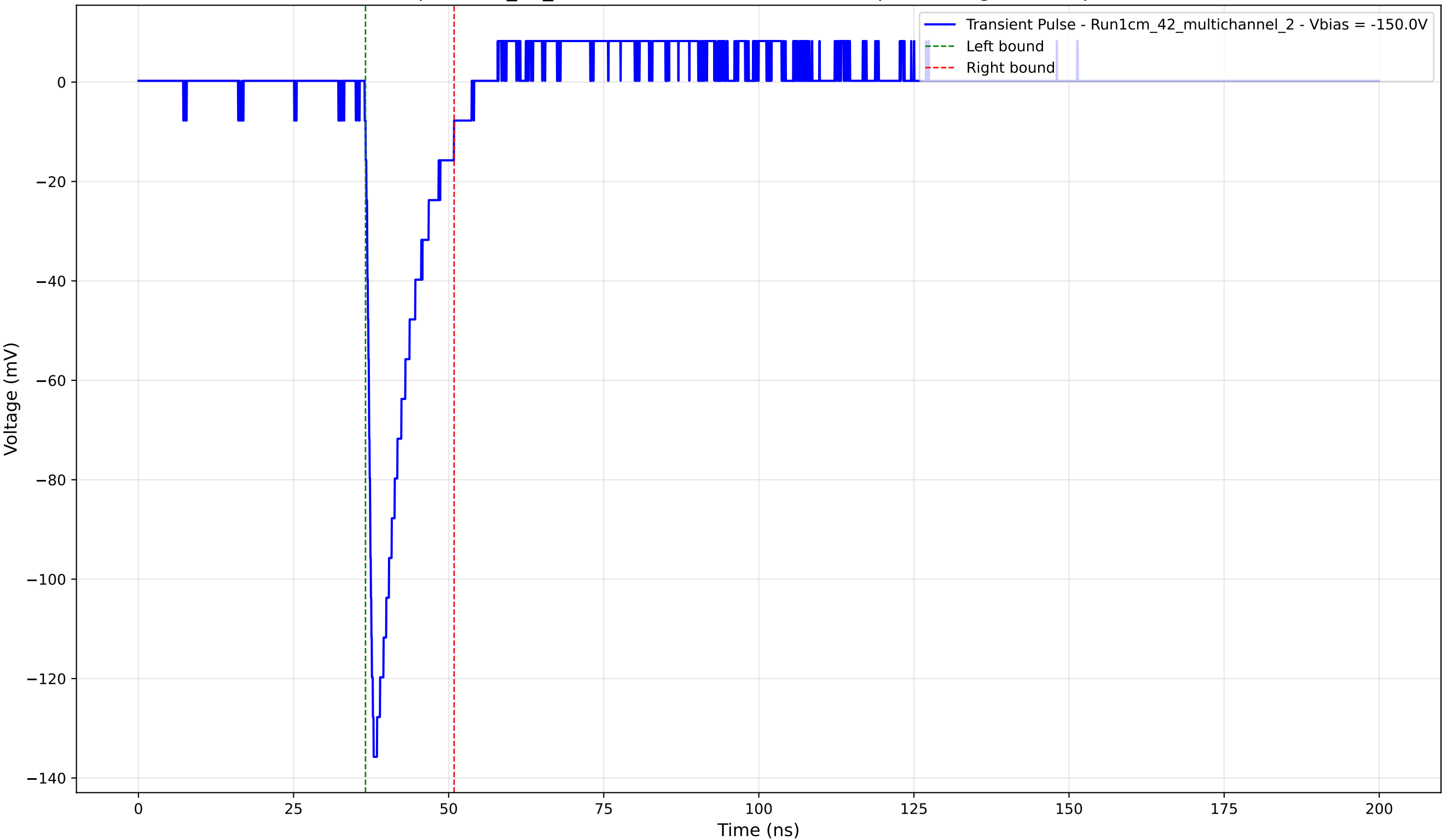
Transient Pulse - Sample: 1cm_42_multichannel - Position: 3480.0 \mu\text{m} - Charge: 16.75 pC - Rise Time: 1.17 ns
