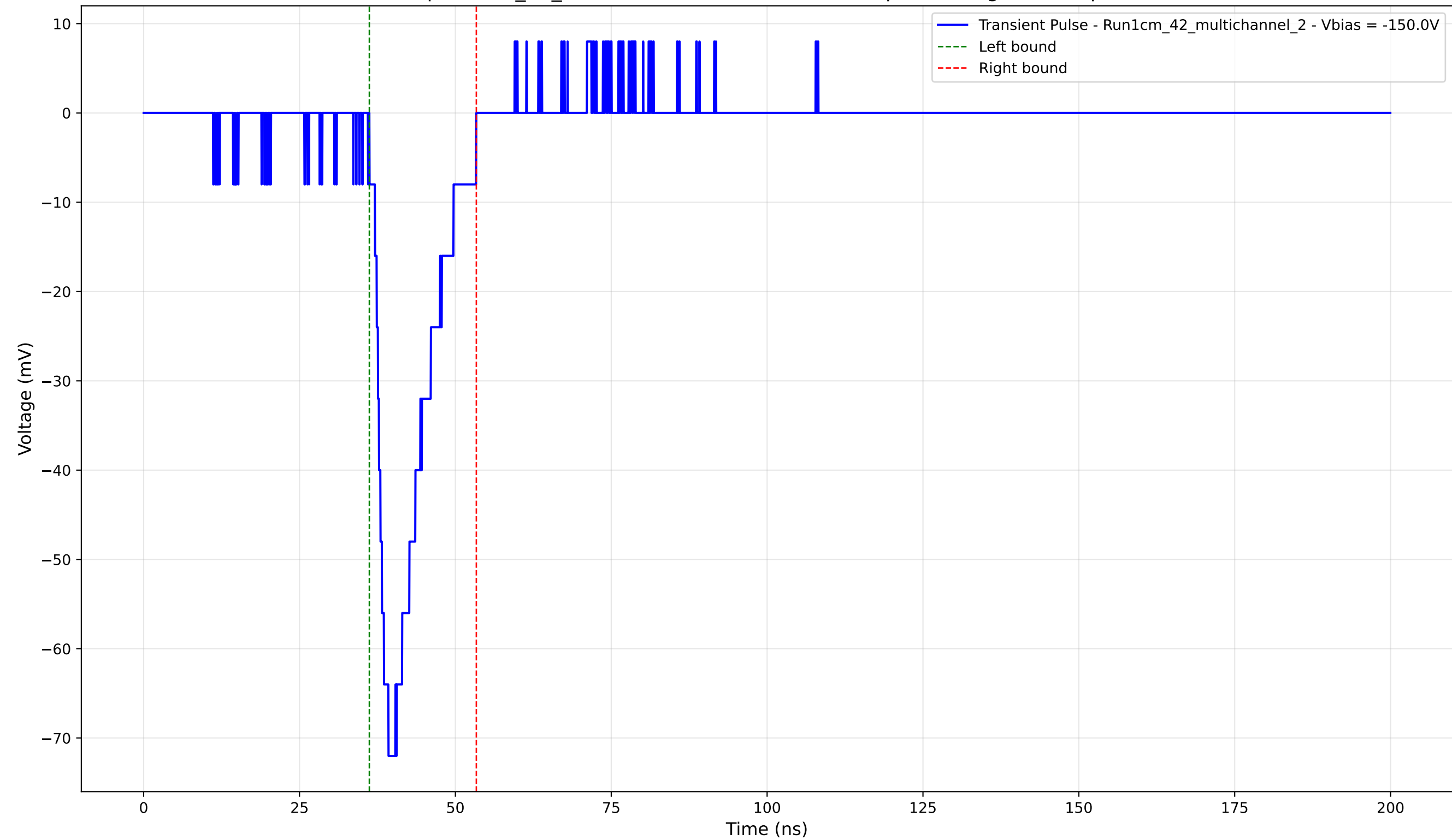
Transient Pulse - Sample: 1cm_42_multichannel - Position: 4680.0 \mu\text{m} - Charge: 11.12 pC - Rise Time: 3.04 ns
