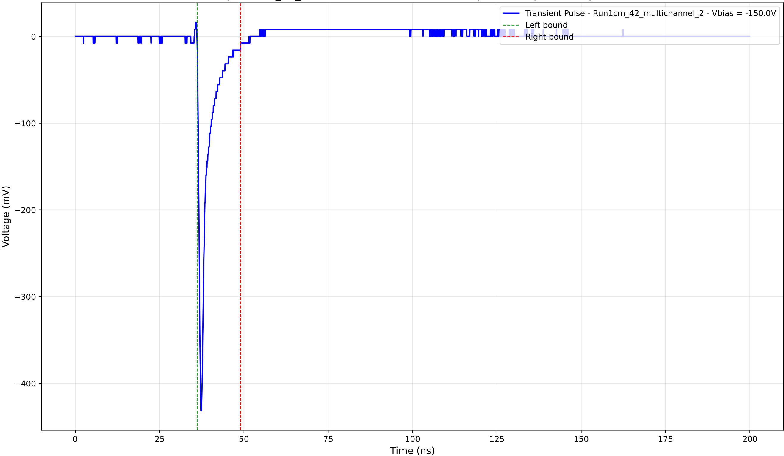
Transient Pulse - Sample: 1cm_42_multichannel - Position: 2695.0 \mu\text{m} - Charge: 24.87 pC - Rise Time: 0.78 ns
