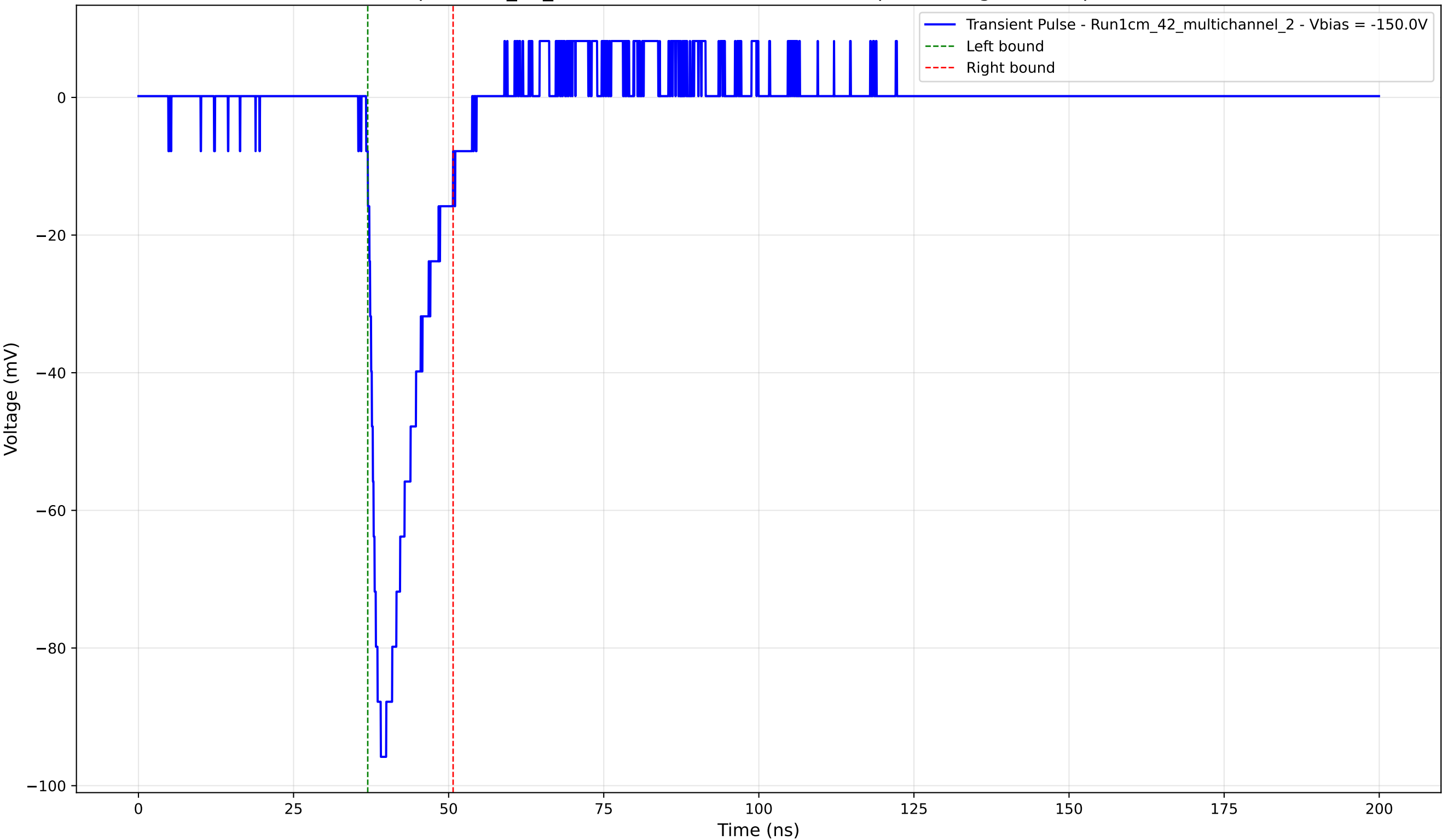
Transient Pulse - Sample: 1cm_42_multichannel - Position: 3990.0 \mu\text{m} - Charge: 13.62 pC - Rise Time: 1.59 ns
