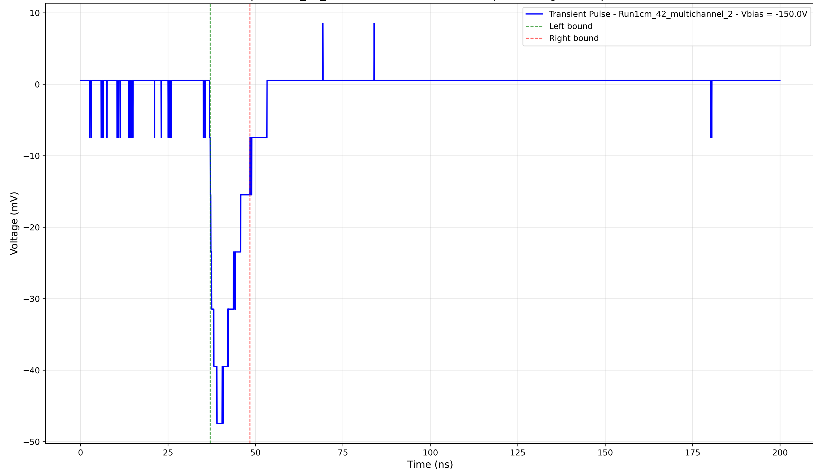
Transient Pulse - Sample: 1cm_42_multichannel - Position: 80.0 \mu\text{m} - Charge: 6.78 pC - Rise Time: 2.18 ns
