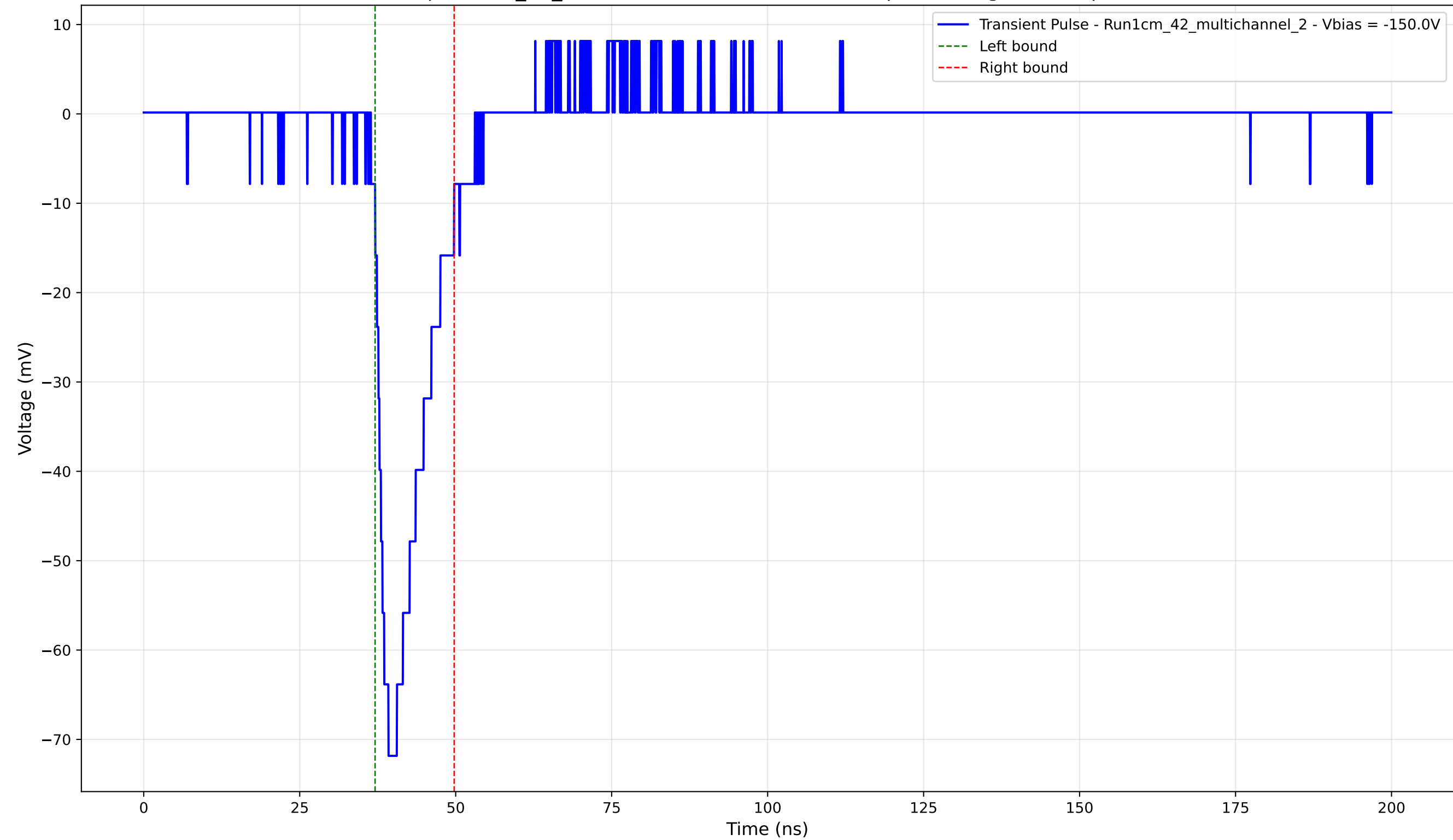
Transient Pulse - Sample: 1cm_42_multichannel - Position: 4650.0 \mu\text{m} - Charge: 10.41 pC - Rise Time: 2.80 ns
