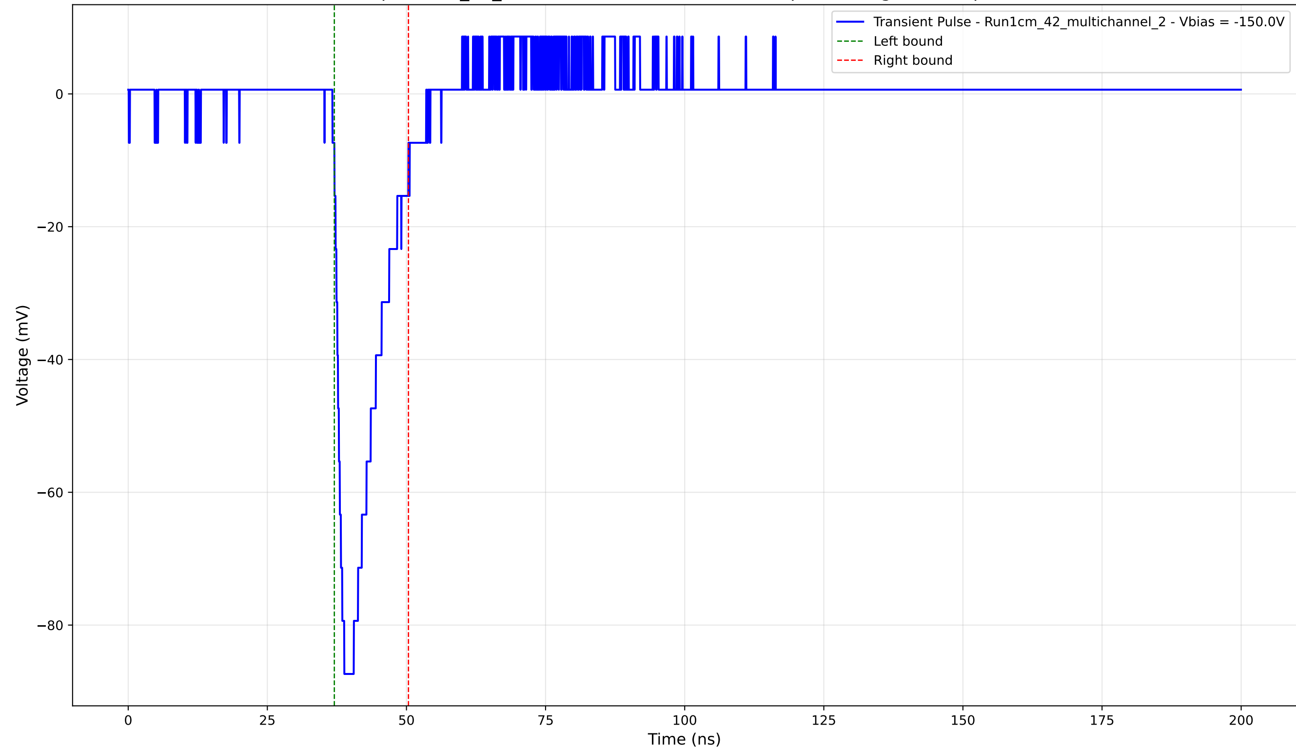
Transient Pulse - Sample: 1cm_42_multichannel - Position: 4065.0 \mu\text{m} - Charge: 12.76 pC - Rise Time: 1.43 ns
