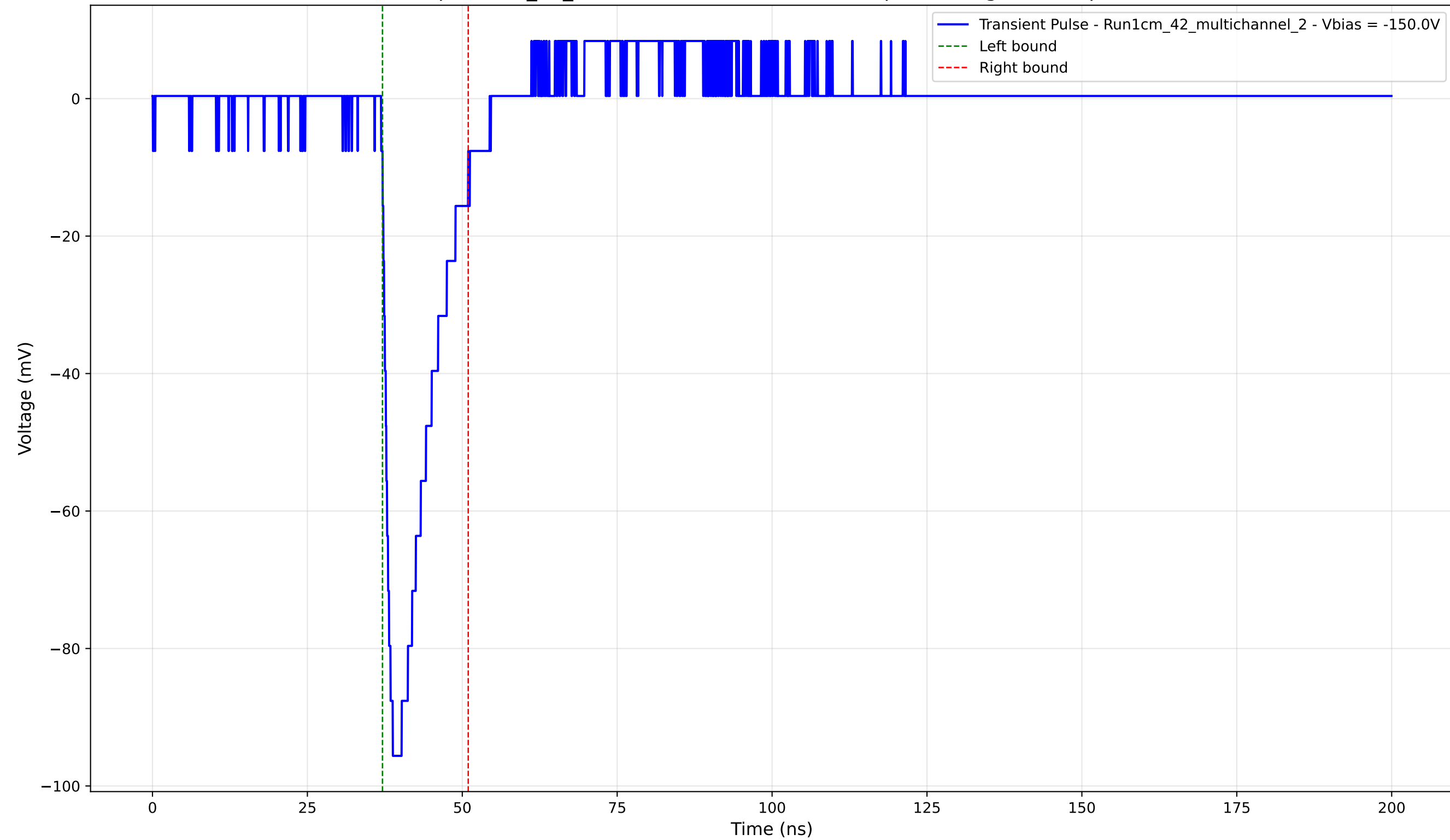
Transient Pulse - Sample: 1cm_42_multichannel - Position: 570.0 \mu\text{m} - Charge: 14.24 pC - Rise Time: 1.31 ns
