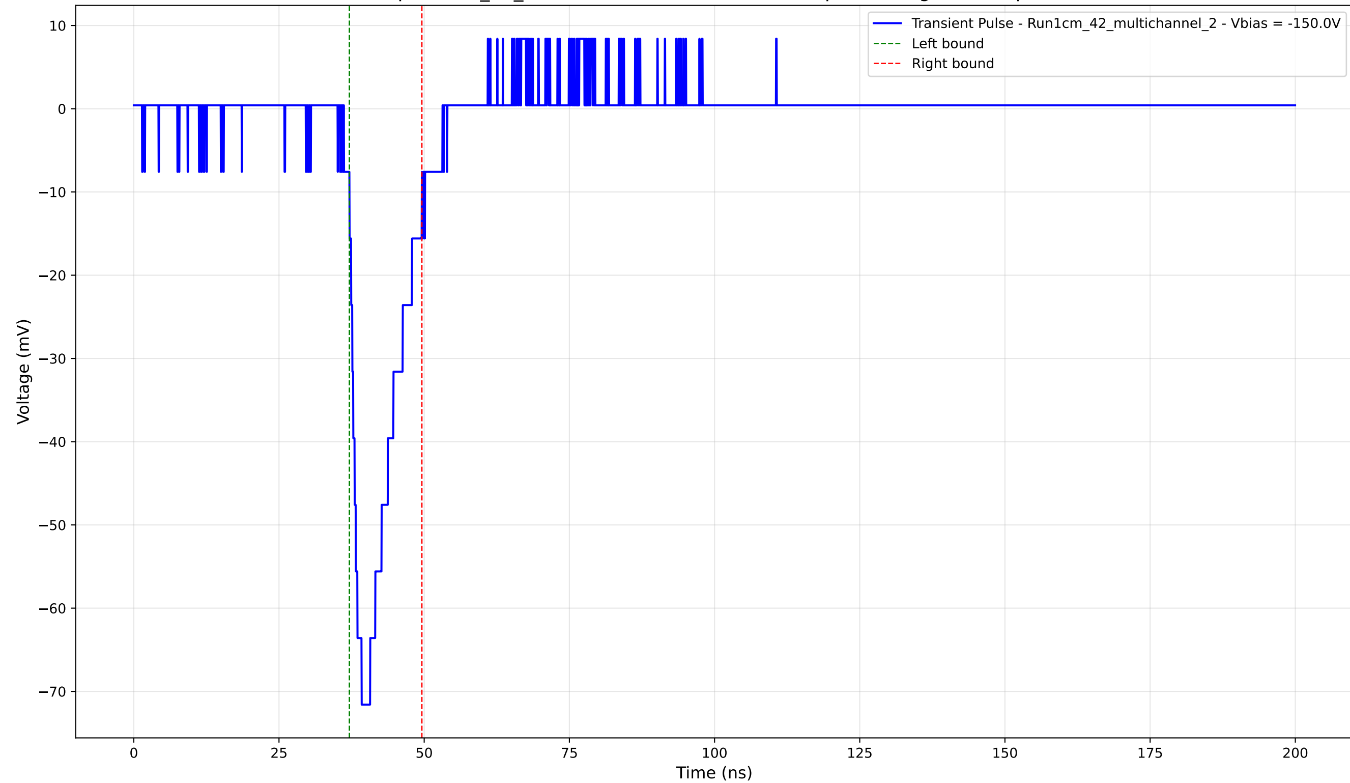
Transient Pulse - Sample: 1cm_42_multichannel - Position: 4600.0 \mu\text{m} - Charge: 10.41 pC - Rise Time: 3.04 ns
