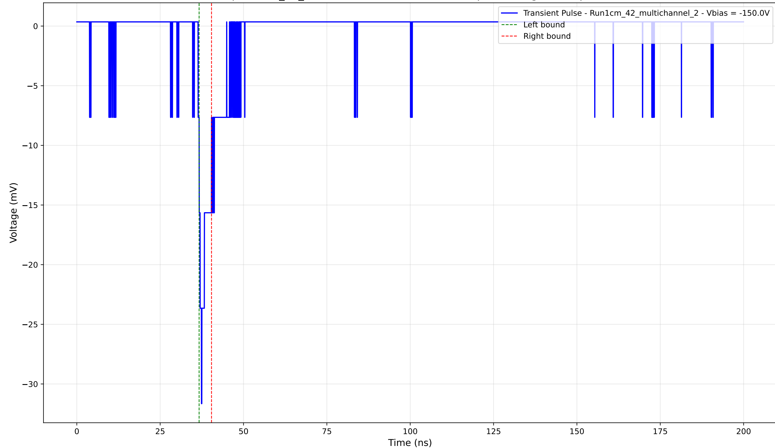
Transient Pulse - Sample: 1cm_42_multichannel - Position: 2900.0 \mu\text{m} - Charge: 1.38 pC - Rise Time: 1.02 ns
