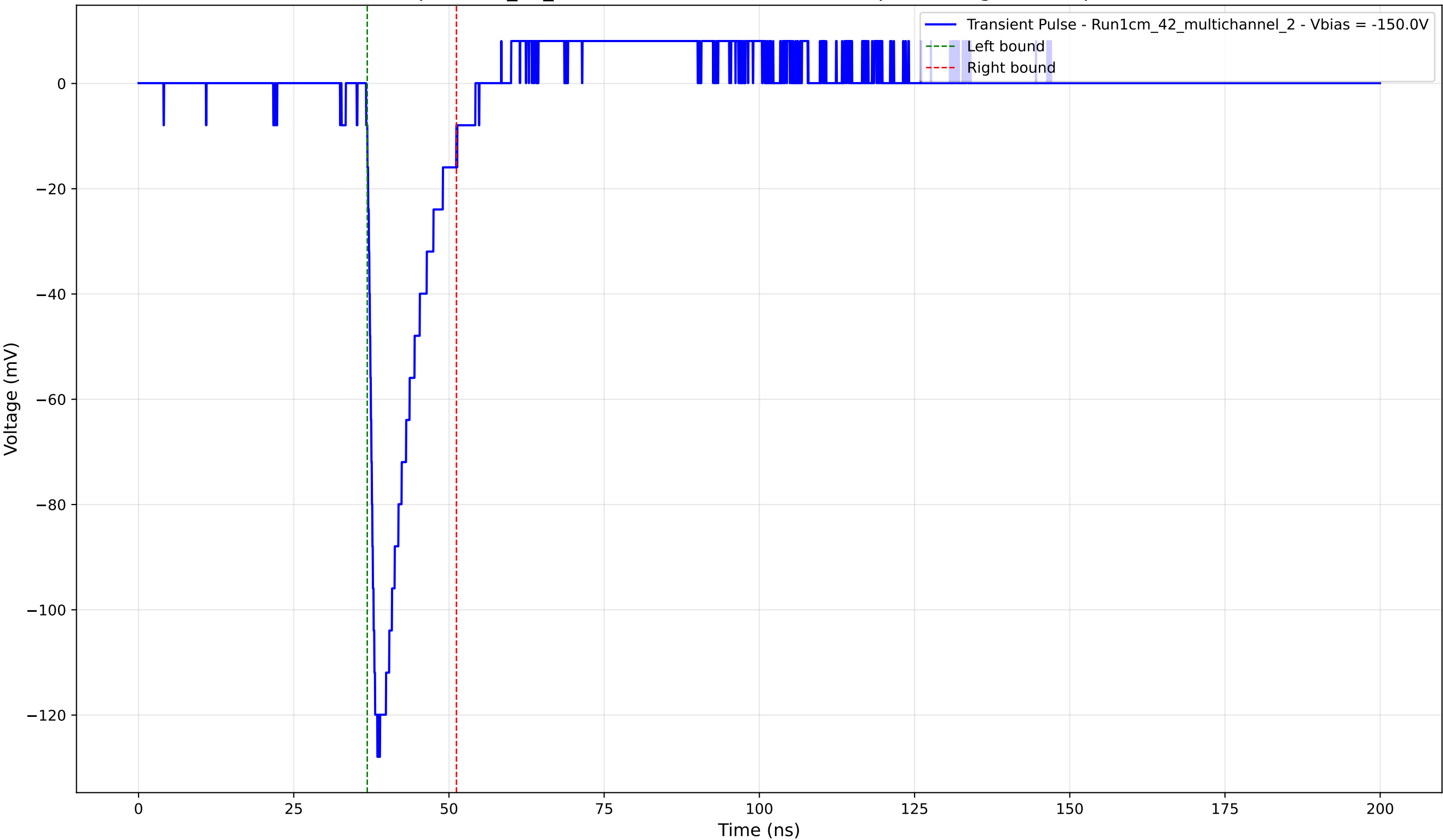
Transient Pulse - Sample: 1cm_42_multichannel - Position: 1000.0 \mu\text{m} - Charge: 17.15 pC - Rise Time: 1.26 ns
