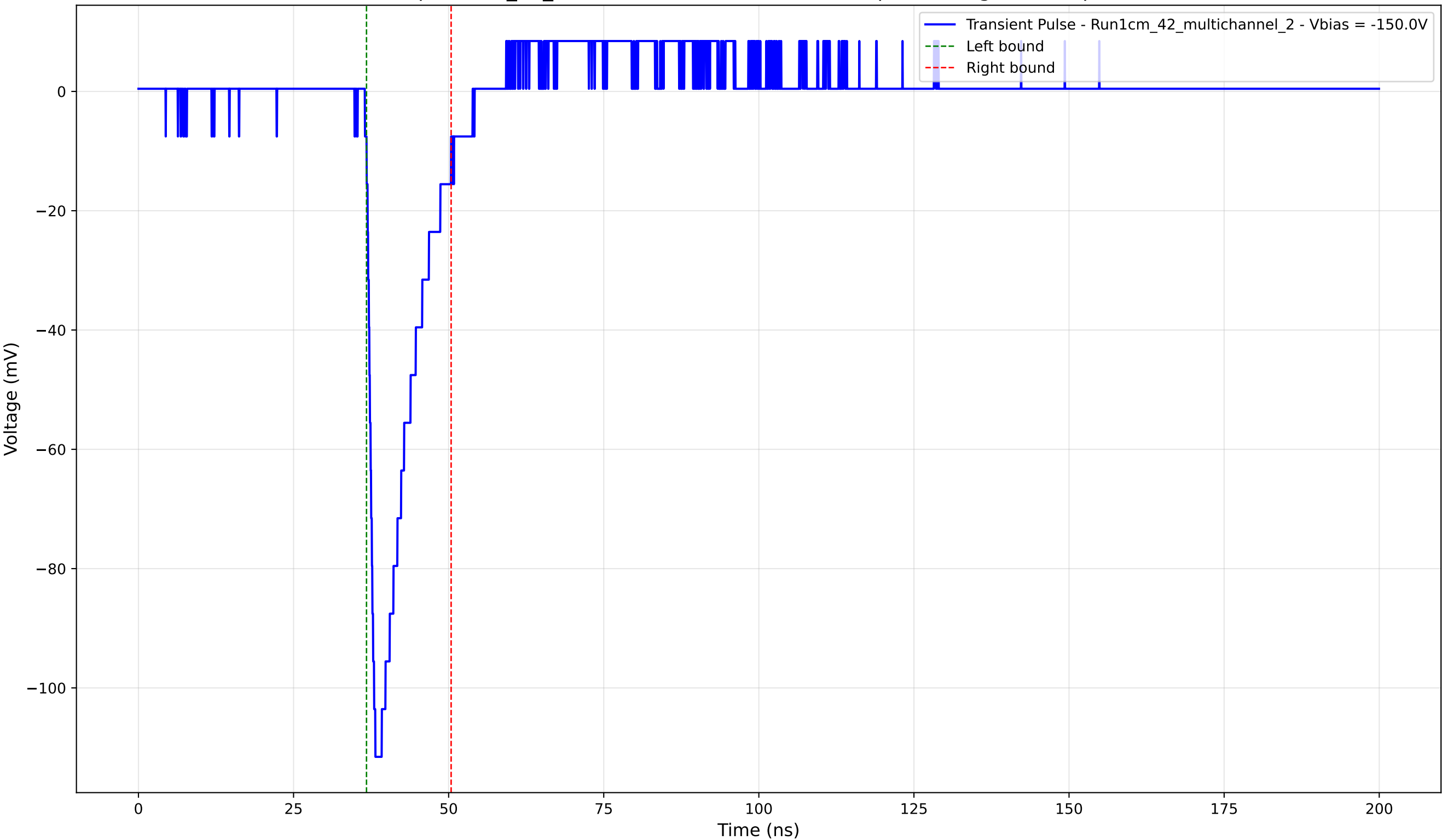
Transient Pulse - Sample: 1cm_42_multichannel - Position: 3670.0 \mu\text{m} - Charge: 15.03 pC - Rise Time: 1.22 ns
