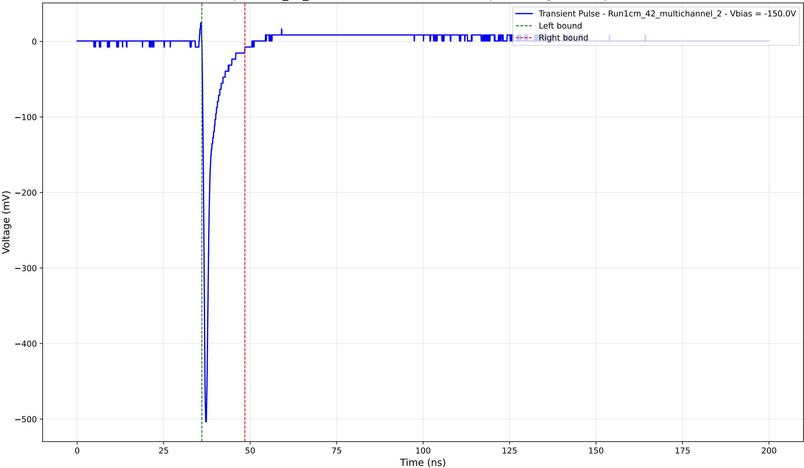
Transient Pulse - Sample: 1cm_42_multichannel - Position: 2560.0 \mu\text{m} - Charge: 25.06 pC - Rise Time: 0.74 ns
