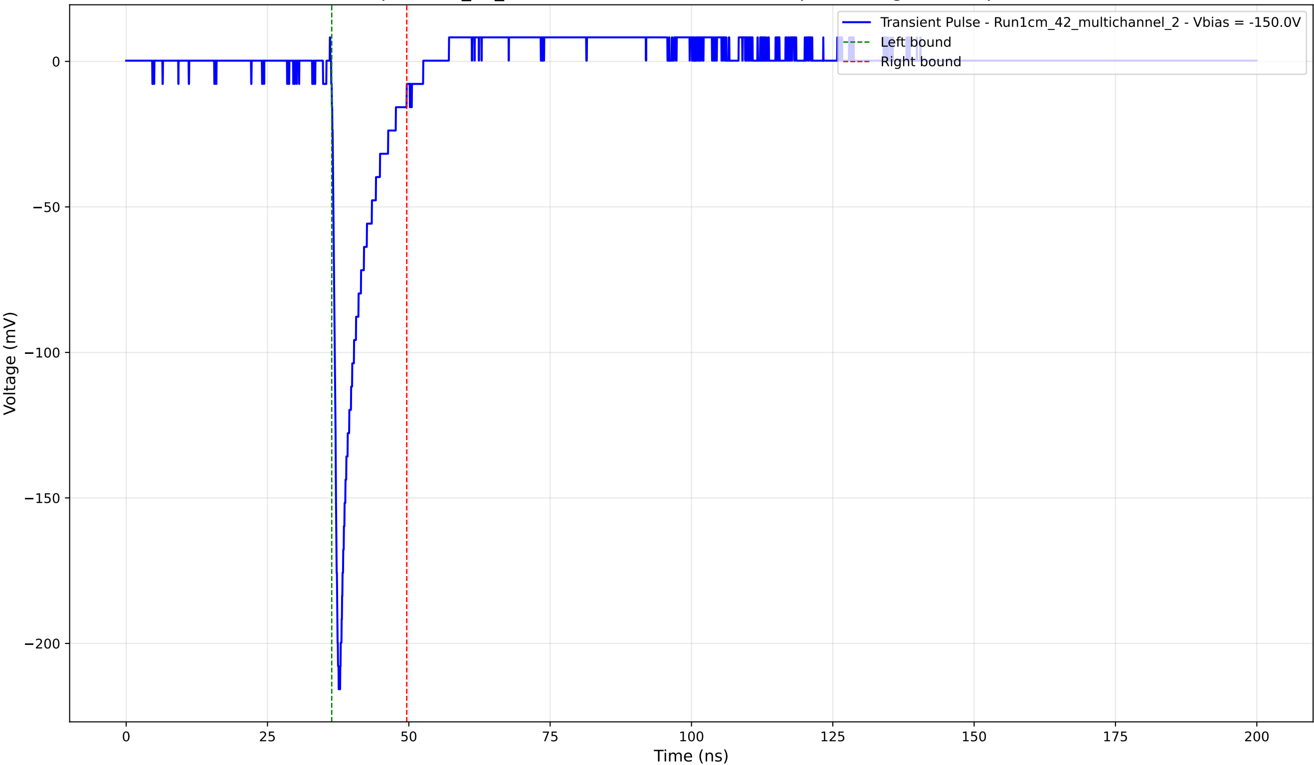
Transient Pulse - Sample: 1cm_42_multichannel - Position: 3105.0 \mu\text{m} - Charge: 18.95 pC - Rise Time: 0.93 ns
