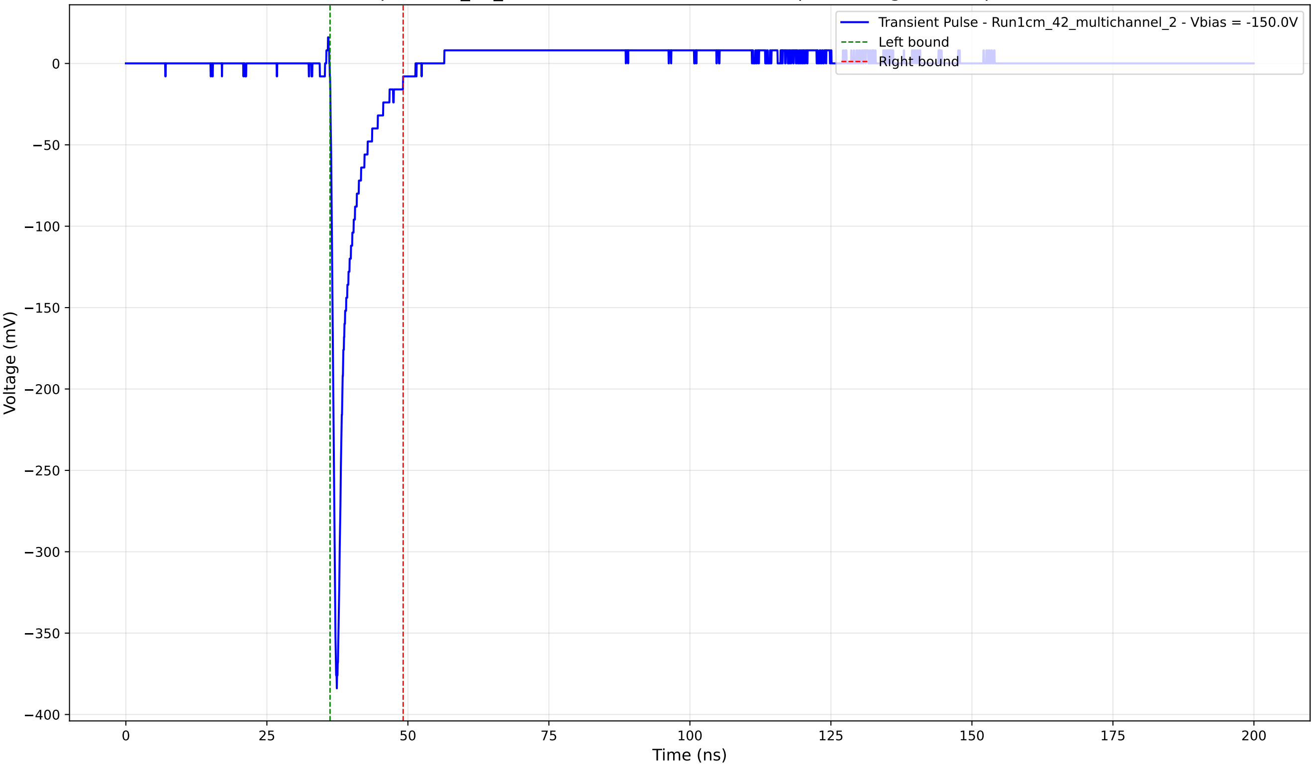
Transient Pulse - Sample: 1cm_42_multichannel - Position: 2770.0 \mu\text{m} - Charge: 23.59 pC - Rise Time: 0.82 ns
