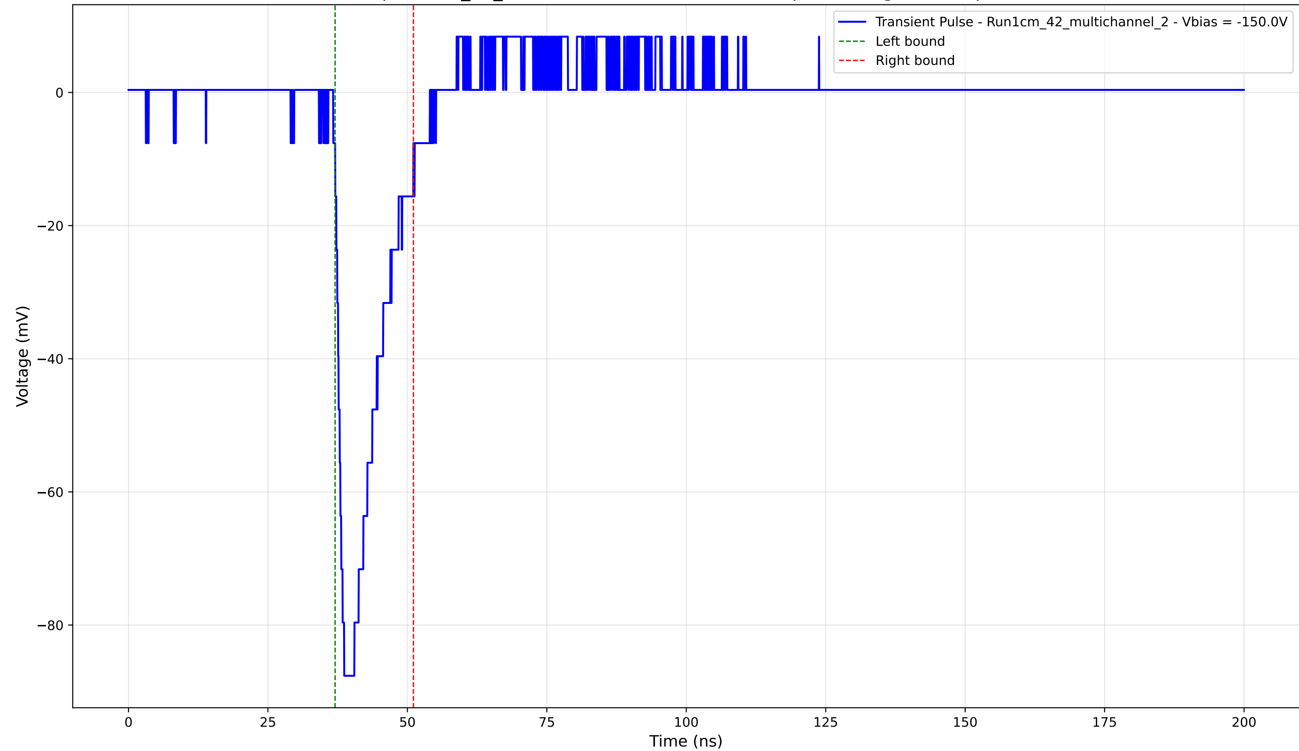
Transient Pulse - Sample: 1cm_42_multichannel - Position: 4030.0 \mu\text{m} - Charge: 13.22 pC - Rise Time: 1.35 ns
