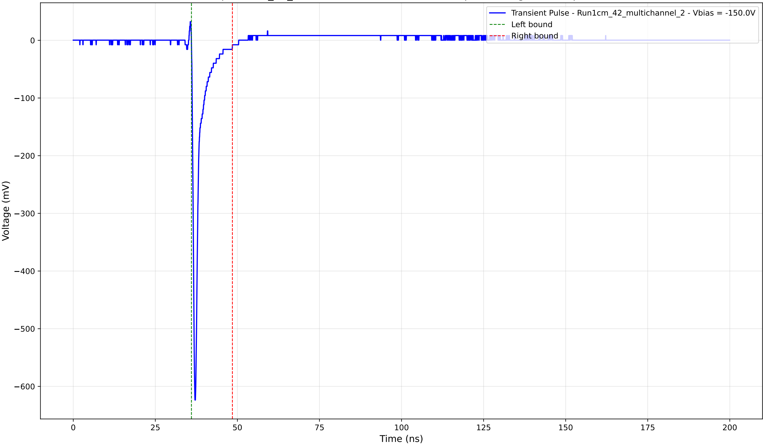
Transient Pulse - Sample: 1cm_42_multichannel - Position: 2455.0 \mu\text{m} - Charge: 28.04 pC - Rise Time: 0.73 ns
