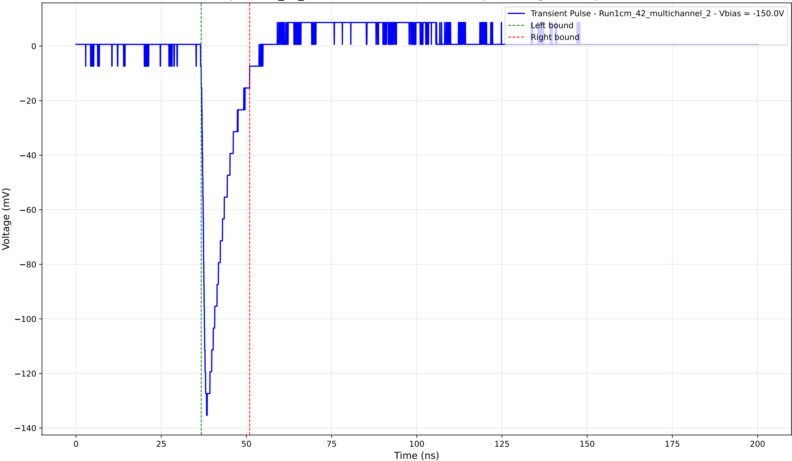
Transient Pulse - Sample: 1cm_42_multichannel - Position: 1105.0 \mu\text{m} - Charge: 17.32 pC - Rise Time: 1.29 ns
