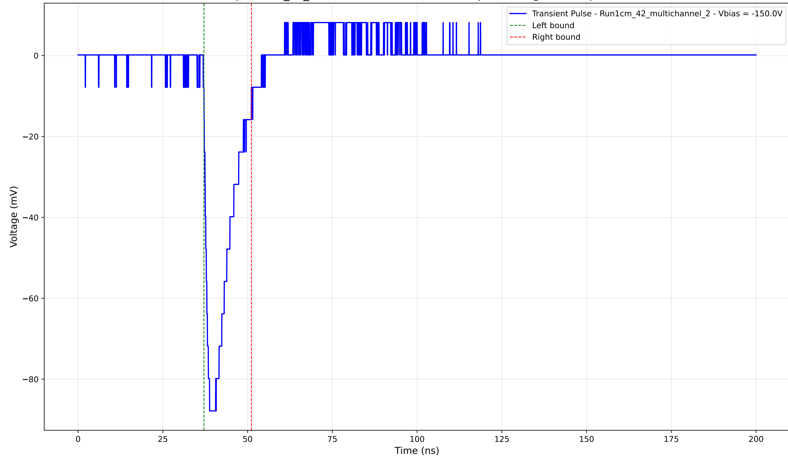
Transient Pulse - Sample: 1cm_42_multichannel - Position: 445.0 \mu\text{m} - Charge: 13.66 pC - Rise Time: 1.32 ns
