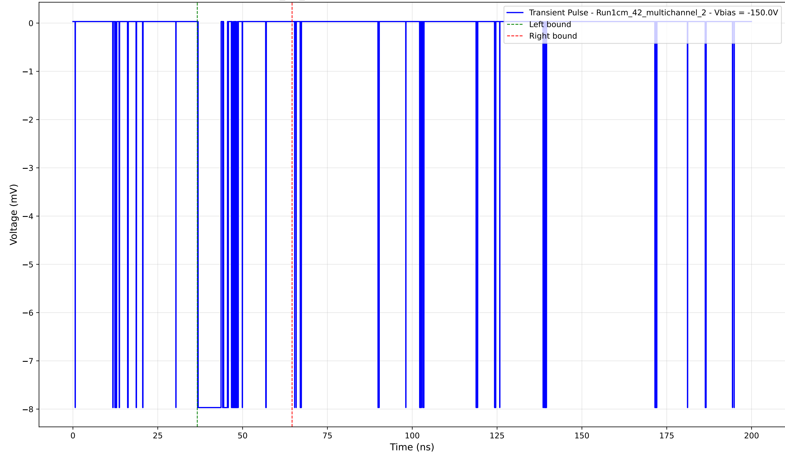
Transient Pulse - Sample: 1cm_42_multichannel - Position: 1355.0 \mu\text{m} - Charge: 1.50 pC - Rise Time: 0.04 ns
