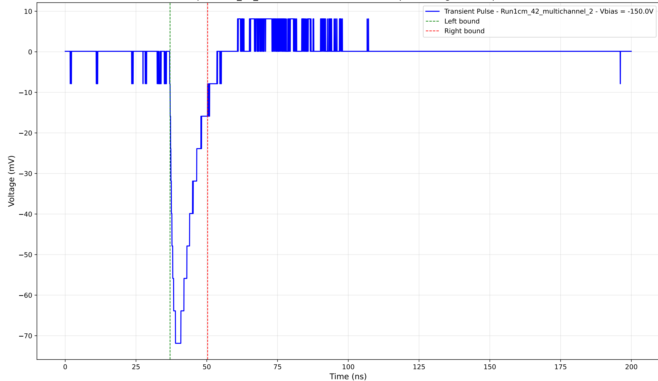
Transient Pulse - Sample: 1cm_42_multichannel - Position: 215.0 \mu\text{m} - Charge: 11.32 pC - Rise Time: 2.04 ns
