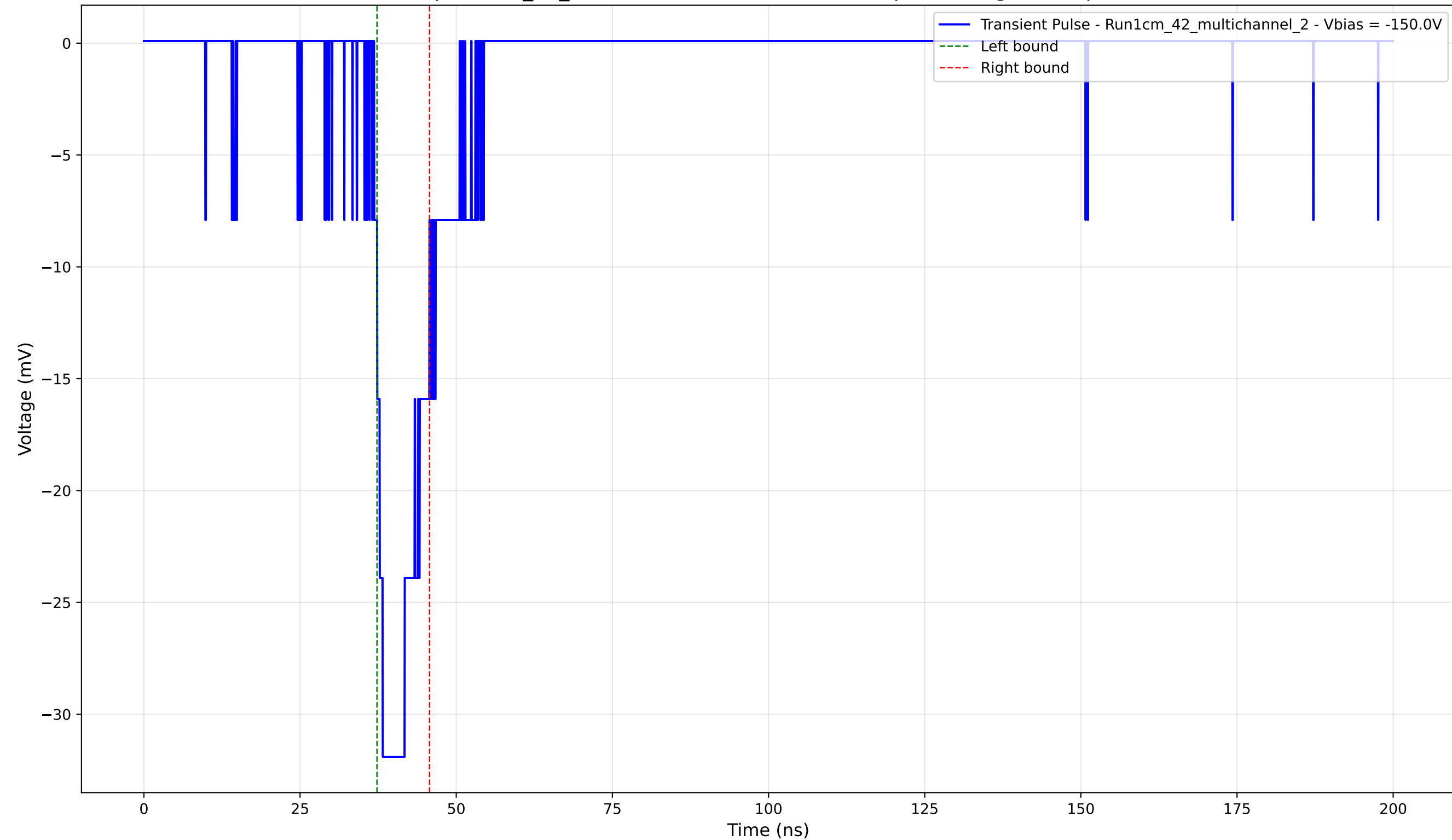
Transient Pulse - Sample: 1cm_42_multichannel - Position: 3930.0 \mu\text{m} - Charge: 4.21 pC - Rise Time: 1.38 ns
