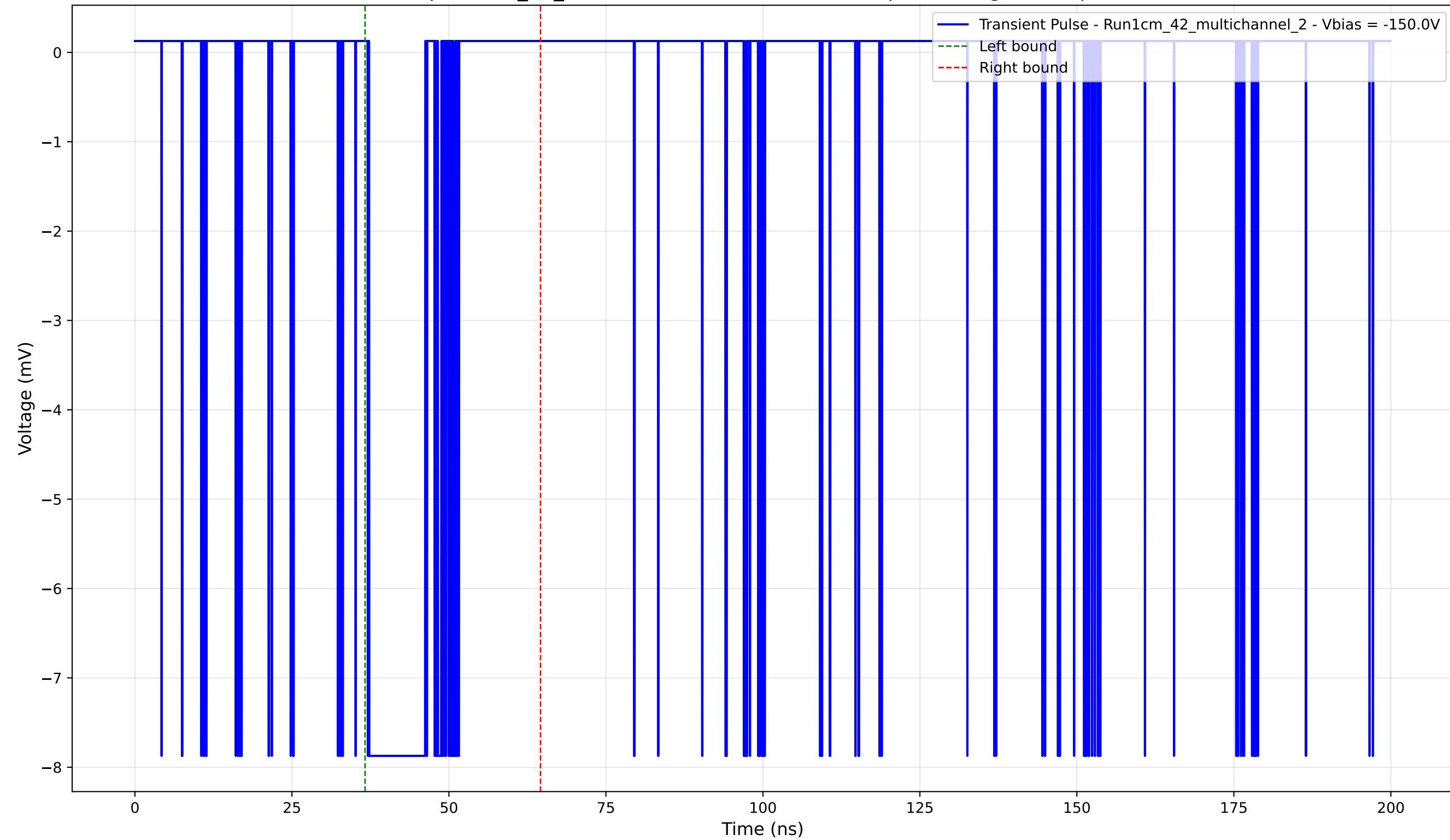
Transient Pulse - Sample: 1cm_42_multichannel - Position: 4875.0 \mu\text{m} - Charge: 1.70 pC - Rise Time: 0.04 ns
