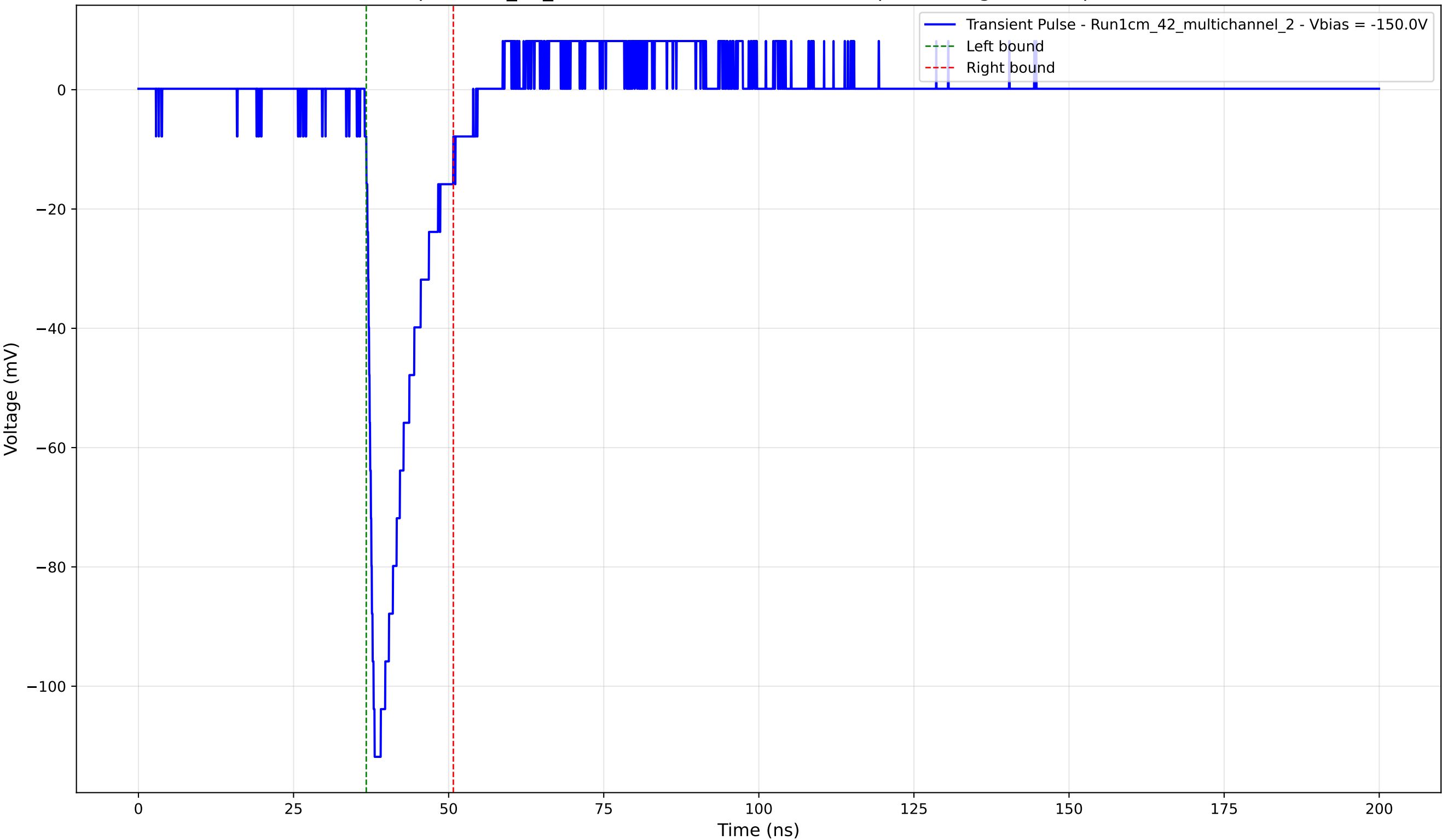
Transient Pulse - Sample: 1cm_42_multichannel - Position: 3615.0 \mu\text{m} - Charge: 15.08 pC - Rise Time: 1.18 ns
