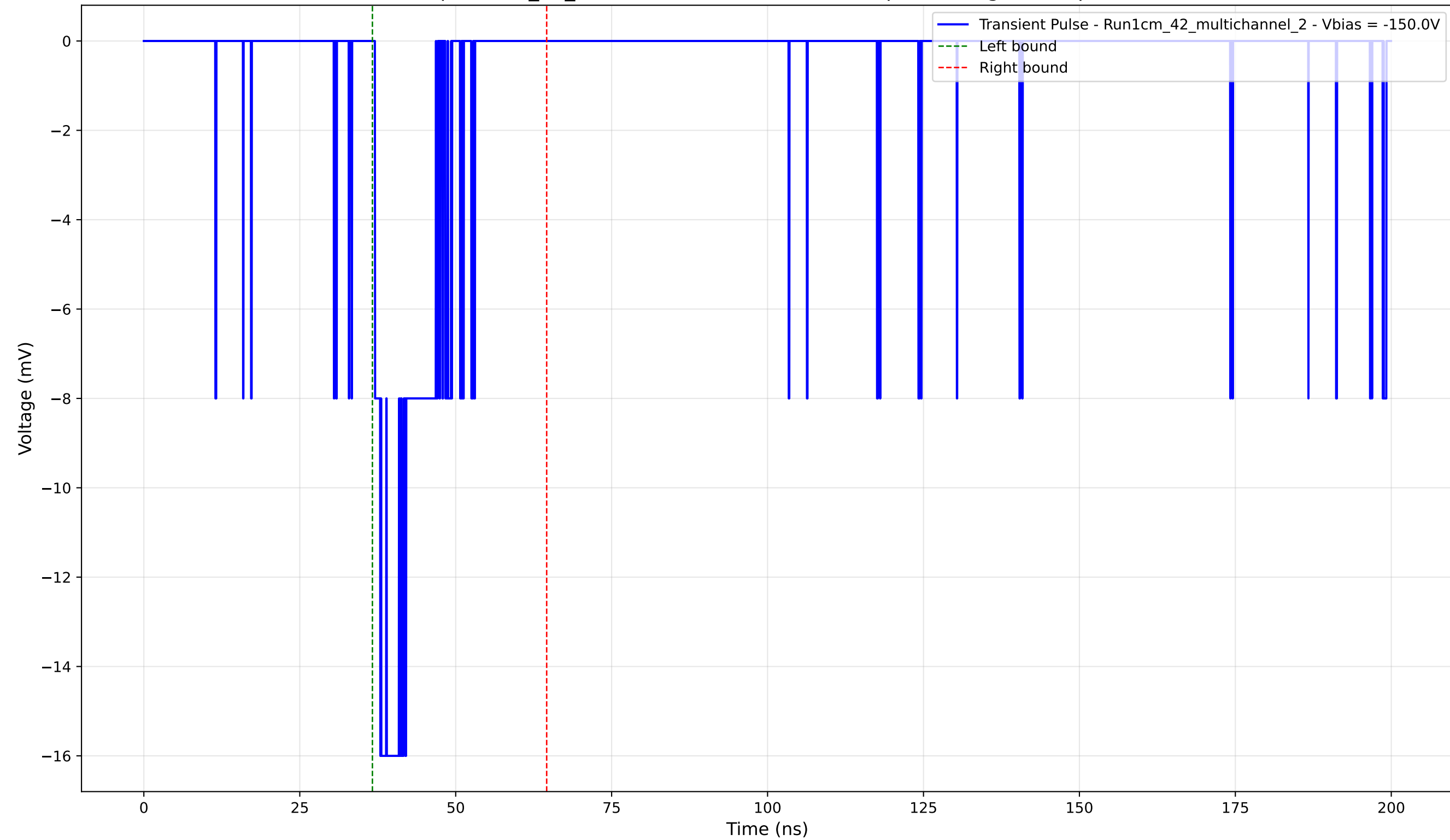
Transient Pulse - Sample: 1cm_42_multichannel - Position: 825.0 \mu\text{m} - Charge: 2.49 pC - Rise Time: 0.87 ns
