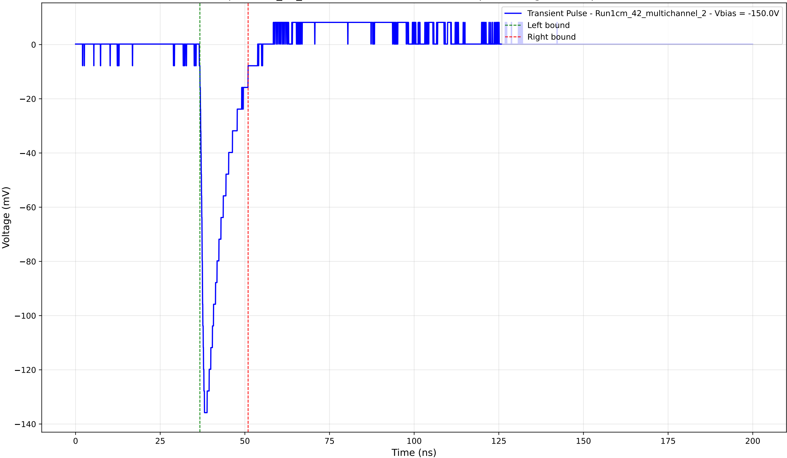
Transient Pulse - Sample: 1cm_42_multichannel - Position: 1140.0 \mu\text{m} - Charge: 17.83 pC - Rise Time: 1.17 ns
