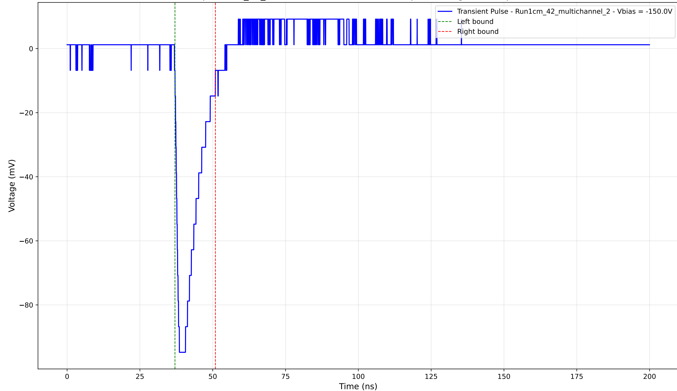
Transient Pulse - Sample: 1cm_42_multichannel - Position: 620.0 \mu\text{m} - Charge: 14.43 pC - Rise Time: 1.23 ns
