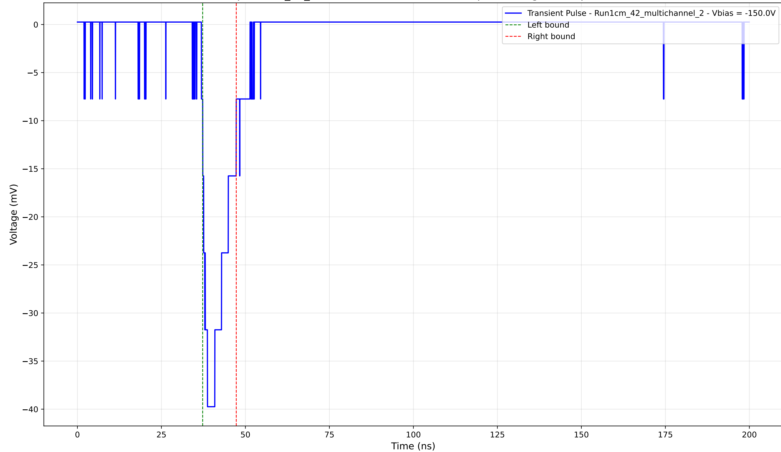
Transient Pulse - Sample: 1cm_42_multichannel - Position: 295.0 \mu\text{m} - Charge: 5.45 pC - Rise Time: 1.82 ns
