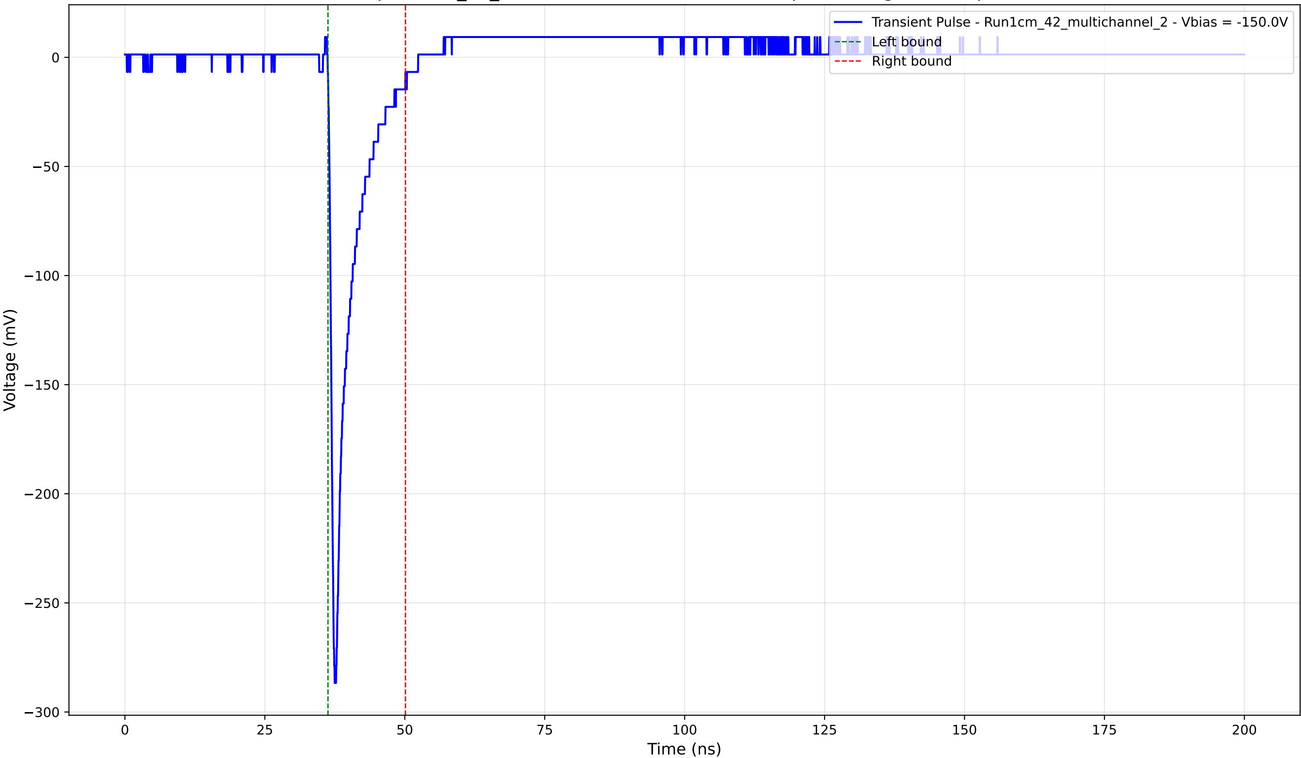
Transient Pulse - Sample: 1cm_42_multichannel - Position: 1760.0 \mu\text{m} - Charge: 22.48 pC - Rise Time: 0.83 ns
