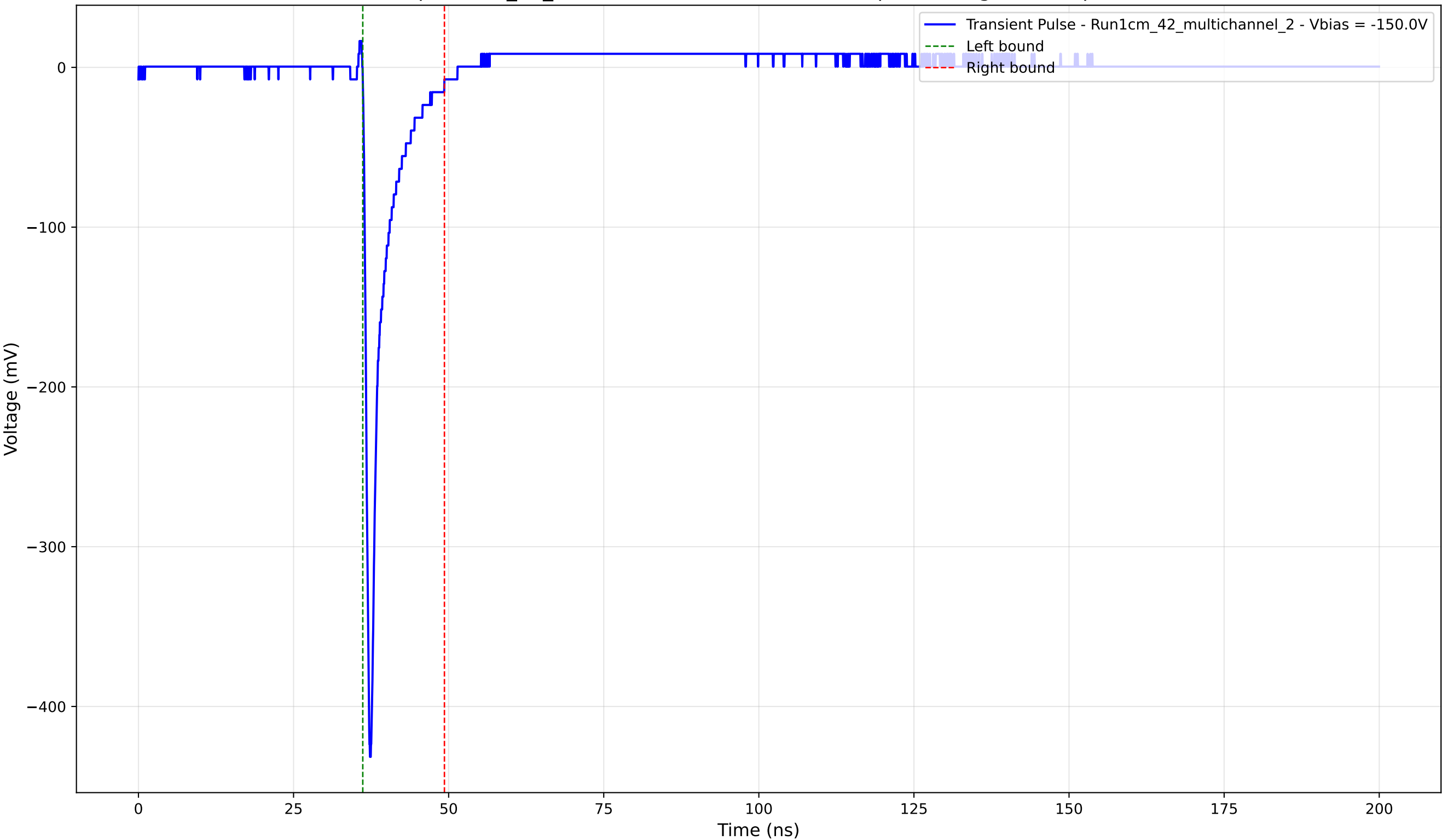
Transient Pulse - Sample: 1cm_42_multichannel - Position: 2005.0 \mu\text{m} - Charge: 25.72 pC - Rise Time: 0.81 ns
