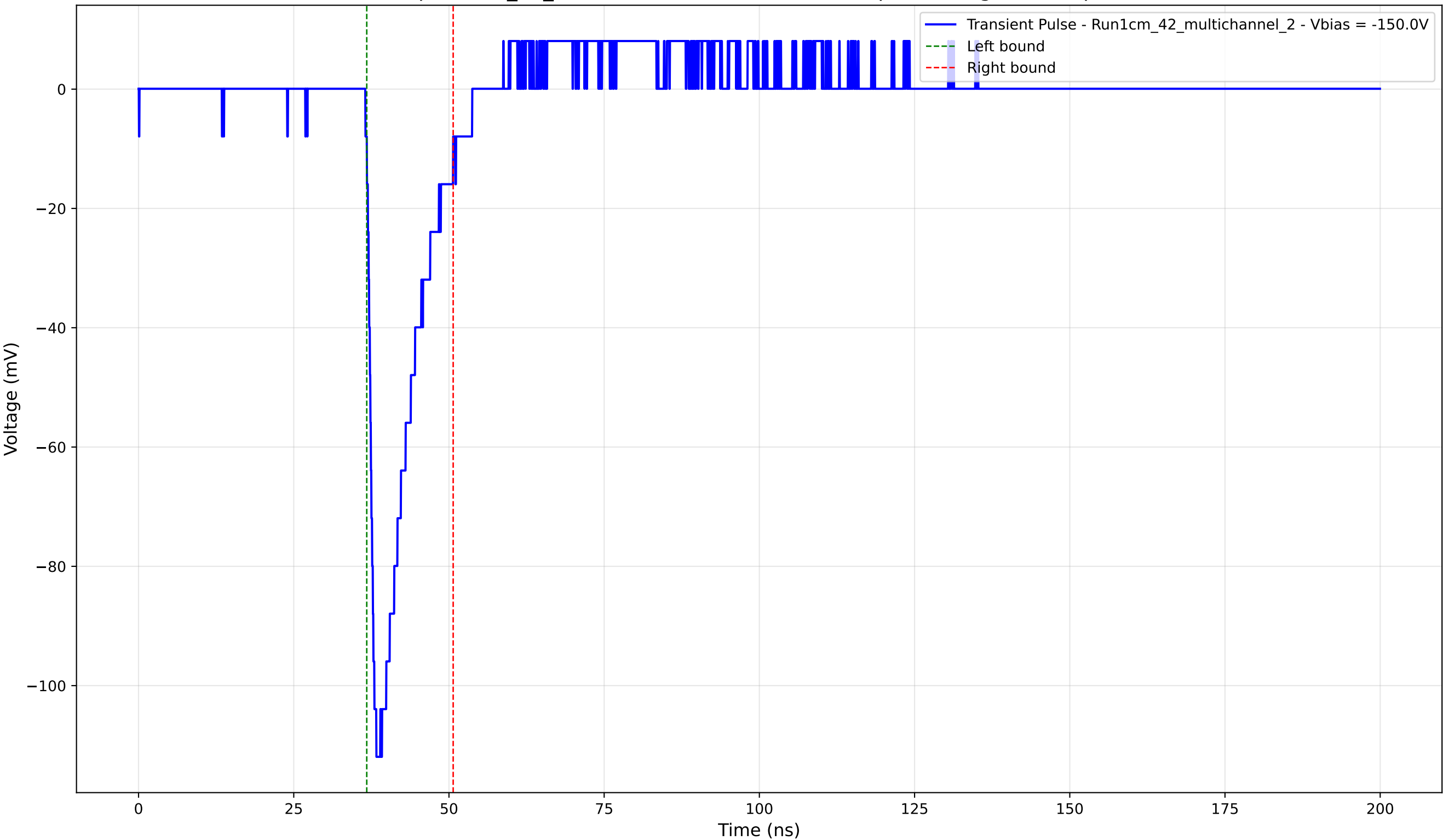
Transient Pulse - Sample: 1cm_42_multichannel - Position: 3675.0 \mu\text{m} - Charge: 15.16 pC - Rise Time: 1.22 ns
