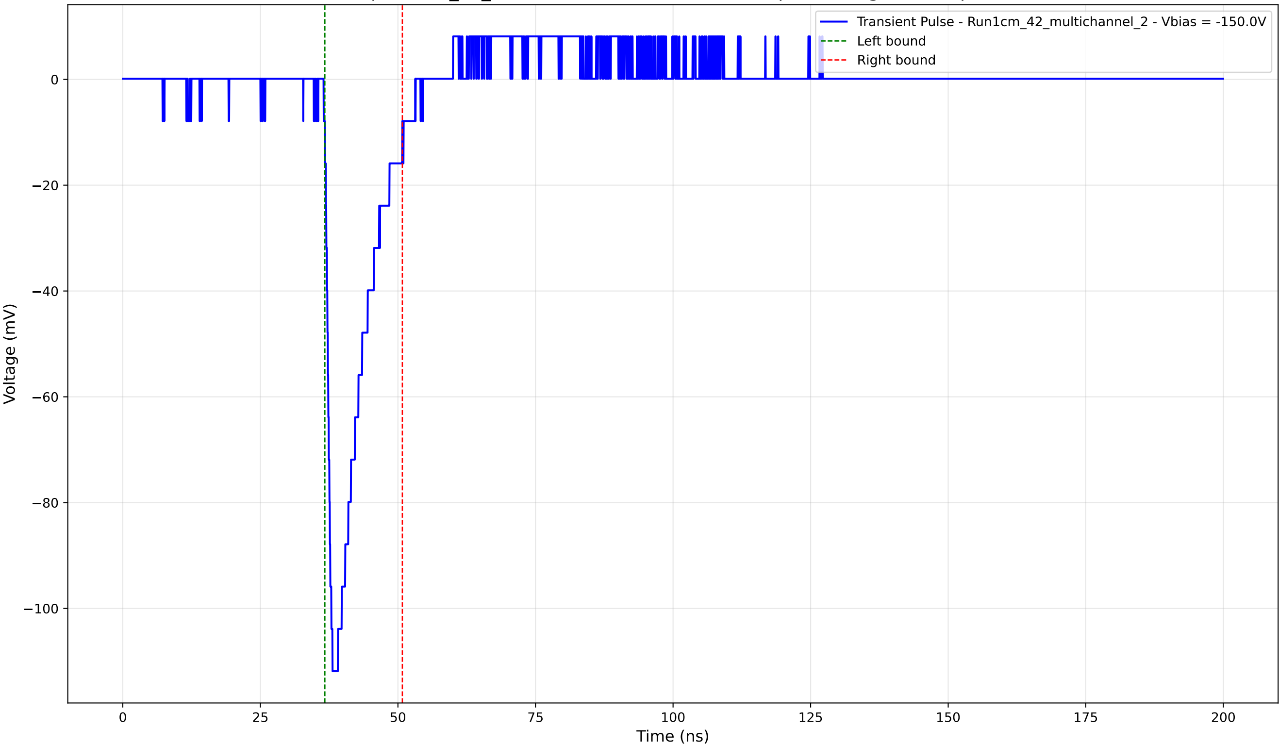
Transient Pulse - Sample: 1cm_42_multichannel - Position: 3610.0 \mu\text{m} - Charge: 15.09 pC - Rise Time: 1.18 ns
