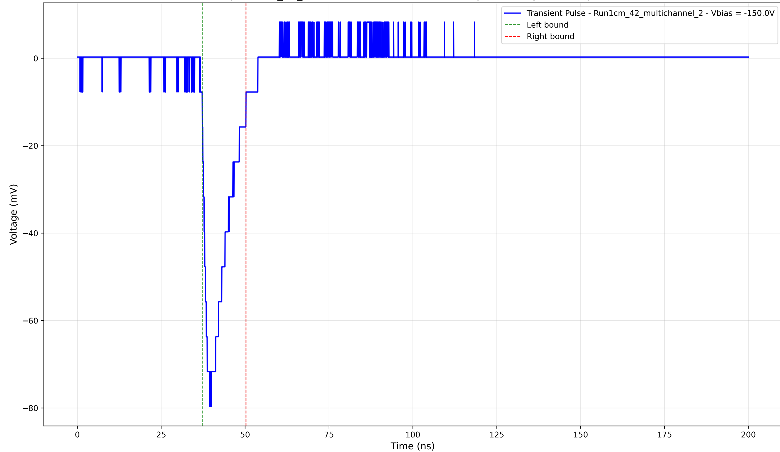
Transient Pulse - Sample: 1cm_42_multichannel - Position: 4265.0 \mu\text{m} - Charge: 11.25 pC - Rise Time: 2.24 ns
