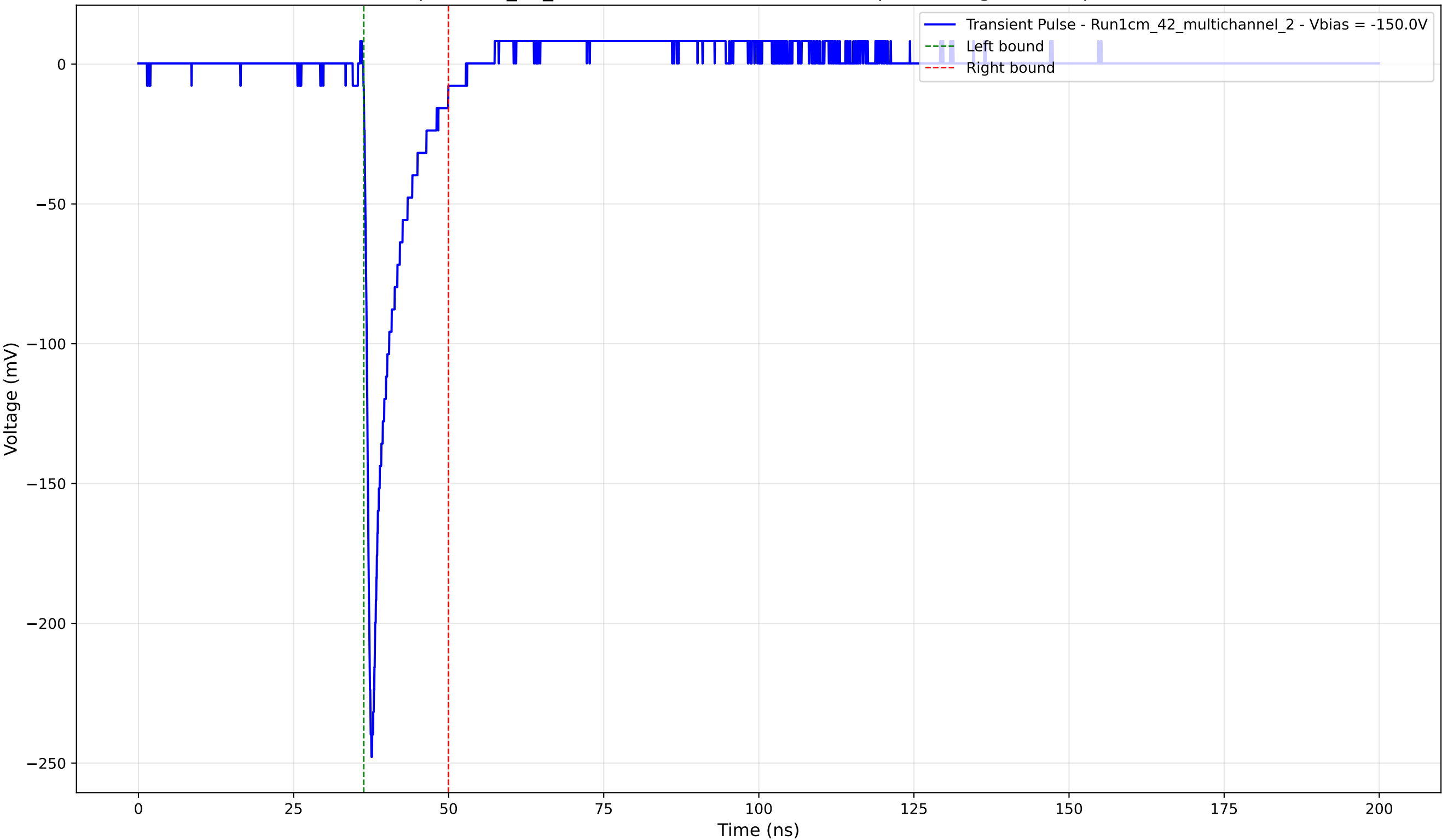
Transient Pulse - Sample: 1cm_42_multichannel - Position: 3035.0 \mu\text{m} - Charge: 20.42 pC - Rise Time: 0.87 ns
