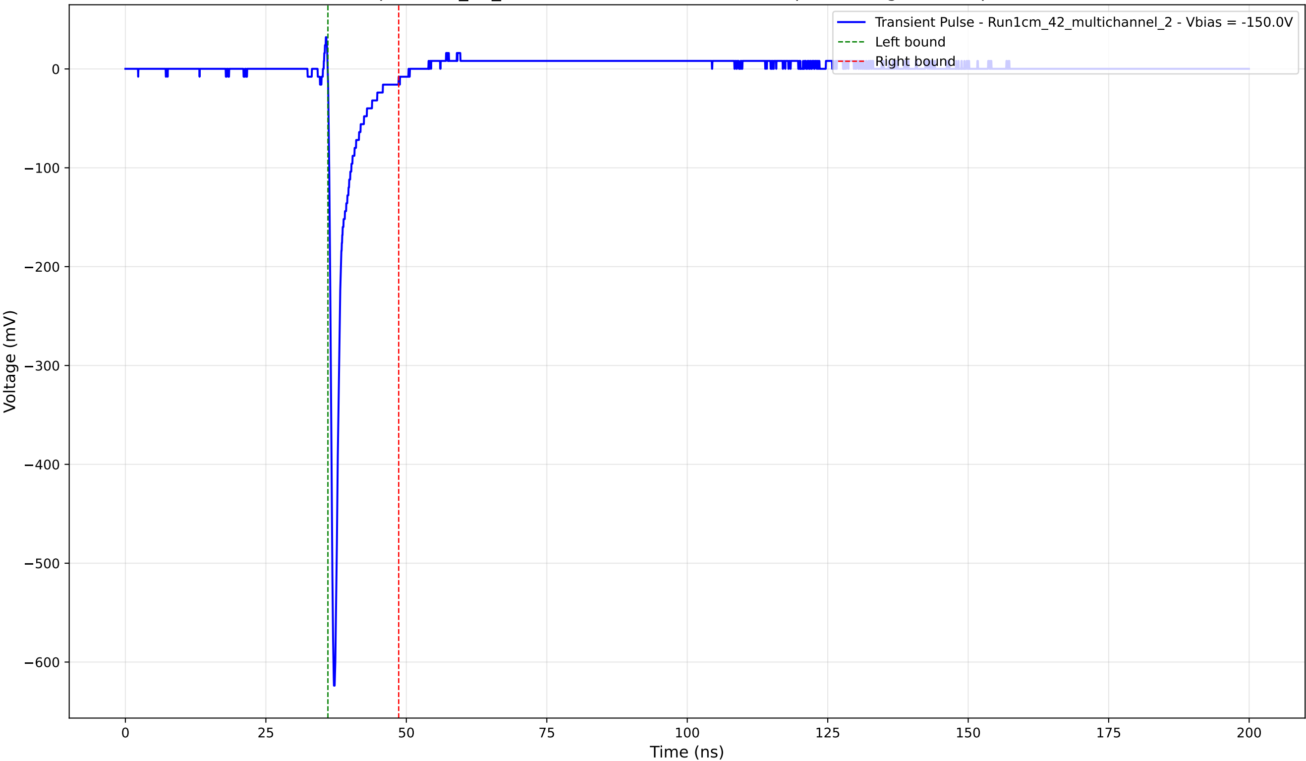
Transient Pulse - Sample: 1cm_42_multichannel - Position: 2245.0 \mu\text{m} - Charge: 29.08 pC - Rise Time: 0.73 ns
