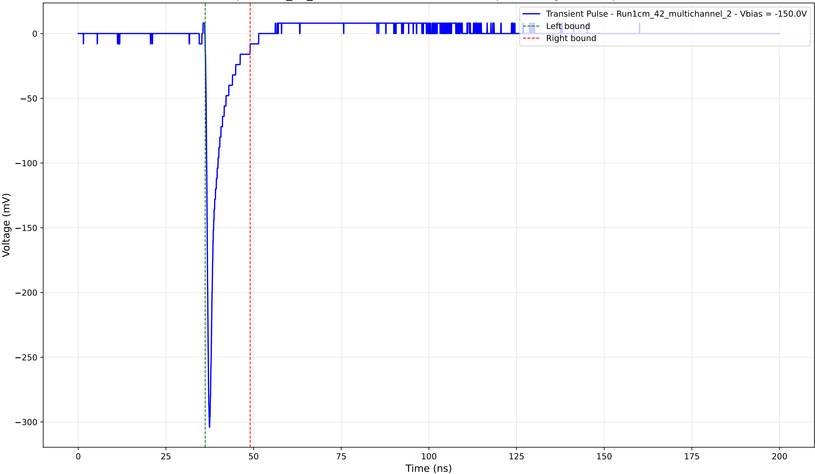
Transient Pulse - Sample: 1cm_42_multichannel - Position: 2805.0 \mu\text{m} - Charge: 19.42 pC - Rise Time: 0.82 ns
