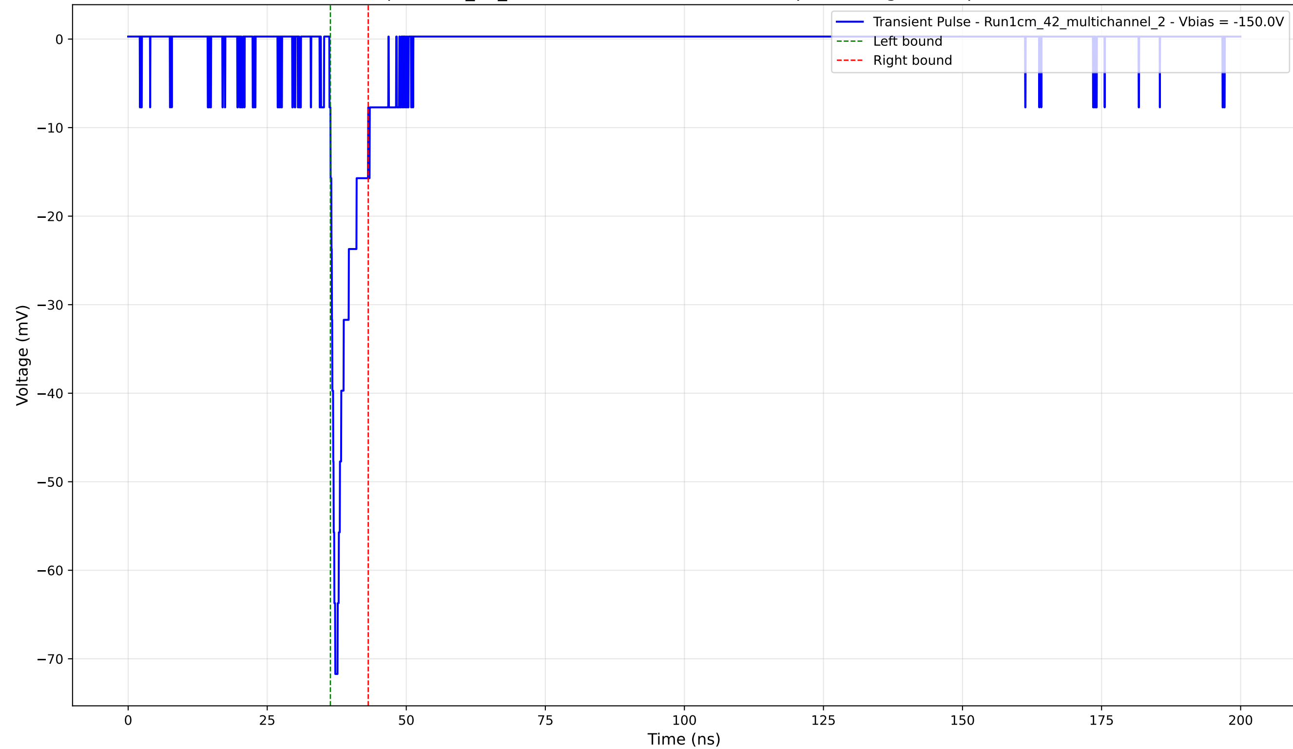
Transient Pulse - Sample: 1cm_42_multichannel - Position: 2840.0 \mu\text{m} - Charge: 4.27 pC - Rise Time: 1.04 ns
