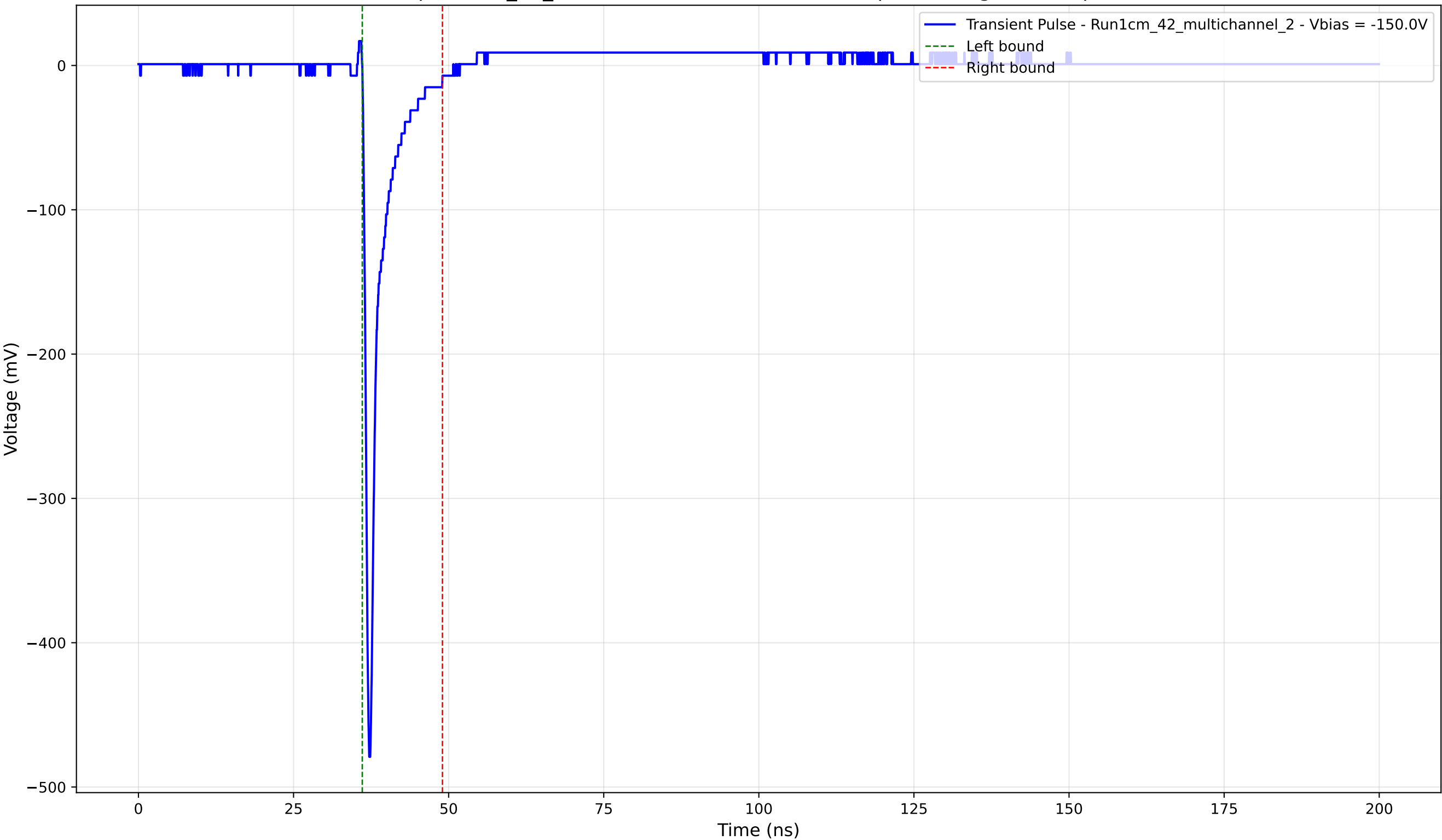
Transient Pulse - Sample: 1cm_42_multichannel - Position: 2605.0 \mu\text{m} - Charge: 24.97 pC - Rise Time: 0.78 ns
