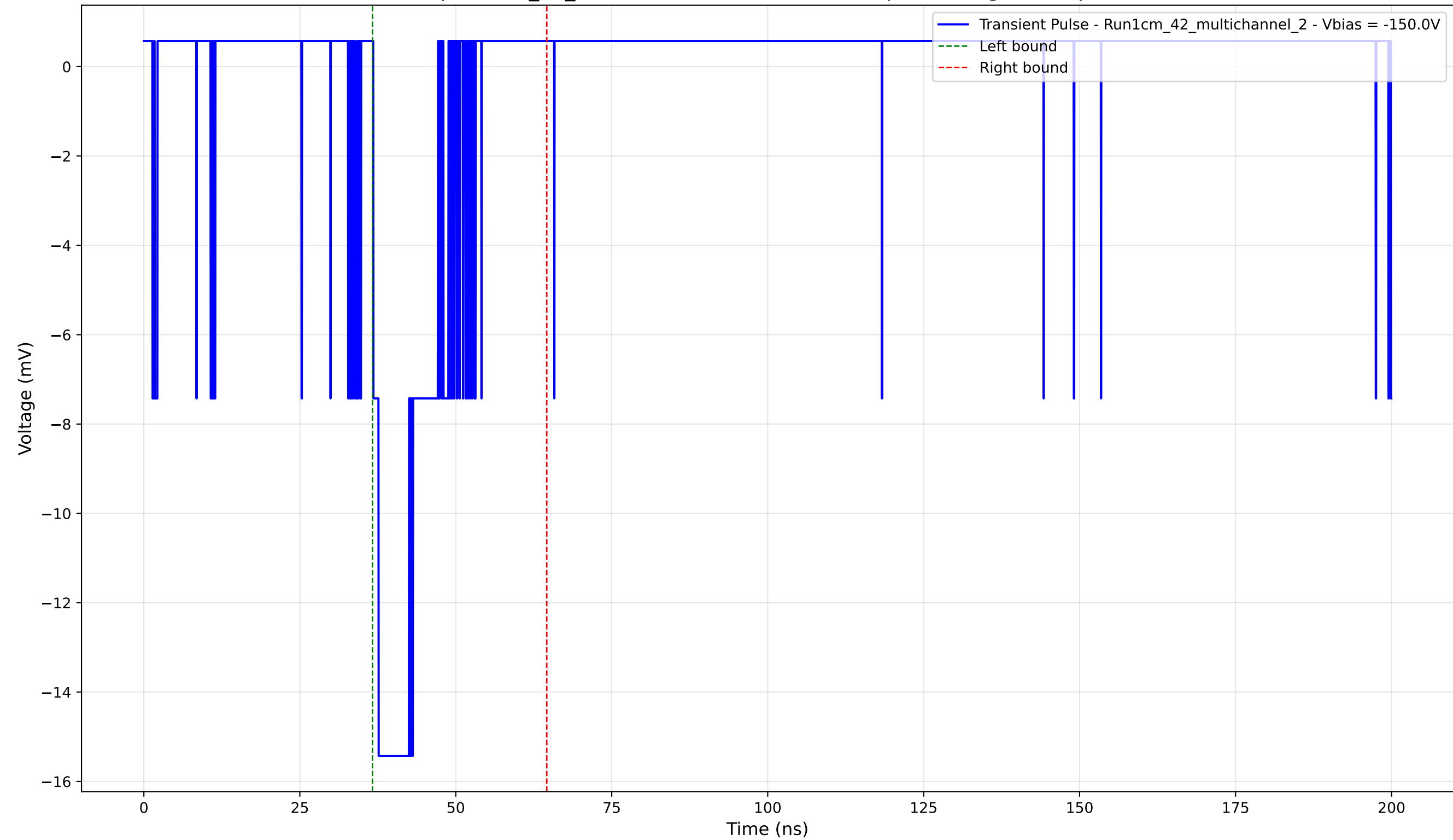
Transient Pulse - Sample: 1cm_42_multichannel - Position: 880.0 \mu\text{m} - Charge: 2.60 pC - Rise Time: 0.87 ns
