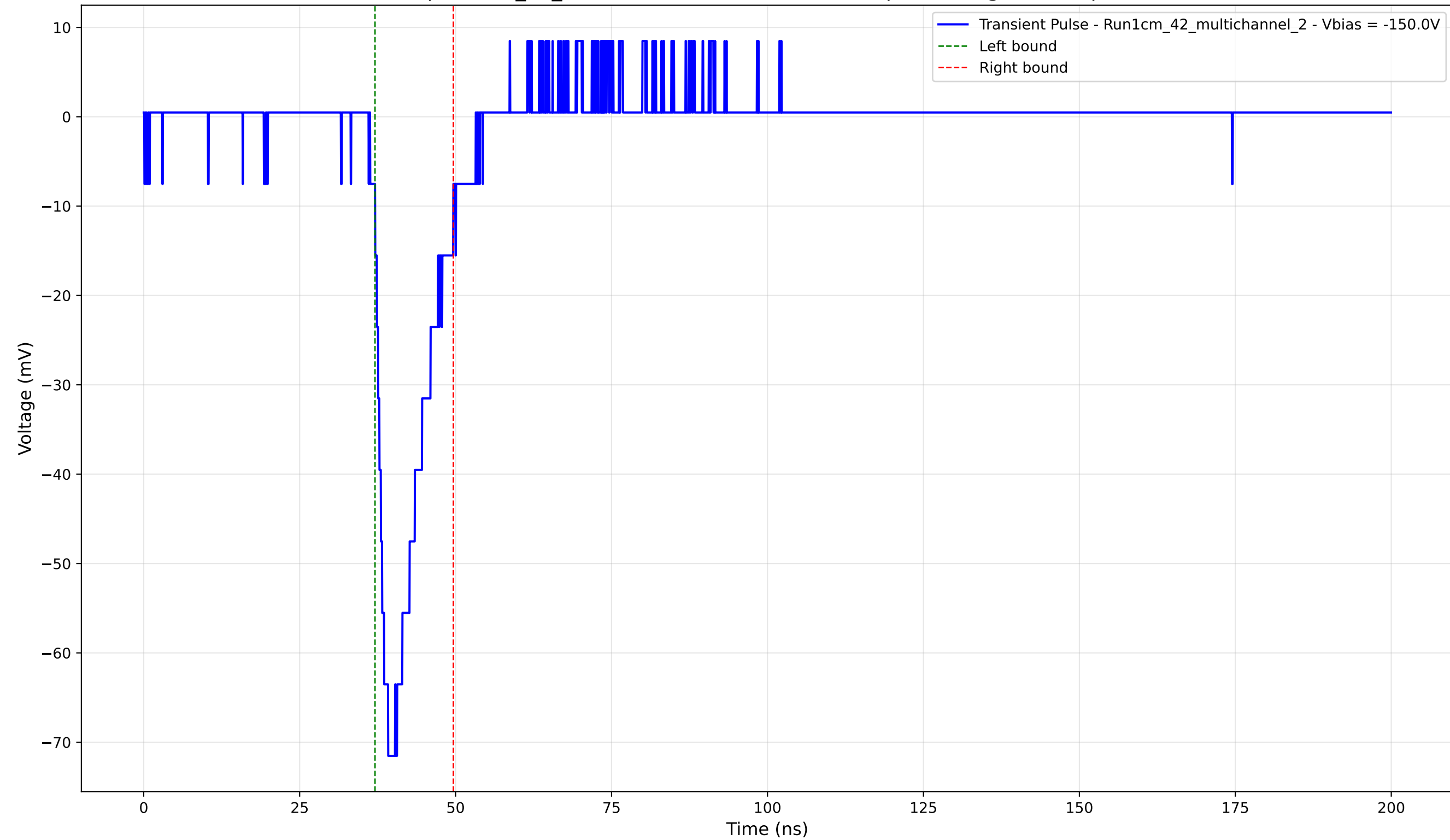
Transient Pulse - Sample: 1cm_42_multichannel - Position: 4665.0 \mu\text{m} - Charge: 10.20 pC - Rise Time: 2.88 ns
