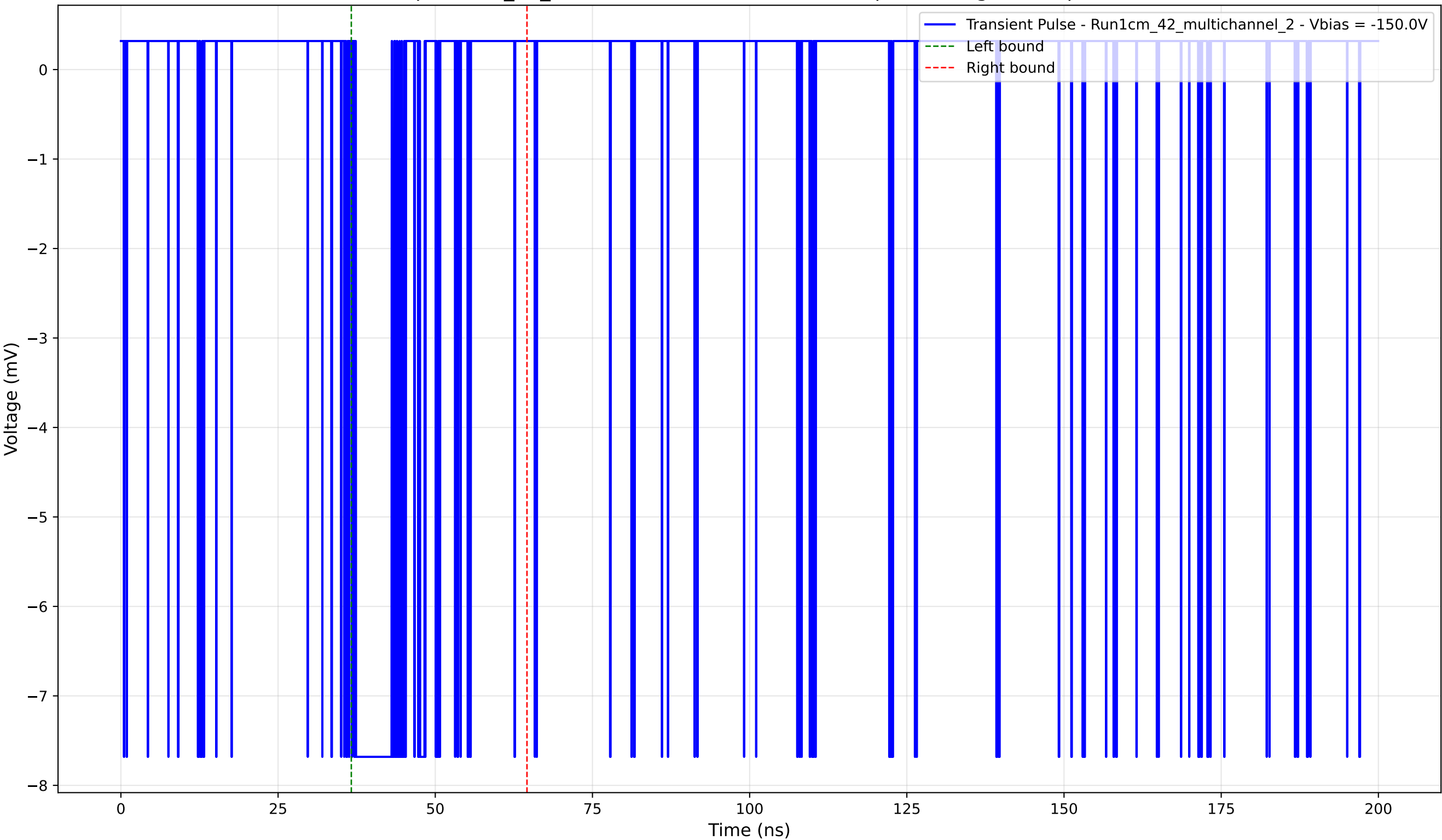
Transient Pulse - Sample: 1cm_42_multichannel - Position: 4880.0 \mu\text{m} - Charge: 1.37 pC - Rise Time: 0.04 ns
