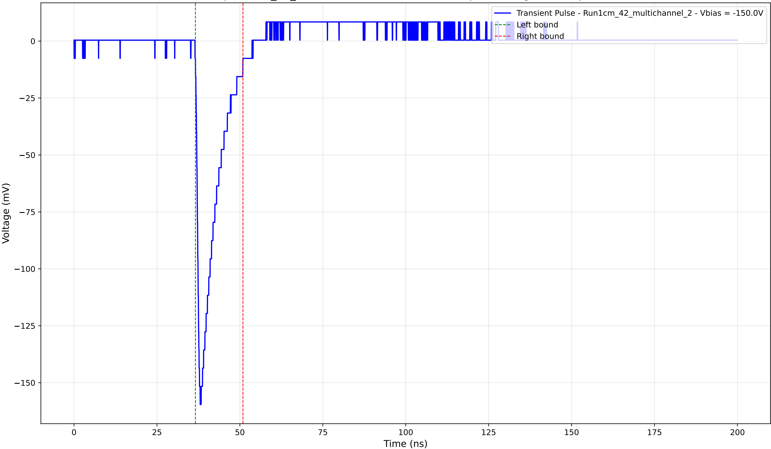
Transient Pulse - Sample: 1cm_42_multichannel - Position: 1260.0 \mu\text{m} - Charge: 18.92 pC - Rise Time: 1.12 ns
