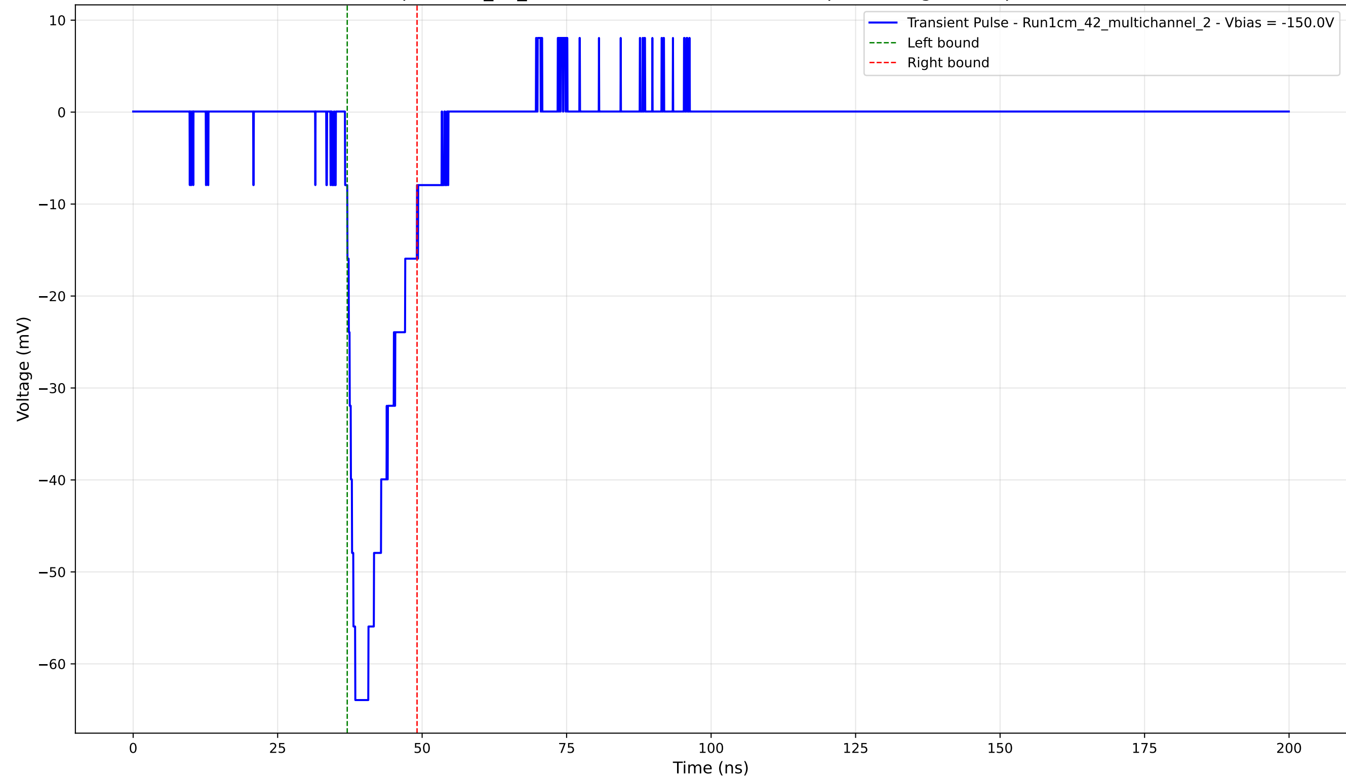
Transient Pulse - Sample: 1cm_42_multichannel - Position: 3945.0 \mu\text{m} - Charge: 9.41 pC - Rise Time: 1.77 ns
