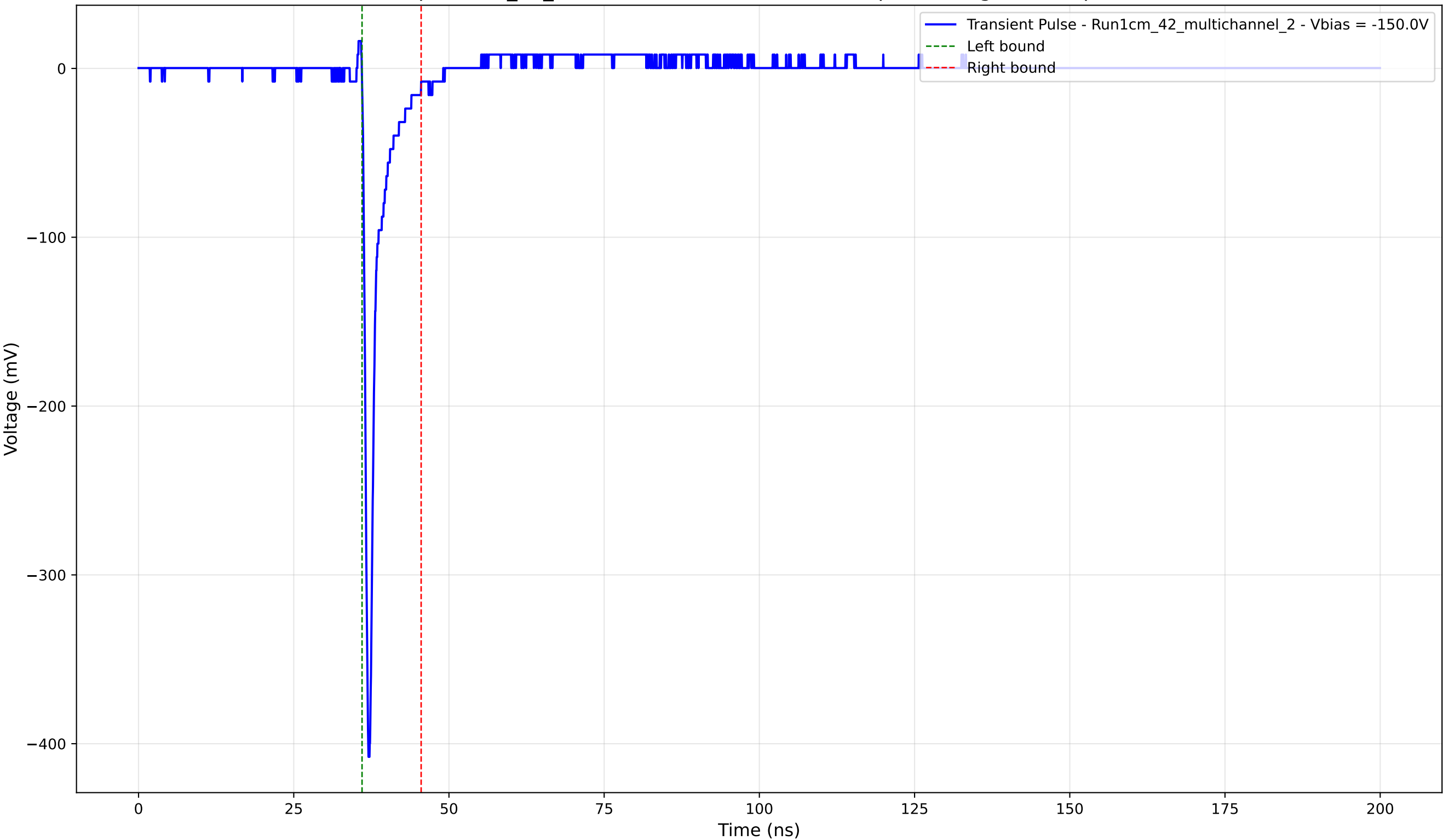
Transient Pulse - Sample: 1cm_42_multichannel - Position: 2425.0 \mu\text{m} - Charge: 17.67 pC - Rise Time: 0.72 ns
