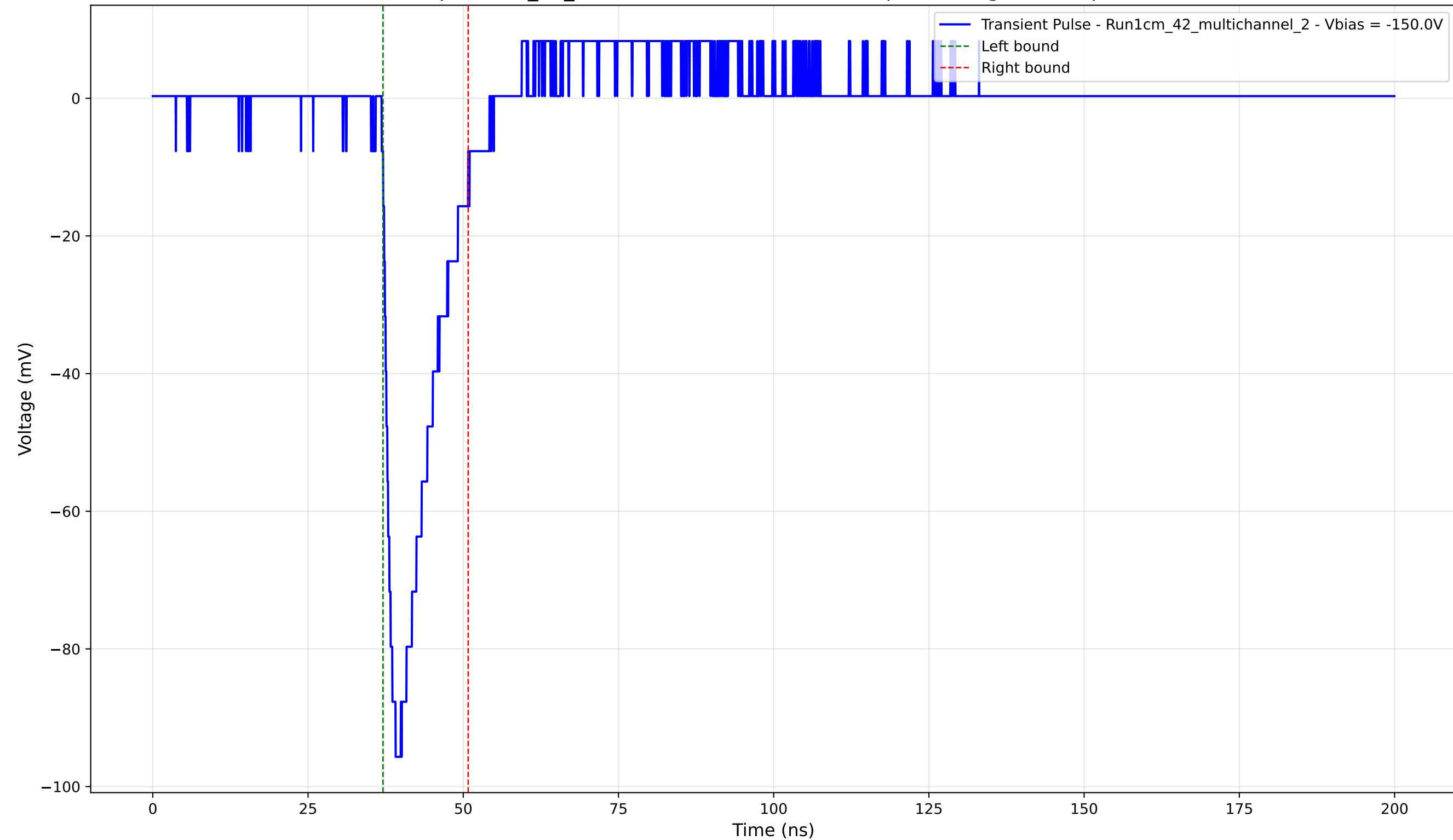
Transient Pulse - Sample: 1cm_42_multichannel - Position: 495.0 \mu\text{m} - Charge: 14.02 pC - Rise Time: 1.51 ns
