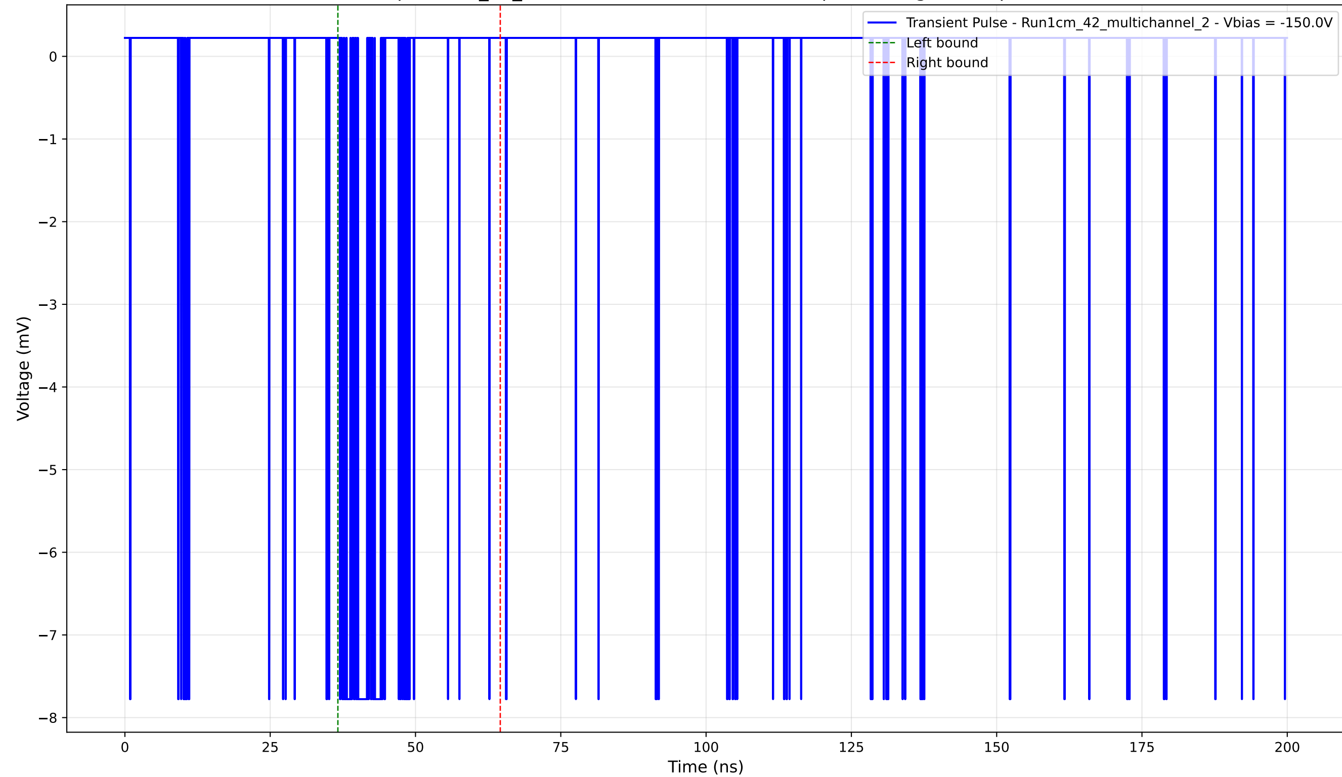
Transient Pulse - Sample: 1cm_42_multichannel - Position: 4915.0 \mu\text{m} - Charge: 0.91 pC - Rise Time: 0.04 ns
