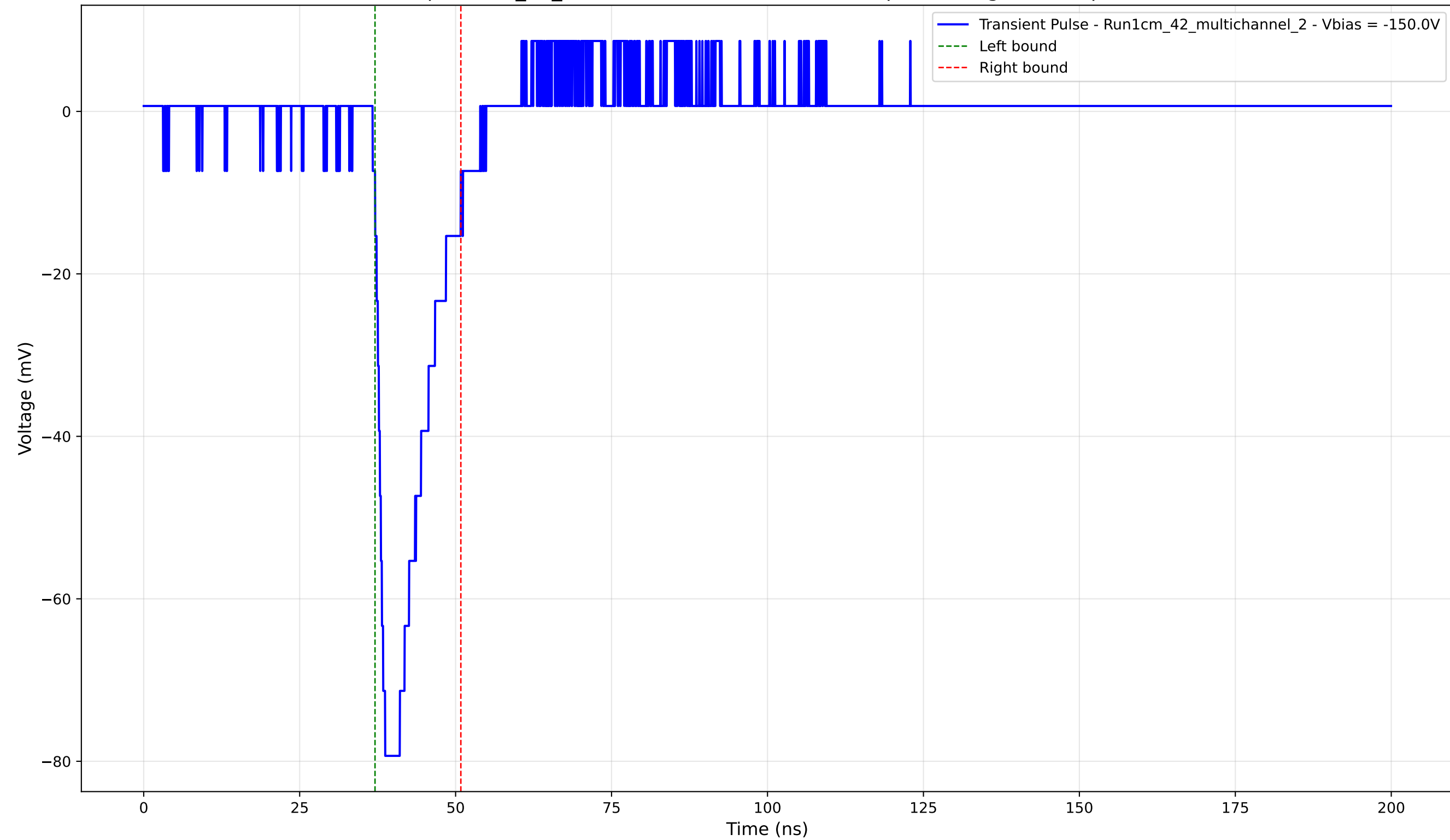
Transient Pulse - Sample: 1cm_42_multichannel - Position: 4185.0 \mu\text{m} - Charge: 12.30 pC - Rise Time: 1.64 ns
