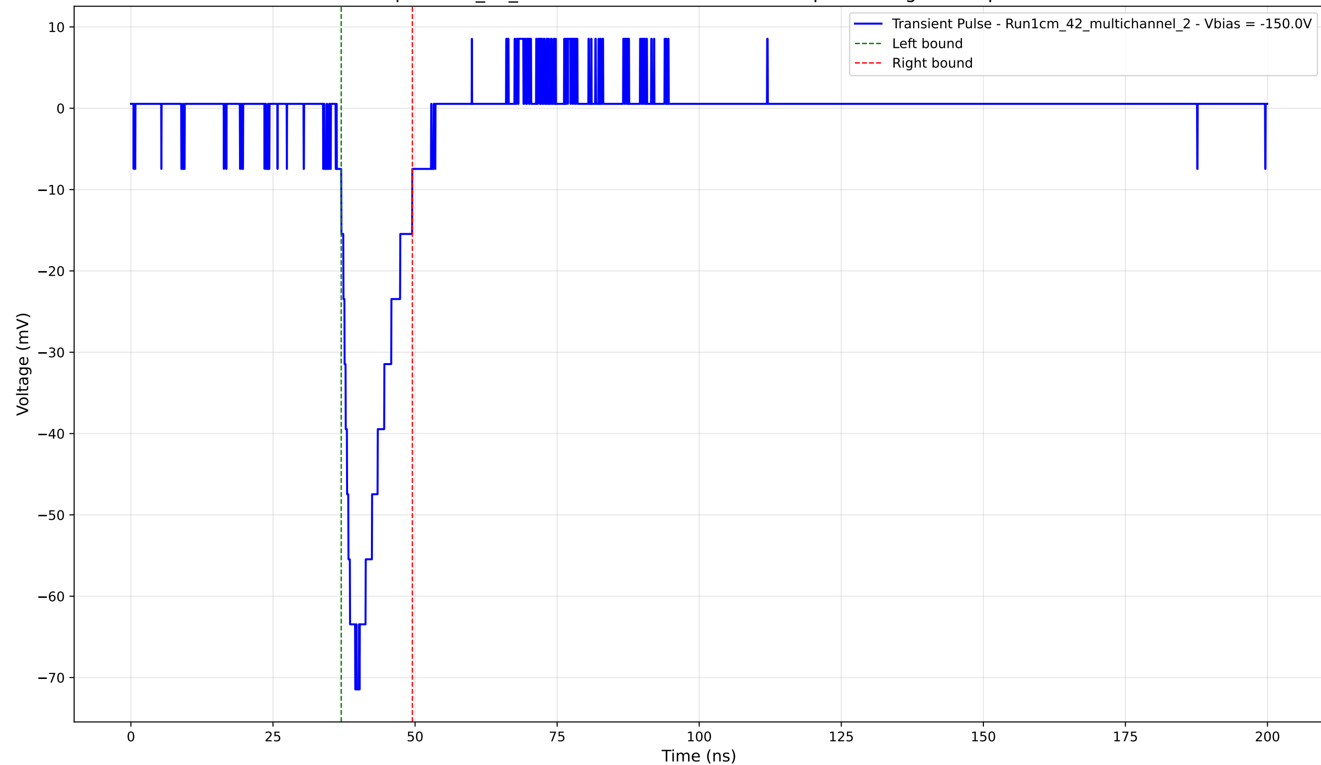
Transient Pulse - Sample: 1cm_42_multichannel - Position: 4710.0 \mu\text{m} - Charge: 9.94 pC - Rise Time: 3.24 ns
