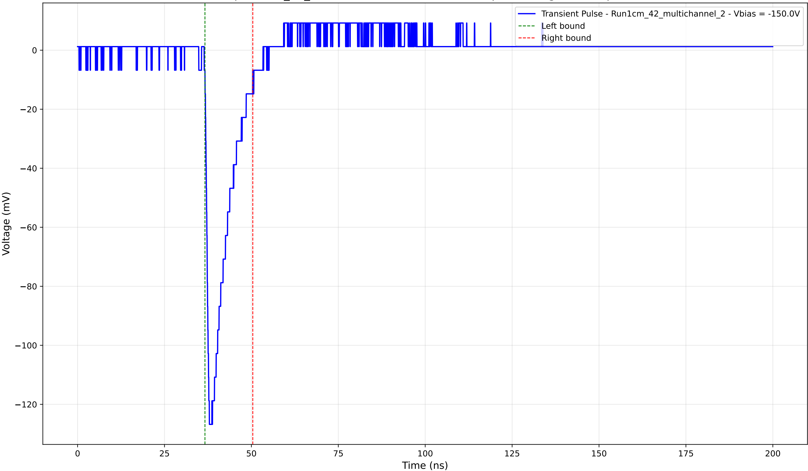
Transient Pulse - Sample: 1cm_42_multichannel - Position: 3515.0 \mu\text{m} - Charge: 16.17 pC - Rise Time: 1.09 ns
