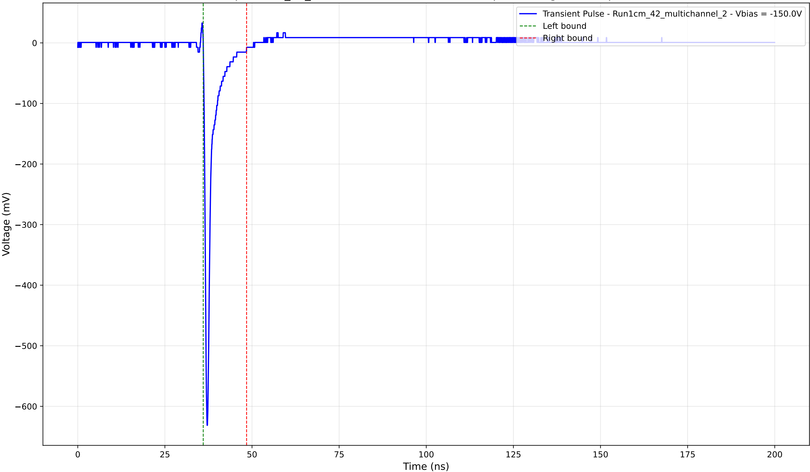
Transient Pulse - Sample: 1cm_42_multichannel - Position: 2280.0 \mu\text{m} - Charge: 28.28 pC - Rise Time: 0.73 ns
