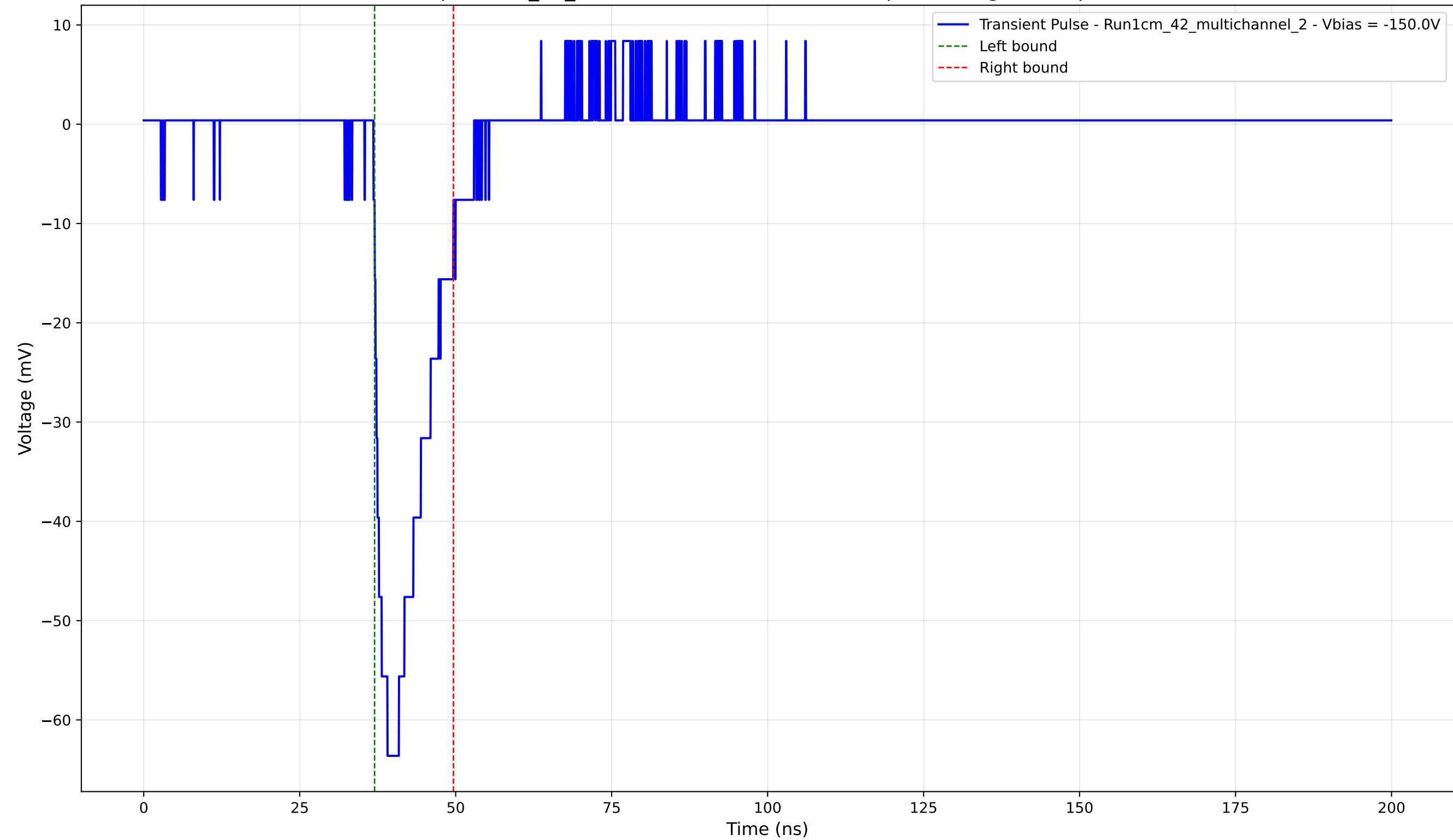
Transient Pulse - Sample: 1cm_42_multichannel - Position: 115.0 \mu\text{m} - Charge: 9.83 pC - Rise Time: 2.25 ns
