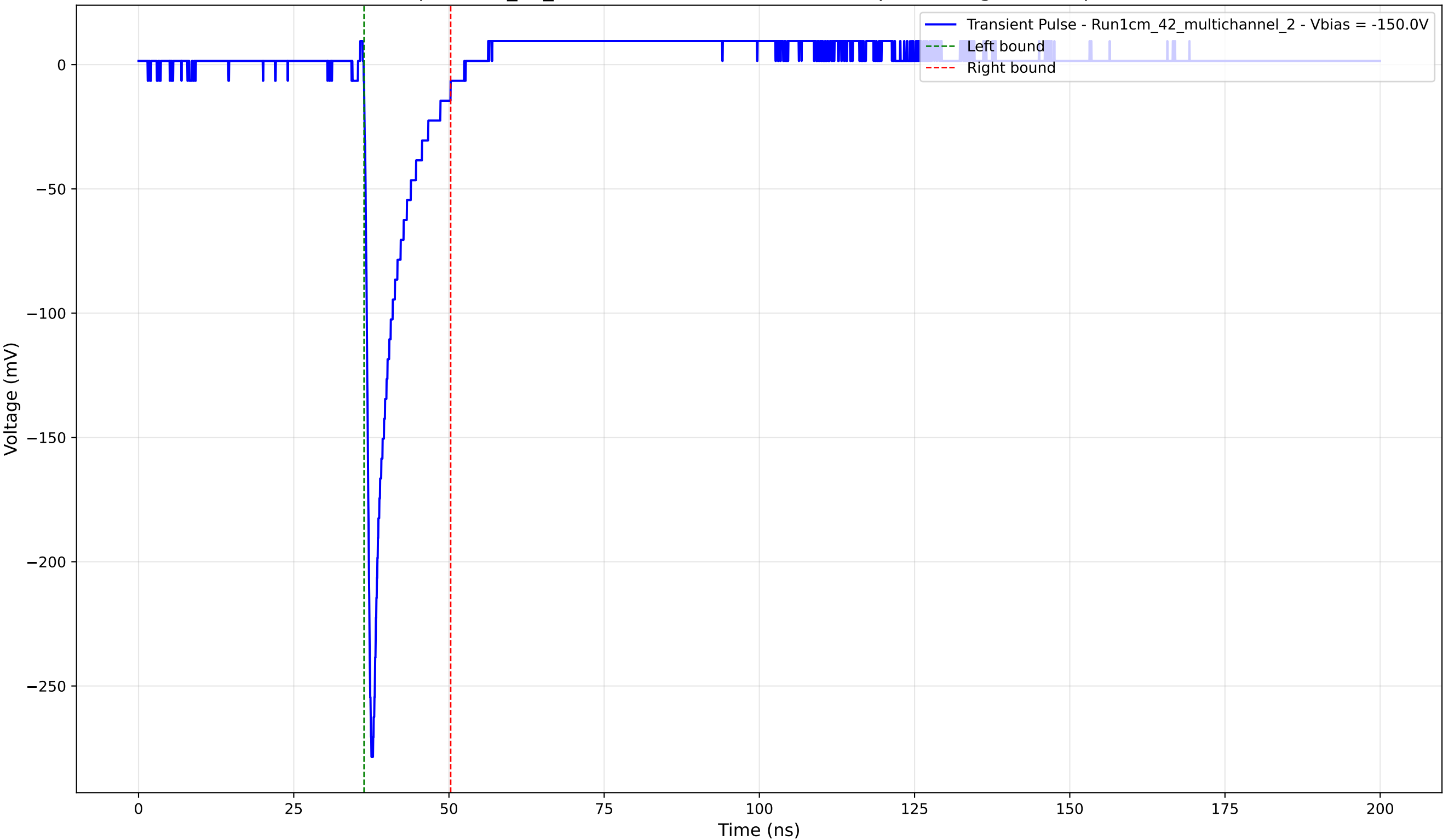
Transient Pulse - Sample: 1cm_42_multichannel - Position: 1705.0 \mu\text{m} - Charge: 22.95 pC - Rise Time: 0.89 ns
