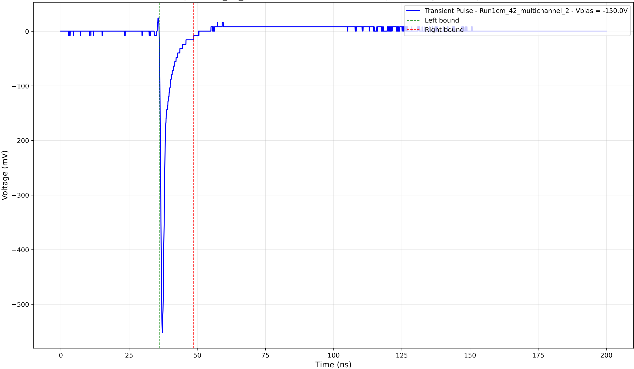
Transient Pulse - Sample: 1cm_42_multichannel - Position: 2525.0 \mu\text{m} - Charge: 26.35 pC - Rise Time: 0.76 ns
