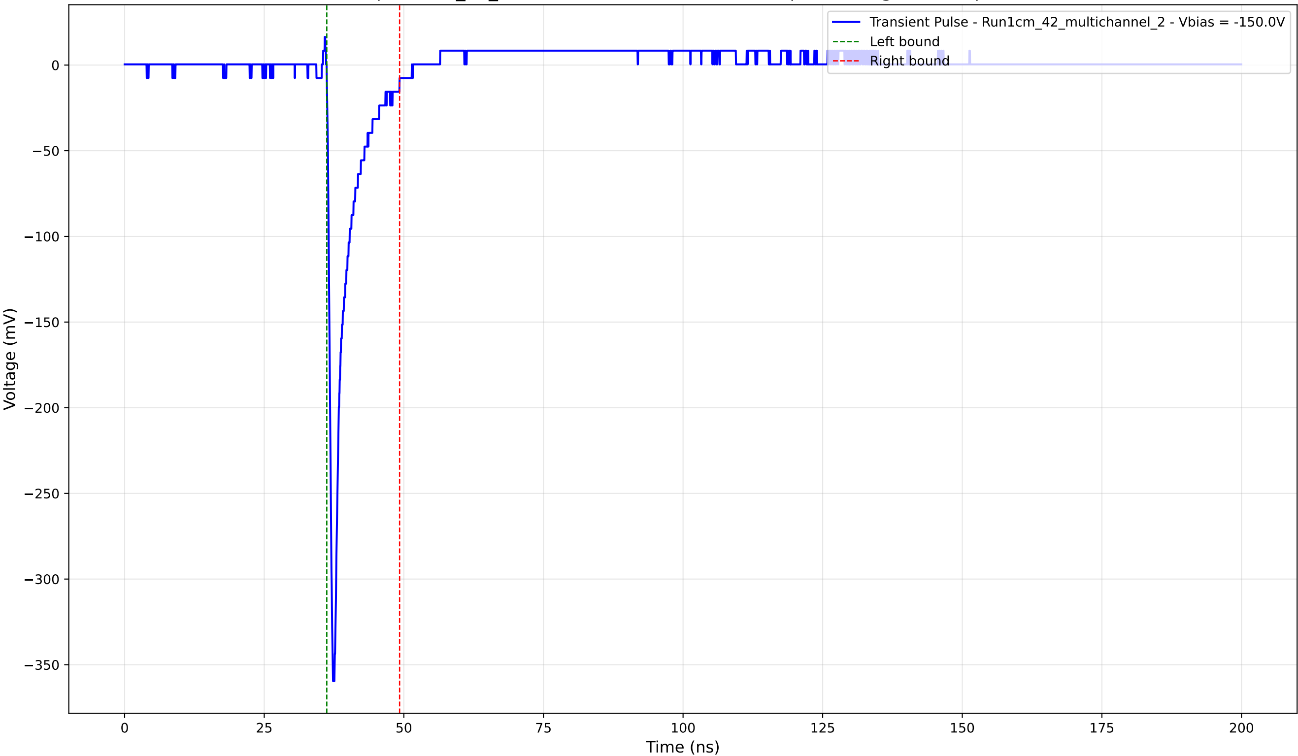
Transient Pulse - Sample: 1cm_42_multichannel - Position: 1945.0 \mu\text{m} - Charge: 23.00 pC - Rise Time: 0.80 ns
