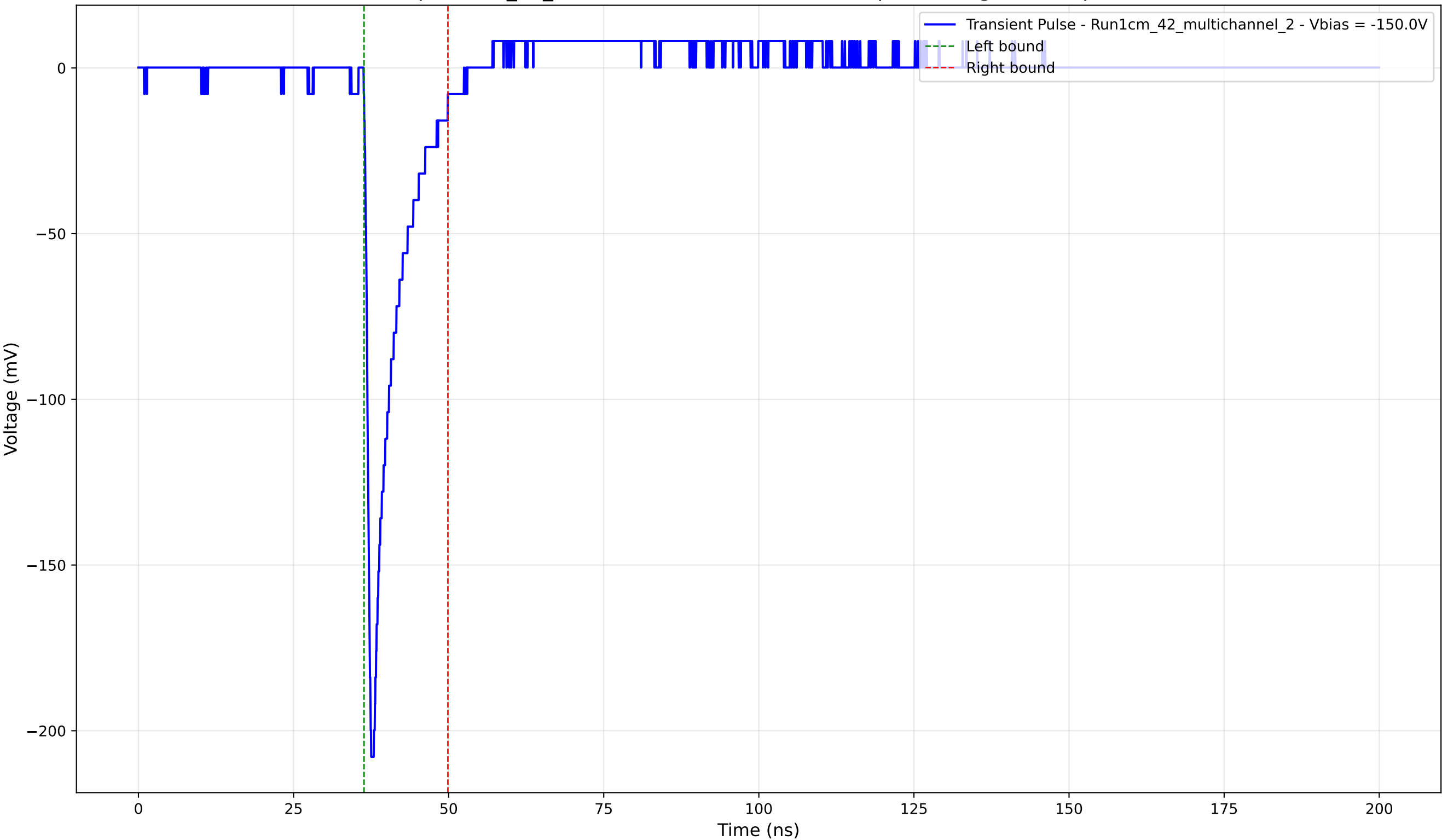
Transient Pulse - Sample: 1cm_42_multichannel - Position: 3115.0 \mu\text{m} - Charge: 19.13 pC - Rise Time: 0.91 ns
