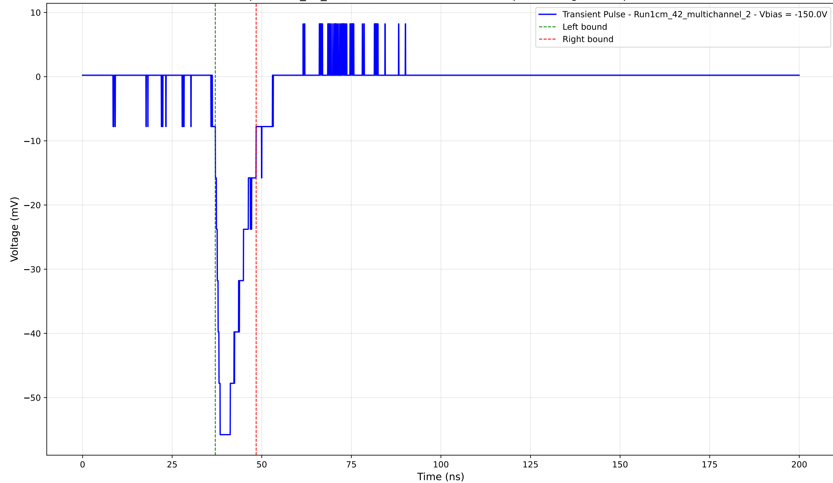
Transient Pulse - Sample: 1cm_42_multichannel - Position: 4805.0 \mu\text{m} - Charge: 8.30 pC - Rise Time: 2.17 ns
