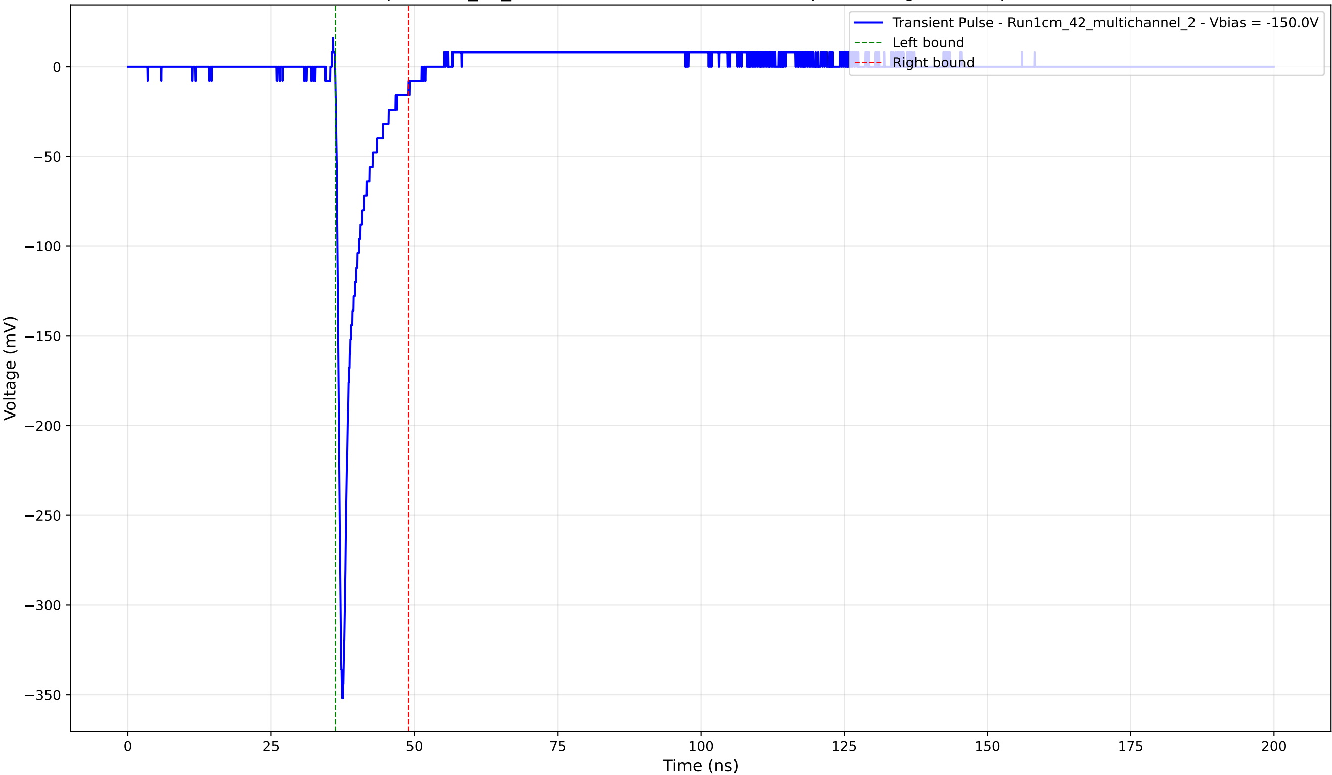
Transient Pulse - Sample: 1cm_42_multichannel - Position: 1940.0 \mu\text{m} - Charge: 22.38 pC - Rise Time: 0.81 ns
