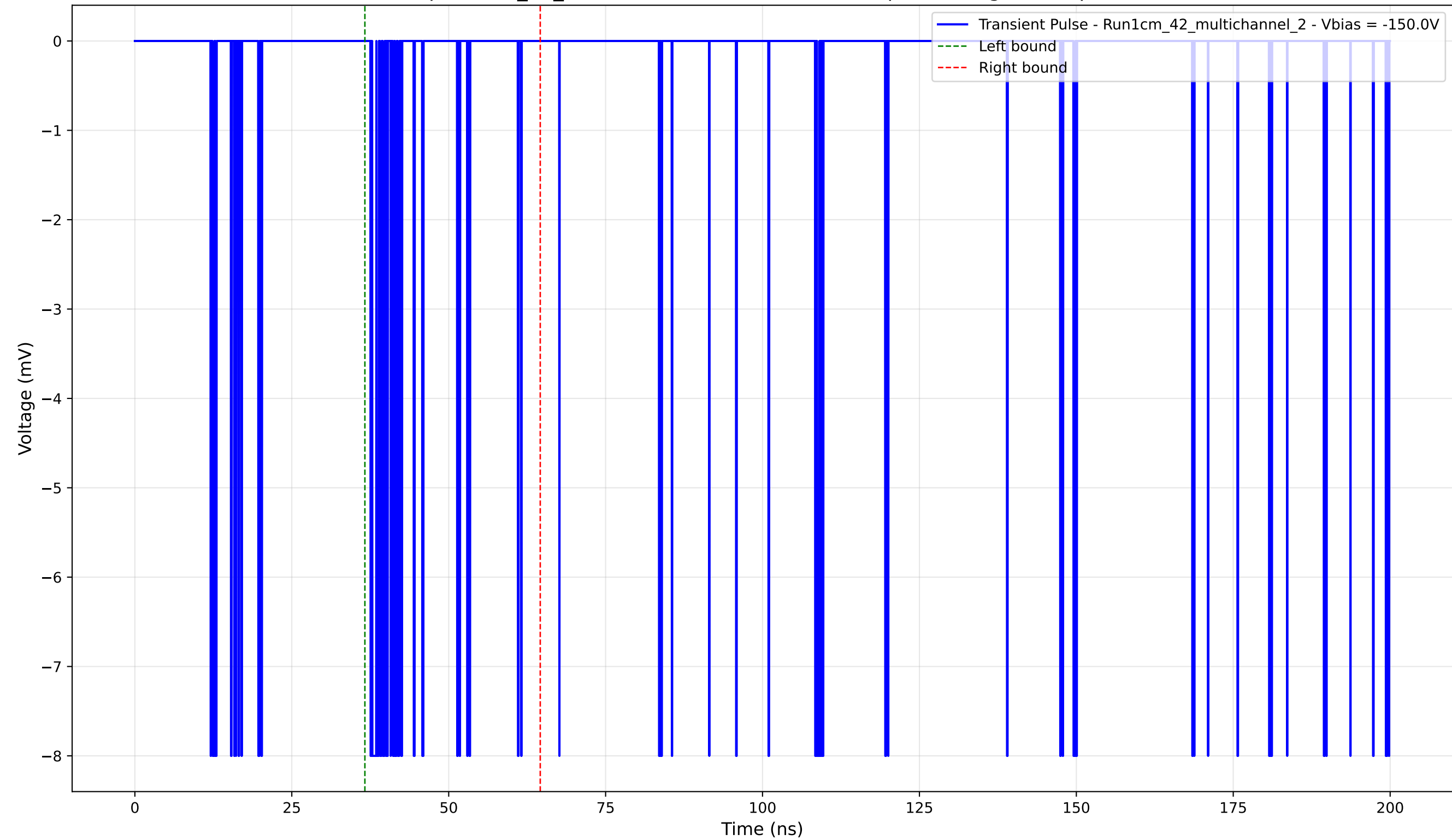
Transient Pulse - Sample: 1cm_42_multichannel - Position: 4900.0 \mu\text{m} - Charge: 0.60 pC - Rise Time: 0.04 ns
