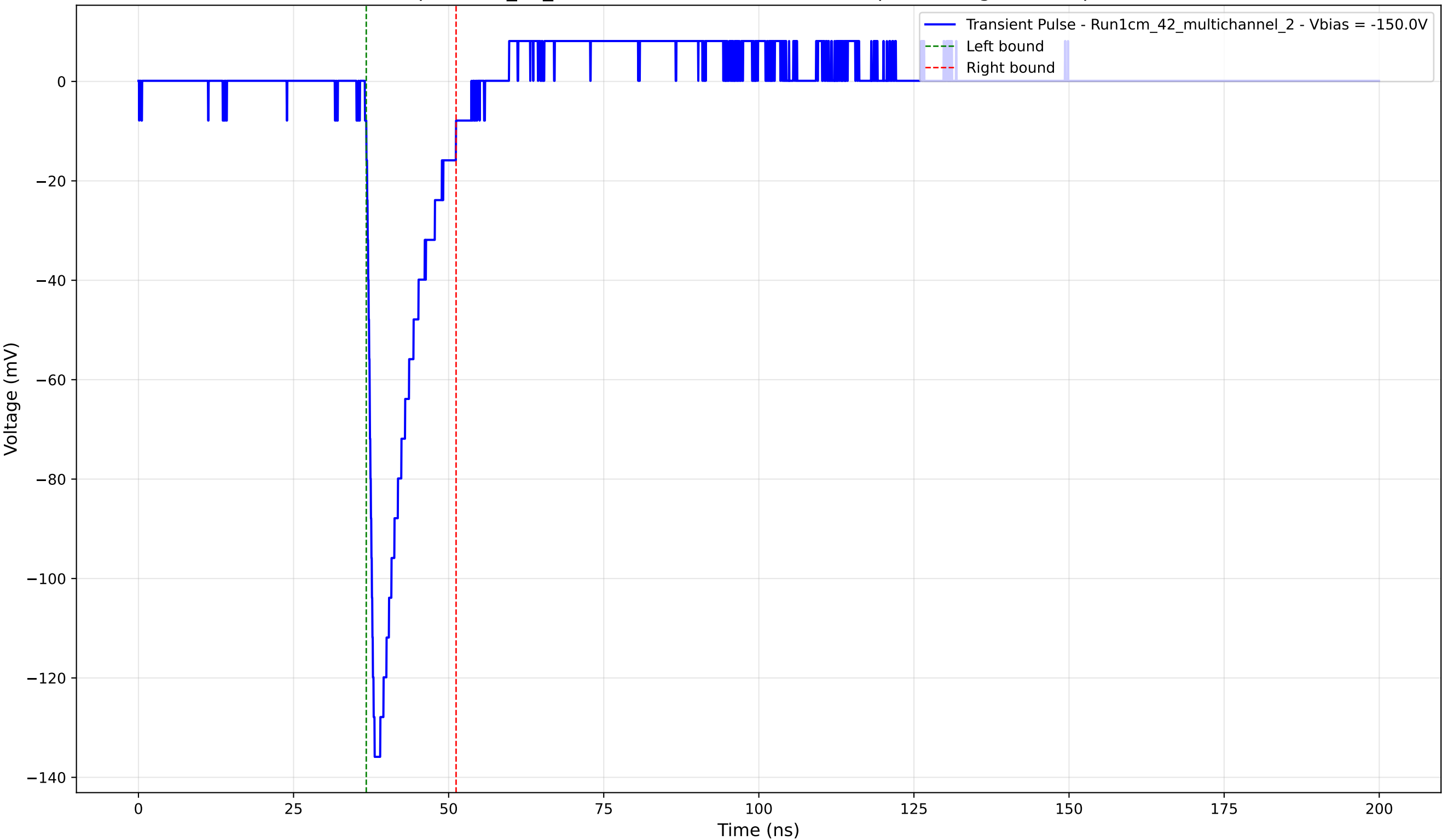
Transient Pulse - Sample: 1cm_42_multichannel - Position: 1135.0 \mu\text{m} - Charge: 17.89 pC - Rise Time: 1.17 ns
