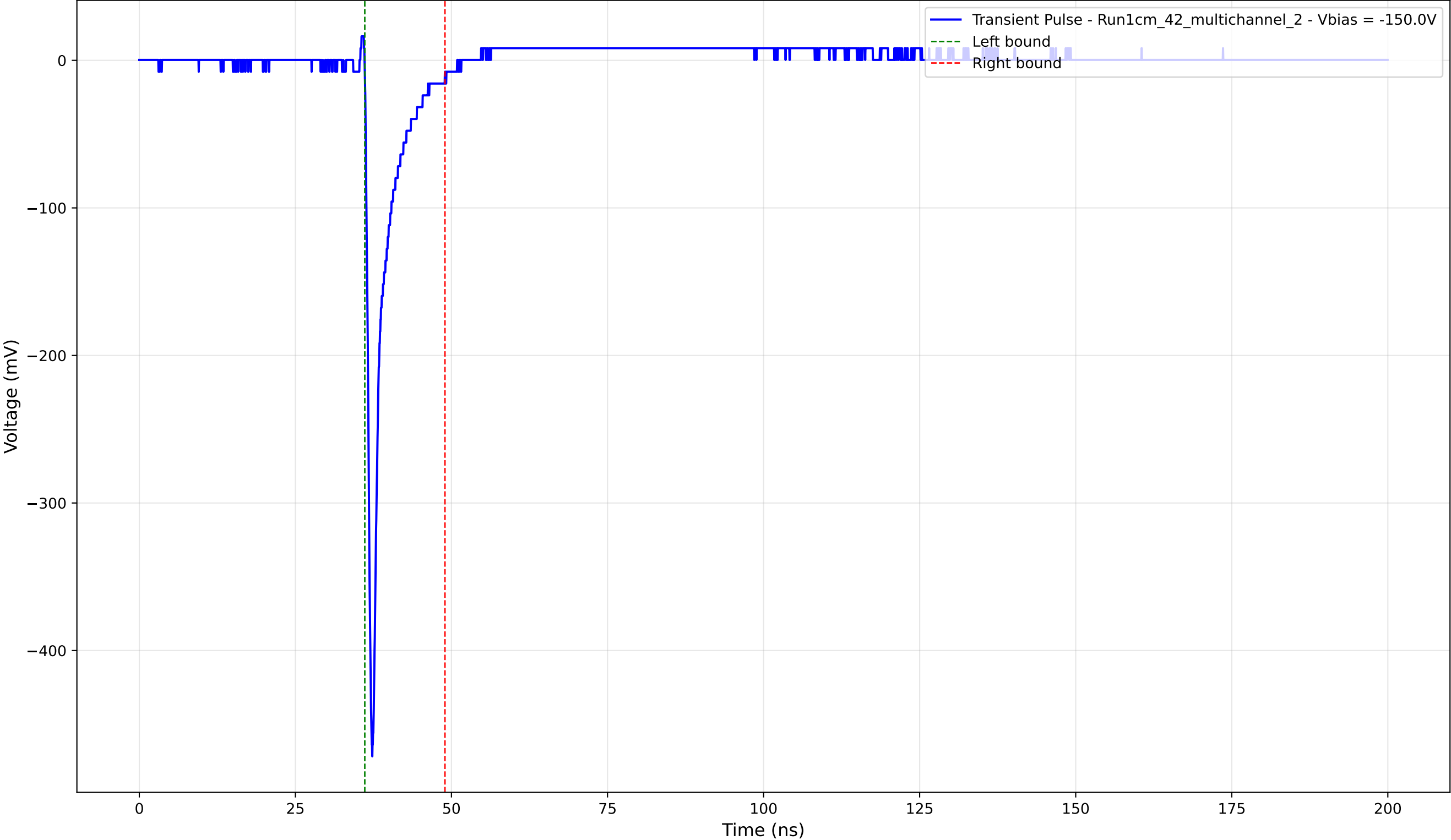
Transient Pulse - Sample: 1cm_42_multichannel - Position: 2070.0 \mu\text{m} - Charge: 25.97 pC - Rise Time: 0.77 ns
