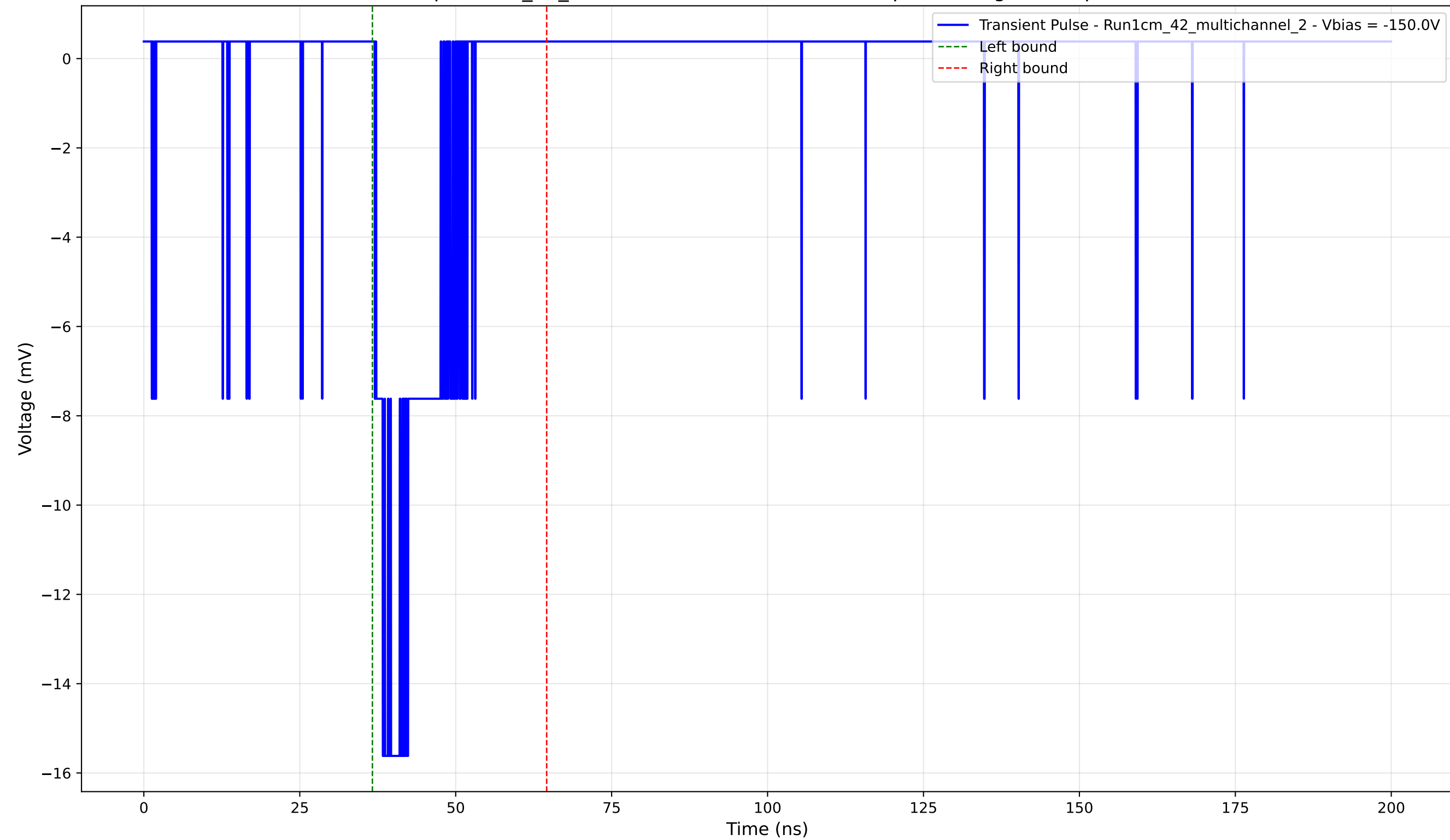
Transient Pulse - Sample: 1cm_42_multichannel - Position: 4355.0 \mu\text{m} - Charge: 2.37 pC - Rise Time: 1.07 ns
