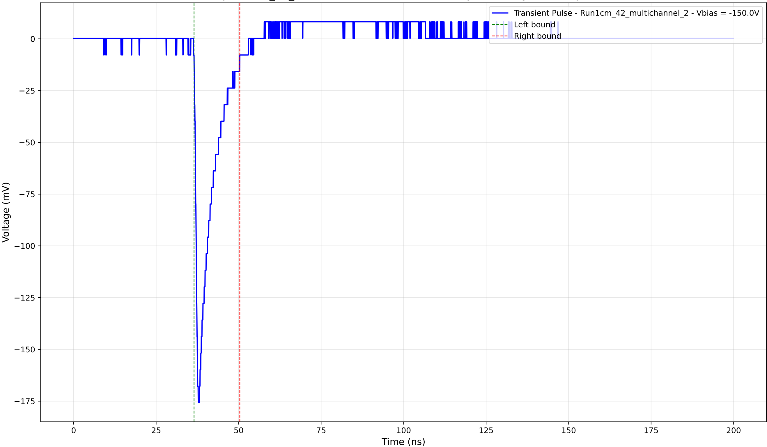
Transient Pulse - Sample: 1cm_42_multichannel - Position: 3275.0 \mu\text{m} - Charge: 18.47 pC - Rise Time: 0.95 ns
