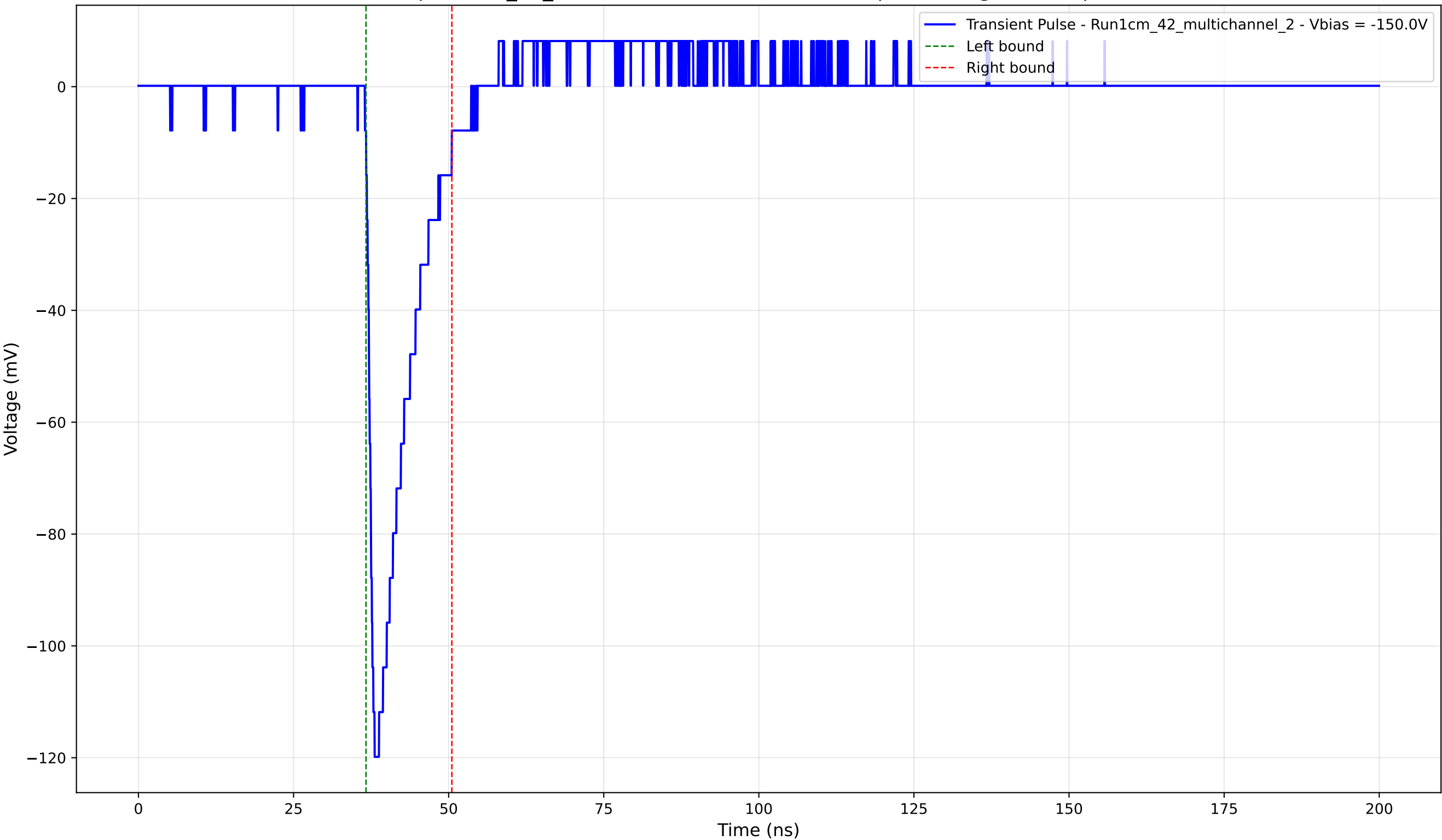
Transient Pulse - Sample: 1cm_42_multichannel - Position: 3565.0 \mu\text{m} - Charge: 15.51 pC - Rise Time: 1.18 ns
