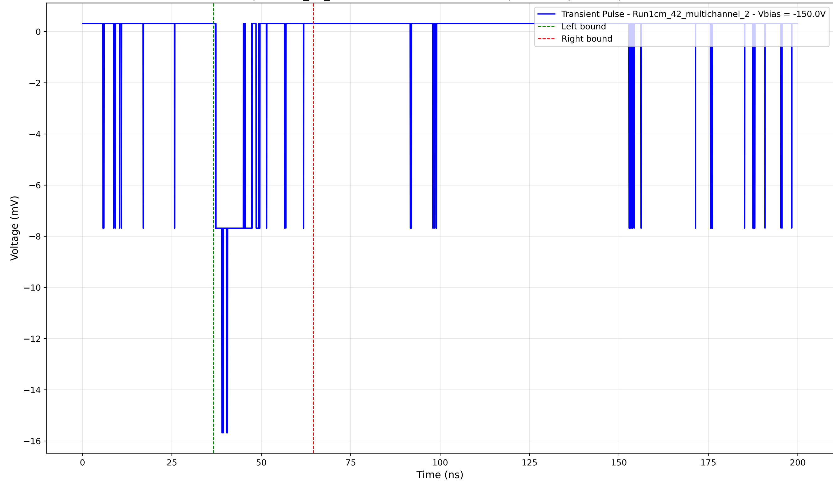
Transient Pulse - Sample: 1cm_42_multichannel - Position: 320.0 \mu\text{m} - Charge: 1.66 pC - Rise Time: 1.71 ns
