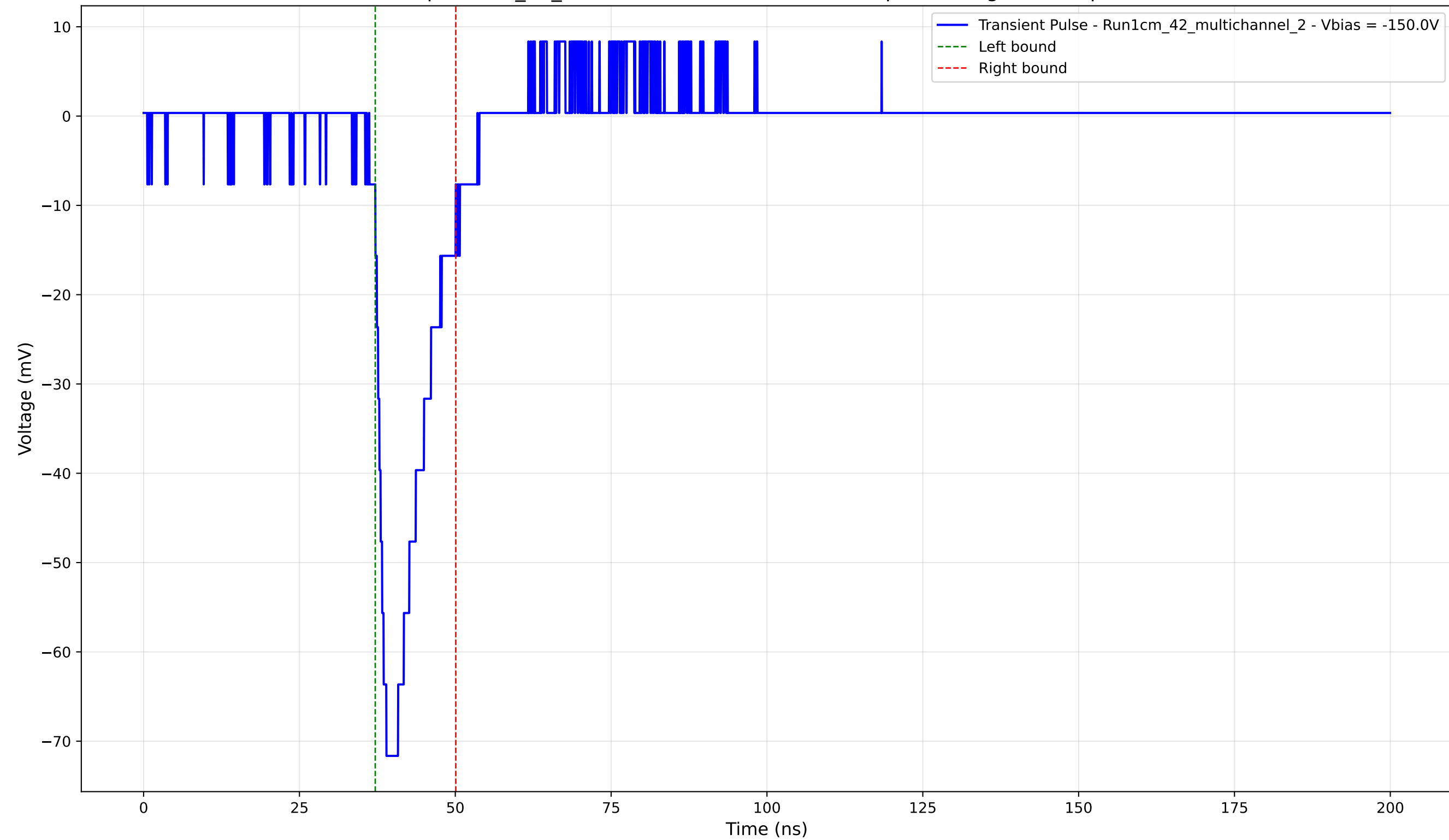
Transient Pulse - Sample: 1cm_42_multichannel - Position: 4555.0 \mu\text{m} - Charge: 10.61 pC - Rise Time: 2.72 ns
