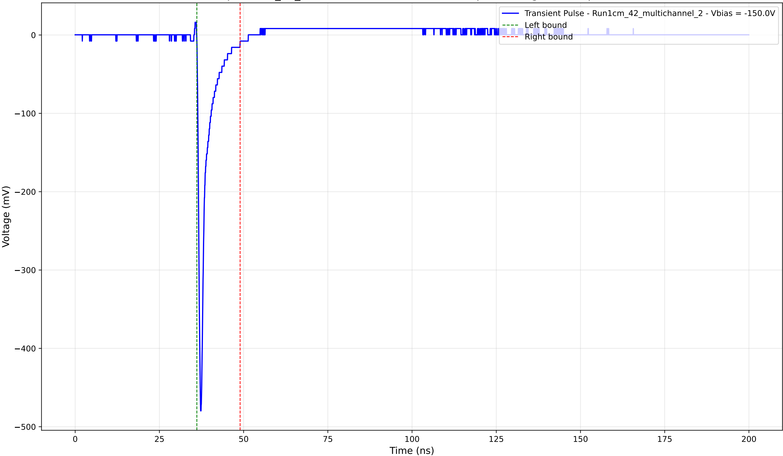
Transient Pulse - Sample: 1cm_42_multichannel - Position: 2090.0 \mu\text{m} - Charge: 26.21 pC - Rise Time: 0.74 ns
