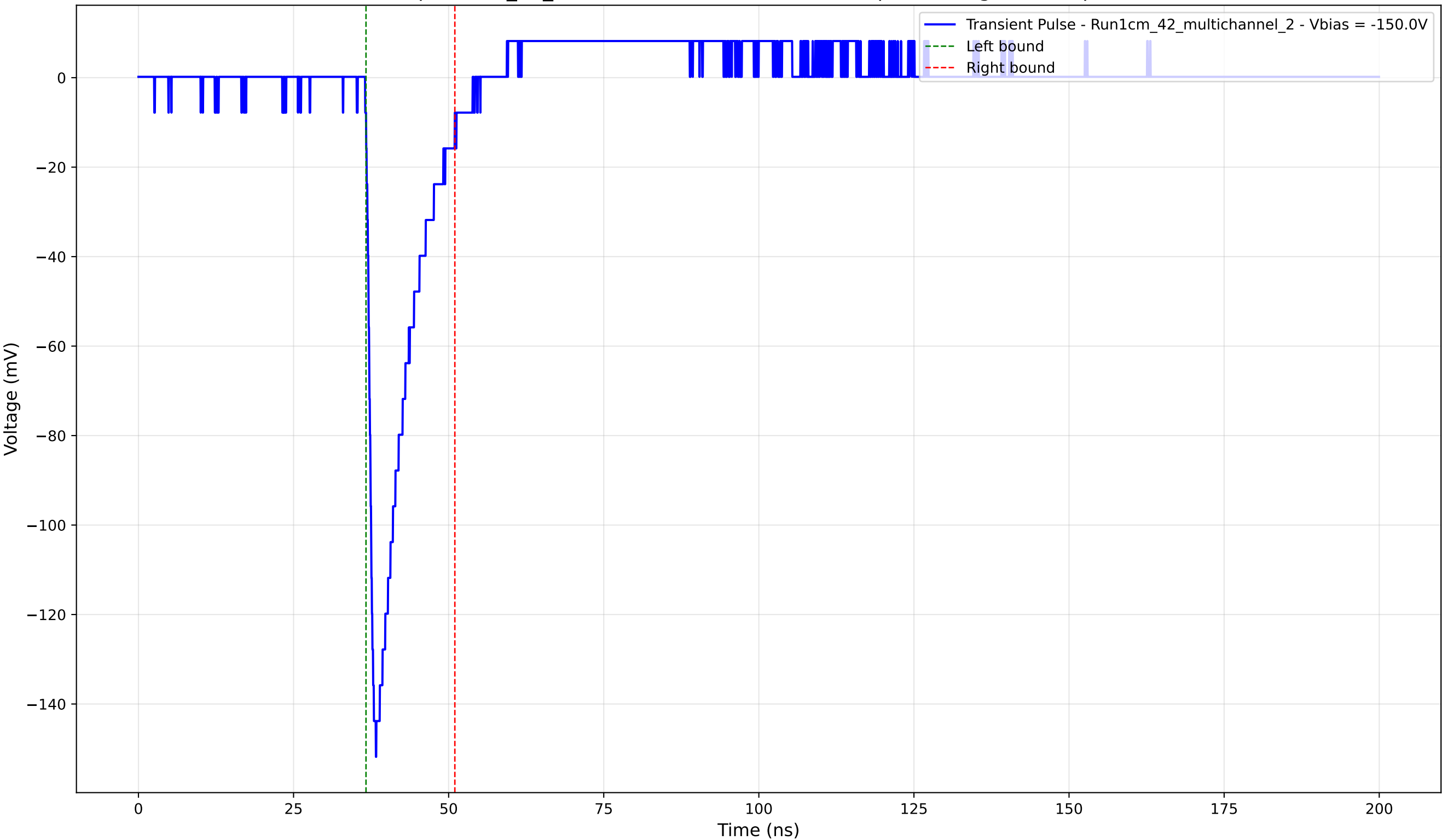
Transient Pulse - Sample: 1cm_42_multichannel - Position: 1185.0 \mu\text{m} - Charge: 18.61 pC - Rise Time: 1.24 ns
