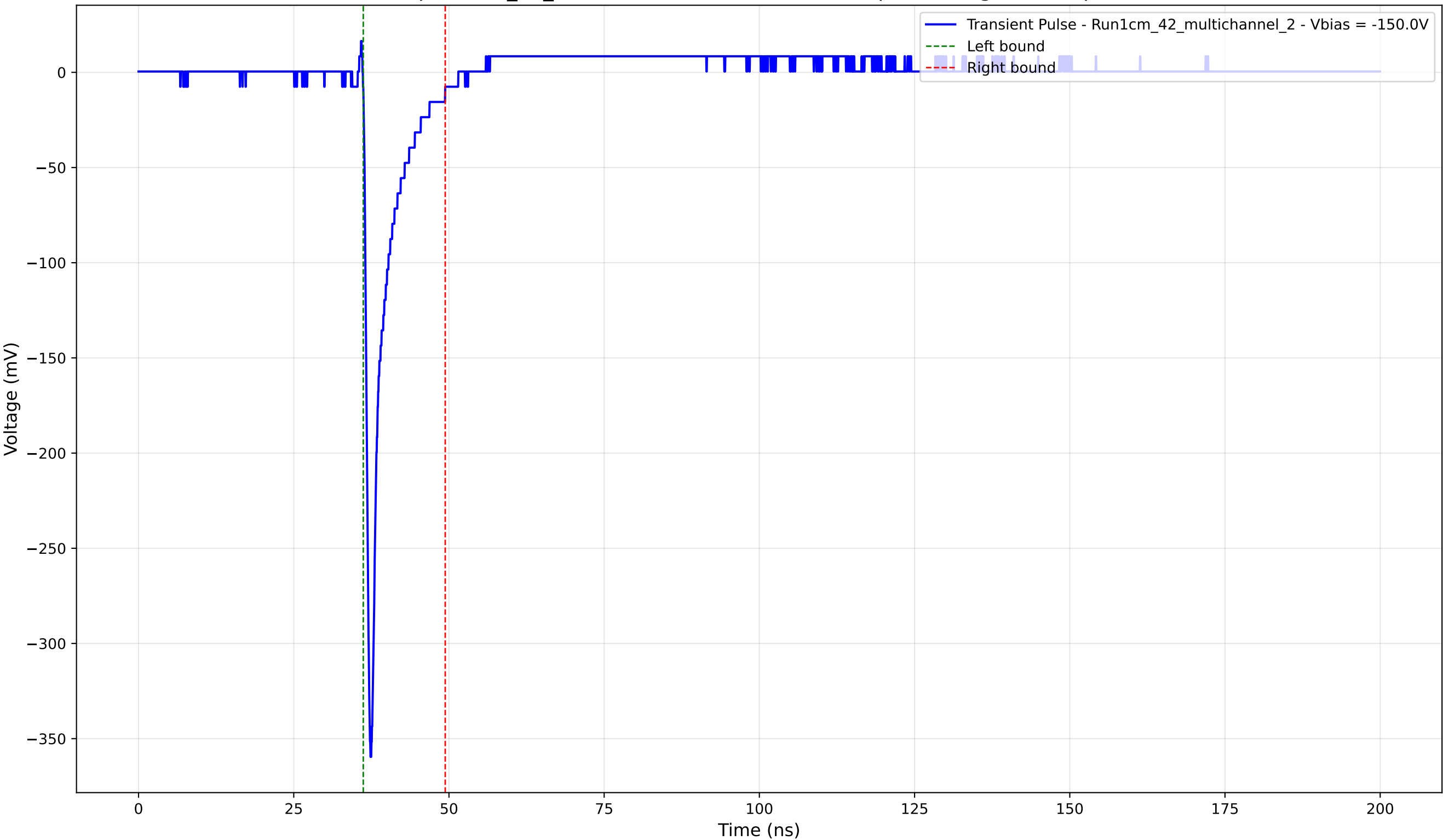
Transient Pulse - Sample: 1cm_42_multichannel - Position: 2785.0 \mu\text{m} - Charge: 22.64 pC - Rise Time: 0.80 ns
