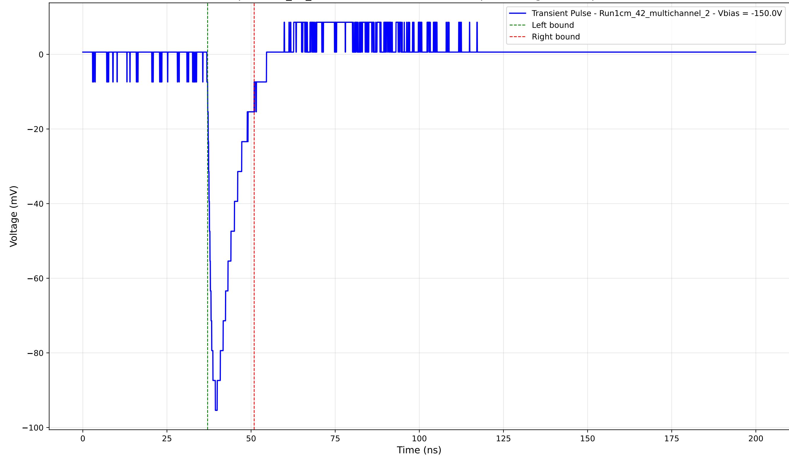
Transient Pulse - Sample: 1cm_42_multichannel - Position: 465.0 \mu\text{m} - Charge: 13.77 pC - Rise Time: 1.59 ns
