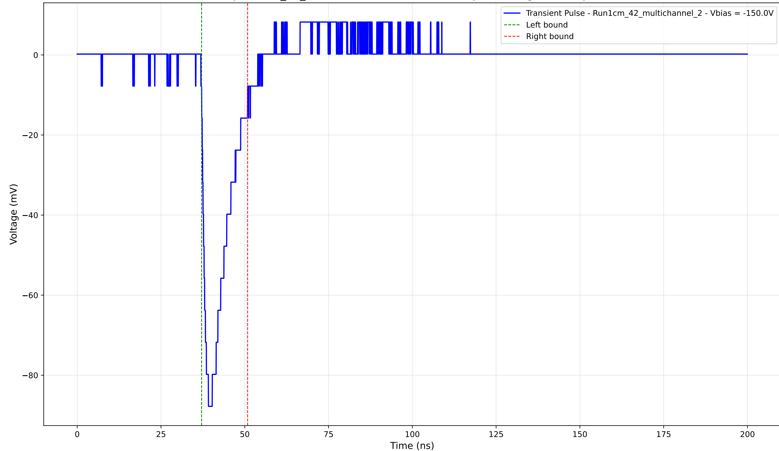
Transient Pulse - Sample: 1cm_42_multichannel - Position: 430.0 \mu\text{m} - Charge: 13.13 pC - Rise Time: 1.43 ns
