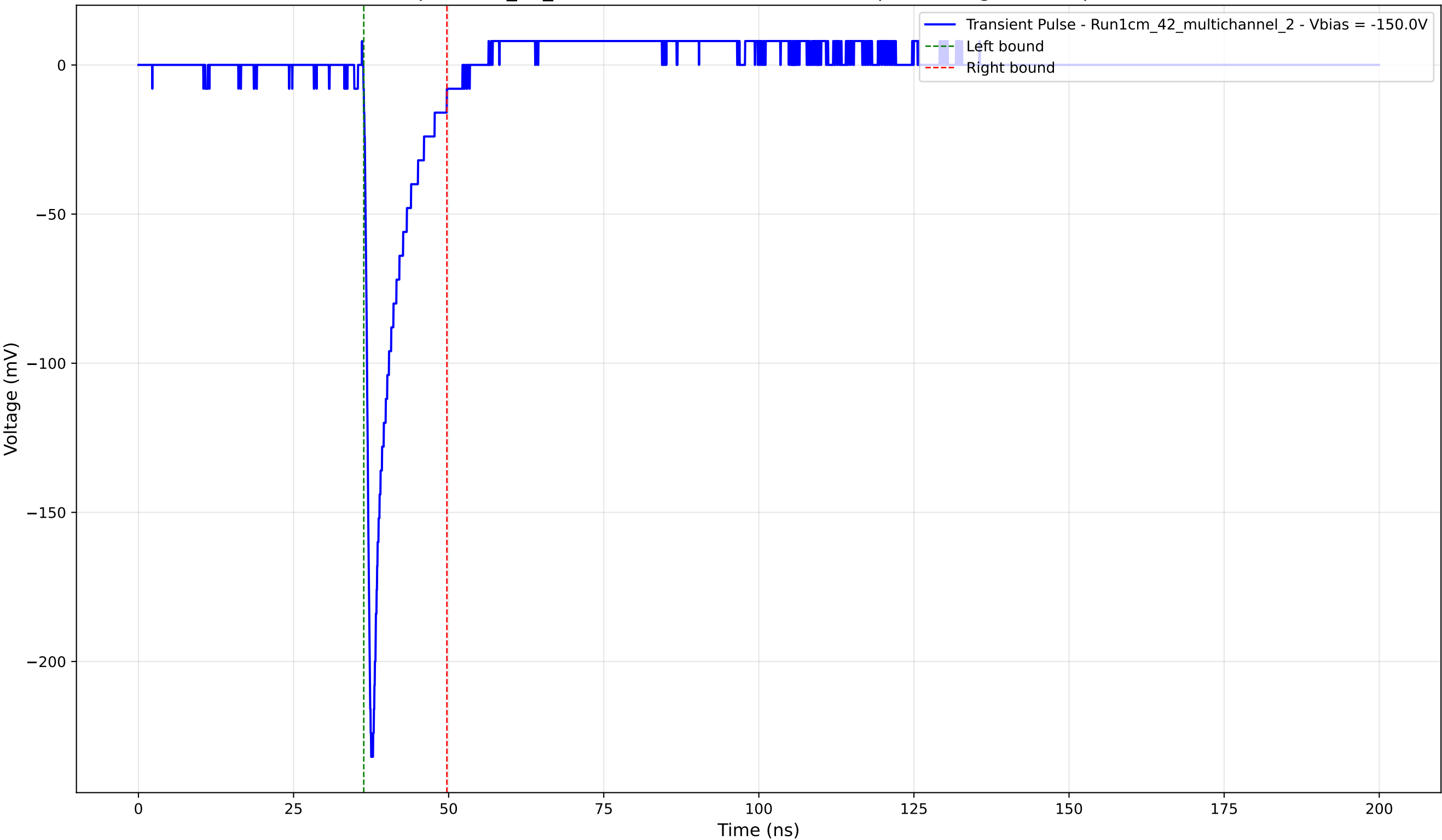
Transient Pulse - Sample: 1cm_42_multichannel - Position: 3055.0 \mu\text{m} - Charge: 19.67 pC - Rise Time: 0.92 ns
