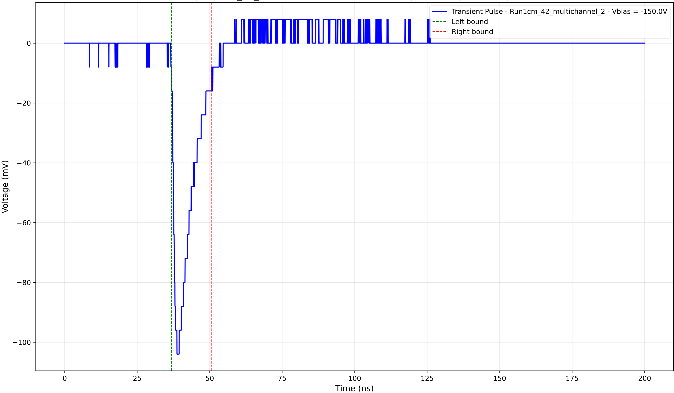
Transient Pulse - Sample: 1cm_42_multichannel - Position: 3795.0 \mu\text{m} - Charge: 14.36 pC - Rise Time: 1.39 ns
