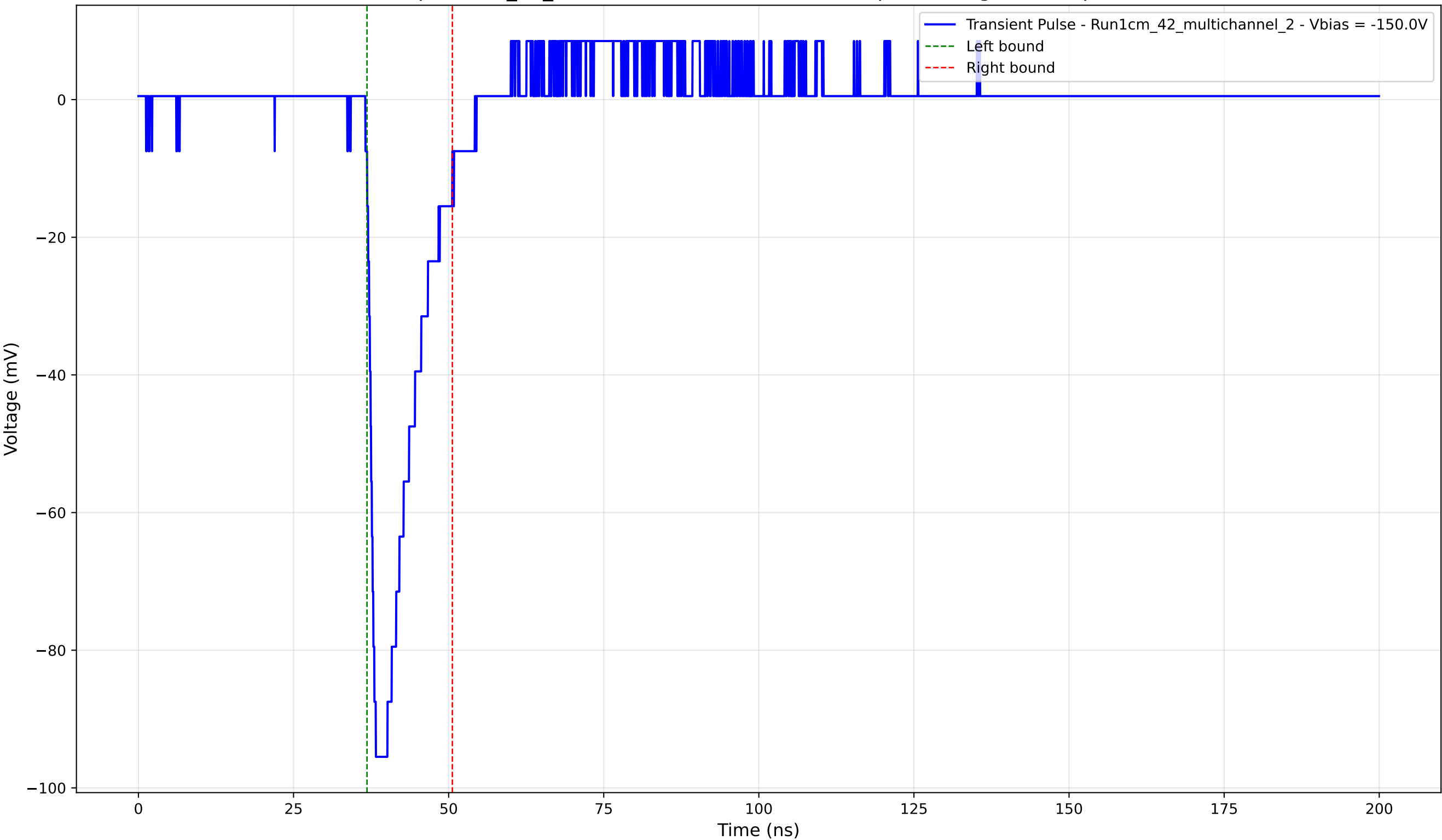
Transient Pulse - Sample: 1cm_42_multichannel - Position: 3800.0 \mu\text{m} - Charge: 13.91 pC - Rise Time: 1.19 ns
