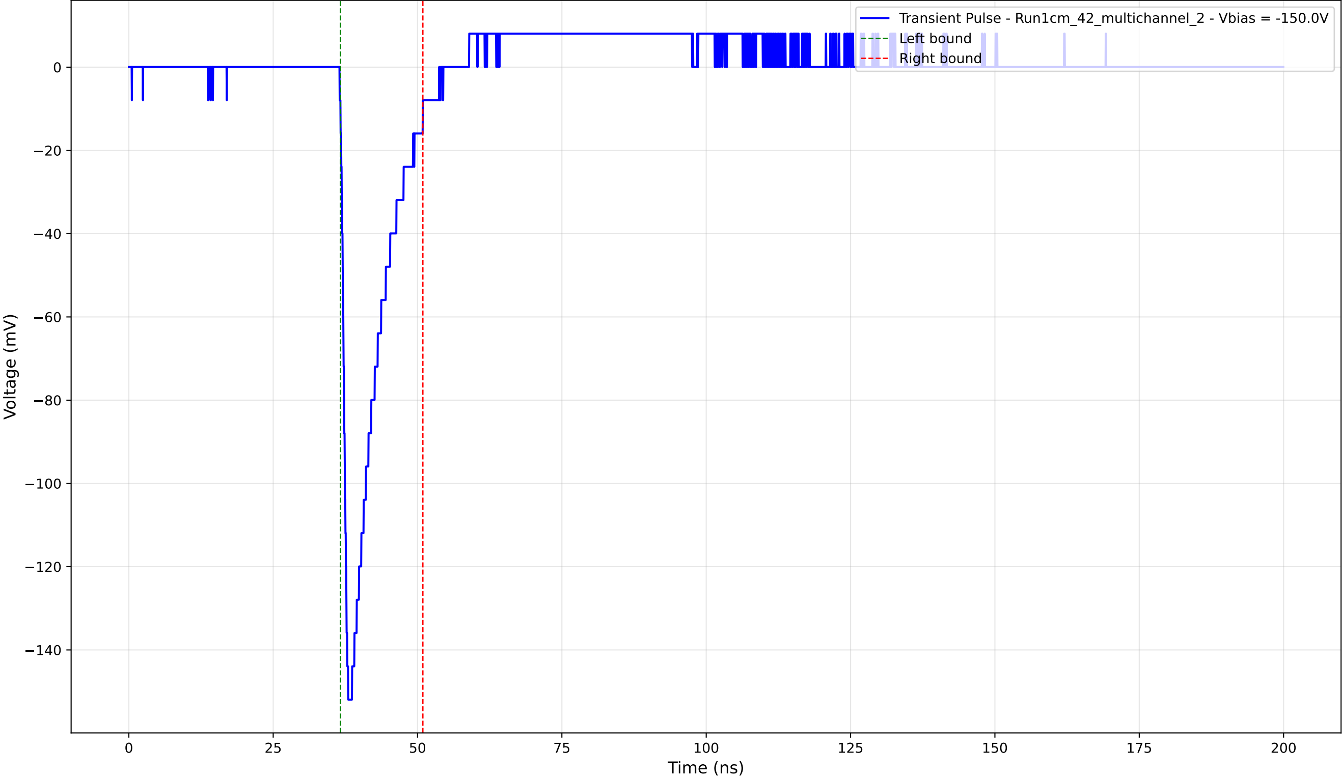
Transient Pulse - Sample: 1cm_42_multichannel - Position: 1220.0 \mu\text{m} - Charge: 18.99 pC - Rise Time: 1.16 ns
