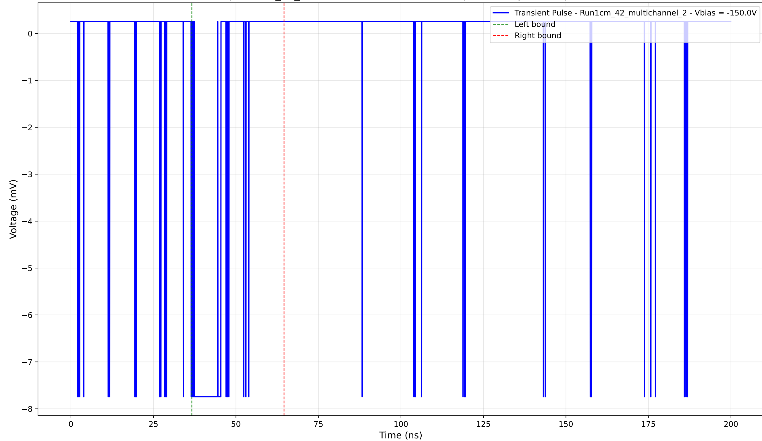
Transient Pulse - Sample: 1cm_42_multichannel - Position: 850.0 \mu\text{m} - Charge: 1.28 pC - Rise Time: 0.04 ns
