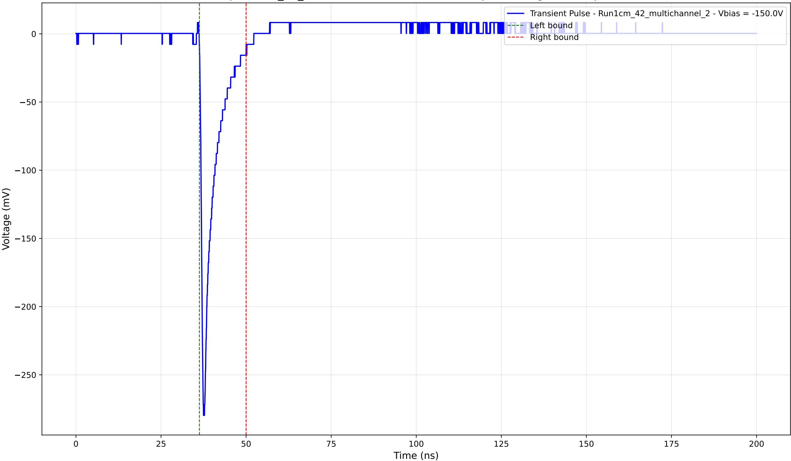
Transient Pulse - Sample: 1cm_42_multichannel - Position: 1720.0 \mu\text{m} - Charge: 22.91 pC - Rise Time: 0.88 ns
