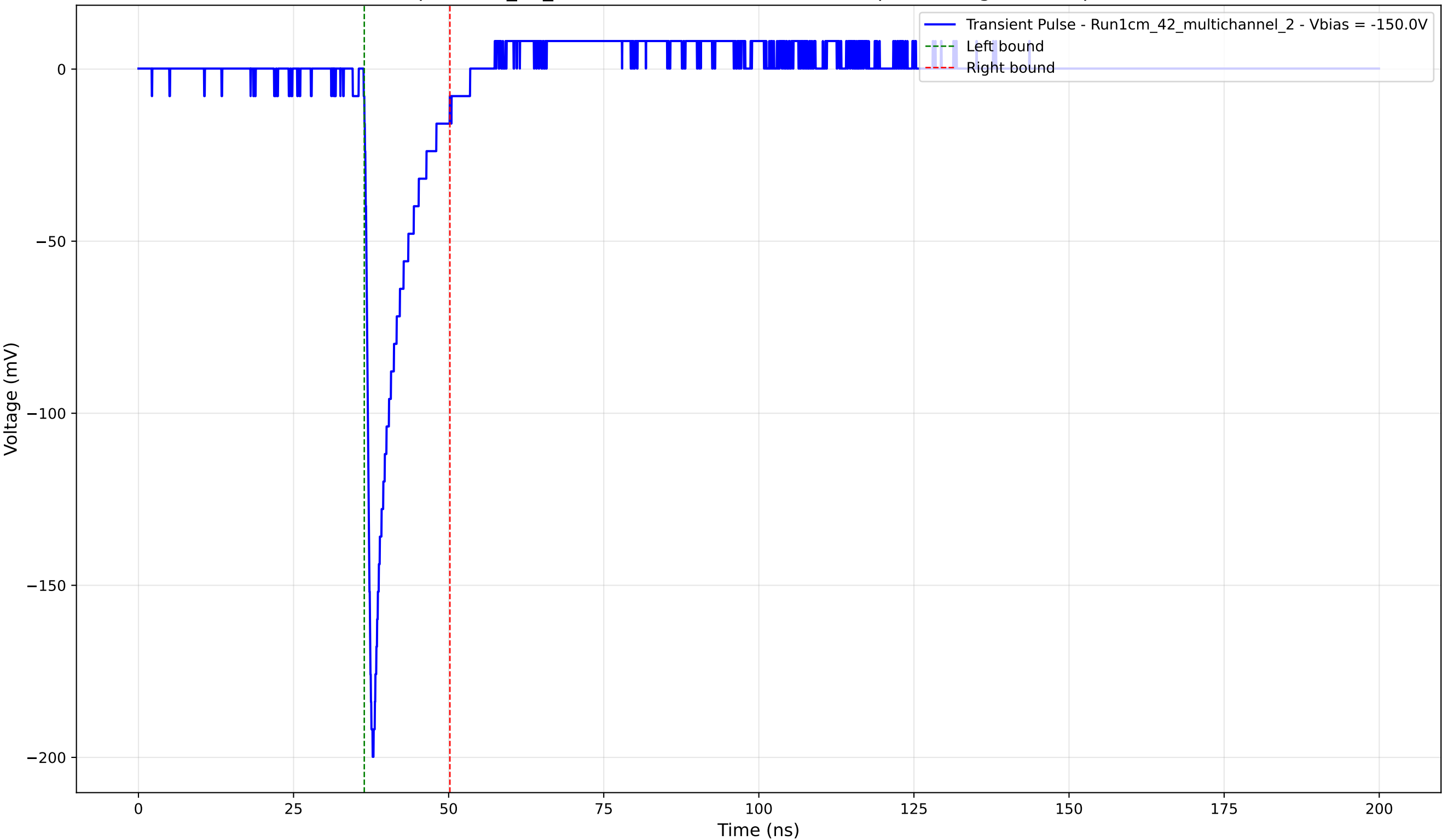
Transient Pulse - Sample: 1cm_42_multichannel - Position: 3170.0 \mu\text{m} - Charge: 18.75 pC - Rise Time: 0.98 ns
