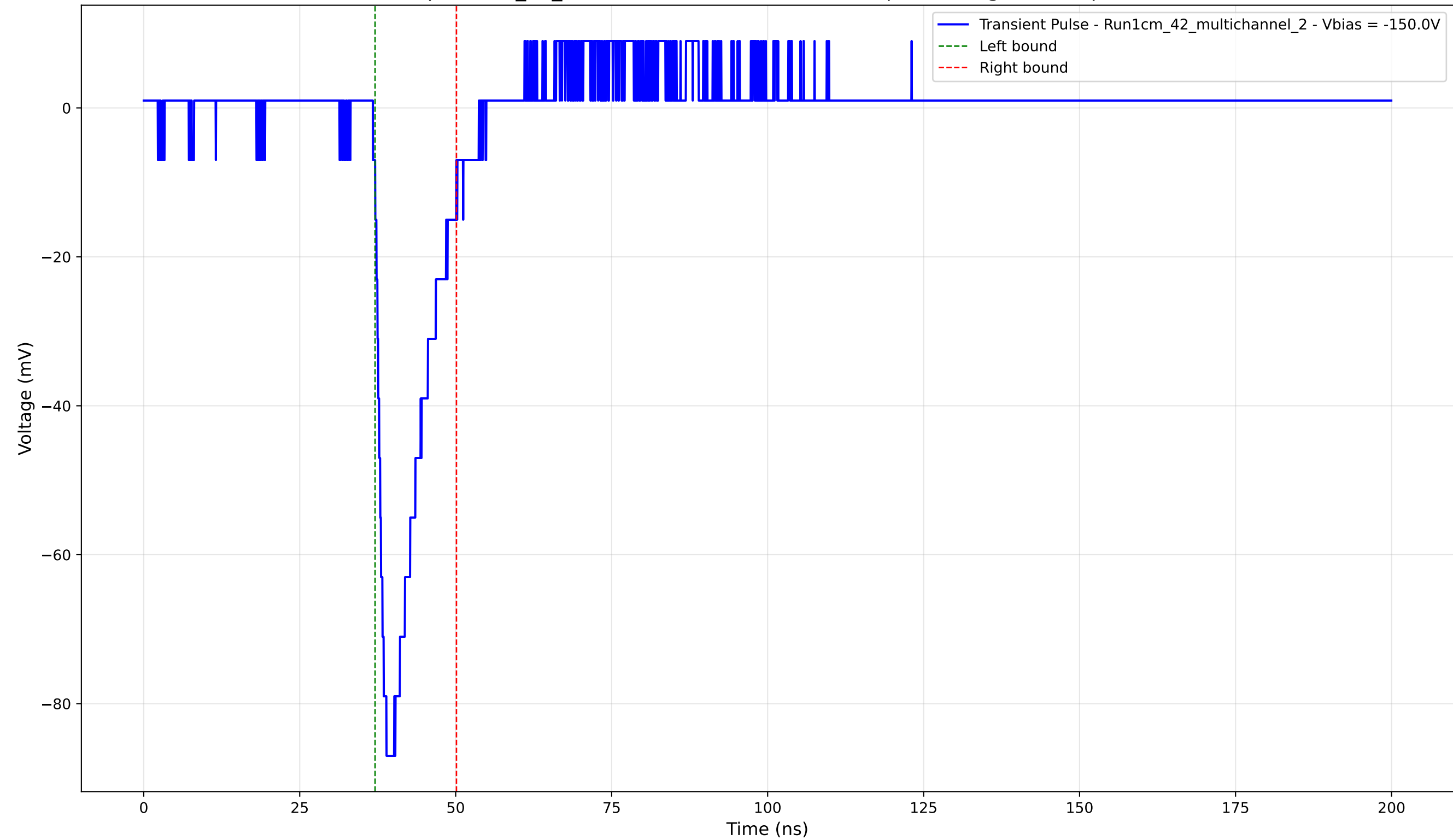
Transient Pulse - Sample: 1cm_42_multichannel - Position: 4080.0 \mu\text{m} - Charge: 12.41 pC - Rise Time: 1.39 ns
