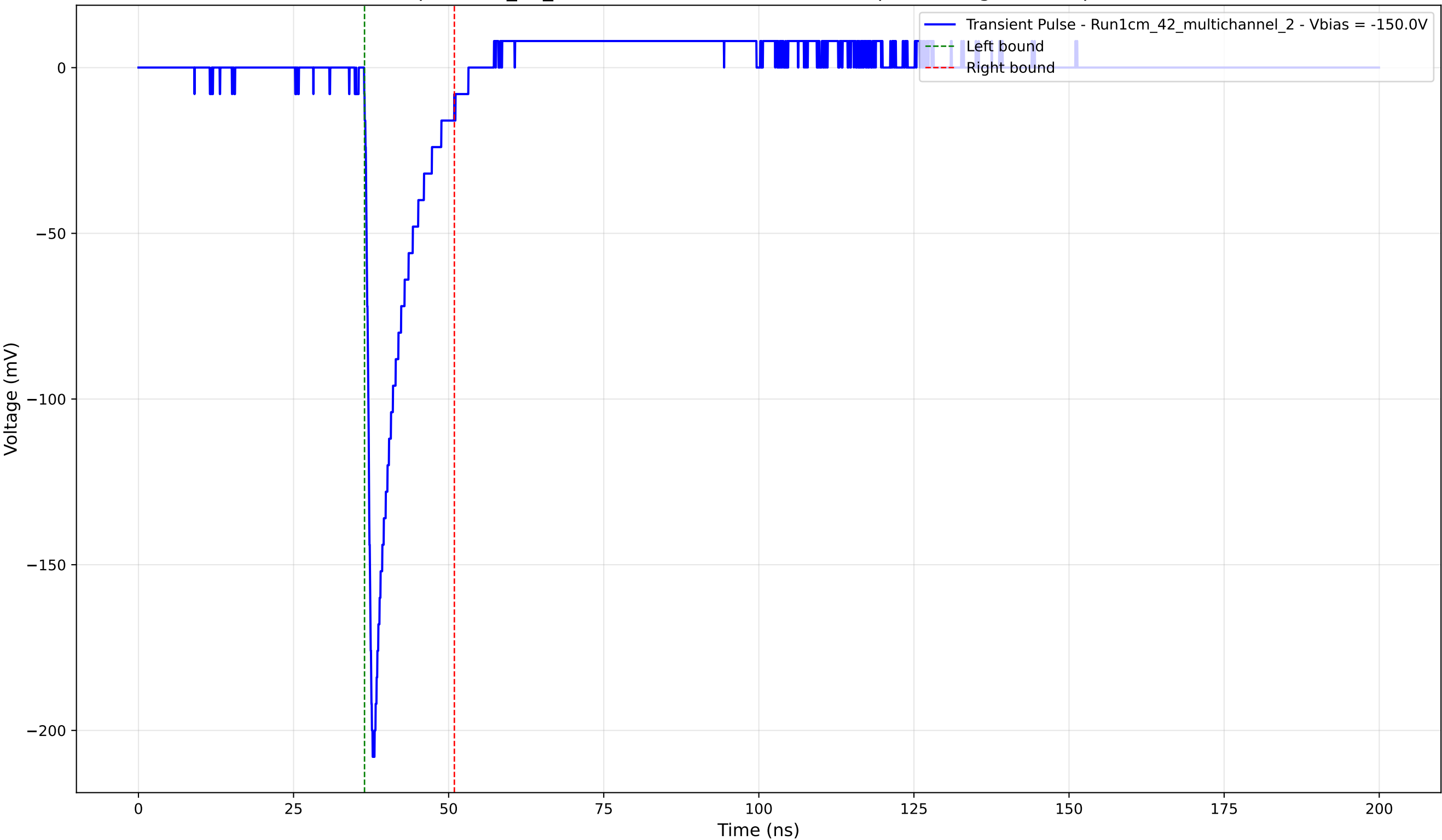
Transient Pulse - Sample: 1cm_42_multichannel - Position: 1480.0 \mu\text{m} - Charge: 21.17 pC - Rise Time: 0.98 ns
