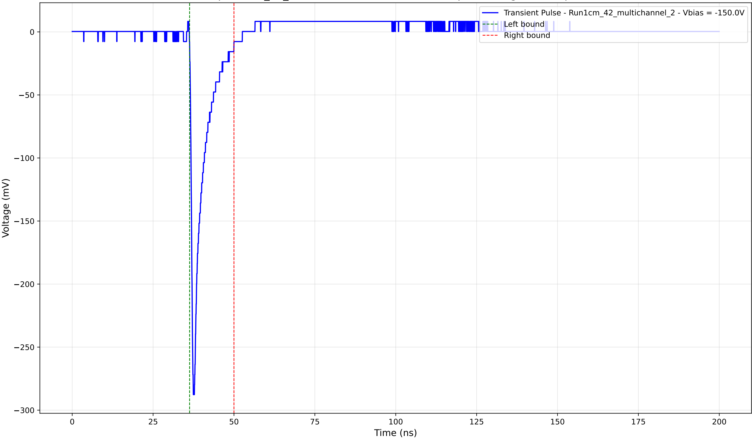
Transient Pulse - Sample: 1cm_42_multichannel - Position: 1750.0 \mu\text{m} - Charge: 23.07 pC - Rise Time: 0.83 ns
