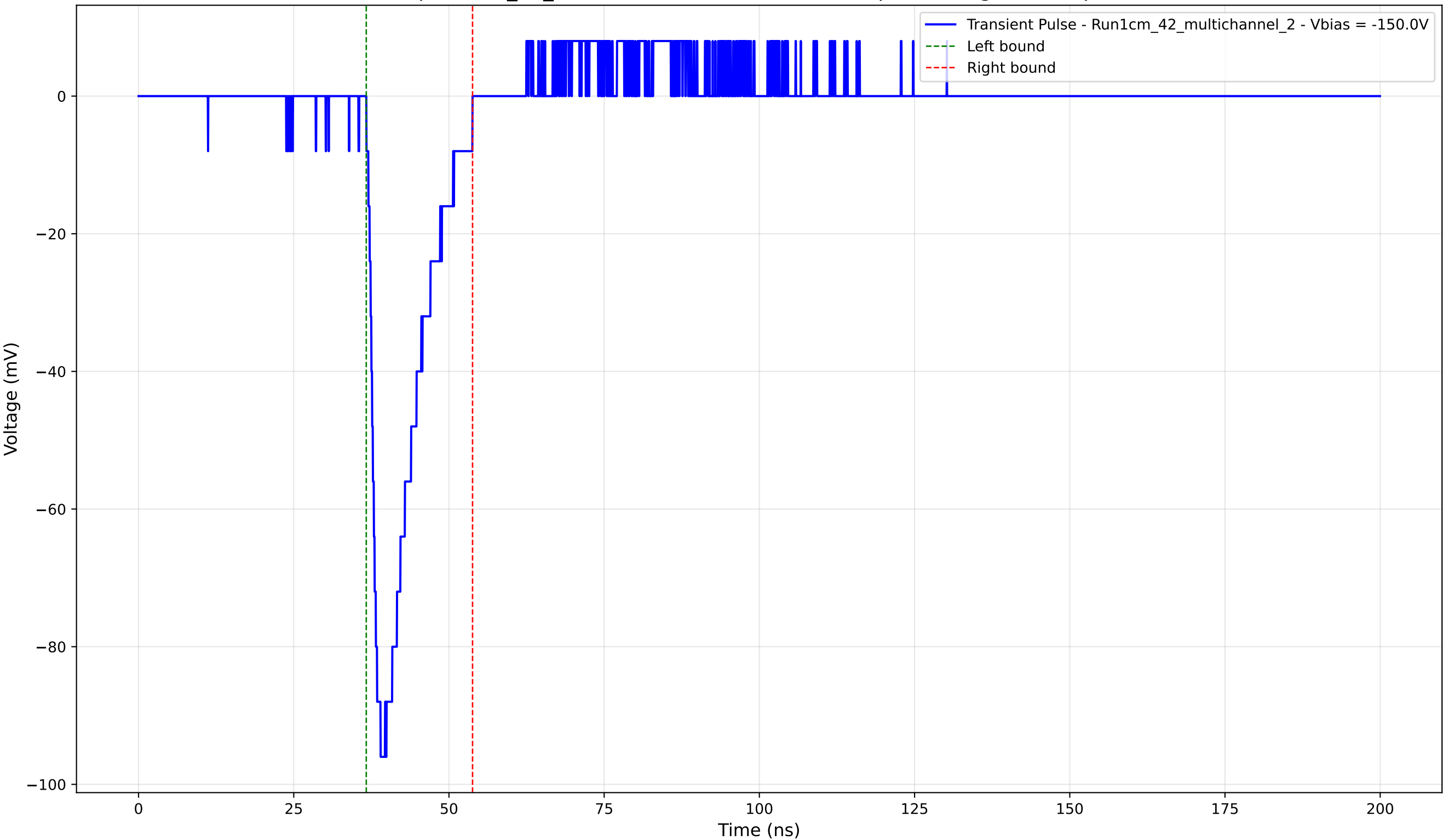
Transient Pulse - Sample: 1cm_42_multichannel - Position: 3995.0 \mu\text{m} - Charge: 14.26 pC - Rise Time: 1.43 ns
