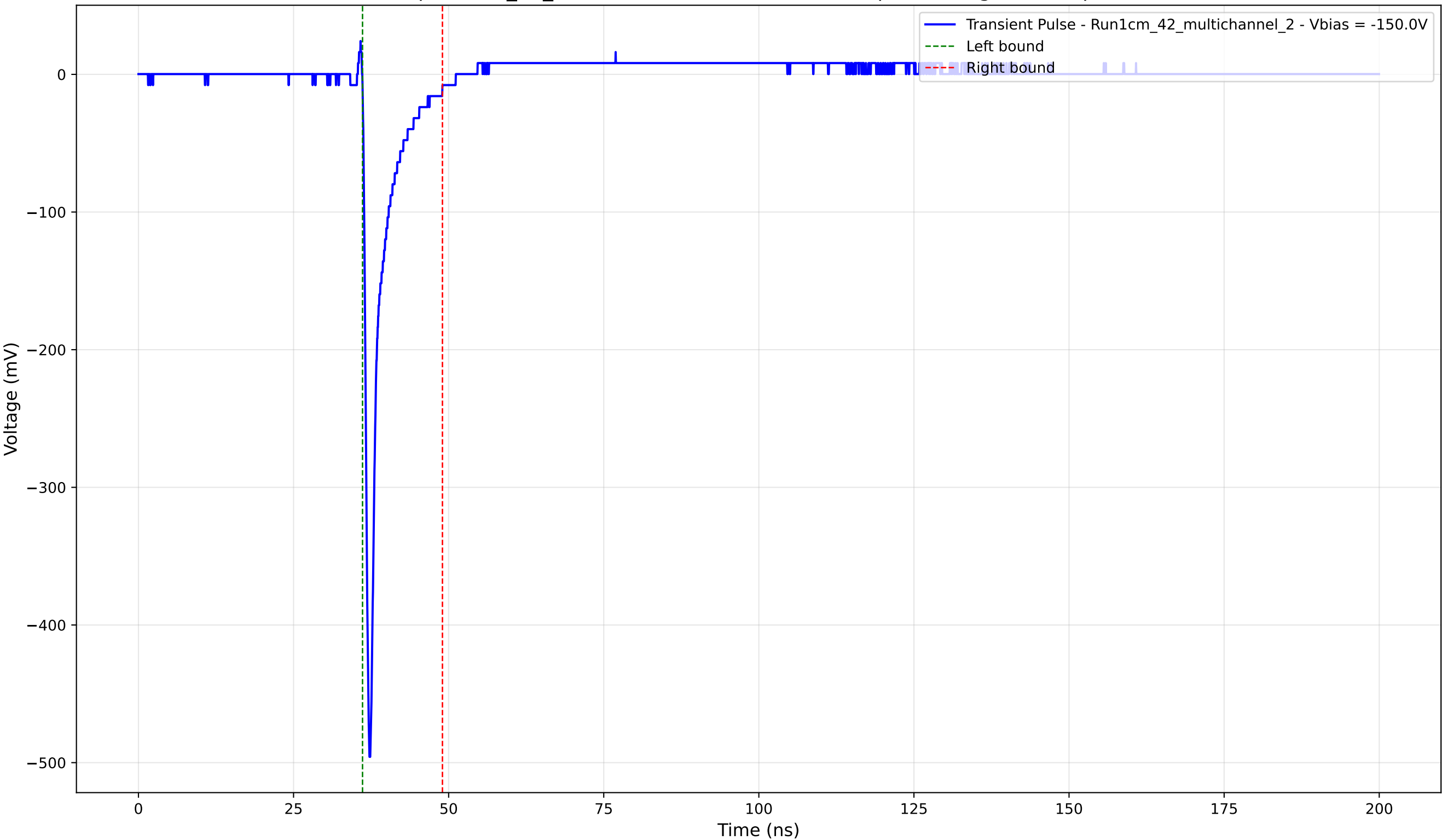
Transient Pulse - Sample: 1cm_42_multichannel - Position: 2105.0 \mu\text{m} - Charge: 26.63 pC - Rise Time: 0.77 ns
