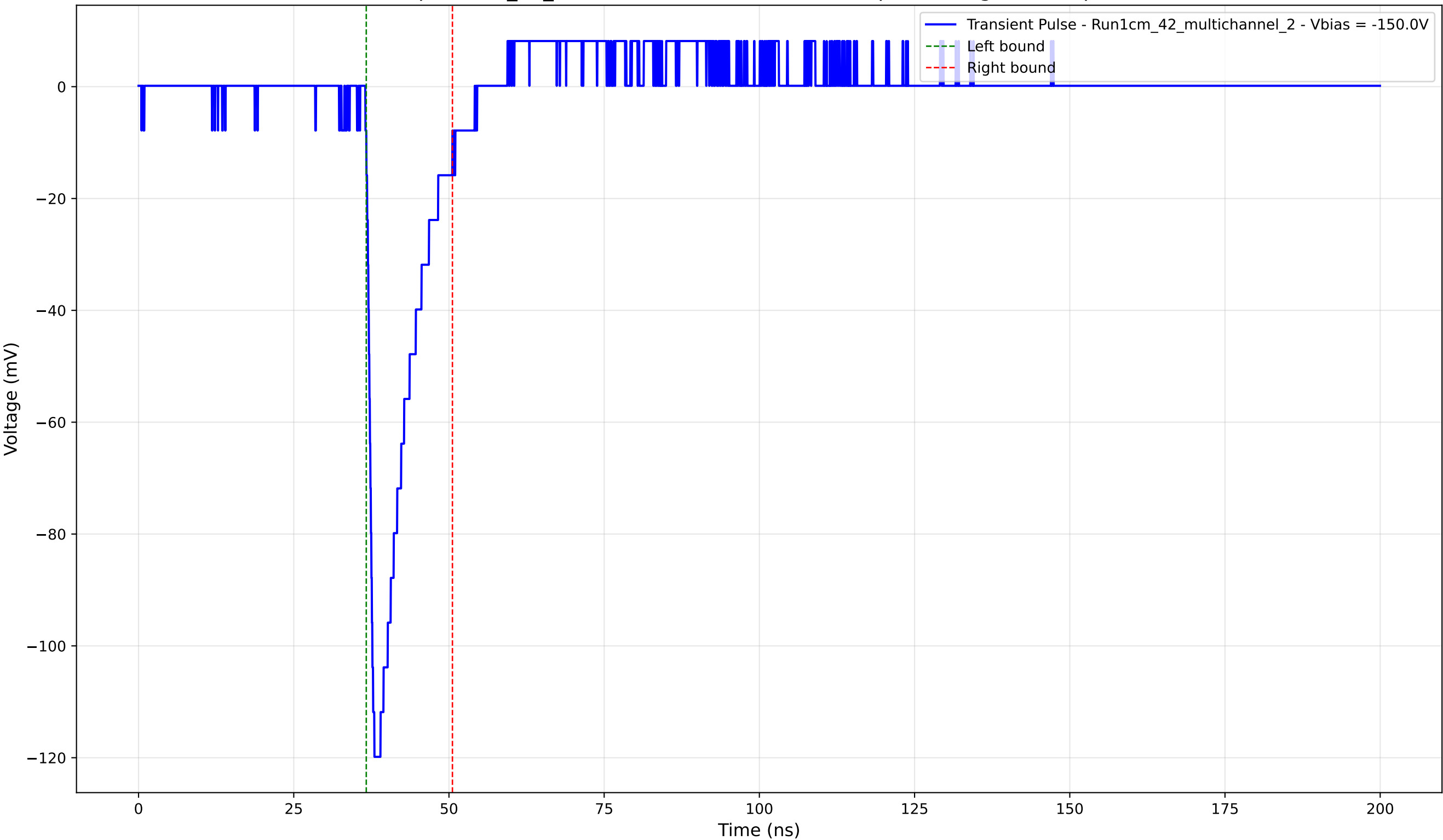
Transient Pulse - Sample: 1cm_42_multichannel - Position: 3555.0 \mu\text{m} - Charge: 15.65 pC - Rise Time: 1.10 ns
