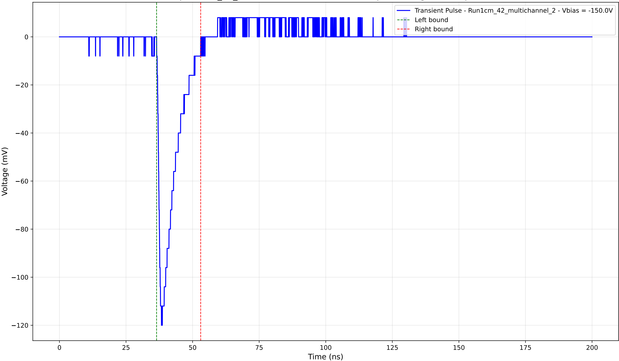
Transient Pulse - Sample: 1cm_42_multichannel - Position: 3595.0 \mu\text{m} - Charge: 15.87 pC - Rise Time: 1.26 ns
