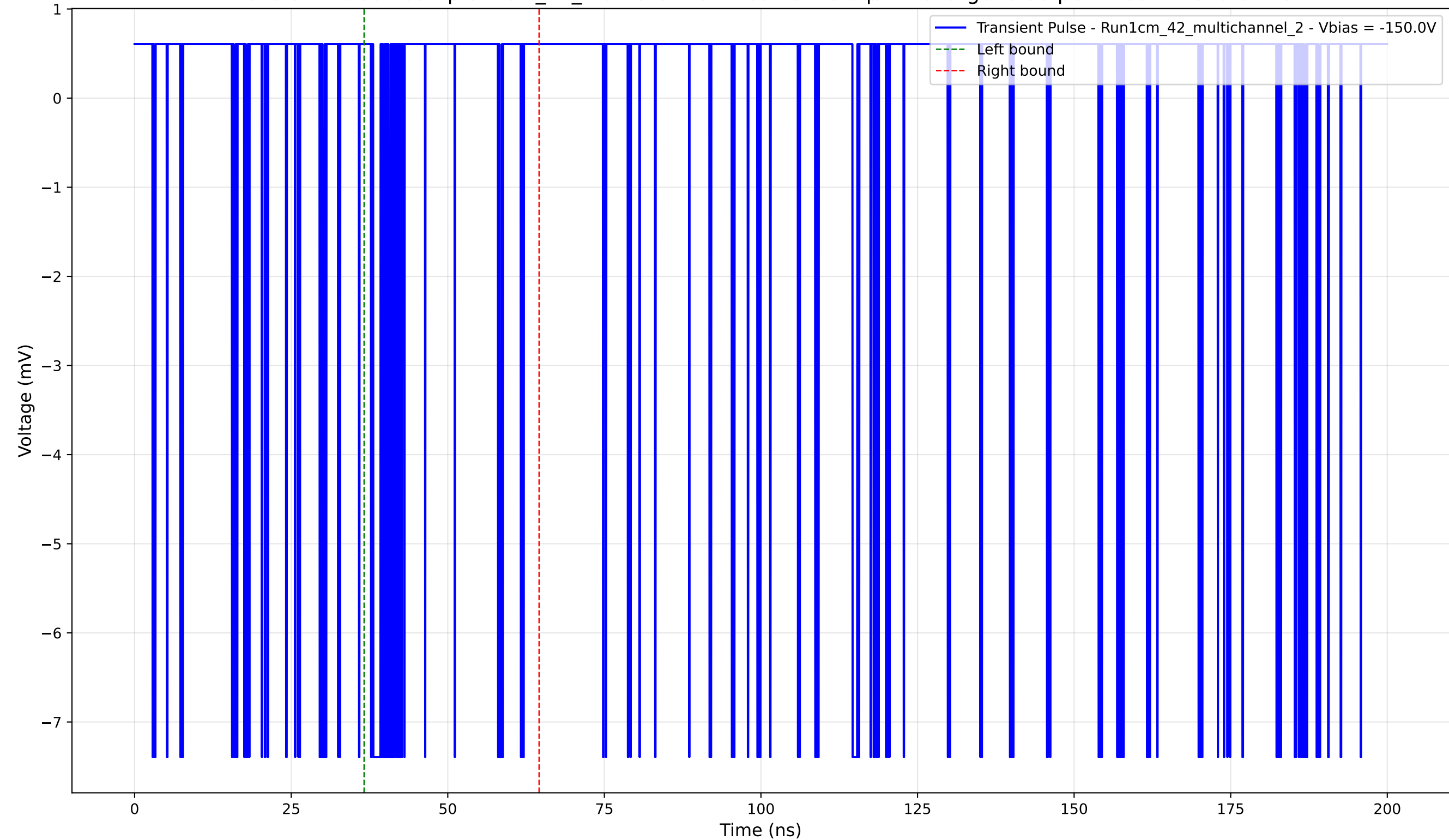
Transient Pulse - Sample: 1cm_42_multichannel - Position: 0.0 \mu\text{m} - Charge: 0.30 pC - Rise Time: 0.04 ns
