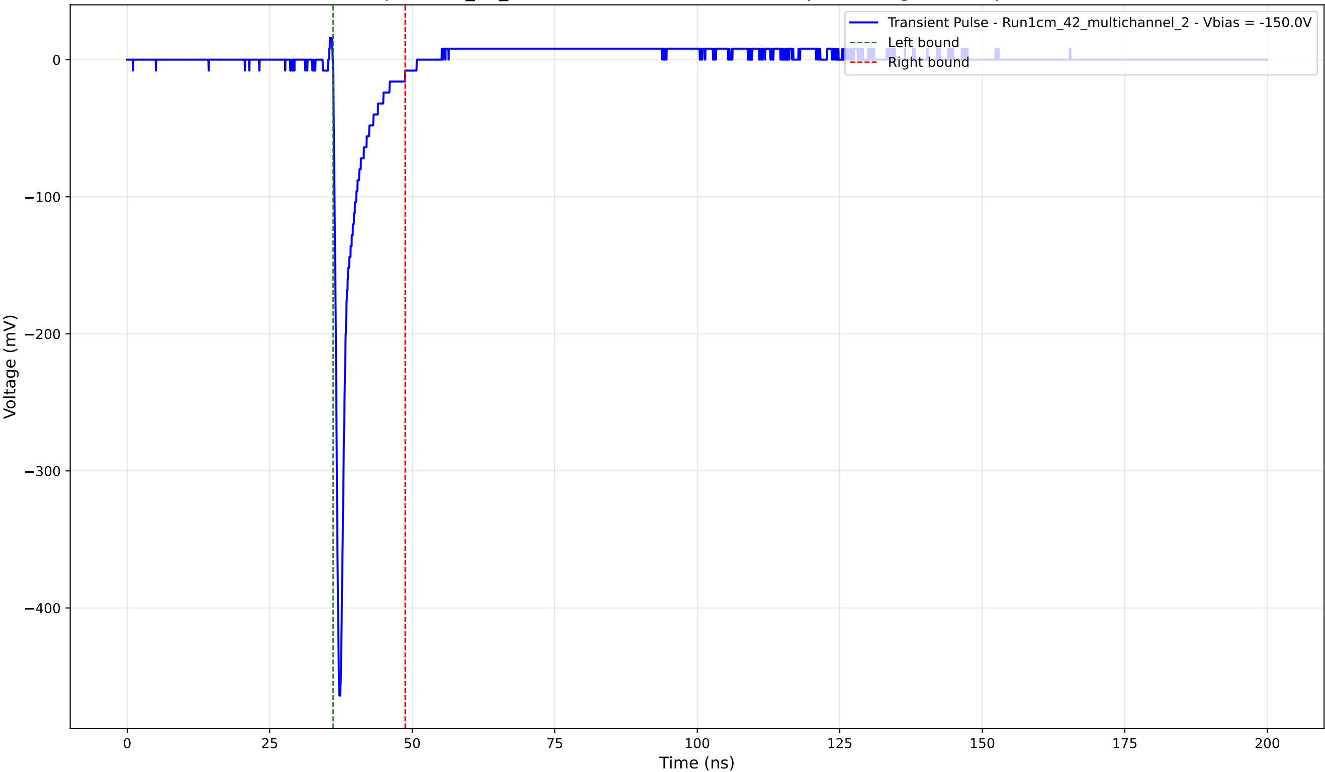
Transient Pulse - Sample: 1cm_42_multichannel - Position: 2635.0 \mu\text{m} - Charge: 24.88 pC - Rise Time: 0.77 ns
