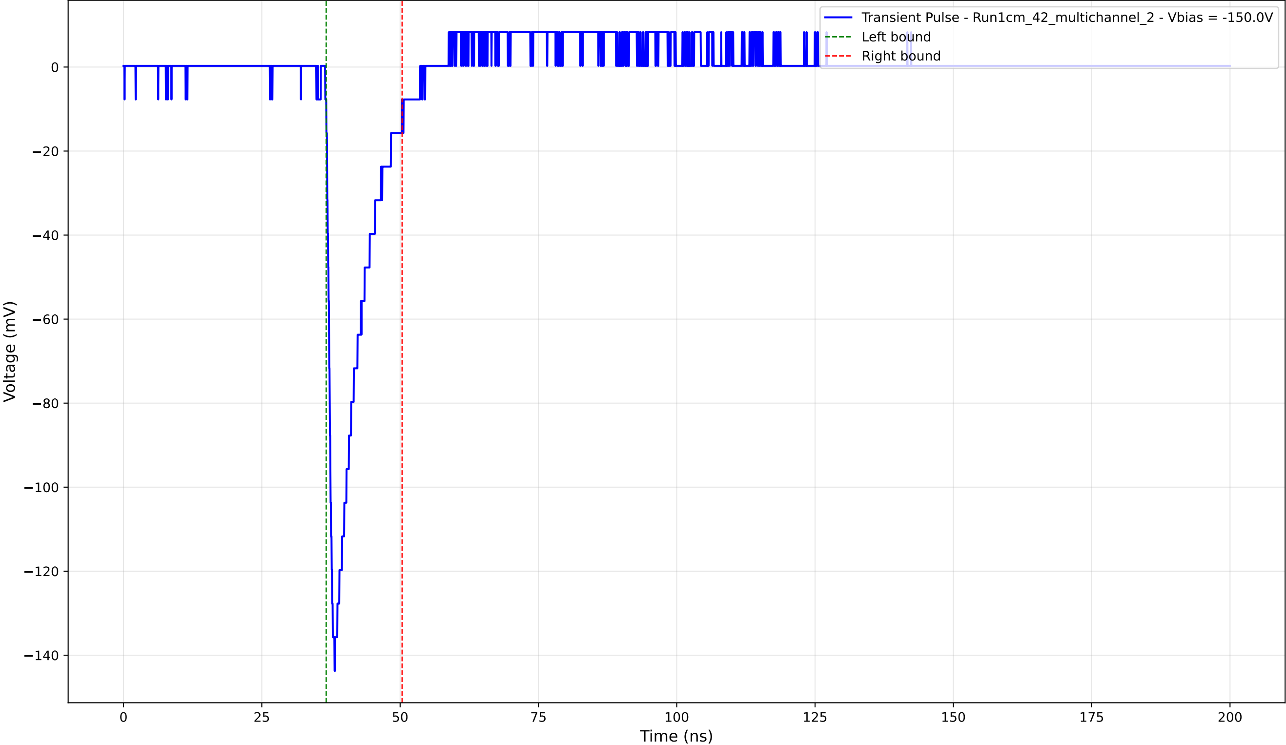
Transient Pulse - Sample: 1cm_42_multichannel - Position: 1285.0 \mu\text{m} - Charge: 16.45 pC - Rise Time: 1.17 ns
