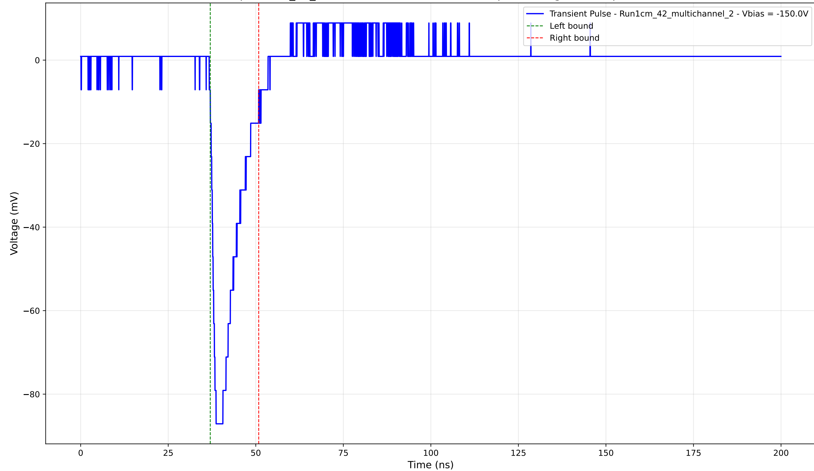
Transient Pulse - Sample: 1cm_42_multichannel - Position: 4045.0 \mu\text{m} - Charge: 13.06 pC - Rise Time: 1.35 ns
