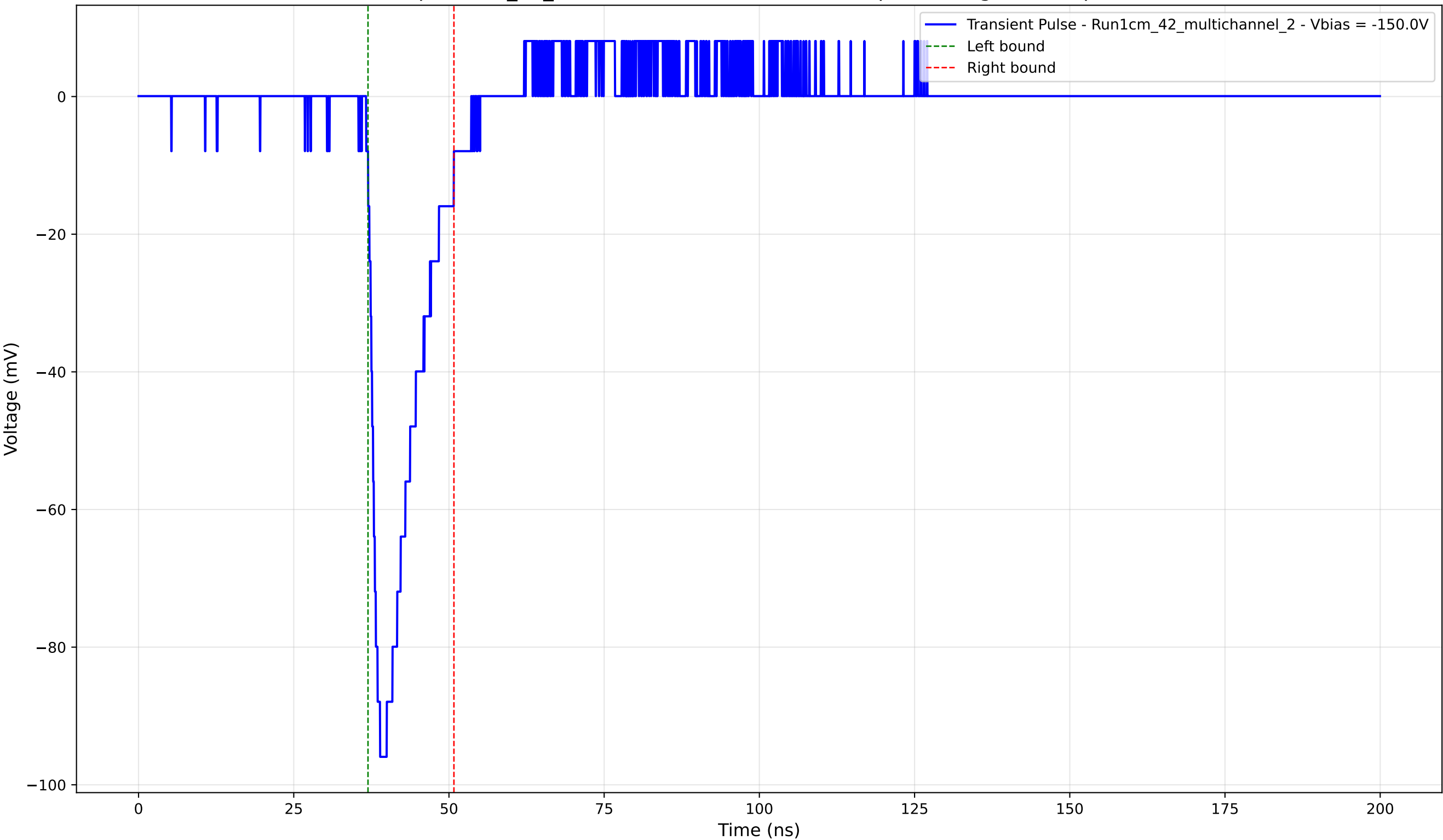
Transient Pulse - Sample: 1cm_42_multichannel - Position: 4010.0 \mu\text{m} - Charge: 13.76 pC - Rise Time: 1.55 ns
