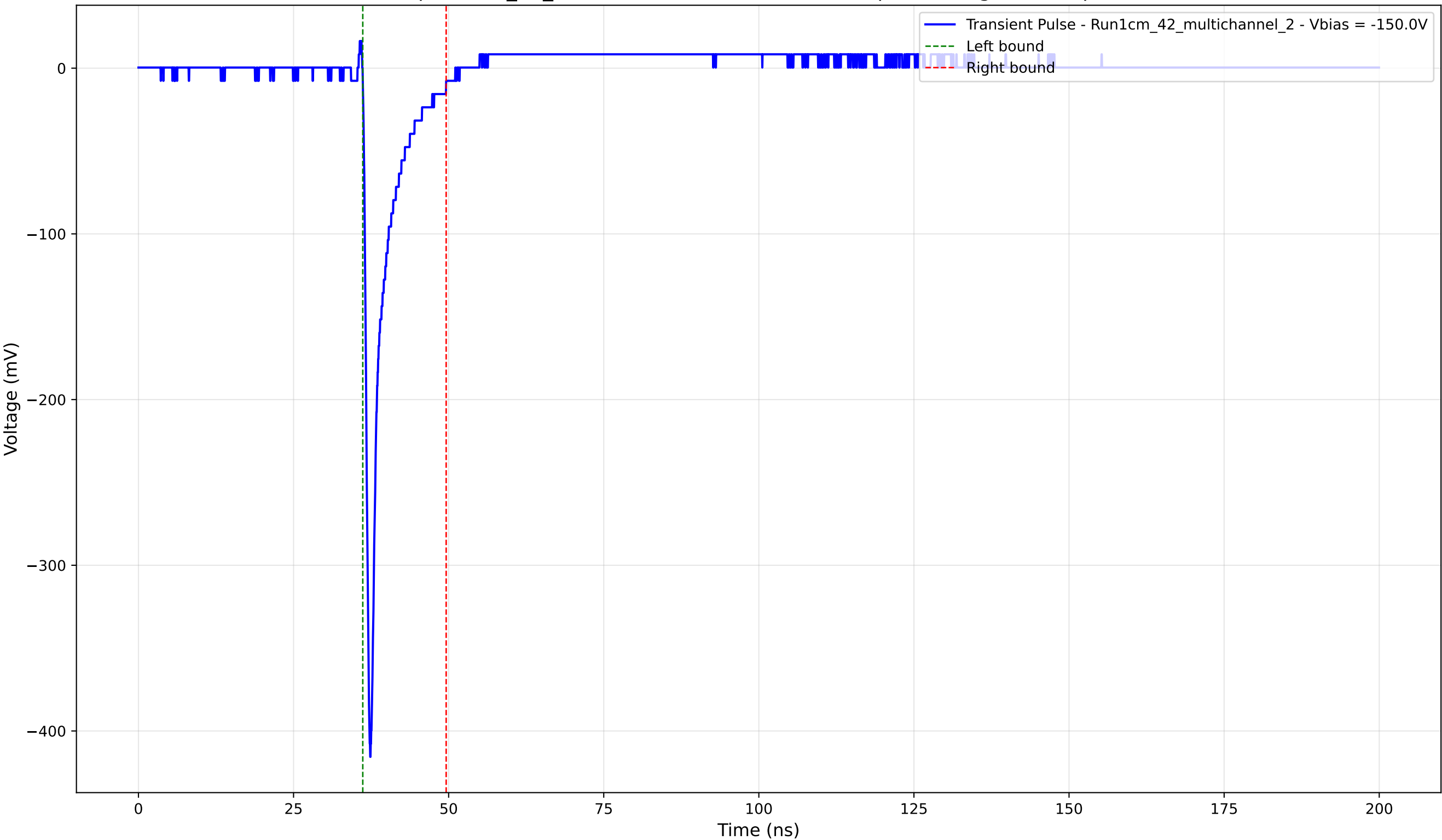
Transient Pulse - Sample: 1cm_42_multichannel - Position: 2740.0 \mu\text{m} - Charge: 24.93 pC - Rise Time: 0.81 ns
