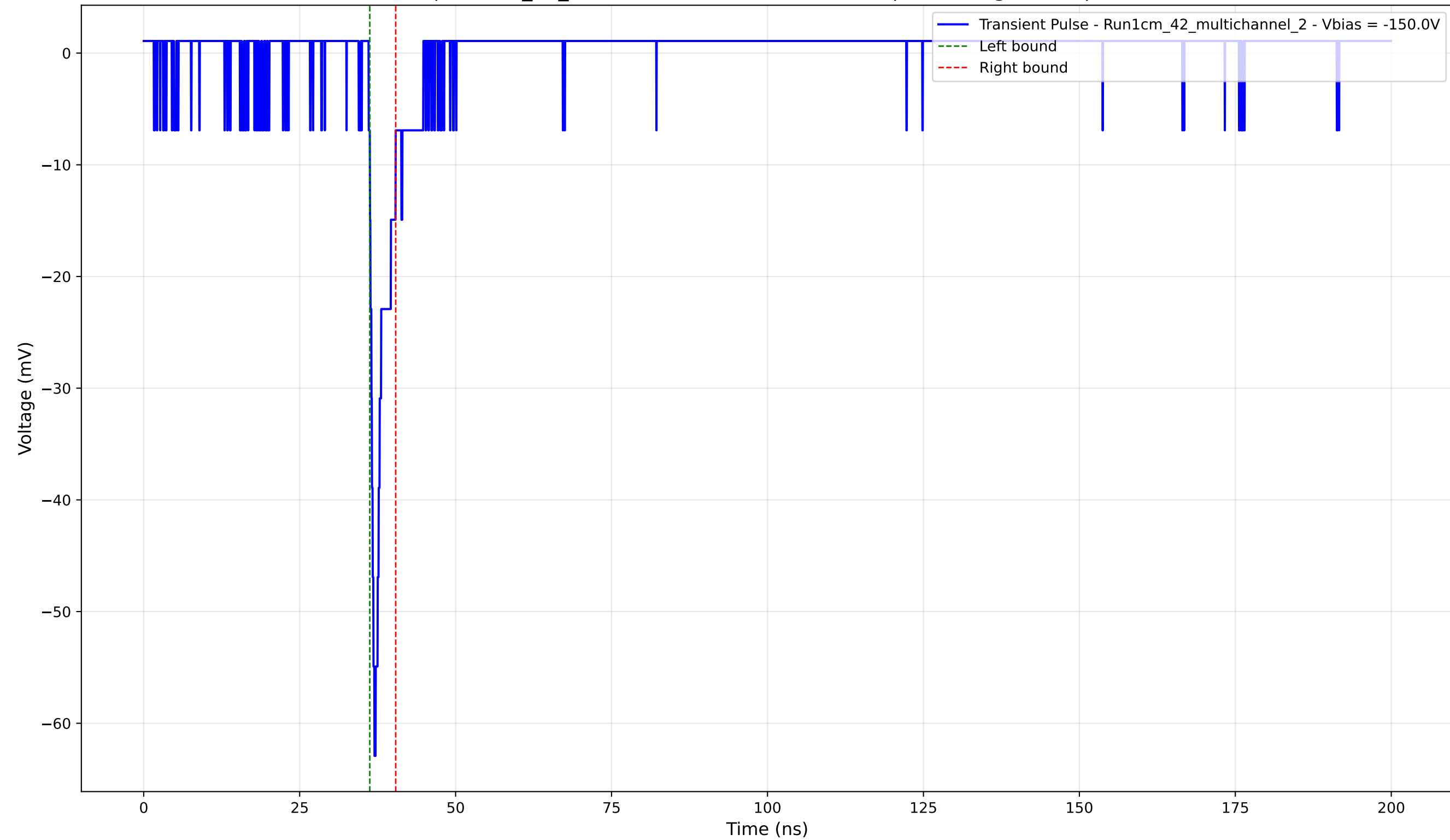
Transient Pulse - Sample: 1cm_42_multichannel - Position: 2395.0 \mu\text{m} - Charge: 2.50 pC - Rise Time: 0.92 ns
