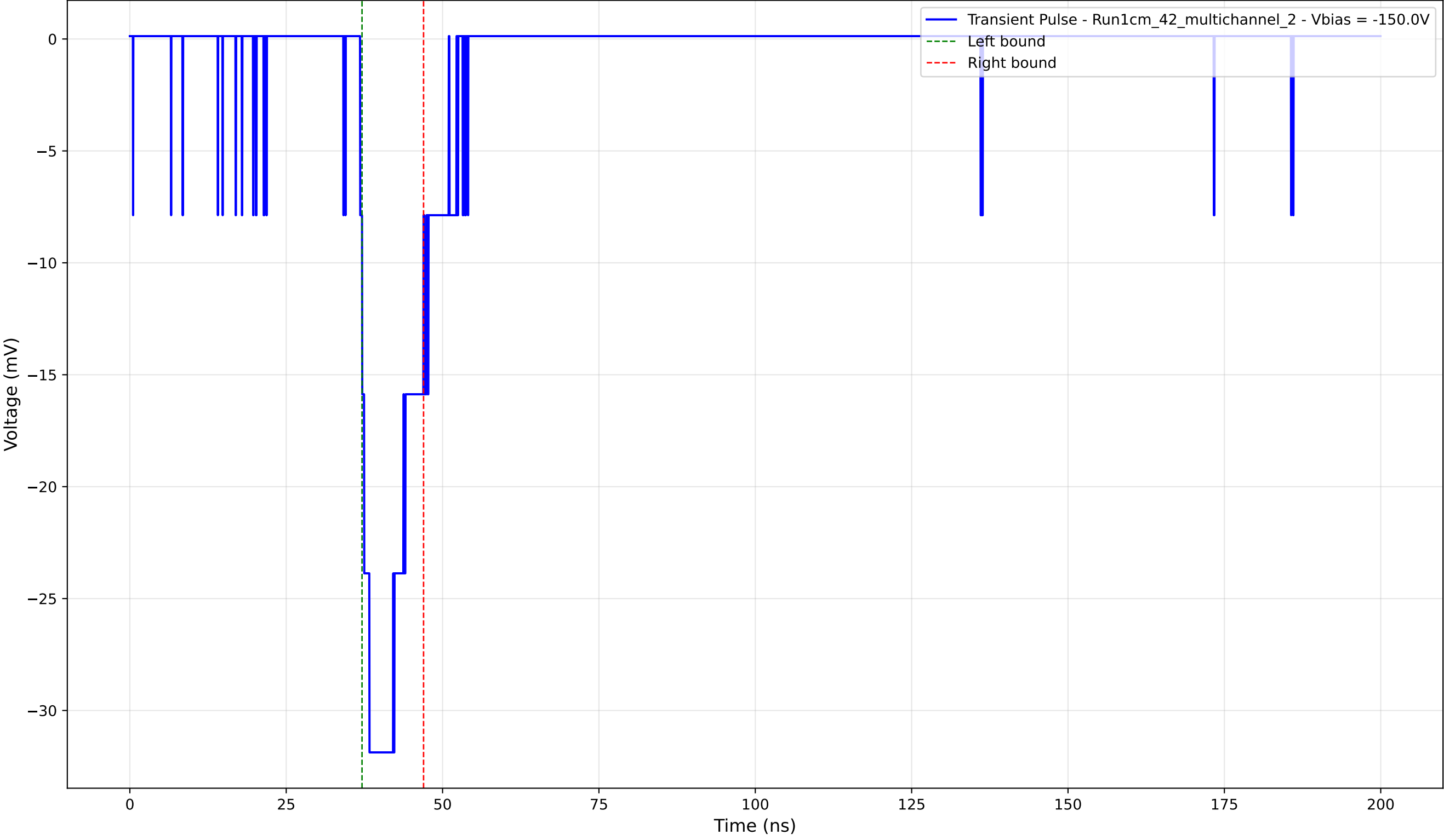
Transient Pulse - Sample: 1cm_42_multichannel - Position: 70.0 \mu\text{m} - Charge: 4.79 pC - Rise Time: 1.50 ns
