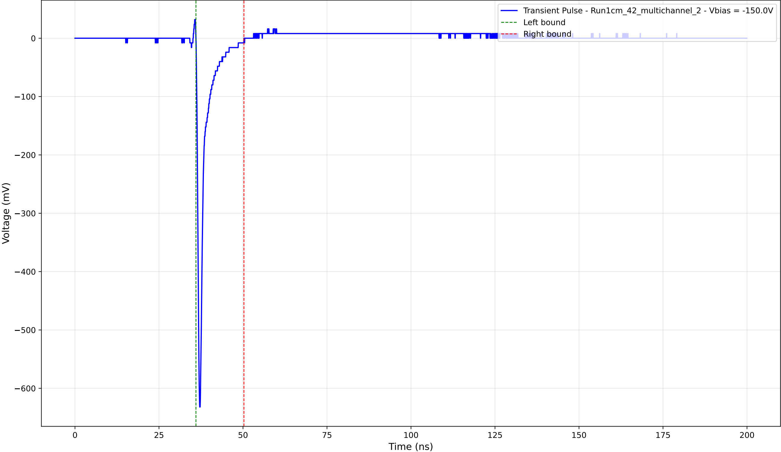
Transient Pulse - Sample: 1cm_42_multichannel - Position: 2255.0 \mu\text{m} - Charge: 29.56 pC - Rise Time: 0.72 ns
