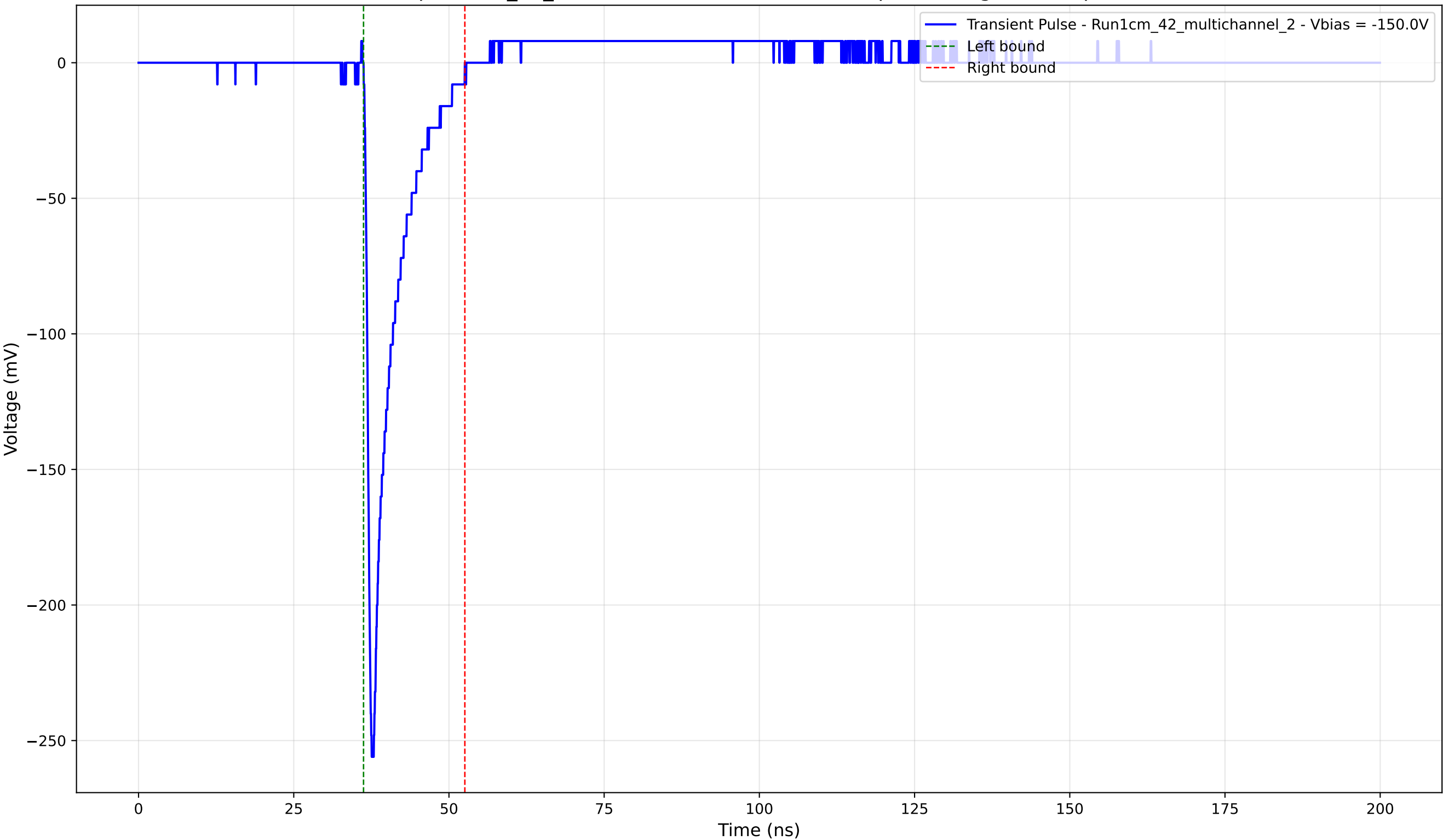
Transient Pulse - Sample: 1cm_42_multichannel - Position: 1655.0 \mu\text{m} - Charge: 22.89 pC - Rise Time: 0.86 ns
