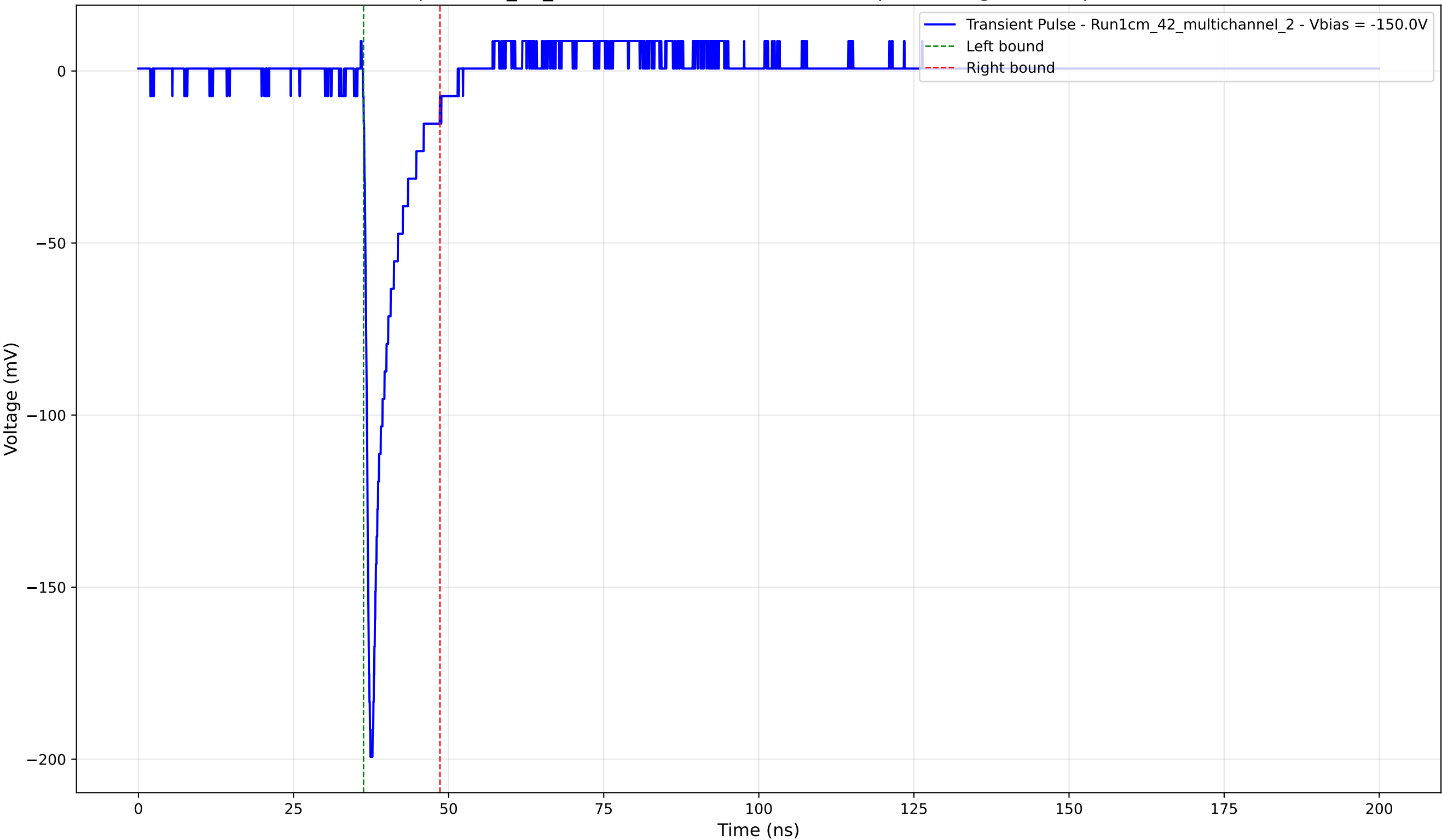
Transient Pulse - Sample: 1cm_42_multichannel - Position: 1805.0 \mu\text{m} - Charge: 15.23 pC - Rise Time: 0.86 ns
