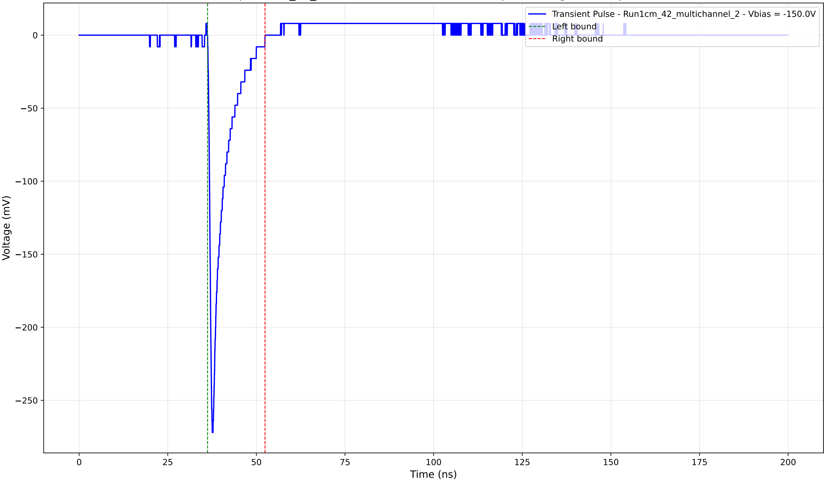
Transient Pulse - Sample: 1cm_42_multichannel - Position: 1685.0 \mu\text{m} - Charge: 23.26 pC - Rise Time: 0.89 ns
