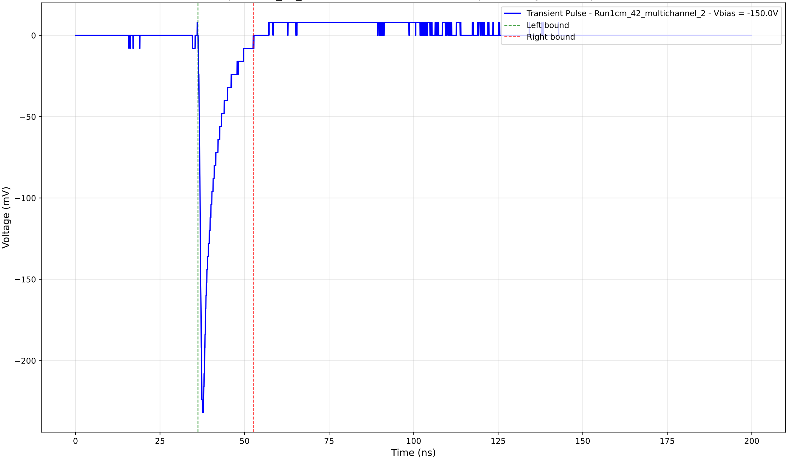
Transient Pulse - Sample: 1cm_42_multichannel - Position: 3050.0 \mu\text{m} - Charge: 20.21 pC - Rise Time: 0.89 ns
