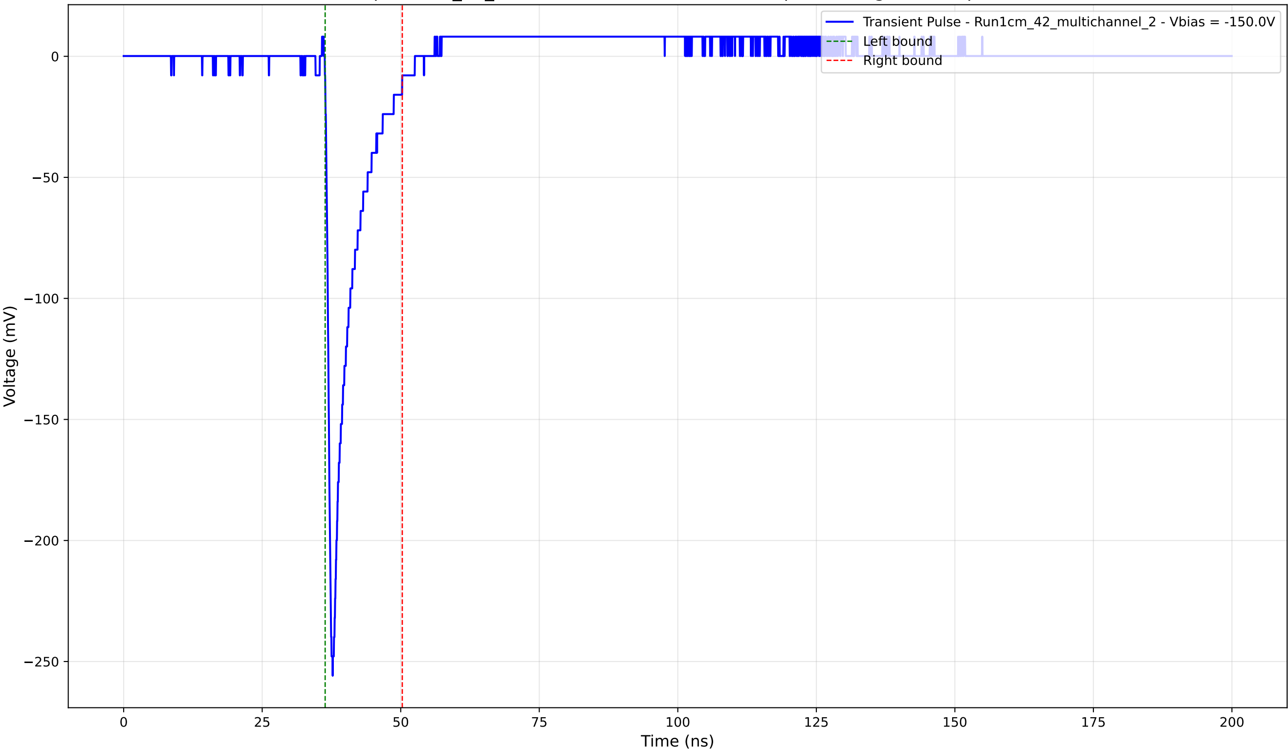
Transient Pulse - Sample: 1cm_42_multichannel - Position: 1645.0 \mu\text{m} - Charge: 22.30 pC - Rise Time: 0.90 ns
