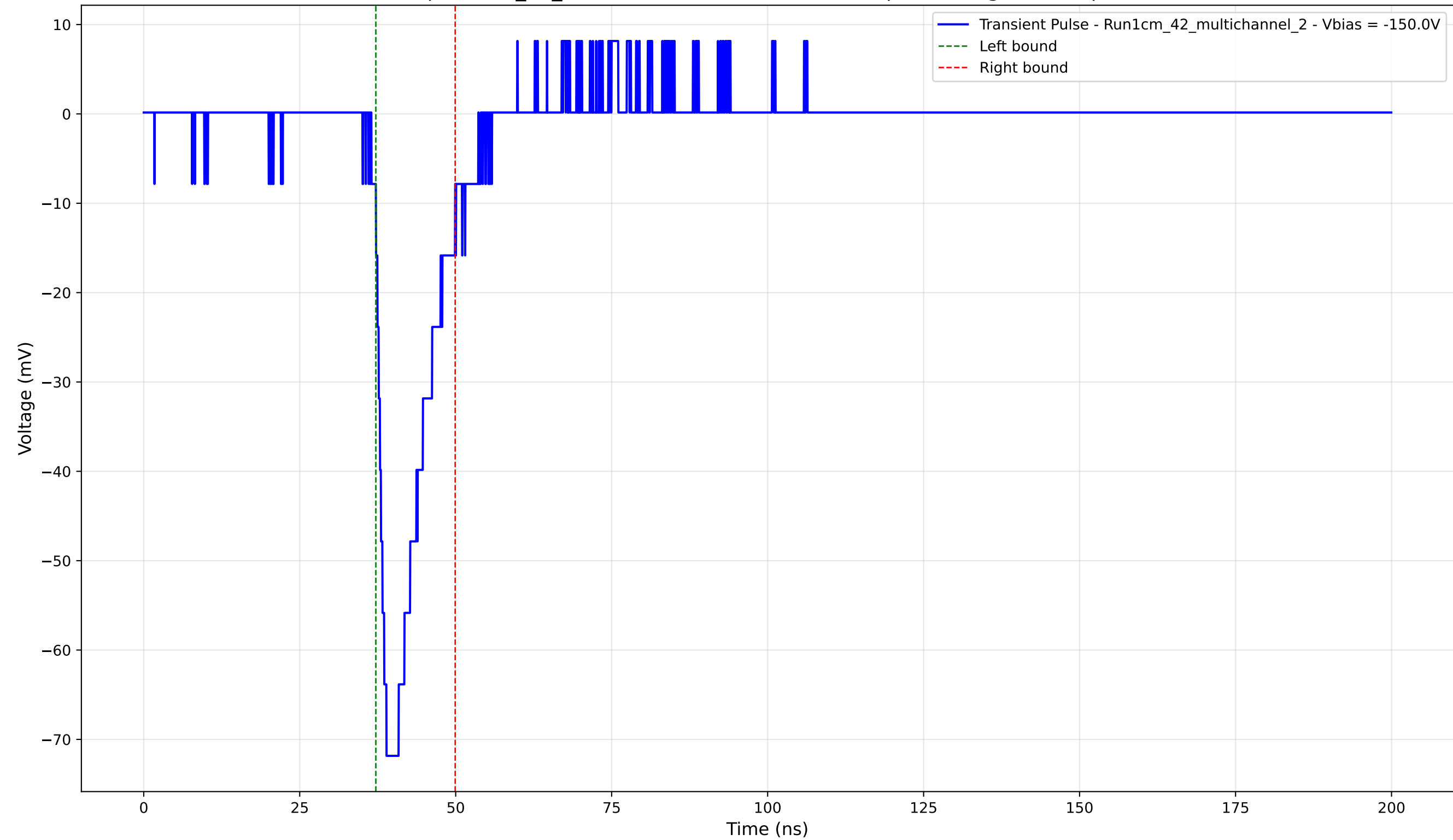
Transient Pulse - Sample: 1cm_42_multichannel - Position: 4520.0 \mu\text{m} - Charge: 10.60 pC - Rise Time: 2.40 ns
