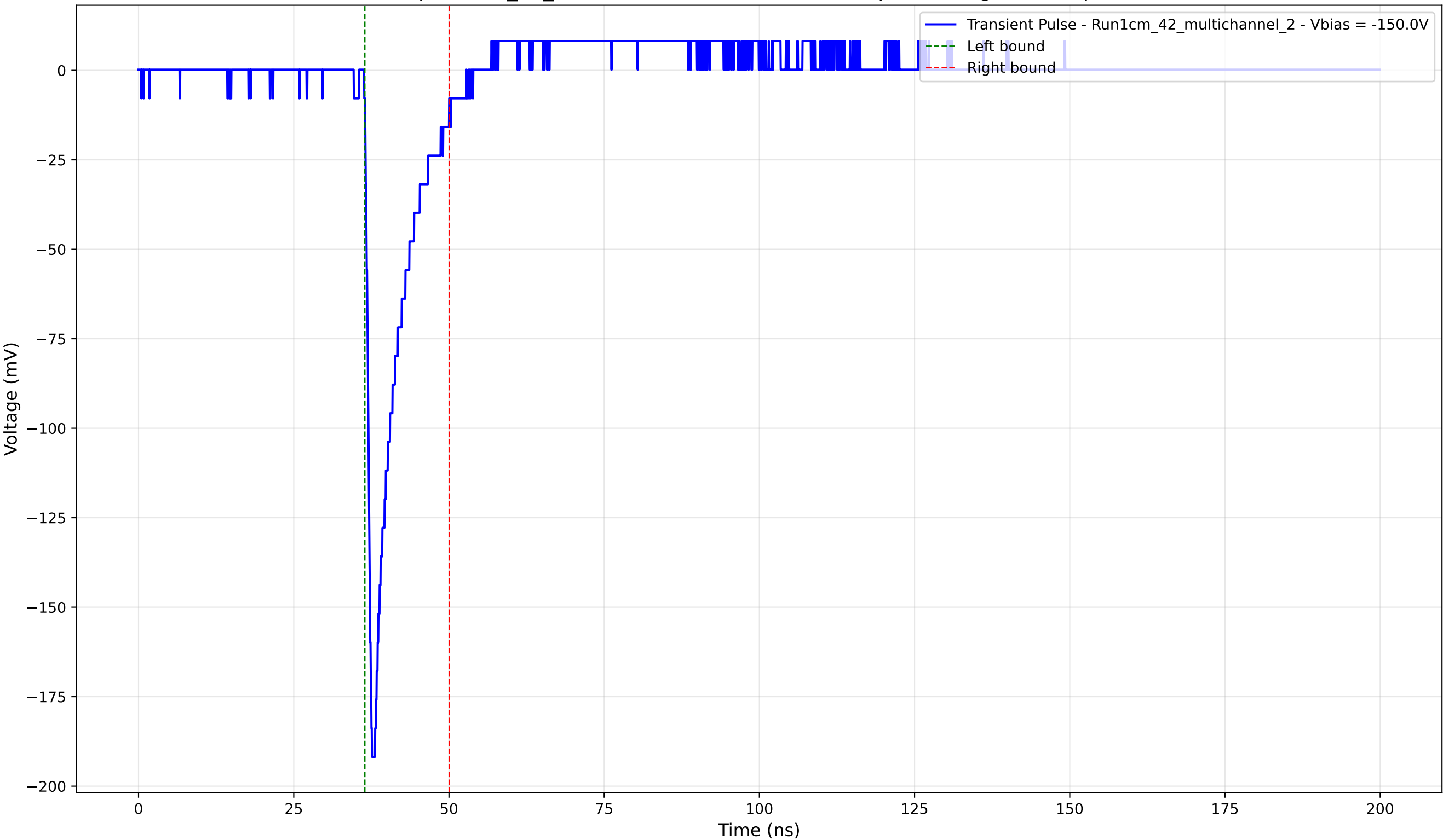
Transient Pulse - Sample: 1cm_42_multichannel - Position: 3195.0 \mu\text{m} - Charge: 19.03 pC - Rise Time: 0.90 ns
