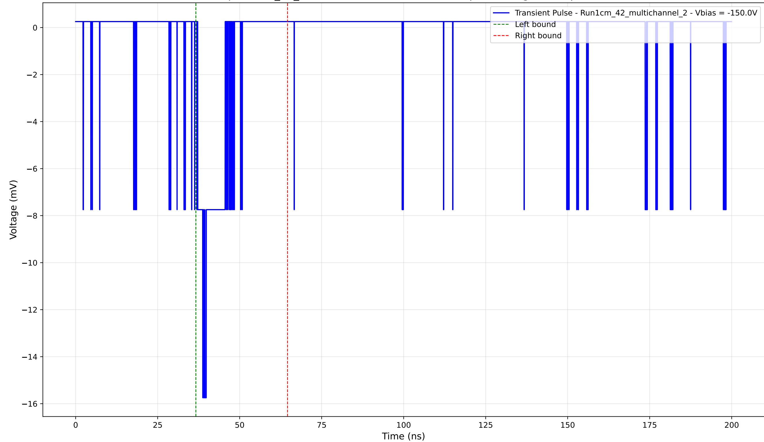
Transient Pulse - Sample: 1cm_42_multichannel - Position: 3910.0 \mu\text{m} - Charge: 1.50 pC - Rise Time: 1.55 ns
