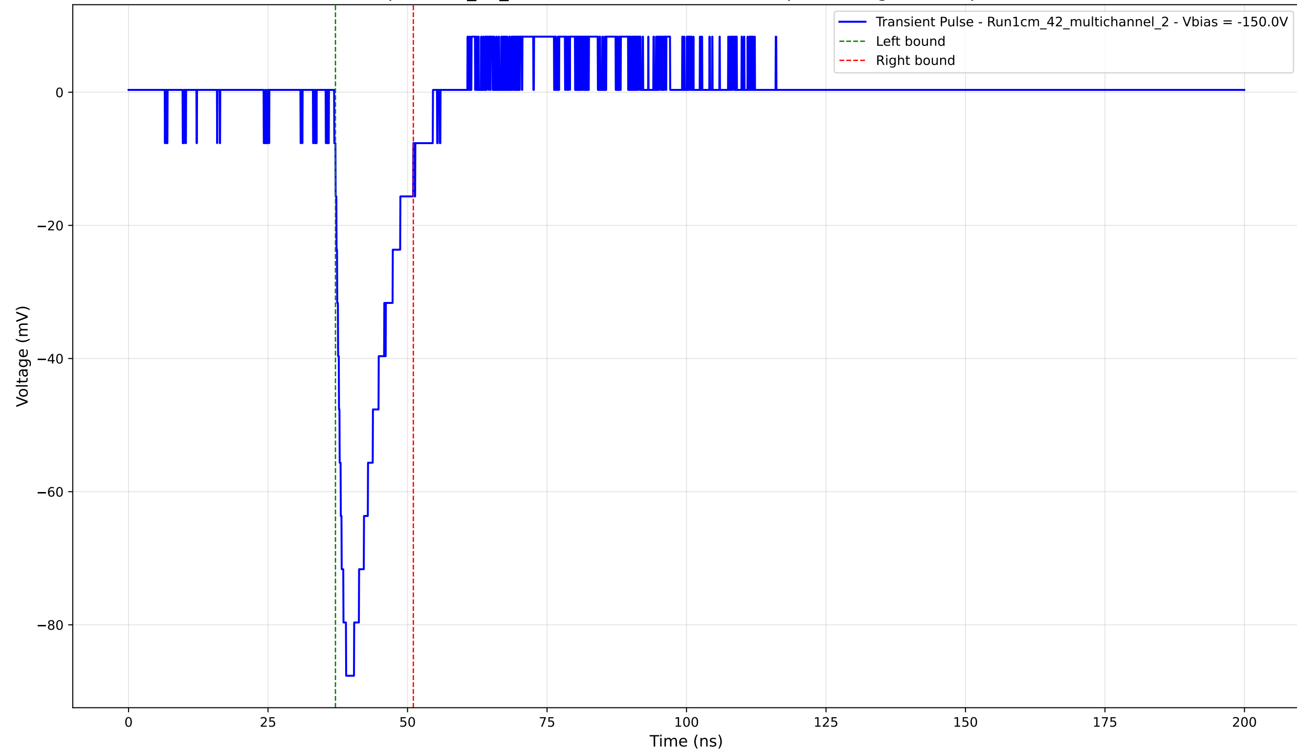
Transient Pulse - Sample: 1cm_42_multichannel - Position: 435.0 \mu\text{m} - Charge: 13.33 pC - Rise Time: 1.43 ns
