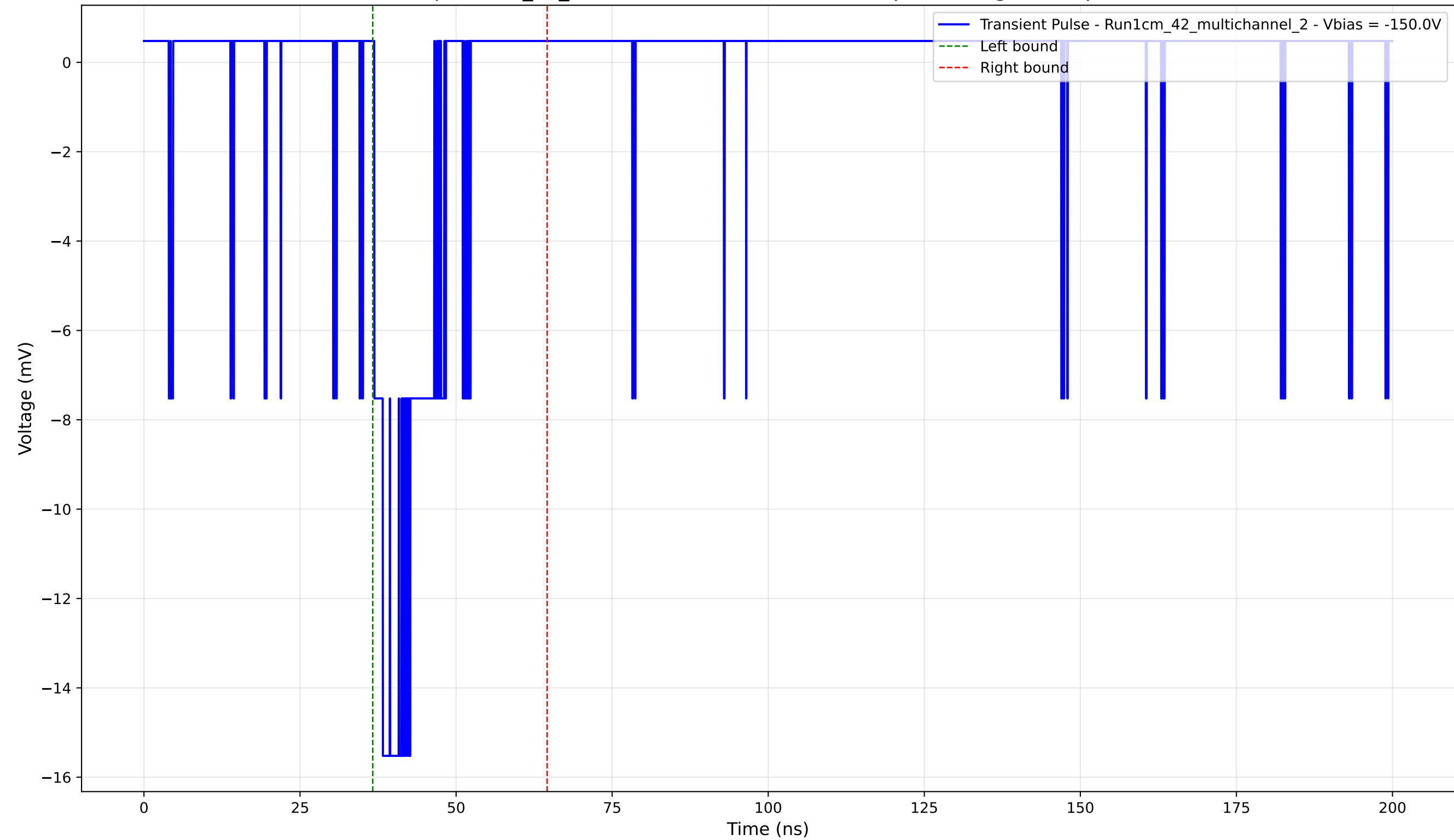
Transient Pulse - Sample: 1cm_42_multichannel - Position: 4865.0 \mu\text{m} - Charge: 2.15 pC - Rise Time: 1.39 ns
