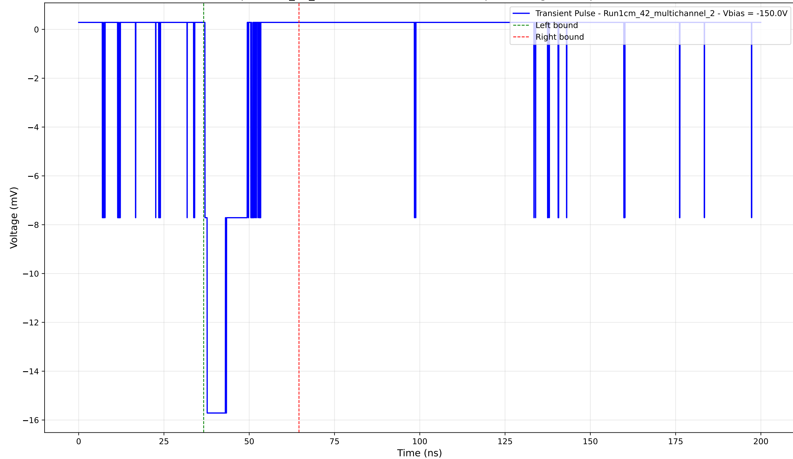
Transient Pulse - Sample: 1cm_42_multichannel - Position: 820.0 \mu\text{m} - Charge: 2.92 pC - Rise Time: 0.67 ns
