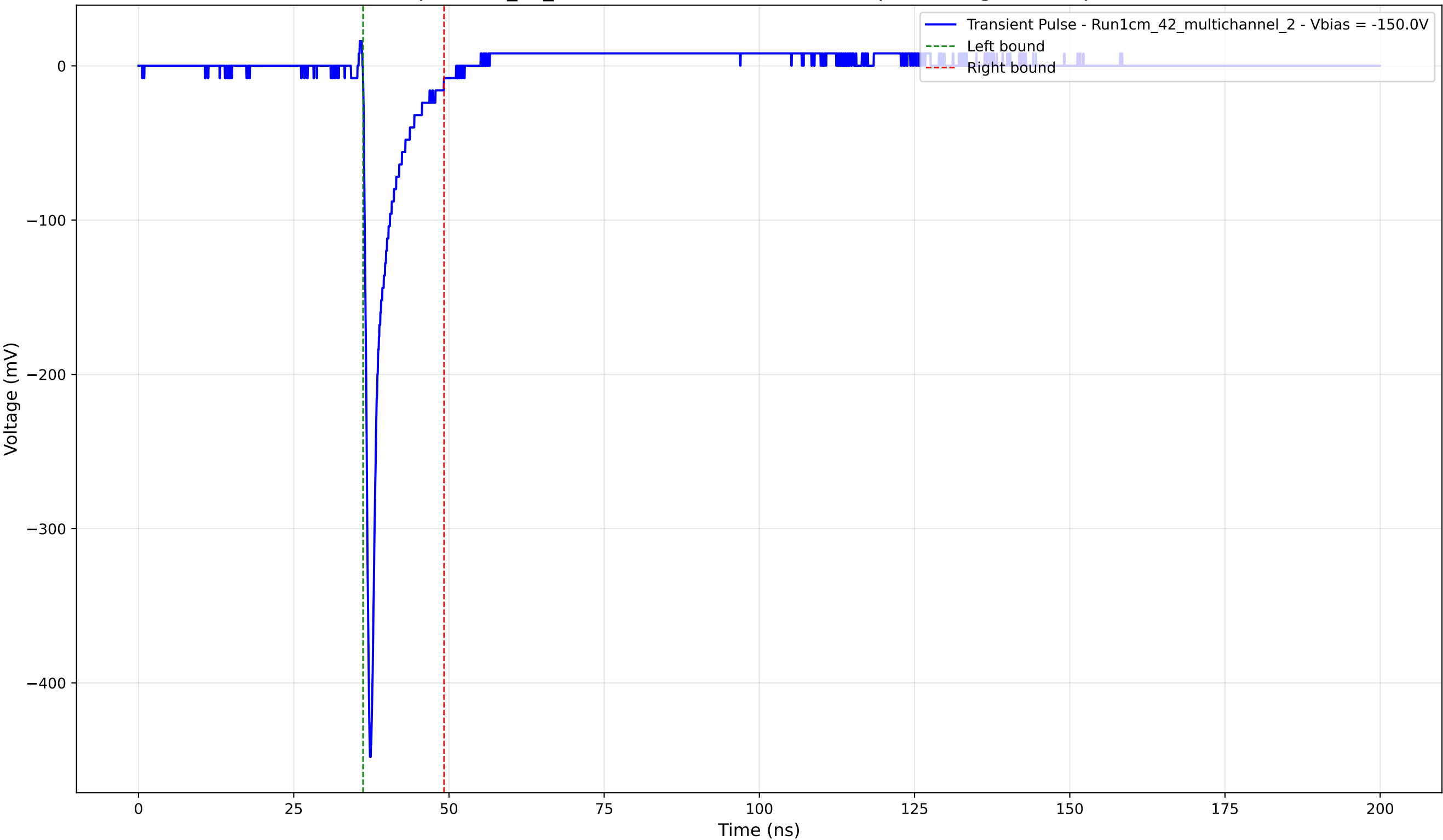
Transient Pulse - Sample: 1cm_42_multichannel - Position: 2030.0 \mu\text{m} - Charge: 26.09 pC - Rise Time: 0.75 ns
