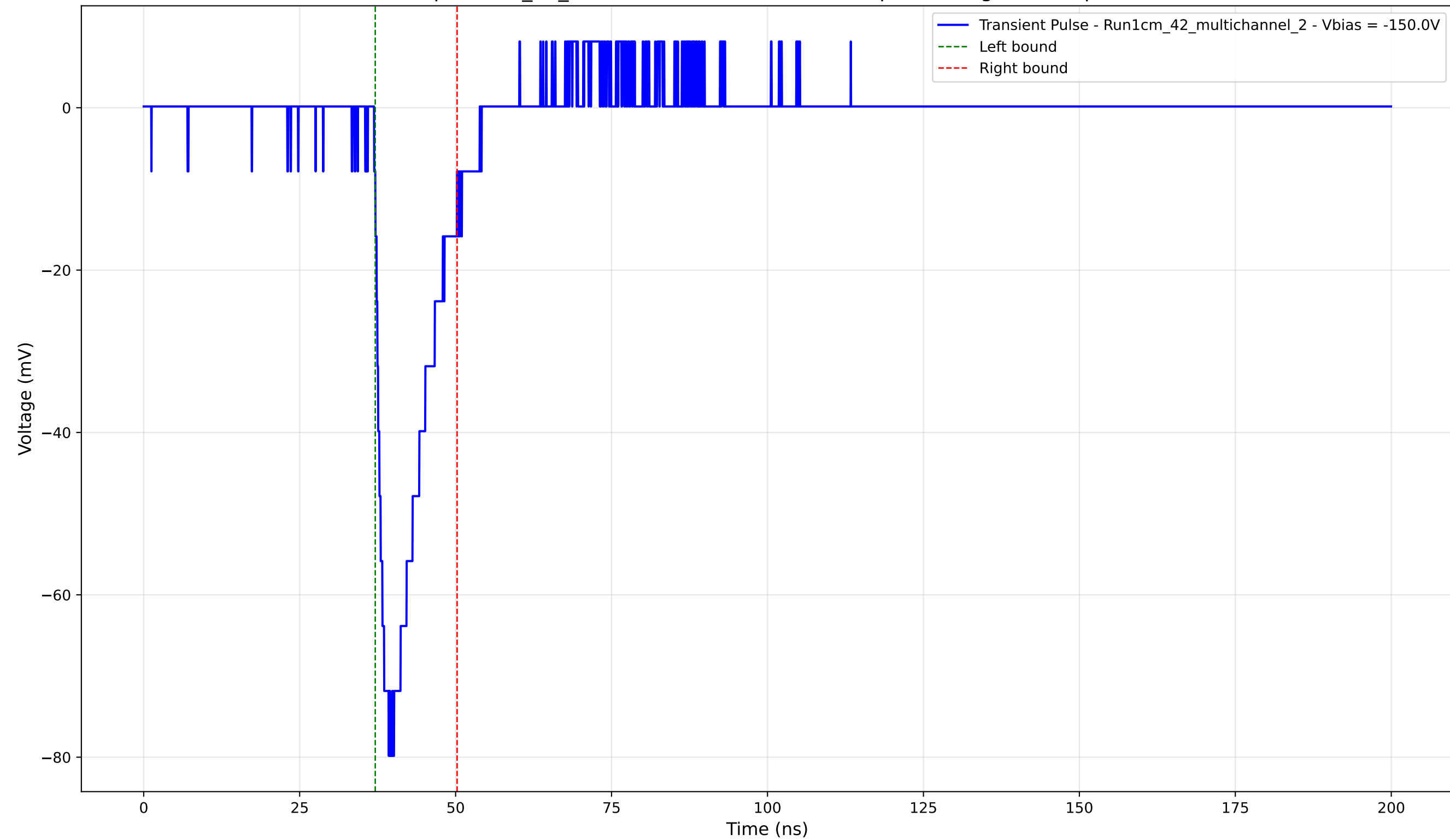
Transient Pulse - Sample: 1cm_42_multichannel - Position: 415.0 \mu\text{m} - Charge: 11.53 pC - Rise Time: 2.16 ns
