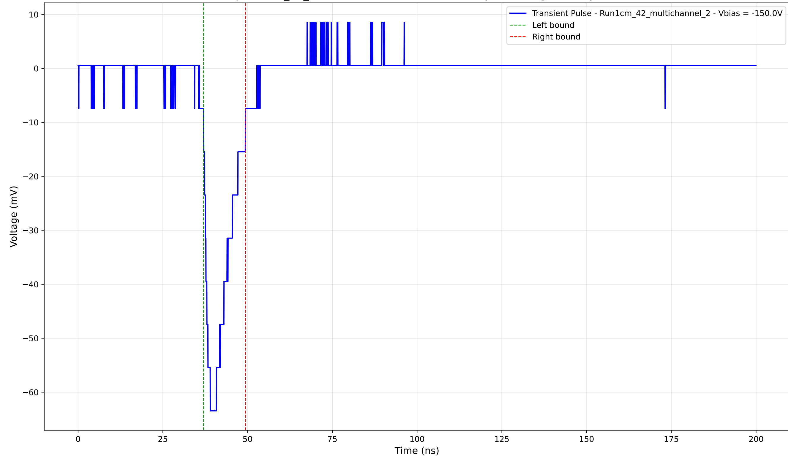
Transient Pulse - Sample: 1cm_42_multichannel - Position: 4775.0 \mu\text{m} - Charge: 9.33 pC - Rise Time: 3.17 ns
