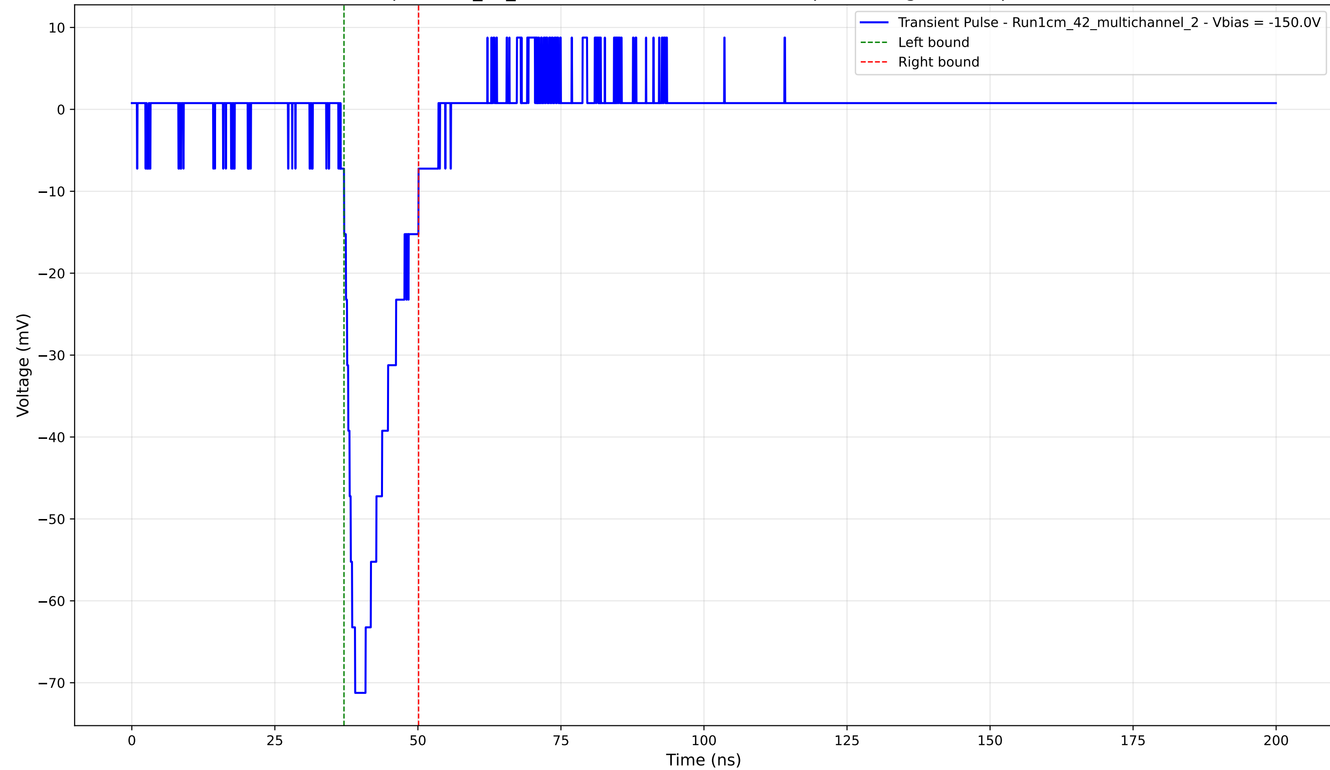
Transient Pulse - Sample: 1cm_42_multichannel - Position: 4575.0 \mu\text{m} - Charge: 10.55 pC - Rise Time: 2.52 ns
