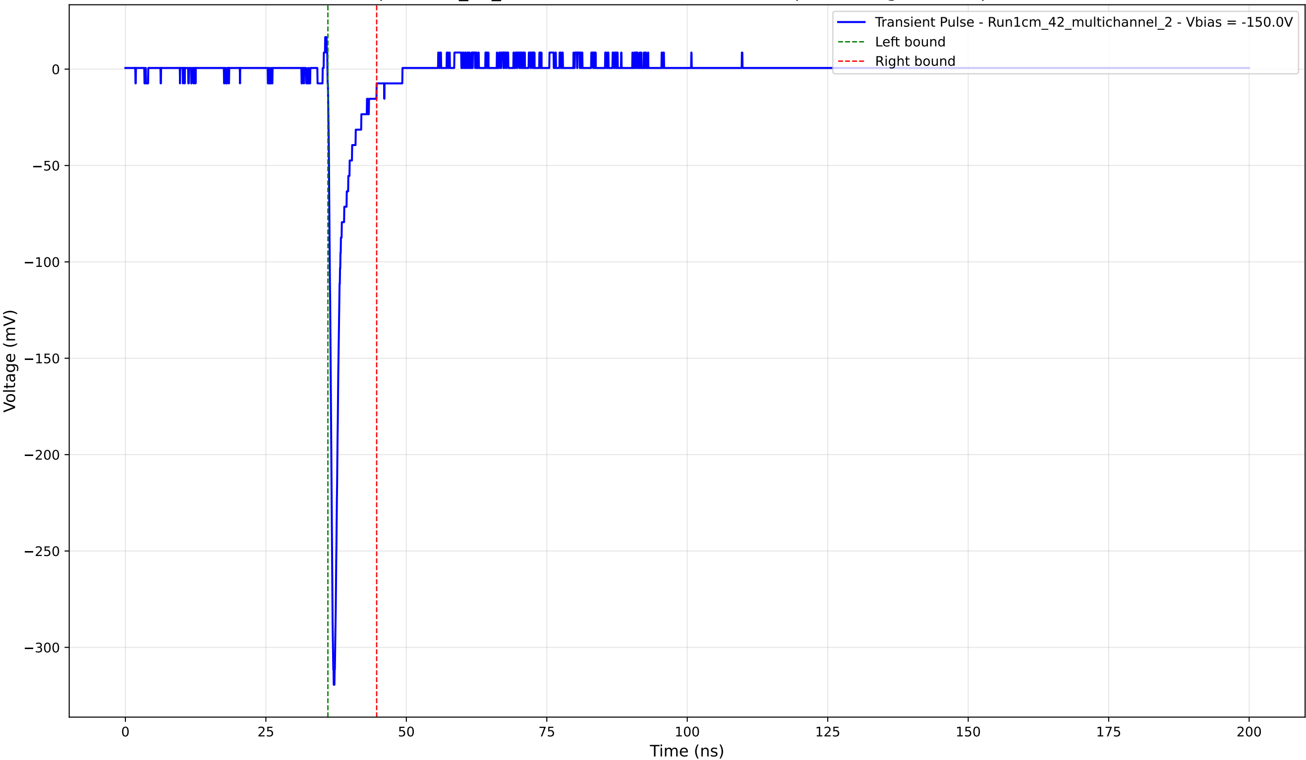
Transient Pulse - Sample: 1cm_42_multichannel - Position: 2420.0 \mu\text{m} - Charge: 13.57 pC - Rise Time: 0.72 ns
