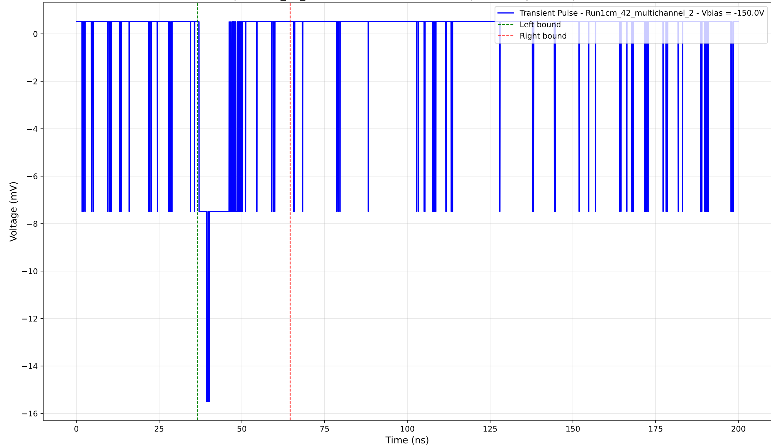
Transient Pulse - Sample: 1cm_42_multichannel - Position: 830.0 \mu\text{m} - Charge: 1.77 pC - Rise Time: 2.23 ns
