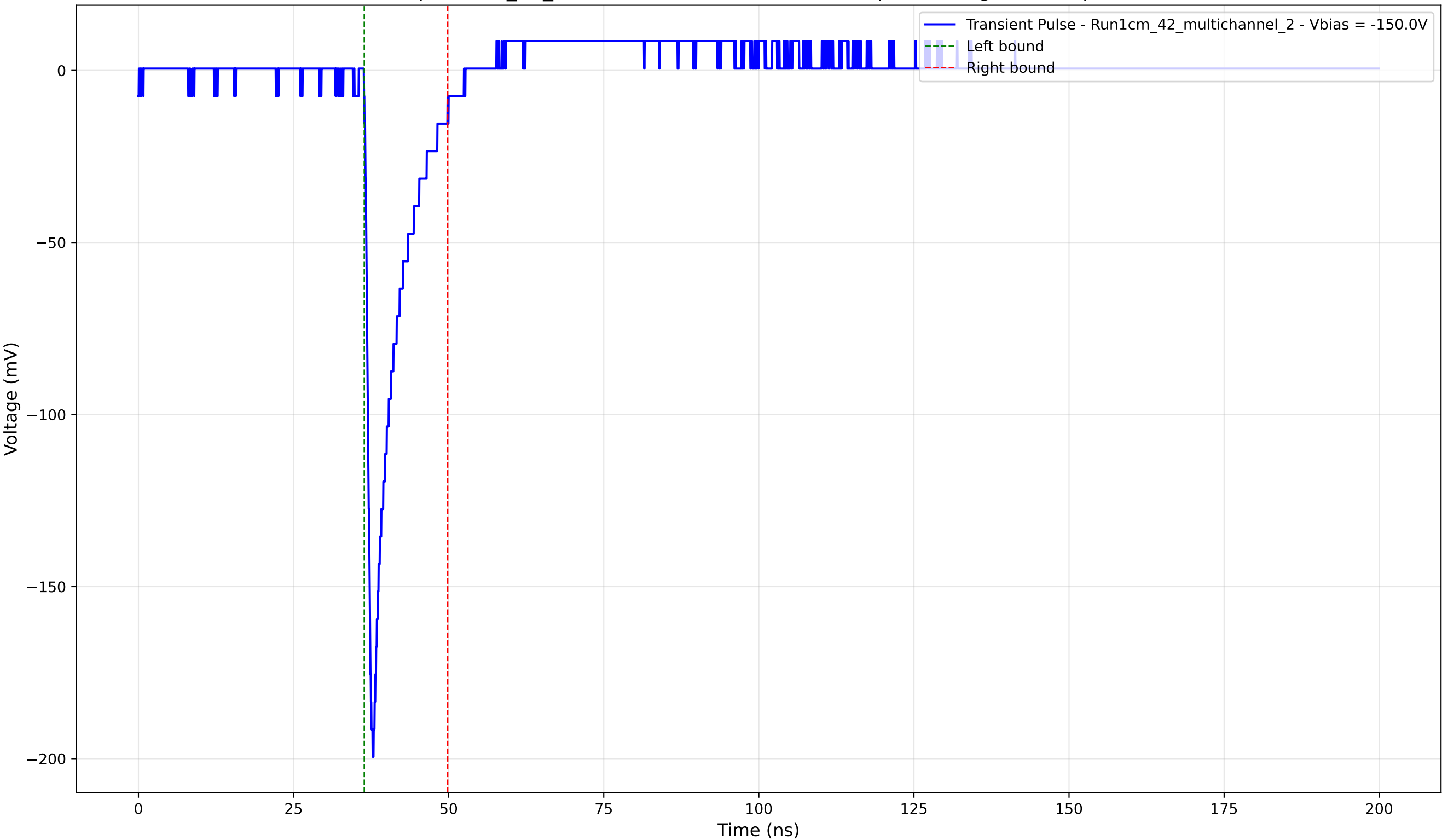
Transient Pulse - Sample: 1cm_42_multichannel - Position: 3175.0 \mu\text{m} - Charge: 18.47 pC - Rise Time: 0.94 ns
