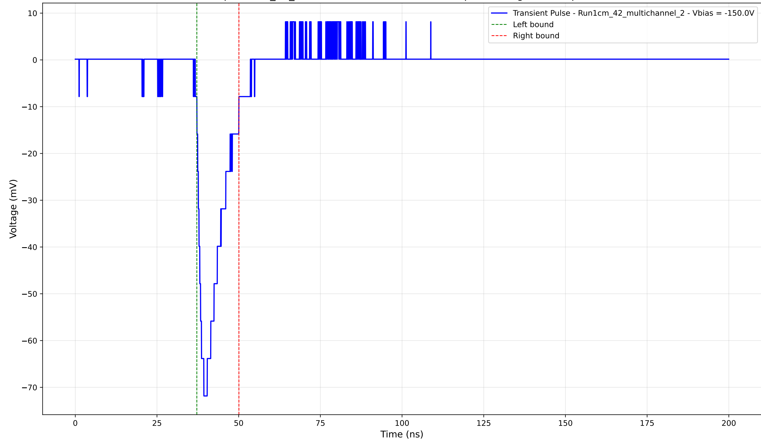
Transient Pulse - Sample: 1cm_42_multichannel - Position: 4300.0 \mu\text{m} - Charge: 10.27 pC - Rise Time: 2.60 ns
