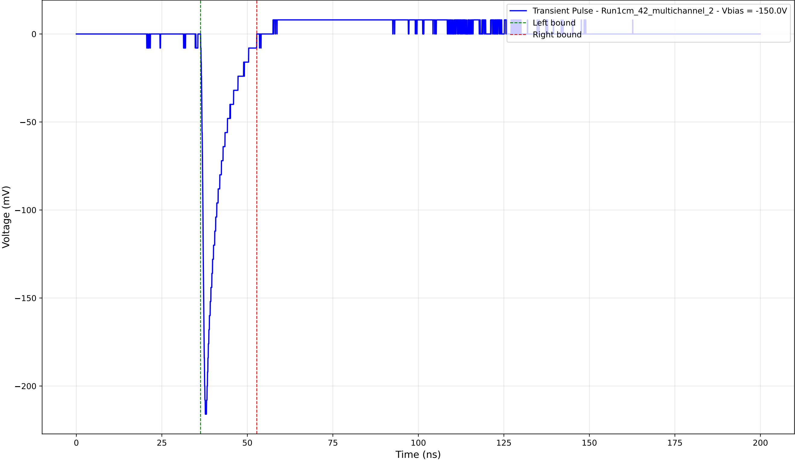
Transient Pulse - Sample: 1cm_42_multichannel - Position: 1510.0 \mu\text{m} - Charge: 21.82 pC - Rise Time: 0.97 ns
