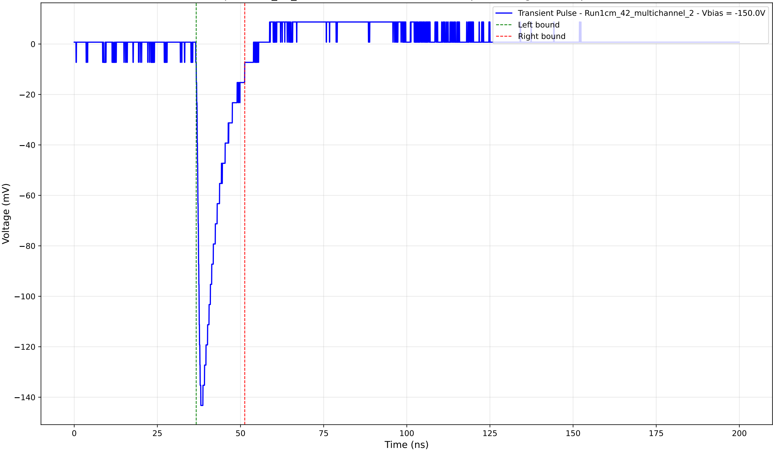
Transient Pulse - Sample: 1cm_42_multichannel - Position: 1170.0 \mu\text{m} - Charge: 18.25 pC - Rise Time: 1.16 ns
