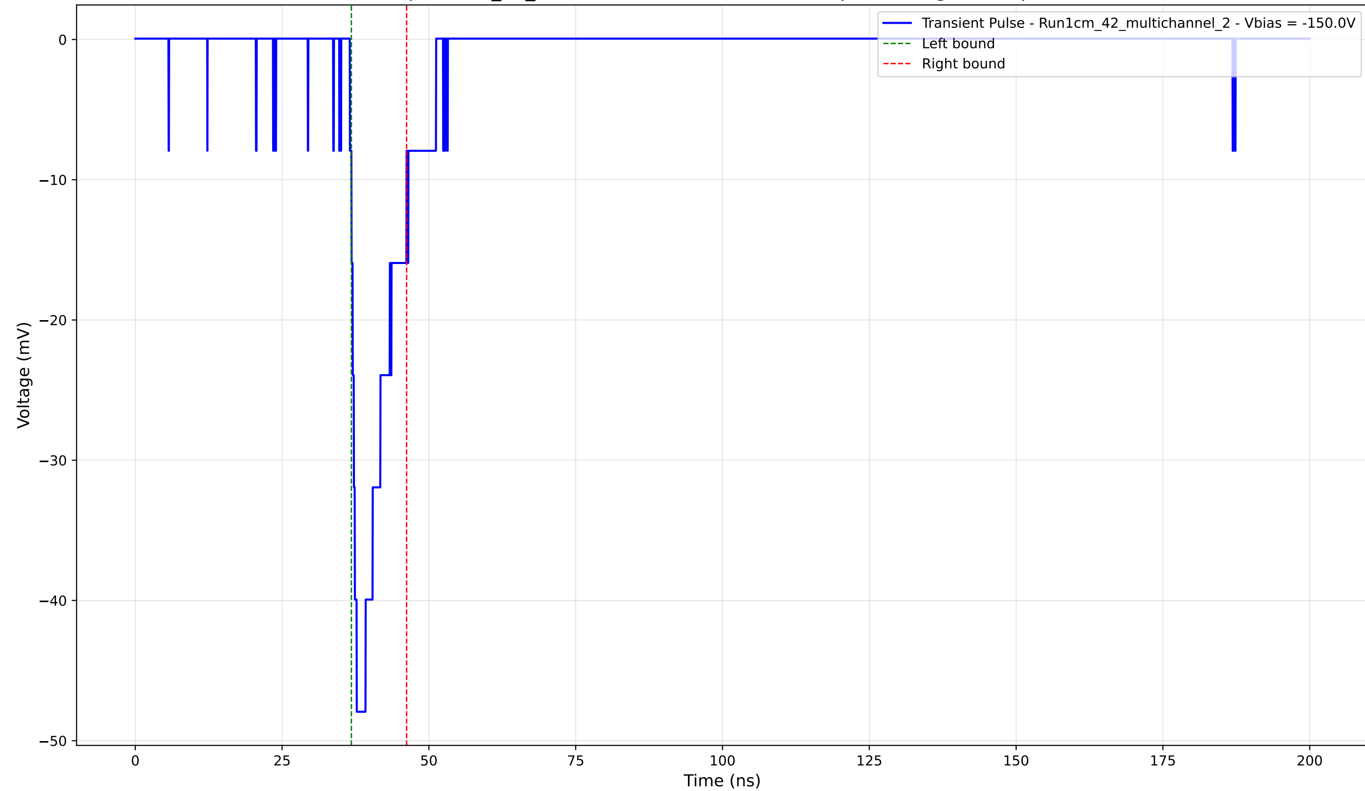
Transient Pulse - Sample: 1cm_42_multichannel - Position: 3425.0 \mu\text{m} - Charge: 5.49 pC - Rise Time: 1.18 ns
