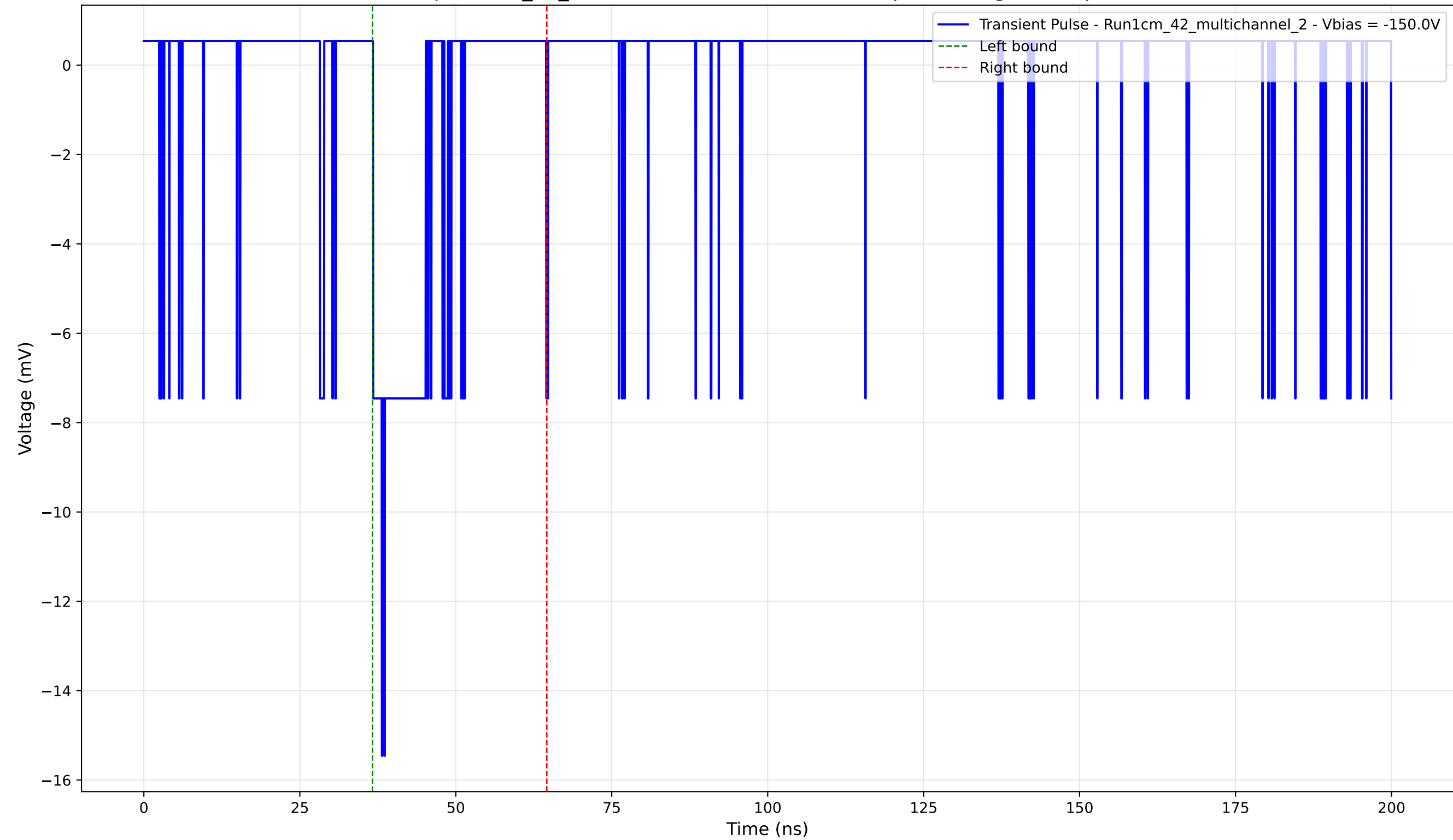
Transient Pulse - Sample: 1cm_42_multichannel - Position: 3370.0 \mu\text{m} - Charge: 1.35 pC - Rise Time: 1.43 ns
