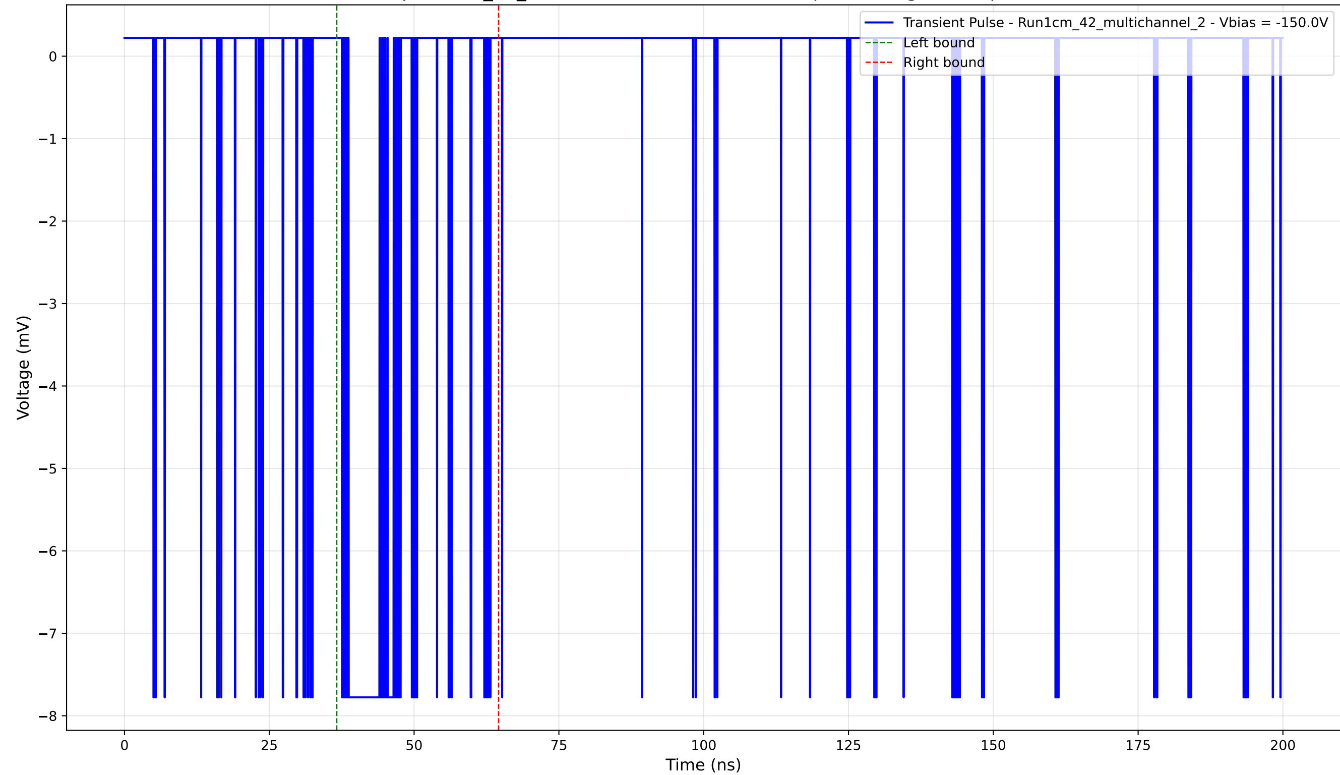
Transient Pulse - Sample: 1cm_42_multichannel - Position: 345.0 \mu\text{m} - Charge: 1.49 pC - Rise Time: 0.04 ns
