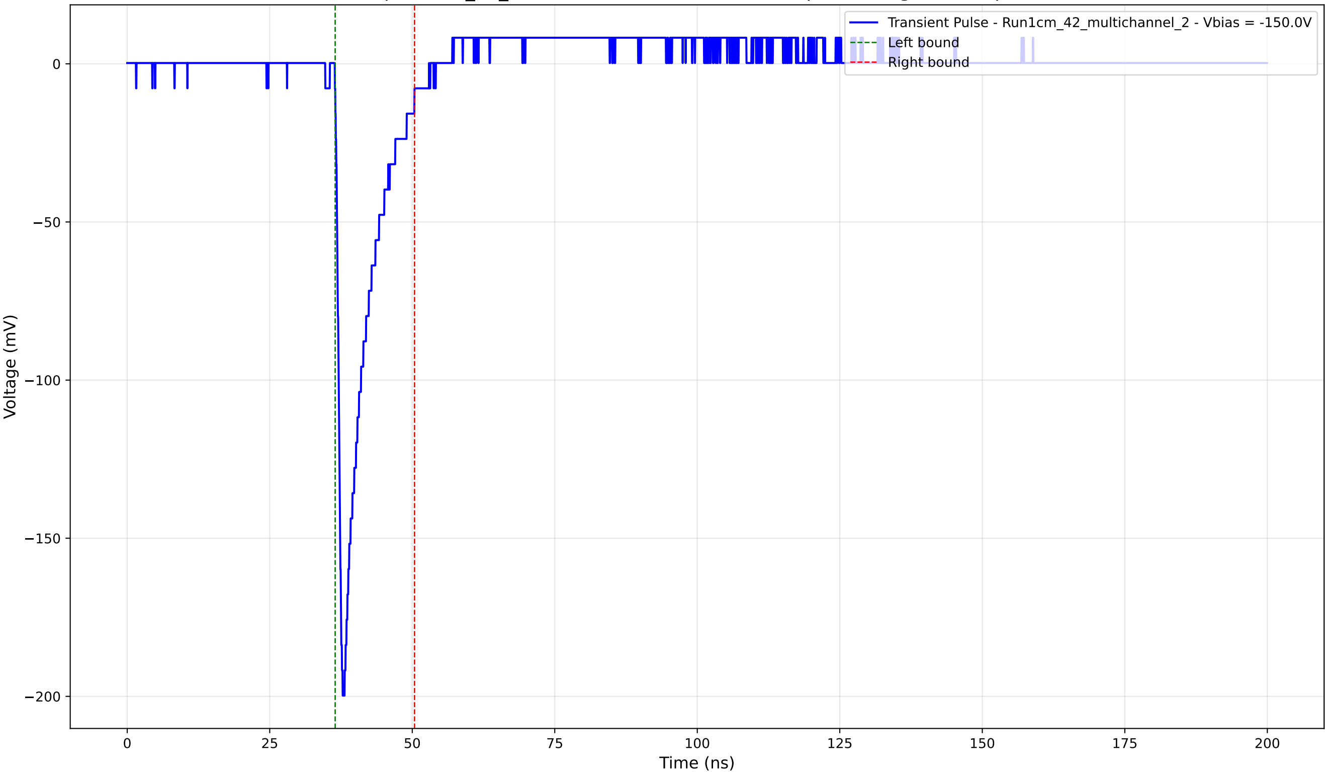
Transient Pulse - Sample: 1cm_42_multichannel - Position: 1460.0 \mu\text{m} - Charge: 20.56 pC - Rise Time: 0.98 ns
