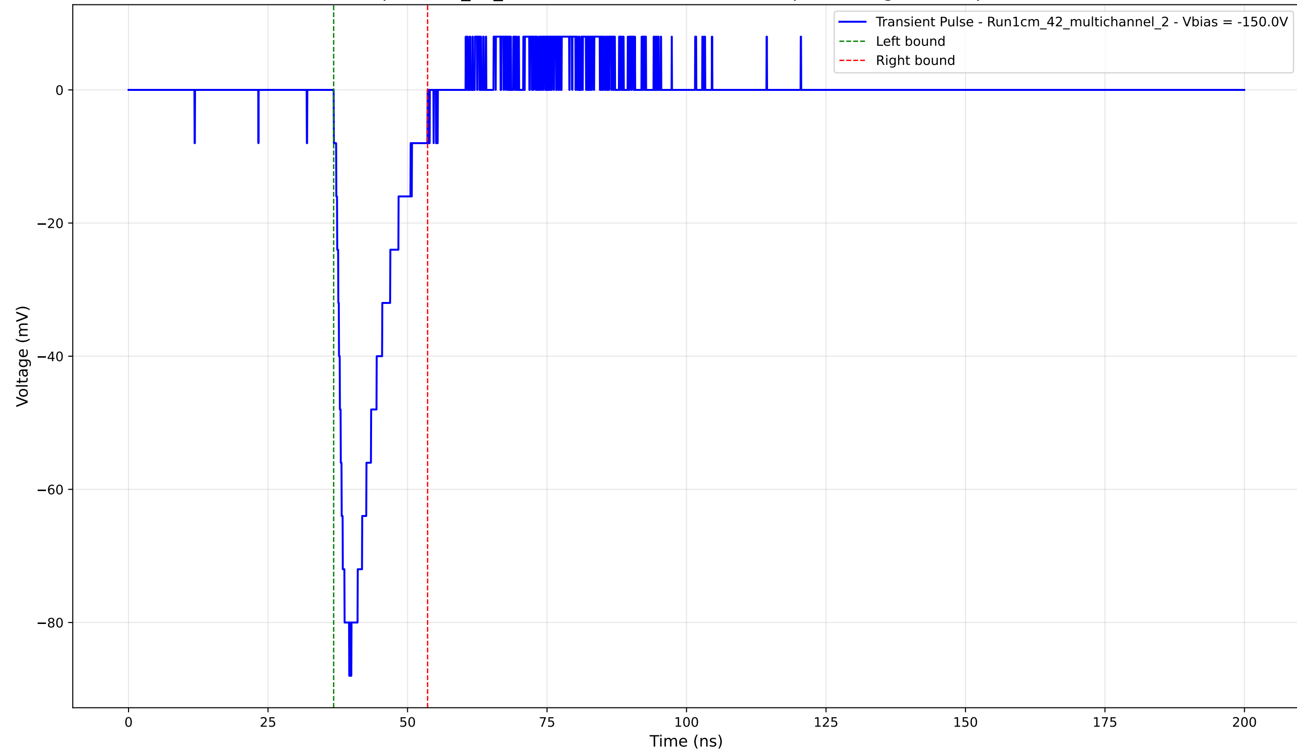
Transient Pulse - Sample: 1cm_42_multichannel - Position: 4180.0 \mu\text{m} - Charge: 12.94 pC - Rise Time: 1.52 ns
