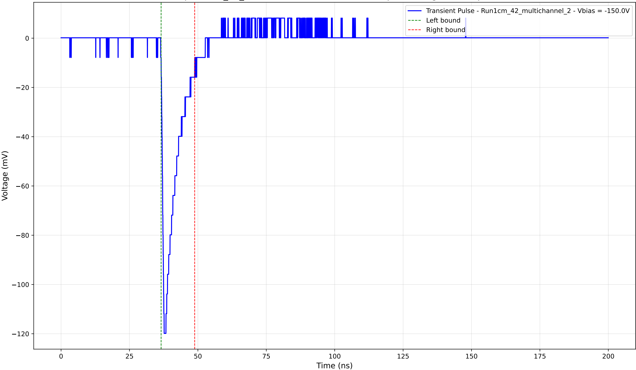
Transient Pulse - Sample: 1cm_42_multichannel - Position: 3320.0 \mu\text{m} - Charge: 12.93 pC - Rise Time: 0.98 ns
