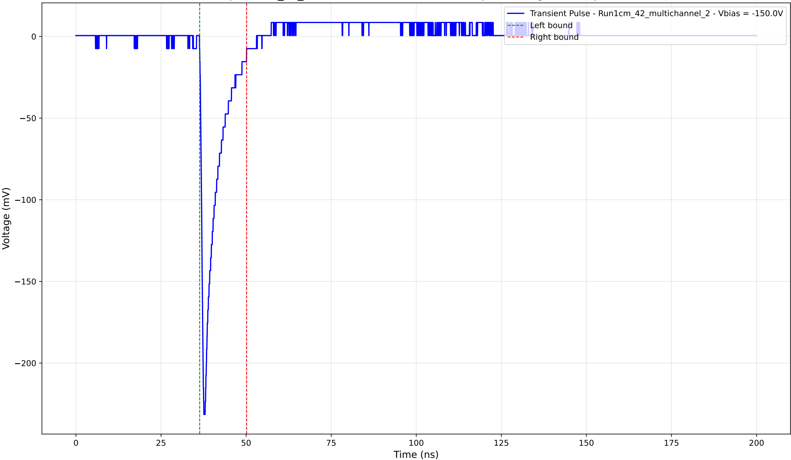
Transient Pulse - Sample: 1cm_42_multichannel - Position: 1595.0 \mu\text{m} - Charge: 21.45 pC - Rise Time: 0.96 ns
