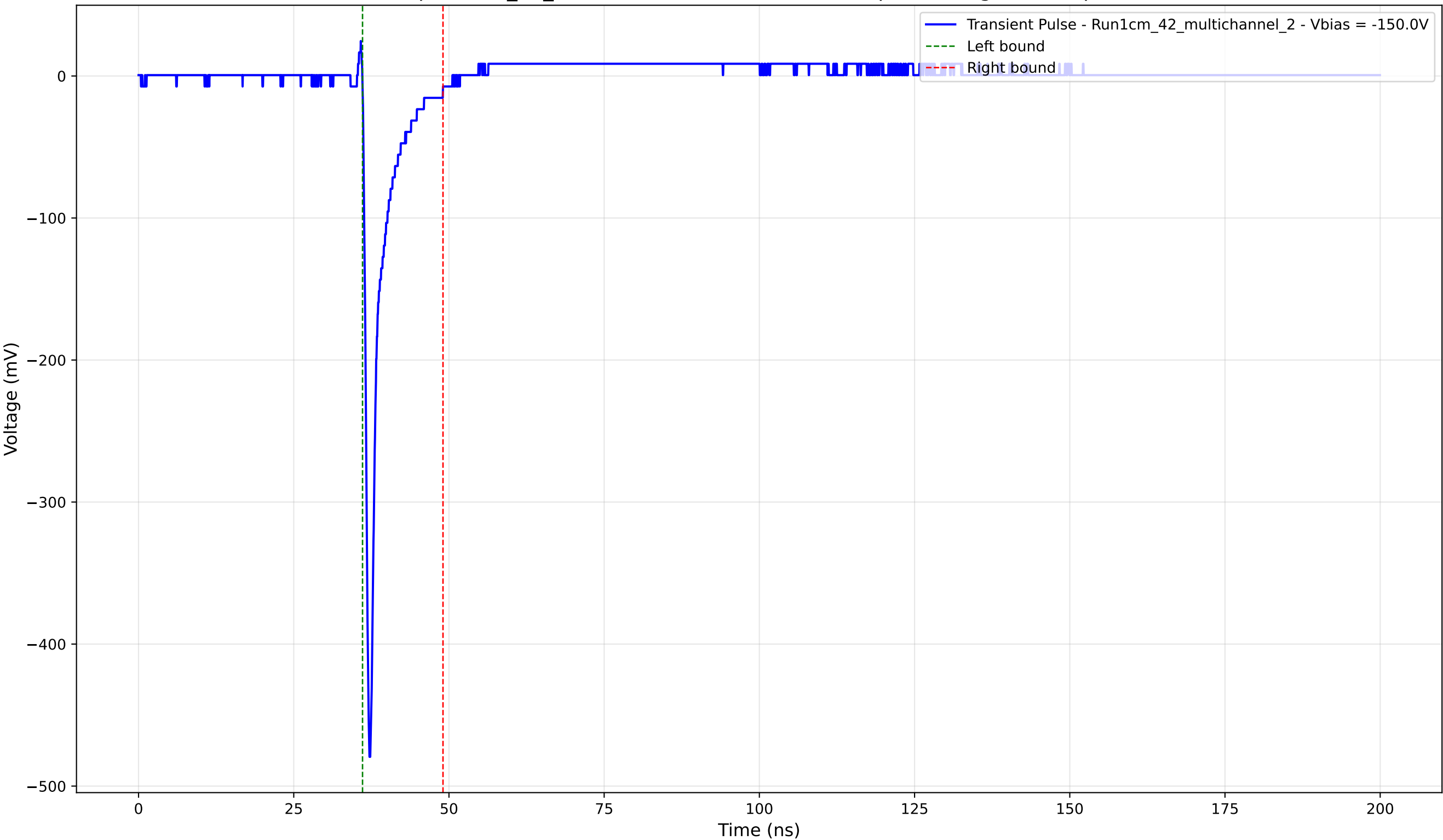
Transient Pulse - Sample: 1cm_42_multichannel - Position: 2600.0 \mu\text{m} - Charge: 24.86 pC - Rise Time: 0.72 ns
