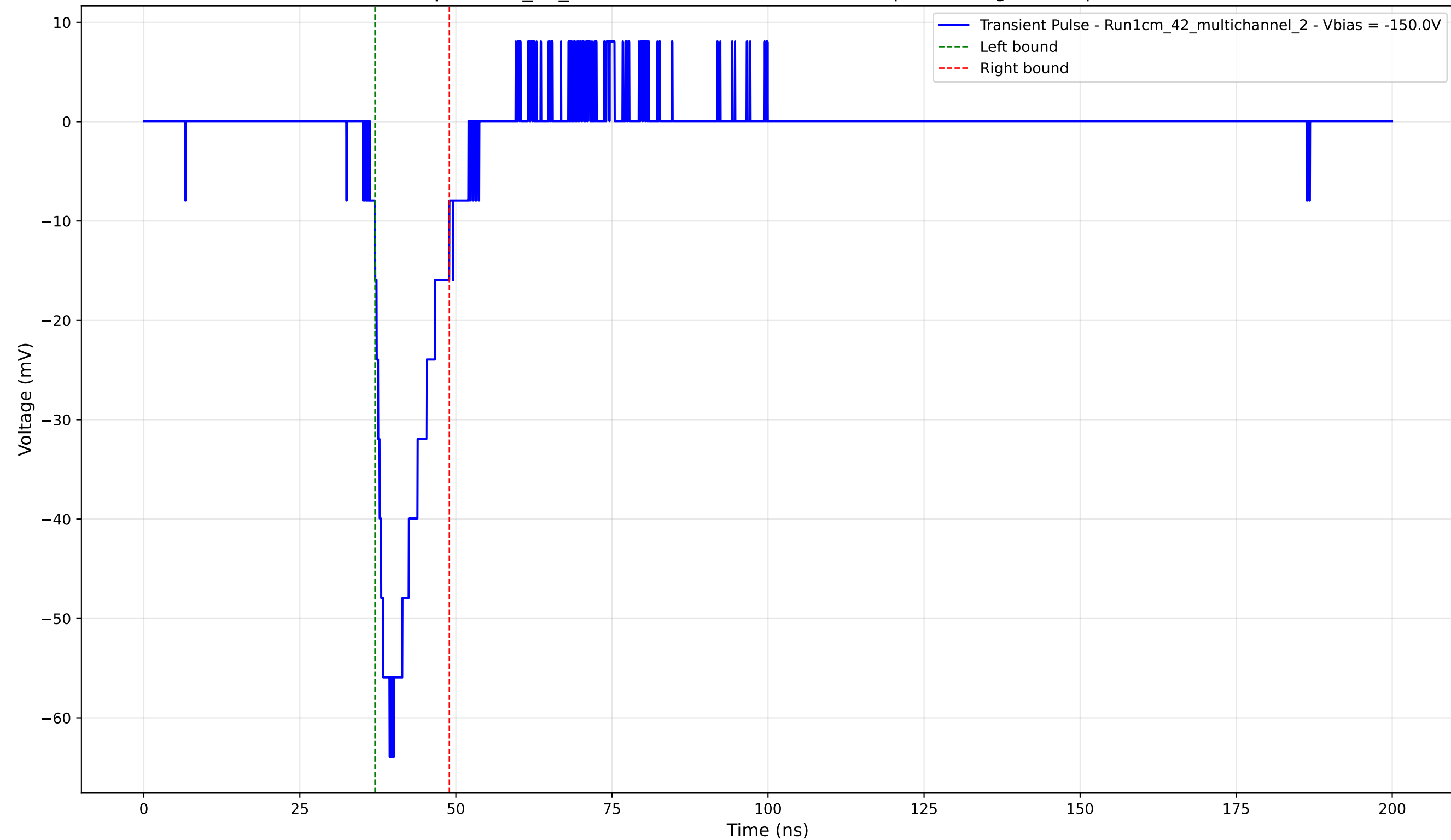
Transient Pulse - Sample: 1cm_42_multichannel - Position: 4795.0 \mu\text{m} - Charge: 8.79 pC - Rise Time: 3.17 ns
