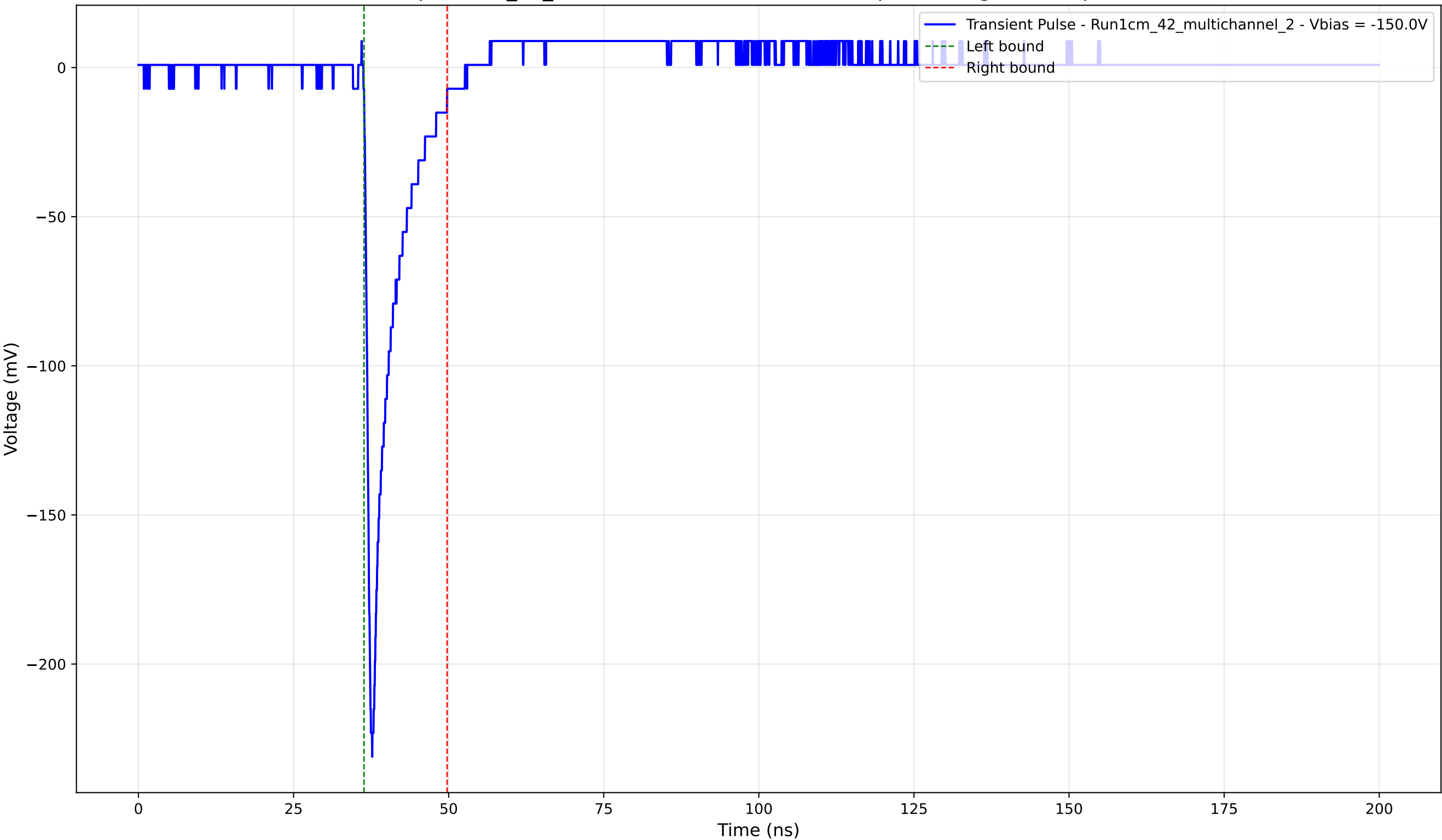
Transient Pulse - Sample: 1cm_42_multichannel - Position: 3065.0 \mu\text{m} - Charge: 19.33 pC - Rise Time: 0.92 ns
