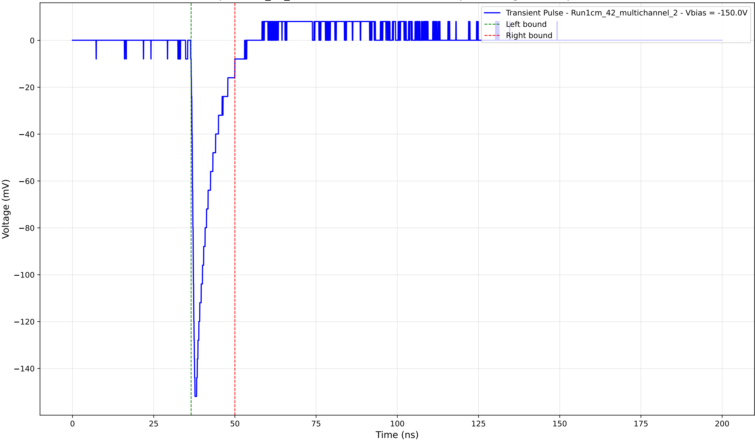
Transient Pulse - Sample: 1cm_42_multichannel - Position: 3305.0 \mu\text{m} - Charge: 16.21 pC - Rise Time: 1.04 ns
