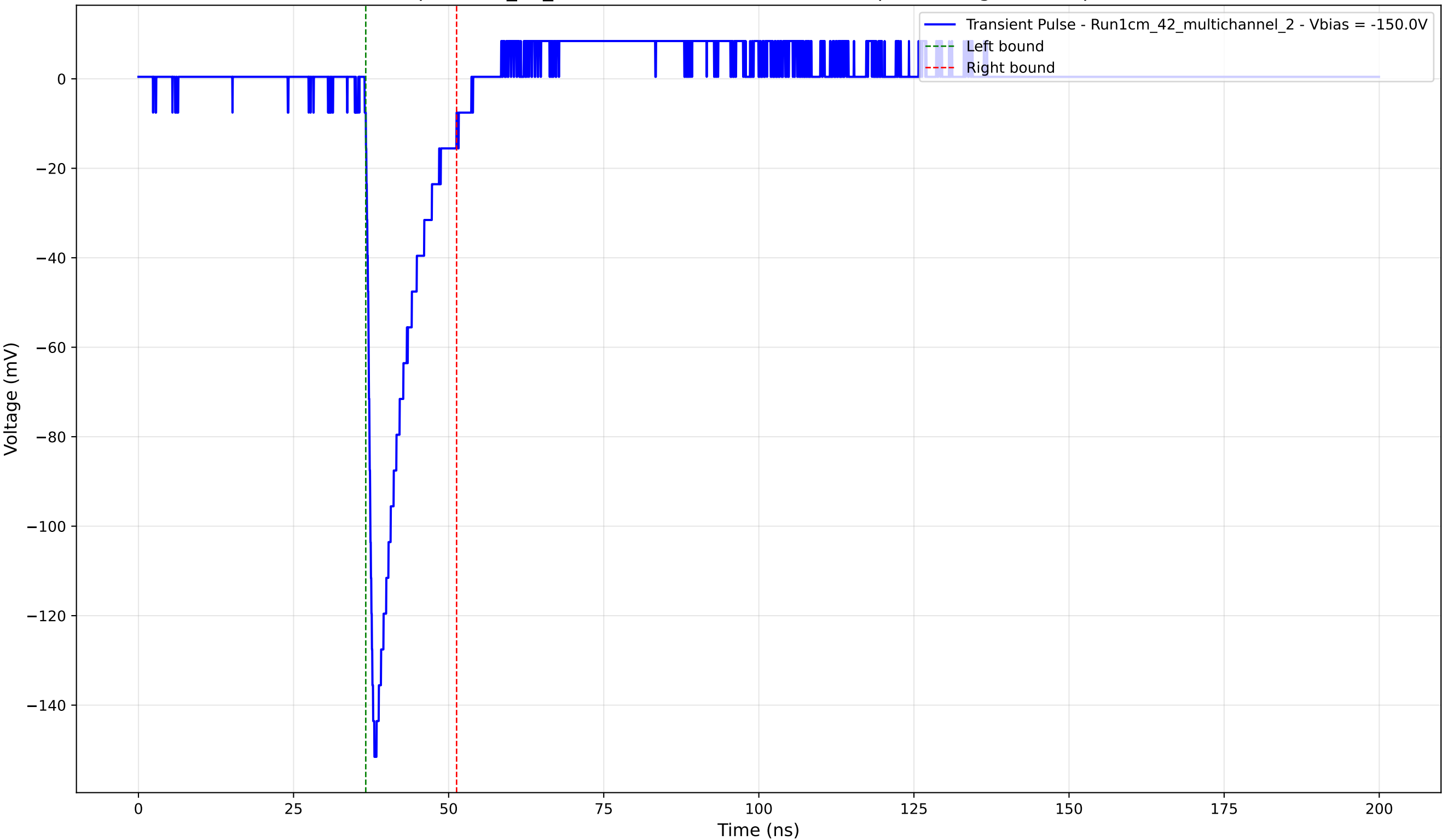
Transient Pulse - Sample: 1cm_42_multichannel - Position: 1275.0 \mu\text{m} - Charge: 18.03 pC - Rise Time: 1.16 ns
