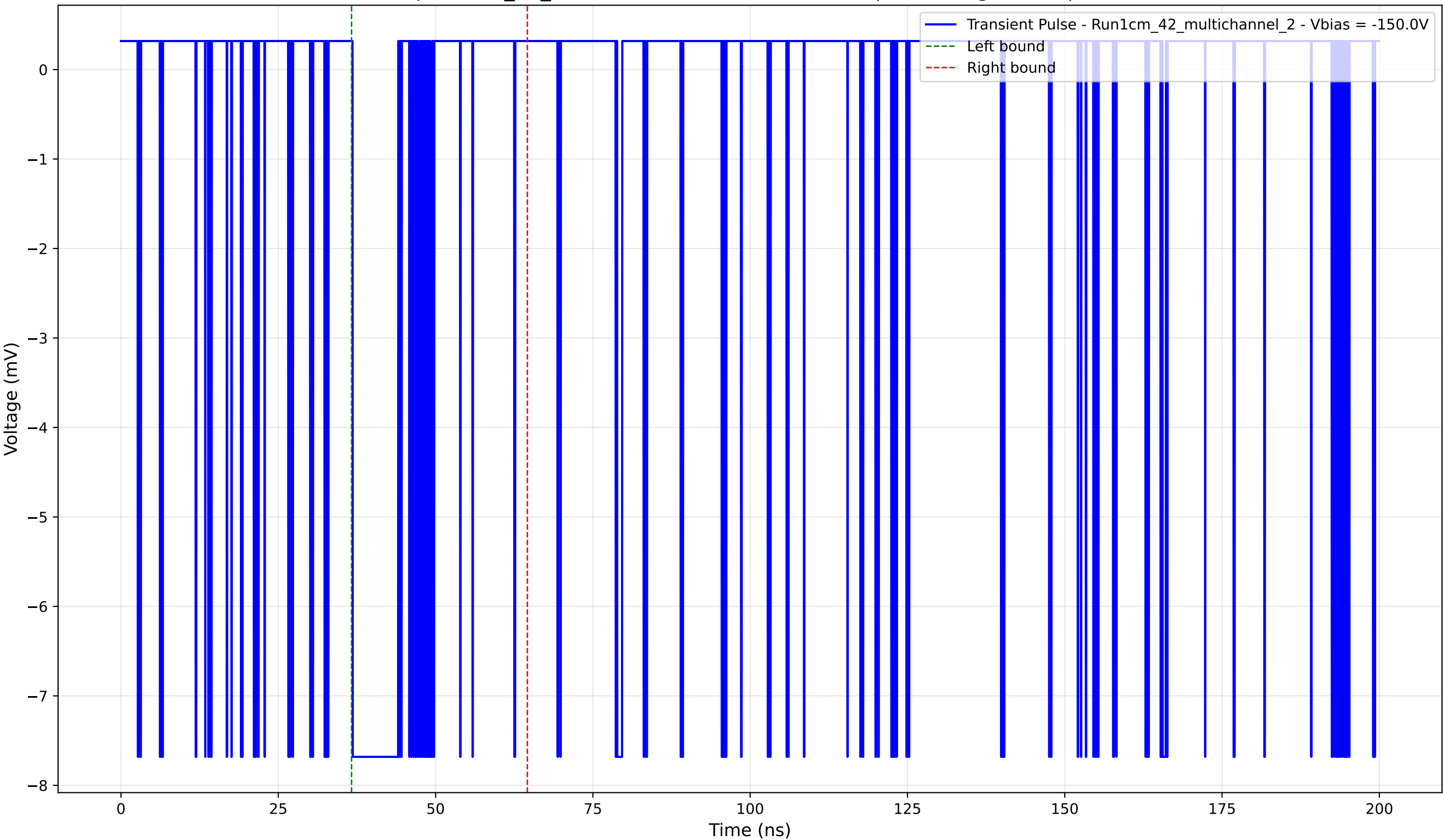
Transient Pulse - Sample: 1cm_42_multichannel - Position: 3380.0 \mu\text{m} - Charge: 1.34 pC - Rise Time: 0.04 ns
