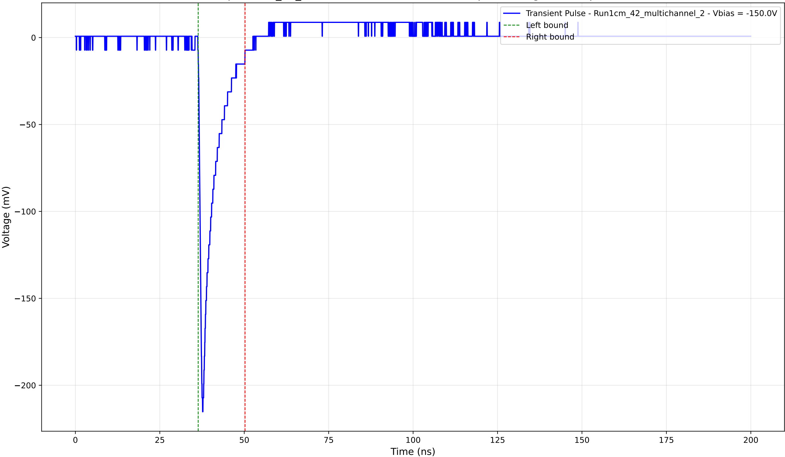
Transient Pulse - Sample: 1cm_42_multichannel - Position: 3110.0 \mu\text{m} - Charge: 18.94 pC - Rise Time: 0.97 ns
