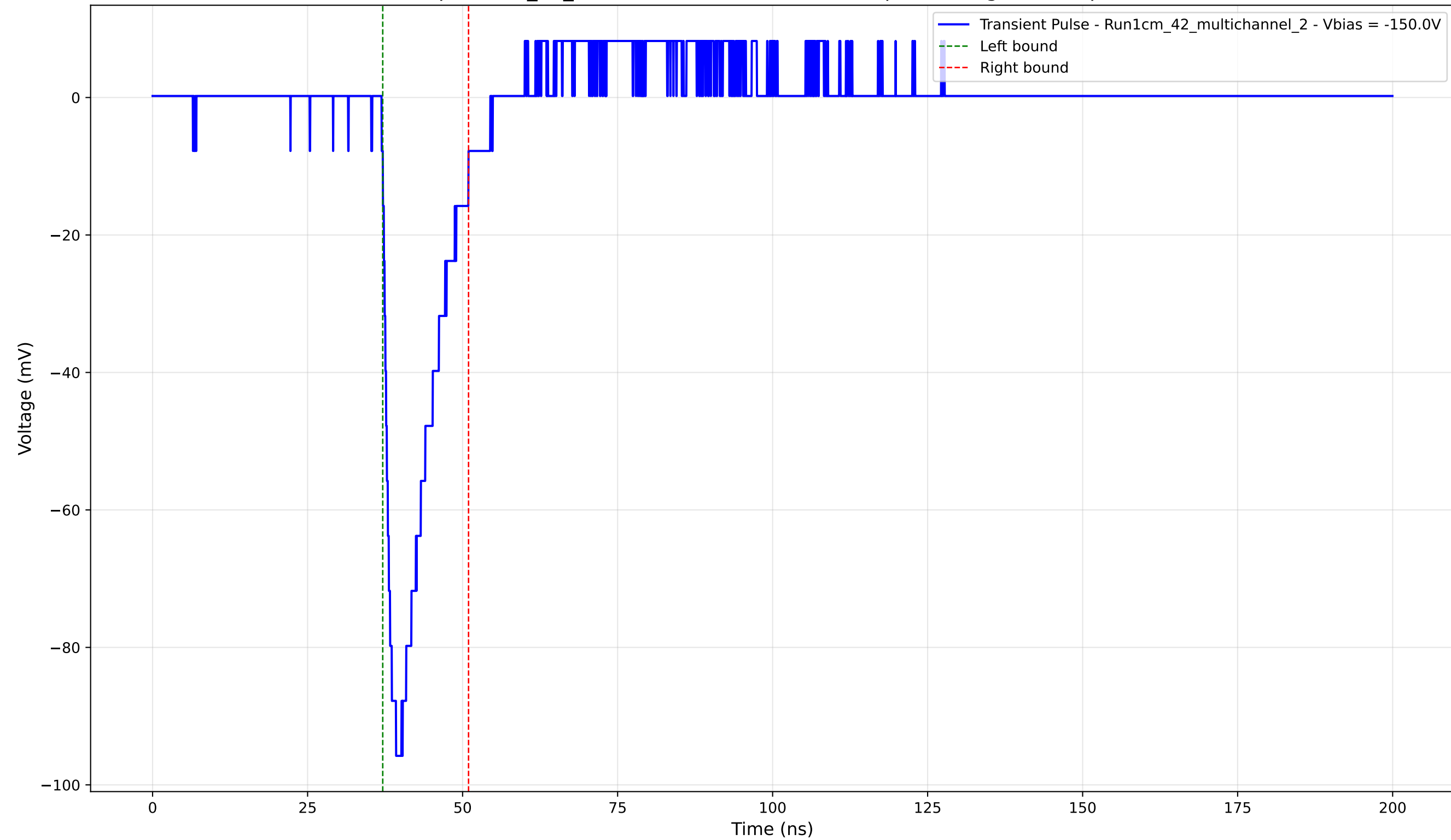
Transient Pulse - Sample: 1cm_42_multichannel - Position: 480.0 \mu\text{m} - Charge: 14.00 pC - Rise Time: 1.47 ns
