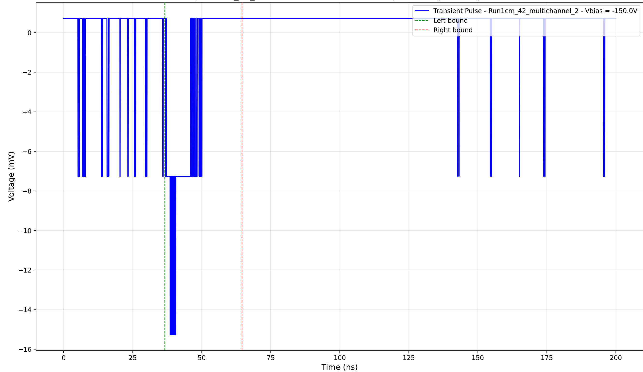
Transient Pulse - Sample: 1cm_42_multichannel - Position: 370.0 \mu\text{m} - Charge: 1.56 pC - Rise Time: 1.36 ns
