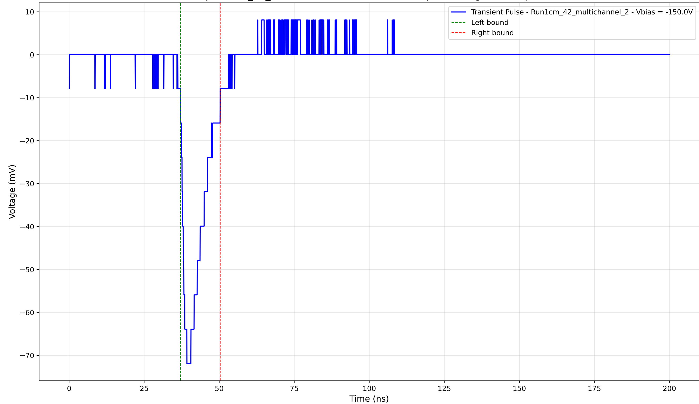
Transient Pulse - Sample: 1cm_42_multichannel - Position: 4625.0 \mu\text{m} - Charge: 10.64 pC - Rise Time: 3.00 ns
