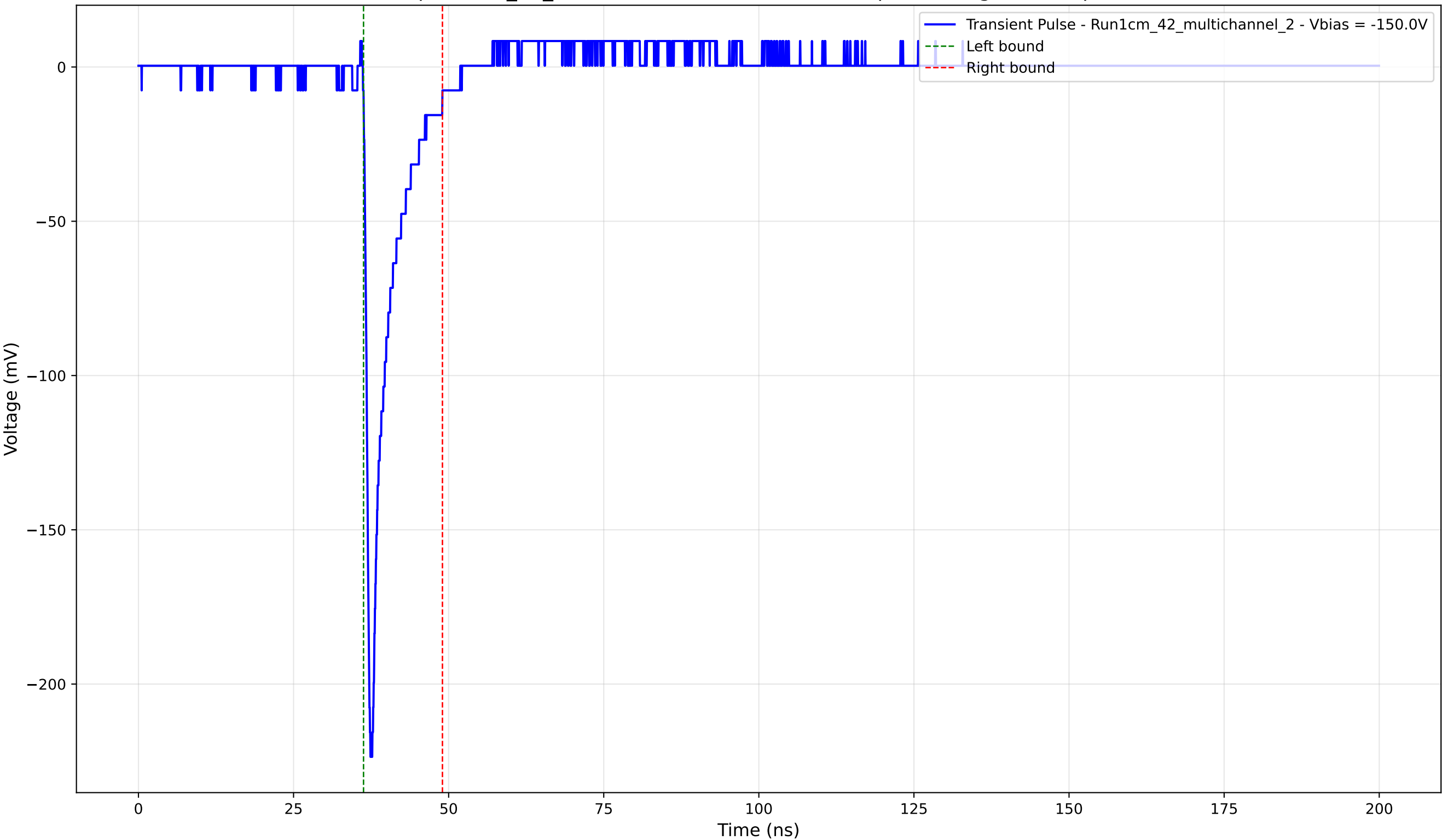
Transient Pulse - Sample: 1cm_42_multichannel - Position: 2940.0 \mu\text{m} - Charge: 16.99 pC - Rise Time: 0.89 ns
