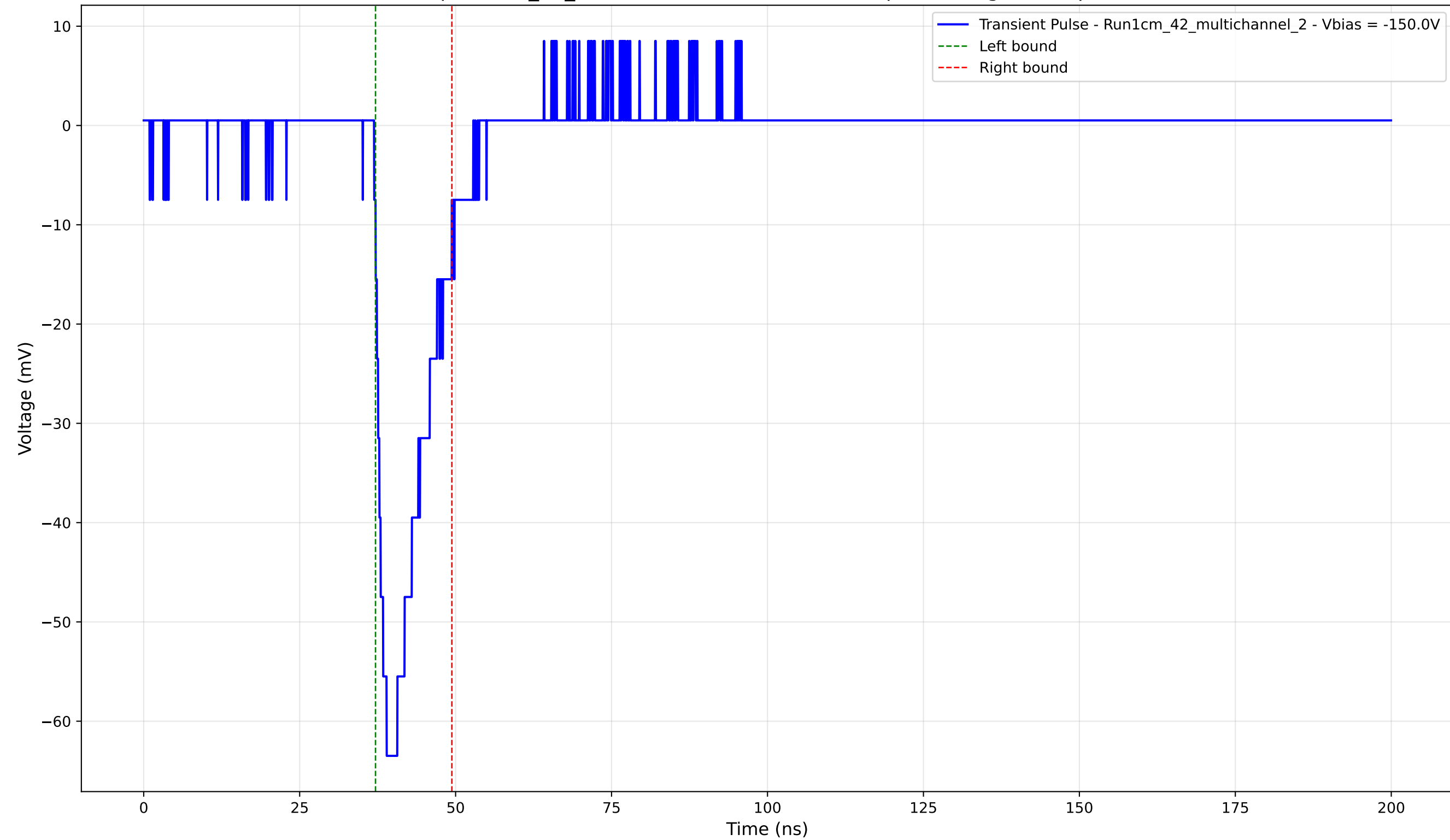
Transient Pulse - Sample: 1cm_42_multichannel - Position: 405.0 \mu\text{m} - Charge: 9.33 pC - Rise Time: 2.01 ns
