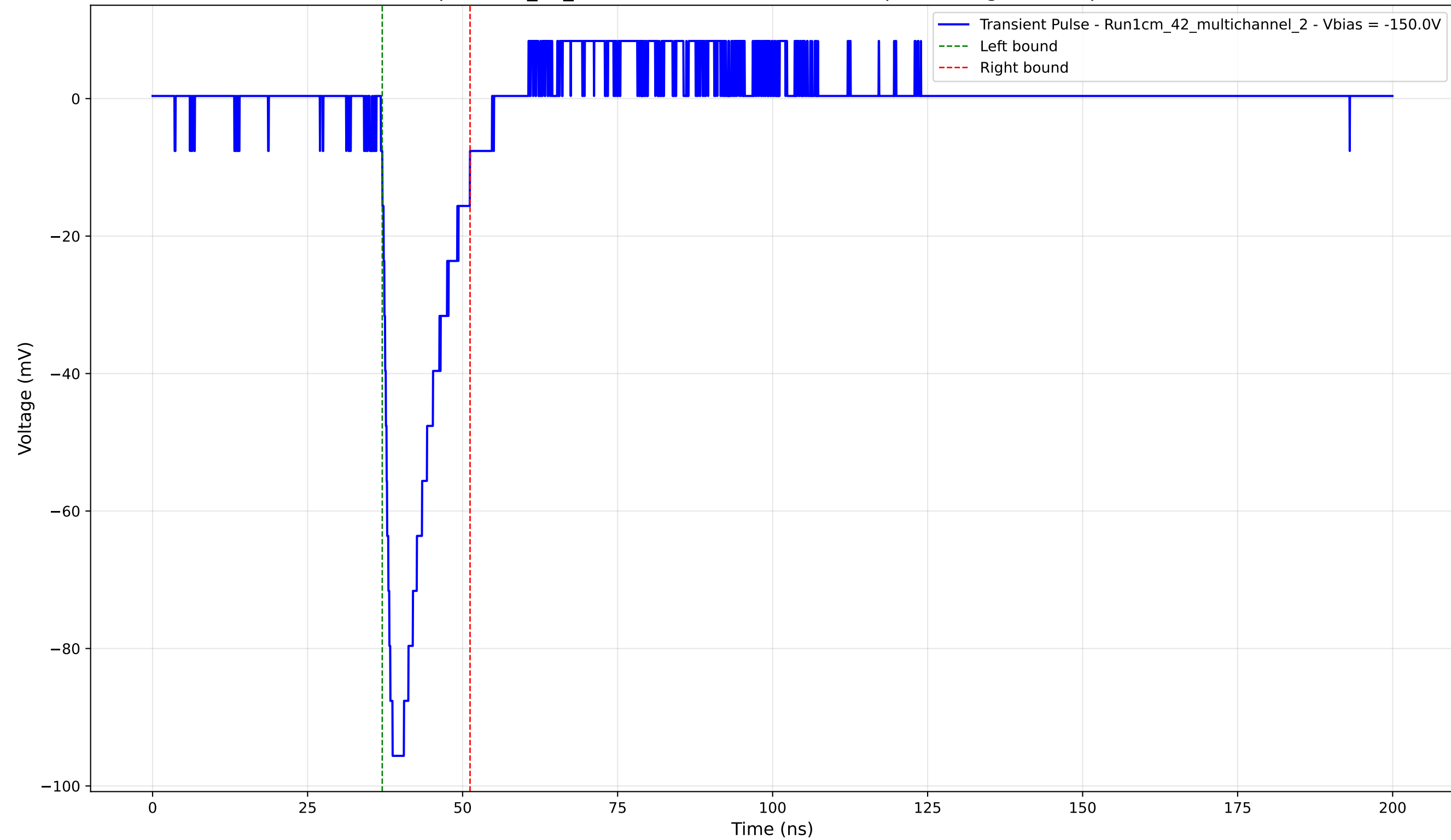
Transient Pulse - Sample: 1cm_42_multichannel - Position: 580.0 \mu\text{m} - Charge: 14.64 pC - Rise Time: 1.31 ns
