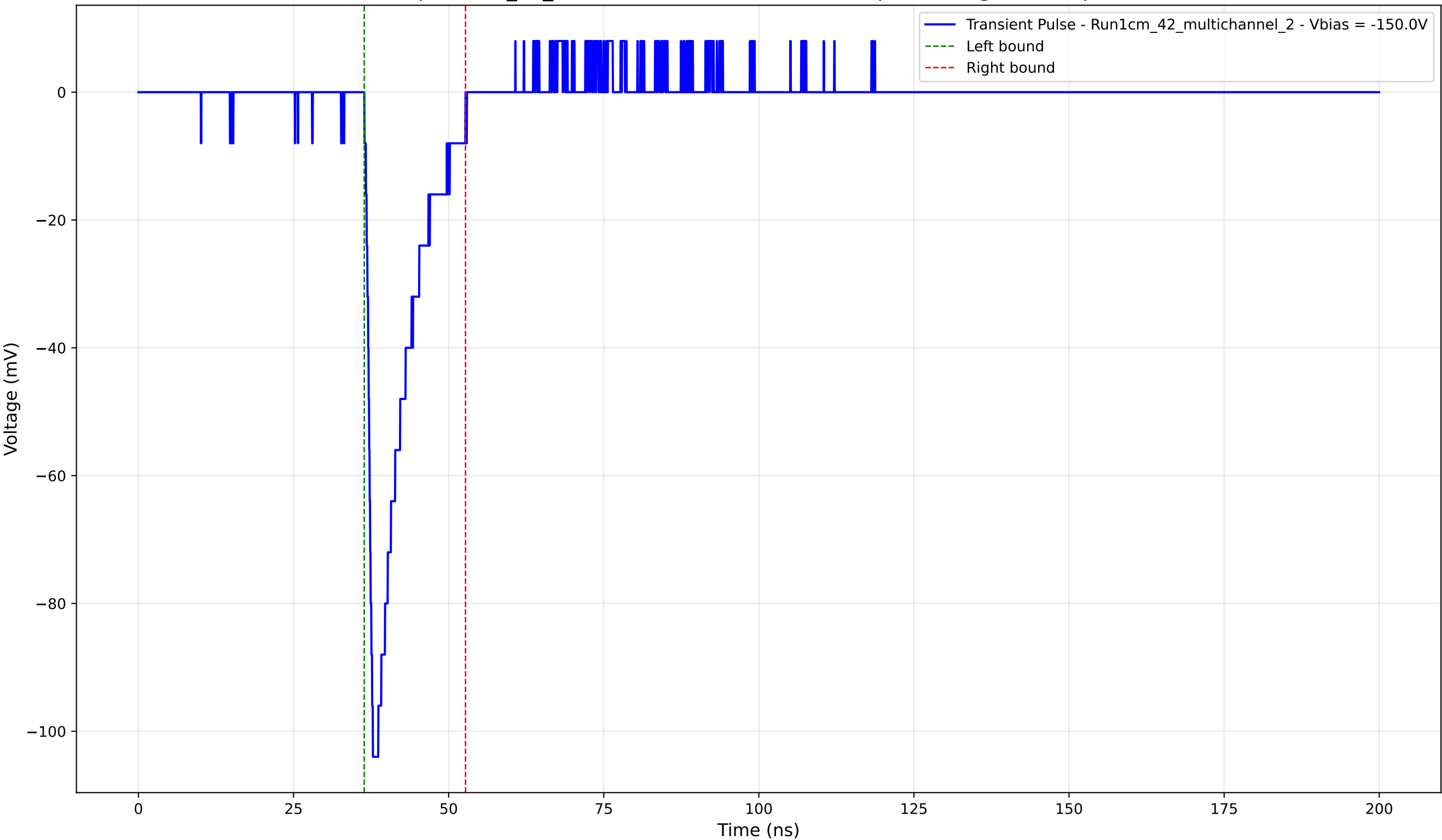
Transient Pulse - Sample: 1cm_42_multichannel - Position: 1300.0 \mu\text{m} - Charge: 12.95 pC - Rise Time: 1.03 ns
