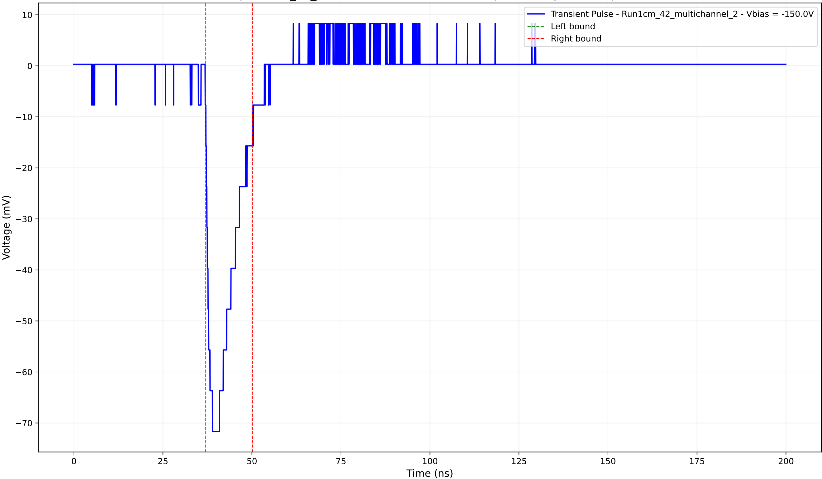
Transient Pulse - Sample: 1cm_42_multichannel - Position: 195.0 \mu\text{m} - Charge: 11.40 pC - Rise Time: 2.04 ns
