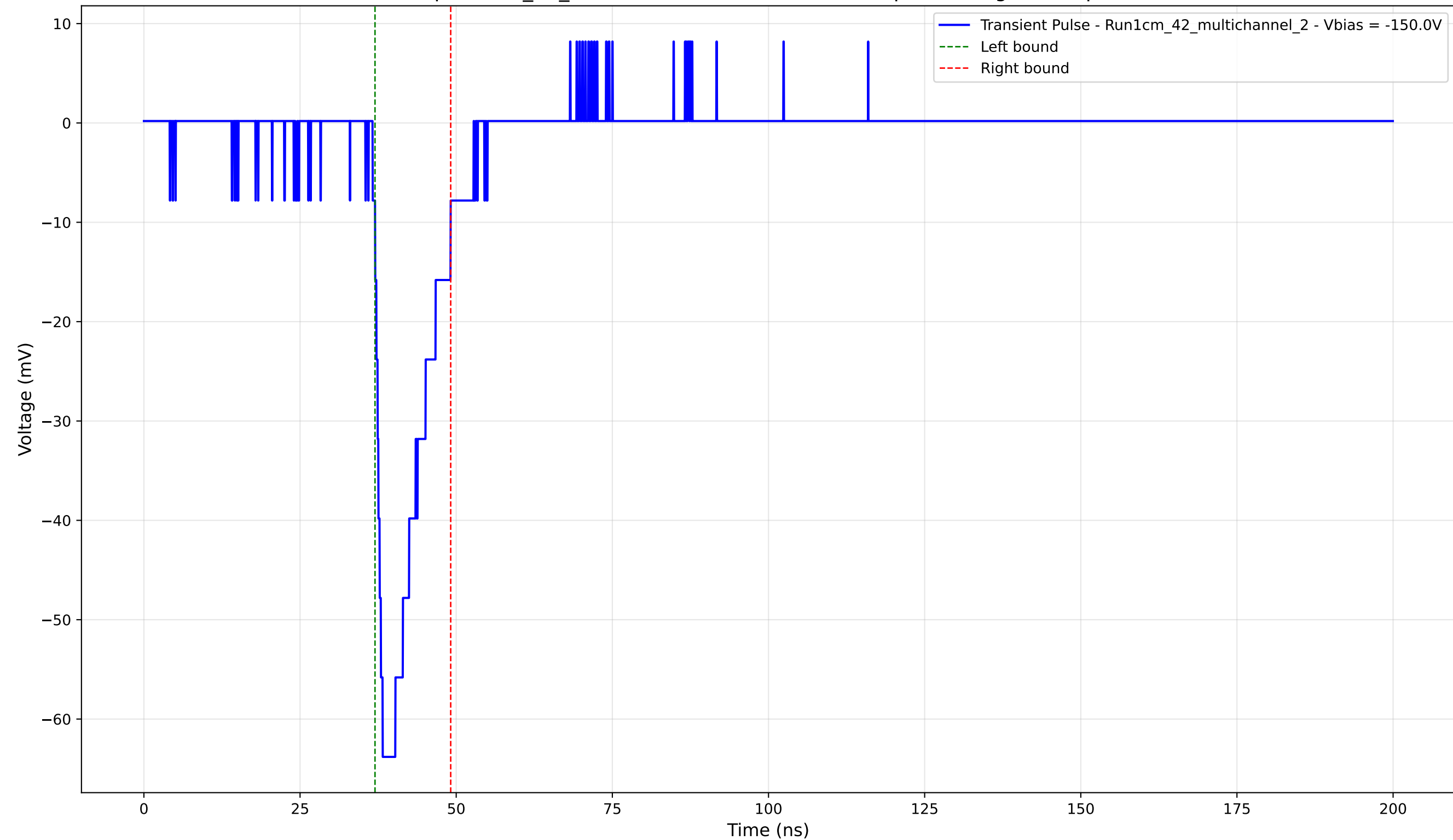
Transient Pulse - Sample: 1cm_42_multichannel - Position: 3830.0 \mu\text{m} - Charge: 9.19 pC - Rise Time: 1.61 ns
