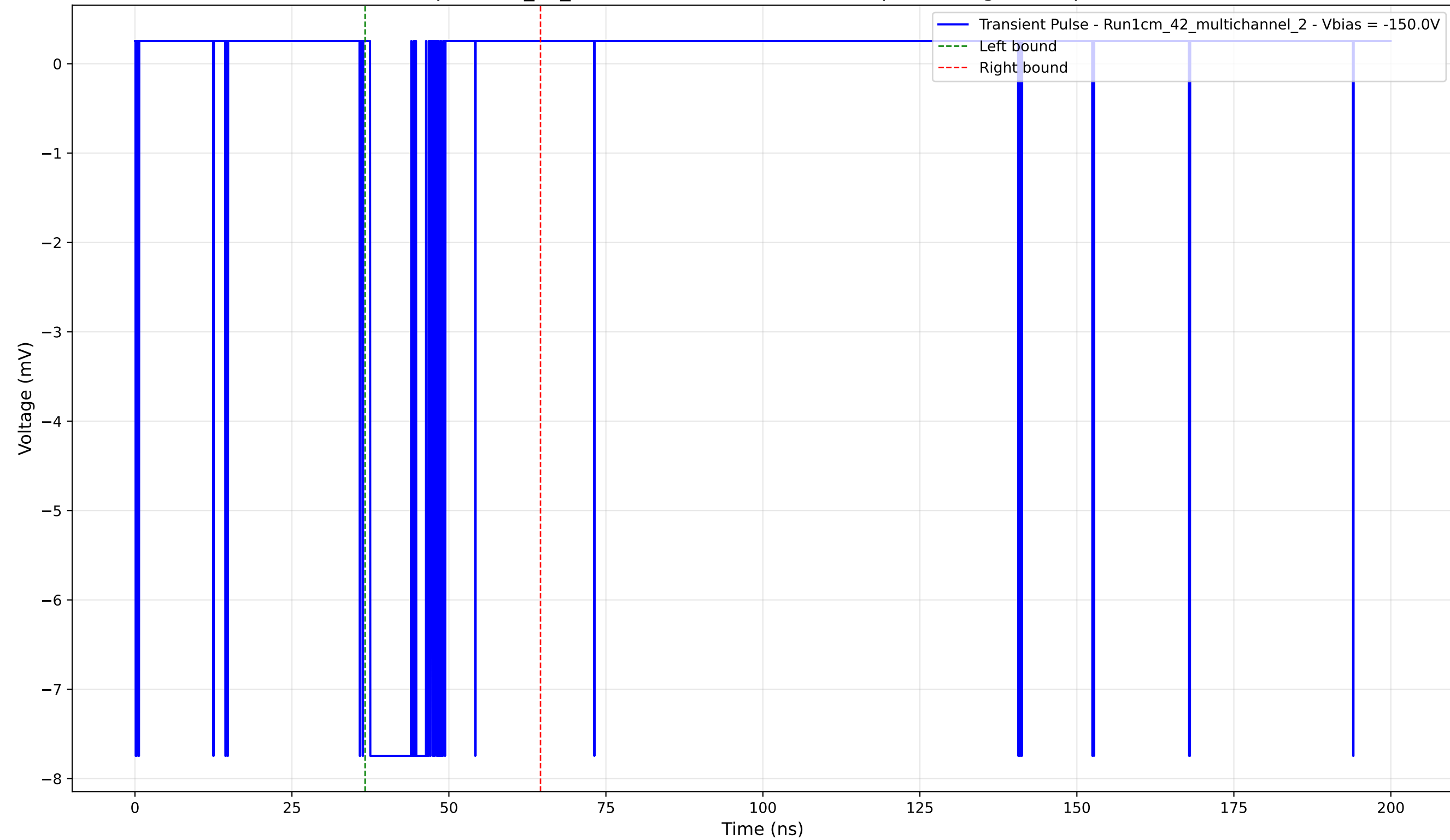
Transient Pulse - Sample: 1cm_42_multichannel - Position: 365.0 \mu\text{m} - Charge: 1.46 pC - Rise Time: 0.04 ns
