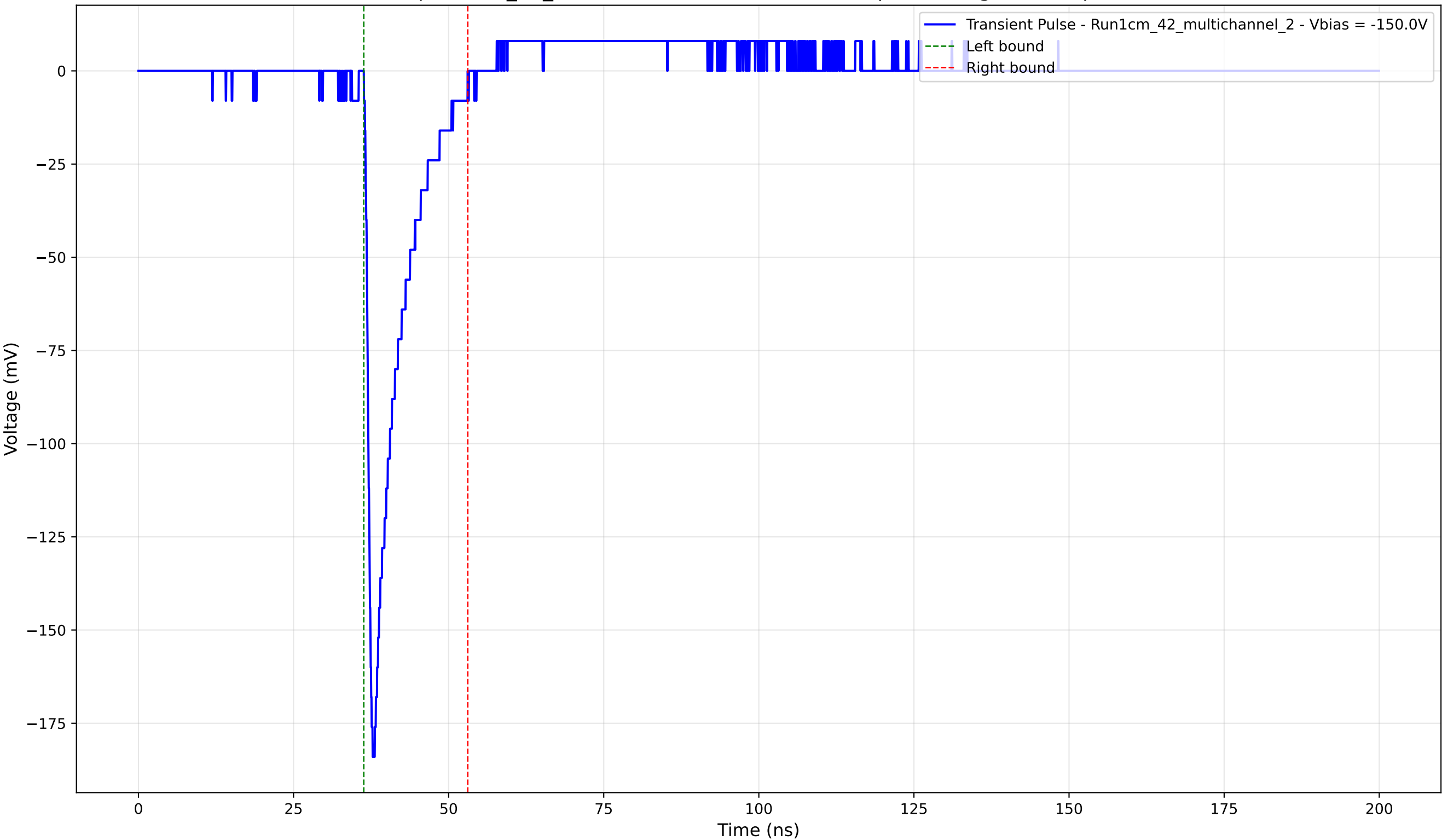
Transient Pulse - Sample: 1cm_42_multichannel - Position: 3250.0 \mu\text{m} - Charge: 19.38 pC - Rise Time: 0.95 ns
