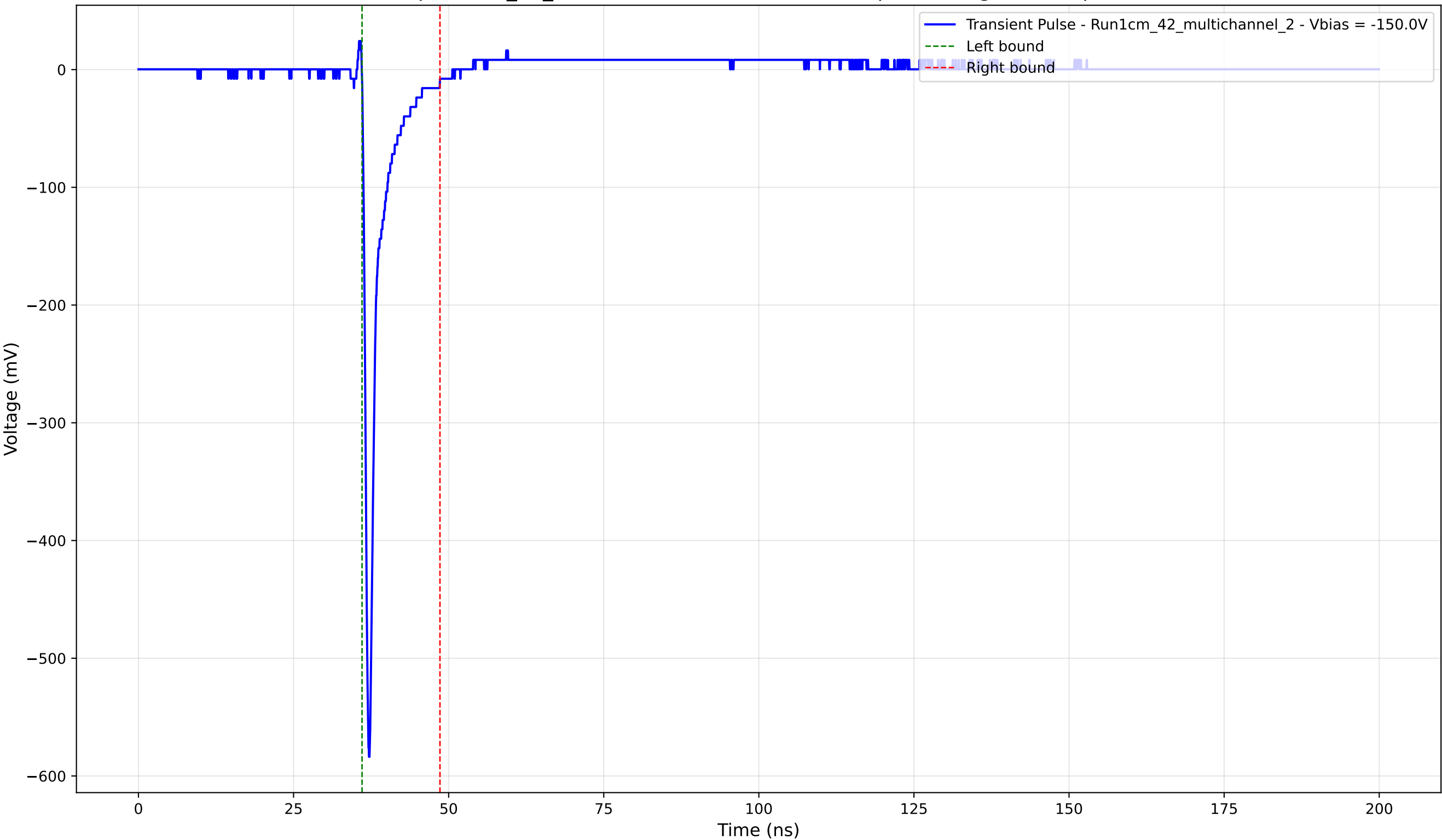
Transient Pulse - Sample: 1cm_42_multichannel - Position: 2505.0 \mu\text{m} - Charge: 27.41 pC - Rise Time: 0.75 ns
