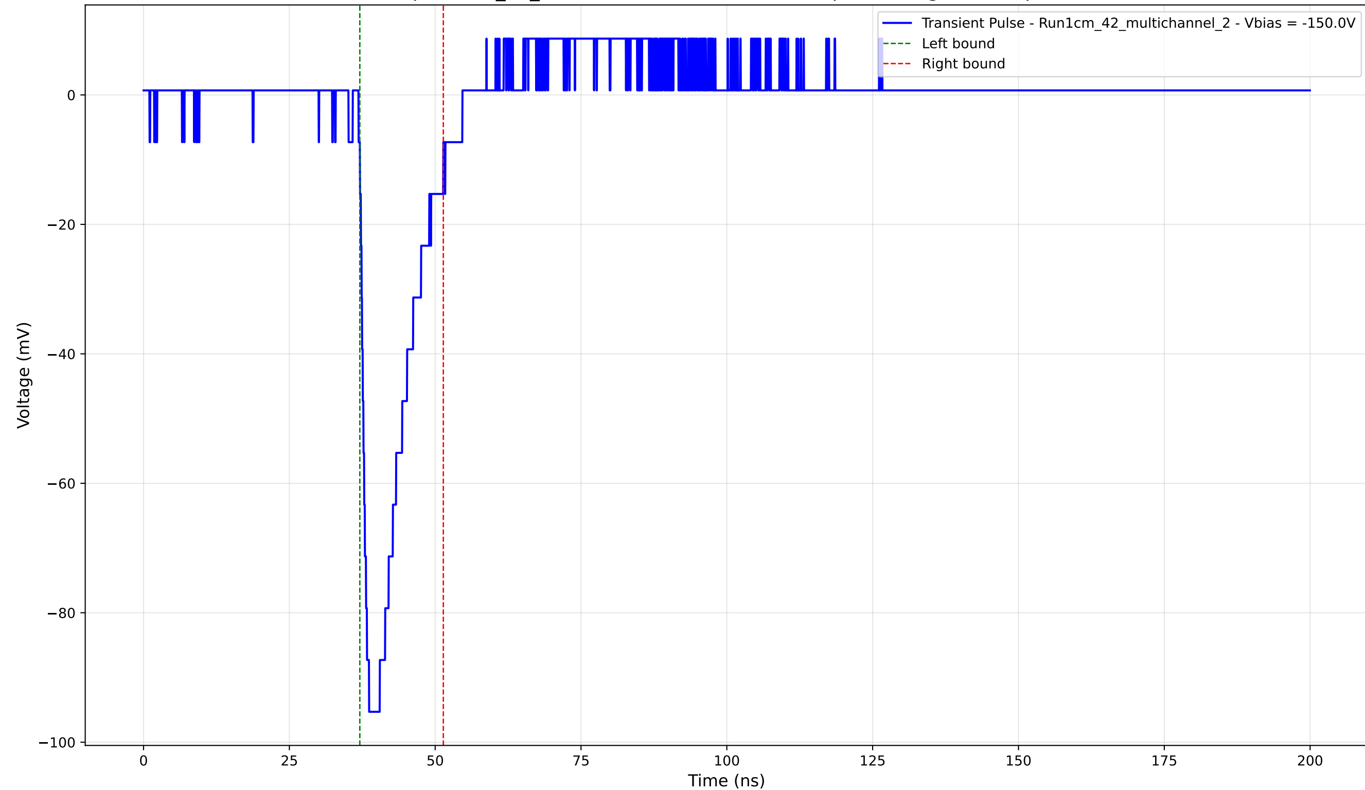
Transient Pulse - Sample: 1cm_42_multichannel - Position: 595.0 \mu\text{m} - Charge: 14.63 pC - Rise Time: 1.23 ns
