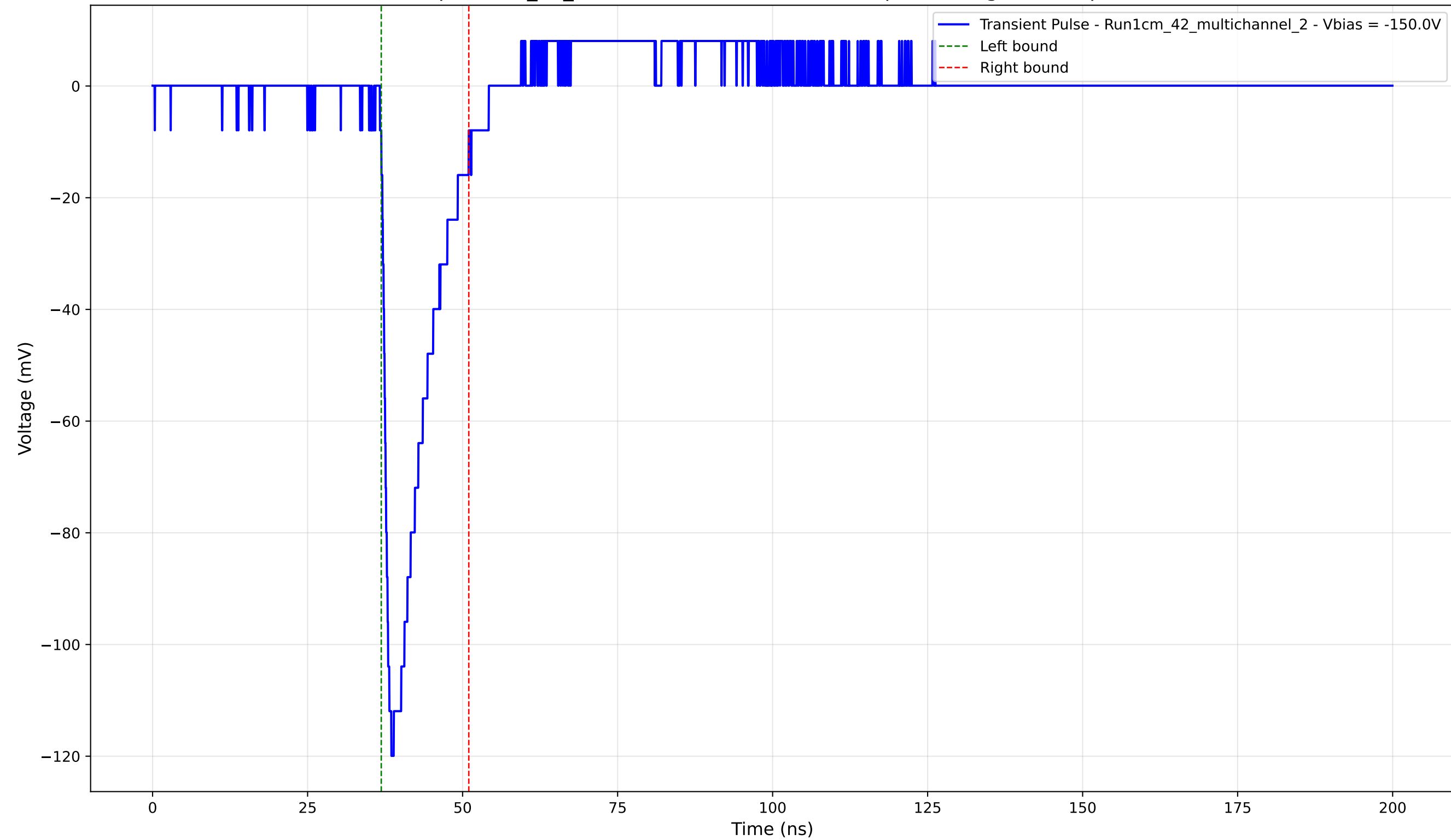
Transient Pulse - Sample: 1cm_42_multichannel - Position: 935.0 \mu\text{m} - Charge: 16.42 pC - Rise Time: 1.30 ns
