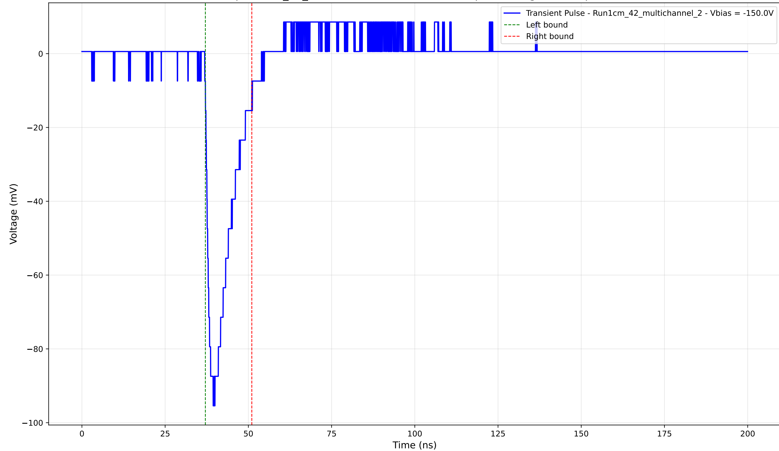
Transient Pulse - Sample: 1cm_42_multichannel - Position: 460.0 \mu\text{m} - Charge: 13.84 pC - Rise Time: 1.59 ns
