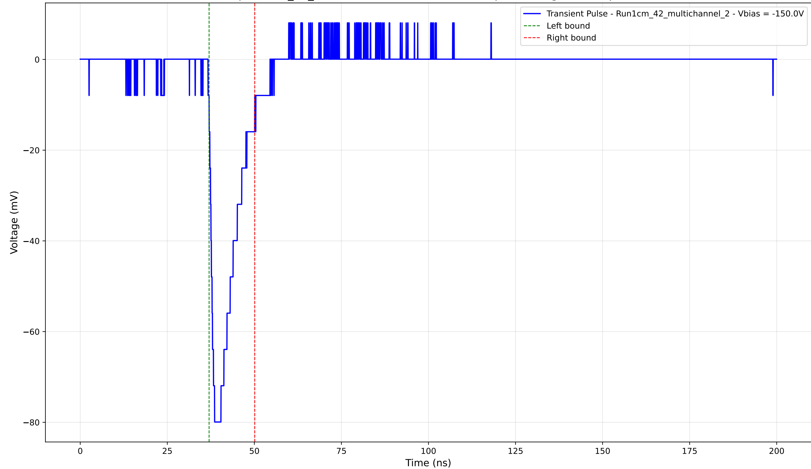
Transient Pulse - Sample: 1cm_42_multichannel - Position: 3955.0 \mu\text{m} - Charge: 11.77 pC - Rise Time: 1.60 ns
