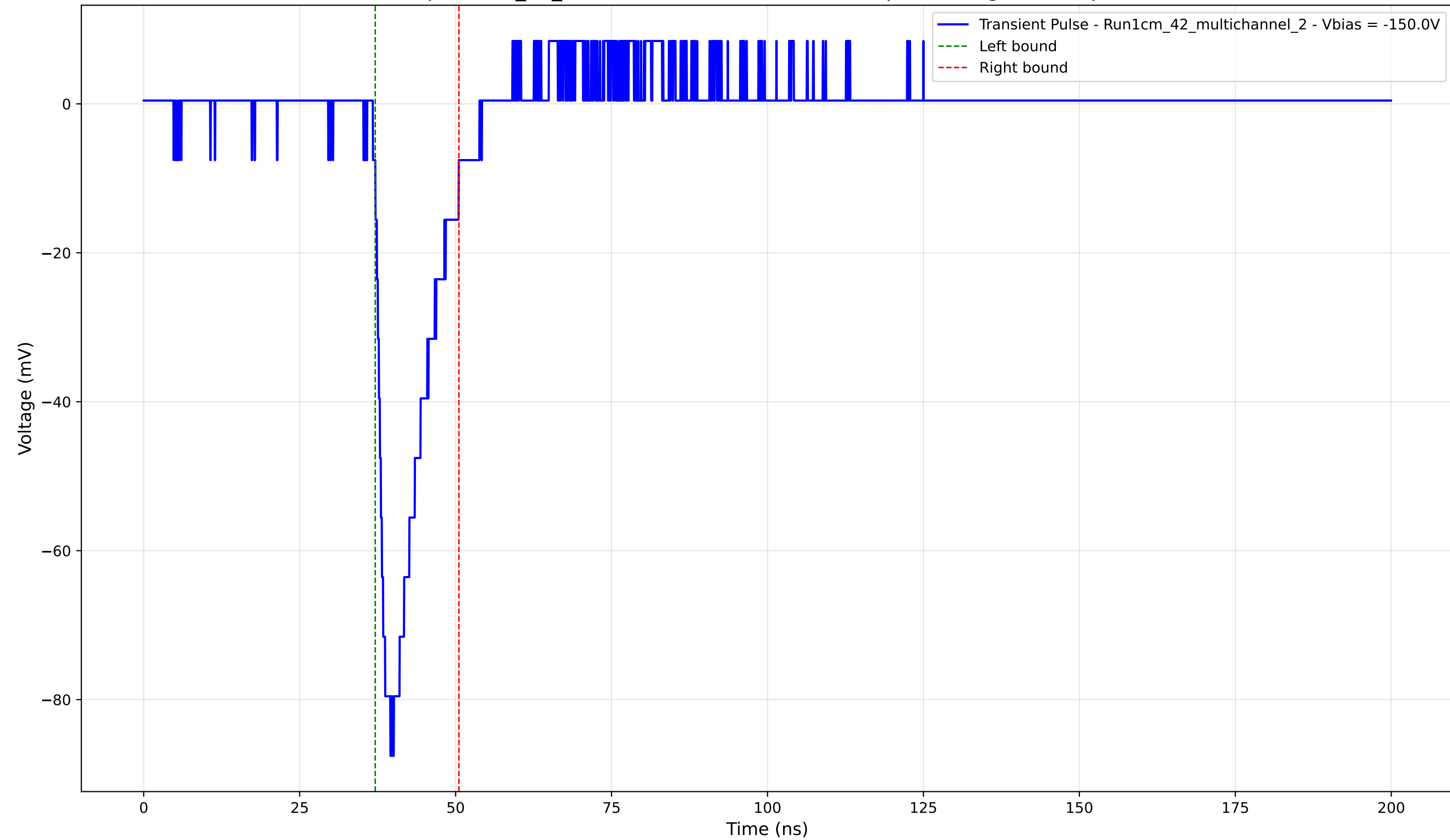
Transient Pulse - Sample: 1cm_42_multichannel - Position: 4190.0 \mu\text{m} - Charge: 12.25 pC - Rise Time: 1.59 ns
