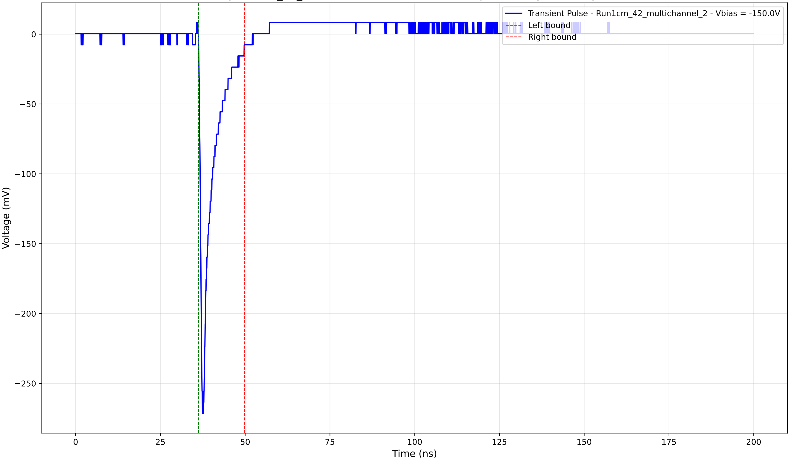
Transient Pulse - Sample: 1cm_42_multichannel - Position: 2965.0 \mu\text{m} - Charge: 21.16 pC - Rise Time: 0.85 ns
