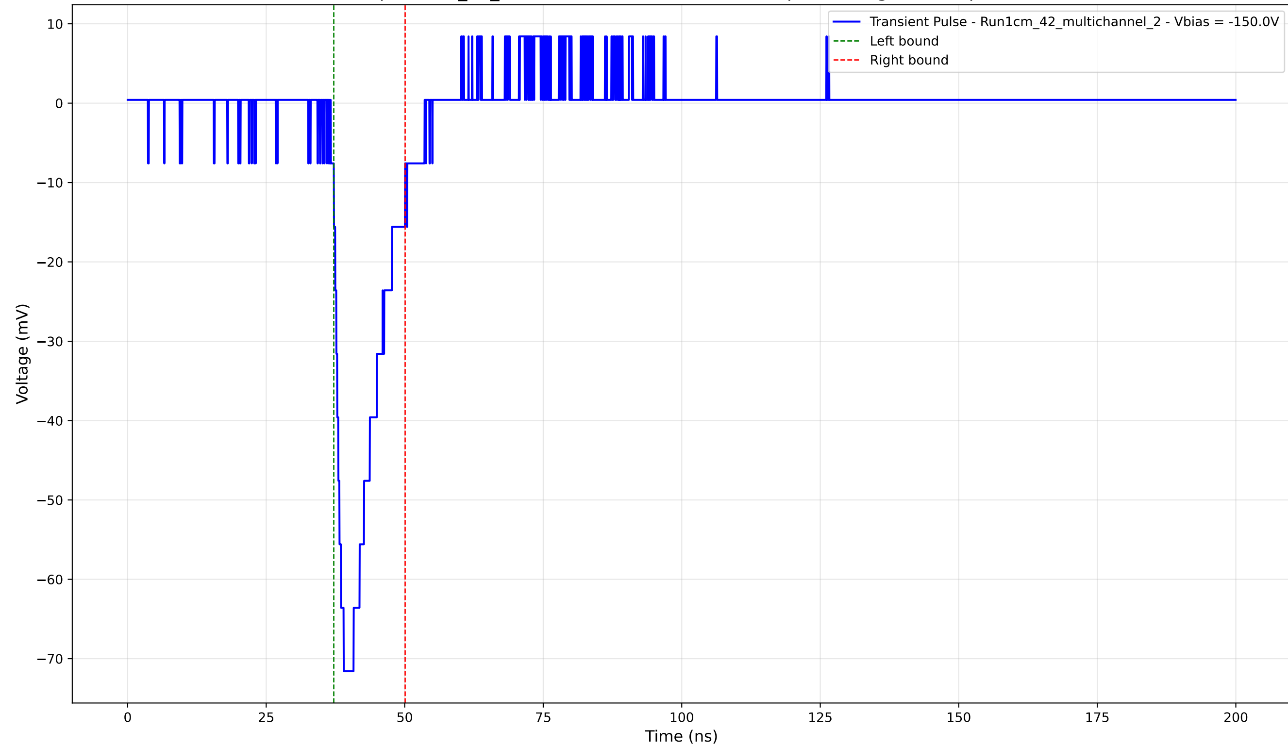
Transient Pulse - Sample: 1cm_42_multichannel - Position: 4510.0 \mu\text{m} - Charge: 10.61 pC - Rise Time: 2.32 ns
