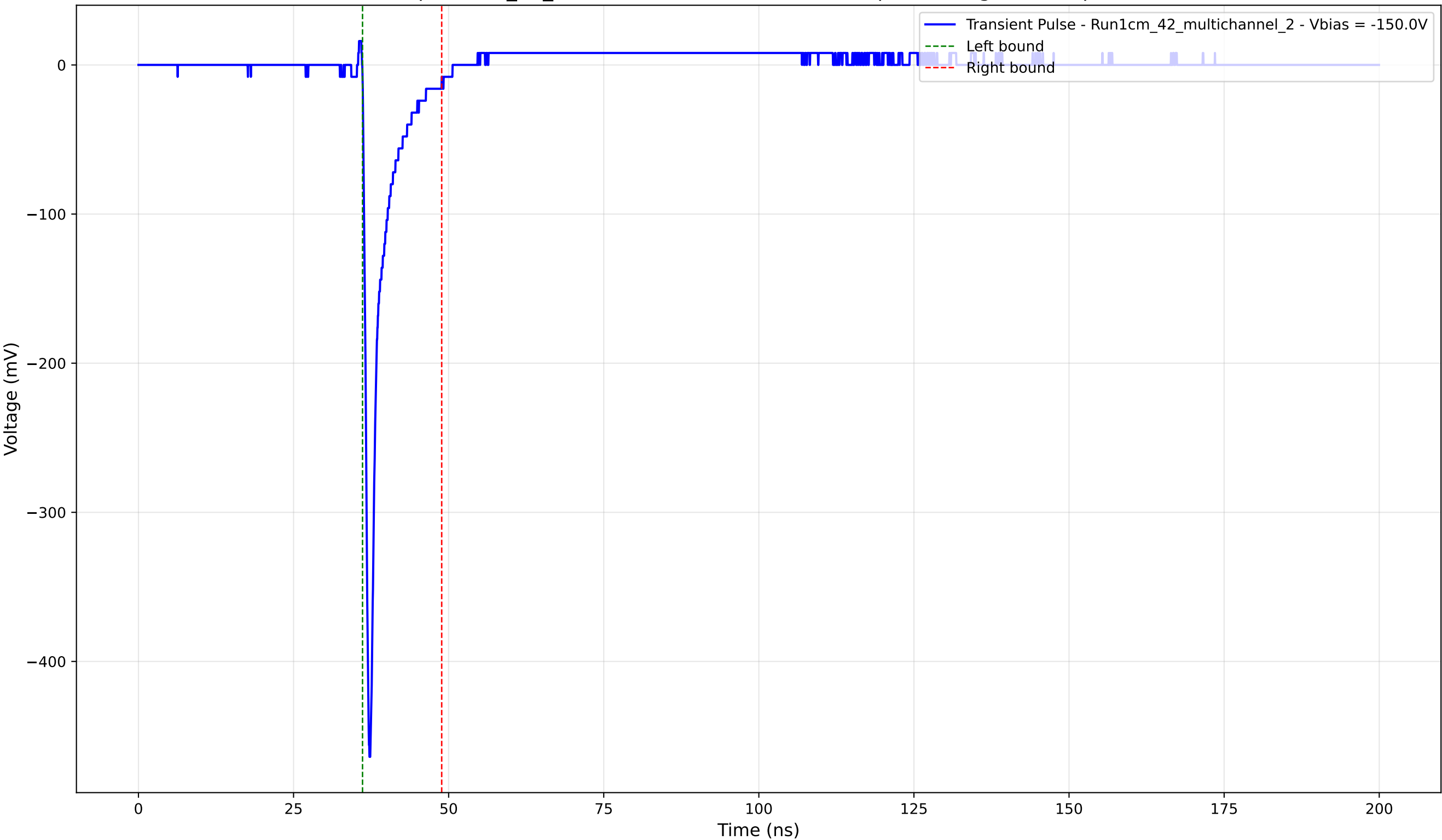
Transient Pulse - Sample: 1cm_42_multichannel - Position: 2640.0 \mu\text{m} - Charge: 25.05 pC - Rise Time: 0.75 ns
