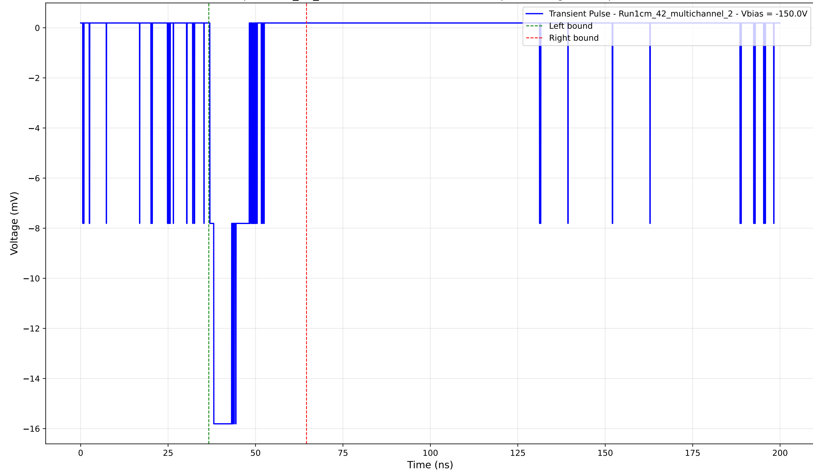
Transient Pulse - Sample: 1cm_42_multichannel - Position: 4425.0 \mu\text{m} - Charge: 2.80 pC - Rise Time: 1.15 ns
