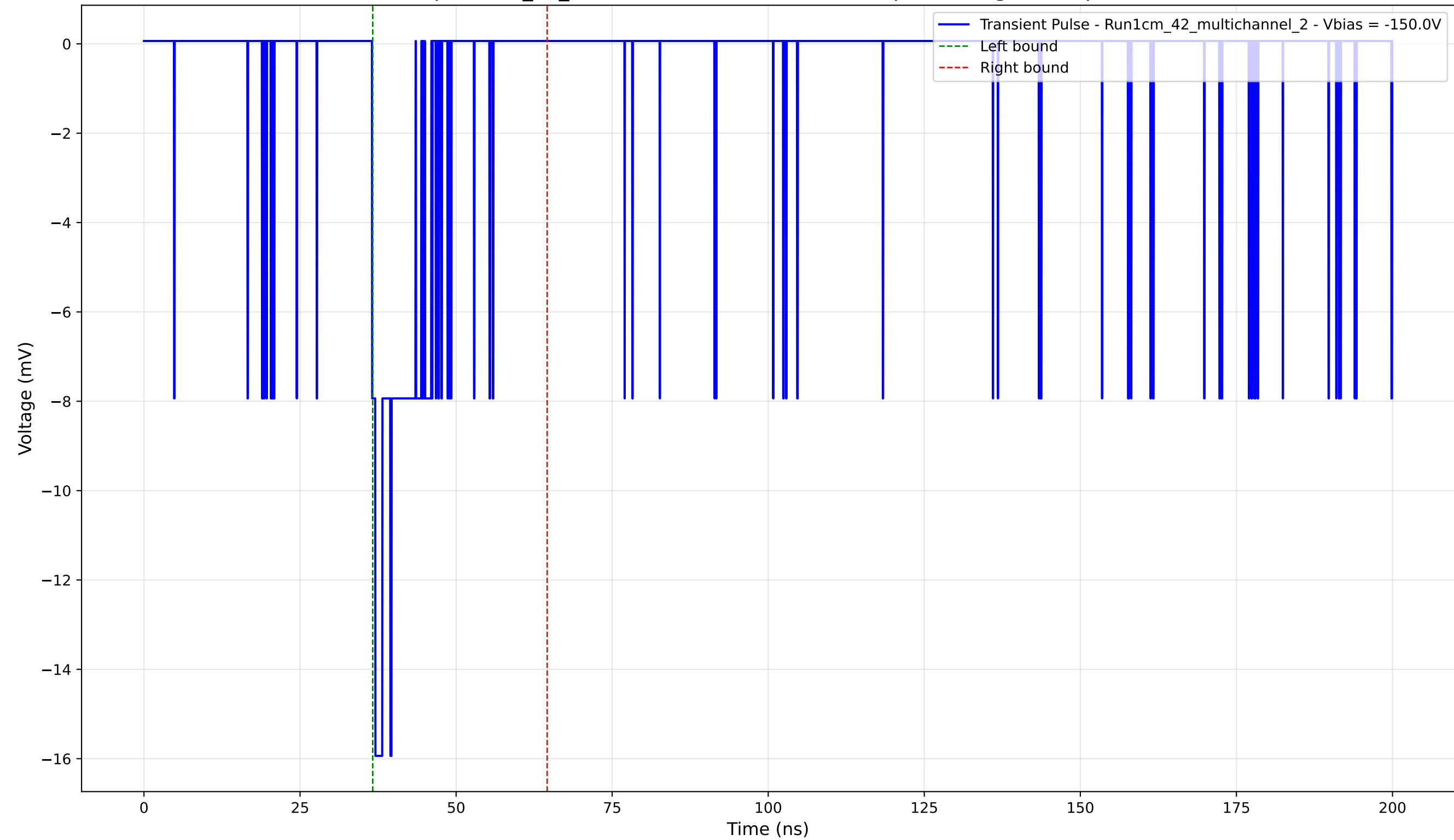
Transient Pulse - Sample: 1cm_42_multichannel - Position: 1865.0 \mu\text{m} - Charge: 1.78 pC - Rise Time: 0.55 ns
