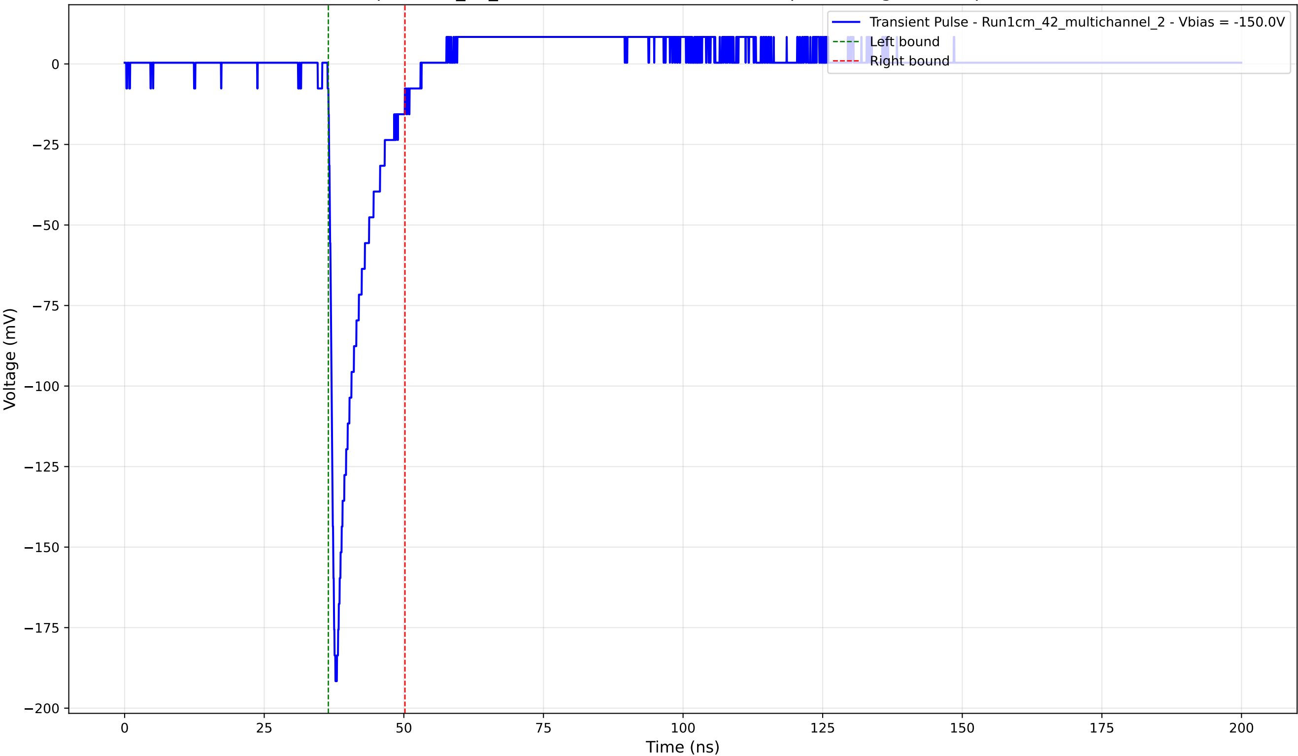
Transient Pulse - Sample: 1cm_42_multichannel - Position: 3235.0 \mu\text{m} - Charge: 19.09 pC - Rise Time: 0.94 ns
