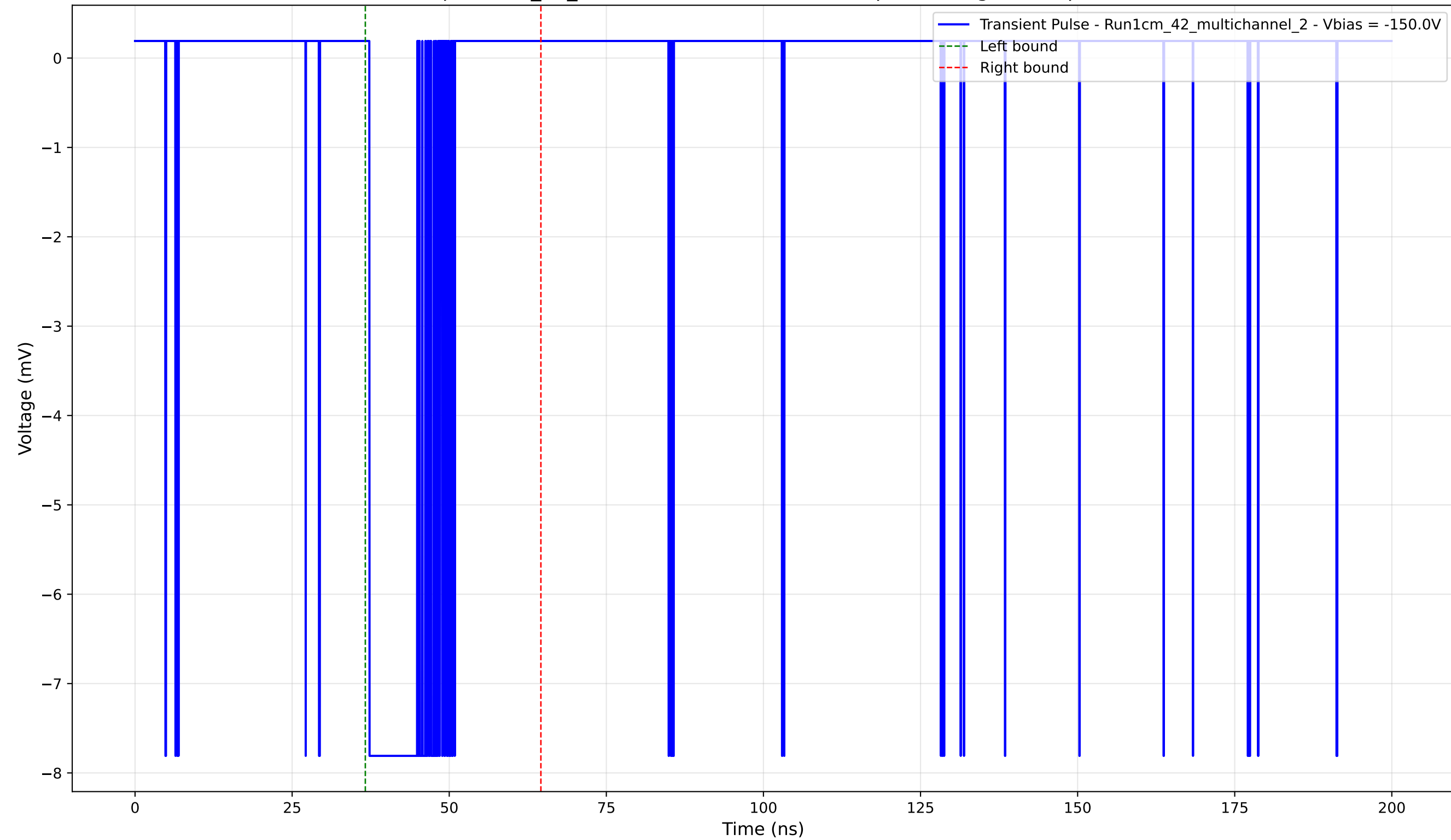
Transient Pulse - Sample: 1cm_42_multichannel - Position: 40.0 \mu\text{m} - Charge: 1.62 pC - Rise Time: 0.04 ns
