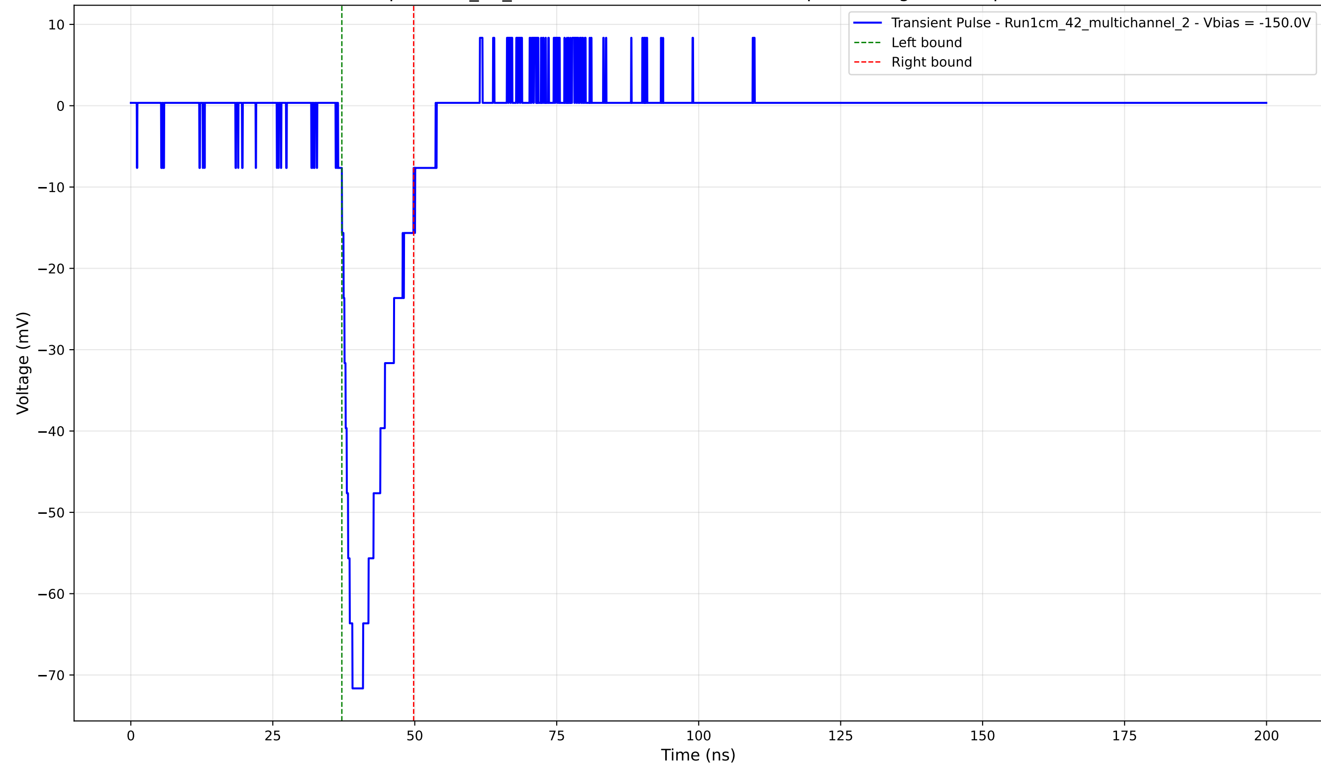
Transient Pulse - Sample: 1cm_42_multichannel - Position: 4505.0 \mu\text{m} - Charge: 10.64 pC - Rise Time: 2.52 ns
