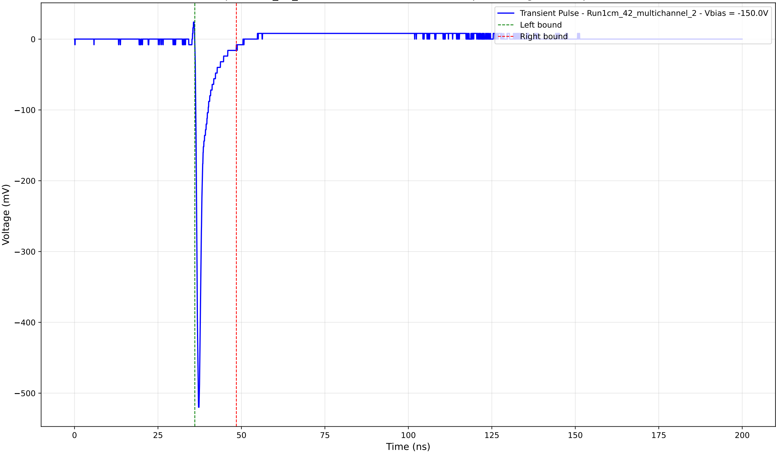
Transient Pulse - Sample: 1cm_42_multichannel - Position: 2545.0 \mu\text{m} - Charge: 25.49 pC - Rise Time: 0.76 ns
