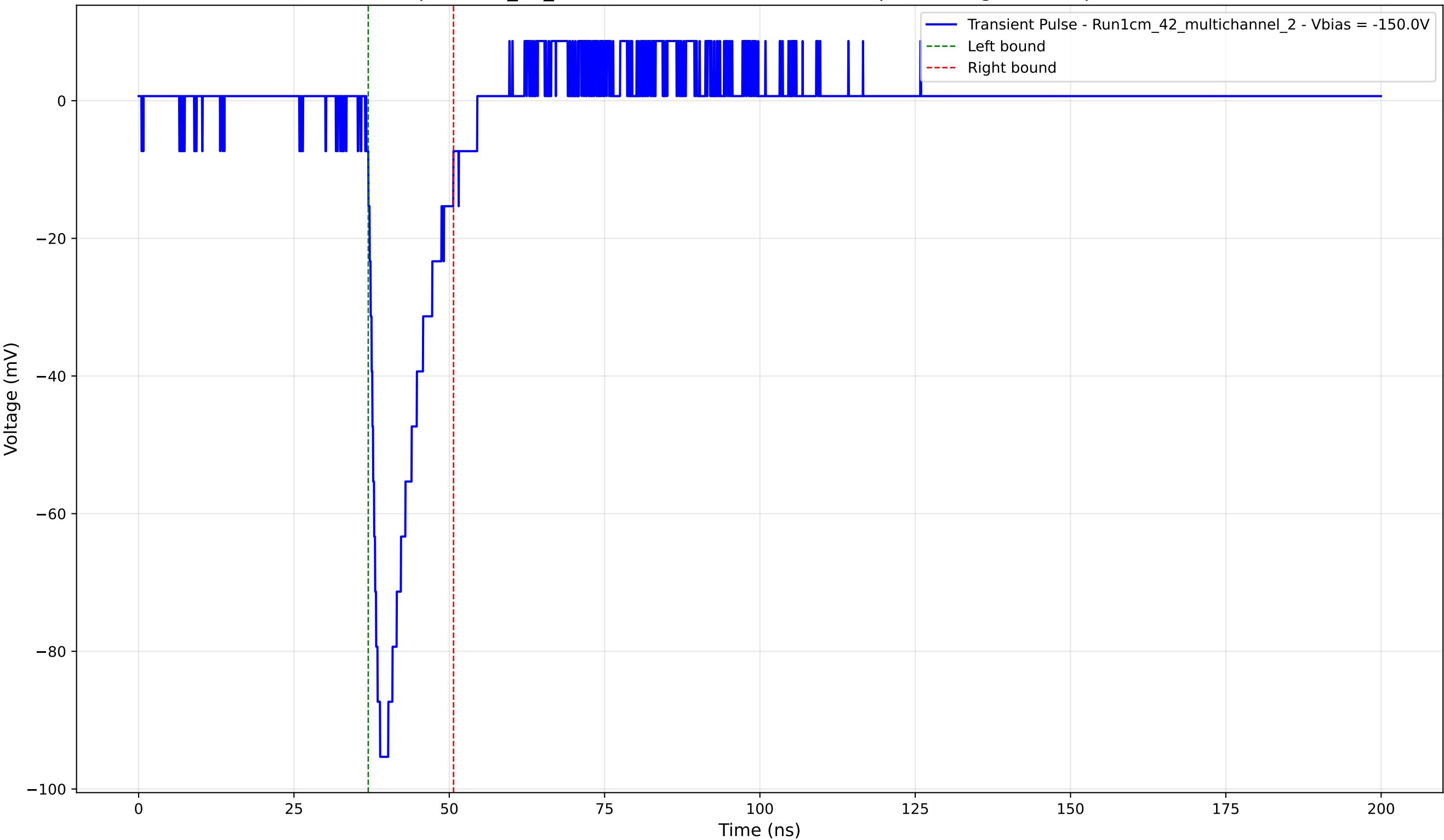
Transient Pulse - Sample: 1cm_42_multichannel - Position: 4000.0 \mu\text{m} - Charge: 13.71 pC - Rise Time: 1.51 ns
