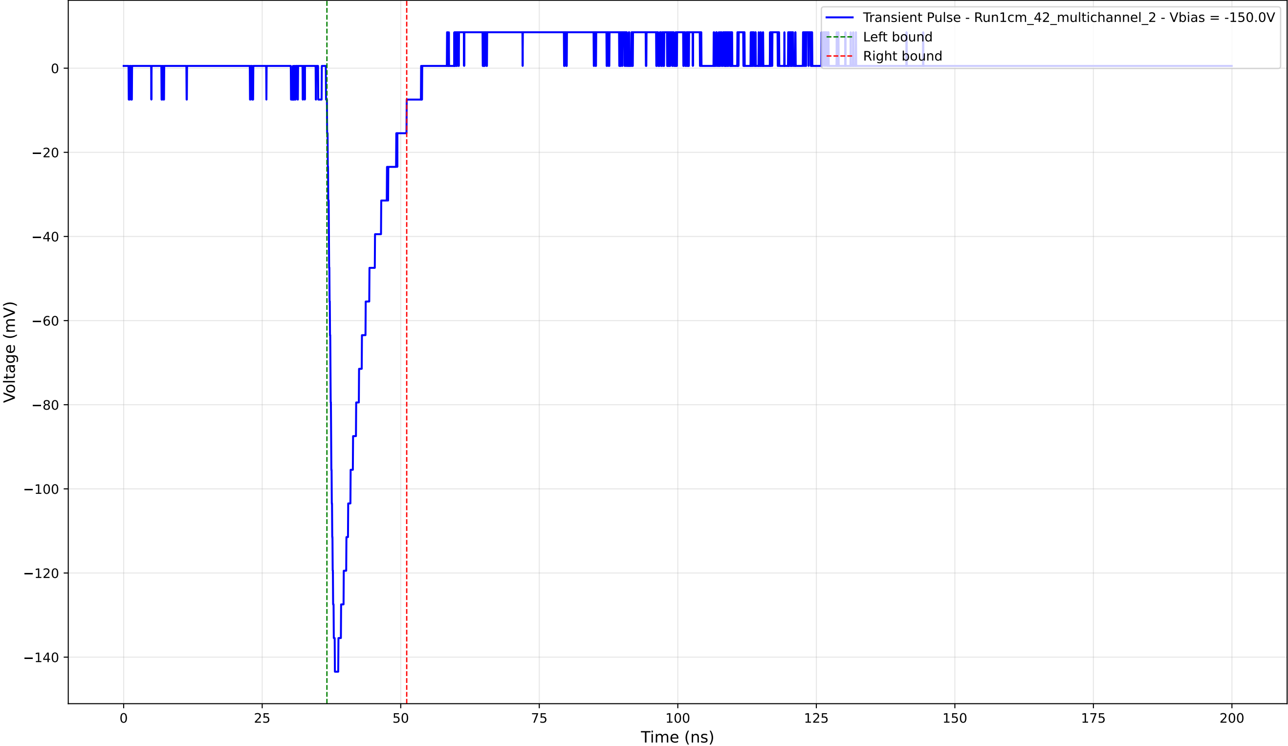
Transient Pulse - Sample: 1cm_42_multichannel - Position: 1165.0 \mu\text{m} - Charge: 18.26 pC - Rise Time: 1.21 ns
