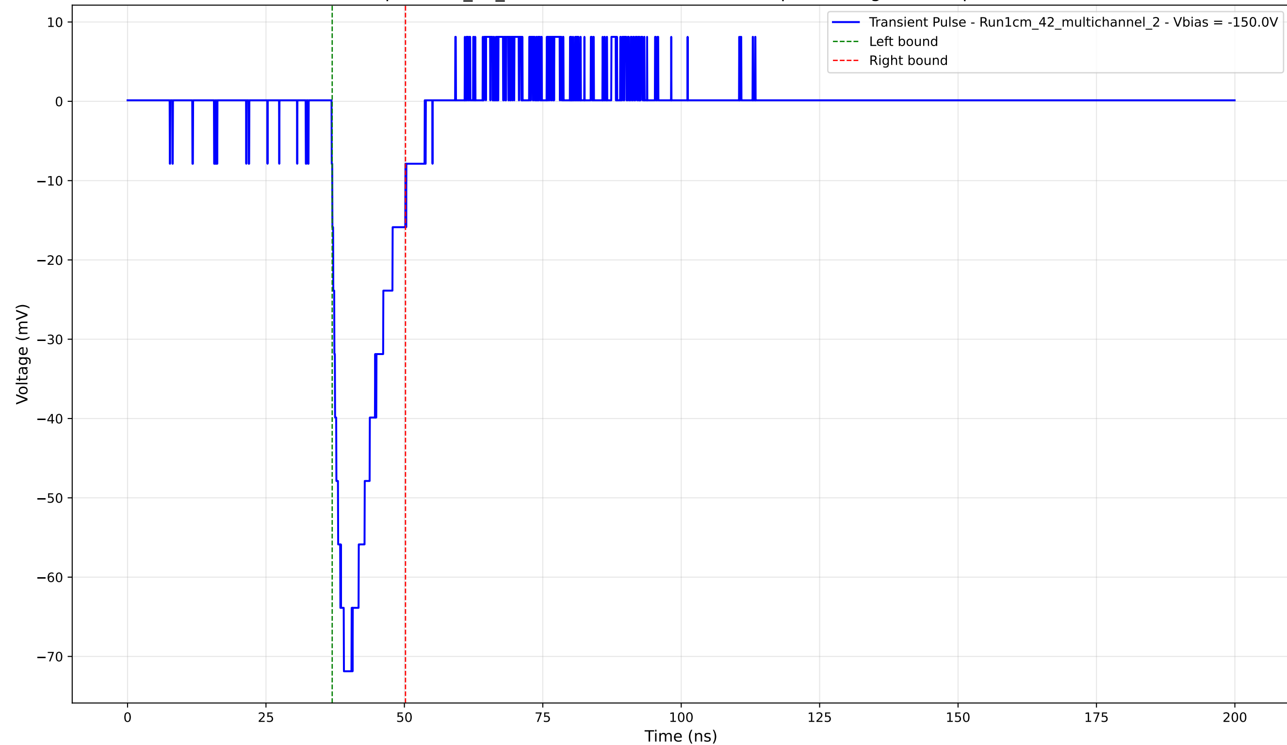
Transient Pulse - Sample: 1cm_42_multichannel - Position: 160.0 \mu\text{m} - Charge: 11.00 pC - Rise Time: 2.20 ns
