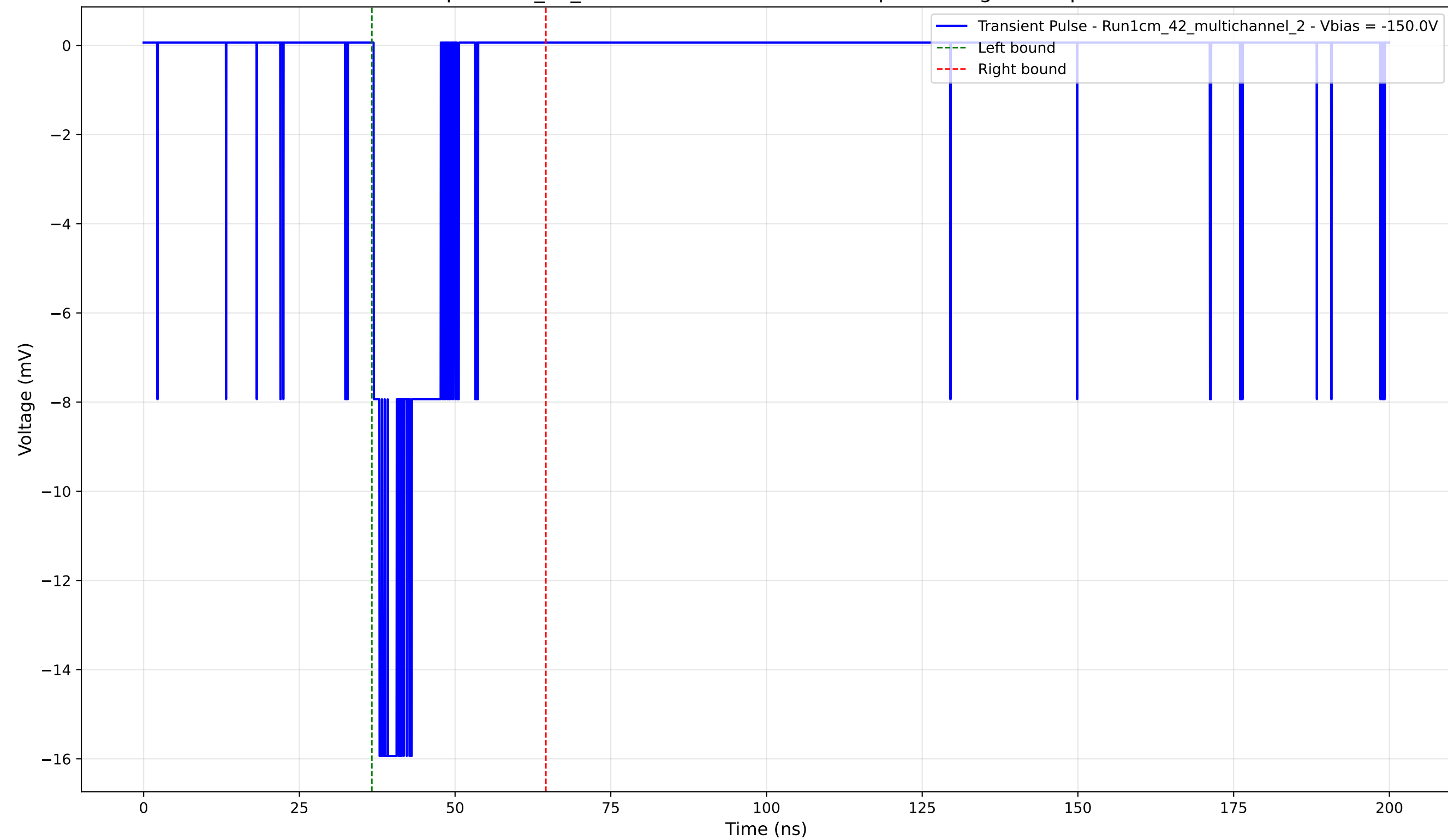
Transient Pulse - Sample: 1cm_42_multichannel - Position: 55.0 \mu\text{m} - Charge: 2.44 pC - Rise Time: 0.95 ns
