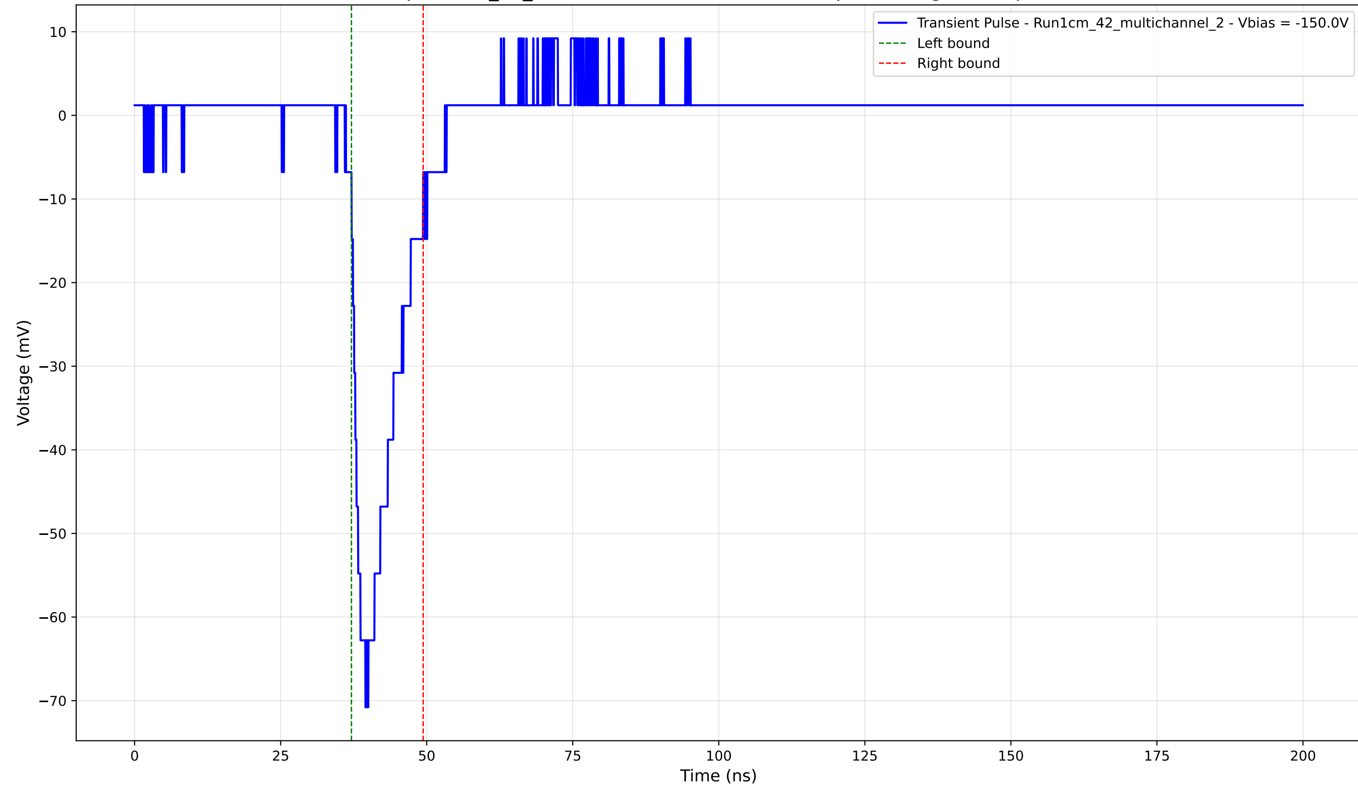
Transient Pulse - Sample: 1cm_42_multichannel - Position: 4735.0 \mu\text{m} - Charge: 9.48 pC - Rise Time: 2.40 ns
