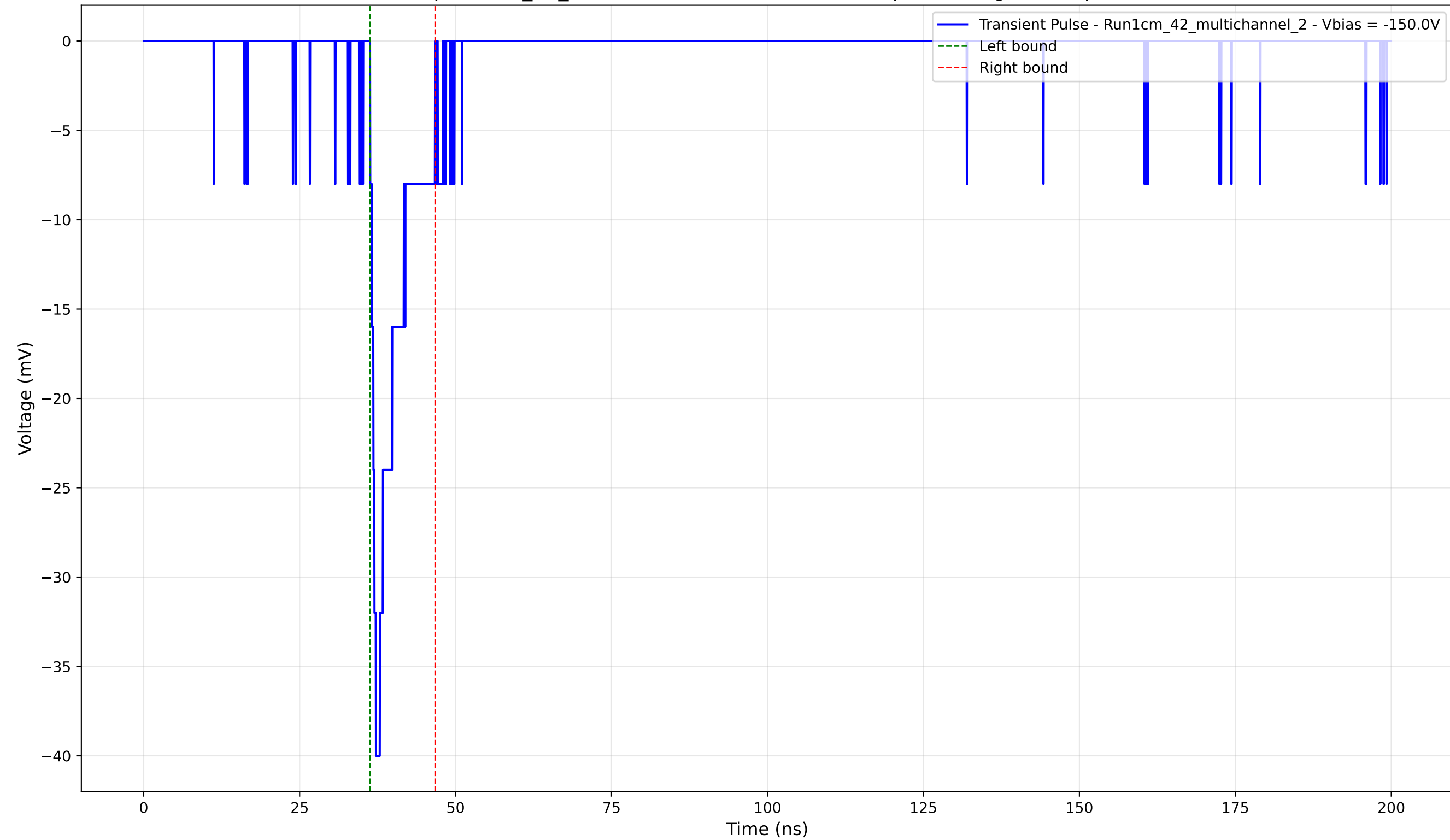
Transient Pulse - Sample: 1cm_42_multichannel - Position: 1835.0 \mu\text{m} - Charge: 3.29 pC - Rise Time: 0.94 ns
