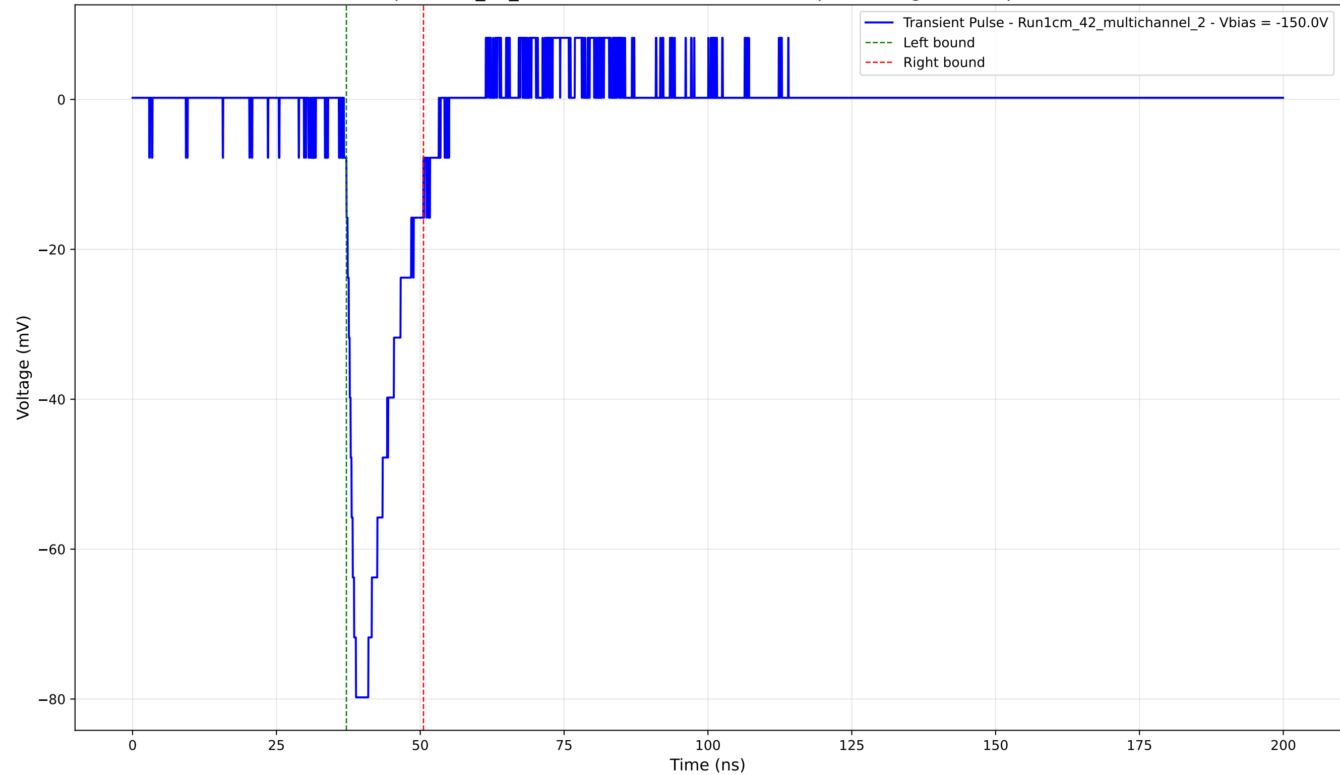
Transient Pulse - Sample: 1cm_42_multichannel - Position: 4235.0 \mu\text{m} - Charge: 12.10 pC - Rise Time: 1.68 ns
