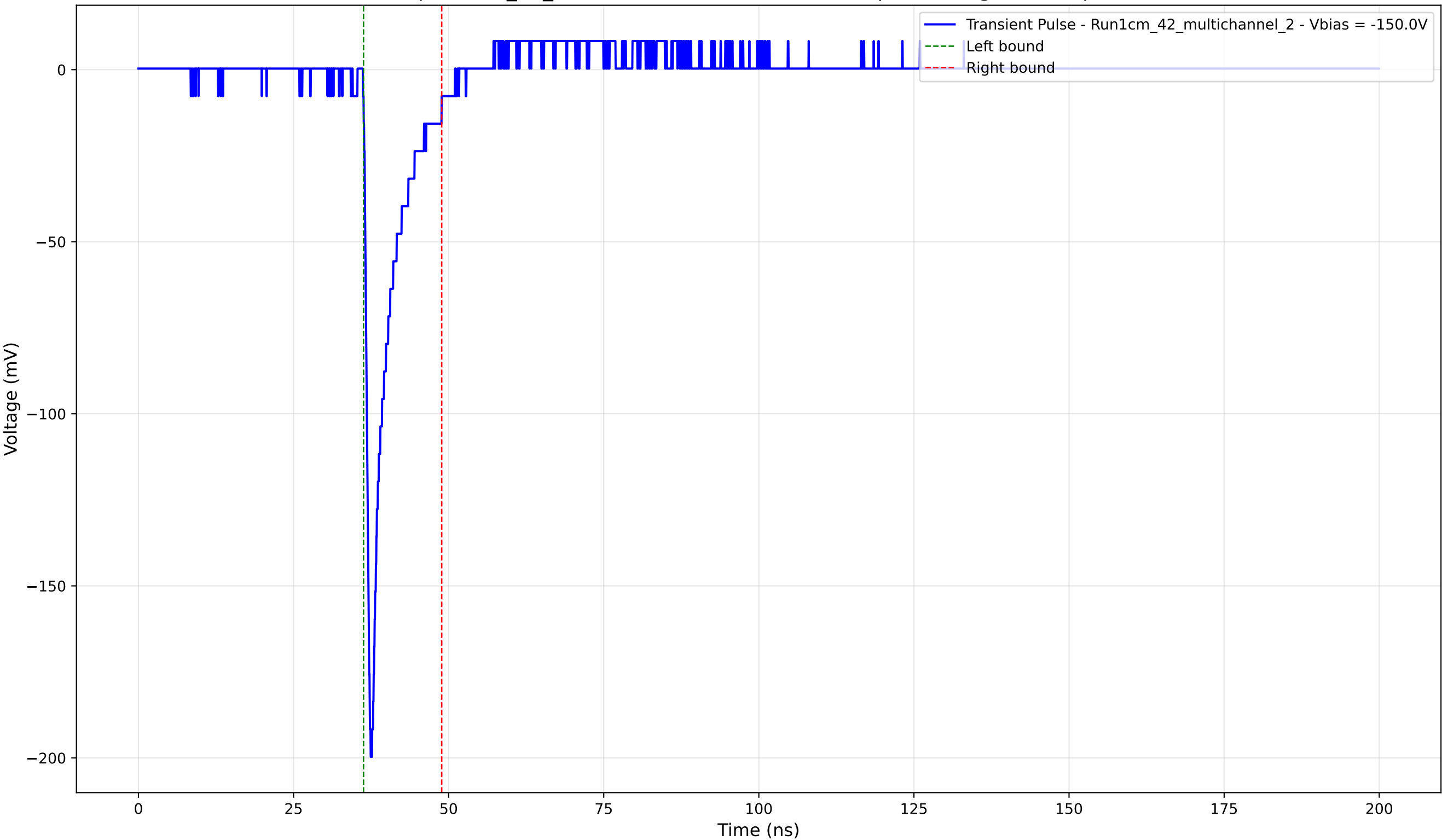
Transient Pulse - Sample: 1cm_42_multichannel - Position: 2935.0 \mu\text{m} - Charge: 15.10 pC - Rise Time: 0.88 ns
