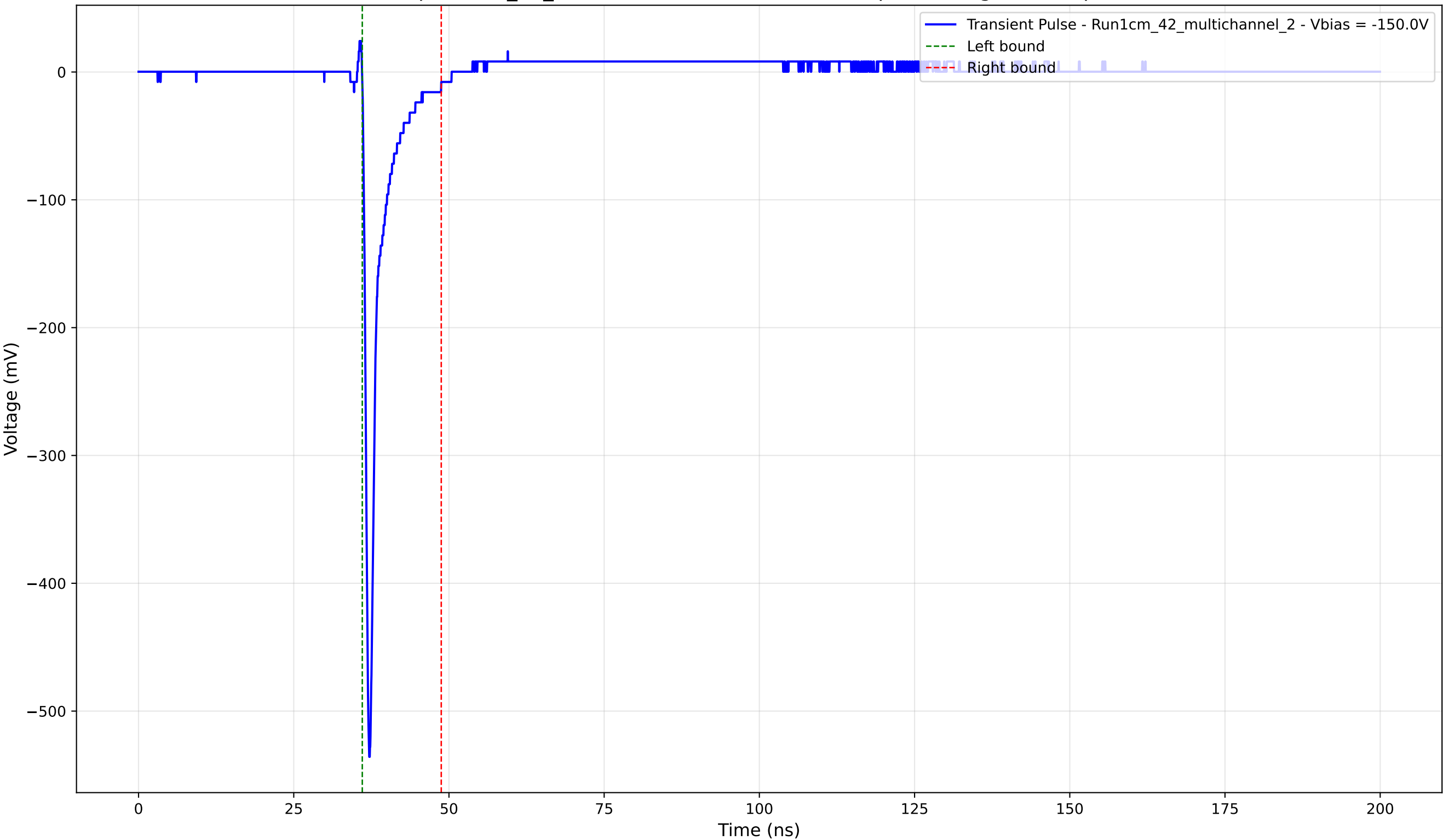
Transient Pulse - Sample: 1cm_42_multichannel - Position: 2535.0 \mu\text{m} - Charge: 25.85 pC - Rise Time: 0.73 ns
