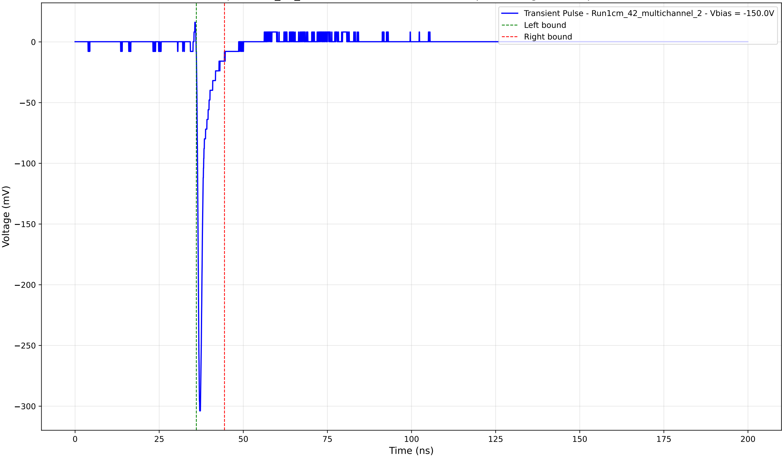
Transient Pulse - Sample: 1cm_42_multichannel - Position: 2320.0 \mu\text{m} - Charge: 12.93 pC - Rise Time: 0.70 ns
