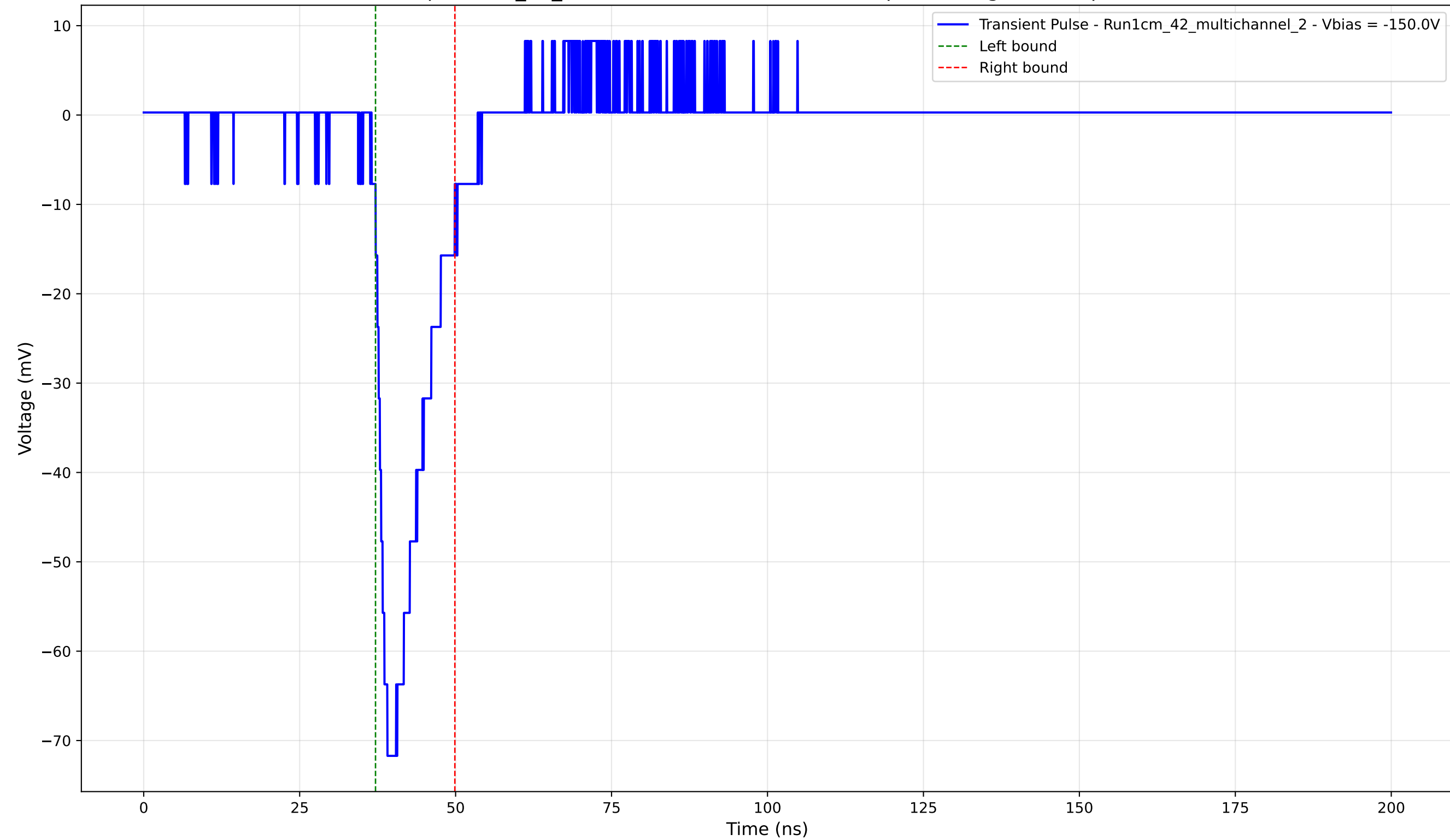
Transient Pulse - Sample: 1cm_42_multichannel - Position: 4495.0 \mu\text{m} - Charge: 10.44 pC - Rise Time: 2.52 ns
