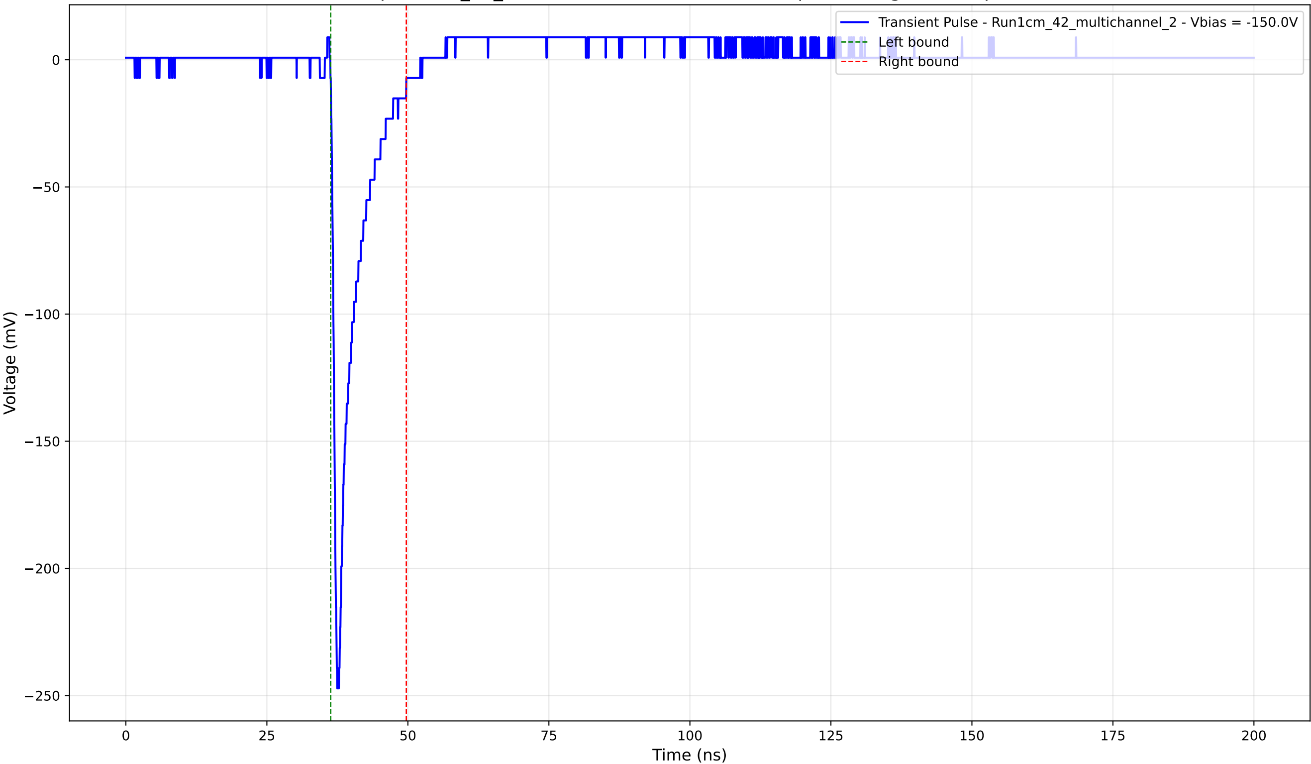
Transient Pulse - Sample: 1cm_42_multichannel - Position: 3025.0 \mu\text{m} - Charge: 20.19 pC - Rise Time: 0.87 ns
