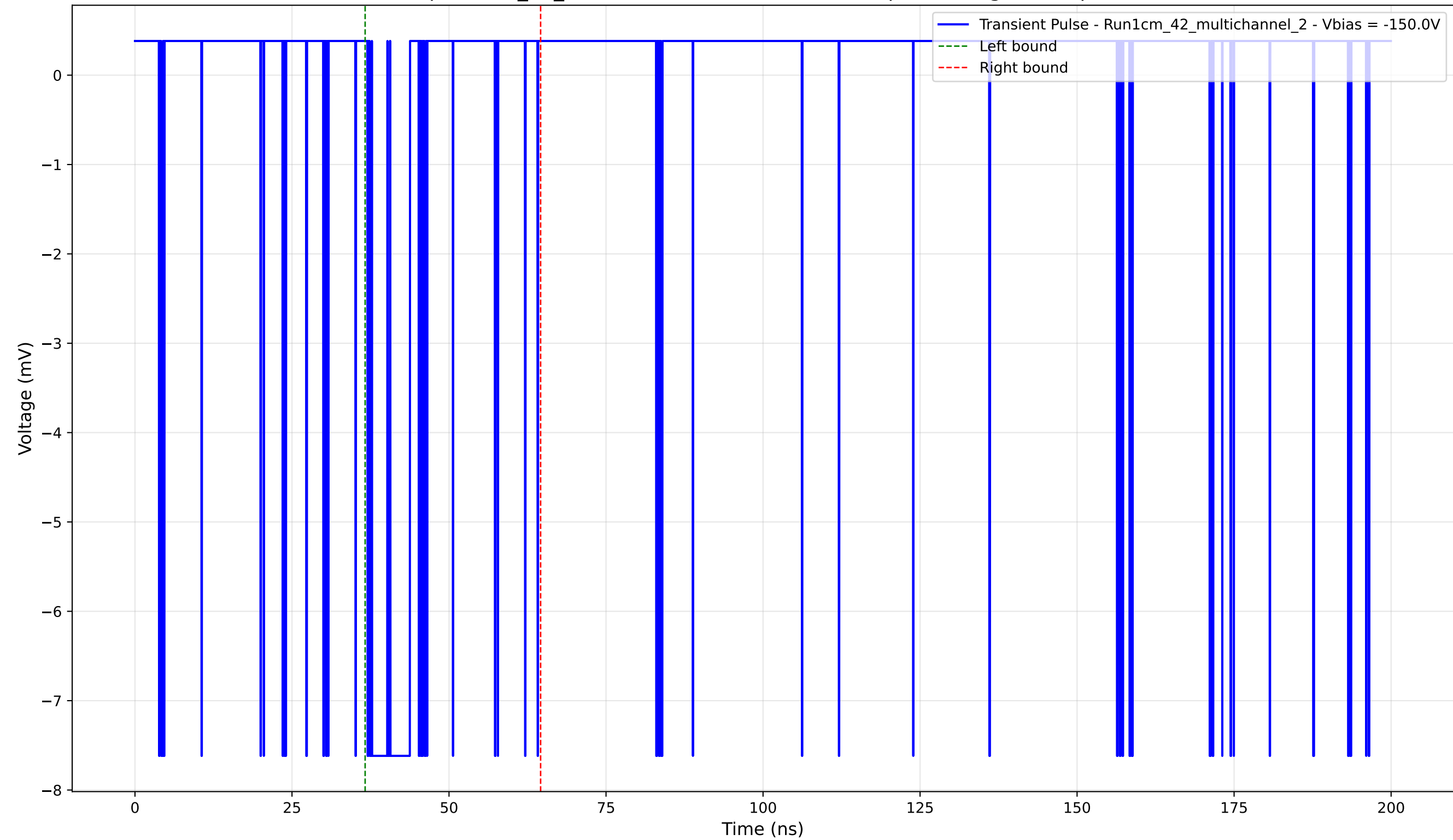
Transient Pulse - Sample: 1cm_42_multichannel - Position: 4380.0 \mu\text{m} - Charge: 0.98 pC - Rise Time: 0.04 ns
