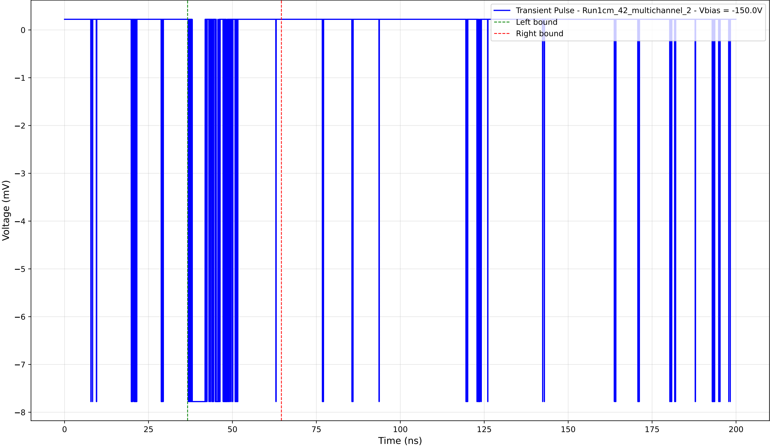
Transient Pulse - Sample: 1cm_42_multichannel - Position: 4400.0 \mu\text{m} - Charge: 1.19 pC - Rise Time: 0.04 ns
