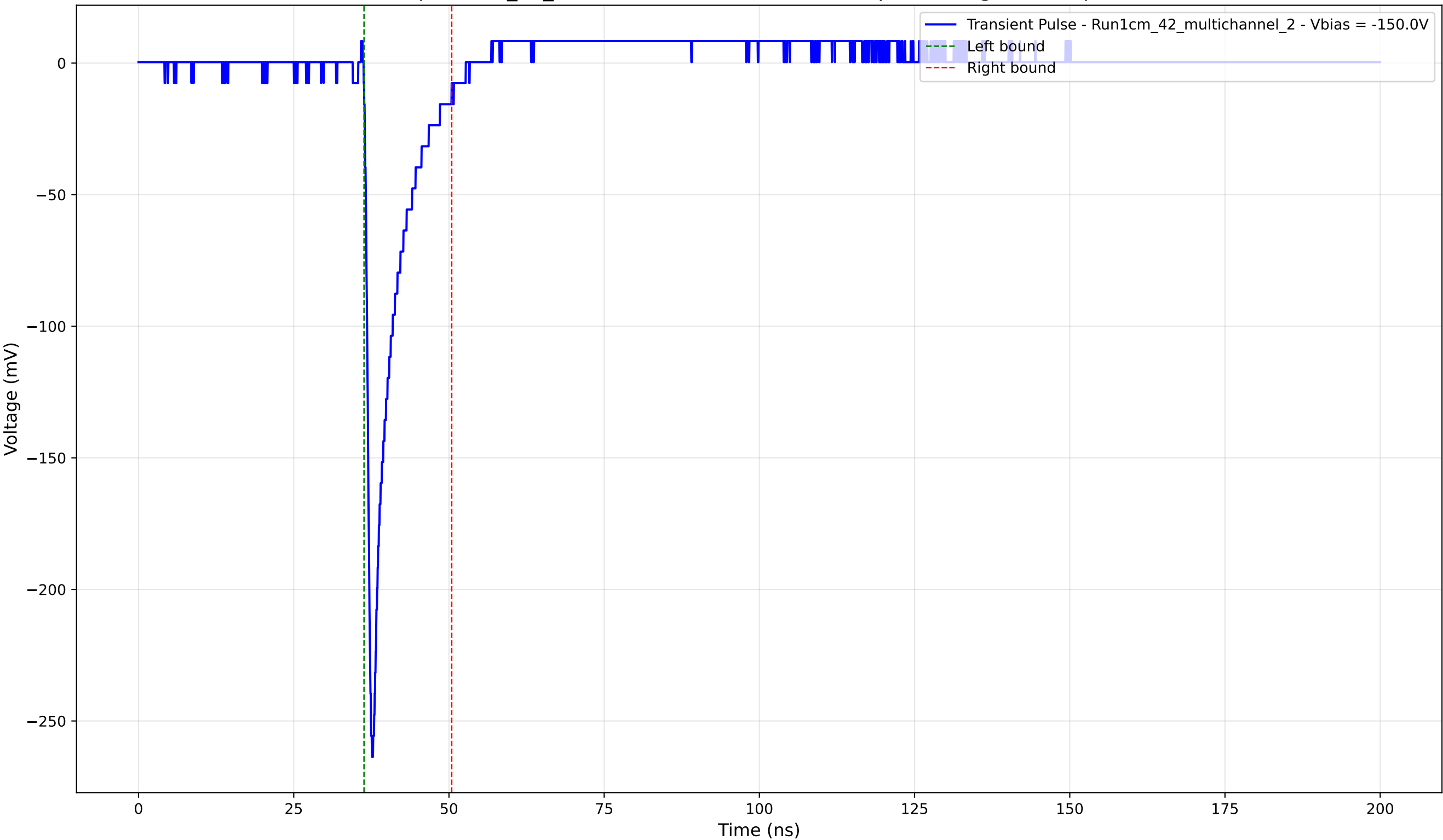
Transient Pulse - Sample: 1cm_42_multichannel - Position: 1665.0 \mu\text{m} - Charge: 22.59 pC - Rise Time: 0.91 ns
