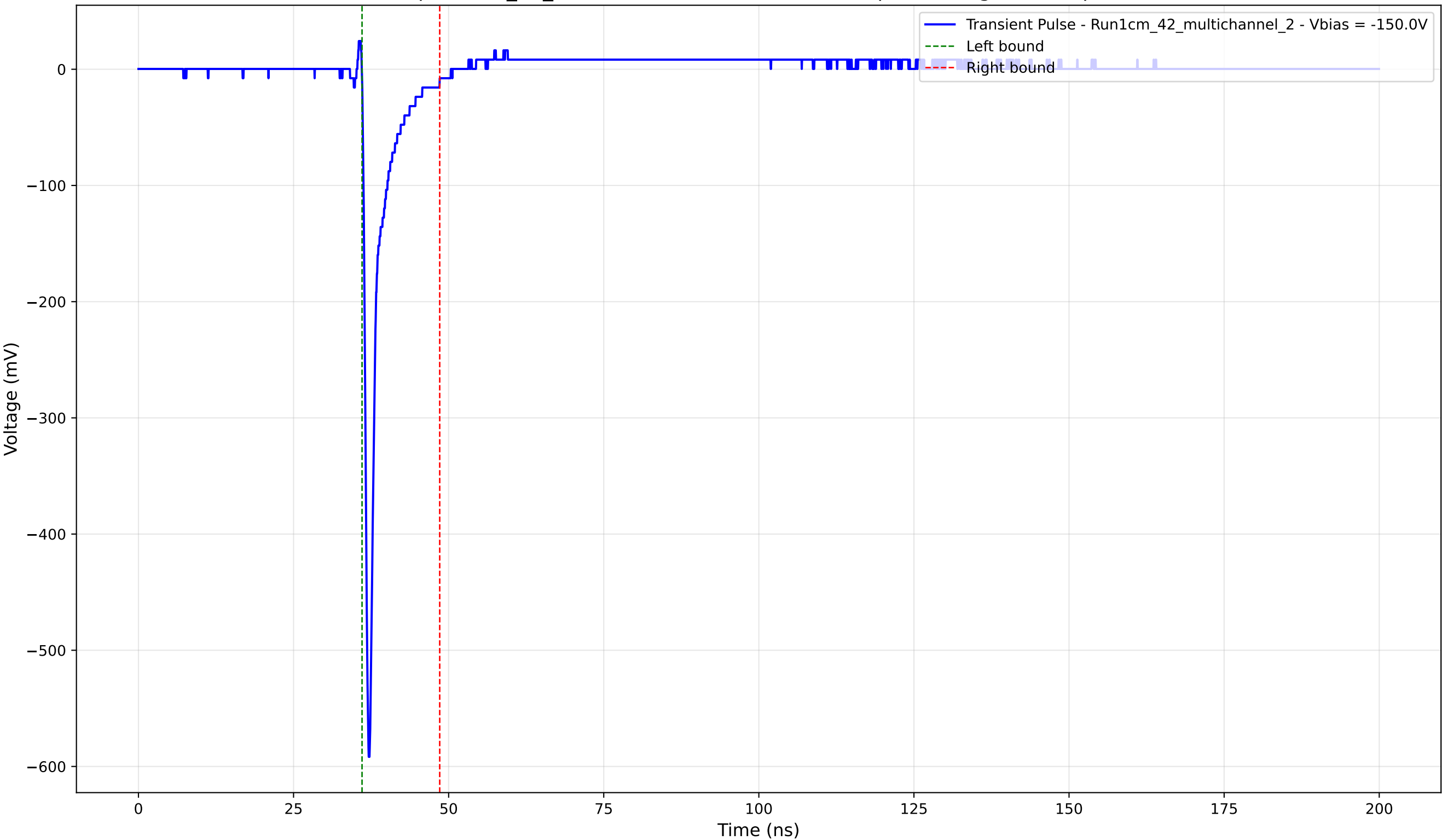
Transient Pulse - Sample: 1cm_42_multichannel - Position: 2495.0 \mu\text{m} - Charge: 27.61 pC - Rise Time: 0.74 ns
