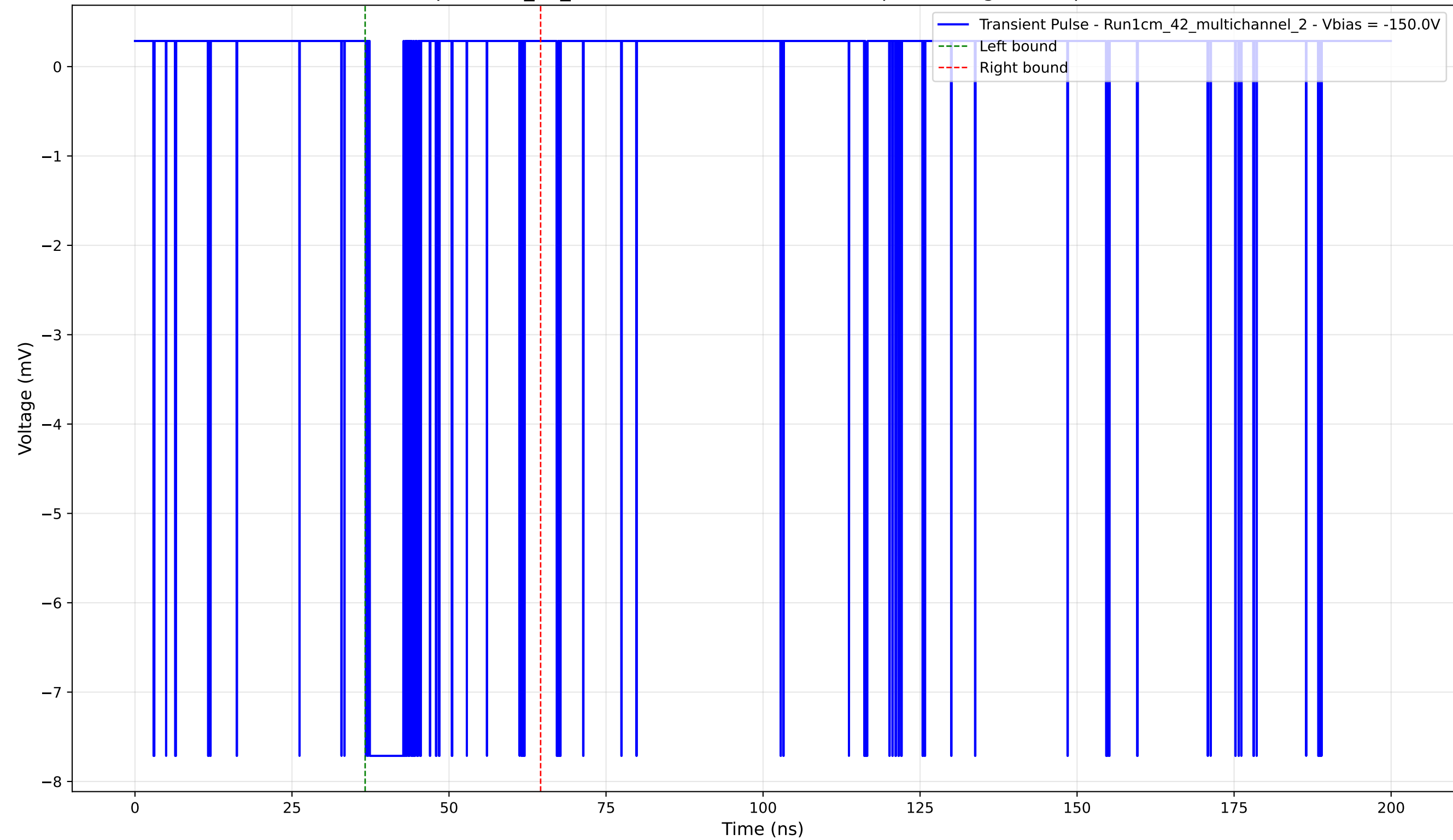
Transient Pulse - Sample: 1cm_42_multichannel - Position: 340.0 \mu\text{m} - Charge: 1.06 pC - Rise Time: 0.04 ns
