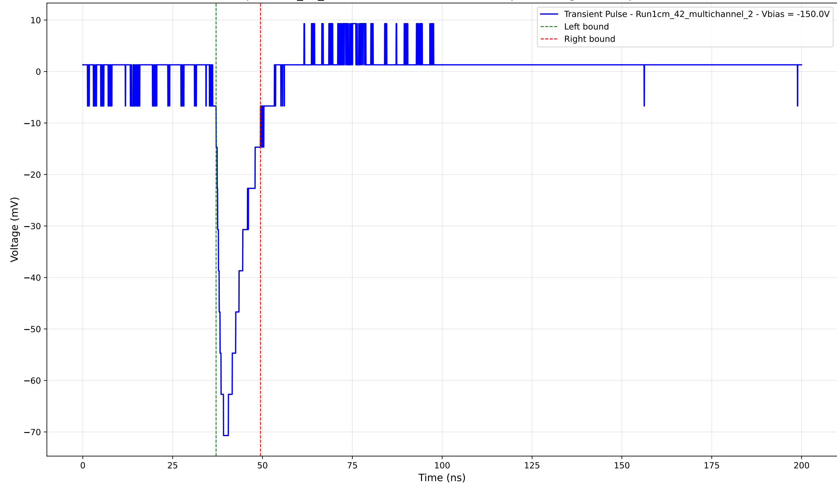
Transient Pulse - Sample: 1cm_42_multichannel - Position: 4700.0 \mu\text{m} - Charge: 10.03 pC - Rise Time: 2.08 ns
