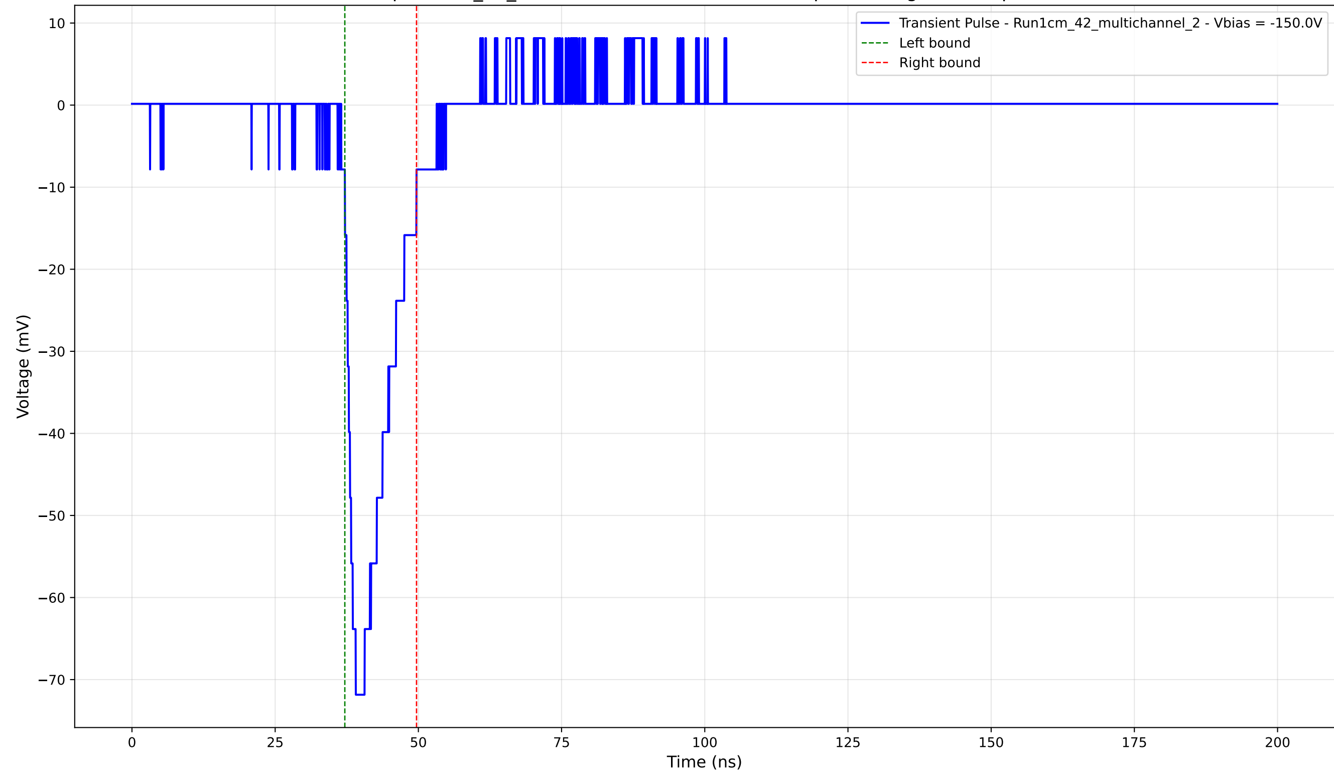
Transient Pulse - Sample: 1cm_42_multichannel - Position: 4500.0 \mu\text{m} - Charge: 10.40 pC - Rise Time: 2.52 ns
