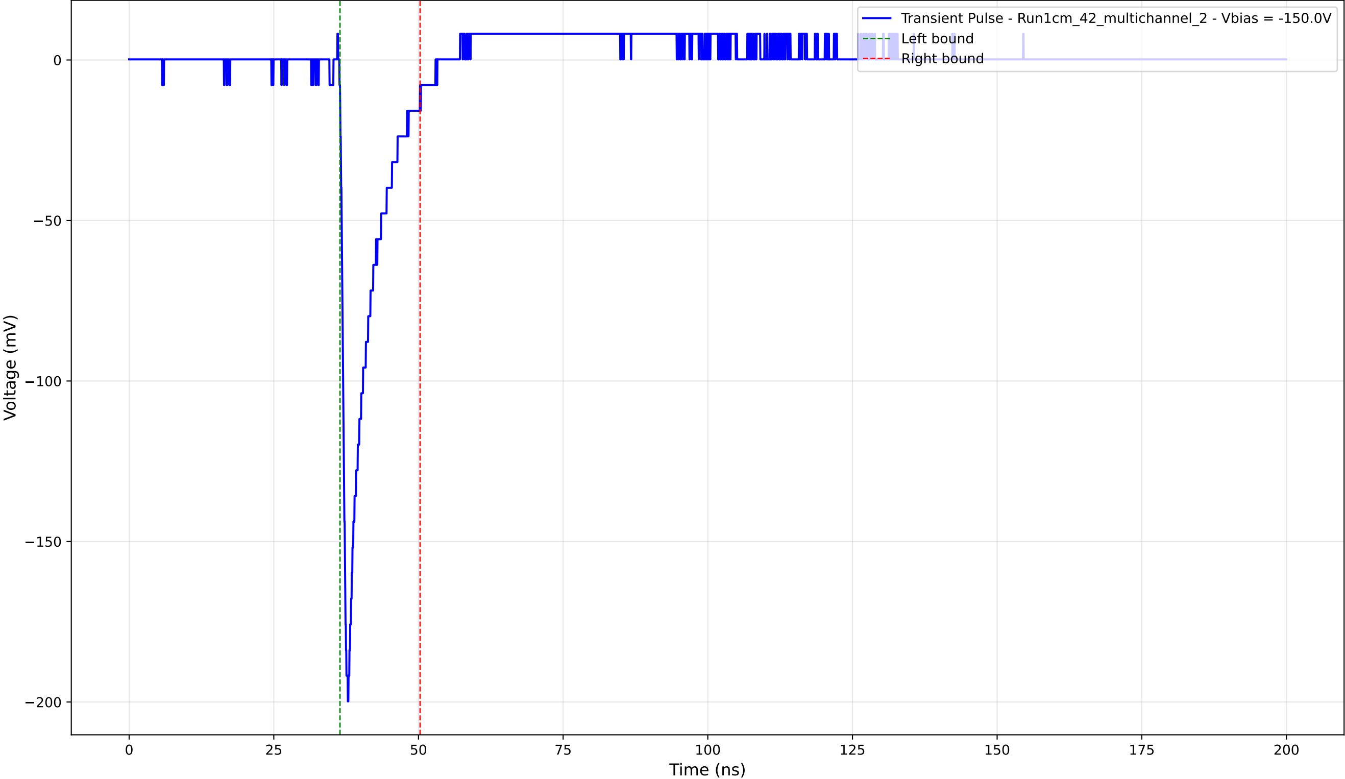
Transient Pulse - Sample: 1cm_42_multichannel - Position: 3185.0 \mu\text{m} - Charge: 18.95 pC - Rise Time: 0.98 ns
