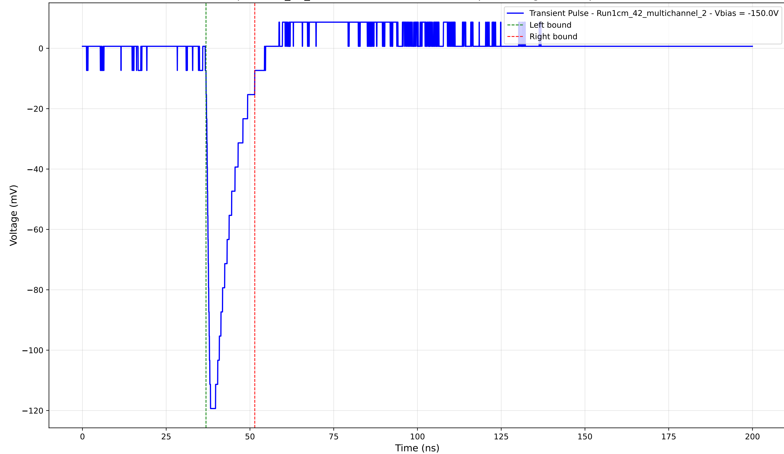
Transient Pulse - Sample: 1cm_42_multichannel - Position: 965.0 \mu\text{m} - Charge: 17.09 pC - Rise Time: 1.14 ns
