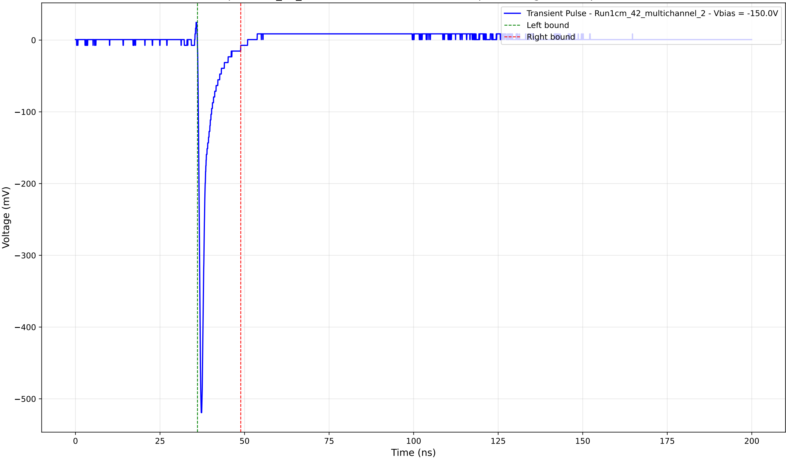
Transient Pulse - Sample: 1cm_42_multichannel - Position: 2145.0 \mu\text{m} - Charge: 26.62 pC - Rise Time: 0.76 ns
