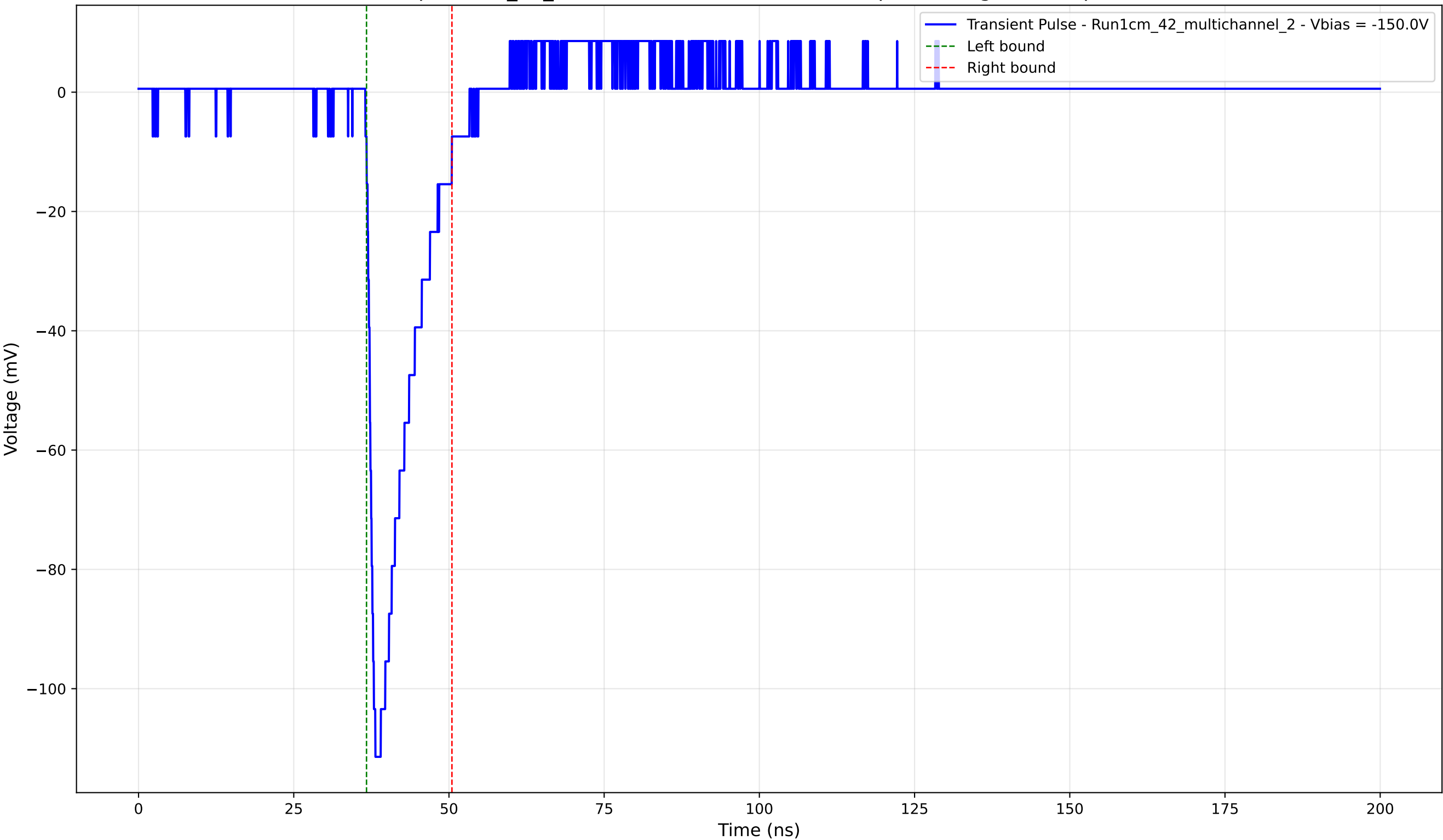
Transient Pulse - Sample: 1cm_42_multichannel - Position: 3625.0 \mu\text{m} - Charge: 14.75 pC - Rise Time: 1.18 ns
