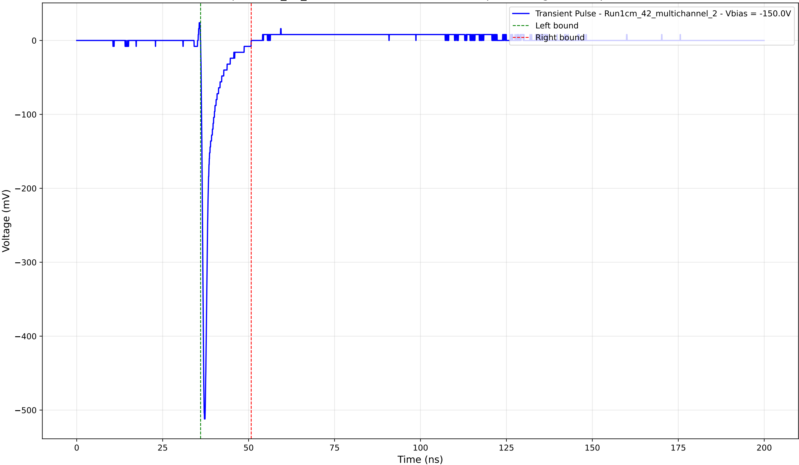
Transient Pulse - Sample: 1cm_42_multichannel - Position: 2555.0 \mu\text{m} - Charge: 25.89 pC - Rise Time: 0.74 ns
