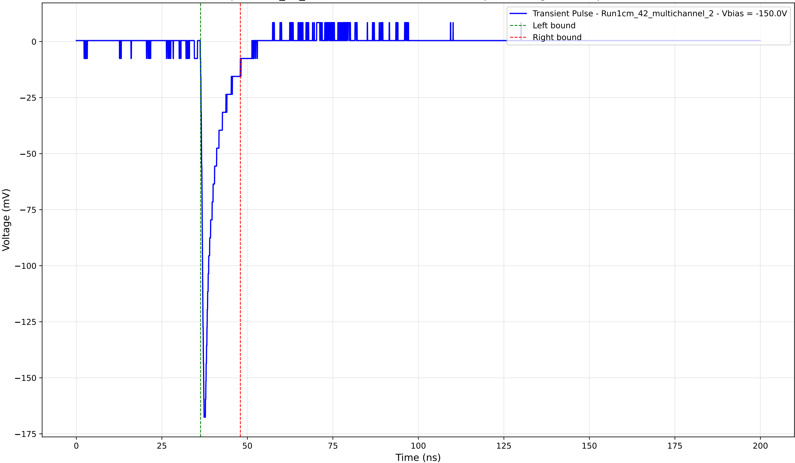
Transient Pulse - Sample: 1cm_42_multichannel - Position: 1810.0 \mu\text{m} - Charge: 12.63 pC - Rise Time: 0.83 ns
