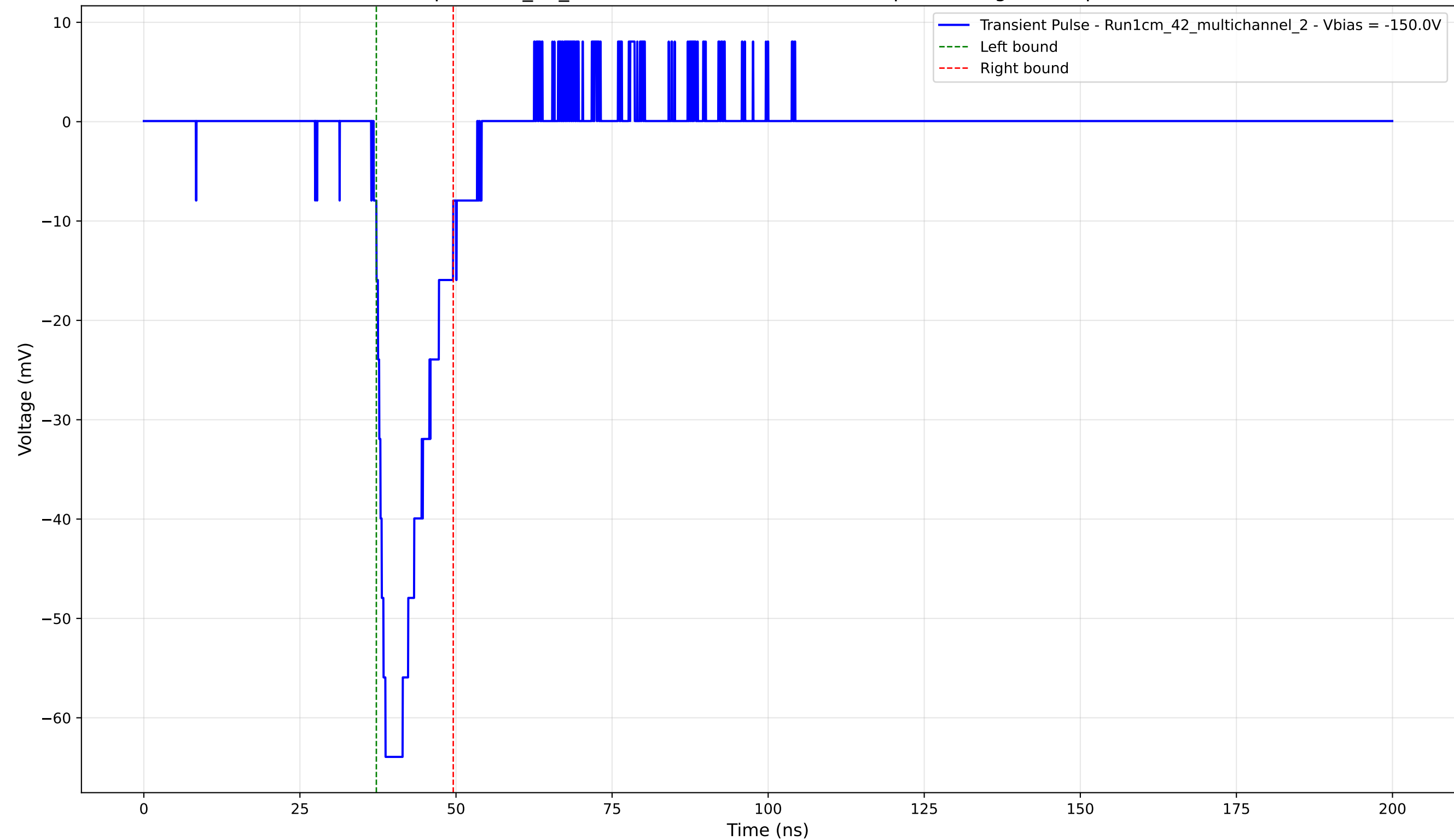
Transient Pulse - Sample: 1cm_42_multichannel - Position: 4475.0 \mu\text{m} - Charge: 9.76 pC - Rise Time: 1.89 ns
