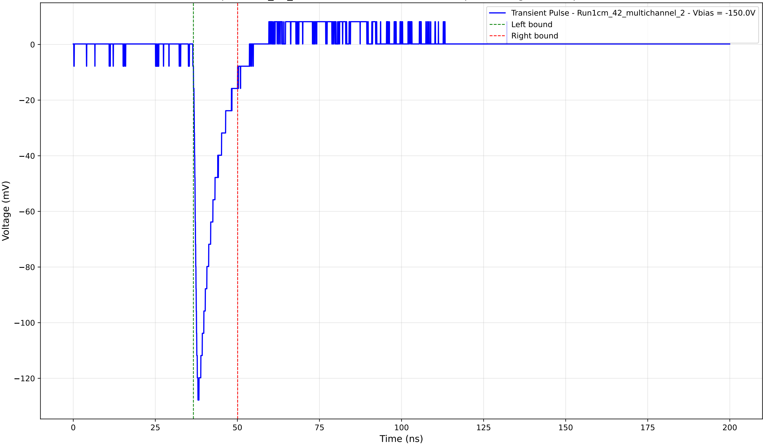
Transient Pulse - Sample: 1cm_42_multichannel - Position: 3455.0 \mu\text{m} - Charge: 15.11 pC - Rise Time: 1.18 ns
