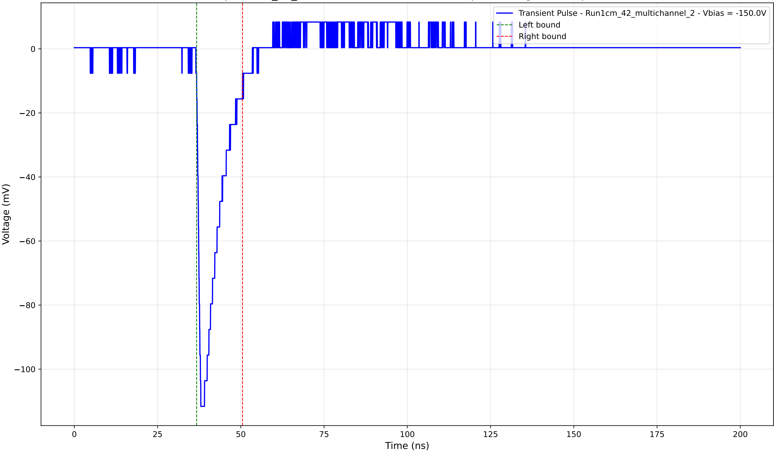
Transient Pulse - Sample: 1cm_42_multichannel - Position: 3600.0 \mu\text{m} - Charge: 15.06 pC - Rise Time: 1.14 ns
