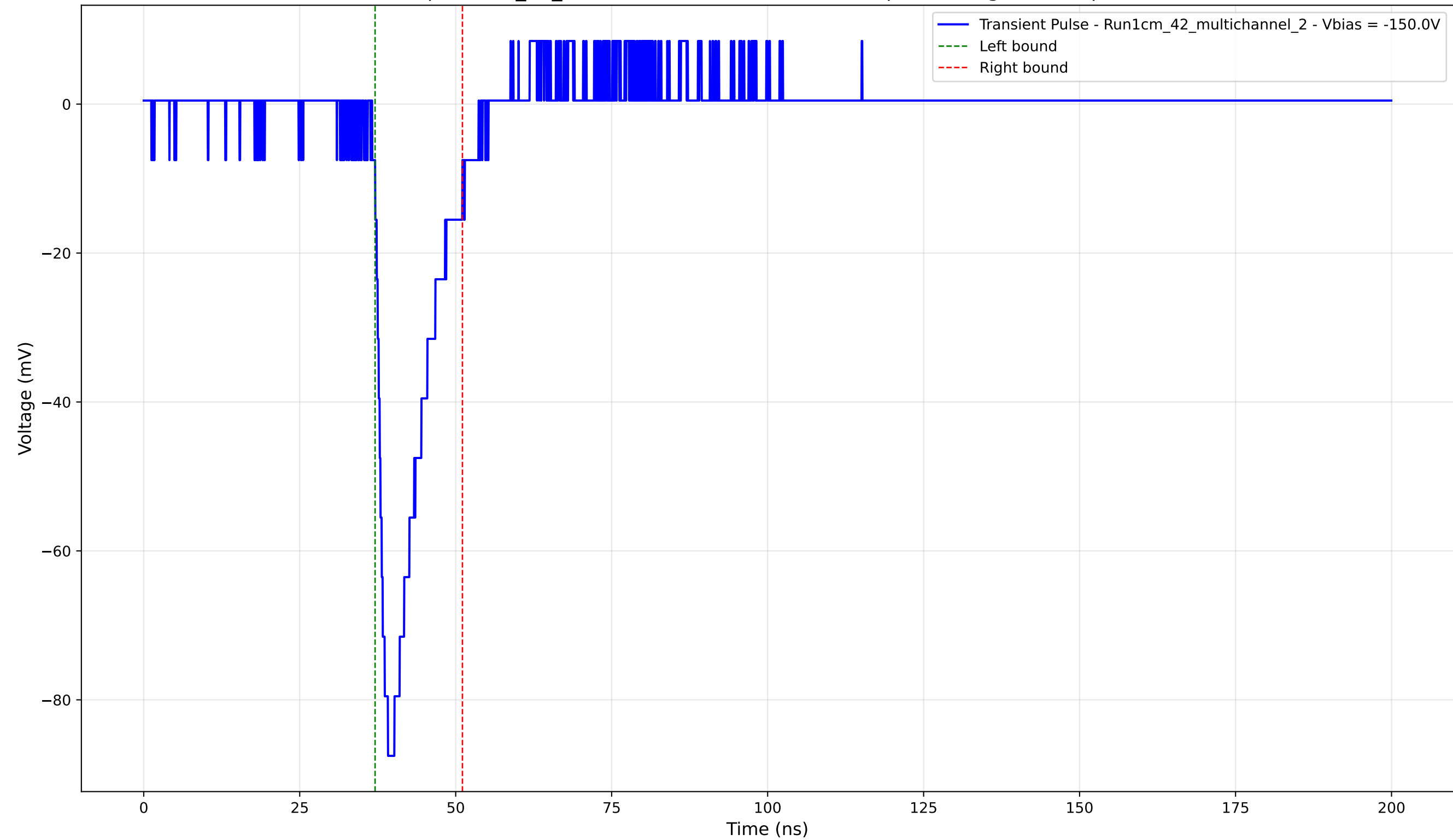
Transient Pulse - Sample: 1cm_42_multichannel - Position: 4115.0 \mu\text{m} - Charge: 12.60 pC - Rise Time: 1.55 ns
