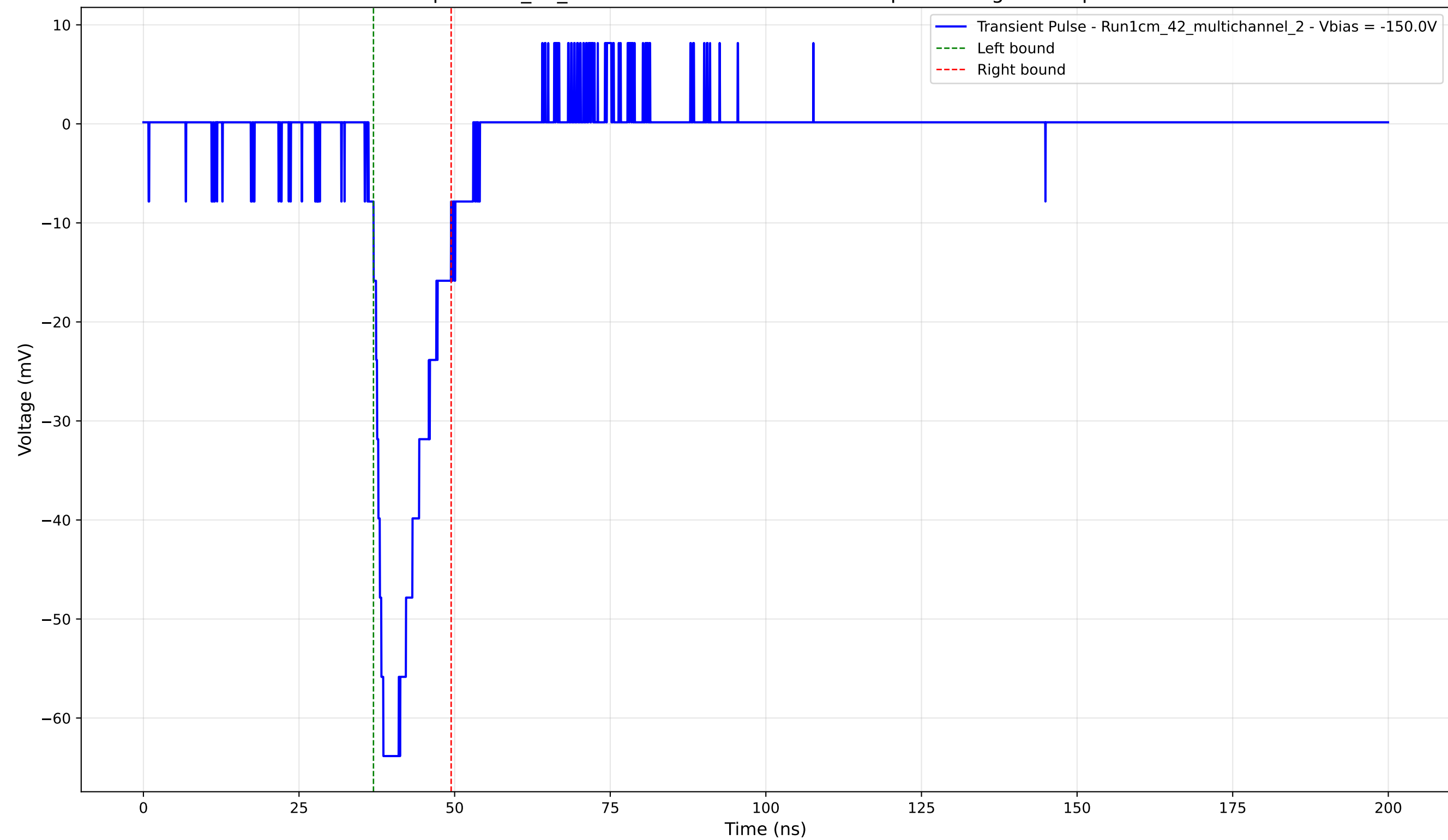
Transient Pulse - Sample: 1cm_42_multichannel - Position: 4745.0 \mu\text{m} - Charge: 9.78 pC - Rise Time: 2.37 ns
