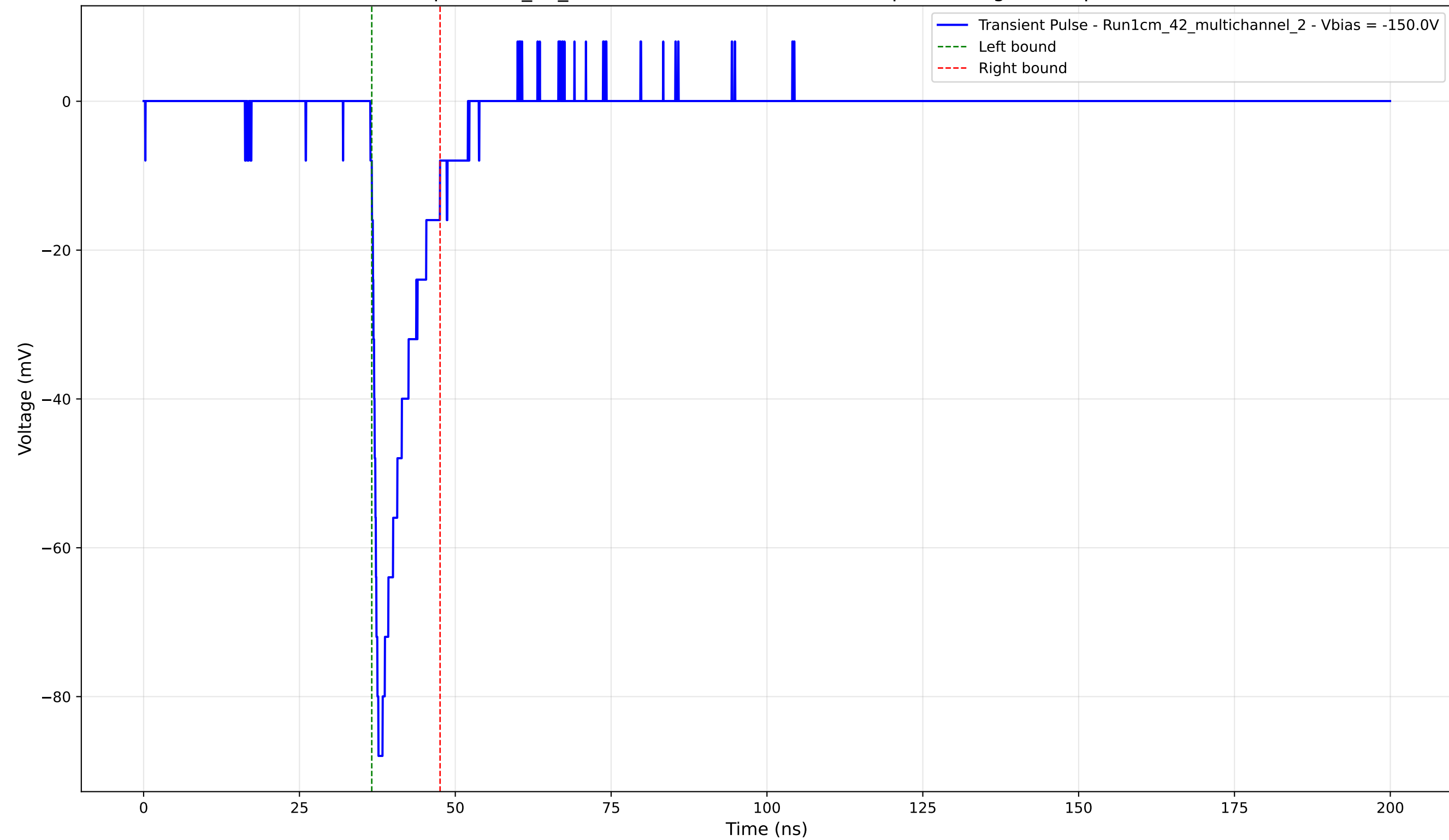
Transient Pulse - Sample: 1cm_42_multichannel - Position: 3330.0 \mu\text{m} - Charge: 9.18 pC - Rise Time: 0.92 ns
