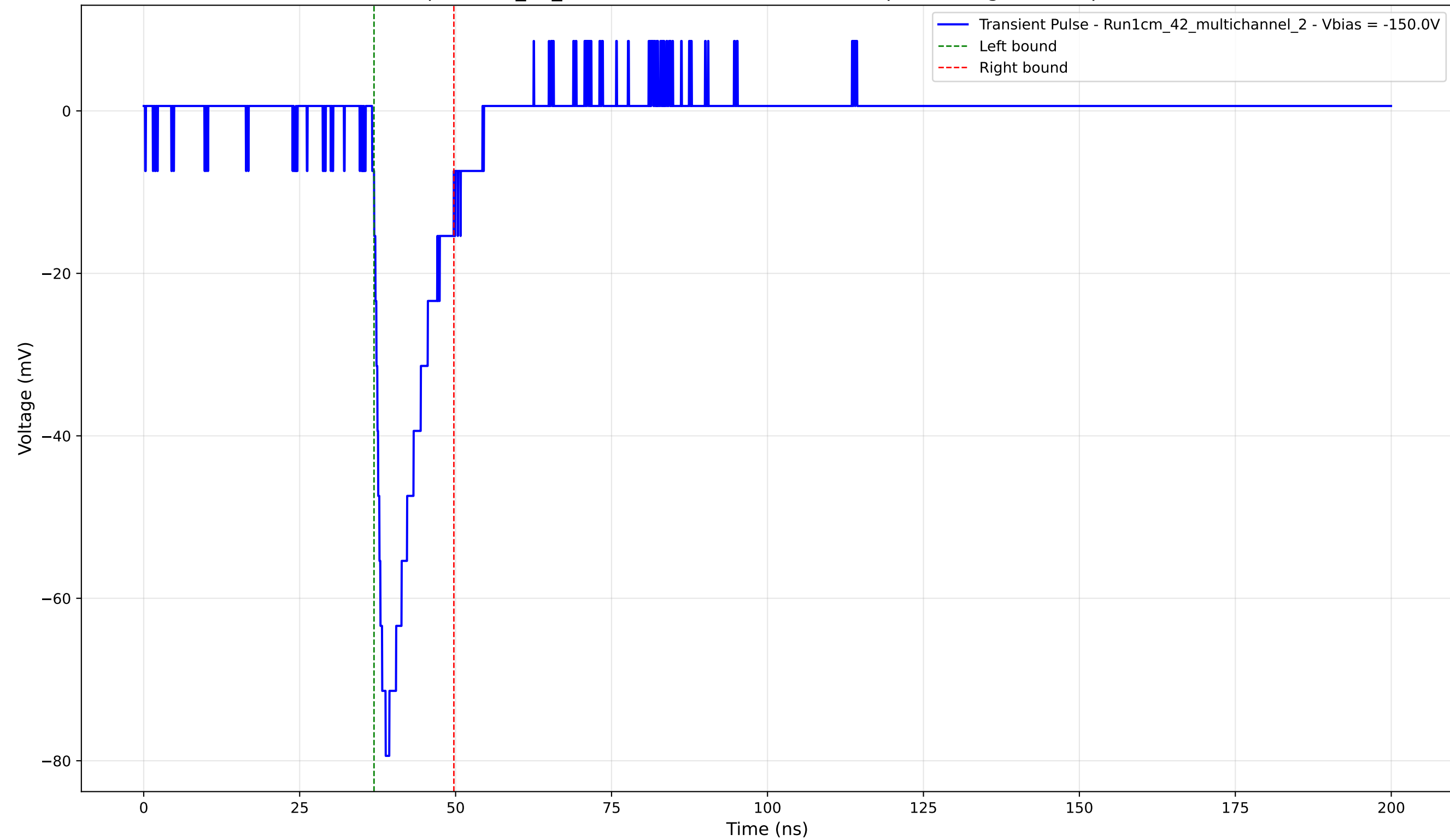
Transient Pulse - Sample: 1cm_42_multichannel - Position: 3825.0 \mu\text{m} - Charge: 10.60 pC - Rise Time: 1.88 ns
