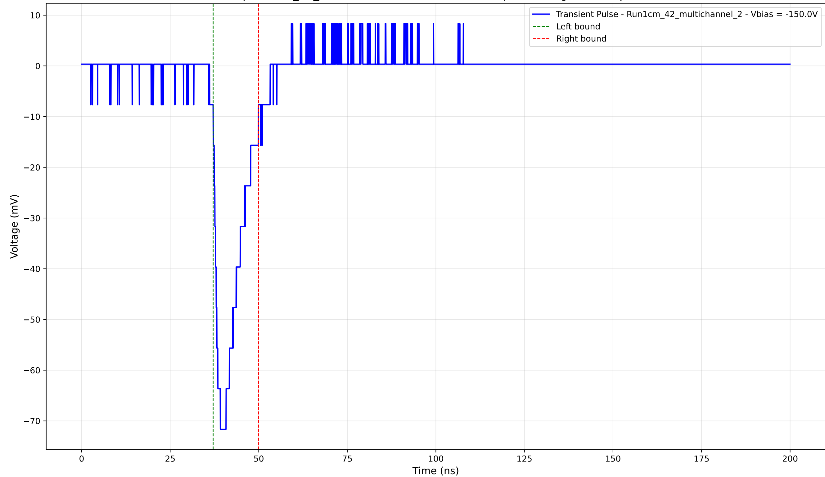
Transient Pulse - Sample: 1cm_42_multichannel - Position: 4585.0 \mu\text{m} - Charge: 10.53 pC - Rise Time: 3.00 ns
