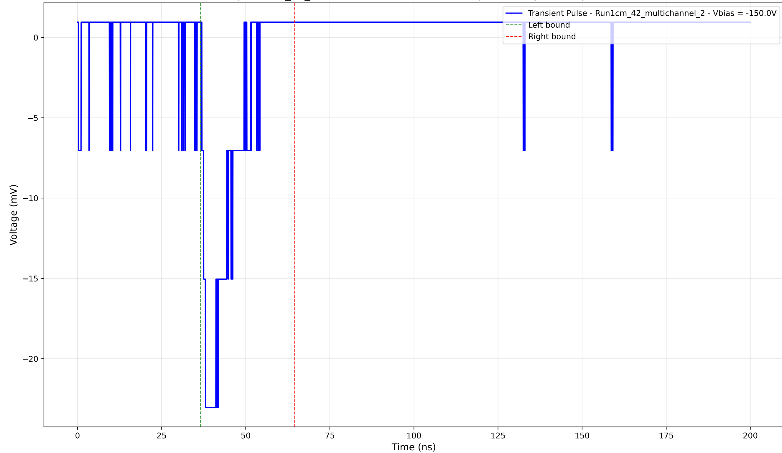
Transient Pulse - Sample: 1cm_42_multichannel - Position: 815.0 \mu\text{m} - Charge: 3.52 pC - Rise Time: 1.07 ns
