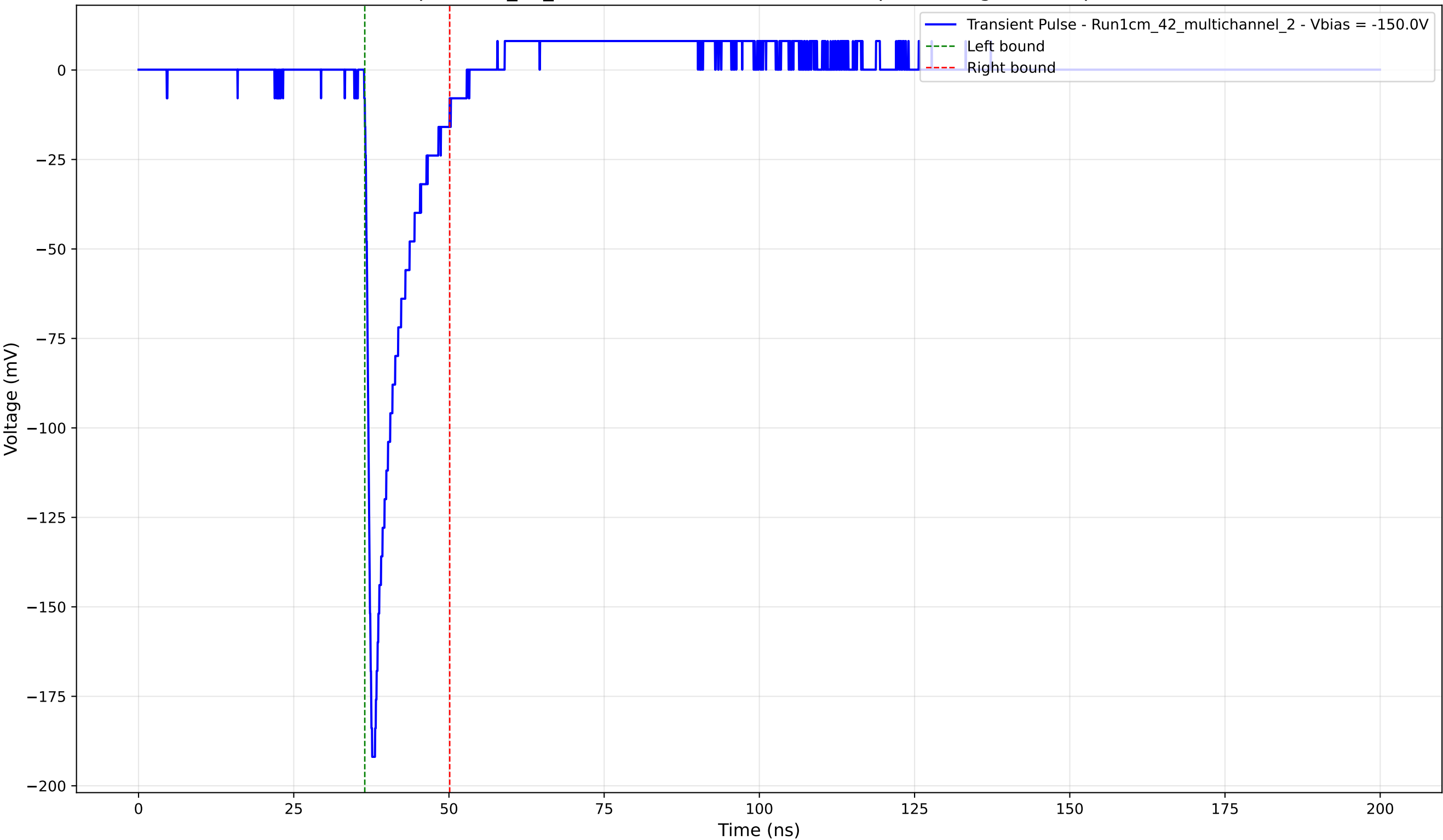
Transient Pulse - Sample: 1cm_42_multichannel - Position: 3205.0 \mu\text{m} - Charge: 19.01 pC - Rise Time: 0.93 ns
