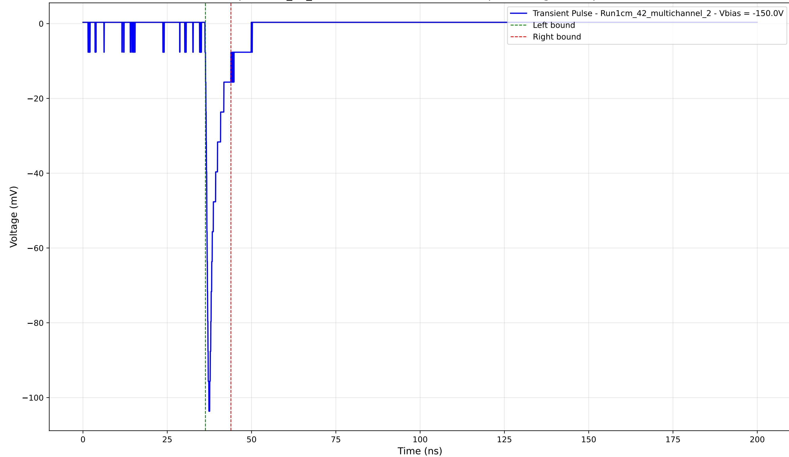
Transient Pulse - Sample: 1cm_42_multichannel - Position: 2835.0 \mu\text{m} - Charge: 6.03 pC - Rise Time: 0.83 ns
