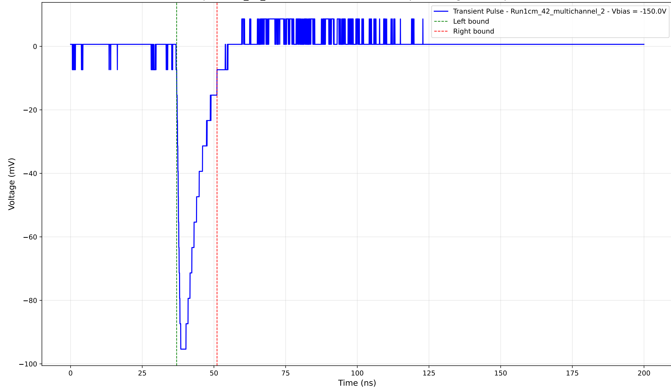
Transient Pulse - Sample: 1cm_42_multichannel - Position: 765.0 \mu\text{m} - Charge: 14.27 pC - Rise Time: 1.15 ns
