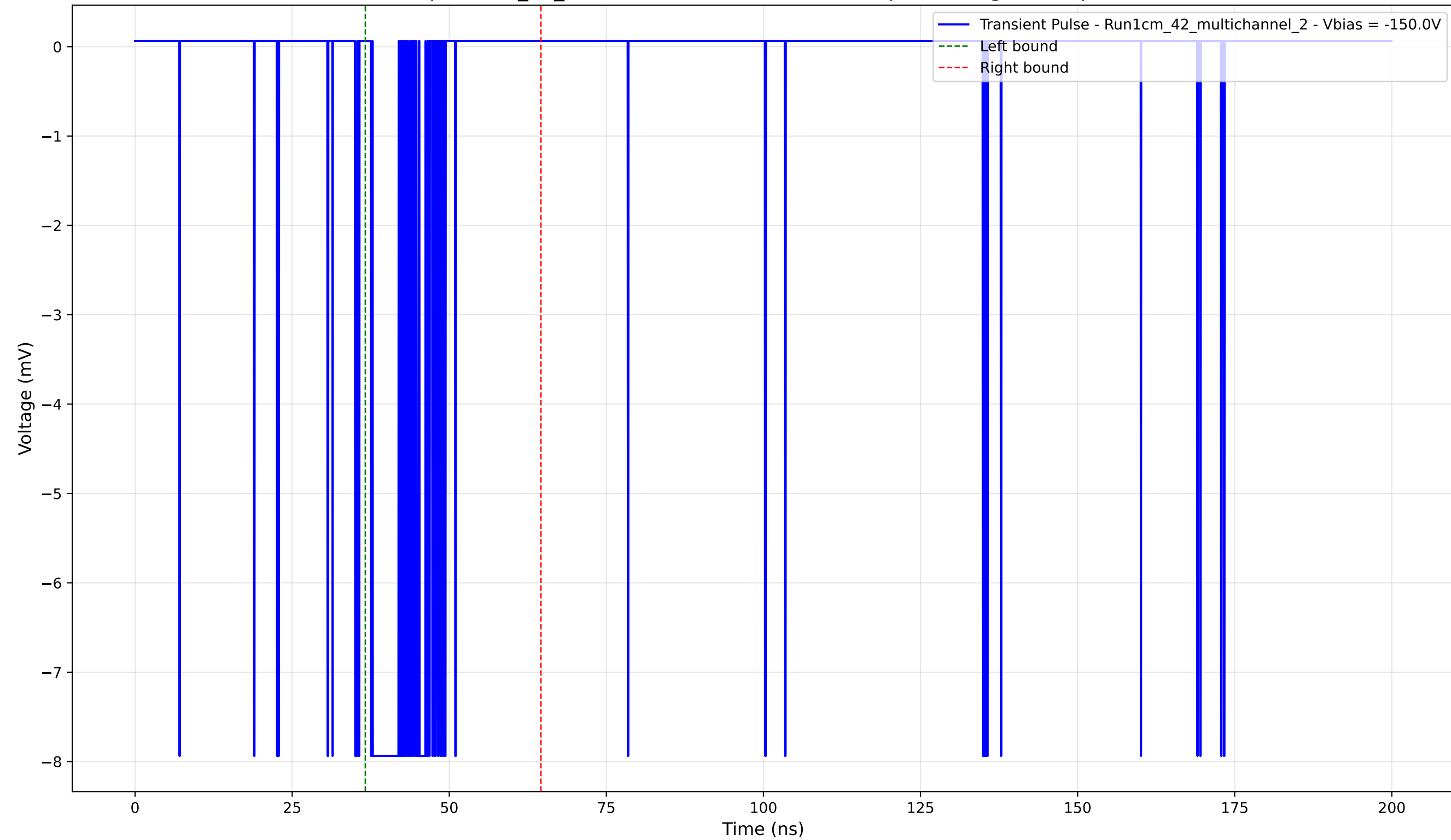
Transient Pulse - Sample: 1cm_42_multichannel - Position: 4405.0 \mu\text{m} - Charge: 1.35 pC - Rise Time: 0.04 ns
