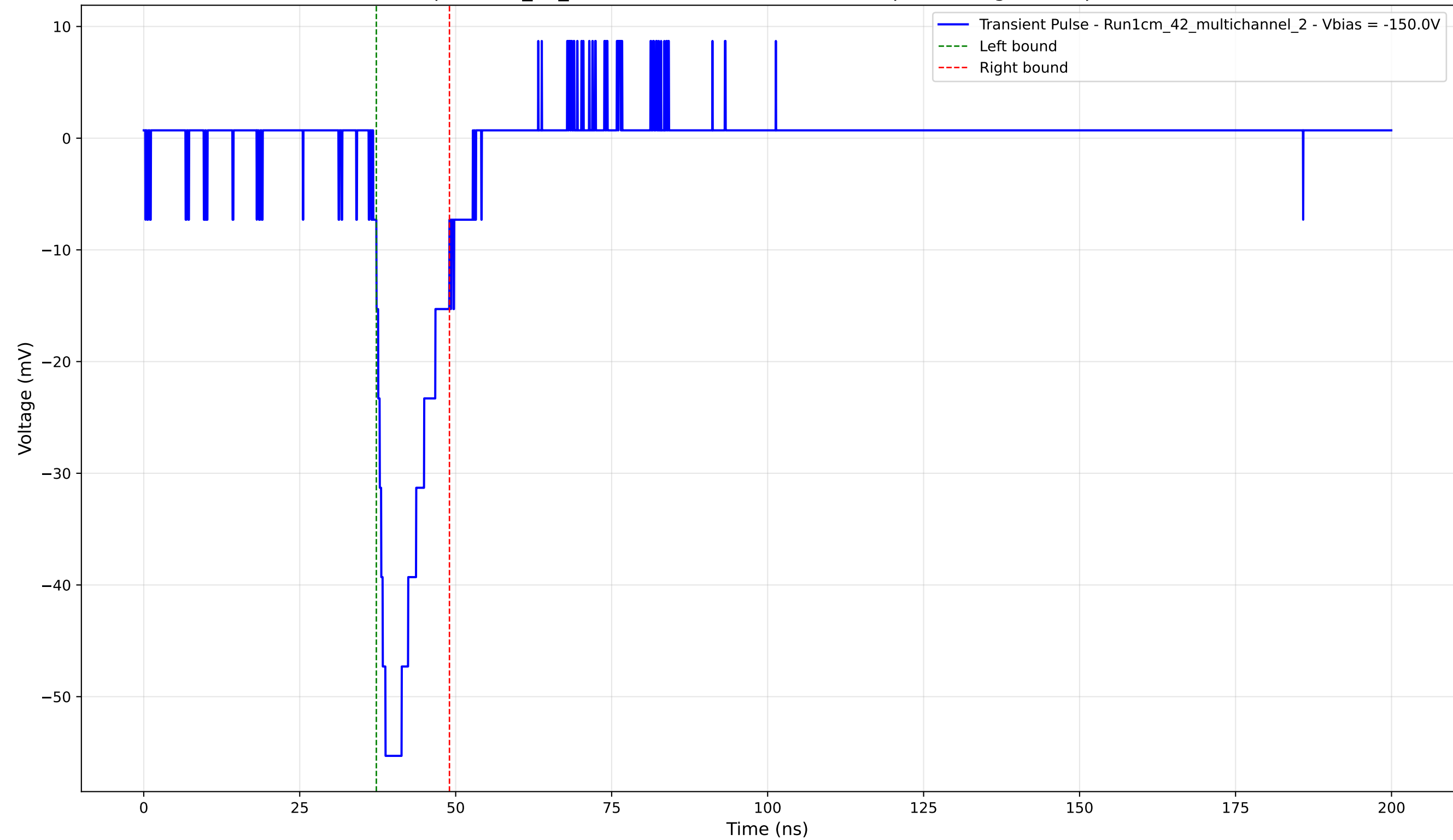
Transient Pulse - Sample: 1cm_42_multichannel - Position: 4455.0 \mu\text{m} - Charge: 8.15 pC - Rise Time: 1.97 ns
