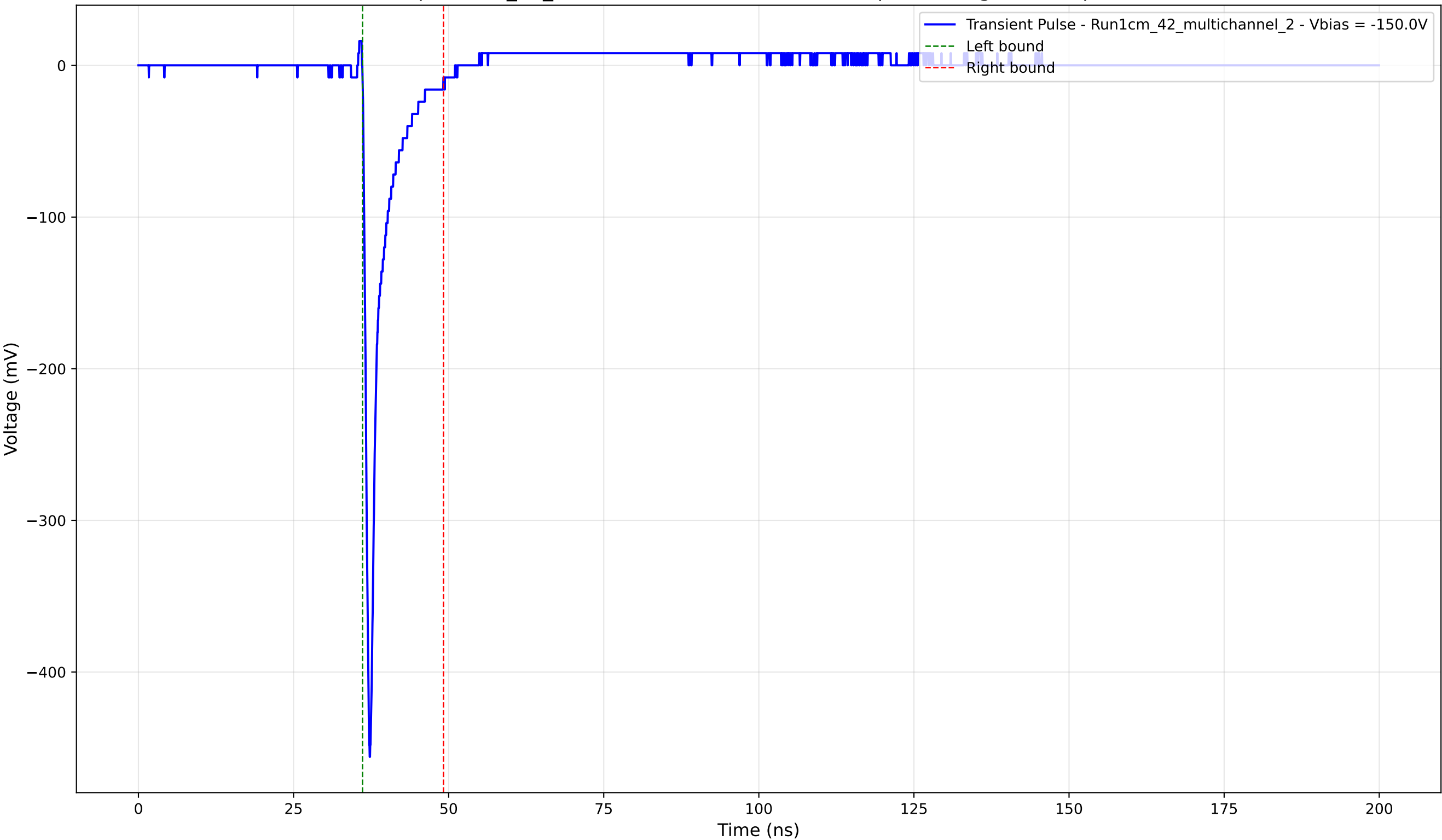
Transient Pulse - Sample: 1cm_42_multichannel - Position: 2650.0 \mu\text{m} - Charge: 24.79 pC - Rise Time: 0.74 ns
