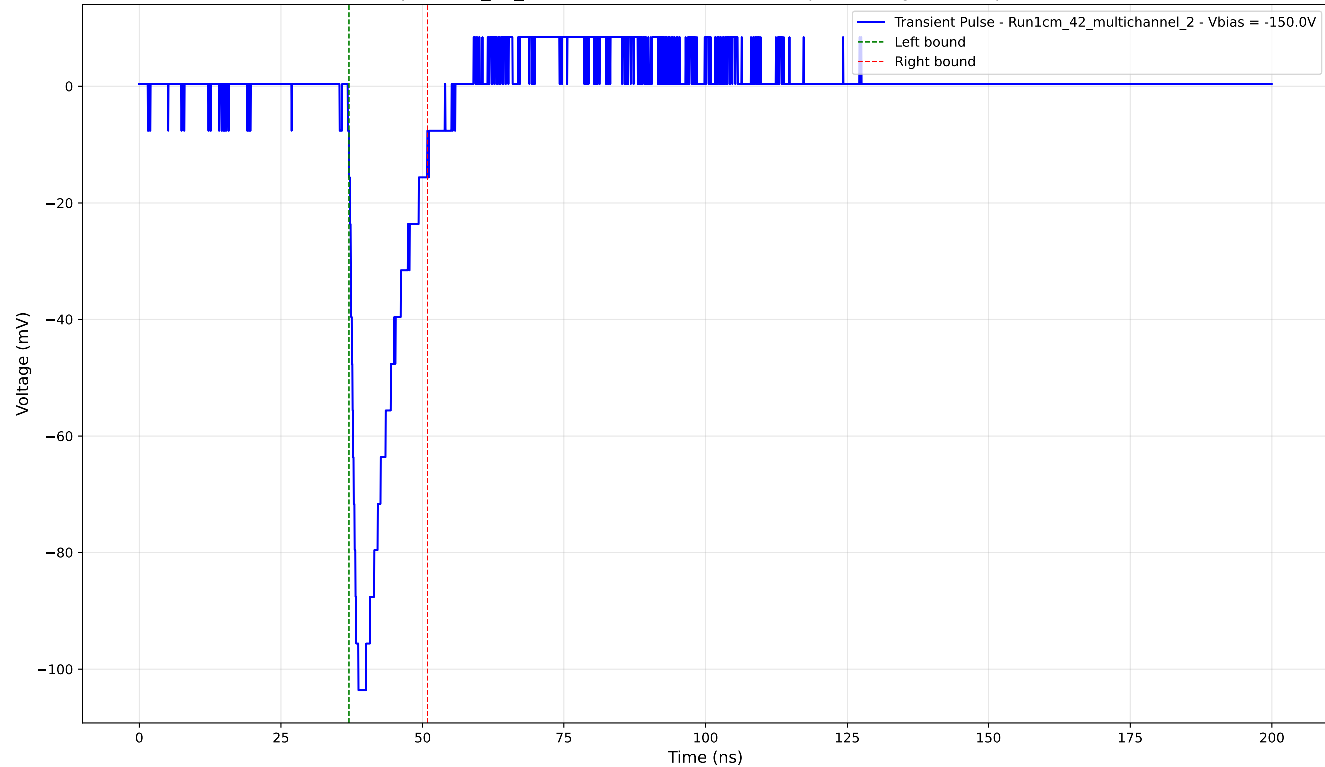
Transient Pulse - Sample: 1cm_42_multichannel - Position: 745.0 \mu\text{m} - Charge: 15.07 pC - Rise Time: 1.27 ns
