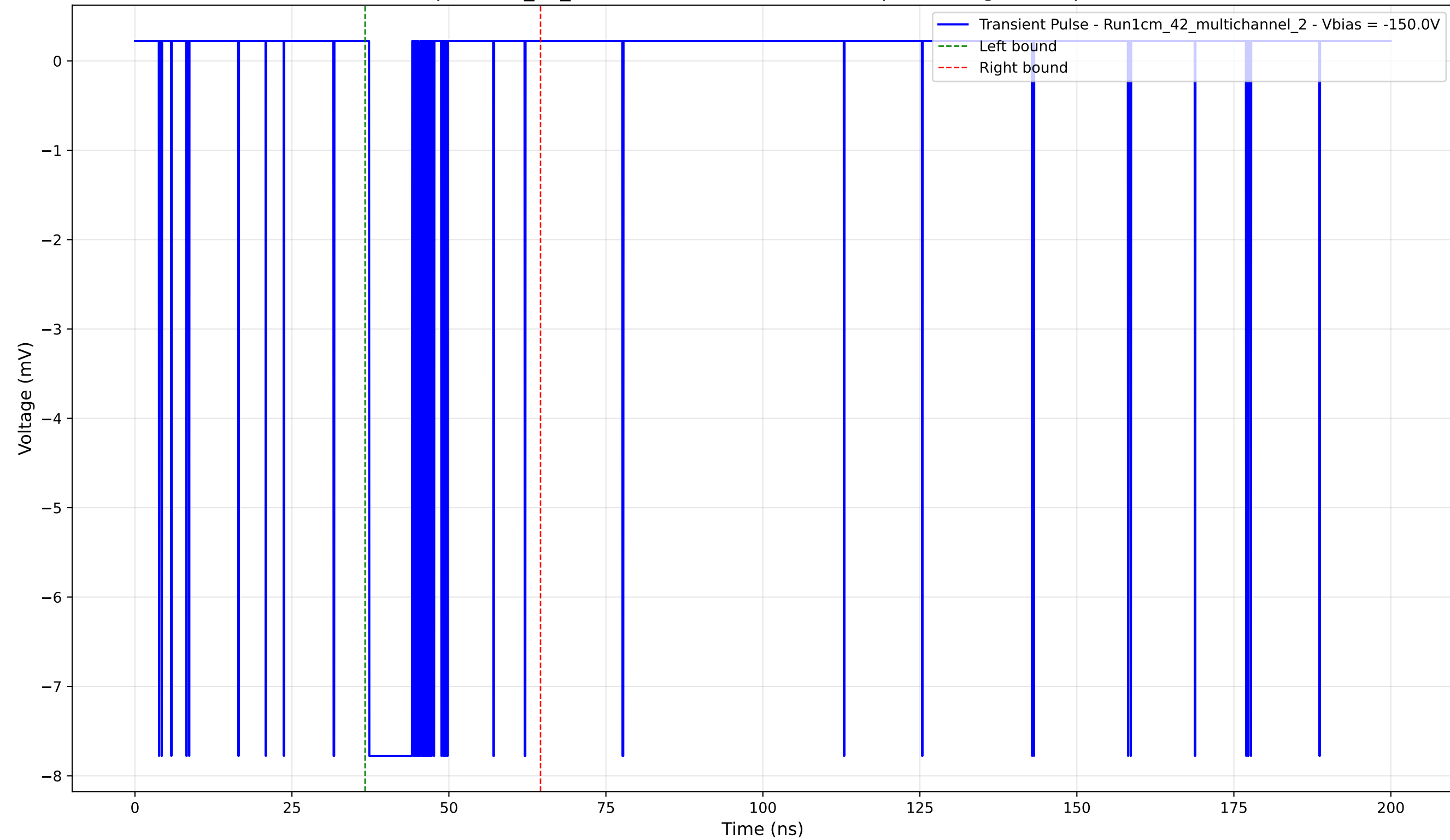
Transient Pulse - Sample: 1cm_42_multichannel - Position: 325.0 \mu\text{m} - Charge: 1.32 pC - Rise Time: 0.04 ns
