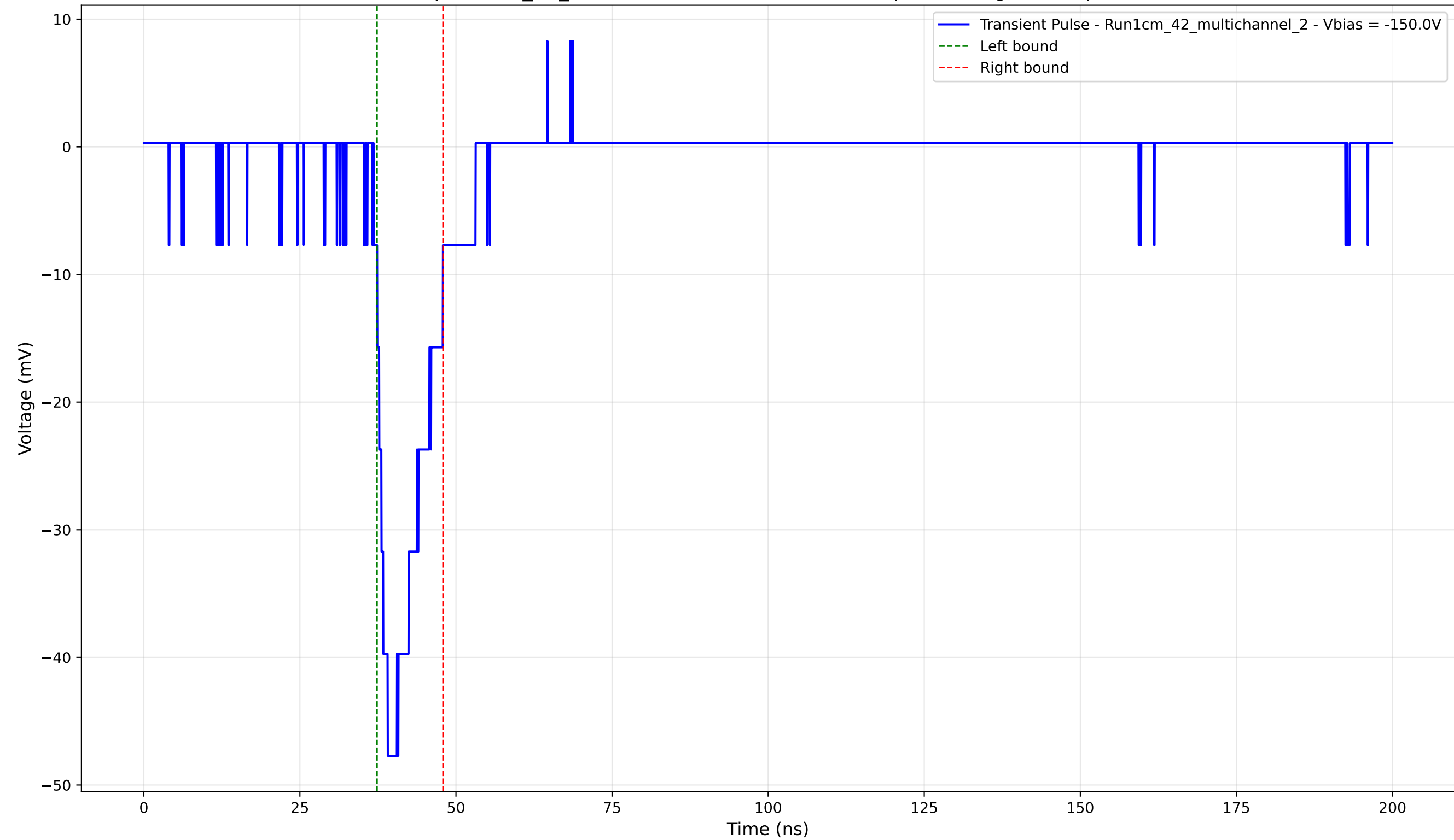
Transient Pulse - Sample: 1cm_42_multichannel - Position: 4445.0 \mu\text{m} - Charge: 6.45 pC - Rise Time: 2.26 ns
