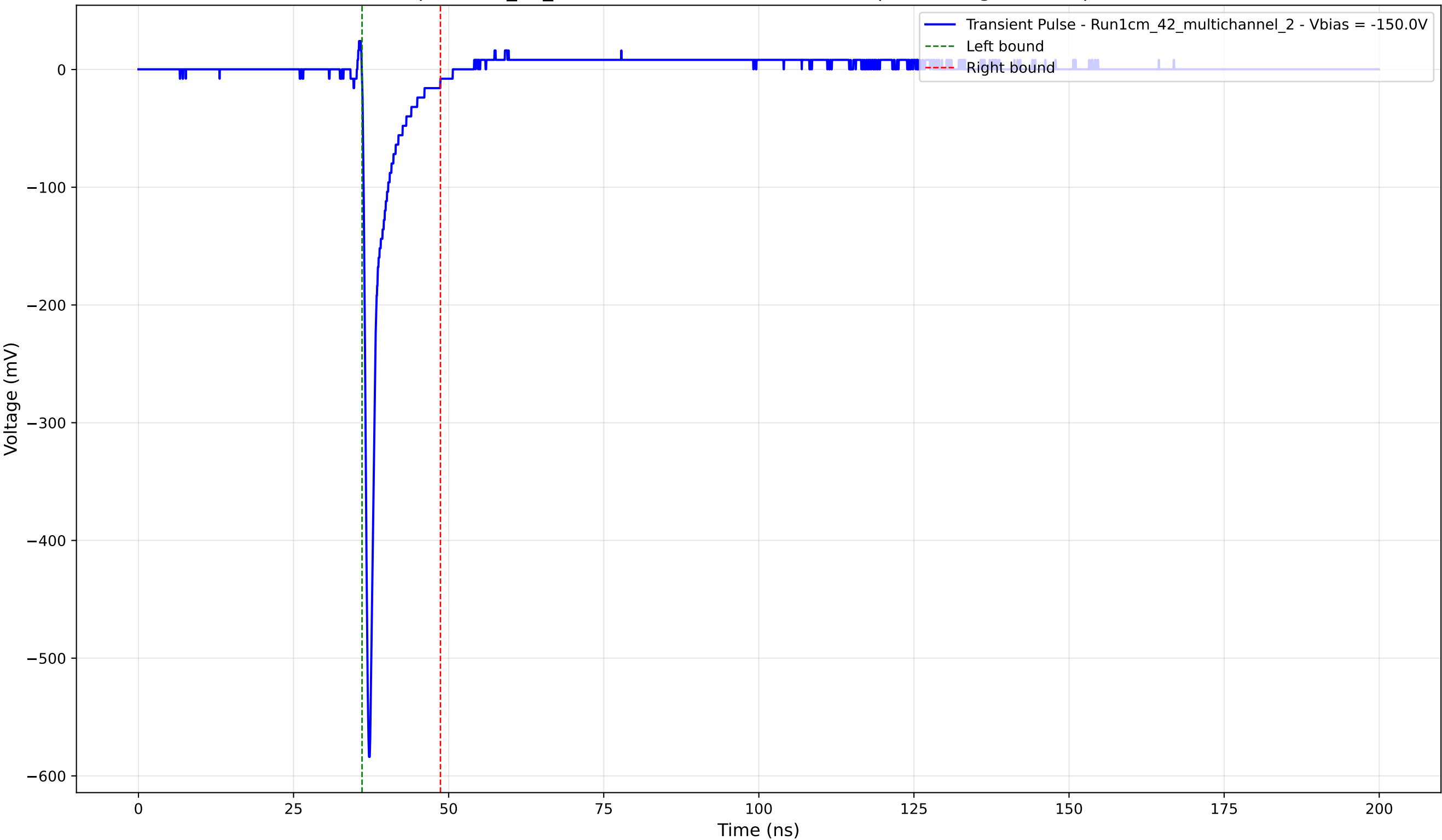
Transient Pulse - Sample: 1cm_42_multichannel - Position: 2205.0 \mu\text{m} - Charge: 28.25 pC - Rise Time: 0.75 ns
