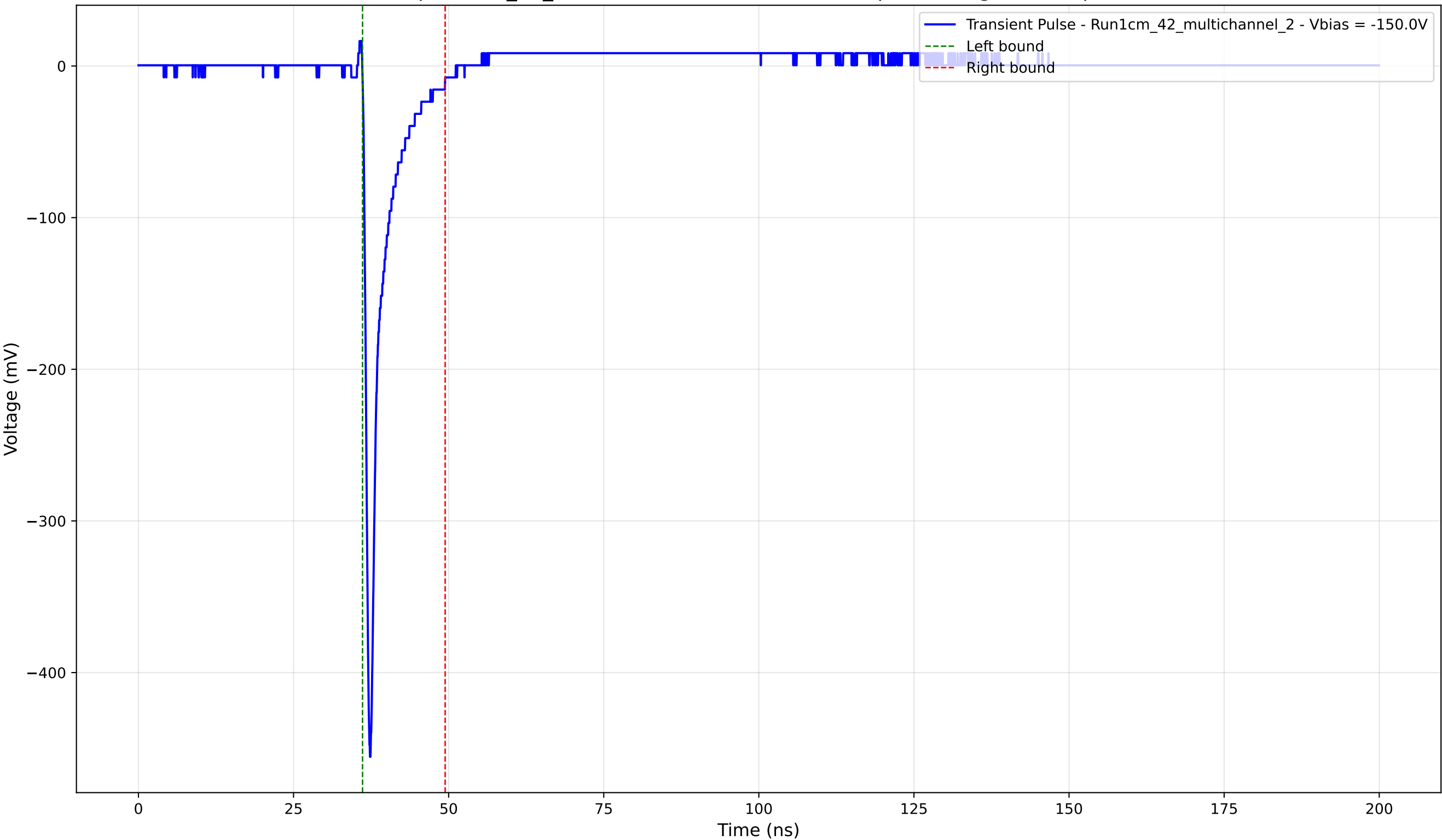
Transient Pulse - Sample: 1cm_42_multichannel - Position: 2040.0 \mu\text{m} - Charge: 26.18 pC - Rise Time: 0.76 ns
