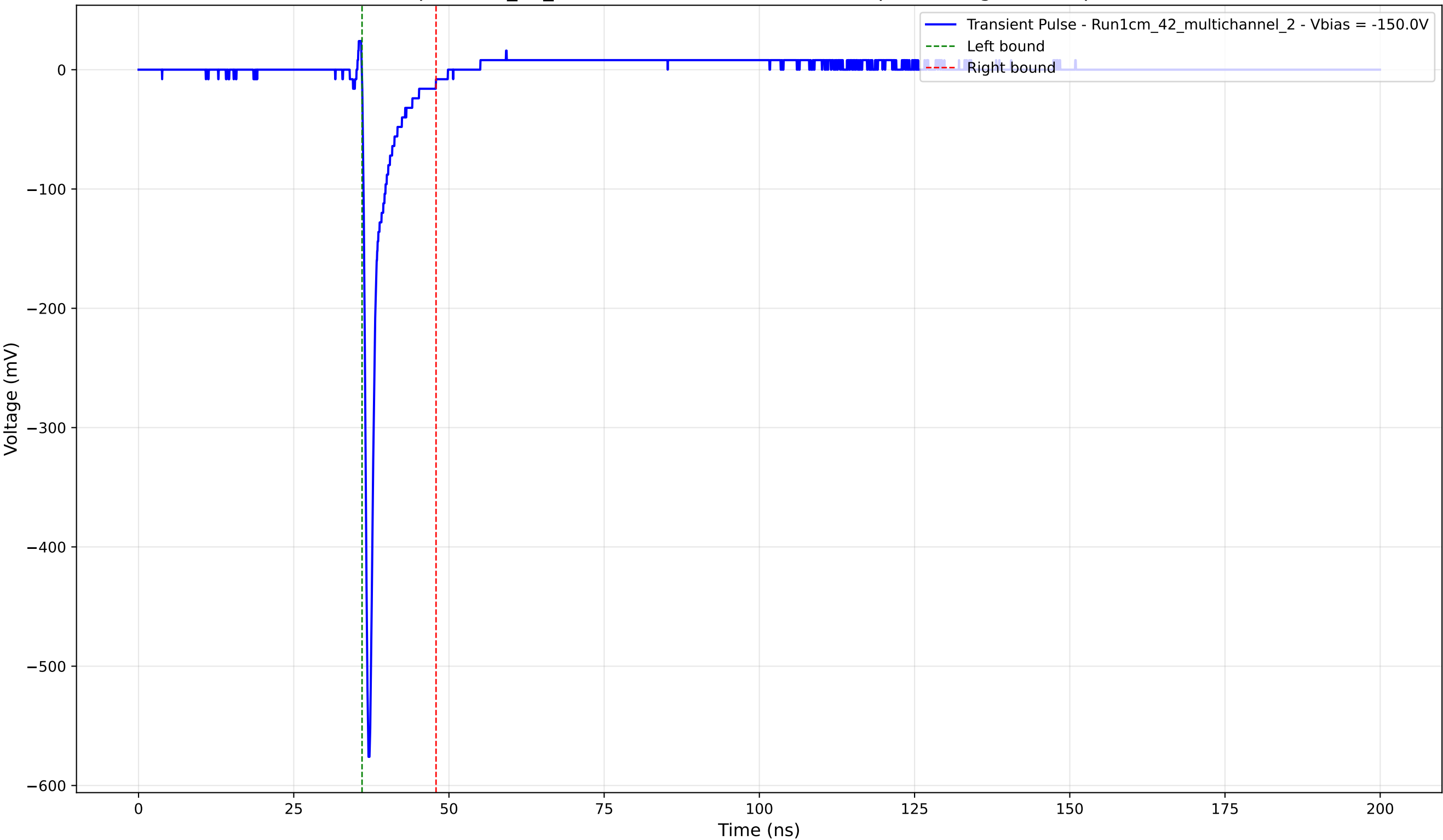
Transient Pulse - Sample: 1cm_42_multichannel - Position: 2440.0 \mu\text{m} - Charge: 25.64 pC - Rise Time: 0.73 ns
