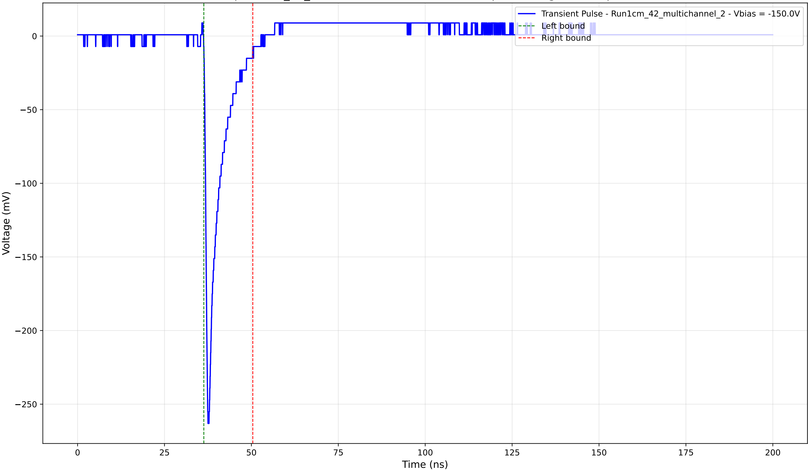
Transient Pulse - Sample: 1cm_42_multichannel - Position: 1675.0 \mu\text{m} - Charge: 22.56 pC - Rise Time: 0.89 ns
