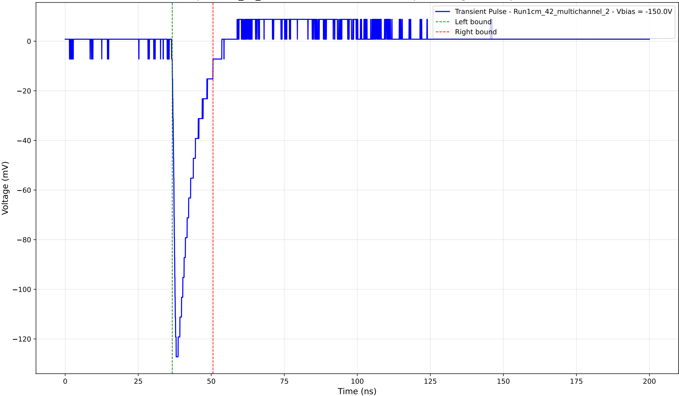
Transient Pulse - Sample: 1cm_42_multichannel - Position: 3525.0 \mu\text{m} - Charge: 16.07 pC - Rise Time: 1.13 ns
