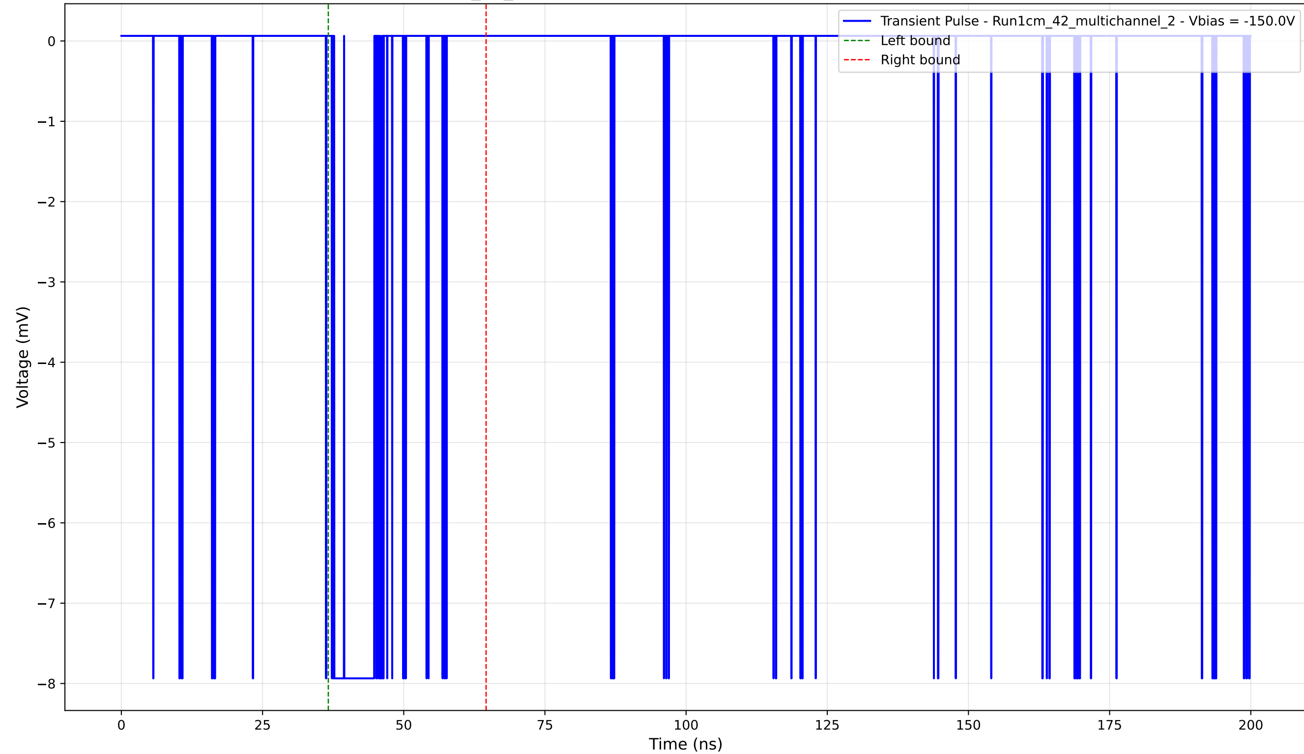
Transient Pulse - Sample: 1cm_42_multichannel - Position: 350.0 \mu\text{m} - Charge: 1.34 pC - Rise Time: 0.04 ns
