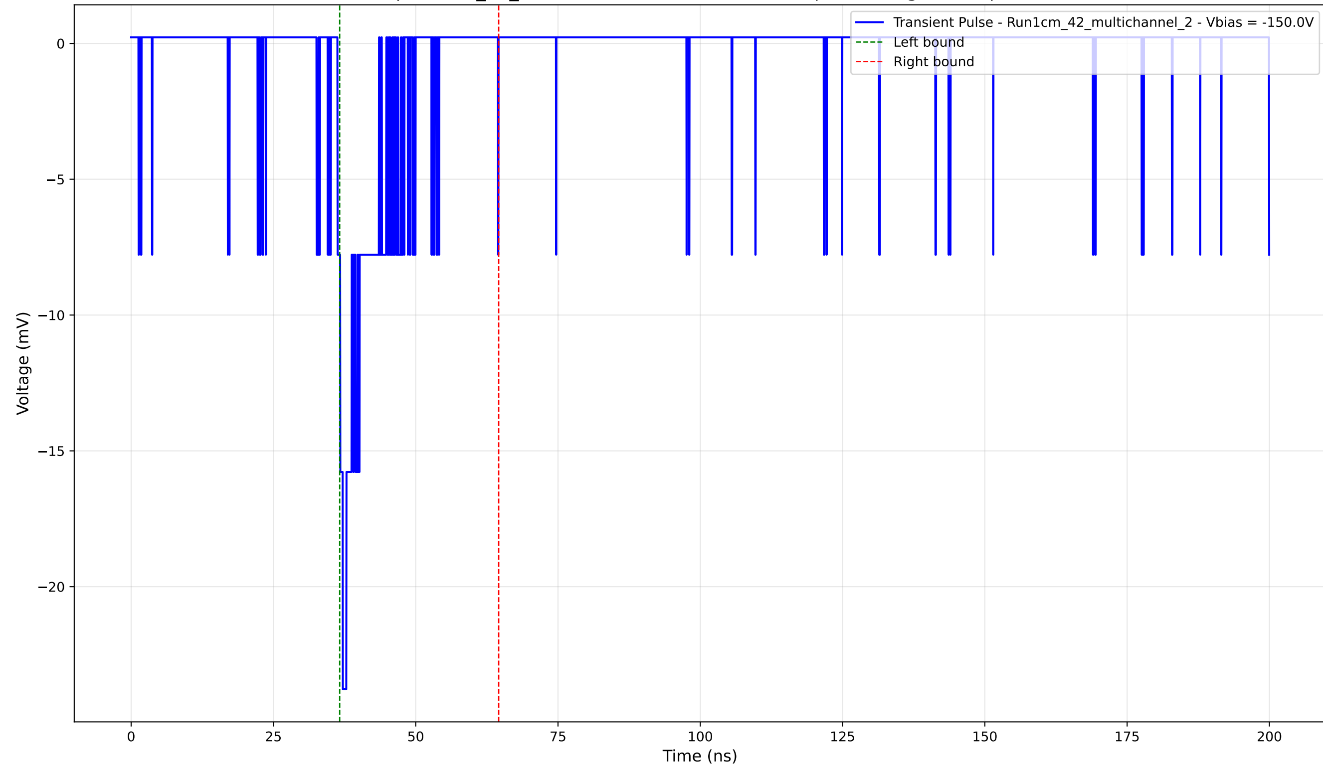
Transient Pulse - Sample: 1cm_42_multichannel - Position: 2860.0 \mu\text{m} - Charge: 2.13 pC - Rise Time: 0.95 ns
