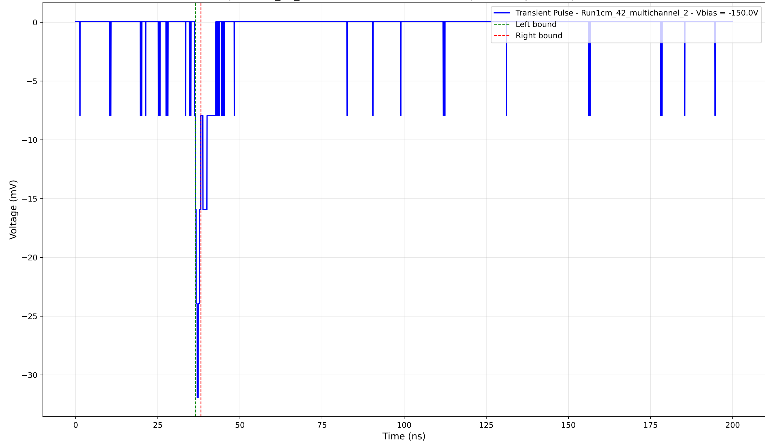
Transient Pulse - Sample: 1cm_42_multichannel - Position: 2380.0 \mu\text{m} - Charge: 0.75 pC - Rise Time: 0.86 ns
