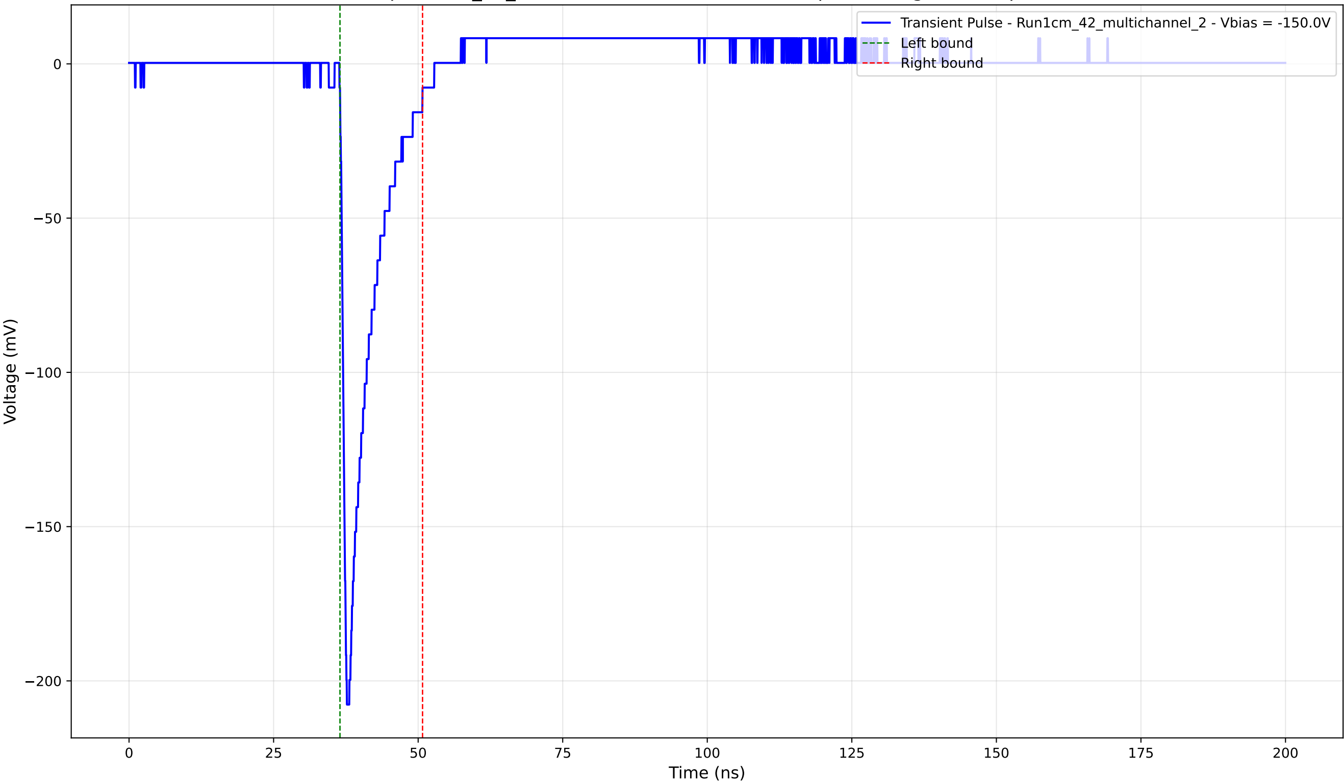
Transient Pulse - Sample: 1cm_42_multichannel - Position: 1495.0 \mu\text{m} - Charge: 21.23 pC - Rise Time: 0.97 ns
