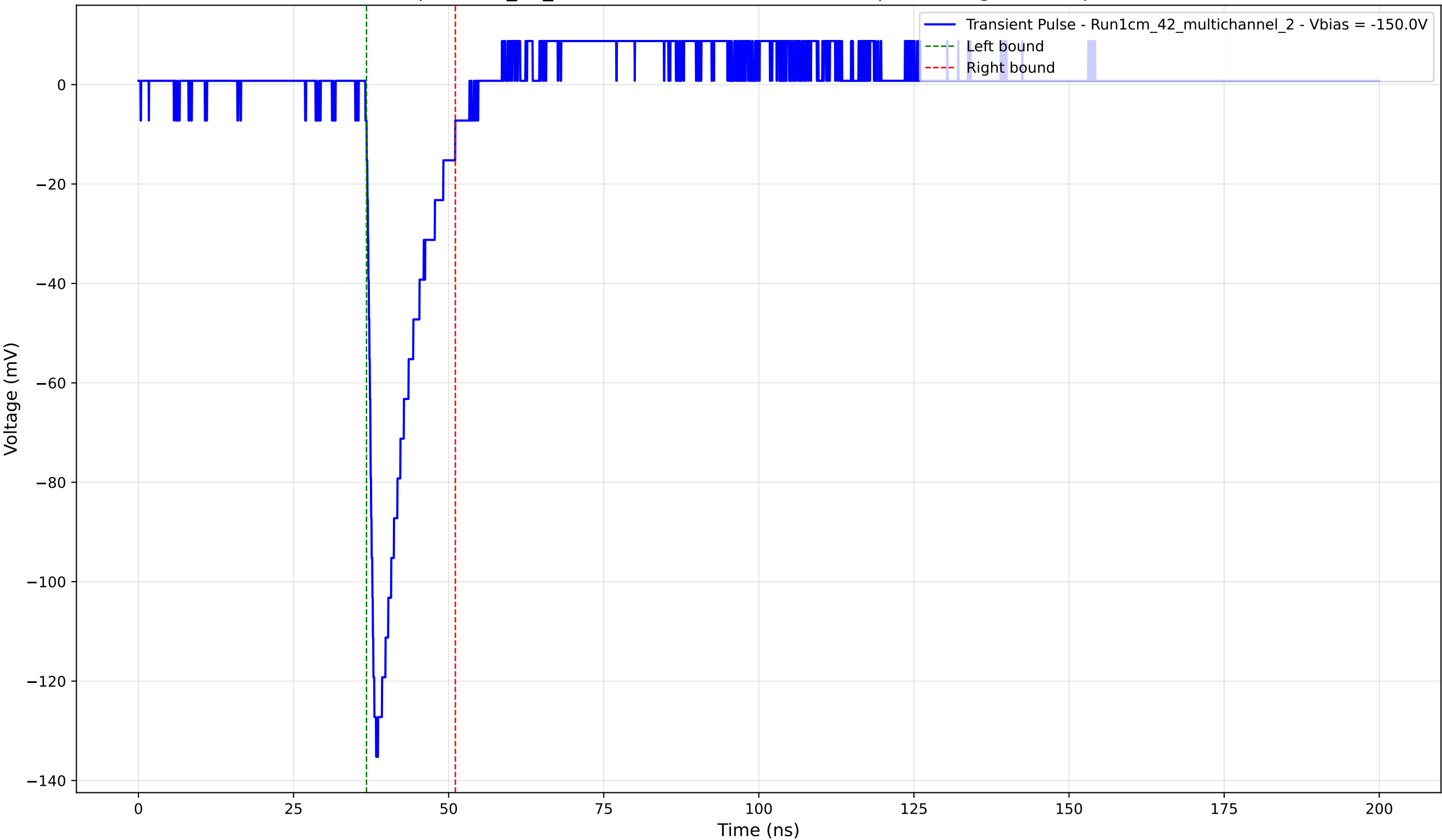
Transient Pulse - Sample: 1cm_42_multichannel - Position: 1100.0 \mu\text{m} - Charge: 17.26 pC - Rise Time: 1.25 ns
