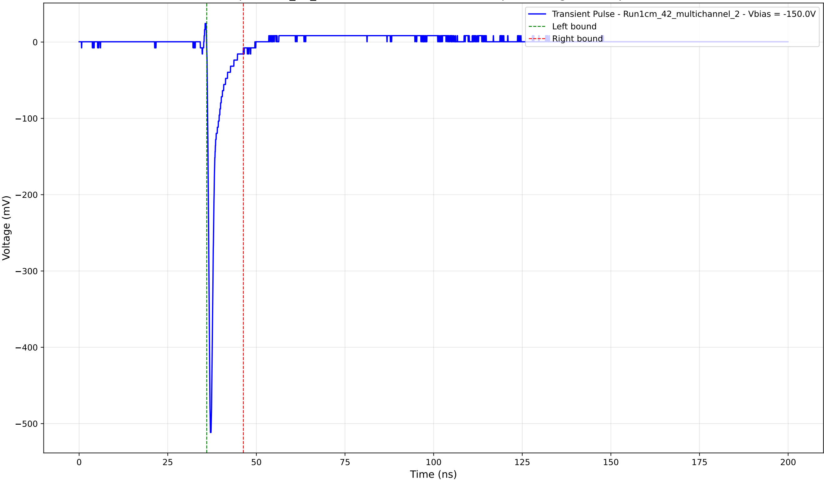
Transient Pulse - Sample: 1cm_42_multichannel - Position: 2305.0 \mu\text{m} - Charge: 22.23 pC - Rise Time: 0.72 ns
