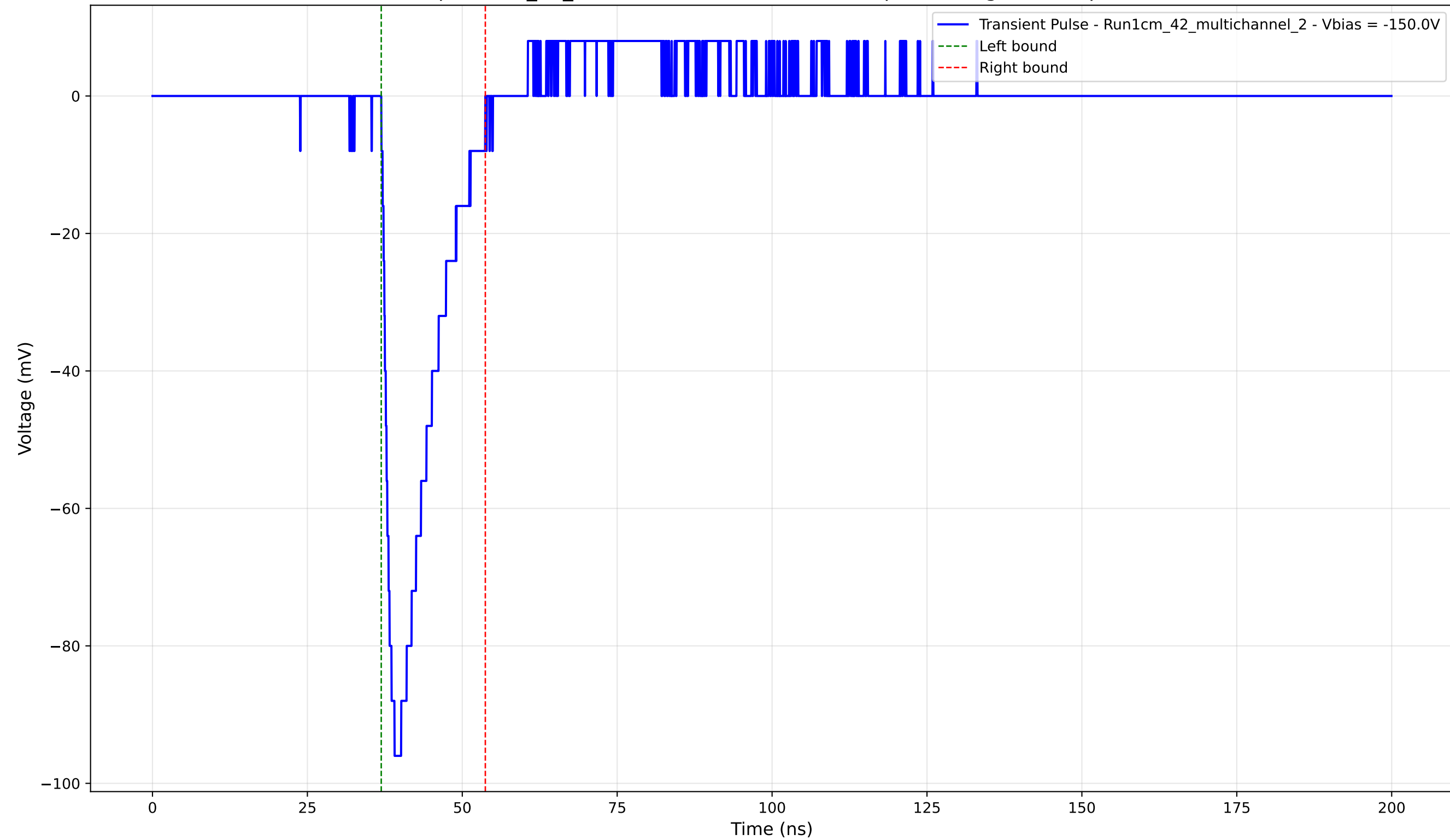
Transient Pulse - Sample: 1cm_42_multichannel - Position: 500.0 \mu\text{m} - Charge: 14.73 pC - Rise Time: 1.47 ns
