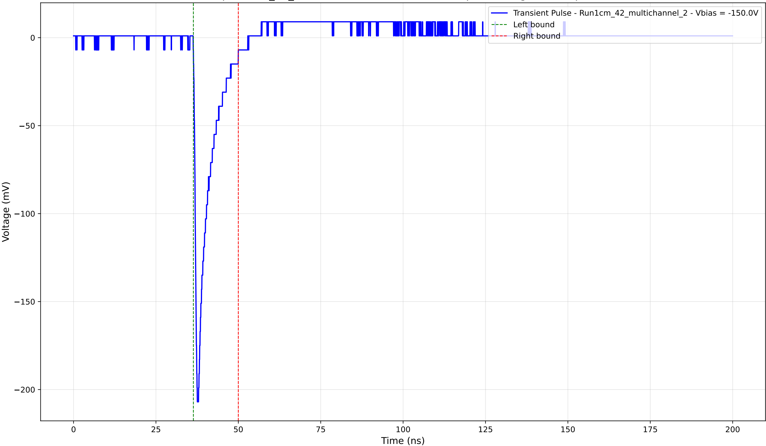
Transient Pulse - Sample: 1cm_42_multichannel - Position: 3120.0 \mu\text{m} - Charge: 18.75 pC - Rise Time: 0.93 ns
