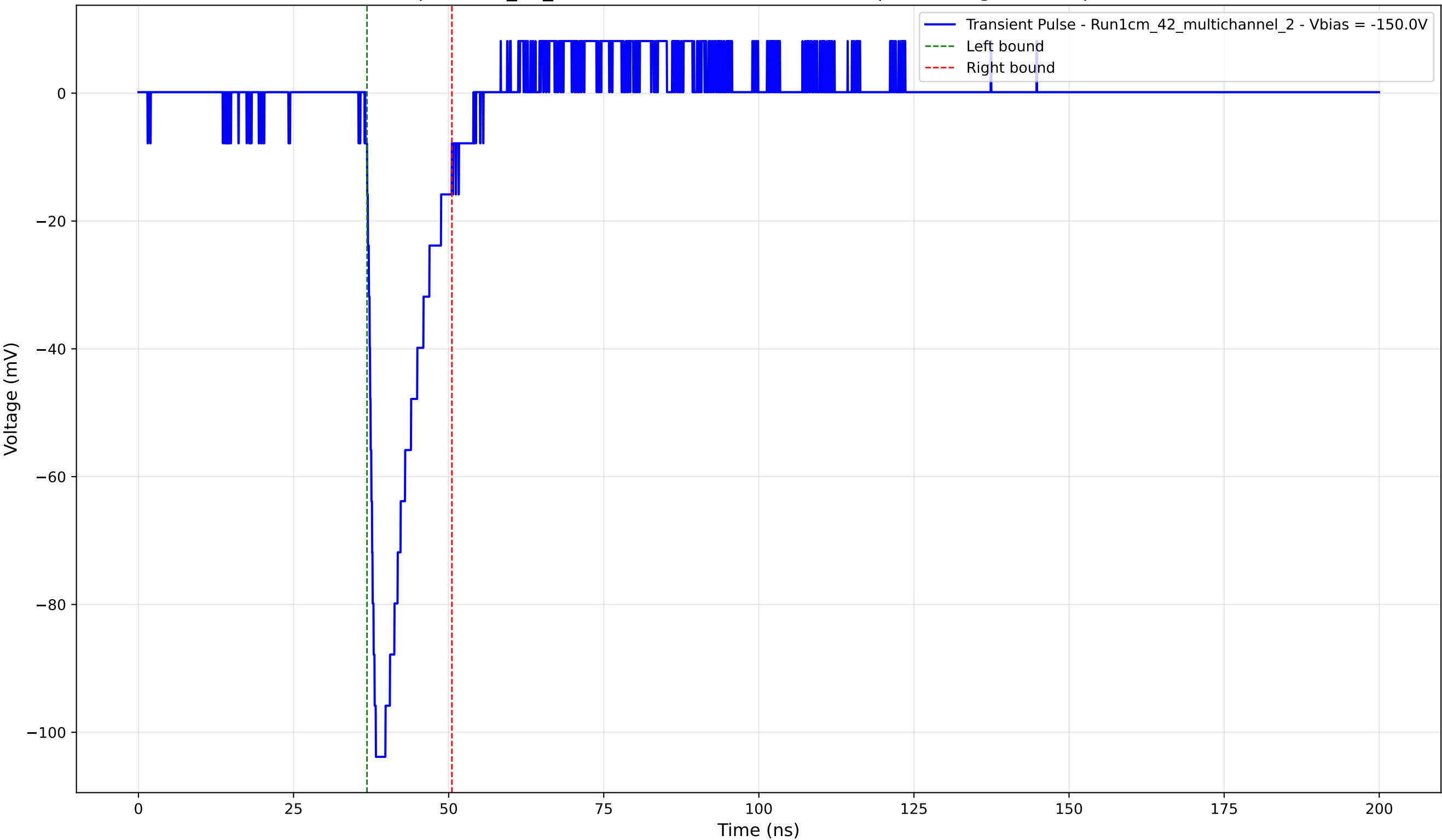
Transient Pulse - Sample: 1cm_42_multichannel - Position: 3765.0 \mu\text{m} - Charge: 14.86 pC - Rise Time: 1.23 ns
