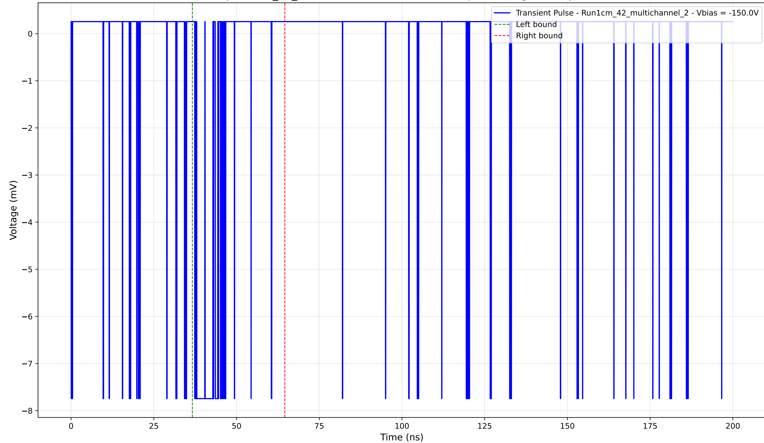
Transient Pulse - Sample: 1cm_42_multichannel - Position: 4390.0 \mu\text{m} - Charge: 0.98 pC - Rise Time: 0.04 ns
