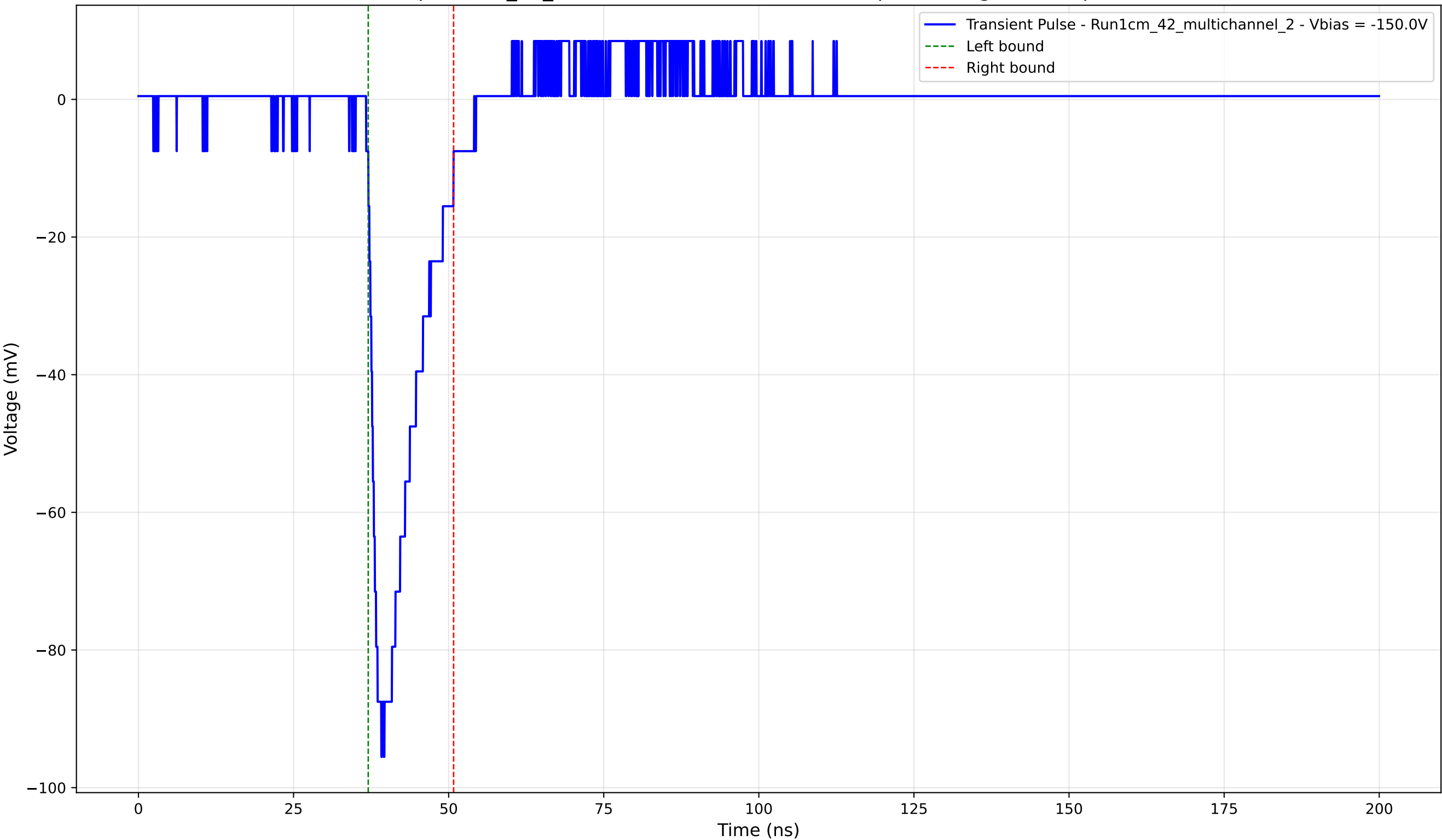
Transient Pulse - Sample: 1cm_42_multichannel - Position: 4020.0 \mu\text{m} - Charge: 13.49 pC - Rise Time: 1.51 ns
