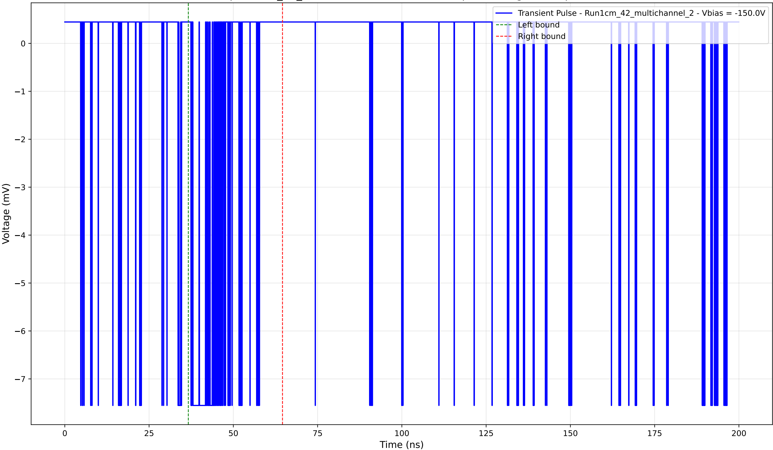
Transient Pulse - Sample: 1cm_42_multichannel - Position: 35.0 \mu\text{m} - Charge: 1.13 pC - Rise Time: 0.04 ns
