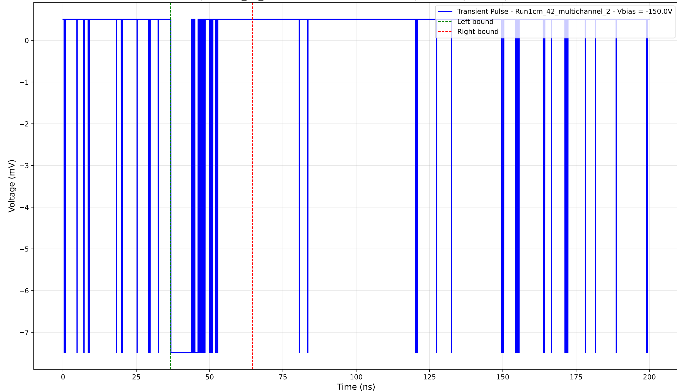
Transient Pulse - Sample: 1cm_42_multichannel - Position: 1365.0 \mu\text{m} - Charge: 1.41 pC - Rise Time: 0.04 ns
