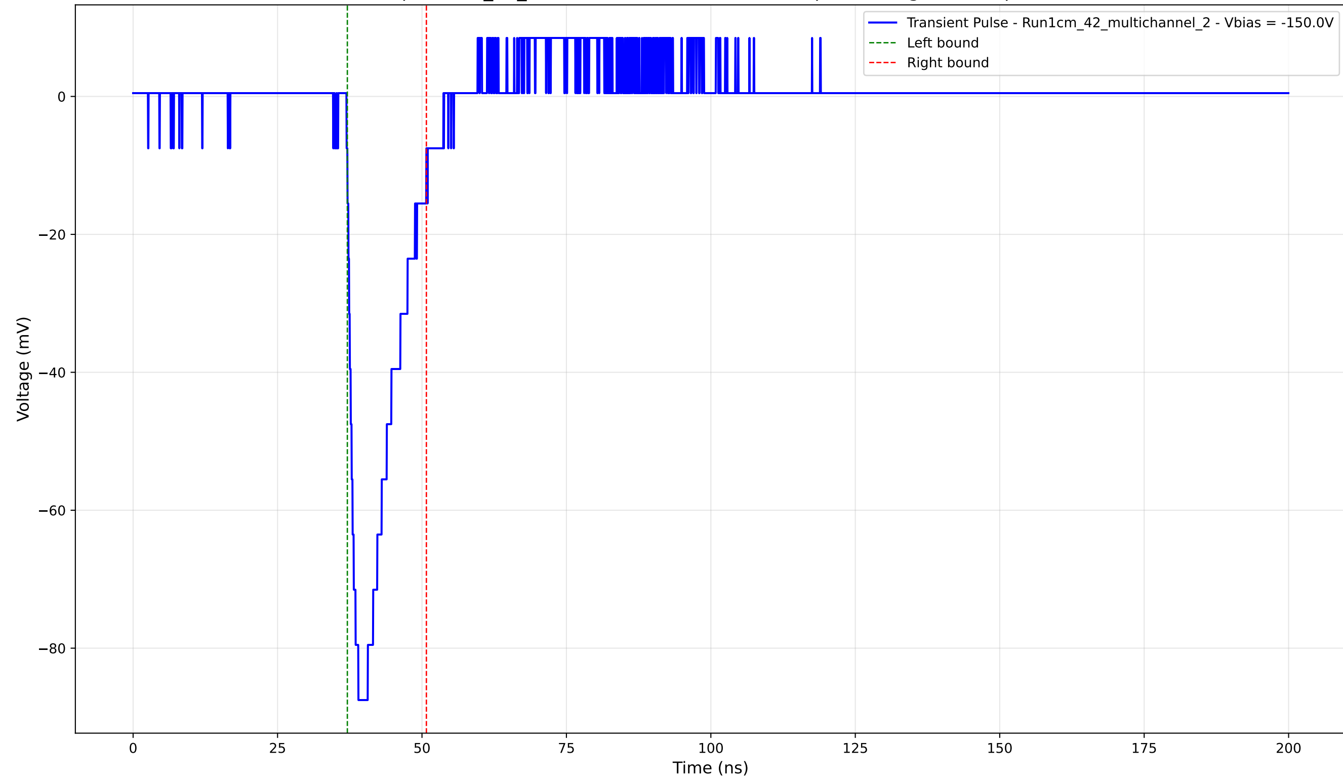
Transient Pulse - Sample: 1cm_42_multichannel - Position: 440.0 \mu\text{m} - Charge: 13.43 pC - Rise Time: 1.43 ns
