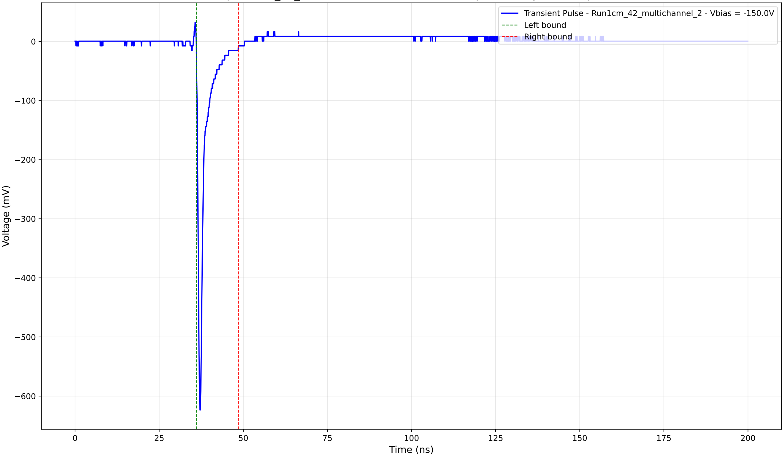
Transient Pulse - Sample: 1cm_42_multichannel - Position: 2465.0 \mu\text{m} - Charge: 28.08 pC - Rise Time: 0.73 ns
