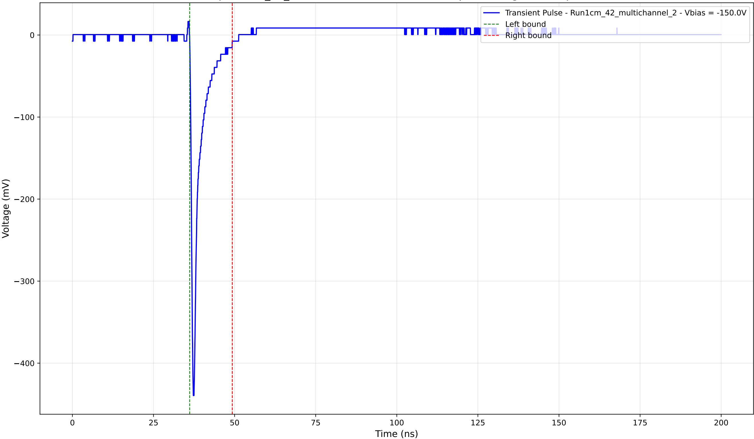
Transient Pulse - Sample: 1cm_42_multichannel - Position: 2020.0 \mu\text{m} - Charge: 25.97 pC - Rise Time: 0.76 ns
