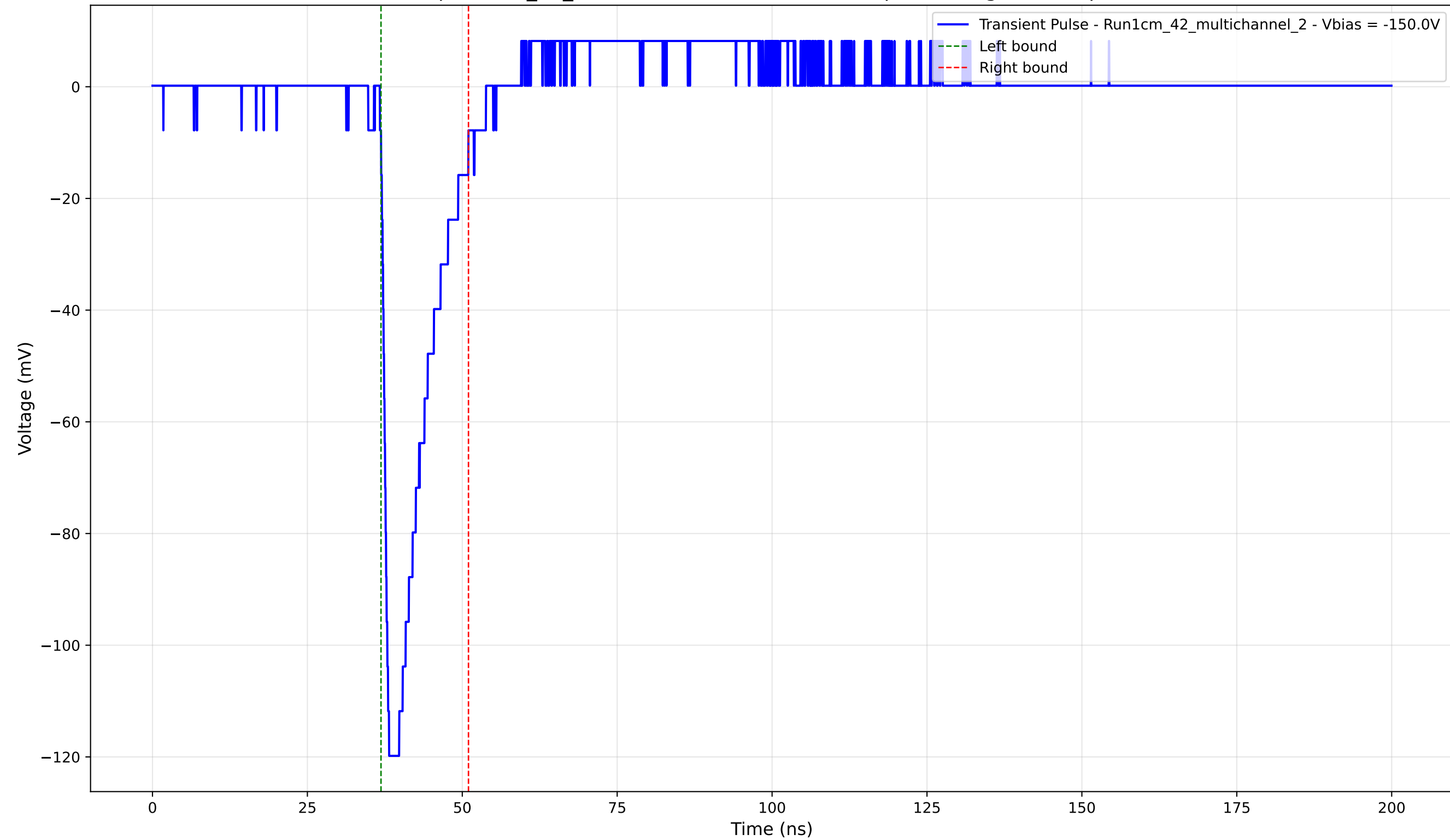
Transient Pulse - Sample: 1cm_42_multichannel - Position: 960.0 \mu\text{m} - Charge: 17.10 pC - Rise Time: 1.14 ns
