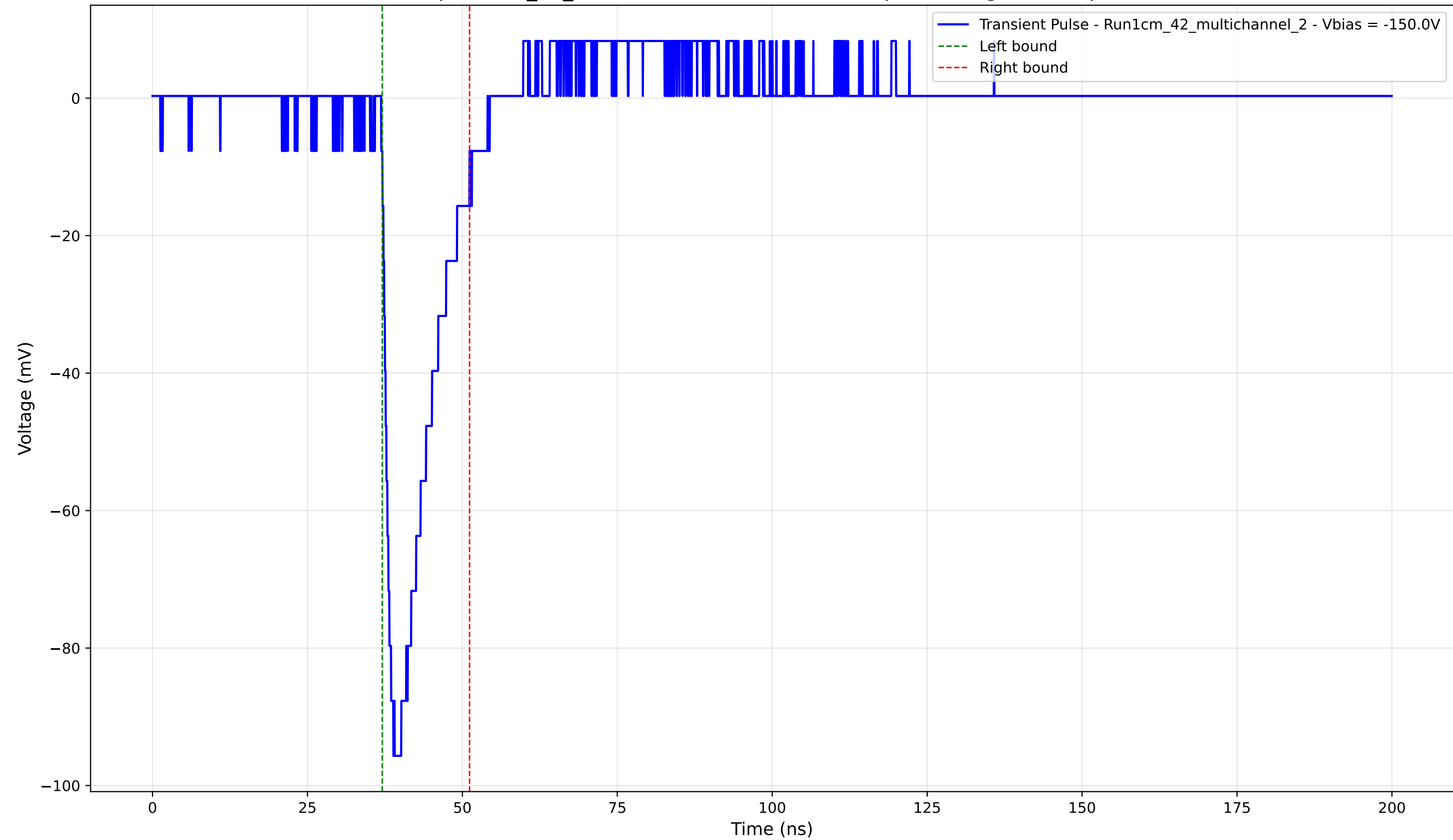
Transient Pulse - Sample: 1cm_42_multichannel - Position: 540.0 \mu\text{m} - Charge: 14.25 pC - Rise Time: 1.43 ns
