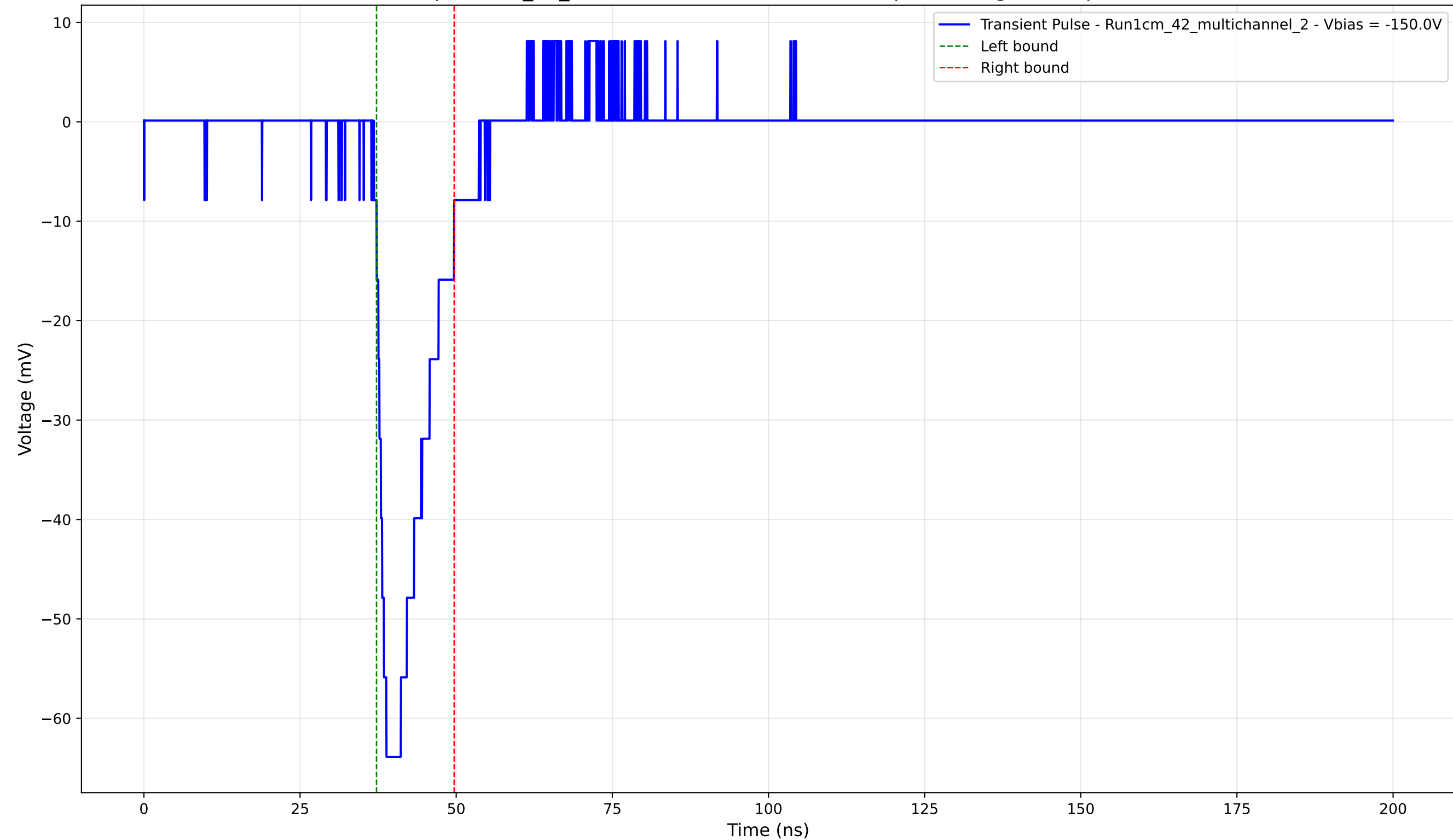
Transient Pulse - Sample: 1cm_42_multichannel - Position: 4470.0 \mu\text{m} - Charge: 9.60 pC - Rise Time: 2.01 ns
