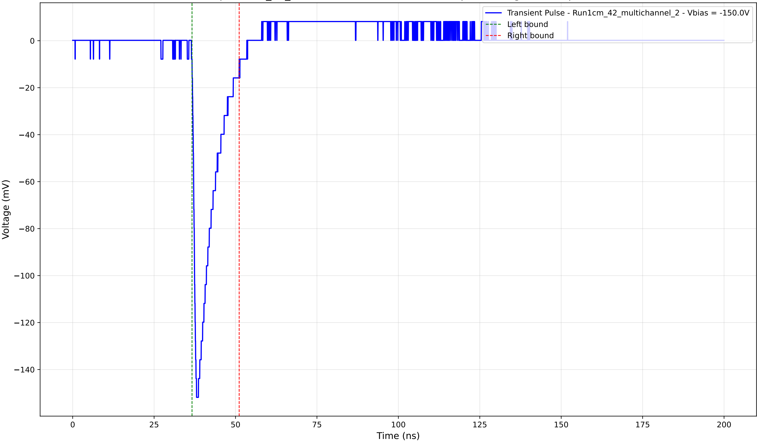
Transient Pulse - Sample: 1cm_42_multichannel - Position: 1210.0 \mu\text{m} - Charge: 19.06 pC - Rise Time: 1.20 ns
