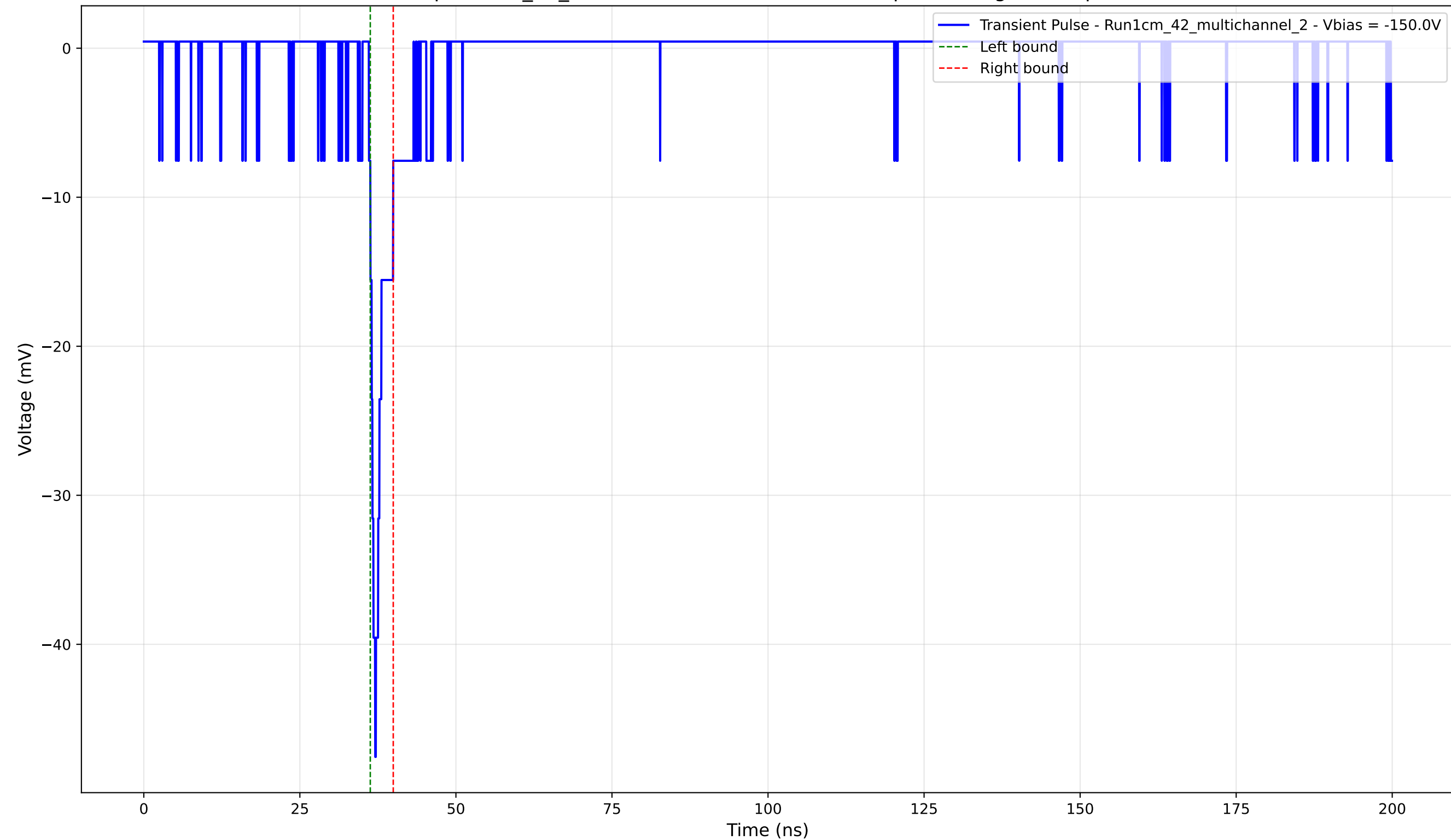
Transient Pulse - Sample: 1cm_42_multichannel - Position: 2350.0 \mu\text{m} - Charge: 1.71 pC - Rise Time: 1.02 ns
