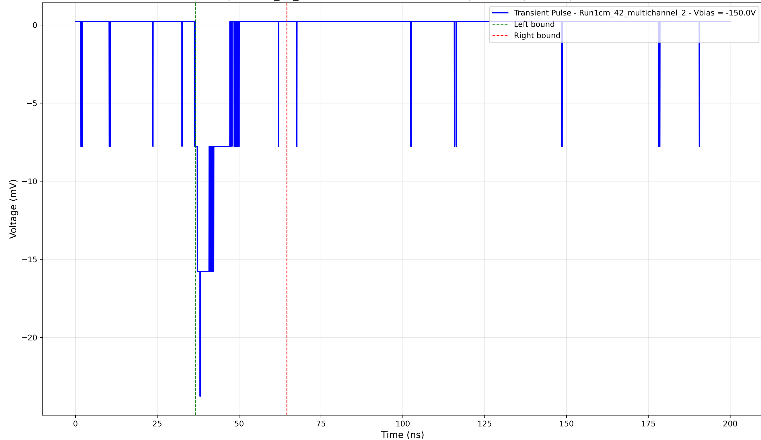
Transient Pulse - Sample: 1cm_42_multichannel - Position: 1380.0 \mu\text{m} - Charge: 2.41 pC - Rise Time: 1.47 ns
