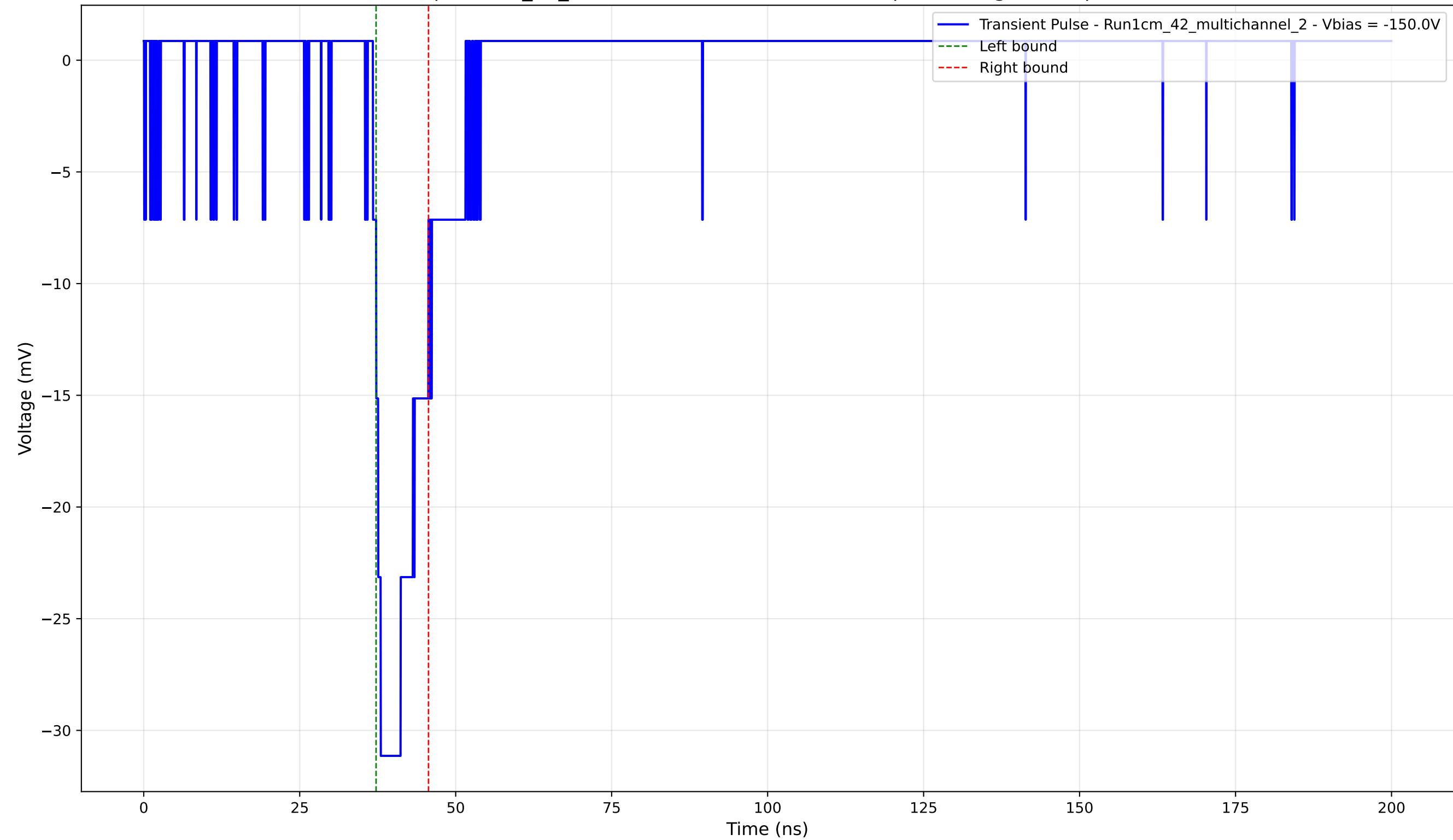
Transient Pulse - Sample: 1cm_42_multichannel - Position: 3845.0 \mu\text{m} - Charge: 3.95 pC - Rise Time: 1.27 ns
