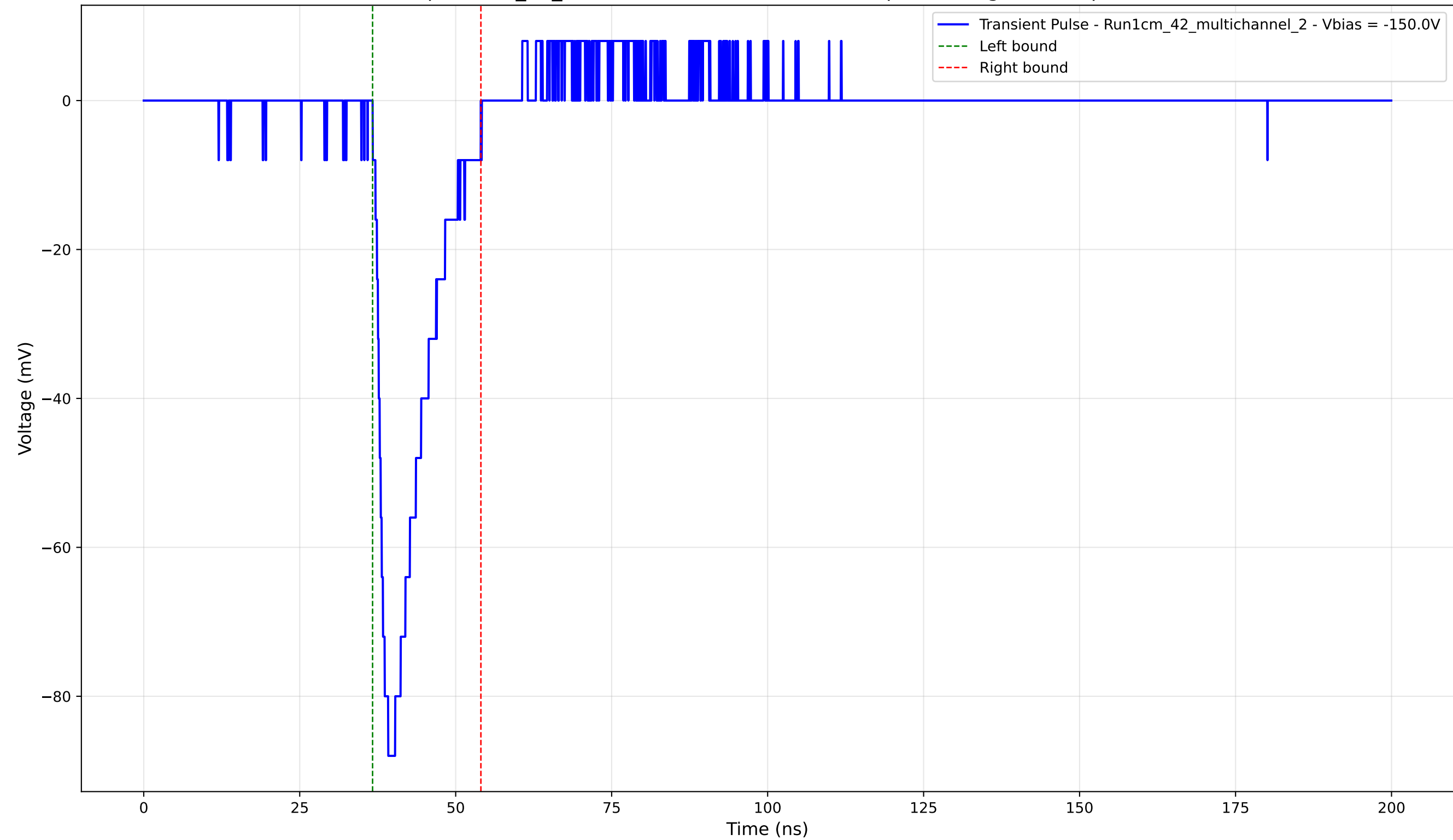
Transient Pulse - Sample: 1cm_42_multichannel - Position: 4175.0 \mu\text{m} - Charge: 13.31 pC - Rise Time: 1.52 ns
