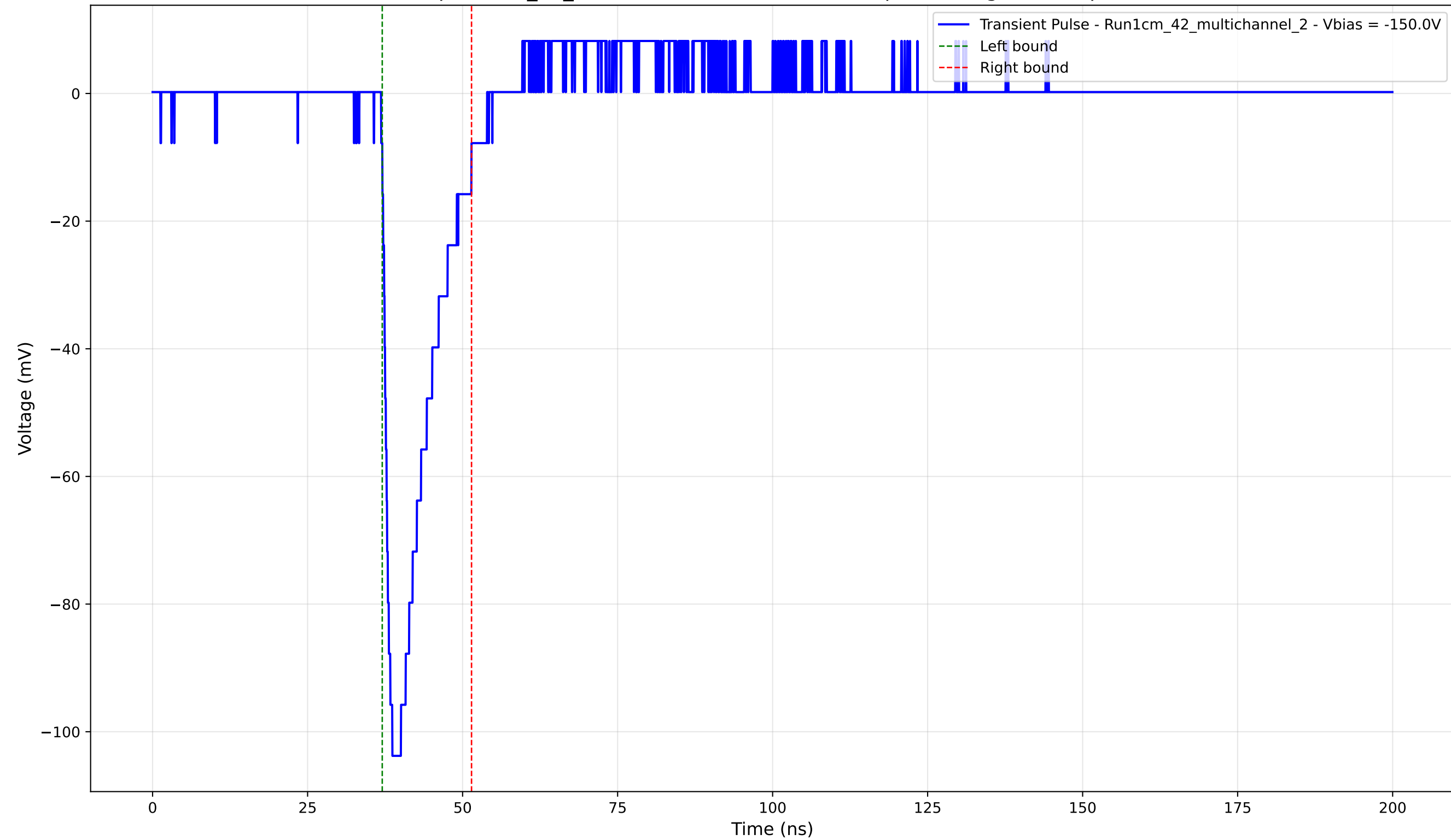
Transient Pulse - Sample: 1cm_42_multichannel - Position: 740.0 \mu\text{m} - Charge: 15.19 pC - Rise Time: 1.31 ns
