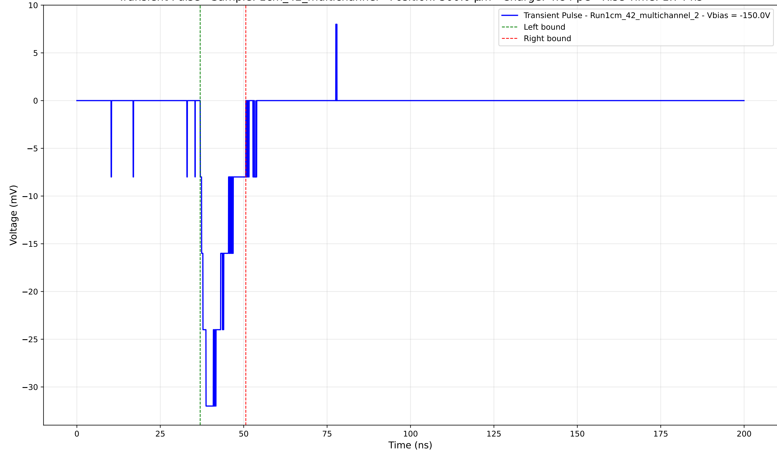
Transient Pulse - Sample: 1cm_42_multichannel - Position: 300.0 \mu\text{m} - Charge: 4.84 pC - Rise Time: 1.74 ns
