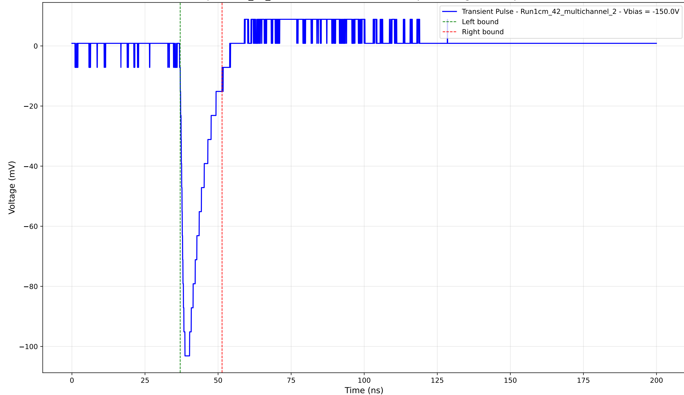
Transient Pulse - Sample: 1cm_42_multichannel - Position: 685.0 \mu\text{m} - Charge: 15.24 pC - Rise Time: 1.26 ns
