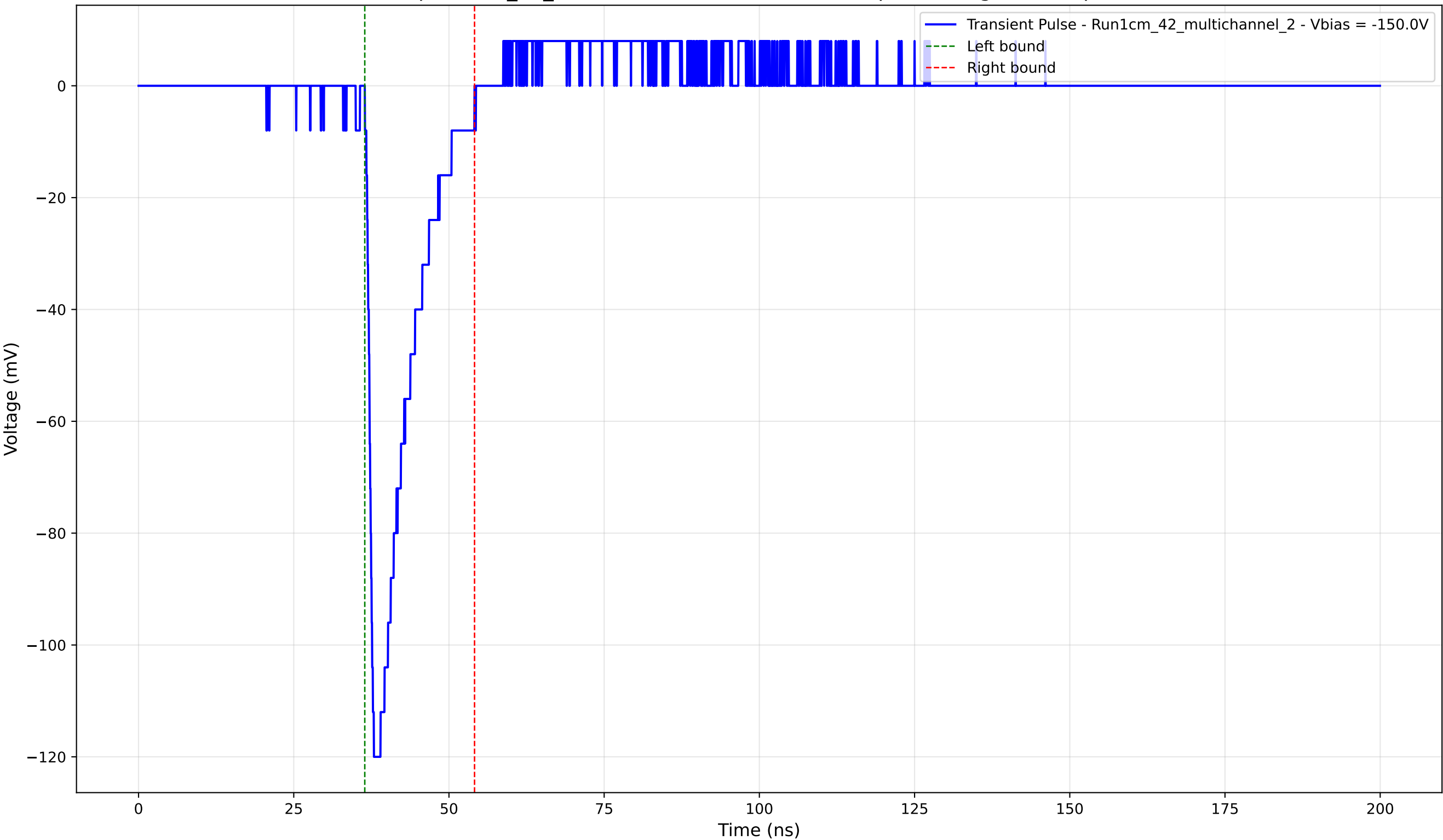
Transient Pulse - Sample: 1cm_42_multichannel - Position: 3545.0 \mu\text{m} - Charge: 16.42 pC - Rise Time: 1.06 ns
