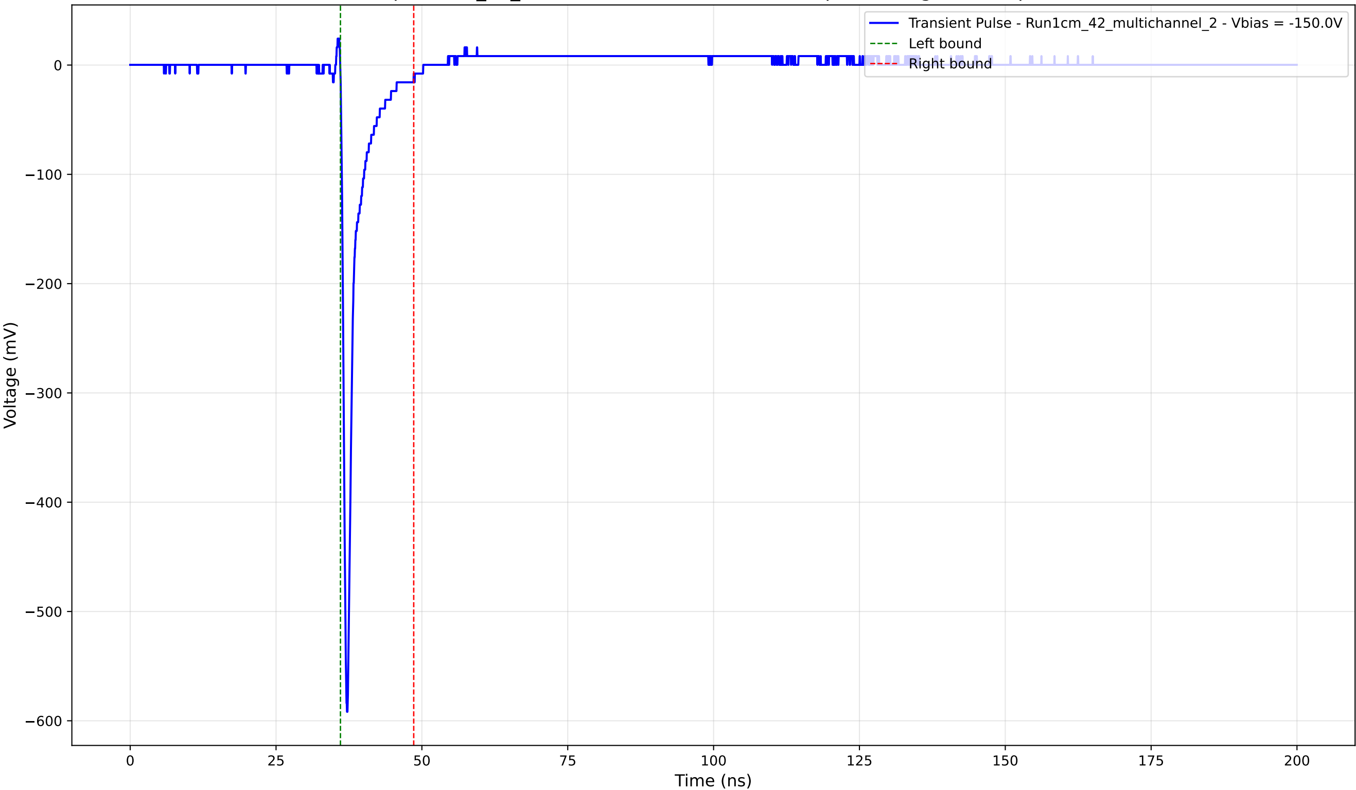
Transient Pulse - Sample: 1cm_42_multichannel - Position: 2500.0 \mu\text{m} - Charge: 27.55 pC - Rise Time: 0.74 ns
