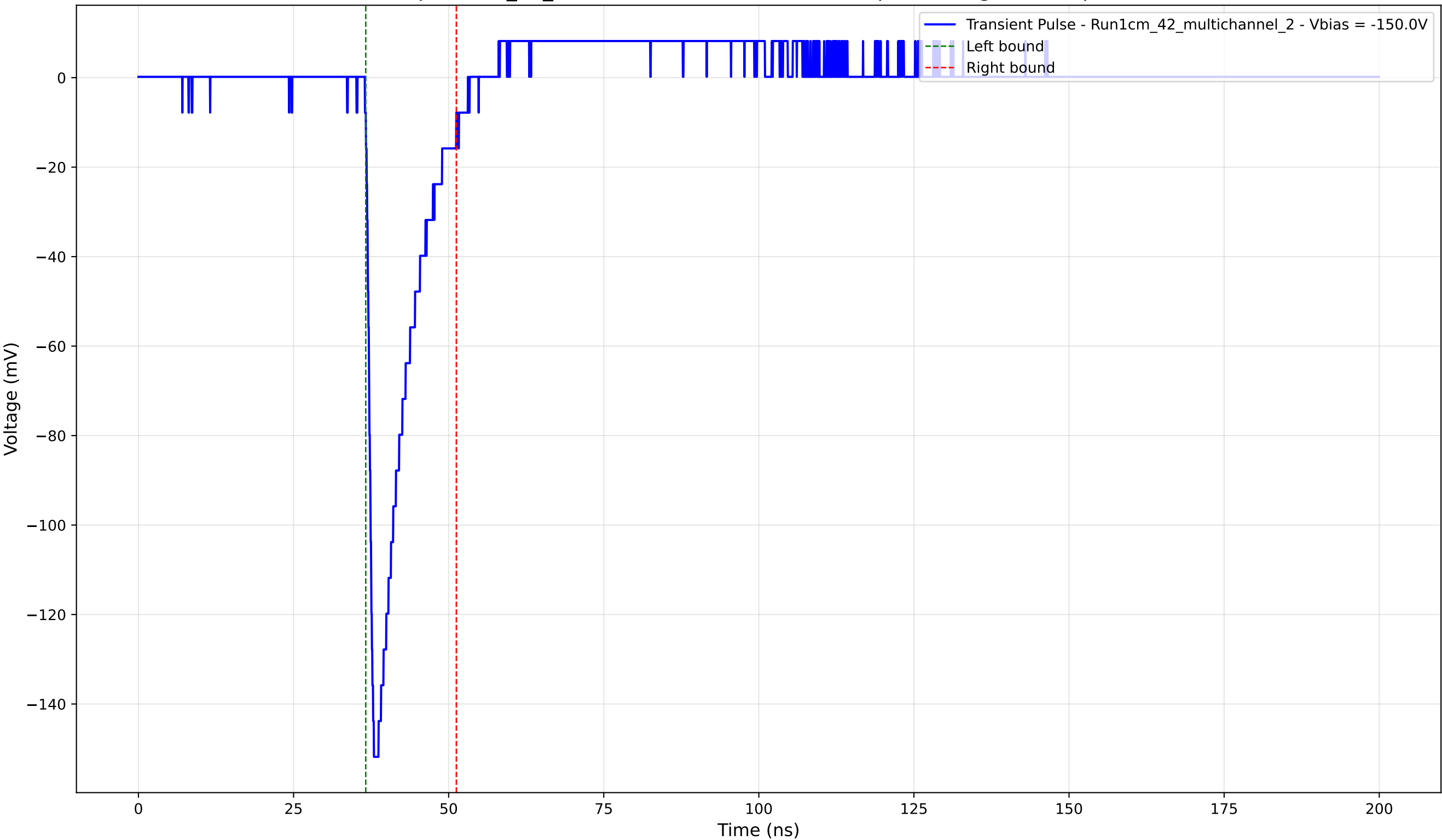
Transient Pulse - Sample: 1cm_42_multichannel - Position: 1225.0 \mu\text{m} - Charge: 19.10 pC - Rise Time: 1.16 ns
