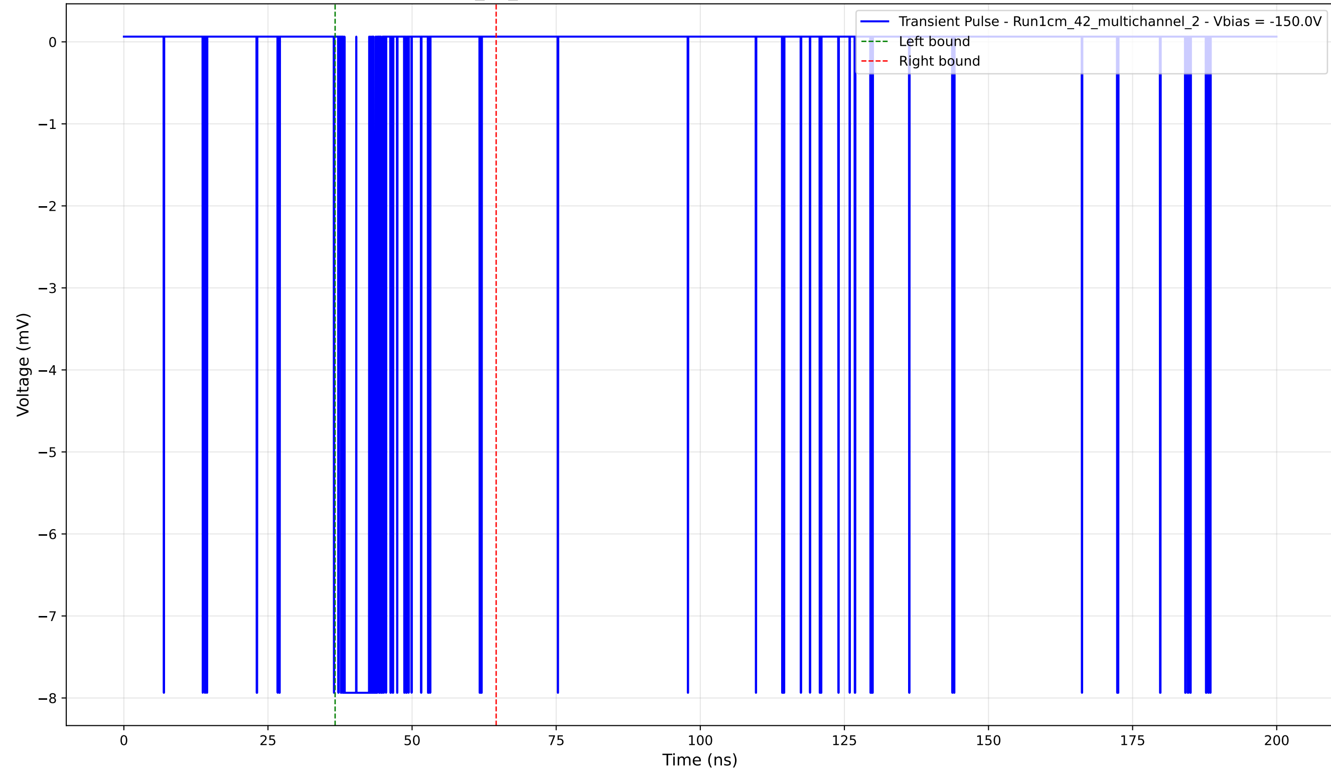
Transient Pulse - Sample: 1cm_42_multichannel - Position: 4385.0 \mu\text{m} - Charge: 1.15 pC - Rise Time: 0.04 ns
