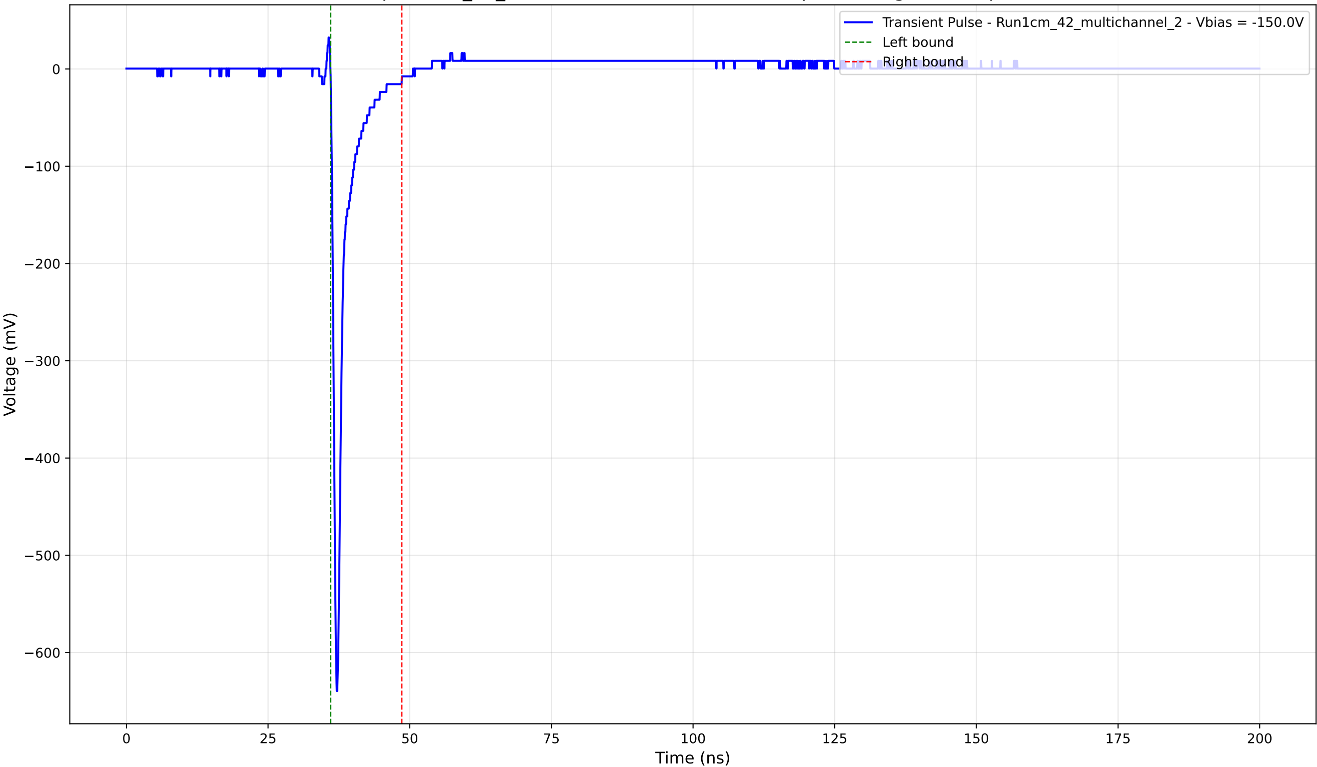
Transient Pulse - Sample: 1cm_42_multichannel - Position: 2265.0 \mu\text{m} - Charge: 29.10 pC - Rise Time: 0.74 ns
