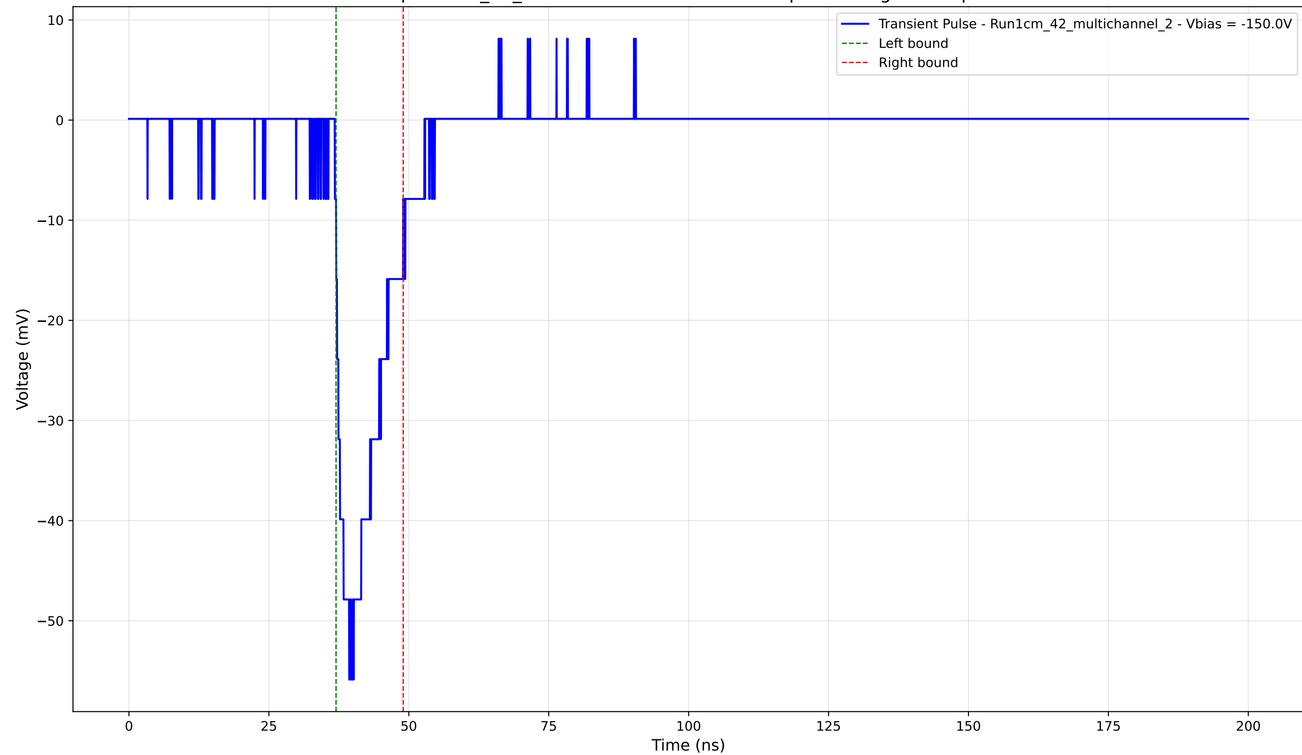
Transient Pulse - Sample: 1cm_42_multichannel - Position: 85.0 \mu\text{m} - Charge: 7.88 pC - Rise Time: 2.57 ns
