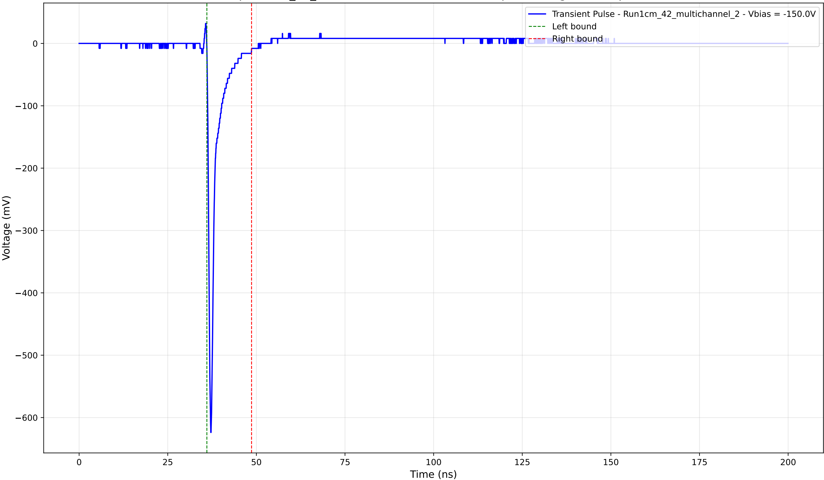
Transient Pulse - Sample: 1cm_42_multichannel - Position: 2240.0 \mu\text{m} - Charge: 29.00 pC - Rise Time: 0.73 ns
