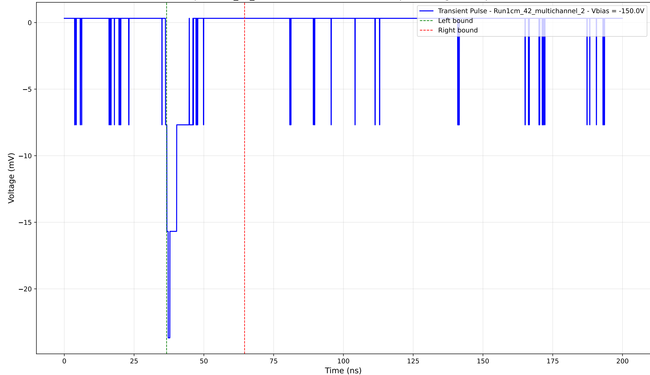
Transient Pulse - Sample: 1cm_42_multichannel - Position: 1880.0 \mu\text{m} - Charge: 2.06 pC - Rise Time: 0.99 ns
