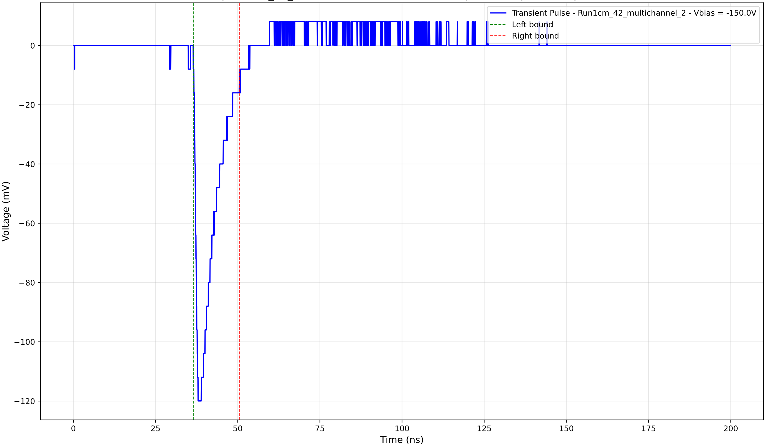
Transient Pulse - Sample: 1cm_42_multichannel - Position: 3550.0 \mu\text{m} - Charge: 15.67 pC - Rise Time: 1.14 ns
