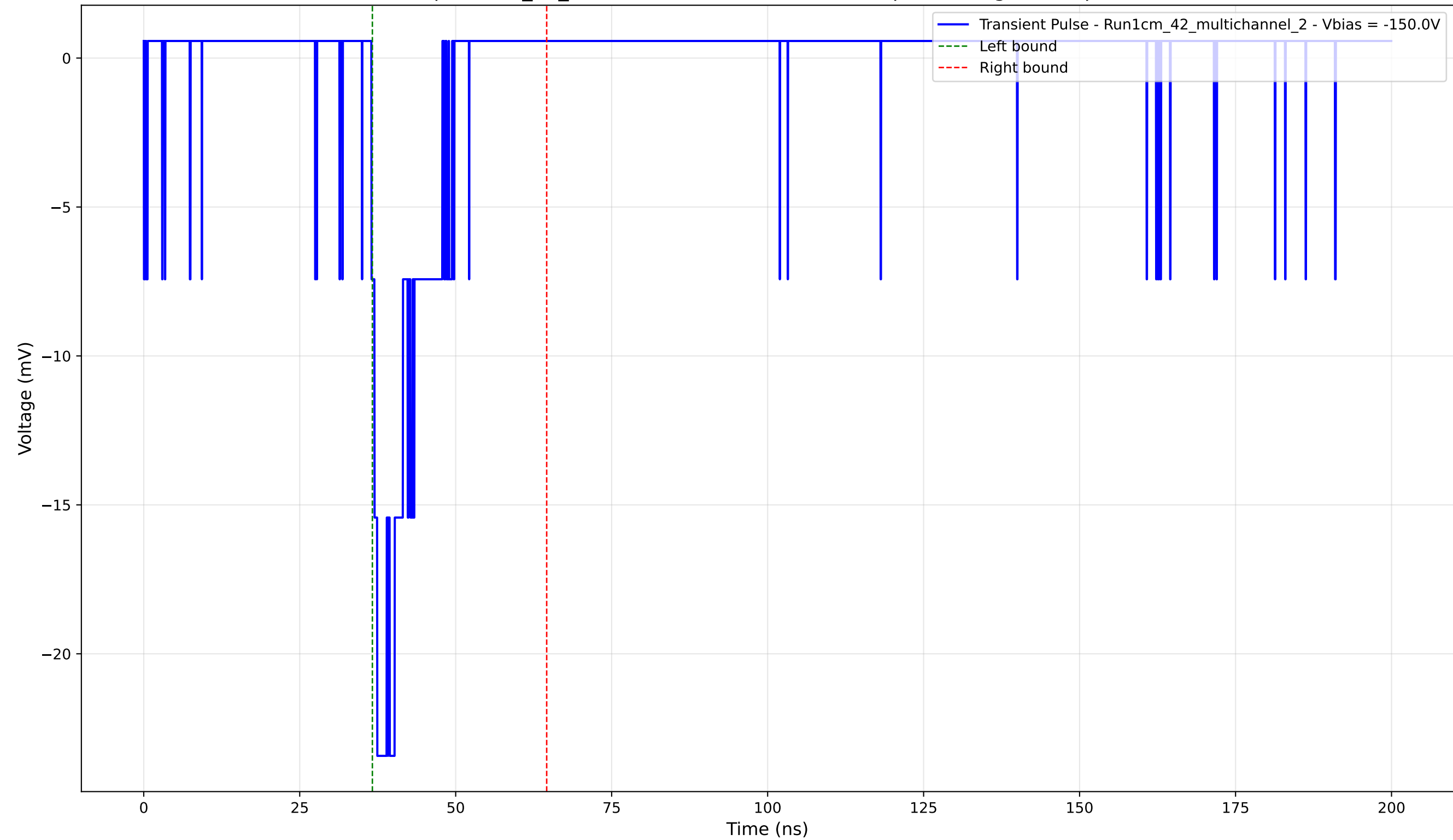
Transient Pulse - Sample: 1cm_42_multichannel - Position: 1385.0 \mu\text{m} - Charge: 2.86 pC - Rise Time: 0.95 ns
