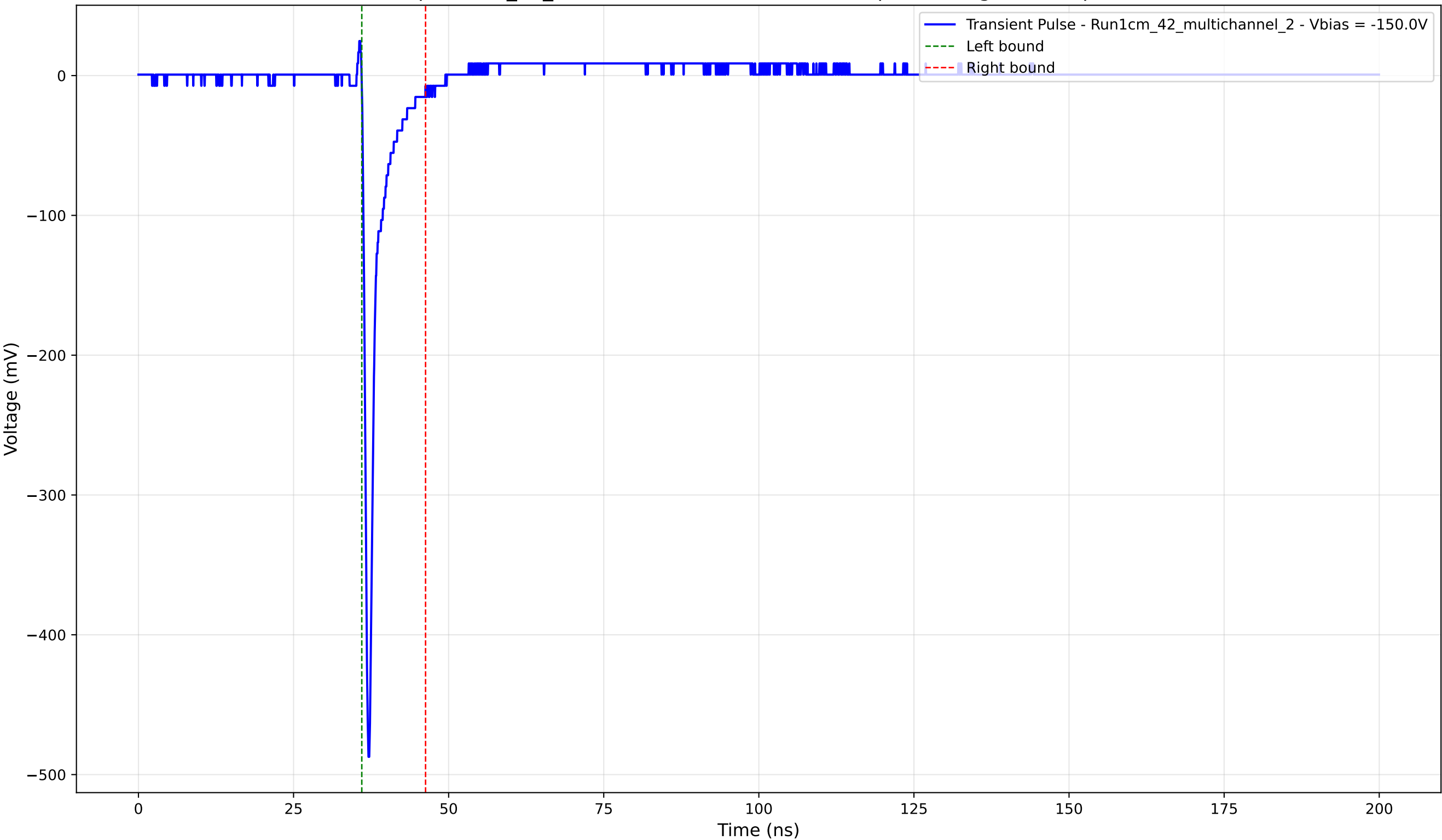
Transient Pulse - Sample: 1cm_42_multichannel - Position: 2430.0 \mu\text{m} - Charge: 21.01 pC - Rise Time: 0.71 ns
