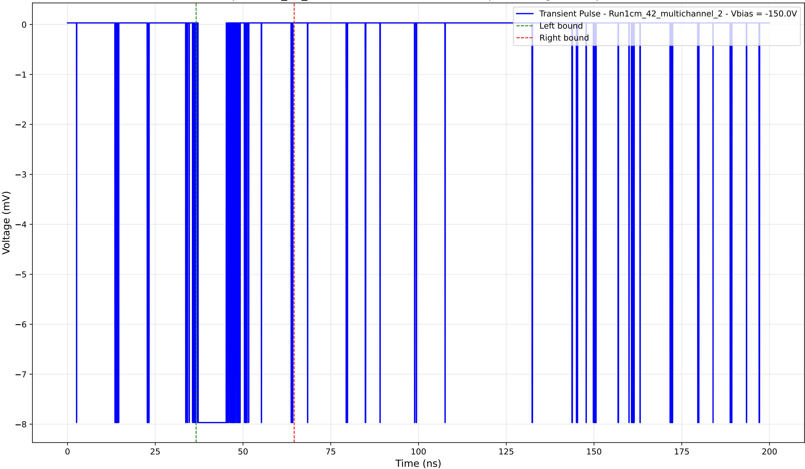
Transient Pulse - Sample: 1cm_42_multichannel - Position: 3900.0 \mu\text{m} - Charge: 1.68 pC - Rise Time: 0.04 ns
