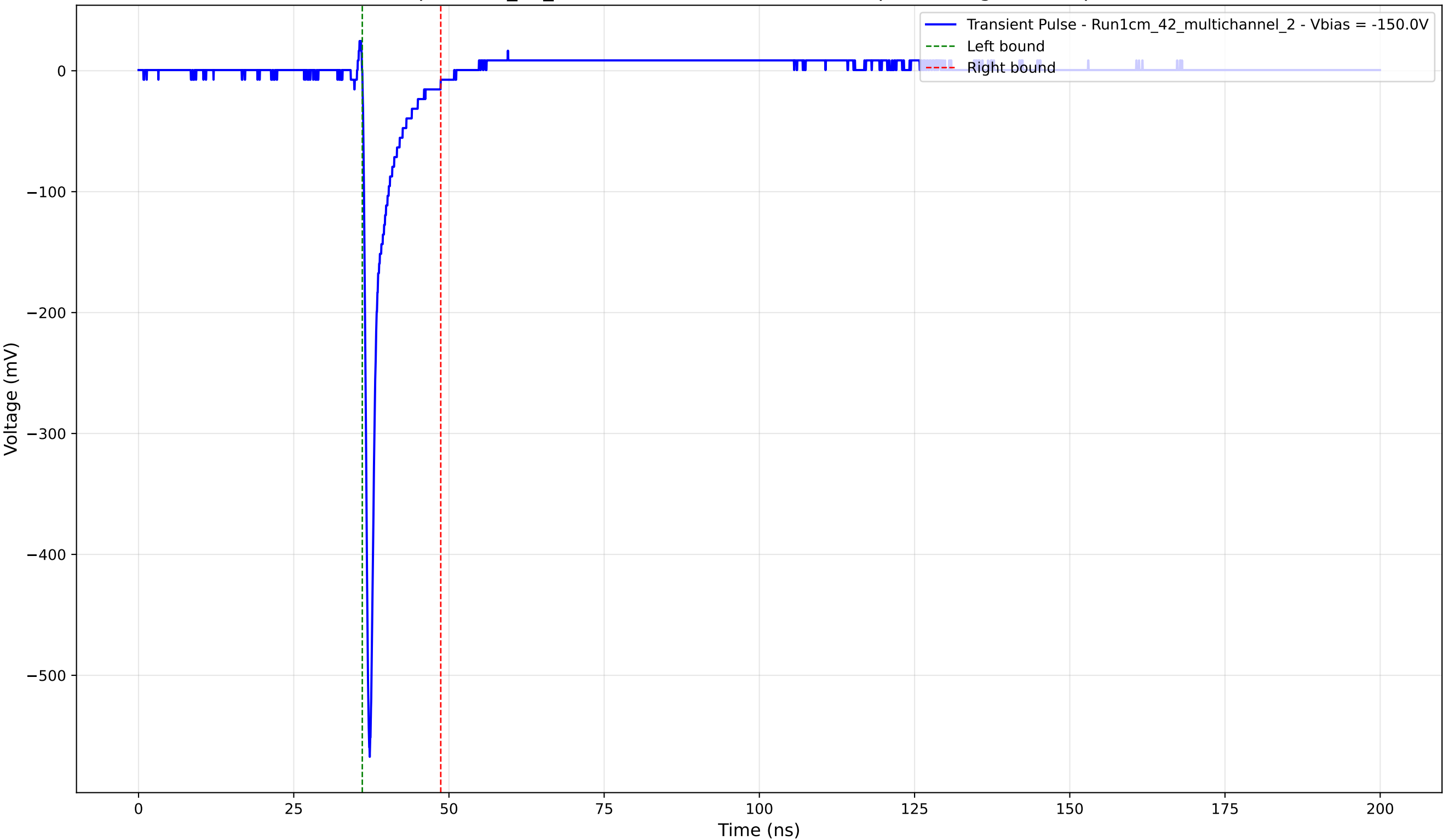
Transient Pulse - Sample: 1cm_42_multichannel - Position: 2185.0 \mu\text{m} - Charge: 27.69 pC - Rise Time: 0.75 ns
