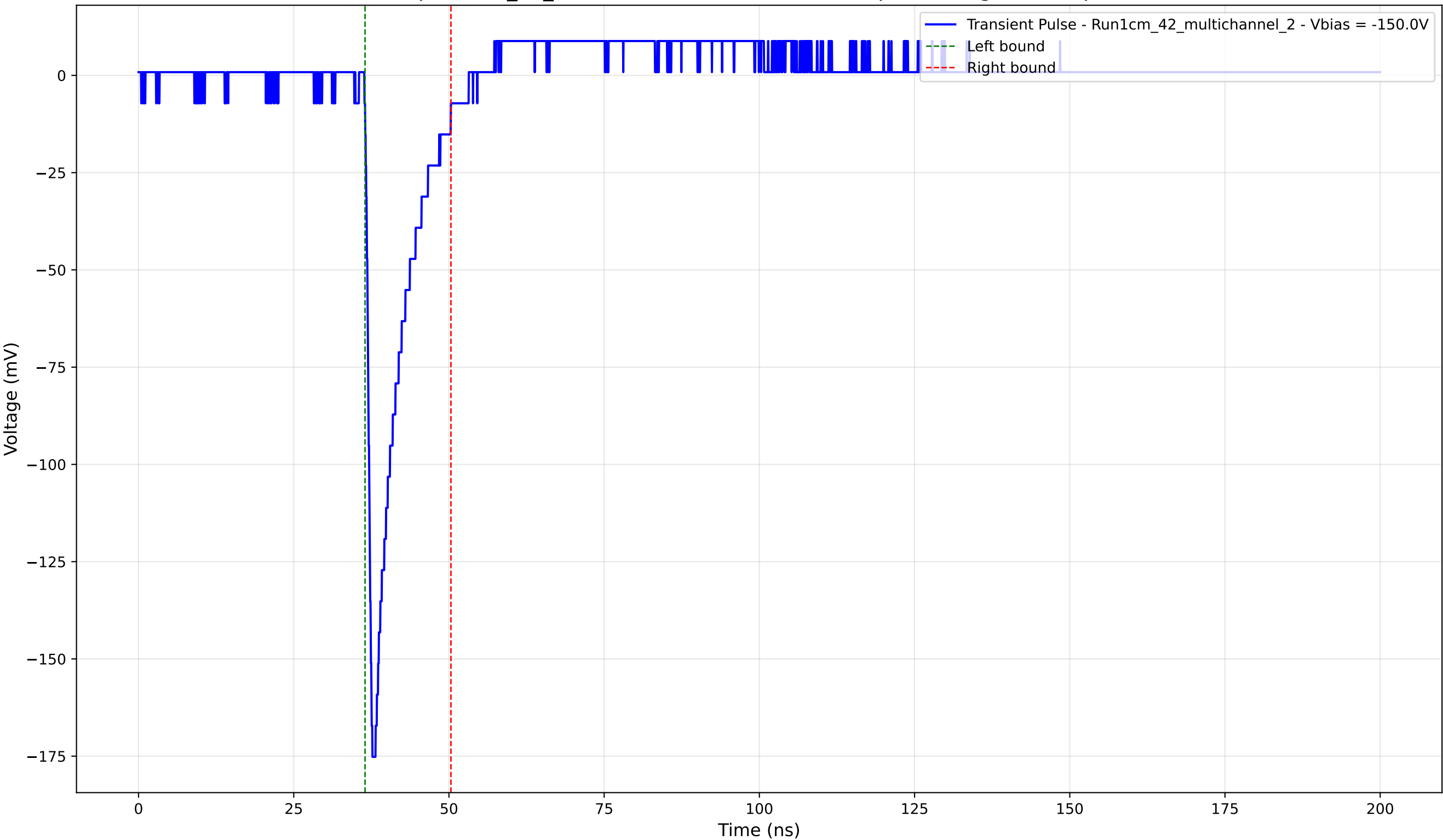
Transient Pulse - Sample: 1cm_42_multichannel - Position: 3270.0 \mu\text{m} - Charge: 18.37 pC - Rise Time: 0.94 ns
