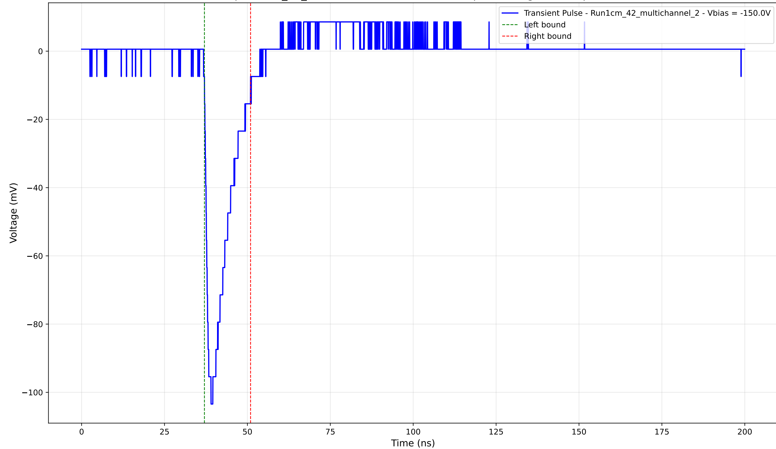
Transient Pulse - Sample: 1cm_42_multichannel - Position: 760.0 \mu\text{m} - Charge: 14.57 pC - Rise Time: 1.31 ns
