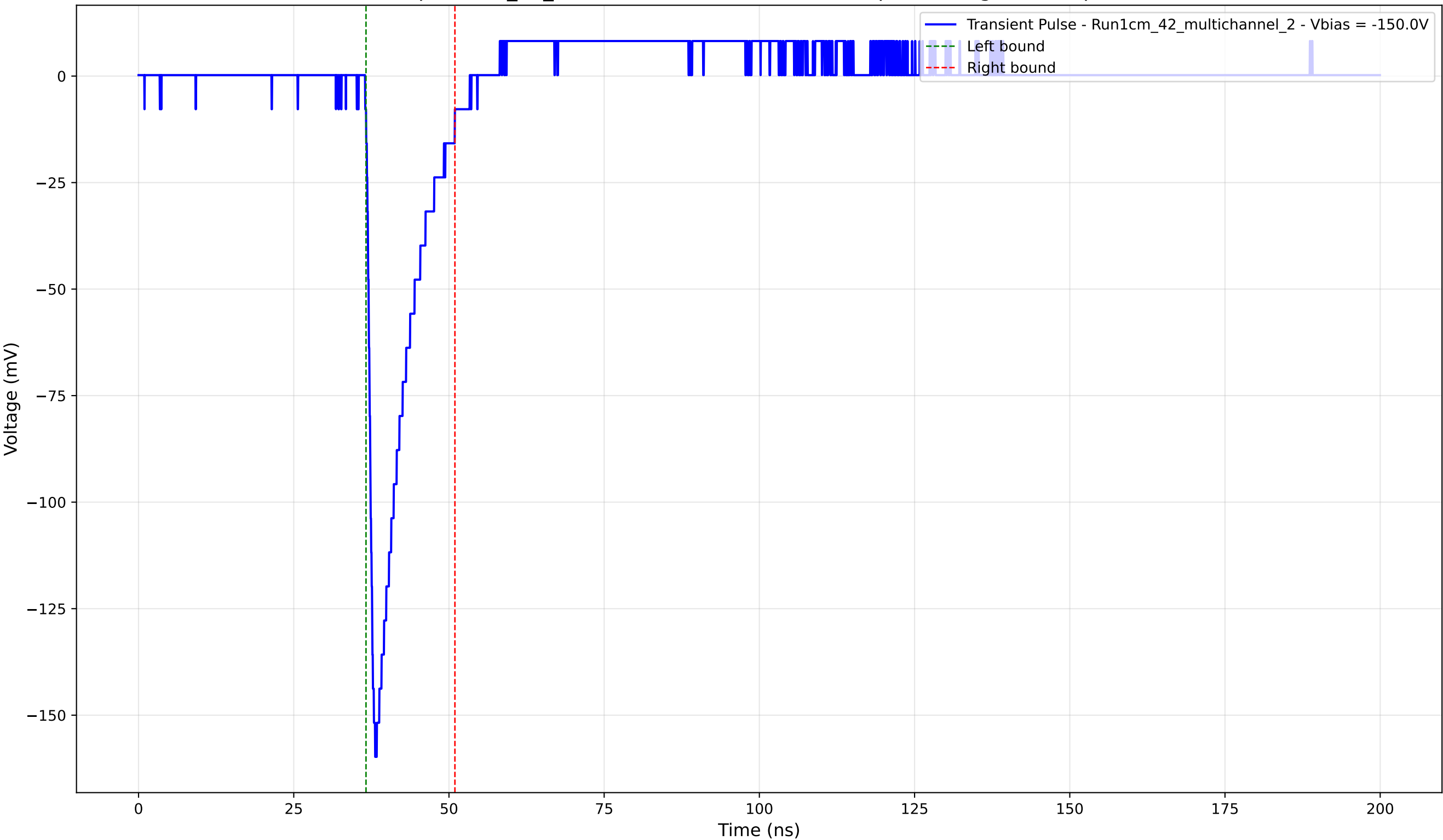
Transient Pulse - Sample: 1cm_42_multichannel - Position: 1230.0 \mu\text{m} - Charge: 19.18 pC - Rise Time: 1.16 ns
