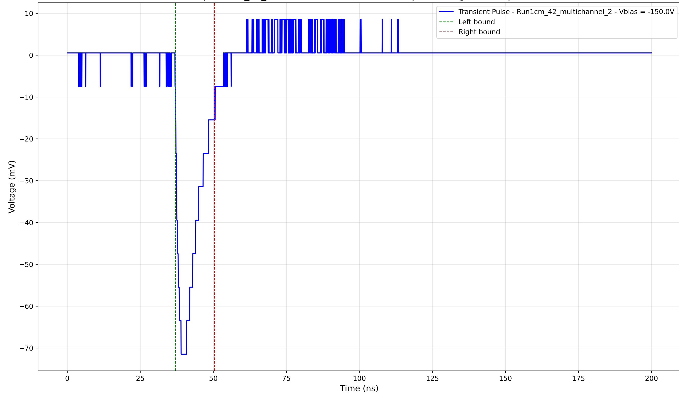
Transient Pulse - Sample: 1cm_42_multichannel - Position: 180.0 \mu\text{m} - Charge: 11.26 pC - Rise Time: 2.08 ns
