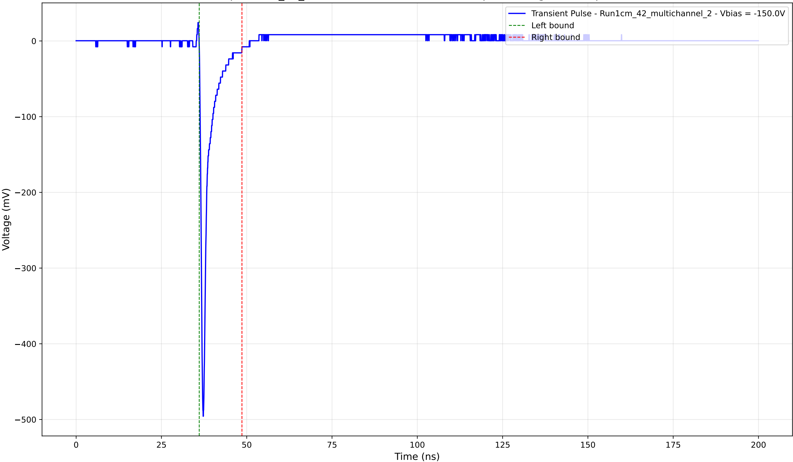
Transient Pulse - Sample: 1cm_42_multichannel - Position: 2585.0 \mu\text{m} - Charge: 25.06 pC - Rise Time: 0.77 ns
