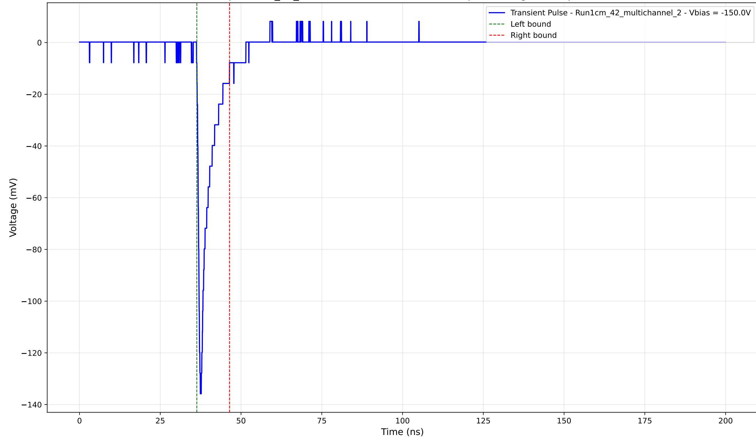
Transient Pulse - Sample: 1cm_42_multichannel - Position: 2925.0 \mu\text{m} - Charge: 9.98 pC - Rise Time: 0.93 ns
