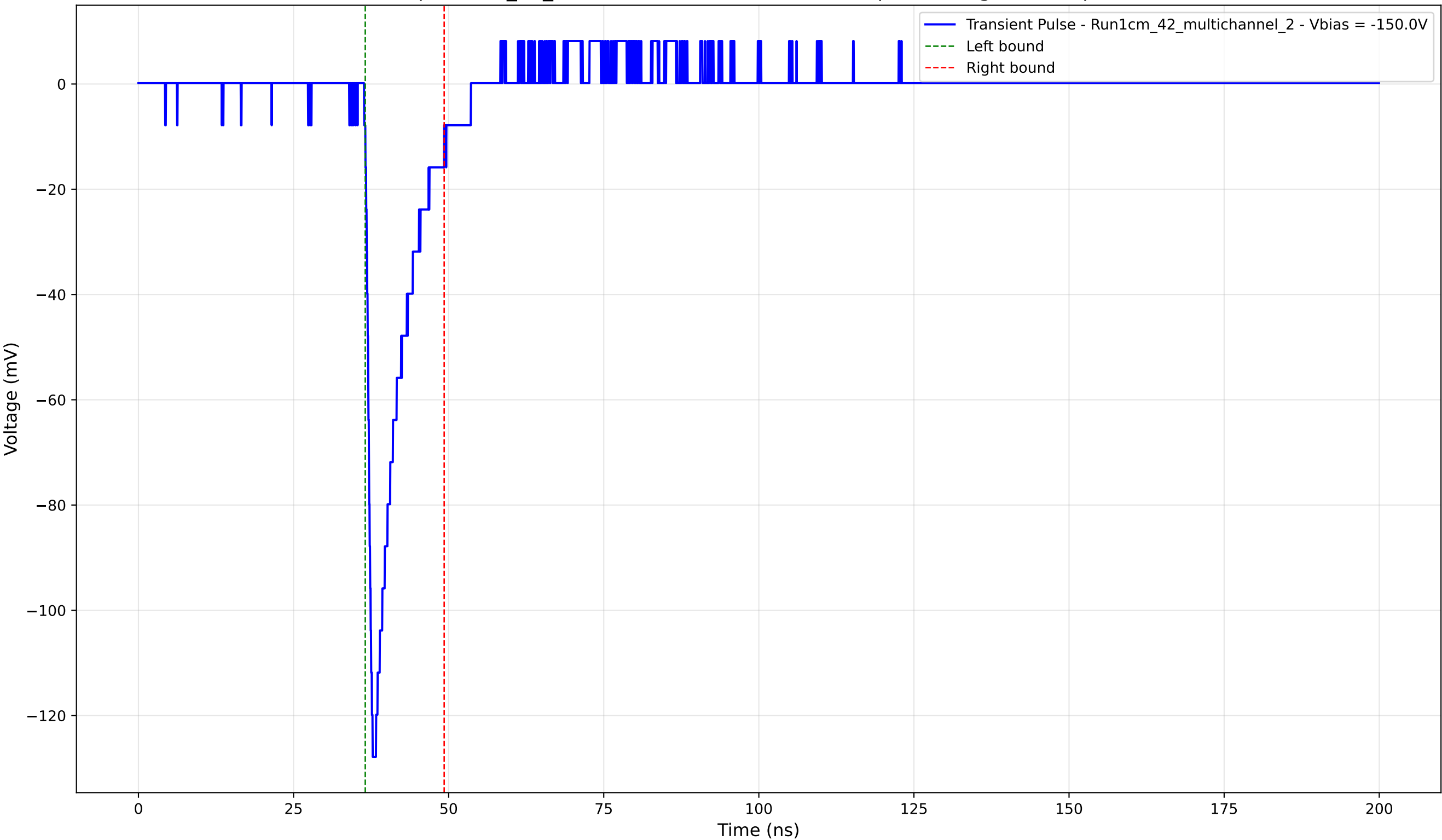
Transient Pulse - Sample: 1cm_42_multichannel - Position: 1415.0 \mu\text{m} - Charge: 13.57 pC - Rise Time: 1.06 ns
