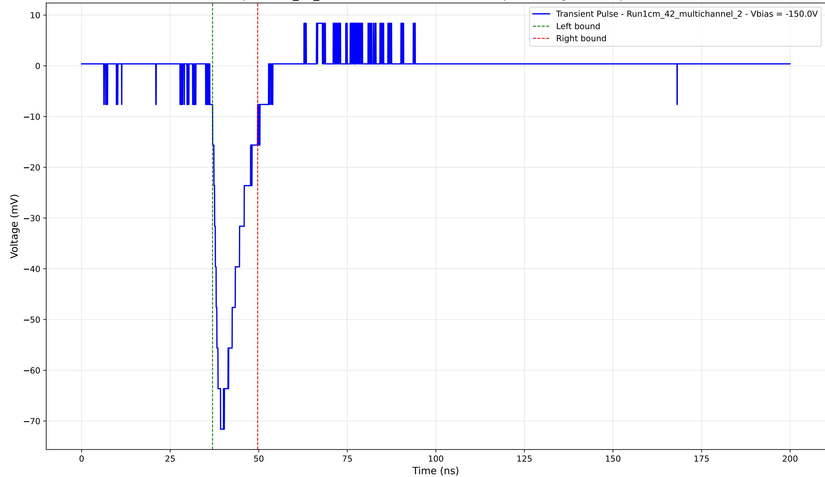
Transient Pulse - Sample: 1cm_42_multichannel - Position: 4715.0 \mu\text{m} - Charge: 10.28 pC - Rise Time: 3.04 ns
