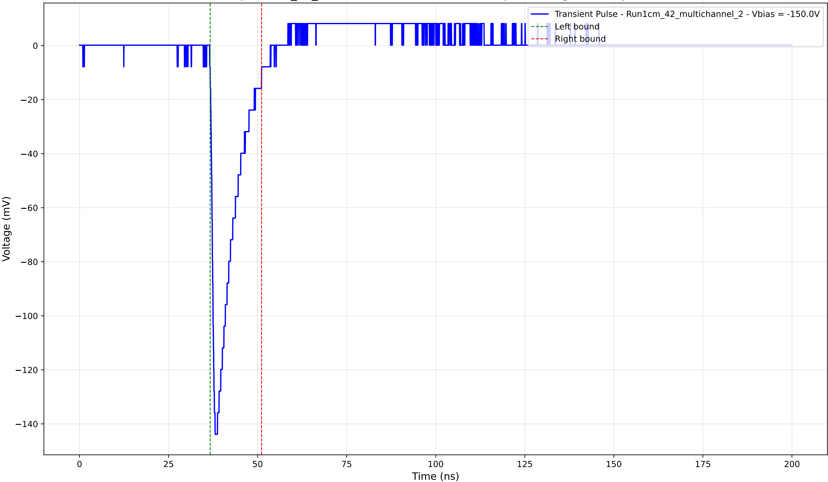
Transient Pulse - Sample: 1cm_42_multichannel - Position: 1180.0 \mu\text{m} - Charge: 18.46 pC - Rise Time: 1.17 ns
