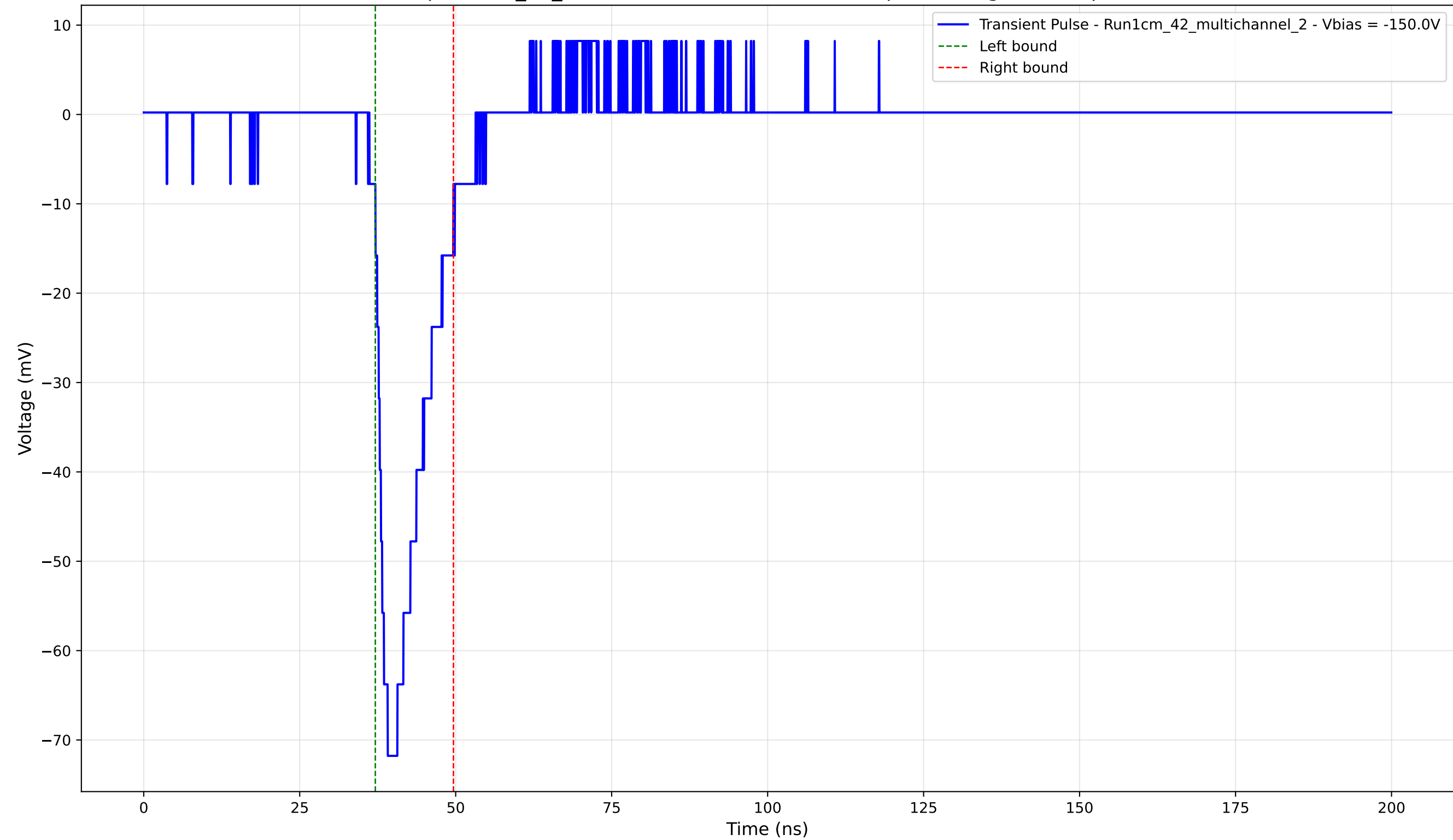
Transient Pulse - Sample: 1cm_42_multichannel - Position: 4570.0 \mu\text{m} - Charge: 10.48 pC - Rise Time: 2.92 ns
