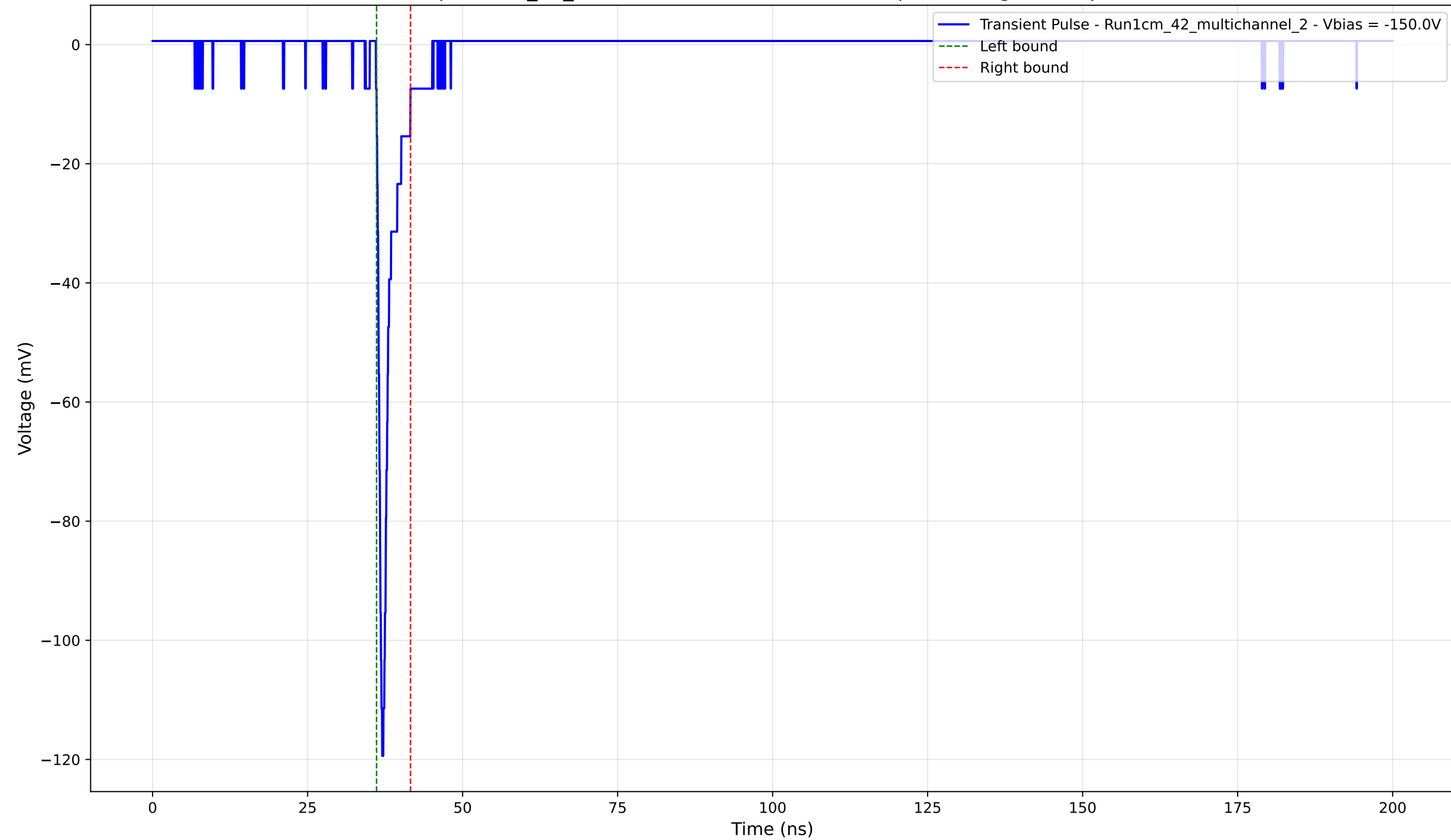
Transient Pulse - Sample: 1cm_42_multichannel - Position: 2335.0 \mu\text{m} - Charge: 4.73 pC - Rise Time: 0.78 ns
