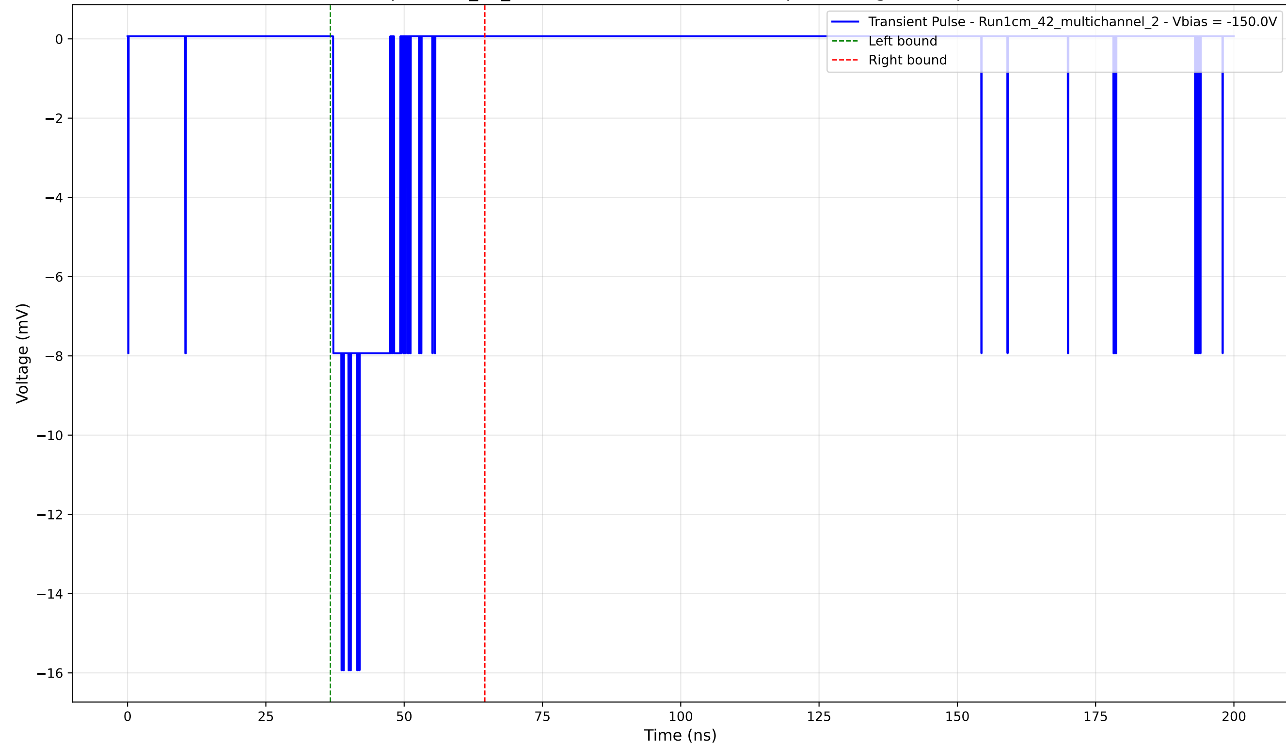
Transient Pulse - Sample: 1cm_42_multichannel - Position: 315.0 \mu\text{m} - Charge: 2.06 pC - Rise Time: 1.51 ns
