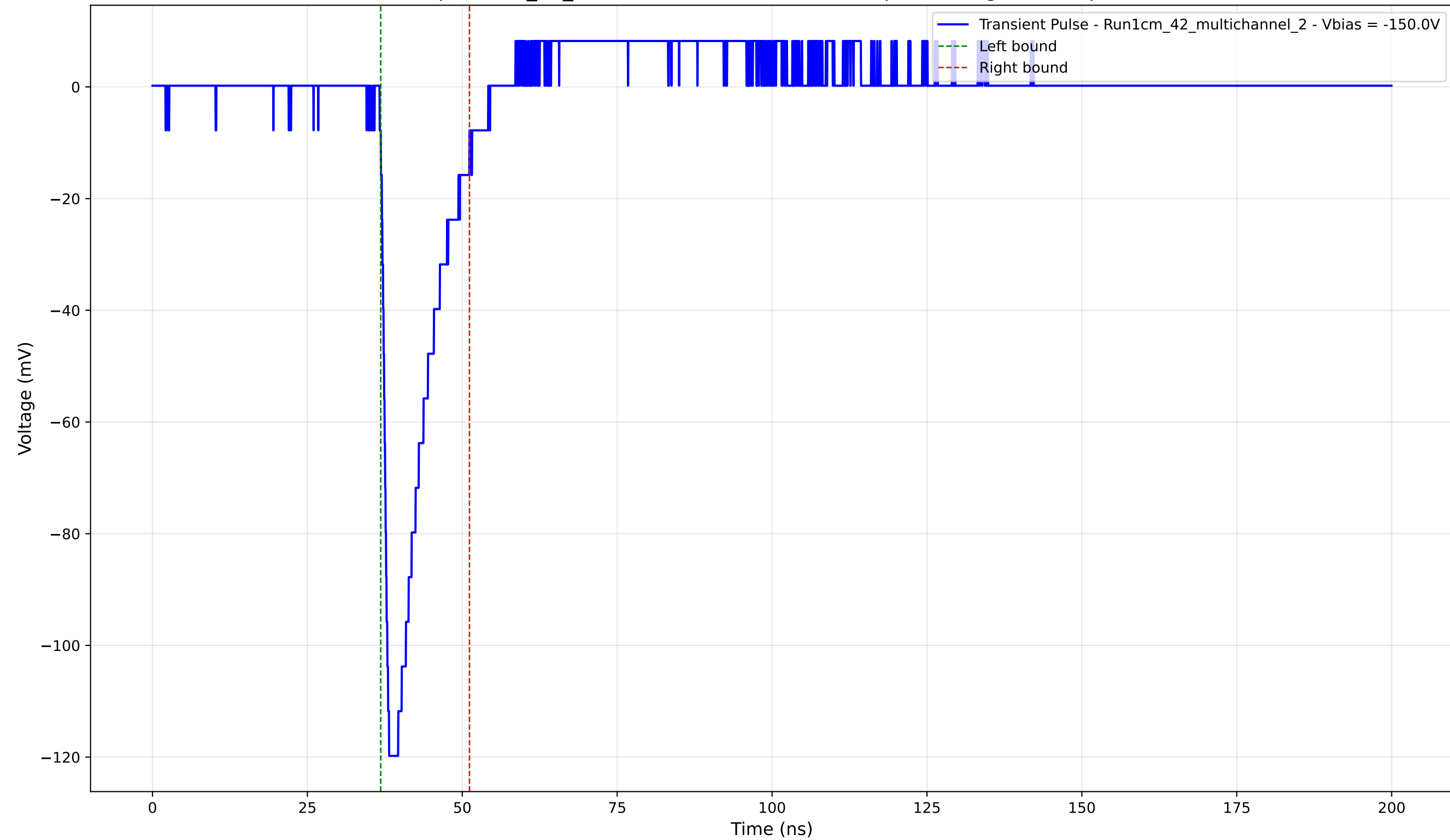
Transient Pulse - Sample: 1cm_42_multichannel - Position: 975.0 \mu\text{m} - Charge: 17.04 pC - Rise Time: 1.18 ns
