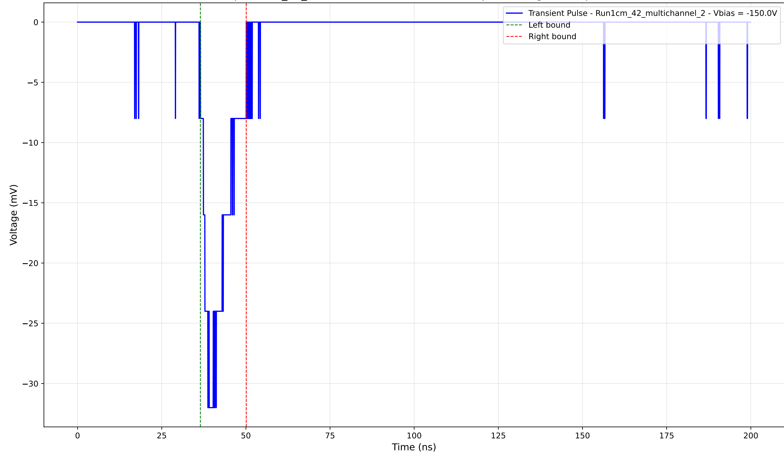
Transient Pulse - Sample: 1cm_42_multichannel - Position: 4850.0 \mu\text{m} - Charge: 4.67 pC - Rise Time: 2.22 ns
