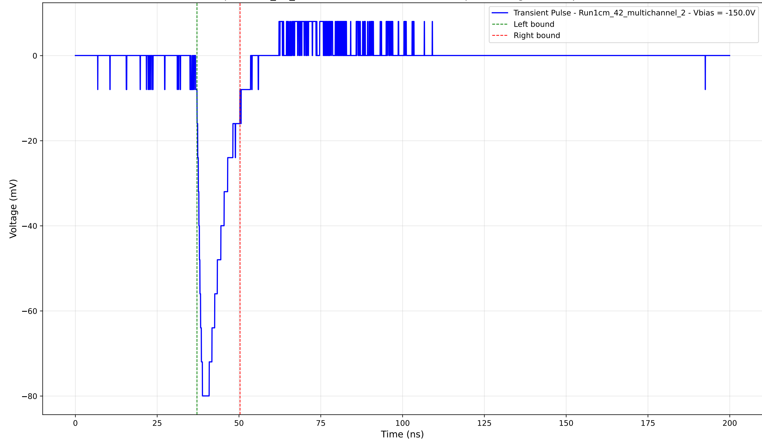
Transient Pulse - Sample: 1cm_42_multichannel - Position: 4230.0 \mu\text{m} - Charge: 12.04 pC - Rise Time: 1.68 ns
