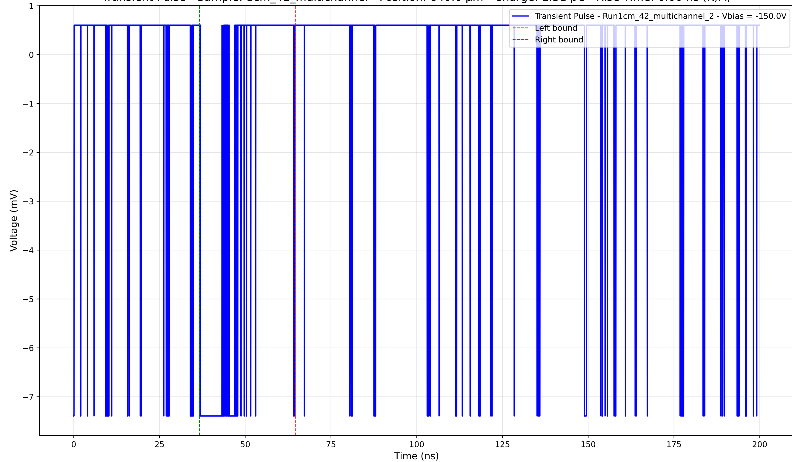
Transient Pulse - Sample: 1cm_42_multichannel - Position: 840.0 \mu\text{m} - Charge: 1.31 pC - Rise Time: 0.00 ns (N/A)
