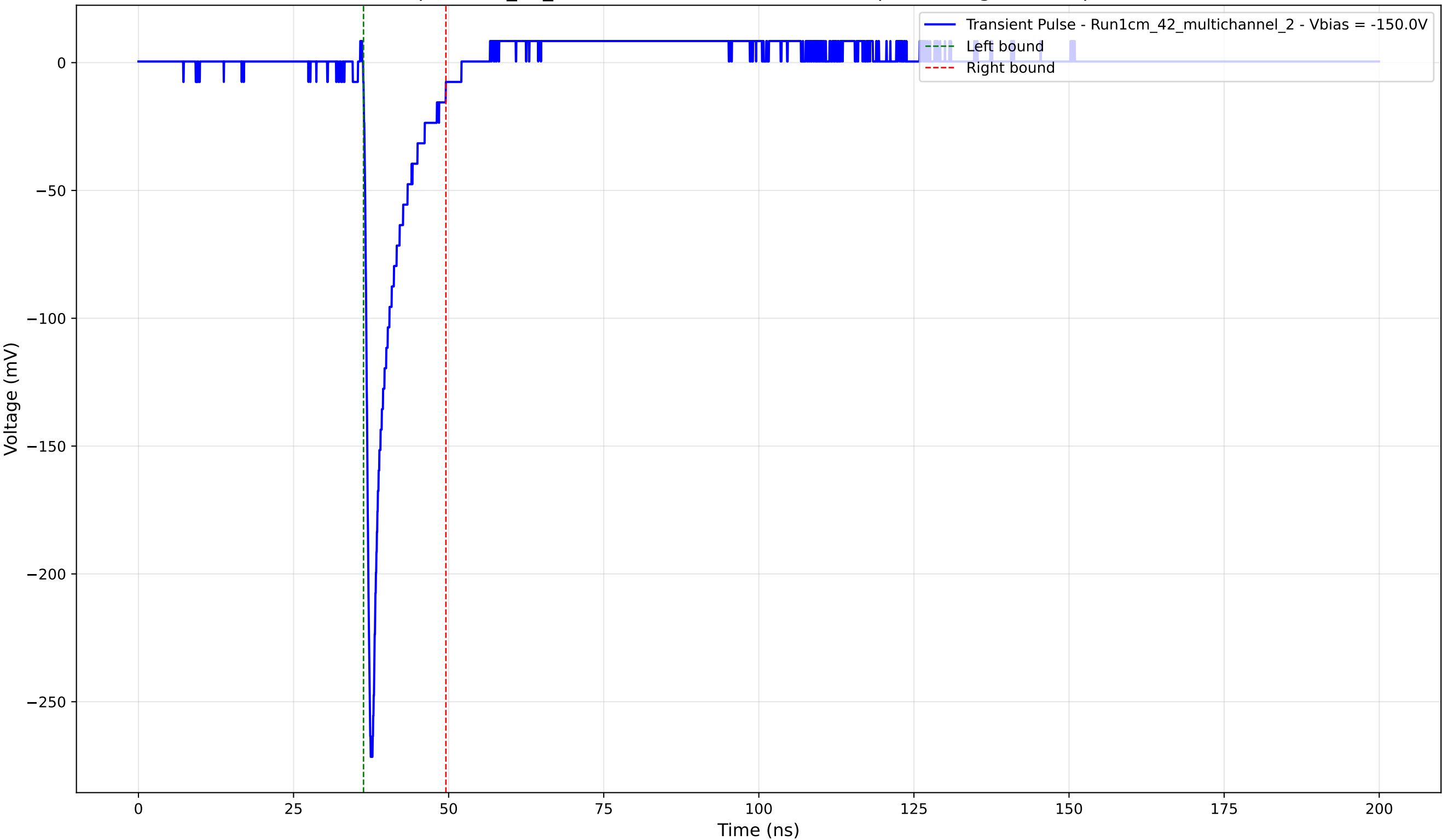
Transient Pulse - Sample: 1cm_42_multichannel - Position: 2970.0 \mu\text{m} - Charge: 21.20 pC - Rise Time: 0.85 ns
