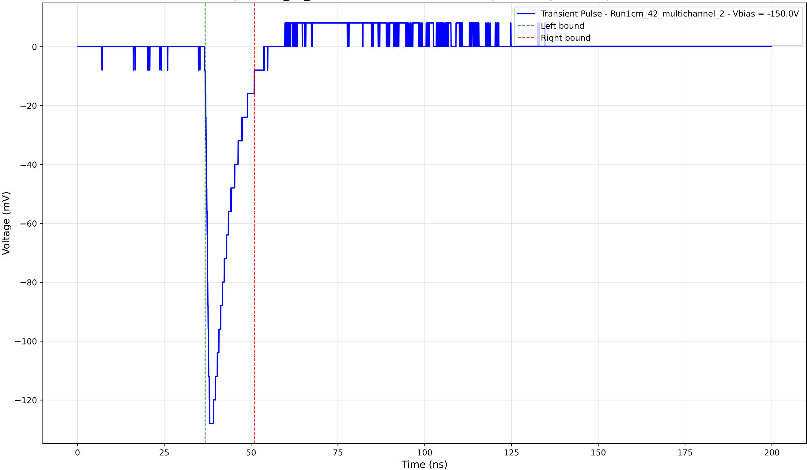
Transient Pulse - Sample: 1cm_42_multichannel - Position: 1085.0 \mu\text{m} - Charge: 17.24 pC - Rise Time: 1.18 ns
