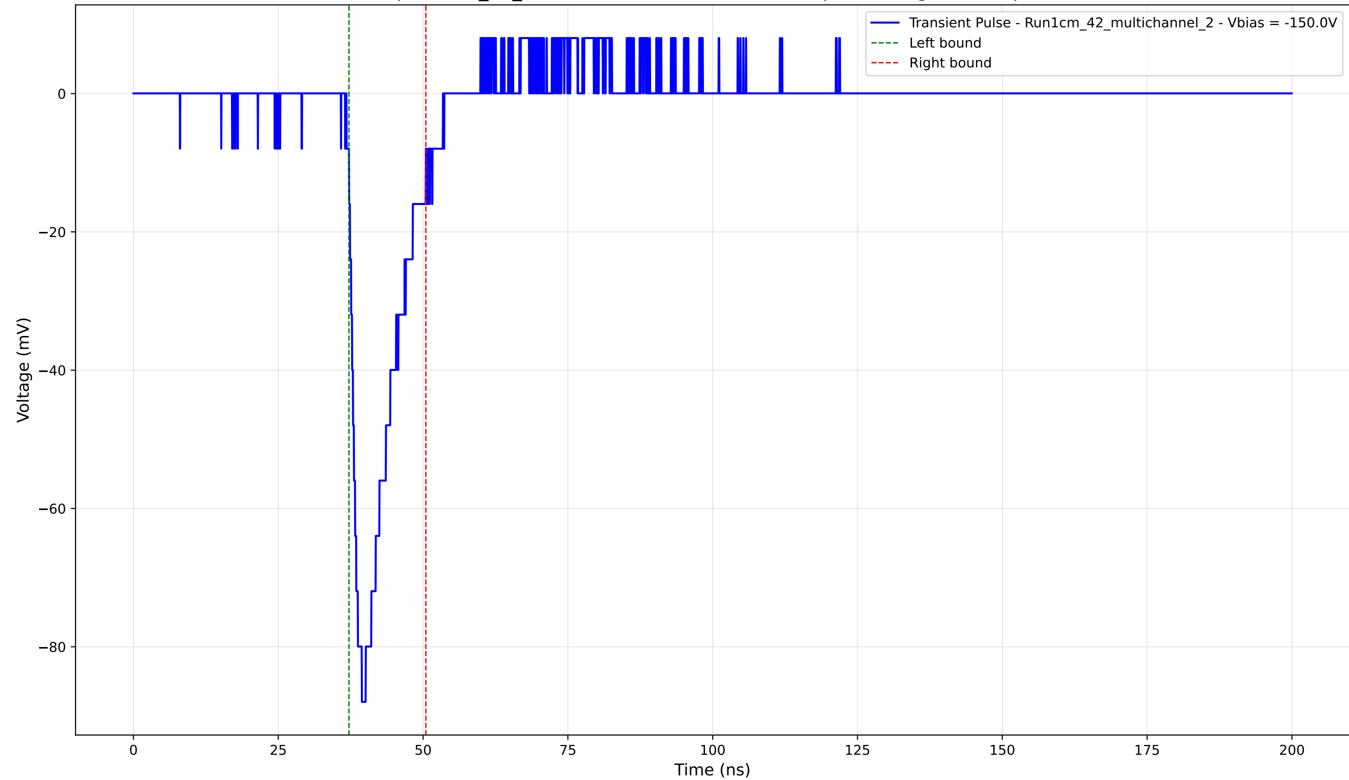
Transient Pulse - Sample: 1cm_42_multichannel - Position: 4225.0 \mu\text{m} - Charge: 12.32 pC - Rise Time: 1.56 ns
