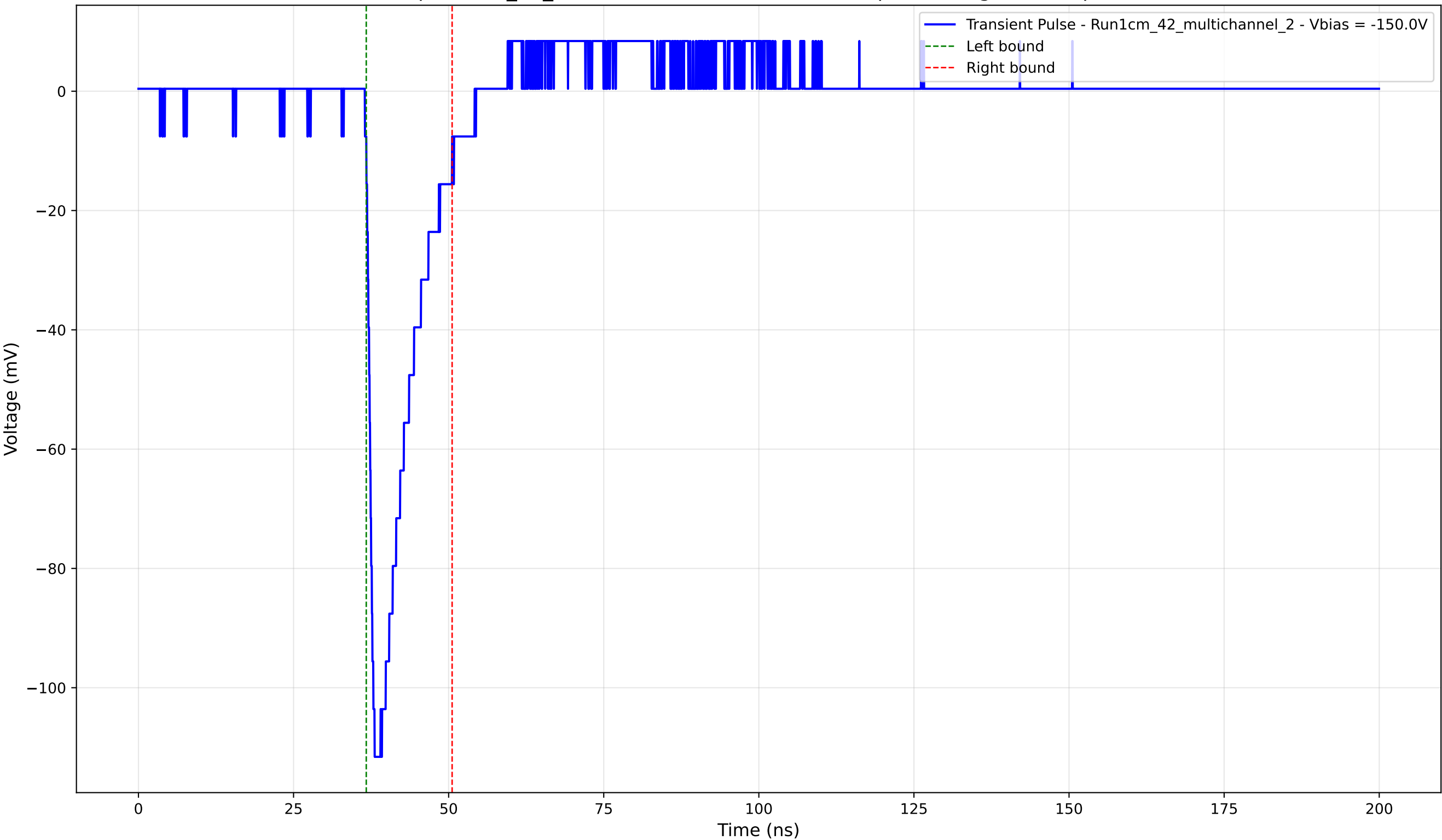
Transient Pulse - Sample: 1cm_42_multichannel - Position: 3605.0 \mu\text{m} - Charge: 15.02 pC - Rise Time: 1.14 ns
