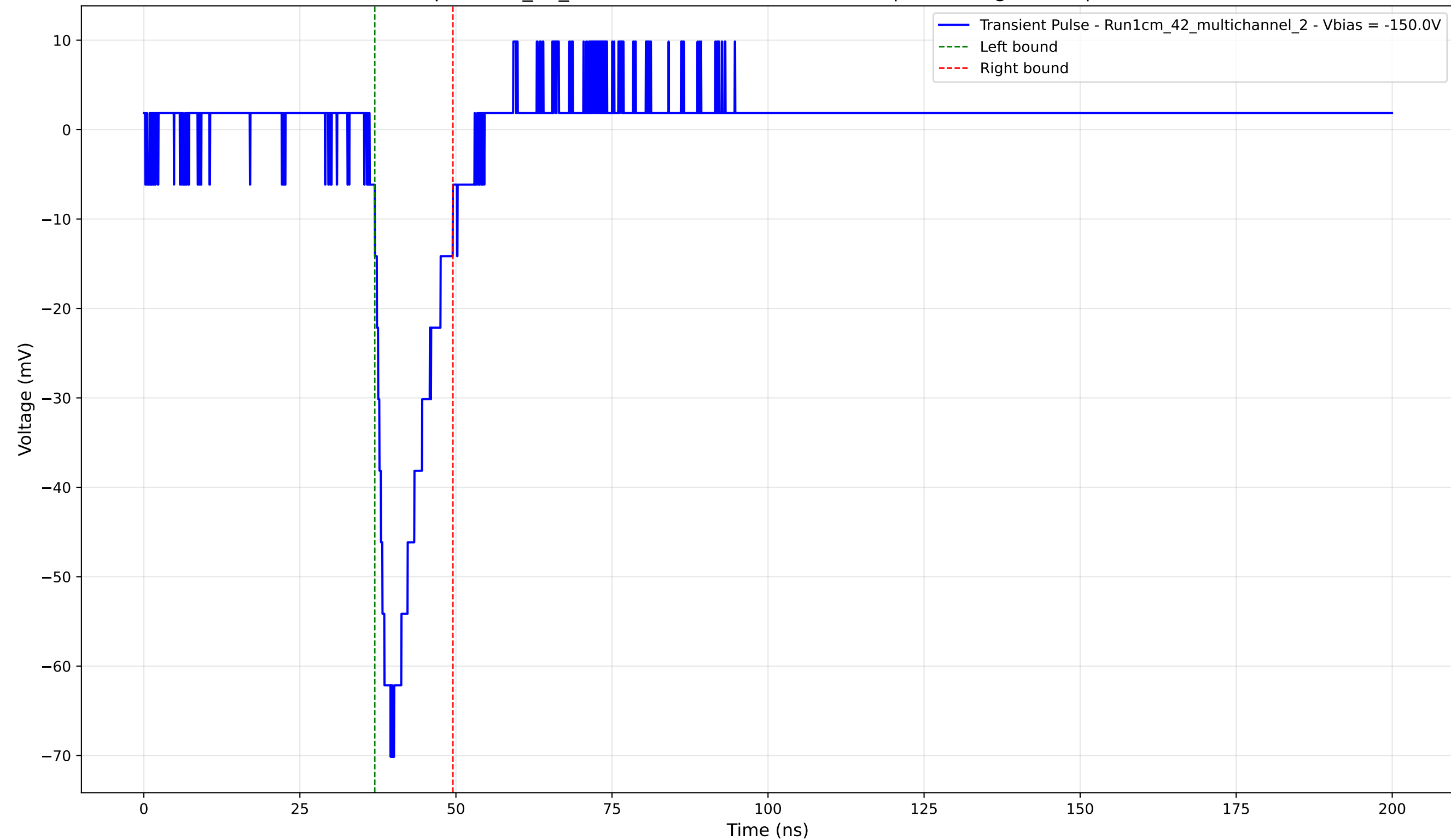
Transient Pulse - Sample: 1cm_42_multichannel - Position: 4725.0 \mu\text{m} - Charge: 9.60 pC - Rise Time: 2.56 ns
