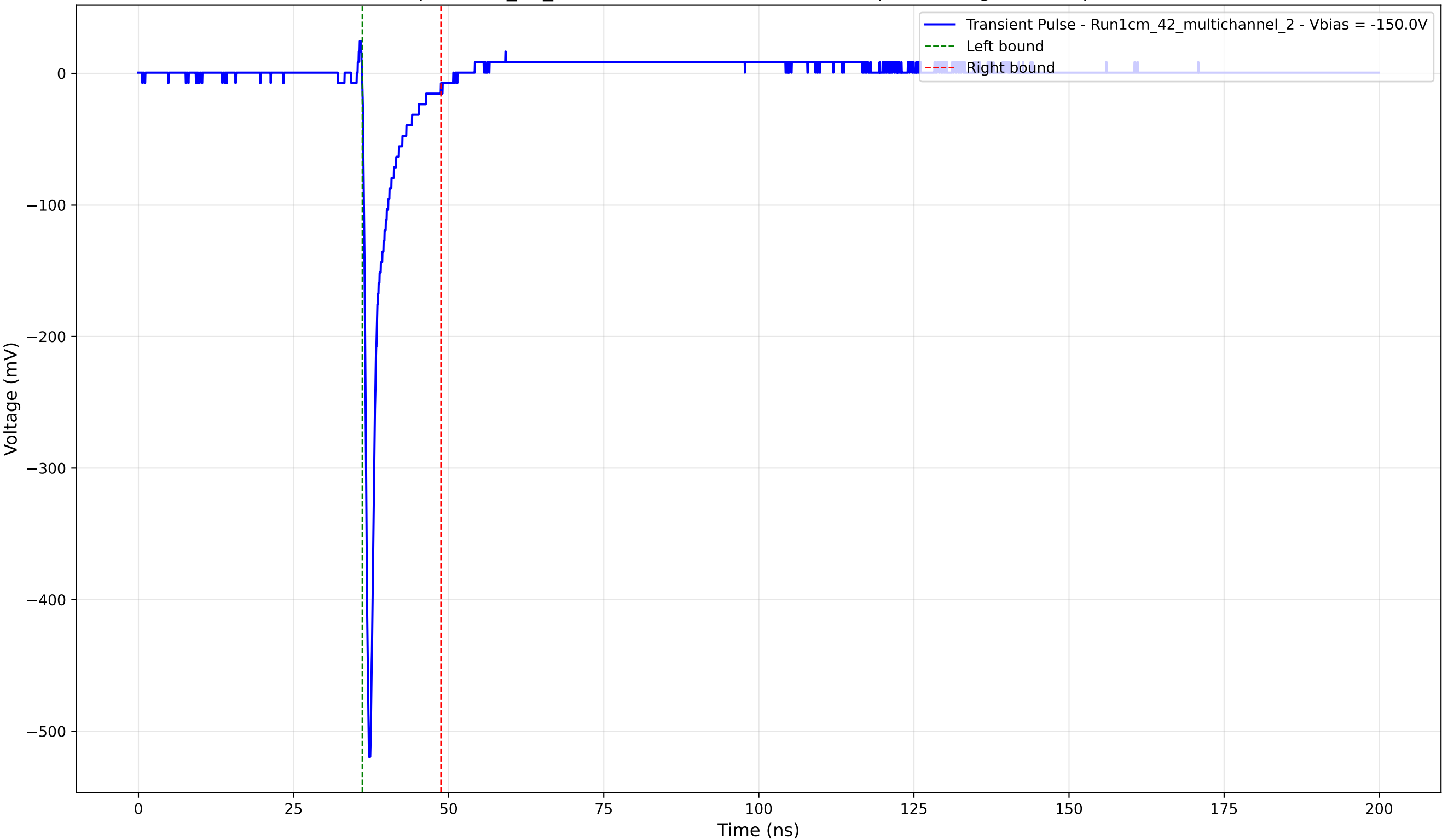
Transient Pulse - Sample: 1cm_42_multichannel - Position: 2150.0 \mu\text{m} - Charge: 26.70 pC - Rise Time: 0.76 ns
