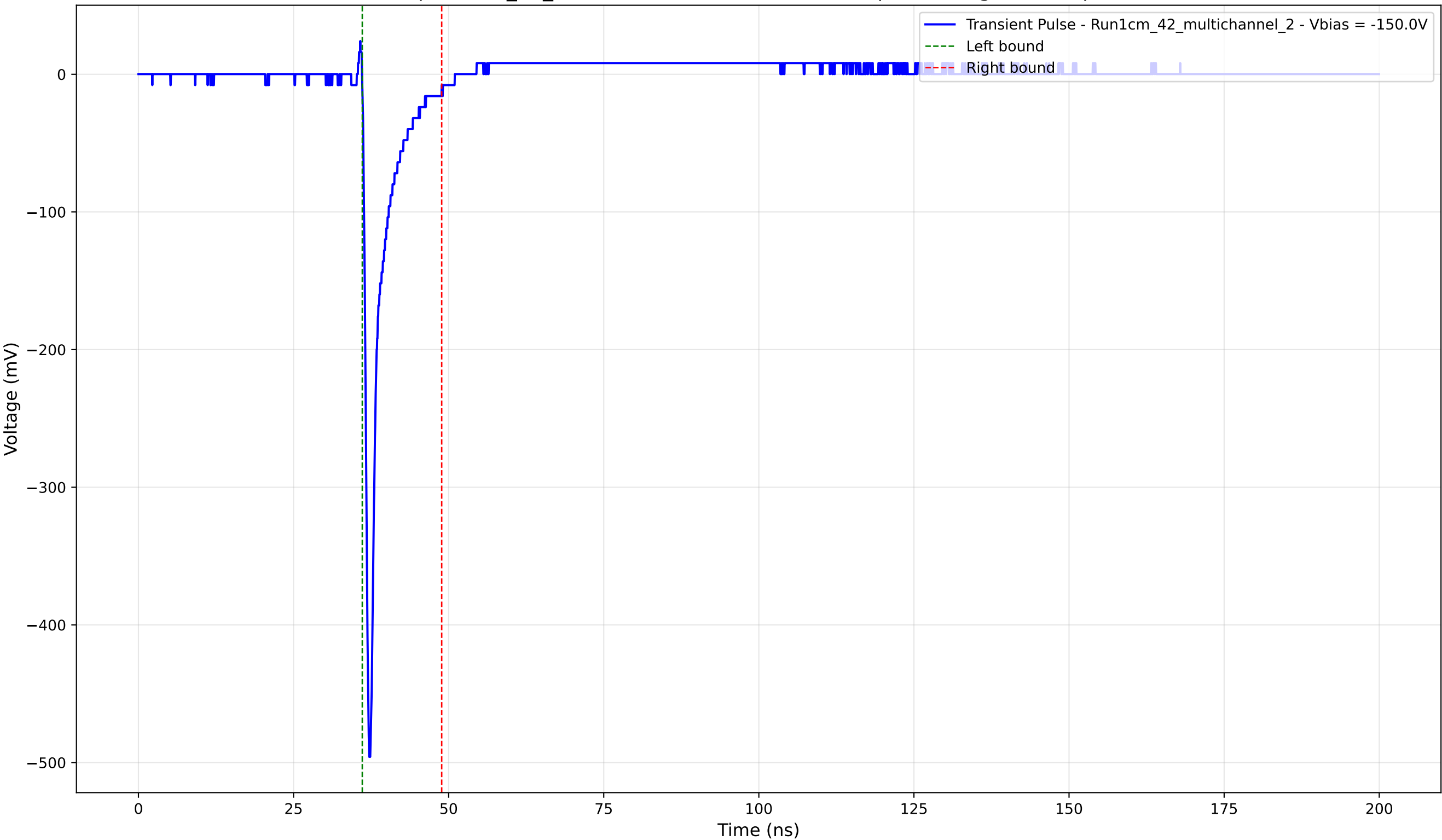
Transient Pulse - Sample: 1cm_42_multichannel - Position: 2110.0 \mu\text{m} - Charge: 26.60 pC - Rise Time: 0.77 ns
