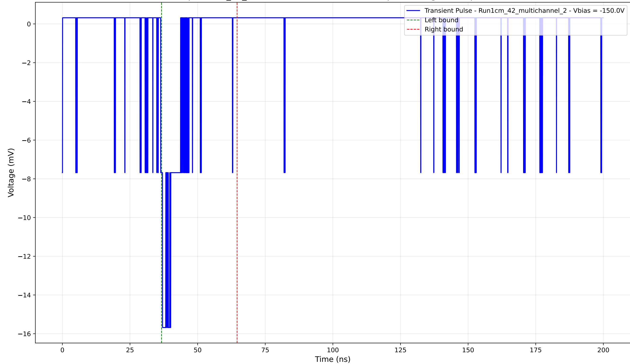
Transient Pulse - Sample: 1cm_42_multichannel - Position: 2890.0 \mu\text{m} - Charge: 1.63 pC - Rise Time: 0.71 ns
