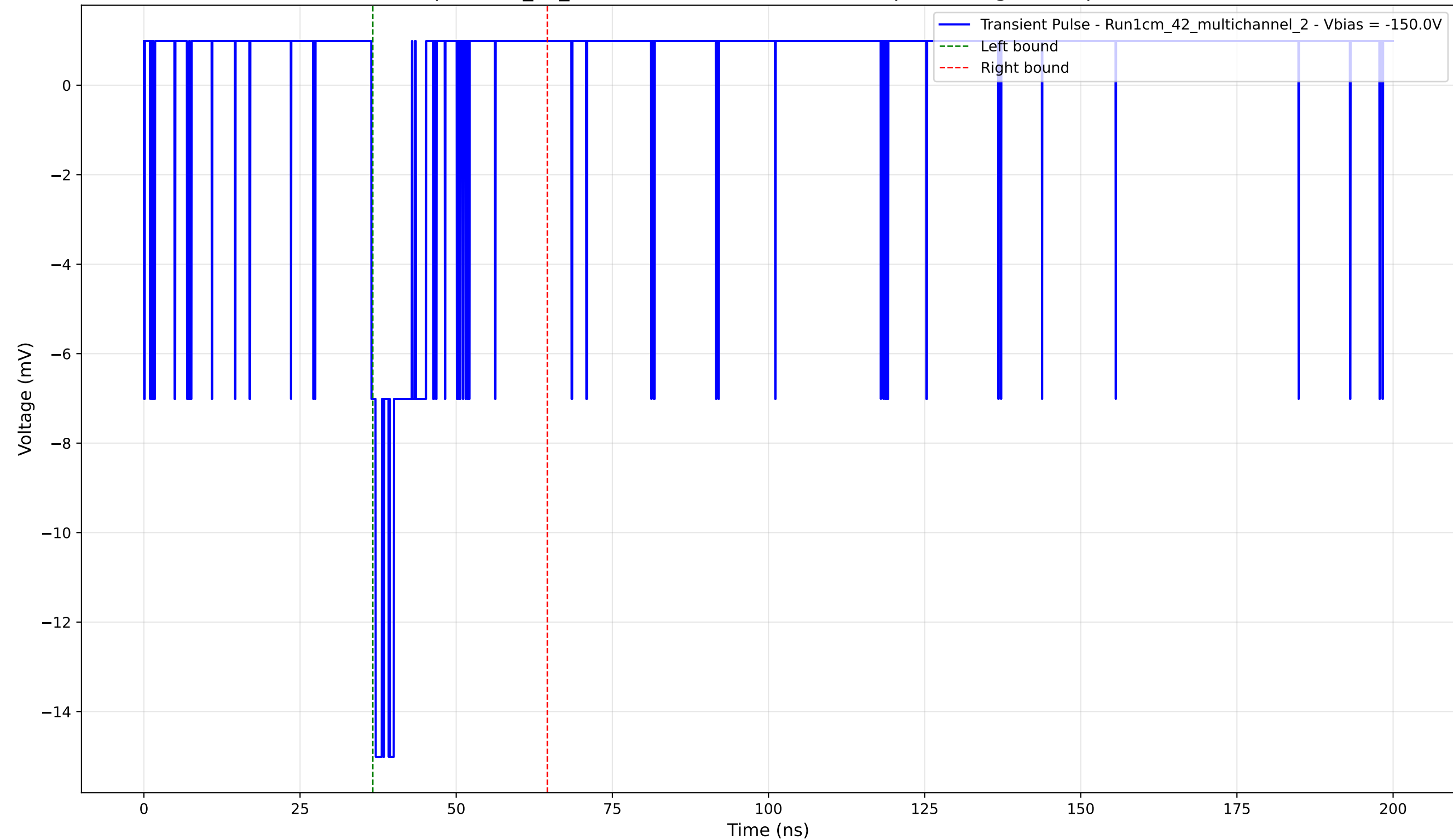
Transient Pulse - Sample: 1cm_42_multichannel - Position: 1860.0 \mu\text{m} - Charge: 1.24 pC - Rise Time: 0.72 ns
