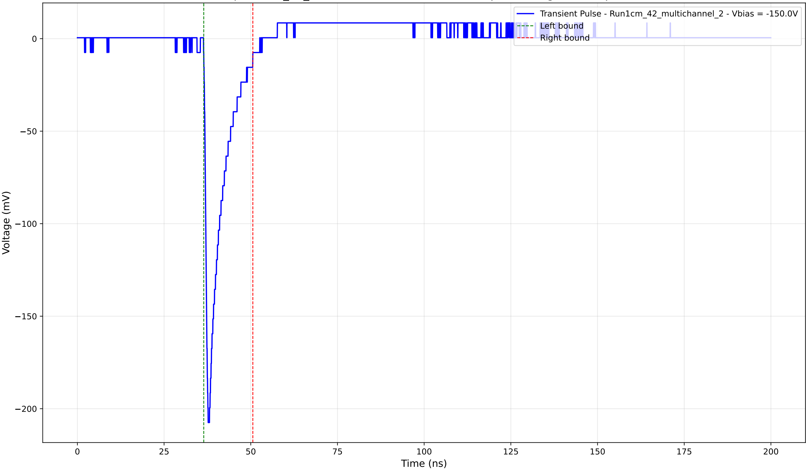
Transient Pulse - Sample: 1cm_42_multichannel - Position: 1490.0 \mu\text{m} - Charge: 20.96 pC - Rise Time: 1.01 ns
