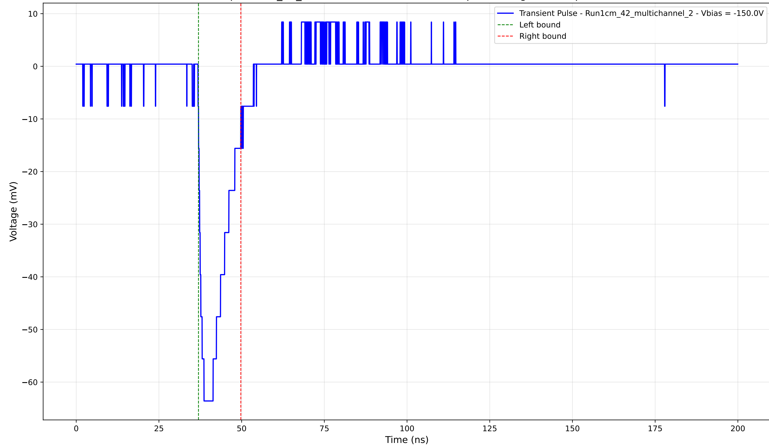
Transient Pulse - Sample: 1cm_42_multichannel - Position: 135.0 \mu\text{m} - Charge: 10.40 pC - Rise Time: 1.81 ns
