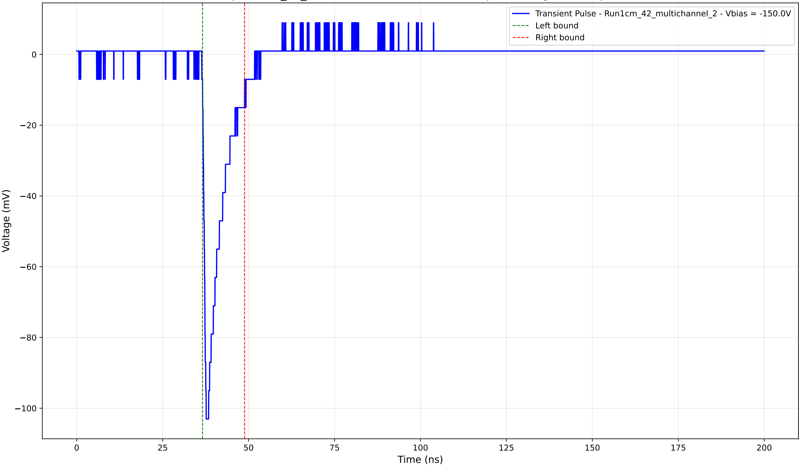
Transient Pulse - Sample: 1cm_42_multichannel - Position: 1410.0 \mu\text{m} - Charge: 11.05 pC - Rise Time: 0.94 ns
