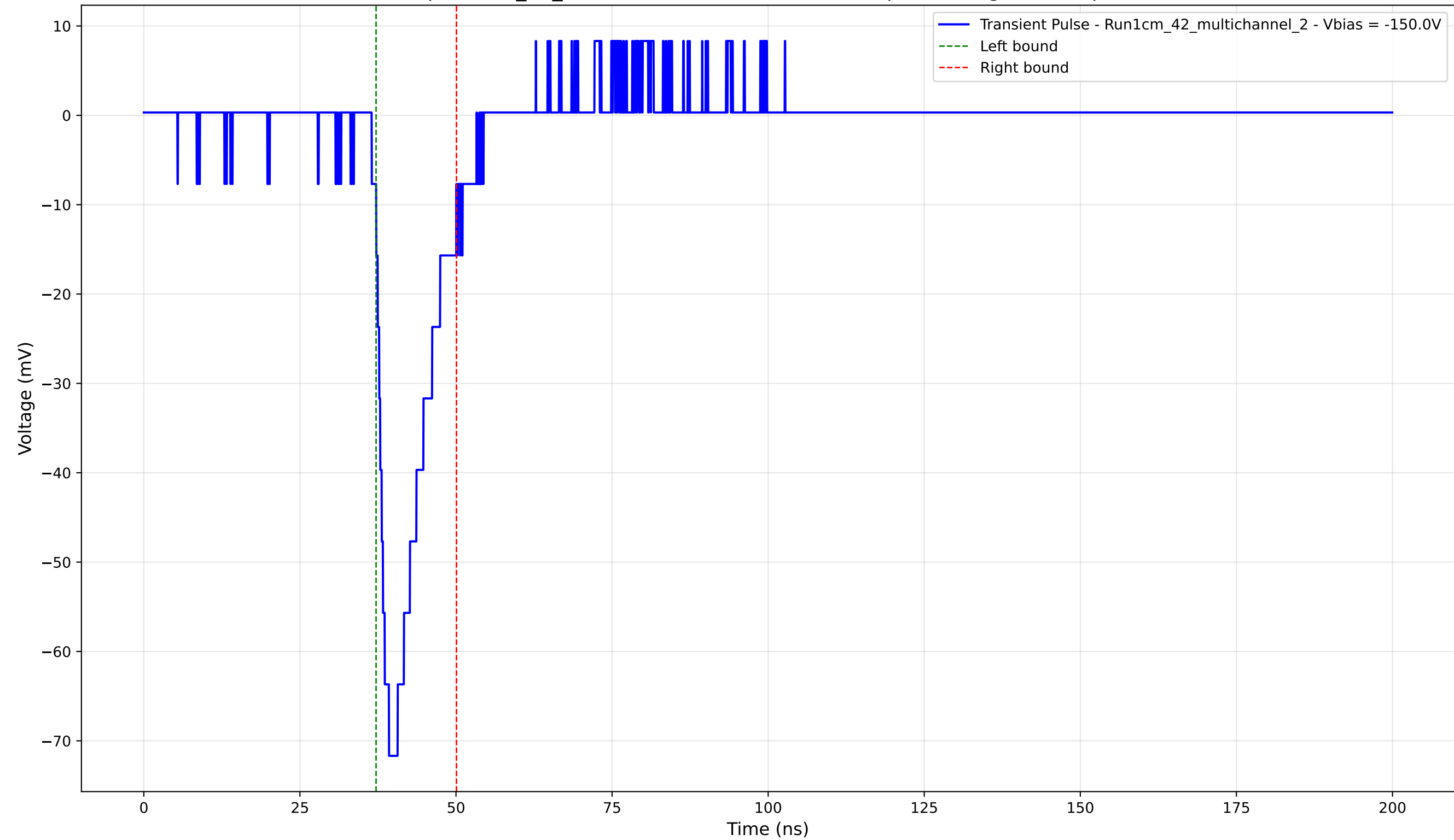
Transient Pulse - Sample: 1cm_42_multichannel - Position: 4485.0 \mu\text{m} - Charge: 10.39 pC - Rise Time: 2.76 ns
