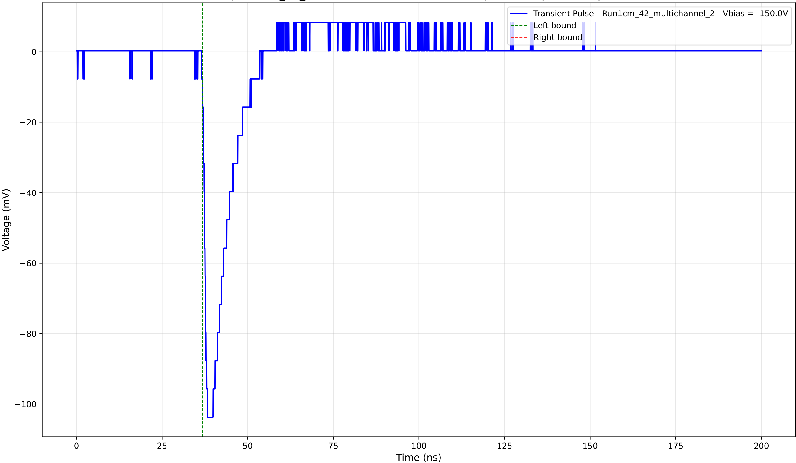
Transient Pulse - Sample: 1cm_42_multichannel - Position: 3745.0 \mu\text{m} - Charge: 14.85 pC - Rise Time: 1.19 ns
