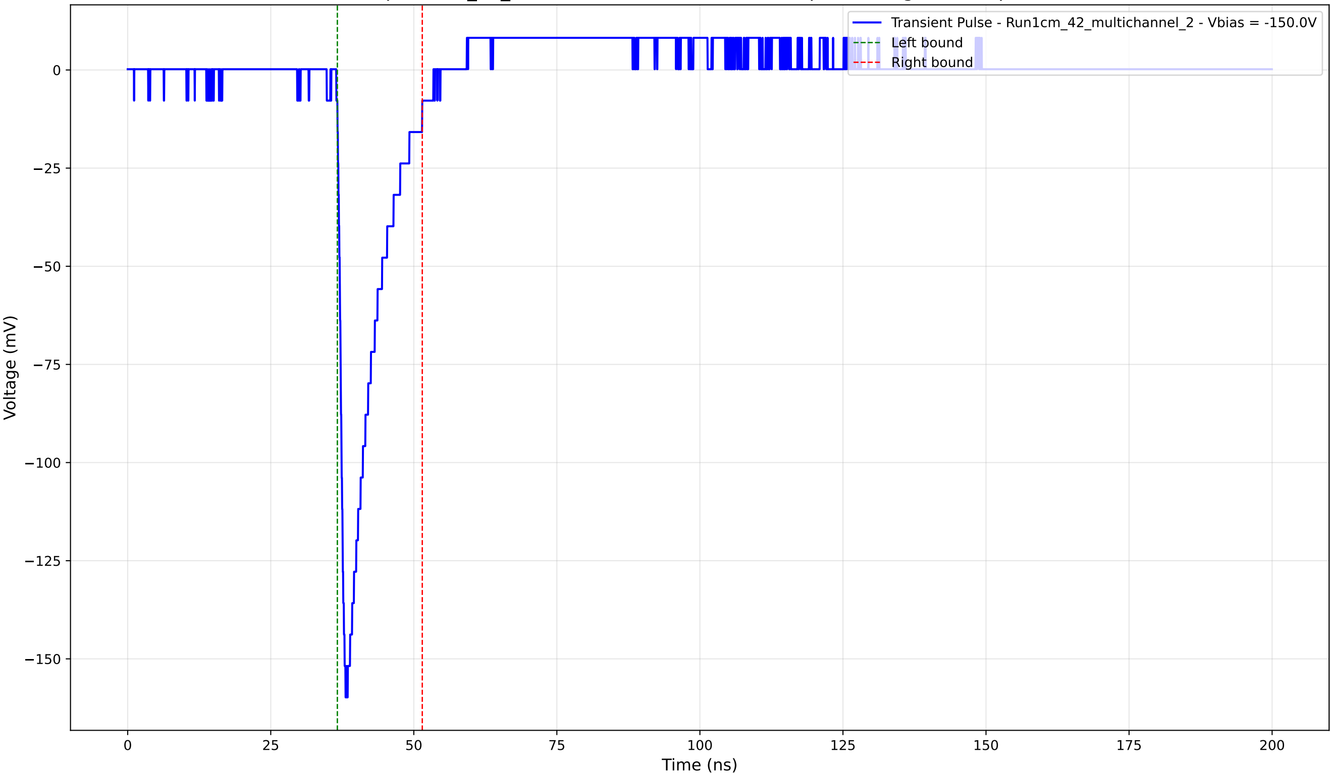
Transient Pulse - Sample: 1cm_42_multichannel - Position: 1235.0 \mu\text{m} - Charge: 19.41 pC - Rise Time: 1.20 ns
