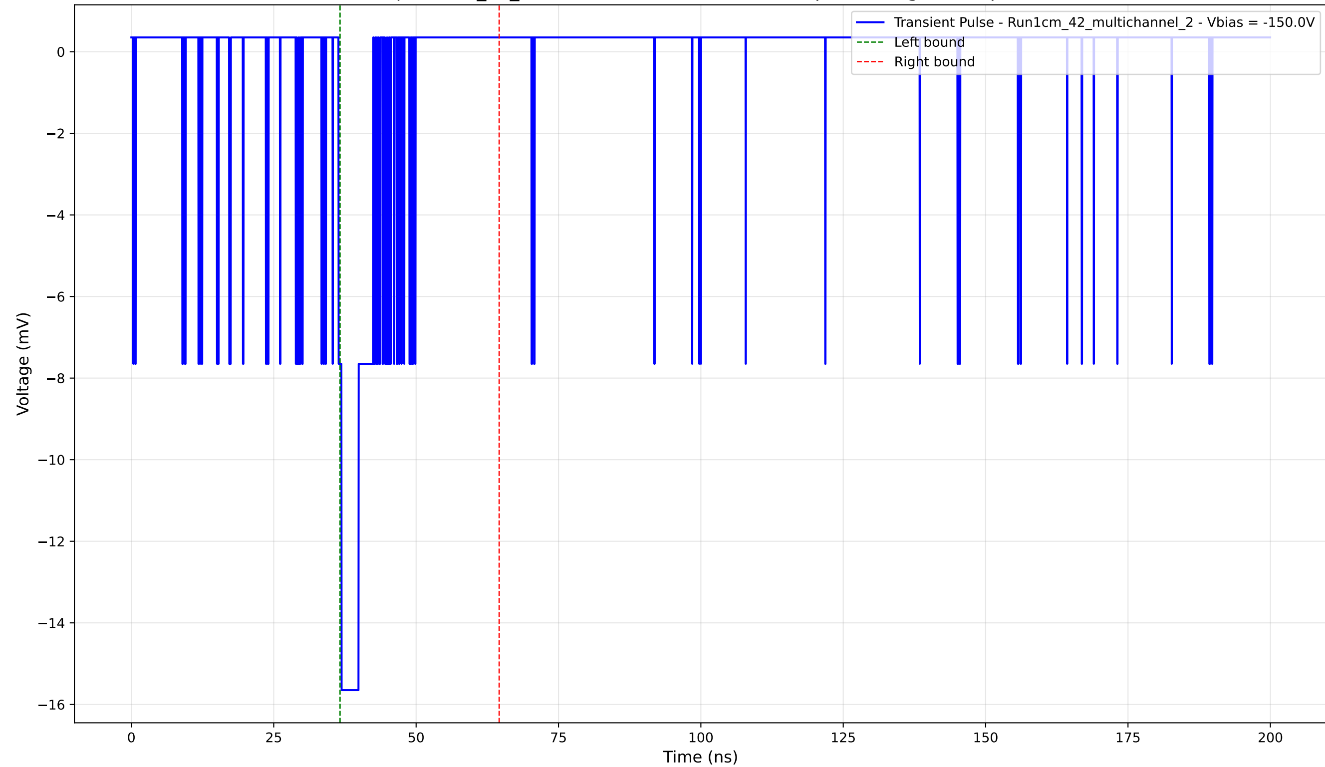
Transient Pulse - Sample: 1cm_42_multichannel - Position: 1850.0 \mu\text{m} - Charge: 1.62 pC - Rise Time: 0.55 ns
