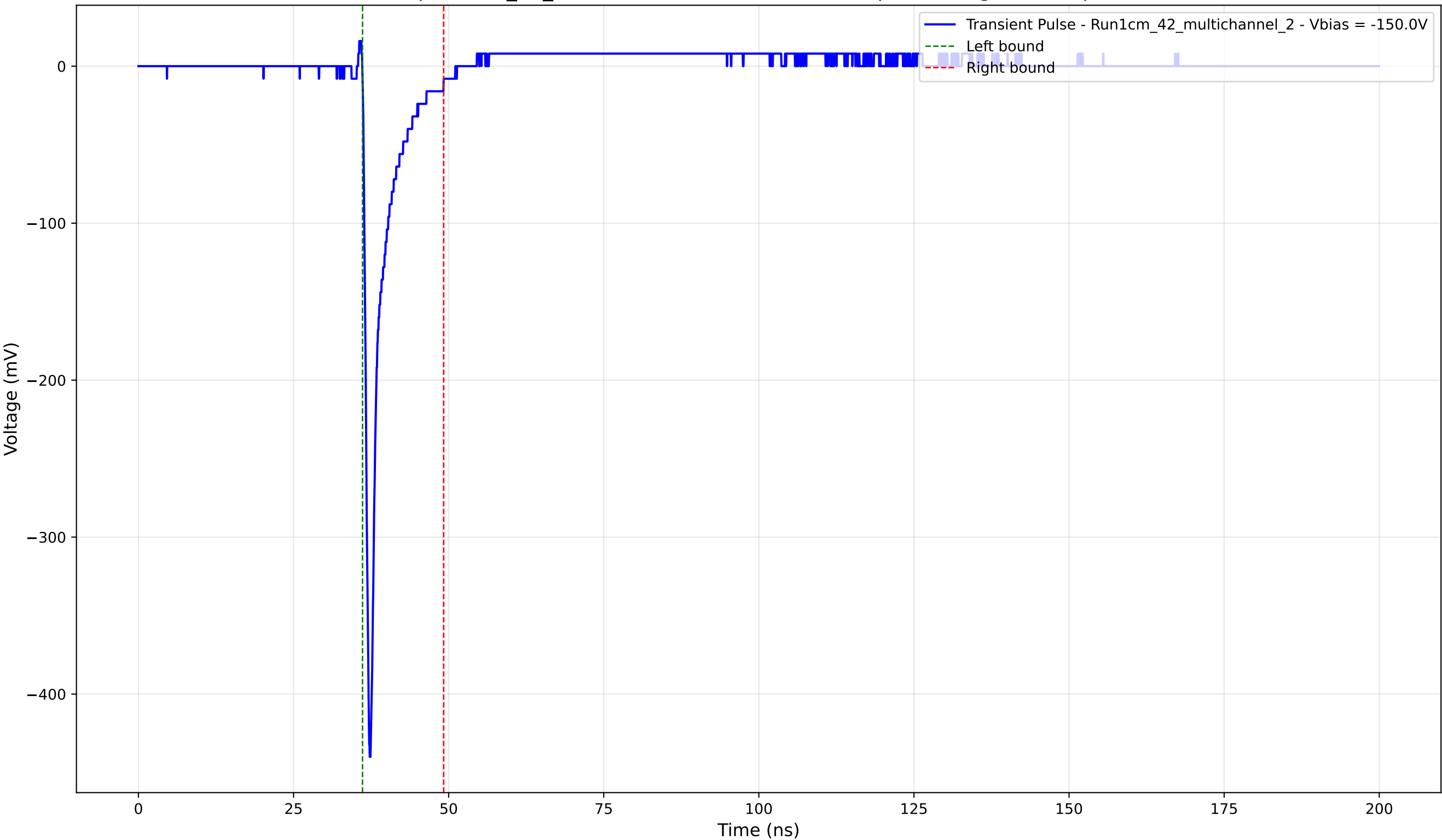
Transient Pulse - Sample: 1cm_42_multichannel - Position: 2675.0 \mu\text{m} - Charge: 24.67 pC - Rise Time: 0.80 ns
