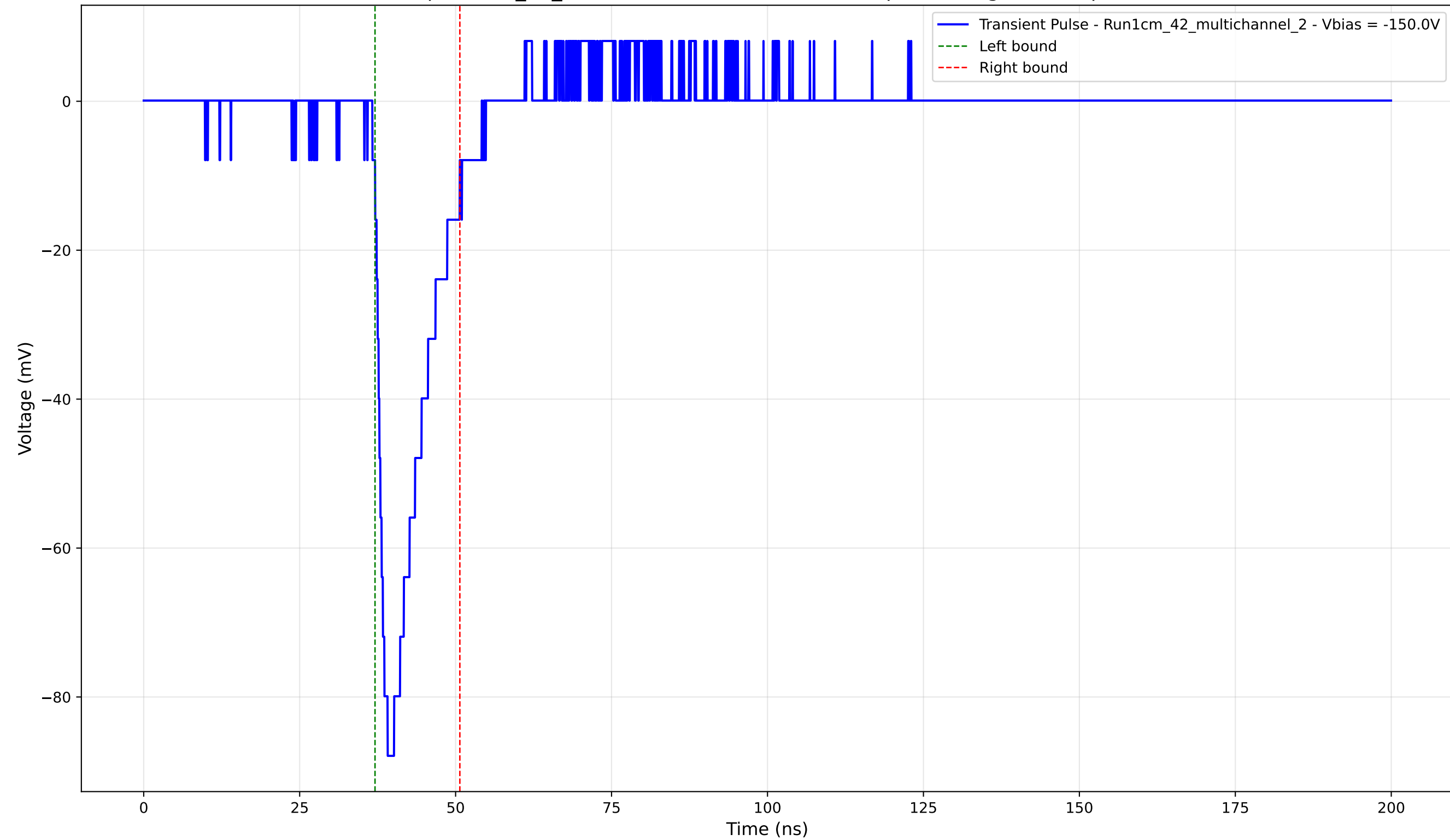
Transient Pulse - Sample: 1cm_42_multichannel - Position: 4135.0 \mu\text{m} - Charge: 12.68 pC - Rise Time: 1.52 ns
