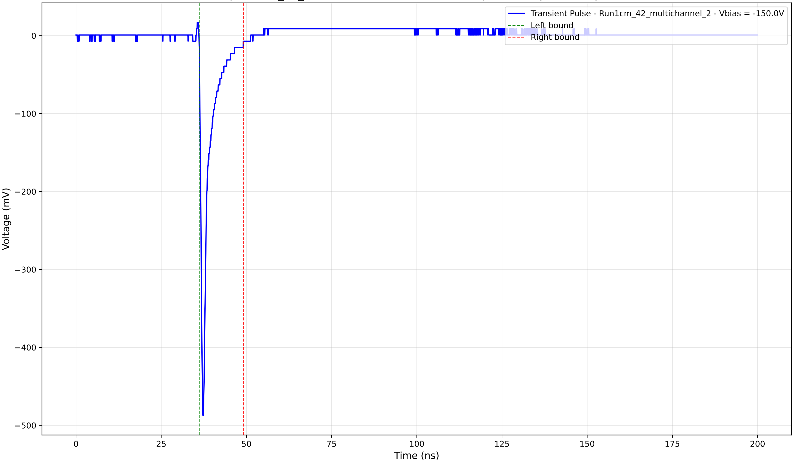
Transient Pulse - Sample: 1cm_42_multichannel - Position: 2100.0 \mu\text{m} - Charge: 26.20 pC - Rise Time: 0.77 ns
