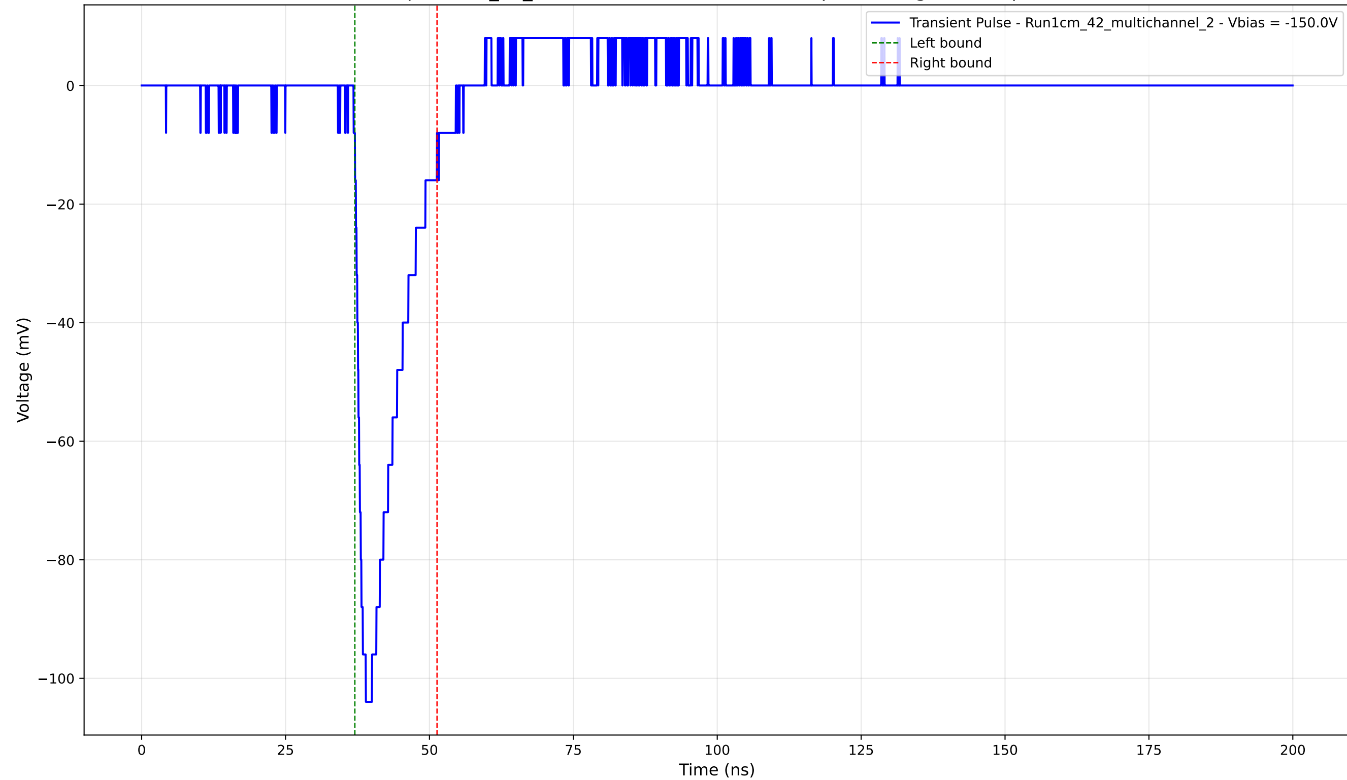
Transient Pulse - Sample: 1cm_42_multichannel - Position: 665.0 \mu\text{m} - Charge: 15.28 pC - Rise Time: 1.39 ns
