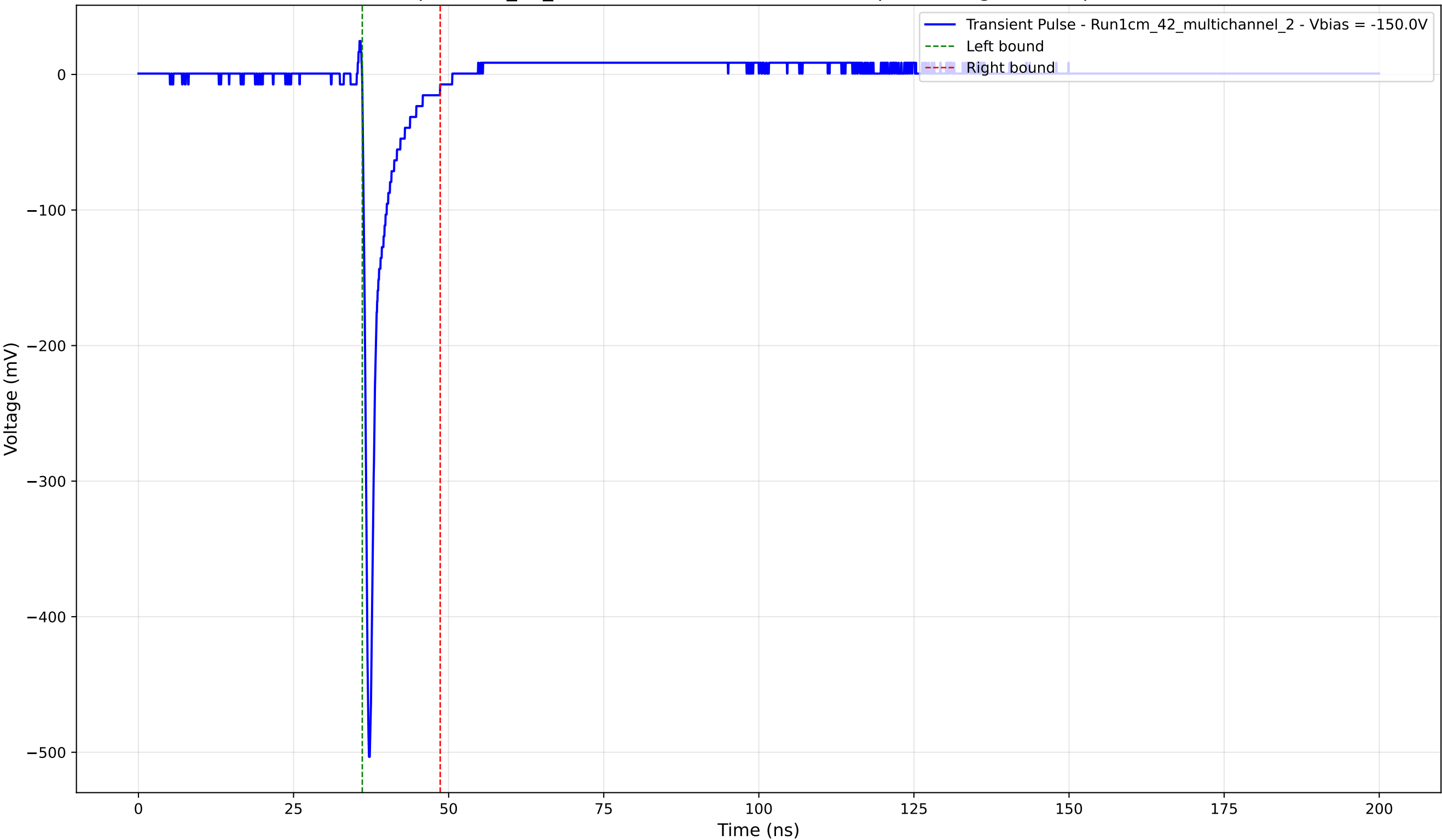
Transient Pulse - Sample: 1cm_42_multichannel - Position: 2565.0 \mu\text{m} - Charge: 25.14 pC - Rise Time: 0.77 ns
