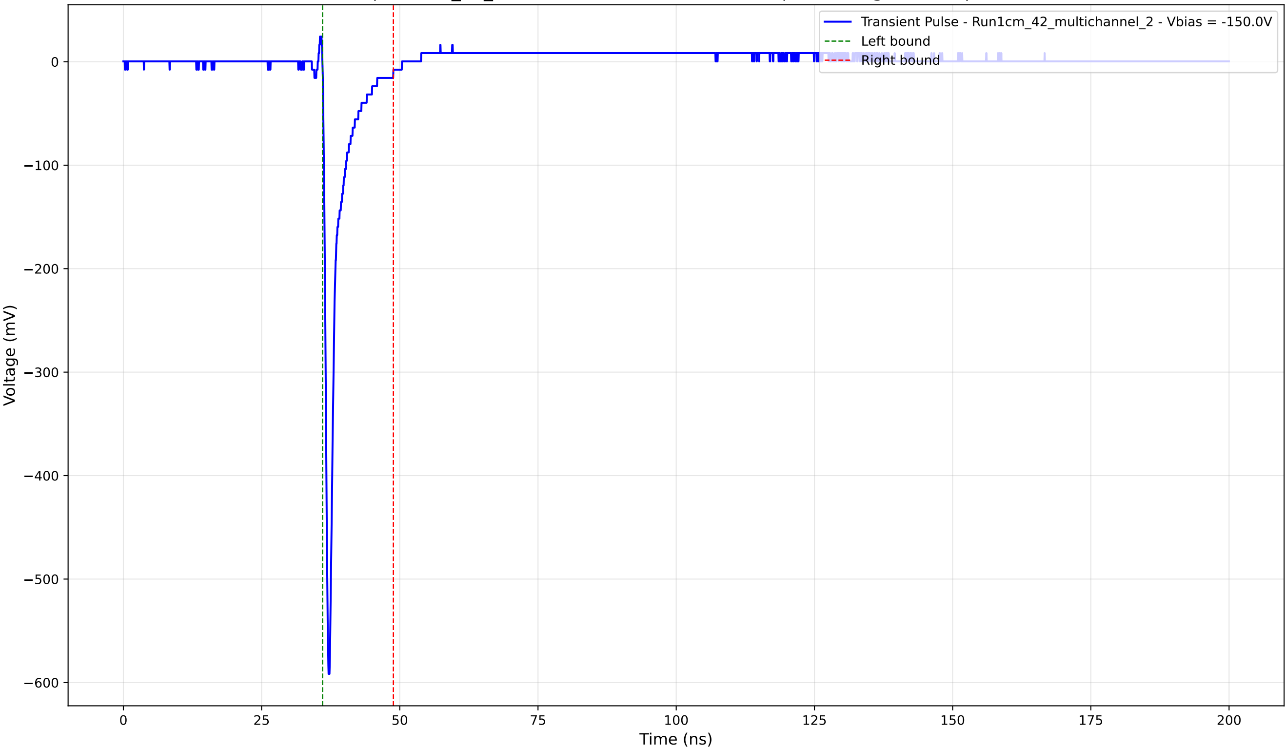
Transient Pulse - Sample: 1cm_42_multichannel - Position: 2215.0 \mu\text{m} - Charge: 28.49 pC - Rise Time: 0.73 ns
