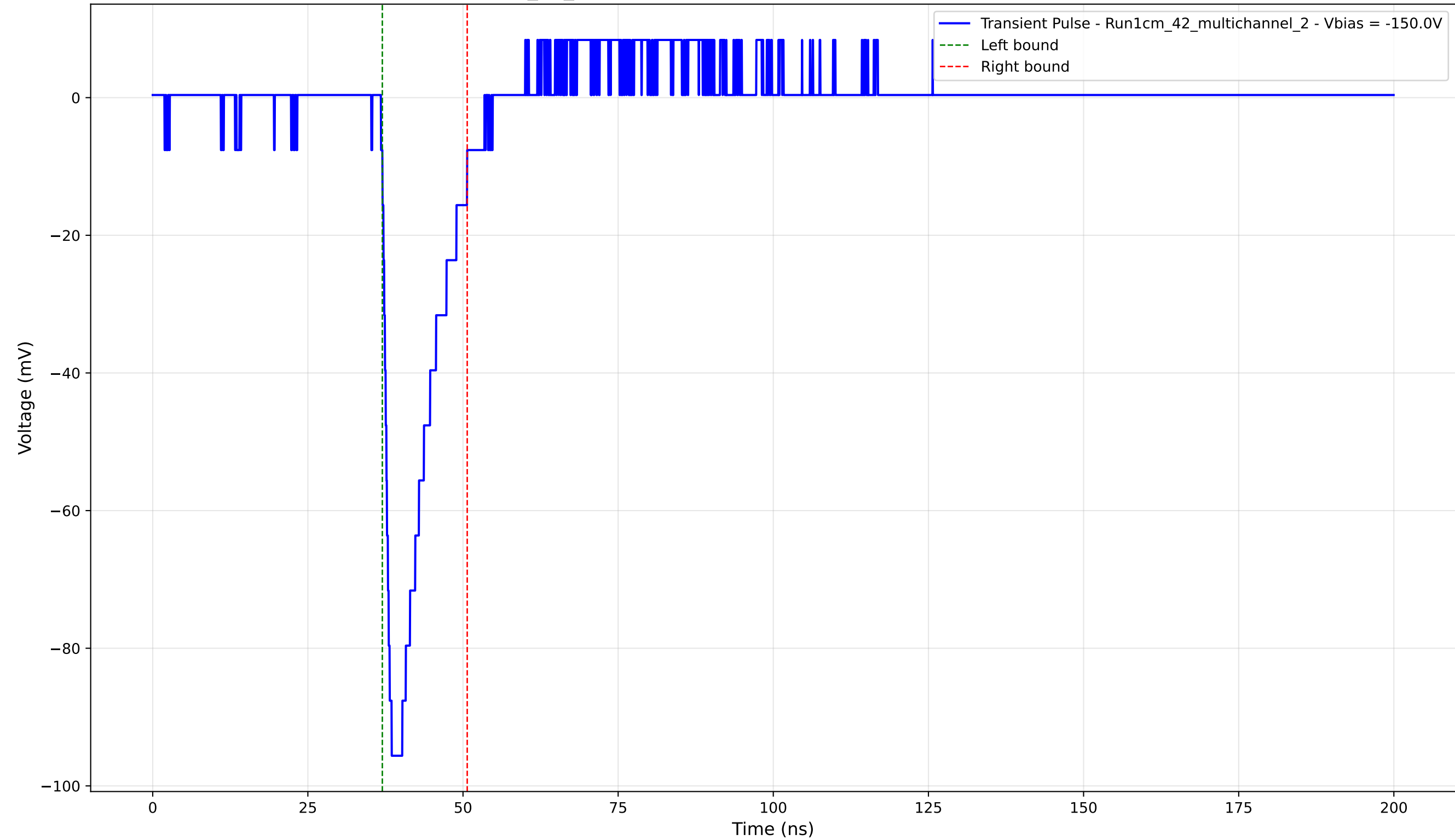
Transient Pulse - Sample: 1cm_42_multichannel - Position: 770.0 \mu\text{m} - Charge: 13.96 pC - Rise Time: 1.19 ns
