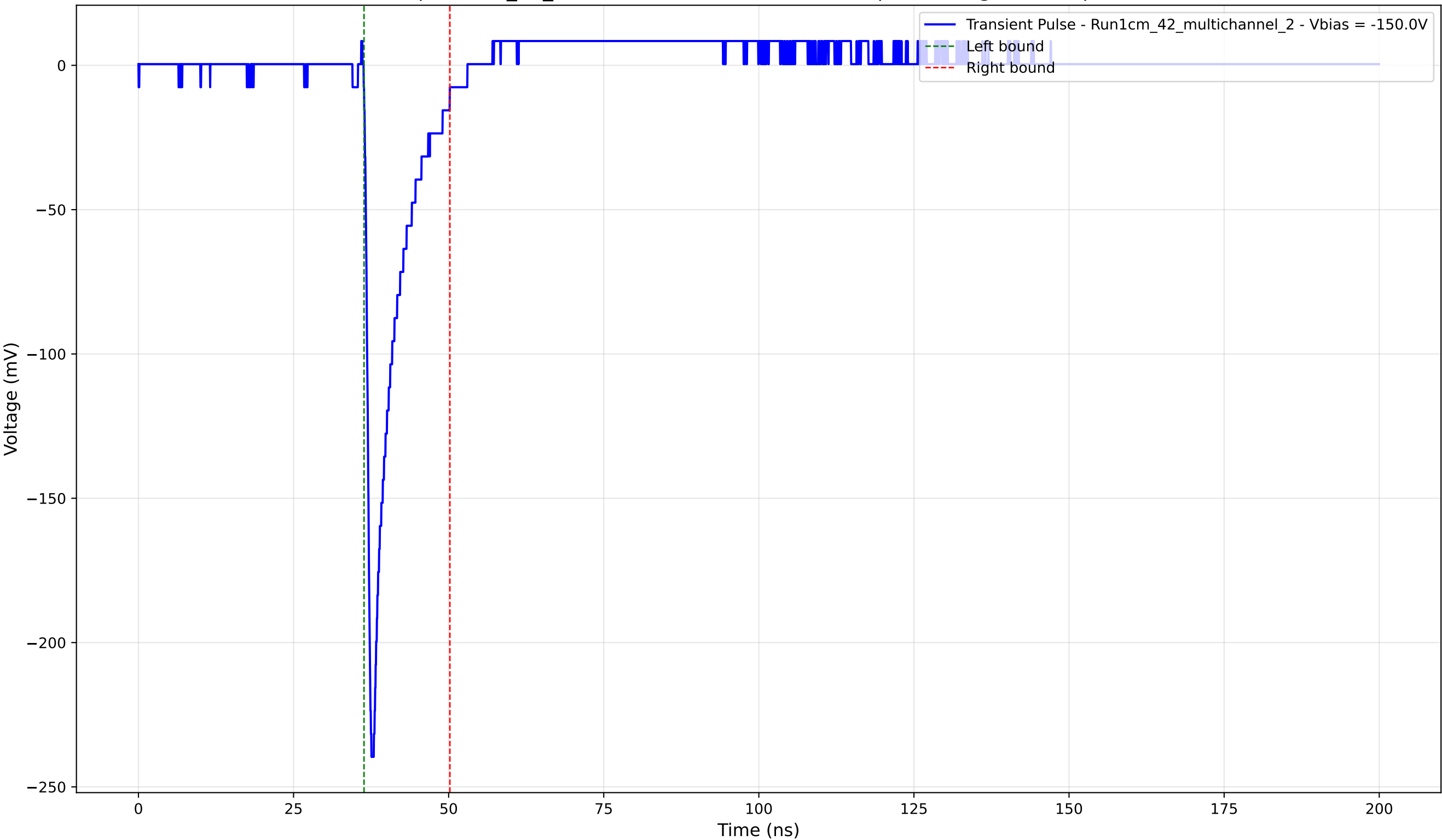
Transient Pulse - Sample: 1cm_42_multichannel - Position: 1620.0 \mu\text{m} - Charge: 21.82 pC - Rise Time: 0.92 ns
