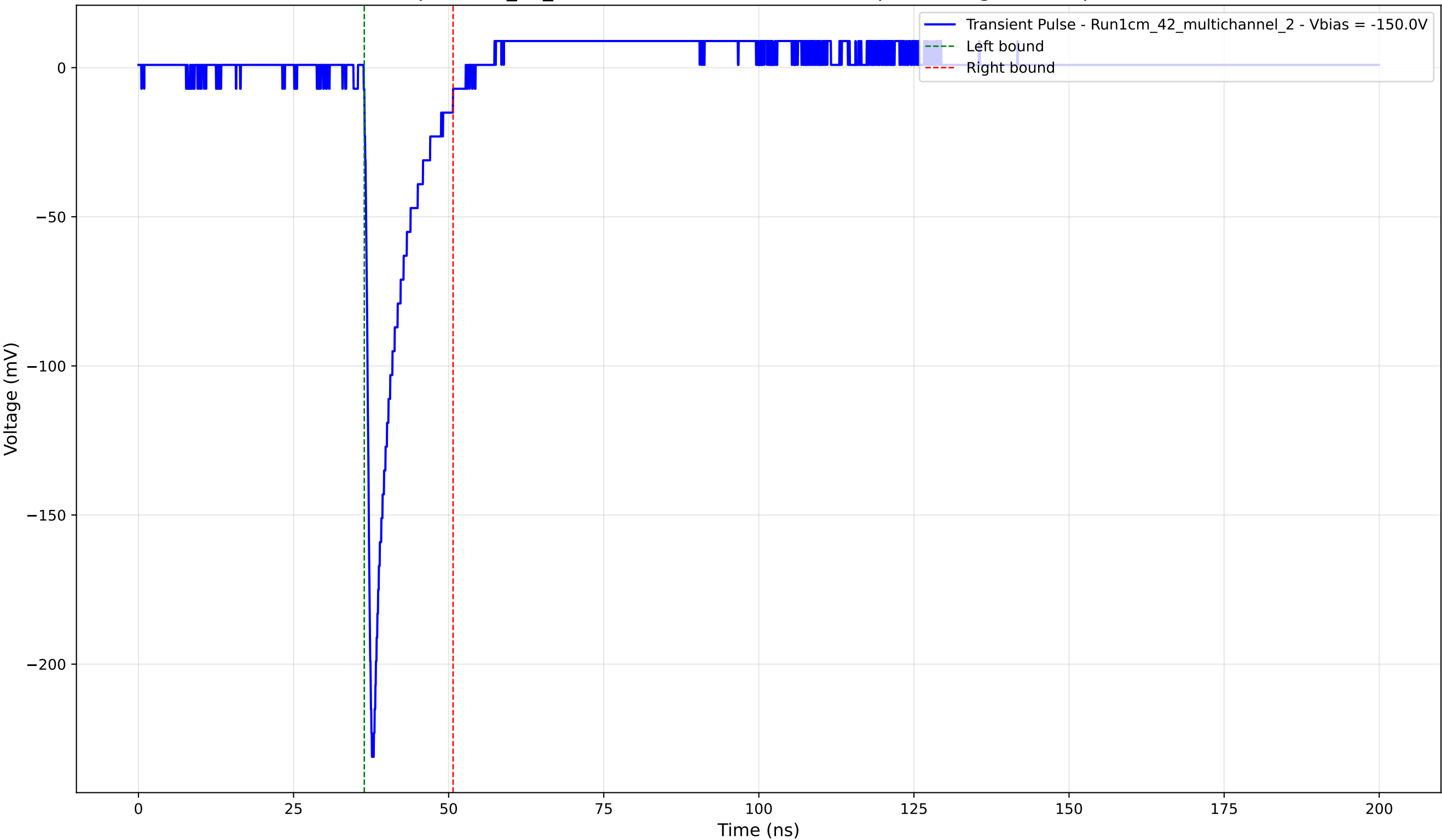
Transient Pulse - Sample: 1cm_42_multichannel - Position: 1580.0 \mu\text{m} - Charge: 21.53 pC - Rise Time: 0.96 ns
