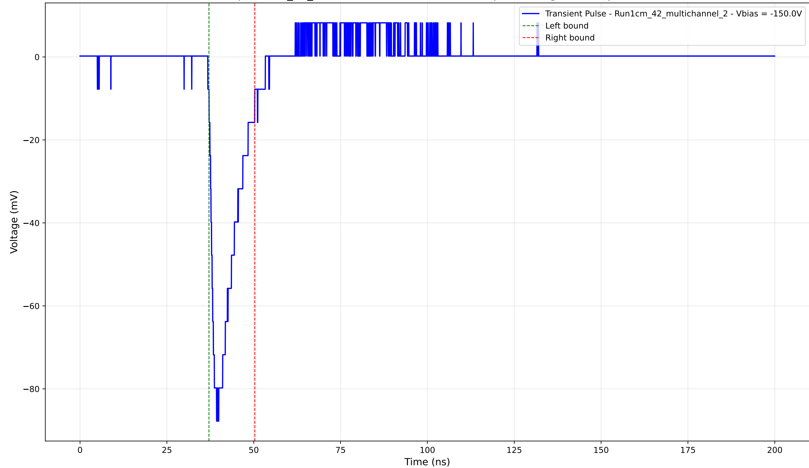
Transient Pulse - Sample: 1cm_42_multichannel - Position: 4195.0 \mu\text{m} - Charge: 12.31 pC - Rise Time: 1.55 ns
