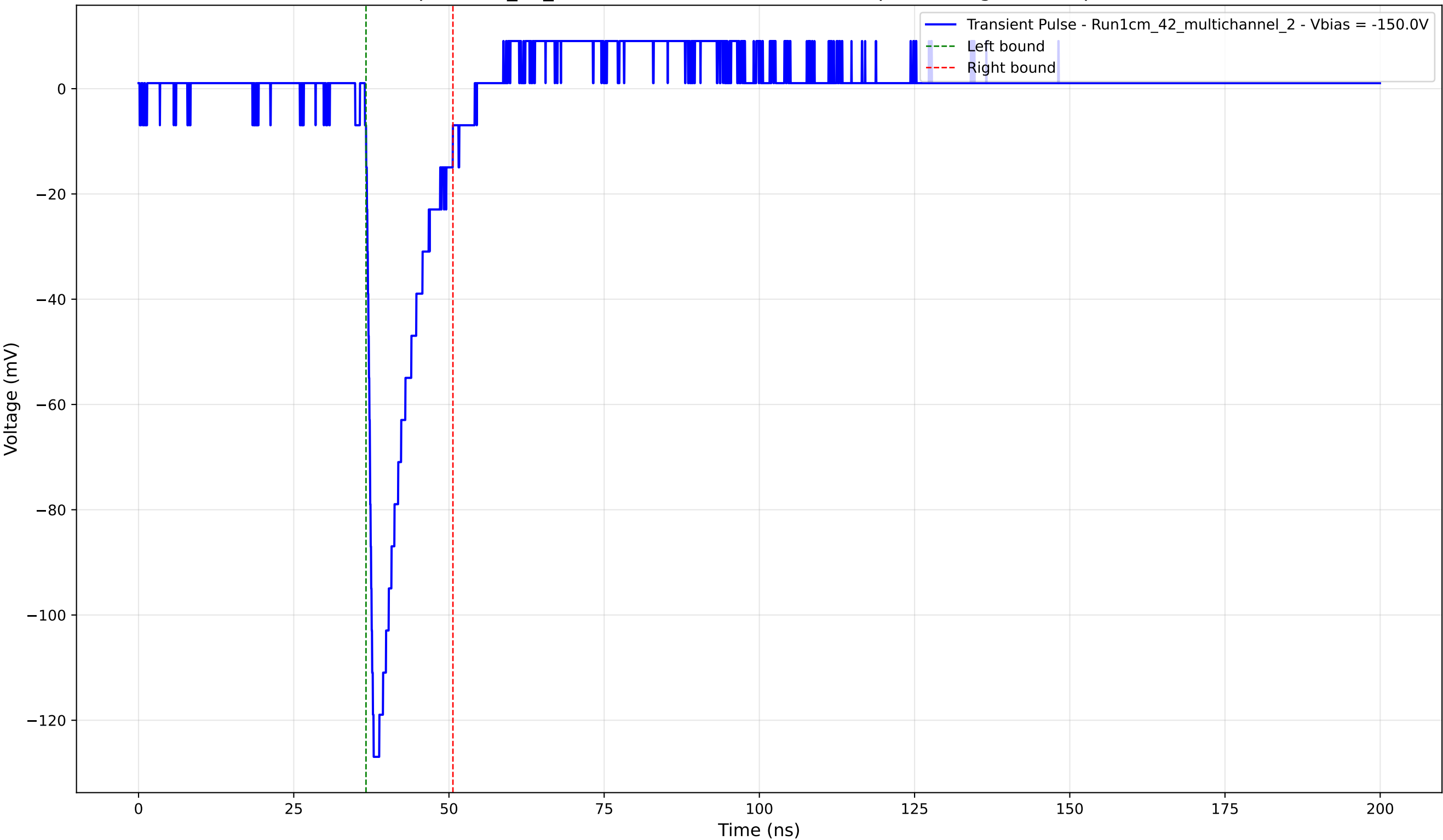
Transient Pulse - Sample: 1cm_42_multichannel - Position: 3510.0 \mu\text{m} - Charge: 16.24 pC - Rise Time: 1.09 ns
