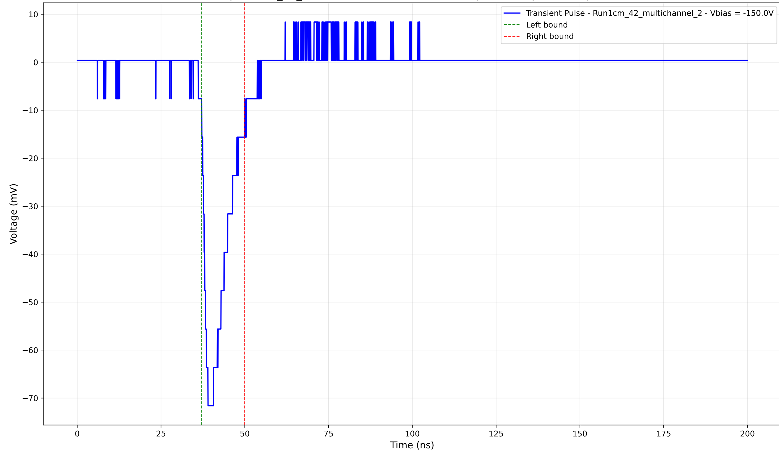
Transient Pulse - Sample: 1cm_42_multichannel - Position: 4525.0 \mu\text{m} - Charge: 10.65 pC - Rise Time: 2.92 ns
