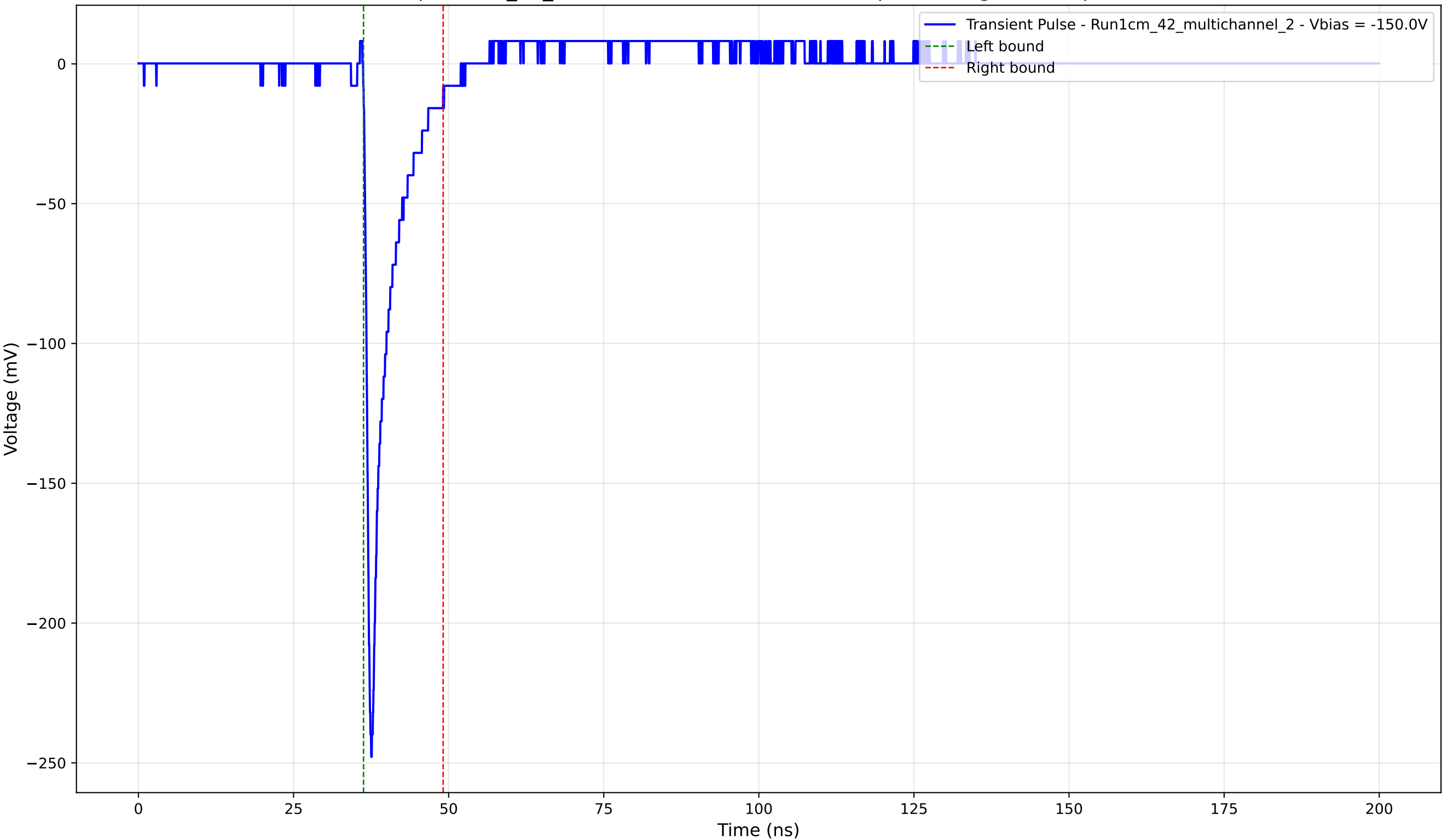
Transient Pulse - Sample: 1cm_42_multichannel - Position: 1795.0 \mu\text{m} - Charge: 18.55 pC - Rise Time: 0.87 ns
