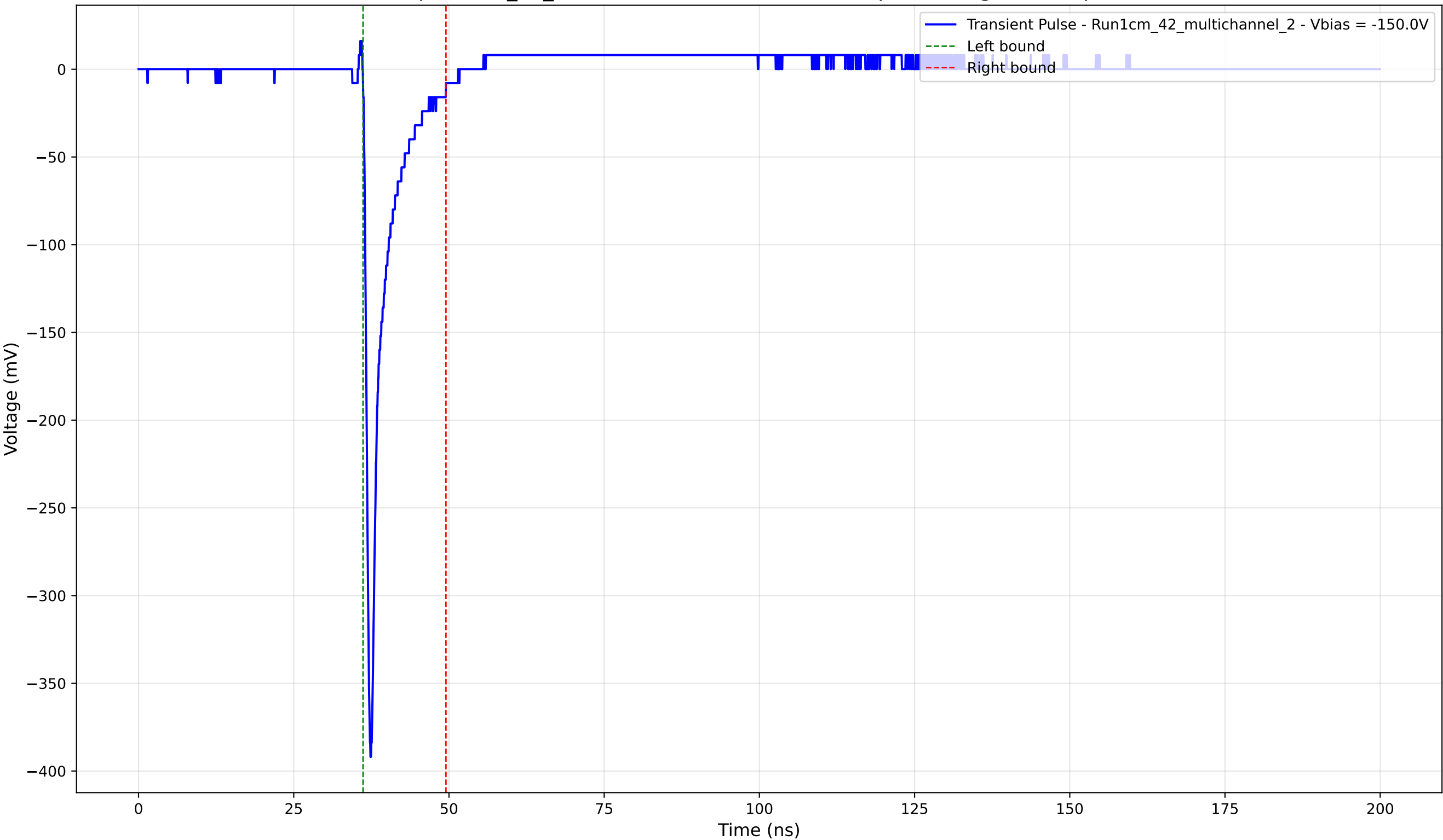
Transient Pulse - Sample: 1cm_42_multichannel - Position: 2760.0 \mu\text{m} - Charge: 24.00 pC - Rise Time: 0.81 ns
