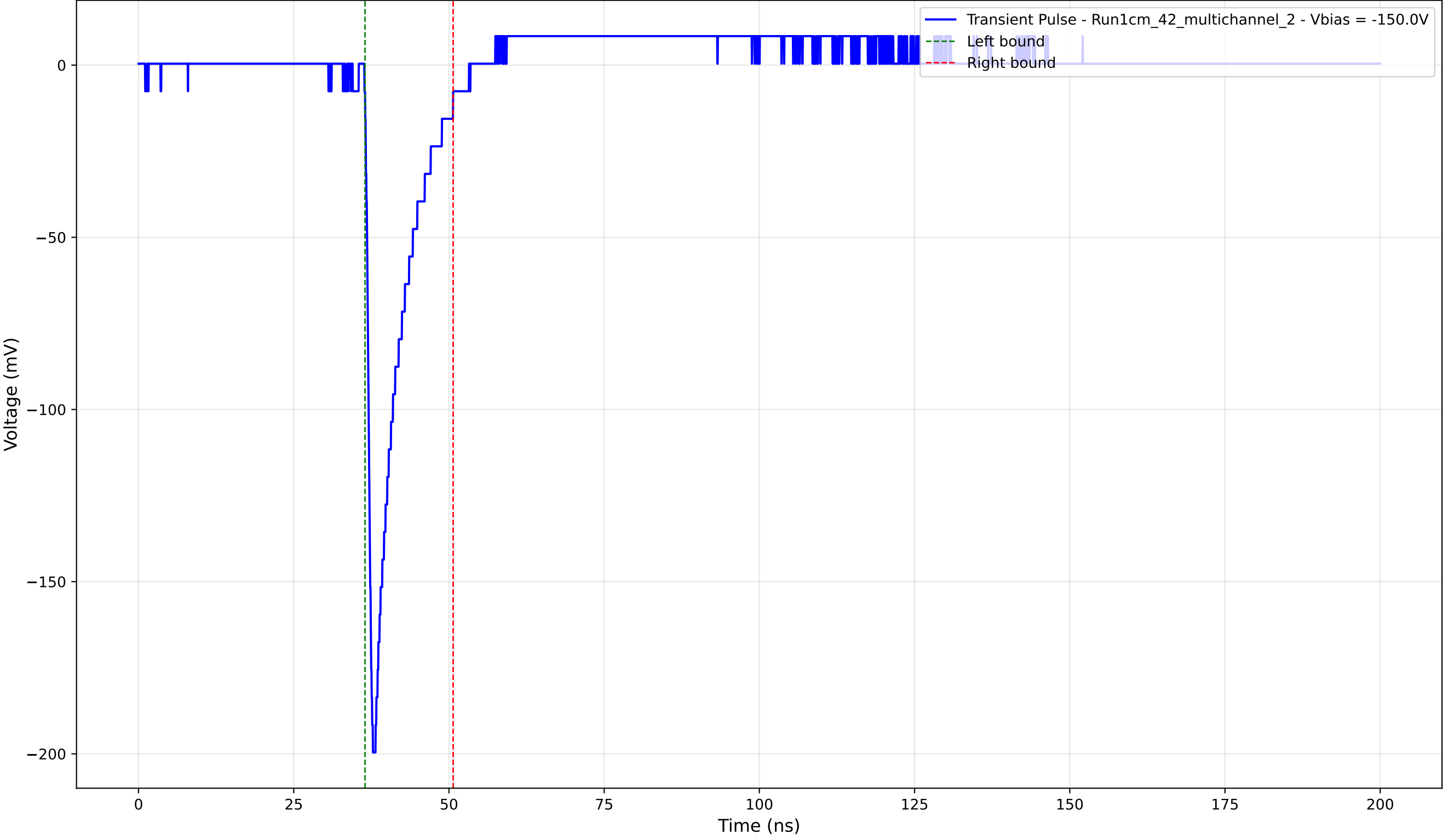
Transient Pulse - Sample: 1cm_42_multichannel - Position: 1465.0 \mu\text{m} - Charge: 20.68 pC - Rise Time: 0.98 ns
