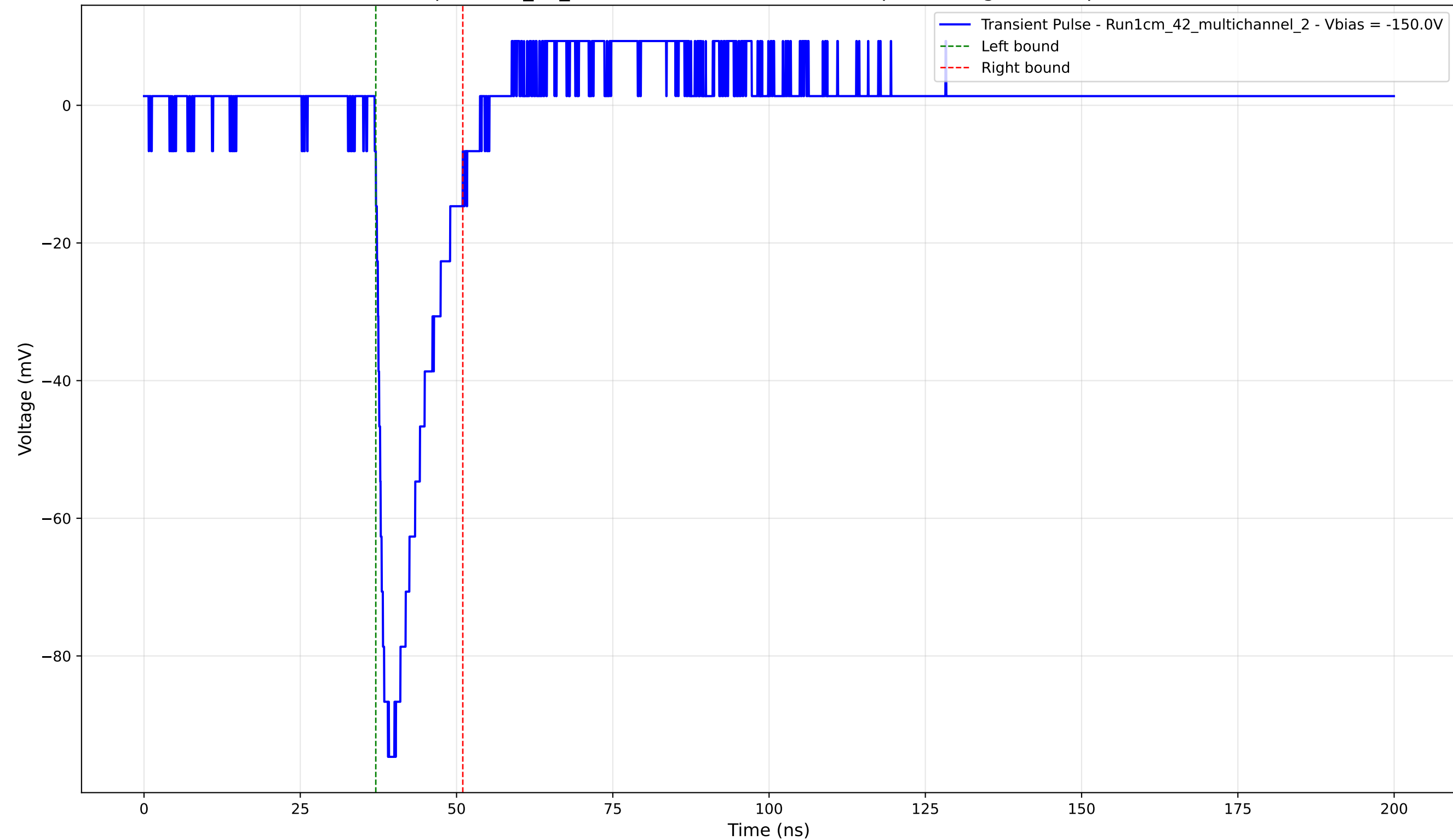
Transient Pulse - Sample: 1cm_42_multichannel - Position: 550.0 \mu\text{m} - Charge: 13.89 pC - Rise Time: 1.35 ns
