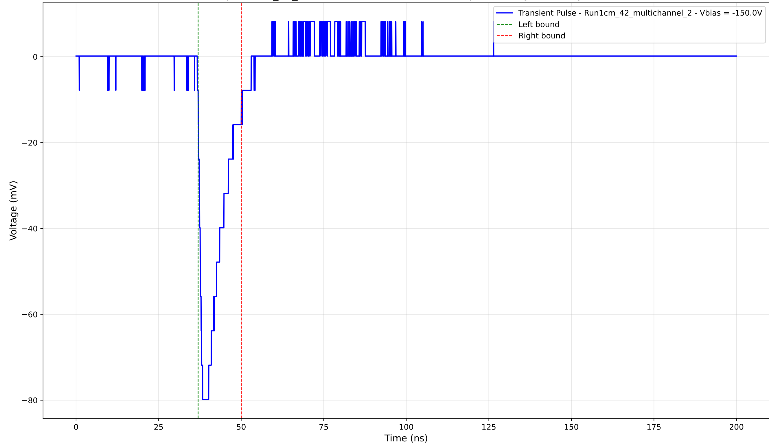
Transient Pulse - Sample: 1cm_42_multichannel - Position: 3820.0 \mu\text{m} - Charge: 11.54 pC - Rise Time: 1.40 ns
