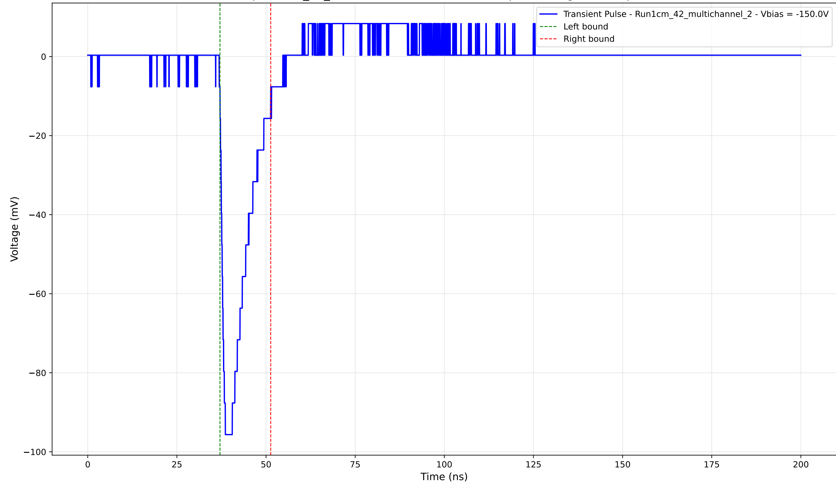
Transient Pulse - Sample: 1cm_42_multichannel - Position: 625.0 \mu\text{m} - Charge: 14.75 pC - Rise Time: 1.23 ns
