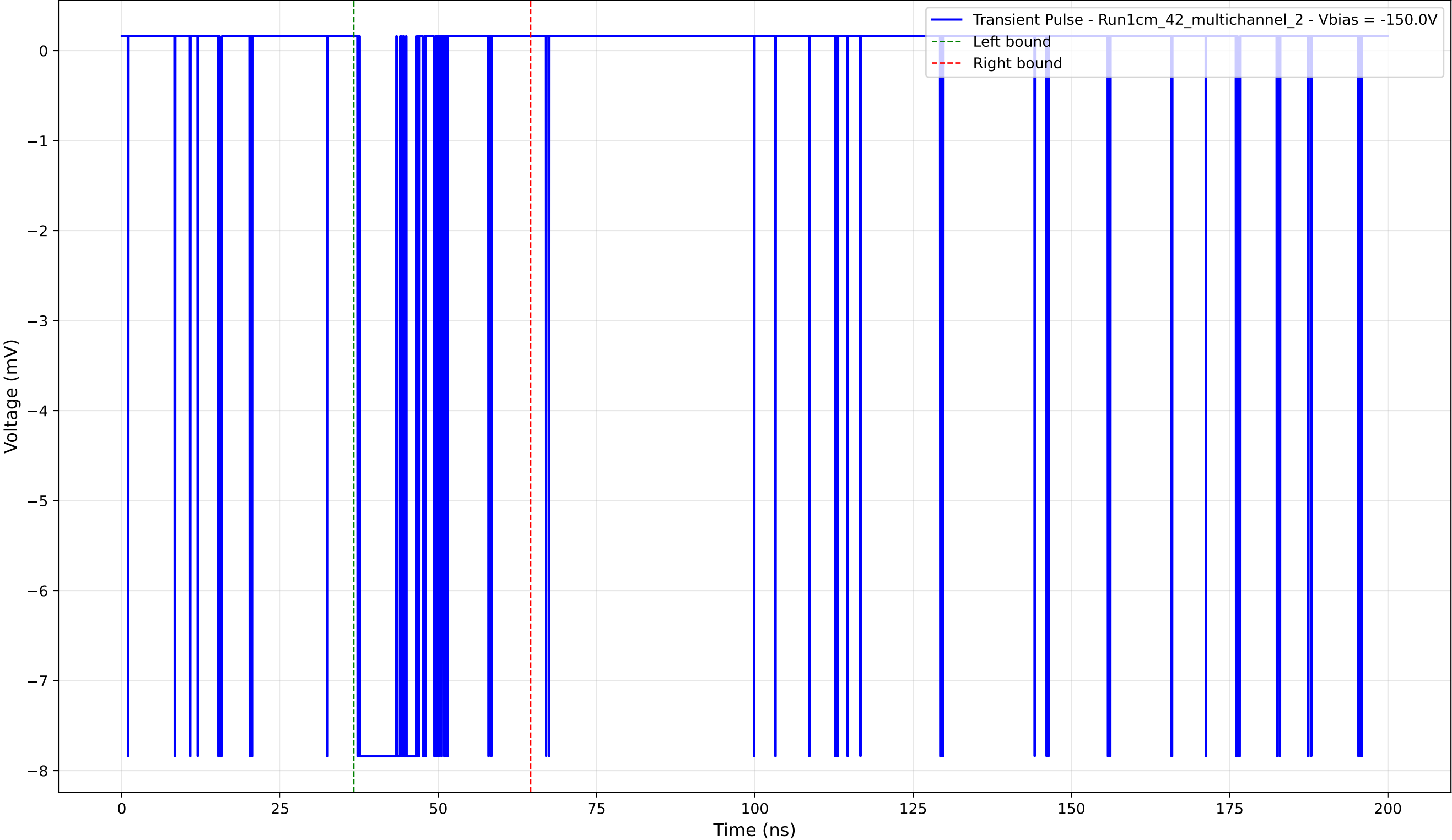
Transient Pulse - Sample: 1cm_42_multichannel - Position: 4375.0 \mu\text{m} - Charge: 1.47 pC - Rise Time: 0.04 ns
