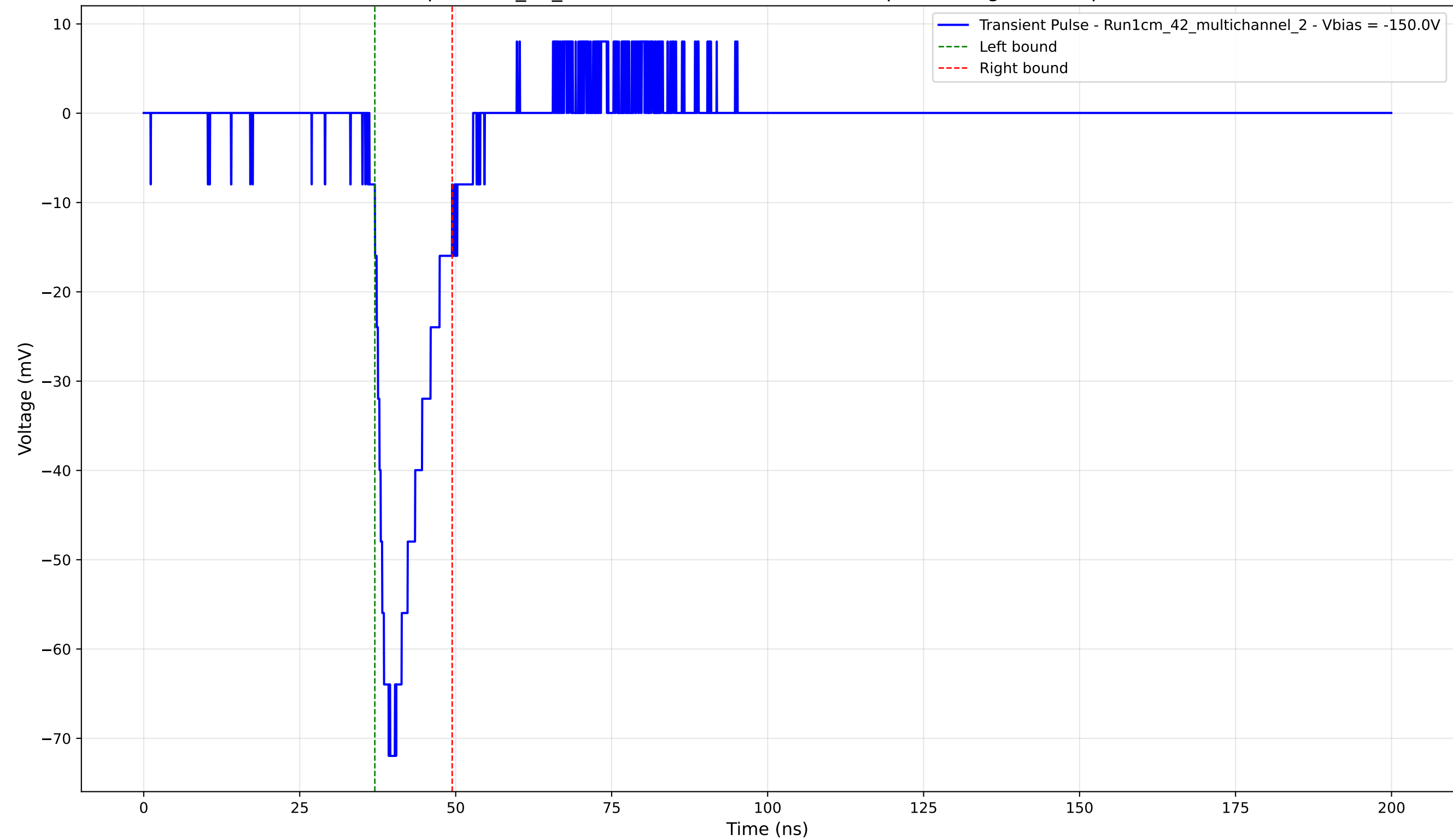
Transient Pulse - Sample: 1cm_42_multichannel - Position: 4705.0 \mu\text{m} - Charge: 10.14 pC - Rise Time: 3.08 ns
