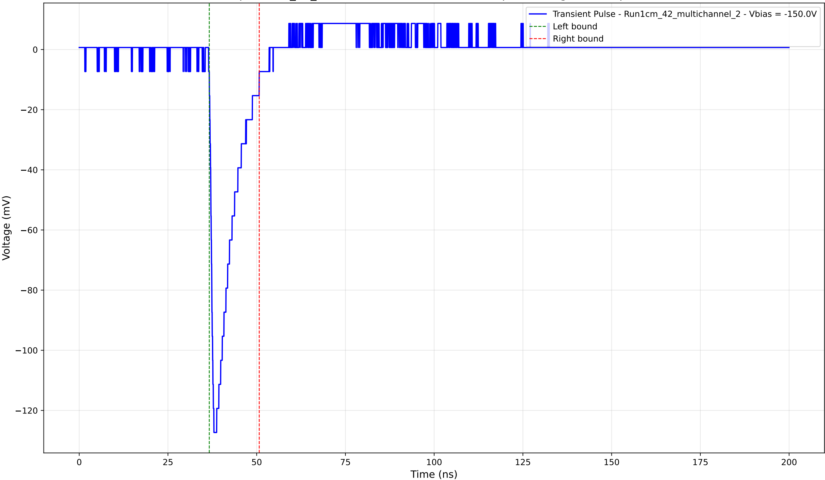
Transient Pulse - Sample: 1cm_42_multichannel - Position: 3520.0 \mu\text{m} - Charge: 16.34 pC - Rise Time: 1.13 ns
