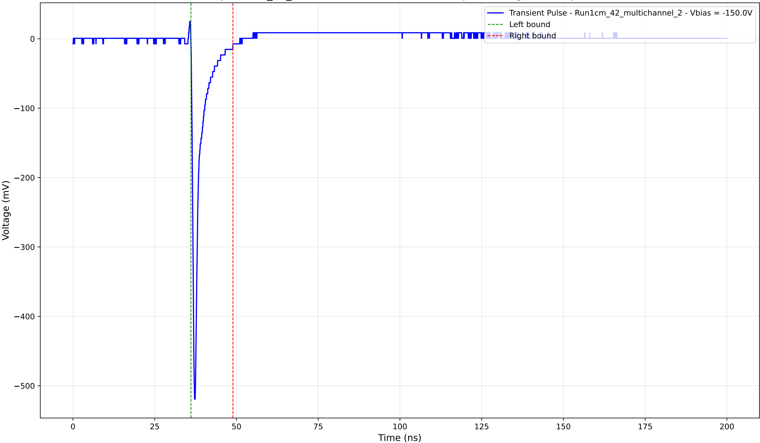
Transient Pulse - Sample: 1cm_42_multichannel - Position: 2140.0 \mu\text{m} - Charge: 26.90 pC - Rise Time: 0.73 ns
