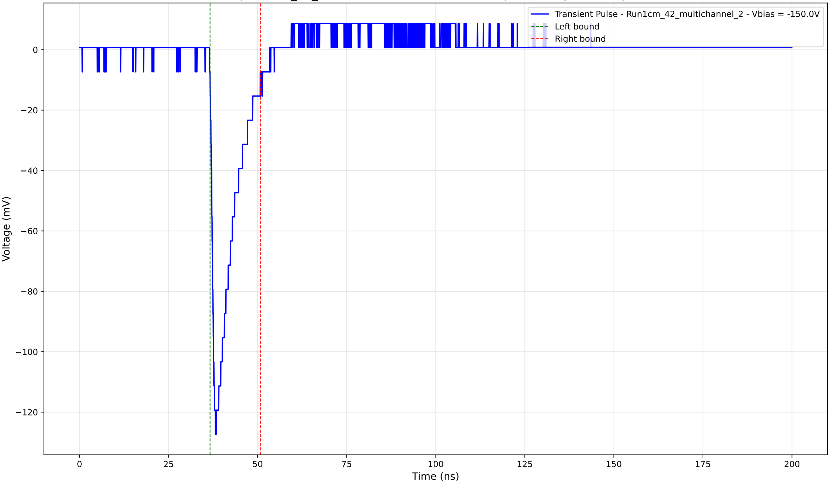
Transient Pulse - Sample: 1cm_42_multichannel - Position: 3540.0 \mu\text{m} - Charge: 15.93 pC - Rise Time: 1.25 ns
