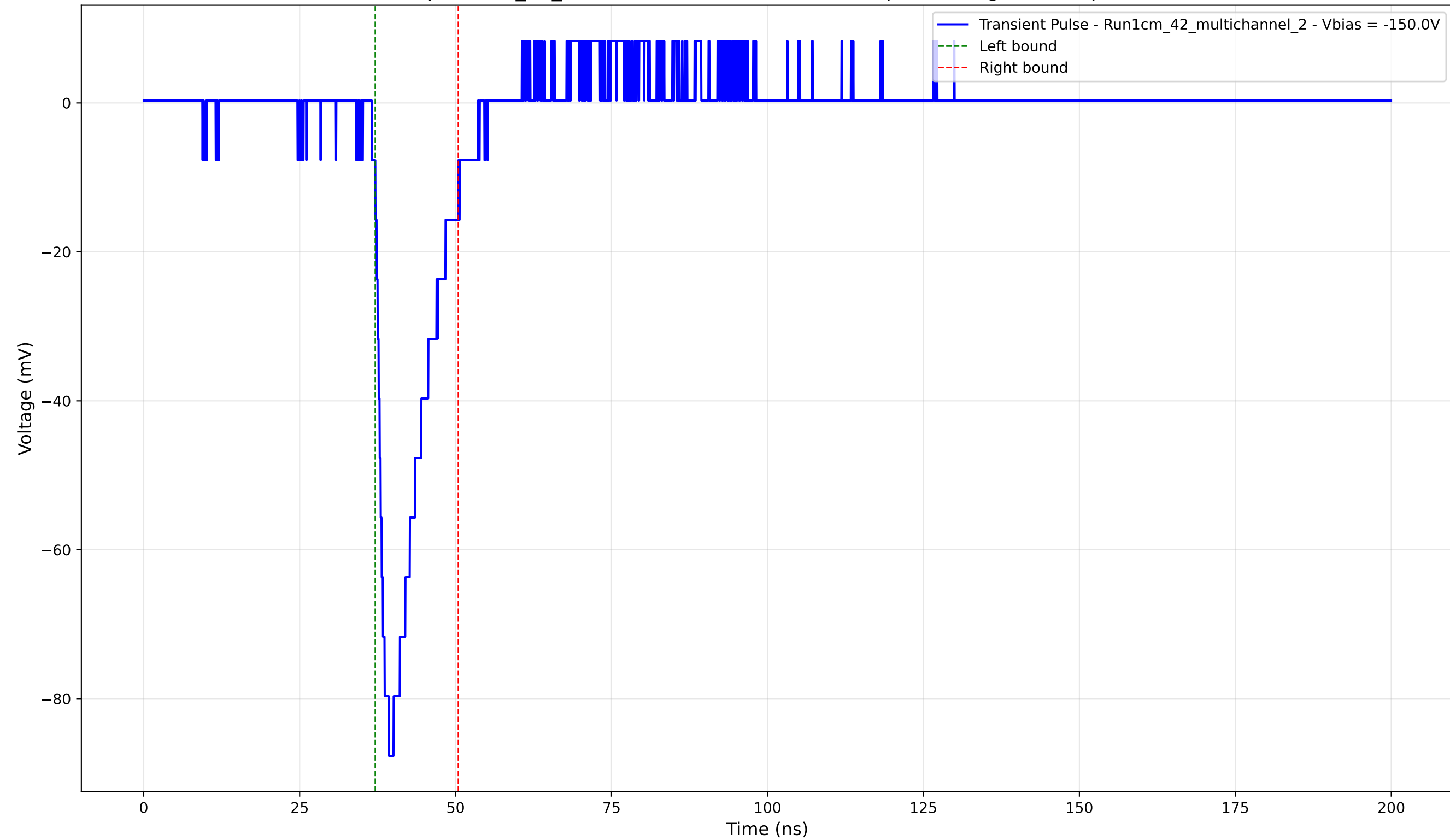
Transient Pulse - Sample: 1cm_42_multichannel - Position: 4170.0 \mu\text{m} - Charge: 12.49 pC - Rise Time: 1.51 ns
