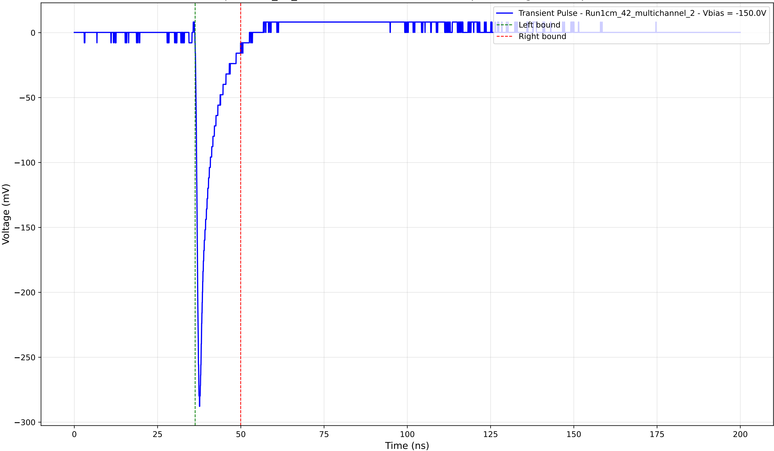
Transient Pulse - Sample: 1cm_42_multichannel - Position: 1725.0 \mu\text{m} - Charge: 23.14 pC - Rise Time: 0.91 ns
