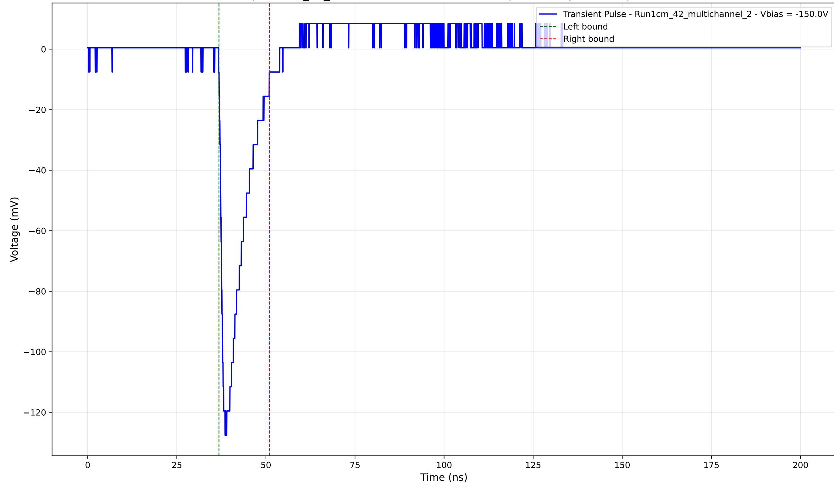
Transient Pulse - Sample: 1cm_42_multichannel - Position: 980.0 \mu\text{m} - Charge: 17.10 pC - Rise Time: 1.29 ns
