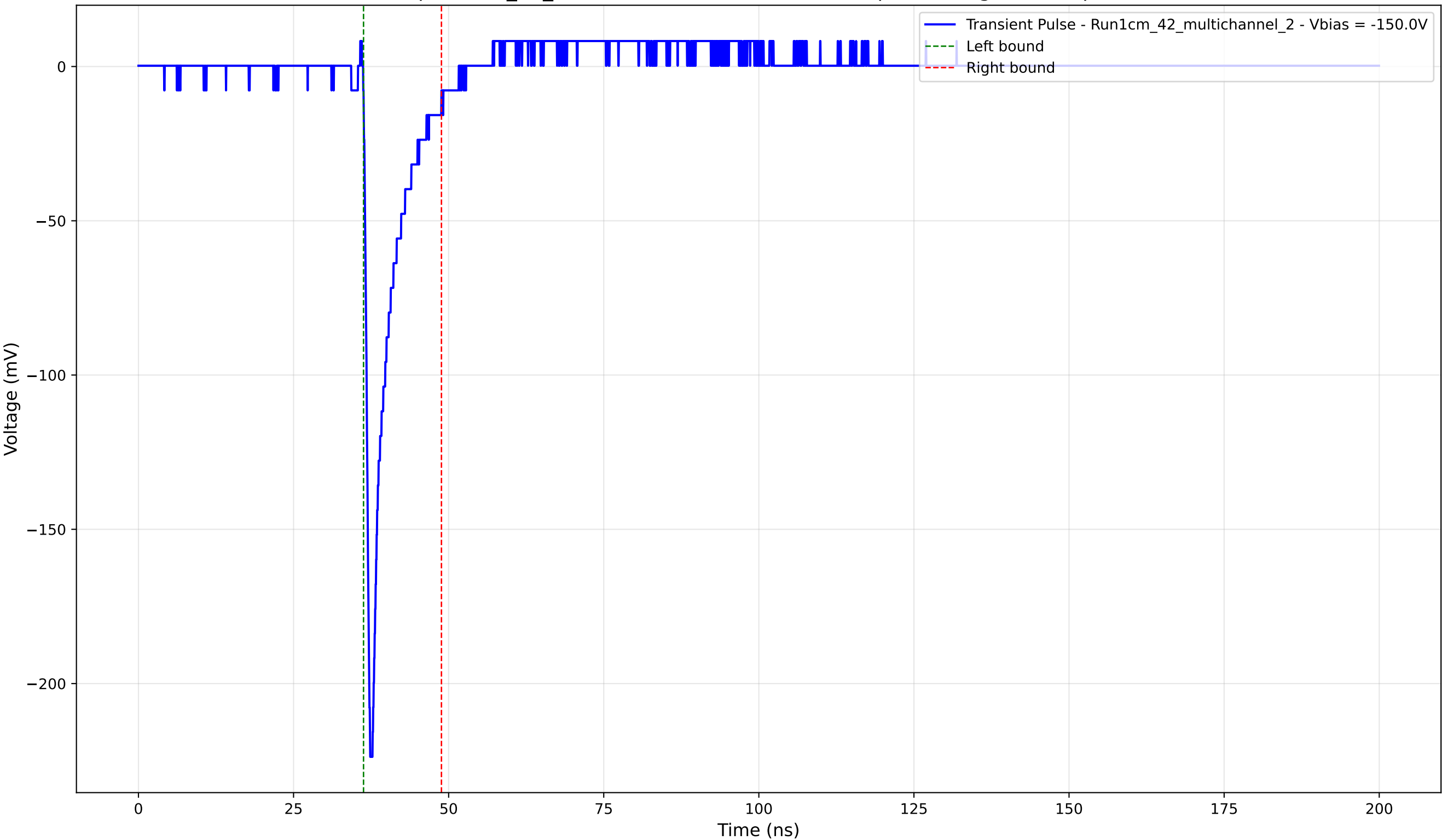
Transient Pulse - Sample: 1cm_42_multichannel - Position: 1800.0 \mu\text{m} - Charge: 17.12 pC - Rise Time: 0.89 ns
