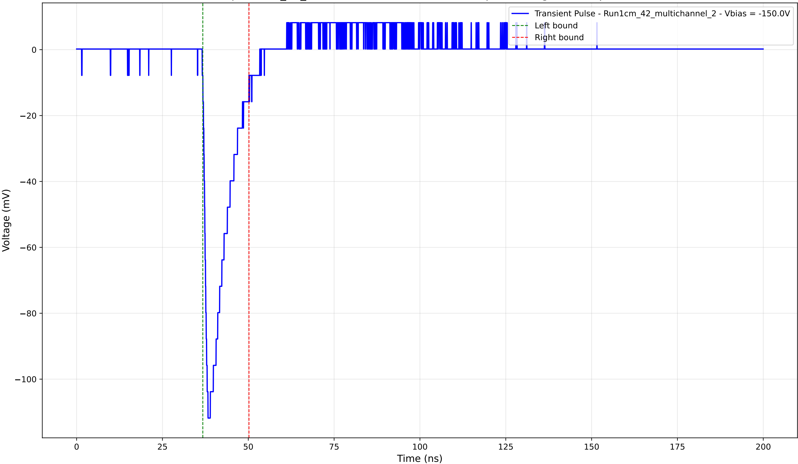
Transient Pulse - Sample: 1cm_42_multichannel - Position: 3680.0 \mu\text{m} - Charge: 14.93 pC - Rise Time: 1.26 ns
