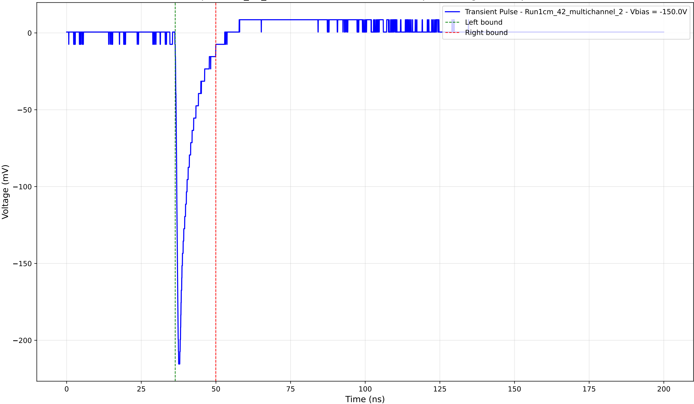
Transient Pulse - Sample: 1cm_42_multichannel - Position: 3090.0 \mu\text{m} - Charge: 19.15 pC - Rise Time: 0.89 ns
