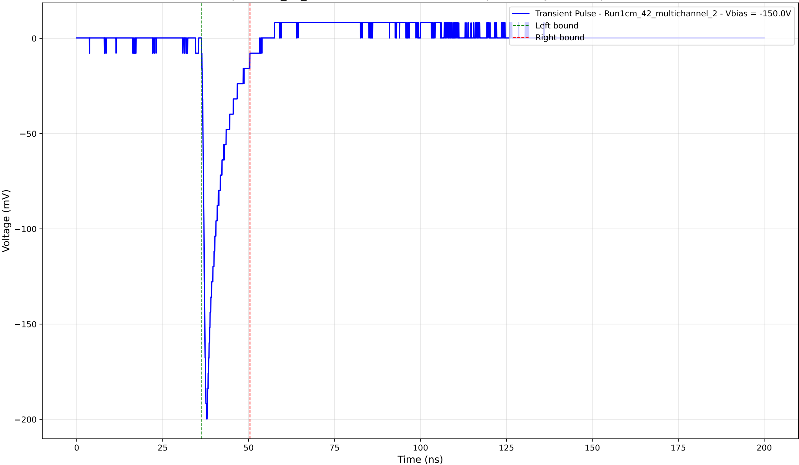
Transient Pulse - Sample: 1cm_42_multichannel - Position: 3190.0 \mu\text{m} - Charge: 19.18 pC - Rise Time: 0.98 ns
