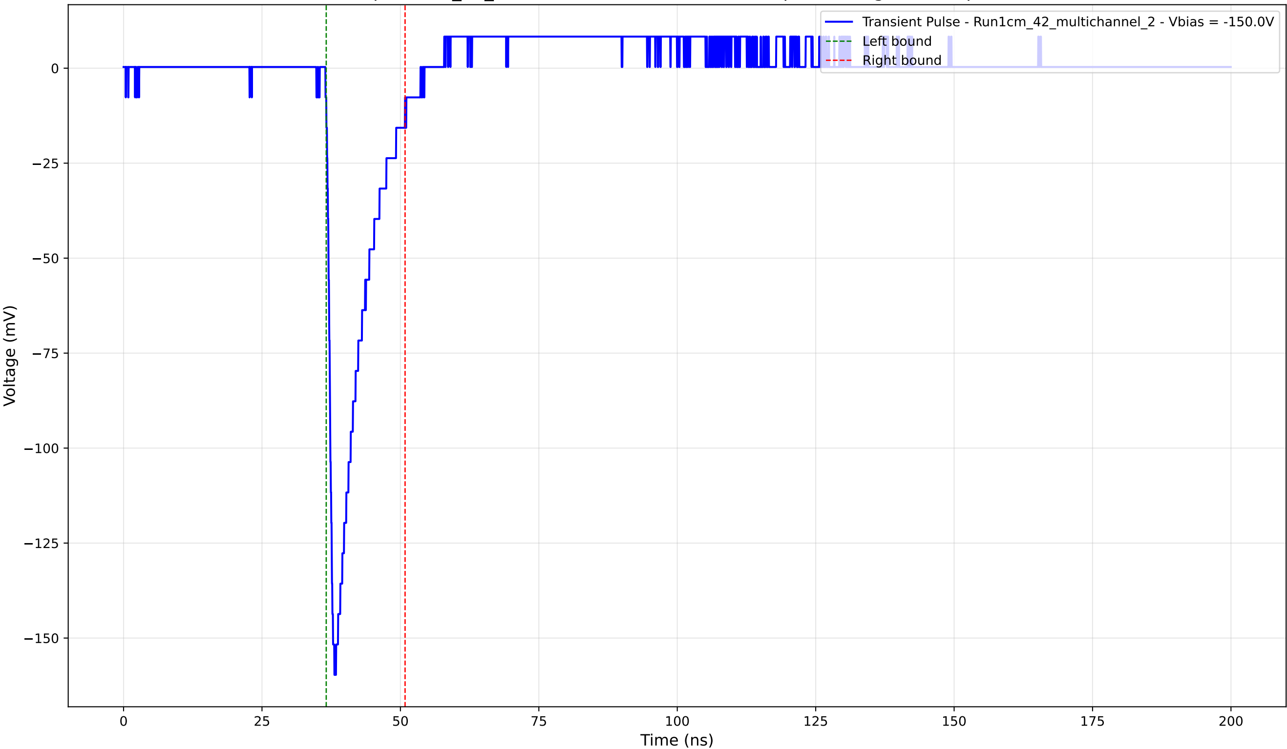
Transient Pulse - Sample: 1cm_42_multichannel - Position: 1250.0 \mu\text{m} - Charge: 19.01 pC - Rise Time: 1.12 ns
