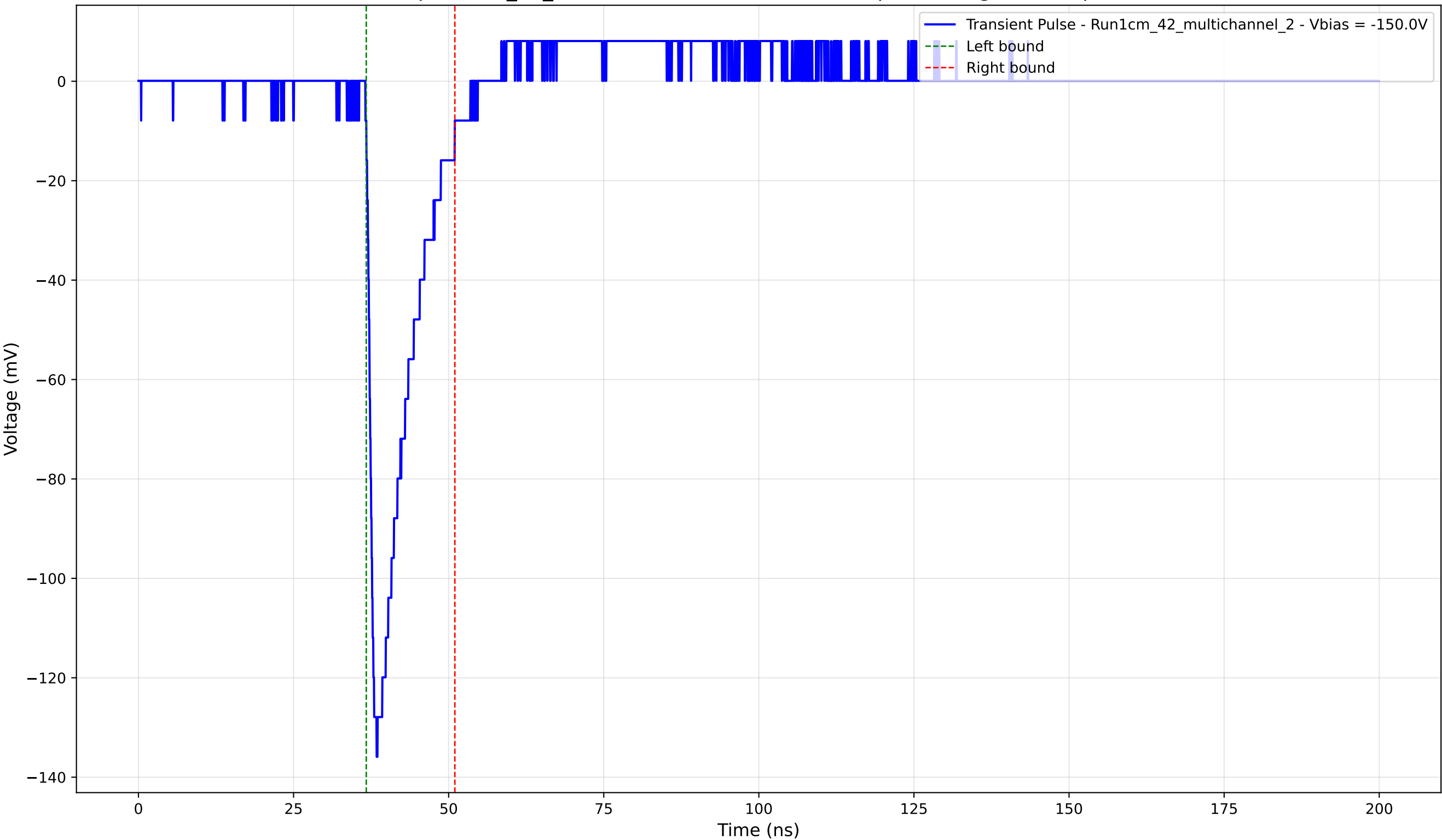
Transient Pulse - Sample: 1cm_42_multichannel - Position: 1115.0 \mu\text{m} - Charge: 17.46 pC - Rise Time: 1.25 ns
