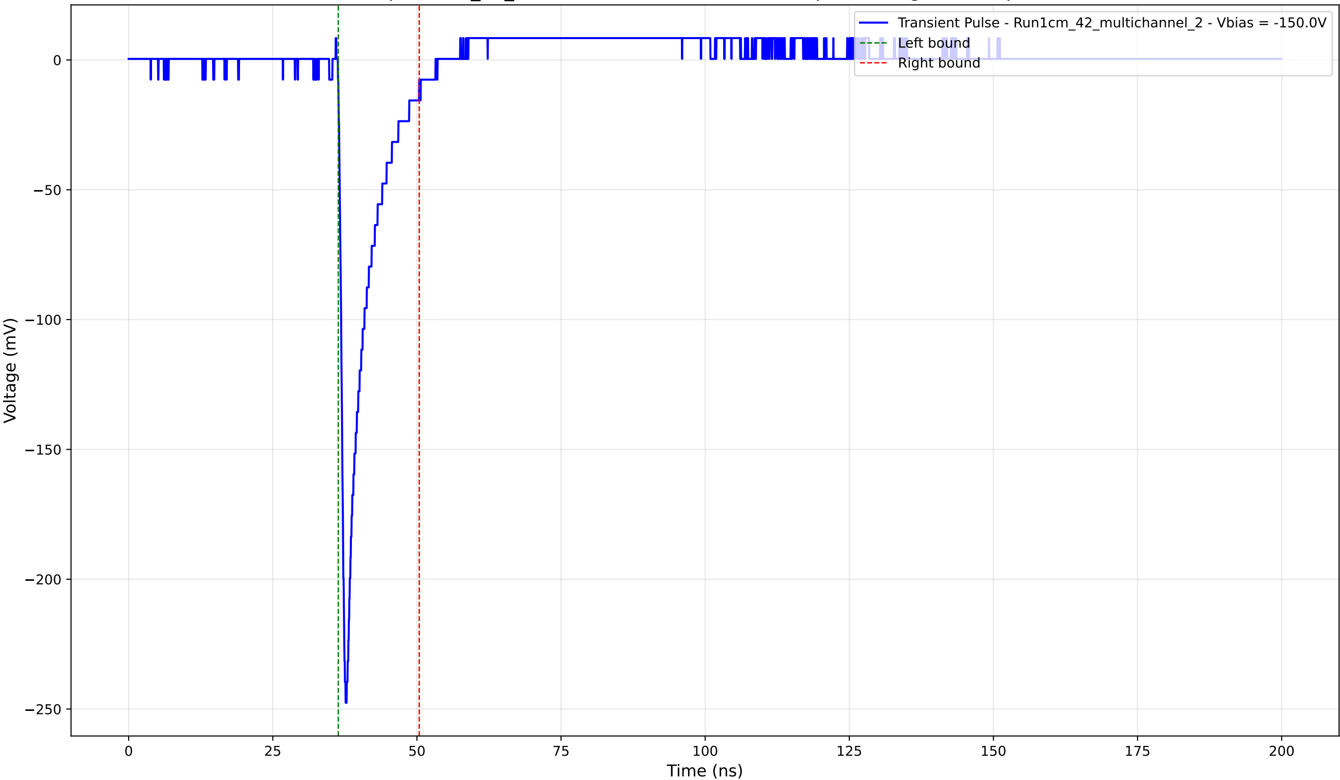
Transient Pulse - Sample: 1cm_42_multichannel - Position: 1635.0 \mu\text{m} - Charge: 22.02 pC - Rise Time: 0.91 ns
