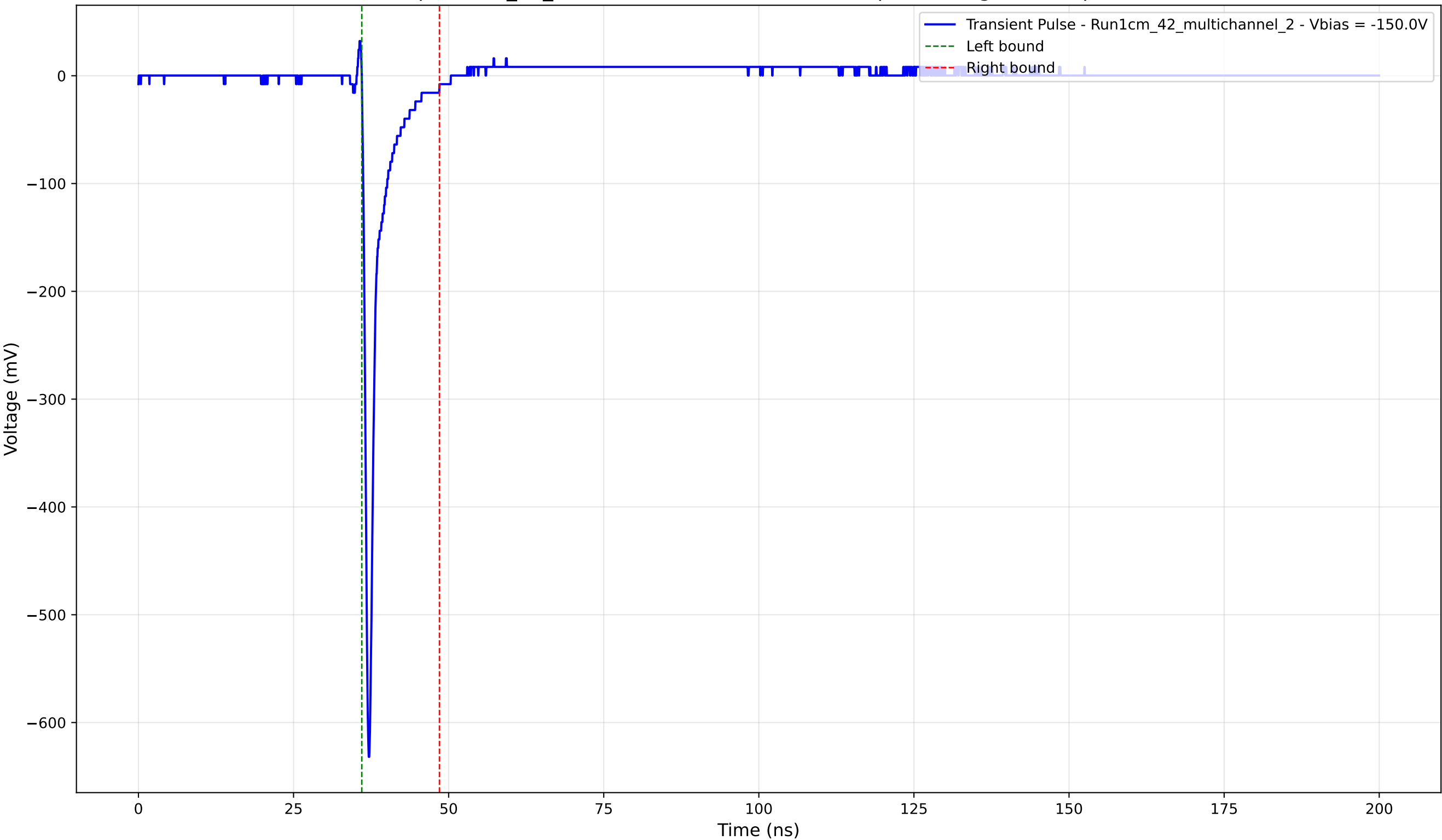
Transient Pulse - Sample: 1cm_42_multichannel - Position: 2275.0 \mu\text{m} - Charge: 28.47 pC - Rise Time: 0.72 ns
