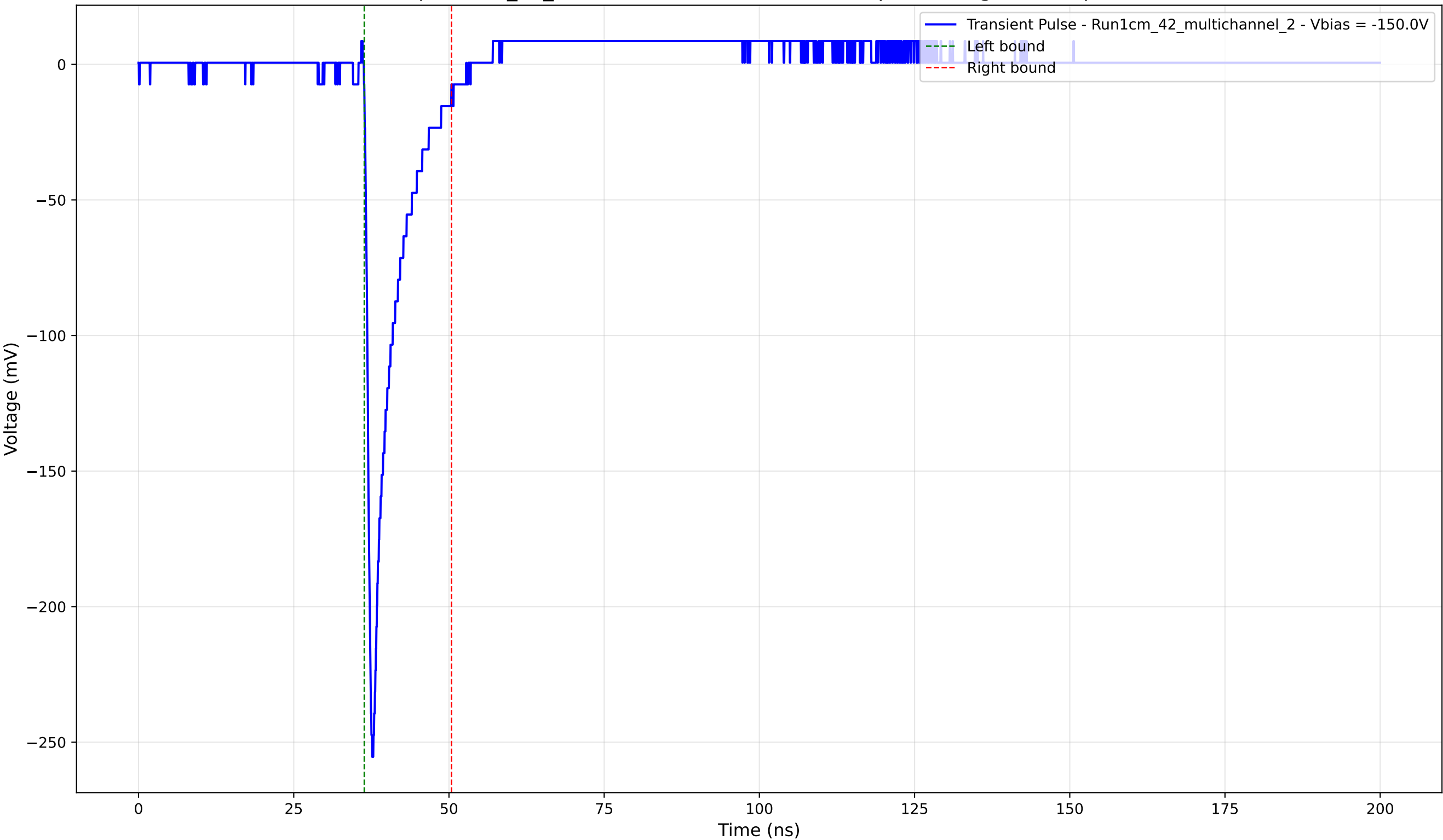
Transient Pulse - Sample: 1cm_42_multichannel - Position: 1650.0 \mu\text{m} - Charge: 22.22 pC - Rise Time: 0.90 ns
