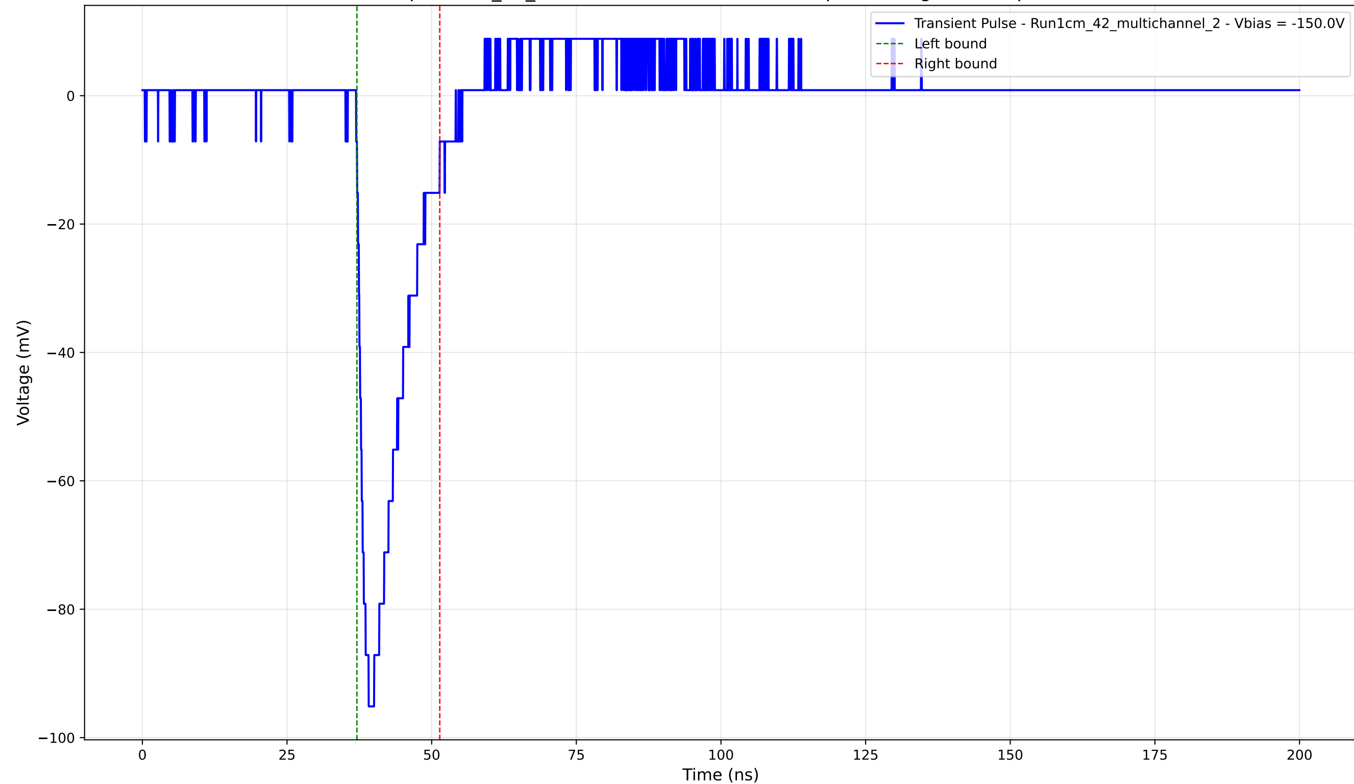
Transient Pulse - Sample: 1cm_42_multichannel - Position: 525.0 \mu\text{m} - Charge: 14.04 pC - Rise Time: 1.51 ns
