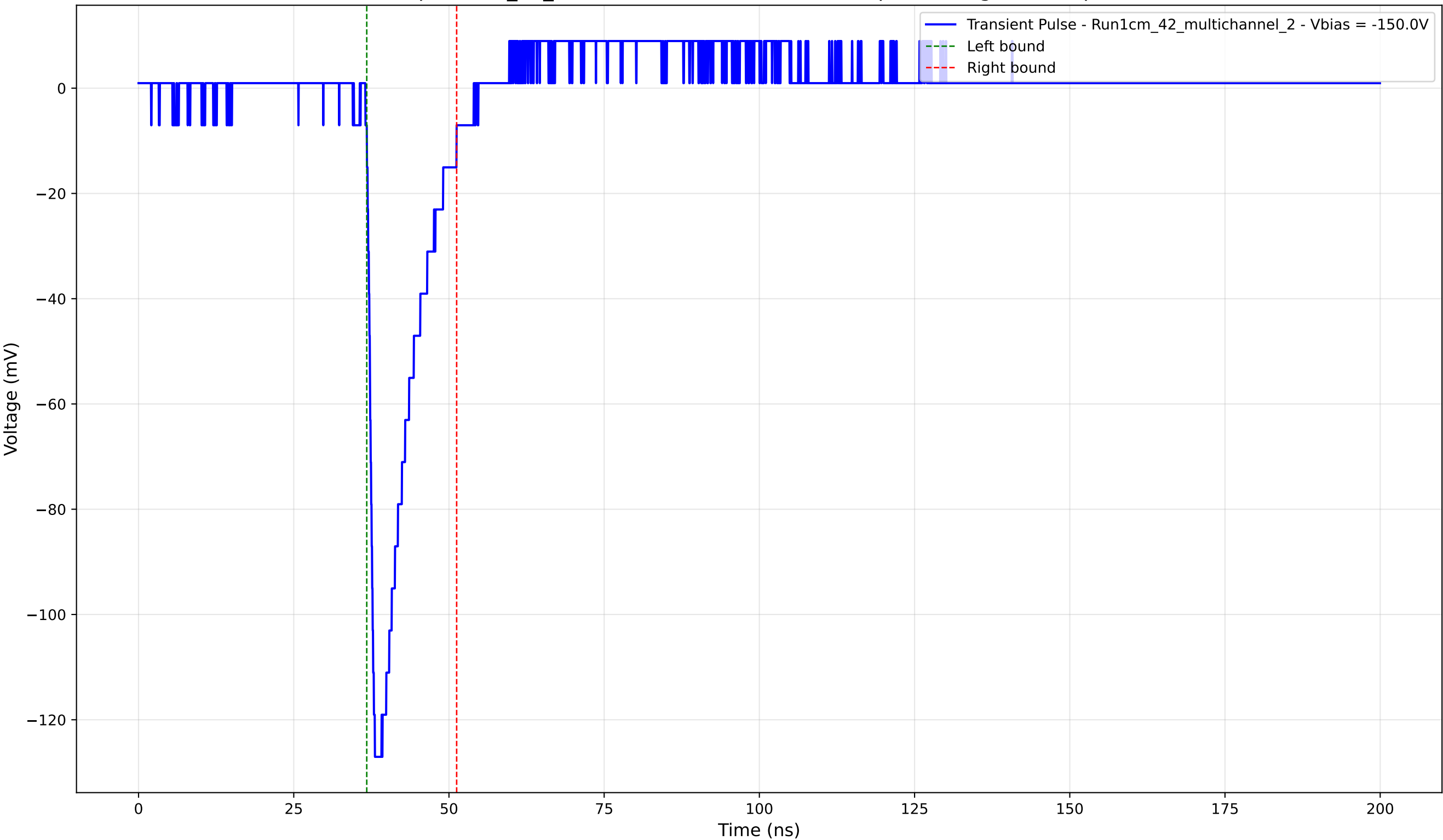
Transient Pulse - Sample: 1cm_42_multichannel - Position: 1080.0 \mu\text{m} - Charge: 17.33 pC - Rise Time: 1.13 ns
