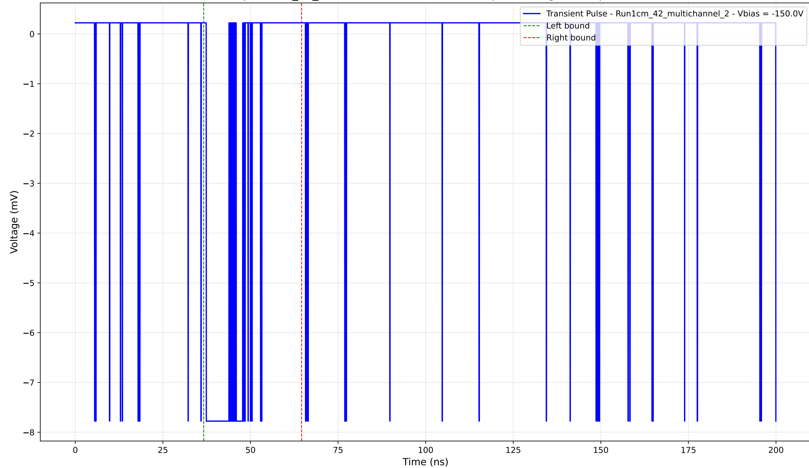
Transient Pulse - Sample: 1cm_42_multichannel - Position: 865.0 \mu\text{m} - Charge: 1.57 pC - Rise Time: 0.04 ns
