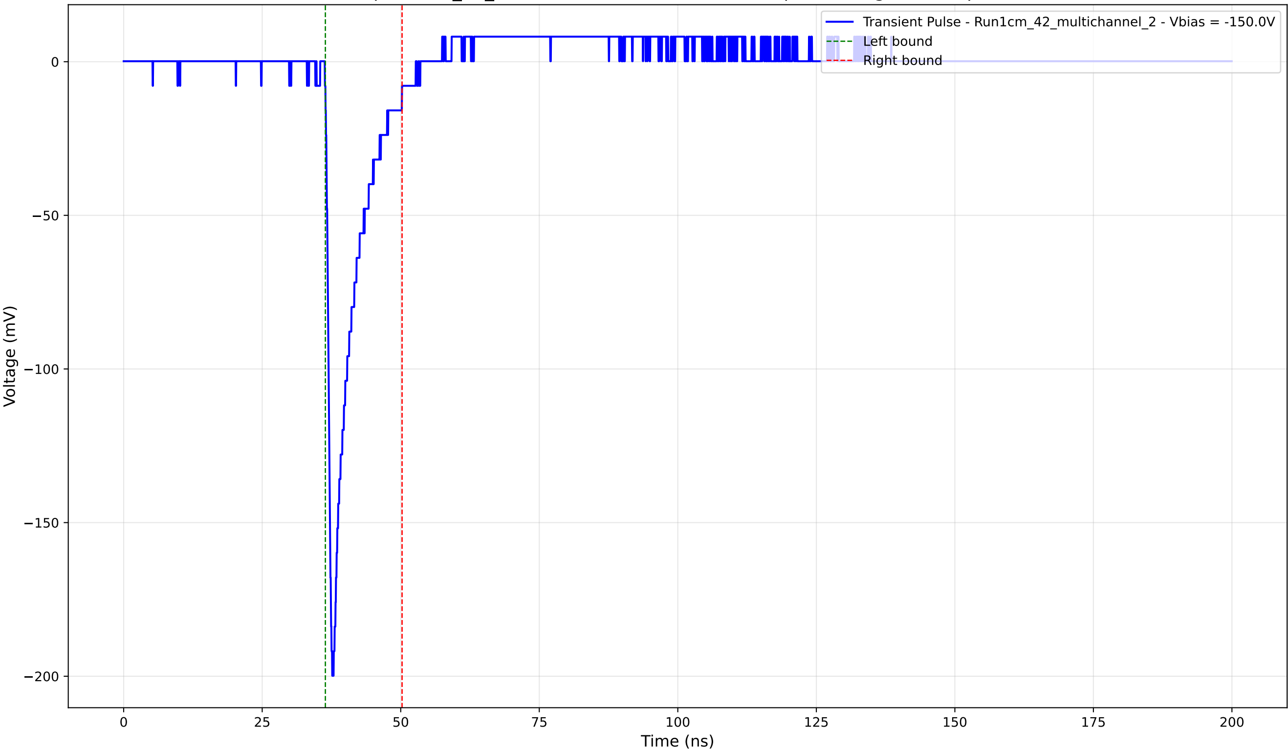
Transient Pulse - Sample: 1cm_42_multichannel - Position: 3155.0 \mu\text{m} - Charge: 18.60 pC - Rise Time: 0.94 ns
