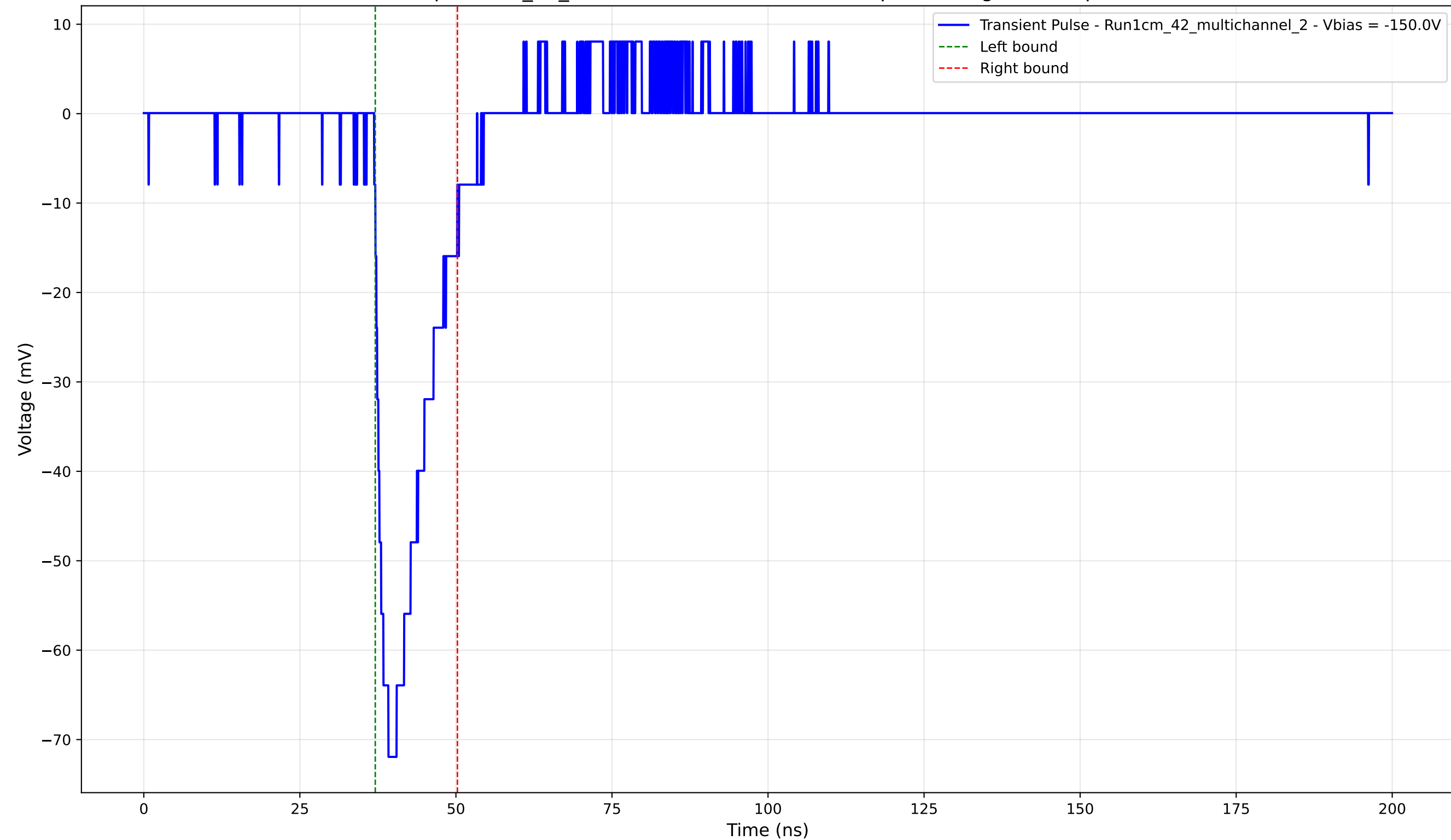
Transient Pulse - Sample: 1cm_42_multichannel - Position: 255.0 \mu\text{m} - Charge: 11.02 pC - Rise Time: 2.28 ns
