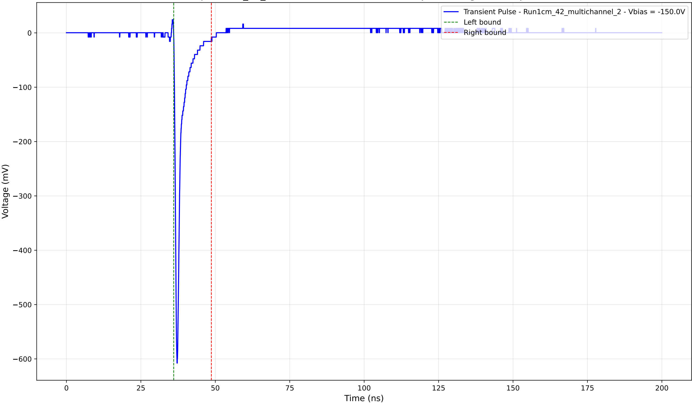
Transient Pulse - Sample: 1cm_42_multichannel - Position: 2225.0 \mu\text{m} - Charge: 28.69 pC - Rise Time: 0.74 ns
