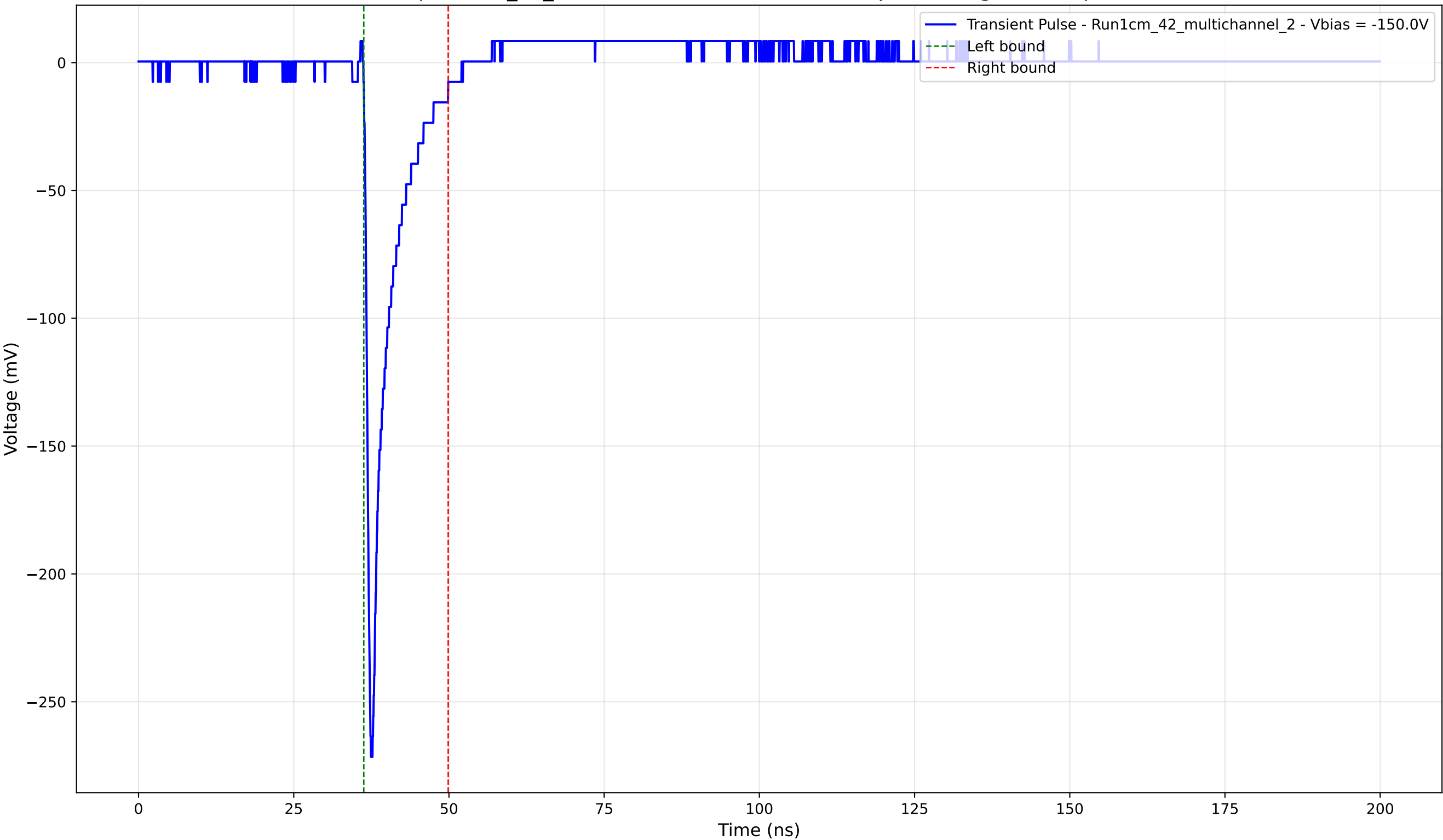
Transient Pulse - Sample: 1cm_42_multichannel - Position: 2960.0 \mu\text{m} - Charge: 20.81 pC - Rise Time: 0.85 ns
