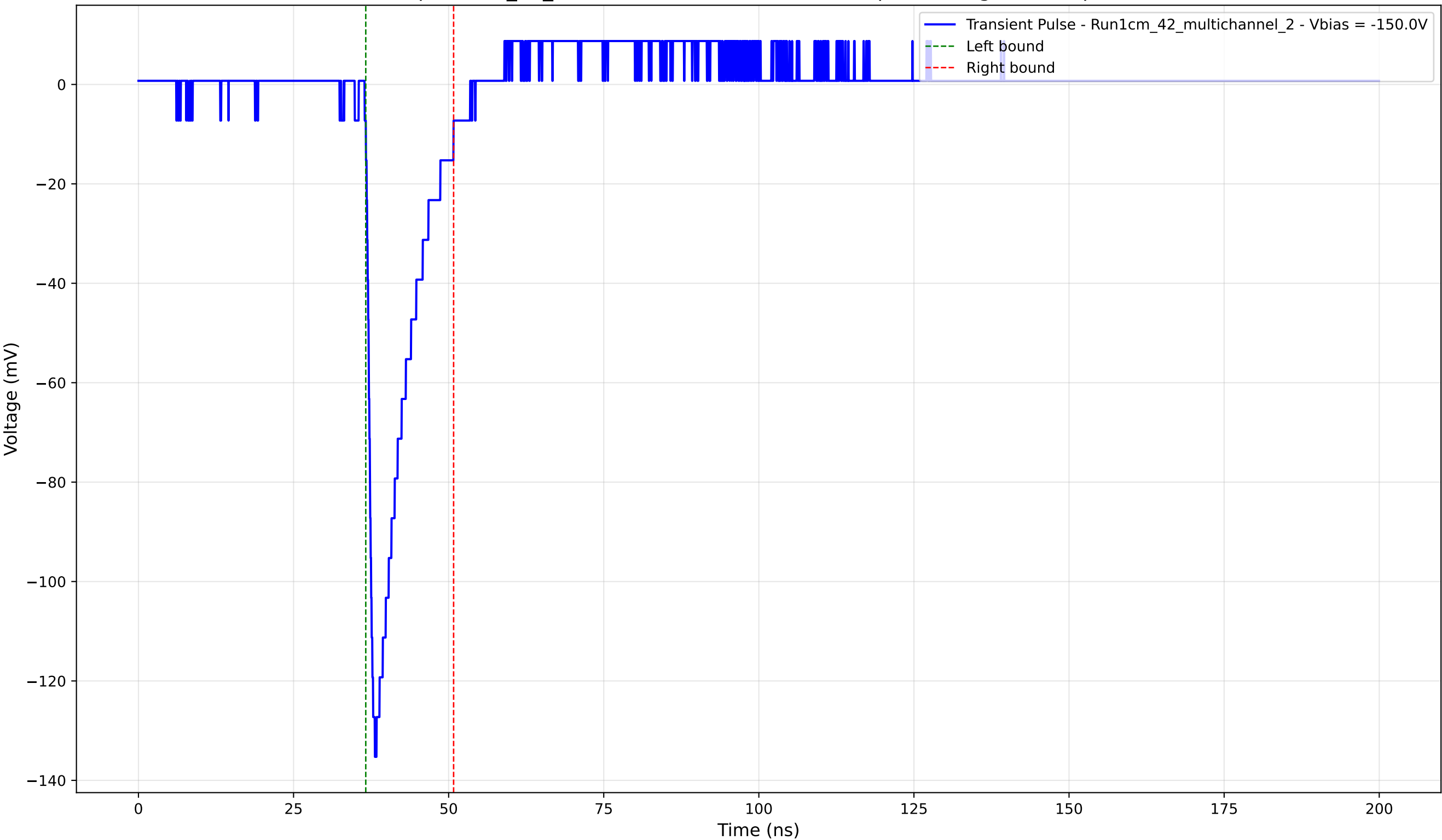
Transient Pulse - Sample: 1cm_42_multichannel - Position: 3495.0 \mu\text{m} - Charge: 16.53 pC - Rise Time: 1.17 ns
