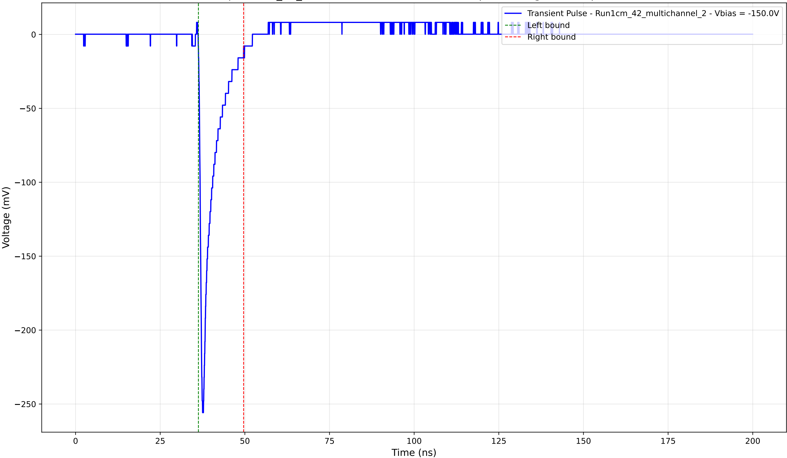
Transient Pulse - Sample: 1cm_42_multichannel - Position: 3015.0 \mu\text{m} - Charge: 20.83 pC - Rise Time: 0.87 ns
