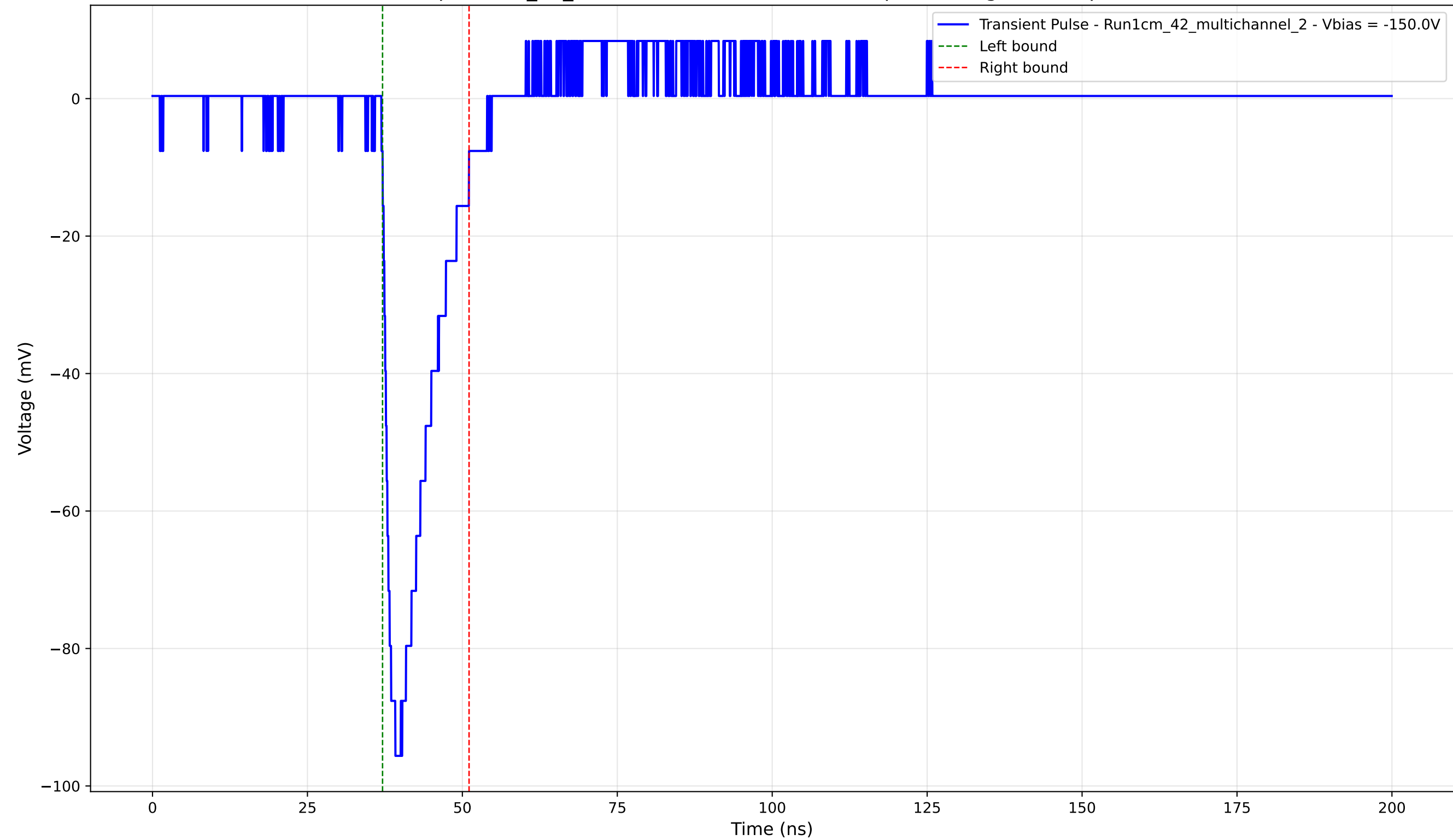
Transient Pulse - Sample: 1cm_42_multichannel - Position: 545.0 \mu\text{m} - Charge: 14.05 pC - Rise Time: 1.39 ns
