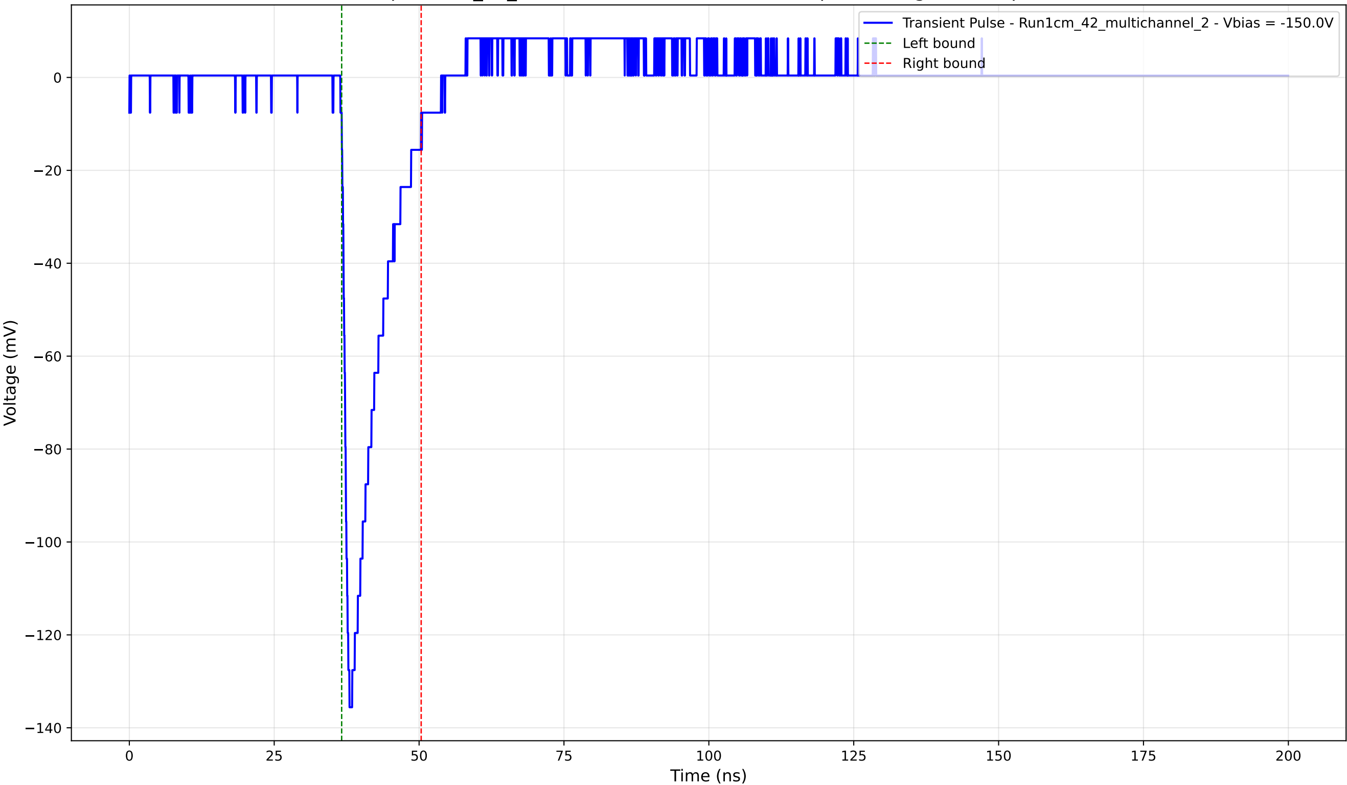
Transient Pulse - Sample: 1cm_42_multichannel - Position: 3475.0 \mu\text{m} - Charge: 16.42 pC - Rise Time: 1.13 ns
