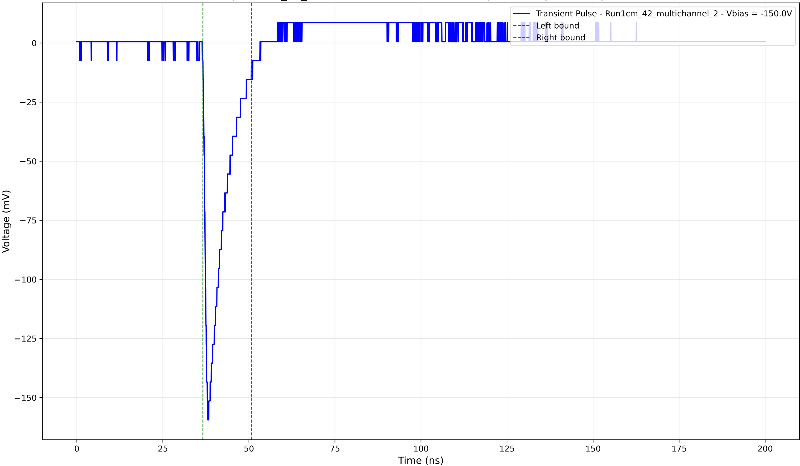
Transient Pulse - Sample: 1cm_42_multichannel - Position: 1240.0 \mu\text{m} - Charge: 18.98 pC - Rise Time: 1.20 ns
