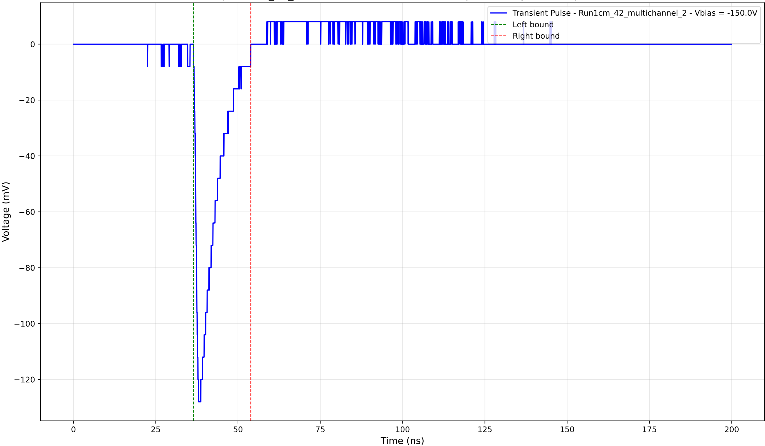
Transient Pulse - Sample: 1cm_42_multichannel - Position: 3530.0 \mu\text{m} - Charge: 16.80 pC - Rise Time: 1.18 ns
