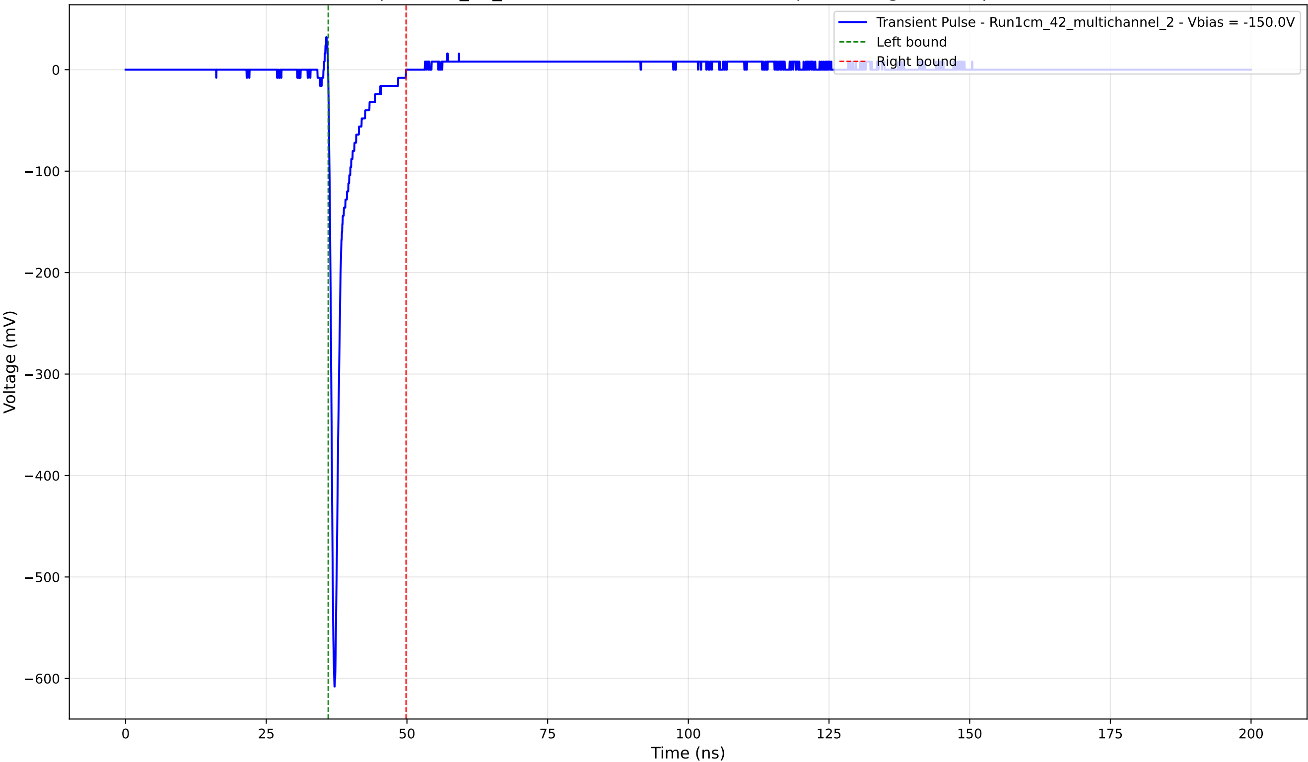
Transient Pulse - Sample: 1cm_42_multichannel - Position: 2445.0 \mu\text{m} - Charge: 27.21 pC - Rise Time: 0.72 ns
