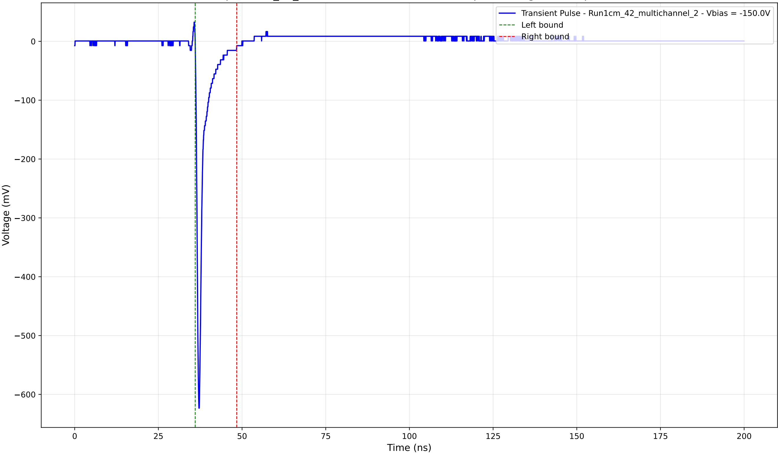
Transient Pulse - Sample: 1cm_42_multichannel - Position: 2285.0 \mu\text{m} - Charge: 27.83 pC - Rise Time: 0.73 ns
