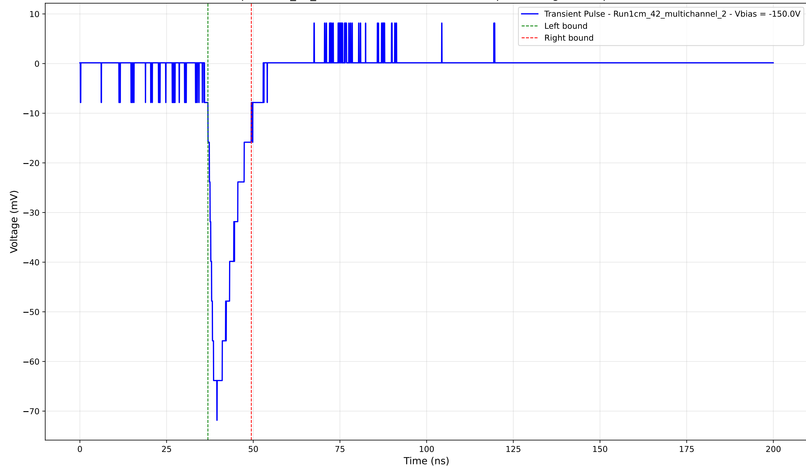
Transient Pulse - Sample: 1cm_42_multichannel - Position: 4740.0 \mu\text{m} - Charge: 9.79 pC - Rise Time: 3.56 ns
