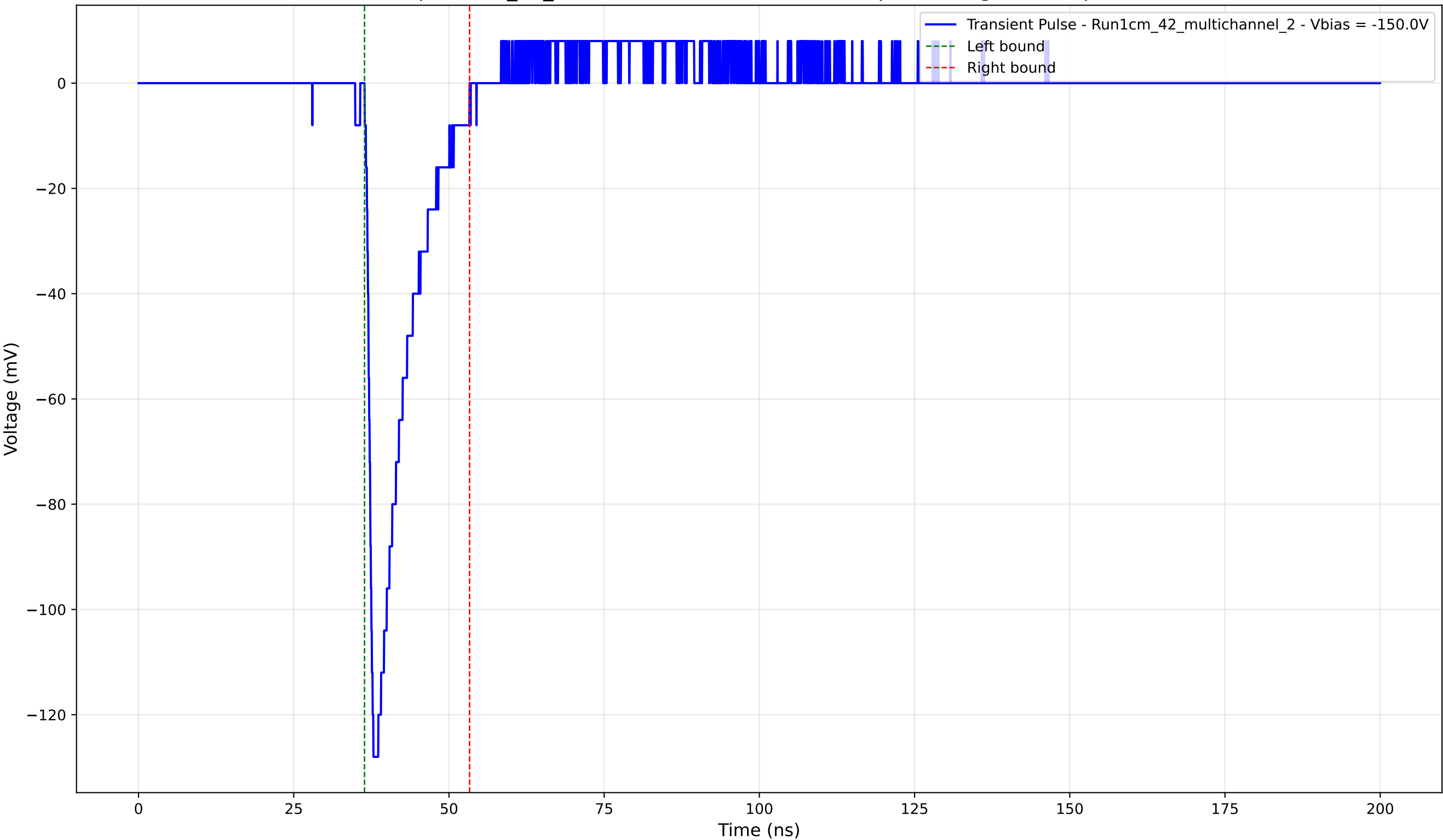
Transient Pulse - Sample: 1cm_42_multichannel - Position: 1290.0 \mu\text{m} - Charge: 16.15 pC - Rise Time: 1.10 ns
