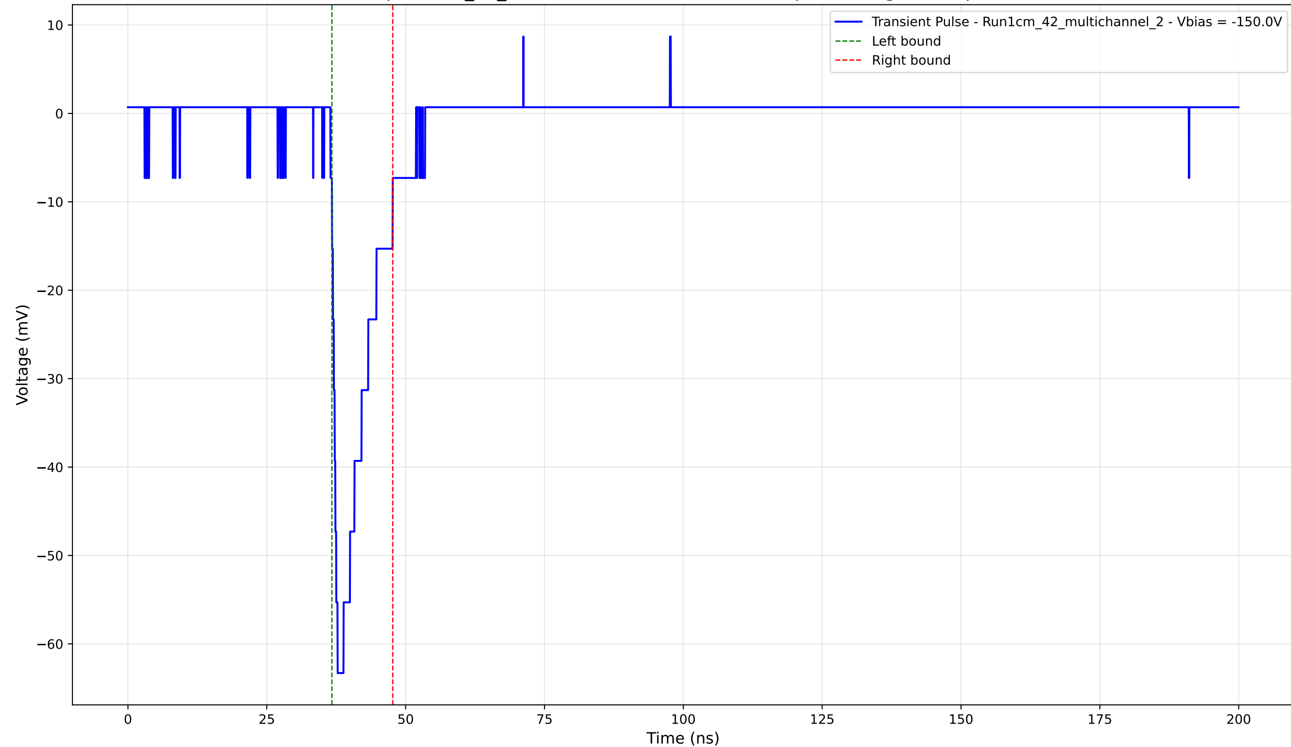
Transient Pulse - Sample: 1cm_42_multichannel - Position: 3430.0 \mu\text{m} - Charge: 7.49 pC - Rise Time: 1.29 ns
