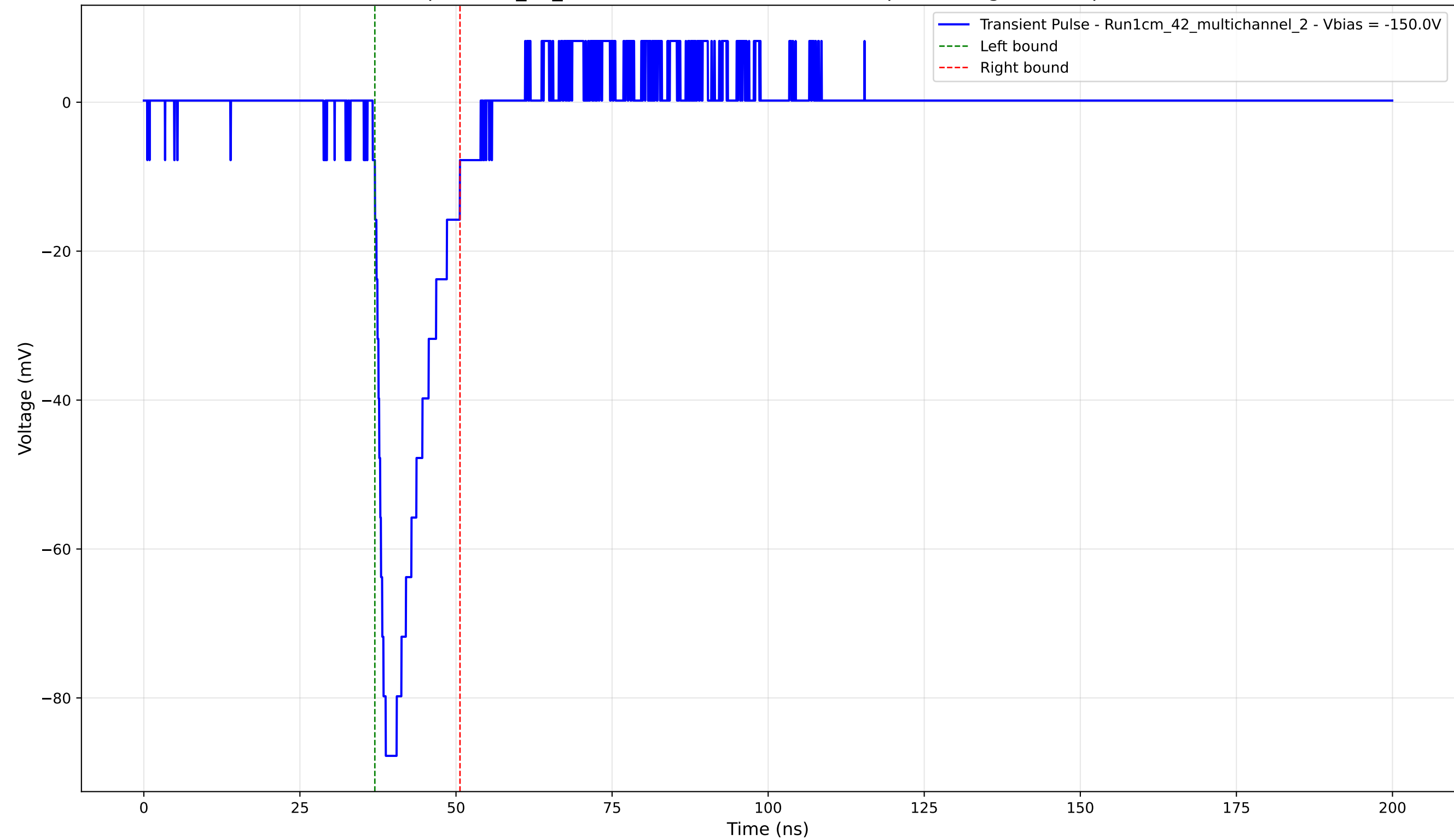
Transient Pulse - Sample: 1cm_42_multichannel - Position: 4055.0 \mu\text{m} - Charge: 13.06 pC - Rise Time: 1.39 ns
