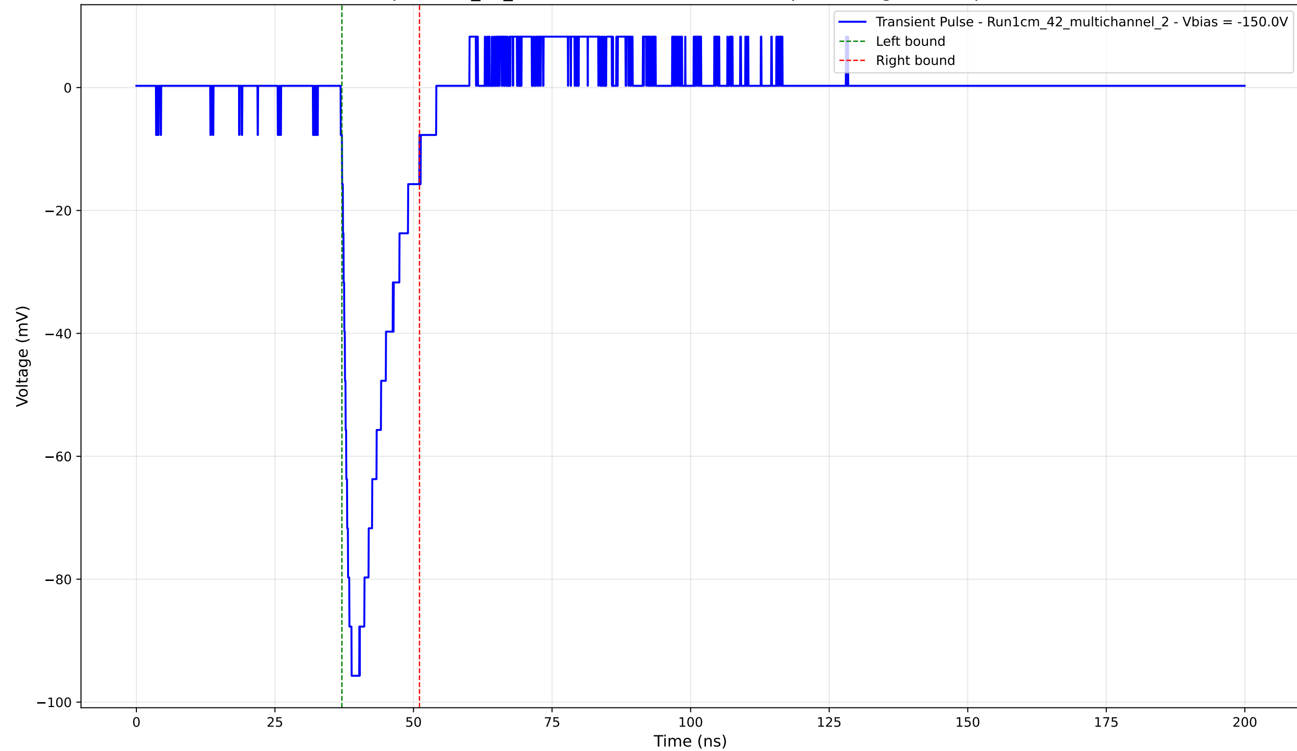
Transient Pulse - Sample: 1cm_42_multichannel - Position: 565.0 \mu\text{m} - Charge: 14.37 pC - Rise Time: 1.35 ns
