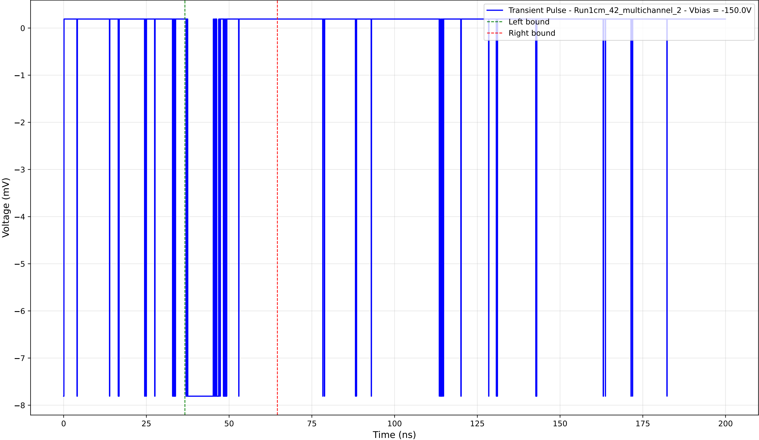
Transient Pulse - Sample: 1cm_42_multichannel - Position: 4365.0 \mu\text{m} - Charge: 1.49 pC - Rise Time: 0.00 ns (N/A)
