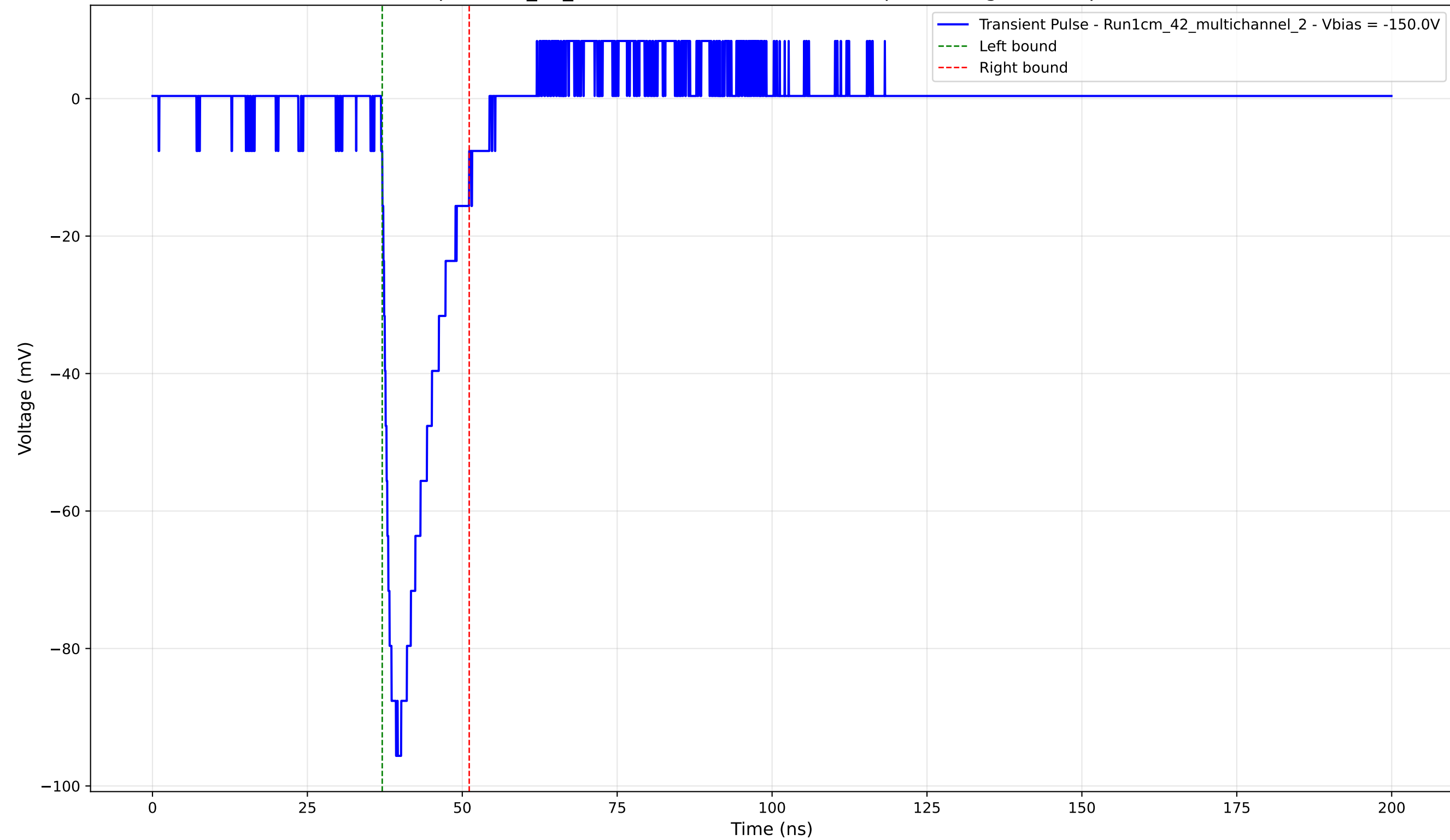
Transient Pulse - Sample: 1cm_42_multichannel - Position: 490.0 \mu\text{m} - Charge: 14.10 pC - Rise Time: 1.51 ns
