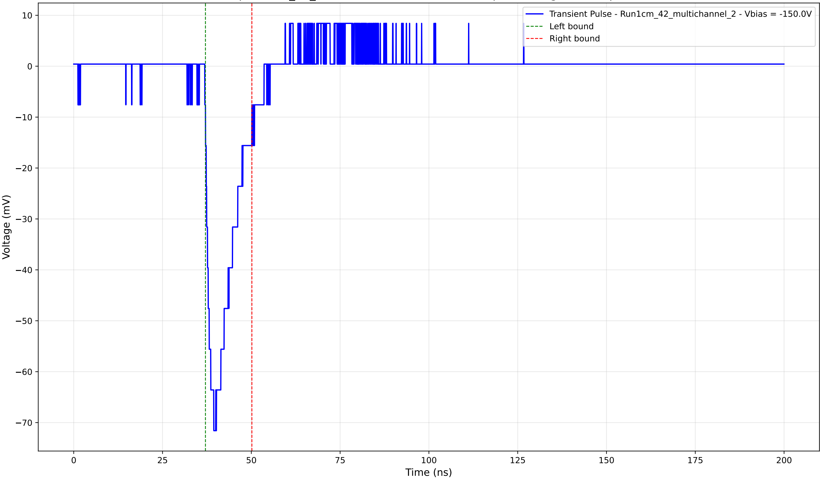
Transient Pulse - Sample: 1cm_42_multichannel - Position: 265.0 \mu\text{m} - Charge: 10.37 pC - Rise Time: 2.52 ns
