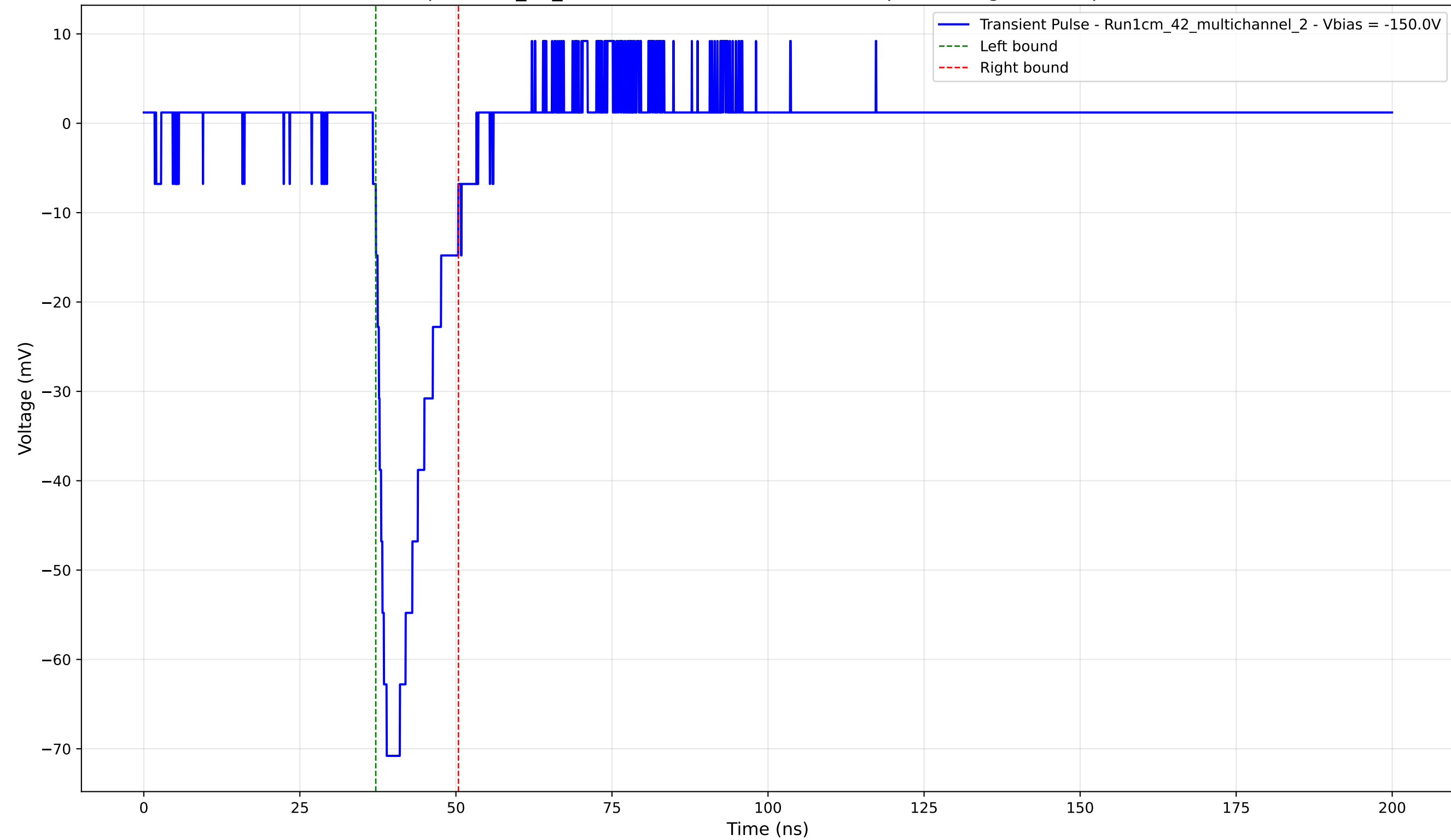
Transient Pulse - Sample: 1cm_42_multichannel - Position: 4280.0 \mu\text{m} - Charge: 10.67 pC - Rise Time: 1.76 ns
