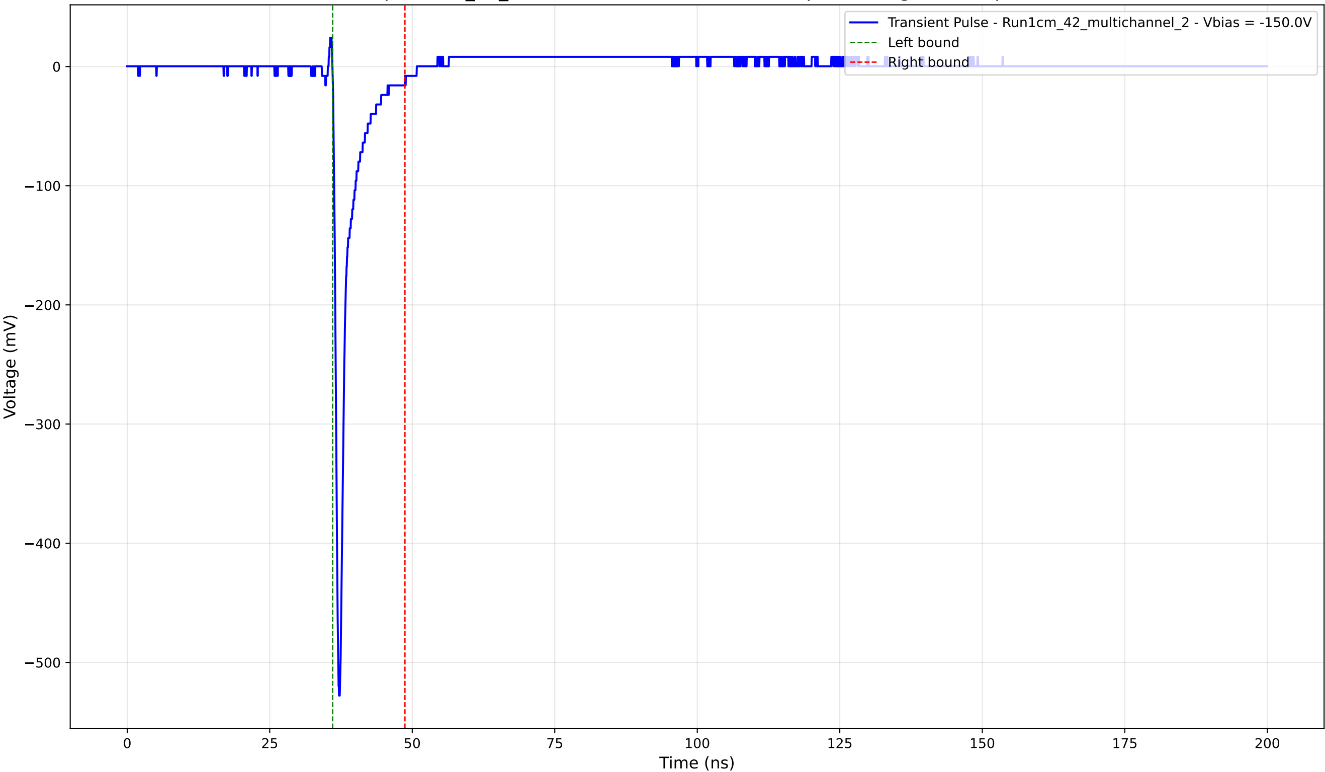
Transient Pulse - Sample: 1cm_42_multichannel - Position: 2540.0 \mu\text{m} - Charge: 25.83 pC - Rise Time: 0.74 ns
