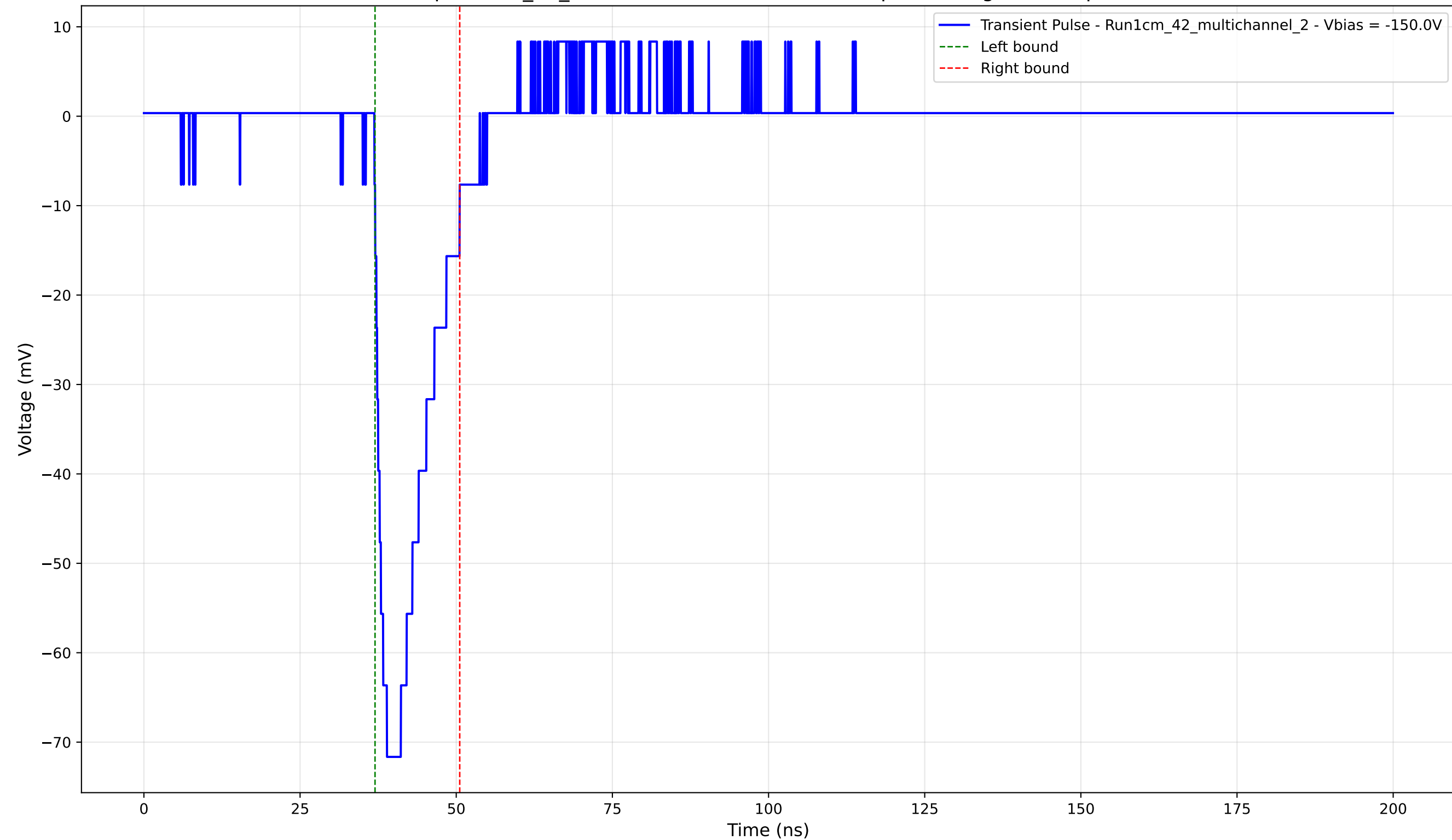
Transient Pulse - Sample: 1cm_42_multichannel - Position: 230.0 \mu\text{m} - Charge: 11.50 pC - Rise Time: 2.00 ns
