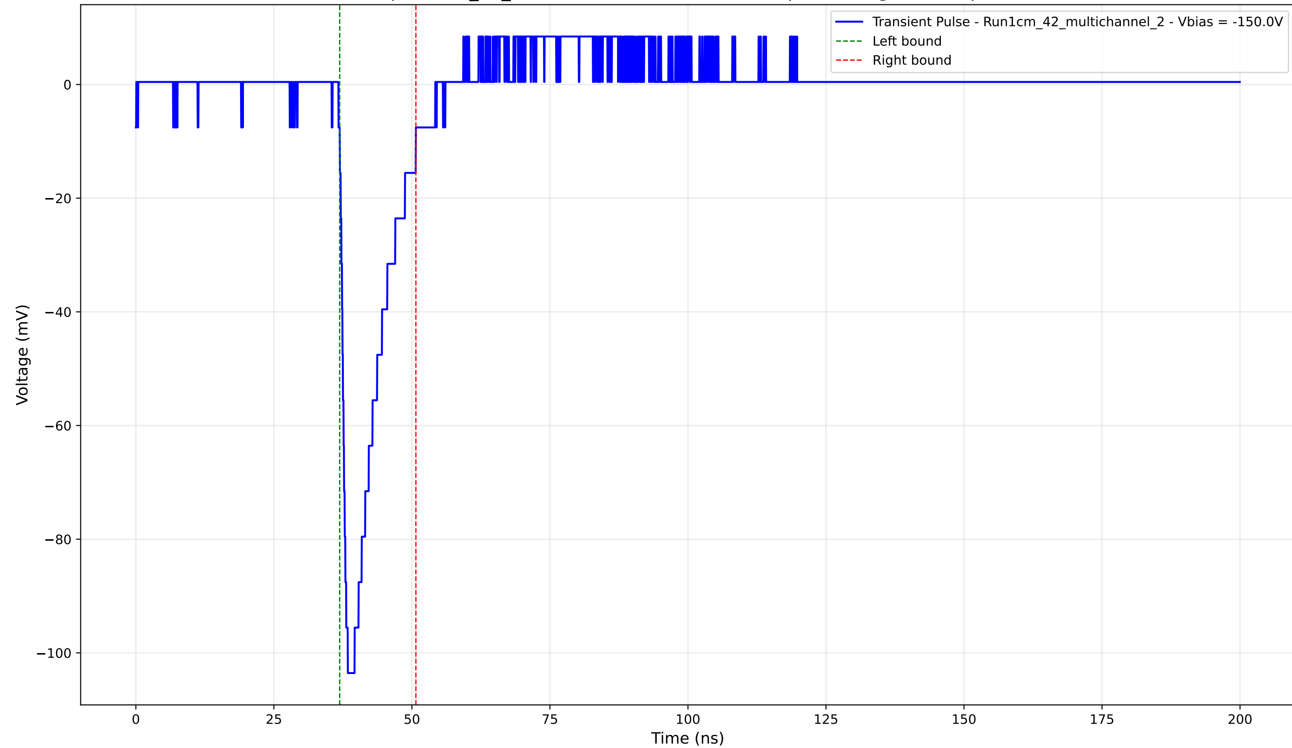
Transient Pulse - Sample: 1cm_42_multichannel - Position: 920.0 \mu\text{m} - Charge: 14.34 pC - Rise Time: 1.19 ns
