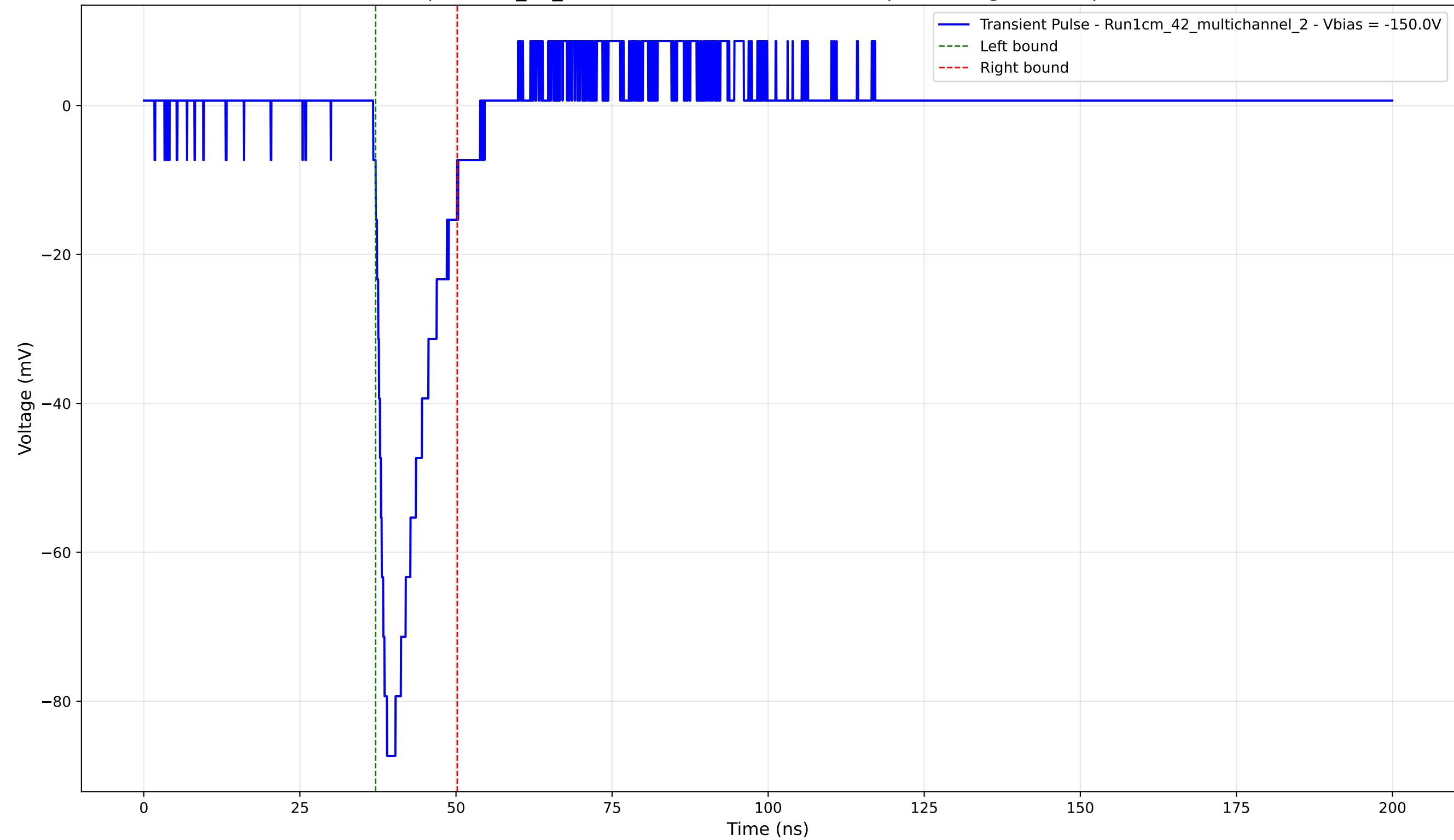
Transient Pulse - Sample: 1cm_42_multichannel - Position: 4150.0 \mu\text{m} - Charge: 12.51 pC - Rise Time: 1.43 ns
