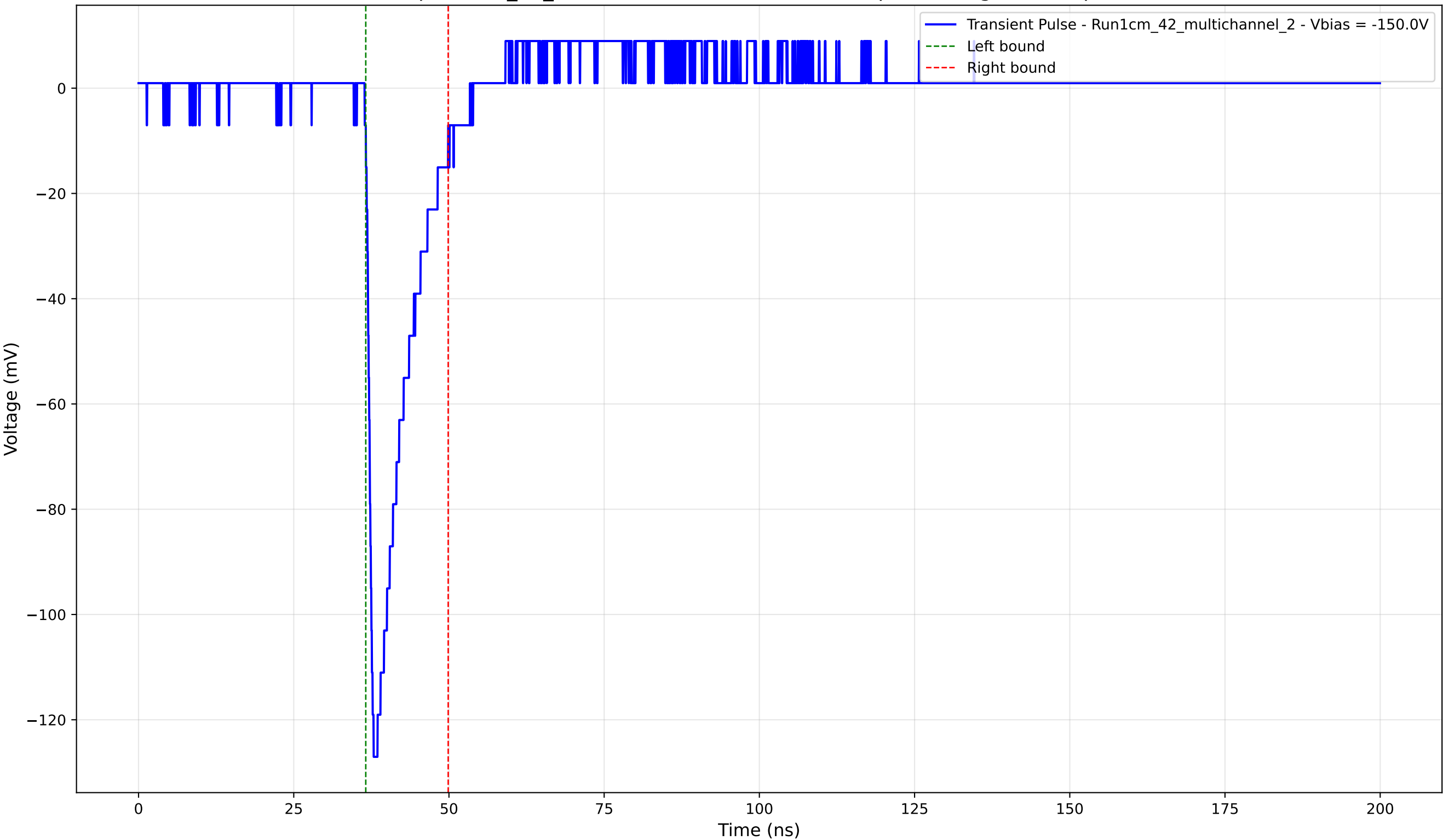
Transient Pulse - Sample: 1cm_42_multichannel - Position: 3460.0 \mu\text{m} - Charge: 15.39 pC - Rise Time: 1.09 ns
