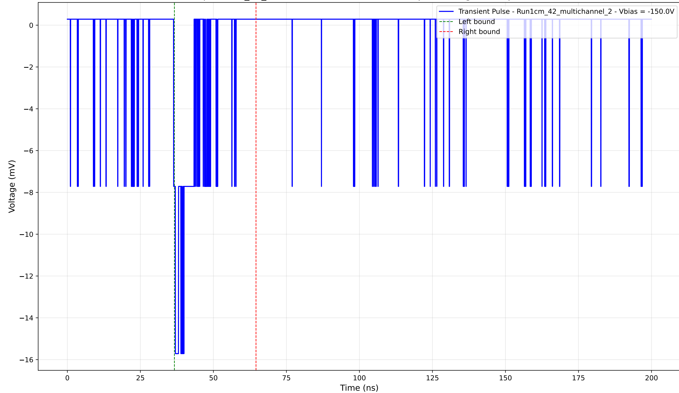
Transient Pulse - Sample: 1cm_42_multichannel - Position: 2885.0 \mu\text{m} - Charge: 1.62 pC - Rise Time: 0.63 ns
