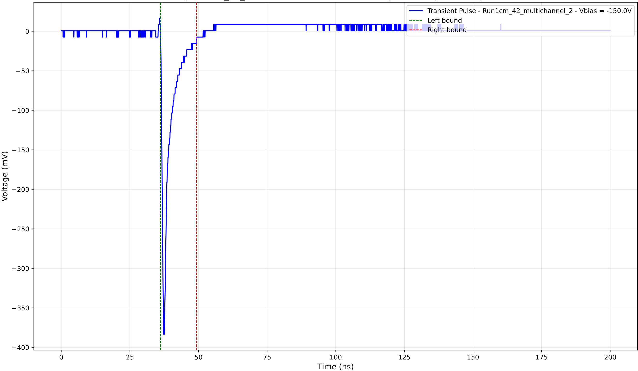
Transient Pulse - Sample: 1cm_42_multichannel - Position: 1960.0 \mu\text{m} - Charge: 24.19 pC - Rise Time: 0.77 ns
