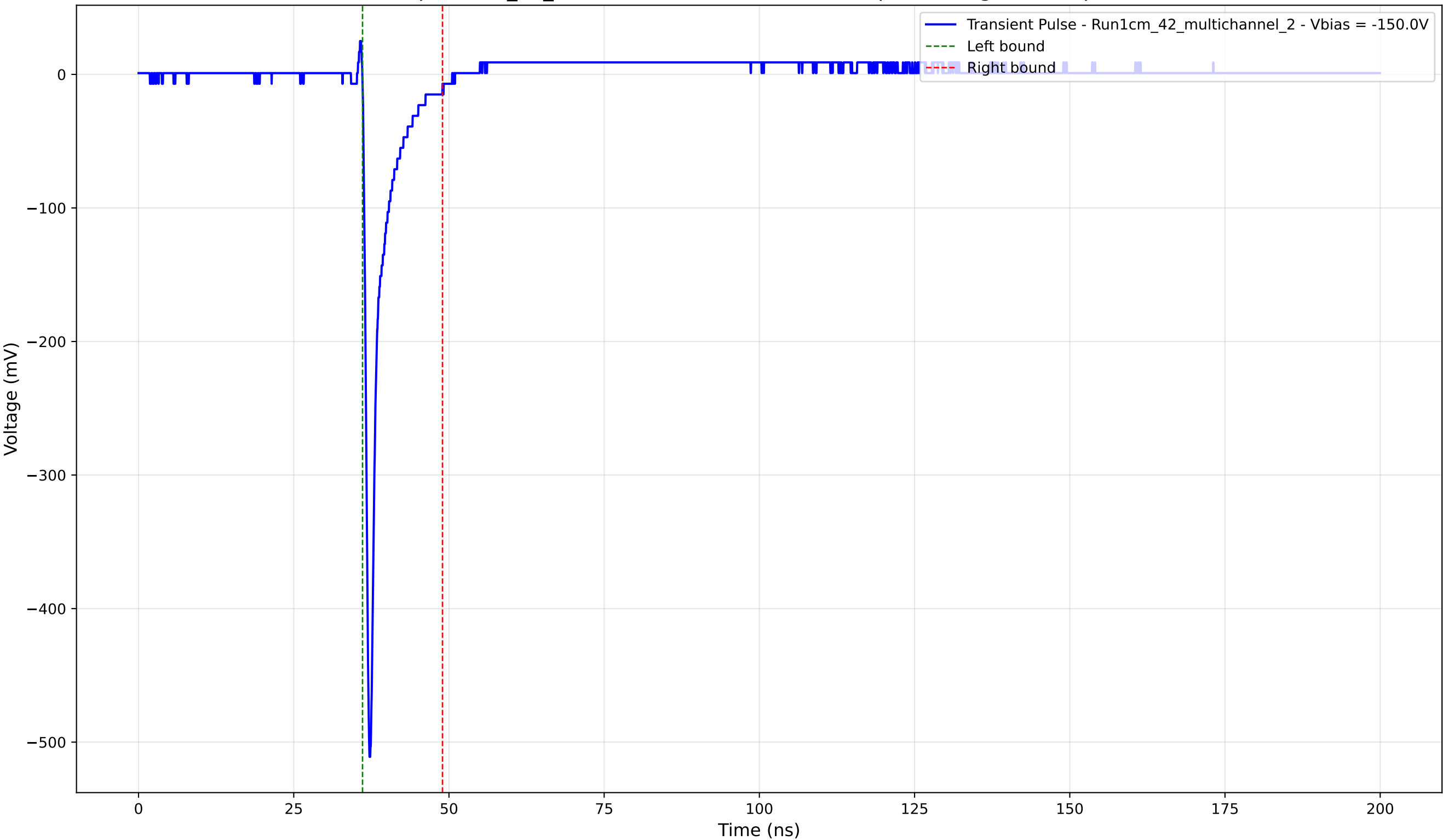
Transient Pulse - Sample: 1cm_42_multichannel - Position: 2130.0 \mu\text{m} - Charge: 26.56 pC - Rise Time: 0.76 ns
