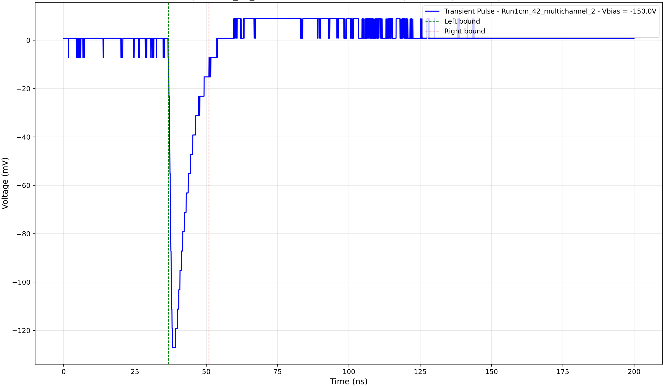
Transient Pulse - Sample: 1cm_42_multichannel - Position: 1065.0 \mu\text{m} - Charge: 17.12 pC - Rise Time: 1.21 ns
