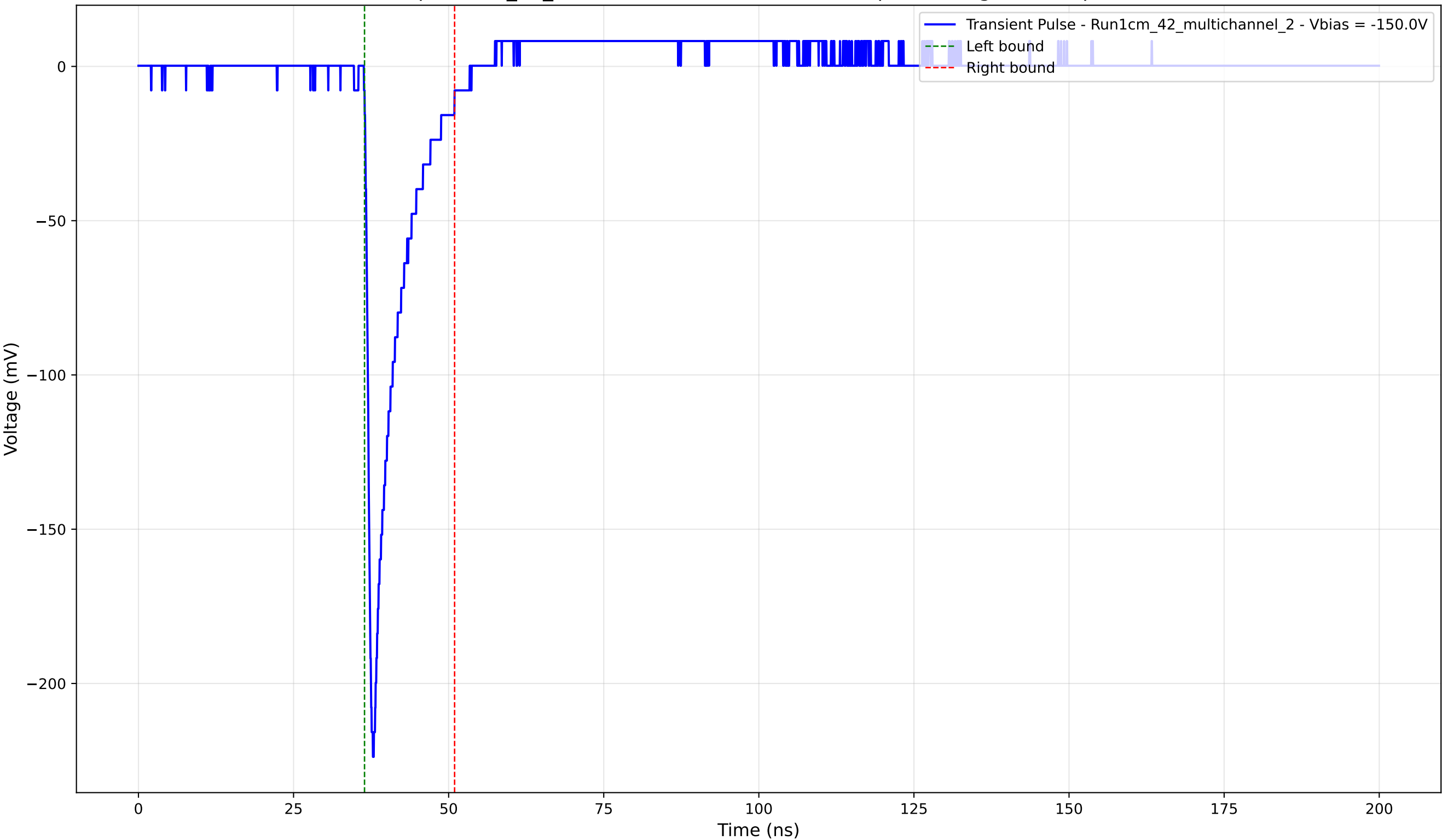
Transient Pulse - Sample: 1cm_42_multichannel - Position: 1550.0 \mu\text{m} - Charge: 21.41 pC - Rise Time: 0.97 ns
