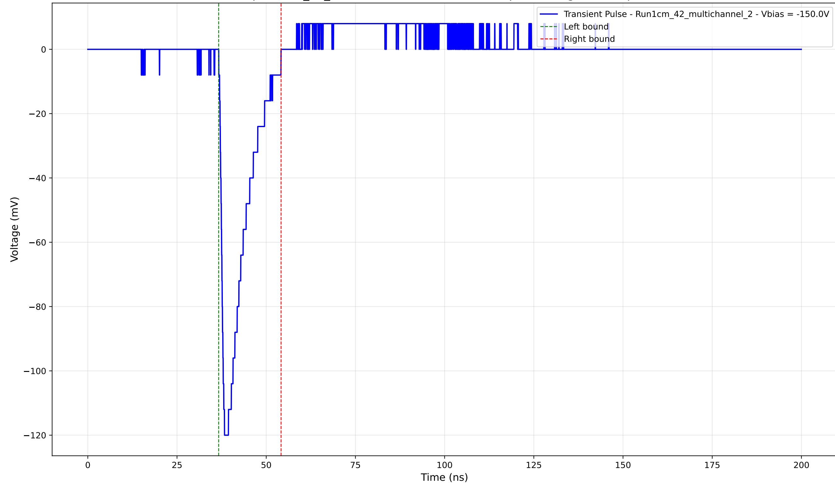
Transient Pulse - Sample: 1cm_42_multichannel - Position: 950.0 \mu\text{m} - Charge: 17.34 pC - Rise Time: 1.18 ns
