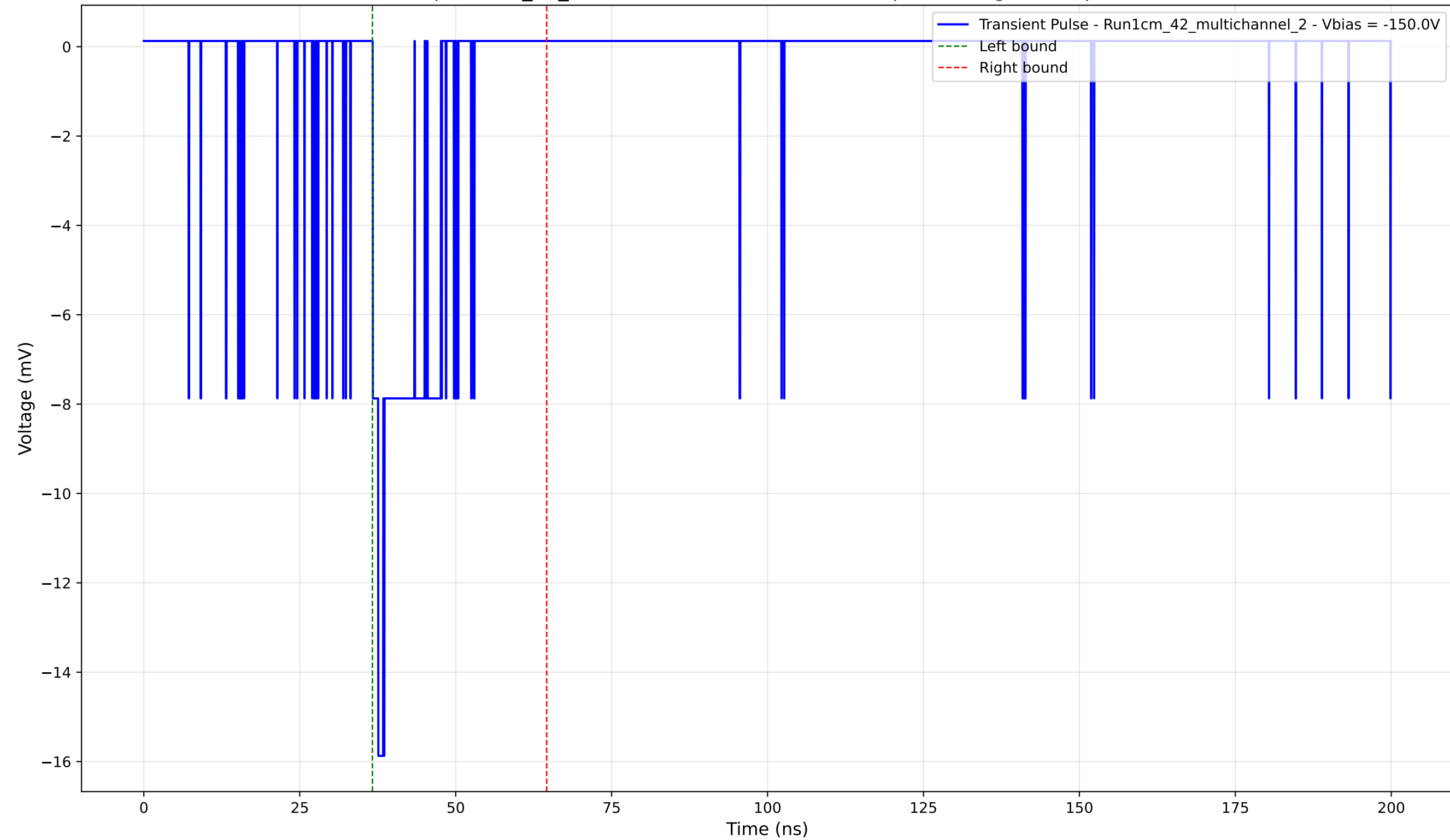
Transient Pulse - Sample: 1cm_42_multichannel - Position: 1370.0 \mu\text{m} - Charge: 1.88 pC - Rise Time: 0.91 ns
