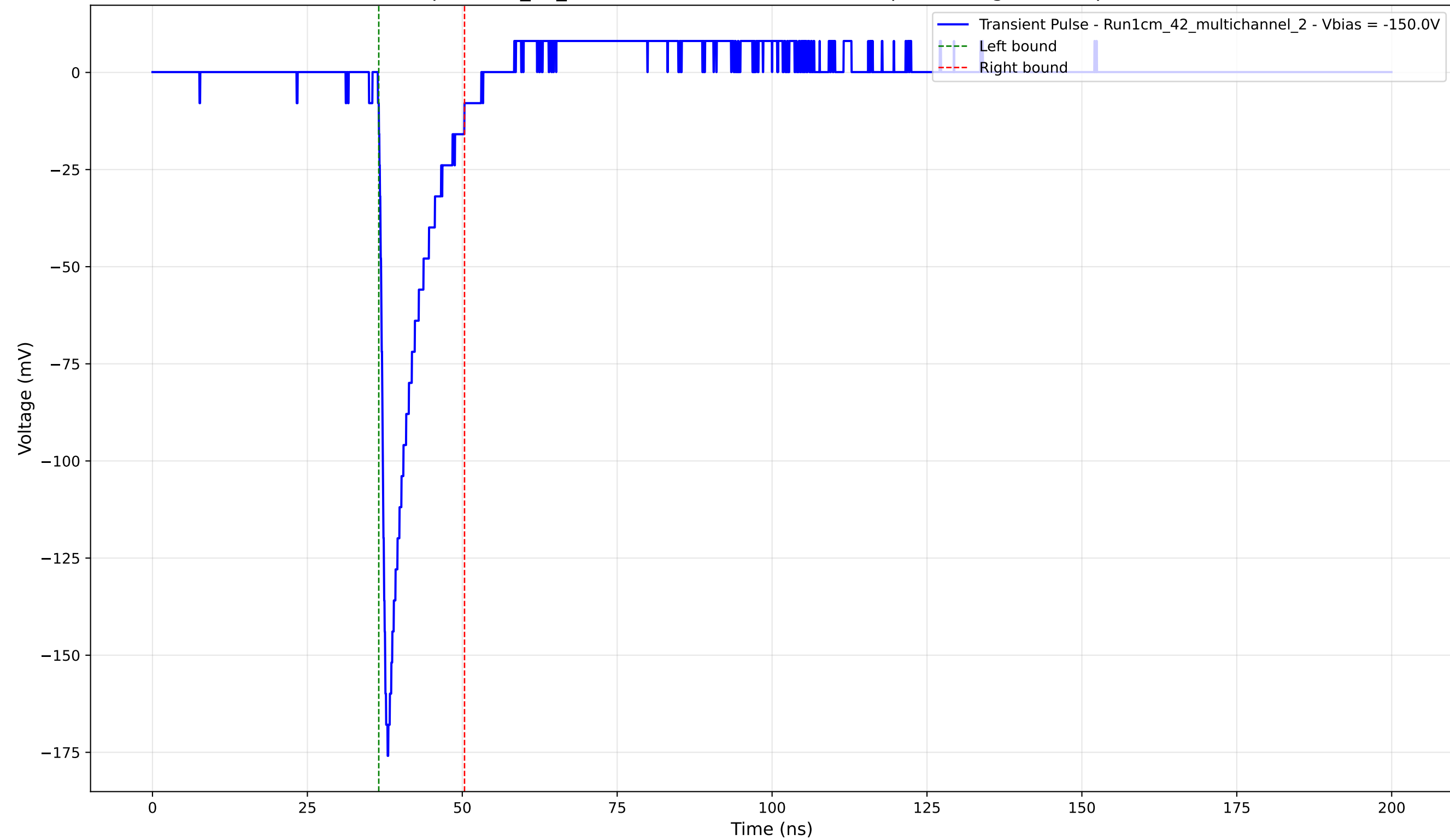
Transient Pulse - Sample: 1cm_42_multichannel - Position: 1430.0 \mu\text{m} - Charge: 18.28 pC - Rise Time: 0.99 ns
