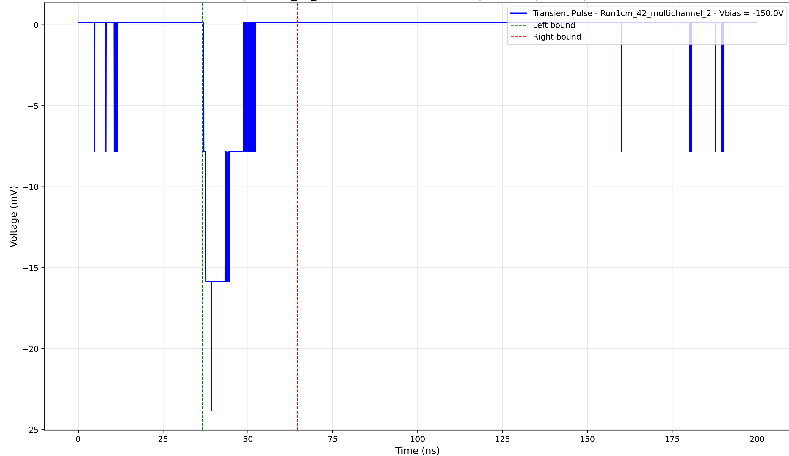
Transient Pulse - Sample: 1cm_42_multichannel - Position: 60.0 \mu\text{m} - Charge: 3.06 pC - Rise Time: 2.31 ns
