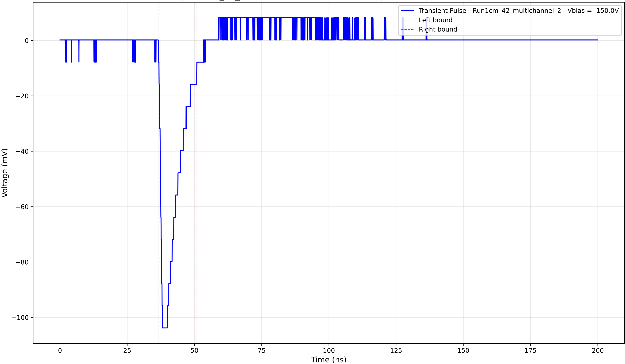
Transient Pulse - Sample: 1cm_42_multichannel - Position: 3730.0 \mu\text{m} - Charge: 15.00 pC - Rise Time: 1.15 ns
