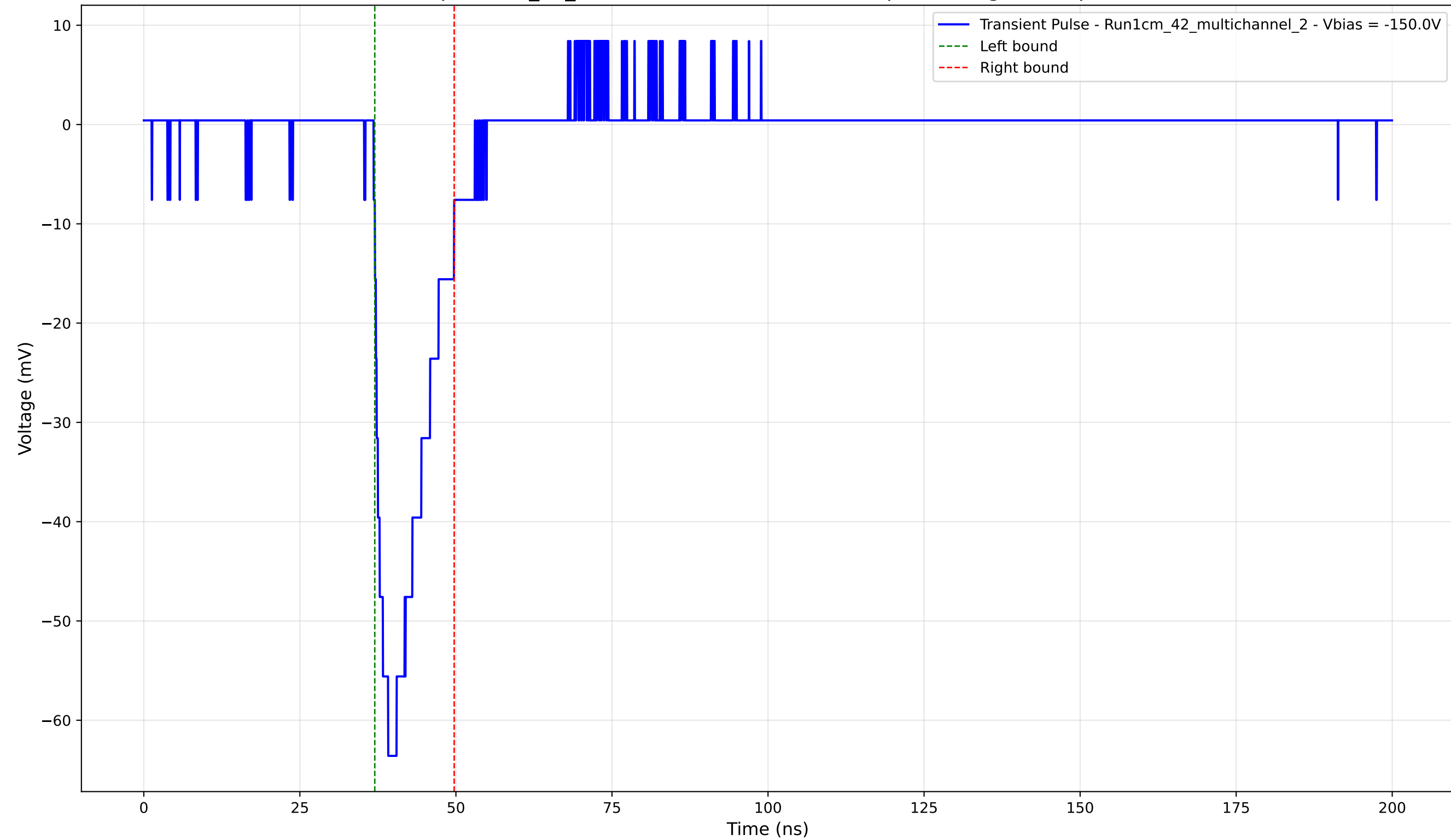
Transient Pulse - Sample: 1cm_42_multichannel - Position: 110.0 \mu\text{m} - Charge: 9.67 pC - Rise Time: 2.33 ns
