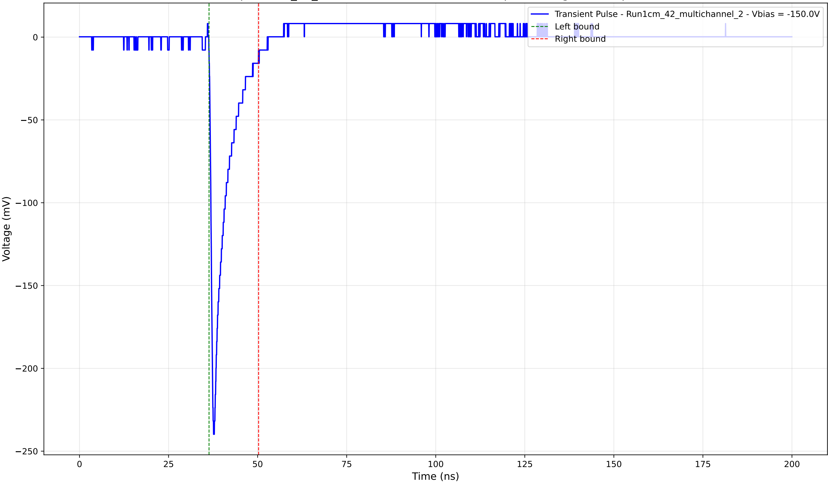
Transient Pulse - Sample: 1cm_42_multichannel - Position: 1615.0 \mu\text{m} - Charge: 21.69 pC - Rise Time: 0.92 ns
