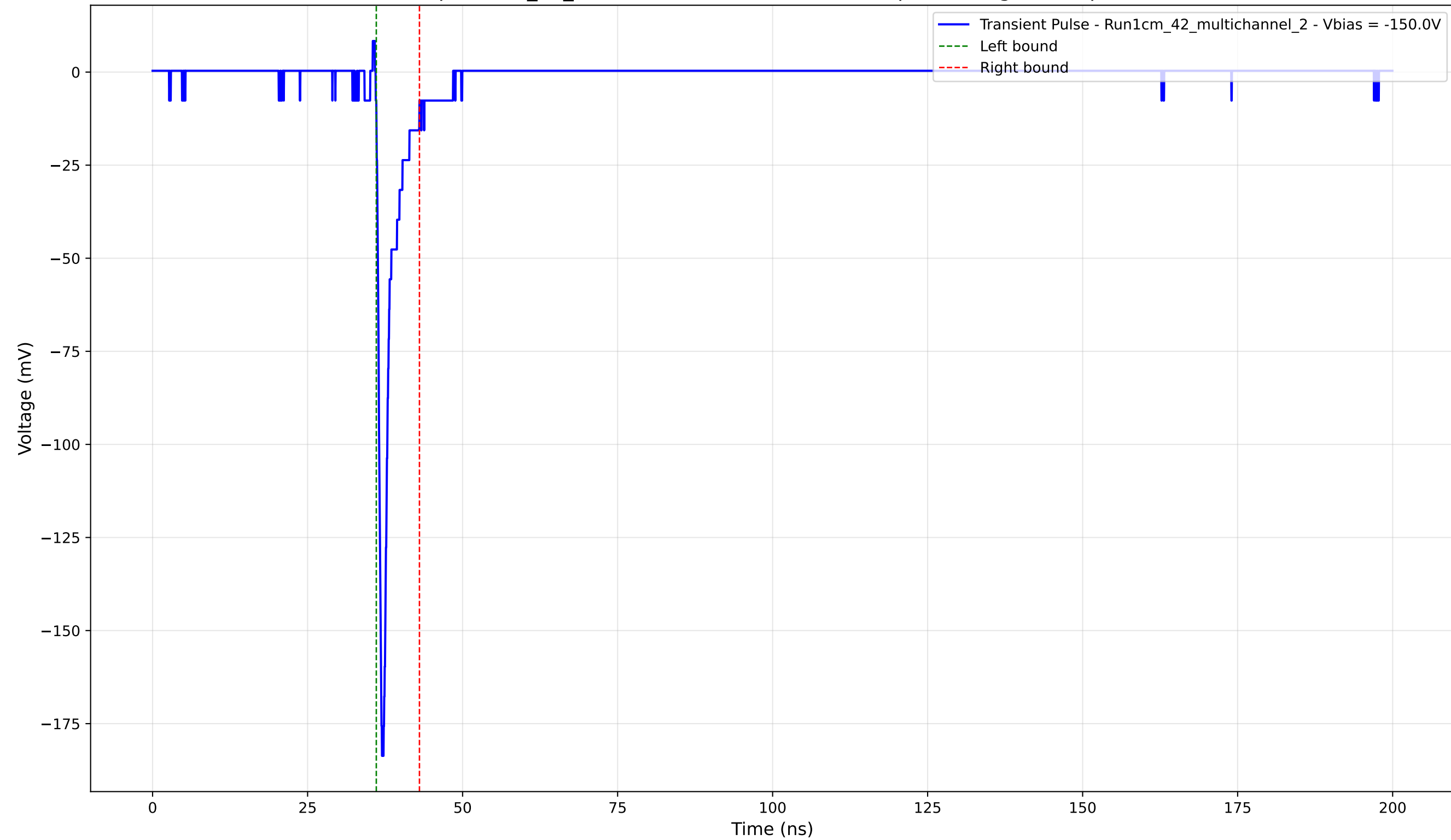
Transient Pulse - Sample: 1cm_42_multichannel - Position: 2410.0 \mu\text{m} - Charge: 7.84 pC - Rise Time: 0.73 ns
