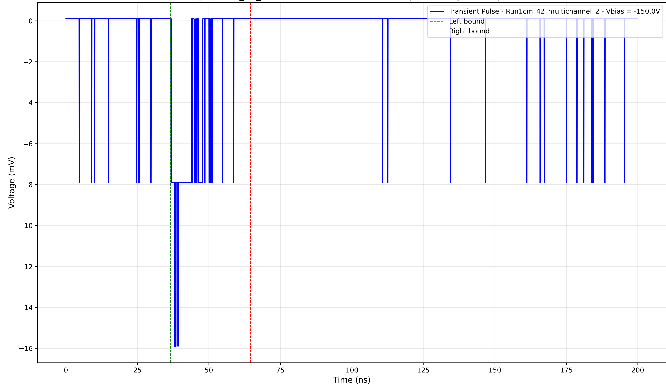
Transient Pulse - Sample: 1cm_42_multichannel - Position: 1345.0 \mu\text{m} - Charge: 1.68 pC - Rise Time: 1.07 ns
