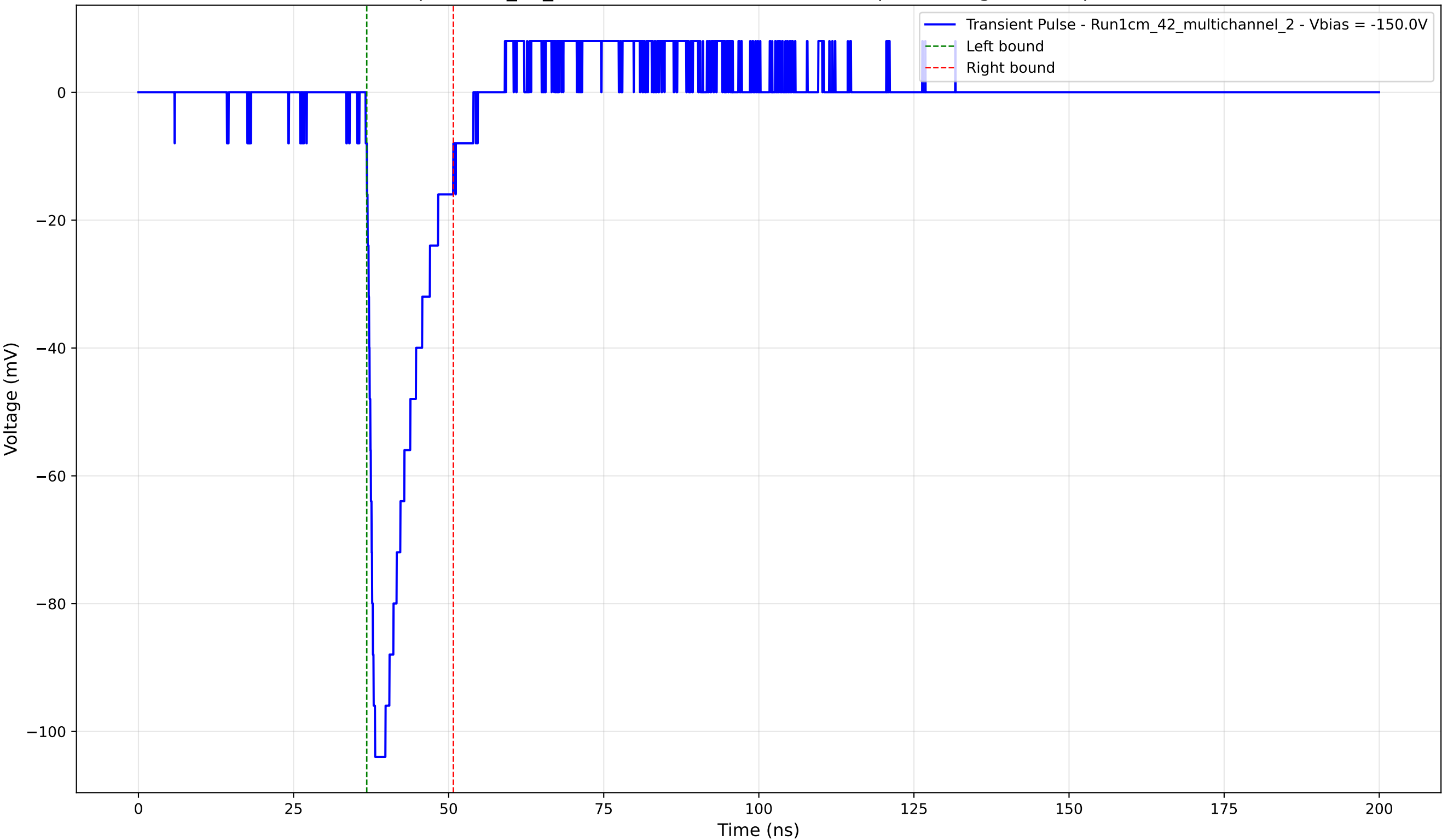
Transient Pulse - Sample: 1cm_42_multichannel - Position: 3705.0 \mu\text{m} - Charge: 14.90 pC - Rise Time: 1.11 ns
