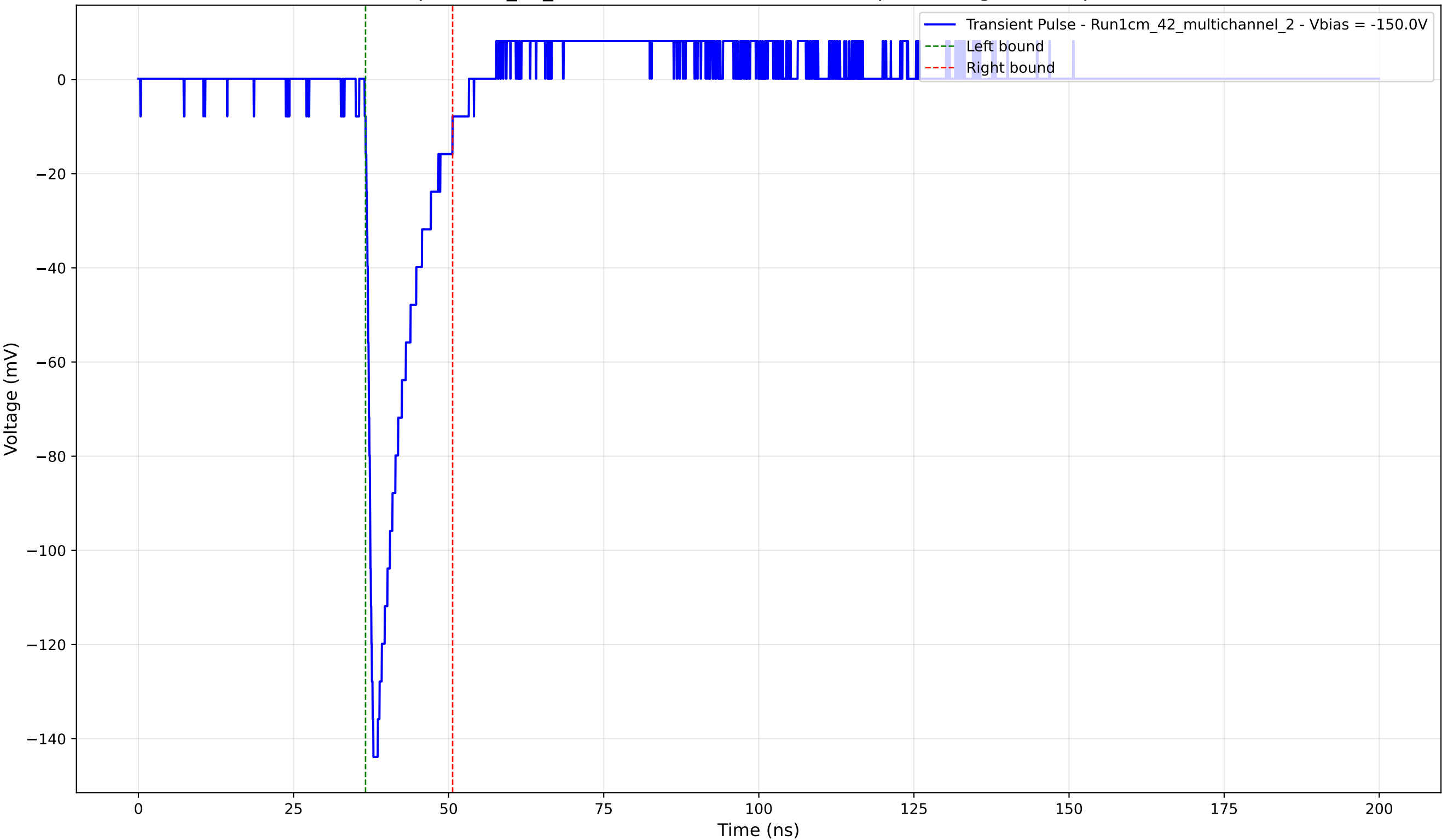
Transient Pulse - Sample: 1cm_42_multichannel - Position: 1280.0 \mu\text{m} - Charge: 17.35 pC - Rise Time: 1.13 ns
