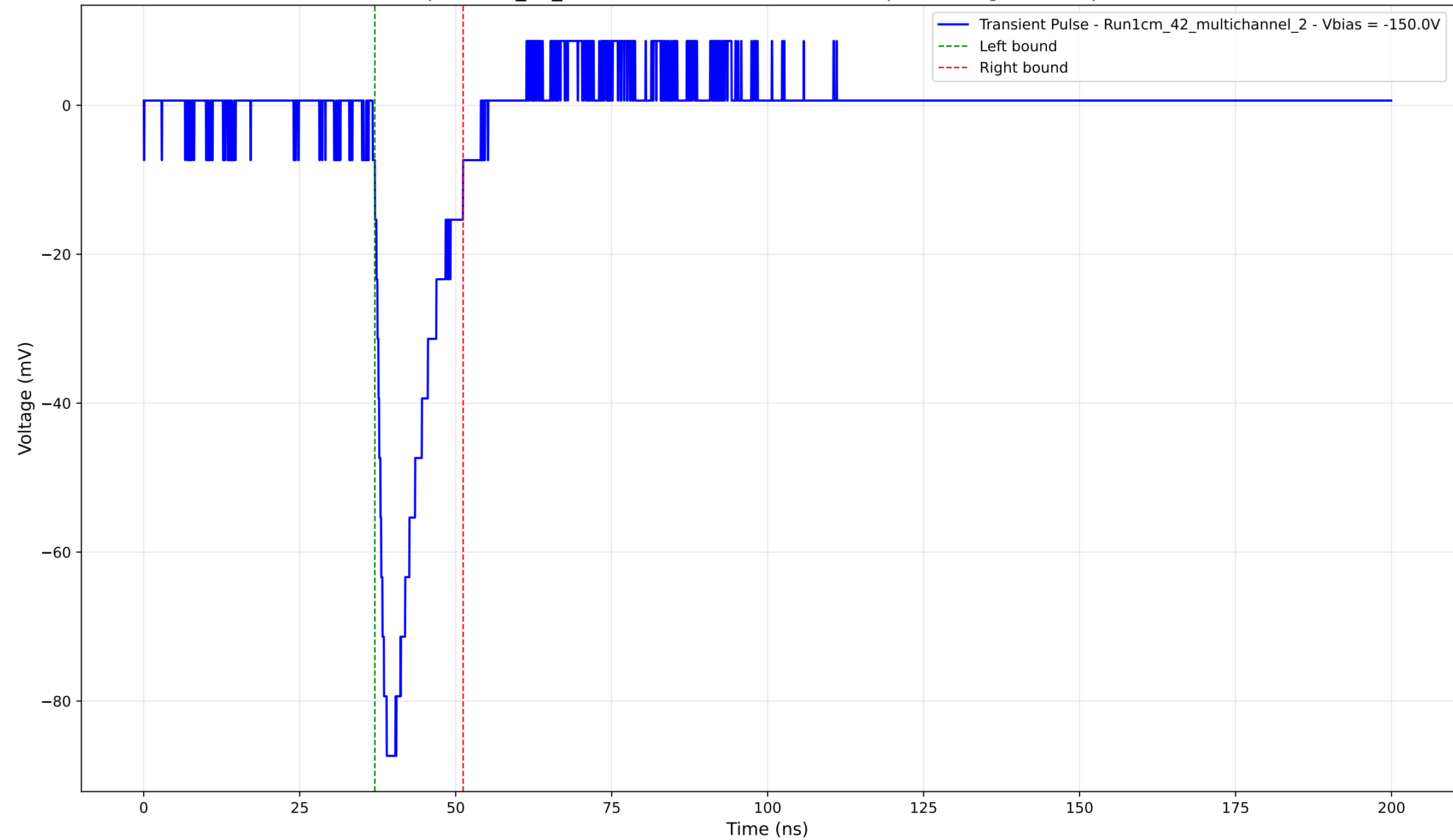
Transient Pulse - Sample: 1cm_42_multichannel - Position: 4095.0 \mu\text{m} - Charge: 12.89 pC - Rise Time: 1.47 ns
