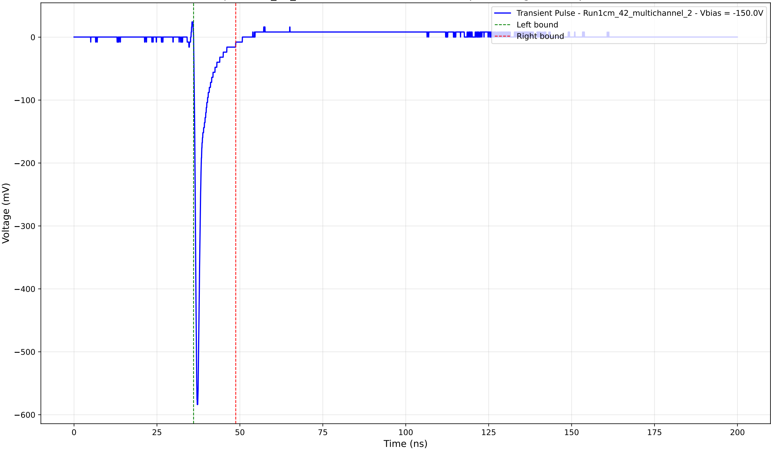
Transient Pulse - Sample: 1cm_42_multichannel - Position: 2210.0 \mu\text{m} - Charge: 28.23 pC - Rise Time: 0.73 ns
