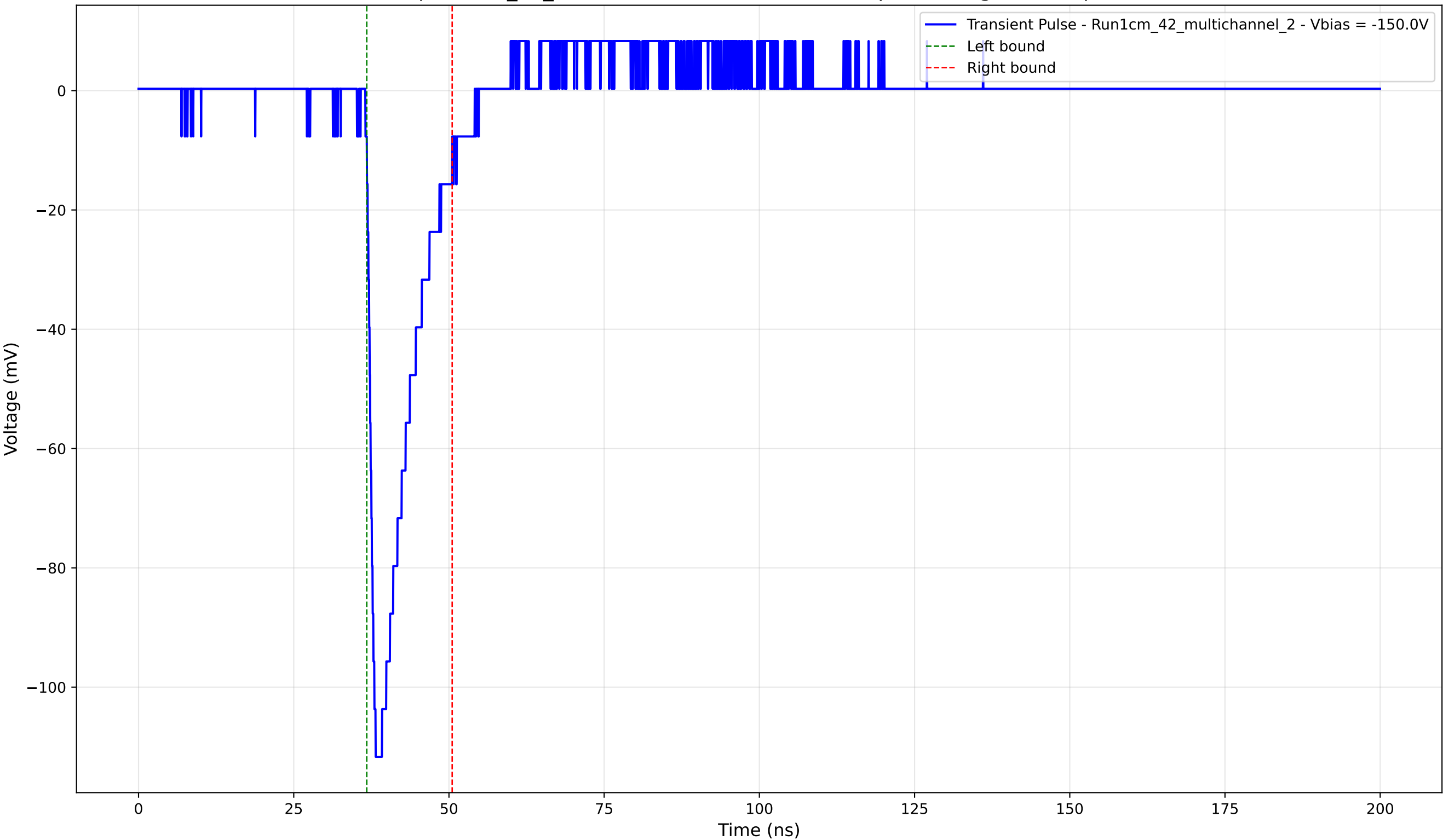
Transient Pulse - Sample: 1cm_42_multichannel - Position: 3660.0 \mu\text{m} - Charge: 15.11 pC - Rise Time: 1.22 ns
