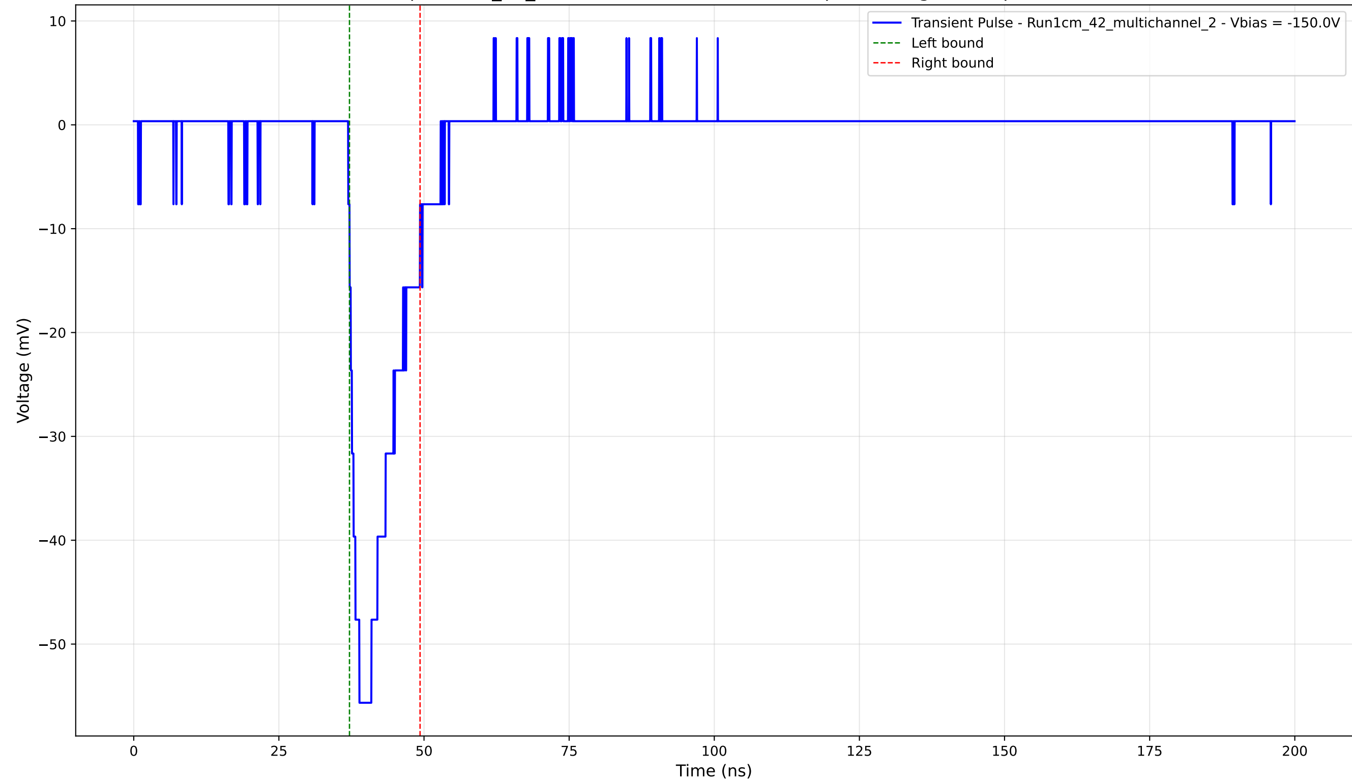
Transient Pulse - Sample: 1cm_42_multichannel - Position: 285.0 \mu\text{m} - Charge: 8.28 pC - Rise Time: 1.93 ns
