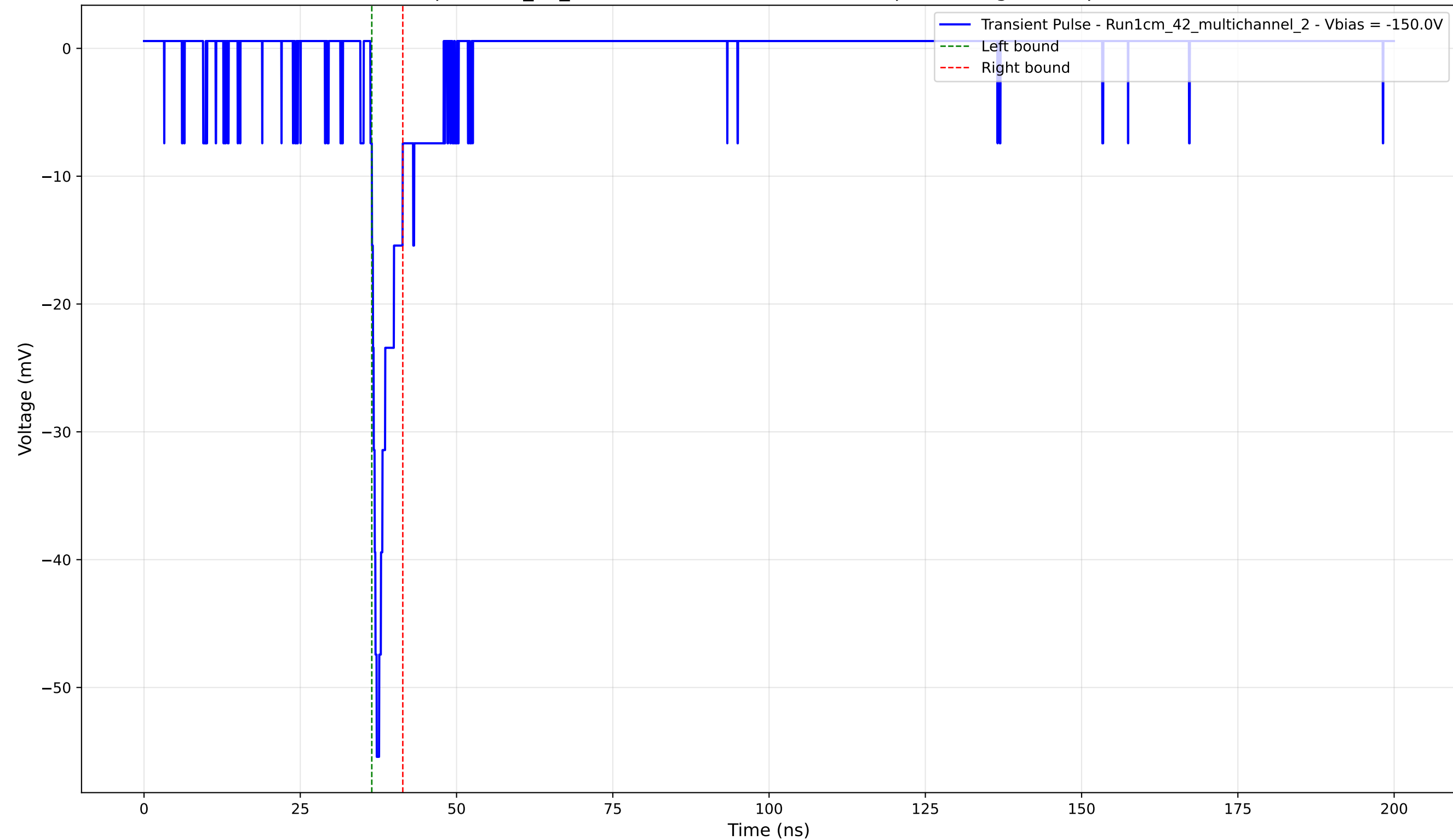
Transient Pulse - Sample: 1cm_42_multichannel - Position: 2845.0 \mu\text{m} - Charge: 2.76 pC - Rise Time: 1.01 ns
