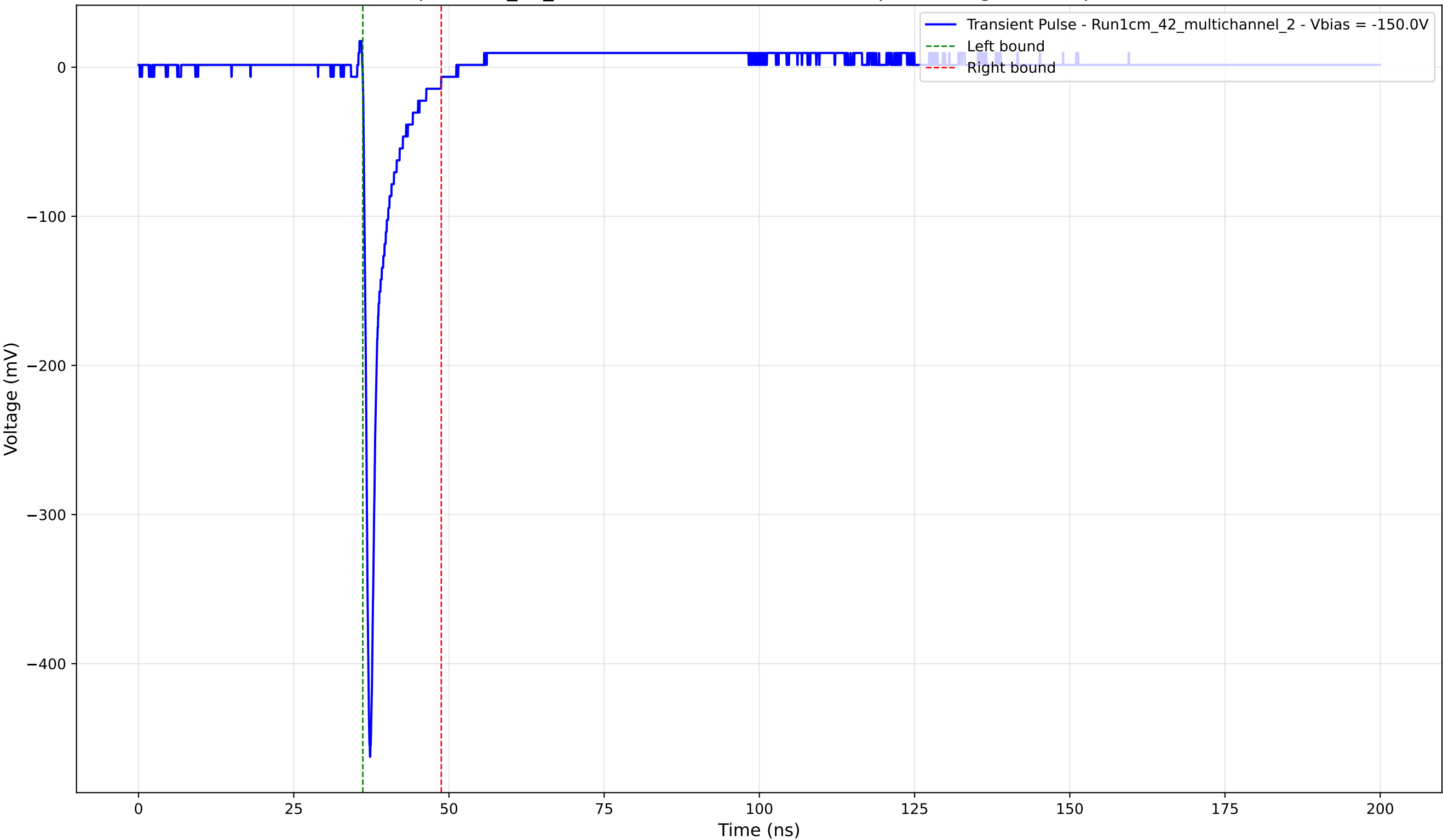
Transient Pulse - Sample: 1cm_42_multichannel - Position: 2645.0 \mu\text{m} - Charge: 24.62 pC - Rise Time: 0.73 ns
