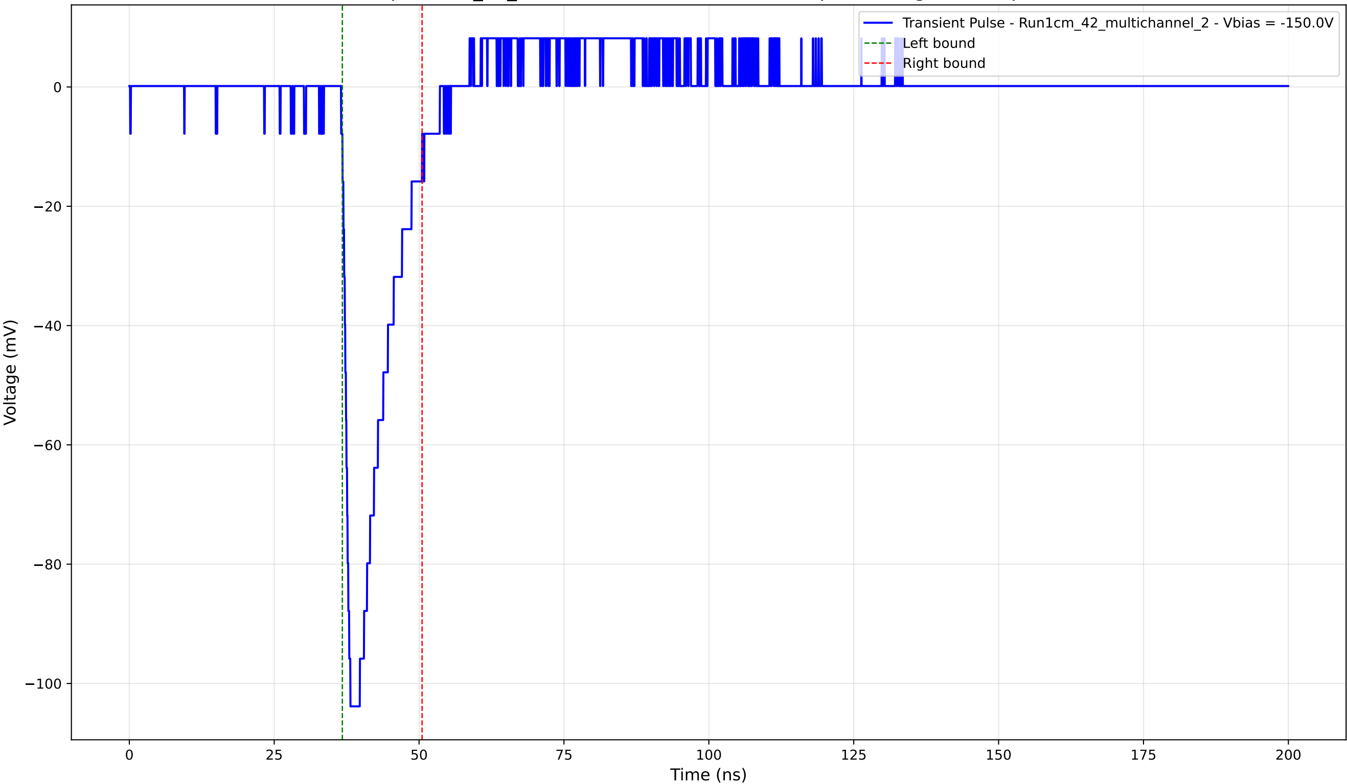
Transient Pulse - Sample: 1cm_42_multichannel - Position: 3710.0 \mu\text{m} - Charge: 14.82 pC - Rise Time: 1.19 ns
