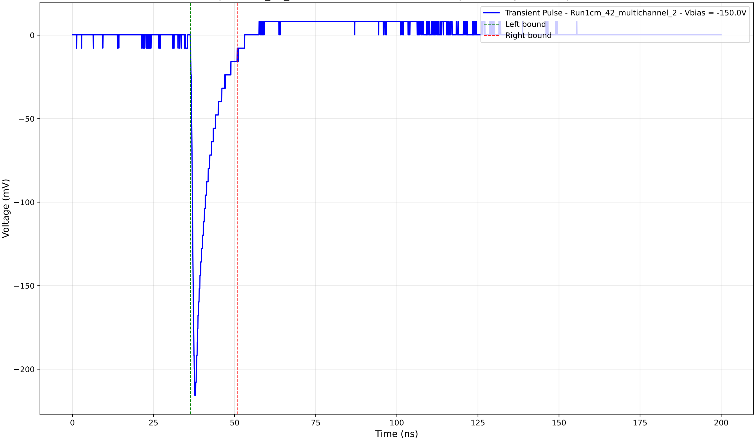
Transient Pulse - Sample: 1cm_42_multichannel - Position: 1515.0 \mu\text{m} - Charge: 21.29 pC - Rise Time: 1.01 ns
