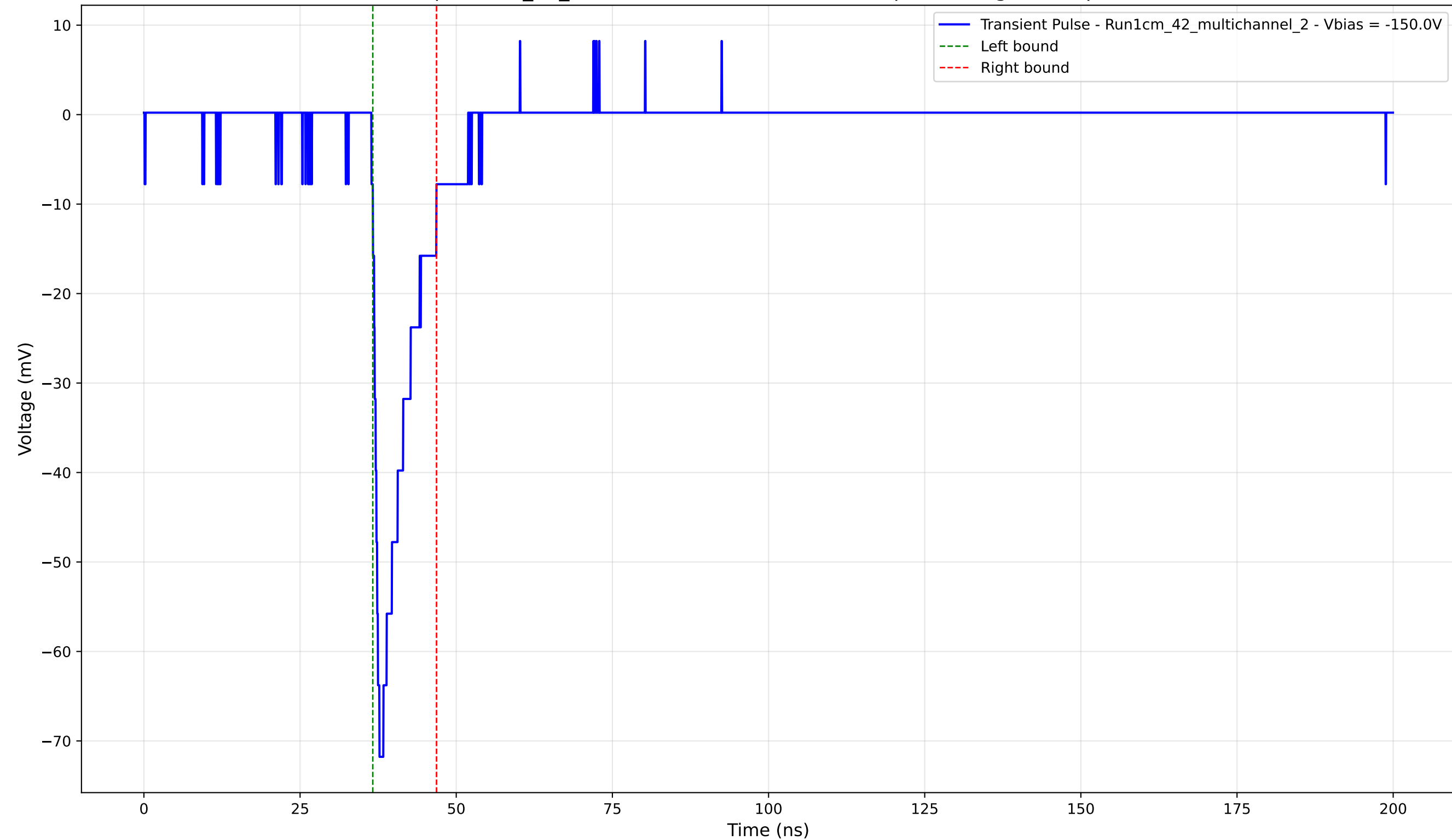
Transient Pulse - Sample: 1cm_42_multichannel - Position: 3335.0 \mu\text{m} - Charge: 7.27 pC - Rise Time: 1.28 ns
