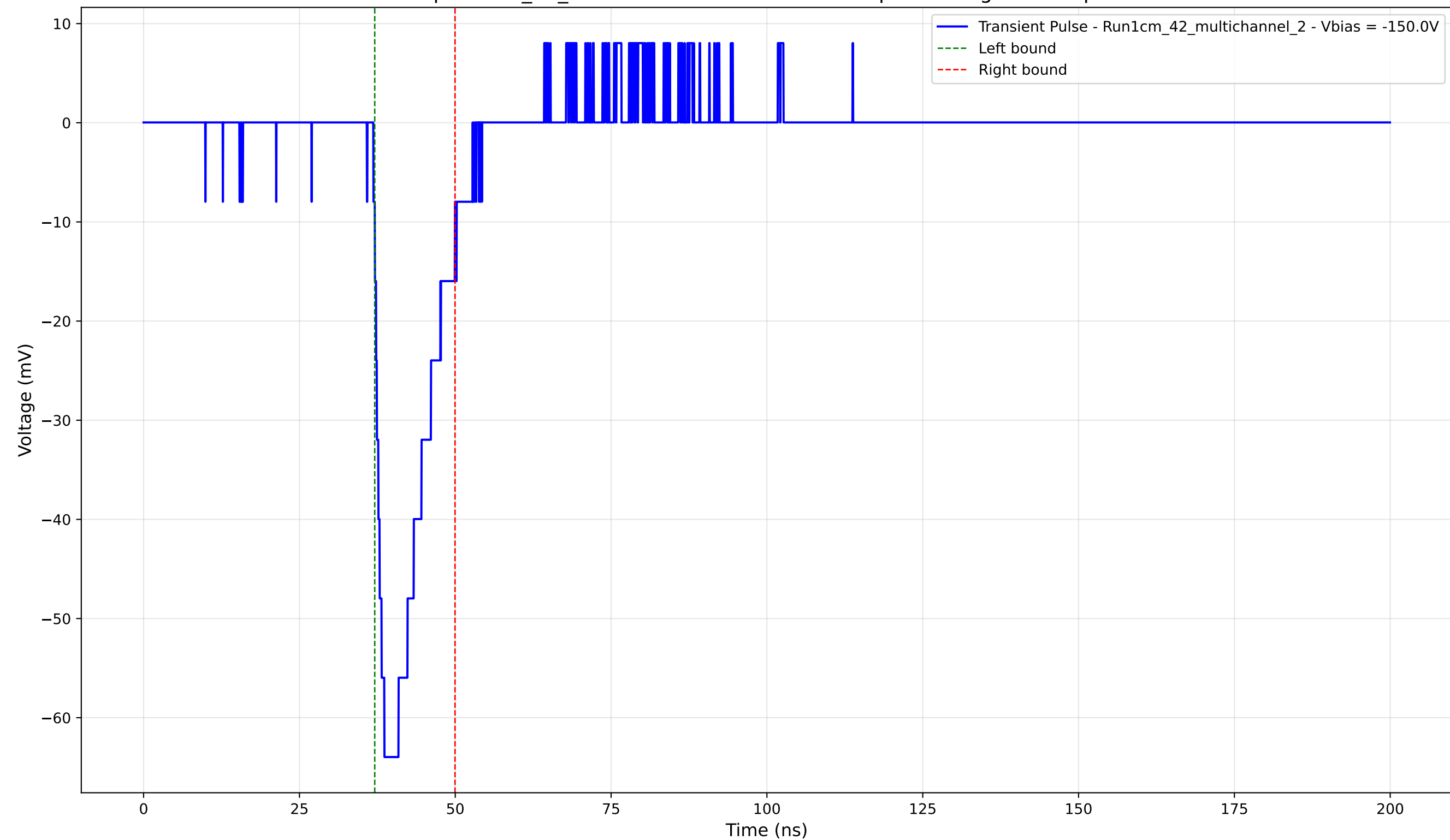
Transient Pulse - Sample: 1cm_42_multichannel - Position: 270.0 \mu\text{m} - Charge: 10.17 pC - Rise Time: 1.77 ns
