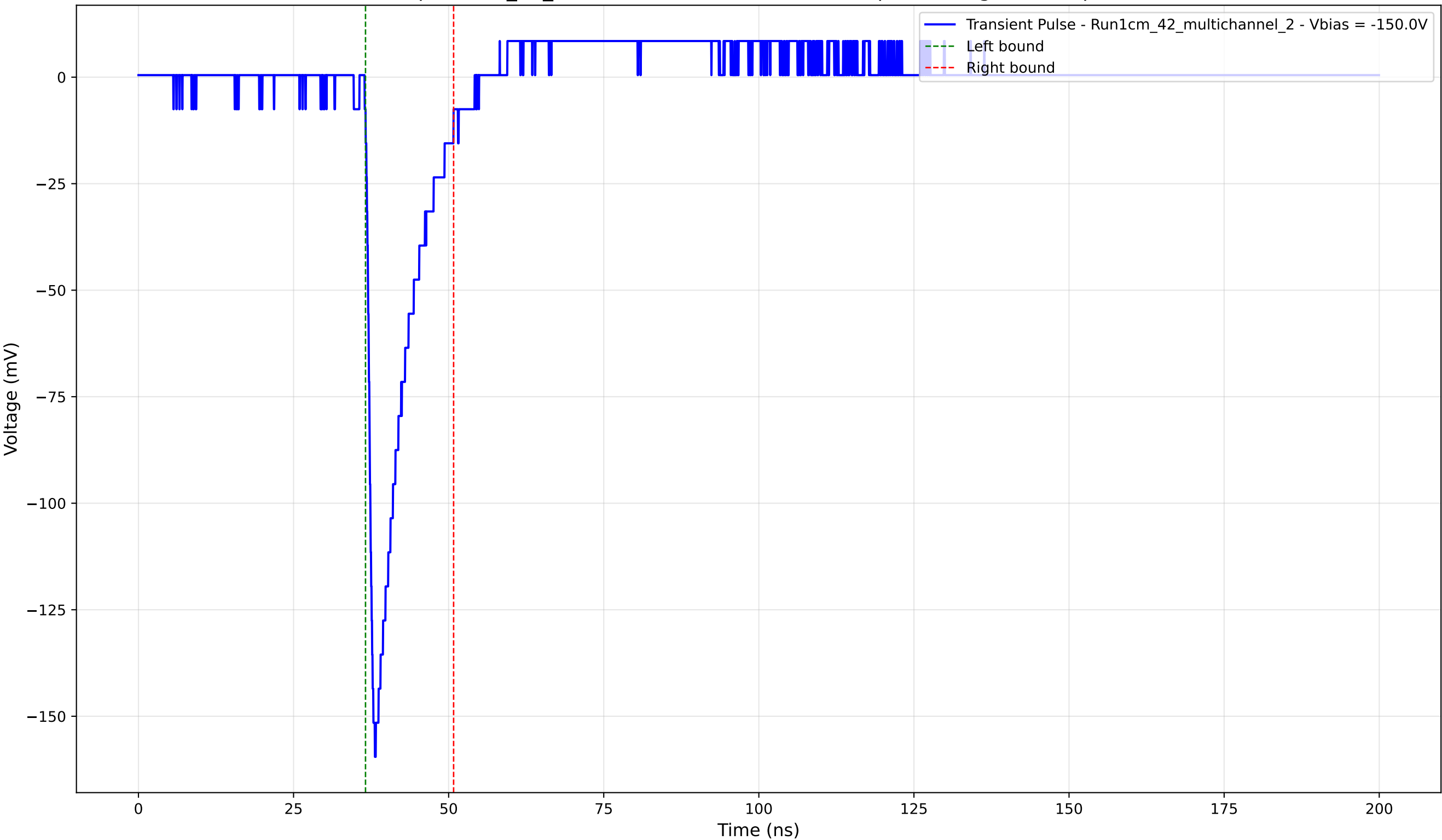
Transient Pulse - Sample: 1cm_42_multichannel - Position: 1255.0 \mu\text{m} - Charge: 18.87 pC - Rise Time: 1.16 ns
