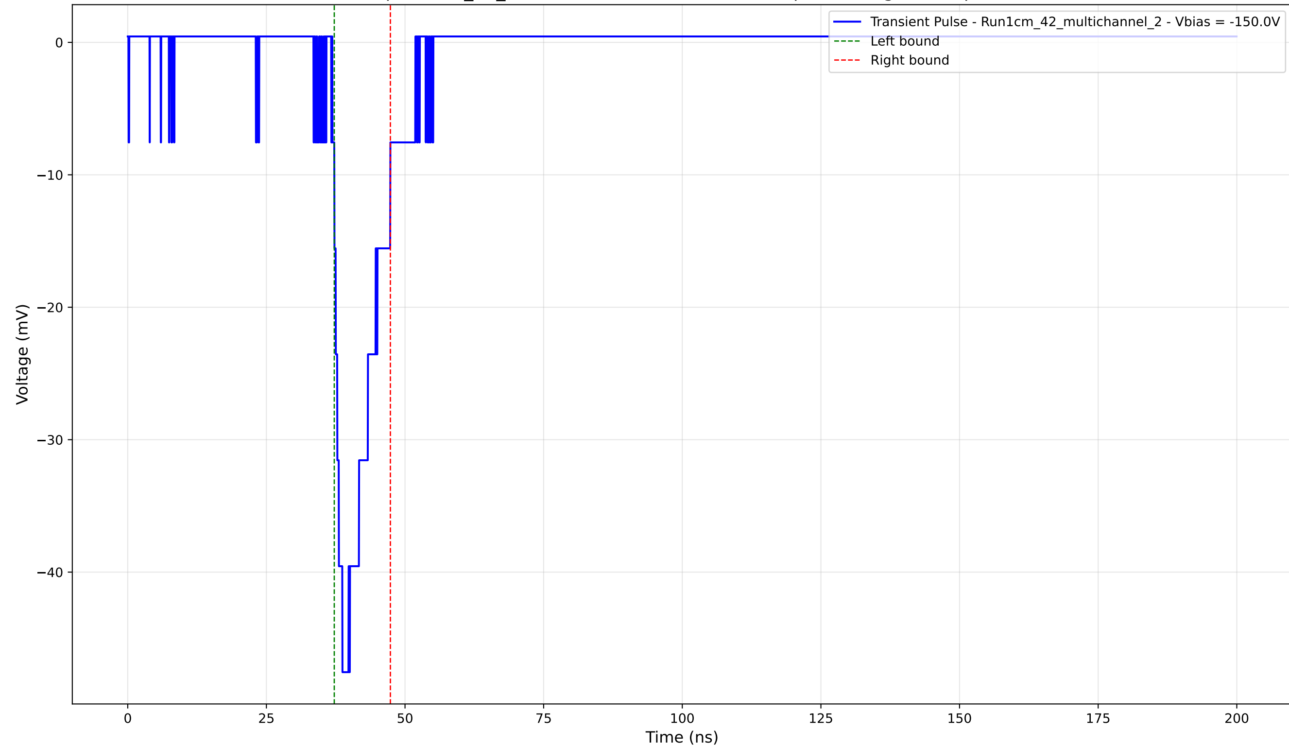
Transient Pulse - Sample: 1cm_42_multichannel - Position: 3935.0 \mu\text{m} - Charge: 5.99 pC - Rise Time: 1.82 ns
