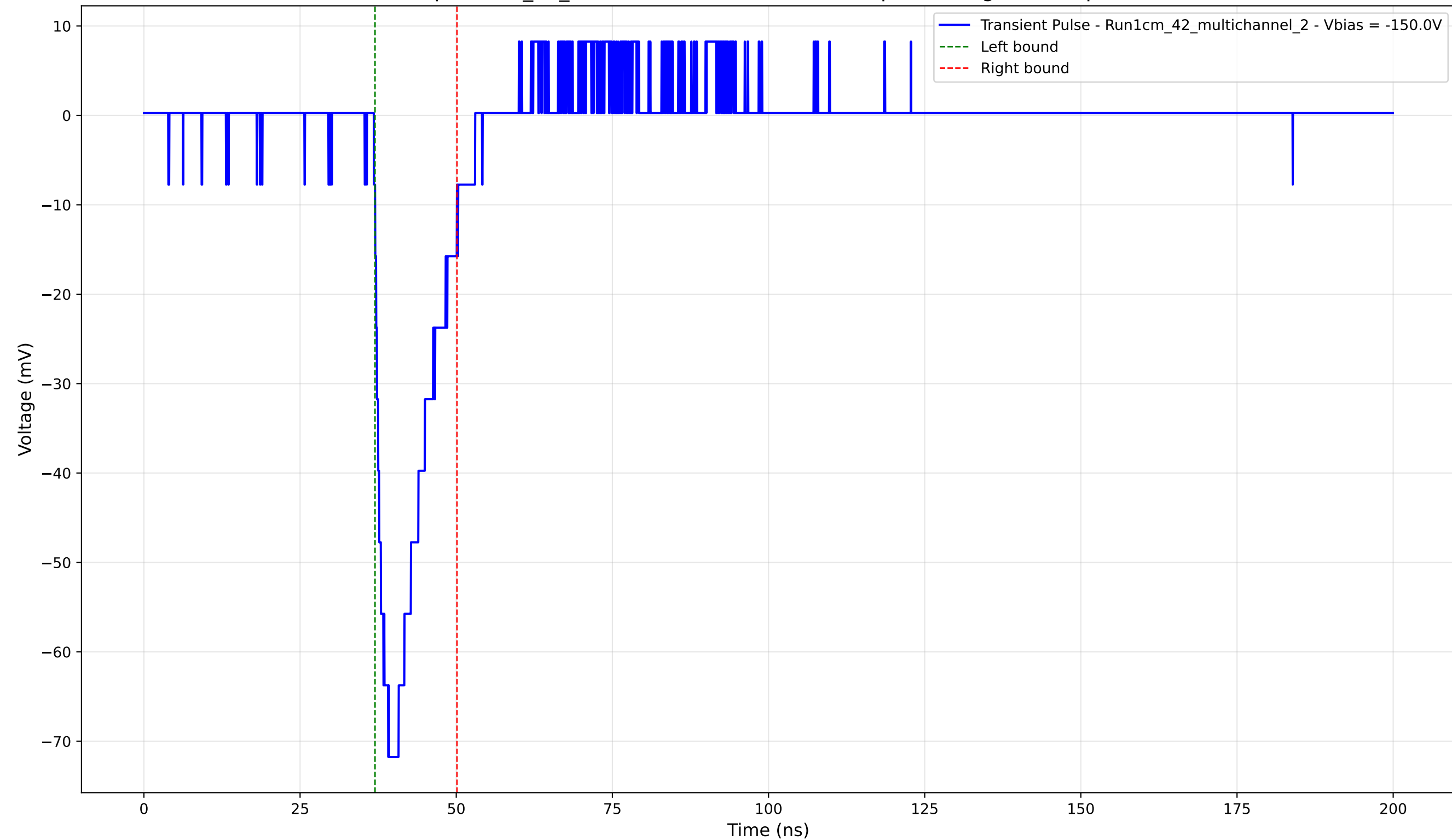
Transient Pulse - Sample: 1cm_42_multichannel - Position: 165.0 \mu\text{m} - Charge: 11.13 pC - Rise Time: 2.28 ns
