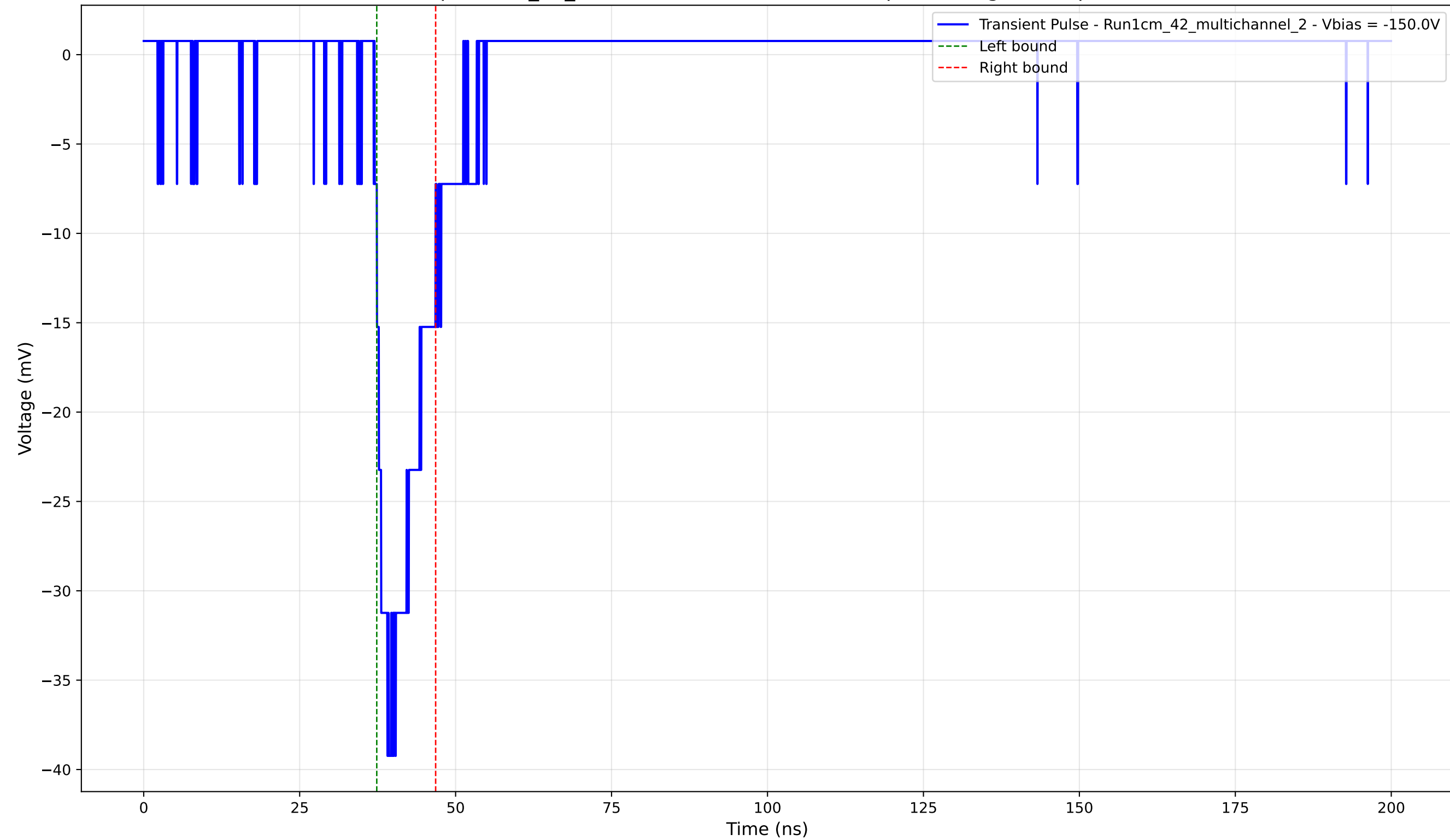
Transient Pulse - Sample: 1cm_42_multichannel - Position: 390.0 \mu\text{m} - Charge: 4.77 pC - Rise Time: 2.06 ns
