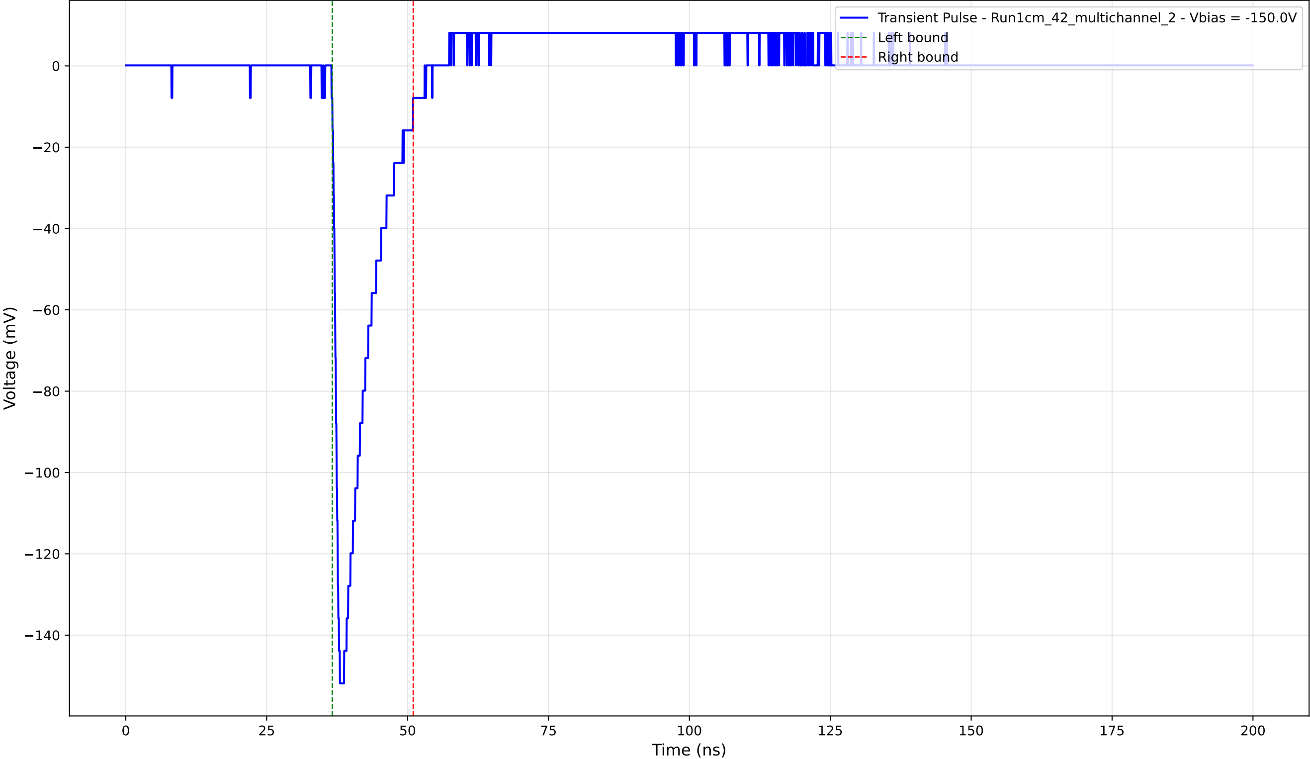
Transient Pulse - Sample: 1cm_42_multichannel - Position: 1215.0 \mu\text{m} - Charge: 19.00 pC - Rise Time: 1.16 ns
