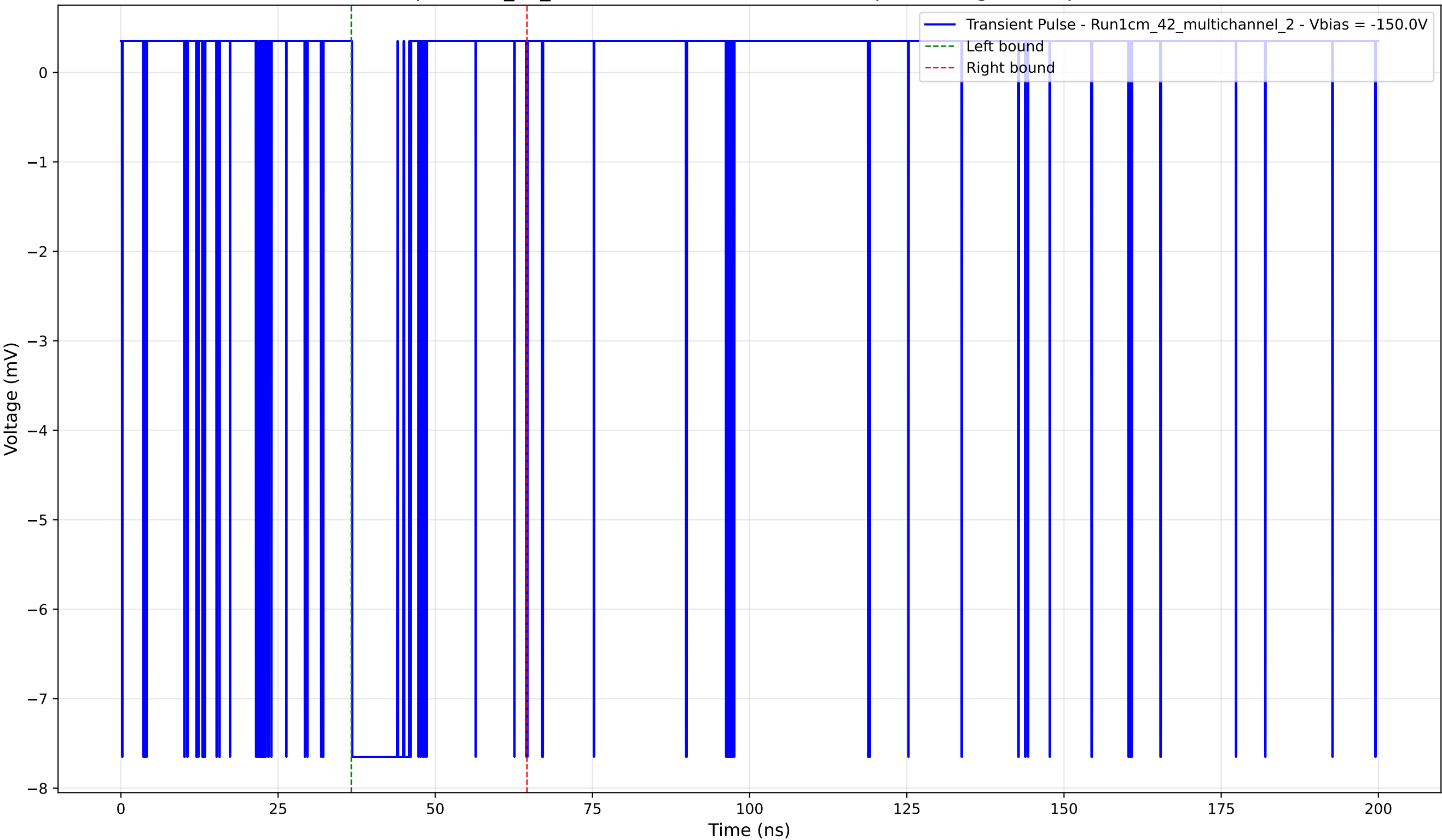
Transient Pulse - Sample: 1cm_42_multichannel - Position: 3385.0 \mu\text{m} - Charge: 1.34 pC - Rise Time: 0.04 ns
