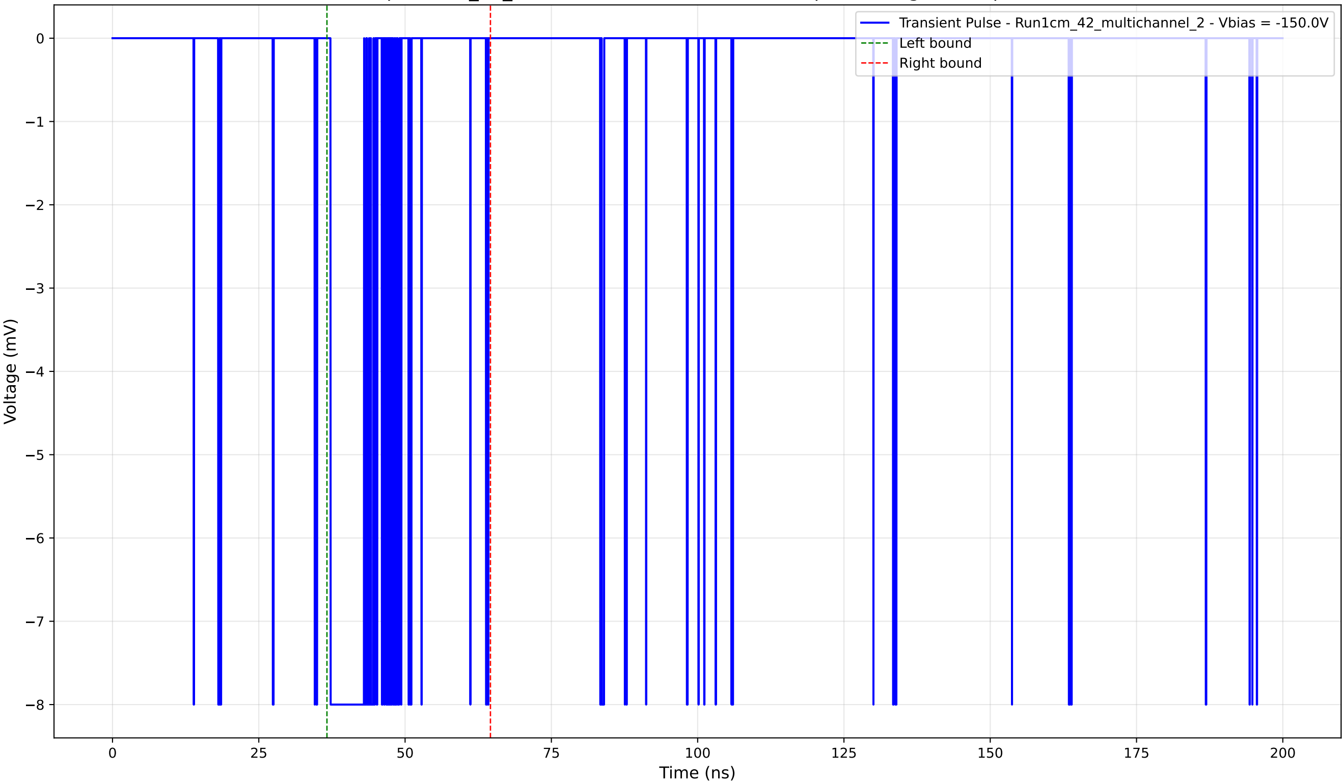
Transient Pulse - Sample: 1cm_42_multichannel - Position: 3885.0 \mu\text{m} - Charge: 1.52 pC - Rise Time: 0.04 ns
