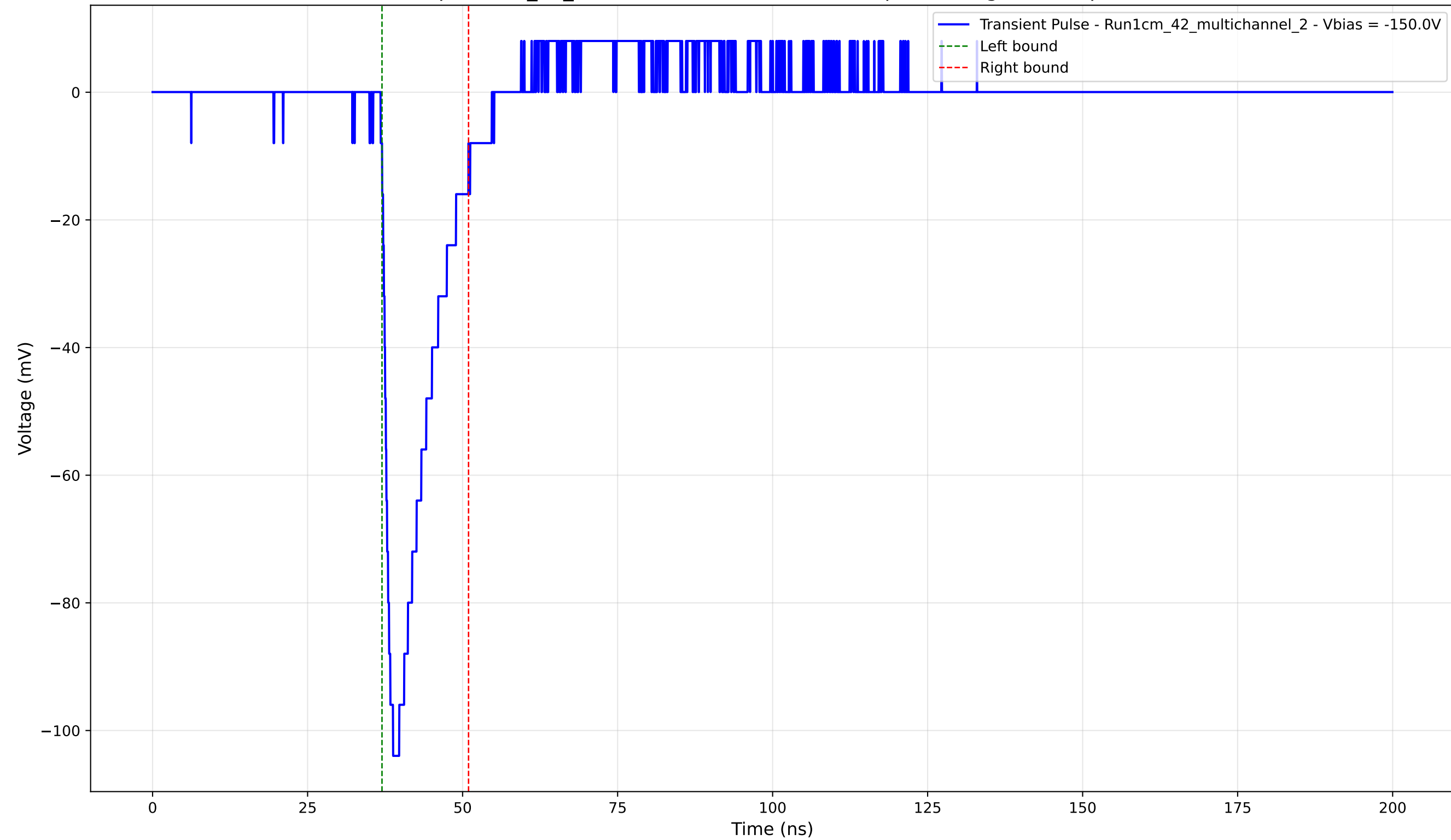
Transient Pulse - Sample: 1cm_42_multichannel - Position: 750.0 \mu\text{m} - Charge: 14.88 pC - Rise Time: 1.35 ns
