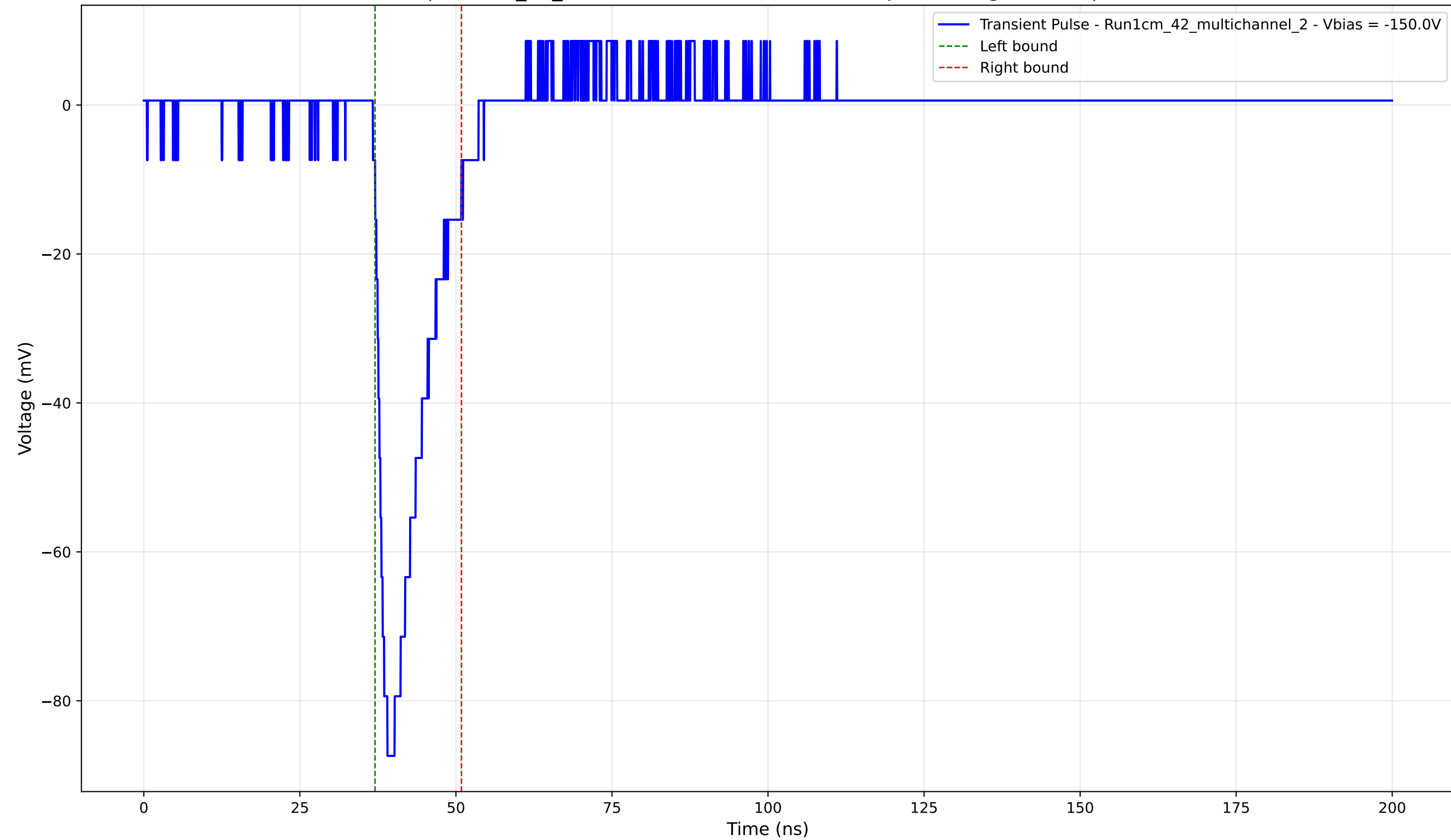
Transient Pulse - Sample: 1cm_42_multichannel - Position: 4085.0 \mu\text{m} - Charge: 12.70 pC - Rise Time: 1.47 ns
