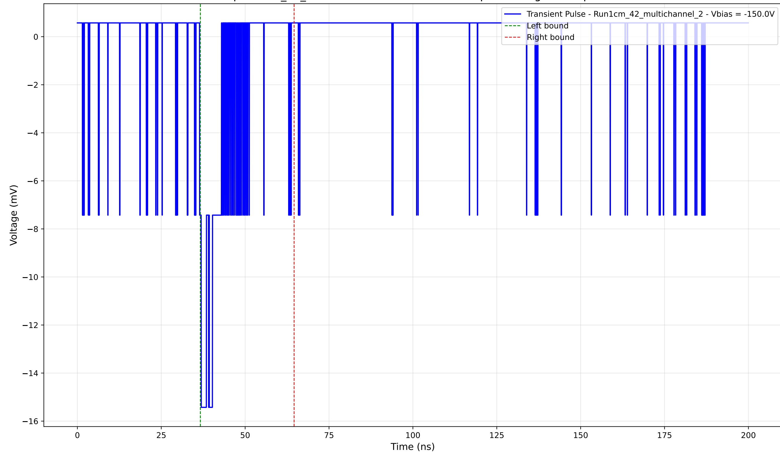
Transient Pulse - Sample: 1cm_42_multichannel - Position: 1875.0 \mu\text{m} - Charge: 1.59 pC - Rise Time: 0.51 ns
