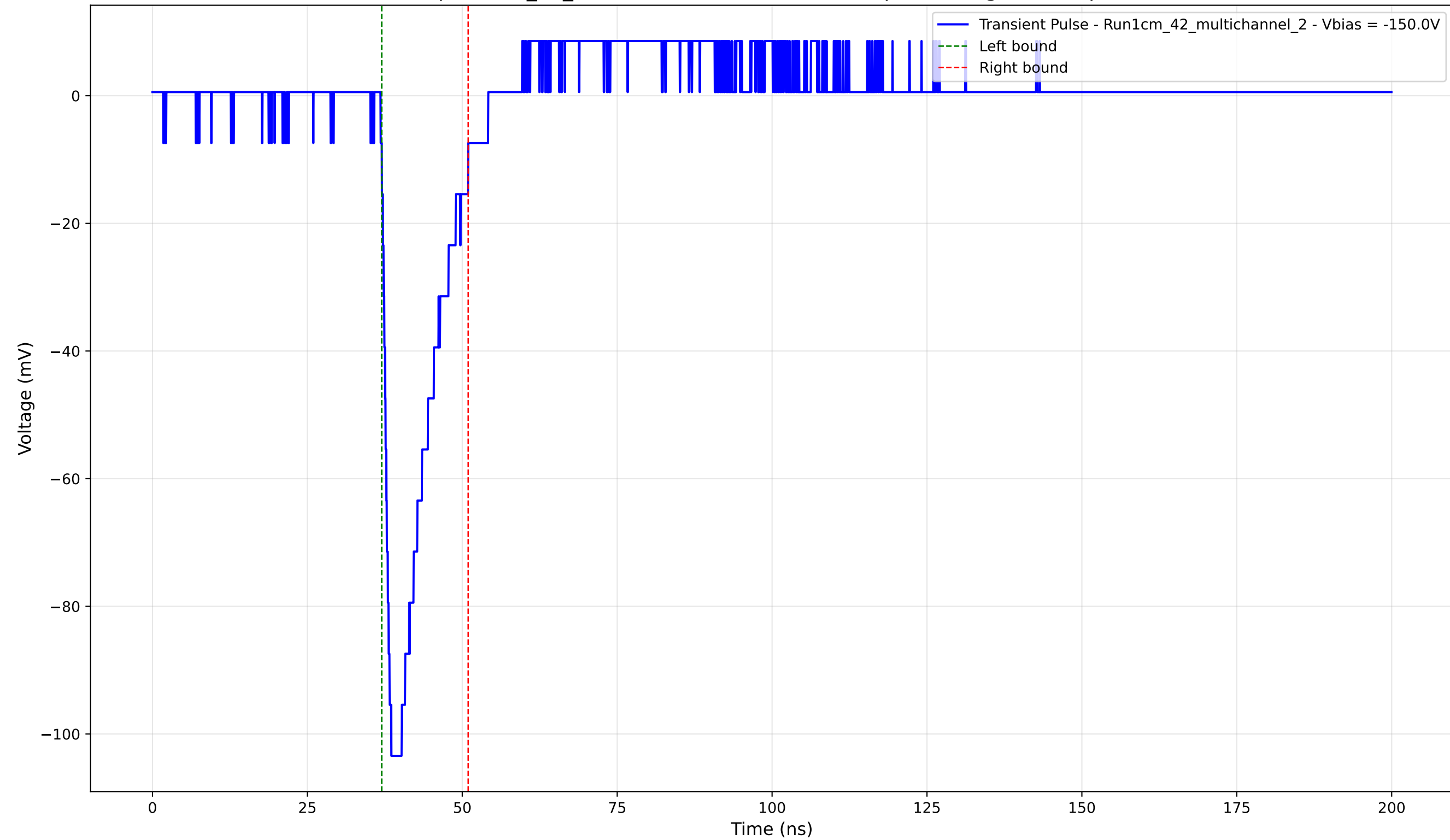
Transient Pulse - Sample: 1cm_42_multichannel - Position: 720.0 \mu\text{m} - Charge: 15.24 pC - Rise Time: 1.27 ns
