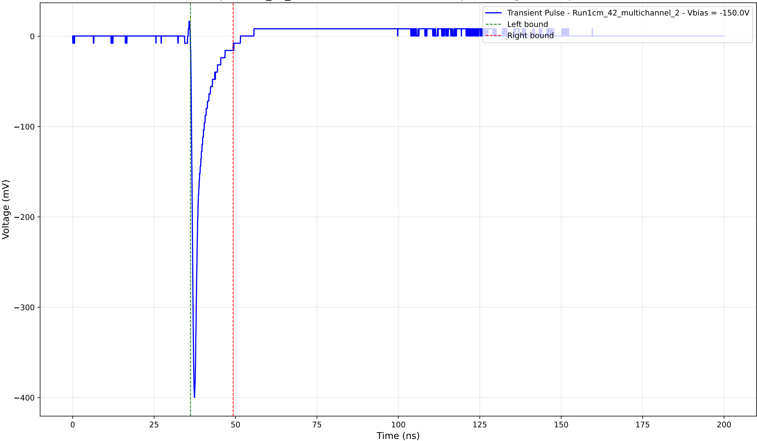
Transient Pulse - Sample: 1cm_42_multichannel - Position: 2755.0 \mu\text{m} - Charge: 24.13 pC - Rise Time: 0.80 ns
