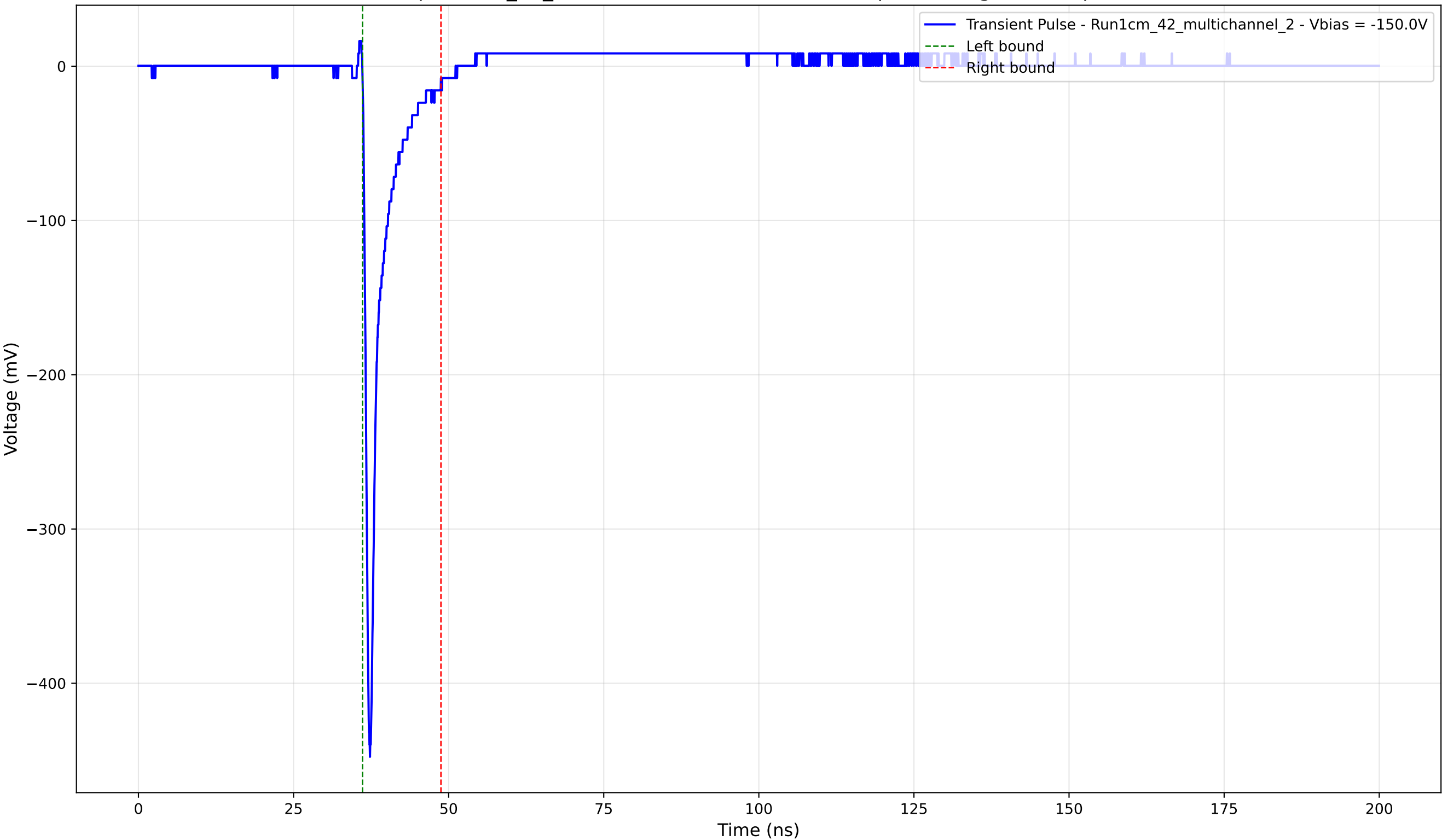
Transient Pulse - Sample: 1cm_42_multichannel - Position: 2665.0 \mu\text{m} - Charge: 24.51 pC - Rise Time: 0.80 ns
