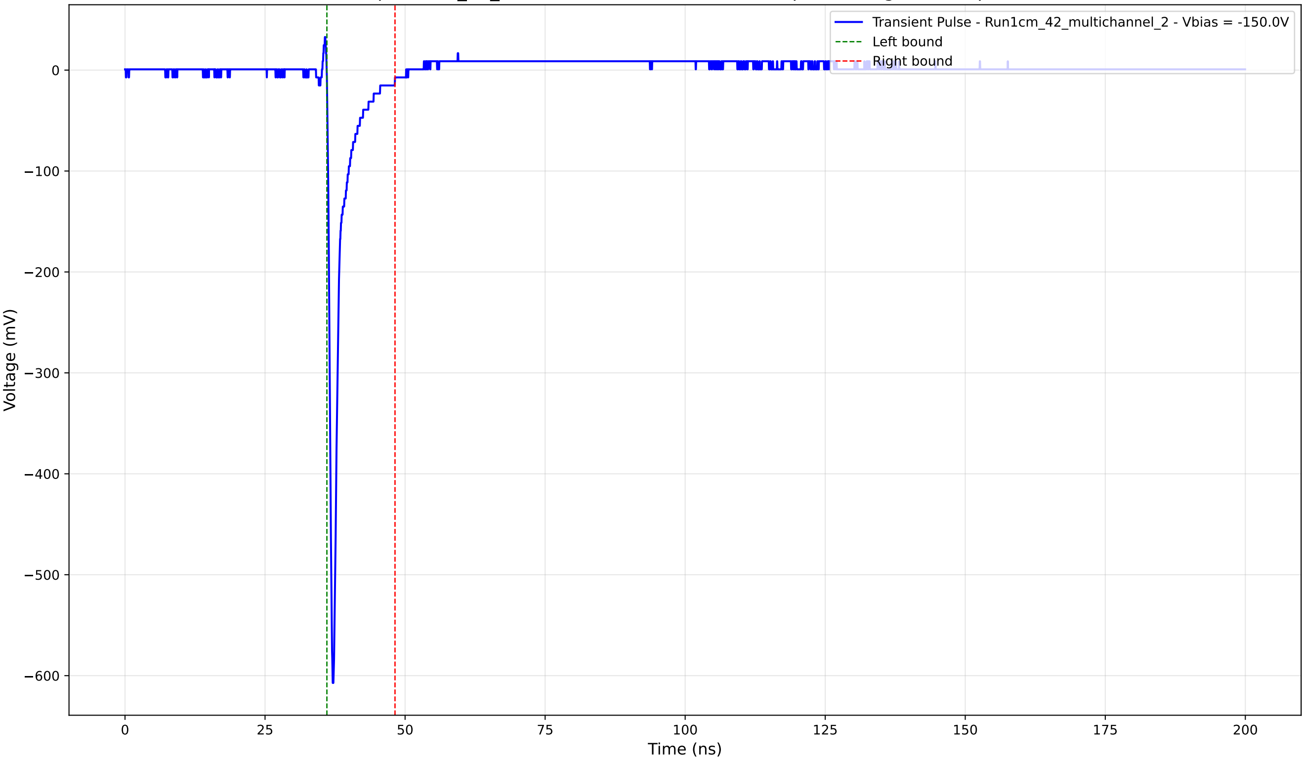
Transient Pulse - Sample: 1cm_42_multichannel - Position: 2290.0 \mu\text{m} - Charge: 27.01 pC - Rise Time: 0.71 ns
