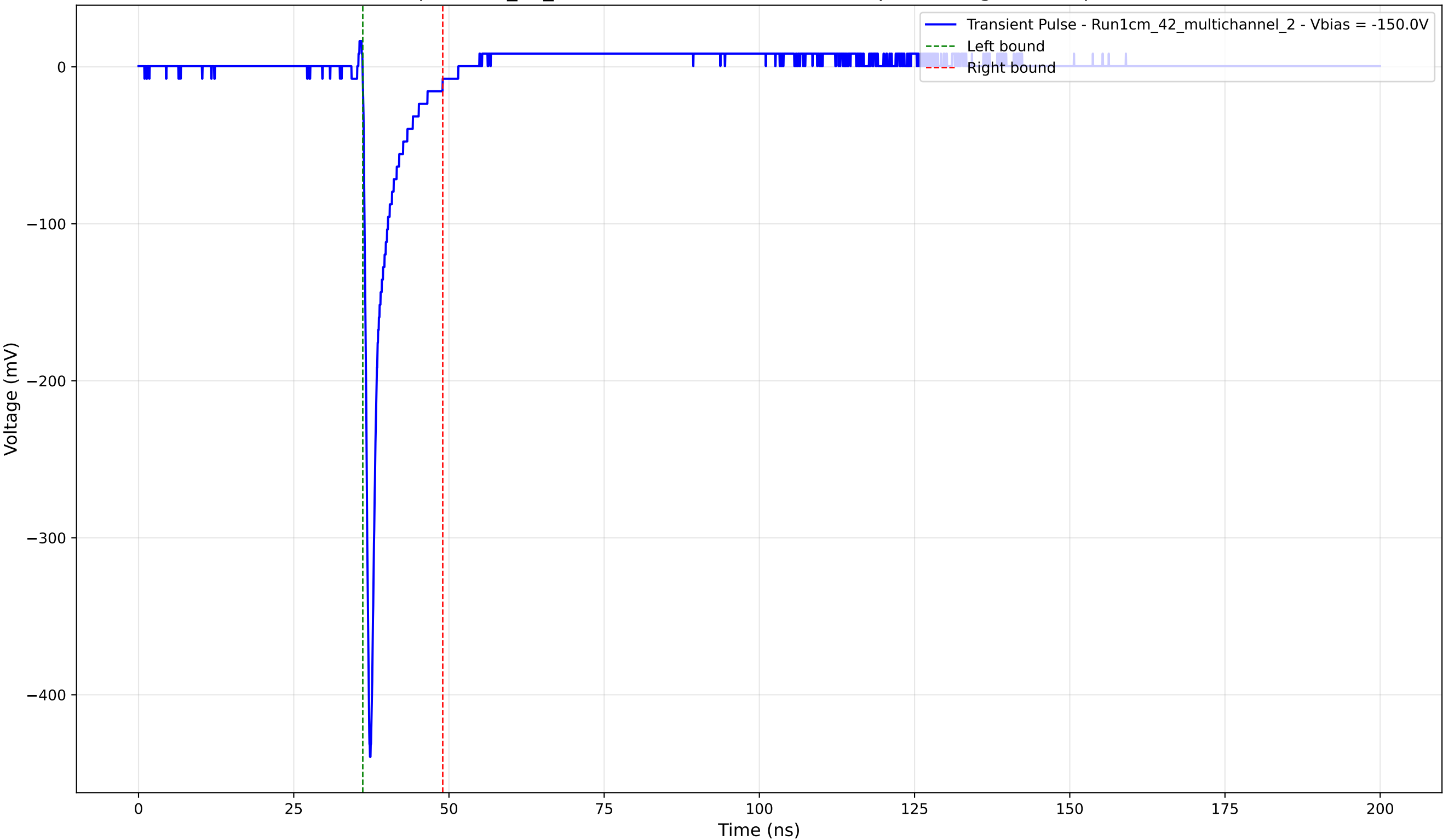
Transient Pulse - Sample: 1cm_42_multichannel - Position: 2670.0 \mu\text{m} - Charge: 24.44 pC - Rise Time: 0.80 ns
