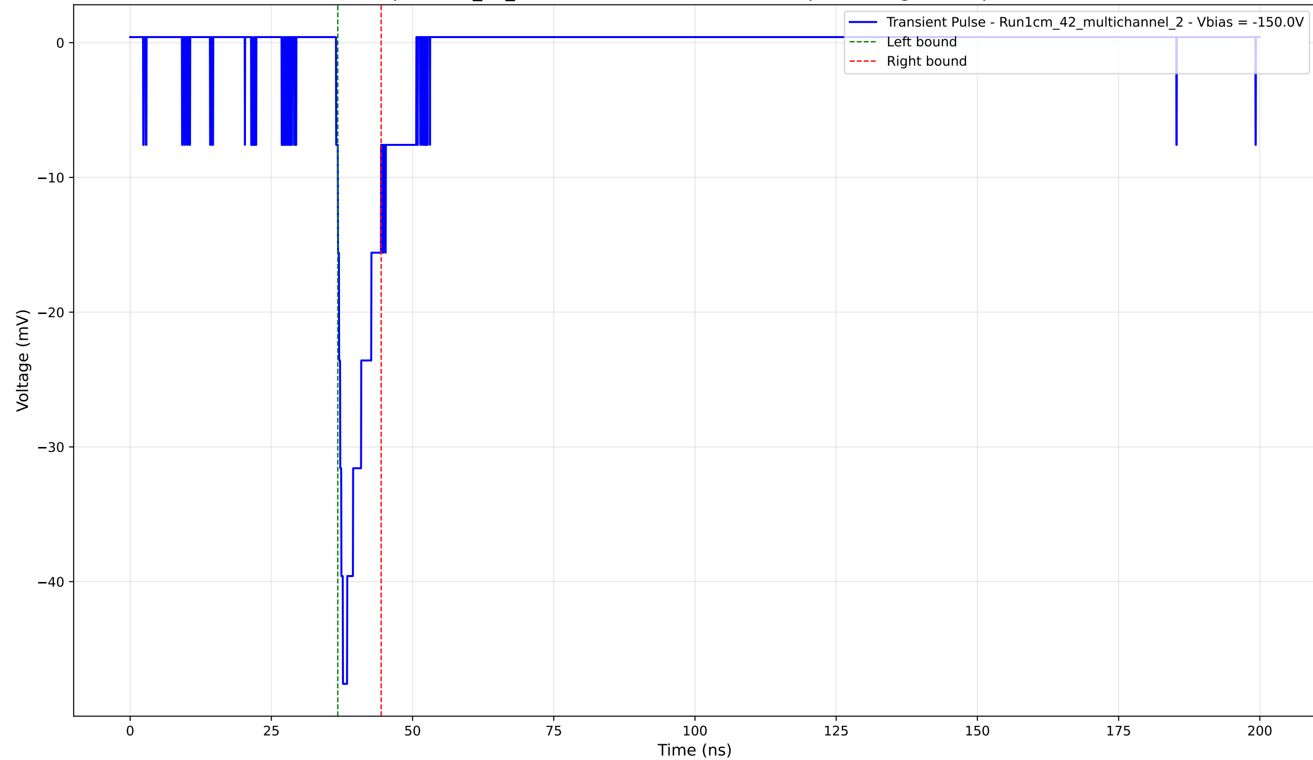
Transient Pulse - Sample: 1cm_42_multichannel - Position: 1395.0 \mu\text{m} - Charge: 4.35 pC - Rise Time: 1.22 ns
