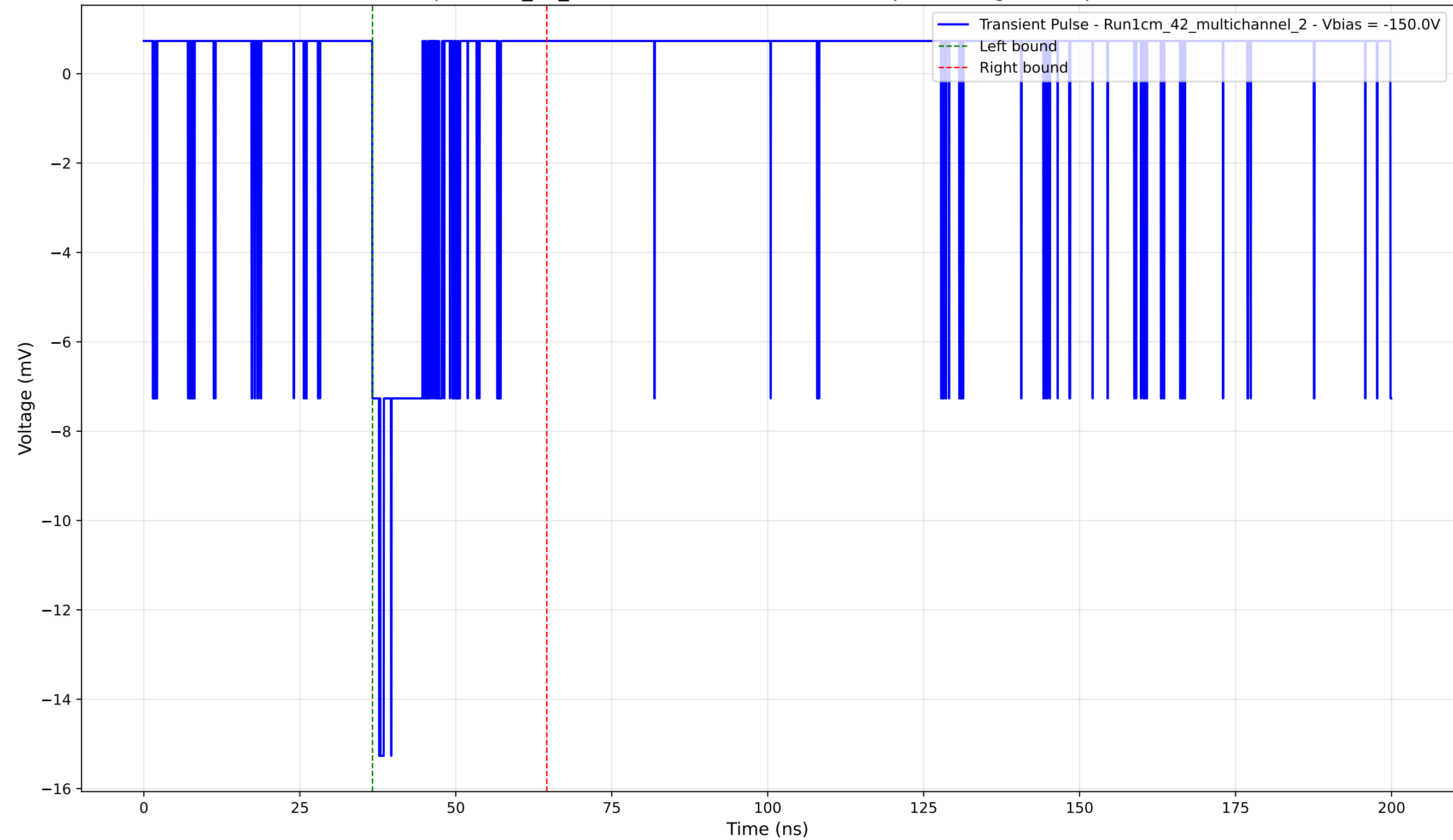
Transient Pulse - Sample: 1cm_42_multichannel - Position: 3400.0 \mu\text{m} - Charge: 1.55 pC - Rise Time: 1.12 ns
