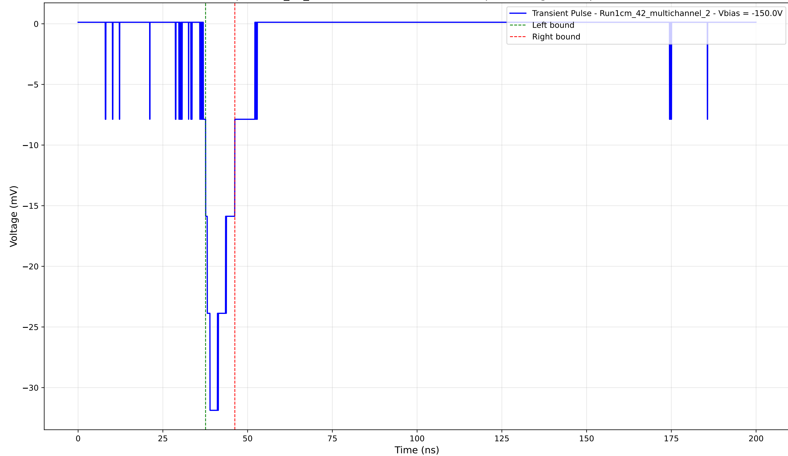
Transient Pulse - Sample: 1cm_42_multichannel - Position: 4435.0 \mu\text{m} - Charge: 3.99 pC - Rise Time: 1.98 ns
