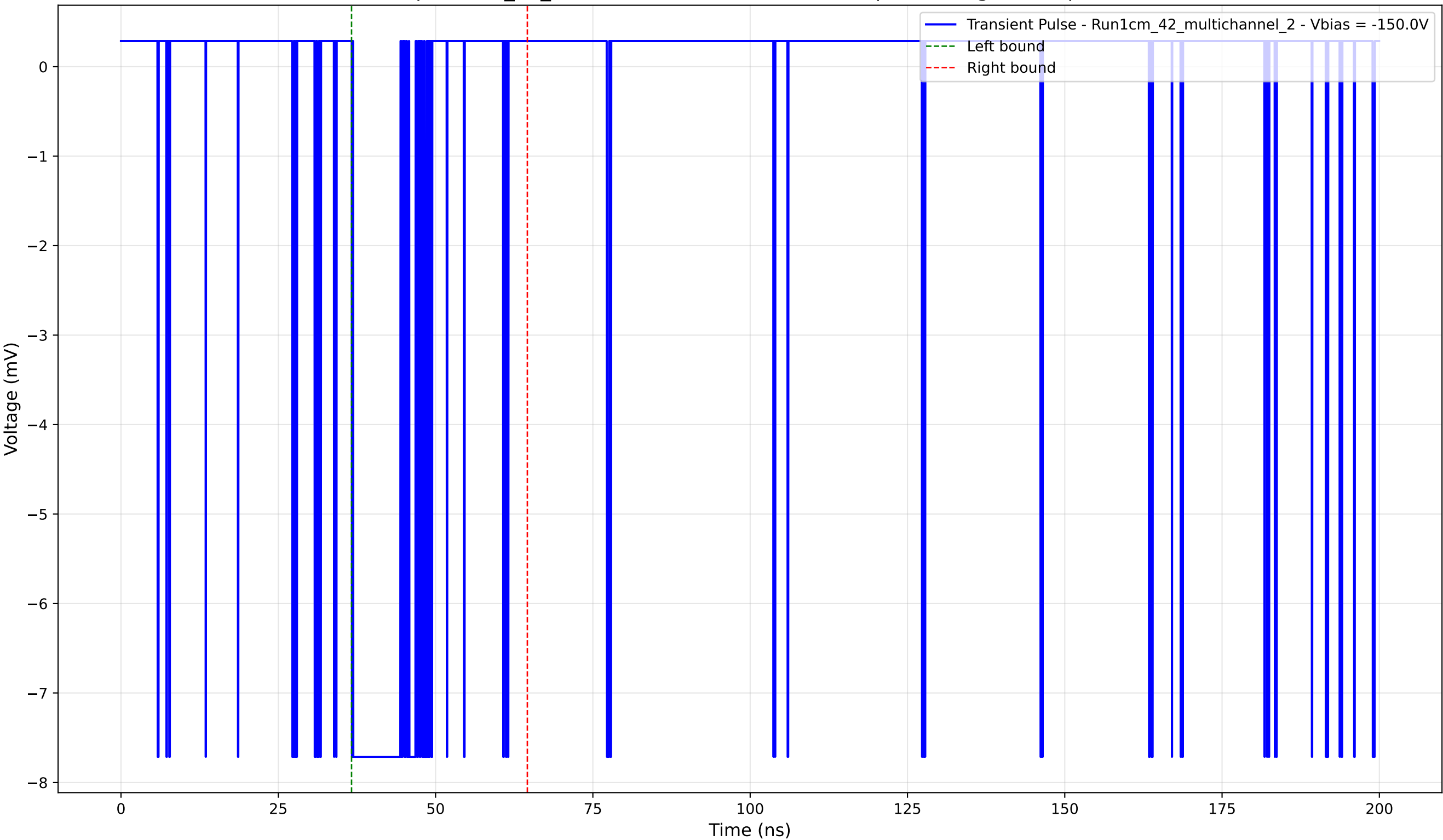
Transient Pulse - Sample: 1cm_42_multichannel - Position: 1360.0 \mu\text{m} - Charge: 1.61 pC - Rise Time: 0.04 ns
