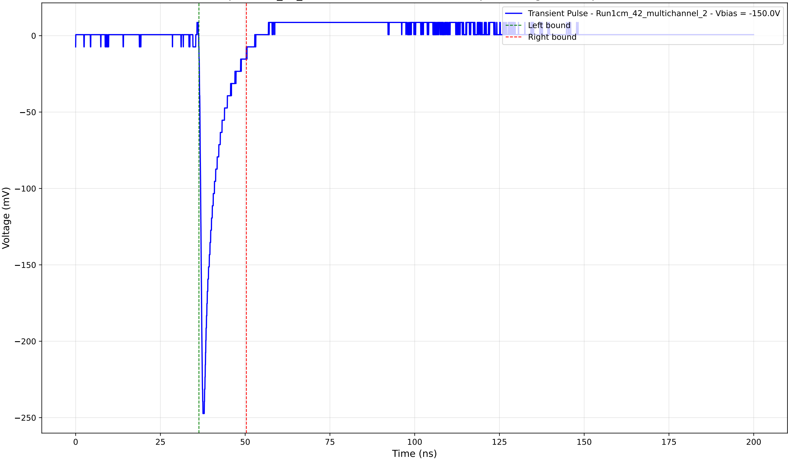
Transient Pulse - Sample: 1cm_42_multichannel - Position: 1640.0 \mu\text{m} - Charge: 22.14 pC - Rise Time: 0.87 ns
