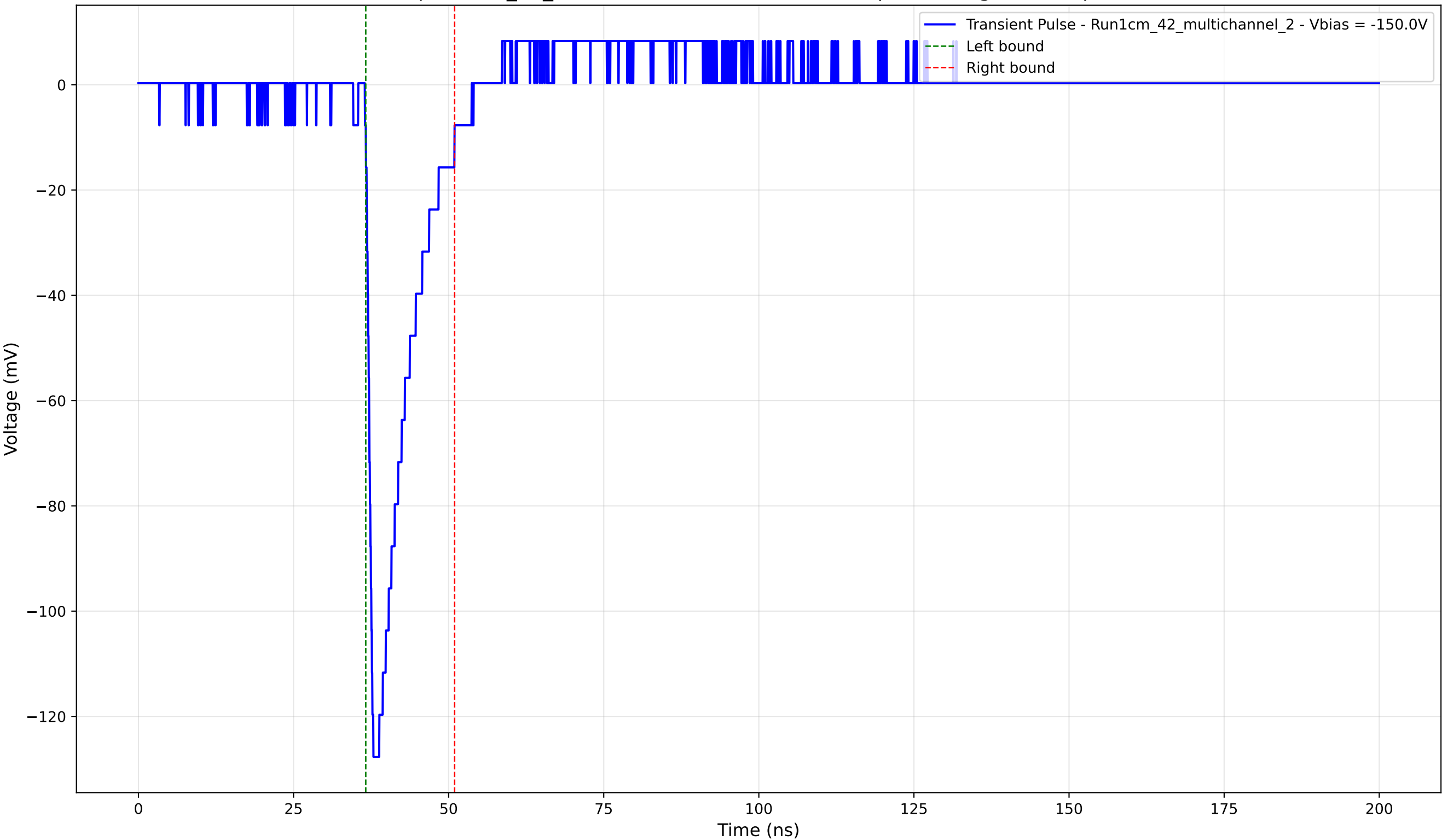
Transient Pulse - Sample: 1cm_42_multichannel - Position: 3505.0 \mu\text{m} - Charge: 16.51 pC - Rise Time: 1.05 ns
