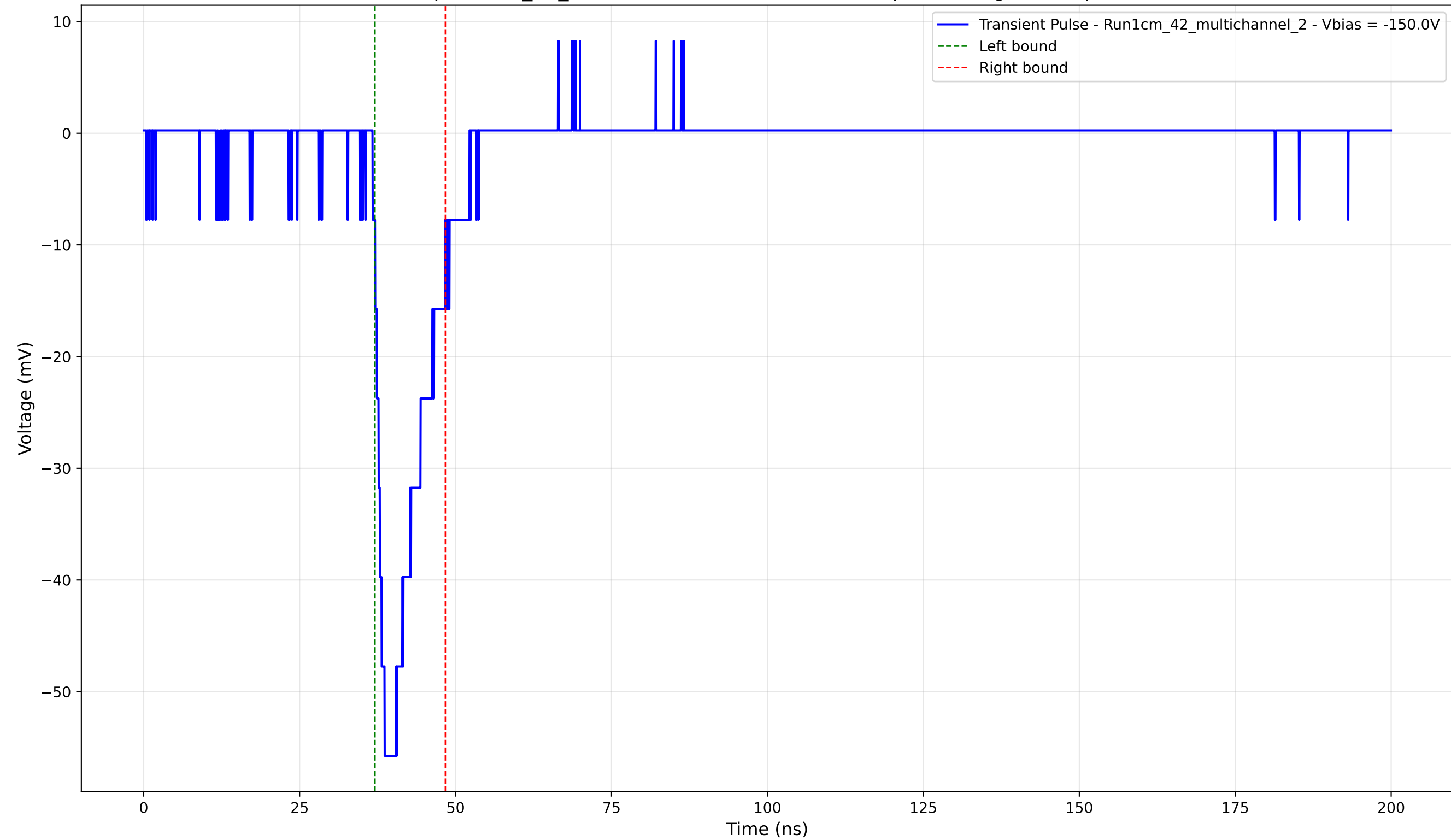
Transient Pulse - Sample: 1cm_42_multichannel - Position: 3940.0 \mu\text{m} - Charge: 7.69 pC - Rise Time: 1.93 ns
