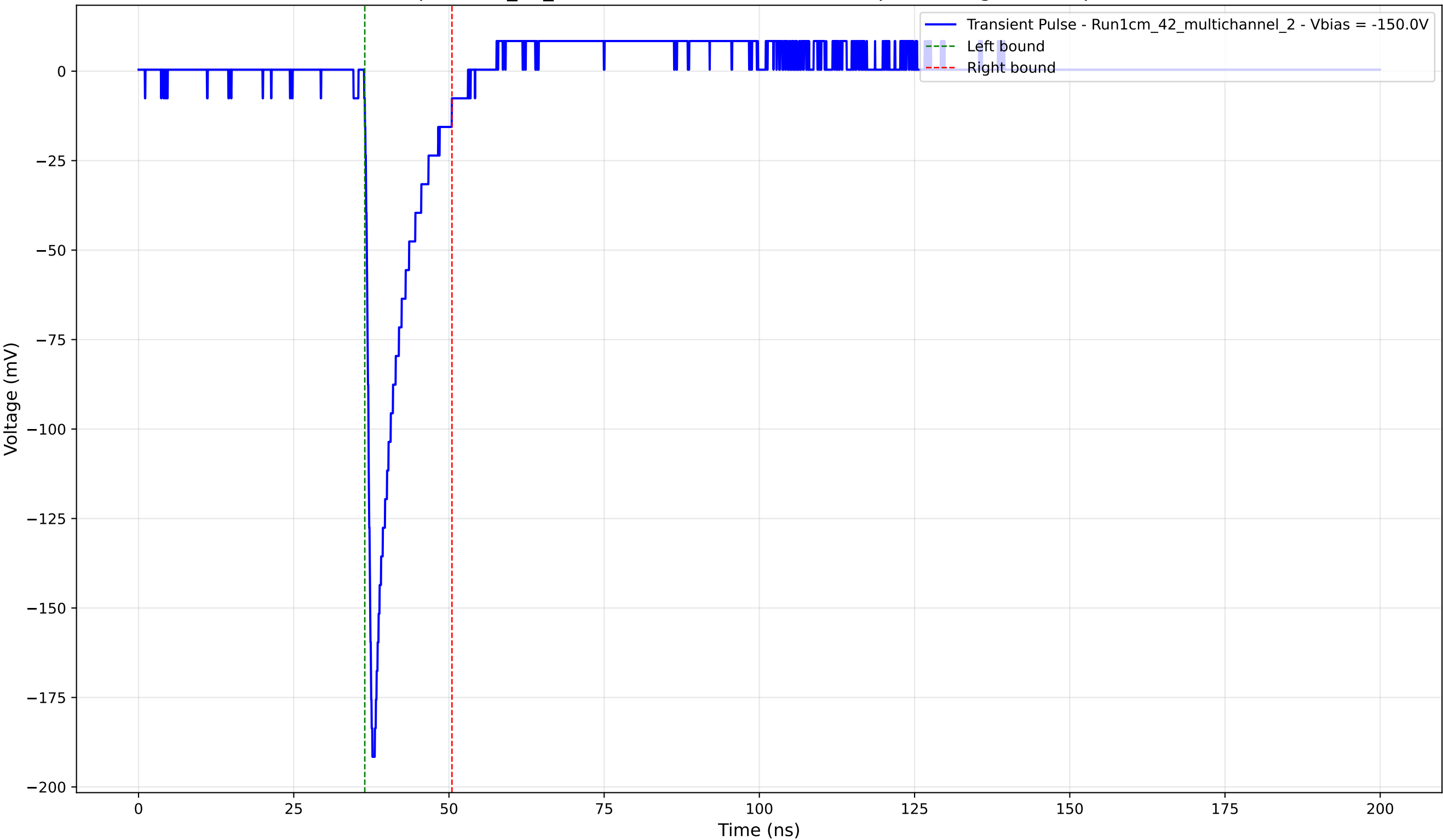
Transient Pulse - Sample: 1cm_42_multichannel - Position: 3225.0 \mu\text{m} - Charge: 19.21 pC - Rise Time: 0.94 ns
