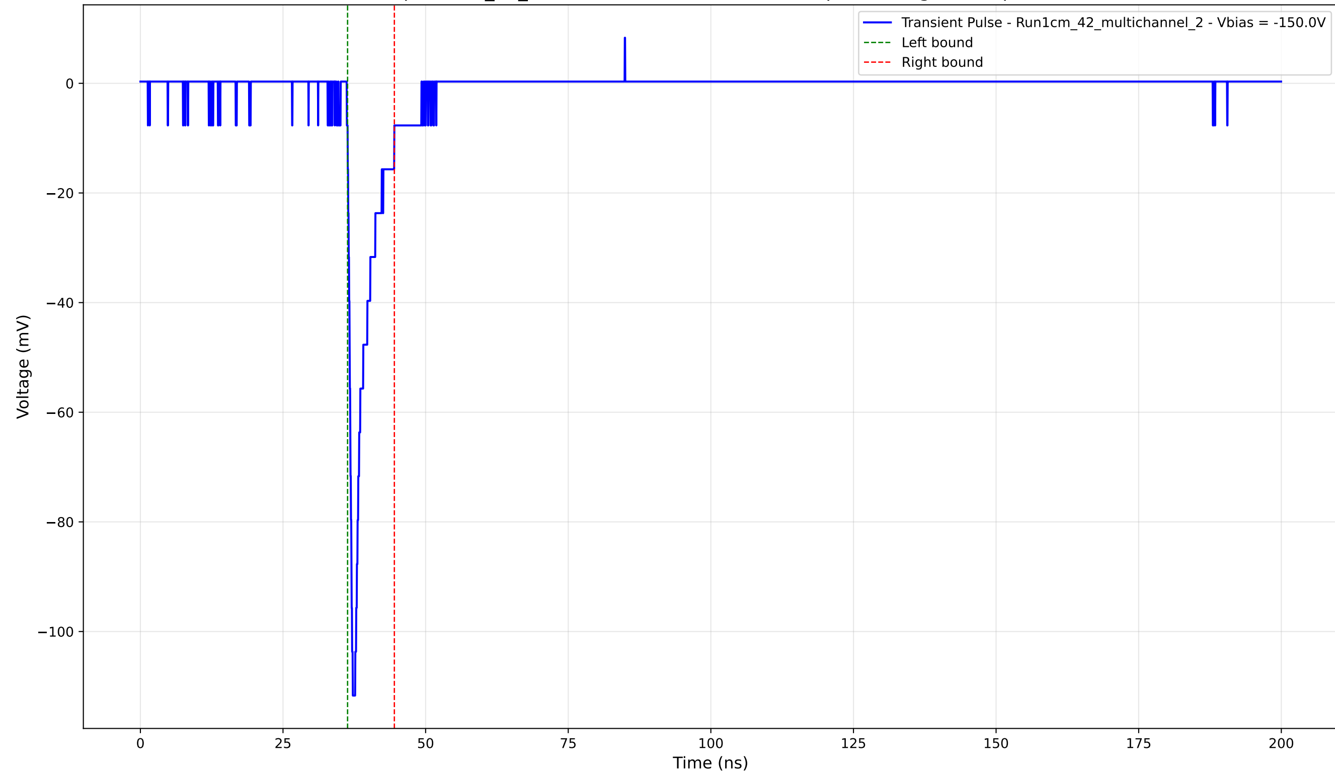
Transient Pulse - Sample: 1cm_42_multichannel - Position: 1905.0 \mu\text{m} - Charge: 6.97 pC - Rise Time: 0.78 ns
