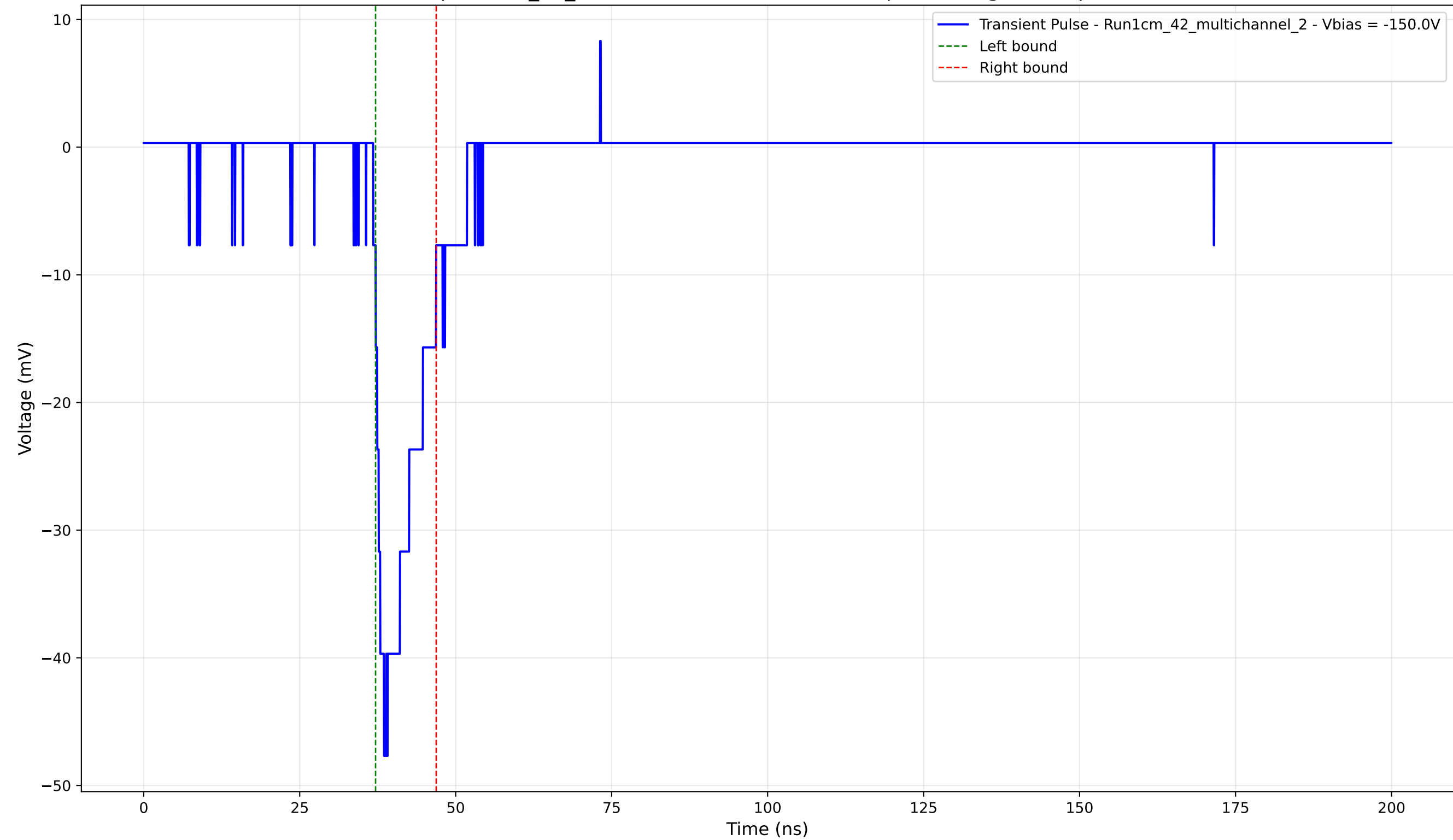
Transient Pulse - Sample: 1cm_42_multichannel - Position: 895.0 \mu\text{m} - Charge: 5.58 pC - Rise Time: 1.74 ns
