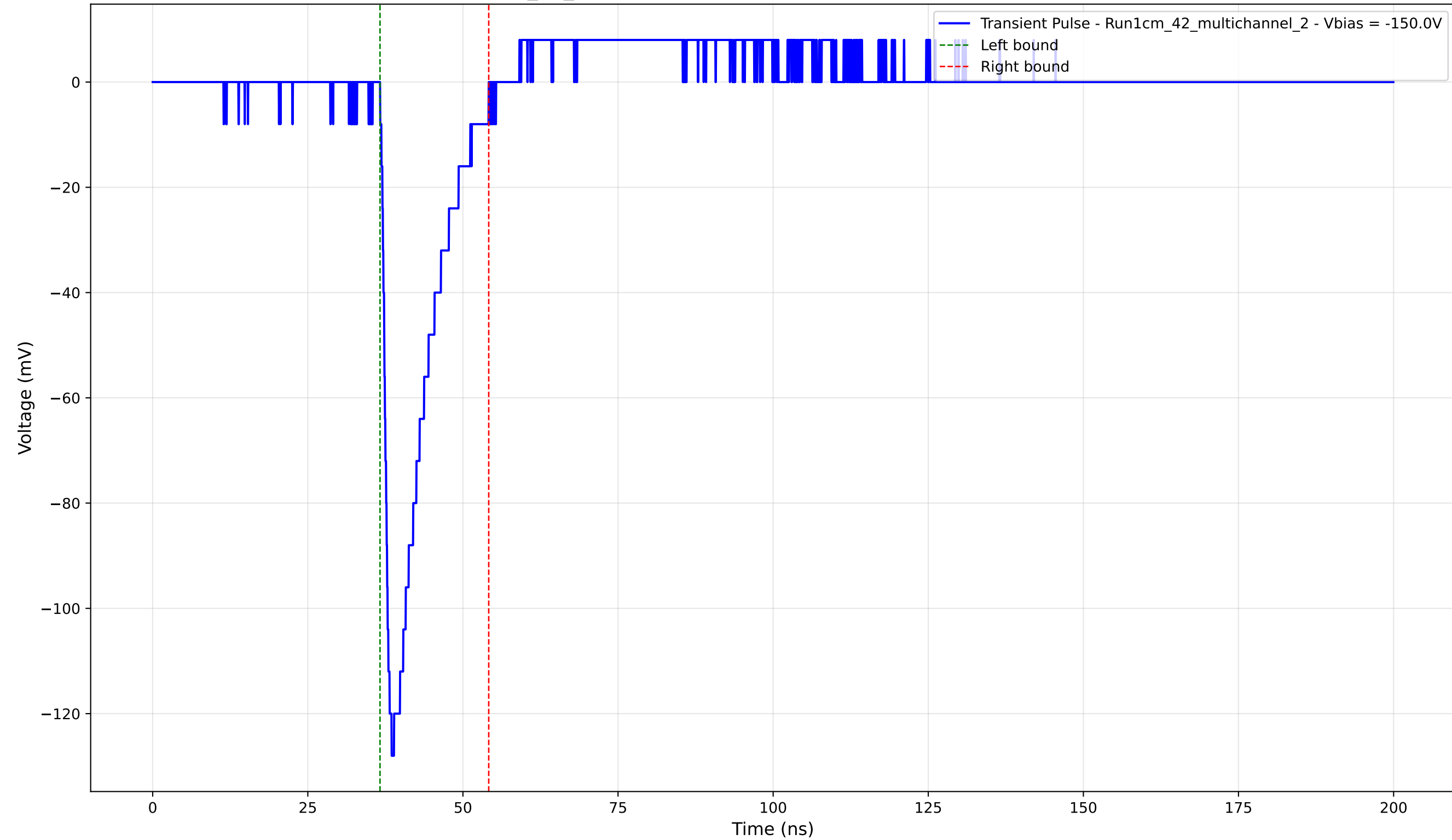
Transient Pulse - Sample: 1cm_42_multichannel - Position: 985.0 \mu\text{m} - Charge: 17.79 pC - Rise Time: 1.34 ns
