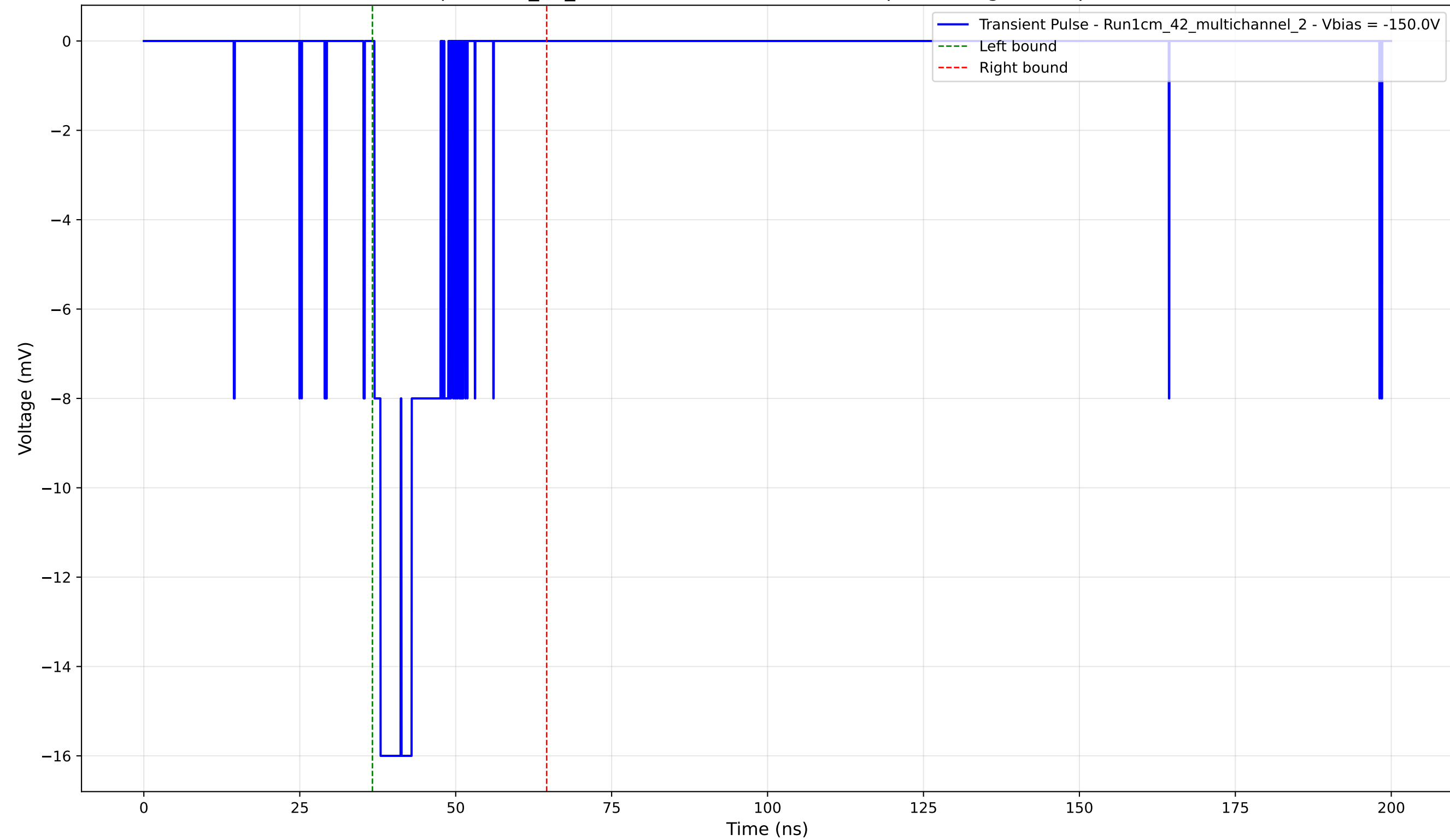
Transient Pulse - Sample: 1cm_42_multichannel - Position: 310.0 \mu\text{m} - Charge: 2.83 pC - Rise Time: 0.99 ns
