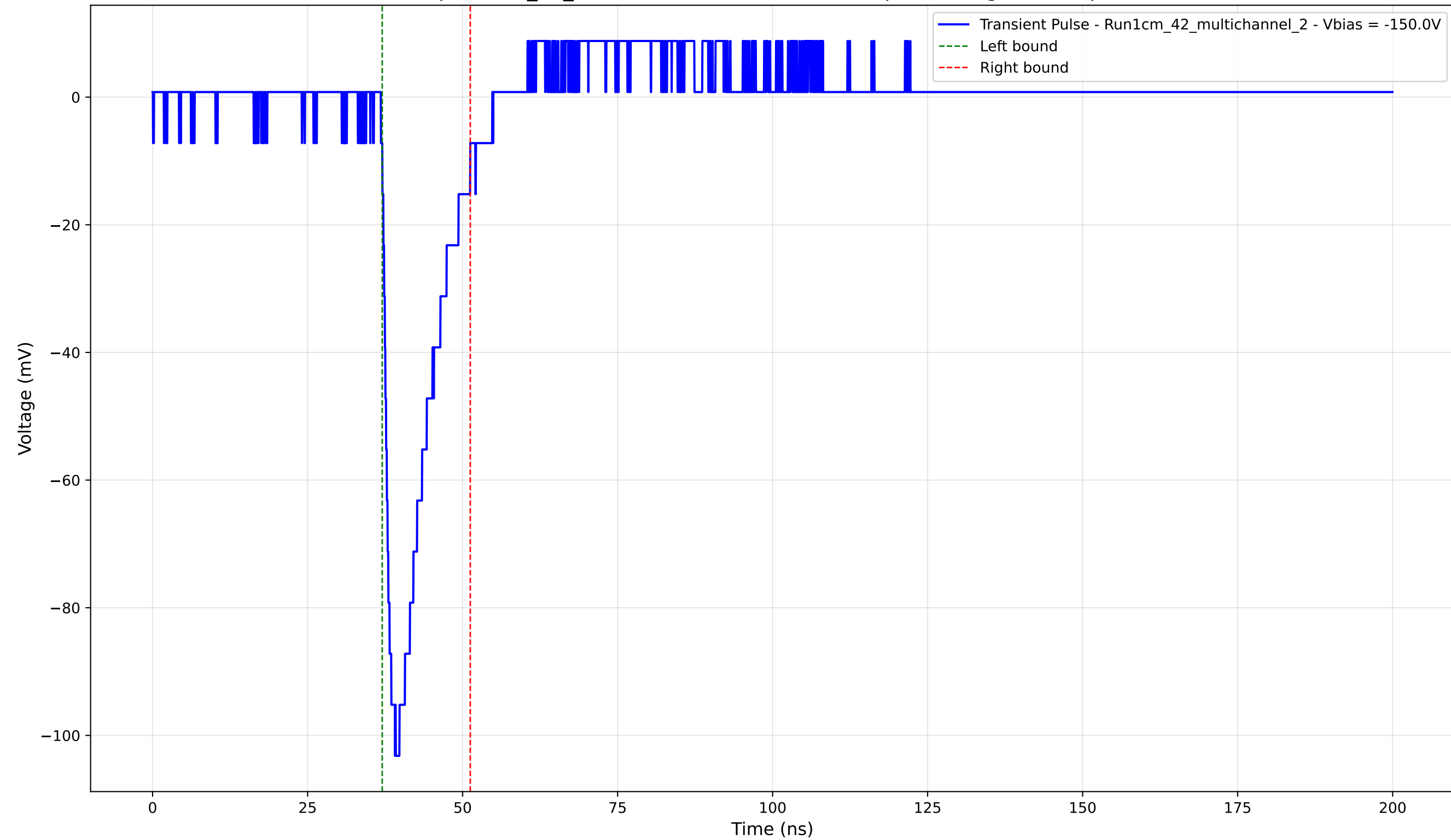
Transient Pulse - Sample: 1cm_42_multichannel - Position: 660.0 \mu\text{m} - Charge: 14.86 pC - Rise Time: 1.46 ns
