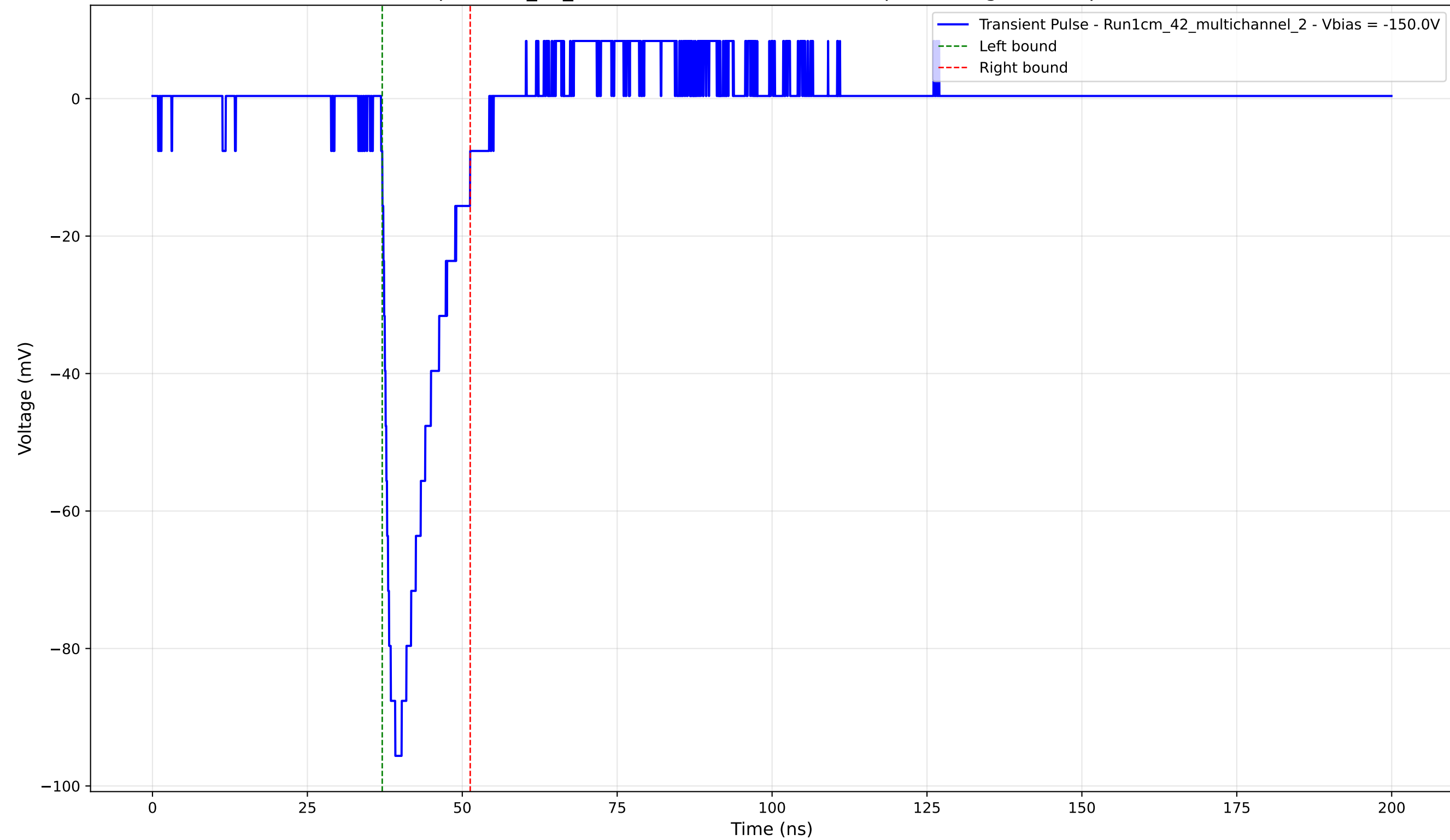
Transient Pulse - Sample: 1cm_42_multichannel - Position: 555.0 \mu\text{m} - Charge: 14.21 pC - Rise Time: 1.39 ns
