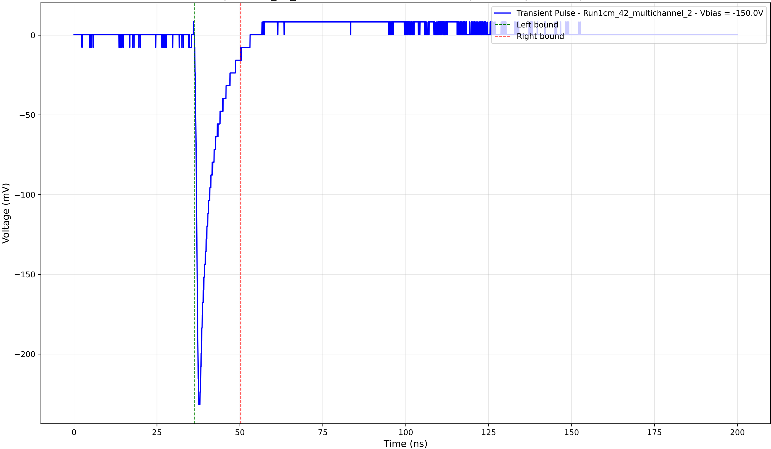
Transient Pulse - Sample: 1cm_42_multichannel - Position: 1590.0 \mu\text{m} - Charge: 21.58 pC - Rise Time: 0.96 ns
