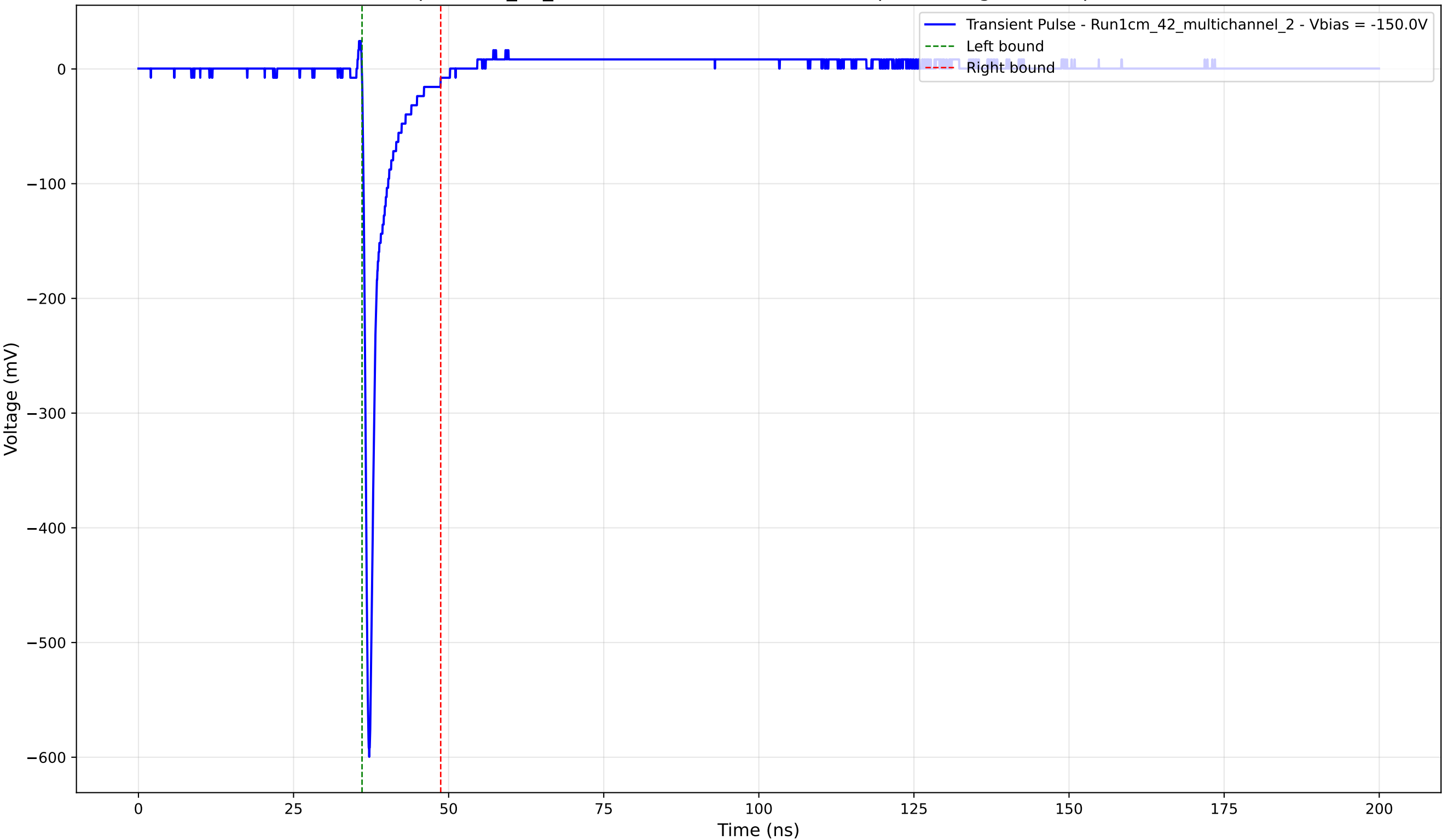
Transient Pulse - Sample: 1cm_42_multichannel - Position: 2220.0 \mu\text{m} - Charge: 28.41 pC - Rise Time: 0.74 ns
