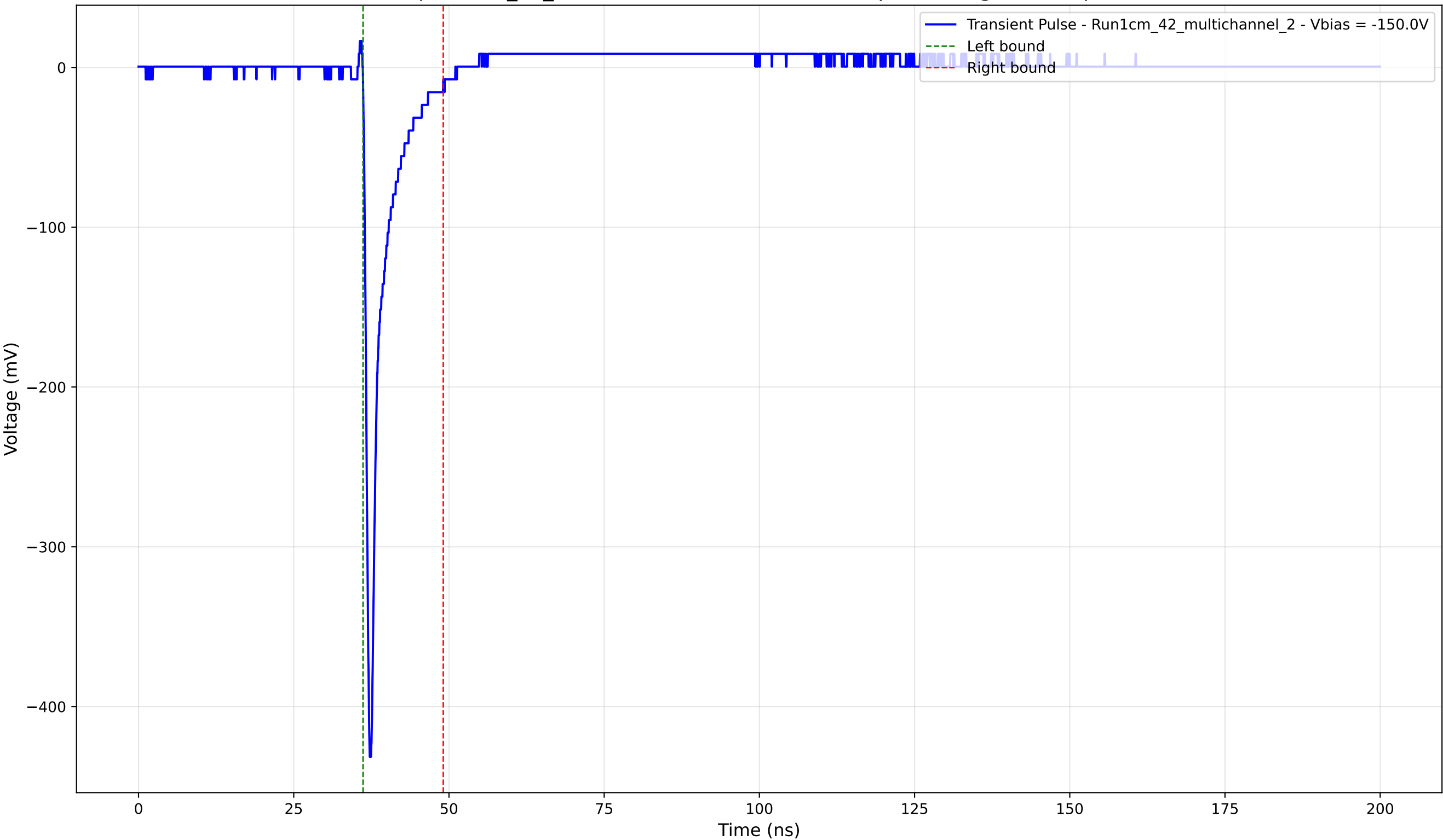
Transient Pulse - Sample: 1cm_42_multichannel - Position: 2700.0 \mu\text{m} - Charge: 24.91 pC - Rise Time: 0.77 ns
