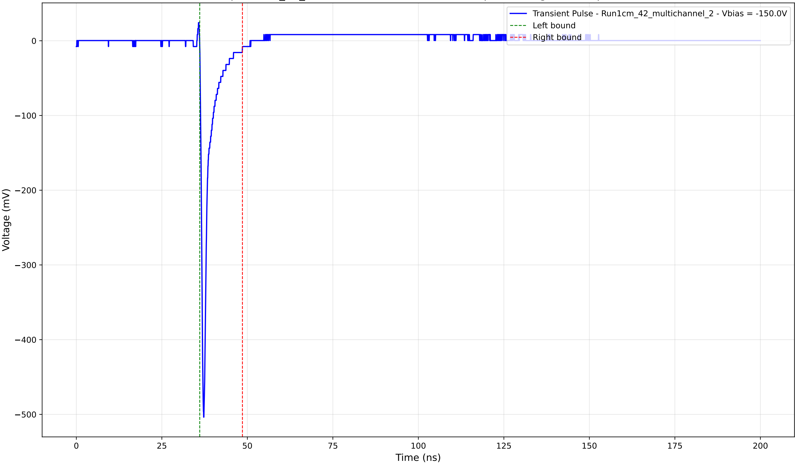
Transient Pulse - Sample: 1cm_42_multichannel - Position: 2570.0 \mu\text{m} - Charge: 25.08 pC - Rise Time: 0.77 ns
