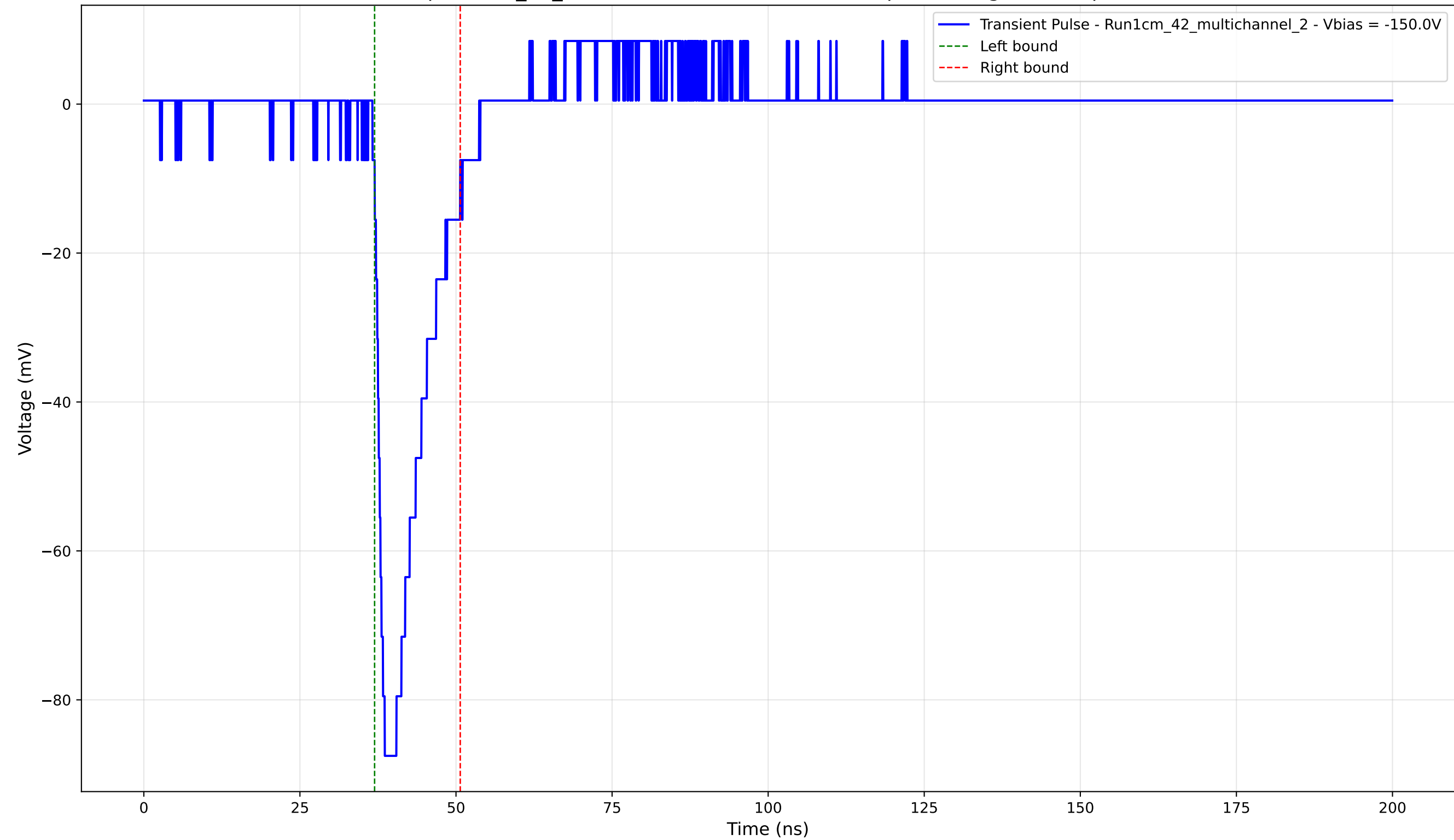
Transient Pulse - Sample: 1cm_42_multichannel - Position: 3965.0 \mu\text{m} - Charge: 12.98 pC - Rise Time: 1.35 ns
