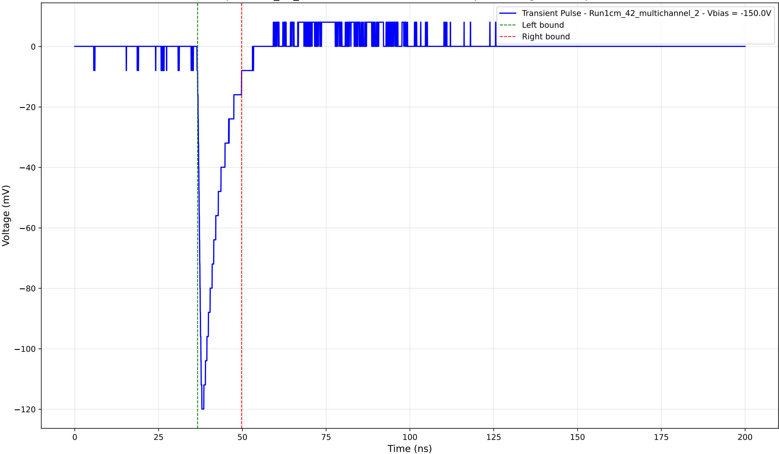
Transient Pulse - Sample: 1cm_42_multichannel - Position: 1295.0 \mu\text{m} - Charge: 14.05 pC - Rise Time: 1.06 ns
