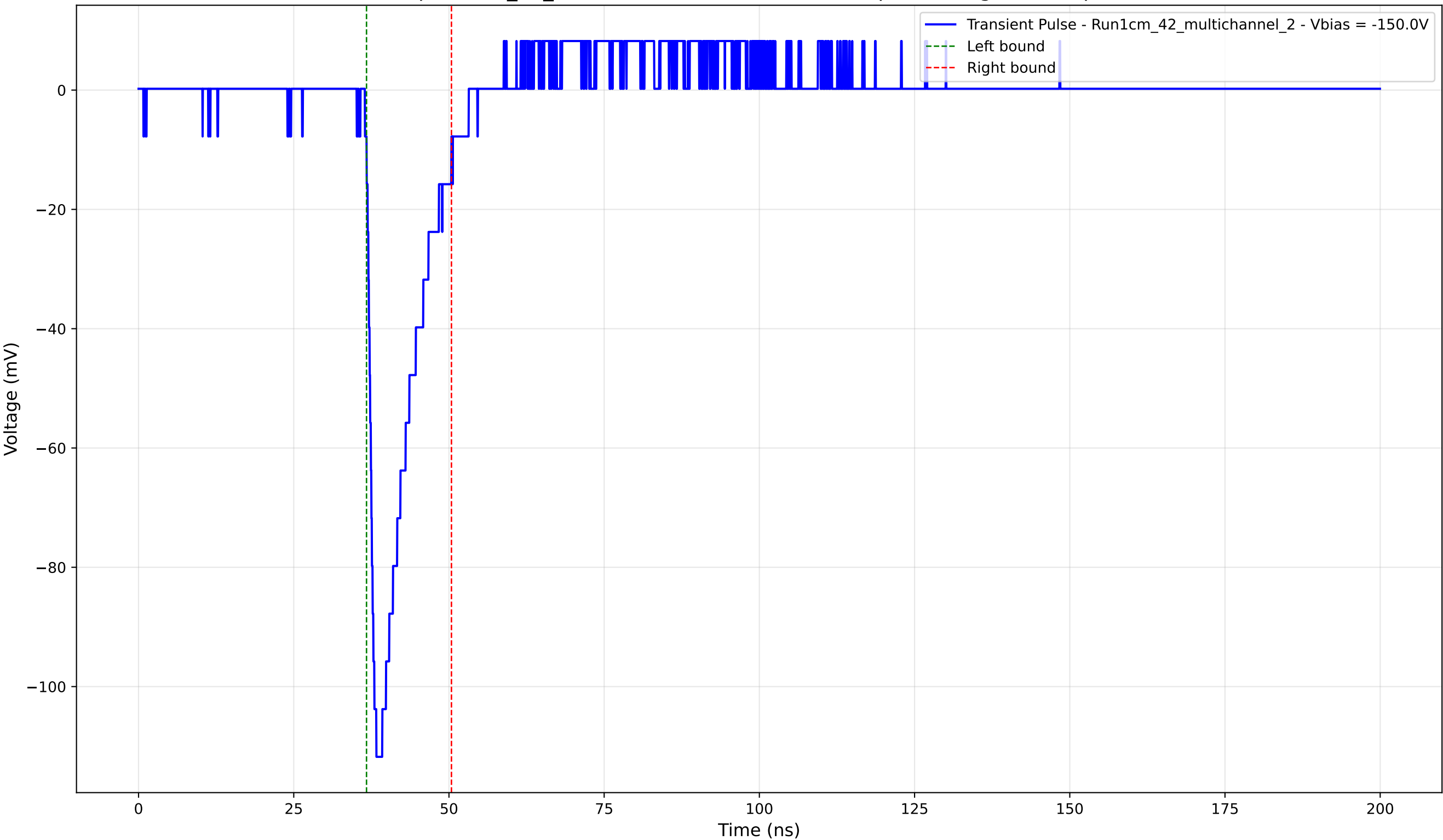
Transient Pulse - Sample: 1cm_42_multichannel - Position: 3655.0 \mu\text{m} - Charge: 14.99 pC - Rise Time: 1.26 ns
