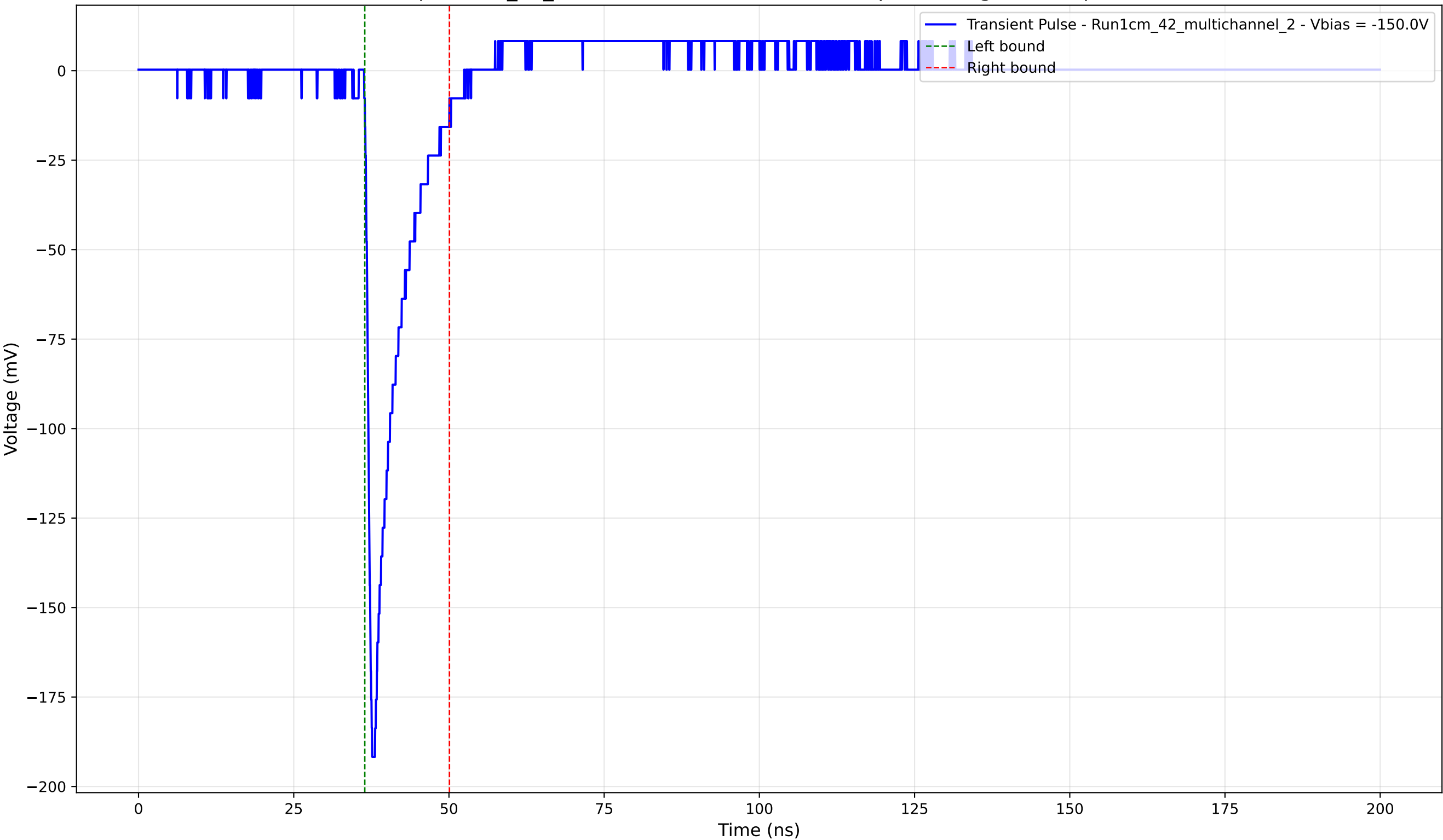
Transient Pulse - Sample: 1cm_42_multichannel - Position: 3210.0 \mu\text{m} - Charge: 19.04 pC - Rise Time: 0.94 ns
