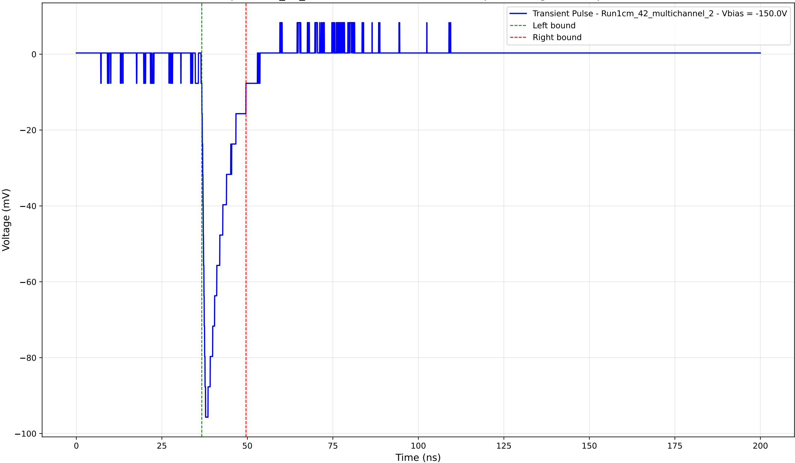
Transient Pulse - Sample: 1cm_42_multichannel - Position: 3440.0 \mu\text{m} - Charge: 11.57 pC - Rise Time: 0.95 ns
