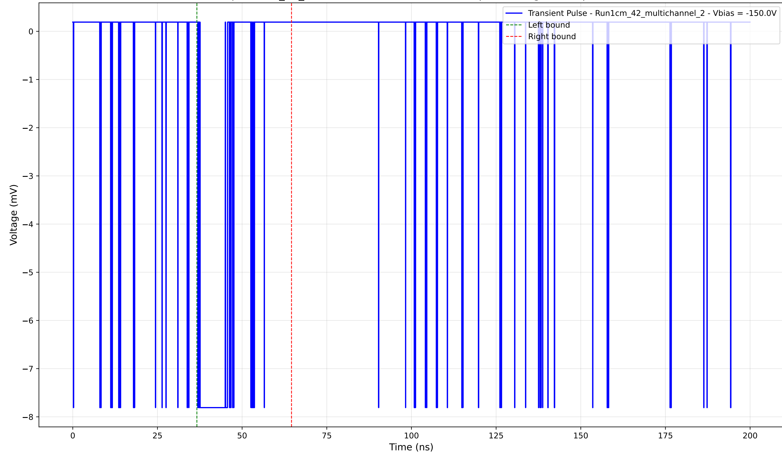
Transient Pulse - Sample: 1cm_42_multichannel - Position: 4410.0 \mu\text{m} - Charge: 1.37 pC - Rise Time: 0.04 ns
