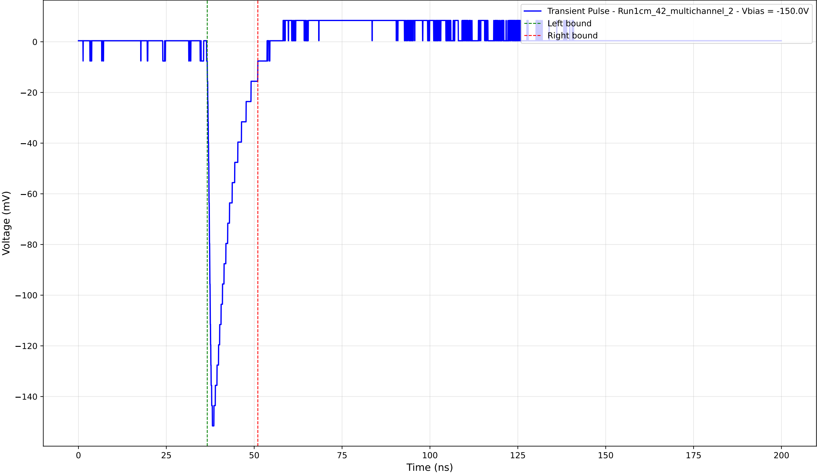
Transient Pulse - Sample: 1cm_42_multichannel - Position: 1205.0 \mu\text{m} - Charge: 18.73 pC - Rise Time: 1.24 ns
