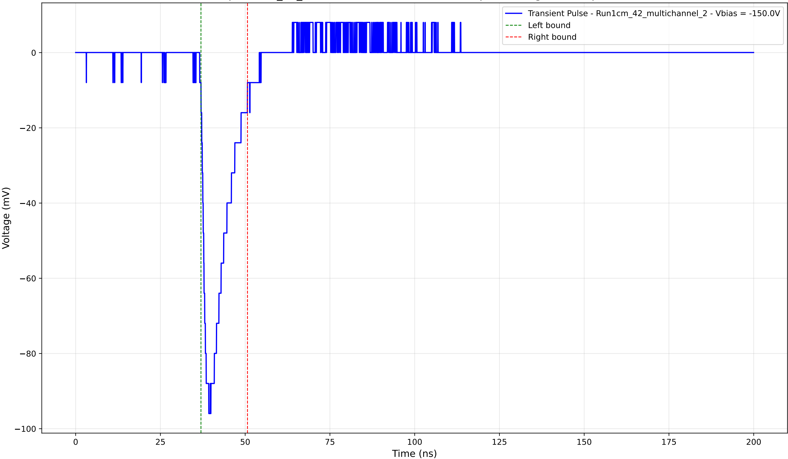
Transient Pulse - Sample: 1cm_42_multichannel - Position: 3980.0 \mu\text{m} - Charge: 13.66 pC - Rise Time: 1.55 ns
