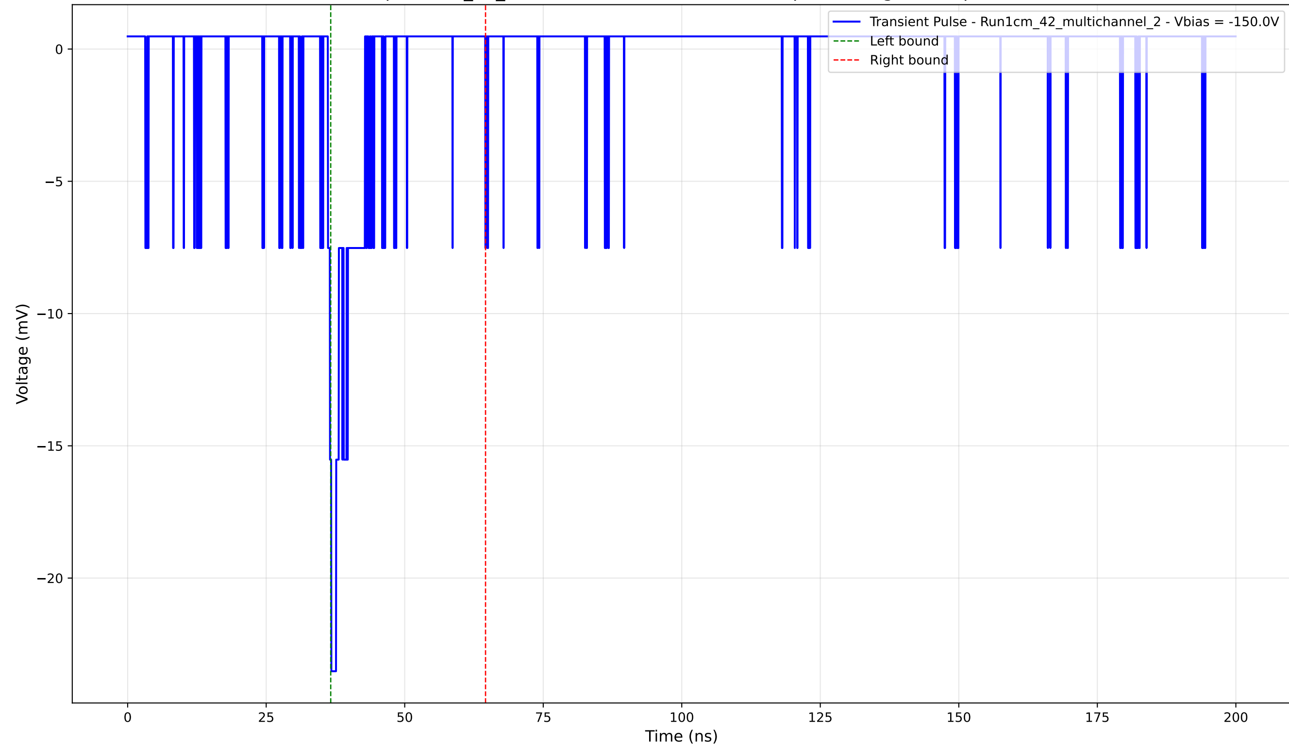
Transient Pulse - Sample: 1cm_42_multichannel - Position: 2365.0 \mu\text{m} - Charge: 1.45 pC - Rise Time: 0.63 ns
