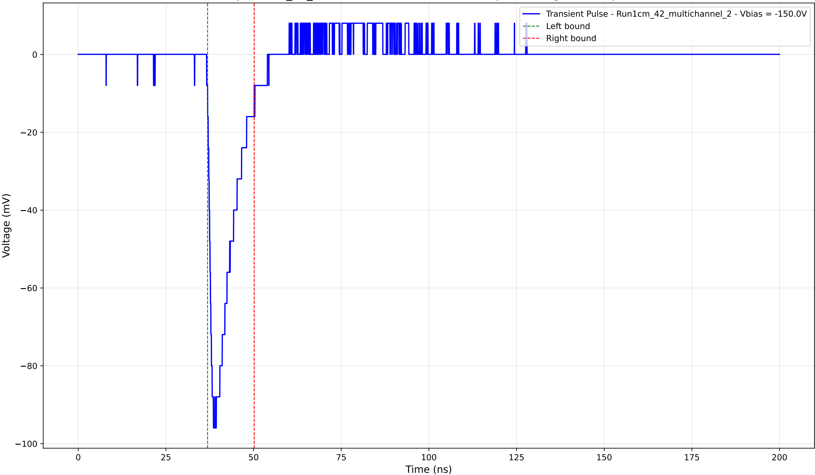
Transient Pulse - Sample: 1cm_42_multichannel - Position: 3810.0 \mu\text{m} - Charge: 13.13 pC - Rise Time: 1.31 ns
