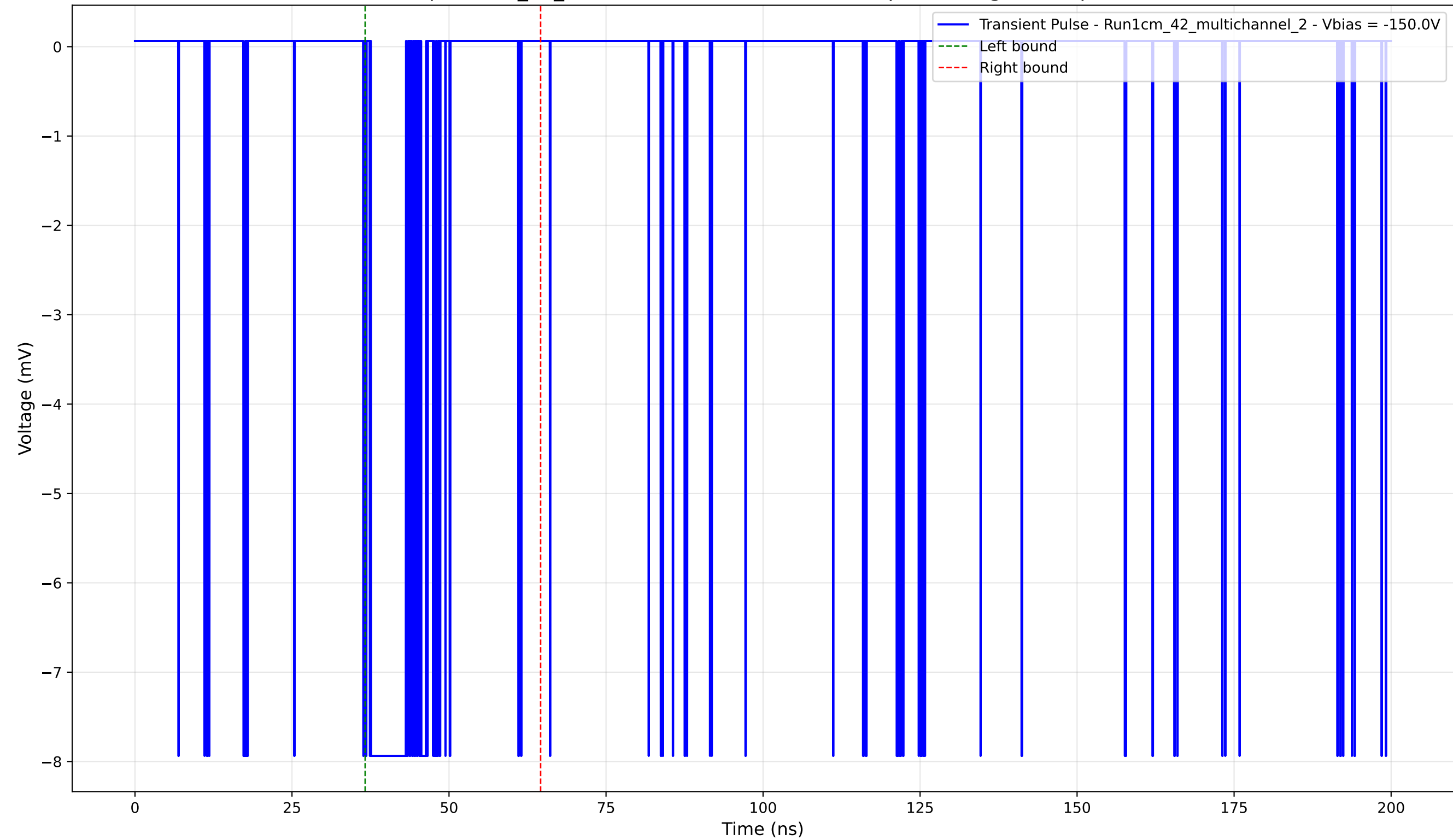
Transient Pulse - Sample: 1cm_42_multichannel - Position: 3895.0 \mu\text{m} - Charge: 1.37 pC - Rise Time: 0.04 ns
