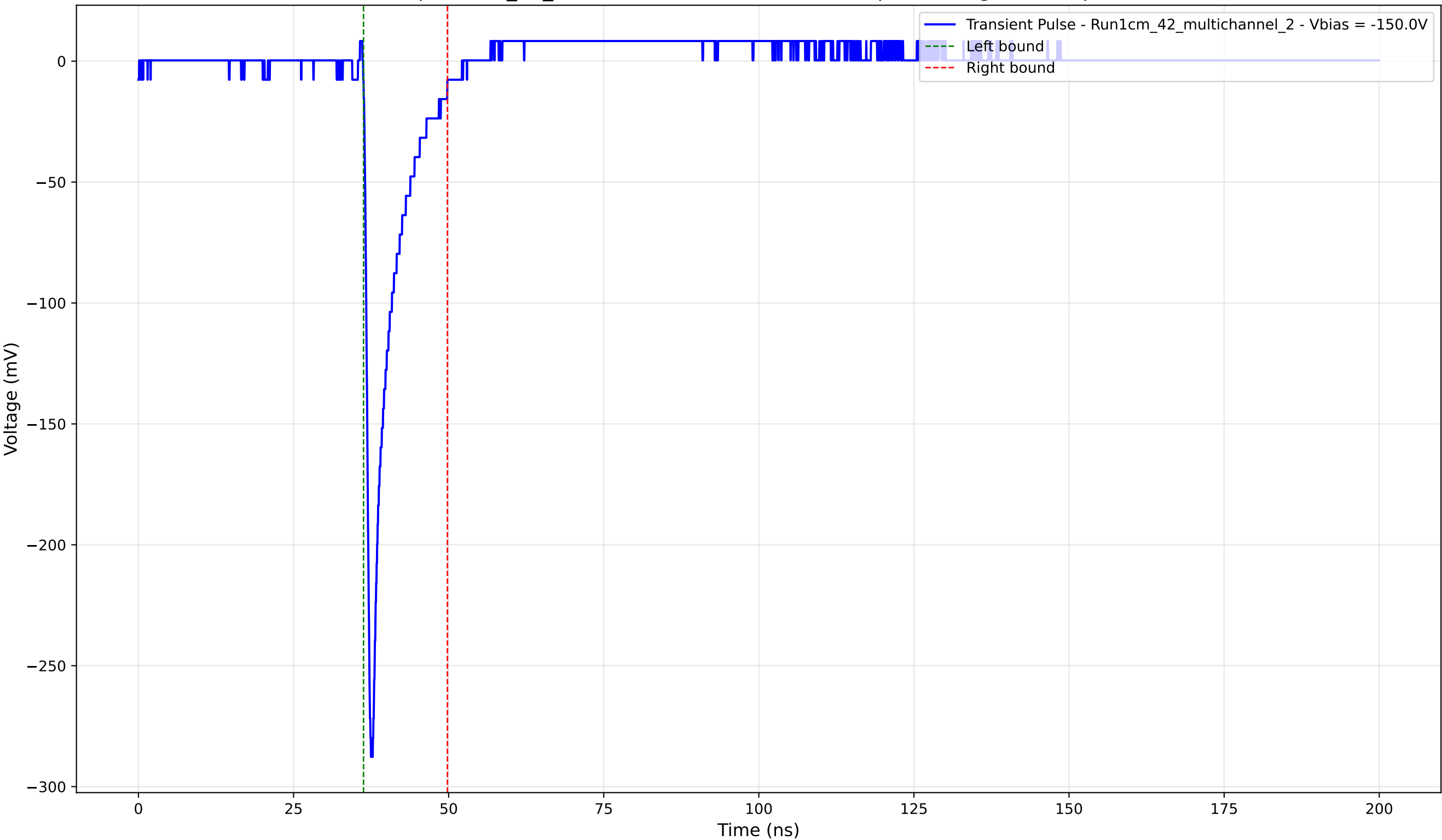
Transient Pulse - Sample: 1cm_42_multichannel - Position: 1745.0 \mu\text{m} - Charge: 23.10 pC - Rise Time: 0.83 ns
