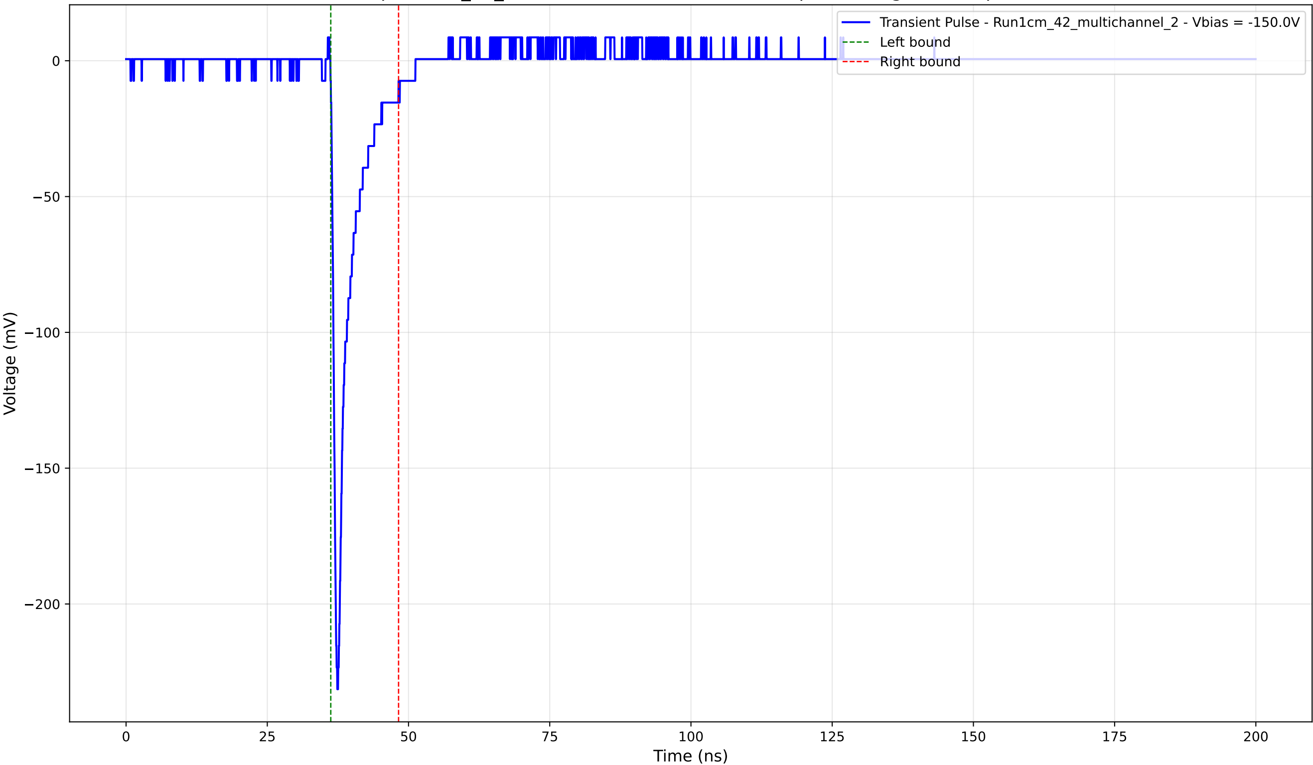
Transient Pulse - Sample: 1cm_42_multichannel - Position: 1920.0 \mu\text{m} - Charge: 14.94 pC - Rise Time: 0.84 ns
