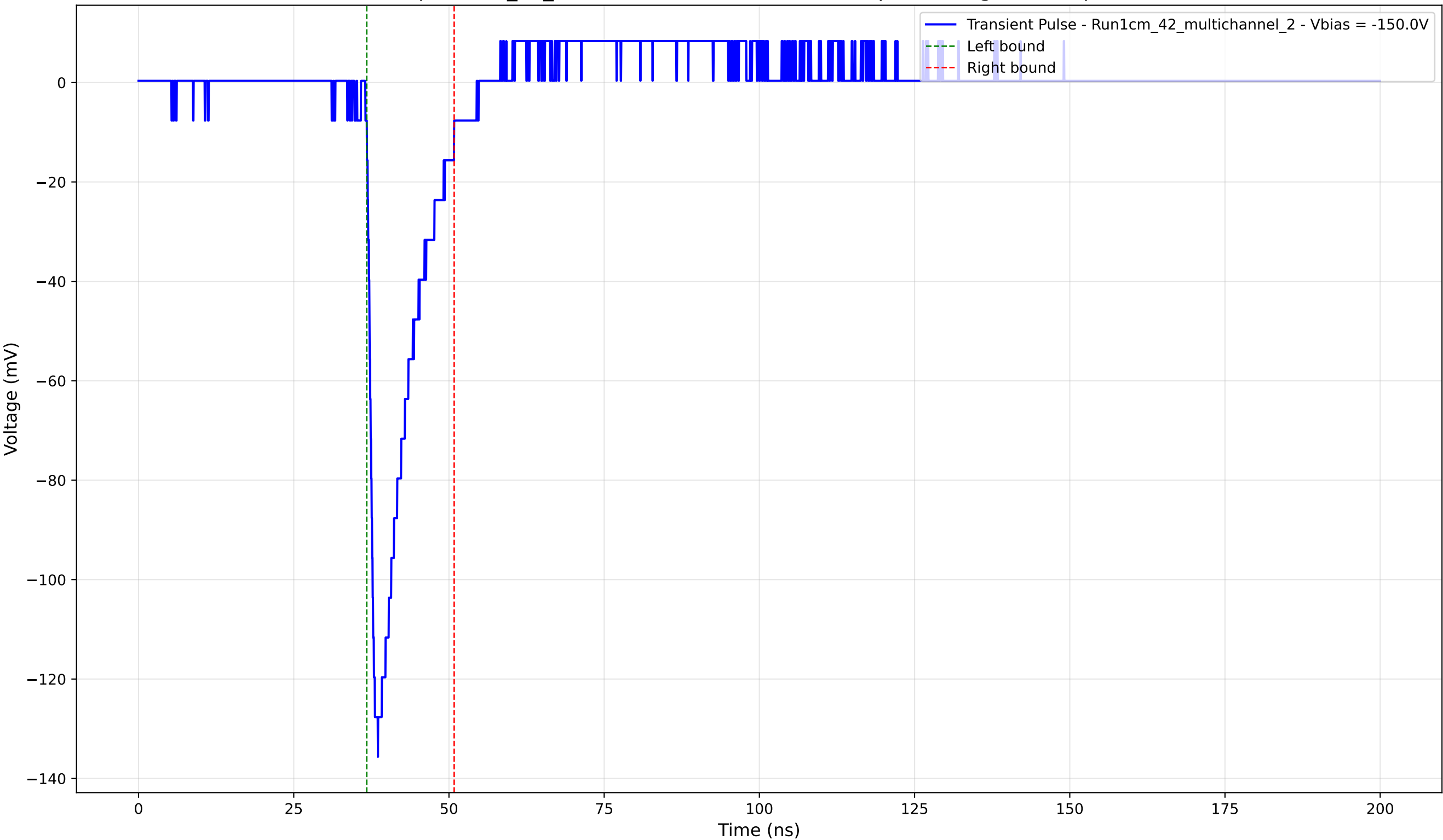
Transient Pulse - Sample: 1cm_42_multichannel - Position: 1095.0 \mu\text{m} - Charge: 17.17 pC - Rise Time: 1.29 ns
