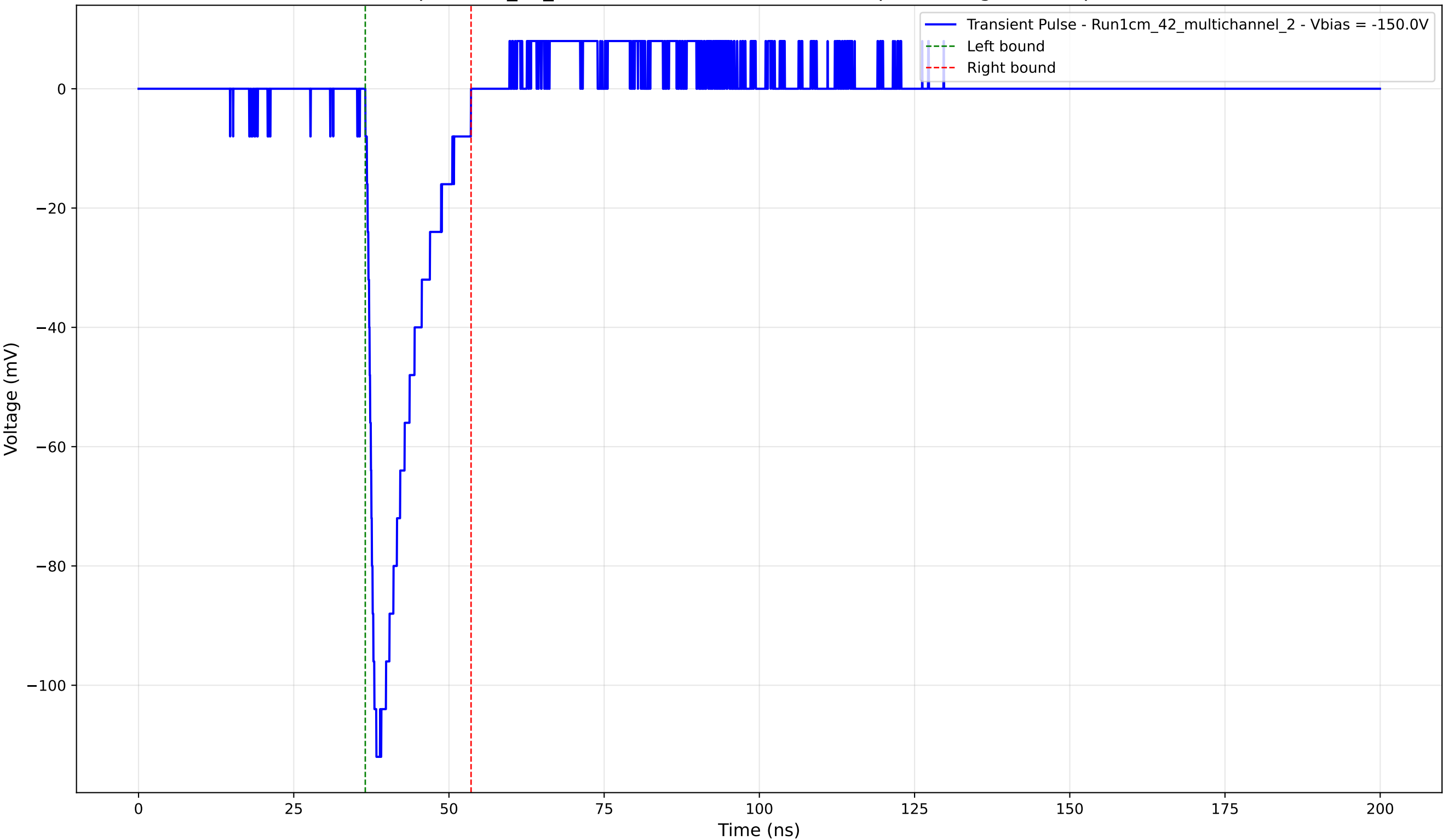
Transient Pulse - Sample: 1cm_42_multichannel - Position: 3650.0 \mu\text{m} - Charge: 15.58 pC - Rise Time: 1.22 ns
