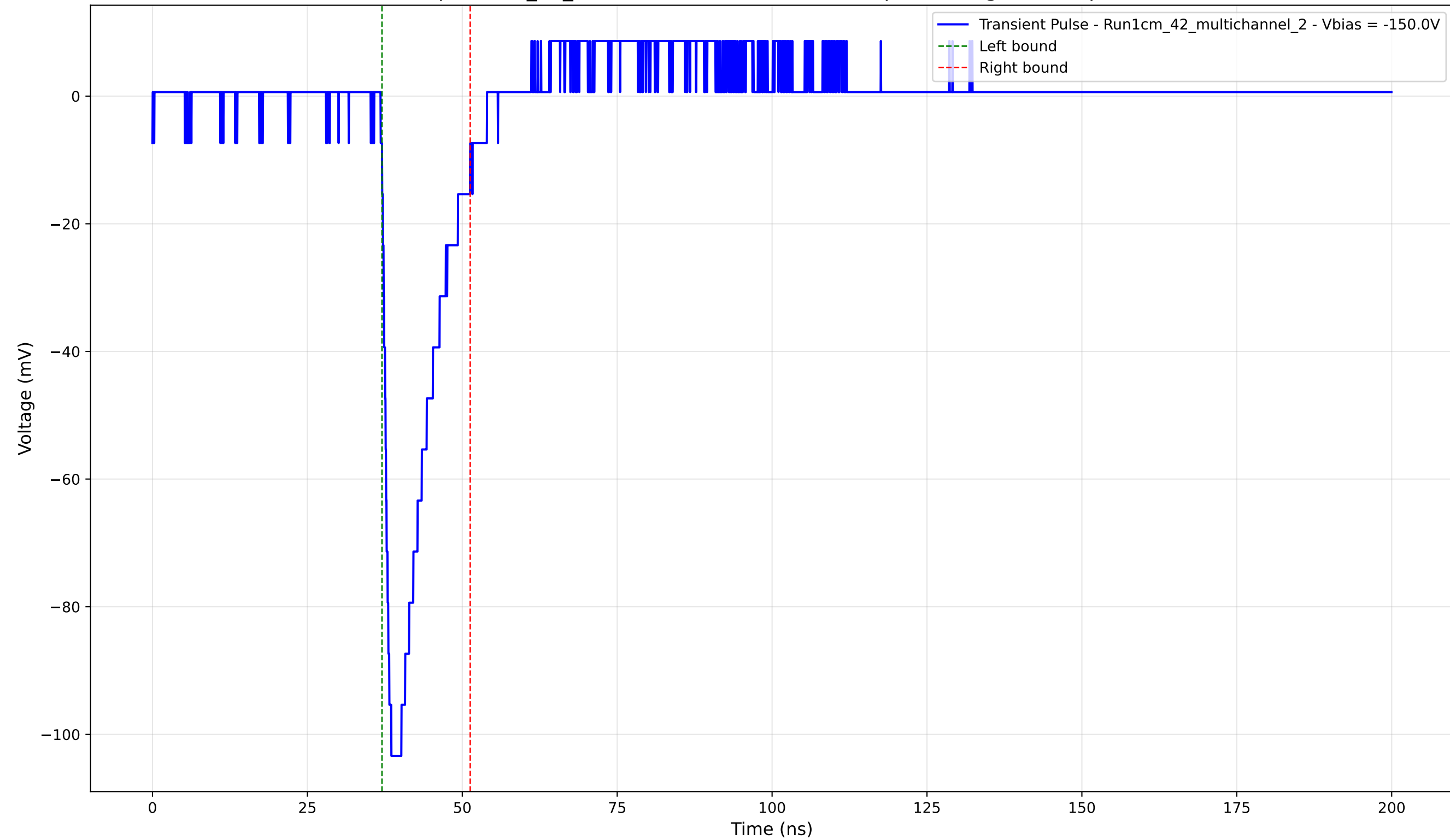
Transient Pulse - Sample: 1cm_42_multichannel - Position: 735.0 \mu\text{m} - Charge: 15.26 pC - Rise Time: 1.19 ns
