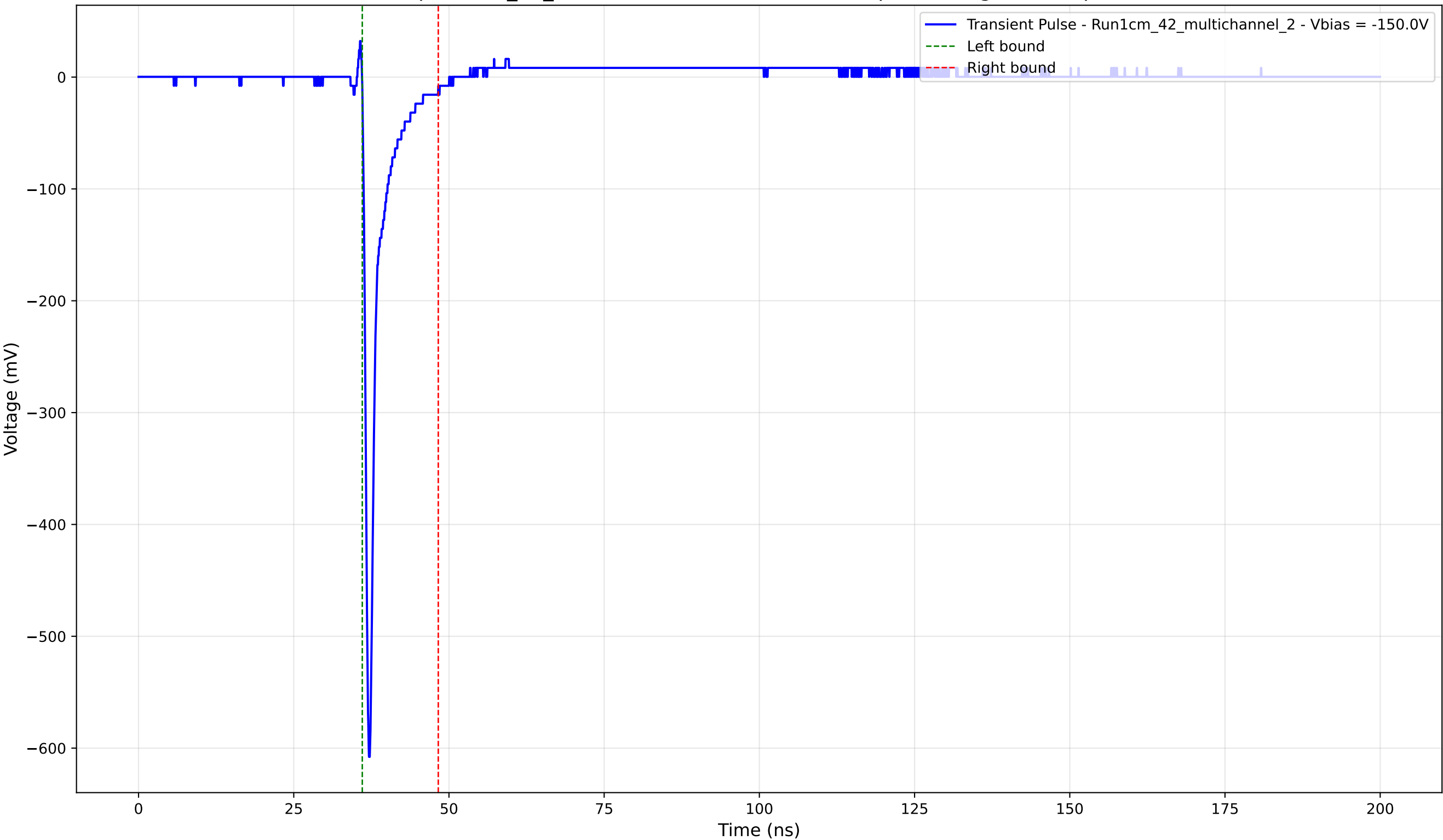
Transient Pulse - Sample: 1cm_42_multichannel - Position: 2485.0 \mu\text{m} - Charge: 27.99 pC - Rise Time: 0.66 ns
