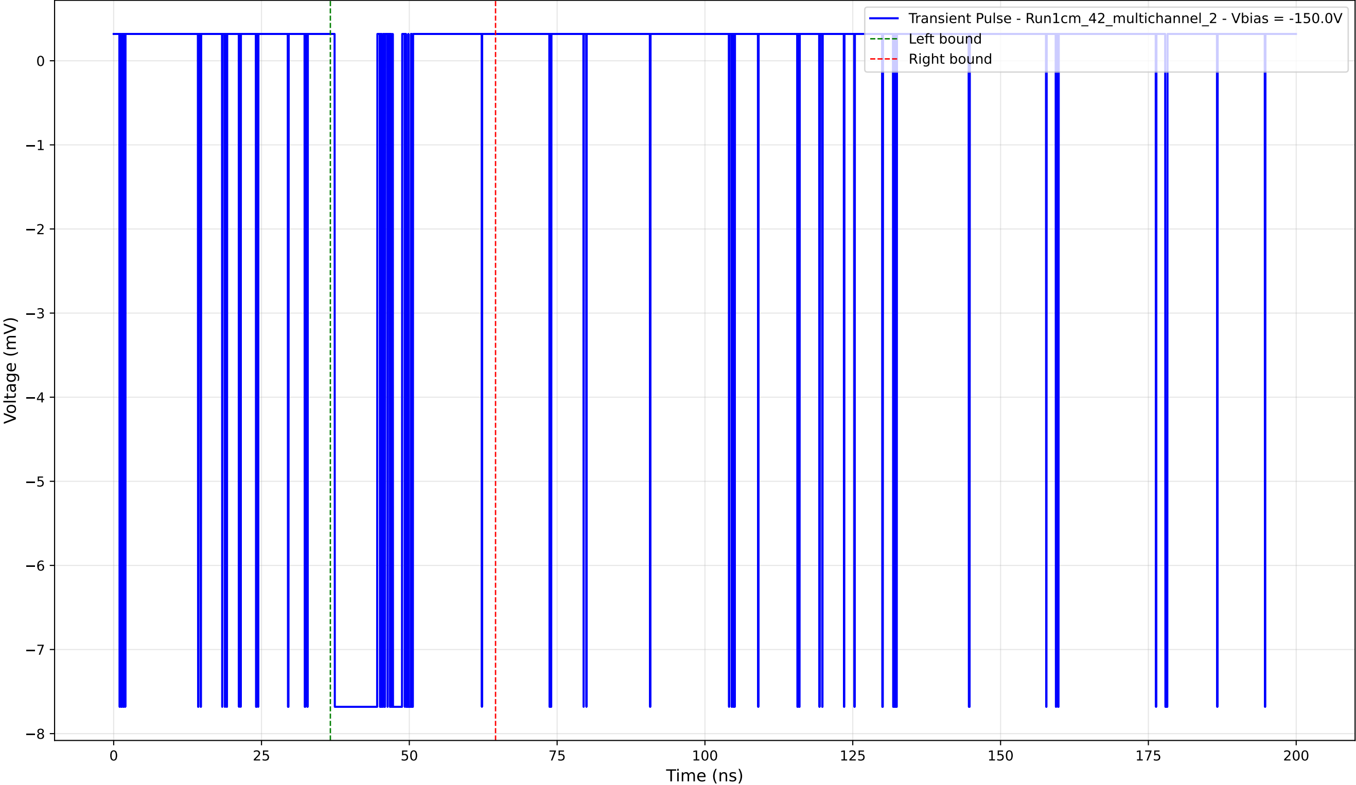
Transient Pulse - Sample: 1cm_42_multichannel - Position: 3905.0 \mu\text{m} - Charge: 1.53 pC - Rise Time: 0.04 ns
