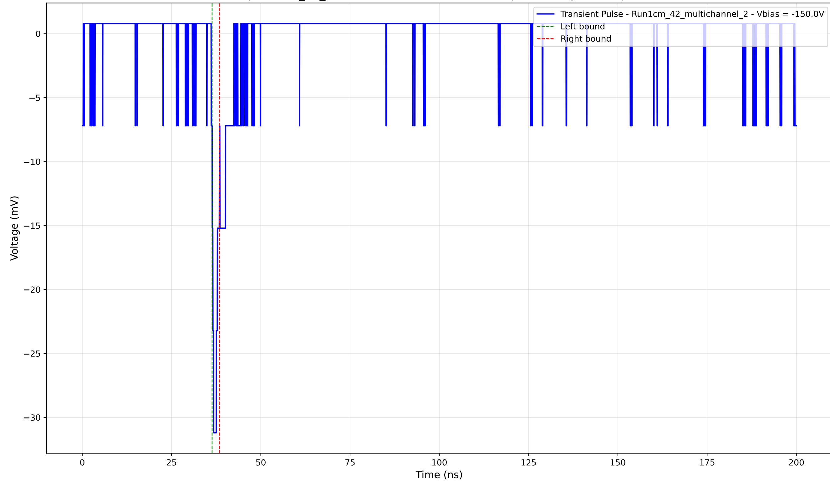
Transient Pulse - Sample: 1cm_42_multichannel - Position: 2385.0 \mu\text{m} - Charge: 0.93 pC - Rise Time: 0.71 ns
