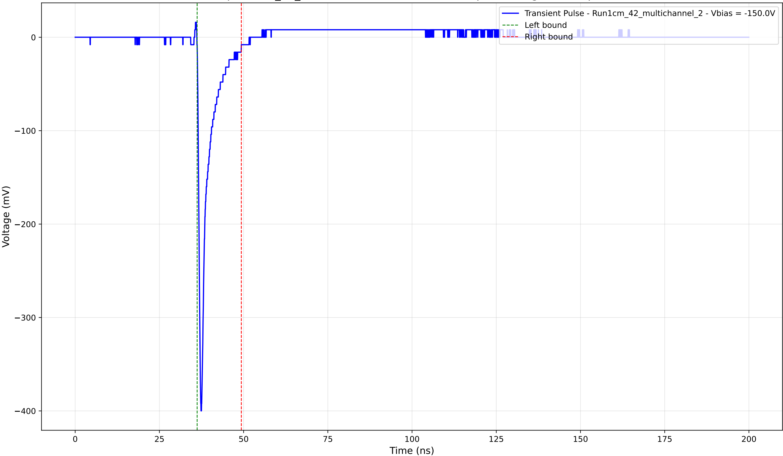
Transient Pulse - Sample: 1cm_42_multichannel - Position: 1970.0 \mu\text{m} - Charge: 24.88 pC - Rise Time: 0.80 ns
