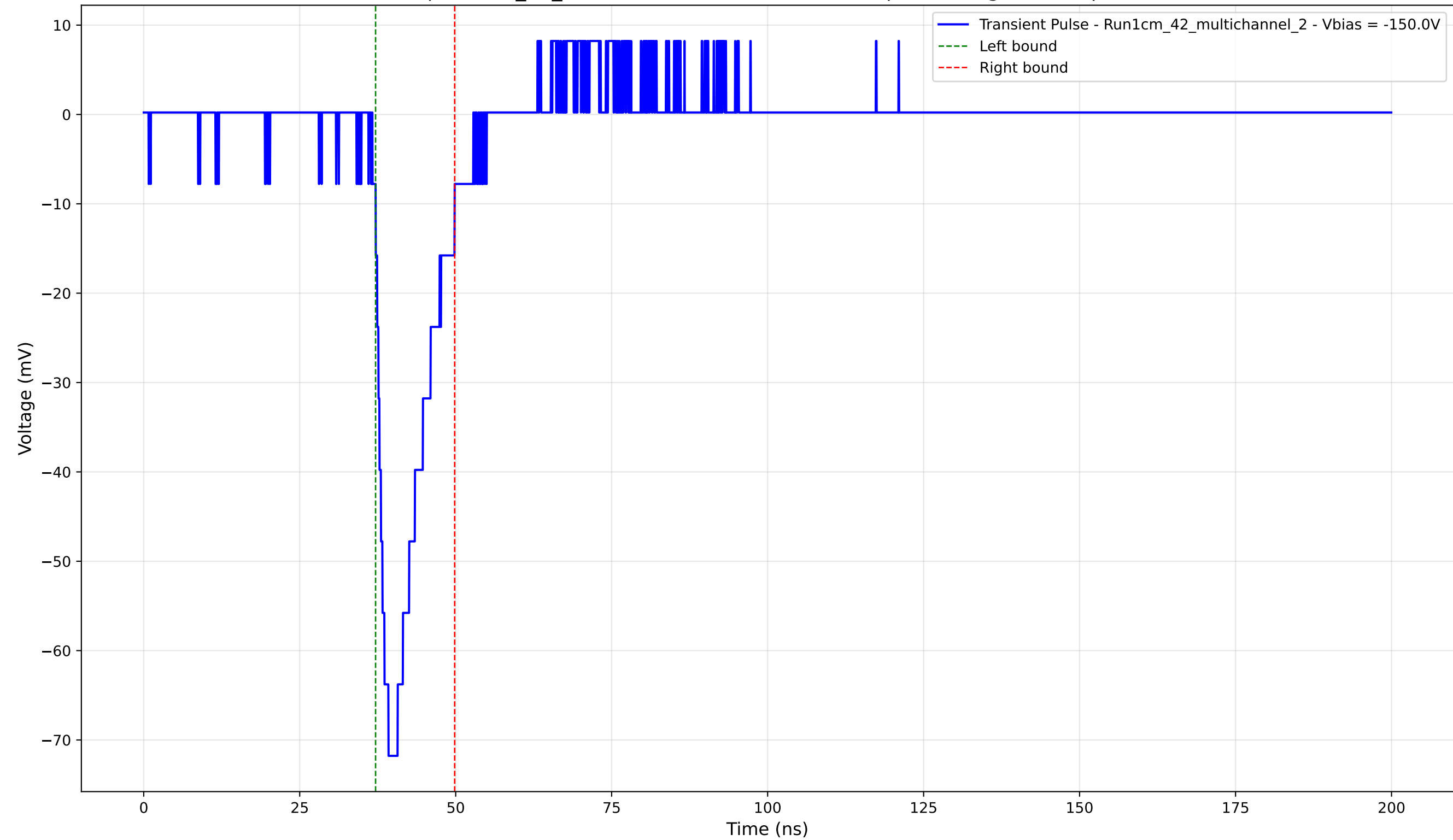
Transient Pulse - Sample: 1cm_42_multichannel - Position: 4635.0 \mu\text{m} - Charge: 10.33 pC - Rise Time: 2.56 ns
