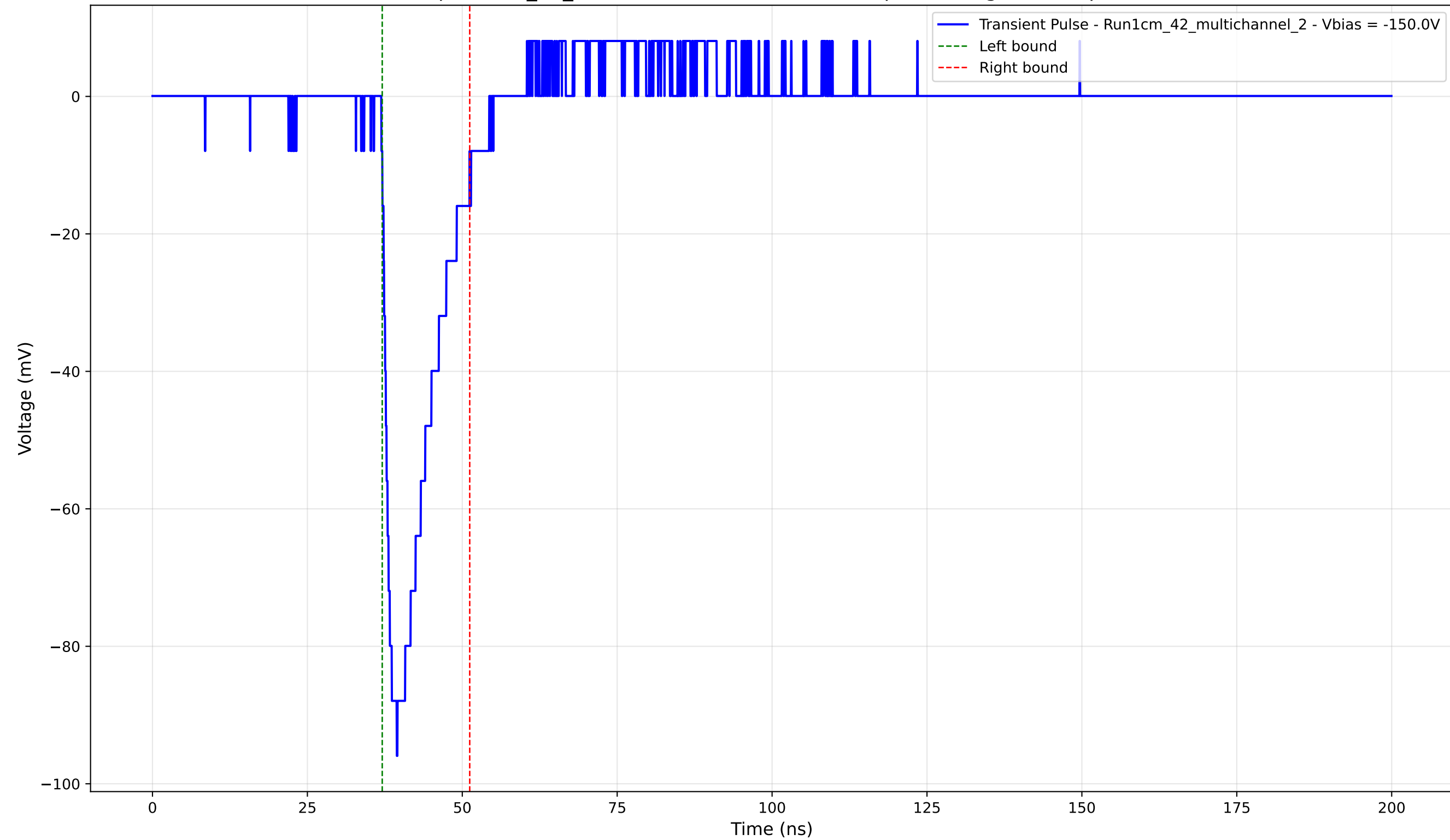
Transient Pulse - Sample: 1cm_42_multichannel - Position: 475.0 \mu\text{m} - Charge: 14.01 pC - Rise Time: 1.55 ns
