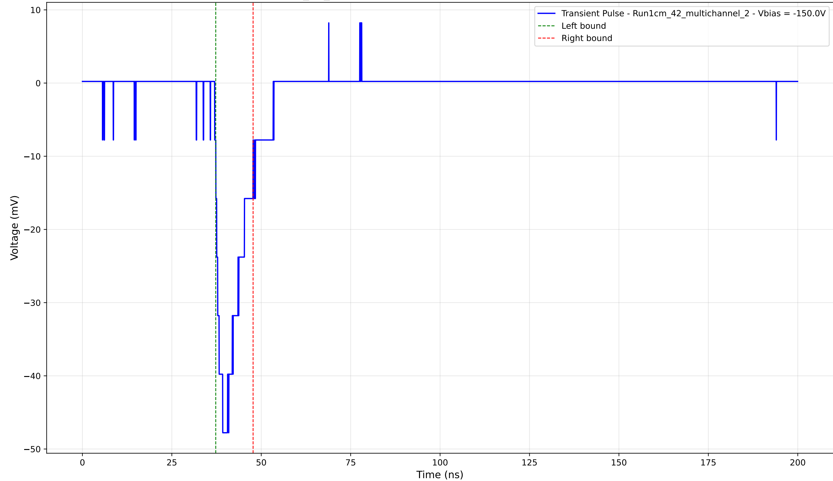
Transient Pulse - Sample: 1cm_42_multichannel - Position: 395.0 \mu\text{m} - Charge: 6.29 pC - Rise Time: 2.26 ns
