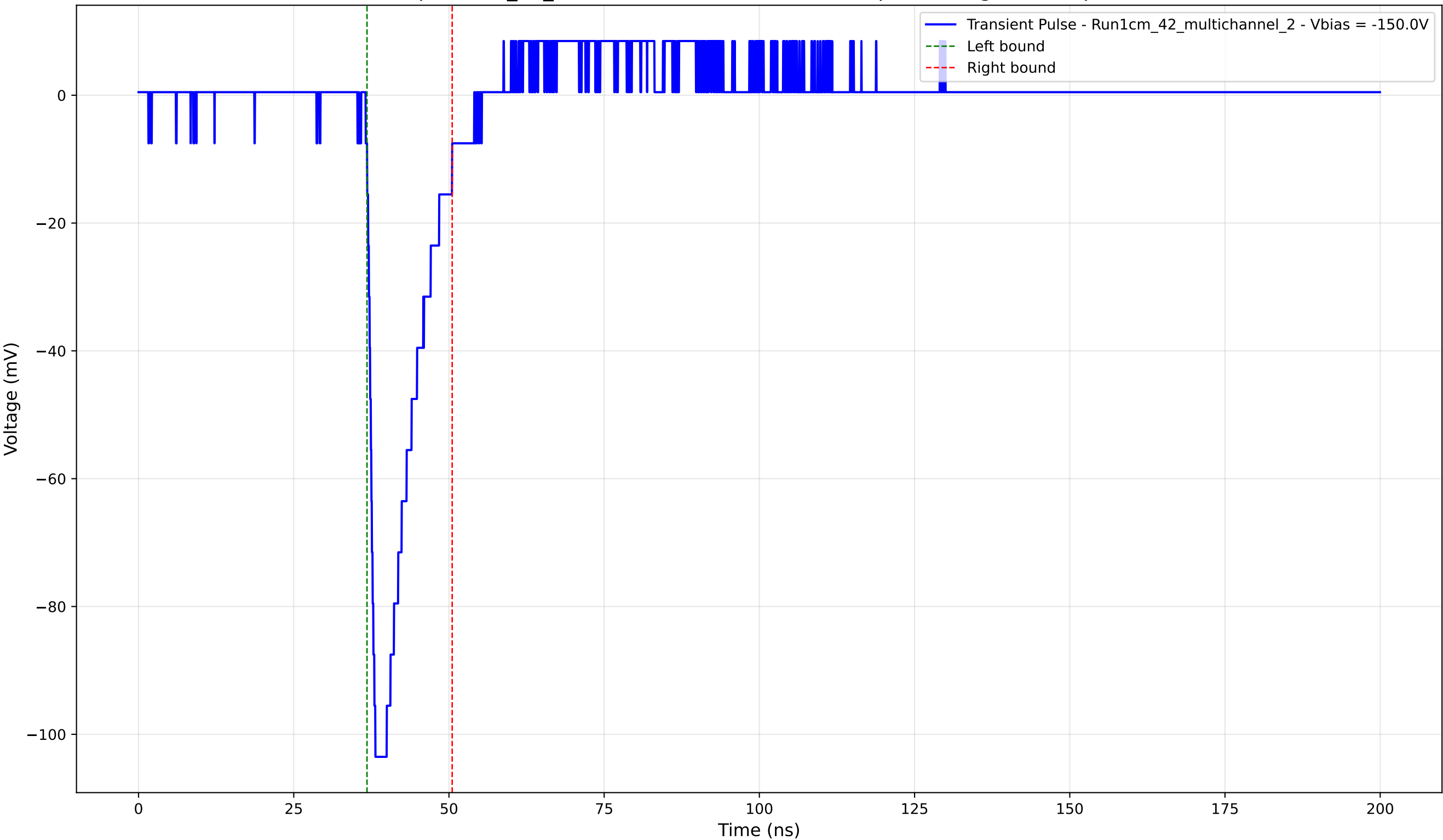
Transient Pulse - Sample: 1cm_42_multichannel - Position: 3740.0 \mu\text{m} - Charge: 14.90 pC - Rise Time: 1.19 ns
