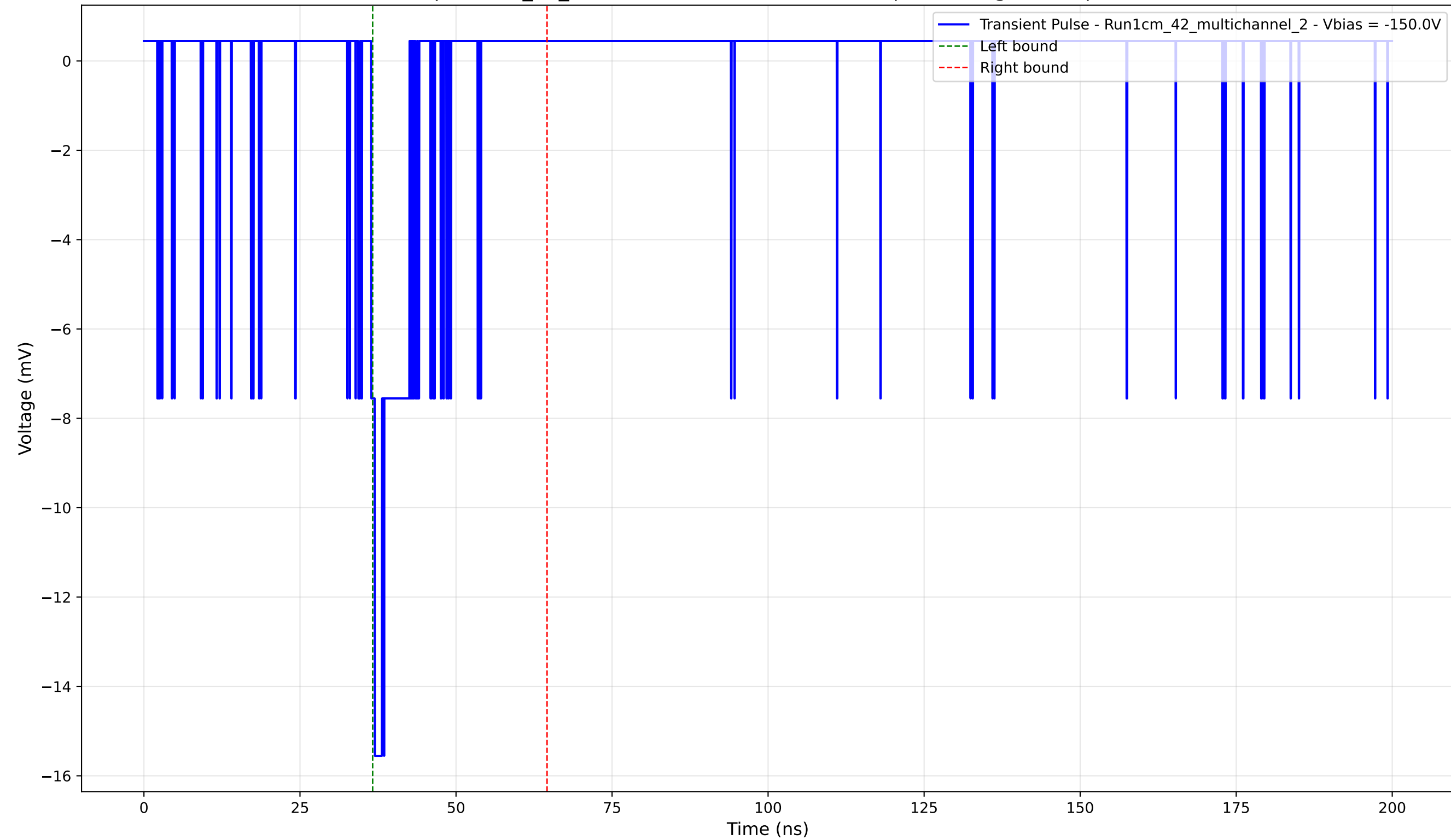
Transient Pulse - Sample: 1cm_42_multichannel - Position: 2870.0 \mu\text{m} - Charge: 1.19 pC - Rise Time: 0.59 ns
