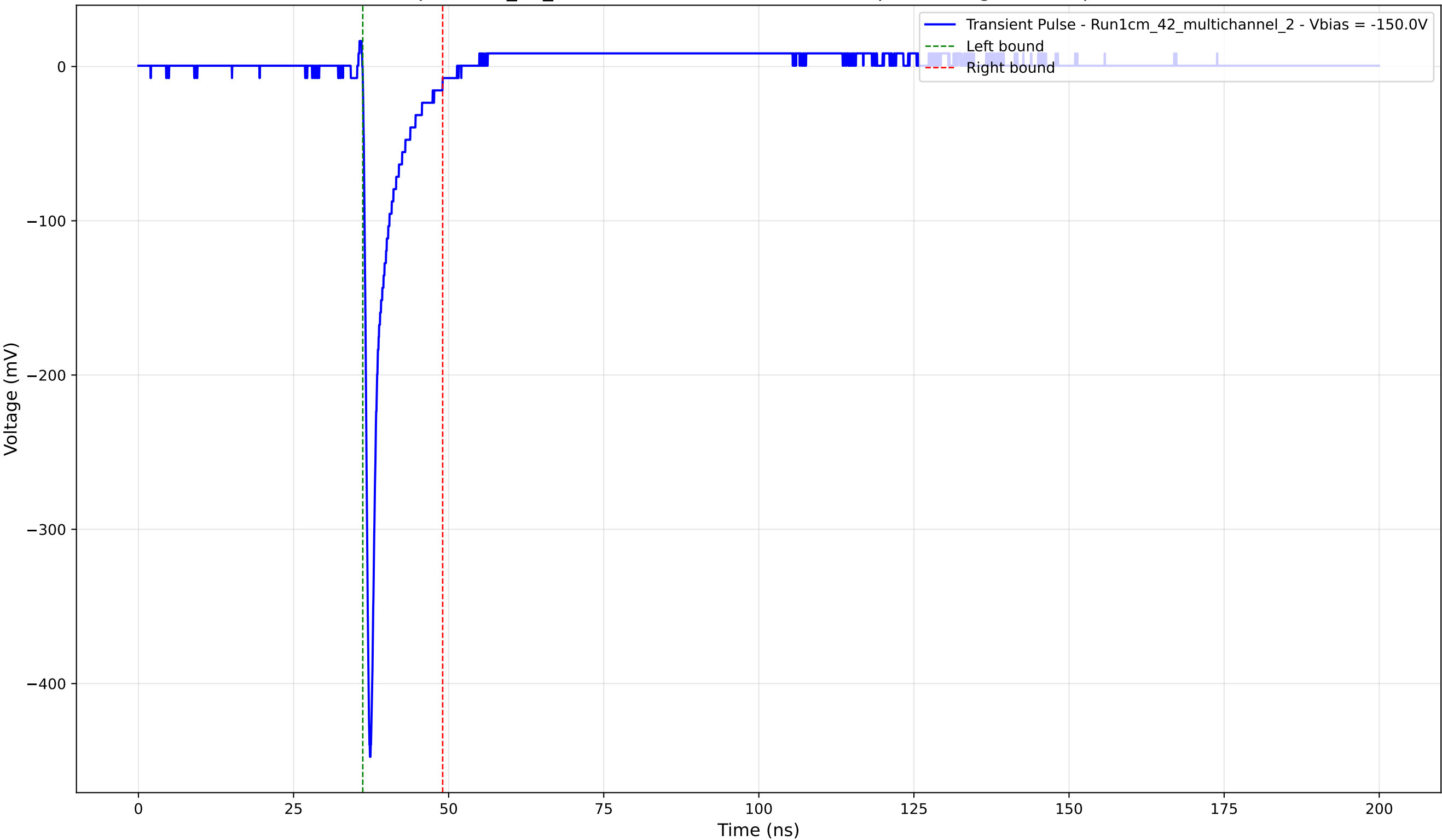
Transient Pulse - Sample: 1cm_42_multichannel - Position: 2025.0 \mu\text{m} - Charge: 26.03 pC - Rise Time: 0.75 ns
