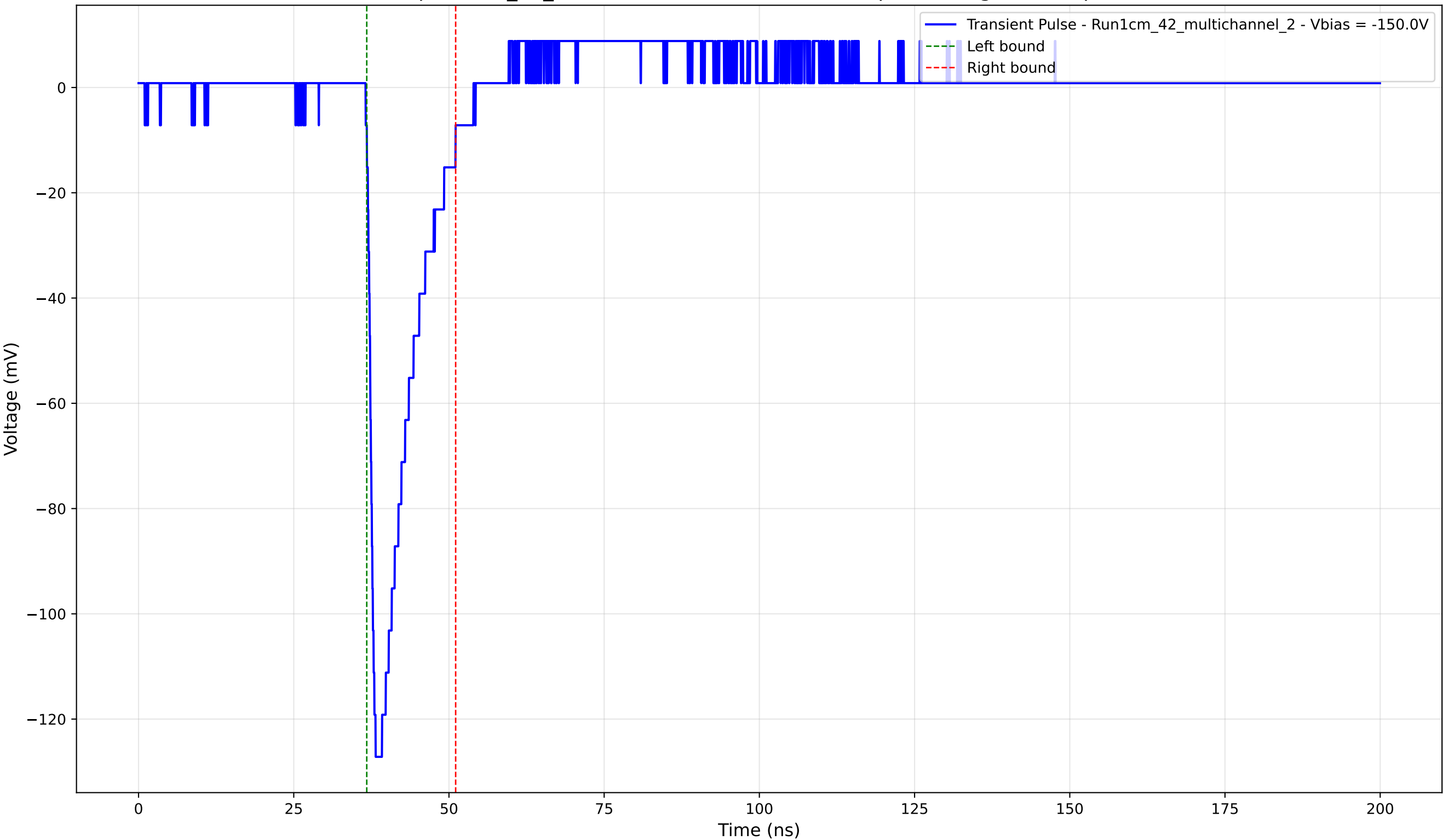
Transient Pulse - Sample: 1cm_42_multichannel - Position: 1055.0 \mu\text{m} - Charge: 17.10 pC - Rise Time: 1.21 ns
