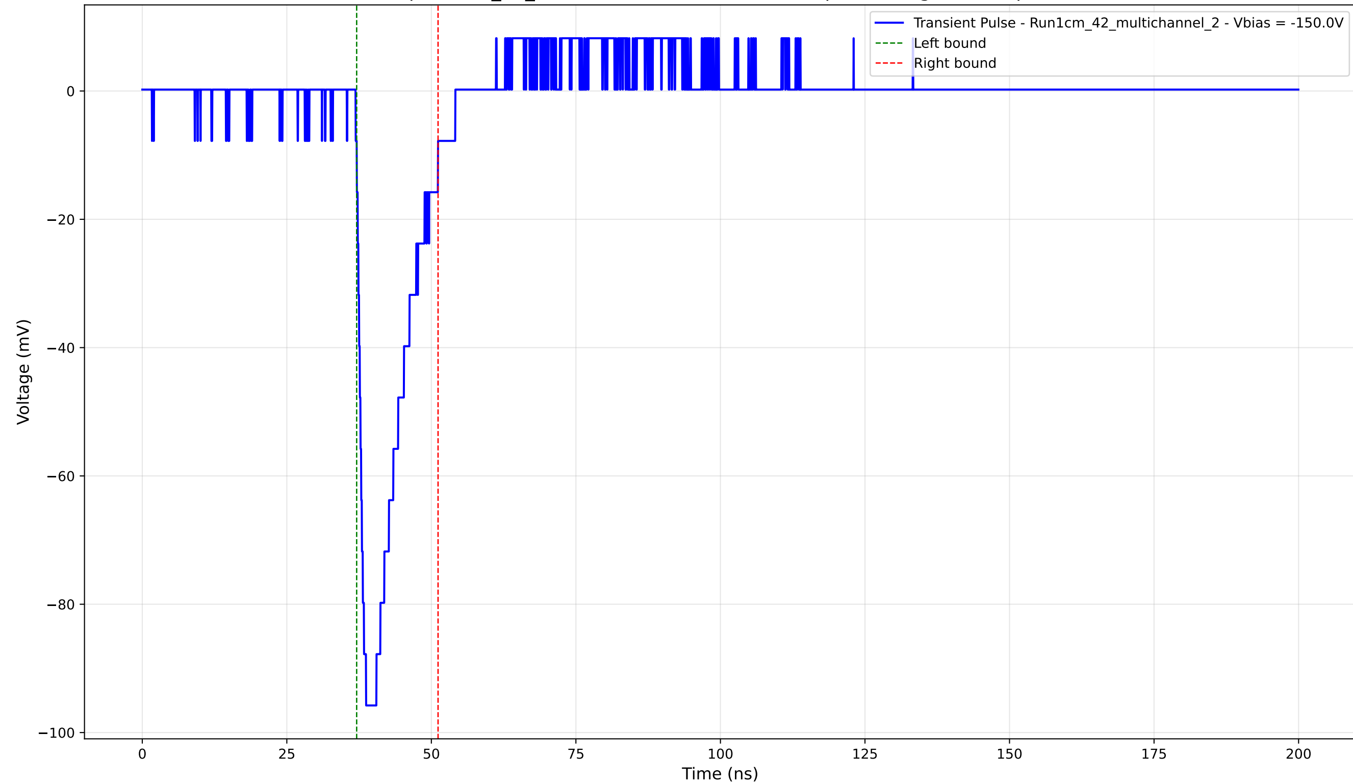
Transient Pulse - Sample: 1cm_42_multichannel - Position: 575.0 \mu\text{m} - Charge: 14.55 pC - Rise Time: 1.27 ns
