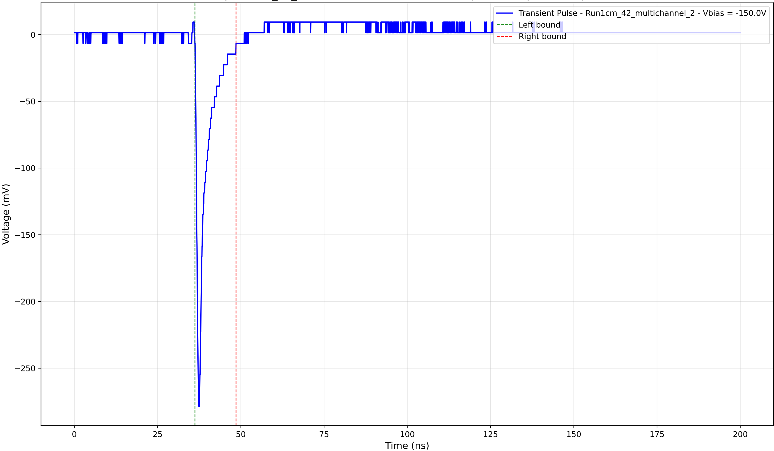
Transient Pulse - Sample: 1cm_42_multichannel - Position: 1925.0 \mu\text{m} - Charge: 17.76 pC - Rise Time: 0.83 ns
