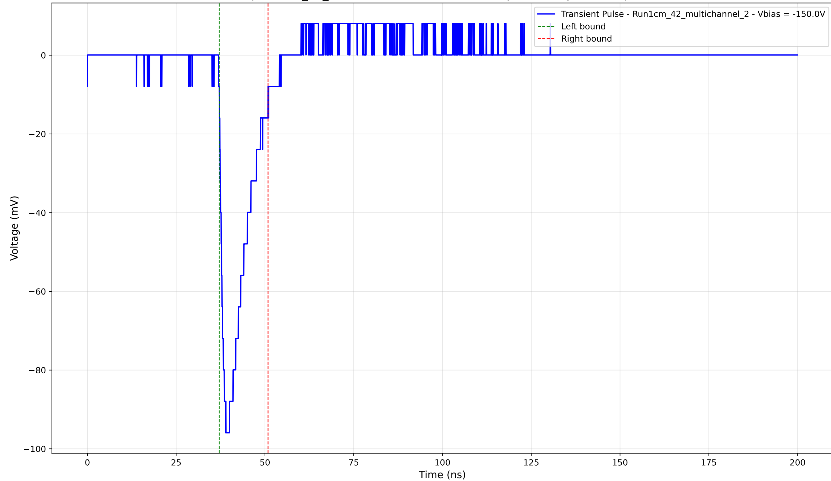
Transient Pulse - Sample: 1cm_42_multichannel - Position: 535.0 \mu\text{m} - Charge: 14.09 pC - Rise Time: 1.43 ns
