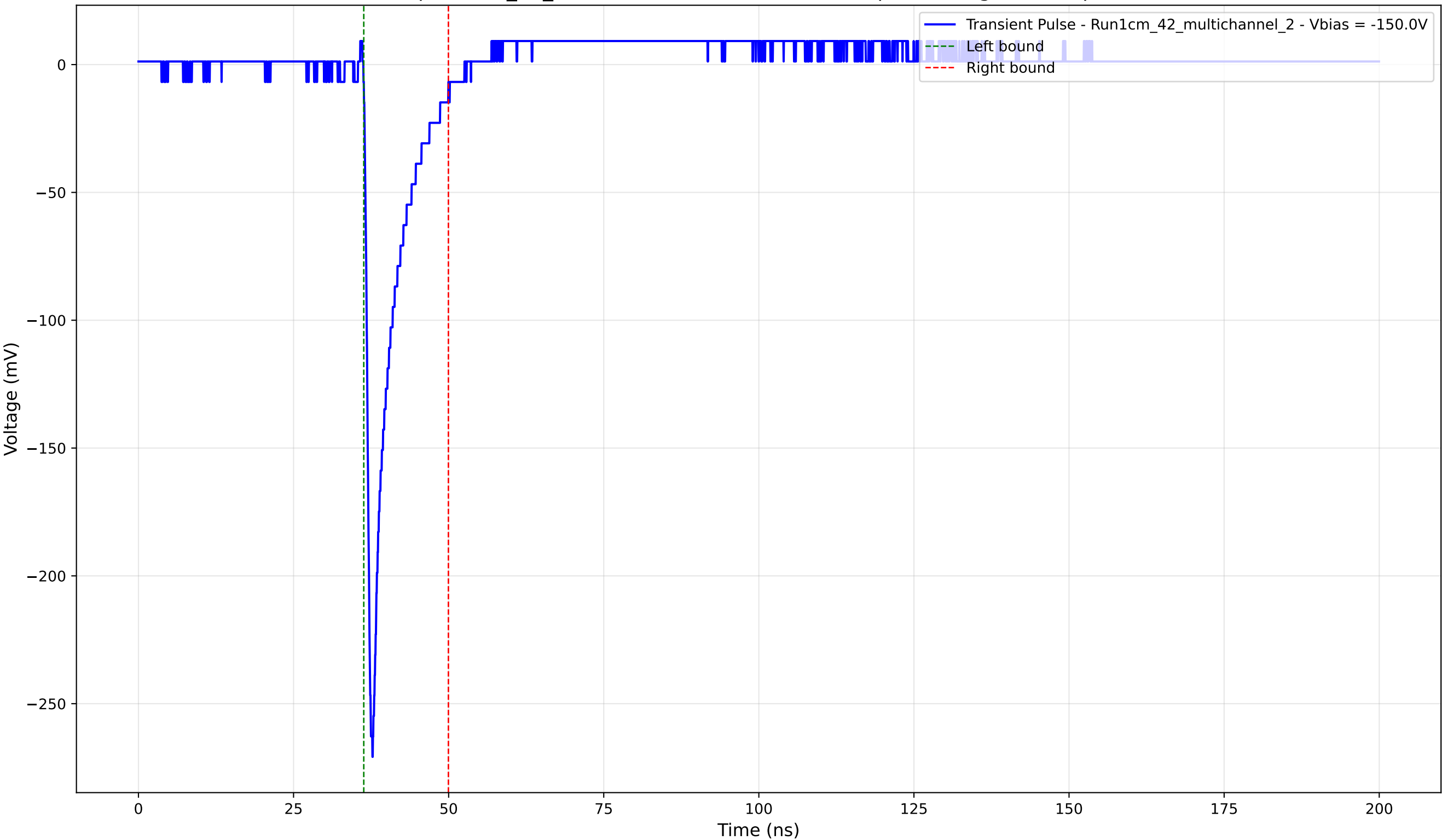
Transient Pulse - Sample: 1cm_42_multichannel - Position: 1680.0 \mu\text{m} - Charge: 22.54 pC - Rise Time: 0.90 ns
