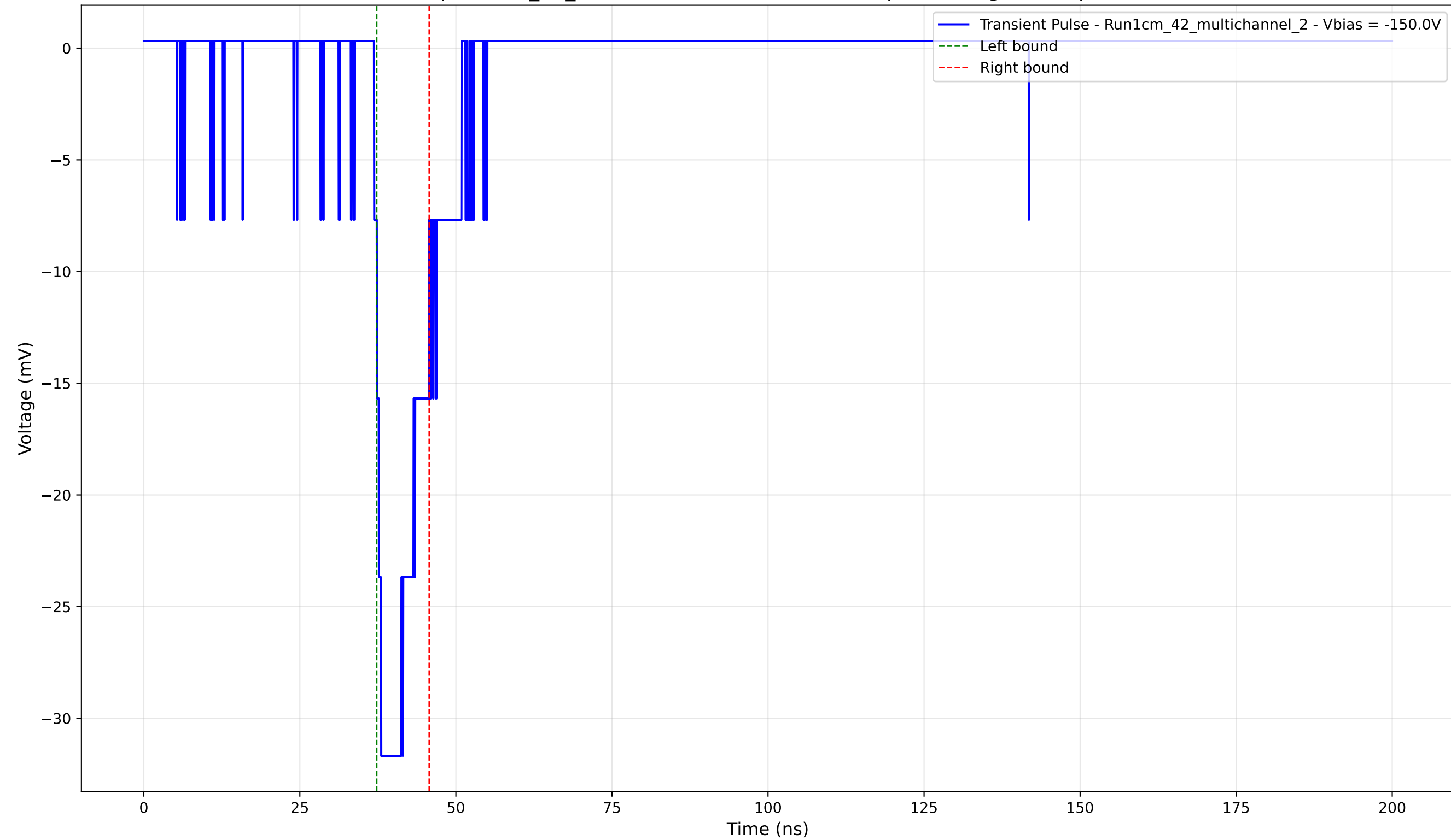
Transient Pulse - Sample: 1cm_42_multichannel - Position: 810.0 \mu\text{m} - Charge: 4.07 pC - Rise Time: 1.14 ns
