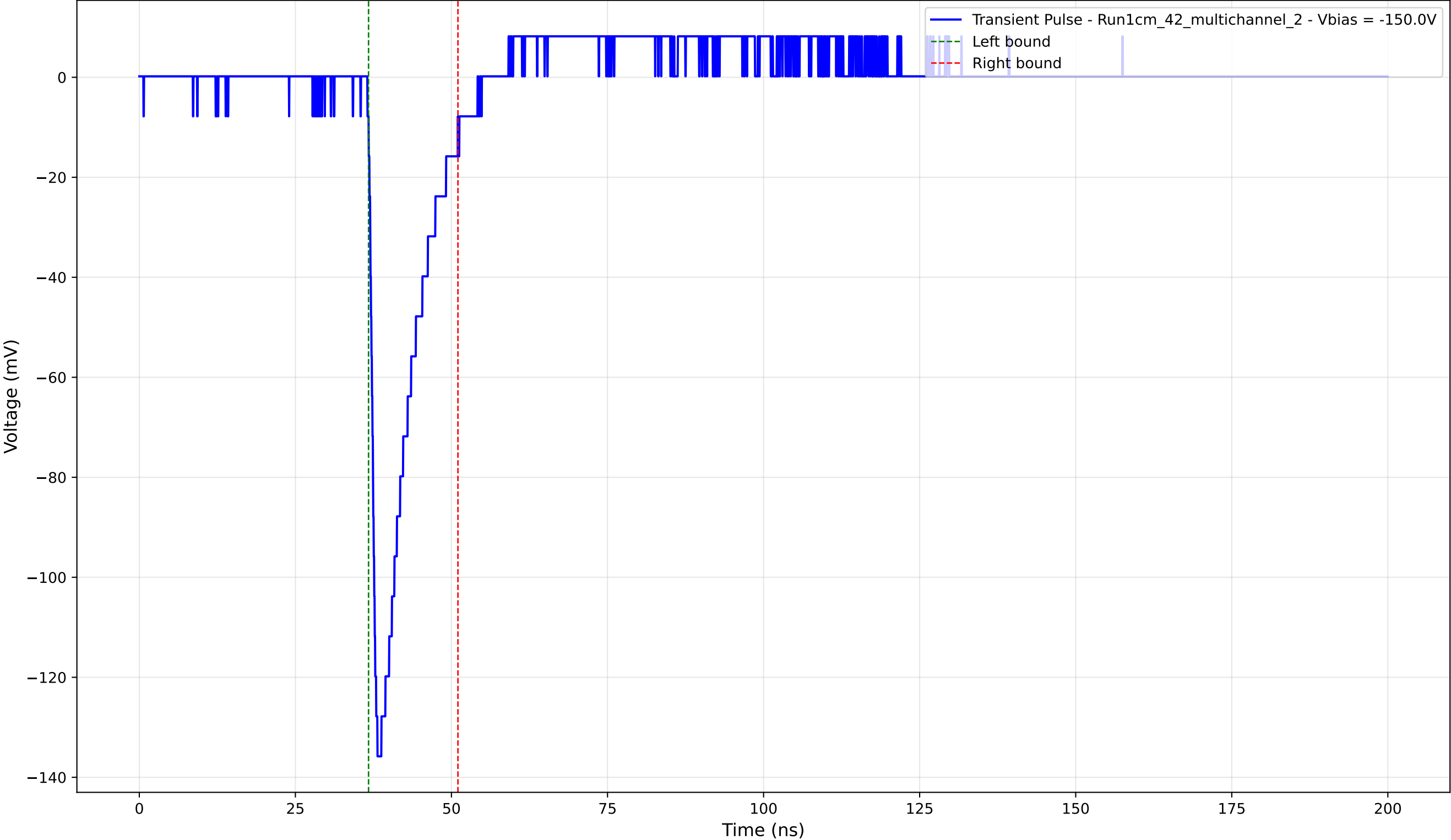
Transient Pulse - Sample: 1cm_42_multichannel - Position: 1125.0 \mu\text{m} - Charge: 17.71 pC - Rise Time: 1.21 ns
