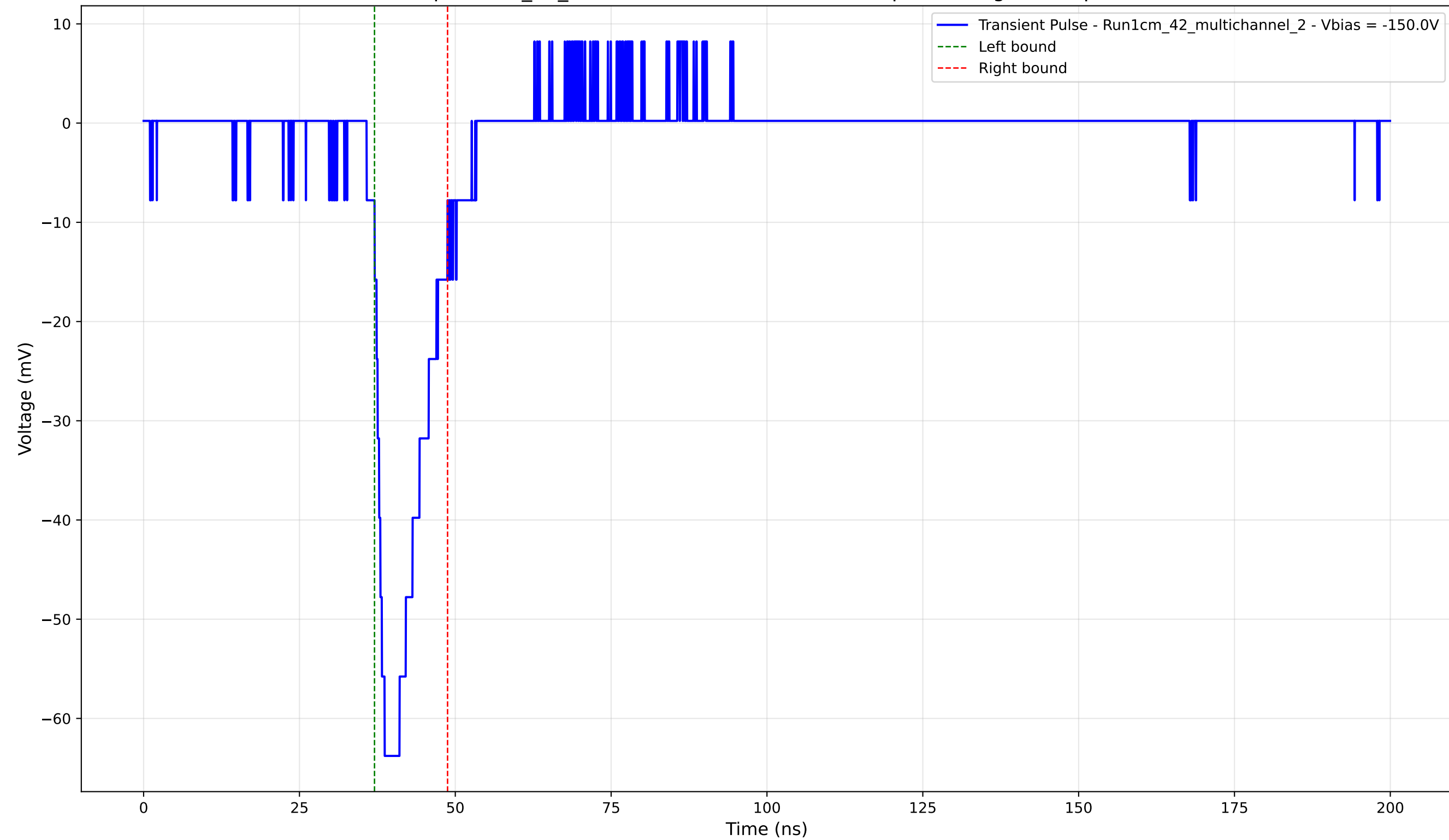
Transient Pulse - Sample: 1cm_42_multichannel - Position: 4750.0 \mu\text{m} - Charge: 9.41 pC - Rise Time: 2.89 ns
