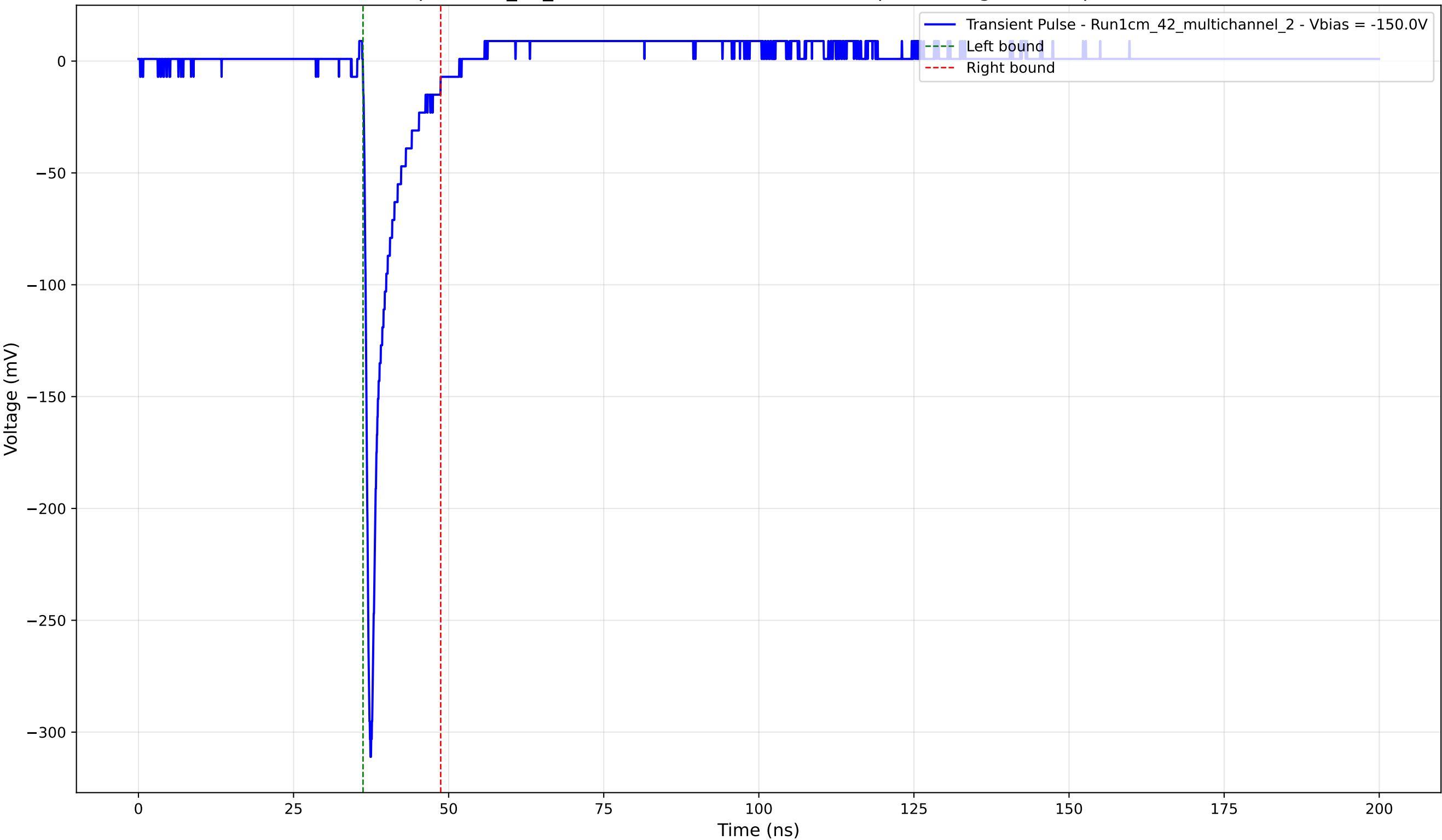
Transient Pulse - Sample: 1cm_42_multichannel - Position: 1930.0 \mu\text{m} - Charge: 19.81 pC - Rise Time: 0.80 ns
