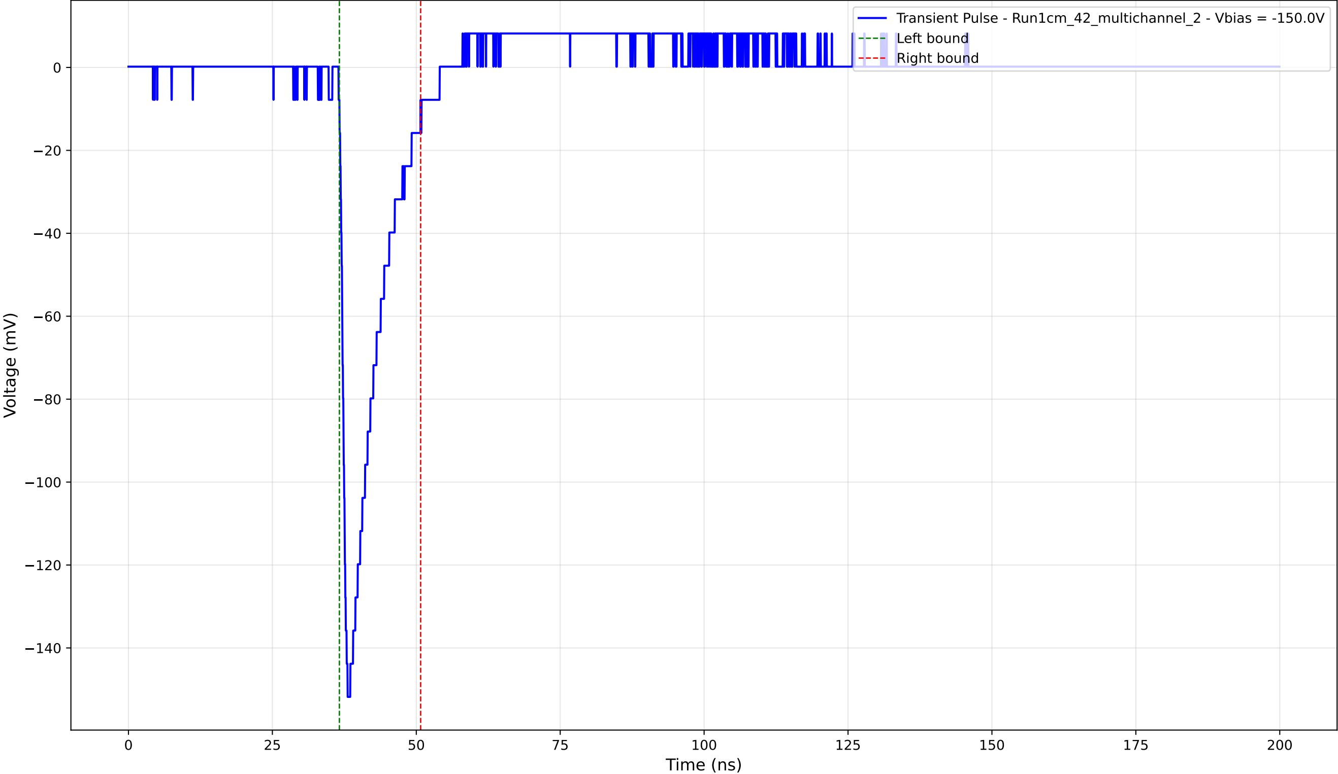
Transient Pulse - Sample: 1cm_42_multichannel - Position: 1200.0 \mu\text{m} - Charge: 18.81 pC - Rise Time: 1.24 ns
