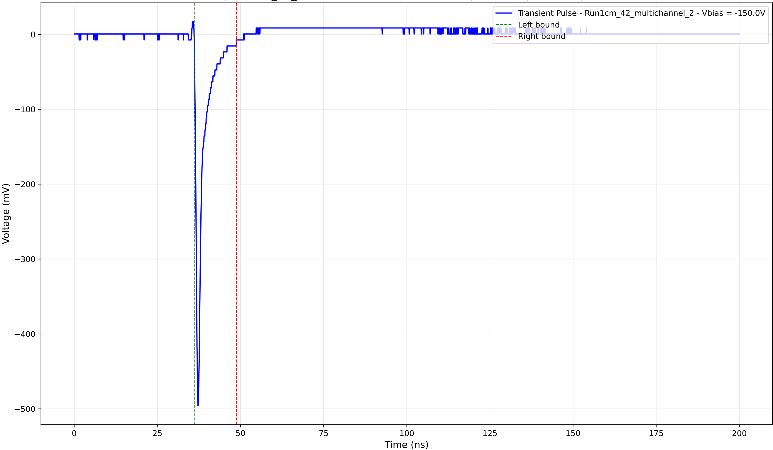
Transient Pulse - Sample: 1cm_42_multichannel - Position: 2580.0 \mu\text{m} - Charge: 25.07 pC - Rise Time: 0.77 ns
