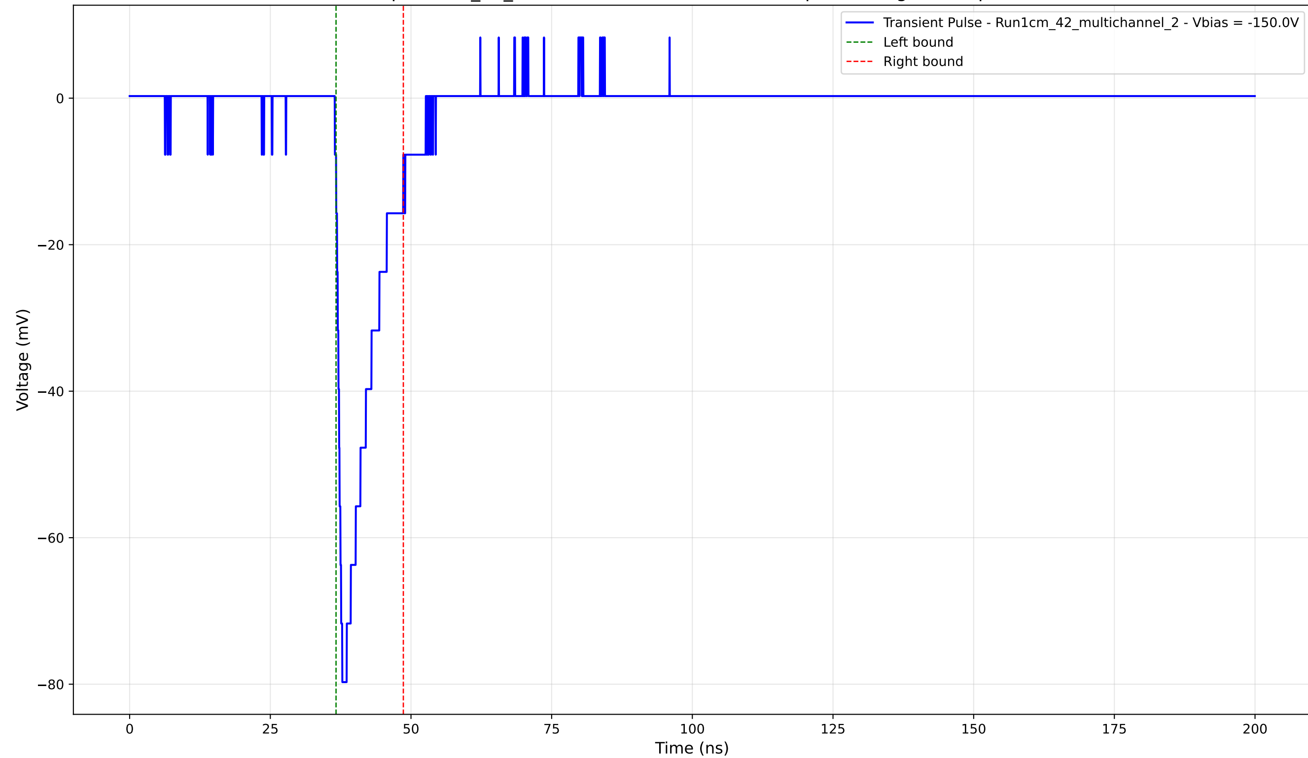
Transient Pulse - Sample: 1cm_42_multichannel - Position: 3435.0 \mu\text{m} - Charge: 9.49 pC - Rise Time: 1.12 ns
