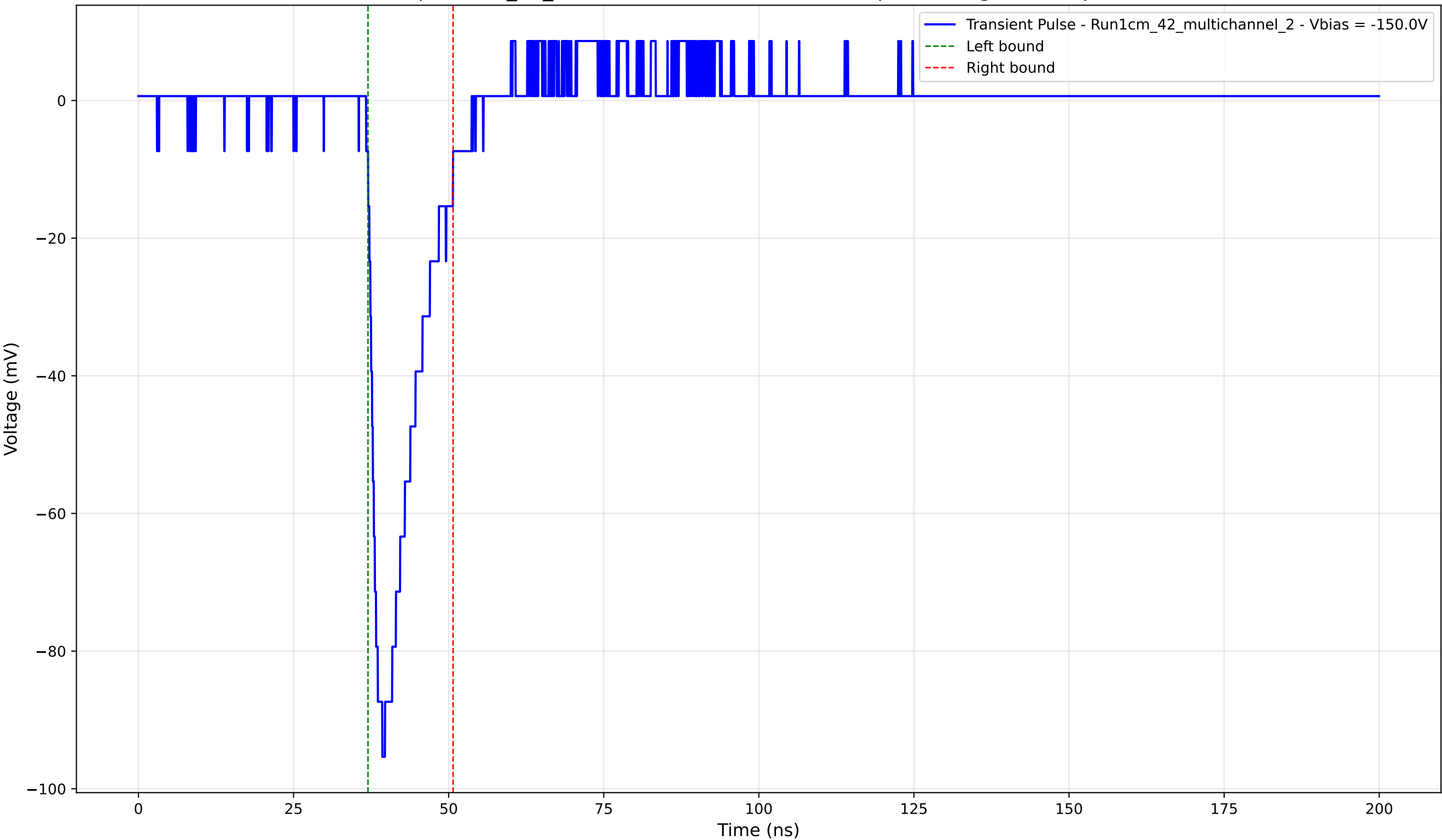
Transient Pulse - Sample: 1cm_42_multichannel - Position: 4015.0 \mu\text{m} - Charge: 13.37 pC - Rise Time: 1.59 ns
