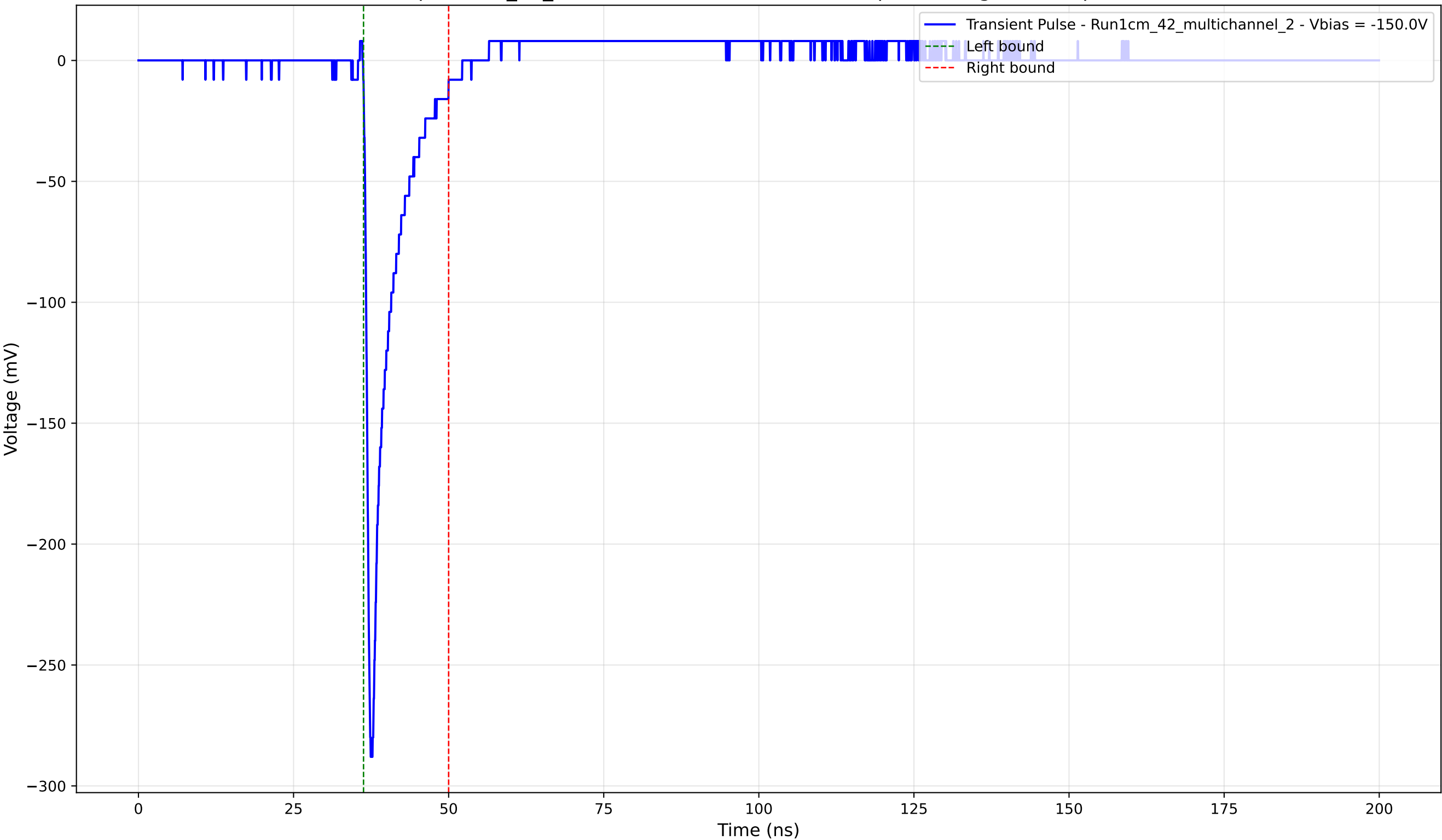
Transient Pulse - Sample: 1cm_42_multichannel - Position: 1765.0 \mu\text{m} - Charge: 22.81 pC - Rise Time: 0.87 ns
