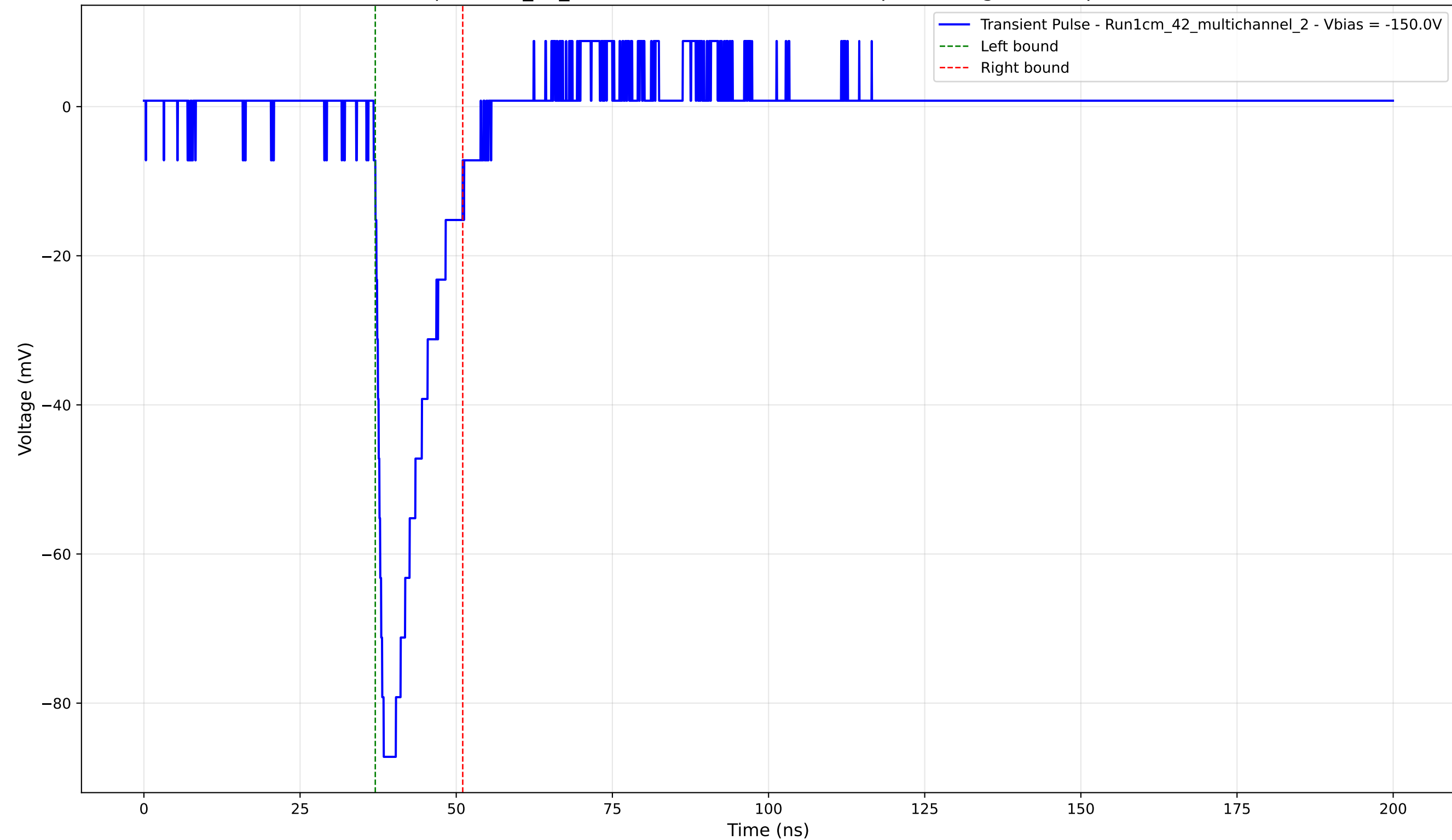
Transient Pulse - Sample: 1cm_42_multichannel - Position: 780.0 \mu\text{m} - Charge: 13.02 pC - Rise Time: 1.11 ns
