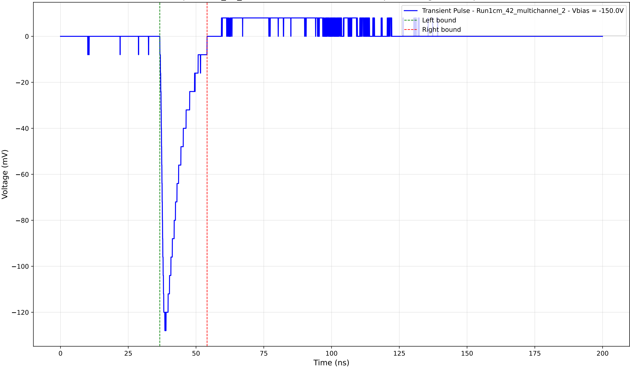
Transient Pulse - Sample: 1cm_42_multichannel - Position: 1005.0 \mu\text{m} - Charge: 17.62 pC - Rise Time: 1.26 ns
