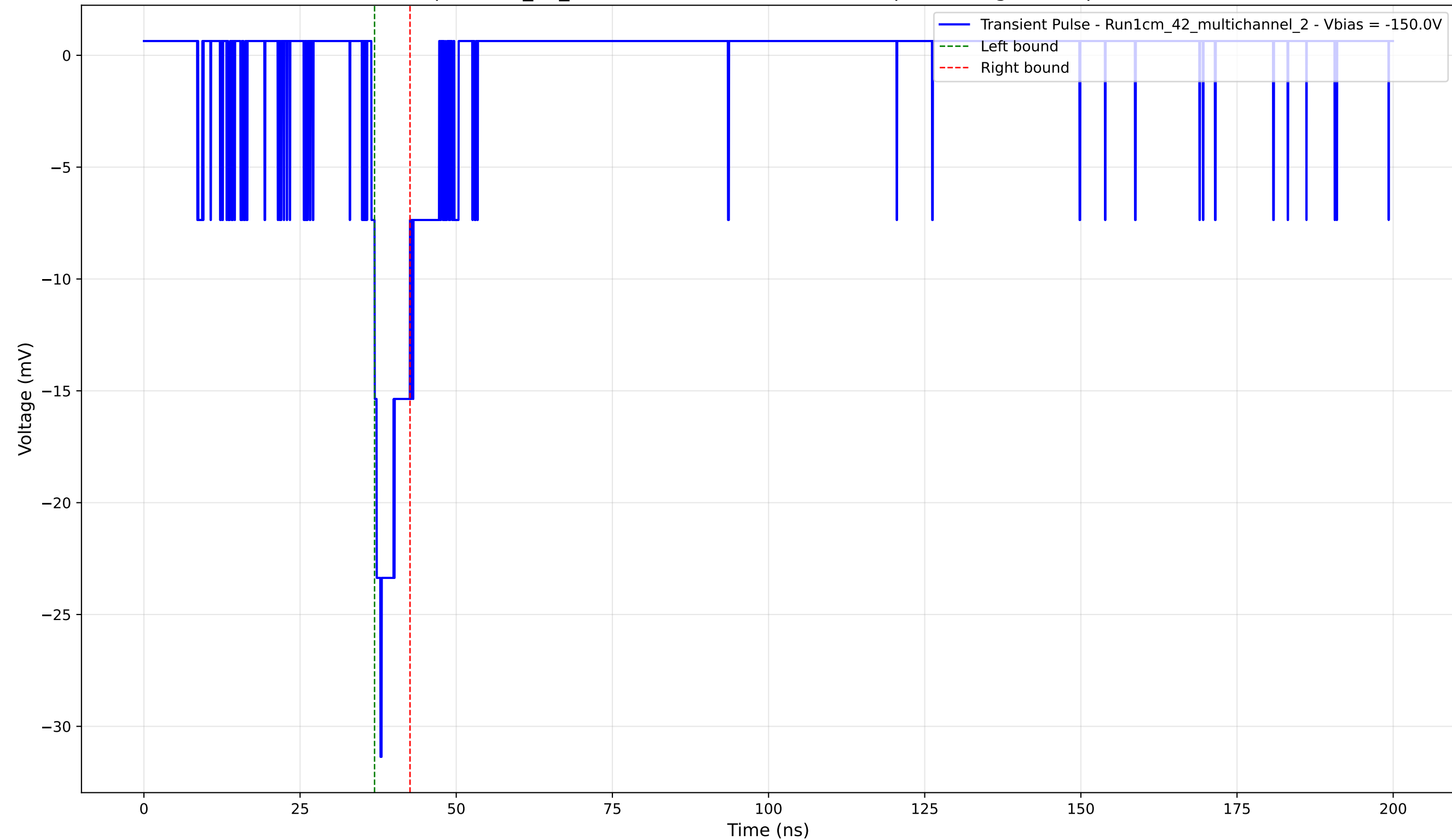
Transient Pulse - Sample: 1cm_42_multichannel - Position: 3350.0 \mu\text{m} - Charge: 2.23 pC - Rise Time: 1.47 ns
