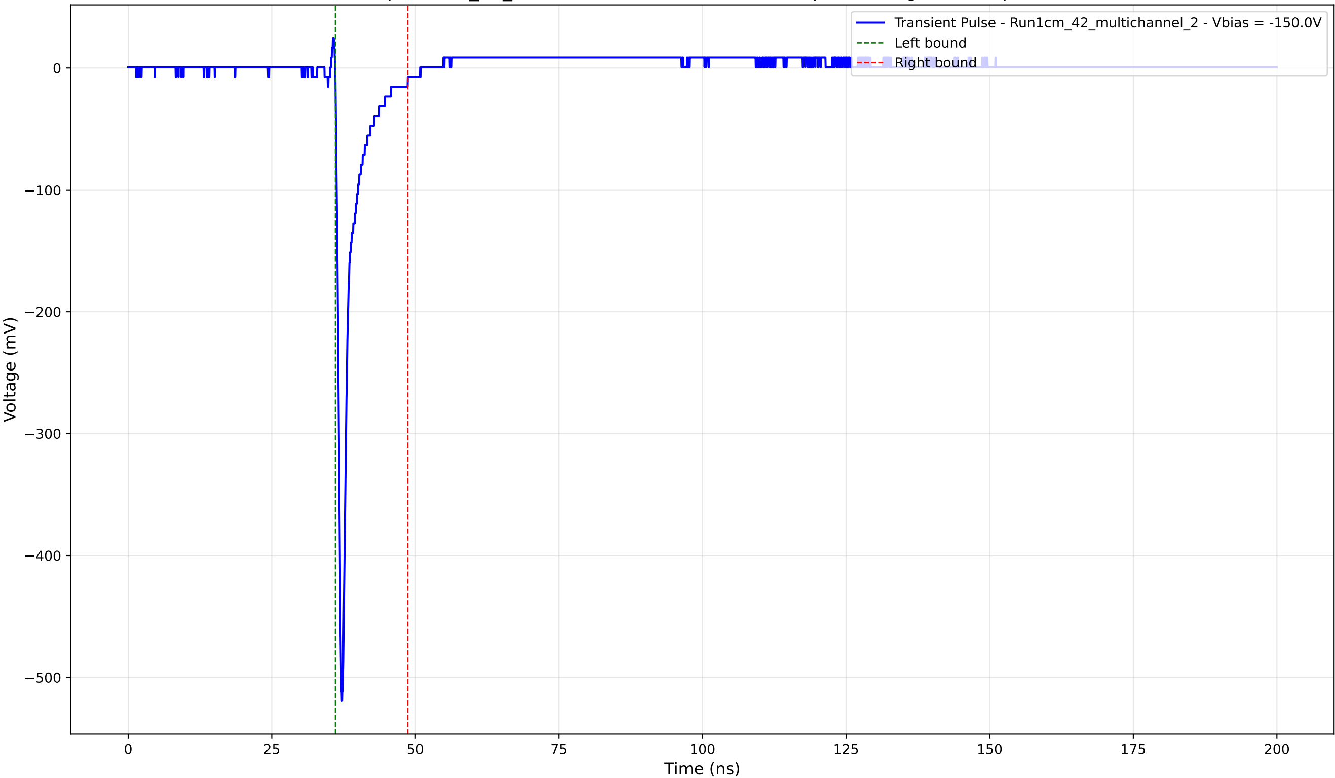
Transient Pulse - Sample: 1cm_42_multichannel - Position: 2550.0 \mu\text{m} - Charge: 25.34 pC - Rise Time: 0.73 ns
