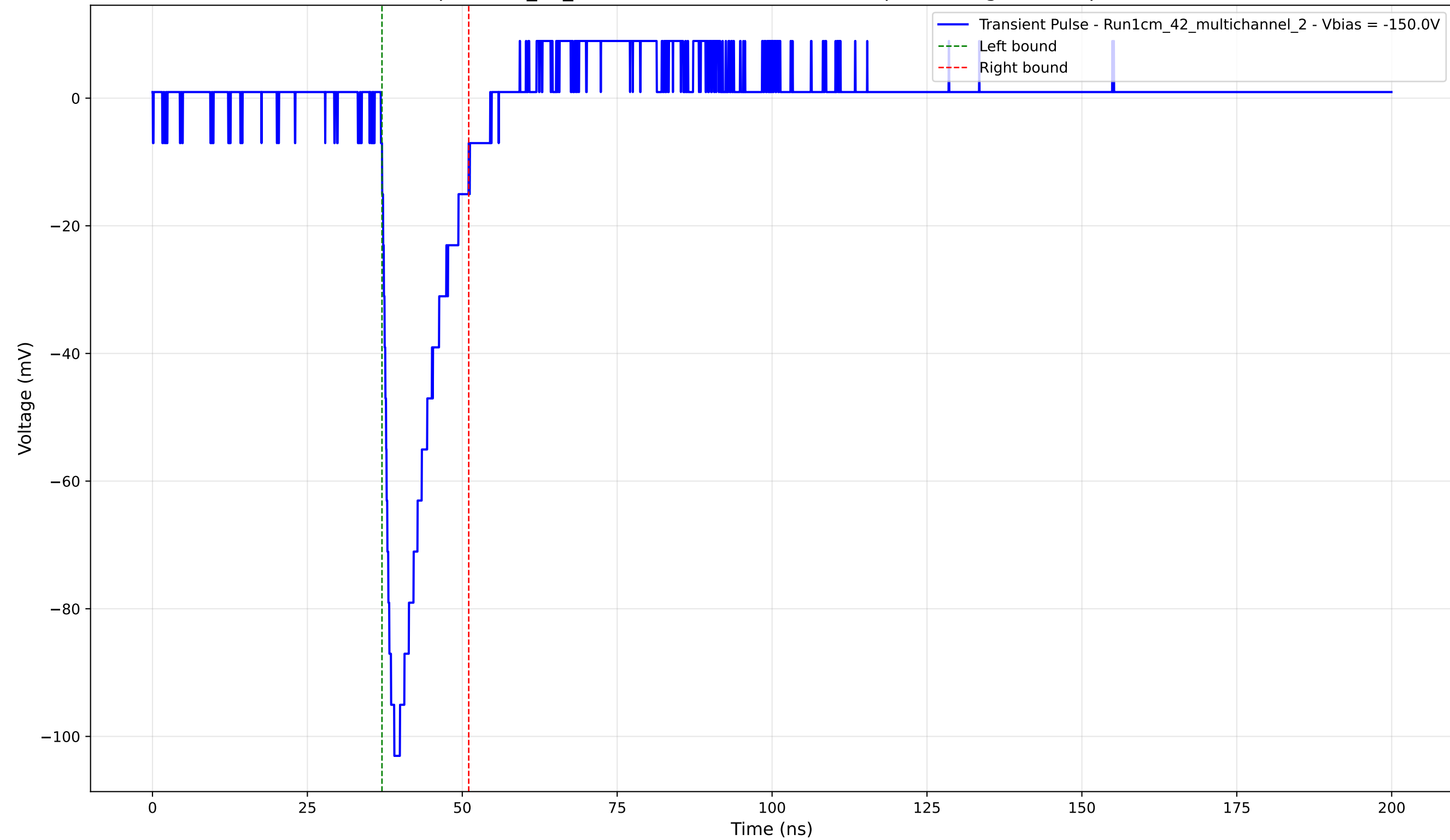
Transient Pulse - Sample: 1cm_42_multichannel - Position: 655.0 \mu\text{m} - Charge: 14.80 pC - Rise Time: 1.46 ns
