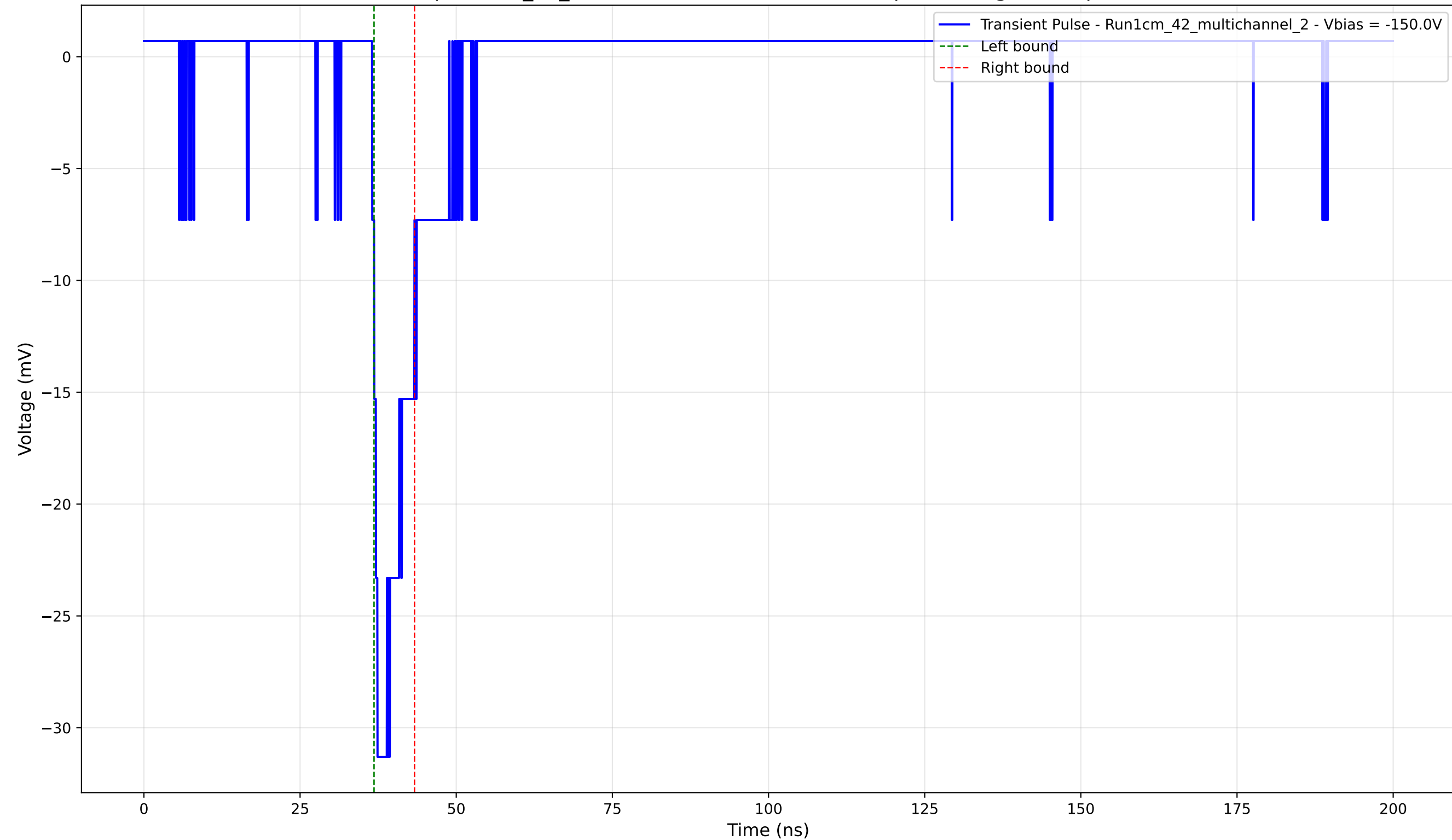
Transient Pulse - Sample: 1cm_42_multichannel - Position: 1390.0 \mu\text{m} - Charge: 2.86 pC - Rise Time: 0.87 ns
