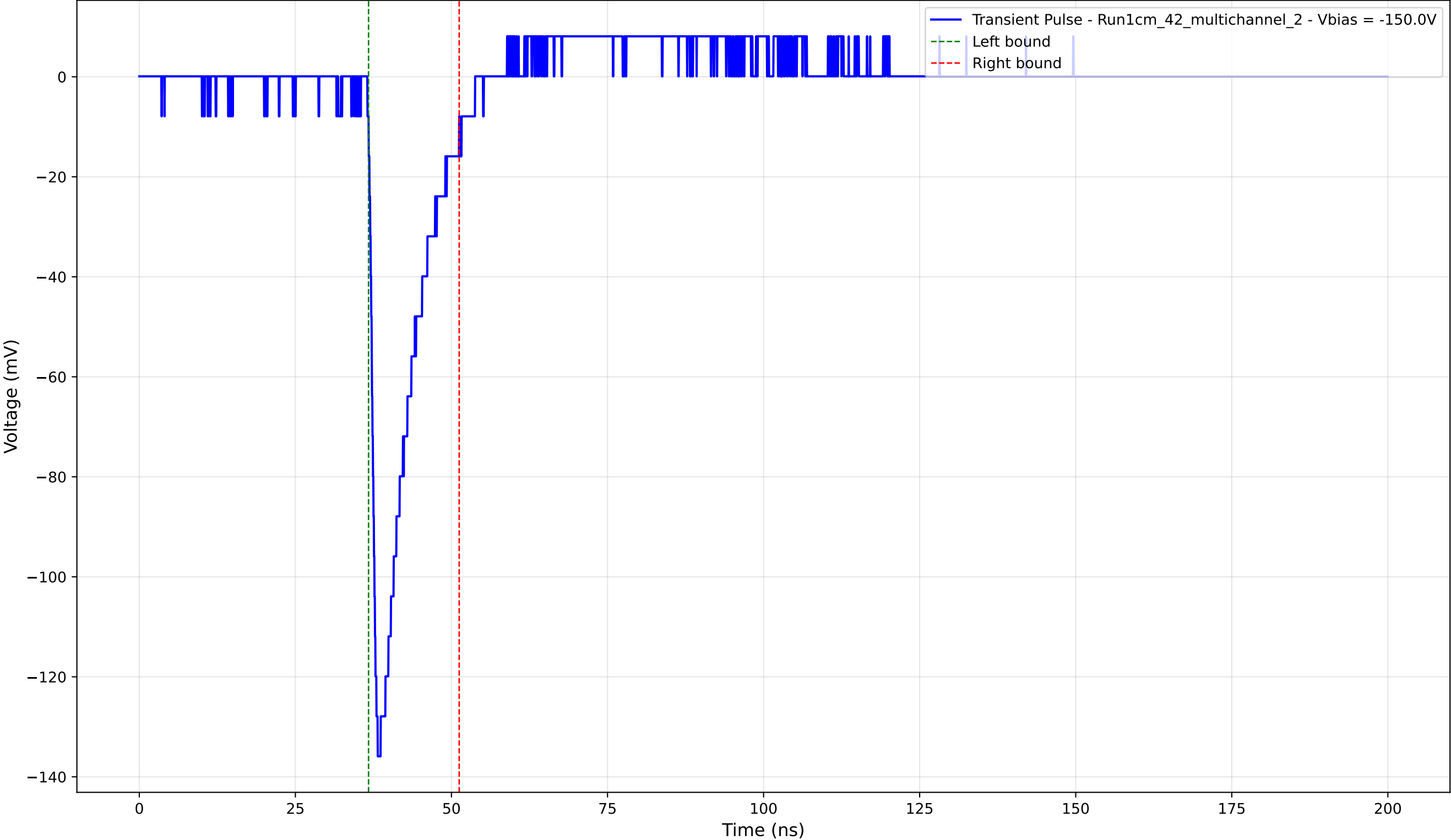
Transient Pulse - Sample: 1cm_42_multichannel - Position: 1120.0 \mu\text{m} - Charge: 17.62 pC - Rise Time: 1.25 ns
