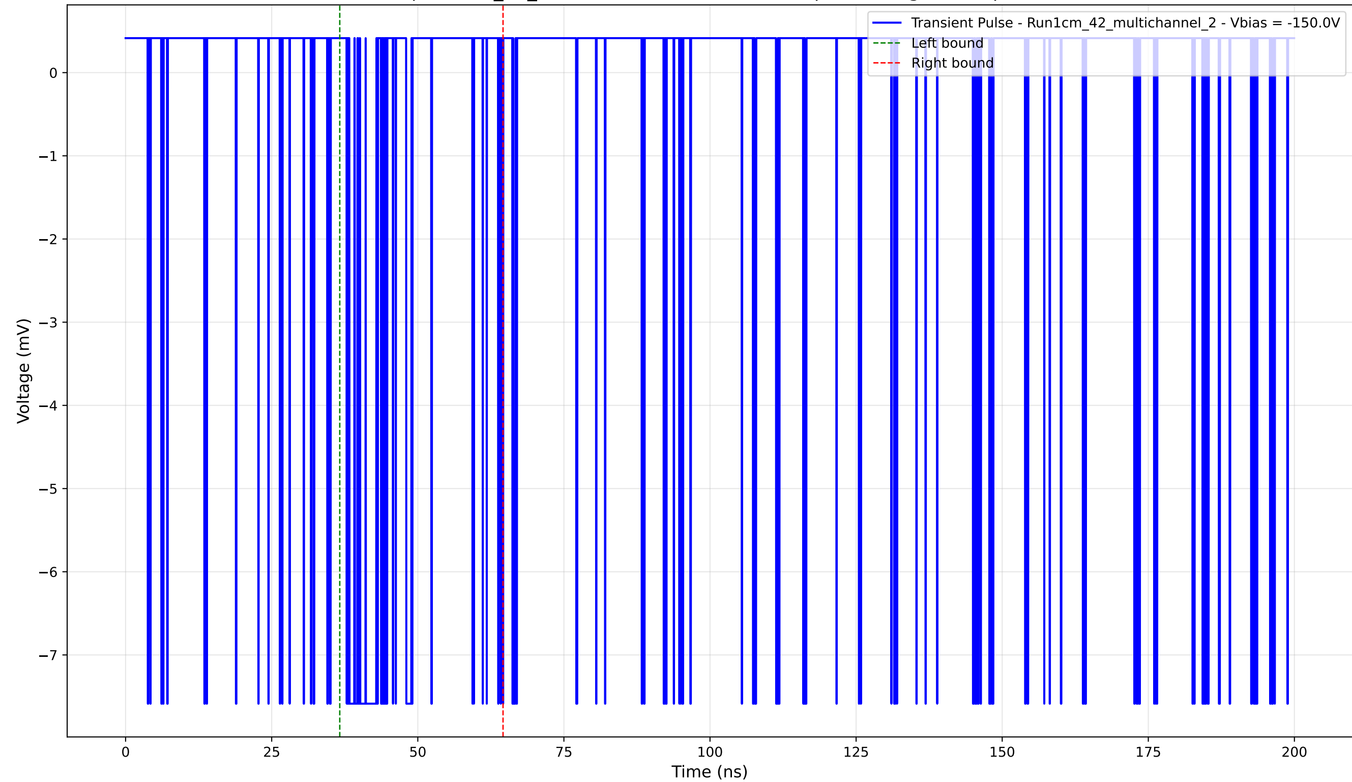
Transient Pulse - Sample: 1cm_42_multichannel - Position: 20.0 \mu\text{m} - Charge: 0.84 pC - Rise Time: 0.04 ns
