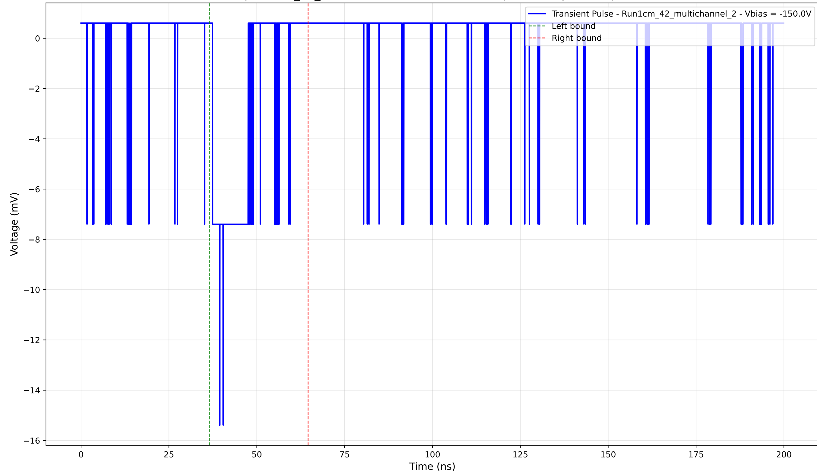
Transient Pulse - Sample: 1cm_42_multichannel - Position: 4415.0 \mu\text{m} - Charge: 1.55 pC - Rise Time: 2.03 ns
