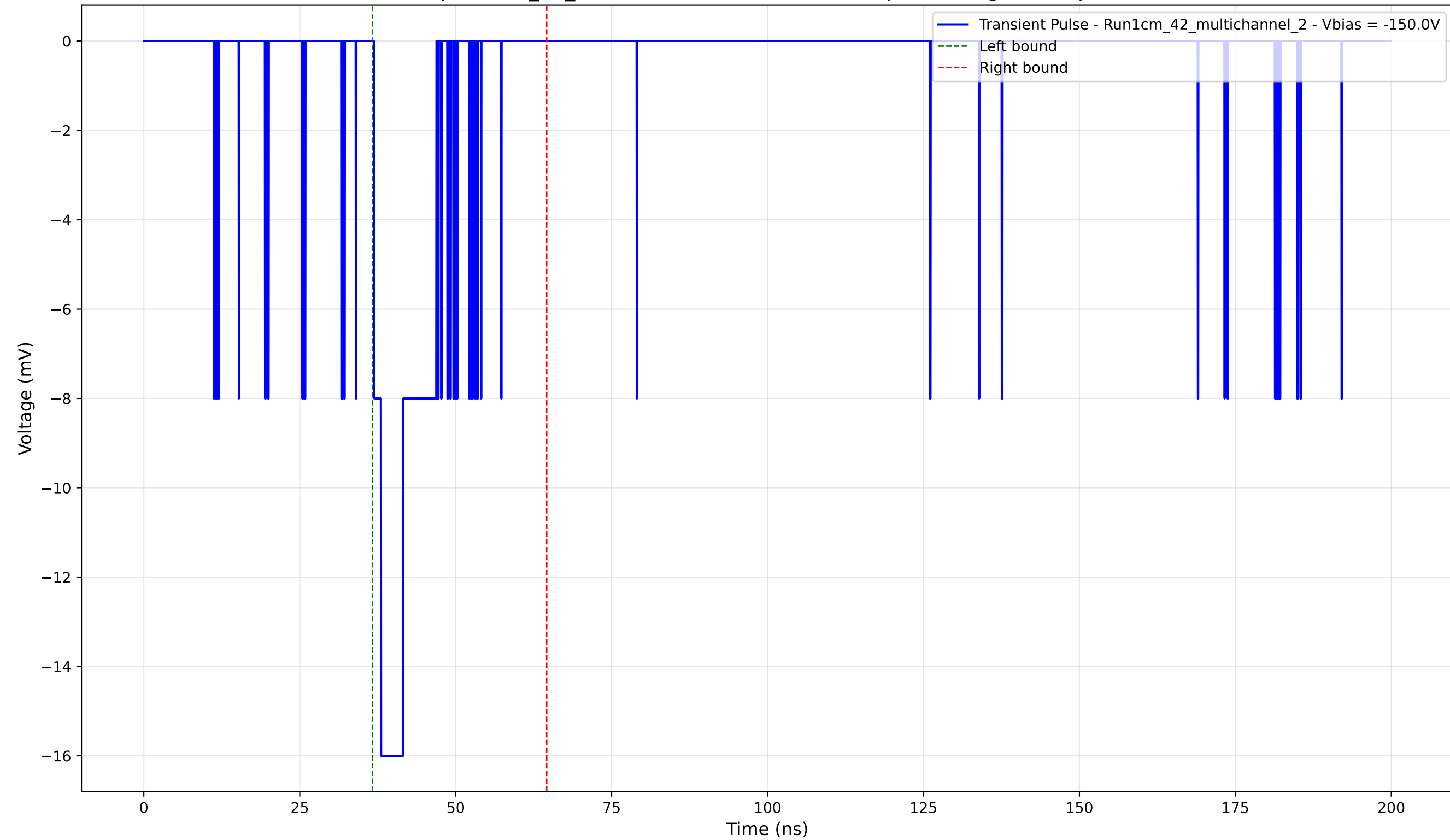
Transient Pulse - Sample: 1cm_42_multichannel - Position: 875.0 \mu\text{m} - Charge: 2.41 pC - Rise Time: 1.11 ns
