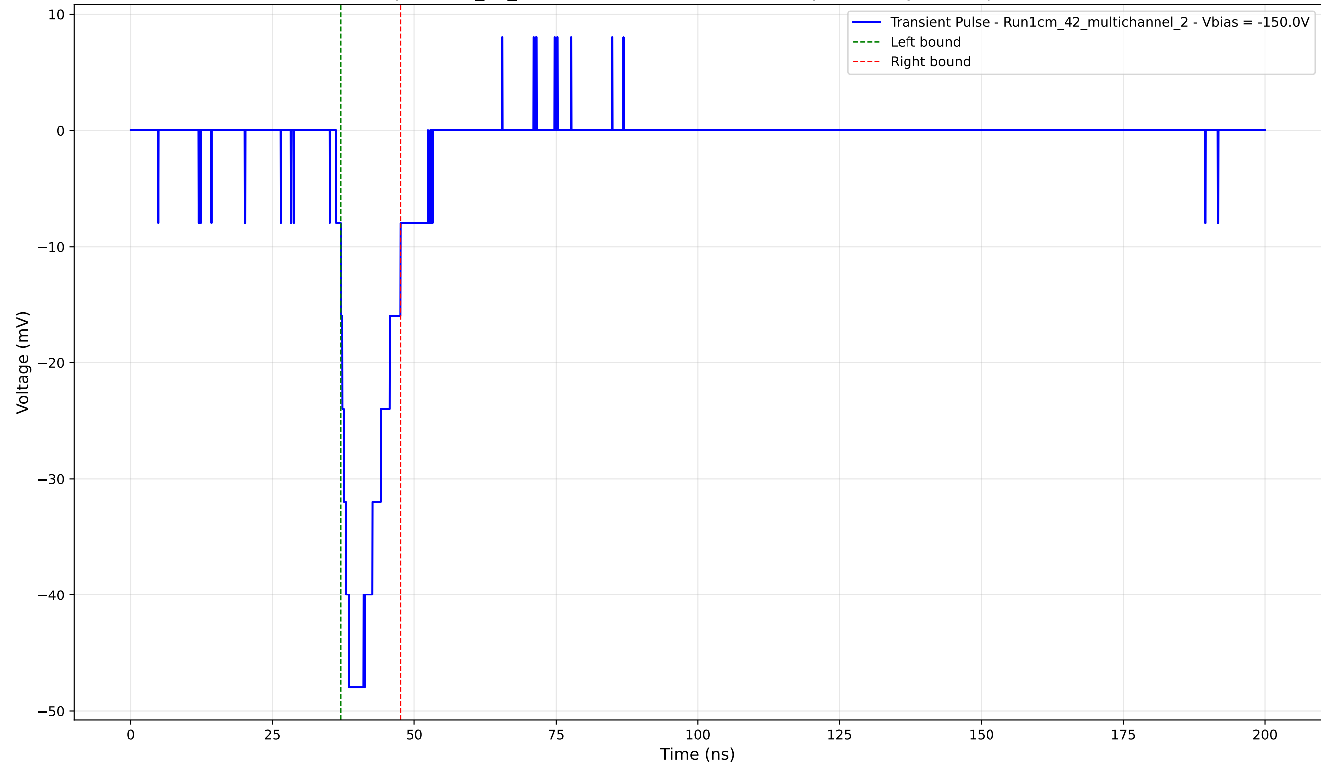
Transient Pulse - Sample: 1cm_42_multichannel - Position: 4830.0 \mu\text{m} - Charge: 6.89 pC - Rise Time: 2.26 ns
