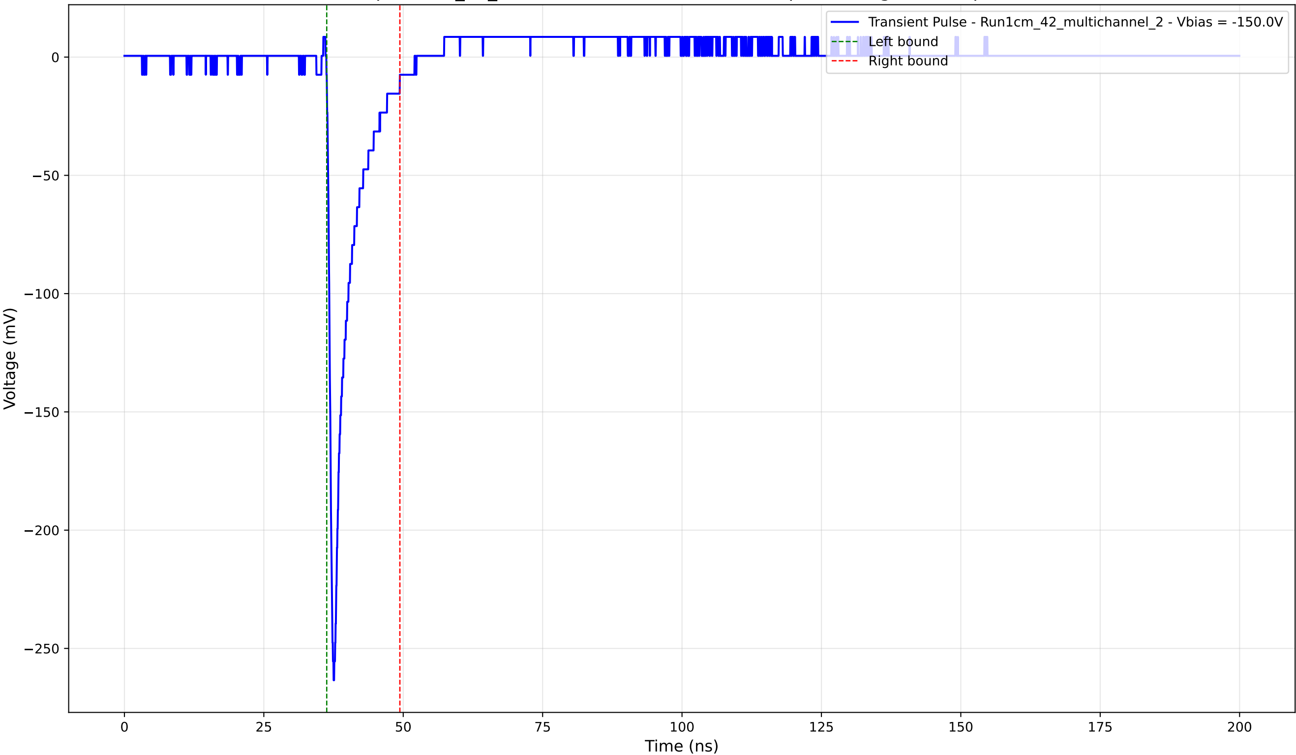
Transient Pulse - Sample: 1cm_42_multichannel - Position: 1790.0 \mu\text{m} - Charge: 19.74 pC - Rise Time: 0.85 ns
