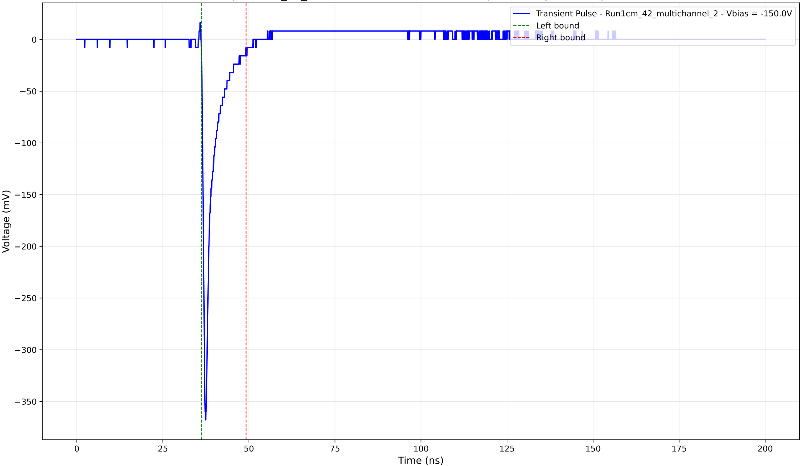
Transient Pulse - Sample: 1cm_42_multichannel - Position: 2780.0 \mu\text{m} - Charge: 23.06 pC - Rise Time: 0.79 ns
