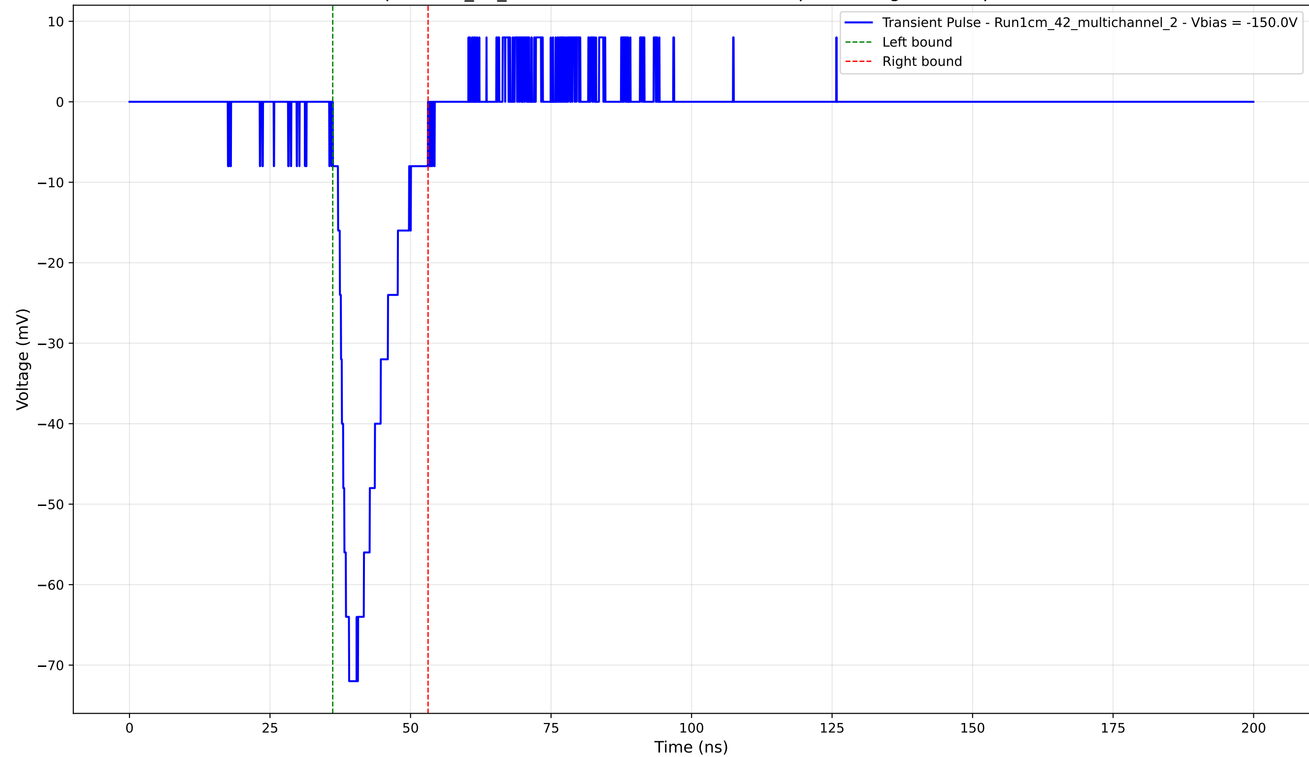
Transient Pulse - Sample: 1cm_42_multichannel - Position: 4620.0 \mu\text{m} - Charge: 11.24 pC - Rise Time: 2.88 ns
