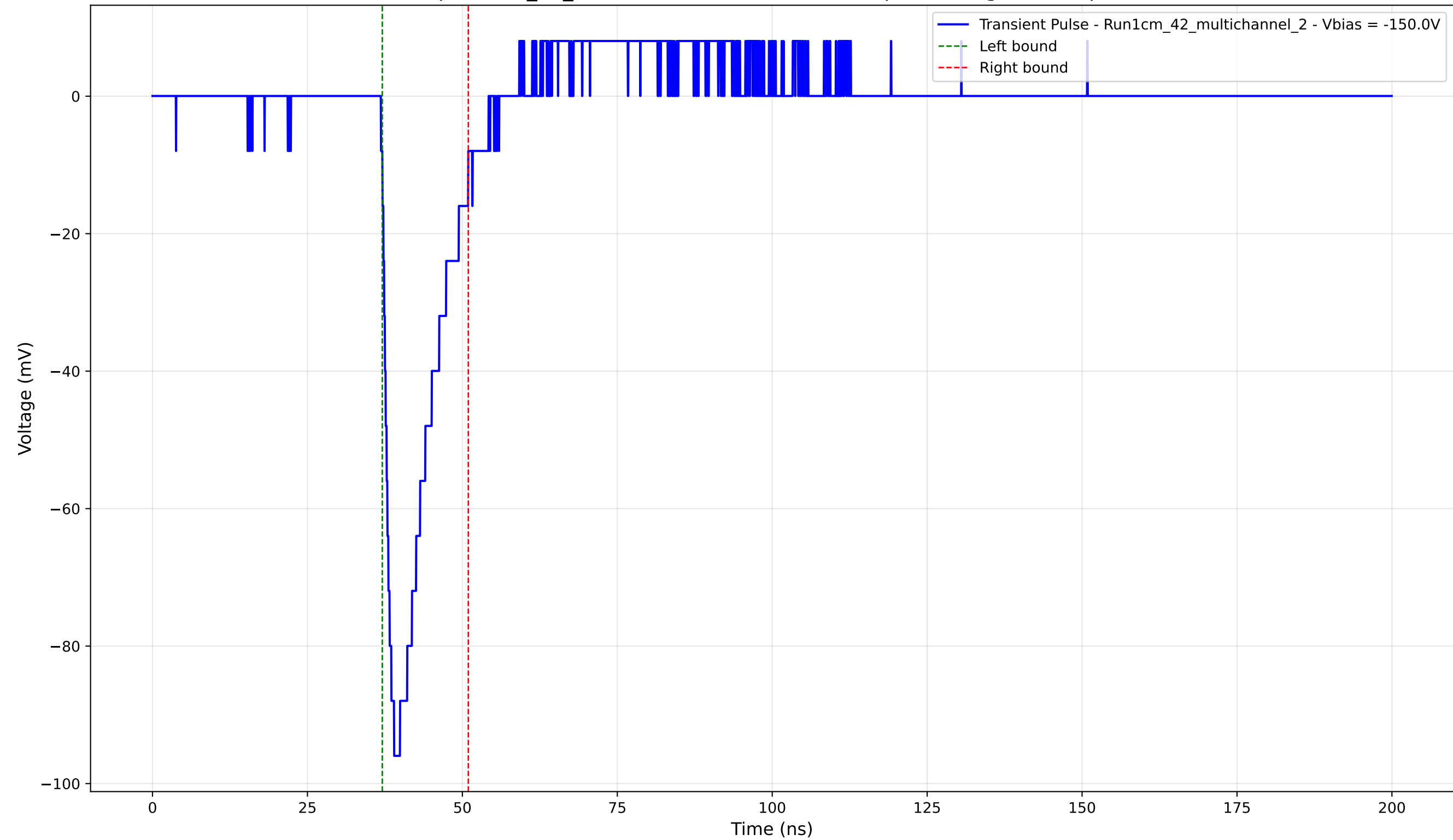
Transient Pulse - Sample: 1cm_42_multichannel - Position: 530.0 \mu\text{m} - Charge: 14.26 pC - Rise Time: 1.47 ns
