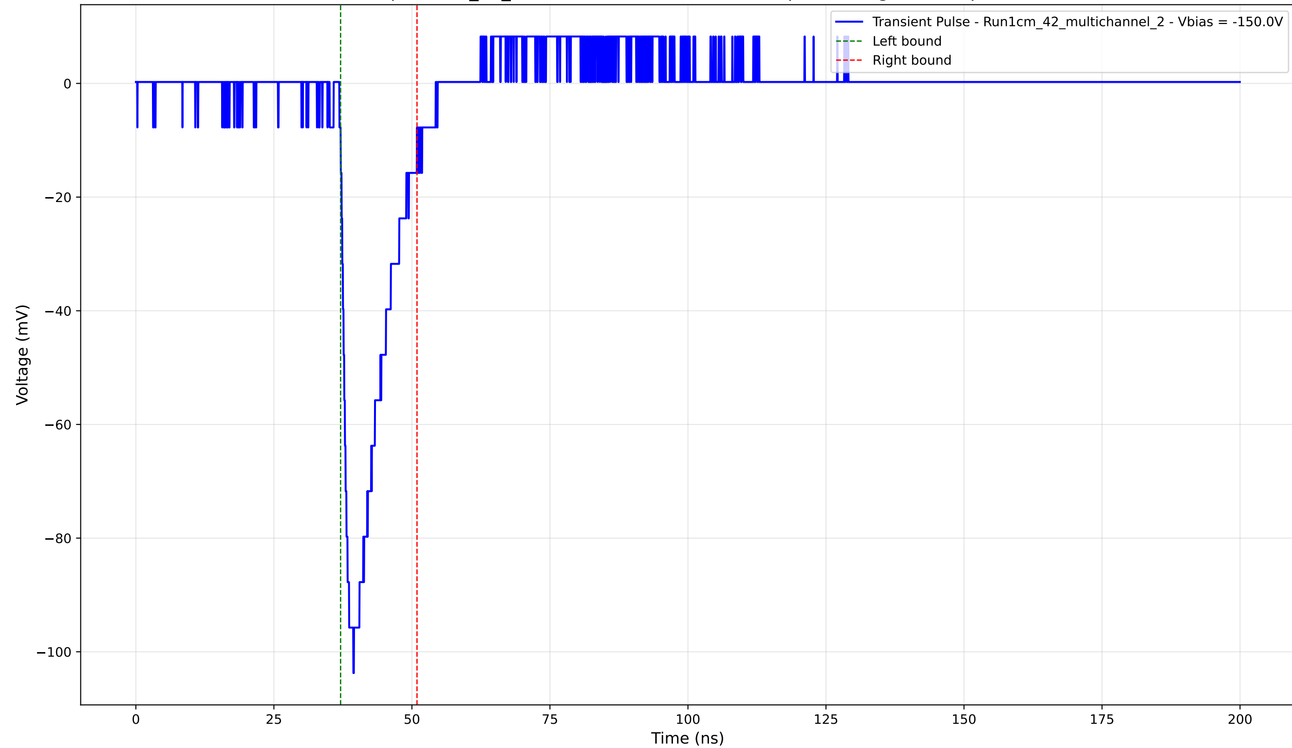
Transient Pulse - Sample: 1cm_42_multichannel - Position: 585.0 \mu\text{m} - Charge: 14.60 pC - Rise Time: 1.55 ns
