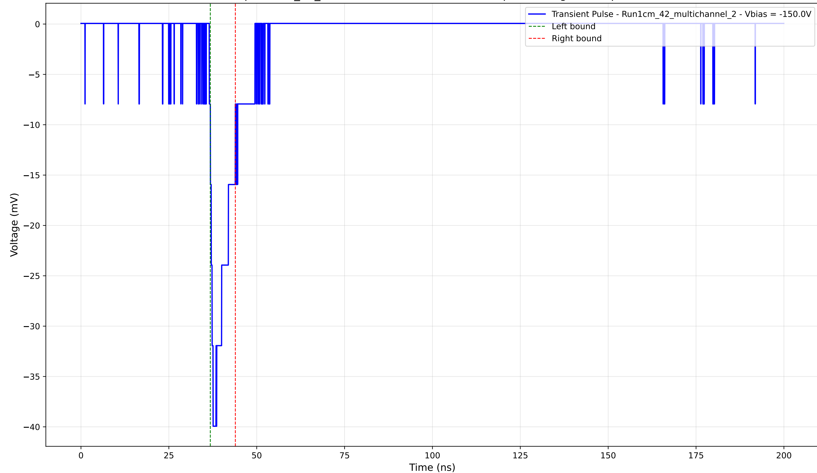
Transient Pulse - Sample: 1cm_42_multichannel - Position: 3345.0 \mu\text{m} - Charge: 3.63 pC - Rise Time: 1.10 ns
