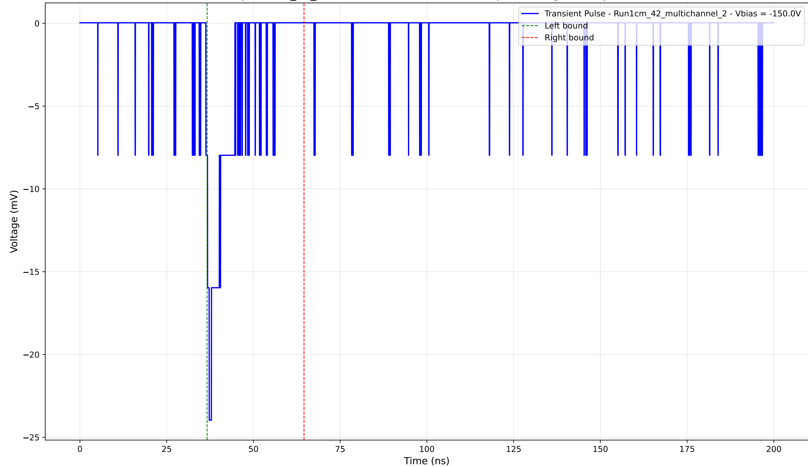
Transient Pulse - Sample: 1cm_42_multichannel - Position: 1845.0 \mu\text{m} - Charge: 2.21 pC - Rise Time: 0.99 ns
