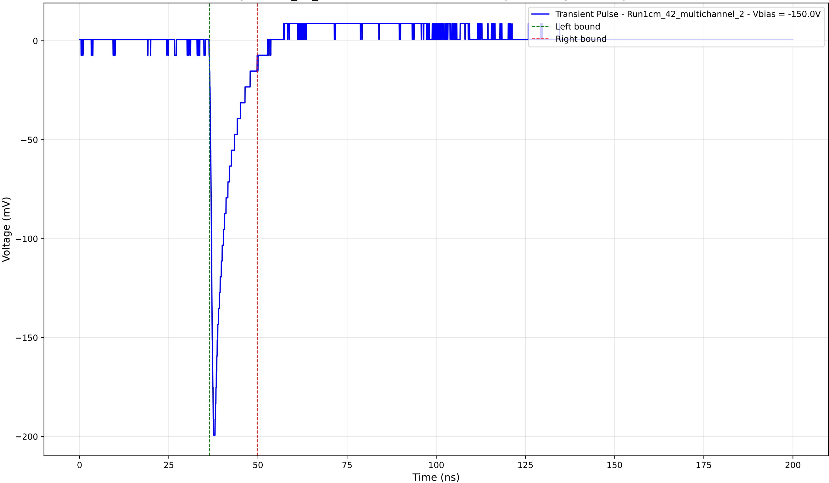
Transient Pulse - Sample: 1cm_42_multichannel - Position: 3150.0 \mu\text{m} - Charge: 18.44 pC - Rise Time: 0.92 ns
