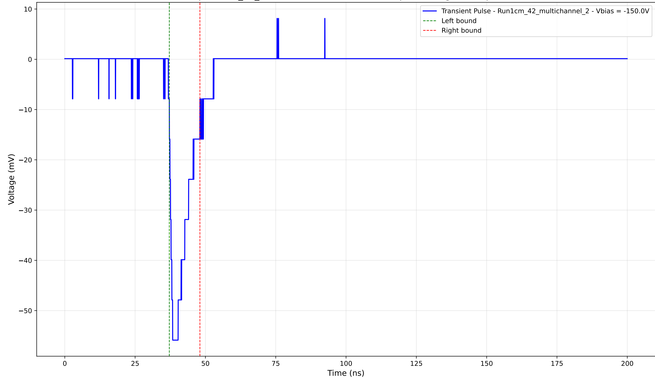
Transient Pulse - Sample: 1cm_42_multichannel - Position: 800.0 \mu\text{m} - Charge: 7.45 pC - Rise Time: 1.53 ns
