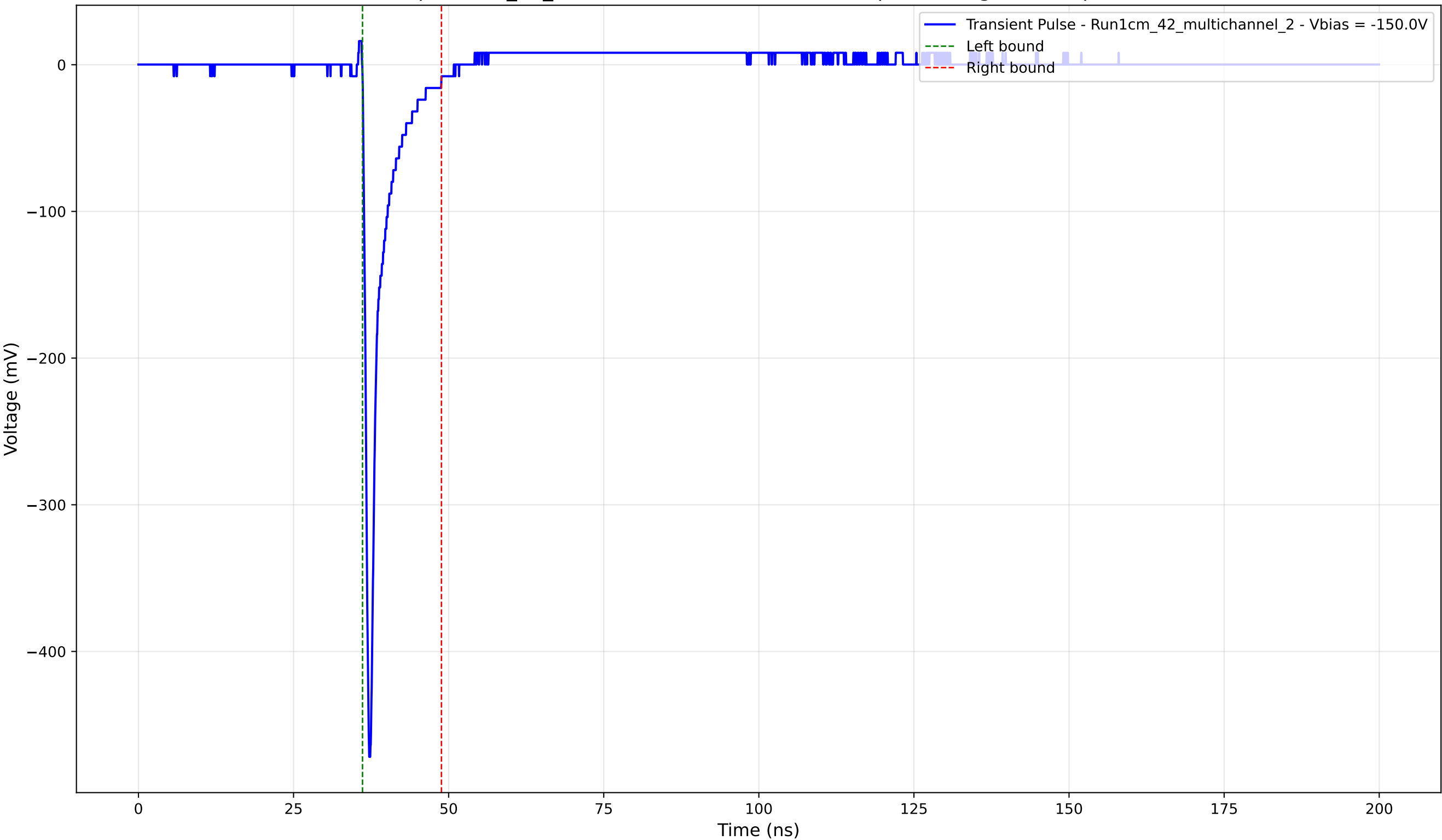
Transient Pulse - Sample: 1cm_42_multichannel - Position: 2625.0 \mu\text{m} - Charge: 25.27 pC - Rise Time: 0.76 ns
