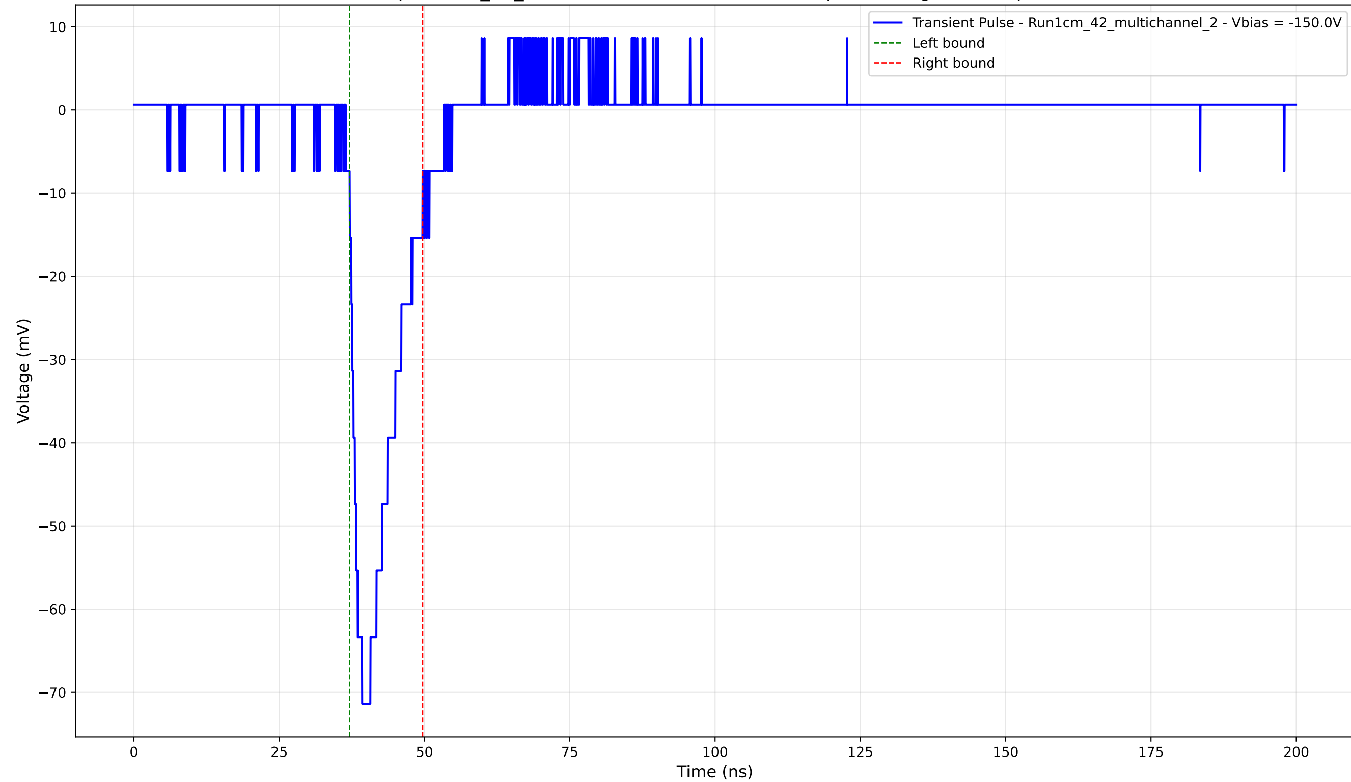
Transient Pulse - Sample: 1cm_42_multichannel - Position: 4615.0 \mu\text{m} - Charge: 10.37 pC - Rise Time: 2.80 ns
