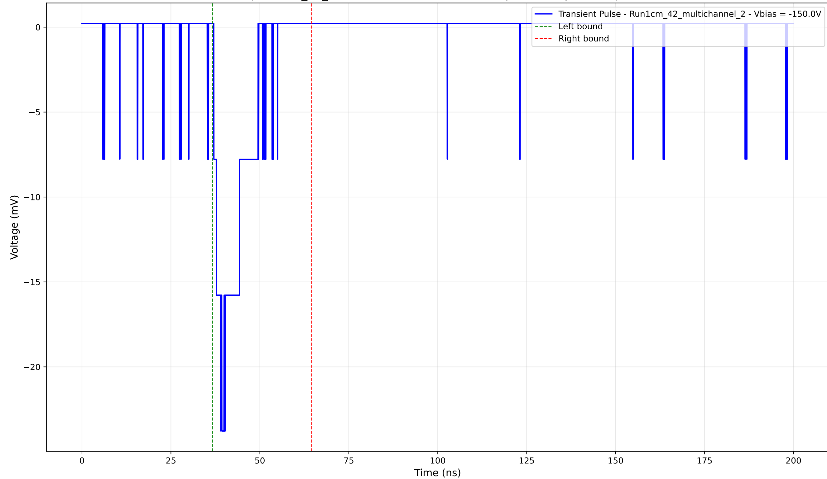
Transient Pulse - Sample: 1cm_42_multichannel - Position: 380.0 \mu\text{m} - Charge: 3.20 pC - Rise Time: 1.99 ns
