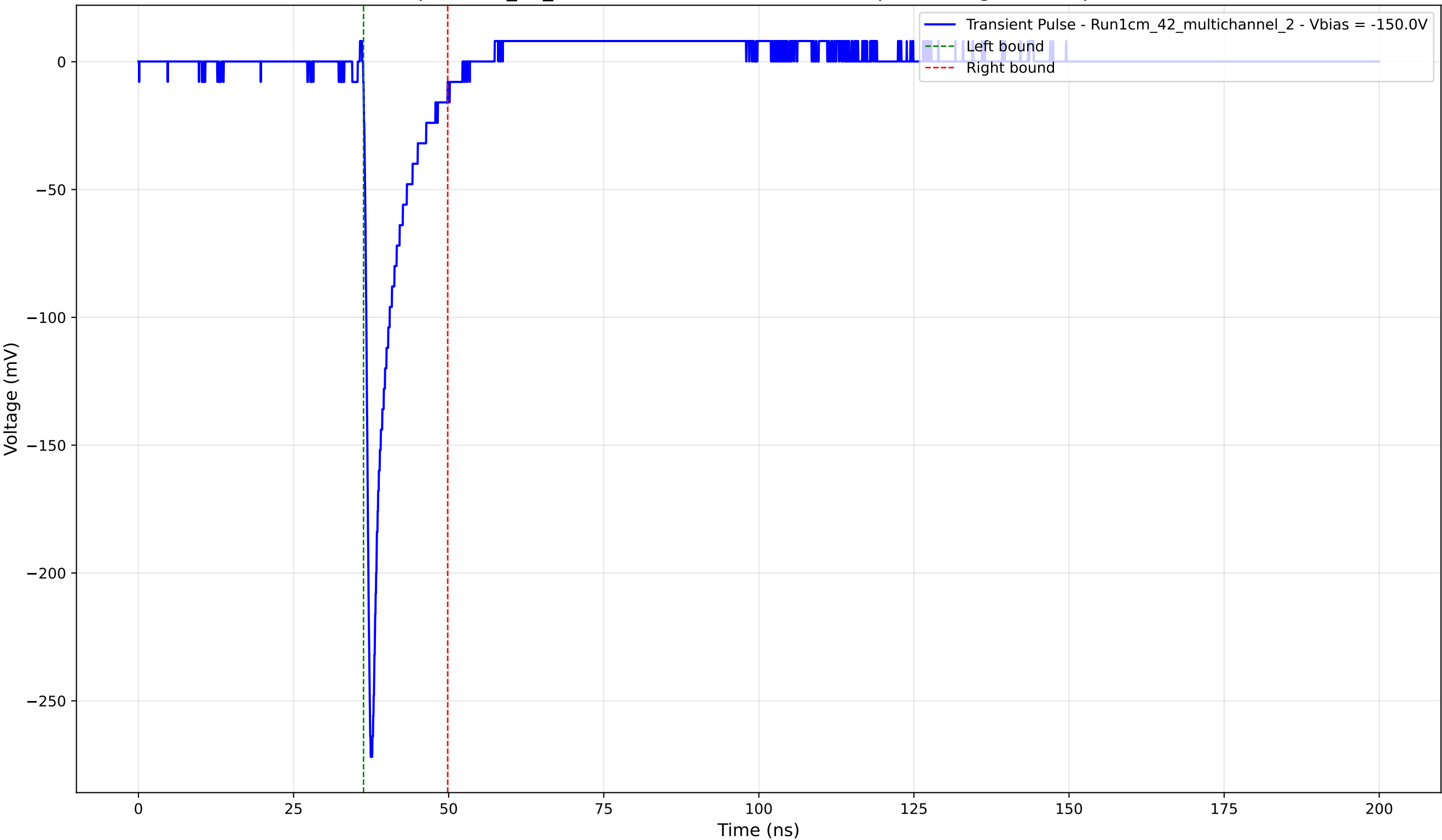
Transient Pulse - Sample: 1cm_42_multichannel - Position: 2980.0 \mu\text{m} - Charge: 21.51 pC - Rise Time: 0.85 ns
