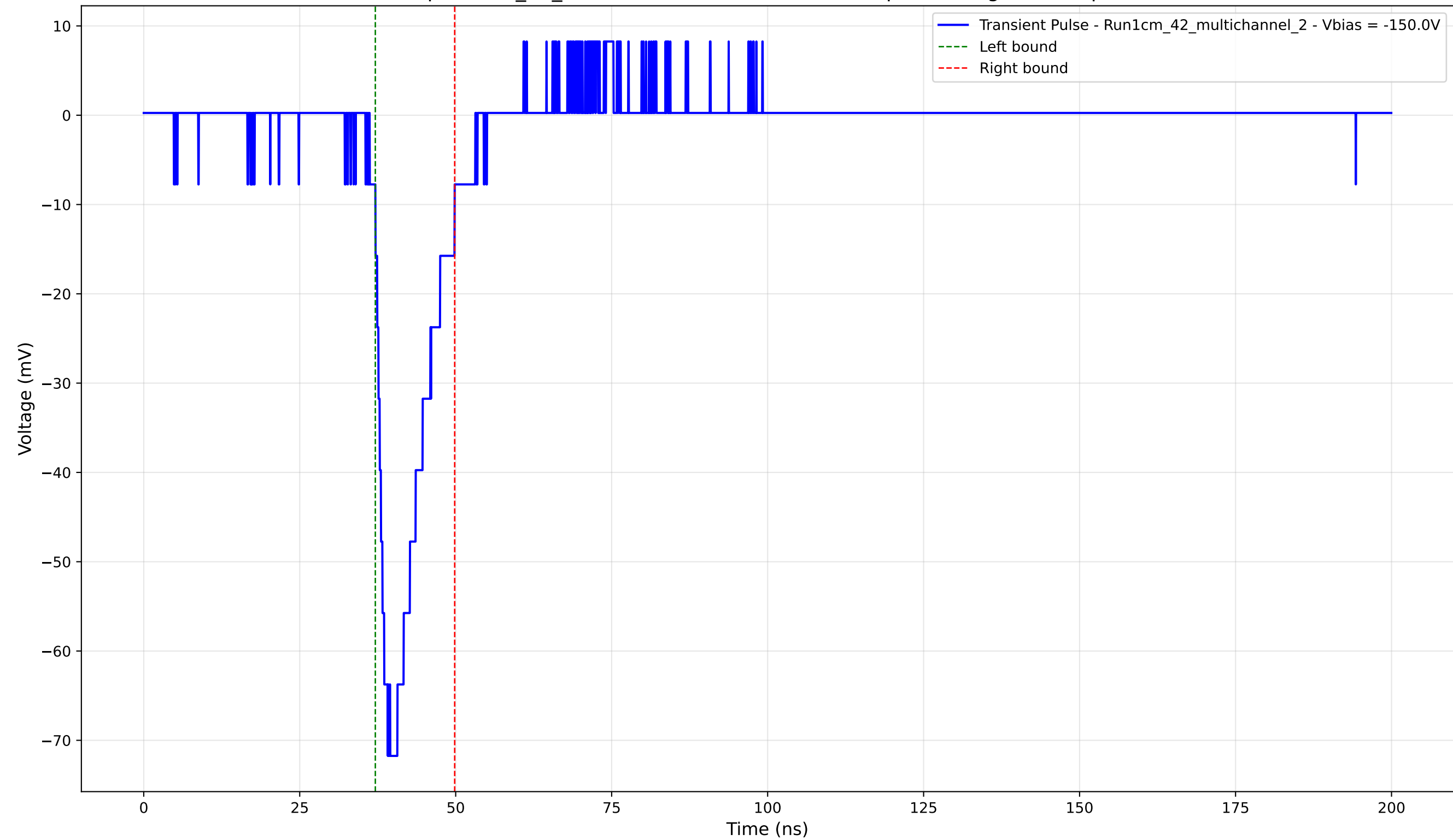
Transient Pulse - Sample: 1cm_42_multichannel - Position: 4630.0 \mu\text{m} - Charge: 10.37 pC - Rise Time: 2.88 ns
