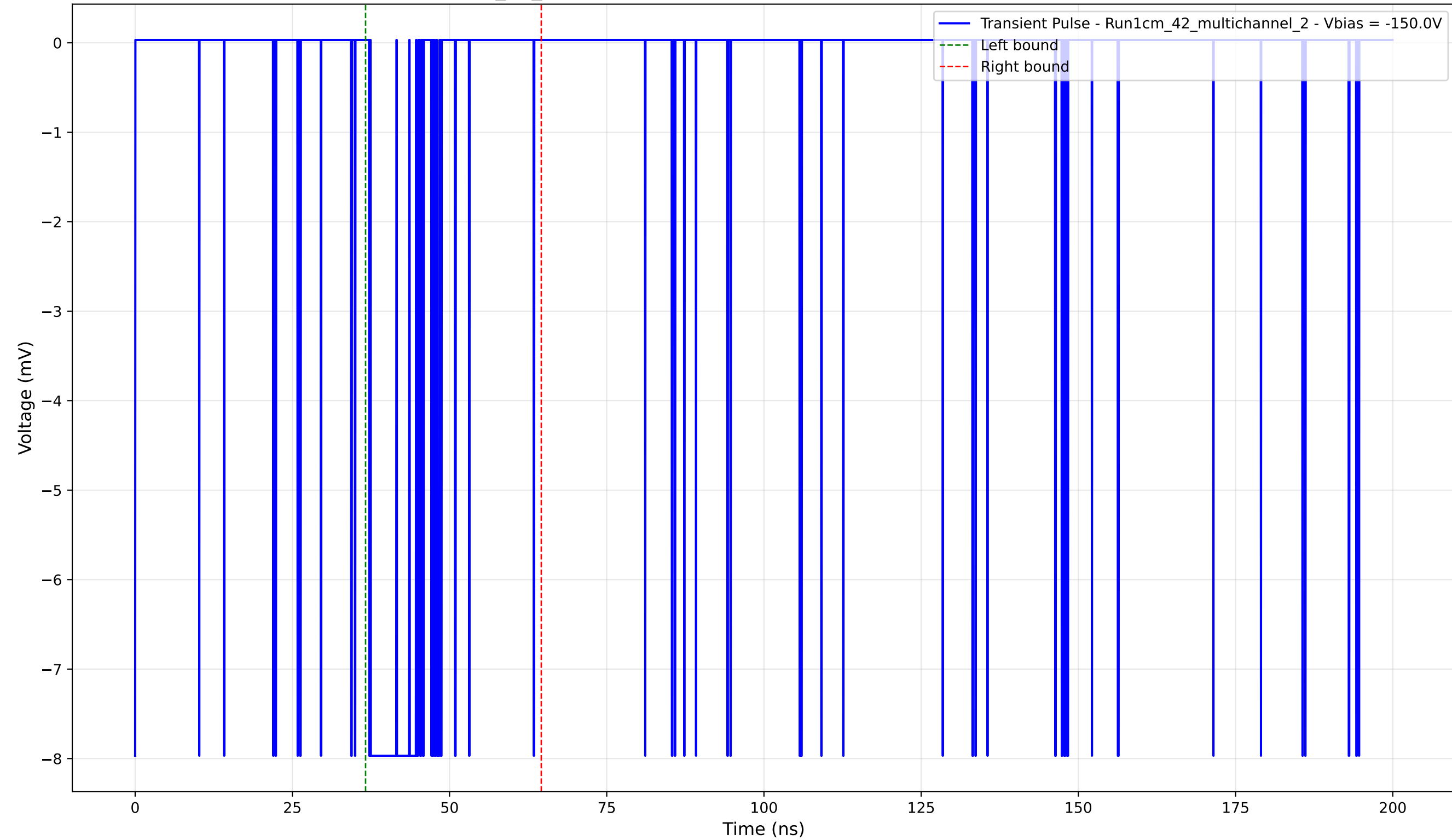
Transient Pulse - Sample: 1cm_42_multichannel - Position: 330.0 \mu\text{m} - Charge: 1.42 pC - Rise Time: 0.00 ns (N/A)
