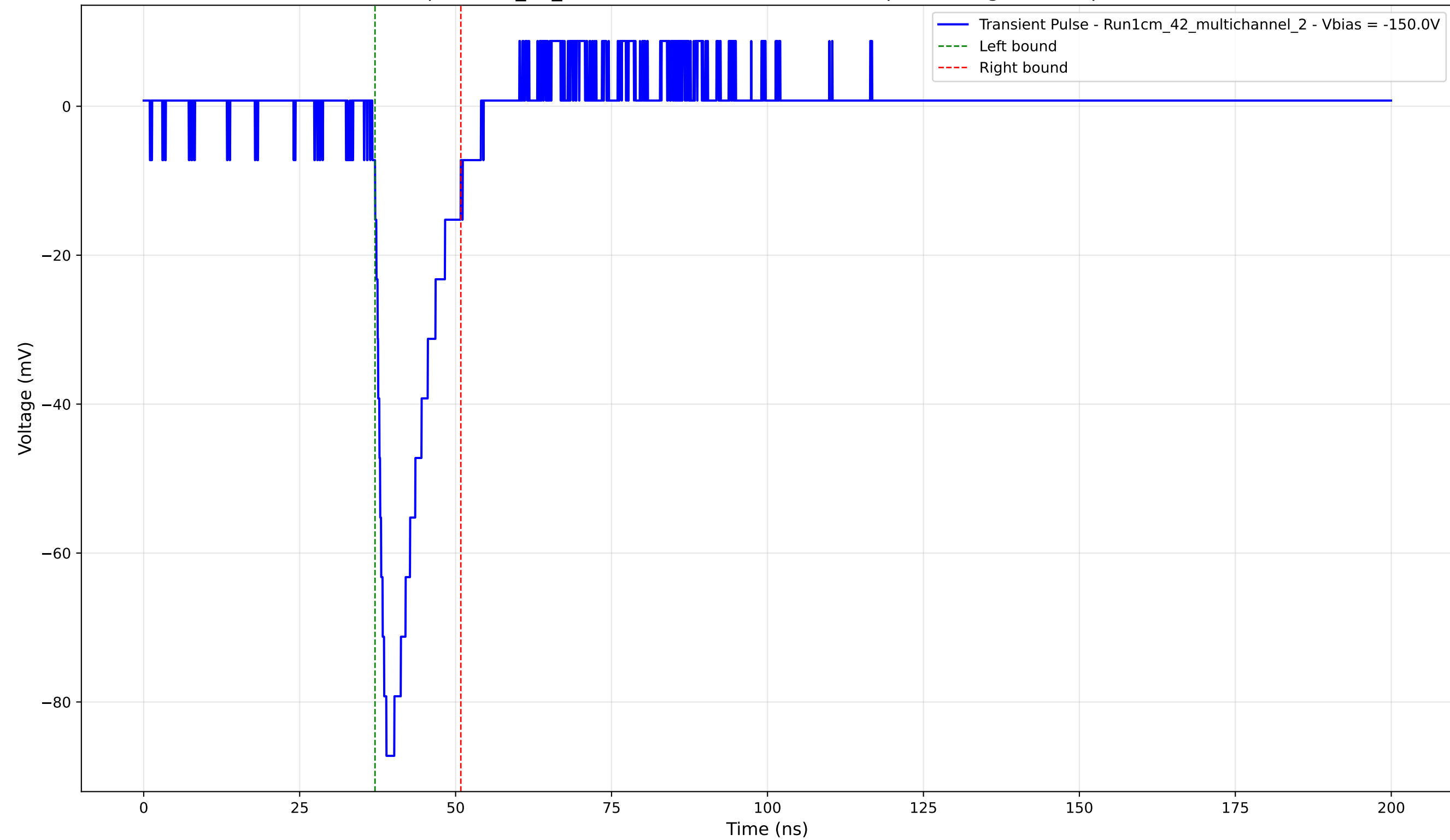
Transient Pulse - Sample: 1cm_42_multichannel - Position: 4105.0 \mu\text{m} - Charge: 12.65 pC - Rise Time: 1.47 ns
