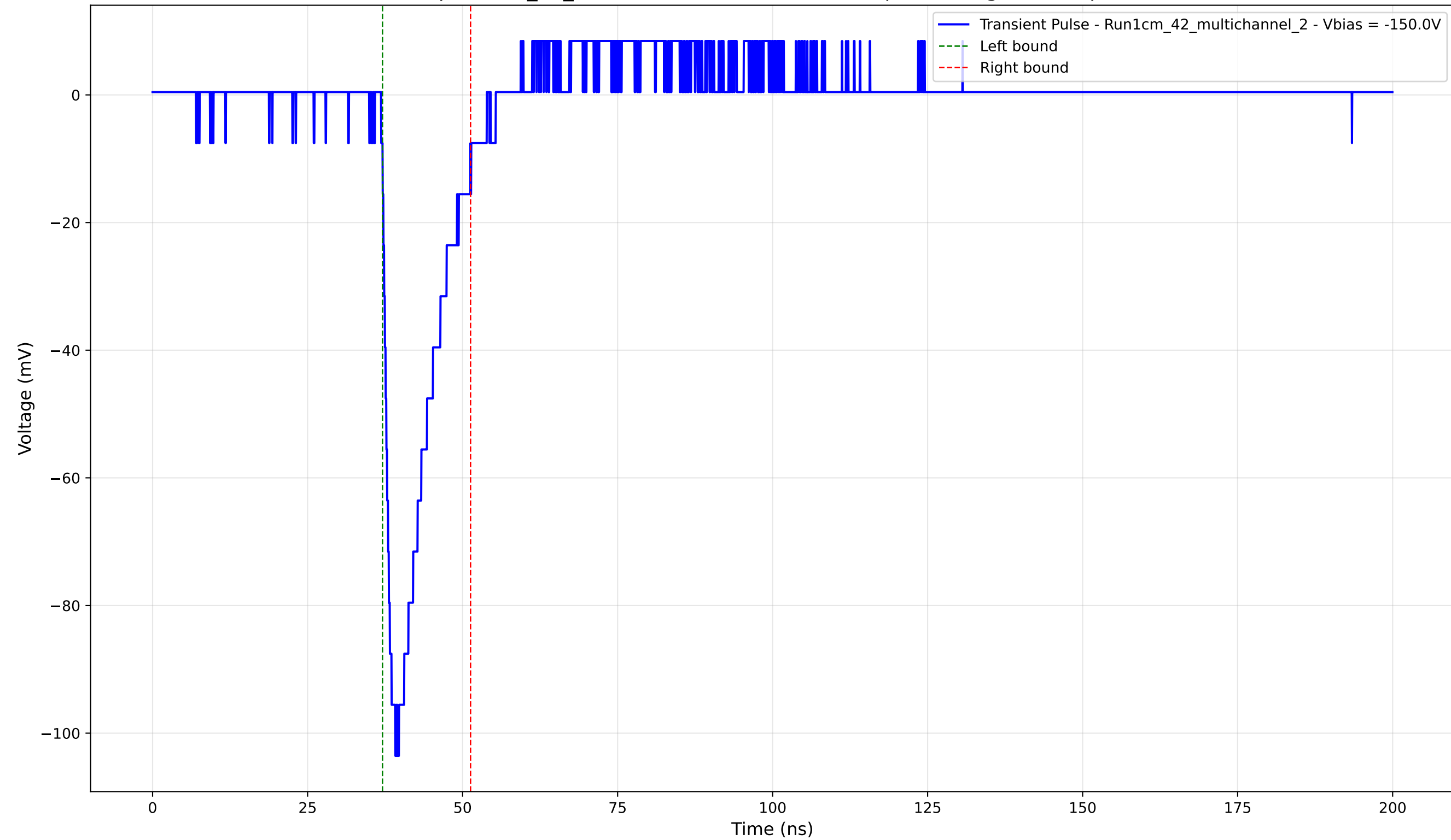
Transient Pulse - Sample: 1cm_42_multichannel - Position: 600.0 \mu\text{m} - Charge: 14.81 pC - Rise Time: 1.47 ns
