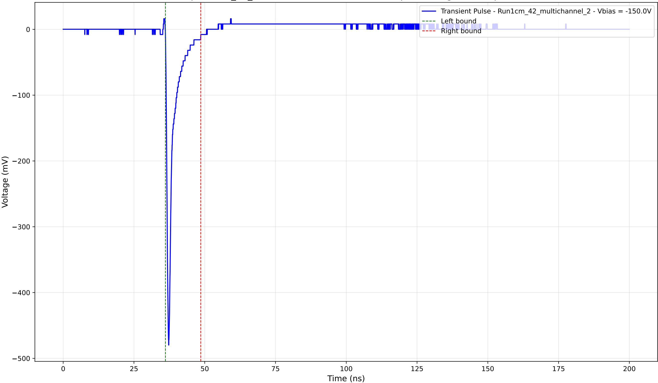
Transient Pulse - Sample: 1cm_42_multichannel - Position: 2615.0 \mu\text{m} - Charge: 24.89 pC - Rise Time: 0.76 ns
