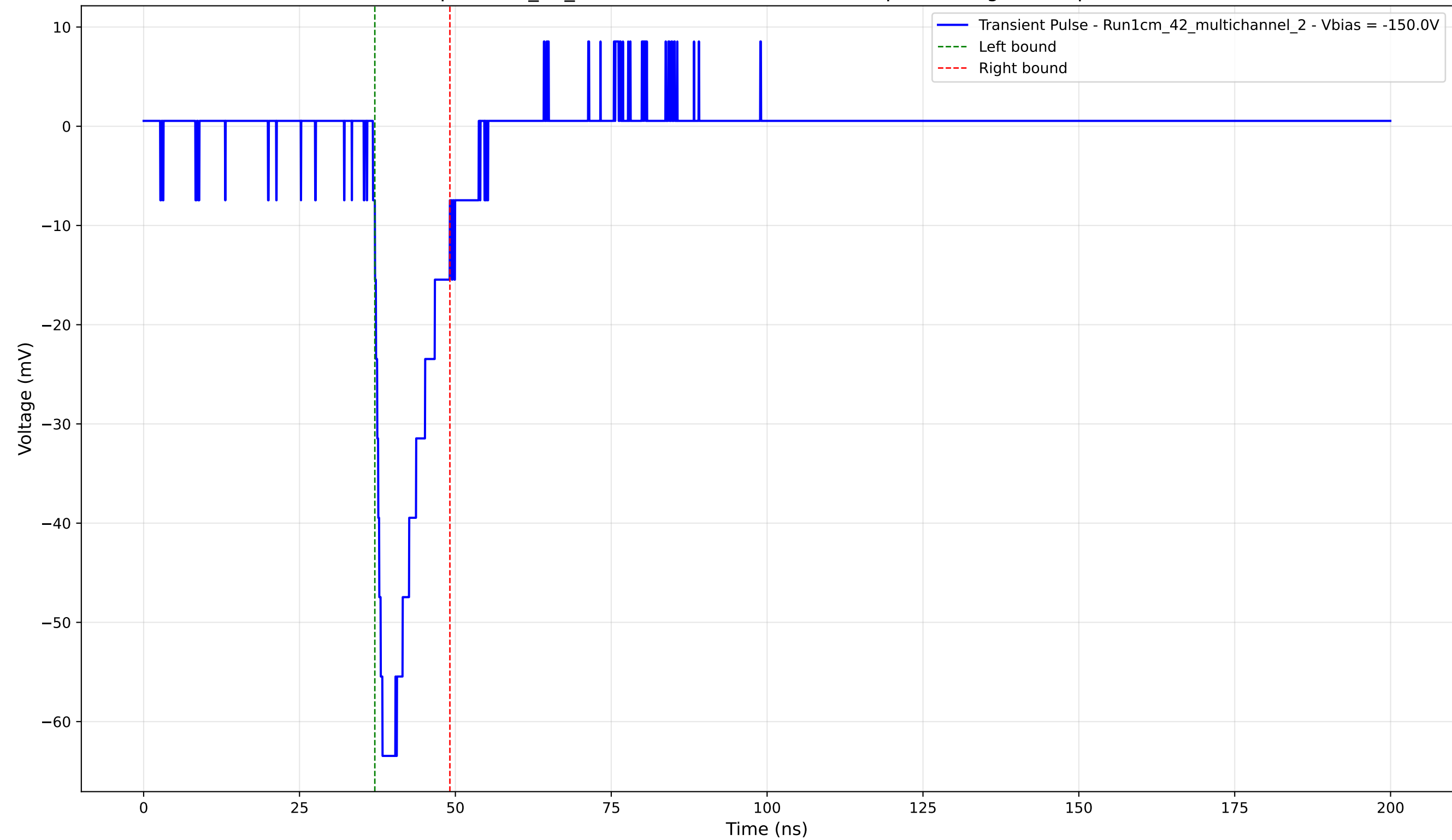
Transient Pulse - Sample: 1cm_42_multichannel - Position: 795.0 \mu\text{m} - Charge: 9.11 pC - Rise Time: 1.53 ns
