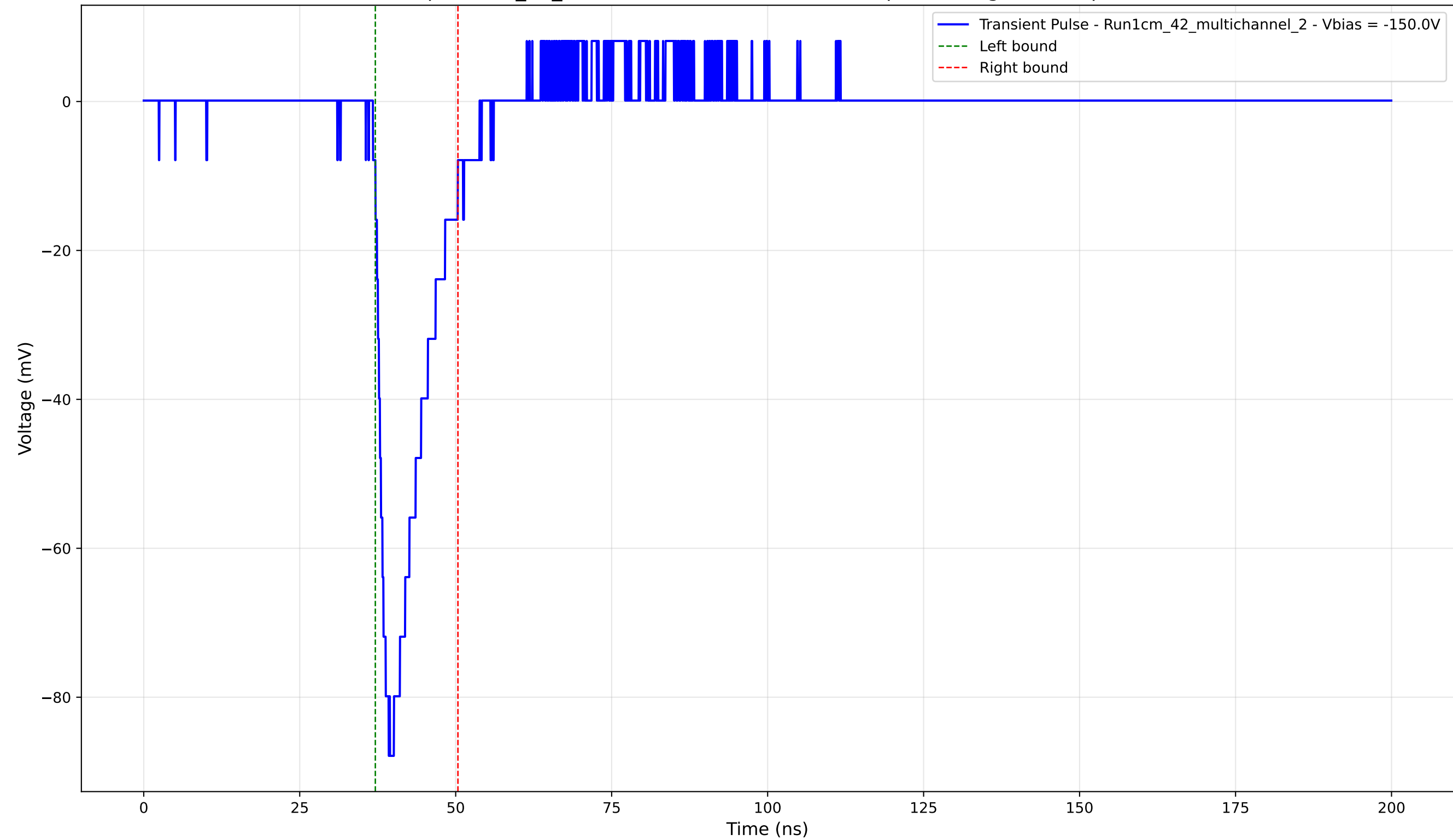
Transient Pulse - Sample: 1cm_42_multichannel - Position: 4215.0 \mu\text{m} - Charge: 12.36 pC - Rise Time: 1.68 ns
