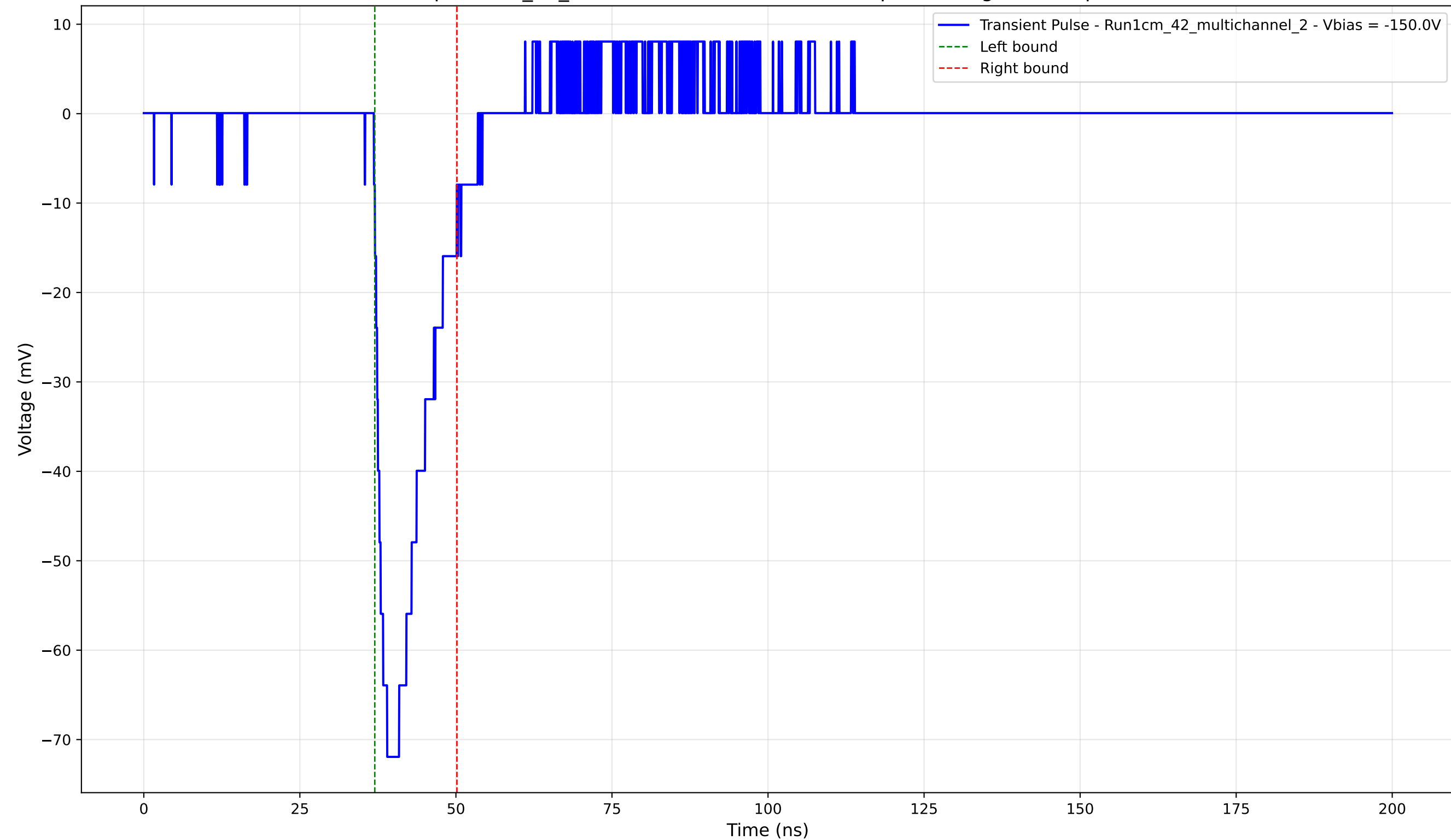
Transient Pulse - Sample: 1cm_42_multichannel - Position: 225.0 \mu\text{m} - Charge: 11.22 pC - Rise Time: 2.12 ns
