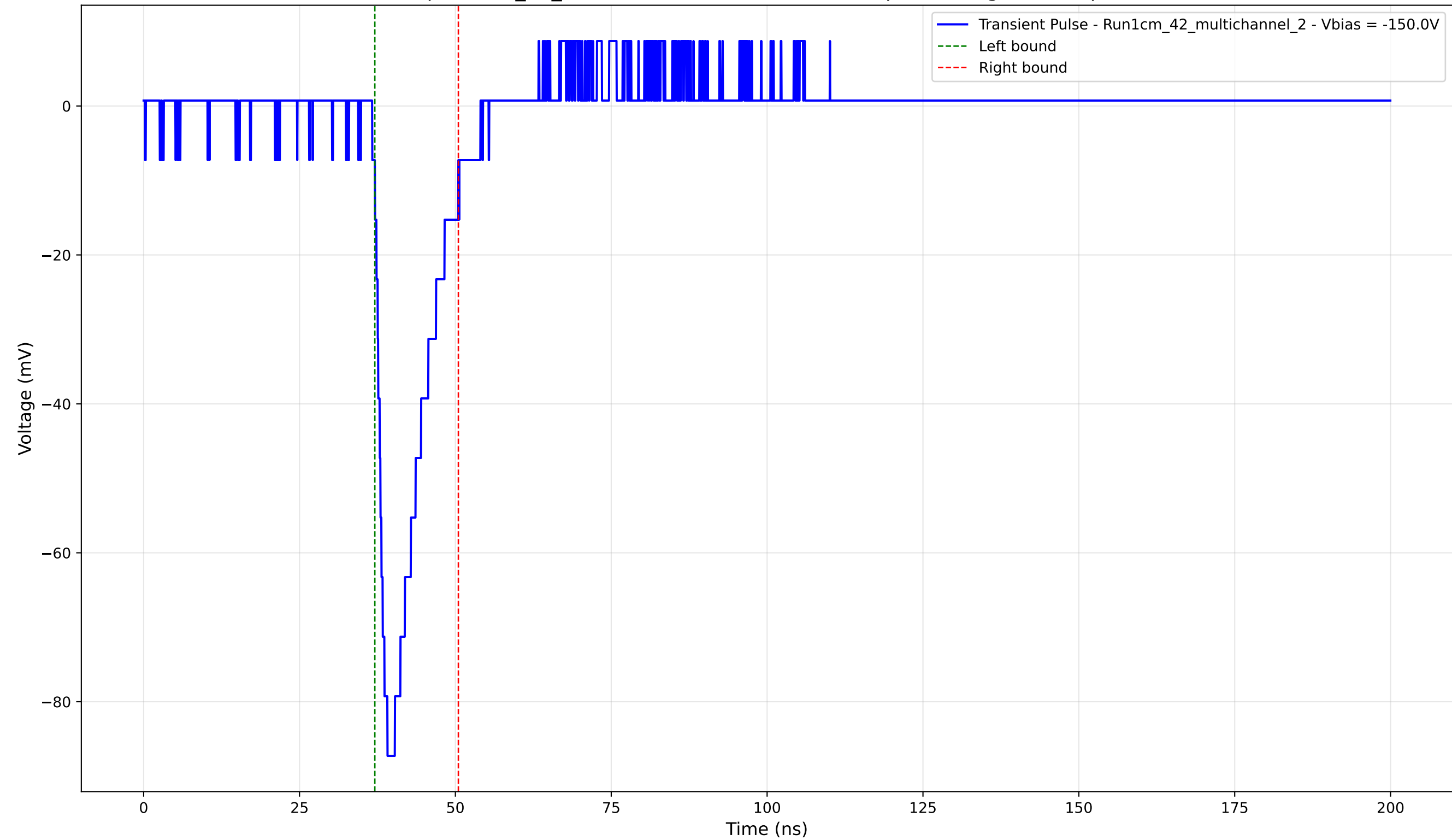
Transient Pulse - Sample: 1cm_42_multichannel - Position: 4155.0 \mu\text{m} - Charge: 12.51 pC - Rise Time: 1.55 ns
