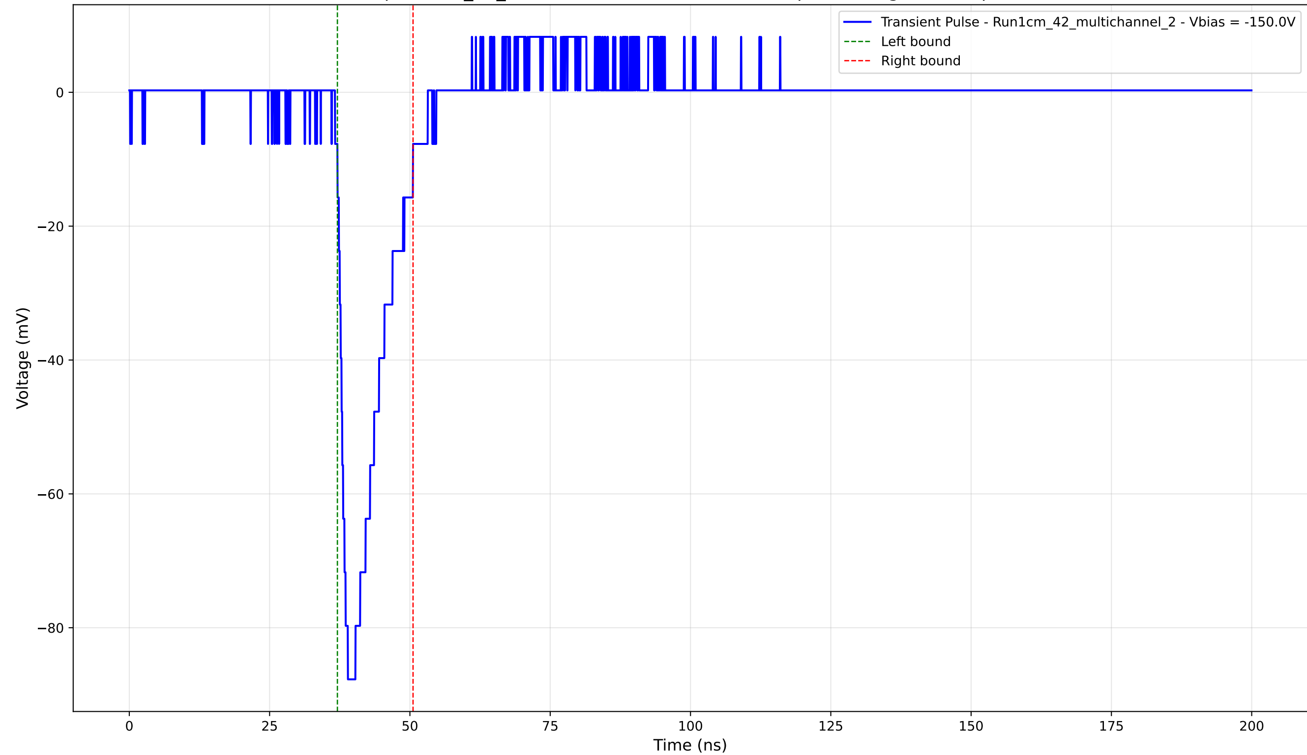
Transient Pulse - Sample: 1cm_42_multichannel - Position: 4160.0 \mu\text{m} - Charge: 12.81 pC - Rise Time: 1.47 ns
