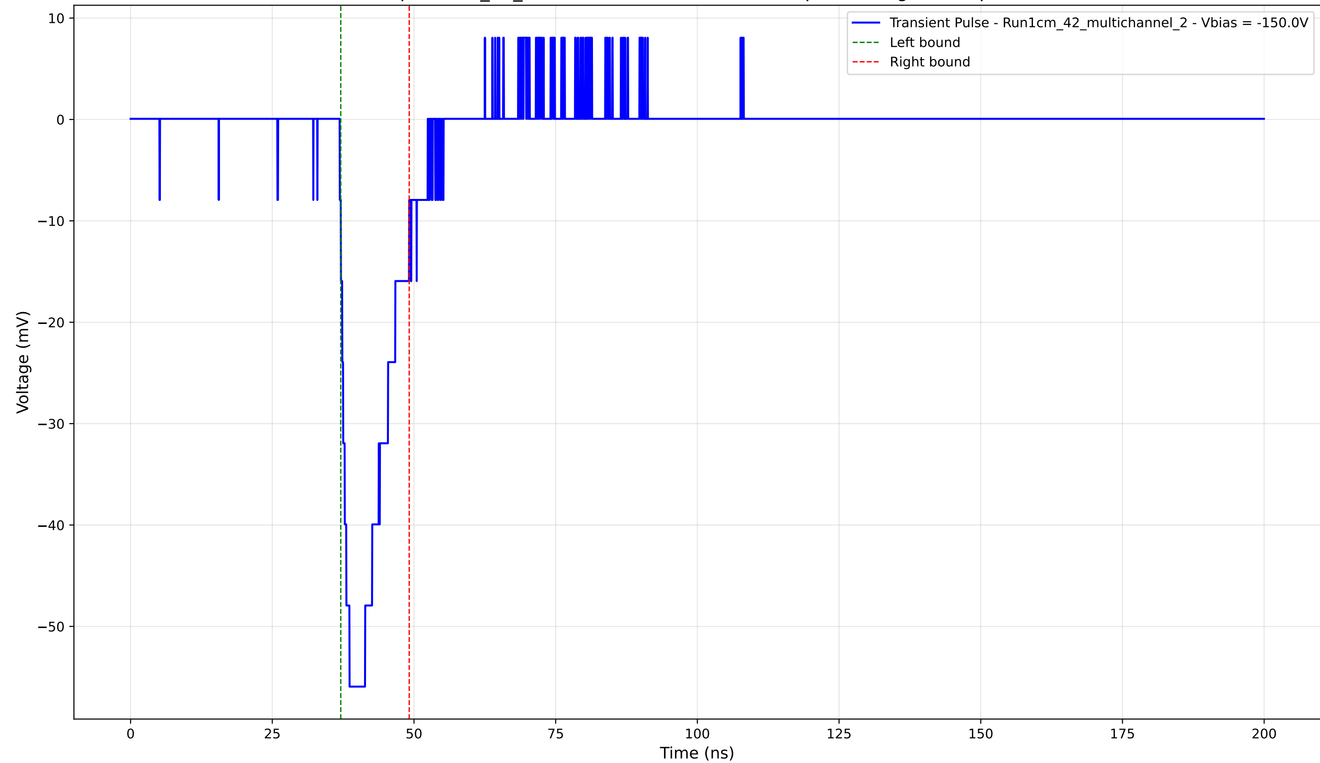
Transient Pulse - Sample: 1cm_42_multichannel - Position: 280.0 \mu\text{m} - Charge: 8.77 pC - Rise Time: 1.73 ns
