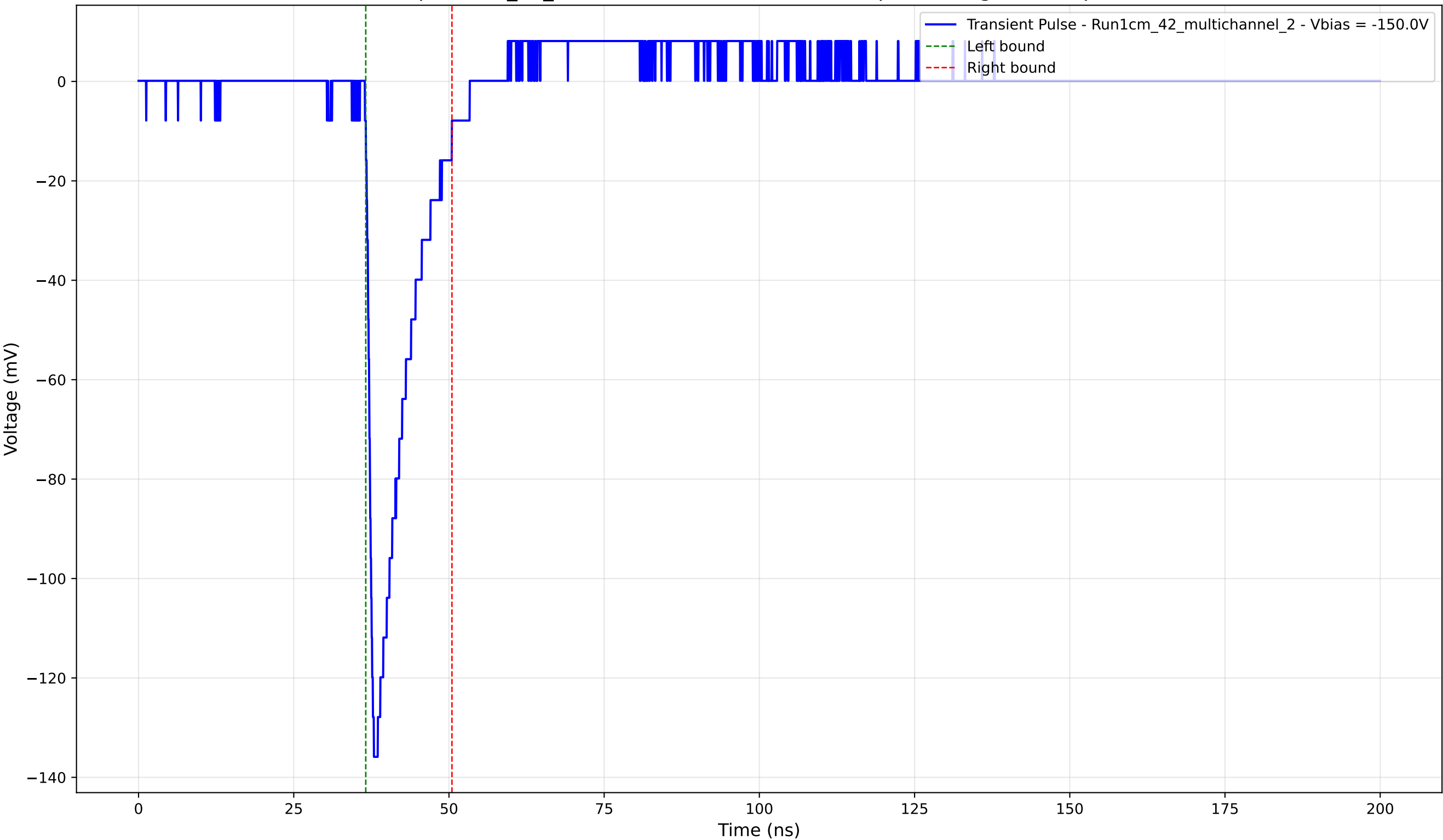
Transient Pulse - Sample: 1cm_42_multichannel - Position: 3485.0 \mu\text{m} - Charge: 16.87 pC - Rise Time: 1.13 ns
