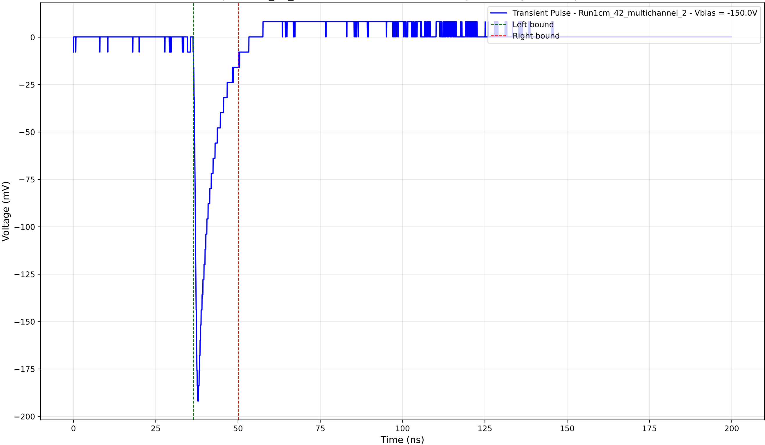
Transient Pulse - Sample: 1cm_42_multichannel - Position: 3230.0 \mu\text{m} - Charge: 19.04 pC - Rise Time: 0.94 ns
