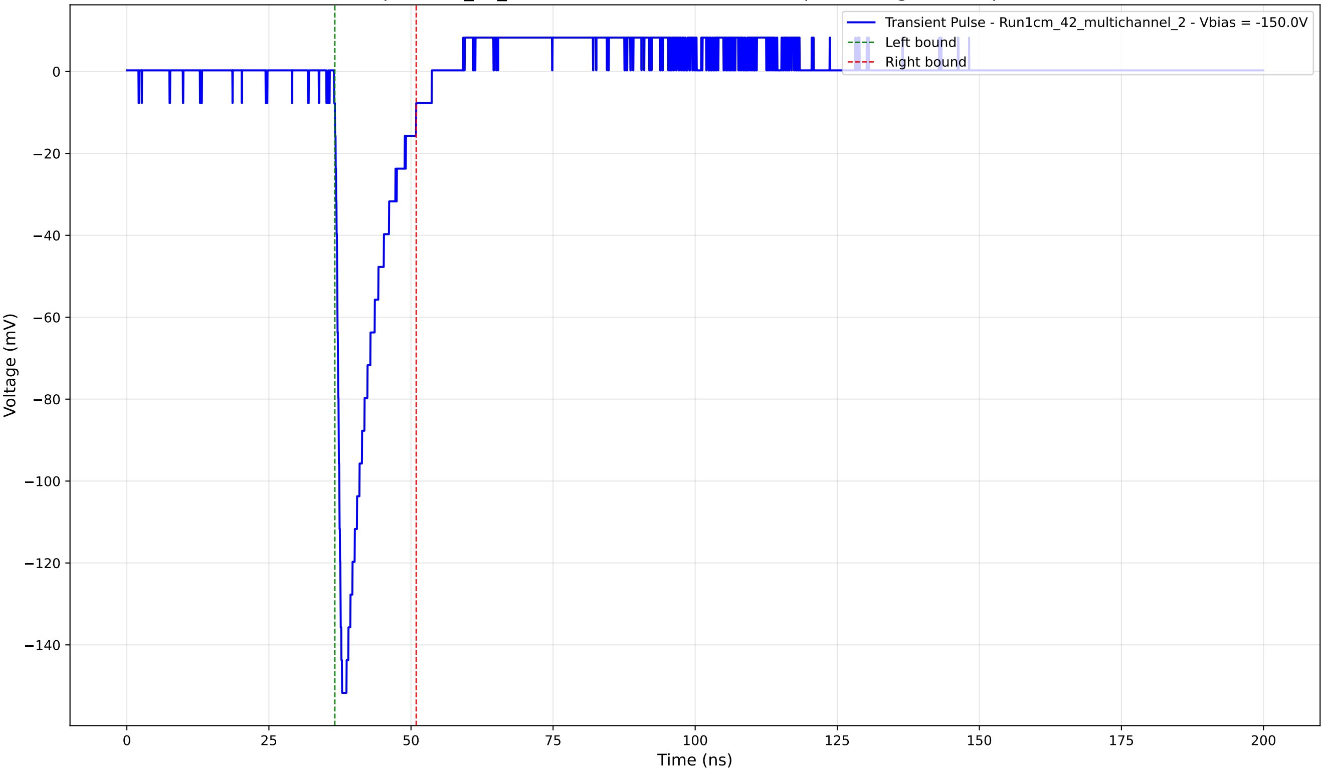
Transient Pulse - Sample: 1cm_42_multichannel - Position: 1265.0 \mu\text{m} - Charge: 18.70 pC - Rise Time: 1.12 ns
