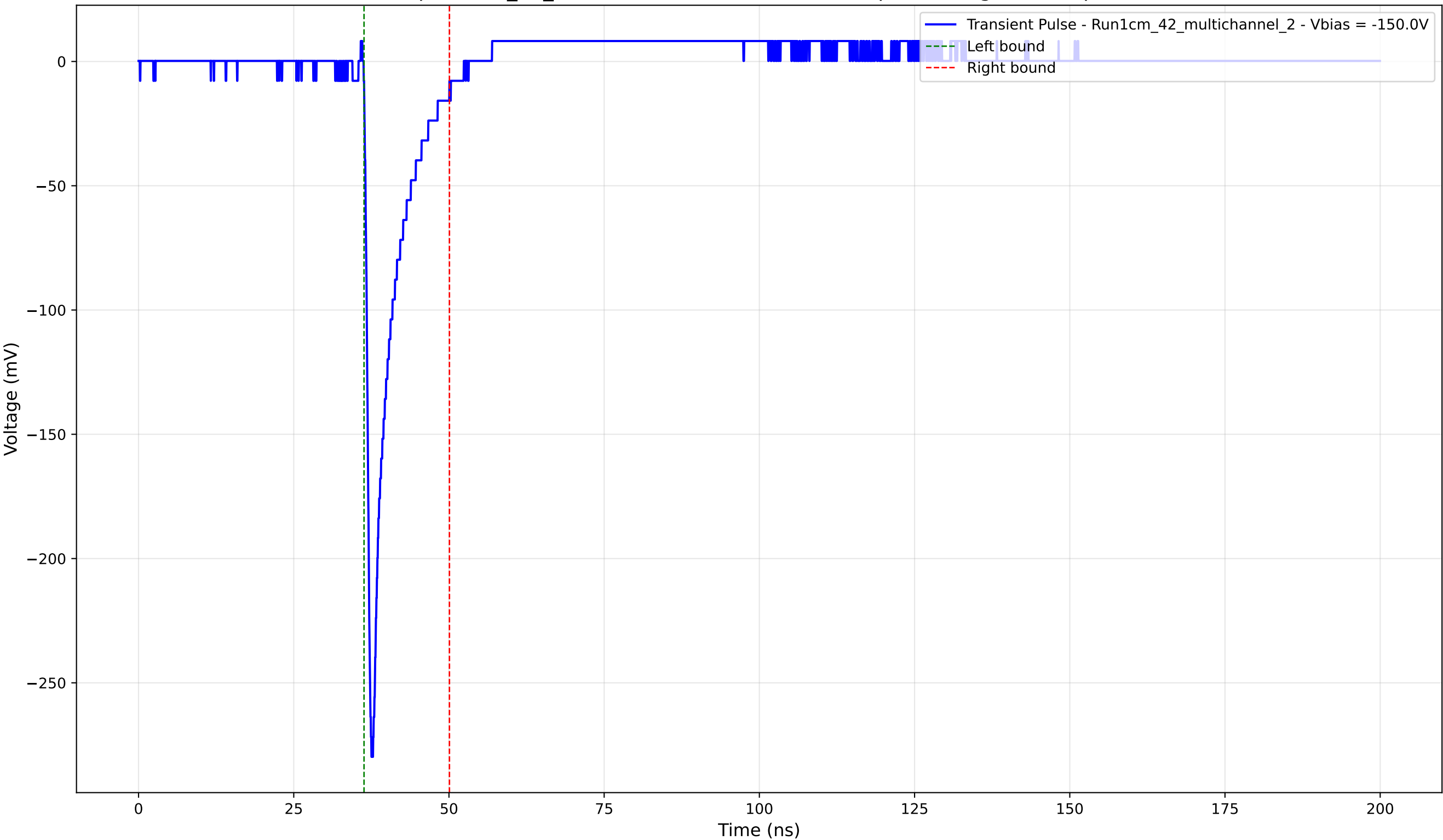
Transient Pulse - Sample: 1cm_42_multichannel - Position: 1715.0 \mu\text{m} - Charge: 23.06 pC - Rise Time: 0.88 ns
