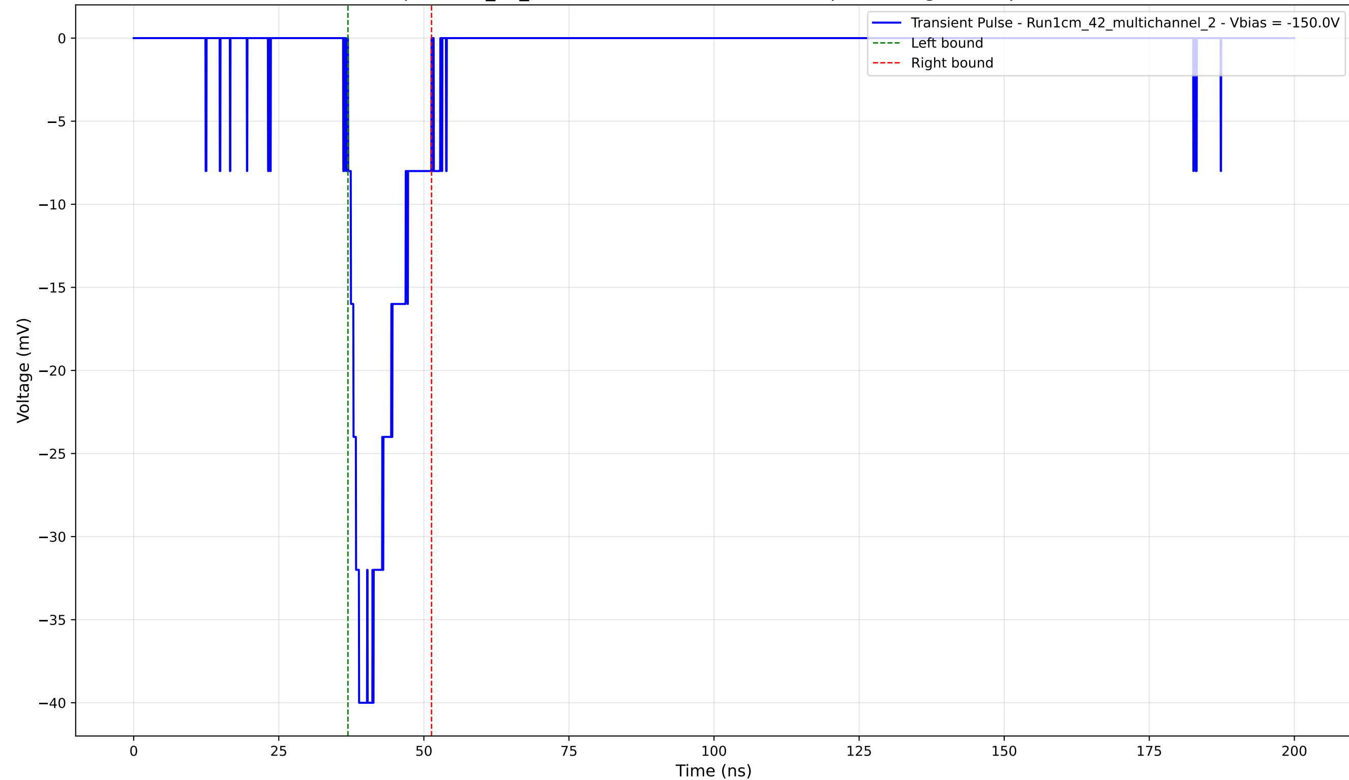
Transient Pulse - Sample: 1cm_42_multichannel - Position: 4440.0 \mu\text{m} - Charge: 6.02 pC - Rise Time: 1.90 ns
