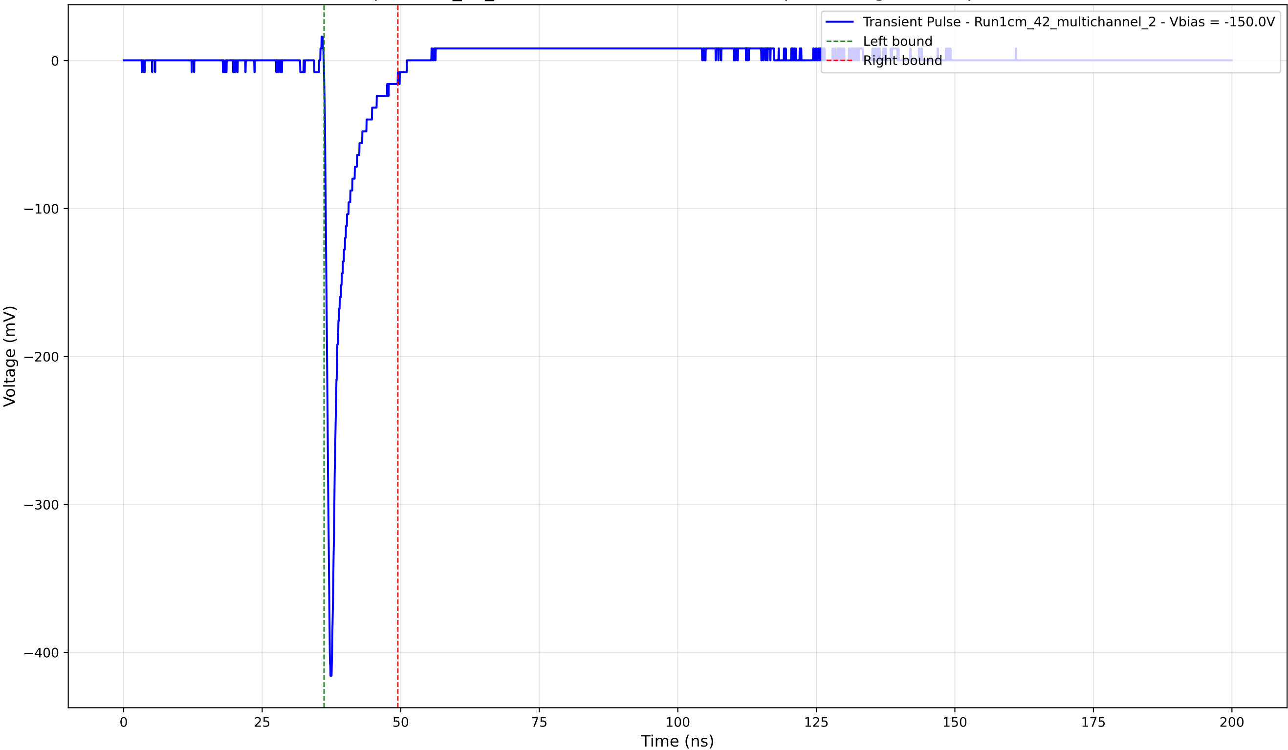
Transient Pulse - Sample: 1cm_42_multichannel - Position: 1980.0 \mu\text{m} - Charge: 25.74 pC - Rise Time: 0.79 ns
