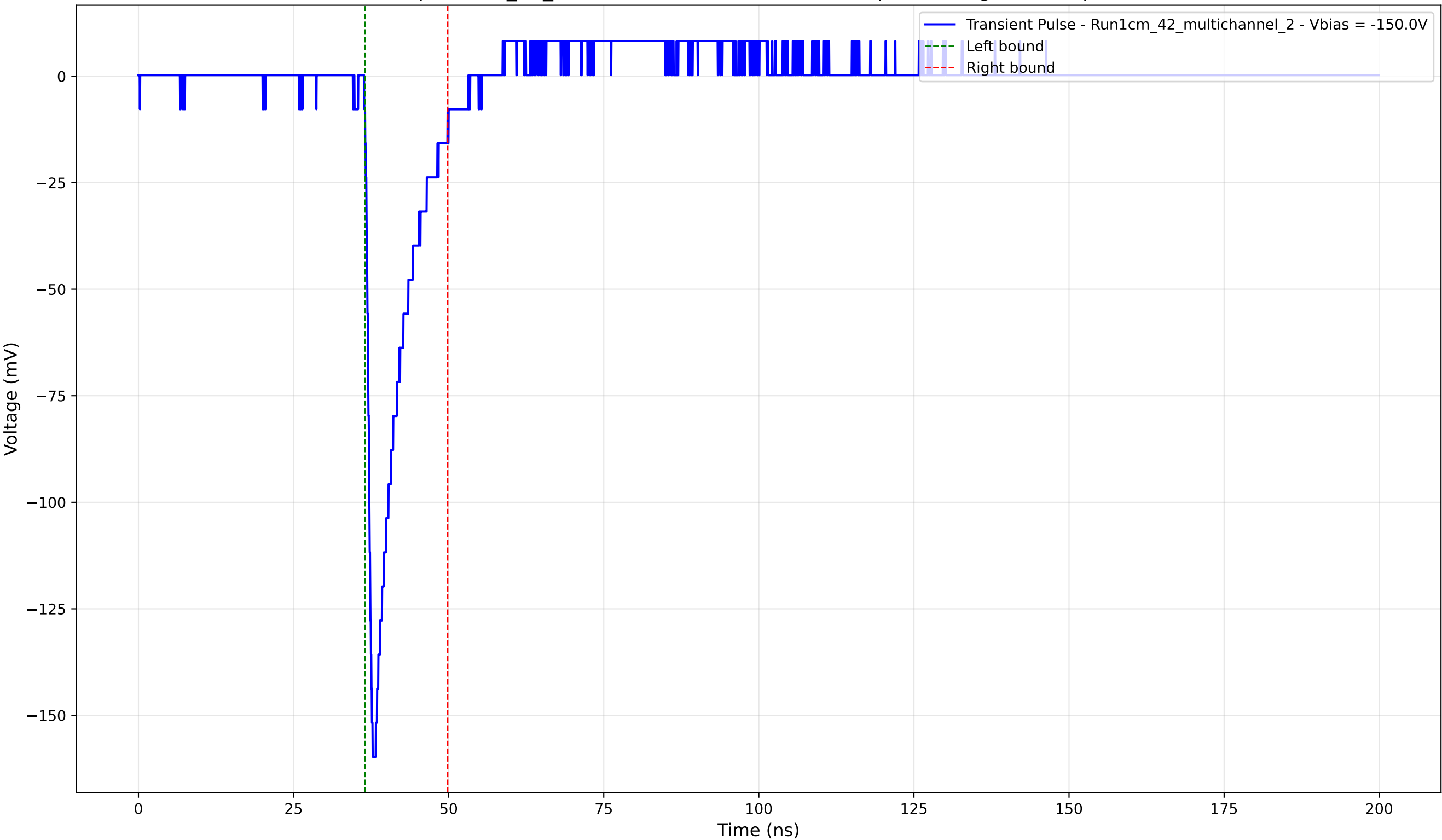
Transient Pulse - Sample: 1cm_42_multichannel - Position: 1425.0 \mu\text{m} - Charge: 17.06 pC - Rise Time: 1.04 ns
