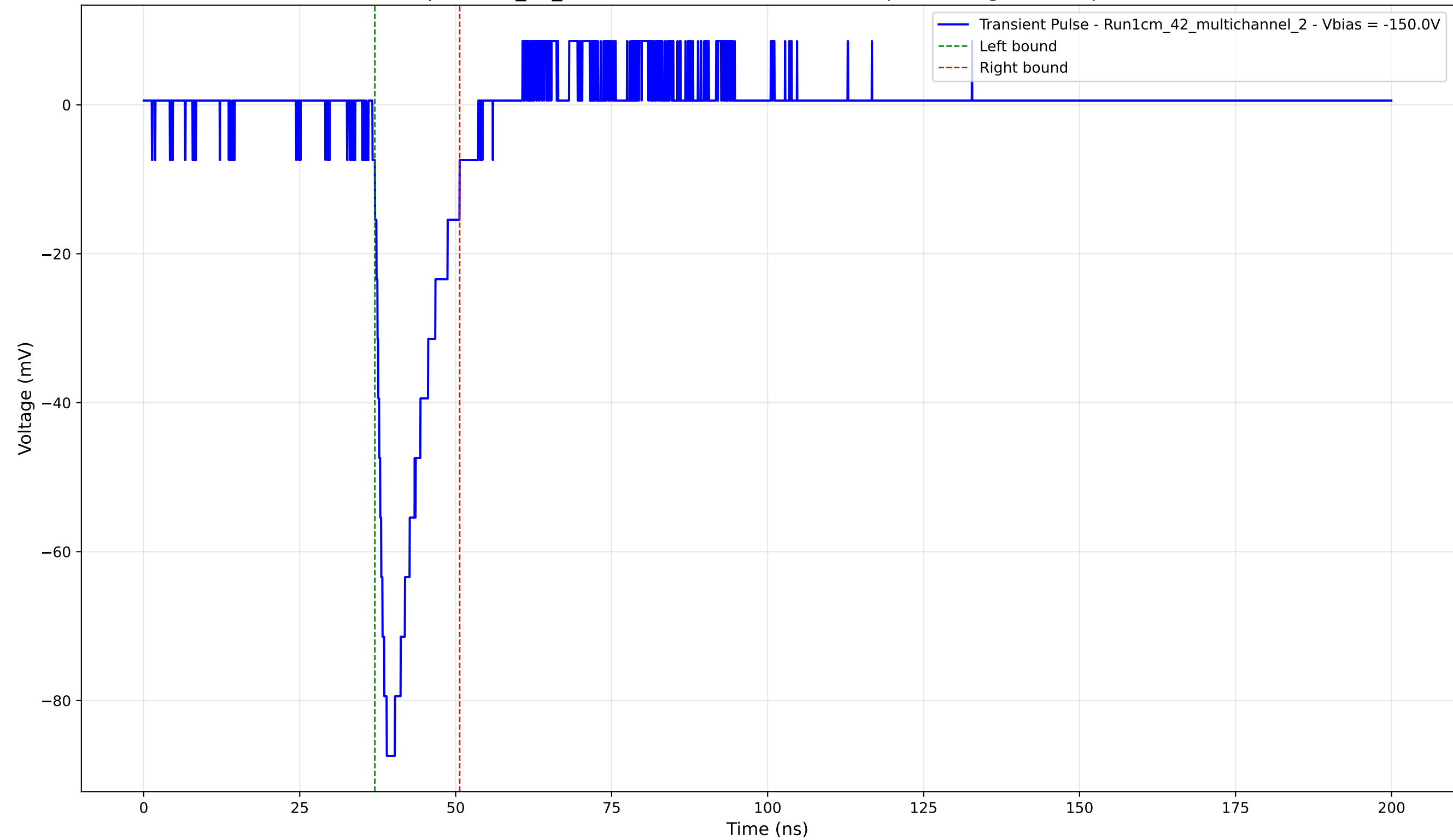
Transient Pulse - Sample: 1cm_42_multichannel - Position: 4090.0 \mu\text{m} - Charge: 12.68 pC - Rise Time: 1.51 ns
