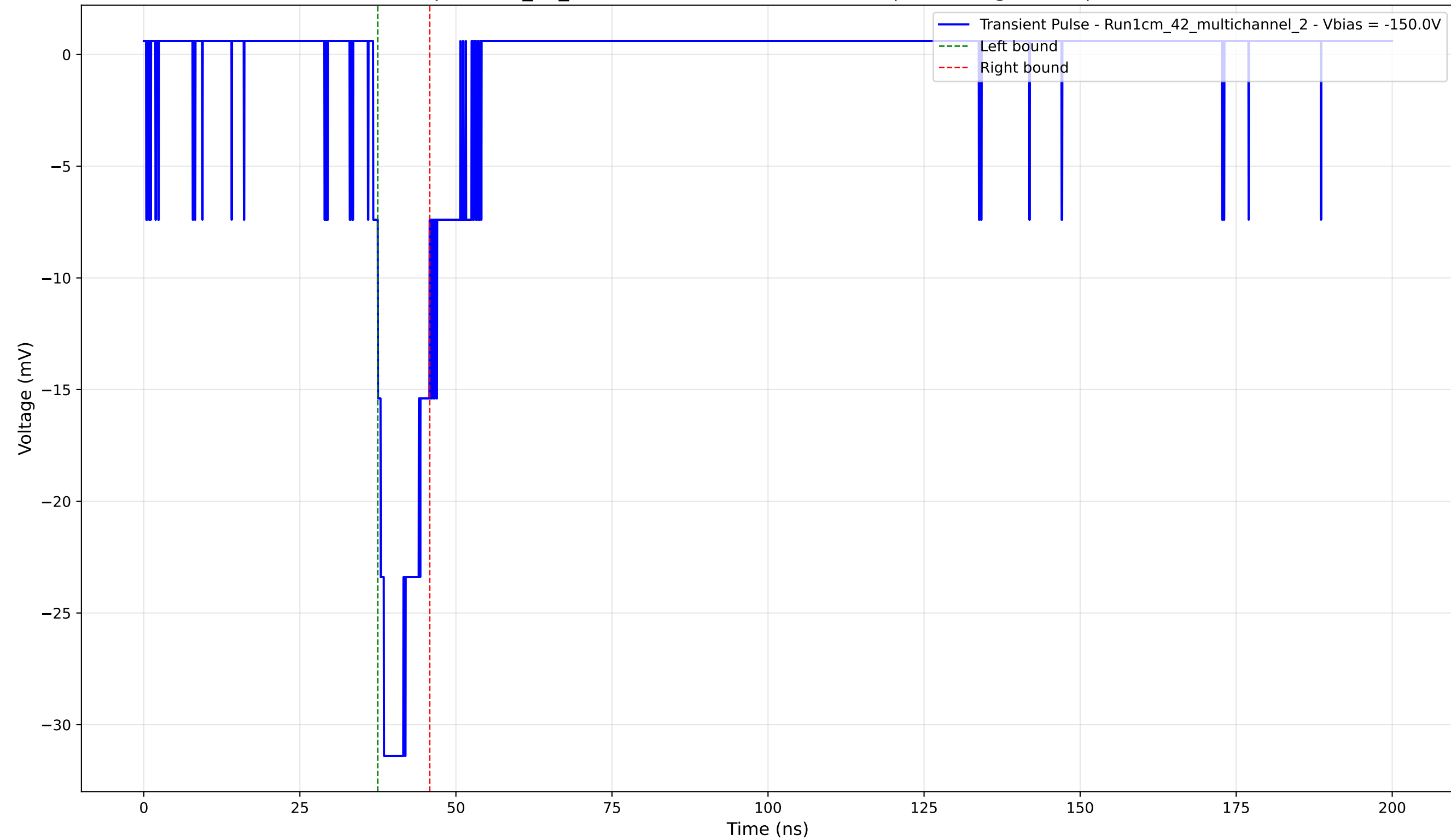
Transient Pulse - Sample: 1cm_42_multichannel - Position: 4340.0 \mu\text{m} - Charge: 4.07 pC - Rise Time: 1.75 ns
