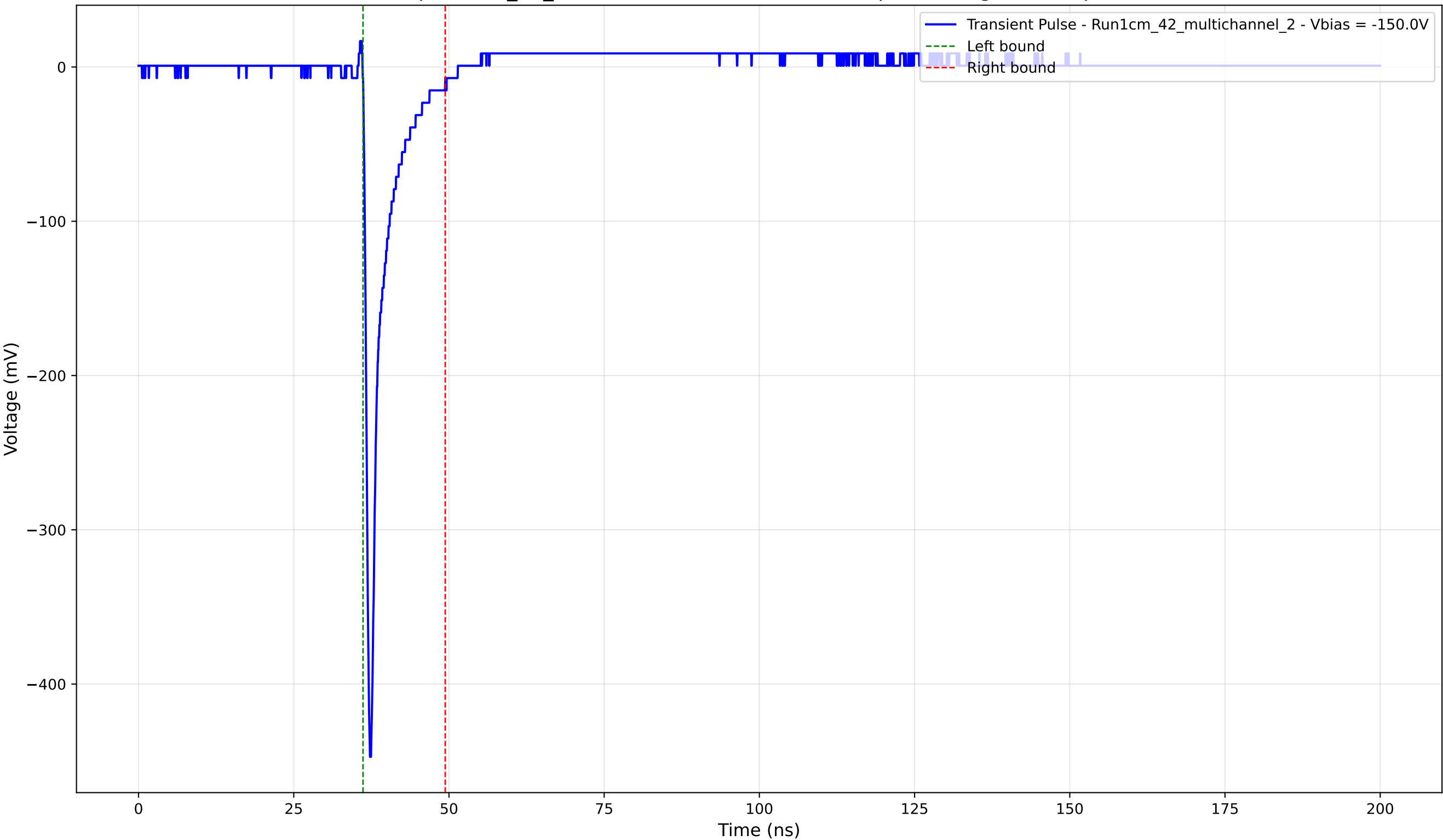
Transient Pulse - Sample: 1cm_42_multichannel - Position: 2035.0 \mu\text{m} - Charge: 25.85 pC - Rise Time: 0.76 ns
