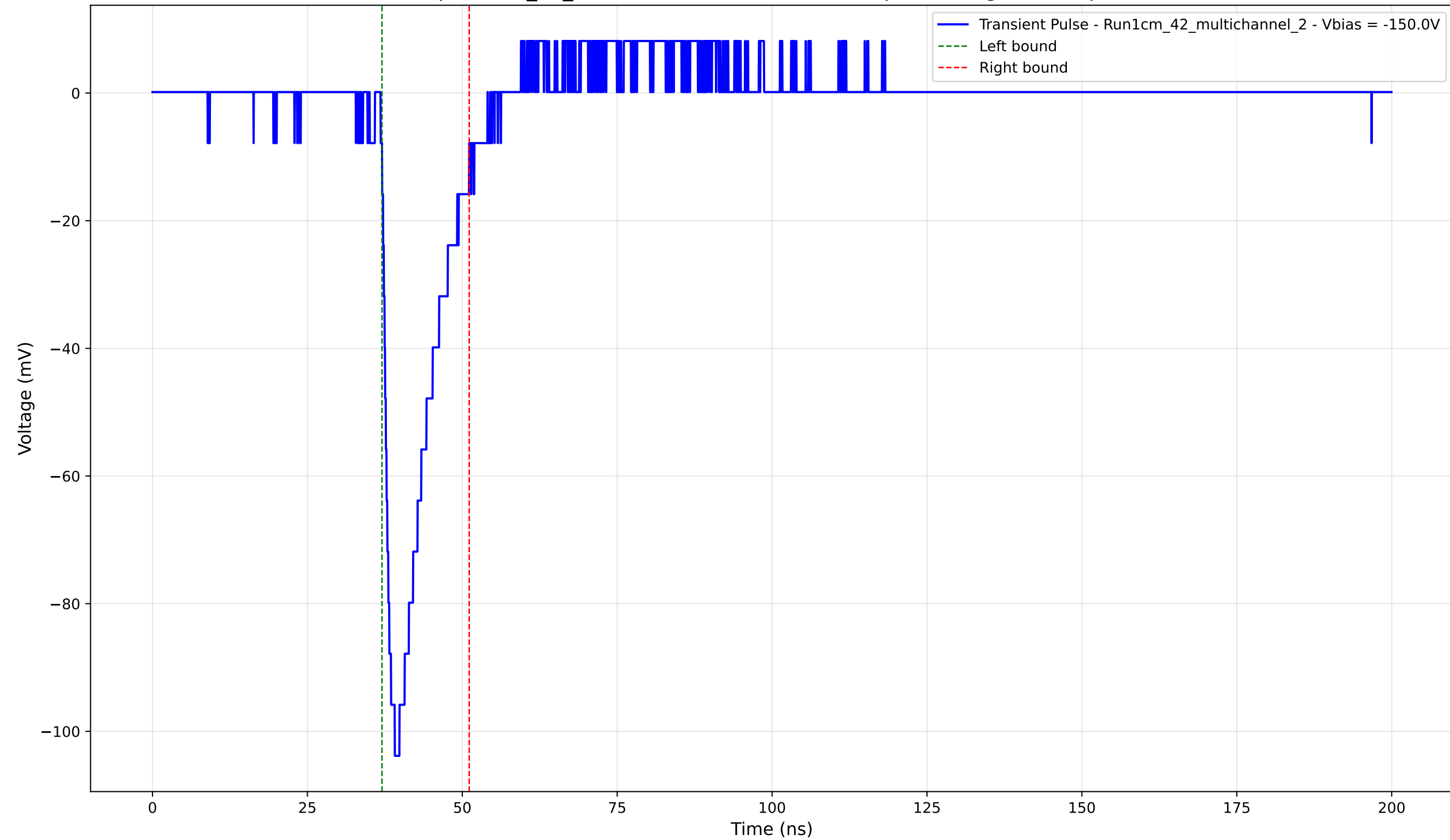
Transient Pulse - Sample: 1cm_42_multichannel - Position: 640.0 \mu\text{m} - Charge: 15.01 pC - Rise Time: 1.47 ns
