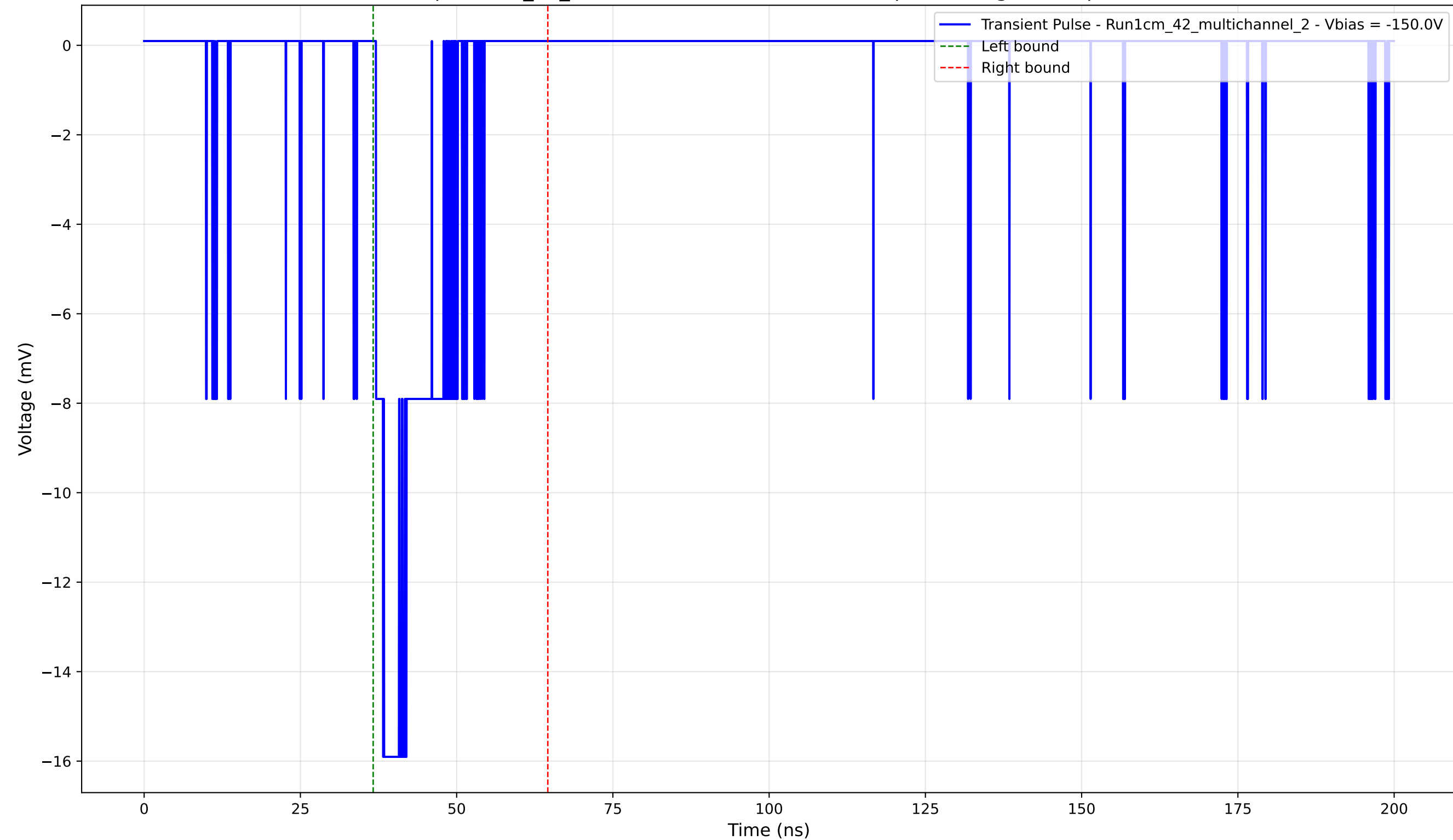
Transient Pulse - Sample: 1cm_42_multichannel - Position: 3915.0 \mu\text{m} - Charge: 2.58 pC - Rise Time: 1.15 ns
