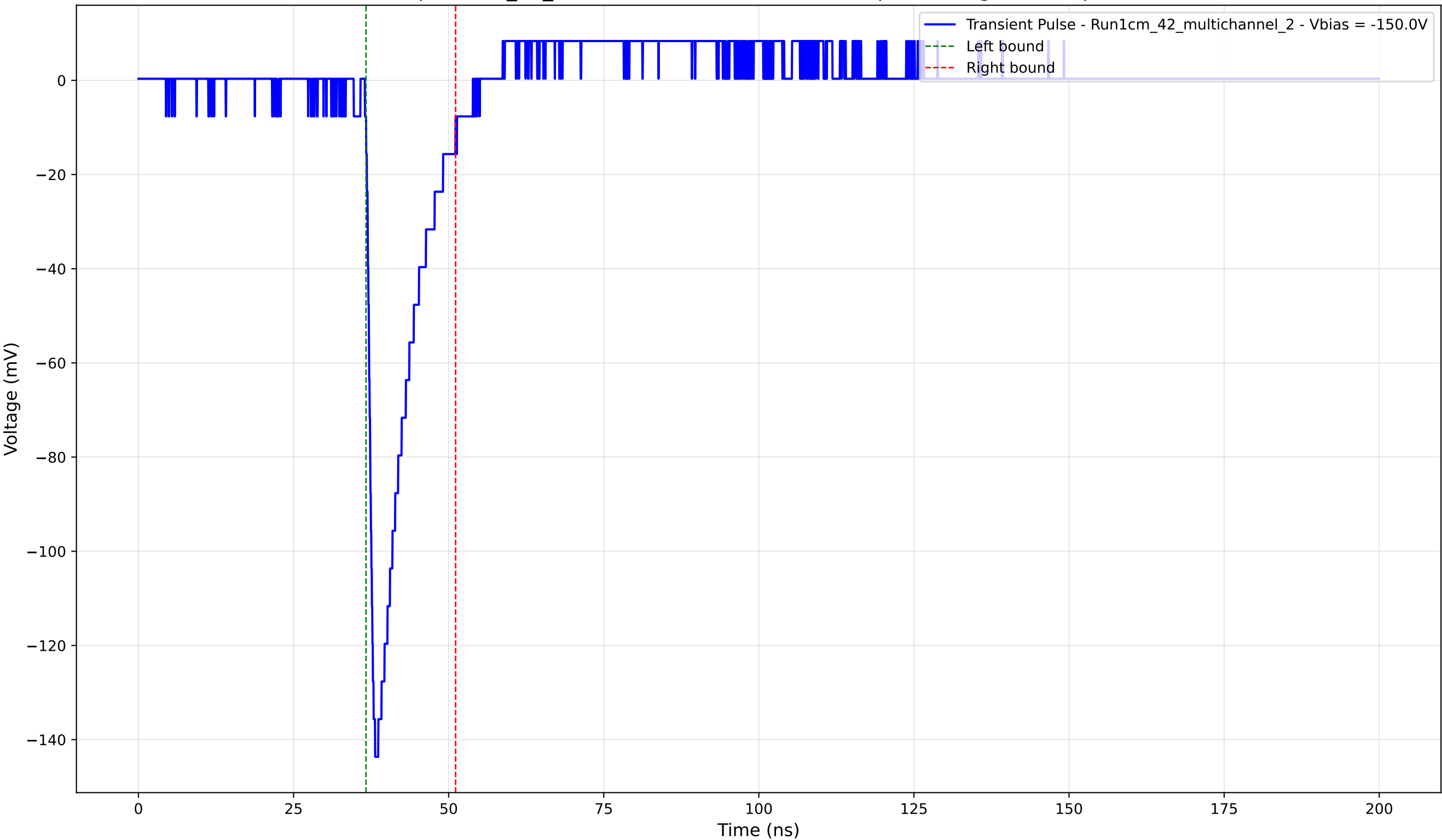
Transient Pulse - Sample: 1cm_42_multichannel - Position: 1160.0 \mu\text{m} - Charge: 18.29 pC - Rise Time: 1.21 ns
