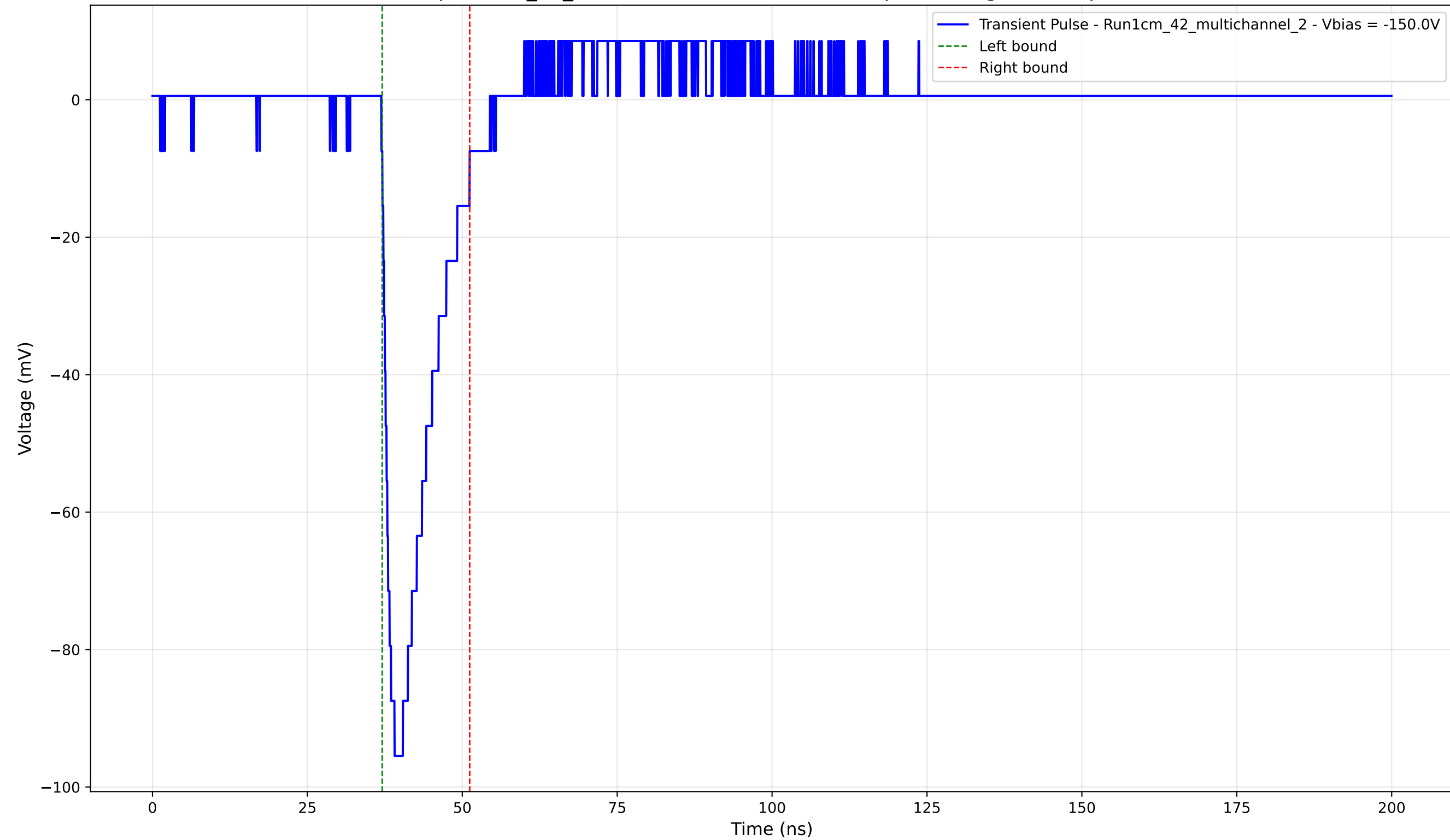
Transient Pulse - Sample: 1cm_42_multichannel - Position: 515.0 \mu\text{m} - Charge: 14.36 pC - Rise Time: 1.43 ns
