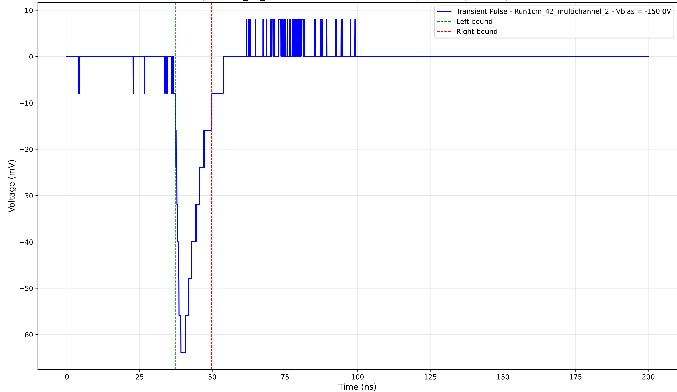
Transient Pulse - Sample: 1cm_42_multichannel - Position: 4465.0 \mu\text{m} - Charge: 9.27 pC - Rise Time: 2.49 ns
