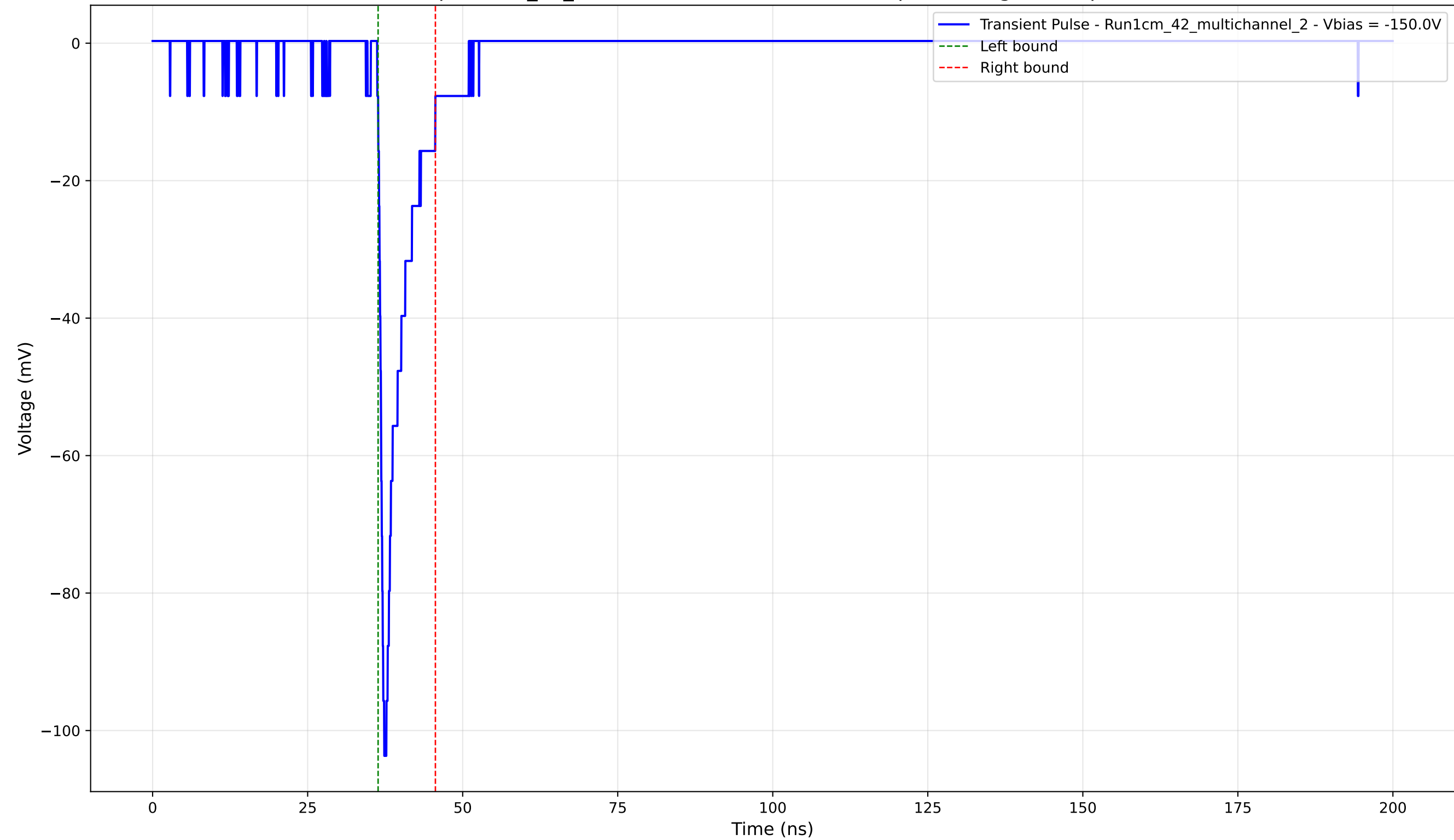
Transient Pulse - Sample: 1cm_42_multichannel - Position: 2920.0 \mu\text{m} - Charge: 7.47 pC - Rise Time: 0.83 ns
