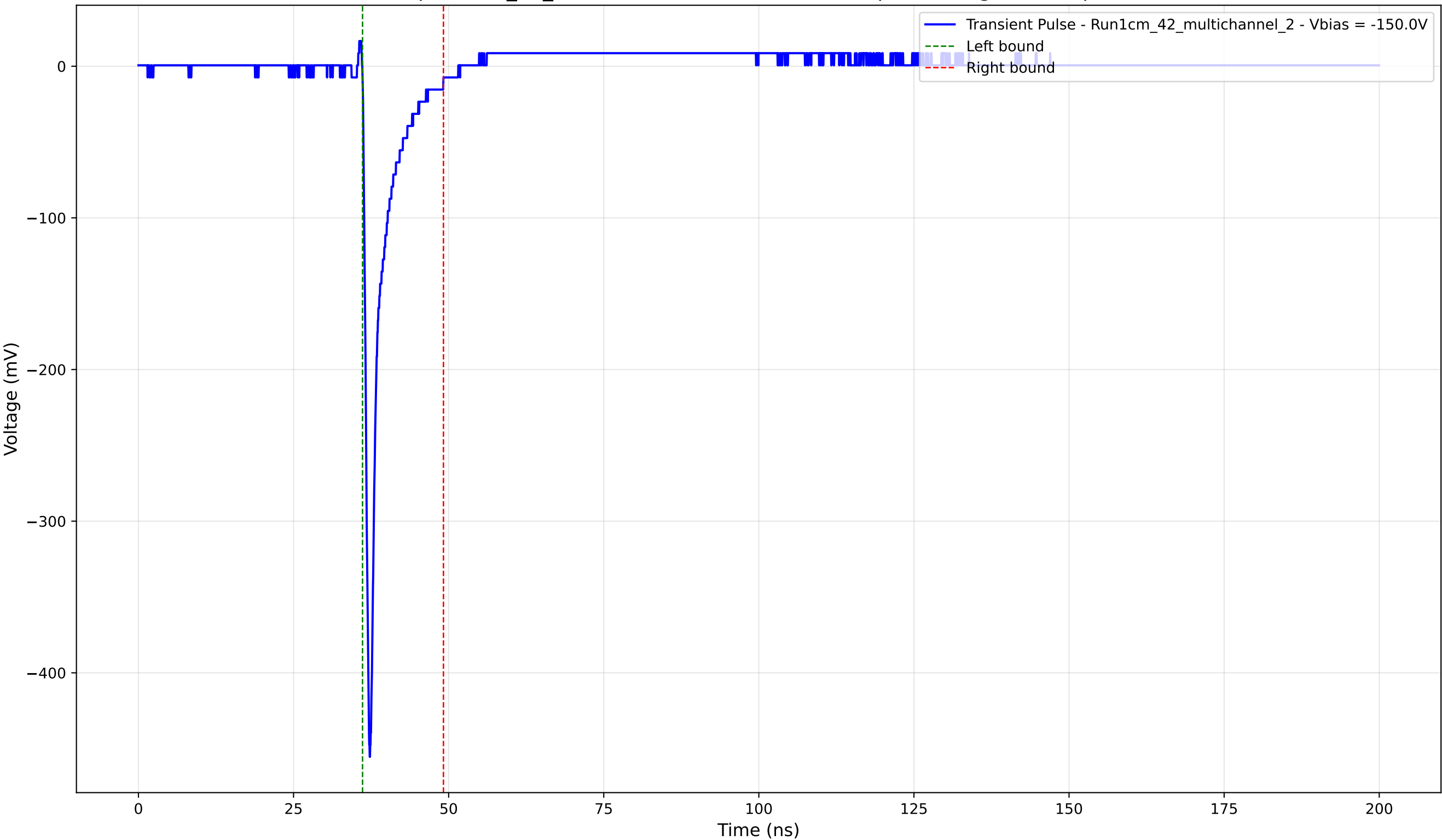
Transient Pulse - Sample: 1cm_42_multichannel - Position: 2655.0 \mu\text{m} - Charge: 24.82 pC - Rise Time: 0.74 ns
