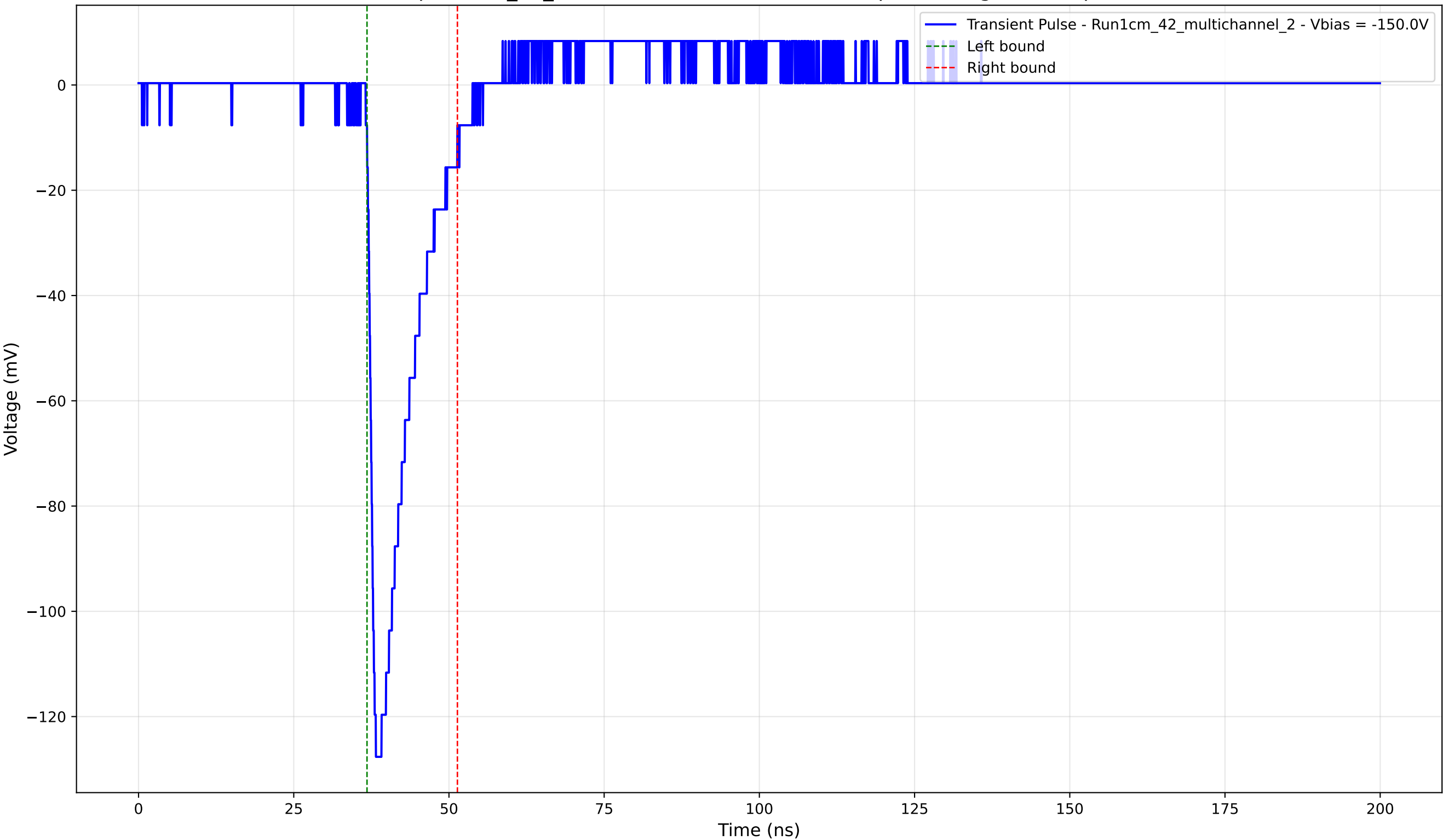
Transient Pulse - Sample: 1cm_42_multichannel - Position: 1045.0 \mu\text{m} - Charge: 17.40 pC - Rise Time: 1.21 ns
