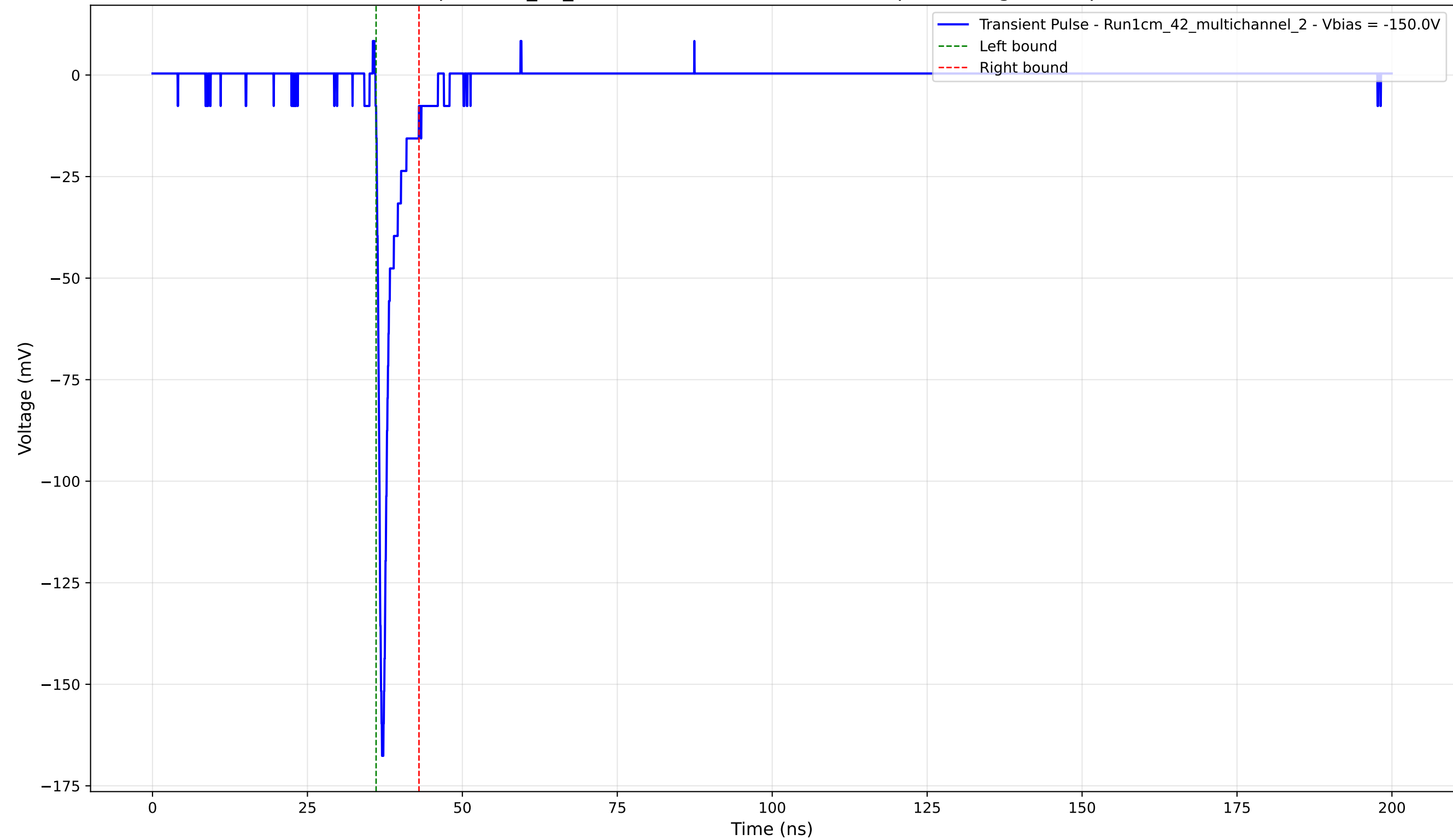
Transient Pulse - Sample: 1cm_42_multichannel - Position: 2330.0 \mu\text{m} - Charge: 7.06 pC - Rise Time: 0.71 ns
