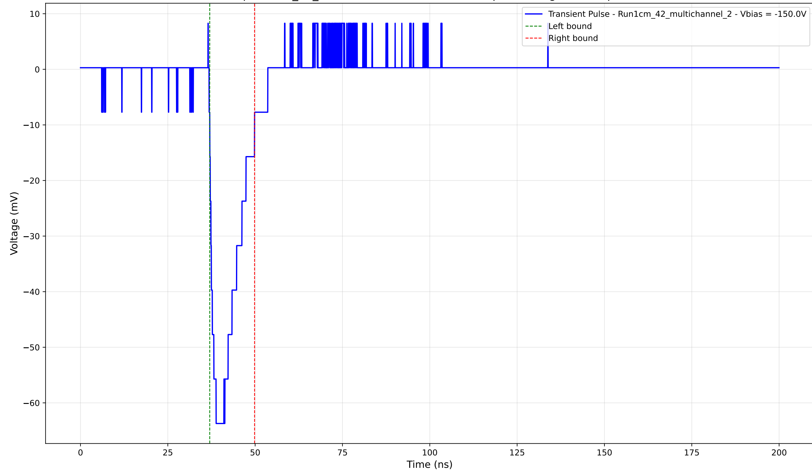
Transient Pulse - Sample: 1cm_42_multichannel - Position: 125.0 \mu\text{m} - Charge: 10.18 pC - Rise Time: 2.01 ns
