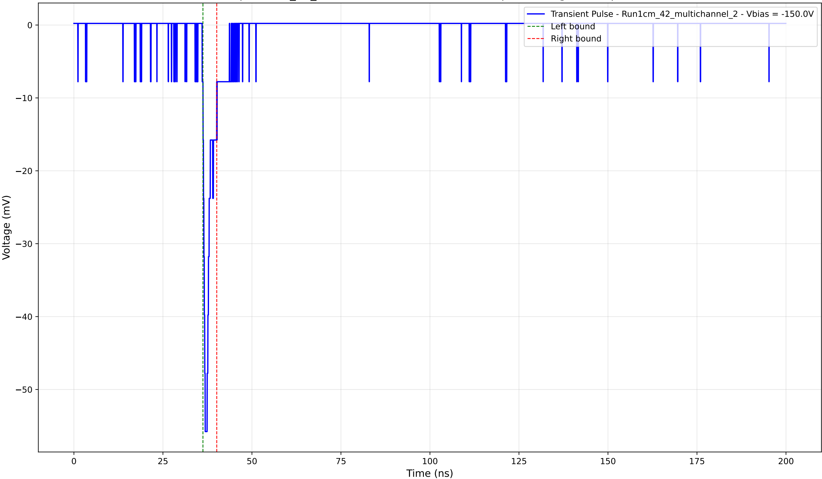
Transient Pulse - Sample: 1cm_42_multichannel - Position: 2345.0 \mu\text{m} - Charge: 2.21 pC - Rise Time: 0.85 ns
