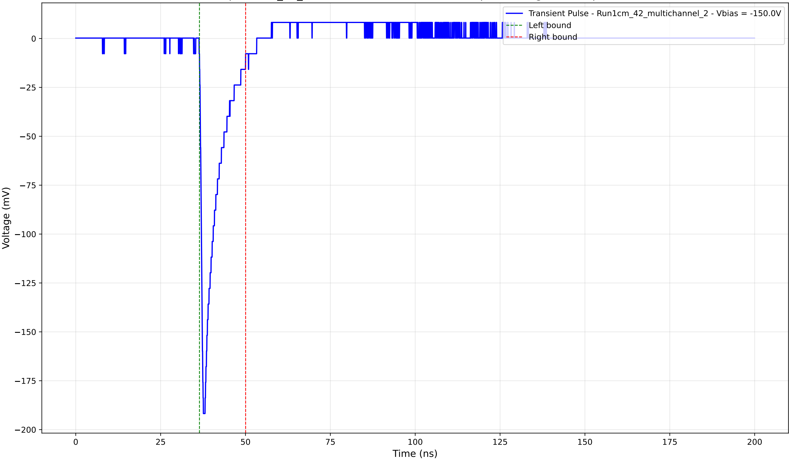
Transient Pulse - Sample: 1cm_42_multichannel - Position: 3200.0 \mu\text{m} - Charge: 18.98 pC - Rise Time: 0.90 ns
