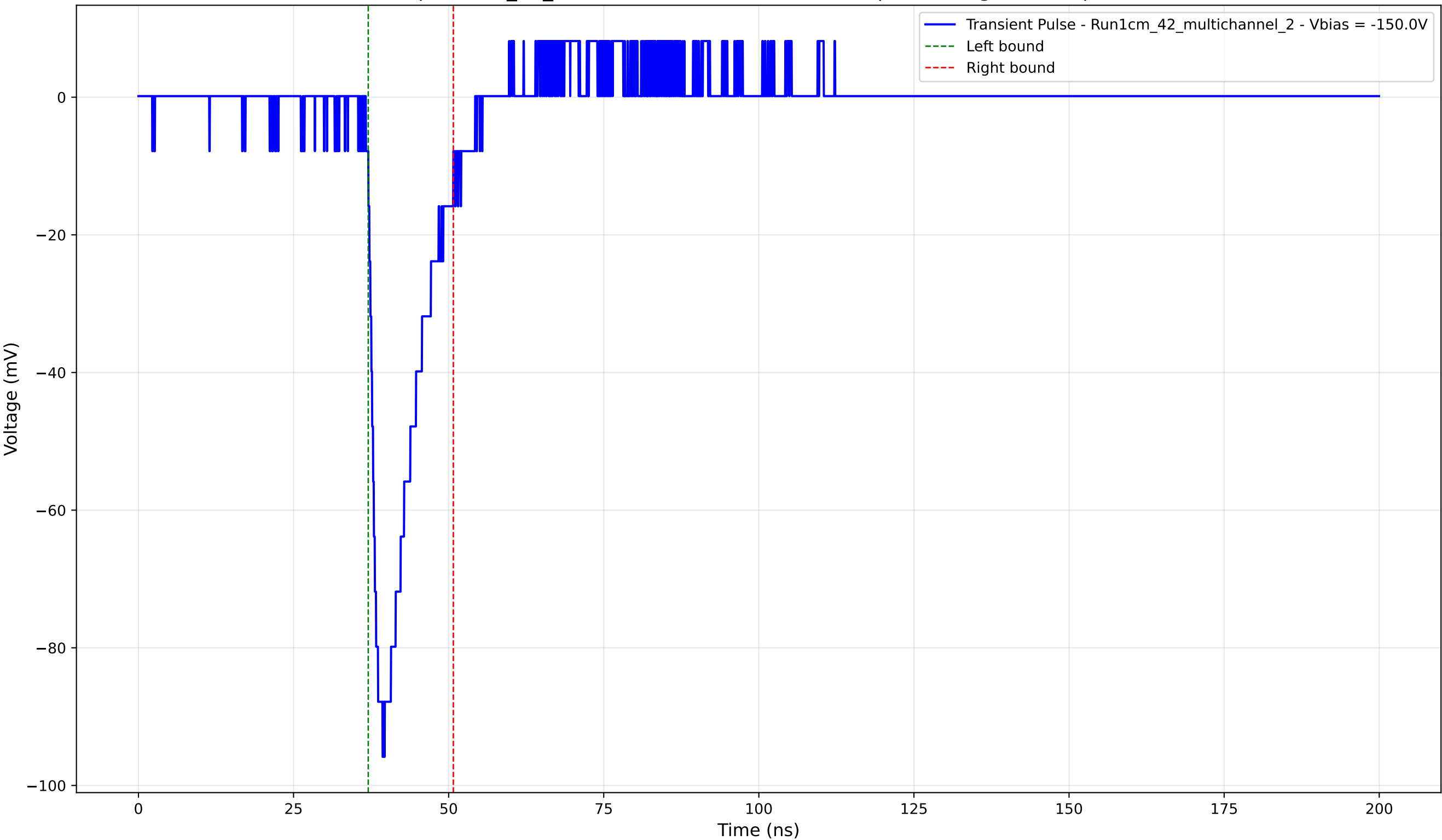
Transient Pulse - Sample: 1cm_42_multichannel - Position: 4025.0 \mu\text{m} - Charge: 13.49 pC - Rise Time: 1.59 ns
