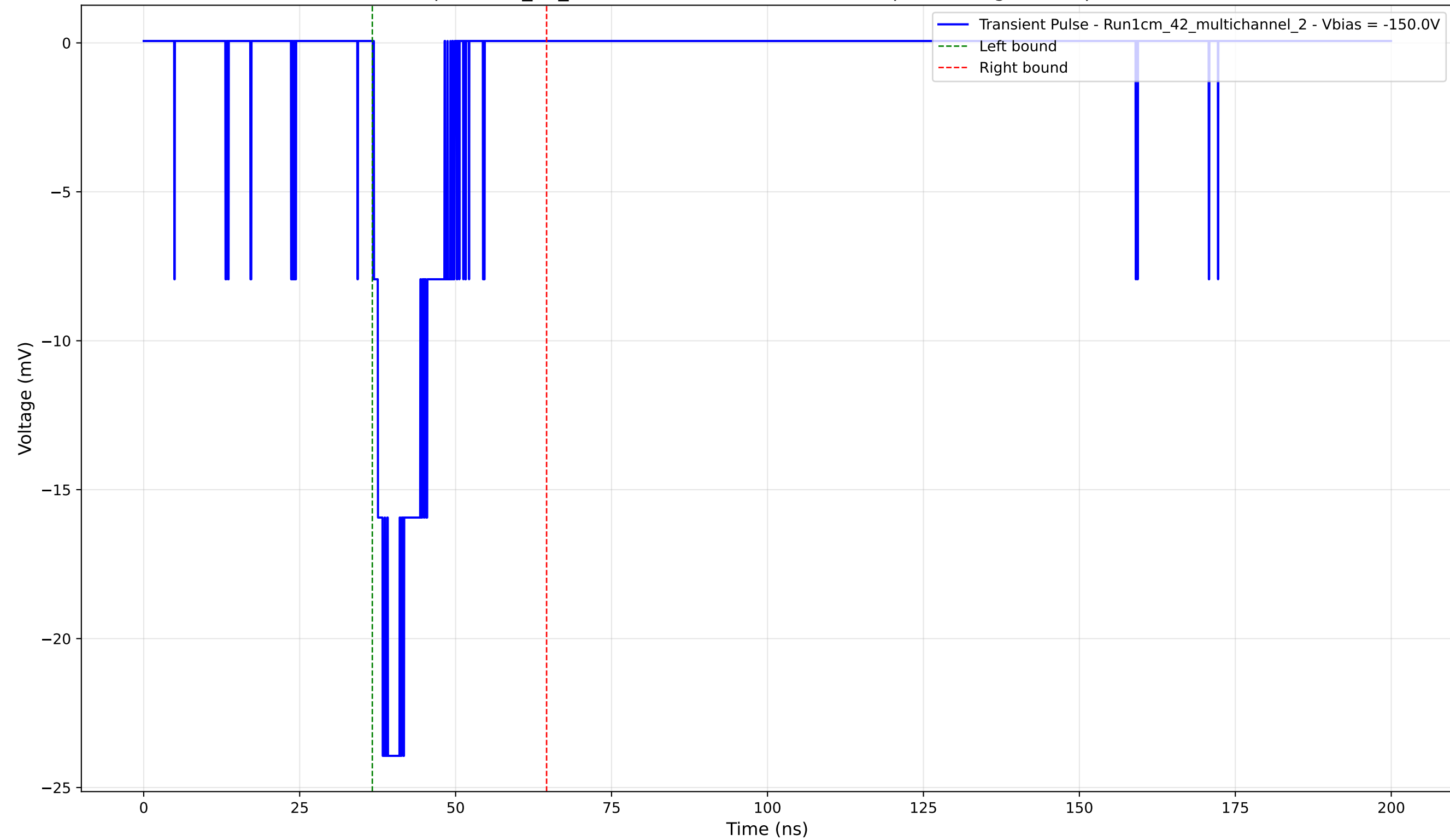
Transient Pulse - Sample: 1cm_42_multichannel - Position: 4855.0 \mu\text{m} - Charge: 3.71 pC - Rise Time: 1.43 ns
