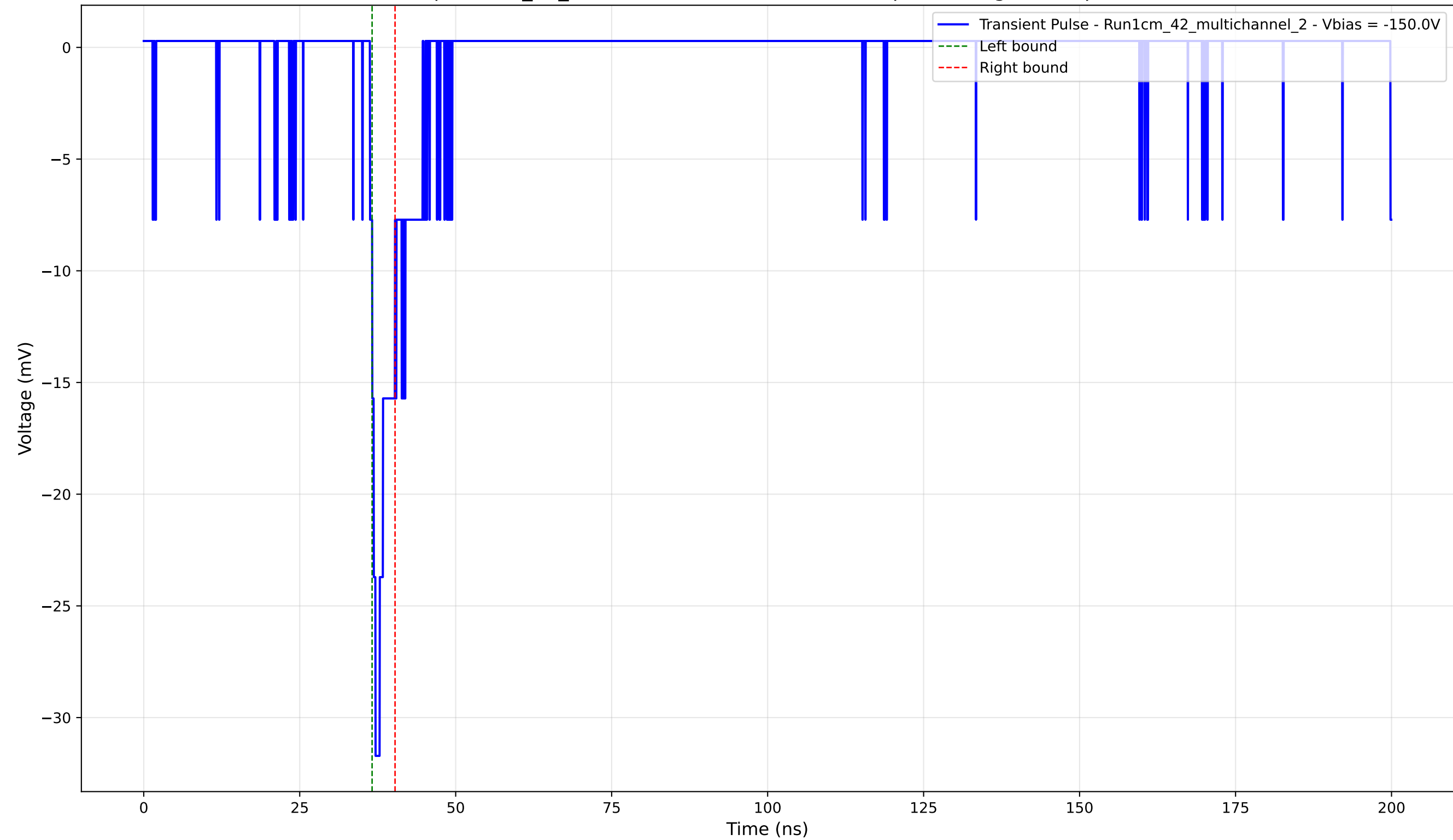
Transient Pulse - Sample: 1cm_42_multichannel - Position: 1885.0 \mu\text{m} - Charge: 1.50 pC - Rise Time: 0.90 ns
