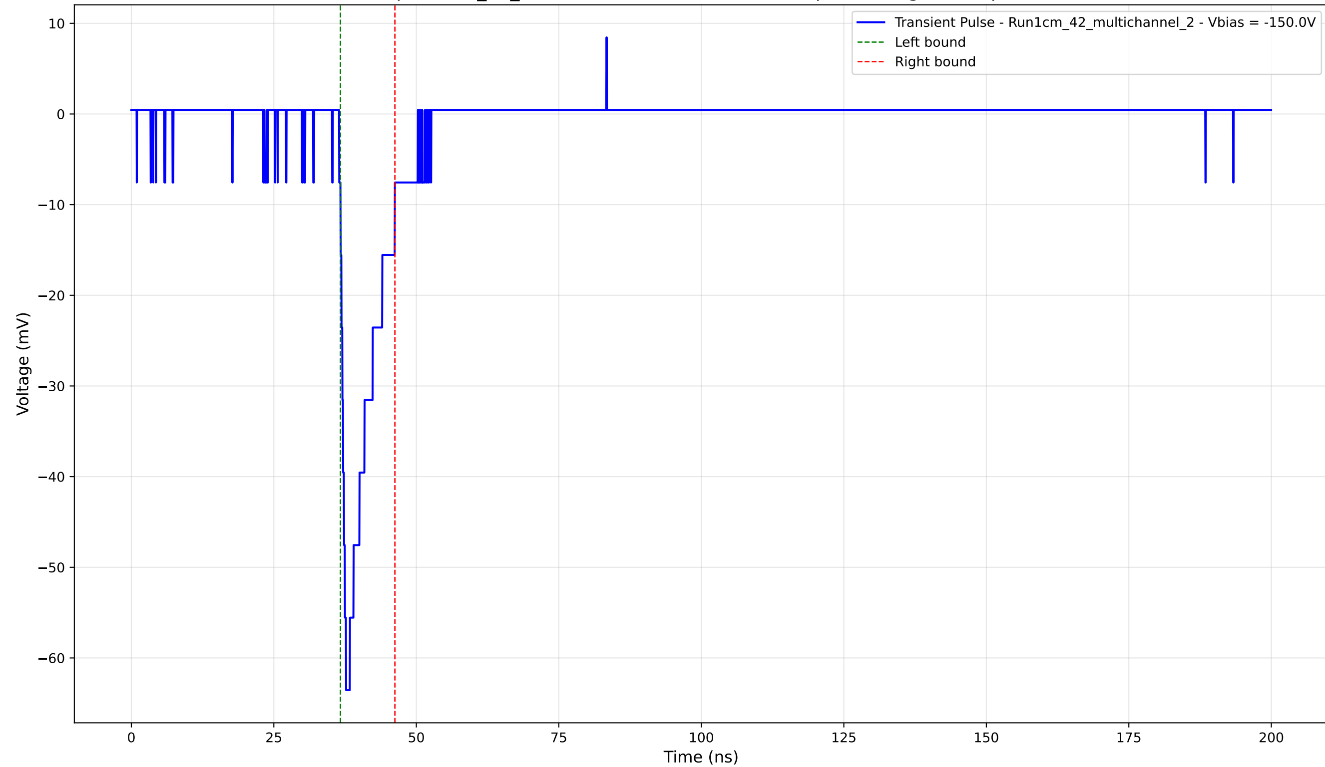
Transient Pulse - Sample: 1cm_42_multichannel - Position: 1400.0 \mu\text{m} - Charge: 6.35 pC - Rise Time: 1.21 ns
