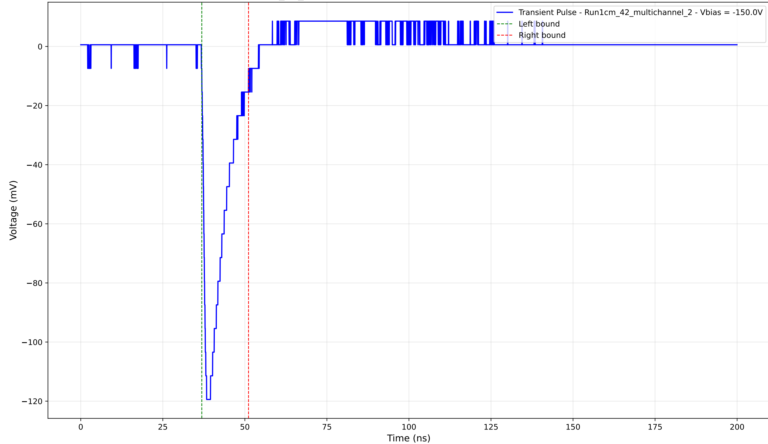
Transient Pulse - Sample: 1cm_42_multichannel - Position: 945.0 \mu\text{m} - Charge: 16.71 pC - Rise Time: 1.22 ns
