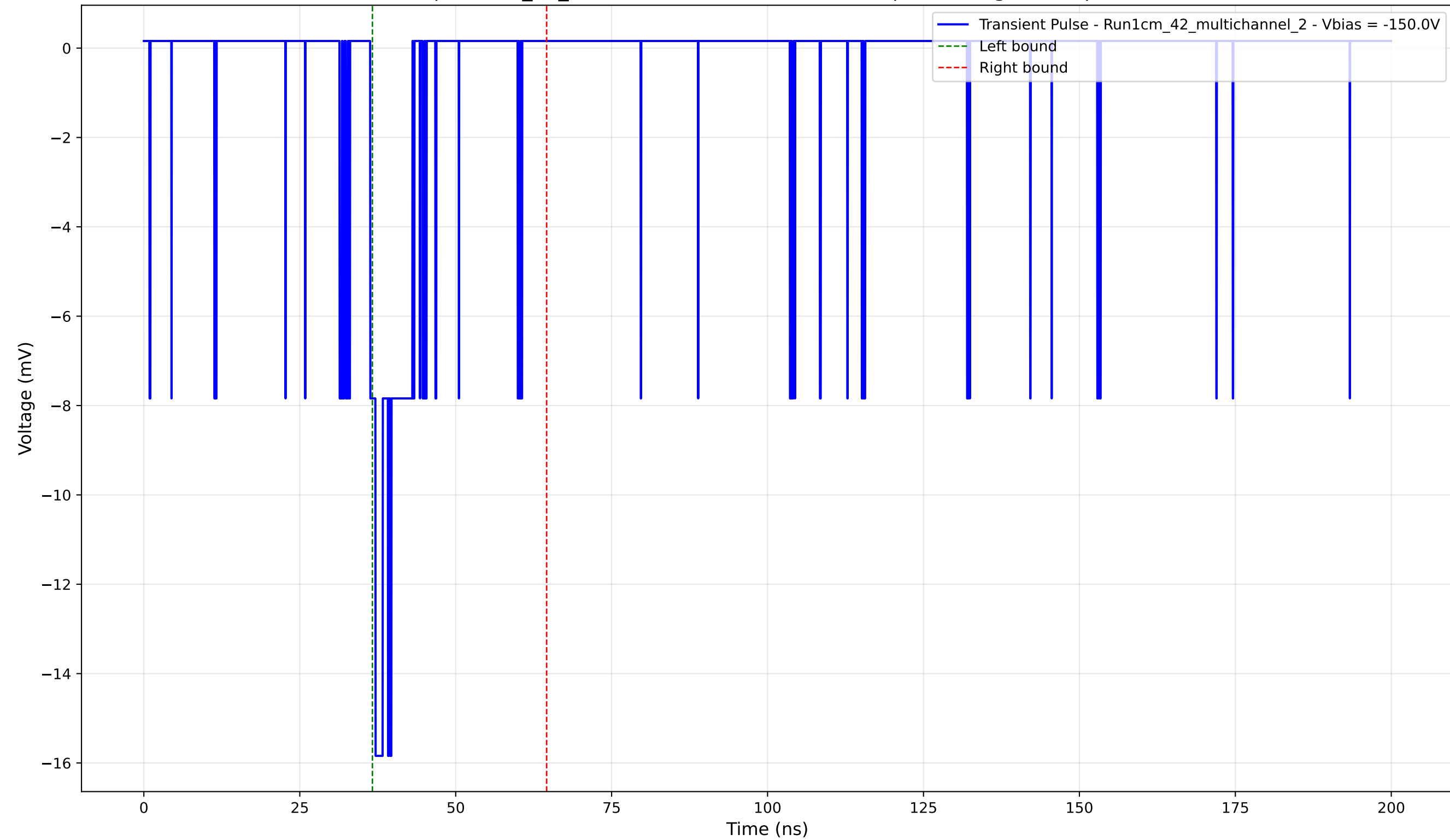
Transient Pulse - Sample: 1cm_42_multichannel - Position: 2875.0 \mu\text{m} - Charge: 1.41 pC - Rise Time: 0.87 ns
