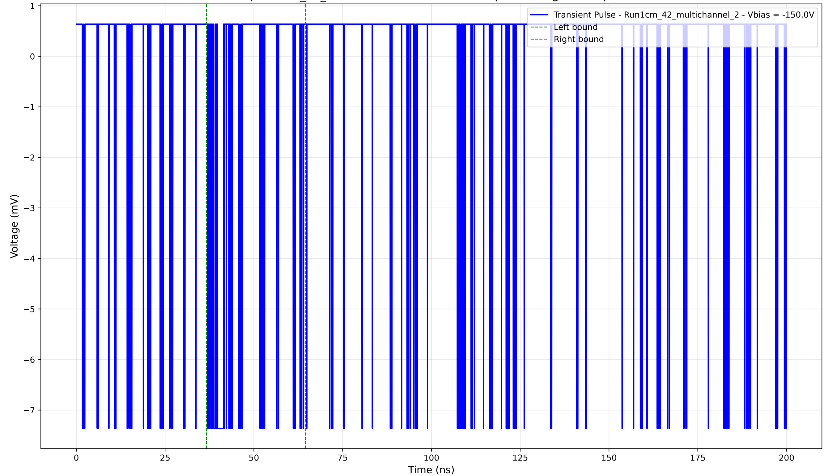
Transient Pulse - Sample: 1cm_42_multichannel - Position: 10.0 \mu\text{m} - Charge: 0.64 pC - Rise Time: 0.04 ns
