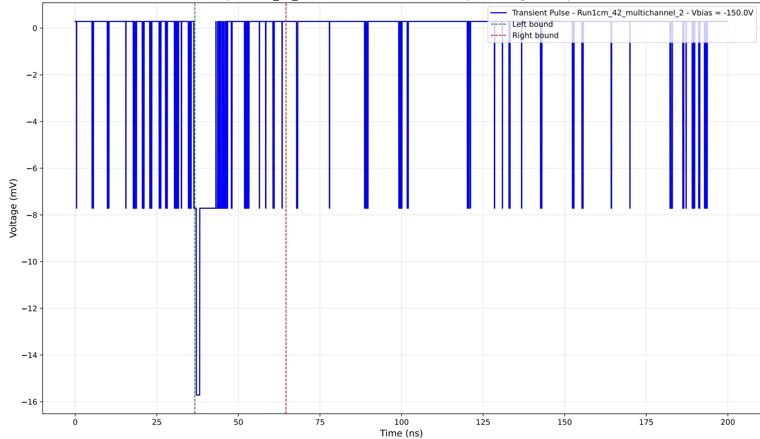
Transient Pulse - Sample: 1cm_42_multichannel - Position: 2880.0 \mu\text{m} - Charge: 1.70 pC - Rise Time: 0.79 ns
