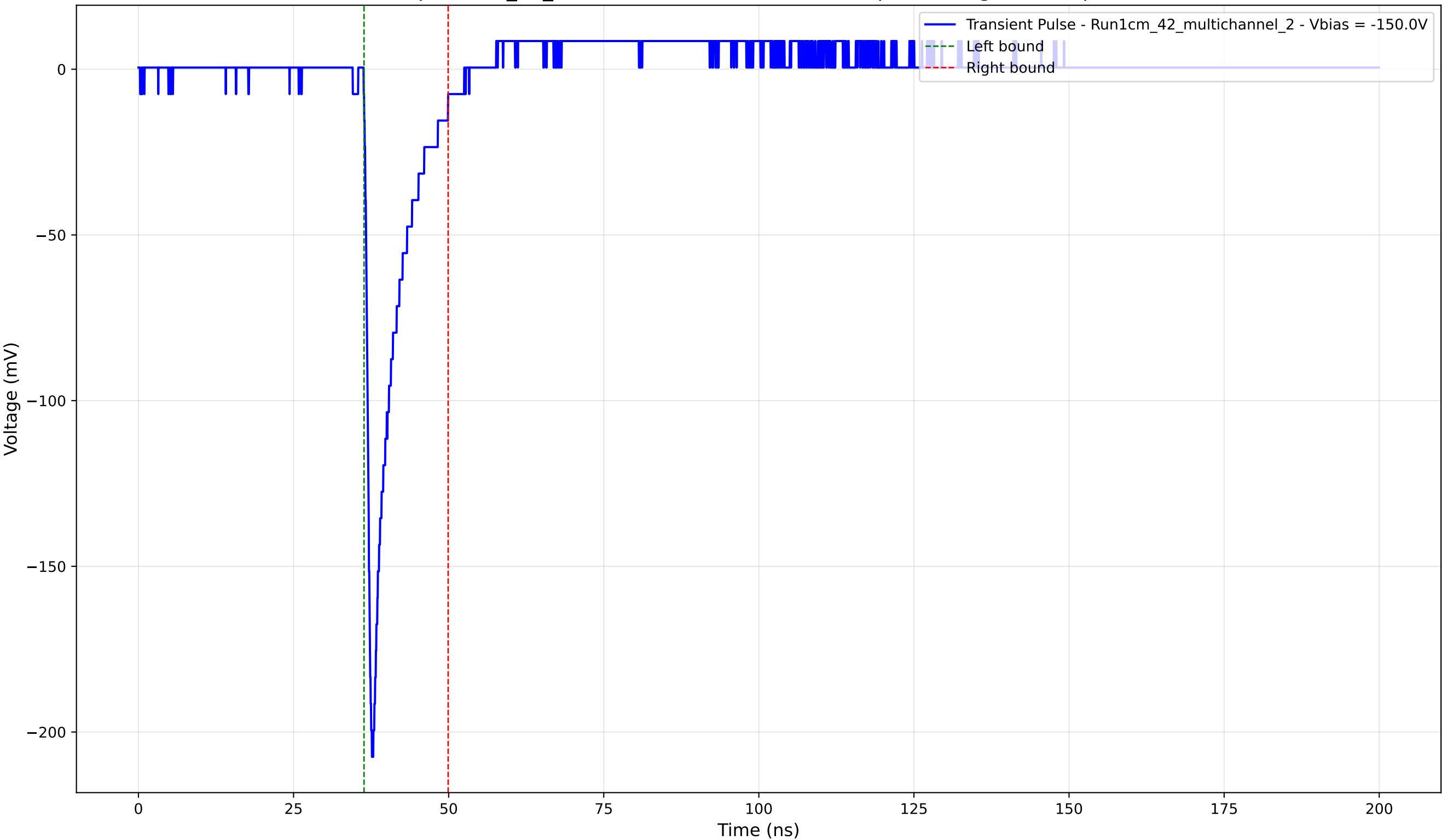
Transient Pulse - Sample: 1cm_42_multichannel - Position: 3130.0 \mu\text{m} - Charge: 18.76 pC - Rise Time: 0.97 ns
