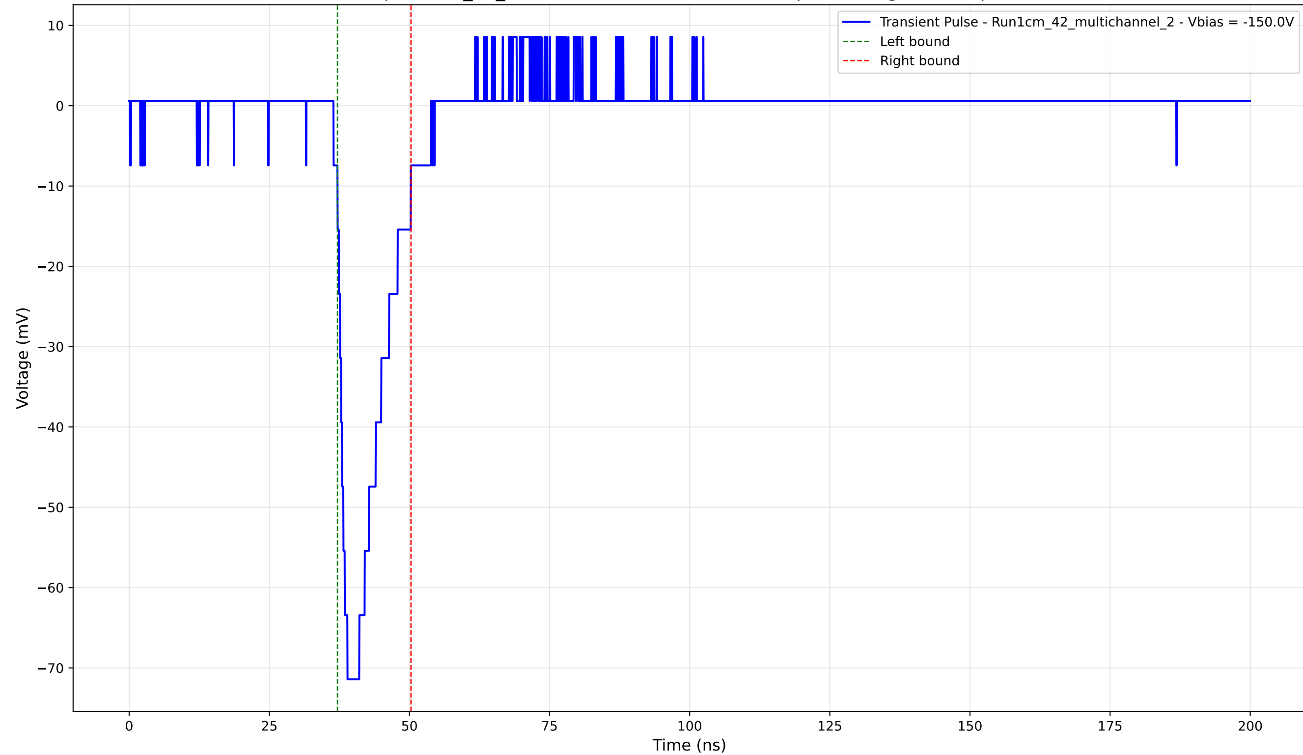
Transient Pulse - Sample: 1cm_42_multichannel - Position: 4535.0 \mu\text{m} - Charge: 10.86 pC - Rise Time: 2.48 ns
