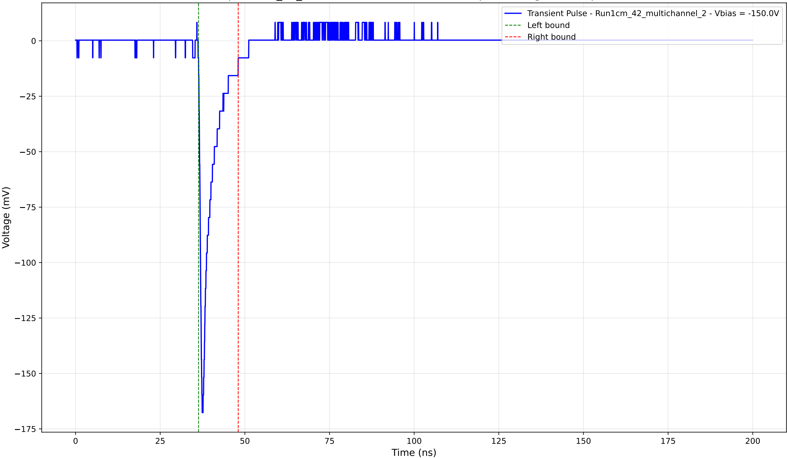
Transient Pulse - Sample: 1cm_42_multichannel - Position: 2930.0 \mu\text{m} - Charge: 12.49 pC - Rise Time: 0.83 ns
