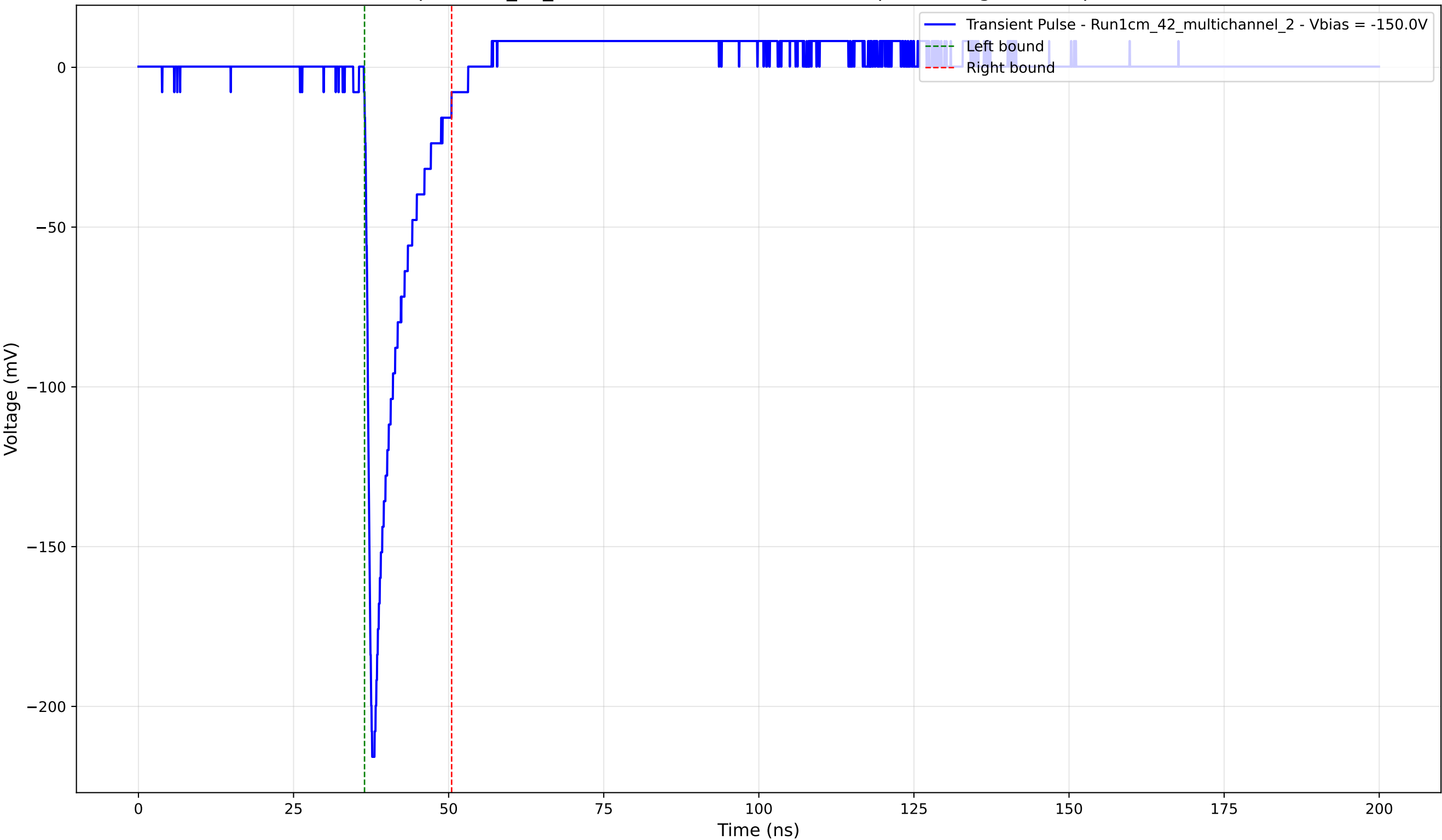
Transient Pulse - Sample: 1cm_42_multichannel - Position: 1520.0 \mu\text{m} - Charge: 21.26 pC - Rise Time: 0.97 ns
