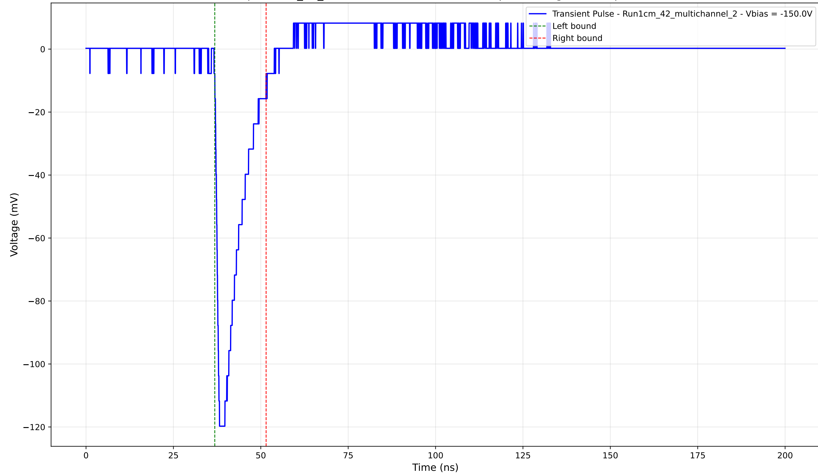
Transient Pulse - Sample: 1cm_42_multichannel - Position: 970.0 \mu\text{m} - Charge: 17.27 pC - Rise Time: 1.18 ns
