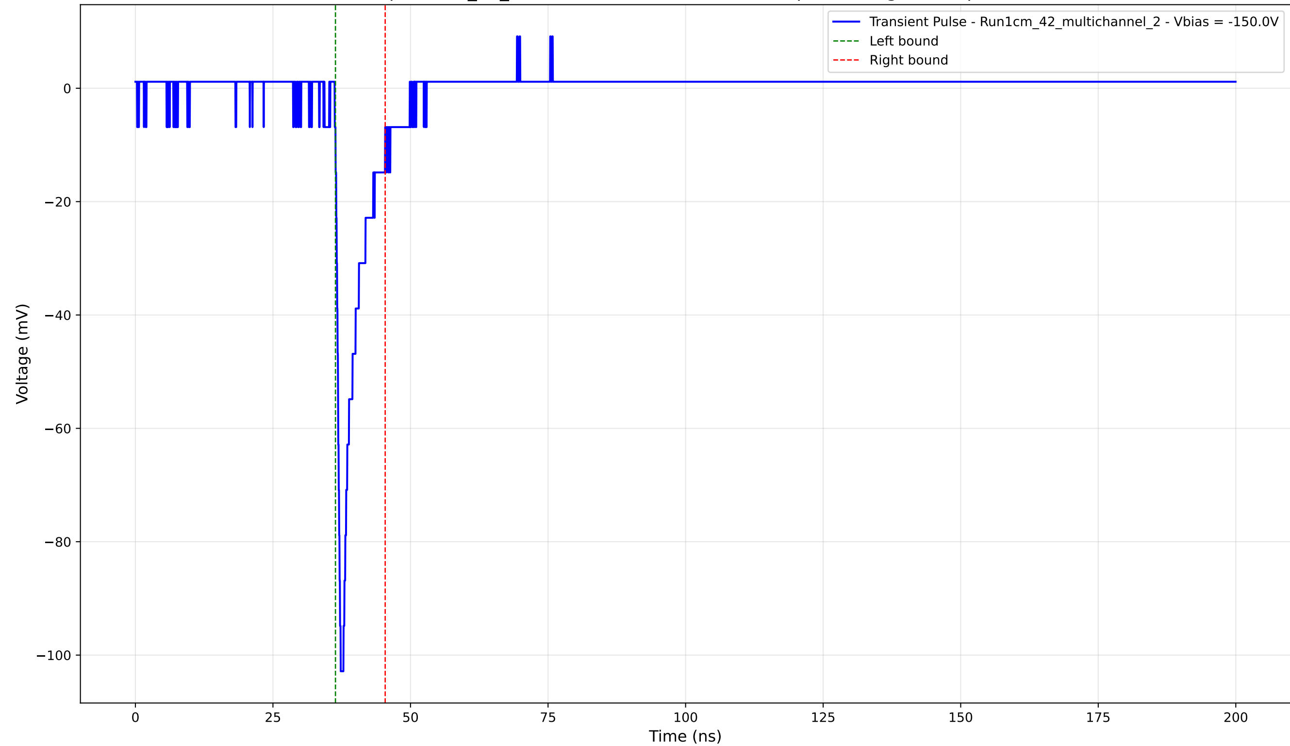
Transient Pulse - Sample: 1cm_42_multichannel - Position: 1820.0 \mu\text{m} - Charge: 7.33 pC - Rise Time: 0.82 ns
