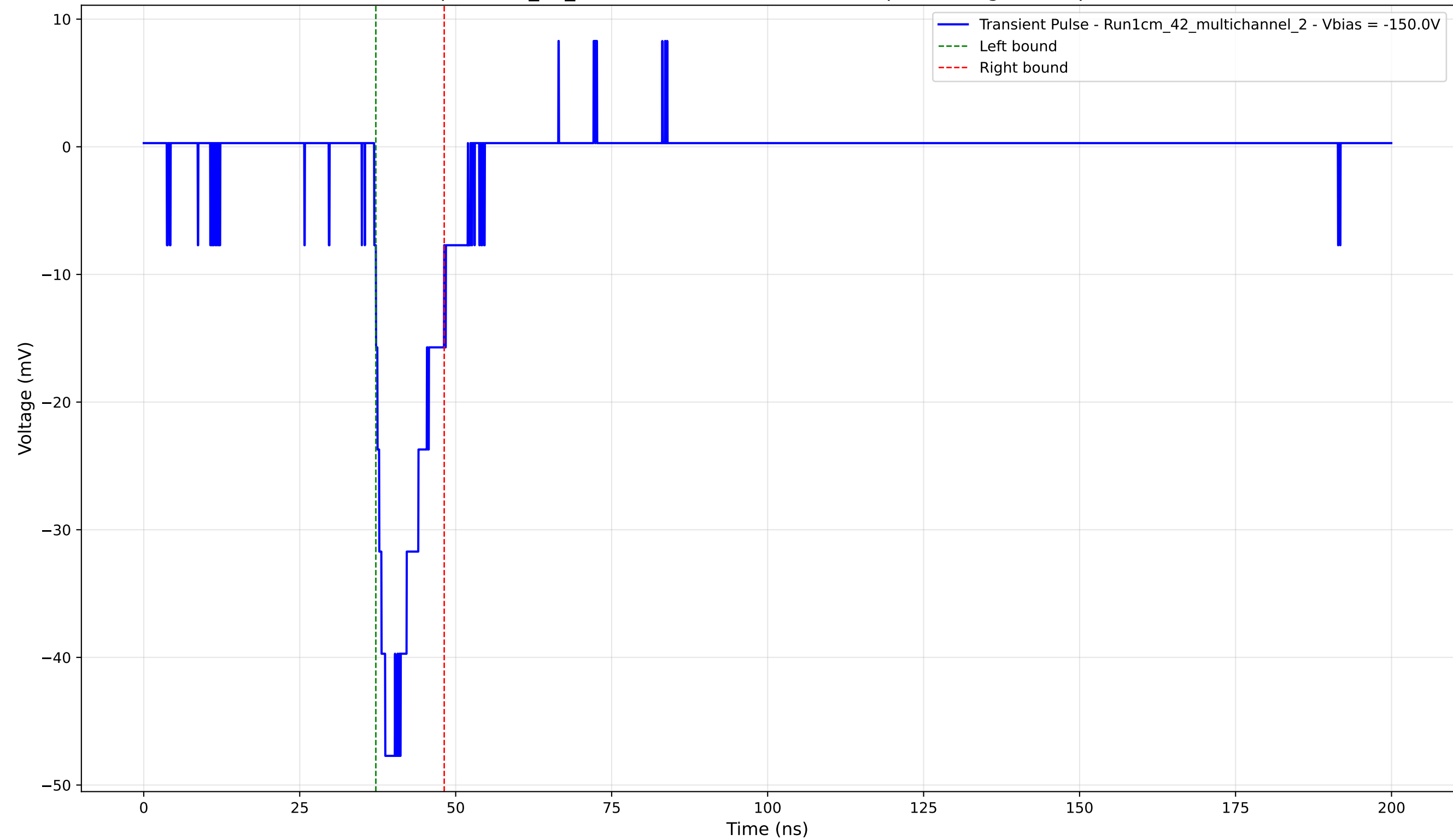
Transient Pulse - Sample: 1cm_42_multichannel - Position: 290.0 \mu\text{m} - Charge: 6.75 pC - Rise Time: 1.78 ns
