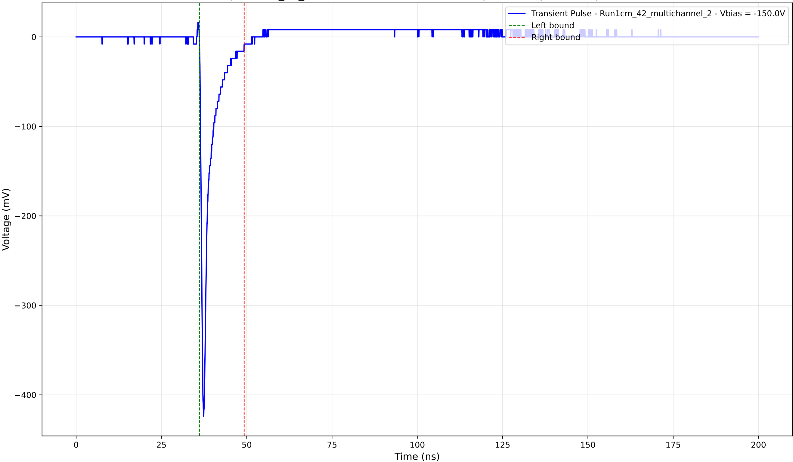
Transient Pulse - Sample: 1cm_42_multichannel - Position: 2725.0 \mu\text{m} - Charge: 24.83 pC - Rise Time: 0.81 ns
