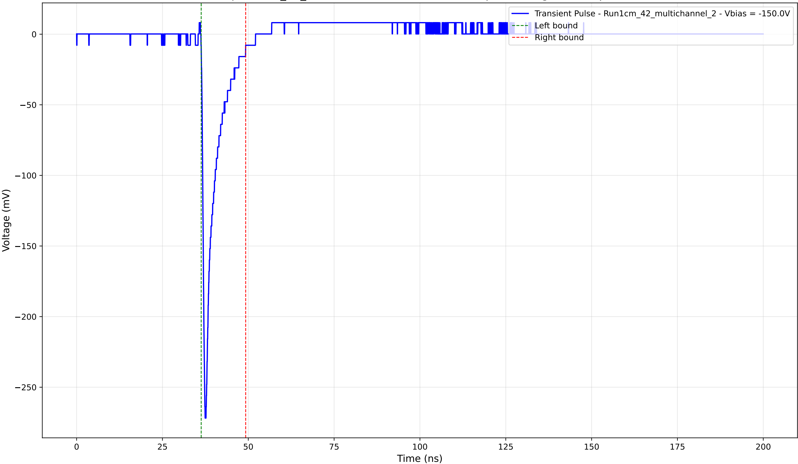
Transient Pulse - Sample: 1cm_42_multichannel - Position: 1785.0 \mu\text{m} - Charge: 20.64 pC - Rise Time: 0.85 ns
