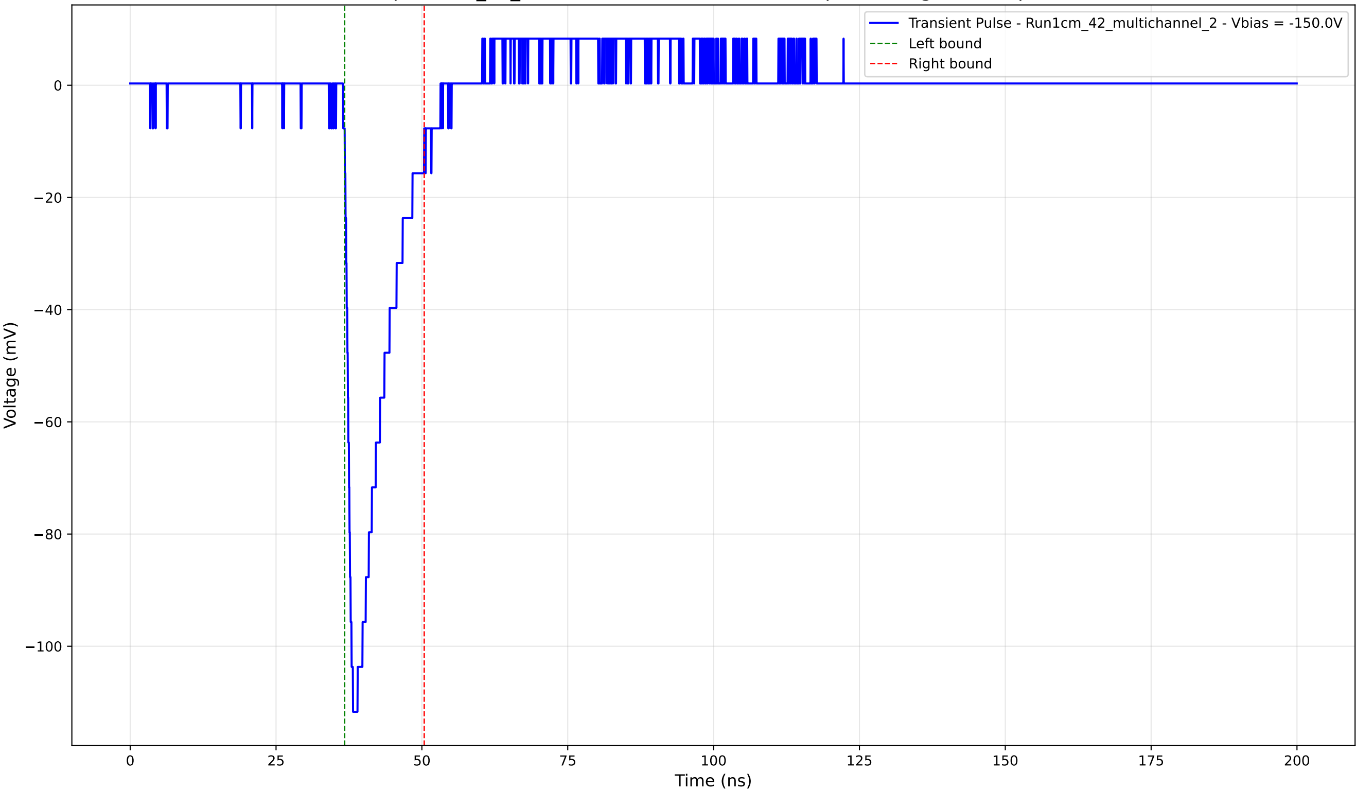
Transient Pulse - Sample: 1cm_42_multichannel - Position: 3640.0 \mu\text{m} - Charge: 14.77 pC - Rise Time: 1.18 ns
