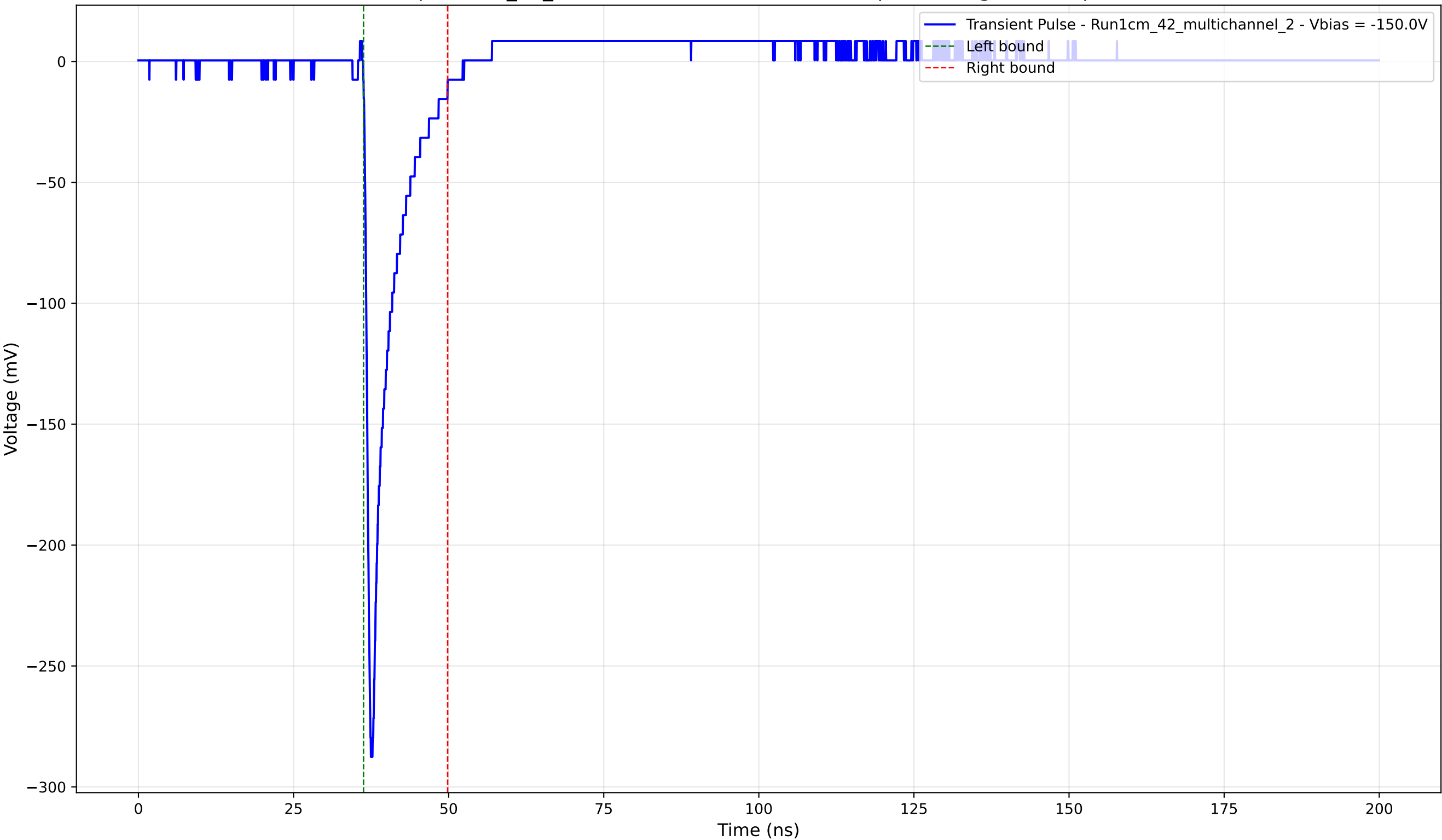
Transient Pulse - Sample: 1cm_42_multichannel - Position: 1735.0 \mu\text{m} - Charge: 23.17 pC - Rise Time: 0.87 ns
