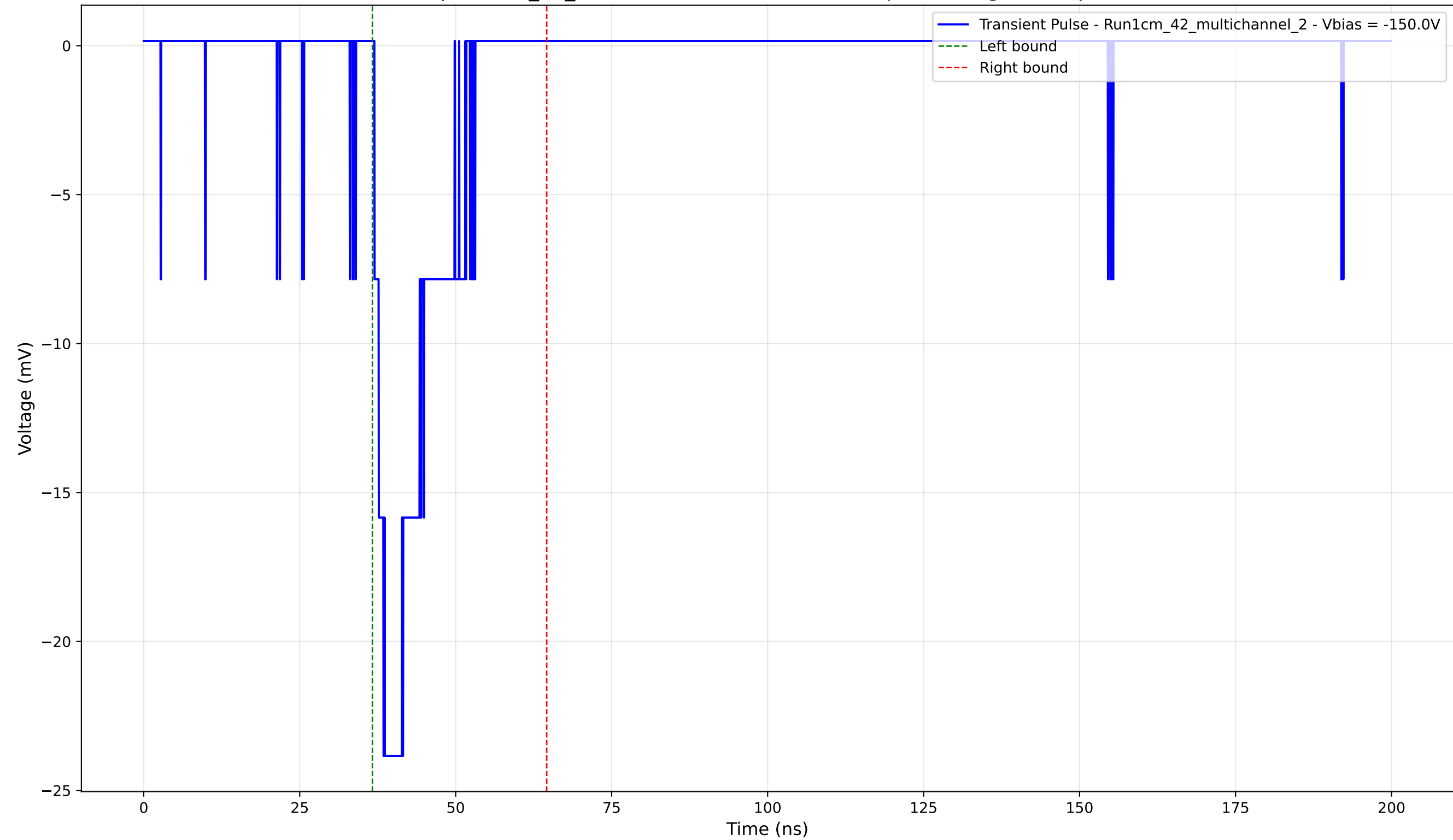
Transient Pulse - Sample: 1cm_42_multichannel - Position: 305.0 \mu\text{m} - Charge: 3.86 pC - Rise Time: 1.47 ns
