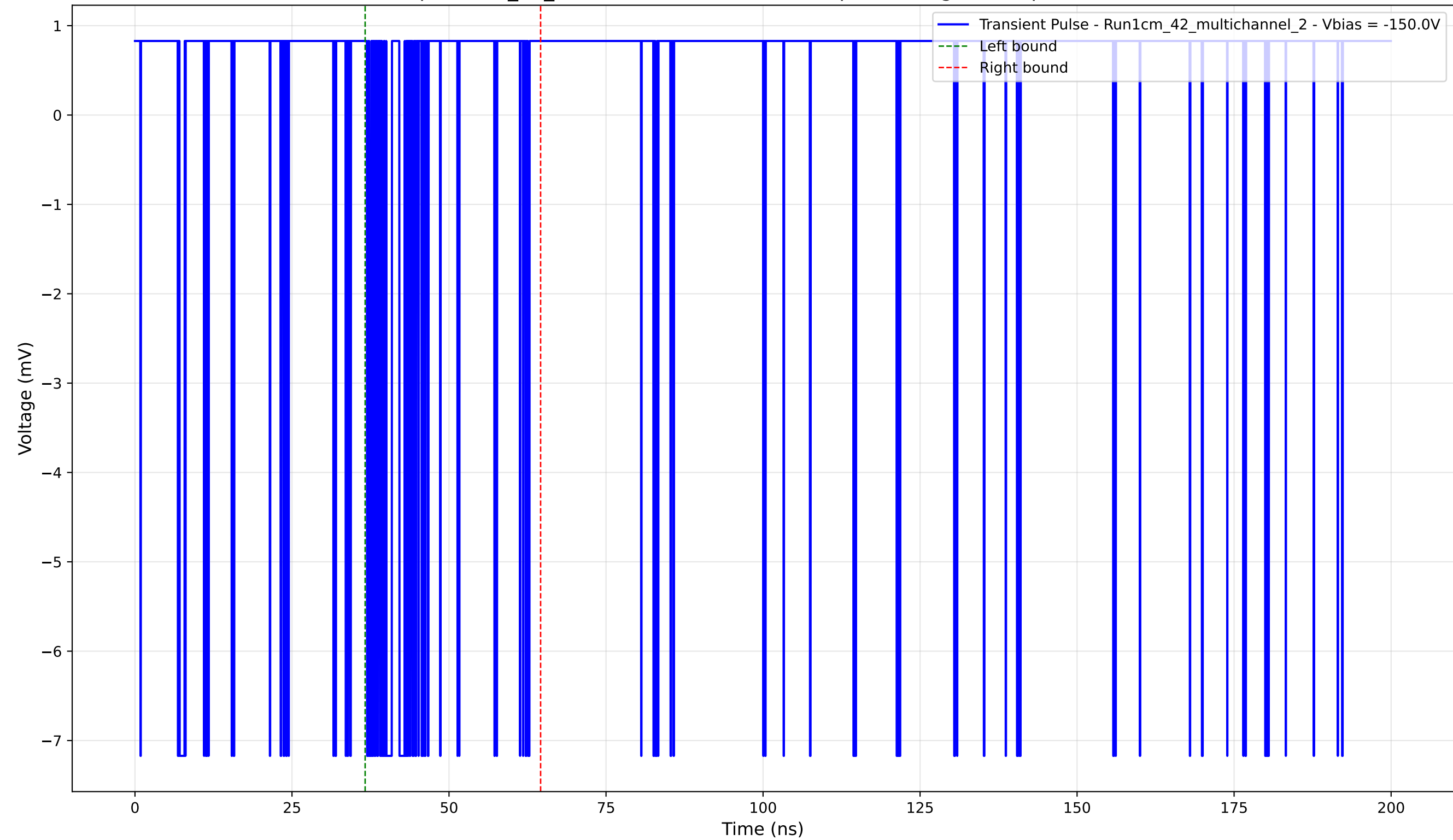
Transient Pulse - Sample: 1cm_42_multichannel - Position: 5.0 \mu\text{m} - Charge: 0.41 pC - Rise Time: 0.00 ns (N/A)
