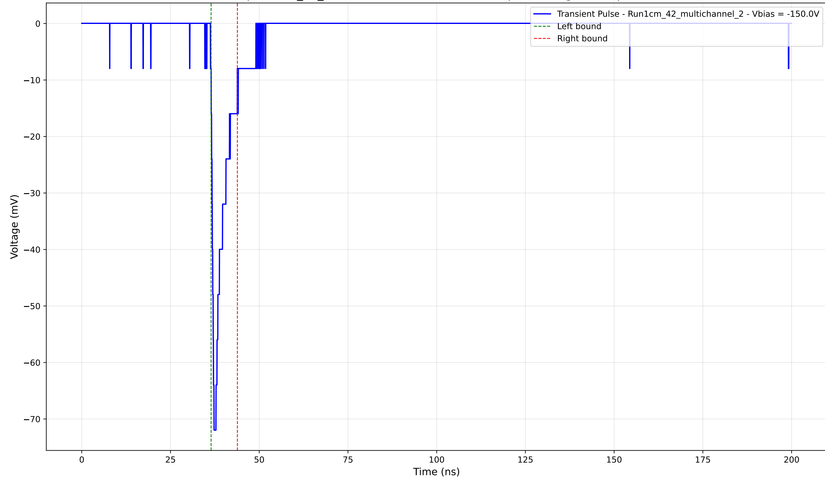
Transient Pulse - Sample: 1cm_42_multichannel - Position: 1825.0 \mu\text{m} - Charge: 5.04 pC - Rise Time: 1.00 ns
