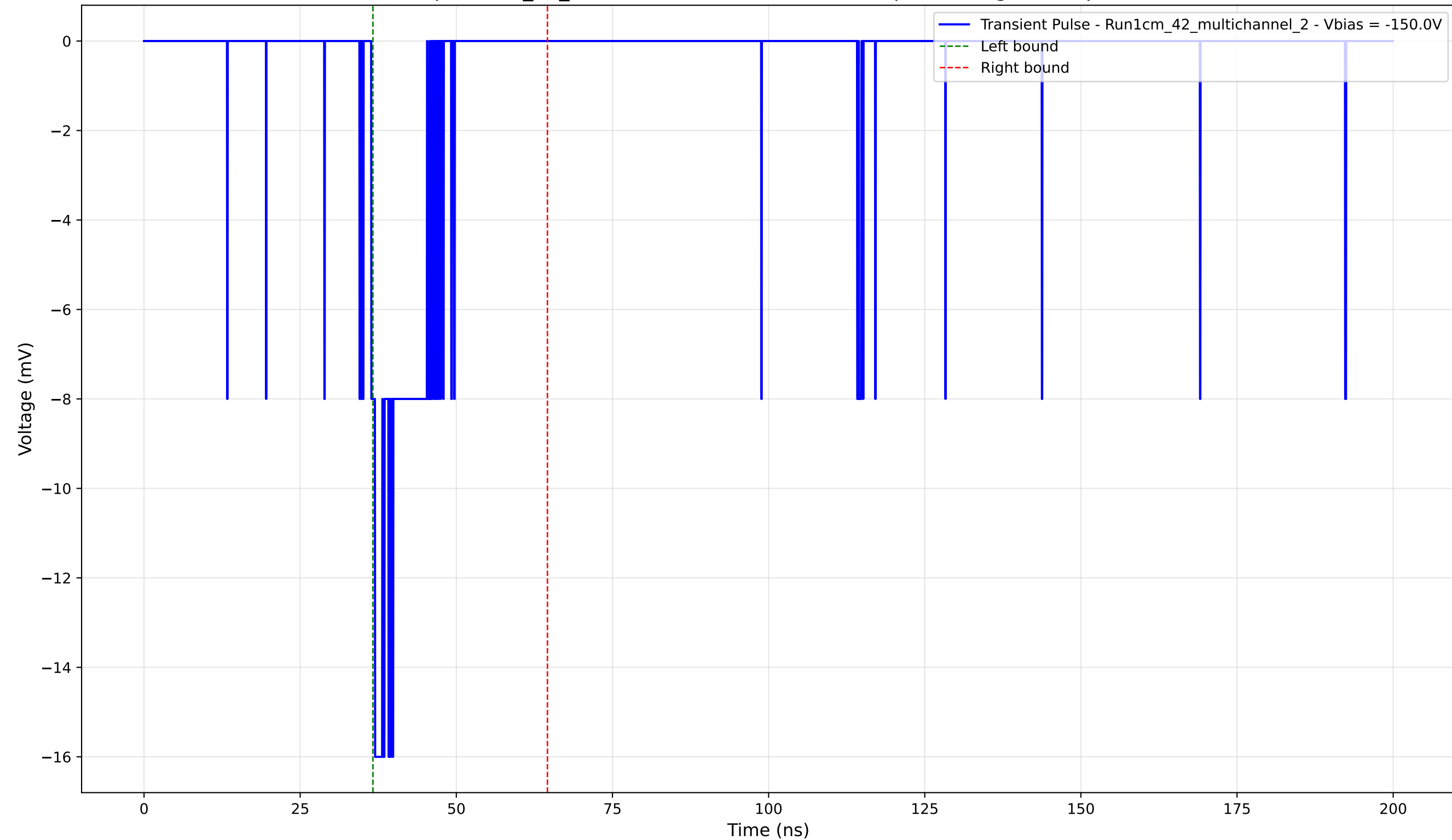
Transient Pulse - Sample: 1cm_42_multichannel - Position: 1855.0 \mu\text{m} - Charge: 1.87 pC - Rise Time: 0.63 ns
