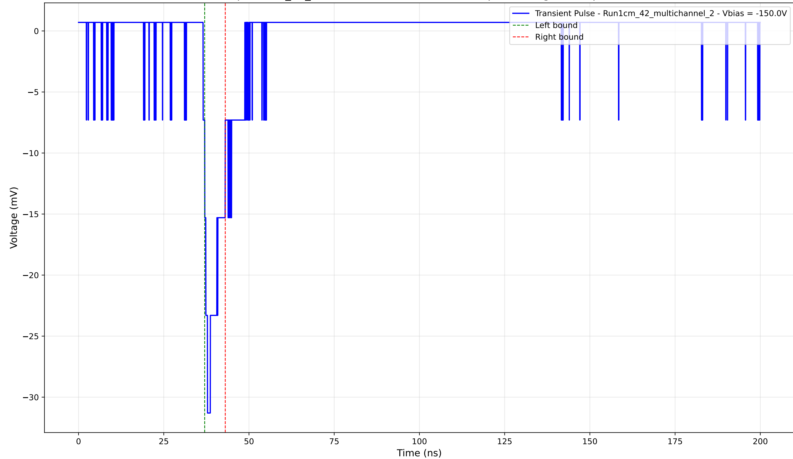
Transient Pulse - Sample: 1cm_42_multichannel - Position: 1325.0 \mu\text{m} - Charge: 2.51 pC - Rise Time: 1.31 ns
