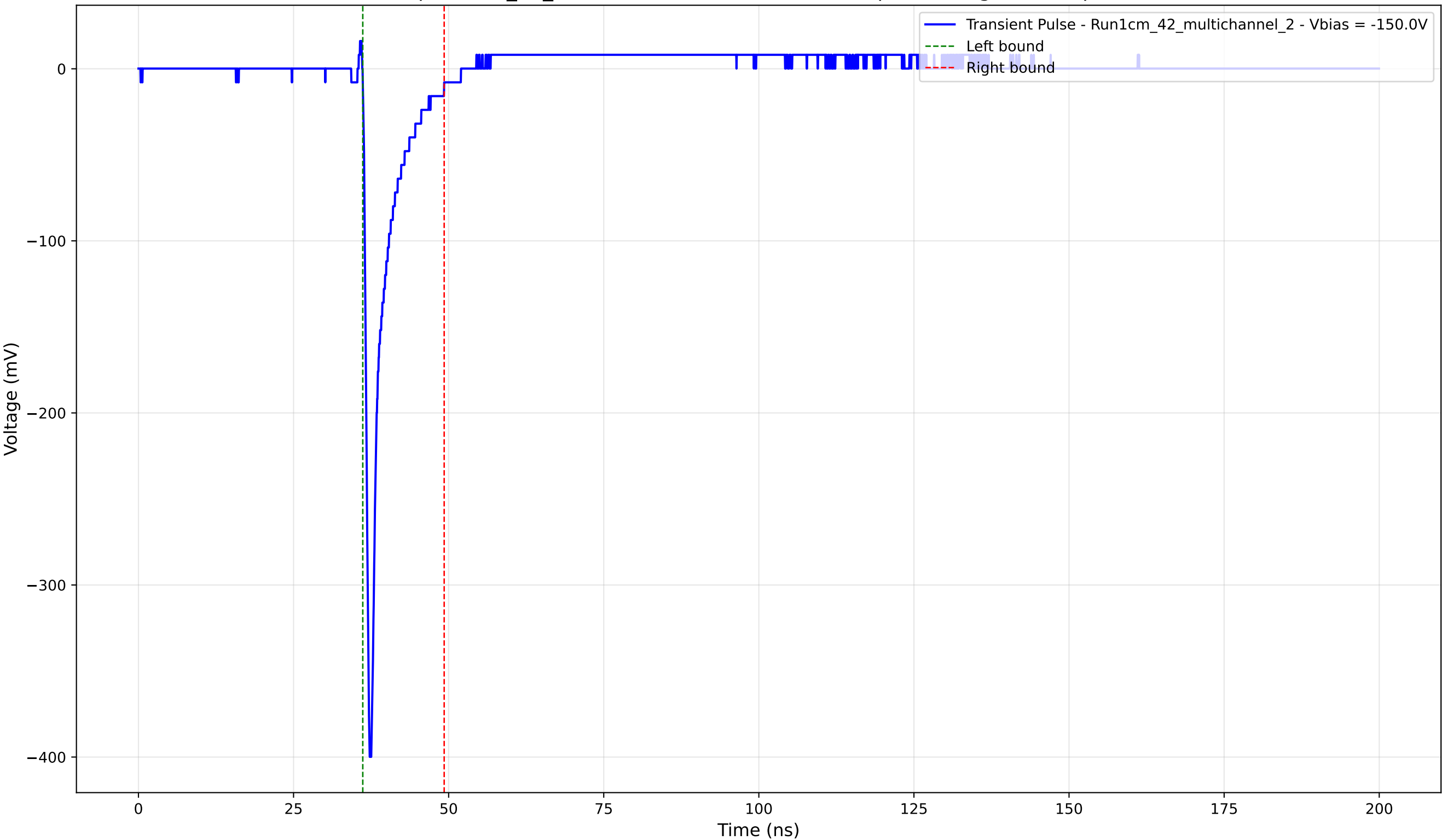
Transient Pulse - Sample: 1cm_42_multichannel - Position: 2750.0 \mu\text{m} - Charge: 24.38 pC - Rise Time: 0.76 ns
