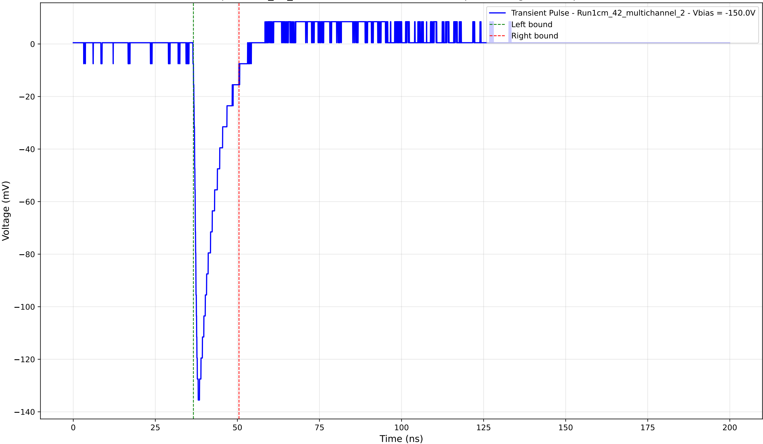
Transient Pulse - Sample: 1cm_42_multichannel - Position: 3470.0 \mu\text{m} - Charge: 16.39 pC - Rise Time: 1.17 ns
