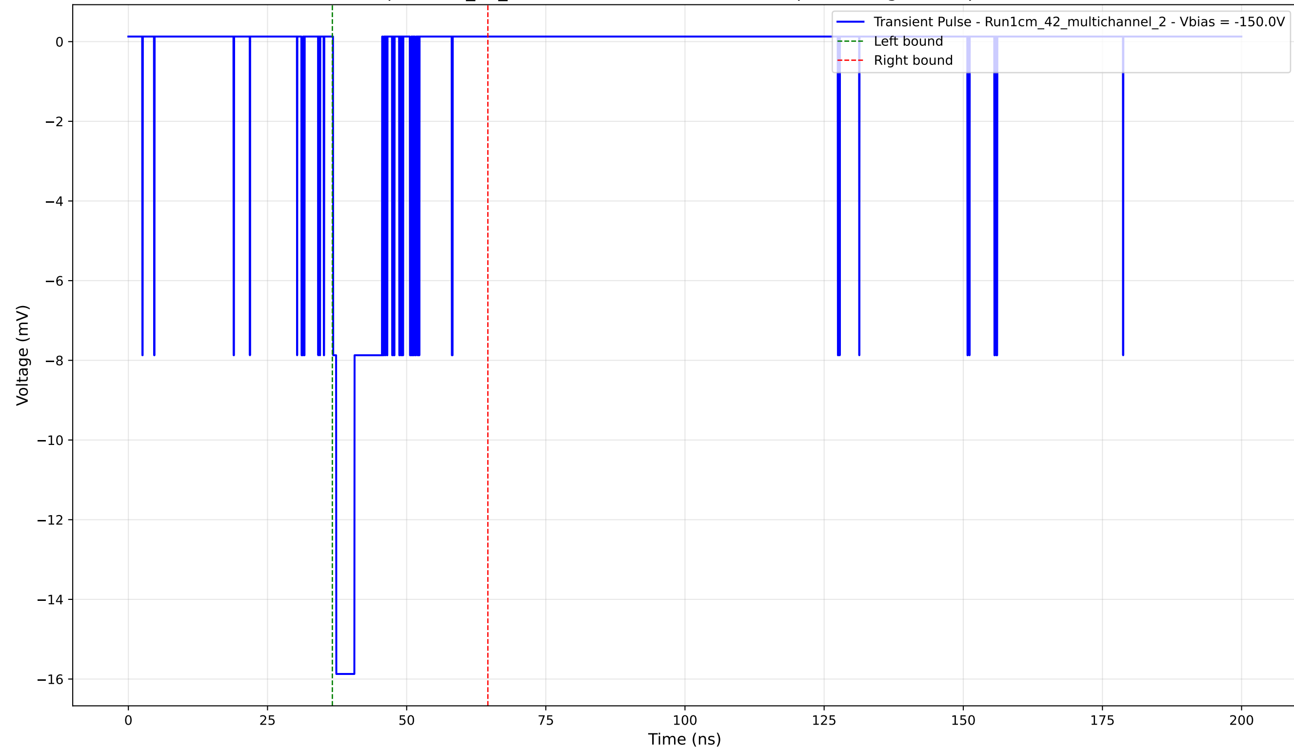
Transient Pulse - Sample: 1cm_42_multichannel - Position: 1335.0 \mu\text{m} - Charge: 2.19 pC - Rise Time: 0.59 ns
