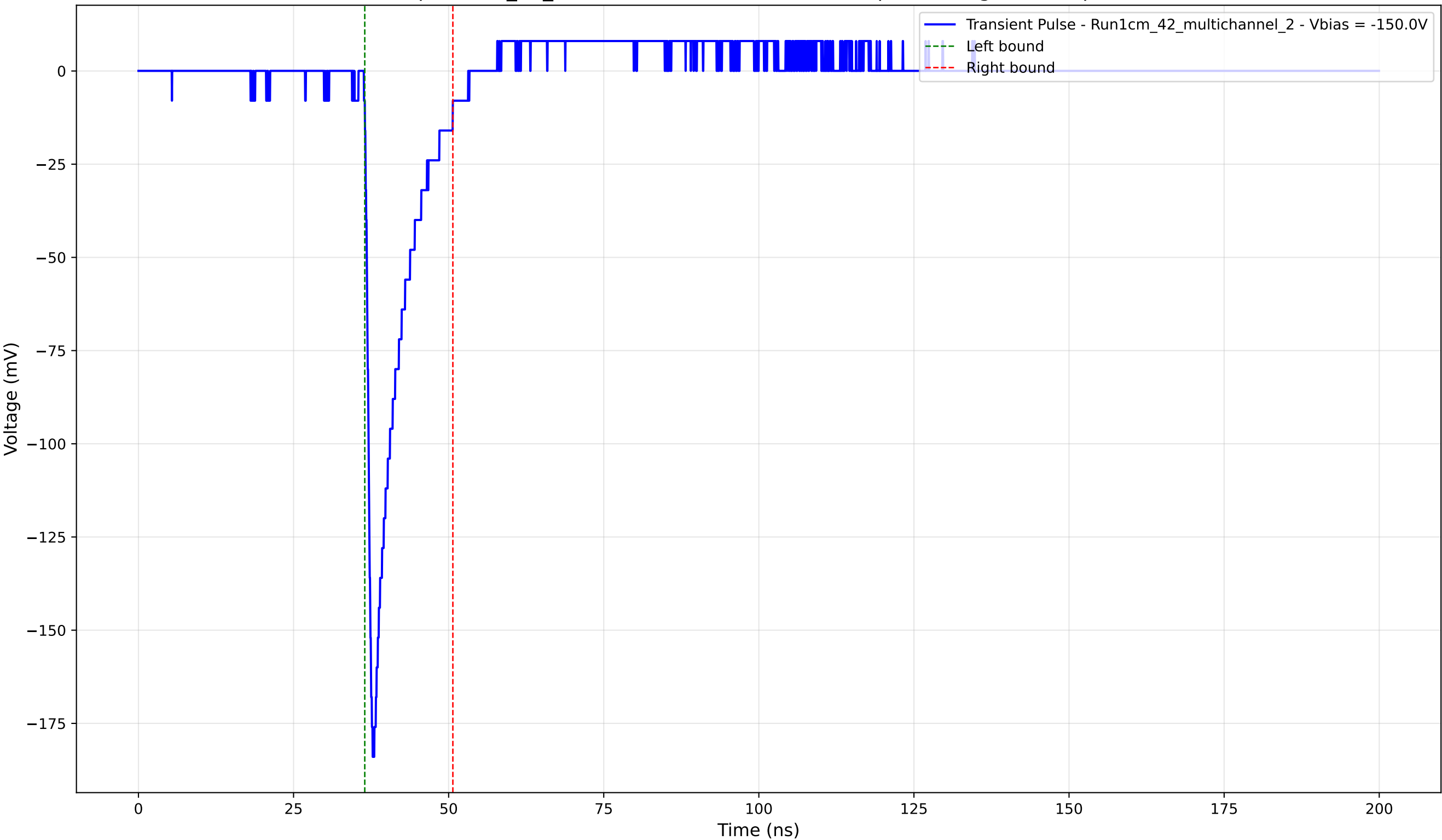
Transient Pulse - Sample: 1cm_42_multichannel - Position: 3260.0 \mu\text{m} - Charge: 18.90 pC - Rise Time: 0.95 ns
