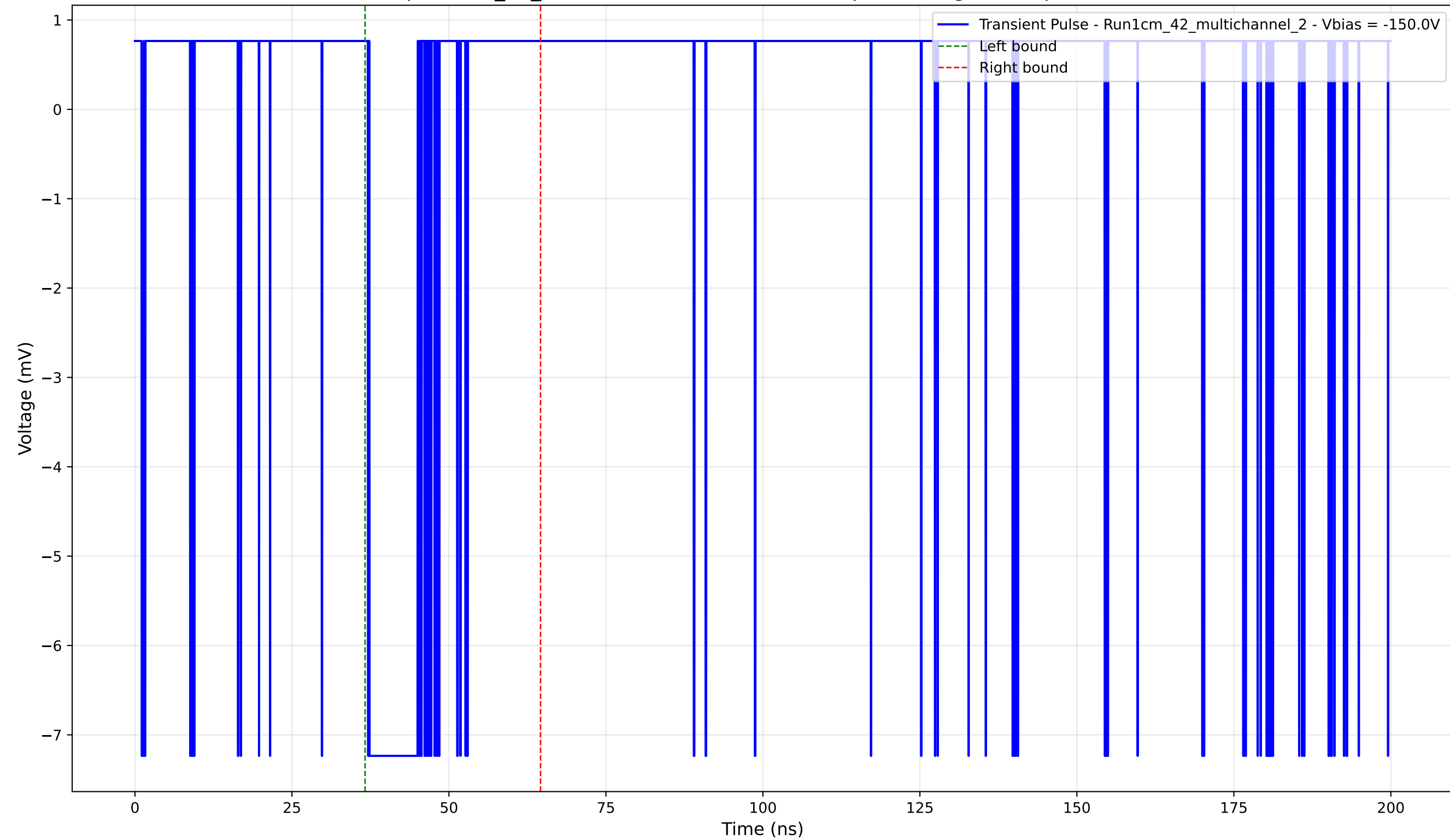
Transient Pulse - Sample: 1cm_42_multichannel - Position: 835.0 \mu\text{m} - Charge: 1.06 pC - Rise Time: 0.00 ns (N/A)
