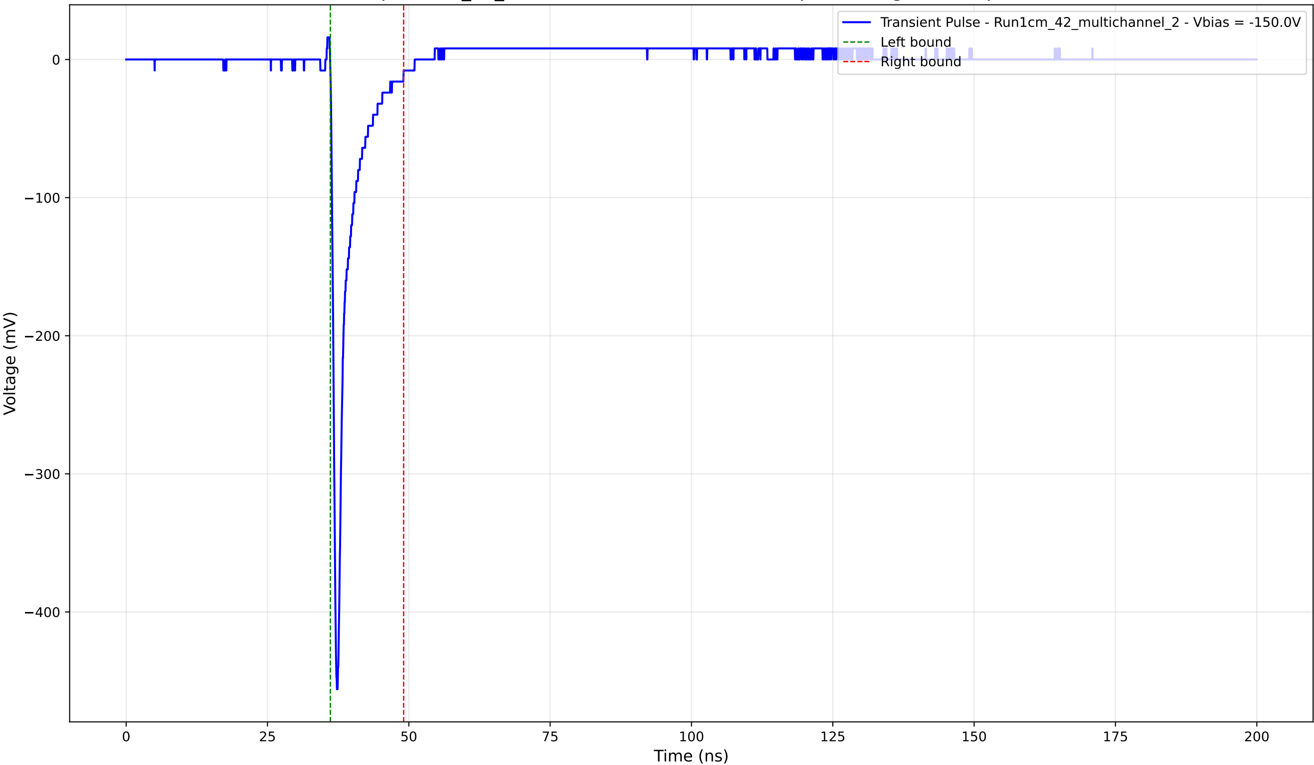
Transient Pulse - Sample: 1cm_42_multichannel - Position: 2055.0 \mu\text{m} - Charge: 25.86 pC - Rise Time: 0.79 ns
