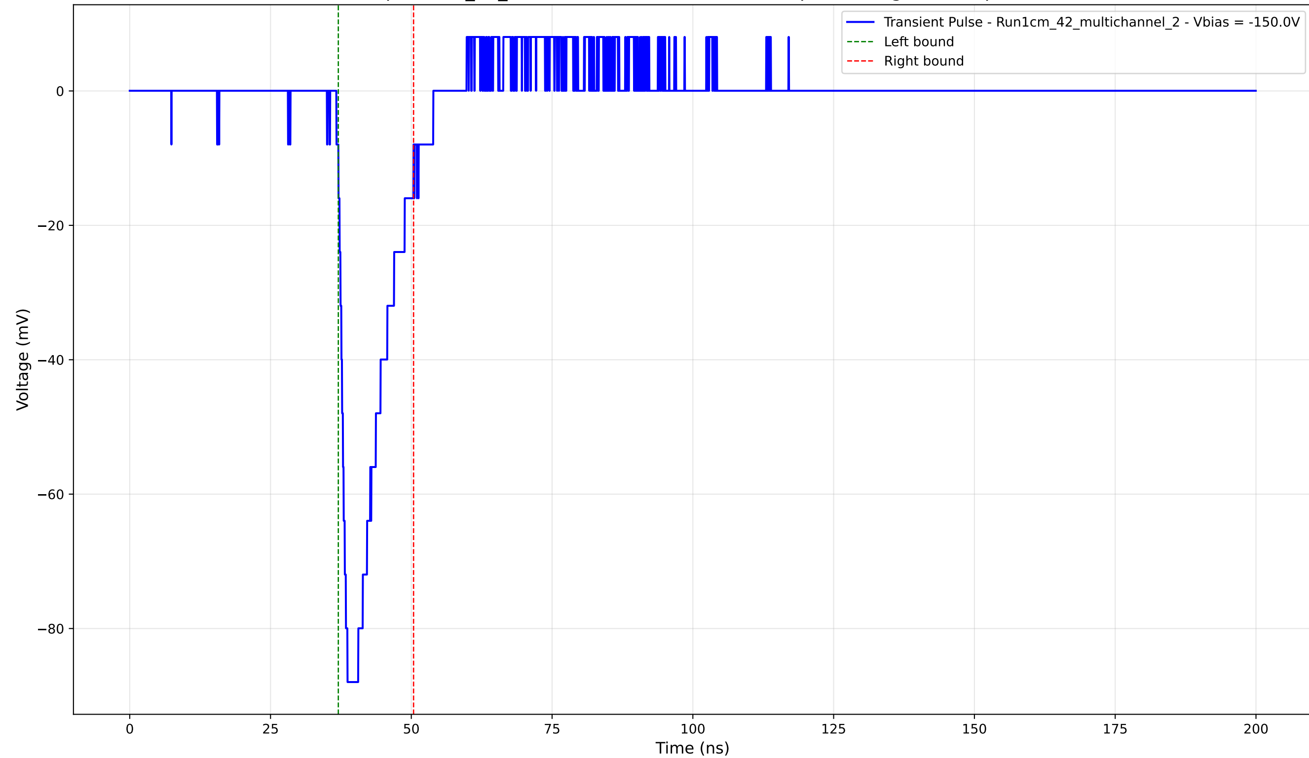
Transient Pulse - Sample: 1cm_42_multichannel - Position: 4050.0 \mu\text{m} - Charge: 13.16 pC - Rise Time: 1.36 ns
