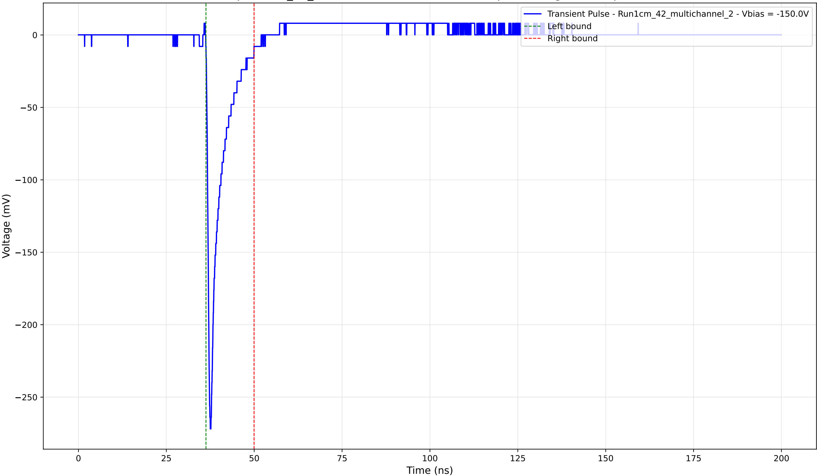
Transient Pulse - Sample: 1cm_42_multichannel - Position: 2985.0 \mu\text{m} - Charge: 21.45 pC - Rise Time: 0.85 ns
