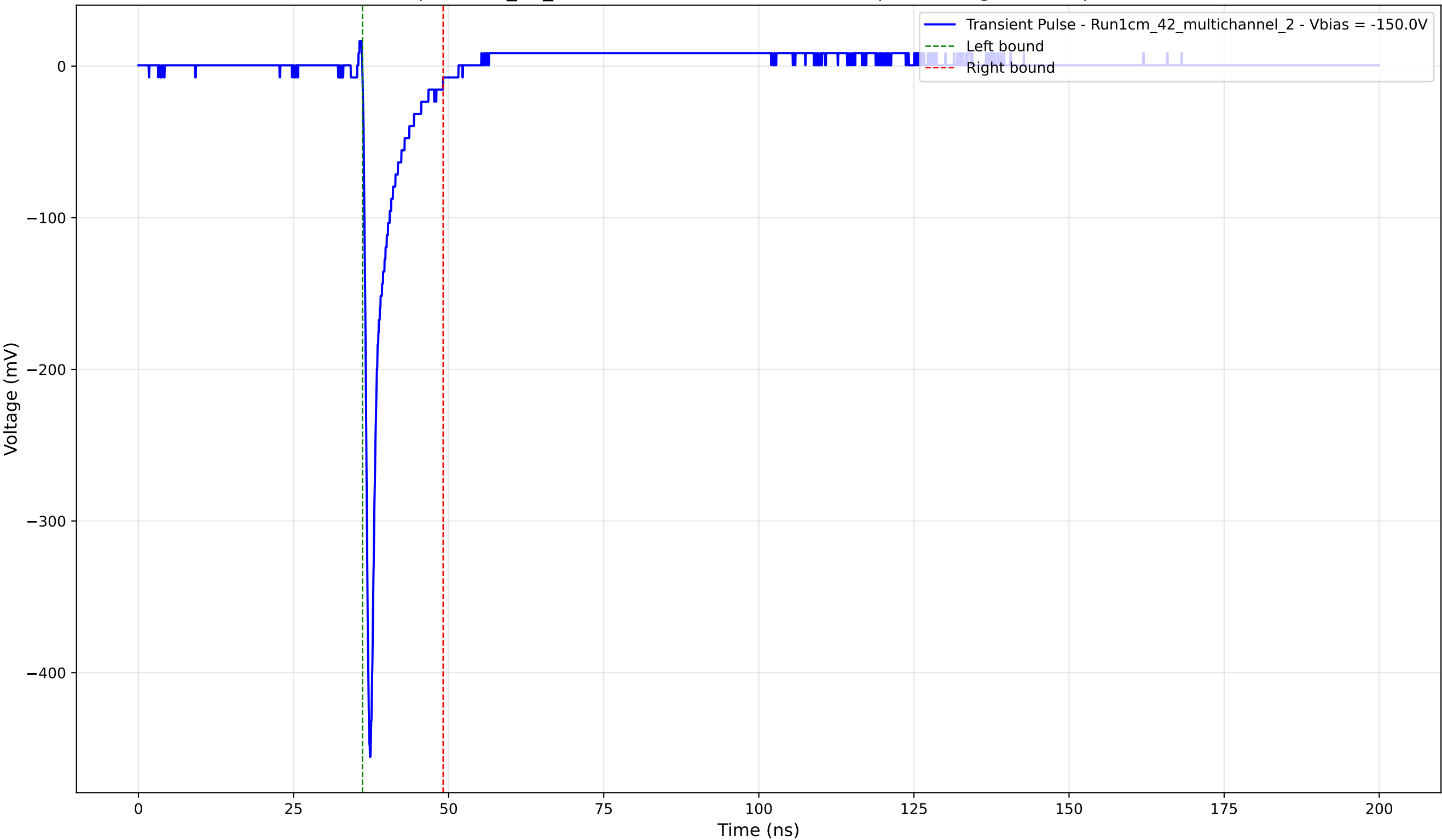
Transient Pulse - Sample: 1cm_42_multichannel - Position: 2045.0 \mu\text{m} - Charge: 25.86 pC - Rise Time: 0.76 ns
