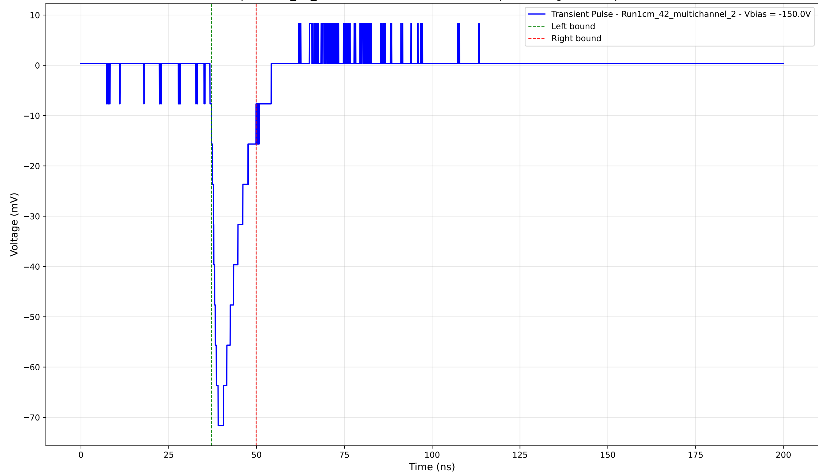
Transient Pulse - Sample: 1cm_42_multichannel - Position: 4295.0 \mu\text{m} - Charge: 10.30 pC - Rise Time: 2.32 ns
