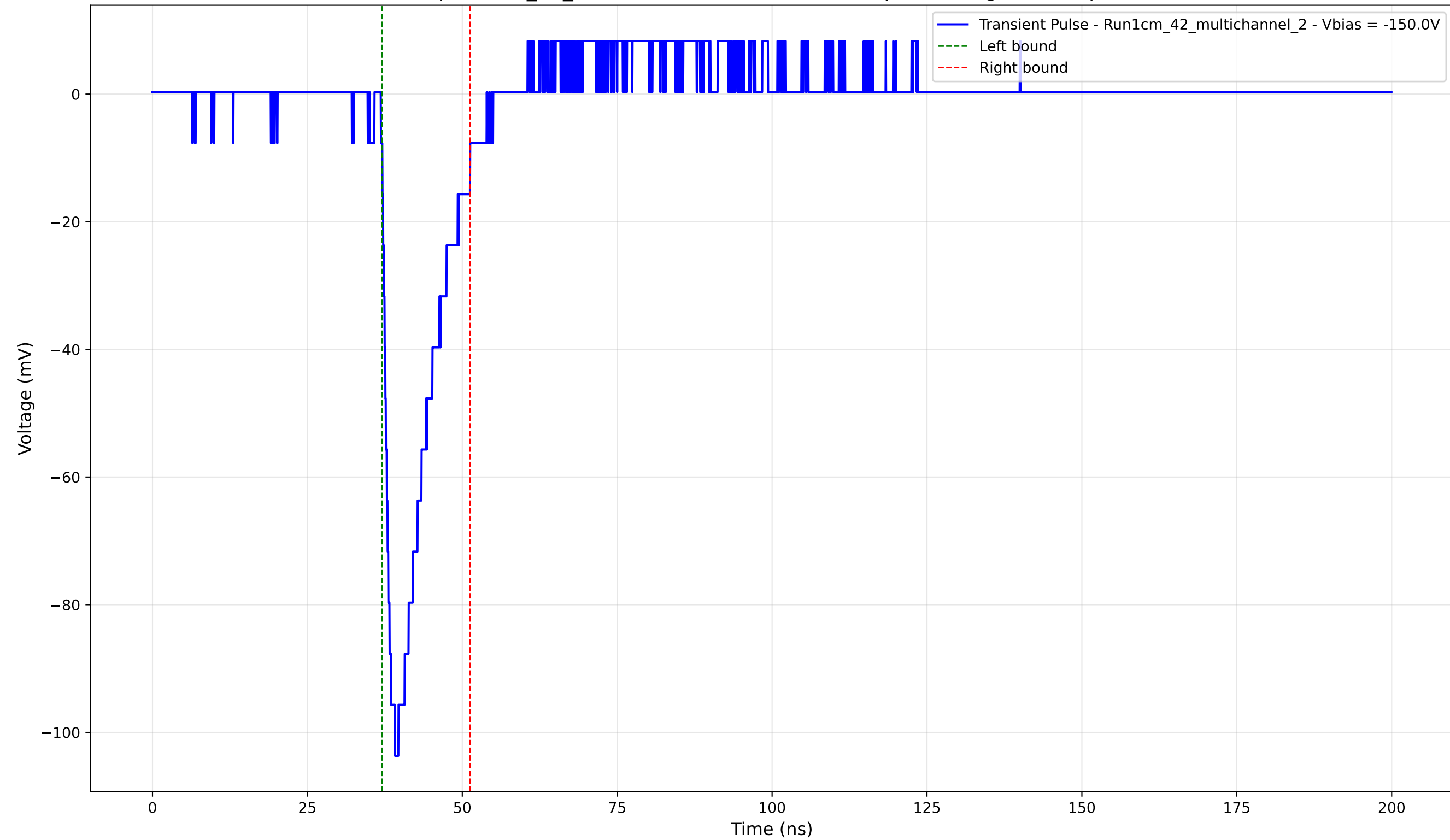
Transient Pulse - Sample: 1cm_42_multichannel - Position: 635.0 \mu\text{m} - Charge: 14.94 pC - Rise Time: 1.43 ns
