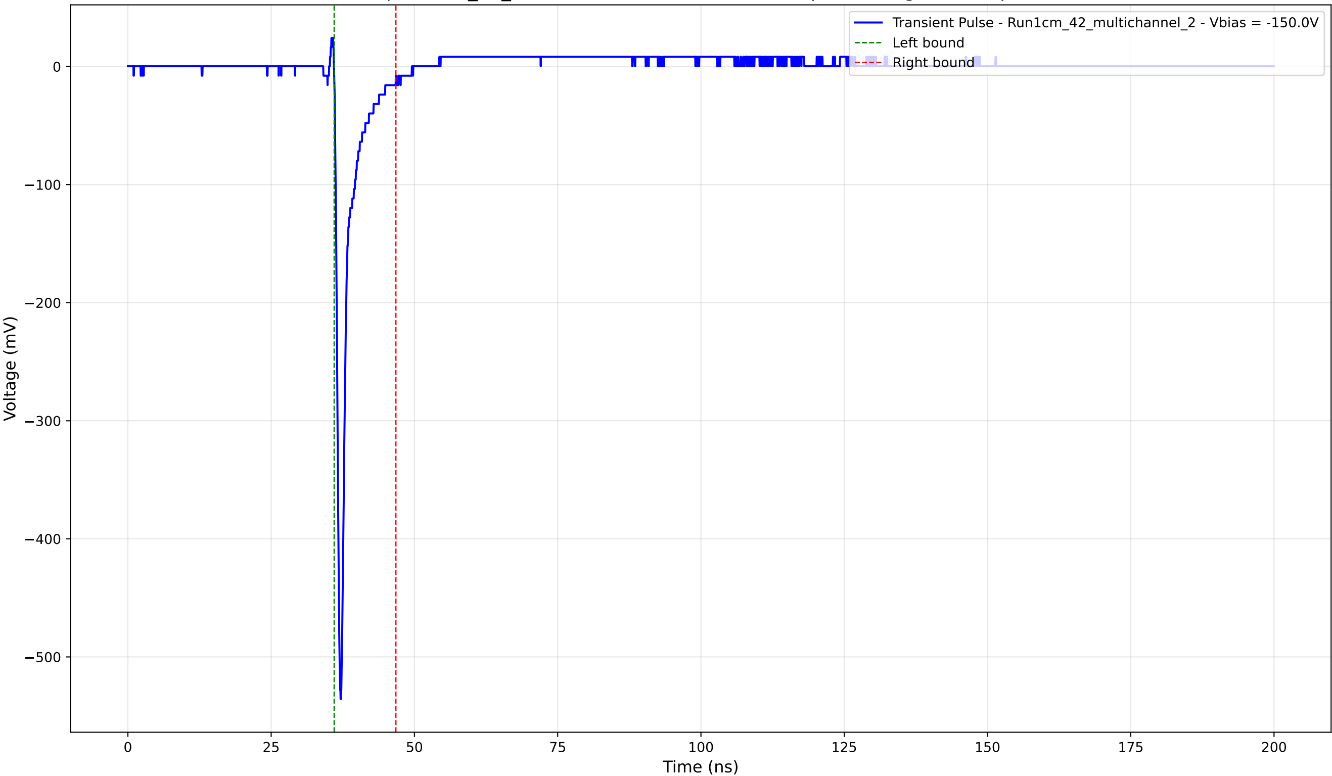
Transient Pulse - Sample: 1cm_42_multichannel - Position: 2435.0 \mu\text{m} - Charge: 23.22 pC - Rise Time: 0.70 ns
