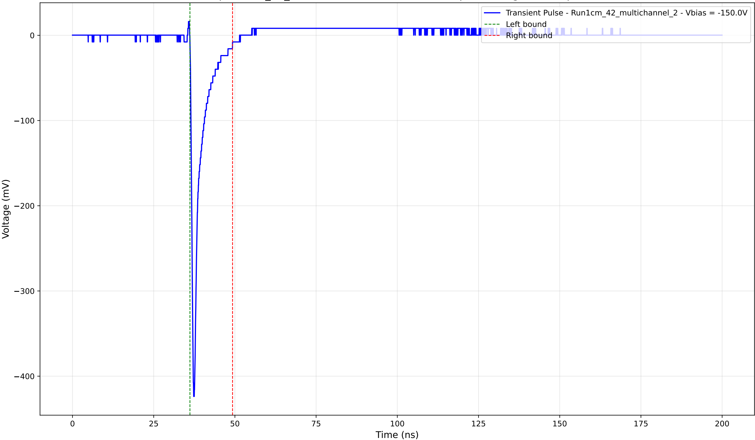
Transient Pulse - Sample: 1cm_42_multichannel - Position: 1990.0 \mu\text{m} - Charge: 25.89 pC - Rise Time: 0.78 ns
