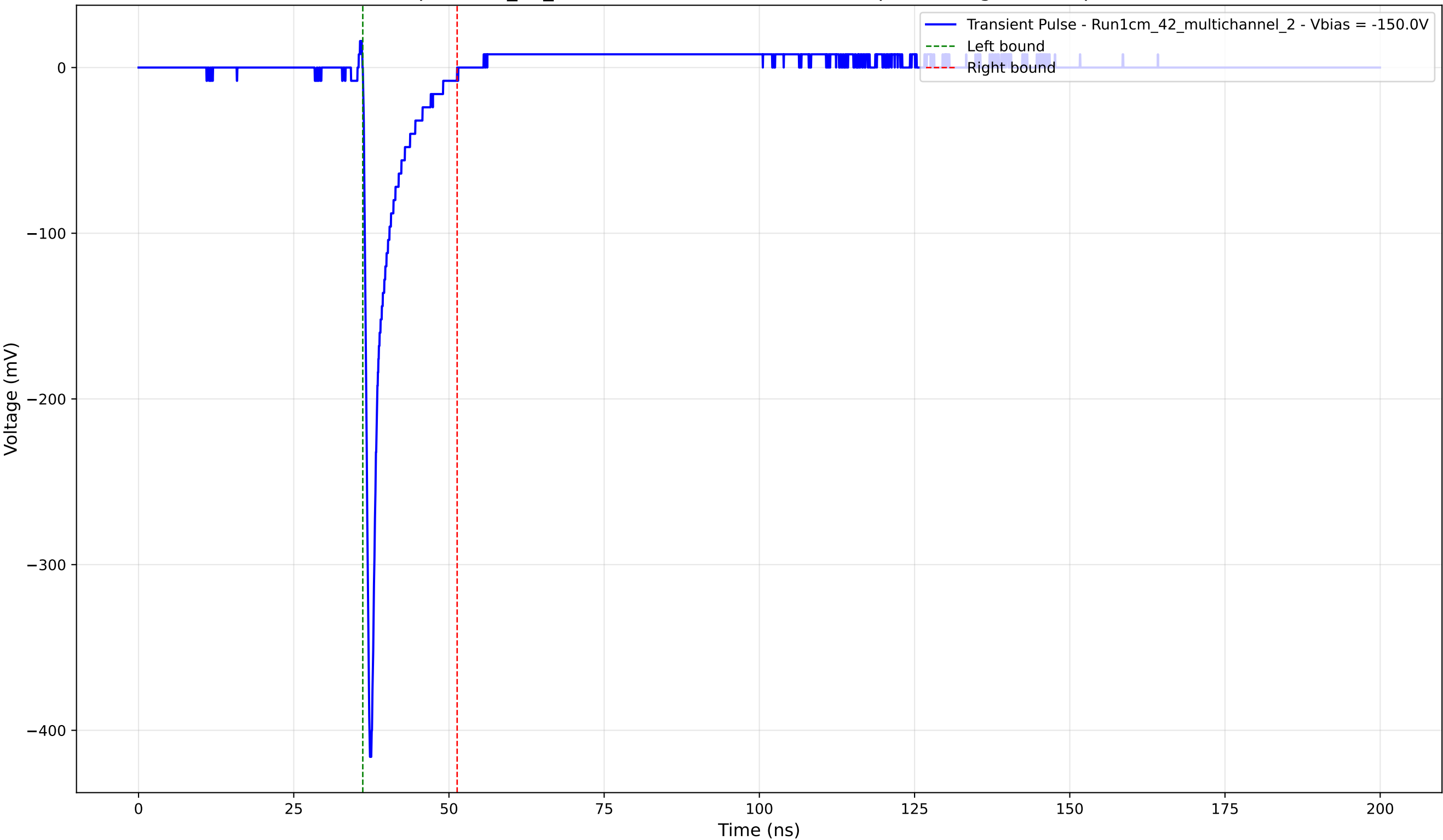
Transient Pulse - Sample: 1cm_42_multichannel - Position: 2730.0 \mu\text{m} - Charge: 25.34 pC - Rise Time: 0.77 ns
