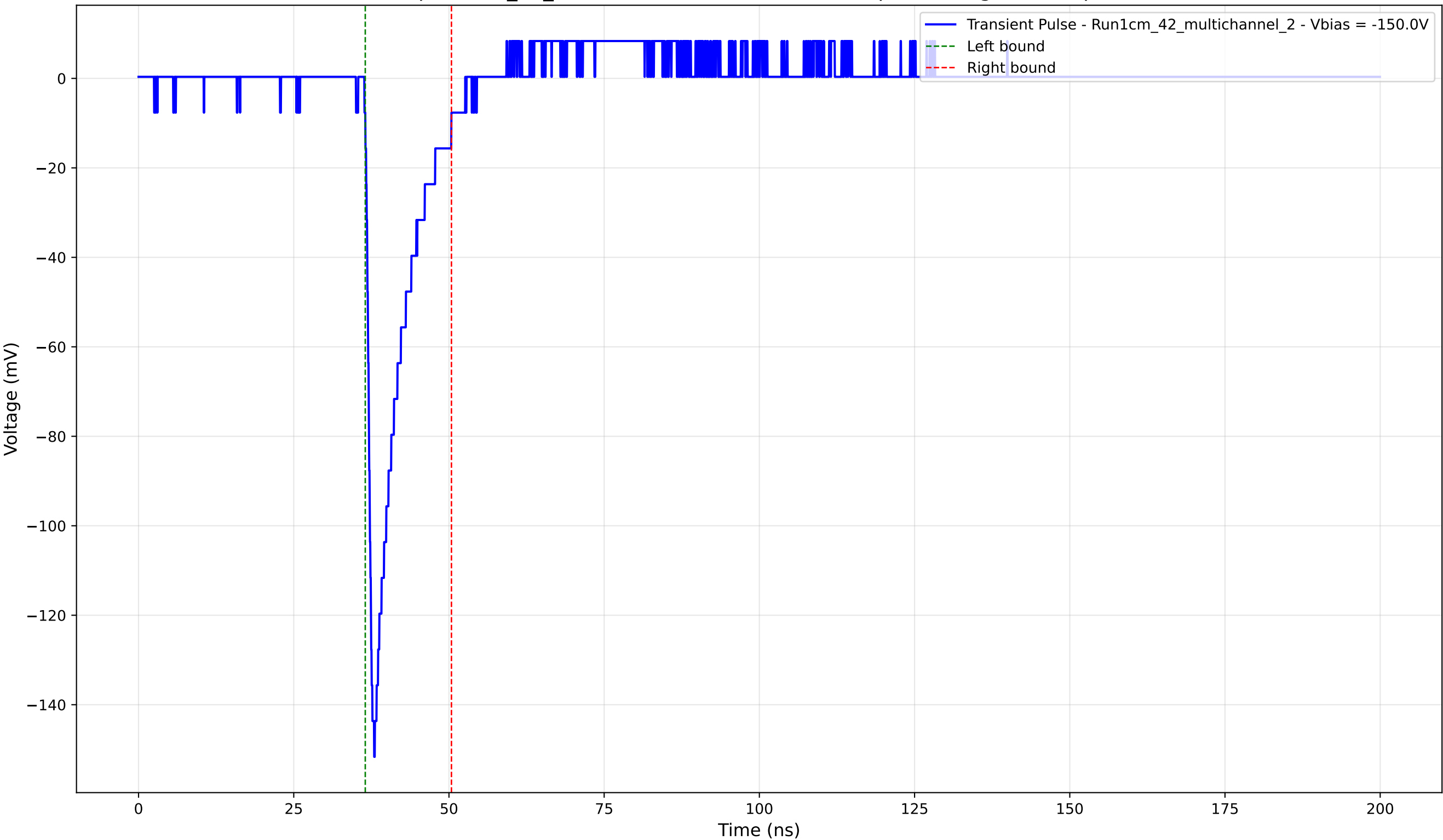
Transient Pulse - Sample: 1cm_42_multichannel - Position: 1420.0 \mu\text{m} - Charge: 15.85 pC - Rise Time: 1.12 ns
