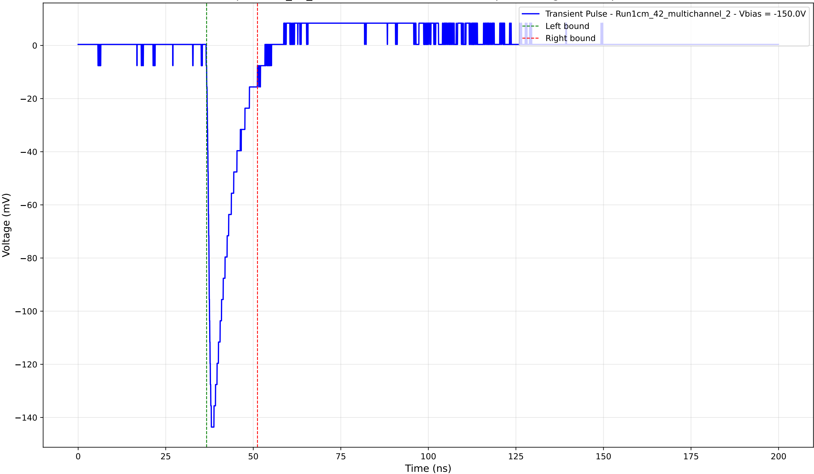
Transient Pulse - Sample: 1cm_42_multichannel - Position: 1175.0 \mu\text{m} - Charge: 18.39 pC - Rise Time: 1.17 ns
