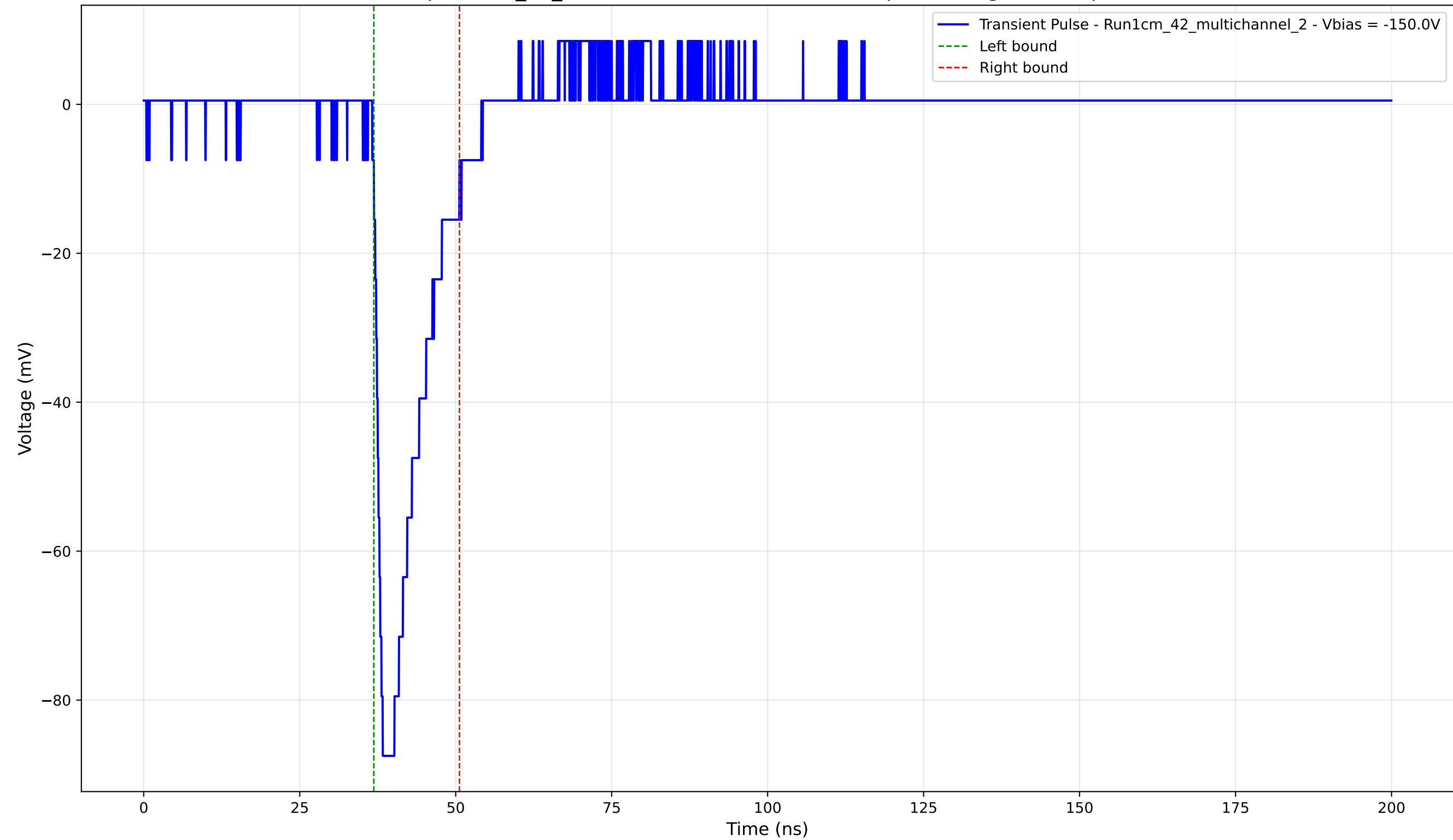
Transient Pulse - Sample: 1cm_42_multichannel - Position: 3815.0 \mu\text{m} - Charge: 12.64 pC - Rise Time: 1.23 ns
