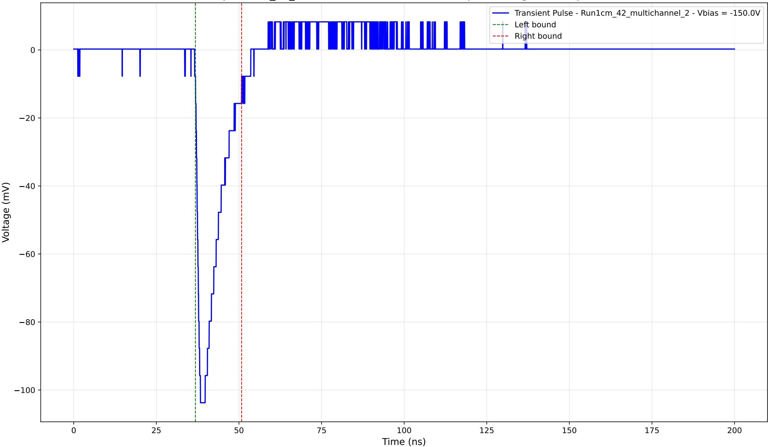
Transient Pulse - Sample: 1cm_42_multichannel - Position: 3775.0 \mu\text{m} - Charge: 14.73 pC - Rise Time: 1.27 ns
