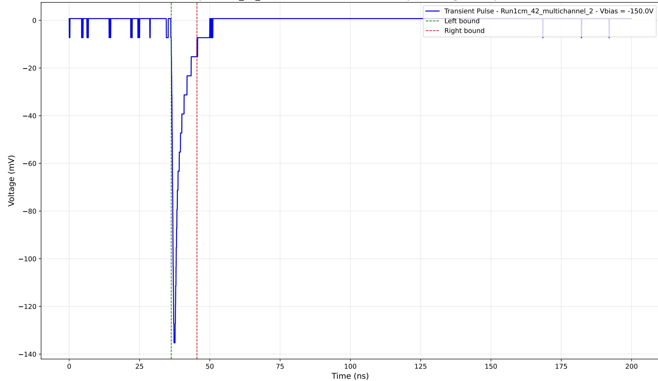
Transient Pulse - Sample: 1cm_42_multichannel - Position: 2830.0 \mu\text{m} - Charge: 8.52 pC - Rise Time: 0.85 ns
