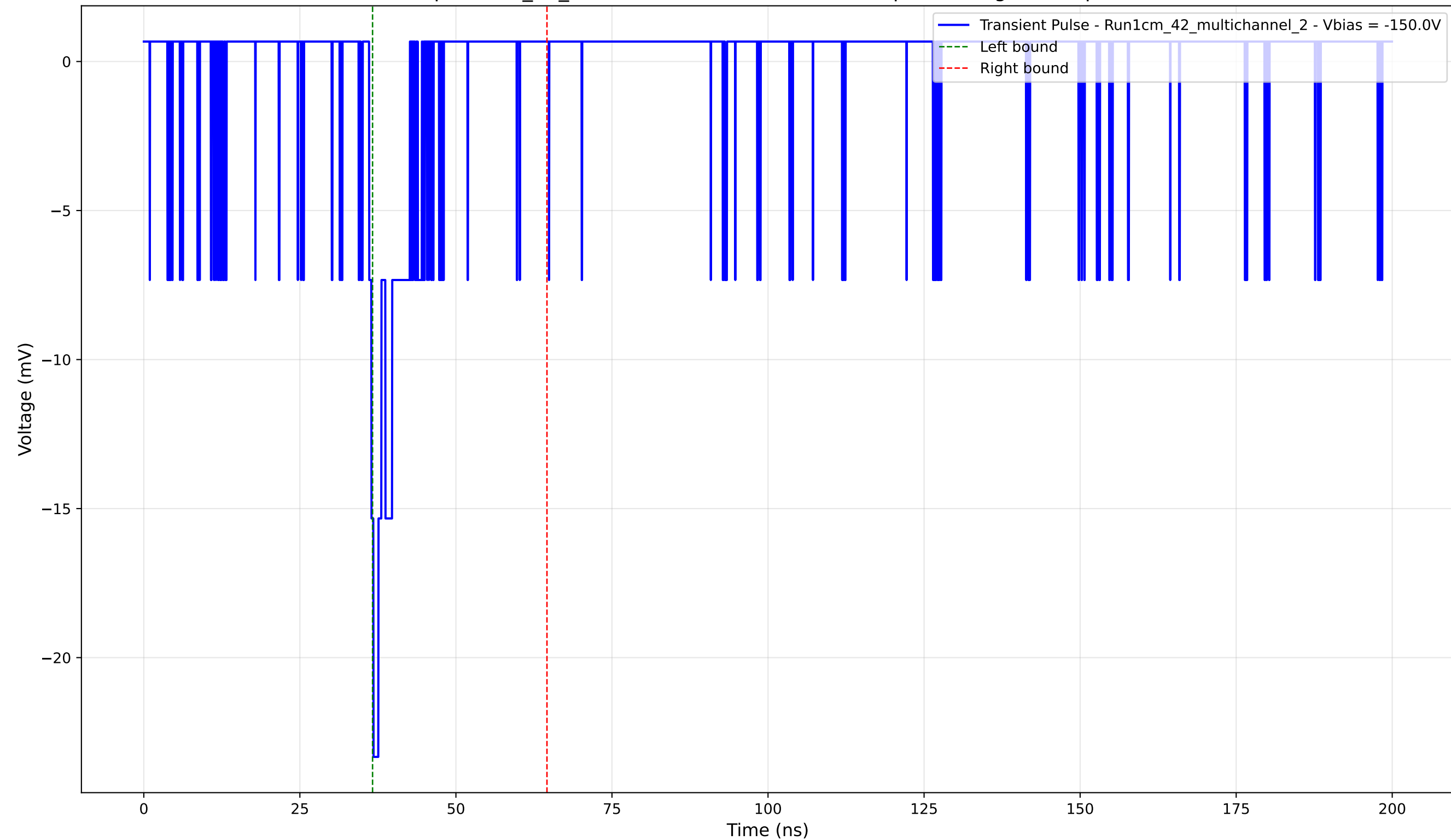
Transient Pulse - Sample: 1cm_42_multichannel - Position: 2370.0 \mu\text{m} - Charge: 1.49 pC - Rise Time: 0.71 ns
