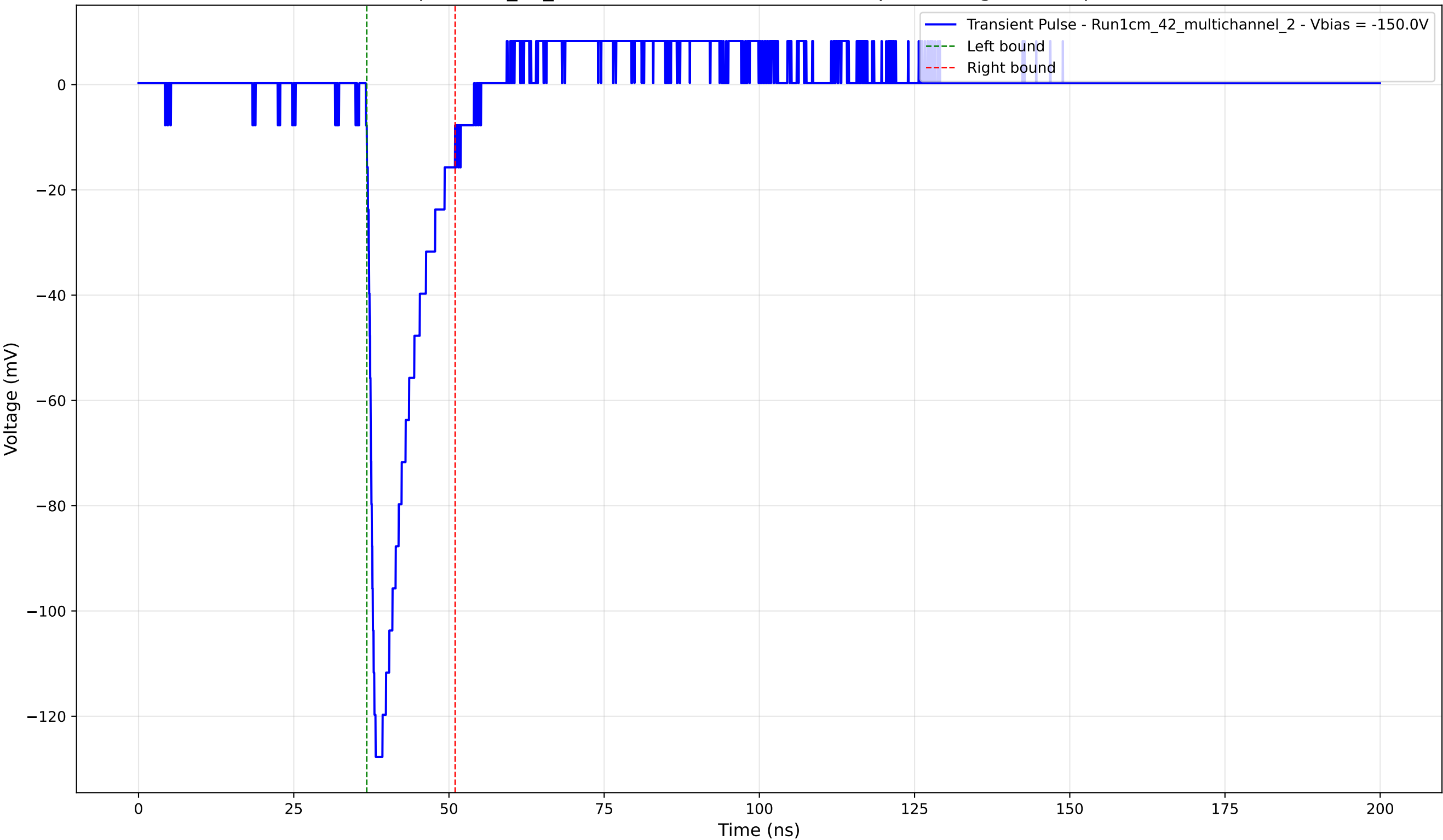
Transient Pulse - Sample: 1cm_42_multichannel - Position: 1050.0 \mu\text{m} - Charge: 17.41 pC - Rise Time: 1.21 ns
