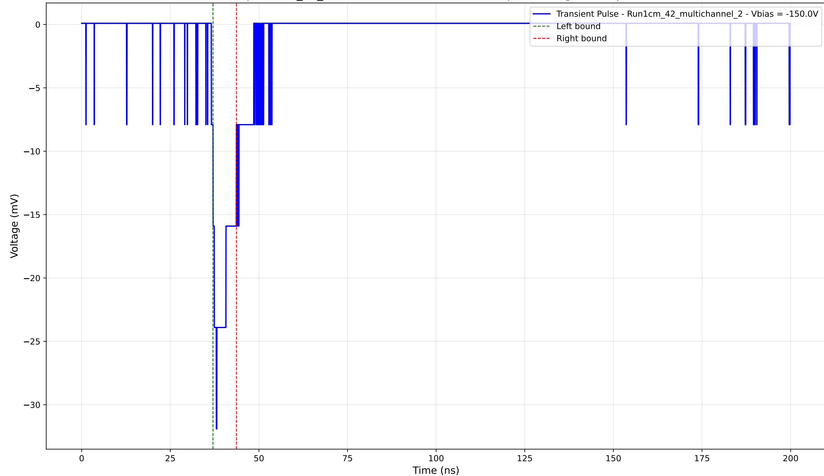
Transient Pulse - Sample: 1cm_42_multichannel - Position: 3415.0 \mu\text{m} - Charge: 2.64 pC - Rise Time: 1.42 ns
