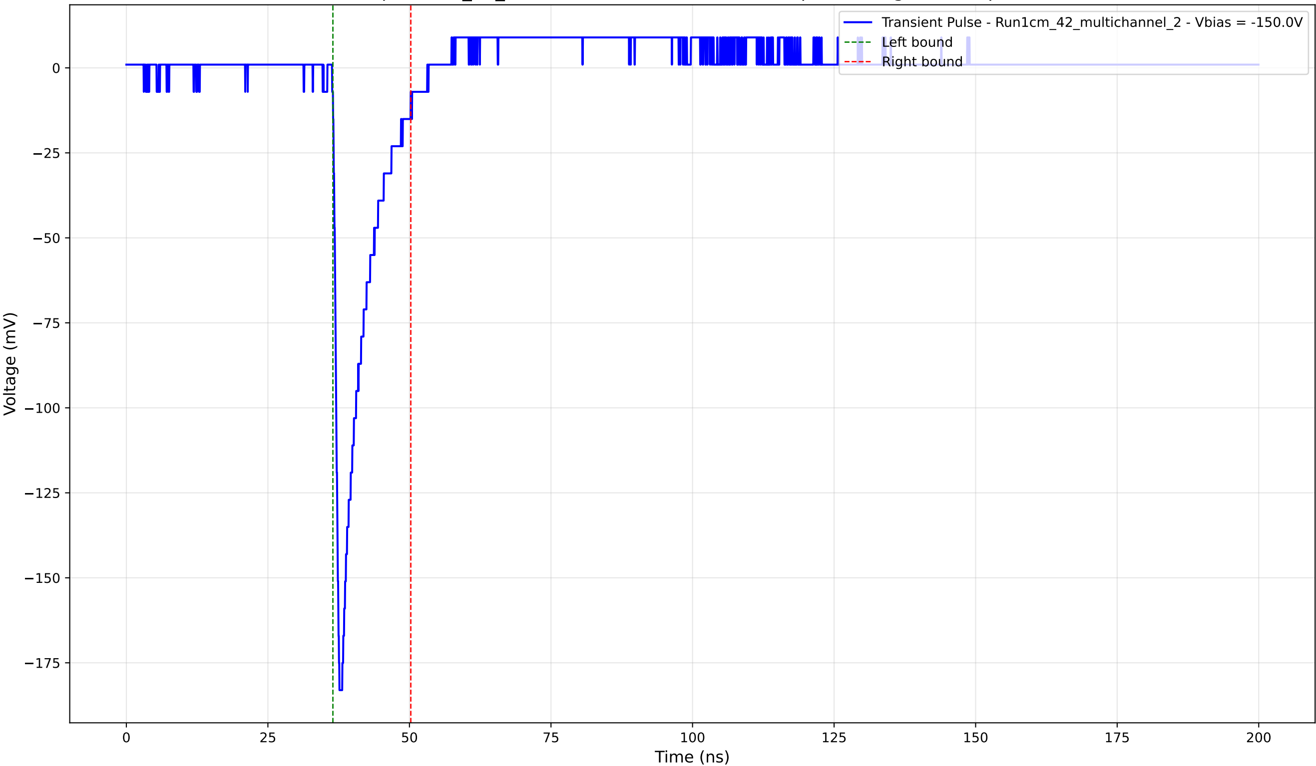
Transient Pulse - Sample: 1cm_42_multichannel - Position: 3245.0 \mu\text{m} - Charge: 18.74 pC - Rise Time: 0.90 ns
