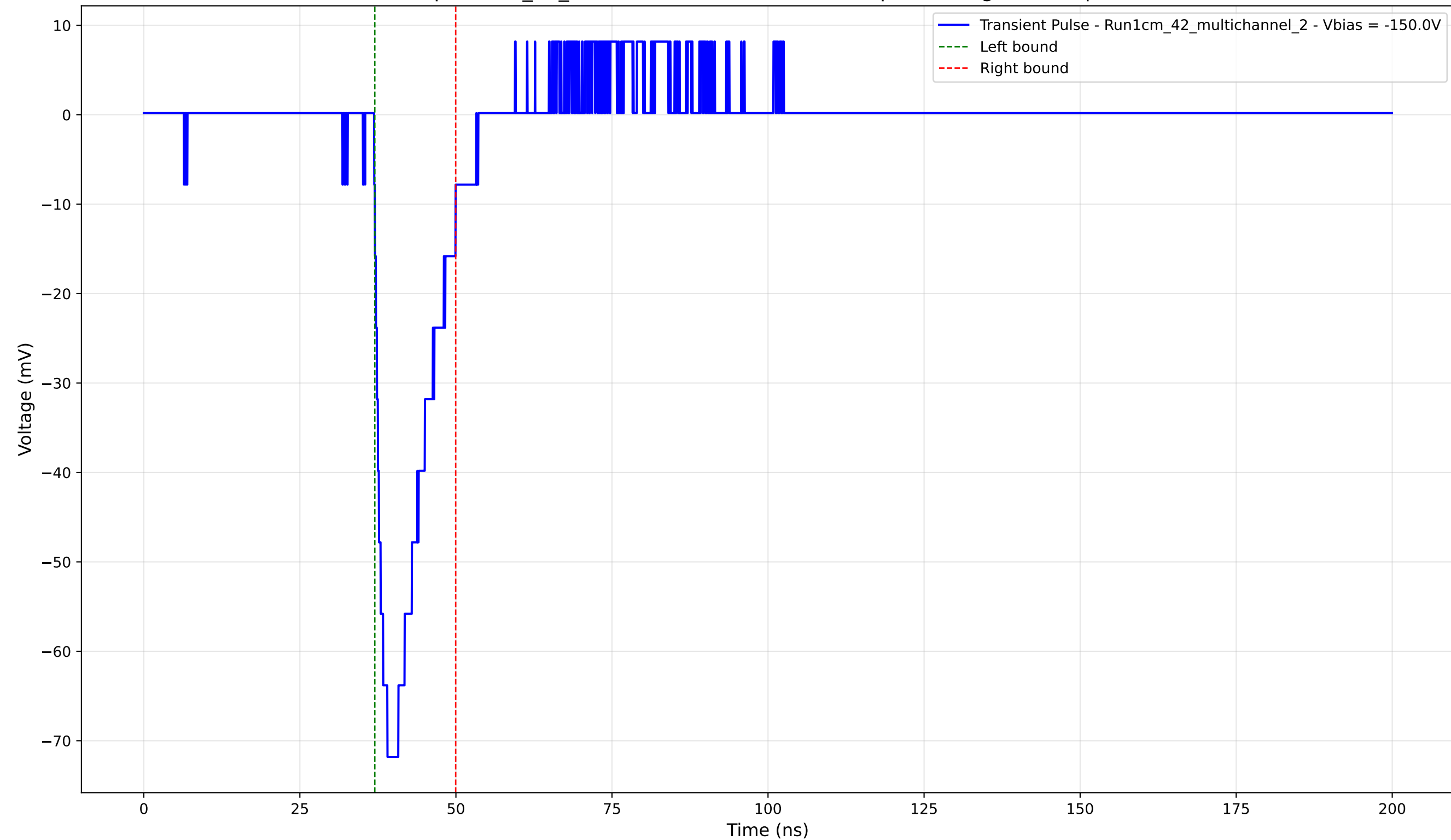
Transient Pulse - Sample: 1cm_42_multichannel - Position: 175.0 \mu\text{m} - Charge: 11.16 pC - Rise Time: 2.12 ns
