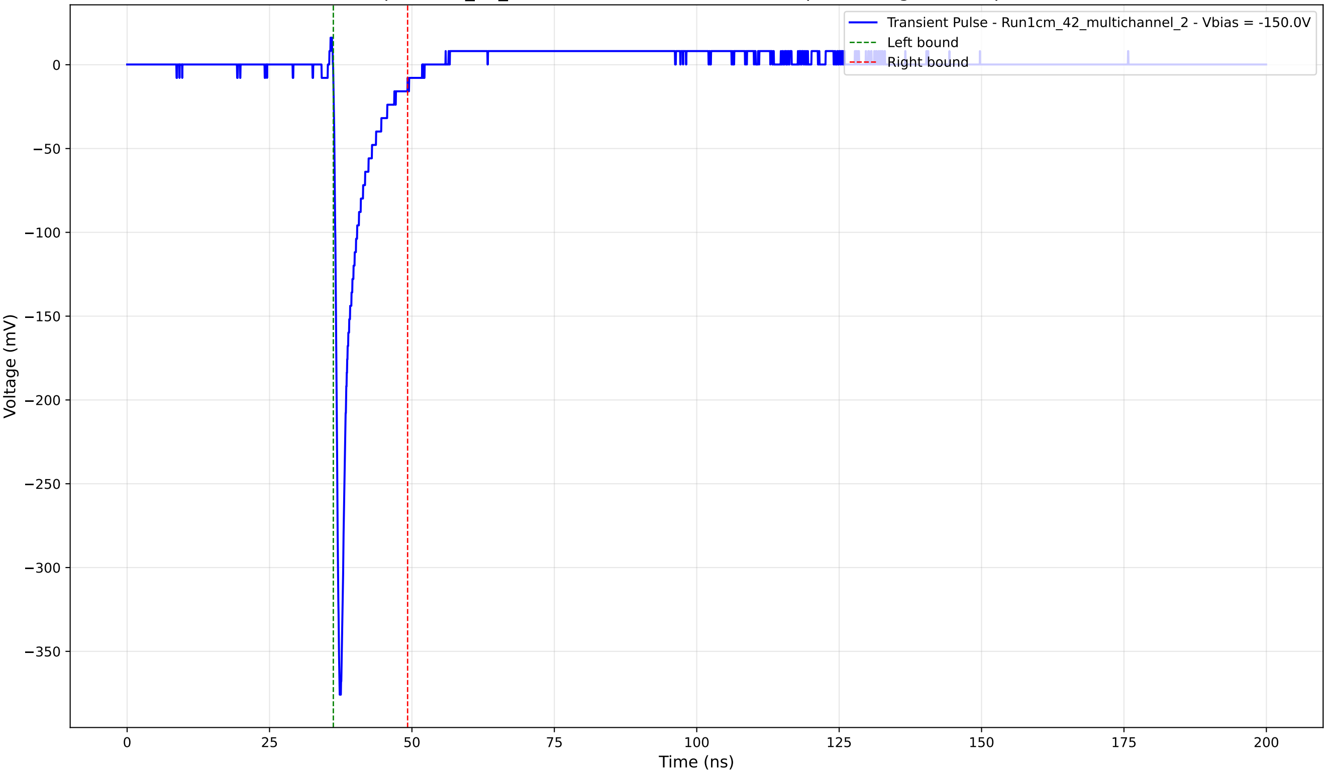
Transient Pulse - Sample: 1cm_42_multichannel - Position: 1955.0 \mu\text{m} - Charge: 23.72 pC - Rise Time: 0.78 ns
