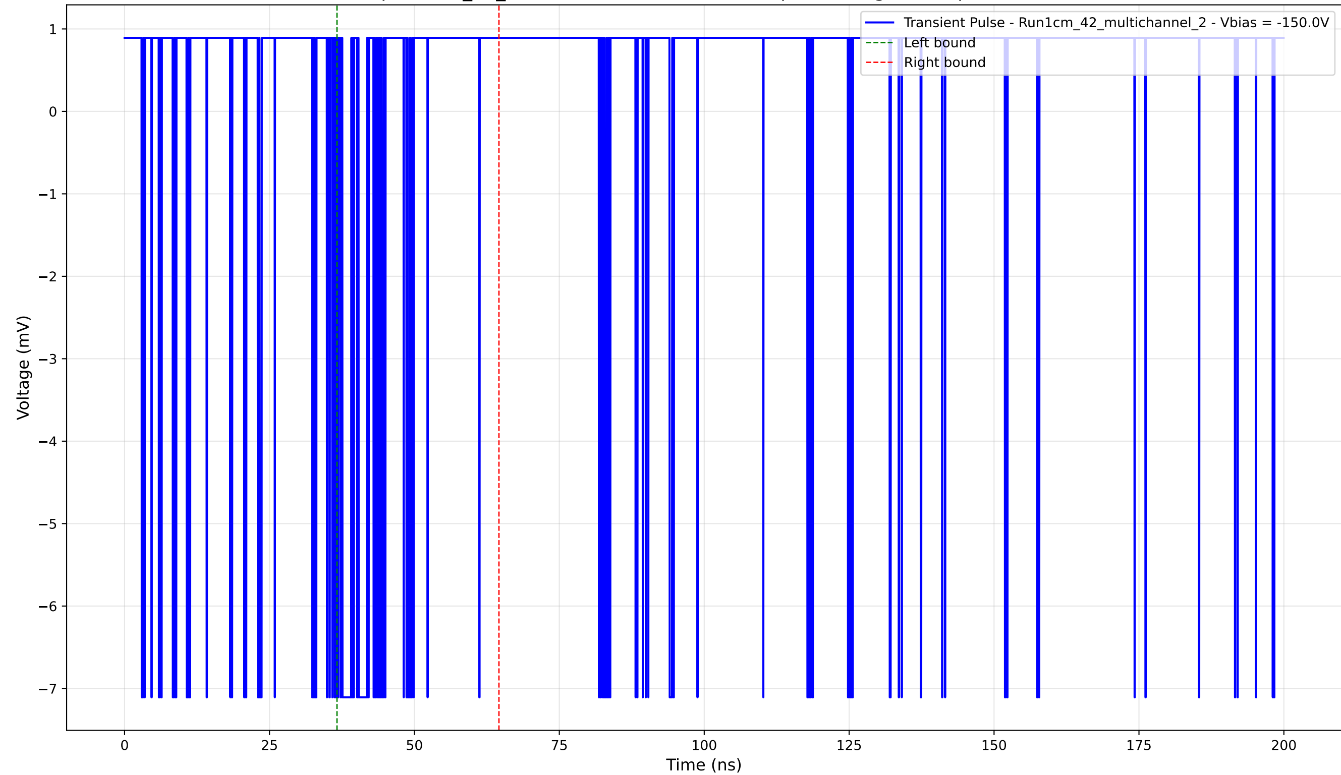
Transient Pulse - Sample: 1cm_42_multichannel - Position: 25.0 \mu\text{m} - Charge: 0.44 pC - Rise Time: 0.00 ns (N/A)
