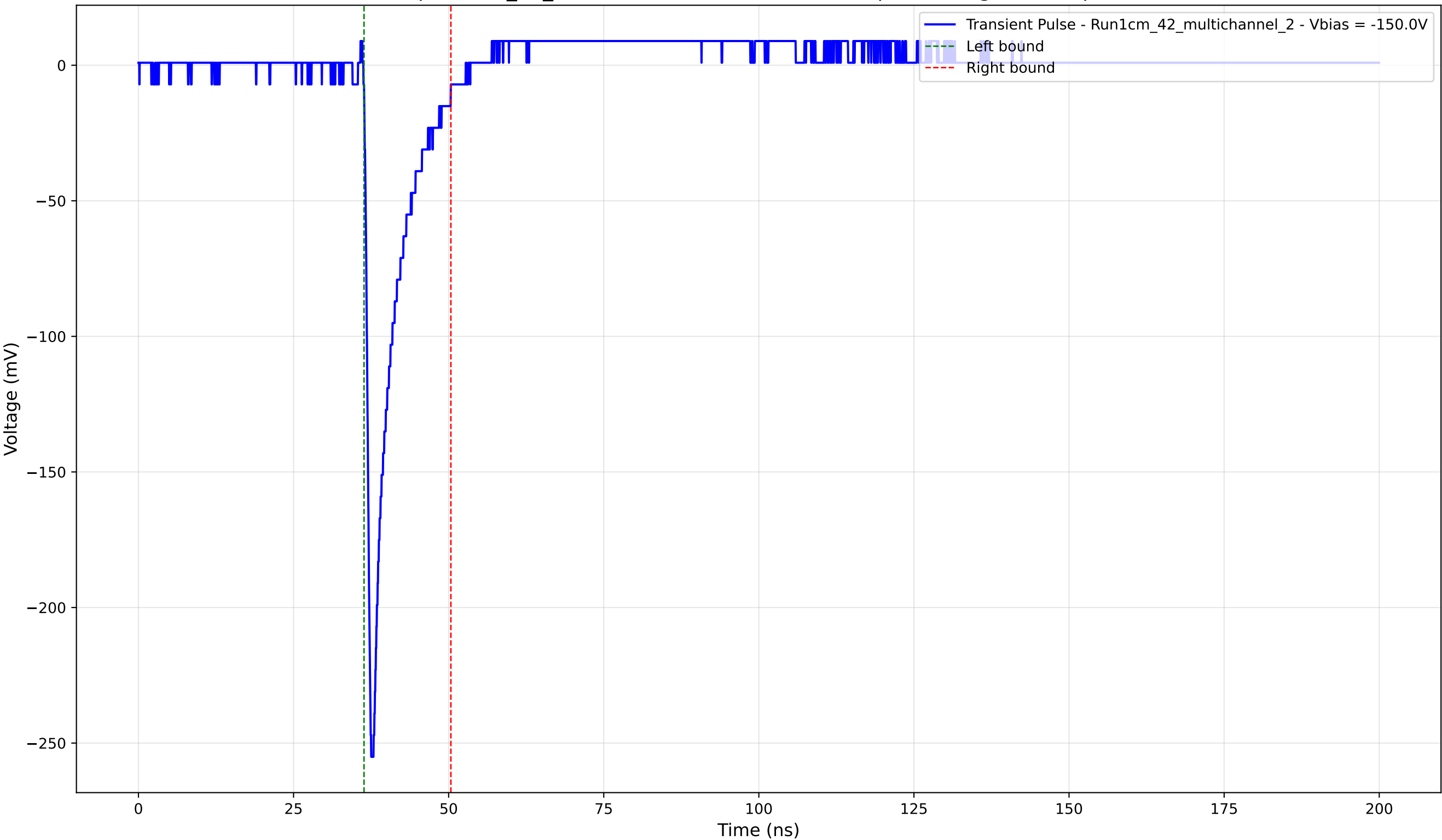
Transient Pulse - Sample: 1cm_42_multichannel - Position: 1660.0 \mu\text{m} - Charge: 22.38 pC - Rise Time: 0.90 ns
