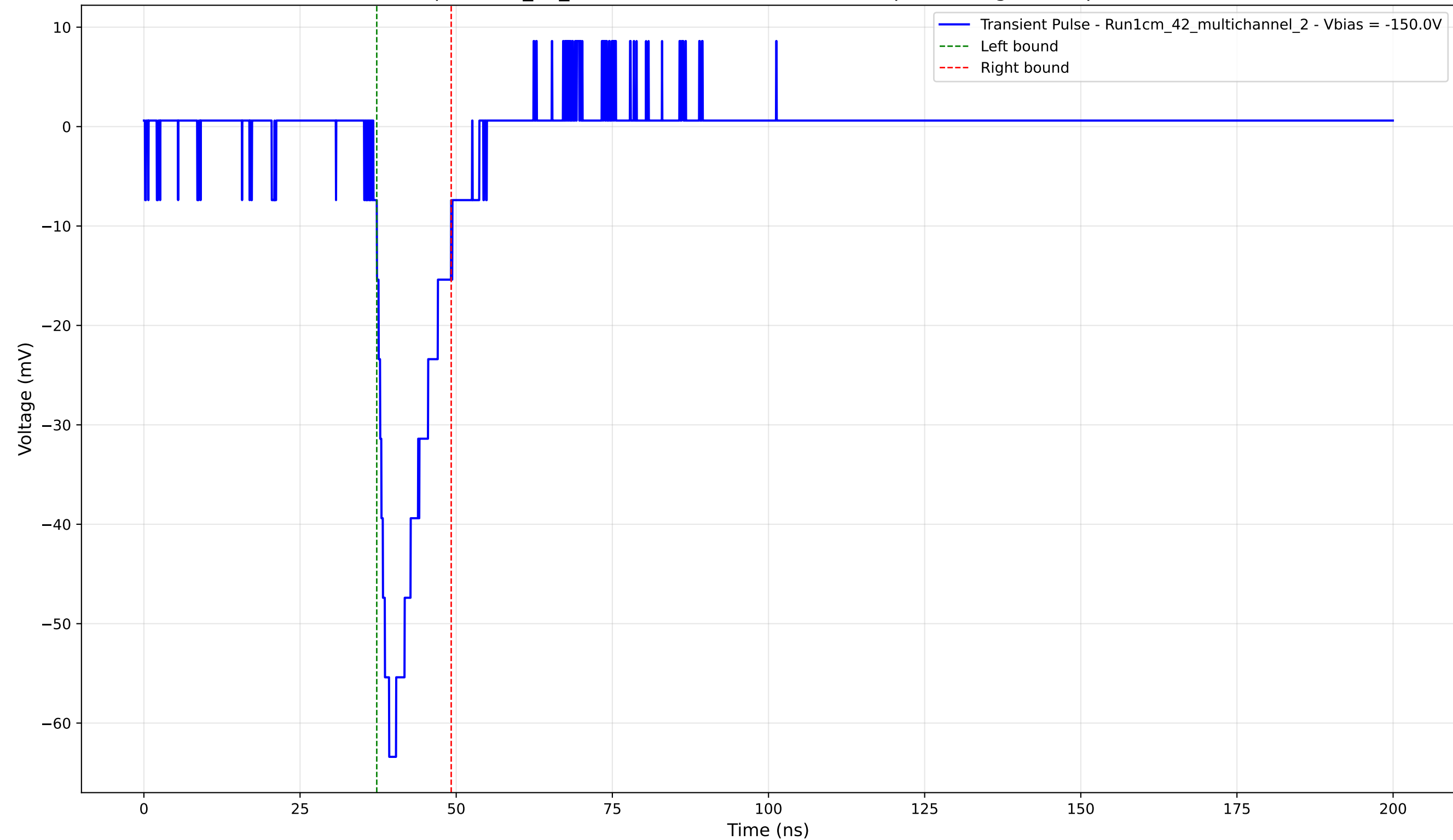
Transient Pulse - Sample: 1cm_42_multichannel - Position: 4460.0 \mu\text{m} - Charge: 8.76 pC - Rise Time: 2.53 ns
