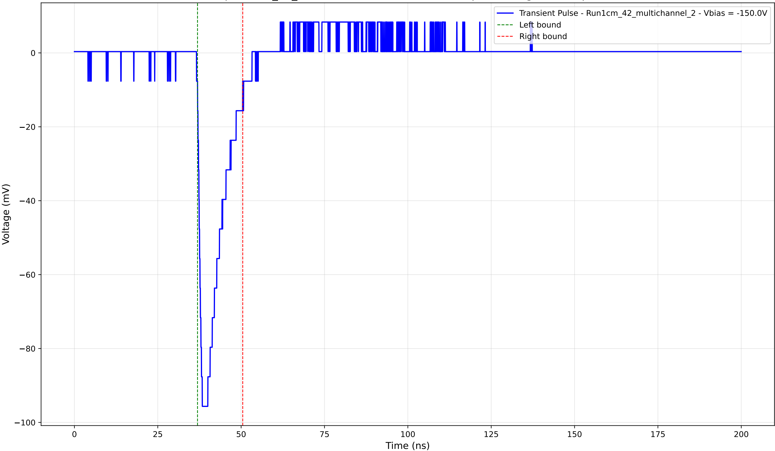
Transient Pulse - Sample: 1cm_42_multichannel - Position: 3805.0 \mu\text{m} - Charge: 13.66 pC - Rise Time: 1.19 ns
