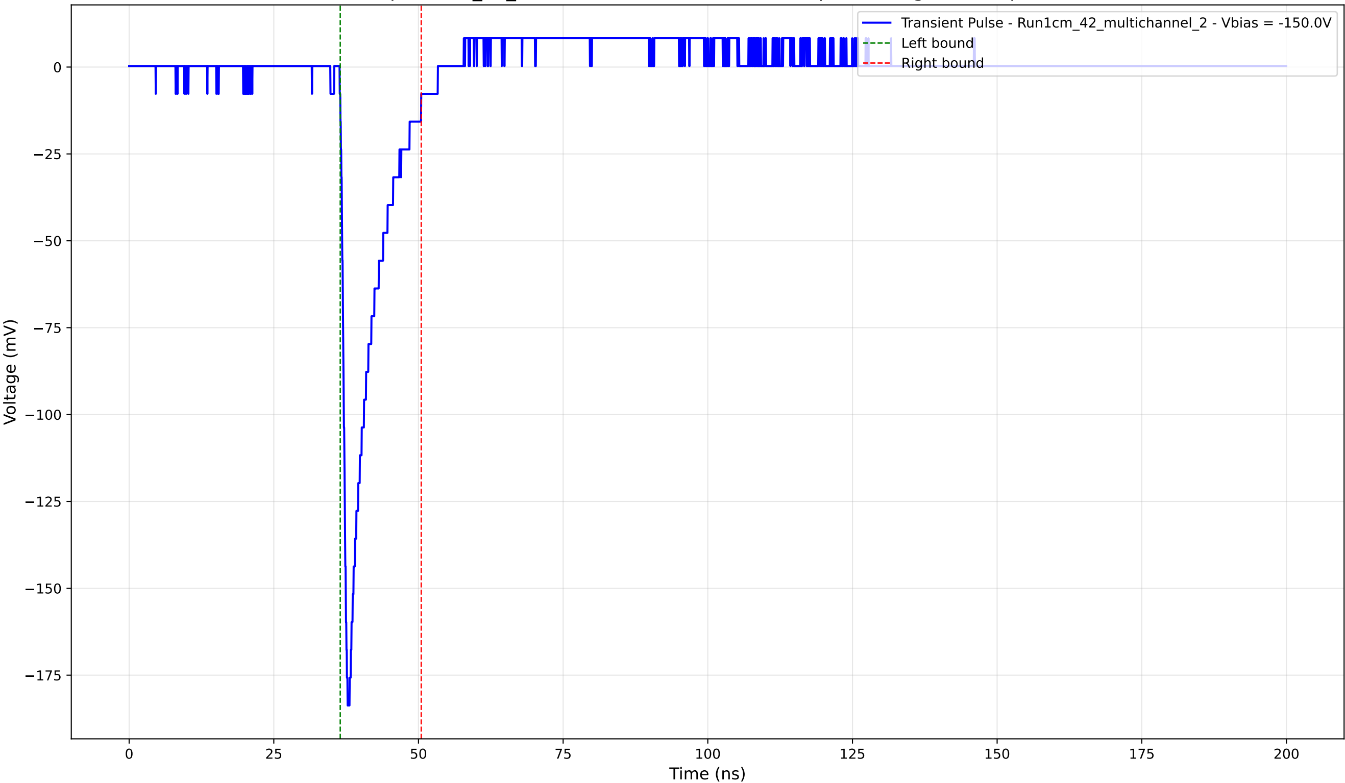
Transient Pulse - Sample: 1cm_42_multichannel - Position: 3265.0 \mu\text{m} - Charge: 18.81 pC - Rise Time: 0.99 ns
