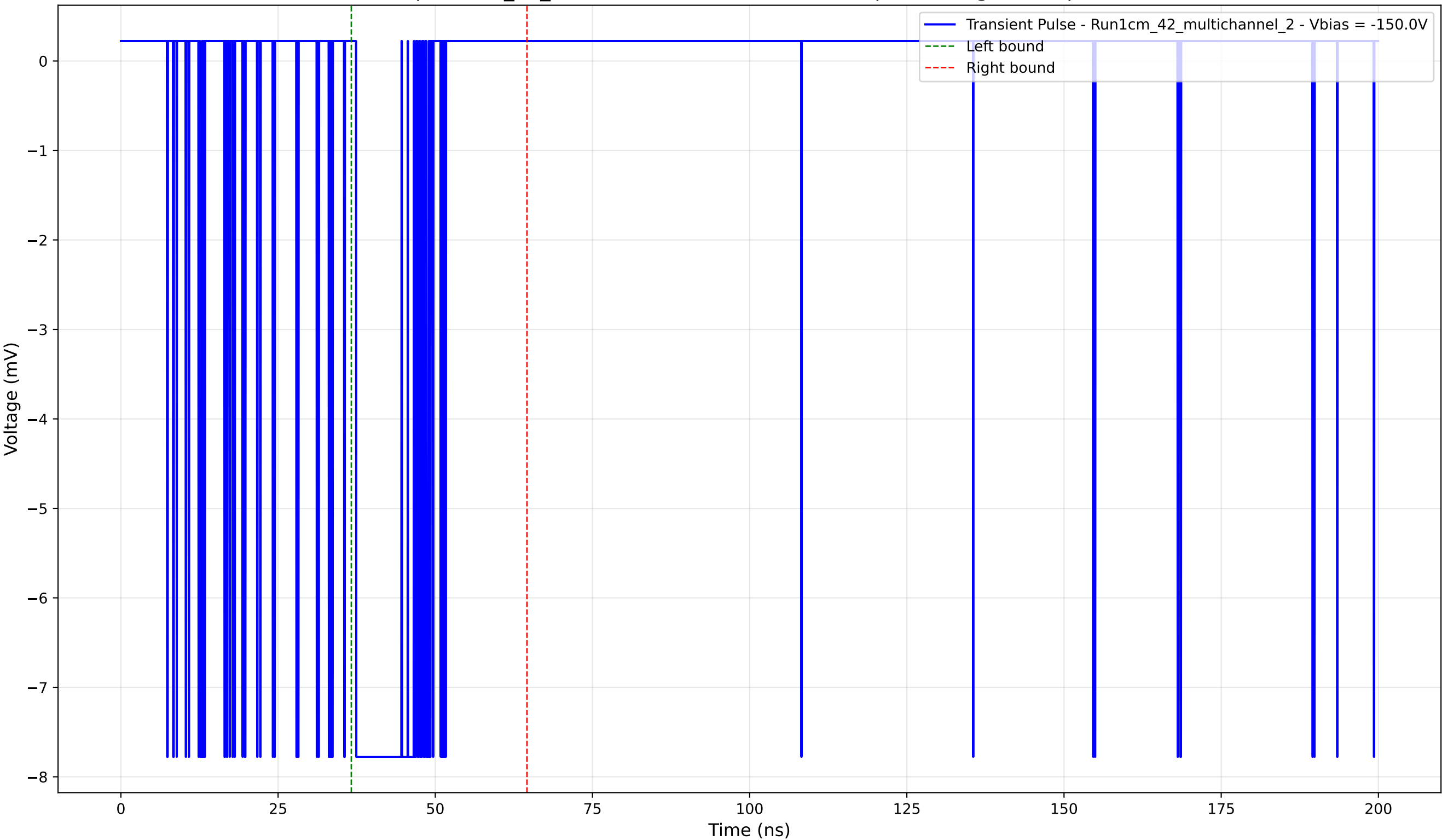
Transient Pulse - Sample: 1cm_42_multichannel - Position: 4360.0 \mu\text{m} - Charge: 1.65 pC - Rise Time: 0.04 ns
