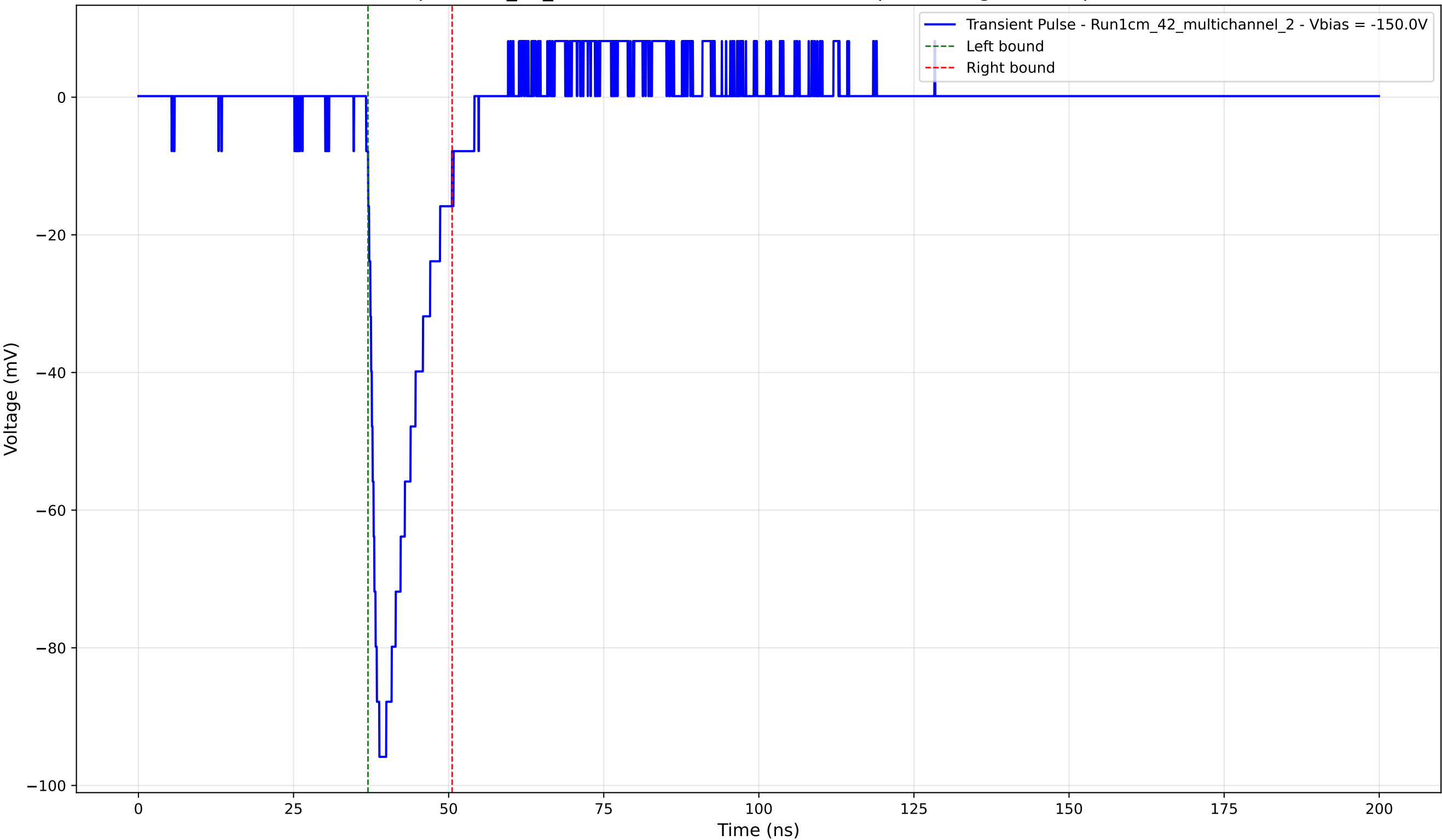
Transient Pulse - Sample: 1cm_42_multichannel - Position: 4005.0 \mu\text{m} - Charge: 13.67 pC - Rise Time: 1.43 ns
