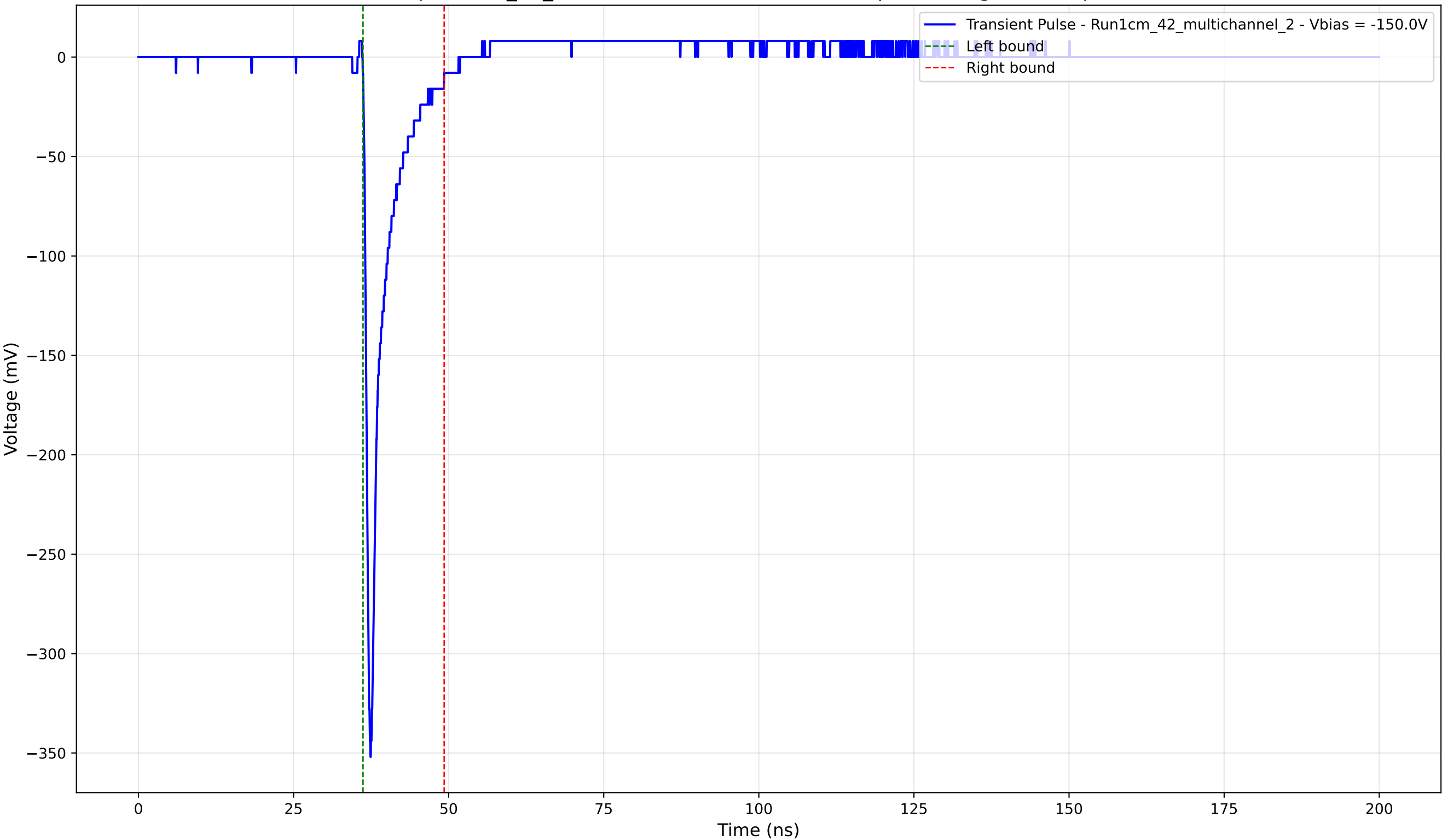
Transient Pulse - Sample: 1cm_42_multichannel - Position: 2790.0 \mu\text{m} - Charge: 22.18 pC - Rise Time: 0.81 ns
