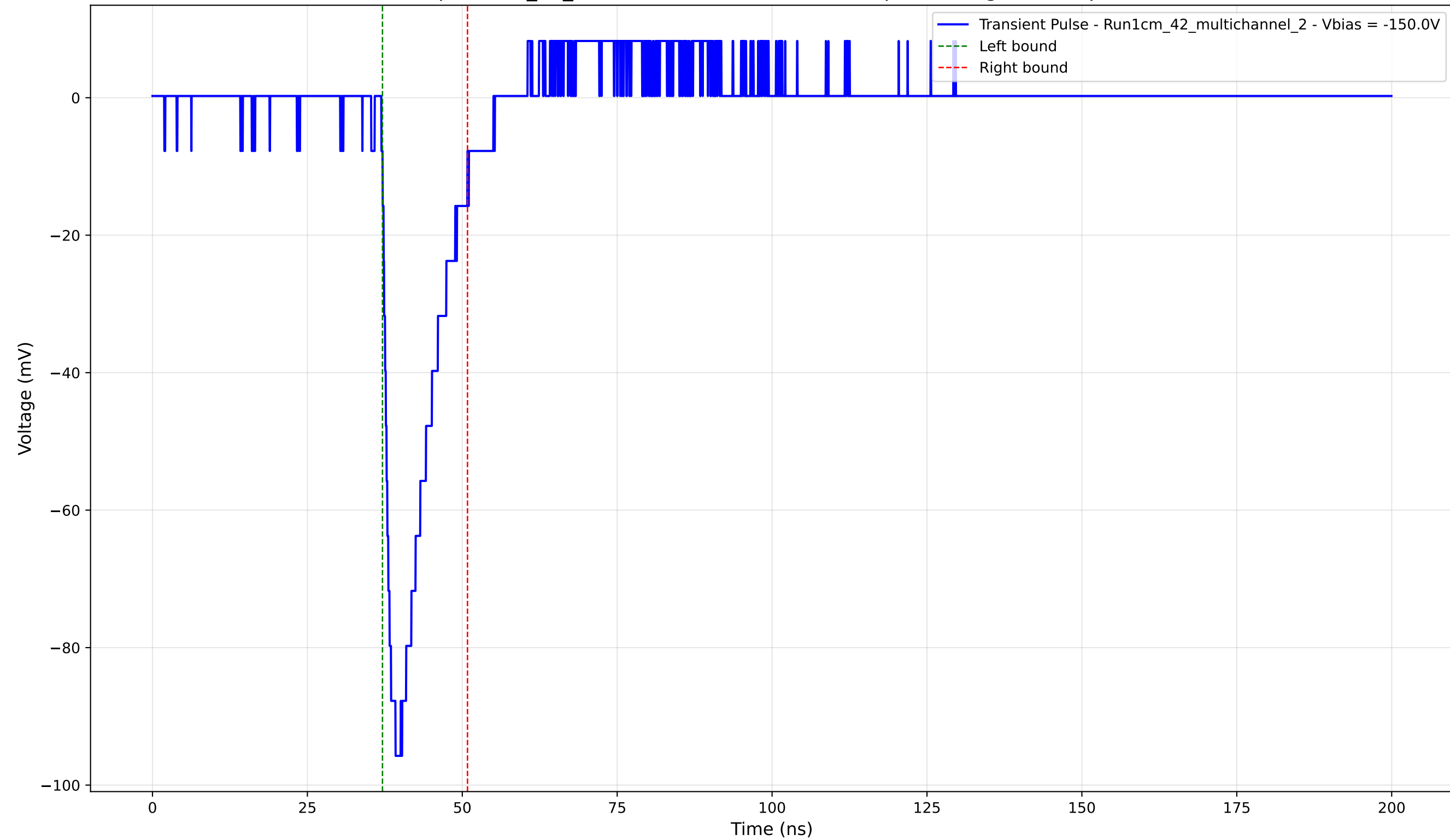
Transient Pulse - Sample: 1cm_42_multichannel - Position: 520.0 \mu\text{m} - Charge: 14.04 pC - Rise Time: 1.39 ns
