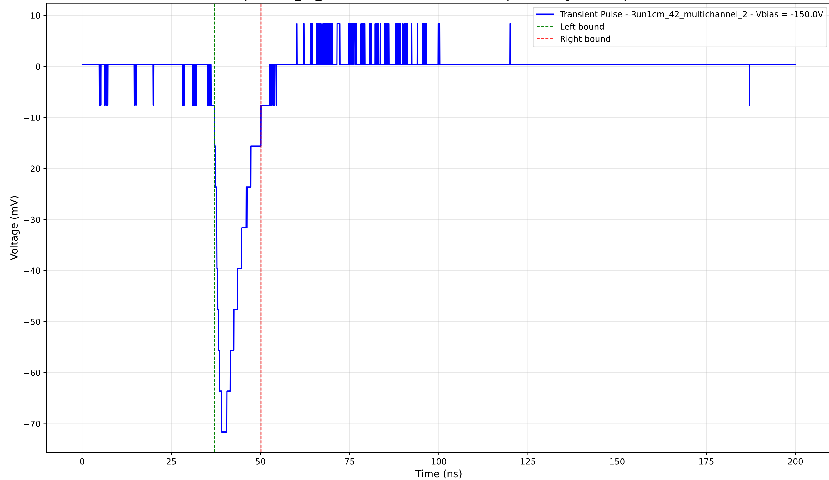
Transient Pulse - Sample: 1cm_42_multichannel - Position: 4655.0 \mu\text{m} - Charge: 10.40 pC - Rise Time: 2.96 ns
