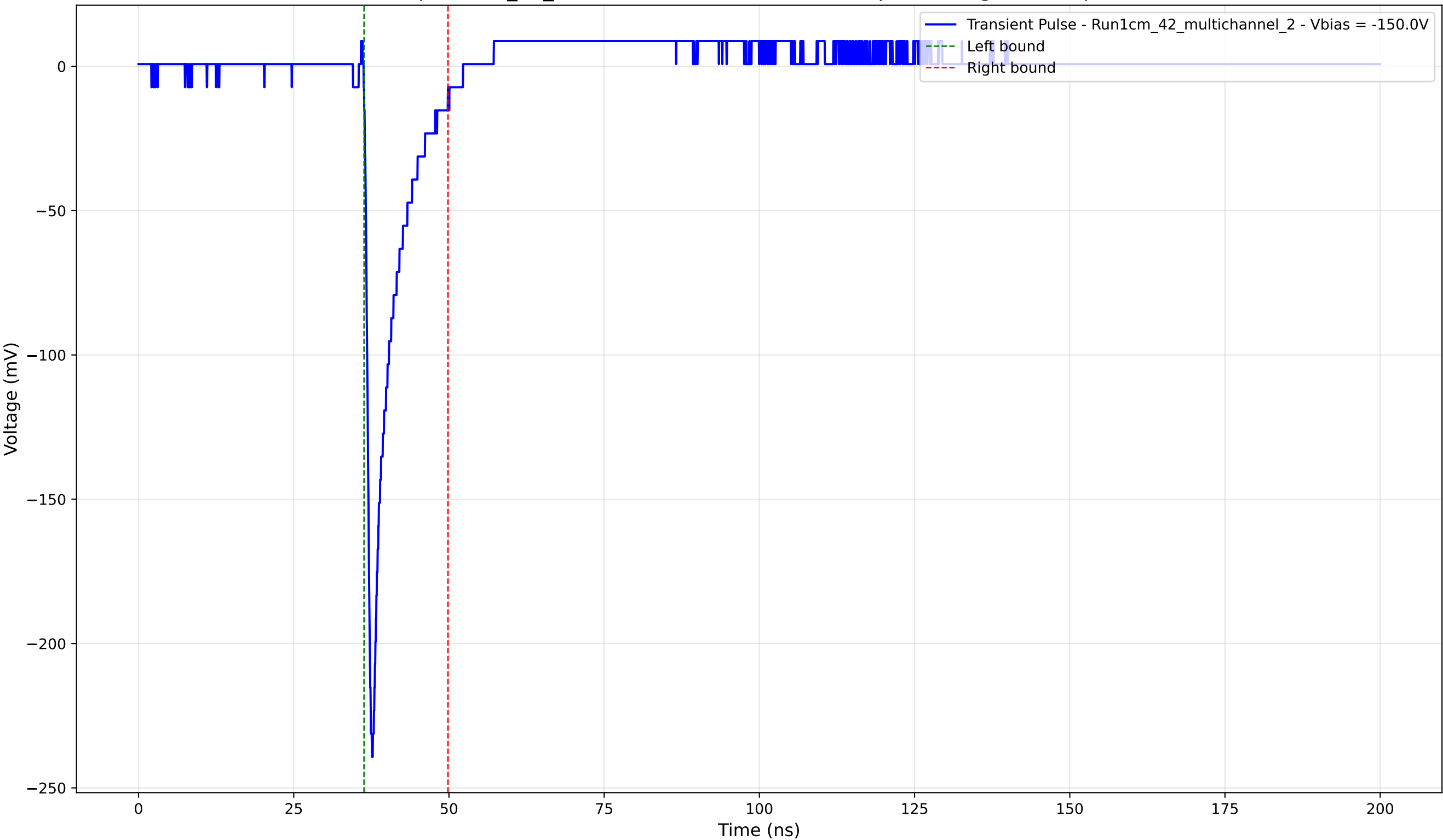
Transient Pulse - Sample: 1cm_42_multichannel - Position: 3045.0 \mu\text{m} - Charge: 19.74 pC - Rise Time: 0.92 ns
