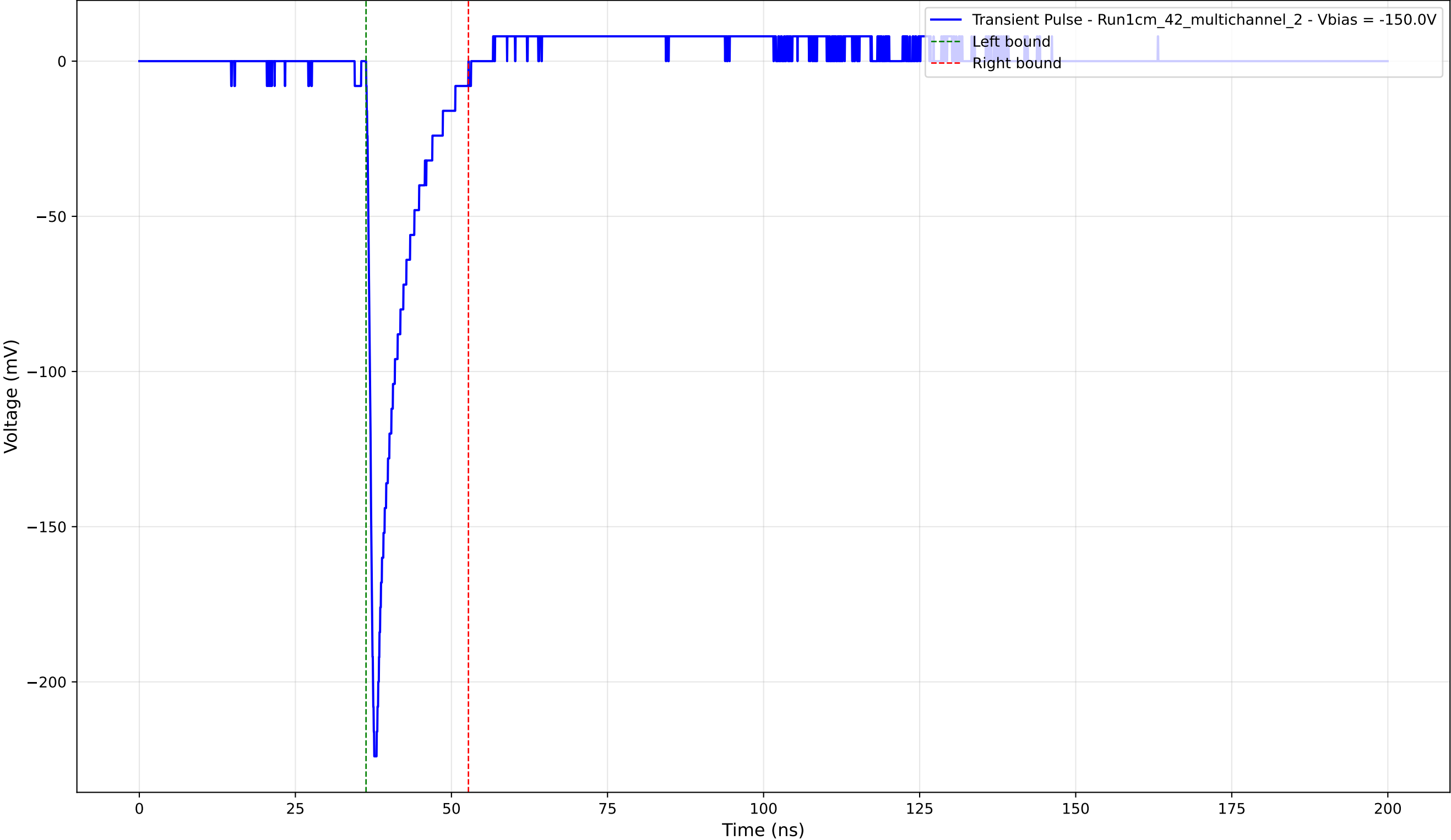
Transient Pulse - Sample: 1cm_42_multichannel - Position: 1555.0 \mu\text{m} - Charge: 21.89 pC - Rise Time: 0.97 ns
