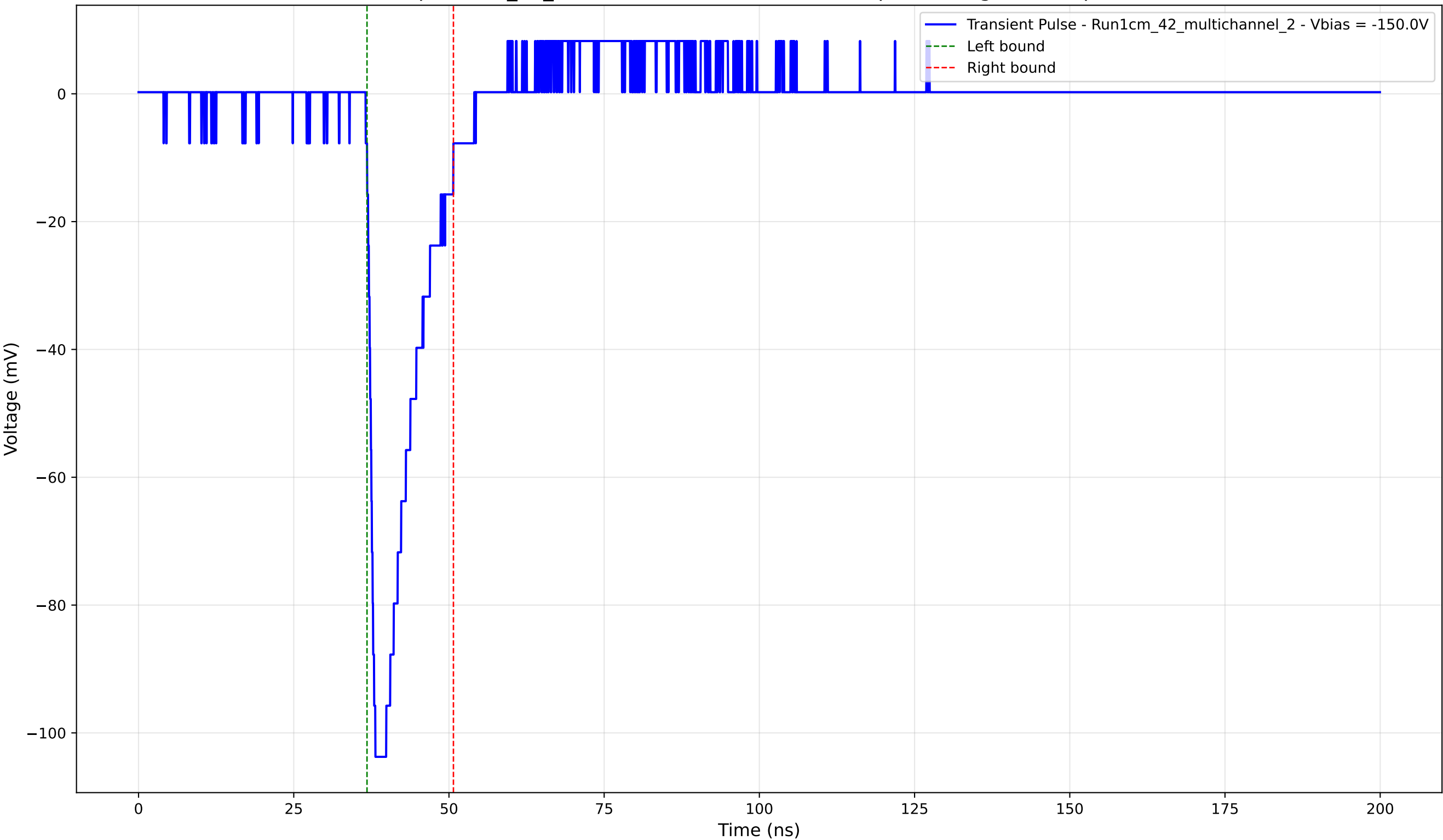
Transient Pulse - Sample: 1cm_42_multichannel - Position: 3725.0 \mu\text{m} - Charge: 14.95 pC - Rise Time: 1.15 ns
