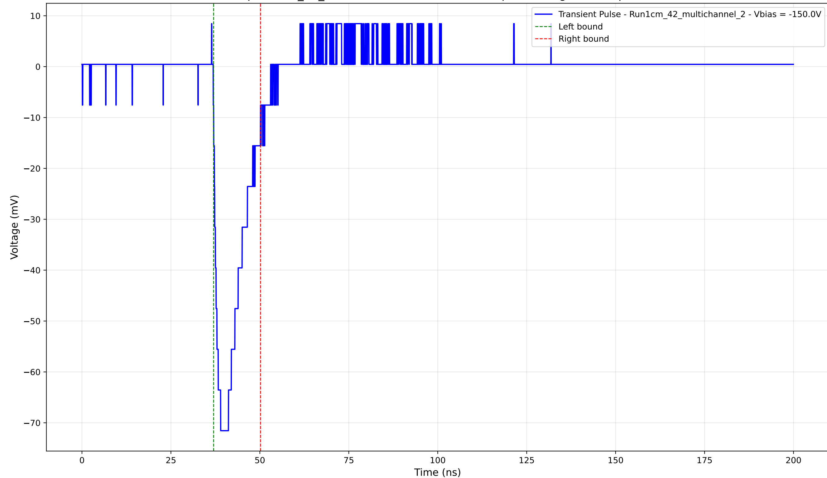
Transient Pulse - Sample: 1cm_42_multichannel - Position: 200.0 \mu\text{m} - Charge: 11.28 pC - Rise Time: 2.08 ns
