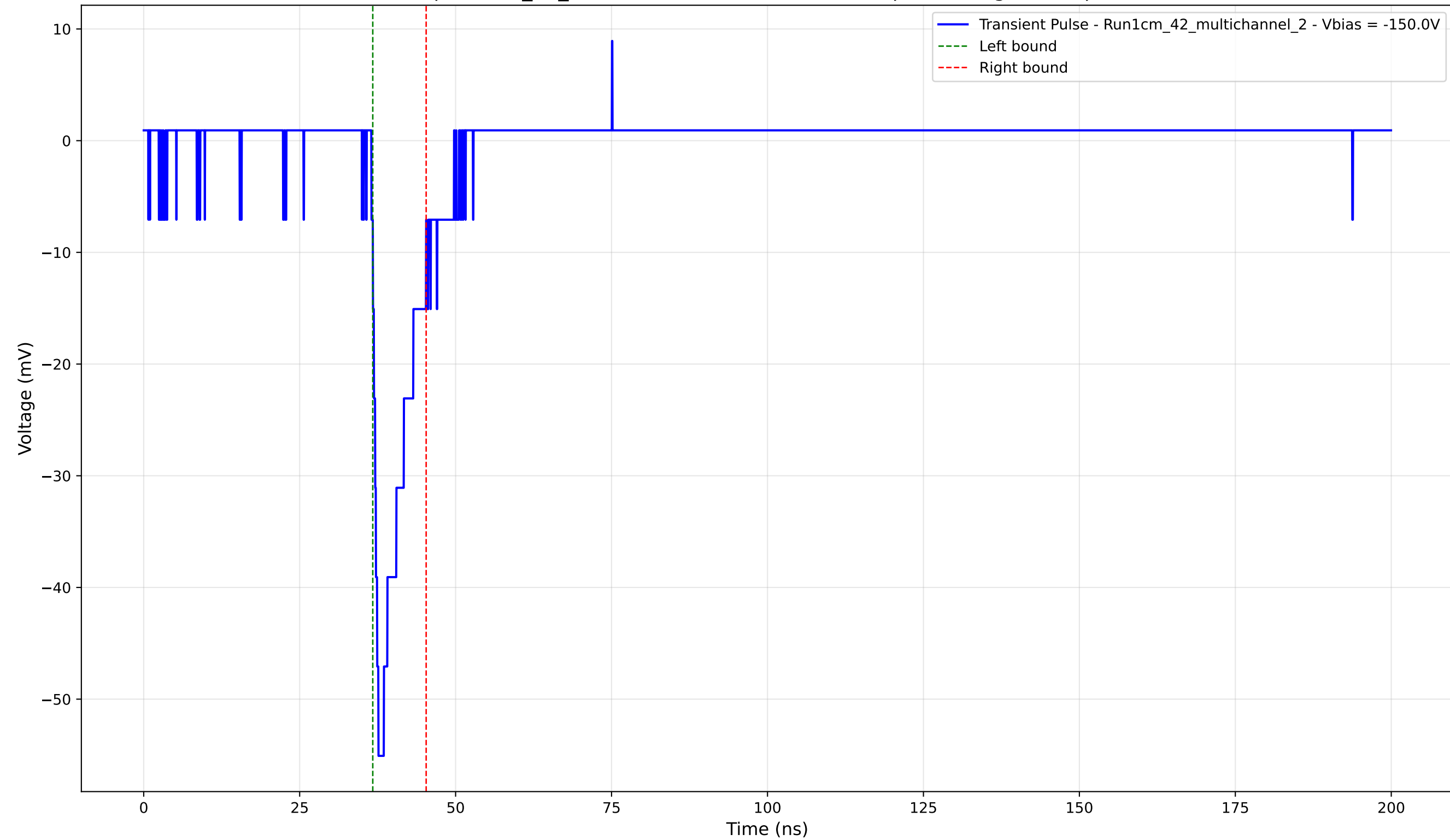
Transient Pulse - Sample: 1cm_42_multichannel - Position: 3340.0 \mu\text{m} - Charge: 5.25 pC - Rise Time: 1.13 ns
