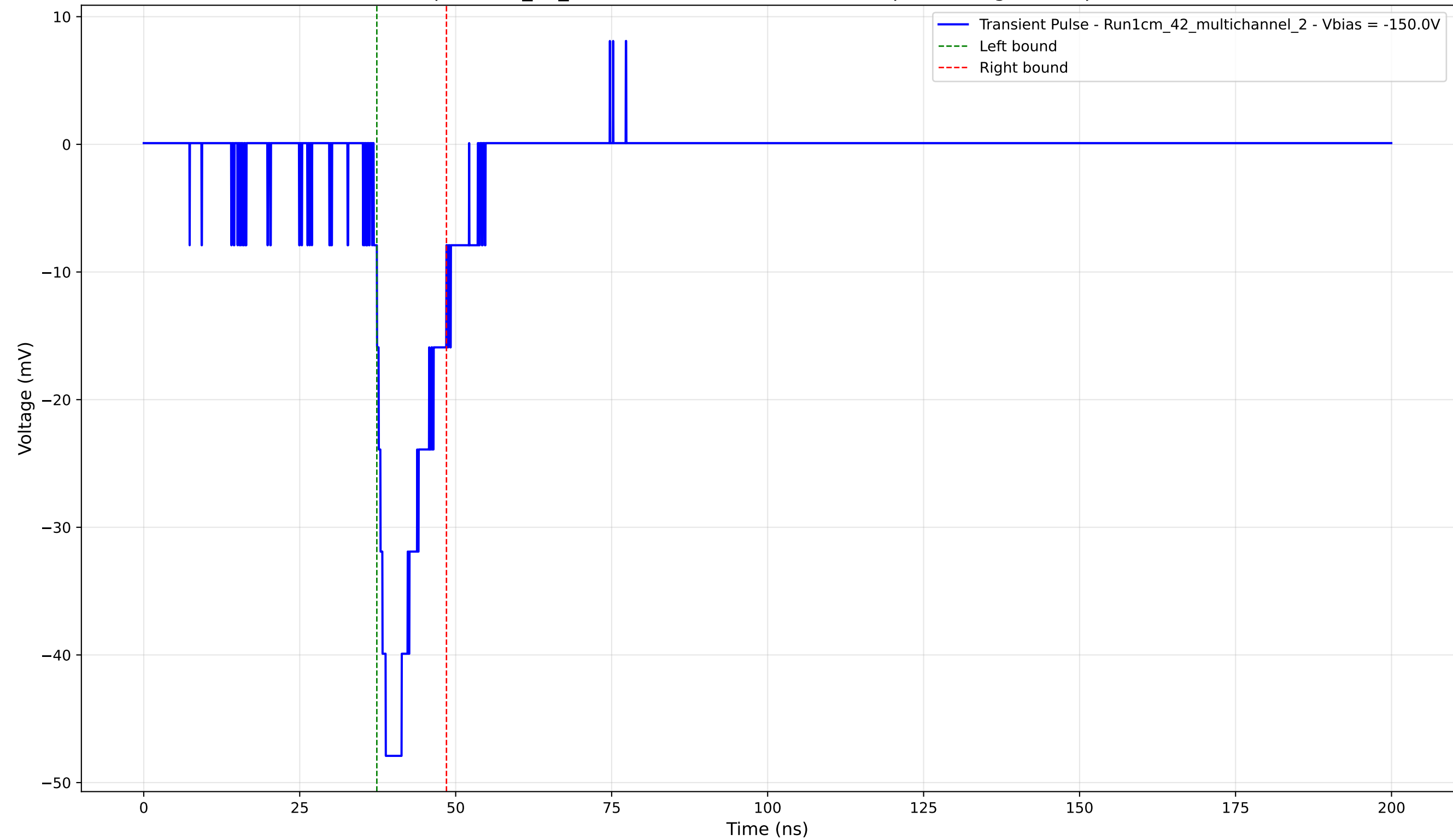
Transient Pulse - Sample: 1cm_42_multichannel - Position: 4330.0 \mu\text{m} - Charge: 6.98 pC - Rise Time: 1.94 ns
