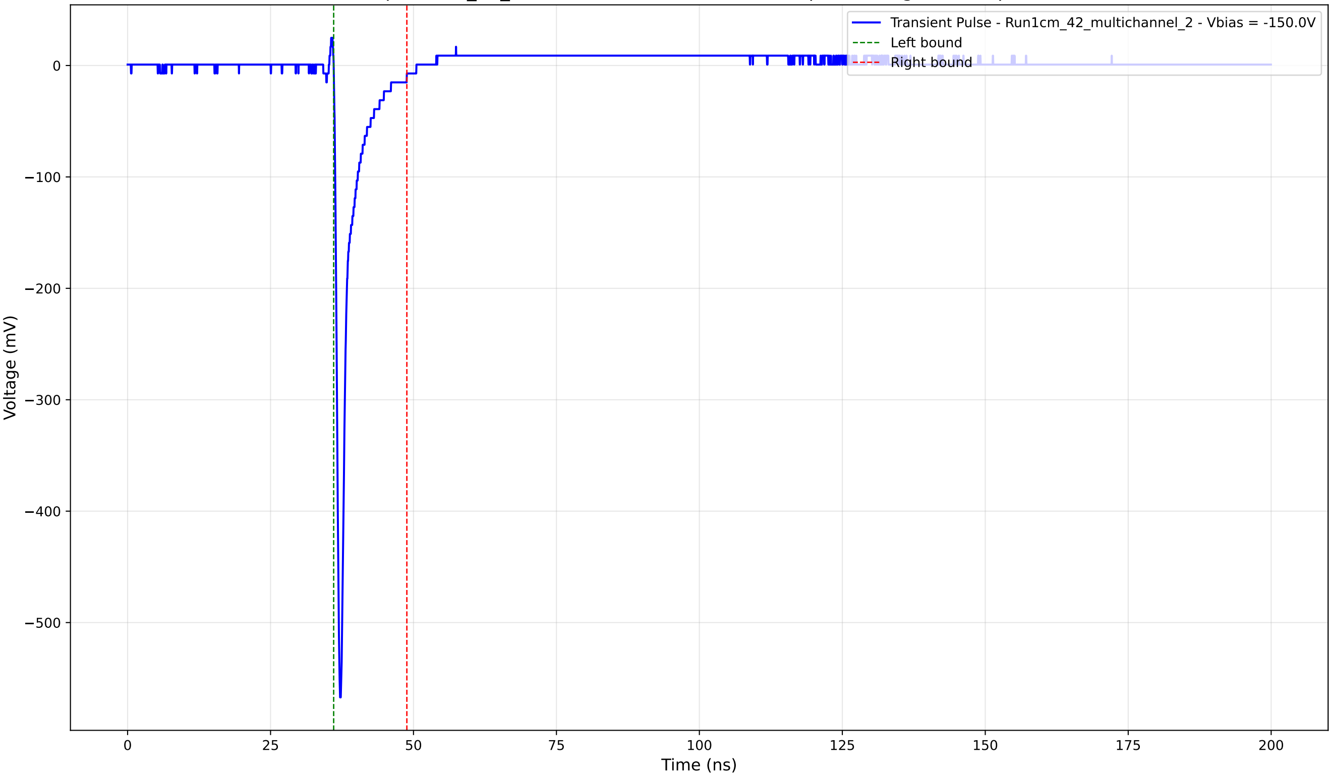
Transient Pulse - Sample: 1cm_42_multichannel - Position: 2195.0 \mu\text{m} - Charge: 27.65 pC - Rise Time: 0.74 ns
