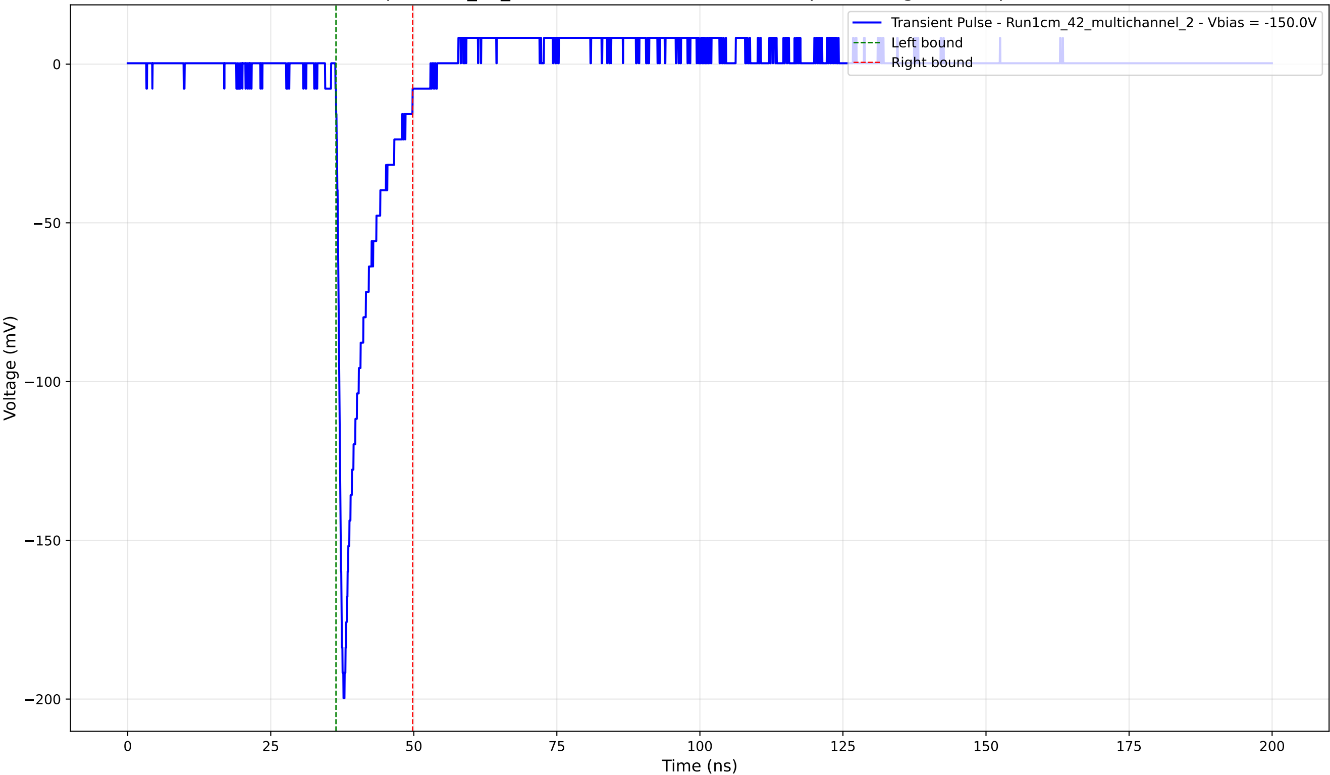
Transient Pulse - Sample: 1cm_42_multichannel - Position: 3165.0 \mu\text{m} - Charge: 18.65 pC - Rise Time: 0.94 ns
