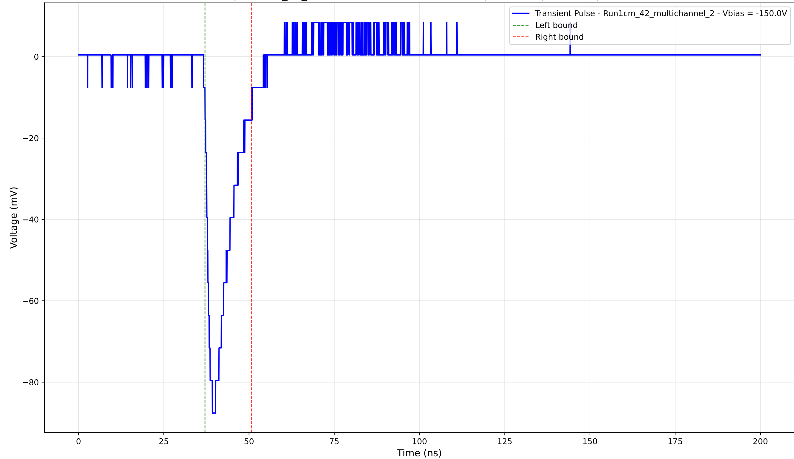
Transient Pulse - Sample: 1cm_42_multichannel - Position: 4120.0 \mu\text{m} - Charge: 12.64 pC - Rise Time: 1.51 ns
