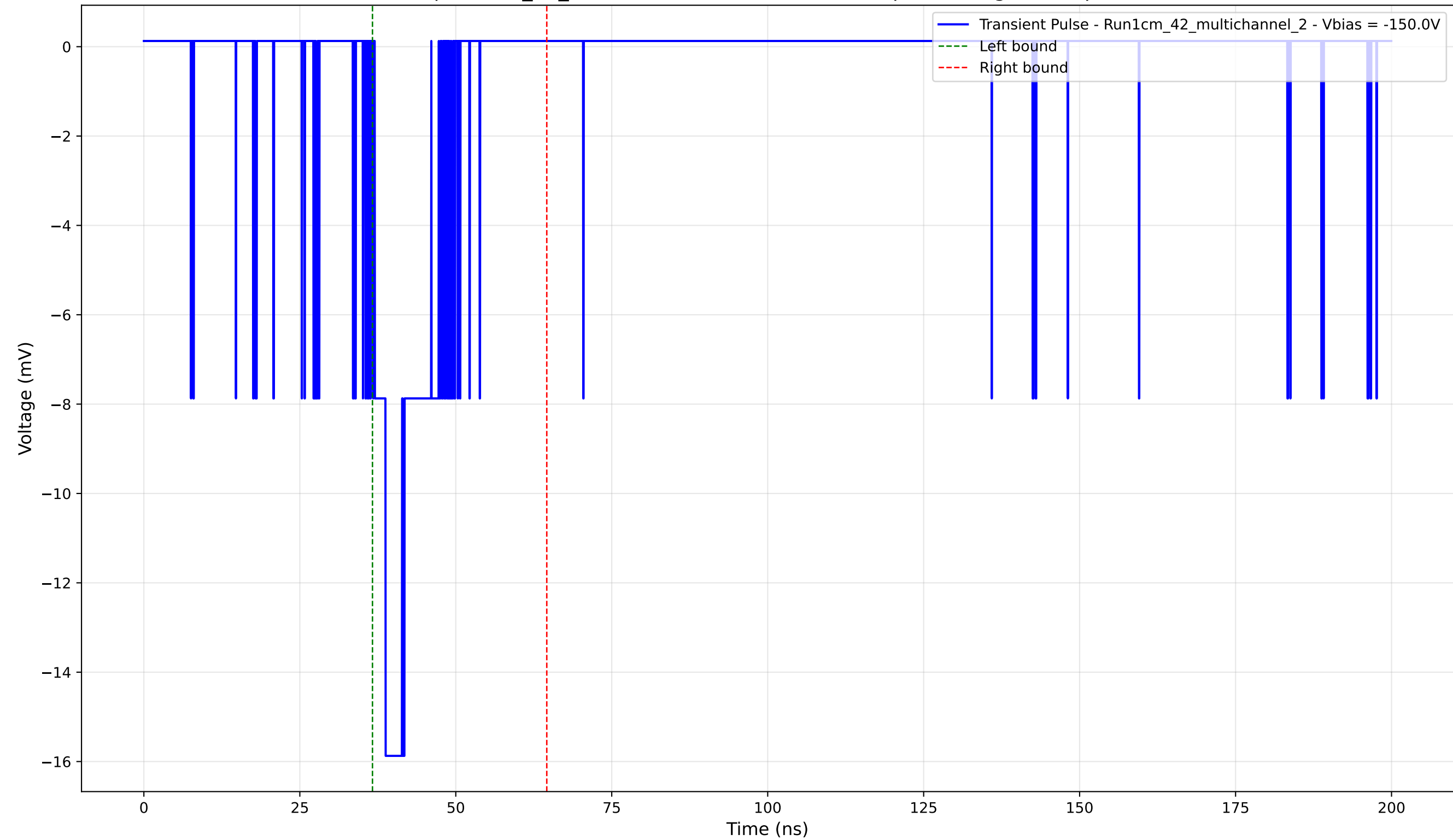
Transient Pulse - Sample: 1cm_42_multichannel - Position: 4420.0 \mu\text{m} - Charge: 2.32 pC - Rise Time: 1.75 ns
