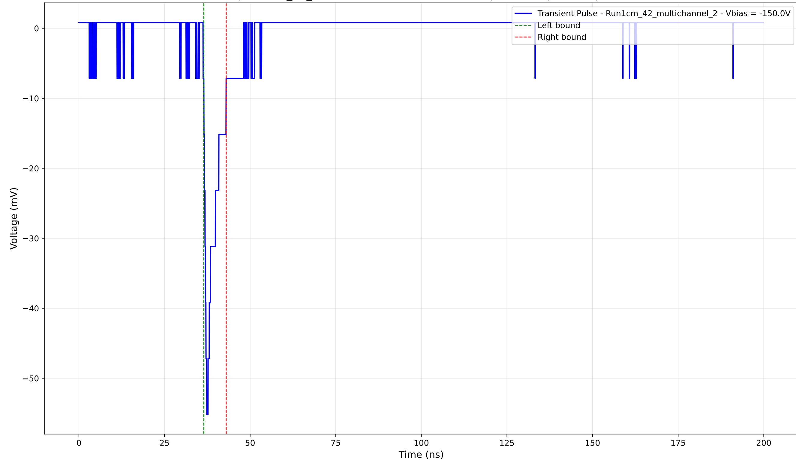
Transient Pulse - Sample: 1cm_42_multichannel - Position: 2910.0 \mu\text{m} - Charge: 3.58 pC - Rise Time: 1.09 ns
