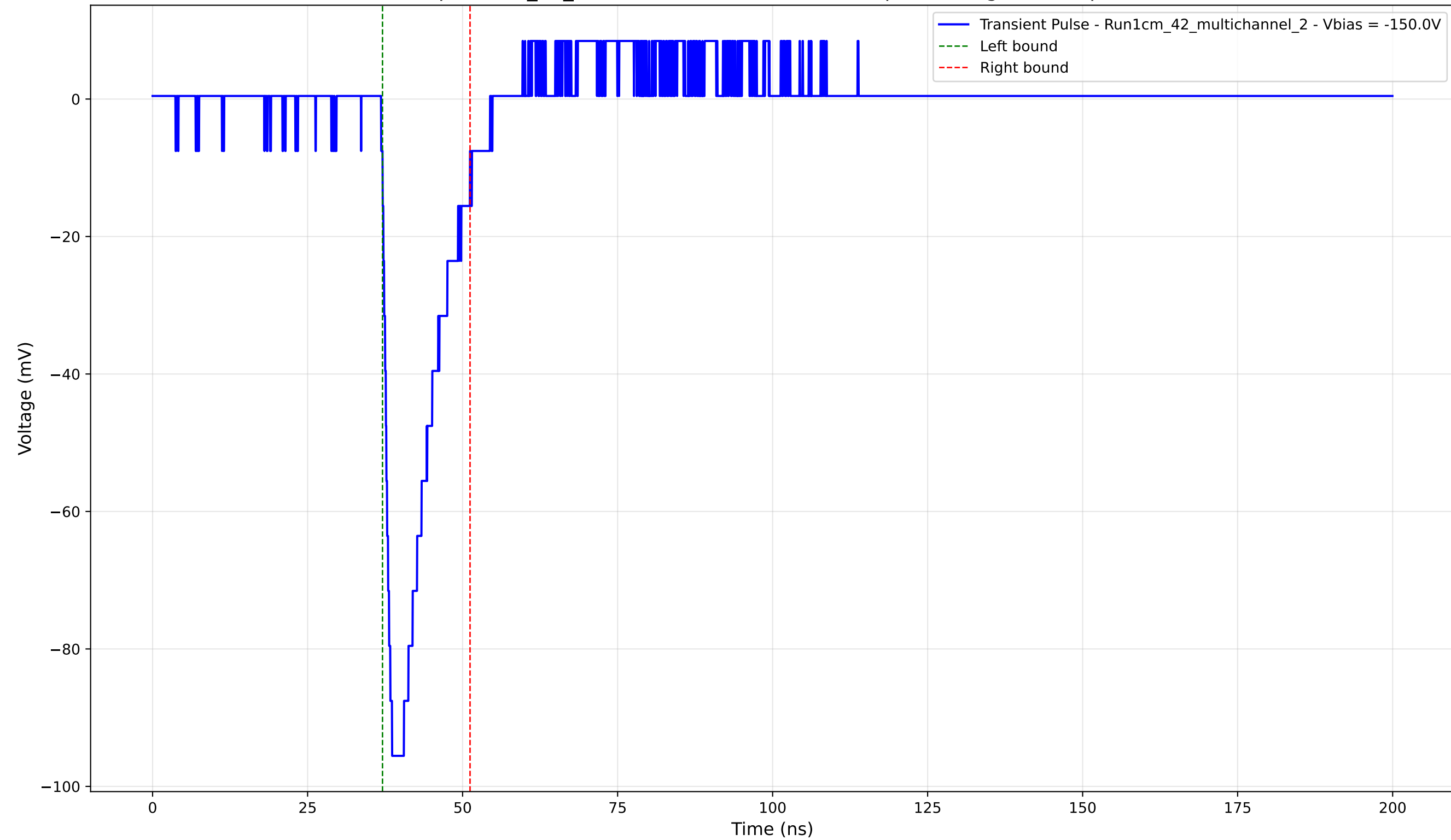
Transient Pulse - Sample: 1cm_42_multichannel - Position: 590.0 \mu\text{m} - Charge: 14.61 pC - Rise Time: 1.27 ns
