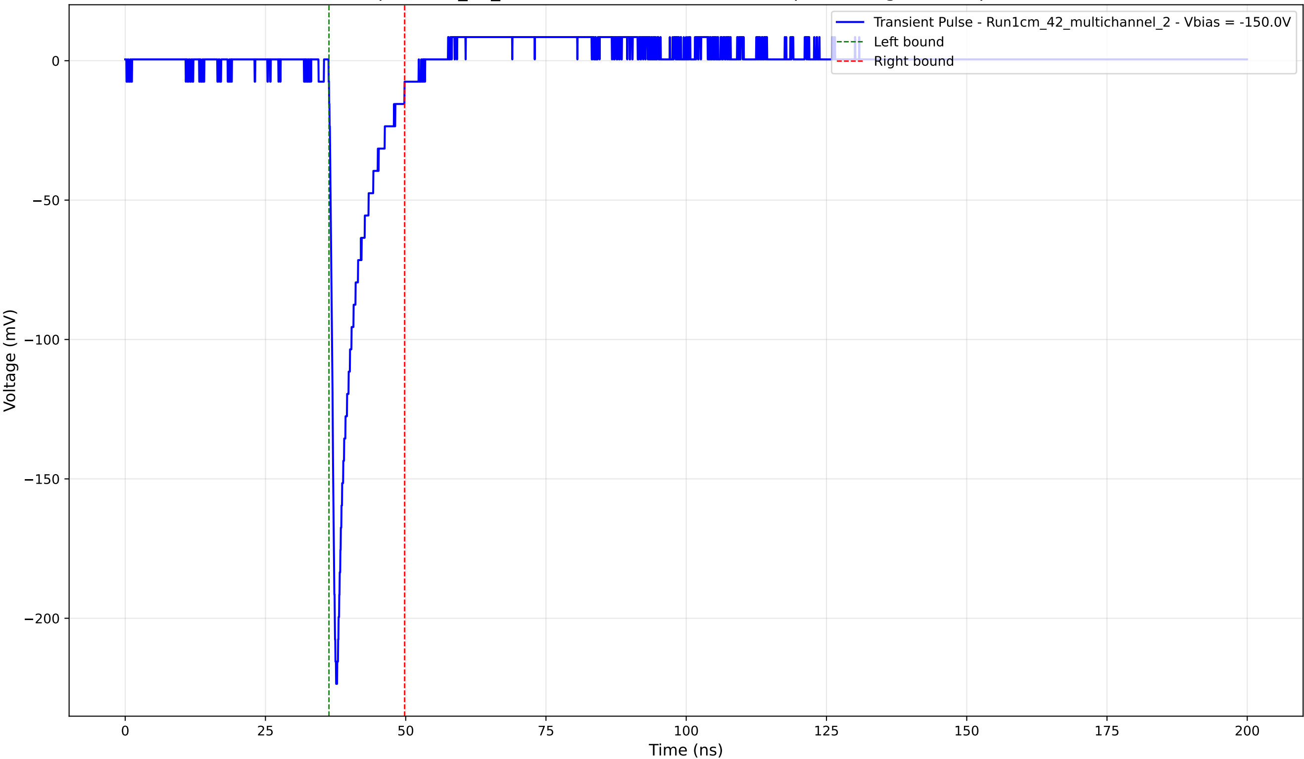
Transient Pulse - Sample: 1cm_42_multichannel - Position: 3080.0 \mu\text{m} - Charge: 19.42 pC - Rise Time: 0.97 ns
