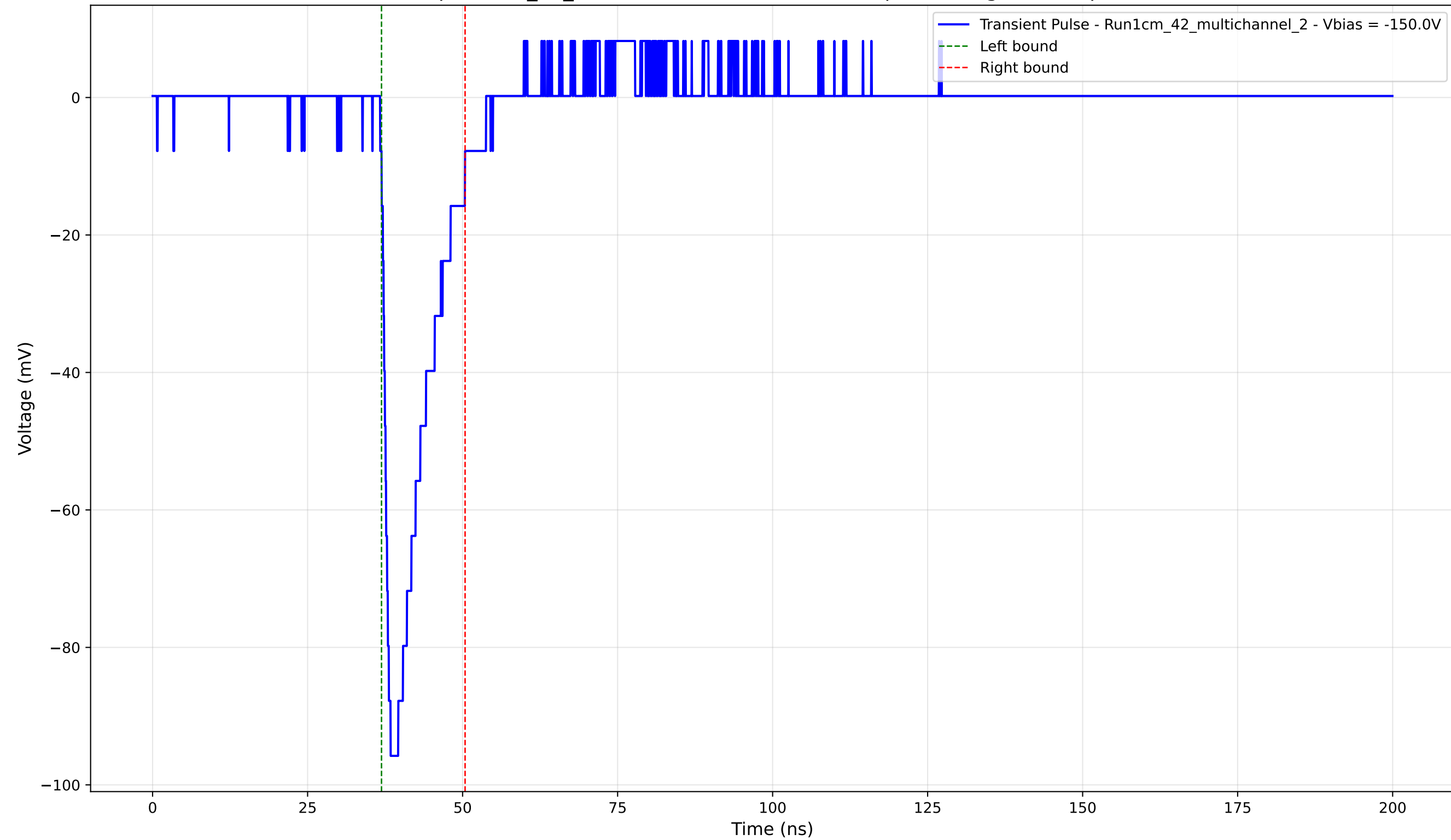
Transient Pulse - Sample: 1cm_42_multichannel - Position: 915.0 \mu\text{m} - Charge: 13.22 pC - Rise Time: 1.19 ns
