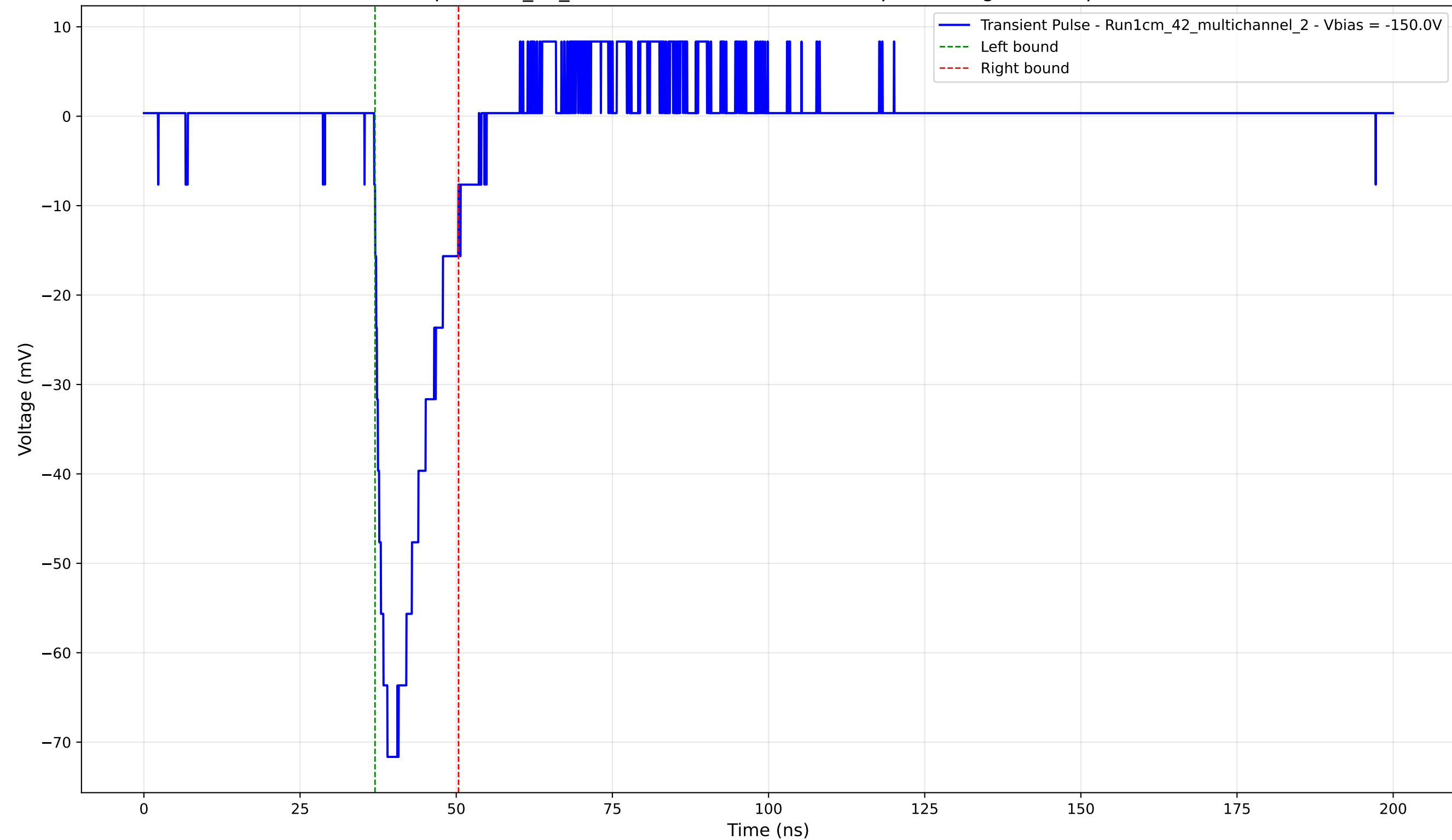
Transient Pulse - Sample: 1cm_42_multichannel - Position: 185.0 \mu\text{m} - Charge: 11.25 pC - Rise Time: 2.12 ns
