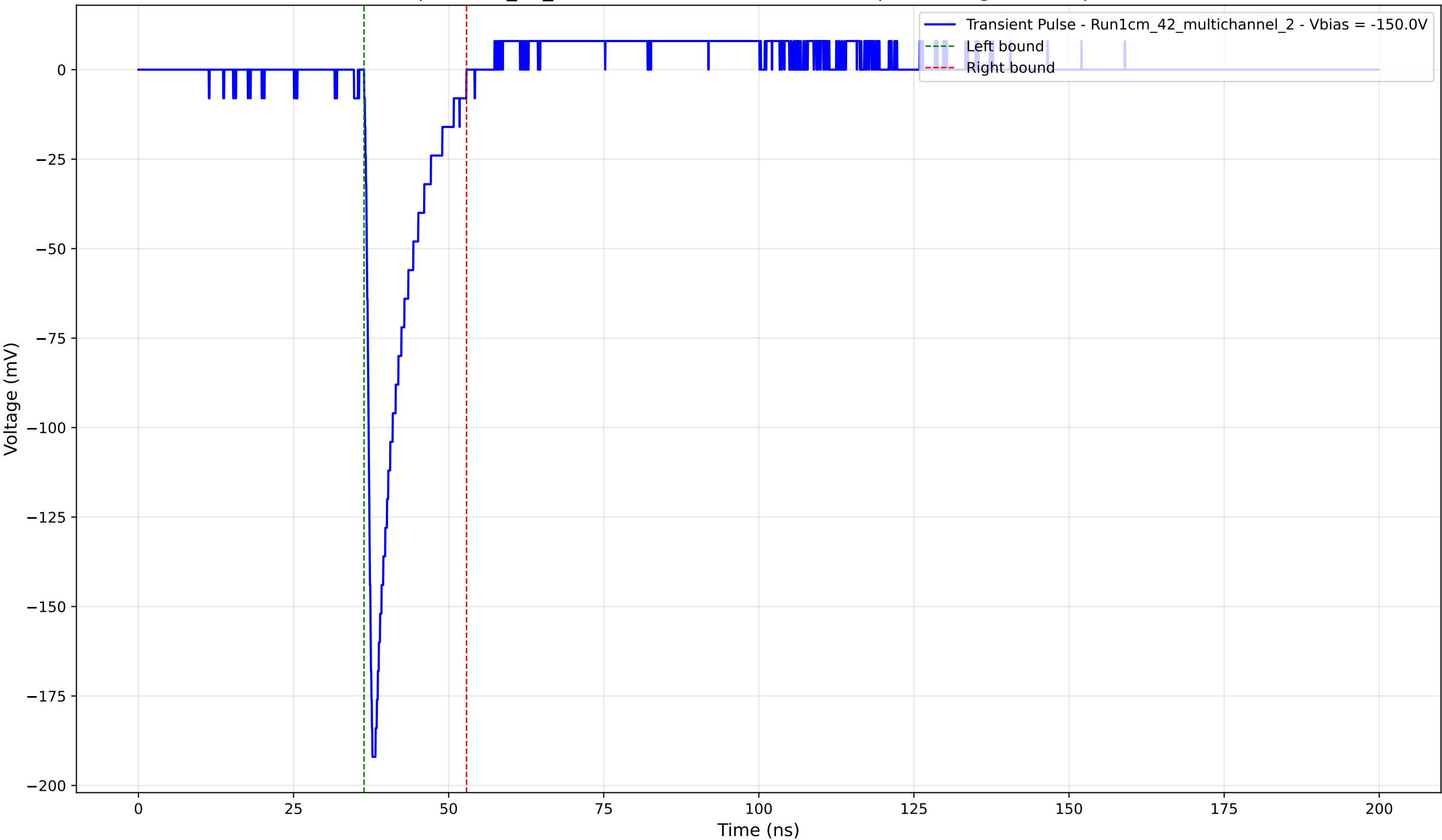
Transient Pulse - Sample: 1cm_42_multichannel - Position: 1450.0 \mu\text{m} - Charge: 20.95 pC - Rise Time: 0.98 ns
