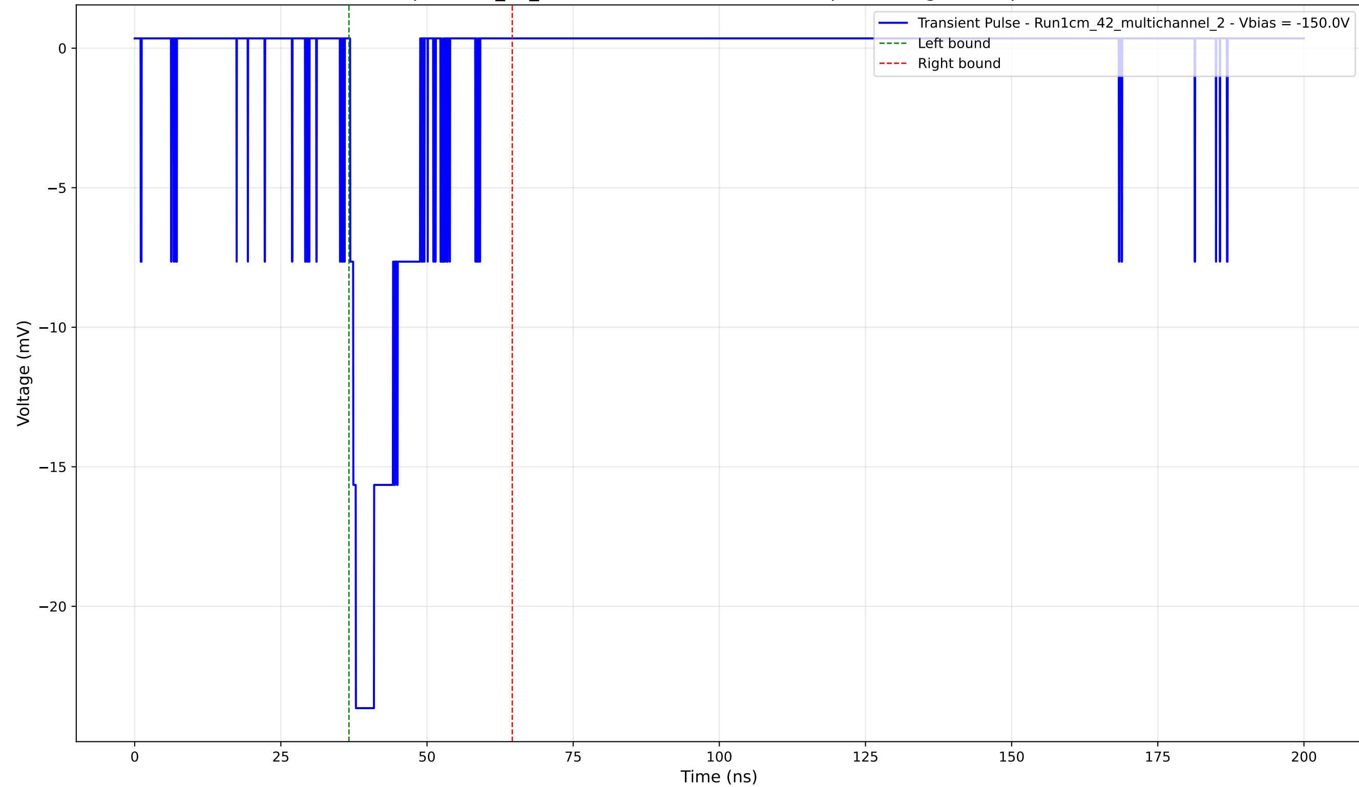
Transient Pulse - Sample: 1cm_42_multichannel - Position: 885.0 \mu\text{m} - Charge: 3.64 pC - Rise Time: 0.99 ns
