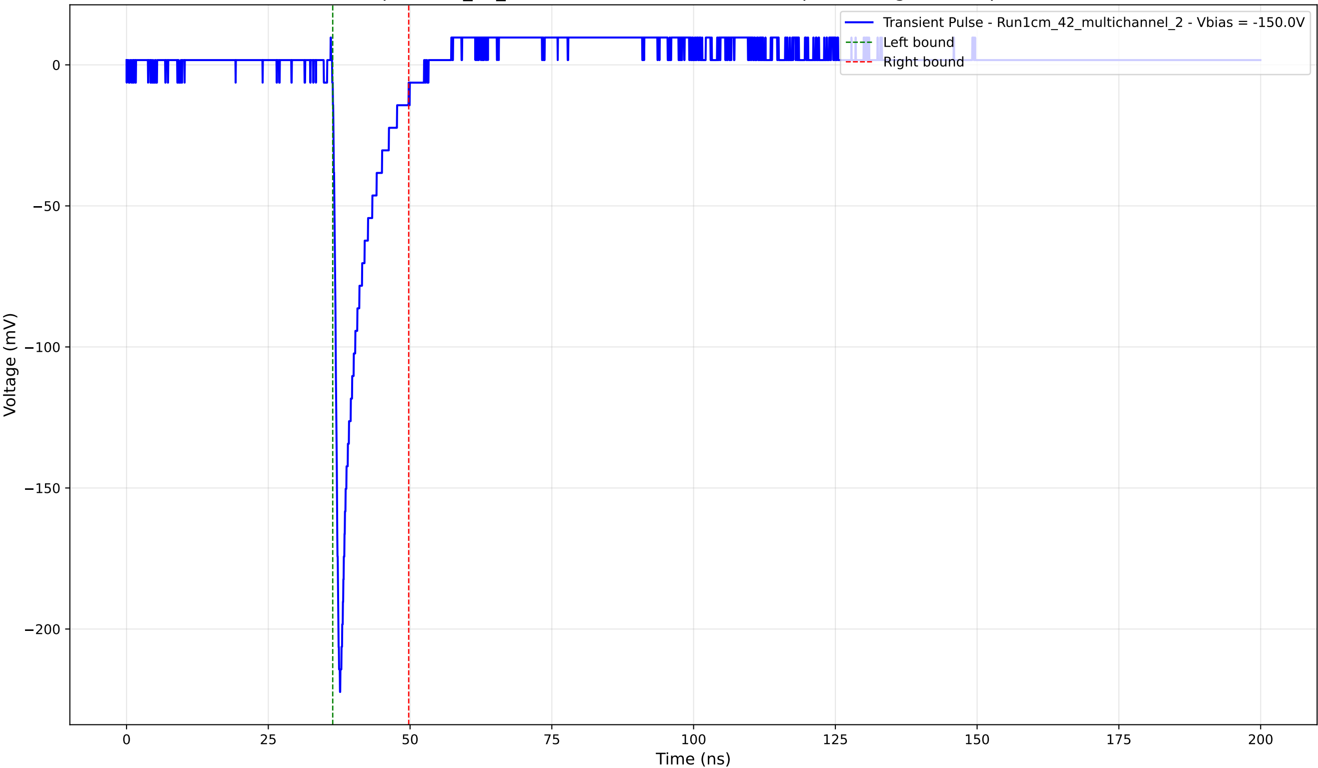
Transient Pulse - Sample: 1cm_42_multichannel - Position: 3085.0 \mu\text{m} - Charge: 18.80 pC - Rise Time: 0.92 ns
