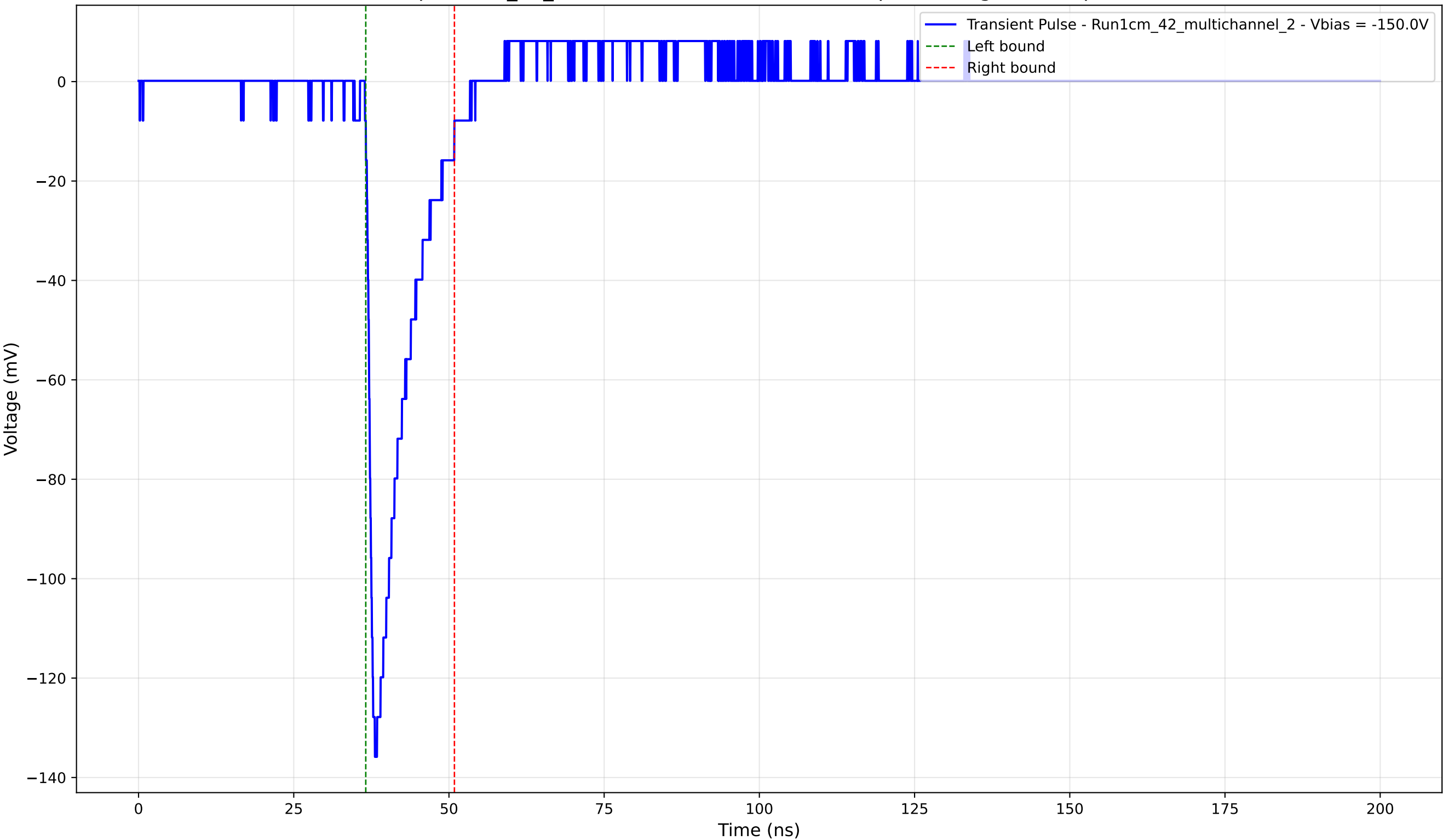
Transient Pulse - Sample: 1cm_42_multichannel - Position: 3490.0 \mu\text{m} - Charge: 16.77 pC - Rise Time: 1.17 ns
