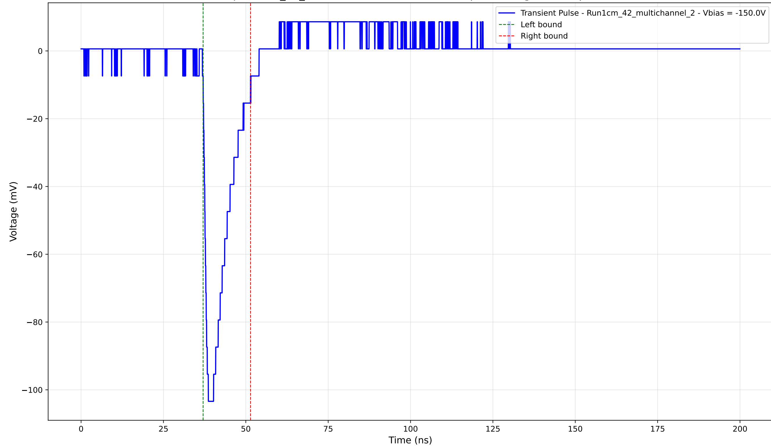
Transient Pulse - Sample: 1cm_42_multichannel - Position: 695.0 \mu\text{m} - Charge: 15.39 pC - Rise Time: 1.27 ns
