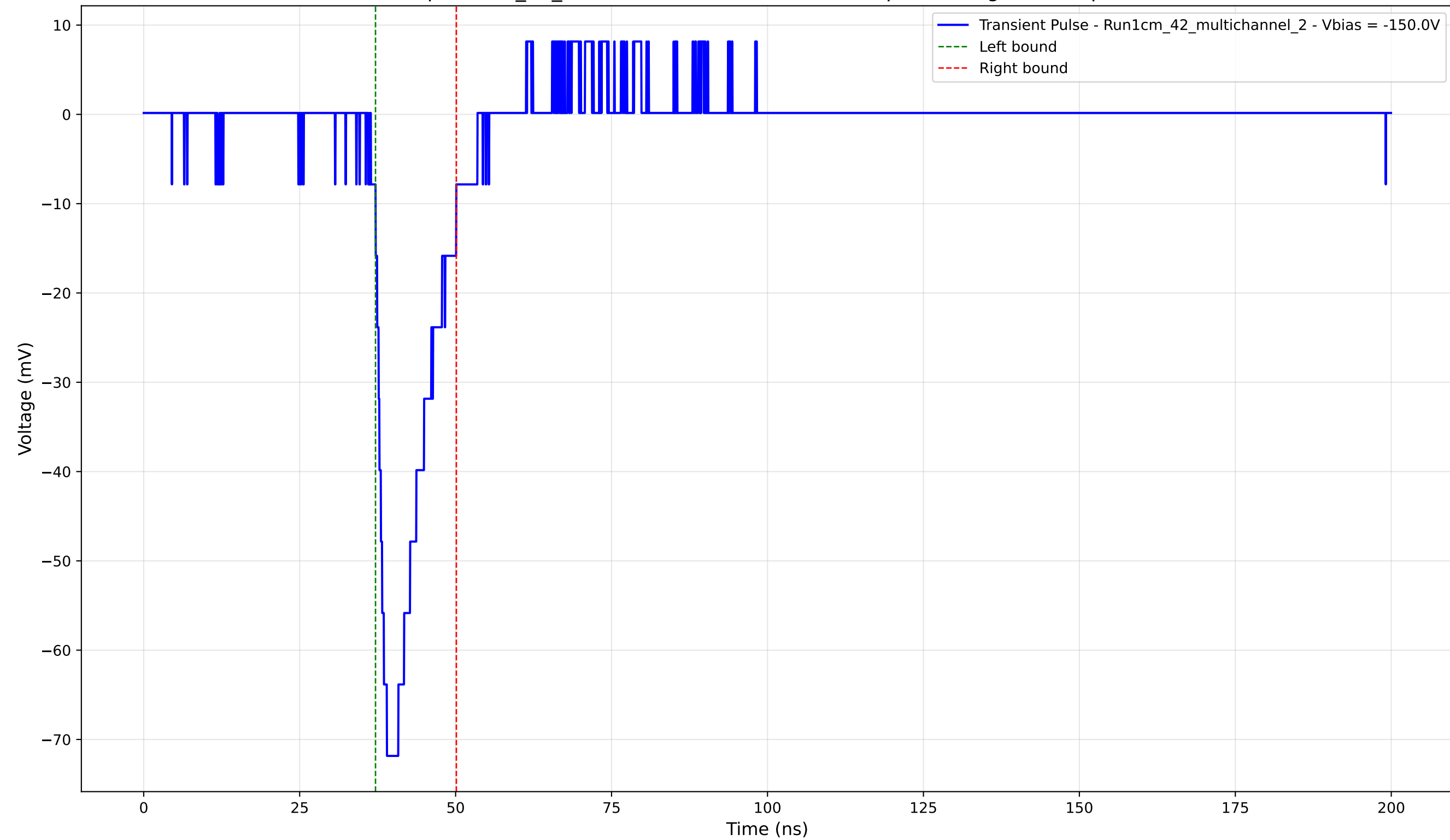
Transient Pulse - Sample: 1cm_42_multichannel - Position: 4540.0 \mu\text{m} - Charge: 10.73 pC - Rise Time: 2.56 ns
