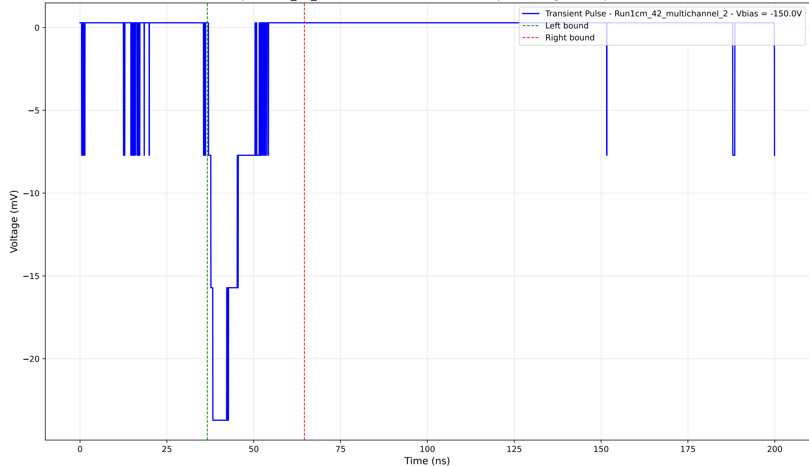
Transient Pulse - Sample: 1cm_42_multichannel - Position: 4345.0 \mu\text{m} - Charge: 4.22 pC - Rise Time: 1.27 ns
