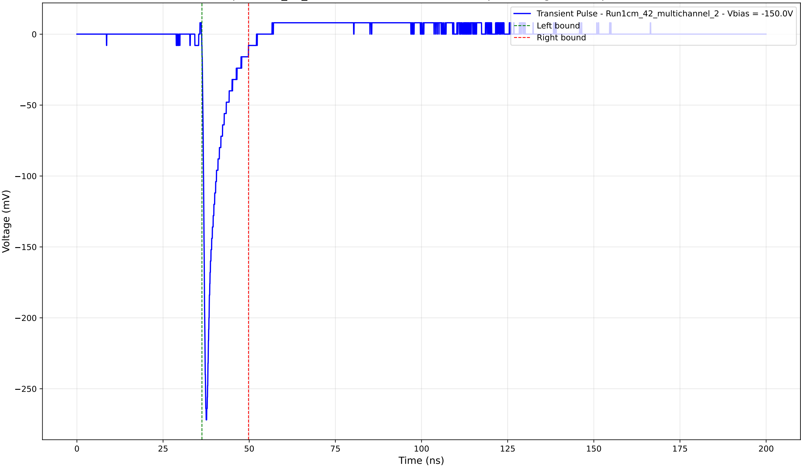
Transient Pulse - Sample: 1cm_42_multichannel - Position: 2990.0 \mu\text{m} - Charge: 21.49 pC - Rise Time: 0.89 ns
