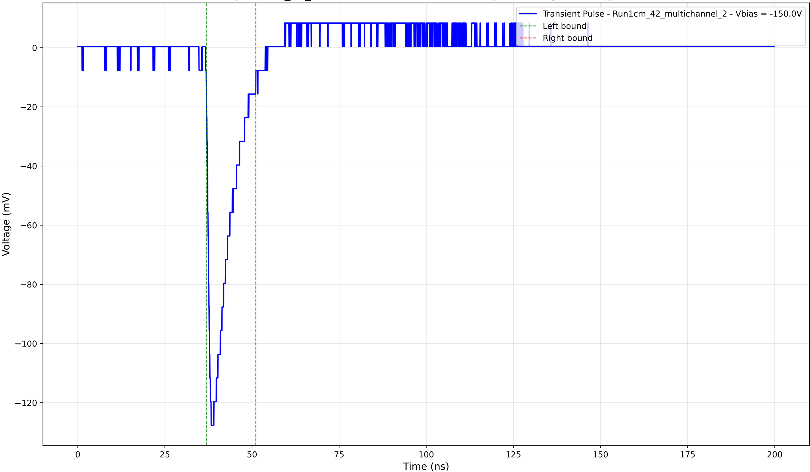
Transient Pulse - Sample: 1cm_42_multichannel - Position: 1025.0 \mu\text{m} - Charge: 17.26 pC - Rise Time: 1.17 ns
