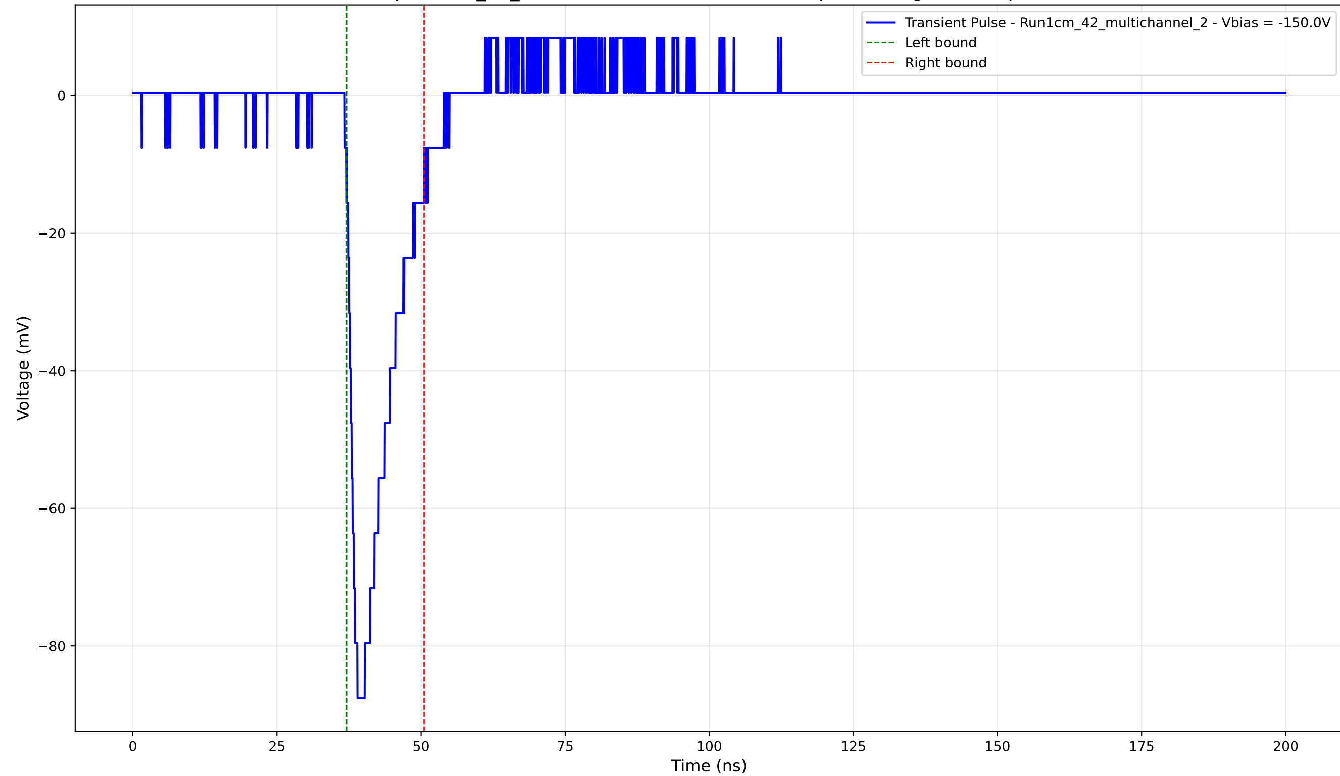
Transient Pulse - Sample: 1cm_42_multichannel - Position: 4140.0 \mu\text{m} - Charge: 12.75 pC - Rise Time: 1.43 ns
