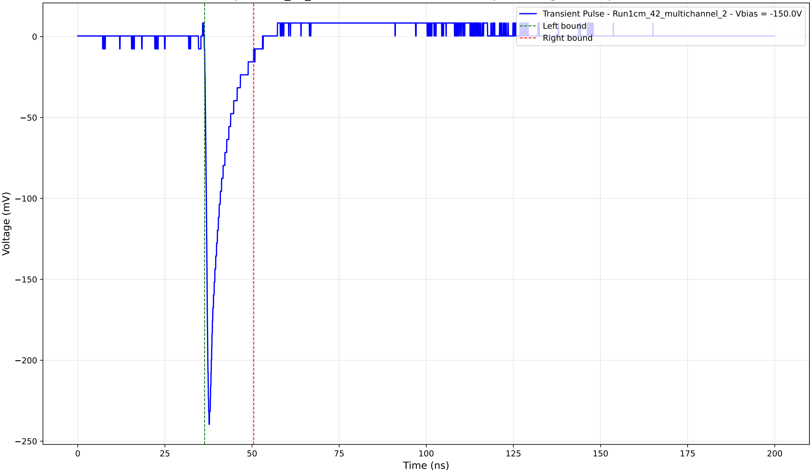
Transient Pulse - Sample: 1cm_42_multichannel - Position: 1600.0 \mu\text{m} - Charge: 21.71 pC - Rise Time: 0.96 ns
