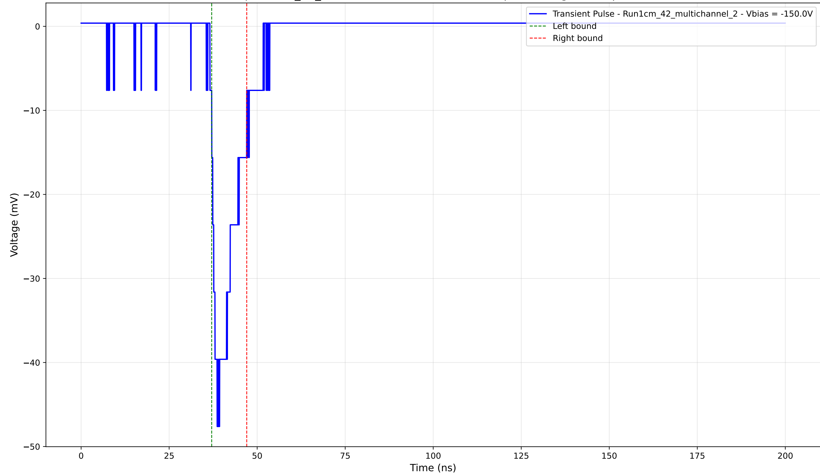
Transient Pulse - Sample: 1cm_42_multichannel - Position: 3840.0 \mu\text{m} - Charge: 5.66 pC - Rise Time: 2.06 ns
