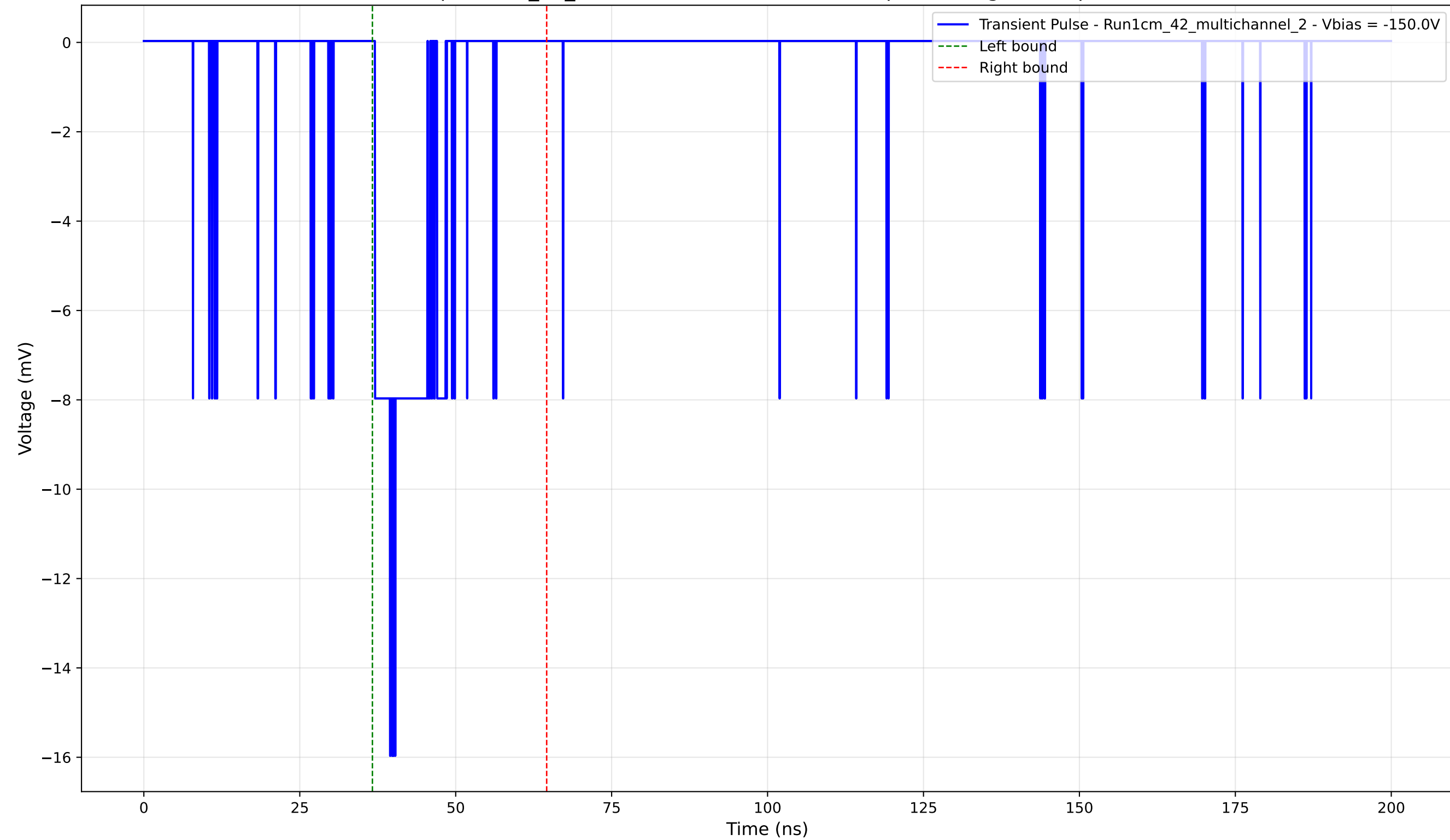
Transient Pulse - Sample: 1cm_42_multichannel - Position: 870.0 \mu\text{m} - Charge: 1.79 pC - Rise Time: 2.43 ns
