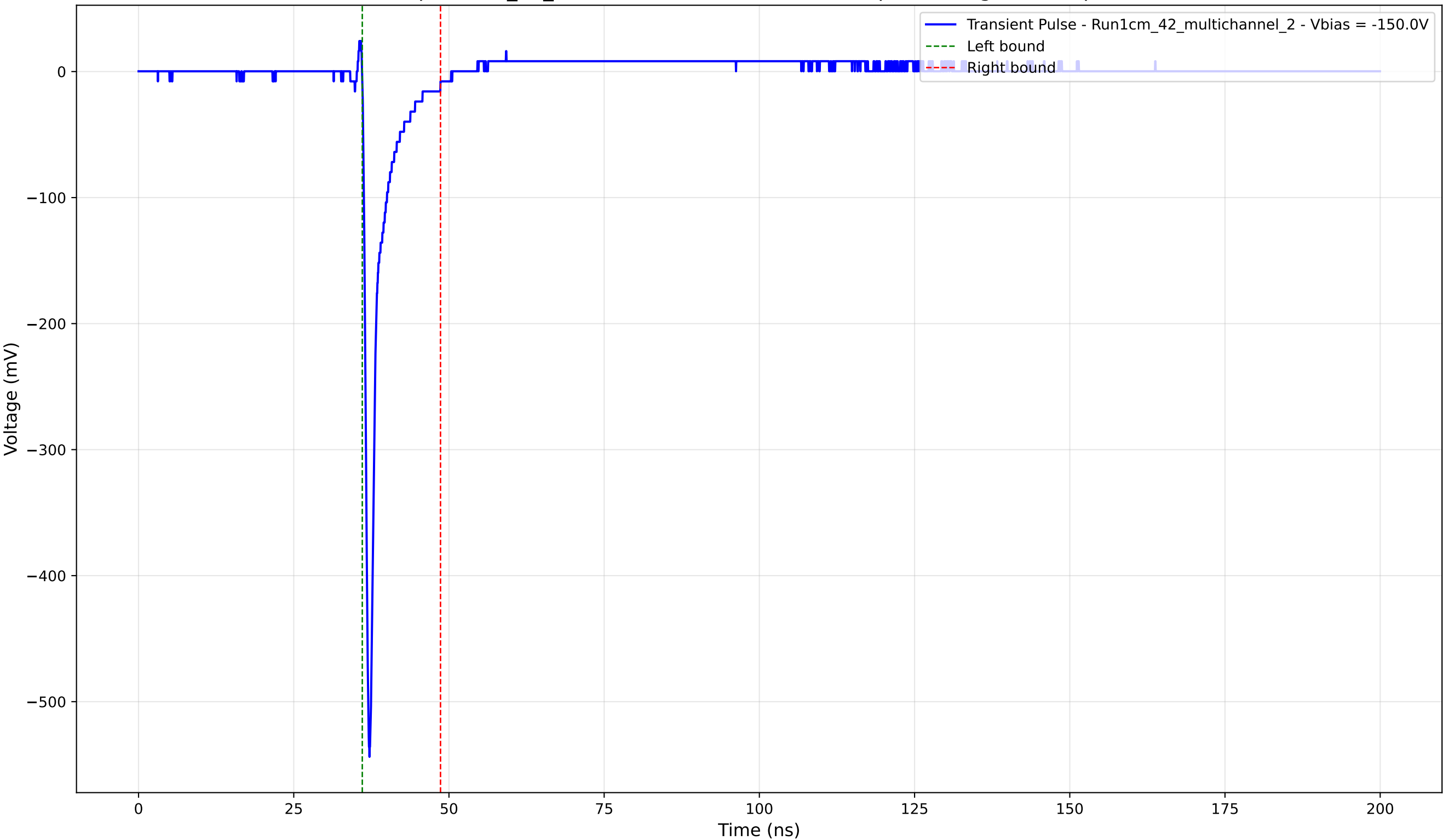
Transient Pulse - Sample: 1cm_42_multichannel - Position: 2530.0 \mu\text{m} - Charge: 26.00 pC - Rise Time: 0.75 ns
