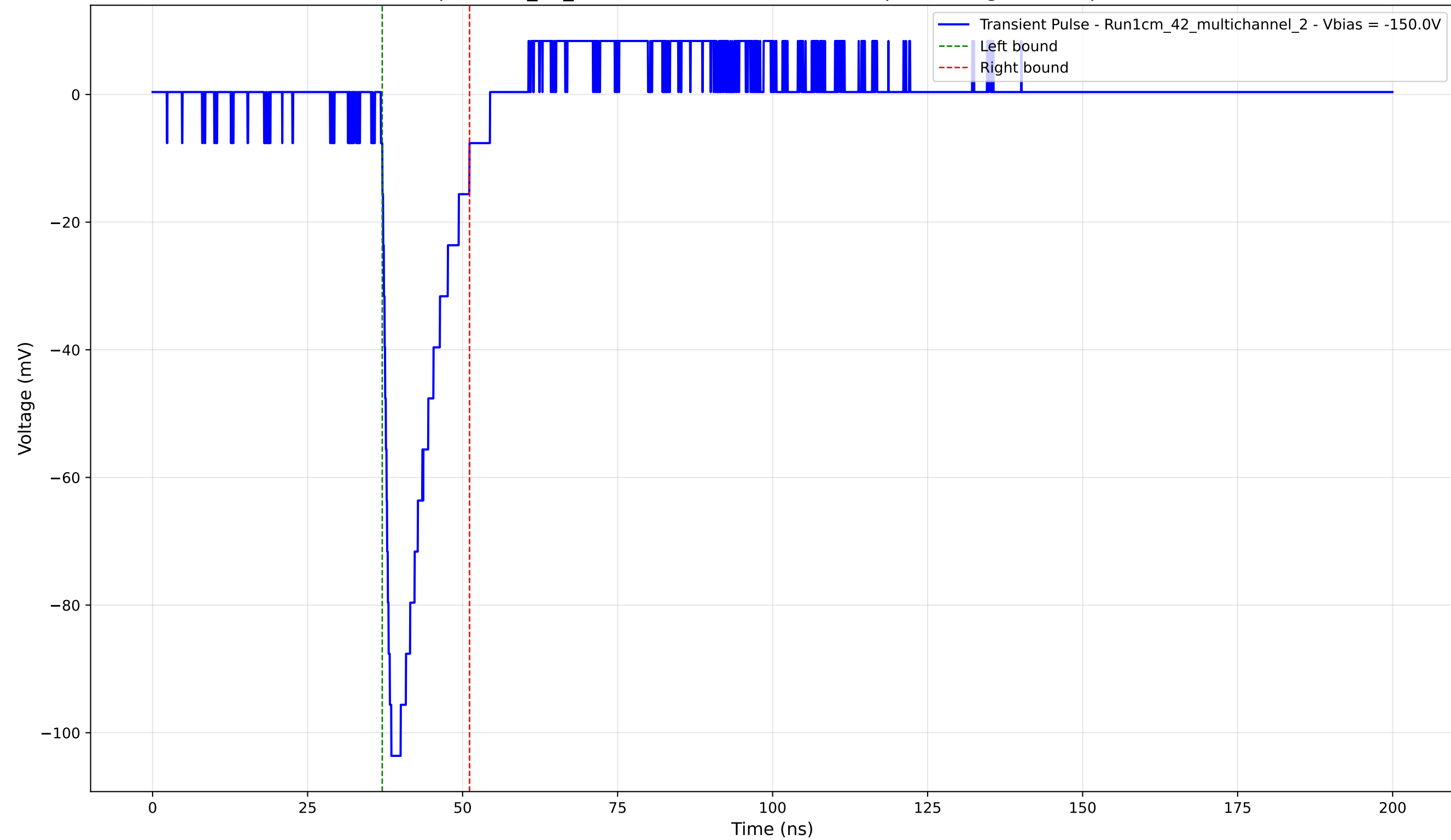
Transient Pulse - Sample: 1cm_42_multichannel - Position: 725.0 \mu\text{m} - Charge: 15.39 pC - Rise Time: 1.23 ns
