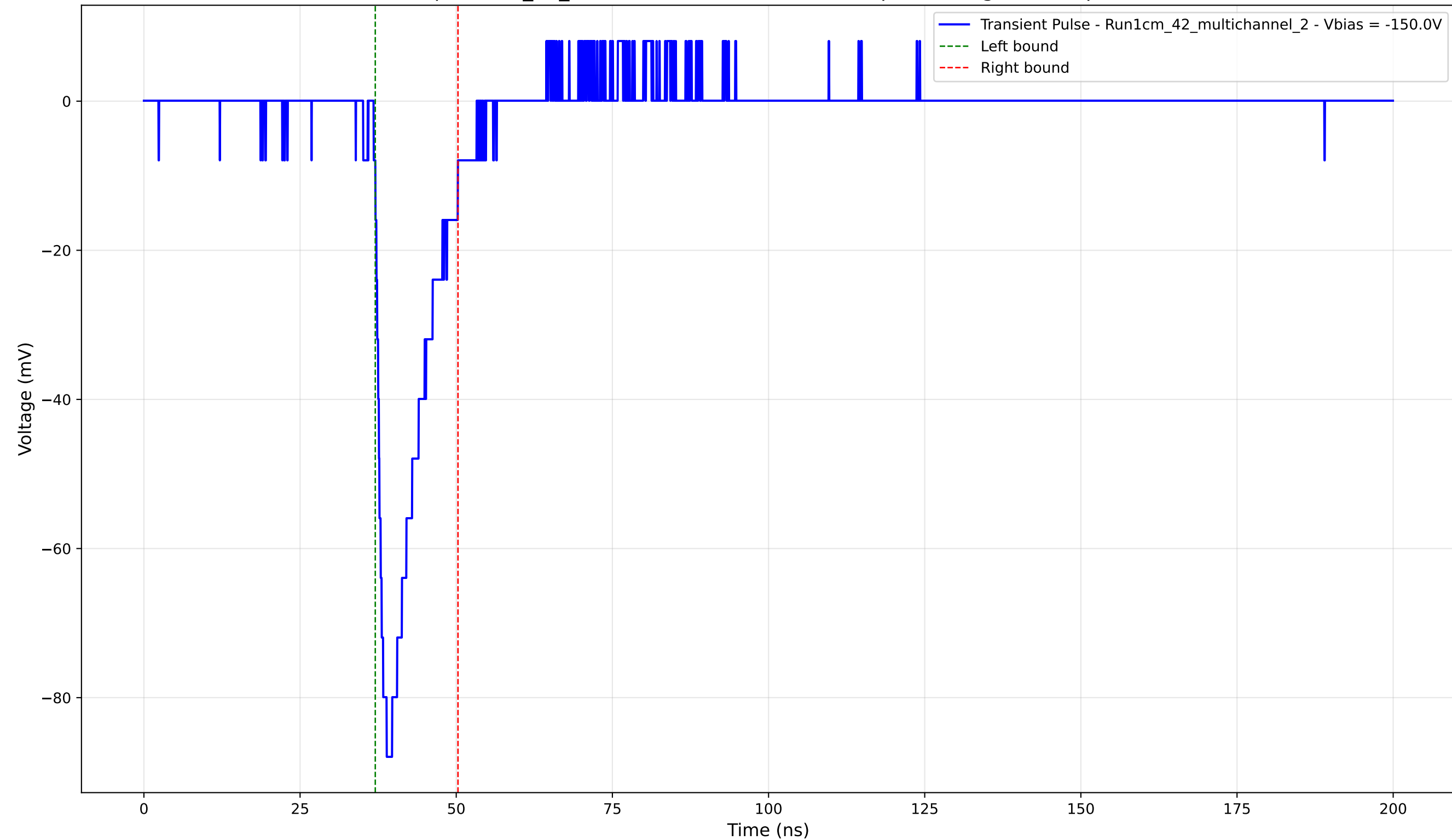
Transient Pulse - Sample: 1cm_42_multichannel - Position: 785.0 \mu\text{m} - Charge: 12.11 pC - Rise Time: 1.28 ns
