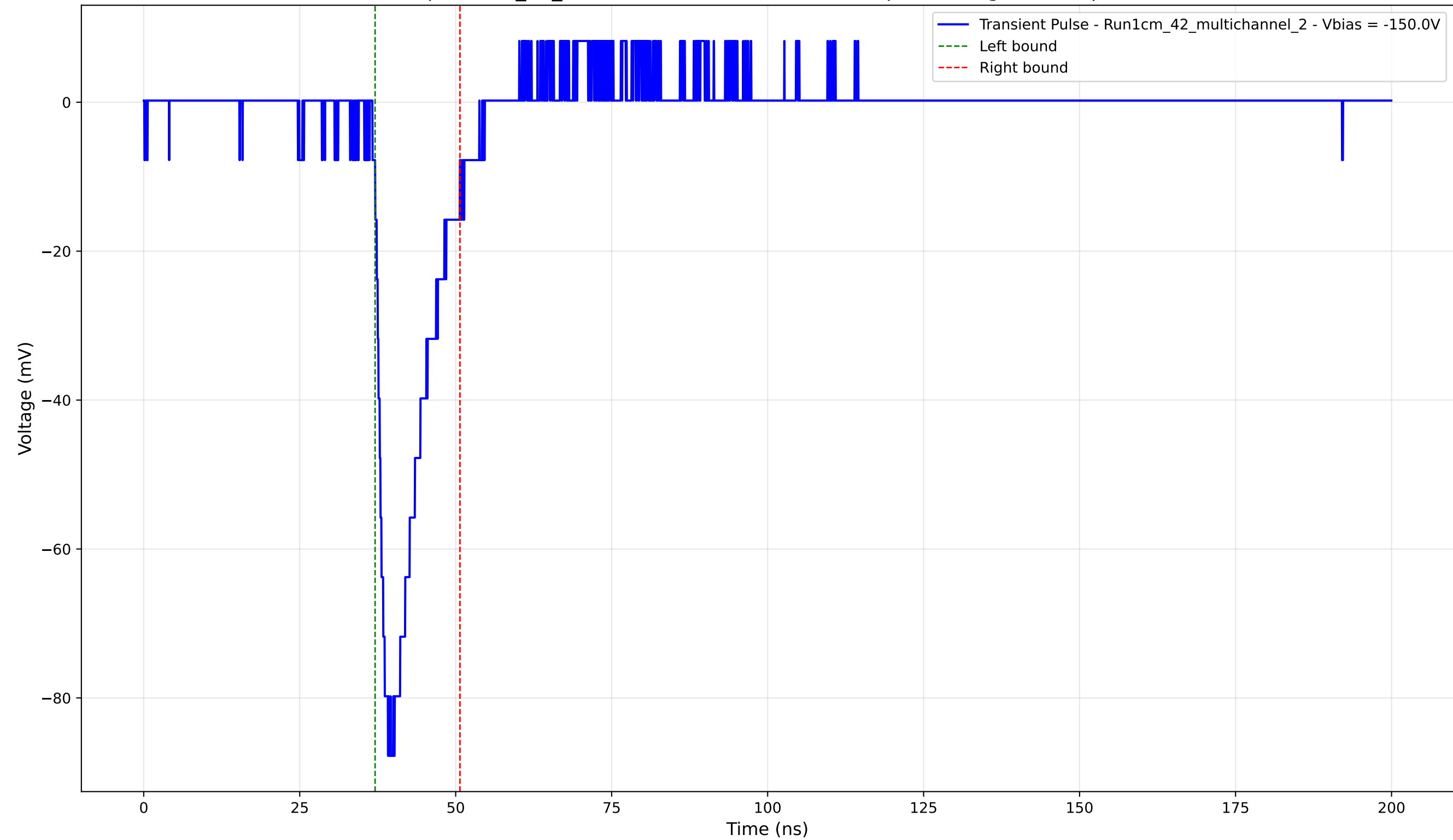
Transient Pulse - Sample: 1cm_42_multichannel - Position: 4125.0 \mu\text{m} - Charge: 12.53 pC - Rise Time: 1.55 ns
