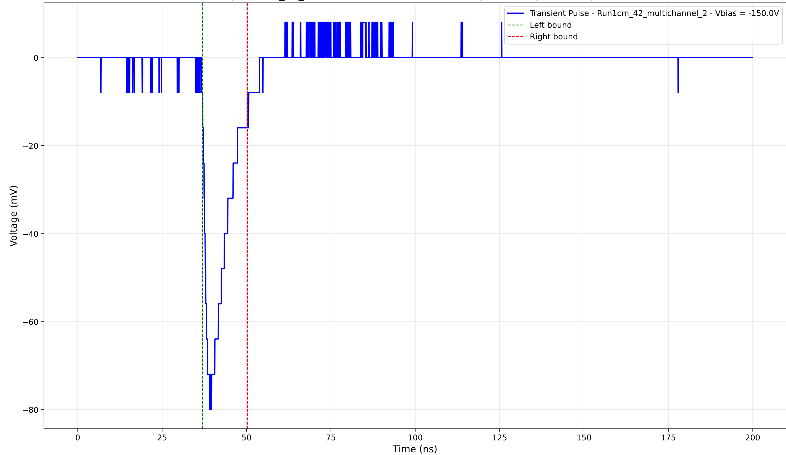
Transient Pulse - Sample: 1cm_42_multichannel - Position: 3950.0 \mu\text{m} - Charge: 10.95 pC - Rise Time: 2.12 ns
