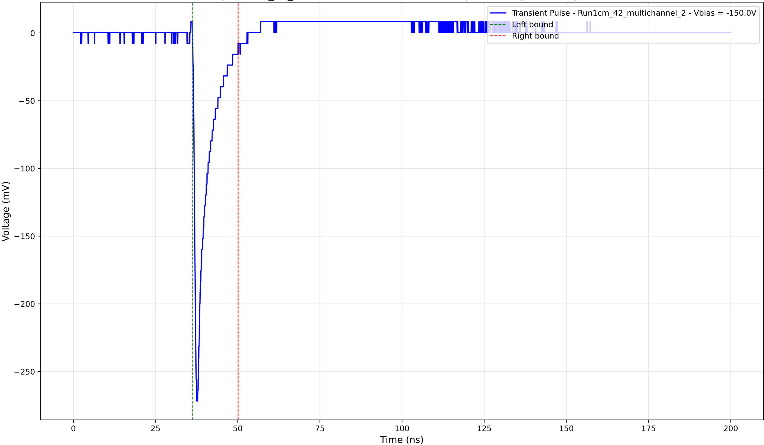
Transient Pulse - Sample: 1cm_42_multichannel - Position: 1695.0 \mu\text{m} - Charge: 23.11 pC - Rise Time: 0.85 ns
