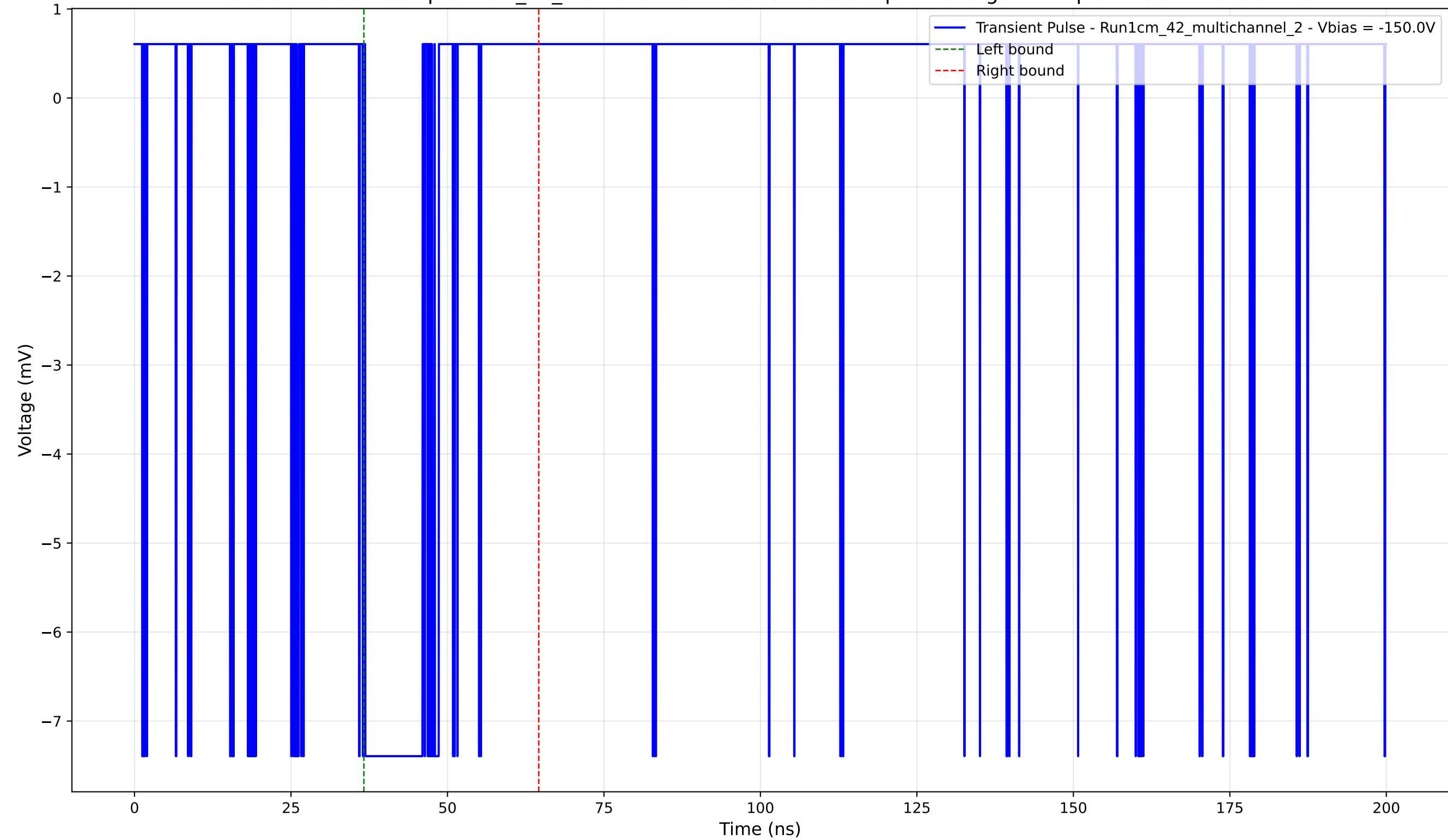
Transient Pulse - Sample: 1cm_42_multichannel - Position: 3395.0 \mu\text{m} - Charge: 1.41 pC - Rise Time: 0.04 ns
