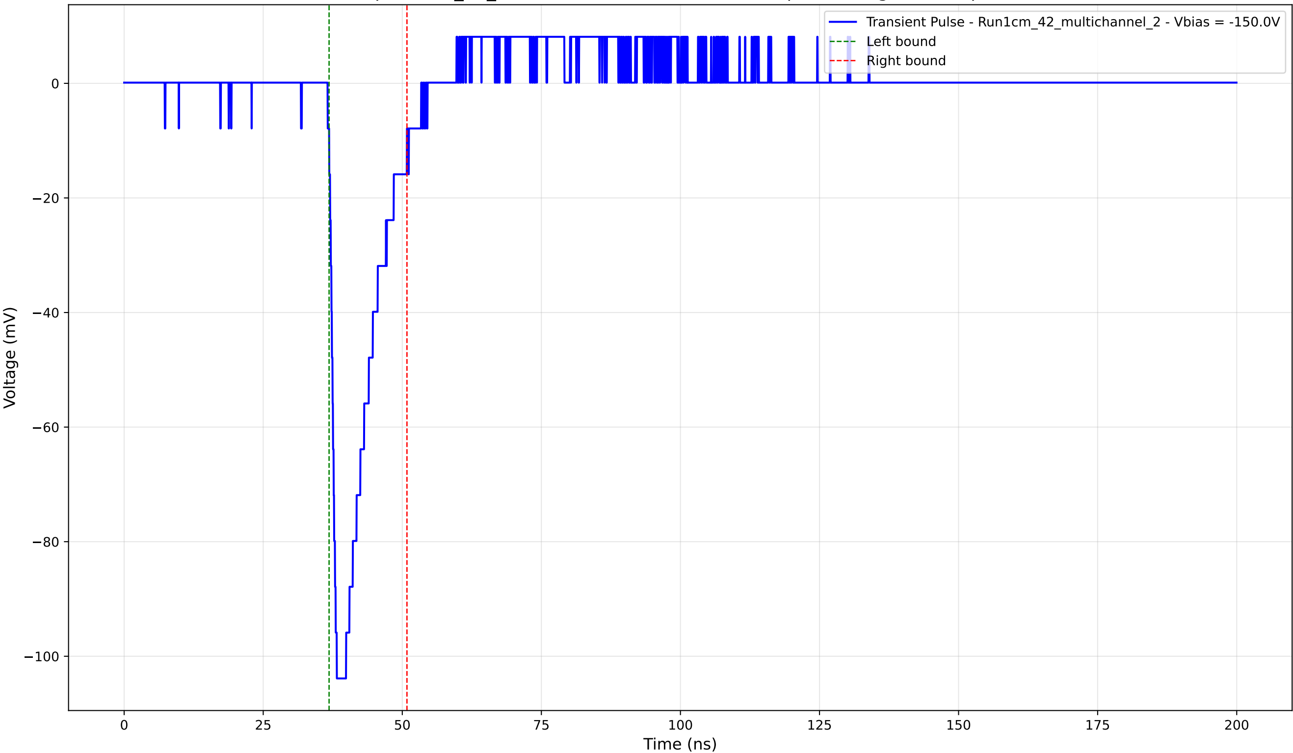
Transient Pulse - Sample: 1cm_42_multichannel - Position: 3760.0 \mu\text{m} - Charge: 14.91 pC - Rise Time: 1.19 ns
