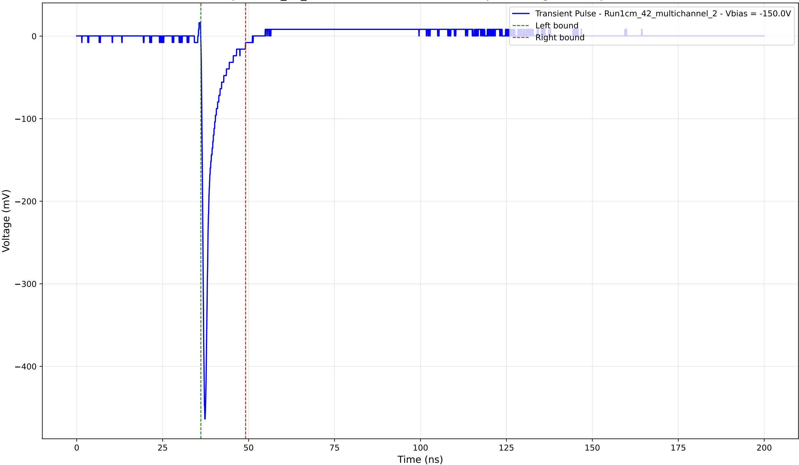
Transient Pulse - Sample: 1cm_42_multichannel - Position: 2065.0 \mu\text{m} - Charge: 25.79 pC - Rise Time: 0.77 ns
