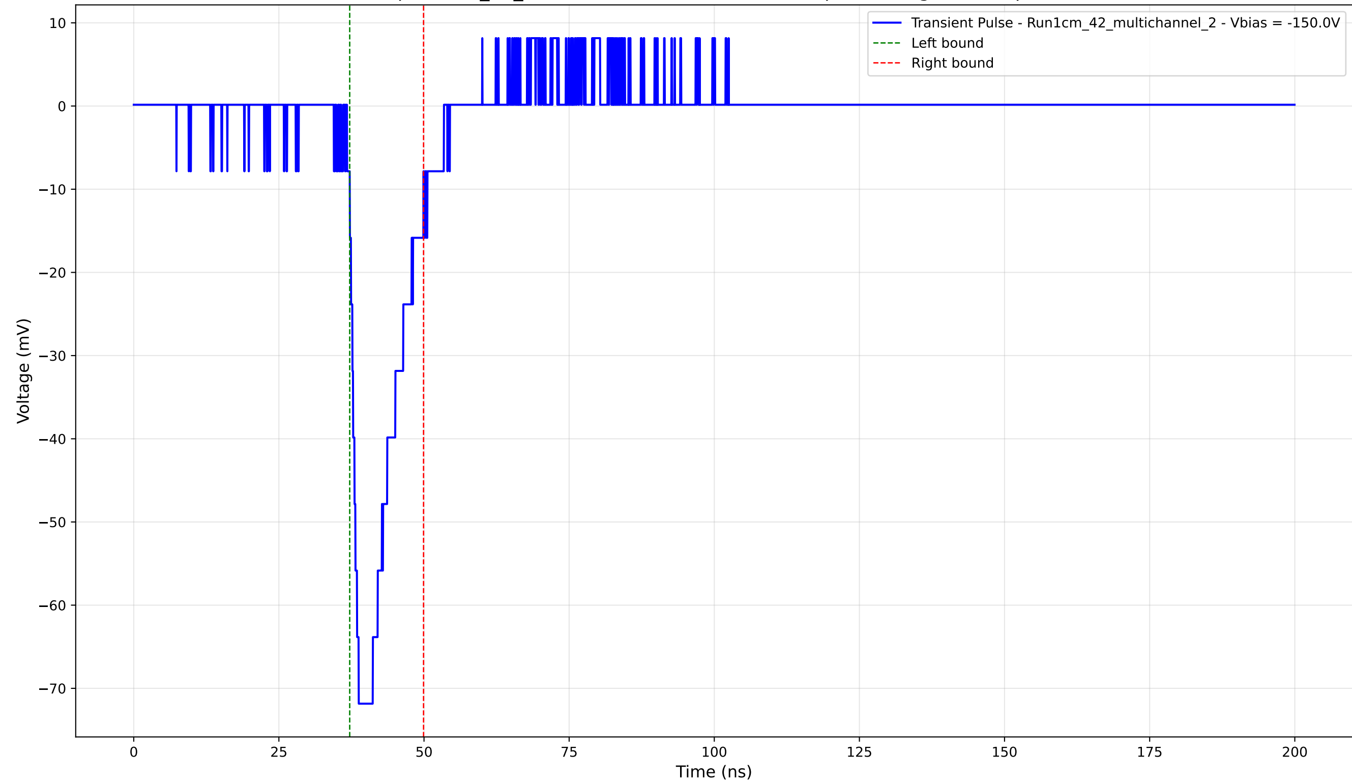
Transient Pulse - Sample: 1cm_42_multichannel - Position: 4275.0 \mu\text{m} - Charge: 10.88 pC - Rise Time: 2.00 ns
