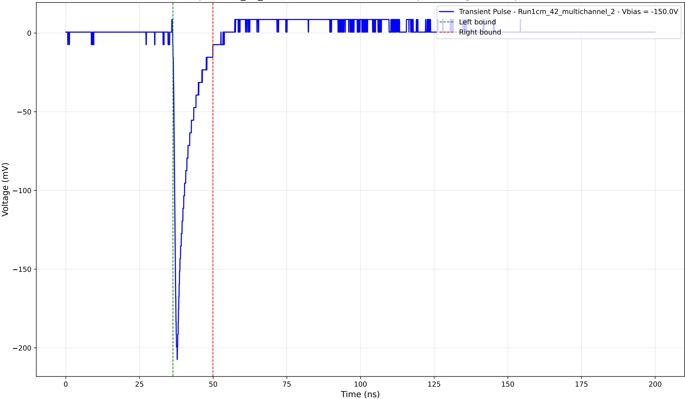
Transient Pulse - Sample: 1cm_42_multichannel - Position: 3140.0 \mu\text{m} - Charge: 18.58 pC - Rise Time: 0.97 ns
