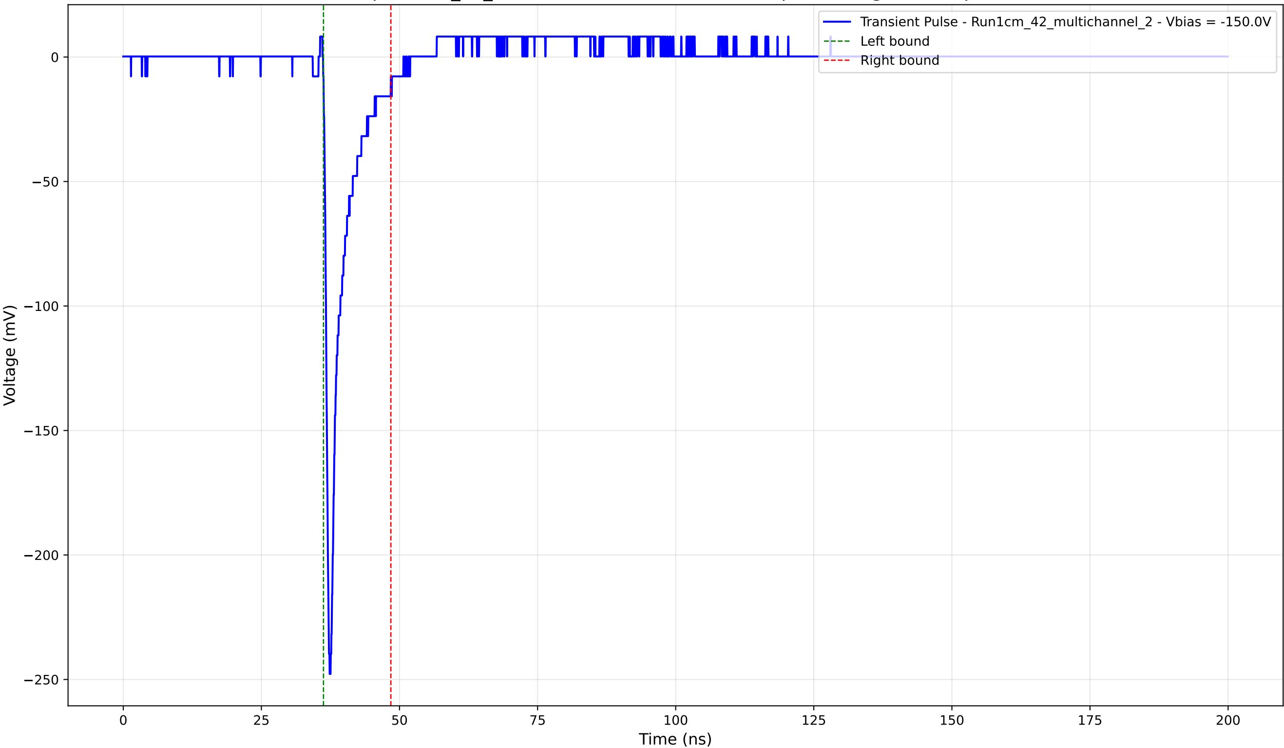
Transient Pulse - Sample: 1cm_42_multichannel - Position: 2815.0 \mu\text{m} - Charge: 16.11 pC - Rise Time: 0.79 ns
