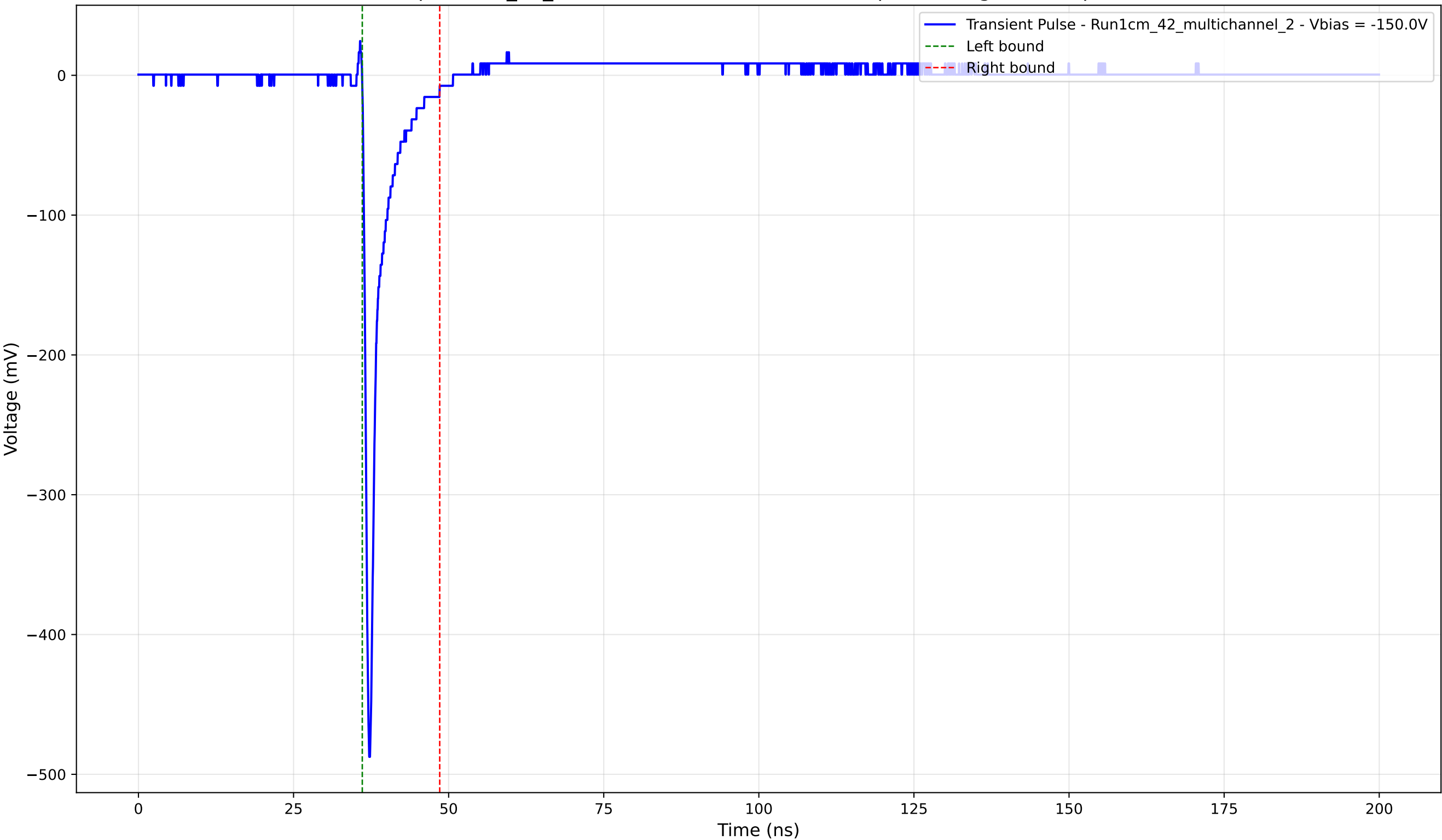
Transient Pulse - Sample: 1cm_42_multichannel - Position: 2590.0 \mu\text{m} - Charge: 24.97 pC - Rise Time: 0.75 ns
