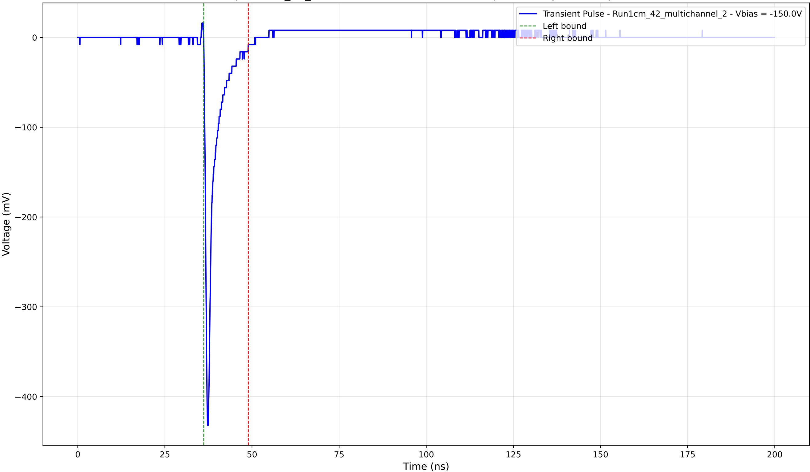
Transient Pulse - Sample: 1cm_42_multichannel - Position: 2690.0 \mu\text{m} - Charge: 24.66 pC - Rise Time: 0.78 ns
