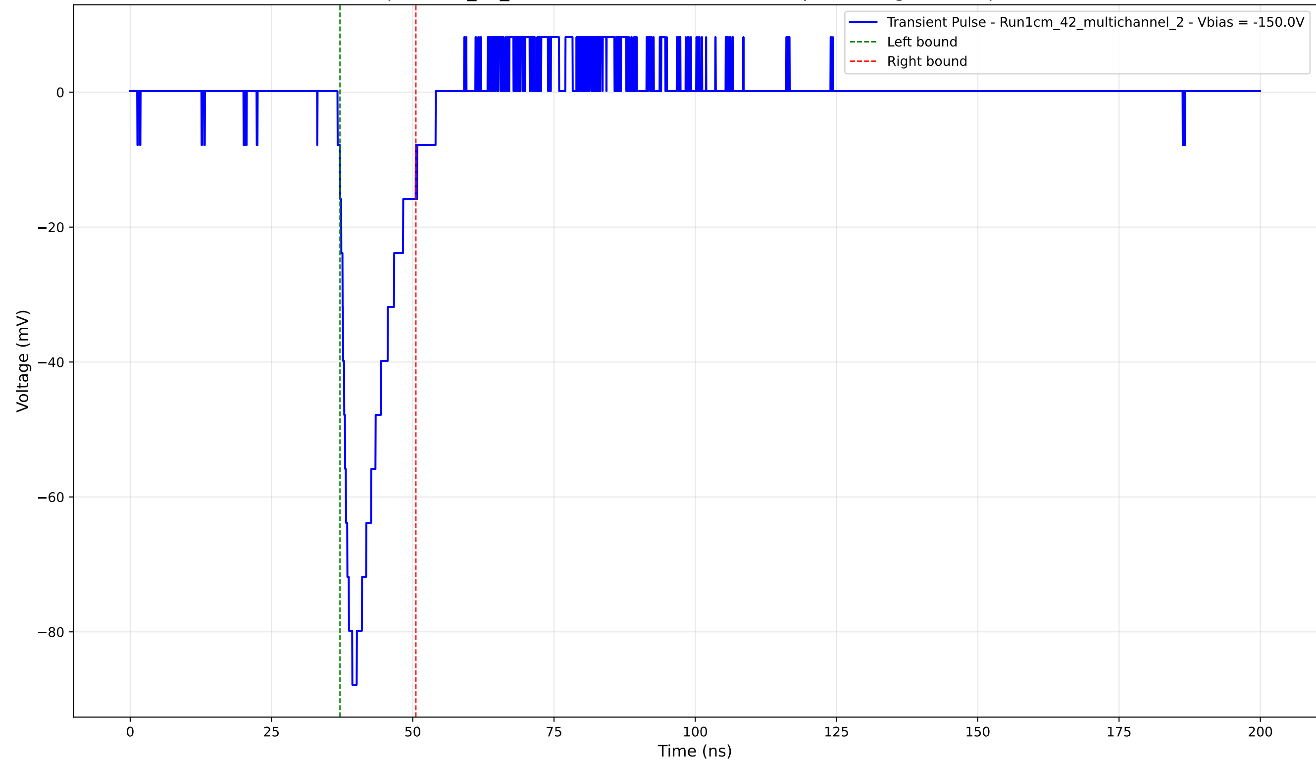
Transient Pulse - Sample: 1cm_42_multichannel - Position: 4205.0 \mu\text{m} - Charge: 12.39 pC - Rise Time: 1.60 ns
