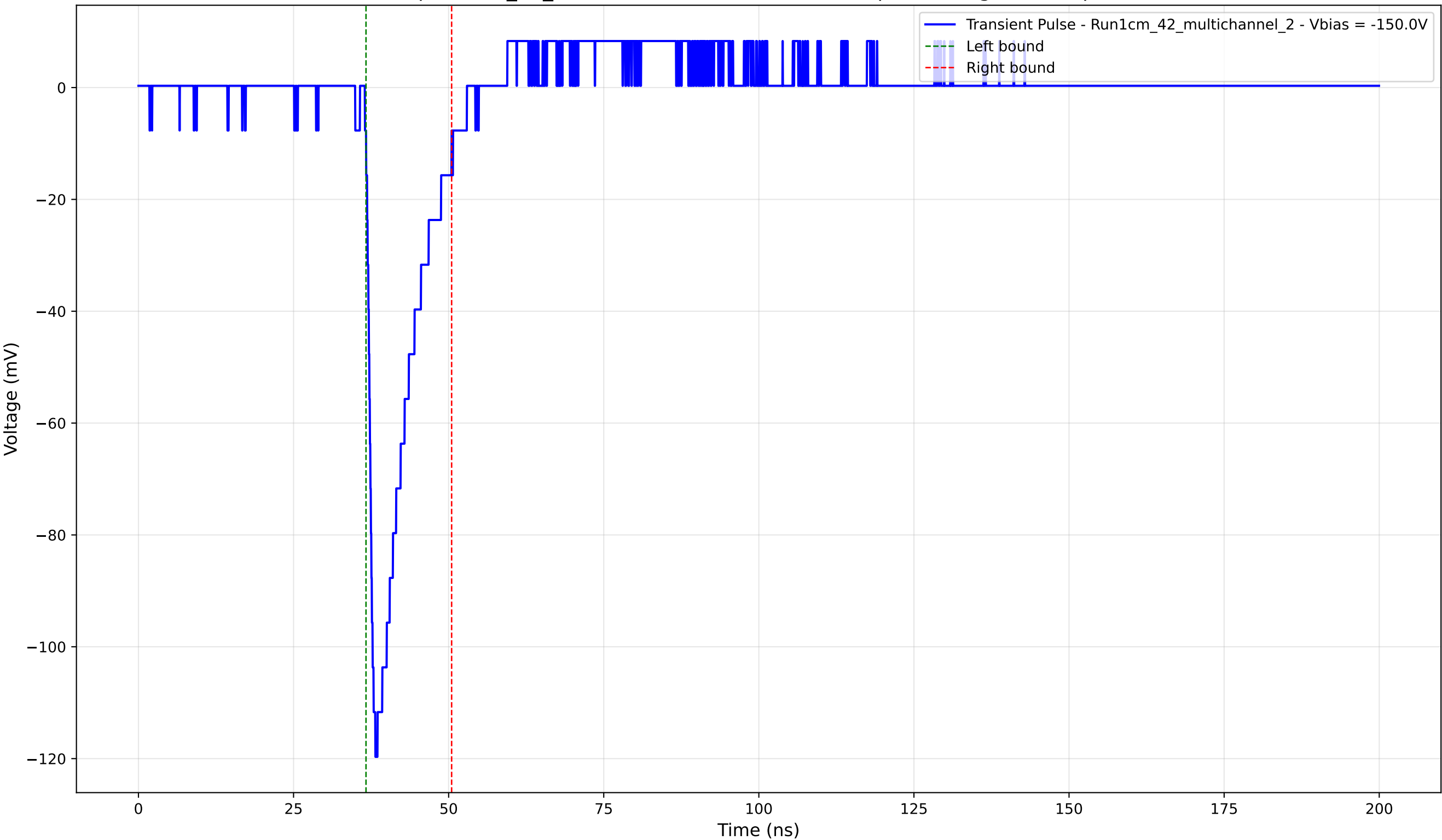
Transient Pulse - Sample: 1cm_42_multichannel - Position: 3575.0 \mu\text{m} - Charge: 15.35 pC - Rise Time: 1.22 ns
