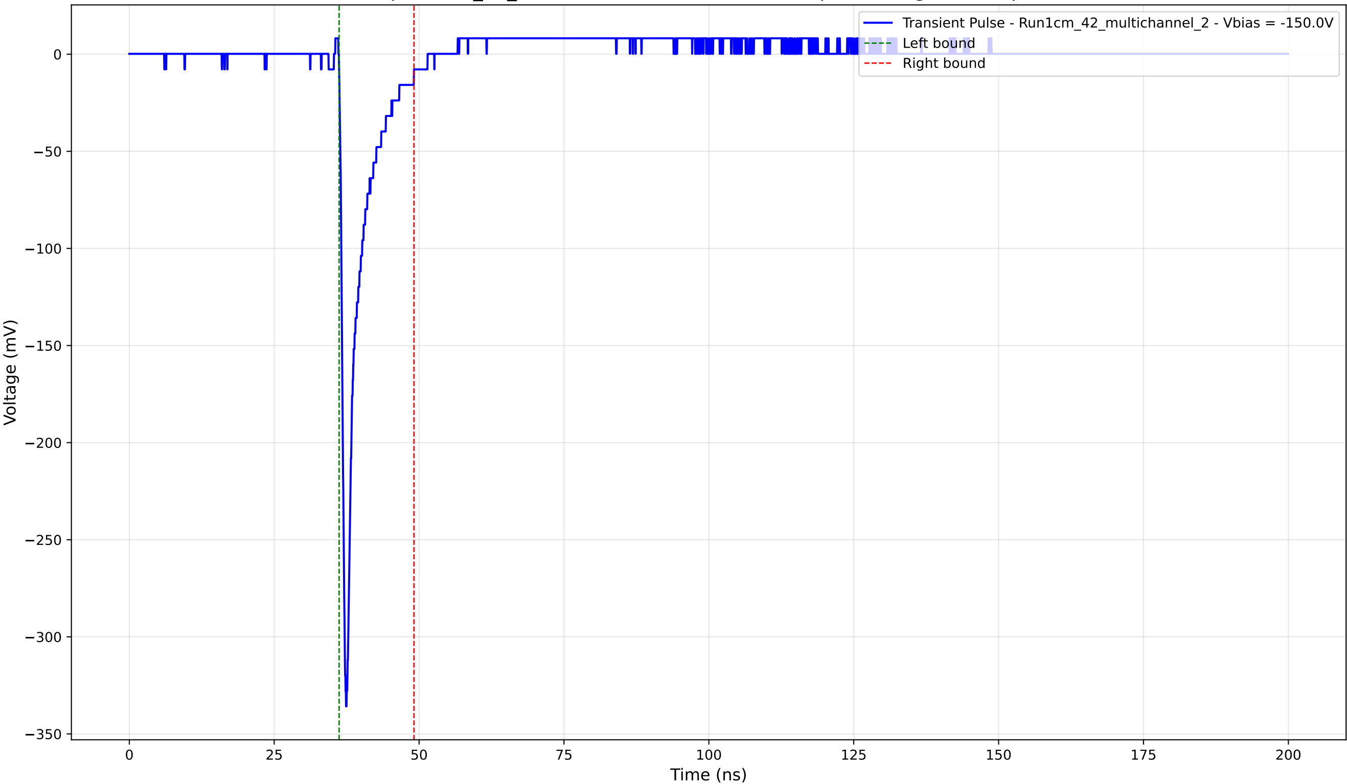
Transient Pulse - Sample: 1cm_42_multichannel - Position: 1935.0 \mu\text{m} - Charge: 21.51 pC - Rise Time: 0.82 ns
