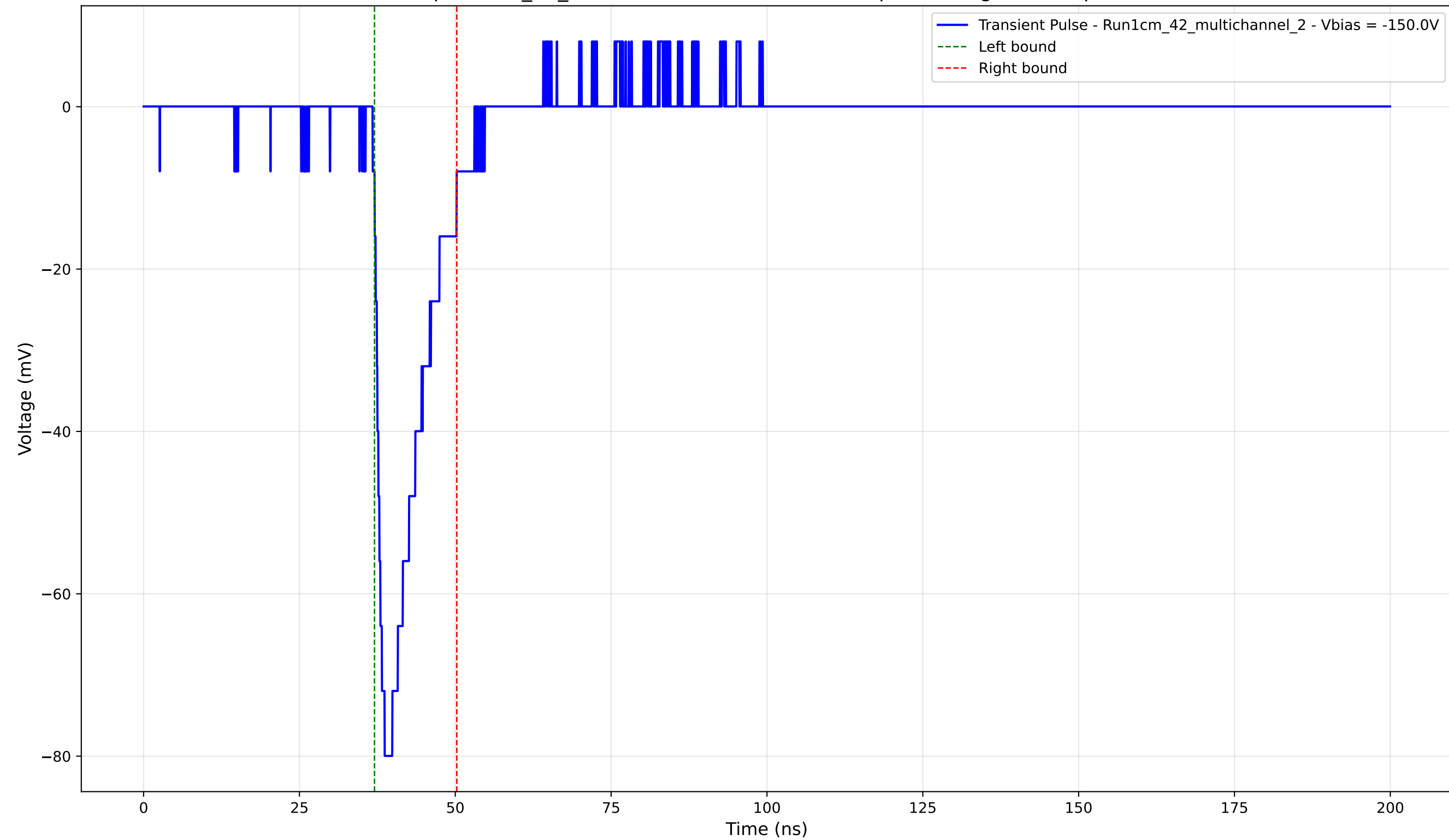
Transient Pulse - Sample: 1cm_42_multichannel - Position: 790.0 \mu\text{m} - Charge: 11.26 pC - Rise Time: 1.64 ns
