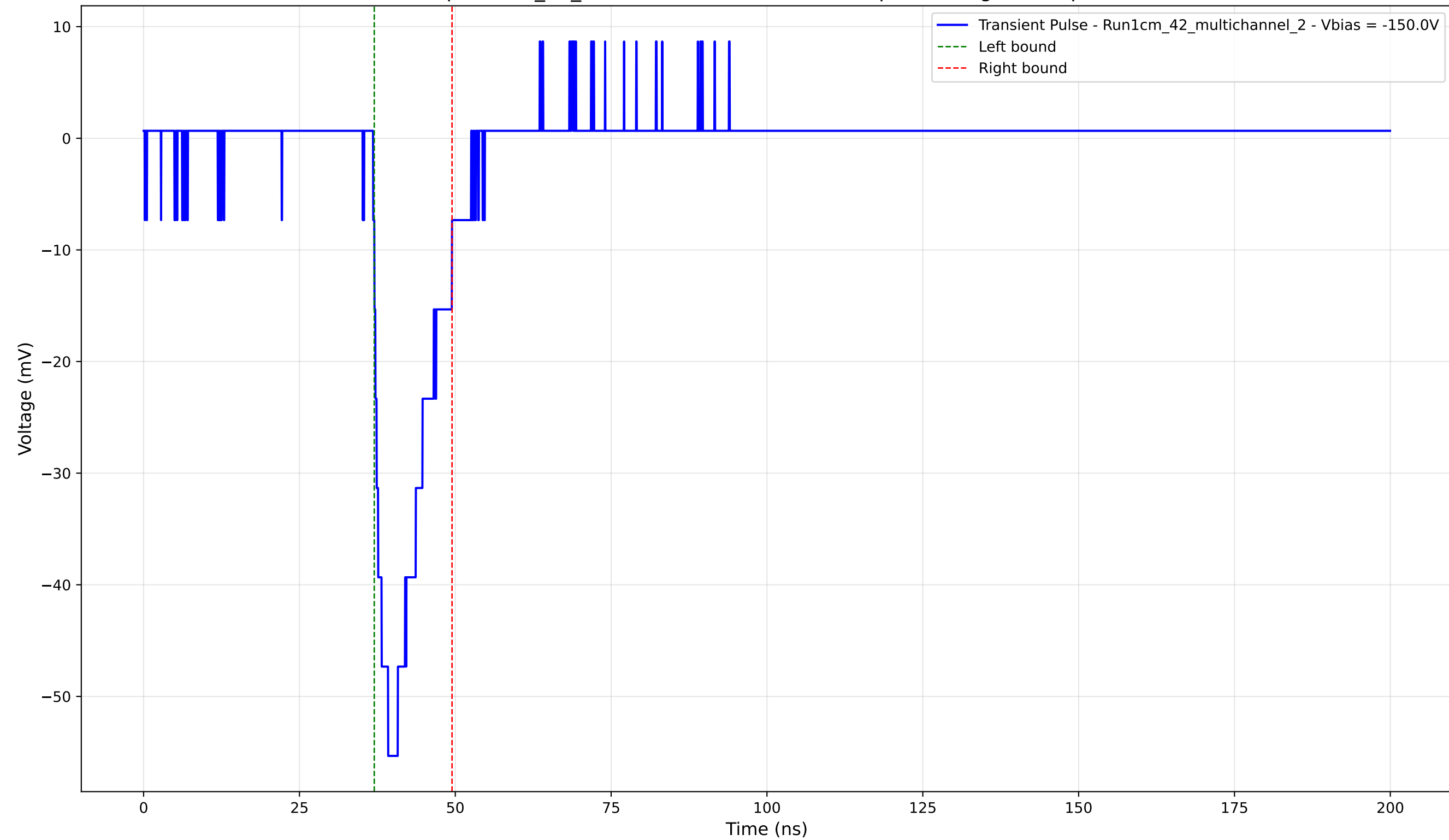
Transient Pulse - Sample: 1cm_42_multichannel - Position: 90.0 \mu\text{m} - Charge: 8.34 pC - Rise Time: 2.41 ns
