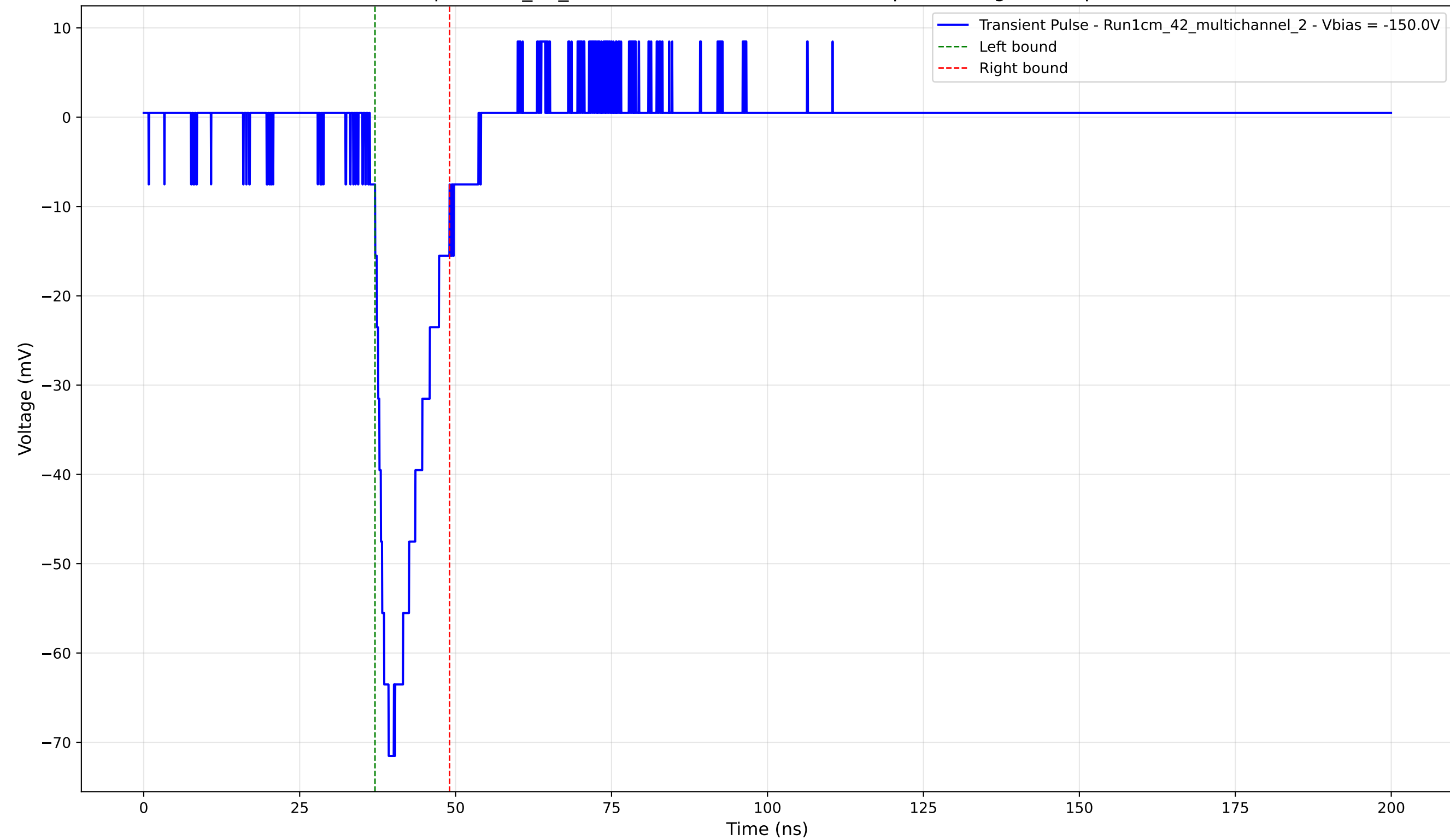
Transient Pulse - Sample: 1cm_42_multichannel - Position: 4690.0 \mu\text{m} - Charge: 9.93 pC - Rise Time: 3.00 ns
