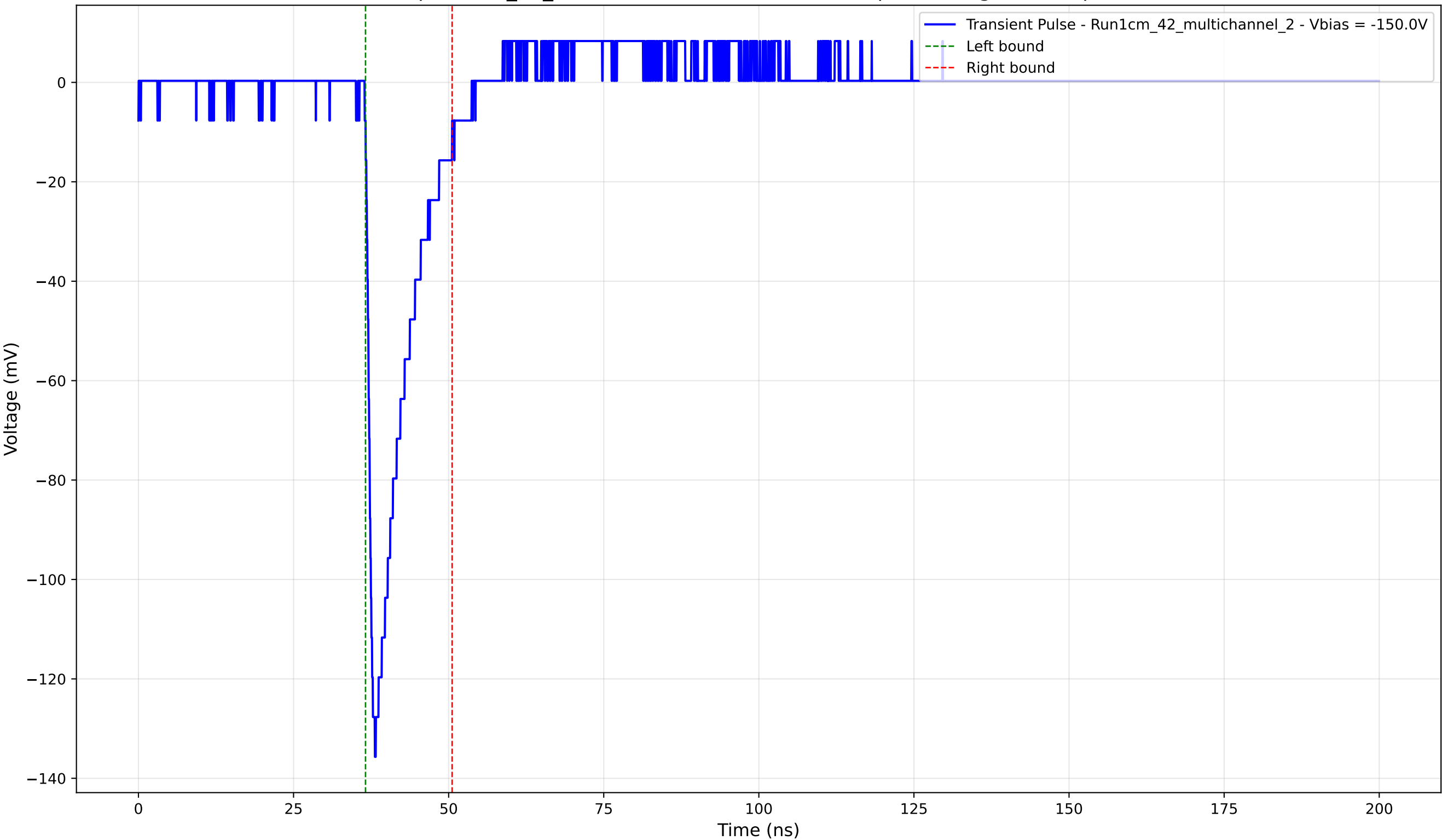
Transient Pulse - Sample: 1cm_42_multichannel - Position: 3465.0 \mu\text{m} - Charge: 16.24 pC - Rise Time: 1.17 ns
