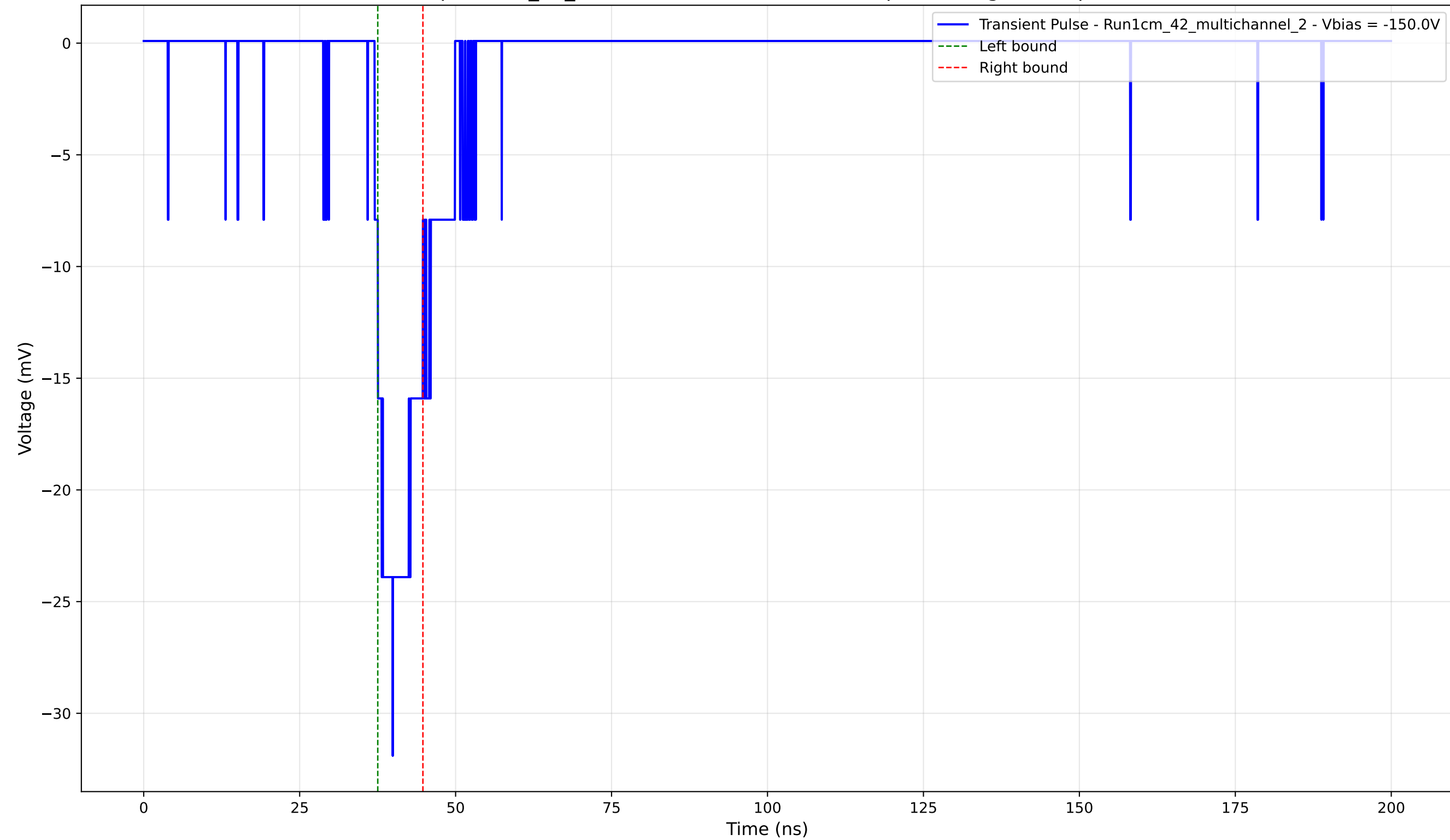
Transient Pulse - Sample: 1cm_42_multichannel - Position: 385.0 \mu\text{m} - Charge: 3.03 pC - Rise Time: 2.90 ns
