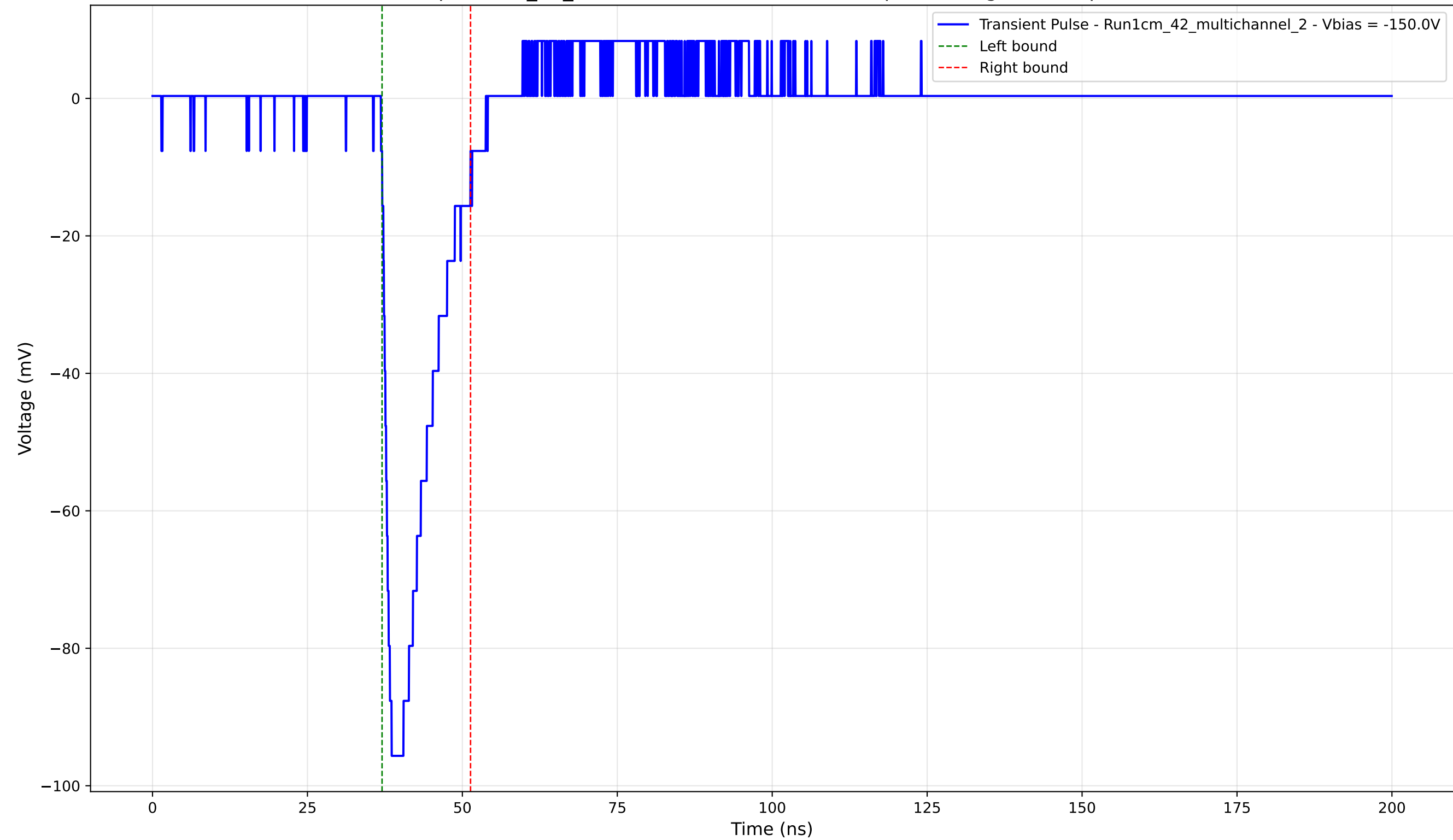
Transient Pulse - Sample: 1cm_42_multichannel - Position: 610.0 \mu\text{m} - Charge: 14.67 pC - Rise Time: 1.27 ns
