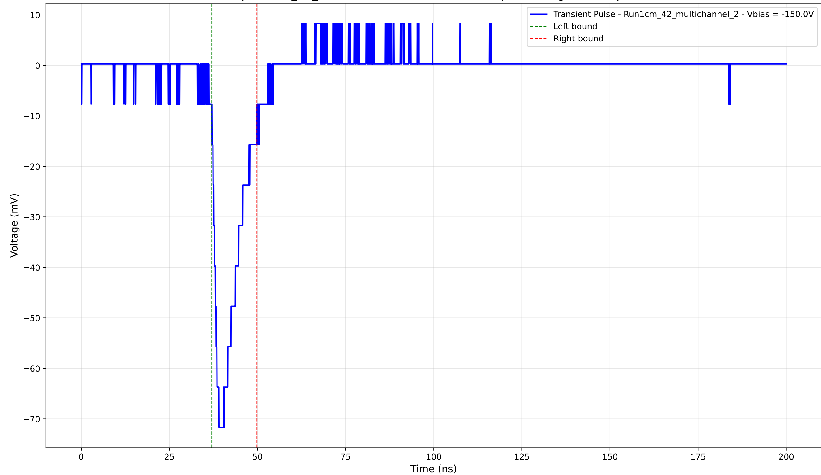
Transient Pulse - Sample: 1cm_42_multichannel - Position: 4640.0 \mu\text{m} - Charge: 10.40 pC - Rise Time: 2.80 ns
