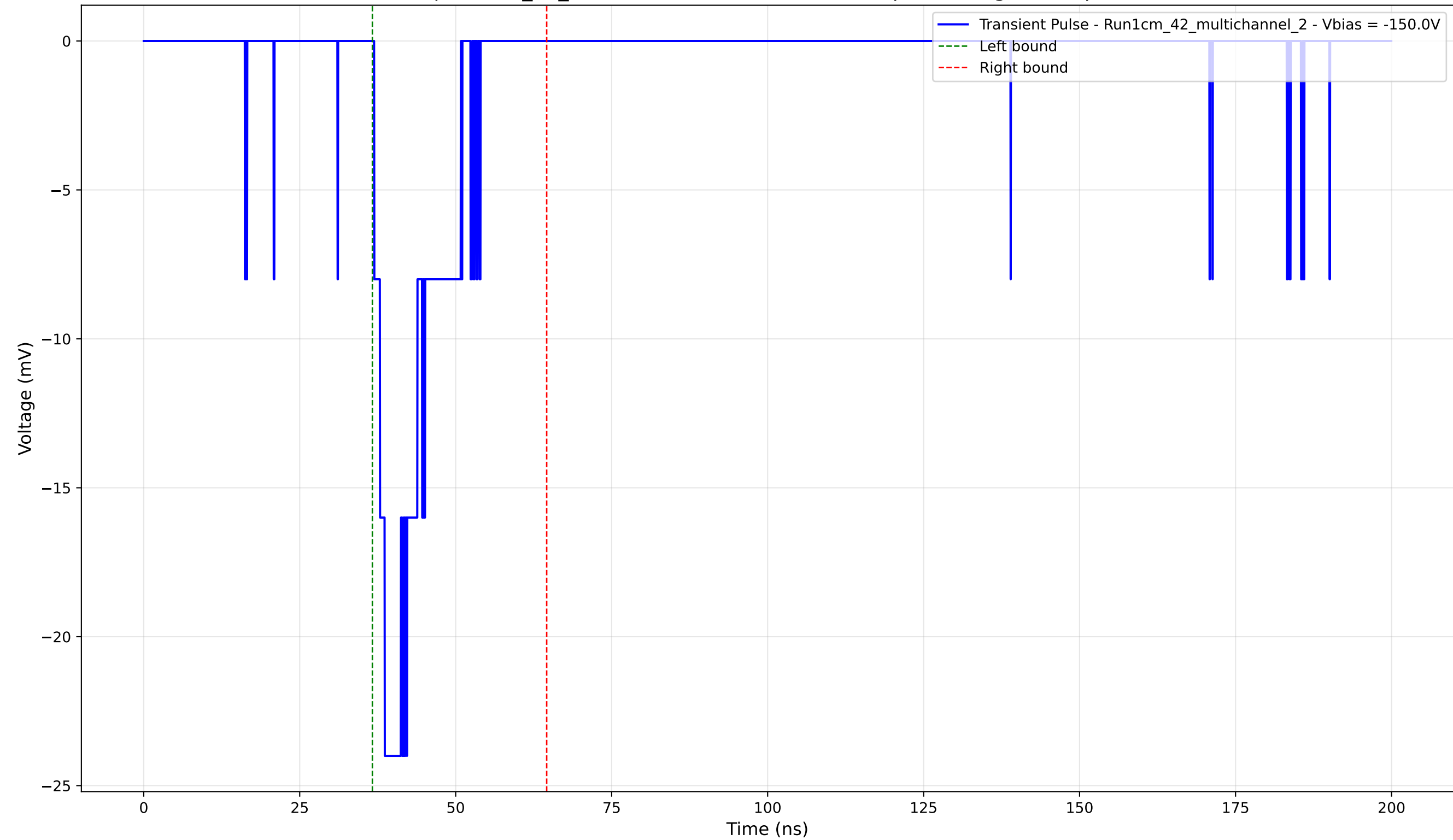
Transient Pulse - Sample: 1cm_42_multichannel - Position: 4430.0 \mu\text{m} - Charge: 3.85 pC - Rise Time: 1.71 ns
