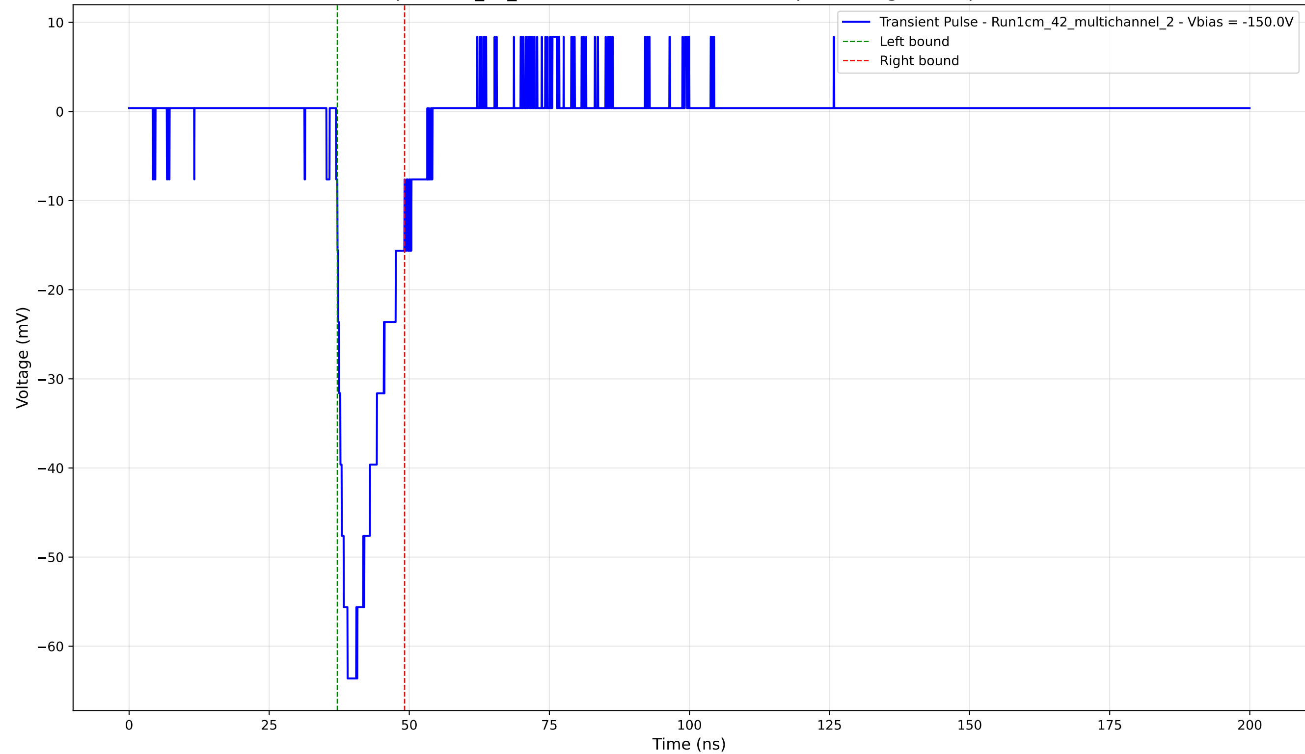
Transient Pulse - Sample: 1cm_42_multichannel - Position: 275.0 \mu\text{m} - Charge: 9.37 pC - Rise Time: 2.05 ns
