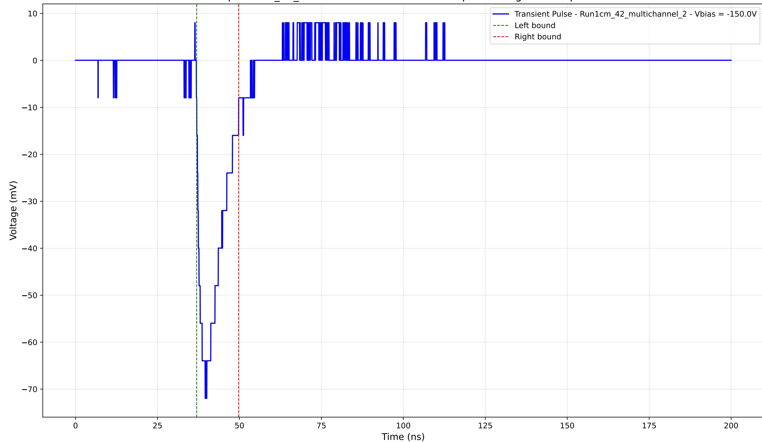
Transient Pulse - Sample: 1cm_42_multichannel - Position: 140.0 \mu\text{m} - Charge: 10.52 pC - Rise Time: 2.68 ns
