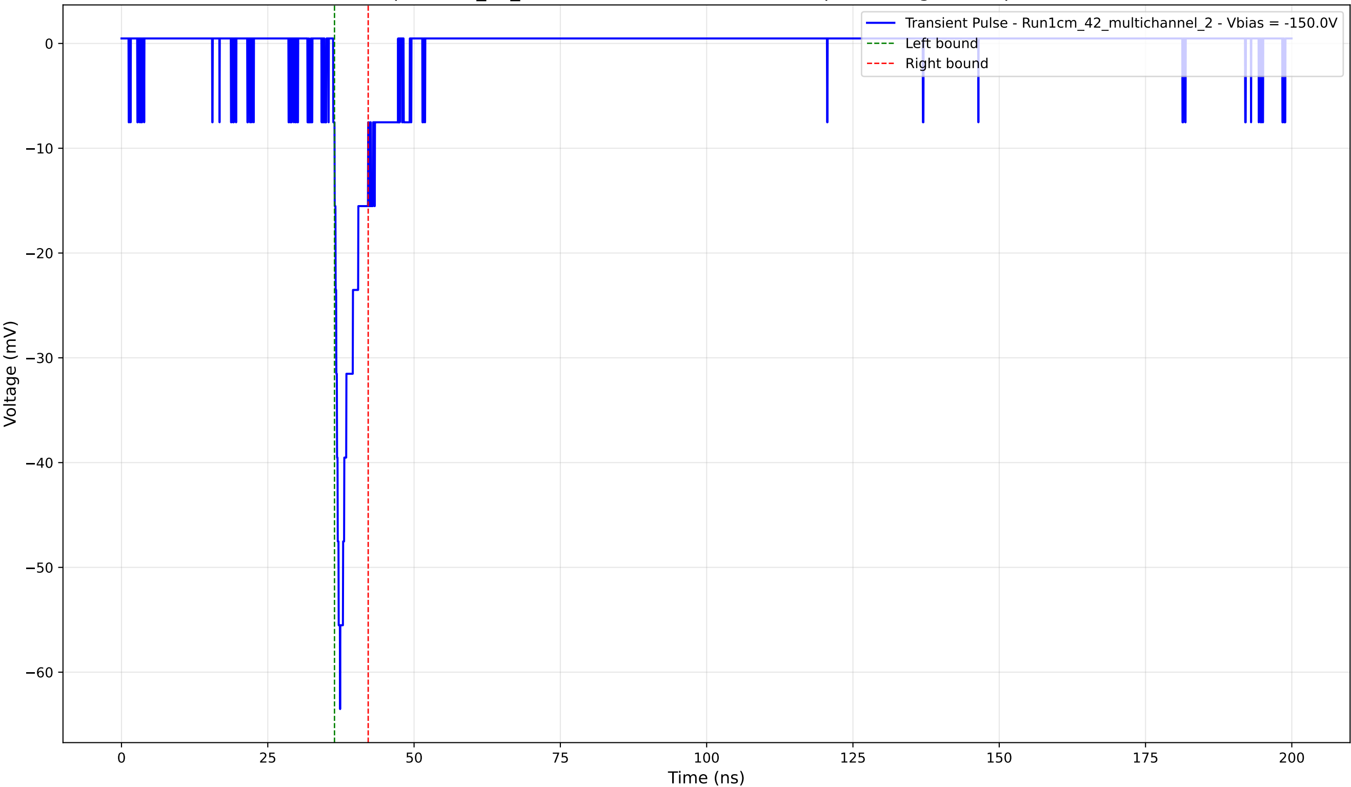
Transient Pulse - Sample: 1cm_42_multichannel - Position: 1895.0 \mu\text{m} - Charge: 3.42 pC - Rise Time: 1.17 ns
