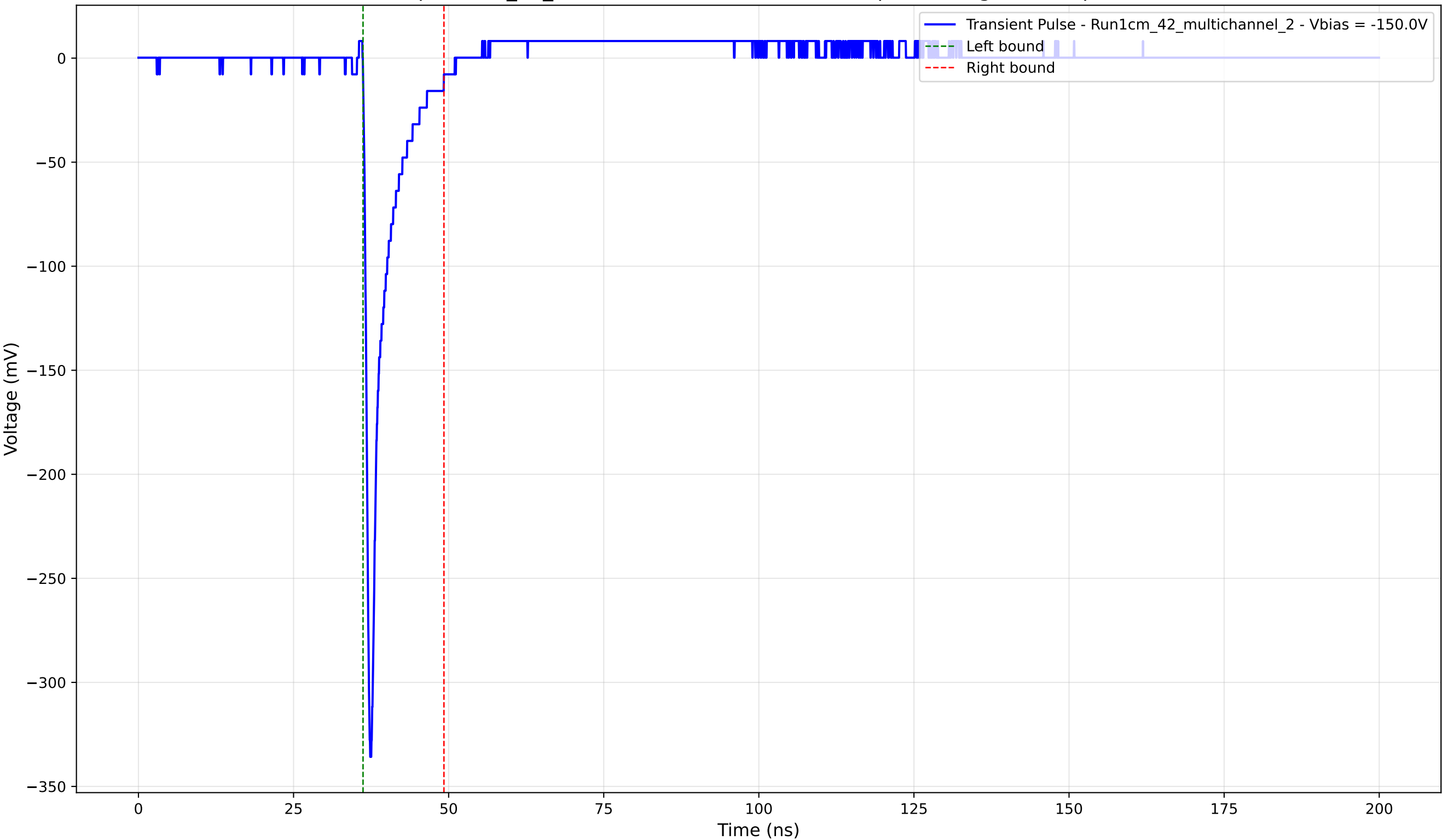
Transient Pulse - Sample: 1cm_42_multichannel - Position: 2795.0 \mu\text{m} - Charge: 21.36 pC - Rise Time: 0.82 ns
