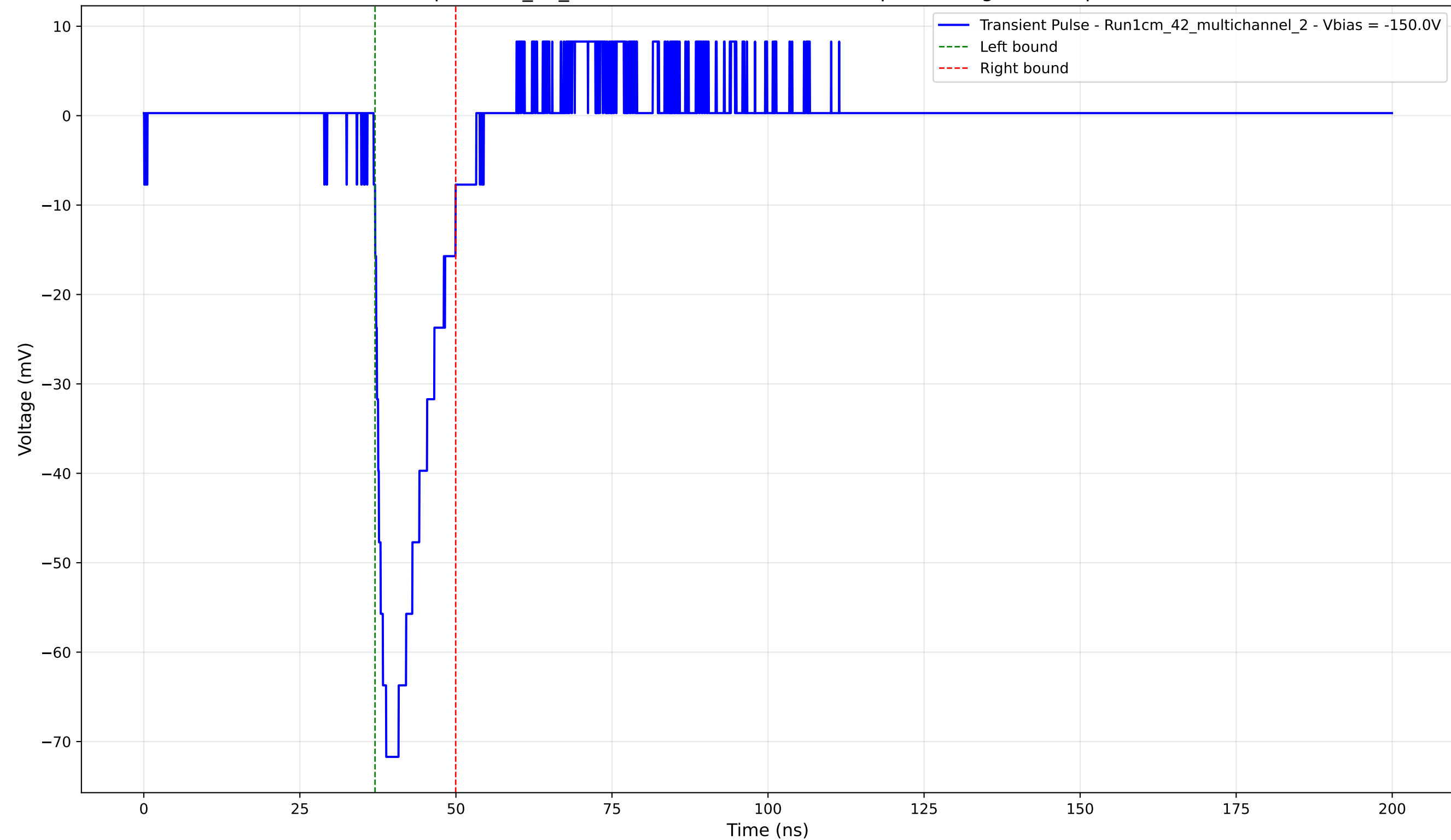
Transient Pulse - Sample: 1cm_42_multichannel - Position: 220.0 \mu\text{m} - Charge: 11.30 pC - Rise Time: 2.00 ns
