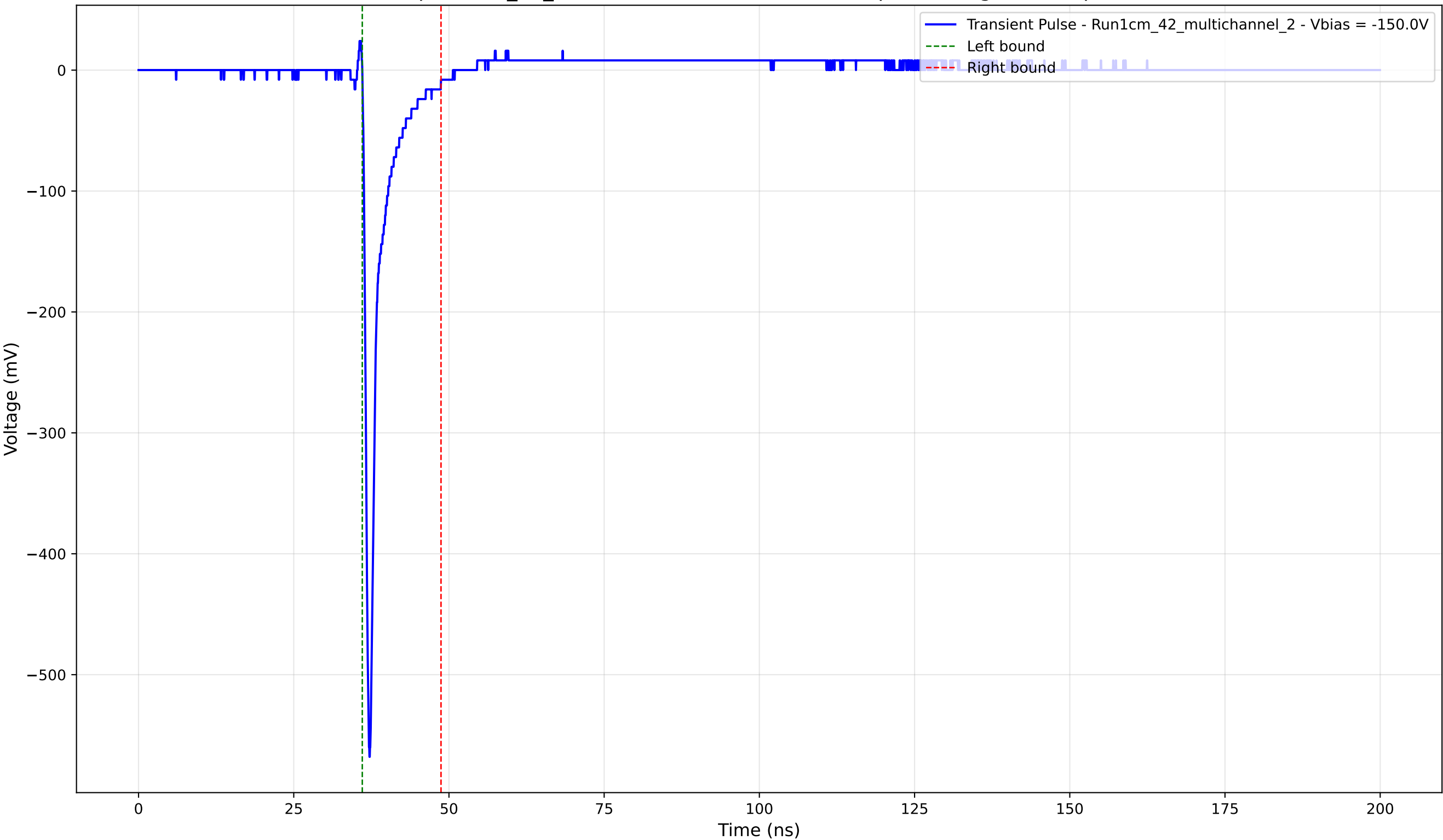
Transient Pulse - Sample: 1cm_42_multichannel - Position: 2190.0 \mu\text{m} - Charge: 27.74 pC - Rise Time: 0.76 ns
