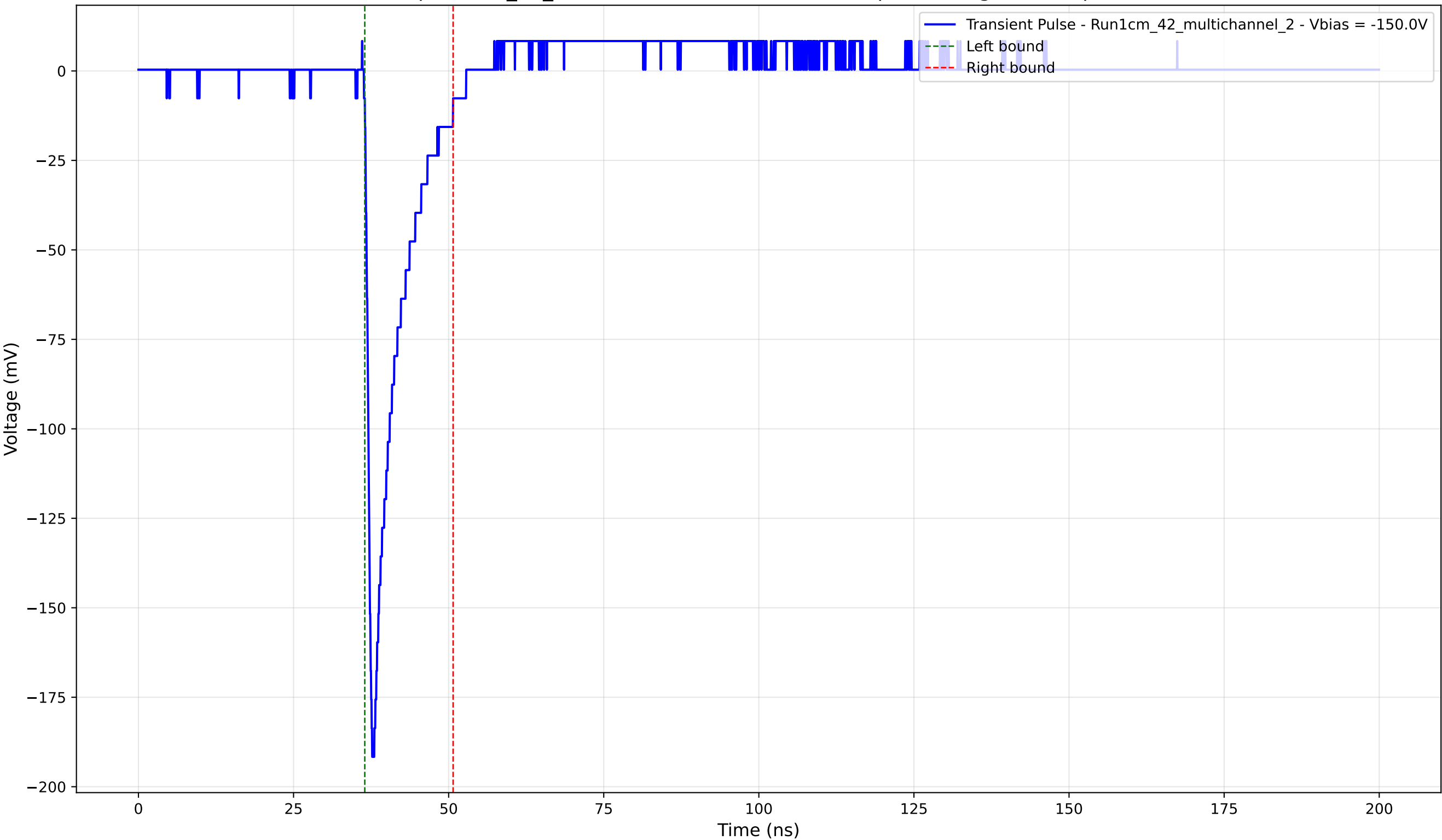
Transient Pulse - Sample: 1cm_42_multichannel - Position: 3220.0 \mu\text{m} - Charge: 19.04 pC - Rise Time: 0.94 ns
