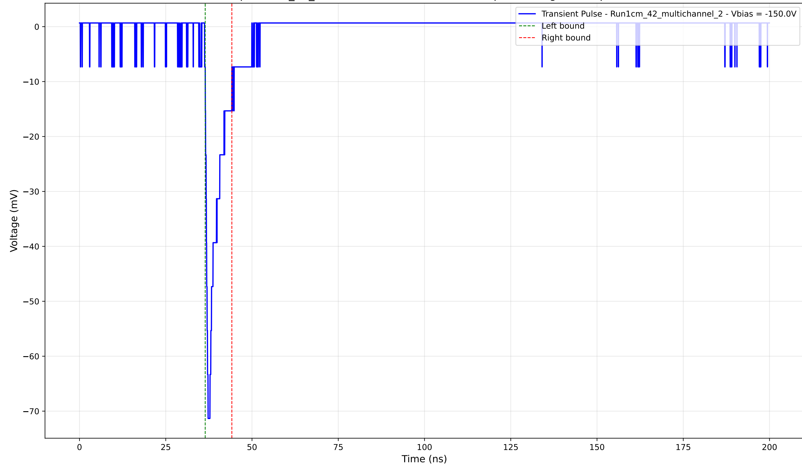
Transient Pulse - Sample: 1cm_42_multichannel - Position: 2915.0 \mu\text{m} - Charge: 5.09 pC - Rise Time: 1.00 ns
