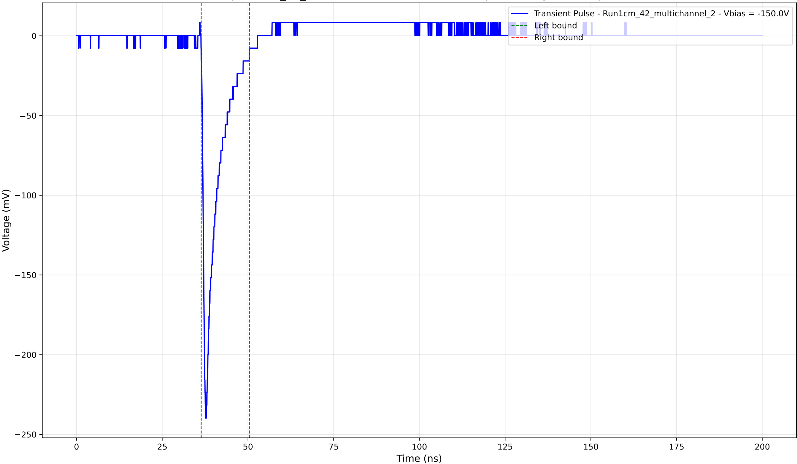
Transient Pulse - Sample: 1cm_42_multichannel - Position: 1605.0 \mu\text{m} - Charge: 21.72 pC - Rise Time: 0.96 ns
