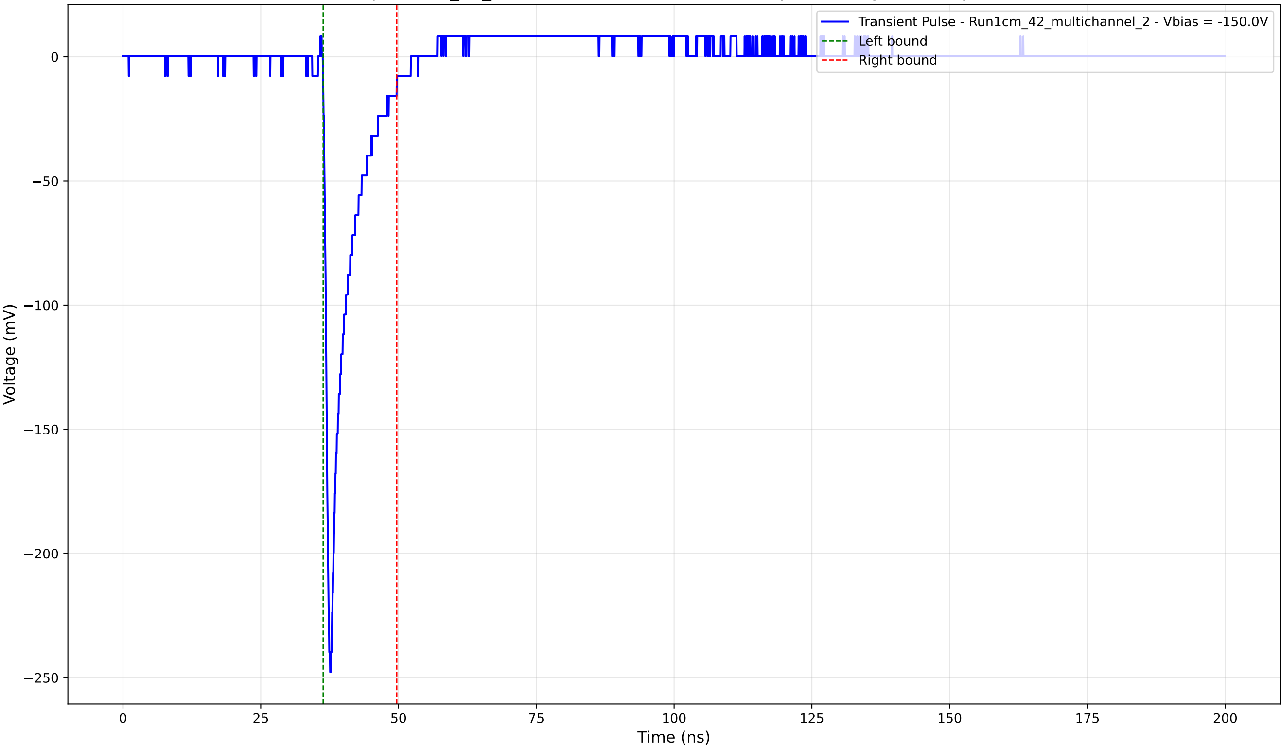
Transient Pulse - Sample: 1cm_42_multichannel - Position: 3030.0 \mu\text{m} - Charge: 20.32 pC - Rise Time: 0.87 ns
