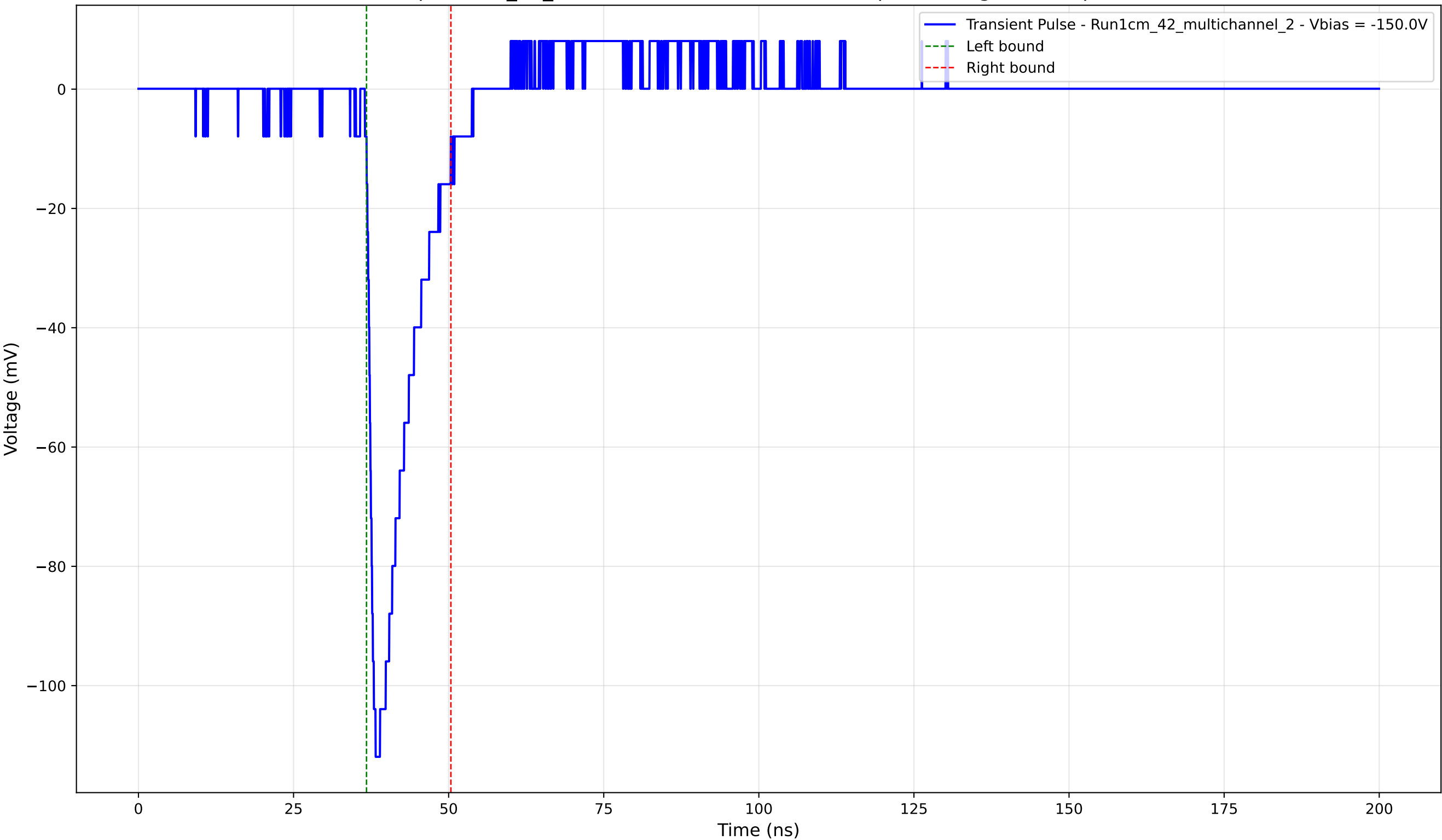
Transient Pulse - Sample: 1cm_42_multichannel - Position: 3635.0 \mu\text{m} - Charge: 14.86 pC - Rise Time: 1.18 ns
