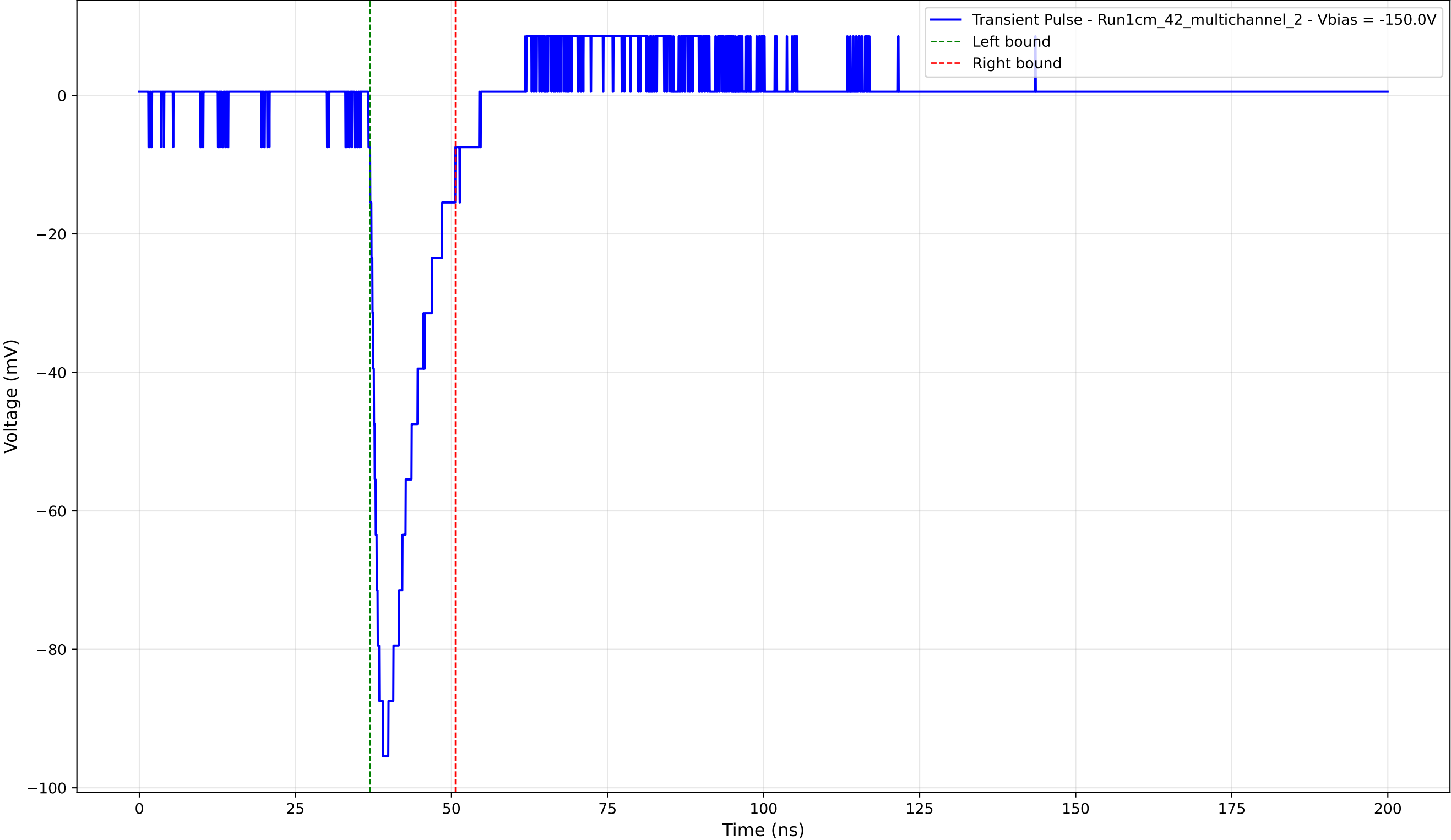
Transient Pulse - Sample: 1cm_42_multichannel - Position: 3975.0 \mu\text{m} - Charge: 13.41 pC - Rise Time: 1.47 ns
