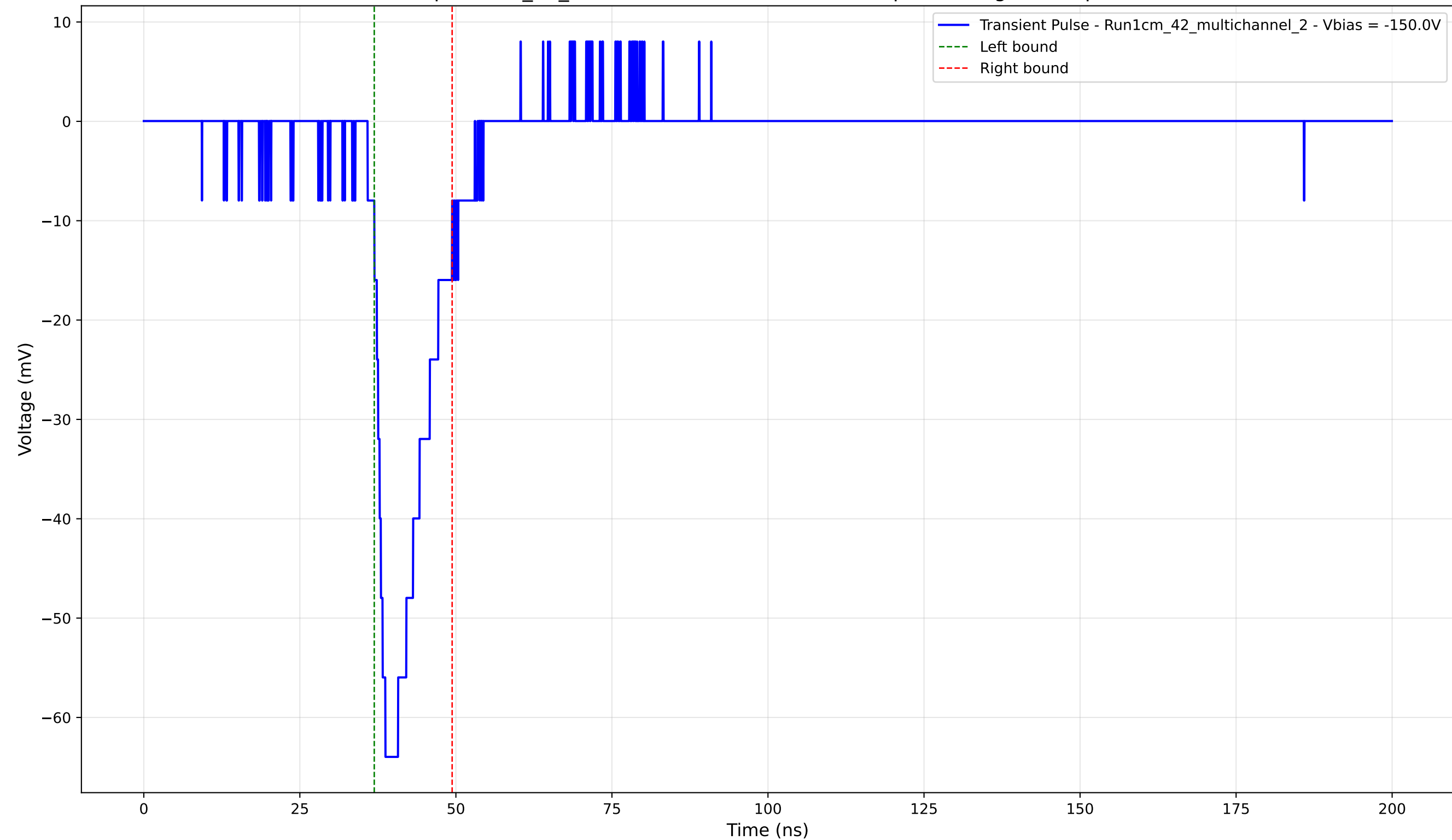
Transient Pulse - Sample: 1cm_42_multichannel - Position: 4755.0 \mu\text{m} - Charge: 9.66 pC - Rise Time: 2.85 ns
