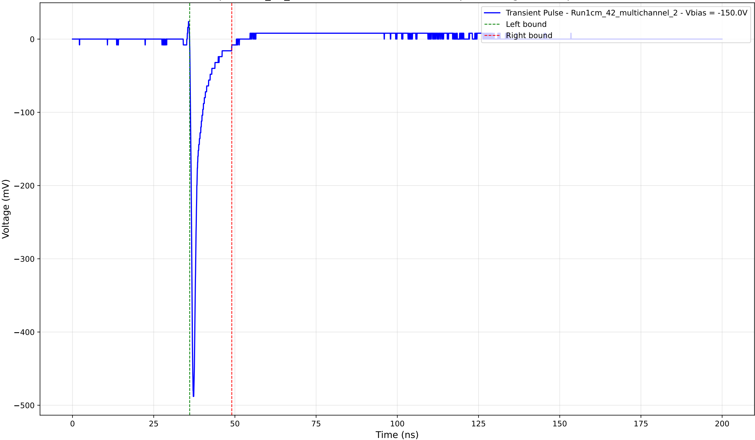
Transient Pulse - Sample: 1cm_42_multichannel - Position: 2595.0 \mu\text{m} - Charge: 25.32 pC - Rise Time: 0.78 ns
