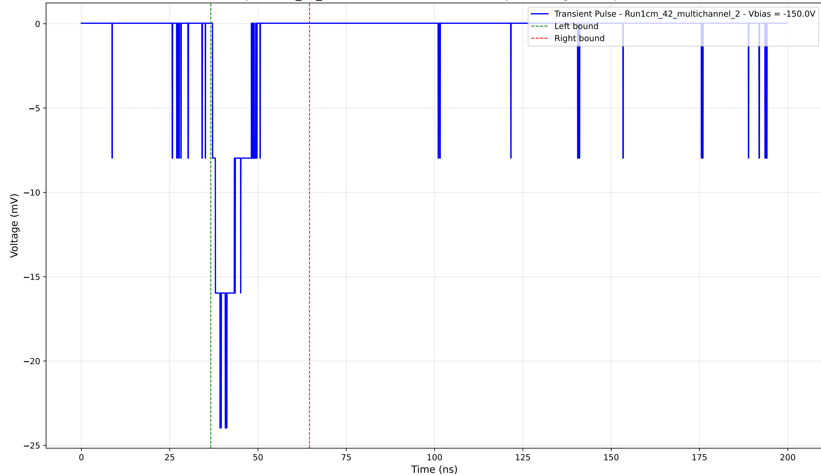
Transient Pulse - Sample: 1cm_42_multichannel - Position: 4350.0 \mu\text{m} - Charge: 2.86 pC - Rise Time: 2.15 ns
