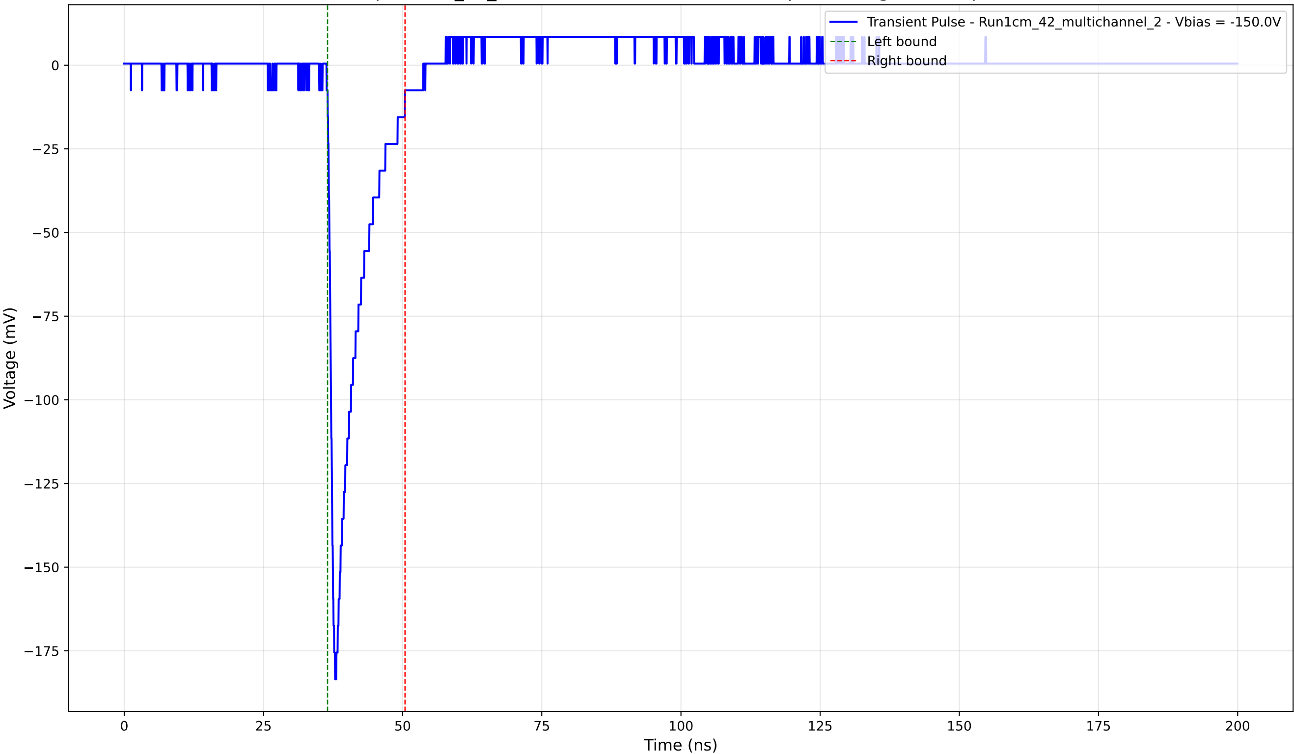
Transient Pulse - Sample: 1cm_42_multichannel - Position: 1435.0 \mu\text{m} - Charge: 19.08 pC - Rise Time: 0.99 ns
