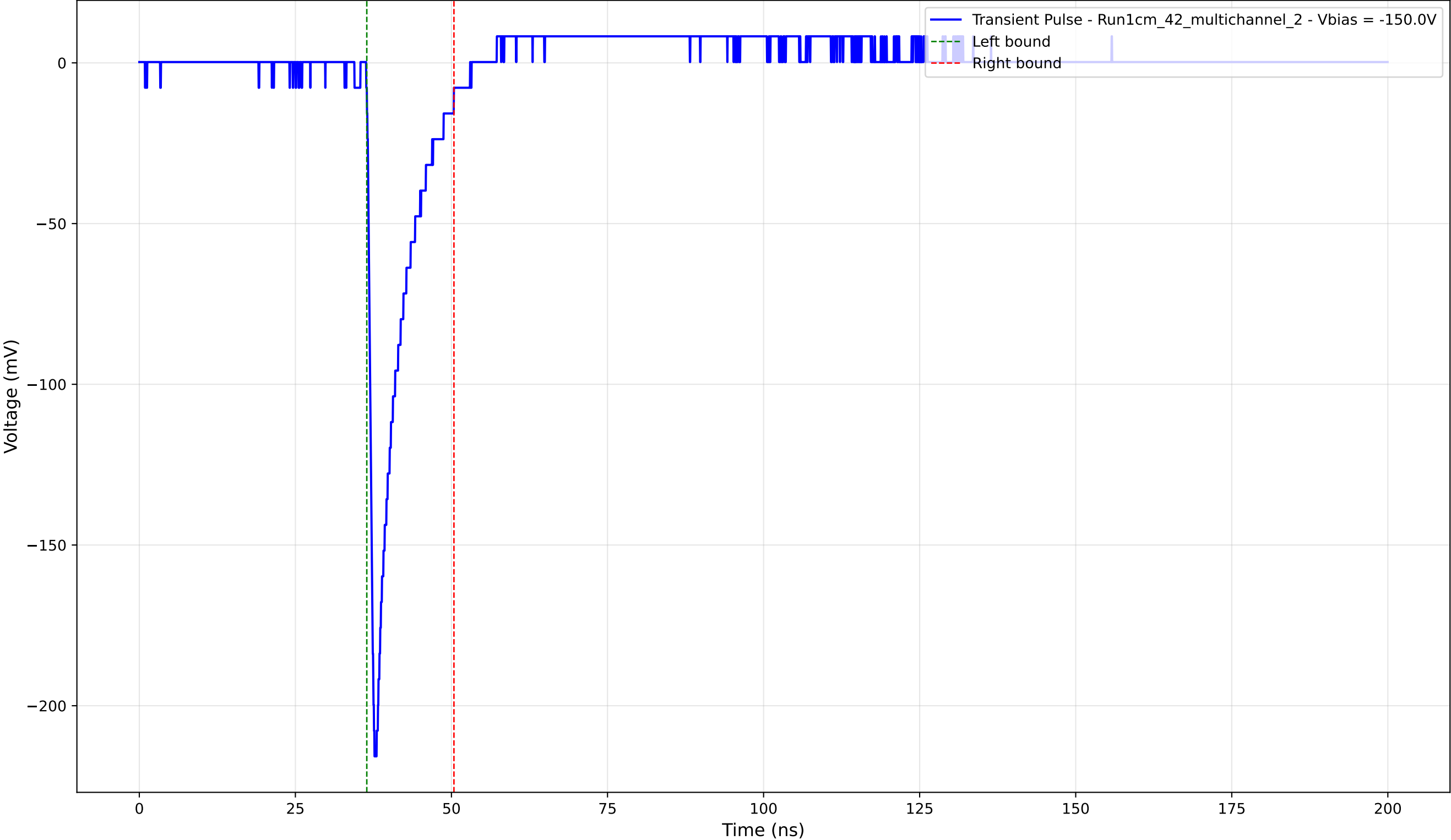
Transient Pulse - Sample: 1cm_42_multichannel - Position: 1525.0 \mu\text{m} - Charge: 21.18 pC - Rise Time: 0.97 ns
