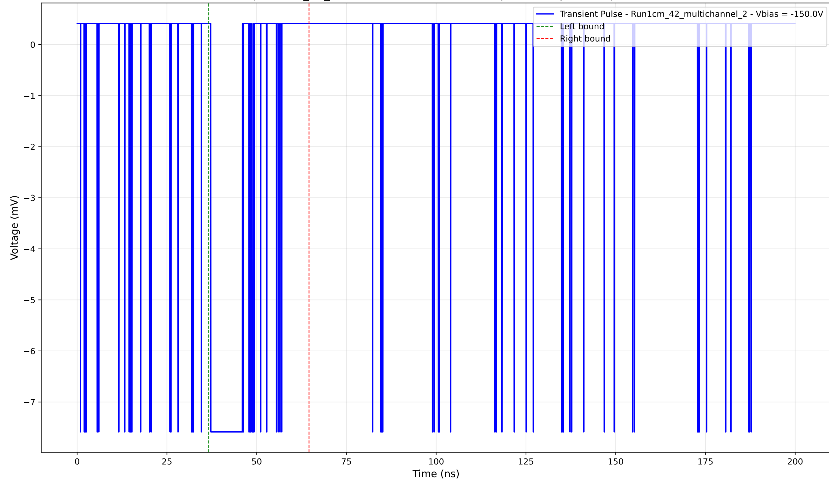
Transient Pulse - Sample: 1cm_42_multichannel - Position: 45.0 \mu\text{m} - Charge: 1.39 pC - Rise Time: 0.04 ns
