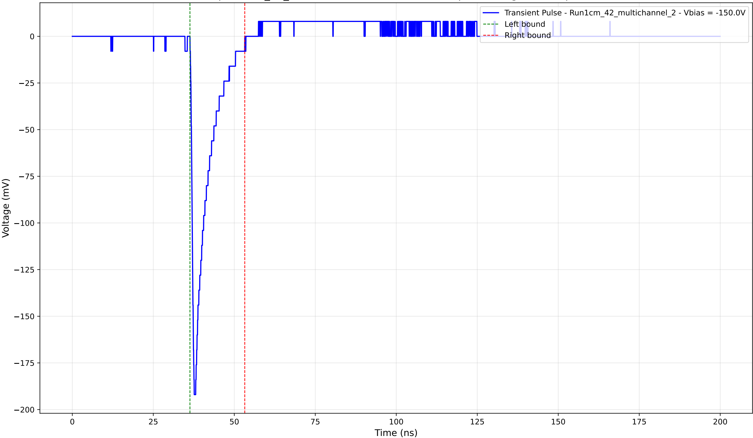
Transient Pulse - Sample: 1cm_42_multichannel - Position: 3215.0 \mu\text{m} - Charge: 19.72 pC - Rise Time: 0.94 ns
