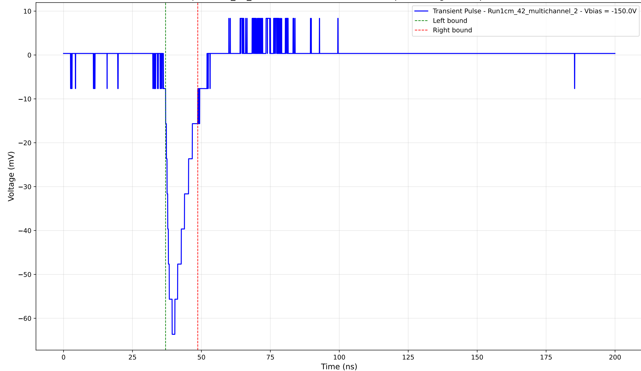
Transient Pulse - Sample: 1cm_42_multichannel - Position: 4800.0 \mu\text{m} - Charge: 8.77 pC - Rise Time: 3.17 ns
