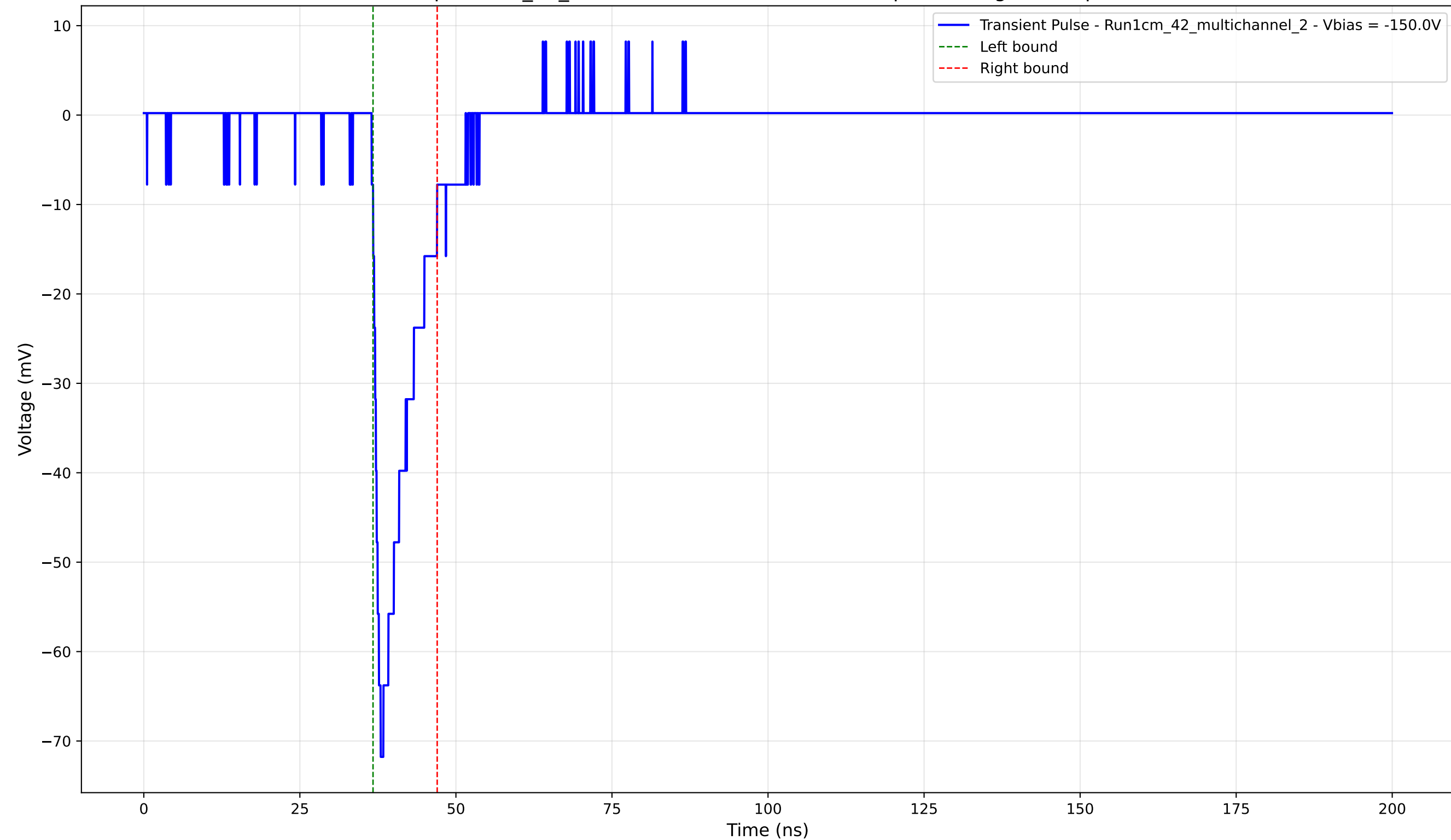
Transient Pulse - Sample: 1cm_42_multichannel - Position: 1310.0 \mu\text{m} - Charge: 7.59 pC - Rise Time: 1.44 ns
