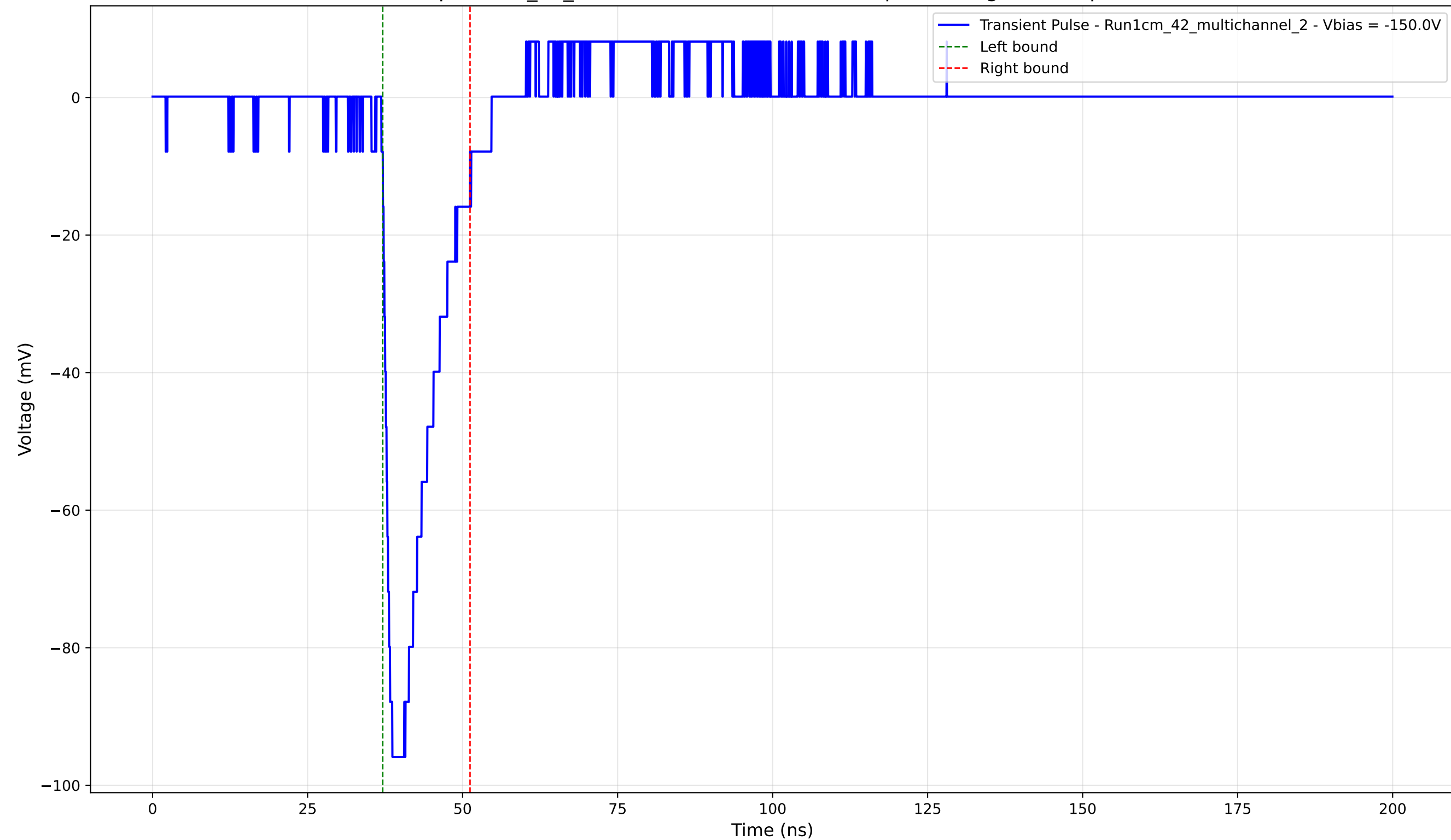
Transient Pulse - Sample: 1cm_42_multichannel - Position: 605.0 \mu\text{m} - Charge: 14.72 pC - Rise Time: 1.19 ns
