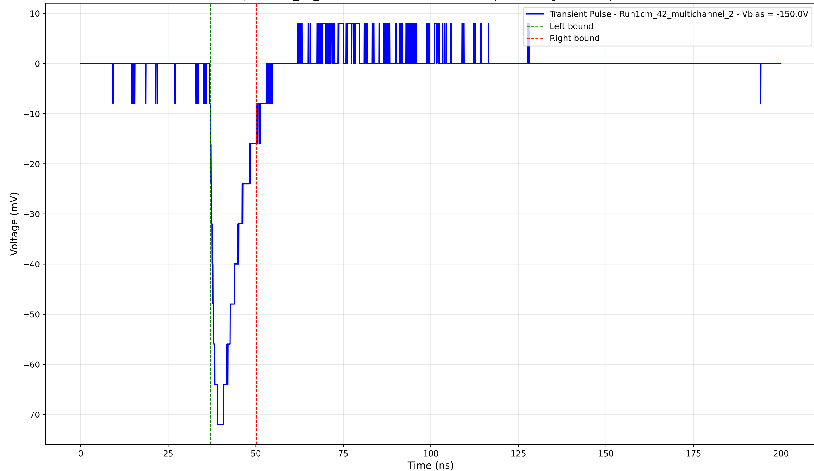
Transient Pulse - Sample: 1cm_42_multichannel - Position: 250.0 \mu\text{m} - Charge: 11.17 pC - Rise Time: 2.16 ns
