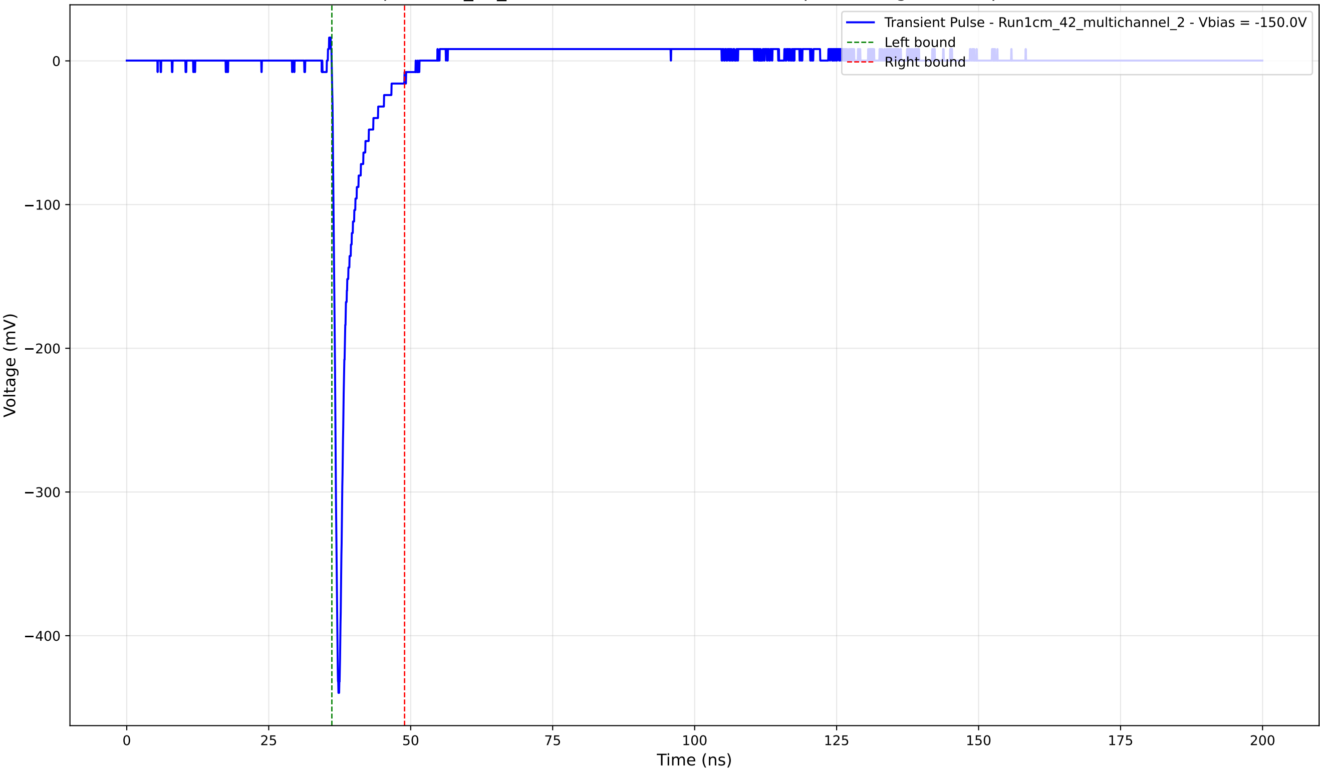
Transient Pulse - Sample: 1cm_42_multichannel - Position: 2680.0 \mu\text{m} - Charge: 24.72 pC - Rise Time: 0.80 ns
