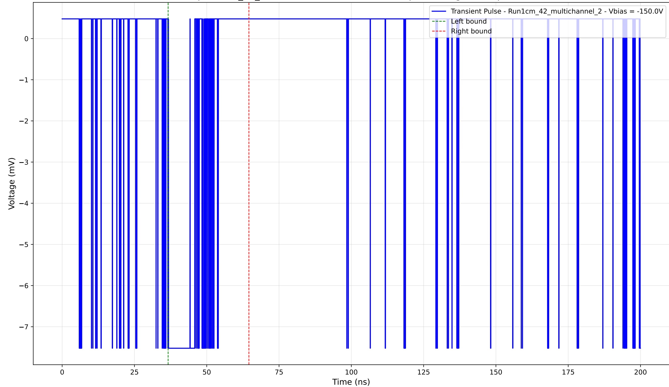
Transient Pulse - Sample: 1cm_42_multichannel - Position: 1350.0 \mu\text{m} - Charge: 1.56 pC - Rise Time: 0.04 ns
