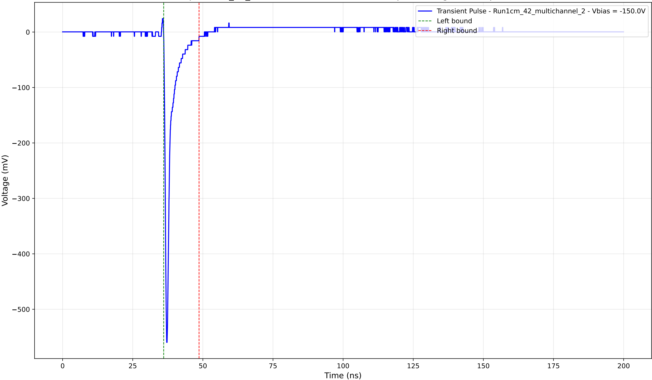
Transient Pulse - Sample: 1cm_42_multichannel - Position: 2520.0 \mu\text{m} - Charge: 26.70 pC - Rise Time: 0.74 ns
