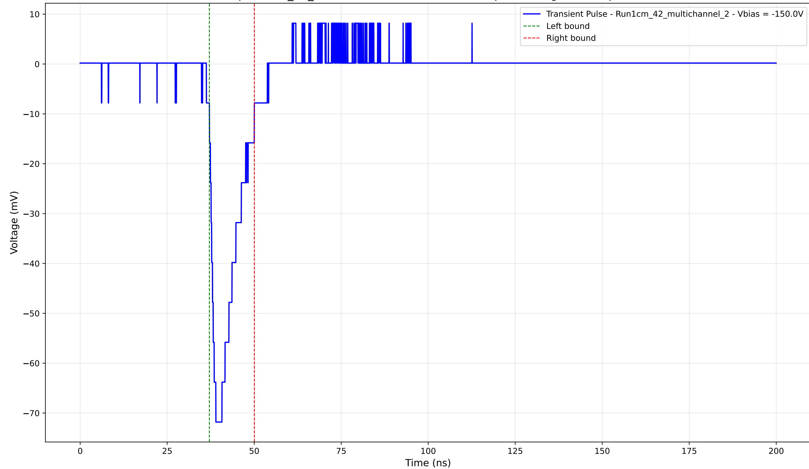
Transient Pulse - Sample: 1cm_42_multichannel - Position: 4580.0 \mu\text{m} - Charge: 10.64 pC - Rise Time: 2.72 ns
