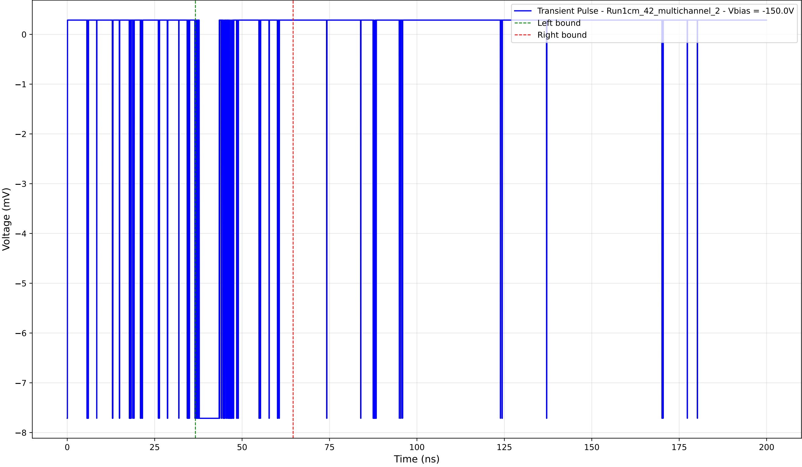
Transient Pulse - Sample: 1cm_42_multichannel - Position: 3890.0 \mu\text{m} - Charge: 1.28 pC - Rise Time: 0.00 ns (N/A)
