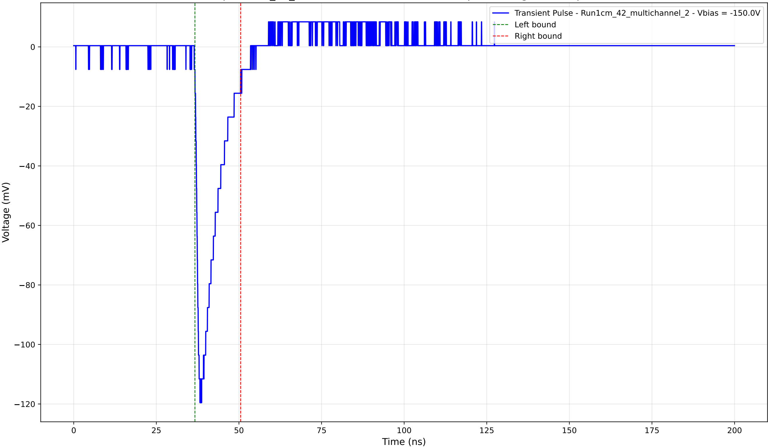
Transient Pulse - Sample: 1cm_42_multichannel - Position: 3585.0 \mu\text{m} - Charge: 15.23 pC - Rise Time: 1.26 ns
