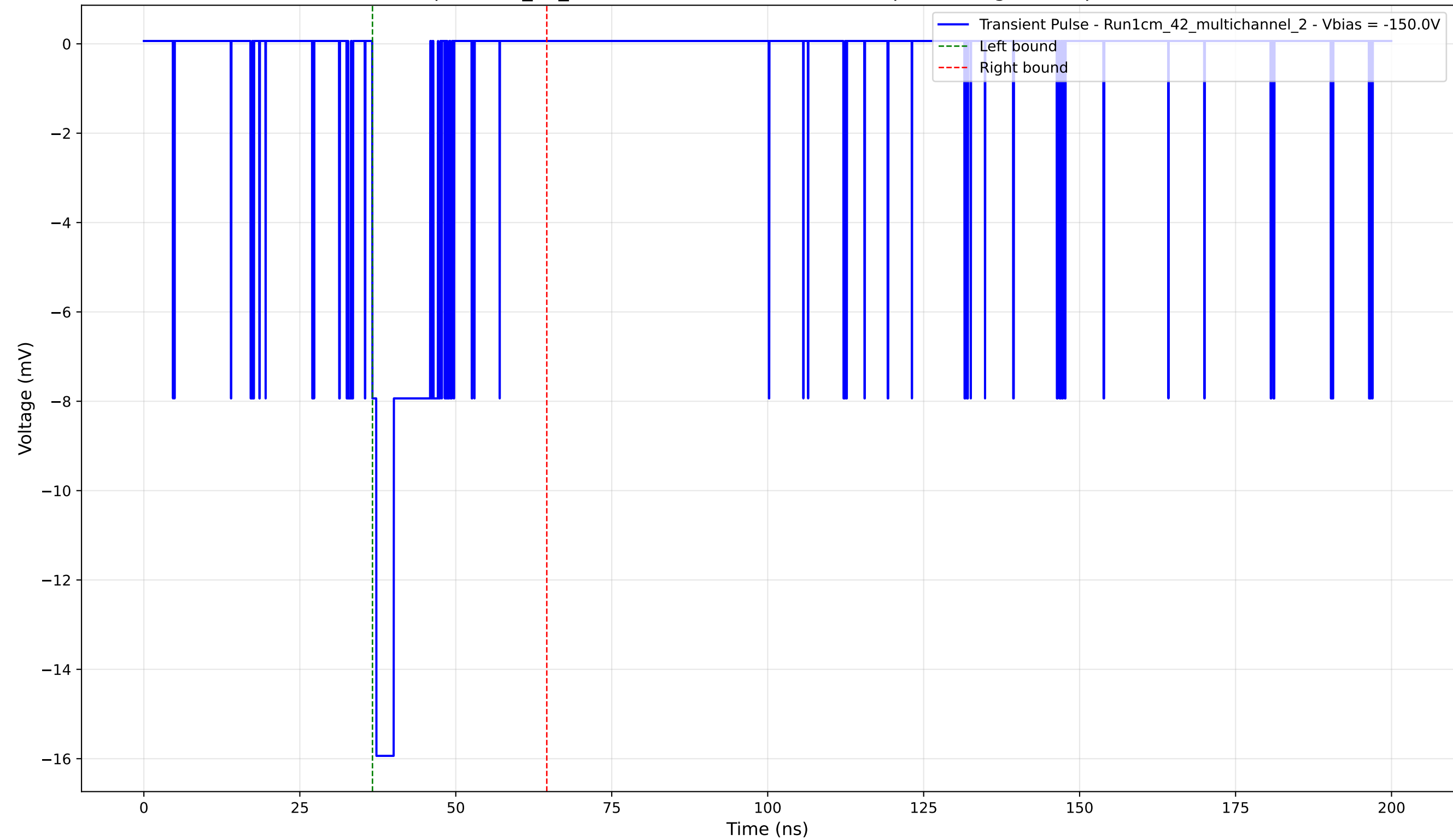
Transient Pulse - Sample: 1cm_42_multichannel - Position: 3360.0 \mu\text{m} - Charge: 2.24 pC - Rise Time: 0.67 ns
