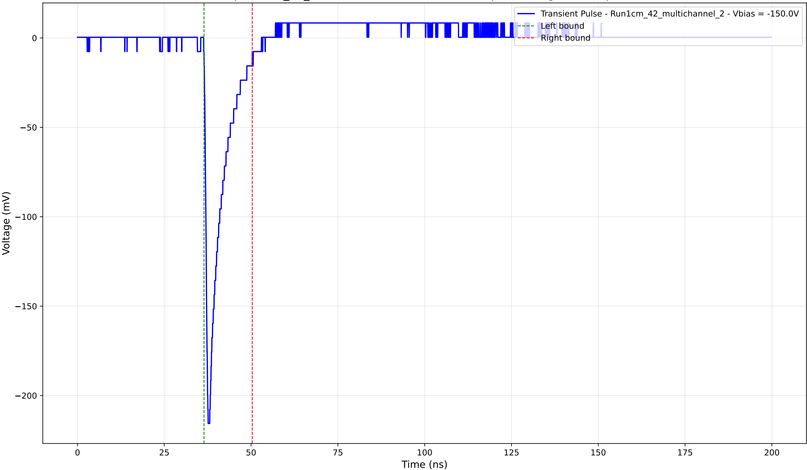
Transient Pulse - Sample: 1cm_42_multichannel - Position: 1535.0 \mu\text{m} - Charge: 21.16 pC - Rise Time: 0.93 ns
