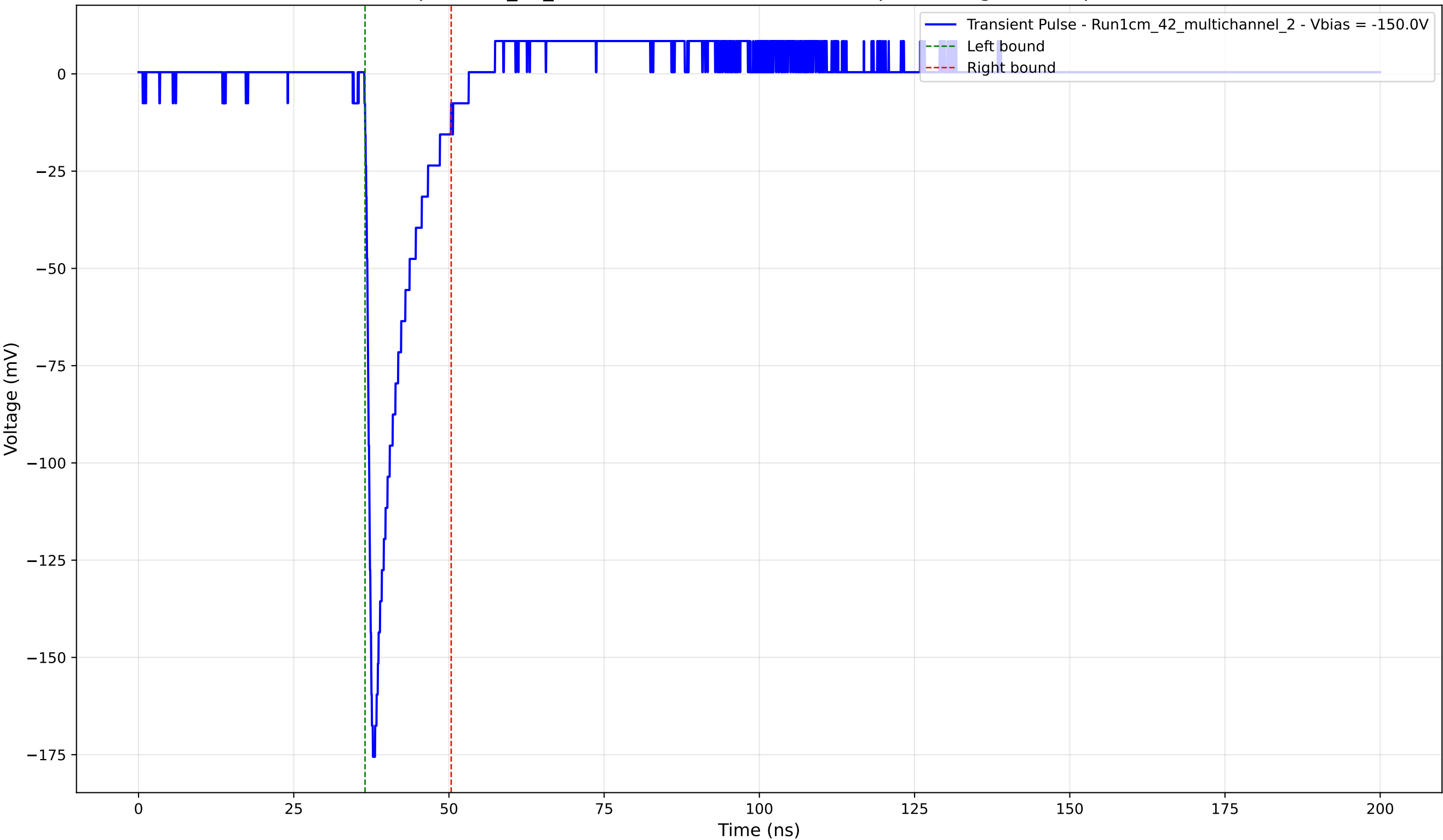
Transient Pulse - Sample: 1cm_42_multichannel - Position: 3280.0 \mu\text{m} - Charge: 18.35 pC - Rise Time: 0.95 ns
