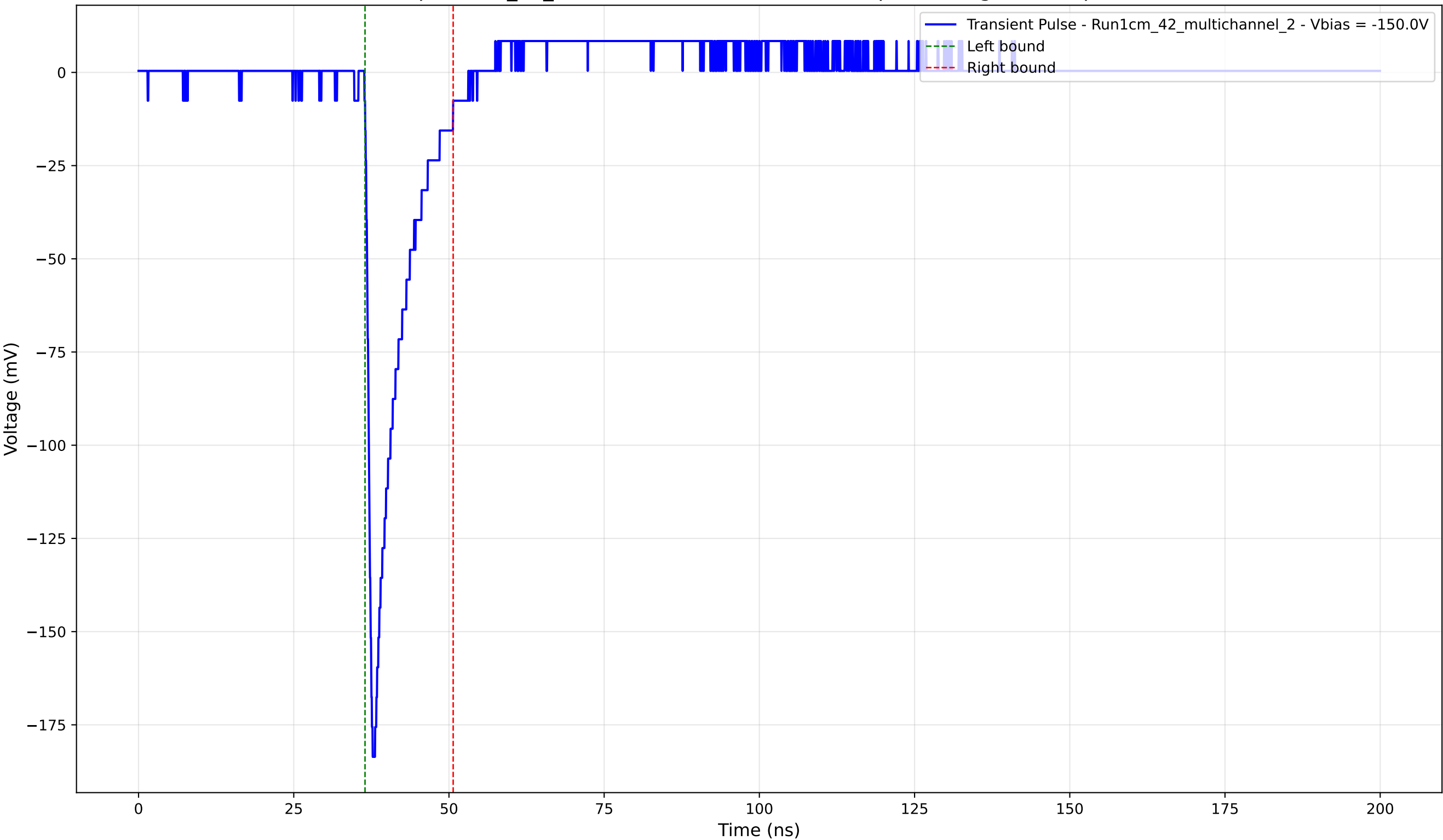
Transient Pulse - Sample: 1cm_42_multichannel - Position: 3255.0 \mu\text{m} - Charge: 18.84 pC - Rise Time: 0.95 ns
