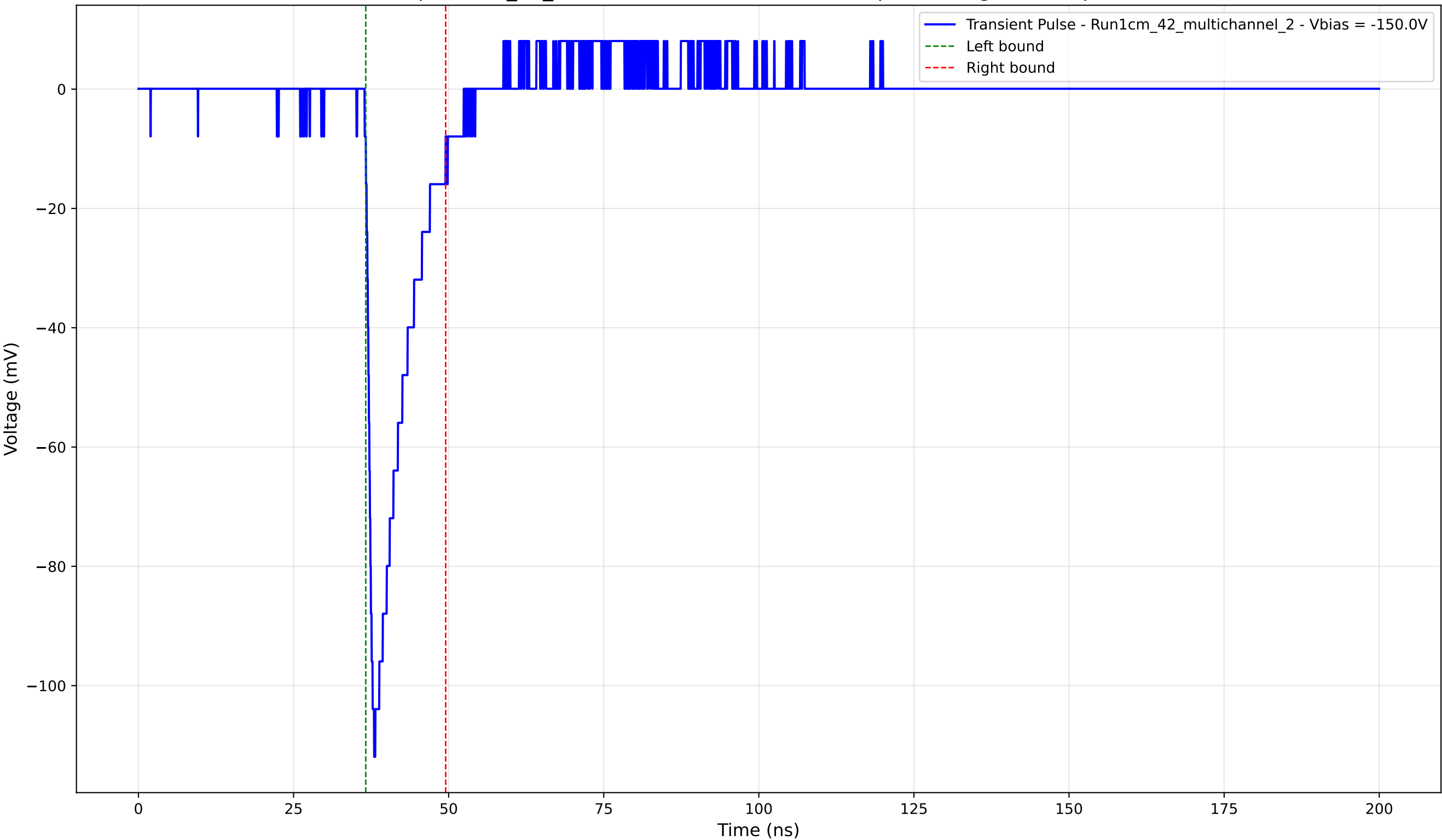
Transient Pulse - Sample: 1cm_42_multichannel - Position: 3445.0 \mu\text{m} - Charge: 12.95 pC - Rise Time: 1.10 ns
