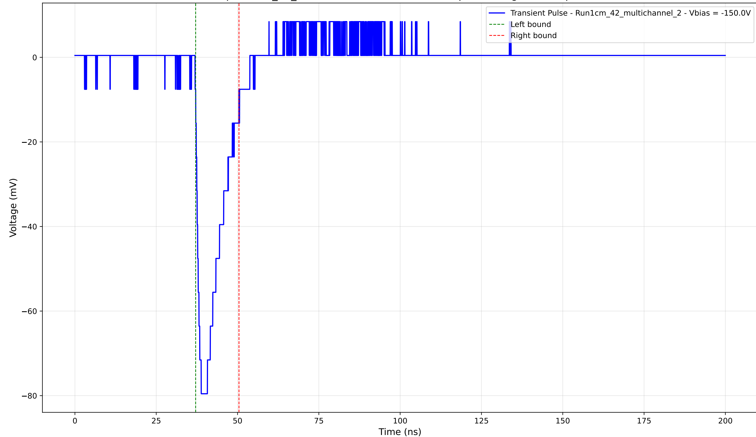
Transient Pulse - Sample: 1cm_42_multichannel - Position: 420.0 \mu\text{m} - Charge: 12.23 pC - Rise Time: 1.72 ns
