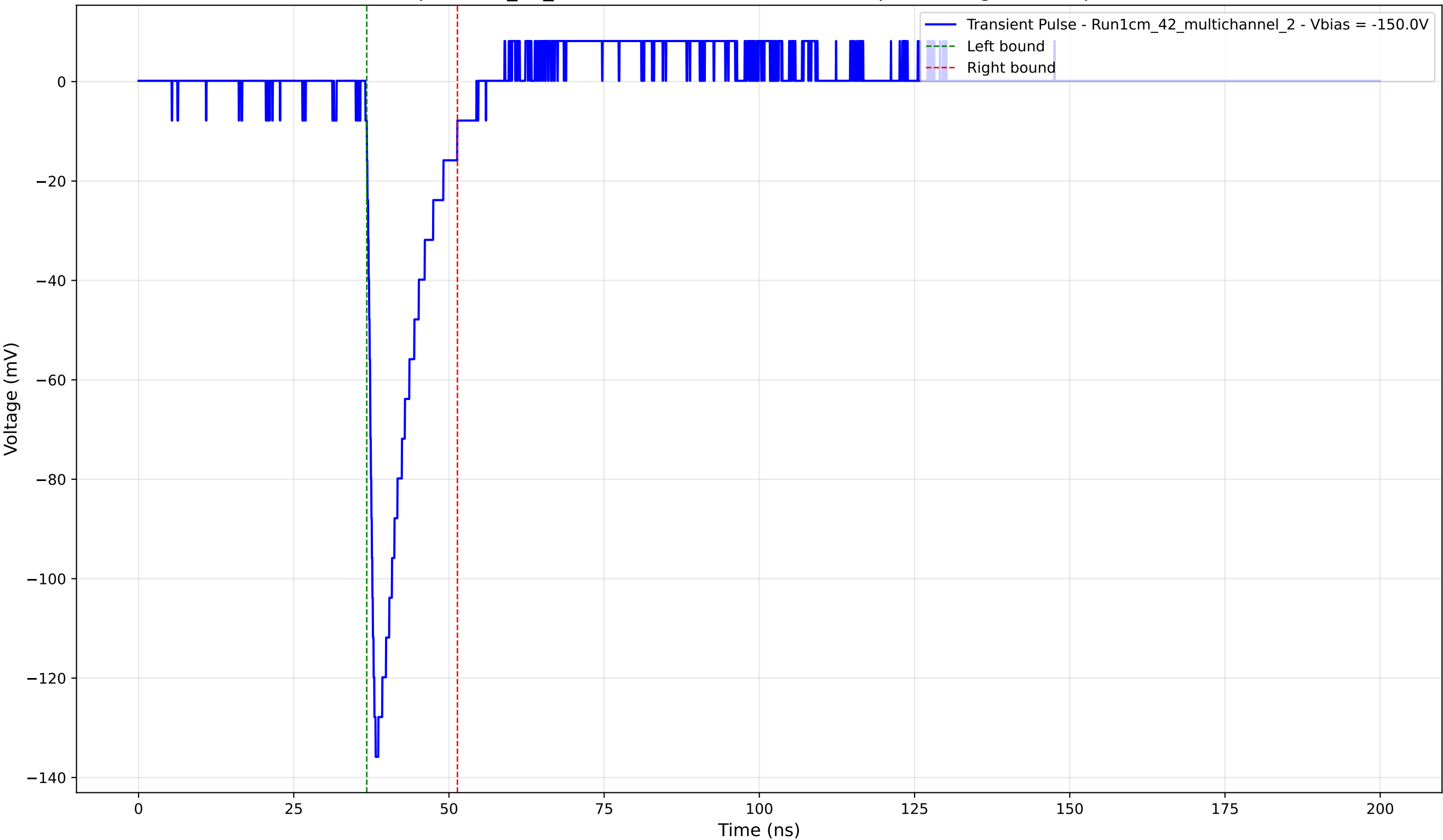
Transient Pulse - Sample: 1cm_42_multichannel - Position: 1110.0 \mu\text{m} - Charge: 17.61 pC - Rise Time: 1.21 ns
