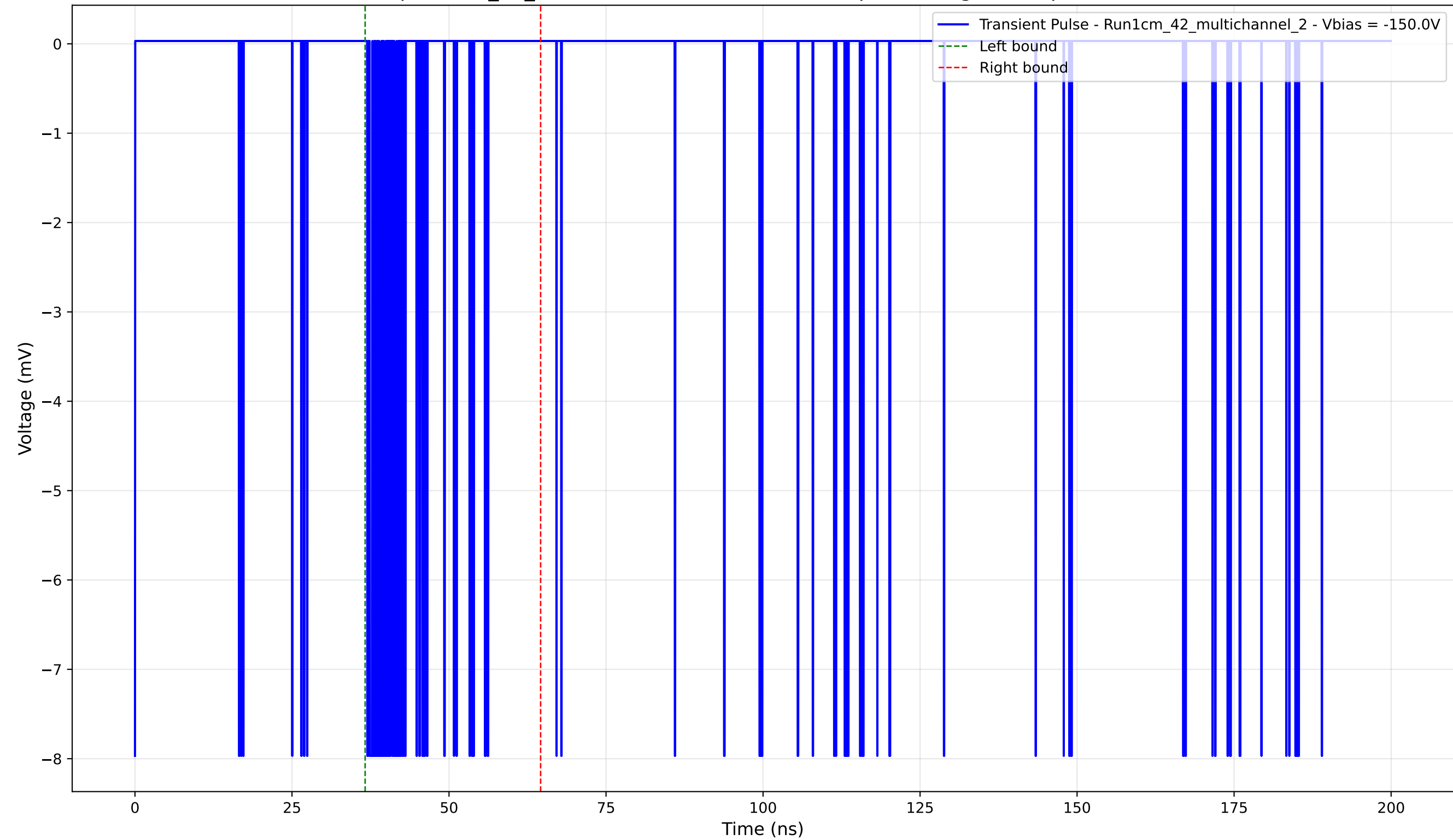
Transient Pulse - Sample: 1cm_42_multichannel - Position: 4890.0 \mu\text{m} - Charge: 0.82 pC - Rise Time: 0.00 ns (N/A)
