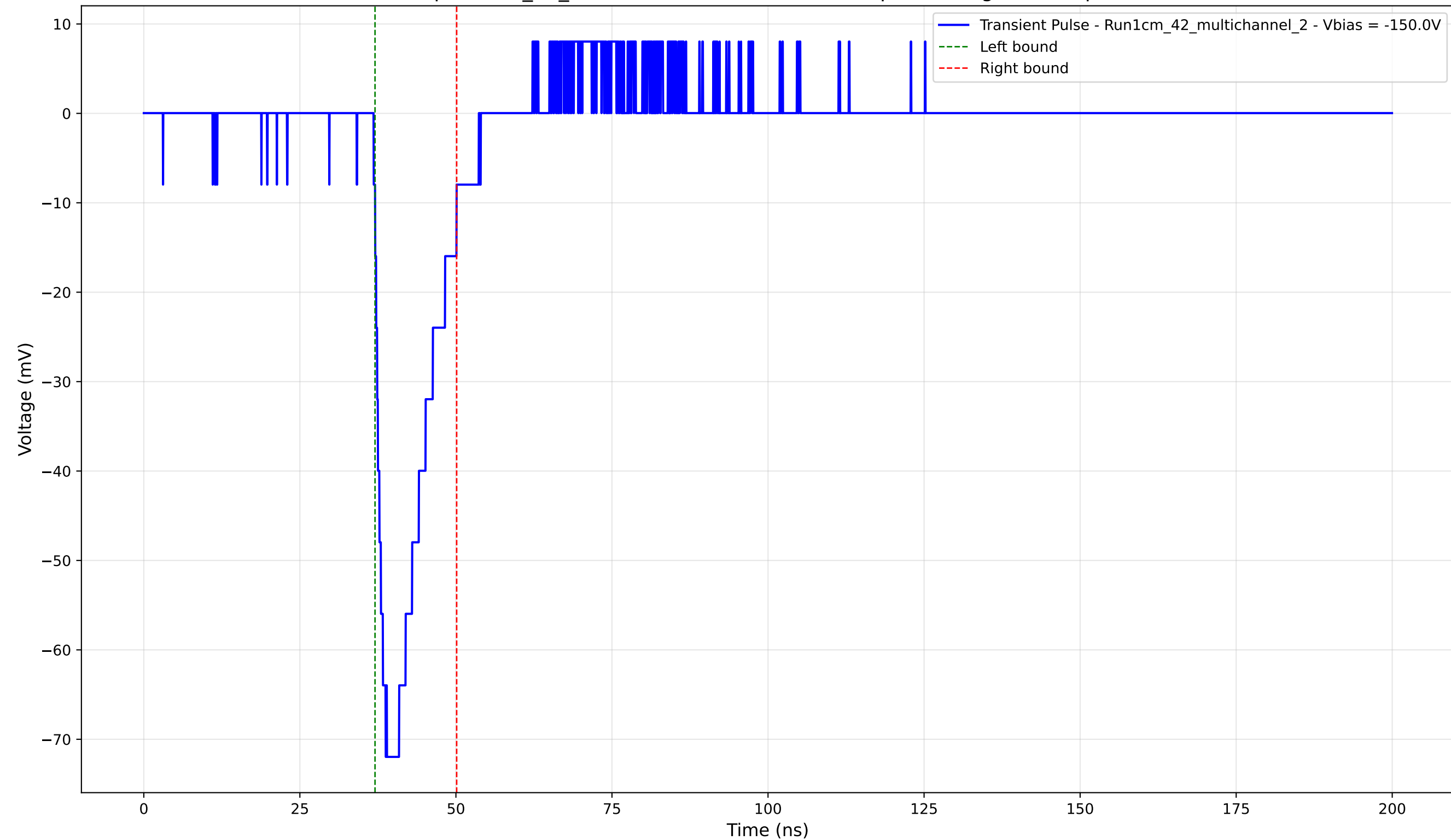
Transient Pulse - Sample: 1cm_42_multichannel - Position: 245.0 \mu\text{m} - Charge: 11.31 pC - Rise Time: 1.92 ns
