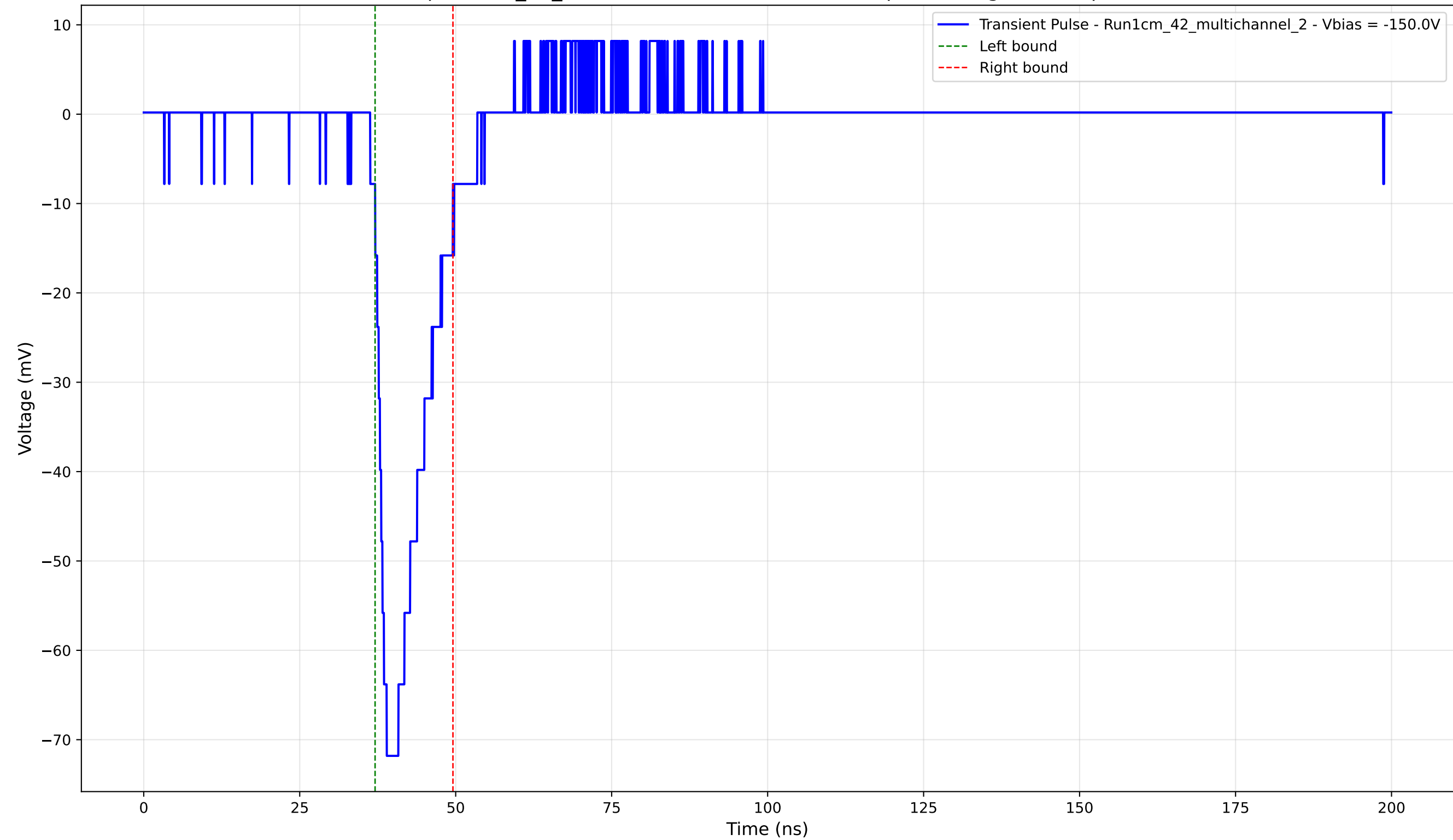
Transient Pulse - Sample: 1cm_42_multichannel - Position: 4550.0 \mu\text{m} - Charge: 10.56 pC - Rise Time: 2.64 ns
