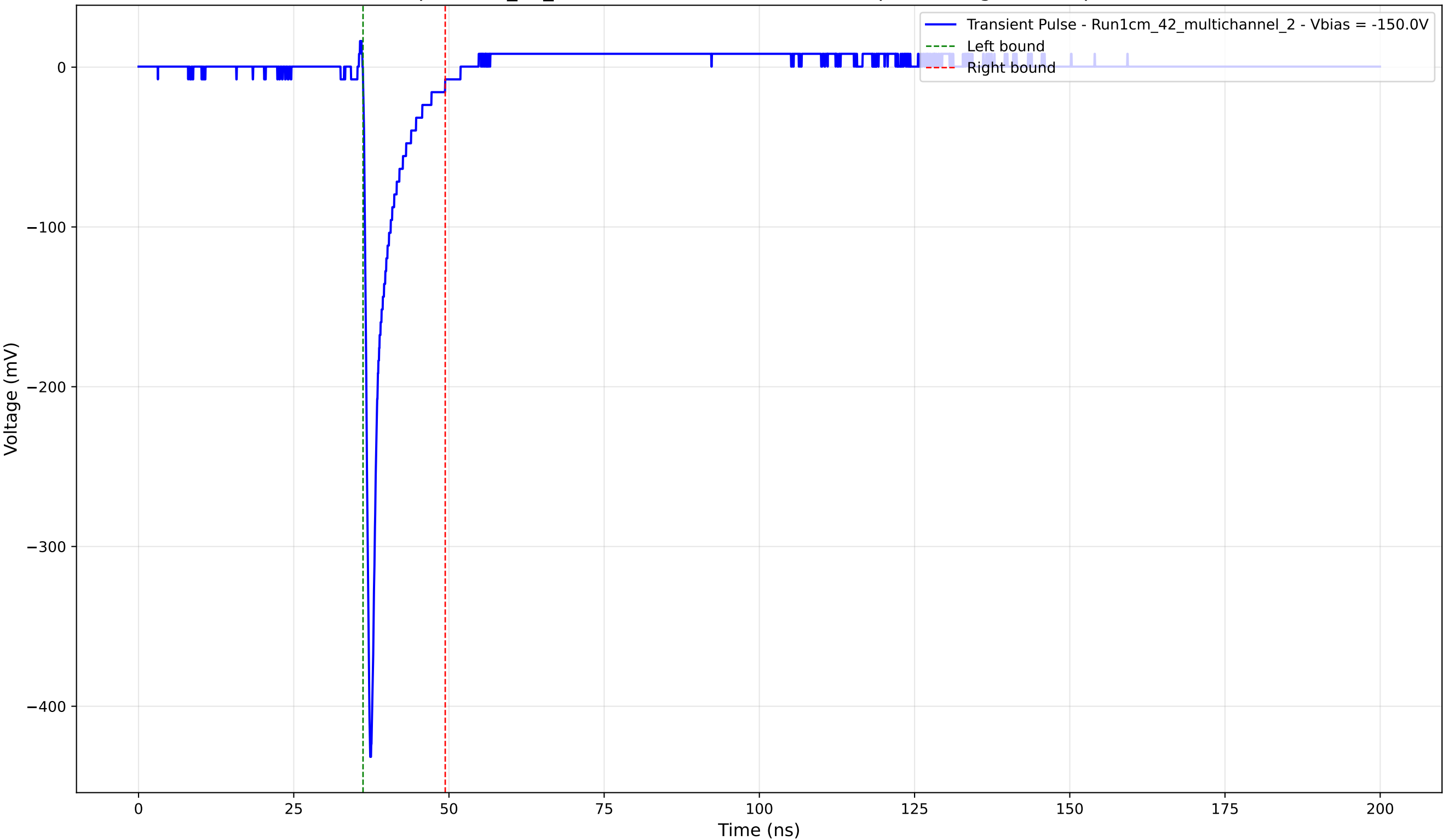
Transient Pulse - Sample: 1cm_42_multichannel - Position: 2000.0 \mu\text{m} - Charge: 25.88 pC - Rise Time: 0.78 ns
