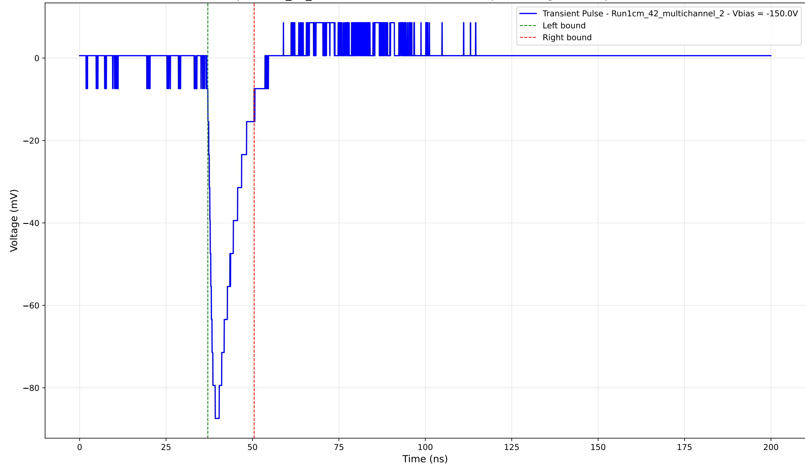
Transient Pulse - Sample: 1cm_42_multichannel - Position: 4145.0 \mu\text{m} - Charge: 12.53 pC - Rise Time: 1.47 ns
