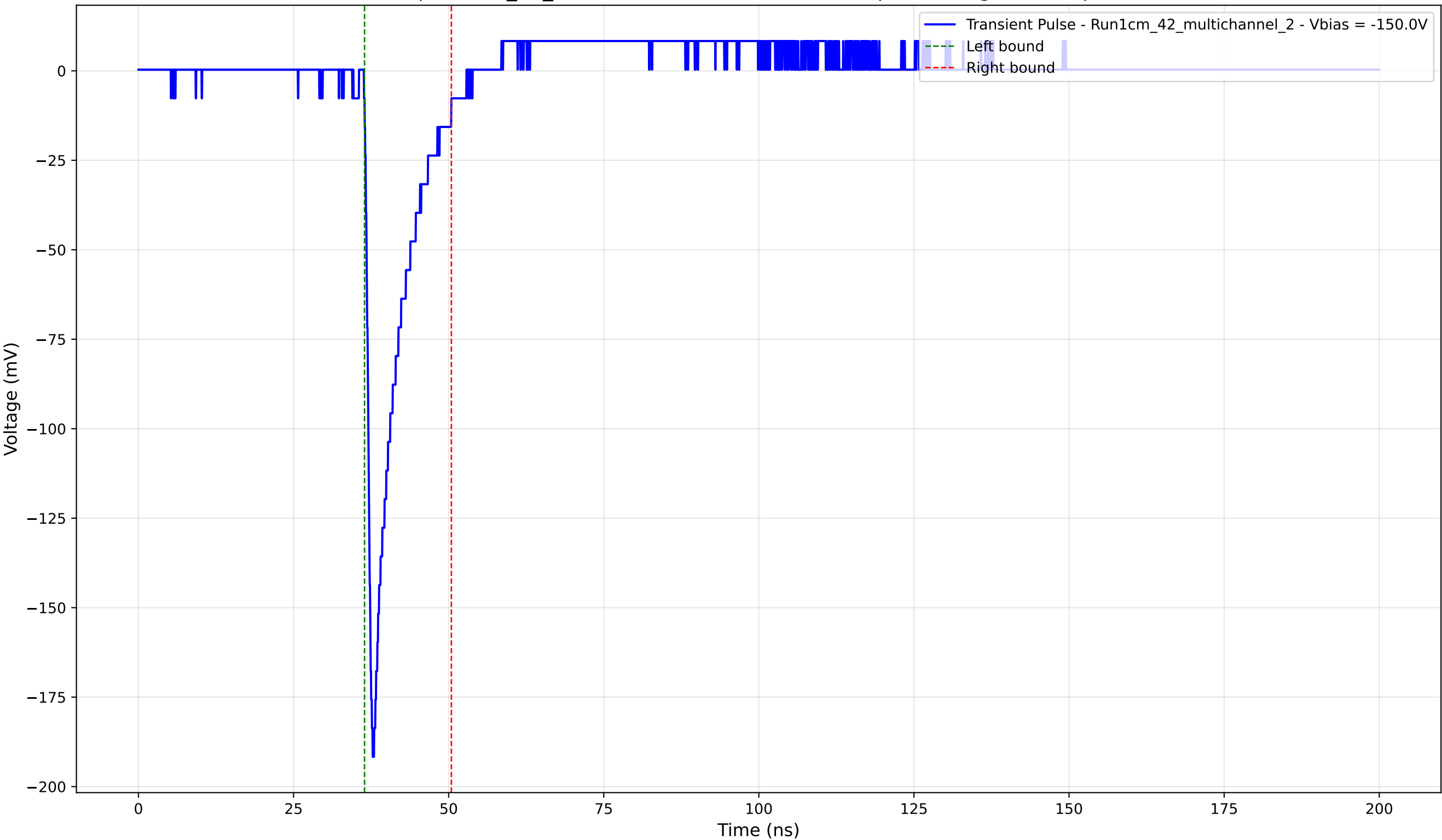
Transient Pulse - Sample: 1cm_42_multichannel - Position: 3240.0 \mu\text{m} - Charge: 19.10 pC - Rise Time: 0.98 ns
