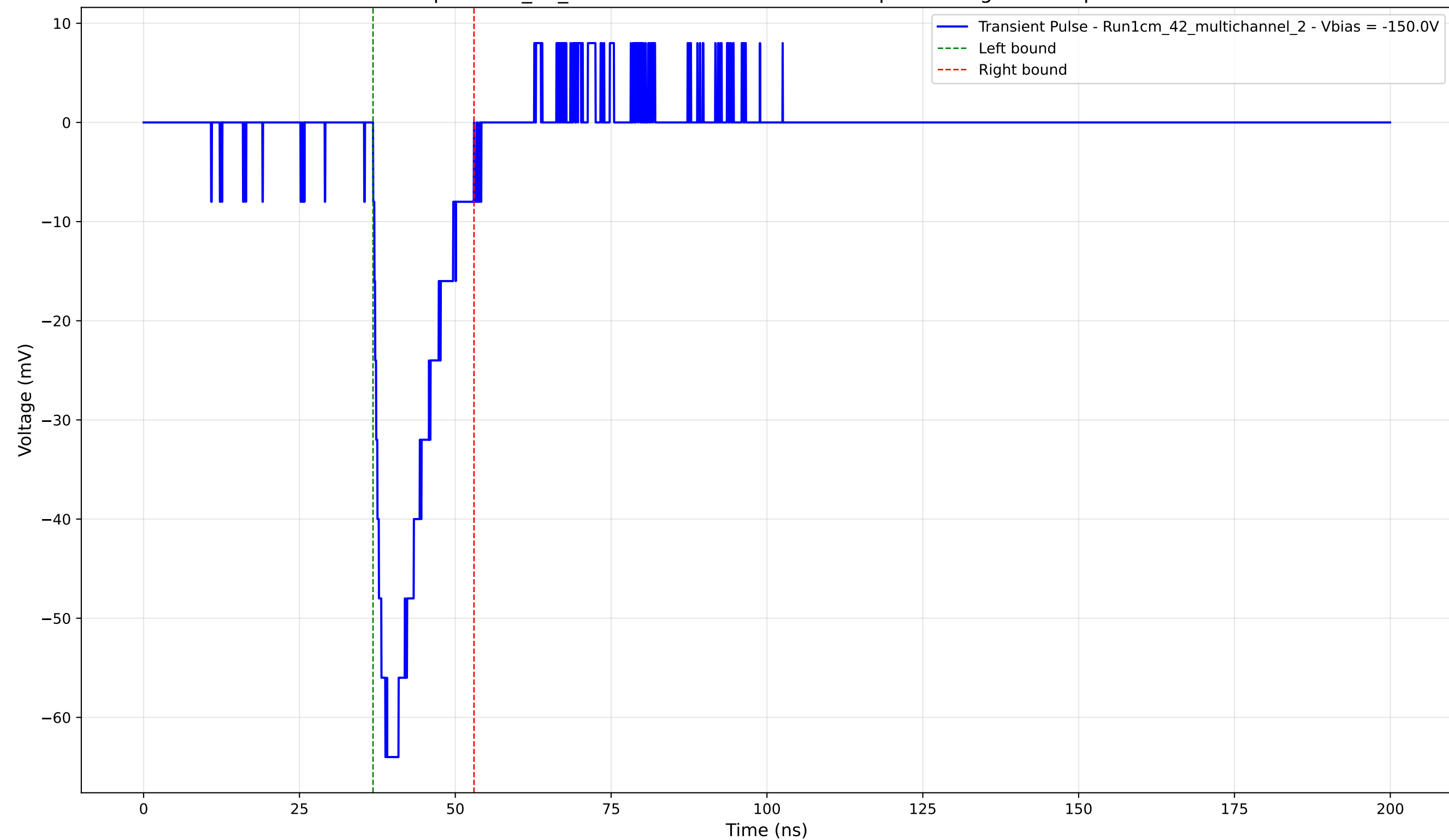
Transient Pulse - Sample: 1cm_42_multichannel - Position: 120.0 \mu\text{m} - Charge: 10.63 pC - Rise Time: 1.97 ns
