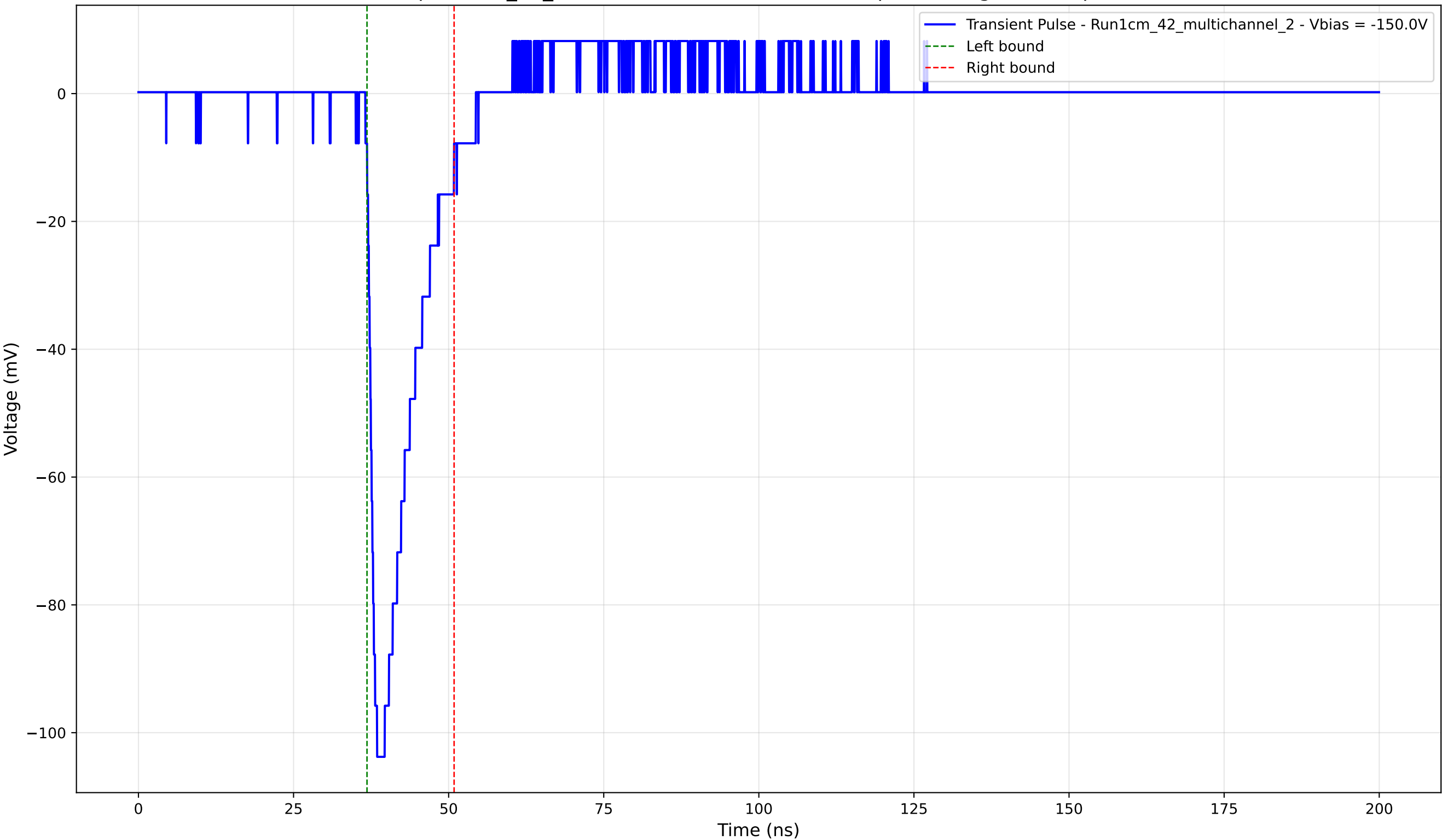
Transient Pulse - Sample: 1cm_42_multichannel - Position: 3780.0 \mu\text{m} - Charge: 14.60 pC - Rise Time: 1.31 ns
