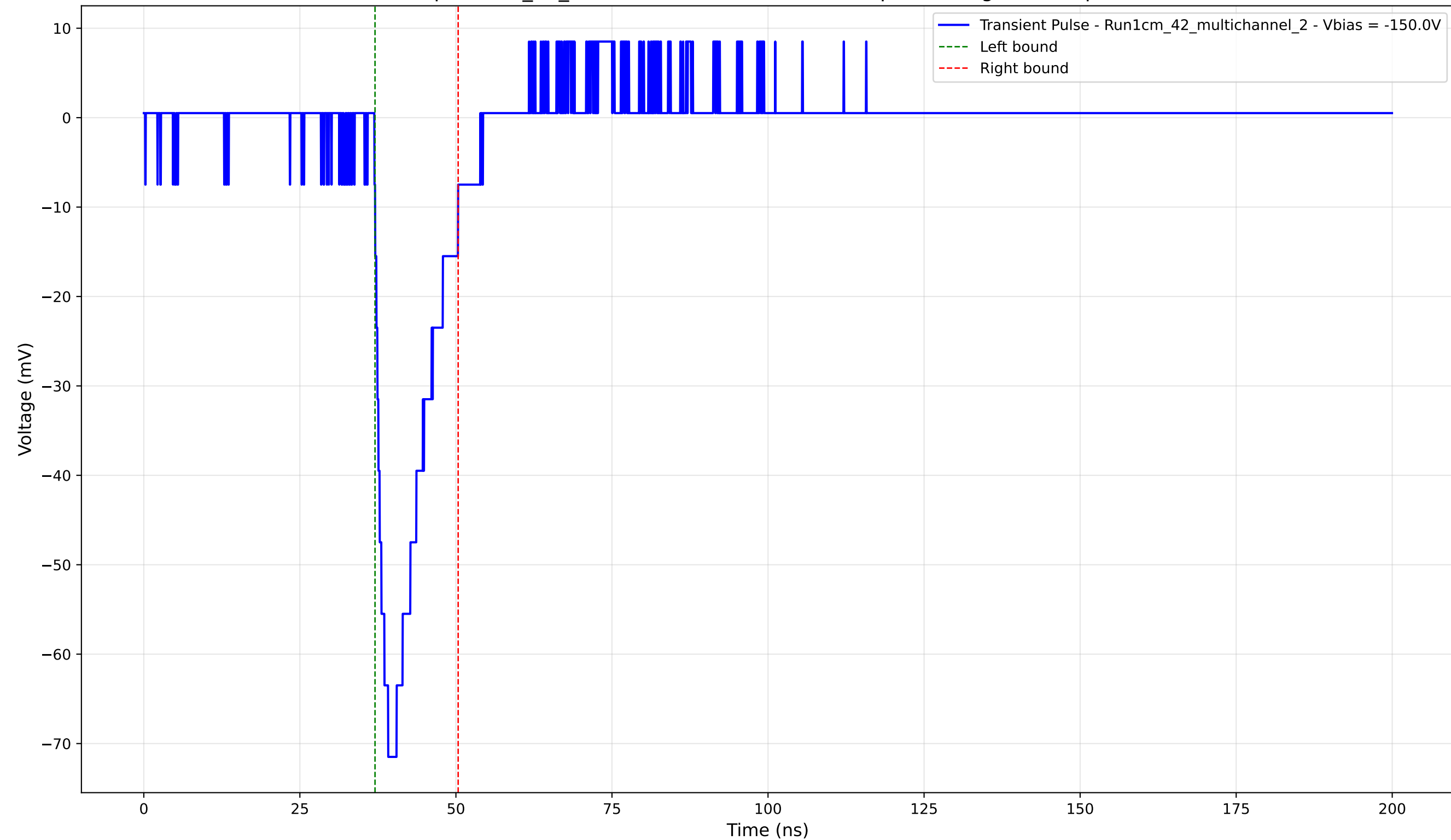
Transient Pulse - Sample: 1cm_42_multichannel - Position: 260.0 \mu\text{m} - Charge: 10.74 pC - Rise Time: 2.20 ns
