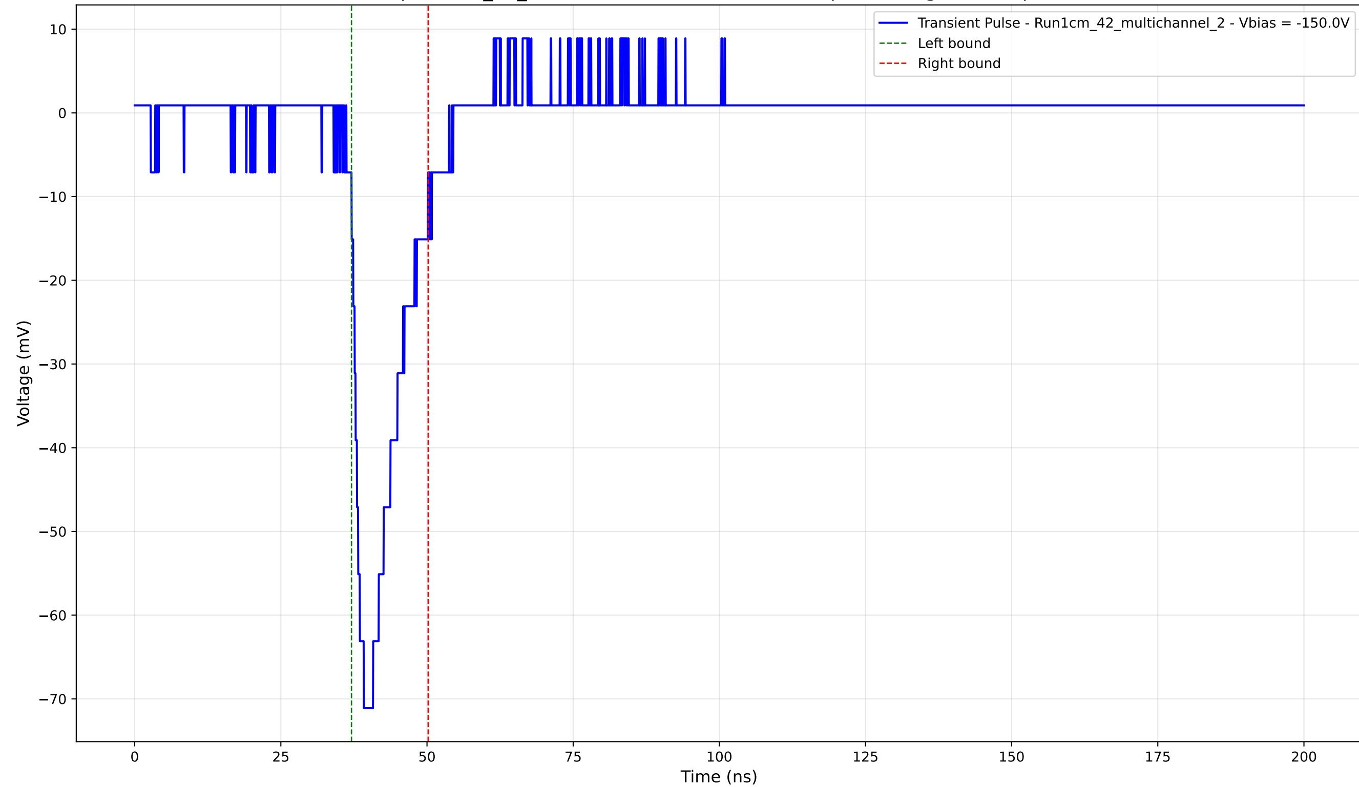
Transient Pulse - Sample: 1cm_42_multichannel - Position: 4590.0 \mu\text{m} - Charge: 10.54 pC - Rise Time: 2.12 ns
