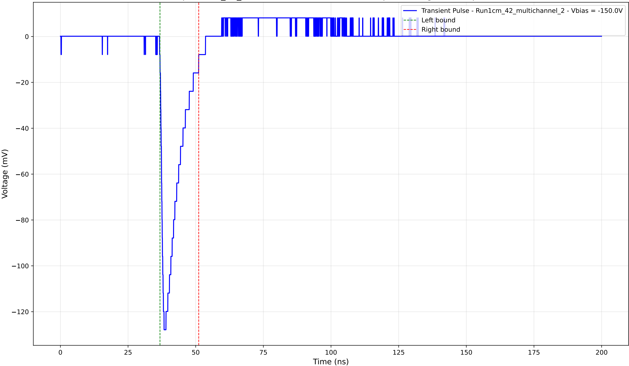
Transient Pulse - Sample: 1cm_42_multichannel - Position: 1020.0 \mu\text{m} - Charge: 17.17 pC - Rise Time: 1.26 ns
