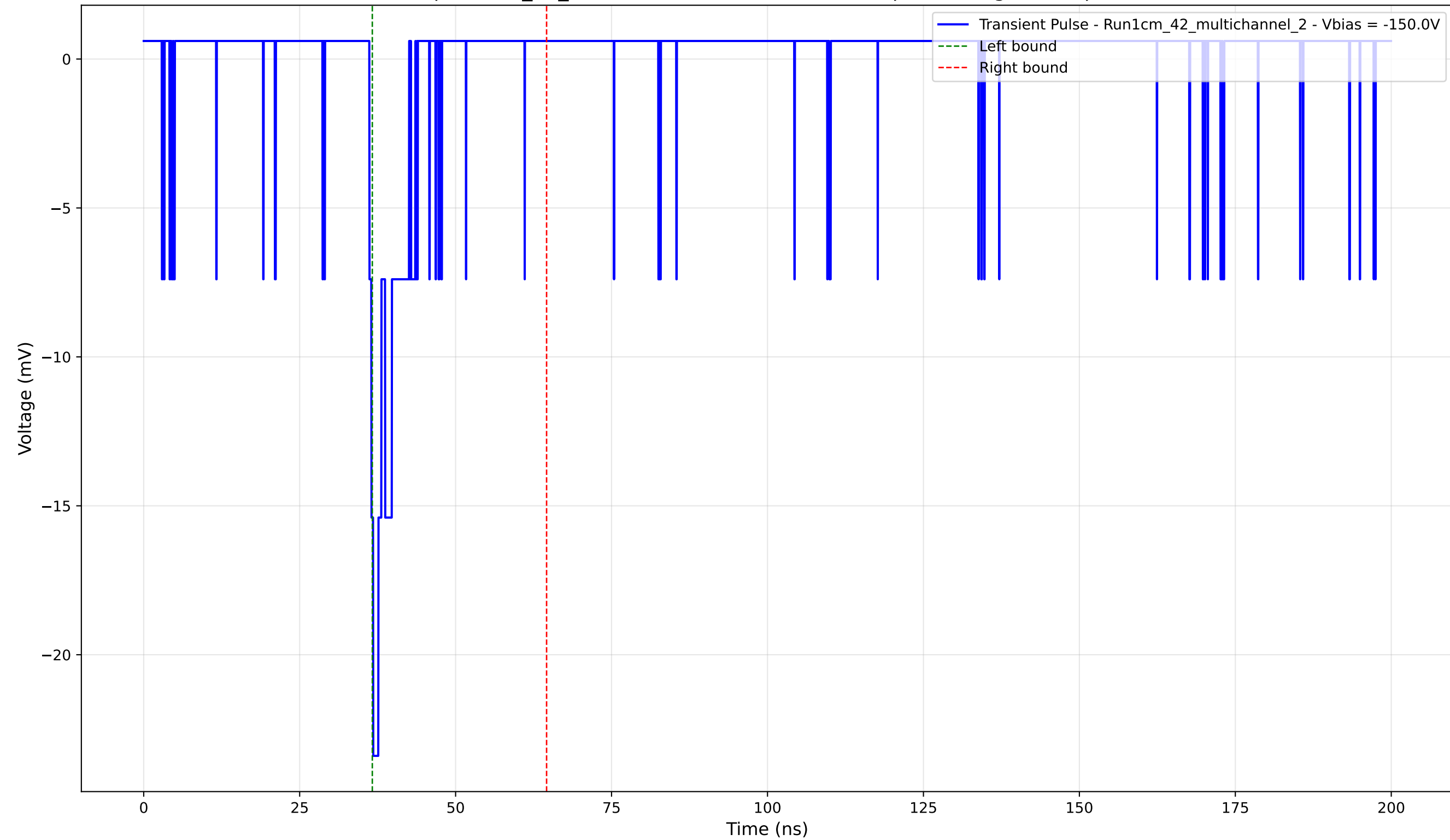
Transient Pulse - Sample: 1cm_42_multichannel - Position: 2375.0 \mu\text{m} - Charge: 1.40 pC - Rise Time: 0.63 ns
