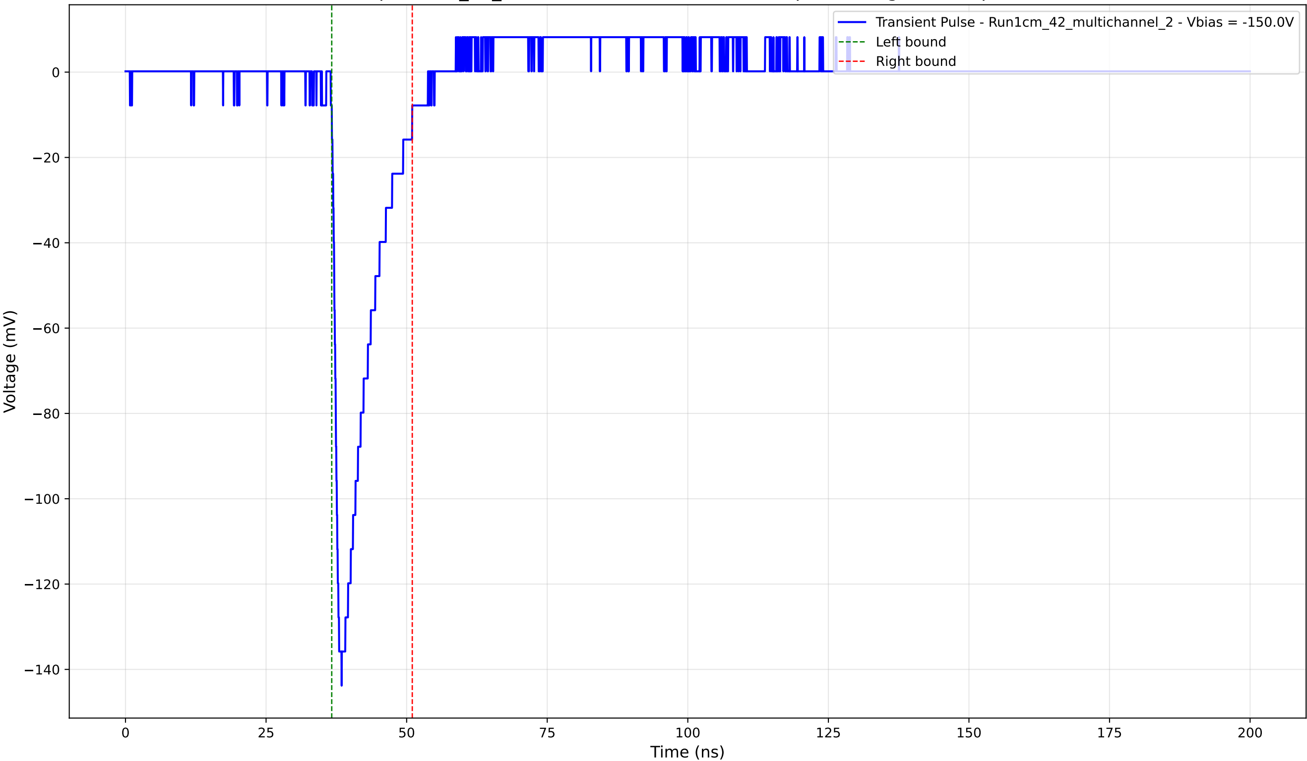
Transient Pulse - Sample: 1cm_42_multichannel - Position: 1145.0 \mu\text{m} - Charge: 18.03 pC - Rise Time: 1.29 ns
