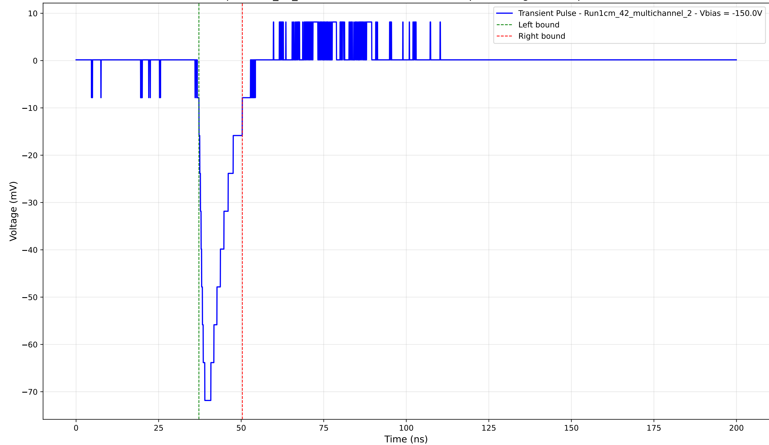
Transient Pulse - Sample: 1cm_42_multichannel - Position: 4515.0 \mu\text{m} - Charge: 10.66 pC - Rise Time: 2.28 ns
