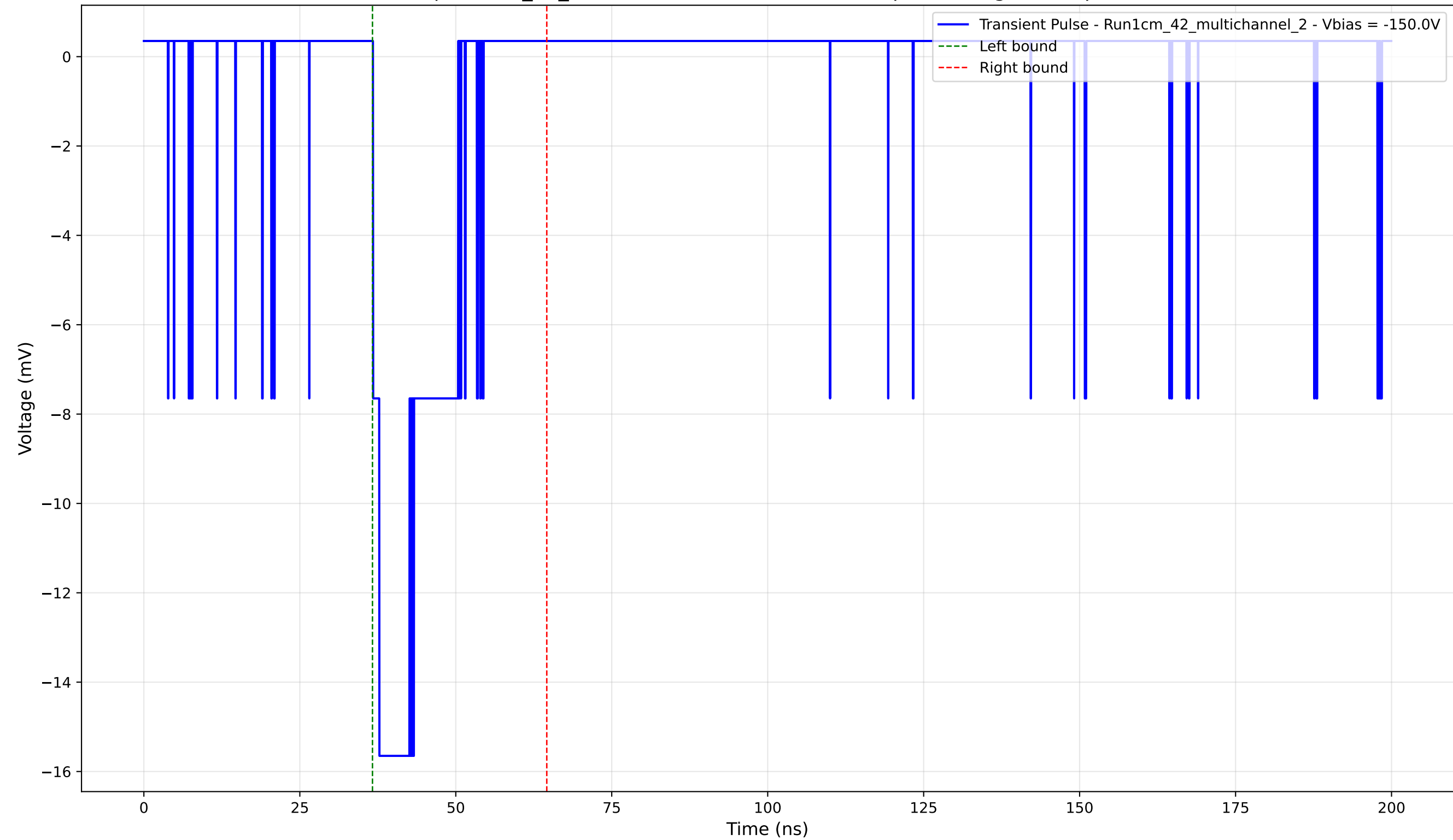
Transient Pulse - Sample: 1cm_42_multichannel - Position: 3855.0 \mu\text{m} - Charge: 2.94 pC - Rise Time: 1.03 ns
