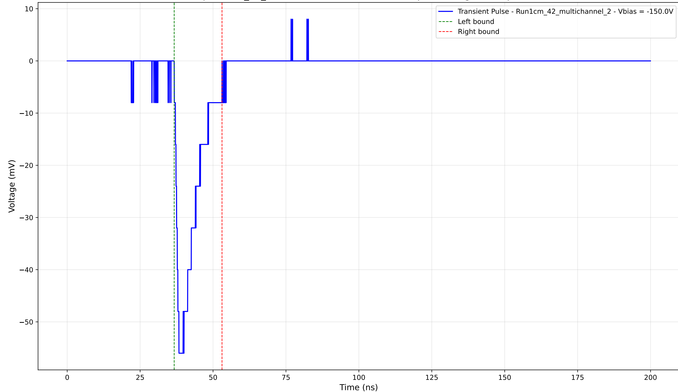
Transient Pulse - Sample: 1cm_42_multichannel - Position: 3835.0 \mu\text{m} - Charge: 8.34 pC - Rise Time: 1.61 ns
