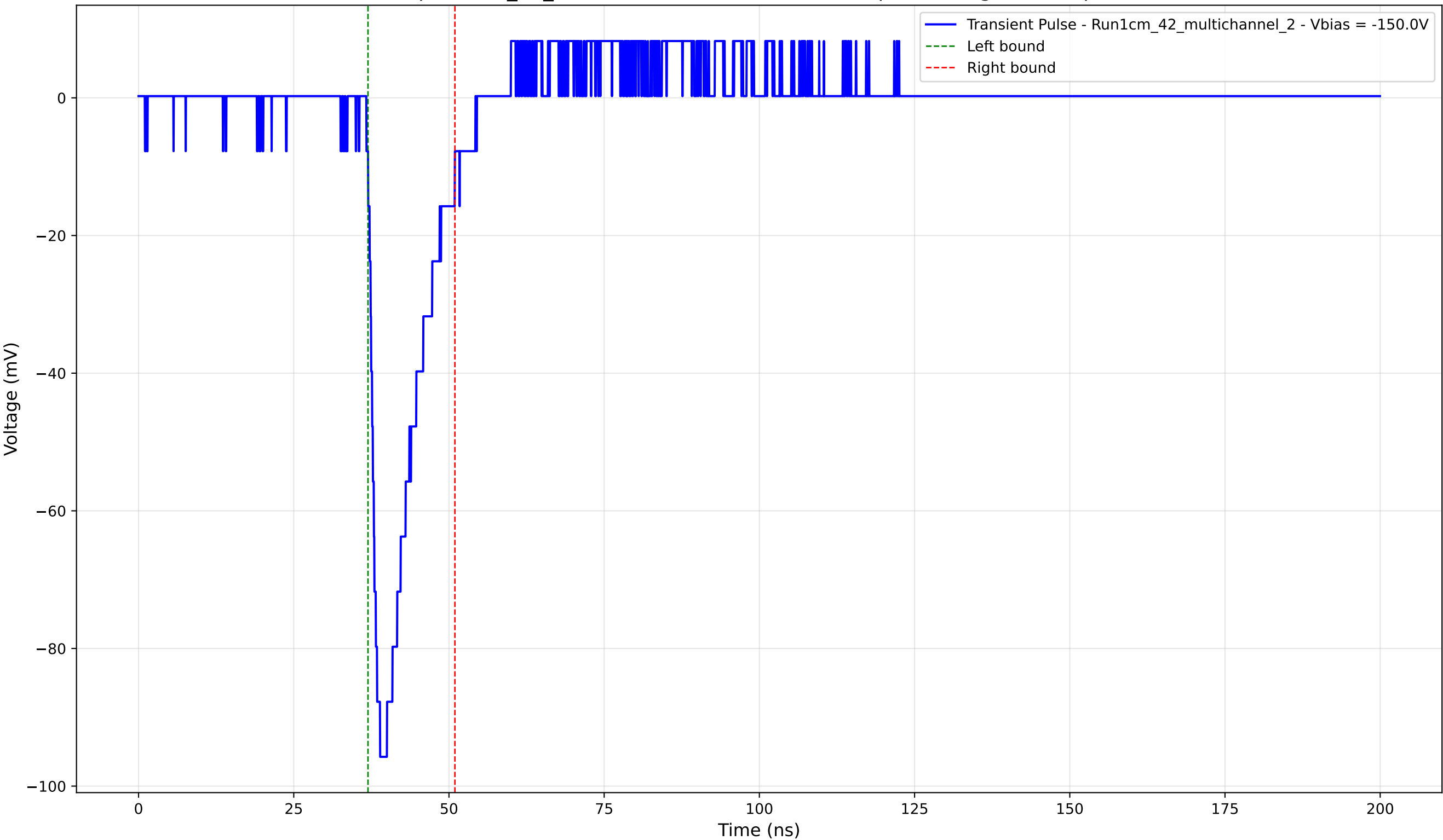
Transient Pulse - Sample: 1cm_42_multichannel - Position: 3985.0 \mu\text{m} - Charge: 13.89 pC - Rise Time: 1.47 ns
