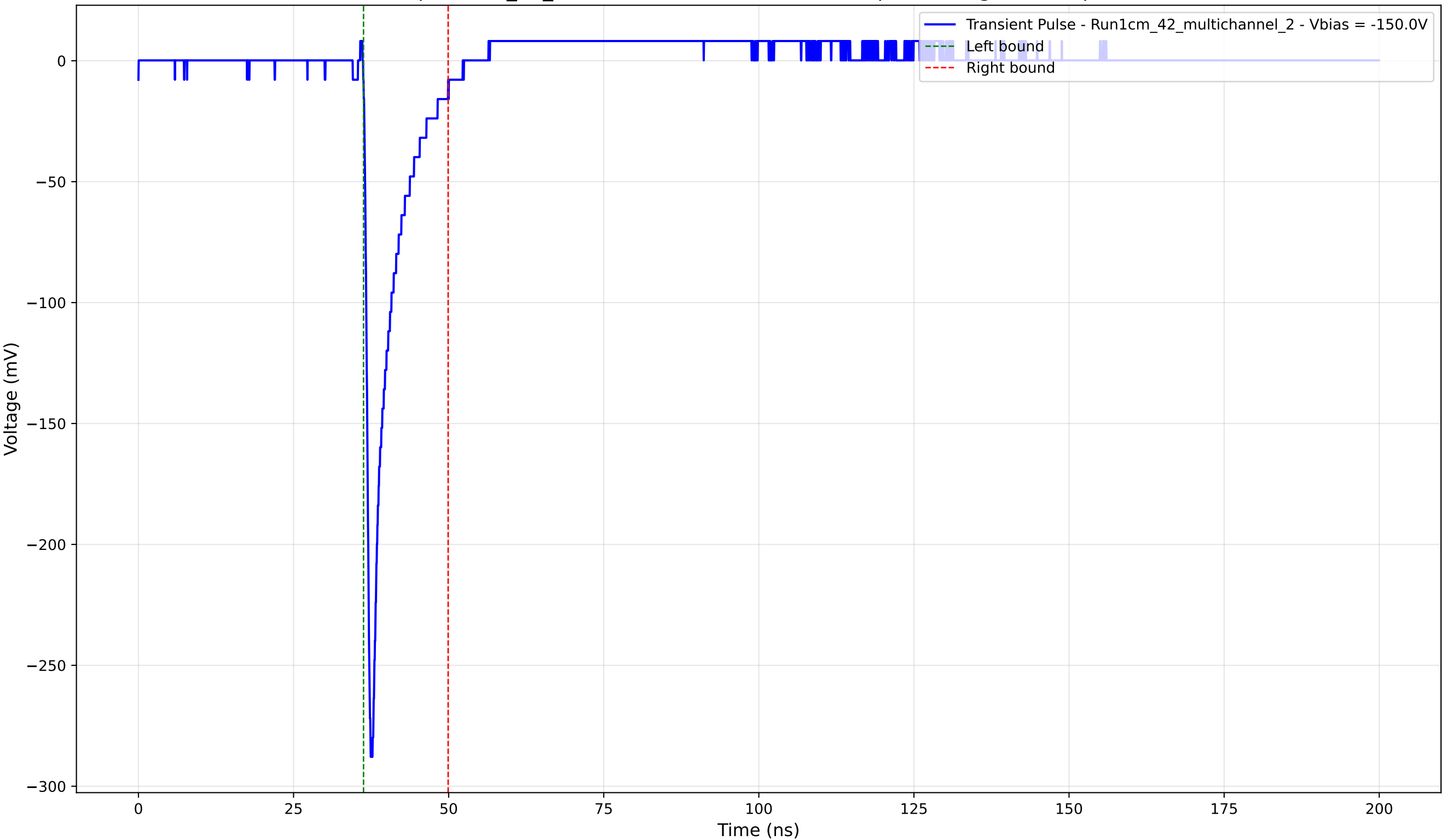
Transient Pulse - Sample: 1cm_42_multichannel - Position: 1755.0 \mu\text{m} - Charge: 22.87 pC - Rise Time: 0.83 ns
