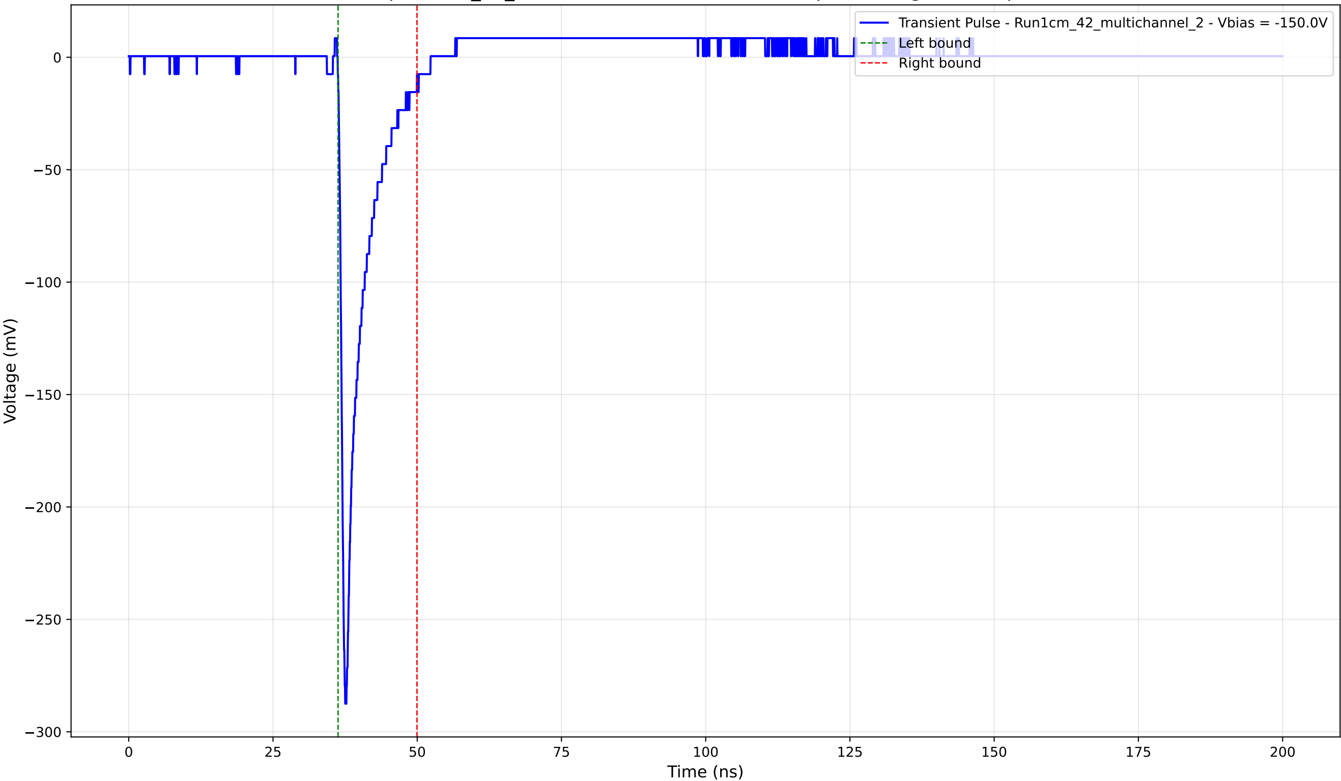
Transient Pulse - Sample: 1cm_42_multichannel - Position: 1730.0 \mu\text{m} - Charge: 23.11 pC - Rise Time: 0.89 ns
