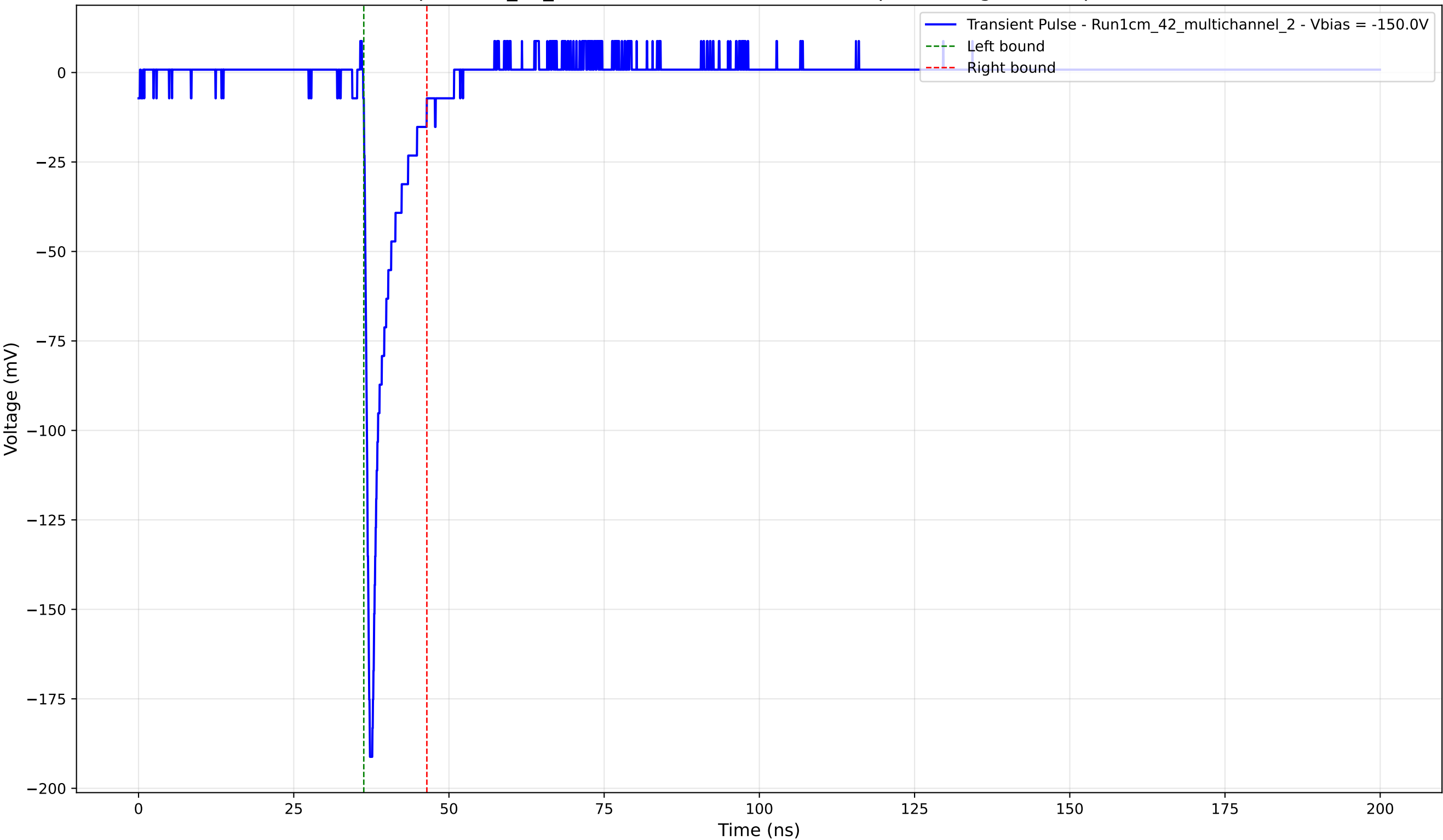
Transient Pulse - Sample: 1cm_42_multichannel - Position: 1915.0 \mu\text{m} - Charge: 12.34 pC - Rise Time: 0.82 ns
