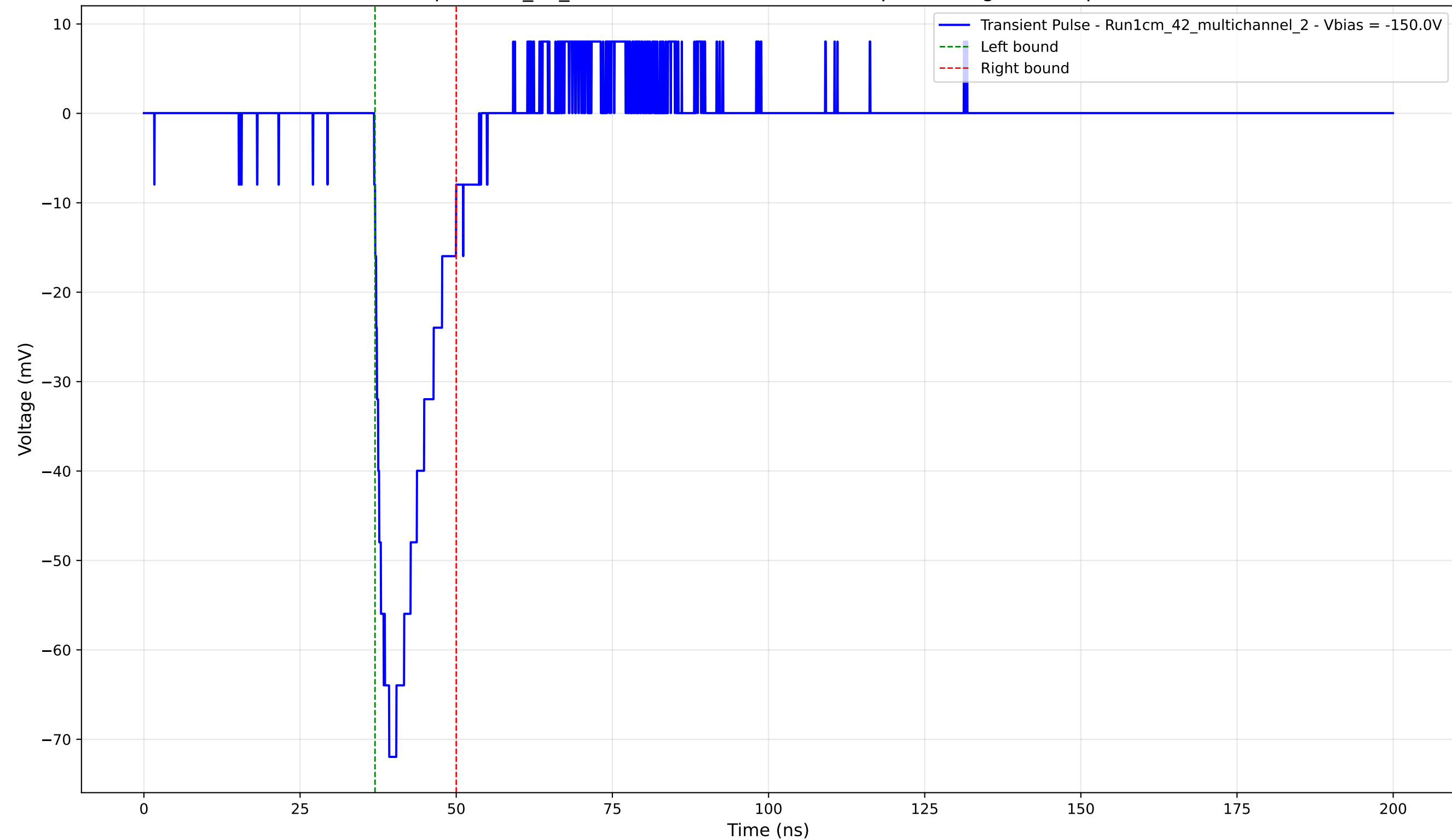
Transient Pulse - Sample: 1cm_42_multichannel - Position: 155.0 \mu\text{m} - Charge: 10.89 pC - Rise Time: 2.40 ns
