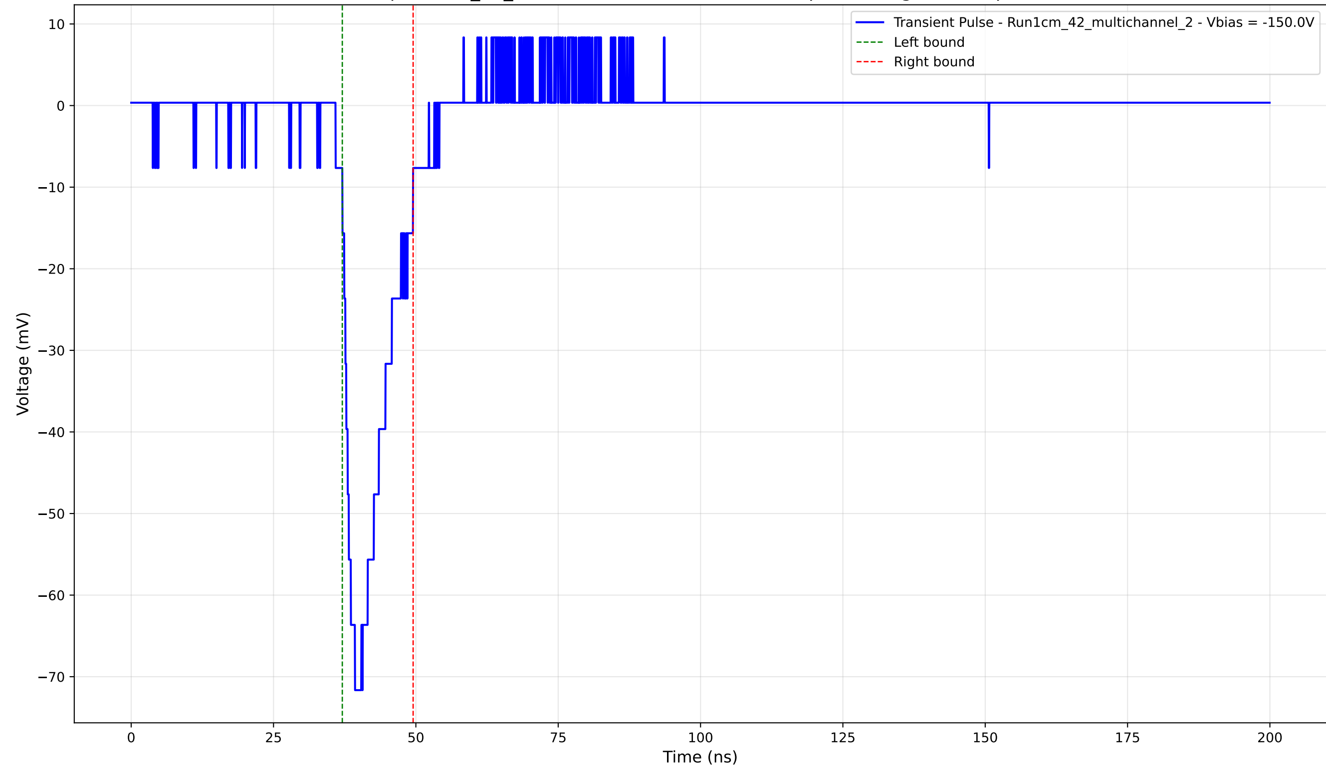
Transient Pulse - Sample: 1cm_42_multichannel - Position: 4670.0 \mu\text{m} - Charge: 10.19 pC - Rise Time: 3.40 ns
