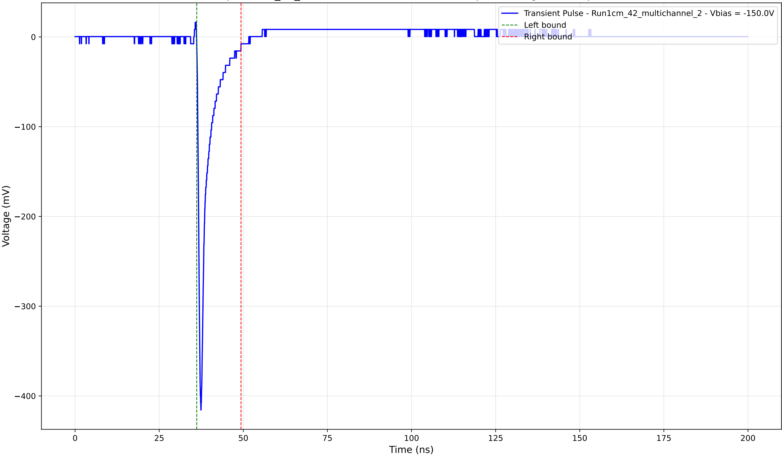
Transient Pulse - Sample: 1cm_42_multichannel - Position: 1975.0 \mu\text{m} - Charge: 25.49 pC - Rise Time: 0.78 ns
