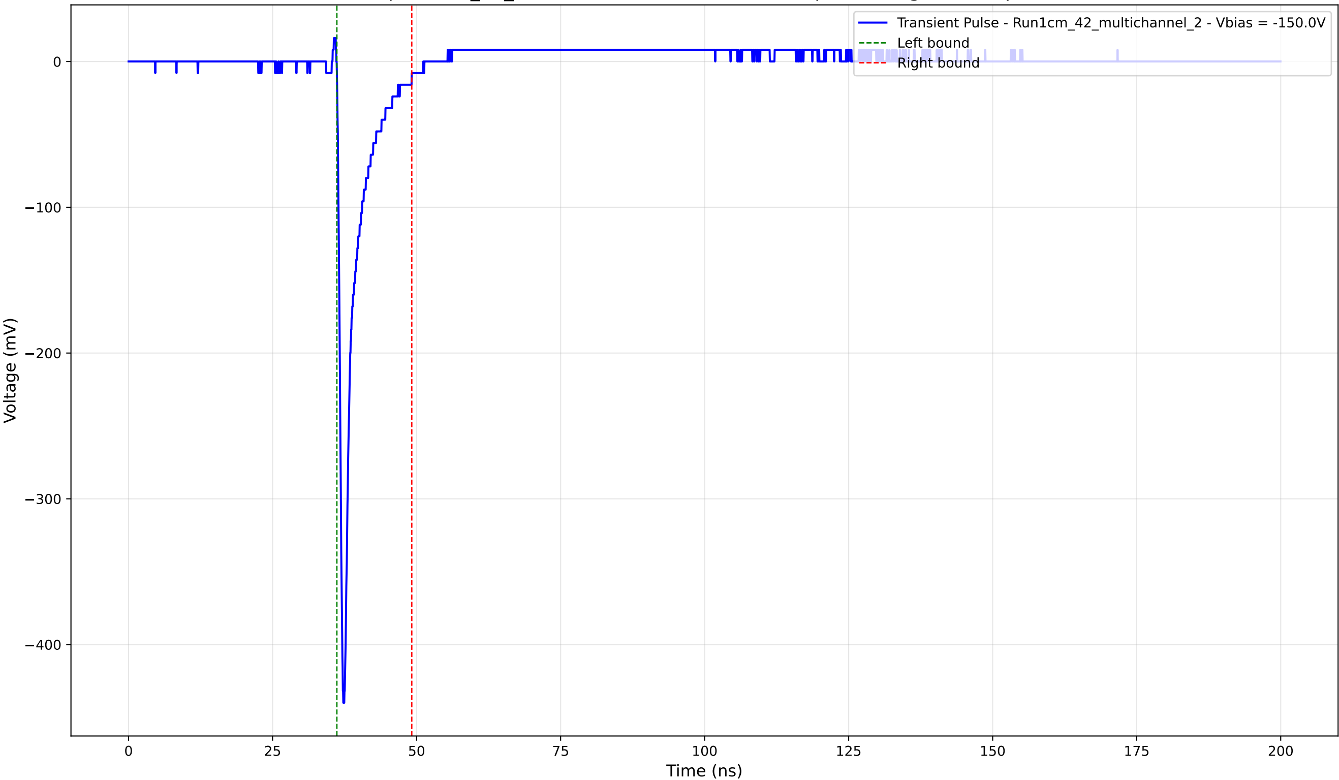
Transient Pulse - Sample: 1cm_42_multichannel - Position: 2015.0 \mu\text{m} - Charge: 26.13 pC - Rise Time: 0.76 ns
