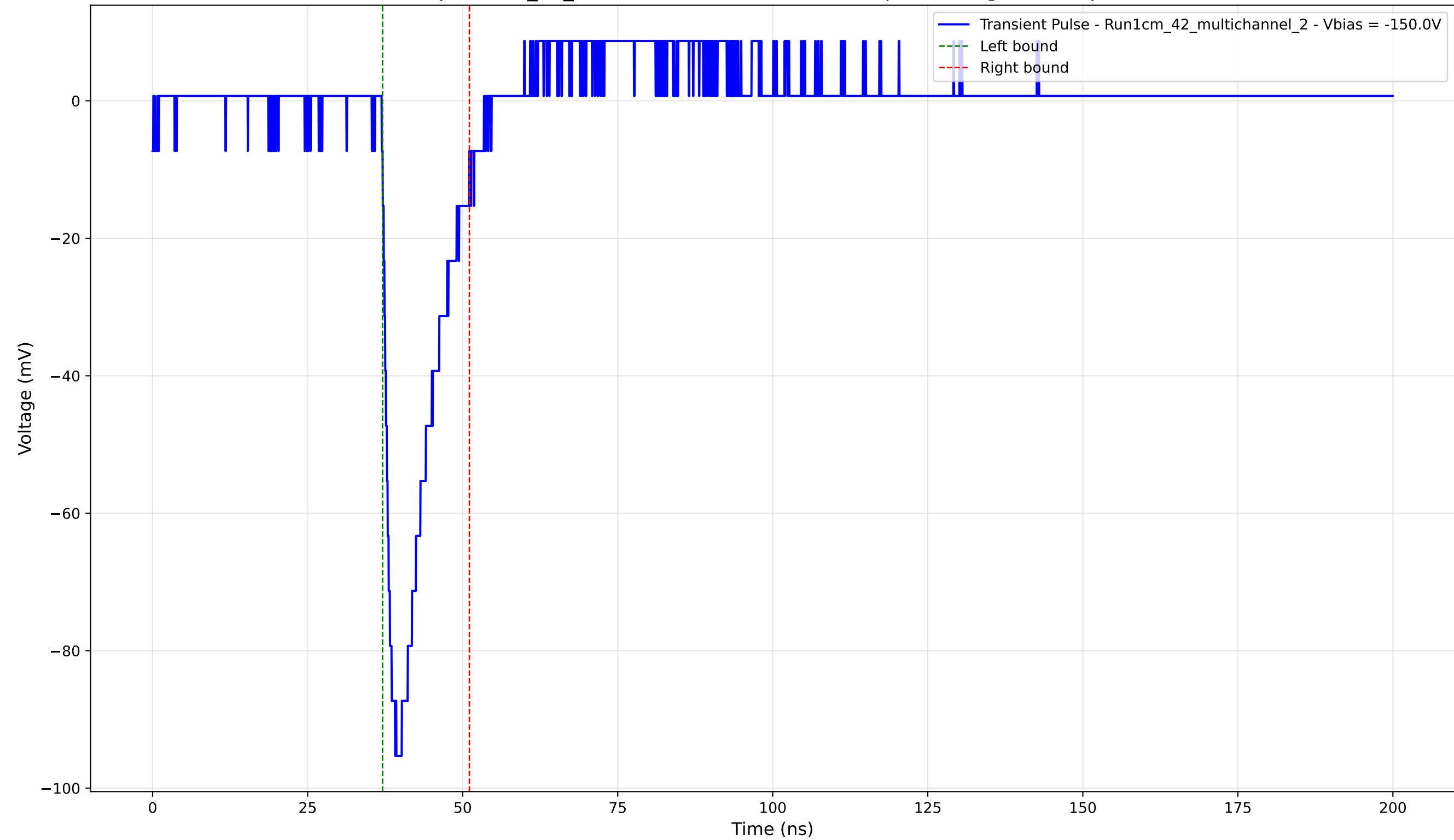
Transient Pulse - Sample: 1cm_42_multichannel - Position: 510.0 \mu\text{m} - Charge: 14.09 pC - Rise Time: 1.47 ns
