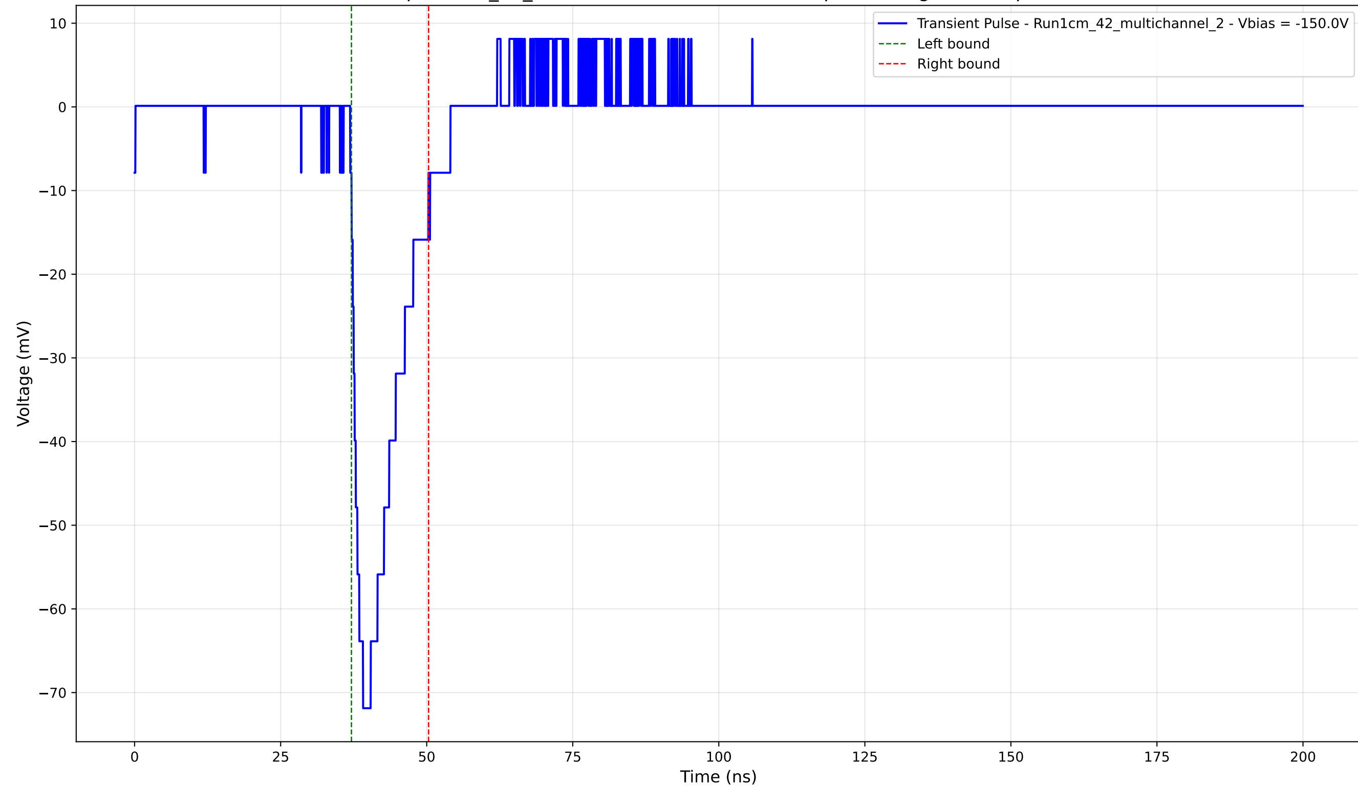
Transient Pulse - Sample: 1cm_42_multichannel - Position: 410.0 \mu\text{m} - Charge: 10.72 pC - Rise Time: 2.20 ns
