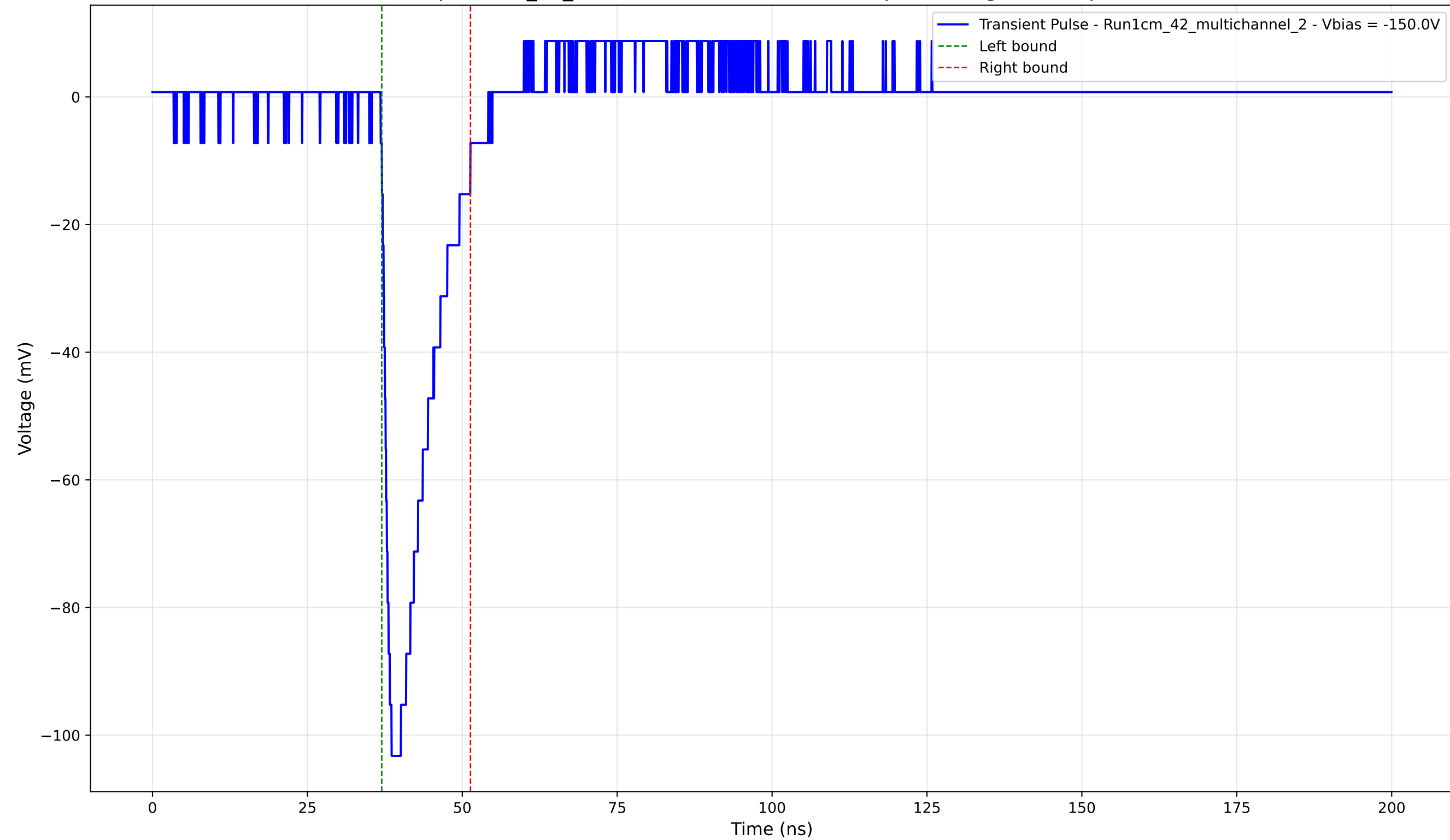
Transient Pulse - Sample: 1cm_42_multichannel - Position: 710.0 \mu\text{m} - Charge: 15.45 pC - Rise Time: 1.30 ns
