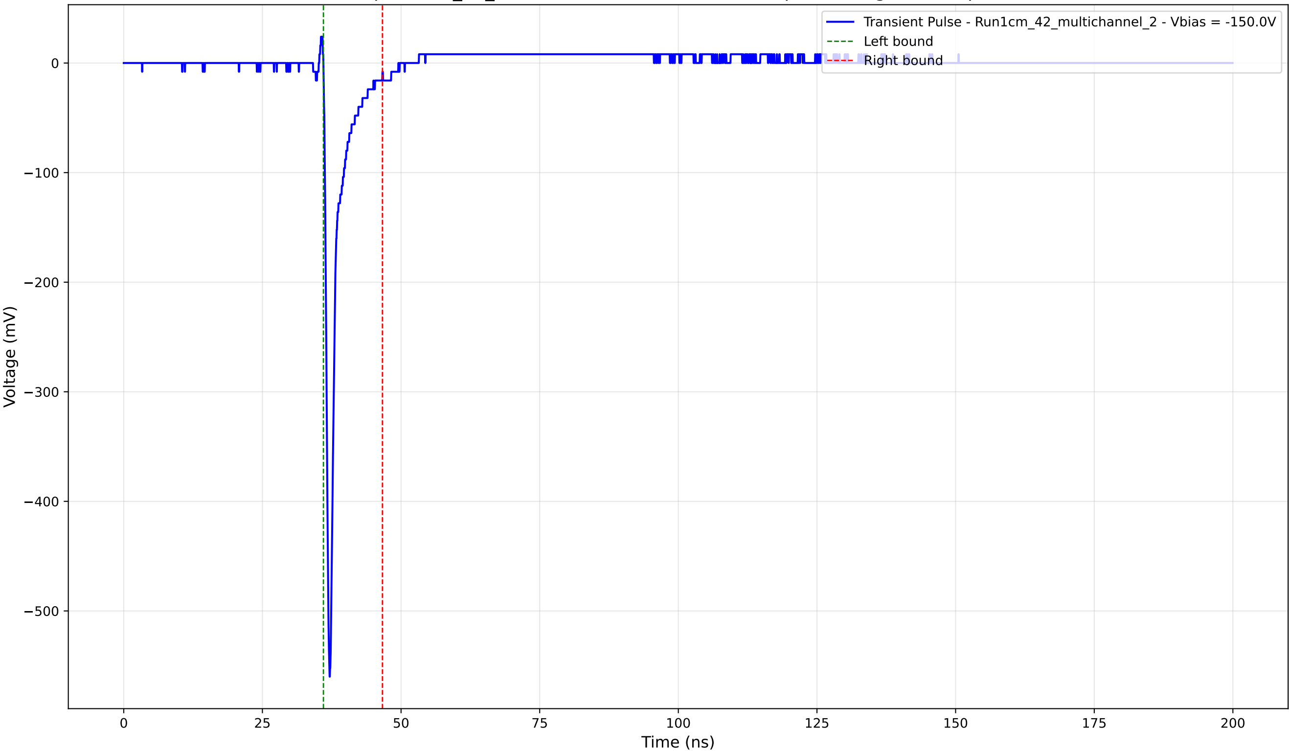
Transient Pulse - Sample: 1cm_42_multichannel - Position: 2300.0 \mu\text{m} - Charge: 24.25 pC - Rise Time: 0.73 ns
