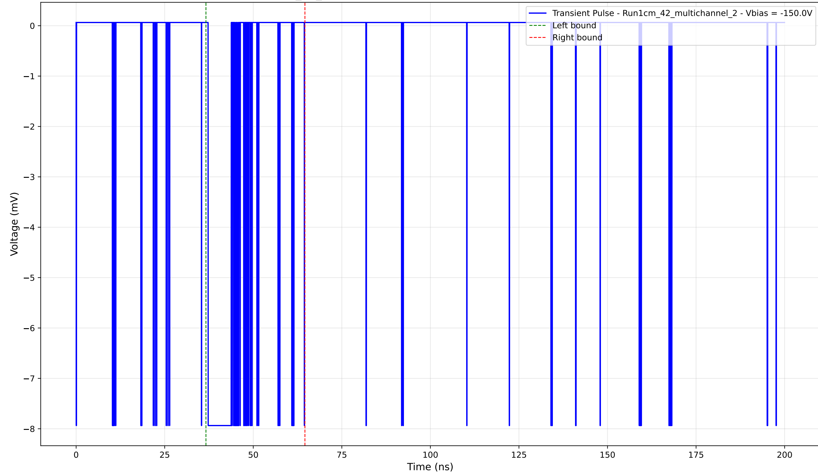
Transient Pulse - Sample: 1cm_42_multichannel - Position: 855.0 \mu\text{m} - Charge: 1.49 pC - Rise Time: 0.04 ns
