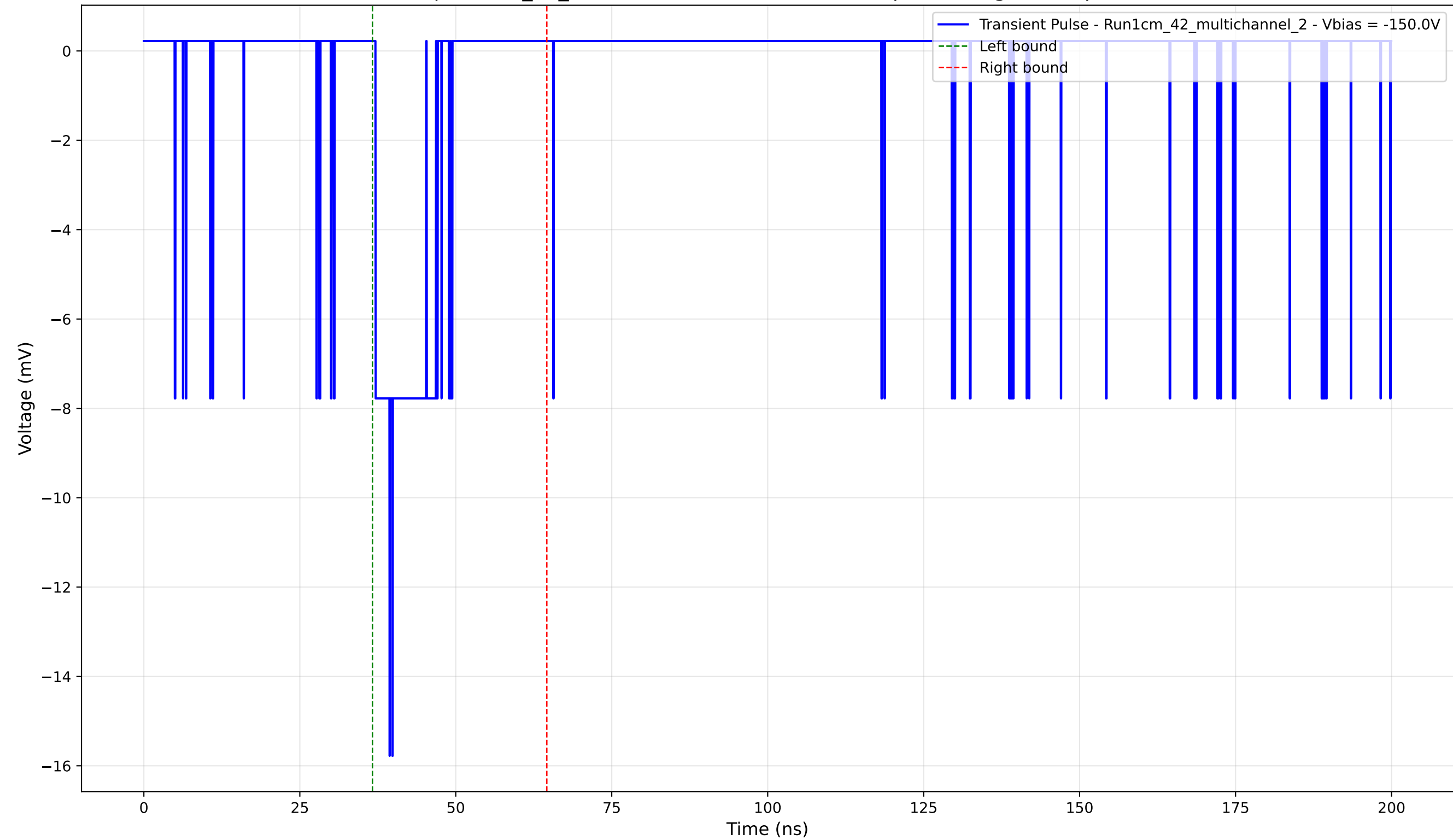
Transient Pulse - Sample: 1cm_42_multichannel - Position: 3865.0 \mu\text{m} - Charge: 1.53 pC - Rise Time: 2.27 ns
