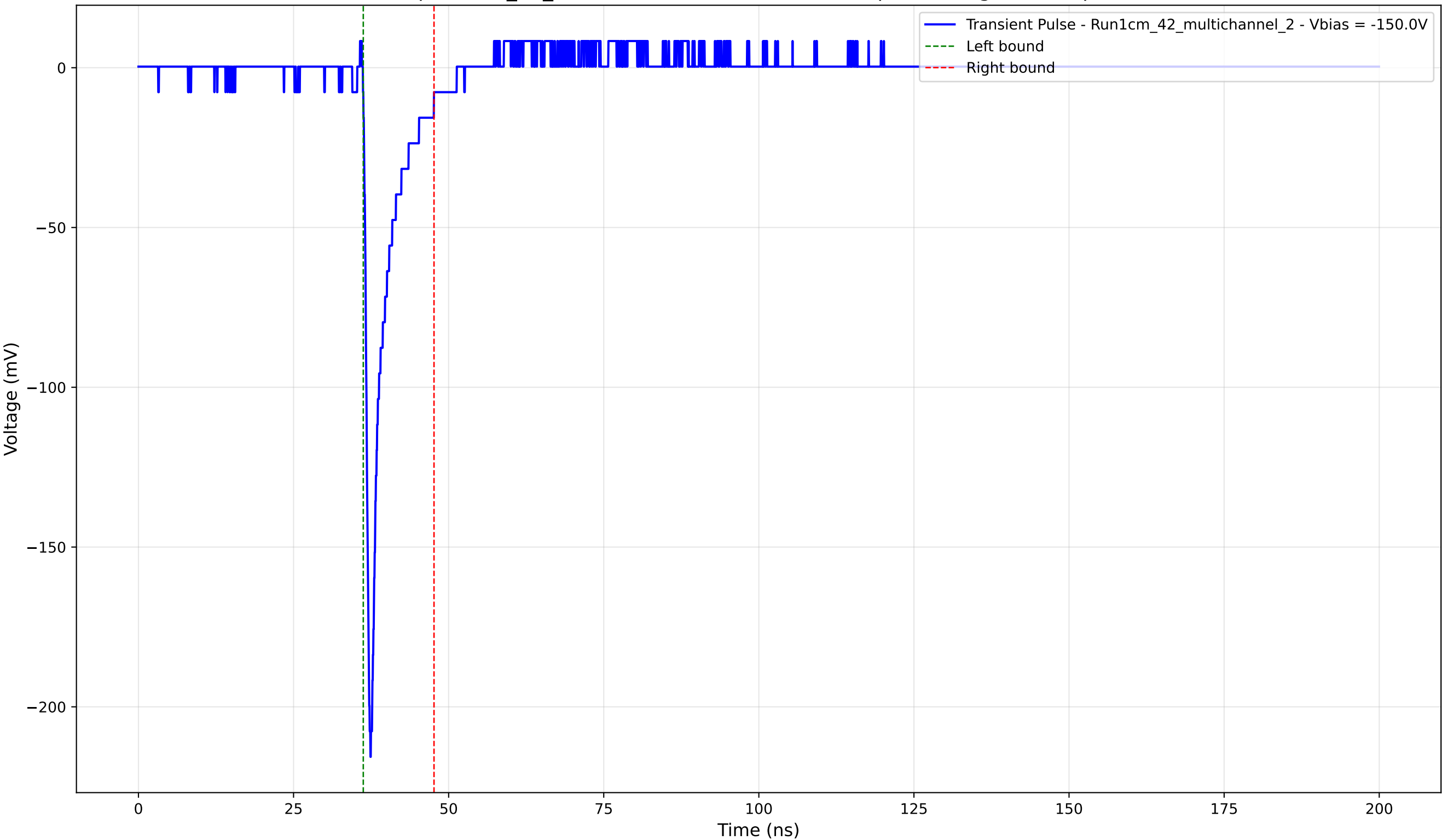
Transient Pulse - Sample: 1cm_42_multichannel - Position: 2820.0 \mu\text{m} - Charge: 13.65 pC - Rise Time: 0.85 ns
