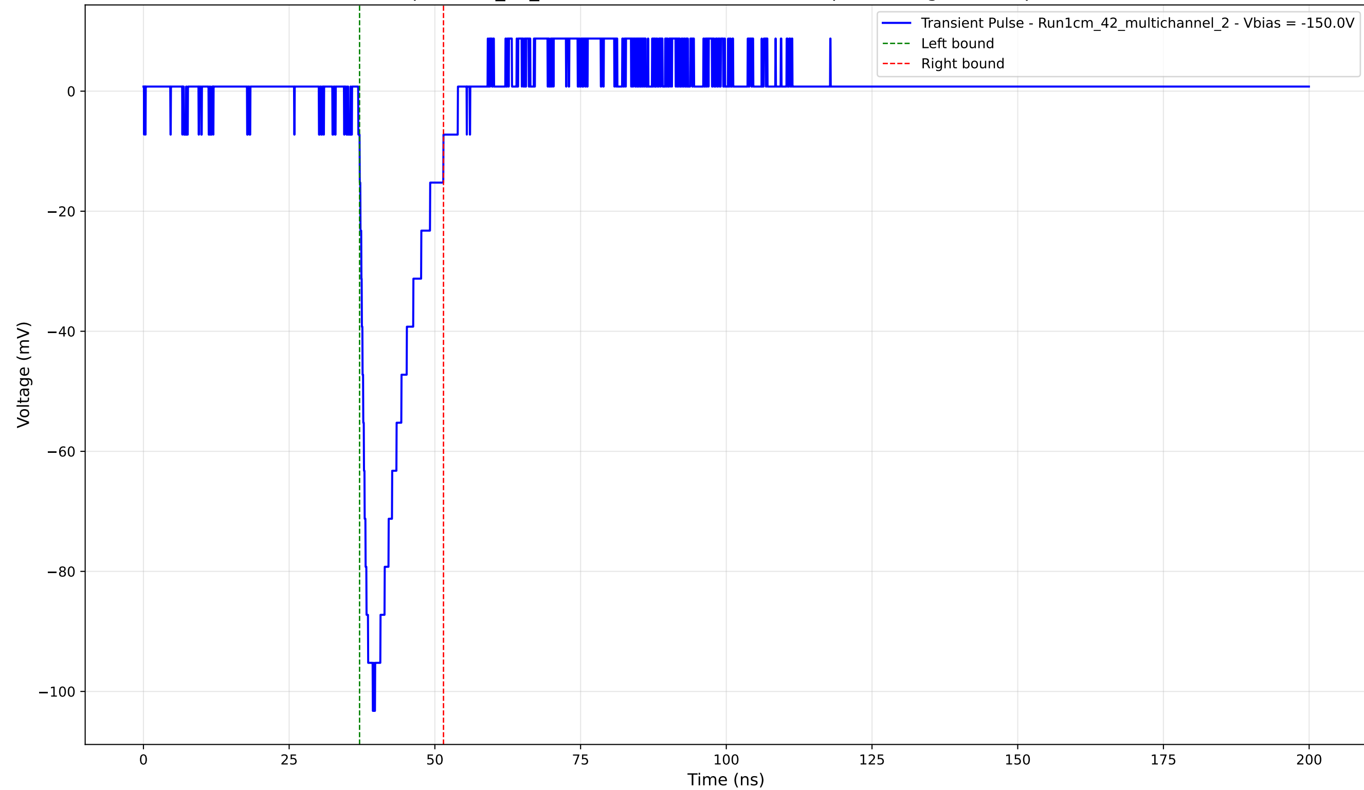
Transient Pulse - Sample: 1cm_42_multichannel - Position: 645.0 \mu\text{m} - Charge: 14.79 pC - Rise Time: 1.46 ns
