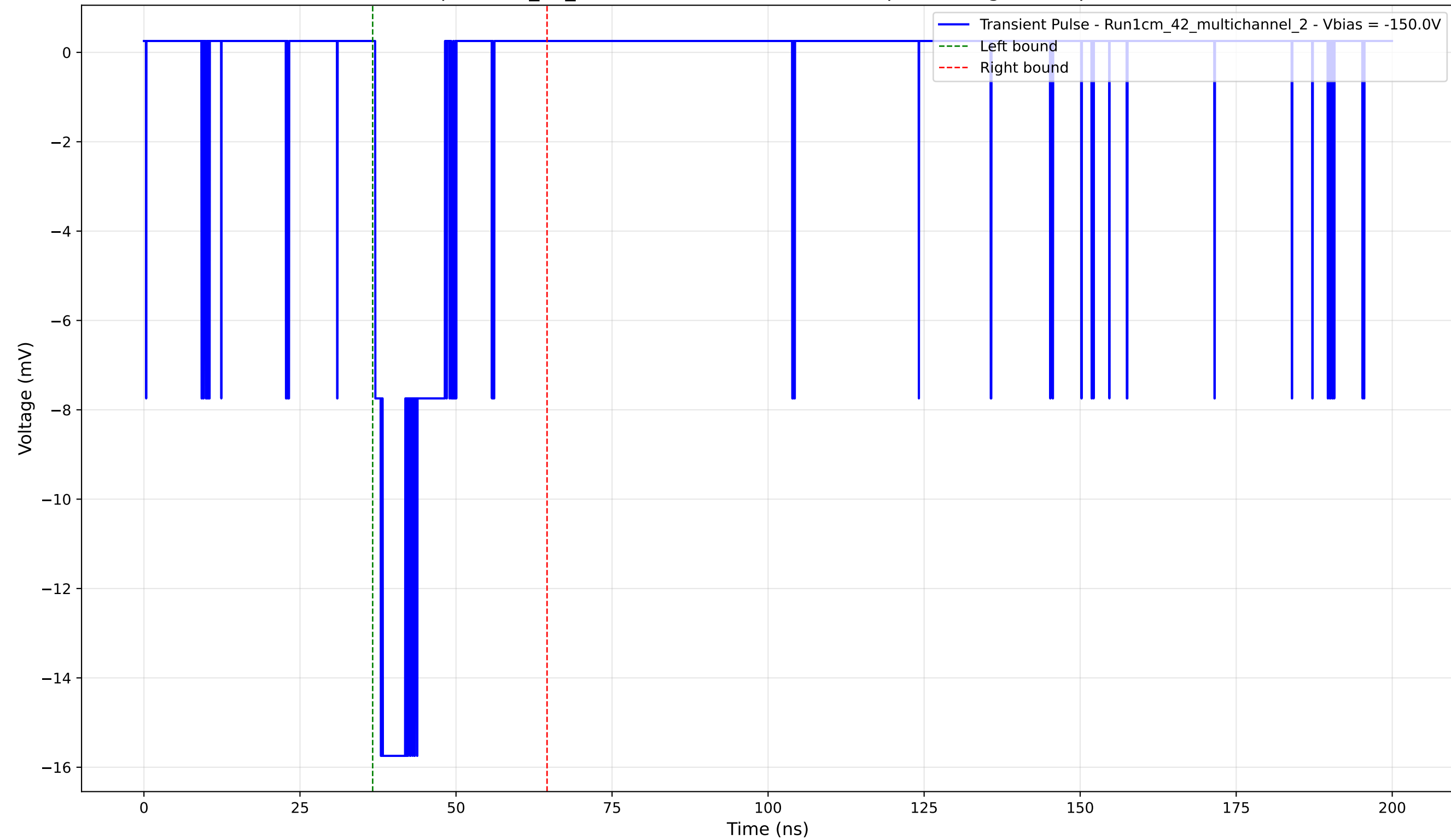
Transient Pulse - Sample: 1cm_42_multichannel - Position: 375.0 \mu\text{m} - Charge: 2.48 pC - Rise Time: 0.91 ns
