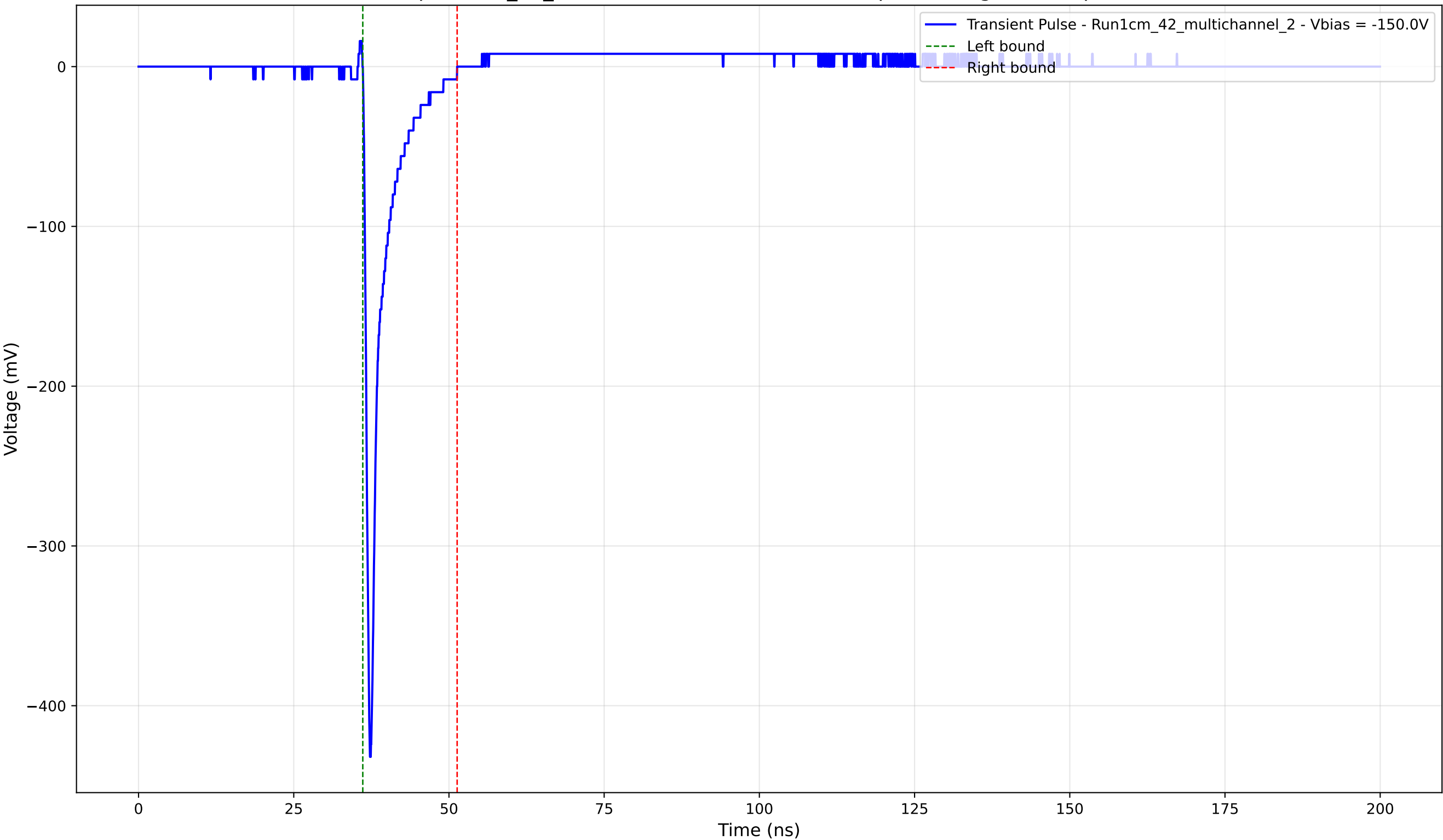
Transient Pulse - Sample: 1cm_42_multichannel - Position: 2705.0 \mu\text{m} - Charge: 25.33 pC - Rise Time: 0.77 ns
