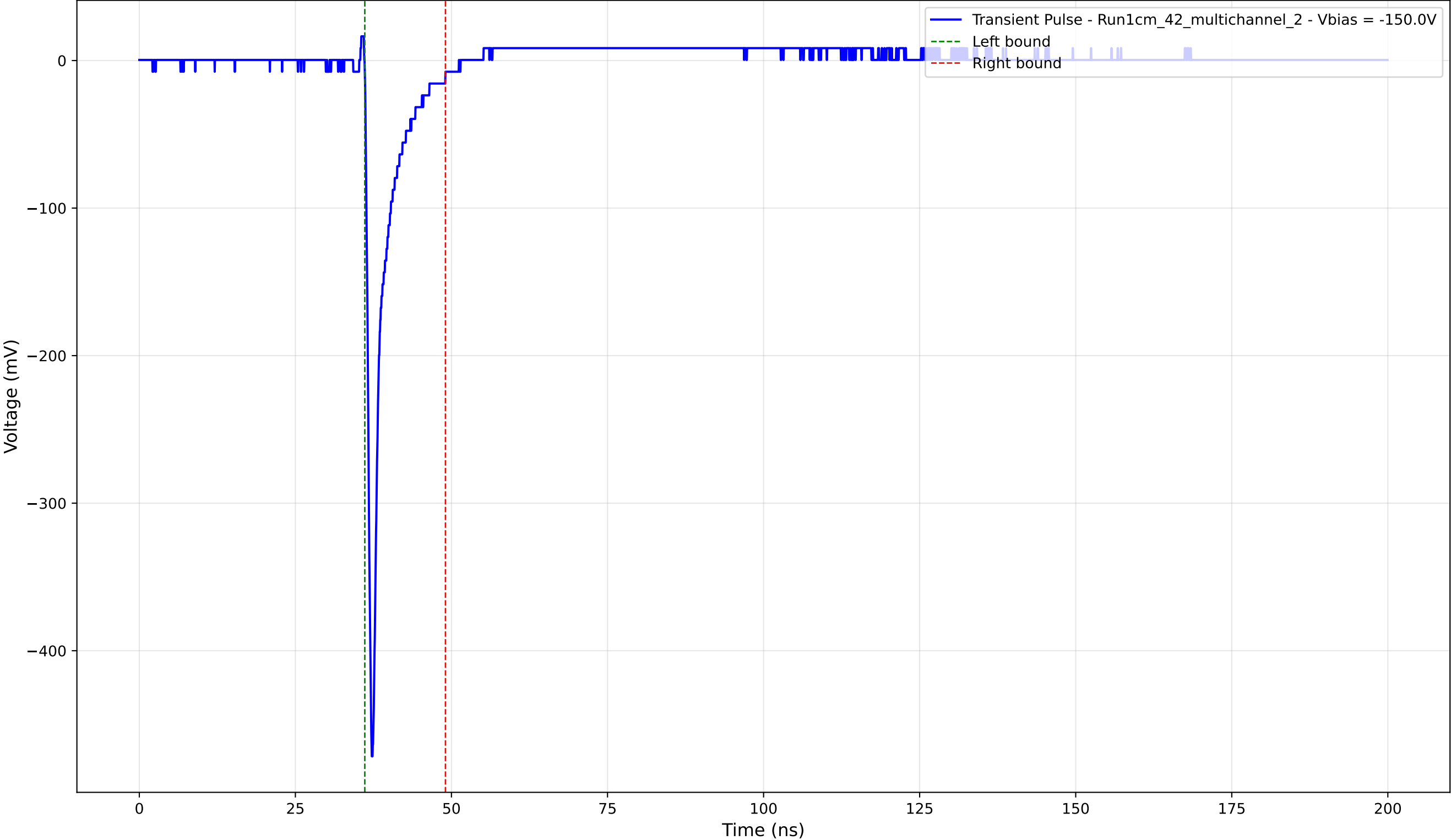
Transient Pulse - Sample: 1cm_42_multichannel - Position: 2080.0 \mu\text{m} - Charge: 25.81 pC - Rise Time: 0.78 ns
