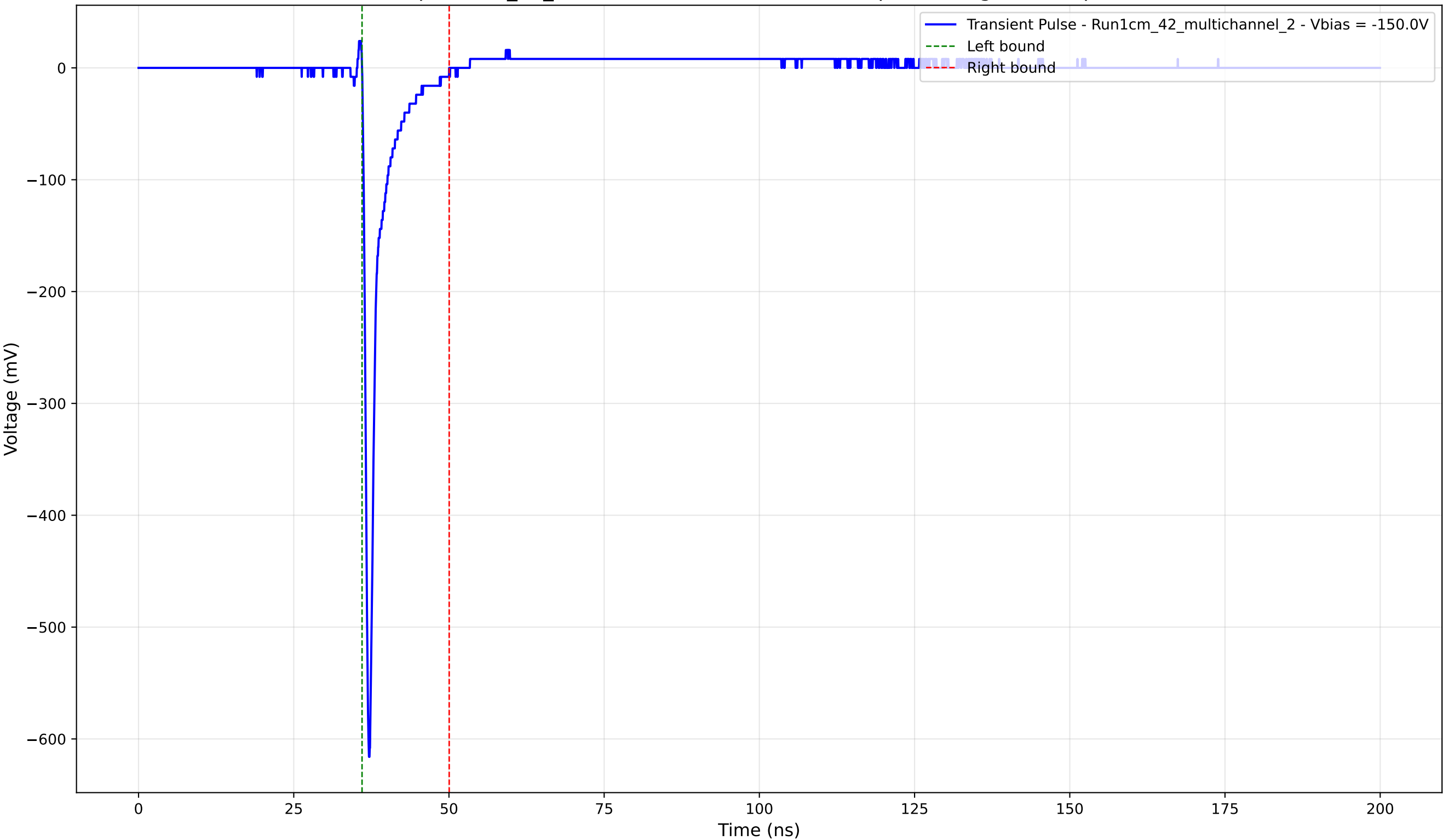
Transient Pulse - Sample: 1cm_42_multichannel - Position: 2480.0 \mu\text{m} - Charge: 28.52 pC - Rise Time: 0.73 ns
