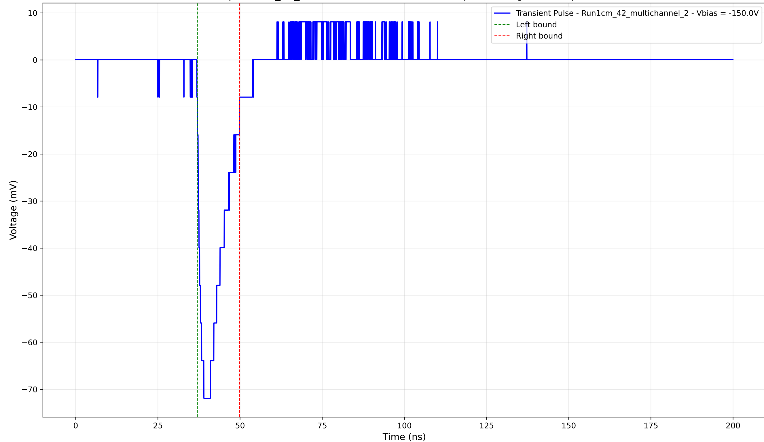
Transient Pulse - Sample: 1cm_42_multichannel - Position: 190.0 \mu\text{m} - Charge: 11.25 pC - Rise Time: 2.12 ns
