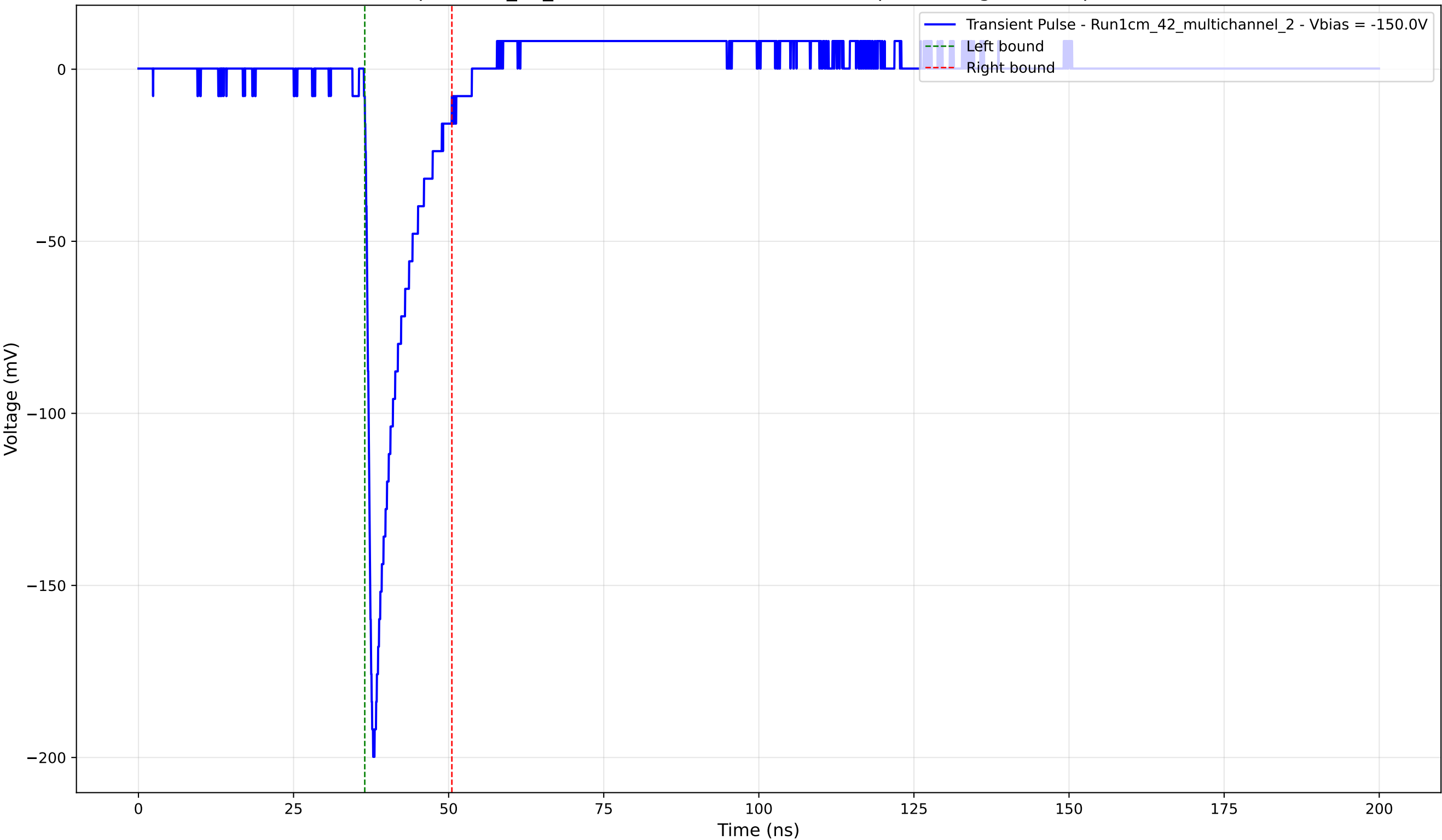
Transient Pulse - Sample: 1cm_42_multichannel - Position: 1455.0 \mu\text{m} - Charge: 20.64 pC - Rise Time: 1.02 ns
