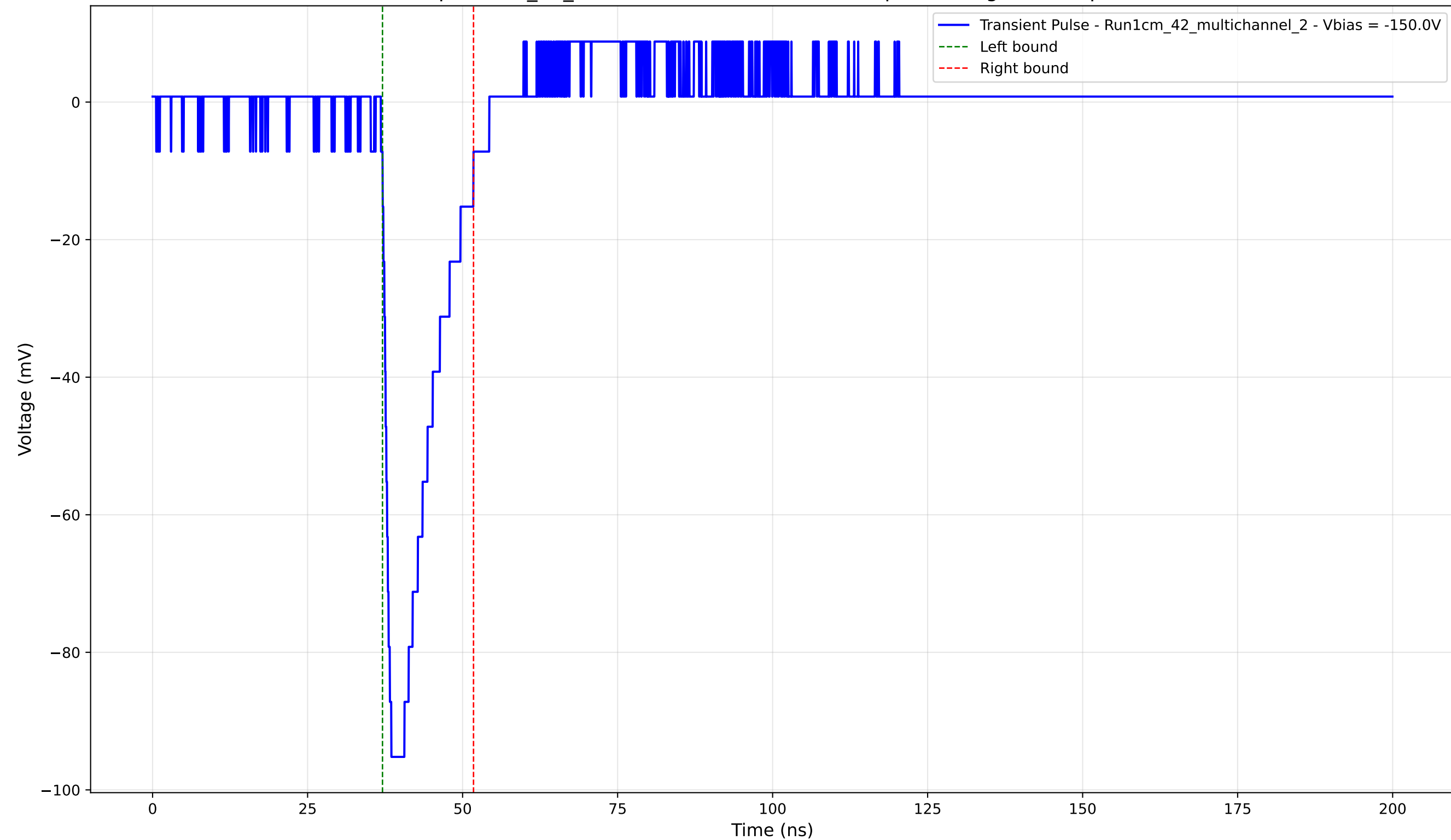
Transient Pulse - Sample: 1cm_42_multichannel - Position: 630.0 \mu\text{m} - Charge: 14.96 pC - Rise Time: 1.19 ns
