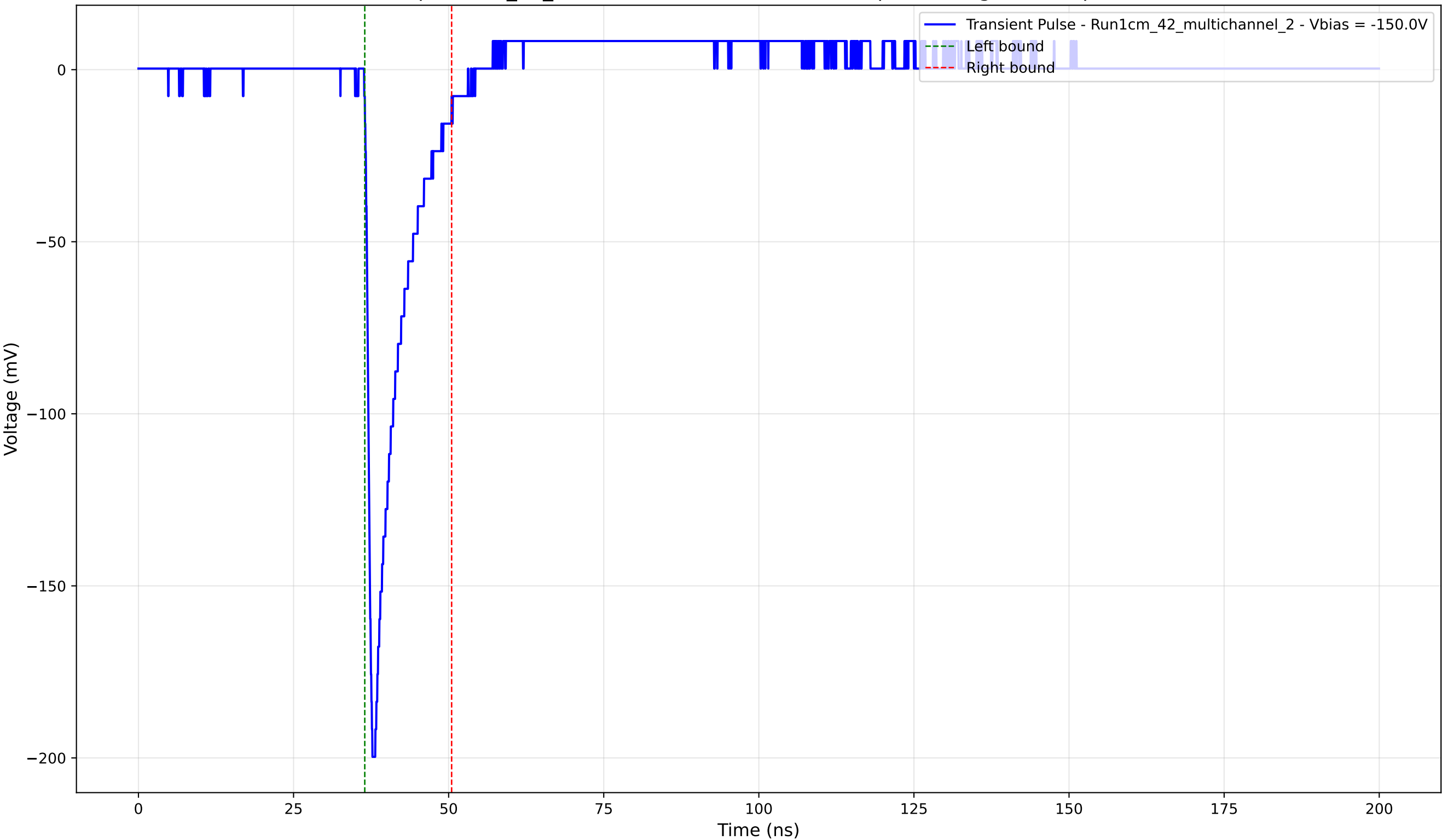
Transient Pulse - Sample: 1cm_42_multichannel - Position: 1470.0 \mu\text{m} - Charge: 20.72 pC - Rise Time: 0.98 ns
