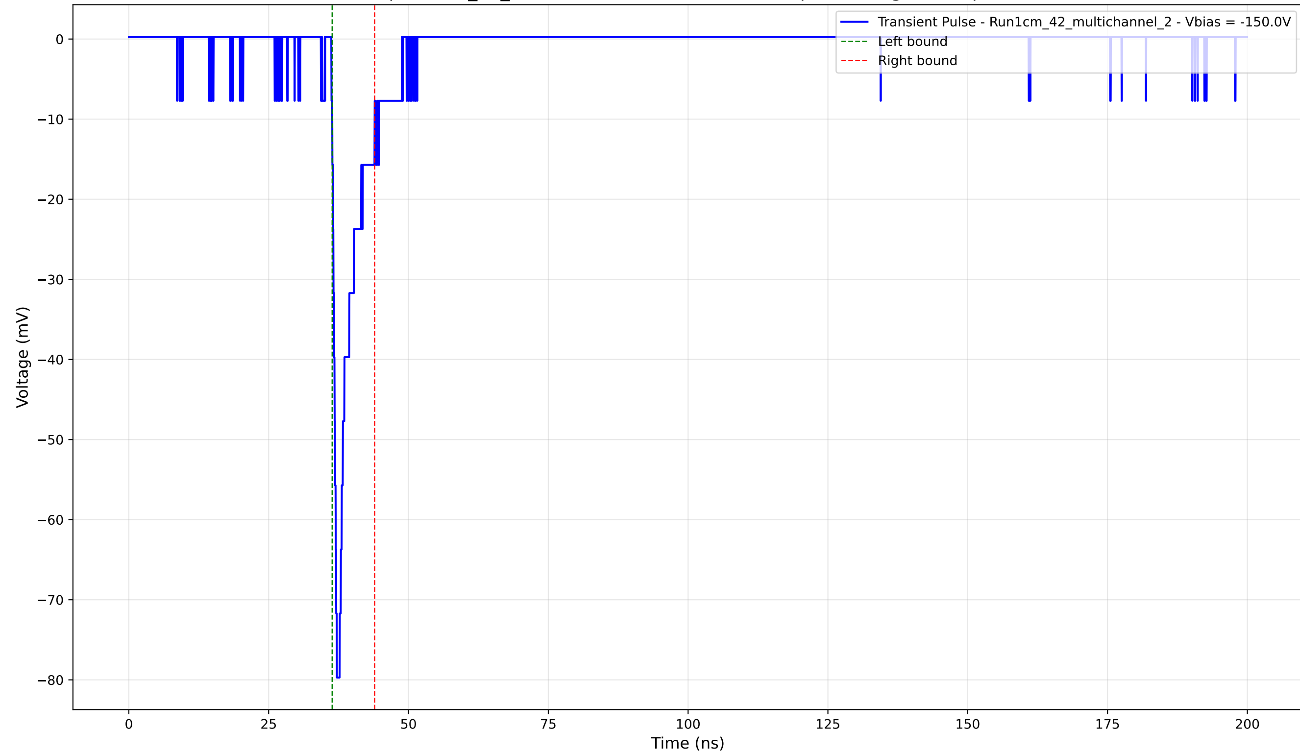
Transient Pulse - Sample: 1cm_42_multichannel - Position: 1900.0 \mu\text{m} - Charge: 5.13 pC - Rise Time: 0.84 ns
