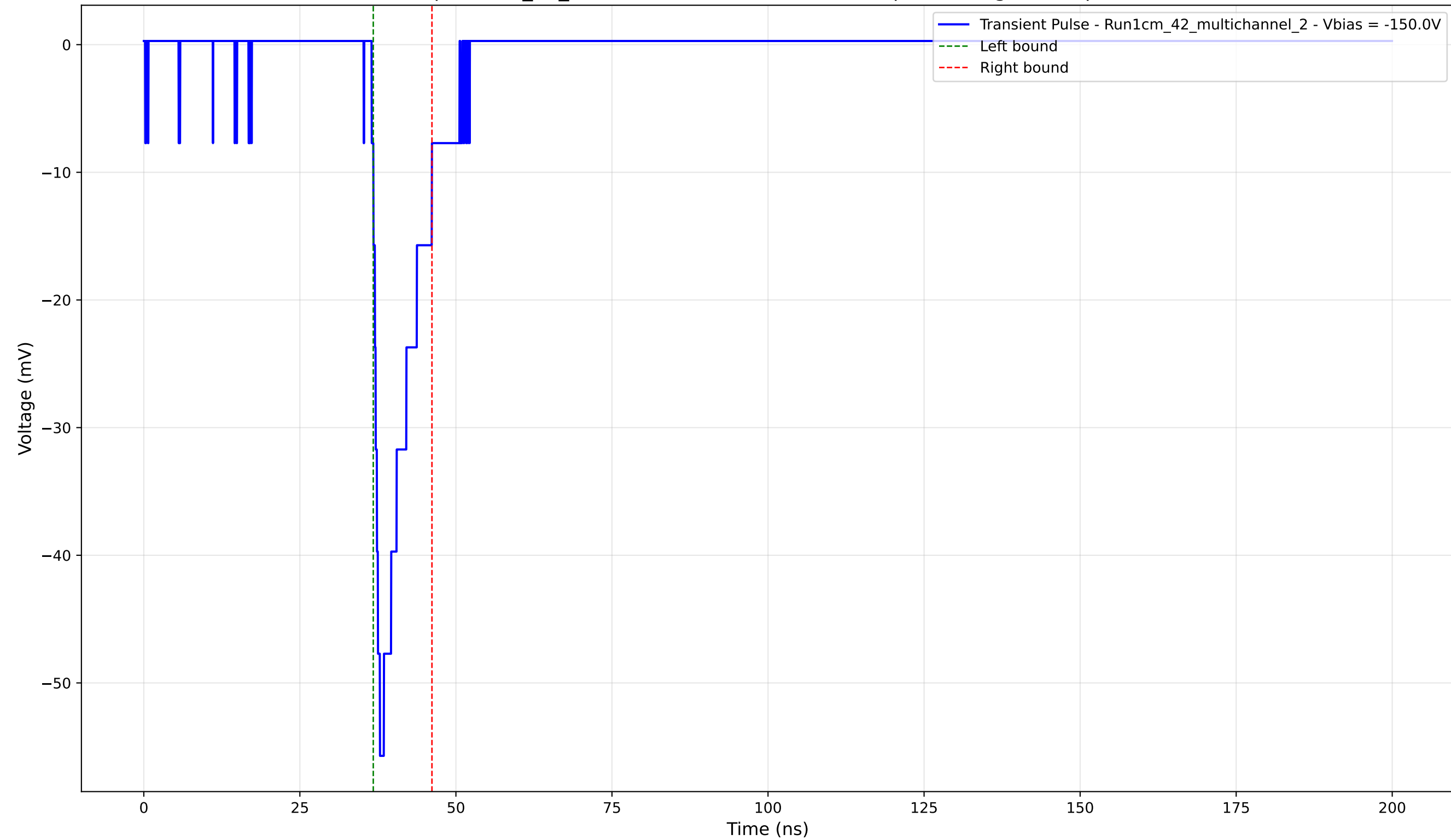
Transient Pulse - Sample: 1cm_42_multichannel - Position: 1315.0 \mu\text{m} - Charge: 5.76 pC - Rise Time: 1.33 ns
