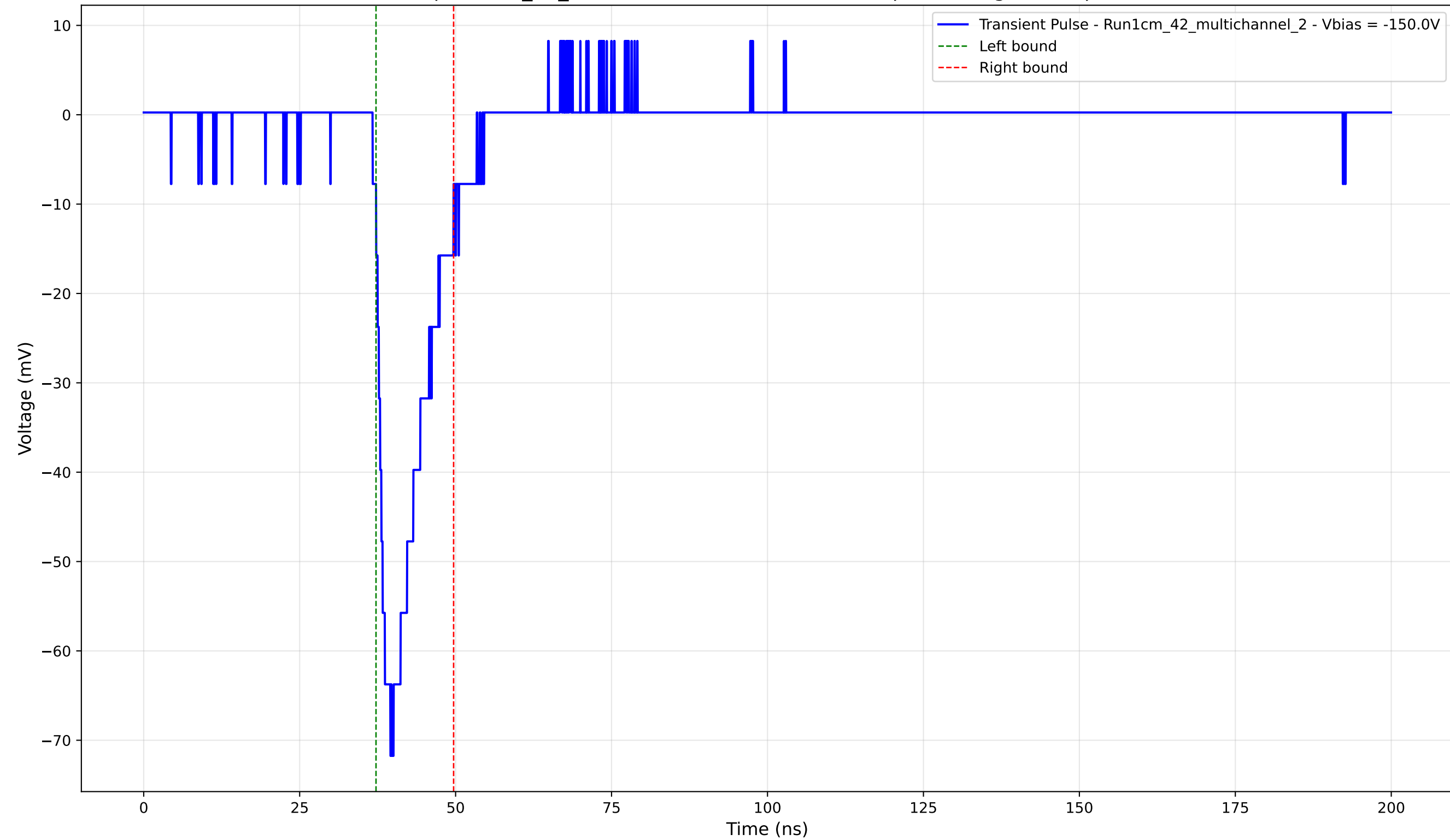
Transient Pulse - Sample: 1cm_42_multichannel - Position: 4305.0 \mu\text{m} - Charge: 9.75 pC - Rise Time: 2.84 ns
