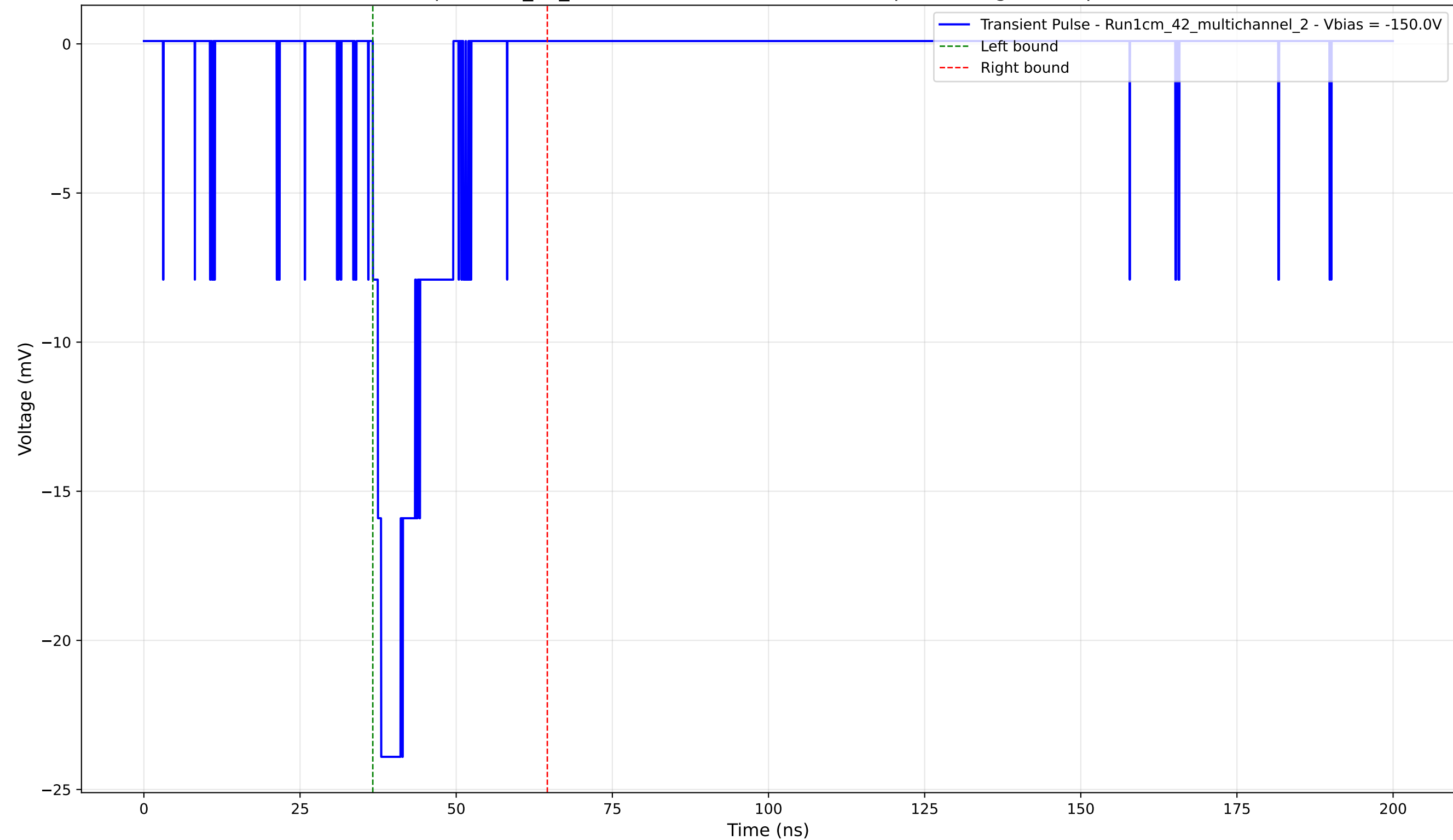
Transient Pulse - Sample: 1cm_42_multichannel - Position: 3850.0 \mu\text{m} - Charge: 3.73 pC - Rise Time: 1.35 ns
