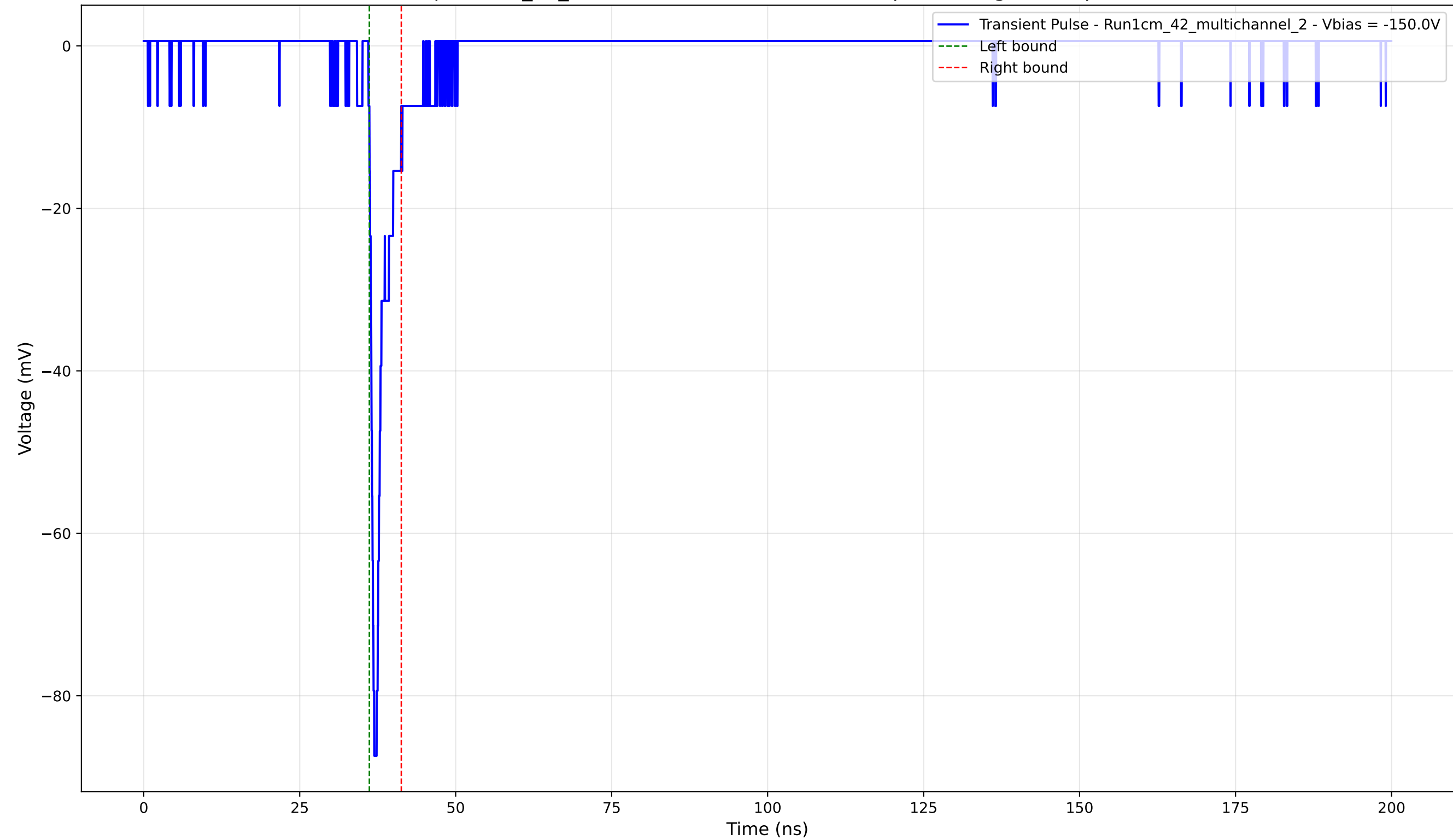
Transient Pulse - Sample: 1cm_42_multichannel - Position: 2400.0 \mu\text{m} - Charge: 3.79 pC - Rise Time: 0.67 ns
