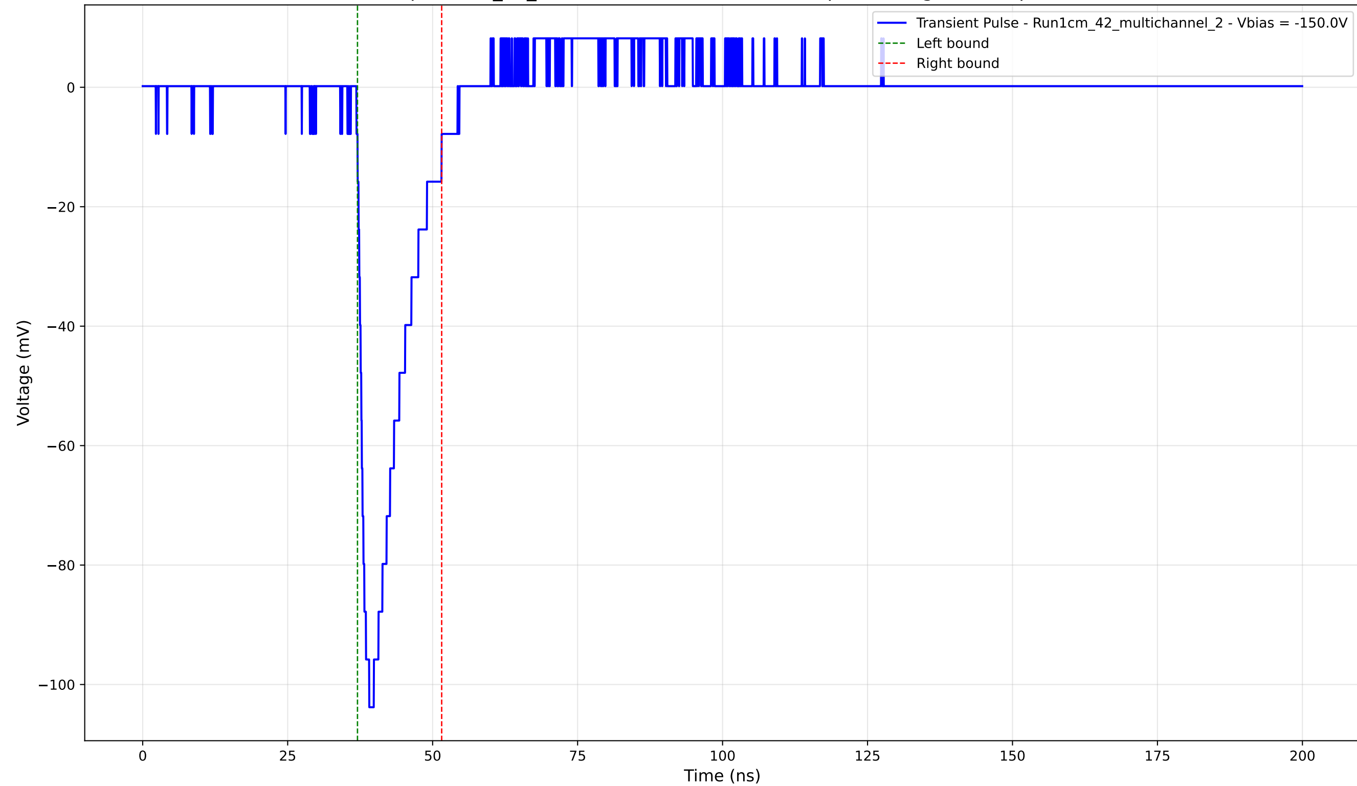
Transient Pulse - Sample: 1cm_42_multichannel - Position: 650.0 \mu\text{m} - Charge: 15.07 pC - Rise Time: 1.47 ns
