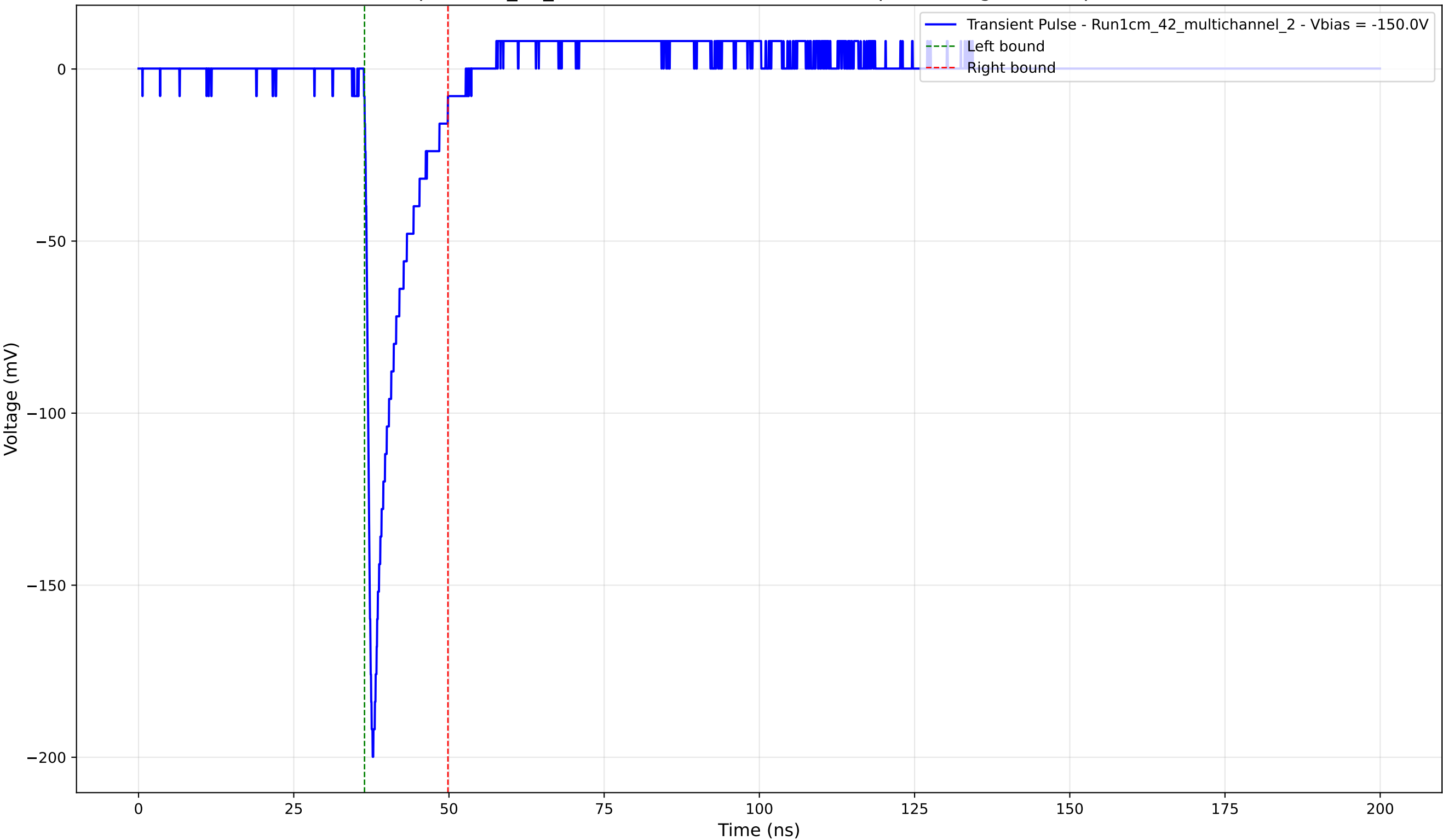
Transient Pulse - Sample: 1cm_42_multichannel - Position: 3160.0 \mu\text{m} - Charge: 18.56 pC - Rise Time: 0.98 ns
