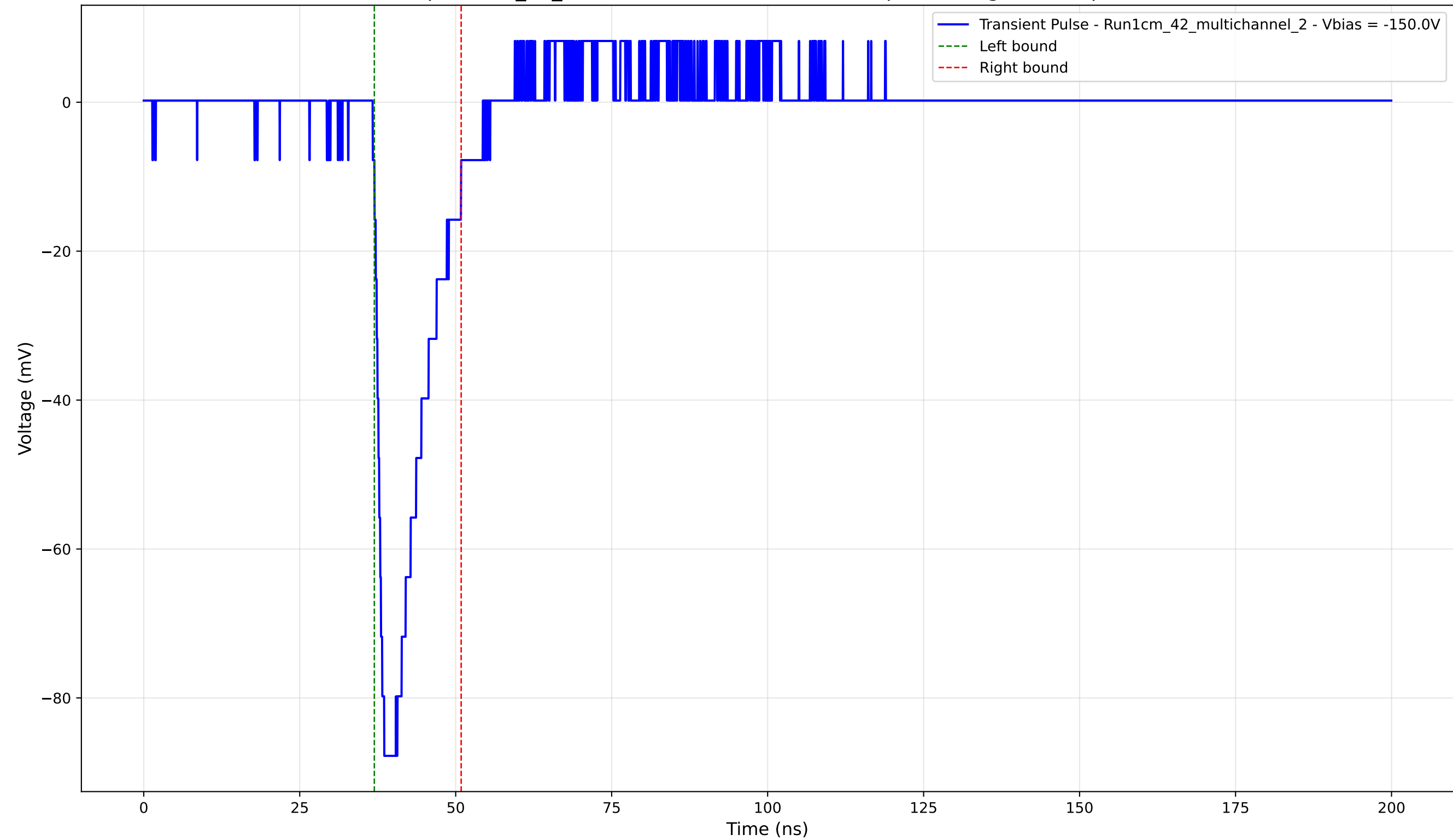
Transient Pulse - Sample: 1cm_42_multichannel - Position: 3970.0 \mu\text{m} - Charge: 13.37 pC - Rise Time: 1.27 ns
