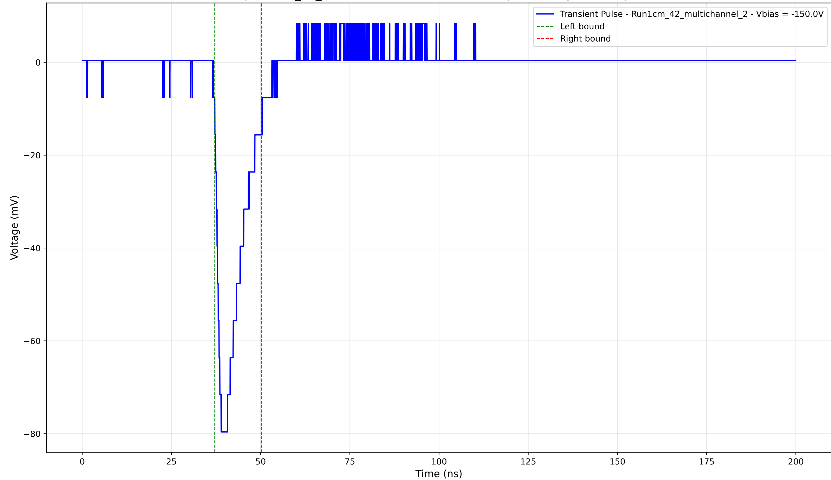
Transient Pulse - Sample: 1cm_42_multichannel - Position: 4250.0 \mu\text{m} - Charge: 11.71 pC - Rise Time: 1.80 ns
