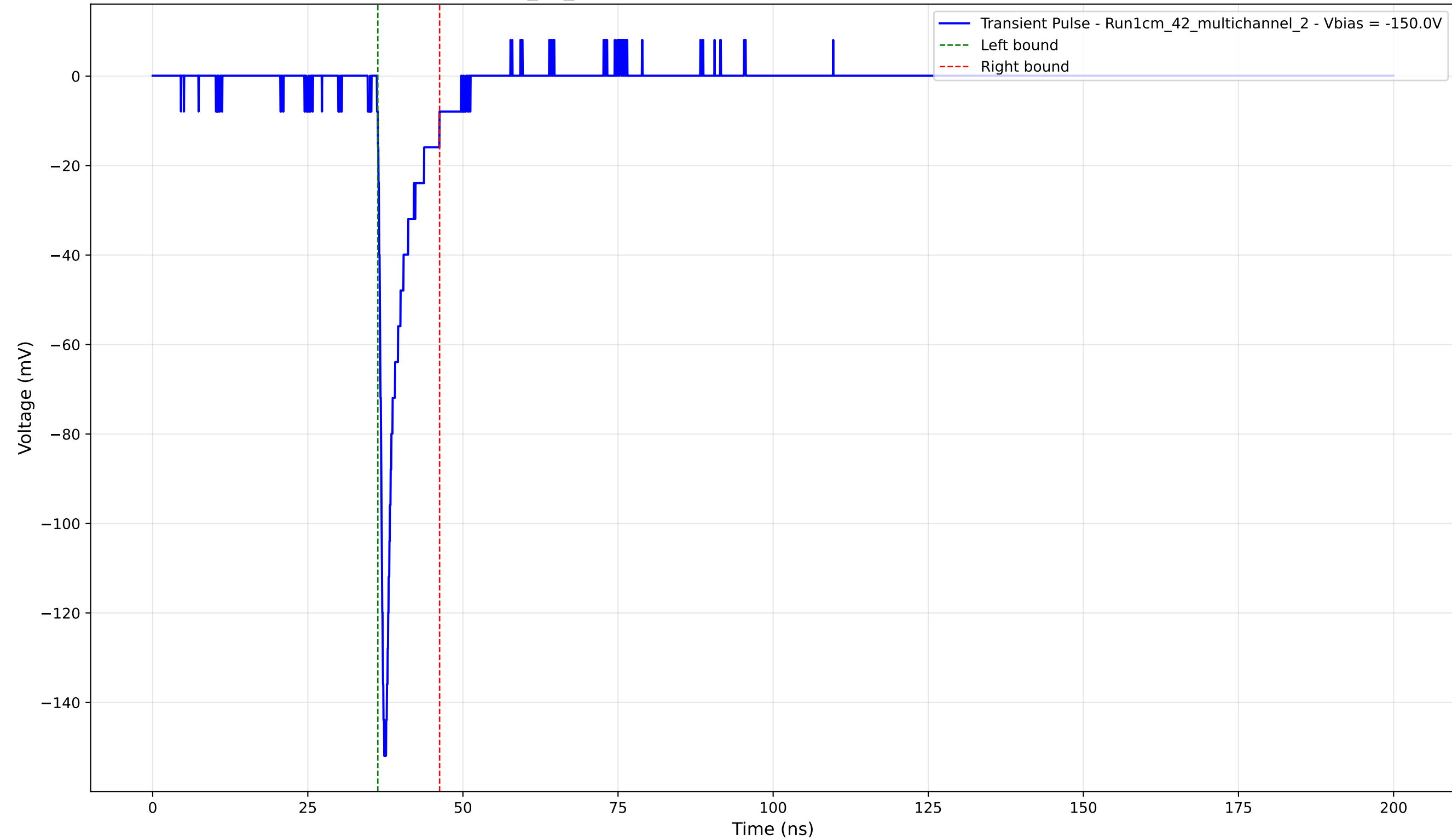
Transient Pulse - Sample: 1cm_42_multichannel - Position: 1910.0 \mu\text{m} - Charge: 9.77 pC - Rise Time: 0.88 ns
