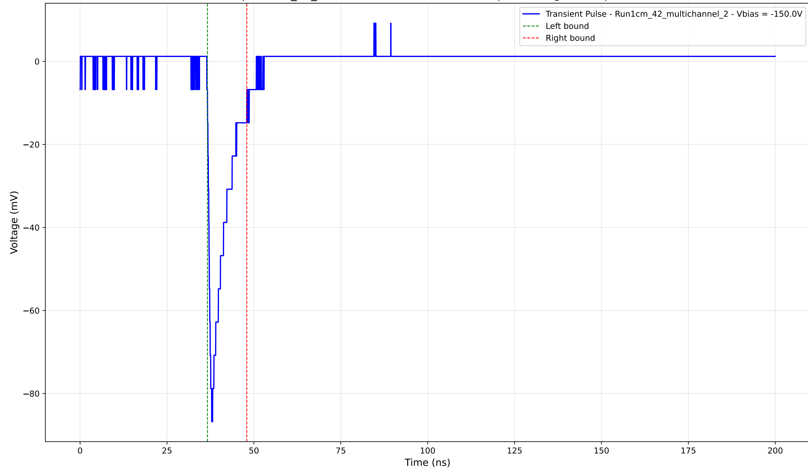
Transient Pulse - Sample: 1cm_42_multichannel - Position: 1405.0 \mu\text{m} - Charge: 8.61 pC - Rise Time: 0.95 ns
