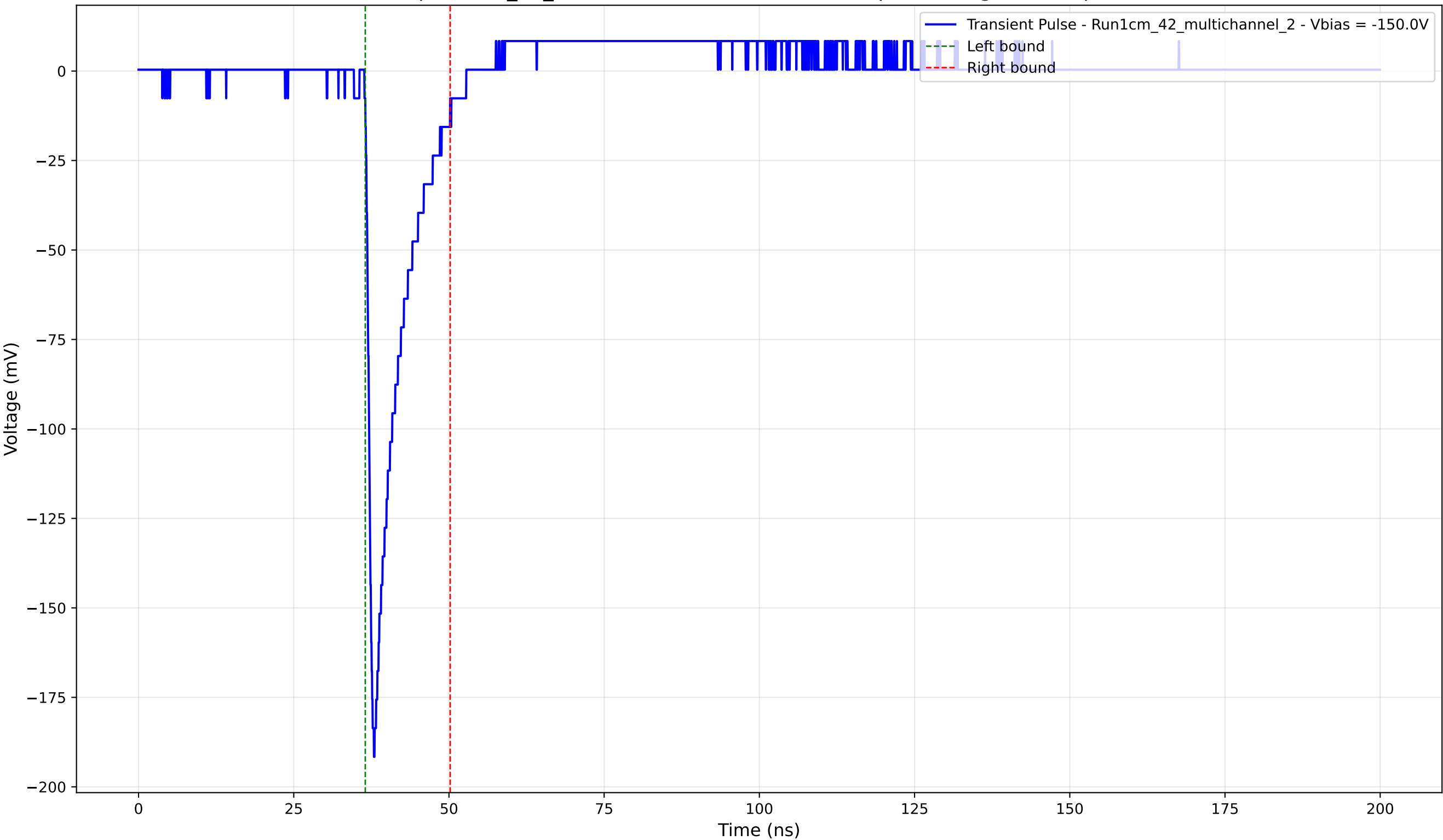
Transient Pulse - Sample: 1cm_42_multichannel - Position: 1440.0 \mu\text{m} - Charge: 19.68 pC - Rise Time: 1.02 ns
