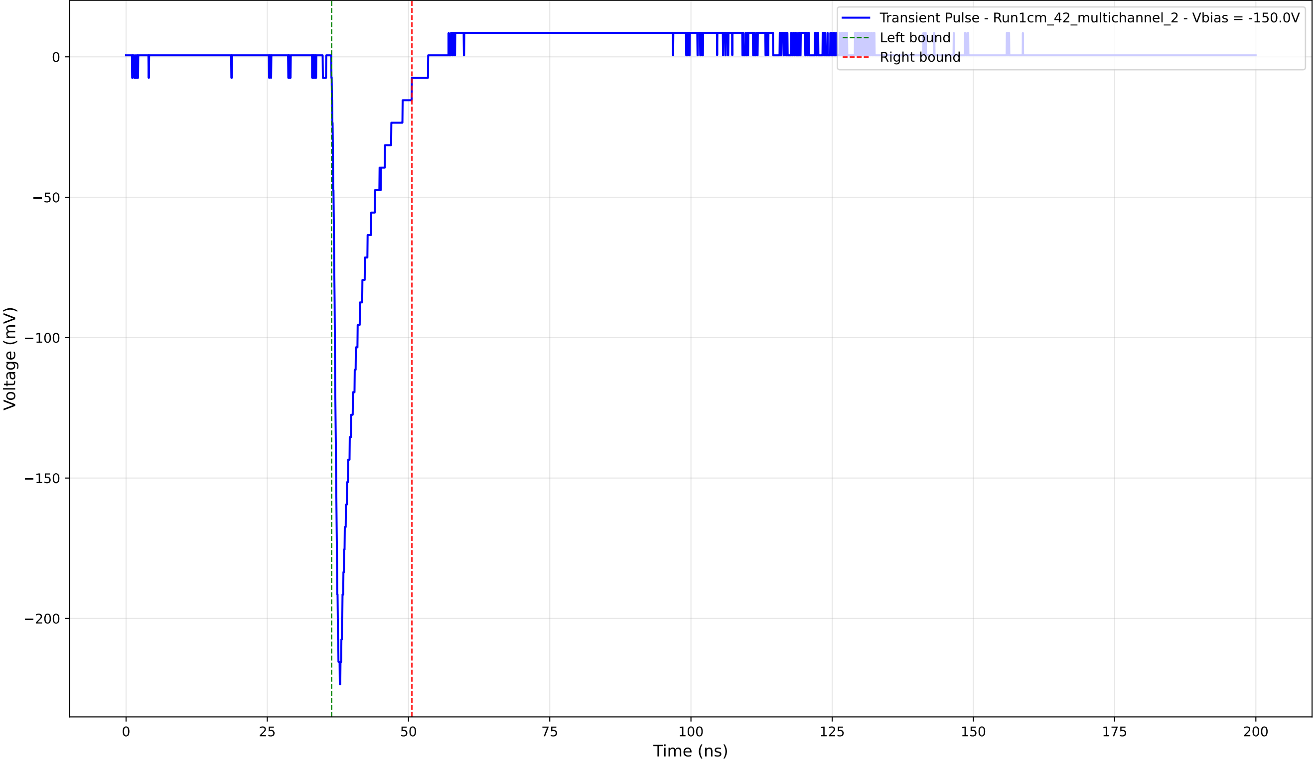
Transient Pulse - Sample: 1cm_42_multichannel - Position: 1540.0 \mu\text{m} - Charge: 21.32 pC - Rise Time: 1.01 ns
