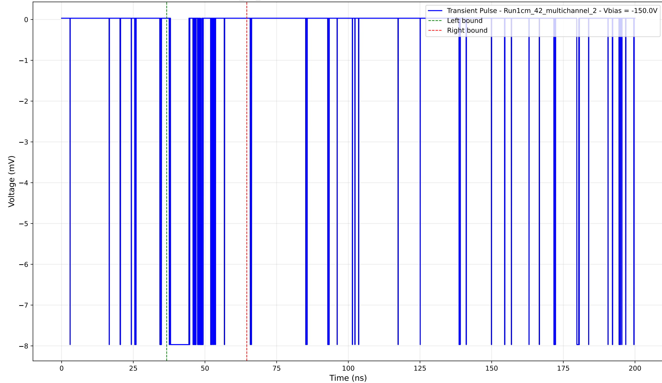
Transient Pulse - Sample: 1cm_42_multichannel - Position: 335.0 \mu\text{m} - Charge: 1.44 pC - Rise Time: 0.04 ns
