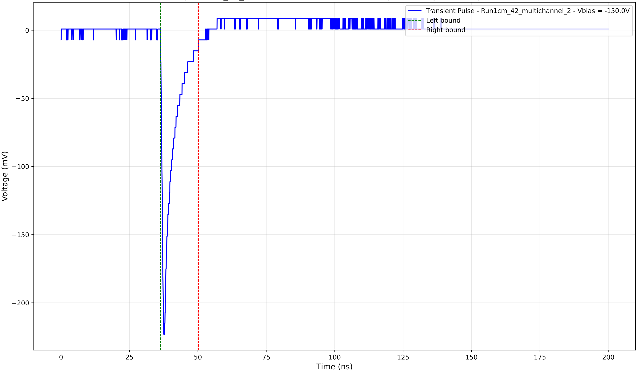
Transient Pulse - Sample: 1cm_42_multichannel - Position: 3075.0 \mu\text{m} - Charge: 19.55 pC - Rise Time: 0.92 ns
