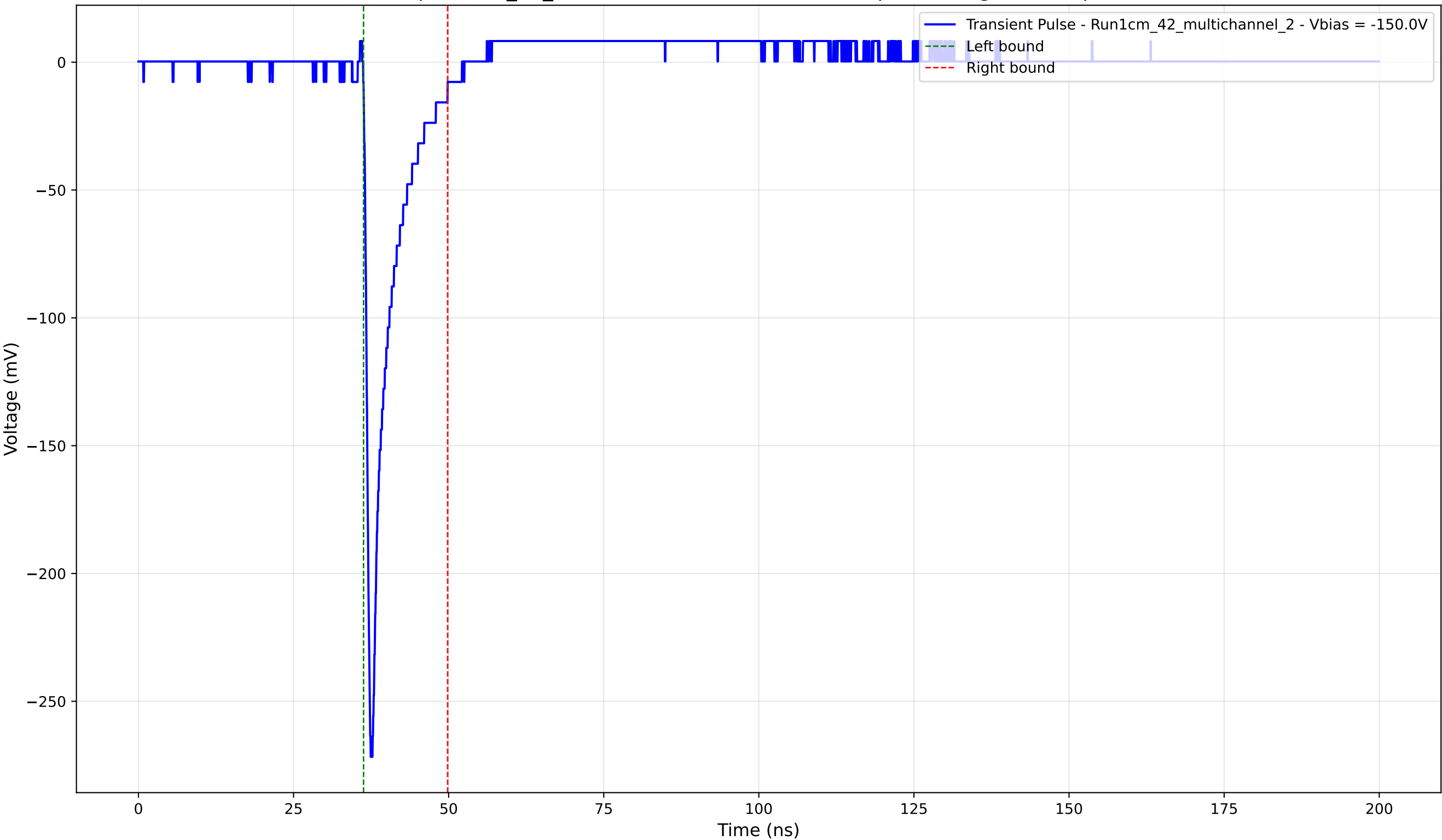
Transient Pulse - Sample: 1cm_42_multichannel - Position: 2975.0 \mu\text{m} - Charge: 21.37 pC - Rise Time: 0.89 ns
