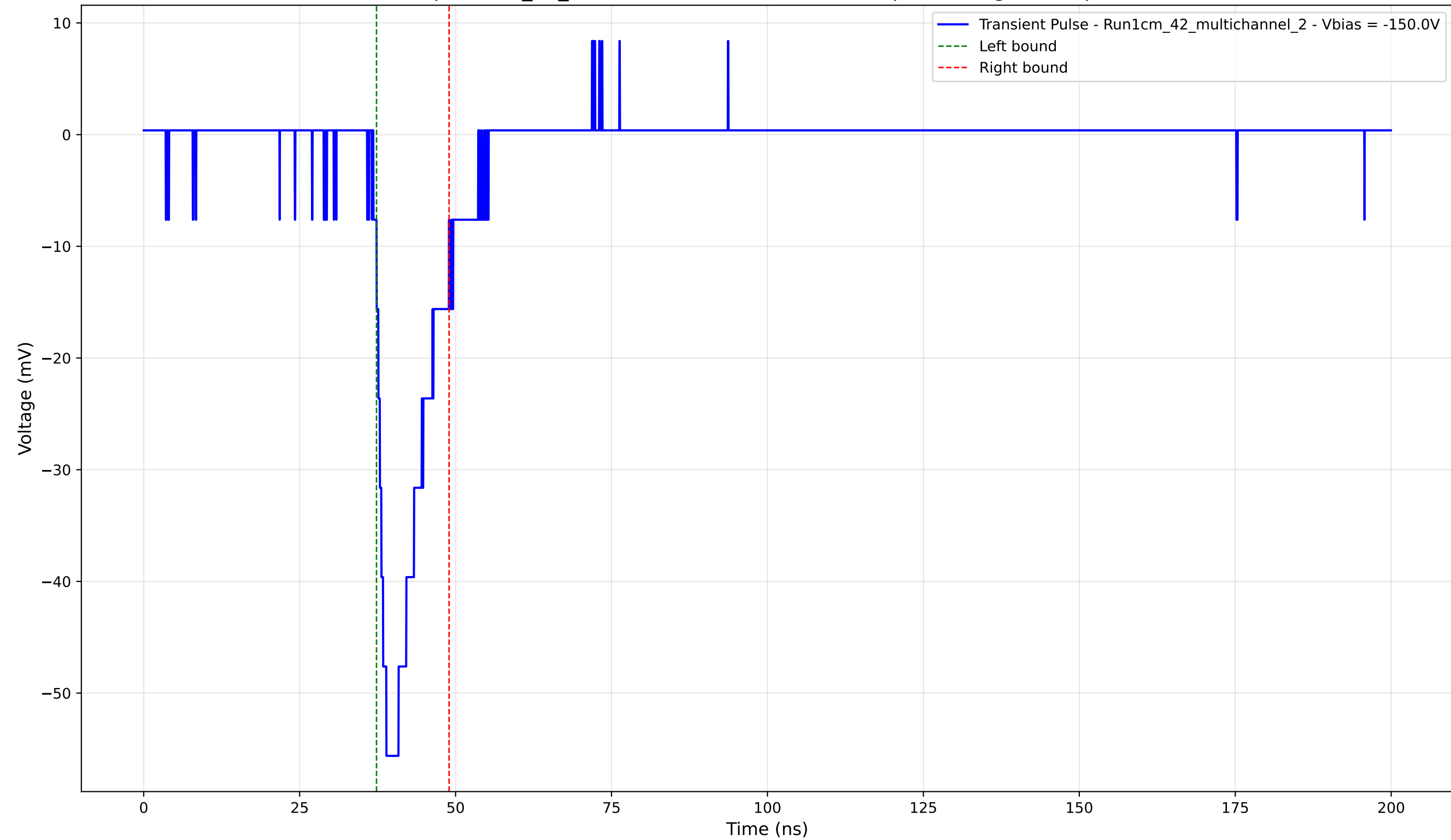
Transient Pulse - Sample: 1cm_42_multichannel - Position: 4325.0 \mu\text{m} - Charge: 7.89 pC - Rise Time: 2.09 ns
