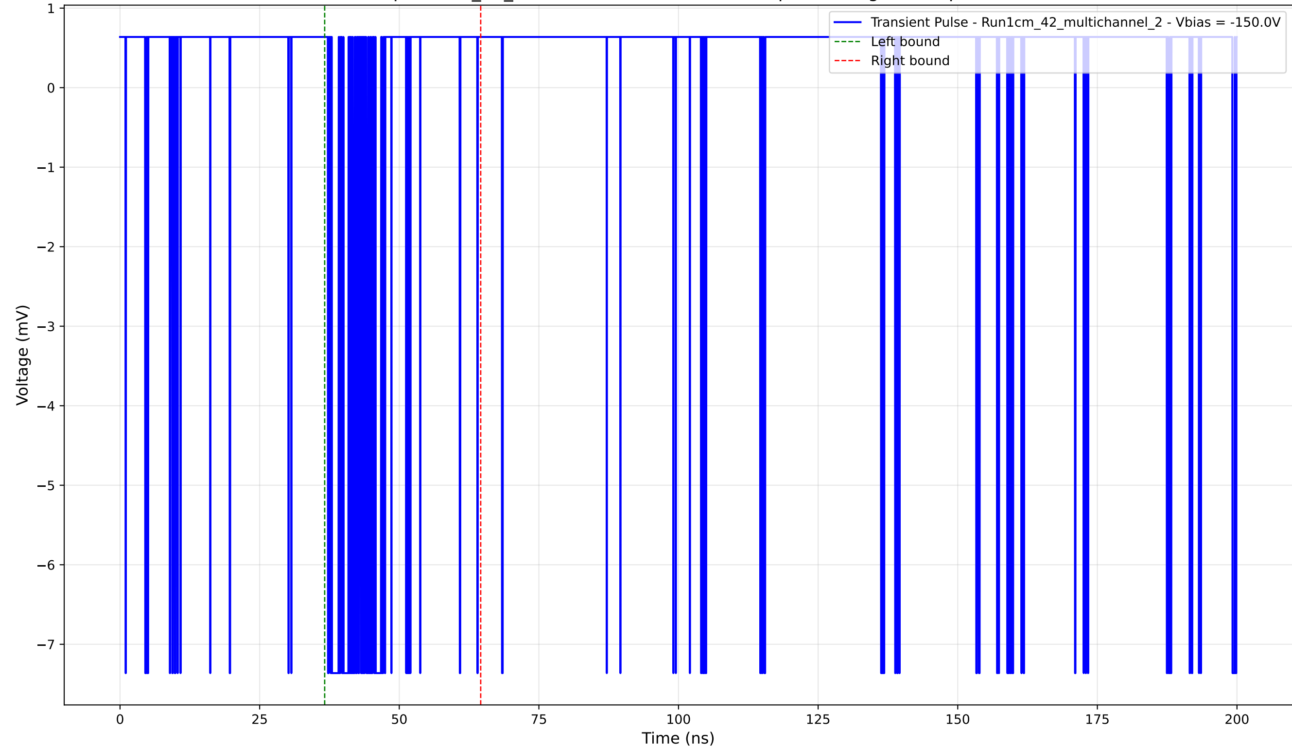
Transient Pulse - Sample: 1cm_42_multichannel - Position: 30.0 \mu\text{m} - Charge: 0.78 pC - Rise Time: 0.04 ns
