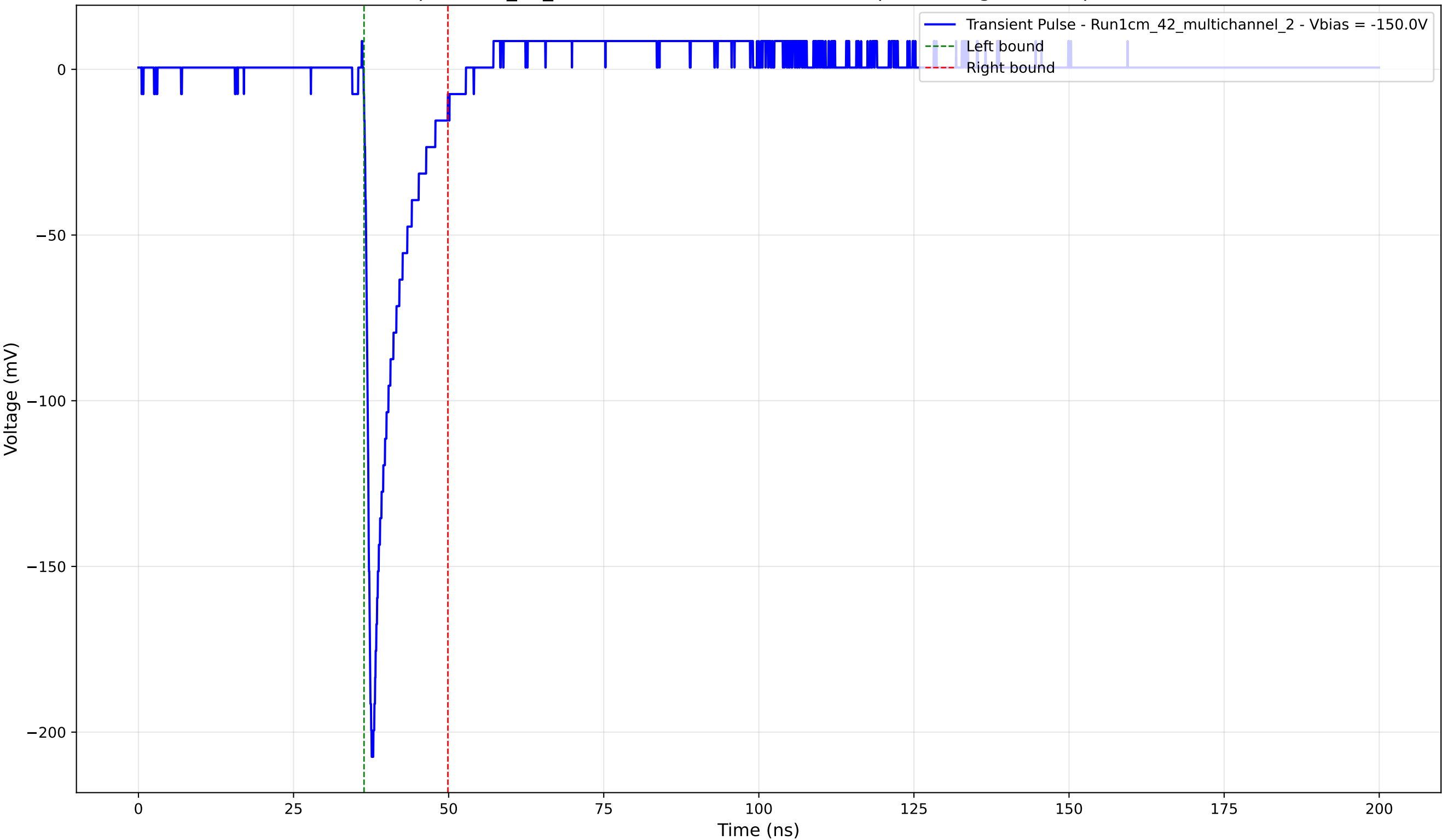
Transient Pulse - Sample: 1cm_42_multichannel - Position: 3125.0 \mu\text{m} - Charge: 18.70 pC - Rise Time: 0.93 ns
