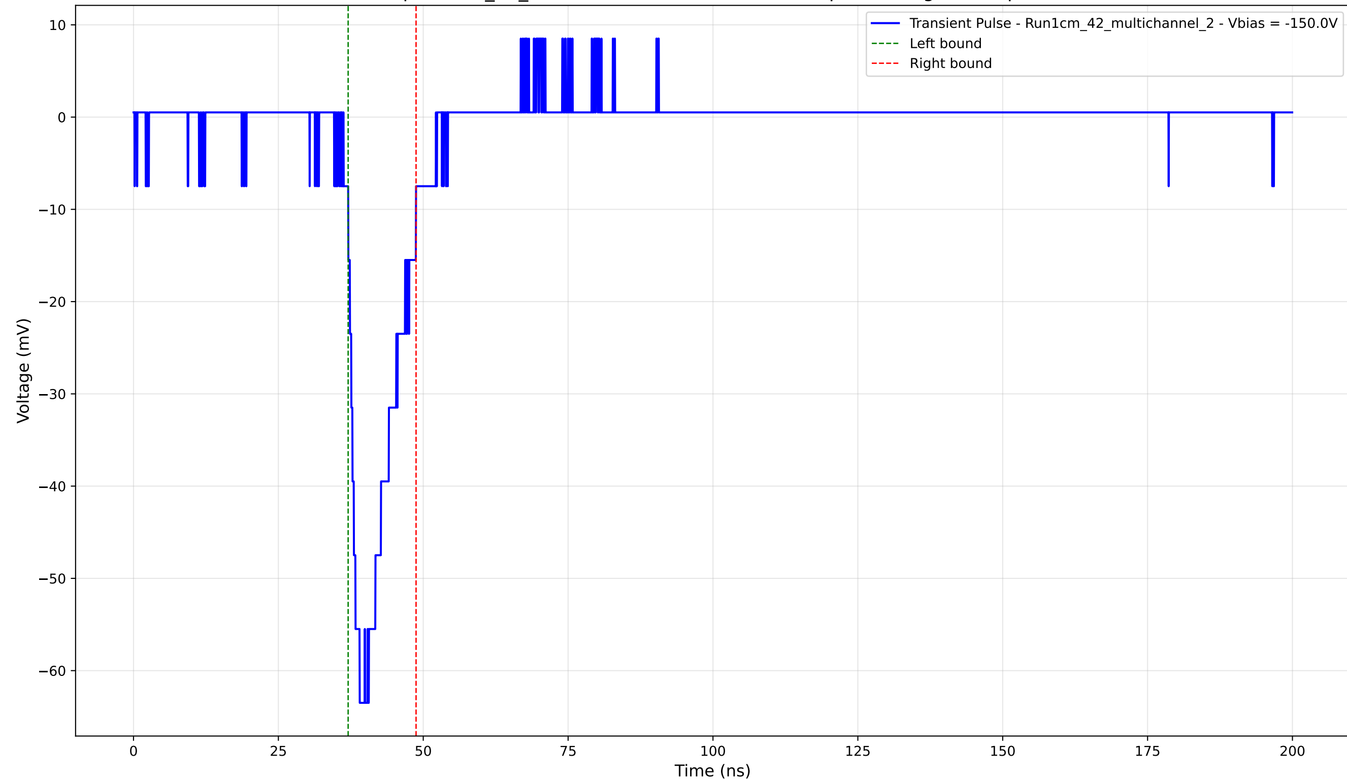
Transient Pulse - Sample: 1cm_42_multichannel - Position: 4790.0 \mu\text{m} - Charge: 8.97 pC - Rise Time: 2.77 ns
