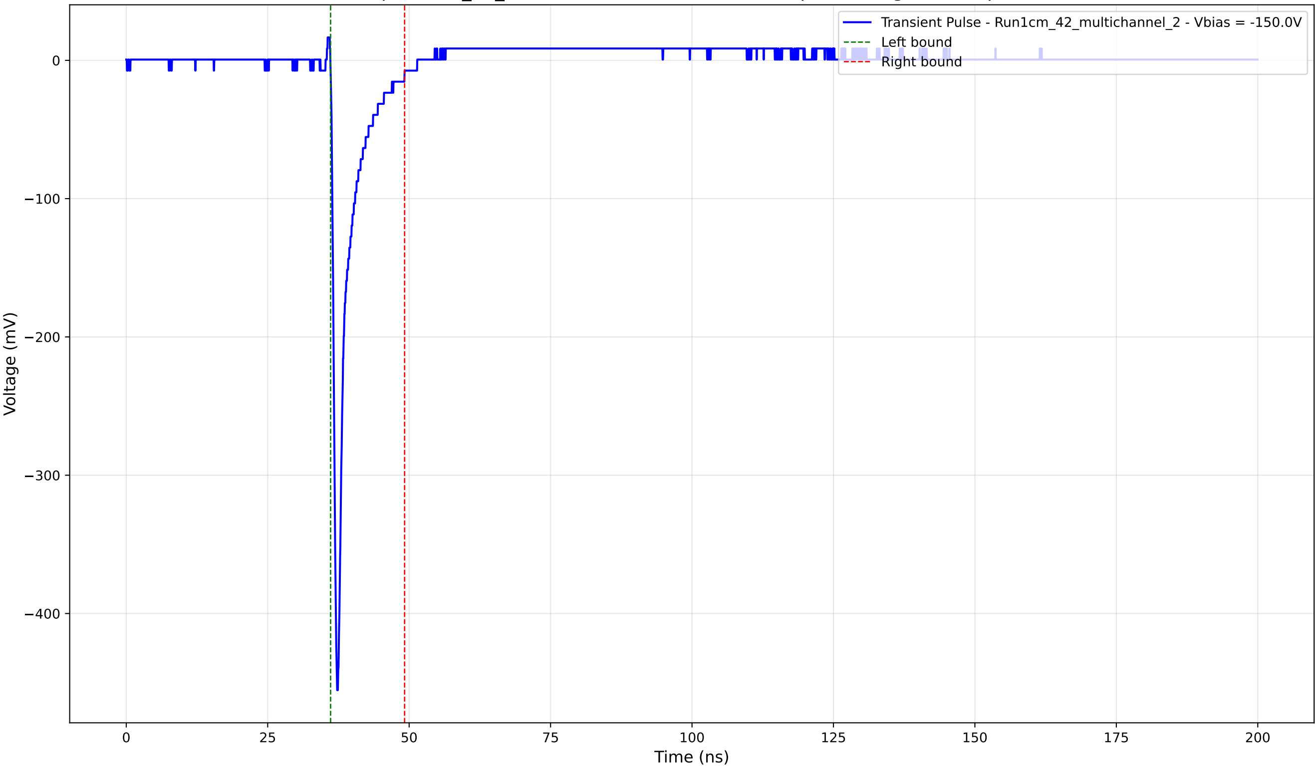
Transient Pulse - Sample: 1cm_42_multichannel - Position: 2050.0 \mu\text{m} - Charge: 25.84 pC - Rise Time: 0.76 ns
