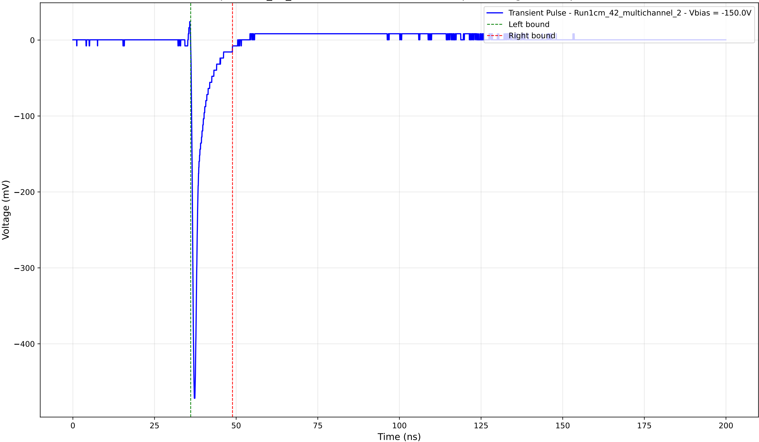
Transient Pulse - Sample: 1cm_42_multichannel - Position: 2620.0 \mu\text{m} - Charge: 25.12 pC - Rise Time: 0.73 ns
