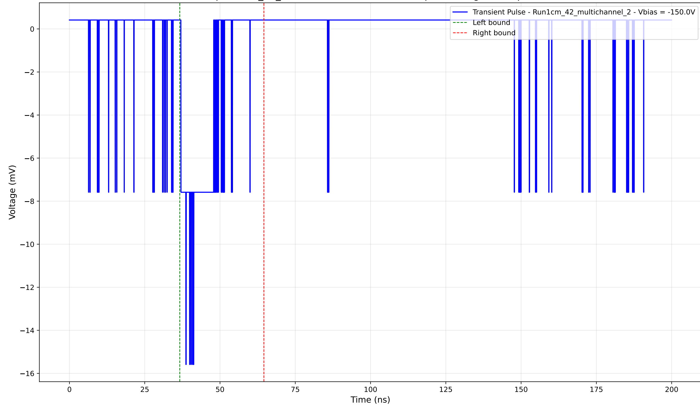
Transient Pulse - Sample: 1cm_42_multichannel - Position: 50.0 \mu\text{m} - Charge: 1.84 pC - Rise Time: 1.67 ns
