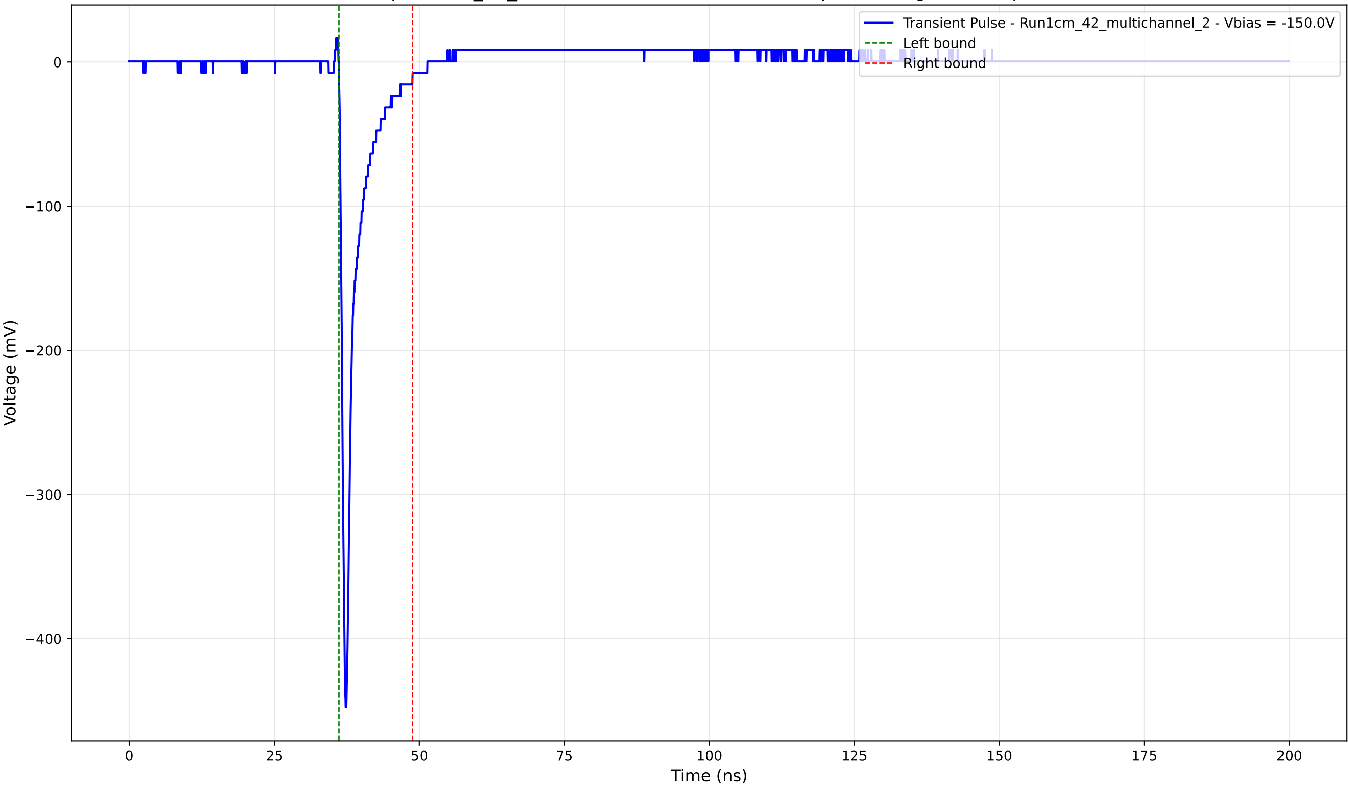
Transient Pulse - Sample: 1cm_42_multichannel - Position: 2660.0 \mu\text{m} - Charge: 24.67 pC - Rise Time: 0.74 ns
