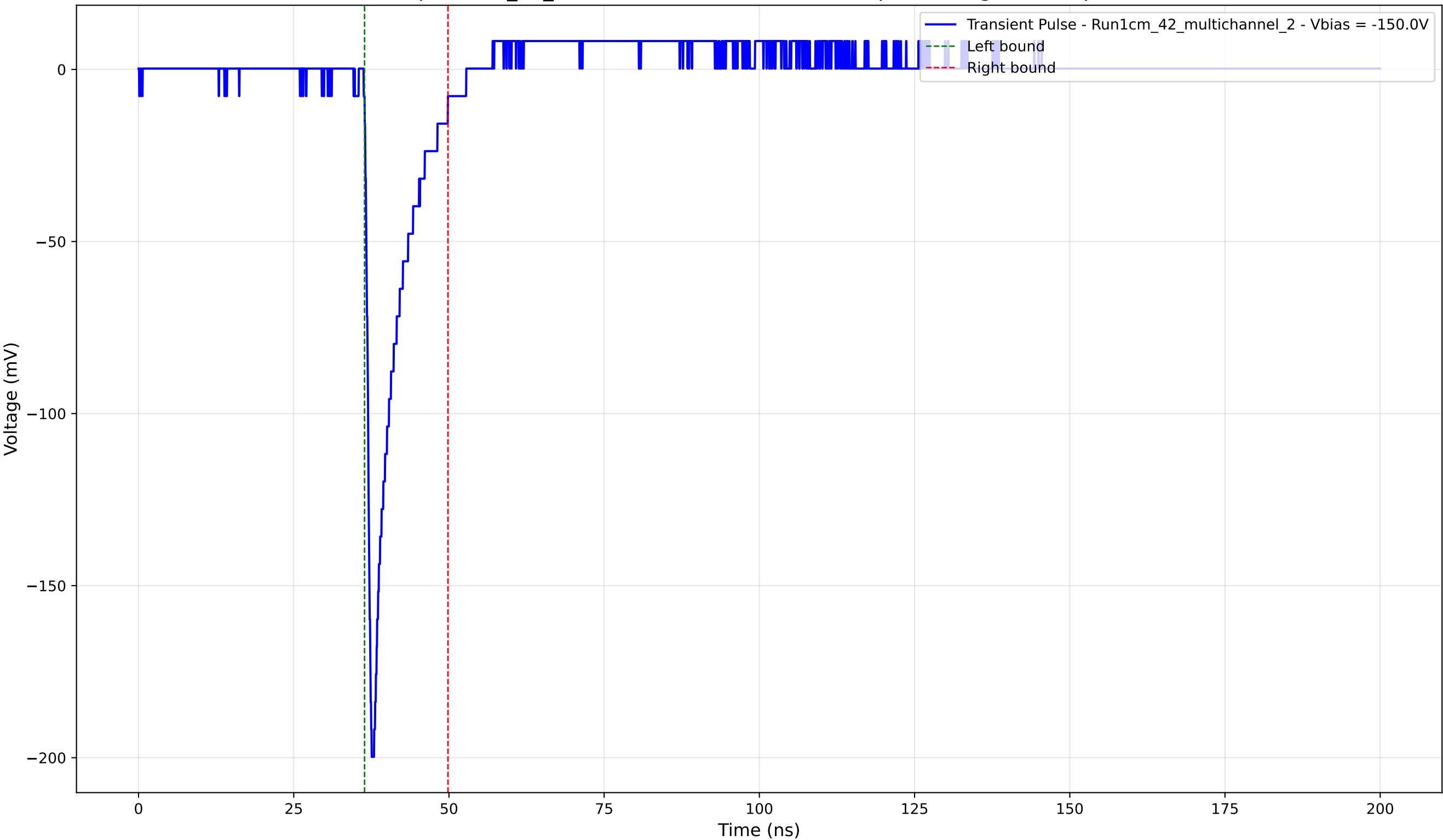
Transient Pulse - Sample: 1cm_42_multichannel - Position: 3145.0 \mu\text{m} - Charge: 18.63 pC - Rise Time: 0.90 ns
