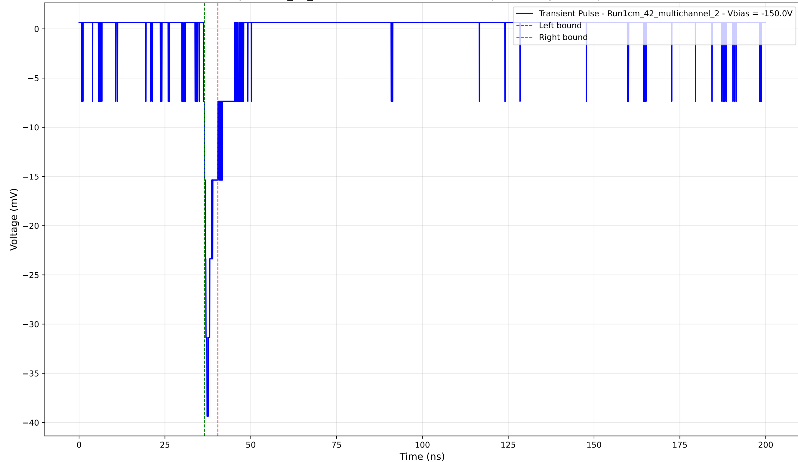
Transient Pulse - Sample: 1cm_42_multichannel - Position: 2850.0 \mu\text{m} - Charge: 1.75 pC - Rise Time: 1.06 ns
