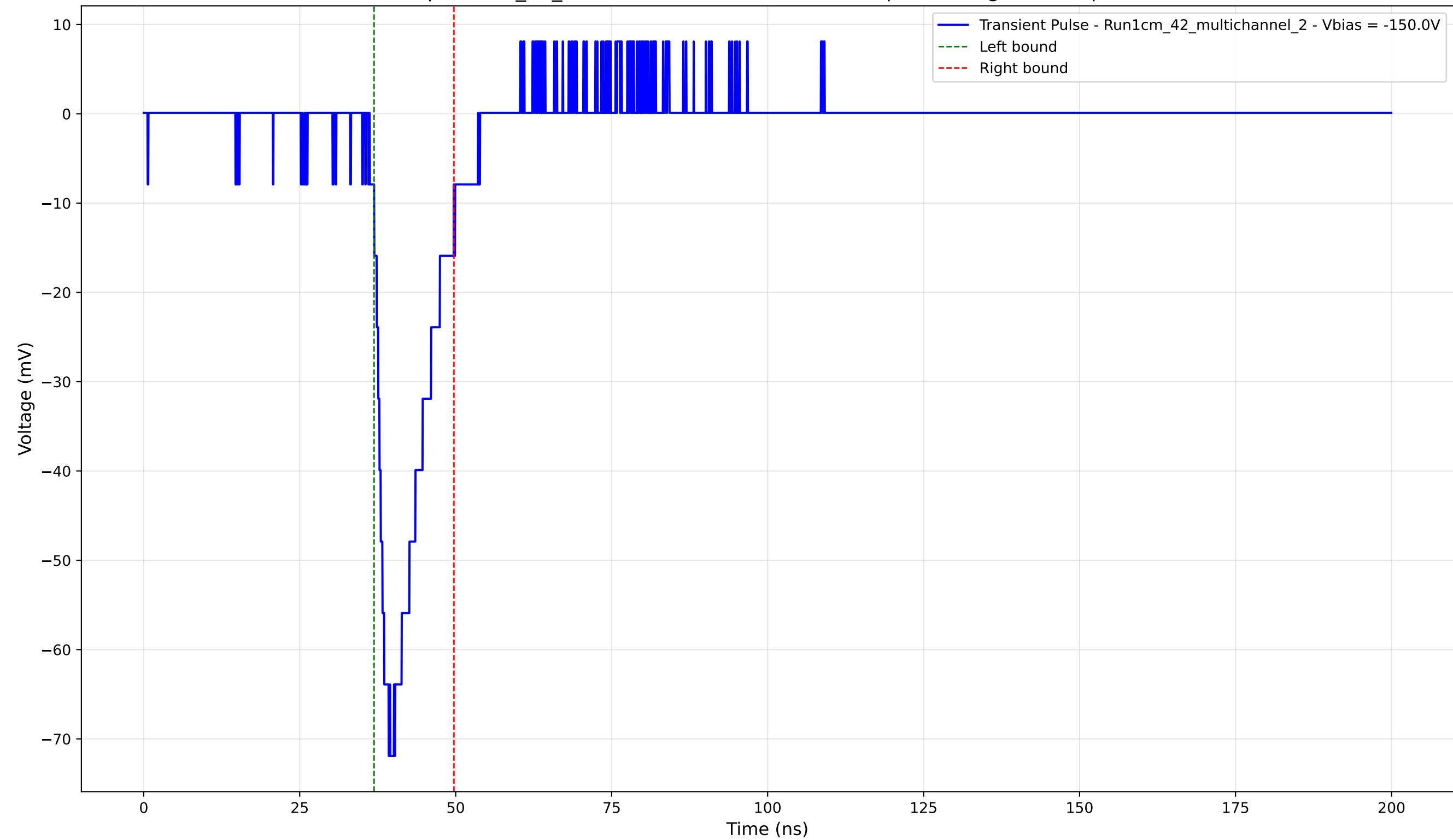
Transient Pulse - Sample: 1cm_42_multichannel - Position: 4685.0 \mu\text{m} - Charge: 10.31 pC - Rise Time: 3.04 ns
