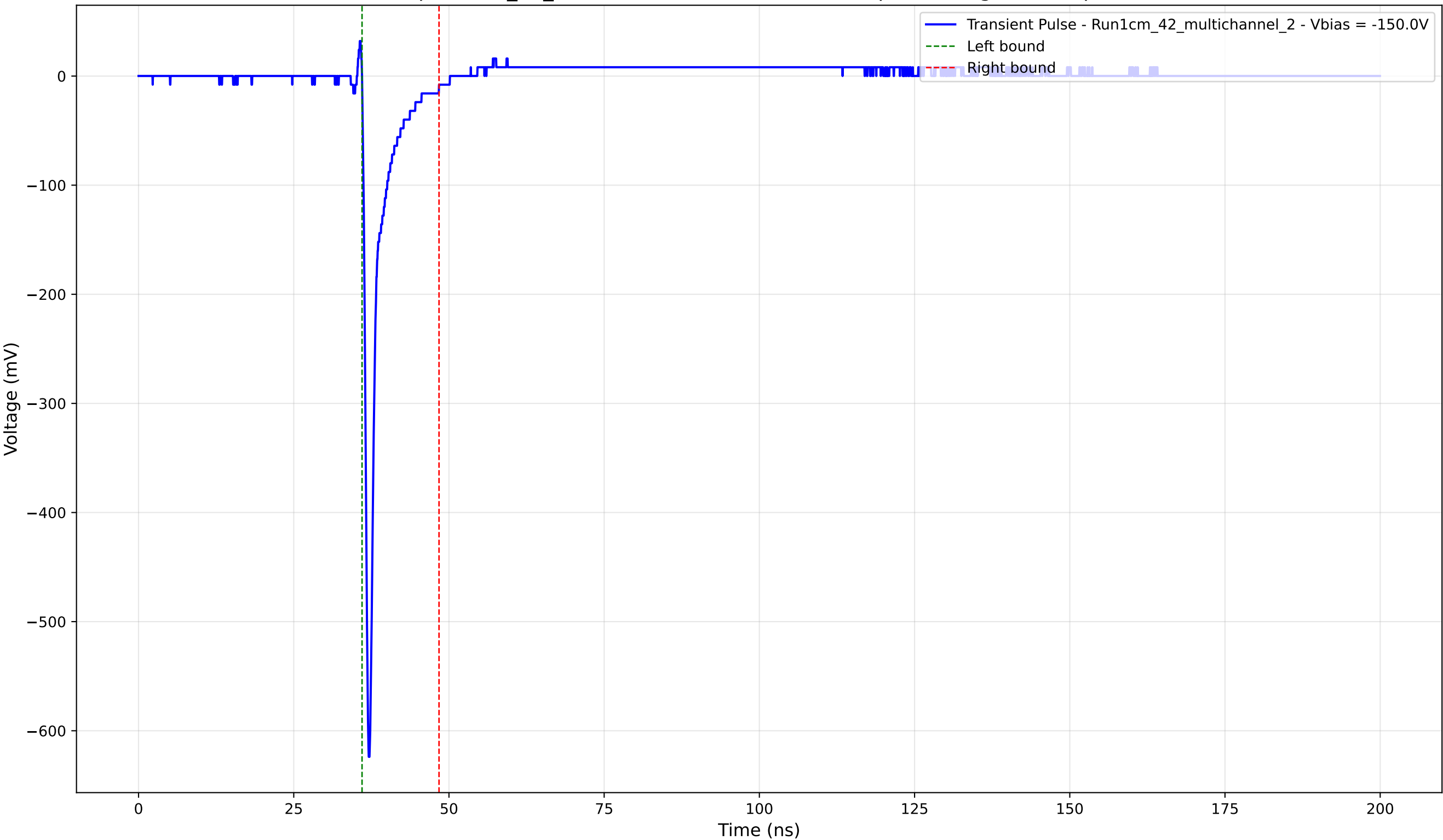
Transient Pulse - Sample: 1cm_42_multichannel - Position: 2460.0 \mu\text{m} - Charge: 28.16 pC - Rise Time: 0.71 ns
