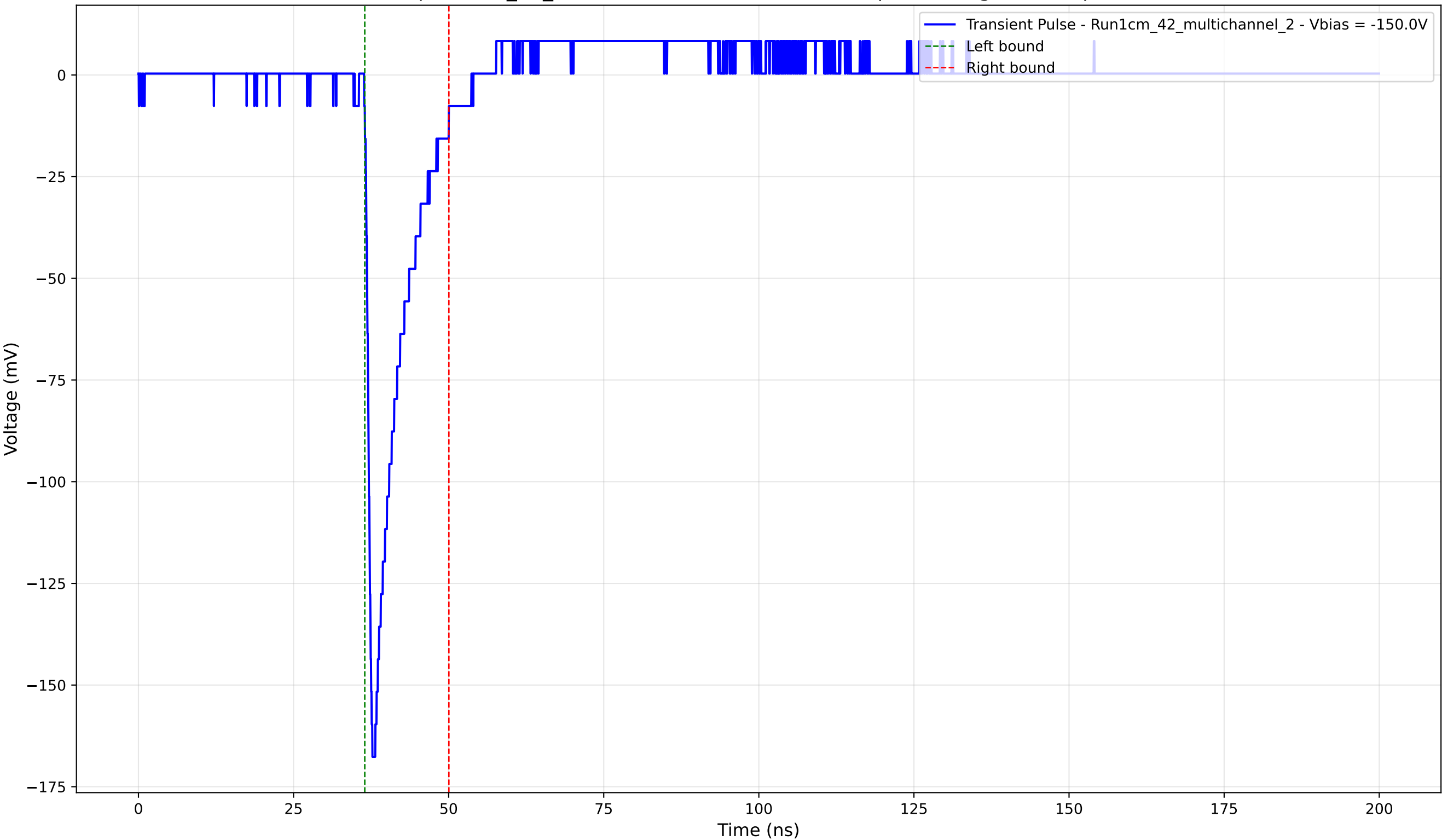
Transient Pulse - Sample: 1cm_42_multichannel - Position: 3290.0 \mu\text{m} - Charge: 17.80 pC - Rise Time: 0.91 ns
