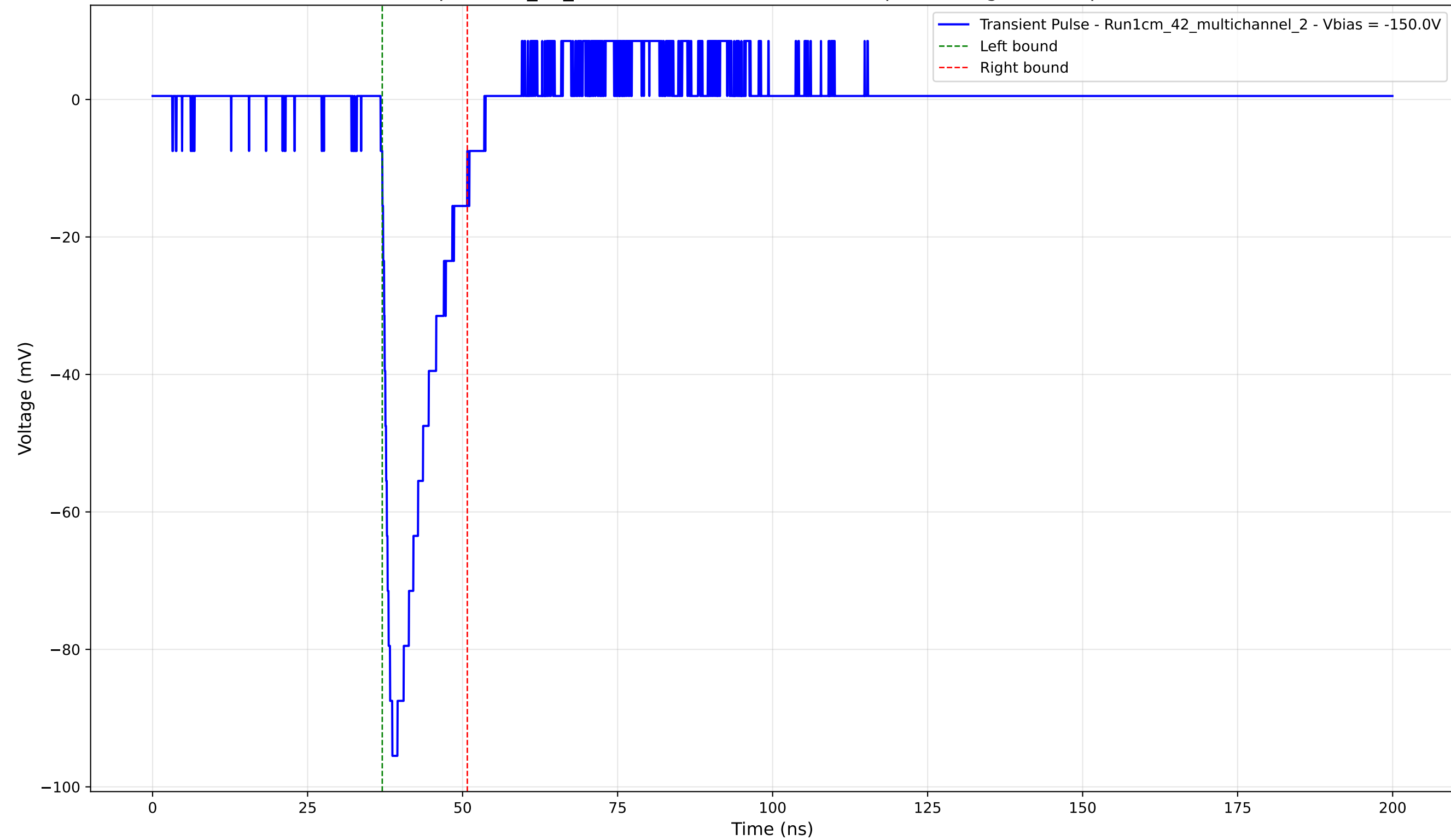
Transient Pulse - Sample: 1cm_42_multichannel - Position: 775.0 \mu\text{m} - Charge: 13.50 pC - Rise Time: 1.27 ns
