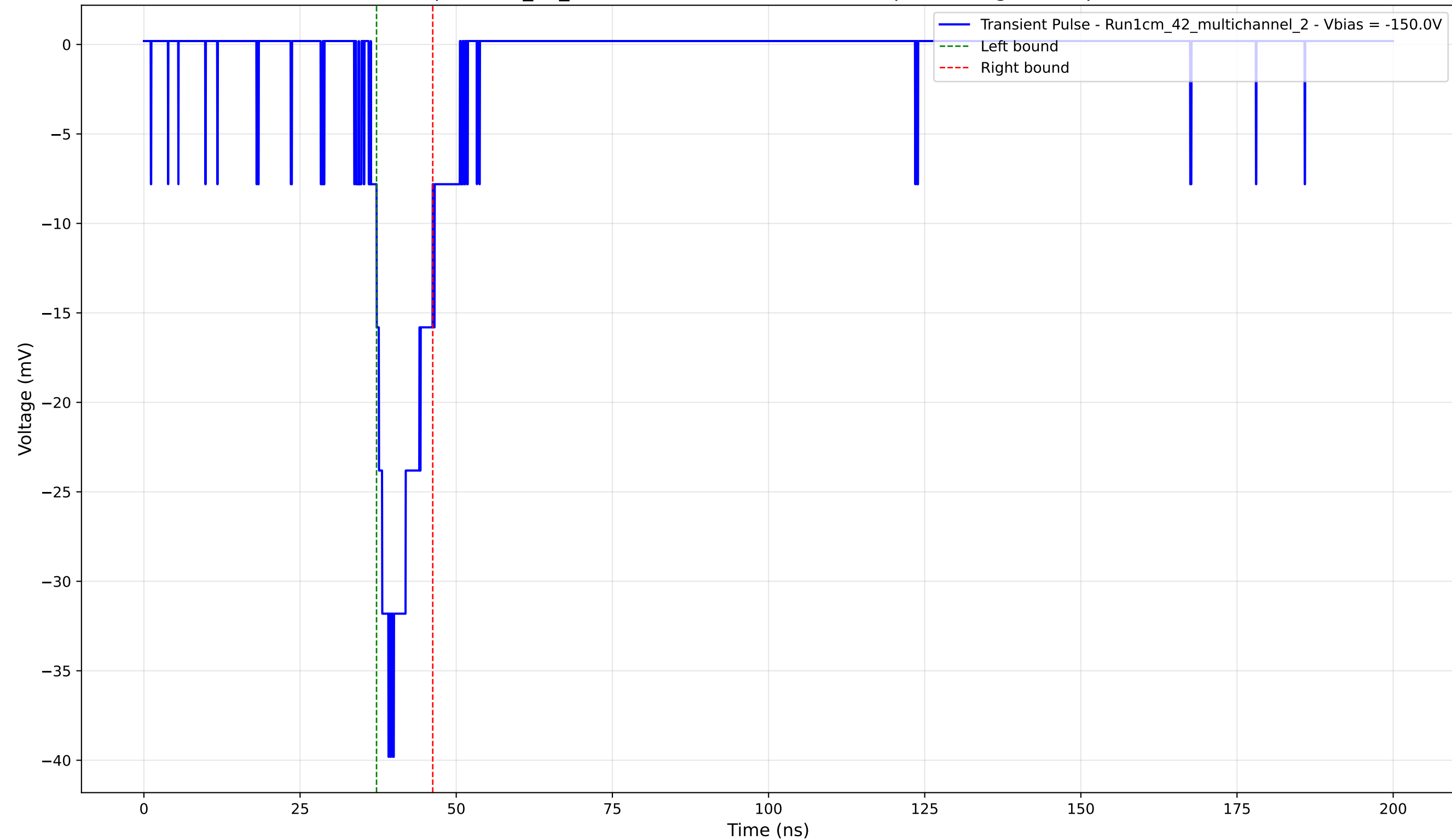
Transient Pulse - Sample: 1cm_42_multichannel - Position: 4845.0 \mu\text{m} - Charge: 4.55 pC - Rise Time: 2.82 ns
