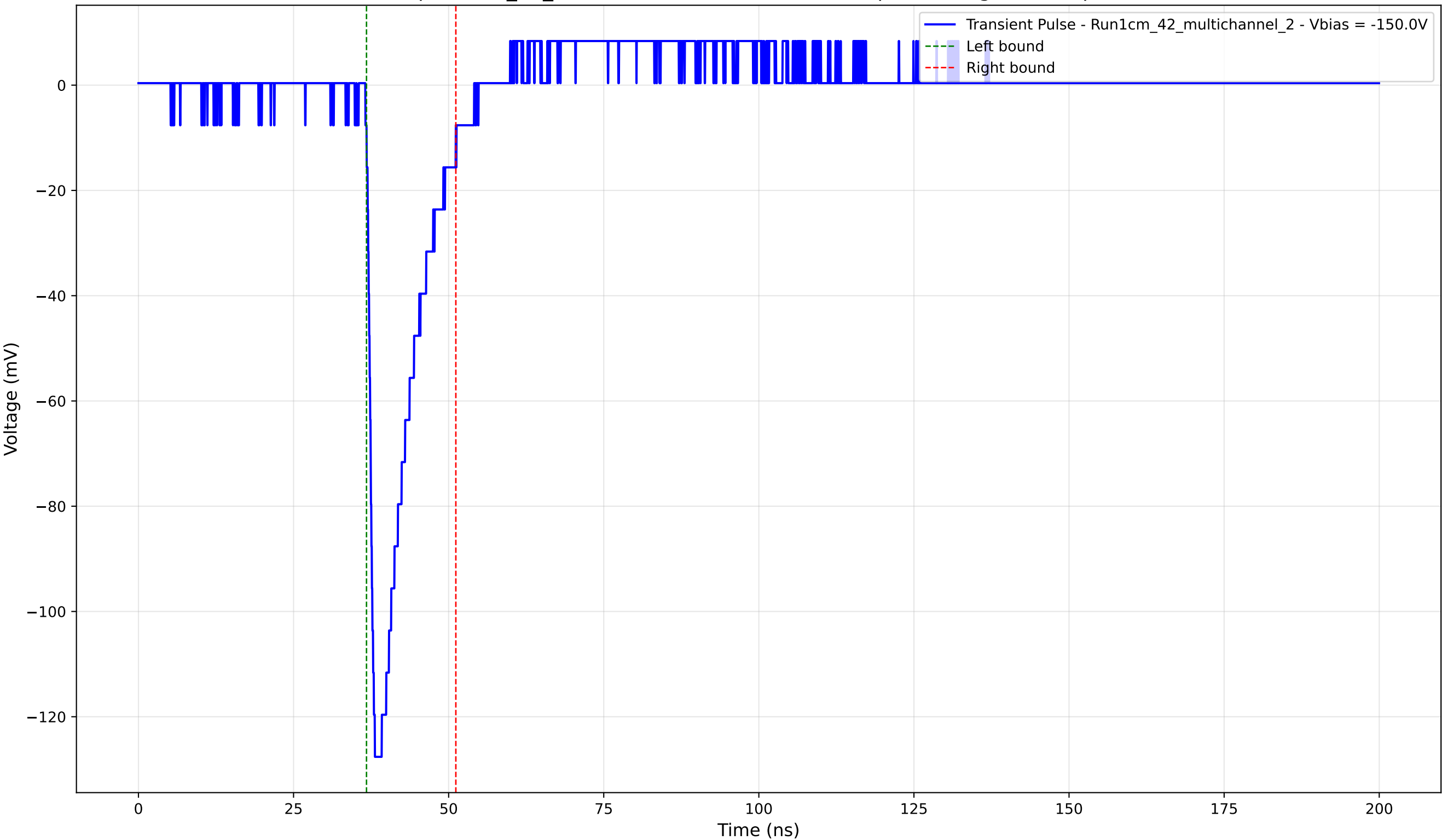
Transient Pulse - Sample: 1cm_42_multichannel - Position: 1070.0 \mu\text{m} - Charge: 17.45 pC - Rise Time: 1.17 ns
