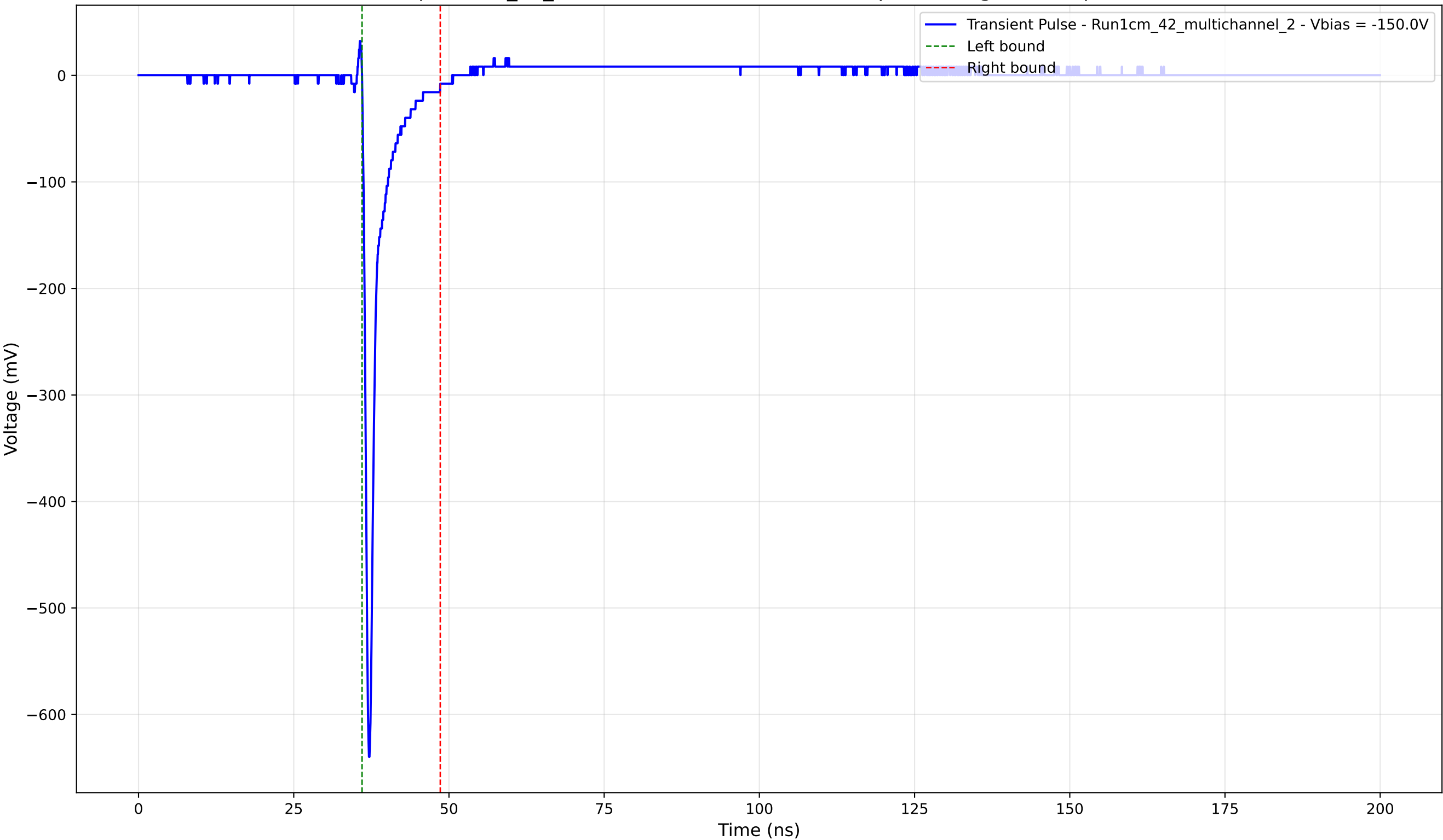
Transient Pulse - Sample: 1cm_42_multichannel - Position: 2270.0 \mu\text{m} - Charge: 29.05 pC - Rise Time: 0.72 ns
