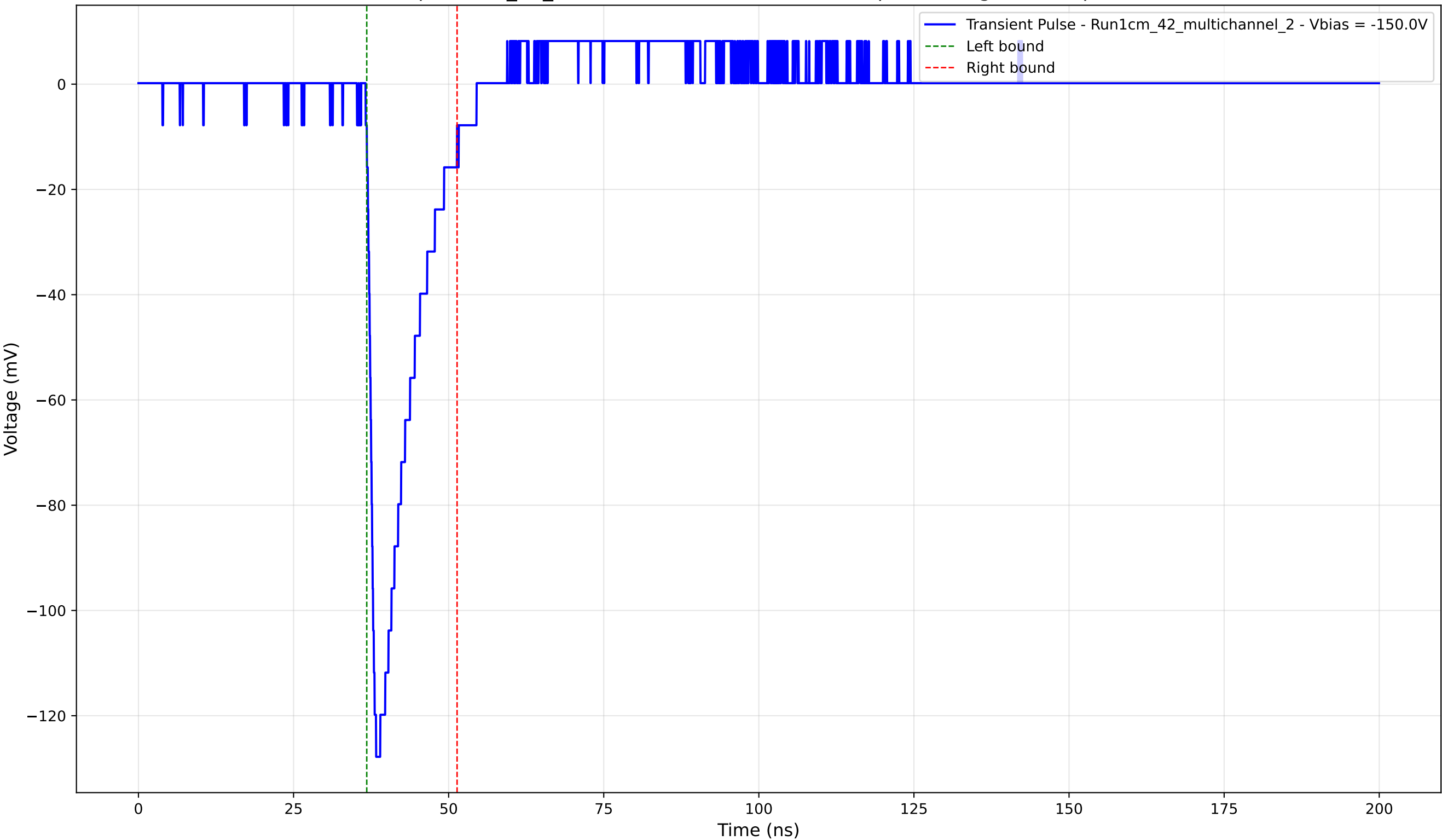
Transient Pulse - Sample: 1cm_42_multichannel - Position: 1010.0 \mu\text{m} - Charge: 17.35 pC - Rise Time: 1.26 ns
