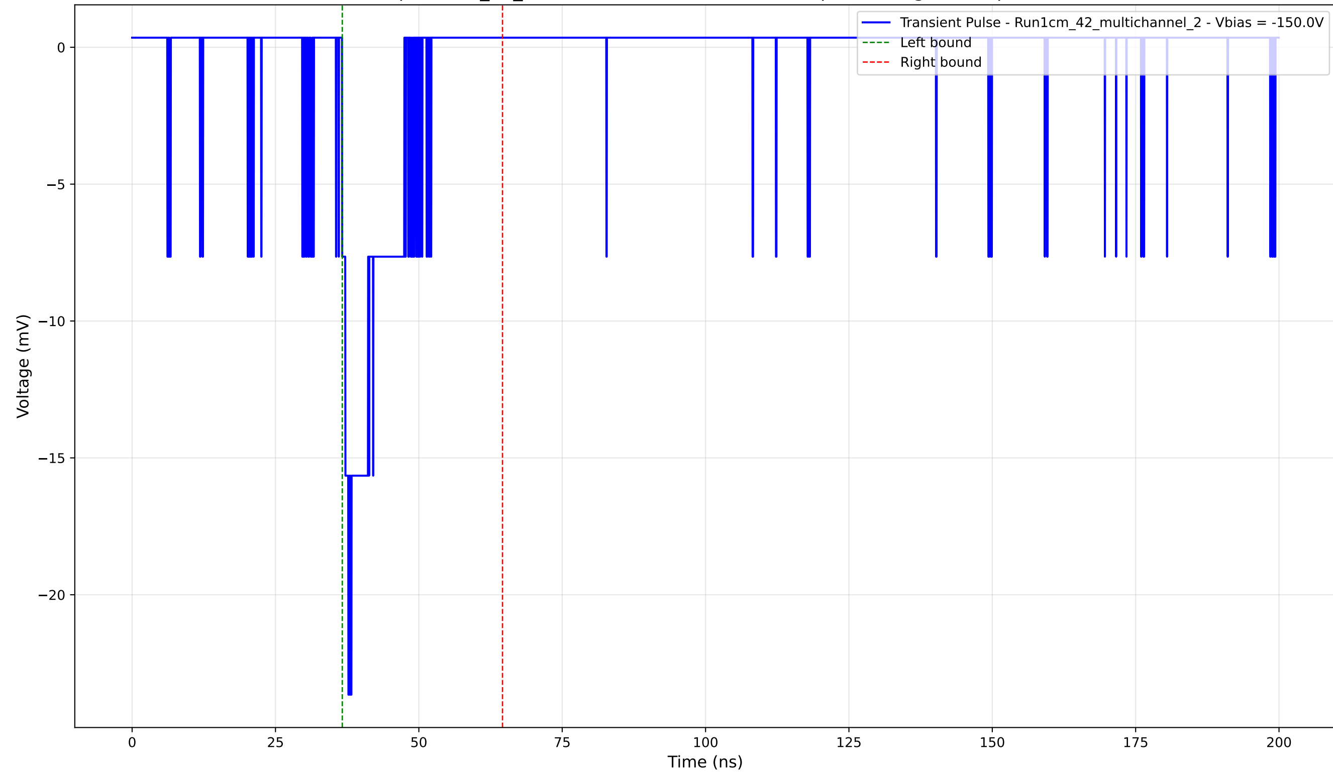
Transient Pulse - Sample: 1cm_42_multichannel - Position: 3355.0 \mu\text{m} - Charge: 2.51 pC - Rise Time: 1.11 ns
