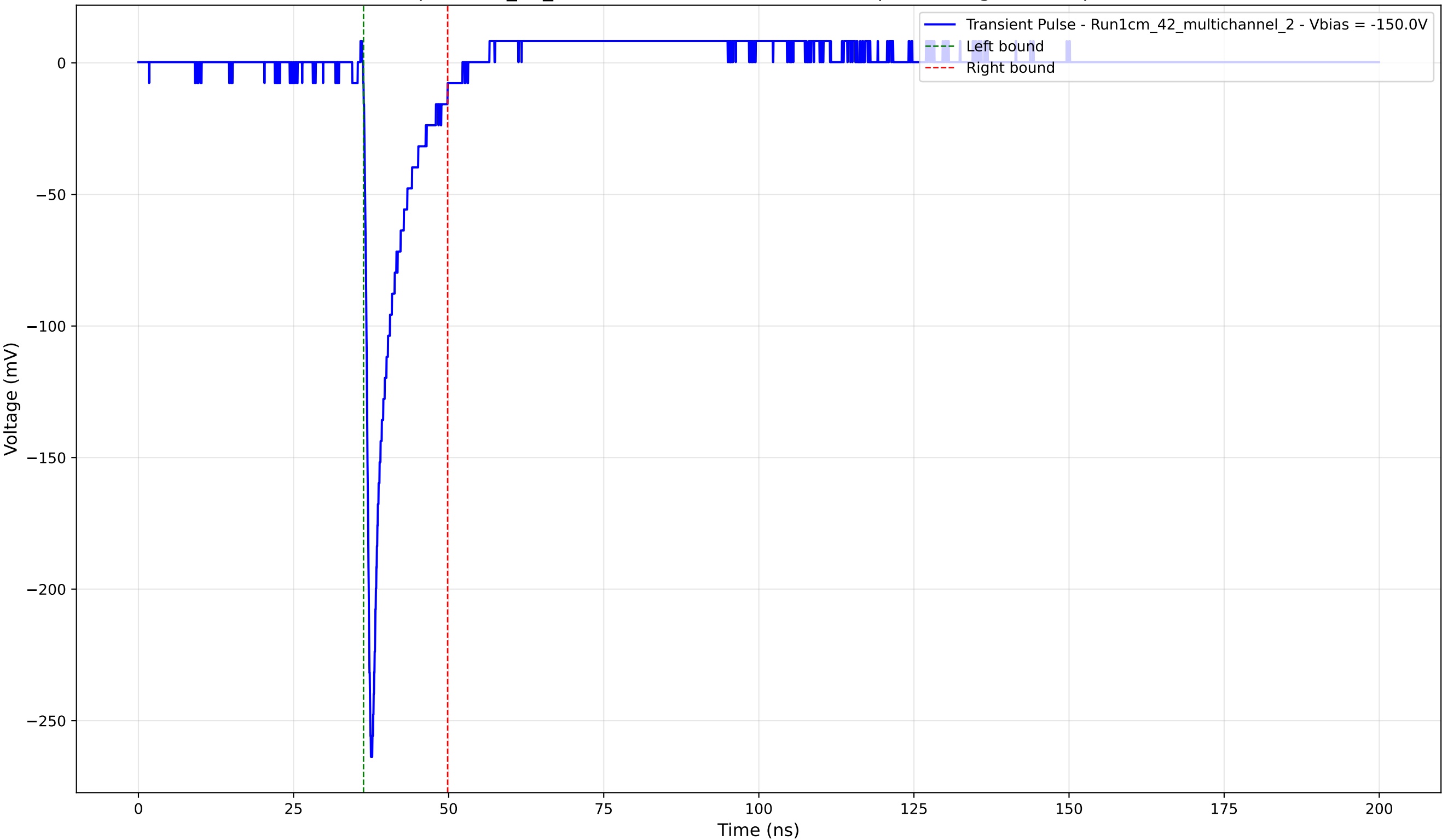
Transient Pulse - Sample: 1cm_42_multichannel - Position: 3000.0 \mu\text{m} - Charge: 21.18 pC - Rise Time: 0.89 ns
