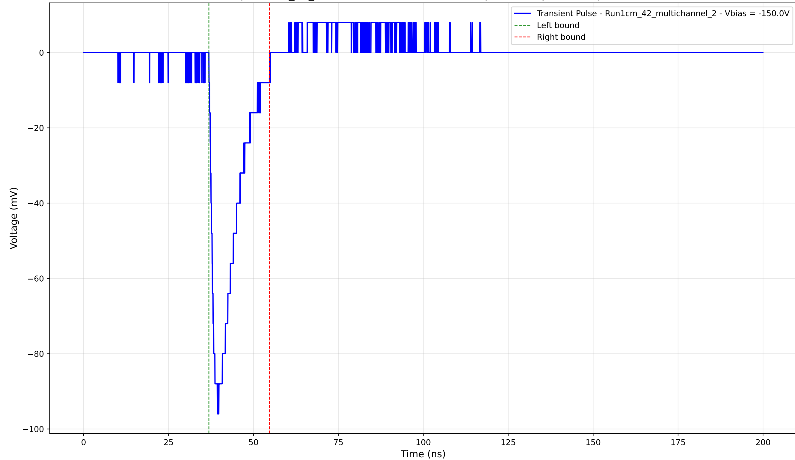
Transient Pulse - Sample: 1cm_42_multichannel - Position: 455.0 \mu\text{m} - Charge: 14.63 pC - Rise Time: 1.59 ns
