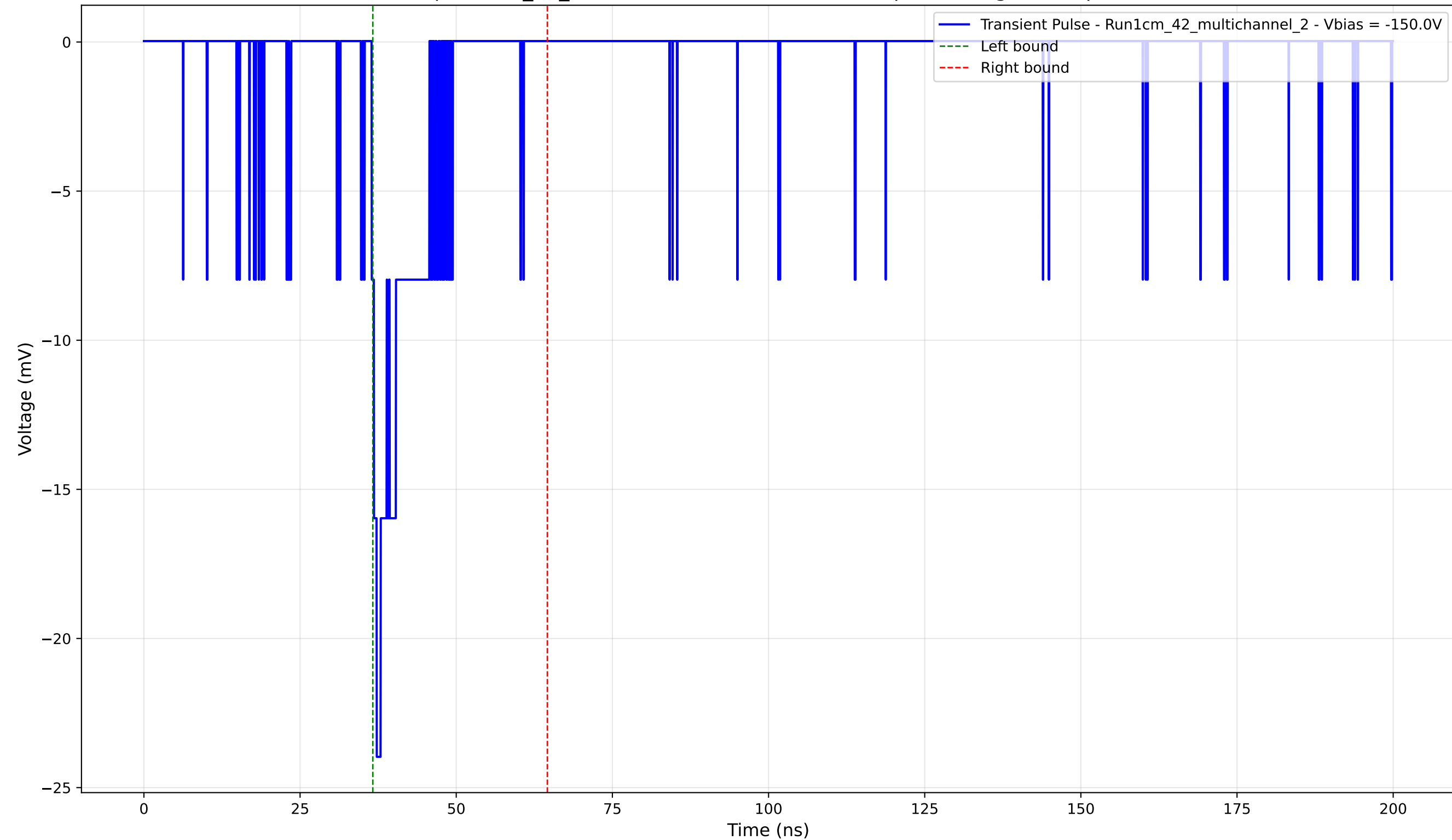
Transient Pulse - Sample: 1cm_42_multichannel - Position: 2895.0 \mu\text{m} - Charge: 2.36 pC - Rise Time: 0.83 ns
