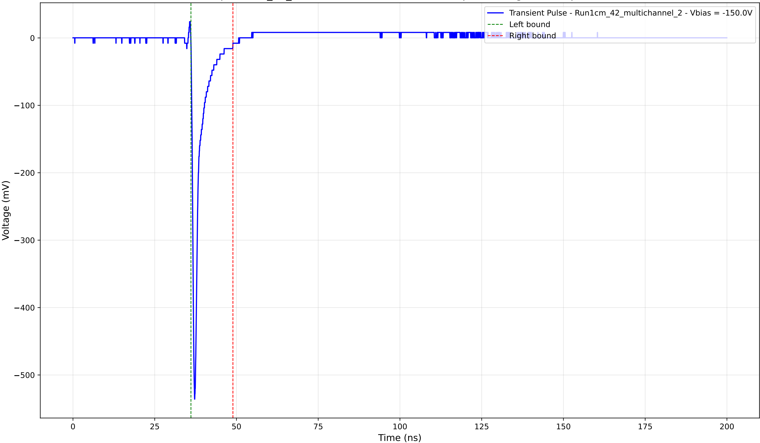
Transient Pulse - Sample: 1cm_42_multichannel - Position: 2160.0 \mu\text{m} - Charge: 27.00 pC - Rise Time: 0.75 ns
