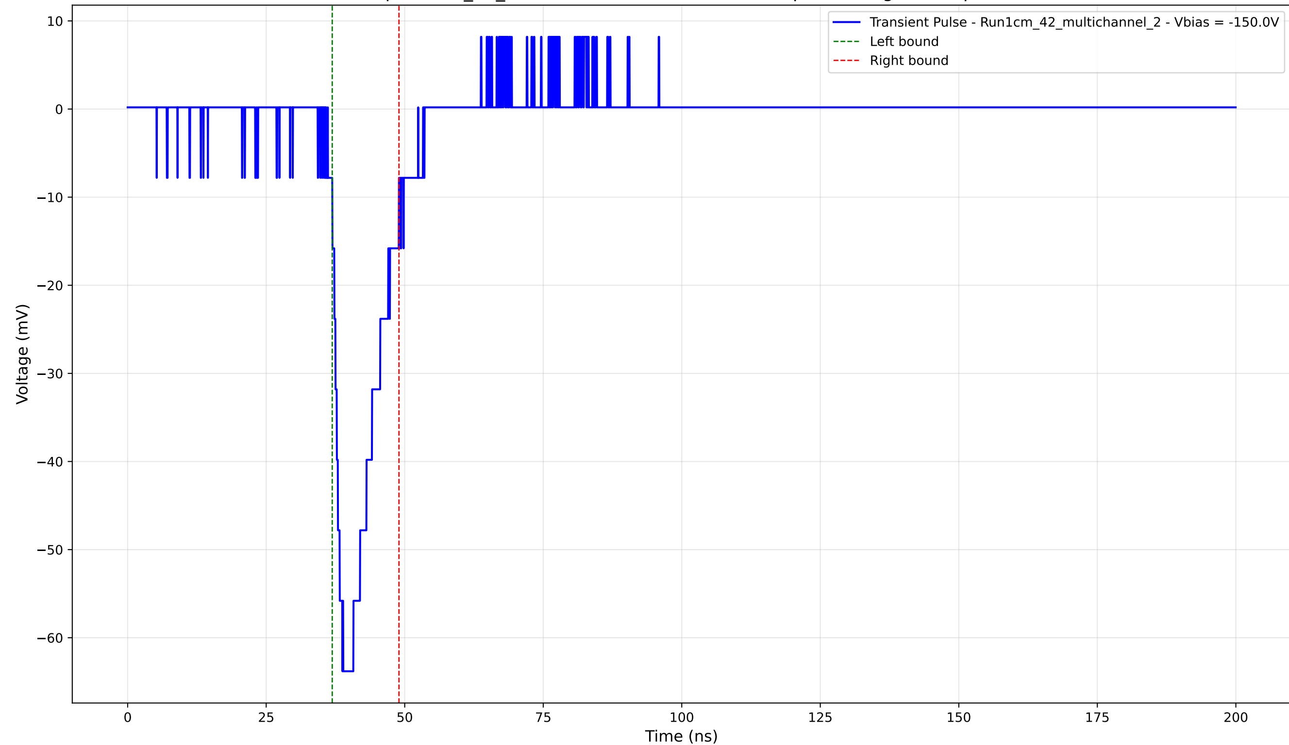
Transient Pulse - Sample: 1cm_42_multichannel - Position: 4770.0 \mu\text{m} - Charge: 9.39 pC - Rise Time: 2.61 ns
