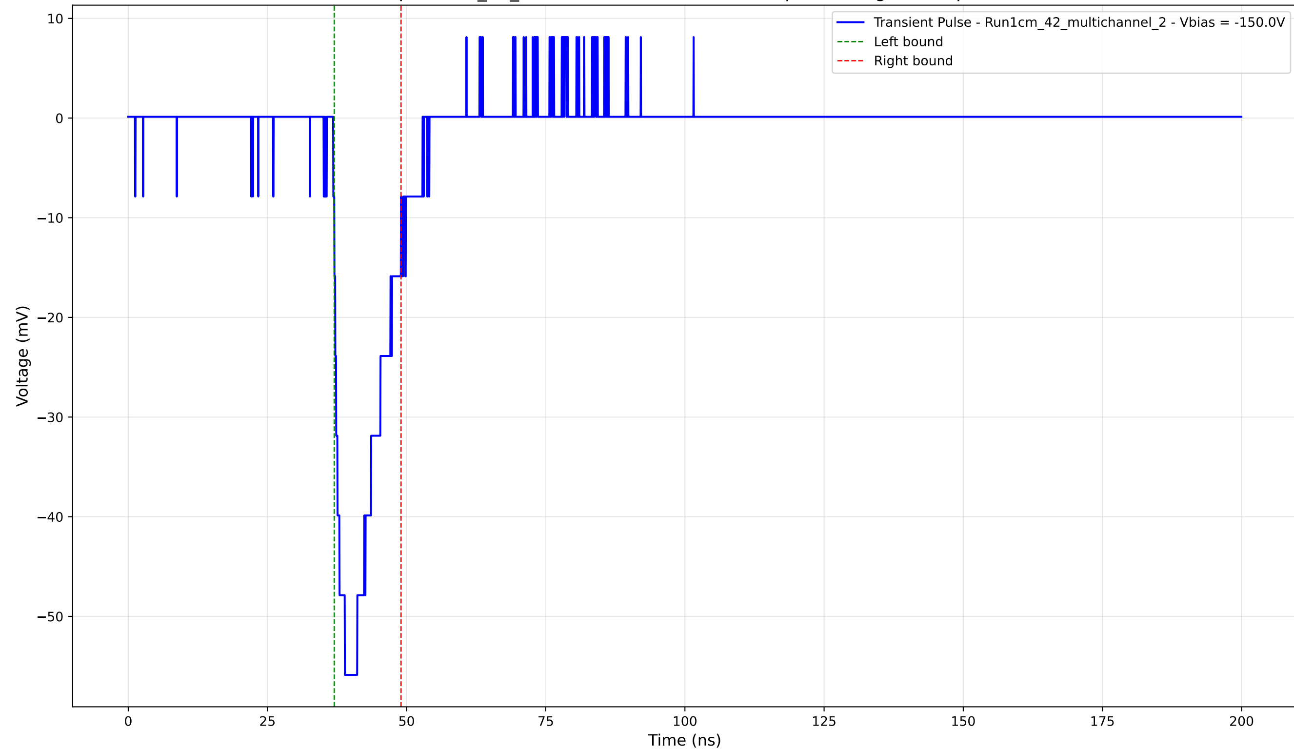
Transient Pulse - Sample: 1cm_42_multichannel - Position: 95.0 \mu\text{m} - Charge: 8.74 pC - Rise Time: 2.09 ns
