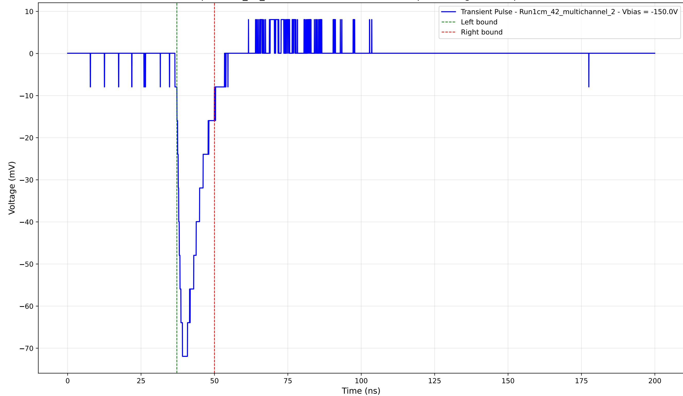
Transient Pulse - Sample: 1cm_42_multichannel - Position: 4530.0 \mu\text{m} - Charge: 10.69 pC - Rise Time: 2.56 ns
