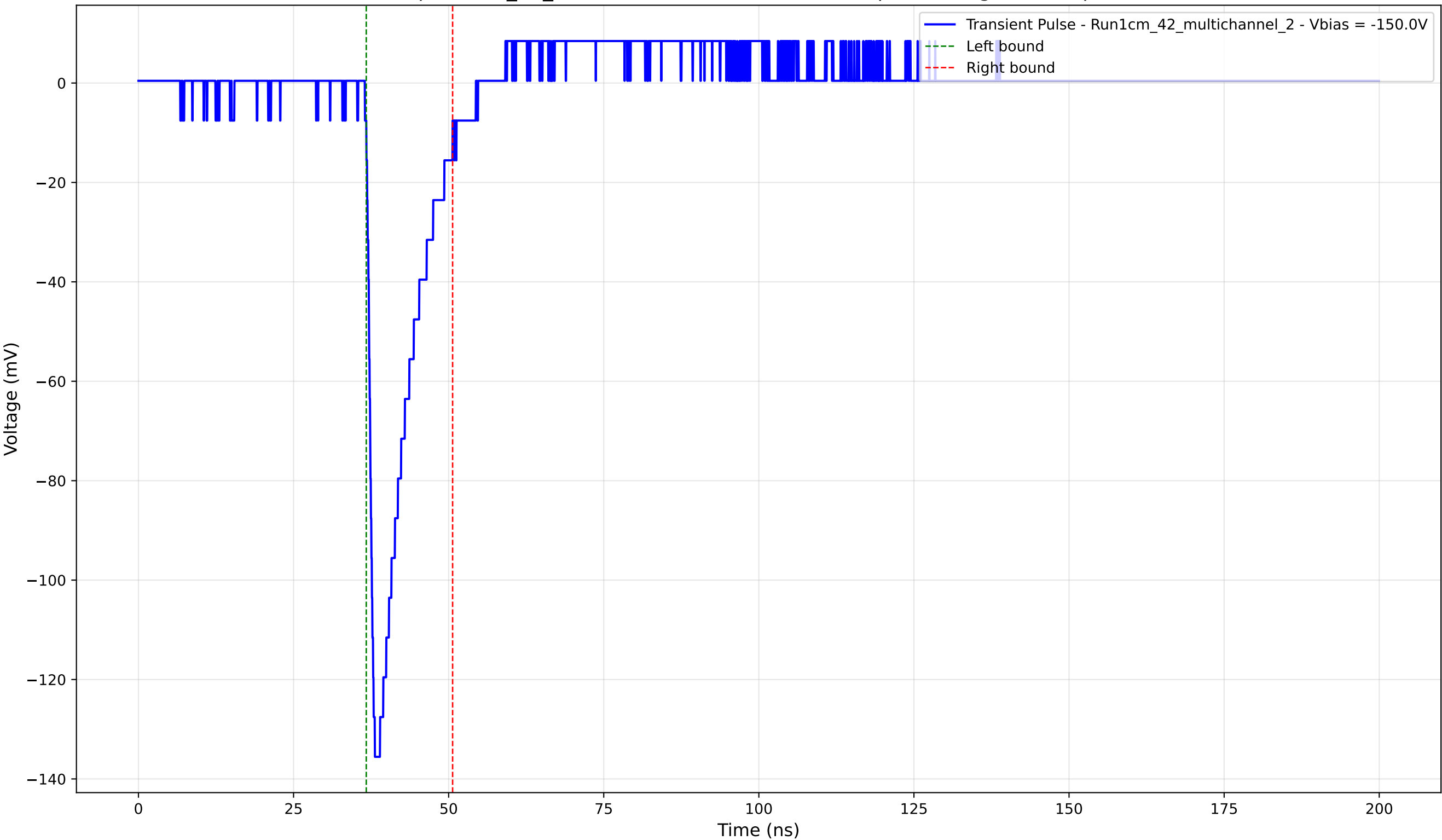
Transient Pulse - Sample: 1cm_42_multichannel - Position: 1130.0 \mu\text{m} - Charge: 17.64 pC - Rise Time: 1.17 ns
