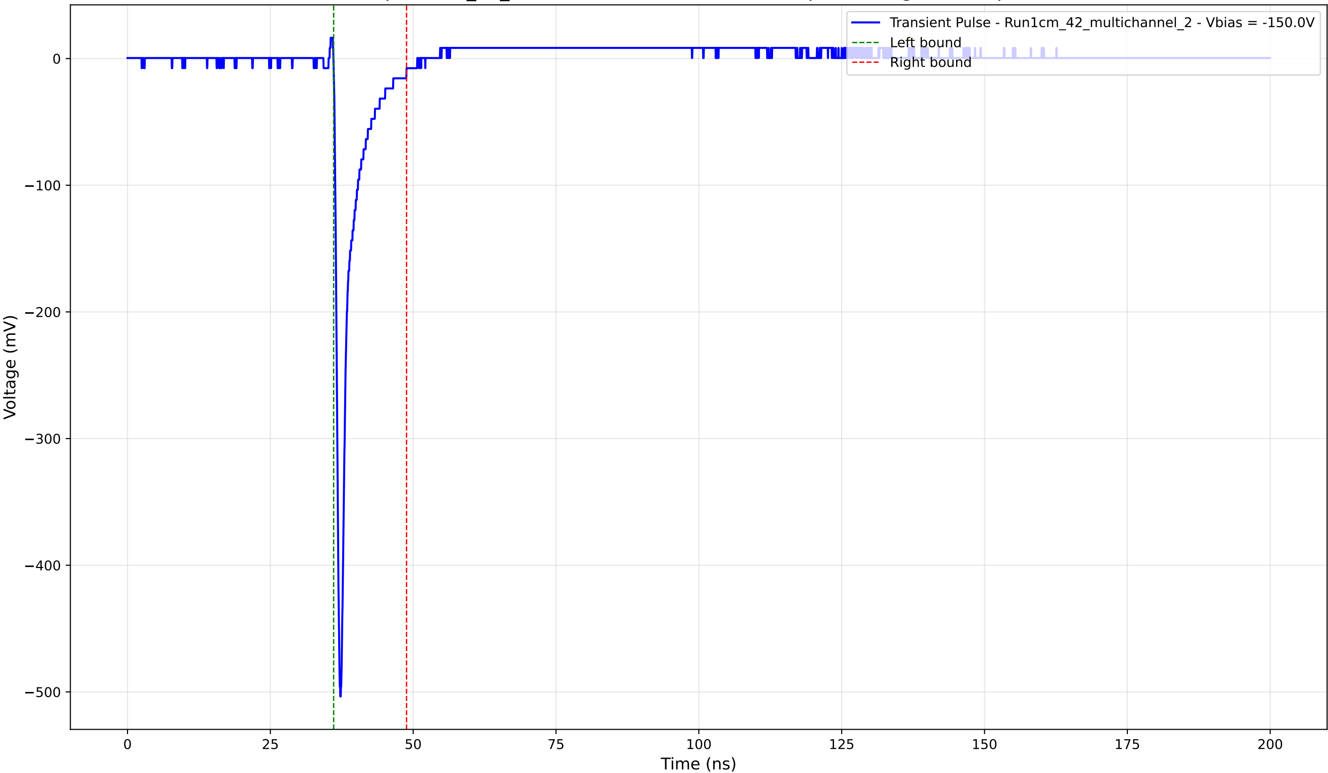
Transient Pulse - Sample: 1cm_42_multichannel - Position: 2115.0 \mu\text{m} - Charge: 26.55 pC - Rise Time: 0.74 ns
