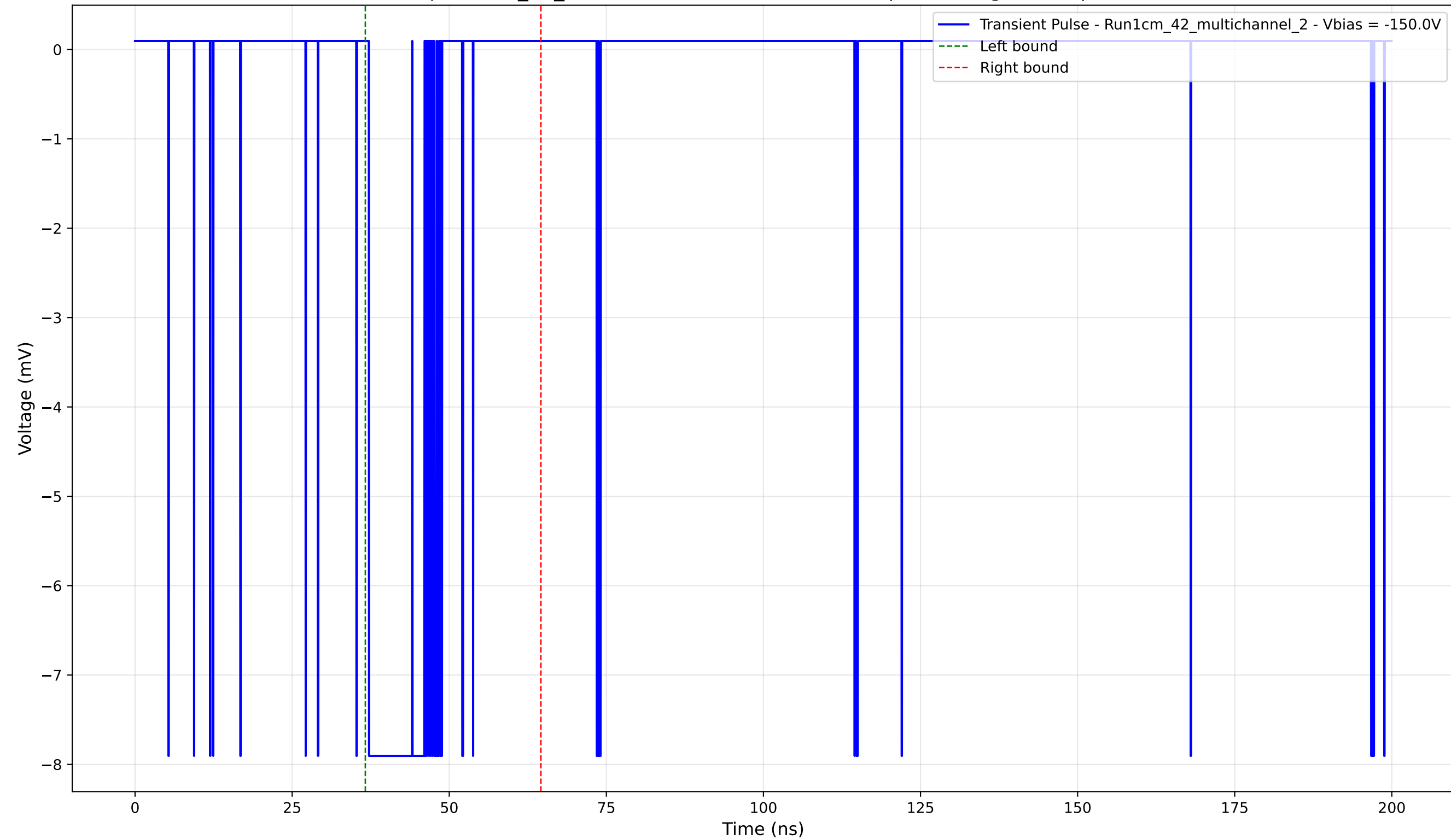
Transient Pulse - Sample: 1cm_42_multichannel - Position: 3870.0 \mu\text{m} - Charge: 1.59 pC - Rise Time: 0.04 ns
