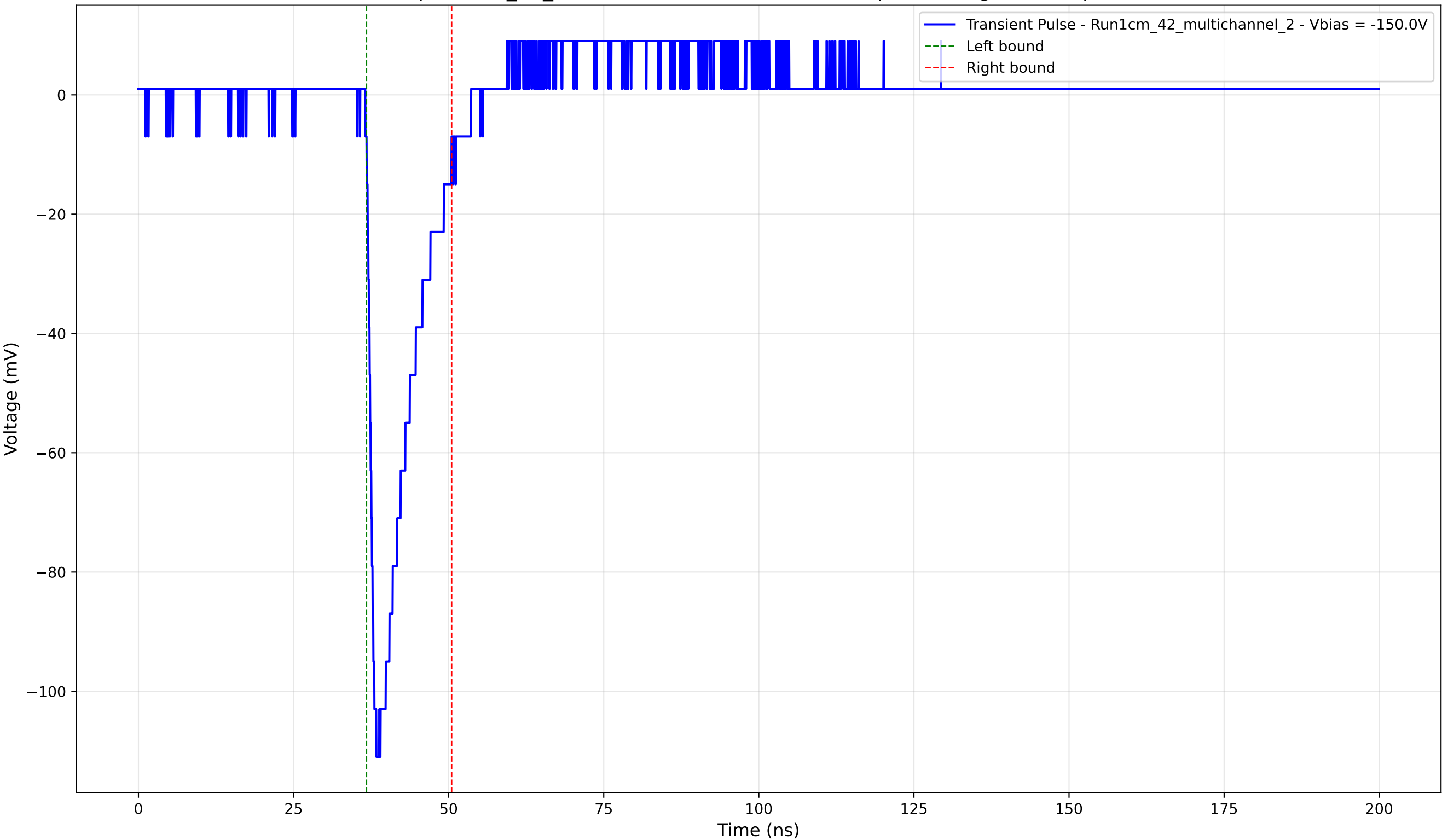
Transient Pulse - Sample: 1cm_42_multichannel - Position: 3685.0 \mu\text{m} - Charge: 14.89 pC - Rise Time: 1.26 ns
