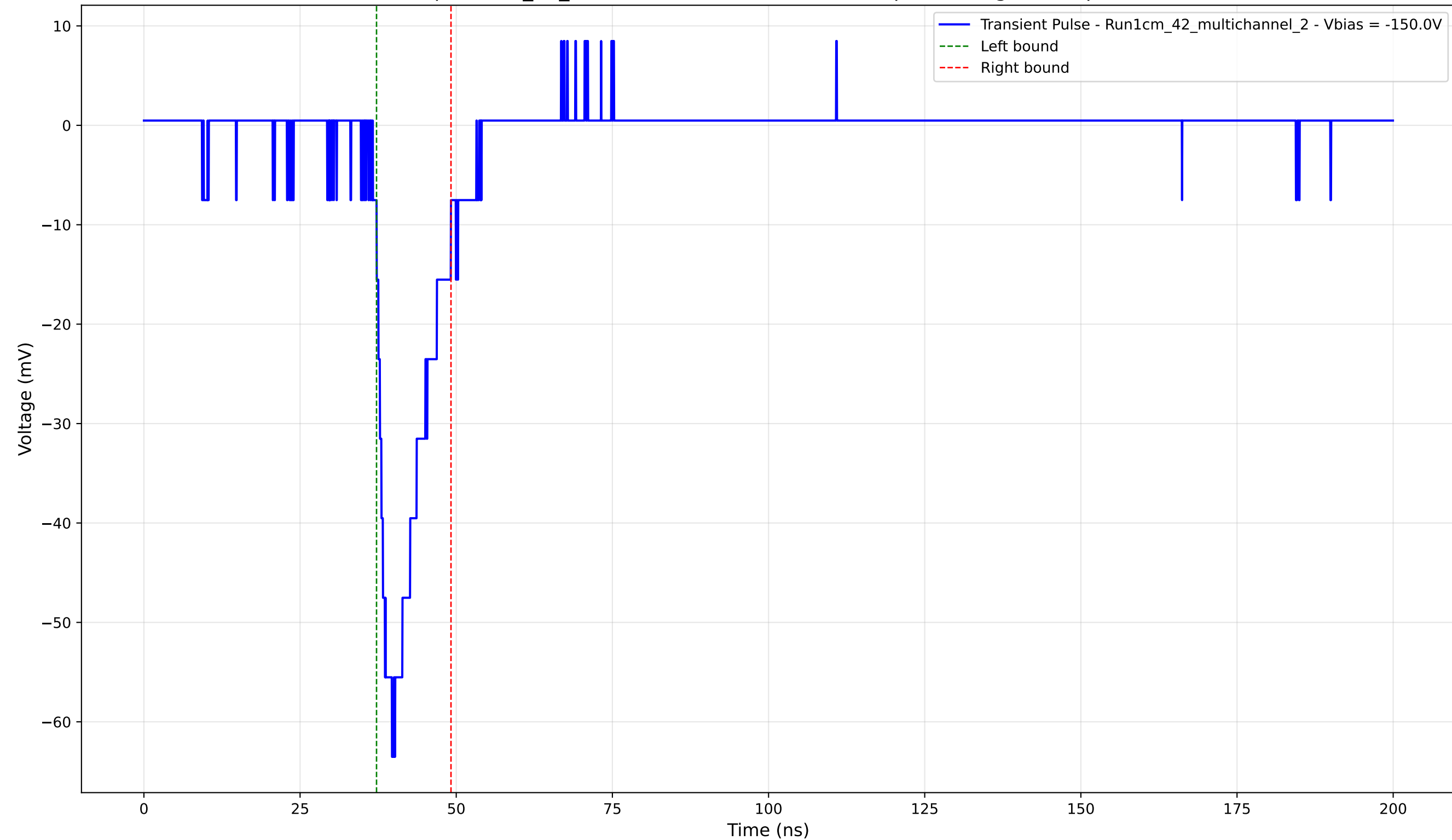
Transient Pulse - Sample: 1cm_42_multichannel - Position: 4320.0 \mu\text{m} - Charge: 8.48 pC - Rise Time: 3.05 ns
