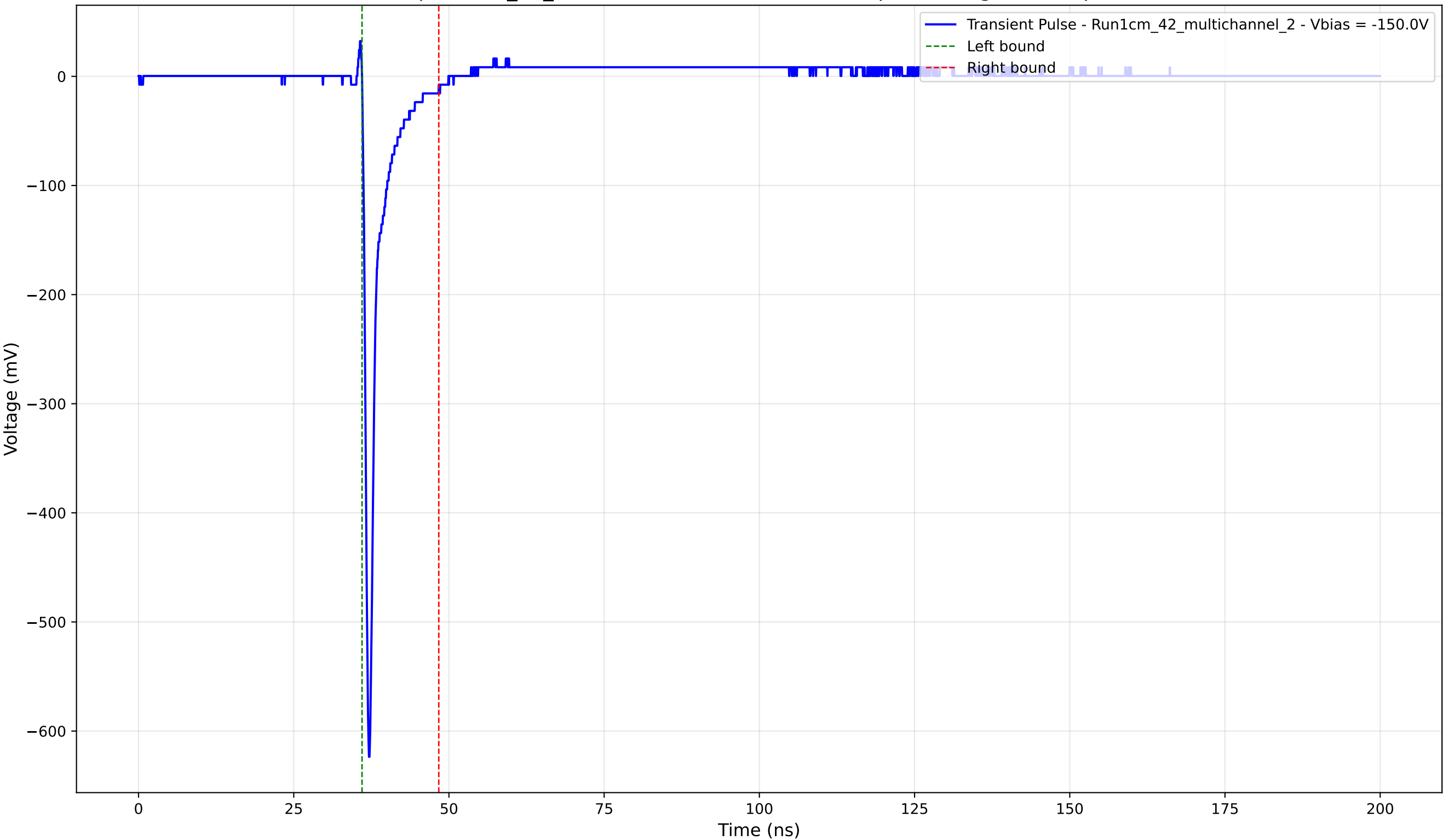
Transient Pulse - Sample: 1cm_42_multichannel - Position: 2470.0 \mu\text{m} - Charge: 28.07 pC - Rise Time: 0.73 ns
