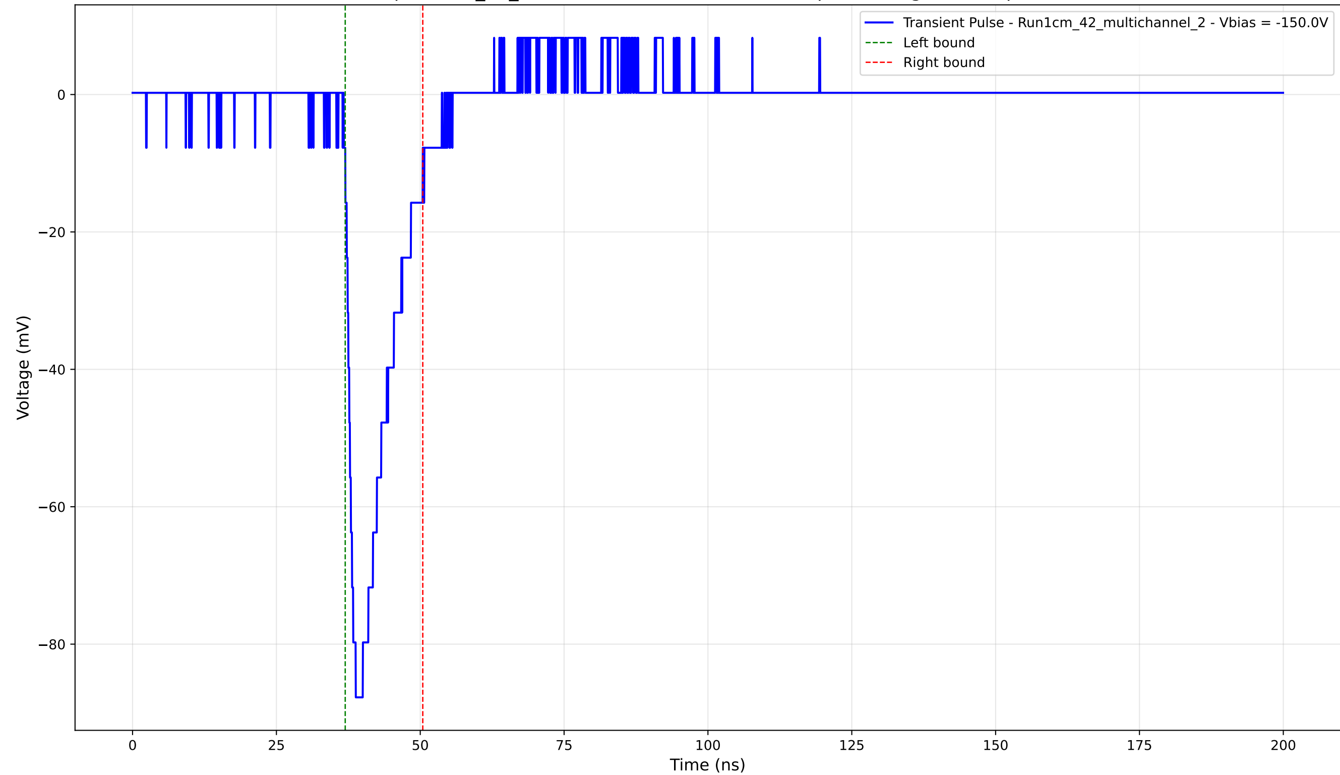
Transient Pulse - Sample: 1cm_42_multichannel - Position: 3960.0 \mu\text{m} - Charge: 12.64 pC - Rise Time: 1.39 ns
