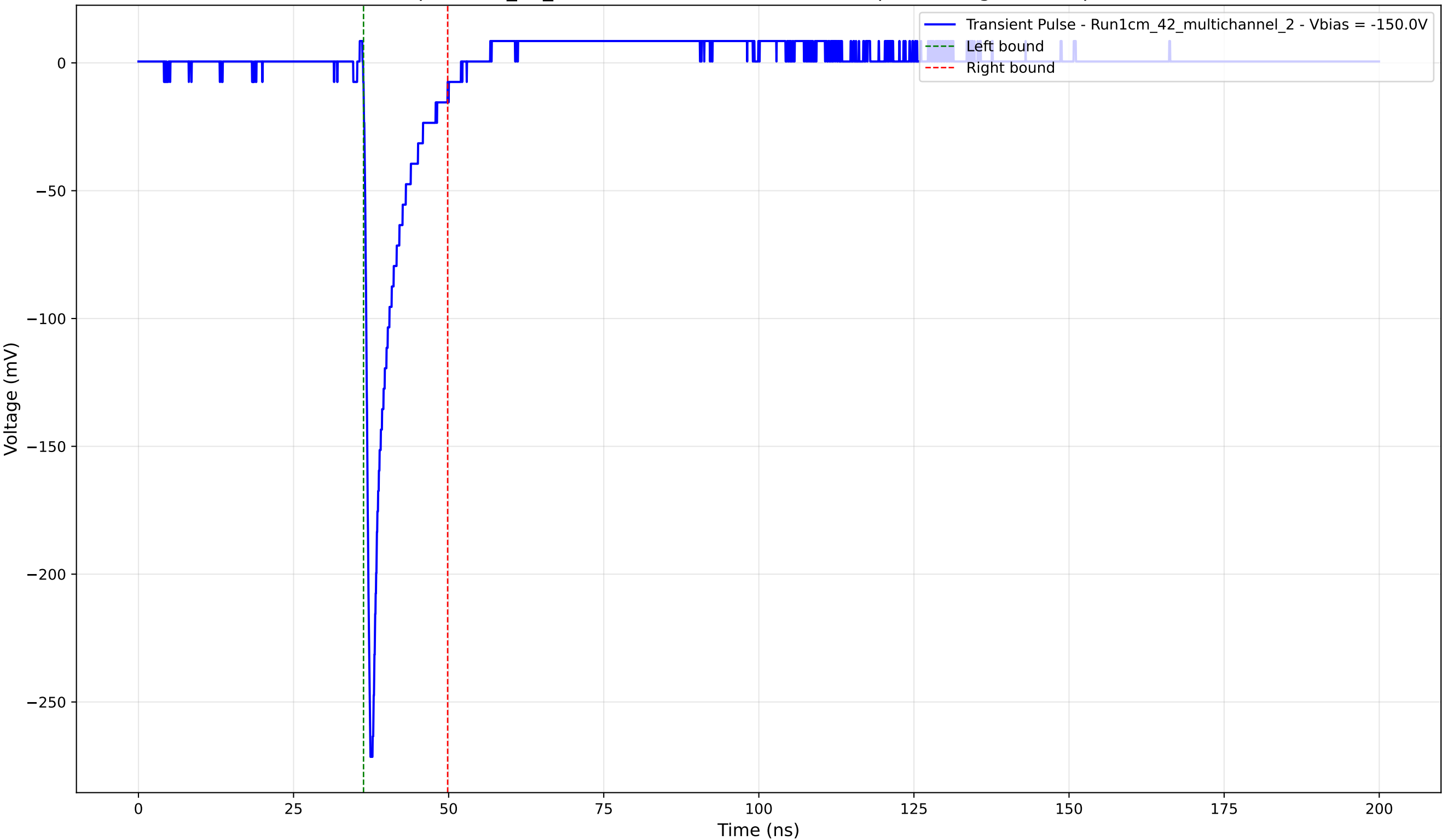
Transient Pulse - Sample: 1cm_42_multichannel - Position: 1780.0 \mu\text{m} - Charge: 21.20 pC - Rise Time: 0.85 ns
