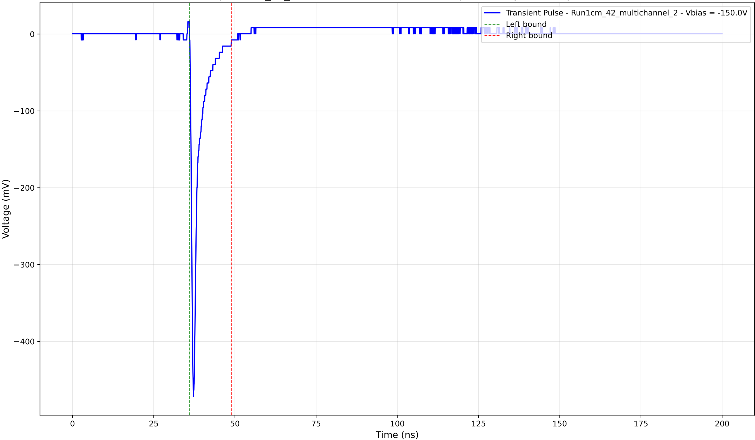
Transient Pulse - Sample: 1cm_42_multichannel - Position: 2630.0 \mu\text{m} - Charge: 24.95 pC - Rise Time: 0.75 ns
