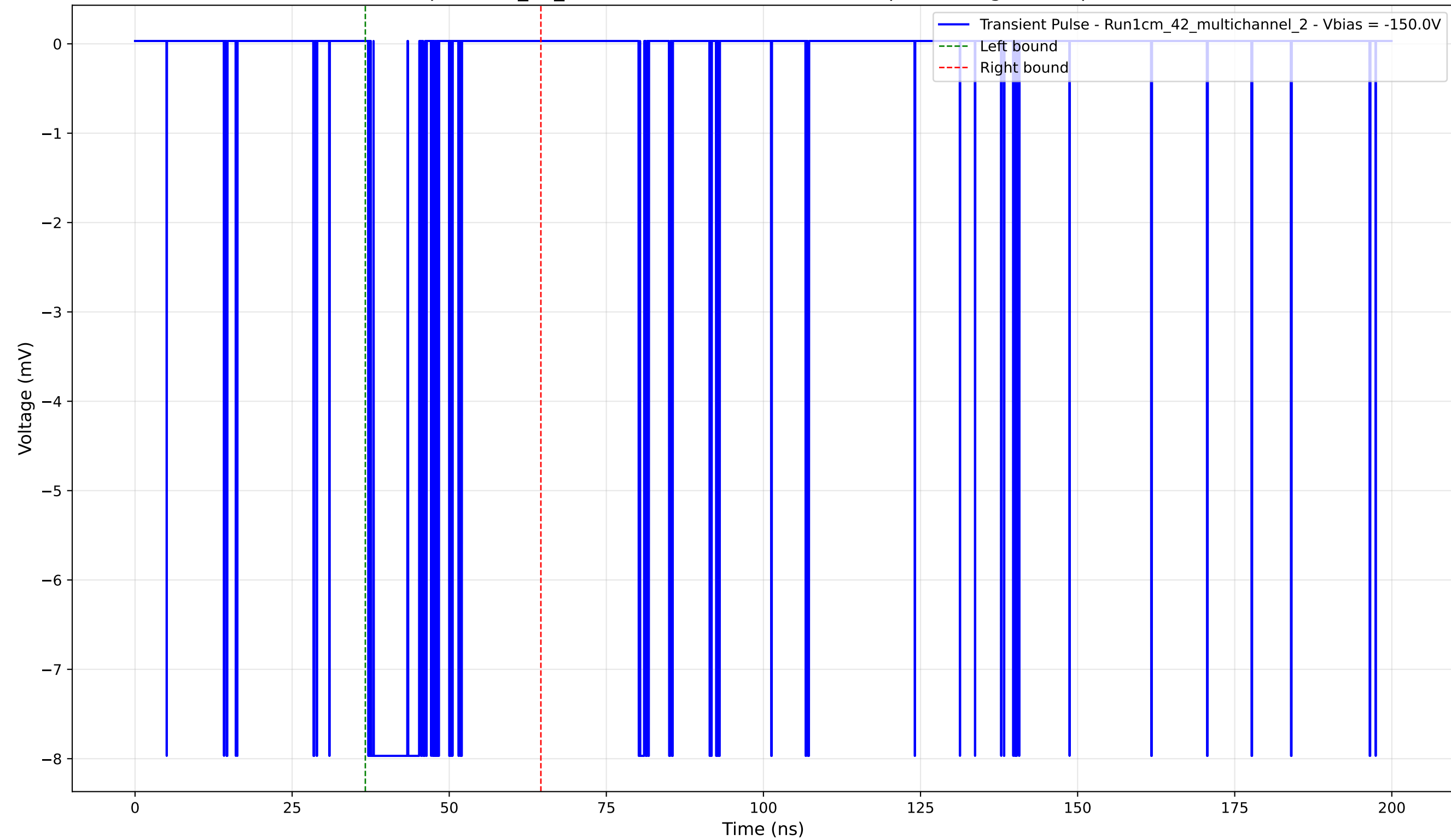
Transient Pulse - Sample: 1cm_42_multichannel - Position: 3880.0 \mu\text{m} - Charge: 1.48 pC - Rise Time: 0.04 ns
