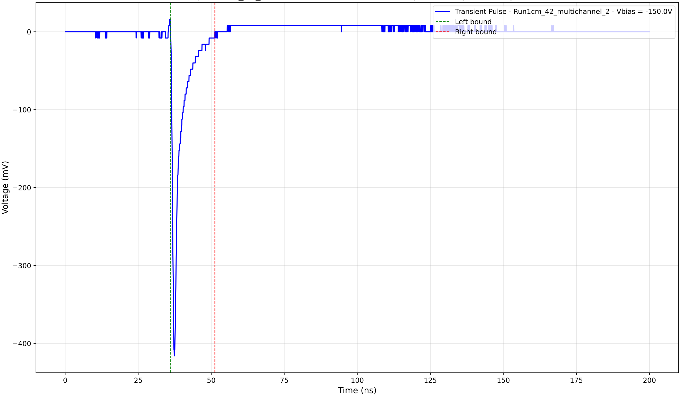
Transient Pulse - Sample: 1cm_42_multichannel - Position: 2735.0 \mu\text{m} - Charge: 25.19 pC - Rise Time: 0.81 ns
