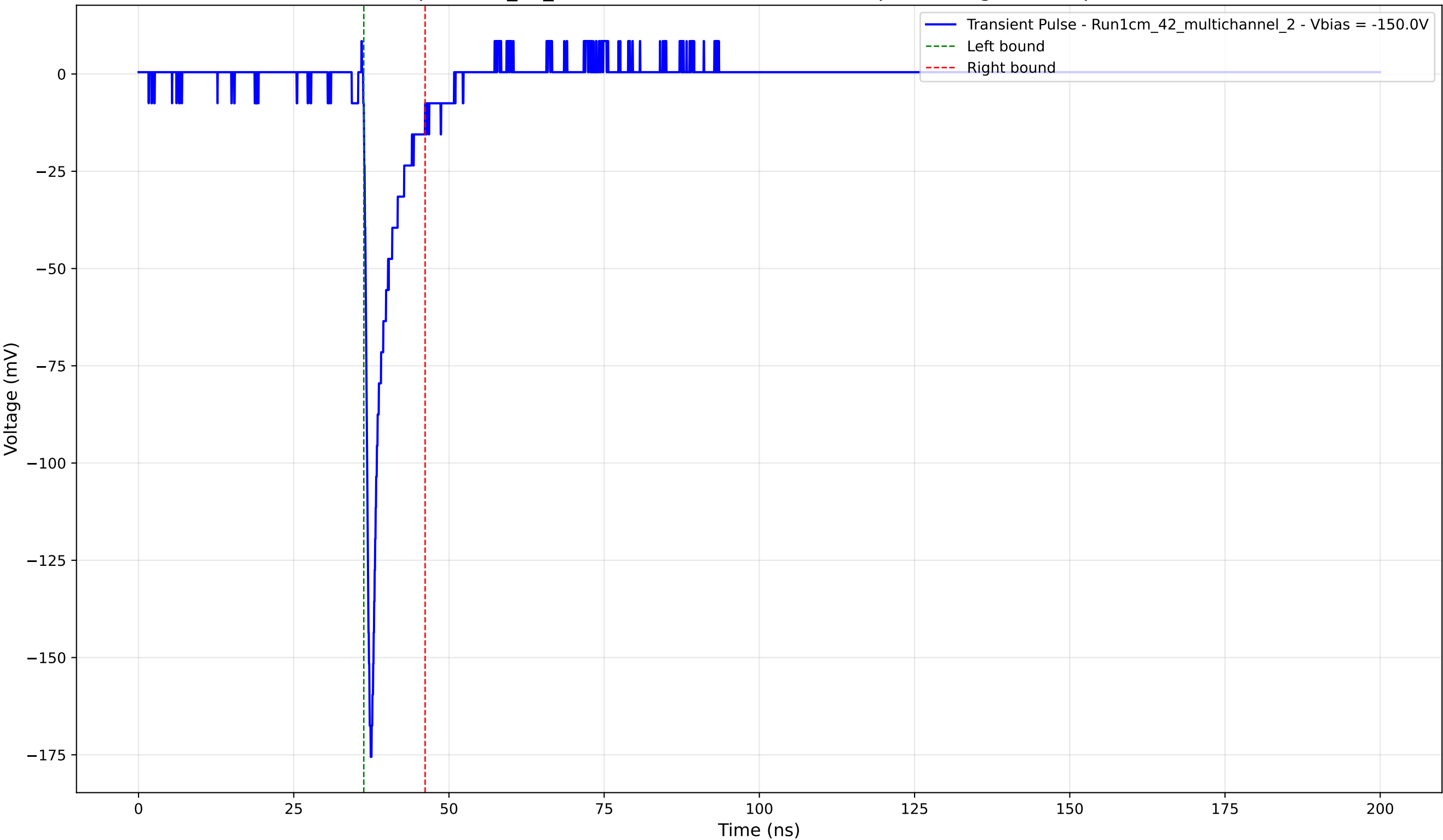
Transient Pulse - Sample: 1cm_42_multichannel - Position: 2825.0 \mu\text{m} - Charge: 10.86 pC - Rise Time: 0.86 ns
