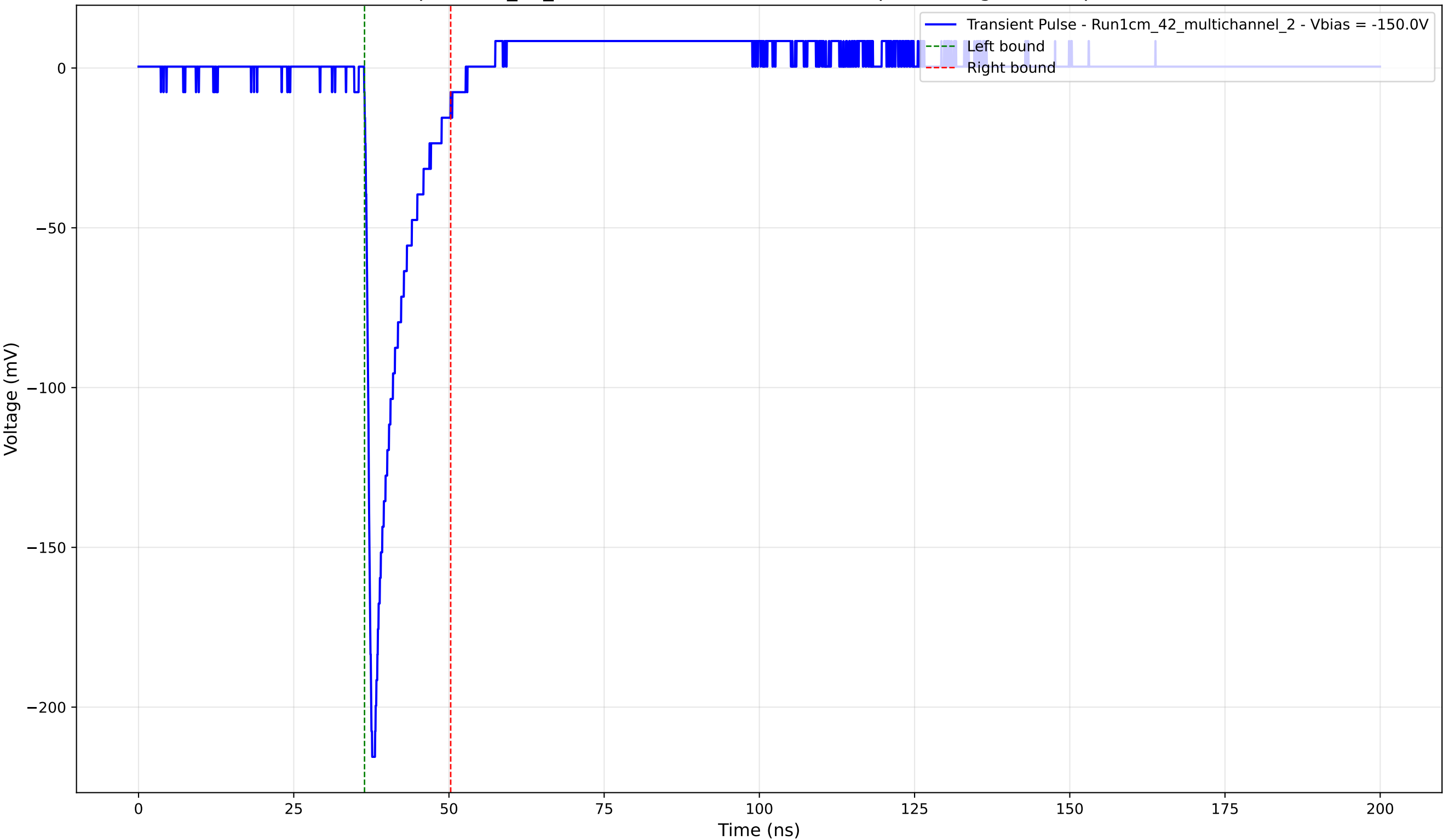
Transient Pulse - Sample: 1cm_42_multichannel - Position: 1545.0 \mu\text{m} - Charge: 21.03 pC - Rise Time: 0.94 ns
