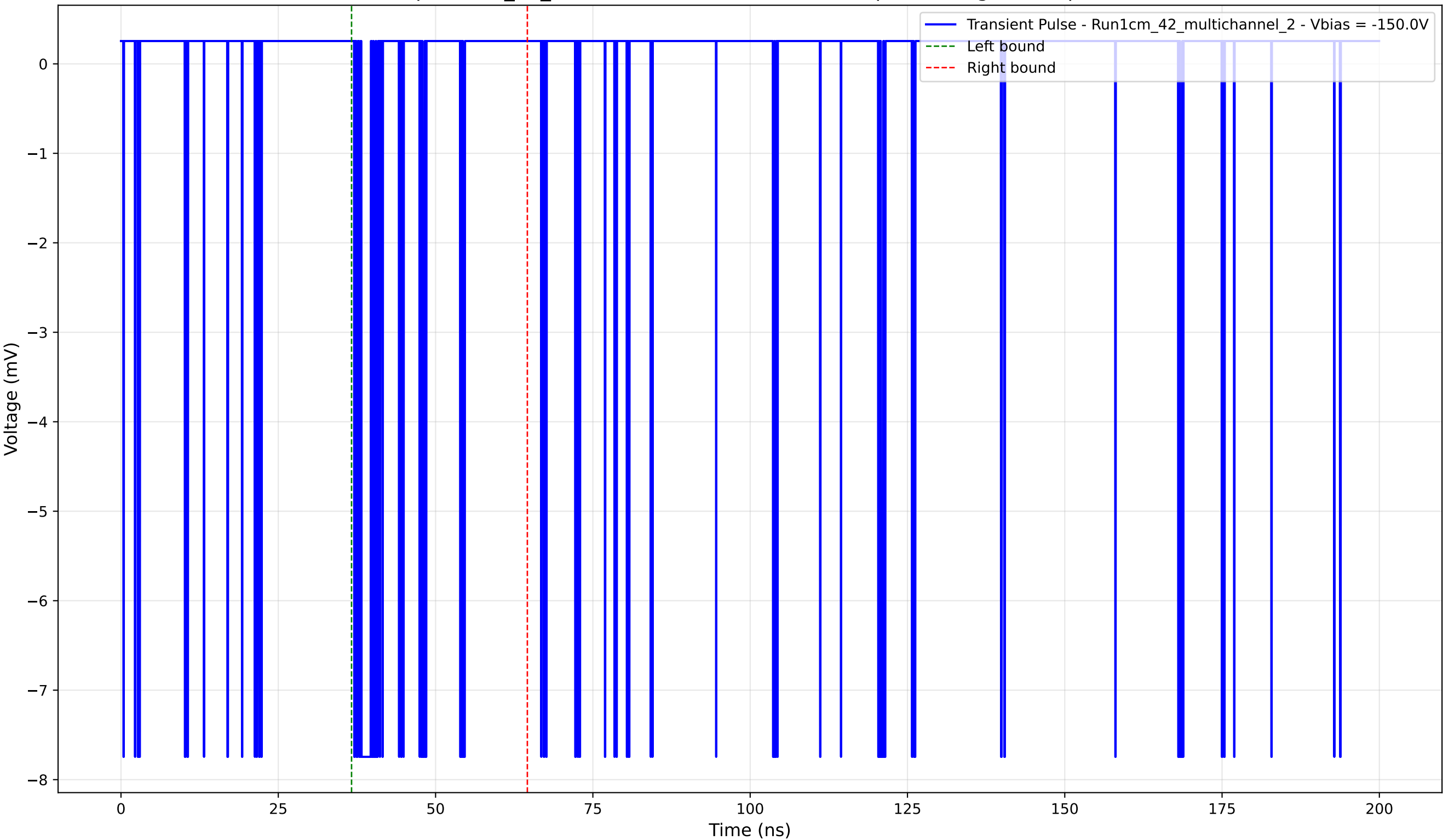
Transient Pulse - Sample: 1cm_42_multichannel - Position: 4925.0 \mu\text{m} - Charge: 0.52 pC - Rise Time: 0.04 ns
