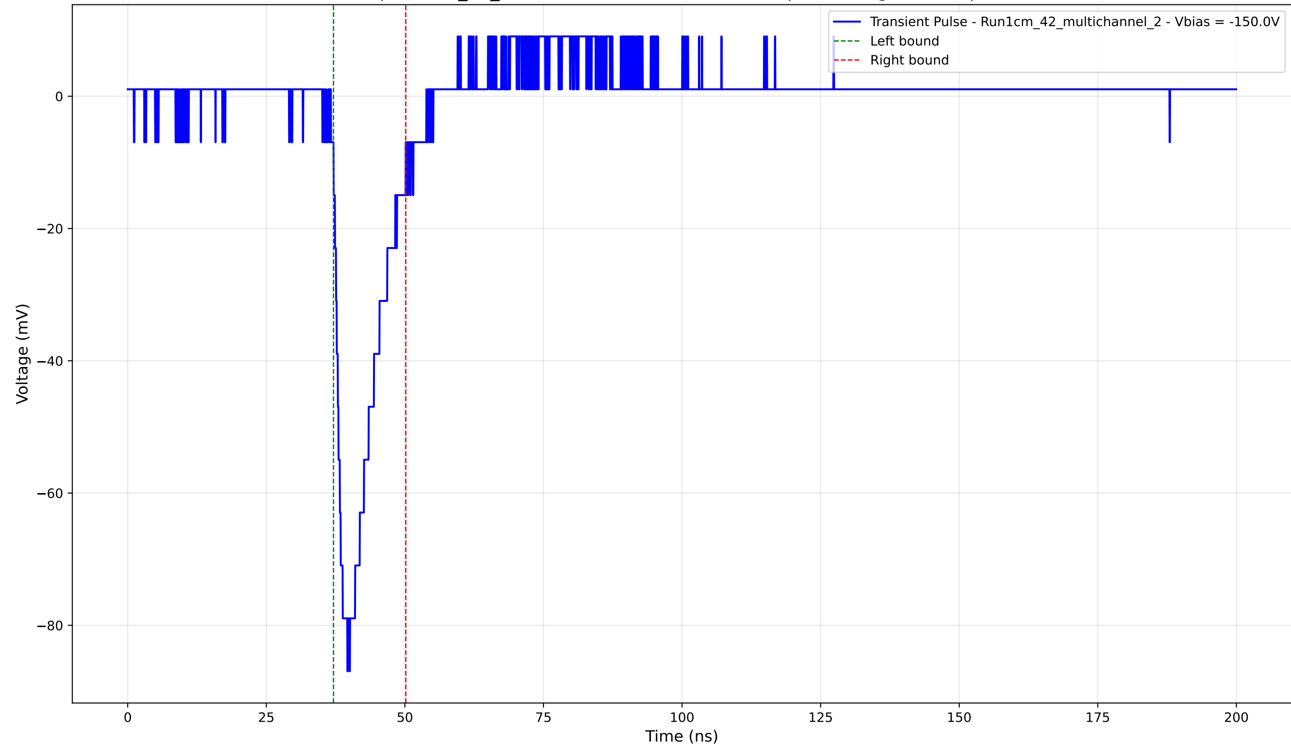
Transient Pulse - Sample: 1cm_42_multichannel - Position: 4220.0 \mu\text{m} - Charge: 11.92 pC - Rise Time: 1.67 ns
