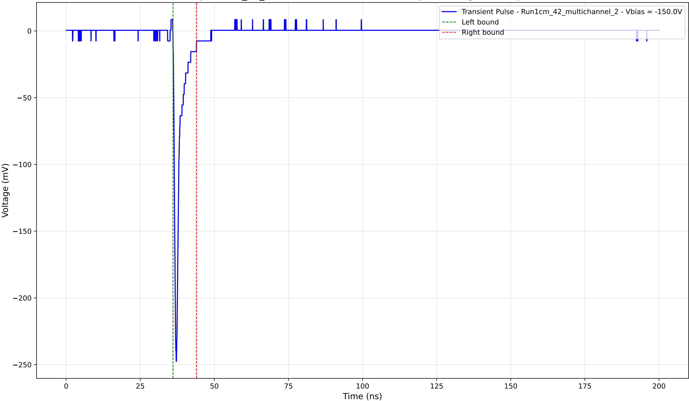
Transient Pulse - Sample: 1cm_42_multichannel - Position: 2415.0 \mu\text{m} - Charge: 10.41 pC - Rise Time: 0.71 ns
