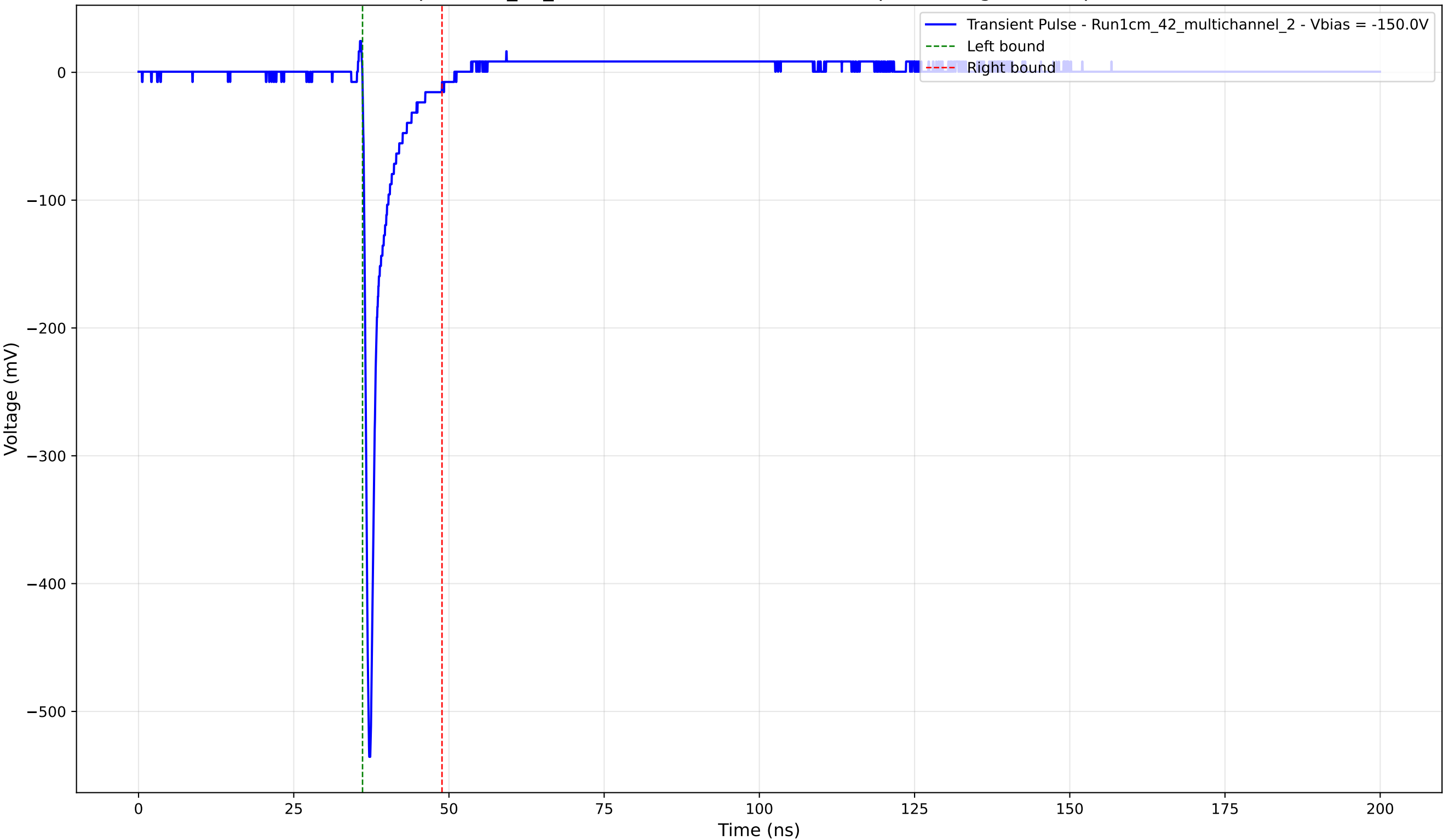
Transient Pulse - Sample: 1cm_42_multichannel - Position: 2165.0 \mu\text{m} - Charge: 27.06 pC - Rise Time: 0.76 ns
