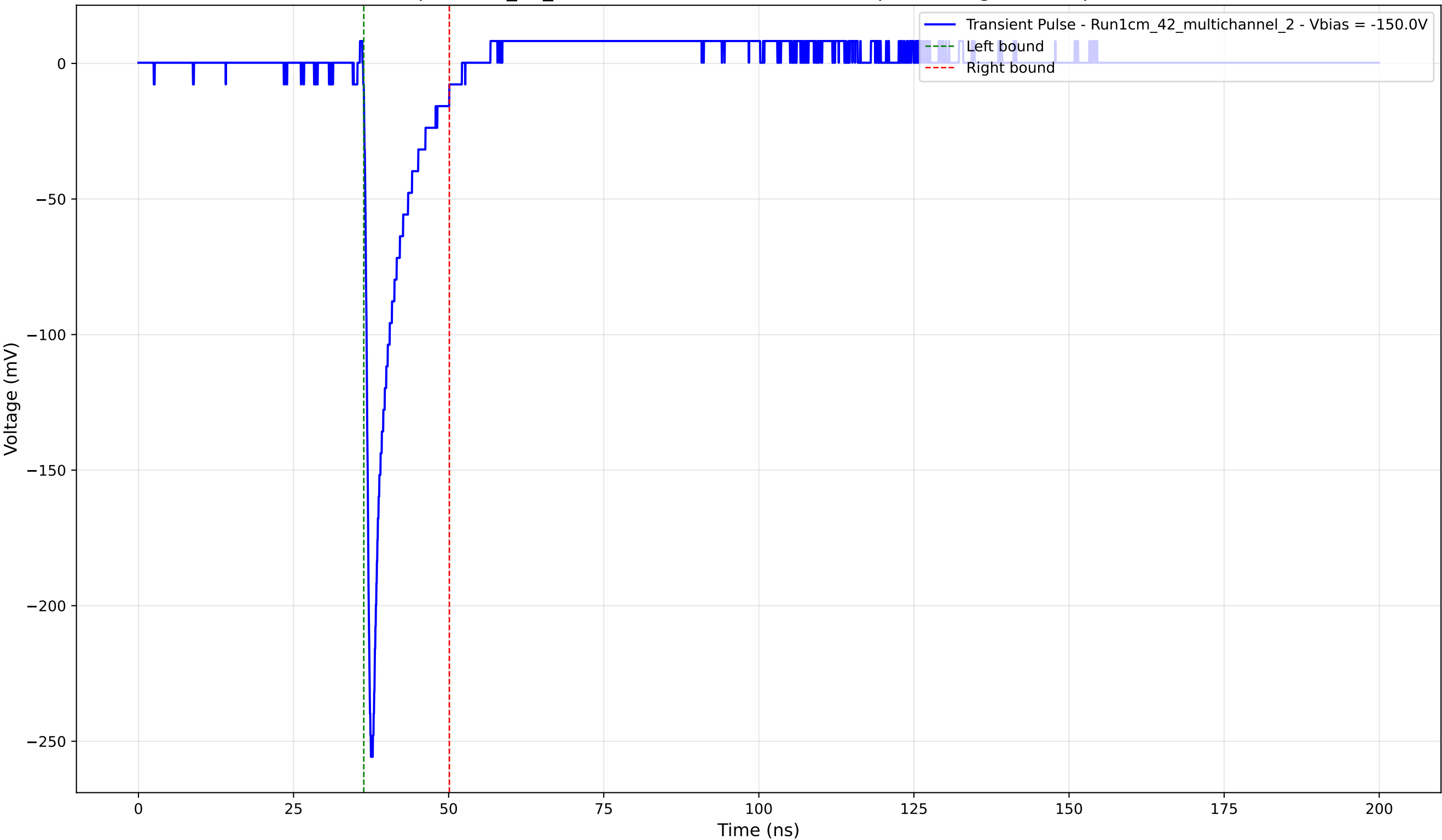
Transient Pulse - Sample: 1cm_42_multichannel - Position: 3010.0 \mu\text{m} - Charge: 21.04 pC - Rise Time: 0.86 ns
