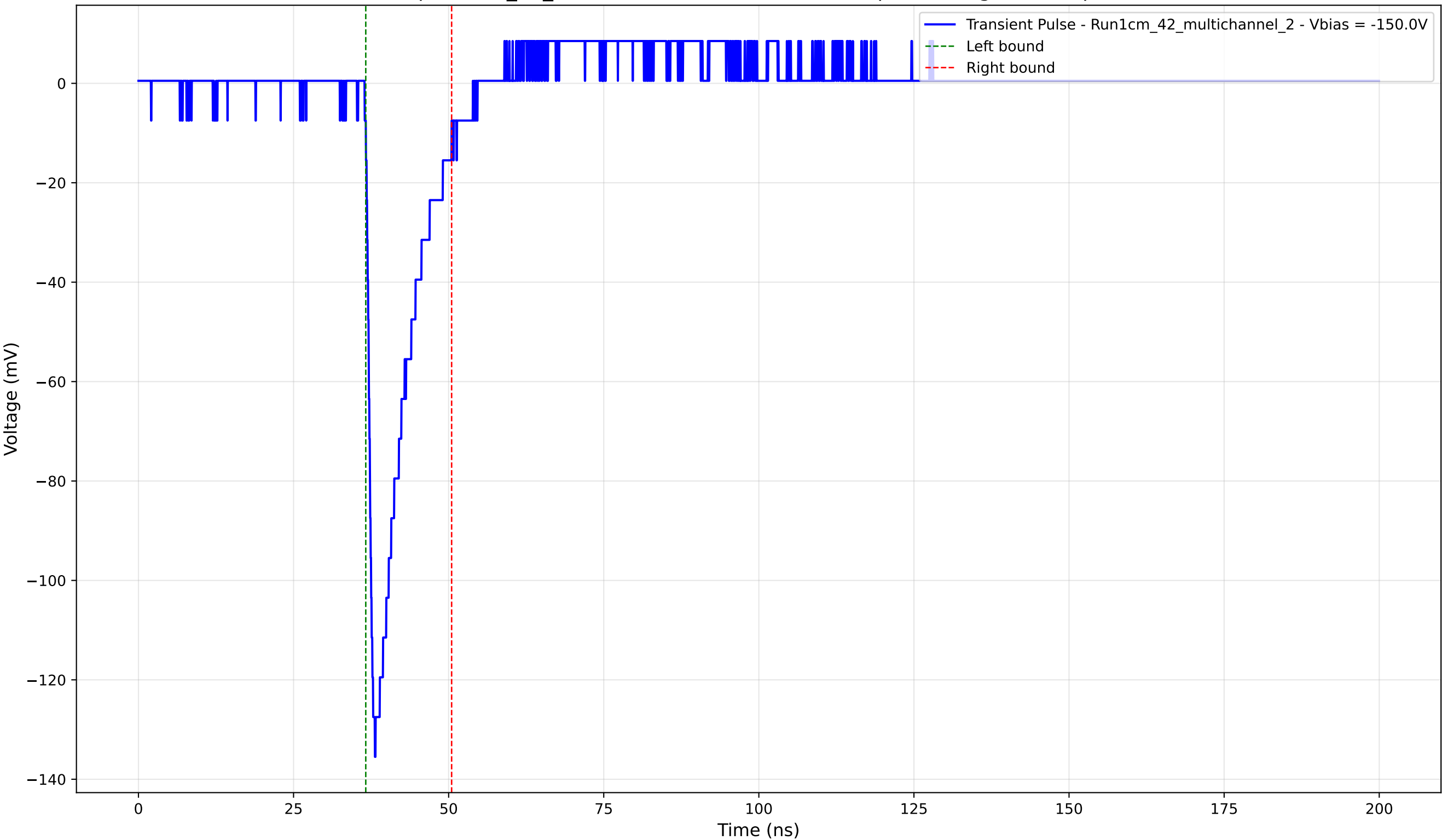
Transient Pulse - Sample: 1cm_42_multichannel - Position: 3500.0 \mu\text{m} - Charge: 16.54 pC - Rise Time: 1.17 ns
