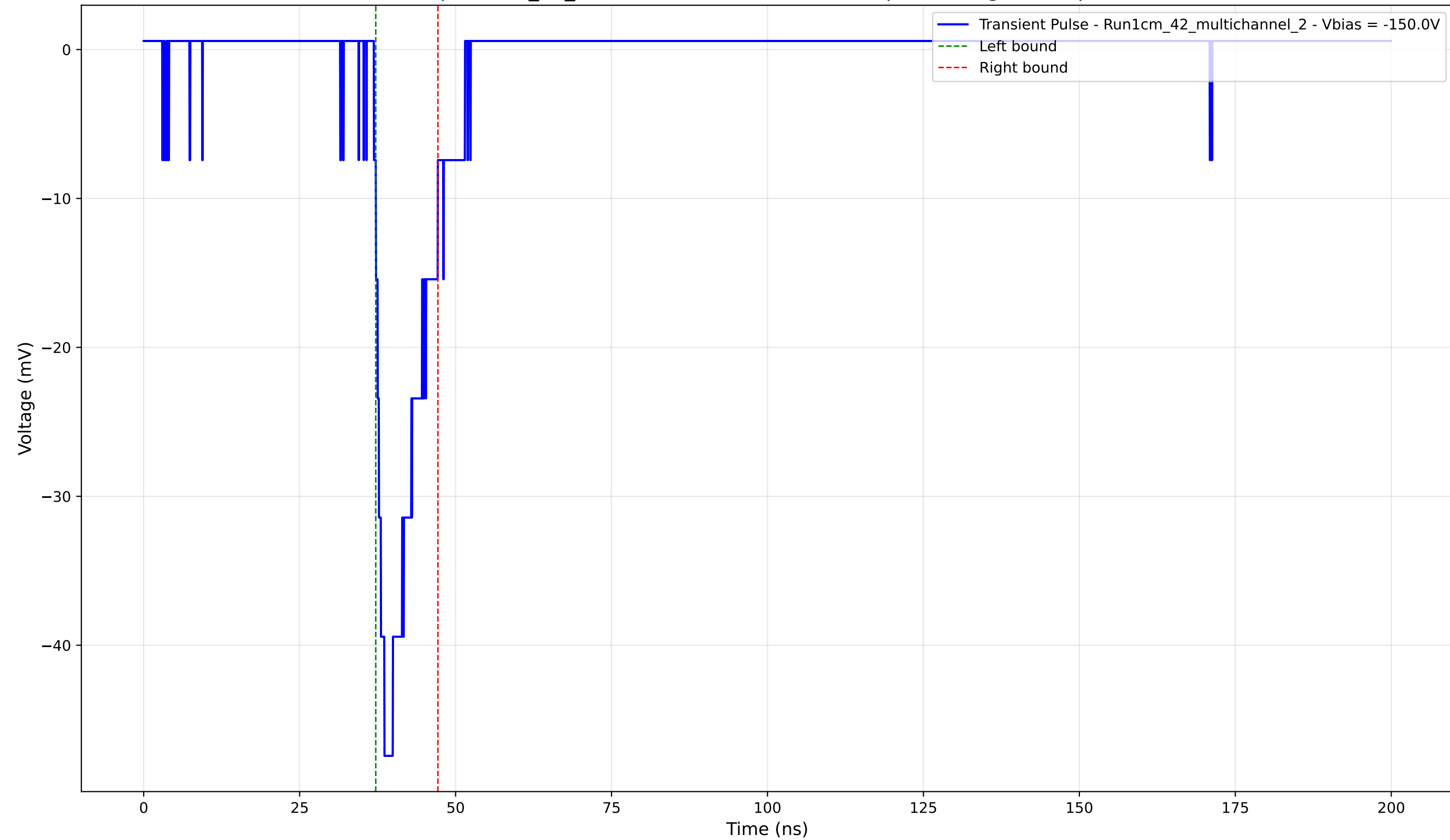
Transient Pulse - Sample: 1cm_42_multichannel - Position: 805.0 \mu\text{m} - Charge: 5.88 pC - Rise Time: 1.70 ns
