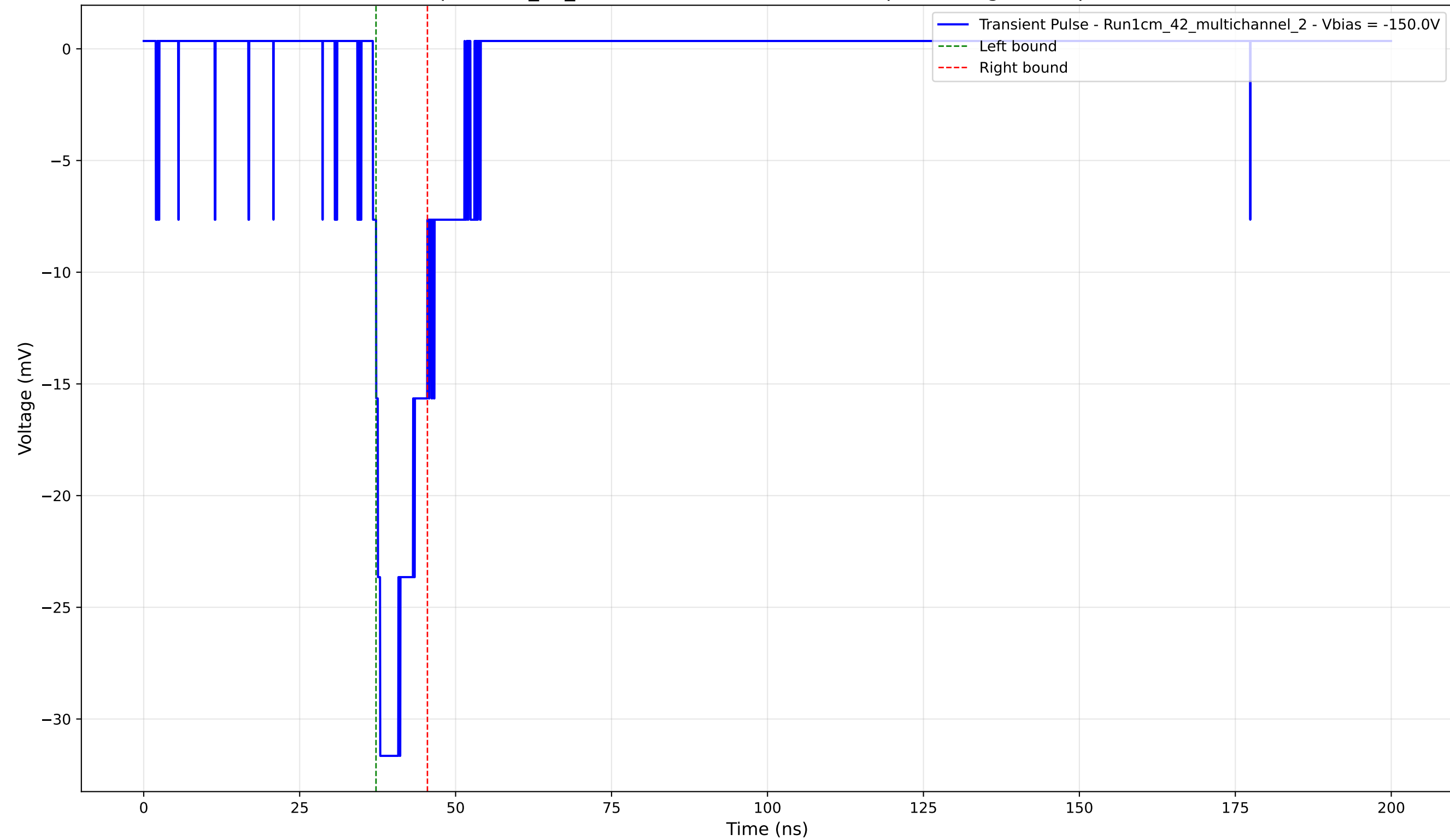
Transient Pulse - Sample: 1cm_42_multichannel - Position: 890.0 \mu\text{m} - Charge: 3.99 pC - Rise Time: 1.18 ns
