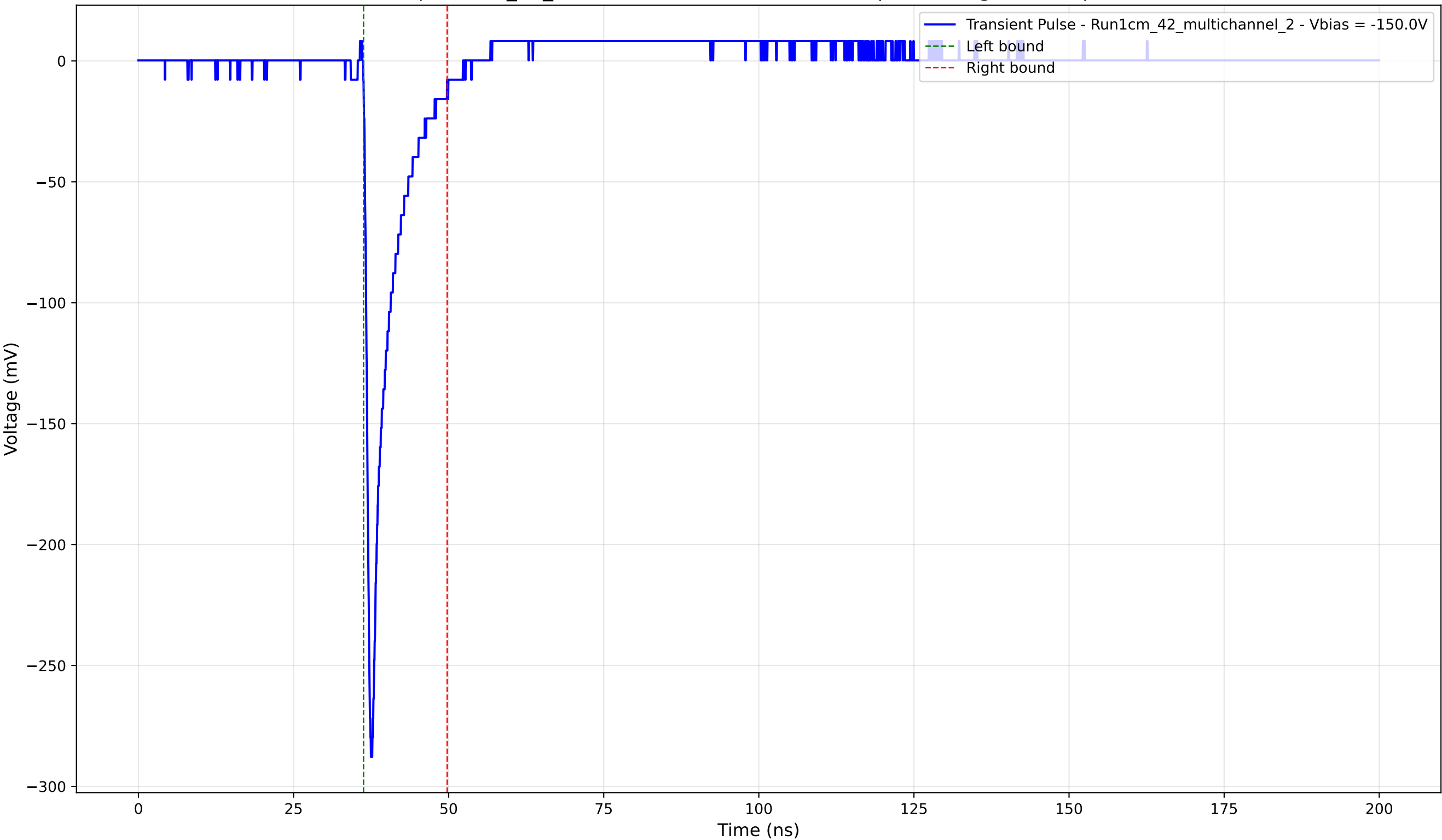
Transient Pulse - Sample: 1cm_42_multichannel - Position: 1770.0 \mu\text{m} - Charge: 22.35 pC - Rise Time: 0.83 ns
