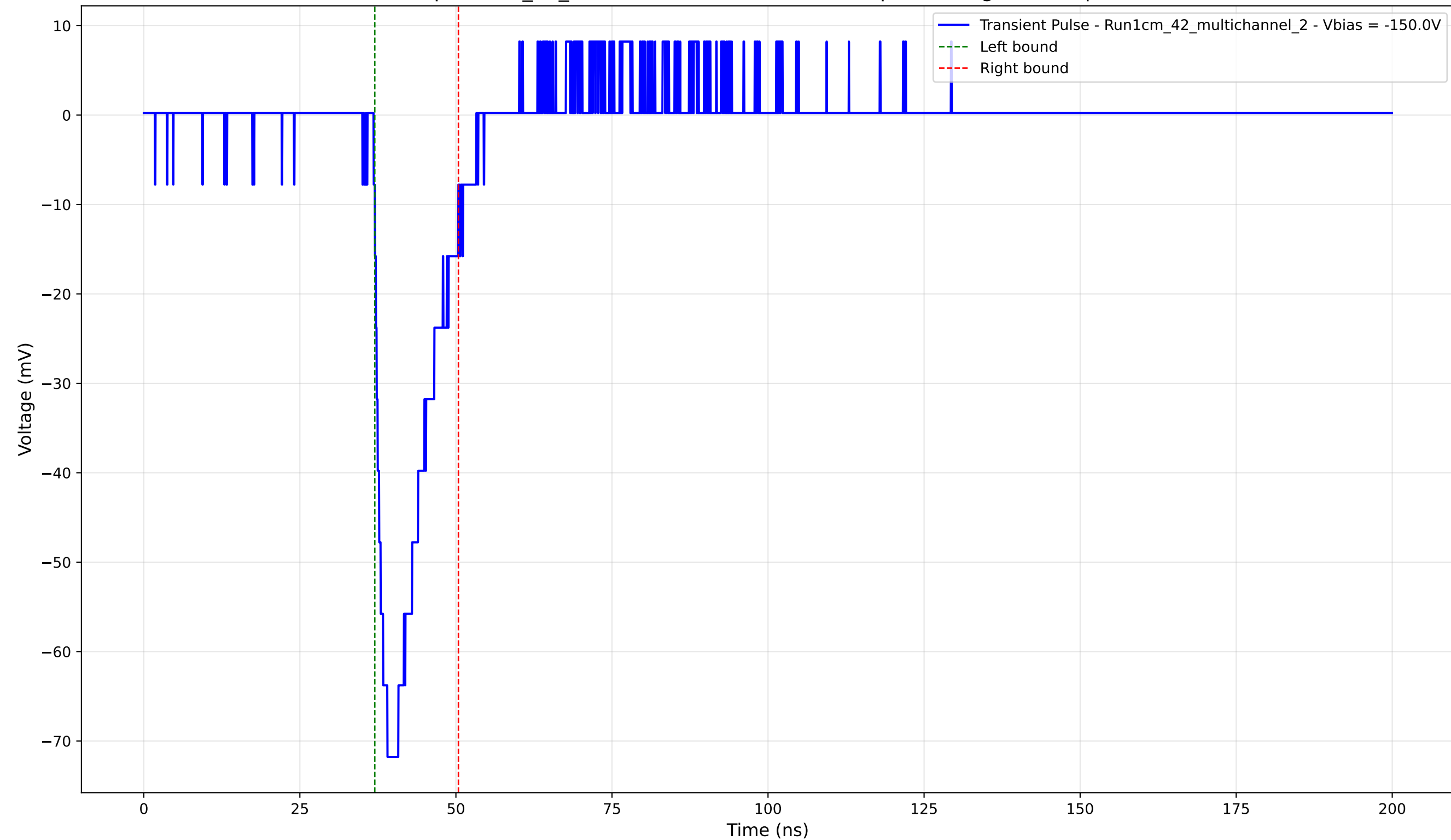
Transient Pulse - Sample: 1cm_42_multichannel - Position: 170.0 \mu\text{m} - Charge: 11.36 pC - Rise Time: 2.20 ns
