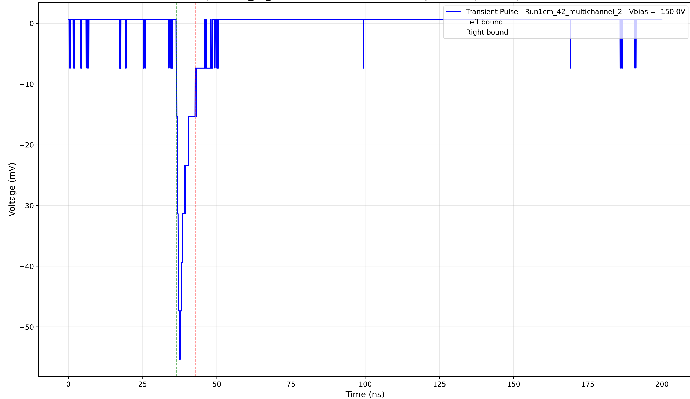
Transient Pulse - Sample: 1cm_42_multichannel - Position: 1830.0 \mu\text{m} - Charge: 3.33 pC - Rise Time: 1.21 ns
