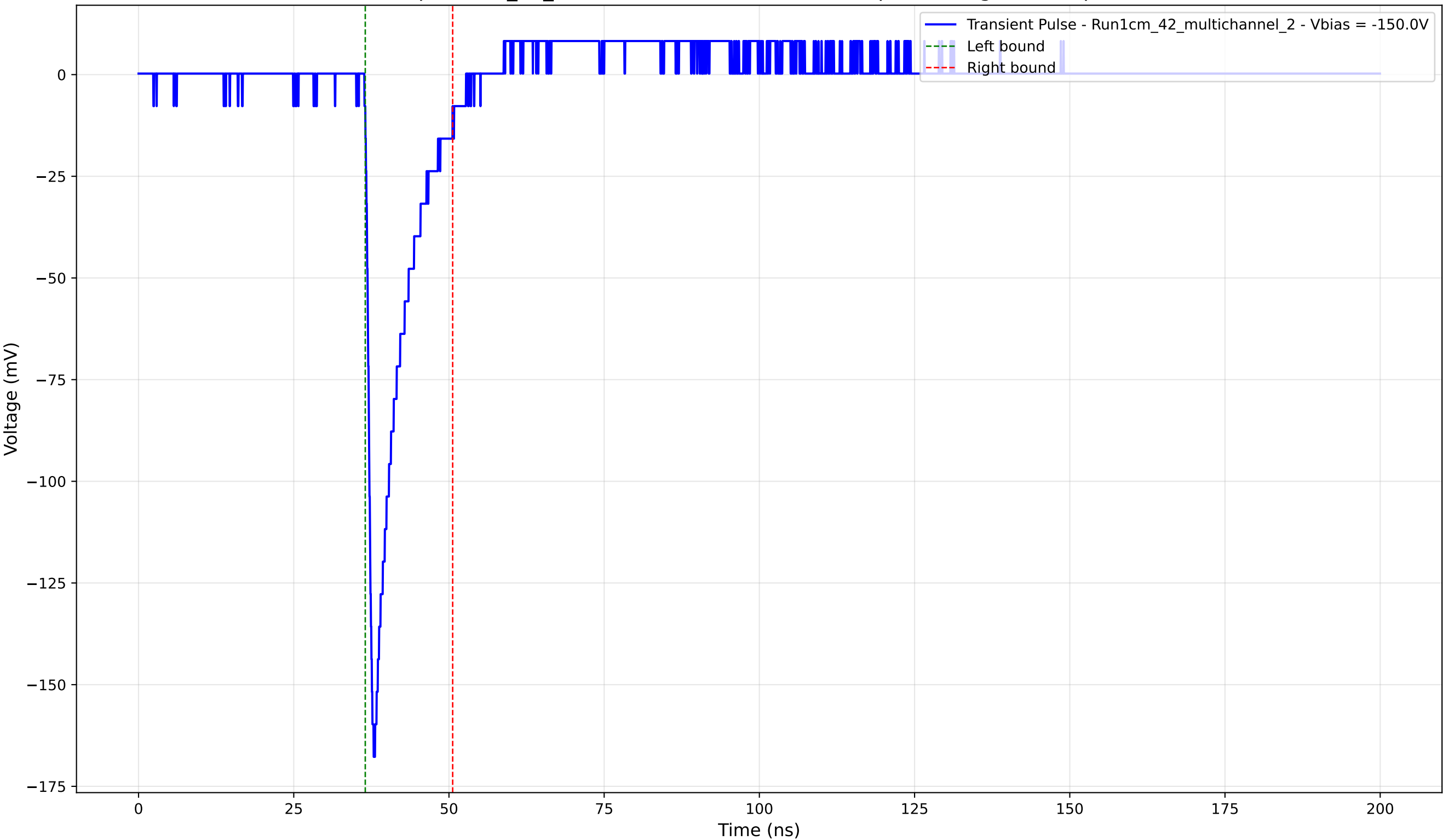
Transient Pulse - Sample: 1cm_42_multichannel - Position: 3295.0 \mu\text{m} - Charge: 17.59 pC - Rise Time: 0.99 ns
