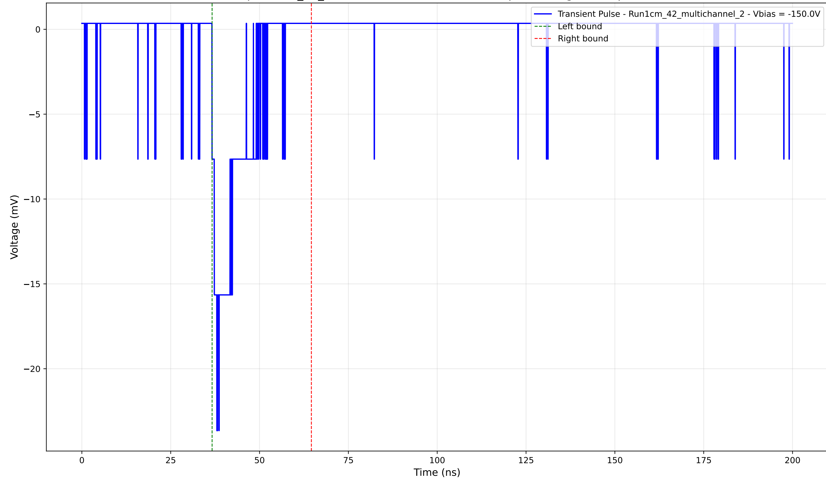
Transient Pulse - Sample: 1cm_42_multichannel - Position: 1330.0 \mu\text{m} - Charge: 2.80 pC - Rise Time: 1.39 ns
