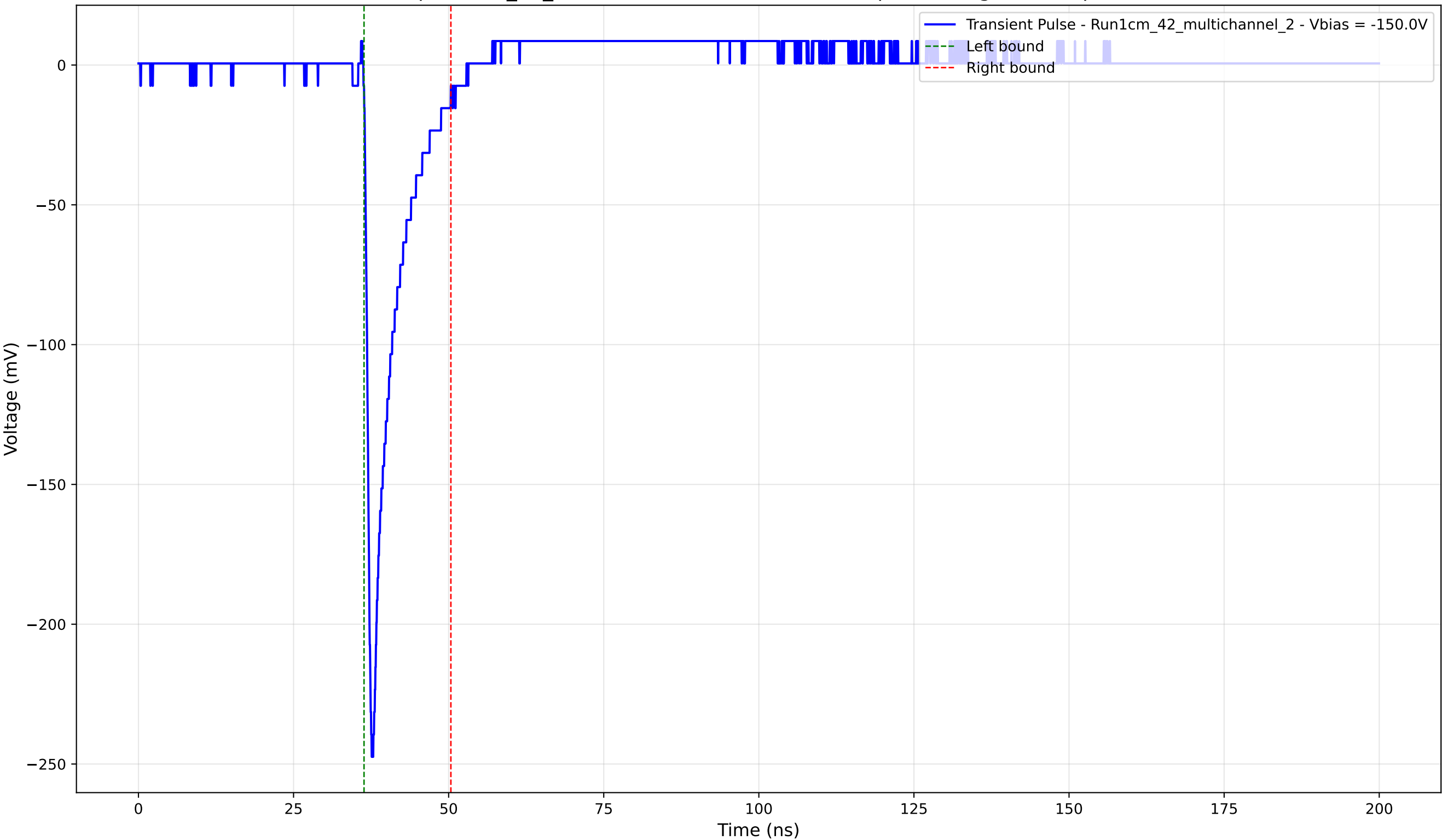
Transient Pulse - Sample: 1cm_42_multichannel - Position: 1630.0 \mu\text{m} - Charge: 22.05 pC - Rise Time: 0.91 ns
