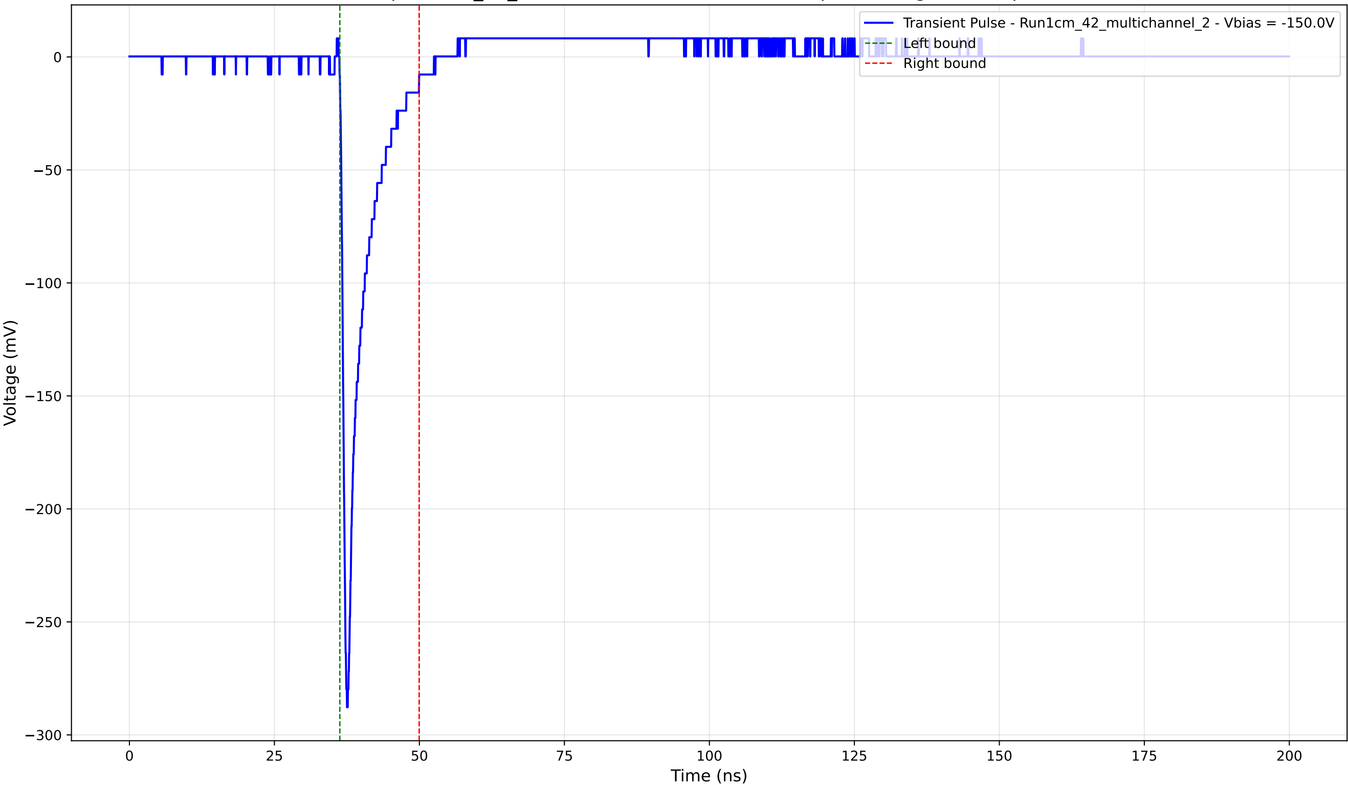
Transient Pulse - Sample: 1cm_42_multichannel - Position: 1775.0 \mu\text{m} - Charge: 22.11 pC - Rise Time: 0.85 ns
