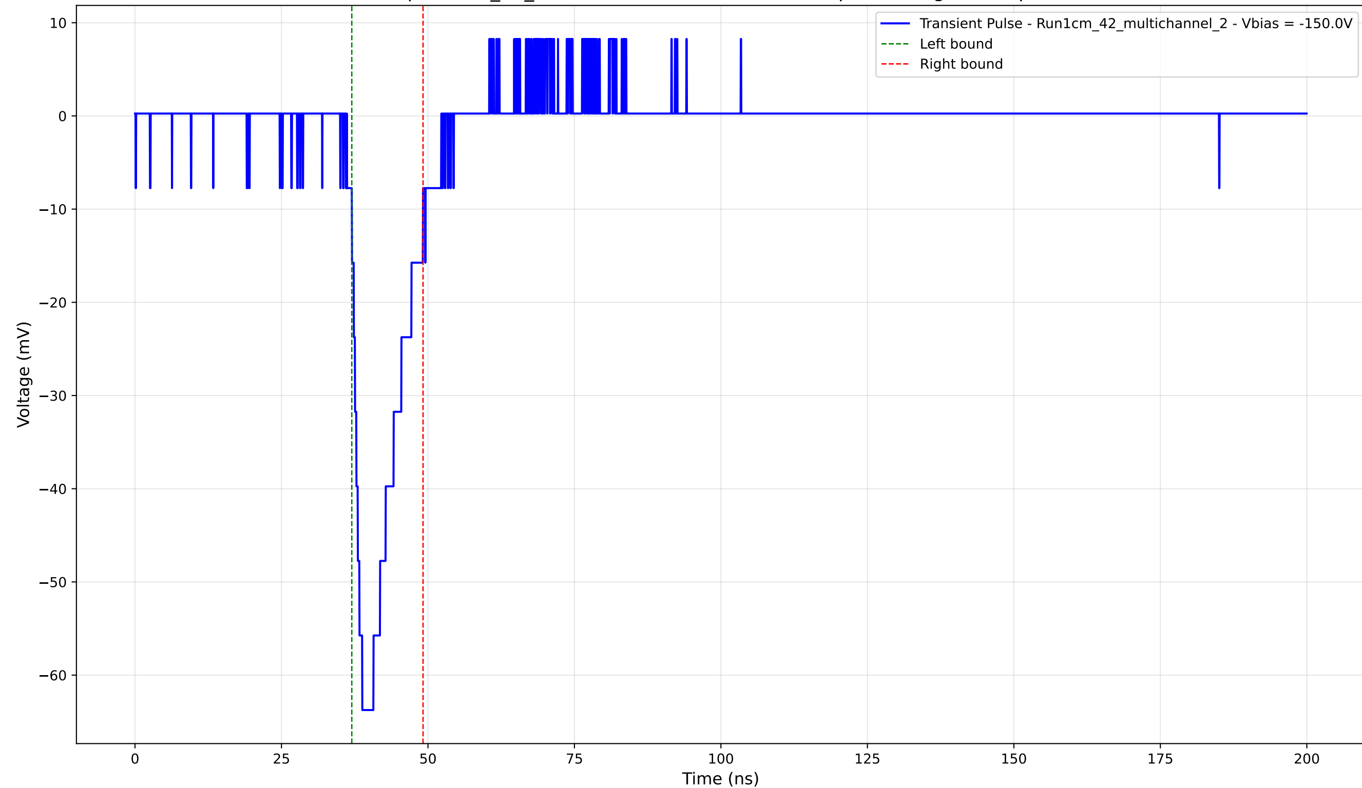
Transient Pulse - Sample: 1cm_42_multichannel - Position: 4780.0 \mu\text{m} - Charge: 9.31 pC - Rise Time: 2.61 ns
