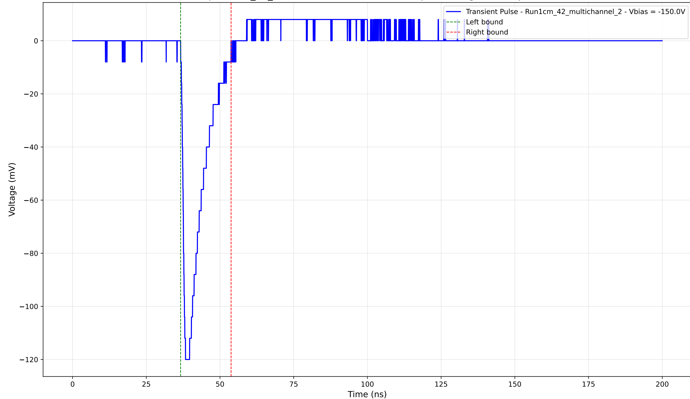
Transient Pulse - Sample: 1cm_42_multichannel - Position: 955.0 \mu\text{m} - Charge: 17.46 pC - Rise Time: 1.18 ns
