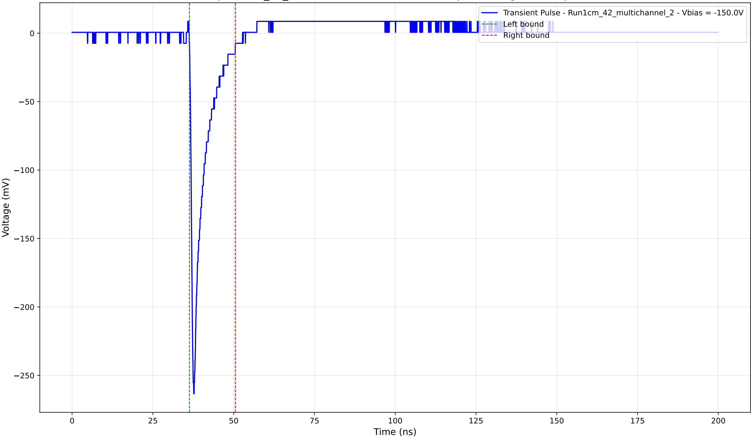
Transient Pulse - Sample: 1cm_42_multichannel - Position: 1670.0 \mu\text{m} - Charge: 22.36 pC - Rise Time: 0.91 ns
