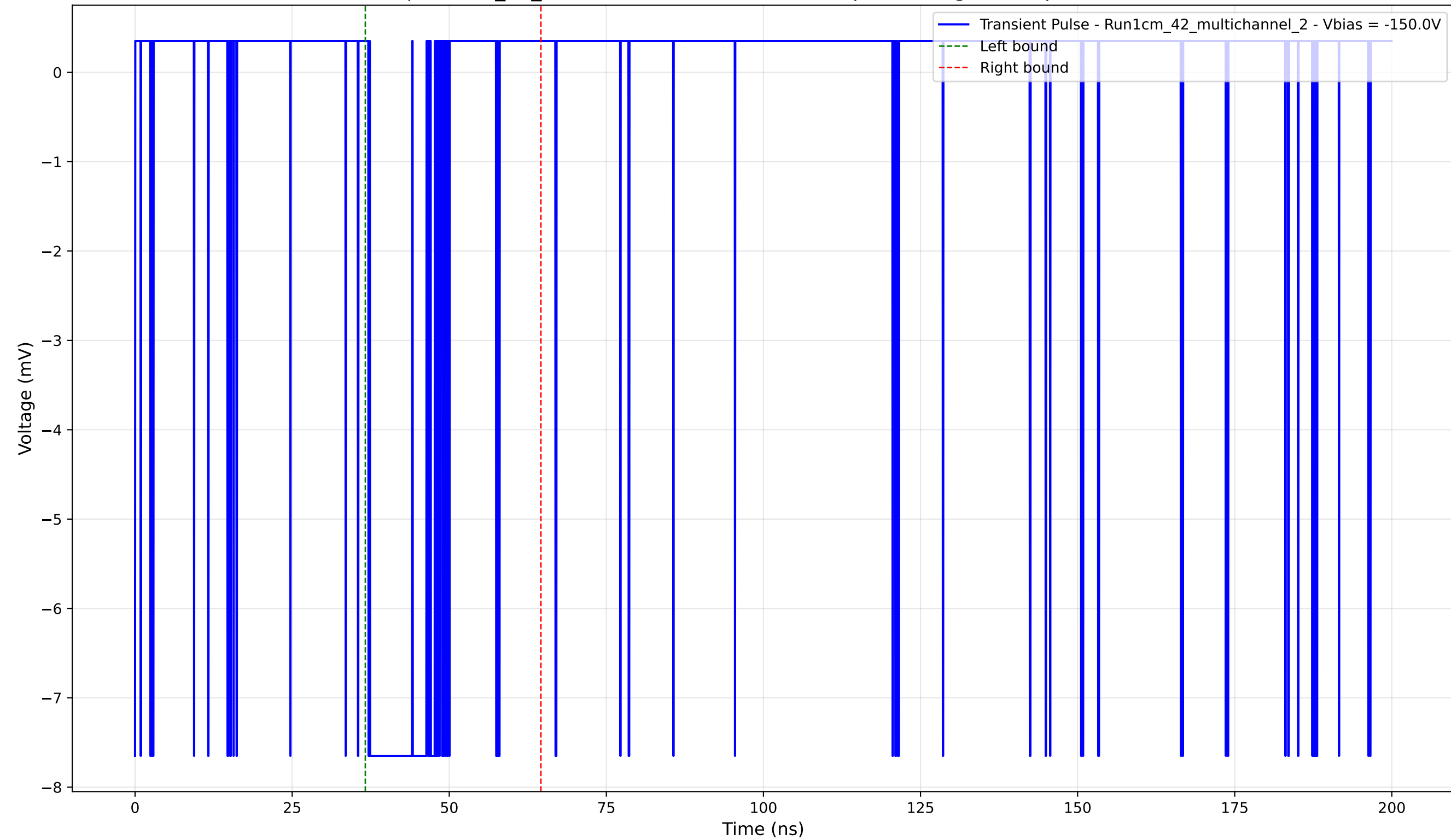
Transient Pulse - Sample: 1cm_42_multichannel - Position: 860.0 \mu\text{m} - Charge: 1.59 pC - Rise Time: 0.00 ns (N/A)
