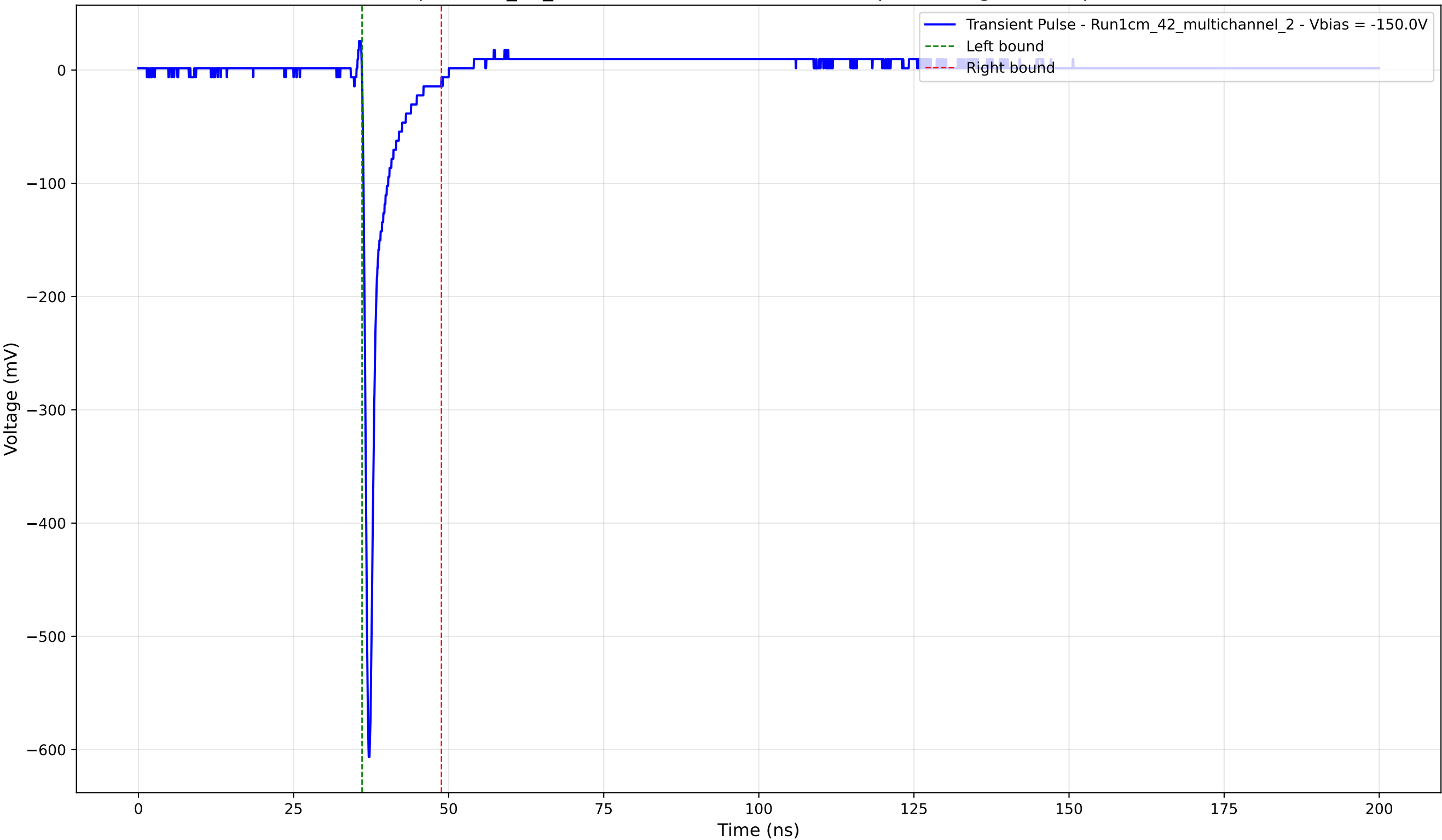
Transient Pulse - Sample: 1cm_42_multichannel - Position: 2230.0 \mu\text{m} - Charge: 28.45 pC - Rise Time: 0.73 ns
