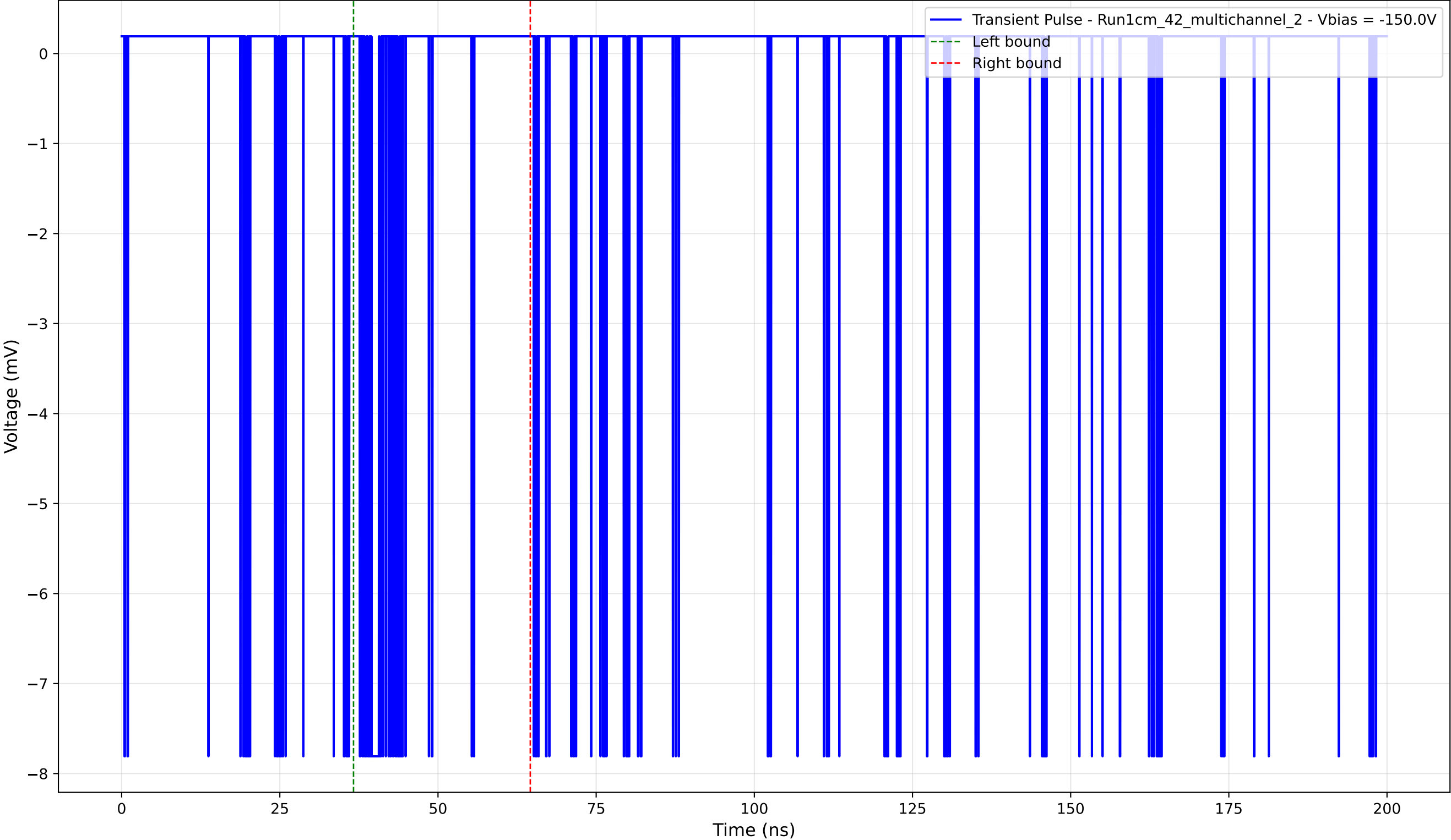
Transient Pulse - Sample: 1cm_42_multichannel - Position: 4905.0 \mu\text{m} - Charge: 0.53 pC - Rise Time: 0.04 ns
