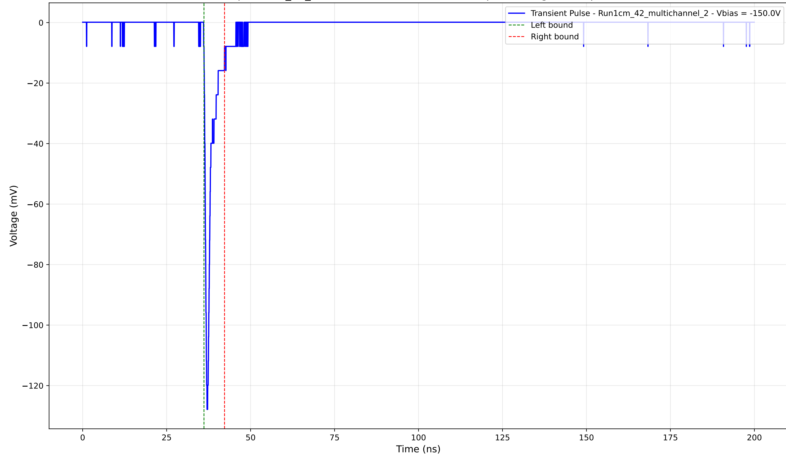
Transient Pulse - Sample: 1cm_42_multichannel - Position: 2405.0 \mu\text{m} - Charge: 5.39 pC - Rise Time: 0.78 ns
