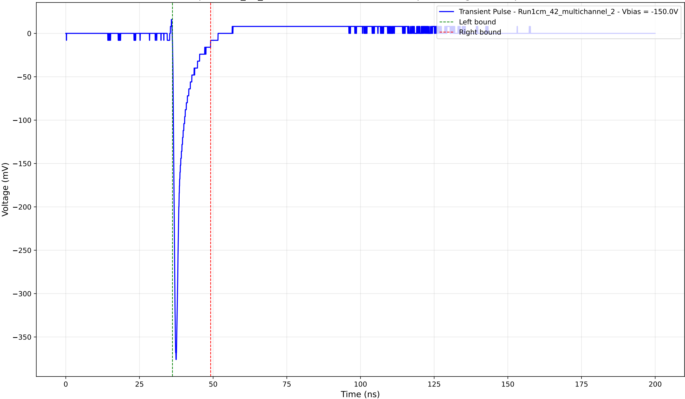
Transient Pulse - Sample: 1cm_42_multichannel - Position: 2775.0 \mu\text{m} - Charge: 23.28 pC - Rise Time: 0.78 ns
