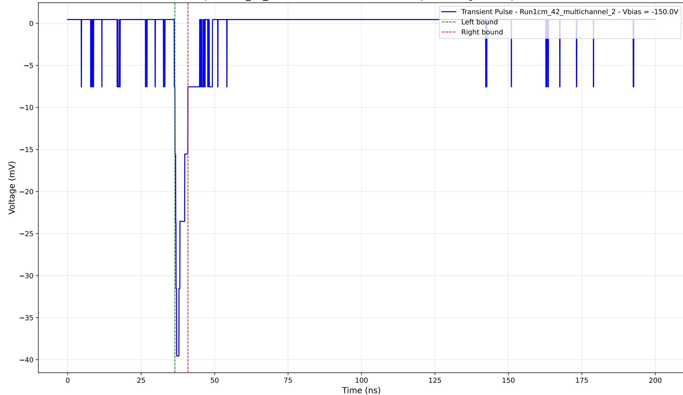
Transient Pulse - Sample: 1cm_42_multichannel - Position: 1890.0 \mu\text{m} - Charge: 2.21 pC - Rise Time: 0.82 ns
