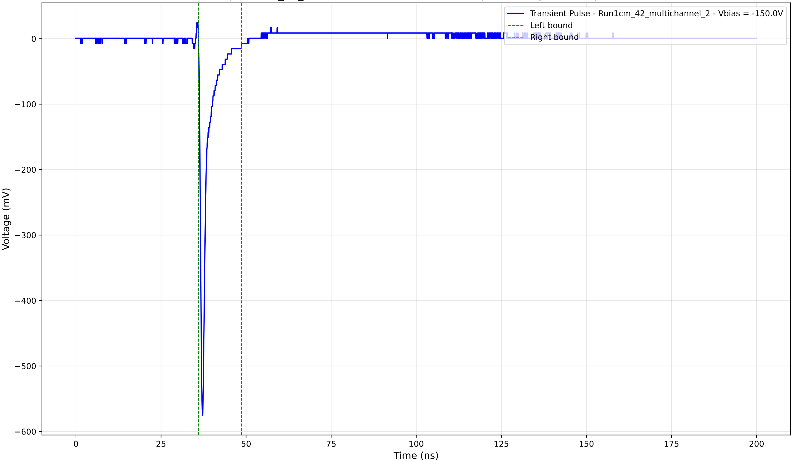
Transient Pulse - Sample: 1cm_42_multichannel - Position: 2510.0 \mu\text{m} - Charge: 26.99 pC - Rise Time: 0.73 ns
