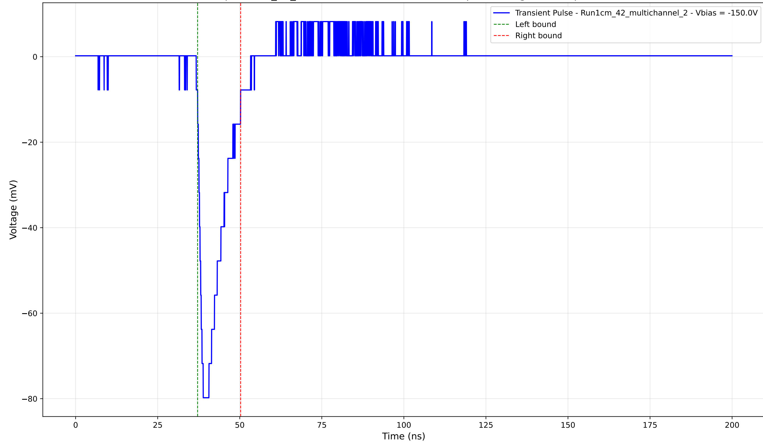
Transient Pulse - Sample: 1cm_42_multichannel - Position: 4245.0 \mu\text{m} - Charge: 11.67 pC - Rise Time: 1.72 ns
