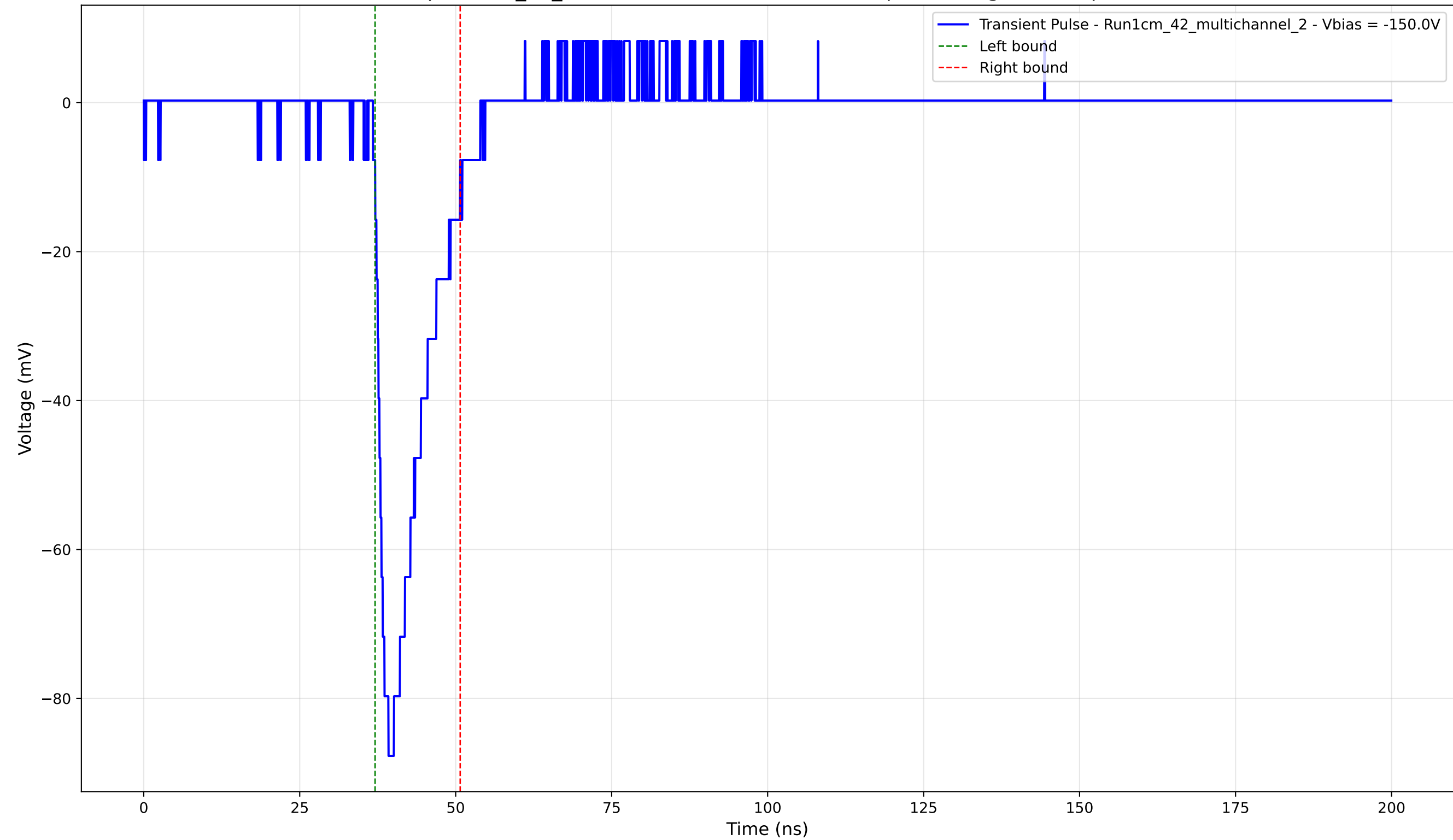
Transient Pulse - Sample: 1cm_42_multichannel - Position: 4100.0 \mu\text{m} - Charge: 12.70 pC - Rise Time: 1.51 ns
