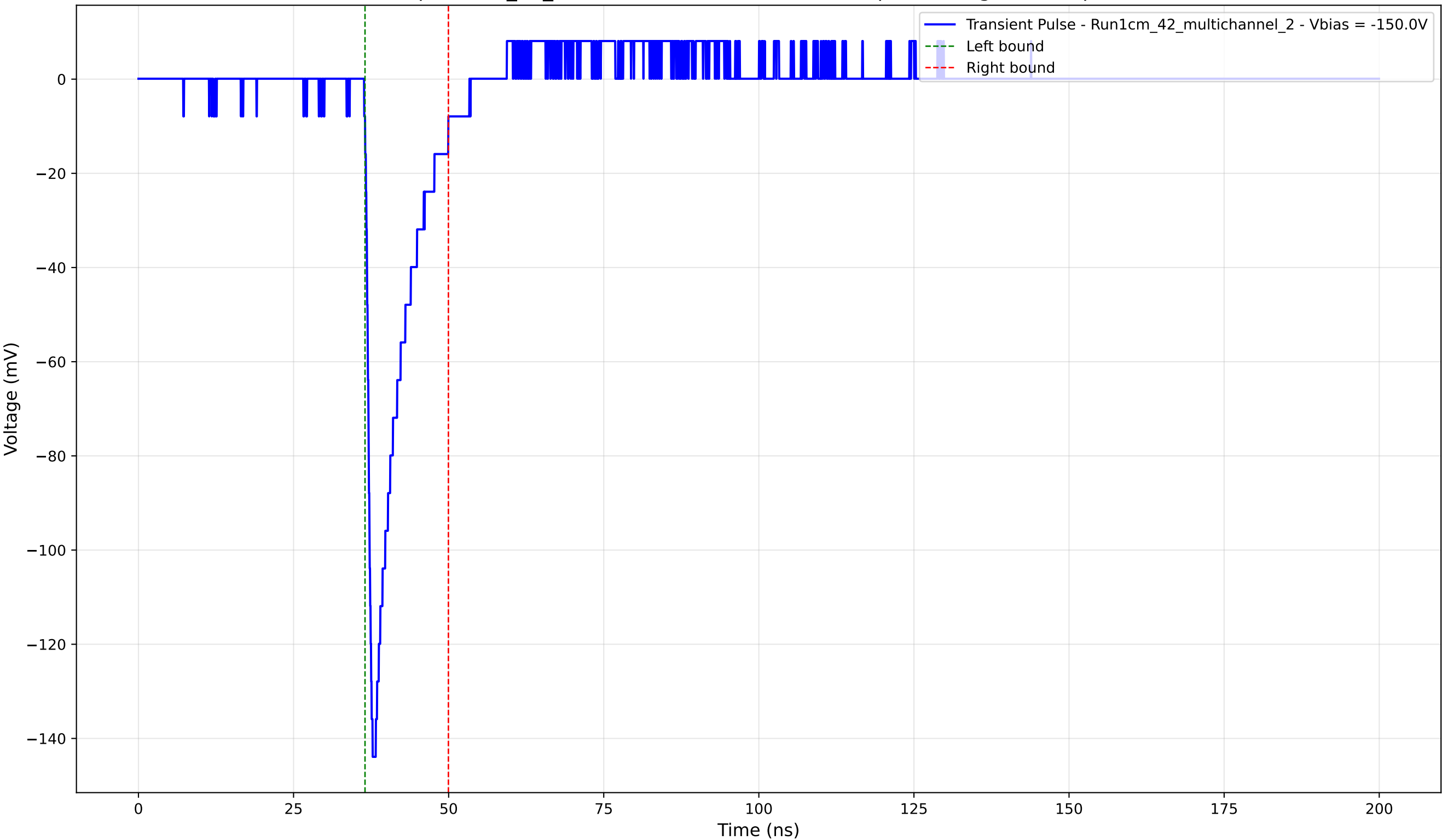
Transient Pulse - Sample: 1cm_42_multichannel - Position: 3310.0 \mu\text{m} - Charge: 15.55 pC - Rise Time: 1.05 ns
