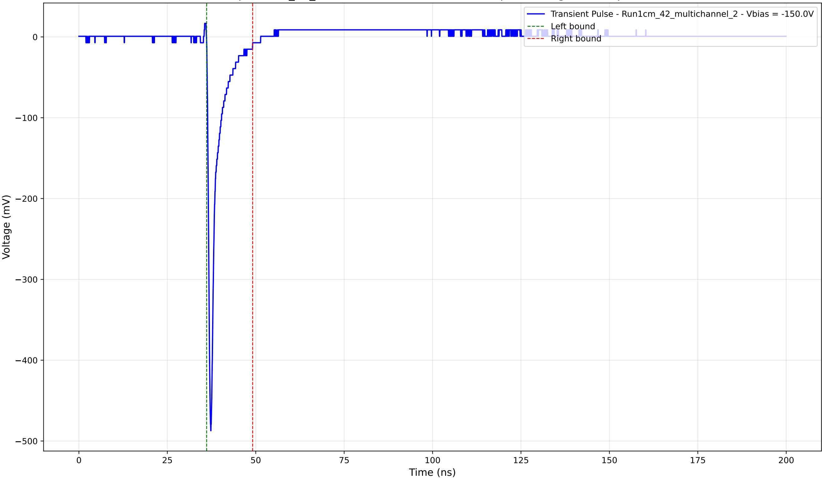
Transient Pulse - Sample: 1cm_42_multichannel - Position: 2095.0 \mu\text{m} - Charge: 26.27 pC - Rise Time: 0.77 ns
