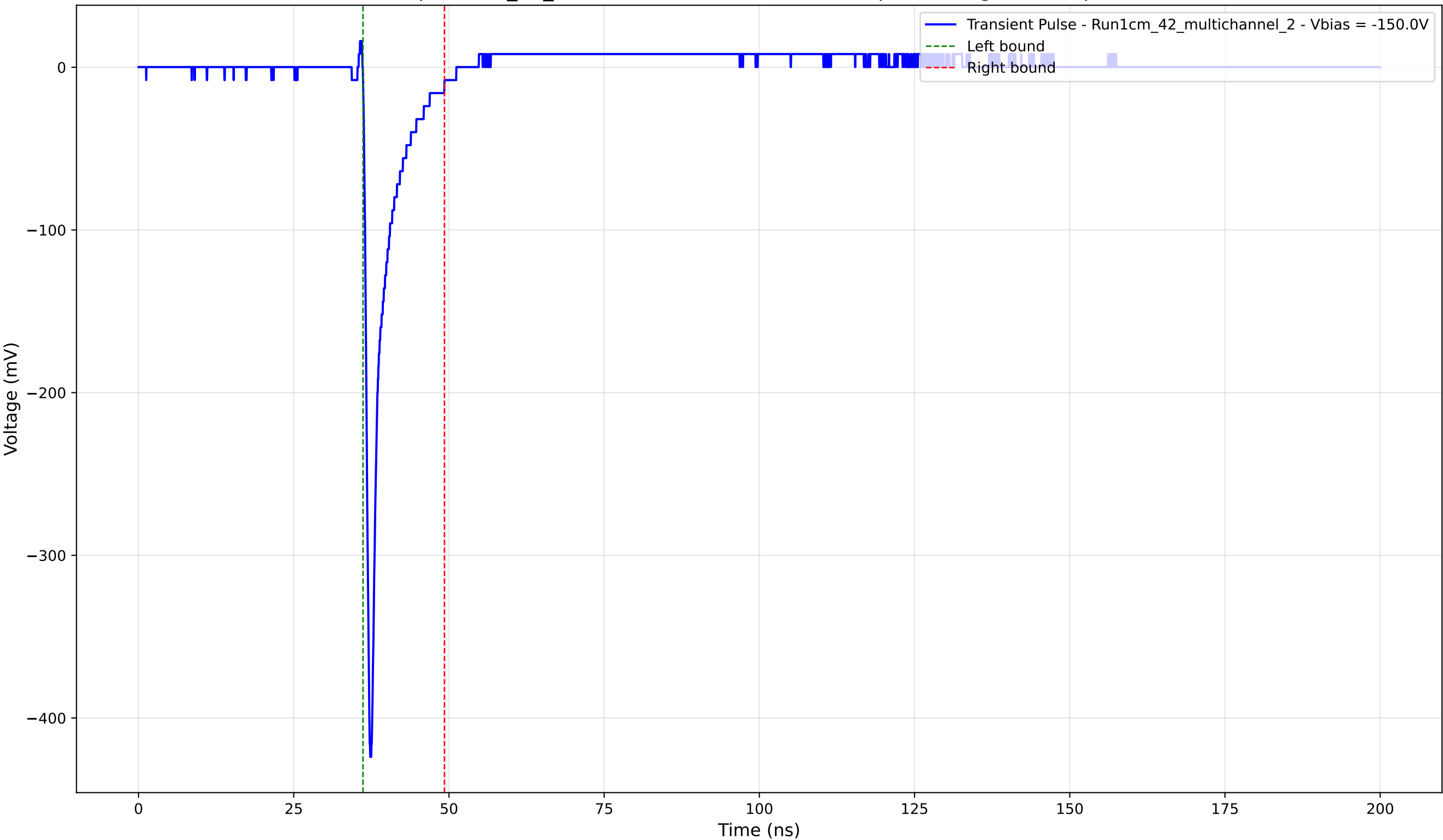
Transient Pulse - Sample: 1cm_42_multichannel - Position: 1995.0 \mu\text{m} - Charge: 25.76 pC - Rise Time: 0.81 ns
