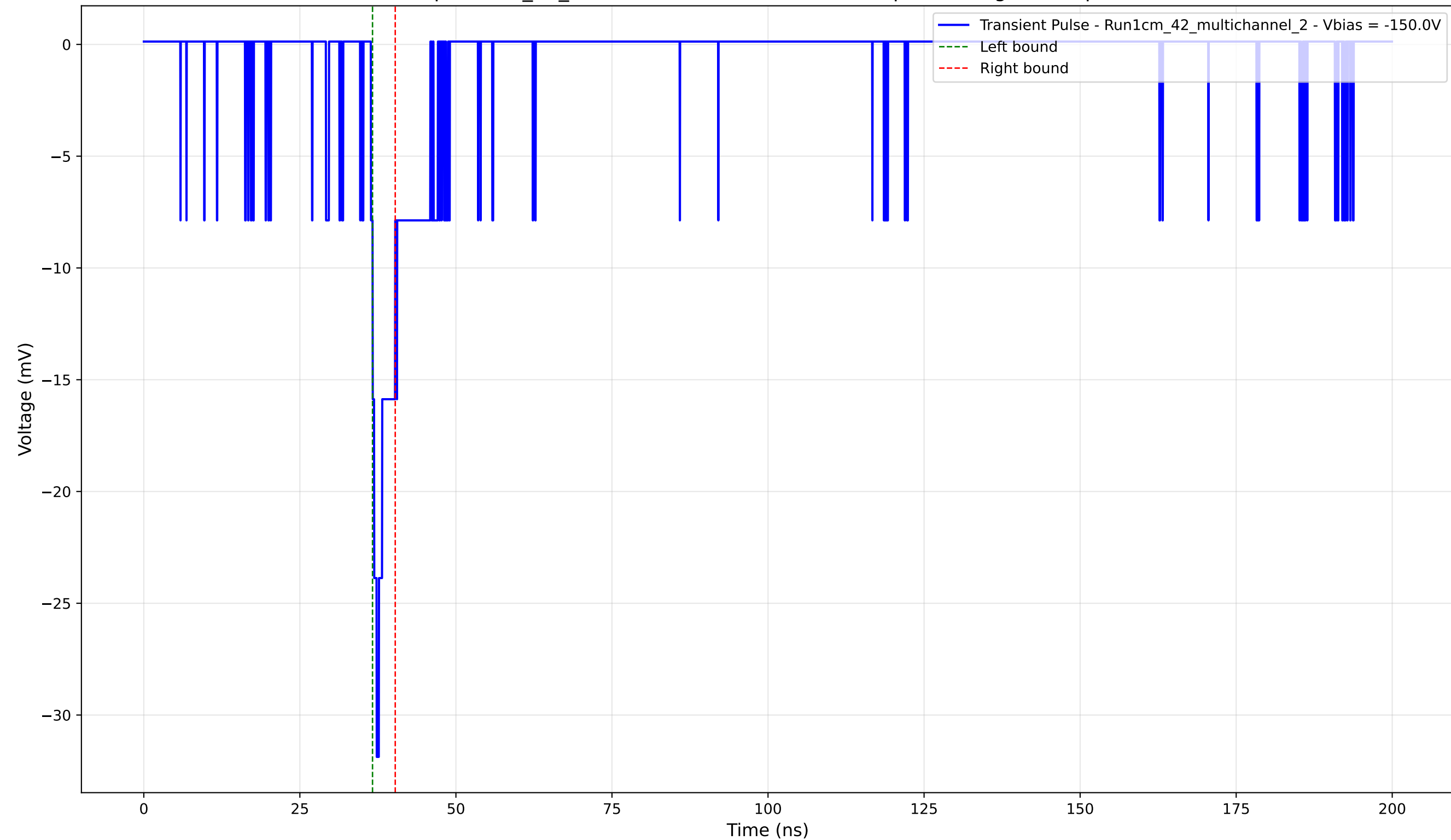
Transient Pulse - Sample: 1cm_42_multichannel - Position: 2855.0 \mu\text{m} - Charge: 1.41 pC - Rise Time: 0.94 ns
