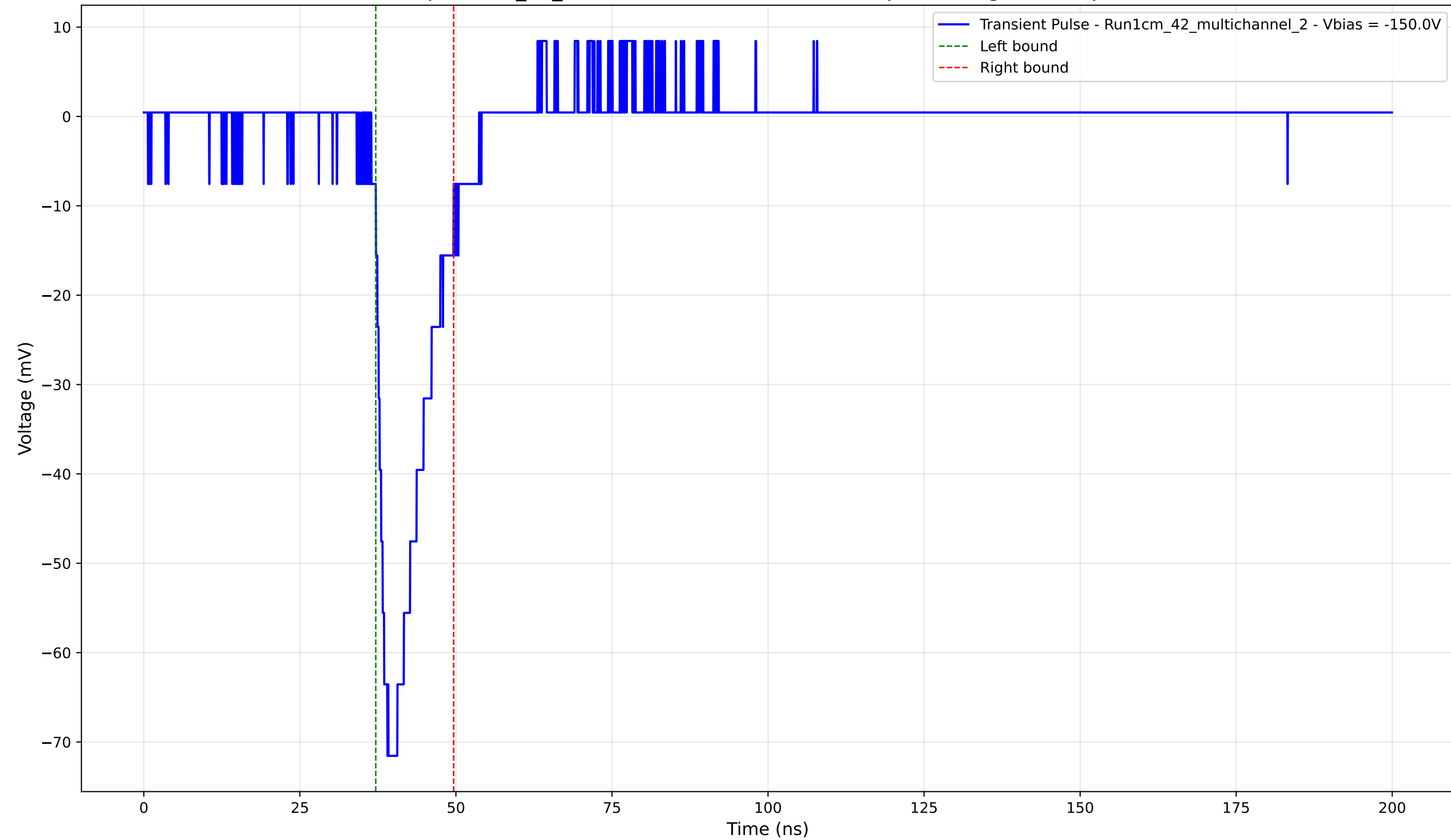
Transient Pulse - Sample: 1cm_42_multichannel - Position: 4605.0 \mu\text{m} - Charge: 10.34 pC - Rise Time: 2.56 ns
