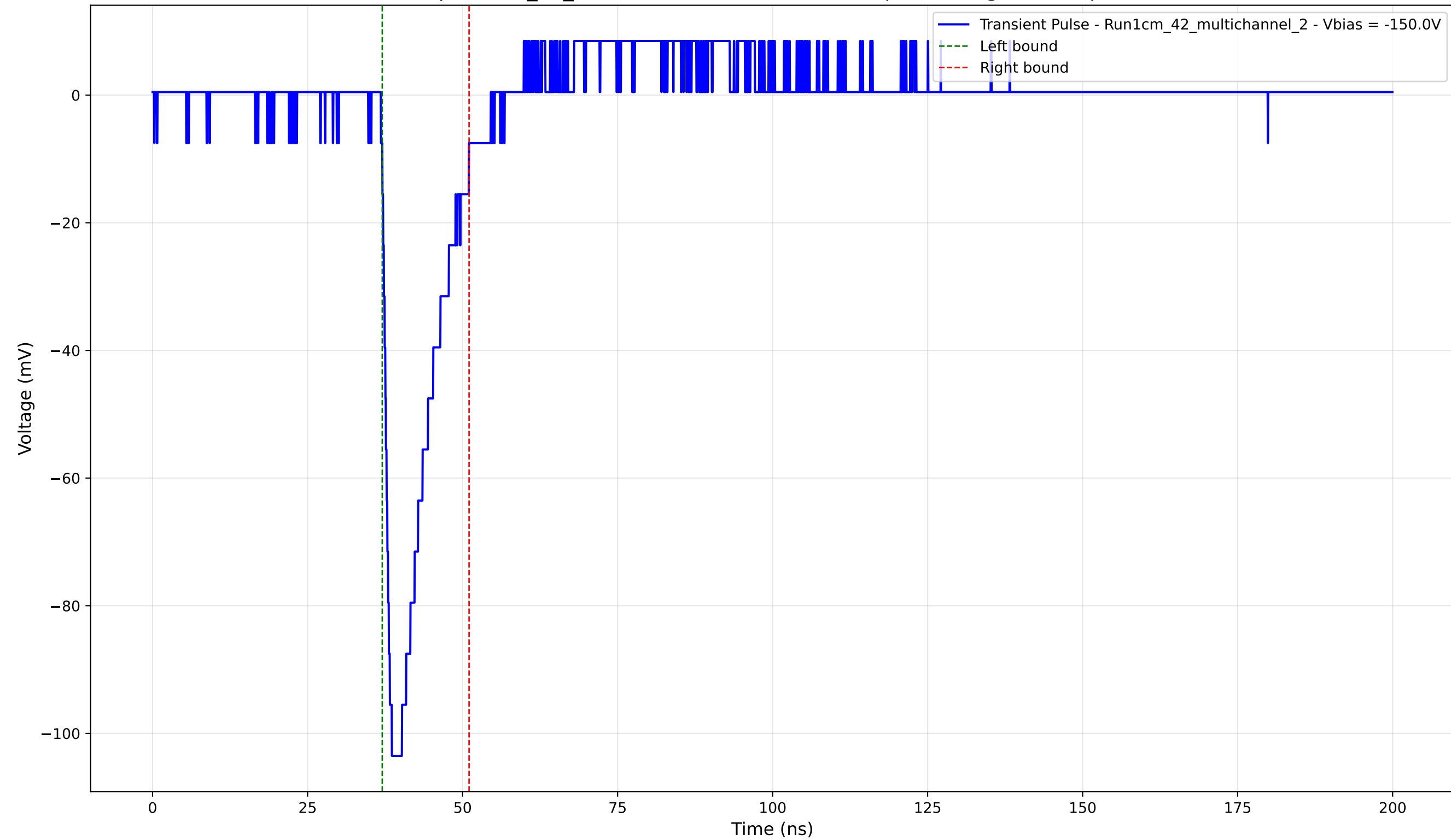
Transient Pulse - Sample: 1cm_42_multichannel - Position: 700.0 \mu\text{m} - Charge: 15.35 pC - Rise Time: 1.23 ns
