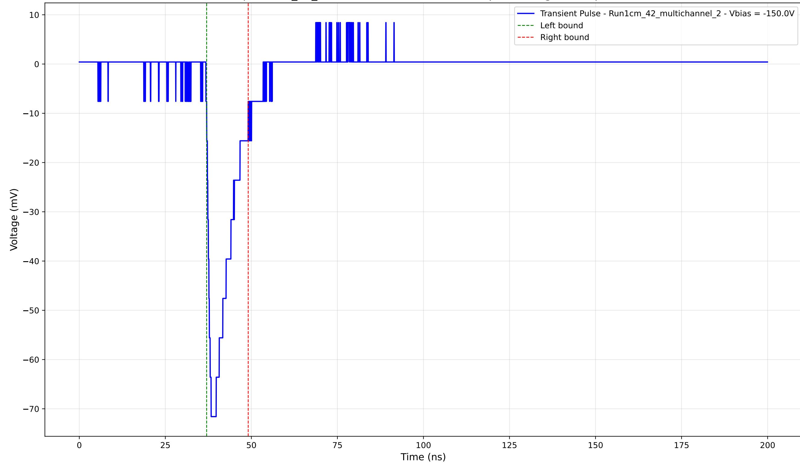
Transient Pulse - Sample: 1cm_42_multichannel - Position: 905.0 \mu\text{m} - Charge: 9.63 pC - Rise Time: 1.52 ns
