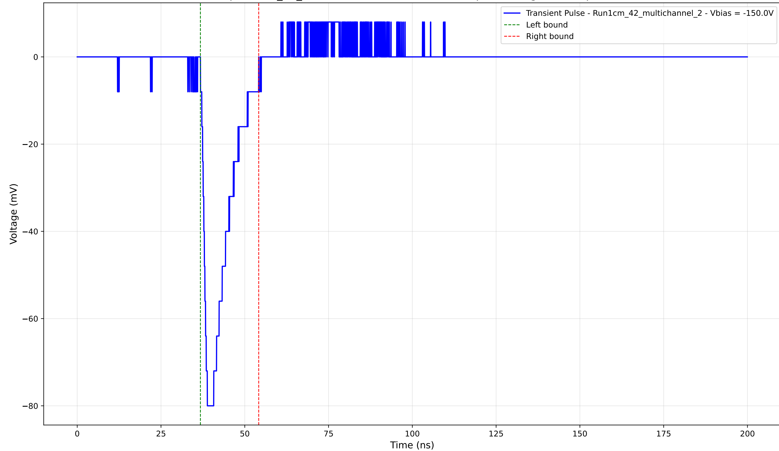
Transient Pulse - Sample: 1cm_42_multichannel - Position: 4240.0 \mu\text{m} - Charge: 12.63 pC - Rise Time: 1.36 ns
