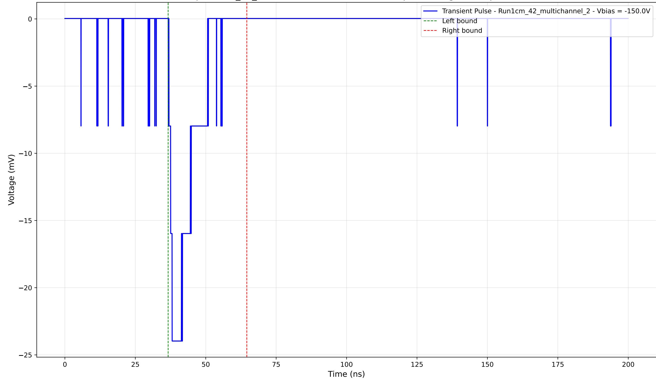
Transient Pulse - Sample: 1cm_42_multichannel - Position: 3925.0 \mu\text{m} - Charge: 3.96 pC - Rise Time: 1.15 ns
