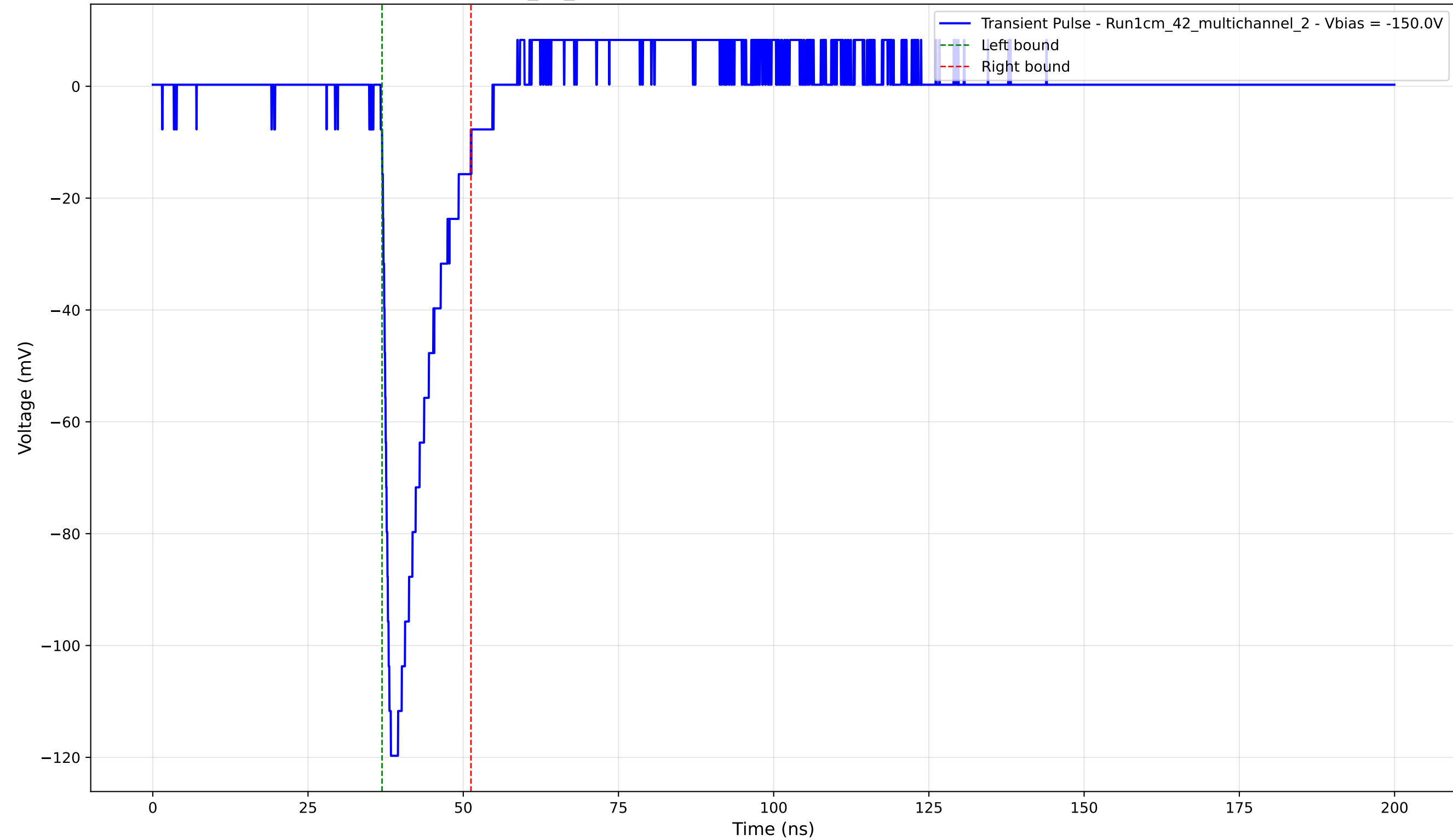
Transient Pulse - Sample: 1cm_42_multichannel - Position: 940.0 \mu\text{m} - Charge: 16.67 pC - Rise Time: 1.18 ns
