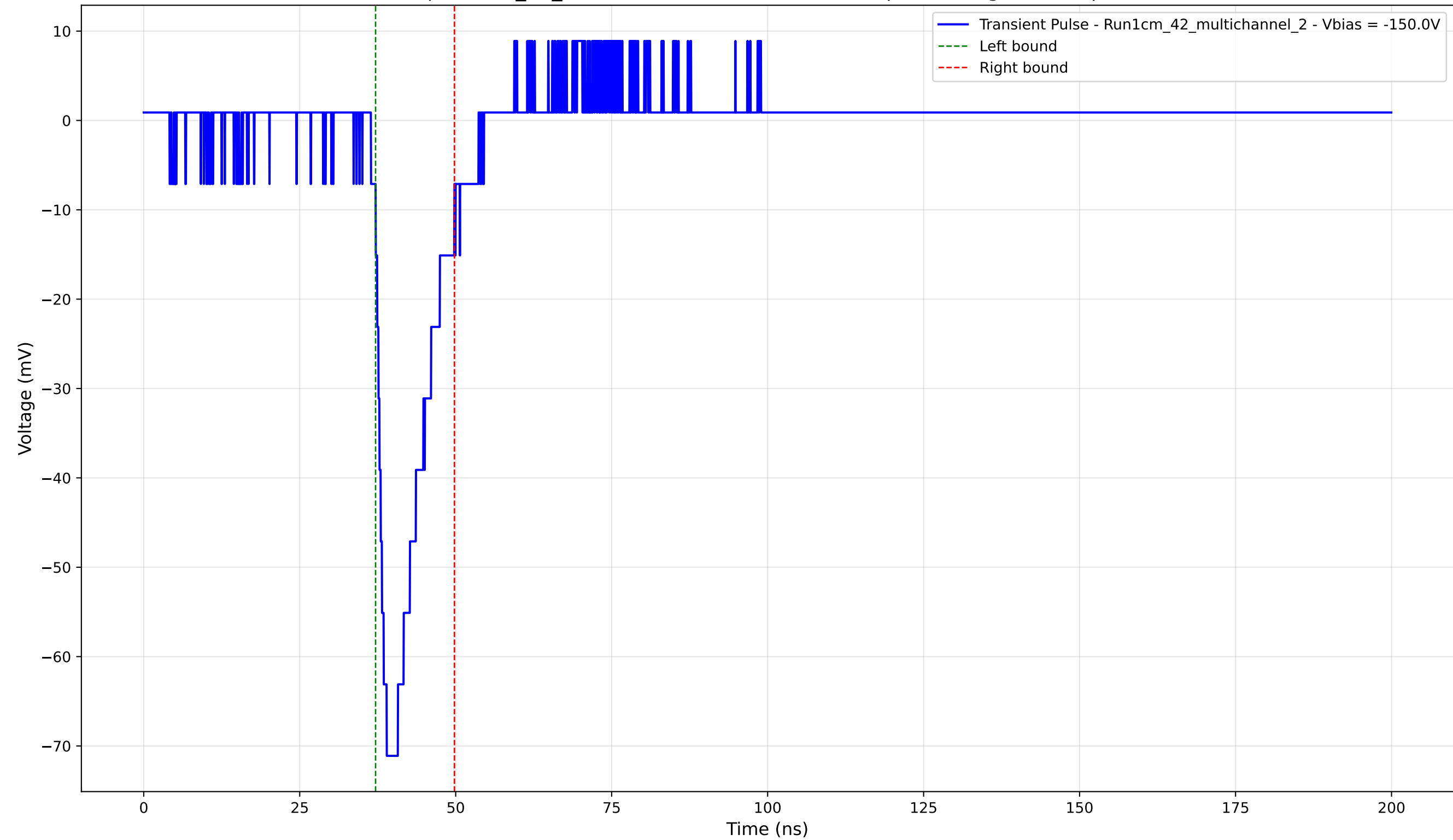
Transient Pulse - Sample: 1cm_42_multichannel - Position: 4610.0 \mu\text{m} - Charge: 10.32 pC - Rise Time: 1.80 ns
