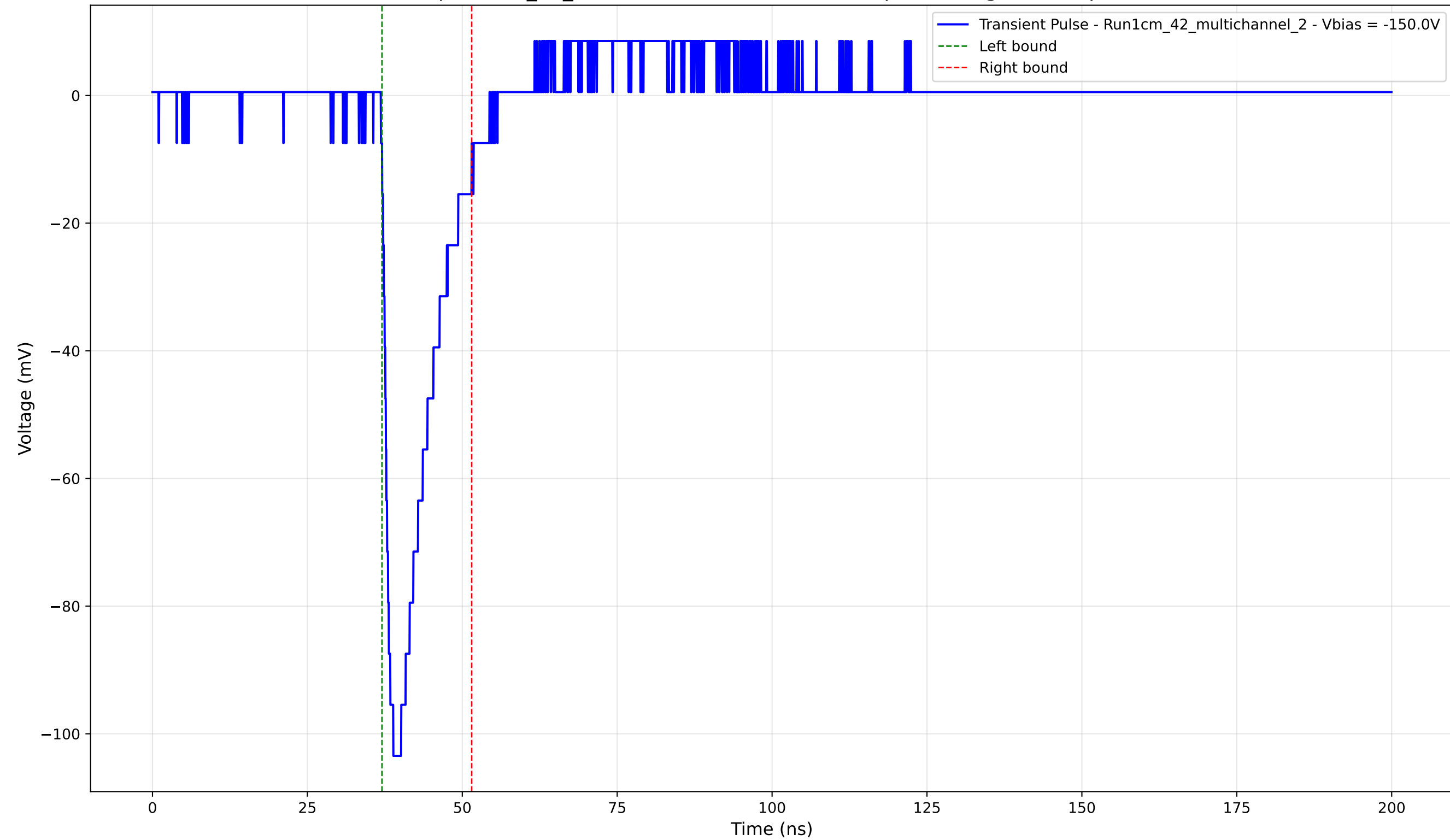
Transient Pulse - Sample: 1cm_42_multichannel - Position: 670.0 \mu\text{m} - Charge: 15.31 pC - Rise Time: 1.35 ns
