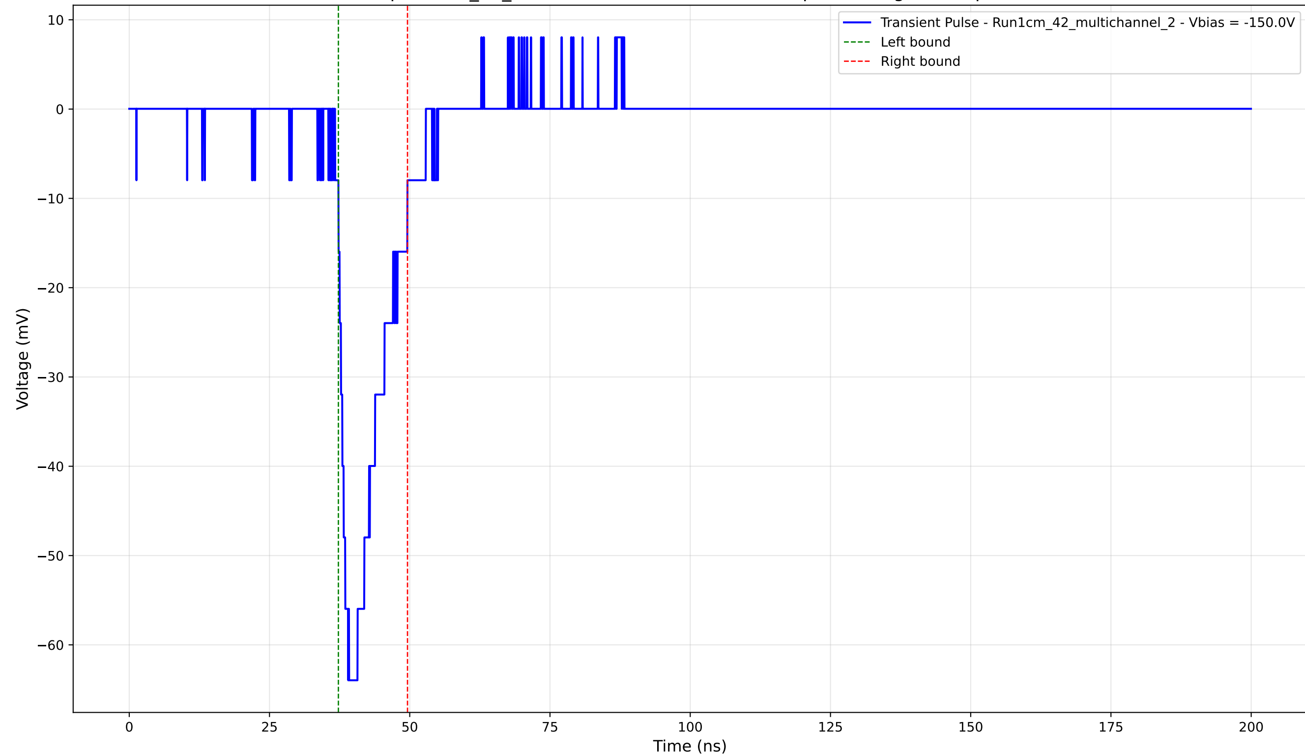
Transient Pulse - Sample: 1cm_42_multichannel - Position: 4315.0 \mu\text{m} - Charge: 9.22 pC - Rise Time: 2.33 ns
