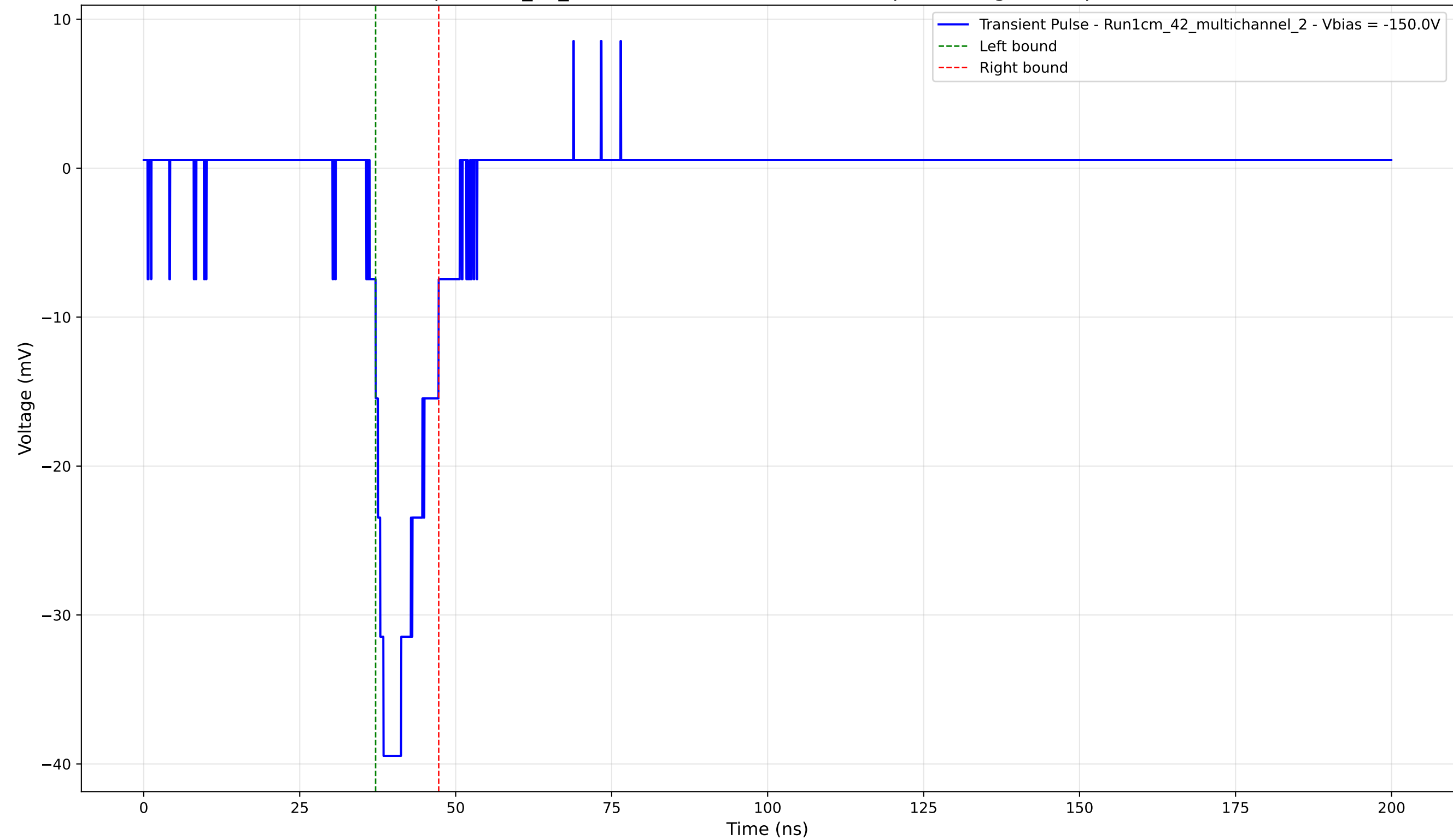
Transient Pulse - Sample: 1cm_42_multichannel - Position: 4840.0 \mu\text{m} - Charge: 5.55 pC - Rise Time: 2.22 ns
