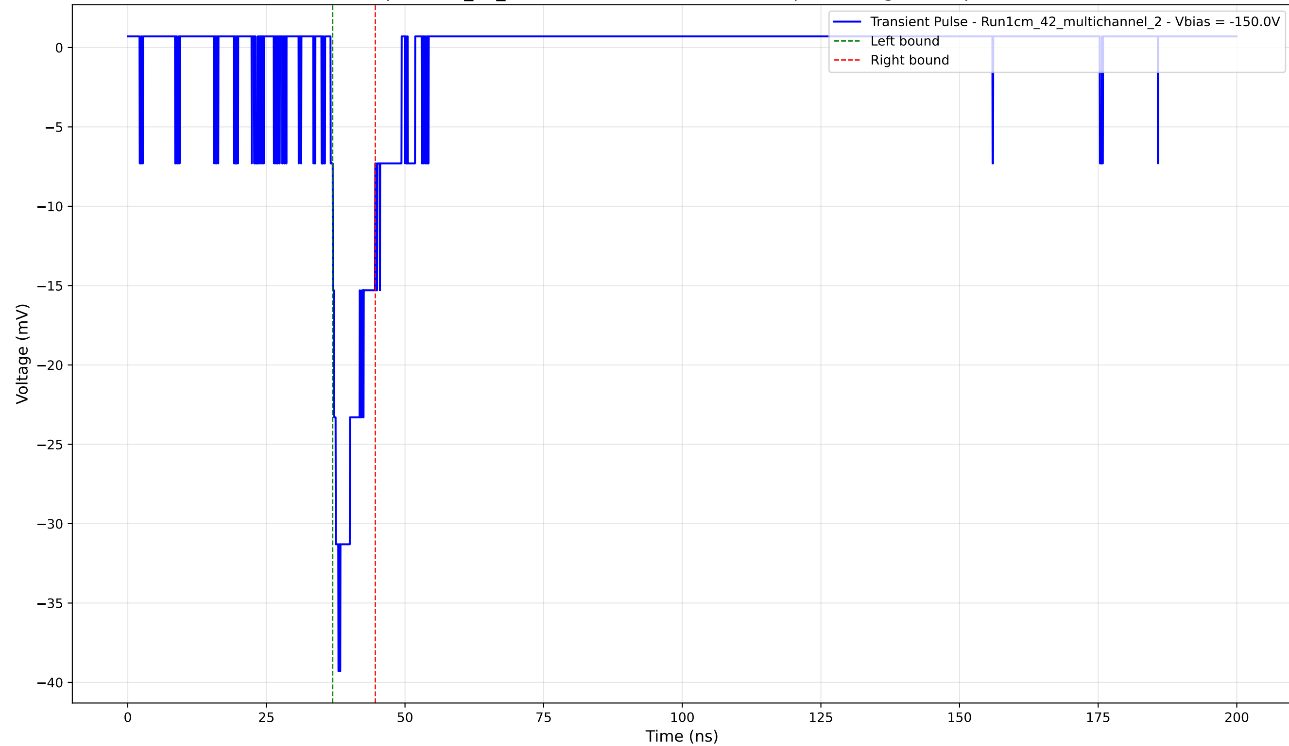
Transient Pulse - Sample: 1cm_42_multichannel - Position: 3420.0 \mu\text{m} - Charge: 3.59 pC - Rise Time: 1.42 ns
