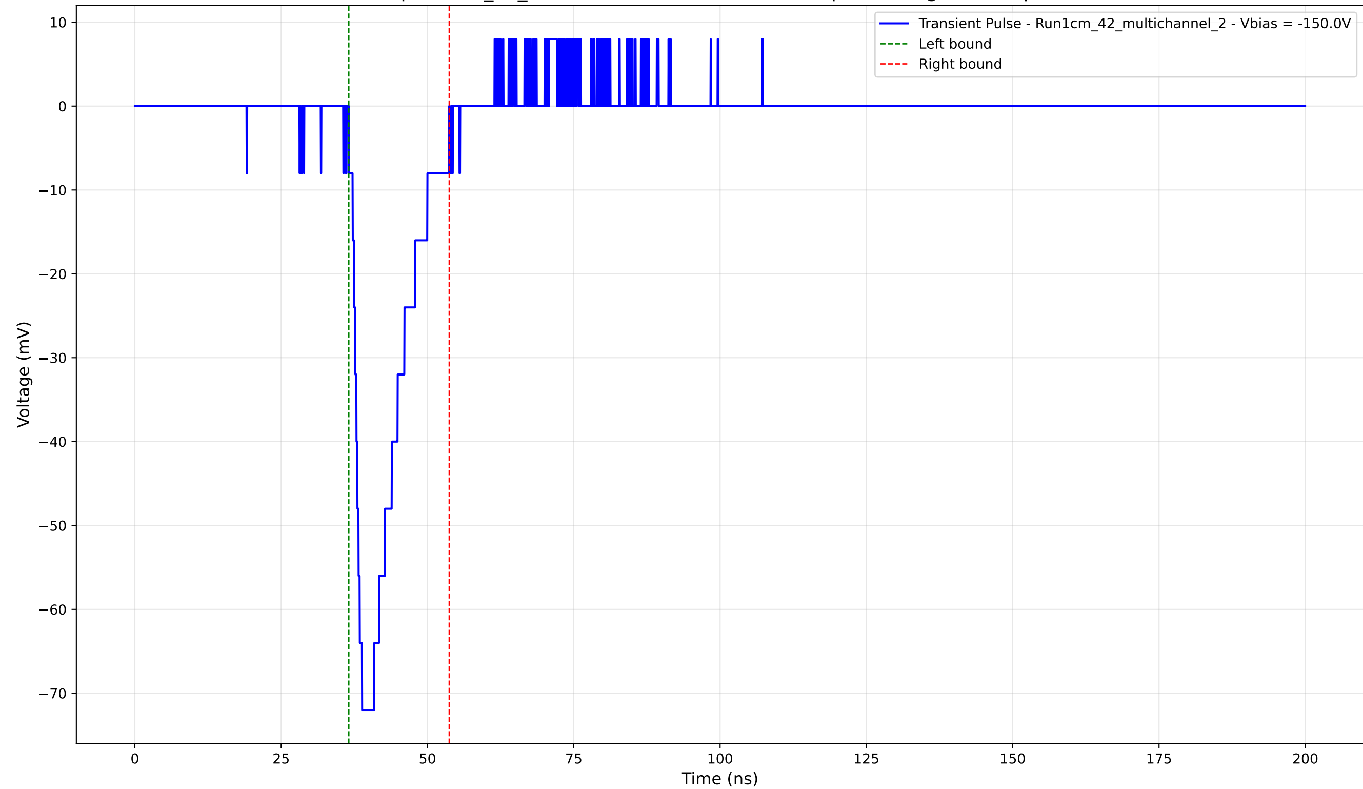
Transient Pulse - Sample: 1cm_42_multichannel - Position: 4285.0 \mu\text{m} - Charge: 11.45 pC - Rise Time: 2.24 ns
