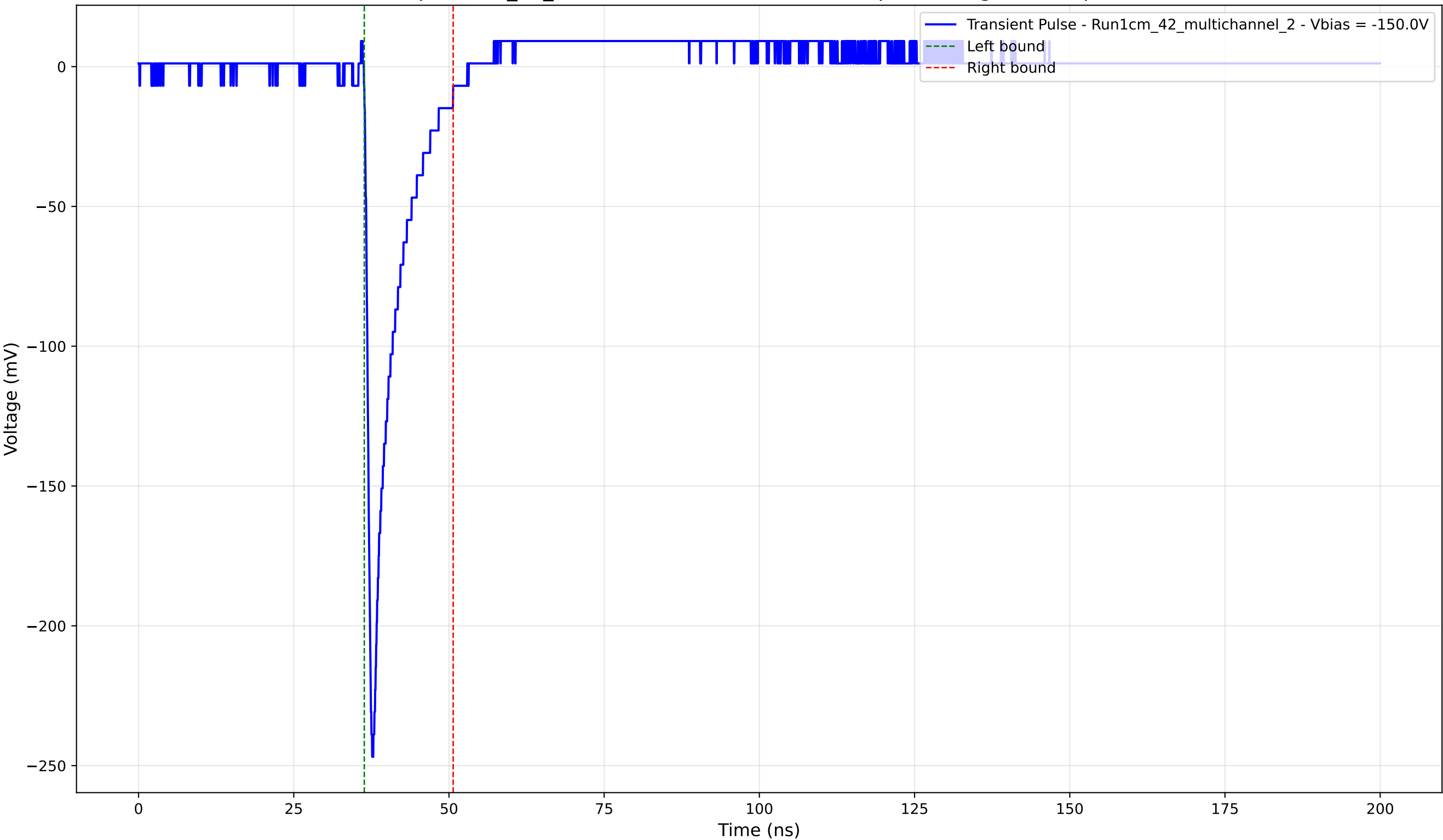
Transient Pulse - Sample: 1cm_42_multichannel - Position: 1625.0 \mu\text{m} - Charge: 21.87 pC - Rise Time: 0.91 ns
