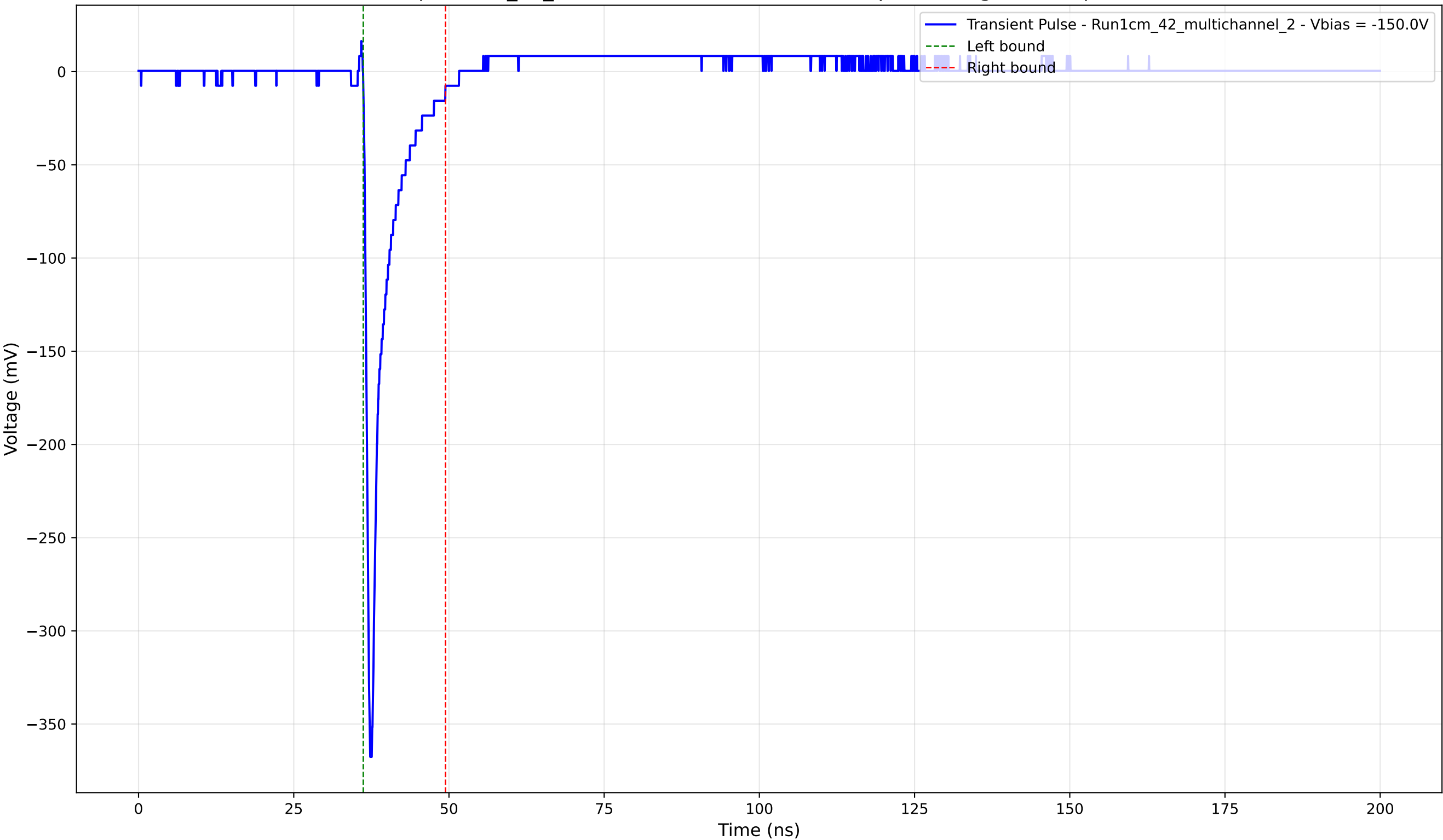
Transient Pulse - Sample: 1cm_42_multichannel - Position: 1950.0 \mu\text{m} - Charge: 23.62 pC - Rise Time: 0.79 ns
