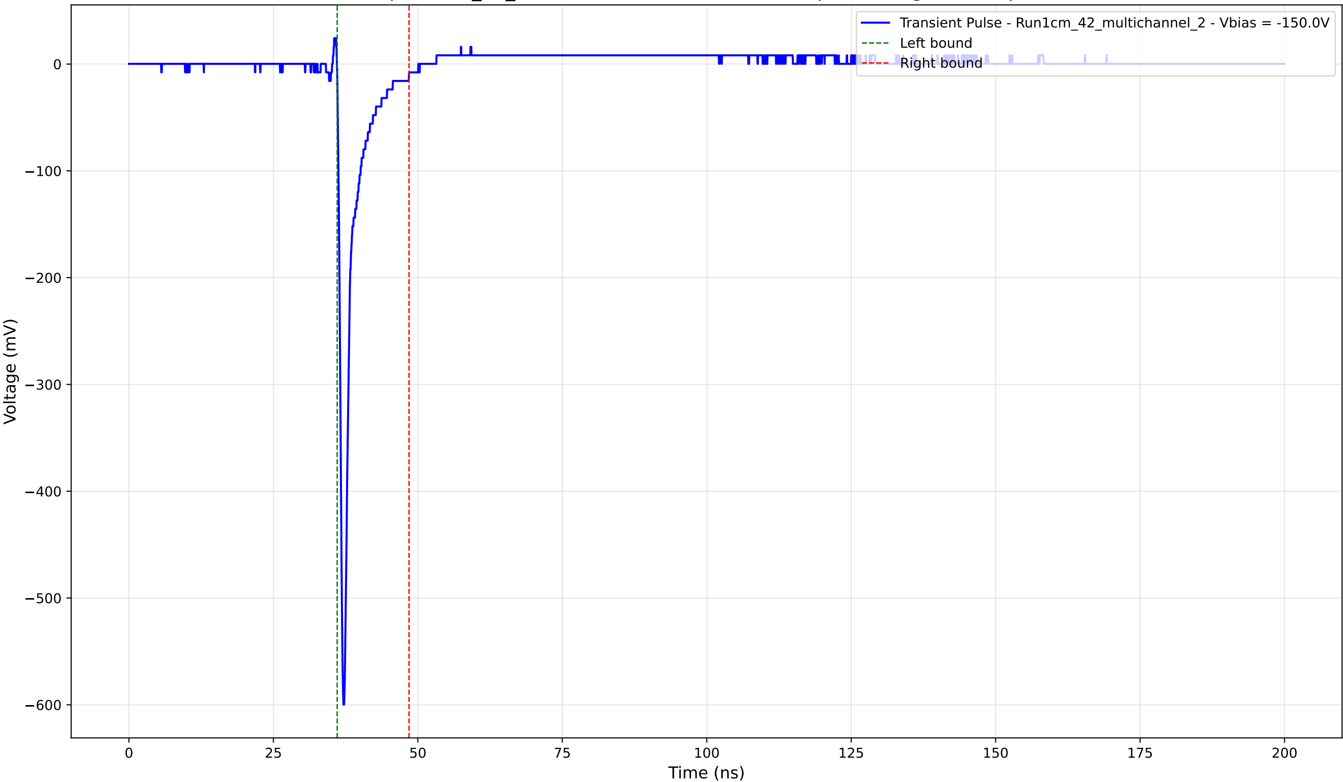
Transient Pulse - Sample: 1cm_42_multichannel - Position: 2490.0 \mu\text{m} - Charge: 27.81 pC - Rise Time: 0.72 ns
