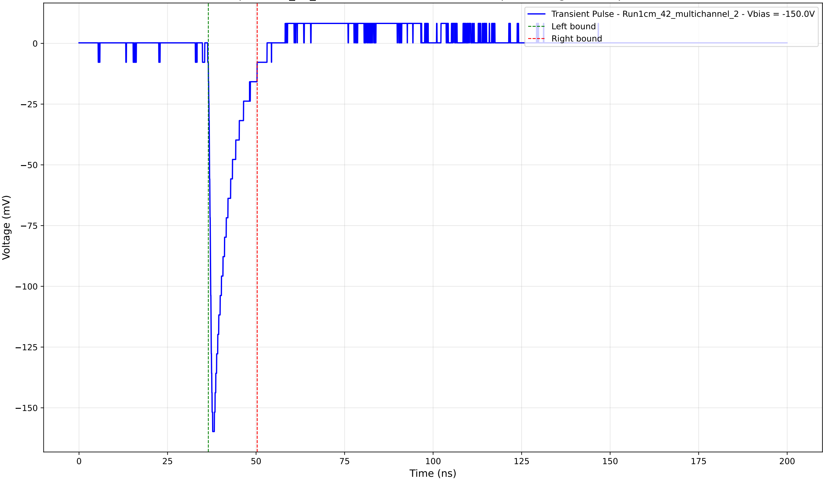
Transient Pulse - Sample: 1cm_42_multichannel - Position: 3300.0 \mu\text{m} - Charge: 17.21 pC - Rise Time: 1.00 ns
