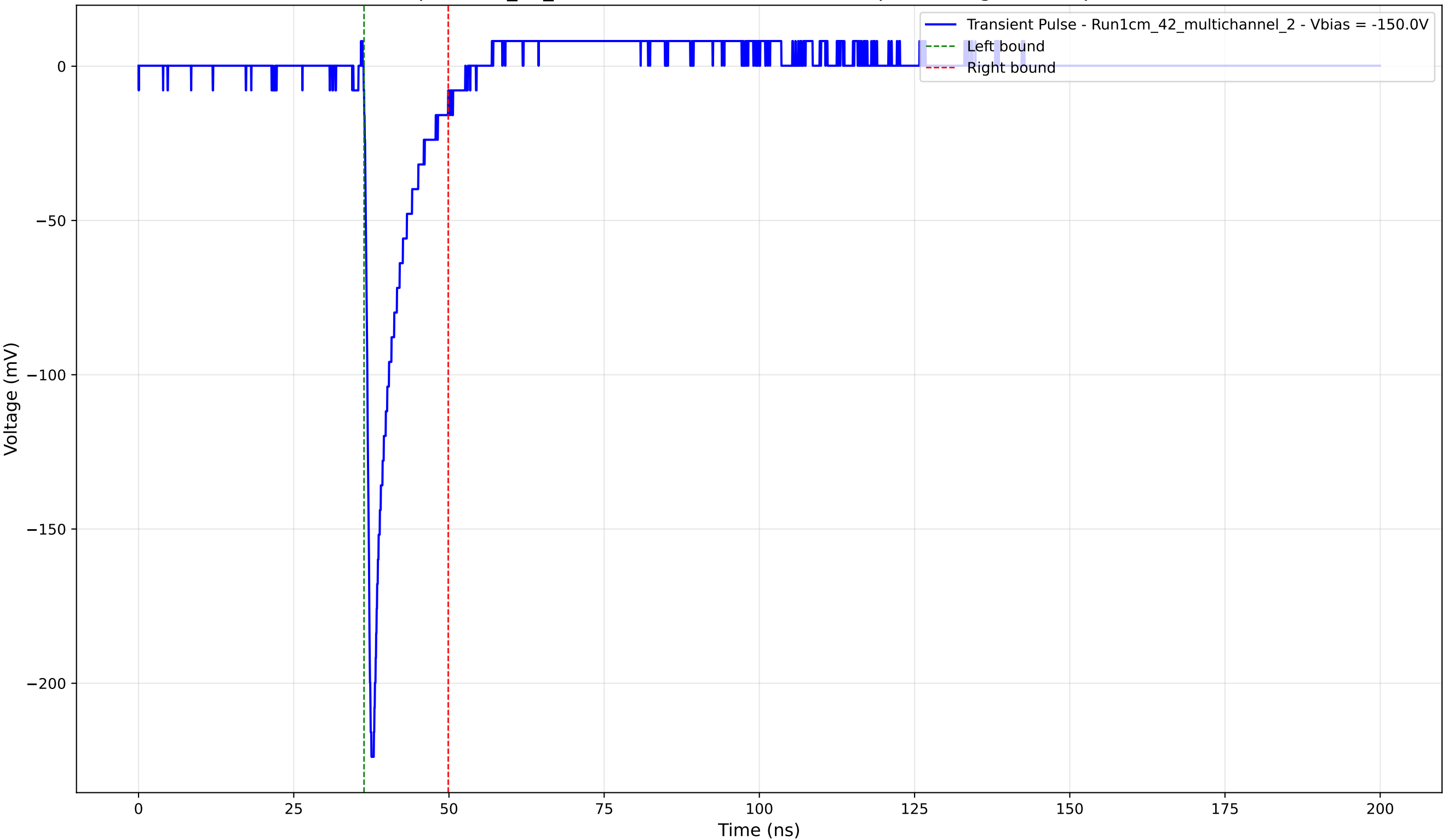
Transient Pulse - Sample: 1cm_42_multichannel - Position: 3070.0 \mu\text{m} - Charge: 19.58 pC - Rise Time: 0.90 ns
