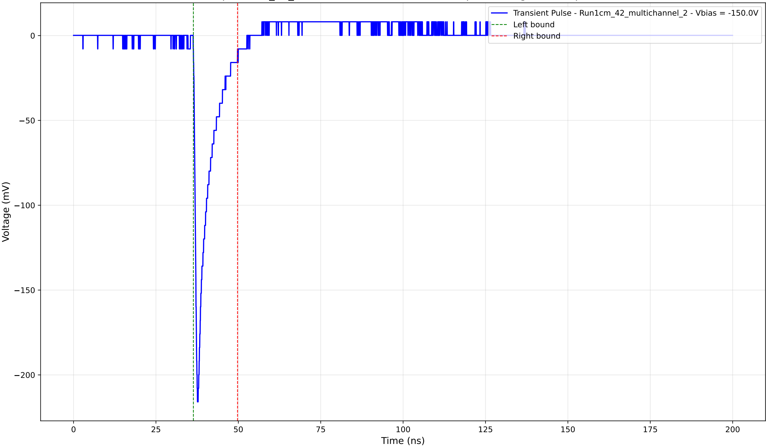
Transient Pulse - Sample: 1cm_42_multichannel - Position: 3100.0 \mu\text{m} - Charge: 19.04 pC - Rise Time: 0.97 ns
