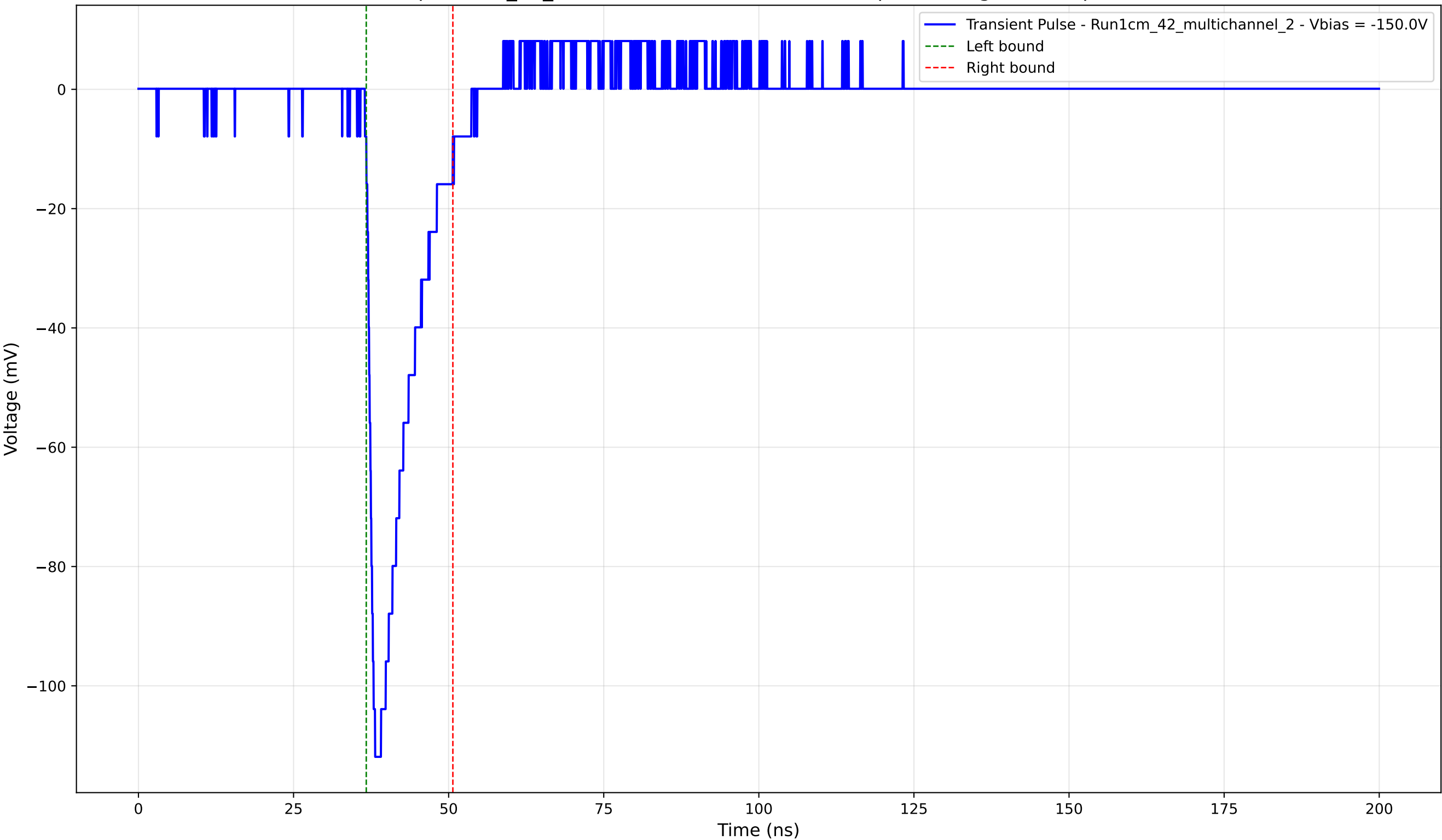
Transient Pulse - Sample: 1cm_42_multichannel - Position: 3620.0 \mu\text{m} - Charge: 14.97 pC - Rise Time: 1.18 ns
