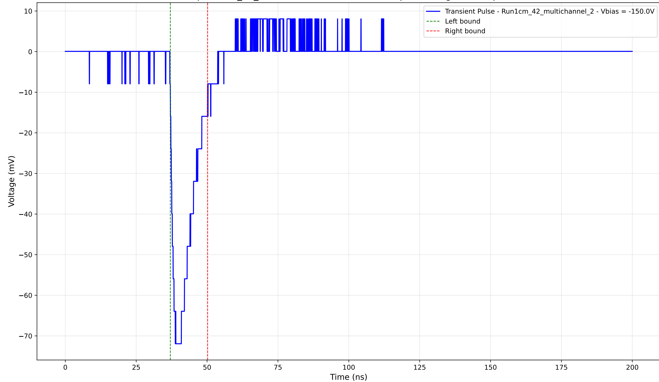
Transient Pulse - Sample: 1cm_42_multichannel - Position: 235.0 \mu\text{m} - Charge: 11.37 pC - Rise Time: 1.92 ns
