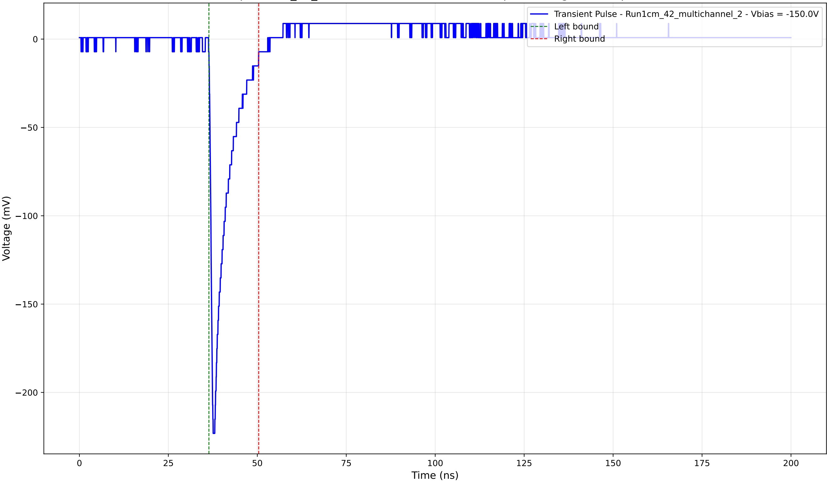
Transient Pulse - Sample: 1cm_42_multichannel - Position: 1565.0 \mu\text{m} - Charge: 21.39 pC - Rise Time: 0.92 ns
