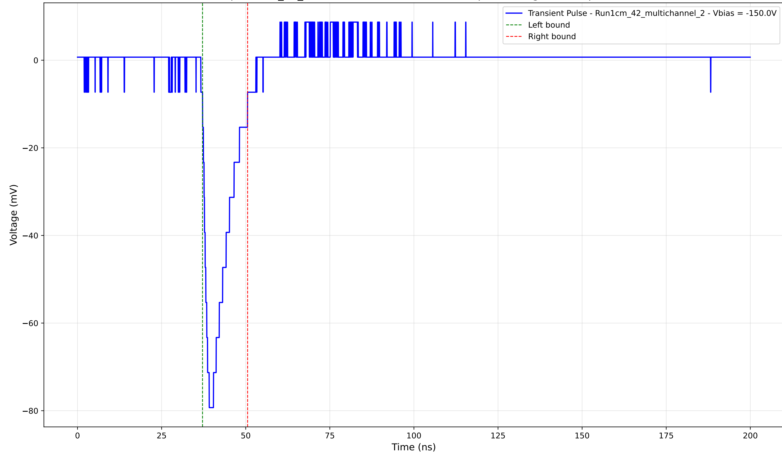
Transient Pulse - Sample: 1cm_42_multichannel - Position: 4260.0 \mu\text{m} - Charge: 11.43 pC - Rise Time: 2.00 ns
