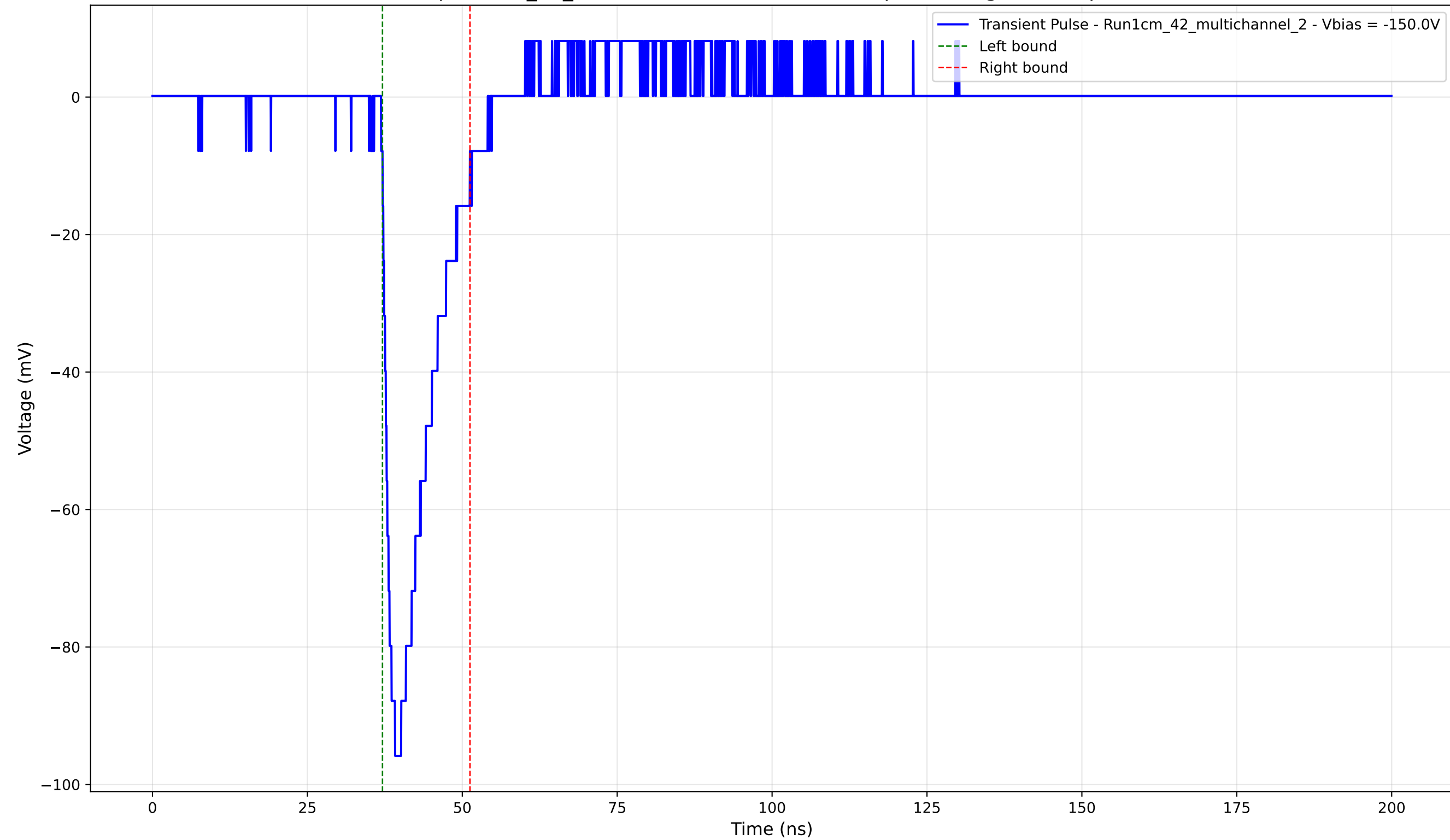
Transient Pulse - Sample: 1cm_42_multichannel - Position: 485.0 \mu\text{m} - Charge: 14.16 pC - Rise Time: 1.47 ns
