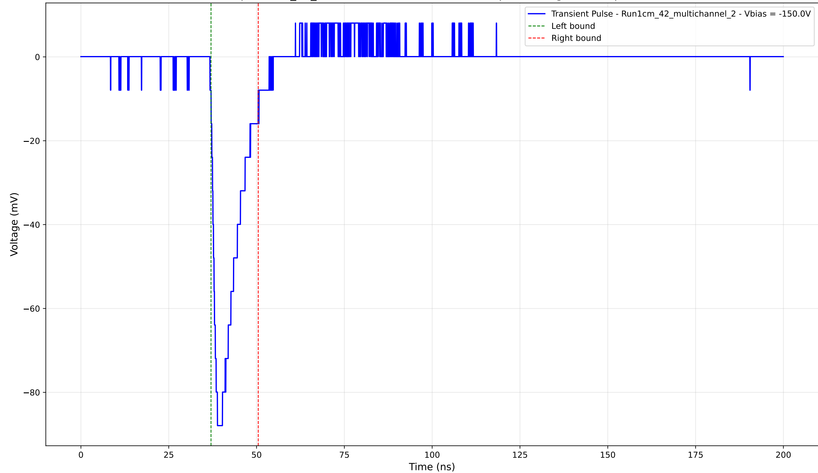
Transient Pulse - Sample: 1cm_42_multichannel - Position: 4070.0 \mu\text{m} - Charge: 12.75 pC - Rise Time: 1.48 ns
