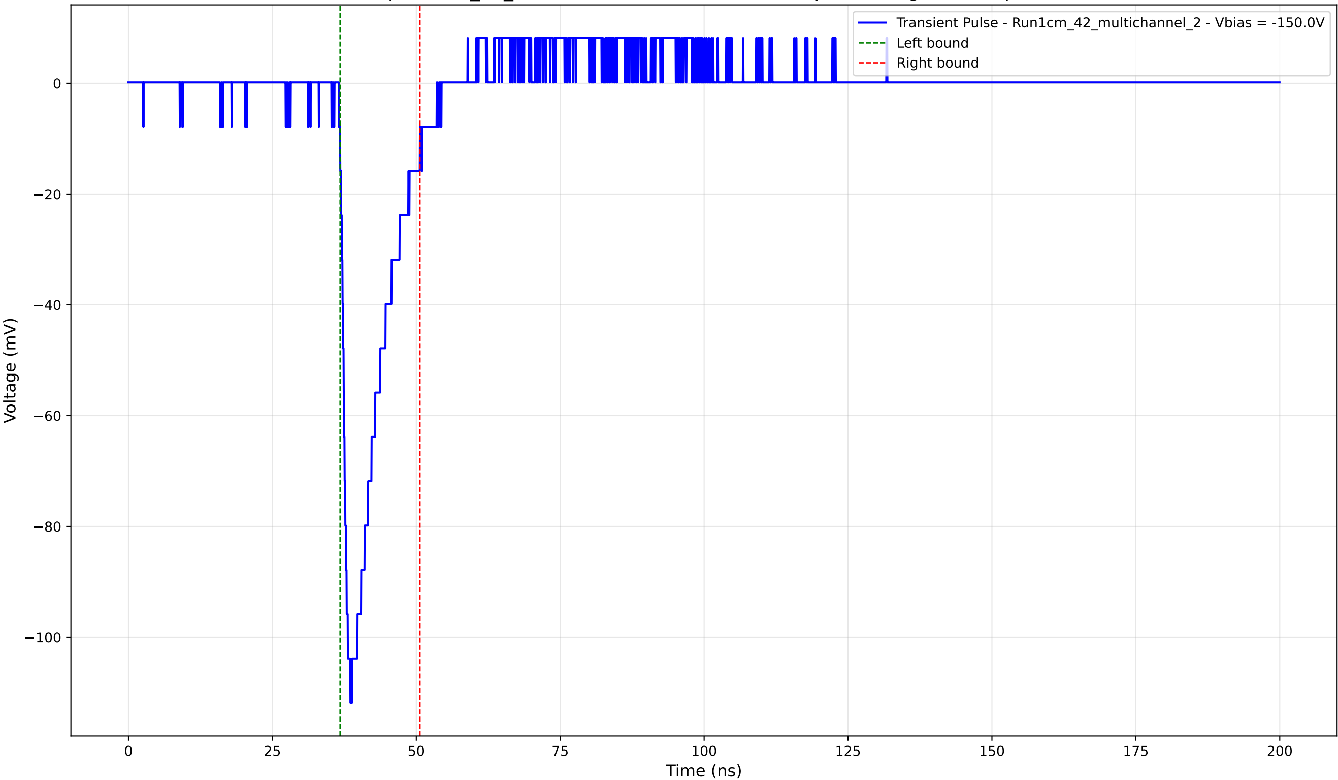
Transient Pulse - Sample: 1cm_42_multichannel - Position: 3695.0 \mu\text{m} - Charge: 14.94 pC - Rise Time: 1.34 ns
