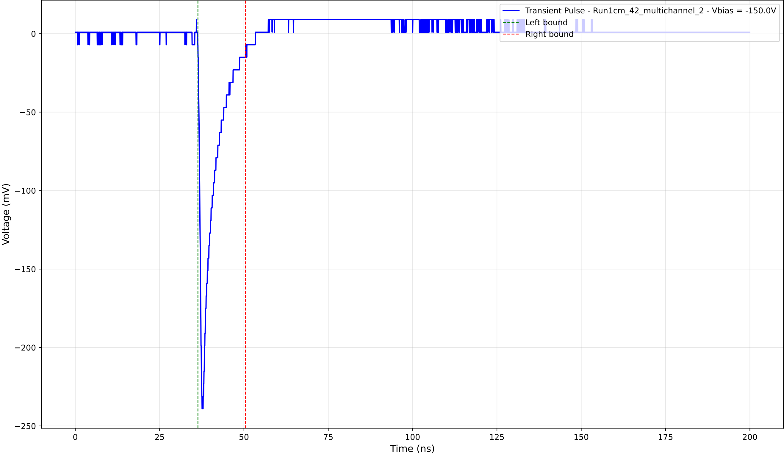
Transient Pulse - Sample: 1cm_42_multichannel - Position: 1610.0 \mu\text{m} - Charge: 21.68 pC - Rise Time: 0.92 ns
