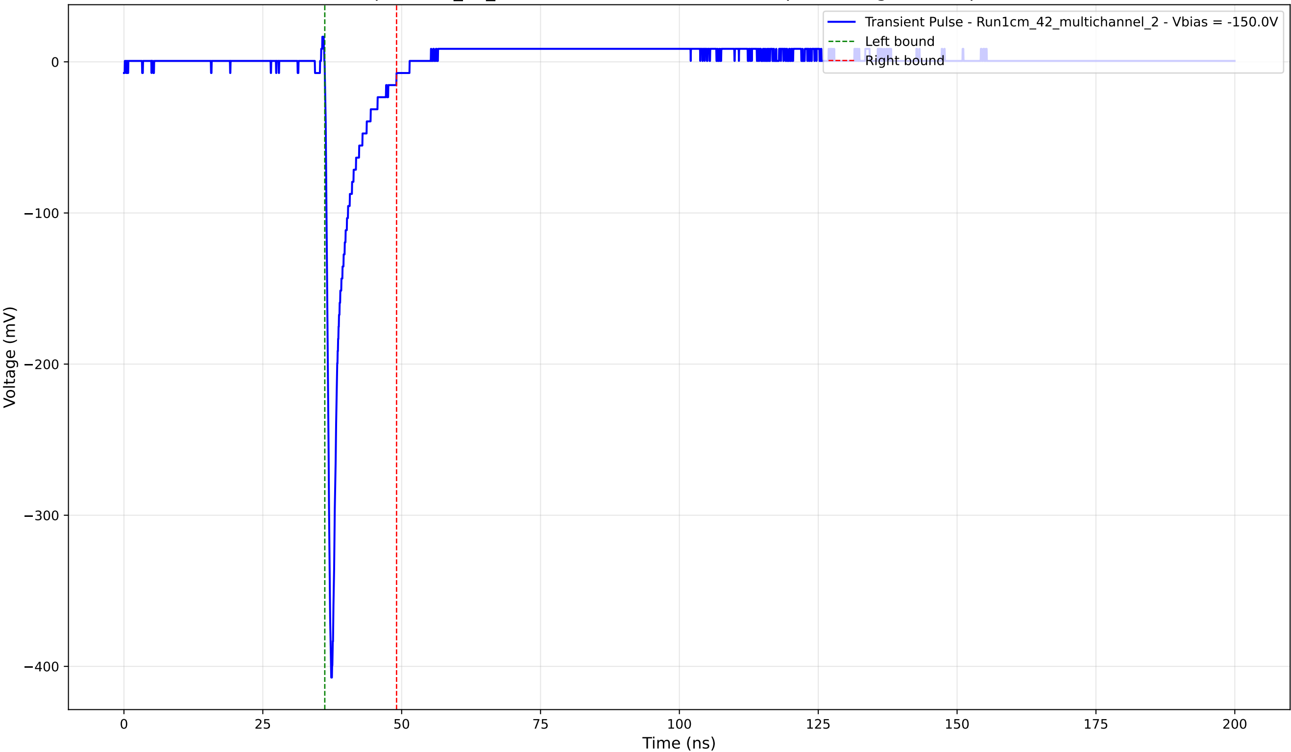
Transient Pulse - Sample: 1cm_42_multichannel - Position: 2745.0 \mu\text{m} - Charge: 24.37 pC - Rise Time: 0.79 ns
