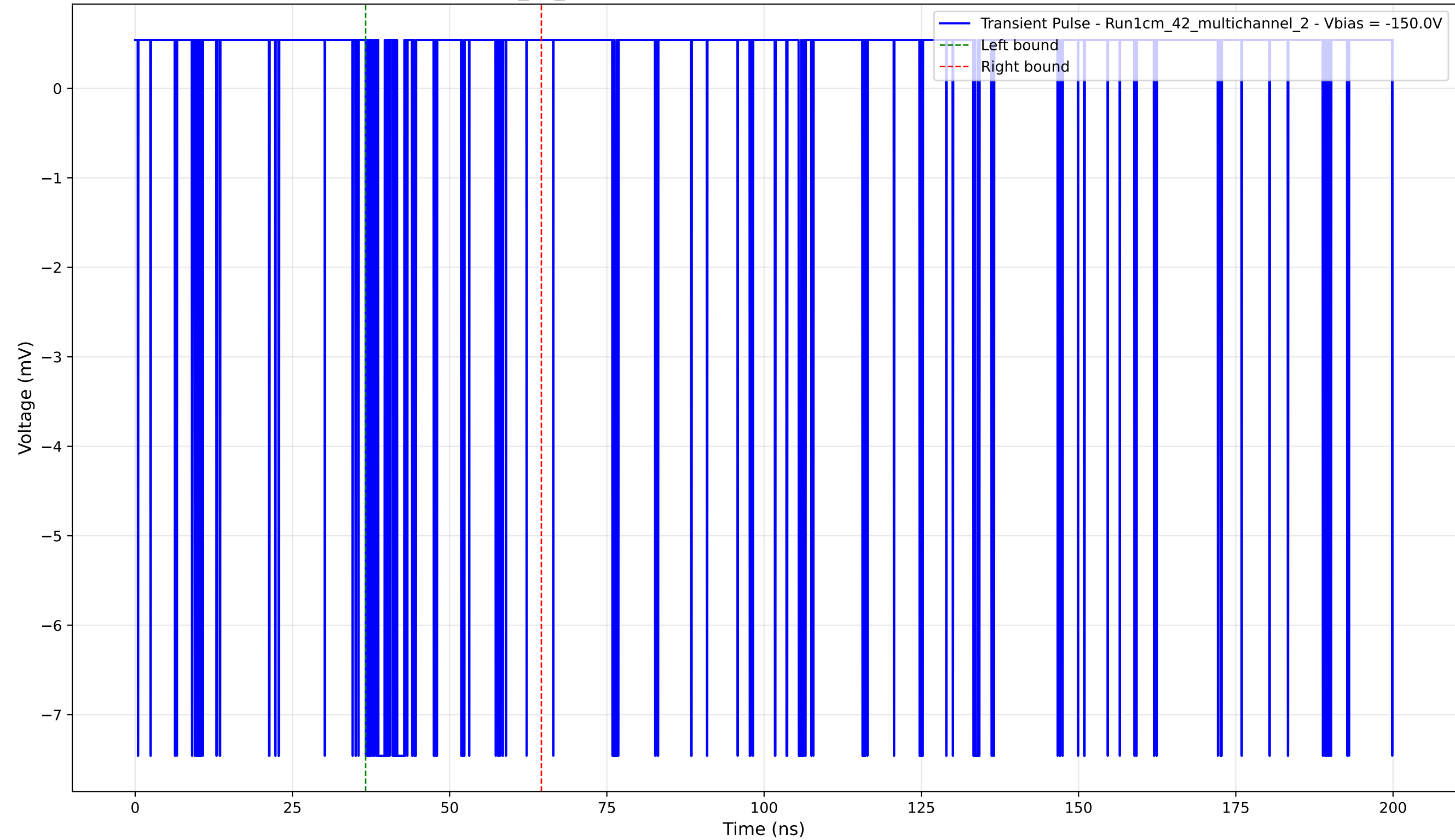
Transient Pulse - Sample: 1cm_42_multichannel - Position: 4920.0 \mu\text{m} - Charge: 0.59 pC - Rise Time: 0.04 ns
