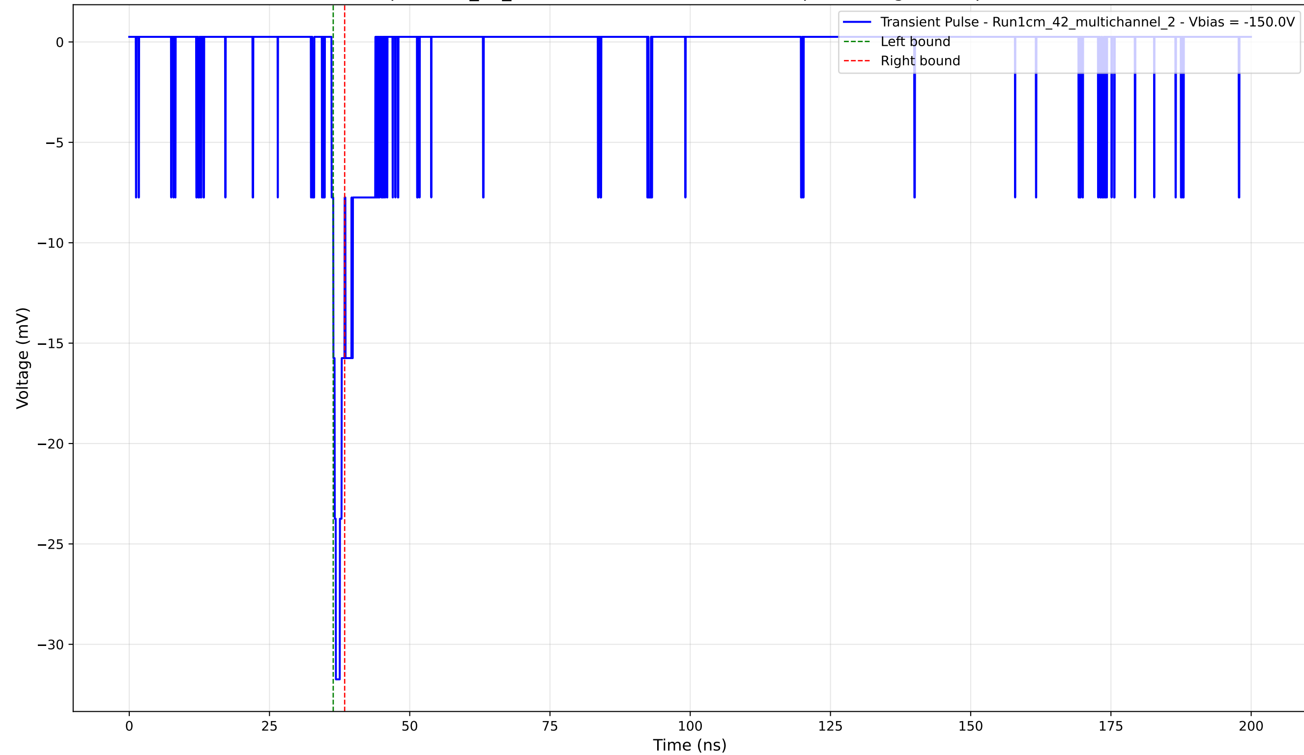
Transient Pulse - Sample: 1cm_42_multichannel - Position: 2355.0 \mu\text{m} - Charge: 0.95 pC - Rise Time: 0.78 ns
