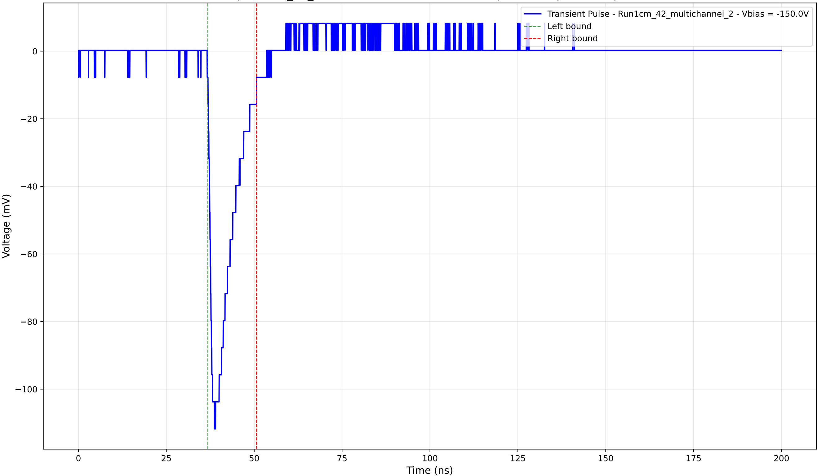
Transient Pulse - Sample: 1cm_42_multichannel - Position: 3735.0 \mu\text{m} - Charge: 15.05 pC - Rise Time: 1.30 ns
