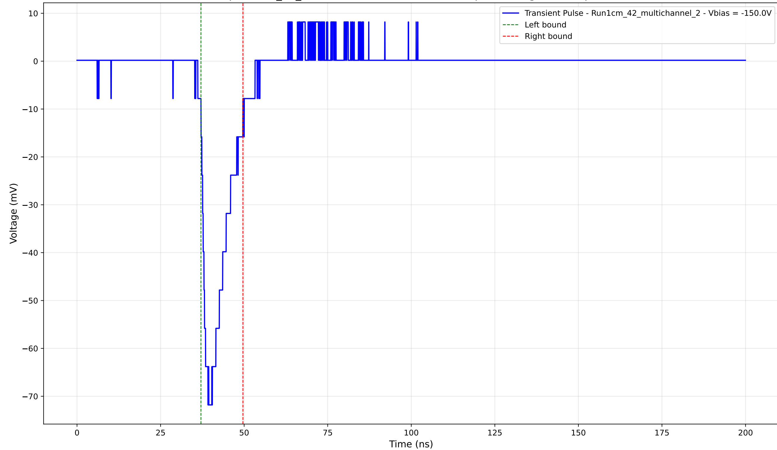
Transient Pulse - Sample: 1cm_42_multichannel - Position: 4695.0 \mu\text{m} - Charge: 10.36 pC - Rise Time: 3.04 ns
