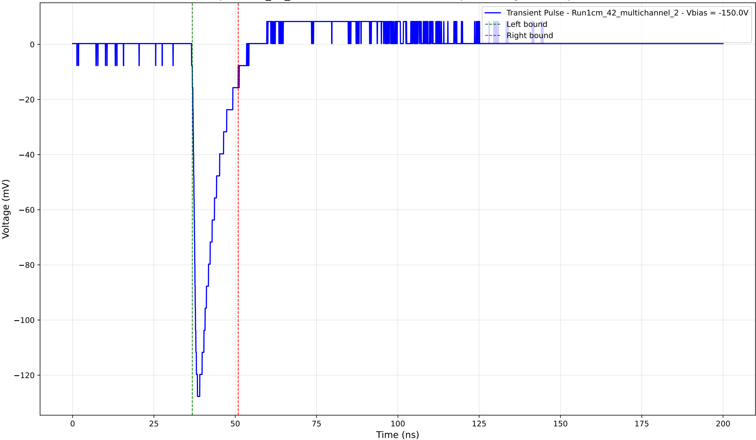
Transient Pulse - Sample: 1cm_42_multichannel - Position: 1030.0 \mu\text{m} - Charge: 17.04 pC - Rise Time: 1.25 ns
