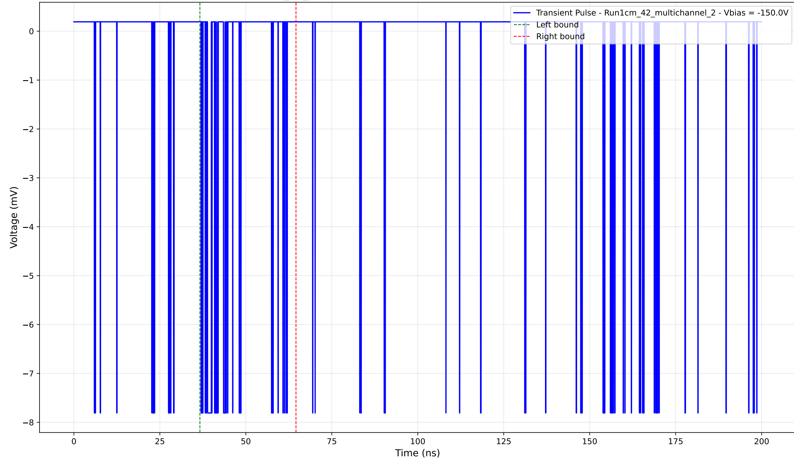
Transient Pulse - Sample: 1cm_42_multichannel - Position: 4895.0 \mu\text{m} - Charge: 0.62 pC - Rise Time: 0.04 ns
