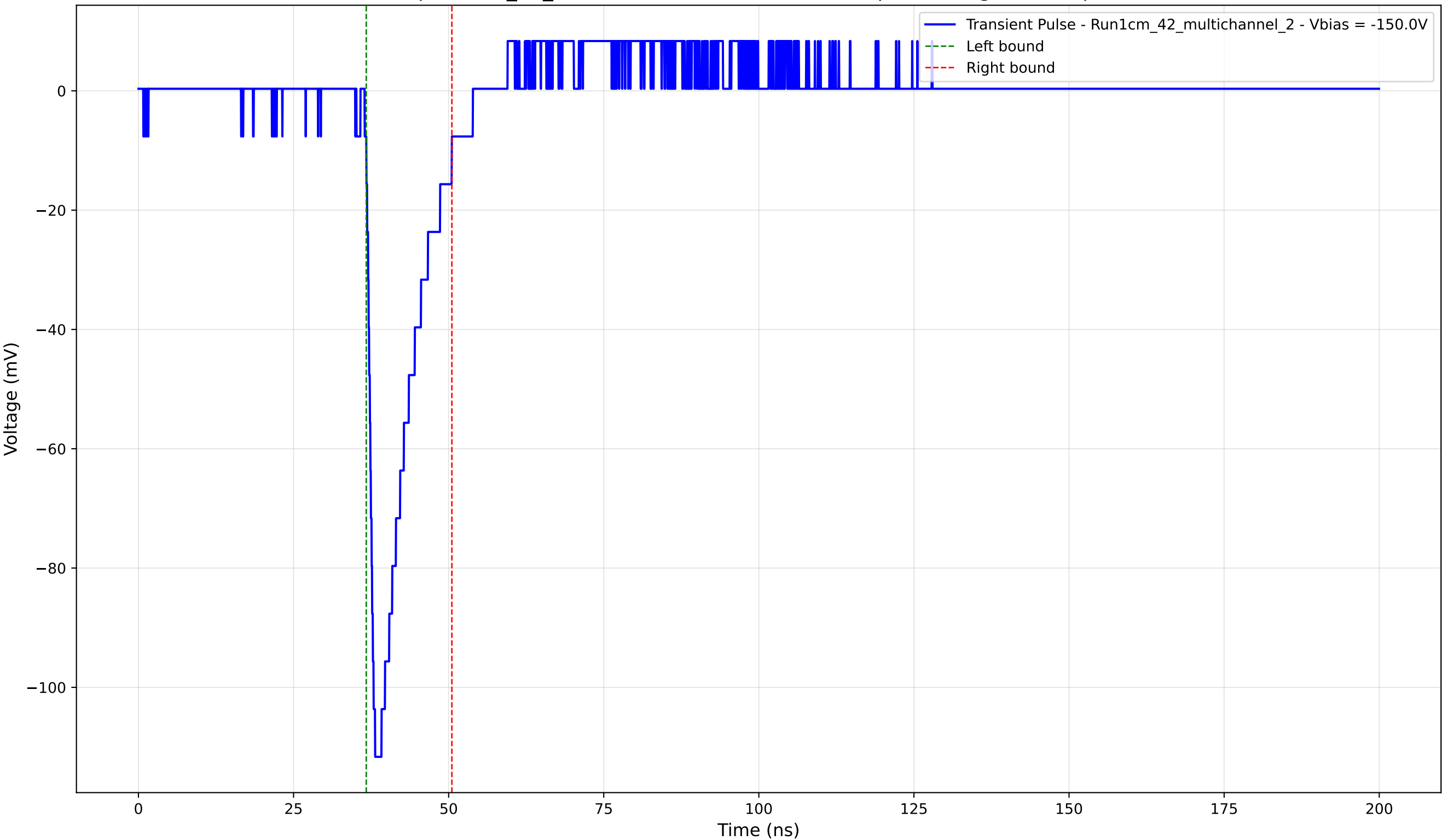
Transient Pulse - Sample: 1cm_42_multichannel - Position: 3630.0 \mu\text{m} - Charge: 14.92 pC - Rise Time: 1.18 ns
