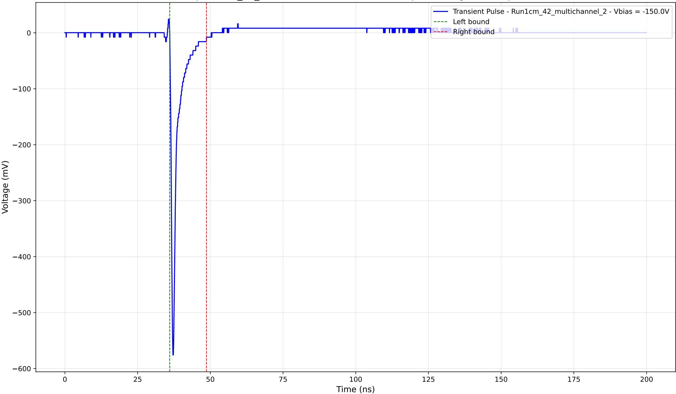
Transient Pulse - Sample: 1cm_42_multichannel - Position: 2200.0 \mu\text{m} - Charge: 28.01 pC - Rise Time: 0.75 ns
