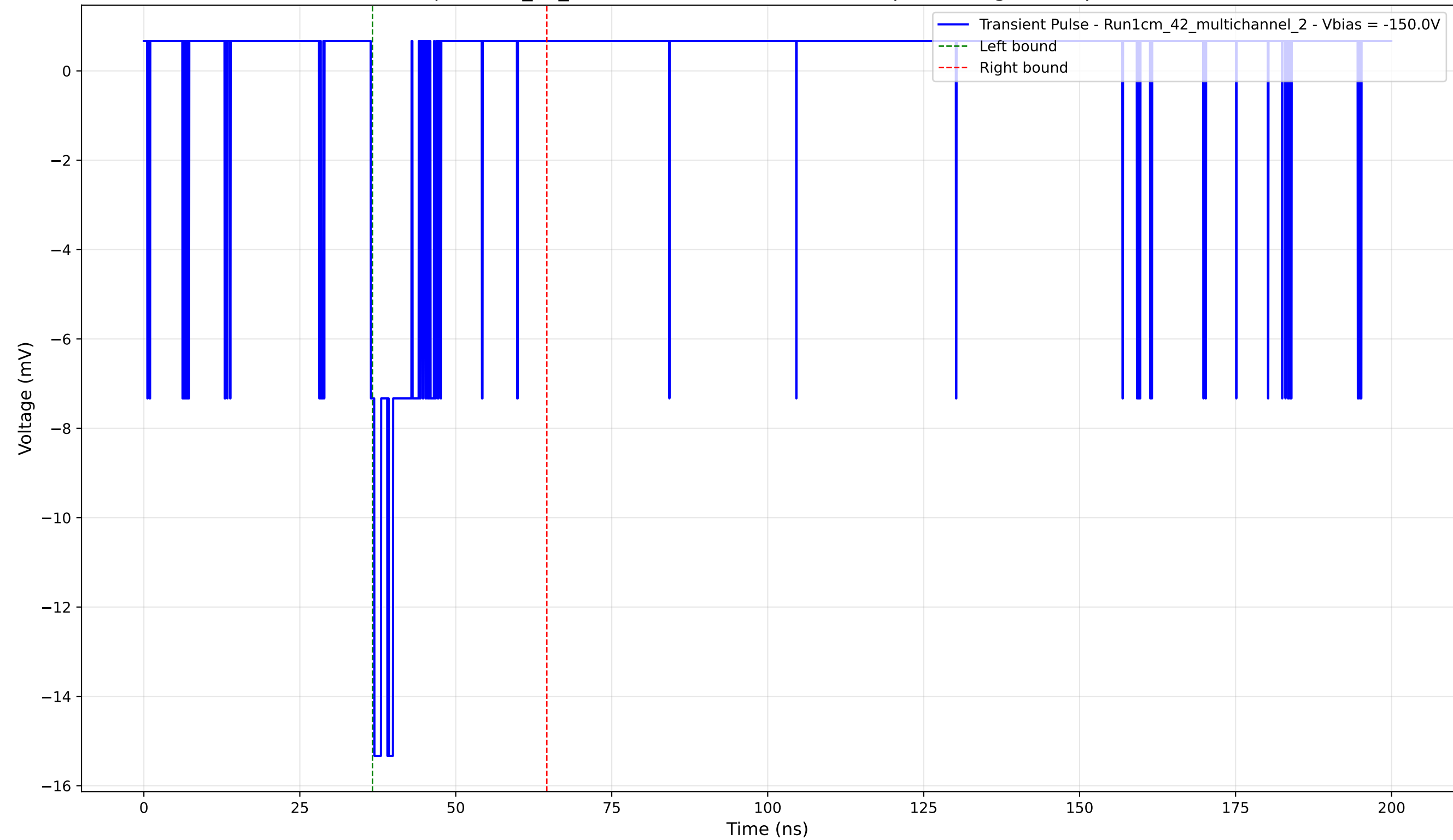
Transient Pulse - Sample: 1cm_42_multichannel - Position: 1870.0 \mu\text{m} - Charge: 1.39 pC - Rise Time: 0.59 ns
