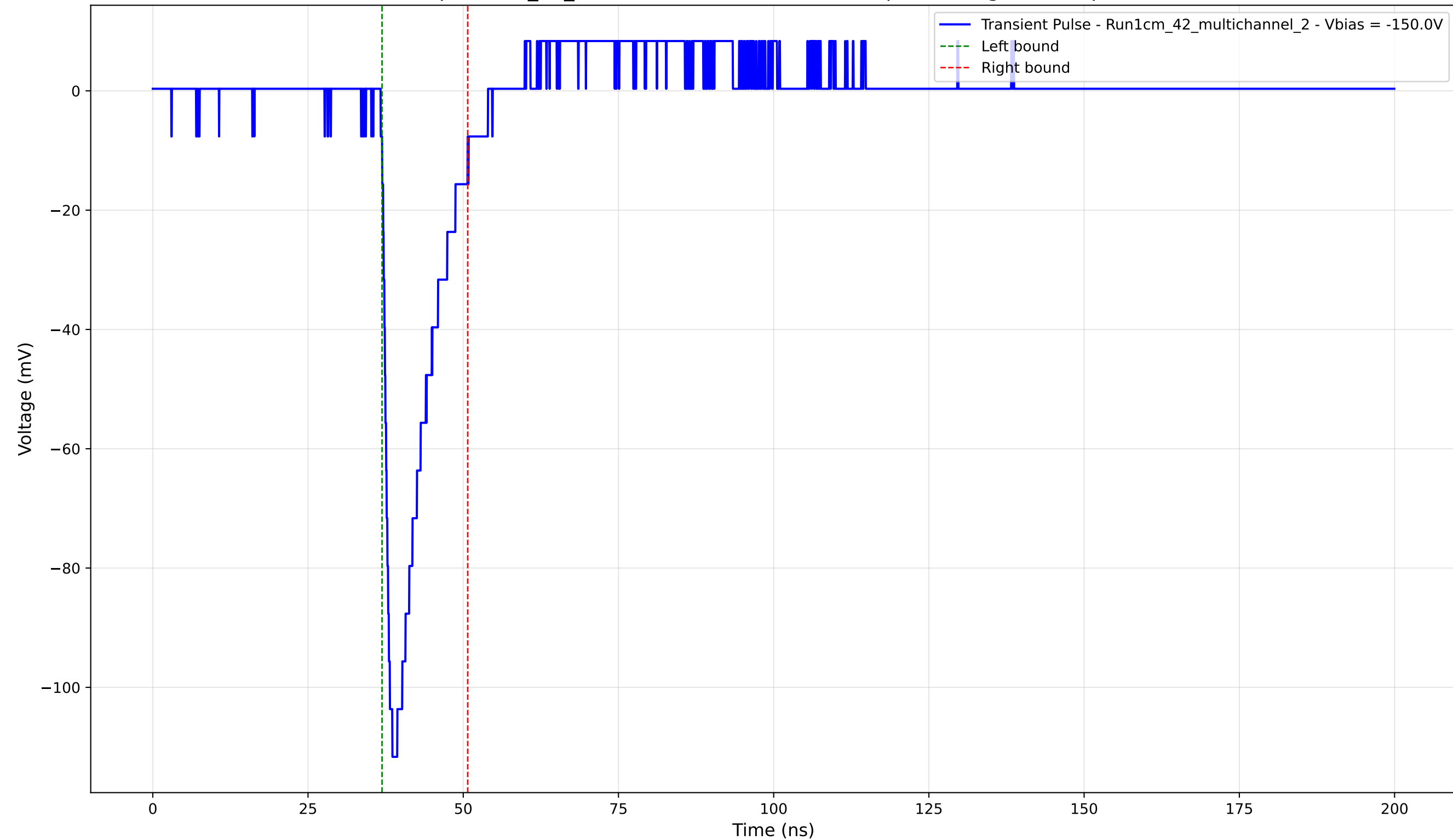
Transient Pulse - Sample: 1cm_42_multichannel - Position: 925.0 \mu\text{m} - Charge: 15.20 pC - Rise Time: 1.26 ns
