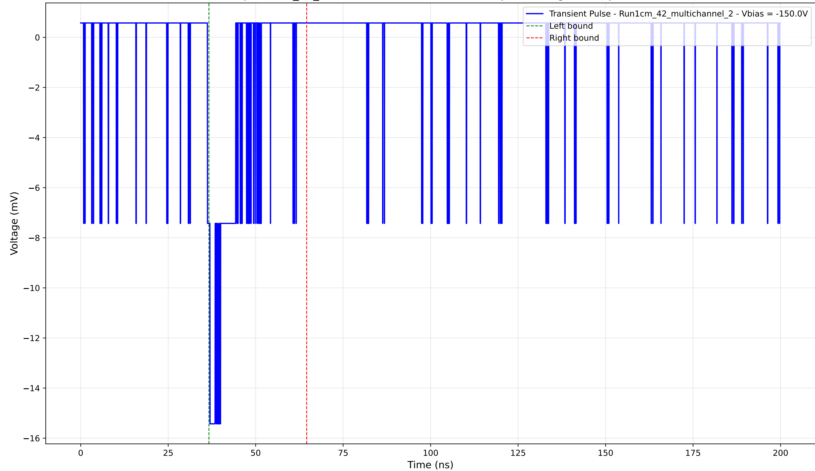
Transient Pulse - Sample: 1cm_42_multichannel - Position: 2865.0 \mu\text{m} - Charge: 1.58 pC - Rise Time: 0.75 ns
