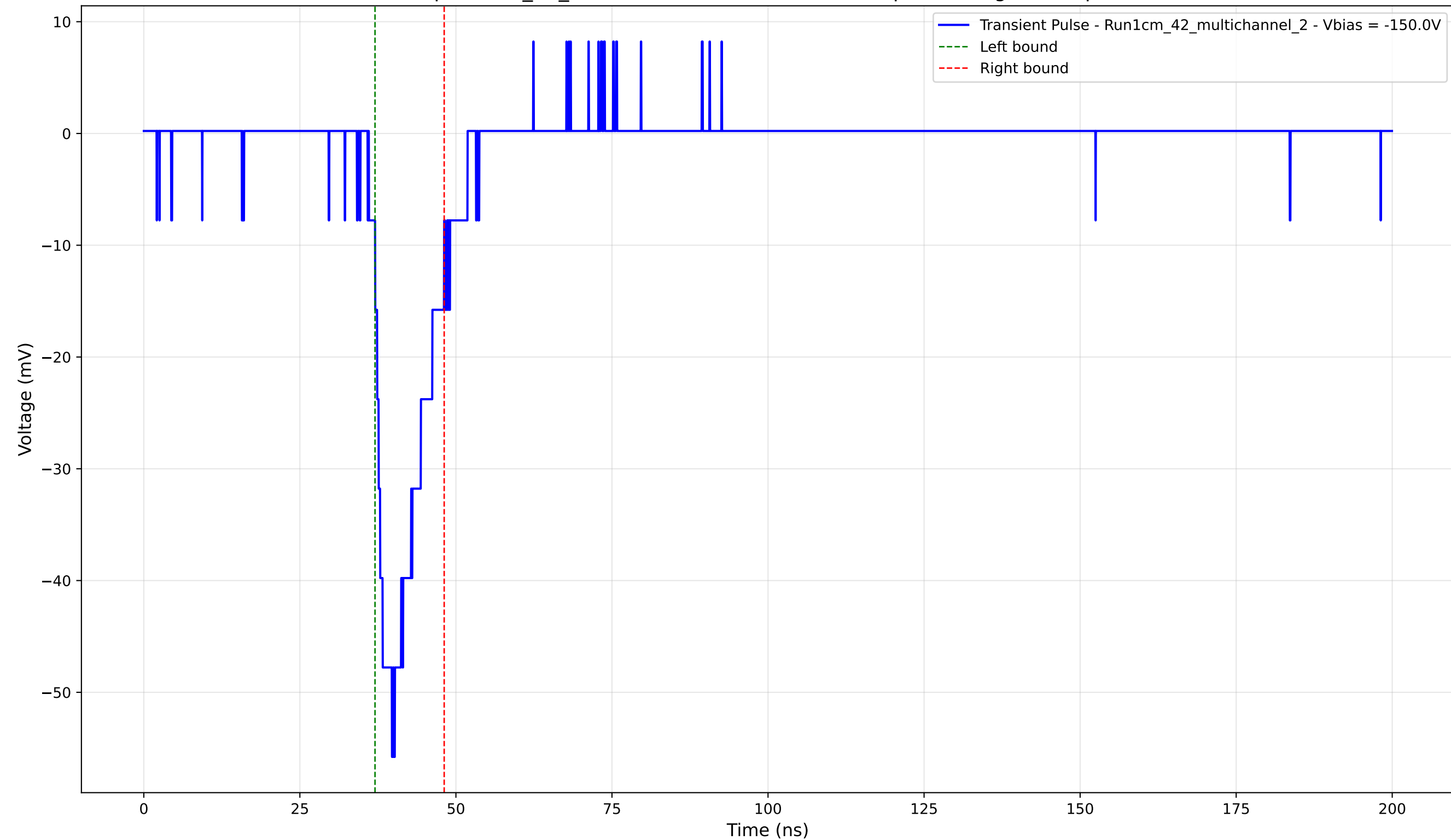
Transient Pulse - Sample: 1cm_42_multichannel - Position: 4825.0 \mu\text{m} - Charge: 7.34 pC - Rise Time: 3.69 ns
