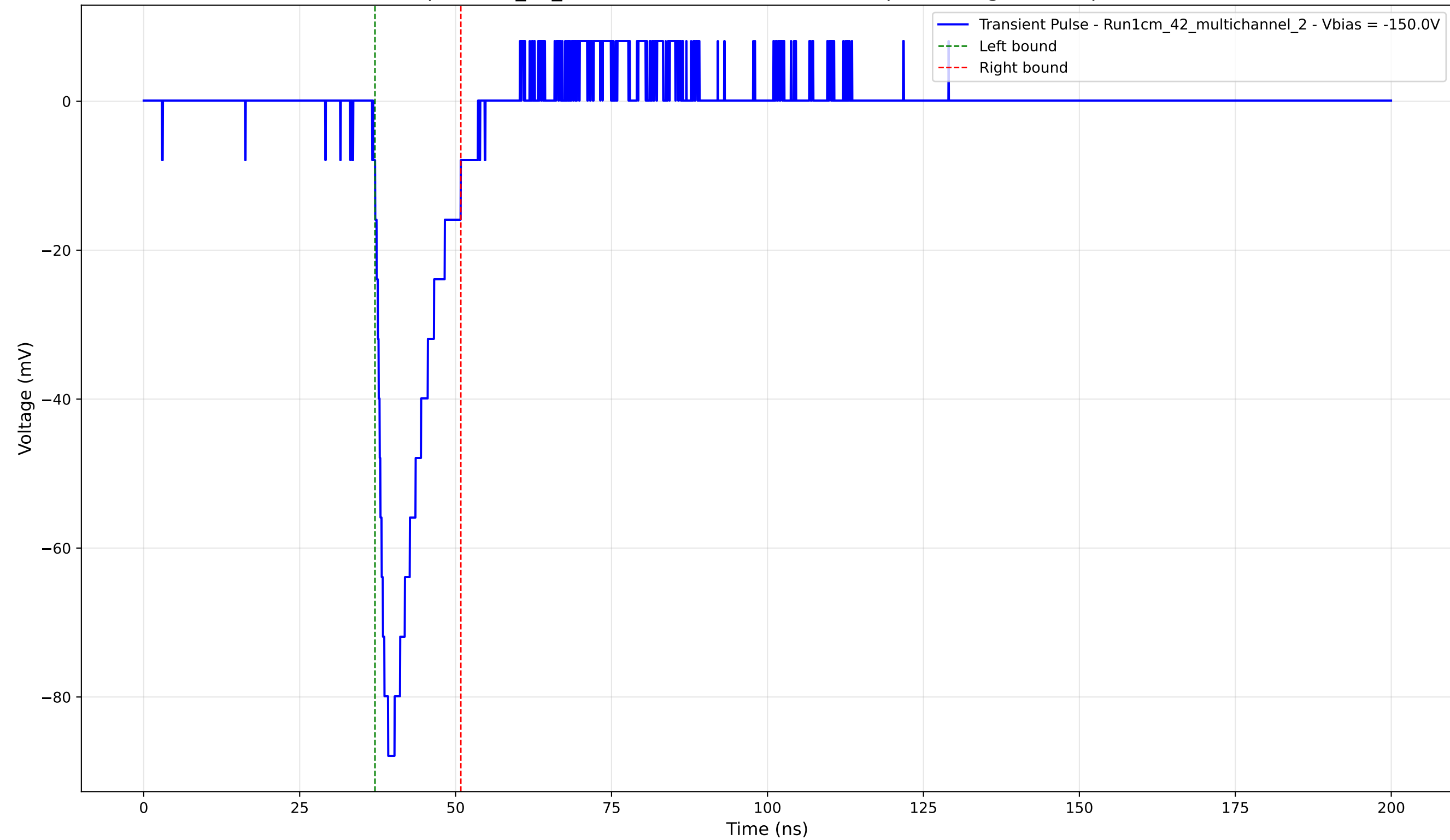
Transient Pulse - Sample: 1cm_42_multichannel - Position: 4130.0 \mu\text{m} - Charge: 12.64 pC - Rise Time: 1.52 ns
