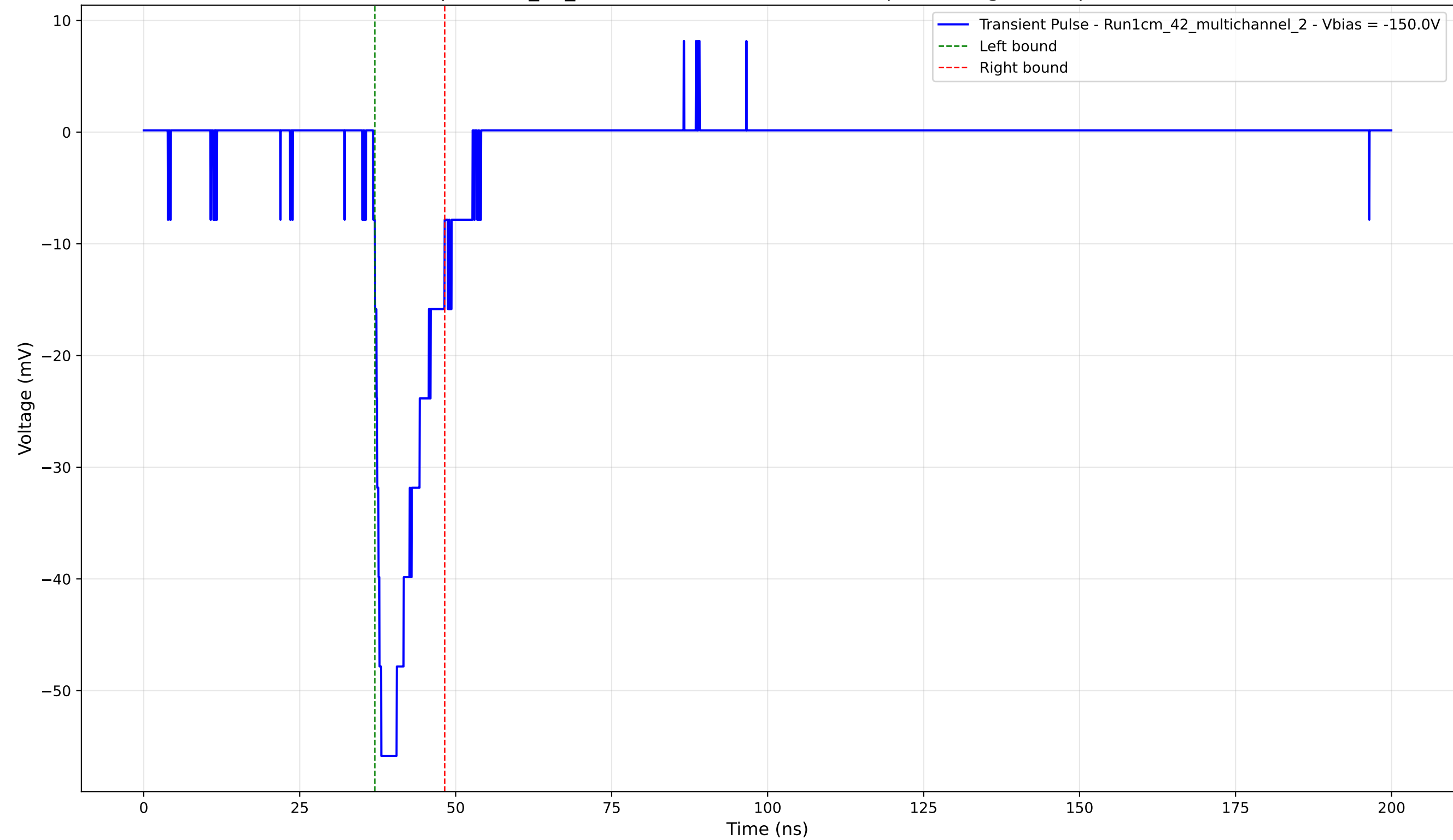
Transient Pulse - Sample: 1cm_42_multichannel - Position: 900.0 \mu\text{m} - Charge: 7.85 pC - Rise Time: 1.29 ns
