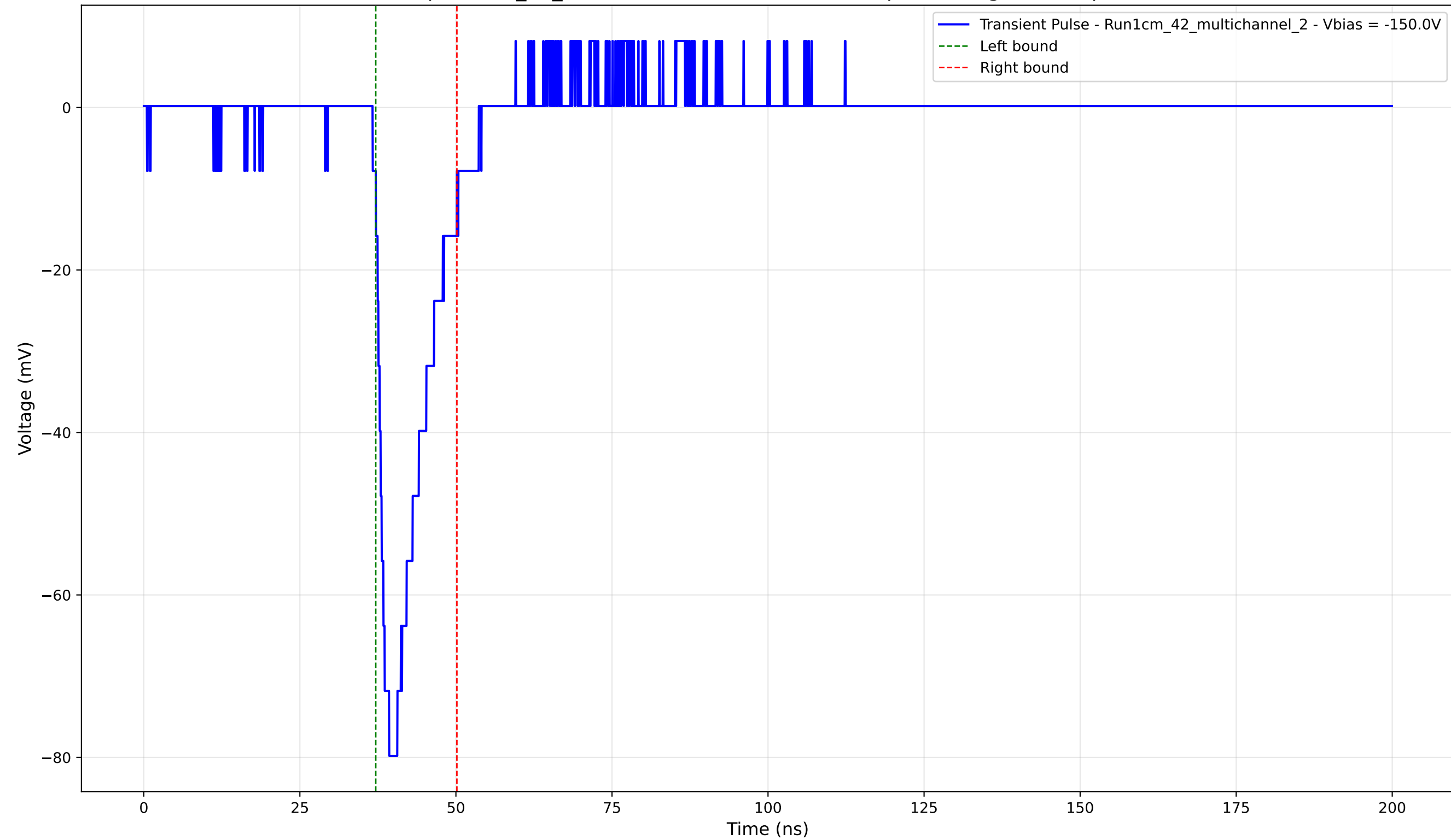
Transient Pulse - Sample: 1cm_42_multichannel - Position: 4255.0 \mu\text{m} - Charge: 11.43 pC - Rise Time: 2.16 ns
