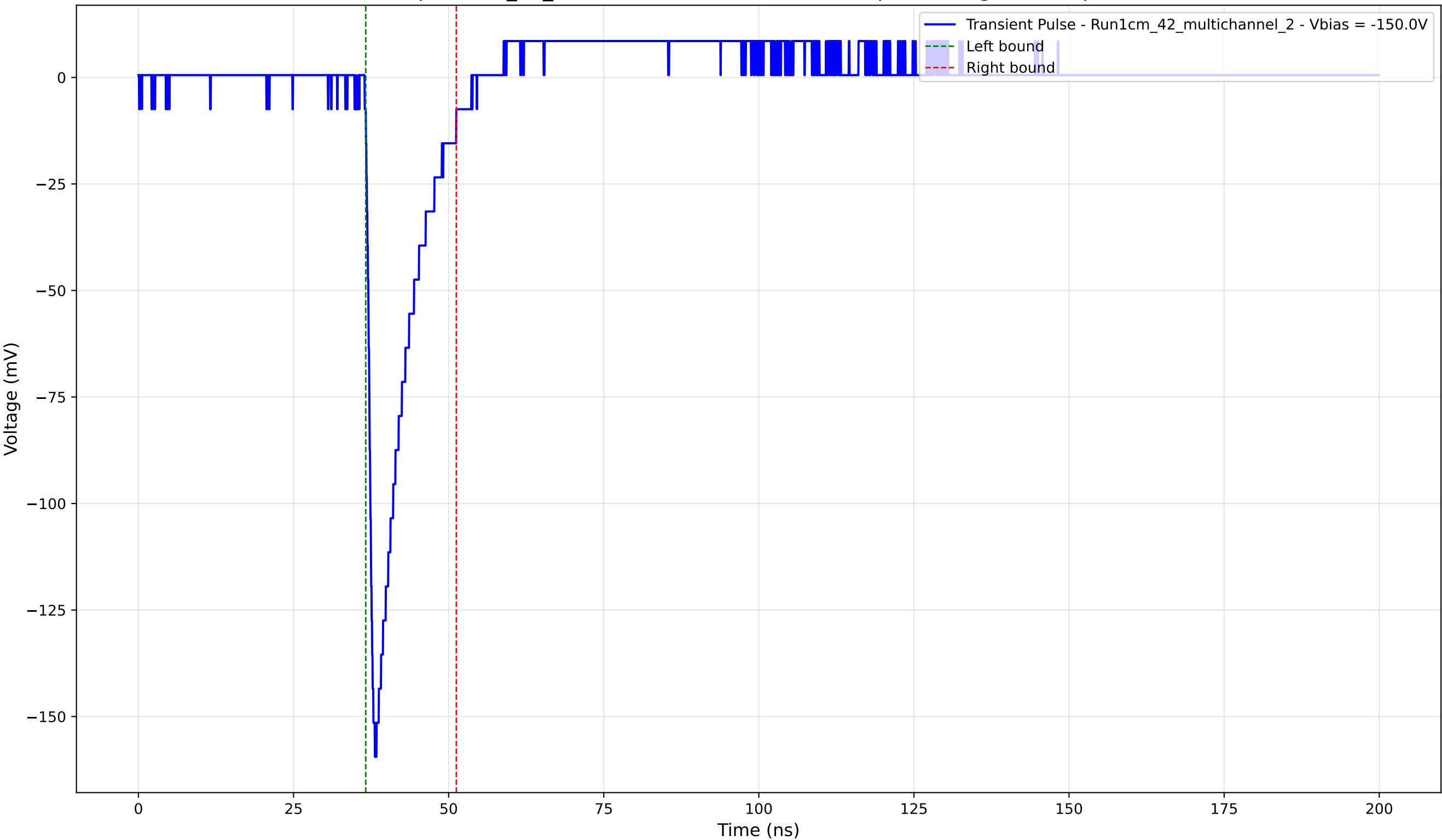
Transient Pulse - Sample: 1cm_42_multichannel - Position: 1245.0 \mu\text{m} - Charge: 19.00 pC - Rise Time: 1.16 ns
