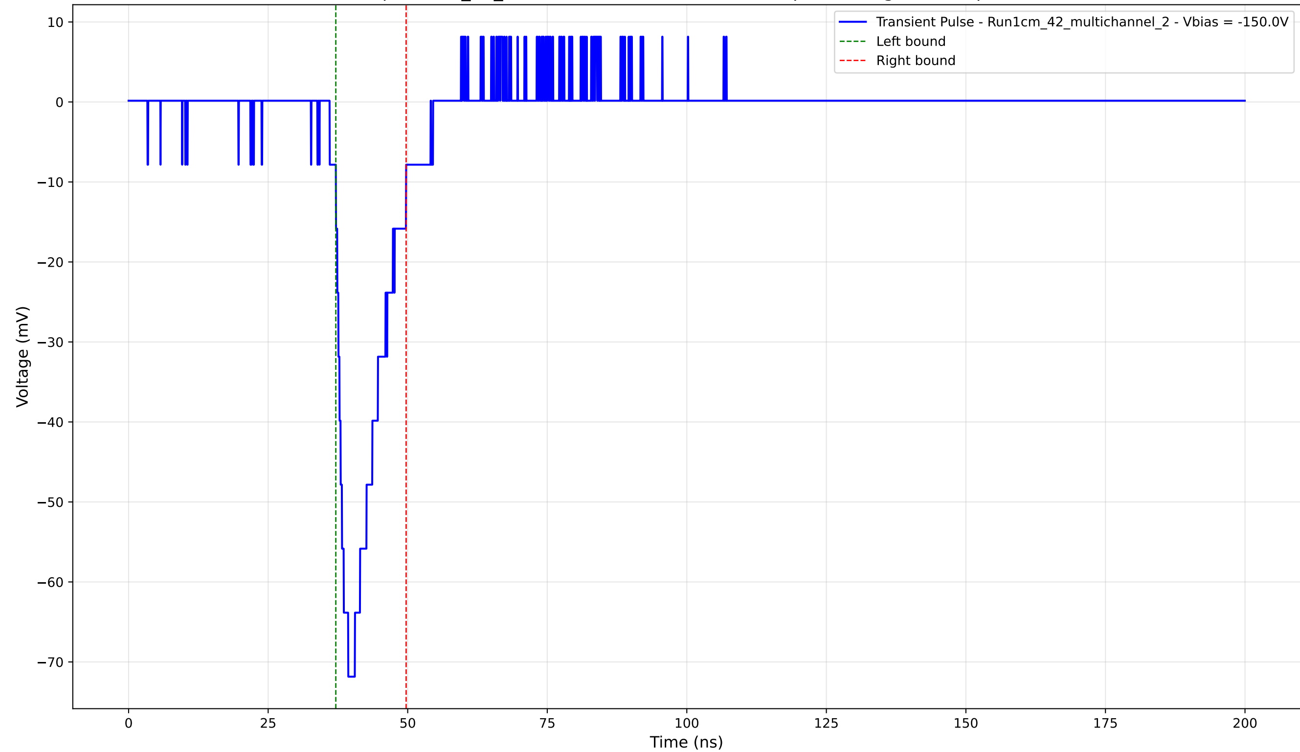
Transient Pulse - Sample: 1cm_42_multichannel - Position: 4645.0 \mu\text{m} - Charge: 10.33 pC - Rise Time: 3.32 ns
