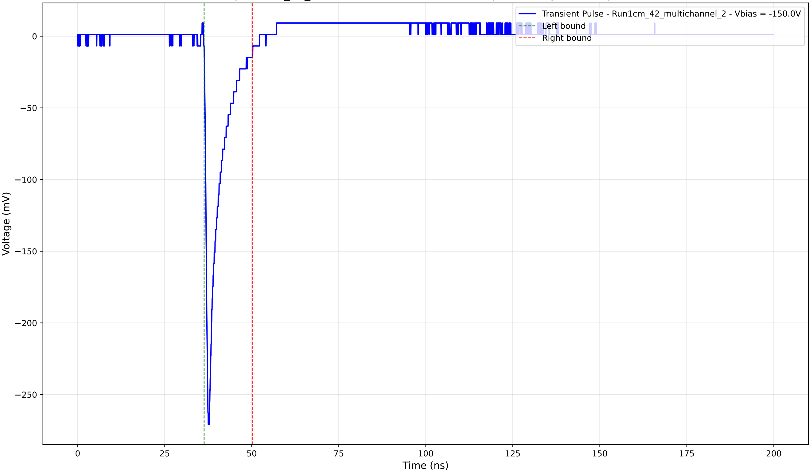
Transient Pulse - Sample: 1cm_42_multichannel - Position: 1690.0 \mu\text{m} - Charge: 22.69 pC - Rise Time: 0.88 ns
