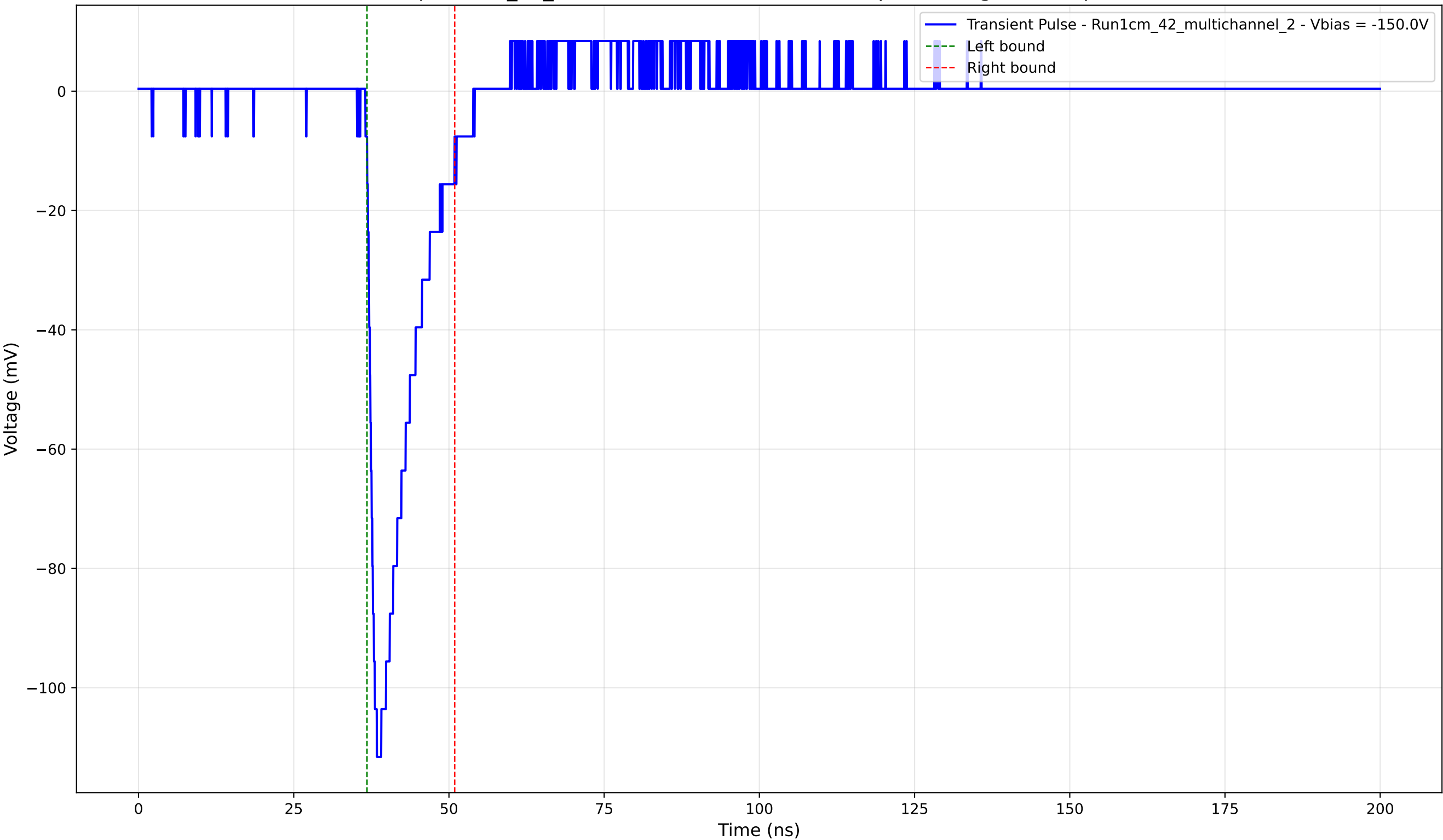
Transient Pulse - Sample: 1cm_42_multichannel - Position: 3690.0 \mu\text{m} - Charge: 15.07 pC - Rise Time: 1.26 ns
