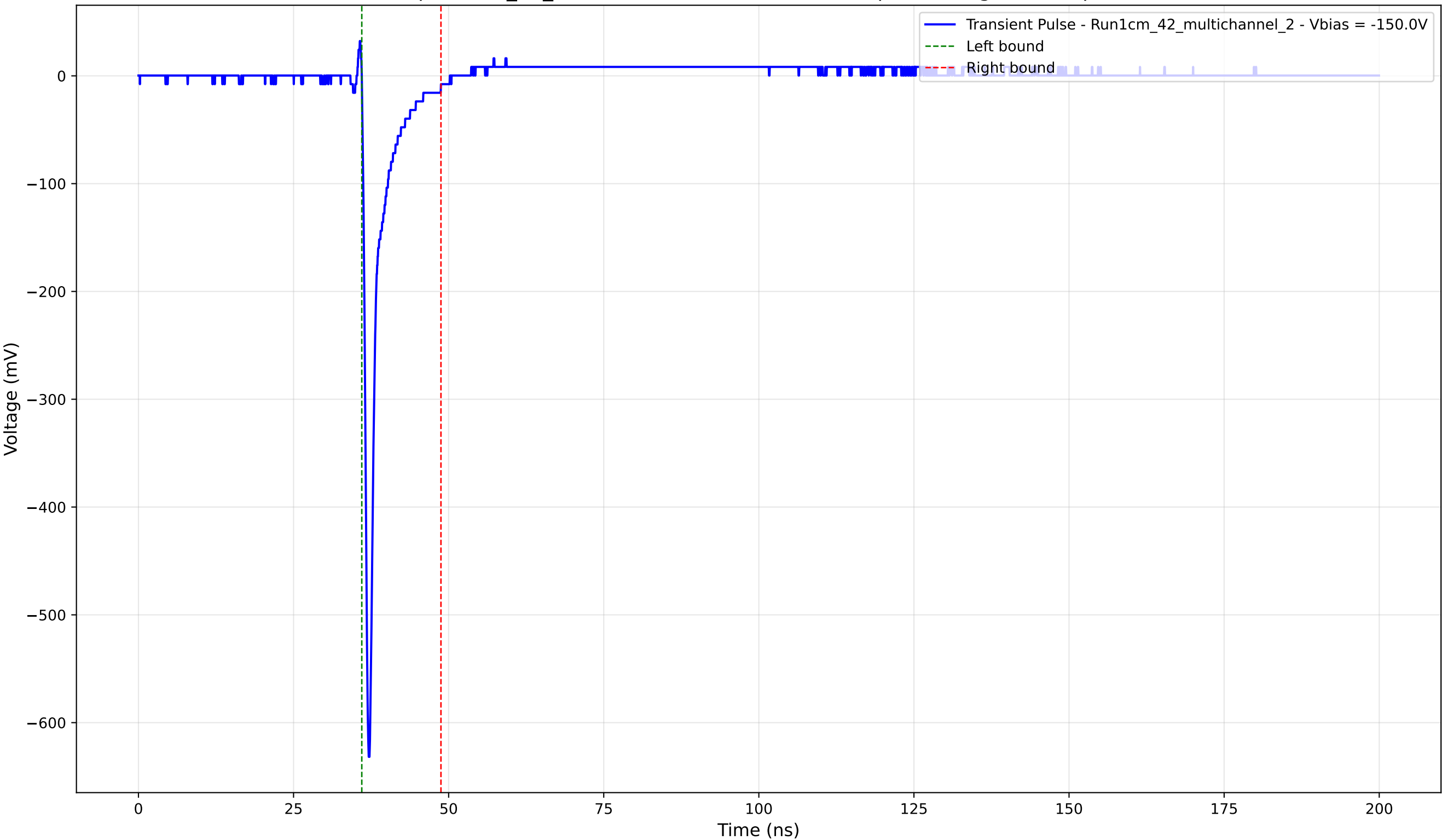
Transient Pulse - Sample: 1cm_42_multichannel - Position: 2260.0 \mu\text{m} - Charge: 29.11 pC - Rise Time: 0.72 ns
