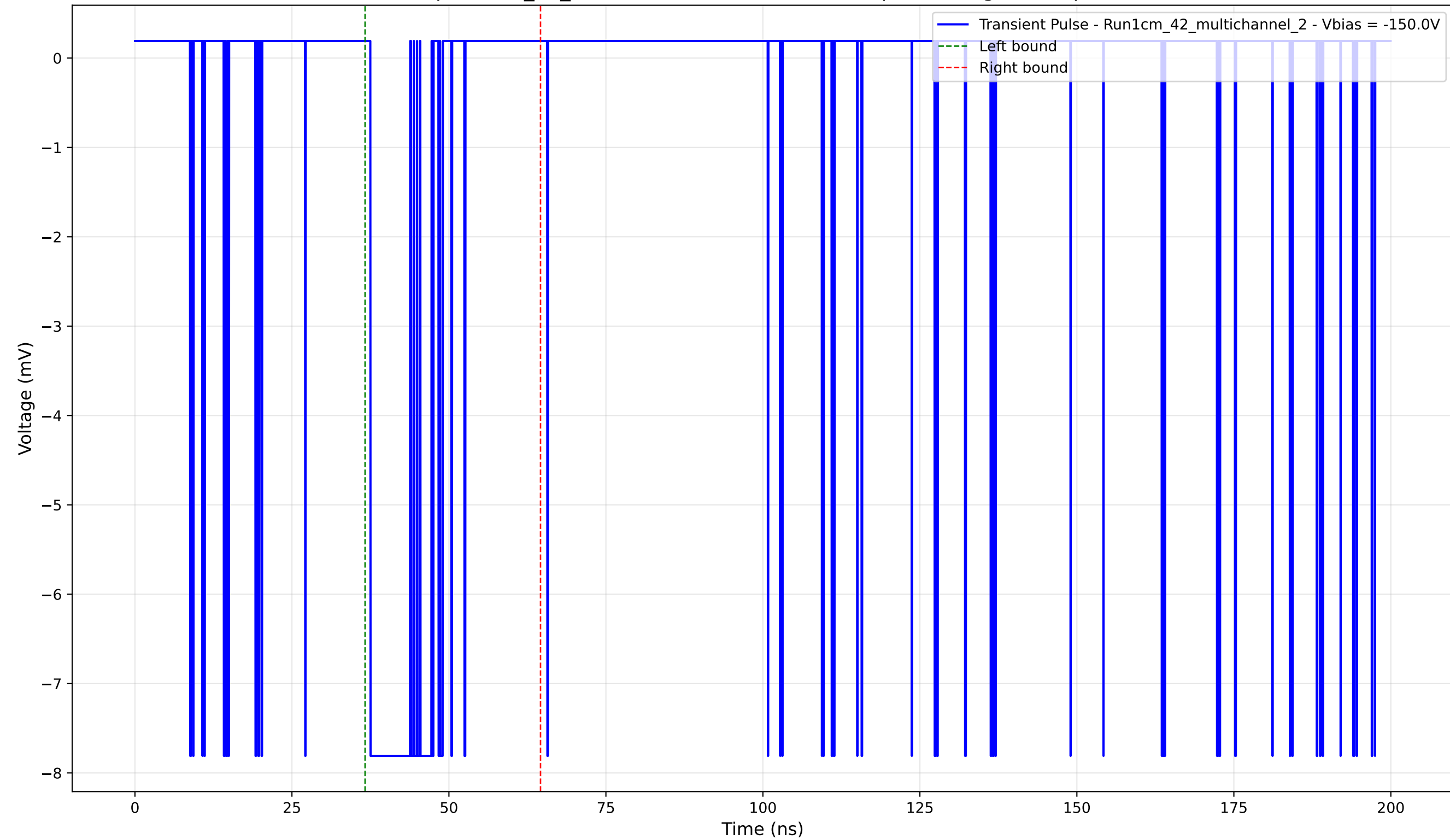
Transient Pulse - Sample: 1cm_42_multichannel - Position: 845.0 \mu\text{m} - Charge: 1.54 pC - Rise Time: 0.04 ns
