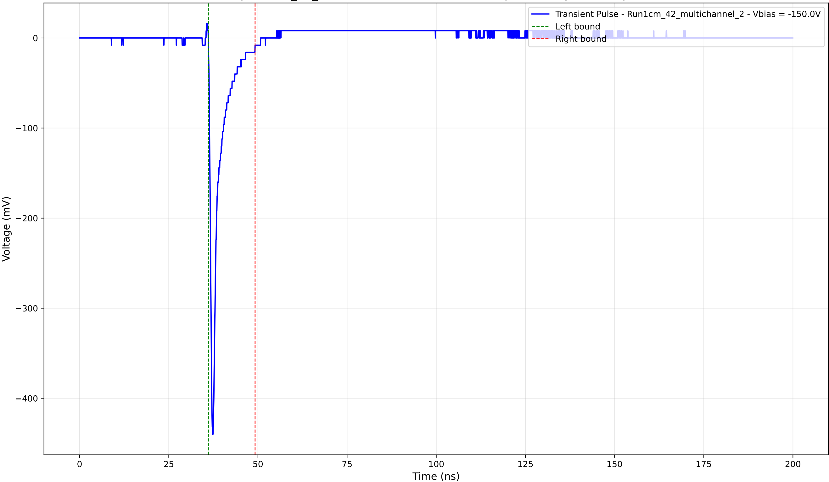
Transient Pulse - Sample: 1cm_42_multichannel - Position: 2685.0 \mu\text{m} - Charge: 25.02 pC - Rise Time: 0.78 ns
