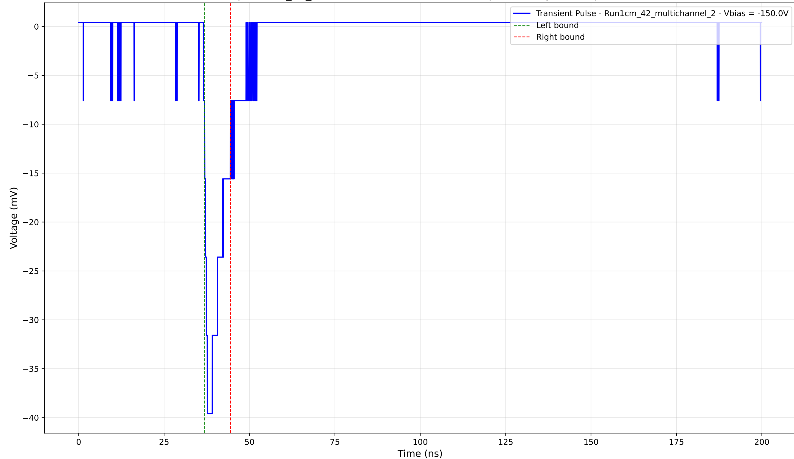
Transient Pulse - Sample: 1cm_42_multichannel - Position: 1320.0 \mu\text{m} - Charge: 3.92 pC - Rise Time: 1.14 ns
