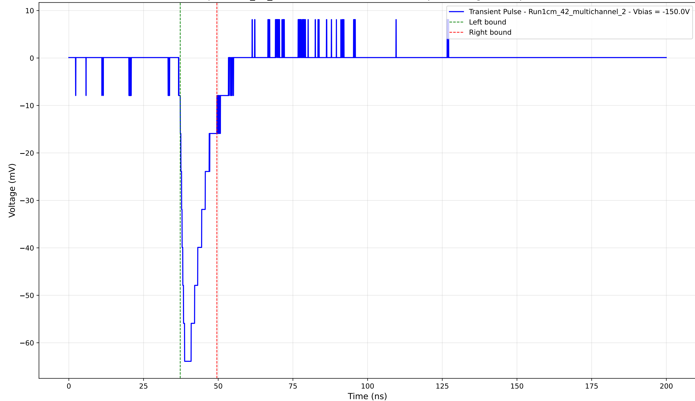
Transient Pulse - Sample: 1cm_42_multichannel - Position: 4310.0 \mu\text{m} - Charge: 9.49 pC - Rise Time: 1.93 ns
