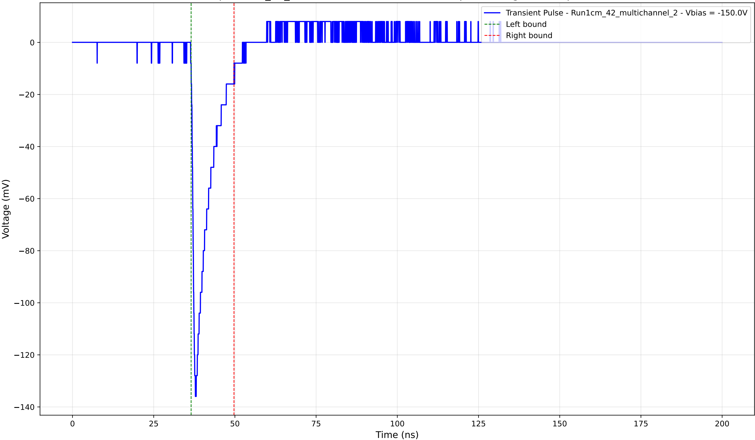
Transient Pulse - Sample: 1cm_42_multichannel - Position: 3315.0 \mu\text{m} - Charge: 14.39 pC - Rise Time: 1.09 ns
