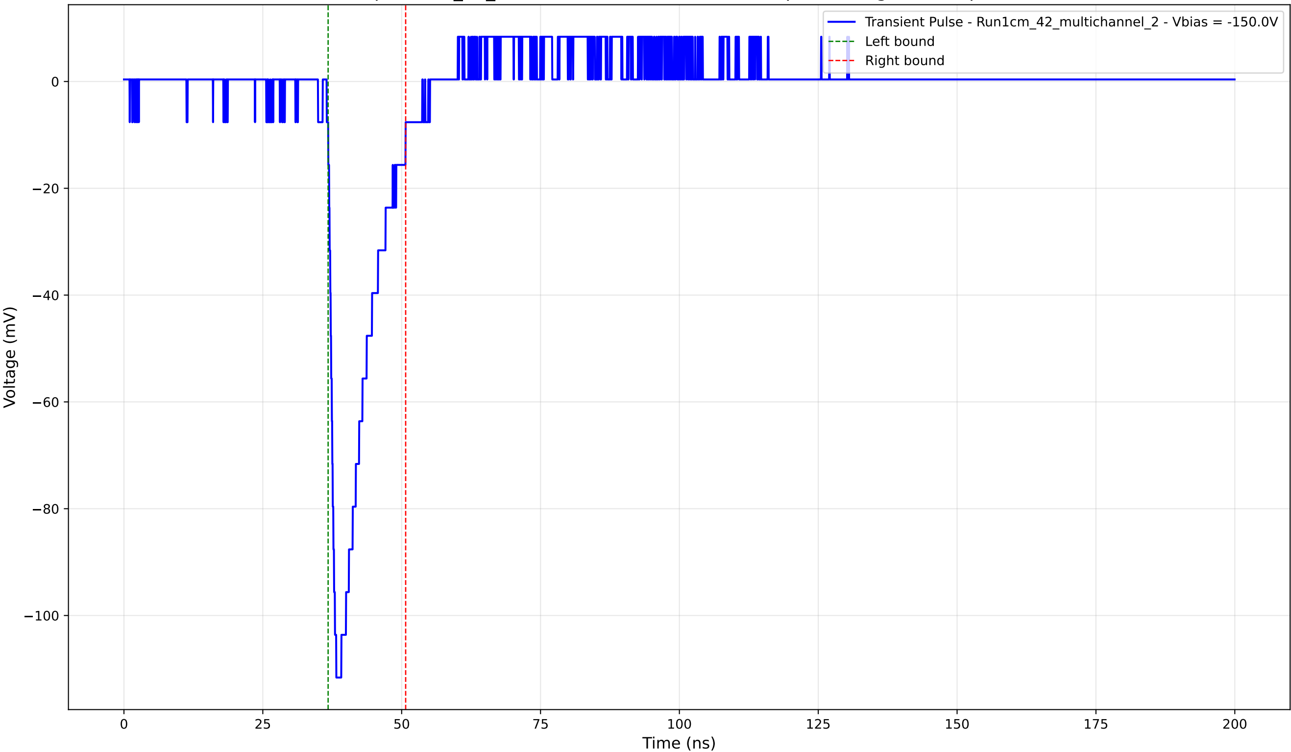
Transient Pulse - Sample: 1cm_42_multichannel - Position: 3665.0 \mu\text{m} - Charge: 15.23 pC - Rise Time: 1.22 ns
