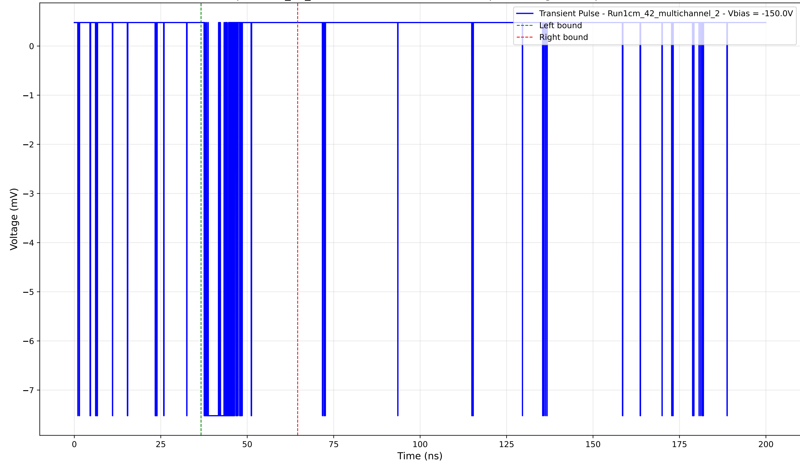
Transient Pulse - Sample: 1cm_42_multichannel - Position: 4395.0 \mu\text{m} - Charge: 0.93 pC - Rise Time: 0.04 ns
