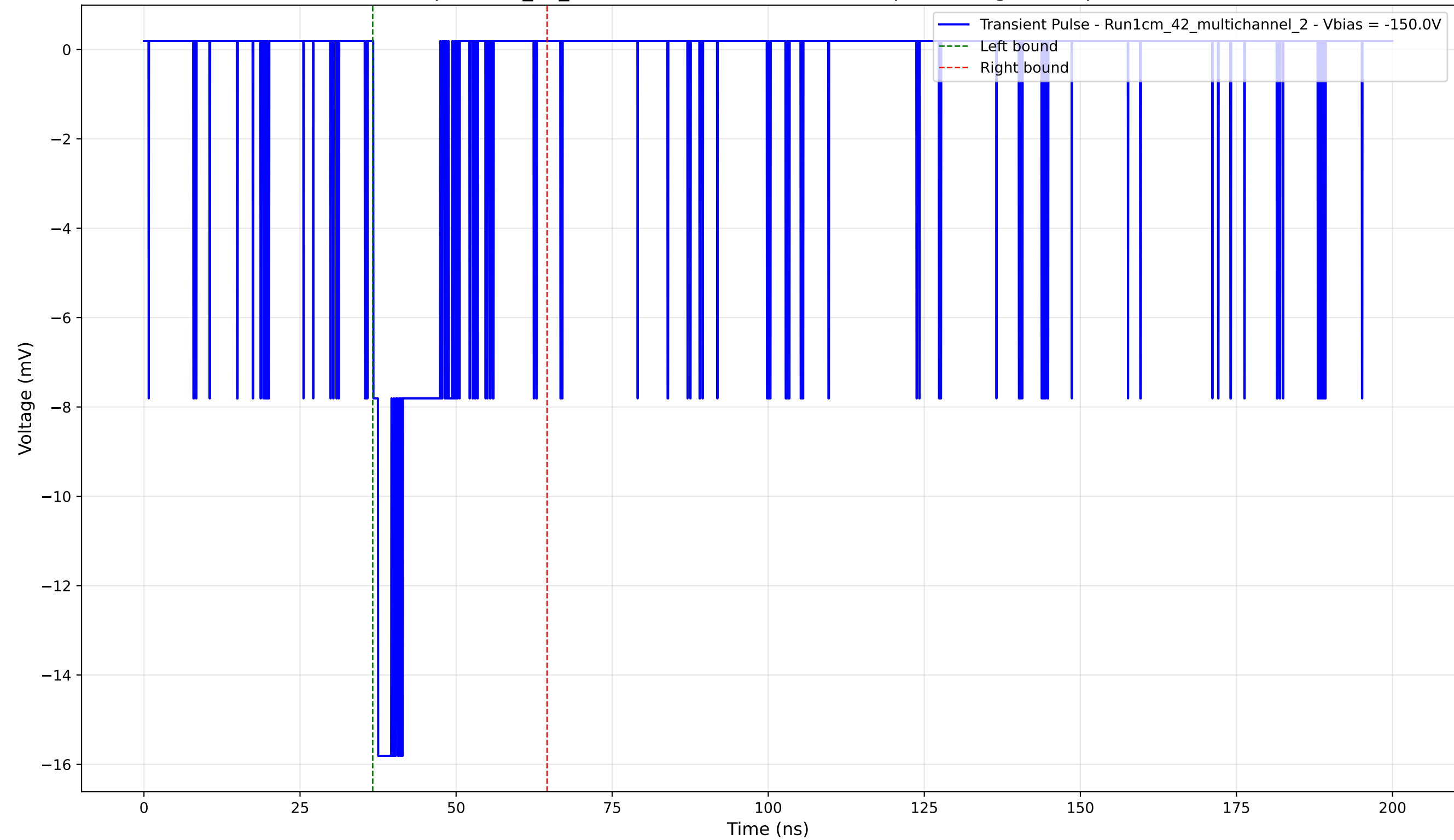
Transient Pulse - Sample: 1cm_42_multichannel - Position: 3405.0 \mu\text{m} - Charge: 2.55 pC - Rise Time: 0.79 ns
