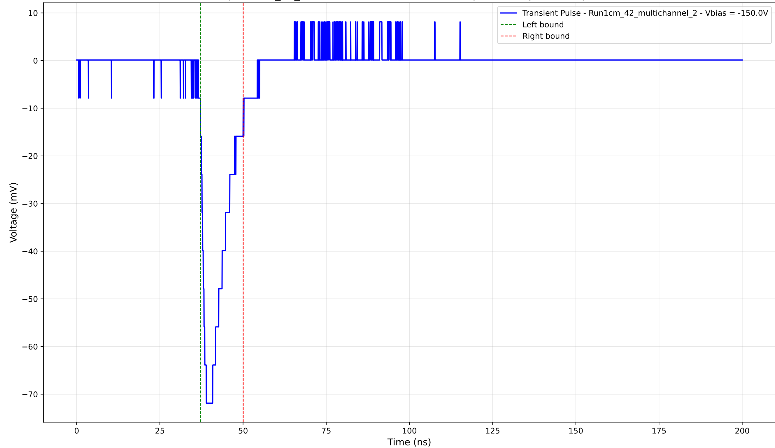
Transient Pulse - Sample: 1cm_42_multichannel - Position: 4290.0 \mu\text{m} - Charge: 10.58 pC - Rise Time: 2.36 ns
