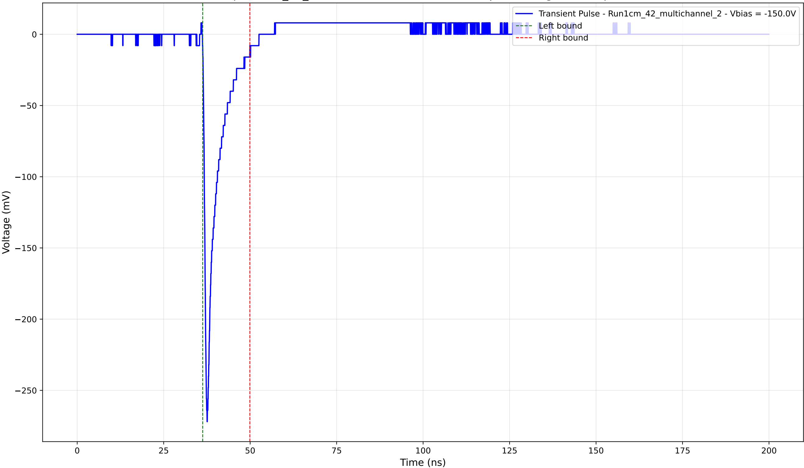
Transient Pulse - Sample: 1cm_42_multichannel - Position: 2995.0 \mu\text{m} - Charge: 21.51 pC - Rise Time: 0.89 ns
