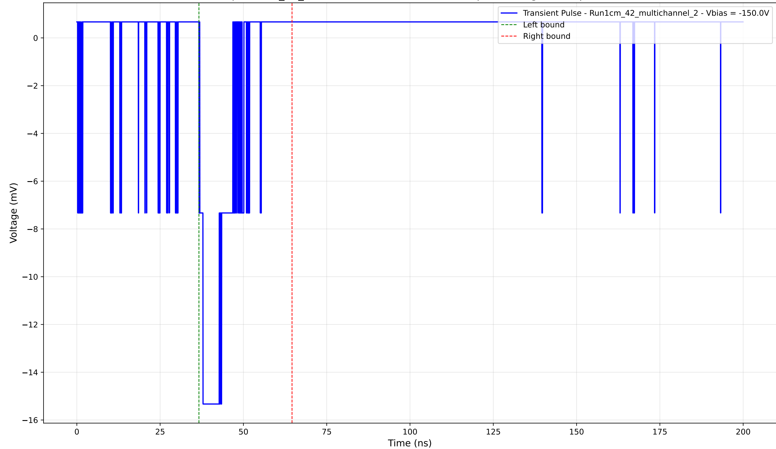
Transient Pulse - Sample: 1cm_42_multichannel - Position: 4860.0 \mu\text{m} - Charge: 2.45 pC - Rise Time: 0.99 ns
