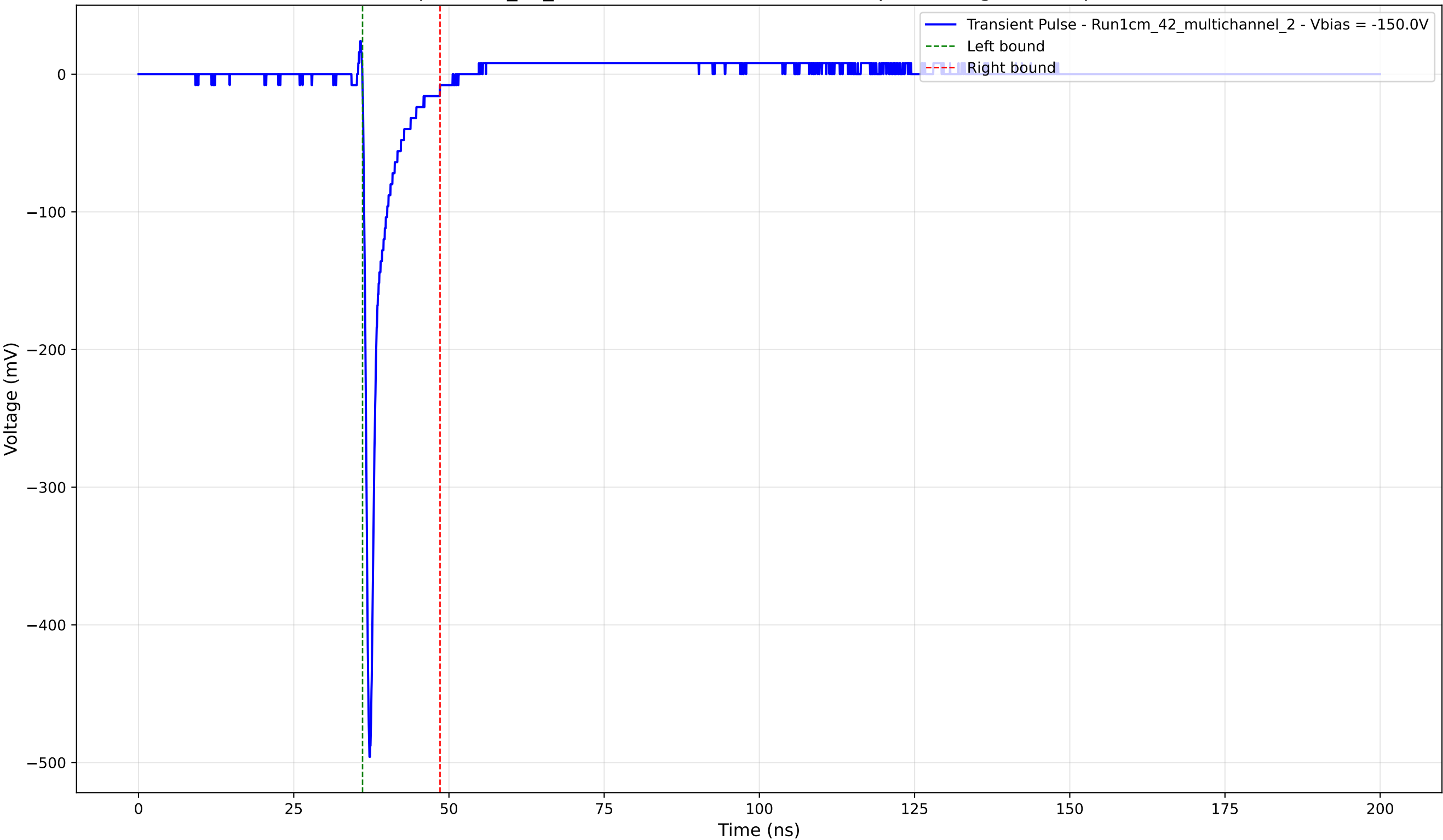
Transient Pulse - Sample: 1cm_42_multichannel - Position: 2575.0 \mu\text{m} - Charge: 24.95 pC - Rise Time: 0.75 ns
