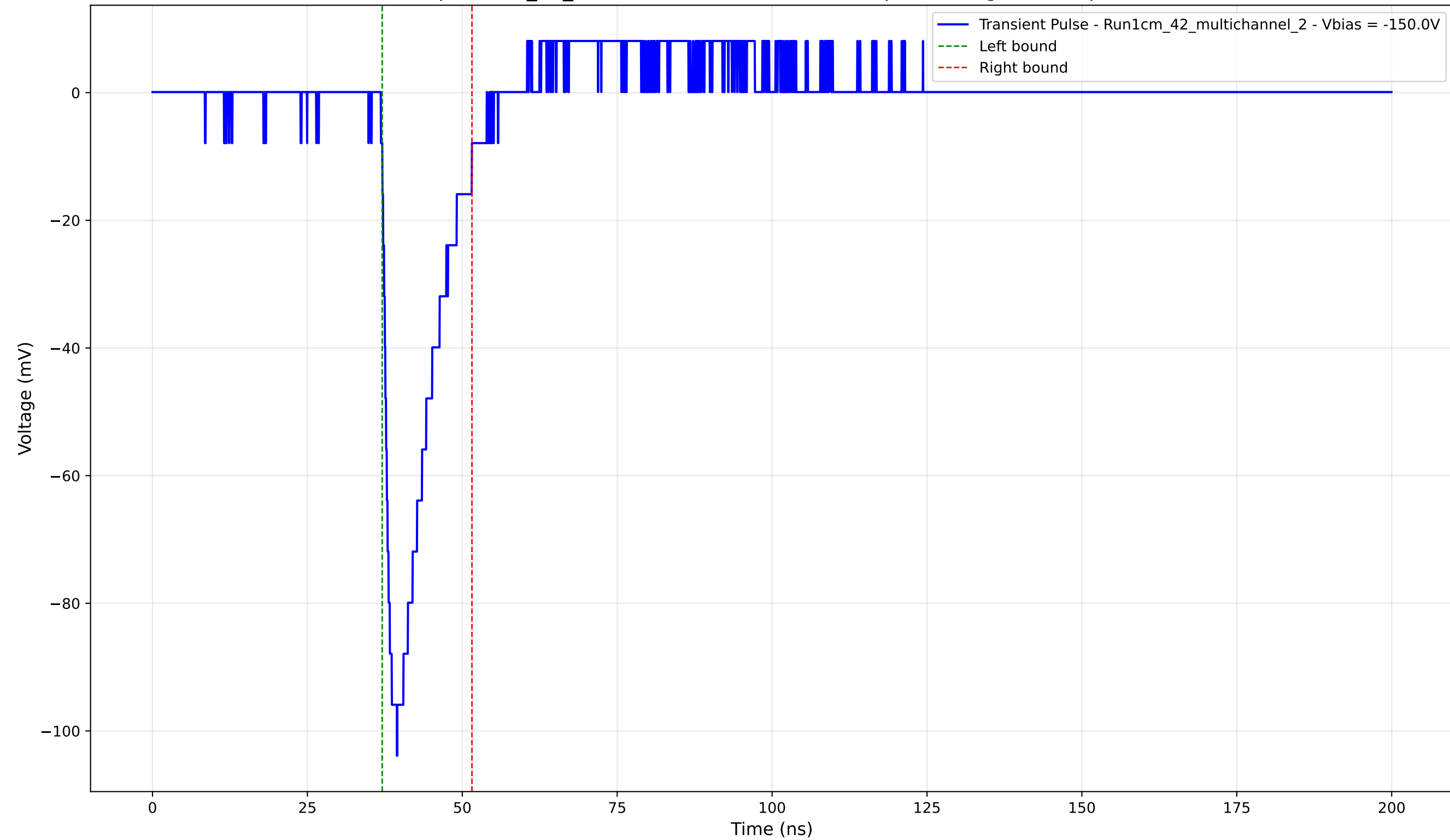
Transient Pulse - Sample: 1cm_42_multichannel - Position: 615.0 \mu\text{m} - Charge: 14.85 pC - Rise Time: 1.55 ns
