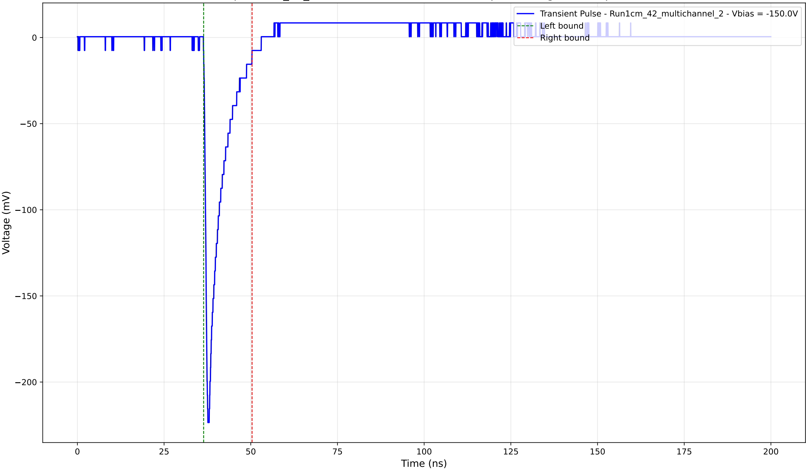
Transient Pulse - Sample: 1cm_42_multichannel - Position: 1560.0 \mu\text{m} - Charge: 21.33 pC - Rise Time: 0.97 ns
