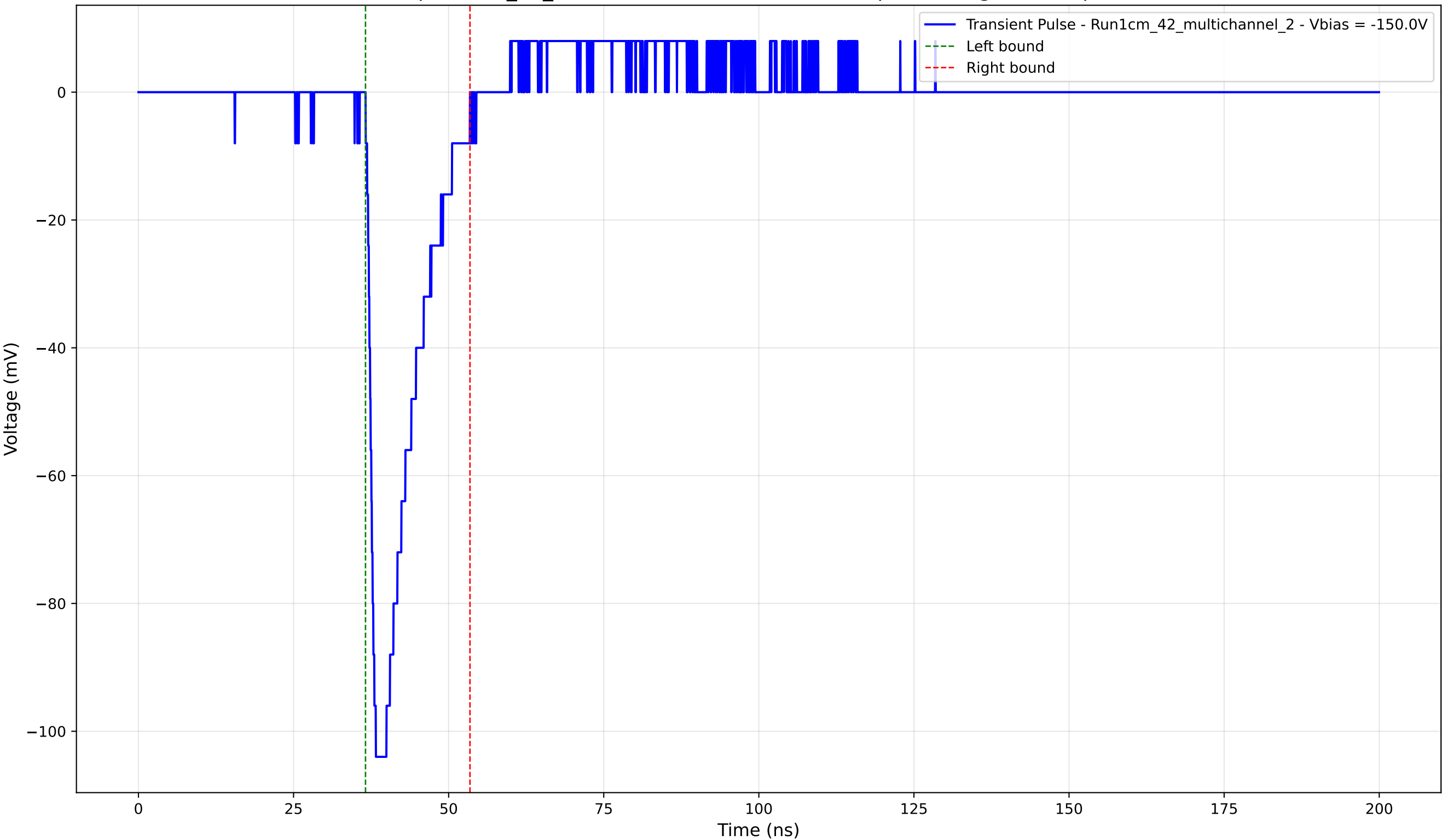
Transient Pulse - Sample: 1cm_42_multichannel - Position: 3755.0 \mu\text{m} - Charge: 15.48 pC - Rise Time: 1.19 ns
