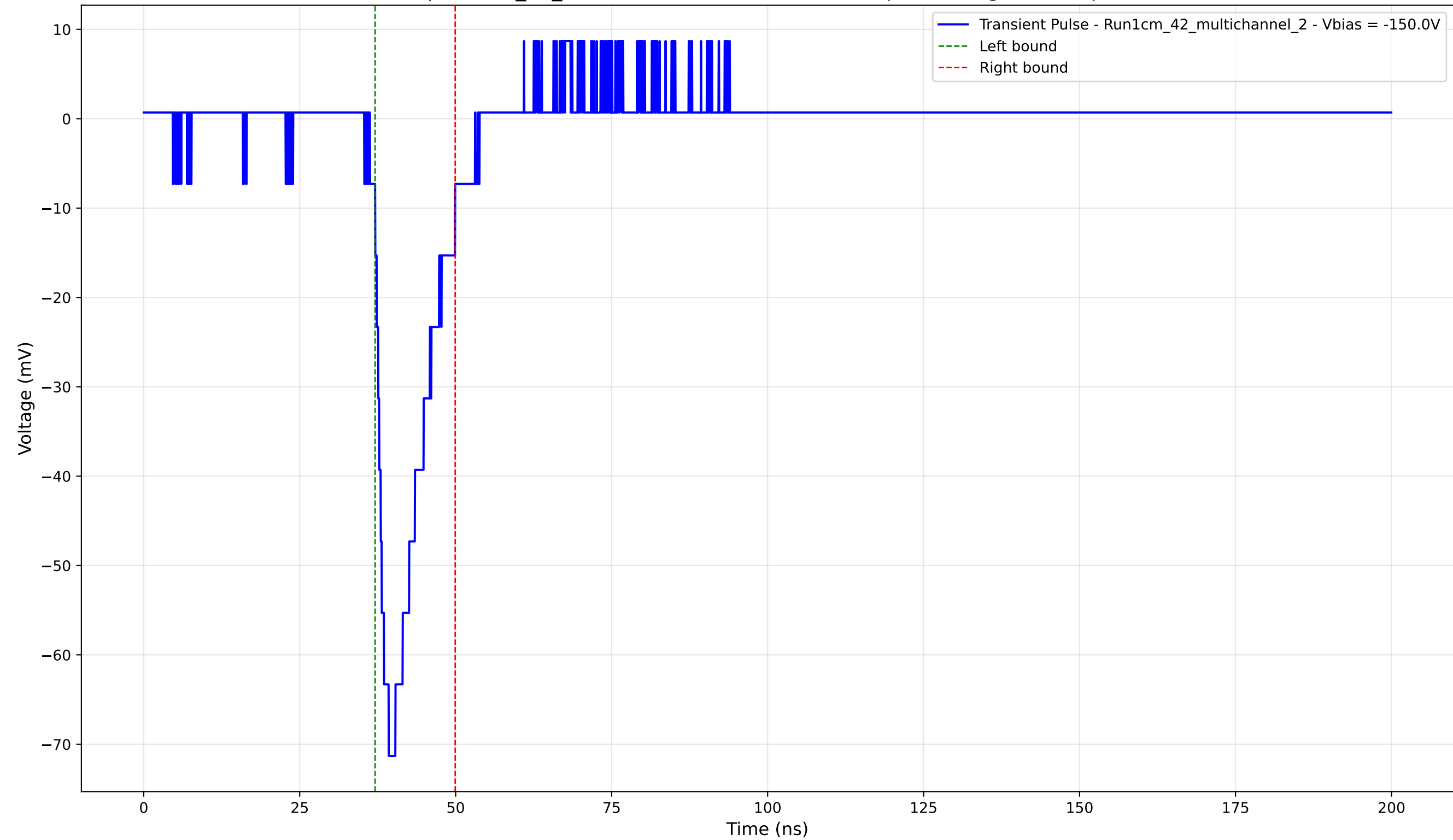
Transient Pulse - Sample: 1cm_42_multichannel - Position: 4675.0 \mu\text{m} - Charge: 10.25 pC - Rise Time: 3.00 ns
