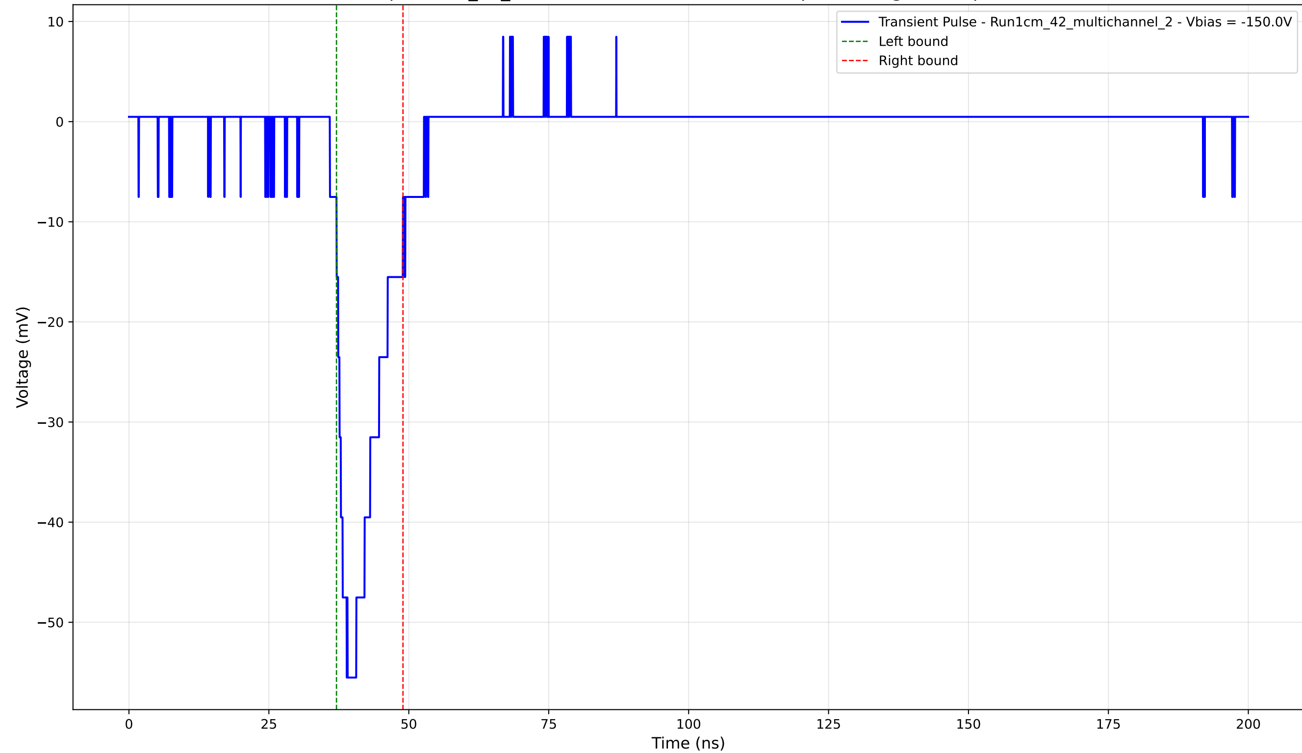
Transient Pulse - Sample: 1cm_42_multichannel - Position: 4820.0 \mu\text{m} - Charge: 7.95 pC - Rise Time: 3.01 ns
