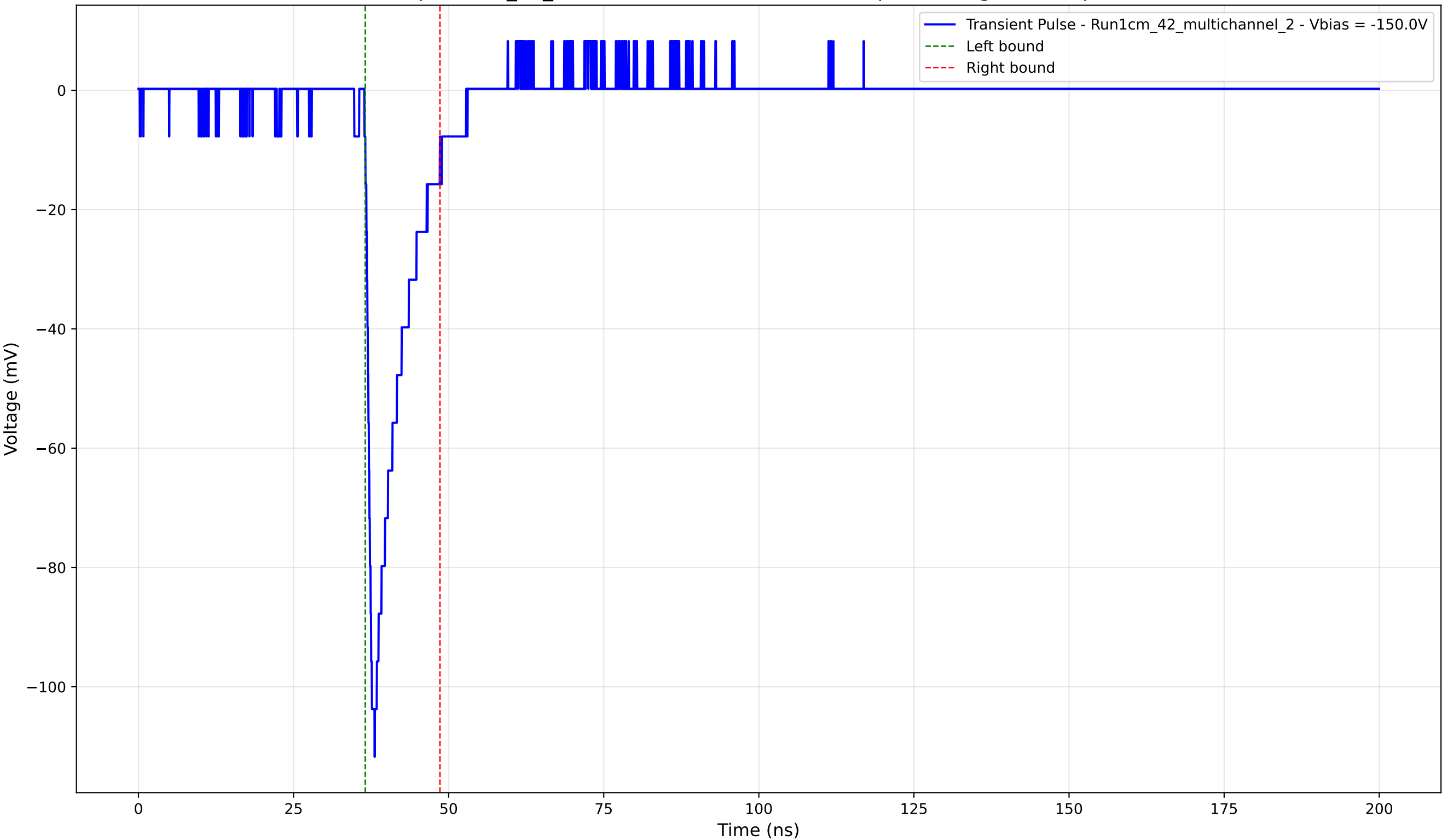
Transient Pulse - Sample: 1cm_42_multichannel - Position: 3325.0 \mu\text{m} - Charge: 11.40 pC - Rise Time: 1.06 ns
