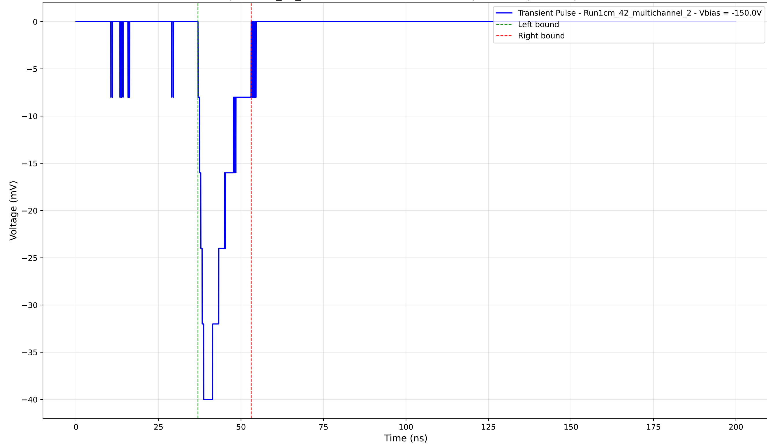
Transient Pulse - Sample: 1cm_42_multichannel - Position: 4335.0 \mu\text{m} - Charge: 6.65 pC - Rise Time: 1.74 ns
