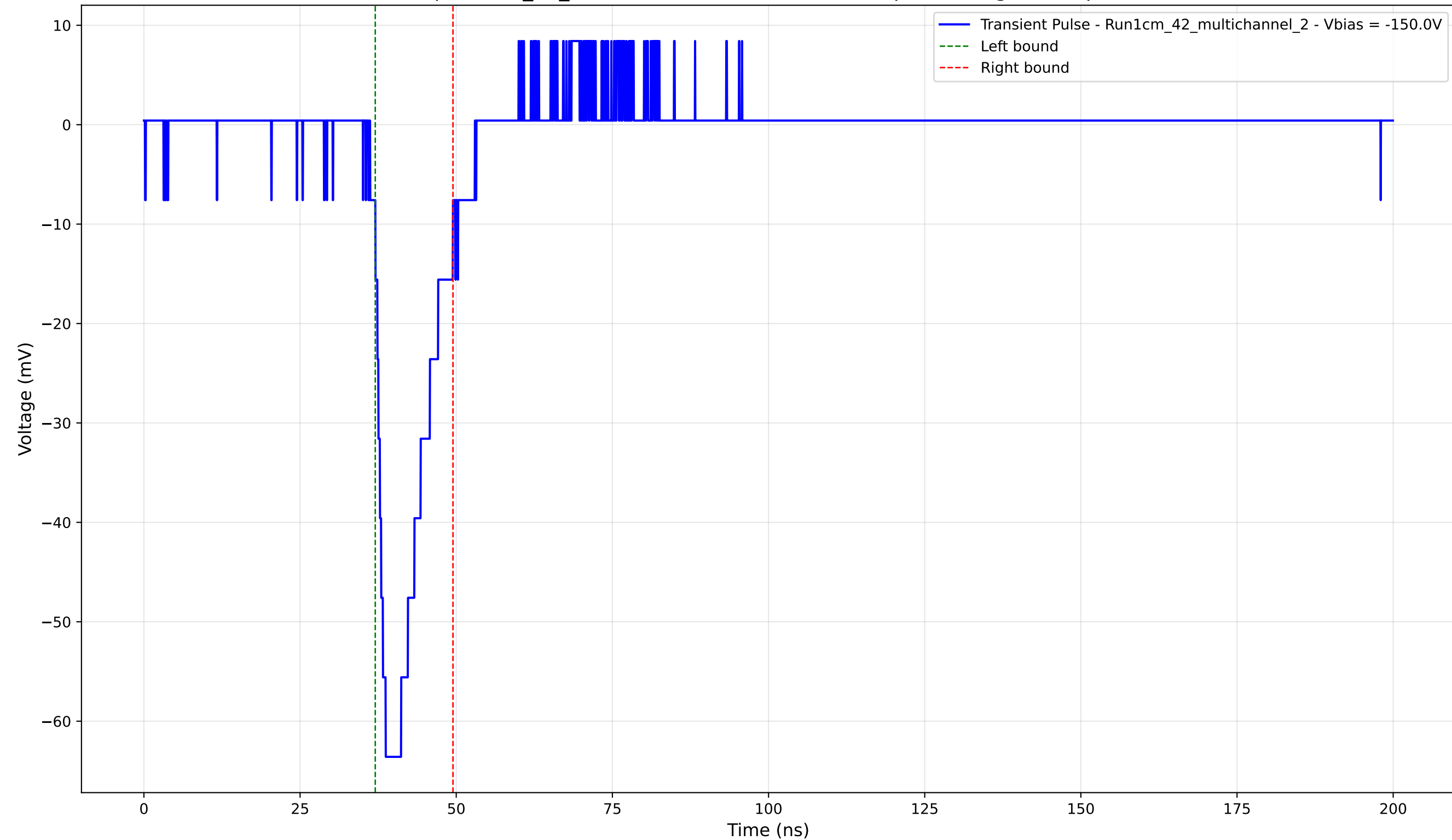
Transient Pulse - Sample: 1cm_42_multichannel - Position: 4730.0 \mu\text{m} - Charge: 9.68 pC - Rise Time: 2.49 ns
