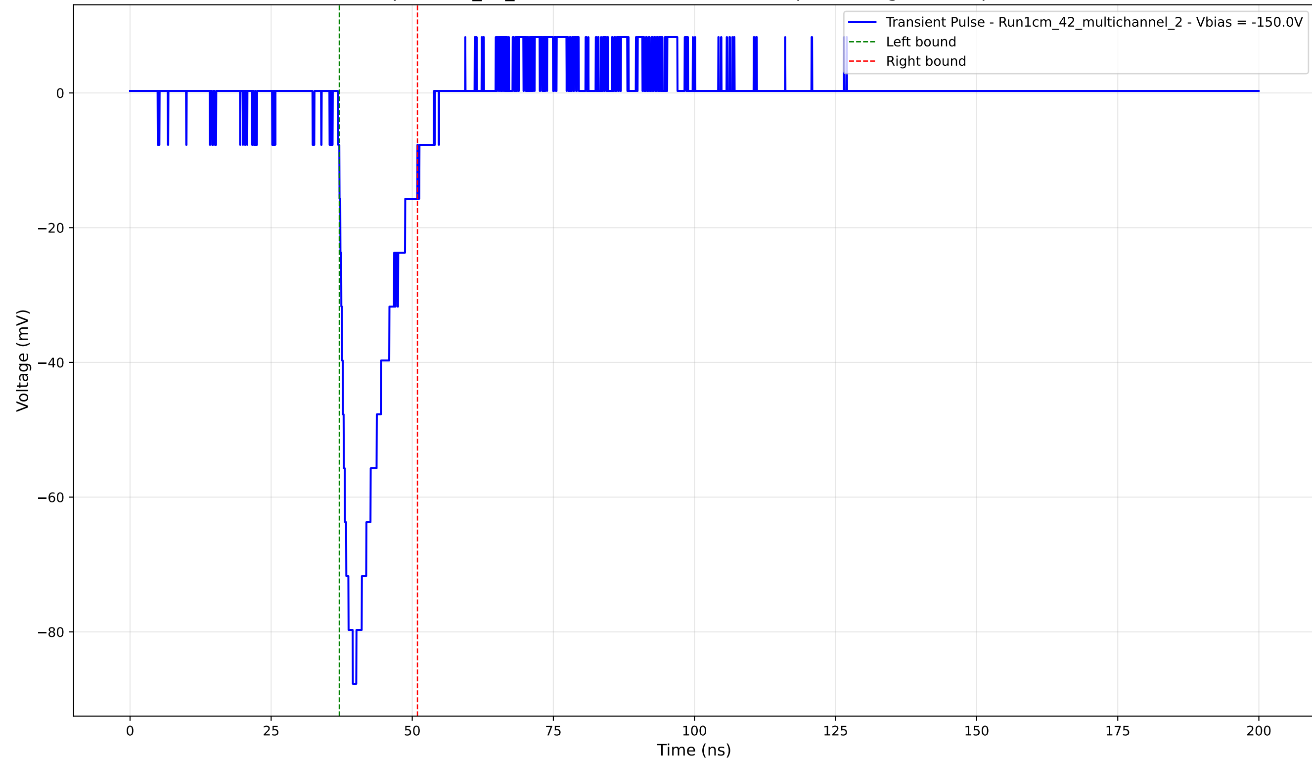
Transient Pulse - Sample: 1cm_42_multichannel - Position: 425.0 \mu\text{m} - Charge: 12.86 pC - Rise Time: 1.63 ns
