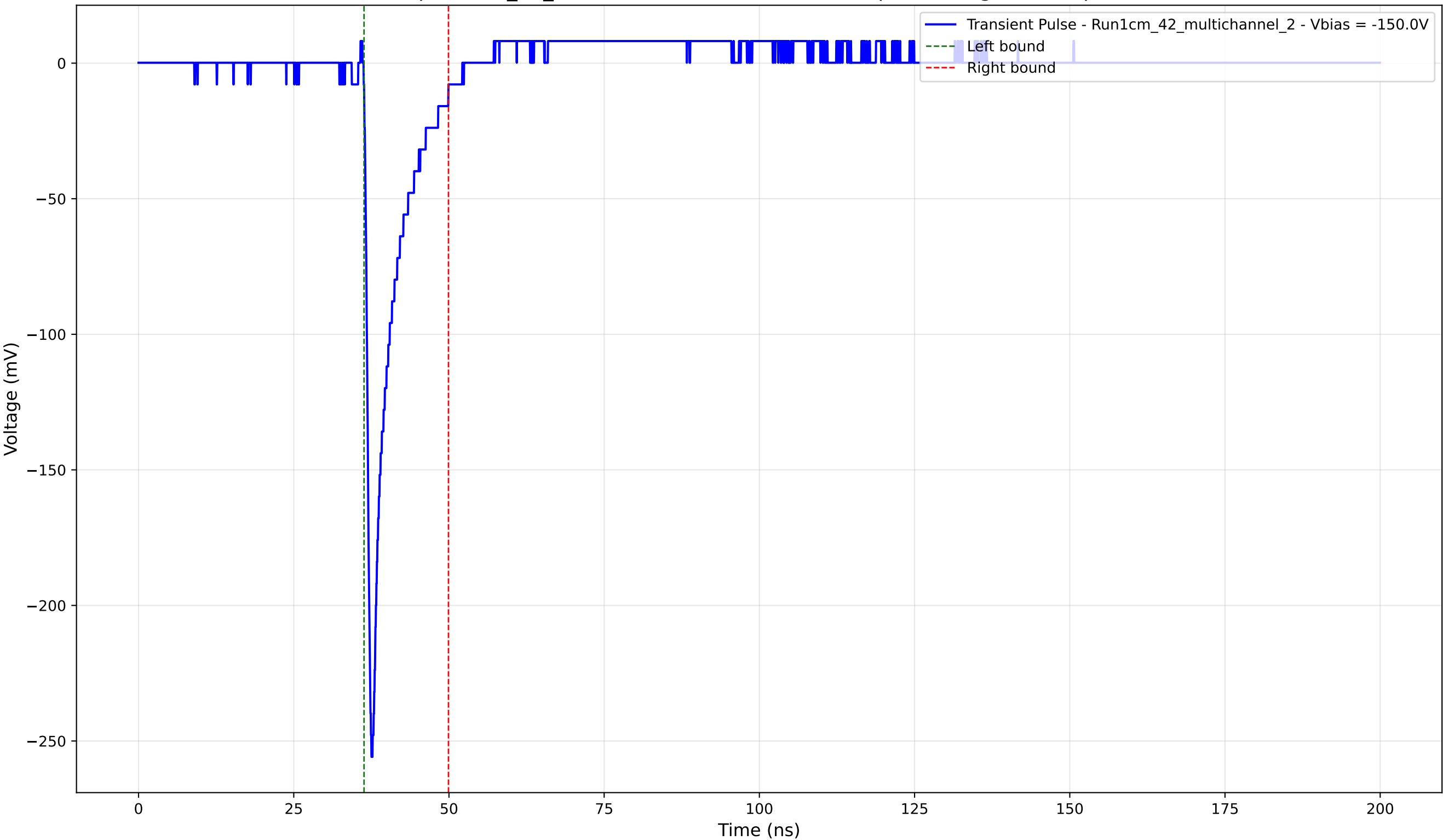
Transient Pulse - Sample: 1cm_42_multichannel - Position: 3020.0 \mu\text{m} - Charge: 20.89 pC - Rise Time: 0.86 ns
