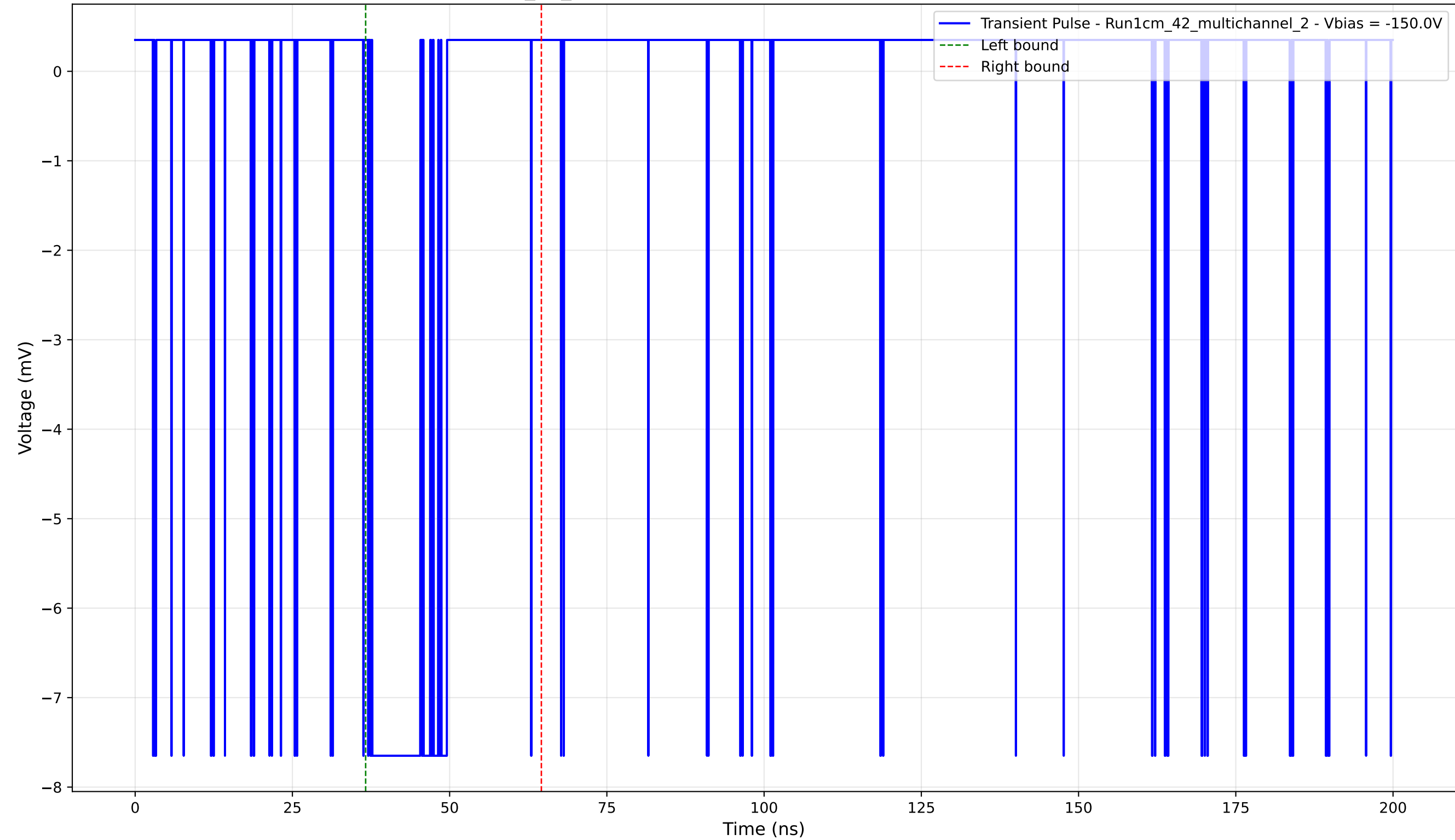
Transient Pulse - Sample: 1cm_42_multichannel - Position: 360.0 \mu\text{m} - Charge: 1.62 pC - Rise Time: 0.04 ns
