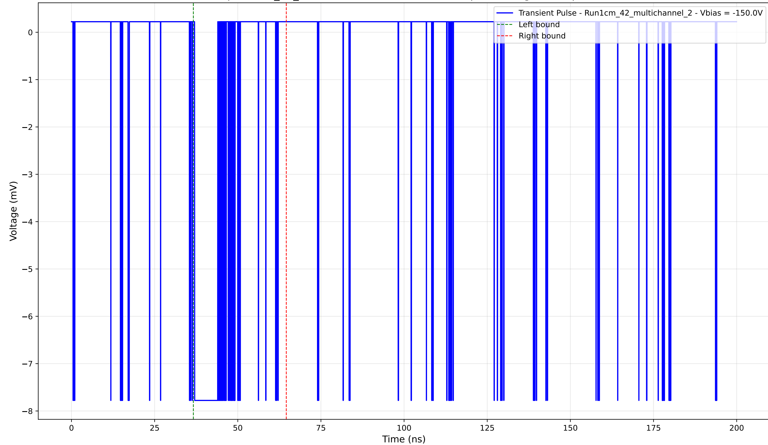
Transient Pulse - Sample: 1cm_42_multichannel - Position: 3375.0 \mu\text{m} - Charge: 1.43 pC - Rise Time: 0.04 ns
