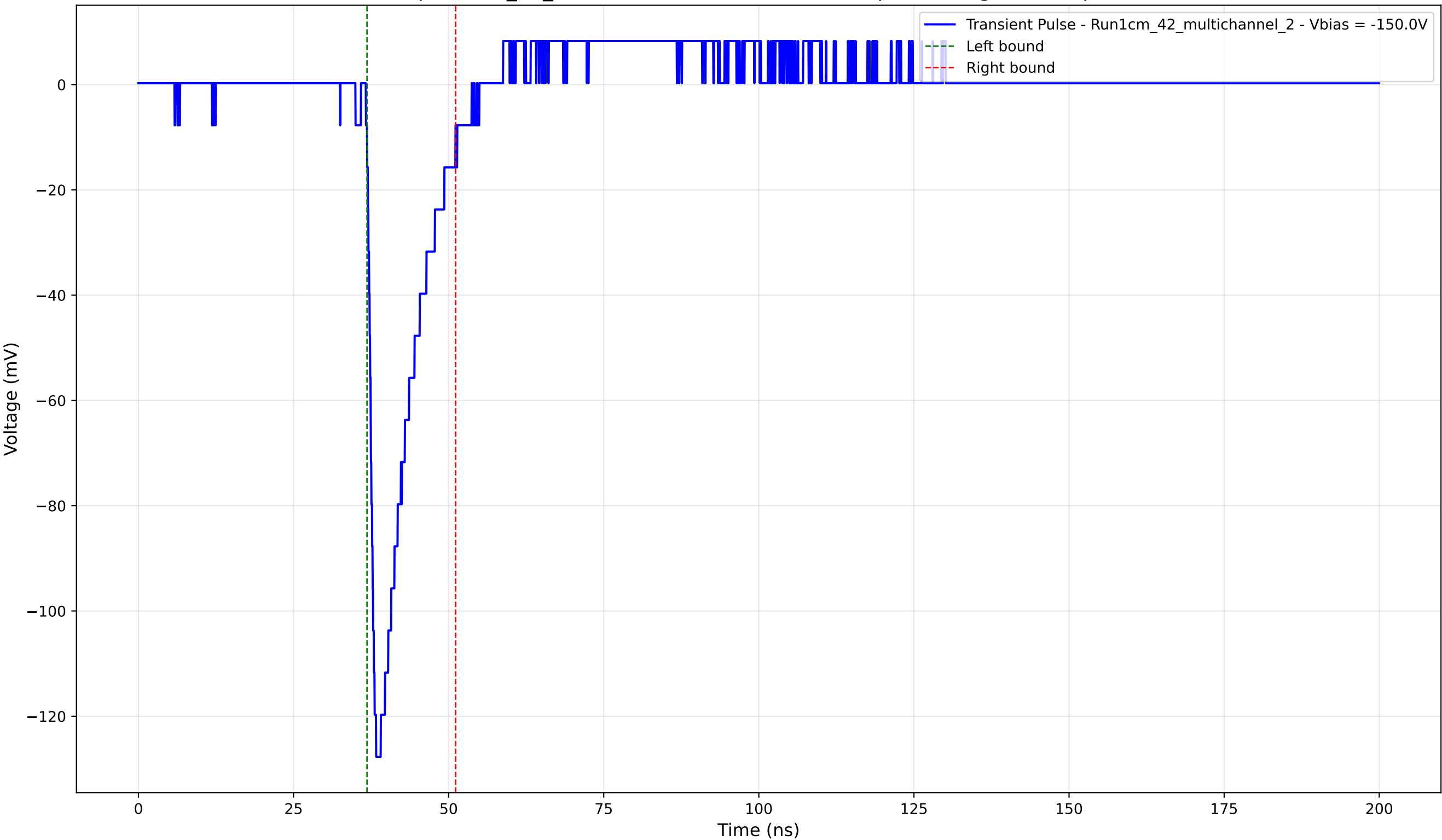
Transient Pulse - Sample: 1cm_42_multichannel - Position: 1015.0 \mu\text{m} - Charge: 17.18 pC - Rise Time: 1.21 ns
