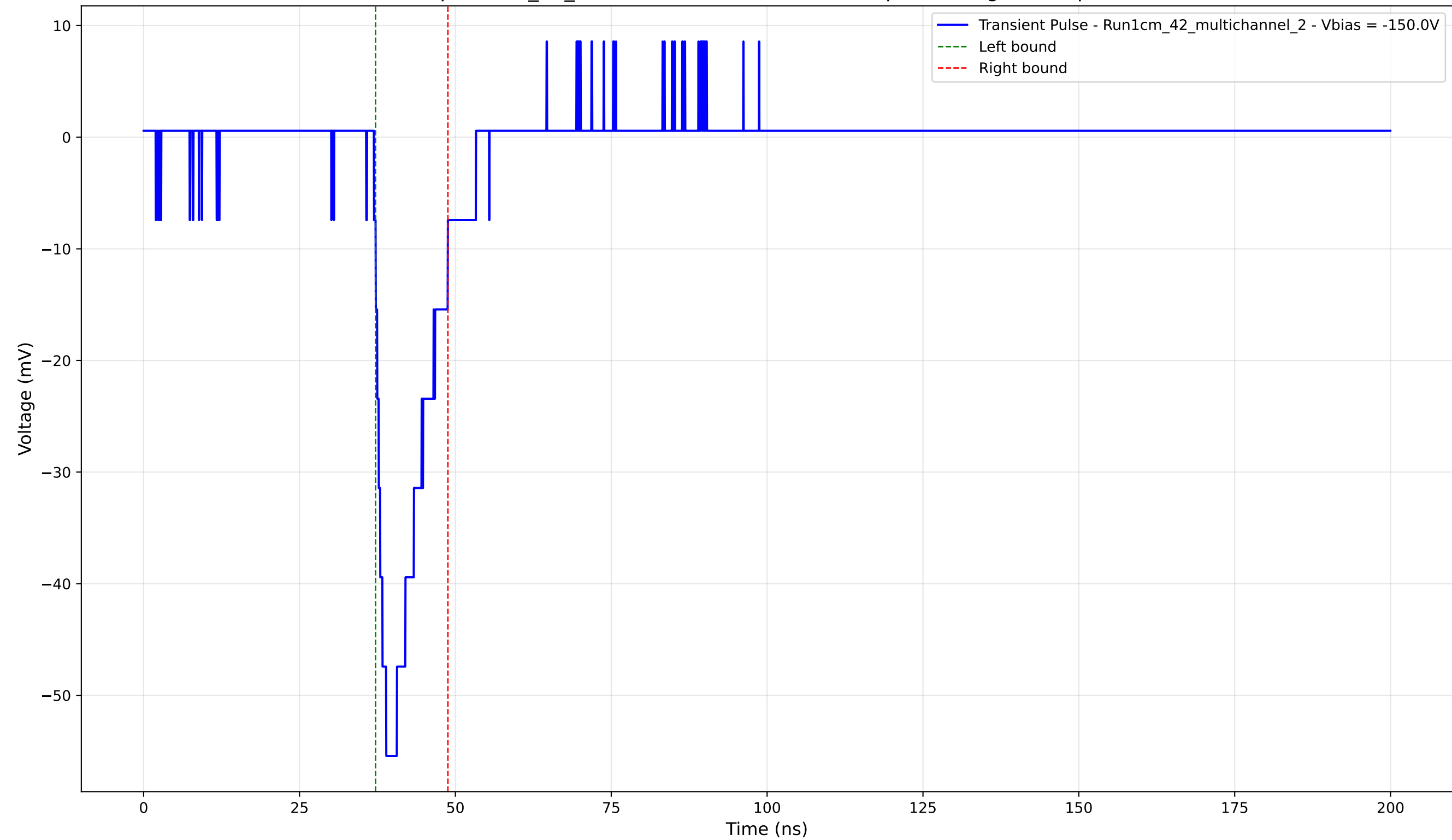
Transient Pulse - Sample: 1cm_42_multichannel - Position: 400.0 \mu\text{m} - Charge: 7.89 pC - Rise Time: 1.97 ns
