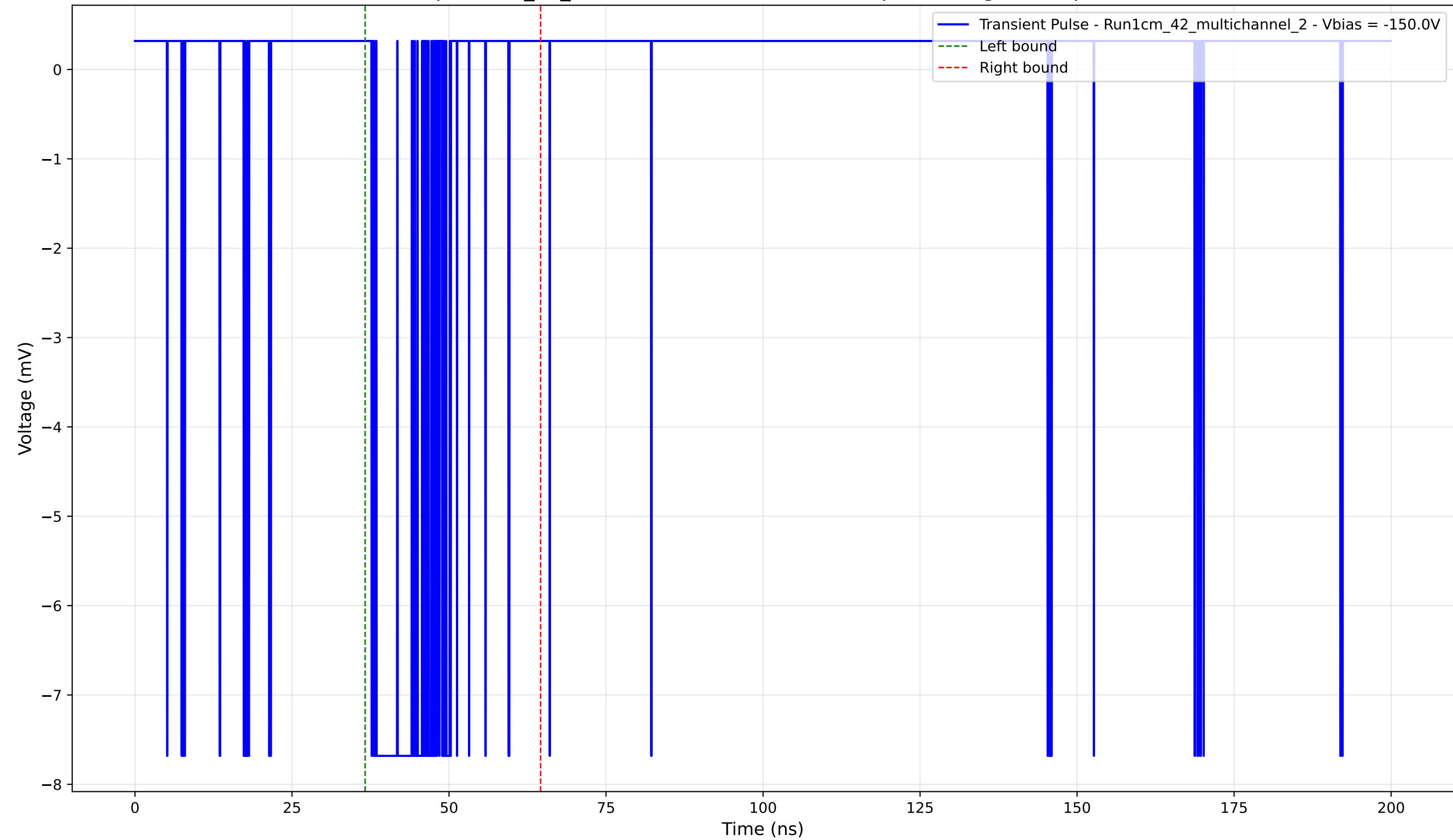
Transient Pulse - Sample: 1cm_42_multichannel - Position: 355.0 \mu\text{m} - Charge: 1.44 pC - Rise Time: 0.04 ns
