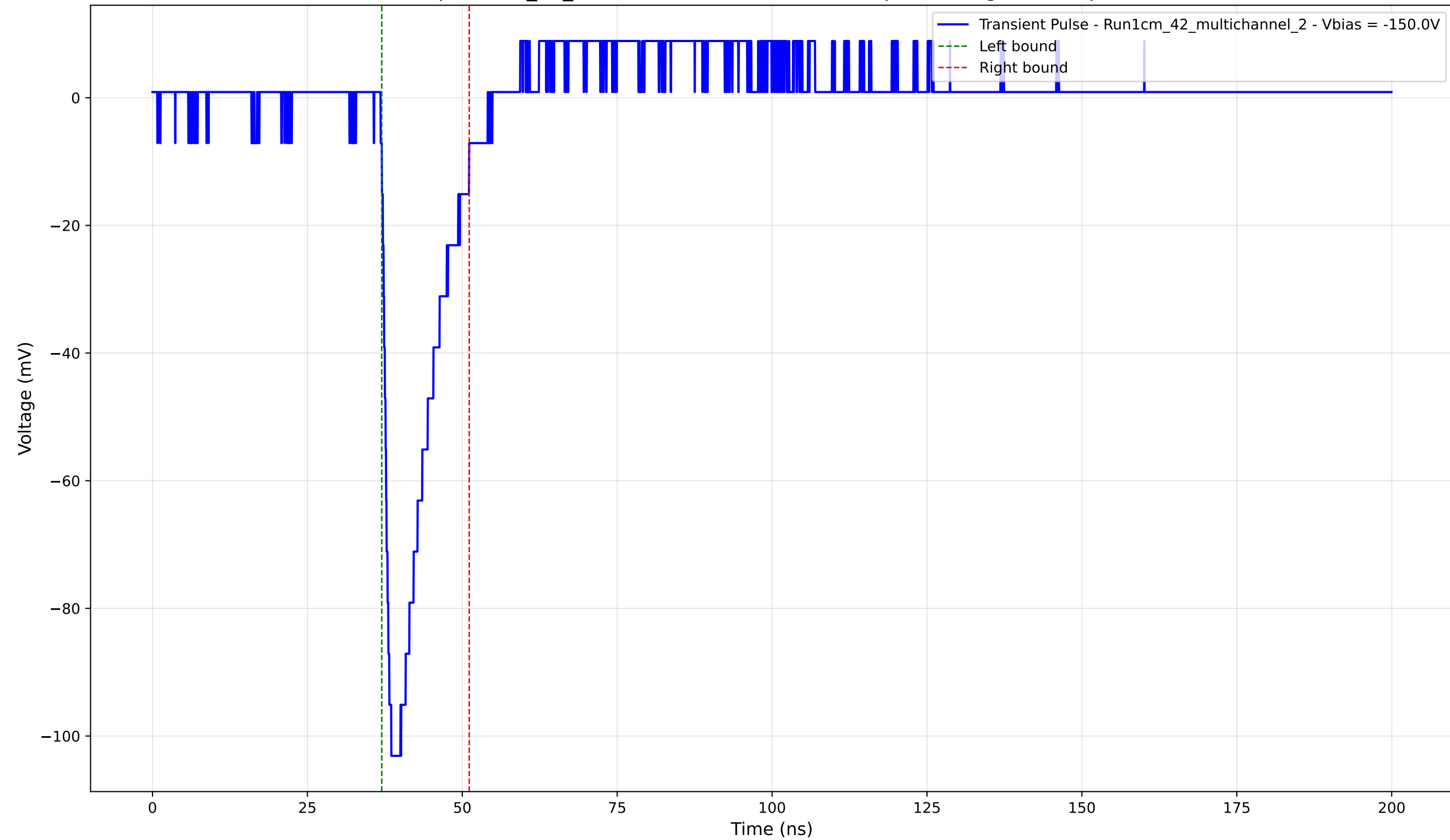
Transient Pulse - Sample: 1cm_42_multichannel - Position: 730.0 \mu\text{m} - Charge: 15.25 pC - Rise Time: 1.22 ns
