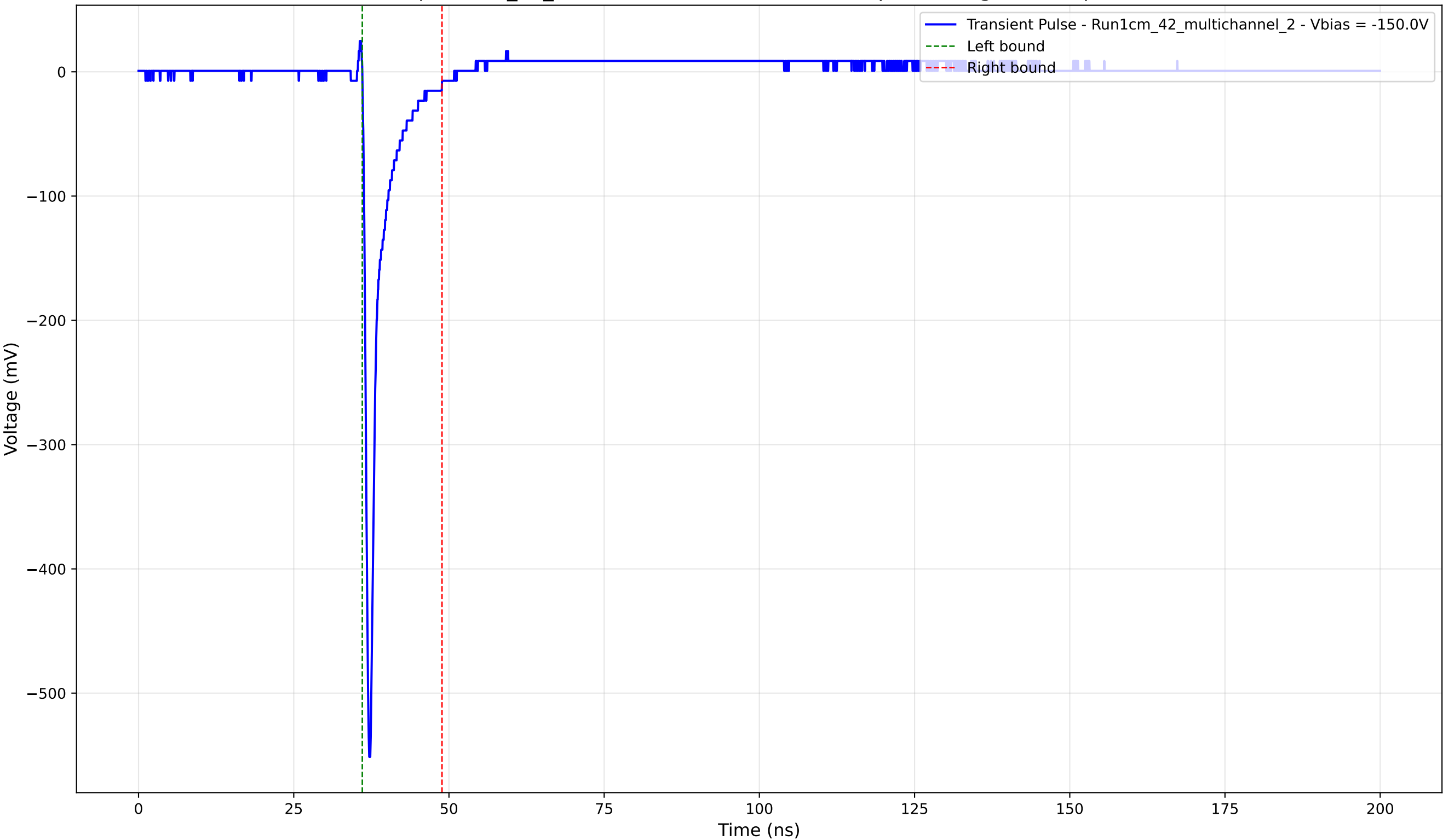
Transient Pulse - Sample: 1cm_42_multichannel - Position: 2175.0 \mu\text{m} - Charge: 27.53 pC - Rise Time: 0.74 ns
