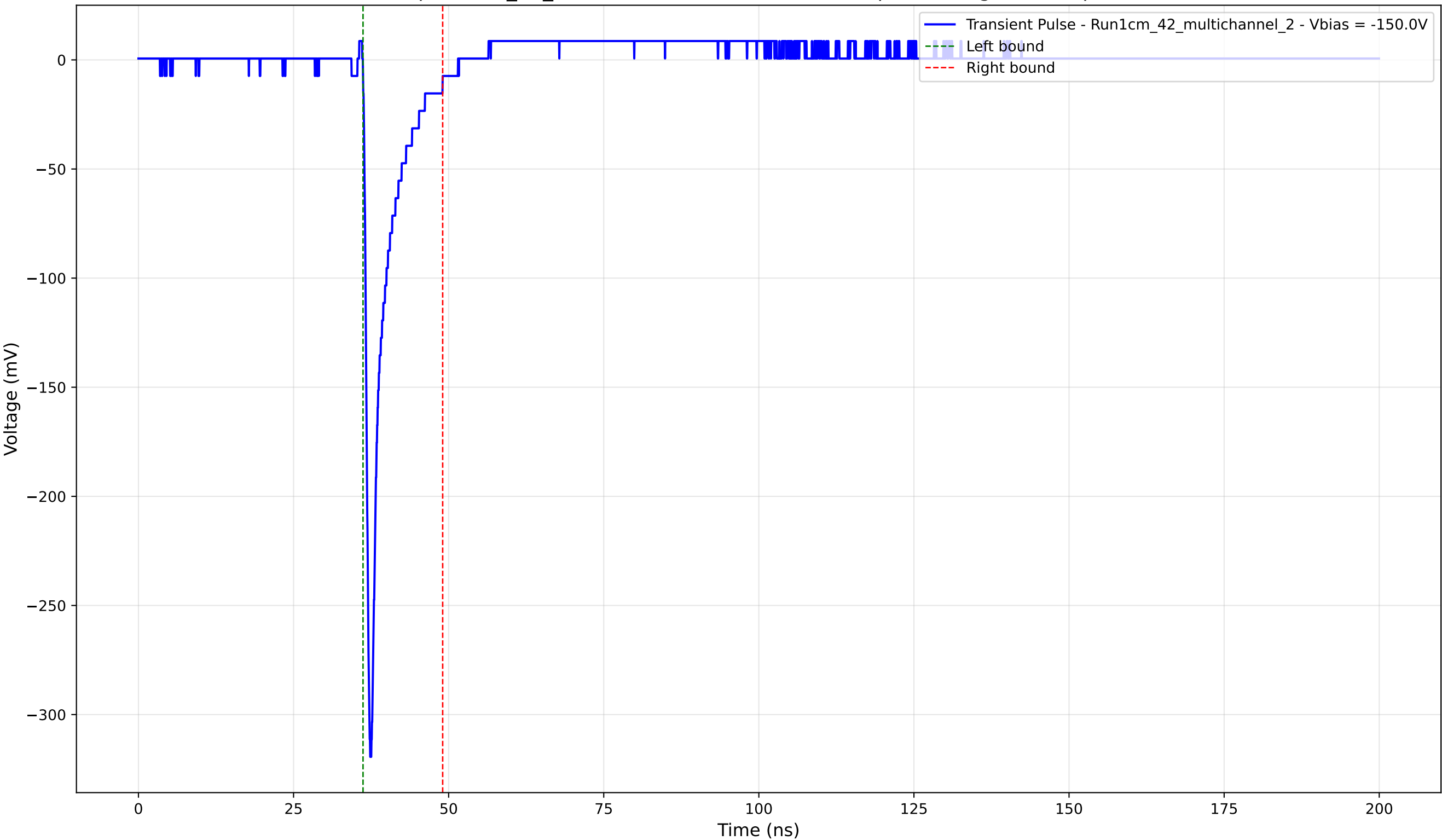
Transient Pulse - Sample: 1cm_42_multichannel - Position: 2800.0 \mu\text{m} - Charge: 20.33 pC - Rise Time: 0.80 ns
