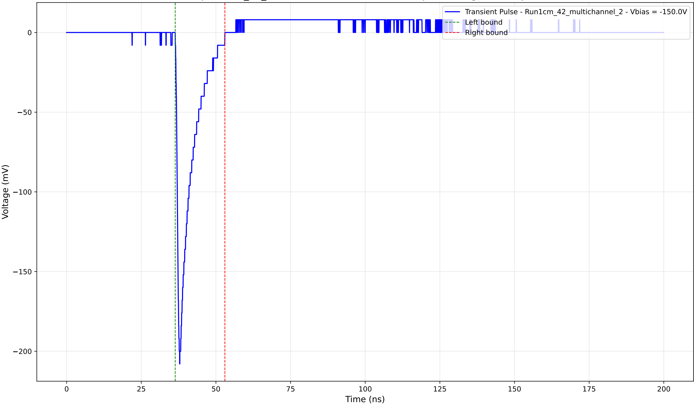
Transient Pulse - Sample: 1cm_42_multichannel - Position: 1475.0 \mu\text{m} - Charge: 21.28 pC - Rise Time: 1.02 ns
