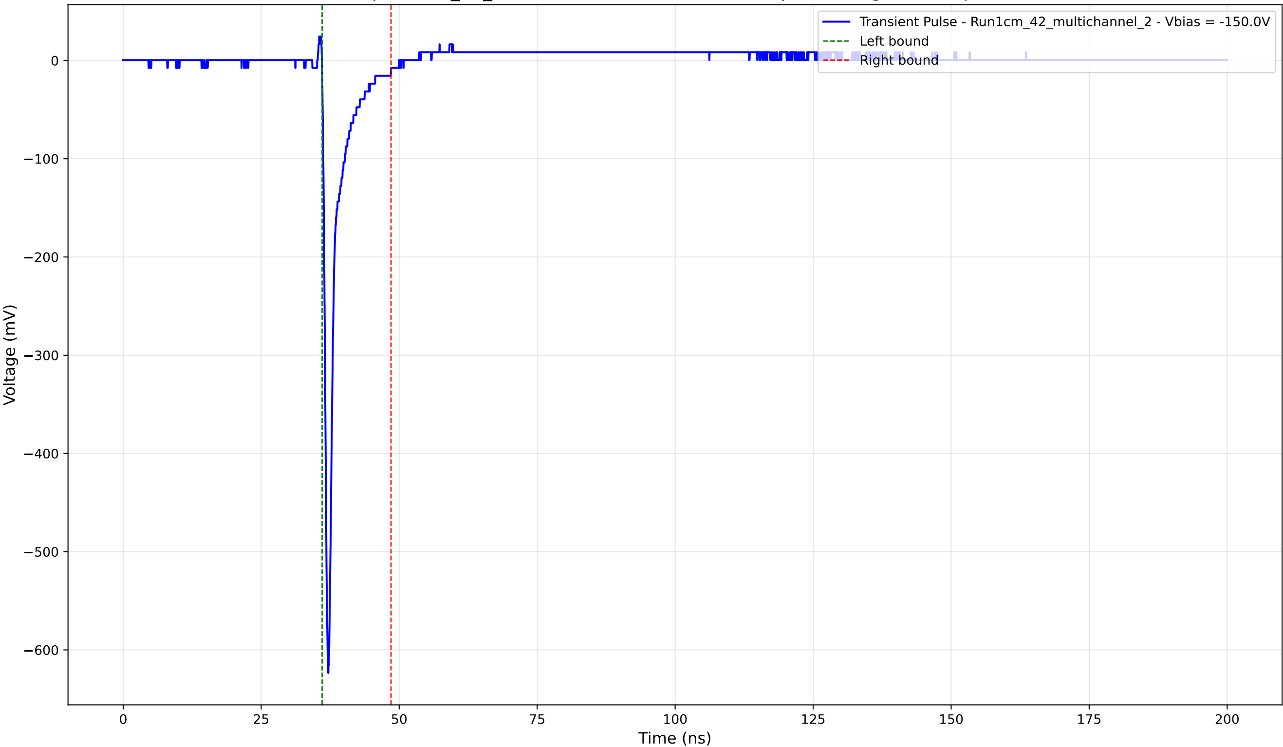
Transient Pulse - Sample: 1cm_42_multichannel - Position: 2475.0 \mu\text{m} - Charge: 28.16 pC - Rise Time: 0.75 ns
