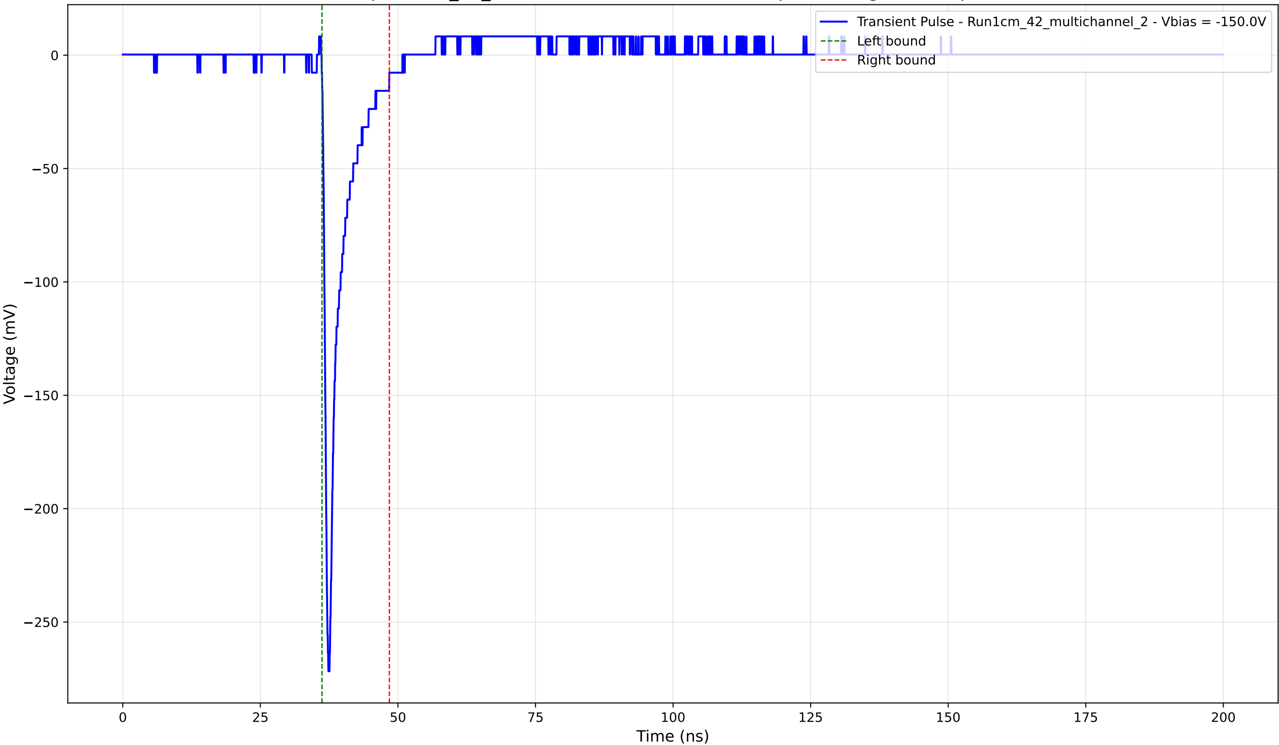
Transient Pulse - Sample: 1cm_42_multichannel - Position: 2810.0 \mu\text{m} - Charge: 17.63 pC - Rise Time: 0.81 ns
