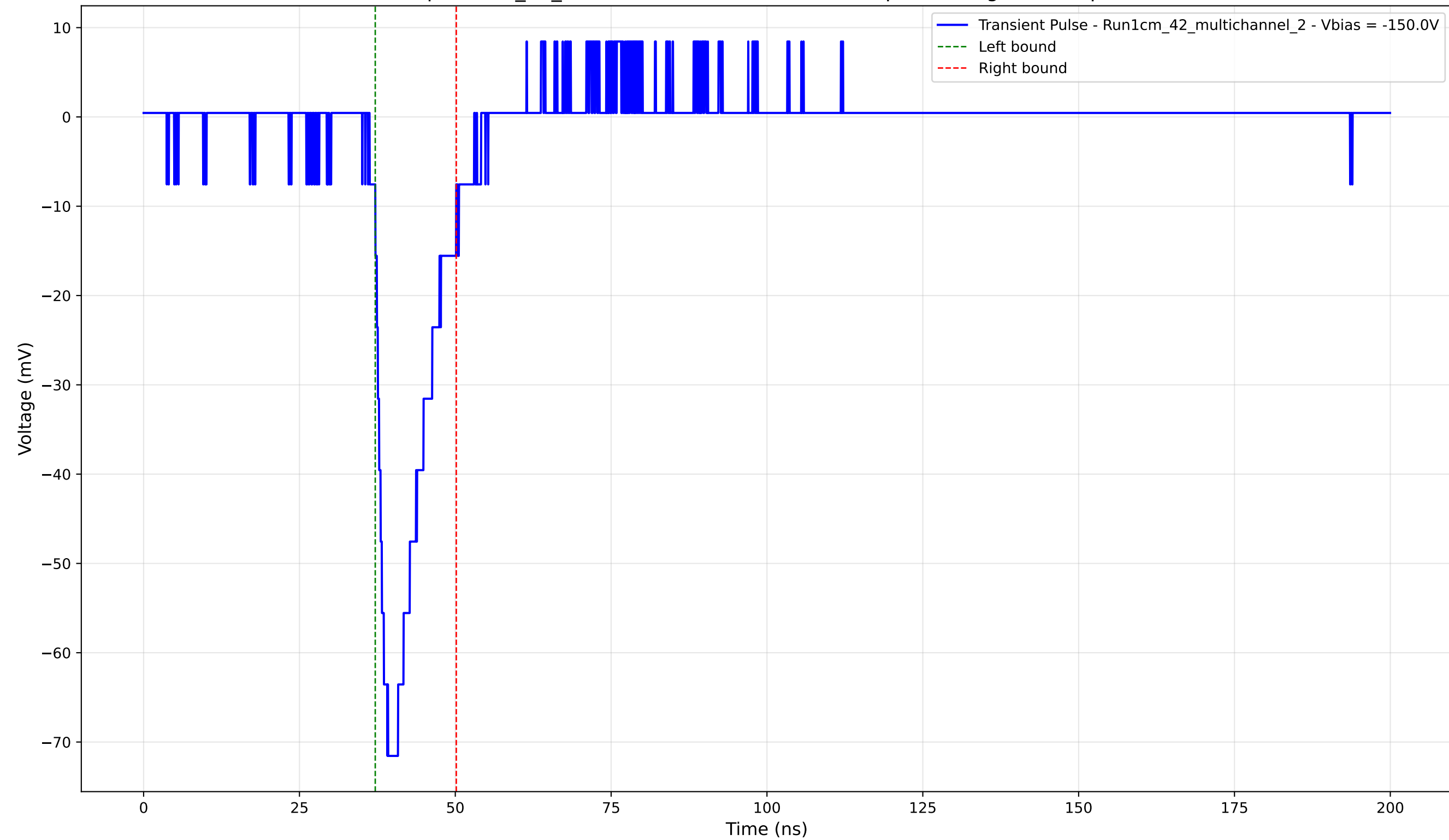
Transient Pulse - Sample: 1cm_42_multichannel - Position: 4595.0 \mu\text{m} - Charge: 10.59 pC - Rise Time: 2.84 ns
