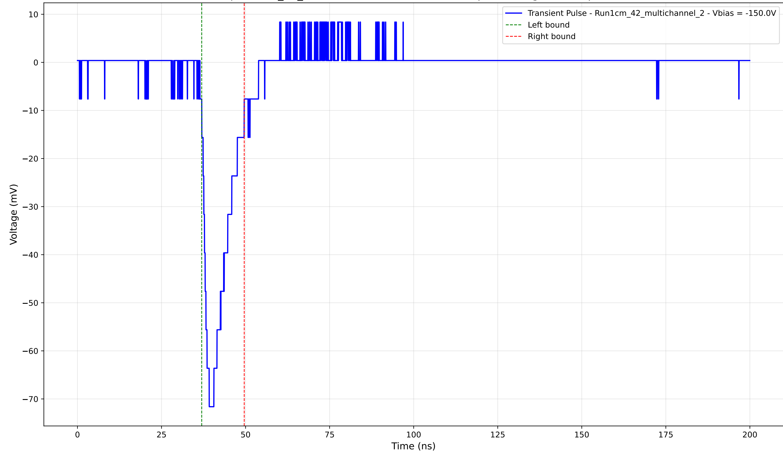
Transient Pulse - Sample: 1cm_42_multichannel - Position: 4660.0 \mu\text{m} - Charge: 10.30 pC - Rise Time: 2.76 ns
