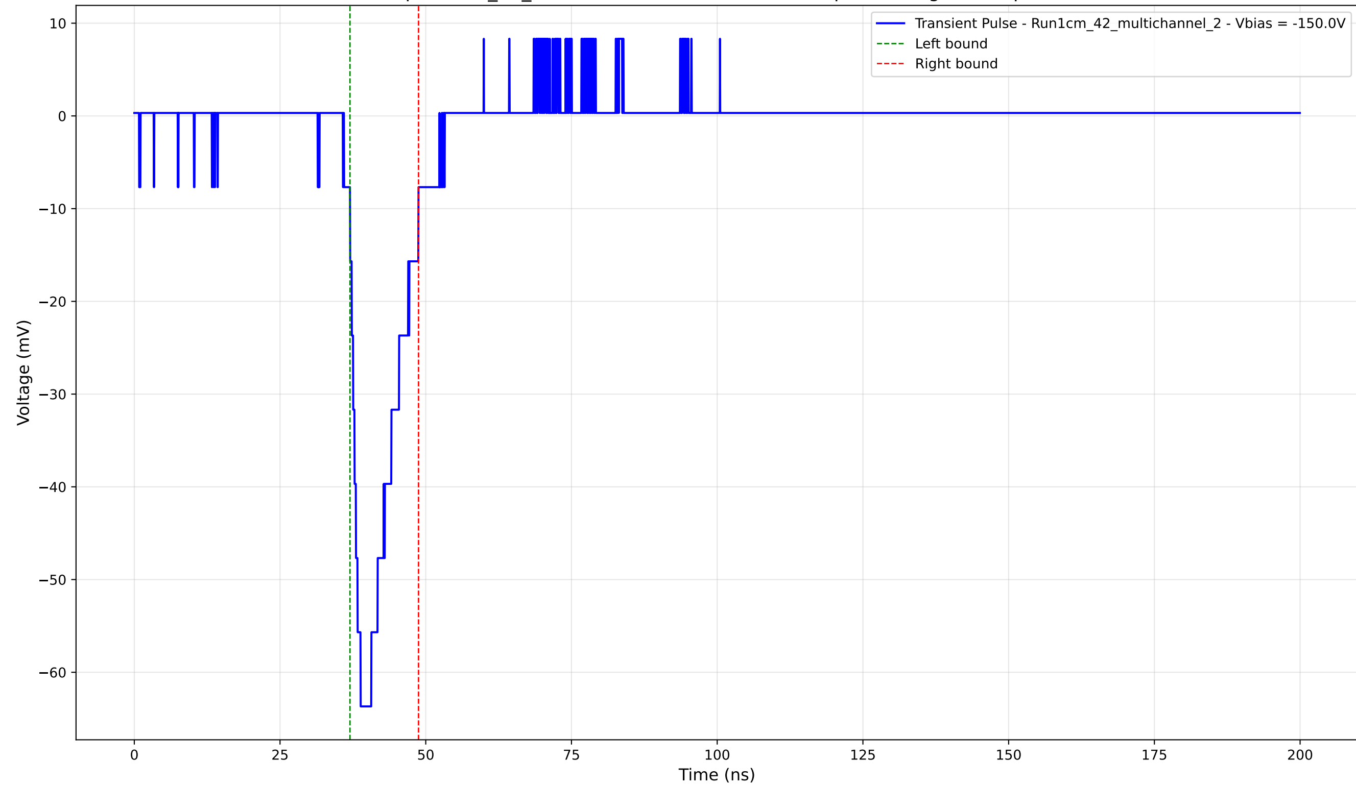
Transient Pulse - Sample: 1cm_42_multichannel - Position: 4785.0 \mu\text{m} - Charge: 9.15 pC - Rise Time: 2.85 ns
