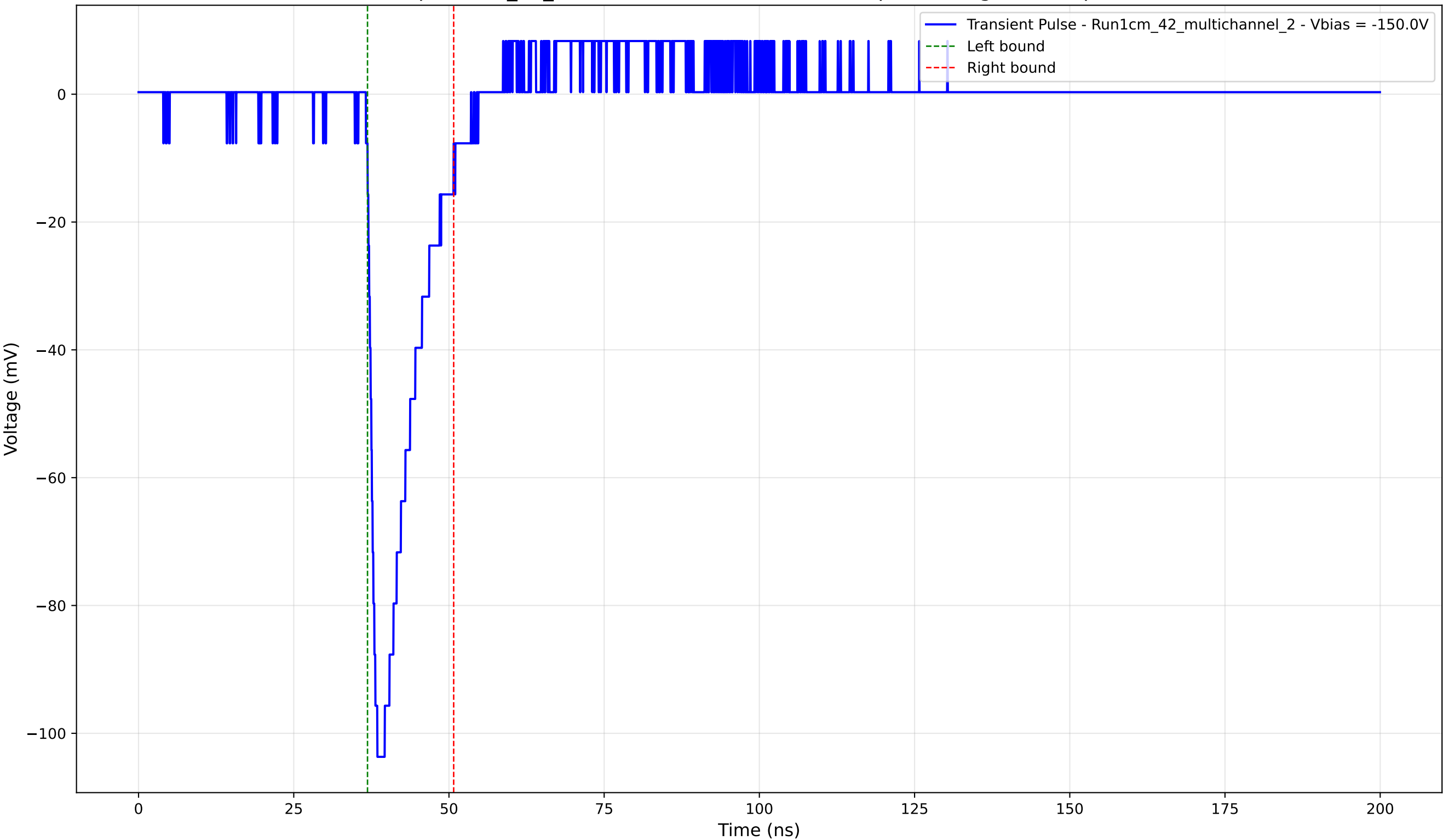
Transient Pulse - Sample: 1cm_42_multichannel - Position: 3785.0 \mu\text{m} - Charge: 14.48 pC - Rise Time: 1.27 ns
