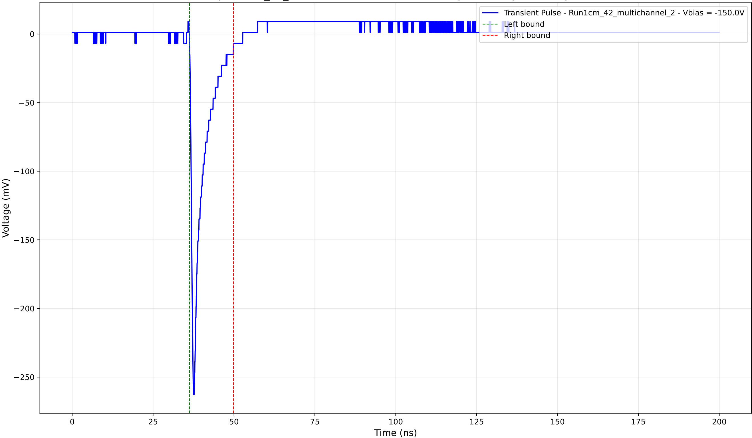
Transient Pulse - Sample: 1cm_42_multichannel - Position: 3005.0 \mu\text{m} - Charge: 20.77 pC - Rise Time: 0.89 ns
