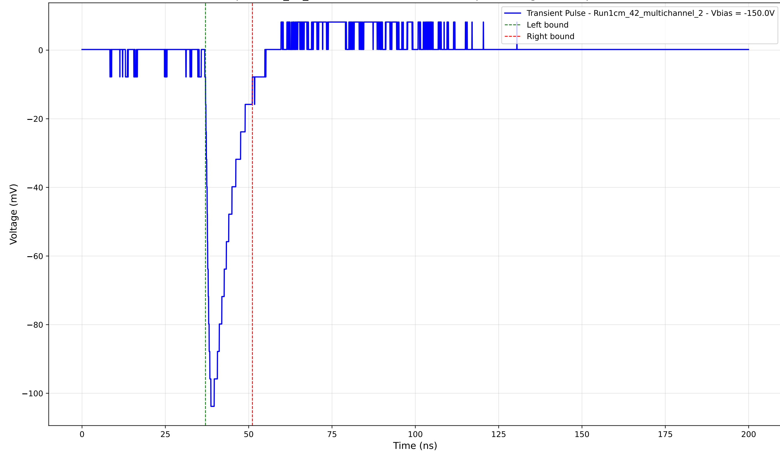
Transient Pulse - Sample: 1cm_42_multichannel - Position: 755.0 \mu\text{m} - Charge: 14.89 pC - Rise Time: 1.31 ns
