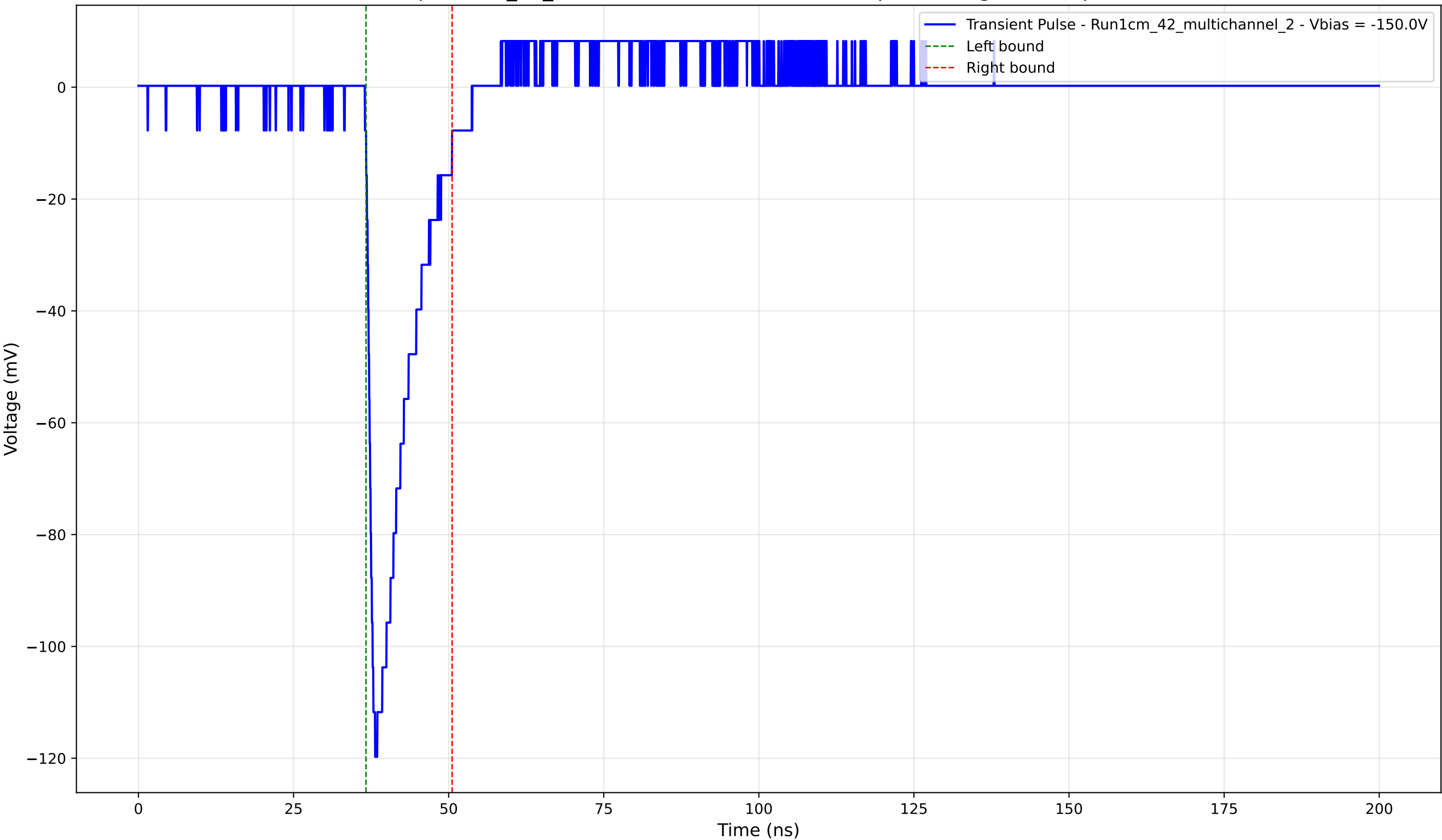
Transient Pulse - Sample: 1cm_42_multichannel - Position: 3570.0 \mu\text{m} - Charge: 15.47 pC - Rise Time: 1.18 ns
