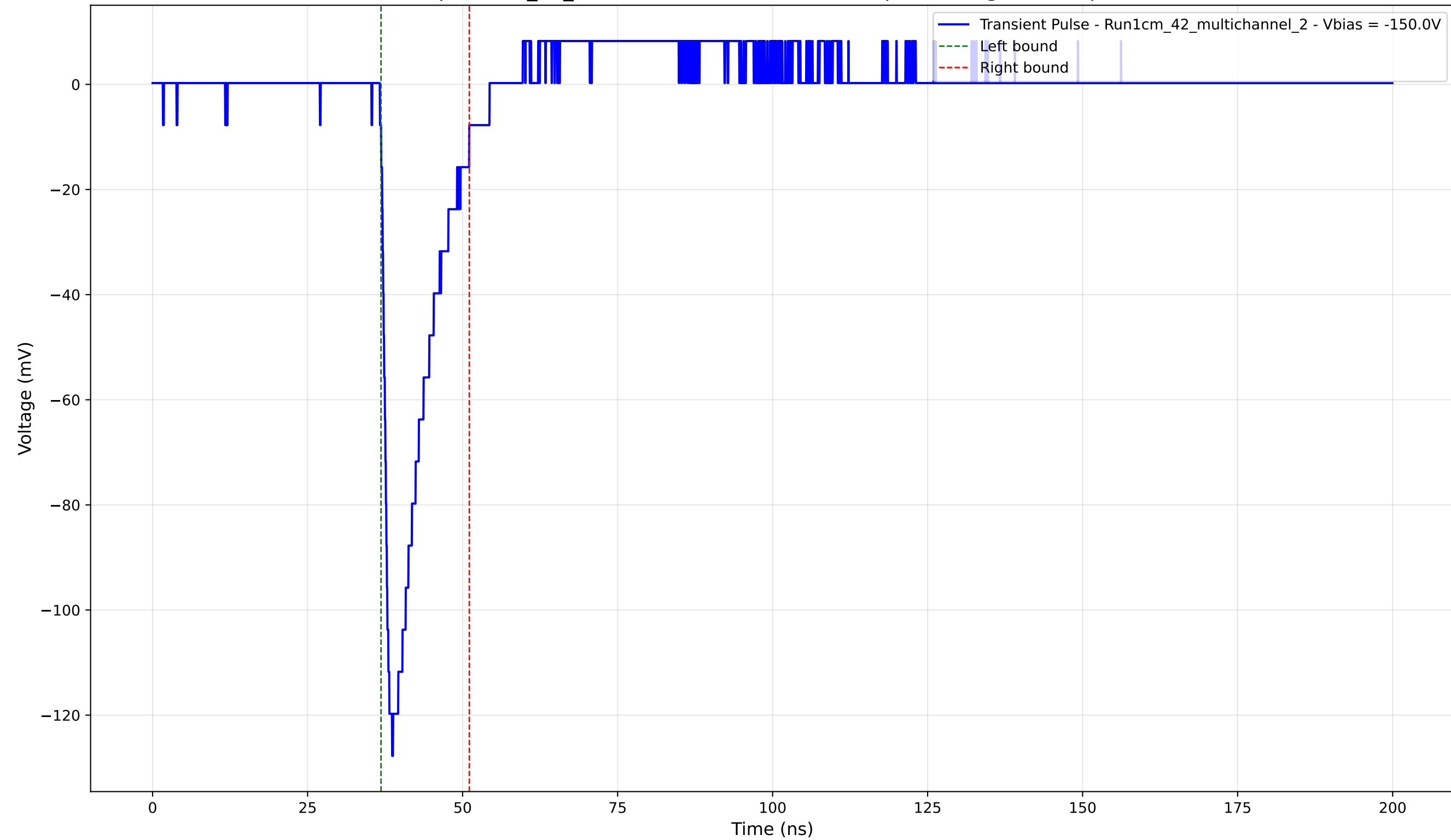
Transient Pulse - Sample: 1cm_42_multichannel - Position: 990.0 \mu\text{m} - Charge: 17.01 pC - Rise Time: 1.33 ns
