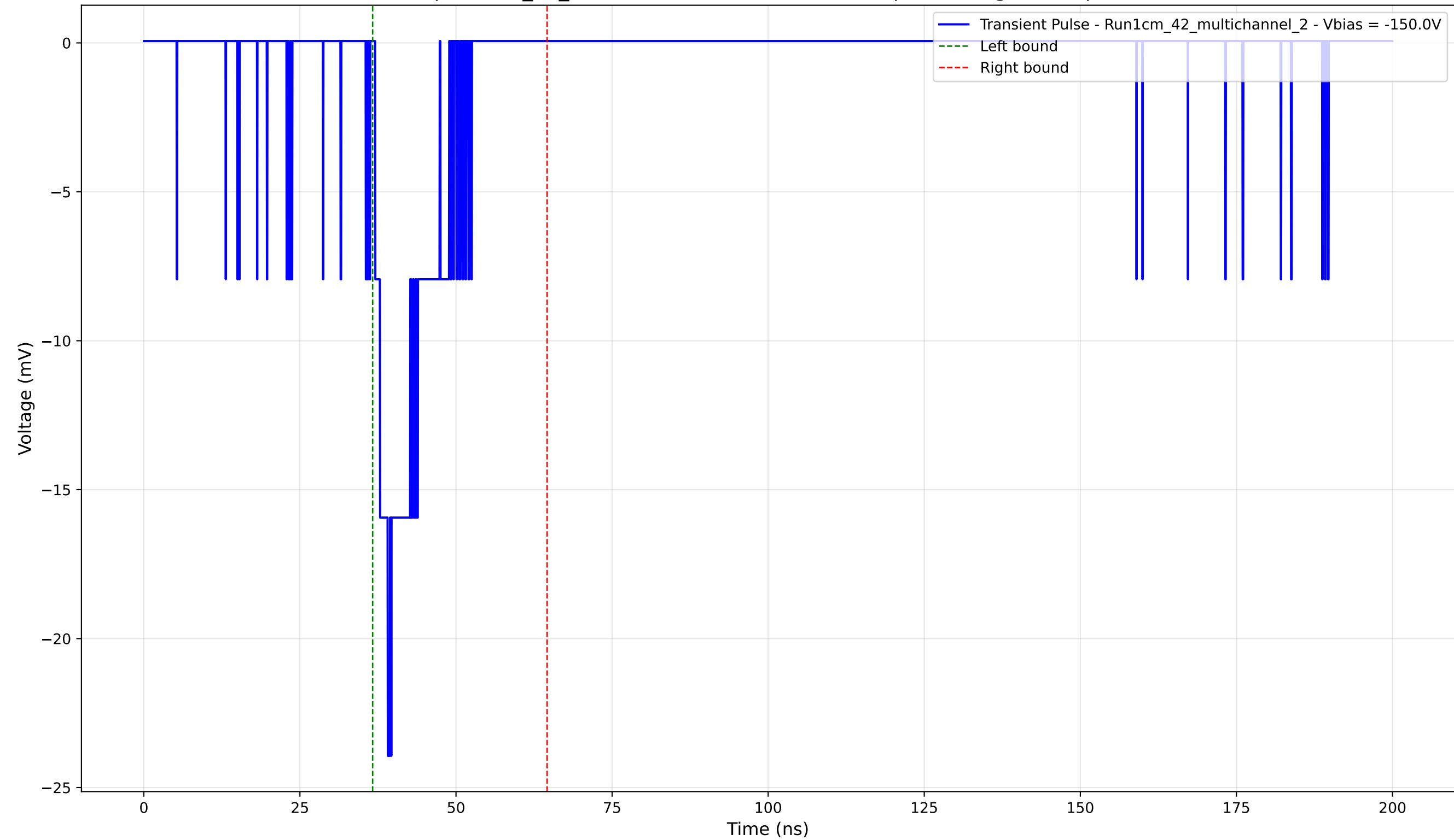
Transient Pulse - Sample: 1cm_42_multichannel - Position: 3920.0 \mu\text{m} - Charge: 2.96 pC - Rise Time: 2.03 ns
