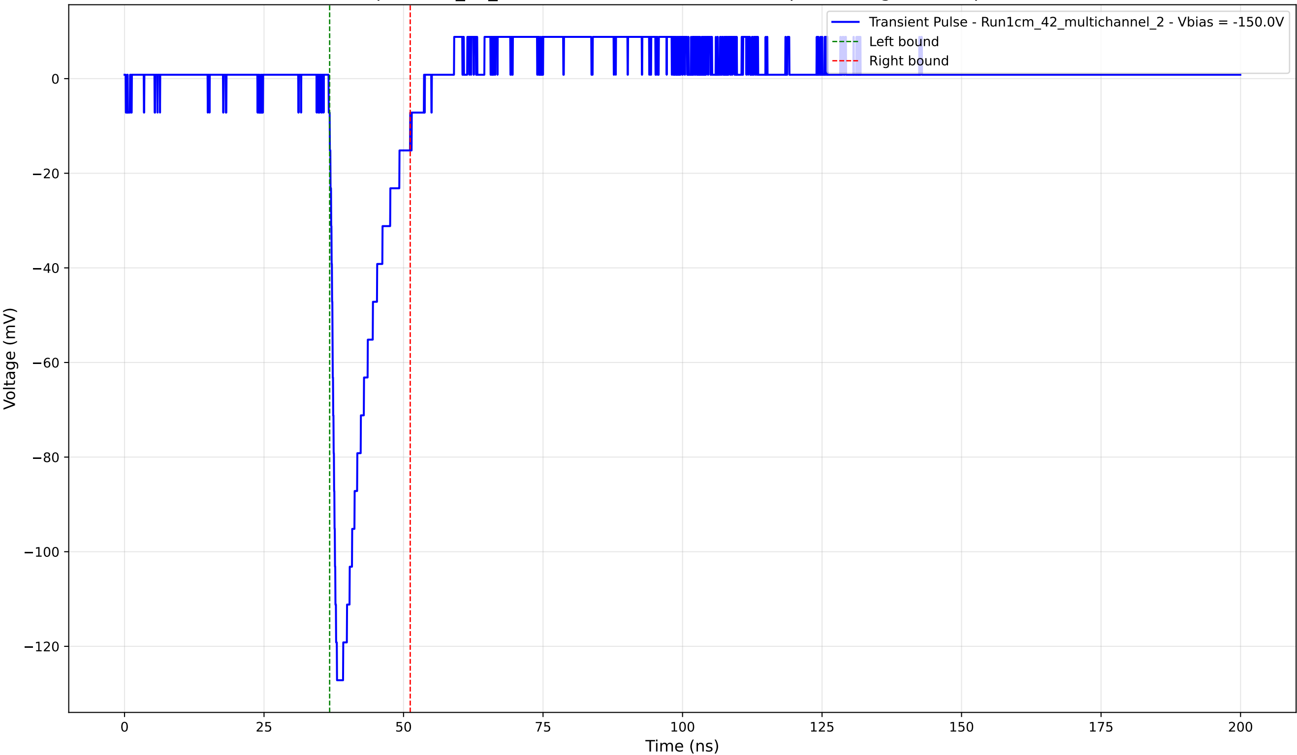
Transient Pulse - Sample: 1cm_42_multichannel - Position: 1075.0 \mu\text{m} - Charge: 17.26 pC - Rise Time: 1.13 ns
