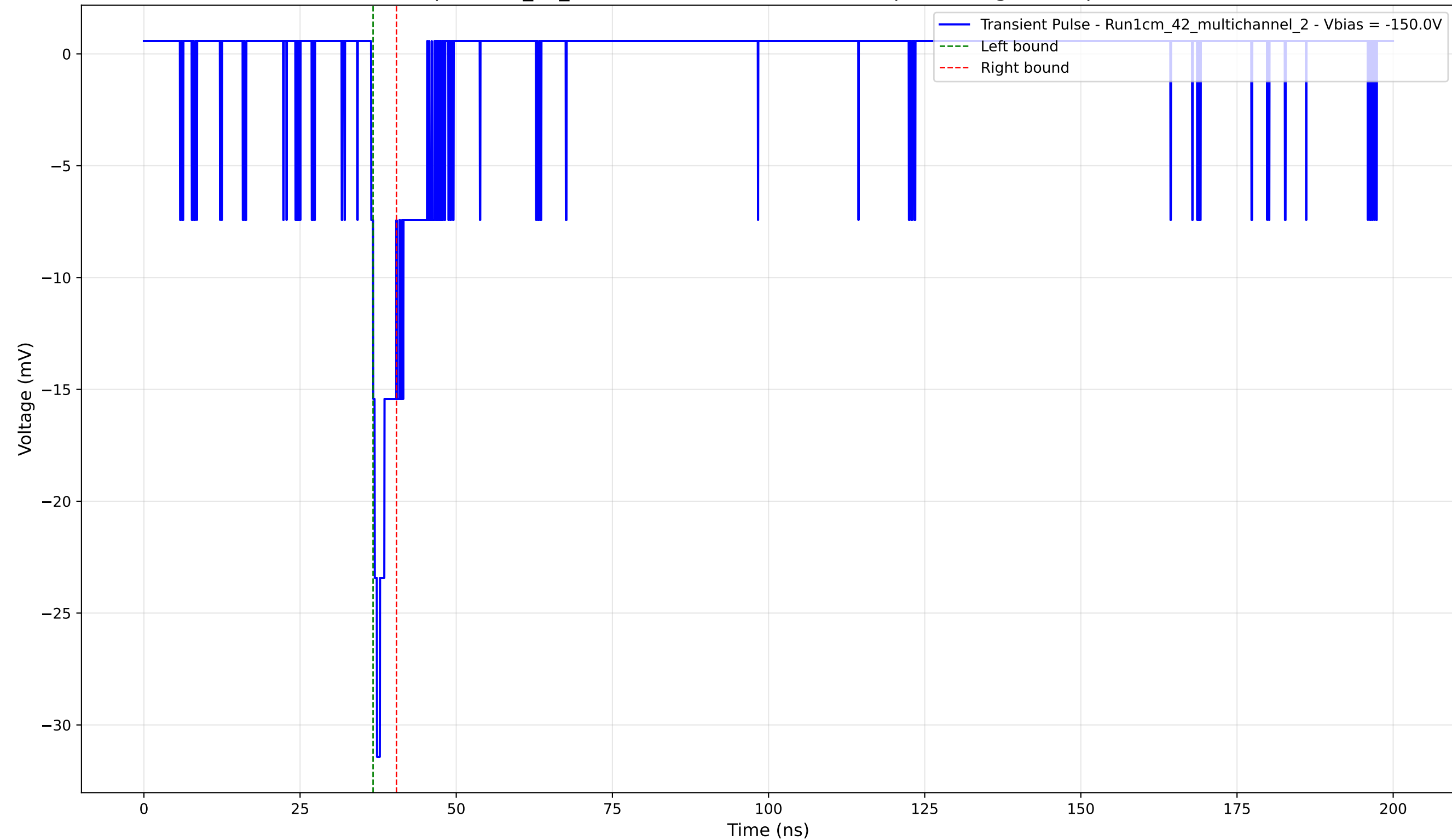
Transient Pulse - Sample: 1cm_42_multichannel - Position: 1840.0 \mu\text{m} - Charge: 1.48 pC - Rise Time: 0.95 ns
