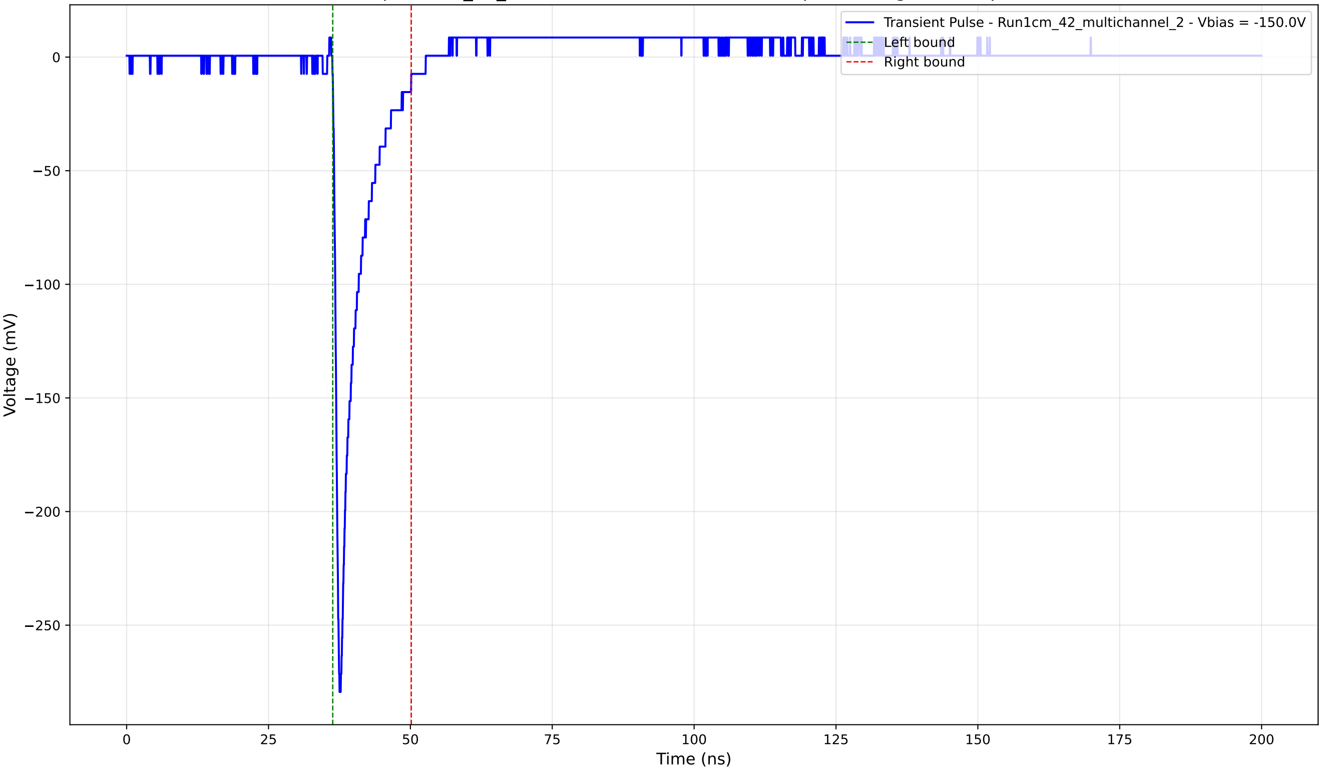
Transient Pulse - Sample: 1cm_42_multichannel - Position: 1710.0 \mu\text{m} - Charge: 22.95 pC - Rise Time: 0.92 ns
