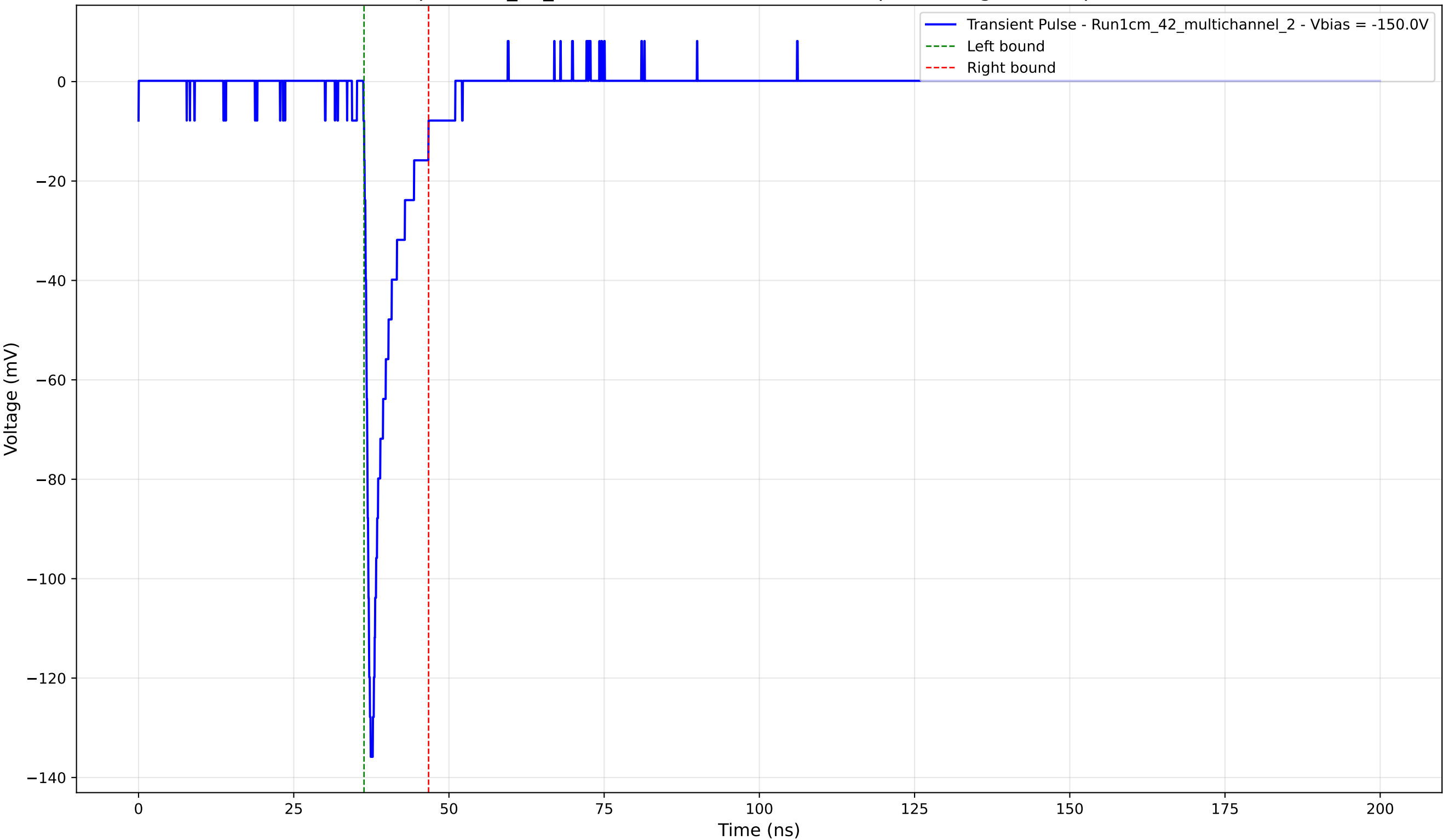
Transient Pulse - Sample: 1cm_42_multichannel - Position: 1815.0 \mu\text{m} - Charge: 10.01 pC - Rise Time: 0.93 ns
