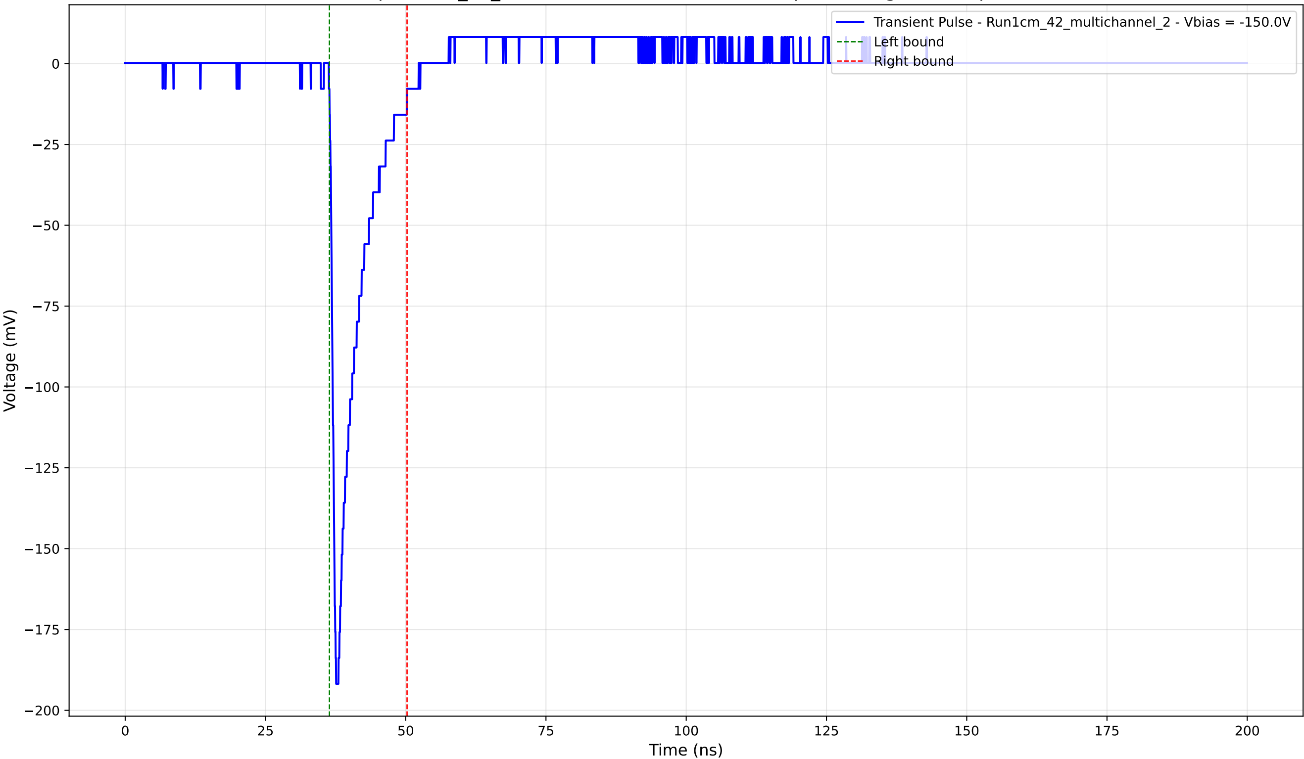
Transient Pulse - Sample: 1cm_42_multichannel - Position: 3180.0 \mu\text{m} - Charge: 18.68 pC - Rise Time: 0.94 ns
