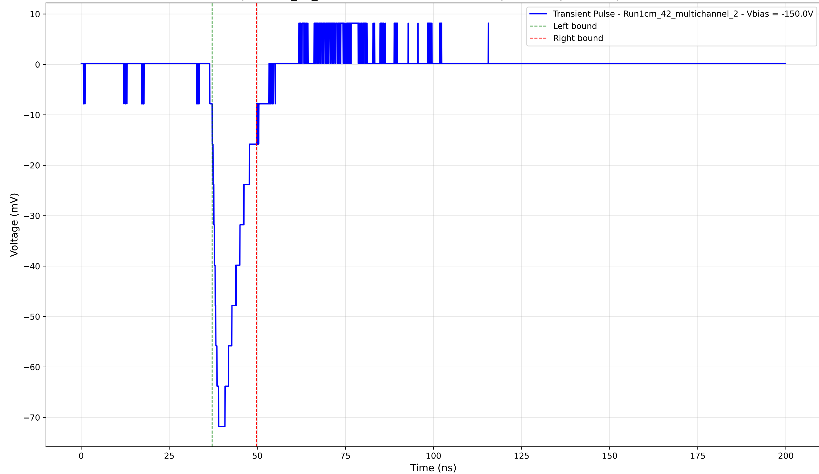
Transient Pulse - Sample: 1cm_42_multichannel - Position: 4565.0 \mu\text{m} - Charge: 10.64 pC - Rise Time: 2.52 ns
