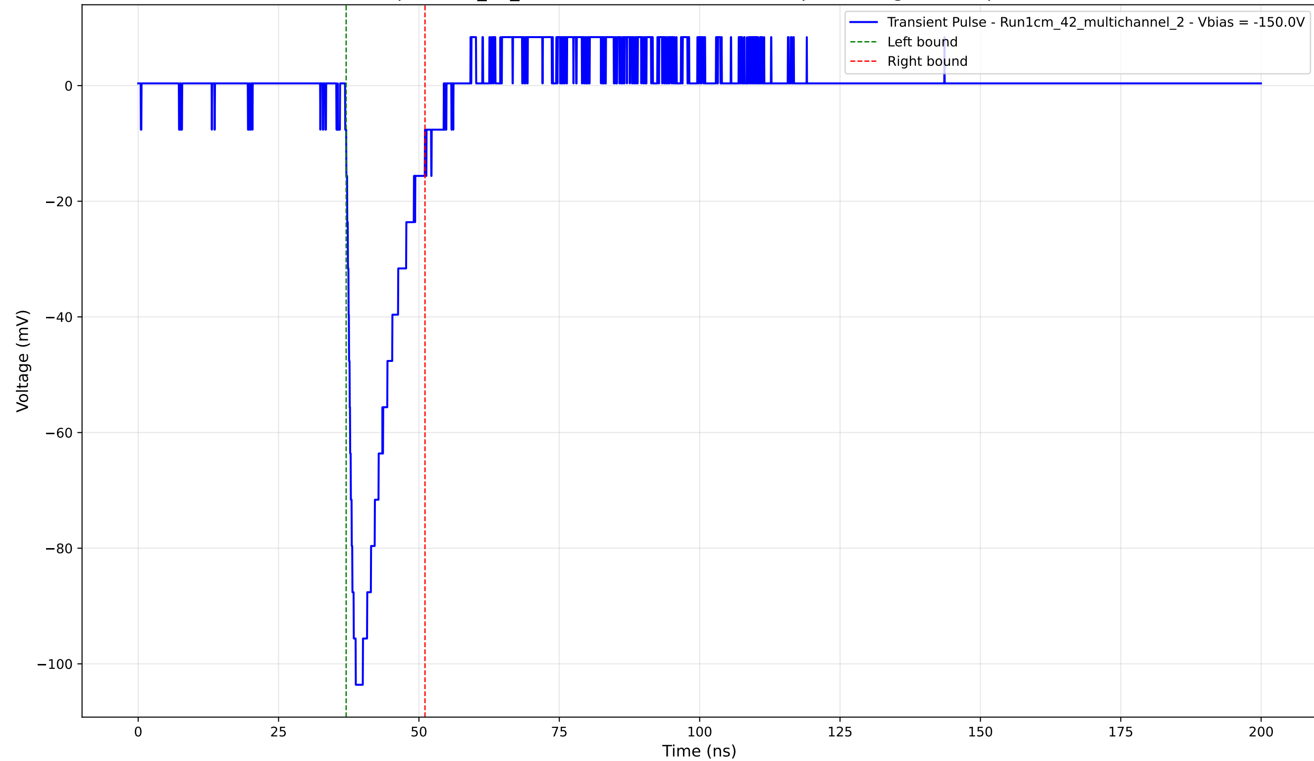
Transient Pulse - Sample: 1cm_42_multichannel - Position: 680.0 \mu\text{m} - Charge: 15.18 pC - Rise Time: 1.35 ns
