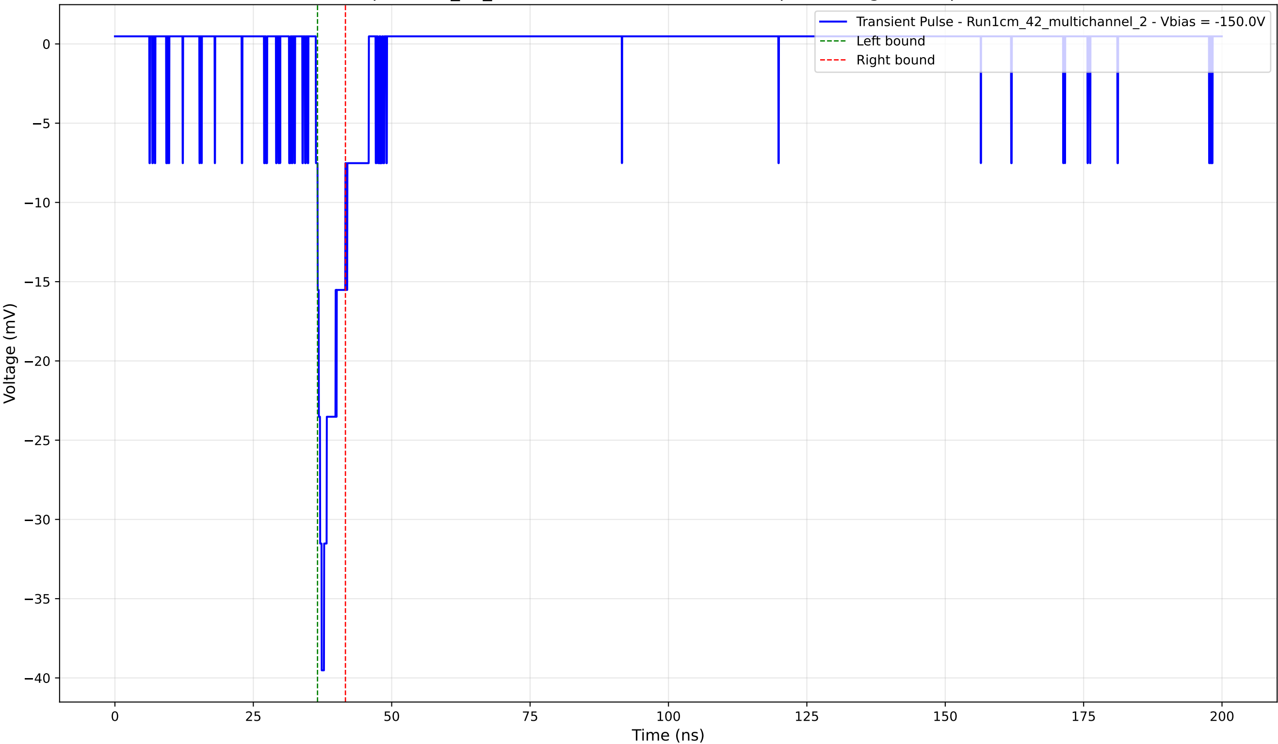
Transient Pulse - Sample: 1cm_42_multichannel - Position: 2905.0 \mu\text{m} - Charge: 2.32 pC - Rise Time: 1.06 ns
