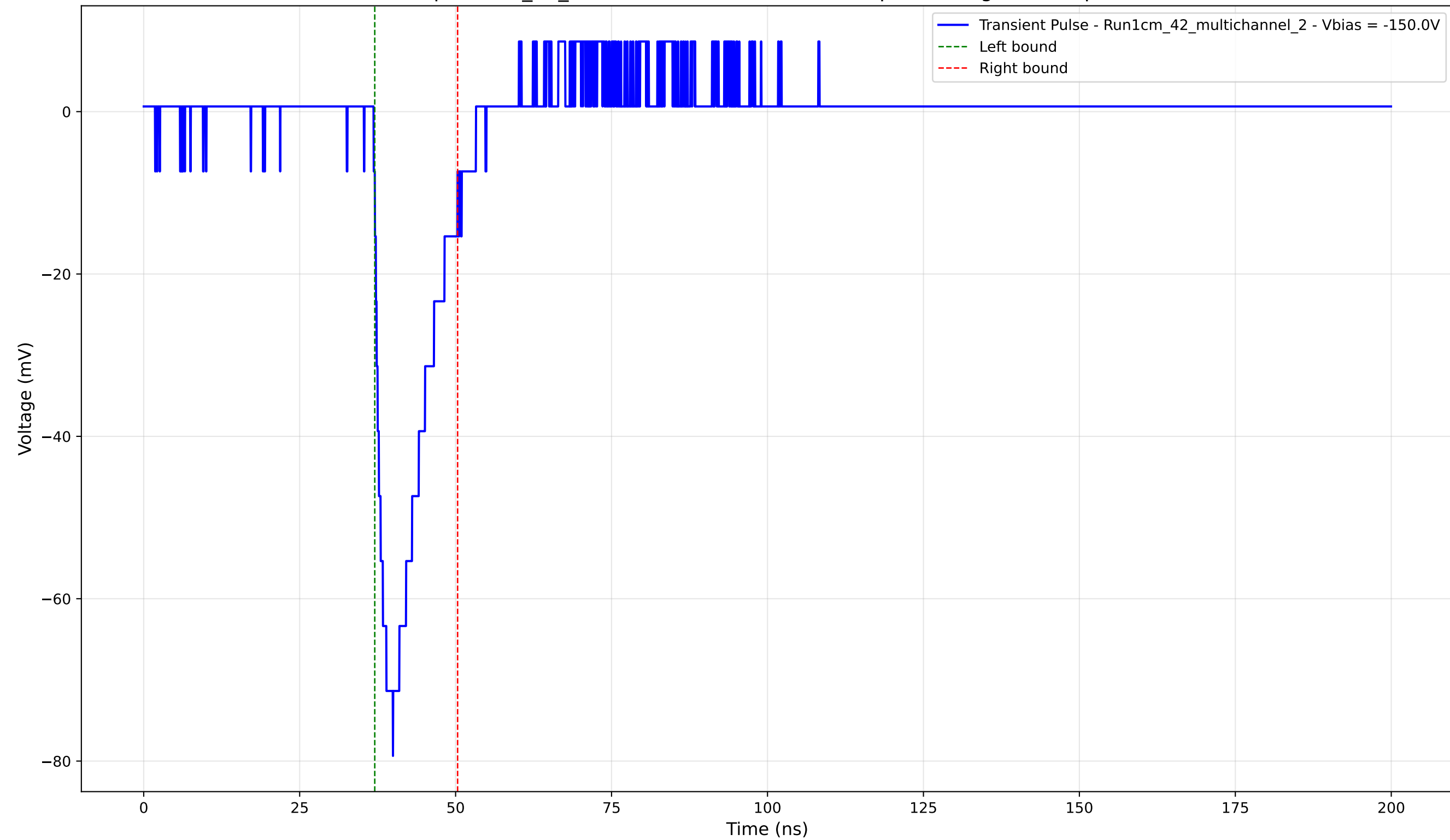
Transient Pulse - Sample: 1cm_42_multichannel - Position: 210.0 \mu\text{m} - Charge: 11.29 pC - Rise Time: 2.92 ns
