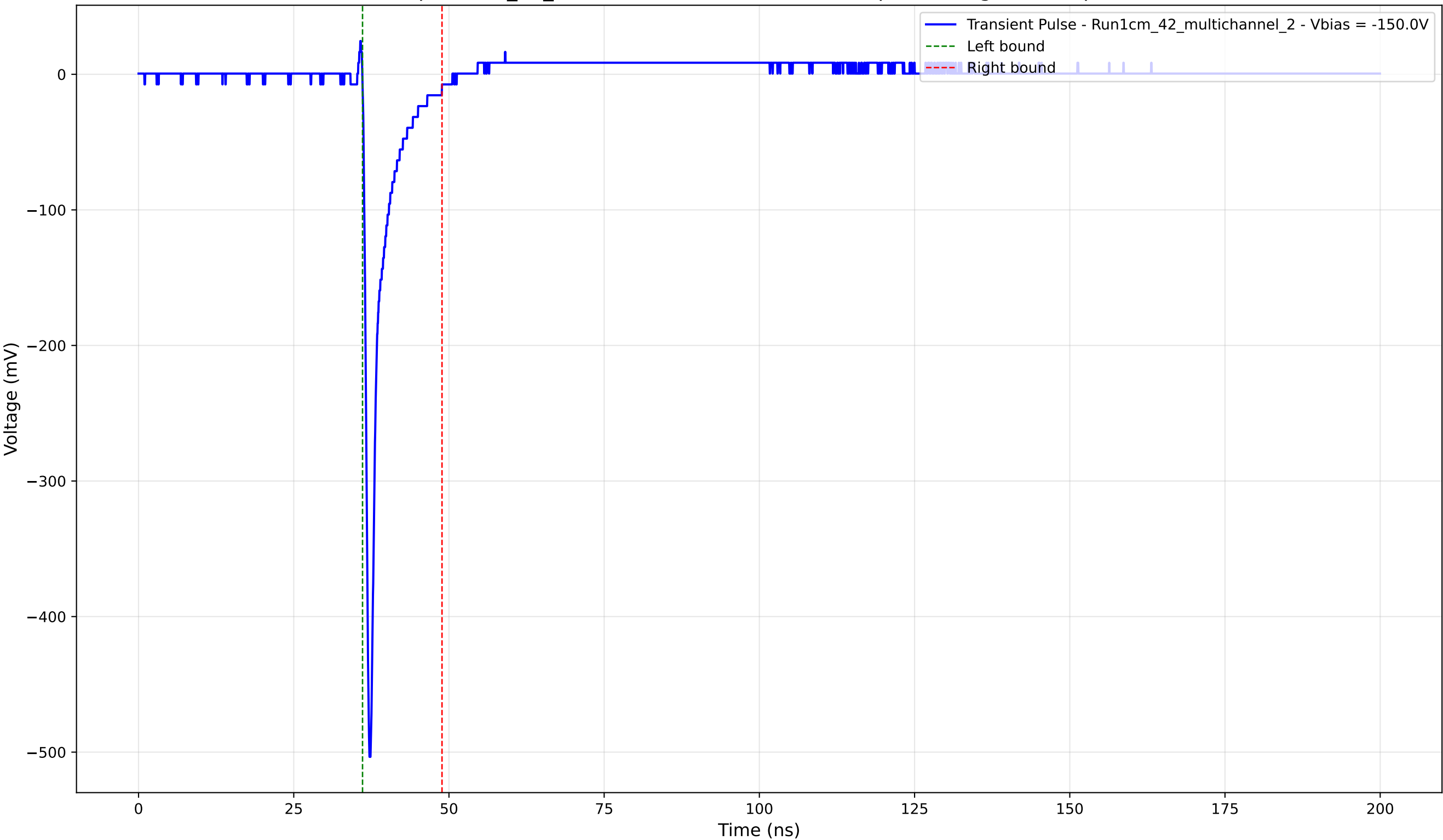
Transient Pulse - Sample: 1cm_42_multichannel - Position: 2125.0 \mu\text{m} - Charge: 26.50 pC - Rise Time: 0.77 ns
