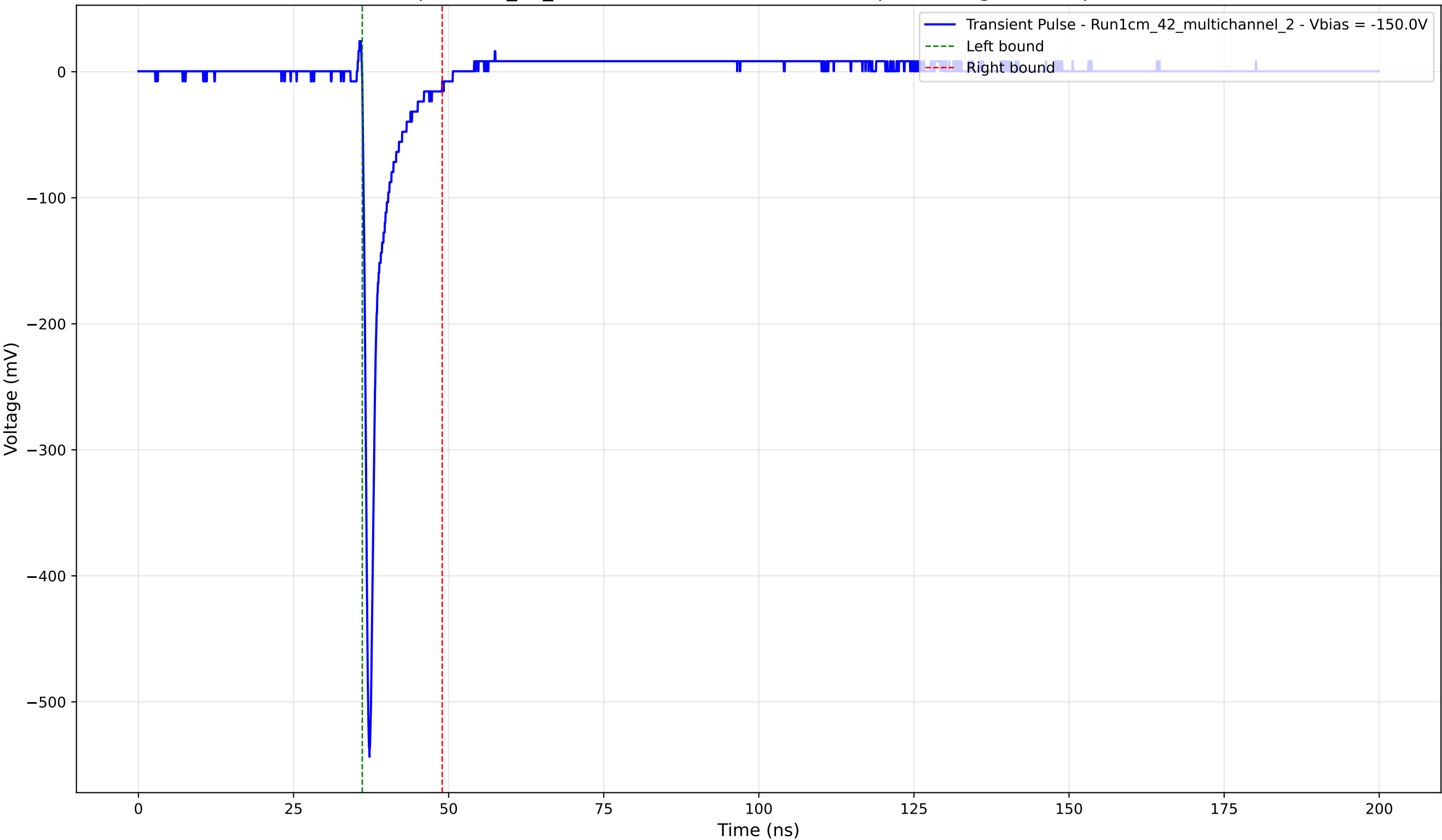
Transient Pulse - Sample: 1cm_42_multichannel - Position: 2170.0 \mu\text{m} - Charge: 27.13 pC - Rise Time: 0.77 ns
