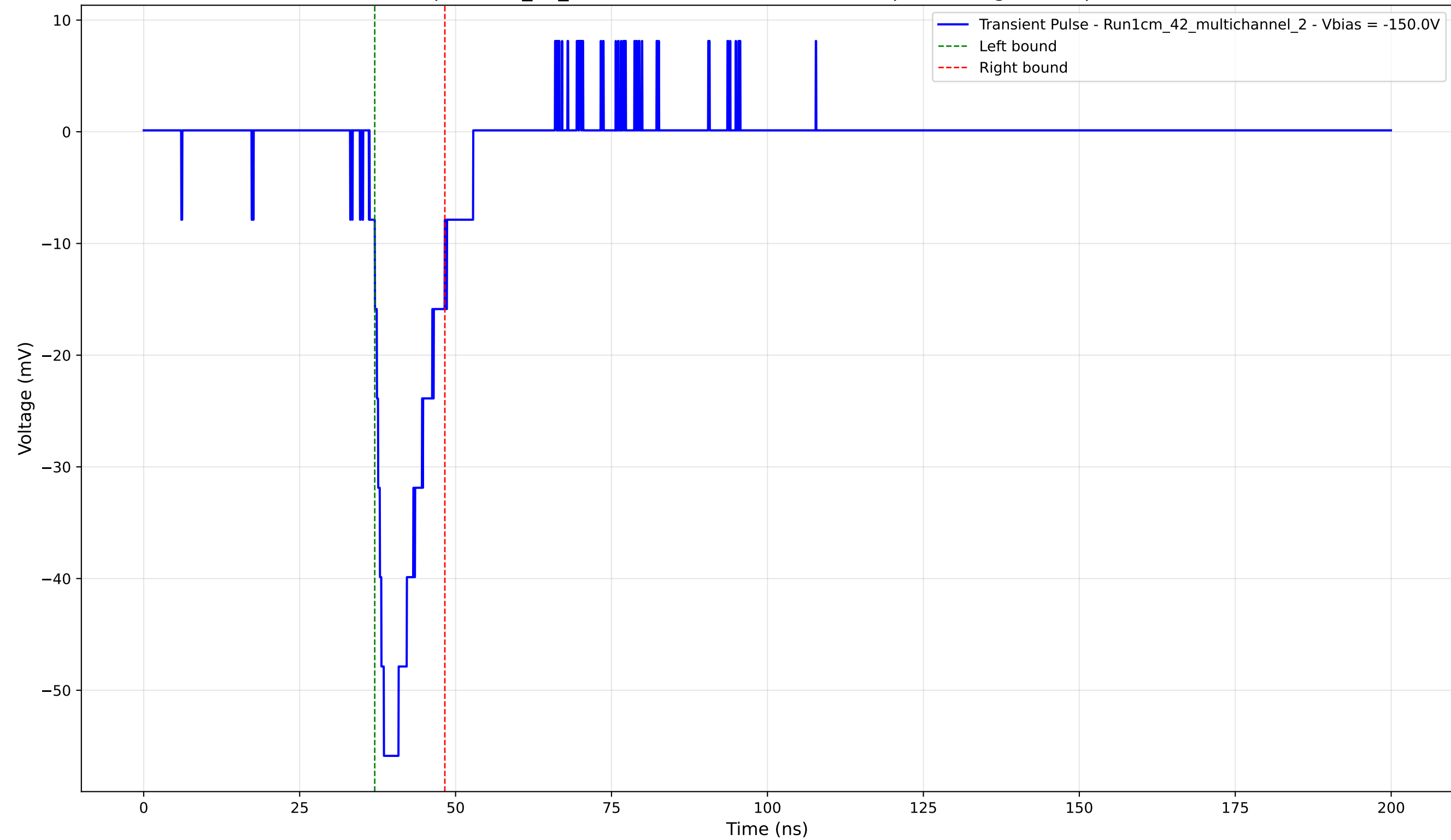
Transient Pulse - Sample: 1cm_42_multichannel - Position: 4815.0 \mu\text{m} - Charge: 8.04 pC - Rise Time: 2.29 ns
