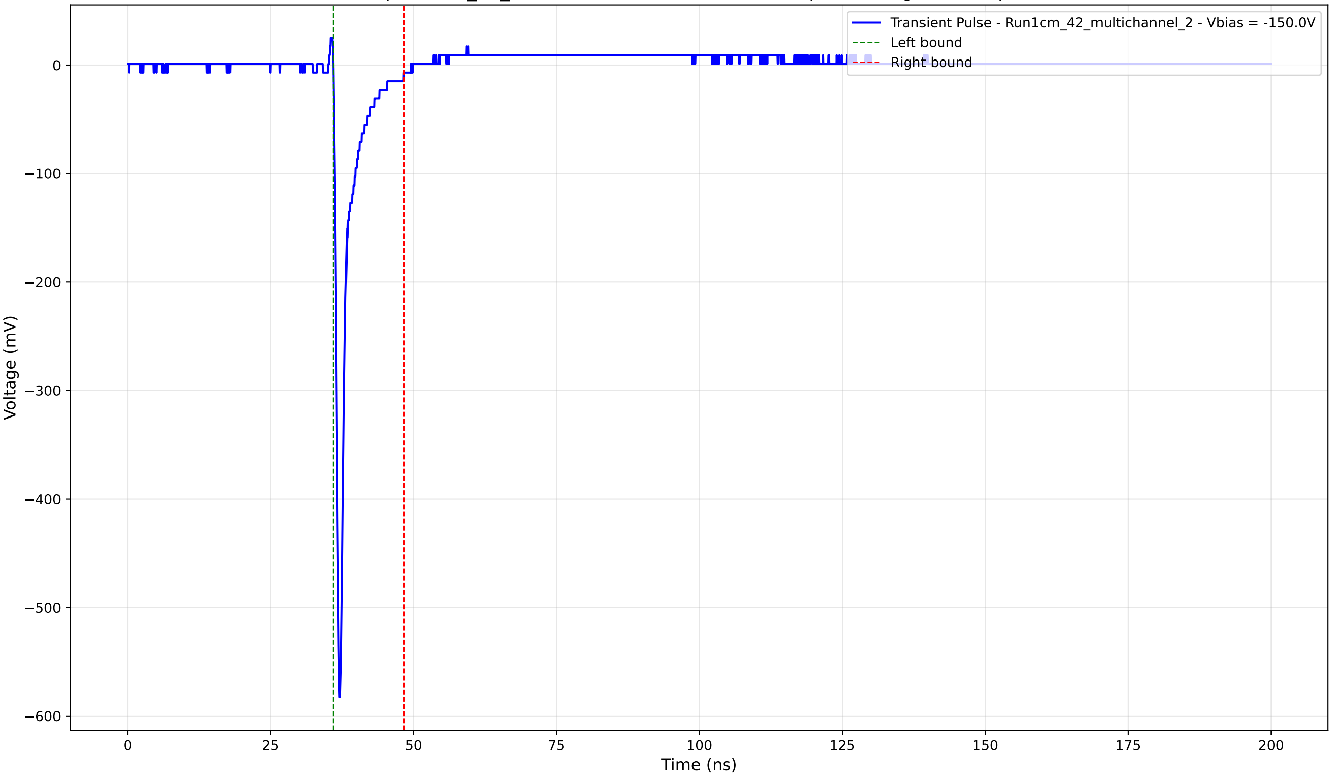
Transient Pulse - Sample: 1cm_42_multichannel - Position: 2295.0 \mu\text{m} - Charge: 25.89 pC - Rise Time: 0.73 ns
