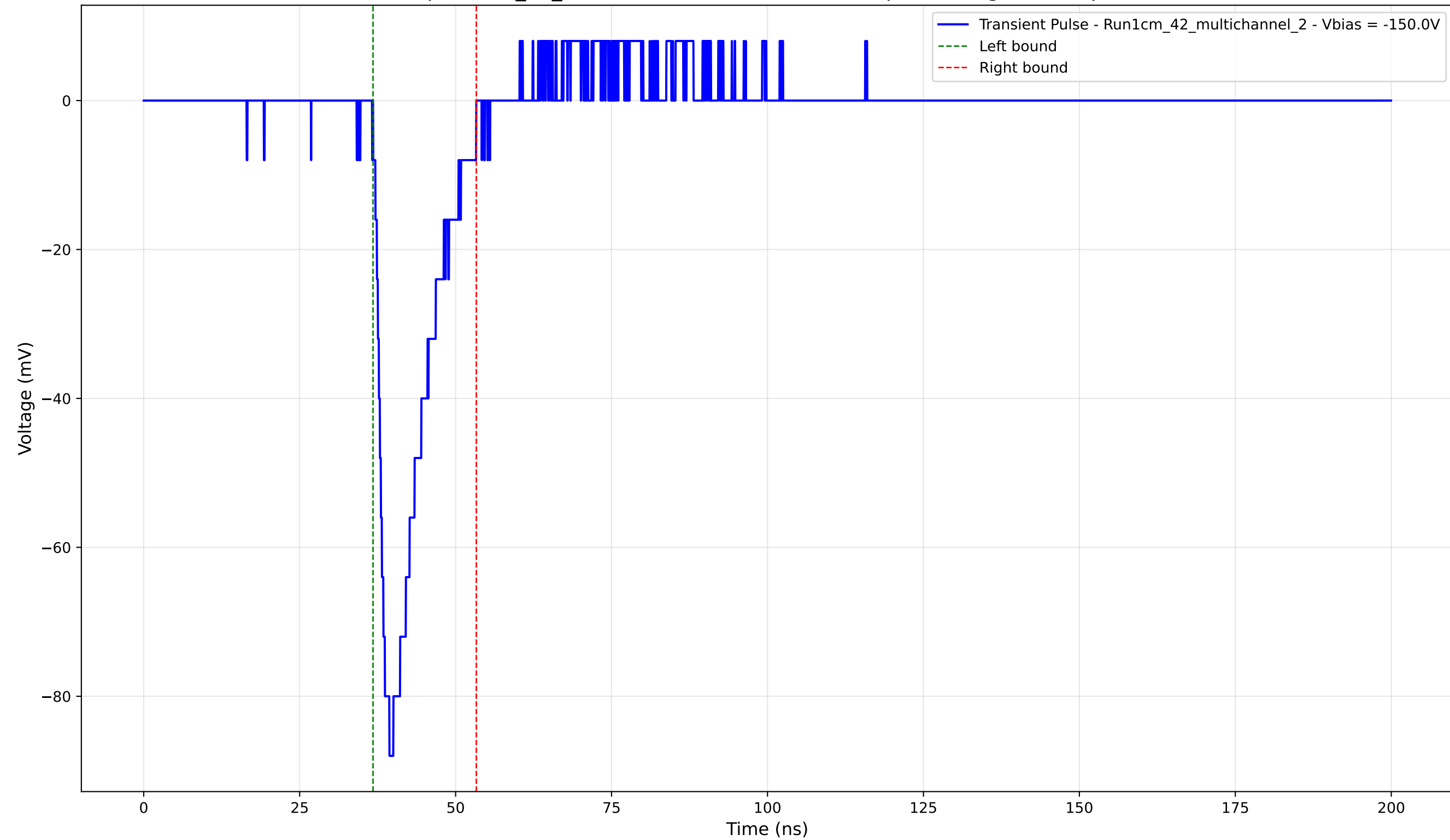
Transient Pulse - Sample: 1cm_42_multichannel - Position: 4200.0 \mu\text{m} - Charge: 13.00 pC - Rise Time: 1.56 ns
