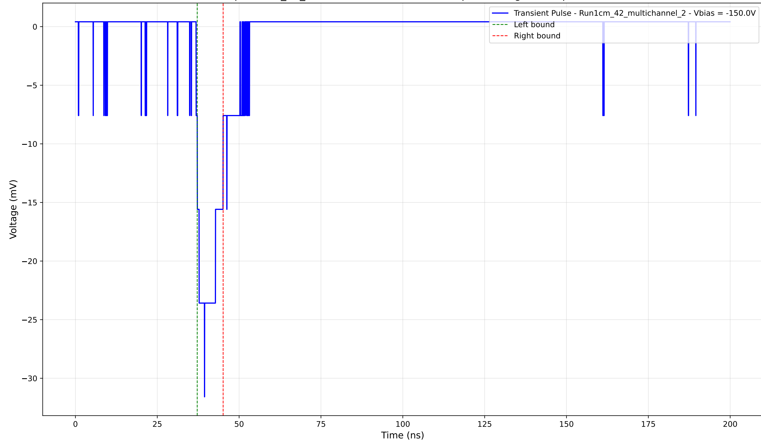
Transient Pulse - Sample: 1cm_42_multichannel - Position: 65.0 \mu\text{m} - Charge: 3.27 pC - Rise Time: 2.58 ns
