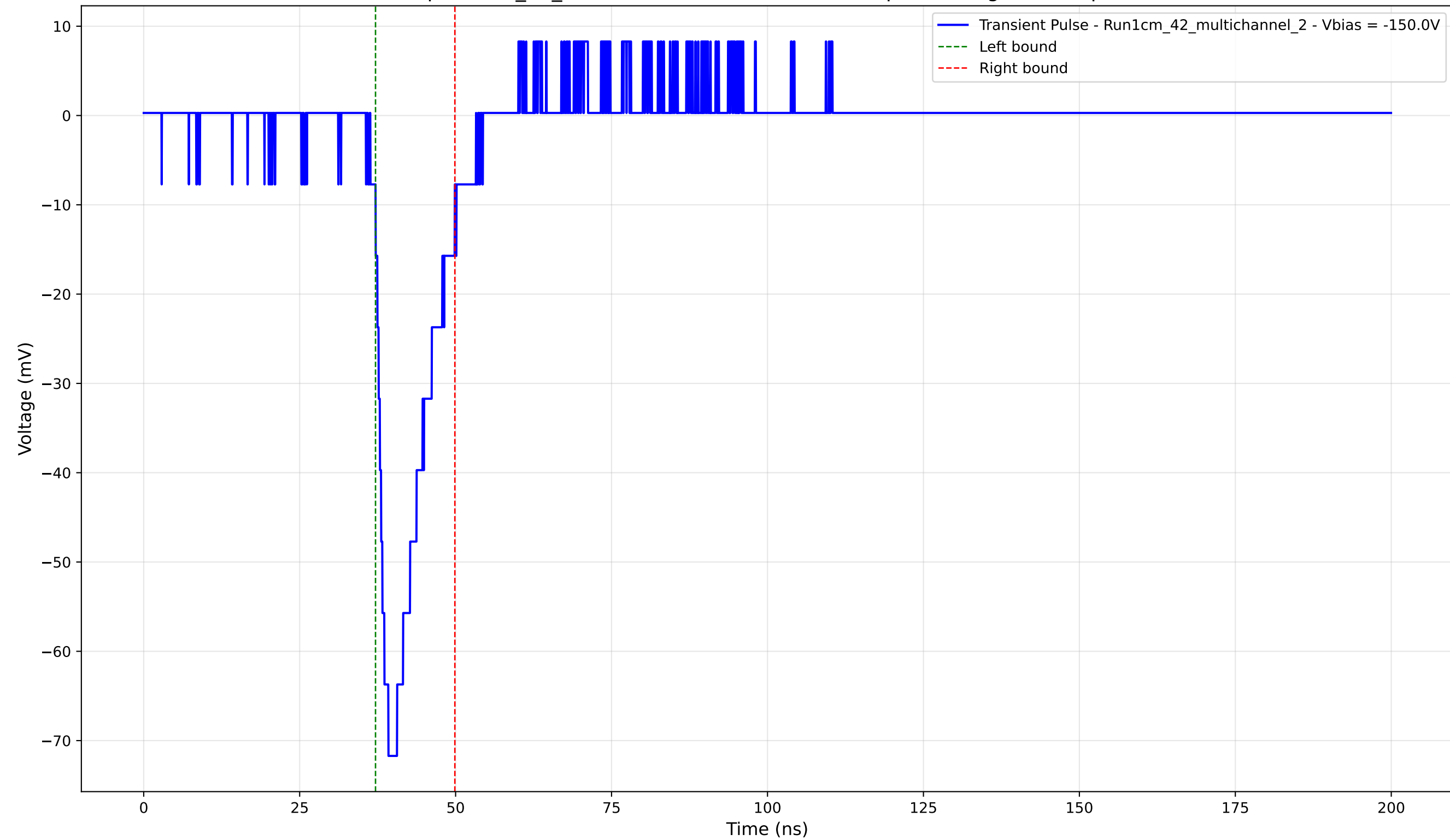
Transient Pulse - Sample: 1cm_42_multichannel - Position: 4490.0 \mu\text{m} - Charge: 10.46 pC - Rise Time: 2.88 ns
