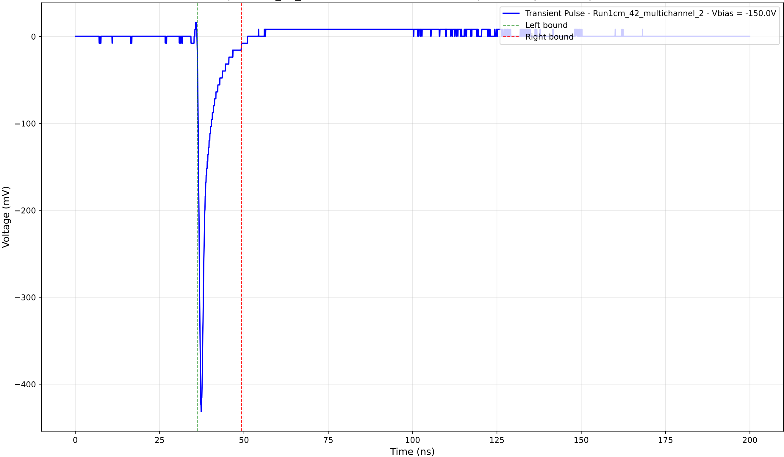
Transient Pulse - Sample: 1cm_42_multichannel - Position: 2710.0 \mu\text{m} - Charge: 24.94 pC - Rise Time: 0.78 ns
