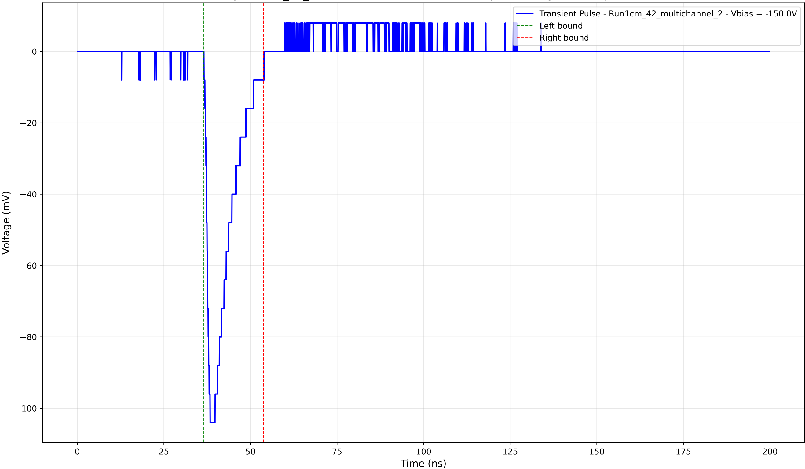
Transient Pulse - Sample: 1cm_42_multichannel - Position: 3770.0 \mu\text{m} - Charge: 15.35 pC - Rise Time: 1.23 ns
