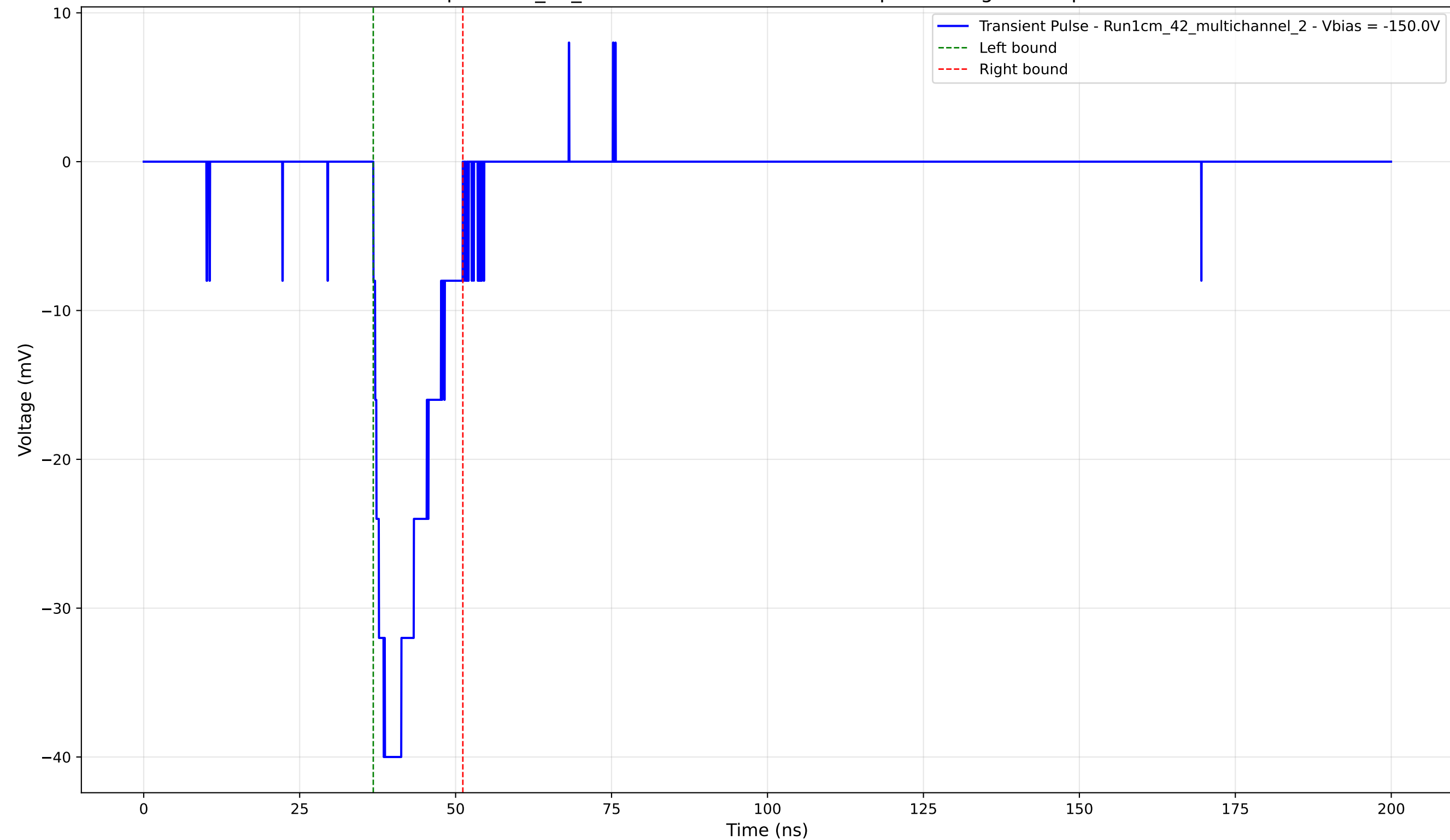
Transient Pulse - Sample: 1cm_42_multichannel - Position: 75.0 \mu\text{m} - Charge: 6.68 pC - Rise Time: 1.66 ns
