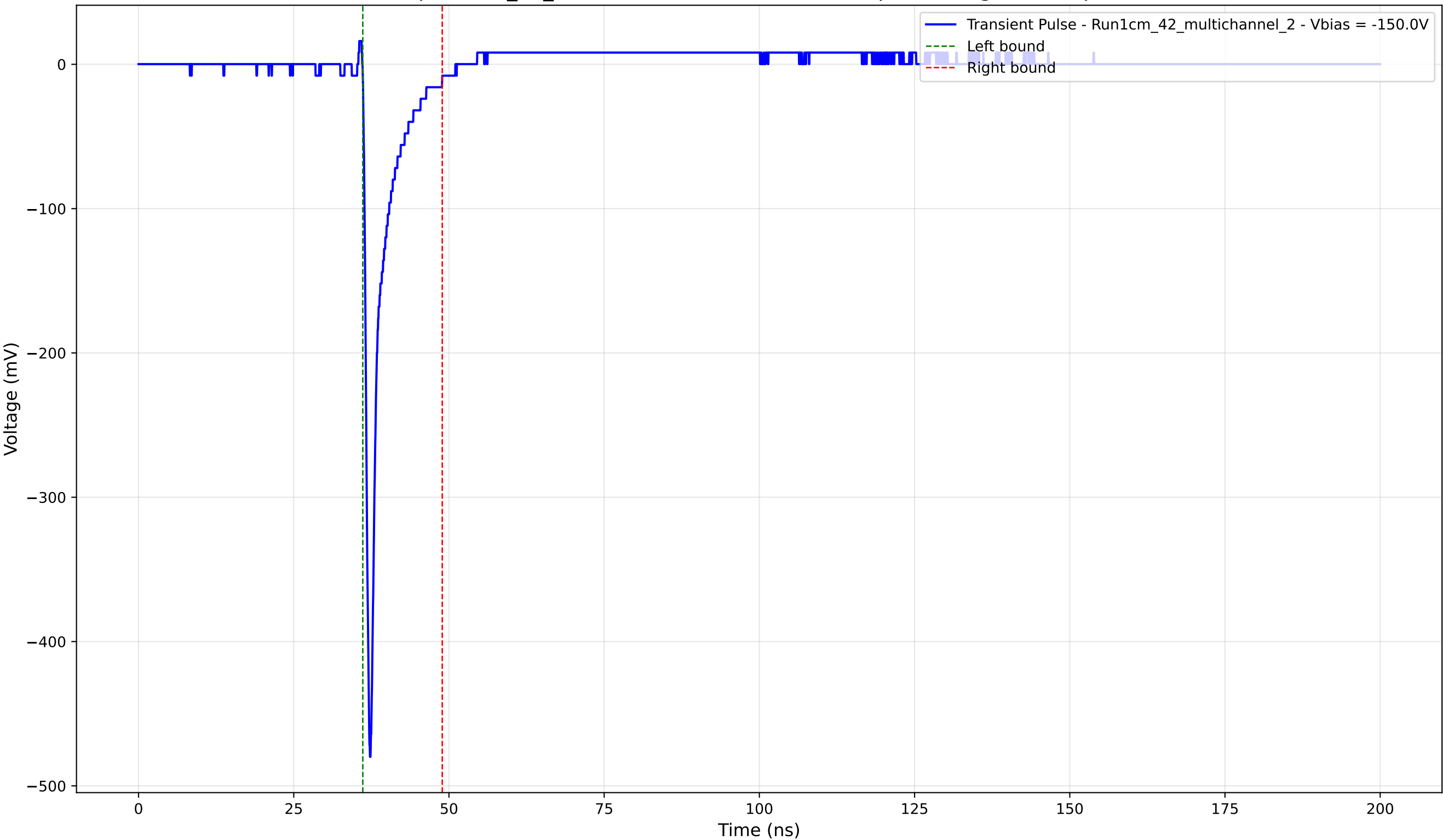
Transient Pulse - Sample: 1cm_42_multichannel - Position: 2085.0 \mu\text{m} - Charge: 26.12 pC - Rise Time: 0.74 ns
