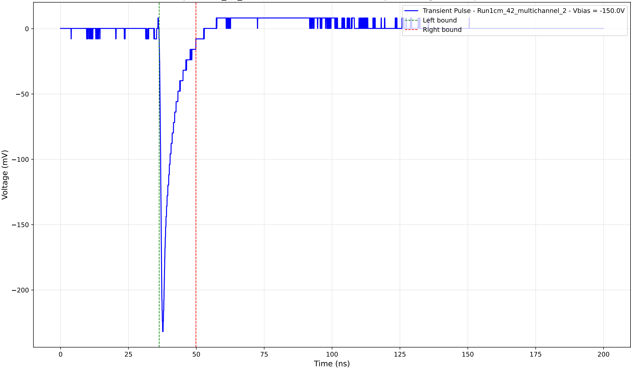
Transient Pulse - Sample: 1cm_42_multichannel - Position: 3060.0 \mu\text{m} - Charge: 19.65 pC - Rise Time: 0.96 ns
