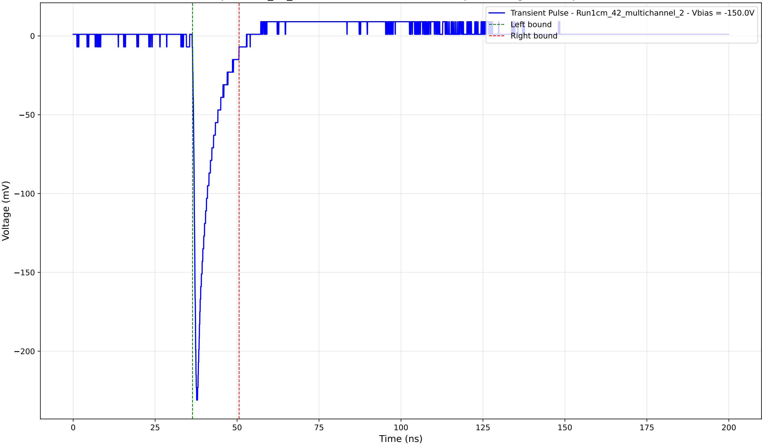
Transient Pulse - Sample: 1cm_42_multichannel - Position: 1575.0 \mu\text{m} - Charge: 21.59 pC - Rise Time: 0.96 ns
