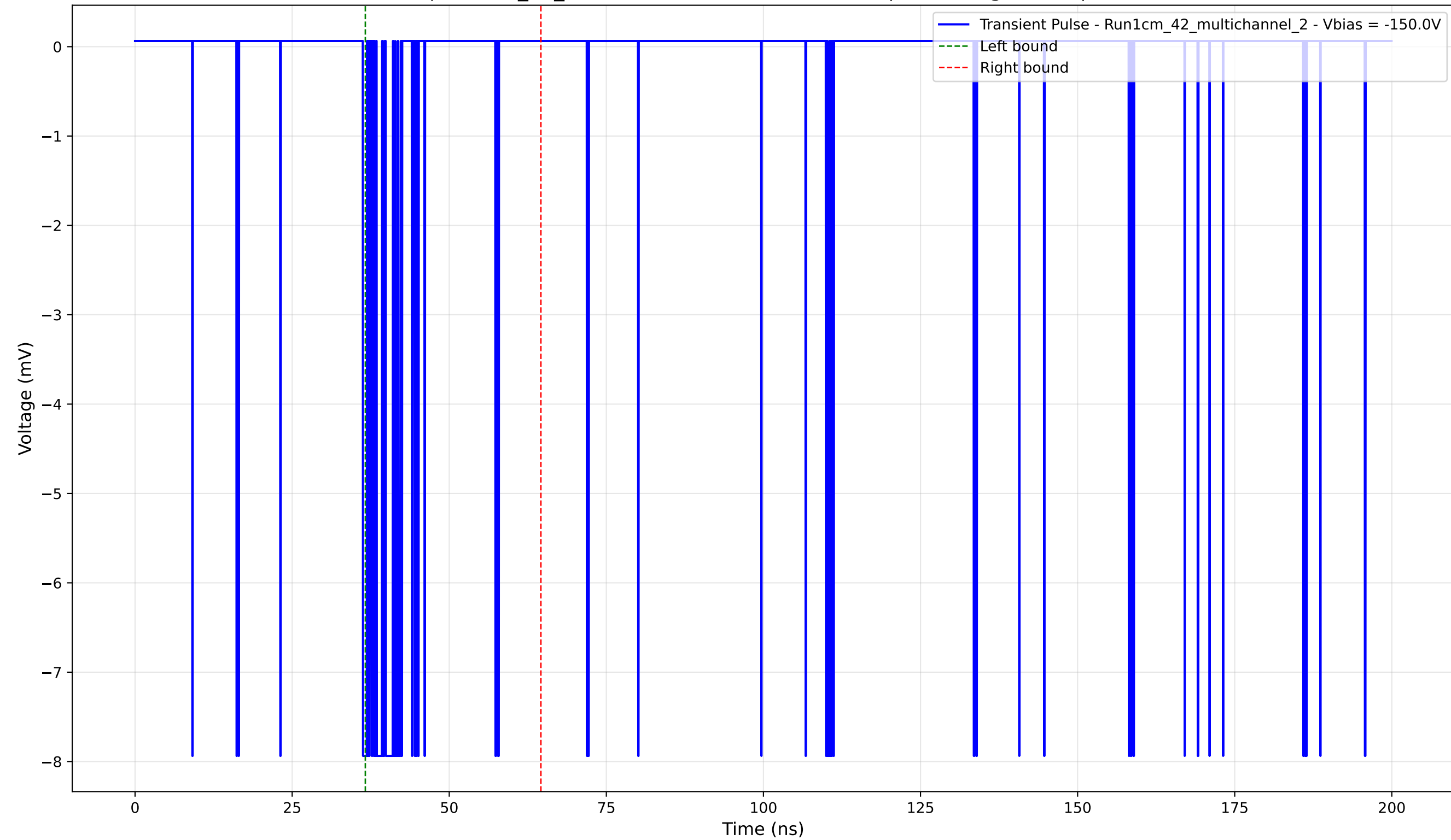
Transient Pulse - Sample: 1cm_42_multichannel - Position: 4910.0 \mu\text{m} - Charge: 0.73 pC - Rise Time: 0.04 ns
