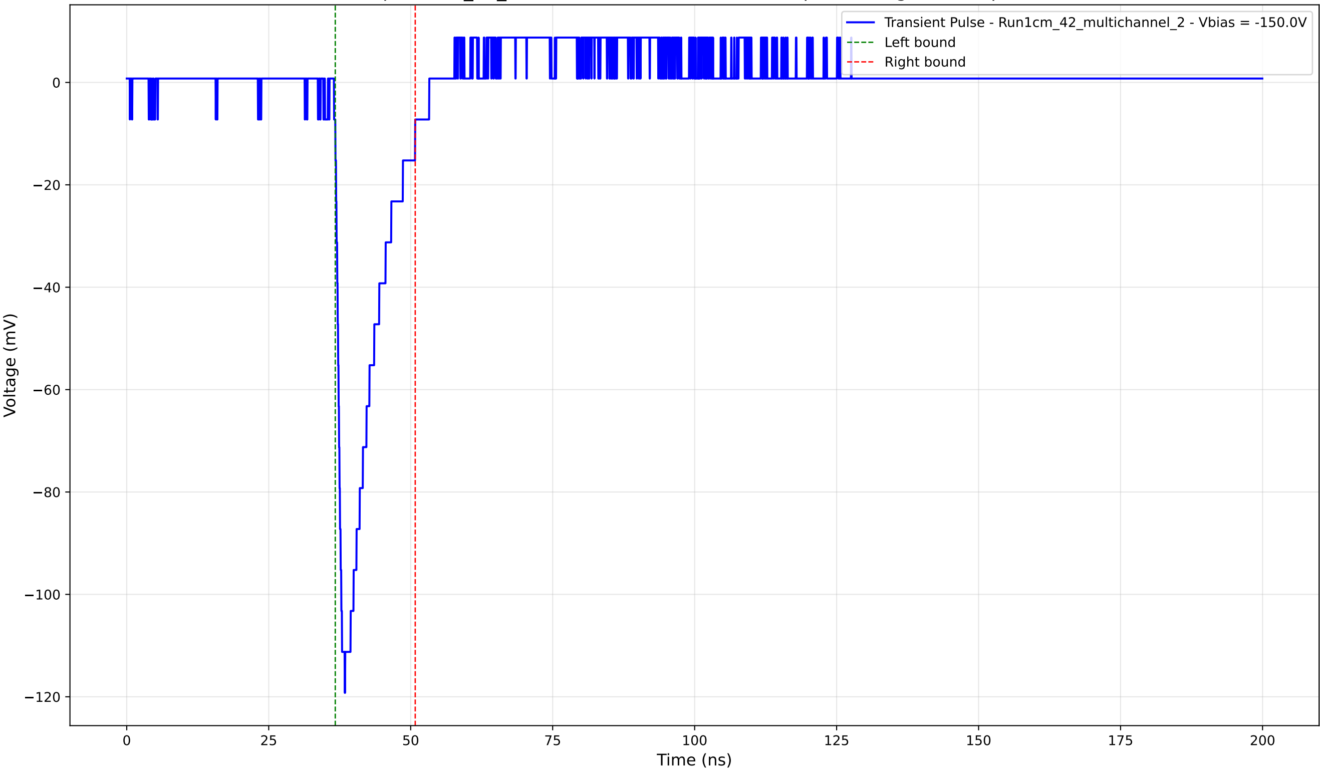
Transient Pulse - Sample: 1cm_42_multichannel - Position: 3590.0 \mu\text{m} - Charge: 15.17 pC - Rise Time: 1.18 ns
