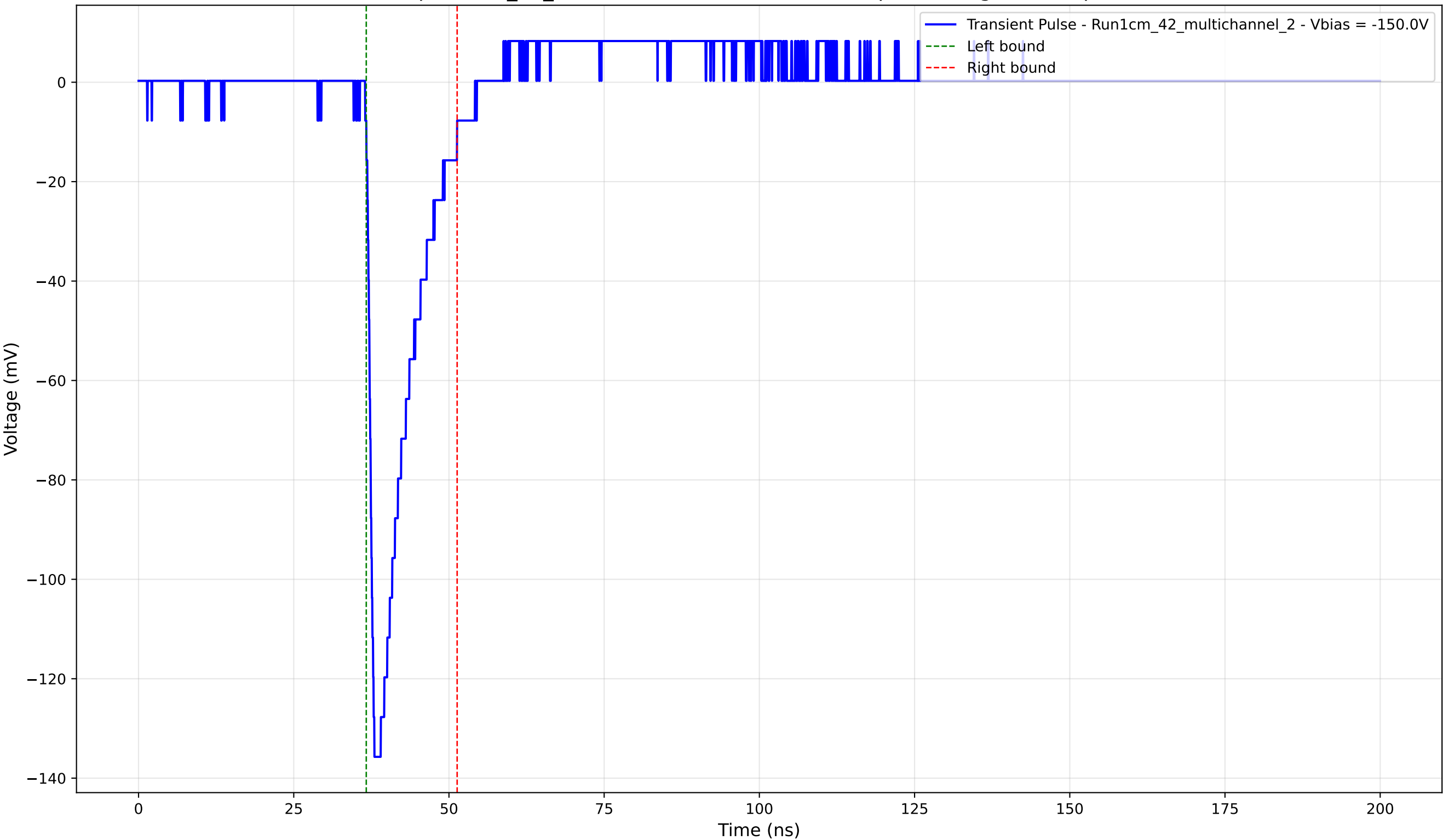
Transient Pulse - Sample: 1cm_42_multichannel - Position: 1150.0 \mu\text{m} - Charge: 18.09 pC - Rise Time: 1.17 ns
