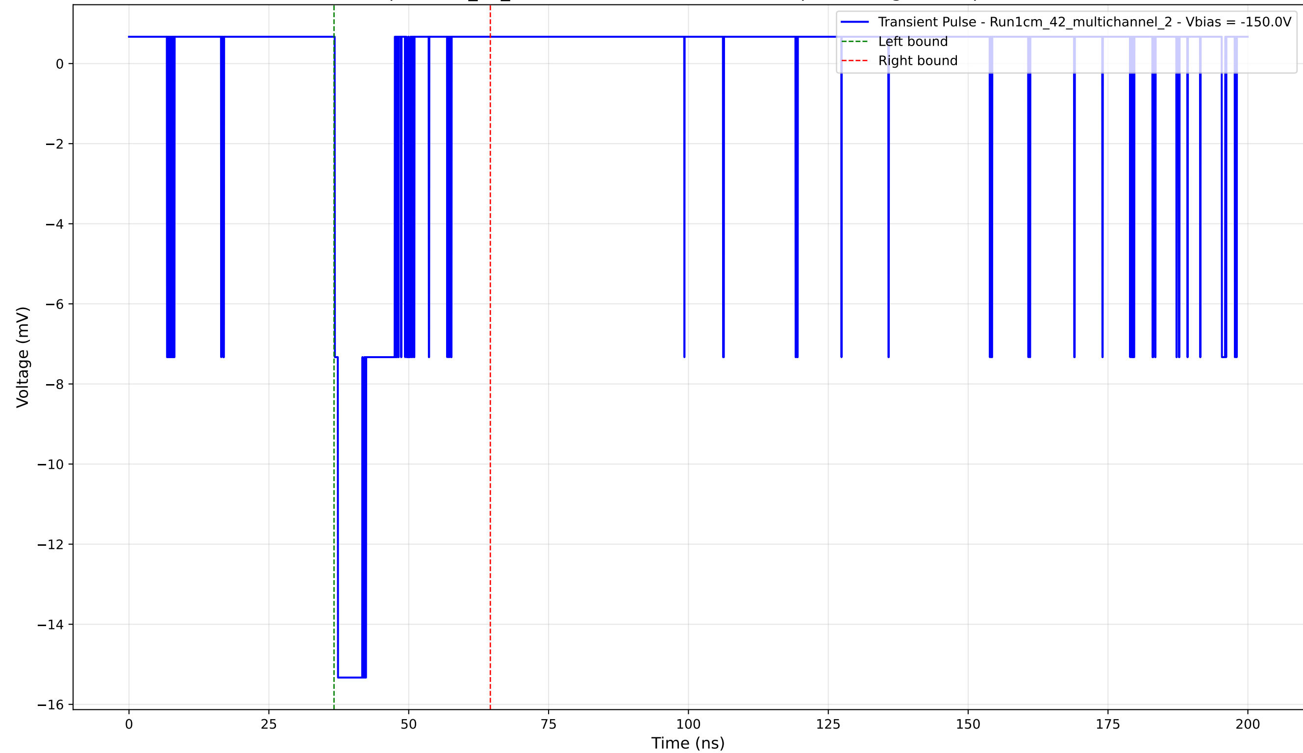
Transient Pulse - Sample: 1cm_42_multichannel - Position: 3410.0 \mu\text{m} - Charge: 2.36 pC - Rise Time: 0.59 ns
