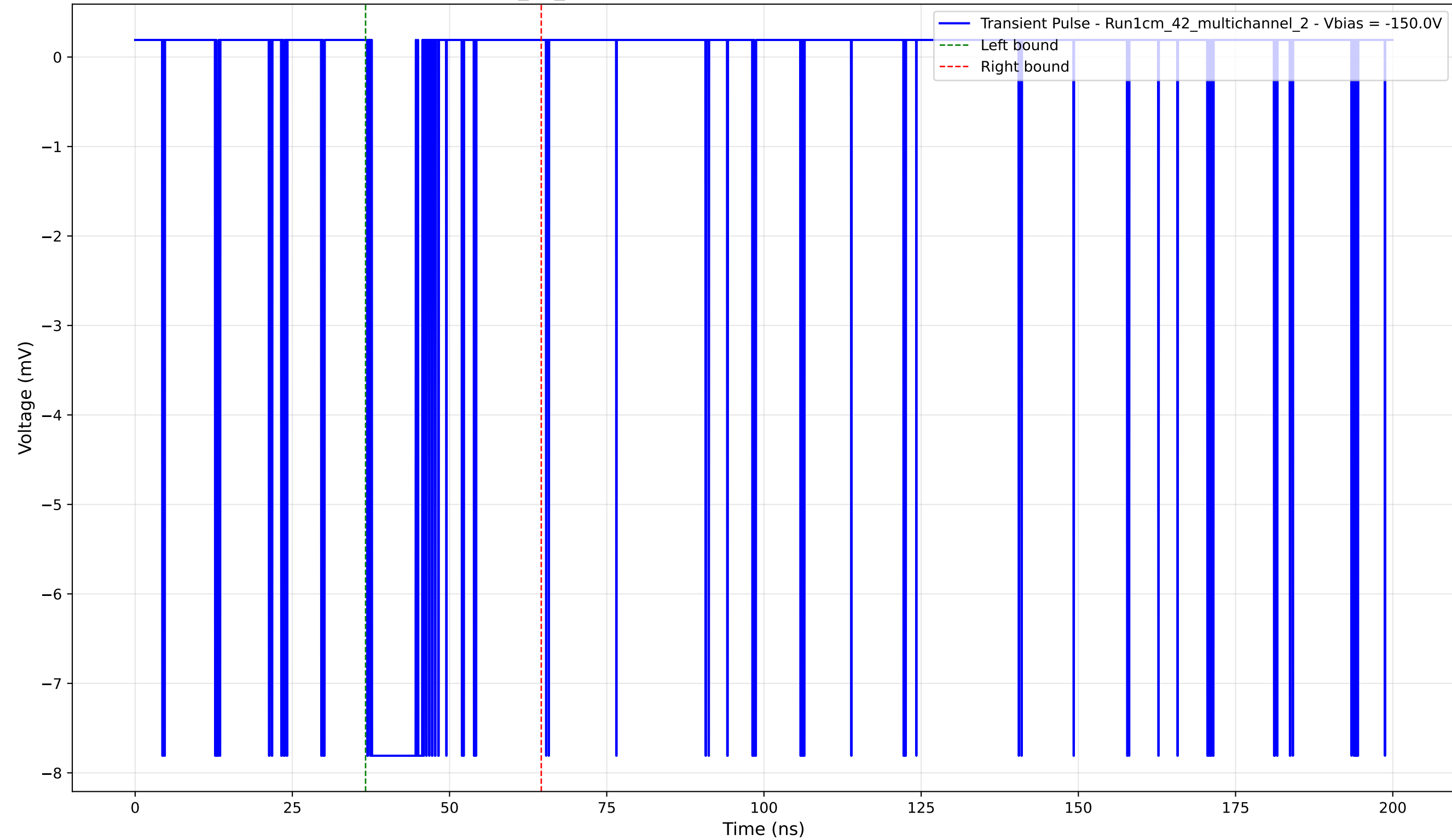
Transient Pulse - Sample: 1cm_42_multichannel - Position: 3875.0 \mu\text{m} - Charge: 1.40 pC - Rise Time: 0.04 ns
