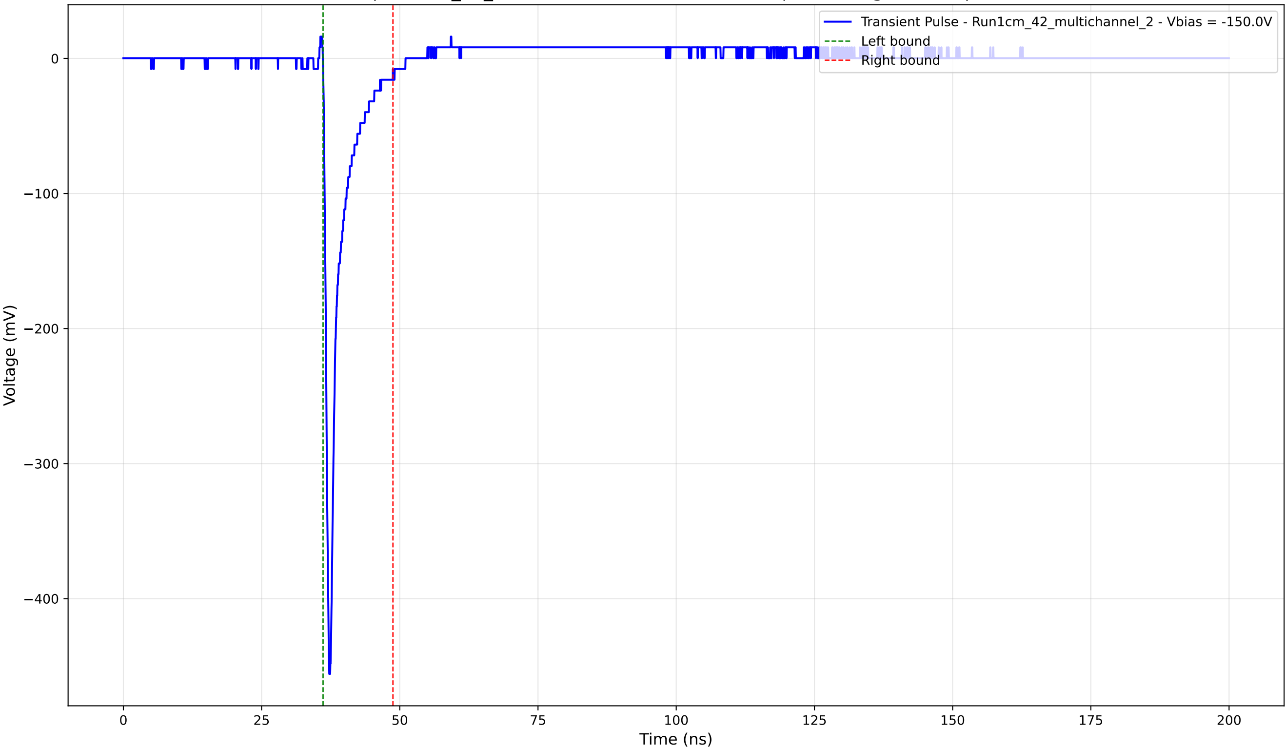
Transient Pulse - Sample: 1cm_42_multichannel - Position: 2060.0 \mu\text{m} - Charge: 25.65 pC - Rise Time: 0.74 ns
