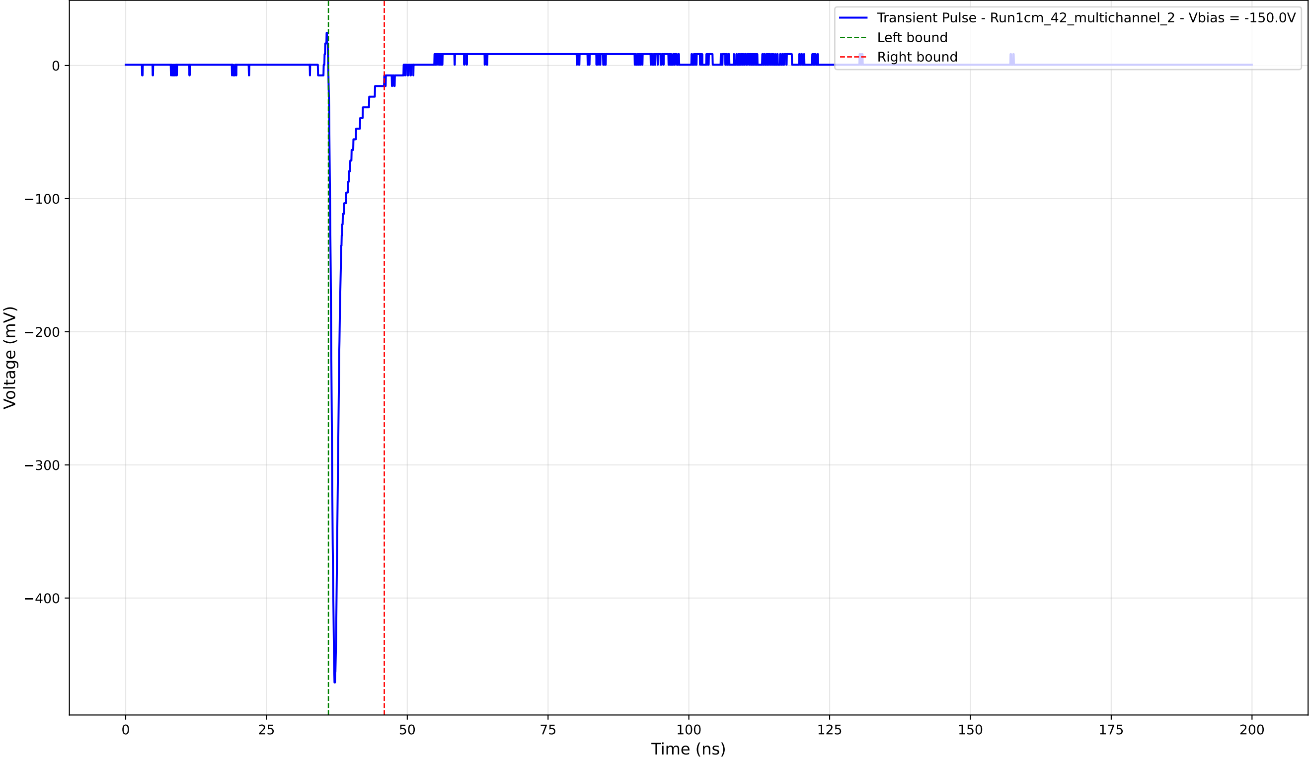
Transient Pulse - Sample: 1cm_42_multichannel - Position: 2310.0 \mu\text{m} - Charge: 19.77 pC - Rise Time: 0.75 ns
