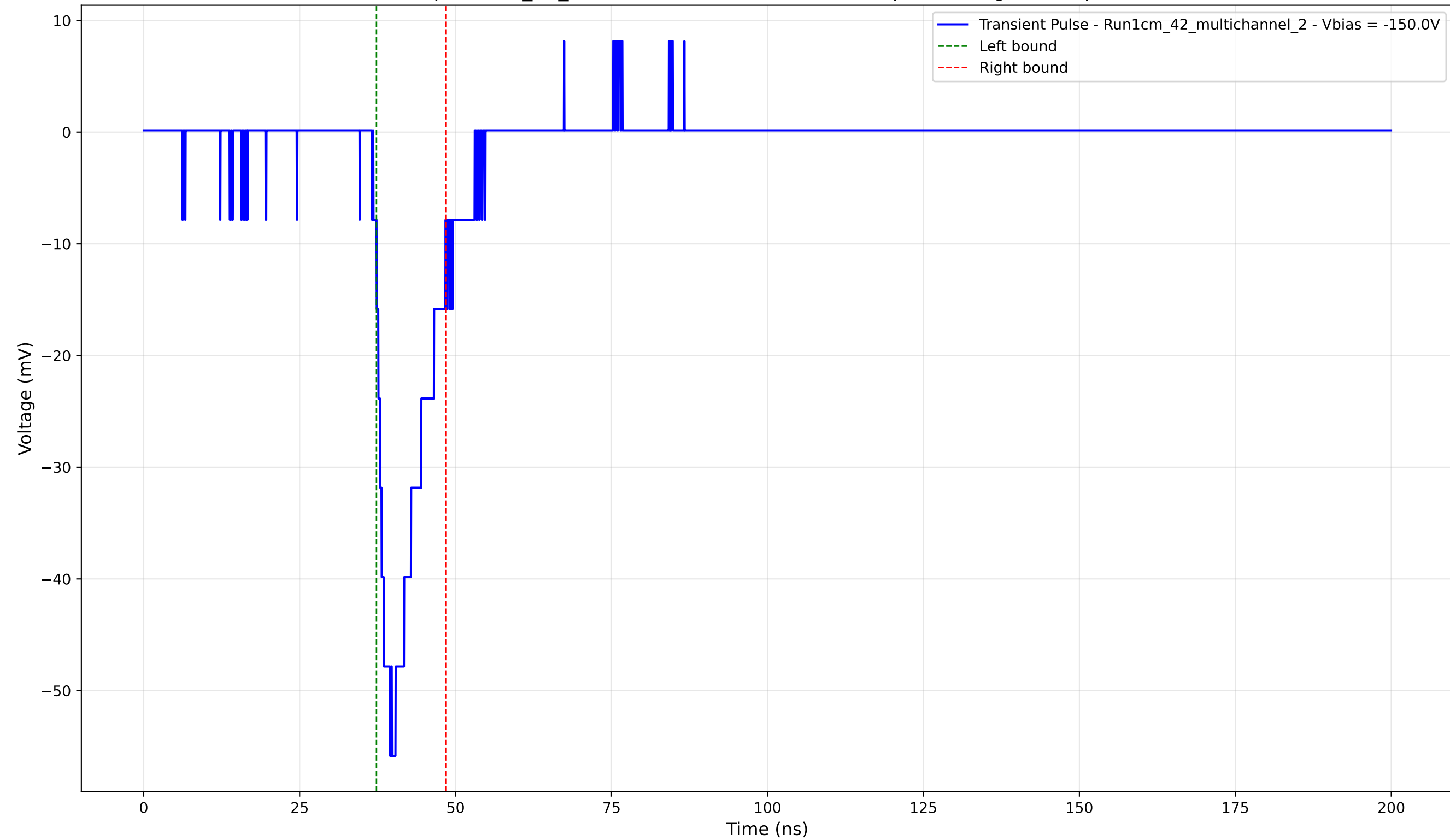
Transient Pulse - Sample: 1cm_42_multichannel - Position: 4450.0 \mu\text{m} - Charge: 7.38 pC - Rise Time: 2.69 ns
