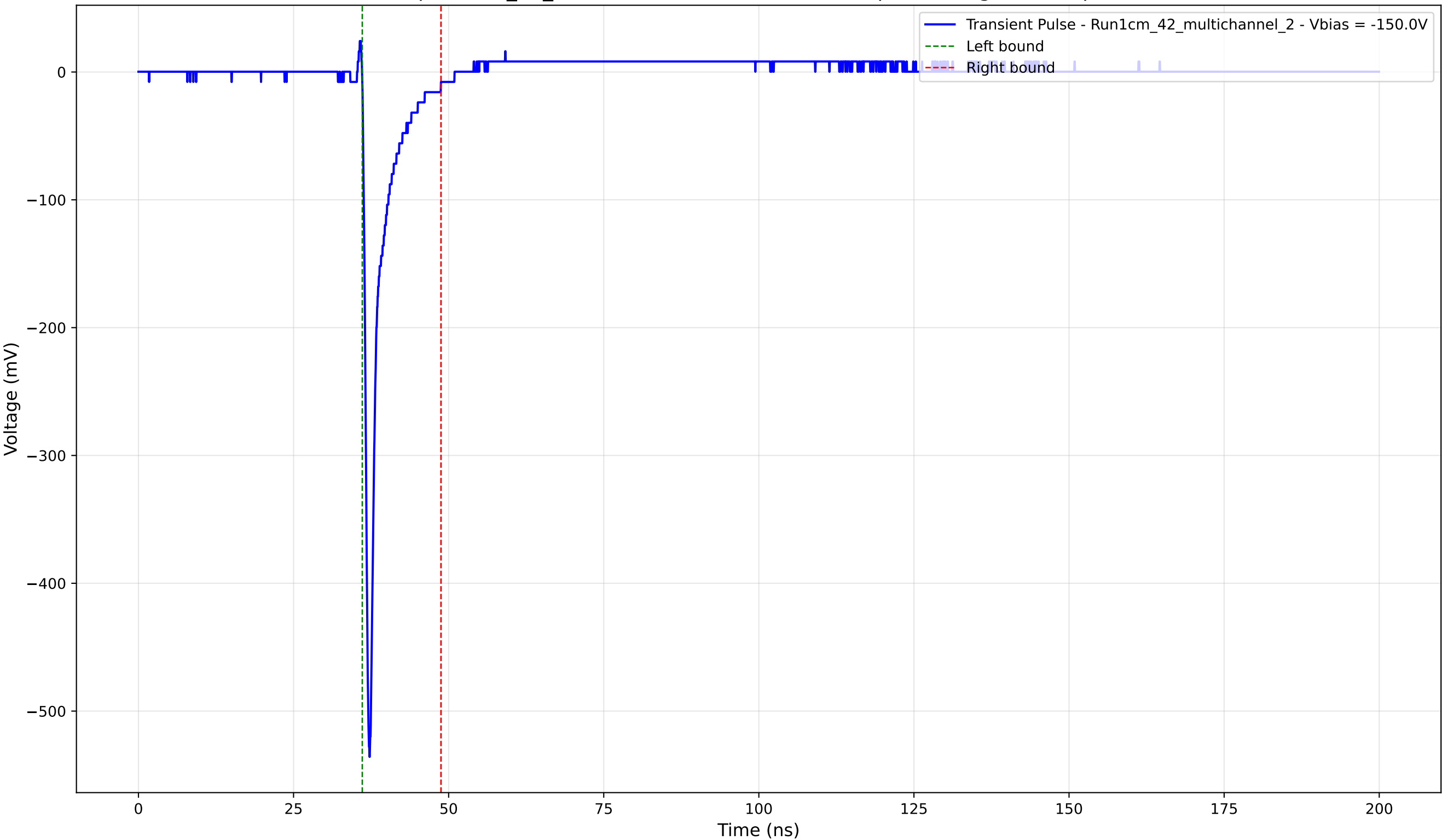
Transient Pulse - Sample: 1cm_42_multichannel - Position: 2155.0 \mu\text{m} - Charge: 27.05 pC - Rise Time: 0.74 ns
