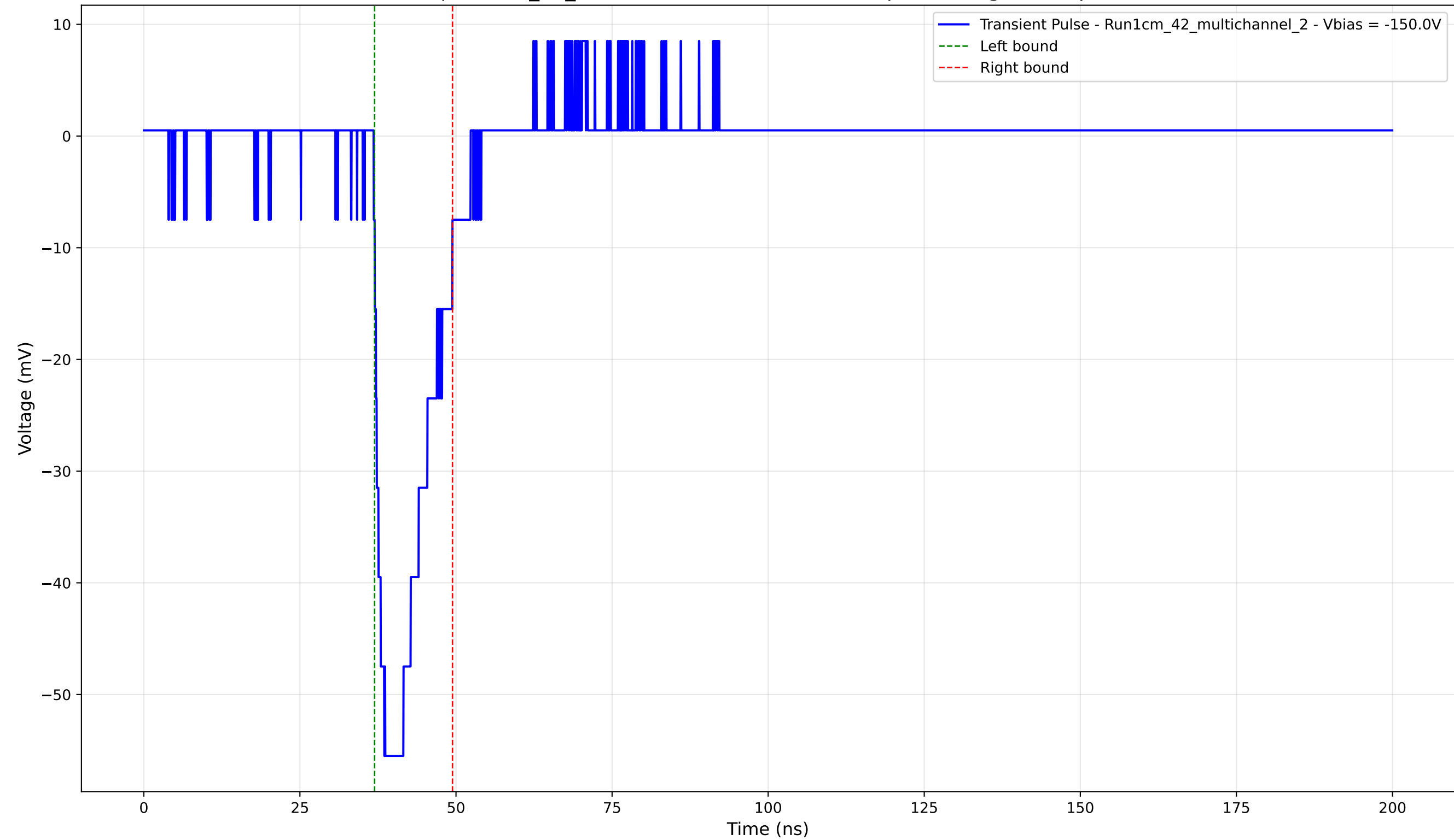
Transient Pulse - Sample: 1cm_42_multichannel - Position: 100.0 \mu\text{m} - Charge: 9.04 pC - Rise Time: 1.69 ns
