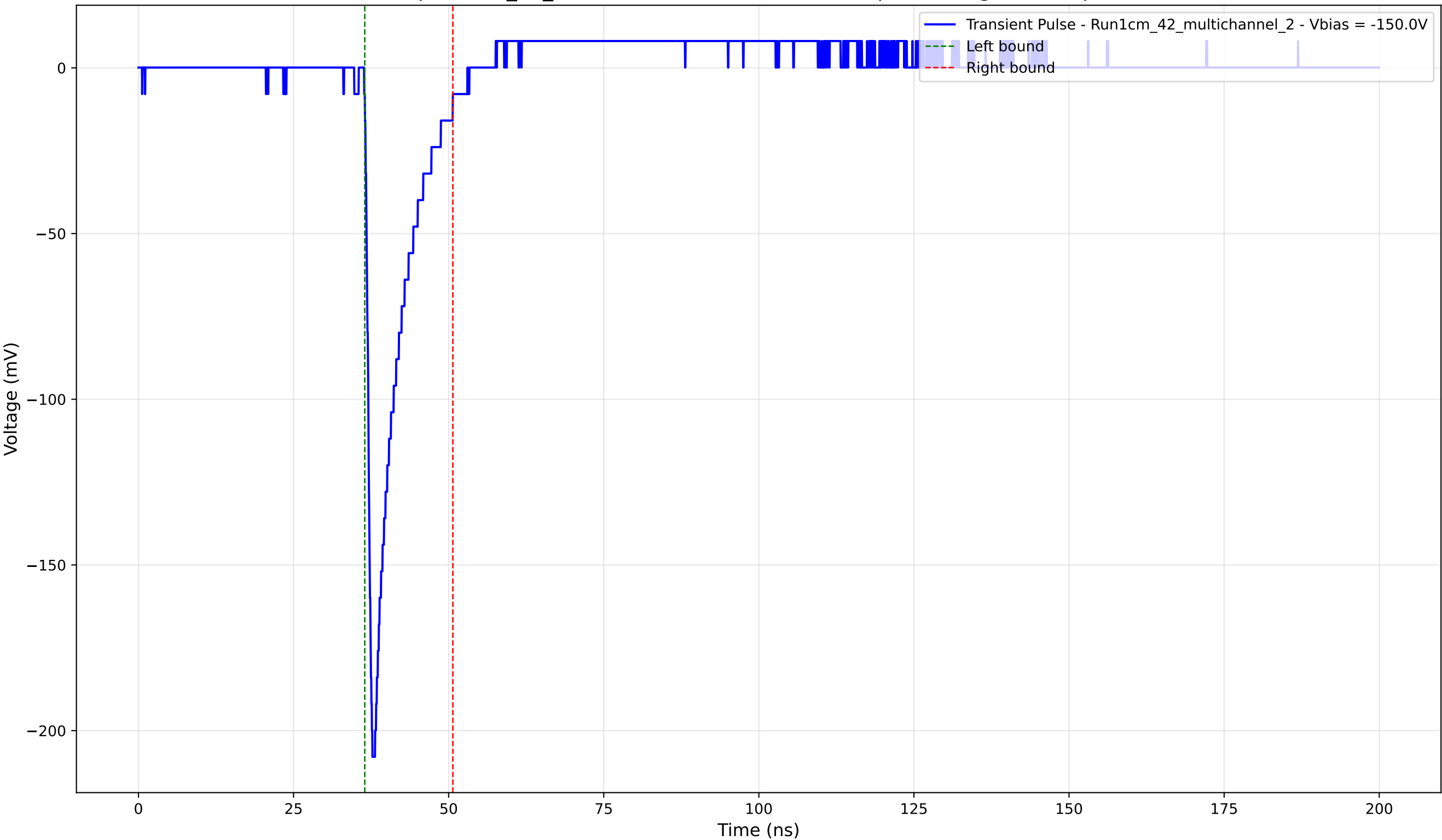
Transient Pulse - Sample: 1cm_42_multichannel - Position: 1485.0 \mu\text{m} - Charge: 21.20 pC - Rise Time: 0.98 ns
