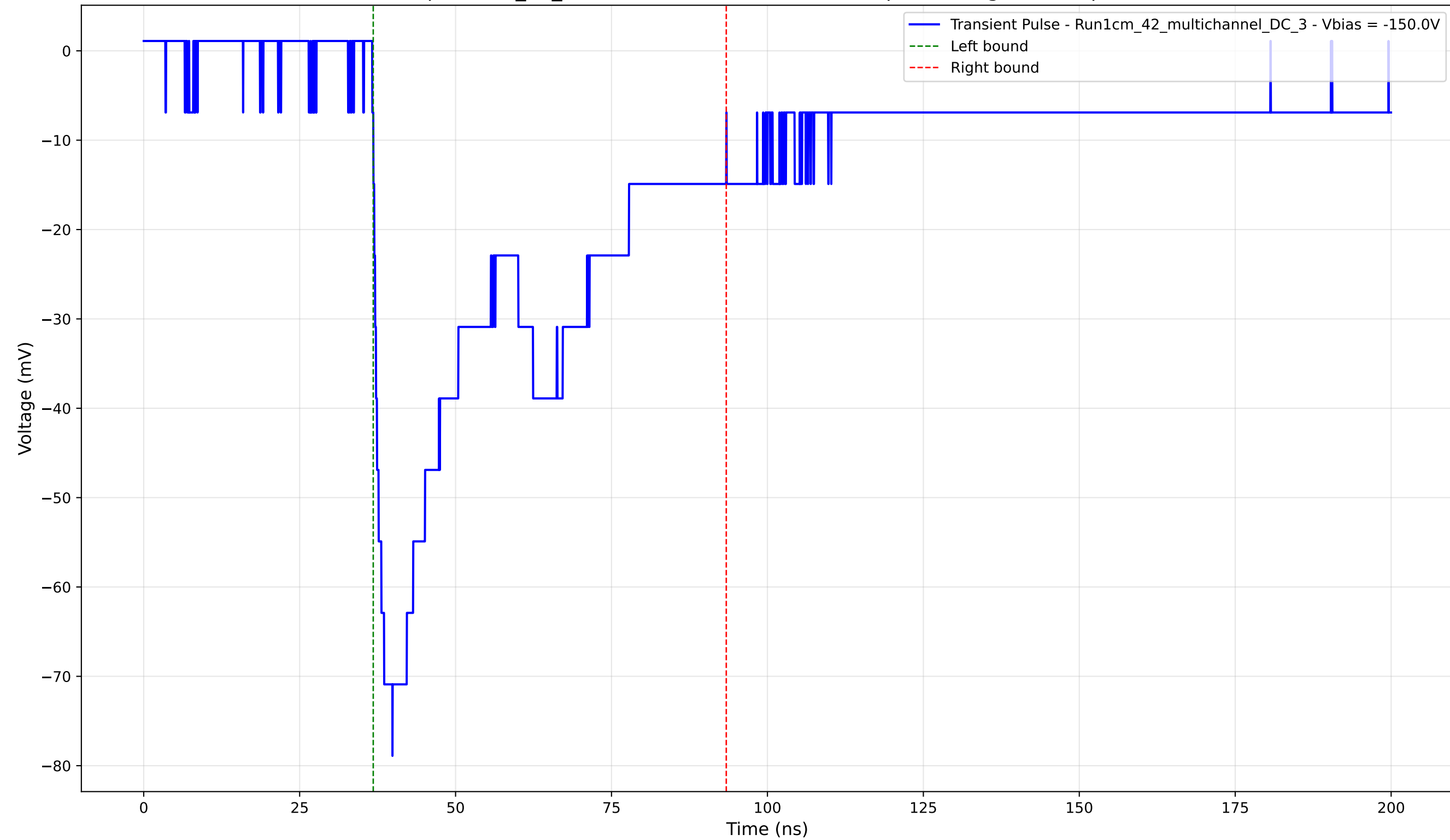
Transient Pulse - Sample: 1cm_42_multichannel - Position: 2450.0 \mu\text{m} - Charge: 35.28 pC - Rise Time: 3.08 ns
