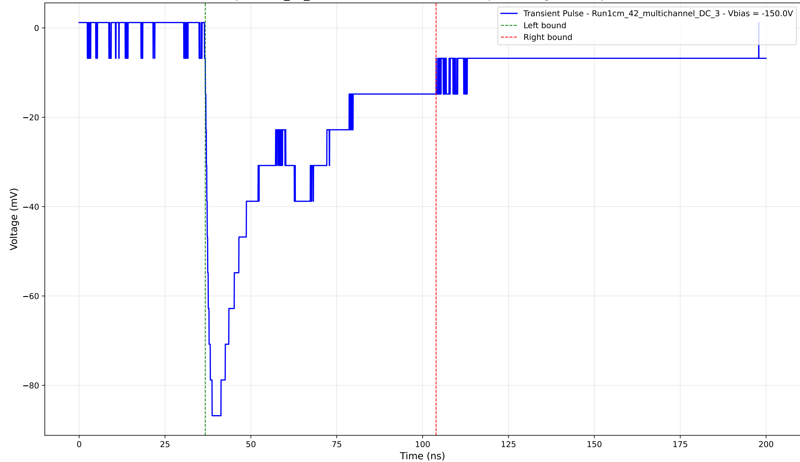
Transient Pulse - Sample: 1cm_42_multichannel - Position: 2135.0 \mu\text{m} - Charge: 41.61 pC - Rise Time: 1.46 ns
