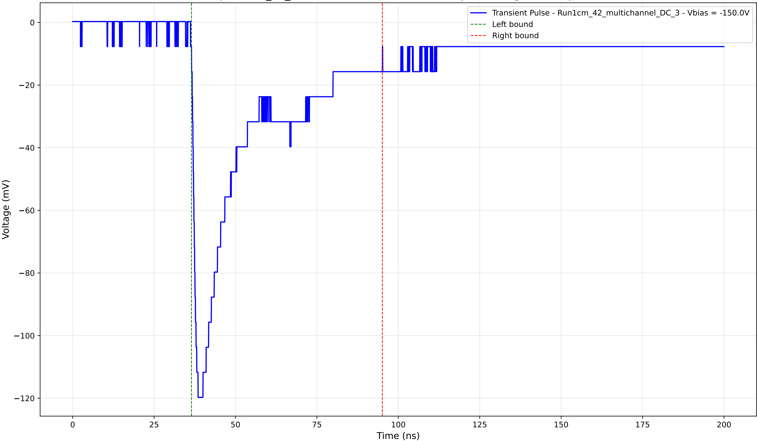
Transient Pulse - Sample: 1cm_42_multichannel - Position: 1690.0 \mu\text{m} - Charge: 44.18 pC - Rise Time: 1.61 ns
