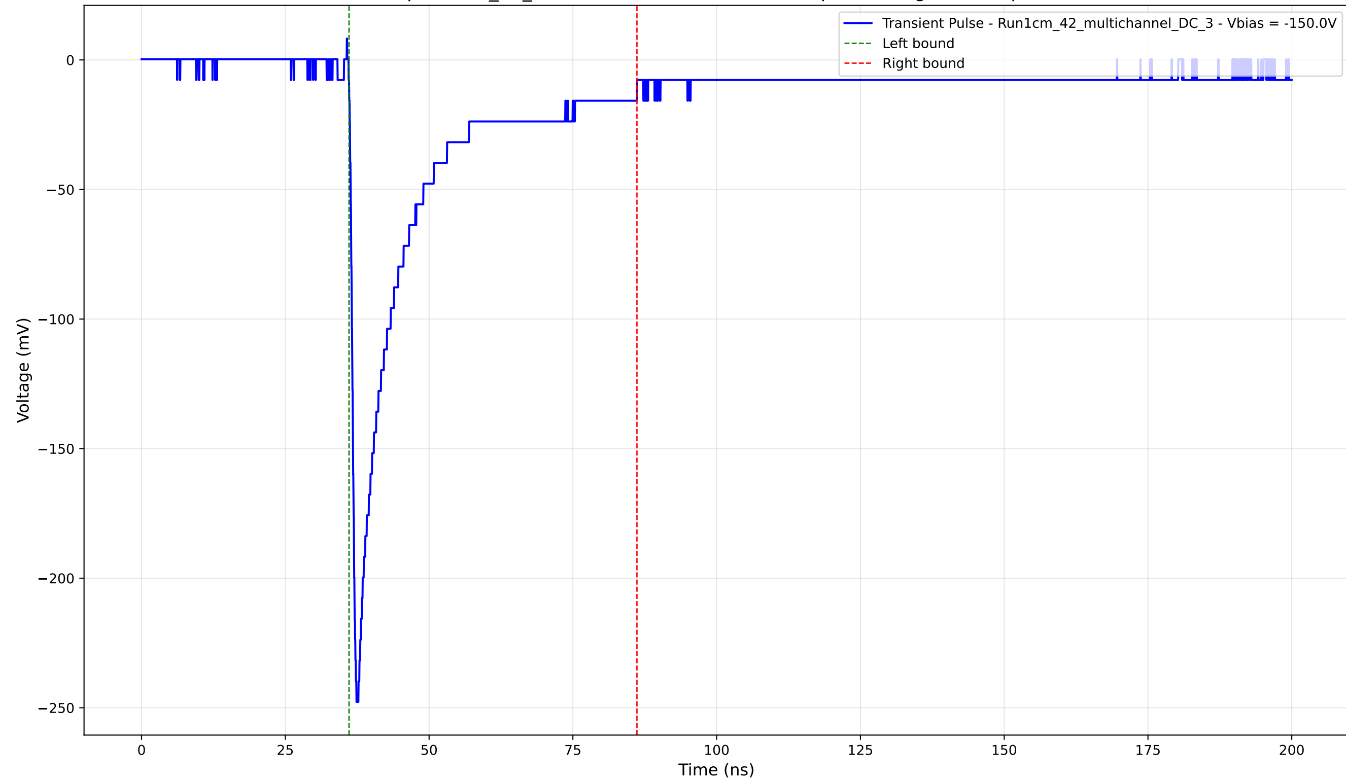
Transient Pulse - Sample: 1cm_42_multichannel - Position: 590.0 \mu\text{m} - Charge: 48.54 pC - Rise Time: 0.90 ns
