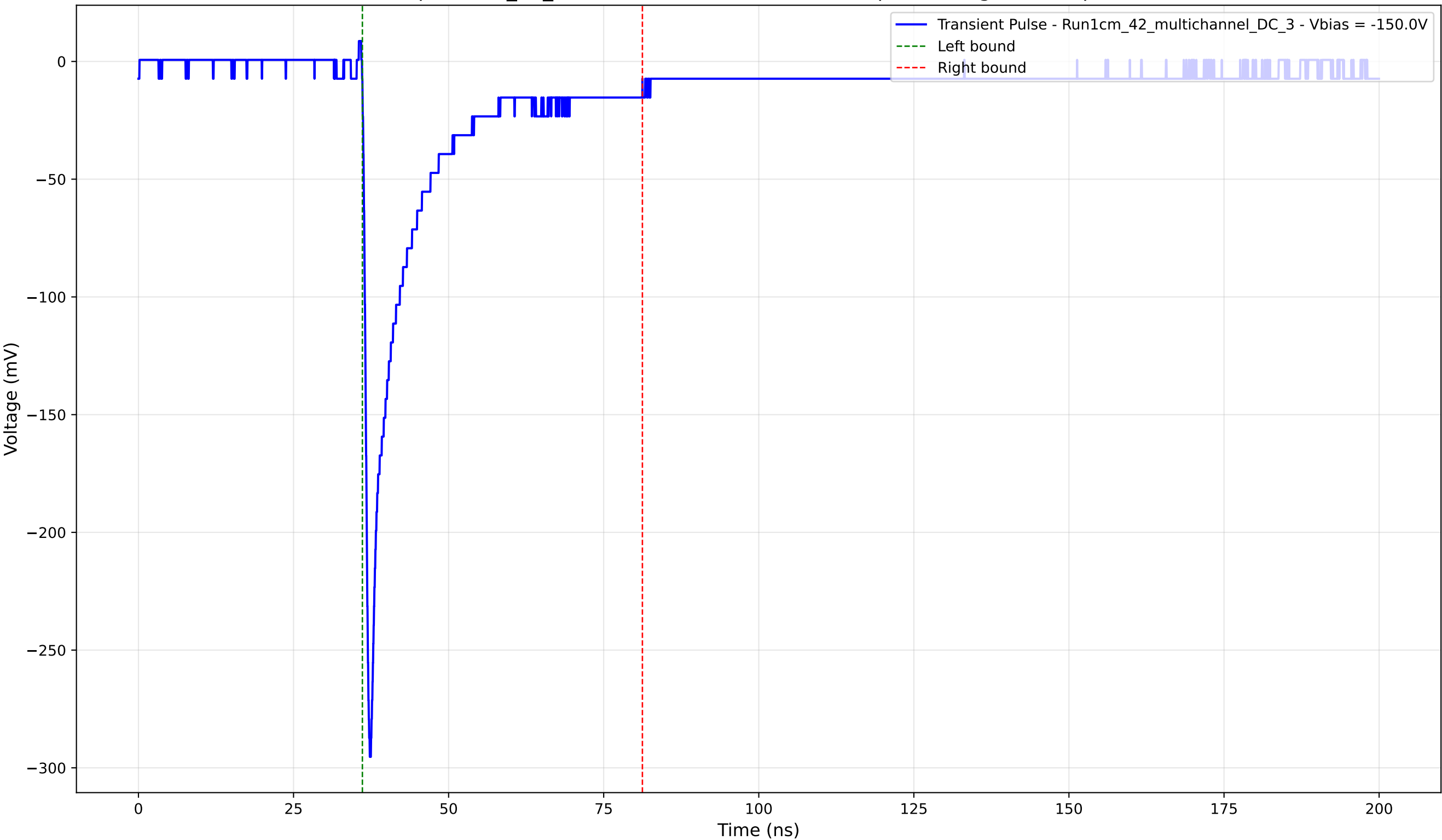
Transient Pulse - Sample: 1cm_42_multichannel - Position: 4590.0 \mu\text{m} - Charge: 41.17 pC - Rise Time: 0.86 ns
