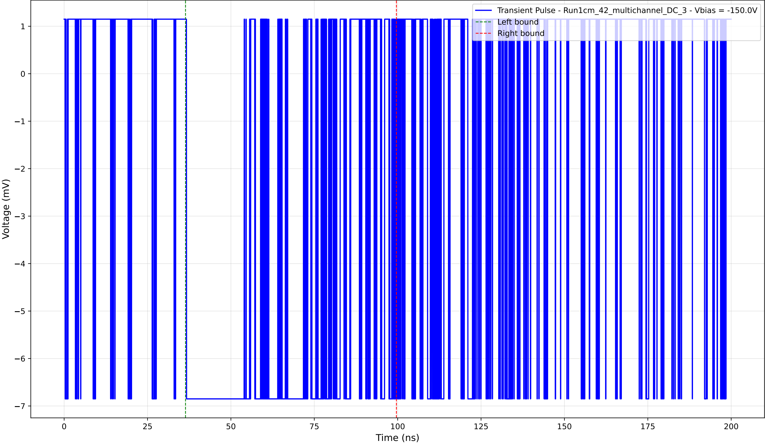
Transient Pulse - Sample: 1cm_42_multichannel - Position: 2885.0 \mu\text{m} - Charge: 5.36 pC - Rise Time: 0.00 ns (N/A)
