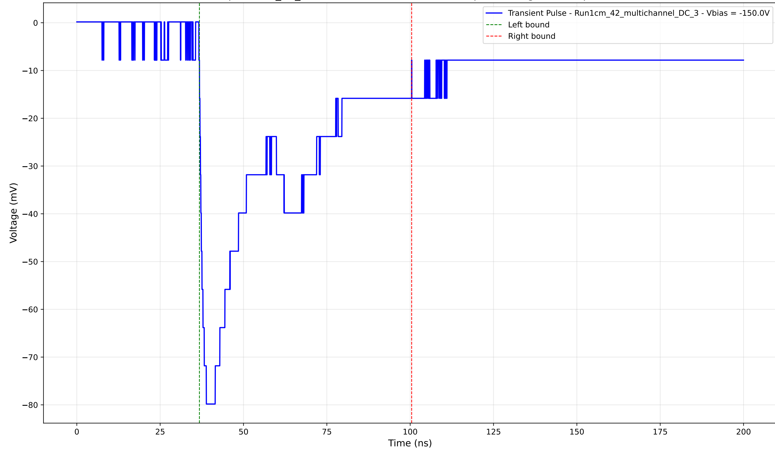
Transient Pulse - Sample: 1cm_42_multichannel - Position: 2475.0 \mu\text{m} - Charge: 40.45 pC - Rise Time: 2.06 ns
