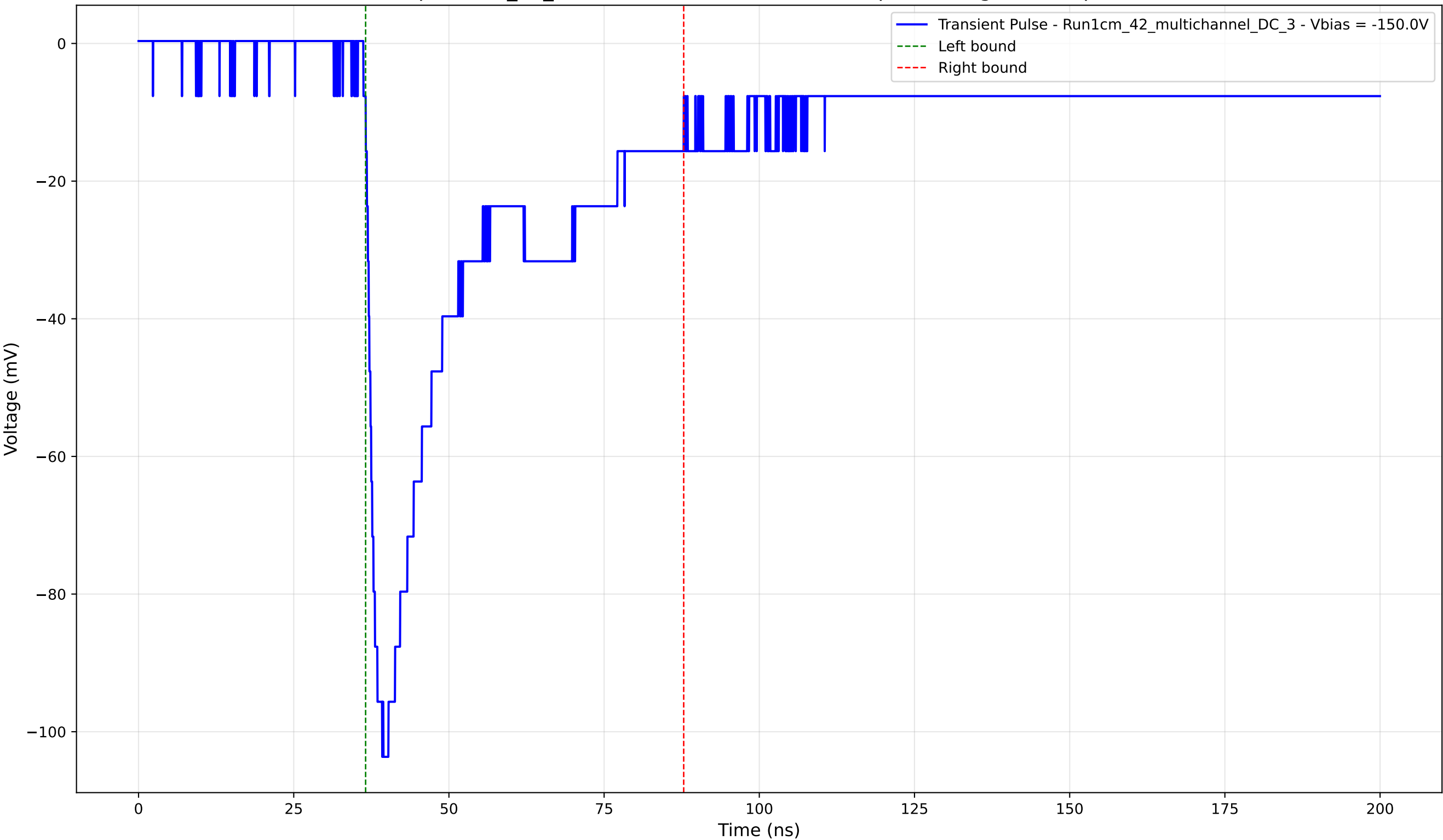
Transient Pulse - Sample: 1cm_42_multichannel - Position: 2980.0 \mu\text{m} - Charge: 37.15 pC - Rise Time: 1.89 ns
