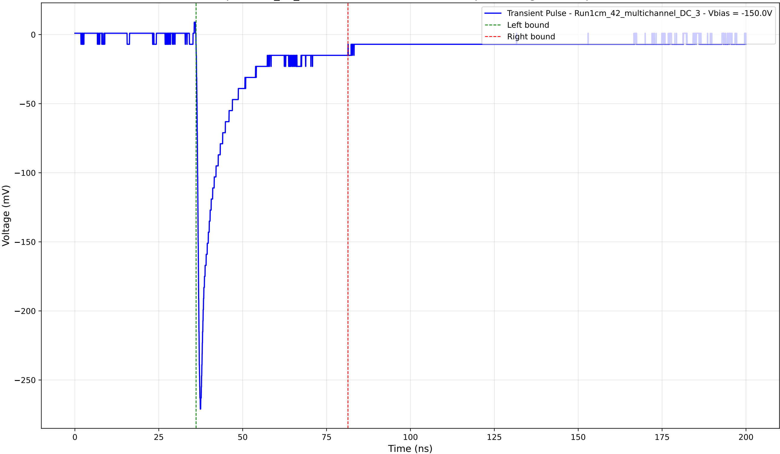
Transient Pulse - Sample: 1cm_42_multichannel - Position: 4520.0 \mu\text{m} - Charge: 40.04 pC - Rise Time: 0.87 ns
