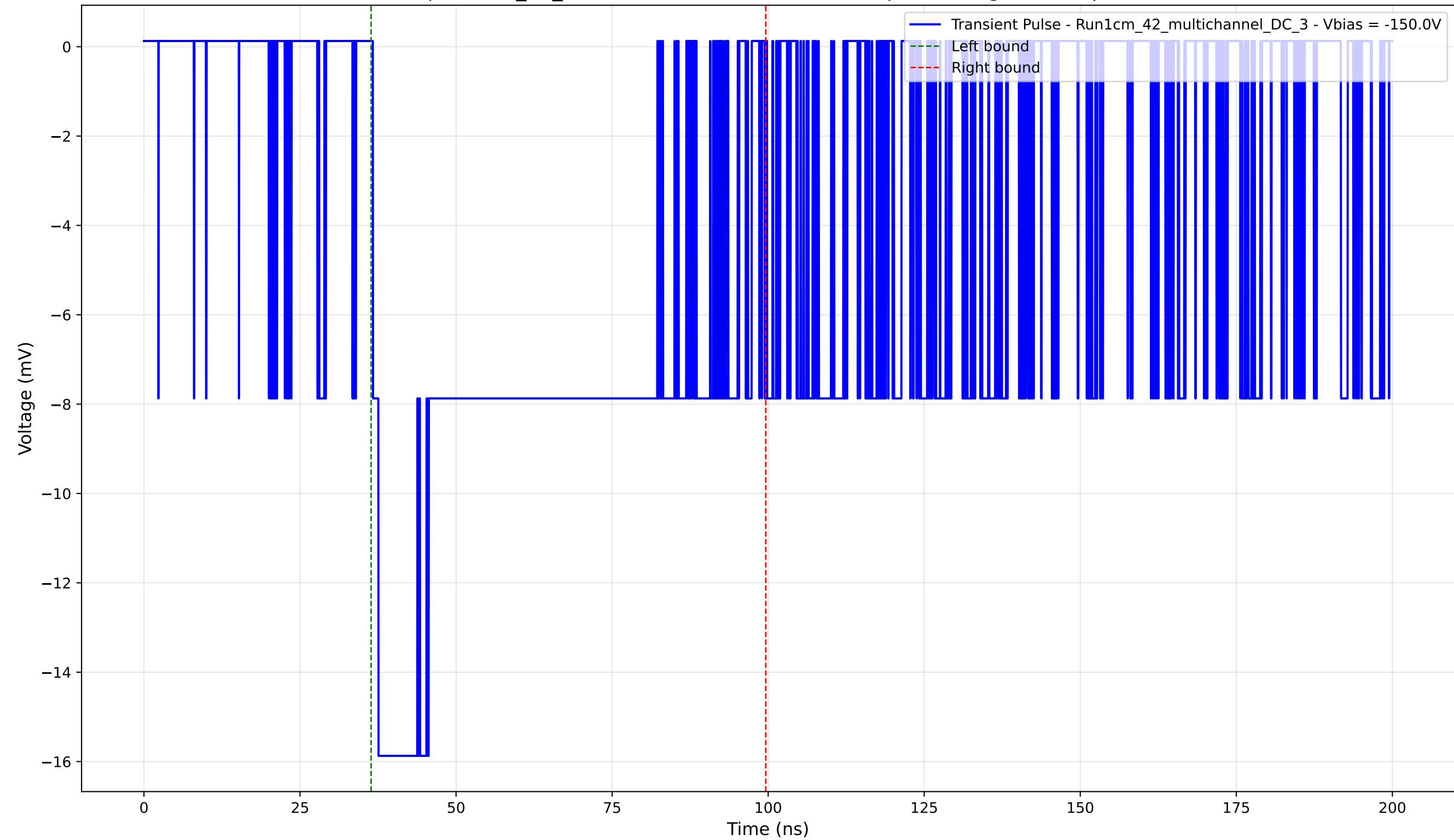
Transient Pulse - Sample: 1cm_42_multichannel - Position: 2910.0 \mu\text{m} - Charge: 10.18 pC - Rise Time: 0.90 ns
