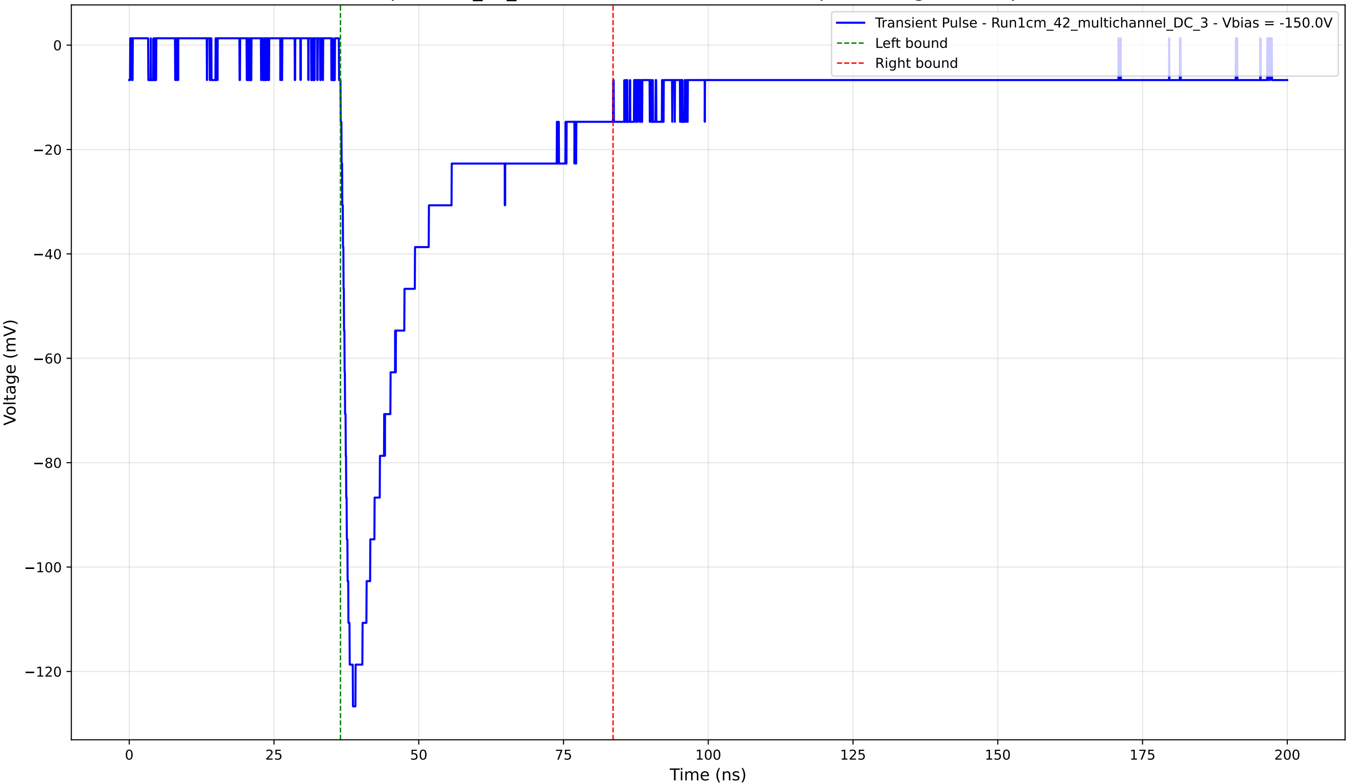
Transient Pulse - Sample: 1cm_42_multichannel - Position: 3505.0 \mu\text{m} - Charge: 36.06 pC - Rise Time: 1.57 ns
