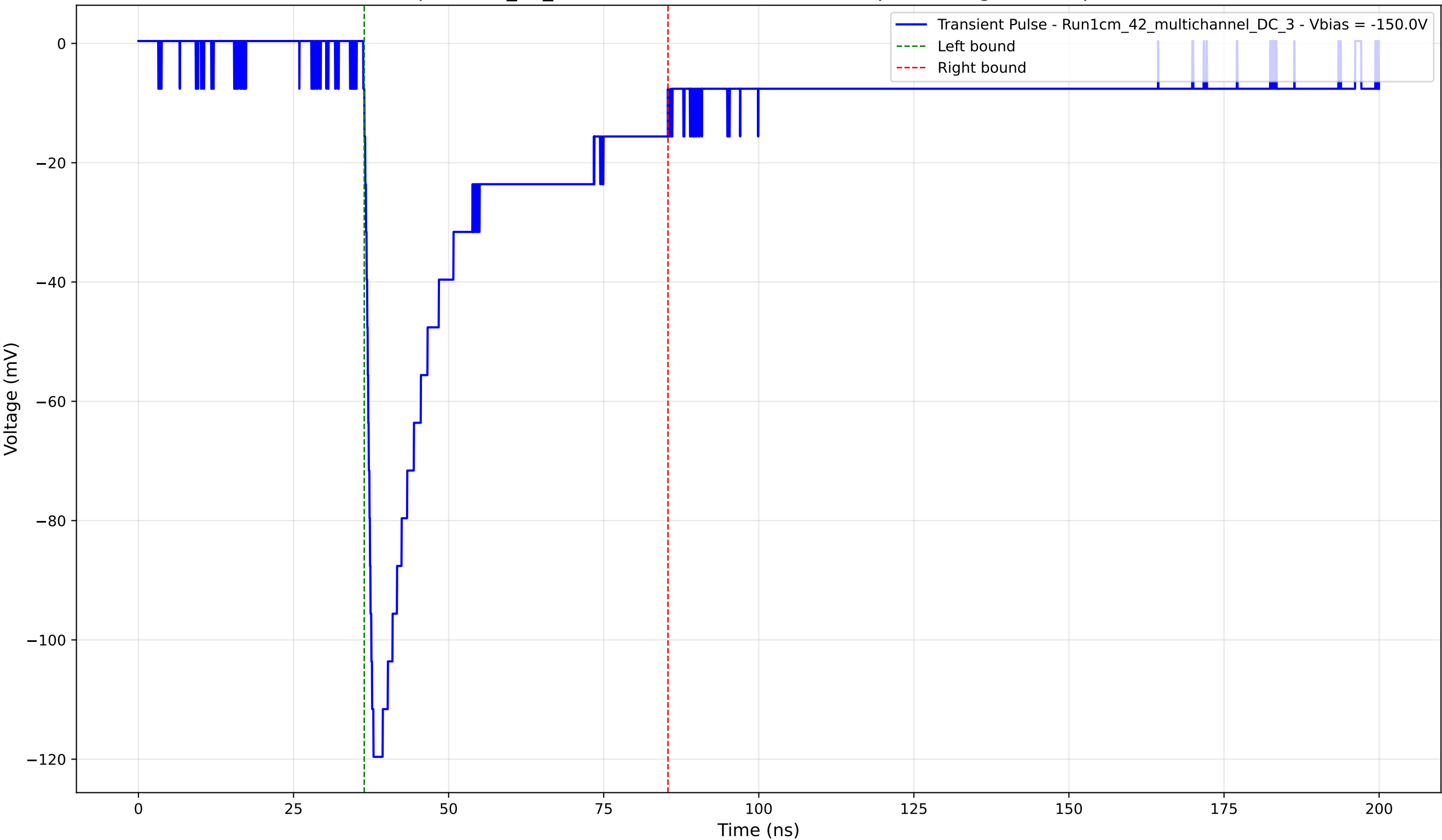
Transient Pulse - Sample: 1cm_42_multichannel - Position: 1295.0 \mu\text{m} - Charge: 35.88 pC - Rise Time: 1.25 ns
