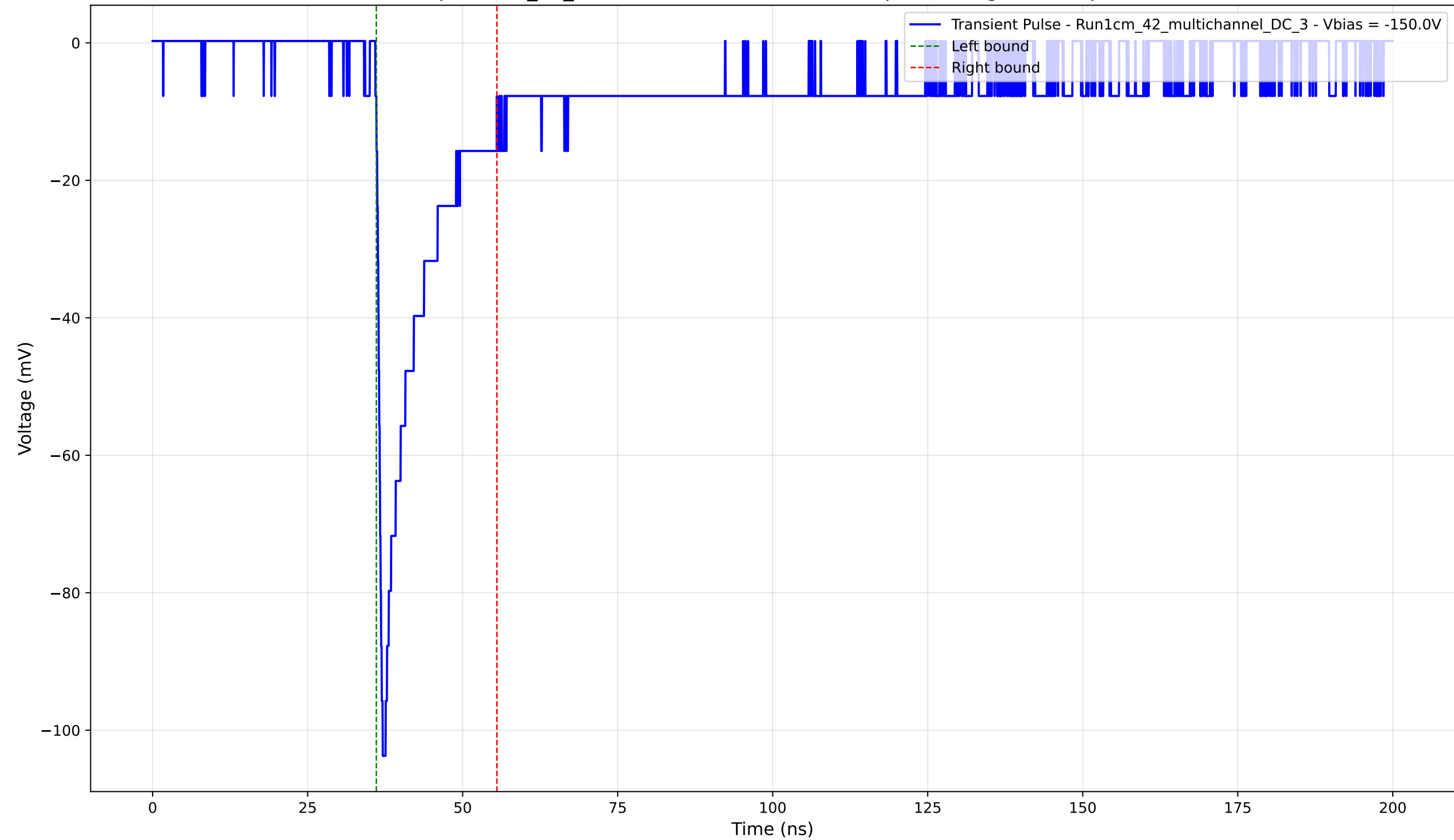
Transient Pulse - Sample: 1cm_42_multichannel - Position: 395.0 \mu\text{m} - Charge: 14.12 pC - Rise Time: 0.85 ns
