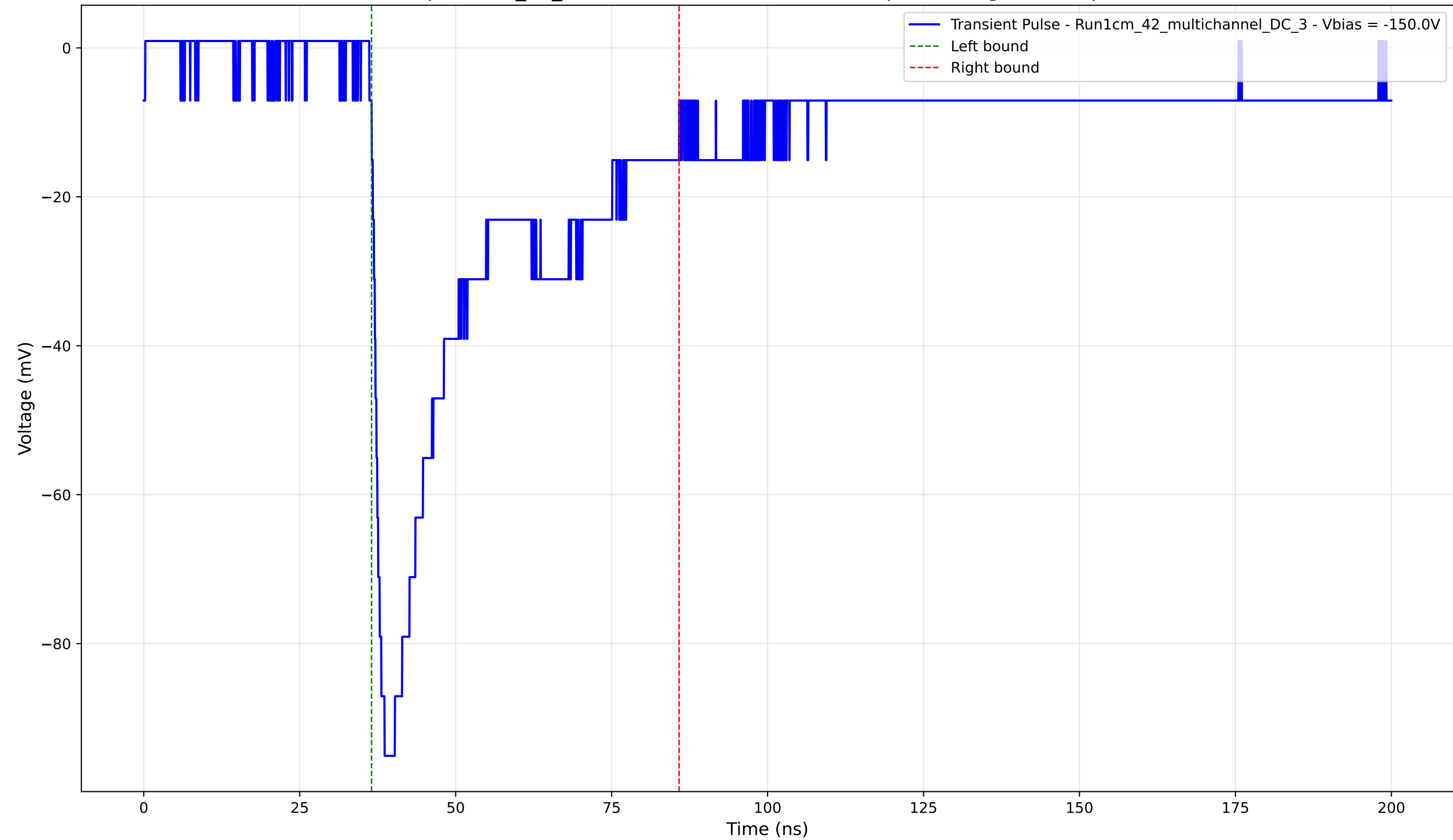
Transient Pulse - Sample: 1cm_42_multichannel - Position: 1795.0 \mu\text{m} - Charge: 34.11 pC - Rise Time: 1.55 ns
