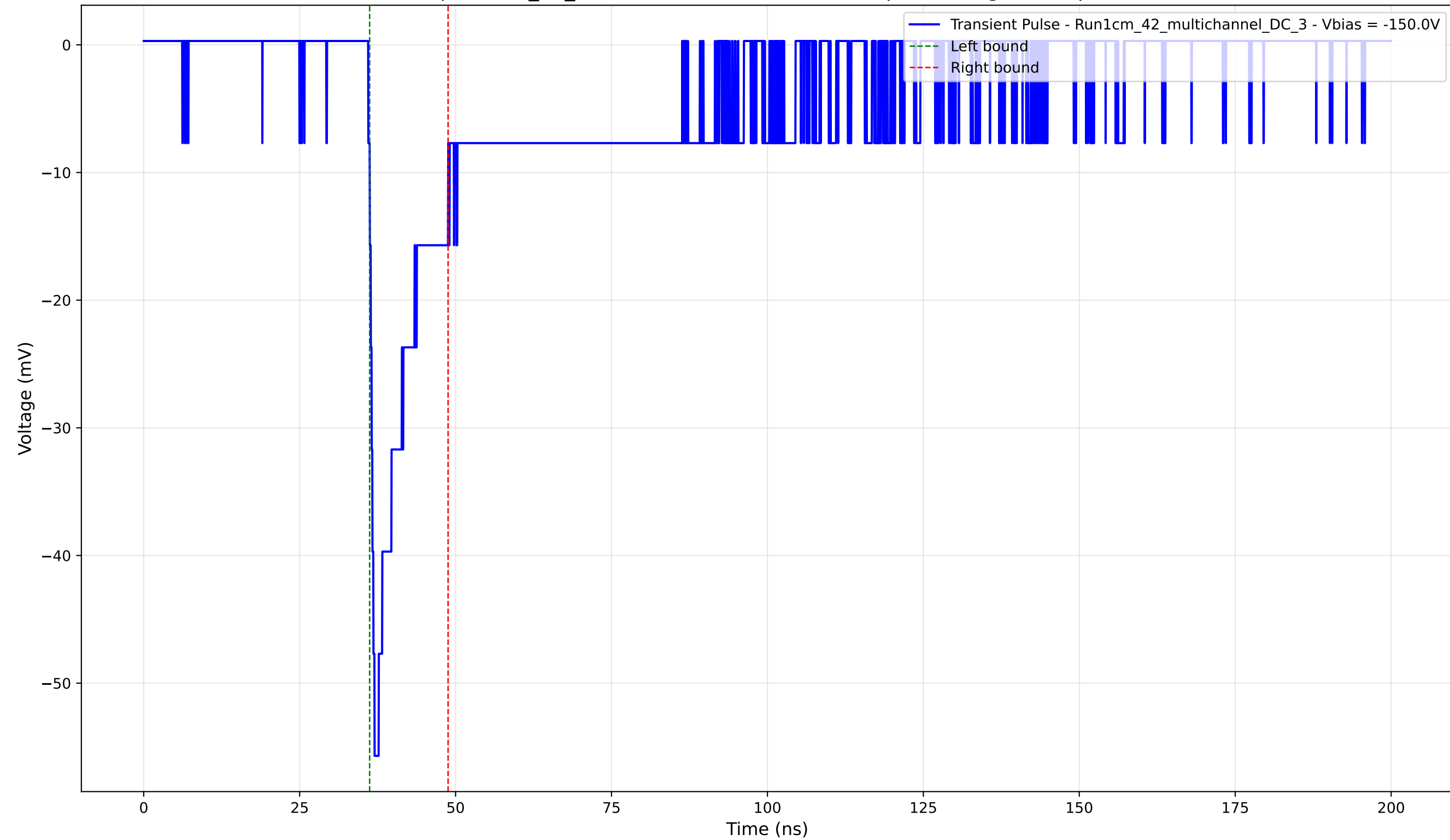
Transient Pulse - Sample: 1cm_42_multichannel - Position: 385.0 \mu\text{m} - Charge: 6.73 pC - Rise Time: 1.01 ns
