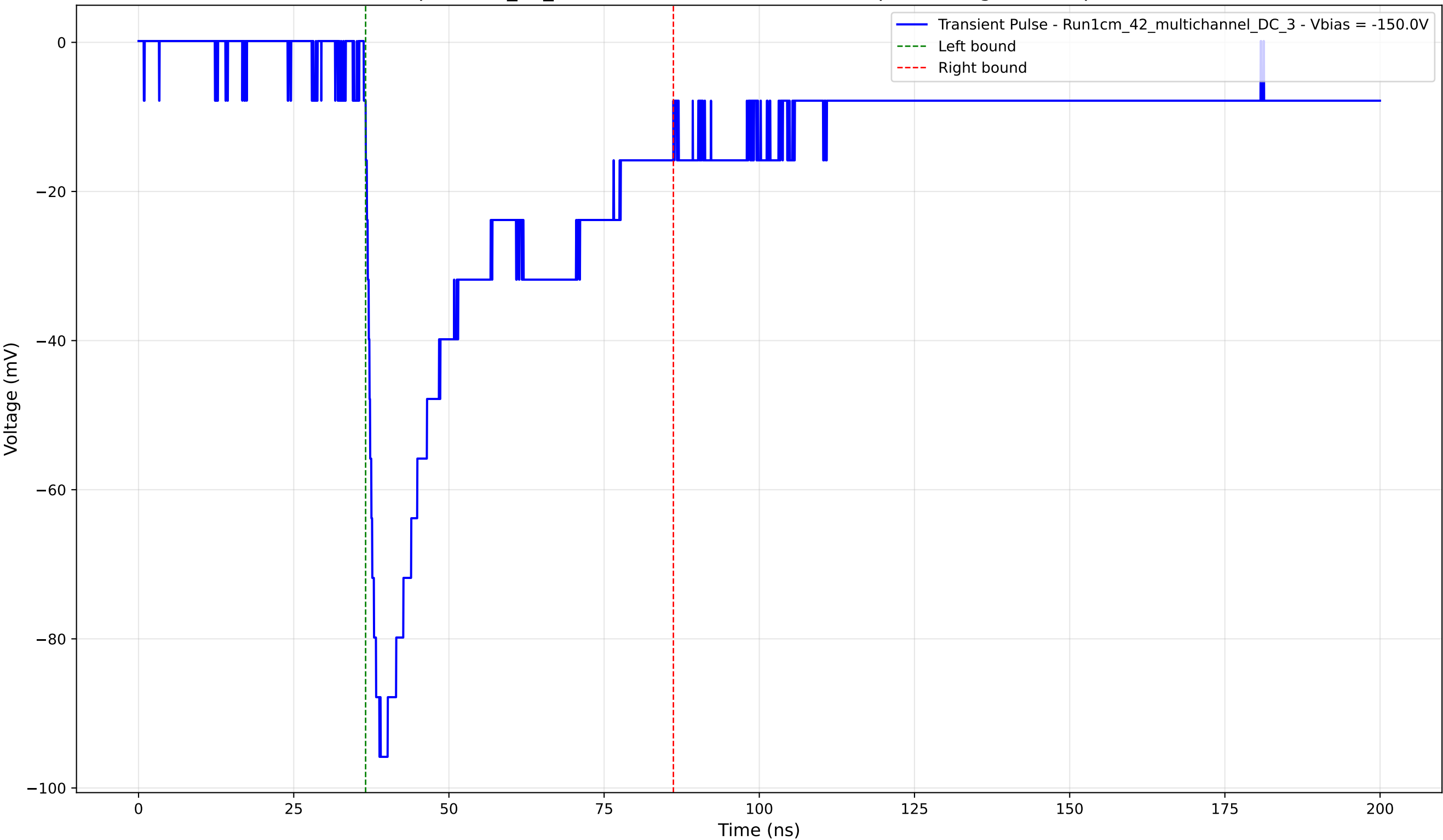
Transient Pulse - Sample: 1cm_42_multichannel - Position: 1950.0 \mu\text{m} - Charge: 36.06 pC - Rise Time: 1.68 ns
