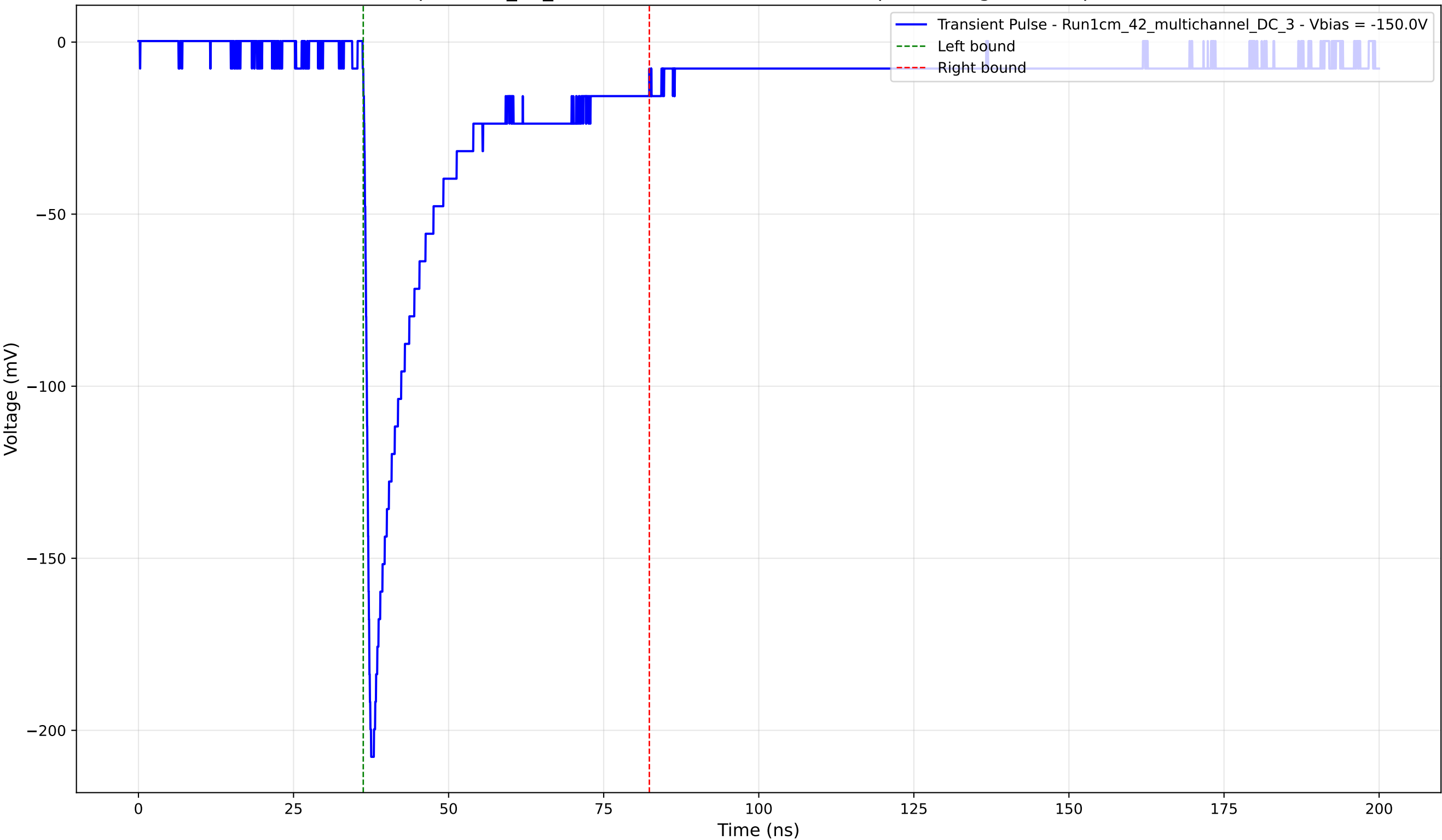
Transient Pulse - Sample: 1cm_42_multichannel - Position: 4235.0 \mu\text{m} - Charge: 41.07 pC - Rise Time: 0.95 ns
