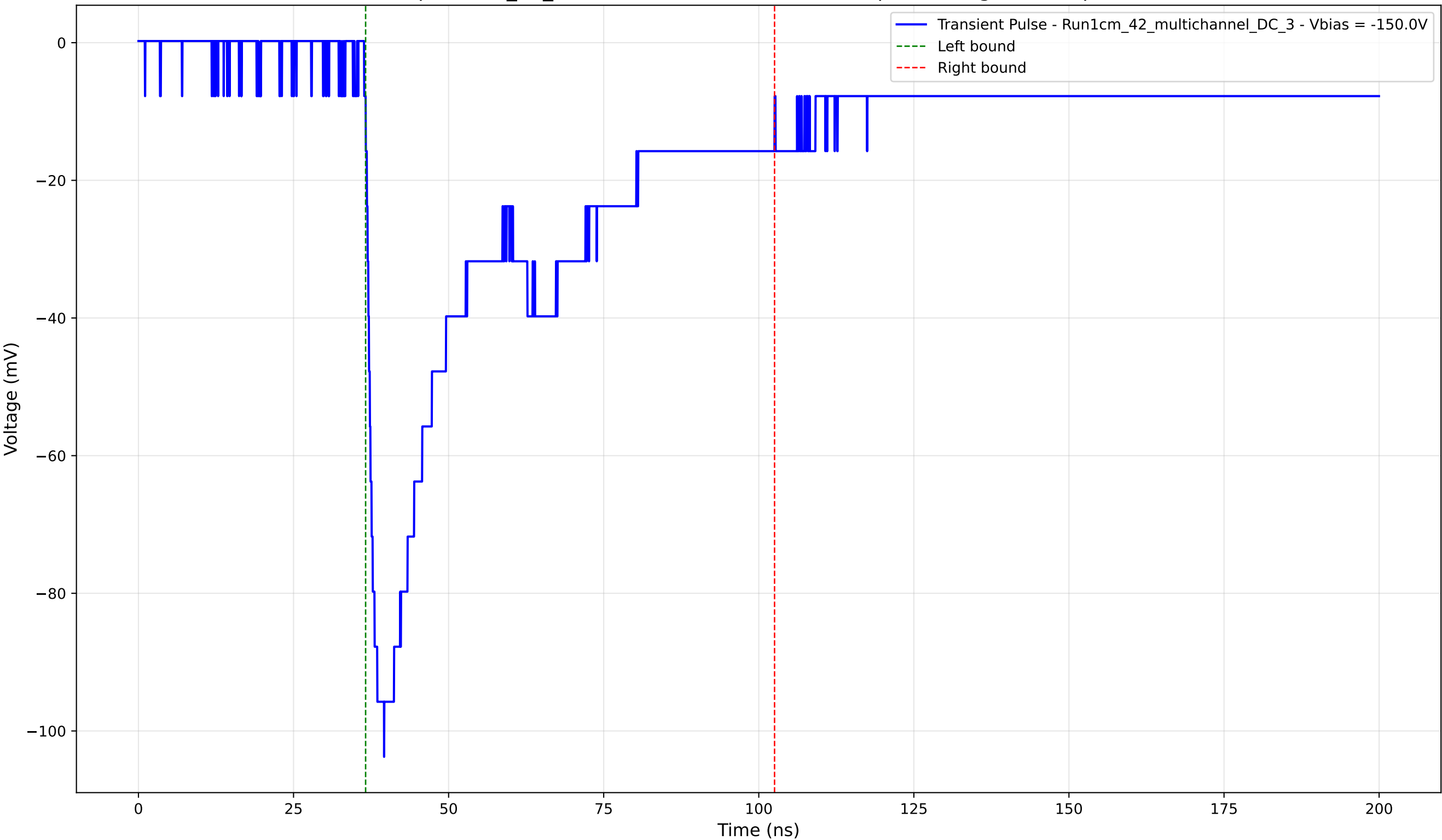
Transient Pulse - Sample: 1cm_42_multichannel - Position: 2000.0 \mu\text{m} - Charge: 44.52 pC - Rise Time: 1.87 ns
