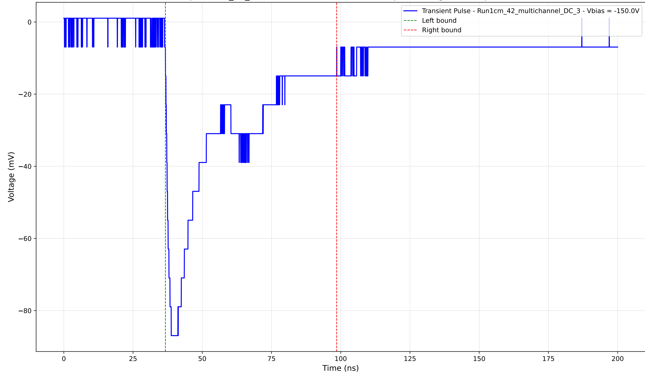
Transient Pulse - Sample: 1cm_42_multichannel - Position: 2700.0 \mu\text{m} - Charge: 38.97 pC - Rise Time: 1.66 ns
