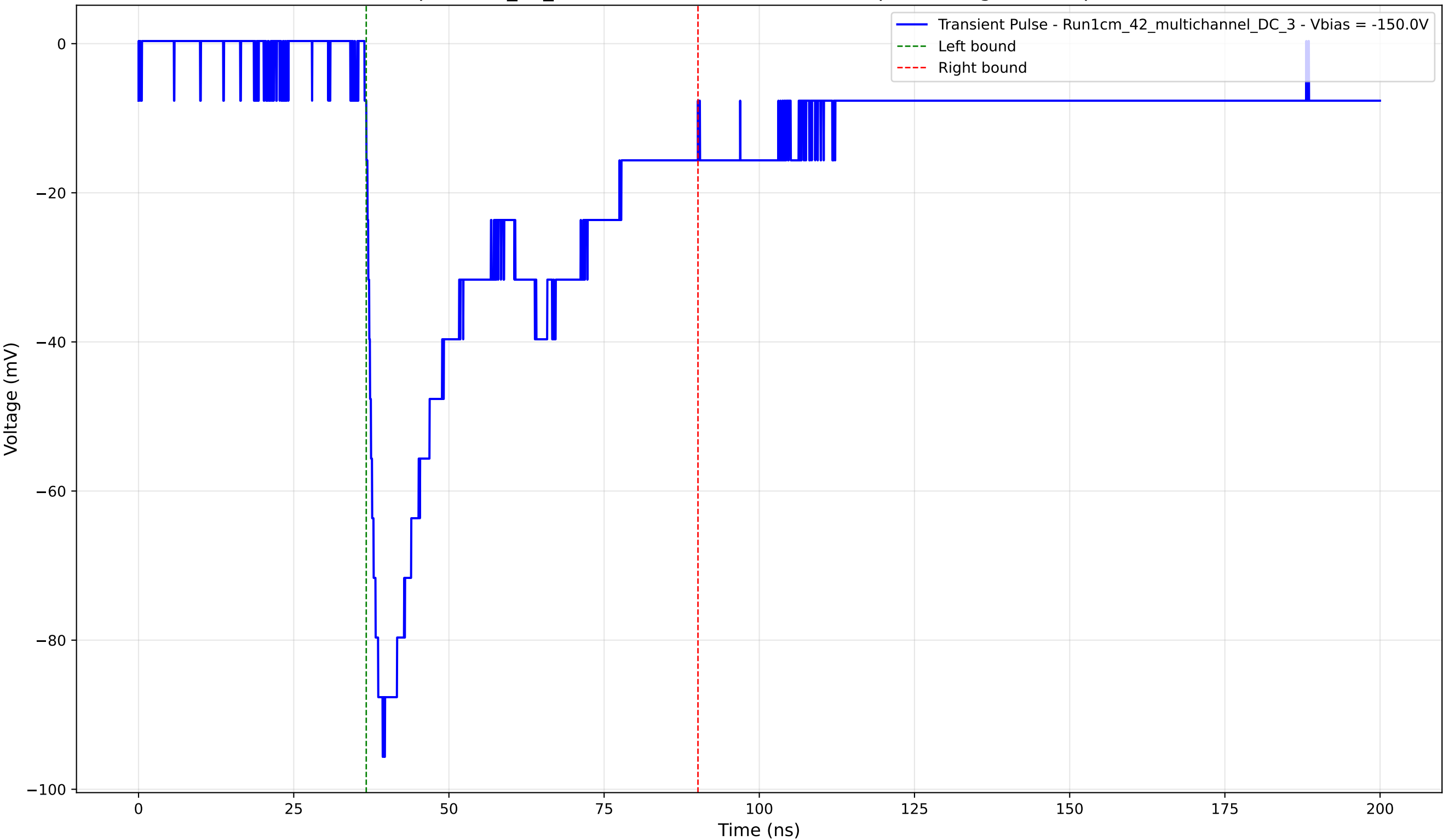
Transient Pulse - Sample: 1cm_42_multichannel - Position: 2725.0 \mu\text{m} - Charge: 37.88 pC - Rise Time: 1.92 ns
