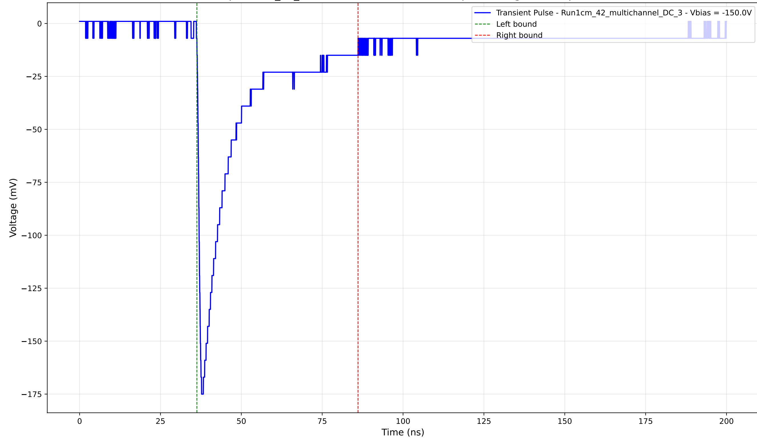
Transient Pulse - Sample: 1cm_42_multichannel - Position: 935.0 \mu\text{m} - Charge: 42.66 pC - Rise Time: 1.03 ns
