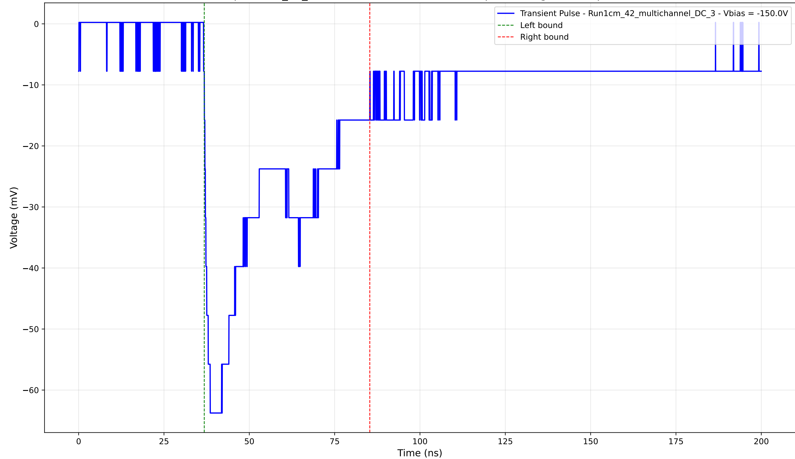
Transient Pulse - Sample: 1cm_42_multichannel - Position: 2440.0 \mu\text{m} - Charge: 30.24 pC - Rise Time: 1.94 ns
