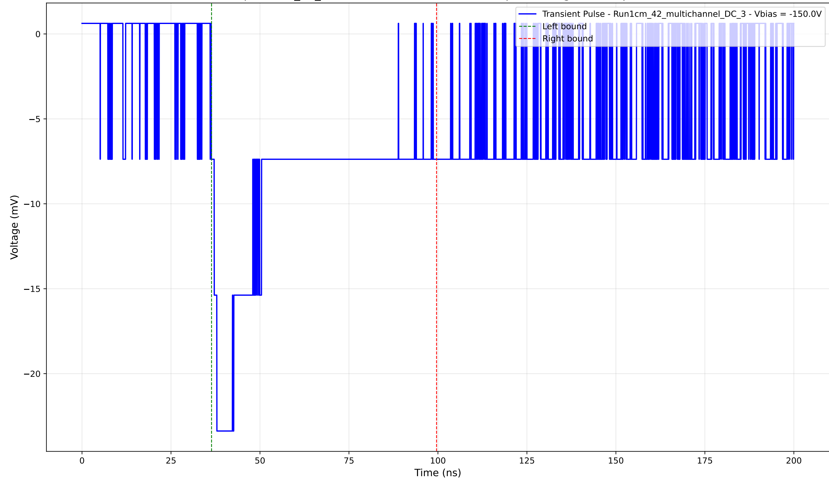
Transient Pulse - Sample: 1cm_42_multichannel - Position: 1835.0 \mu\text{m} - Charge: 11.89 pC - Rise Time: 1.57 ns
