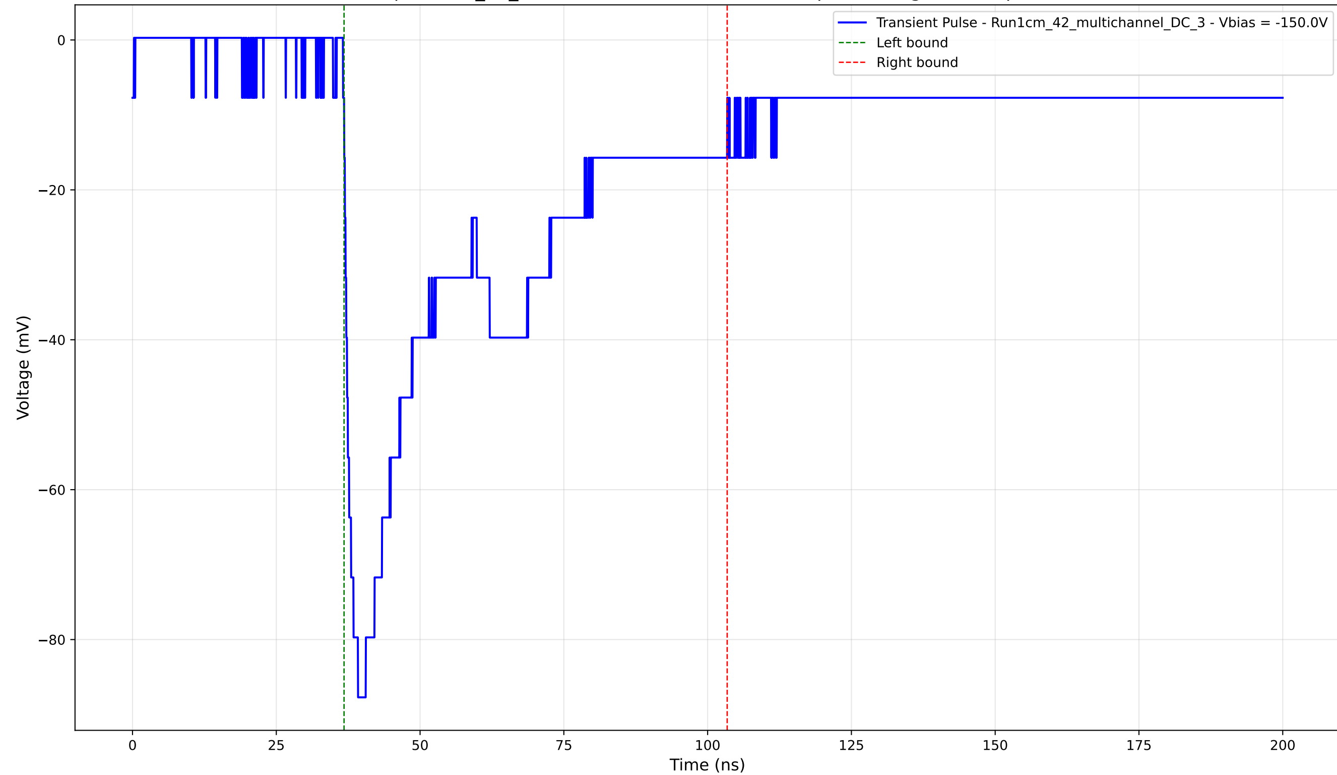
Transient Pulse - Sample: 1cm_42_multichannel - Position: 2255.0 \mu\text{m} - Charge: 42.91 pC - Rise Time: 1.64 ns
