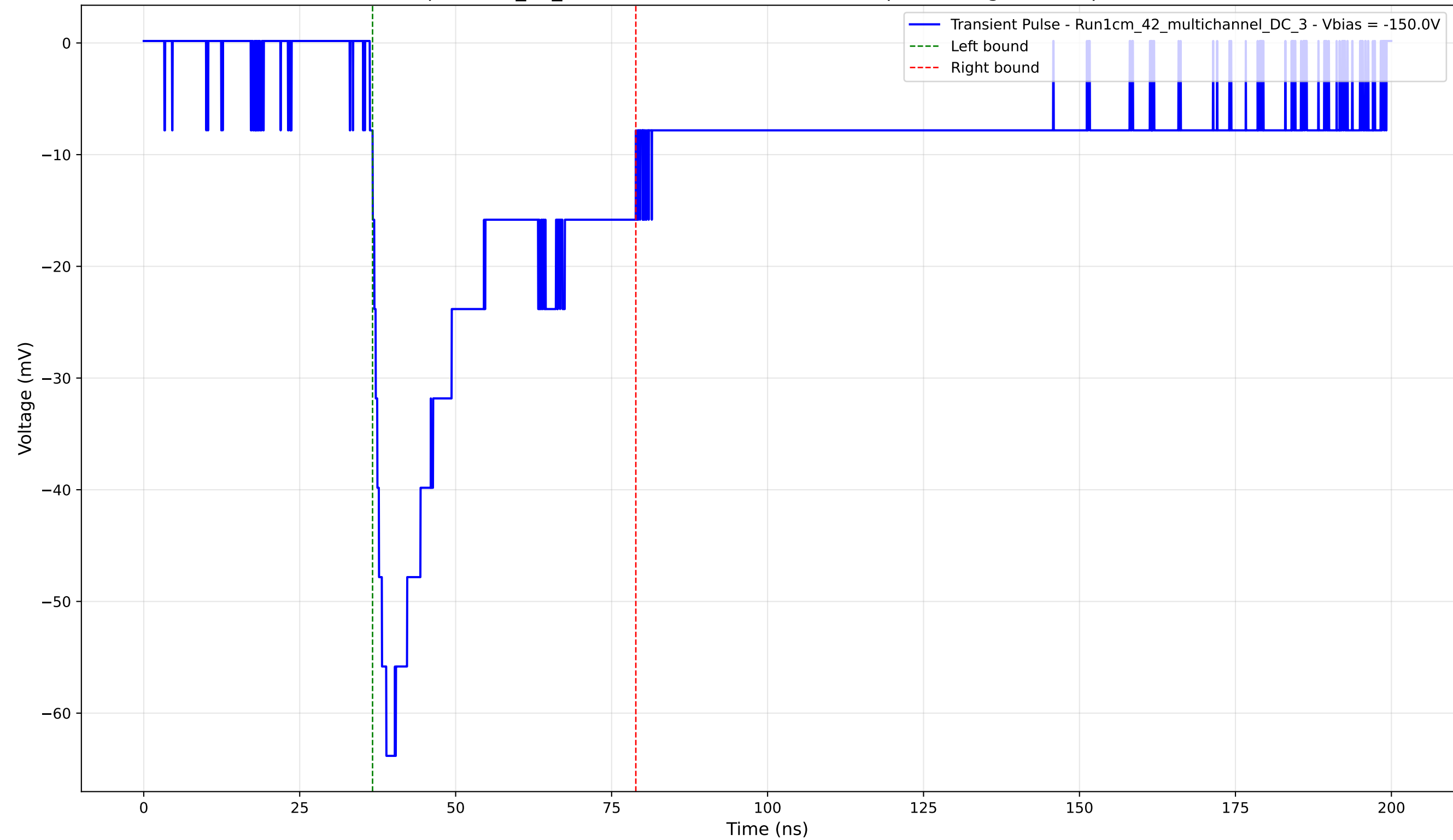
Transient Pulse - Sample: 1cm_42_multichannel - Position: 2935.0 \mu\text{m} - Charge: 21.99 pC - Rise Time: 2.64 ns
