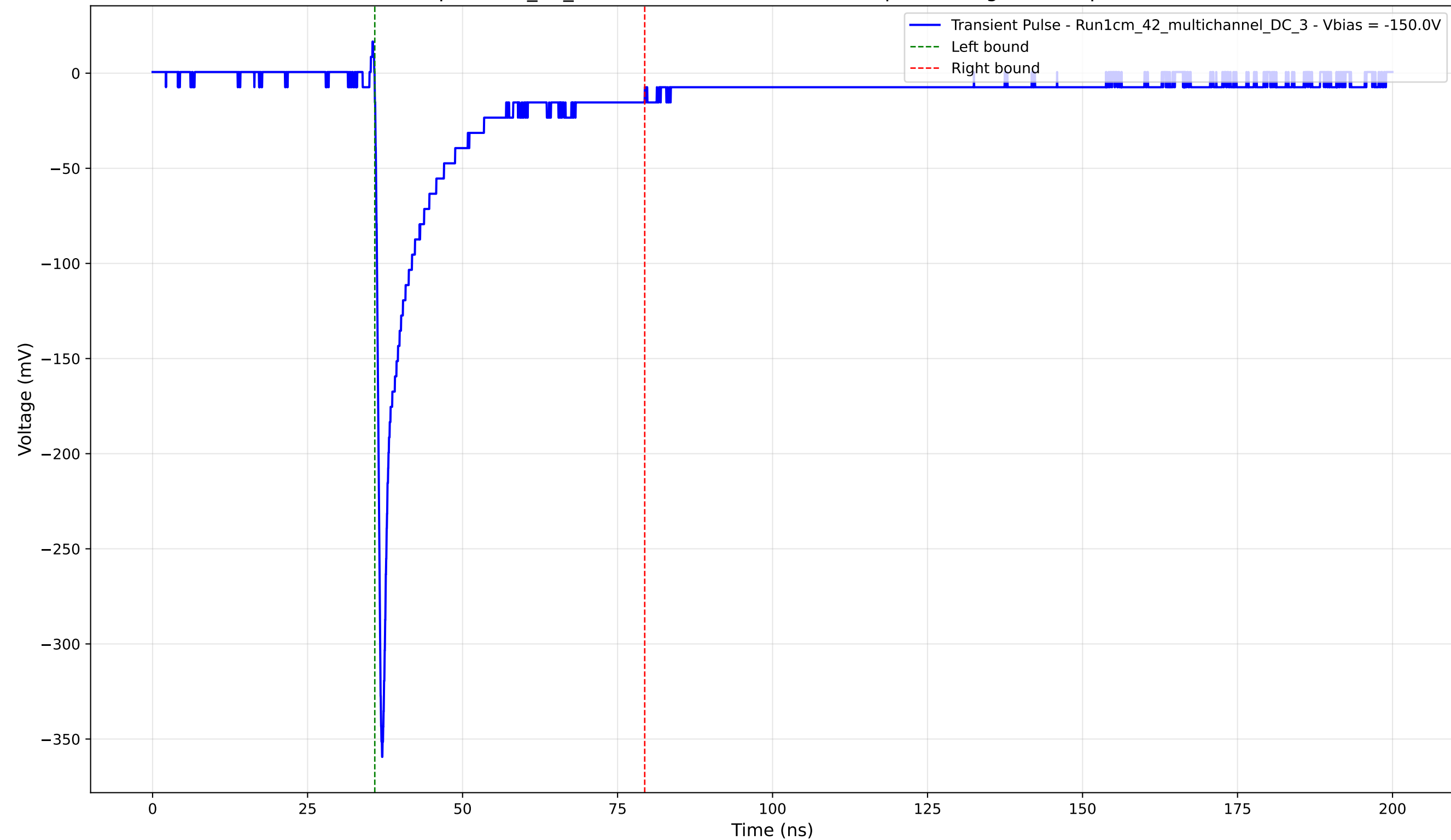
Transient Pulse - Sample: 1cm_42_multichannel - Position: 120.0 \mu\text{m} - Charge: 42.49 pC - Rise Time: 0.81 ns
