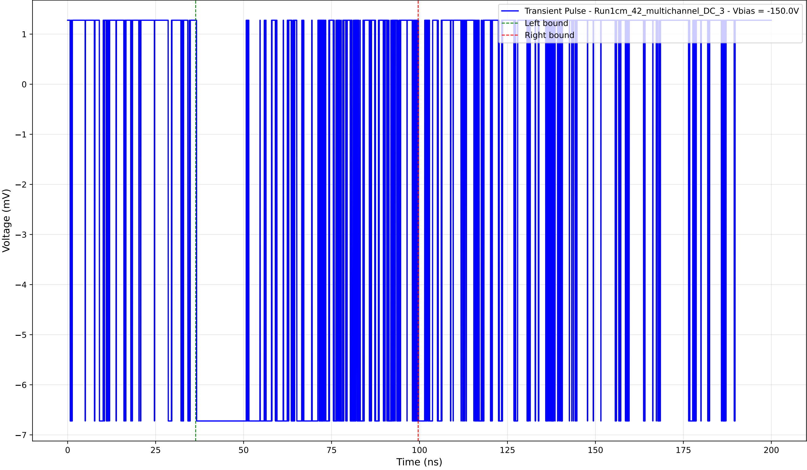
Transient Pulse - Sample: 1cm_42_multichannel - Position: 1370.0 \mu\text{m} - Charge: 4.93 pC - Rise Time: 0.00 ns (N/A)
