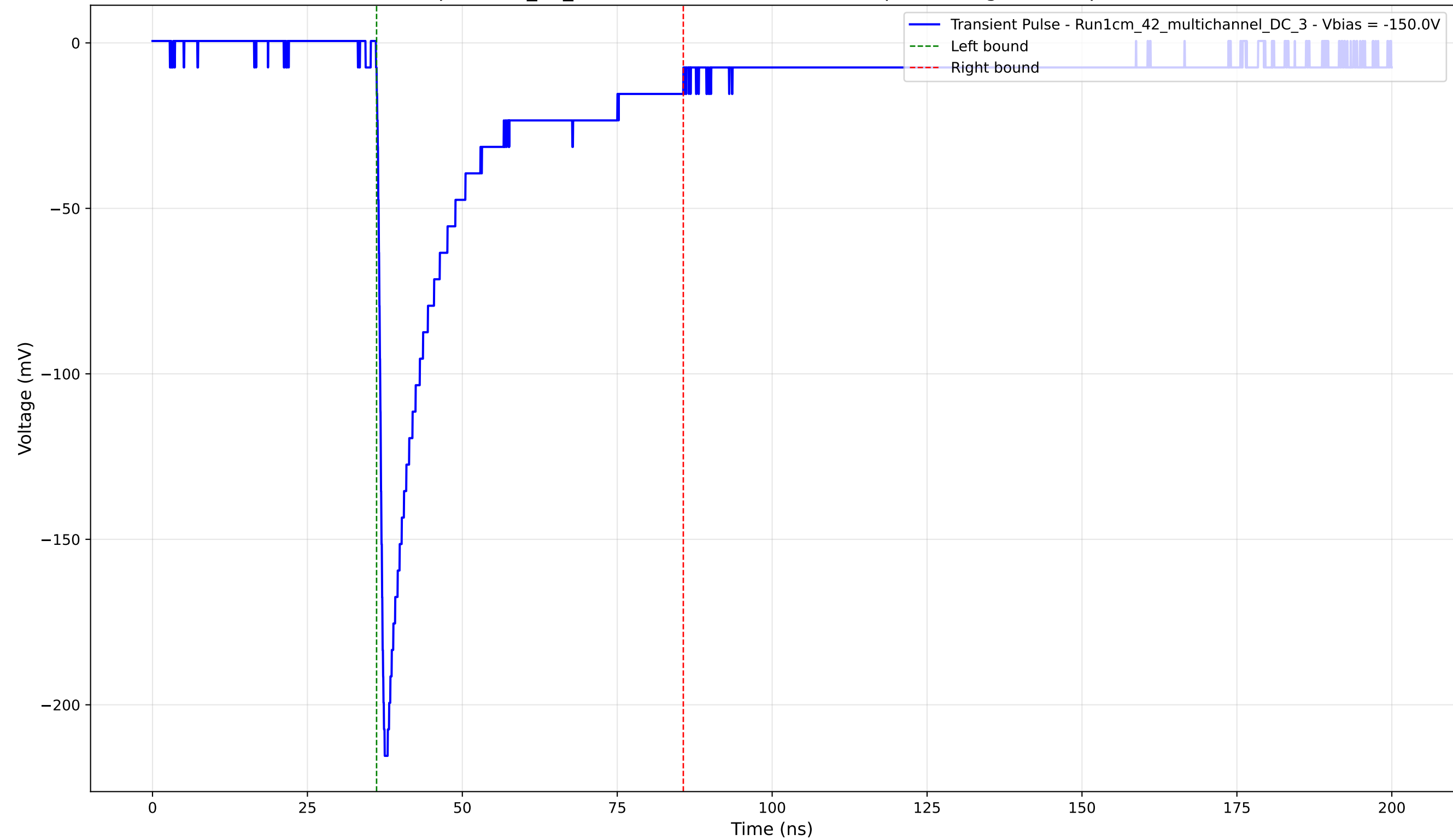
Transient Pulse - Sample: 1cm_42_multichannel - Position: 725.0 \mu\text{m} - Charge: 46.12 pC - Rise Time: 1.00 ns
