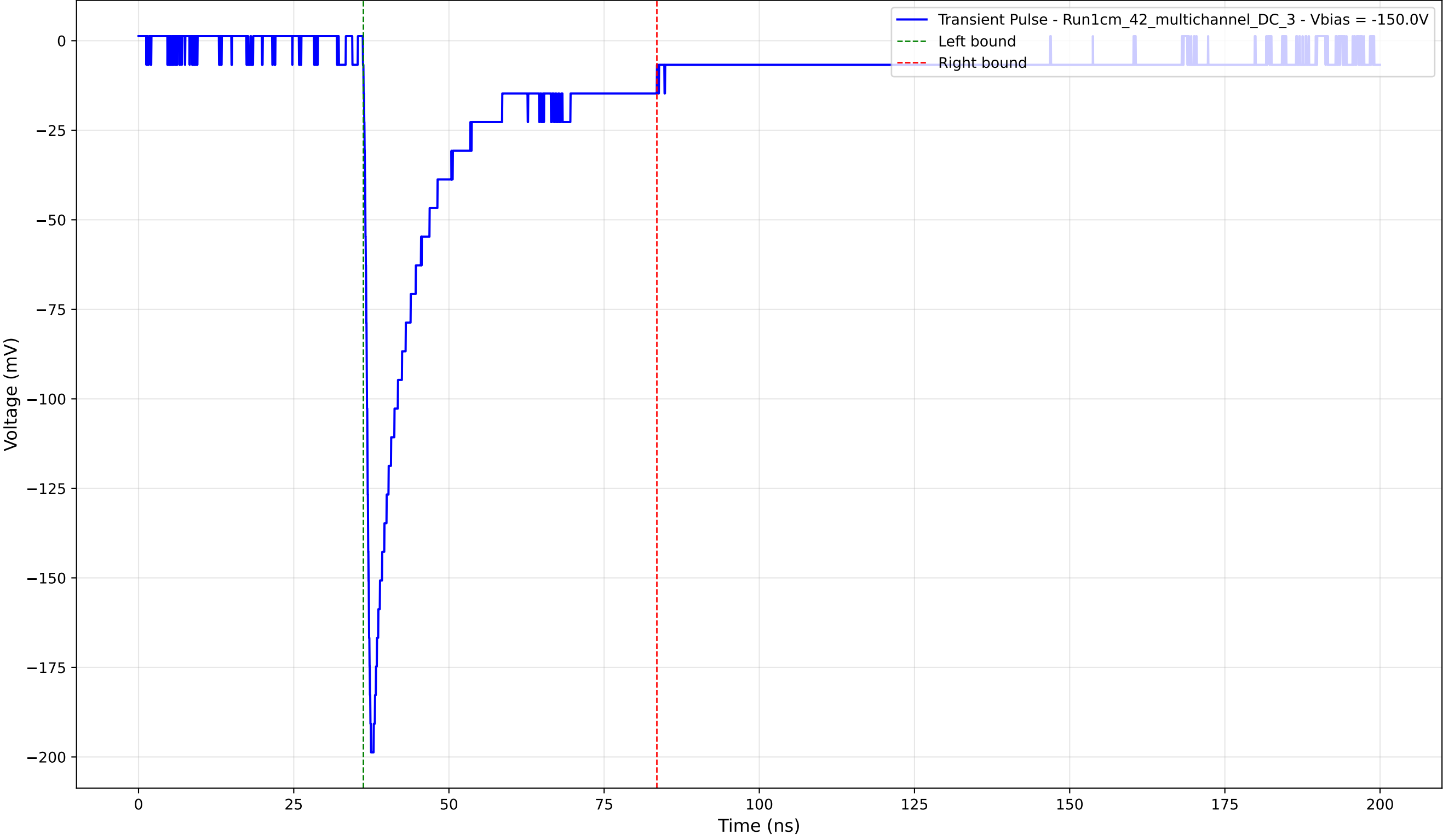
Transient Pulse - Sample: 1cm_42_multichannel - Position: 4285.0 \mu\text{m} - Charge: 37.16 pC - Rise Time: 0.93 ns
