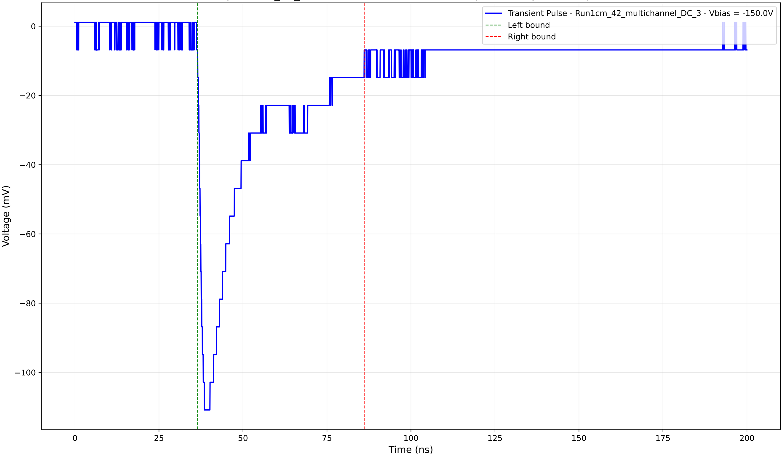
Transient Pulse - Sample: 1cm_42_multichannel - Position: 3230.0 \mu\text{m} - Charge: 36.74 pC - Rise Time: 1.63 ns
