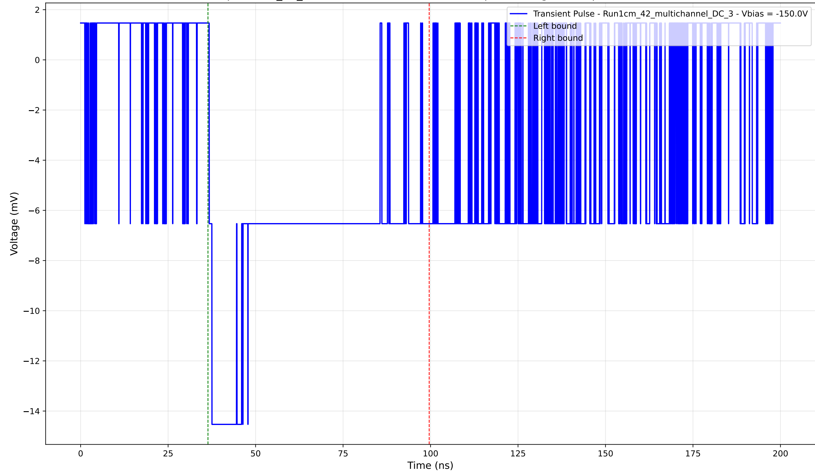
Transient Pulse - Sample: 1cm_42_multichannel - Position: 2405.0 \mu\text{m} - Charge: 9.19 pC - Rise Time: 0.00 ns (N/A)
