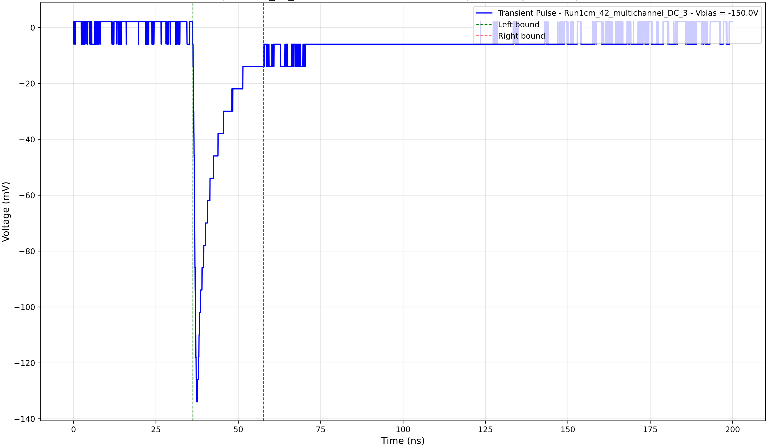
Transient Pulse - Sample: 1cm_42_multichannel - Position: 4445.0 \mu\text{m} - Charge: 17.19 pC - Rise Time: 0.94 ns
