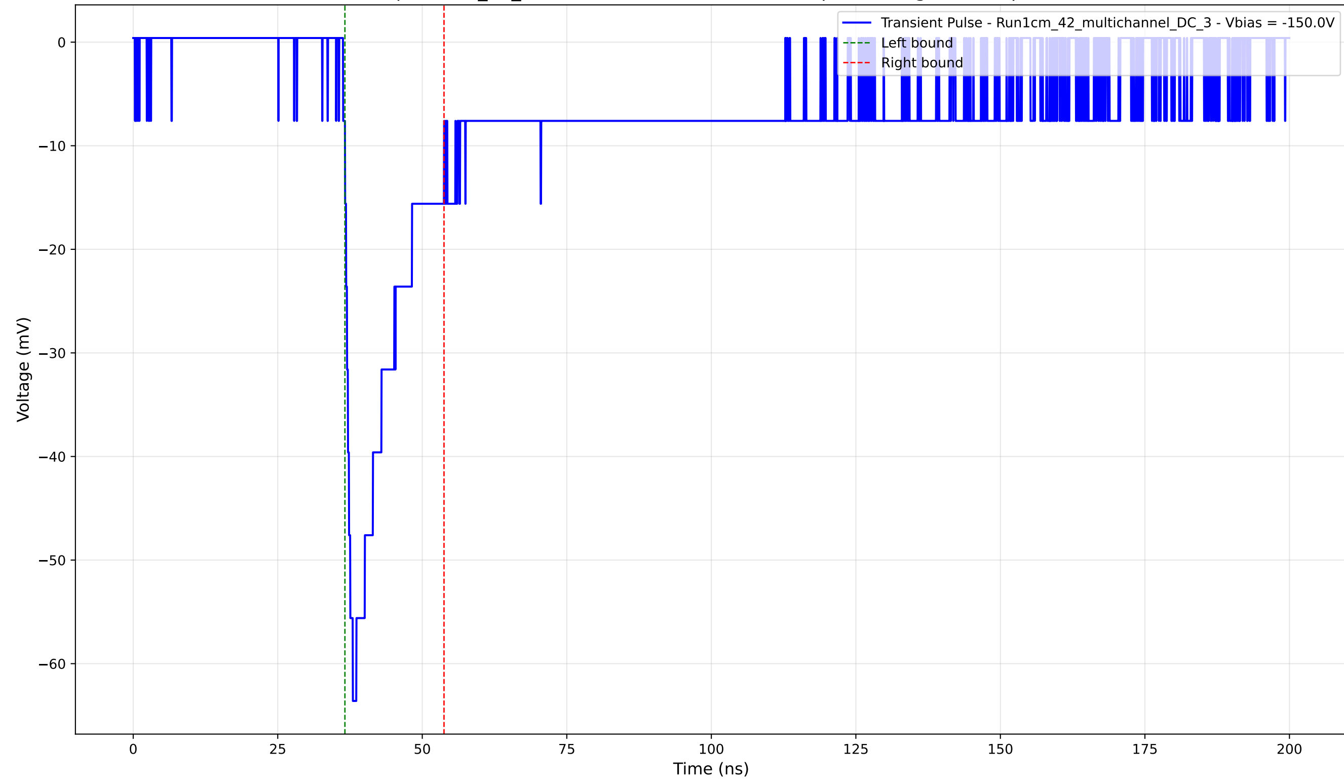
Transient Pulse - Sample: 1cm_42_multichannel - Position: 3845.0 \mu\text{m} - Charge: 10.58 pC - Rise Time: 1.68 ns
