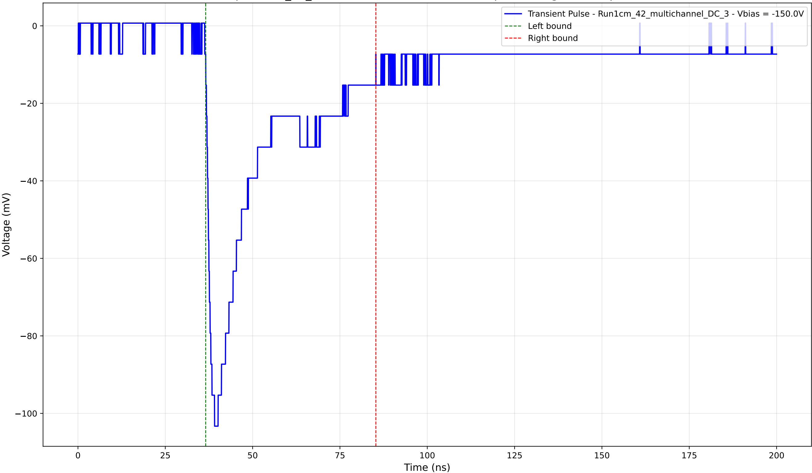
Transient Pulse - Sample: 1cm_42_multichannel - Position: 3095.0 \mu\text{m} - Charge: 35.19 pC - Rise Time: 1.79 ns
