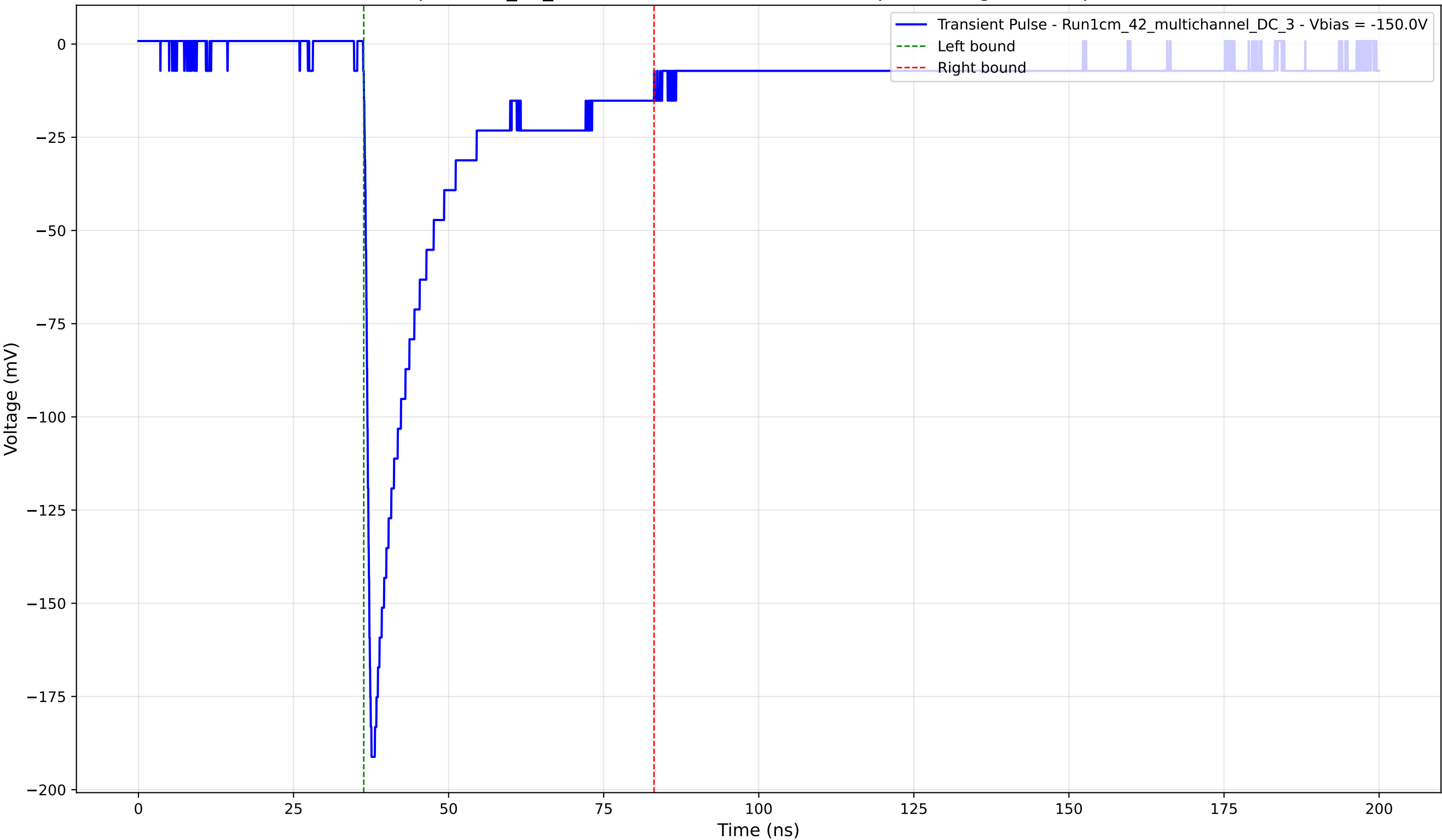
Transient Pulse - Sample: 1cm_42_multichannel - Position: 4155.0 \mu\text{m} - Charge: 40.26 pC - Rise Time: 0.95 ns
