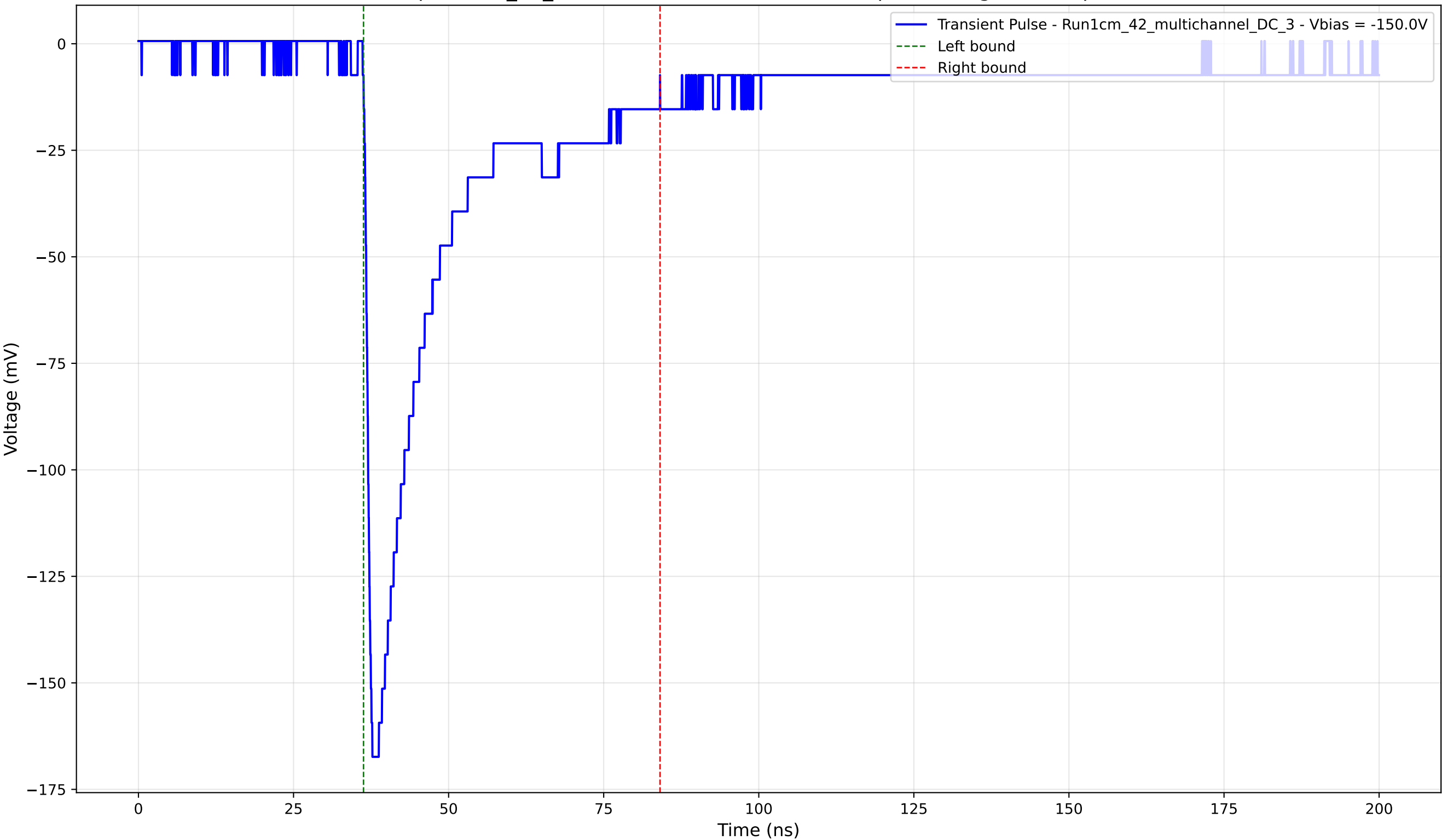
Transient Pulse - Sample: 1cm_42_multichannel - Position: 1030.0 \mu\text{m} - Charge: 43.26 pC - Rise Time: 1.06 ns
