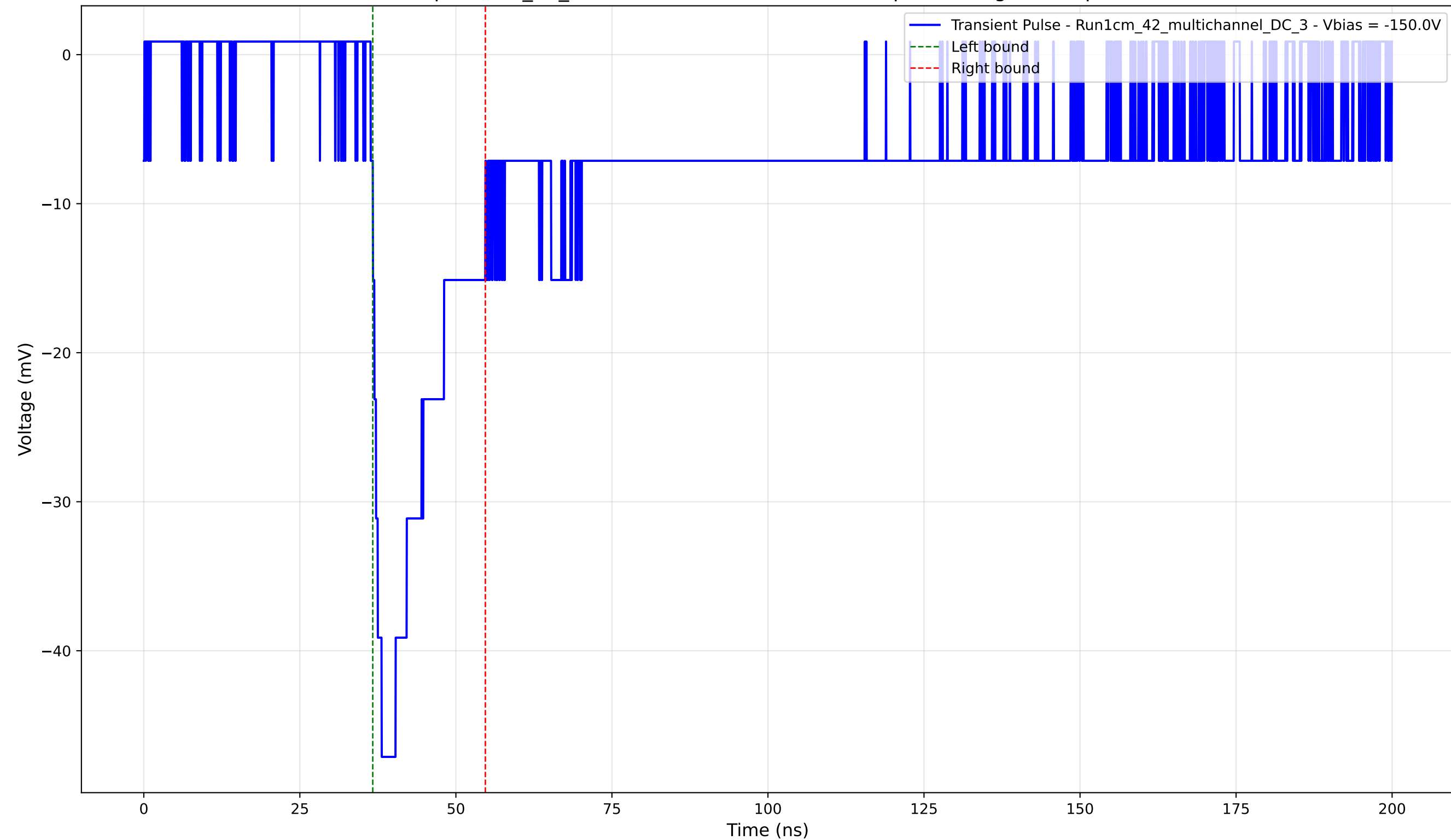
Transient Pulse - Sample: 1cm_42_multichannel - Position: 1405.0 \mu\text{m} - Charge: 9.54 pC - Rise Time: 1.77 ns
