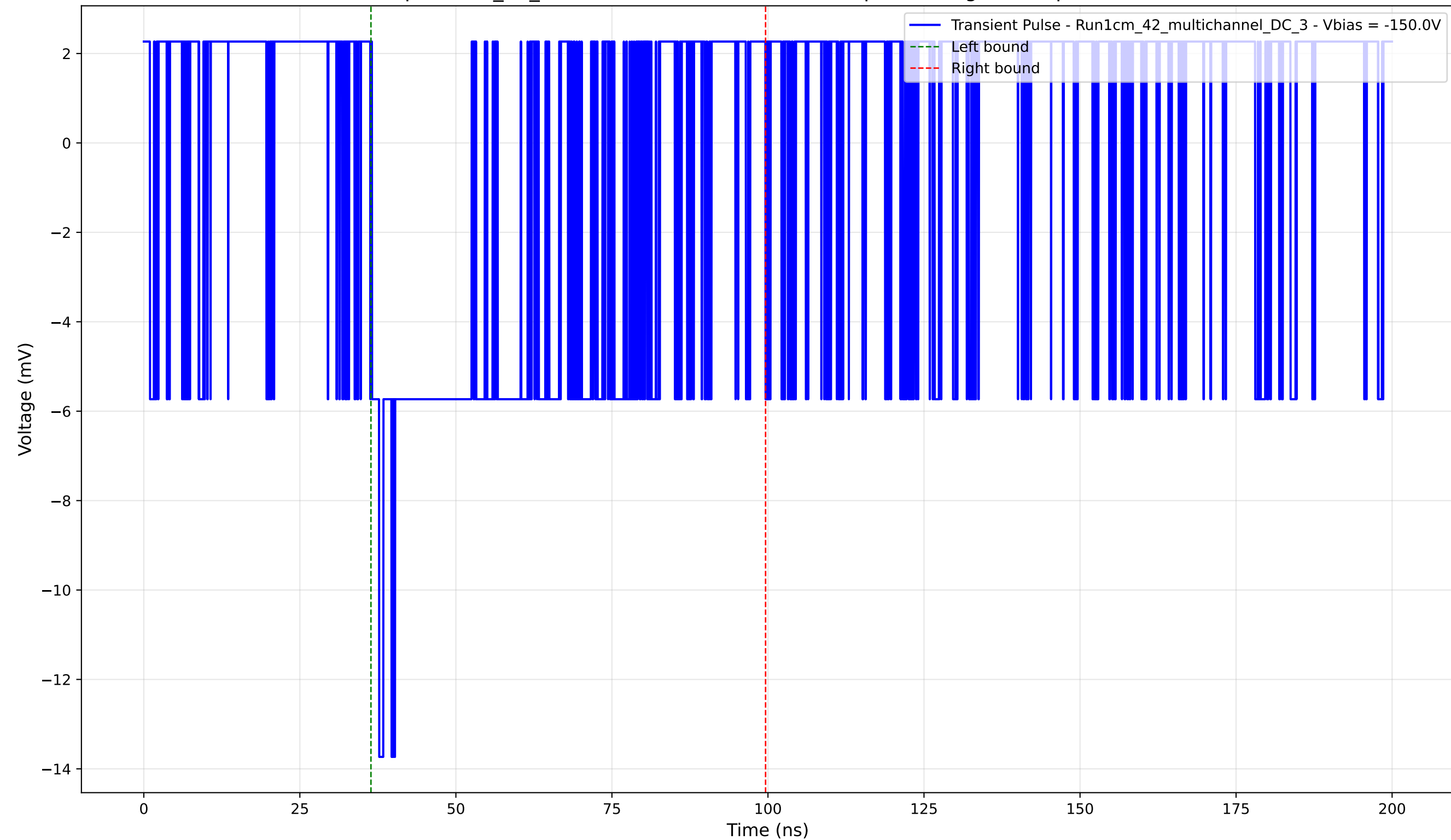
Transient Pulse - Sample: 1cm_42_multichannel - Position: 3905.0 \mu\text{m} - Charge: 3.78 pC - Rise Time: 0.00 ns (N/A)
