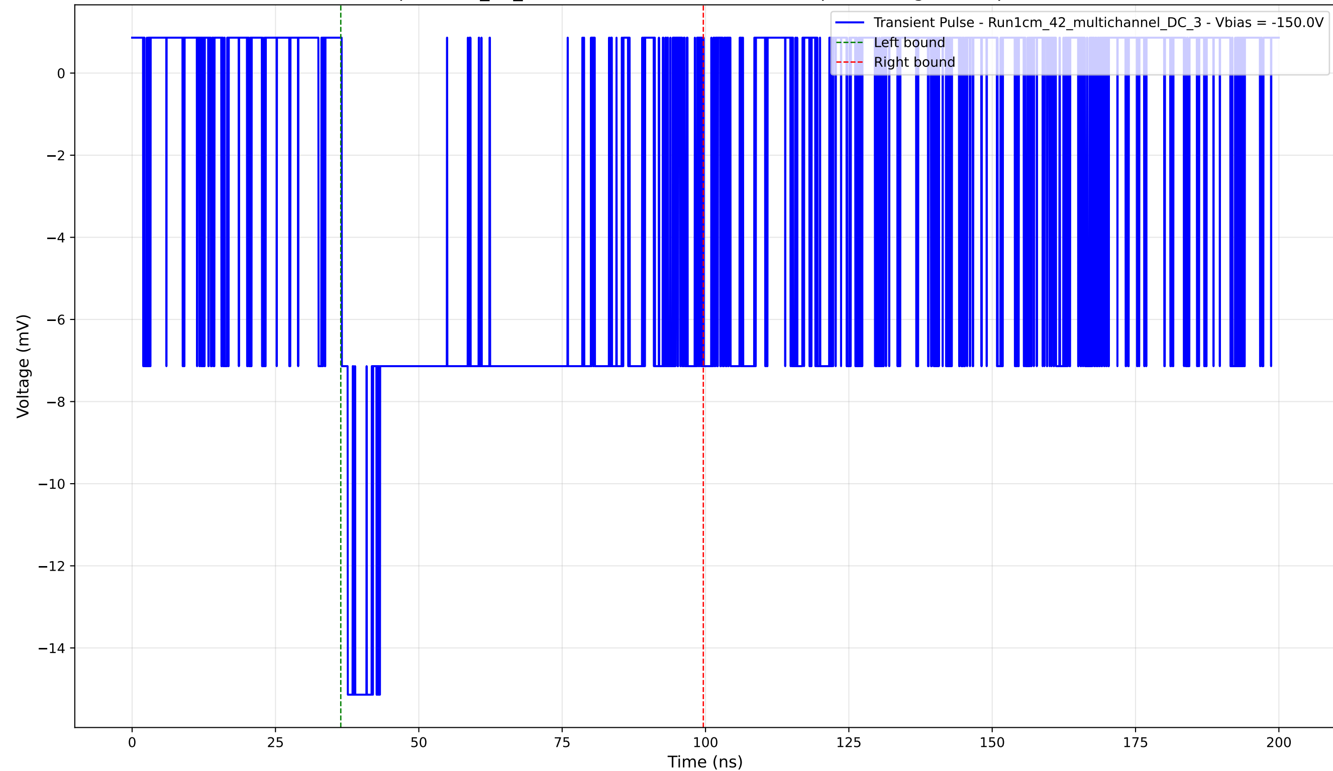
Transient Pulse - Sample: 1cm_42_multichannel - Position: 1845.0 \mu\text{m} - Charge: 8.61 pC - Rise Time: 1.06 ns
