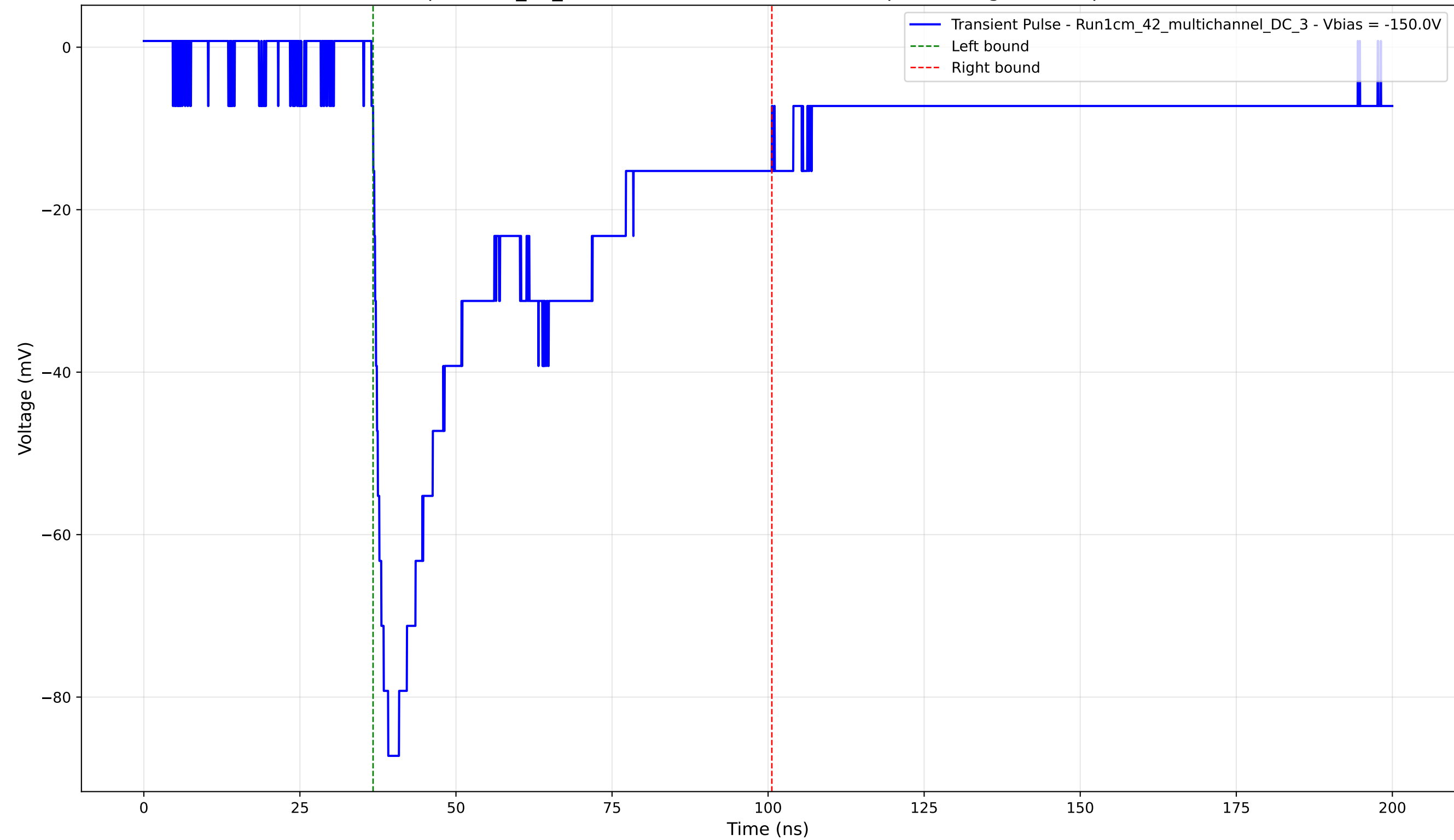
Transient Pulse - Sample: 1cm_42_multichannel - Position: 2675.0 \mu\text{m} - Charge: 39.09 pC - Rise Time: 1.70 ns
