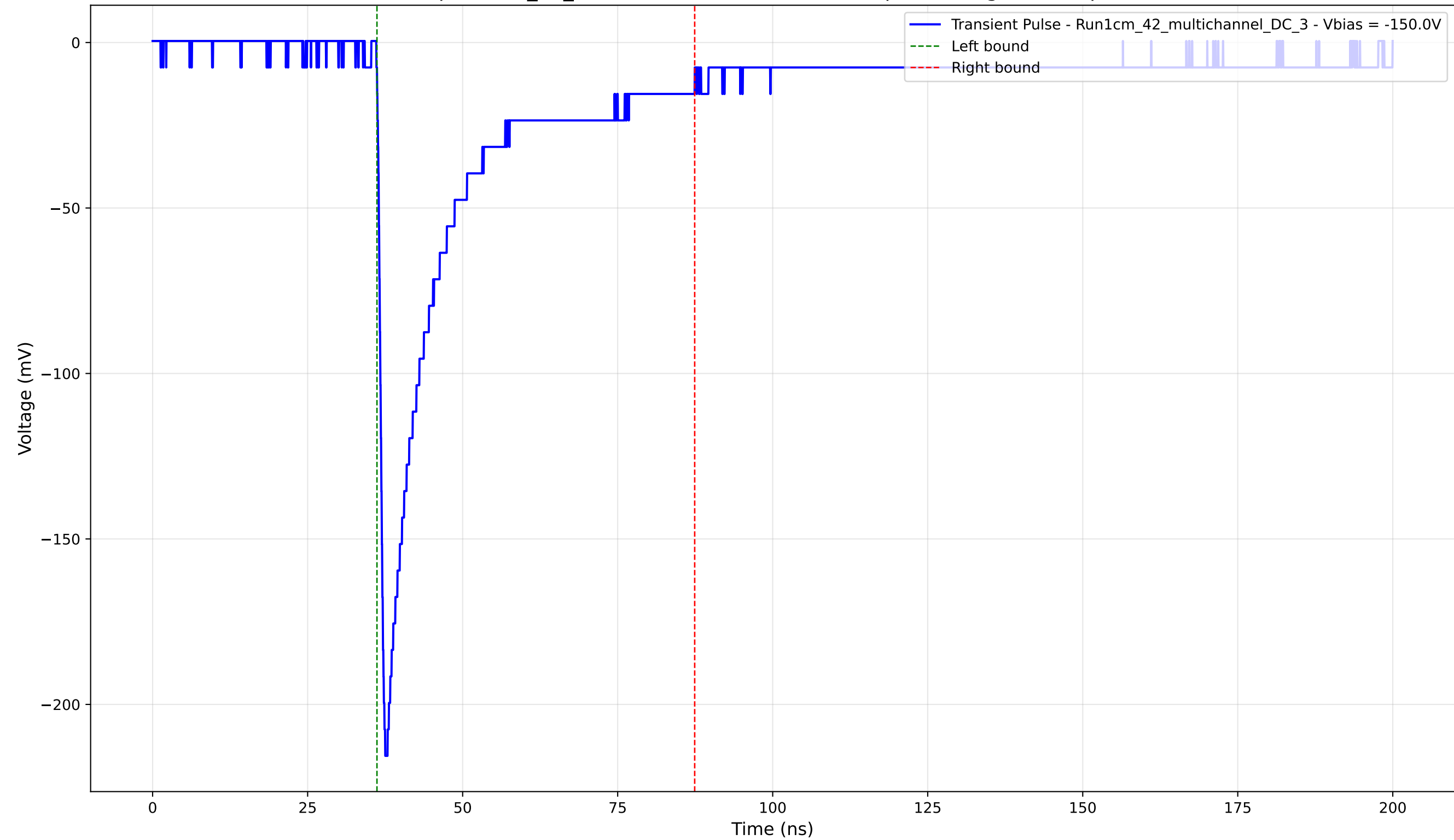
Transient Pulse - Sample: 1cm_42_multichannel - Position: 735.0 \mu\text{m} - Charge: 46.85 pC - Rise Time: 1.02 ns
