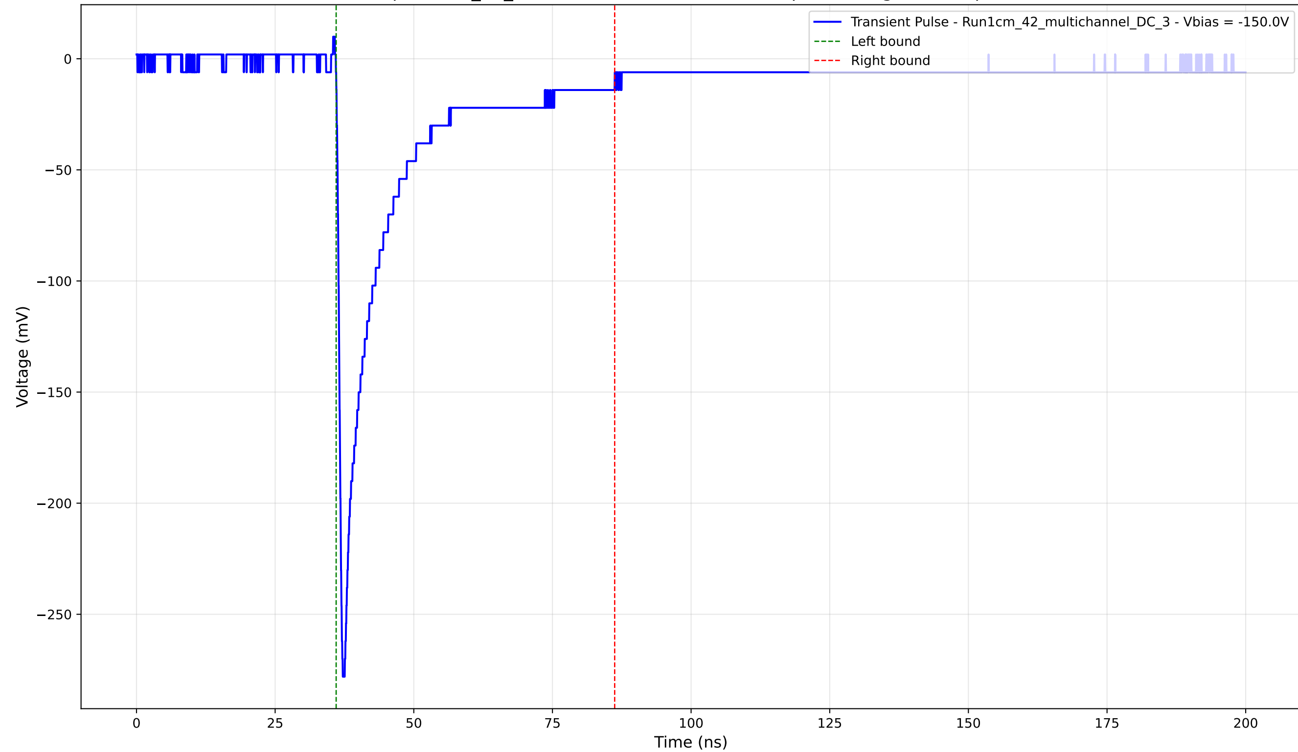
Transient Pulse - Sample: 1cm_42_multichannel - Position: 445.0 \mu\text{m} - Charge: 47.79 pC - Rise Time: 0.89 ns
