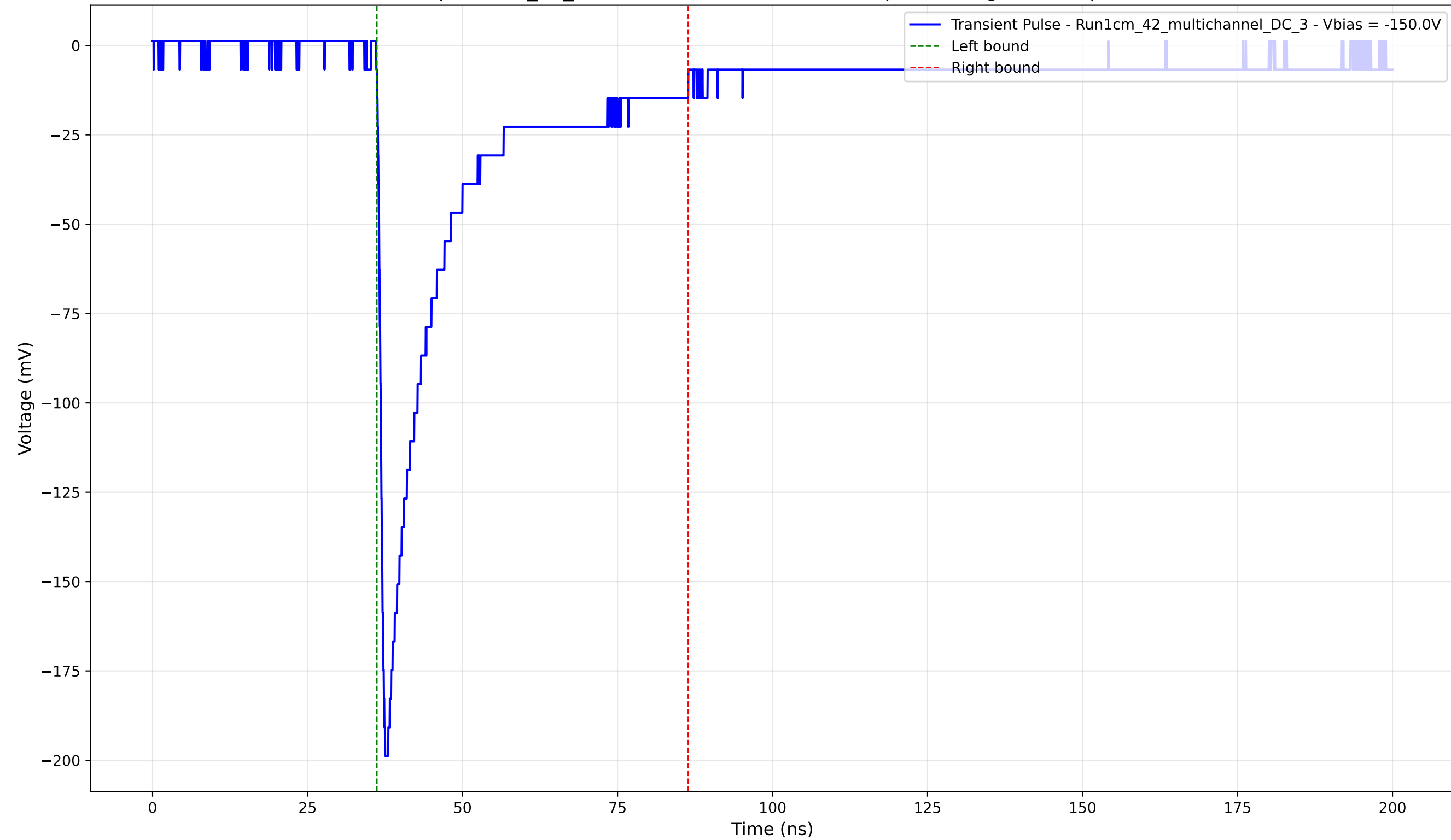
Transient Pulse - Sample: 1cm_42_multichannel - Position: 765.0 \mu\text{m} - Charge: 43.52 pC - Rise Time: 1.01 ns
