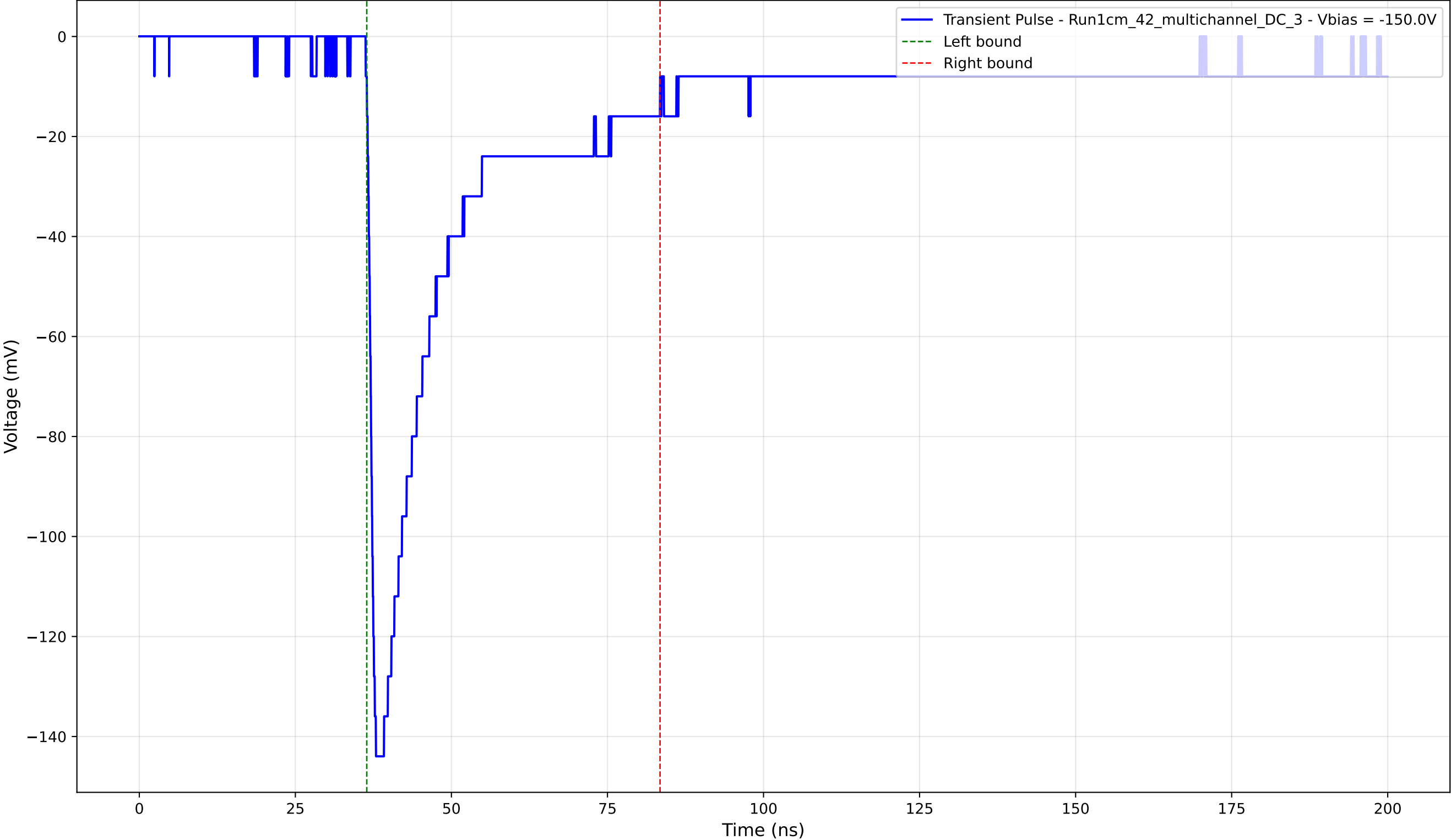
Transient Pulse - Sample: 1cm_42_multichannel - Position: 3770.0 \mu\text{m} - Charge: 39.07 pC - Rise Time: 1.26 ns
