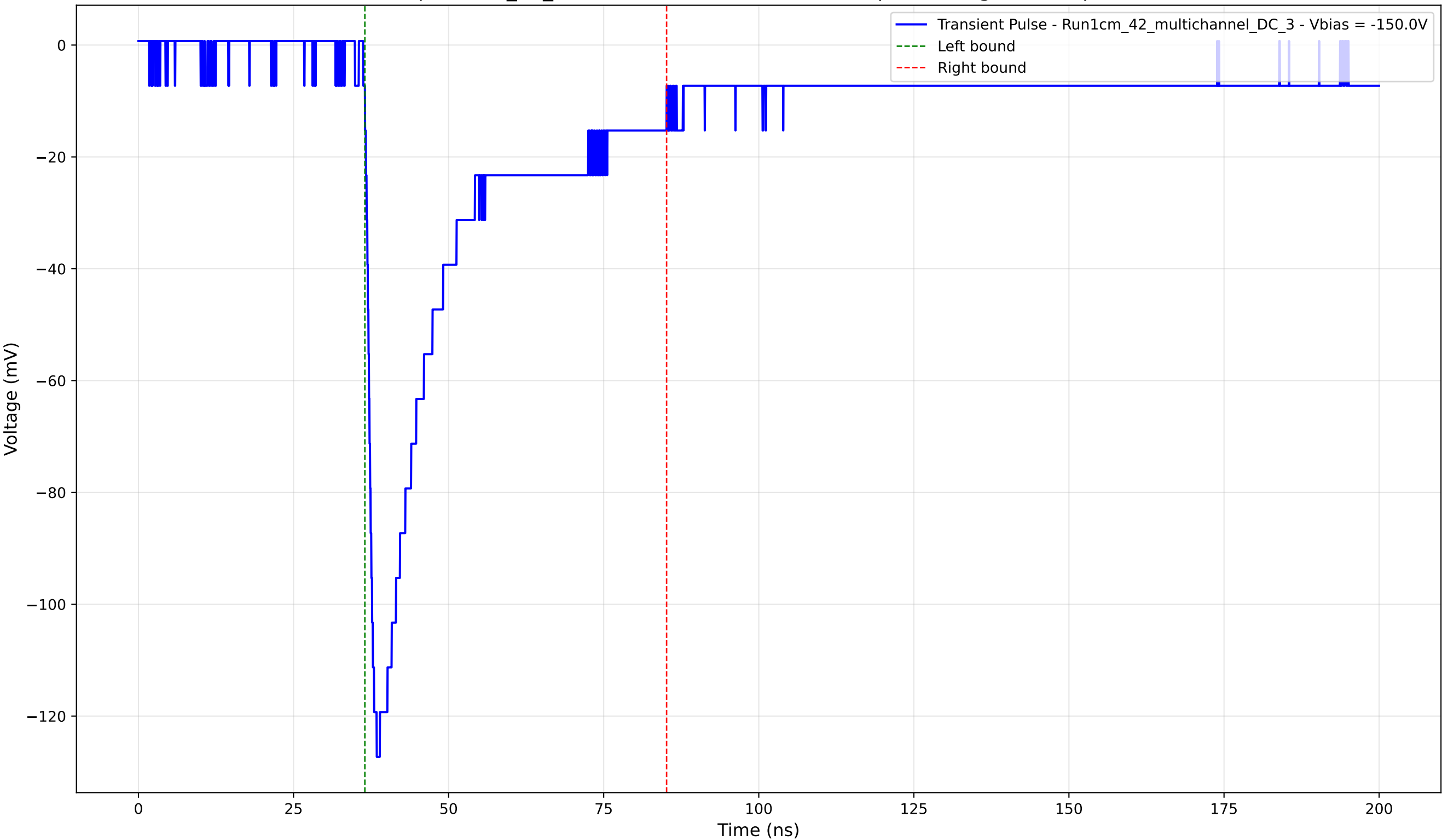
Transient Pulse - Sample: 1cm_42_multichannel - Position: 3555.0 \mu\text{m} - Charge: 36.42 pC - Rise Time: 1.47 ns
