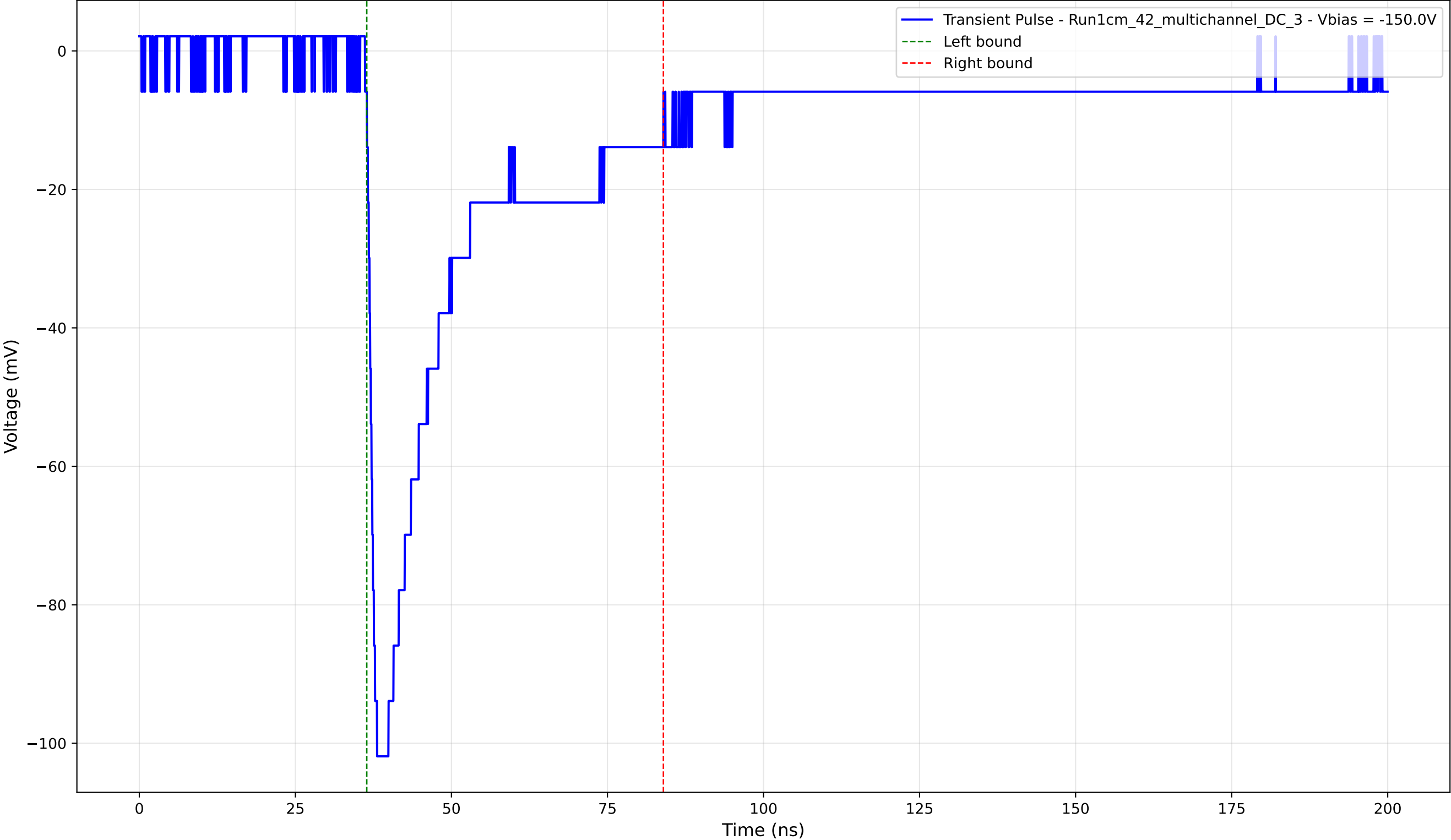
Transient Pulse - Sample: 1cm_42_multichannel - Position: 1425.0 \mu\text{m} - Charge: 31.36 pC - Rise Time: 1.31 ns
