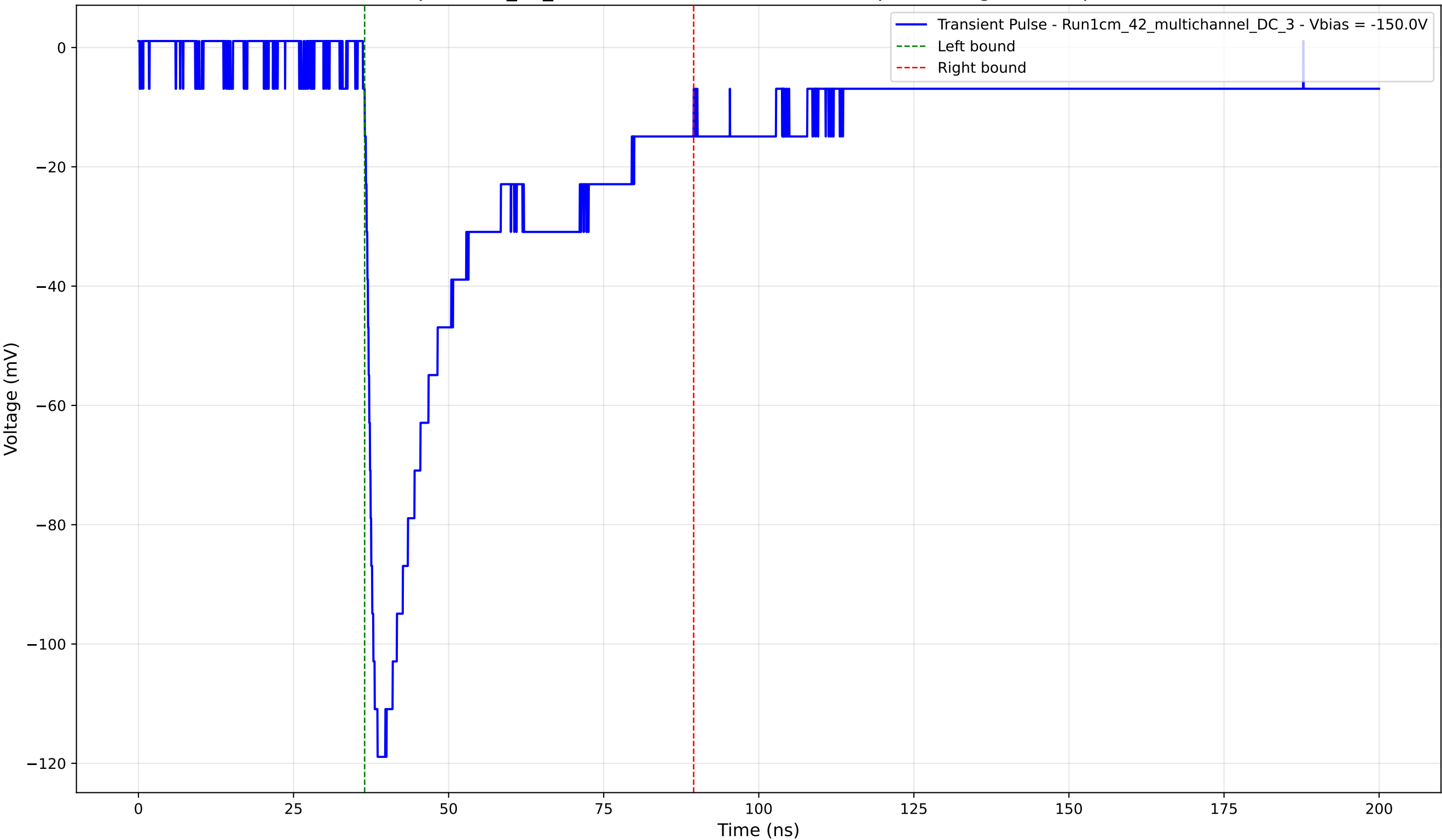
Transient Pulse - Sample: 1cm_42_multichannel - Position: 1680.0 \mu\text{m} - Charge: 41.23 pC - Rise Time: 1.61 ns
