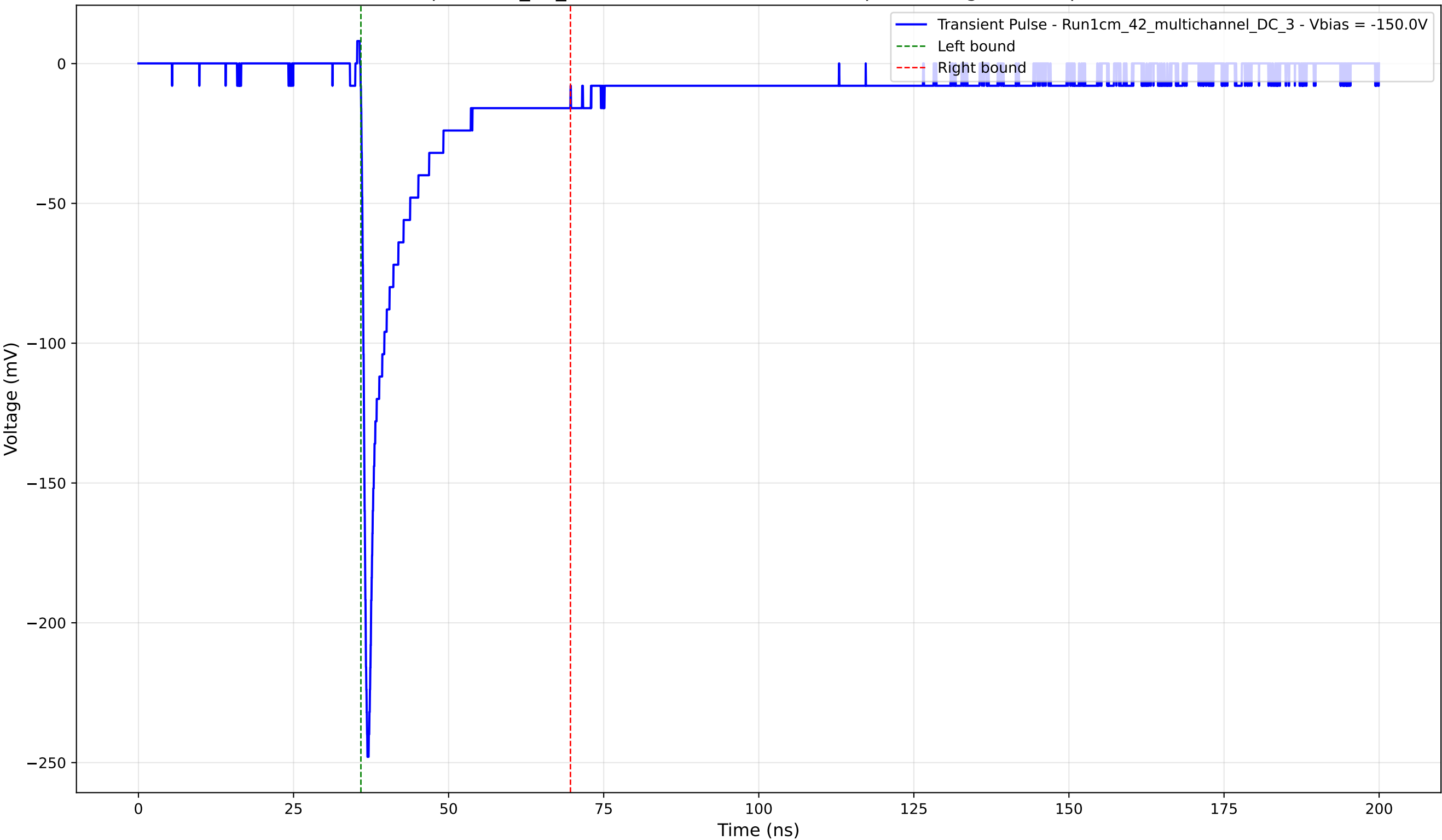
Transient Pulse - Sample: 1cm_42_multichannel - Position: 85.0 \mu\text{m} - Charge: 28.31 pC - Rise Time: 0.76 ns
