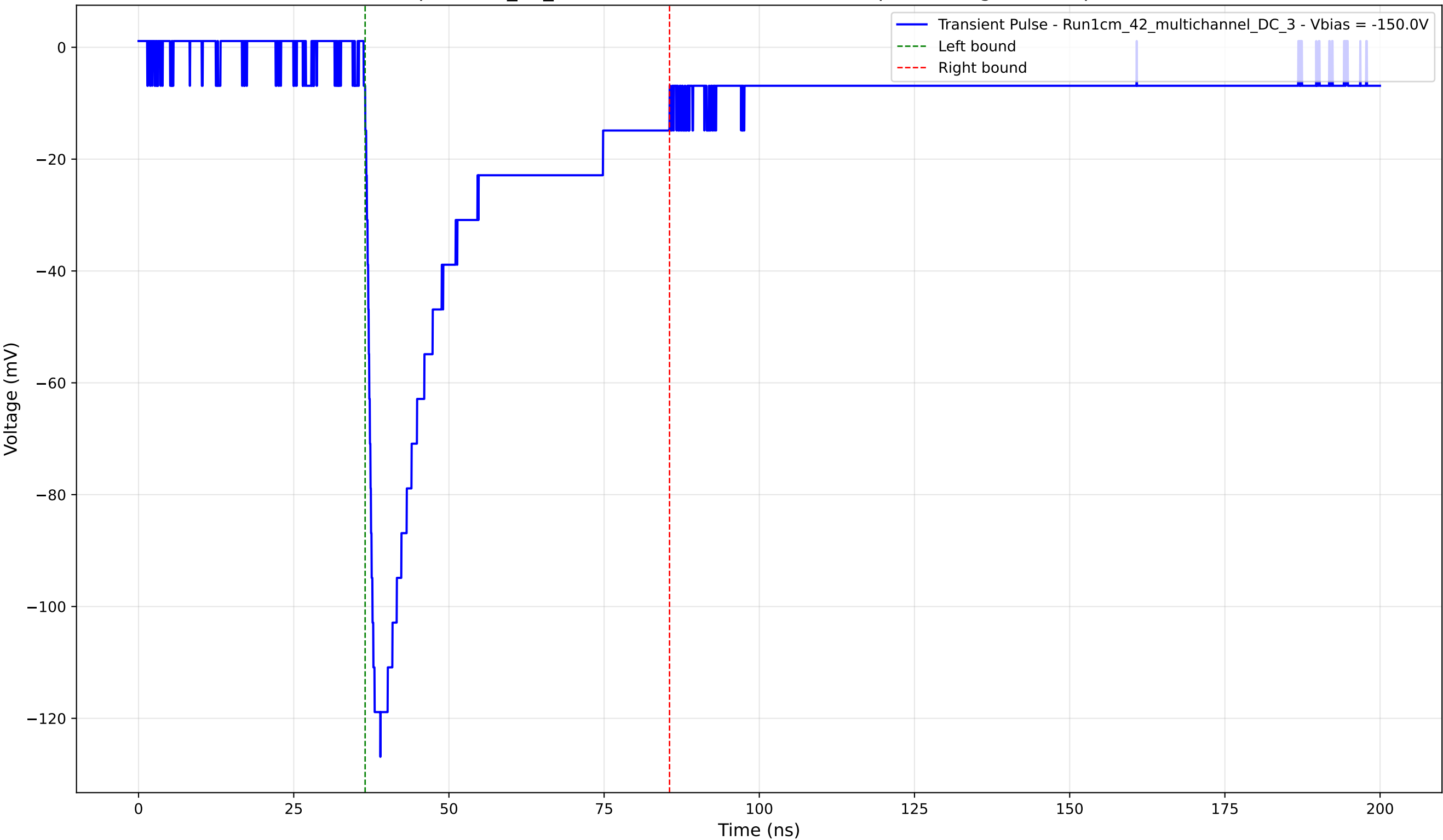
Transient Pulse - Sample: 1cm_42_multichannel - Position: 3520.0 \mu\text{m} - Charge: 36.24 pC - Rise Time: 1.51 ns
