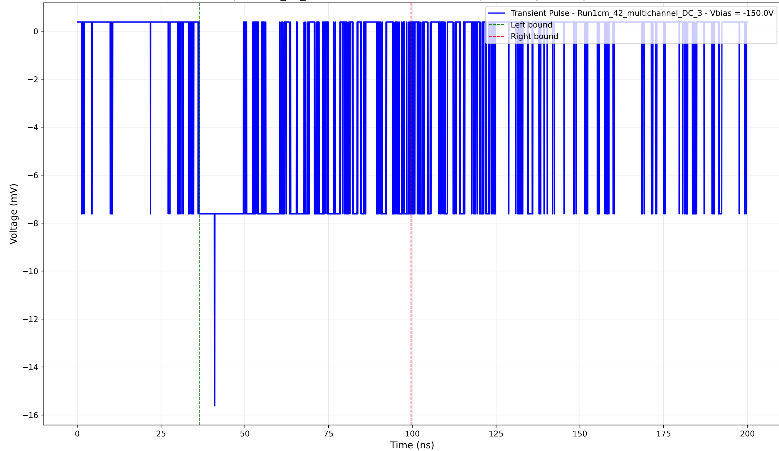
Transient Pulse - Sample: 1cm_42_multichannel - Position: 3400.0 \mu\text{m} - Charge: 6.42 pC - Rise Time: 4.42 ns
