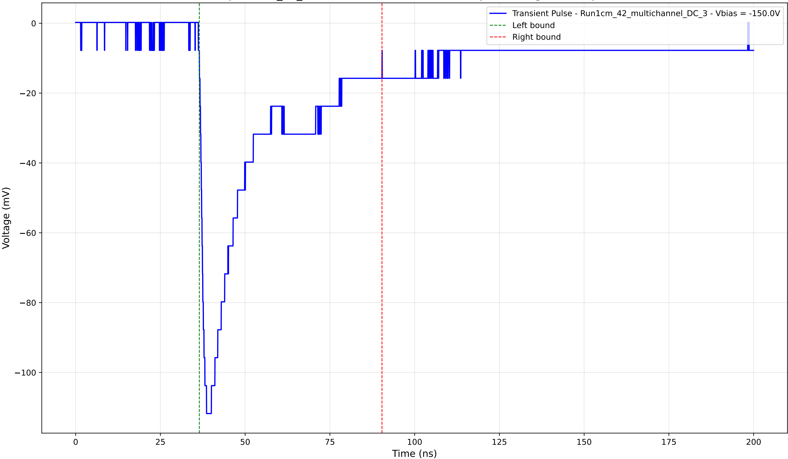
Transient Pulse - Sample: 1cm_42_multichannel - Position: 1765.0 \mu\text{m} - Charge: 40.73 pC - Rise Time: 1.63 ns
