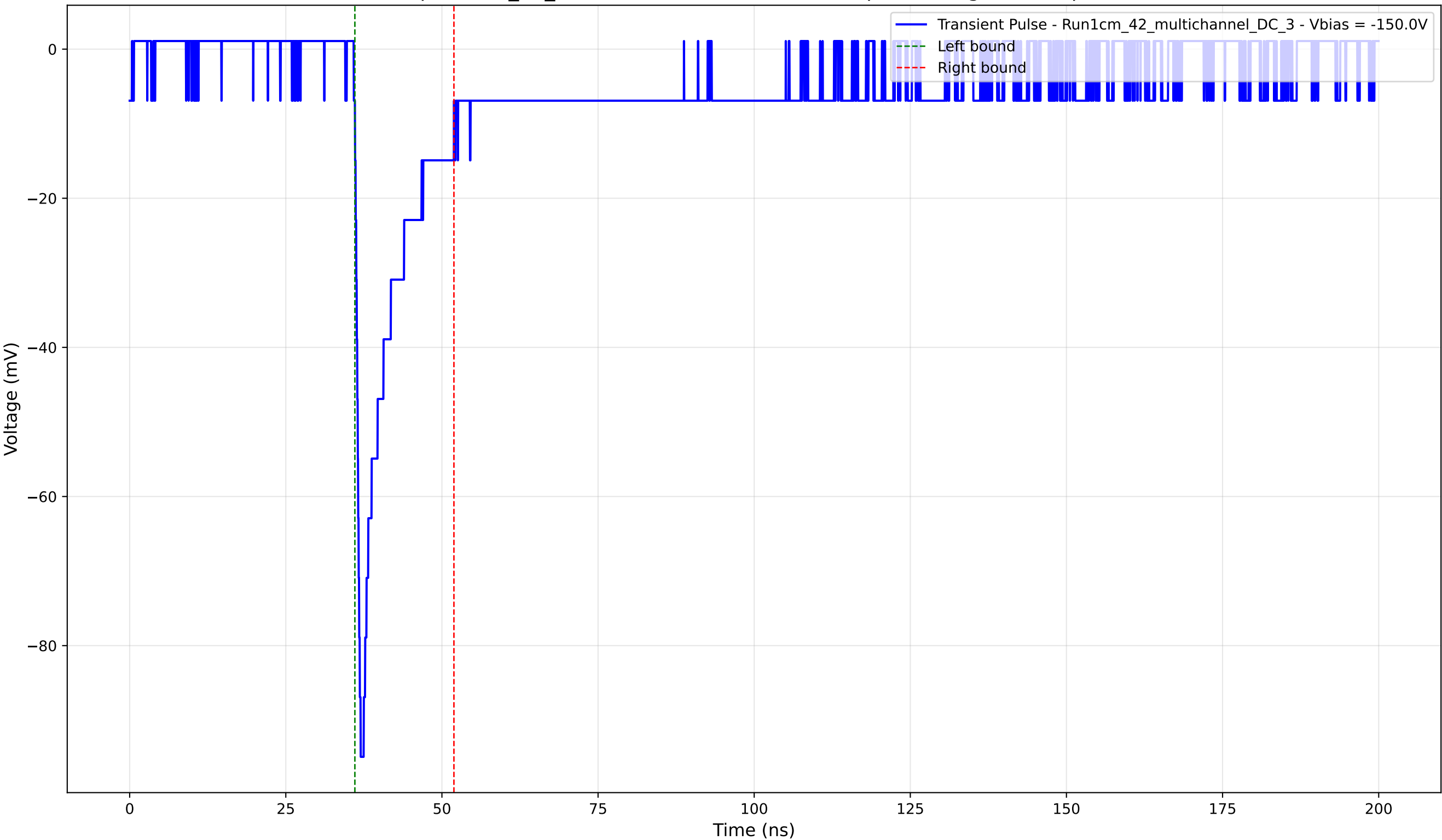
Transient Pulse - Sample: 1cm_42_multichannel - Position: 310.0 \mu\text{m} - Charge: 10.71 pC - Rise Time: 0.77 ns
