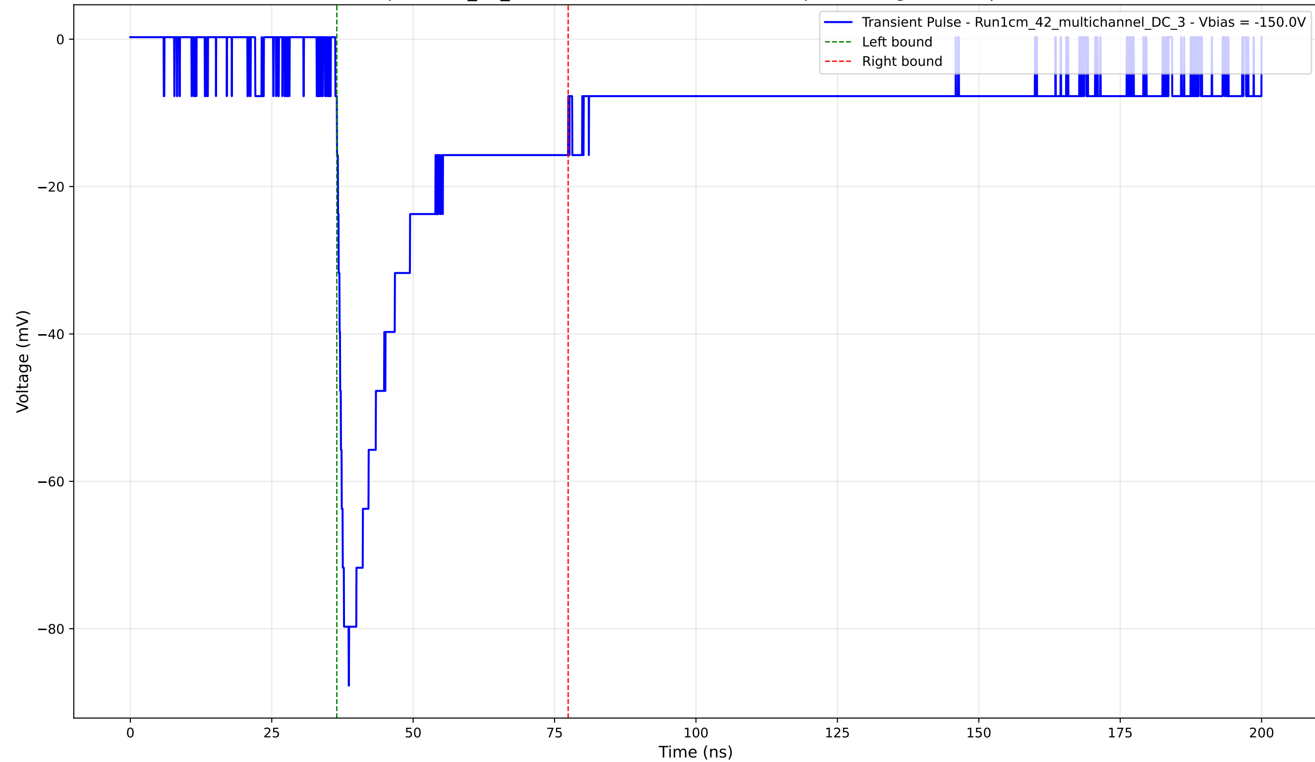
Transient Pulse - Sample: 1cm_42_multichannel - Position: 1310.0 \mu\text{m} - Charge: 23.27 pC - Rise Time: 1.26 ns
