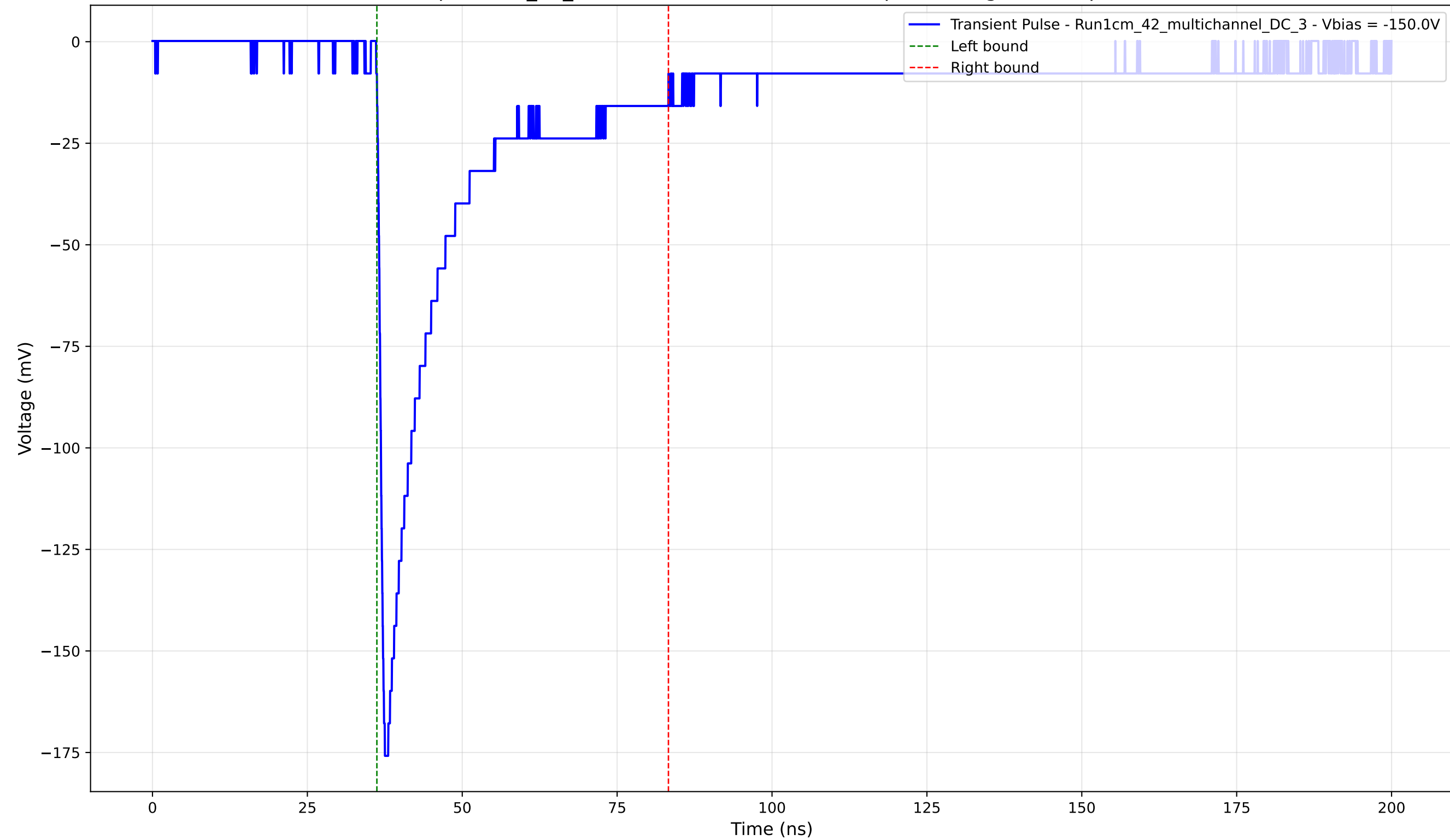
Transient Pulse - Sample: 1cm_42_multichannel - Position: 785.0 \mu\text{m} - Charge: 39.50 pC - Rise Time: 0.98 ns
