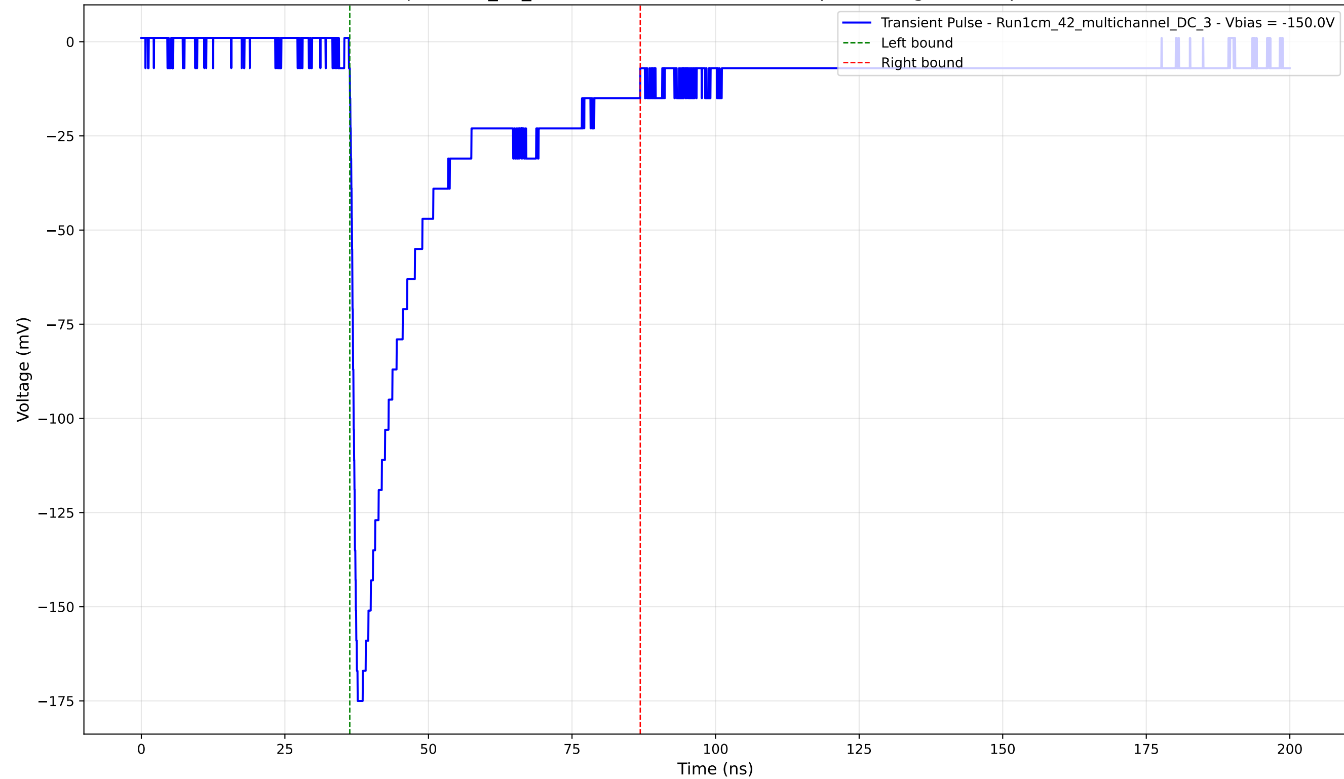
Transient Pulse - Sample: 1cm_42_multichannel - Position: 995.0 \mu\text{m} - Charge: 44.91 pC - Rise Time: 1.03 ns
