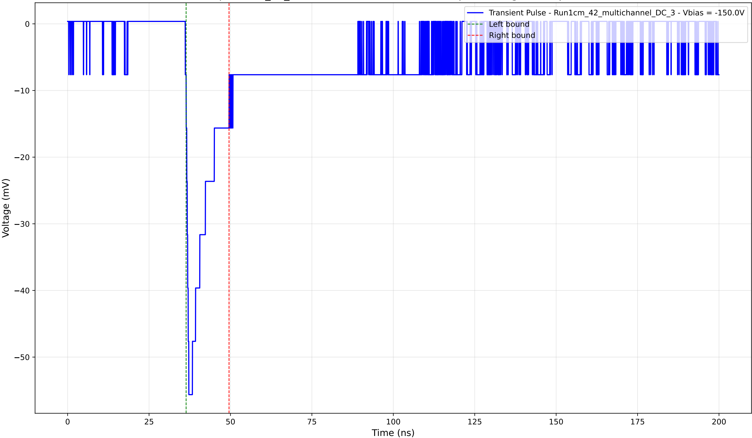
Transient Pulse - Sample: 1cm_42_multichannel - Position: 4350.0 \mu\text{m} - Charge: 7.50 pC - Rise Time: 1.09 ns
