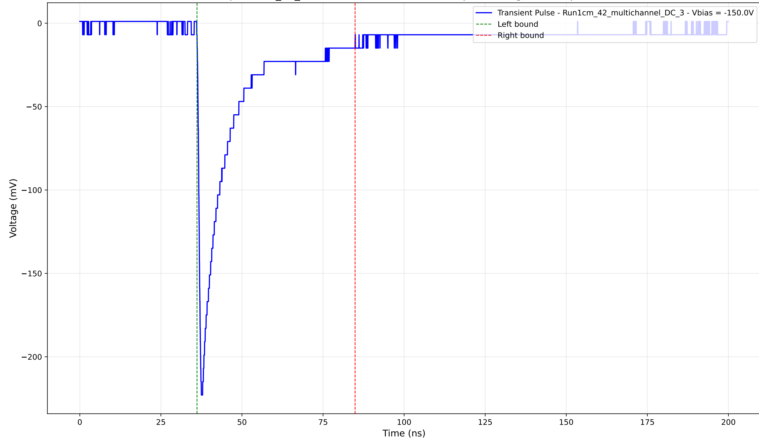
Transient Pulse - Sample: 1cm_42_multichannel - Position: 700.0 \mu\text{m} - Charge: 46.07 pC - Rise Time: 1.02 ns
