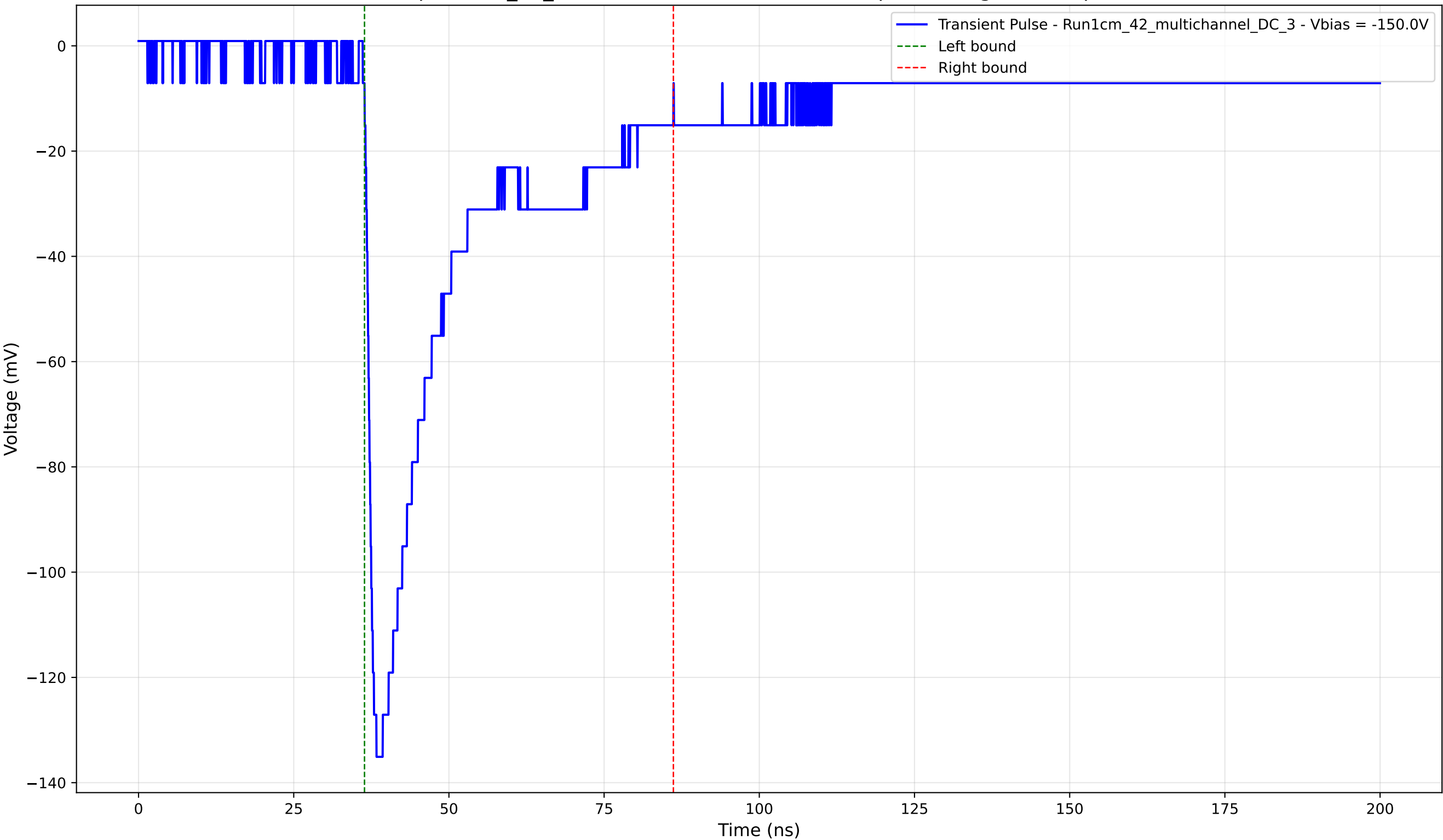
Transient Pulse - Sample: 1cm_42_multichannel - Position: 1460.0 \mu\text{m} - Charge: 42.42 pC - Rise Time: 1.50 ns
