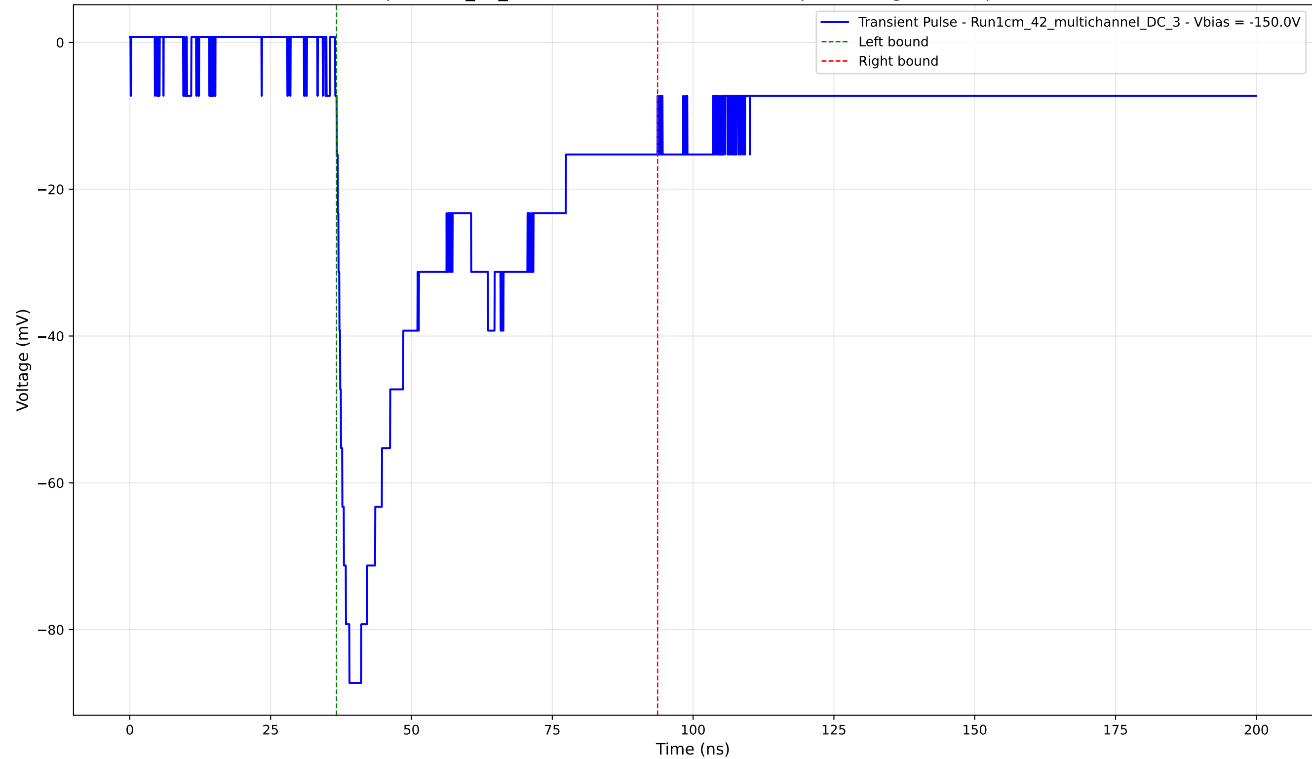
Transient Pulse - Sample: 1cm_42_multichannel - Position: 2680.0 \mu\text{m} - Charge: 37.39 pC - Rise Time: 1.66 ns
