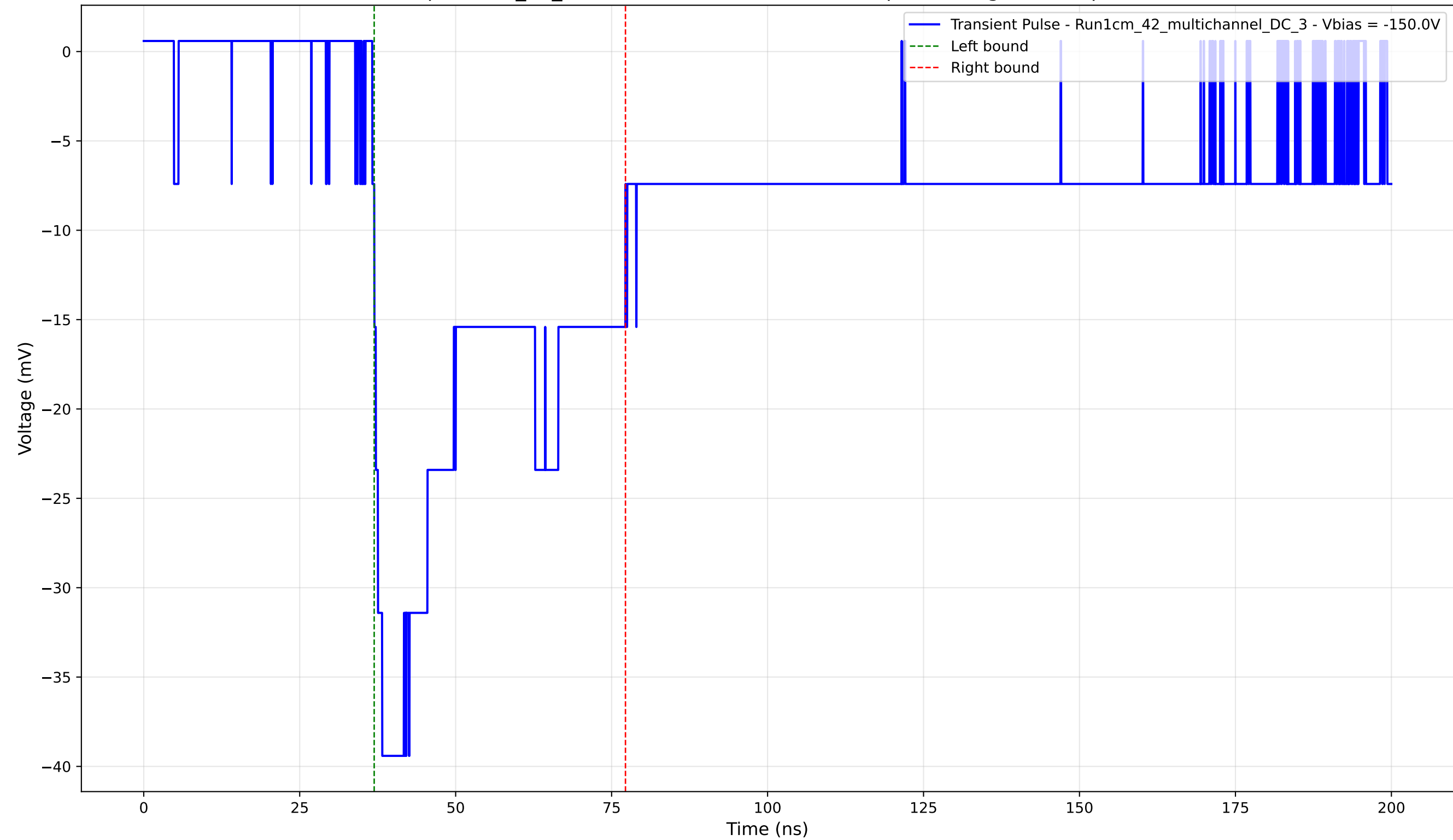
Transient Pulse - Sample: 1cm_42_multichannel - Position: 2325.0 \mu\text{m} - Charge: 16.89 pC - Rise Time: 1.59 ns
