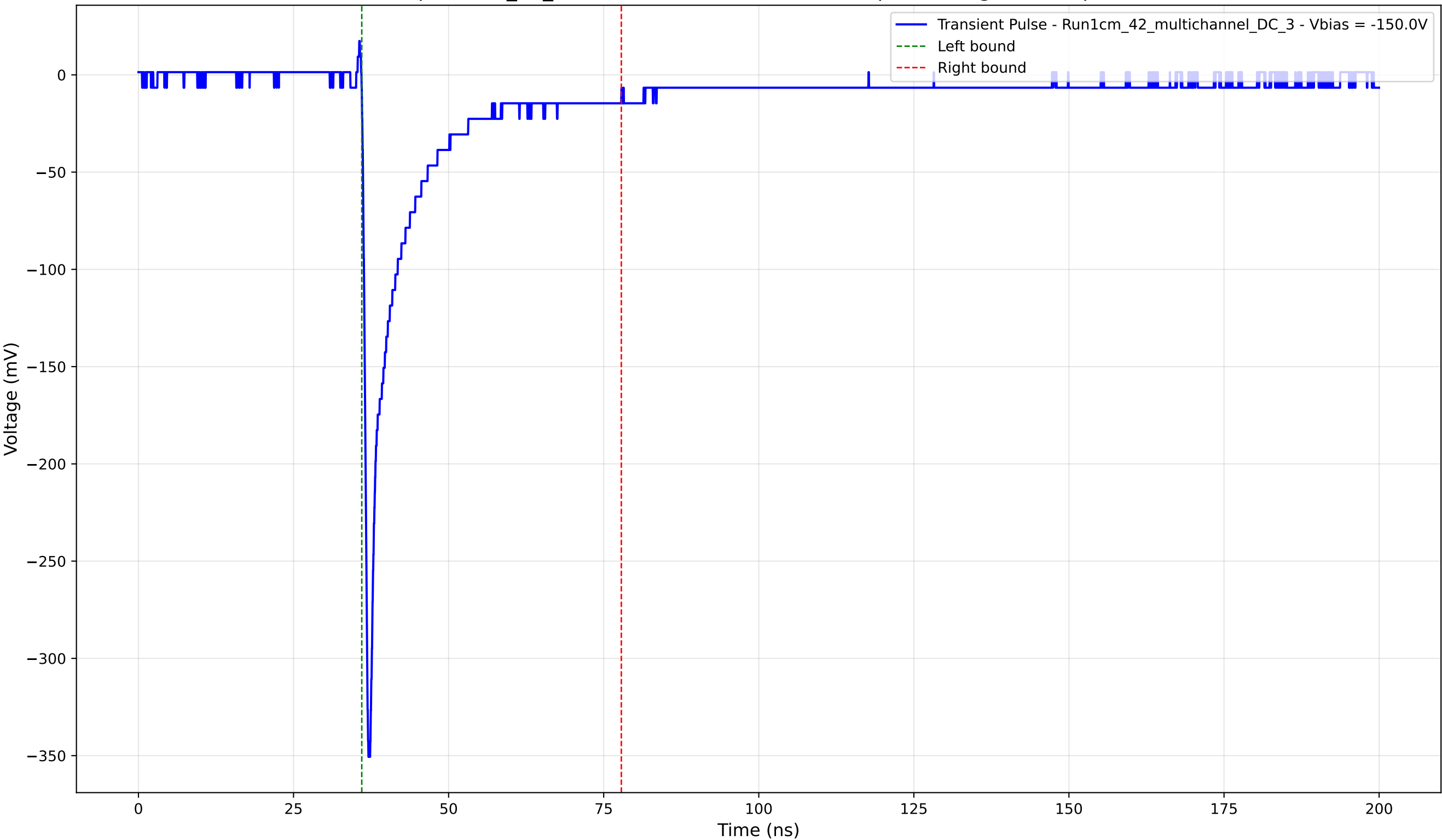
Transient Pulse - Sample: 1cm_42_multichannel - Position: 4760.0 \mu\text{m} - Charge: 40.33 pC - Rise Time: 0.78 ns
