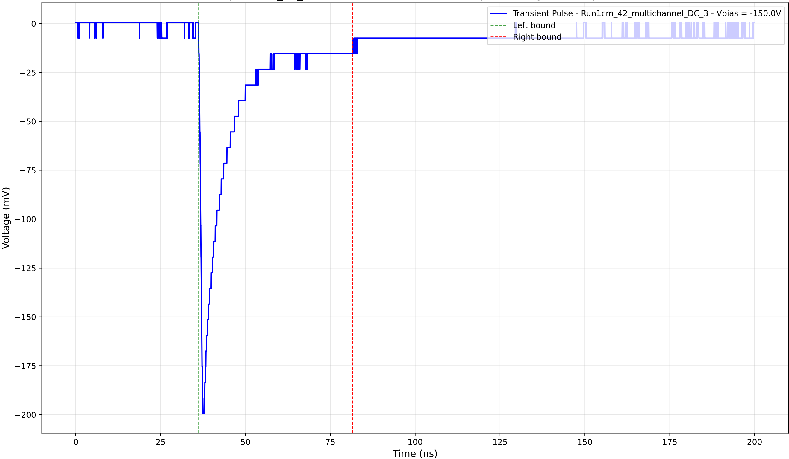
Transient Pulse - Sample: 1cm_42_multichannel - Position: 4290.0 \mu\text{m} - Charge: 36.38 pC - Rise Time: 0.93 ns
