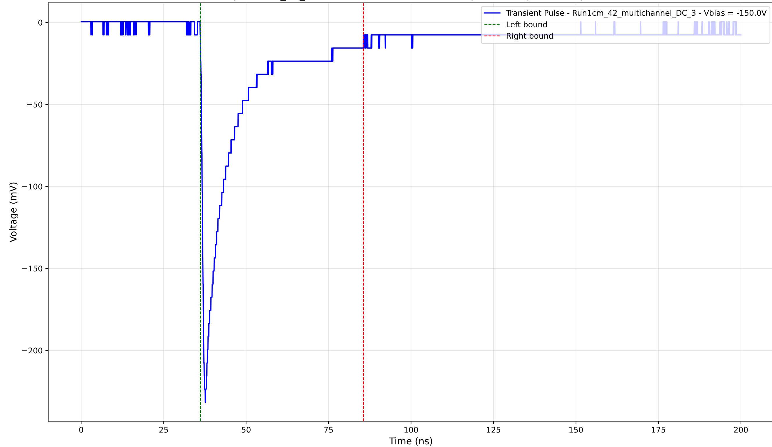
Transient Pulse - Sample: 1cm_42_multichannel - Position: 680.0 \mu\text{m} - Charge: 47.18 pC - Rise Time: 1.04 ns
