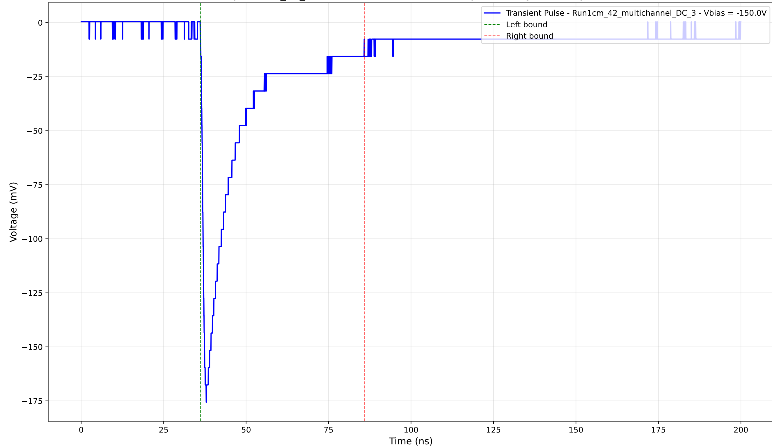
Transient Pulse - Sample: 1cm_42_multichannel - Position: 930.0 \mu\text{m} - Charge: 42.16 pC - Rise Time: 1.08 ns
