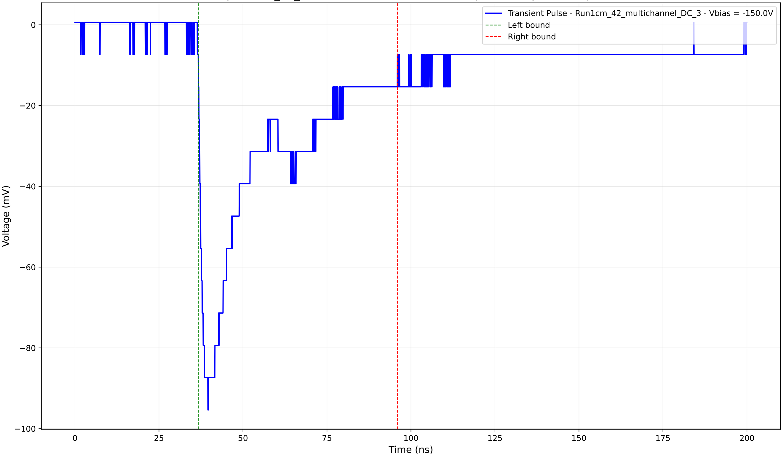
Transient Pulse - Sample: 1cm_42_multichannel - Position: 2730.0 \mu\text{m} - Charge: 39.23 pC - Rise Time: 1.85 ns
