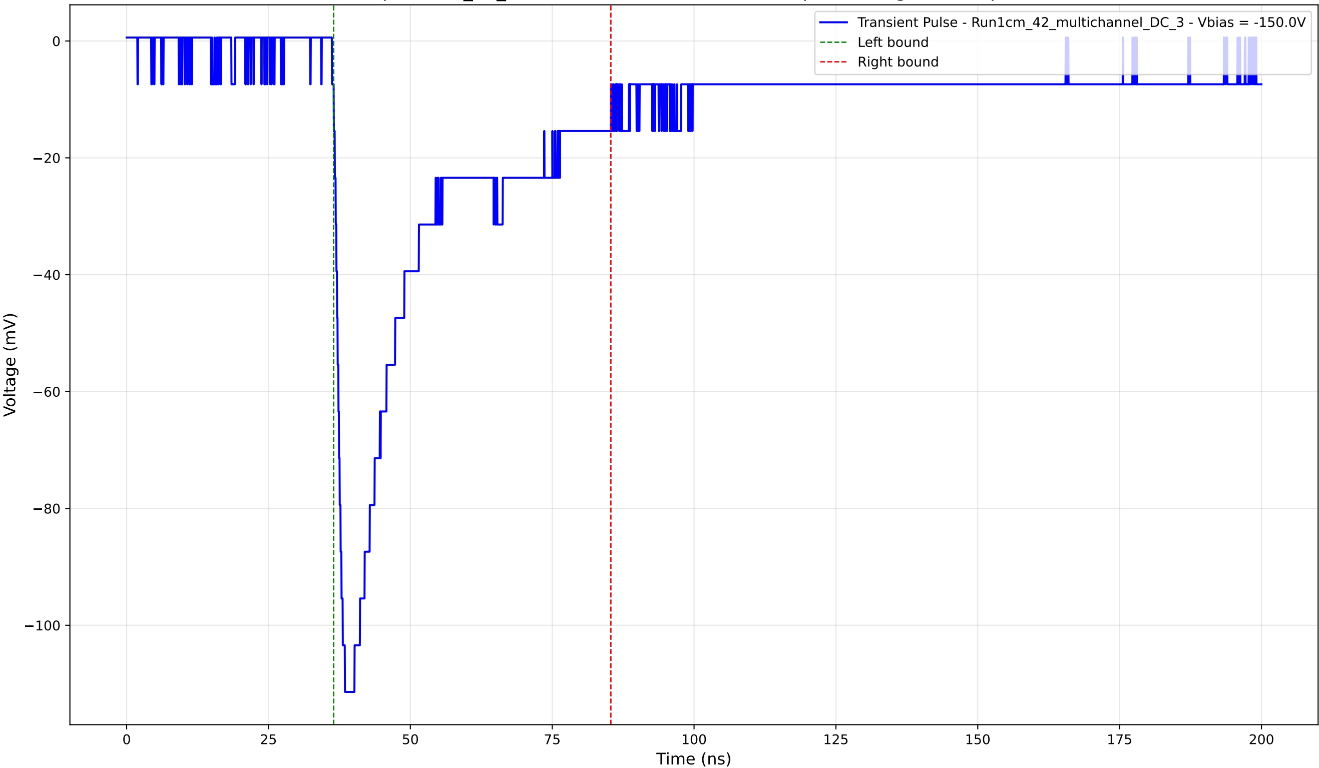
Transient Pulse - Sample: 1cm_42_multichannel - Position: 3300.0 \mu\text{m} - Charge: 36.07 pC - Rise Time: 1.59 ns
