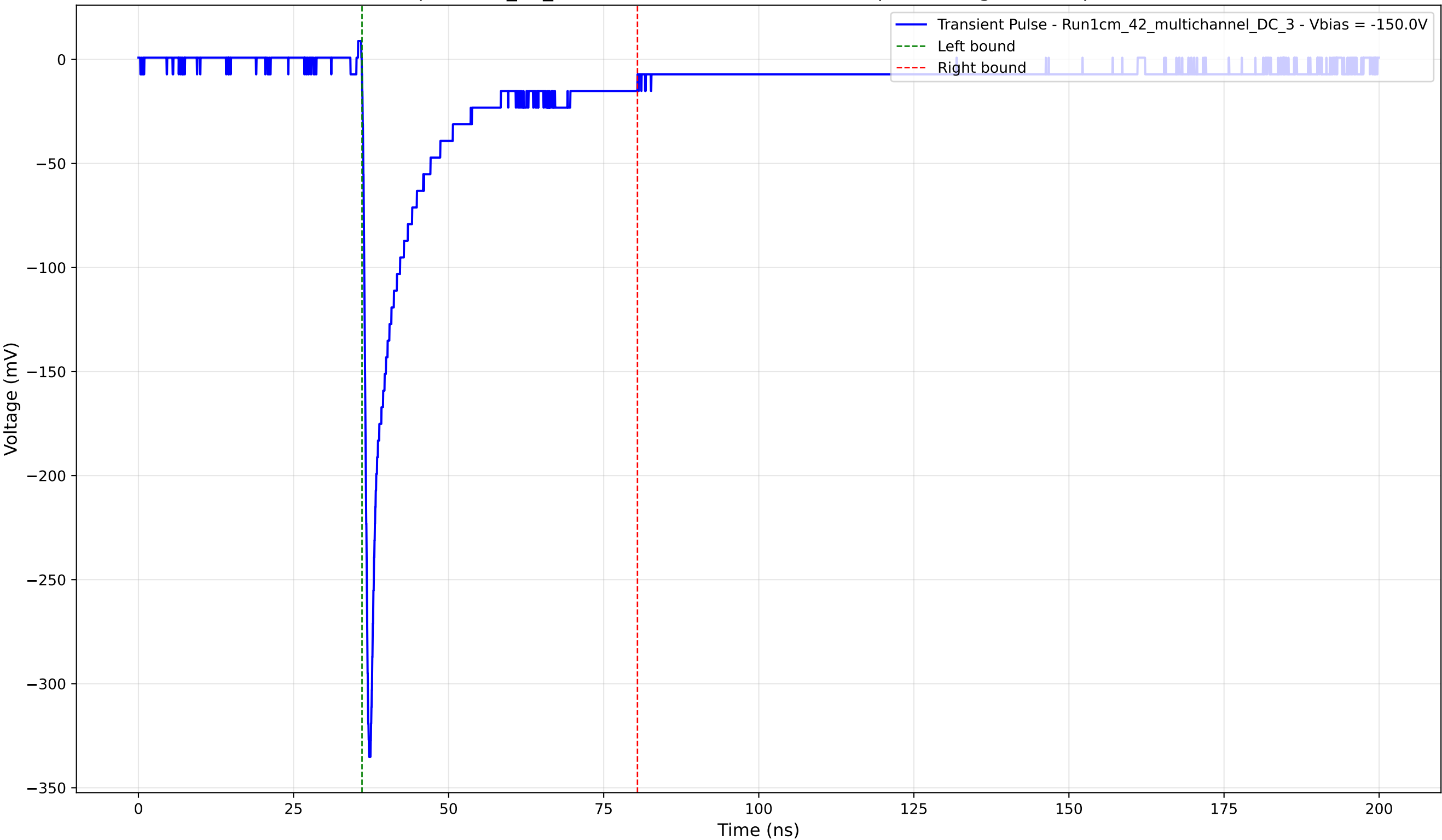
Transient Pulse - Sample: 1cm_42_multichannel - Position: 4680.0 \mu\text{m} - Charge: 42.90 pC - Rise Time: 0.79 ns
