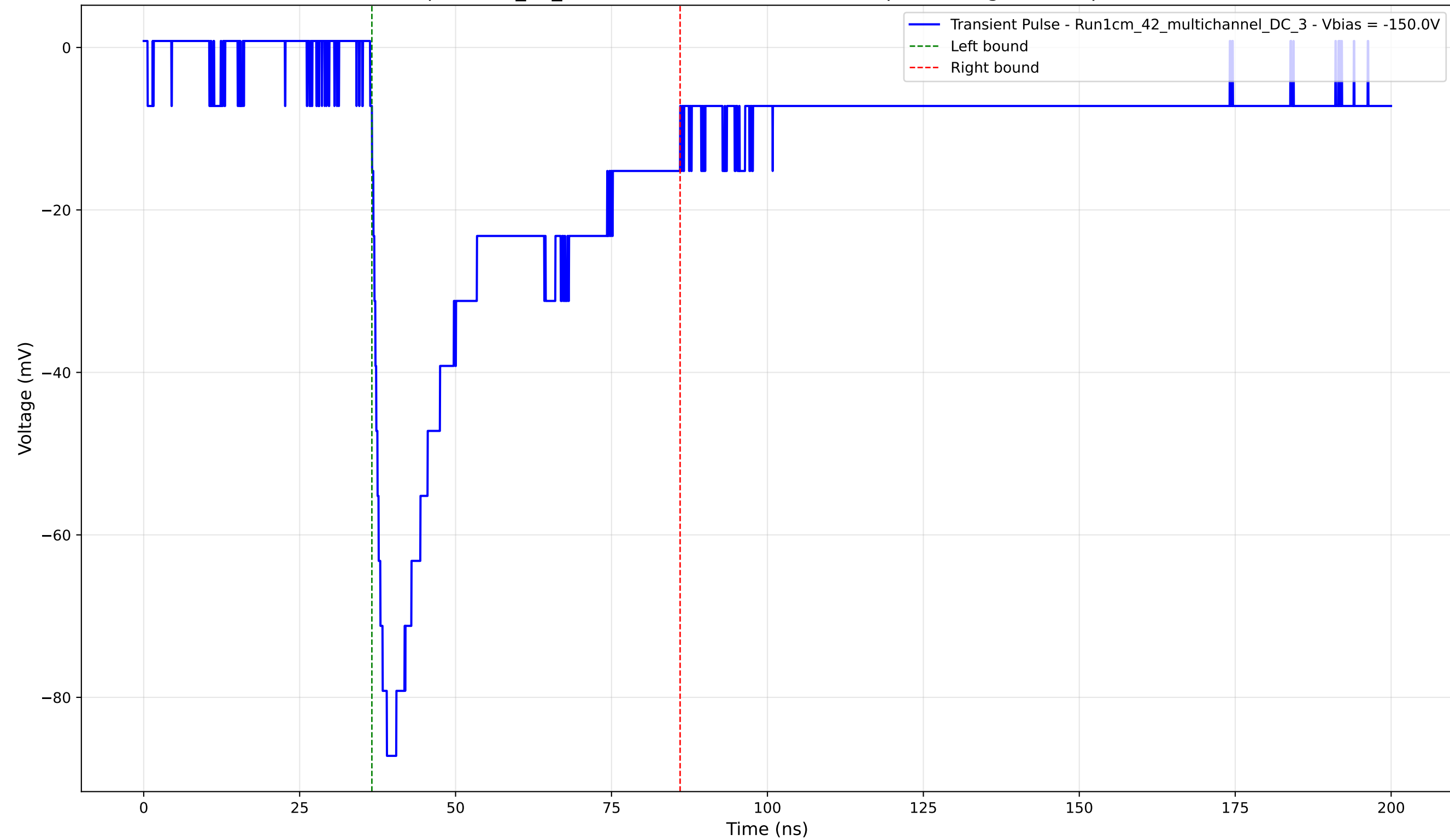
Transient Pulse - Sample: 1cm_42_multichannel - Position: 2950.0 \mu\text{m} - Charge: 31.75 pC - Rise Time: 1.72 ns
