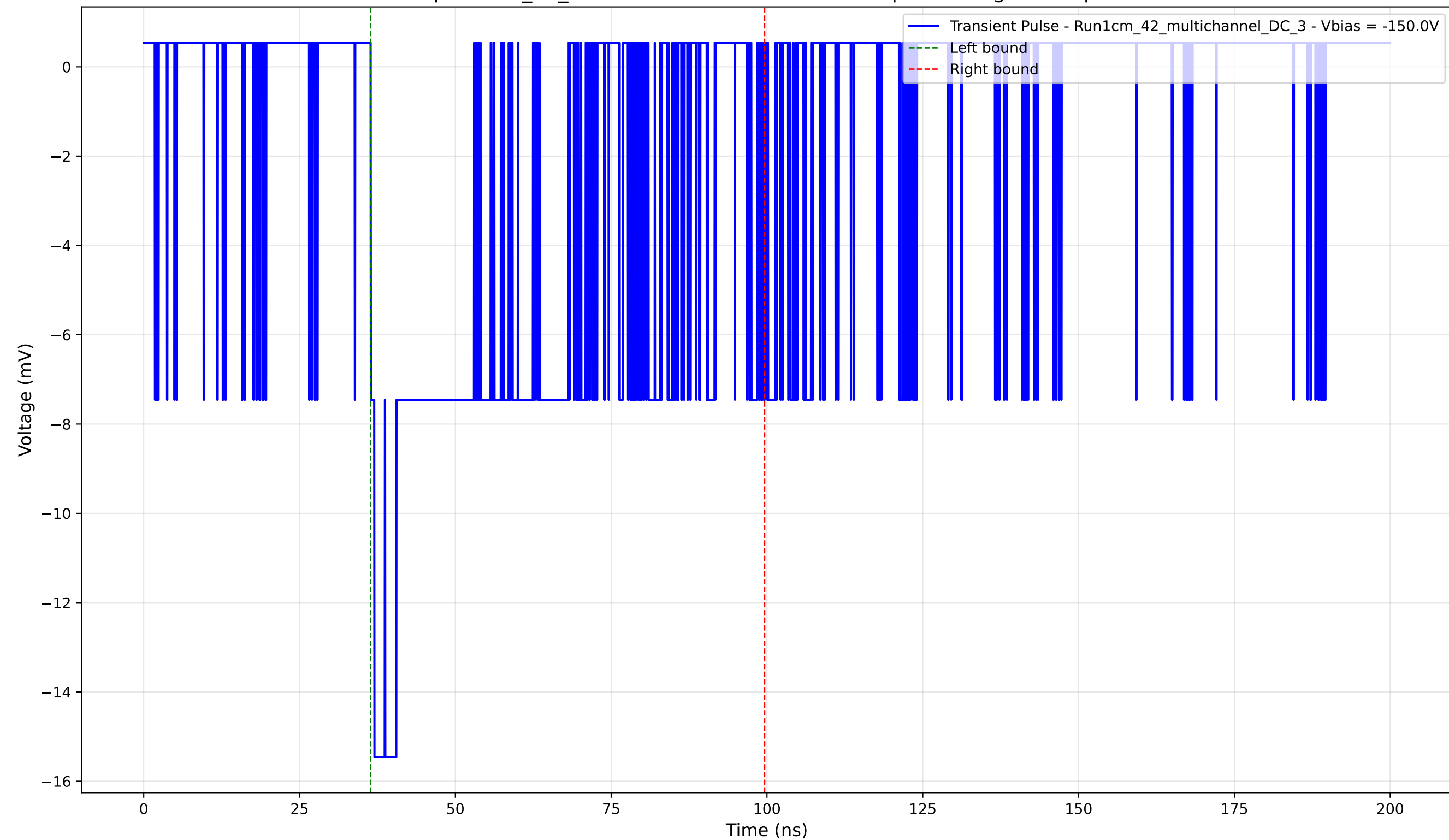
Transient Pulse - Sample: 1cm_42_multichannel - Position: 4375.0 \mu\text{m} - Charge: 6.40 pC - Rise Time: 0.60 ns
