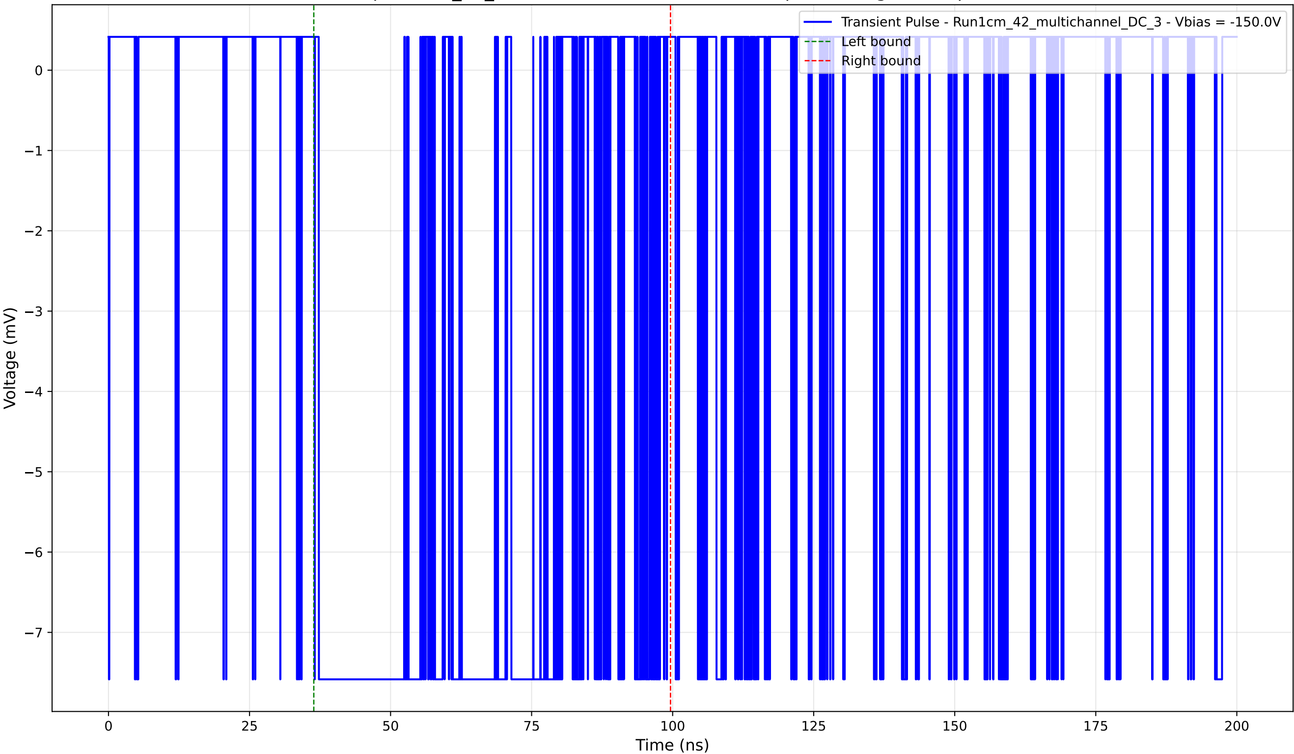
Transient Pulse - Sample: 1cm_42_multichannel - Position: 2365.0 \mu\text{m} - Charge: 6.34 pC - Rise Time: 0.02 ns
