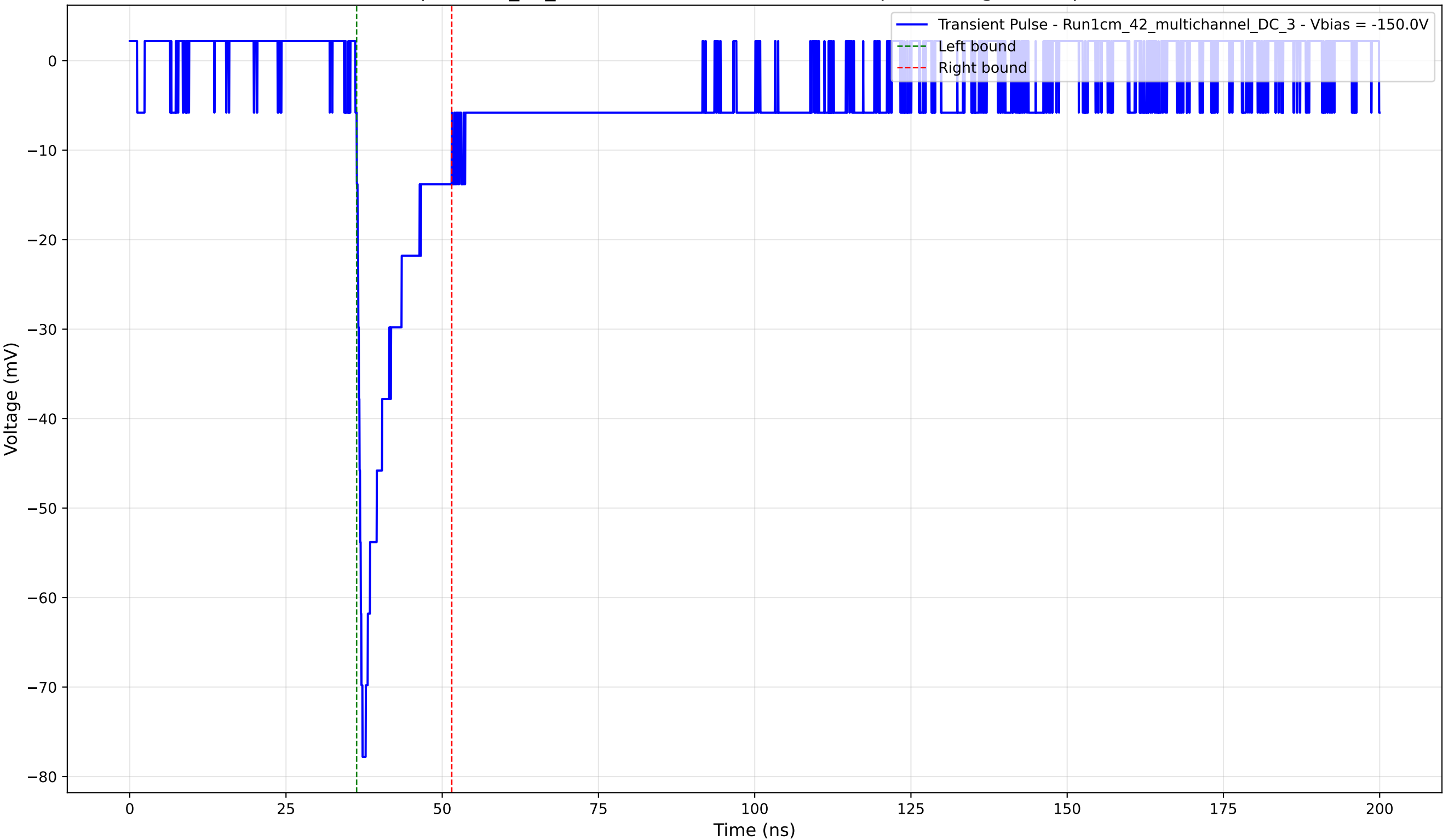
Transient Pulse - Sample: 1cm_42_multichannel - Position: 4435.0 \mu\text{m} - Charge: 9.19 pC - Rise Time: 0.94 ns
