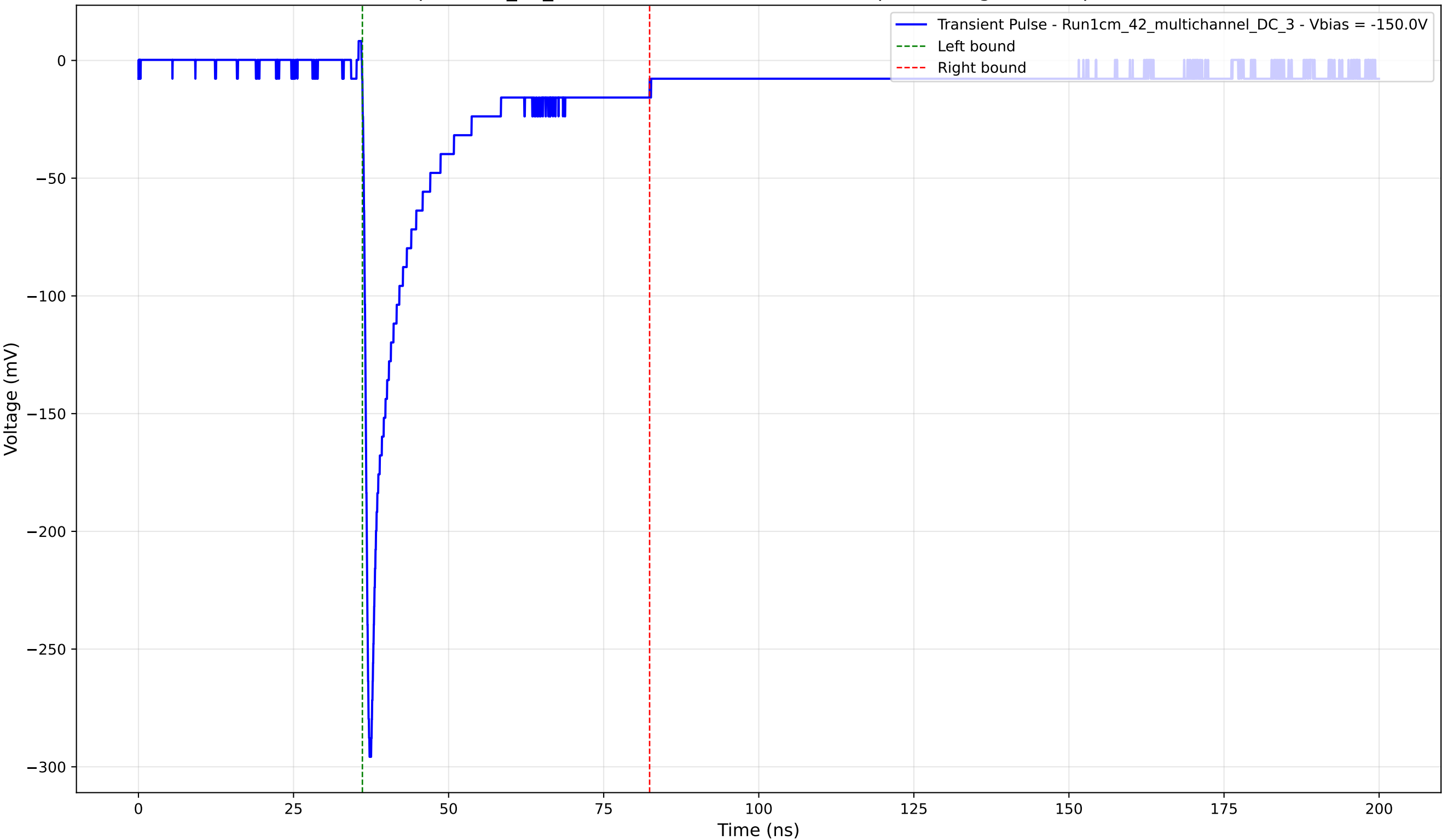
Transient Pulse - Sample: 1cm_42_multichannel - Position: 4595.0 \mu\text{m} - Charge: 41.89 pC - Rise Time: 0.85 ns
