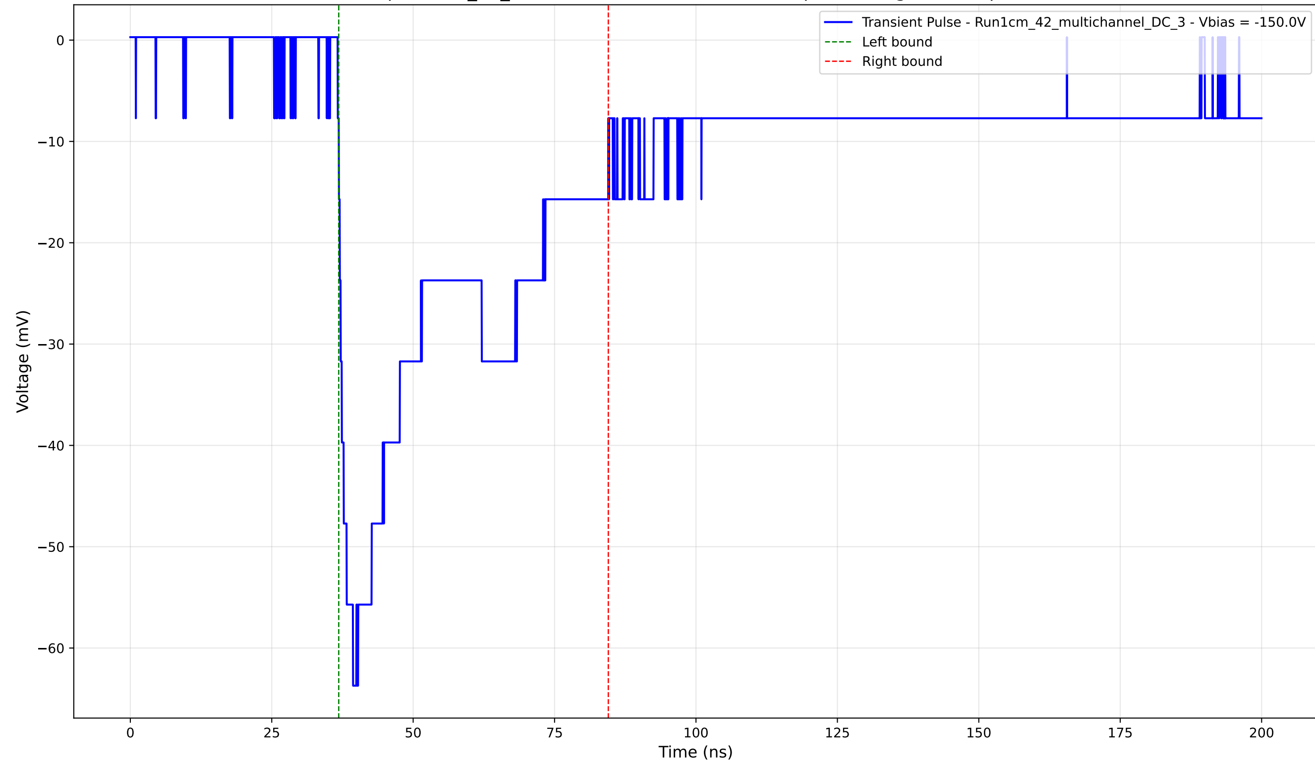
Transient Pulse - Sample: 1cm_42_multichannel - Position: 2435.0 \mu\text{m} - Charge: 27.63 pC - Rise Time: 2.70 ns
