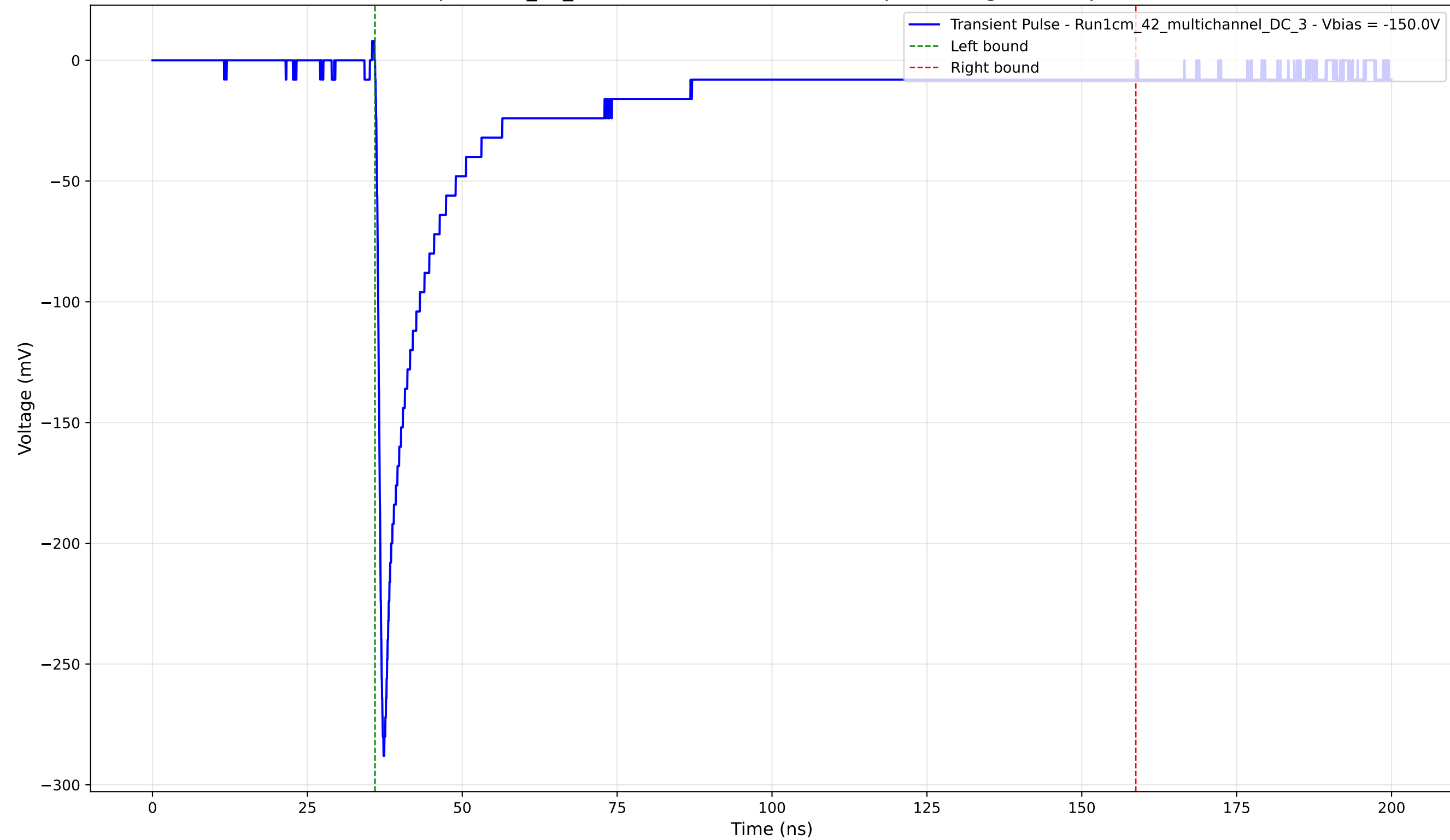
Transient Pulse - Sample: 1cm_42_multichannel - Position: 450.0 \mu\text{m} - Charge: 61.54 pC - Rise Time: 0.91 ns
