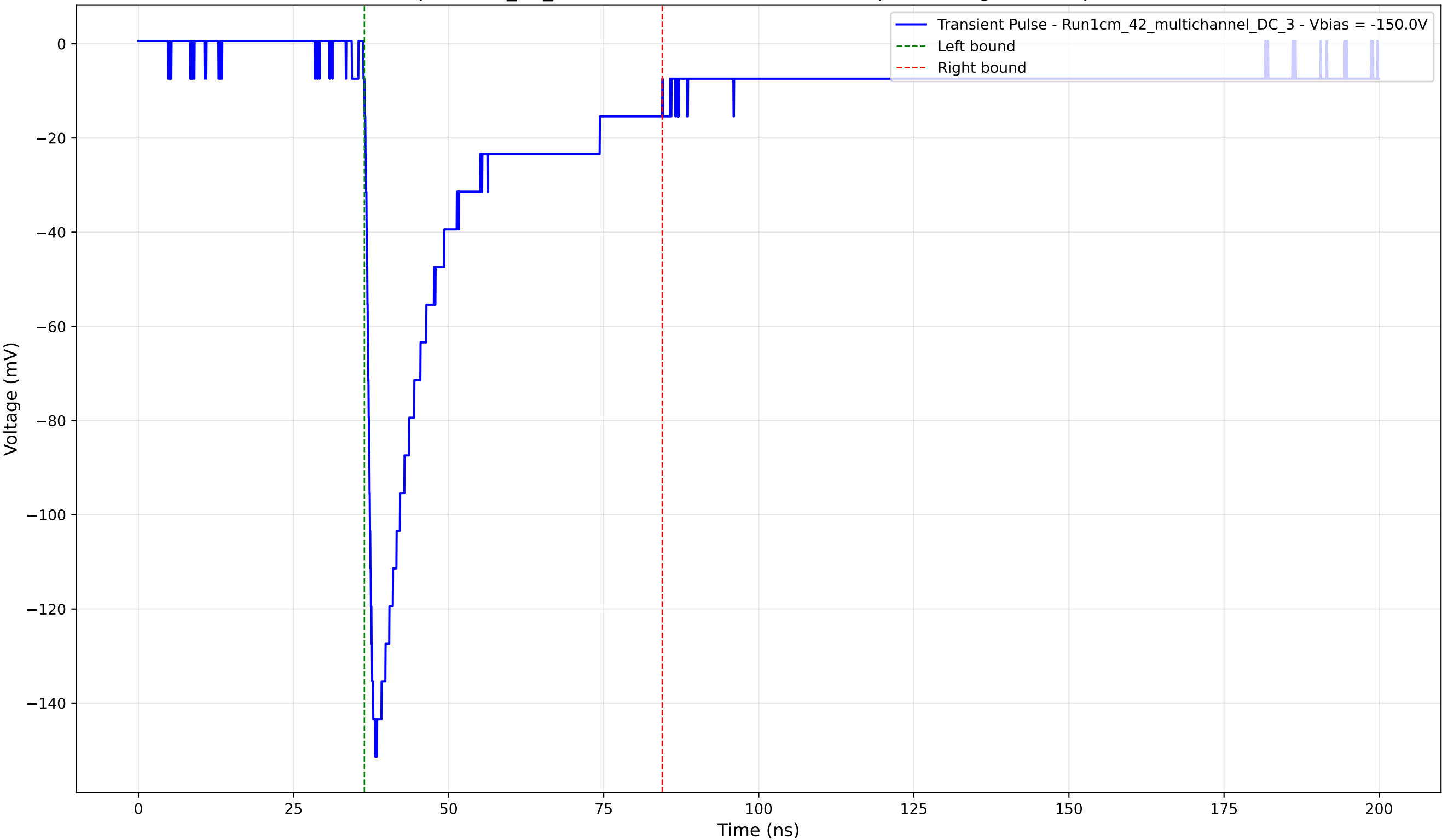
Transient Pulse - Sample: 1cm_42_multichannel - Position: 3780.0 \mu\text{m} - Charge: 38.92 pC - Rise Time: 1.40 ns
