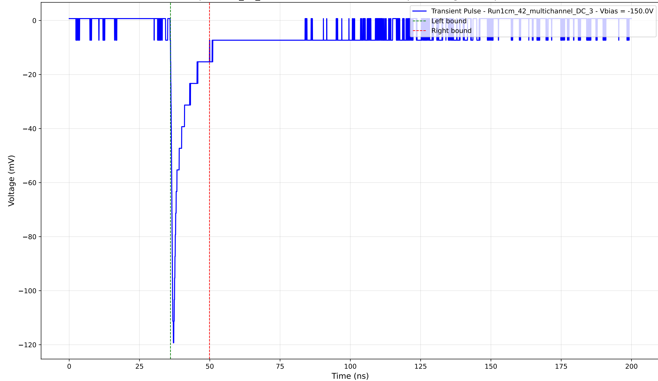
Transient Pulse - Sample: 1cm_42_multichannel - Position: 4860.0 \mu\text{m} - Charge: 9.89 pC - Rise Time: 0.81 ns
