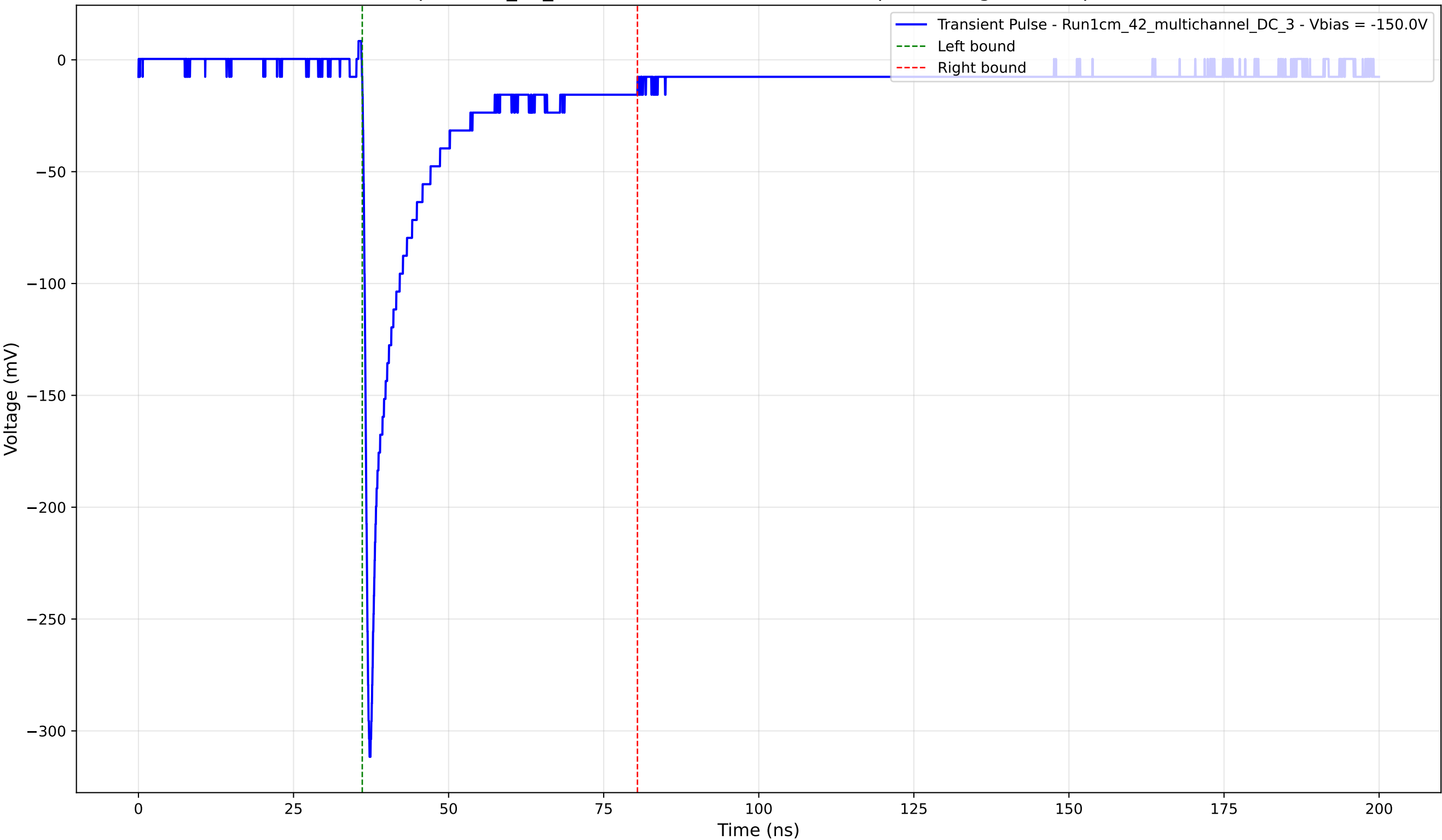
Transient Pulse - Sample: 1cm_42_multichannel - Position: 4630.0 \mu\text{m} - Charge: 41.77 pC - Rise Time: 0.86 ns
