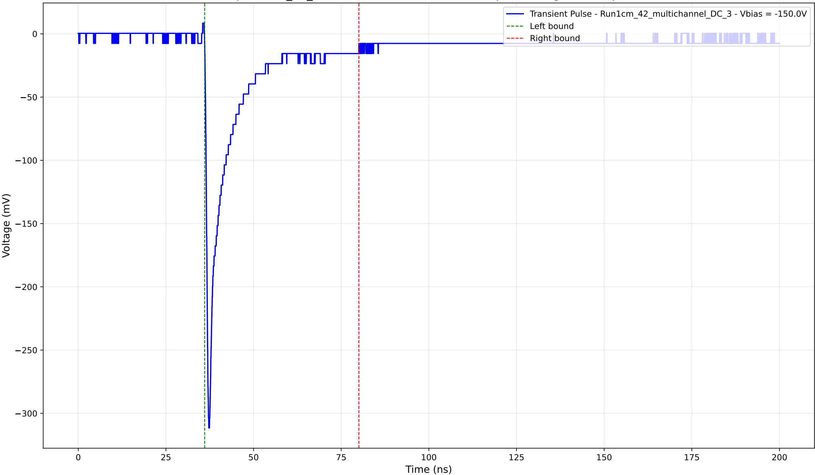
Transient Pulse - Sample: 1cm_42_multichannel - Position: 4625.0 \mu\text{m} - Charge: 41.81 pC - Rise Time: 0.86 ns
