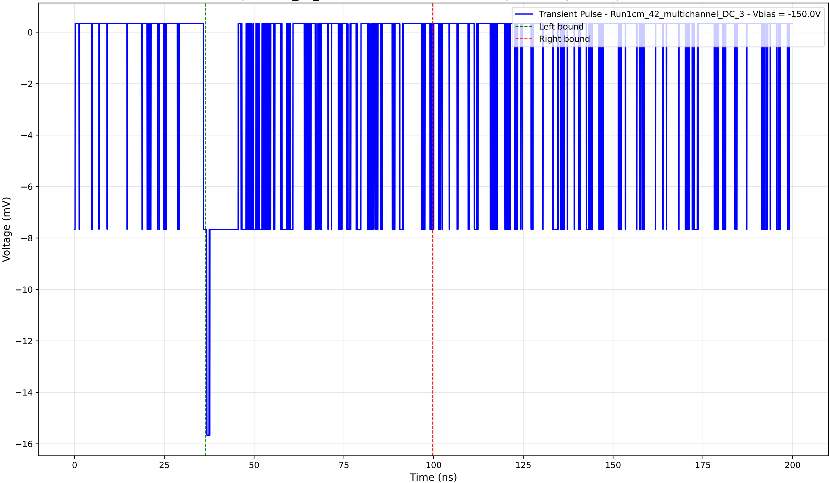
Transient Pulse - Sample: 1cm_42_multichannel - Position: 4925.0 \mu\text{m} - Charge: 3.85 pC - Rise Time: 0.94 ns
