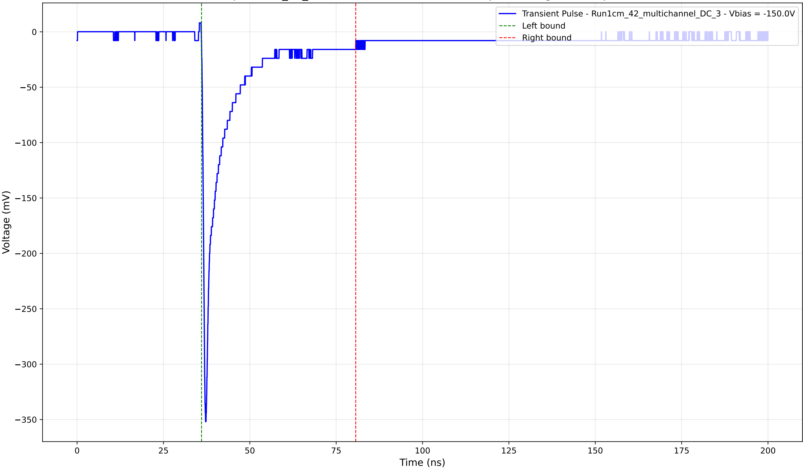
Transient Pulse - Sample: 1cm_42_multichannel - Position: 4705.0 \mu\text{m} - Charge: 43.79 pC - Rise Time: 0.80 ns
