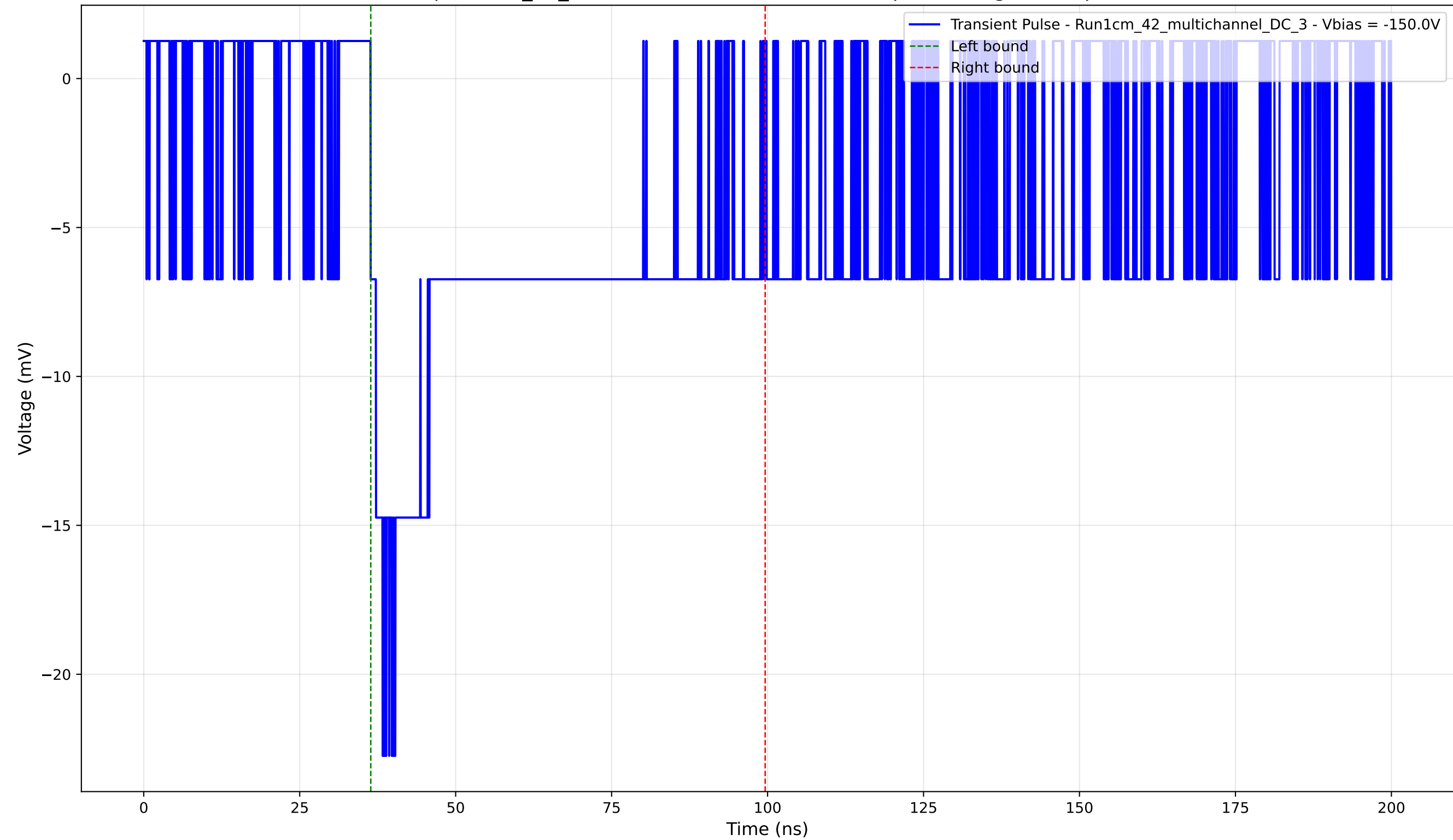
Transient Pulse - Sample: 1cm_42_multichannel - Position: 1390.0 \mu\text{m} - Charge: 9.54 pC - Rise Time: 1.94 ns
