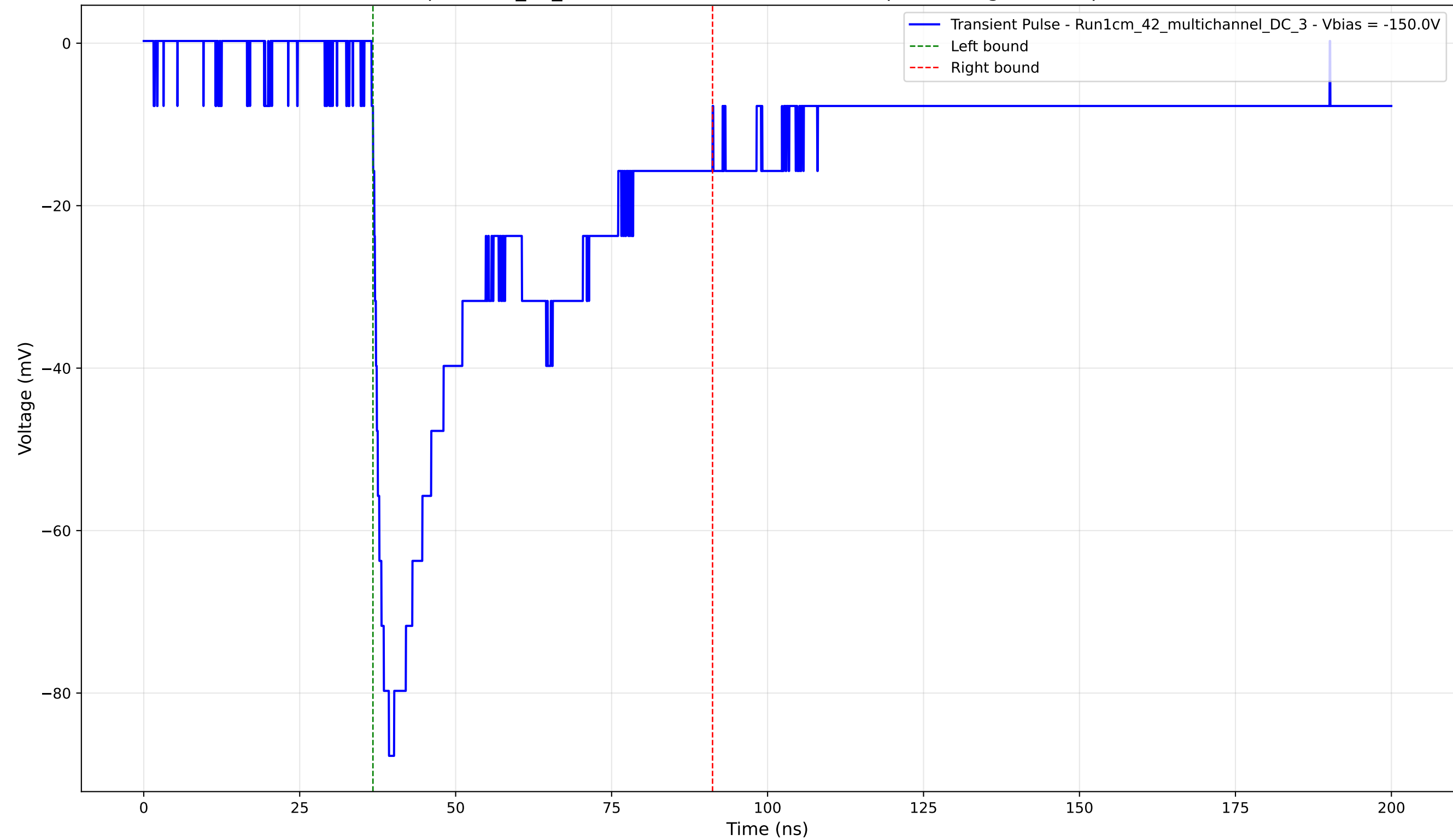
Transient Pulse - Sample: 1cm_42_multichannel - Position: 2660.0 \mu\text{m} - Charge: 36.16 pC - Rise Time: 1.74 ns
