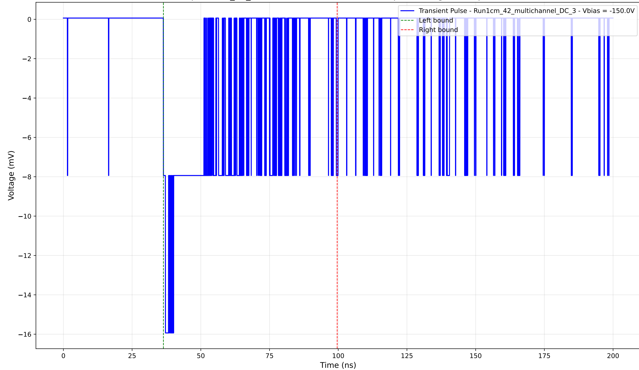
Transient Pulse - Sample: 1cm_42_multichannel - Position: 4380.0 \mu\text{m} - Charge: 5.11 pC - Rise Time: 0.76 ns
