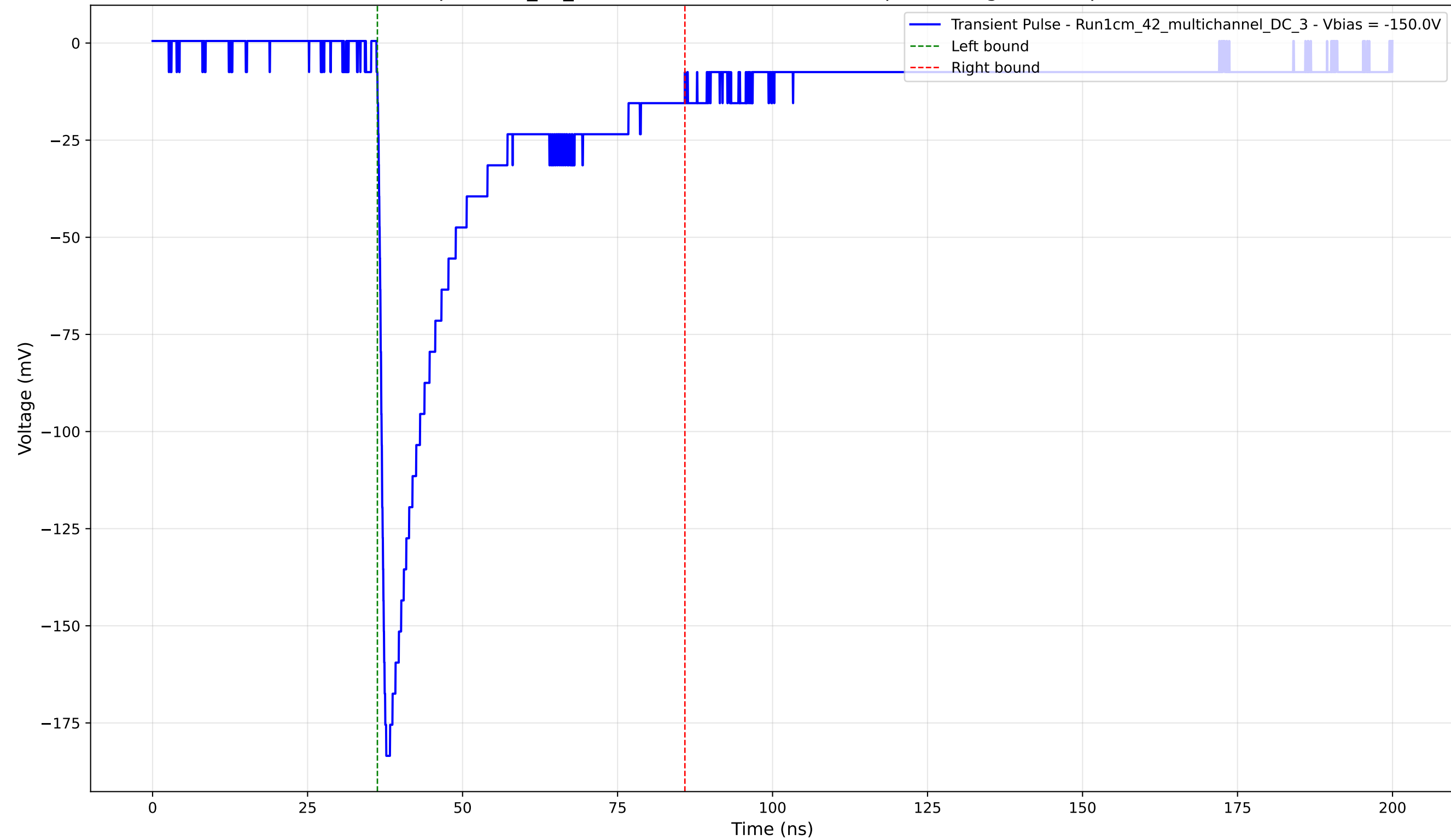
Transient Pulse - Sample: 1cm_42_multichannel - Position: 960.0 \mu\text{m} - Charge: 45.51 pC - Rise Time: 1.05 ns
