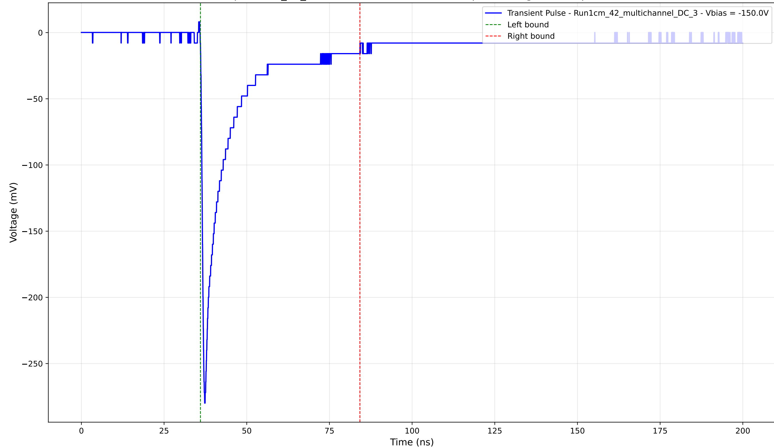
Transient Pulse - Sample: 1cm_42_multichannel - Position: 435.0 \mu\text{m} - Charge: 47.87 pC - Rise Time: 0.91 ns
