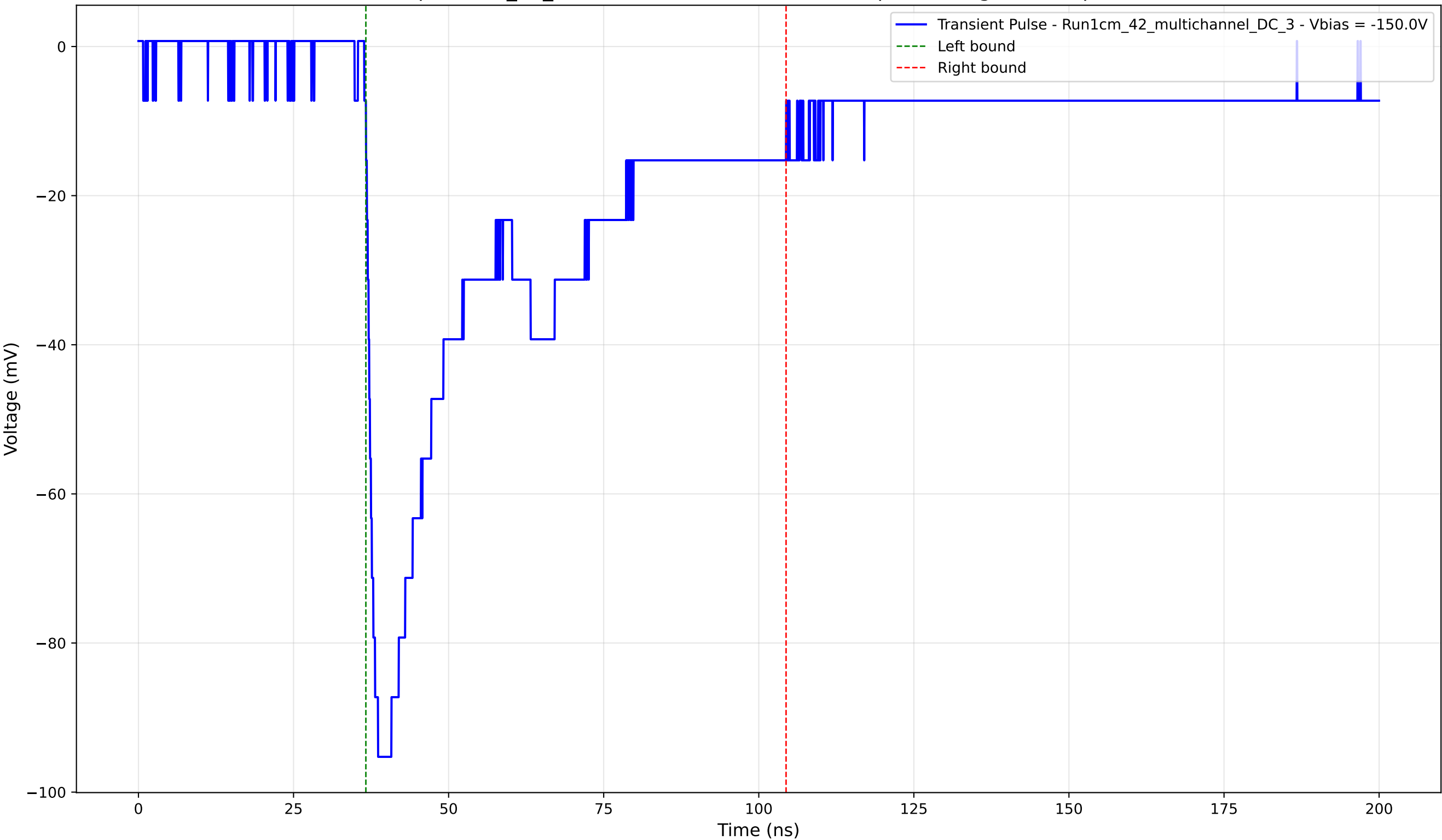
Transient Pulse - Sample: 1cm_42_multichannel - Position: 2030.0 \mu\text{m} - Charge: 43.39 pC - Rise Time: 1.47 ns
