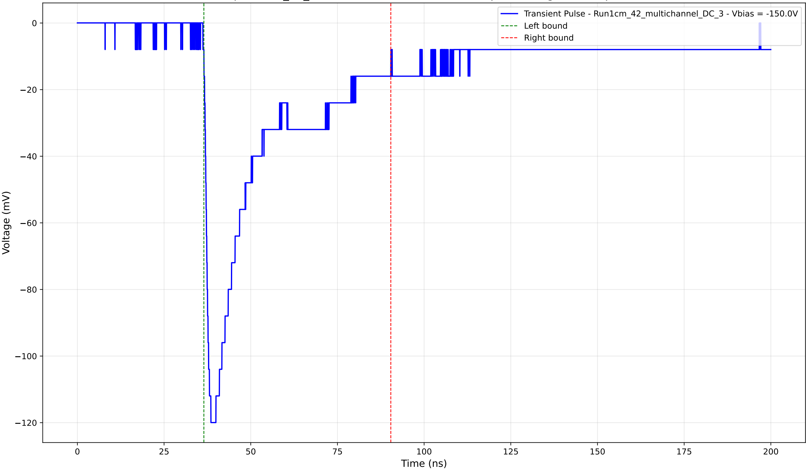
Transient Pulse - Sample: 1cm_42_multichannel - Position: 1685.0 \mu\text{m} - Charge: 43.05 pC - Rise Time: 1.59 ns
