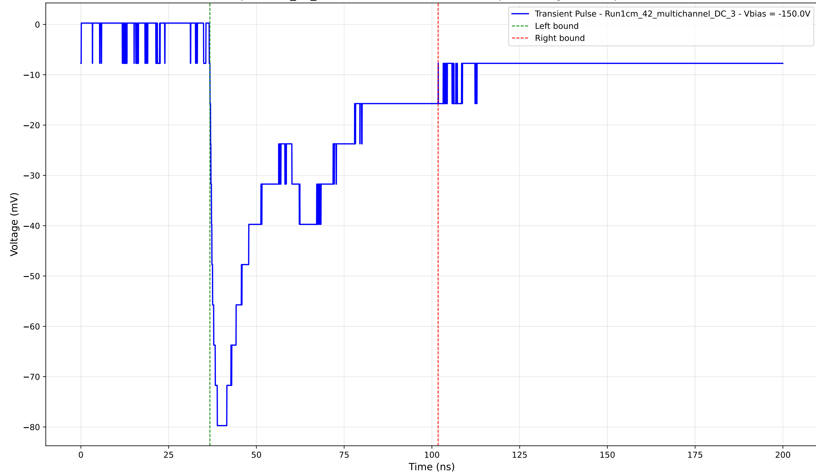
Transient Pulse - Sample: 1cm_42_multichannel - Position: 2480.0 \mu\text{m} - Charge: 40.54 pC - Rise Time: 2.10 ns
