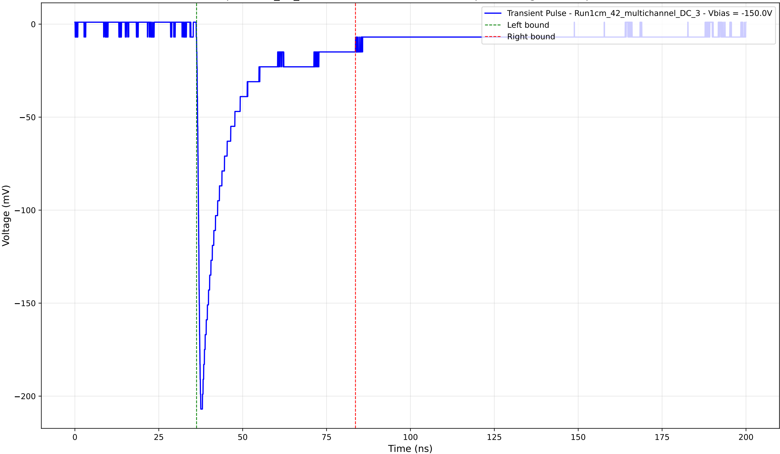
Transient Pulse - Sample: 1cm_42_multichannel - Position: 4220.0 \mu\text{m} - Charge: 41.27 pC - Rise Time: 0.97 ns
