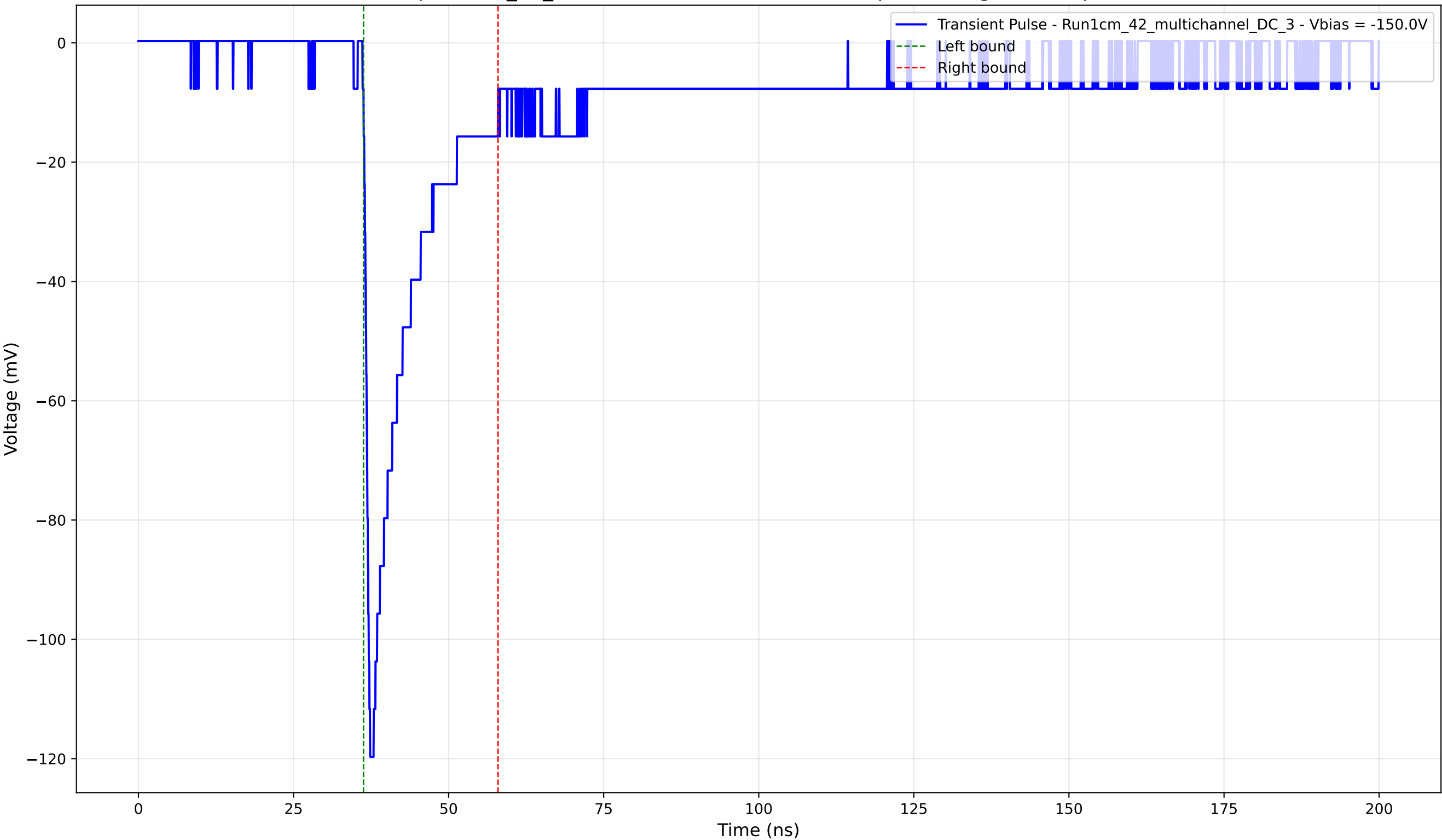
Transient Pulse - Sample: 1cm_42_multichannel - Position: 4335.0 \mu\text{m} - Charge: 17.63 pC - Rise Time: 0.93 ns
