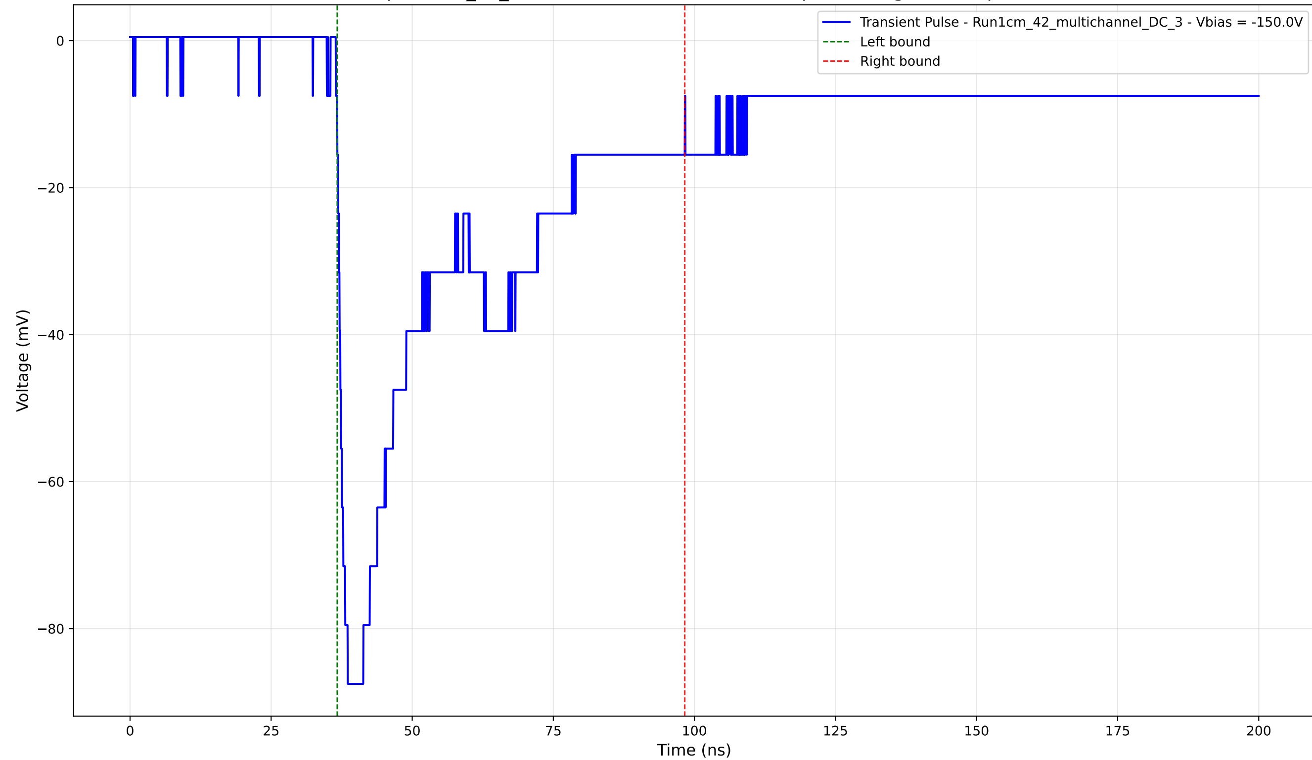
Transient Pulse - Sample: 1cm_42_multichannel - Position: 2115.0 \mu\text{m} - Charge: 41.05 pC - Rise Time: 1.42 ns
