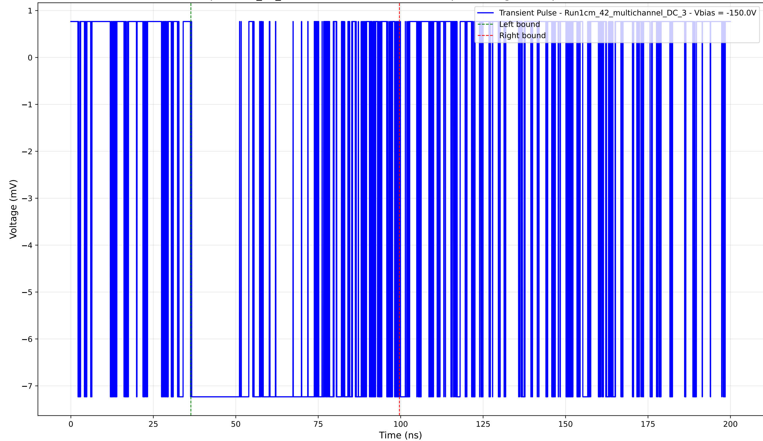
Transient Pulse - Sample: 1cm_42_multichannel - Position: 1880.0 \mu\text{m} - Charge: 6.92 pC - Rise Time: 0.00 ns (N/A)
