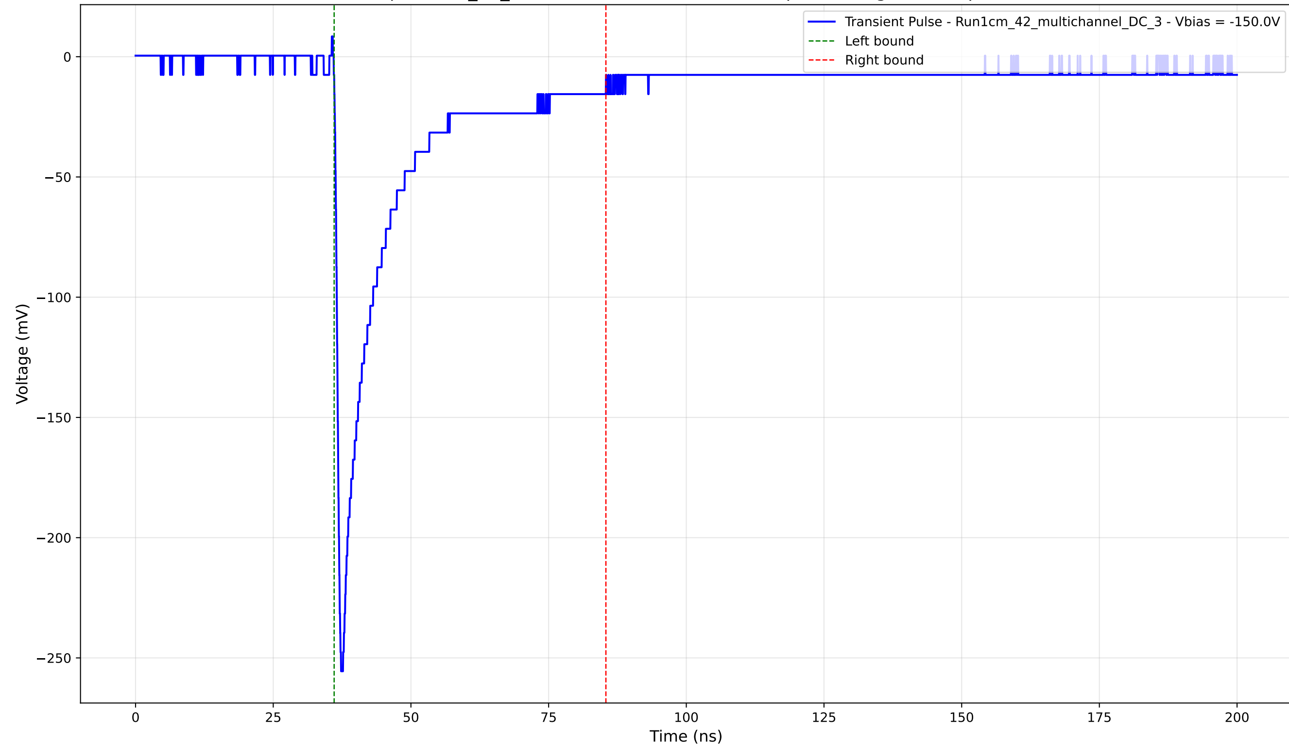
Transient Pulse - Sample: 1cm_42_multichannel - Position: 545.0 \mu\text{m} - Charge: 48.13 pC - Rise Time: 0.89 ns
