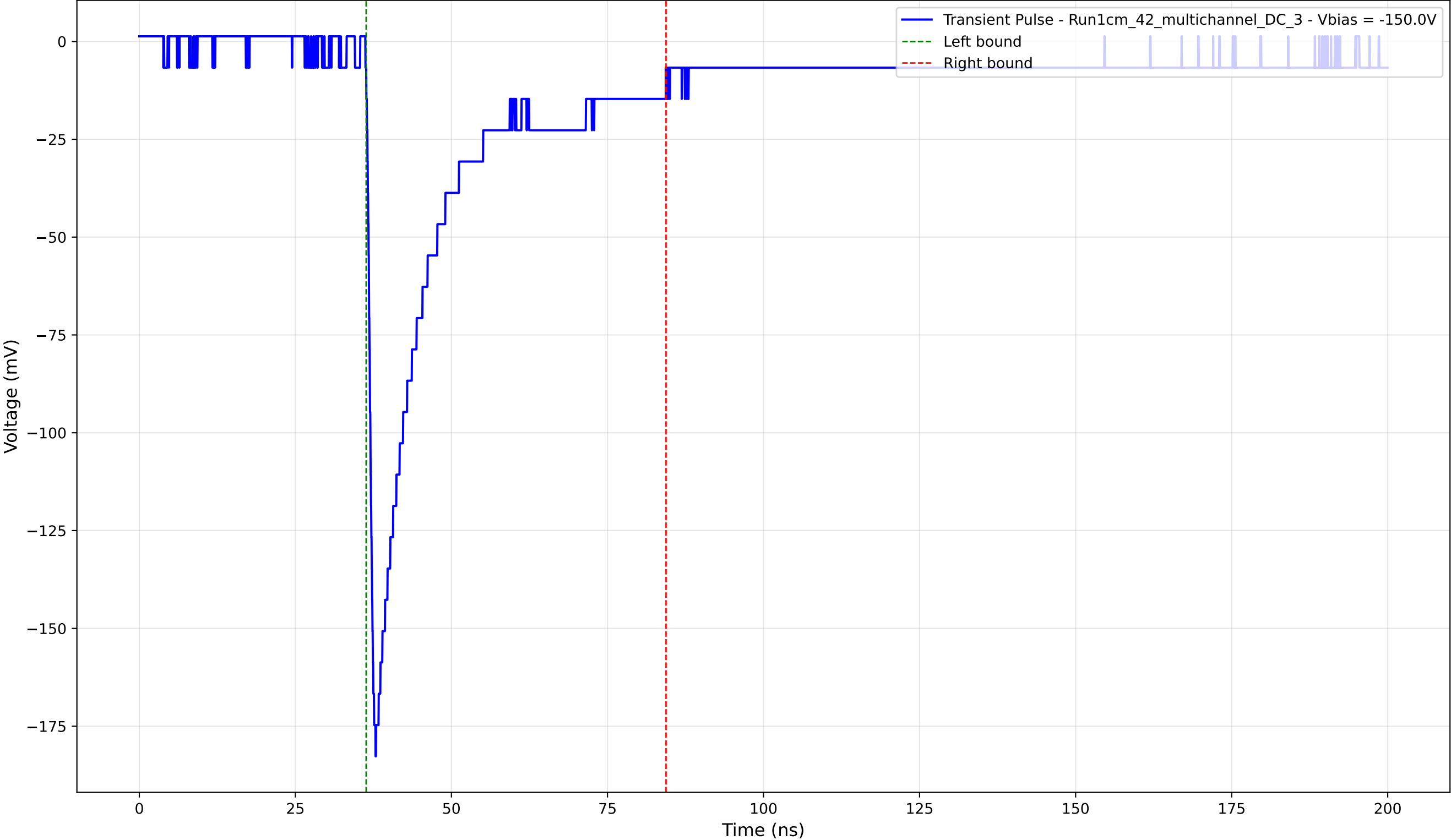
Transient Pulse - Sample: 1cm_42_multichannel - Position: 4075.0 \mu\text{m} - Charge: 39.13 pC - Rise Time: 1.03 ns
