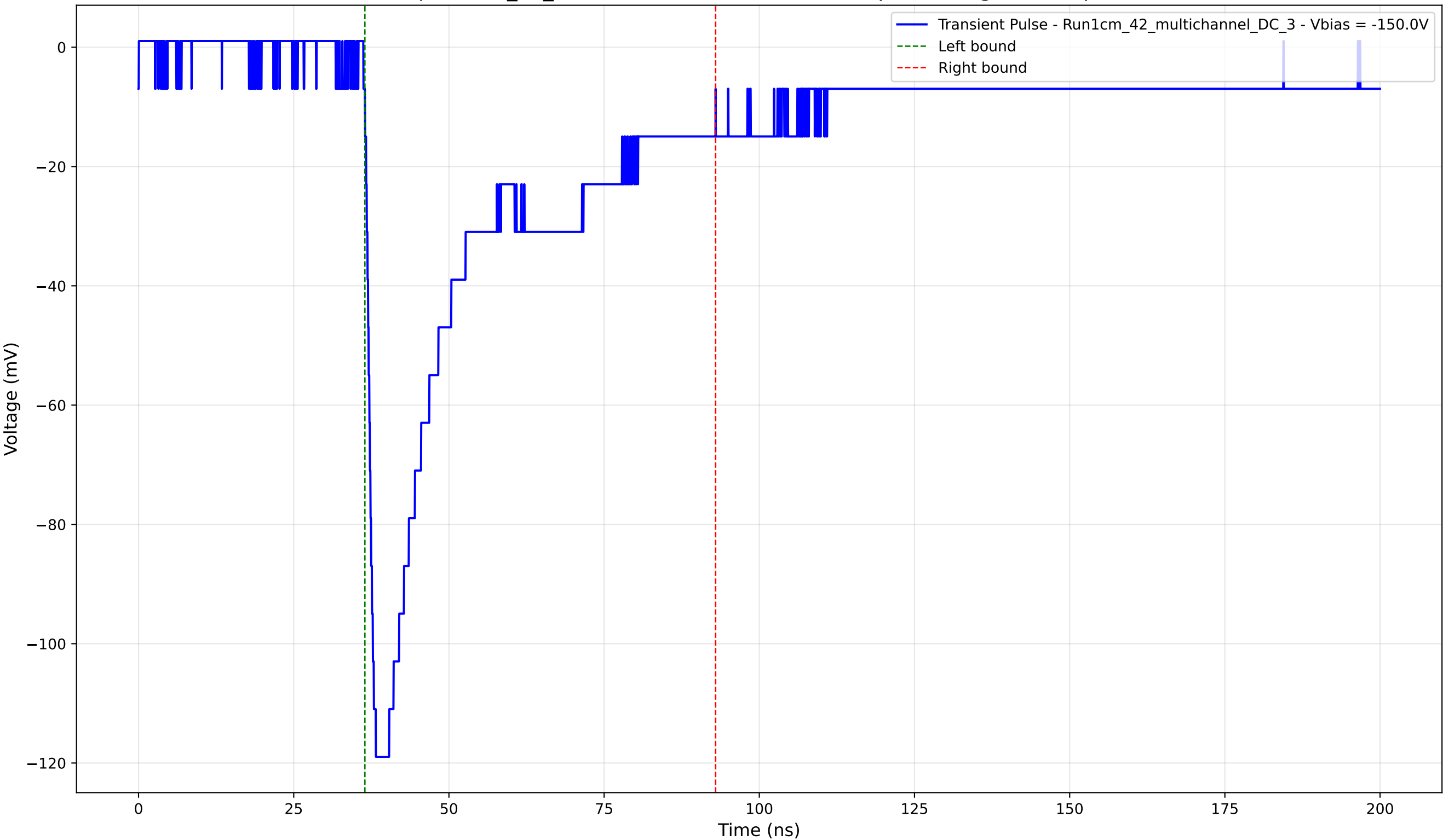
Transient Pulse - Sample: 1cm_42_multichannel - Position: 1595.0 \mu\text{m} - Charge: 42.67 pC - Rise Time: 1.43 ns
