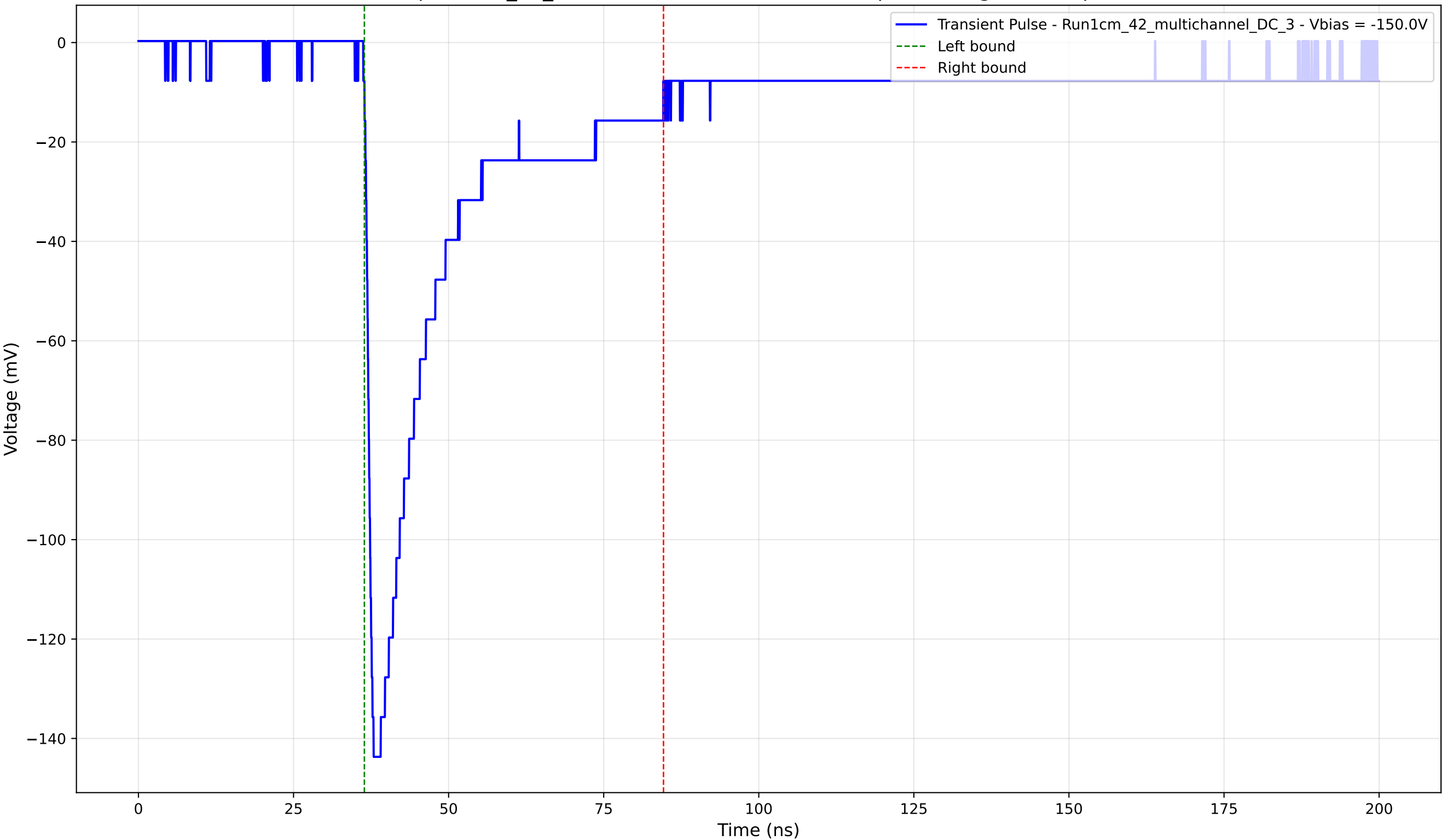
Transient Pulse - Sample: 1cm_42_multichannel - Position: 3760.0 \mu\text{m} - Charge: 39.07 pC - Rise Time: 1.28 ns
