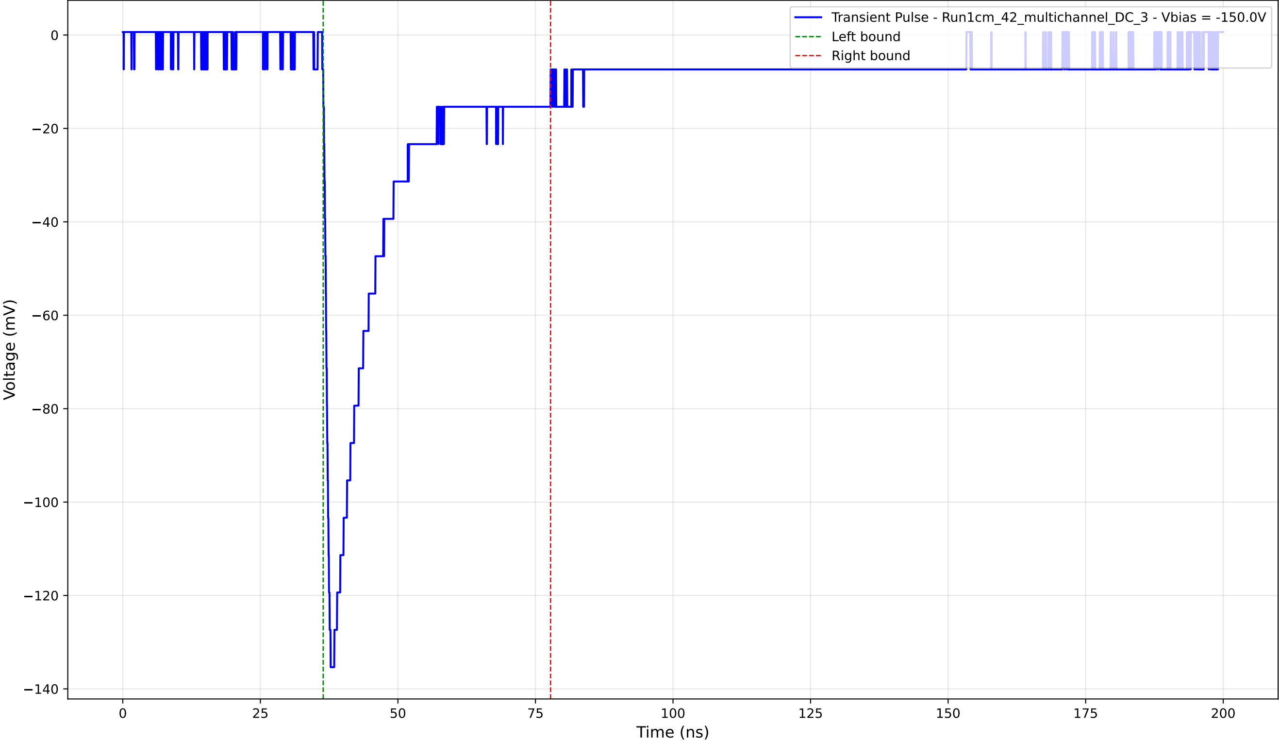
Transient Pulse - Sample: 1cm_42_multichannel - Position: 3955.0 \mu\text{m} - Charge: 30.01 pC - Rise Time: 1.14 ns
