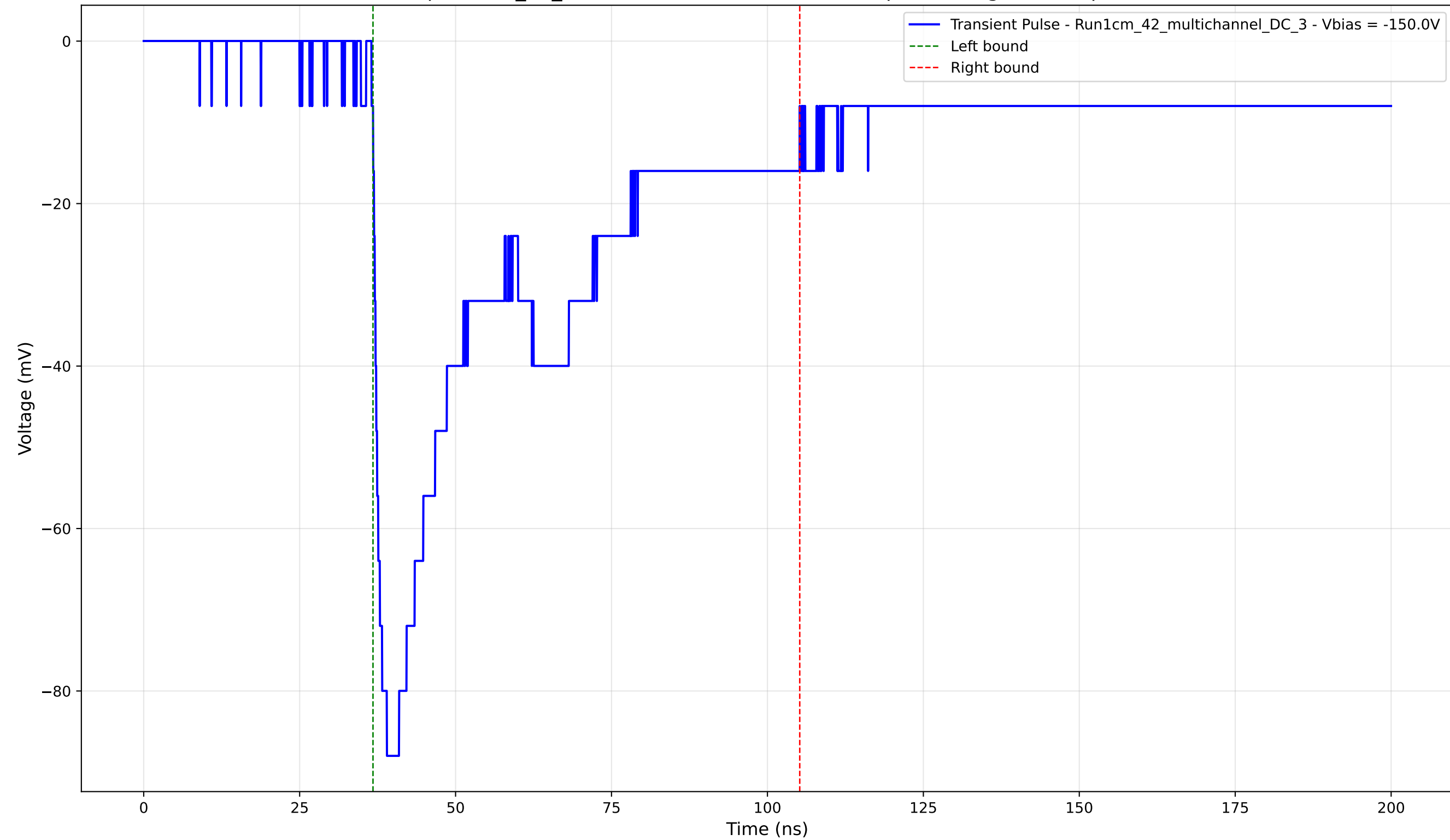
Transient Pulse - Sample: 1cm_42_multichannel - Position: 2185.0 \mu\text{m} - Charge: 43.41 pC - Rise Time: 1.46 ns
