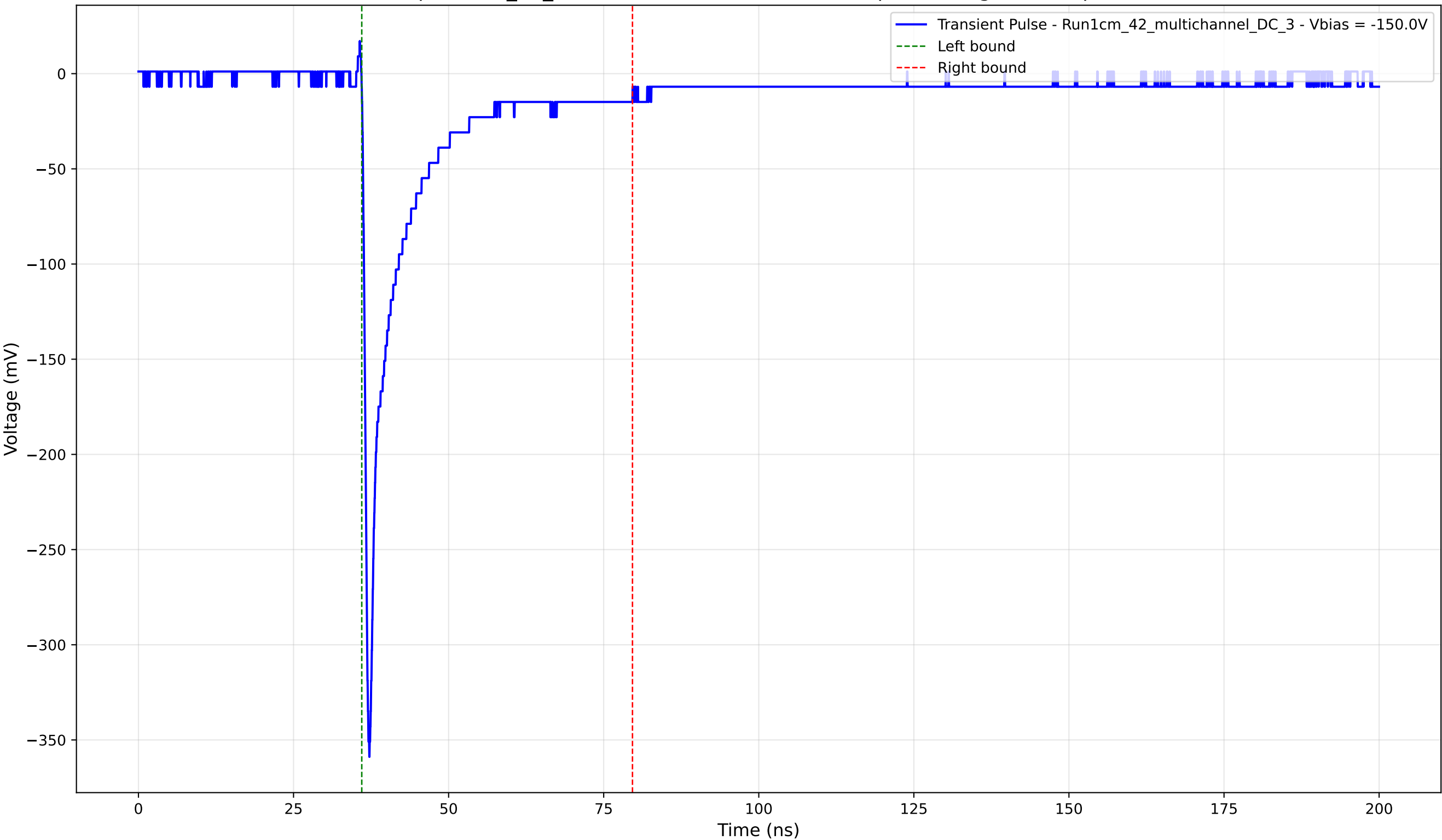
Transient Pulse - Sample: 1cm_42_multichannel - Position: 4740.0 \mu\text{m} - Charge: 41.49 pC - Rise Time: 0.80 ns
