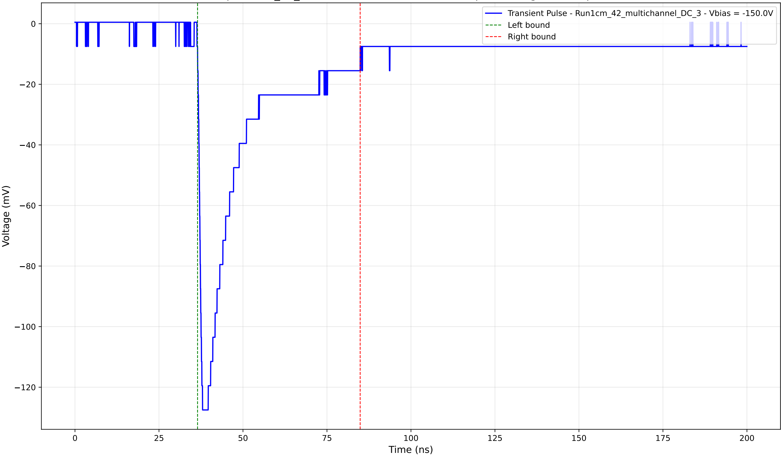
Transient Pulse - Sample: 1cm_42_multichannel - Position: 3650.0 \mu\text{m} - Charge: 36.92 pC - Rise Time: 1.27 ns
