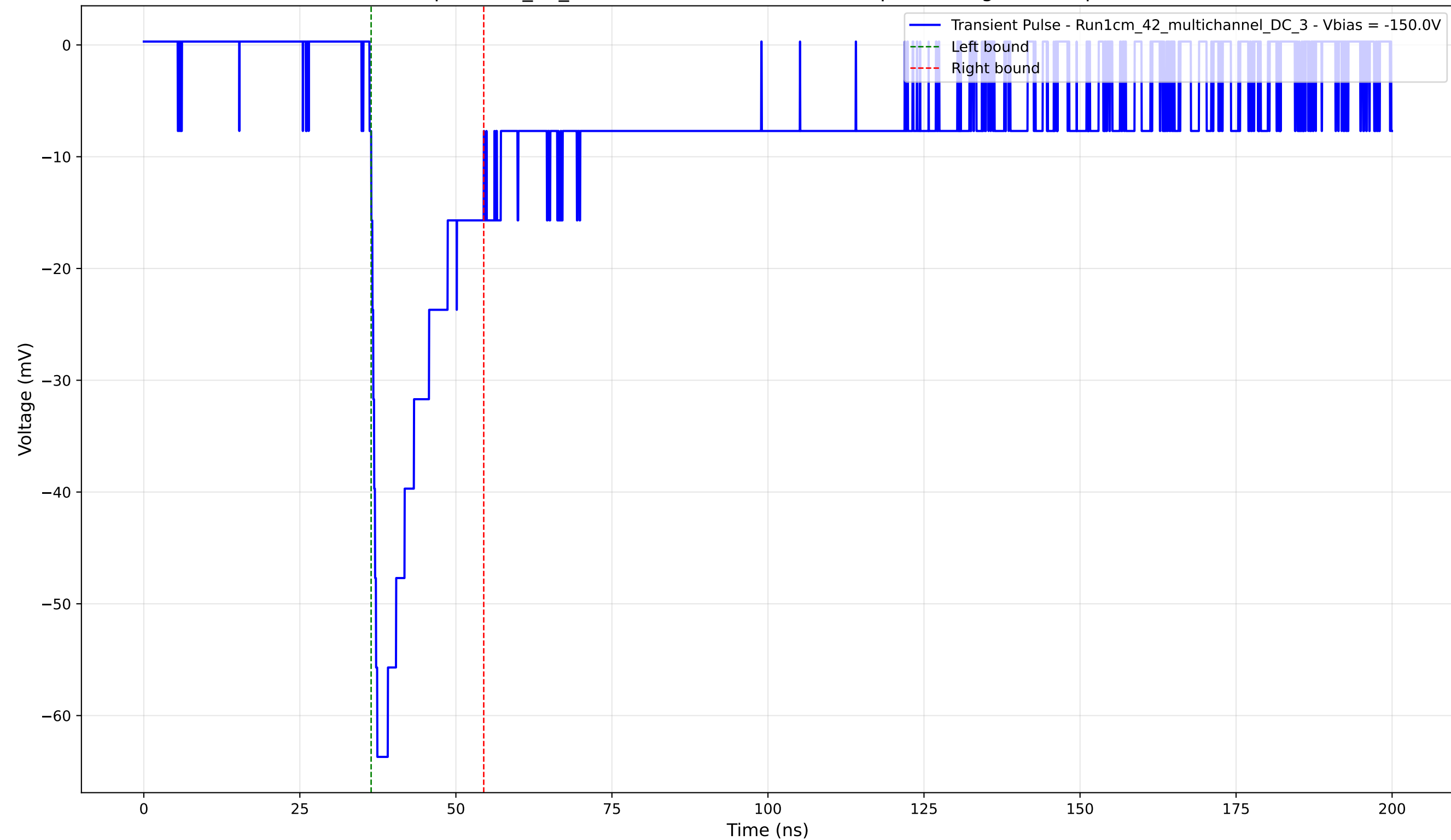
Transient Pulse - Sample: 1cm_42_multichannel - Position: 900.0 \mu\text{m} - Charge: 11.59 pC - Rise Time: 1.24 ns
