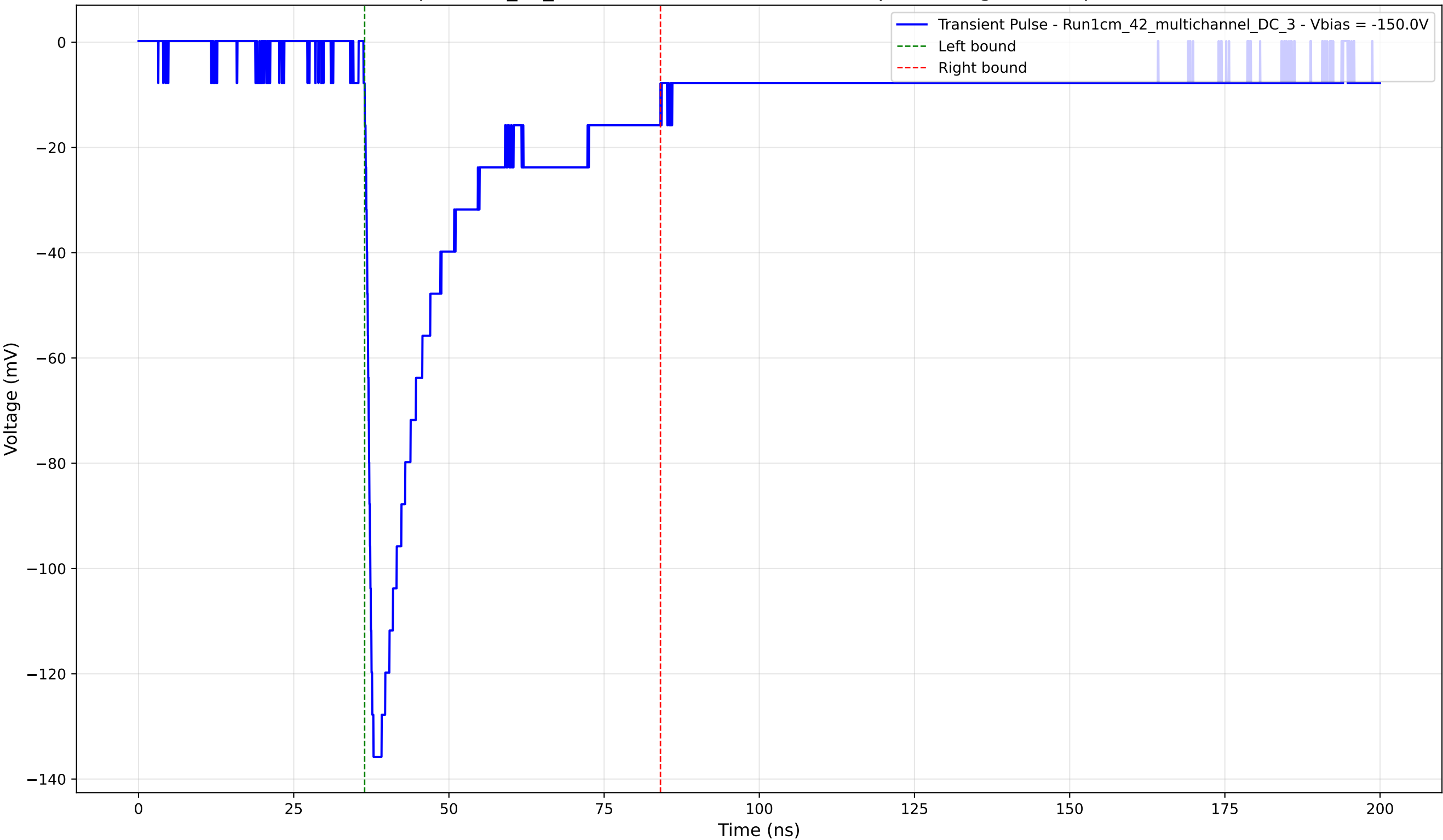
Transient Pulse - Sample: 1cm_42_multichannel - Position: 3810.0 \mu\text{m} - Charge: 36.84 pC - Rise Time: 1.21 ns
