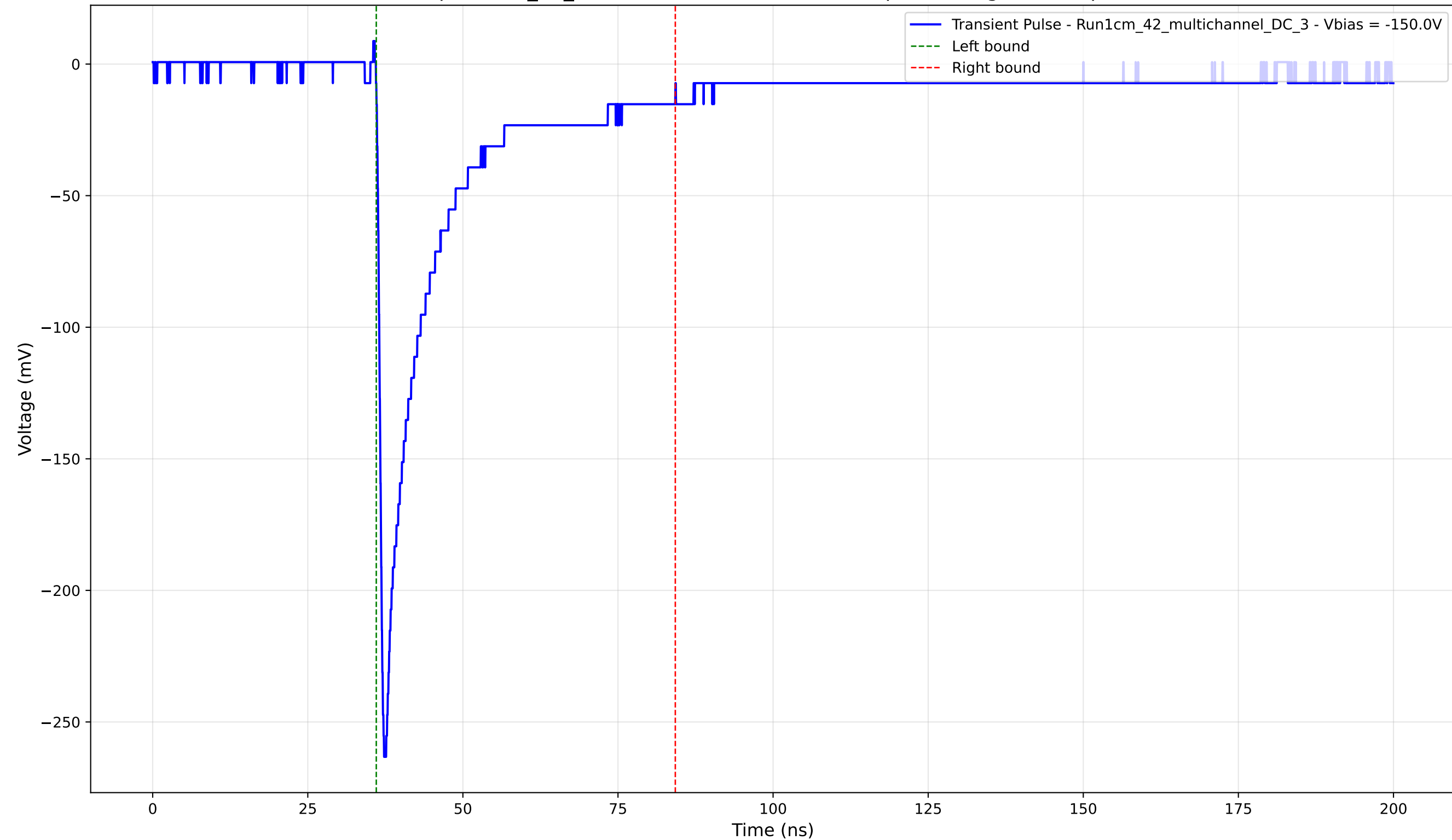
Transient Pulse - Sample: 1cm_42_multichannel - Position: 525.0 \mu\text{m} - Charge: 47.88 pC - Rise Time: 0.91 ns
