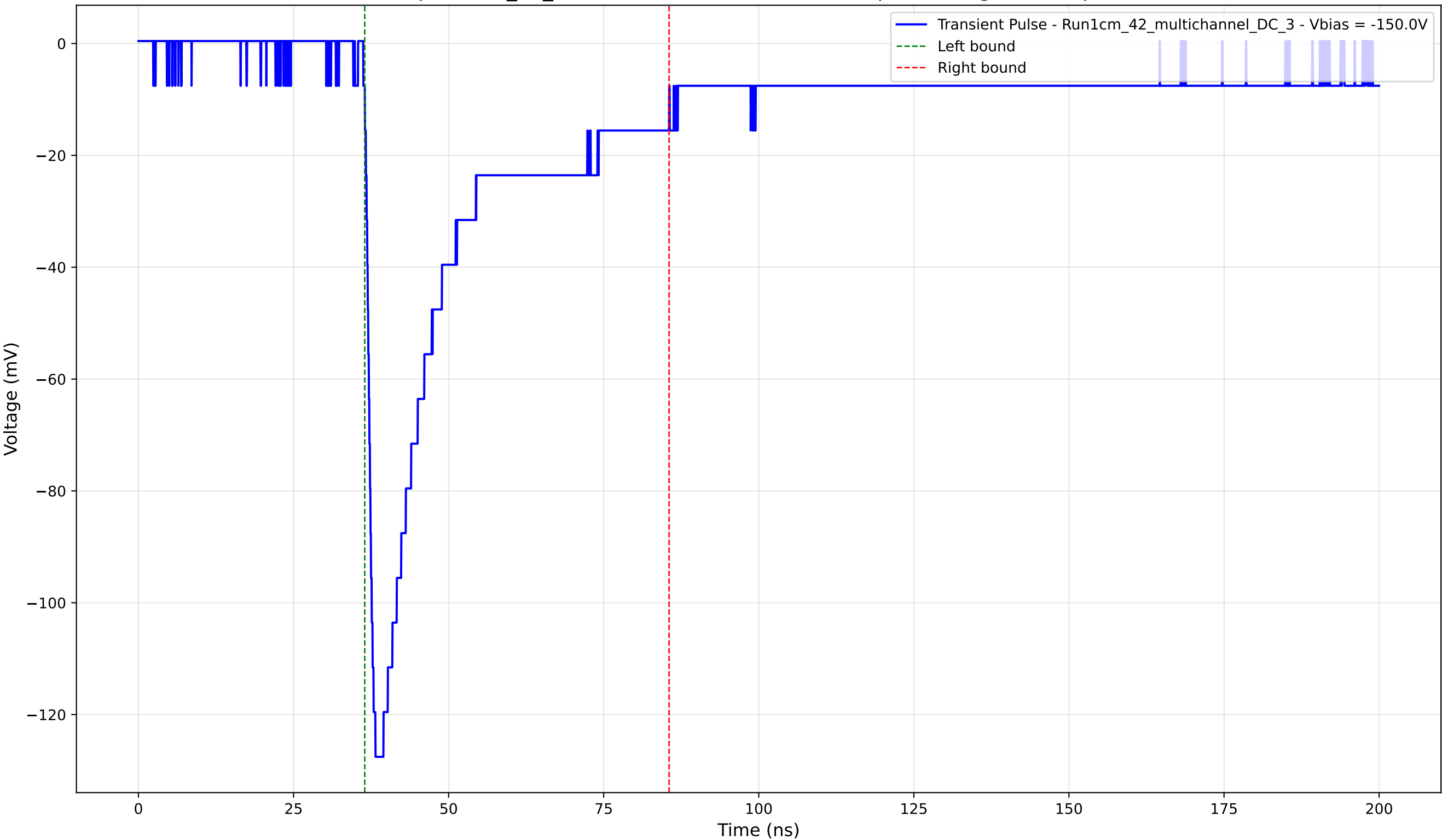
Transient Pulse - Sample: 1cm_42_multichannel - Position: 3580.0 \mu\text{m} - Charge: 37.05 pC - Rise Time: 1.41 ns
