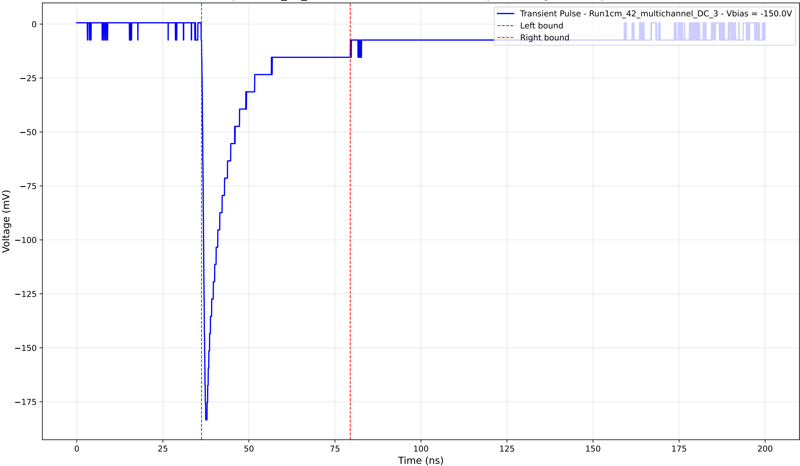
Transient Pulse - Sample: 1cm_42_multichannel - Position: 4310.0 \mu\text{m} - Charge: 32.87 pC - Rise Time: 0.91 ns
