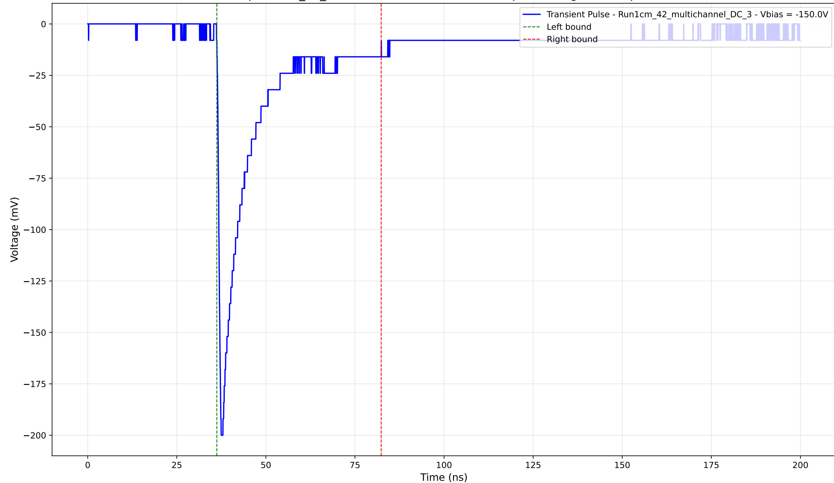
Transient Pulse - Sample: 1cm_42_multichannel - Position: 4255.0 \mu\text{m} - Charge: 38.84 pC - Rise Time: 0.95 ns
