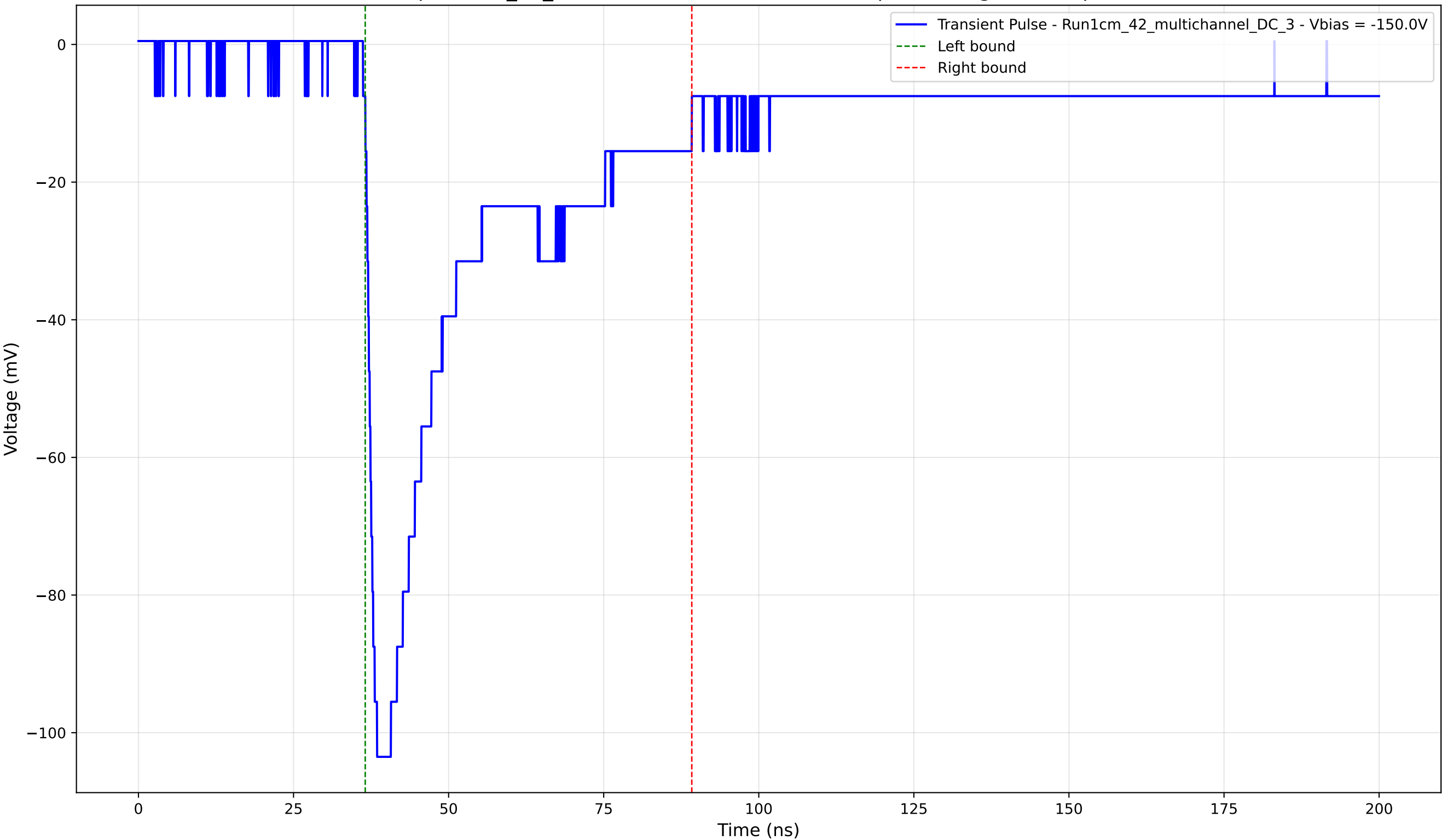
Transient Pulse - Sample: 1cm_42_multichannel - Position: 3185.0 \mu\text{m} - Charge: 36.85 pC - Rise Time: 1.51 ns
