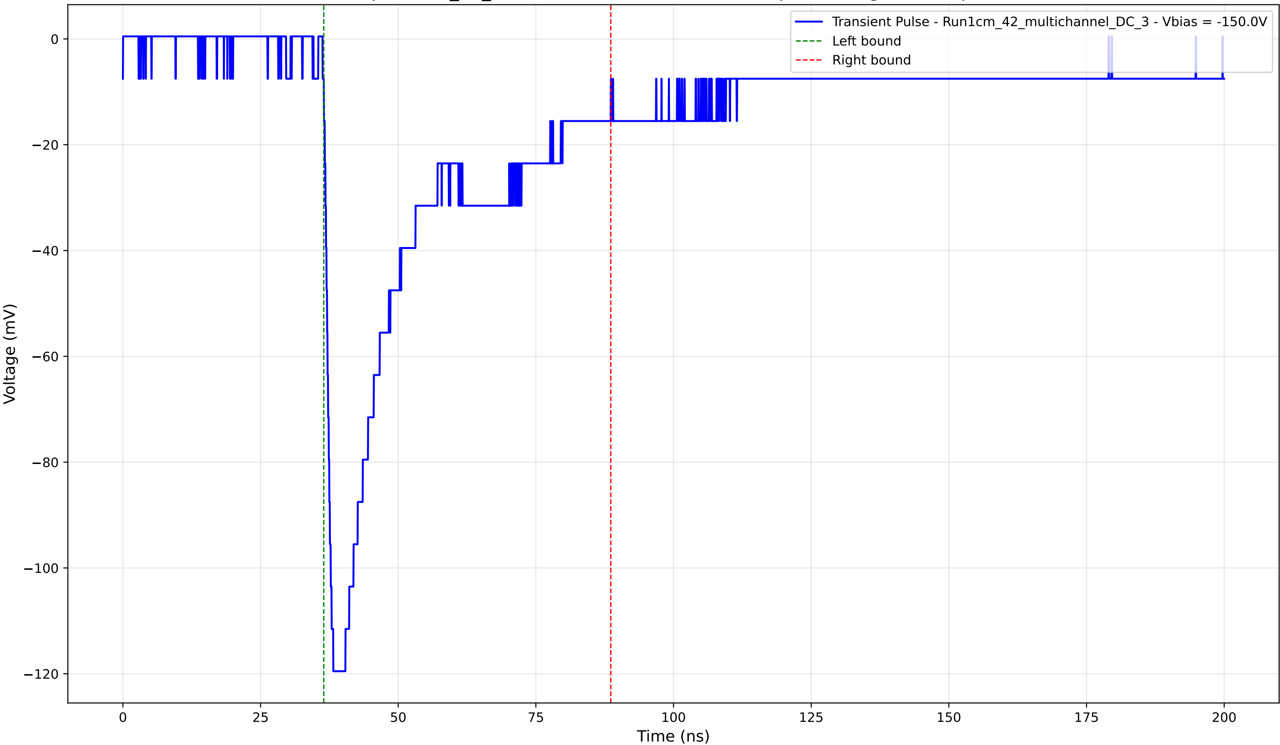
Transient Pulse - Sample: 1cm_42_multichannel - Position: 1605.0 \mu\text{m} - Charge: 41.74 pC - Rise Time: 1.41 ns
