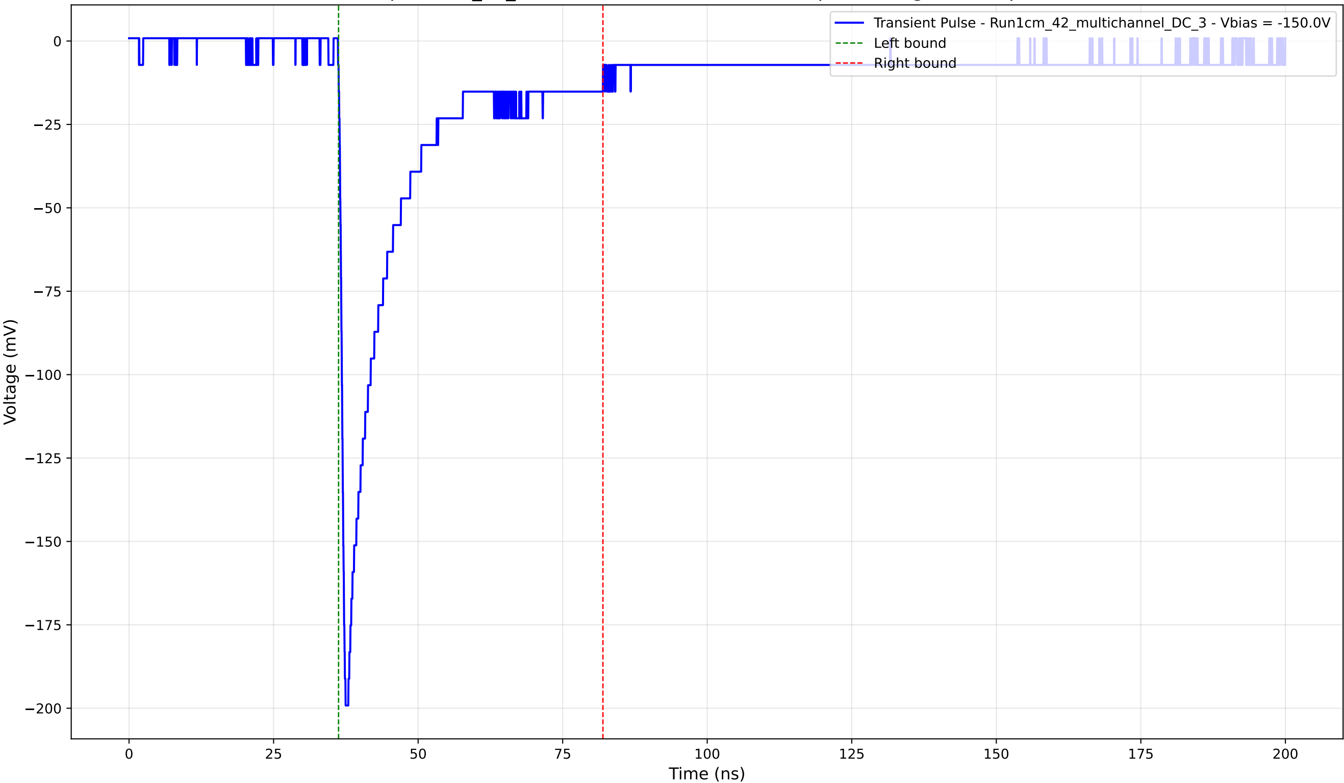
Transient Pulse - Sample: 1cm_42_multichannel - Position: 4275.0 \mu\text{m} - Charge: 37.31 pC - Rise Time: 0.93 ns
