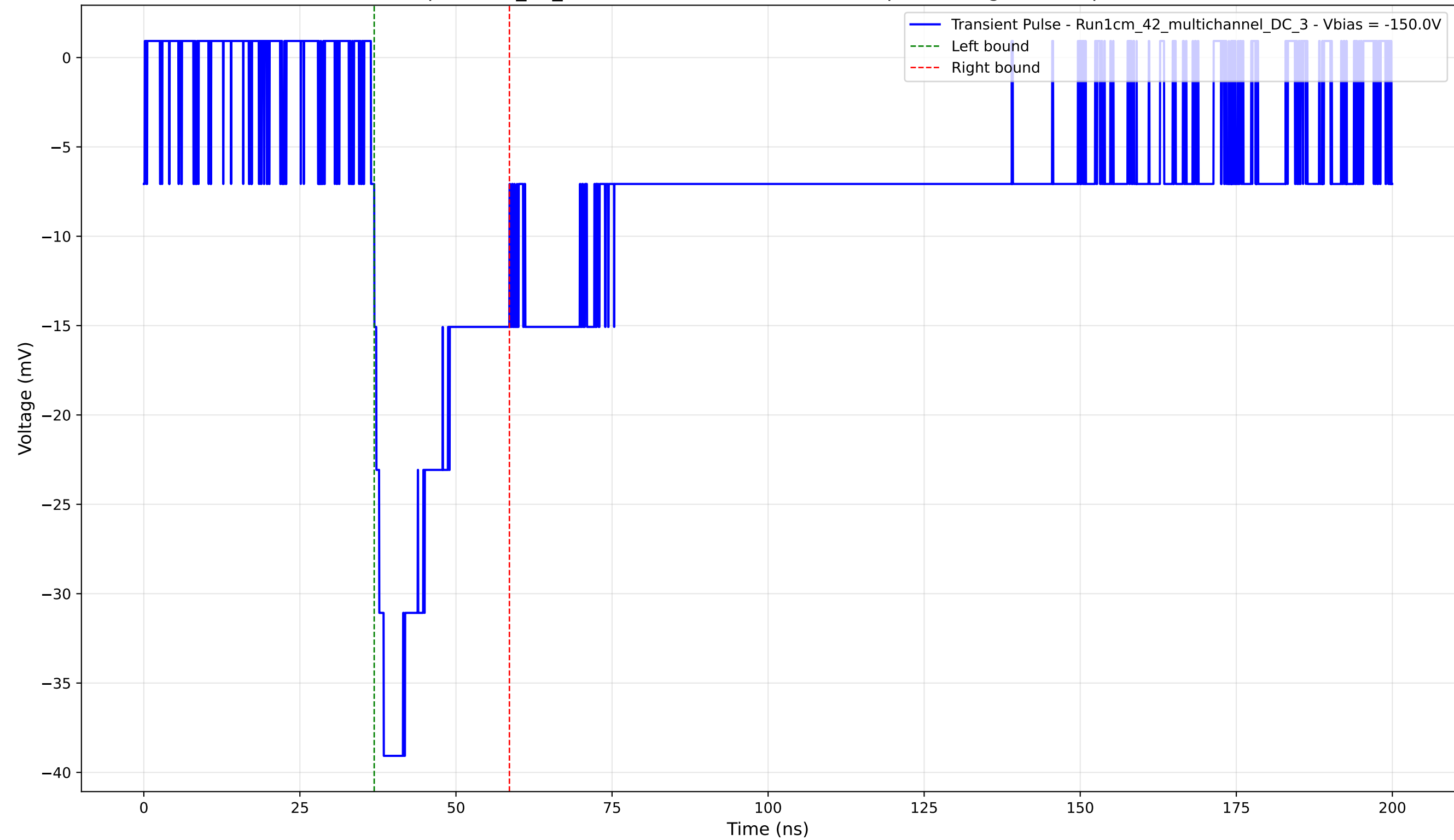
Transient Pulse - Sample: 1cm_42_multichannel - Position: 2835.0 \mu\text{m} - Charge: 10.03 pC - Rise Time: 2.05 ns
