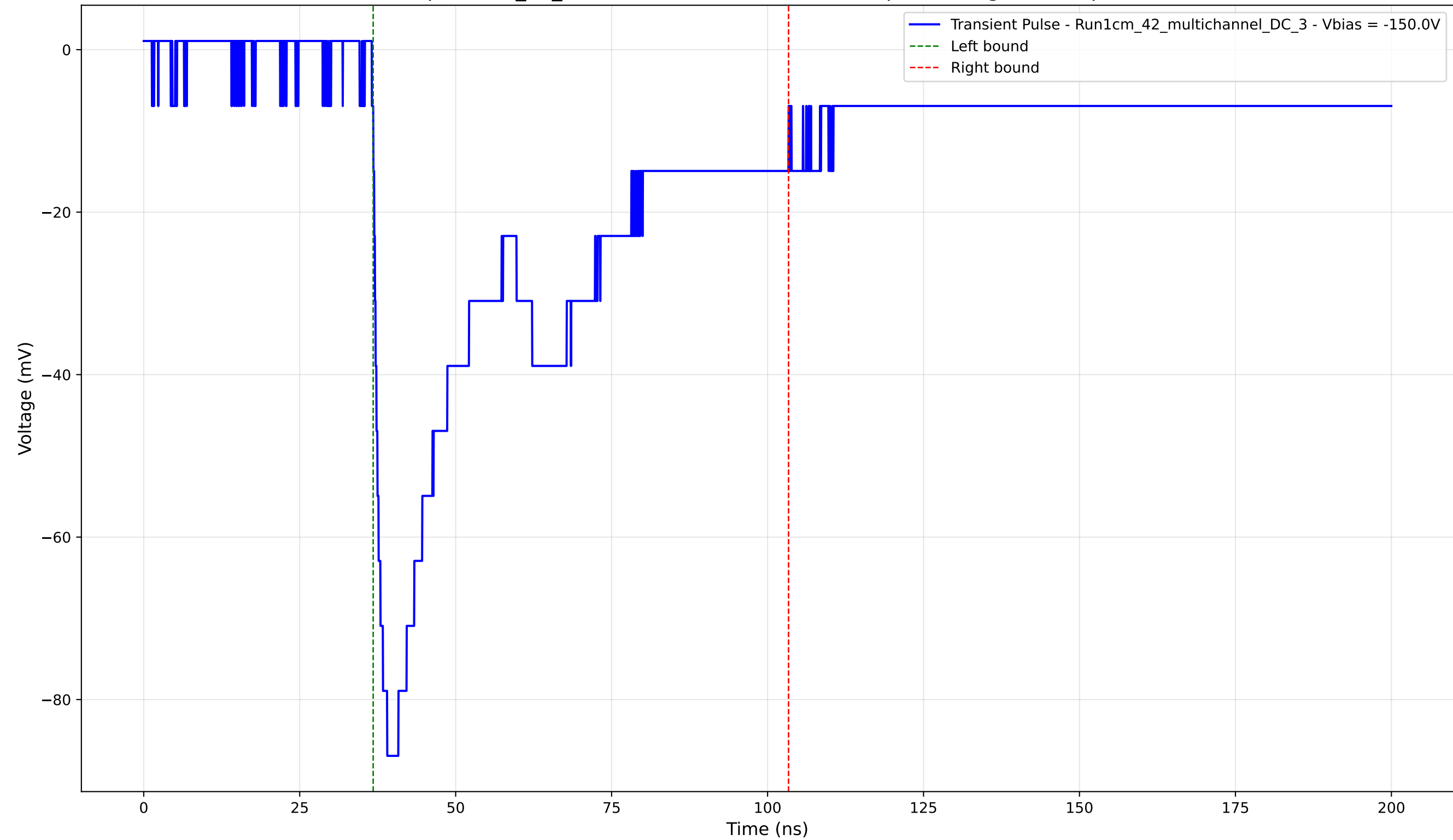
Transient Pulse - Sample: 1cm_42_multichannel - Position: 2215.0 \mu\text{m} - Charge: 41.39 pC - Rise Time: 1.56 ns
