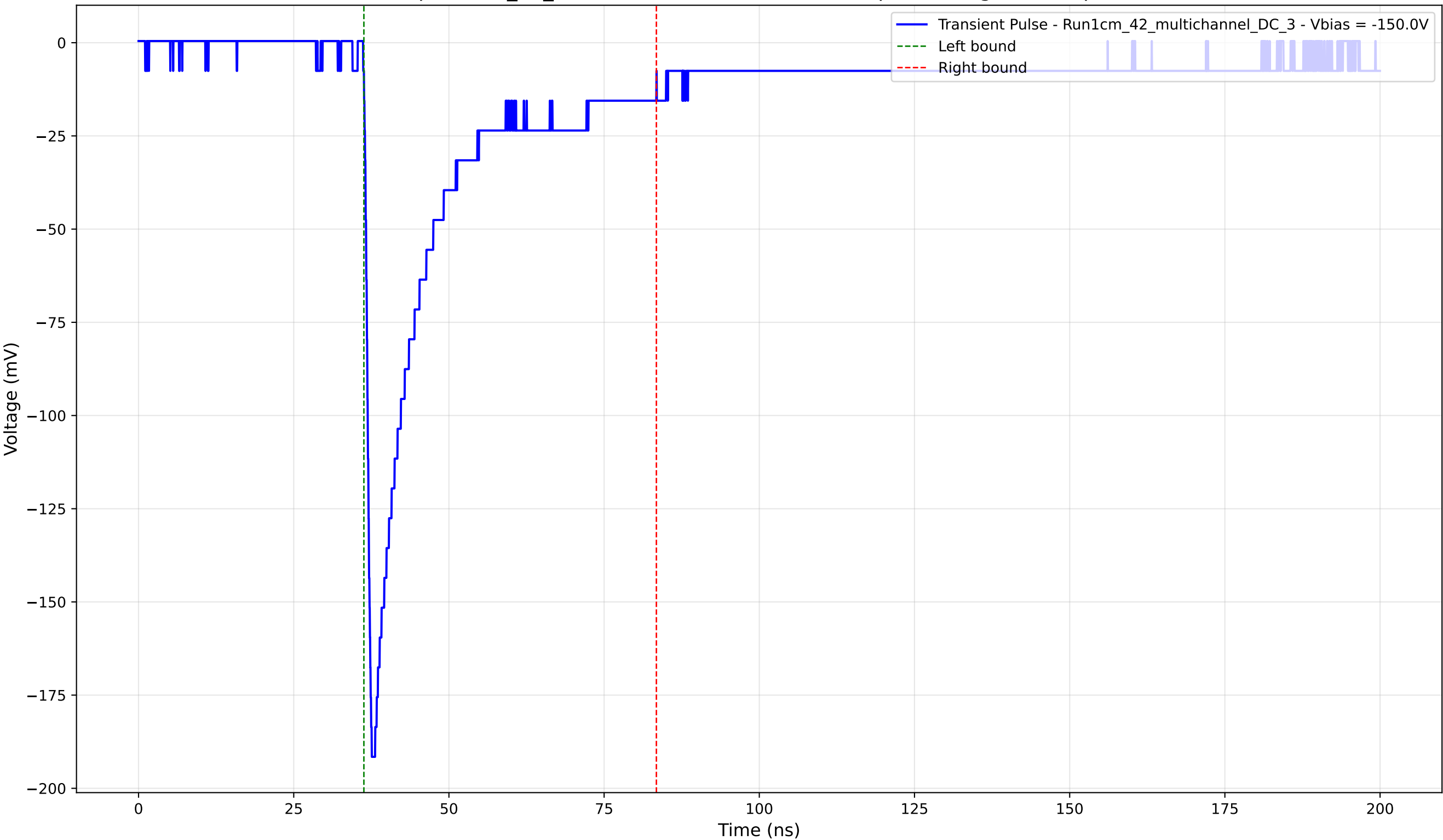
Transient Pulse - Sample: 1cm_42_multichannel - Position: 4150.0 \mu\text{m} - Charge: 40.60 pC - Rise Time: 0.99 ns
