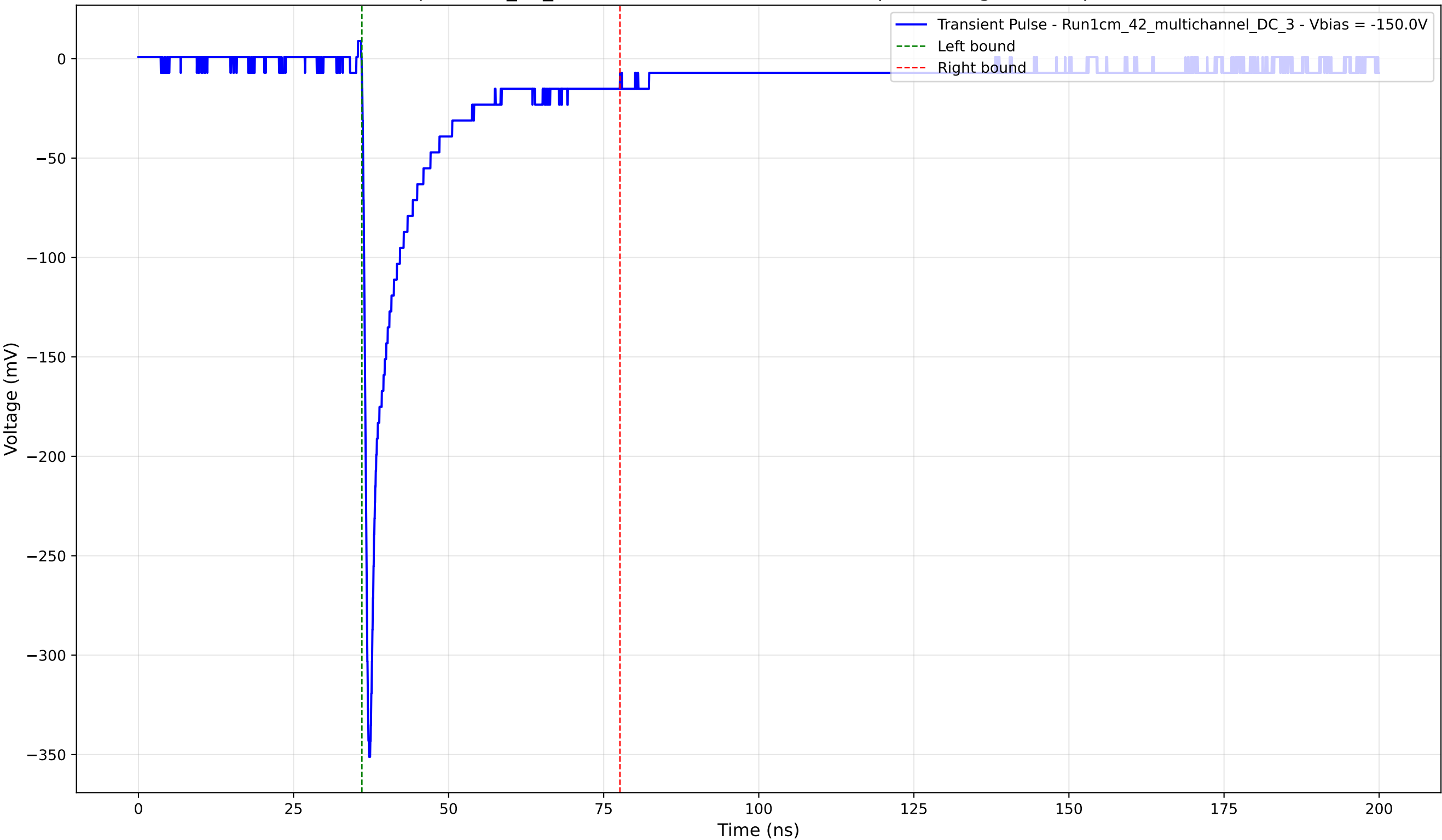
Transient Pulse - Sample: 1cm_42_multichannel - Position: 4710.0 \mu\text{m} - Charge: 42.01 pC - Rise Time: 0.79 ns
