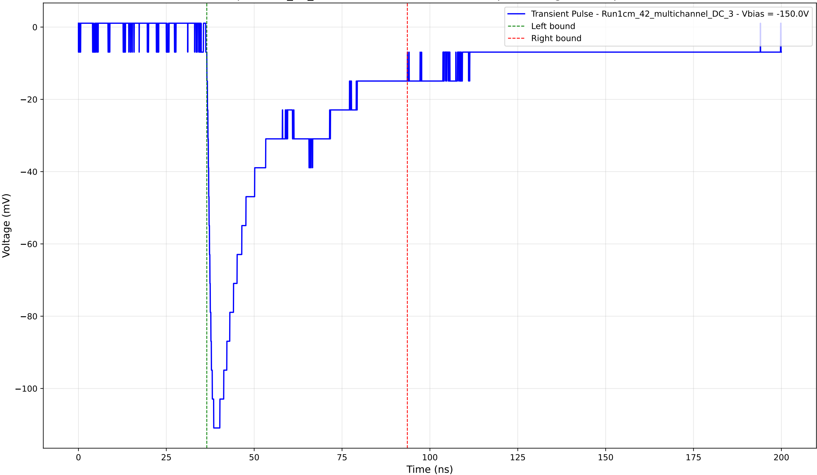
Transient Pulse - Sample: 1cm_42_multichannel - Position: 1755.0 \mu\text{m} - Charge: 41.64 pC - Rise Time: 1.55 ns
