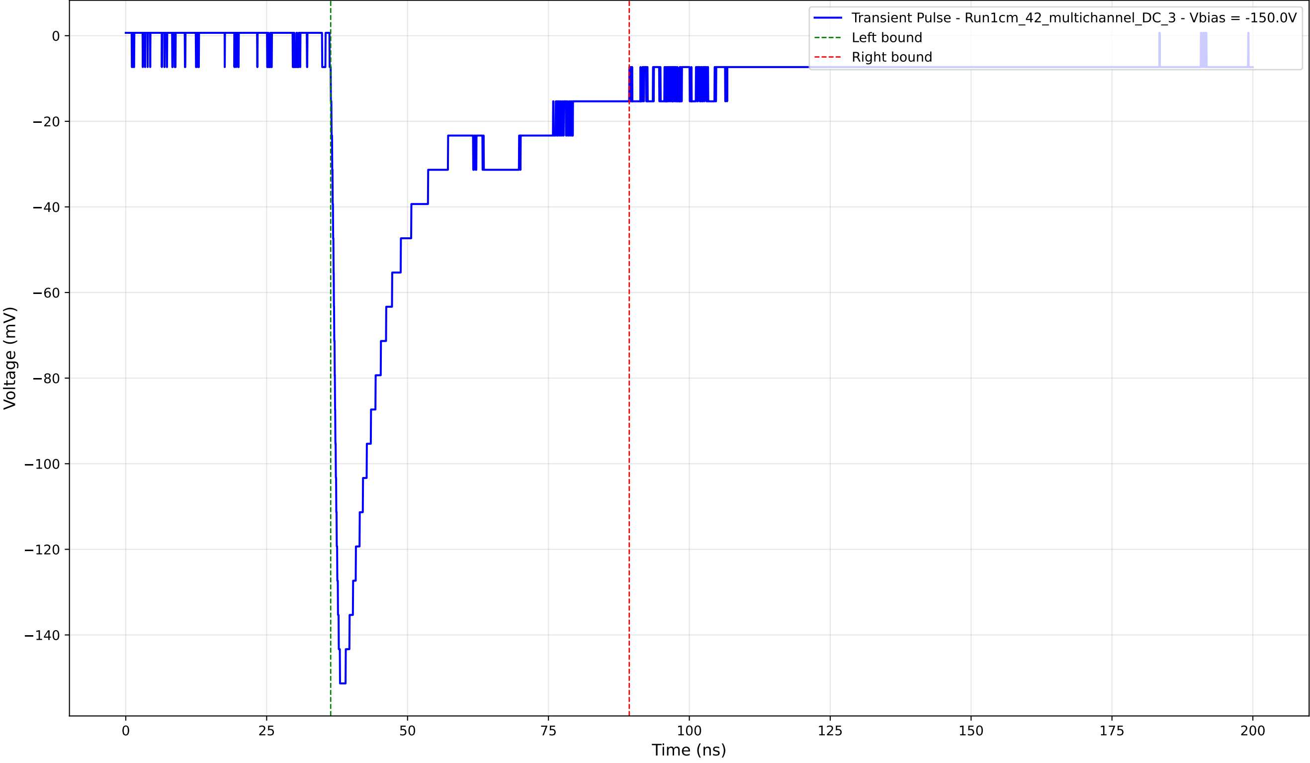
Transient Pulse - Sample: 1cm_42_multichannel - Position: 1260.0 \mu\text{m} - Charge: 44.35 pC - Rise Time: 1.40 ns
