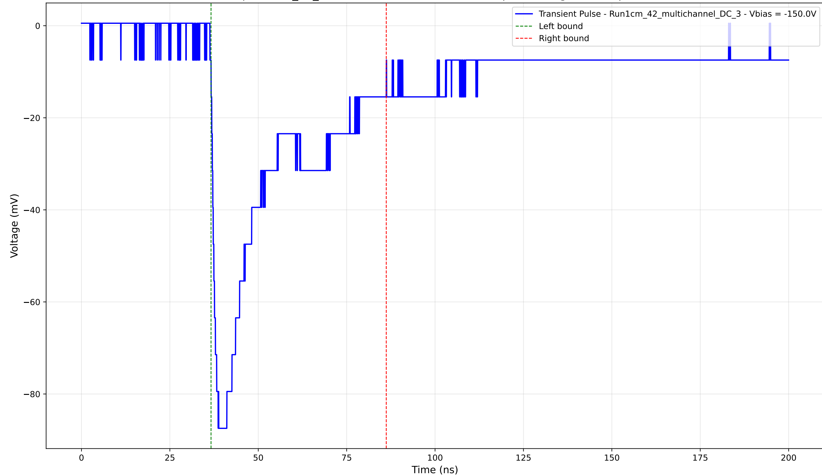
Transient Pulse - Sample: 1cm_42_multichannel - Position: 2790.0 \mu\text{m} - Charge: 34.52 pC - Rise Time: 1.60 ns
