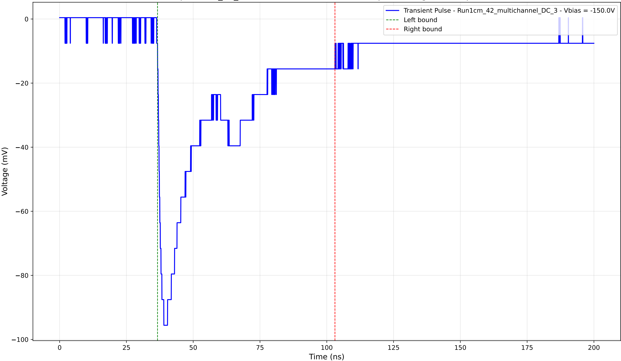
Transient Pulse - Sample: 1cm_42_multichannel - Position: 2050.0 \mu\text{m} - Charge: 43.08 pC - Rise Time: 1.64 ns
