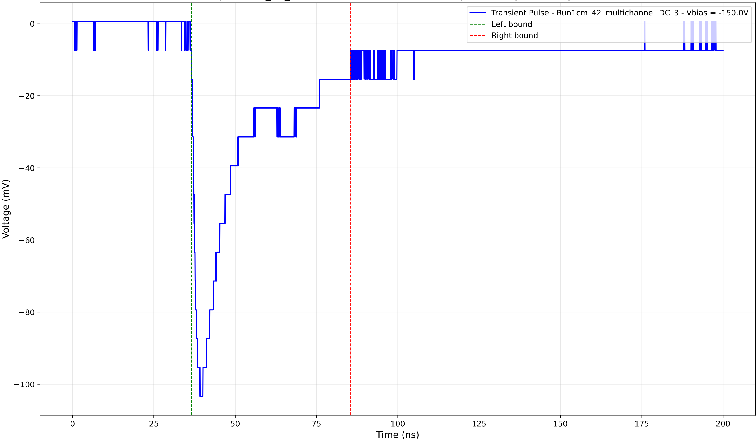
Transient Pulse - Sample: 1cm_42_multichannel - Position: 3070.0 \mu\text{m} - Charge: 35.11 pC - Rise Time: 1.83 ns
