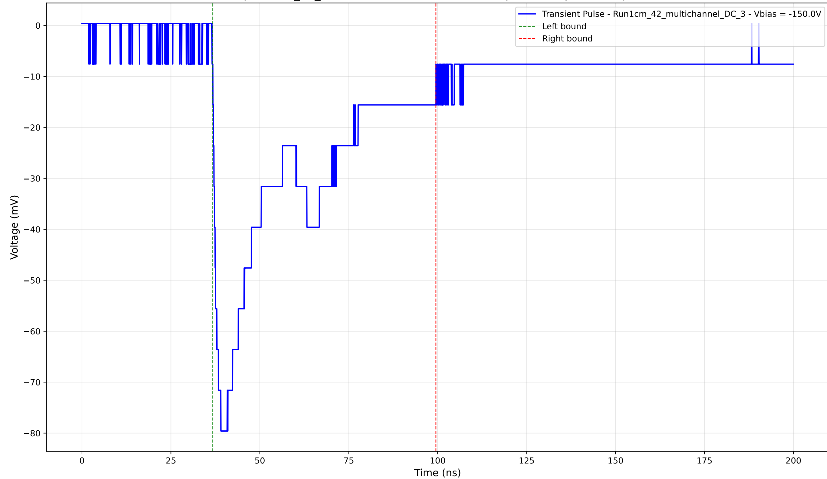
Transient Pulse - Sample: 1cm_42_multichannel - Position: 2545.0 \mu\text{m} - Charge: 38.28 pC - Rise Time: 2.26 ns
