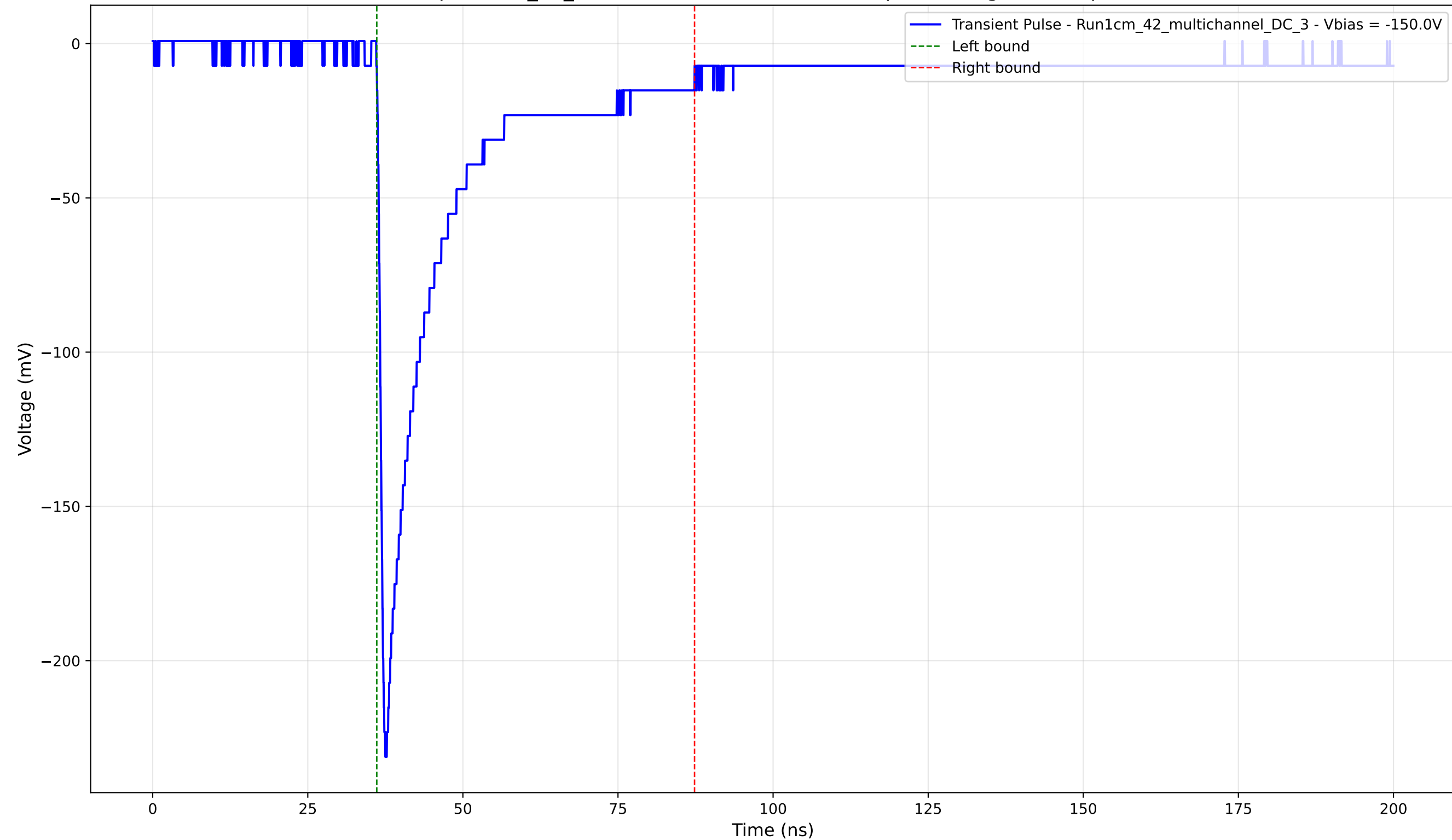
Transient Pulse - Sample: 1cm_42_multichannel - Position: 660.0 \mu\text{m} - Charge: 47.19 pC - Rise Time: 1.02 ns
