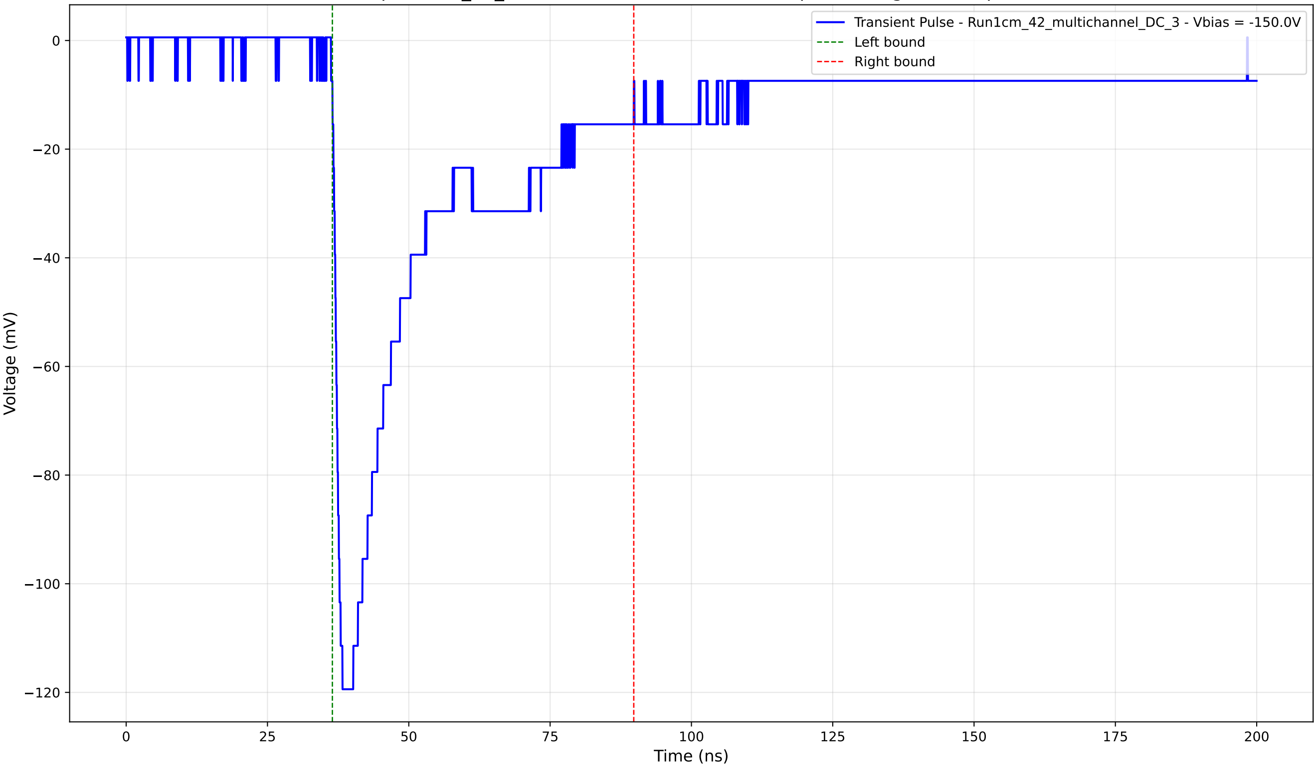
Transient Pulse - Sample: 1cm_42_multichannel - Position: 1625.0 \mu\text{m} - Charge: 41.78 pC - Rise Time: 1.45 ns
