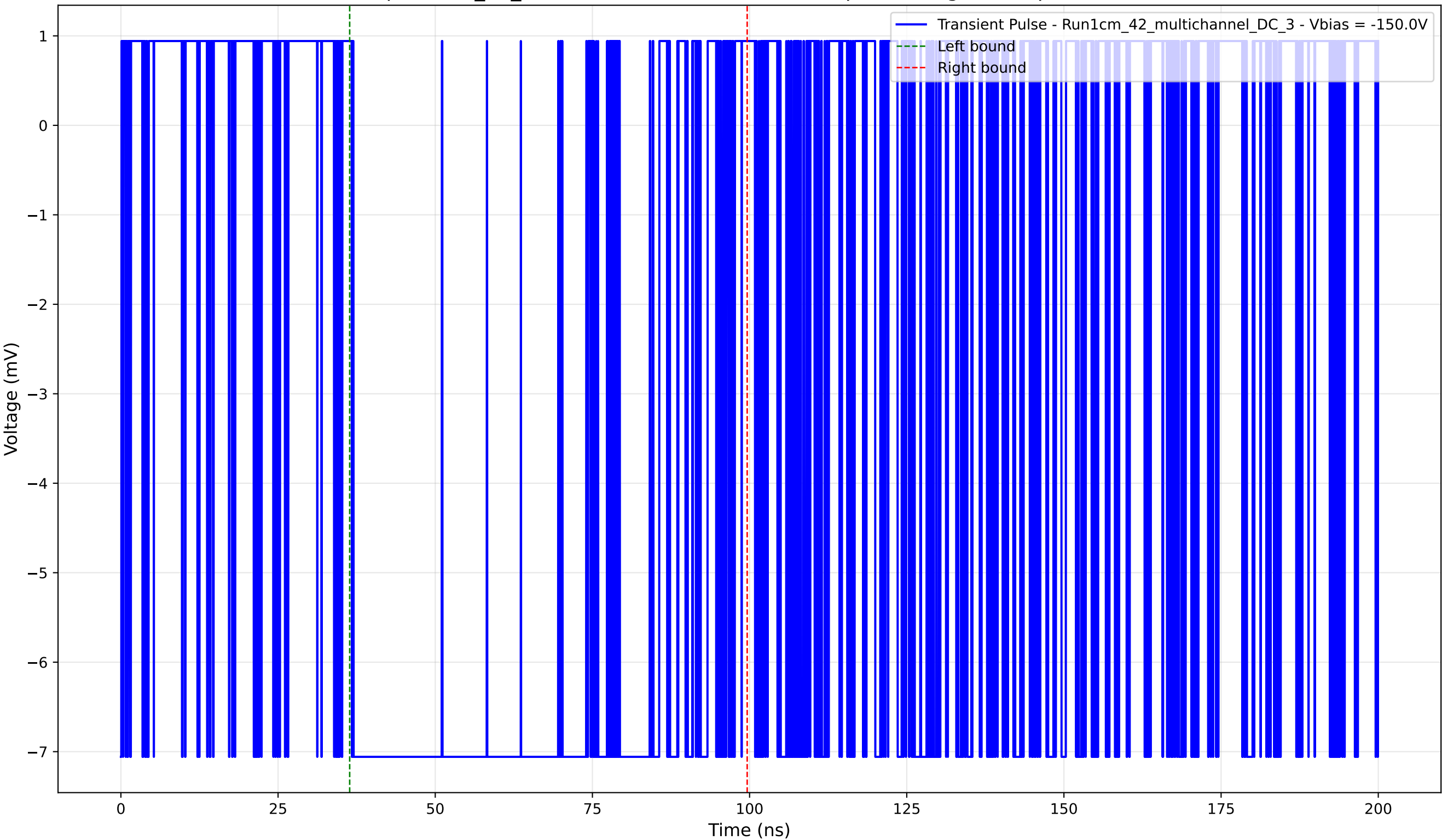
Transient Pulse - Sample: 1cm_42_multichannel - Position: 1855.0 \mu\text{m} - Charge: 7.10 pC - Rise Time: 0.00 ns (N/A)
