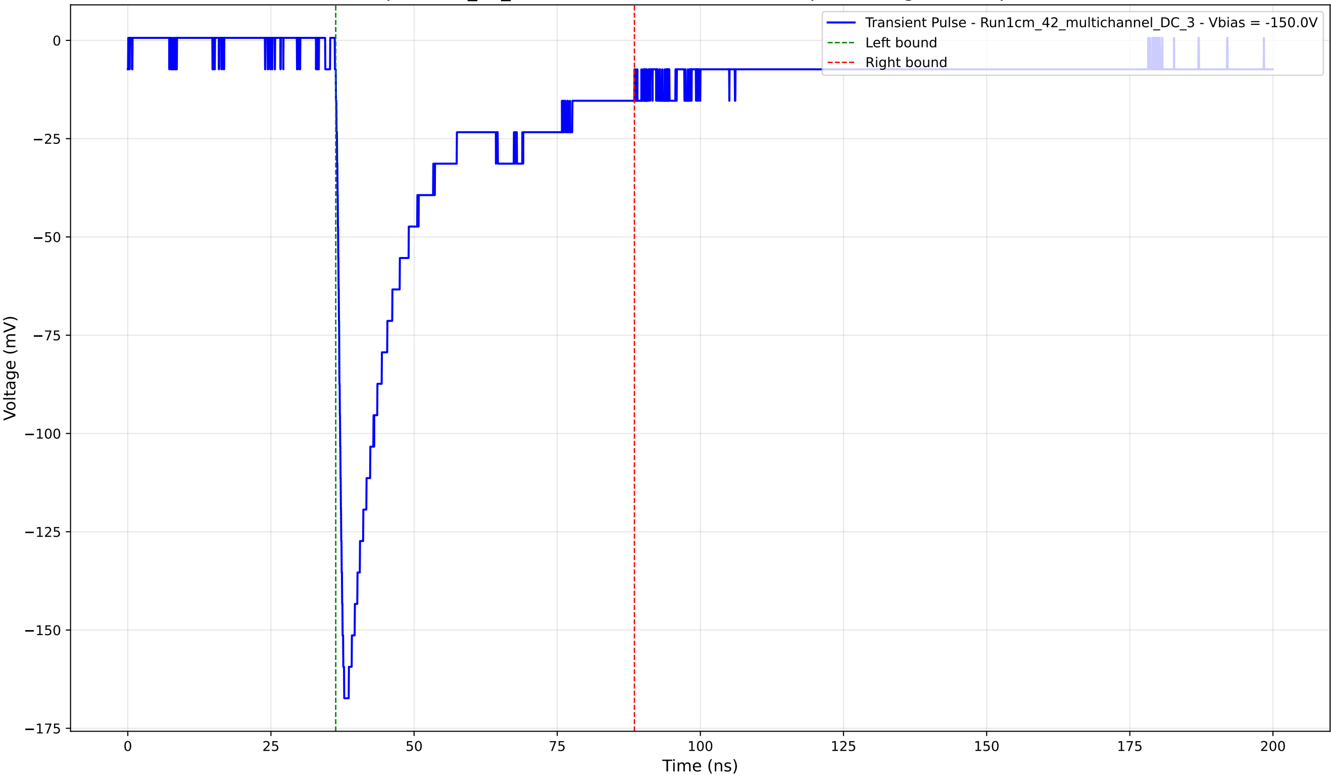
Transient Pulse - Sample: 1cm_42_multichannel - Position: 1070.0 \mu\text{m} - Charge: 45.00 pC - Rise Time: 1.08 ns
