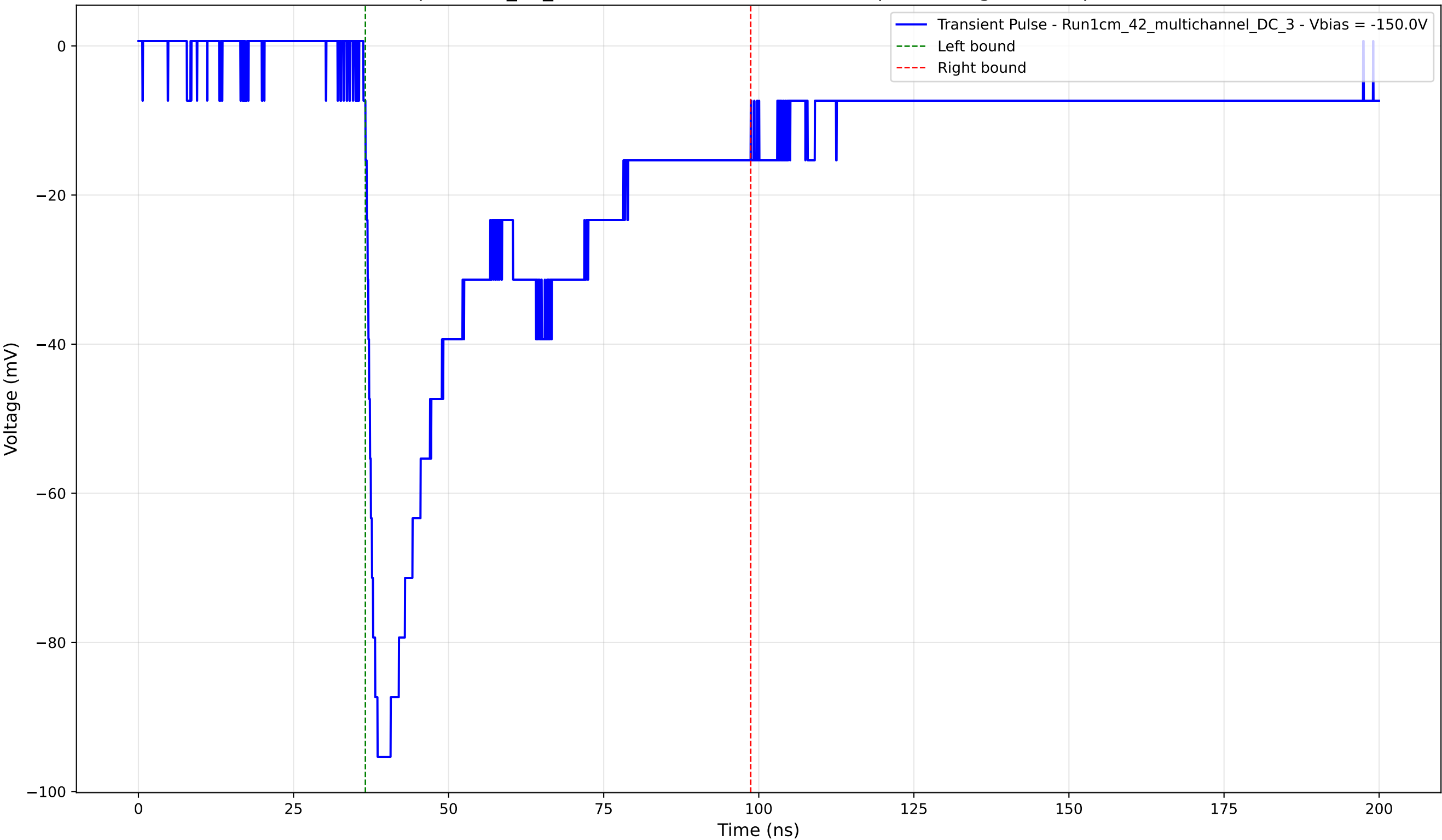
Transient Pulse - Sample: 1cm_42_multichannel - Position: 1970.0 \mu\text{m} - Charge: 41.16 pC - Rise Time: 1.57 ns
