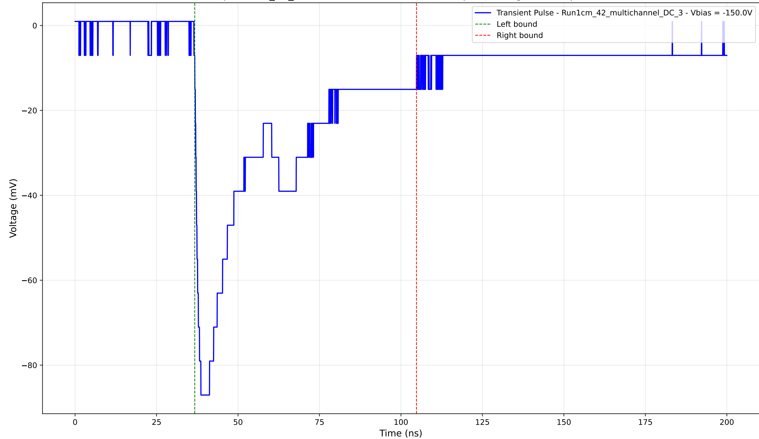
Transient Pulse - Sample: 1cm_42_multichannel - Position: 2125.0 \mu\text{m} - Charge: 42.24 pC - Rise Time: 1.46 ns
