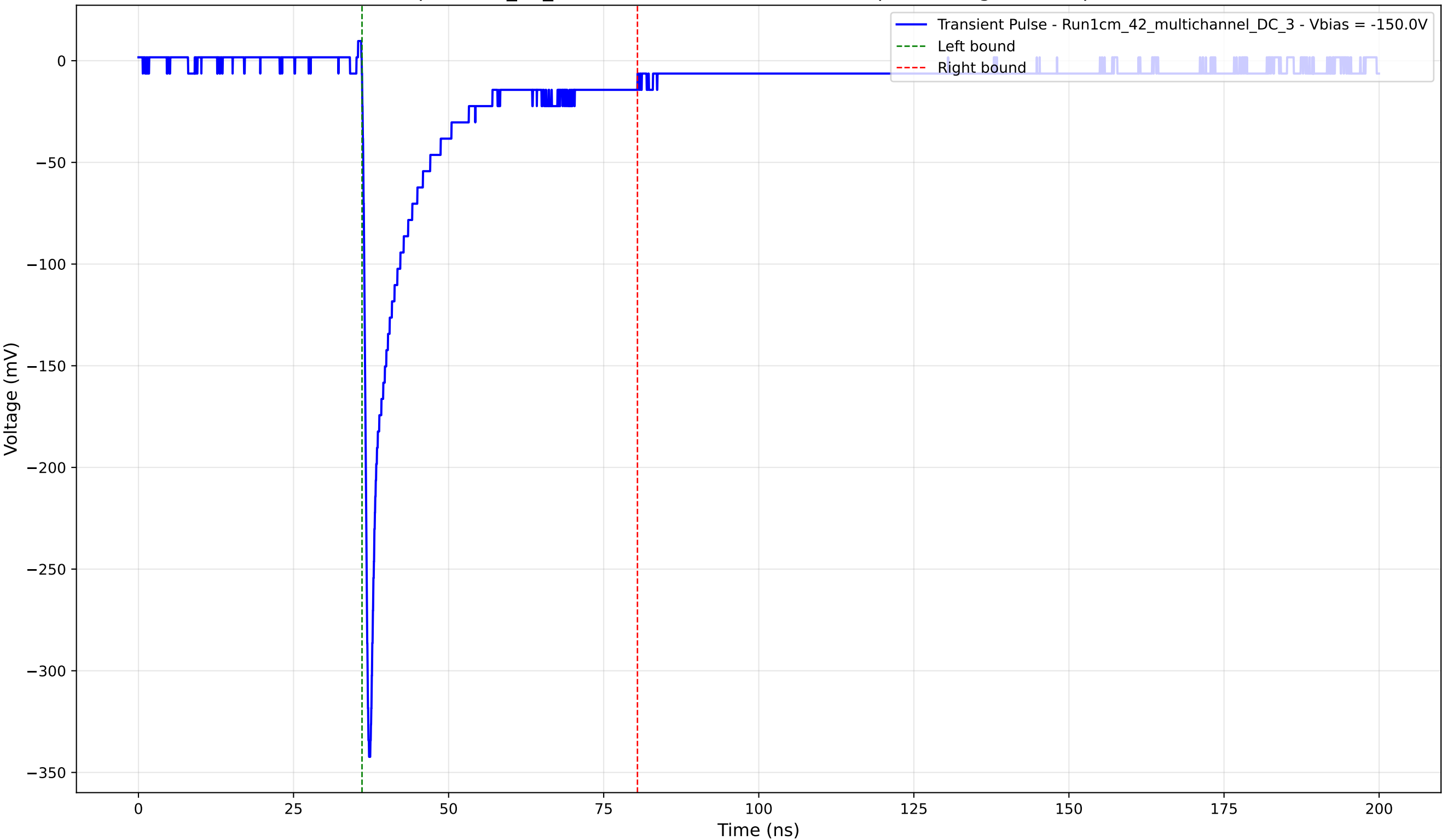
Transient Pulse - Sample: 1cm_42_multichannel - Position: 4695.0 \mu\text{m} - Charge: 41.92 pC - Rise Time: 0.80 ns
