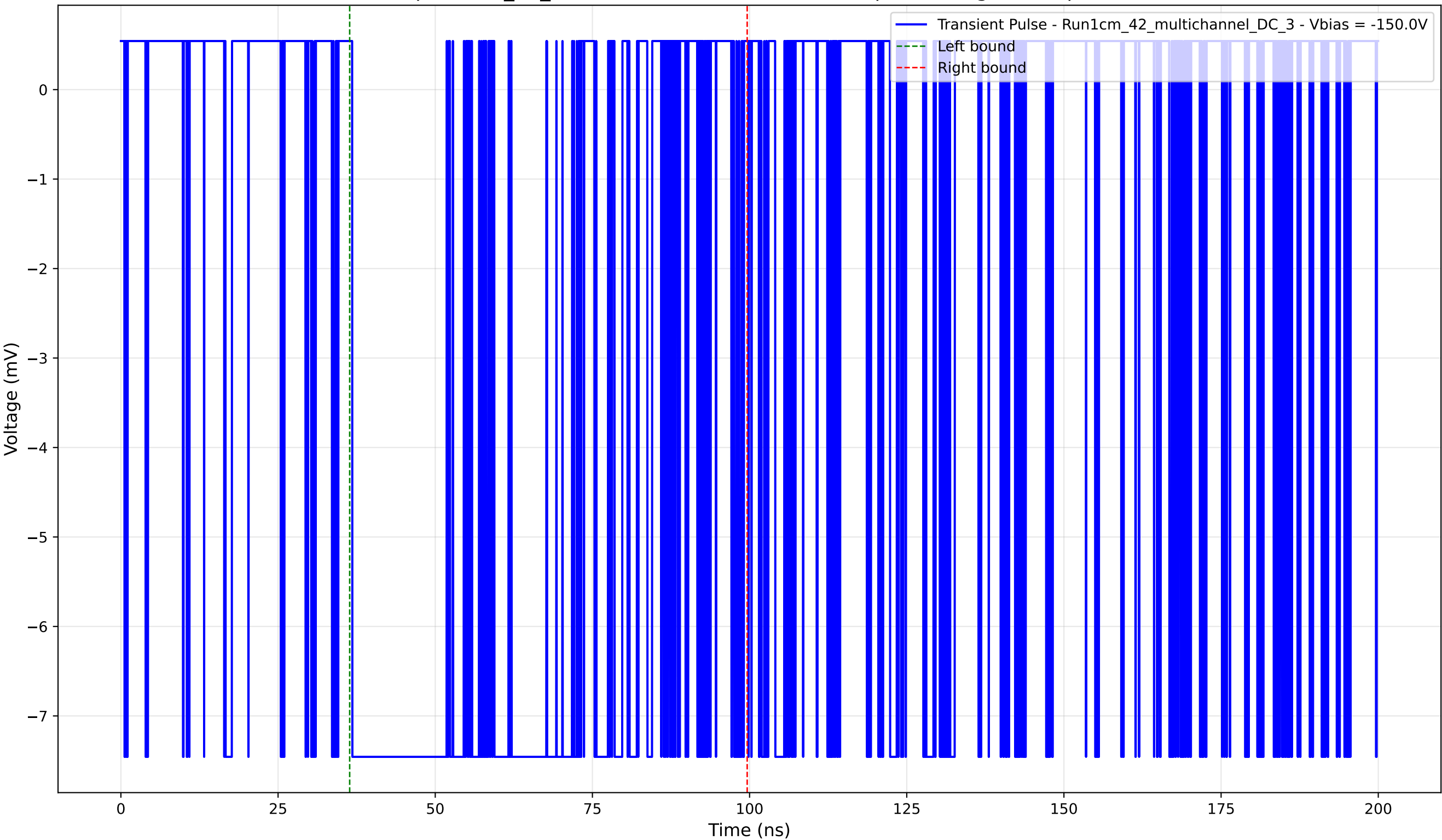
Transient Pulse - Sample: 1cm_42_multichannel - Position: 1355.0 \mu\text{m} - Charge: 6.12 pC - Rise Time: 0.02 ns
