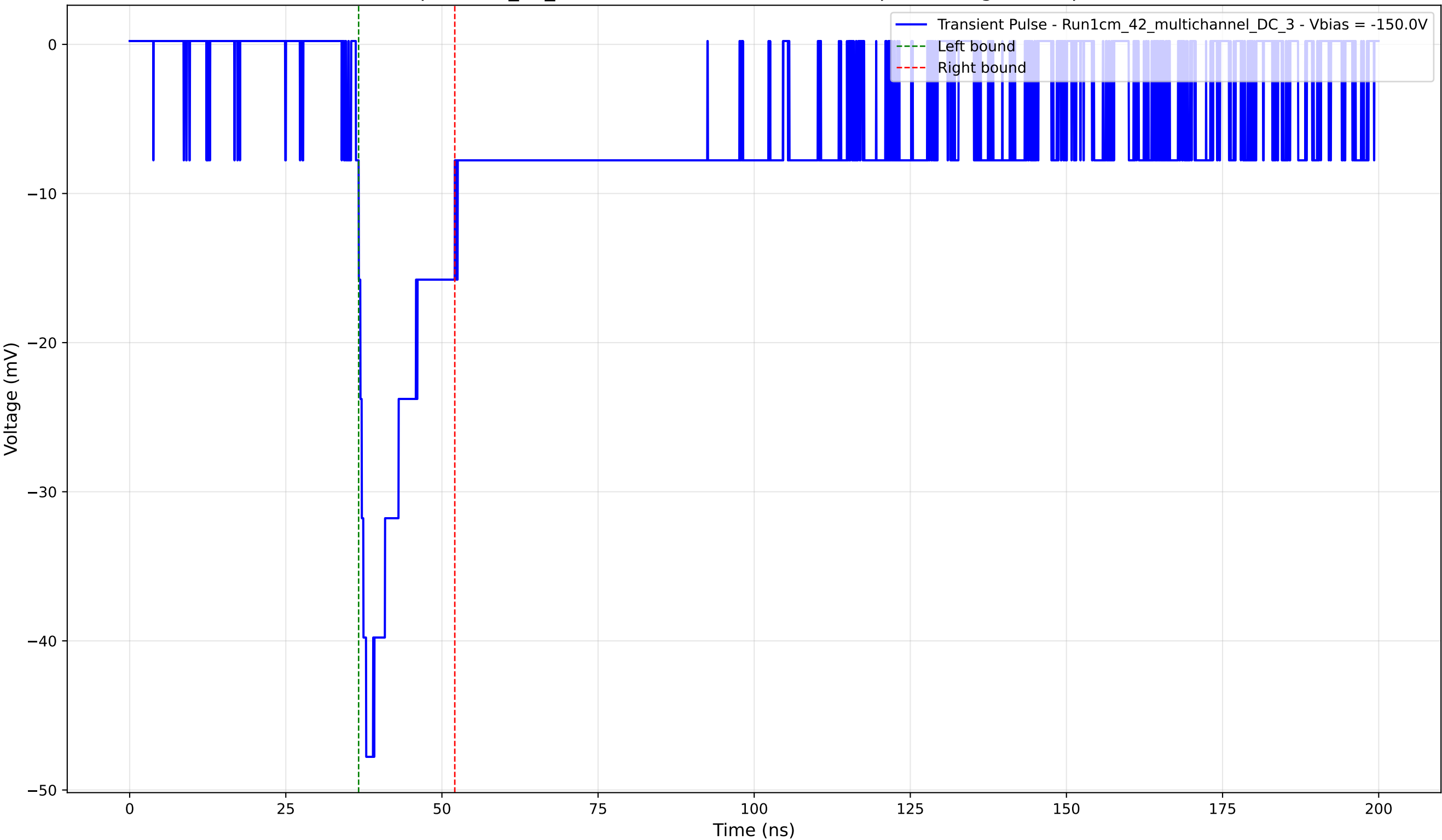
Transient Pulse - Sample: 1cm_42_multichannel - Position: 3850.0 \mu\text{m} - Charge: 7.98 pC - Rise Time: 1.65 ns
