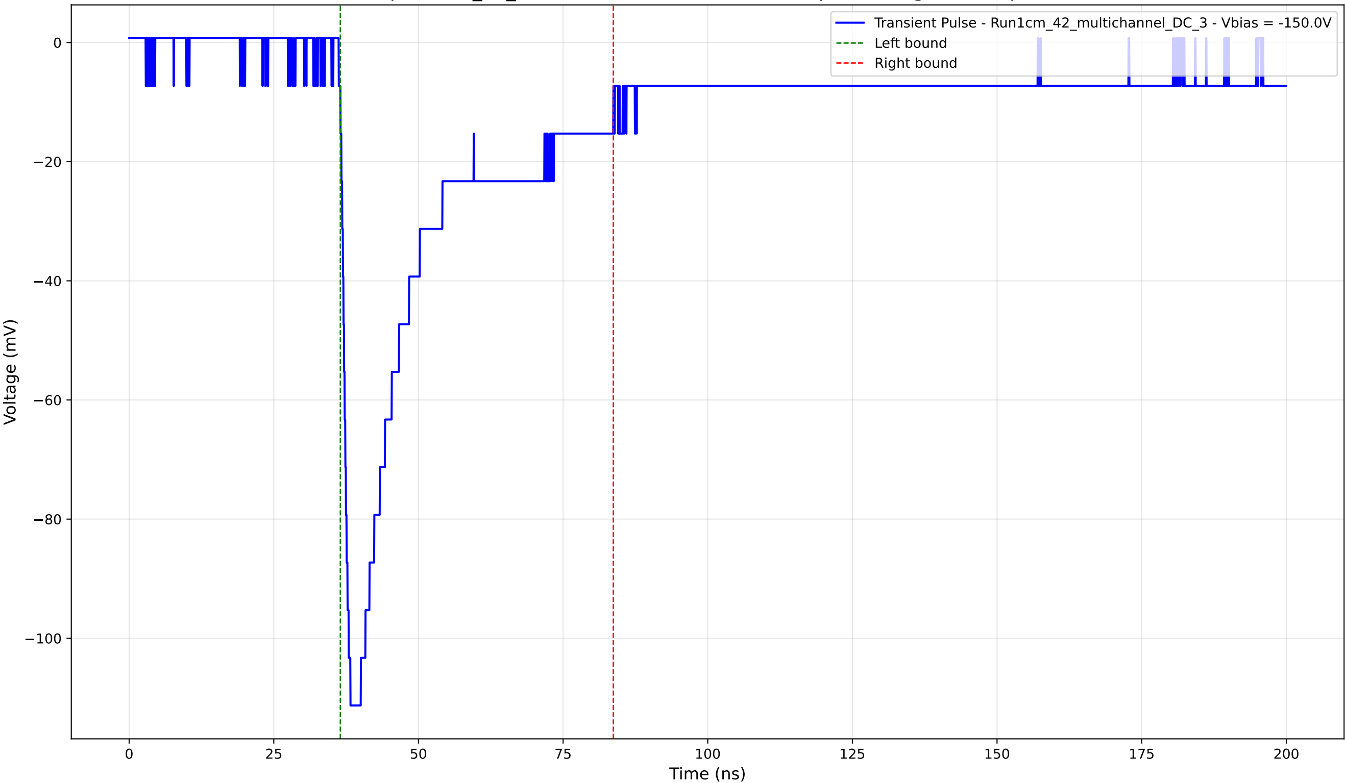
Transient Pulse - Sample: 1cm_42_multichannel - Position: 3460.0 \mu\text{m} - Charge: 33.86 pC - Rise Time: 1.43 ns
