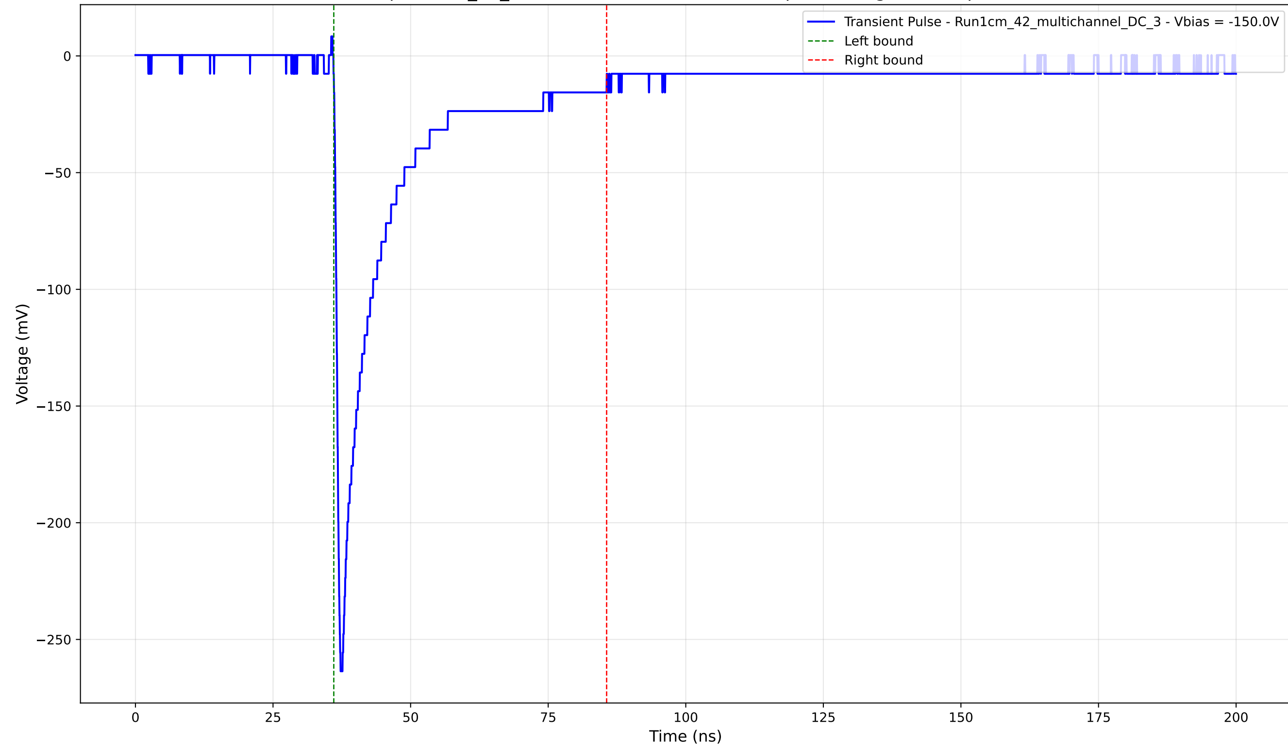
Transient Pulse - Sample: 1cm_42_multichannel - Position: 520.0 \mu\text{m} - Charge: 48.81 pC - Rise Time: 0.89 ns
