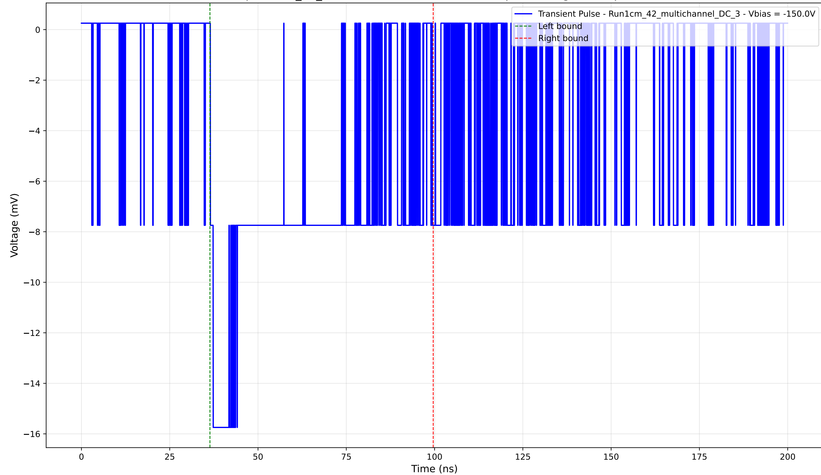
Transient Pulse - Sample: 1cm_42_multichannel - Position: 1340.0 \mu\text{m} - Charge: 8.89 pC - Rise Time: 0.82 ns
