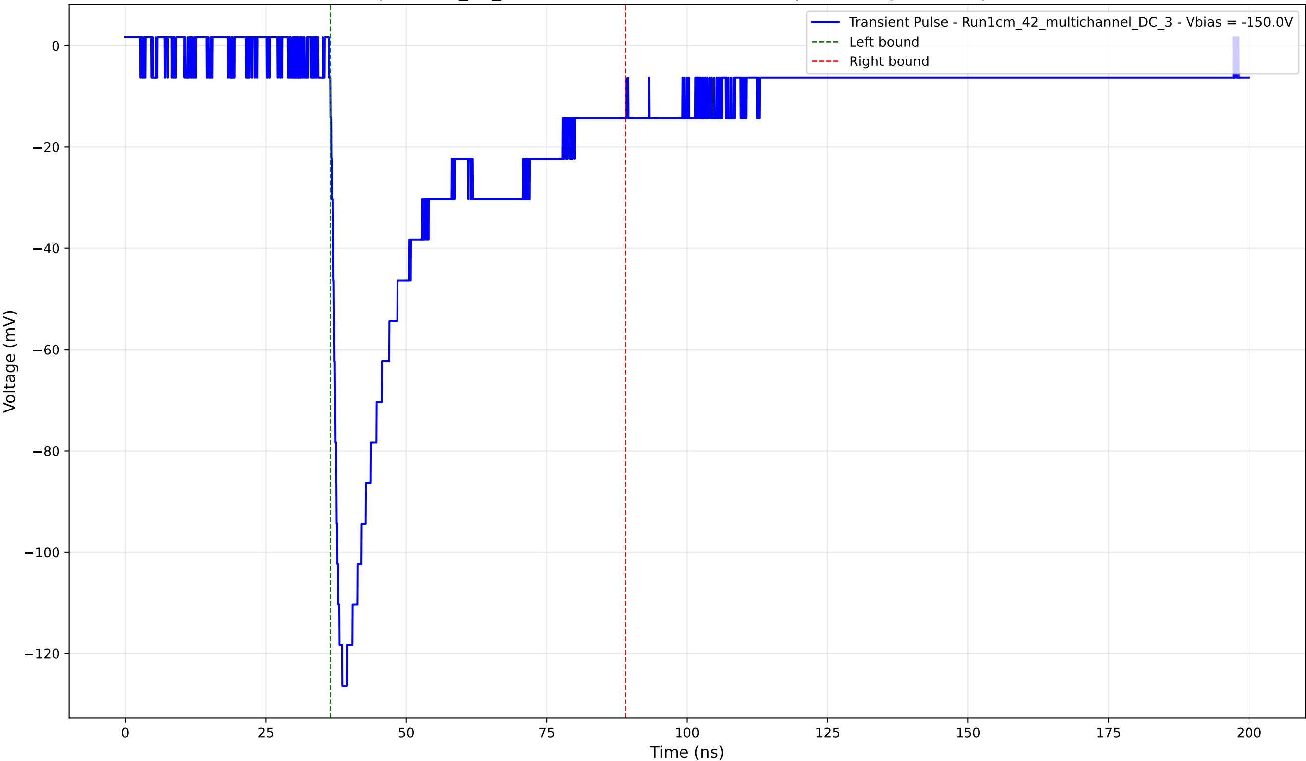
Transient Pulse - Sample: 1cm_42_multichannel - Position: 1565.0 \mu\text{m} - Charge: 41.15 pC - Rise Time: 1.56 ns
