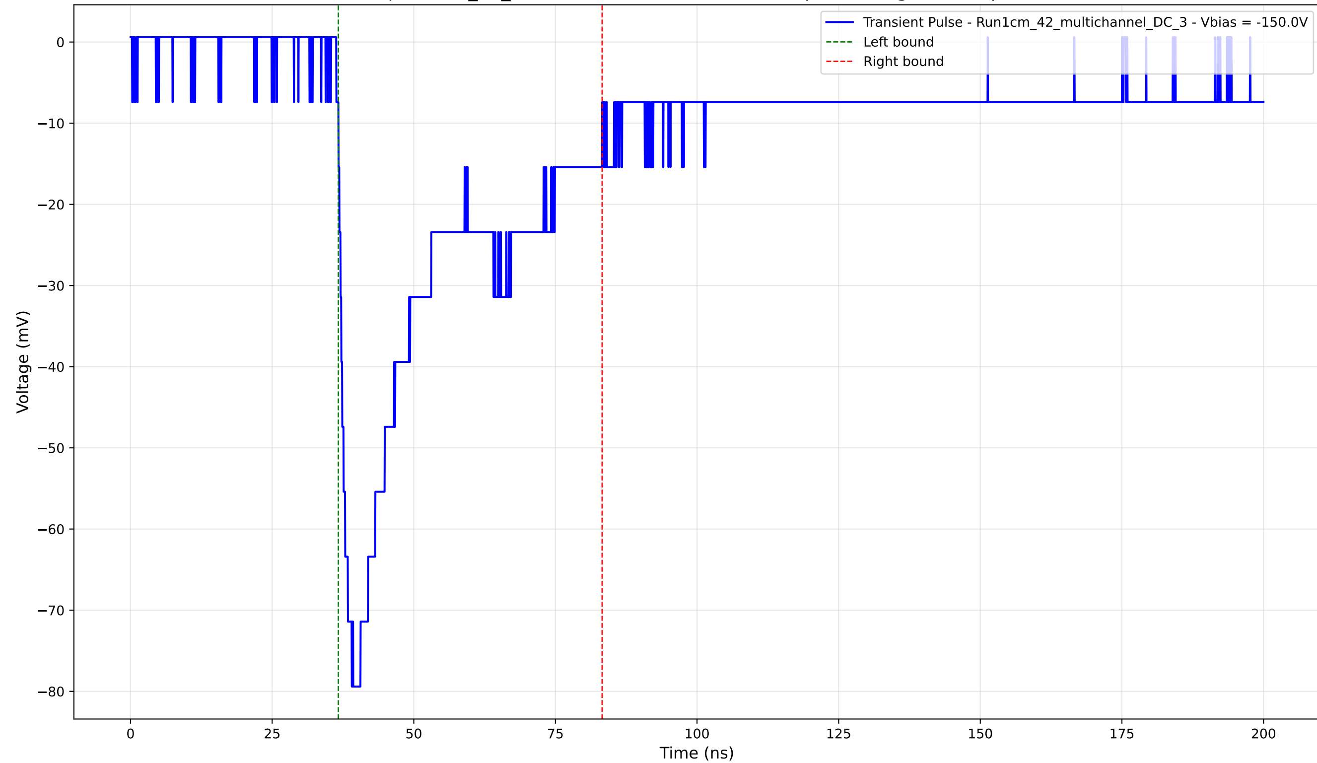
Transient Pulse - Sample: 1cm_42_multichannel - Position: 2810.0 \mu\text{m} - Charge: 29.50 pC - Rise Time: 2.36 ns
