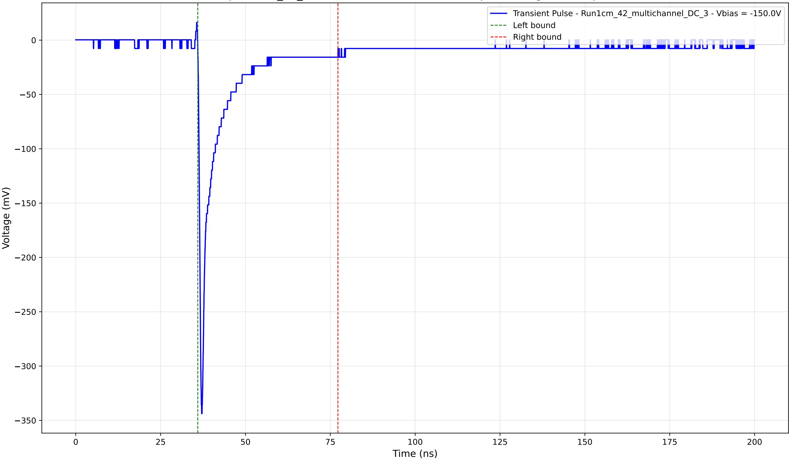
Transient Pulse - Sample: 1cm_42_multichannel - Position: 4815.0 \mu\text{m} - Charge: 37.96 pC - Rise Time: 0.77 ns
