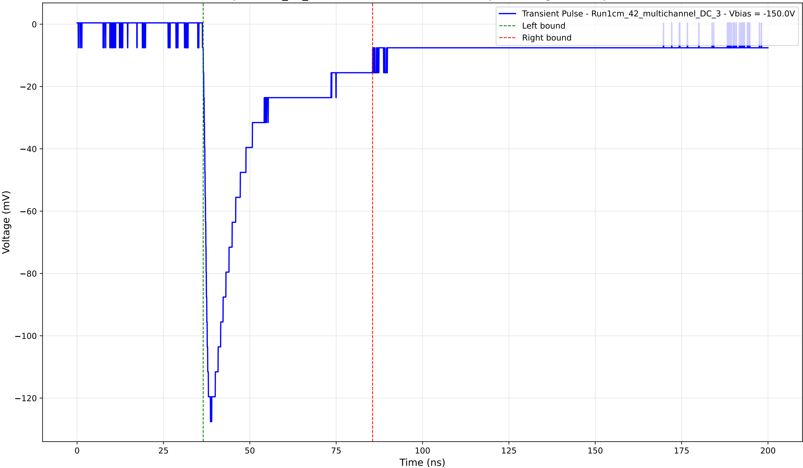
Transient Pulse - Sample: 1cm_42_multichannel - Position: 3560.0 \mu\text{m} - Charge: 36.61 pC - Rise Time: 1.49 ns
