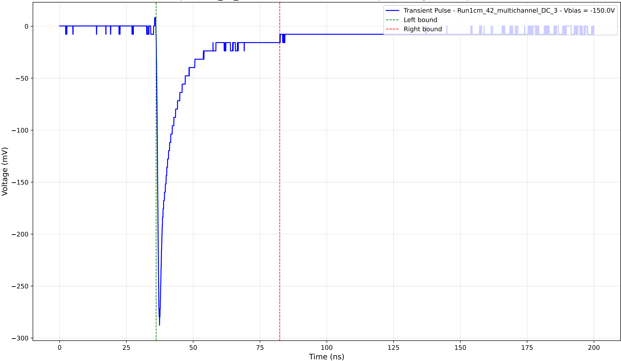
Transient Pulse - Sample: 1cm_42_multichannel - Position: 4550.0 \mu\text{m} - Charge: 41.67 pC - Rise Time: 0.89 ns
