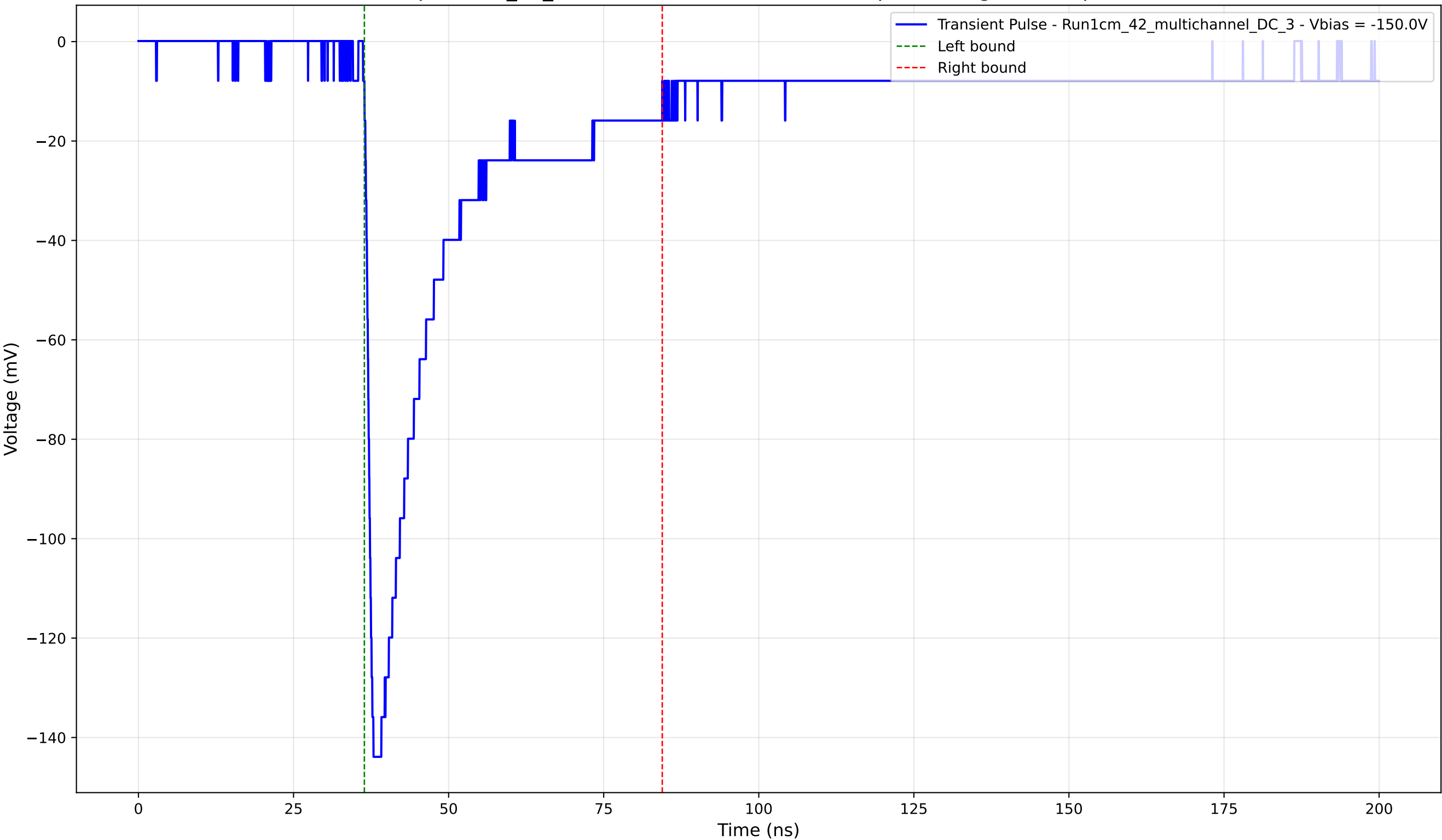
Transient Pulse - Sample: 1cm_42_multichannel - Position: 3775.0 \mu\text{m} - Charge: 39.01 pC - Rise Time: 1.26 ns
