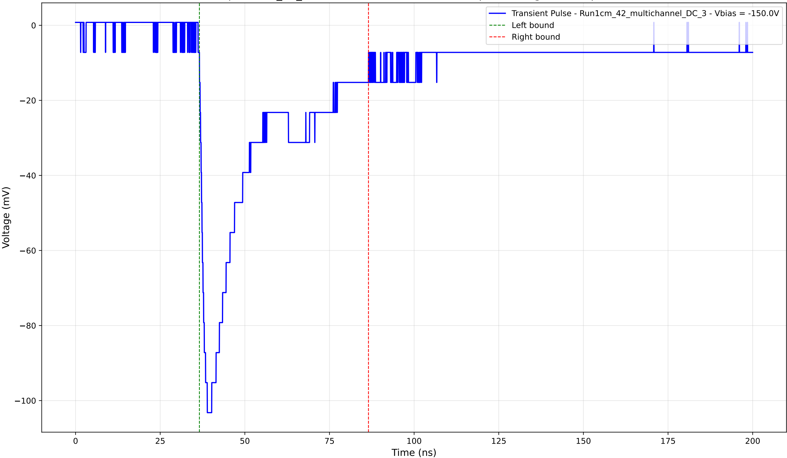
Transient Pulse - Sample: 1cm_42_multichannel - Position: 3020.0 \mu\text{m} - Charge: 36.12 pC - Rise Time: 1.81 ns
