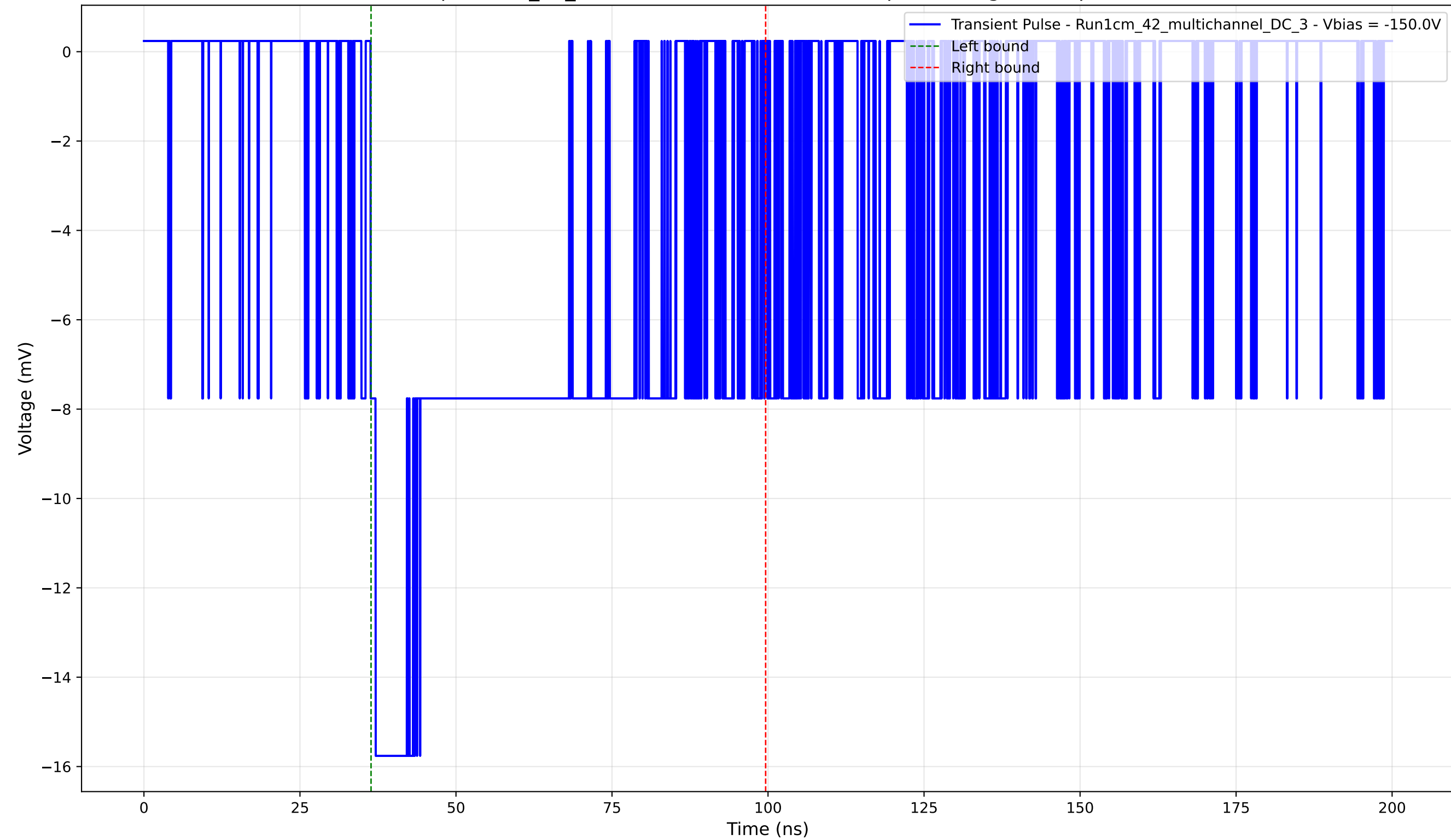
Transient Pulse - Sample: 1cm_42_multichannel - Position: 875.0 \mu\text{m} - Charge: 8.90 pC - Rise Time: 0.82 ns
