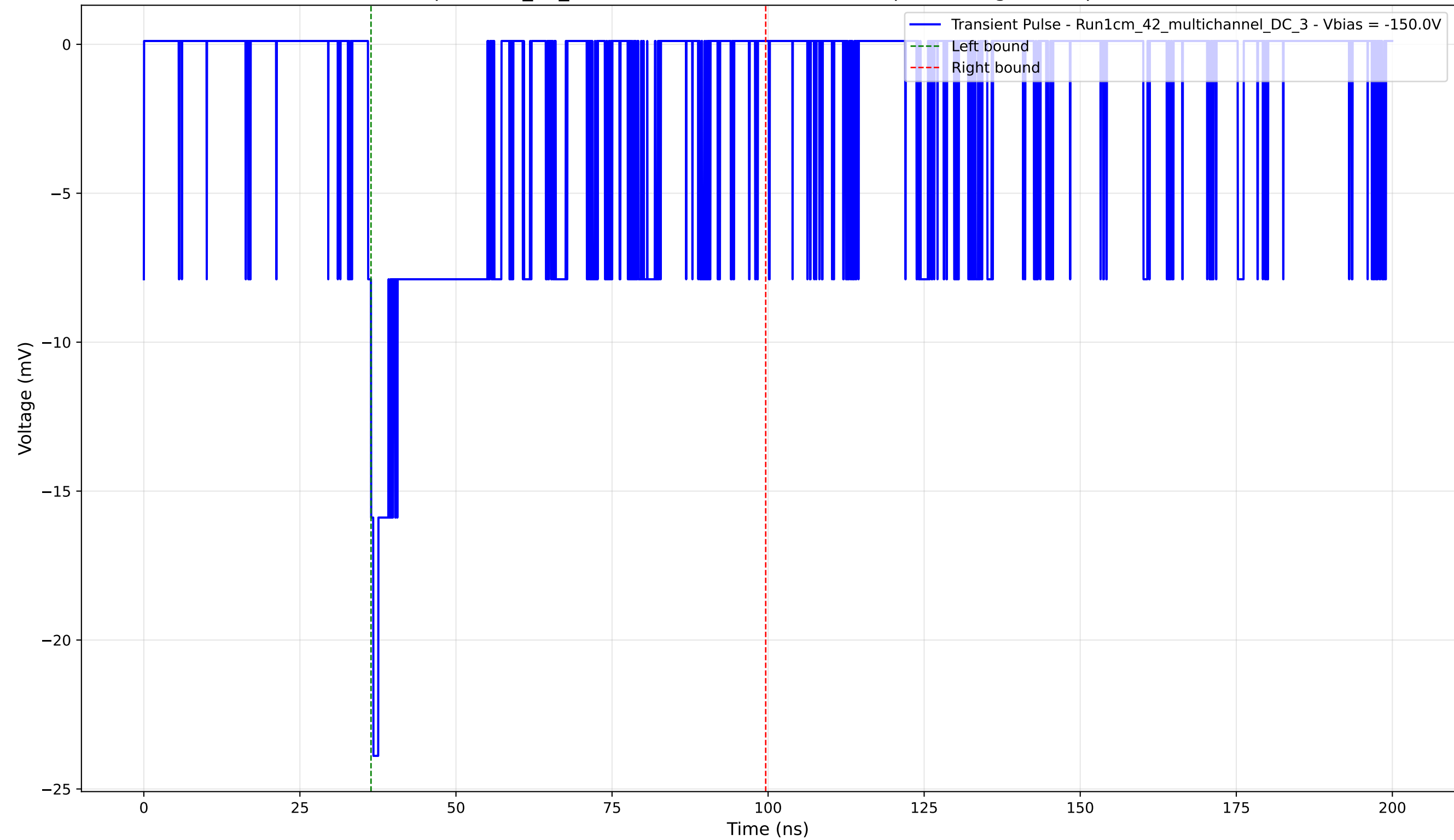
Transient Pulse - Sample: 1cm_42_multichannel - Position: 4885.0 \mu\text{m} - Charge: 5.74 pC - Rise Time: 0.85 ns
