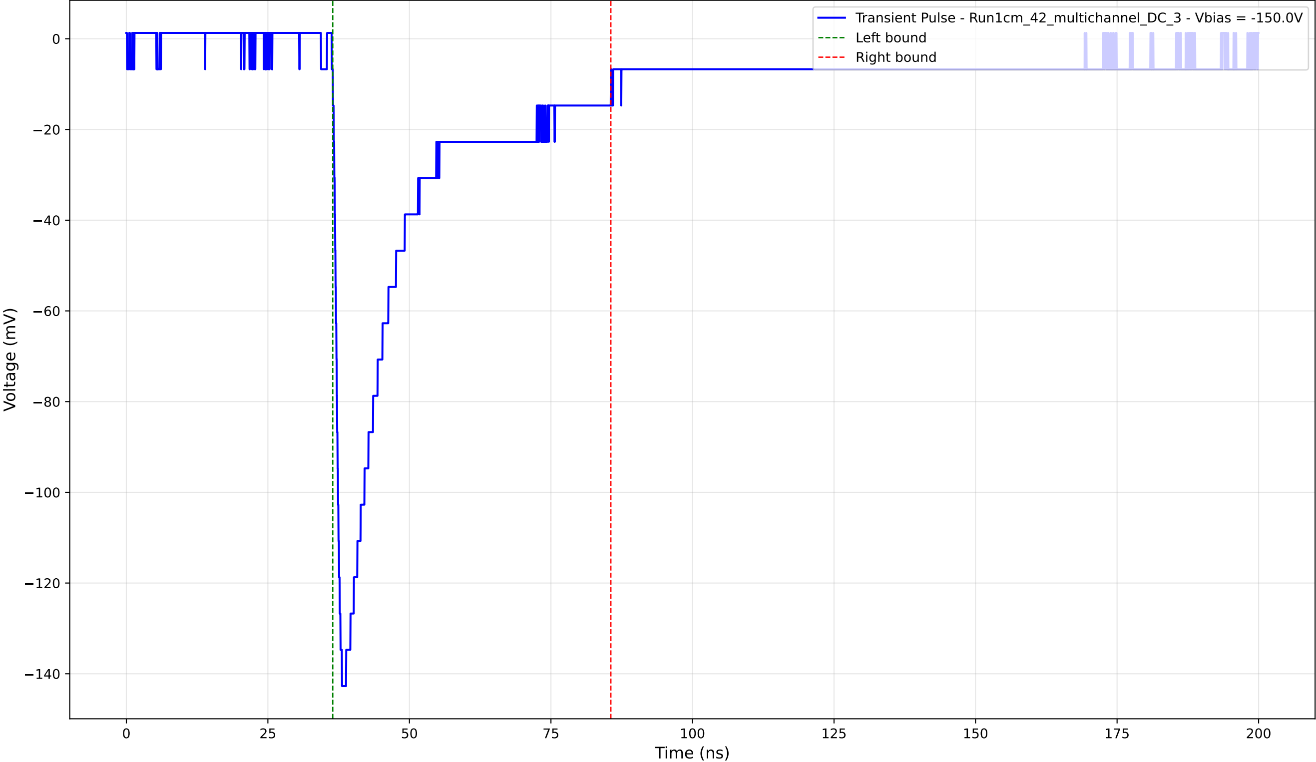
Transient Pulse - Sample: 1cm_42_multichannel - Position: 3730.0 \mu\text{m} - Charge: 37.87 pC - Rise Time: 1.34 ns
