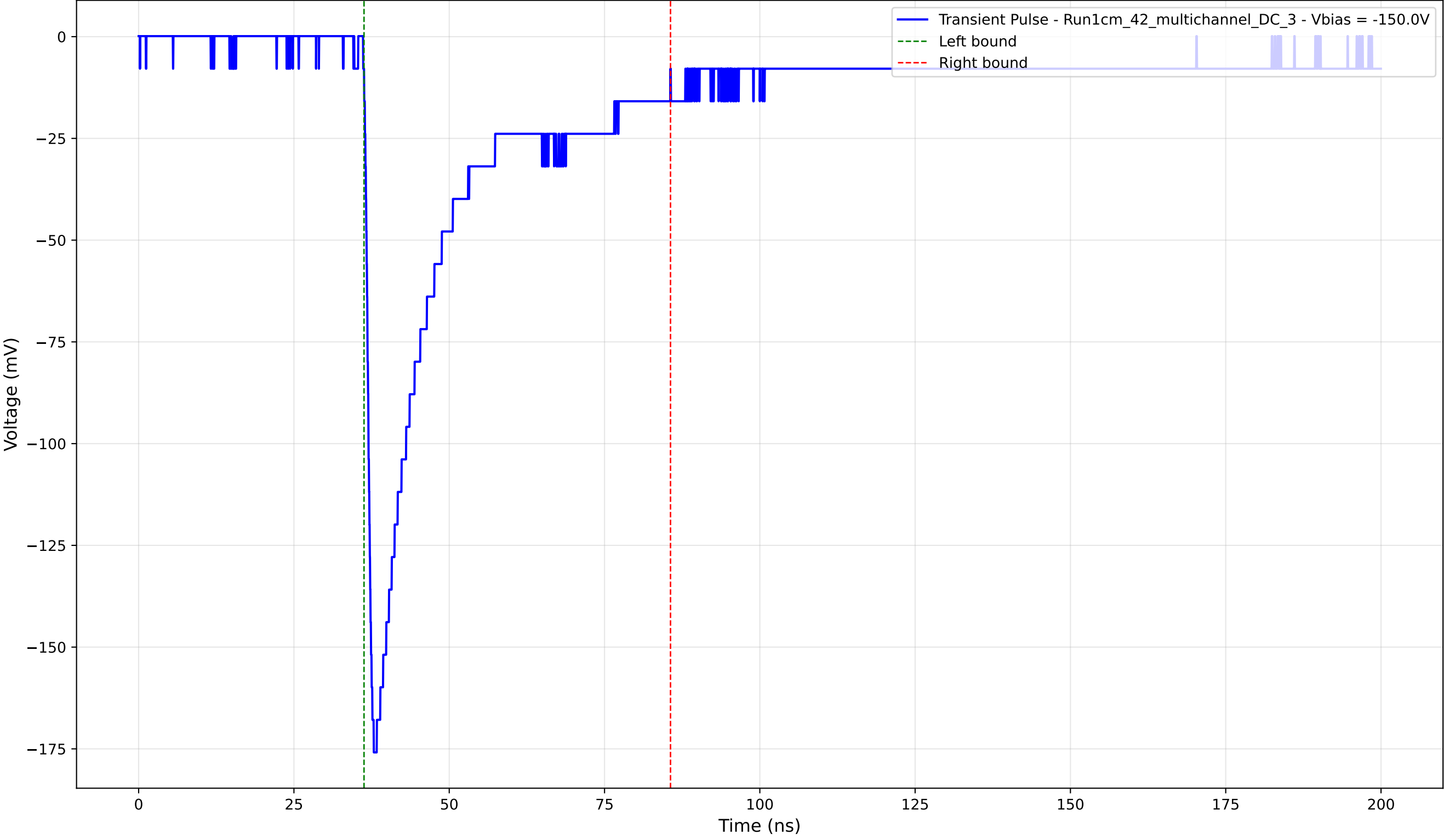
Transient Pulse - Sample: 1cm_42_multichannel - Position: 1020.0 \mu\text{m} - Charge: 44.61 pC - Rise Time: 1.10 ns
