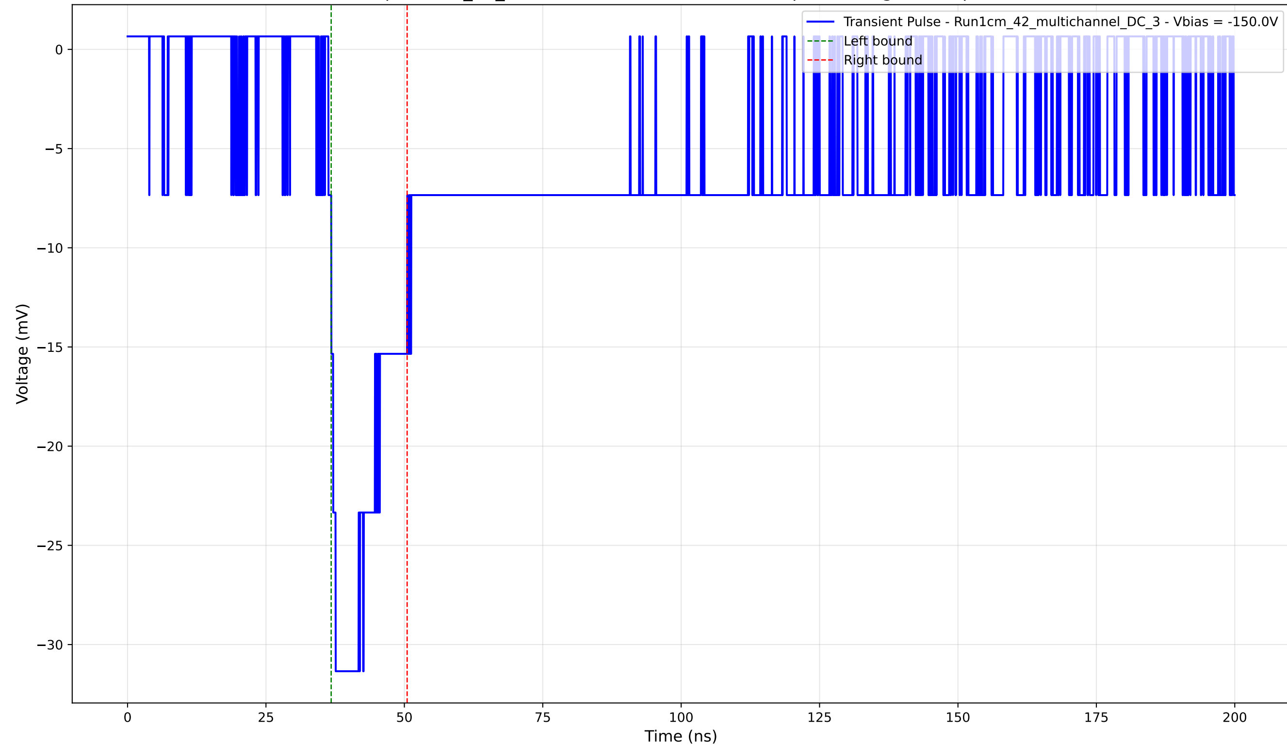
Transient Pulse - Sample: 1cm_42_multichannel - Position: 1400.0 \mu\text{m} - Charge: 6.19 pC - Rise Time: 1.31 ns
