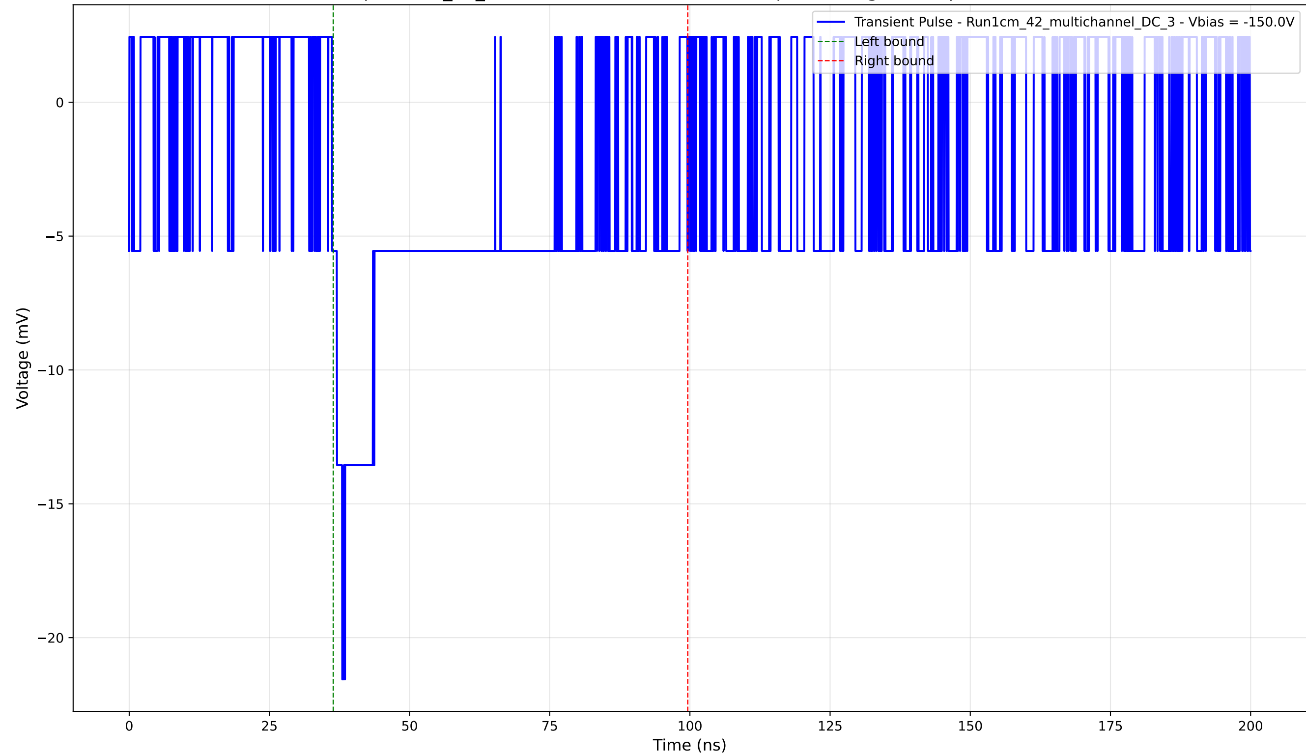
Transient Pulse - Sample: 1cm_42_multichannel - Position: 3915.0 \mu\text{m} - Charge: 6.82 pC - Rise Time: 0.00 ns (N/A)
