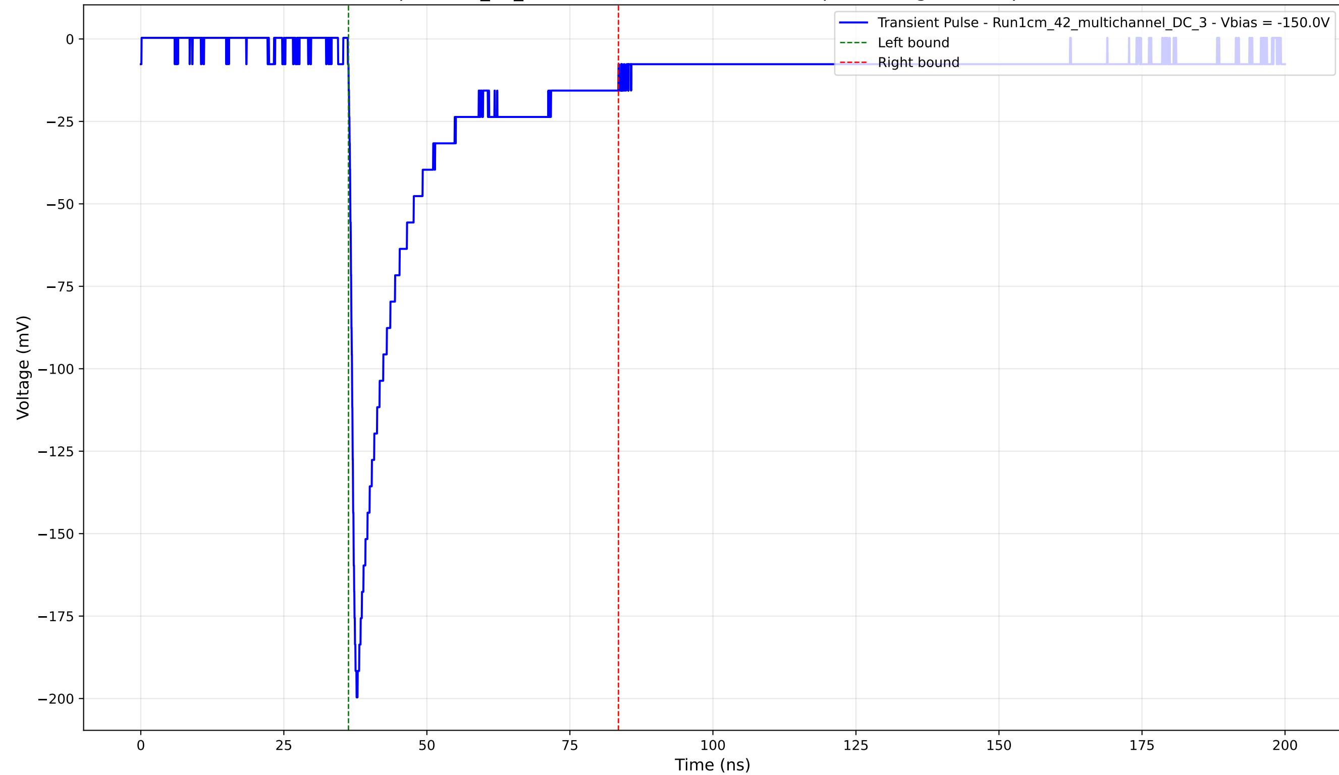
Transient Pulse - Sample: 1cm_42_multichannel - Position: 4165.0 \mu\text{m} - Charge: 40.87 pC - Rise Time: 1.03 ns
