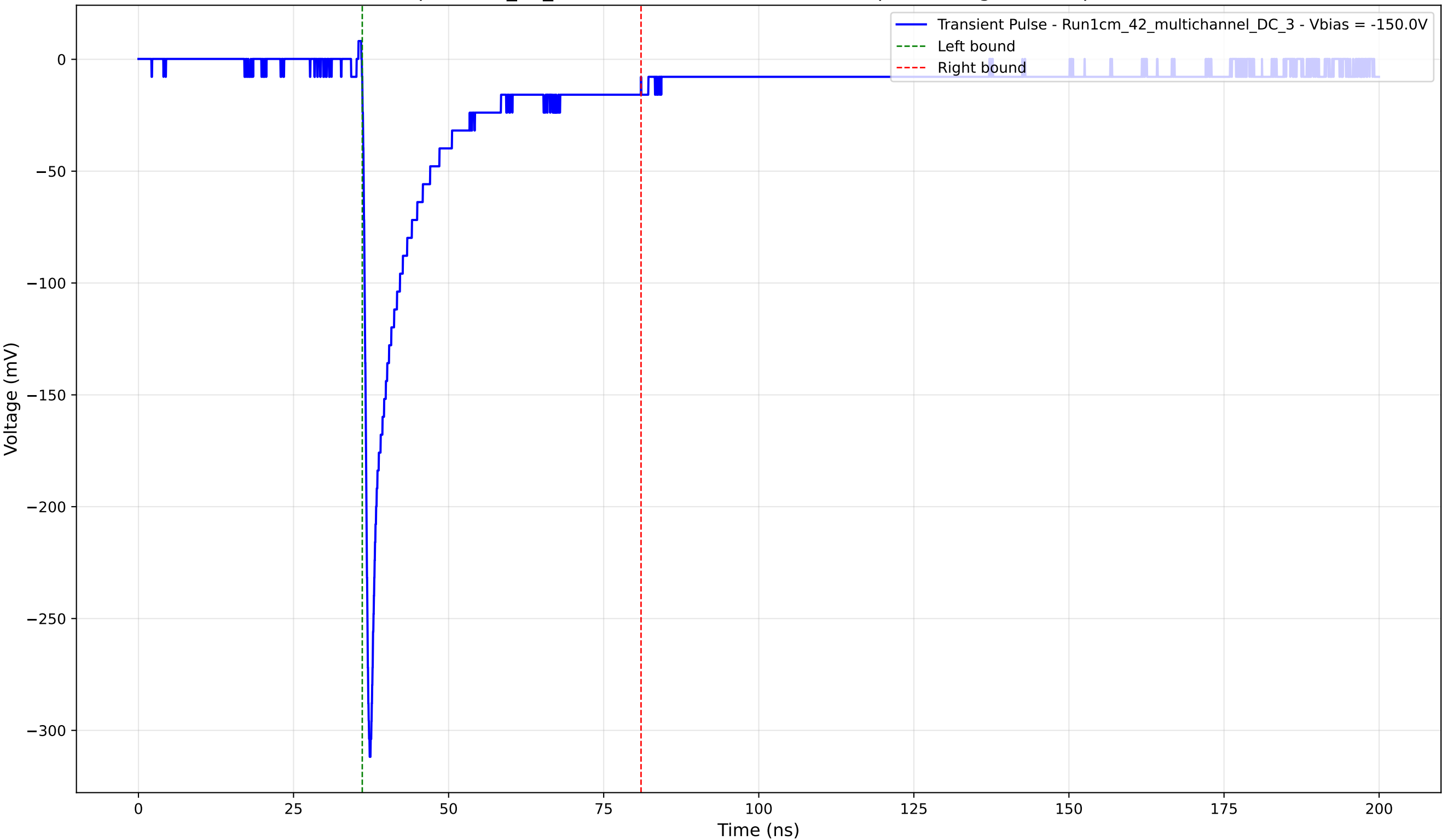
Transient Pulse - Sample: 1cm_42_multichannel - Position: 4620.0 \mu\text{m} - Charge: 42.08 pC - Rise Time: 0.86 ns
