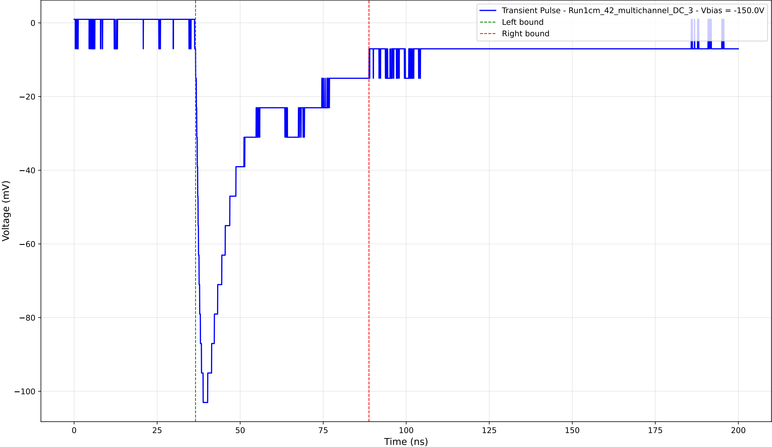
Transient Pulse - Sample: 1cm_42_multichannel - Position: 3105.0 \mu\text{m} - Charge: 35.86 pC - Rise Time: 1.77 ns
