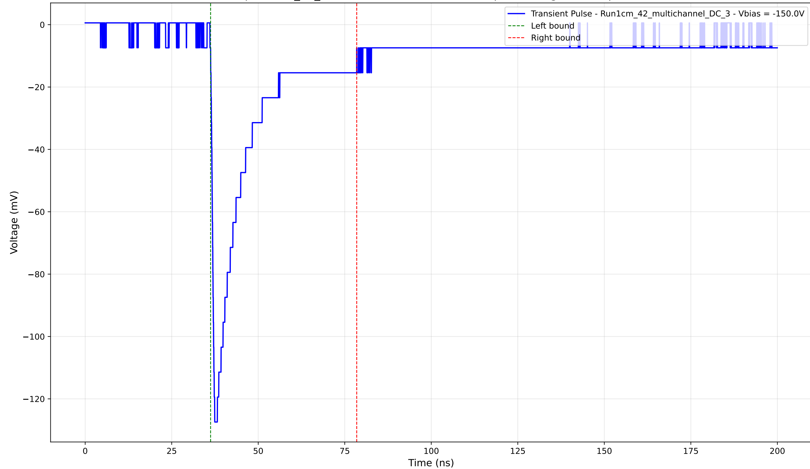
Transient Pulse - Sample: 1cm_42_multichannel - Position: 800.0 \mu\text{m} - Charge: 28.41 pC - Rise Time: 1.03 ns
