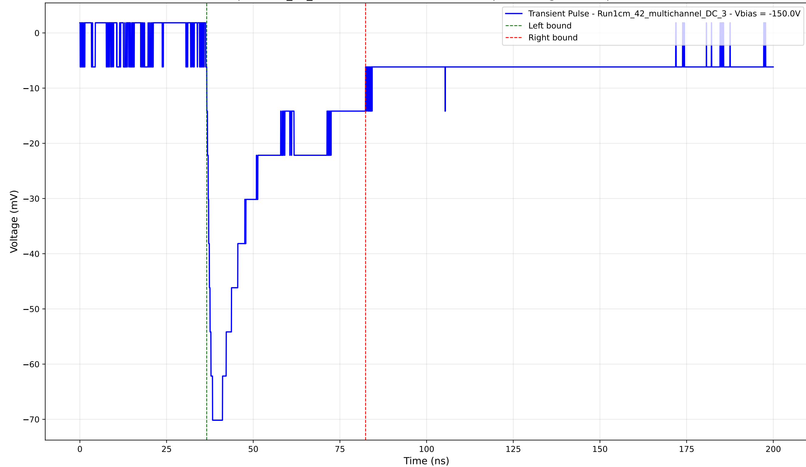
Transient Pulse - Sample: 1cm_42_multichannel - Position: 1810.0 \mu\text{m} - Charge: 25.56 pC - Rise Time: 1.68 ns
