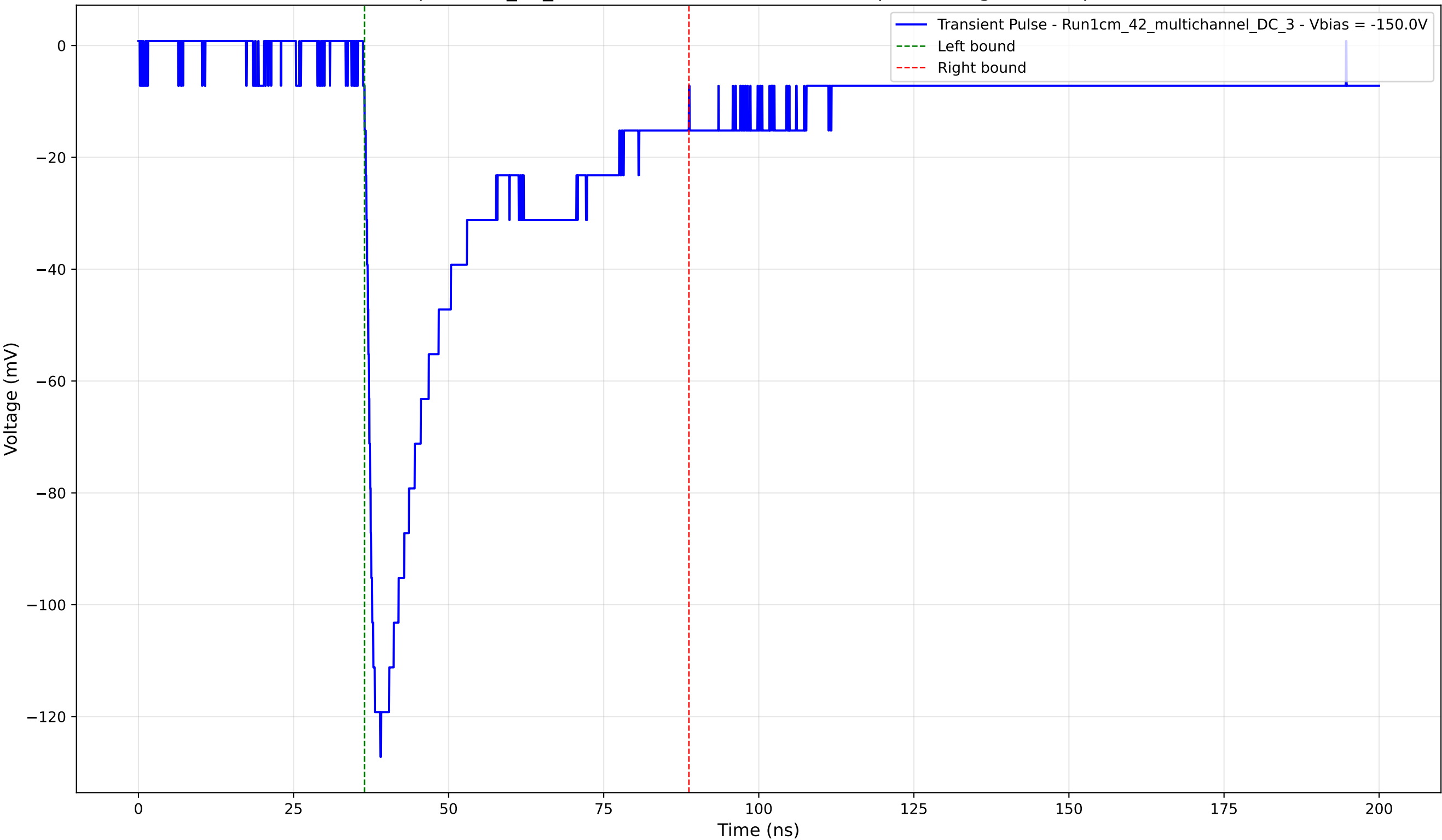
Transient Pulse - Sample: 1cm_42_multichannel - Position: 1575.0 \mu\text{m} - Charge: 41.35 pC - Rise Time: 1.65 ns
