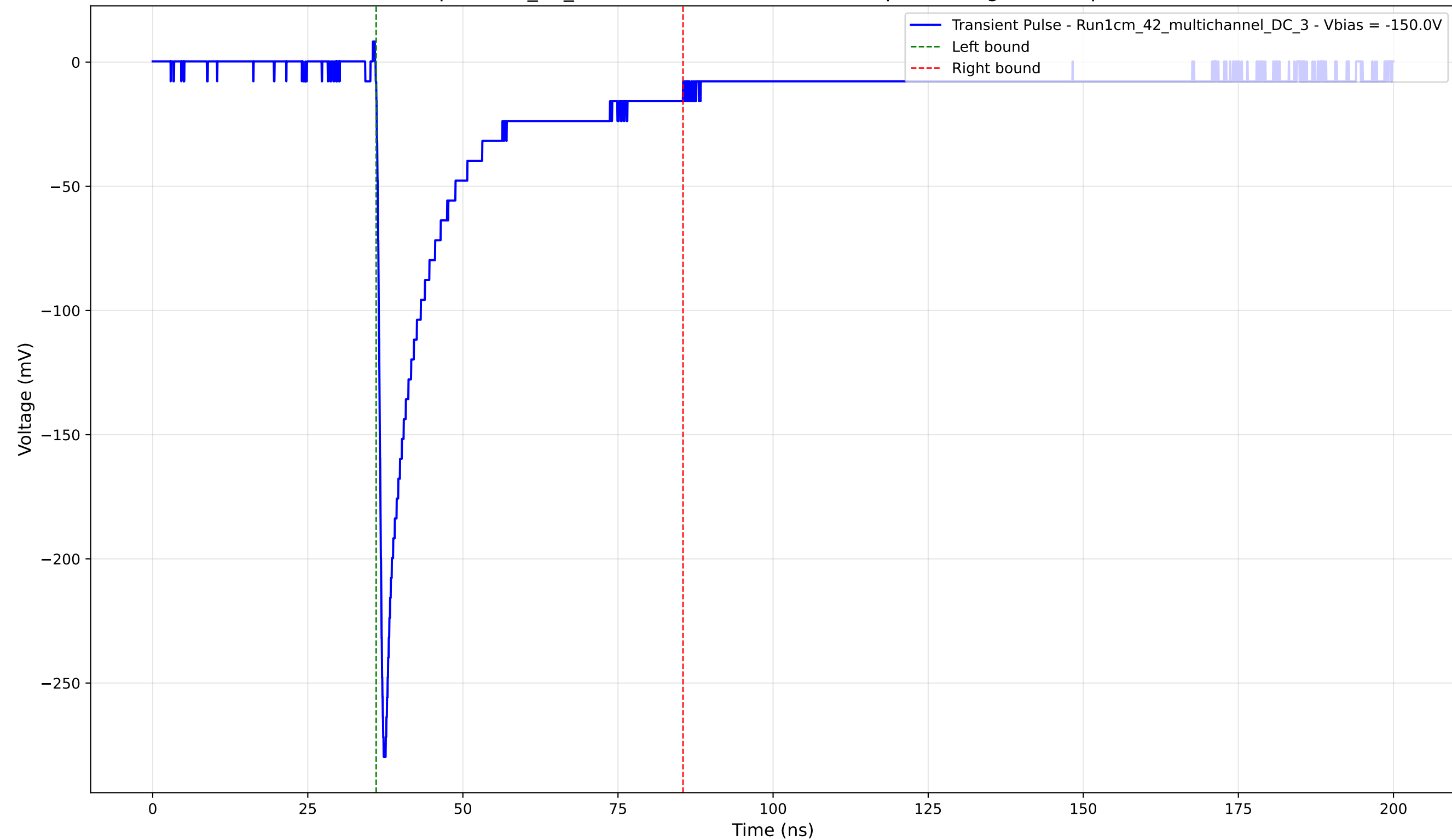
Transient Pulse - Sample: 1cm_42_multichannel - Position: 465.0 \mu\text{m} - Charge: 49.44 pC - Rise Time: 0.89 ns
