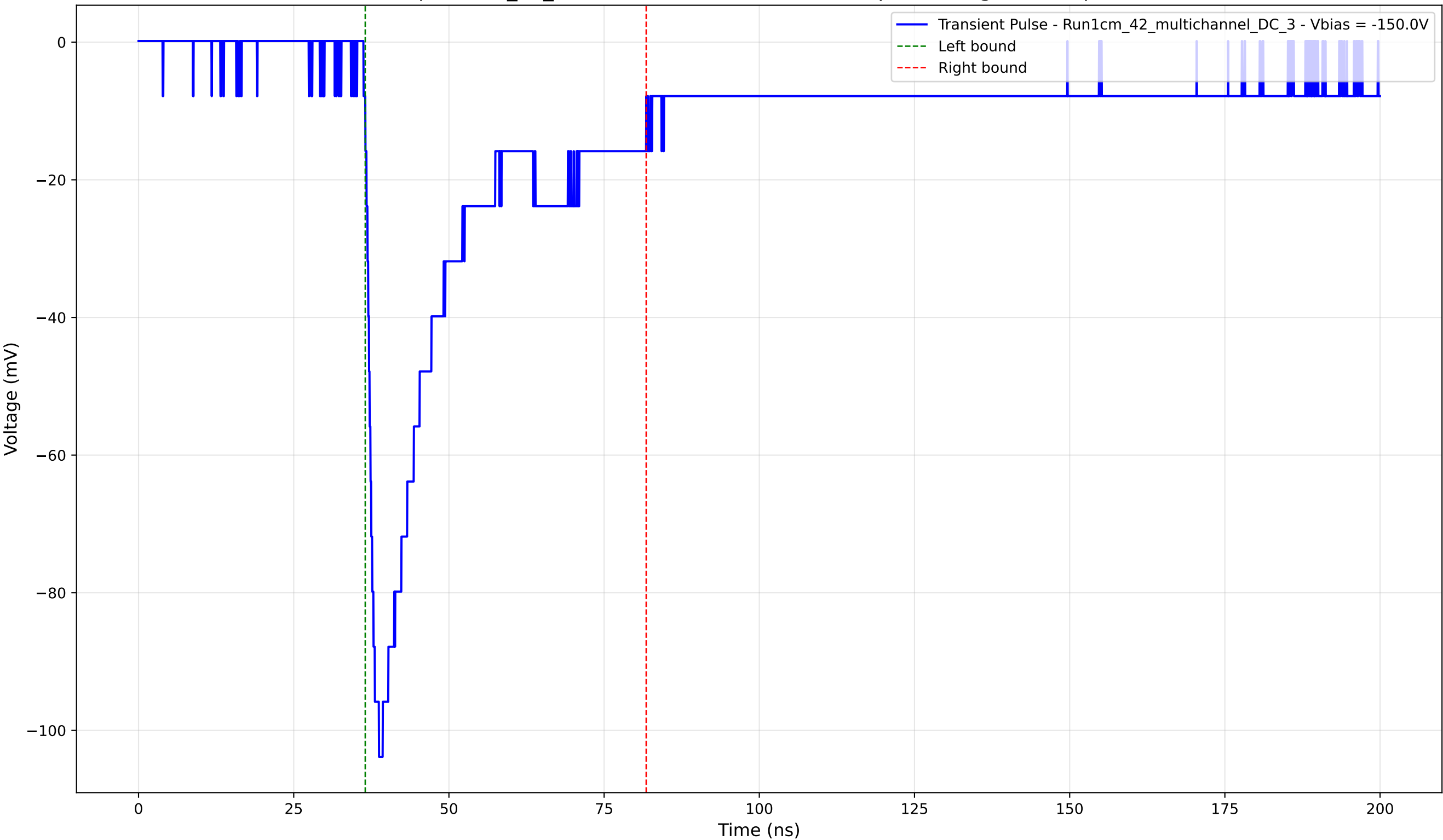
Transient Pulse - Sample: 1cm_42_multichannel - Position: 3450.0 \mu\text{m} - Charge: 29.84 pC - Rise Time: 1.53 ns
