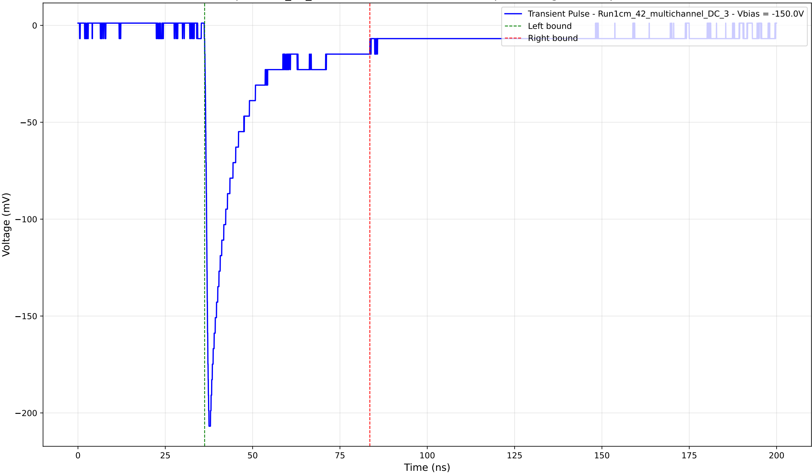
Transient Pulse - Sample: 1cm_42_multichannel - Position: 4245.0 \mu\text{m} - Charge: 39.79 pC - Rise Time: 0.97 ns
