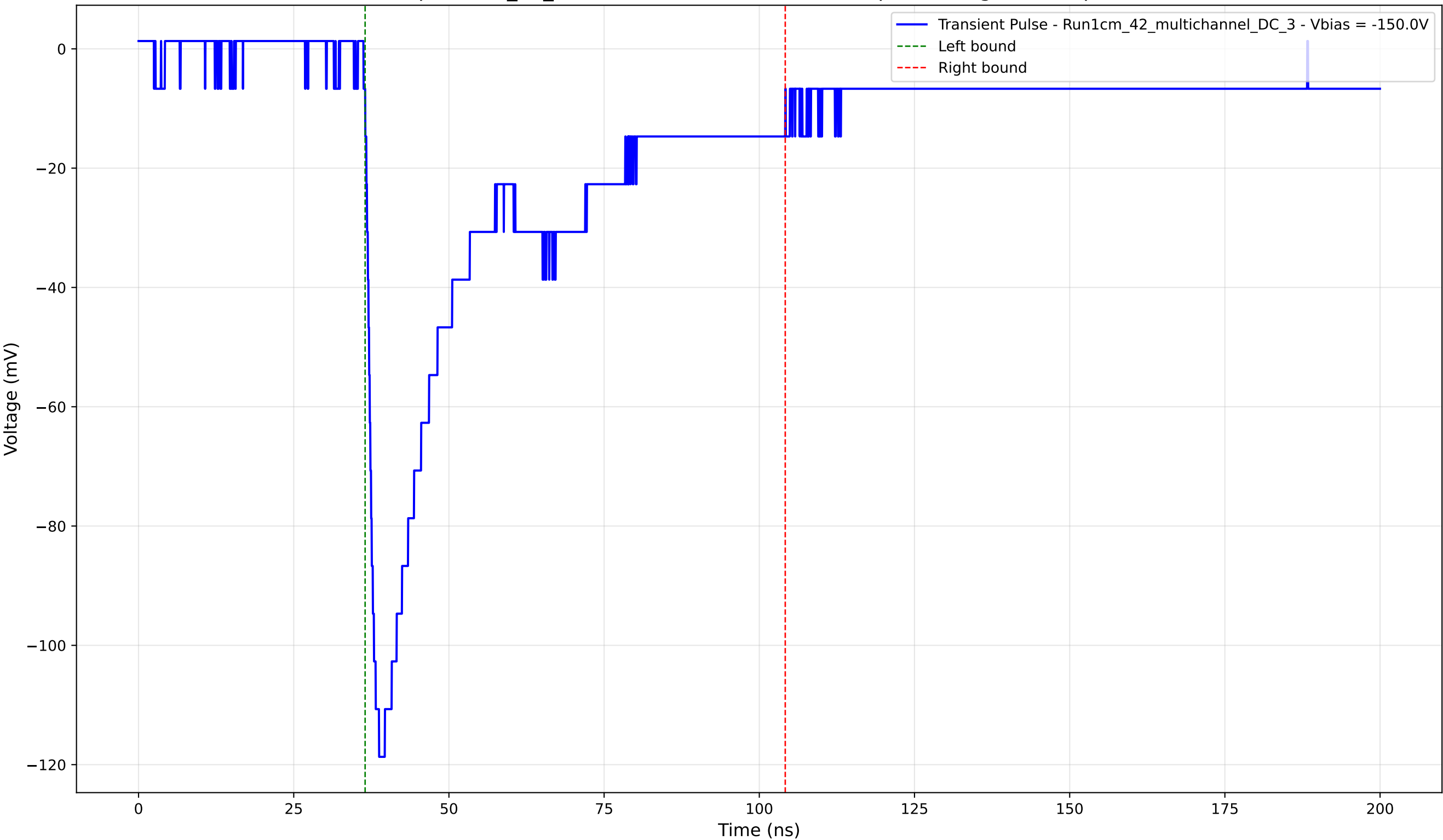
Transient Pulse - Sample: 1cm_42_multichannel - Position: 1710.0 \mu\text{m} - Charge: 45.29 pC - Rise Time: 1.69 ns
