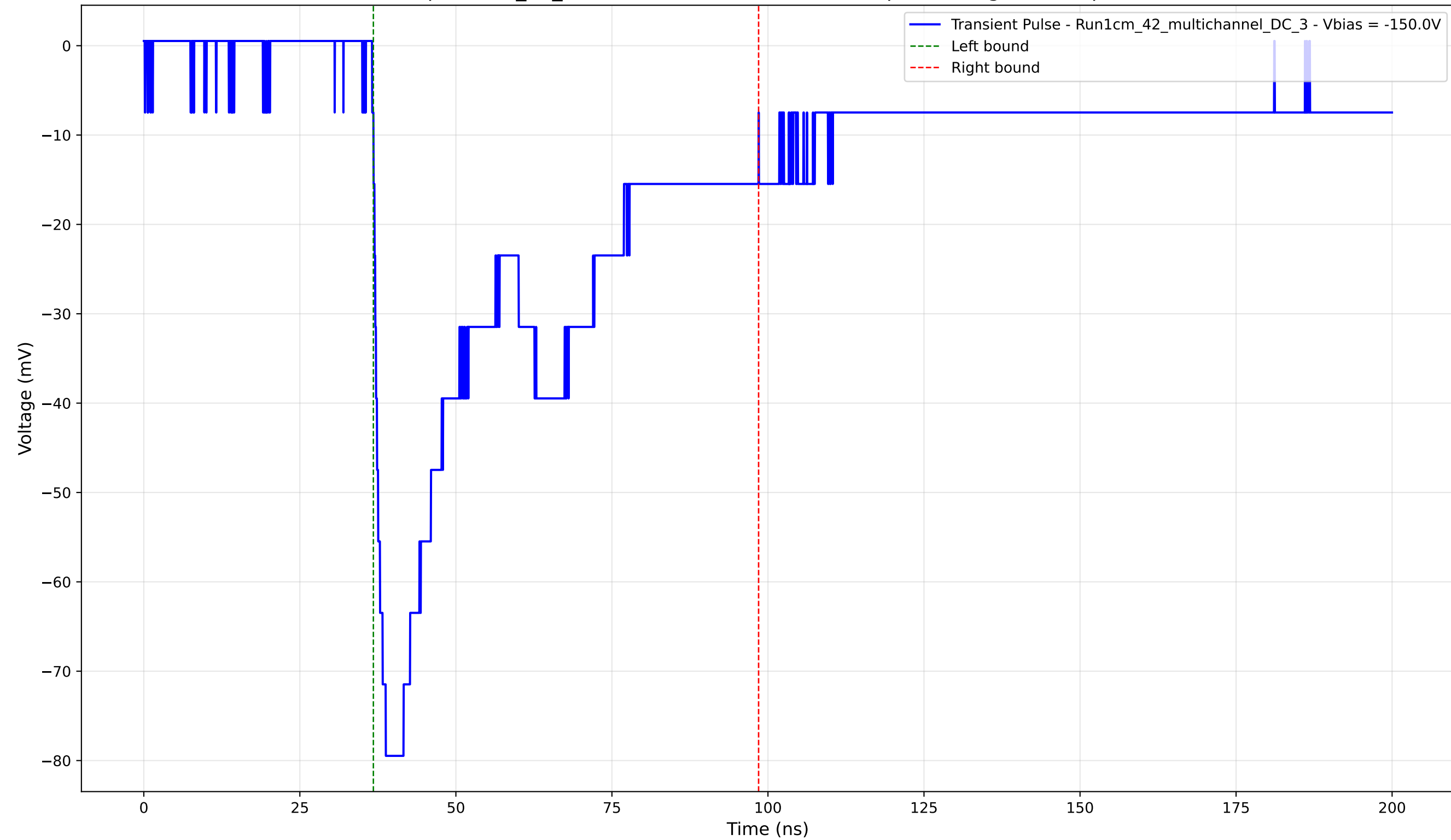
Transient Pulse - Sample: 1cm_42_multichannel - Position: 2510.0 \mu\text{m} - Charge: 38.84 pC - Rise Time: 1.98 ns
