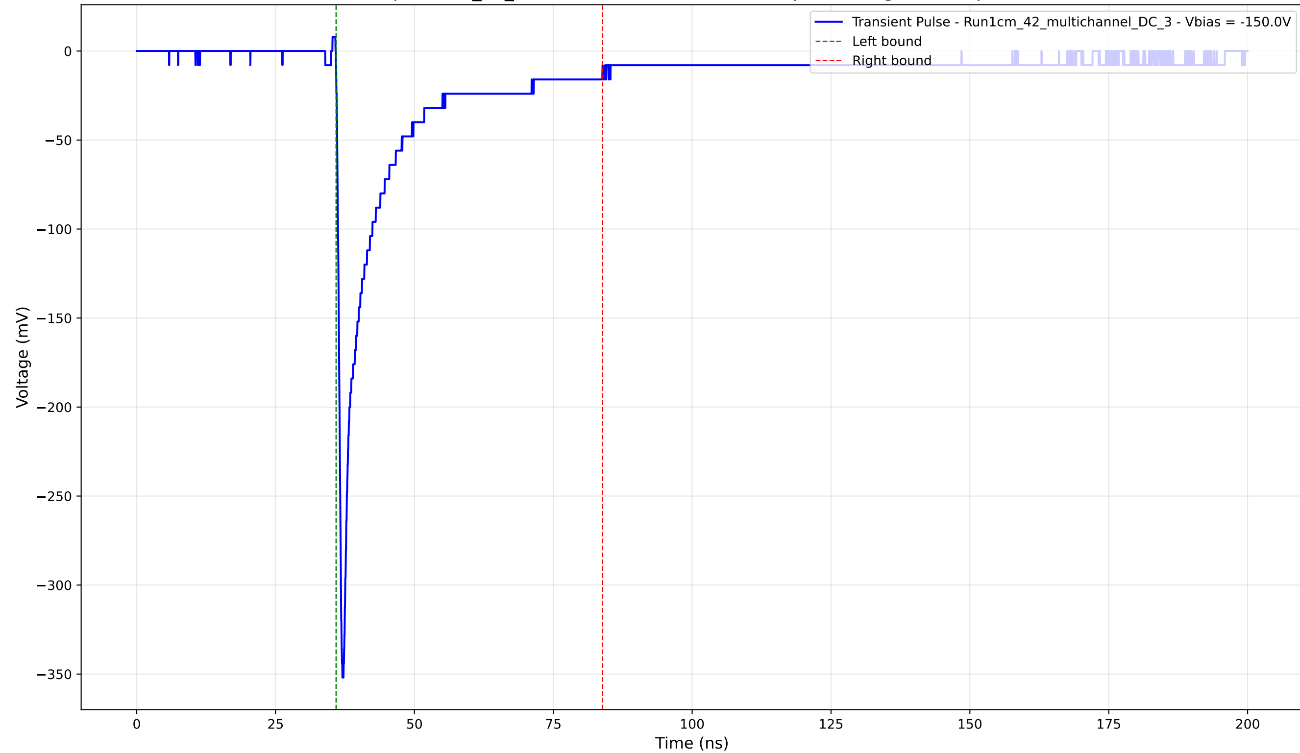
Transient Pulse - Sample: 1cm_42_multichannel - Position: 205.0 \mu\text{m} - Charge: 48.40 pC - Rise Time: 0.79 ns
