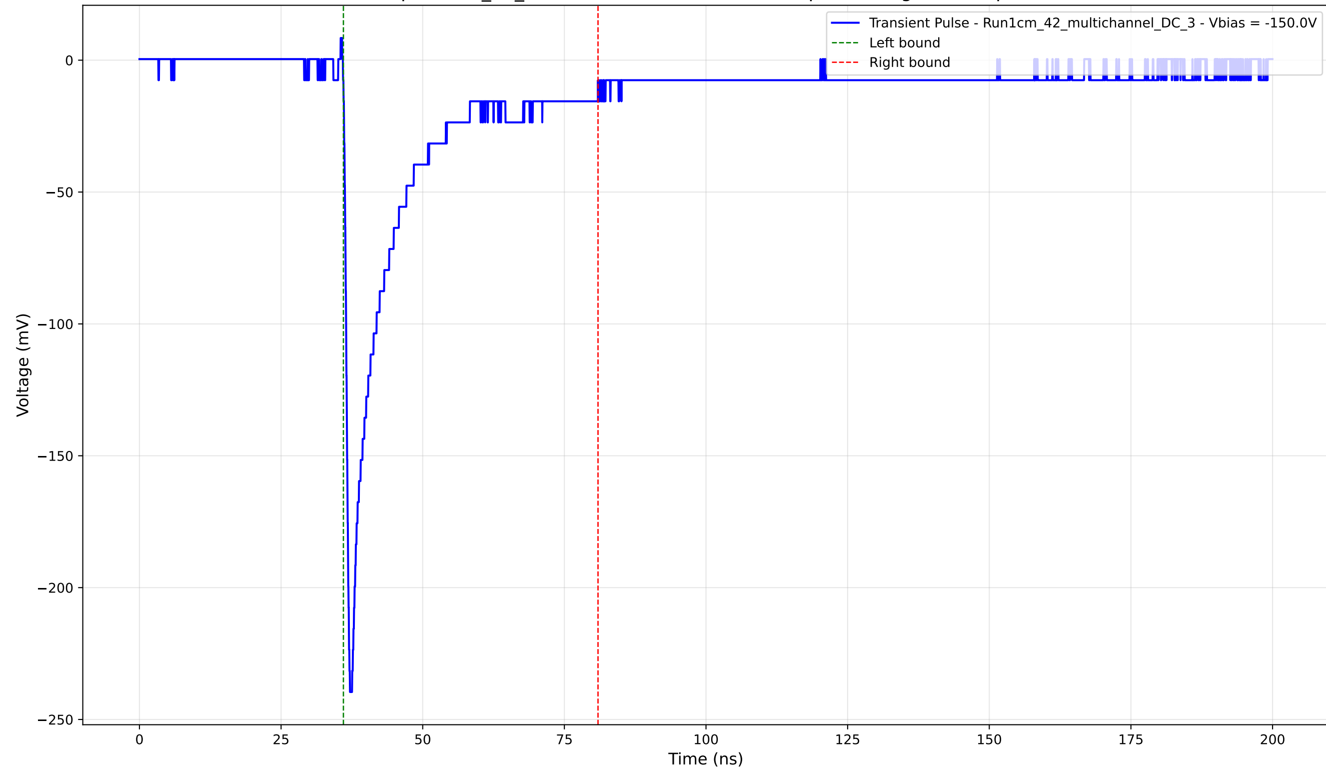
Transient Pulse - Sample: 1cm_42_multichannel - Position: 420.0 \mu\text{m} - Charge: 39.93 pC - Rise Time: 0.88 ns
