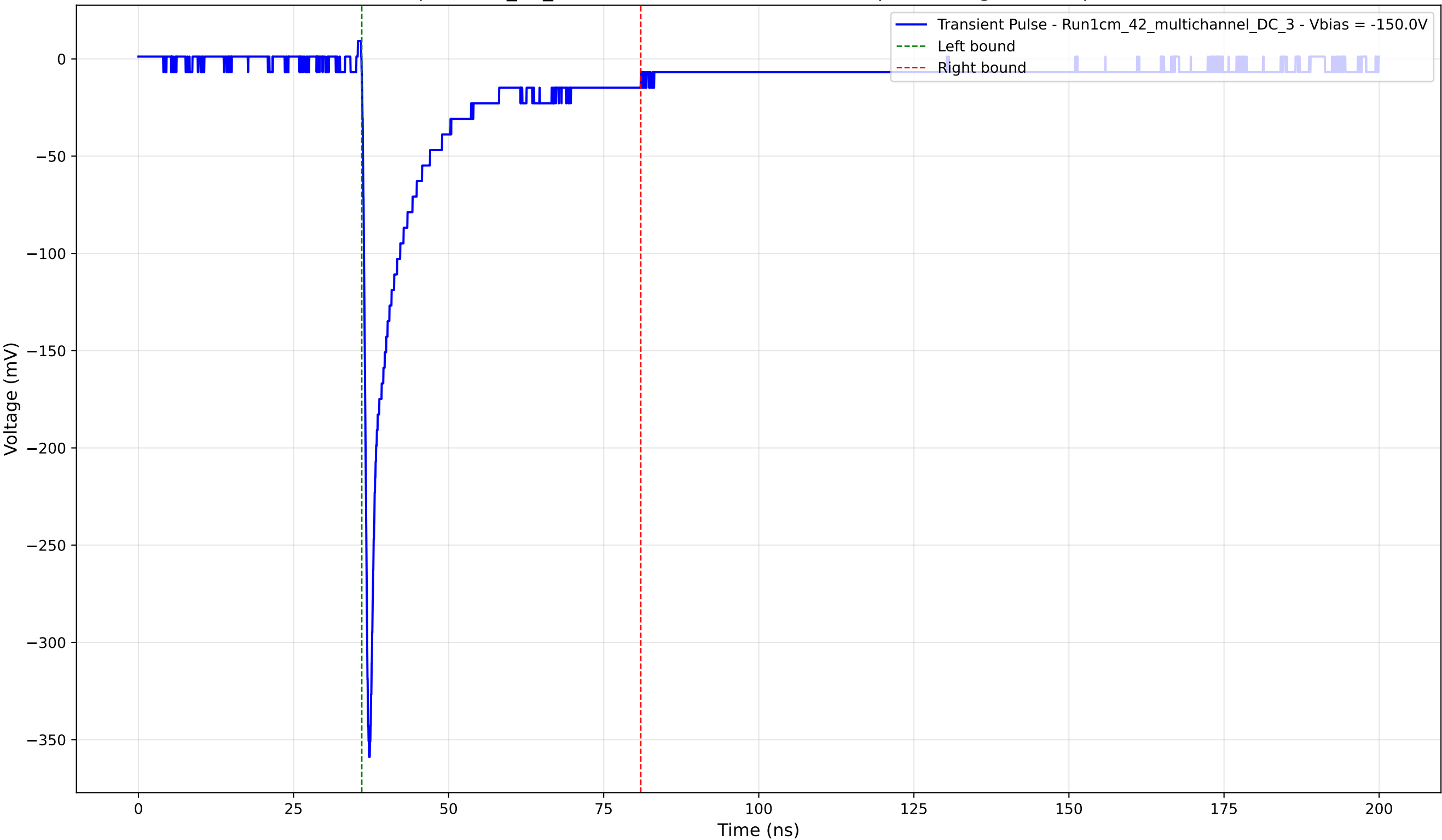
Transient Pulse - Sample: 1cm_42_multichannel - Position: 4730.0 \mu\text{m} - Charge: 43.21 pC - Rise Time: 0.80 ns
