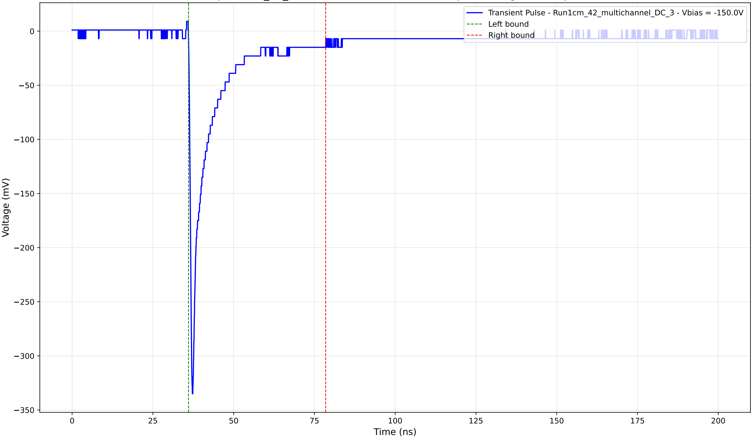
Transient Pulse - Sample: 1cm_42_multichannel - Position: 4670.0 \mu\text{m} - Charge: 41.89 pC - Rise Time: 0.81 ns
