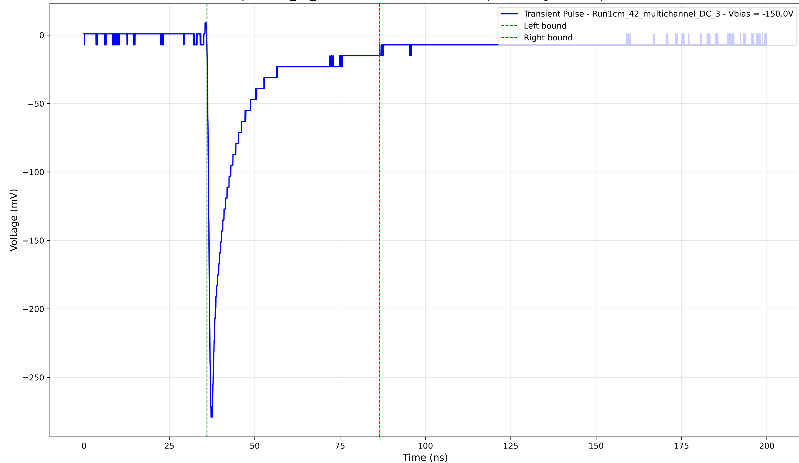
Transient Pulse - Sample: 1cm_42_multichannel - Position: 440.0 \mu\text{m} - Charge: 48.55 pC - Rise Time: 0.87 ns
