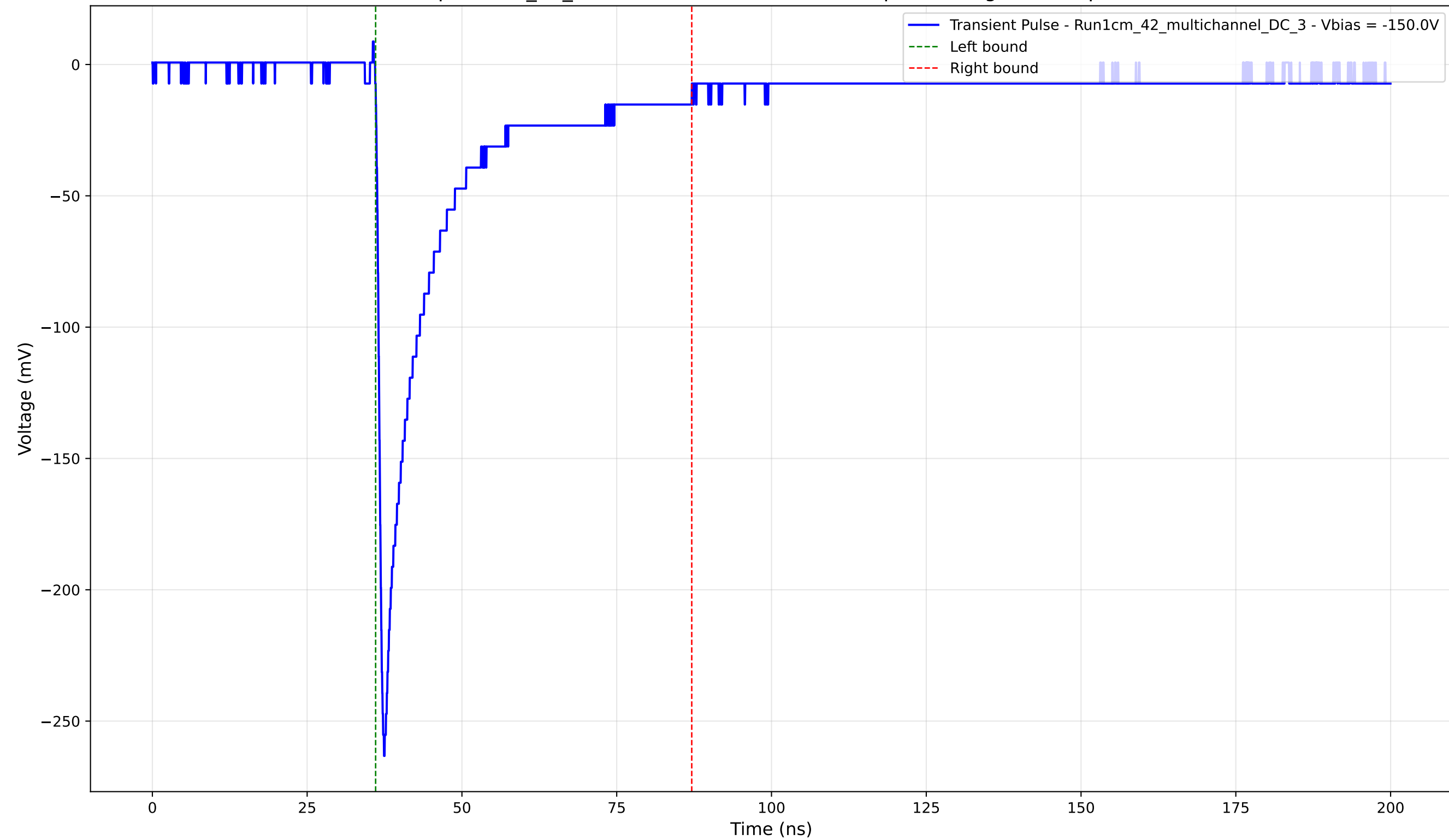
Transient Pulse - Sample: 1cm_42_multichannel - Position: 540.0 \mu\text{m} - Charge: 48.64 pC - Rise Time: 0.93 ns
