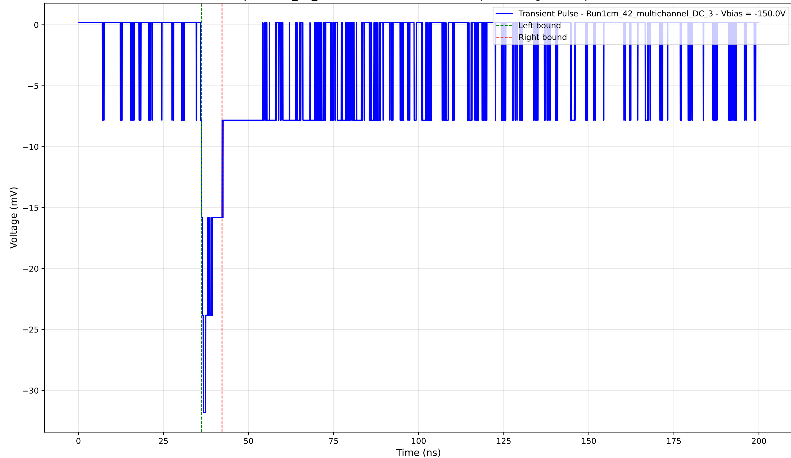
Transient Pulse - Sample: 1cm_42_multichannel - Position: 50.0 \mu\text{m} - Charge: 2.41 pC - Rise Time: 0.85 ns
