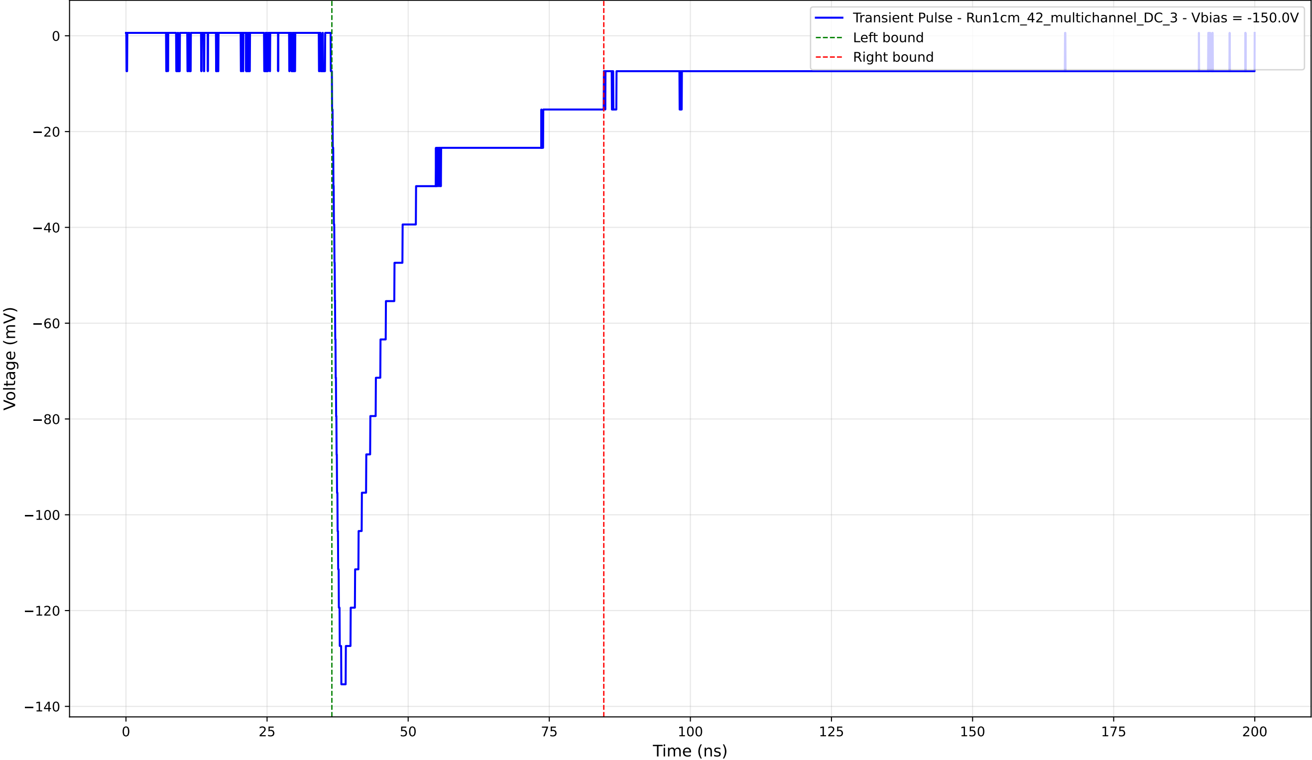
Transient Pulse - Sample: 1cm_42_multichannel - Position: 3675.0 \mu\text{m} - Charge: 37.49 pC - Rise Time: 1.36 ns
