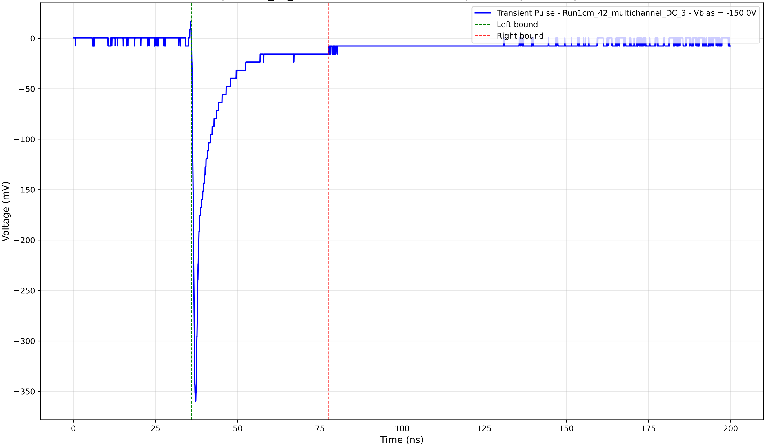
Transient Pulse - Sample: 1cm_42_multichannel - Position: 4790.0 \mu\text{m} - Charge: 40.14 pC - Rise Time: 0.78 ns
