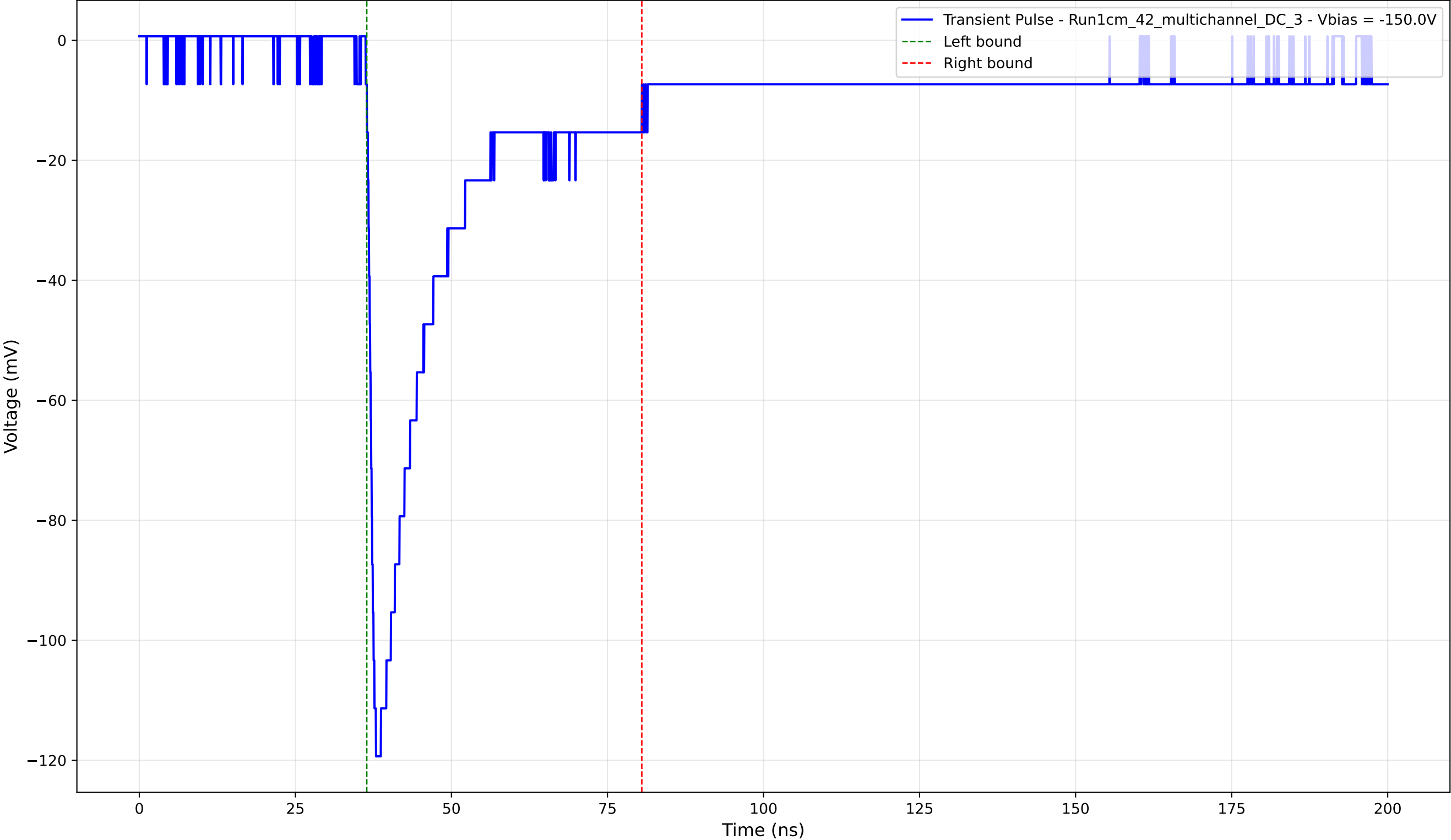
Transient Pulse - Sample: 1cm_42_multichannel - Position: 3825.0 \mu\text{m} - Charge: 29.51 pC - Rise Time: 1.21 ns
