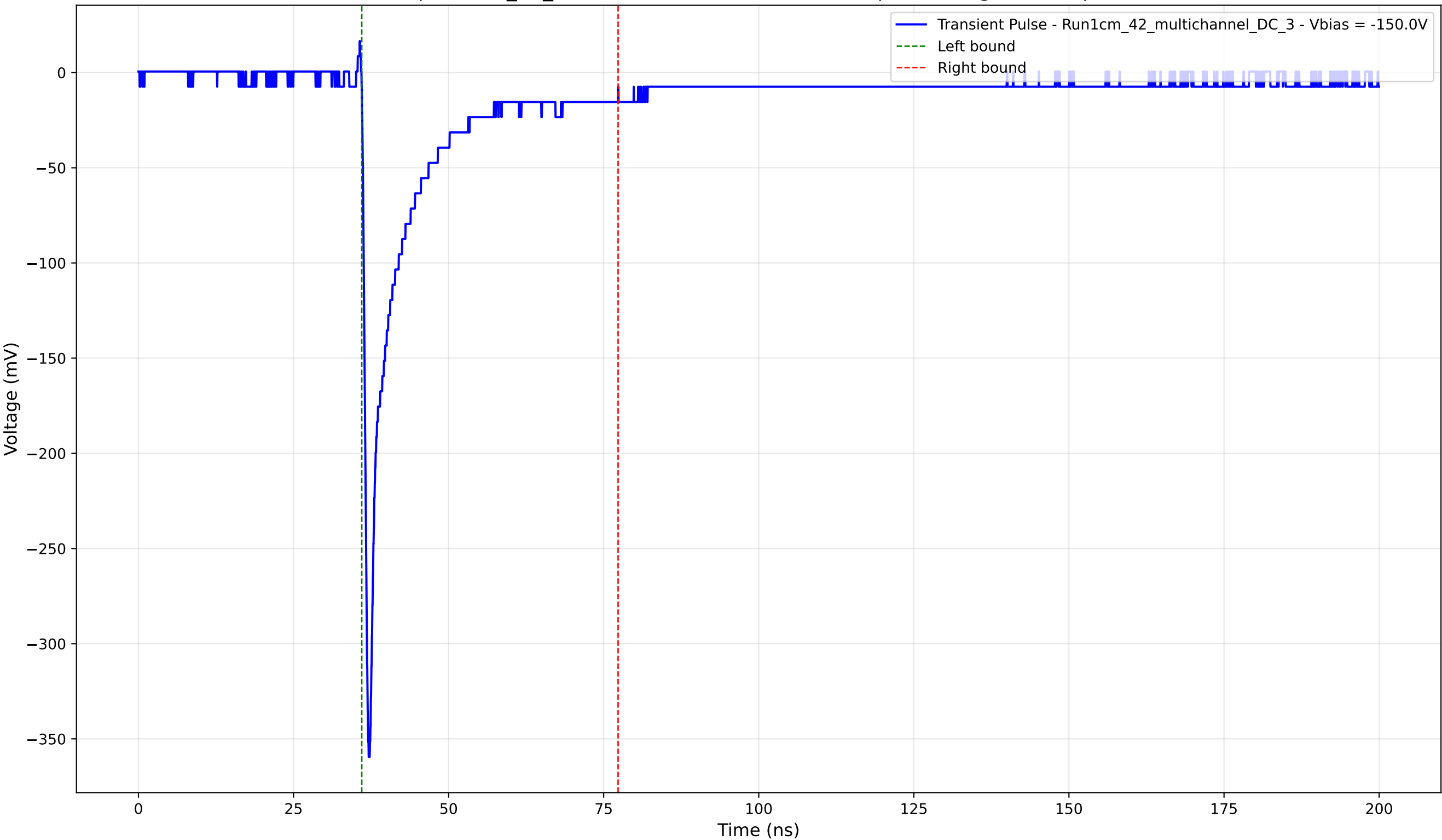
Transient Pulse - Sample: 1cm_42_multichannel - Position: 4755.0 \mu\text{m} - Charge: 41.19 pC - Rise Time: 0.79 ns
