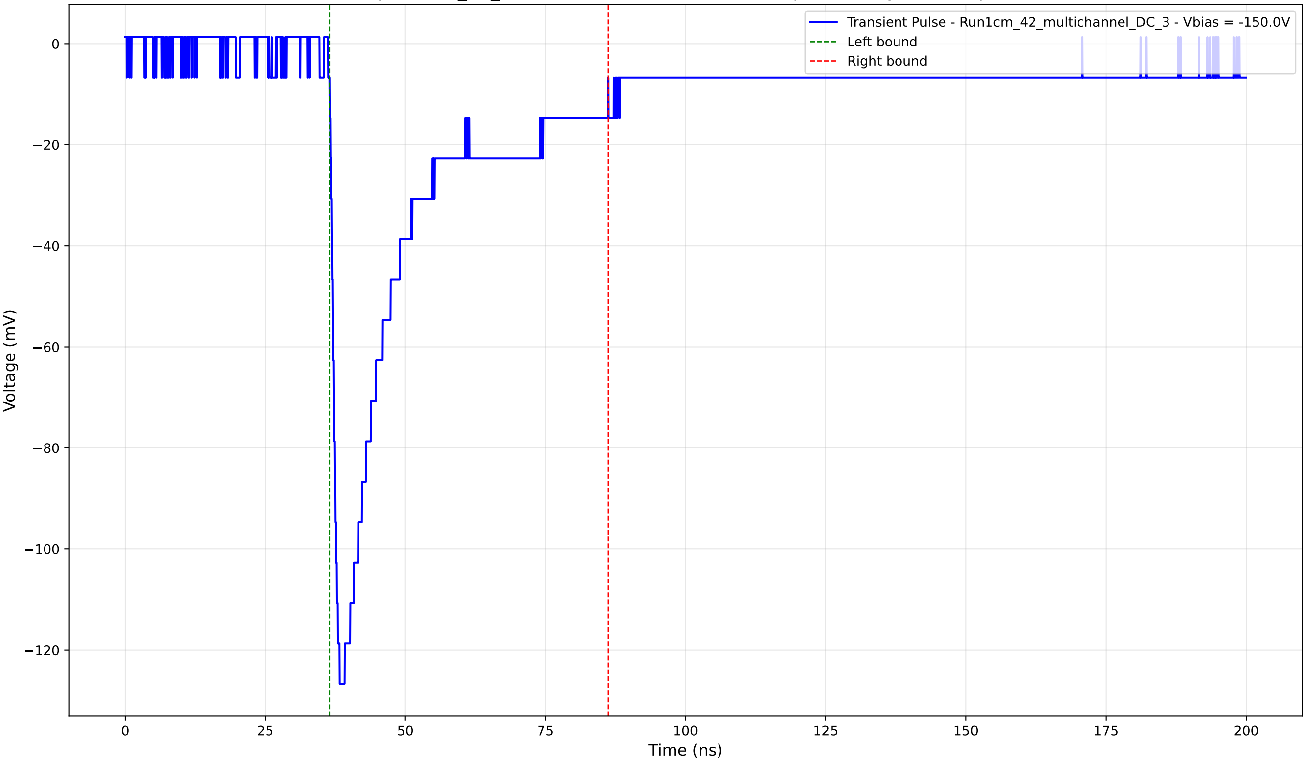
Transient Pulse - Sample: 1cm_42_multichannel - Position: 3600.0 \mu\text{m} - Charge: 36.29 pC - Rise Time: 1.41 ns
