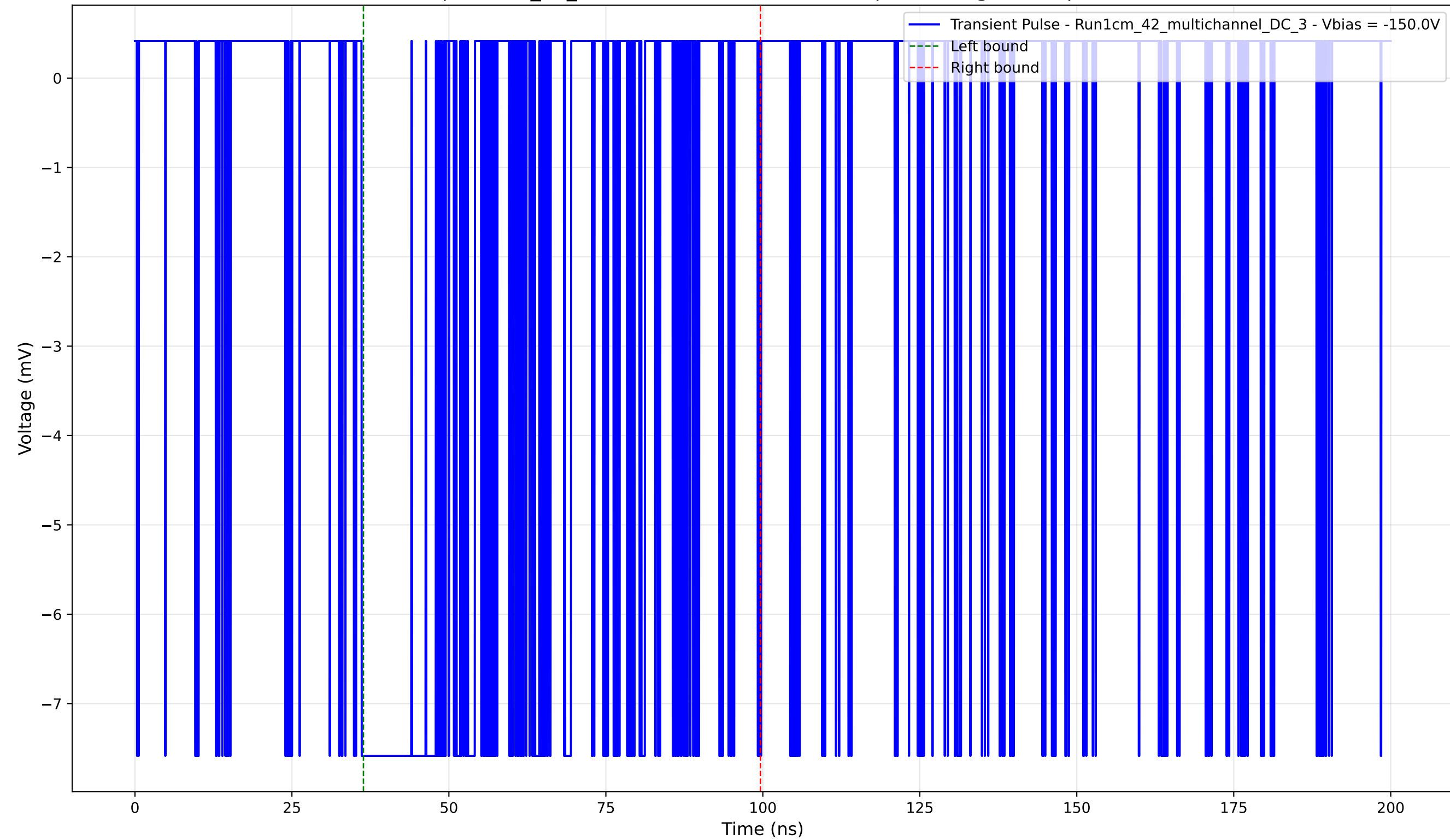
Transient Pulse - Sample: 1cm_42_multichannel - Position: 20.0 \mu\text{m} - Charge: 3.53 pC - Rise Time: 0.02 ns
