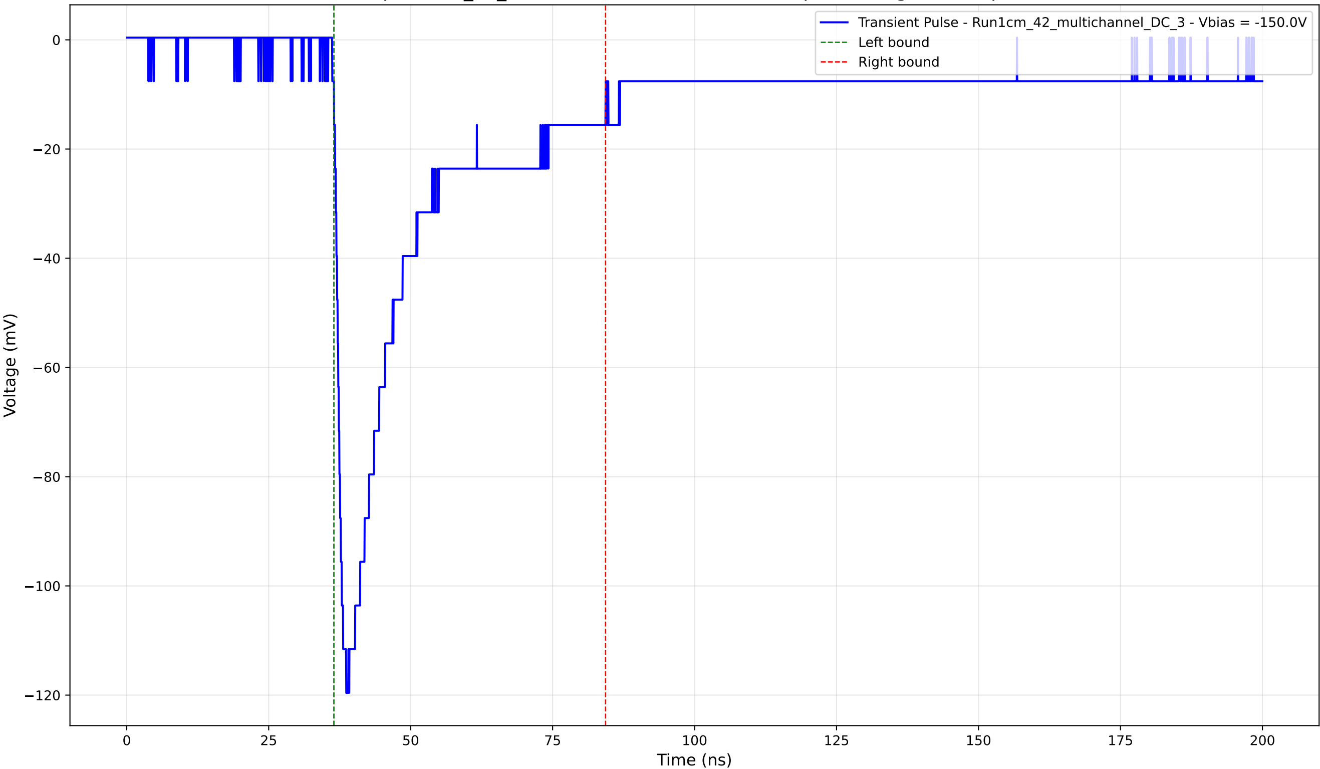
Transient Pulse - Sample: 1cm_42_multichannel - Position: 3465.0 \mu\text{m} - Charge: 35.22 pC - Rise Time: 1.61 ns
