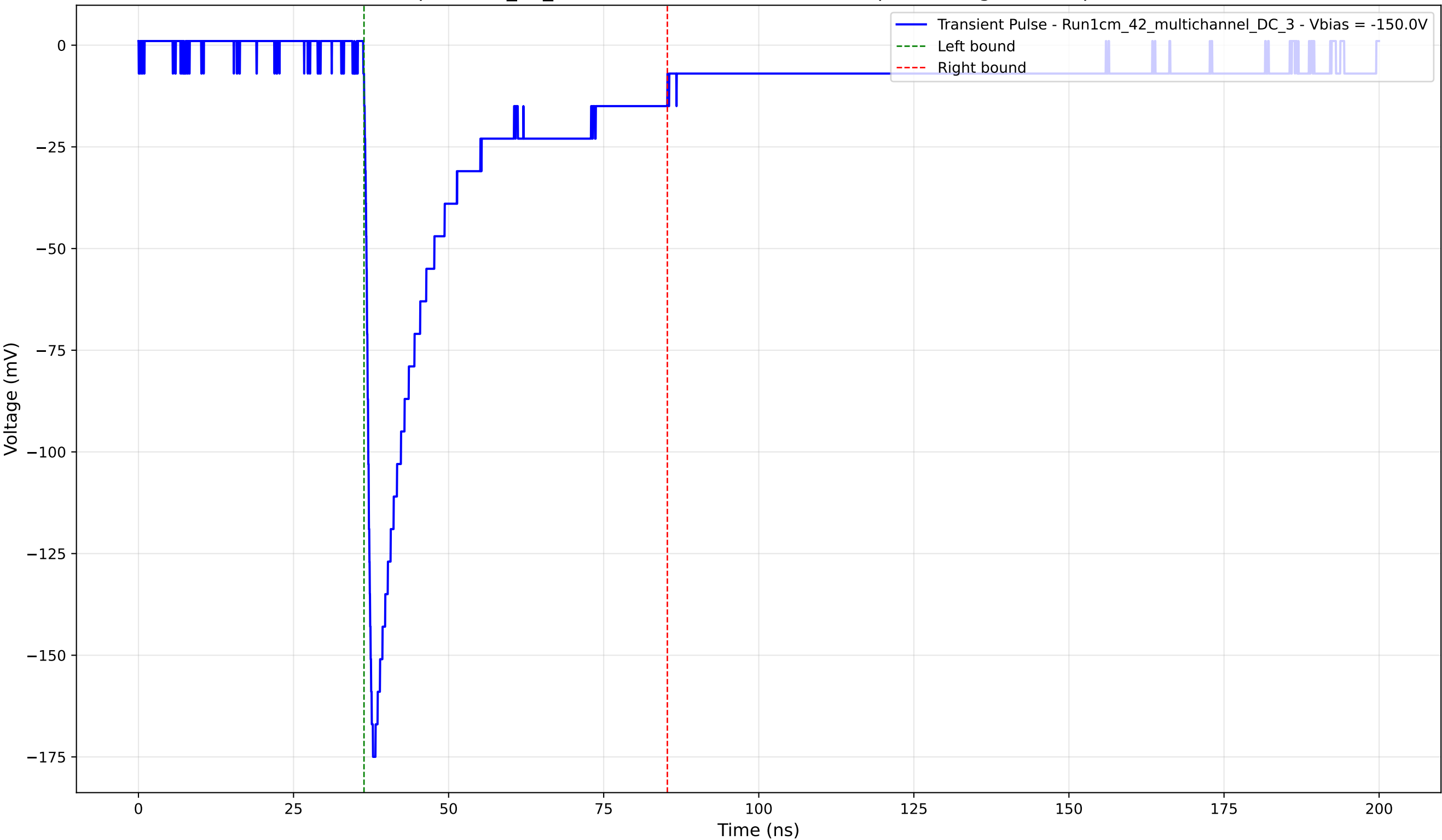
Transient Pulse - Sample: 1cm_42_multichannel - Position: 4025.0 \mu\text{m} - Charge: 40.05 pC - Rise Time: 1.03 ns
