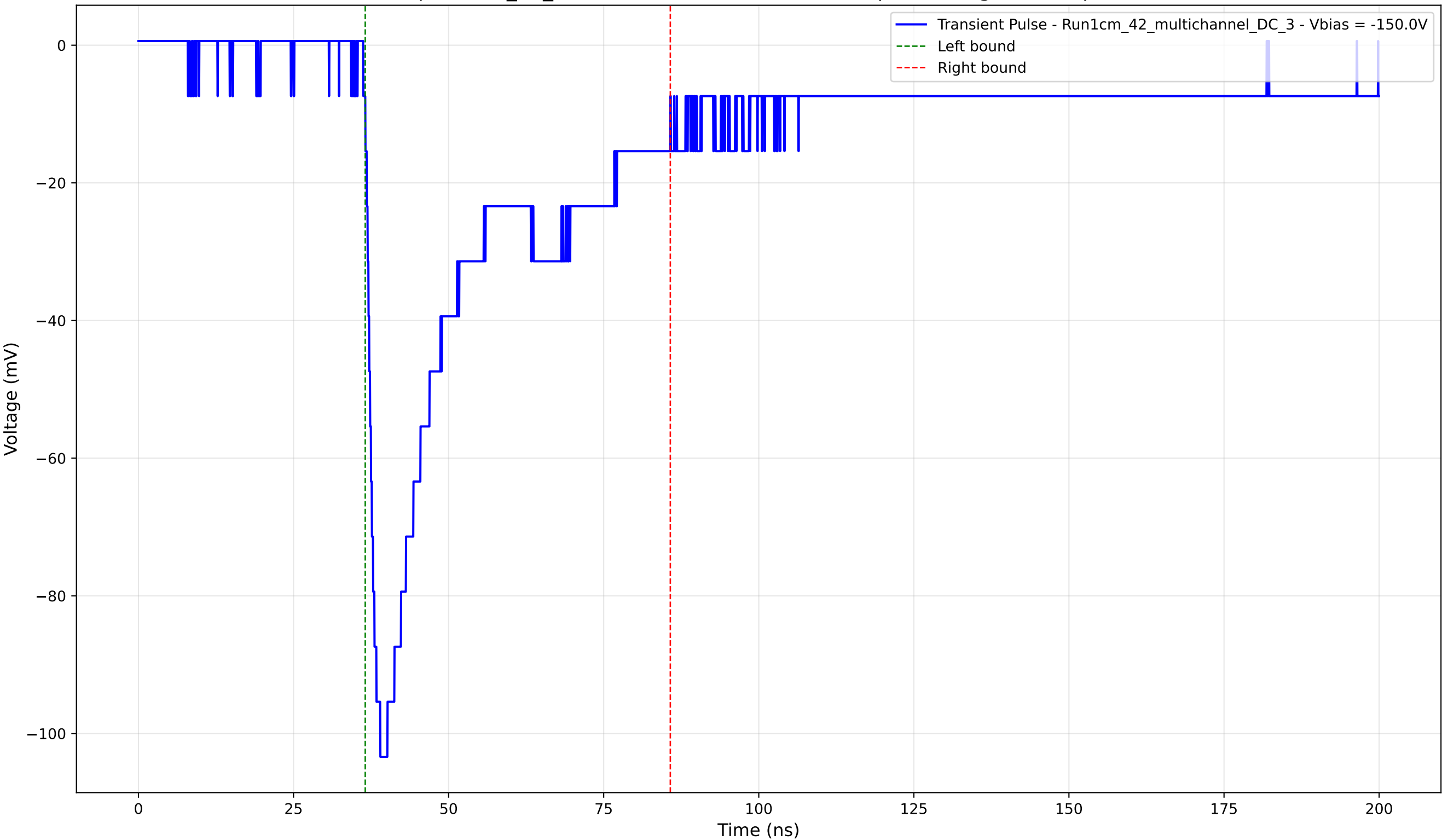
Transient Pulse - Sample: 1cm_42_multichannel - Position: 3065.0 \mu\text{m} - Charge: 35.70 pC - Rise Time: 1.79 ns
