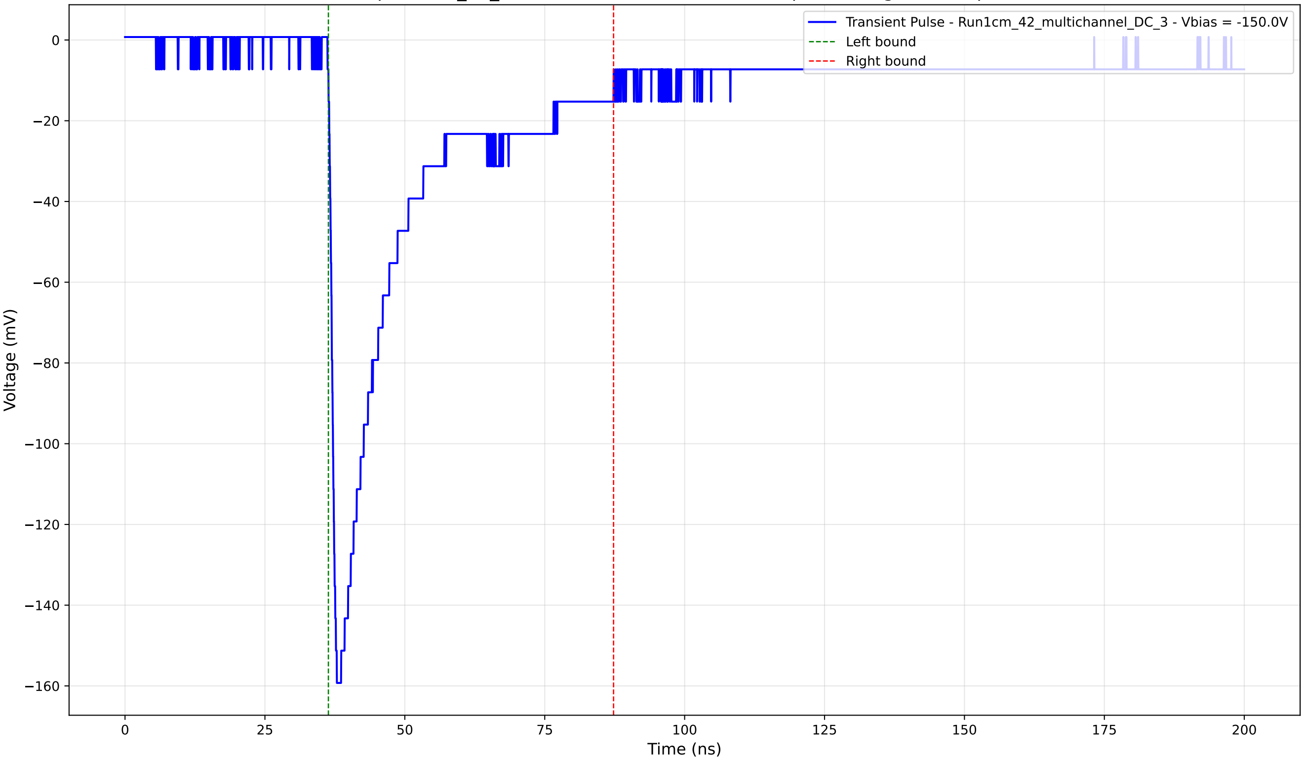
Transient Pulse - Sample: 1cm_42_multichannel - Position: 1120.0 \mu\text{m} - Charge: 43.13 pC - Rise Time: 1.22 ns
