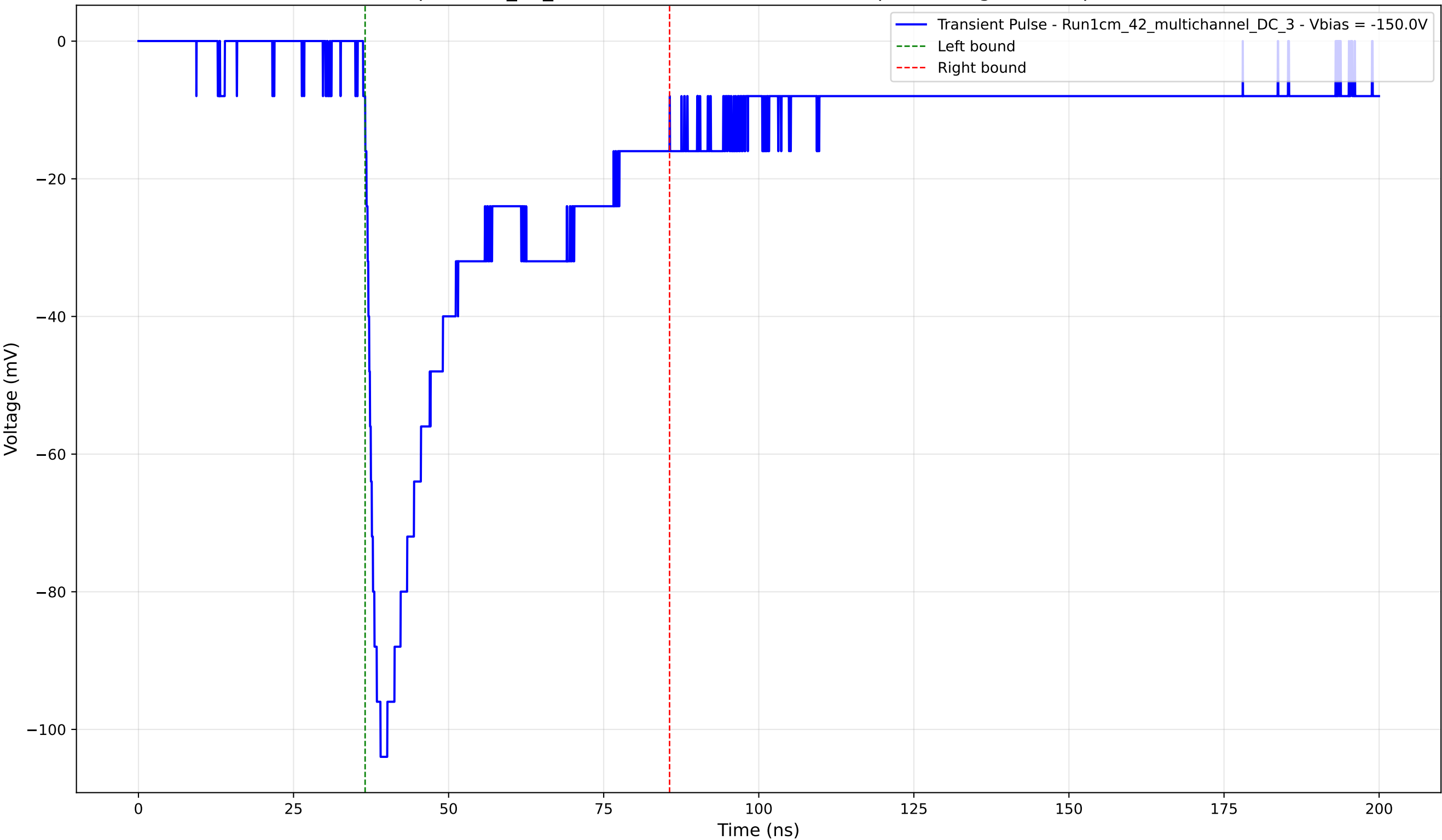
Transient Pulse - Sample: 1cm_42_multichannel - Position: 2995.0 \mu\text{m} - Charge: 36.86 pC - Rise Time: 1.87 ns
