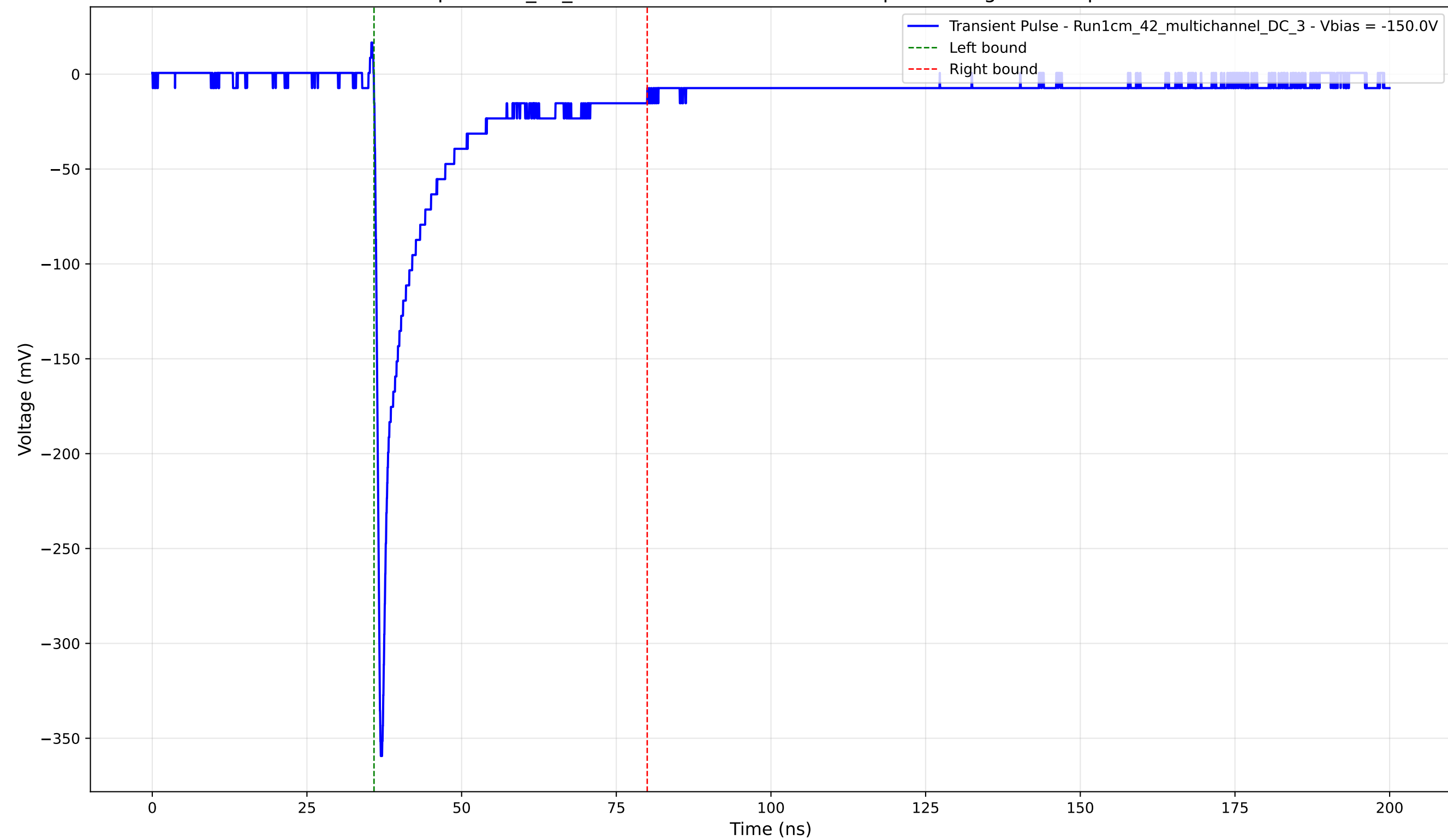
Transient Pulse - Sample: 1cm_42_multichannel - Position: 130.0 \mu\text{m} - Charge: 44.25 pC - Rise Time: 0.79 ns
