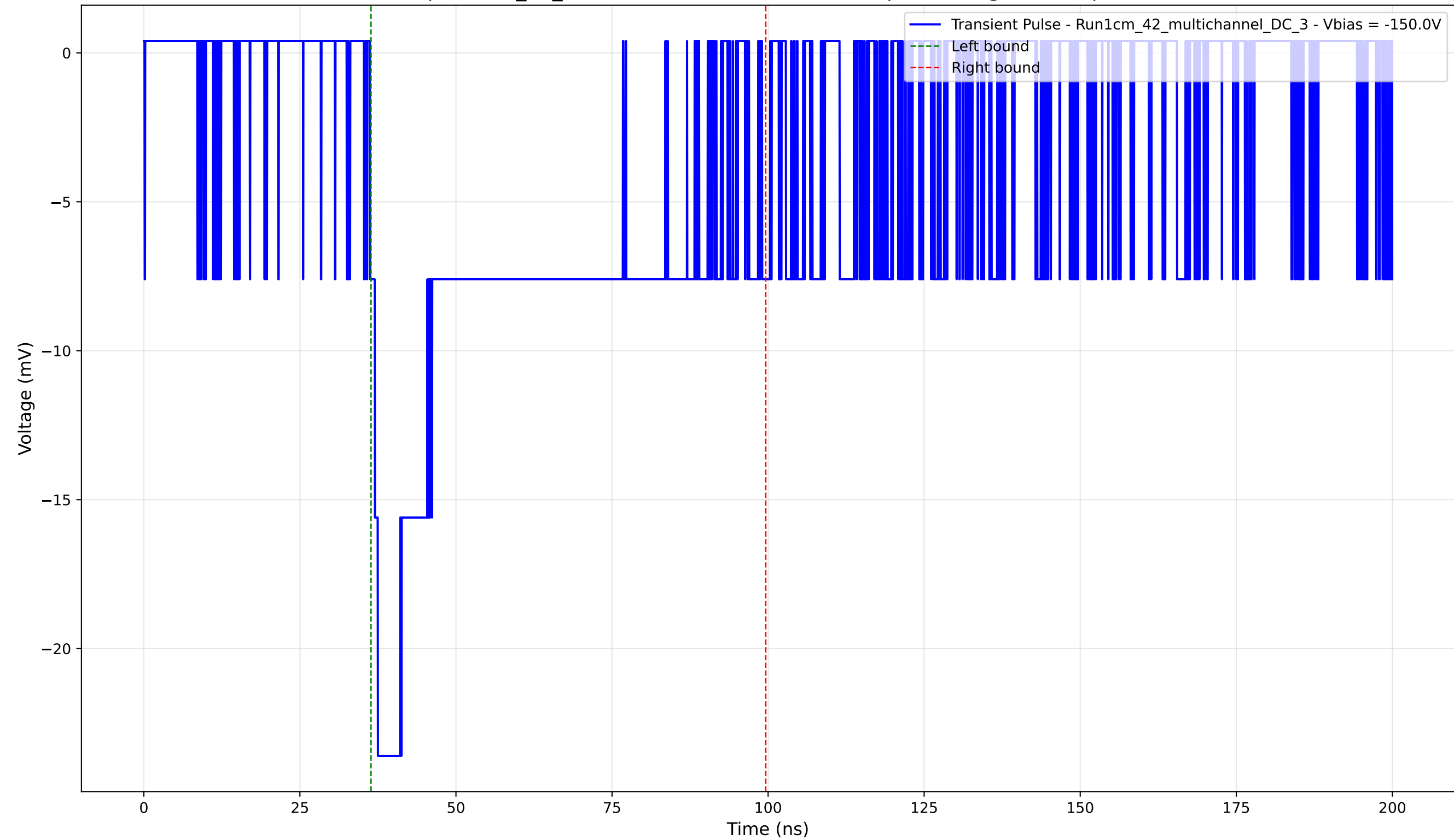
Transient Pulse - Sample: 1cm_42_multichannel - Position: 3860.0 \mu\text{m} - Charge: 10.79 pC - Rise Time: 1.27 ns
