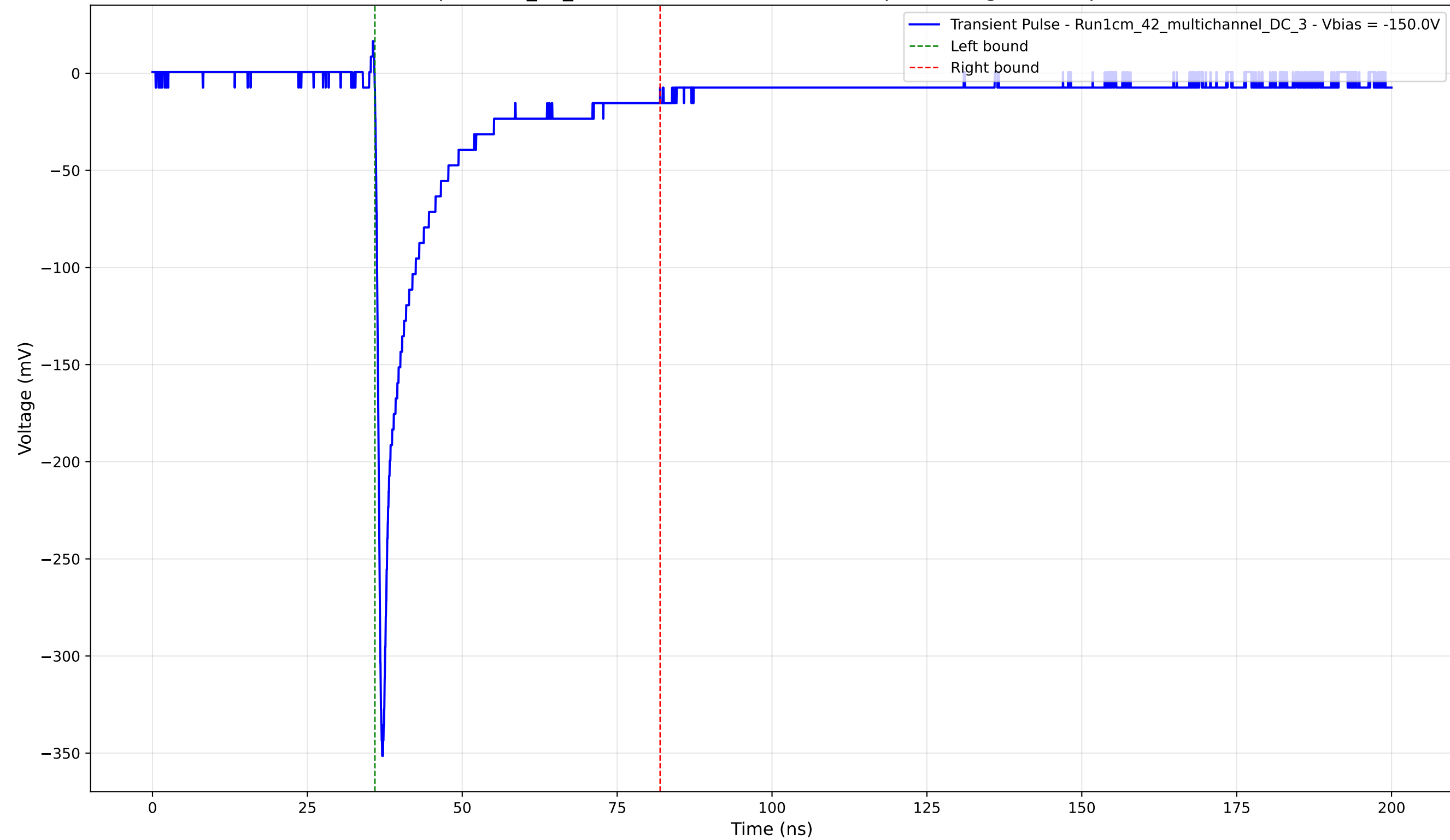
Transient Pulse - Sample: 1cm_42_multichannel - Position: 210.0 \mu\text{m} - Charge: 47.10 pC - Rise Time: 0.82 ns
