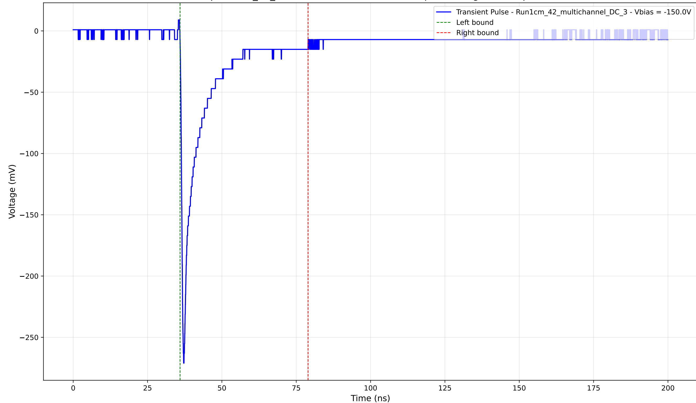
Transient Pulse - Sample: 1cm_42_multichannel - Position: 280.0 \mu\text{m} - Charge: 37.39 pC - Rise Time: 0.83 ns
