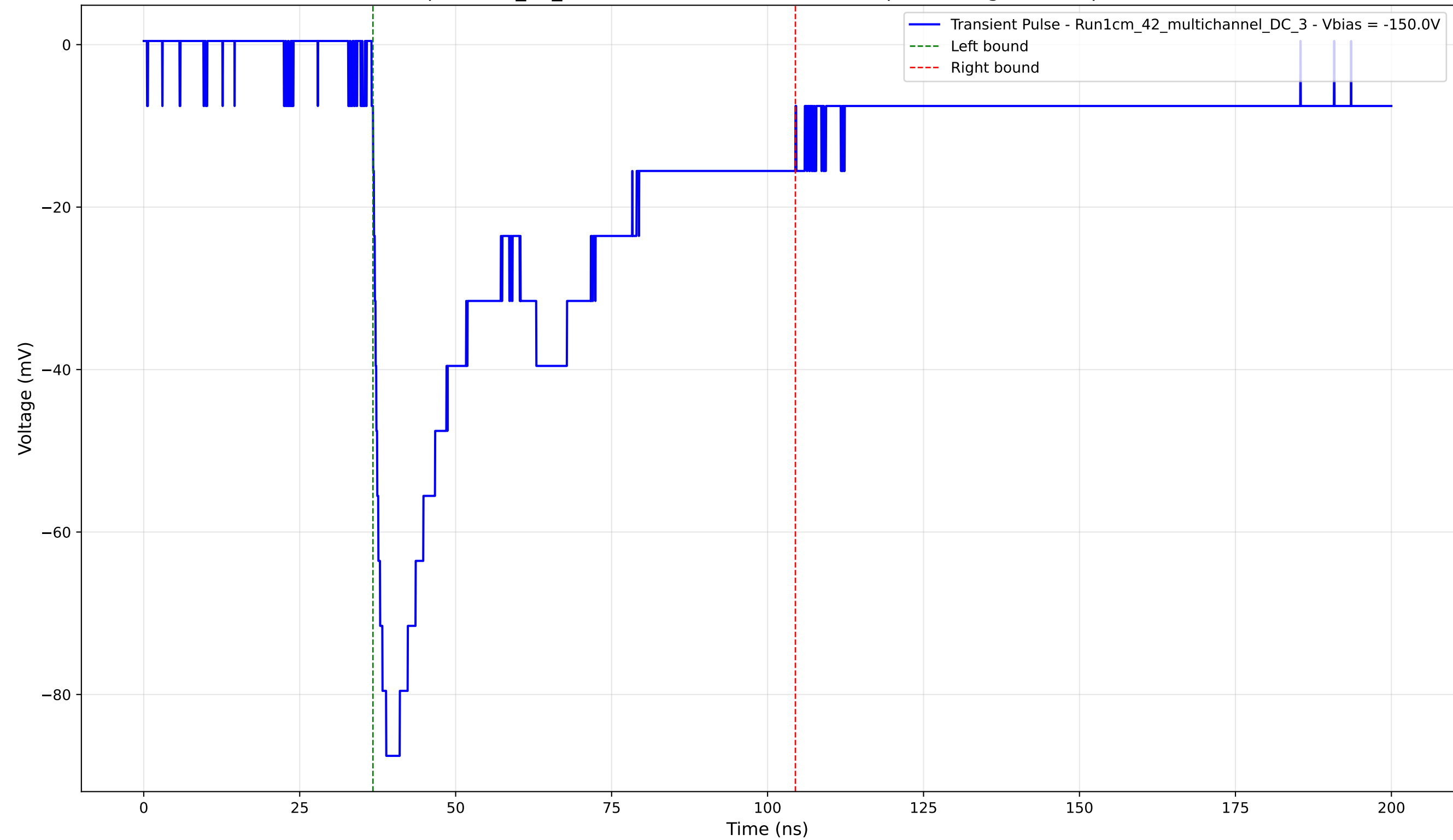
Transient Pulse - Sample: 1cm_42_multichannel - Position: 2140.0 \mu\text{m} - Charge: 42.45 pC - Rise Time: 1.52 ns
