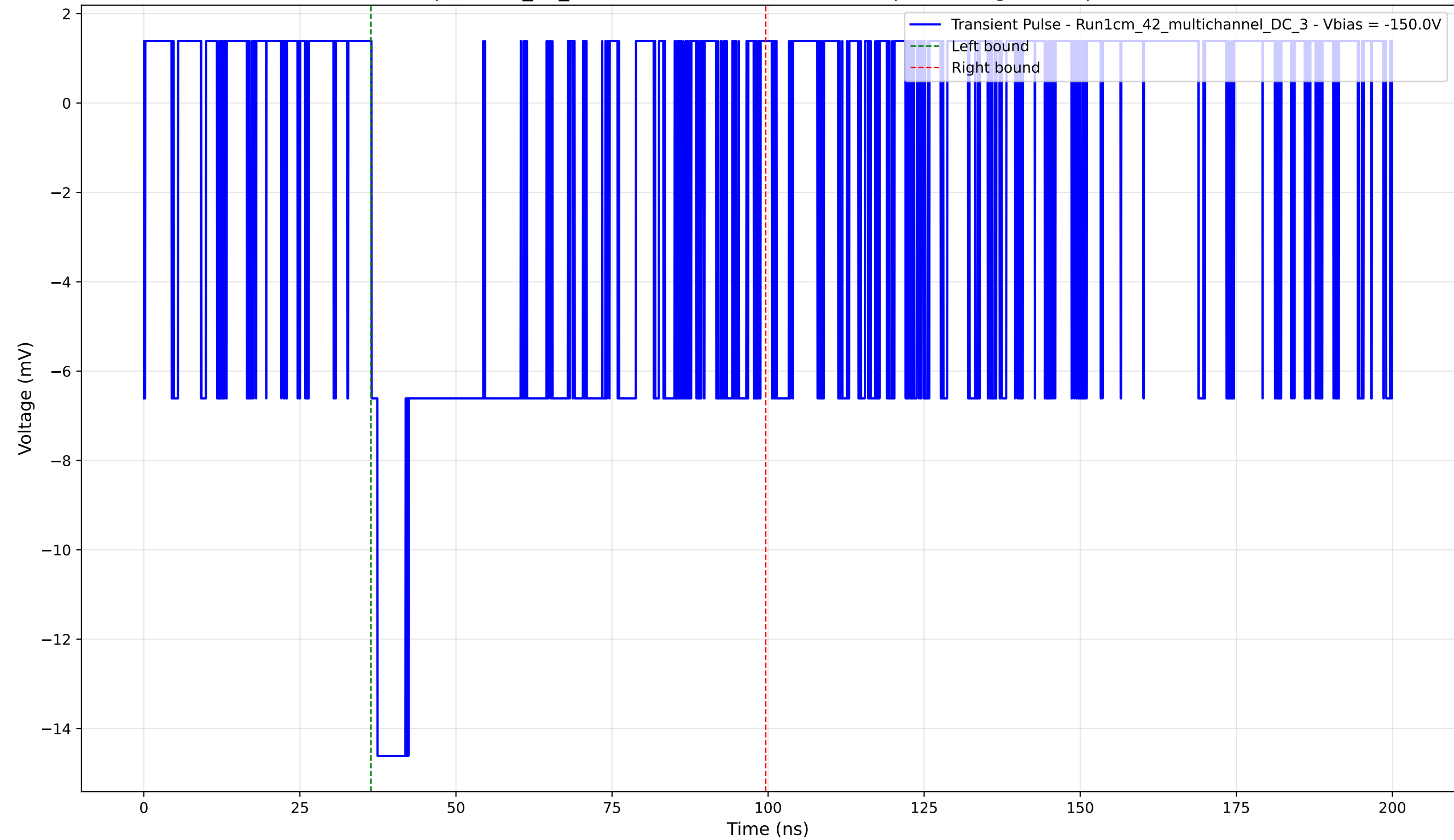
Transient Pulse - Sample: 1cm_42_multichannel - Position: 3910.0 \mu\text{m} - Charge: 6.72 pC - Rise Time: 0.96 ns
