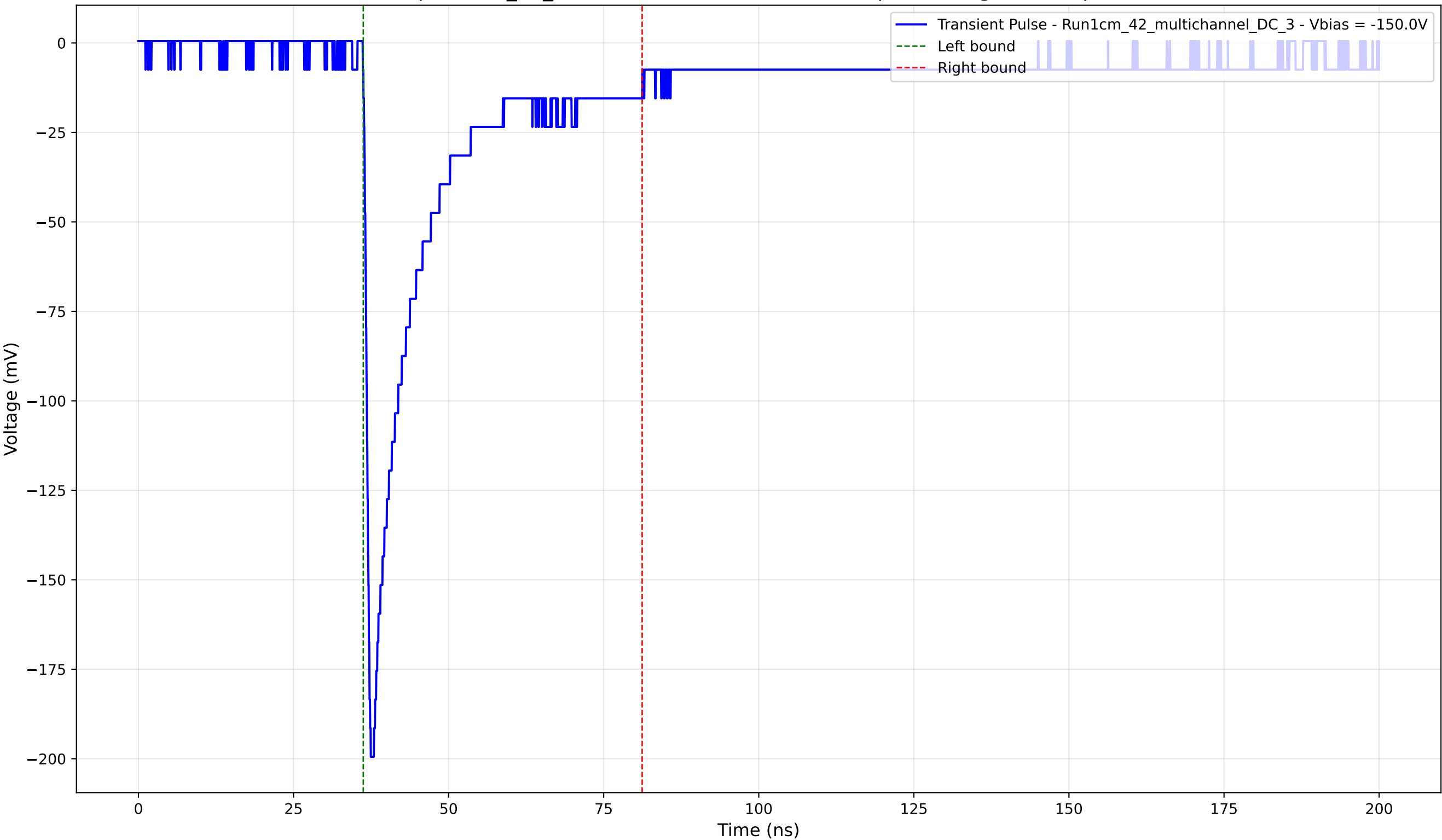
Transient Pulse - Sample: 1cm_42_multichannel - Position: 4270.0 \mu\text{m} - Charge: 37.53 pC - Rise Time: 0.91 ns
