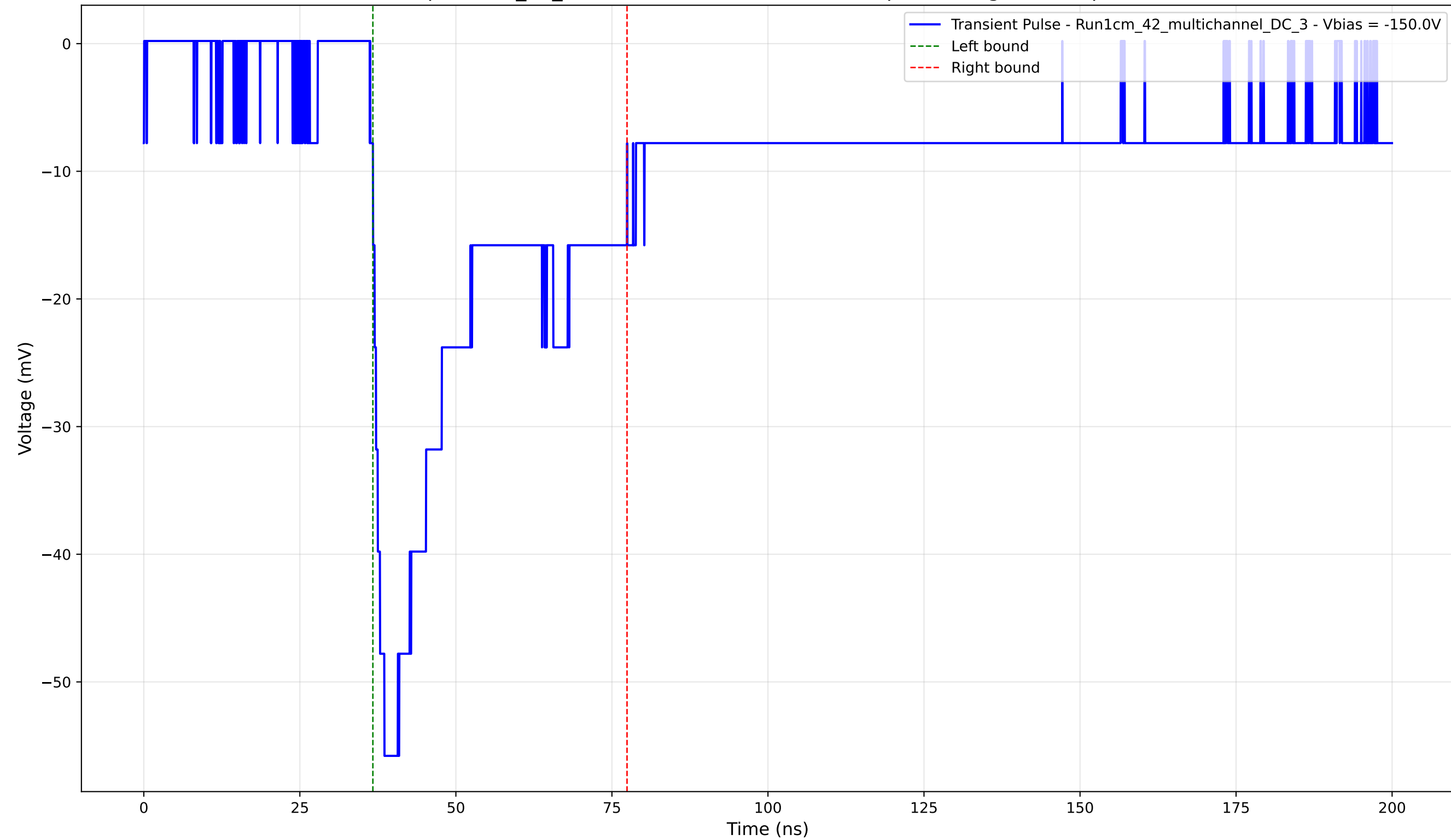
Transient Pulse - Sample: 1cm_42_multichannel - Position: 1920.0 \mu\text{m} - Charge: 19.87 pC - Rise Time: 2.27 ns
