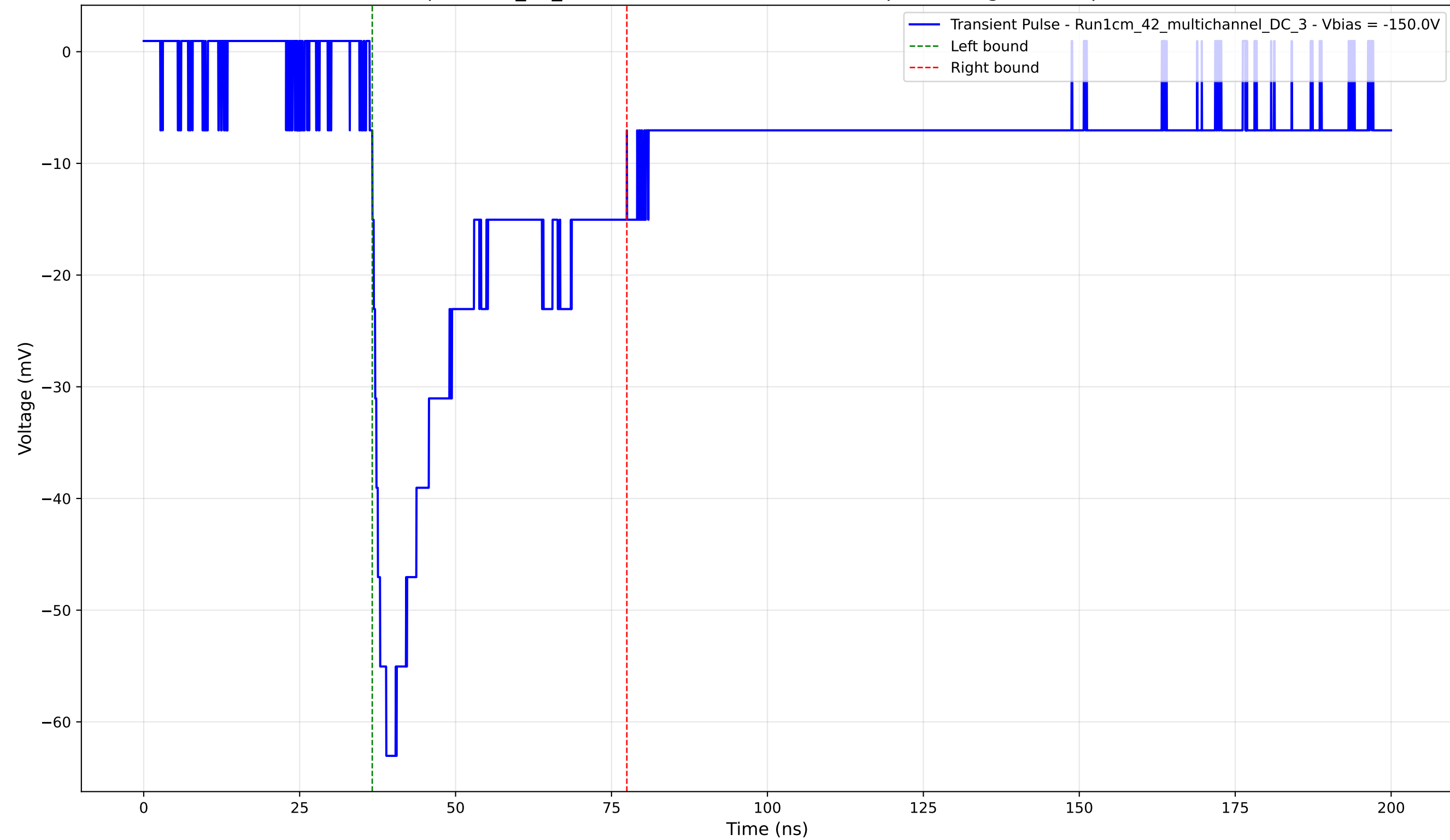
Transient Pulse - Sample: 1cm_42_multichannel - Position: 1815.0 \mu\text{m} - Charge: 20.82 pC - Rise Time: 2.66 ns
