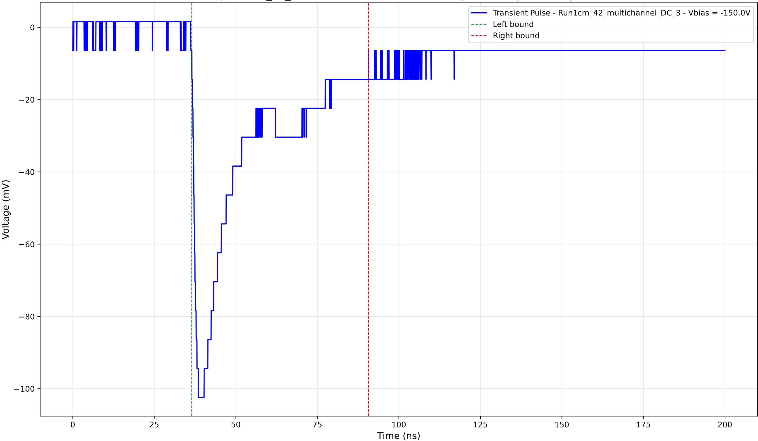
Transient Pulse - Sample: 1cm_42_multichannel - Position: 1785.0 \mu\text{m} - Charge: 37.41 pC - Rise Time: 1.57 ns
