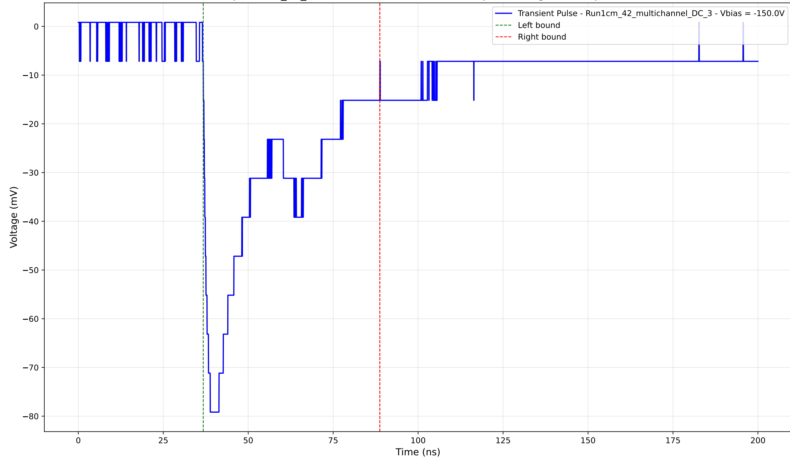
Transient Pulse - Sample: 1cm_42_multichannel - Position: 2580.0 \mu\text{m} - Charge: 34.79 pC - Rise Time: 2.06 ns
