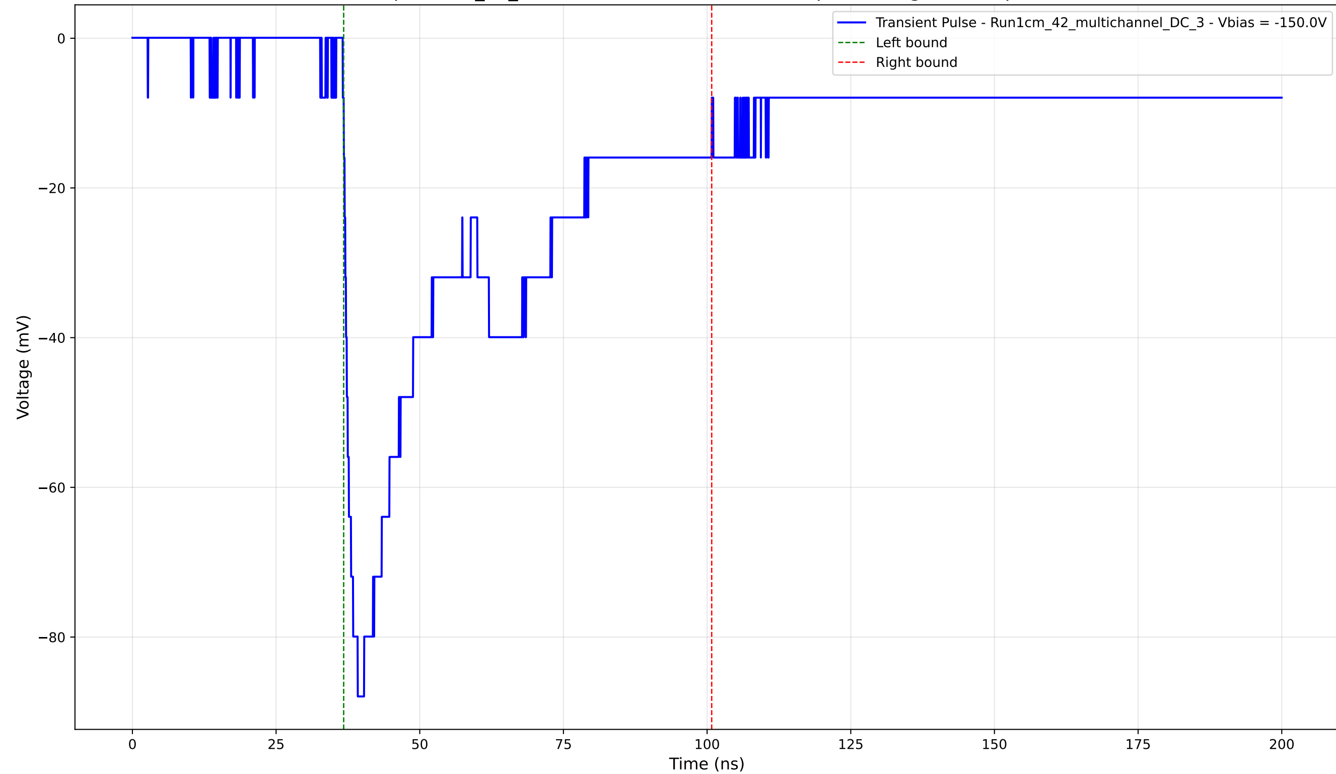
Transient Pulse - Sample: 1cm_42_multichannel - Position: 2260.0 \mu\text{m} - Charge: 42.06 pC - Rise Time: 1.64 ns
