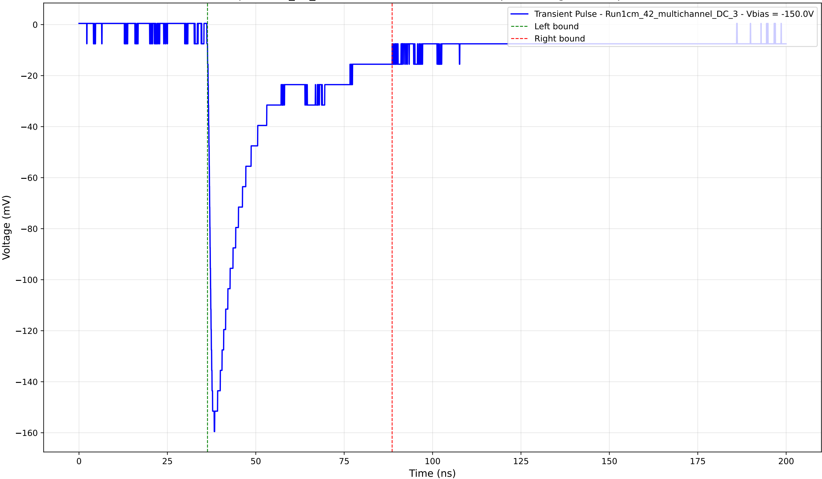
Transient Pulse - Sample: 1cm_42_multichannel - Position: 1175.0 \mu\text{m} - Charge: 44.15 pC - Rise Time: 1.30 ns
