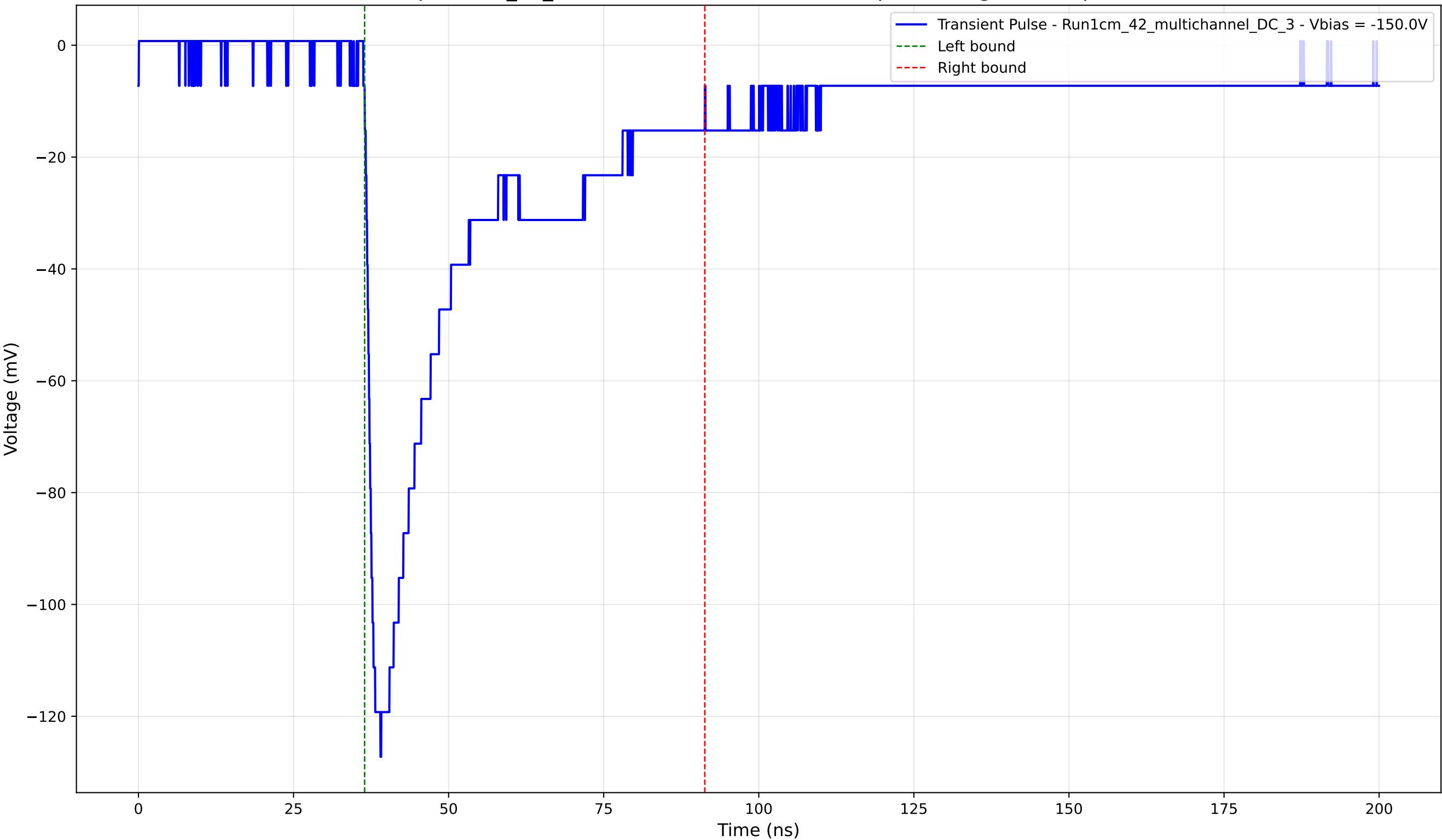
Transient Pulse - Sample: 1cm_42_multichannel - Position: 1590.0 \mu\text{m} - Charge: 42.52 pC - Rise Time: 1.69 ns
