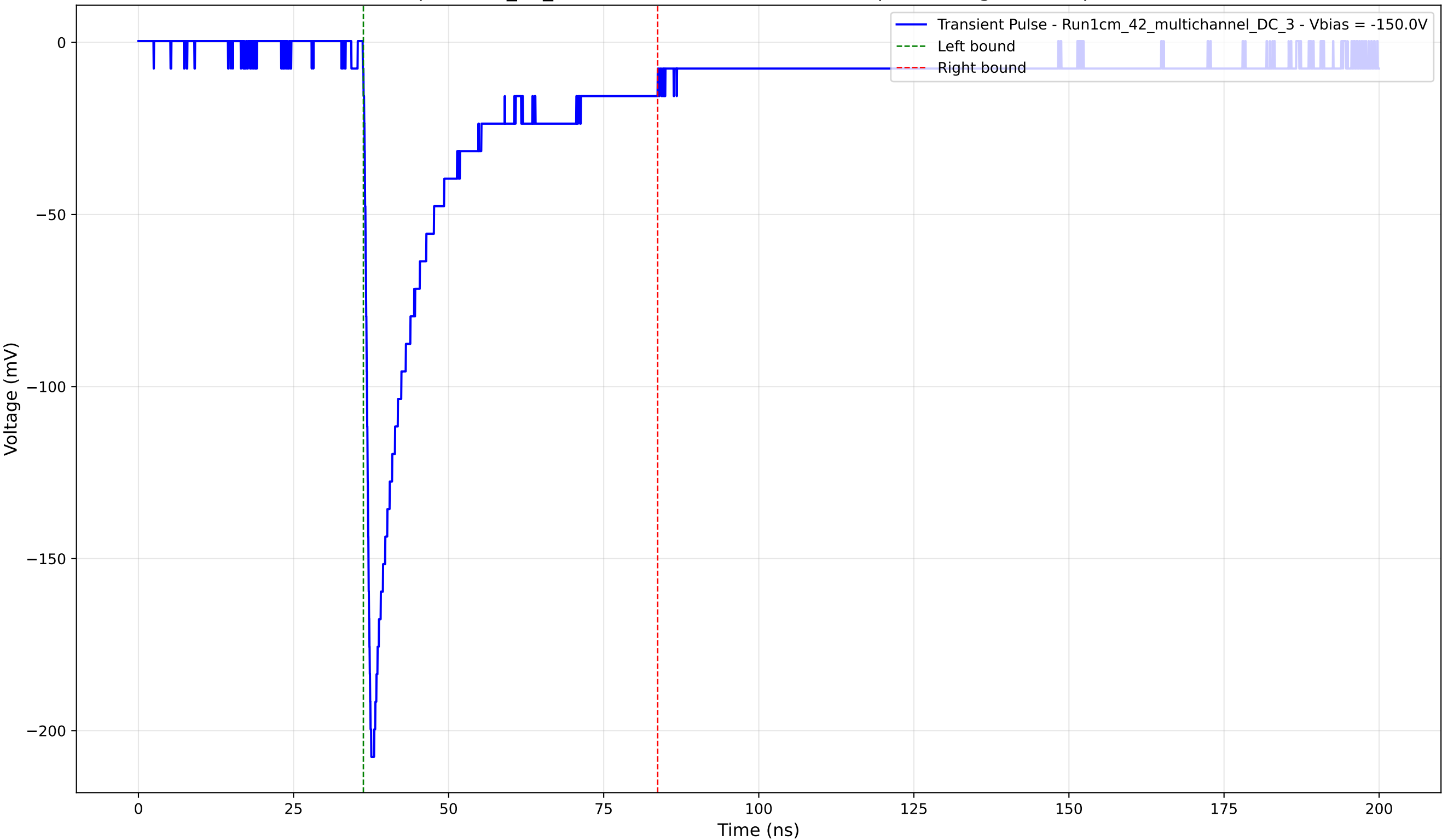
Transient Pulse - Sample: 1cm_42_multichannel - Position: 4215.0 \mu\text{m} - Charge: 41.65 pC - Rise Time: 0.97 ns
