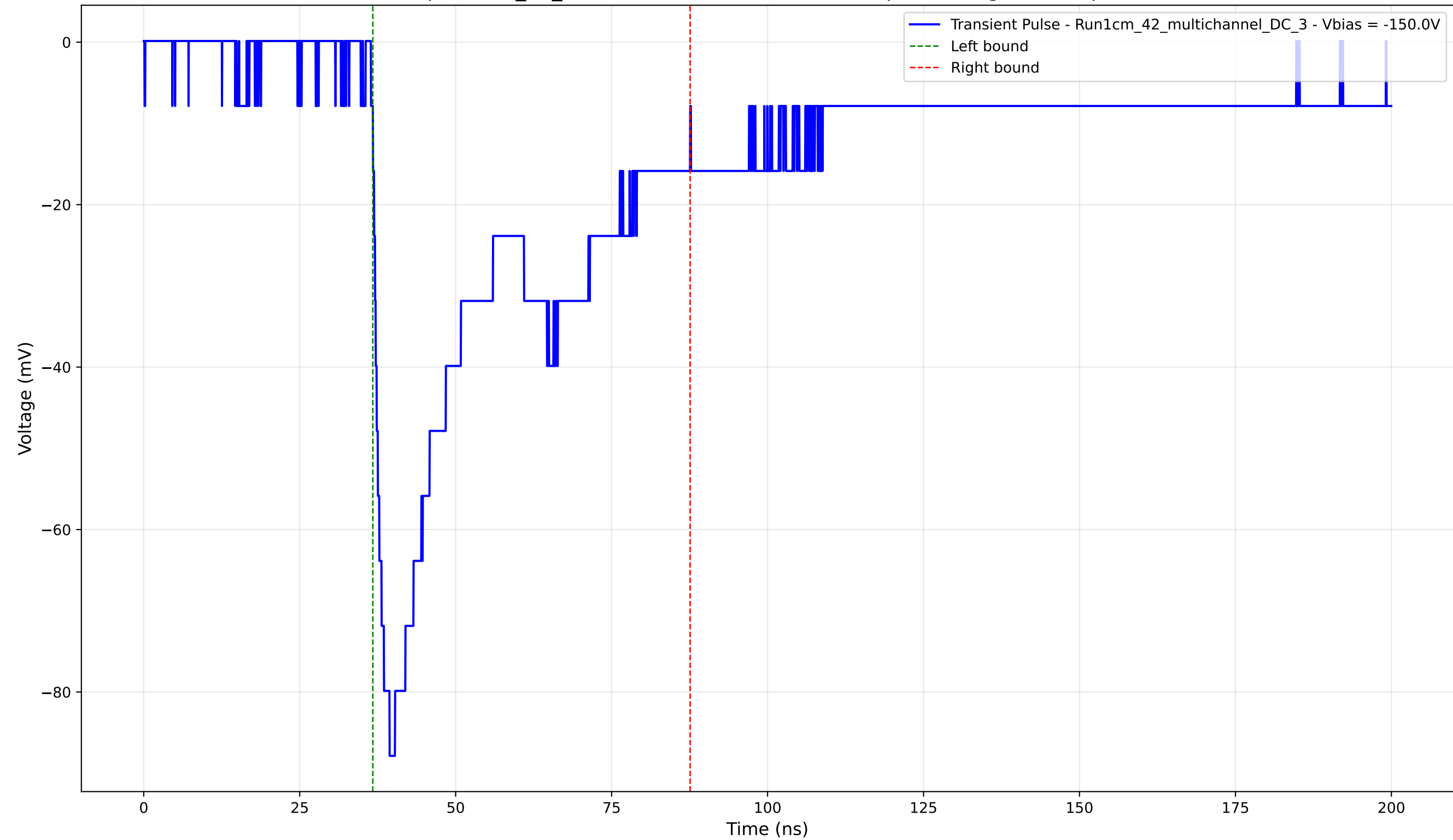
Transient Pulse - Sample: 1cm_42_multichannel - Position: 2640.0 \mu\text{m} - Charge: 35.53 pC - Rise Time: 1.78 ns
