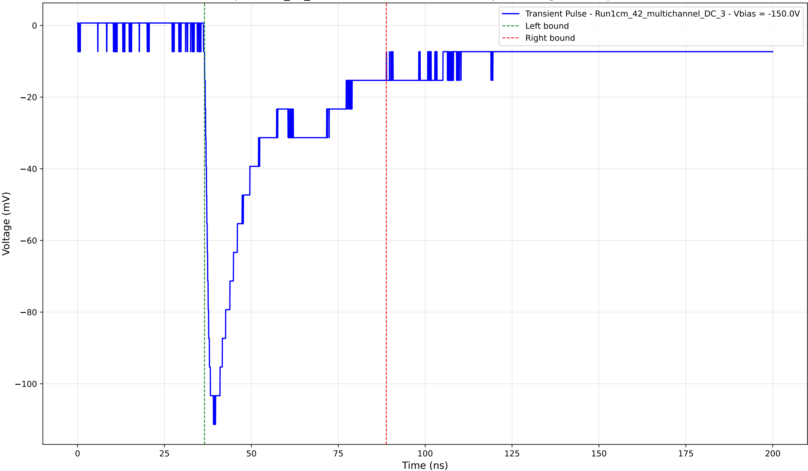
Transient Pulse - Sample: 1cm_42_multichannel - Position: 1775.0 \mu\text{m} - Charge: 39.23 pC - Rise Time: 1.67 ns
