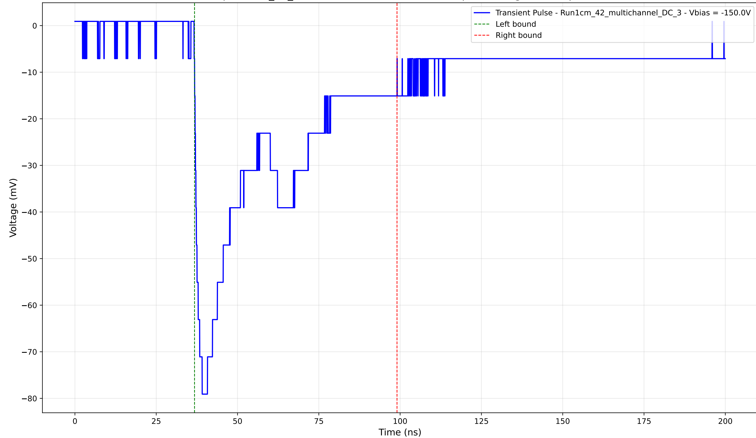
Transient Pulse - Sample: 1cm_42_multichannel - Position: 2290.0 \mu\text{m} - Charge: 38.03 pC - Rise Time: 2.34 ns
