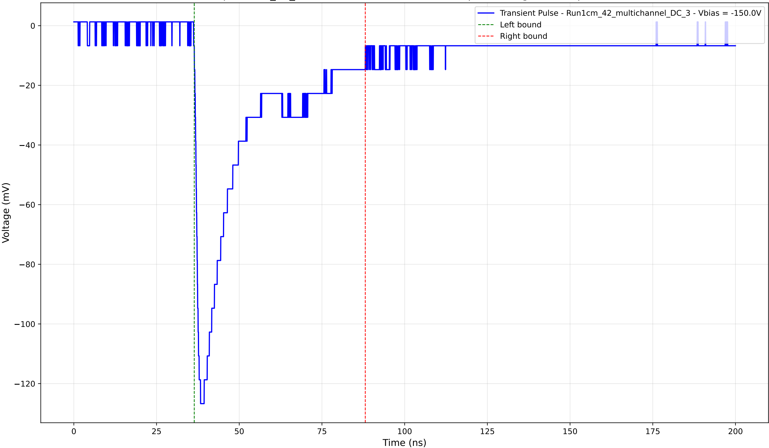
Transient Pulse - Sample: 1cm_42_multichannel - Position: 1440.0 \mu\text{m} - Charge: 39.73 pC - Rise Time: 1.47 ns
