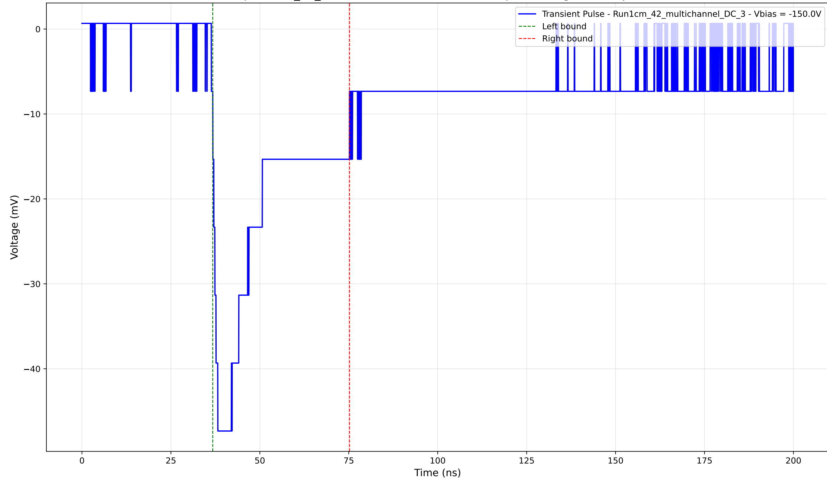
Transient Pulse - Sample: 1cm_42_multichannel - Position: 2930.0 \mu\text{m} - Charge: 17.12 pC - Rise Time: 1.83 ns
