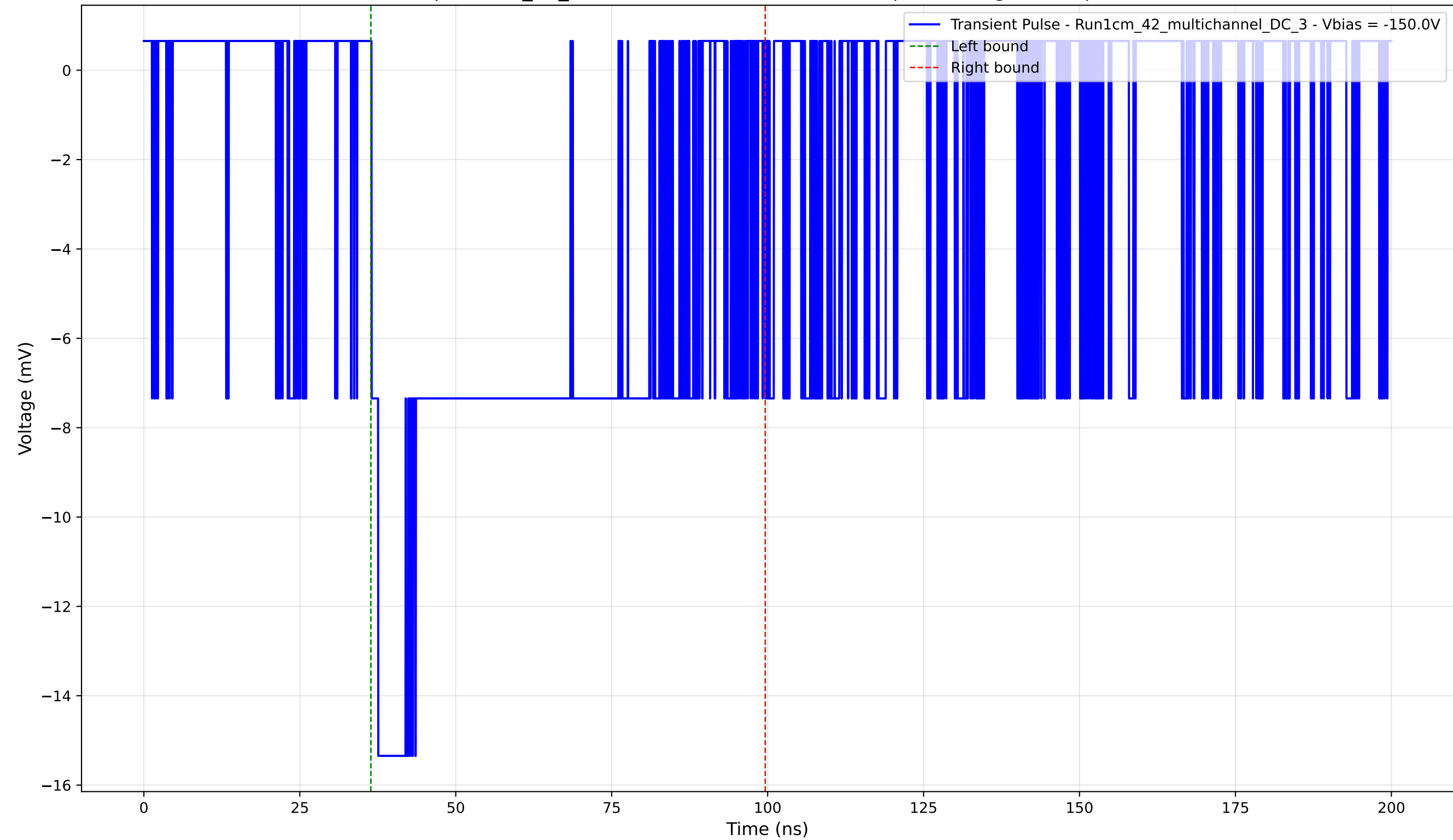
Transient Pulse - Sample: 1cm_42_multichannel - Position: 1385.0 \mu\text{m} - Charge: 8.39 pC - Rise Time: 1.08 ns
