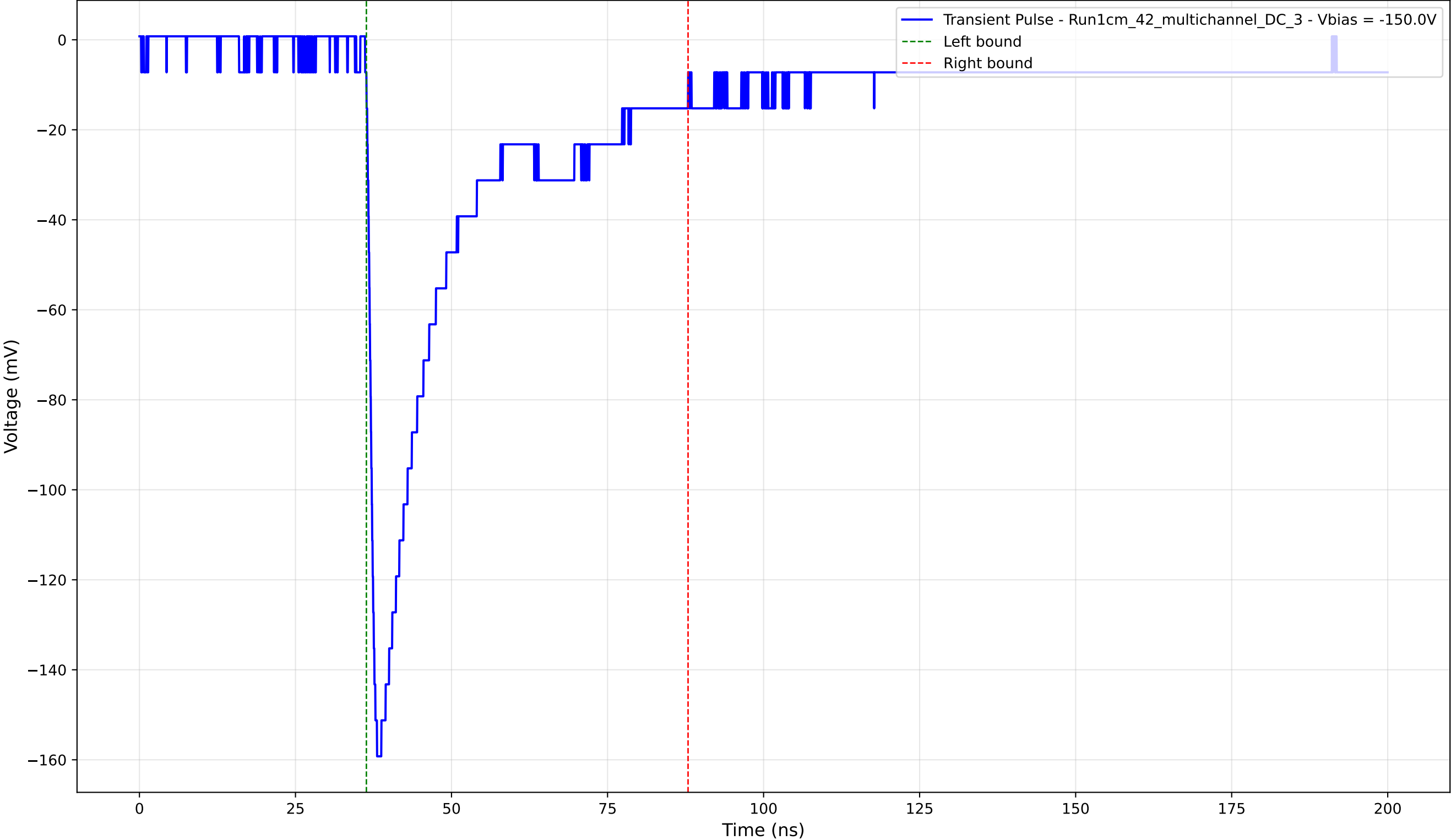
Transient Pulse - Sample: 1cm_42_multichannel - Position: 1215.0 \mu\text{m} - Charge: 44.82 pC - Rise Time: 1.32 ns
