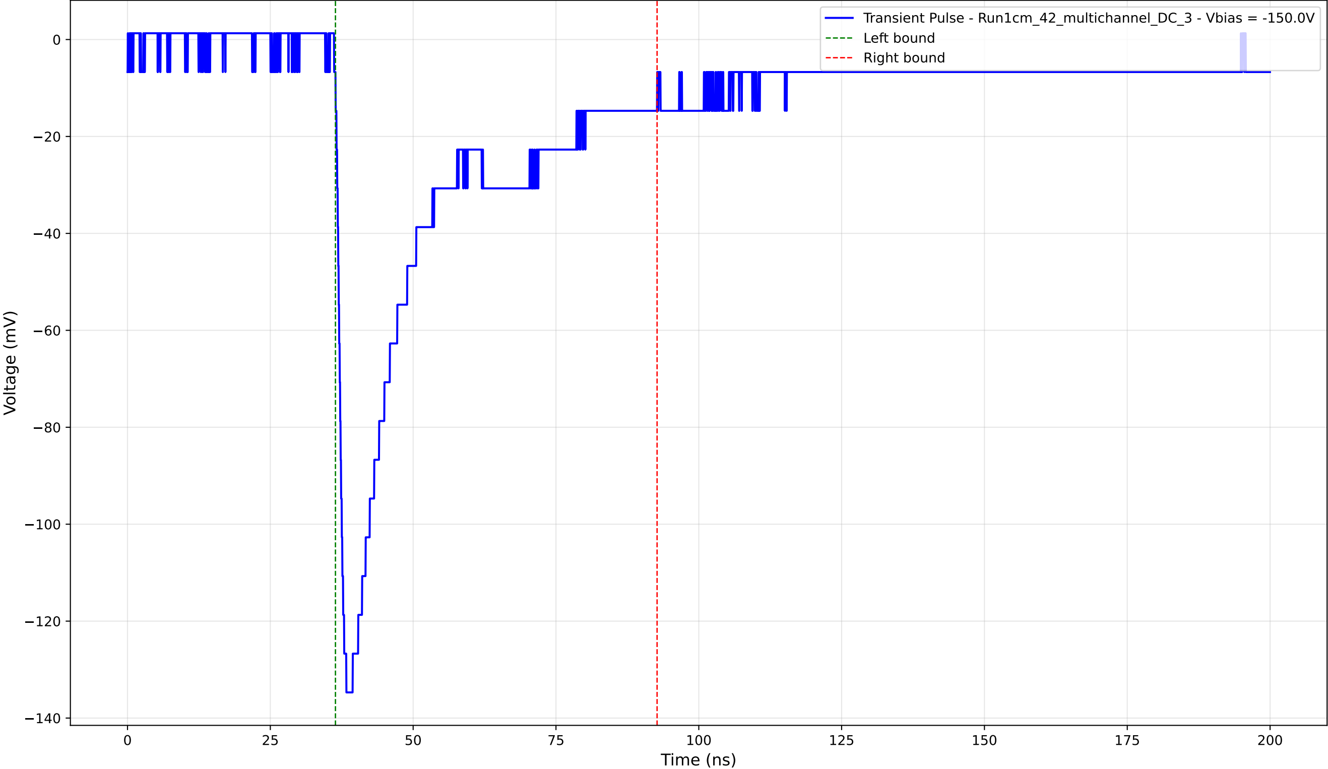
Transient Pulse - Sample: 1cm_42_multichannel - Position: 1470.0 \mu\text{m} - Charge: 43.84 pC - Rise Time: 1.50 ns
