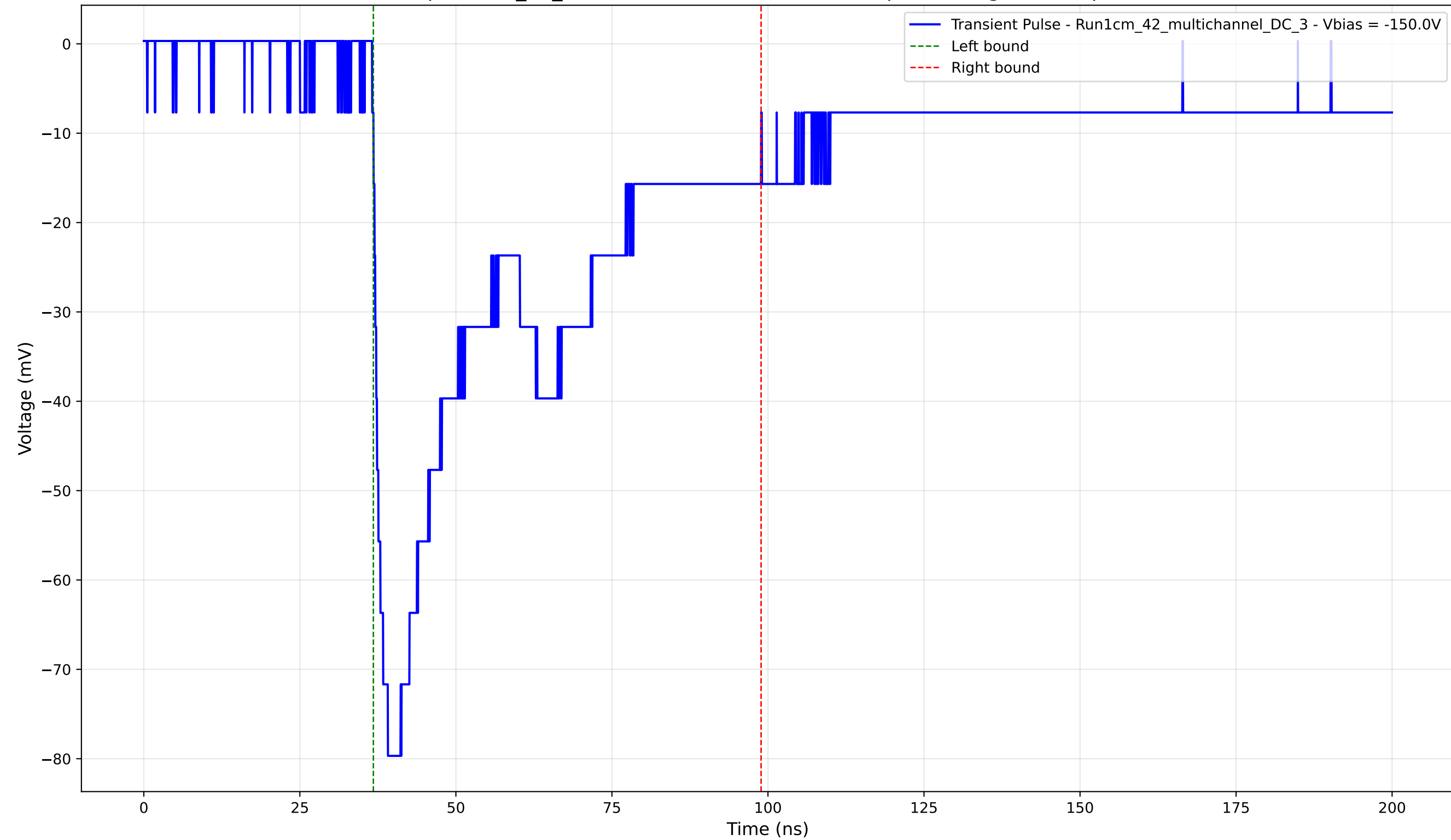
Transient Pulse - Sample: 1cm_42_multichannel - Position: 2525.0 \mu\text{m} - Charge: 38.60 pC - Rise Time: 2.32 ns
