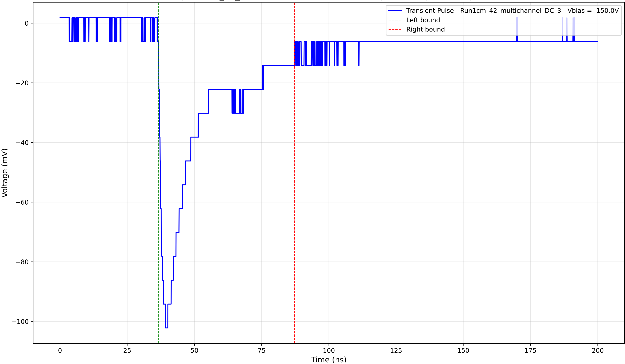
Transient Pulse - Sample: 1cm_42_multichannel - Position: 3075.0 \mu\text{m} - Charge: 34.13 pC - Rise Time: 1.85 ns
