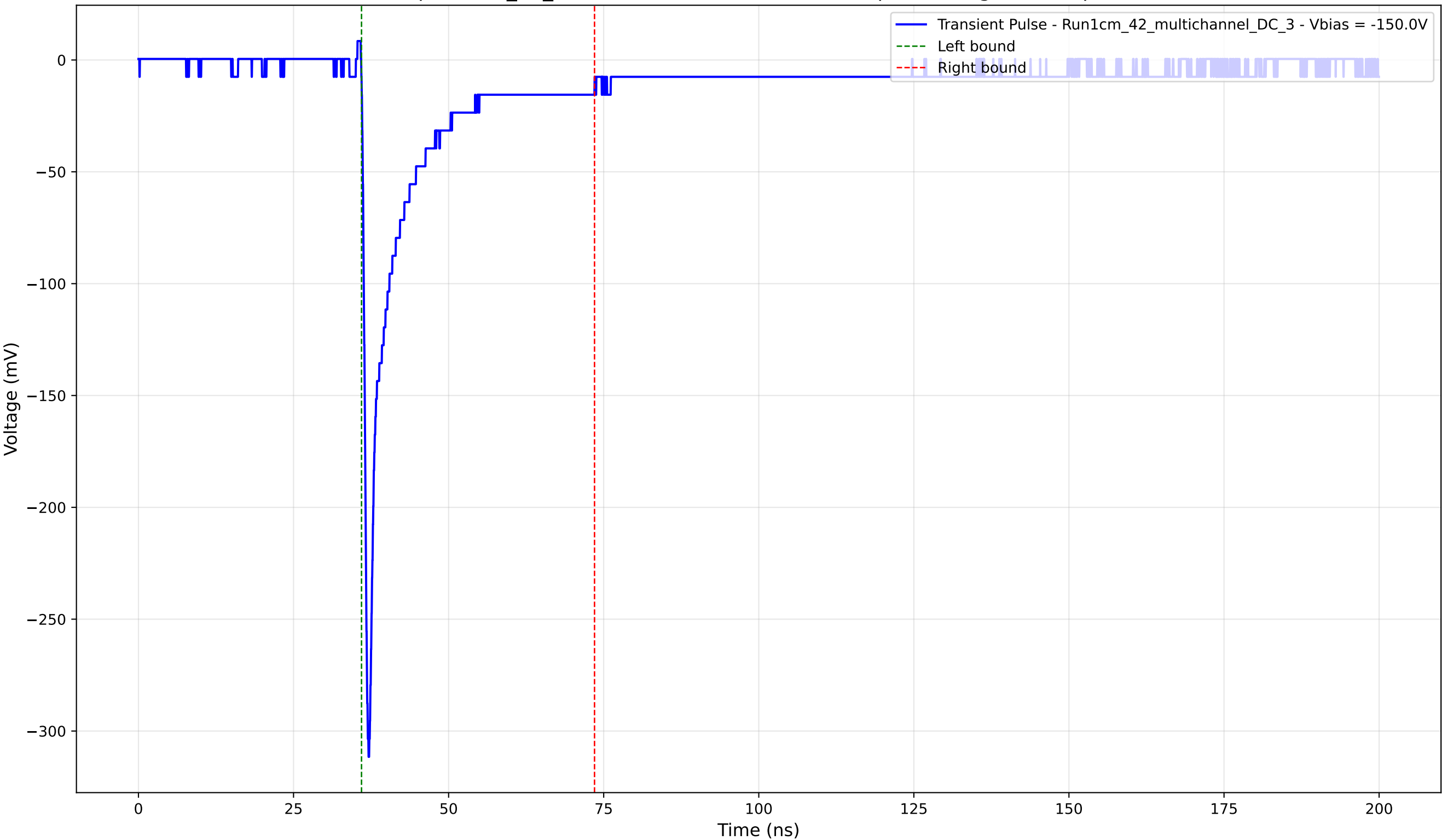
Transient Pulse - Sample: 1cm_42_multichannel - Position: 4830.0 \mu\text{m} - Charge: 33.18 pC - Rise Time: 0.80 ns
