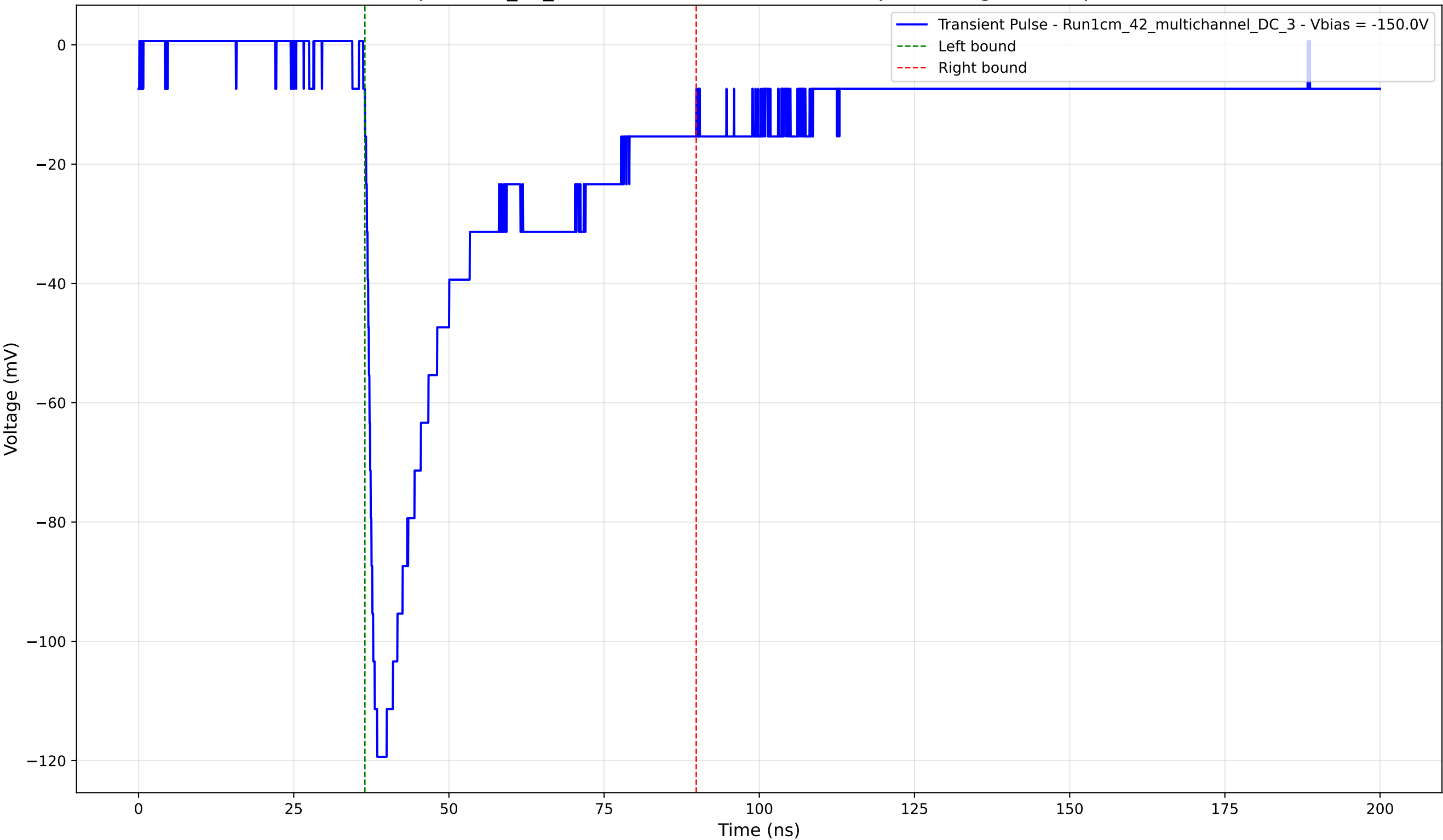
Transient Pulse - Sample: 1cm_42_multichannel - Position: 1645.0 \mu\text{m} - Charge: 41.60 pC - Rise Time: 1.57 ns
