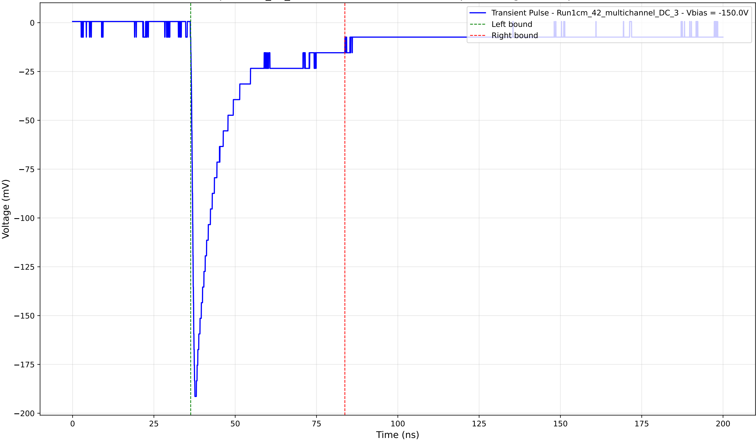
Transient Pulse - Sample: 1cm_42_multichannel - Position: 4145.0 \mu\text{m} - Charge: 40.68 pC - Rise Time: 0.99 ns
