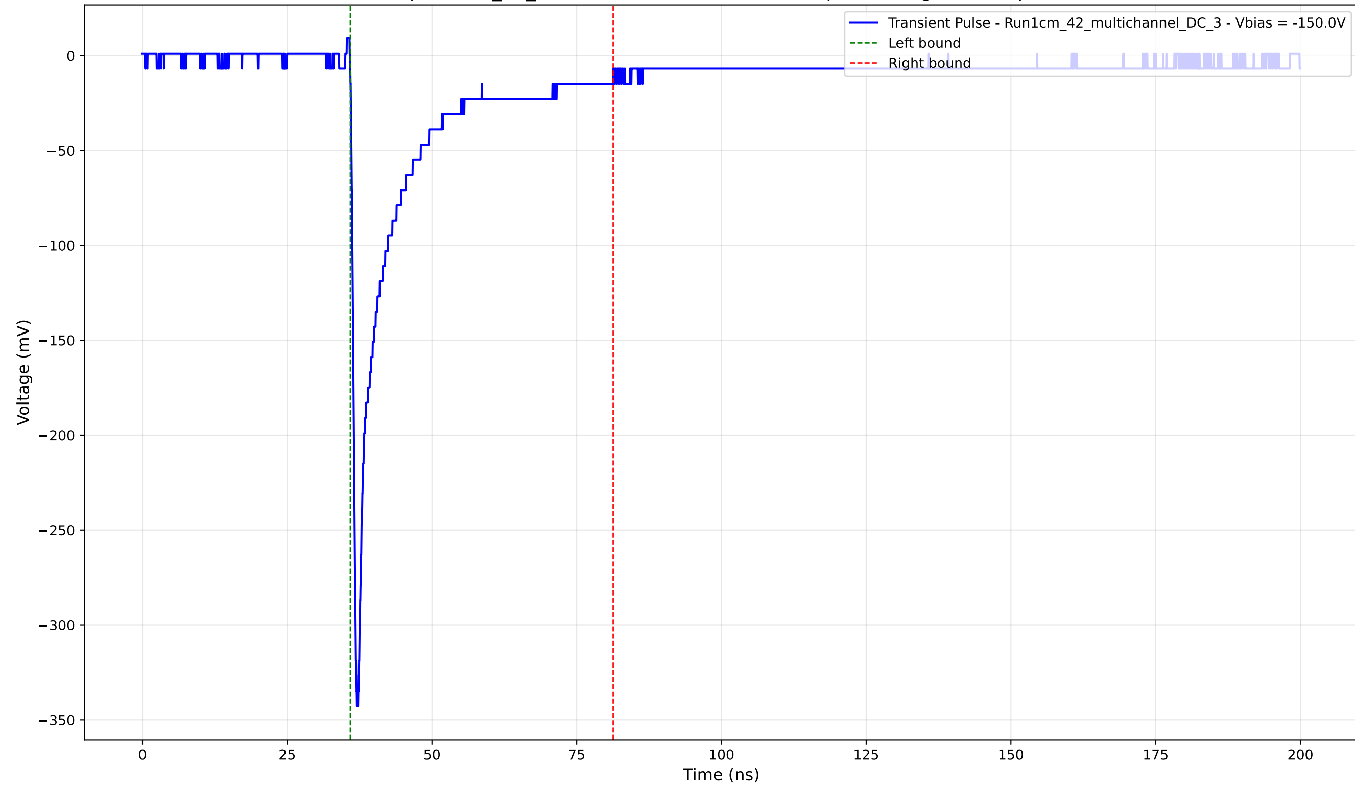
Transient Pulse - Sample: 1cm_42_multichannel - Position: 220.0 \mu\text{m} - Charge: 46.37 pC - Rise Time: 0.81 ns
