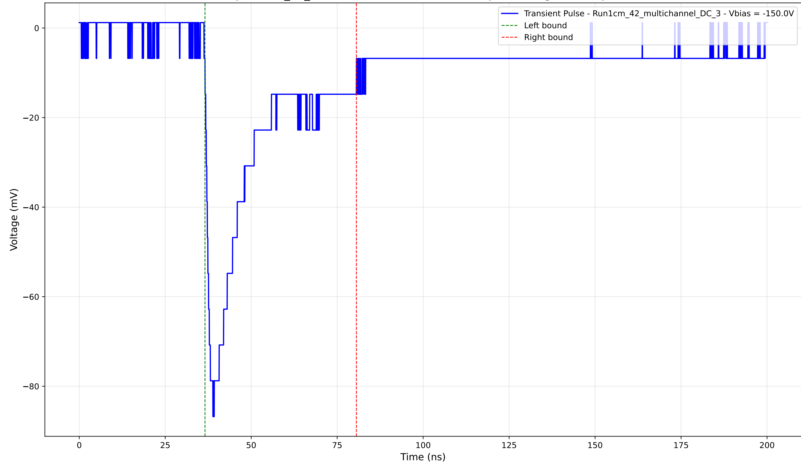
Transient Pulse - Sample: 1cm_42_multichannel - Position: 3325.0 \mu\text{m} - Charge: 25.08 pC - Rise Time: 1.56 ns
