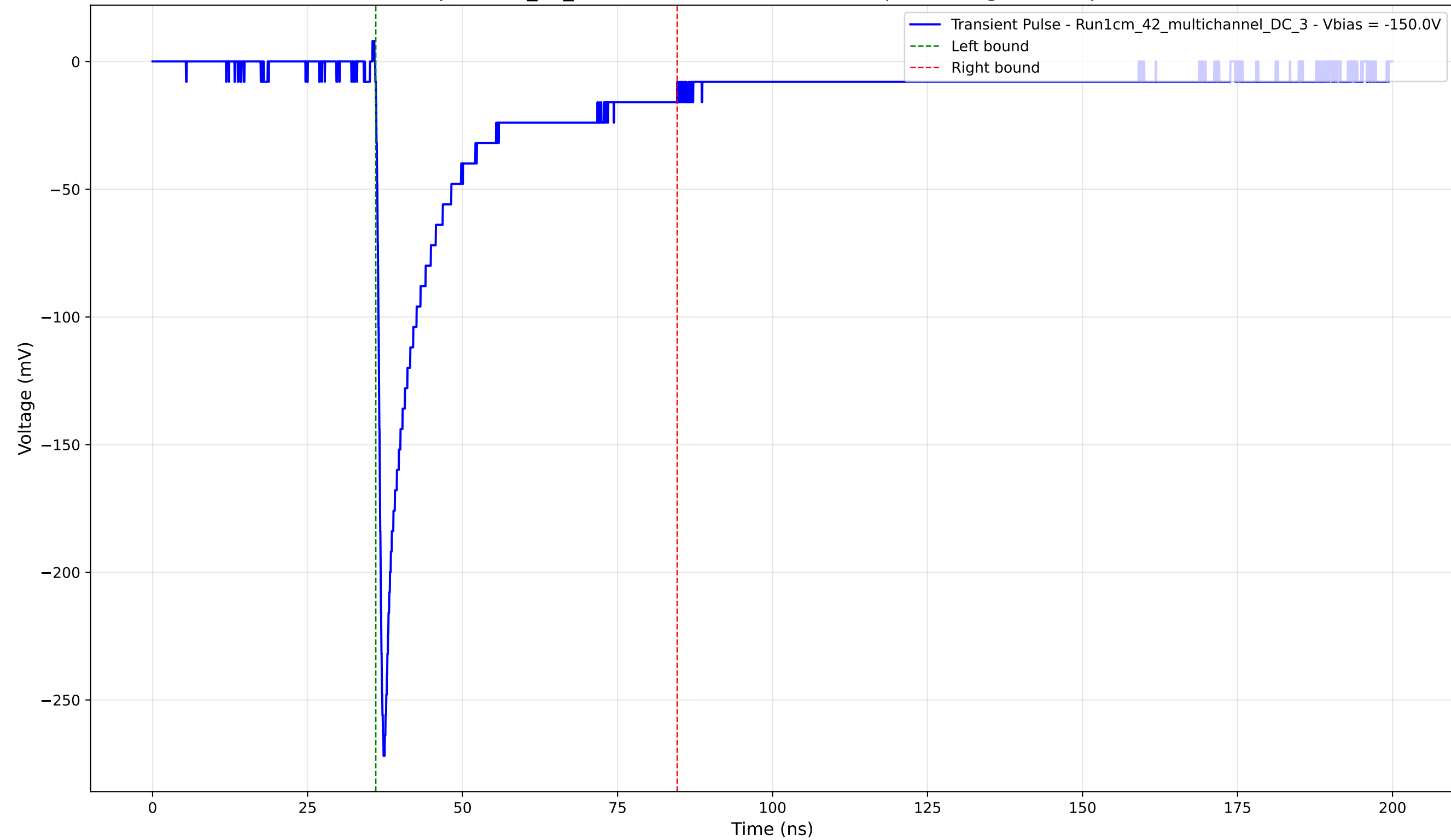
Transient Pulse - Sample: 1cm_42_multichannel - Position: 430.0 \mu\text{m} - Charge: 46.62 pC - Rise Time: 0.89 ns
