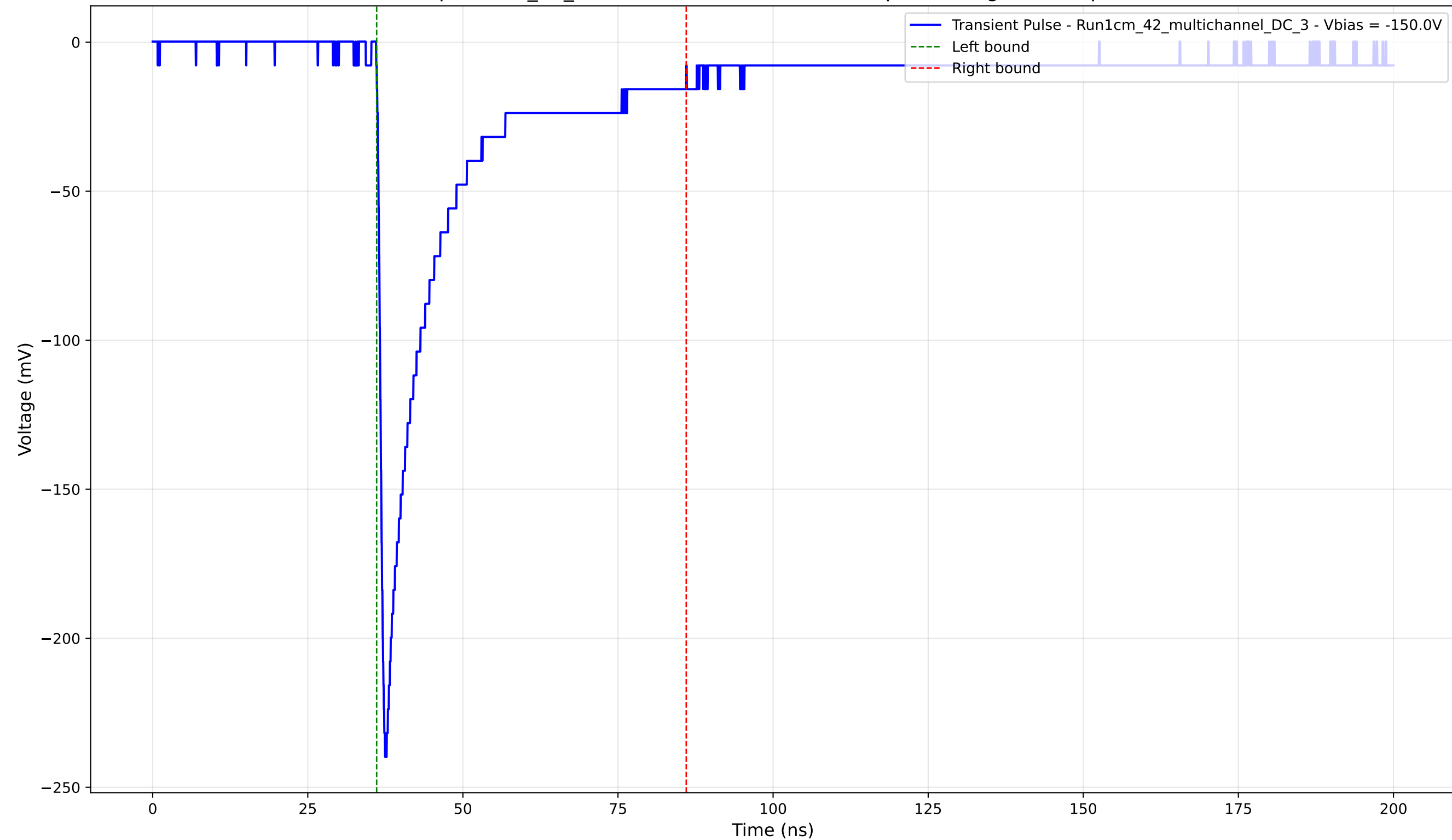
Transient Pulse - Sample: 1cm_42_multichannel - Position: 630.0 \mu\text{m} - Charge: 47.86 pC - Rise Time: 0.98 ns
