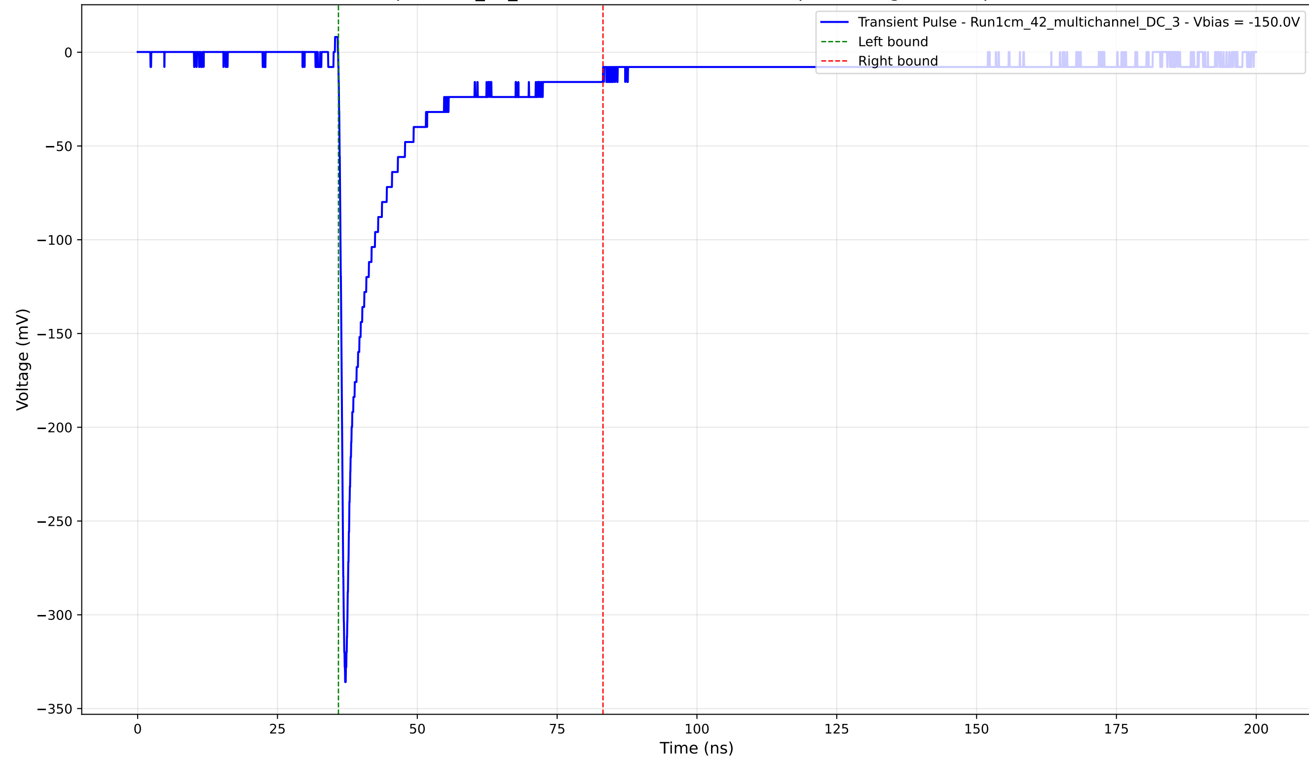
Transient Pulse - Sample: 1cm_42_multichannel - Position: 235.0 \mu\text{m} - Charge: 47.11 pC - Rise Time: 0.82 ns
