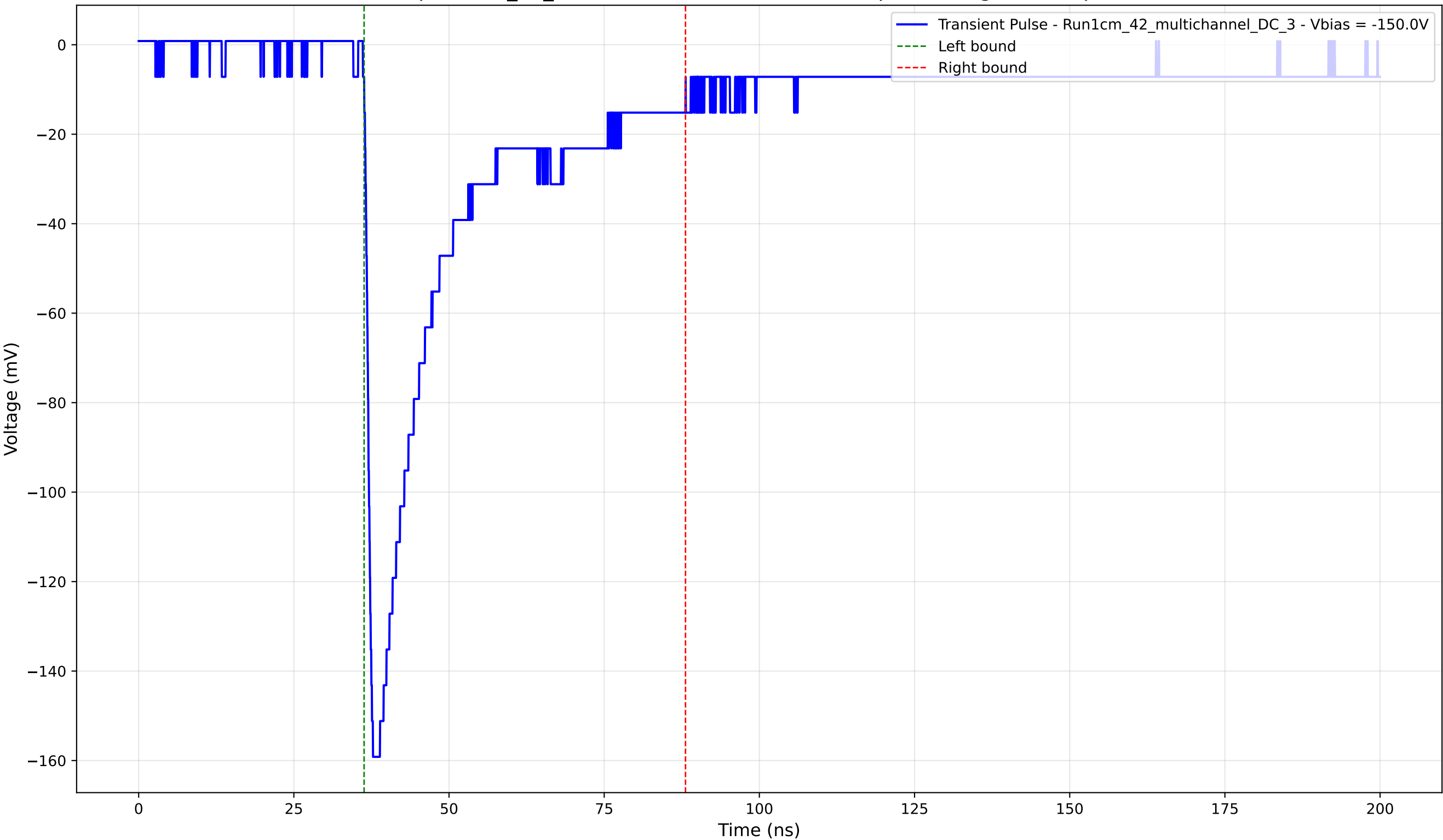
Transient Pulse - Sample: 1cm_42_multichannel - Position: 1090.0 \mu\text{m} - Charge: 43.64 pC - Rise Time: 1.14 ns
