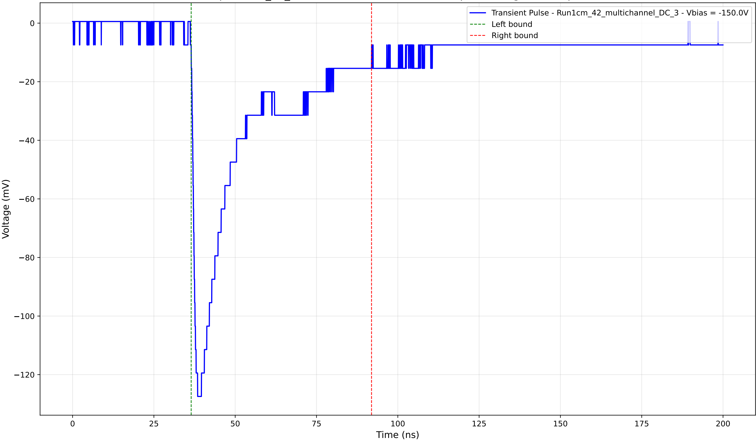
Transient Pulse - Sample: 1cm_42_multichannel - Position: 1550.0 \mu\text{m} - Charge: 43.33 pC - Rise Time: 1.51 ns
