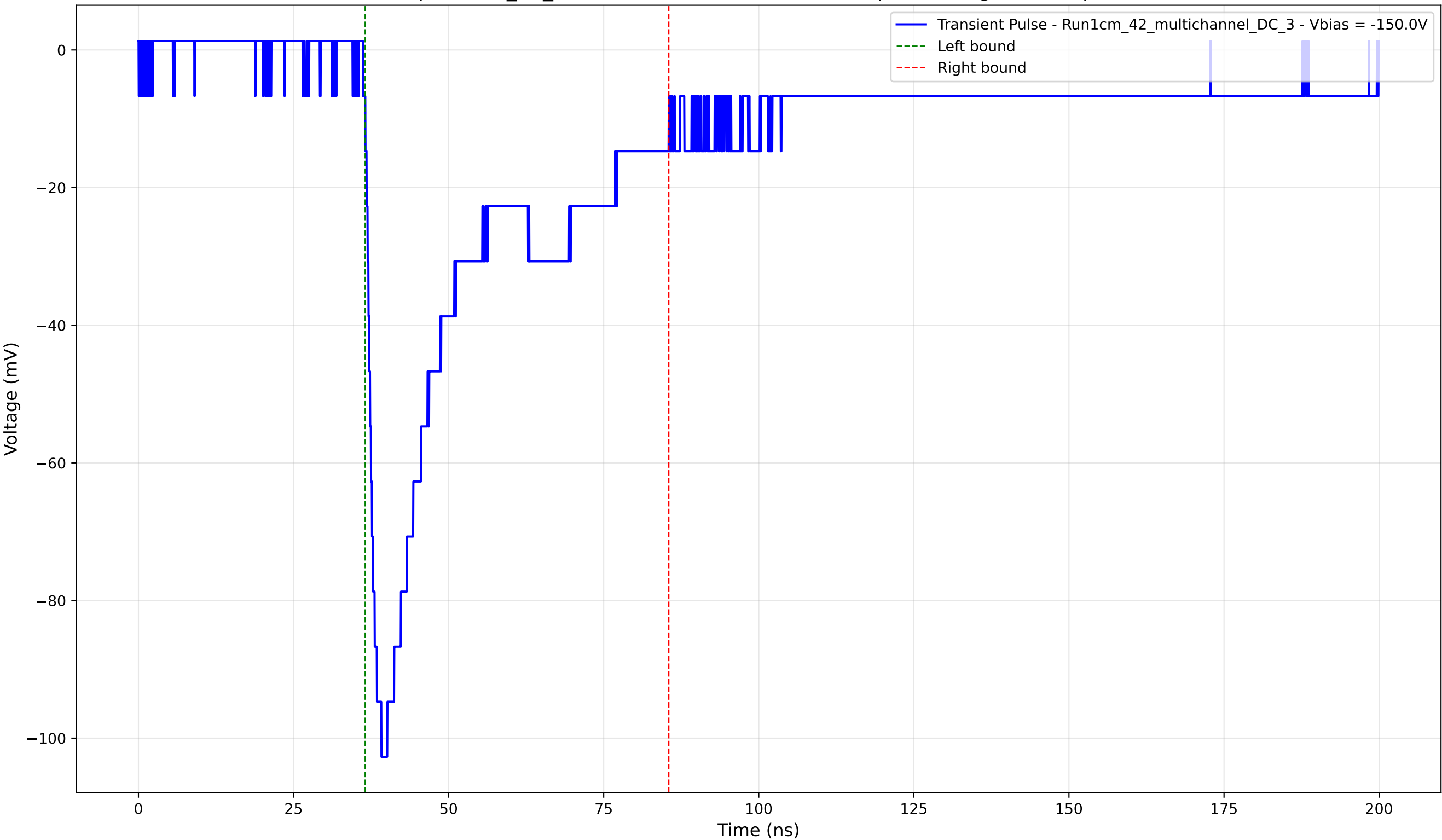
Transient Pulse - Sample: 1cm_42_multichannel - Position: 3040.0 \mu\text{m} - Charge: 35.00 pC - Rise Time: 1.87 ns
