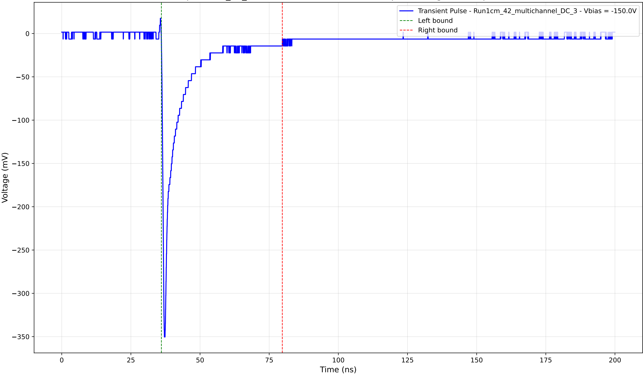
Transient Pulse - Sample: 1cm_42_multichannel - Position: 4735.0 \mu\text{m} - Charge: 41.81 pC - Rise Time: 0.77 ns
