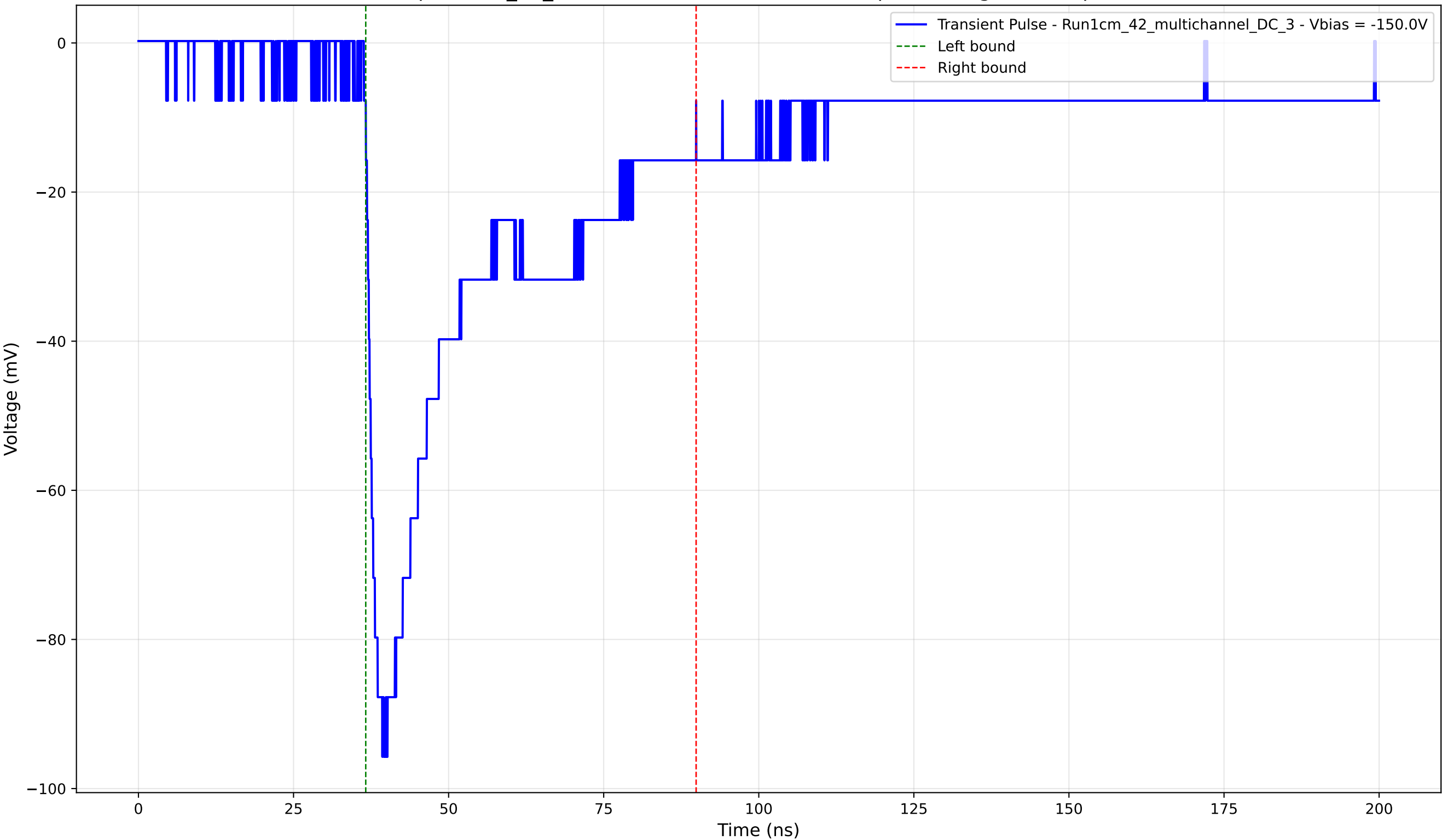
Transient Pulse - Sample: 1cm_42_multichannel - Position: 2785.0 \mu\text{m} - Charge: 37.16 pC - Rise Time: 1.92 ns
