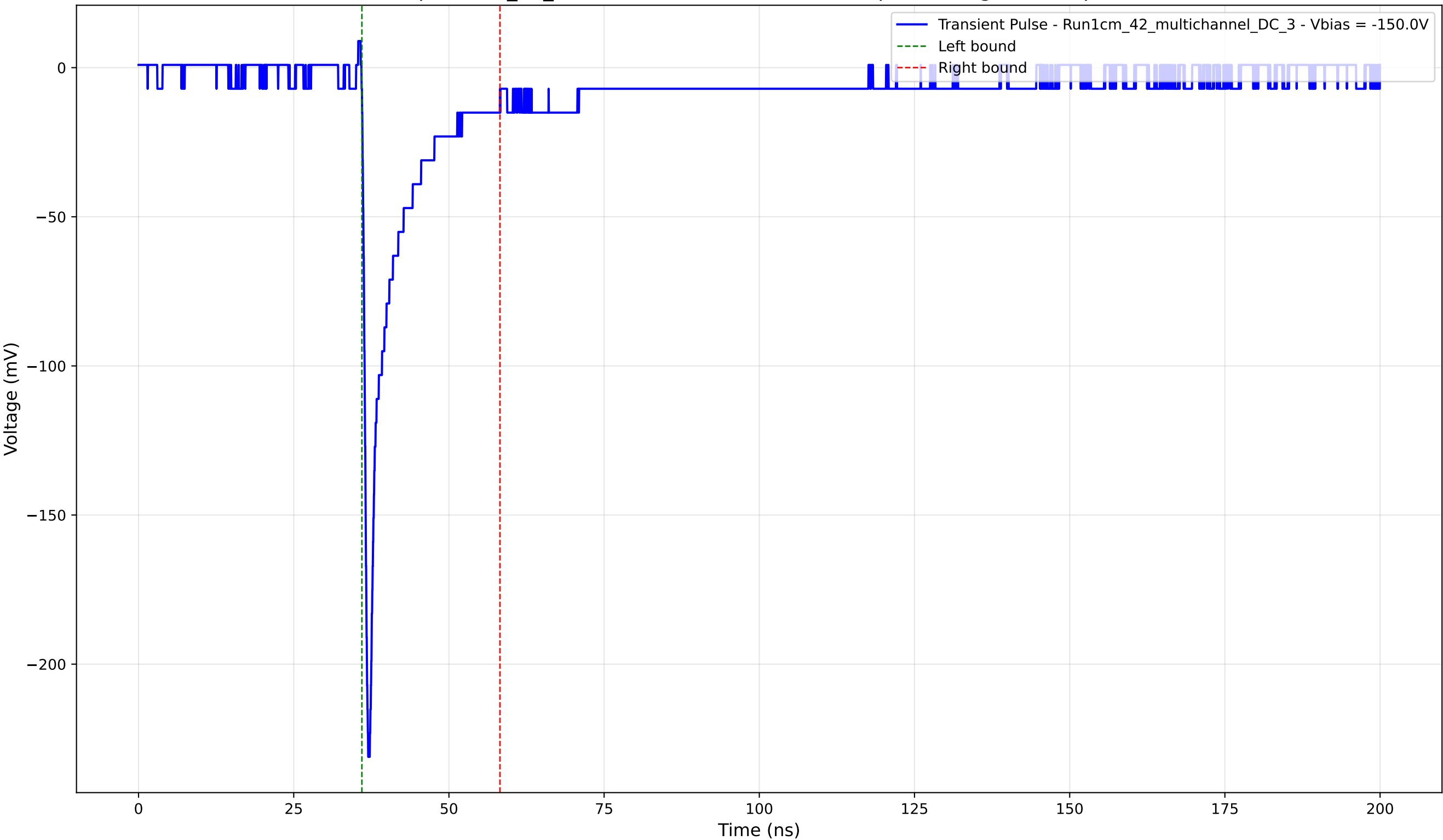
Transient Pulse - Sample: 1cm_42_multichannel - Position: 4845.0 \mu\text{m} - Charge: 21.56 pC - Rise Time: 0.78 ns
