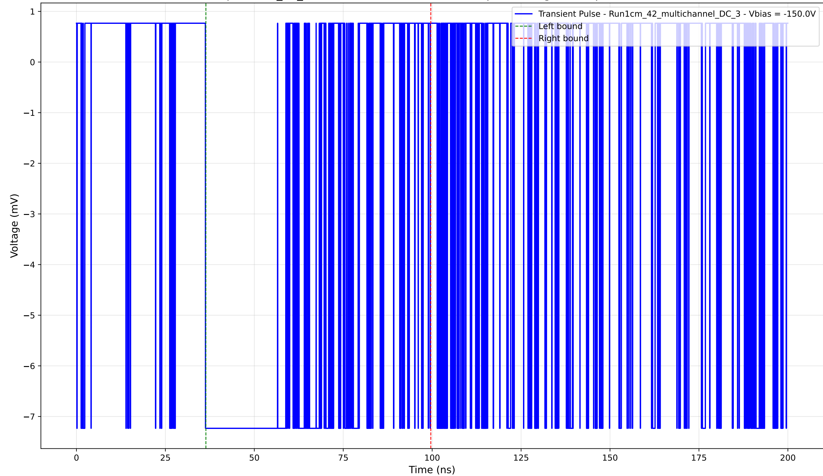
Transient Pulse - Sample: 1cm_42_multichannel - Position: 3880.0 \mu\text{m} - Charge: 5.02 pC - Rise Time: 0.00 ns (N/A)
