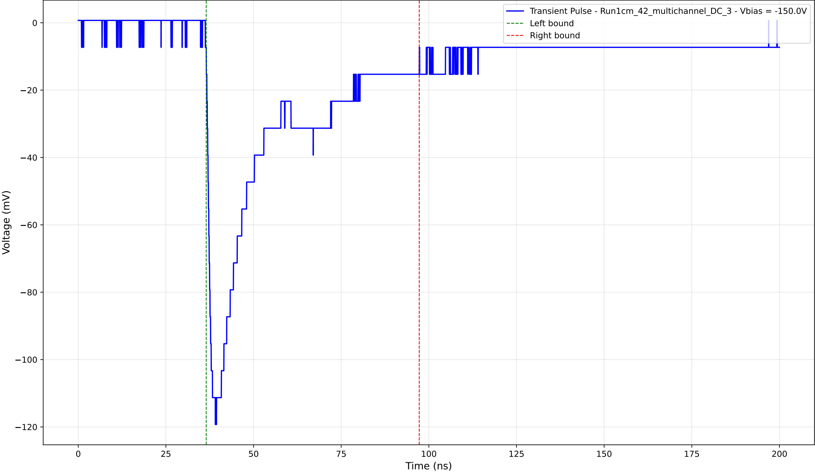
Transient Pulse - Sample: 1cm_42_multichannel - Position: 1730.0 \mu\text{m} - Charge: 43.64 pC - Rise Time: 1.77 ns
