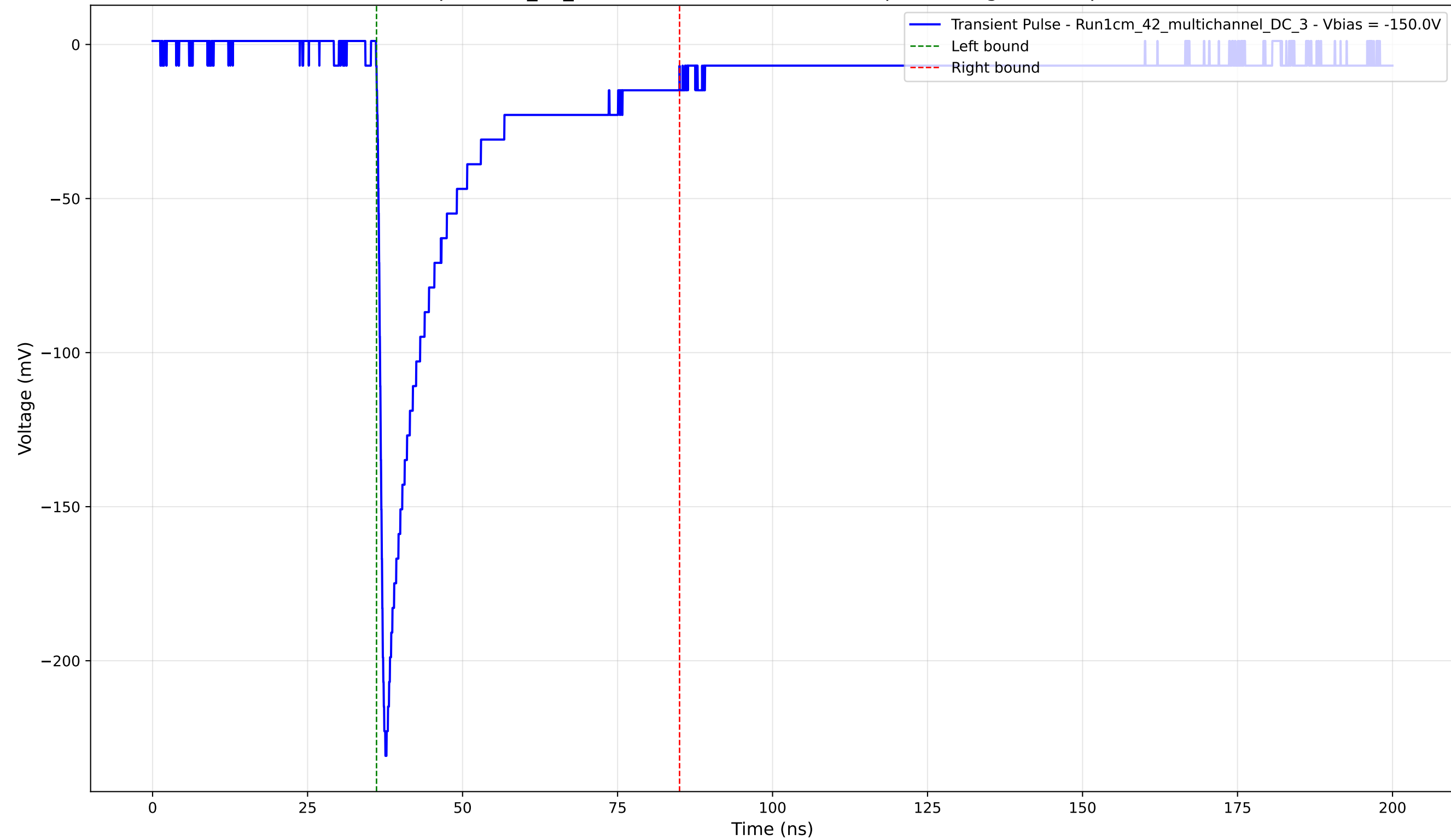
Transient Pulse - Sample: 1cm_42_multichannel - Position: 675.0 \mu\text{m} - Charge: 46.08 pC - Rise Time: 1.00 ns
