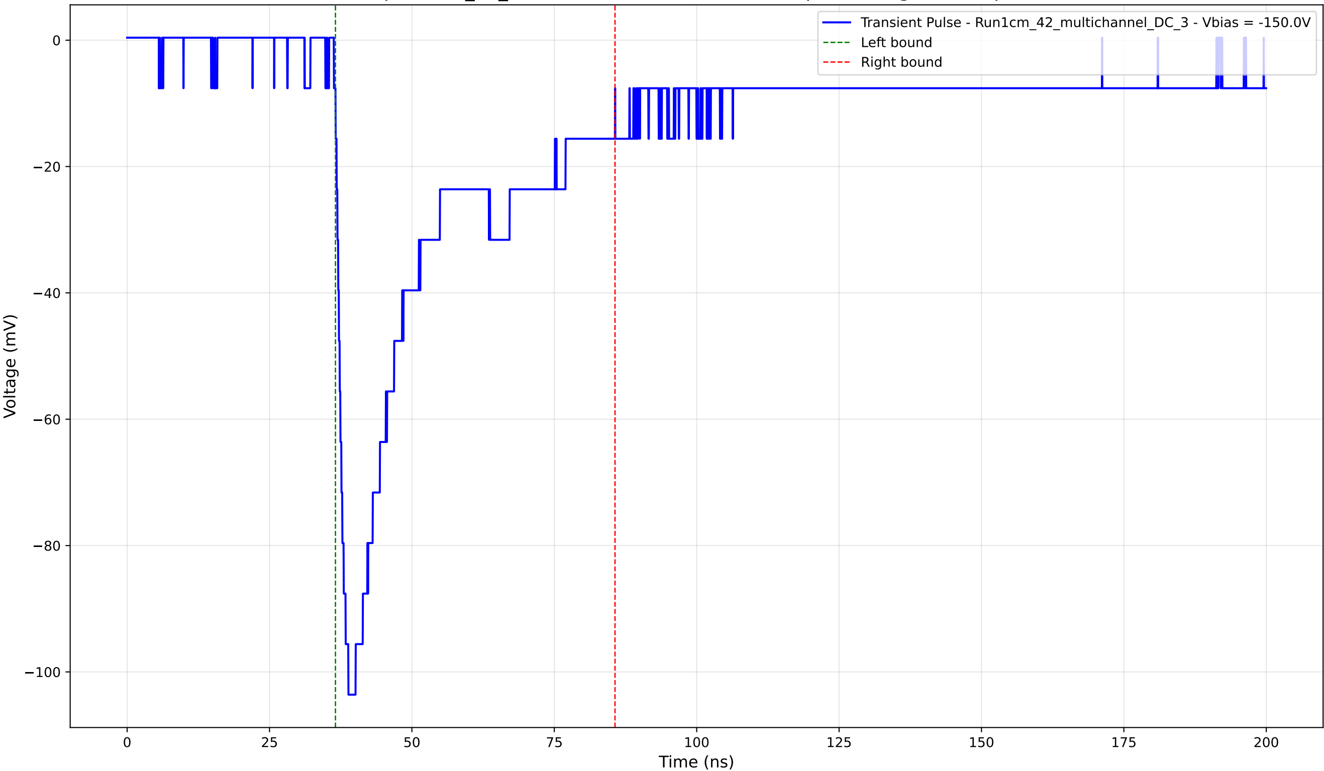
Transient Pulse - Sample: 1cm_42_multichannel - Position: 3110.0 \mu\text{m} - Charge: 35.36 pC - Rise Time: 1.77 ns
