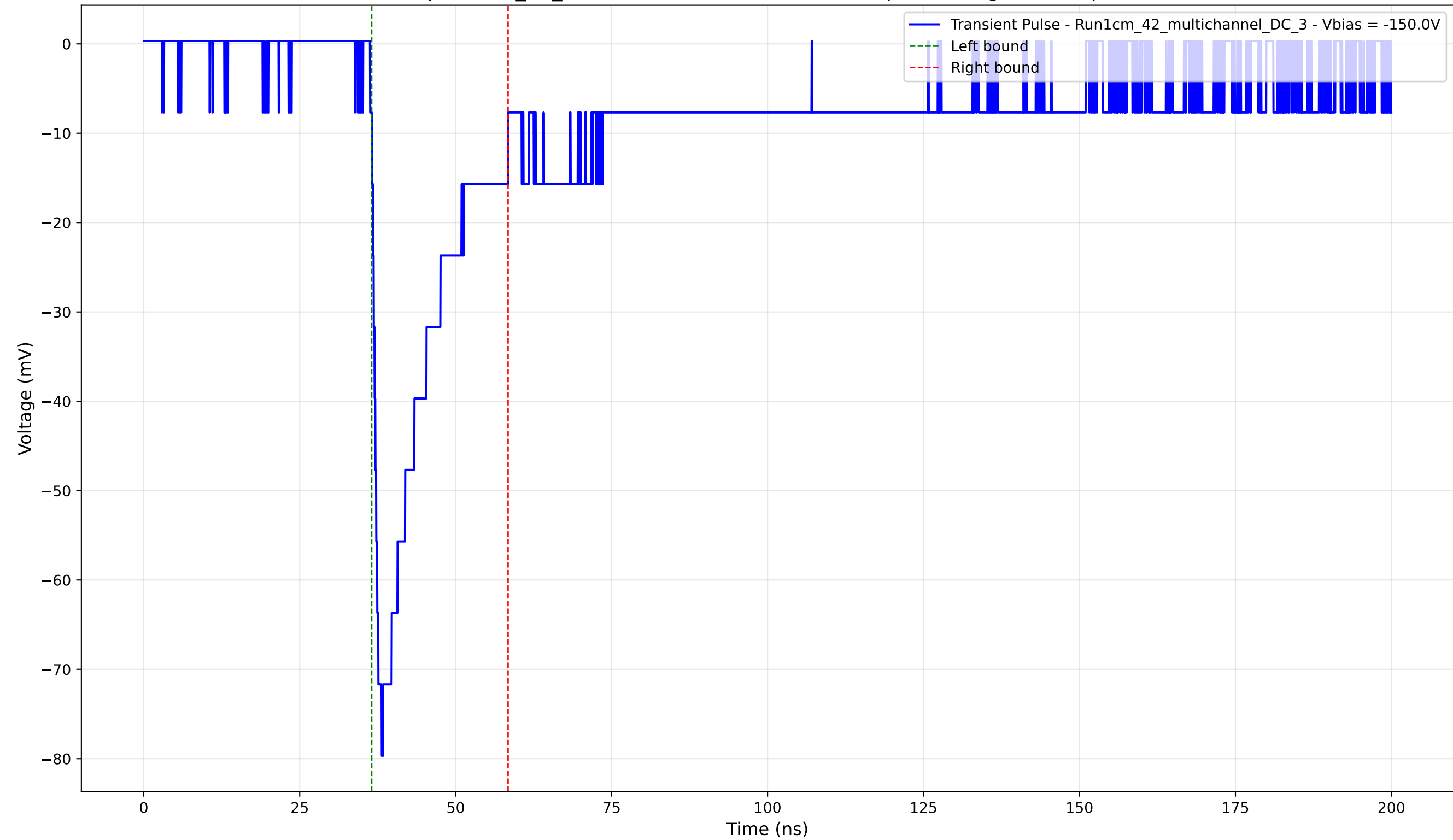
Transient Pulse - Sample: 1cm_42_multichannel - Position: 3840.0 \mu\text{m} - Charge: 14.84 pC - Rise Time: 1.60 ns
