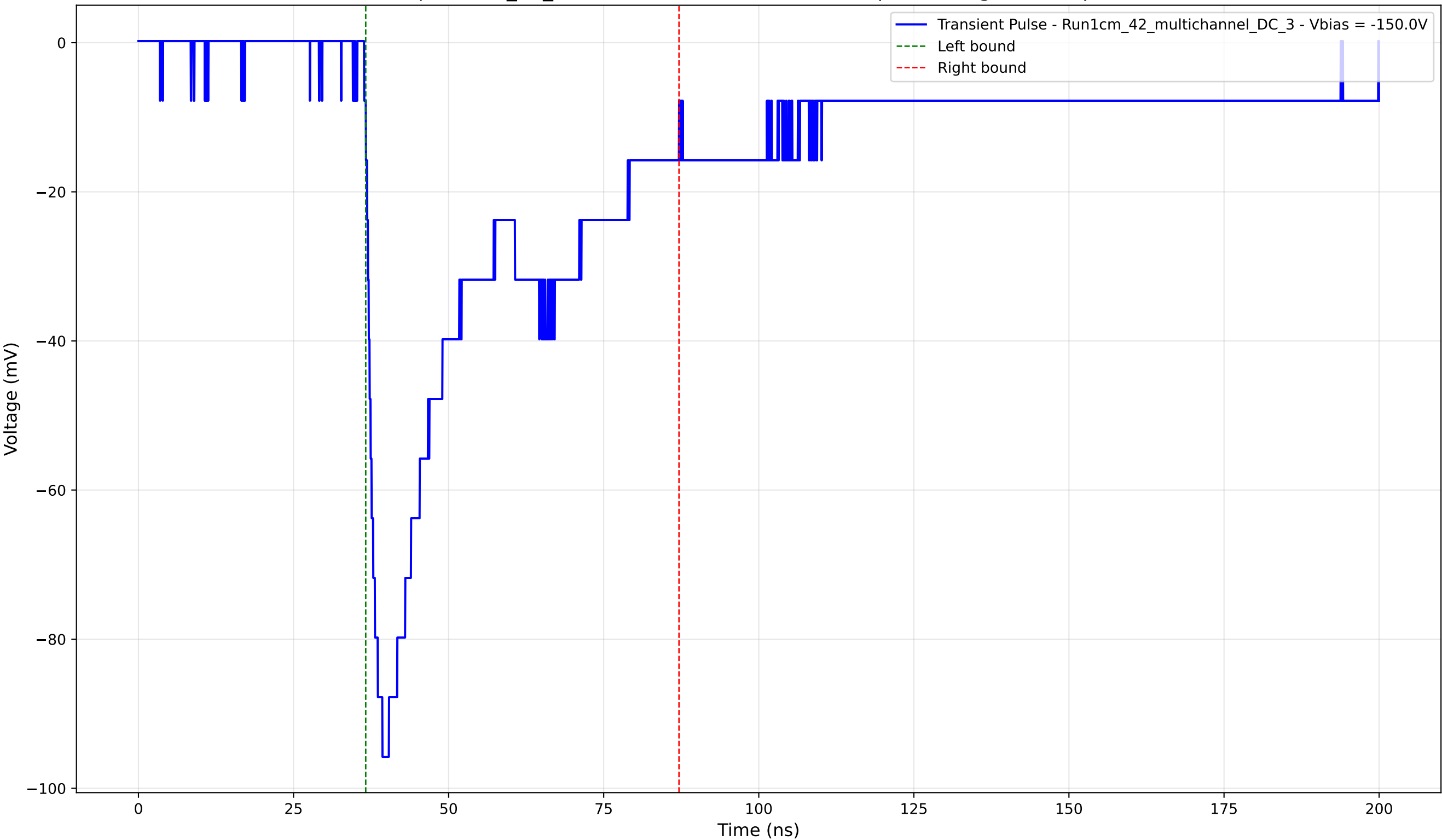
Transient Pulse - Sample: 1cm_42_multichannel - Position: 2745.0 \mu\text{m} - Charge: 37.26 pC - Rise Time: 1.94 ns
