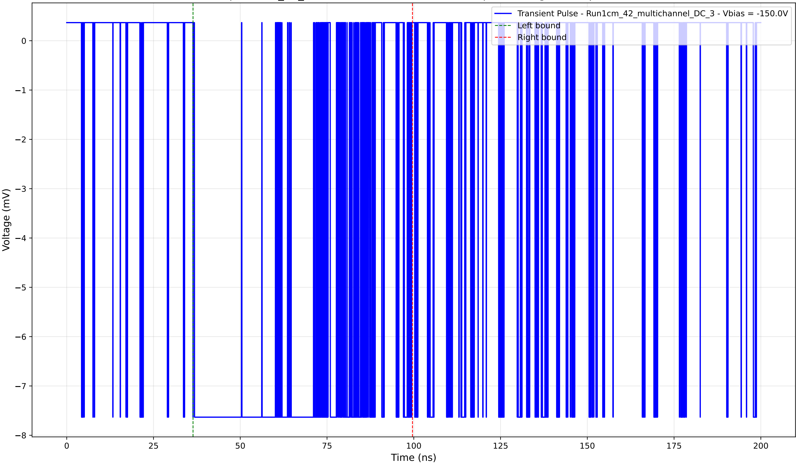
Transient Pulse - Sample: 1cm_42_multichannel - Position: 2865.0 \mu\text{m} - Charge: 7.08 pC - Rise Time: 0.02 ns
