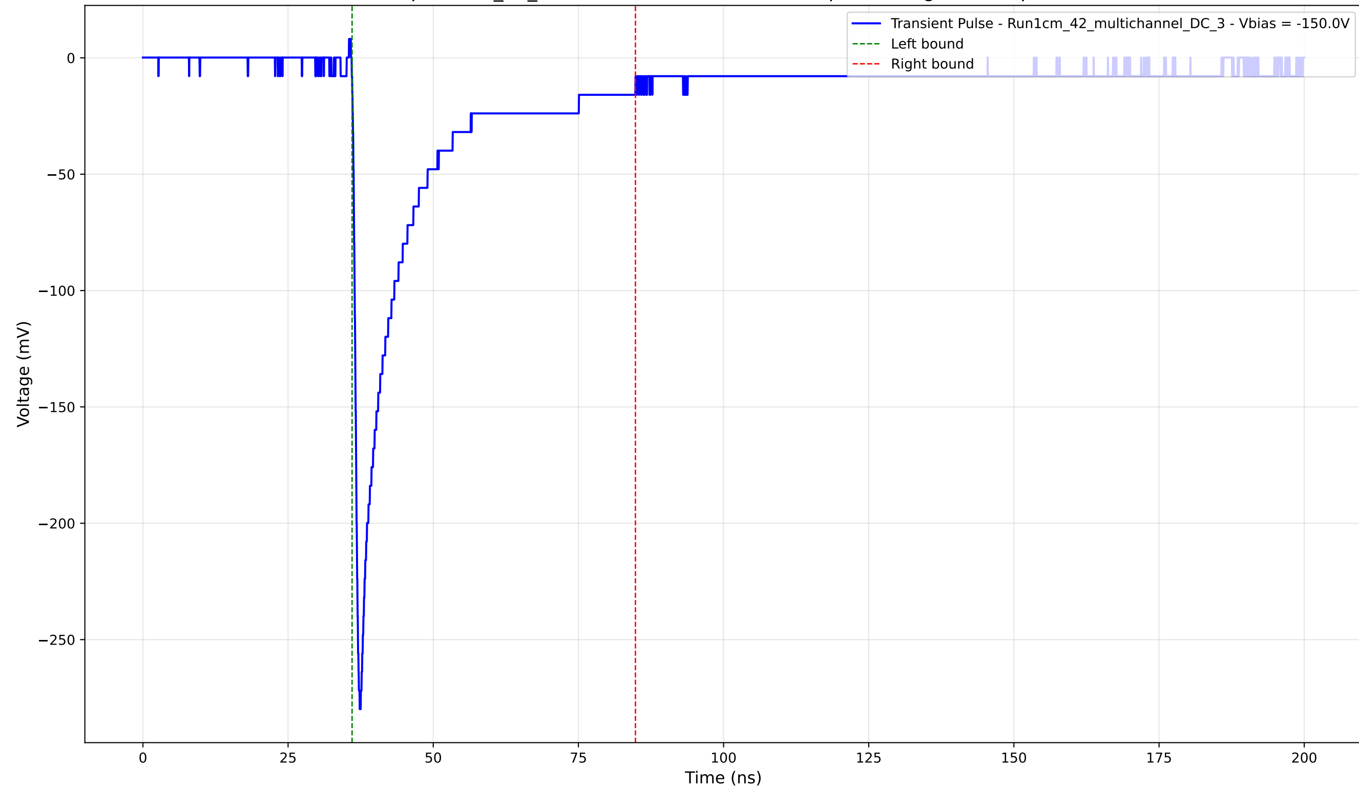
Transient Pulse - Sample: 1cm_42_multichannel - Position: 490.0 \mu\text{m} - Charge: 49.68 pC - Rise Time: 0.91 ns
