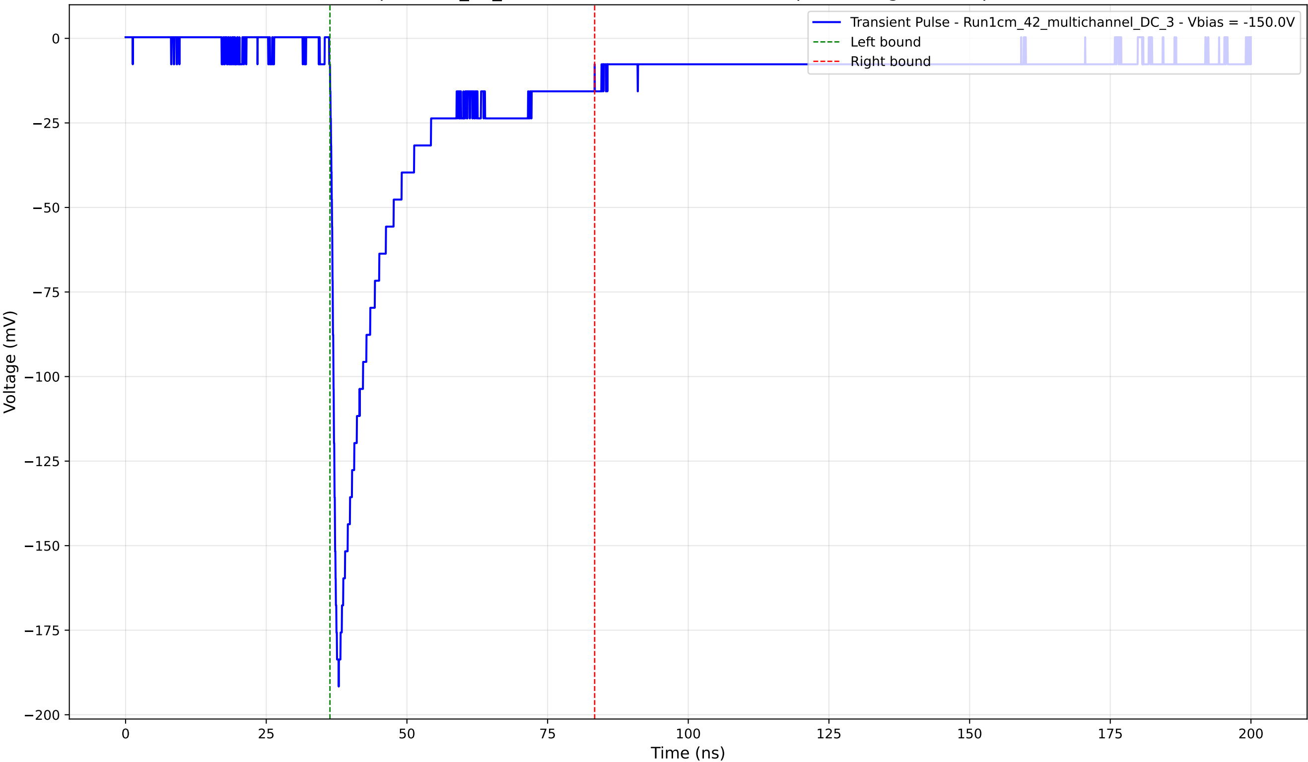
Transient Pulse - Sample: 1cm_42_multichannel - Position: 4135.0 \mu\text{m} - Charge: 39.76 pC - Rise Time: 1.05 ns
