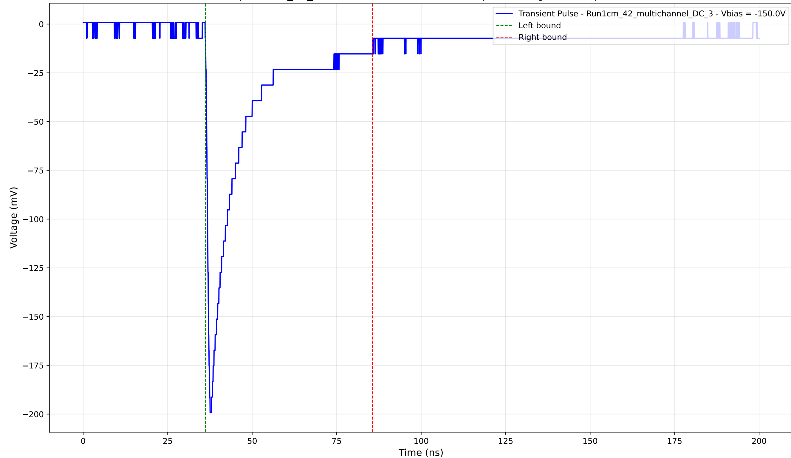
Transient Pulse - Sample: 1cm_42_multichannel - Position: 770.0 \mu\text{m} - Charge: 43.73 pC - Rise Time: 1.05 ns
