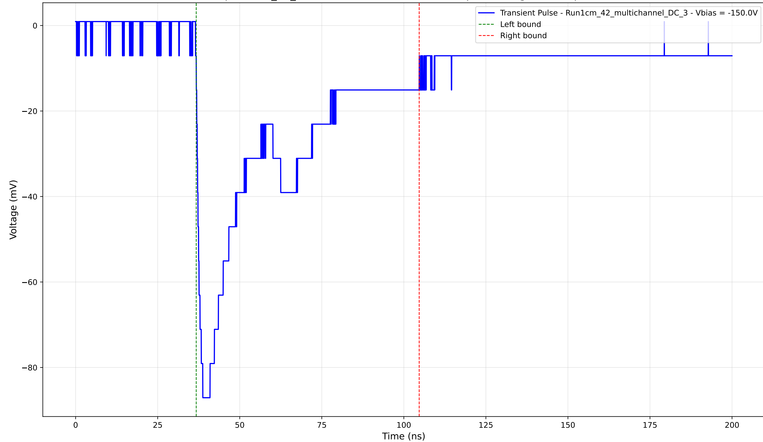
Transient Pulse - Sample: 1cm_42_multichannel - Position: 2145.0 \mu\text{m} - Charge: 41.73 pC - Rise Time: 1.54 ns
