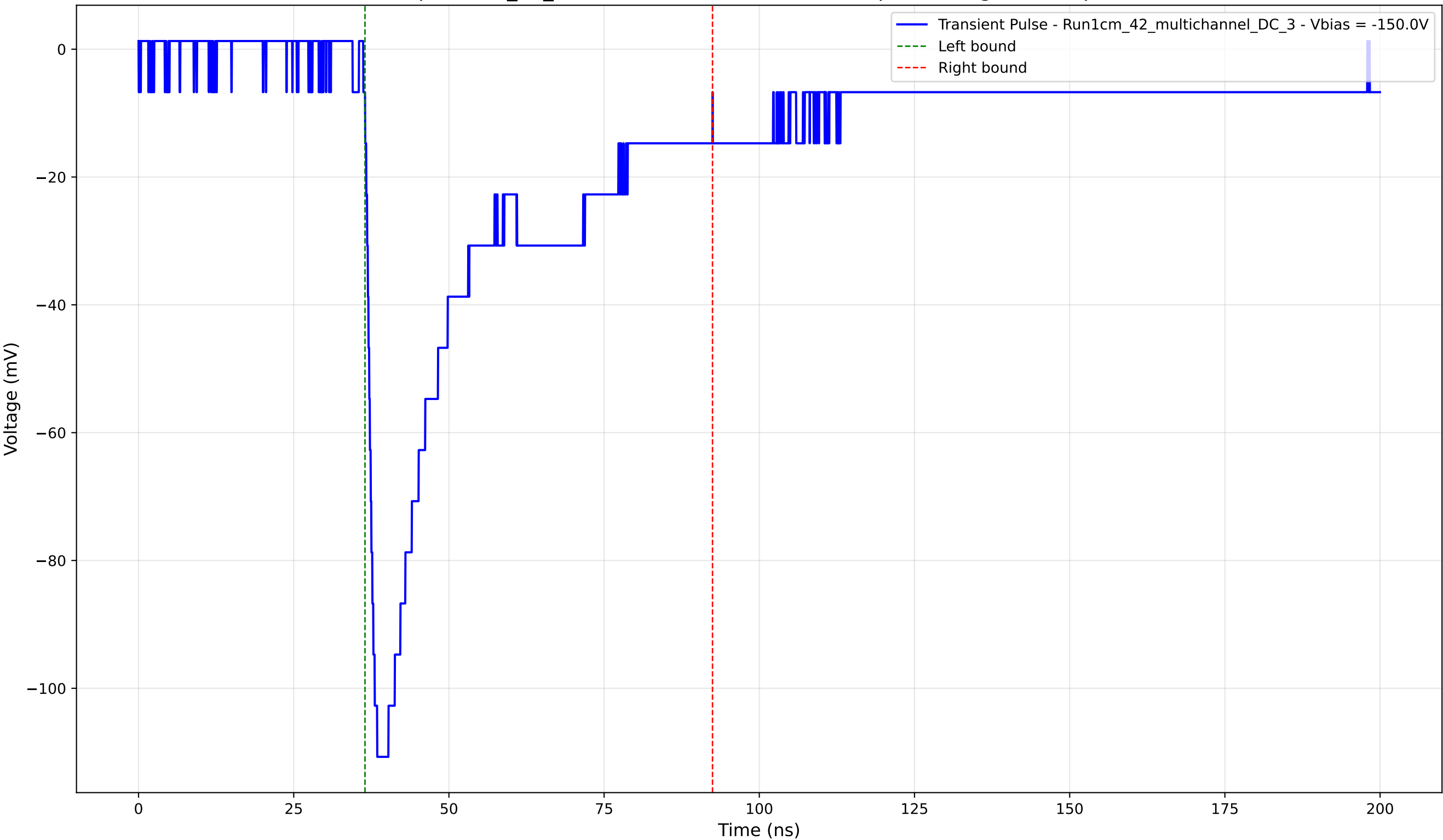
Transient Pulse - Sample: 1cm_42_multichannel - Position: 1760.0 \mu\text{m} - Charge: 40.82 pC - Rise Time: 1.55 ns
