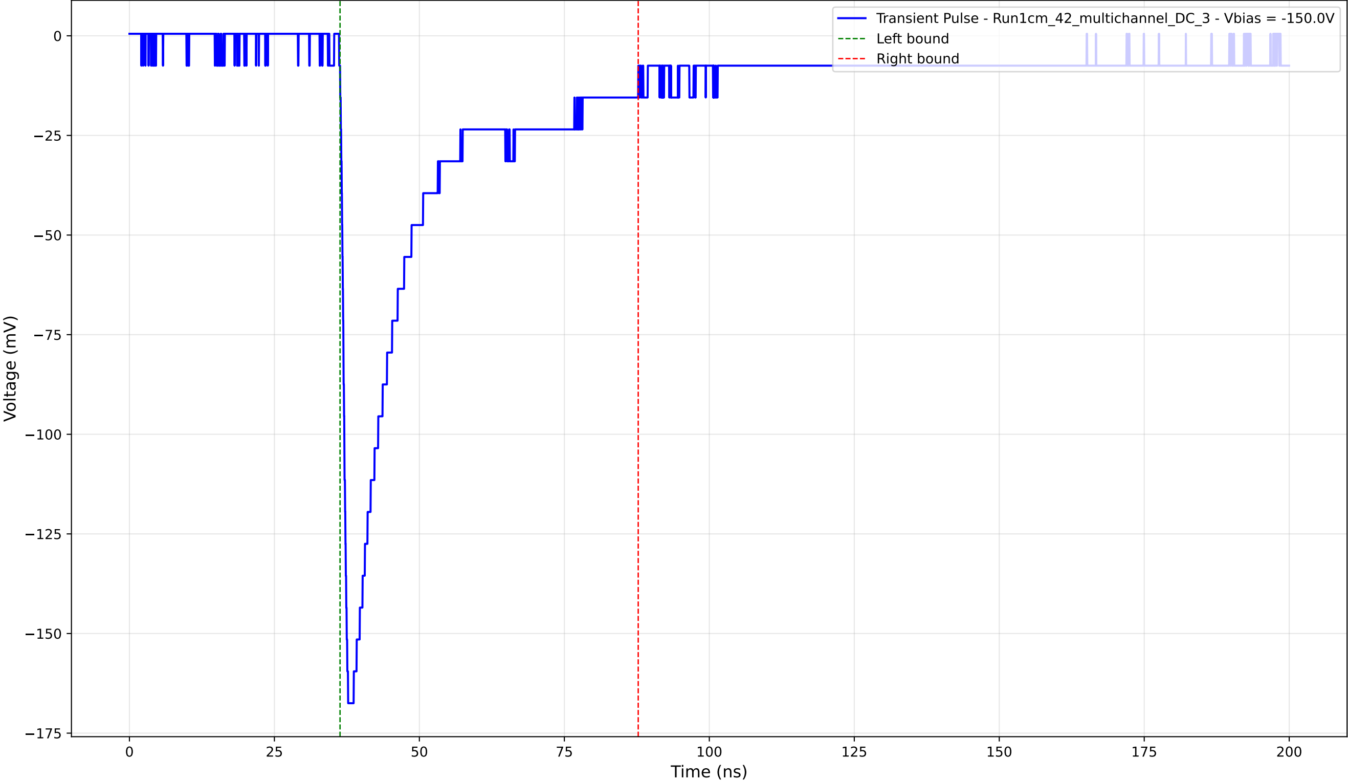
Transient Pulse - Sample: 1cm_42_multichannel - Position: 1040.0 \mu\text{m} - Charge: 44.52 pC - Rise Time: 1.04 ns
