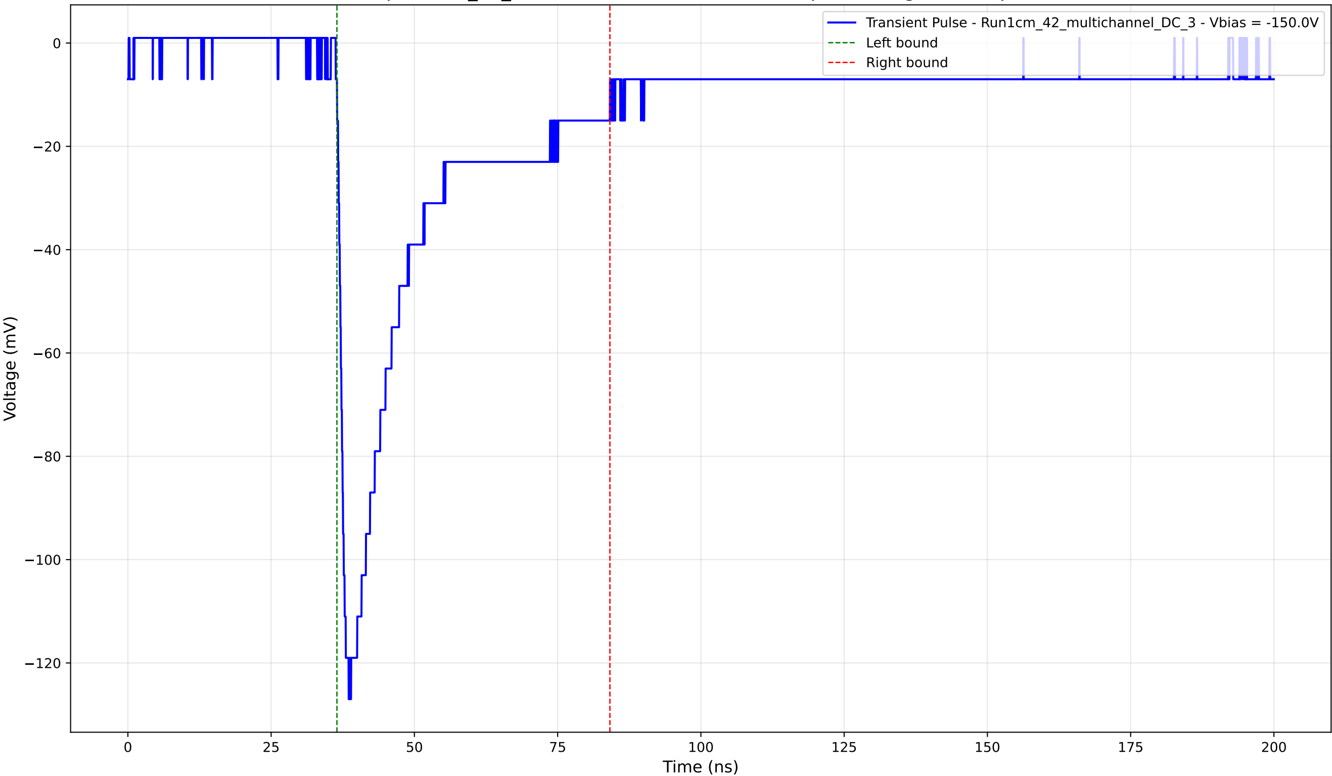
Transient Pulse - Sample: 1cm_42_multichannel - Position: 3540.0 \mu\text{m} - Charge: 36.02 pC - Rise Time: 1.53 ns
