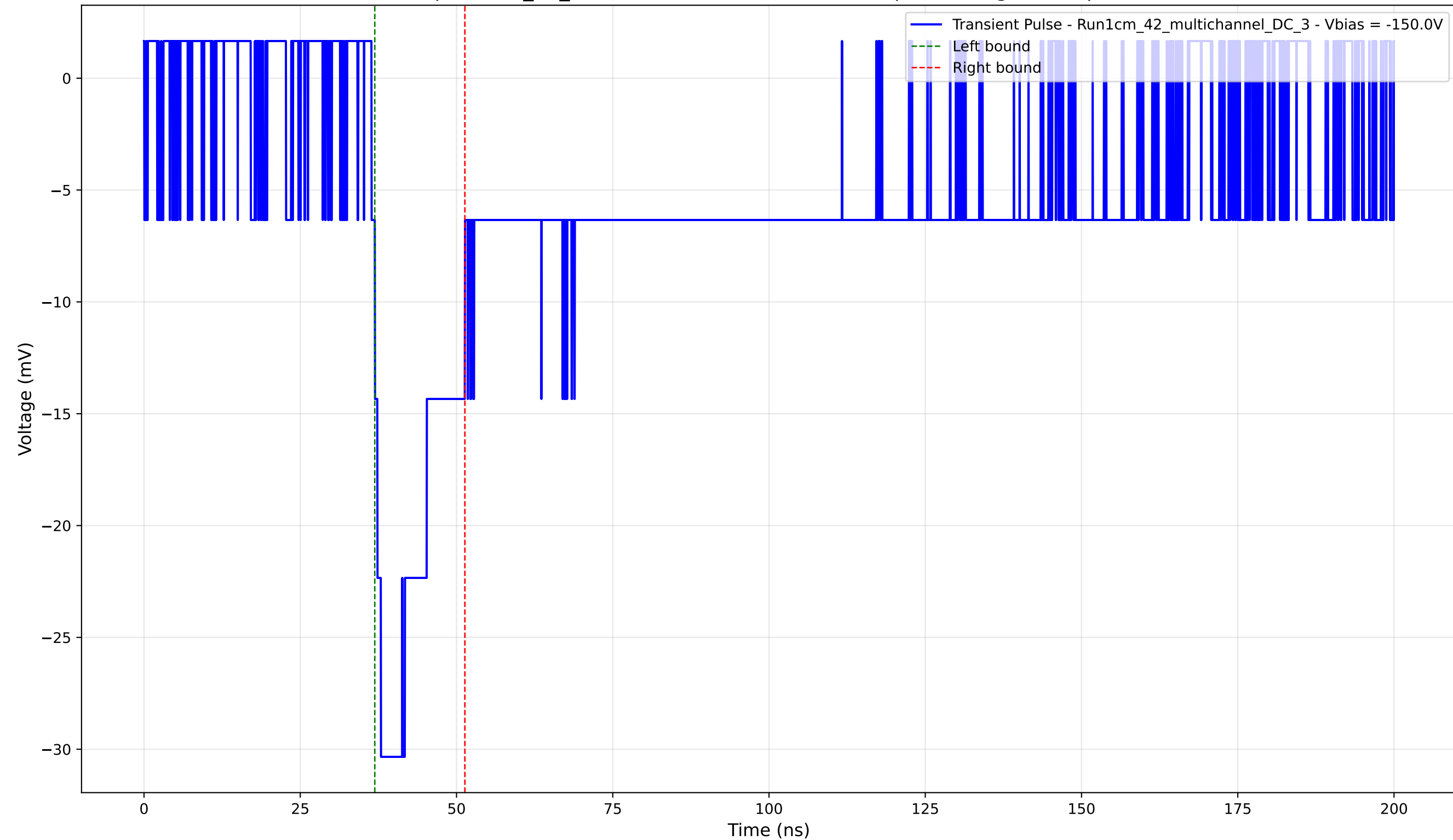
Transient Pulse - Sample: 1cm_42_multichannel - Position: 1830.0 \mu\text{m} - Charge: 6.01 pC - Rise Time: 1.51 ns
