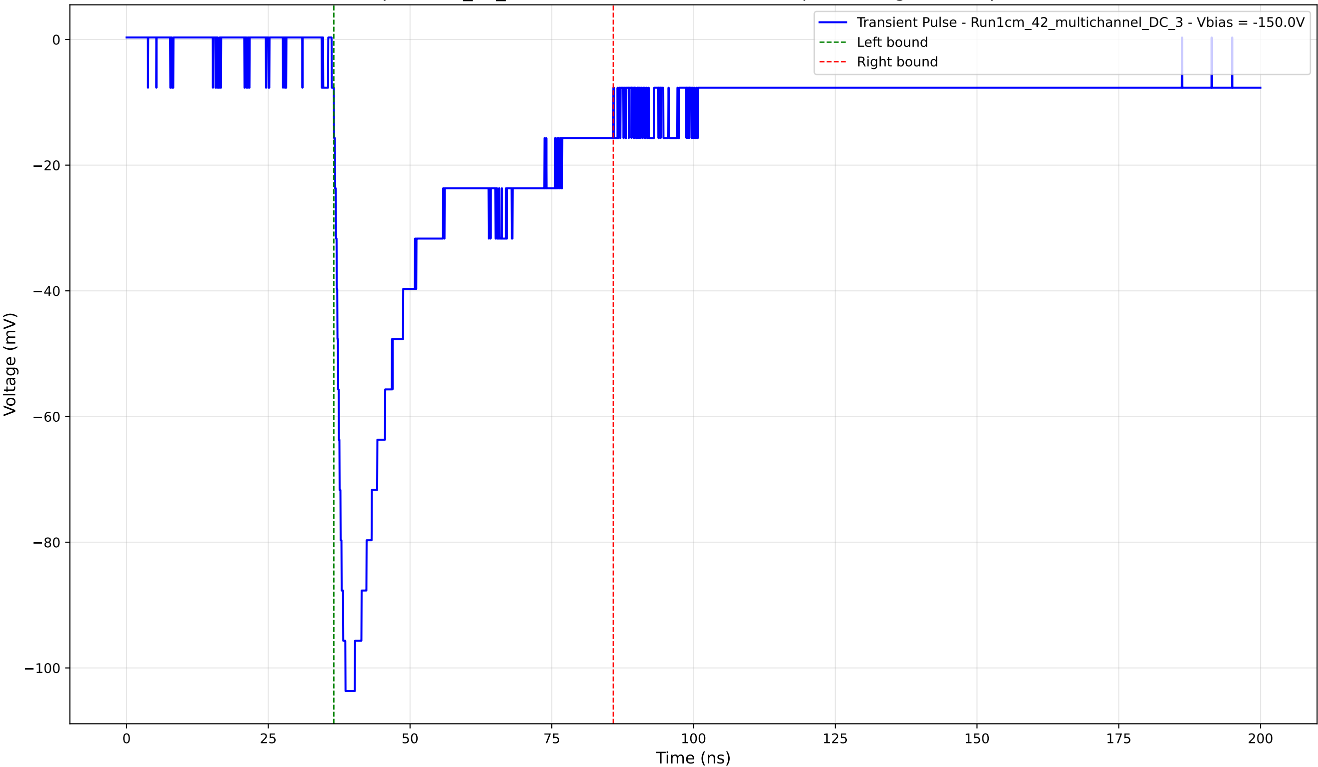
Transient Pulse - Sample: 1cm_42_multichannel - Position: 3165.0 \mu\text{m} - Charge: 35.47 pC - Rise Time: 1.63 ns
