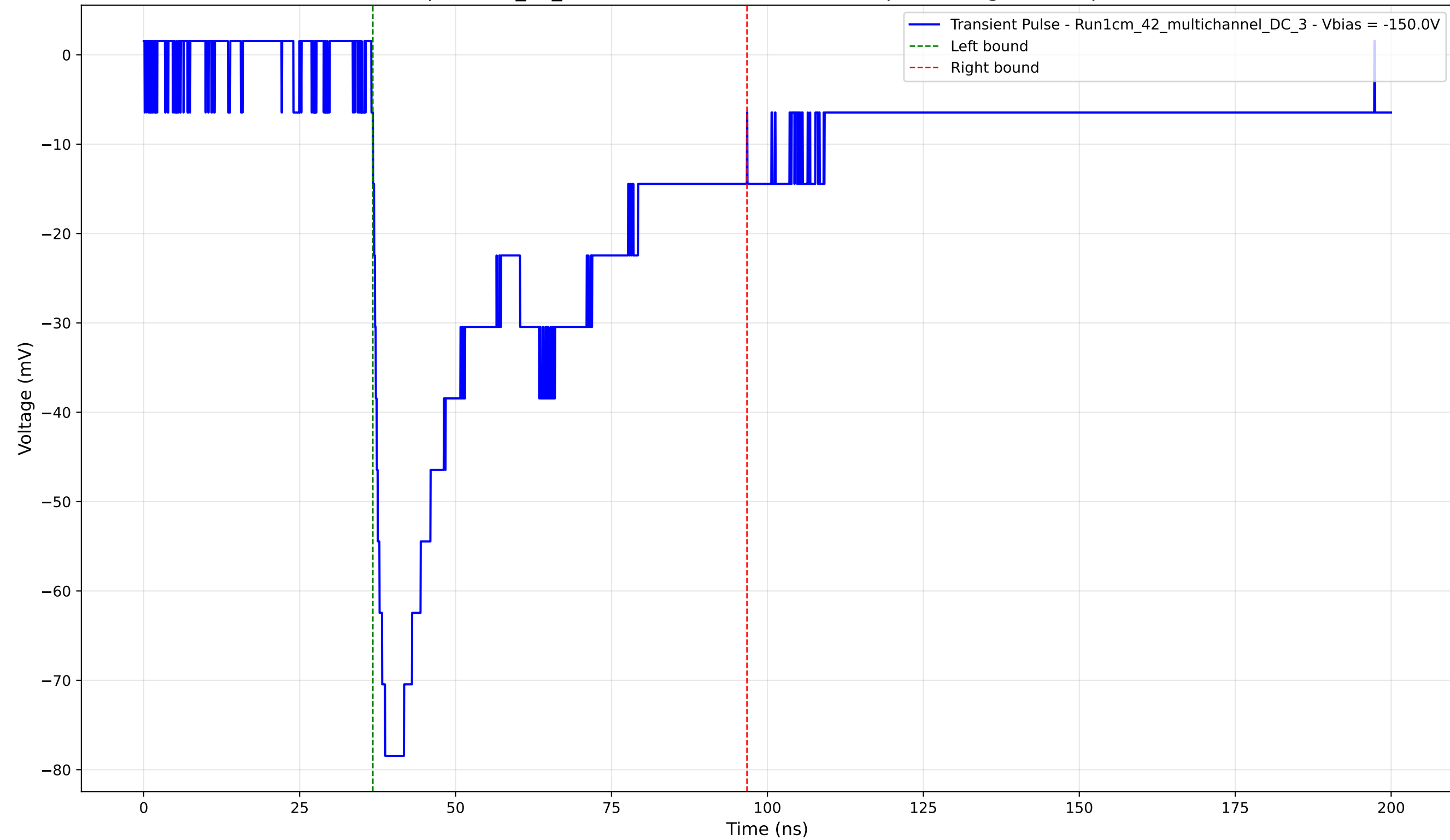
Transient Pulse - Sample: 1cm_42_multichannel - Position: 2610.0 \mu\text{m} - Charge: 36.96 pC - Rise Time: 1.96 ns
