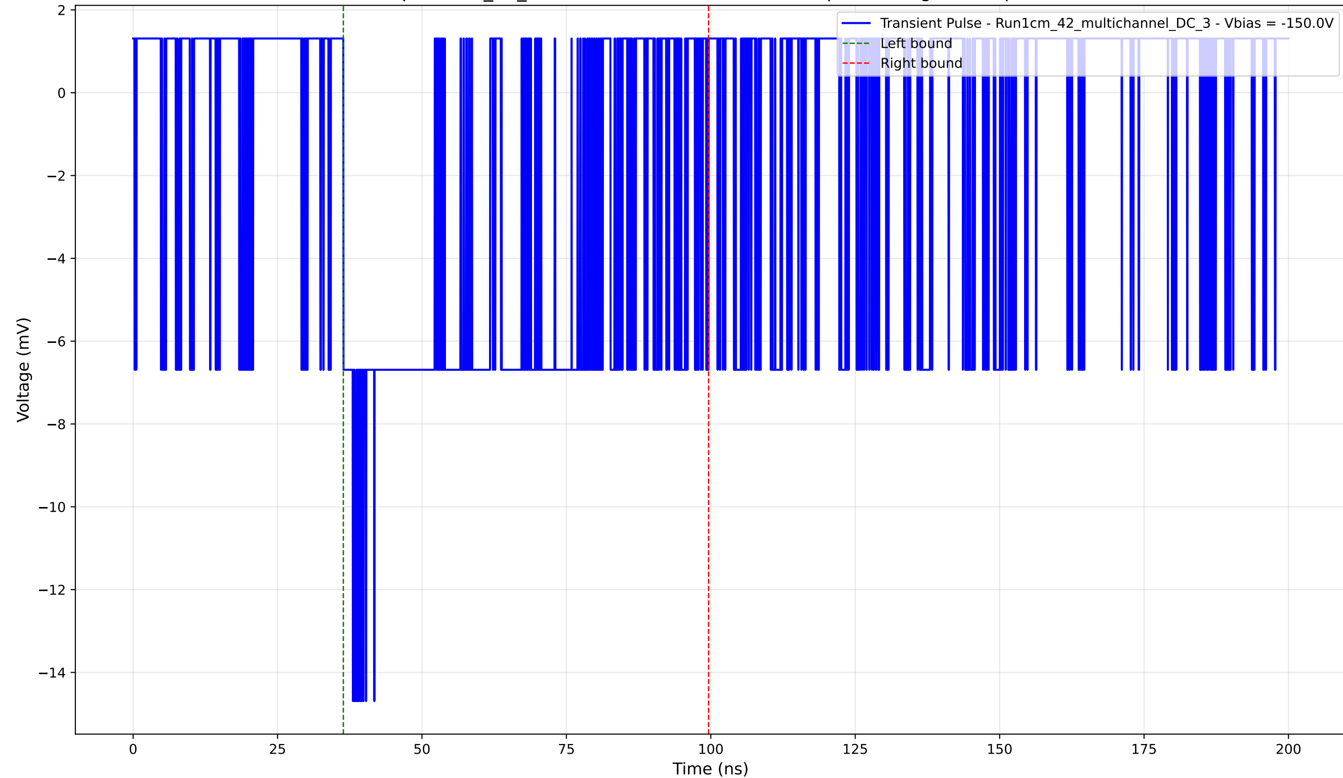
Transient Pulse - Sample: 1cm_42_multichannel - Position: 1350.0 \mu\text{m} - Charge: 5.69 pC - Rise Time: 1.64 ns
