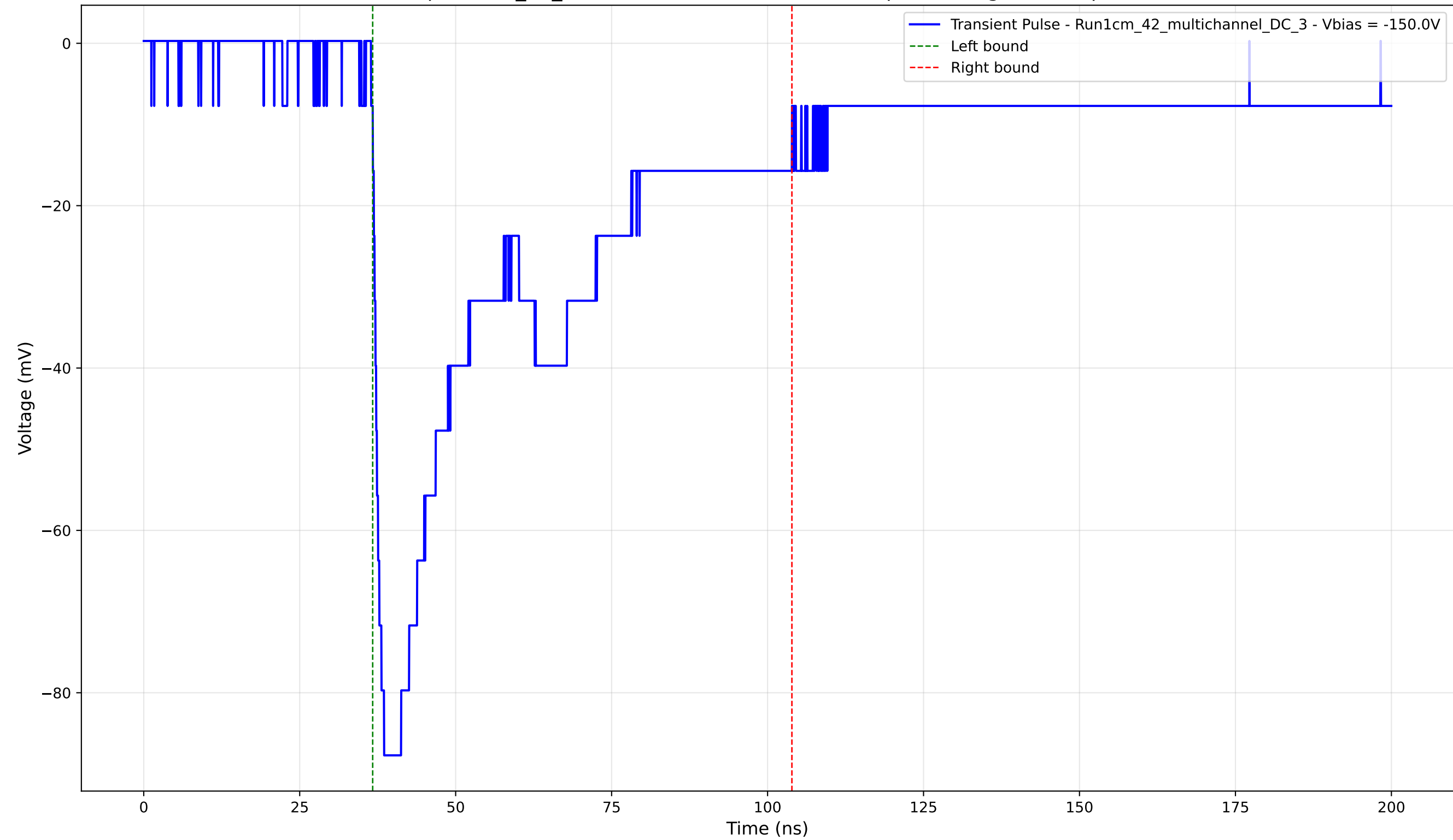
Transient Pulse - Sample: 1cm_42_multichannel - Position: 2100.0 \mu\text{m} - Charge: 43.01 pC - Rise Time: 1.40 ns
