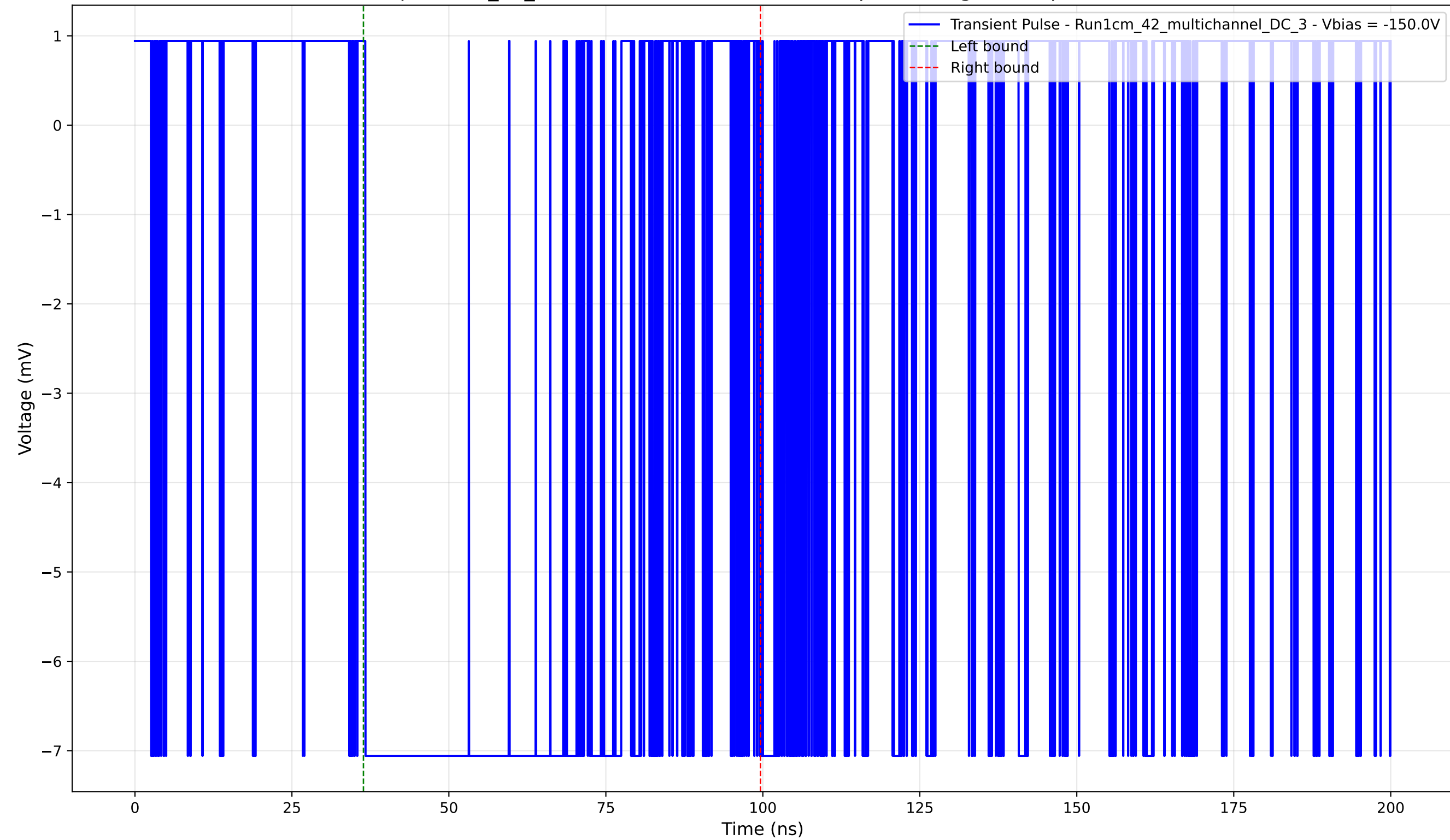
Transient Pulse - Sample: 1cm_42_multichannel - Position: 2385.0 \mu\text{m} - Charge: 5.84 pC - Rise Time: 0.00 ns (N/A)
