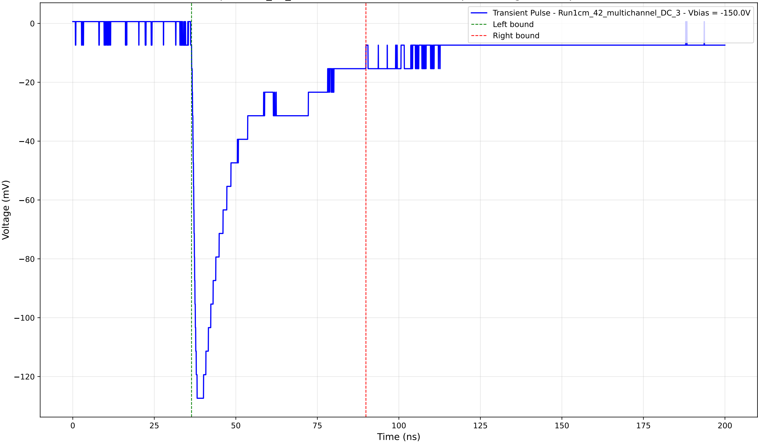
Transient Pulse - Sample: 1cm_42_multichannel - Position: 1525.0 \mu\text{m} - Charge: 43.49 pC - Rise Time: 1.43 ns
