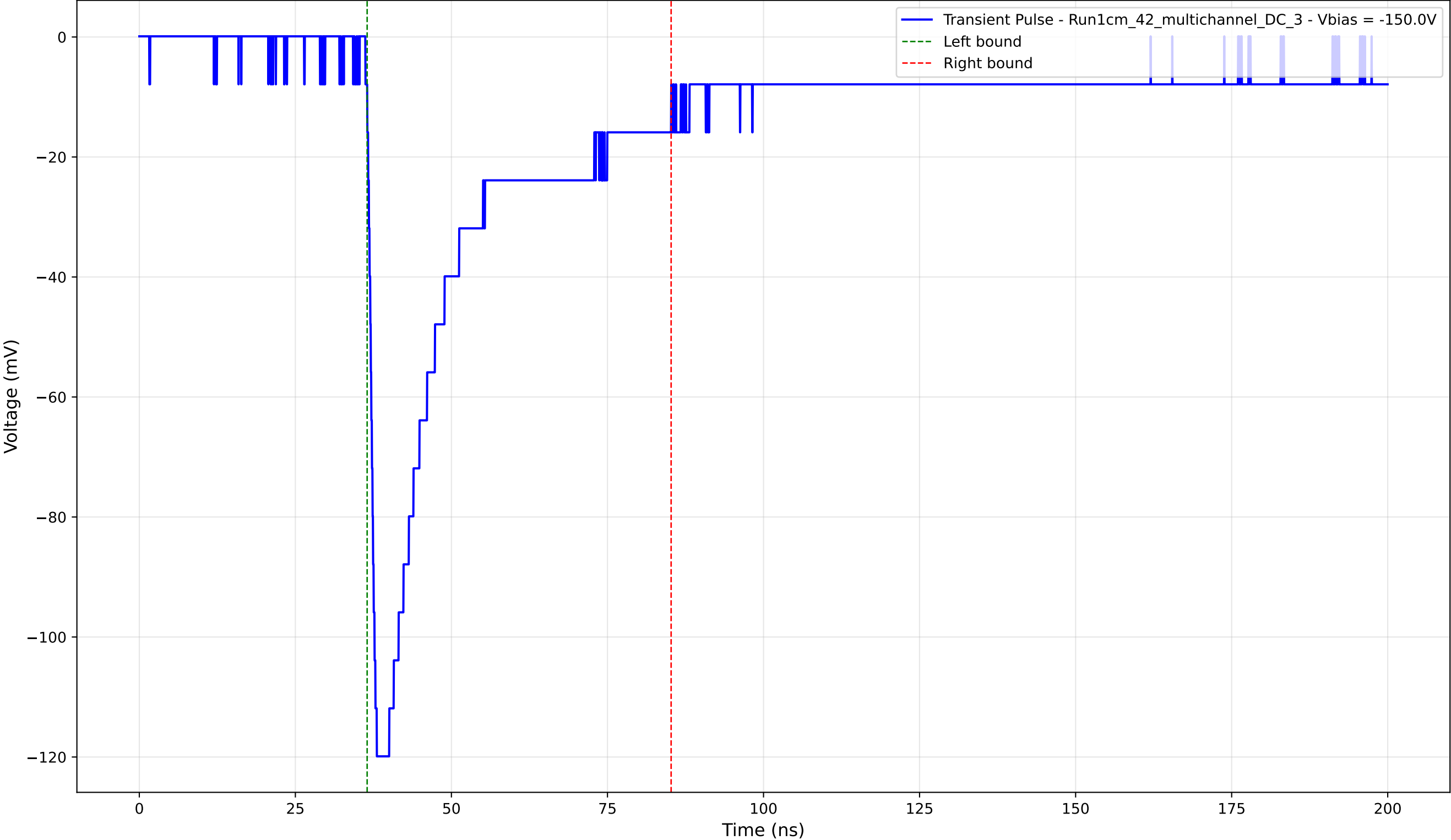
Transient Pulse - Sample: 1cm_42_multichannel - Position: 3535.0 \mu\text{m} - Charge: 37.01 pC - Rise Time: 1.31 ns
