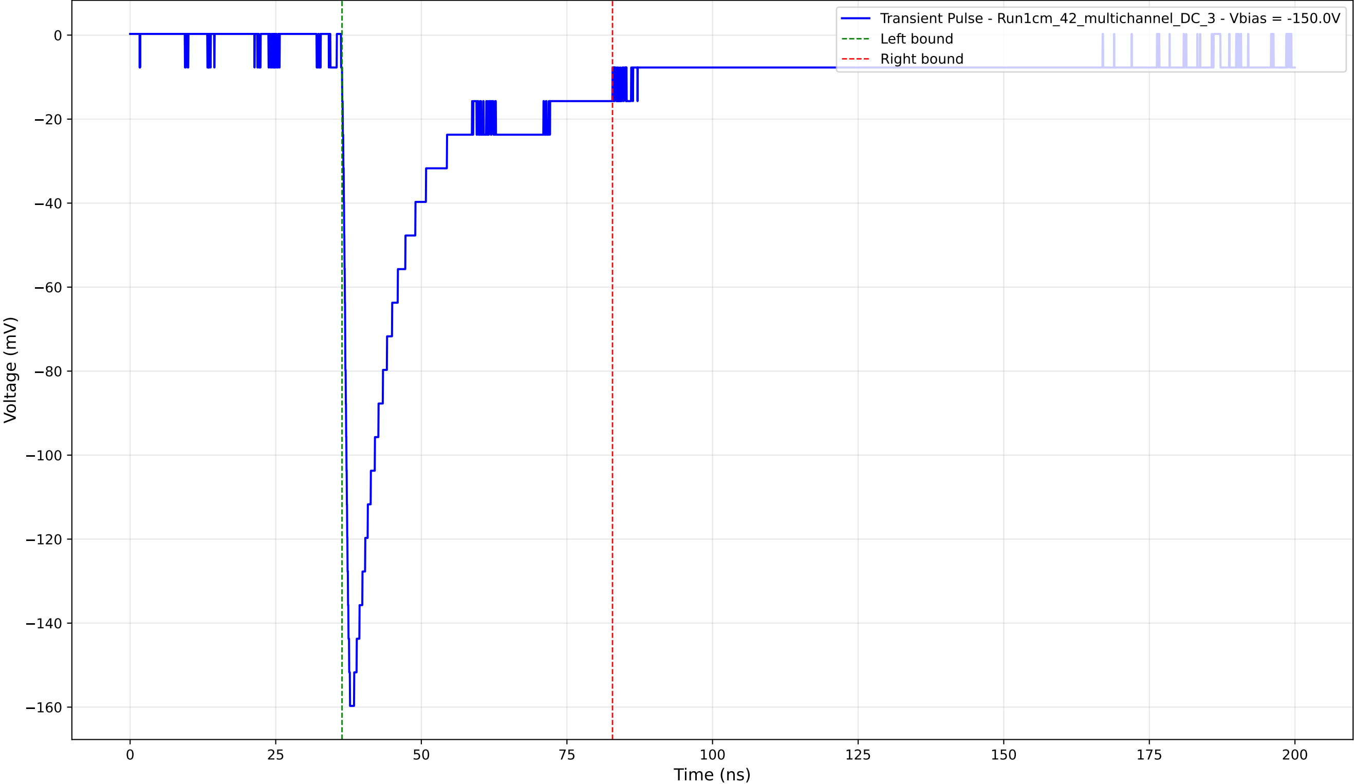
Transient Pulse - Sample: 1cm_42_multichannel - Position: 3970.0 \mu\text{m} - Charge: 37.95 pC - Rise Time: 1.12 ns
