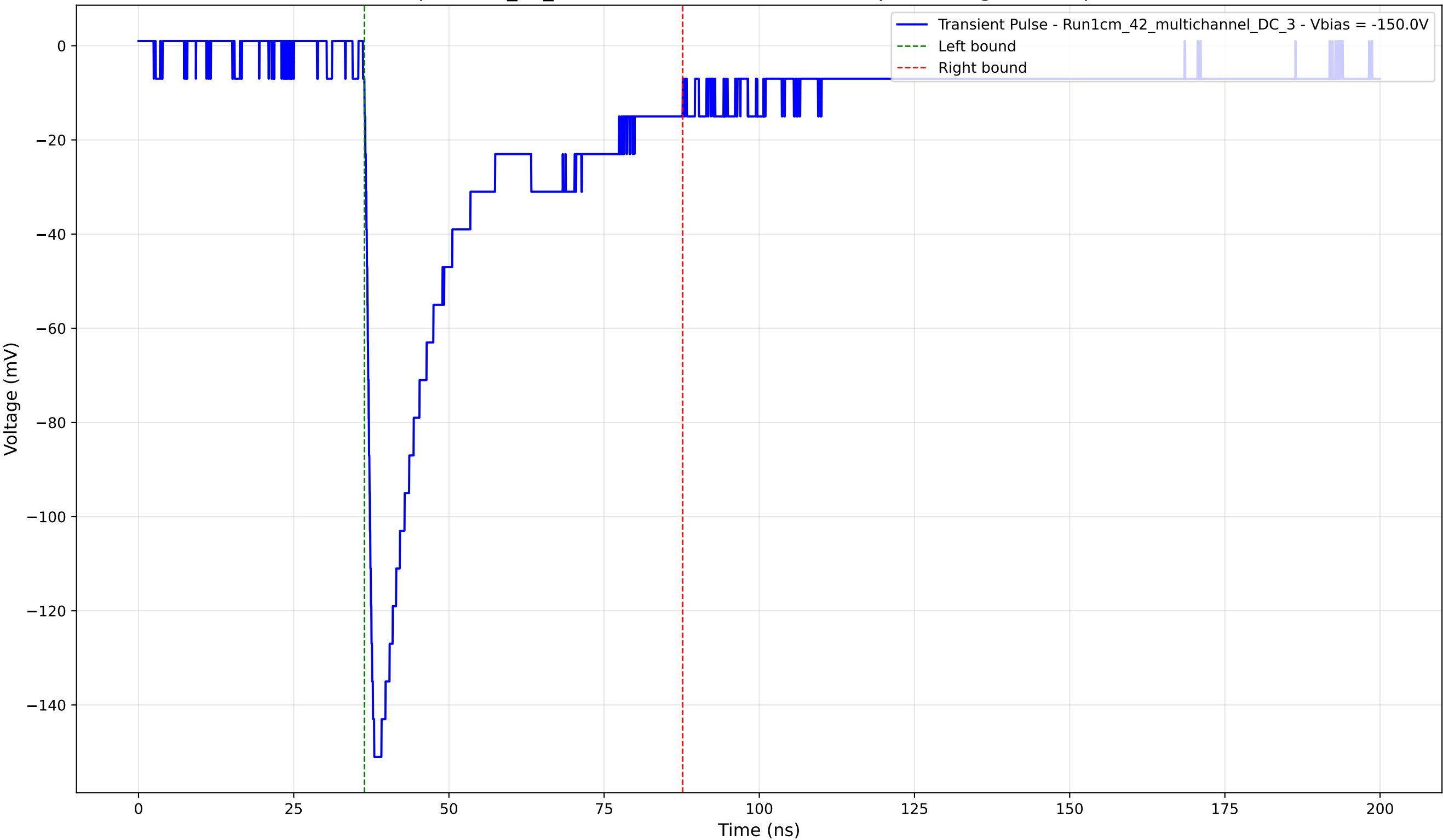
Transient Pulse - Sample: 1cm_42_multichannel - Position: 1255.0 \mu\text{m} - Charge: 43.88 pC - Rise Time: 1.26 ns
