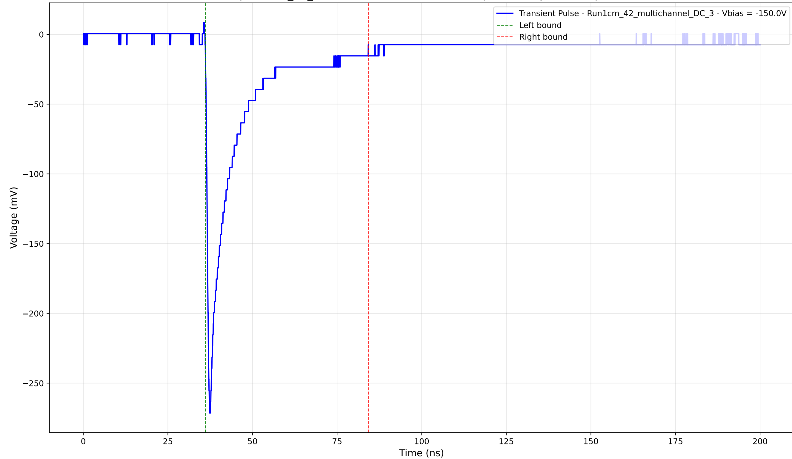
Transient Pulse - Sample: 1cm_42_multichannel - Position: 515.0 \mu\text{m} - Charge: 48.56 pC - Rise Time: 0.91 ns
