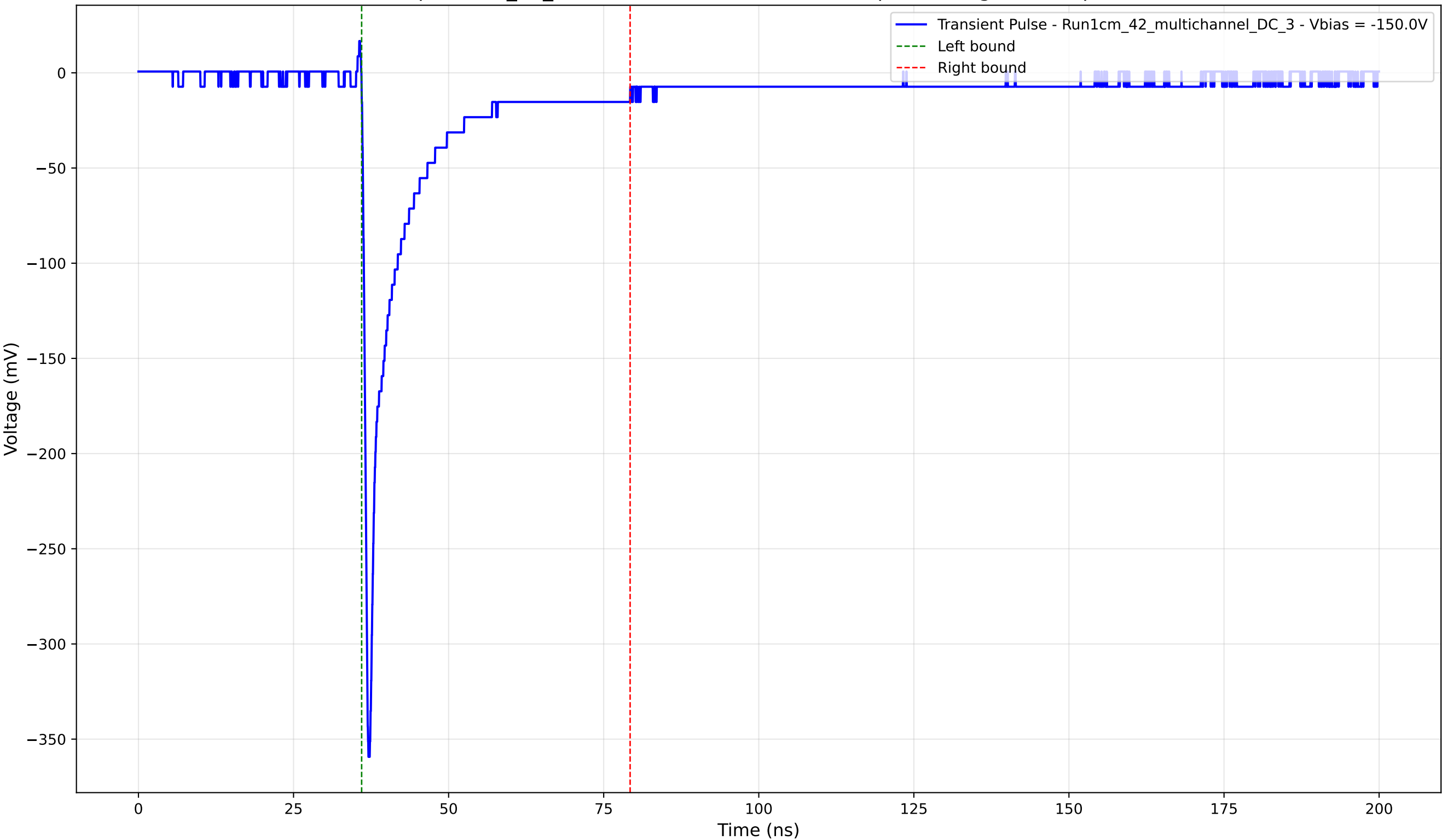
Transient Pulse - Sample: 1cm_42_multichannel - Position: 4780.0 \mu\text{m} - Charge: 40.81 pC - Rise Time: 0.79 ns
