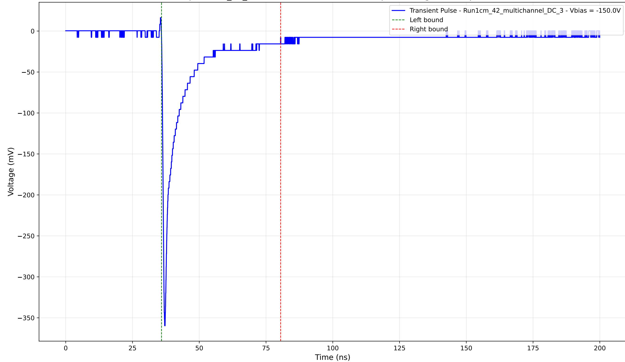
Transient Pulse - Sample: 1cm_42_multichannel - Position: 195.0 \mu\text{m} - Charge: 47.35 pC - Rise Time: 0.82 ns
