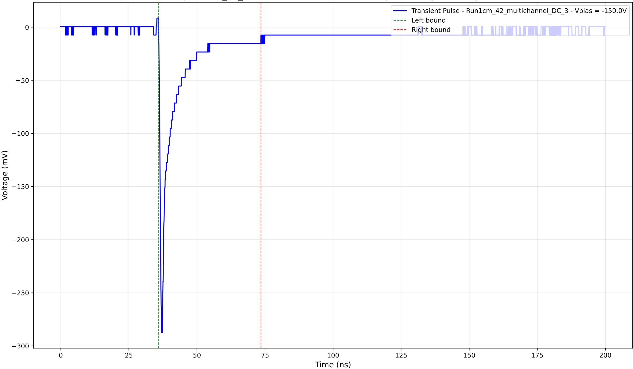
Transient Pulse - Sample: 1cm_42_multichannel - Position: 4835.0 \mu\text{m} - Charge: 31.41 pC - Rise Time: 0.79 ns
