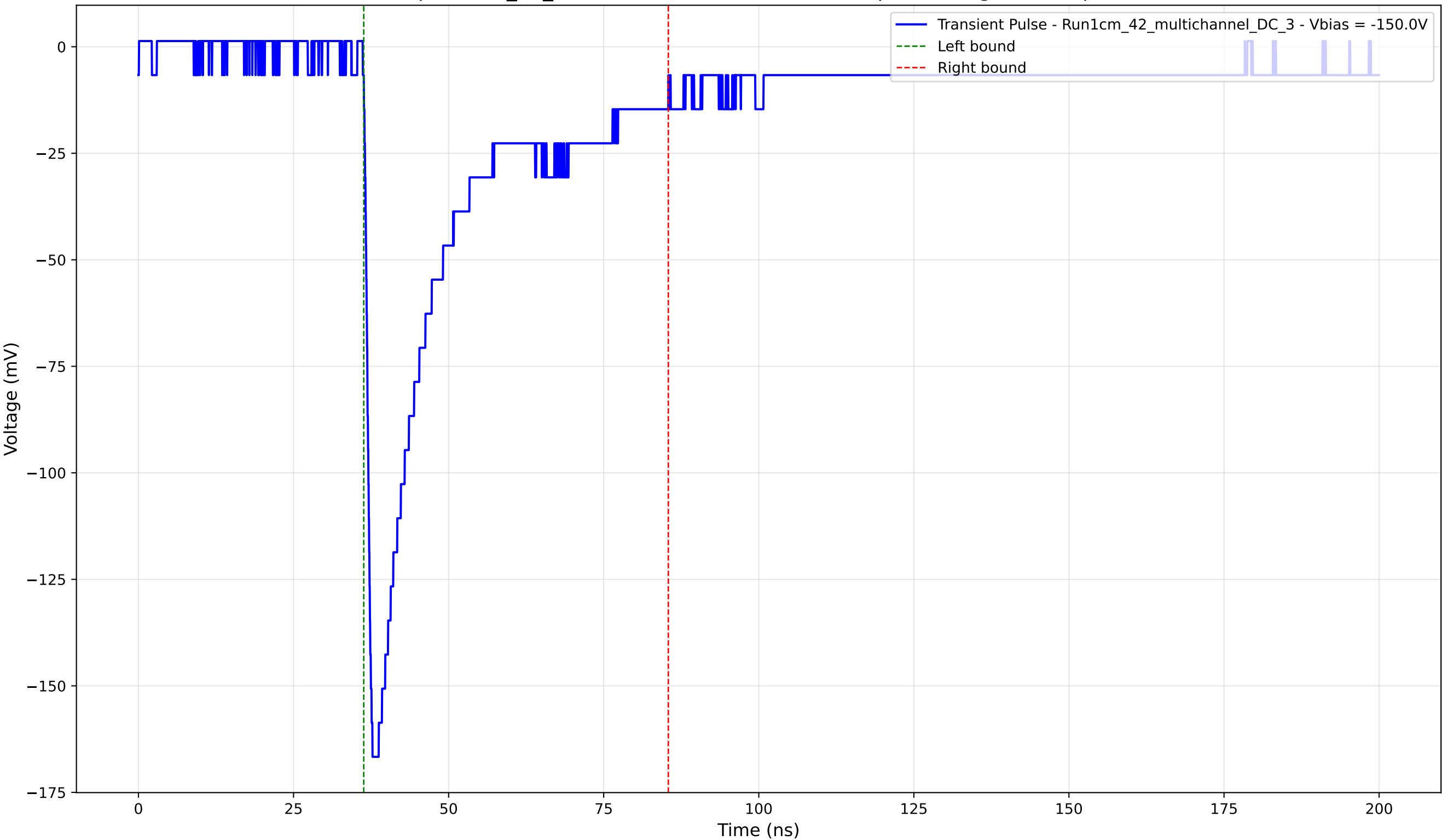
Transient Pulse - Sample: 1cm_42_multichannel - Position: 1050.0 \mu\text{m} - Charge: 43.27 pC - Rise Time: 1.03 ns
