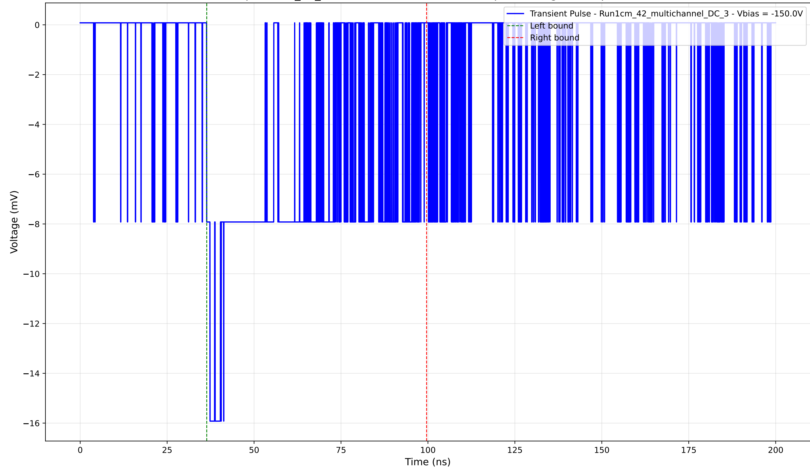
Transient Pulse - Sample: 1cm_42_multichannel - Position: 850.0 \mu\text{m} - Charge: 7.64 pC - Rise Time: 0.98 ns
