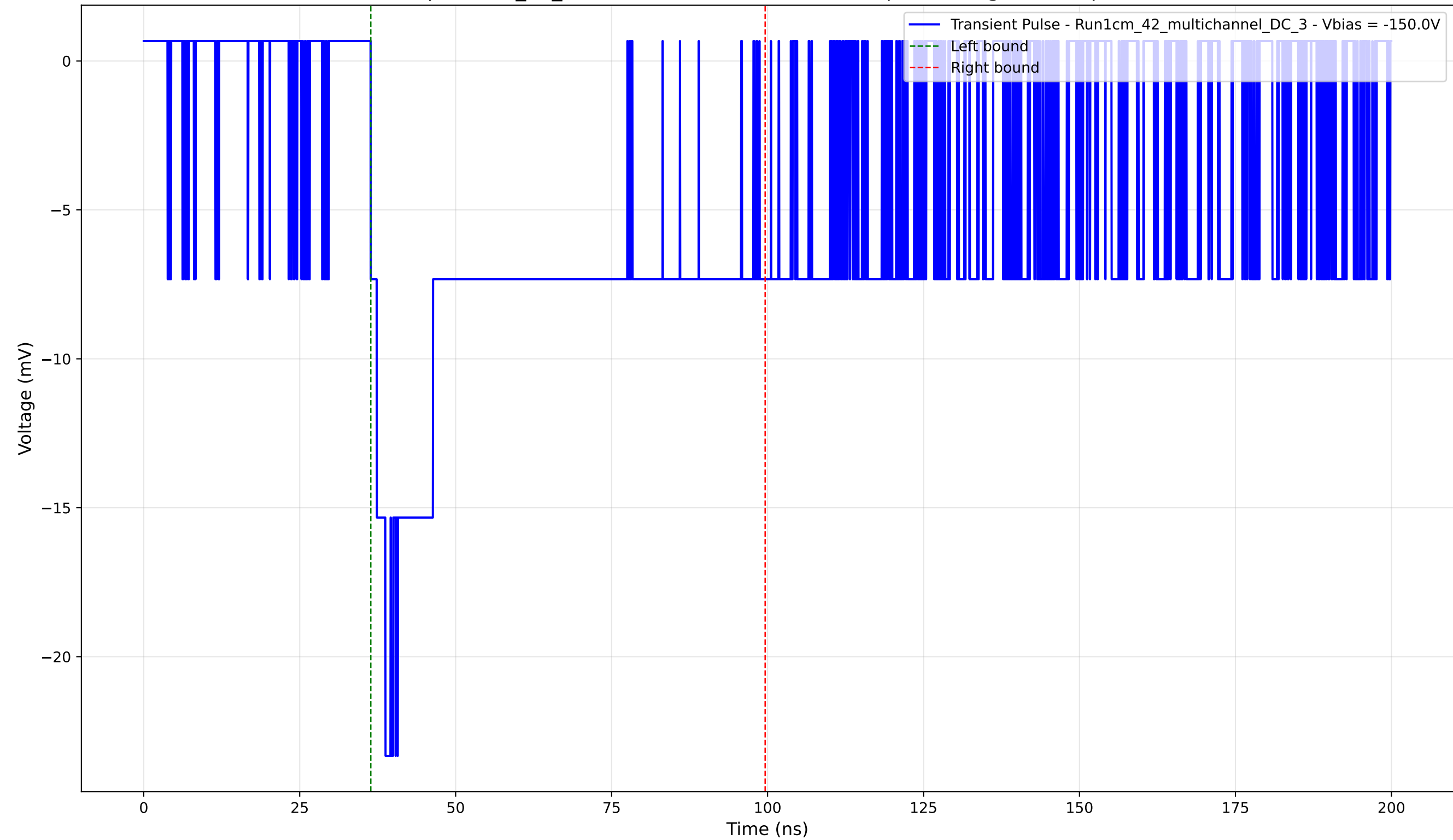
Transient Pulse - Sample: 1cm_42_multichannel - Position: 1900.0 \mu\text{m} - Charge: 10.77 pC - Rise Time: 2.38 ns
