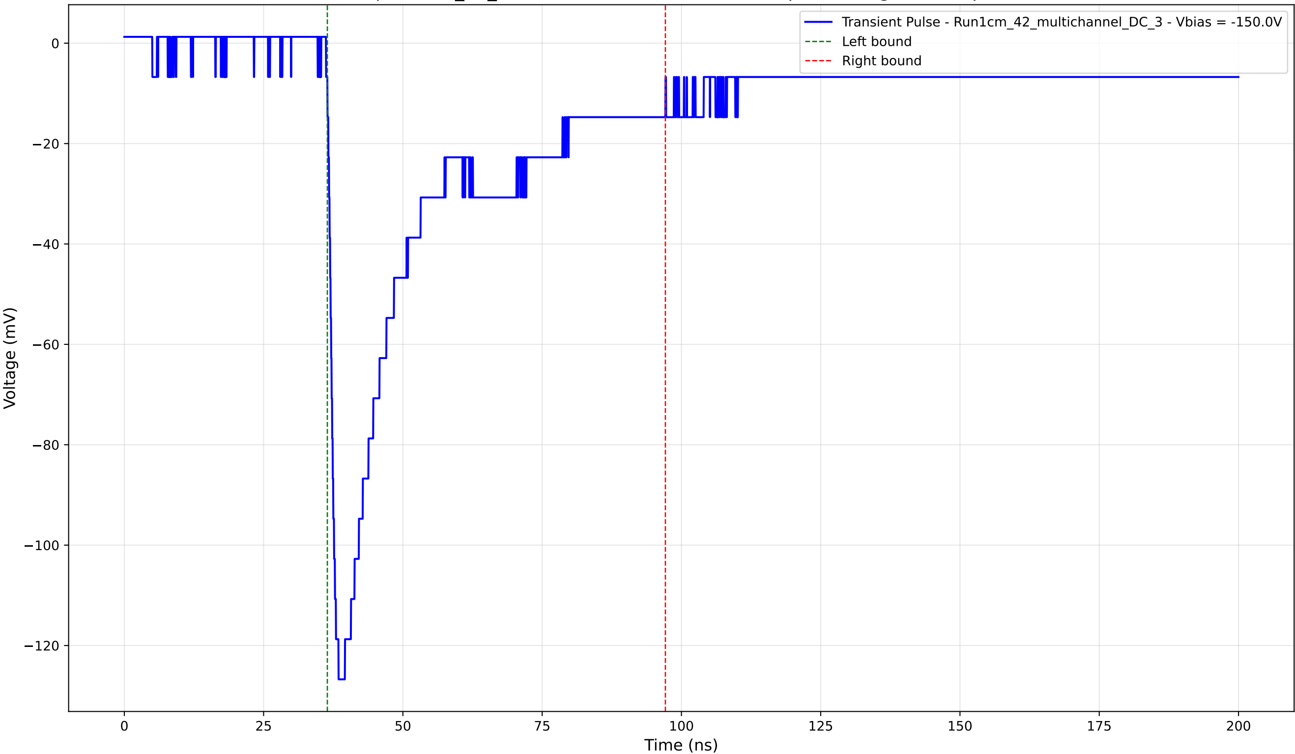
Transient Pulse - Sample: 1cm_42_multichannel - Position: 1560.0 \mu\text{m} - Charge: 44.05 pC - Rise Time: 1.53 ns
