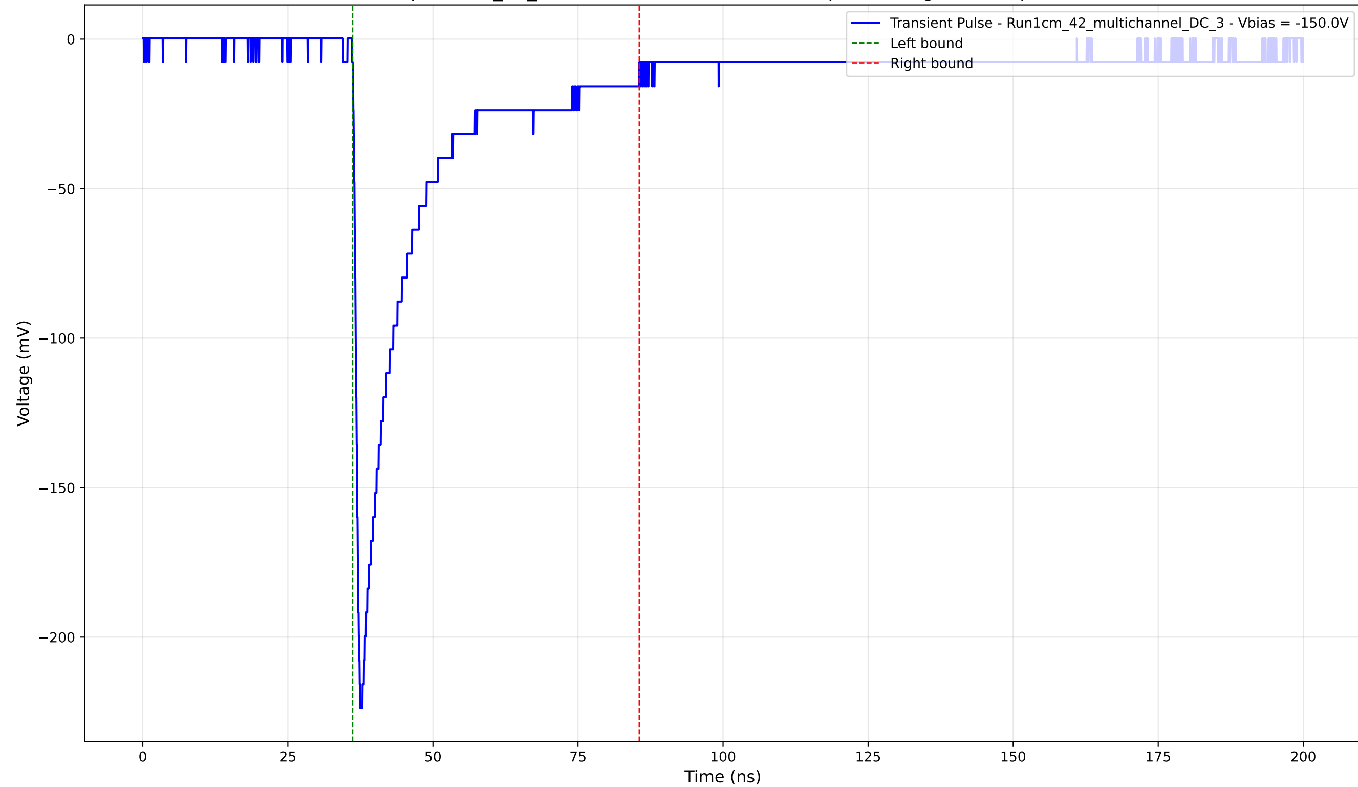
Transient Pulse - Sample: 1cm_42_multichannel - Position: 705.0 \mu\text{m} - Charge: 46.99 pC - Rise Time: 1.00 ns
