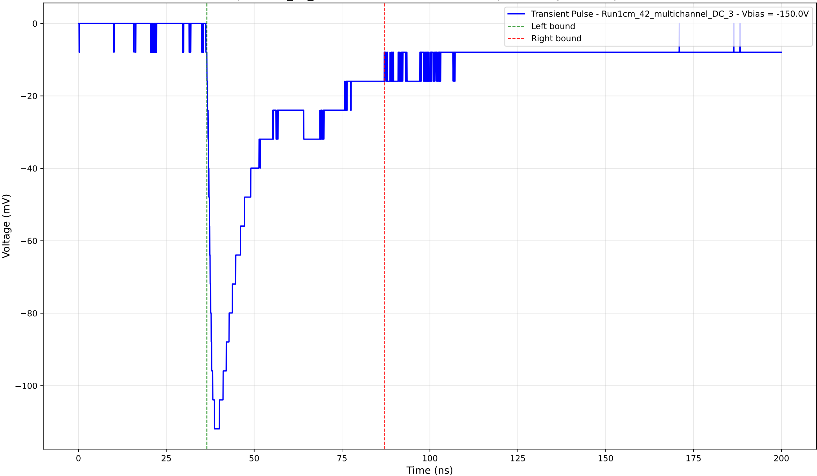
Transient Pulse - Sample: 1cm_42_multichannel - Position: 3205.0 \mu\text{m} - Charge: 37.83 pC - Rise Time: 1.67 ns
