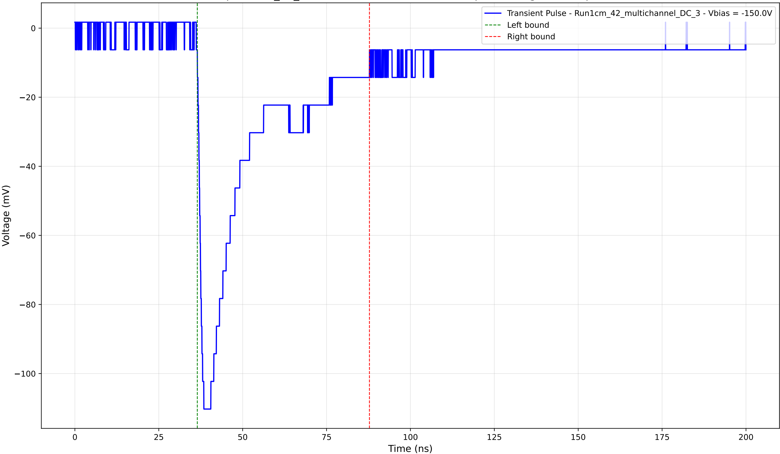
Transient Pulse - Sample: 1cm_42_multichannel - Position: 3255.0 \mu\text{m} - Charge: 36.94 pC - Rise Time: 1.57 ns
