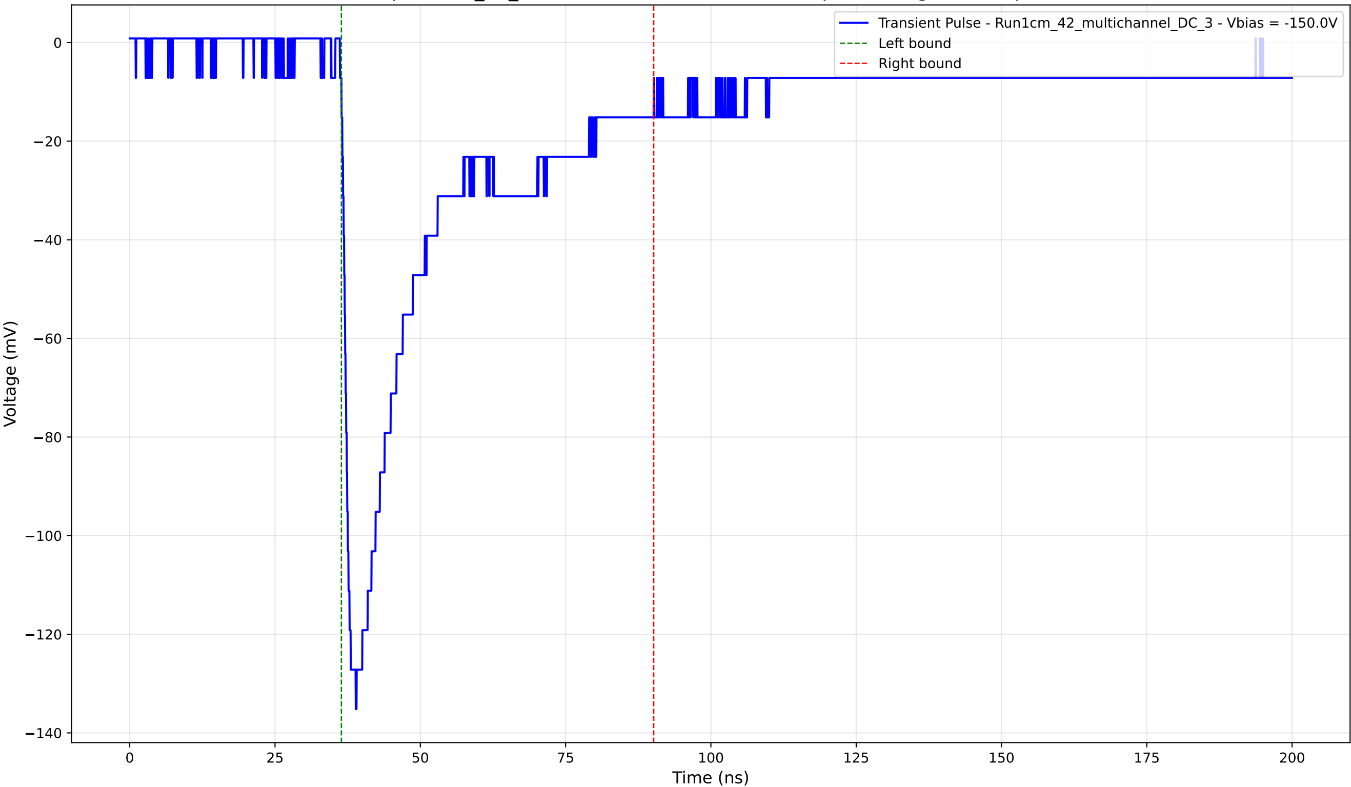
Transient Pulse - Sample: 1cm_42_multichannel - Position: 1495.0 \mu\text{m} - Charge: 42.98 pC - Rise Time: 1.58 ns
