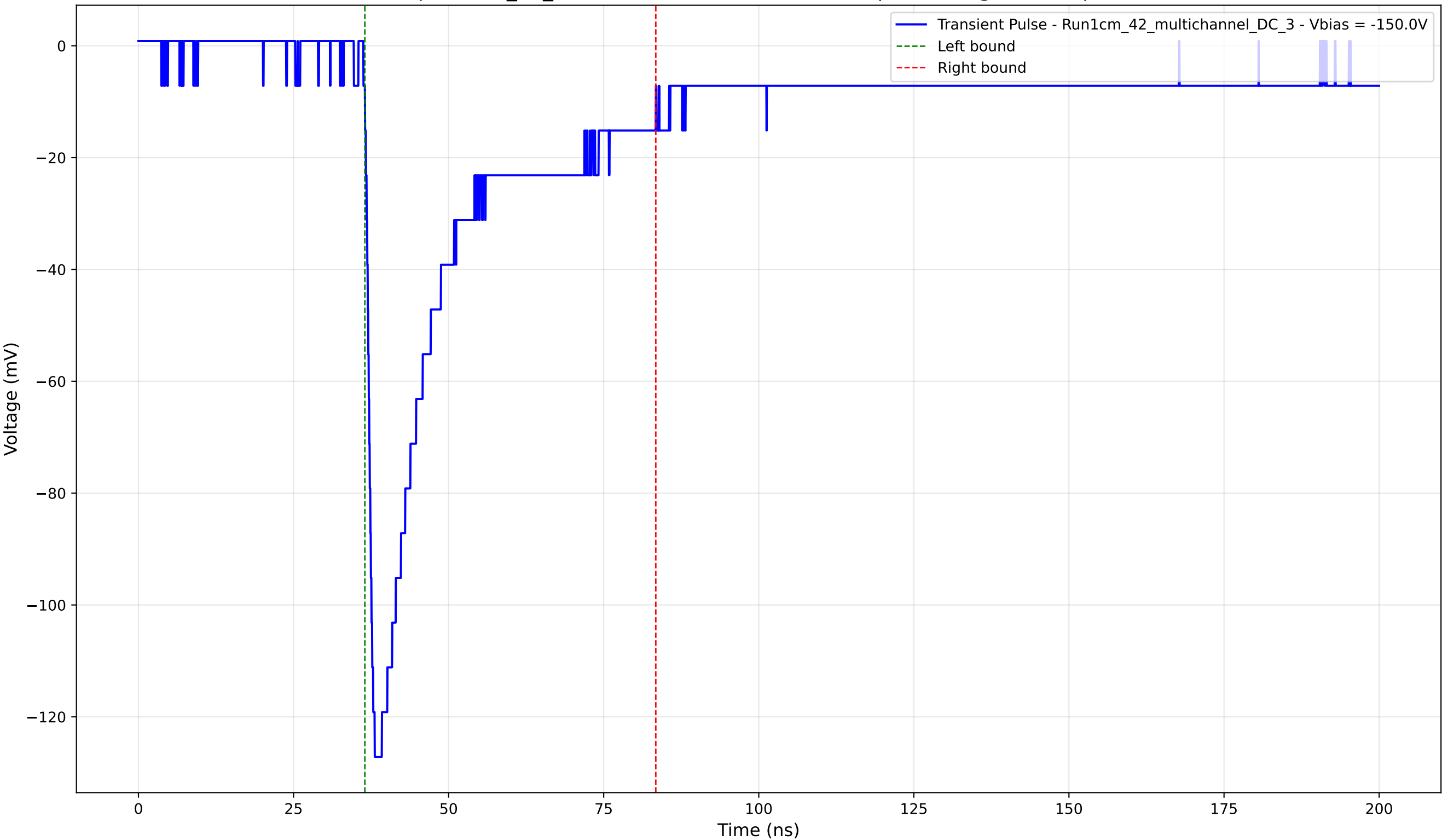
Transient Pulse - Sample: 1cm_42_multichannel - Position: 3640.0 \mu\text{m} - Charge: 35.75 pC - Rise Time: 1.33 ns
