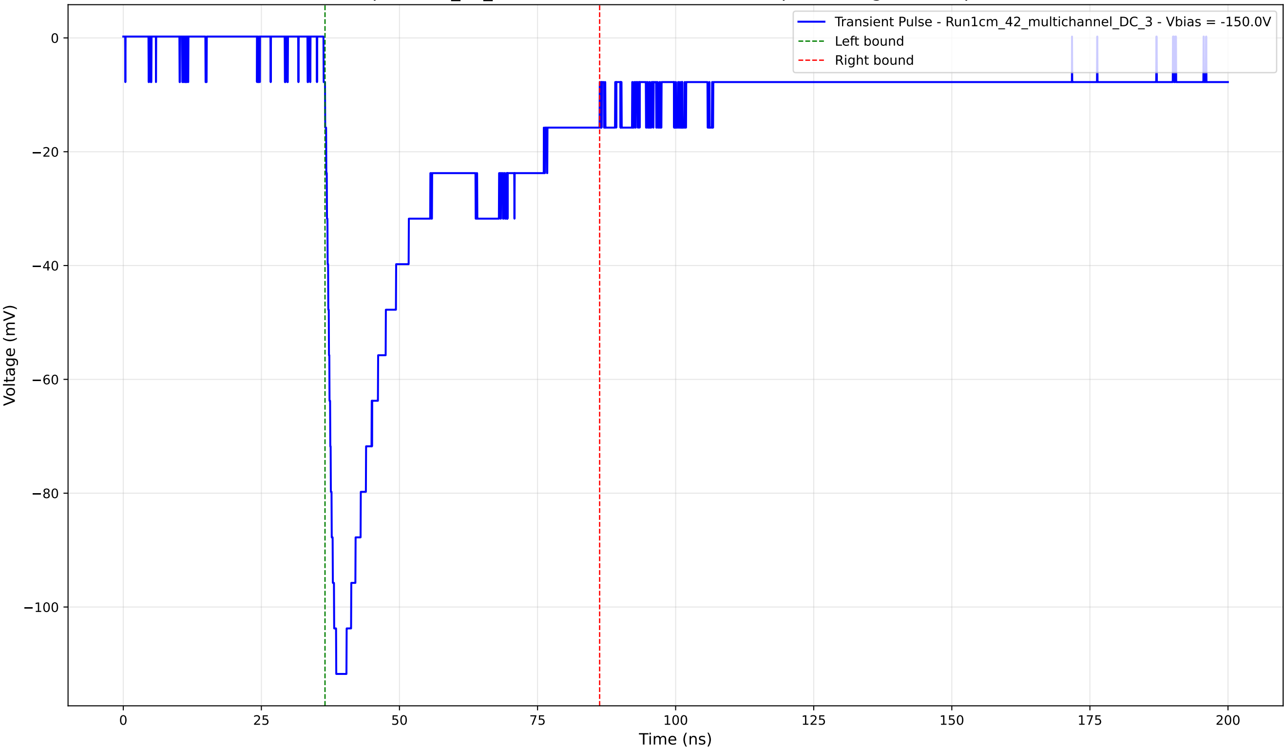
Transient Pulse - Sample: 1cm_42_multichannel - Position: 3220.0 \mu\text{m} - Charge: 37.68 pC - Rise Time: 1.63 ns
