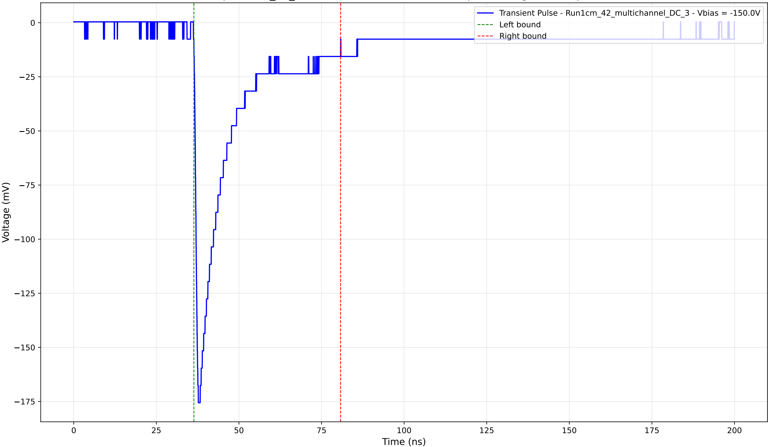
Transient Pulse - Sample: 1cm_42_multichannel - Position: 4045.0 \mu\text{m} - Charge: 39.23 pC - Rise Time: 1.00 ns
