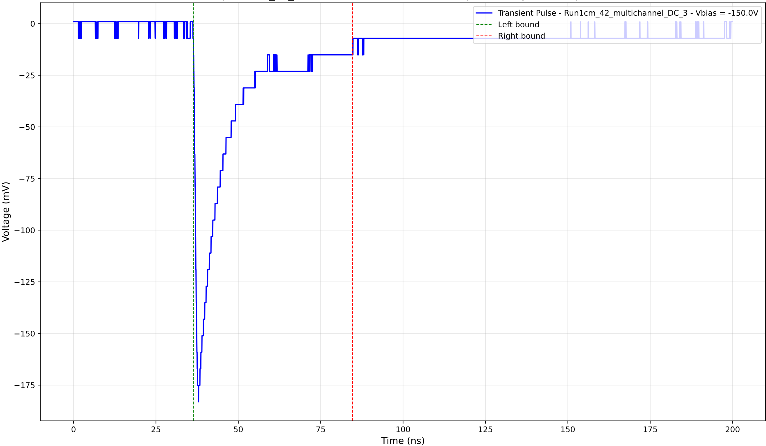
Transient Pulse - Sample: 1cm_42_multichannel - Position: 4060.0 \mu\text{m} - Charge: 39.88 pC - Rise Time: 1.03 ns
