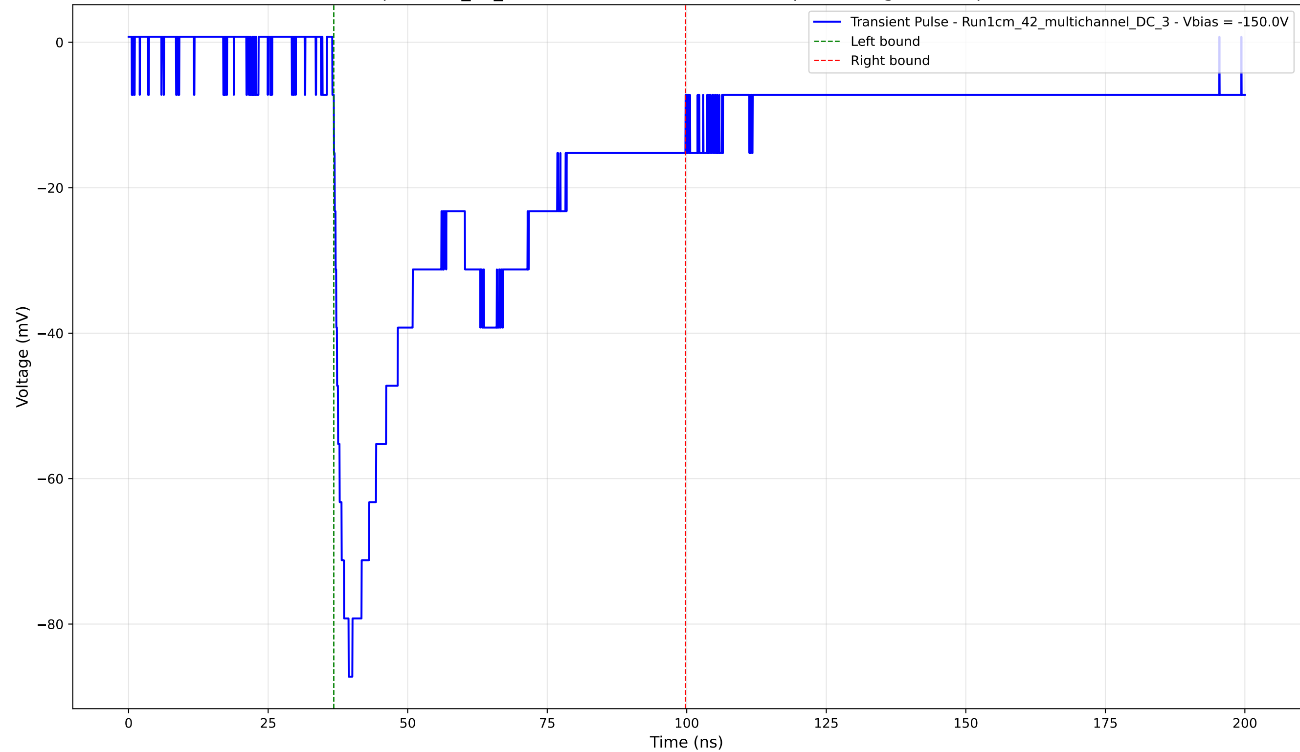
Transient Pulse - Sample: 1cm_42_multichannel - Position: 2615.0 \mu\text{m} - Charge: 38.97 pC - Rise Time: 1.84 ns
