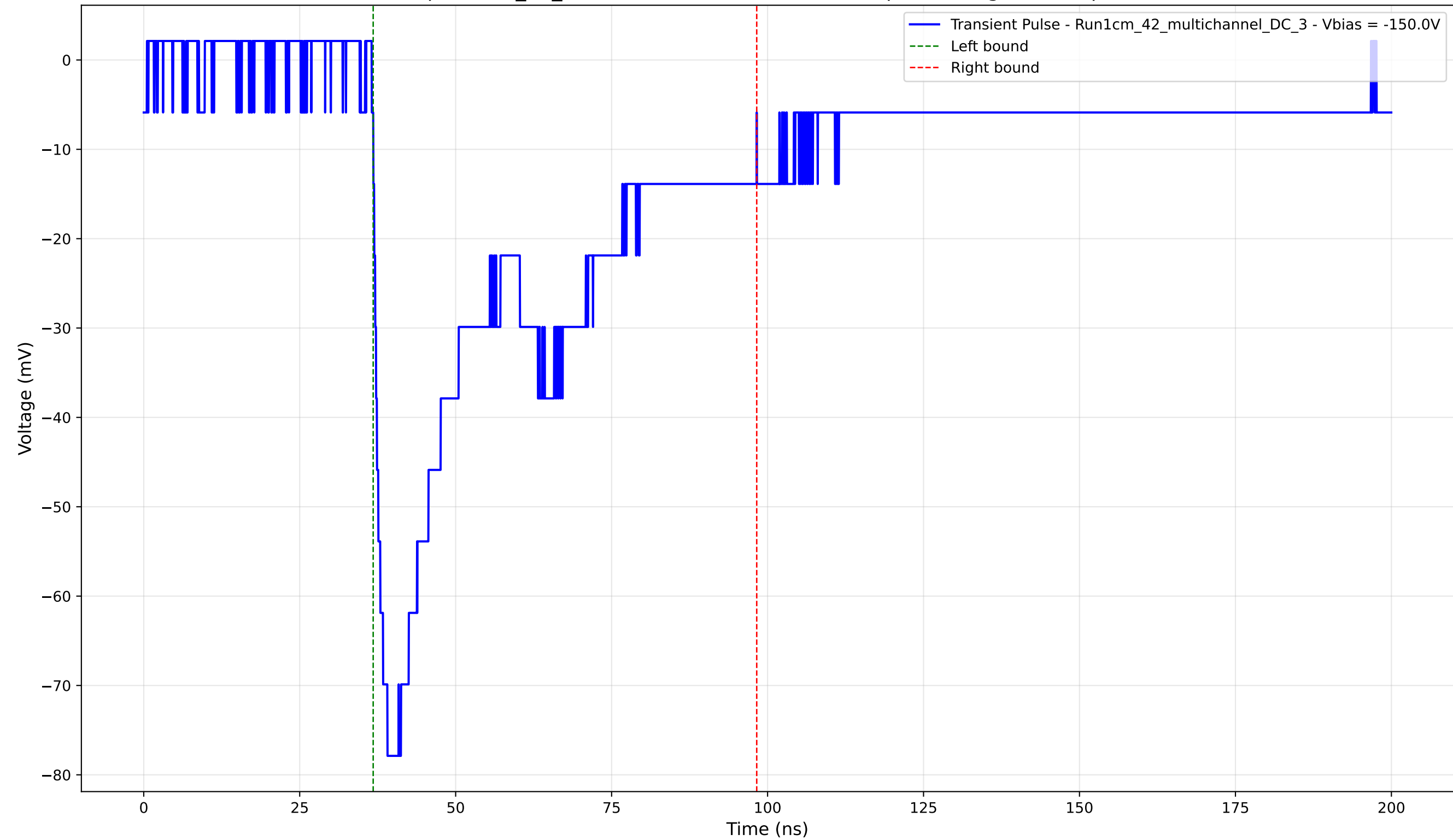
Transient Pulse - Sample: 1cm_42_multichannel - Position: 2555.0 \mu\text{m} - Charge: 35.83 pC - Rise Time: 2.28 ns
