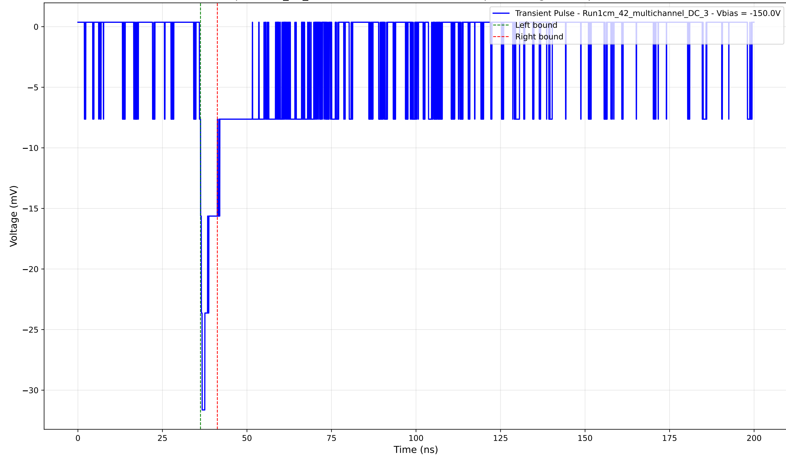
Transient Pulse - Sample: 1cm_42_multichannel - Position: 4880.0 \mu\text{m} - Charge: 2.01 pC - Rise Time: 0.81 ns
