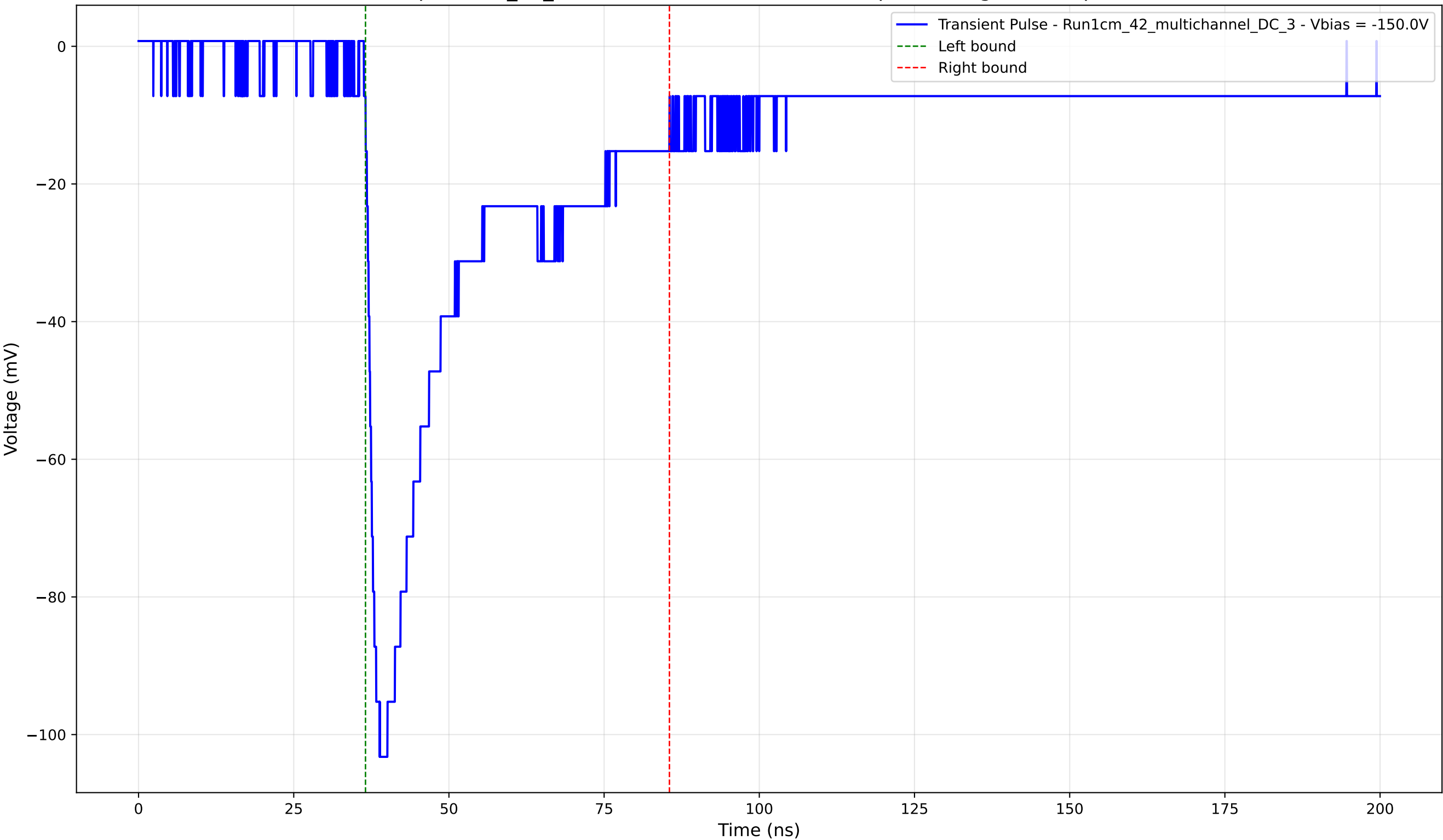
Transient Pulse - Sample: 1cm_42_multichannel - Position: 3120.0 \mu\text{m} - Charge: 34.75 pC - Rise Time: 1.71 ns
