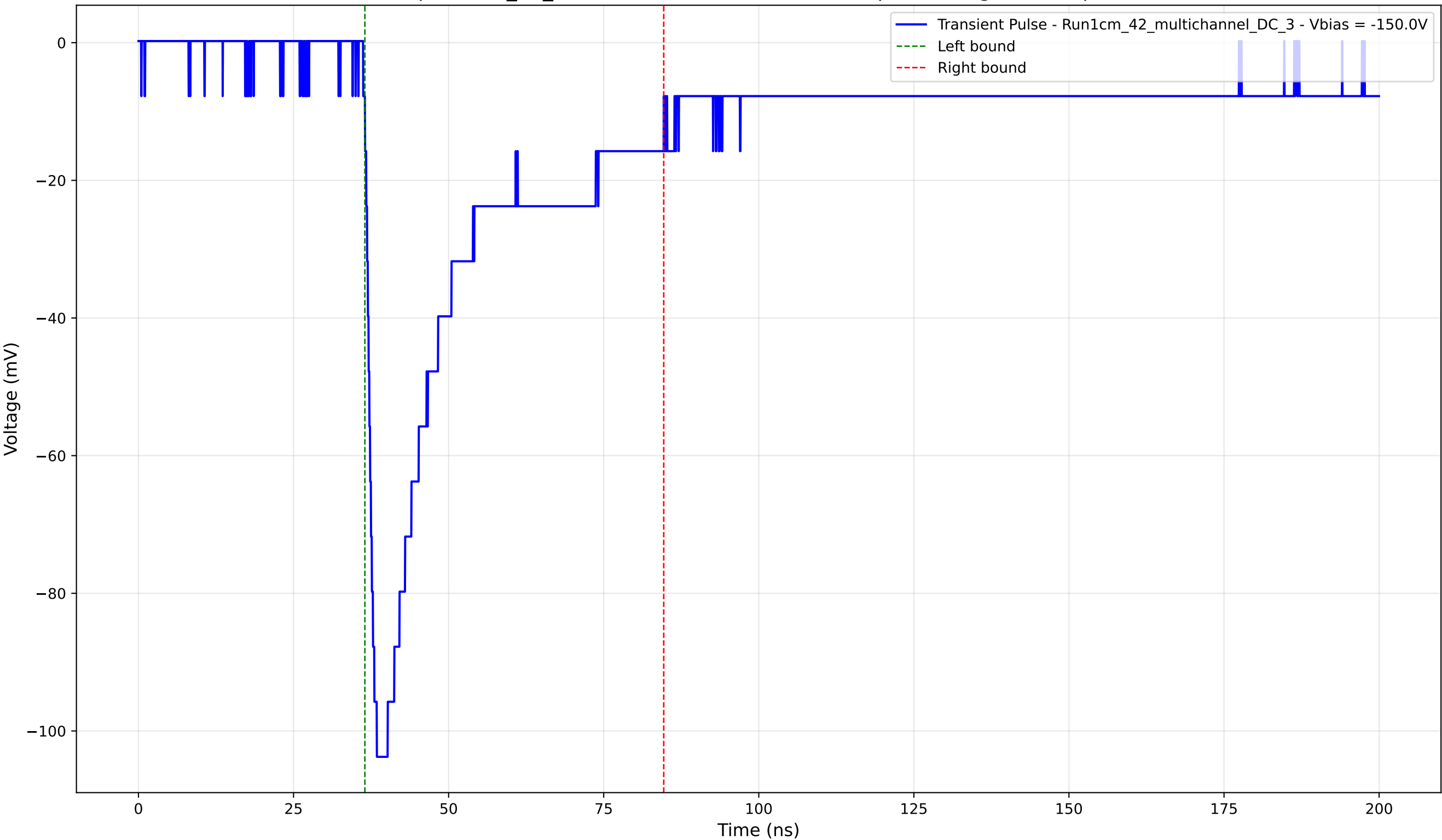
Transient Pulse - Sample: 1cm_42_multichannel - Position: 3310.0 \mu\text{m} - Charge: 33.91 pC - Rise Time: 1.51 ns
