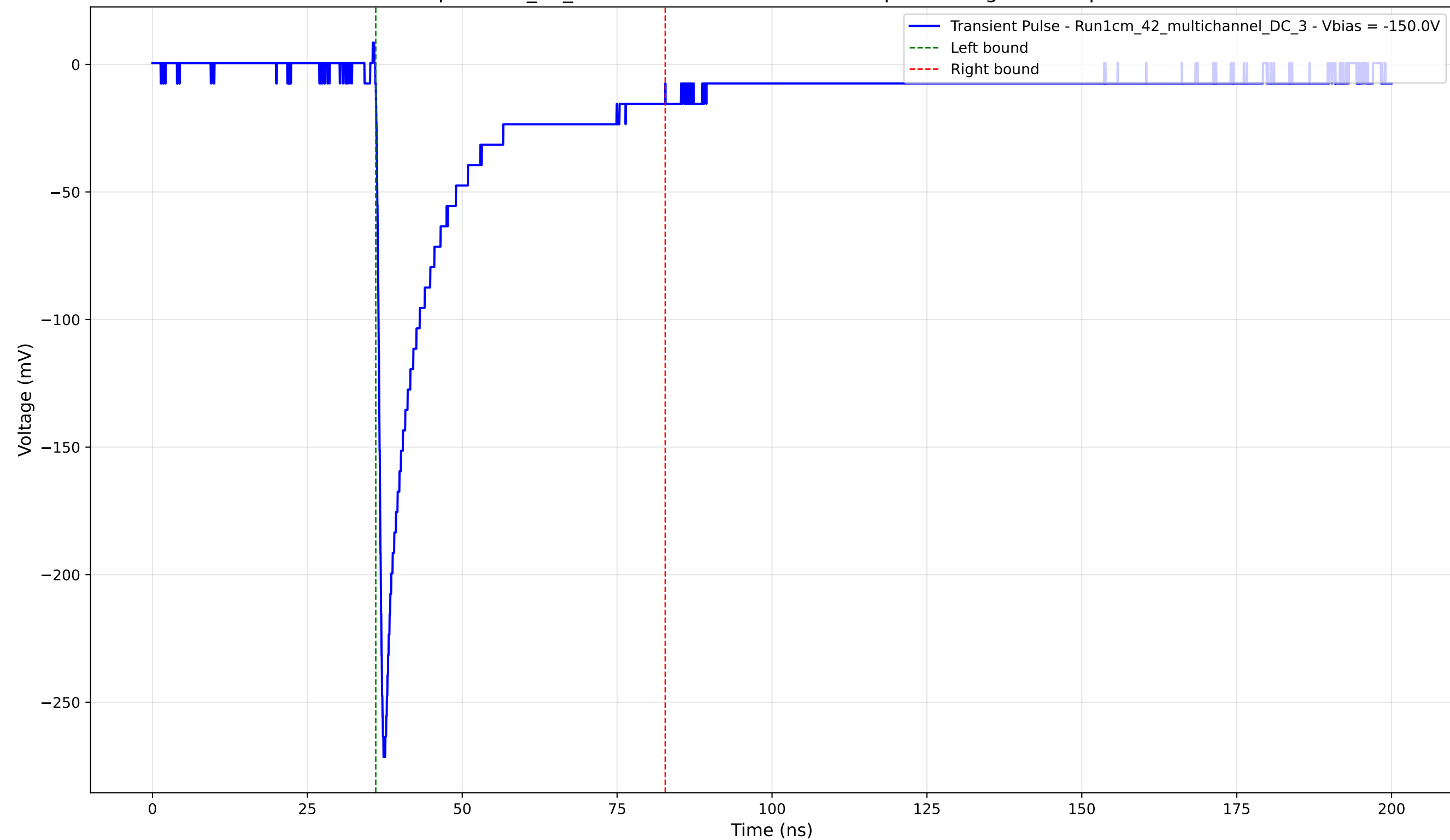
Transient Pulse - Sample: 1cm_42_multichannel - Position: 500.0 \mu\text{m} - Charge: 48.20 pC - Rise Time: 0.89 ns
