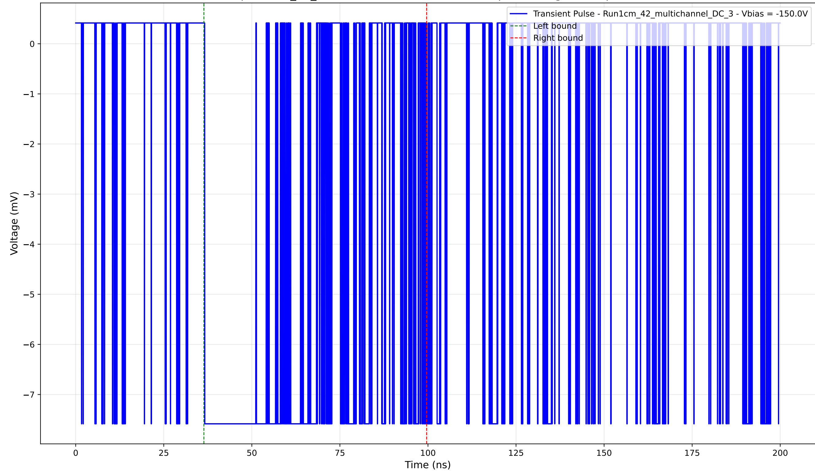
Transient Pulse - Sample: 1cm_42_multichannel - Position: 2875.0 \mu\text{m} - Charge: 5.93 pC - Rise Time: 0.02 ns
