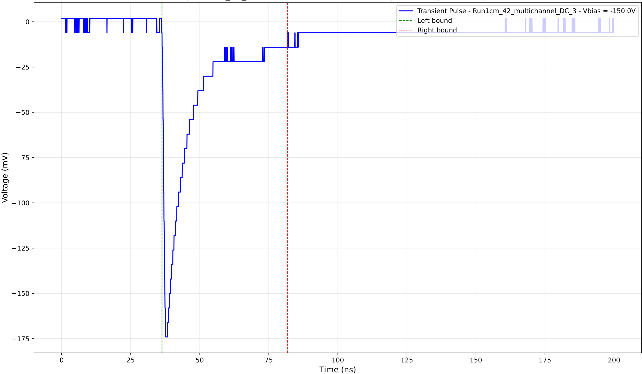
Transient Pulse - Sample: 1cm_42_multichannel - Position: 4055.0 \mu\text{m} - Charge: 38.33 pC - Rise Time: 0.97 ns
