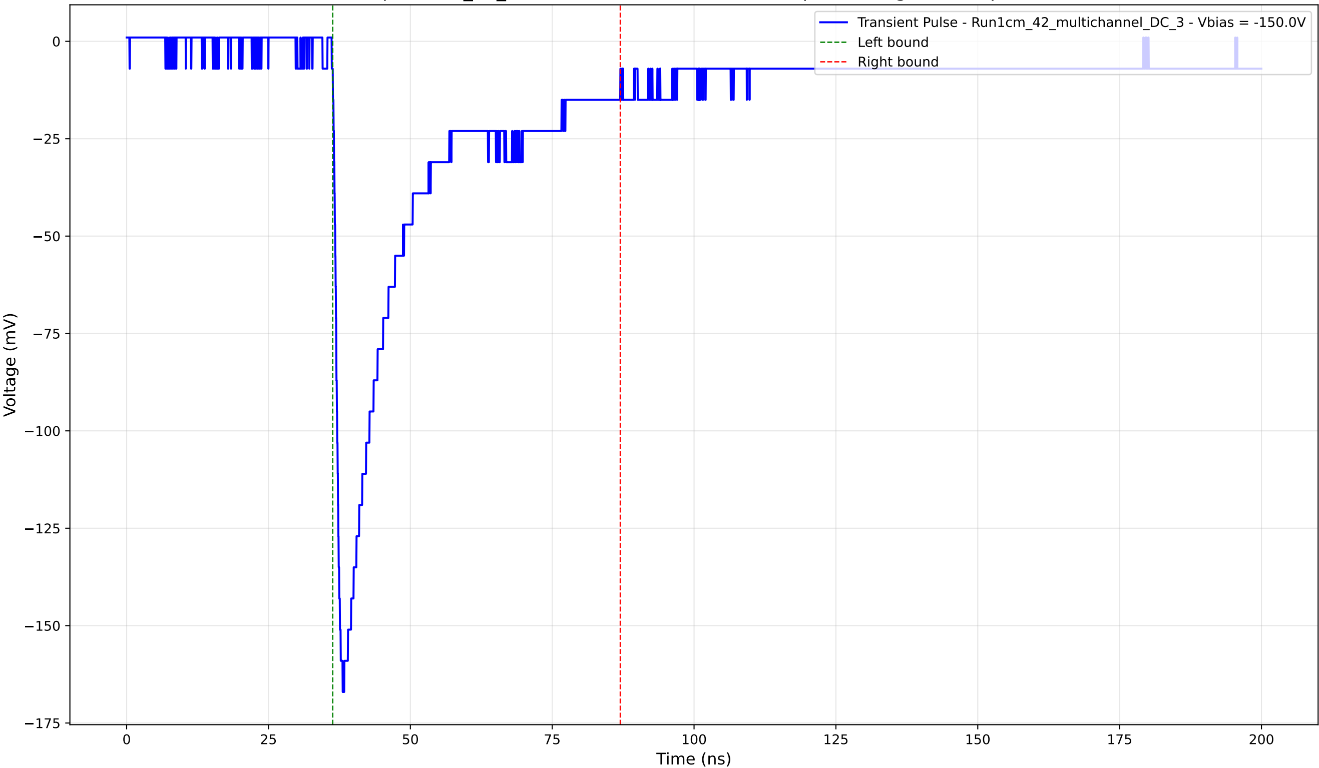
Transient Pulse - Sample: 1cm_42_multichannel - Position: 1080.0 \mu\text{m} - Charge: 43.38 pC - Rise Time: 1.14 ns
