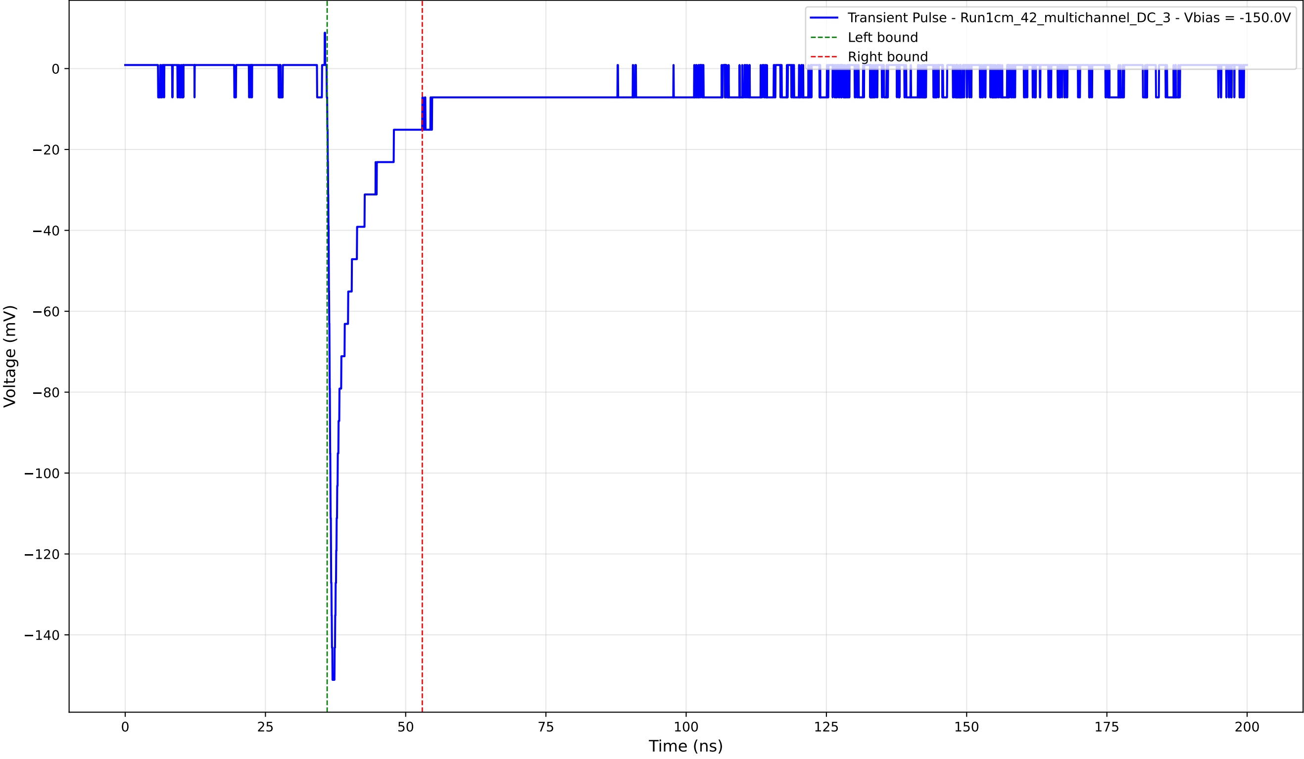
Transient Pulse - Sample: 1cm_42_multichannel - Position: 4855.0 \mu\text{m} - Charge: 13.66 pC - Rise Time: 0.82 ns
