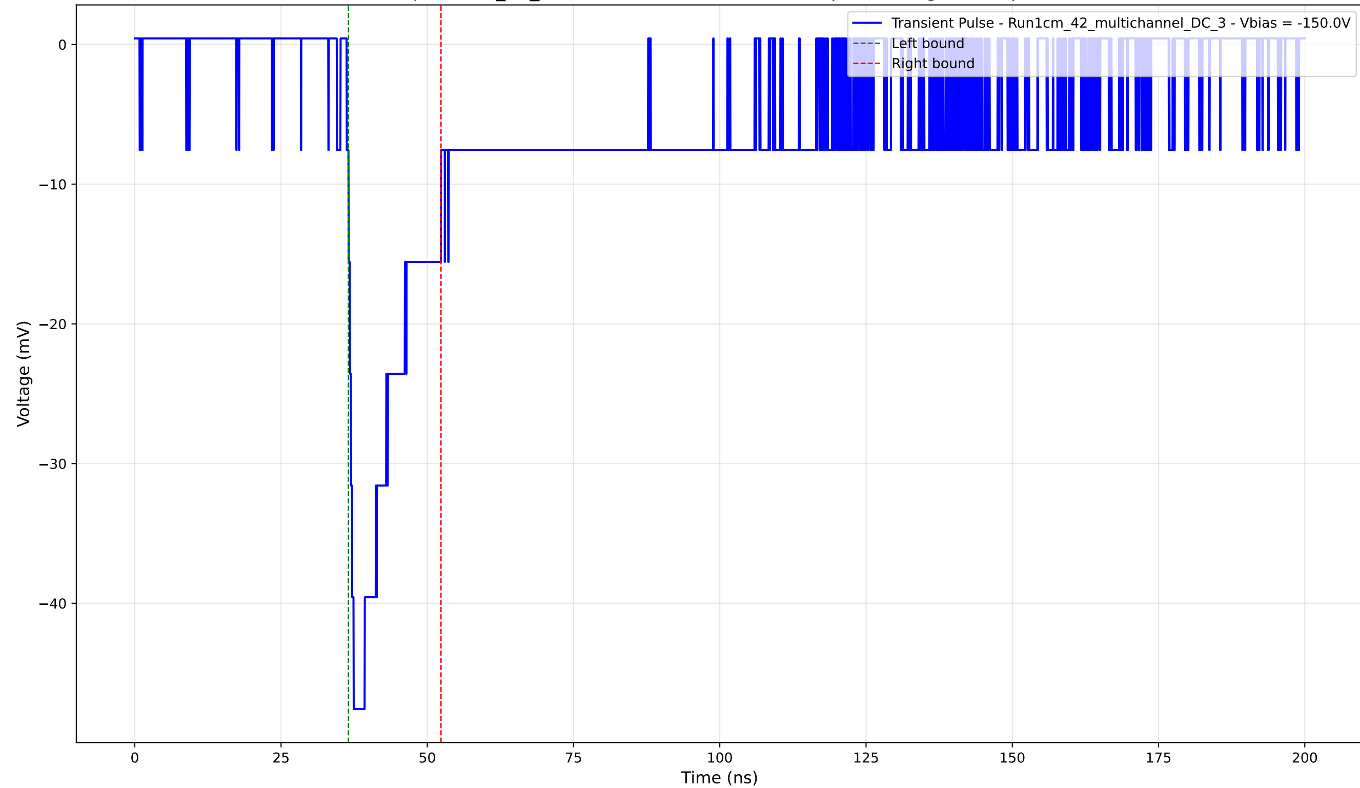
Transient Pulse - Sample: 1cm_42_multichannel - Position: 895.0 \mu\text{m} - Charge: 8.39 pC - Rise Time: 1.19 ns
