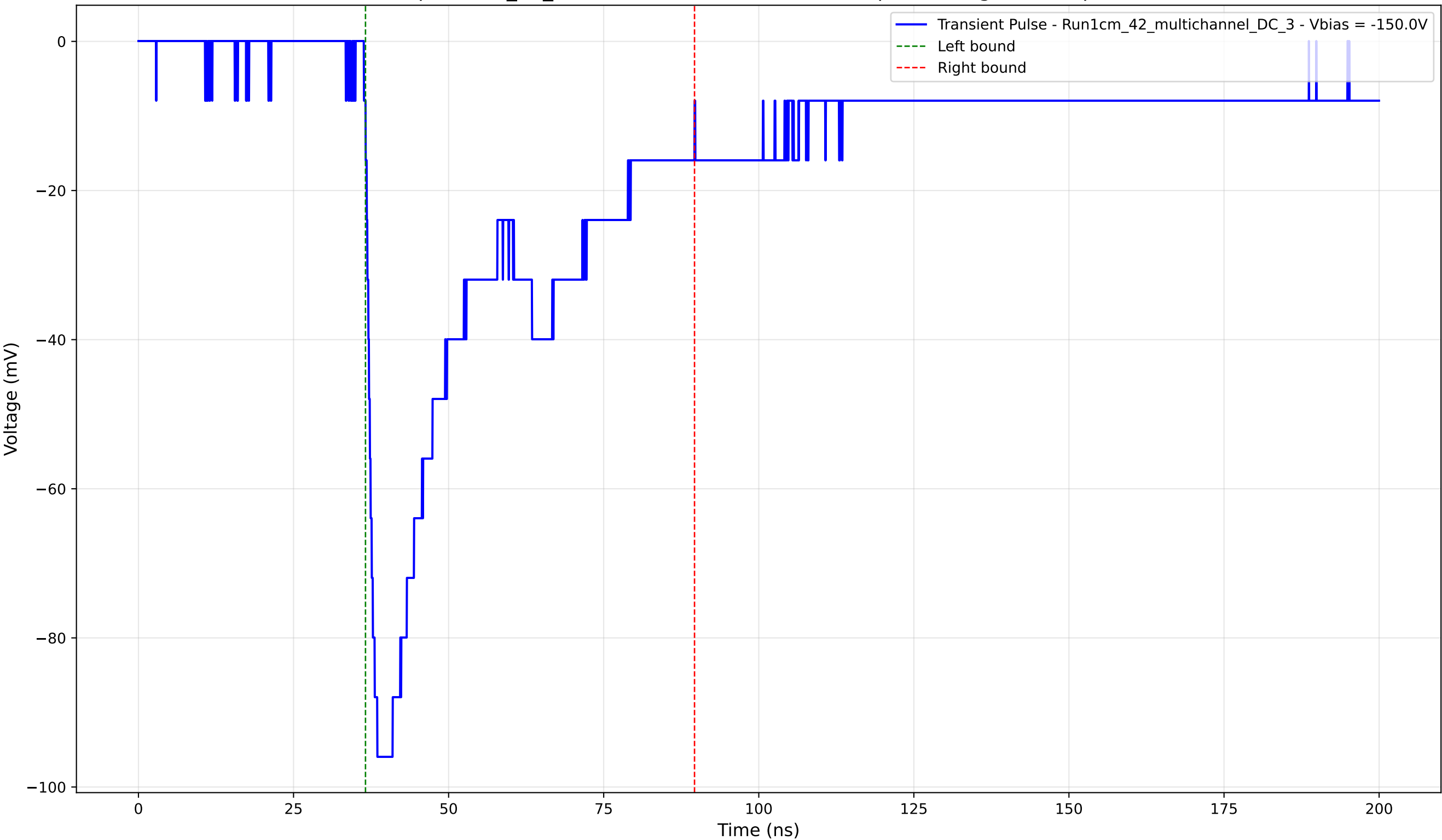
Transient Pulse - Sample: 1cm_42_multichannel - Position: 1990.0 \mu\text{m} - Charge: 39.92 pC - Rise Time: 1.48 ns
