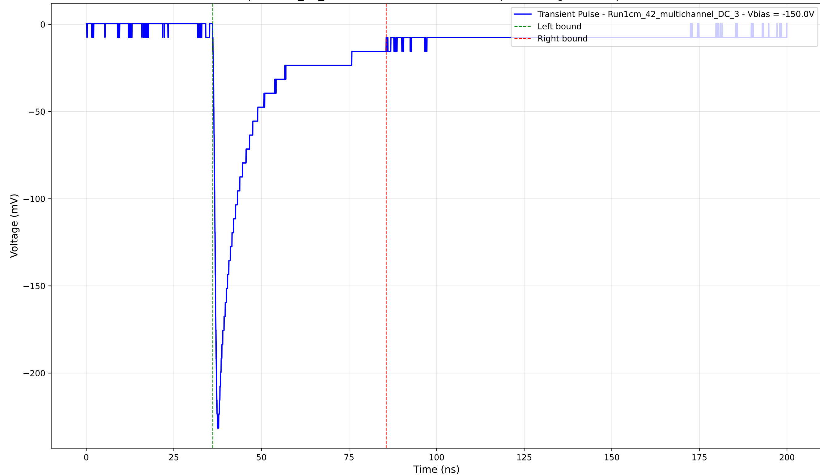
Transient Pulse - Sample: 1cm_42_multichannel - Position: 665.0 \mu\text{m} - Charge: 47.40 pC - Rise Time: 1.00 ns
