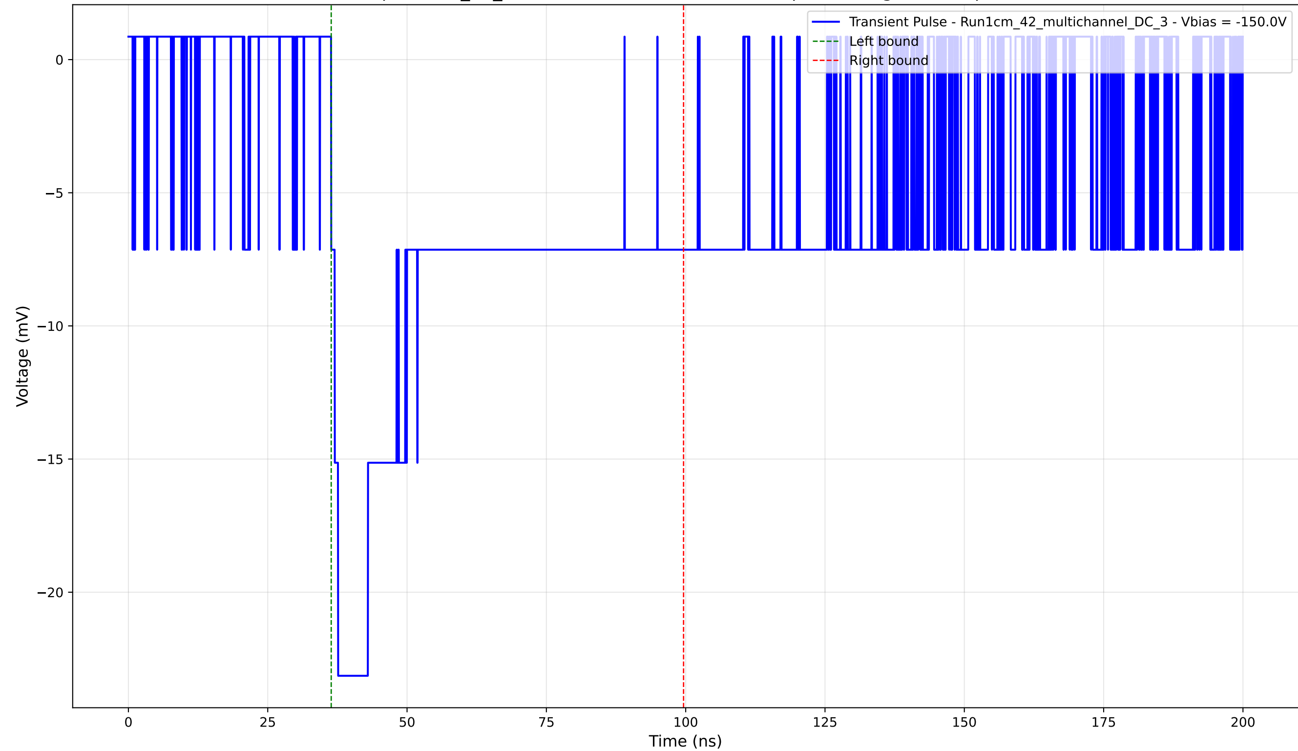
Transient Pulse - Sample: 1cm_42_multichannel - Position: 1905.0 \mu\text{m} - Charge: 11.89 pC - Rise Time: 1.26 ns
