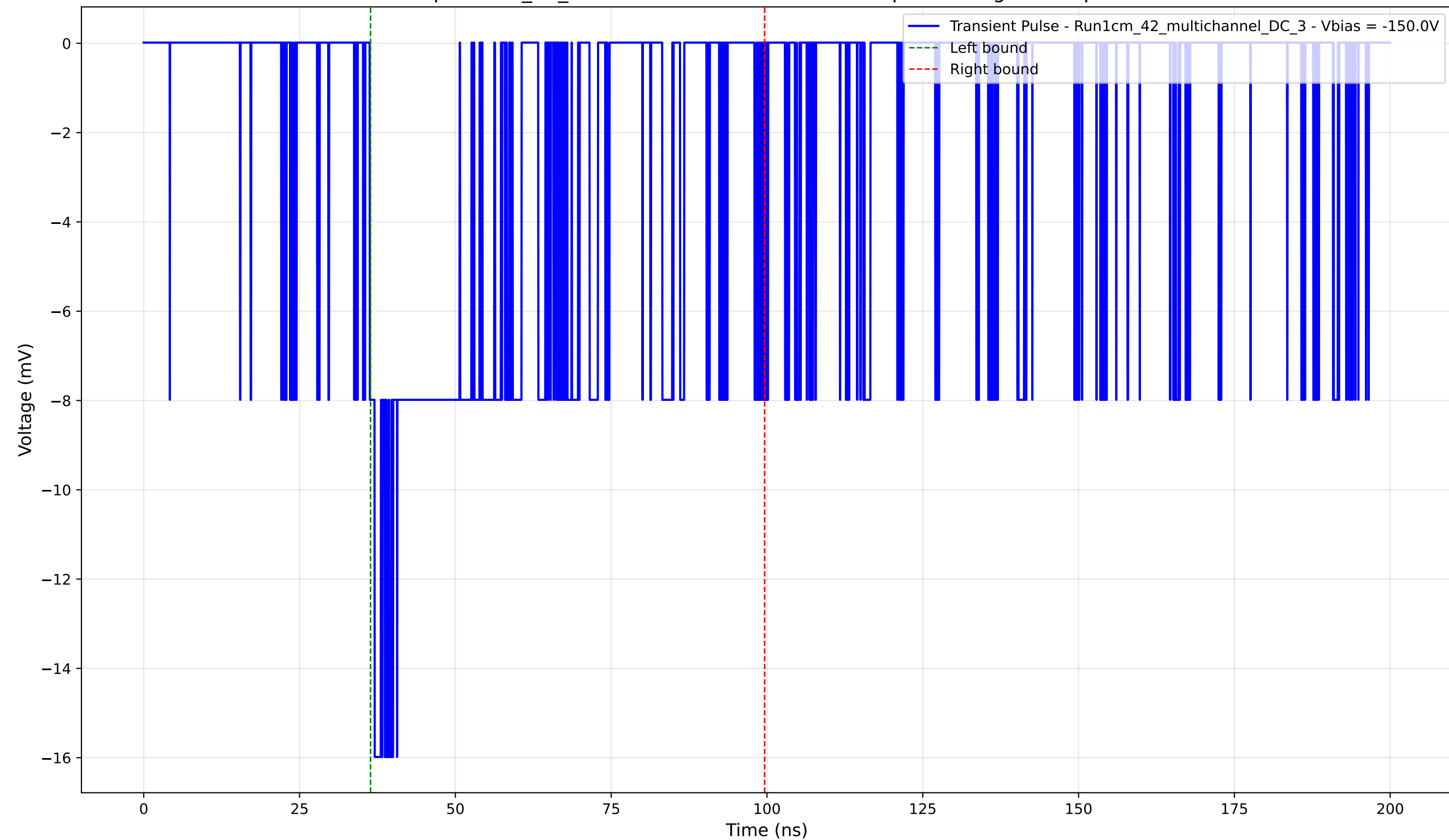
Transient Pulse - Sample: 1cm_42_multichannel - Position: 4400.0 \mu\text{m} - Charge: 5.62 pC - Rise Time: 0.80 ns
