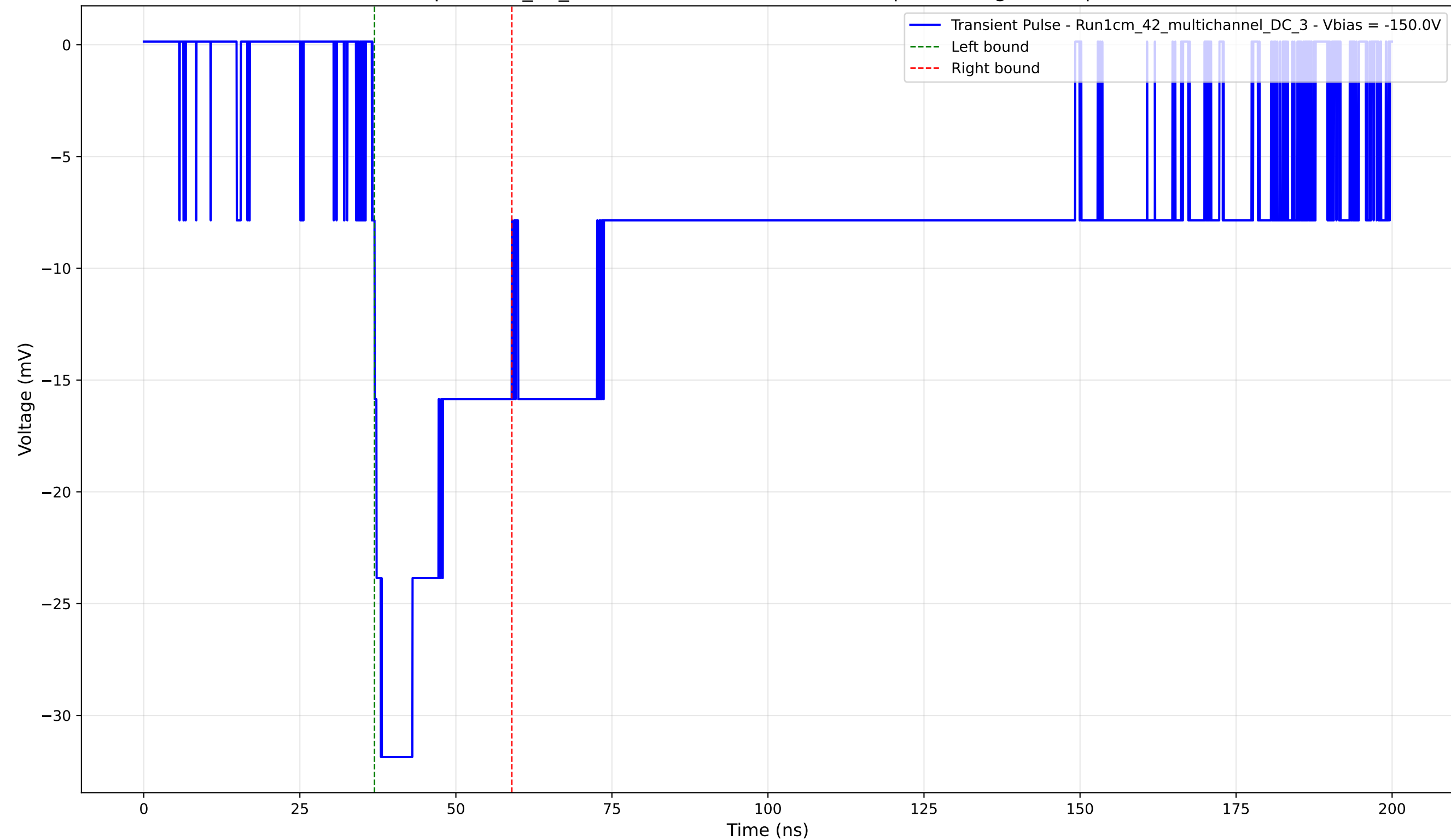
Transient Pulse - Sample: 1cm_42_multichannel - Position: 2330.0 \mu\text{m} - Charge: 9.44 pC - Rise Time: 1.35 ns
