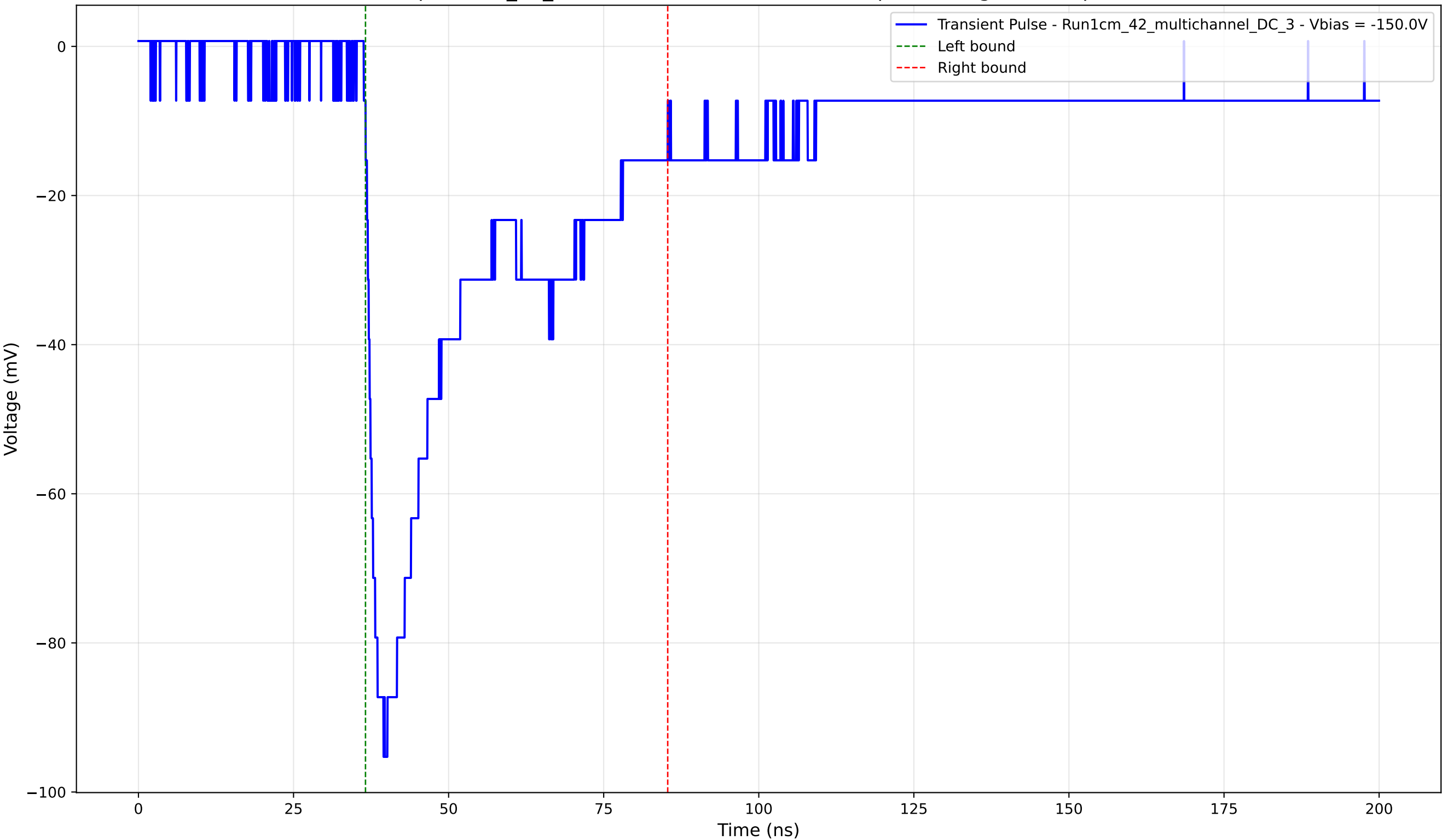
Transient Pulse - Sample: 1cm_42_multichannel - Position: 2770.0 \mu\text{m} - Charge: 35.51 pC - Rise Time: 1.93 ns
