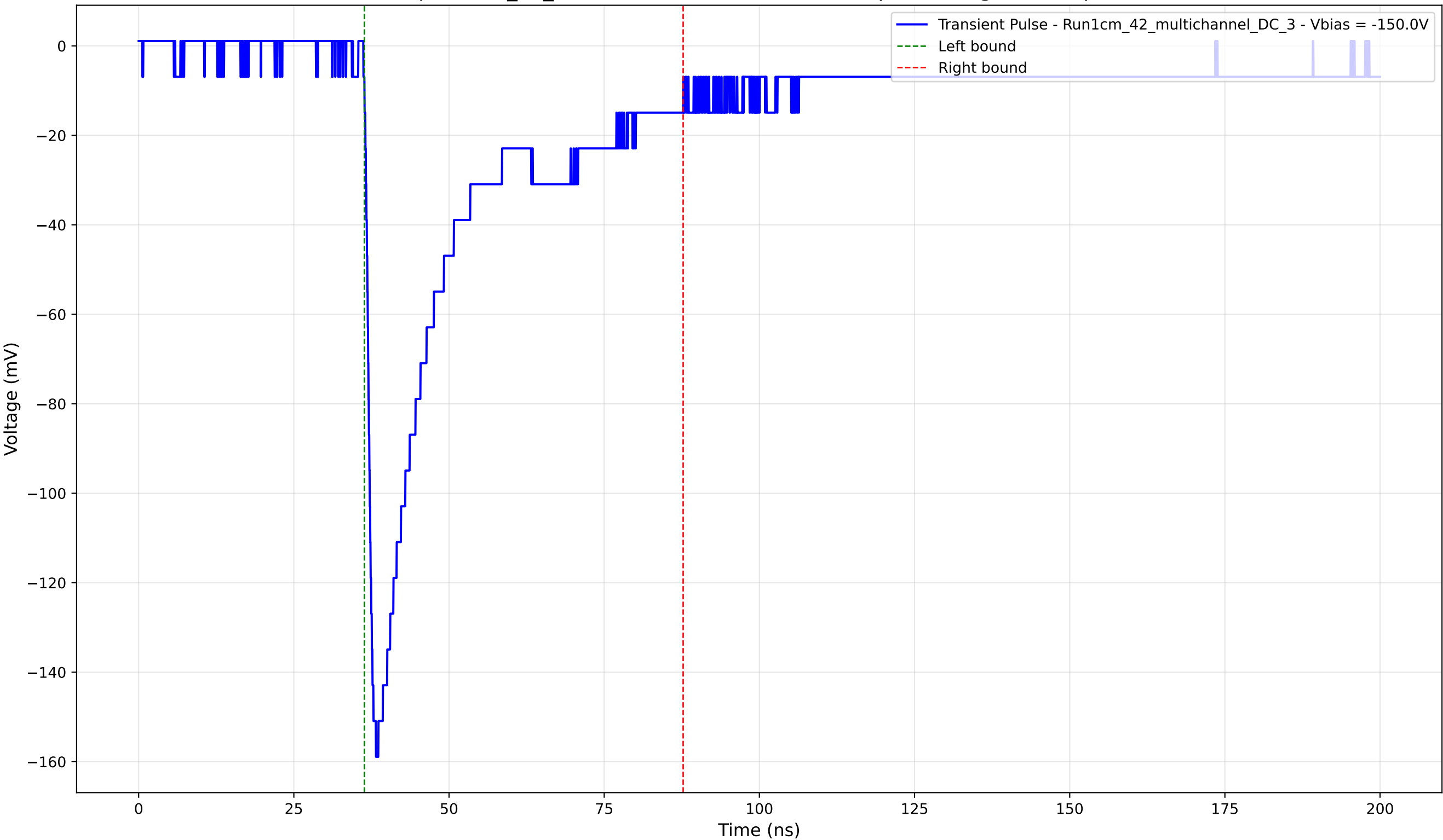
Transient Pulse - Sample: 1cm_42_multichannel - Position: 1225.0 \mu\text{m} - Charge: 44.51 pC - Rise Time: 1.32 ns
