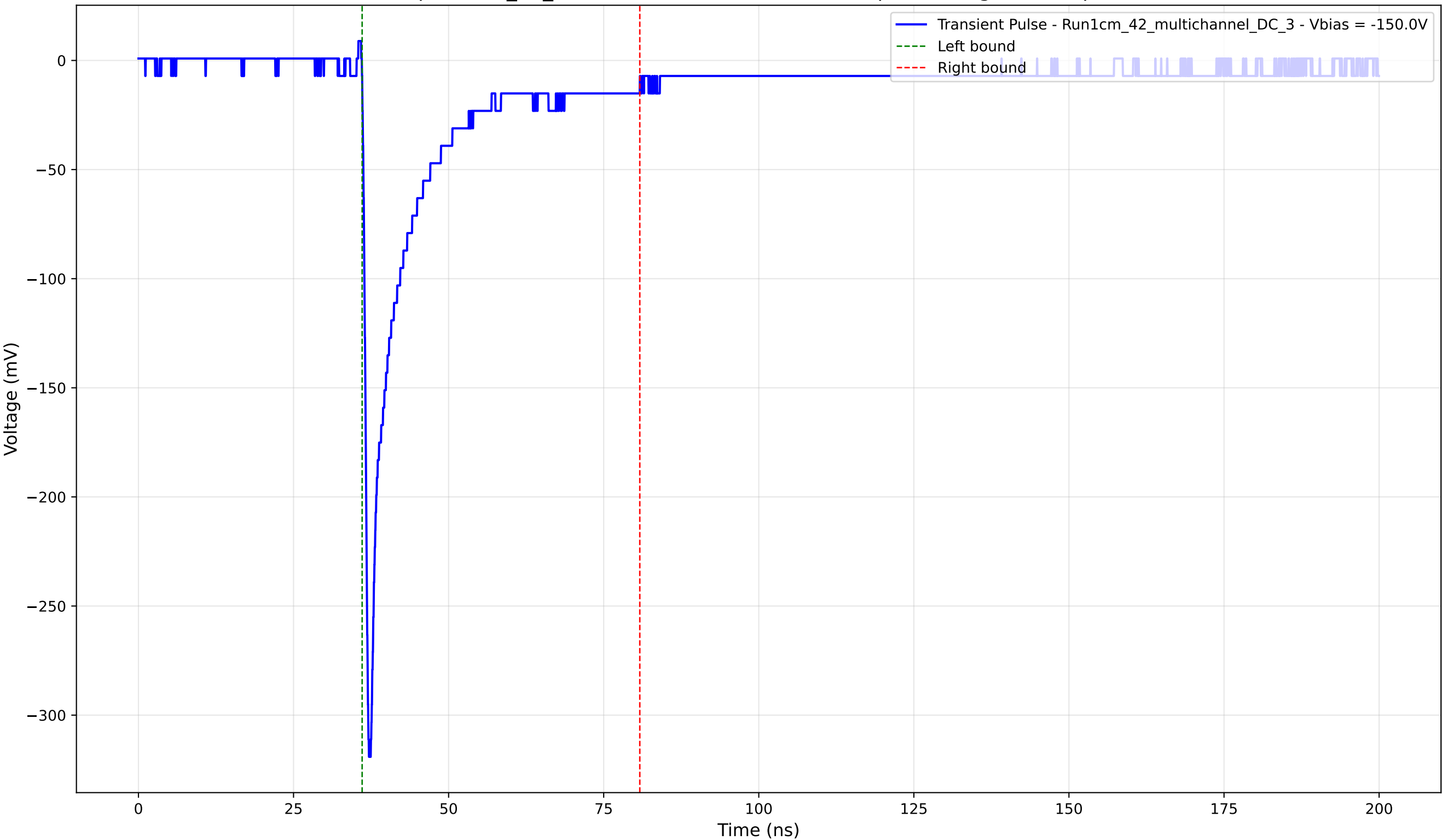
Transient Pulse - Sample: 1cm_42_multichannel - Position: 4655.0 \mu\text{m} - Charge: 41.96 pC - Rise Time: 0.82 ns
