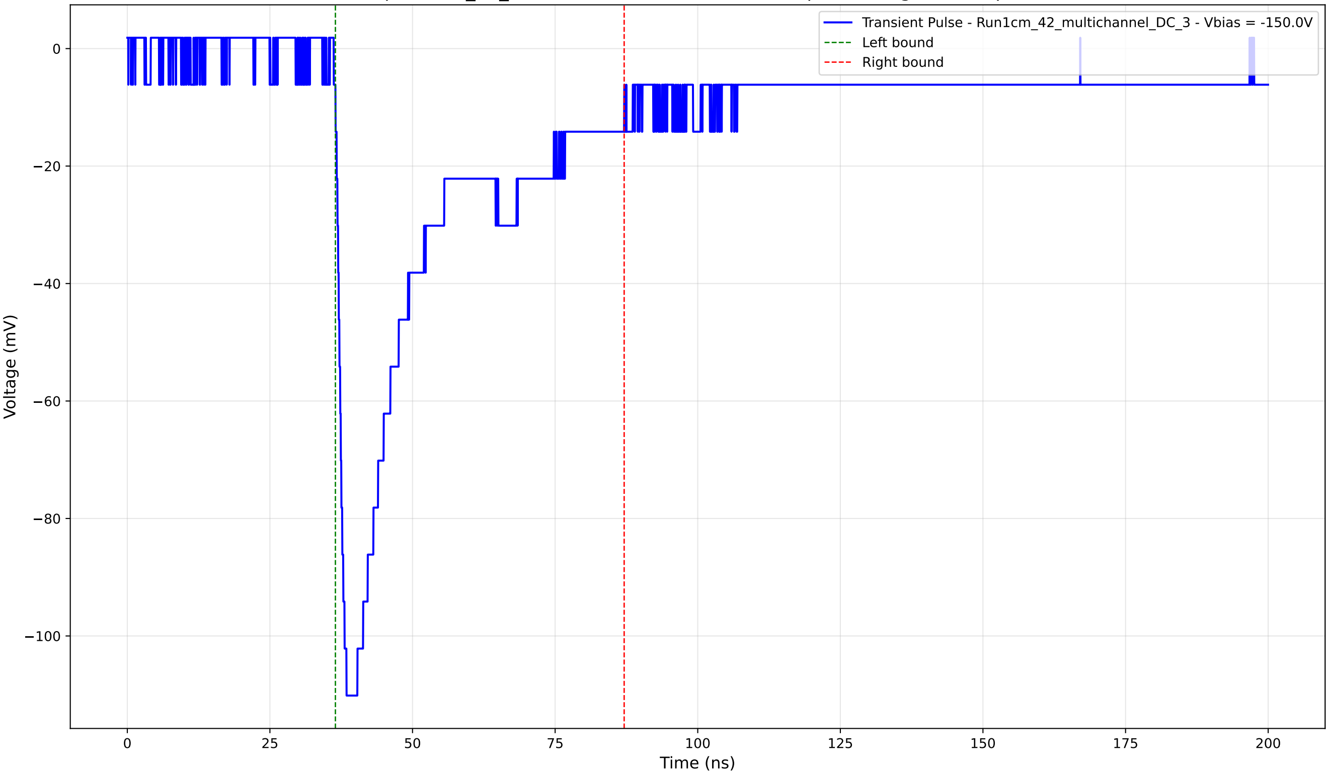
Transient Pulse - Sample: 1cm_42_multichannel - Position: 3260.0 \mu\text{m} - Charge: 36.24 pC - Rise Time: 1.59 ns
