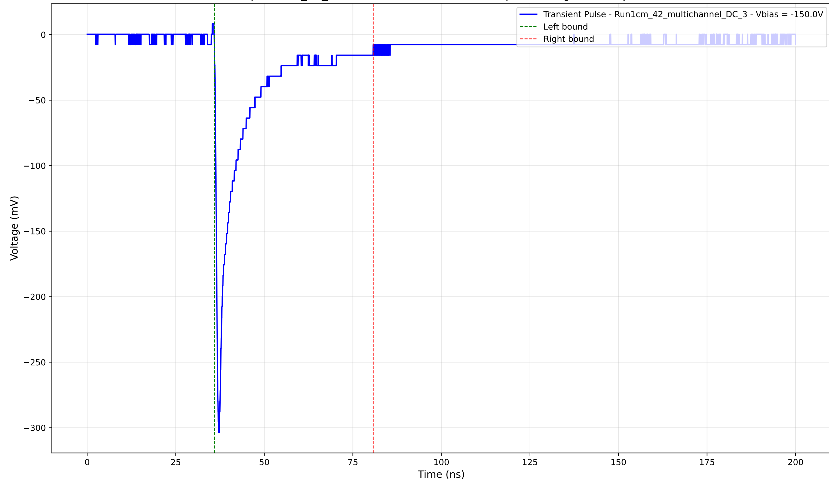
Transient Pulse - Sample: 1cm_42_multichannel - Position: 265.0 \mu\text{m} - Charge: 43.20 pC - Rise Time: 0.84 ns
