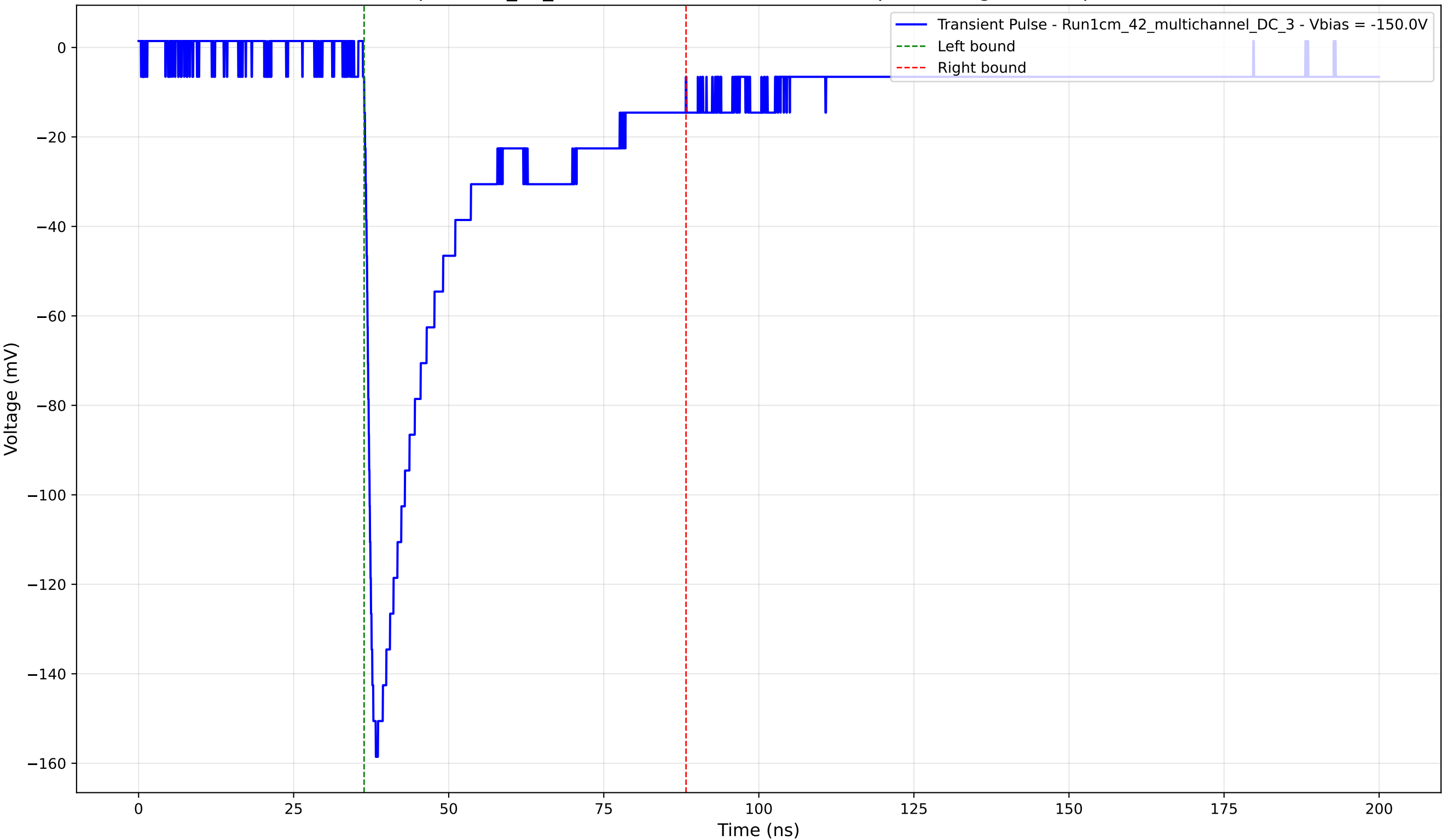
Transient Pulse - Sample: 1cm_42_multichannel - Position: 1240.0 \mu\text{m} - Charge: 44.34 pC - Rise Time: 1.36 ns
