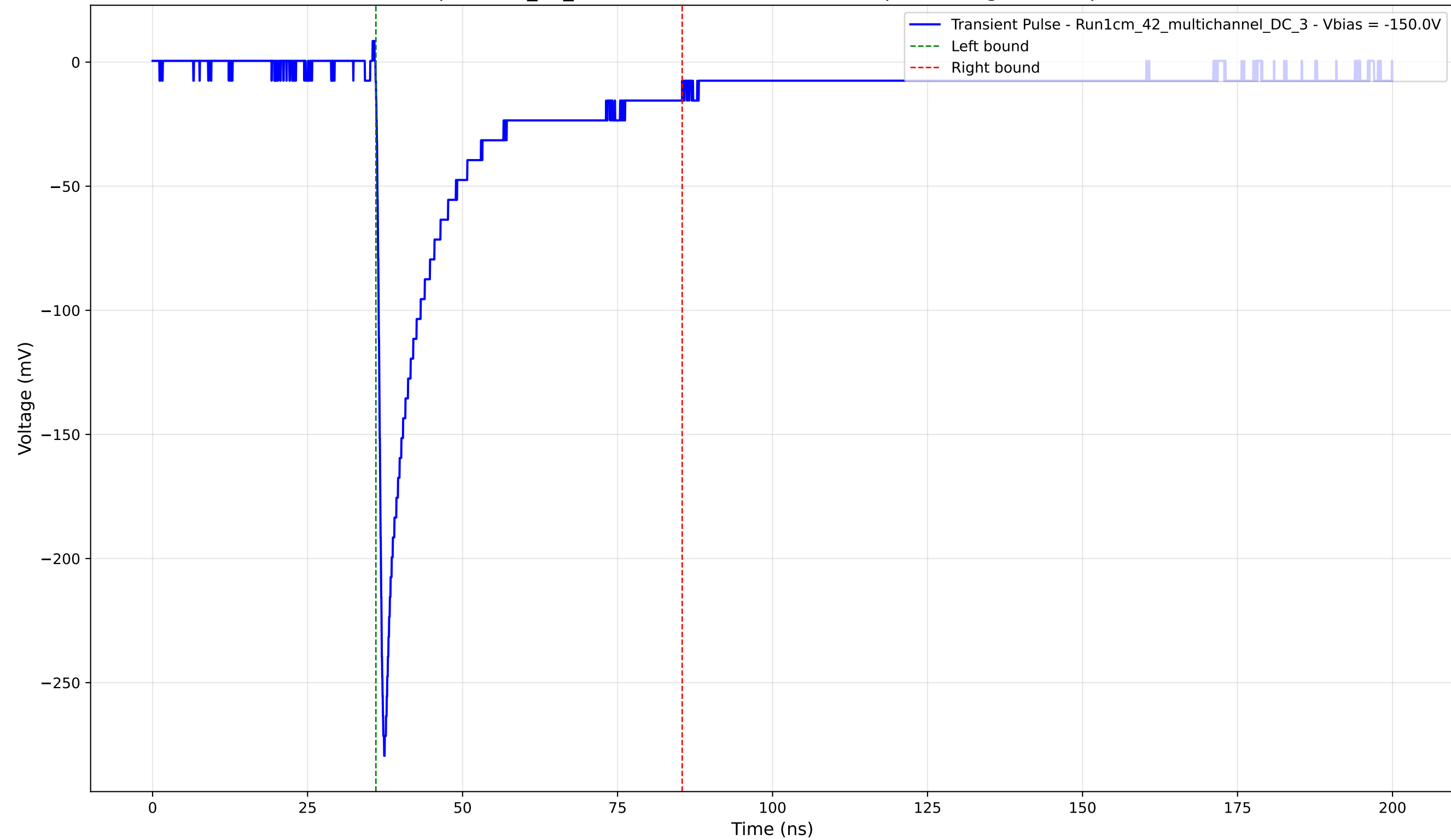
Transient Pulse - Sample: 1cm_42_multichannel - Position: 485.0 \mu\text{m} - Charge: 49.16 pC - Rise Time: 0.93 ns
