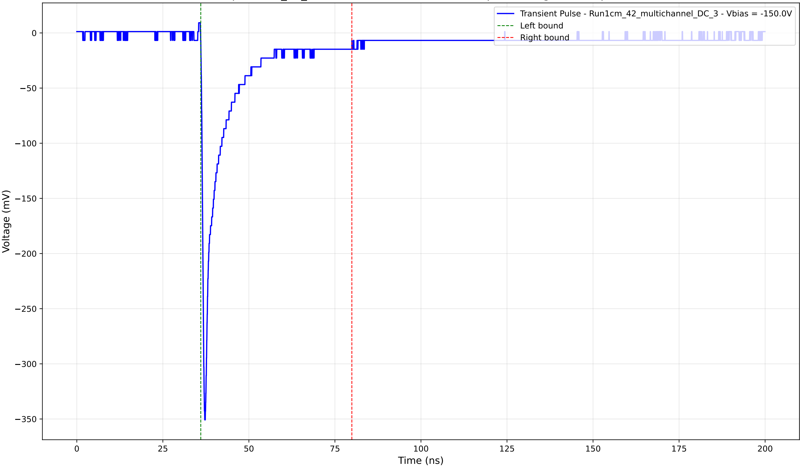
Transient Pulse - Sample: 1cm_42_multichannel - Position: 4715.0 \mu\text{m} - Charge: 42.24 pC - Rise Time: 0.81 ns
