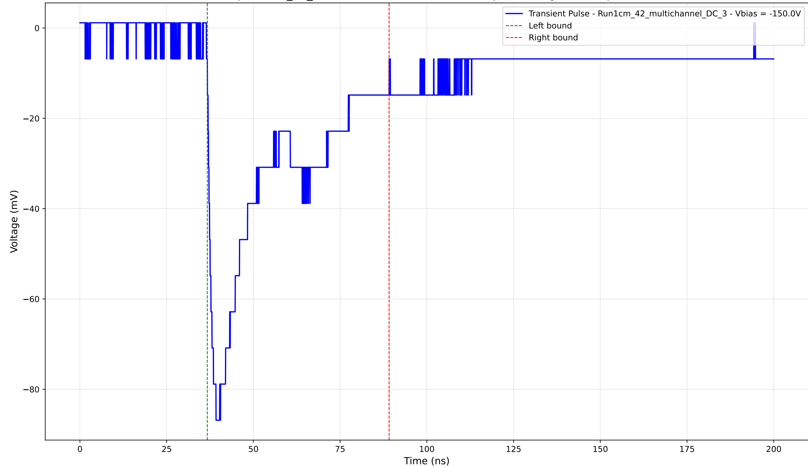
Transient Pulse - Sample: 1cm_42_multichannel - Position: 2655.0 \mu\text{m} - Charge: 35.16 pC - Rise Time: 1.76 ns
