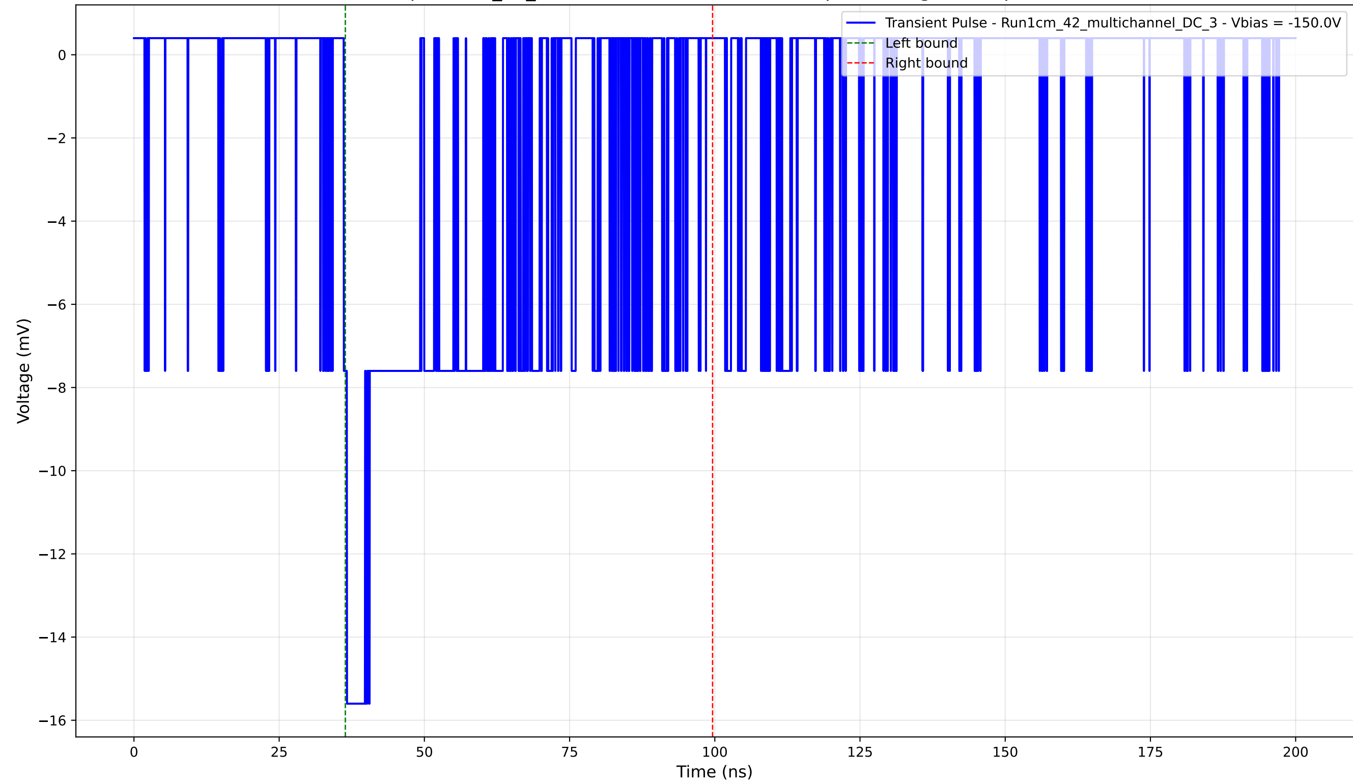
Transient Pulse - Sample: 1cm_42_multichannel - Position: 340.0 \mu\text{m} - Charge: 5.61 pC - Rise Time: 0.56 ns
