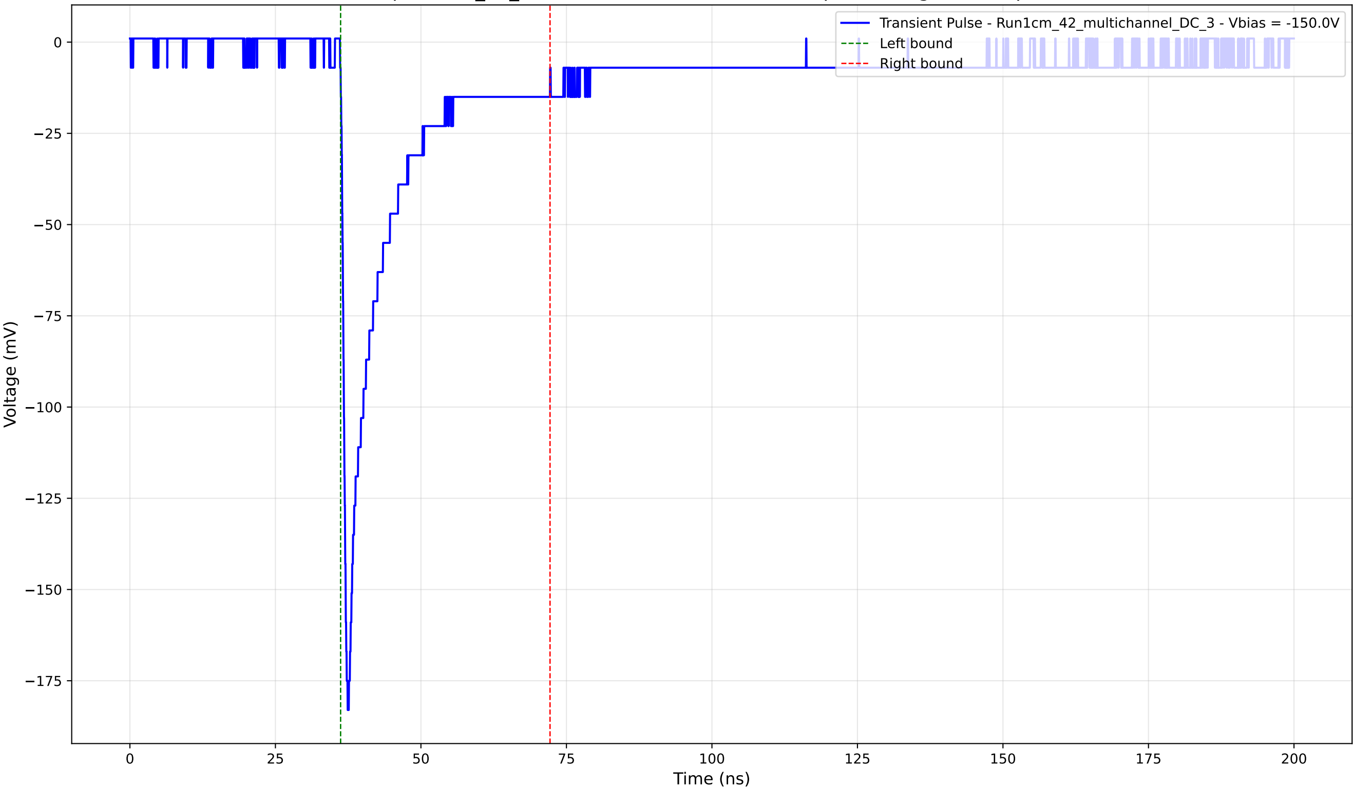
Transient Pulse - Sample: 1cm_42_multichannel - Position: 4455.0 \mu\text{m} - Charge: 27.53 pC - Rise Time: 0.87 ns
