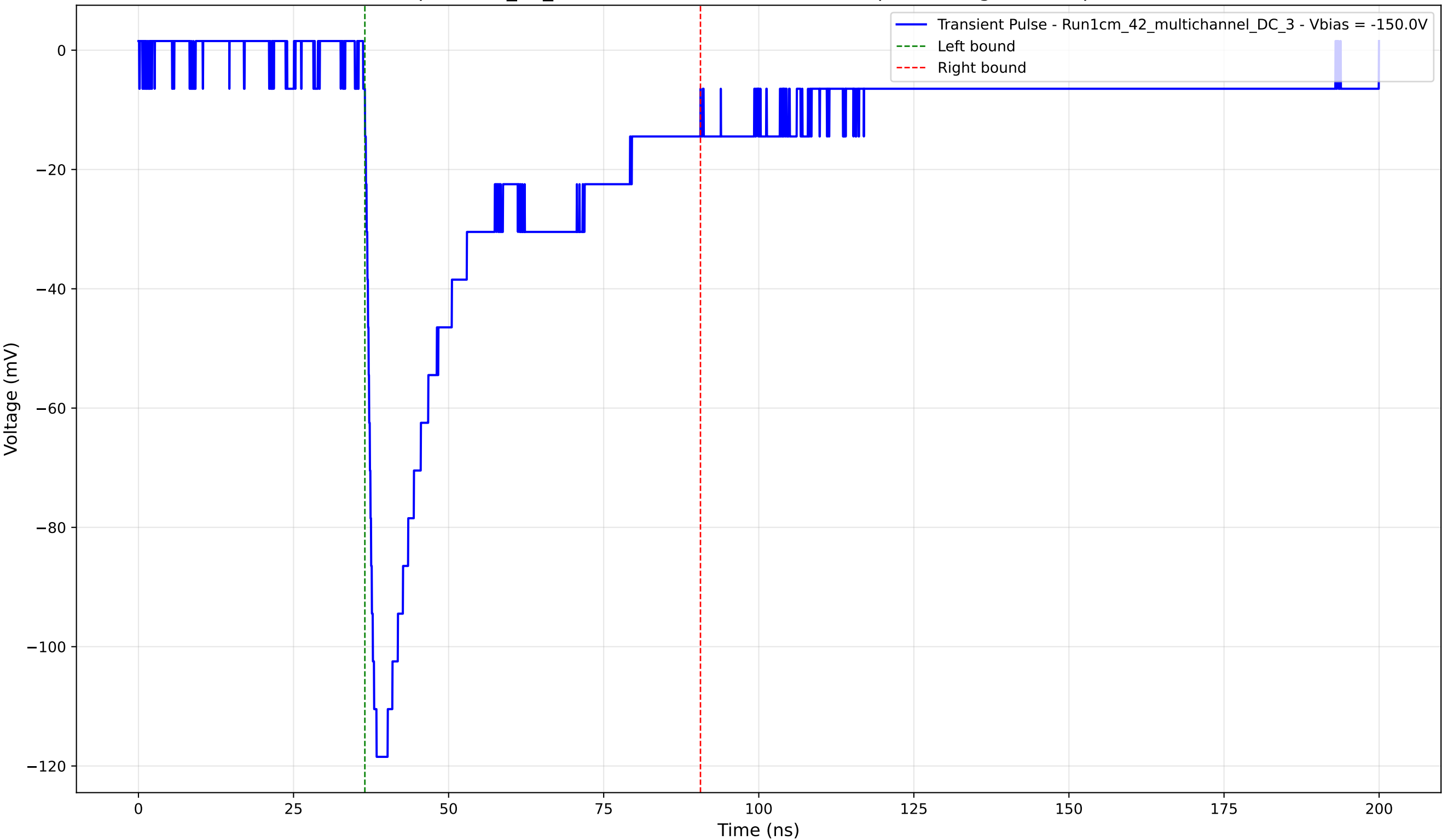
Transient Pulse - Sample: 1cm_42_multichannel - Position: 1635.0 \mu\text{m} - Charge: 41.16 pC - Rise Time: 1.47 ns
