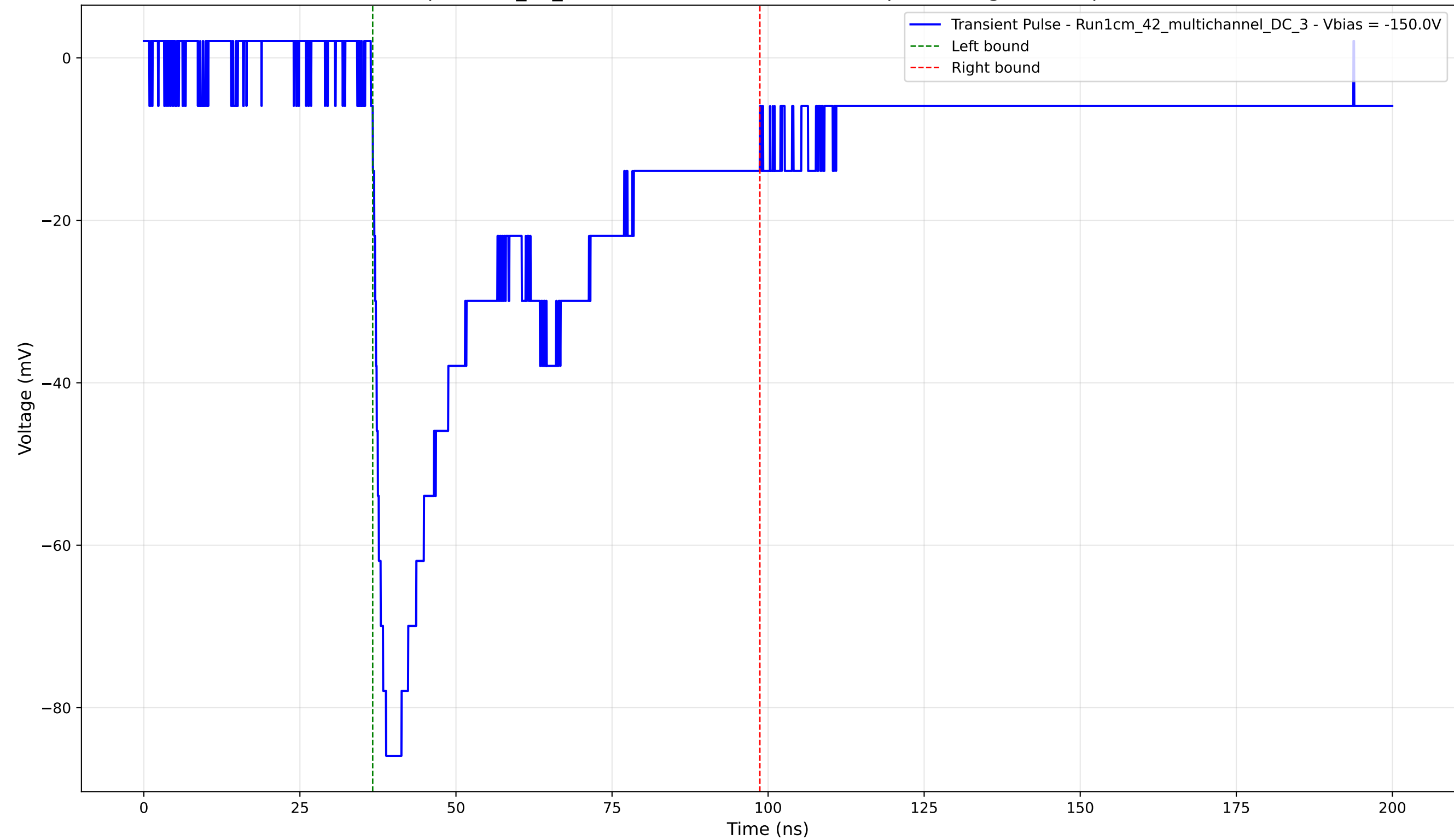
Transient Pulse - Sample: 1cm_42_multichannel - Position: 2690.0 \mu\text{m} - Charge: 37.90 pC - Rise Time: 1.65 ns
