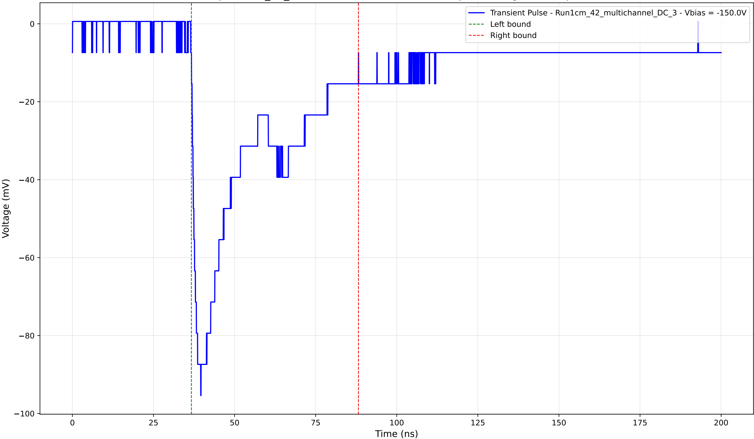
Transient Pulse - Sample: 1cm_42_multichannel - Position: 2705.0 \mu\text{m} - Charge: 36.97 pC - Rise Time: 1.89 ns
