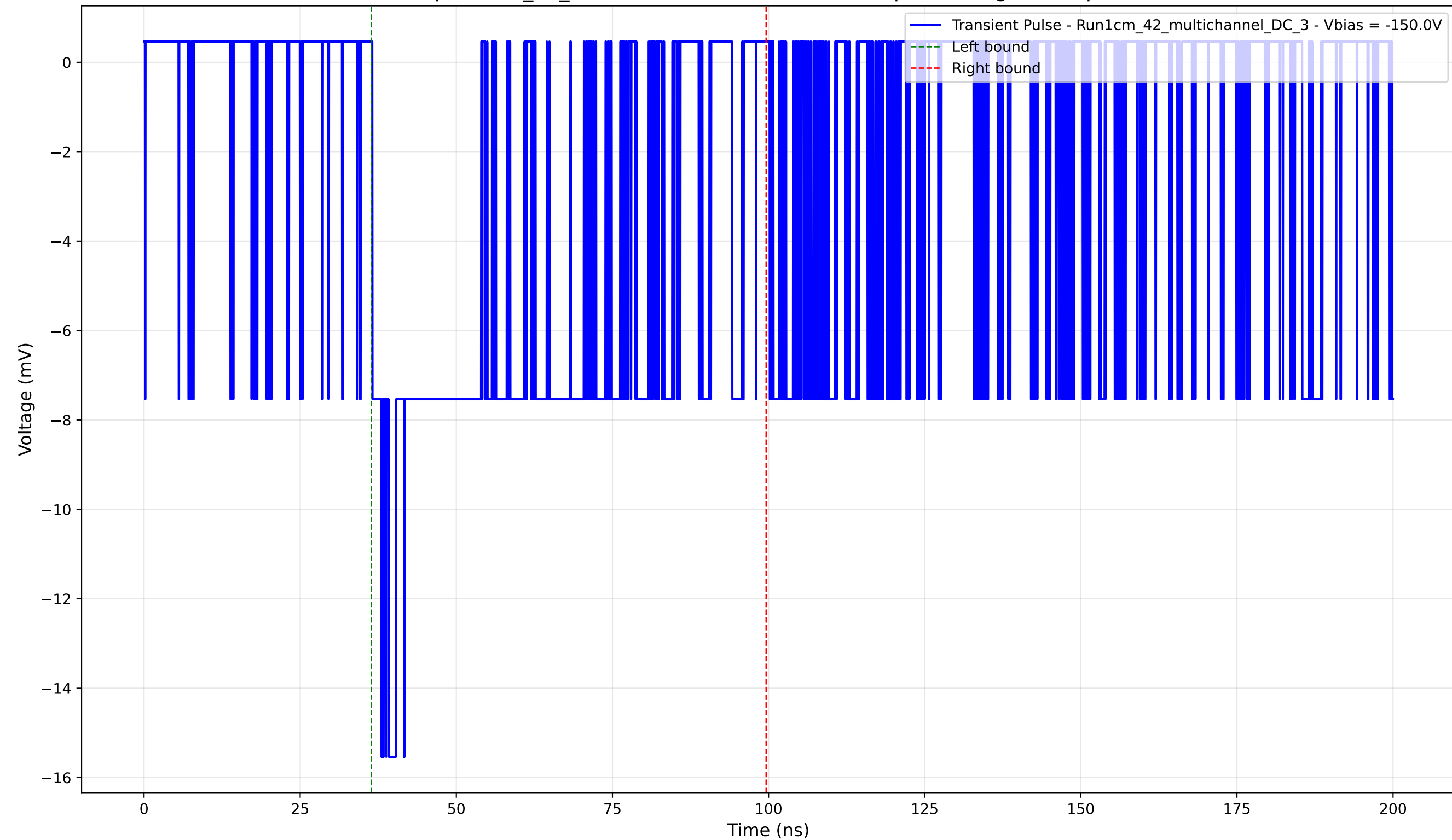
Transient Pulse - Sample: 1cm_42_multichannel - Position: 1375.0 \mu\text{m} - Charge: 6.67 pC - Rise Time: 1.46 ns
