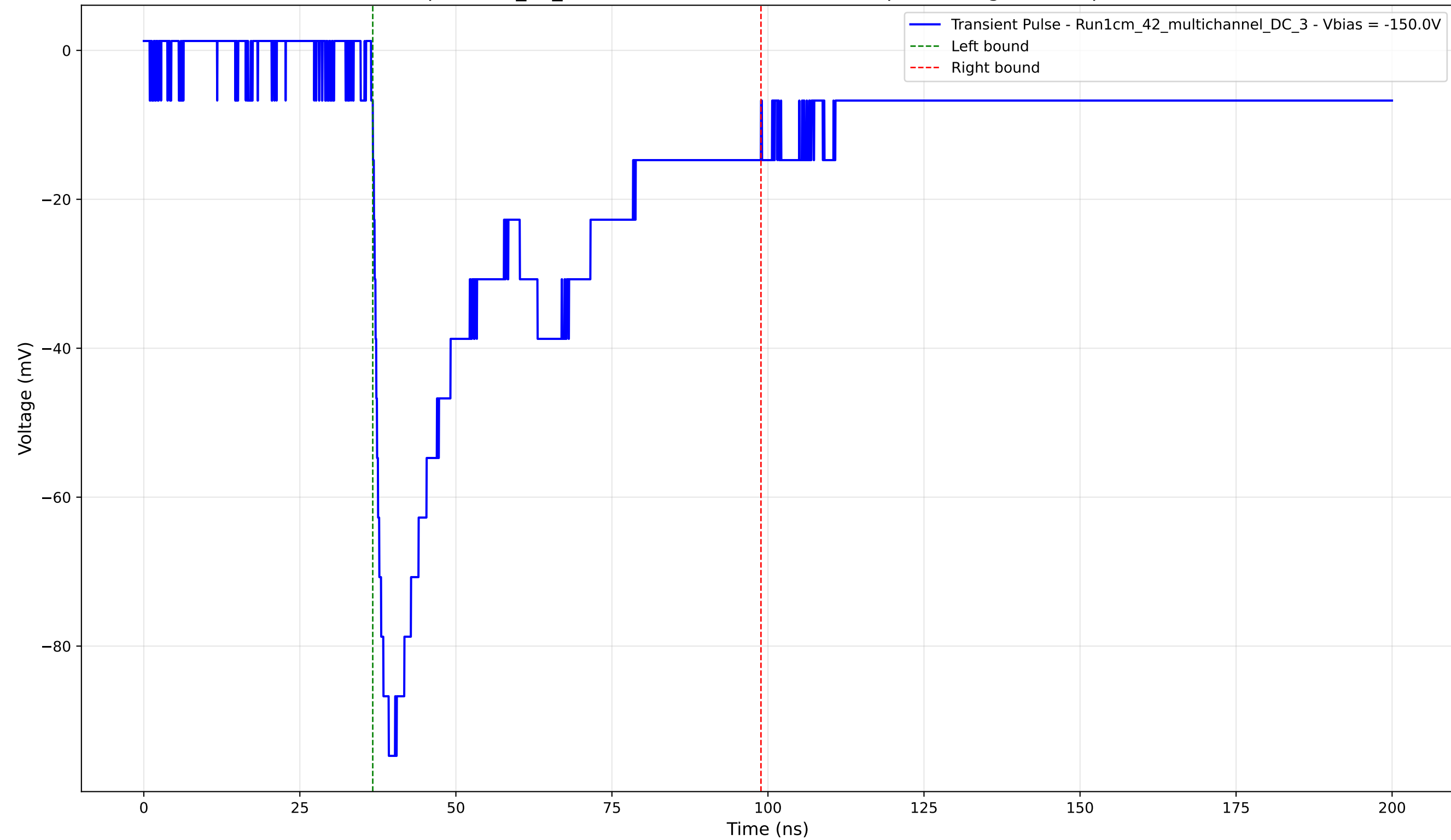
Transient Pulse - Sample: 1cm_42_multichannel - Position: 2065.0 \mu\text{m} - Charge: 40.57 pC - Rise Time: 1.69 ns
