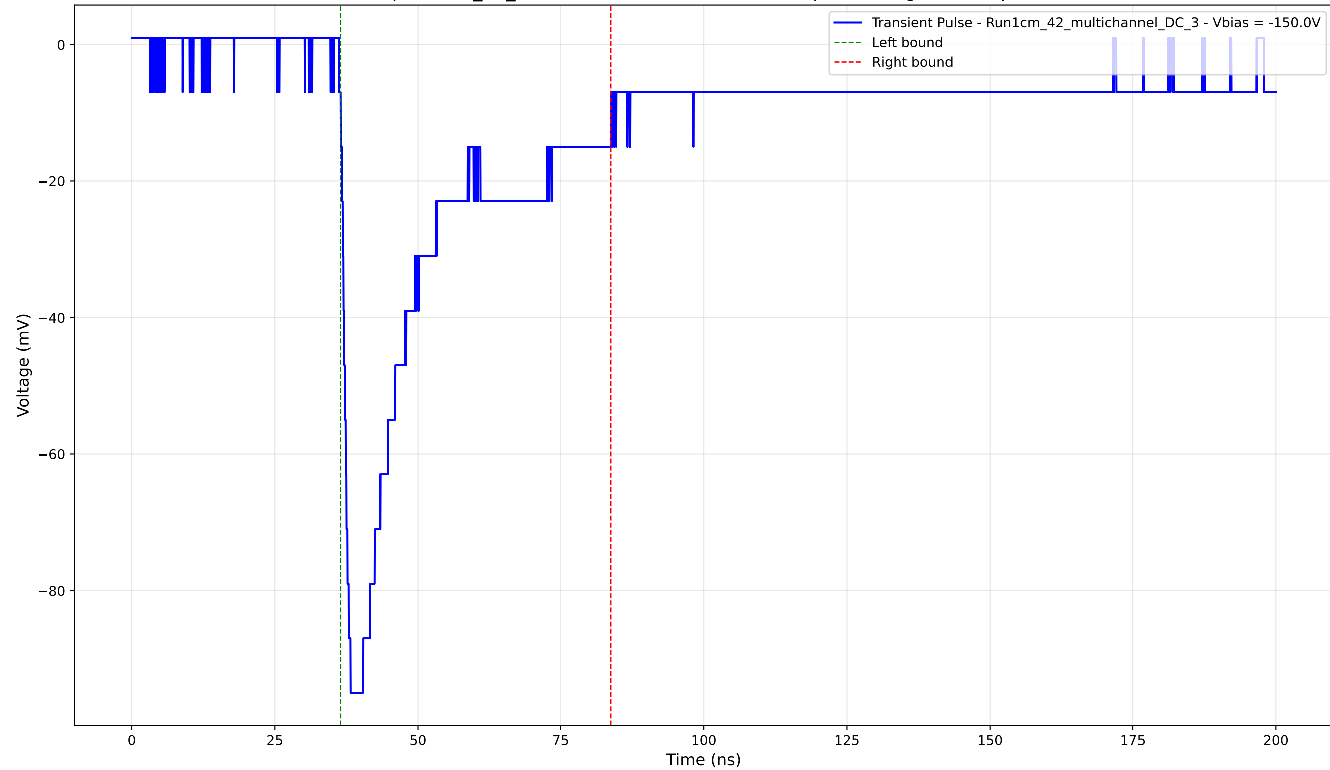
Transient Pulse - Sample: 1cm_42_multichannel - Position: 3315.0 \mu\text{m} - Charge: 31.19 pC - Rise Time: 1.41 ns
