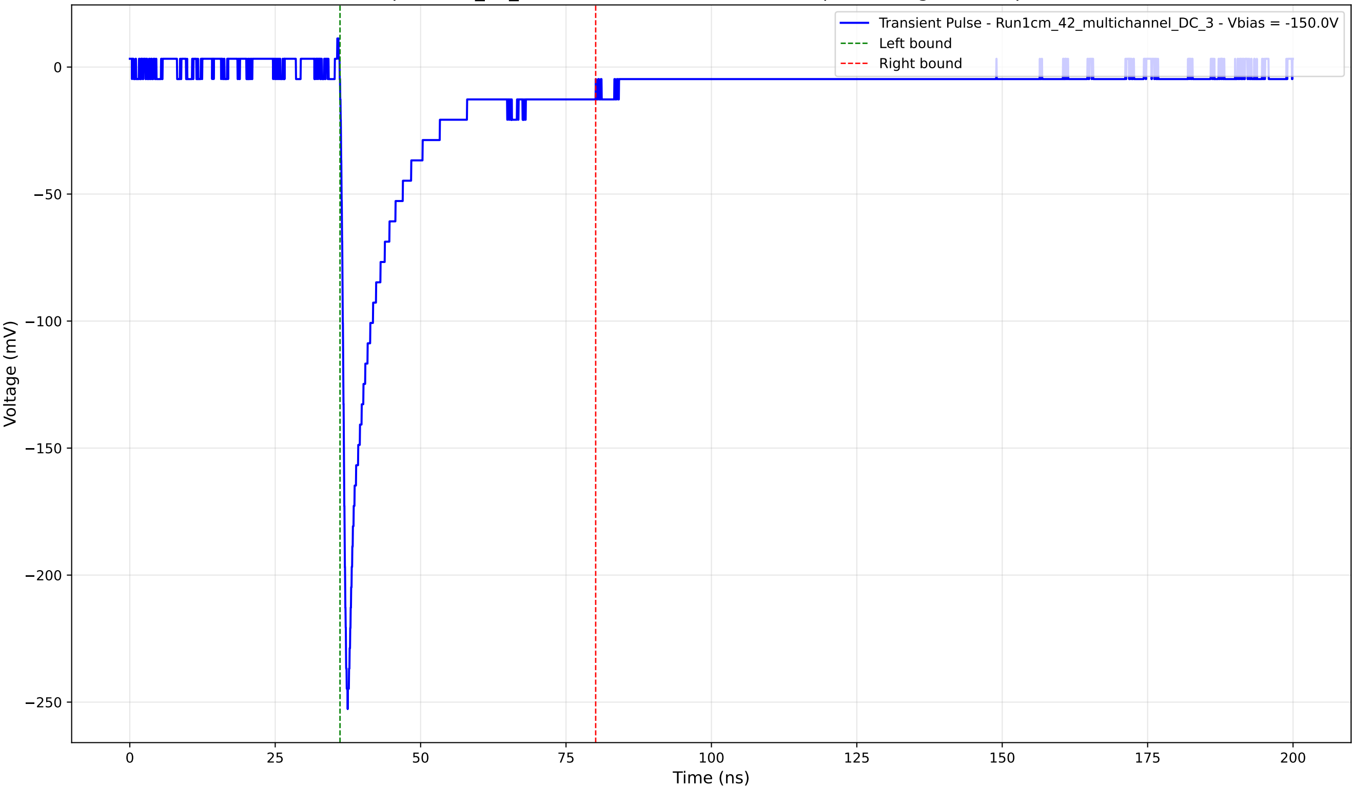
Transient Pulse - Sample: 1cm_42_multichannel - Position: 4490.0 \mu\text{m} - Charge: 36.20 pC - Rise Time: 0.87 ns
