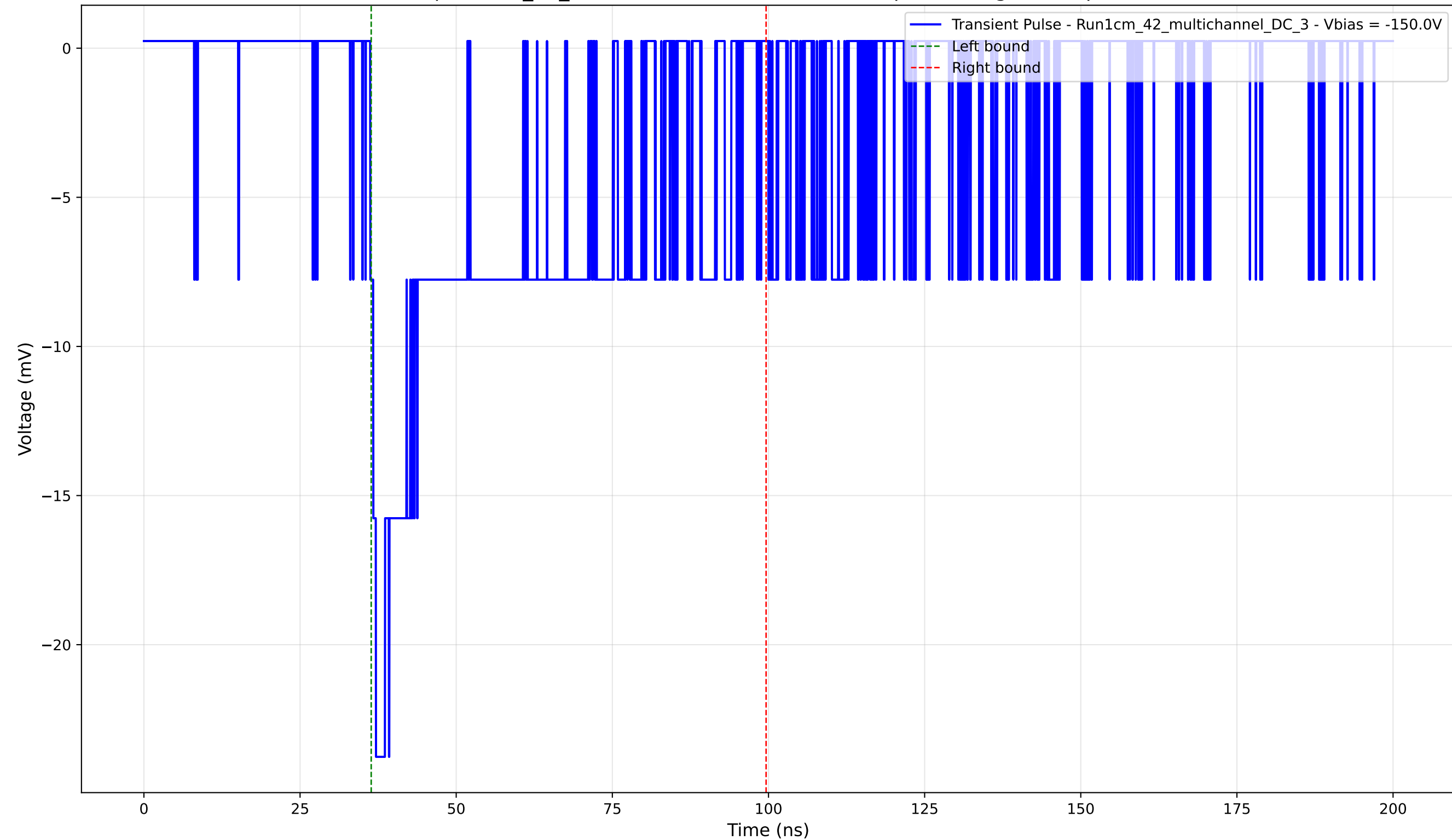
Transient Pulse - Sample: 1cm_42_multichannel - Position: 4365.0 \mu\text{m} - Charge: 8.57 pC - Rise Time: 0.91 ns
