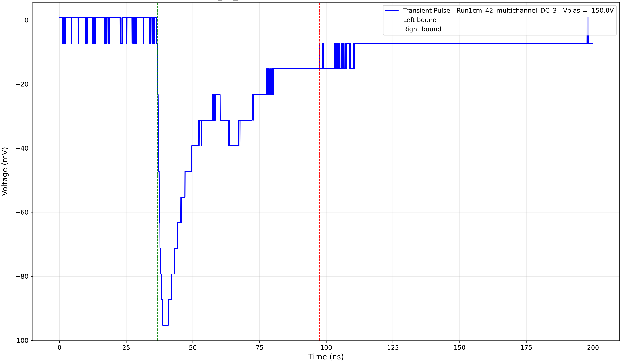
Transient Pulse - Sample: 1cm_42_multichannel - Position: 2025.0 \mu\text{m} - Charge: 41.32 pC - Rise Time: 1.53 ns
