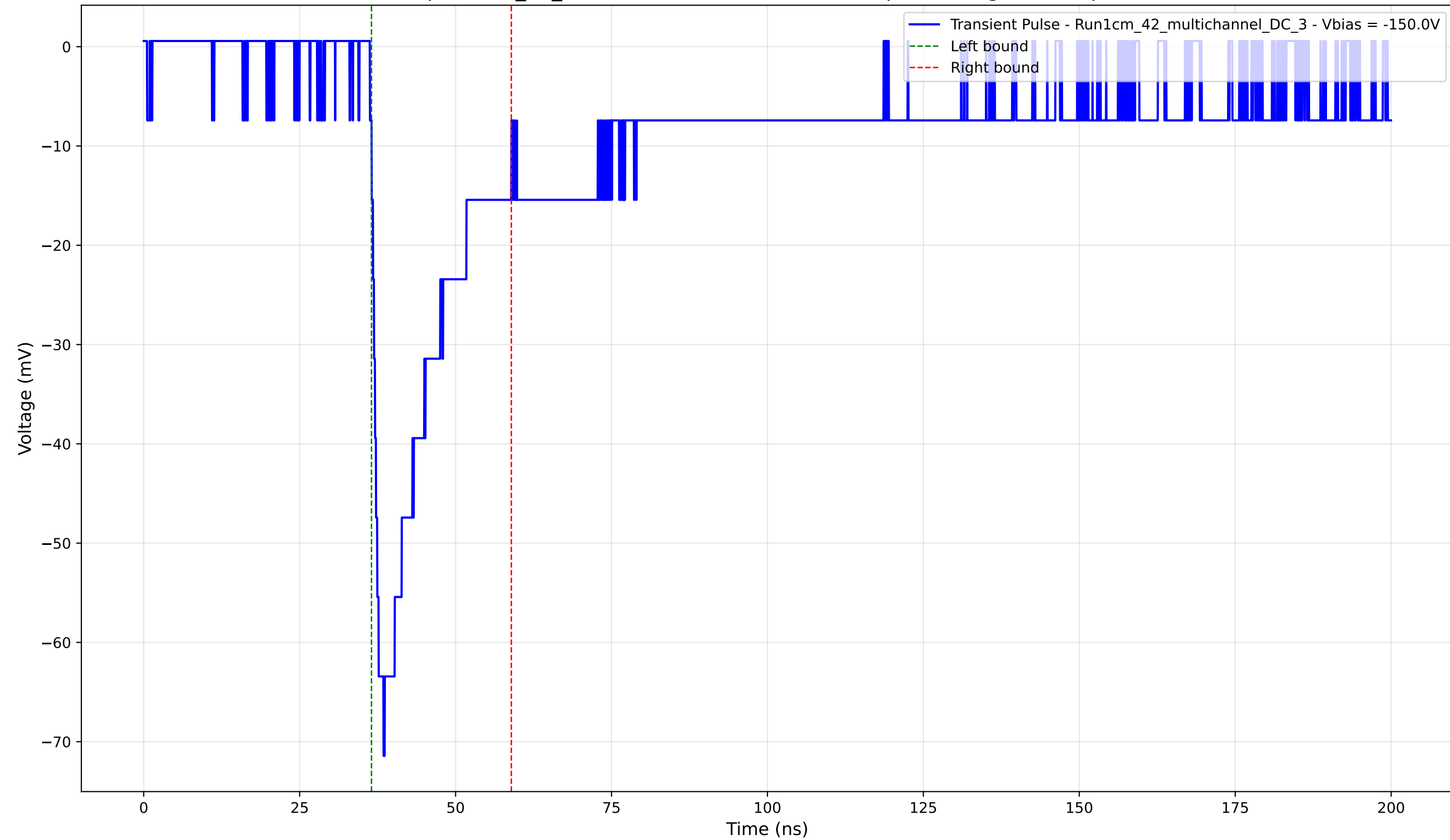
Transient Pulse - Sample: 1cm_42_multichannel - Position: 1315.0 \mu\text{m} - Charge: 14.34 pC - Rise Time: 2.18 ns
