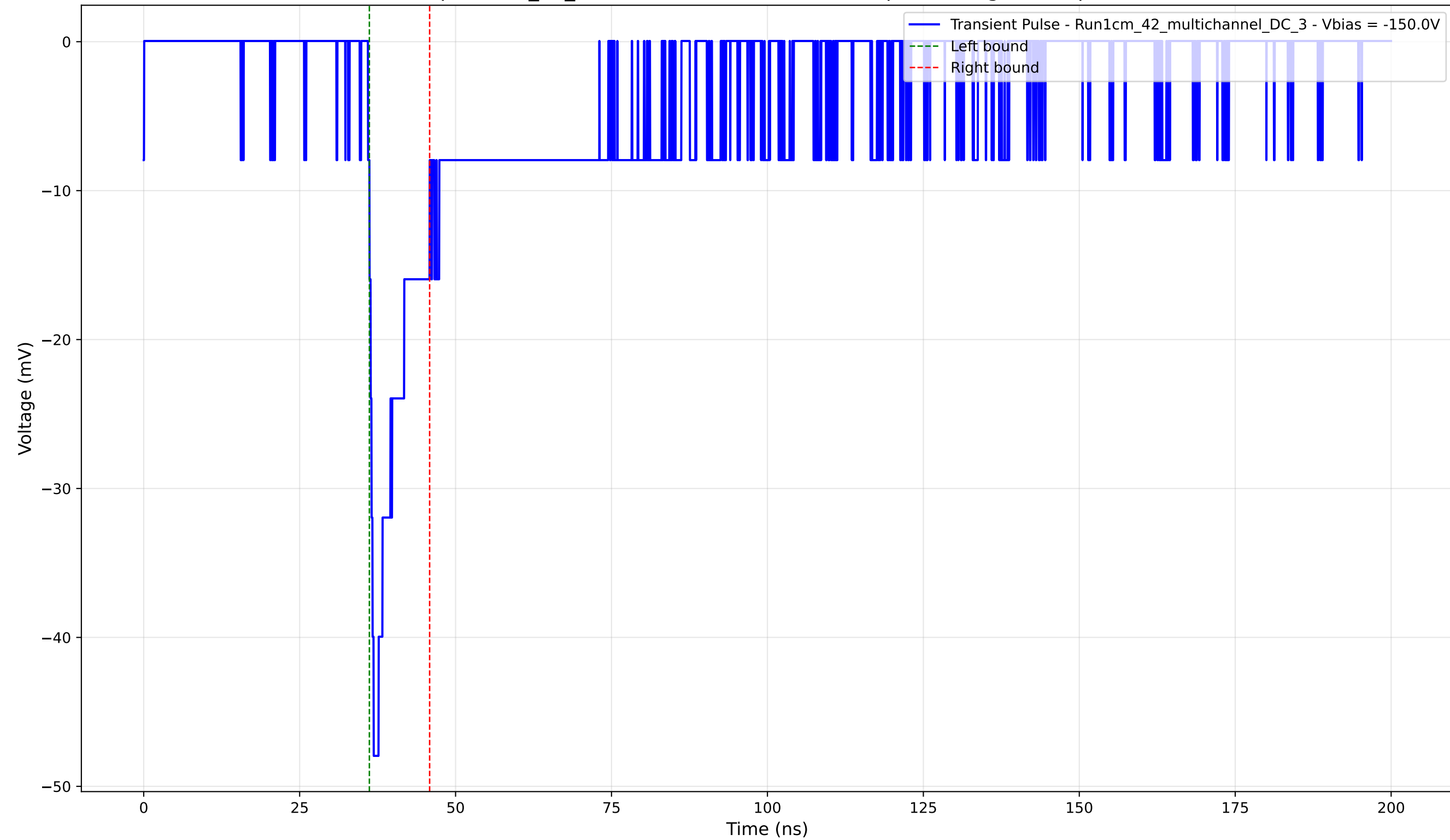
Transient Pulse - Sample: 1cm_42_multichannel - Position: 320.0 \mu\text{m} - Charge: 4.83 pC - Rise Time: 0.91 ns
