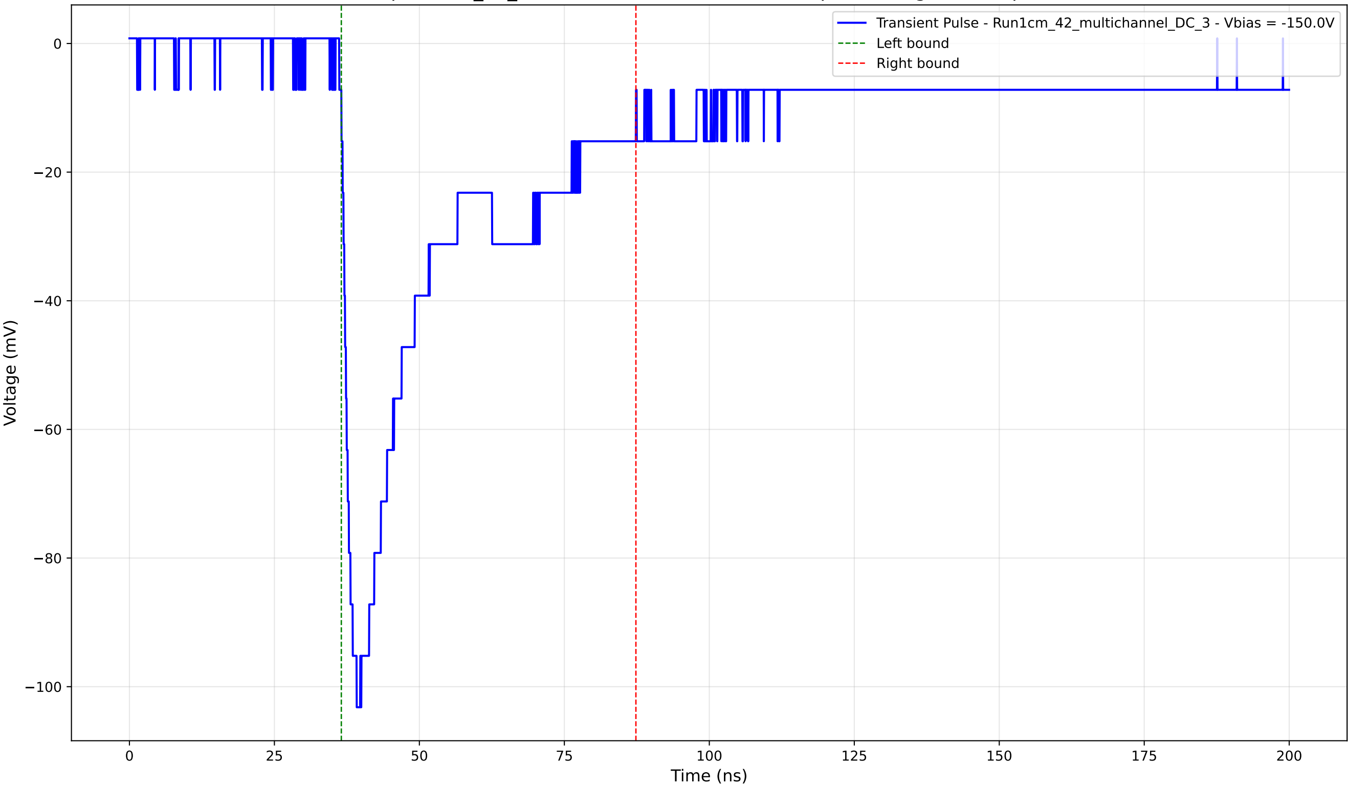
Transient Pulse - Sample: 1cm_42_multichannel - Position: 2975.0 \mu\text{m} - Charge: 36.52 pC - Rise Time: 1.95 ns
