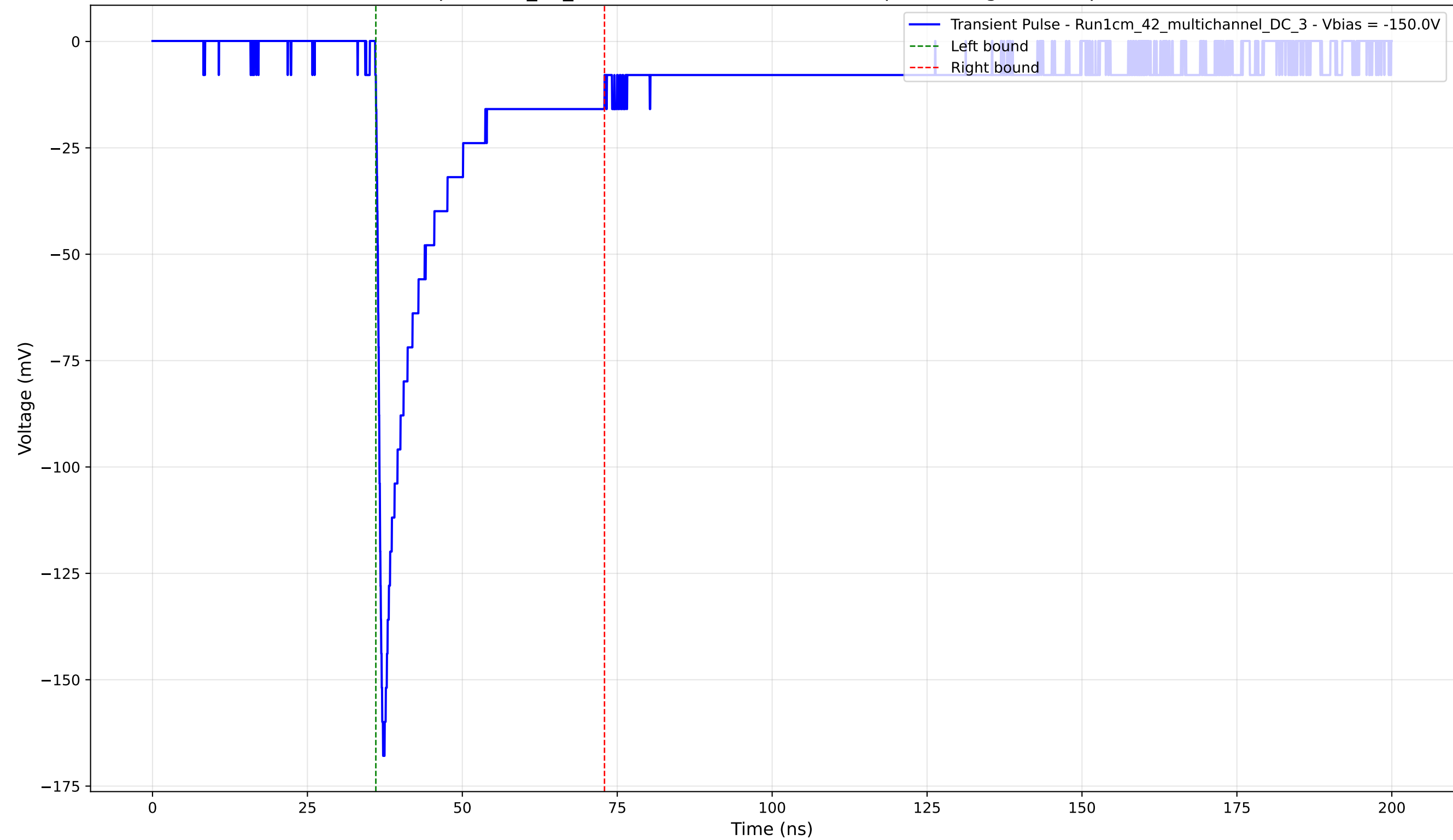
Transient Pulse - Sample: 1cm_42_multichannel - Position: 405.0 \mu\text{m} - Charge: 27.16 pC - Rise Time: 0.86 ns
