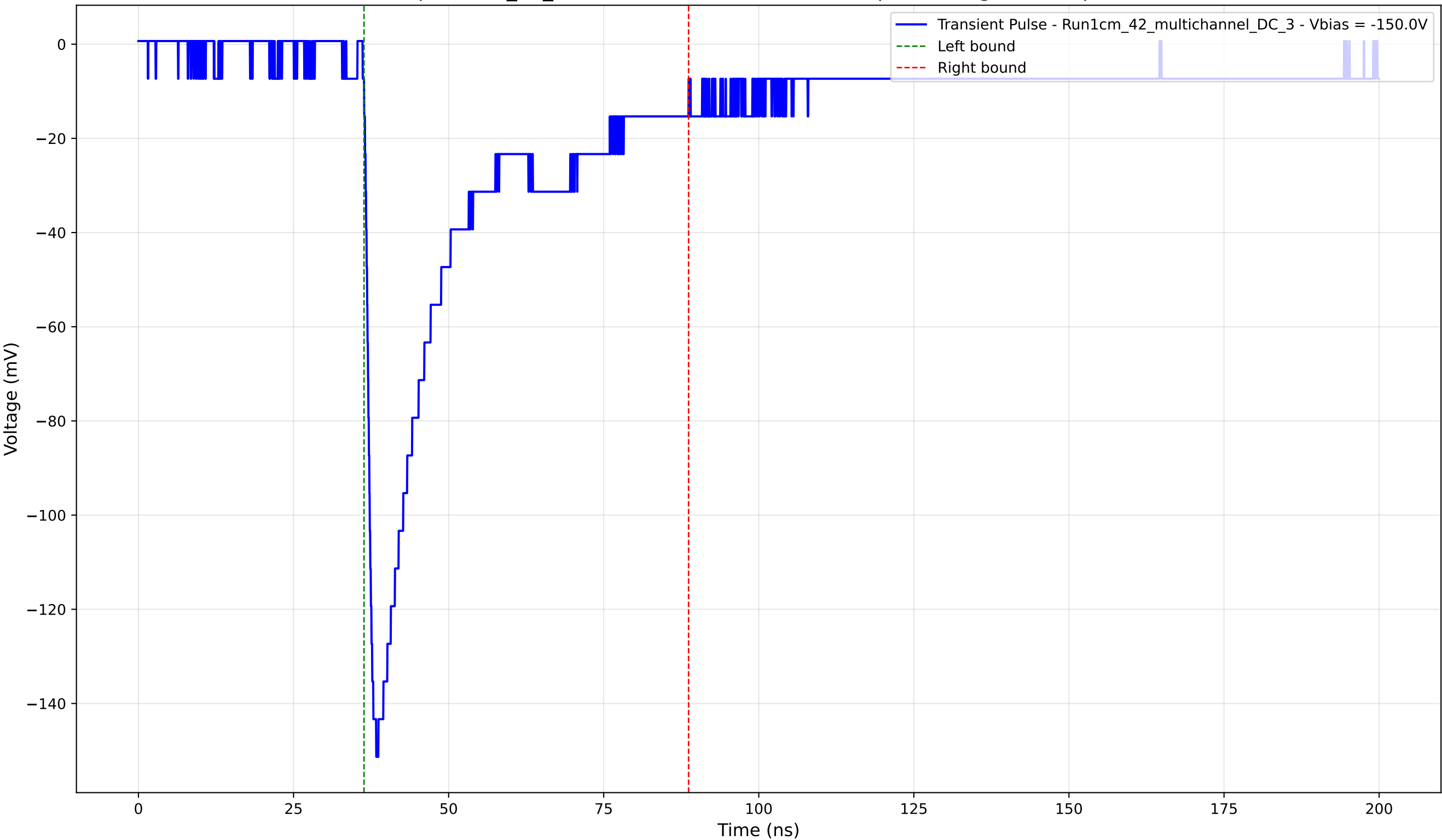
Transient Pulse - Sample: 1cm_42_multichannel - Position: 1270.0 \mu\text{m} - Charge: 43.60 pC - Rise Time: 1.48 ns
