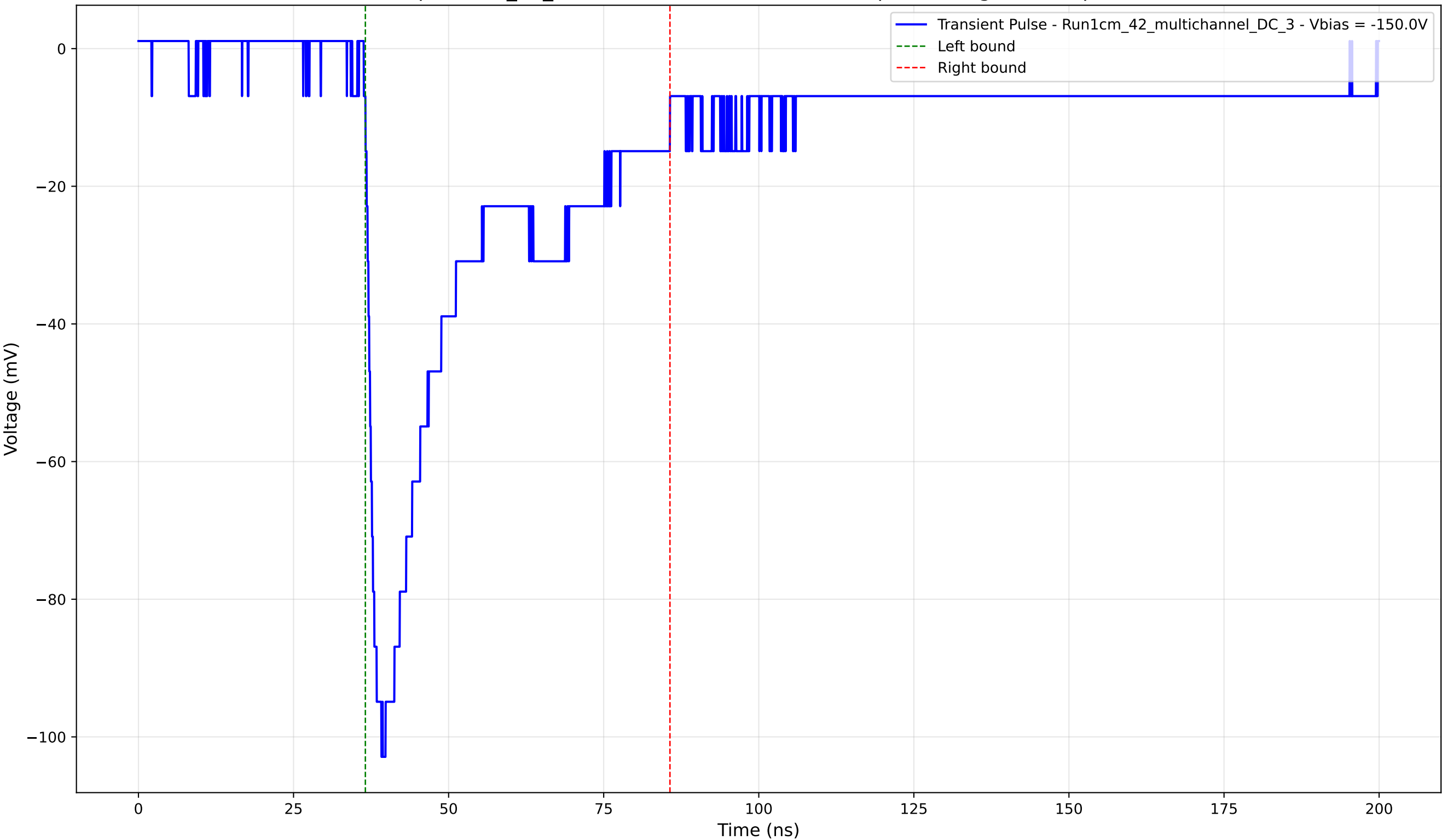
Transient Pulse - Sample: 1cm_42_multichannel - Position: 3050.0 \mu\text{m} - Charge: 34.80 pC - Rise Time: 1.81 ns
