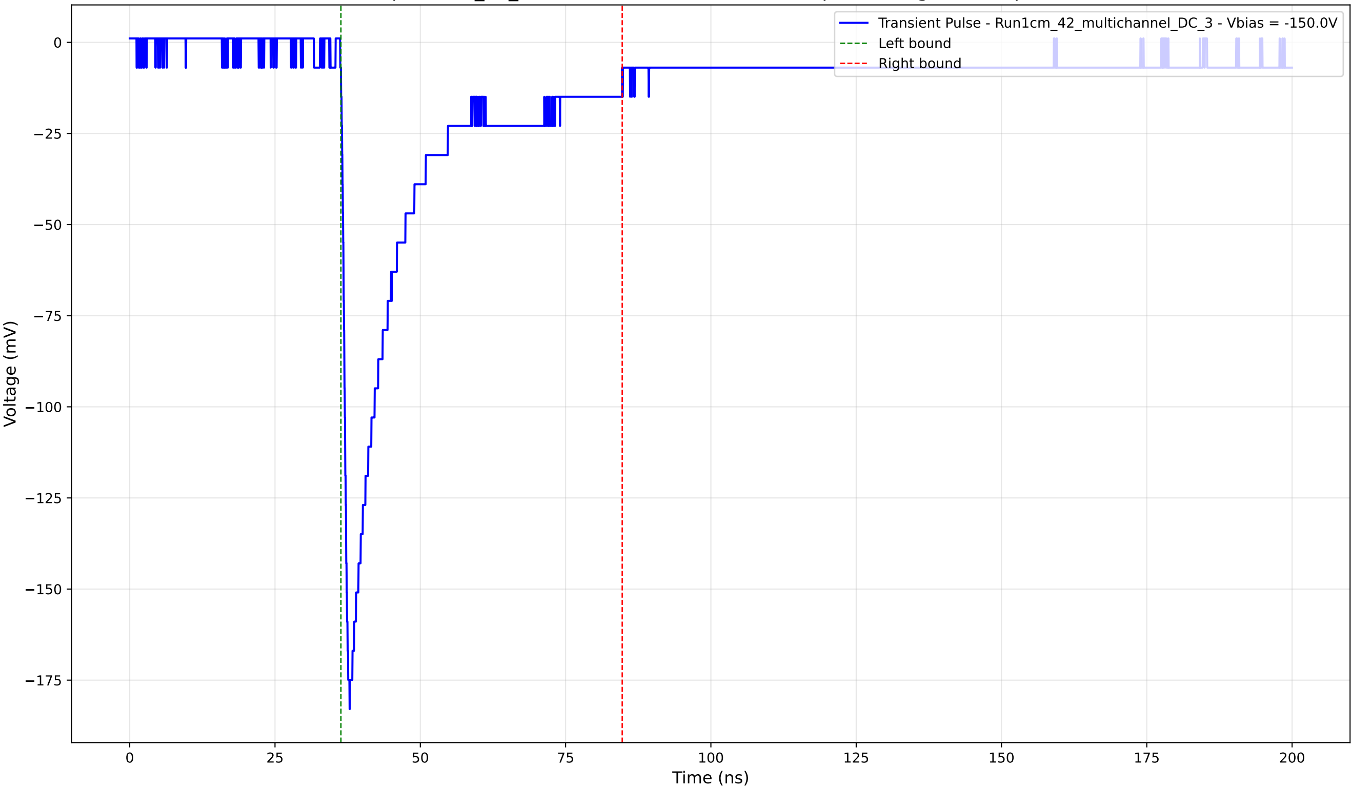
Transient Pulse - Sample: 1cm_42_multichannel - Position: 4095.0 \mu\text{m} - Charge: 39.35 pC - Rise Time: 1.03 ns
