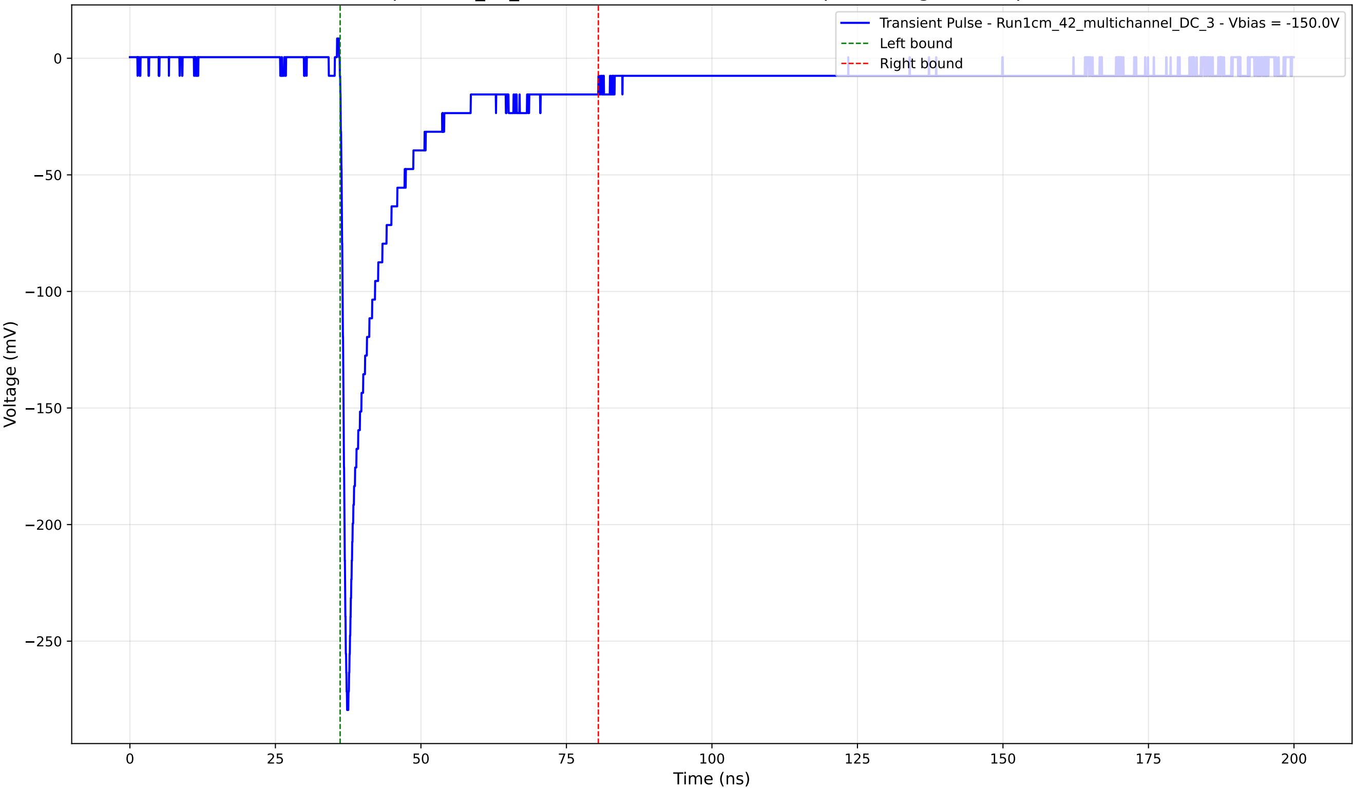
Transient Pulse - Sample: 1cm_42_multichannel - Position: 4540.0 \mu\text{m} - Charge: 40.95 pC - Rise Time: 0.87 ns
