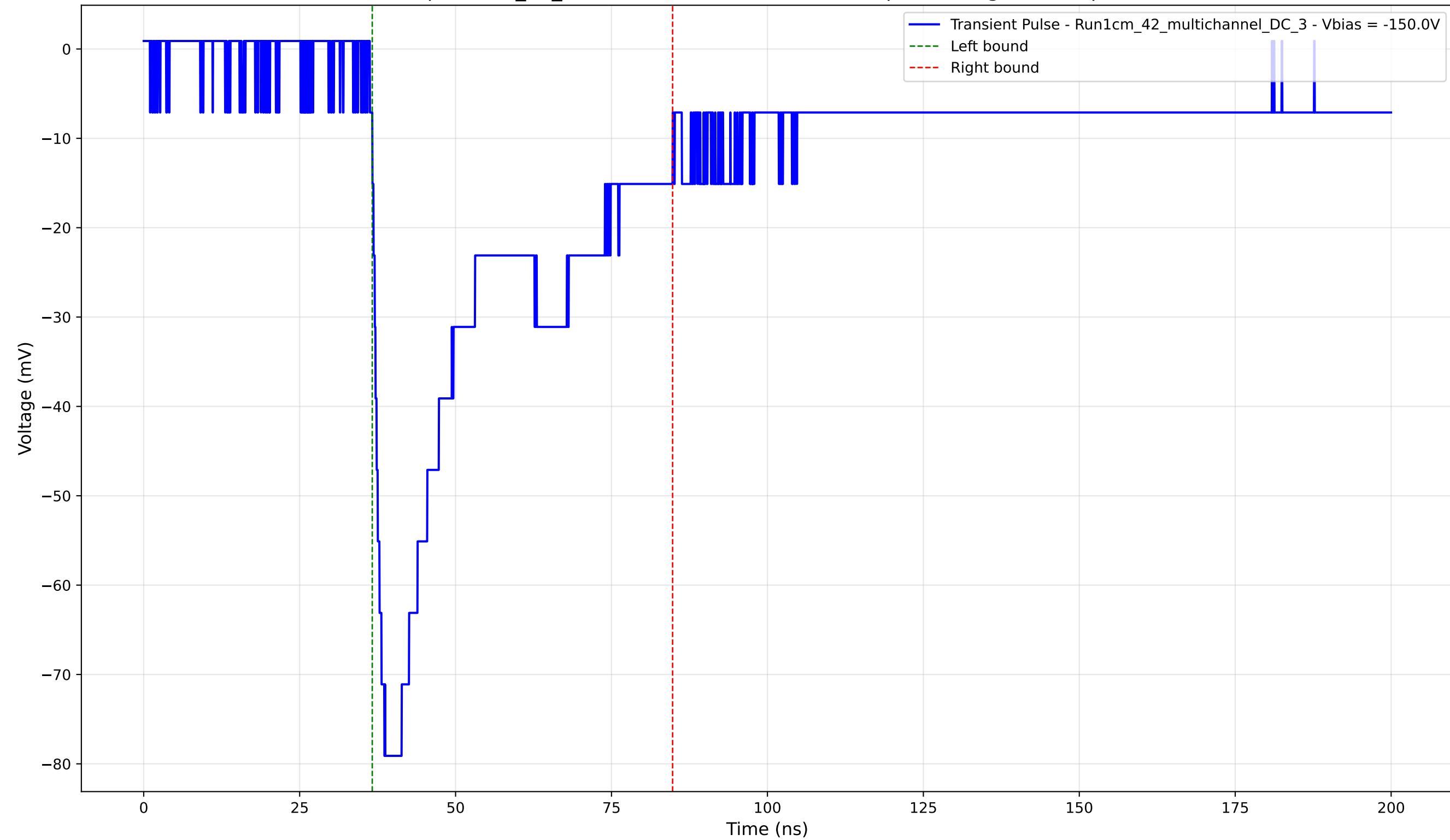
Transient Pulse - Sample: 1cm_42_multichannel - Position: 2805.0 \mu\text{m} - Charge: 30.98 pC - Rise Time: 1.94 ns
