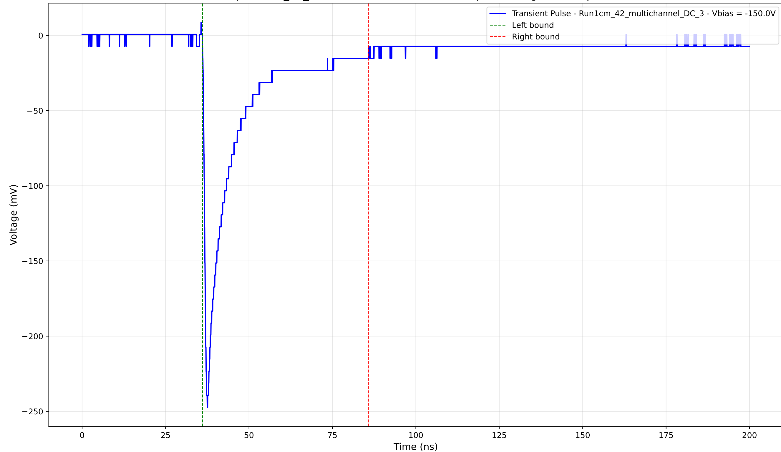
Transient Pulse - Sample: 1cm_42_multichannel - Position: 610.0 \mu\text{m} - Charge: 47.84 pC - Rise Time: 0.92 ns
