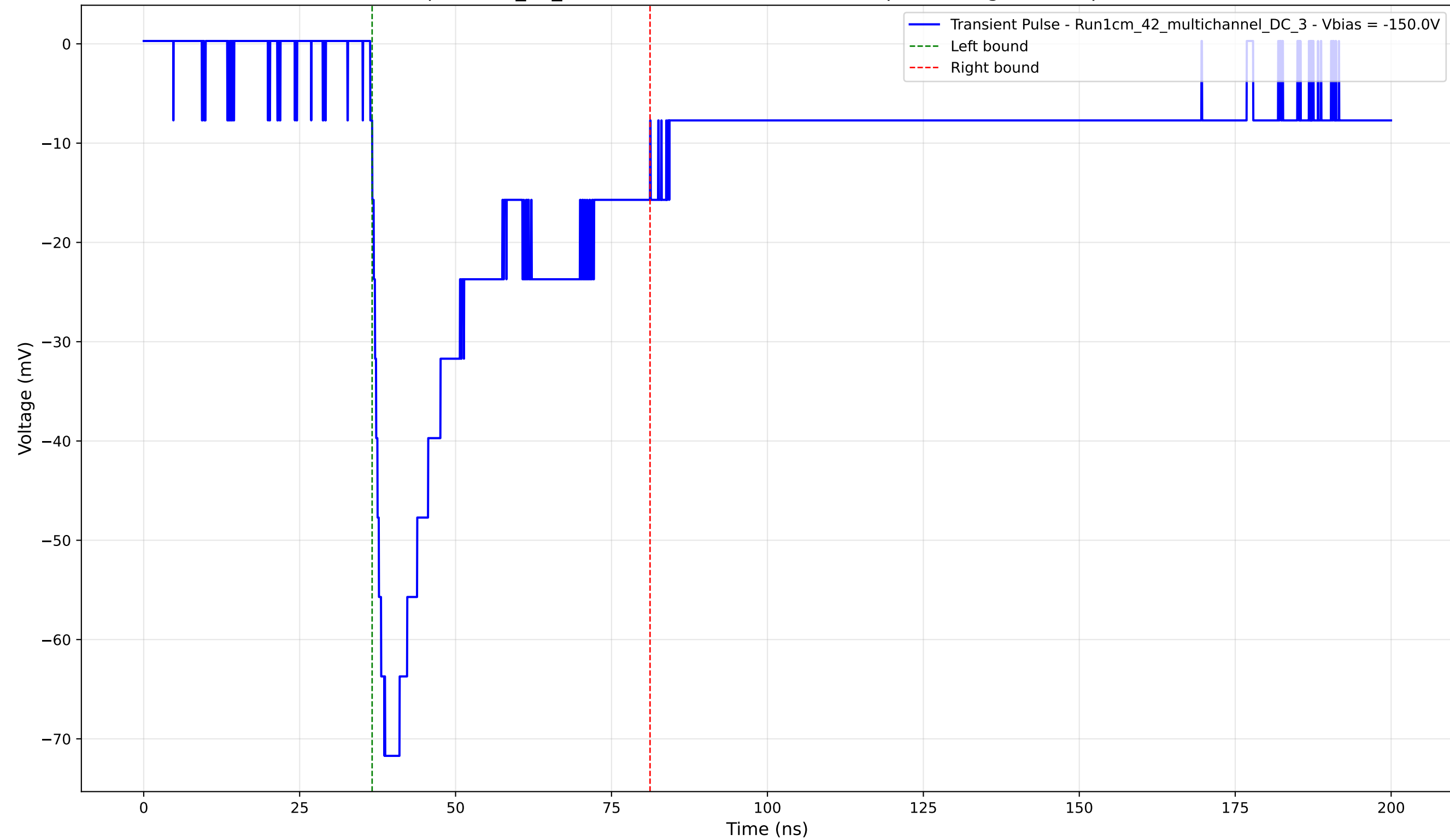
Transient Pulse - Sample: 1cm_42_multichannel - Position: 2940.0 \mu\text{m} - Charge: 26.14 pC - Rise Time: 2.26 ns
