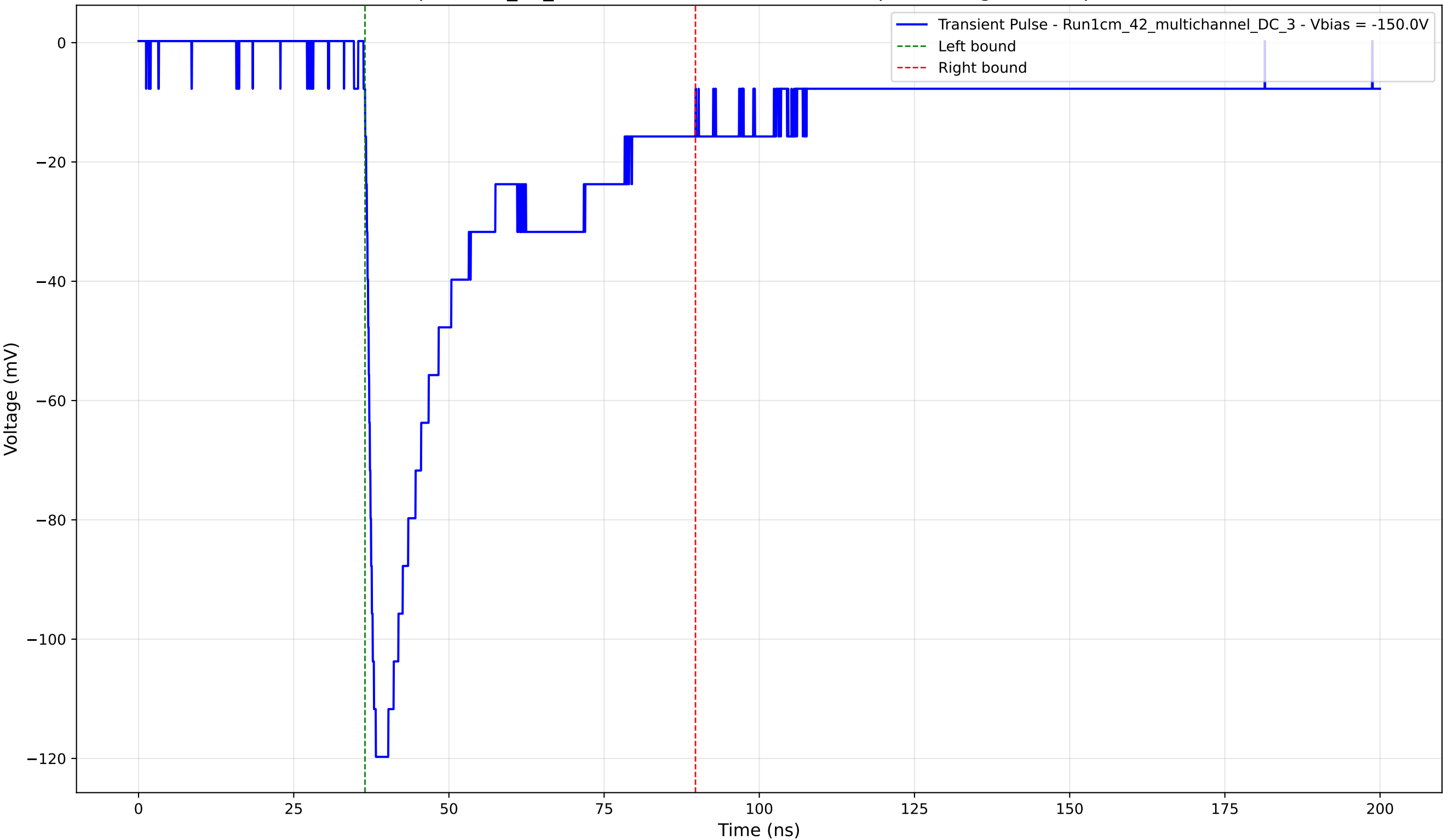
Transient Pulse - Sample: 1cm_42_multichannel - Position: 1600.0 \mu\text{m} - Charge: 42.24 pC - Rise Time: 1.43 ns
