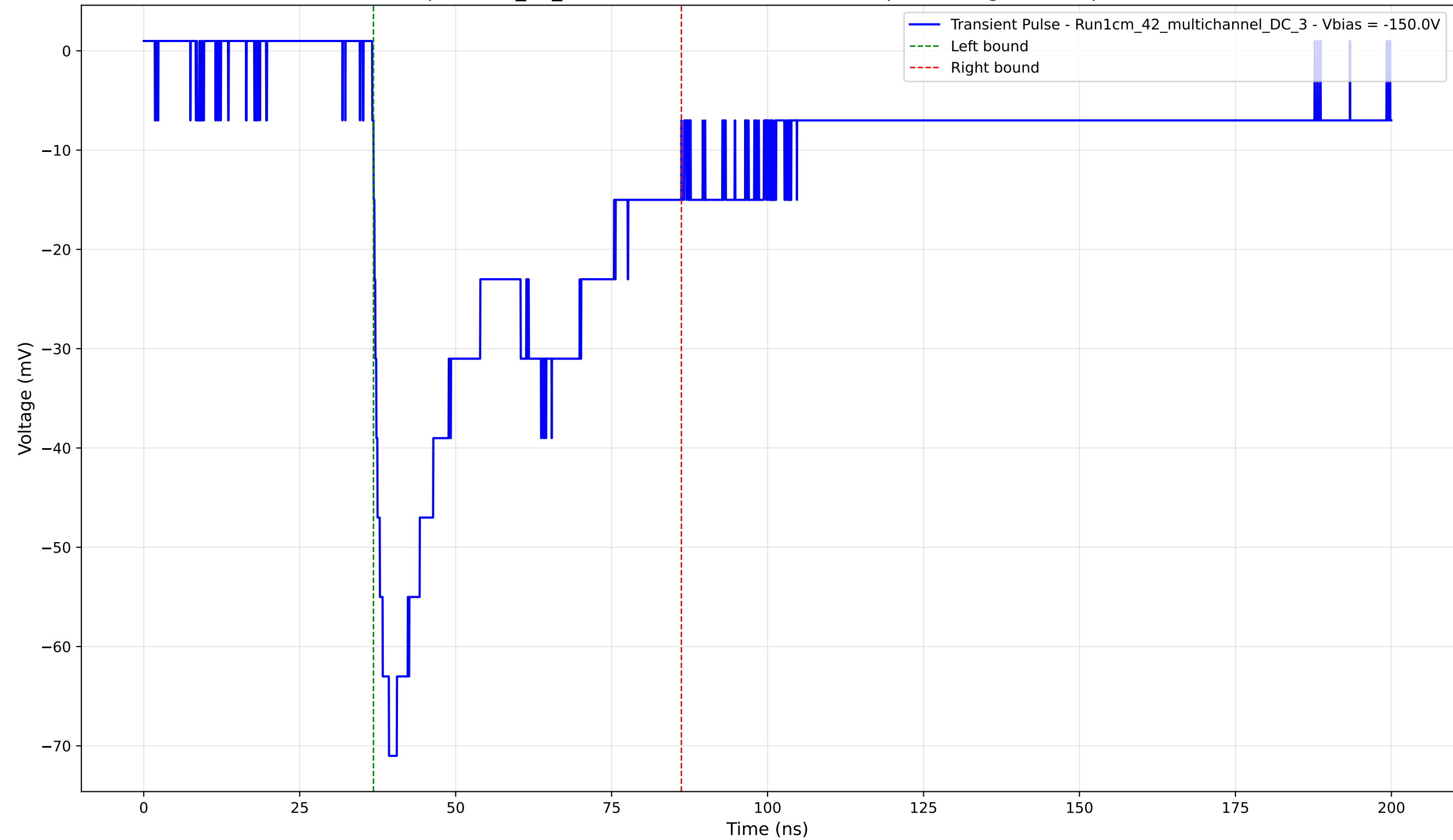
Transient Pulse - Sample: 1cm_42_multichannel - Position: 2305.0 \mu\text{m} - Charge: 30.42 pC - Rise Time: 2.48 ns
