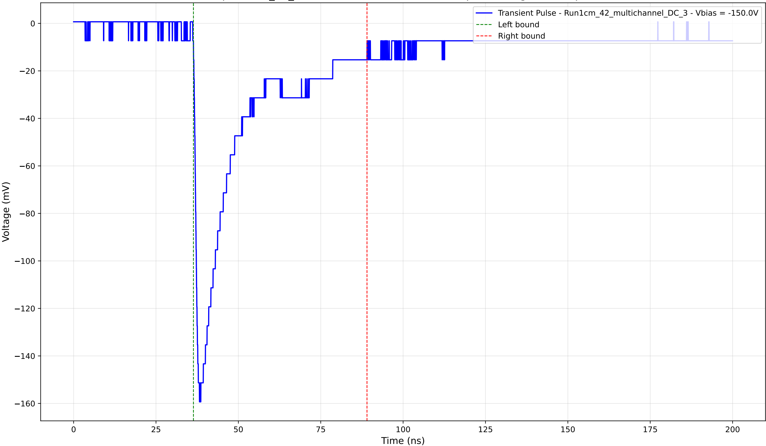
Transient Pulse - Sample: 1cm_42_multichannel - Position: 1235.0 \mu\text{m} - Charge: 45.55 pC - Rise Time: 1.36 ns
