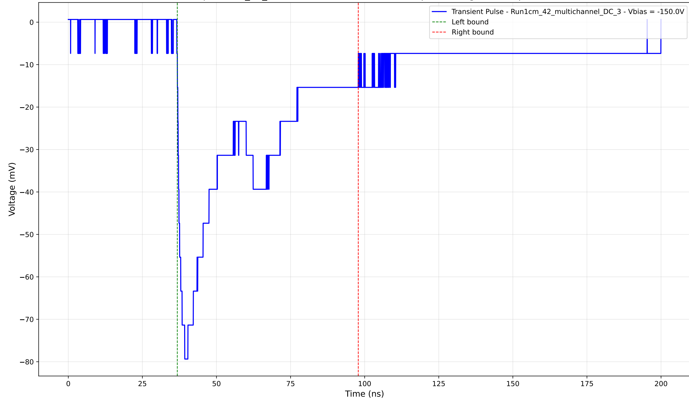
Transient Pulse - Sample: 1cm_42_multichannel - Position: 2295.0 \mu\text{m} - Charge: 37.48 pC - Rise Time: 2.50 ns
