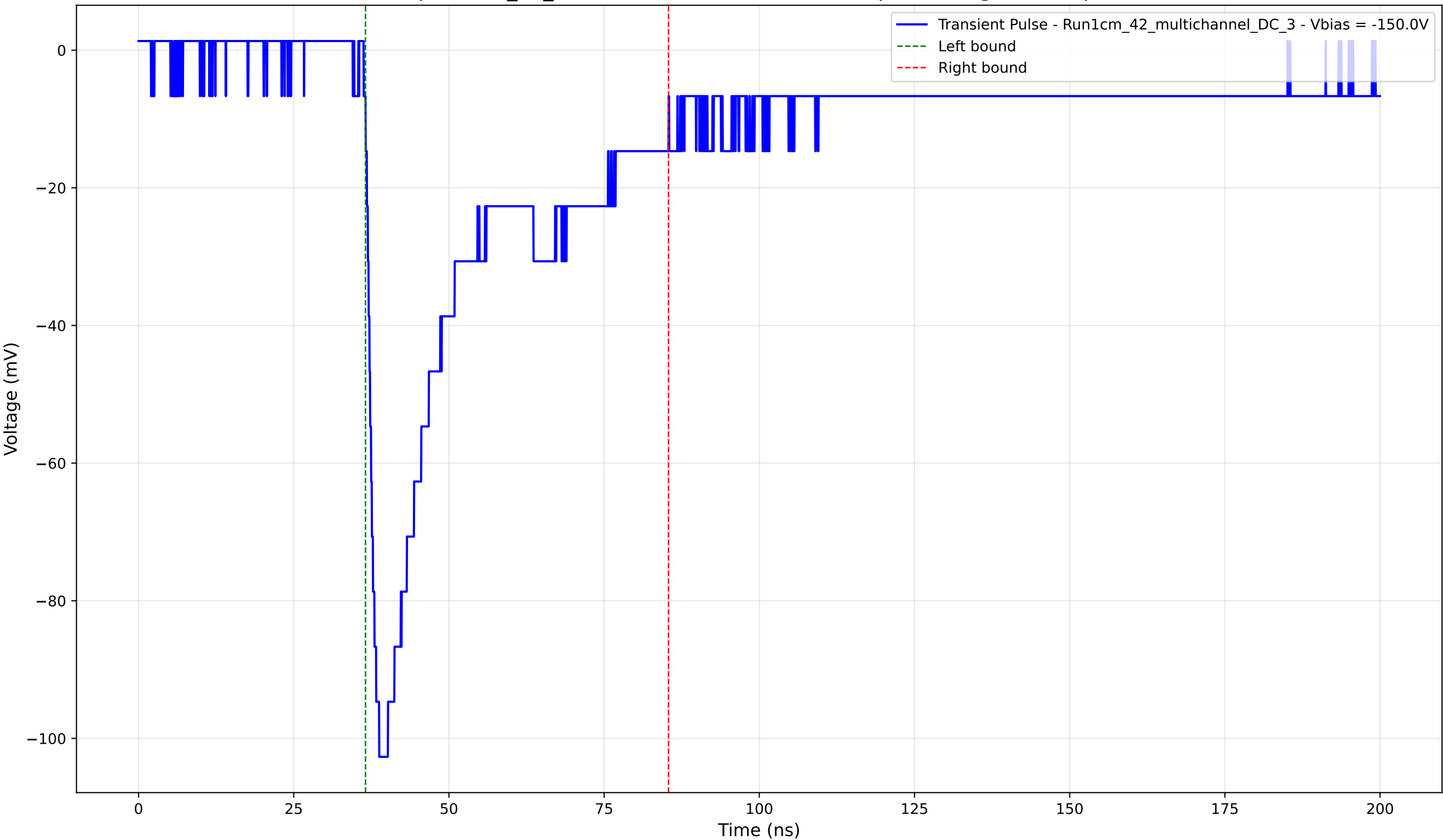
Transient Pulse - Sample: 1cm_42_multichannel - Position: 3125.0 \mu\text{m} - Charge: 34.55 pC - Rise Time: 1.71 ns
