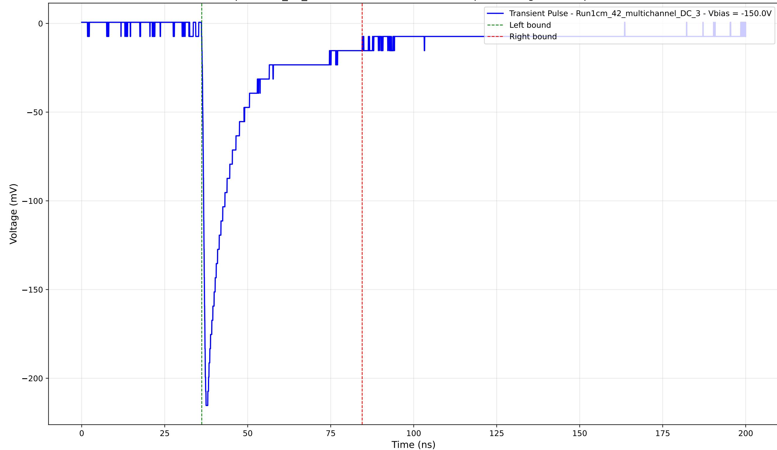
Transient Pulse - Sample: 1cm_42_multichannel - Position: 720.0 \mu\text{m} - Charge: 45.69 pC - Rise Time: 0.98 ns
