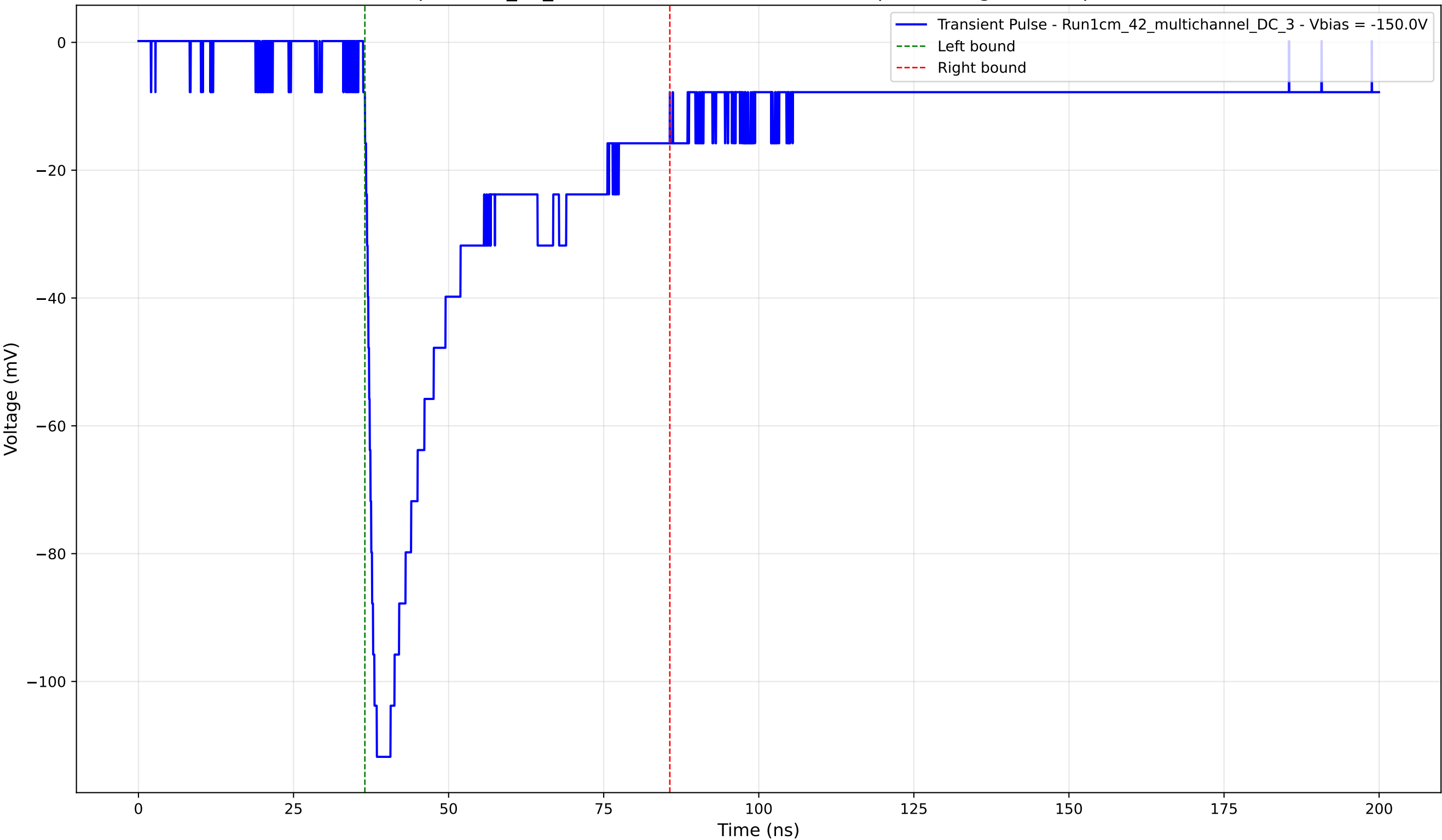
Transient Pulse - Sample: 1cm_42_multichannel - Position: 3270.0 \mu\text{m} - Charge: 37.66 pC - Rise Time: 1.53 ns
