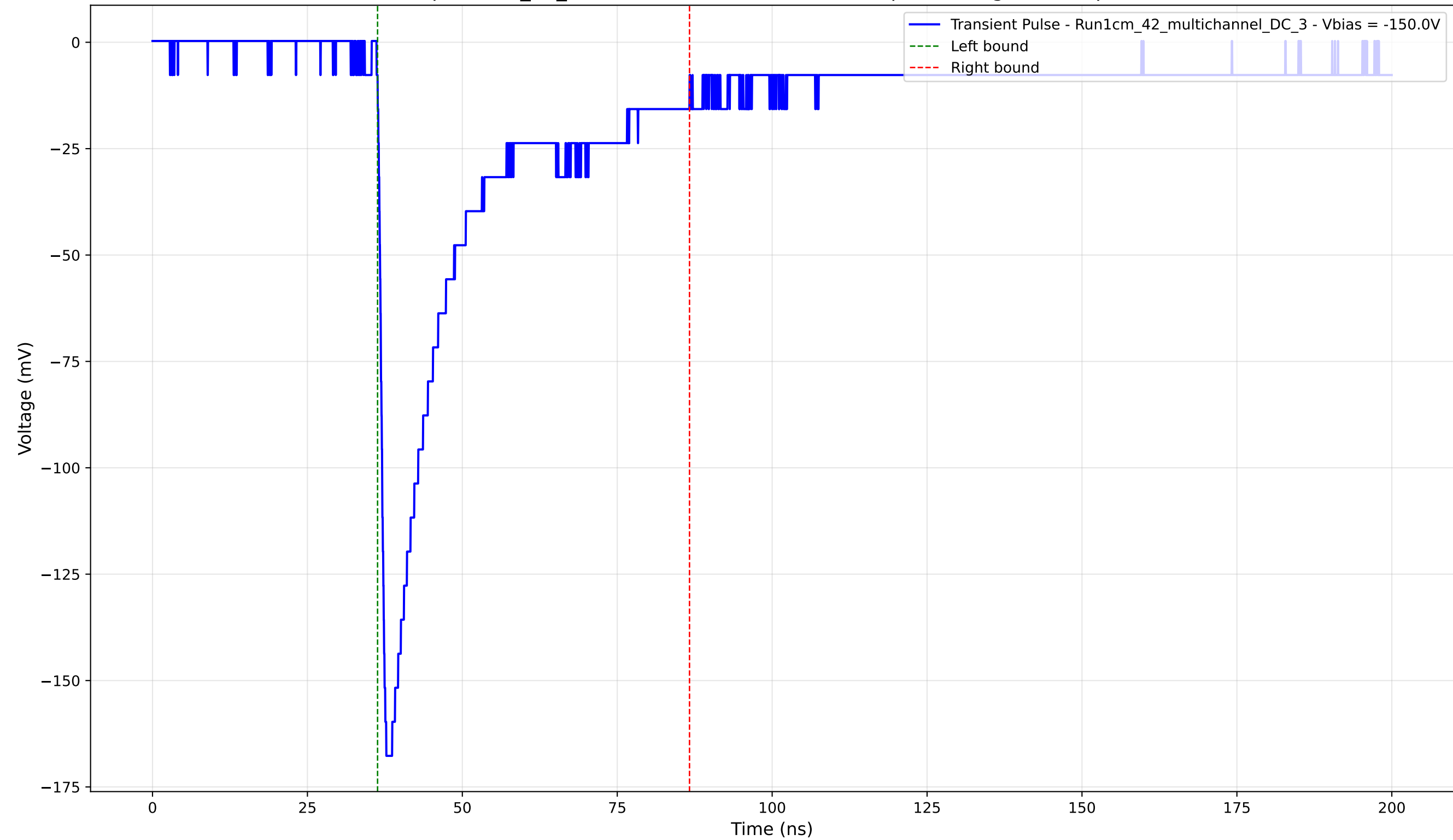
Transient Pulse - Sample: 1cm_42_multichannel - Position: 1035.0 \mu\text{m} - Charge: 44.48 pC - Rise Time: 1.02 ns
