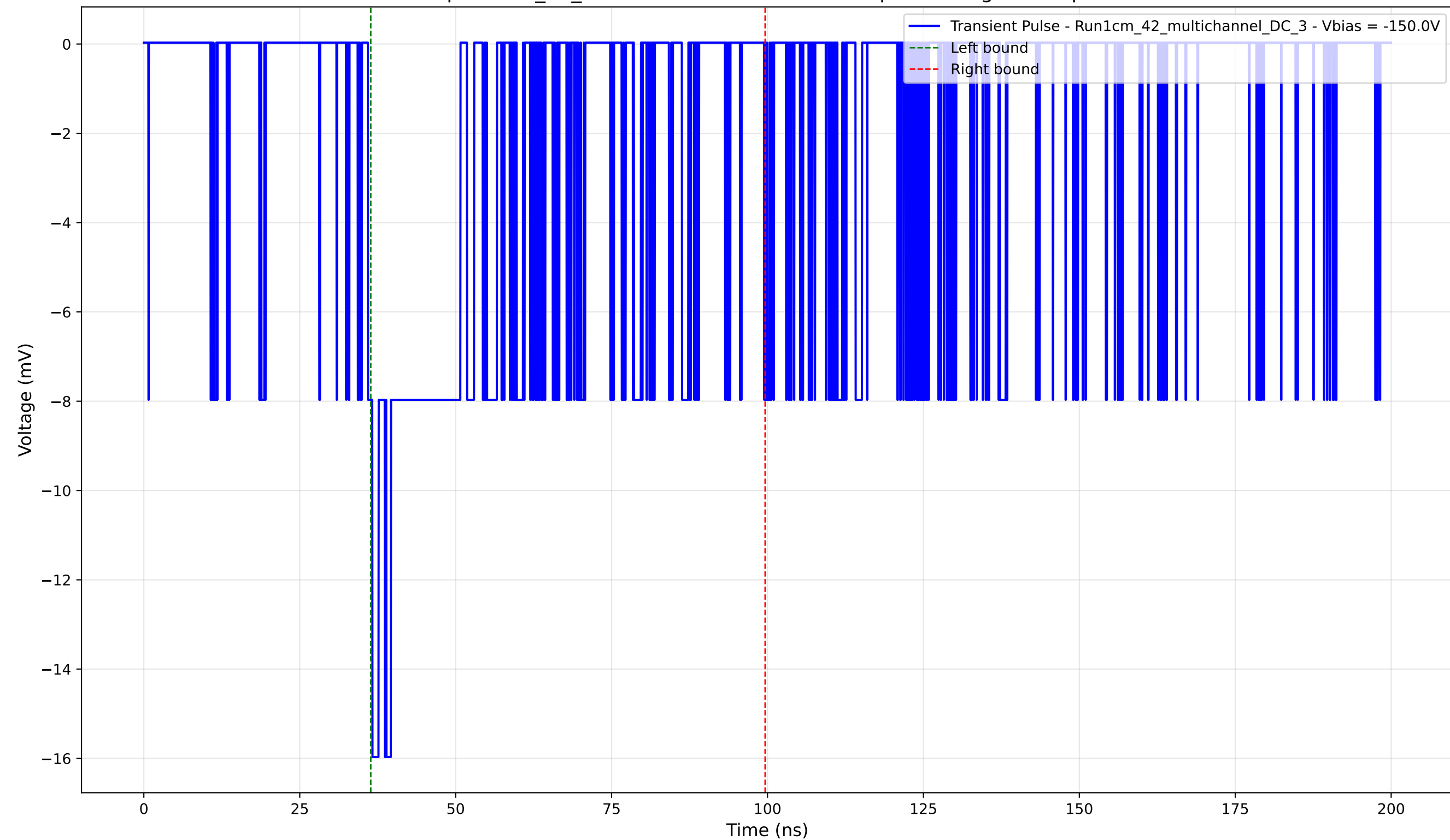
Transient Pulse - Sample: 1cm_42_multichannel - Position: 35.0 \mu\text{m} - Charge: 4.73 pC - Rise Time: 0.72 ns
