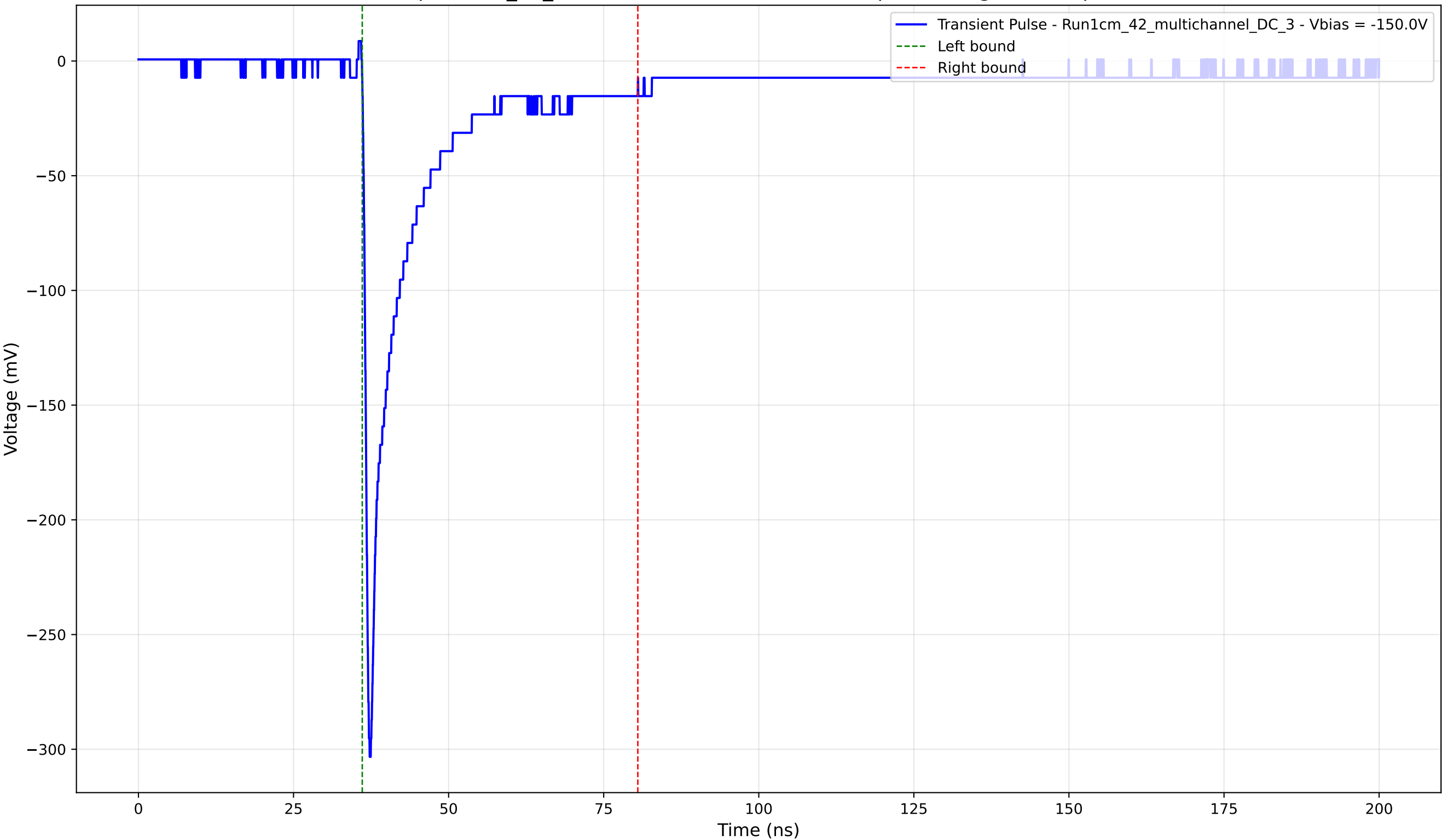
Transient Pulse - Sample: 1cm_42_multichannel - Position: 4605.0 \mu\text{m} - Charge: 41.69 pC - Rise Time: 0.86 ns
