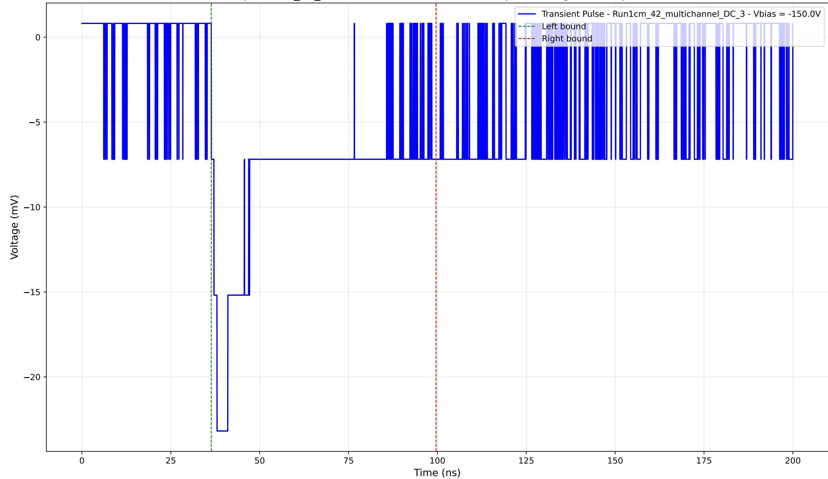
Transient Pulse - Sample: 1cm_42_multichannel - Position: 3355.0 \mu\text{m} - Charge: 10.56 pC - Rise Time: 1.62 ns
