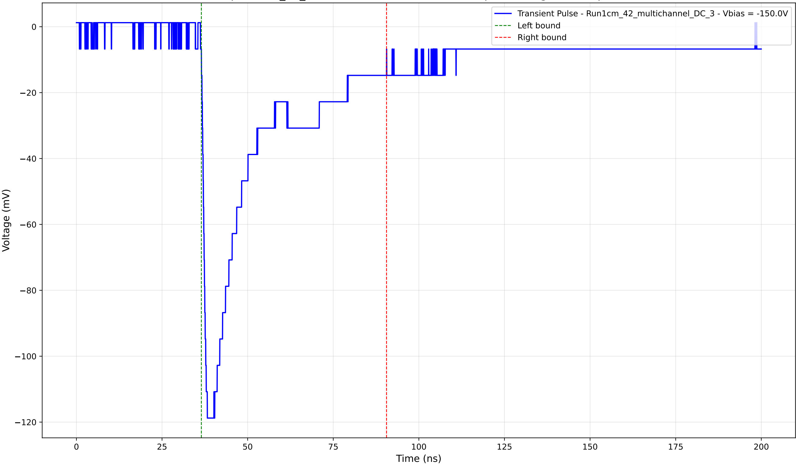
Transient Pulse - Sample: 1cm_42_multichannel - Position: 1610.0 \mu\text{m} - Charge: 41.37 pC - Rise Time: 1.41 ns
