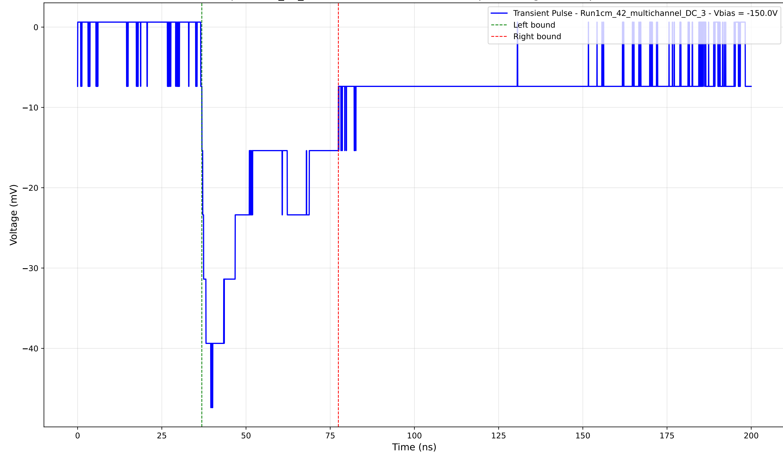
Transient Pulse - Sample: 1cm_42_multichannel - Position: 2425.0 \mu\text{m} - Charge: 18.20 pC - Rise Time: 2.99 ns
