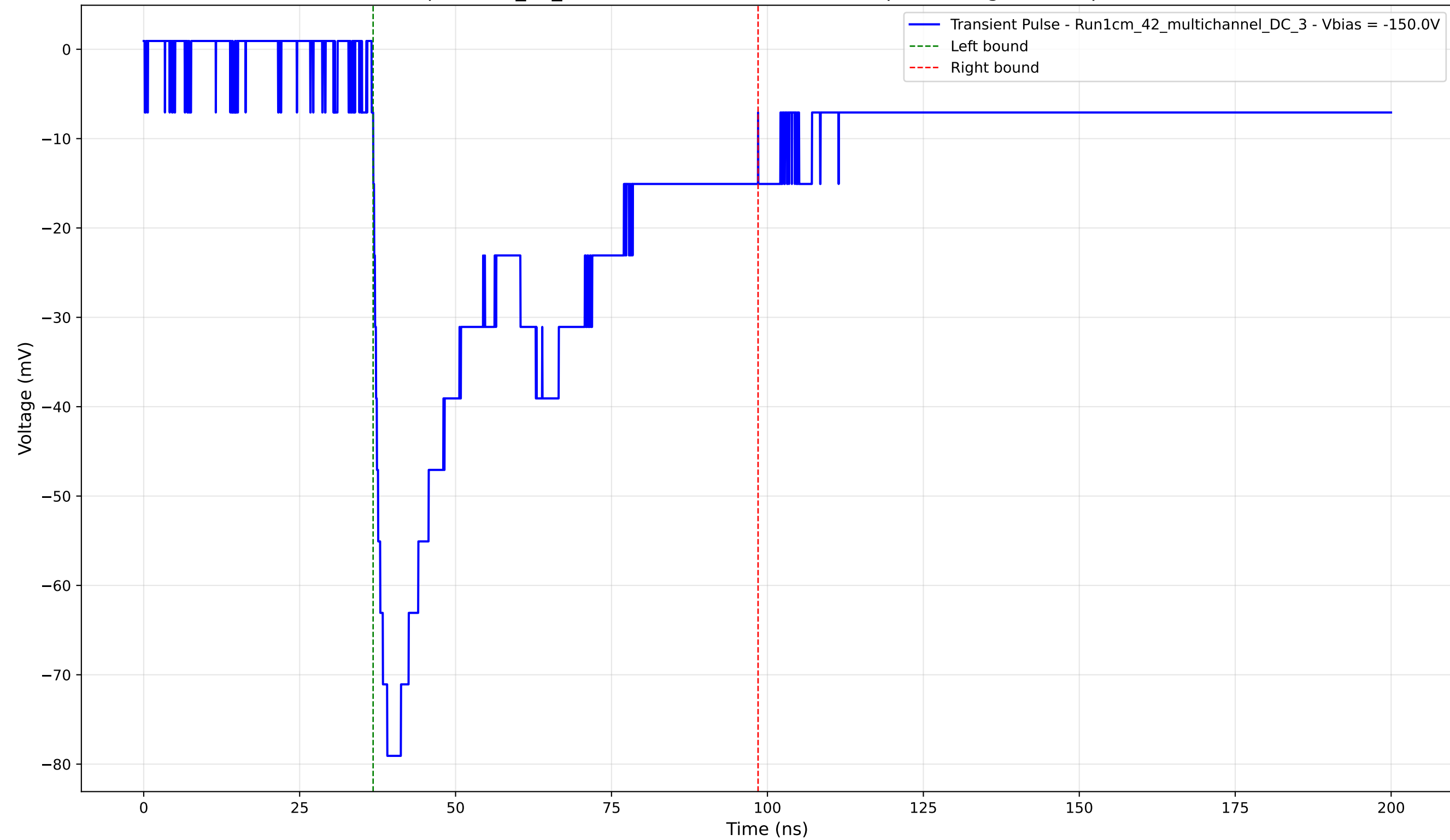
Transient Pulse - Sample: 1cm_42_multichannel - Position: 2550.0 \mu\text{m} - Charge: 37.64 pC - Rise Time: 2.26 ns
