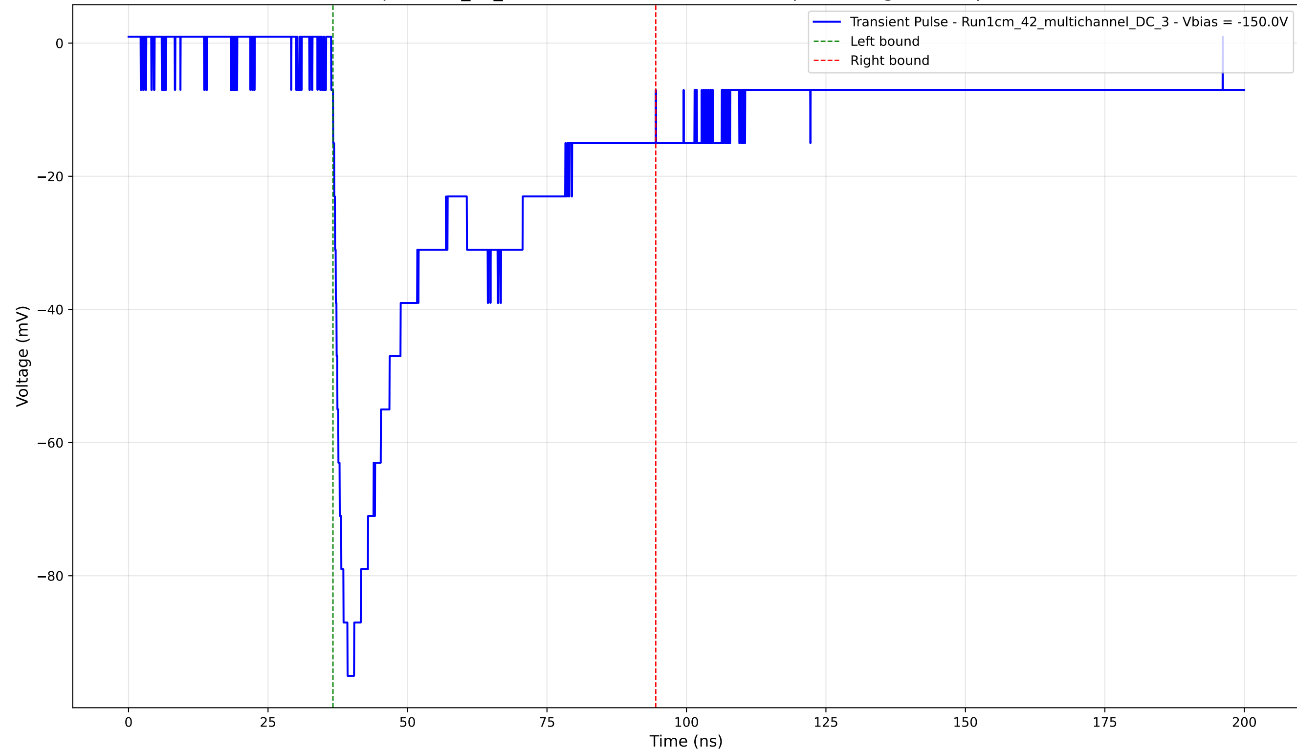
Transient Pulse - Sample: 1cm_42_multichannel - Position: 2760.0 \mu\text{m} - Charge: 38.31 pC - Rise Time: 1.87 ns
