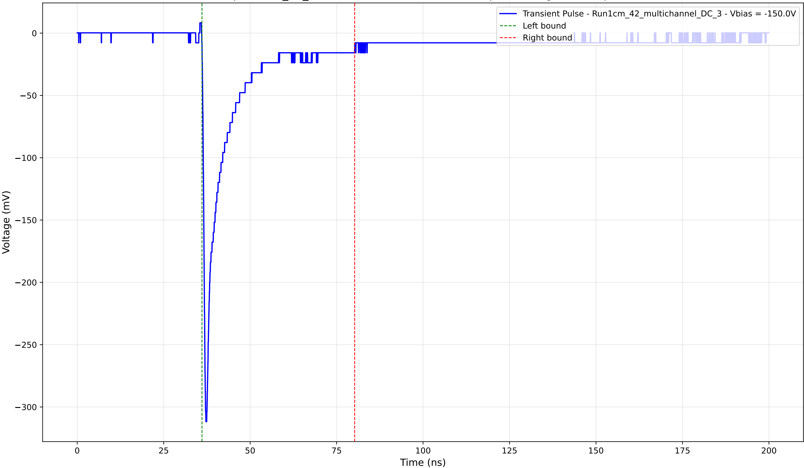
Transient Pulse - Sample: 1cm_42_multichannel - Position: 4635.0 \mu\text{m} - Charge: 41.96 pC - Rise Time: 0.86 ns
