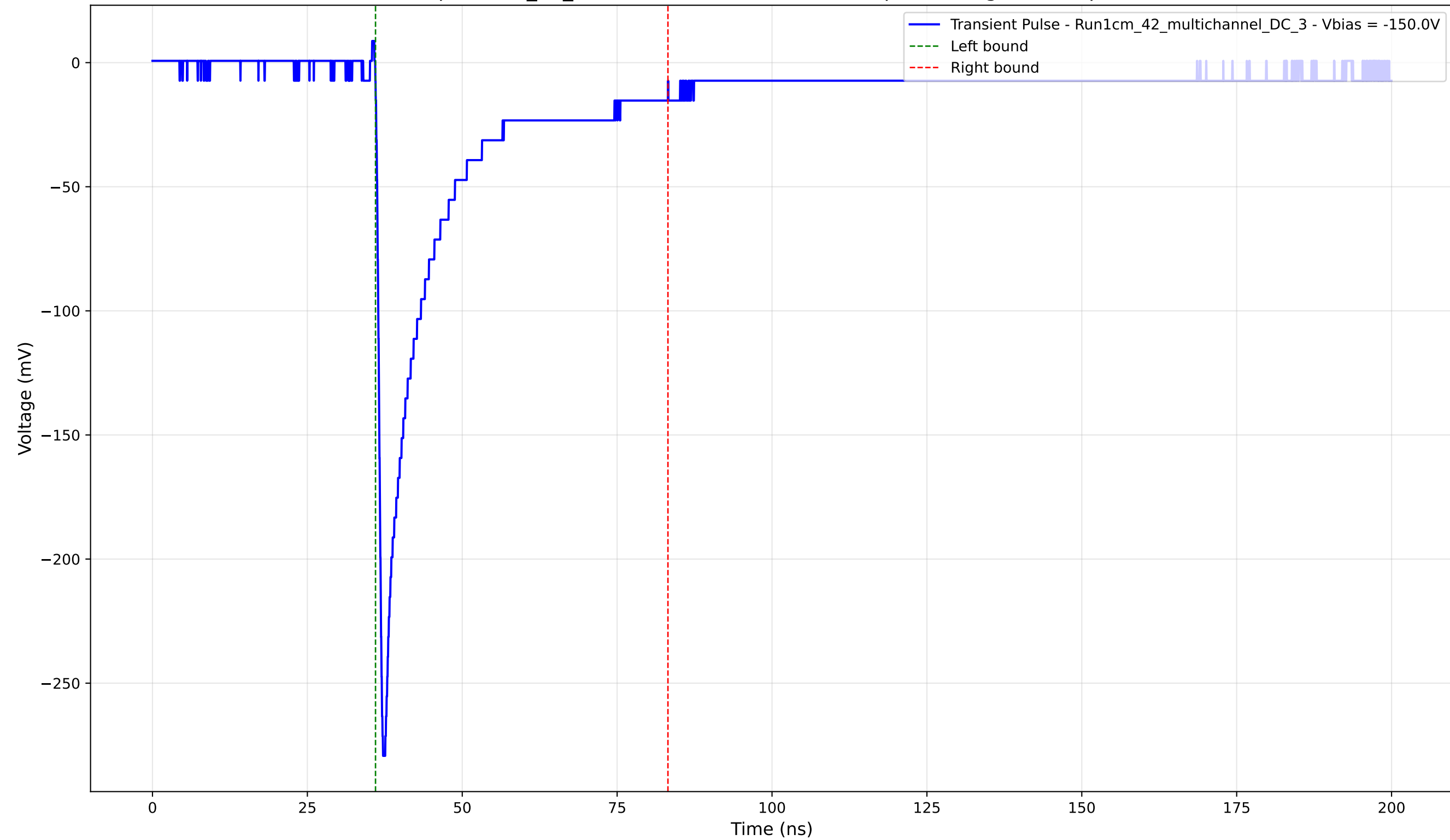
Transient Pulse - Sample: 1cm_42_multichannel - Position: 470.0 \mu\text{m} - Charge: 48.55 pC - Rise Time: 0.89 ns
