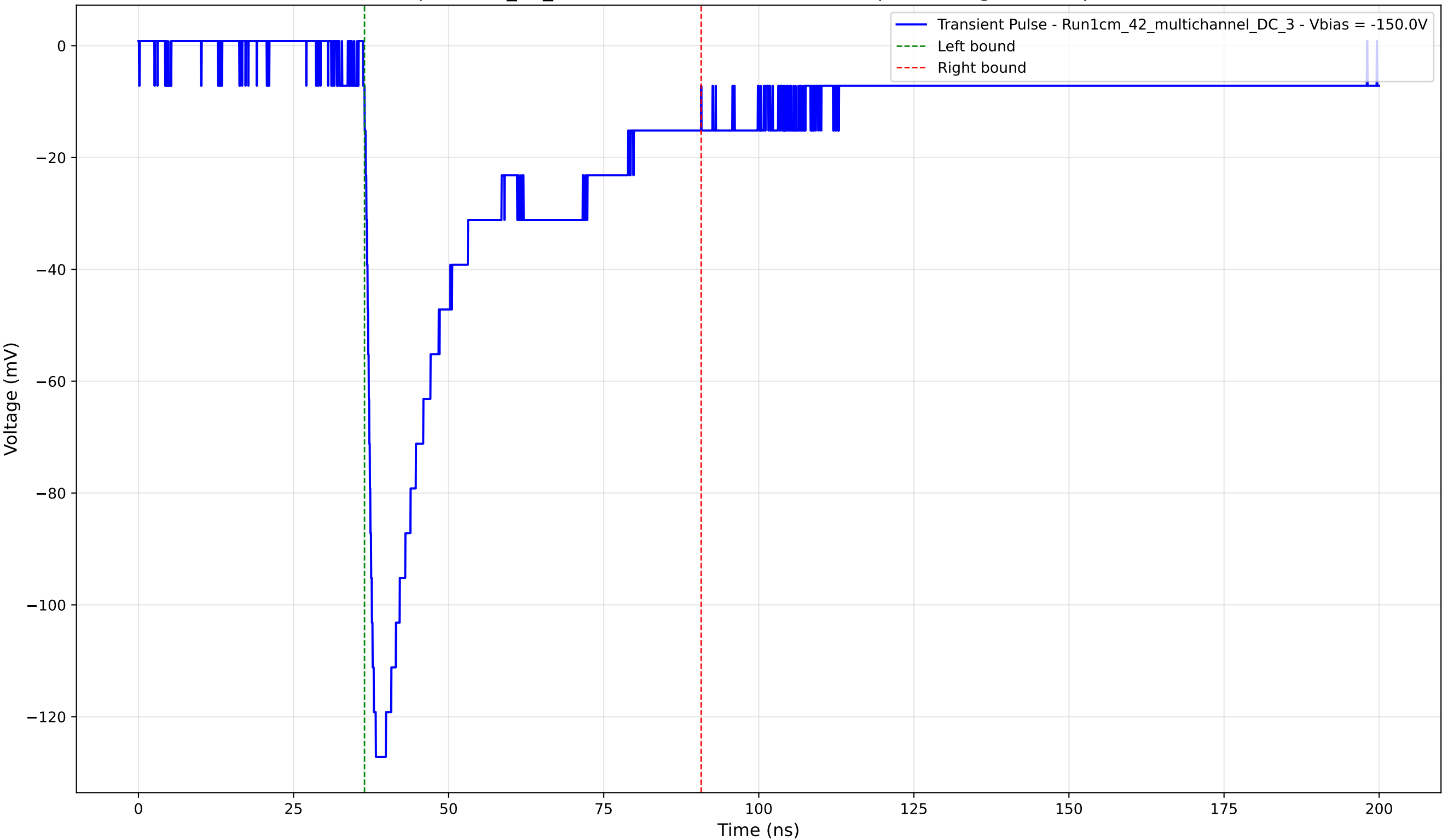
Transient Pulse - Sample: 1cm_42_multichannel - Position: 1540.0 \mu\text{m} - Charge: 43.20 pC - Rise Time: 1.49 ns
