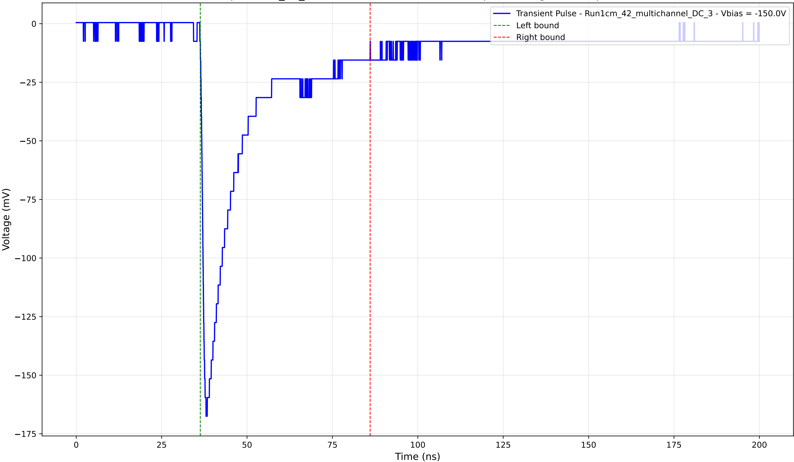
Transient Pulse - Sample: 1cm_42_multichannel - Position: 1085.0 \mu\text{m} - Charge: 43.37 pC - Rise Time: 1.14 ns
