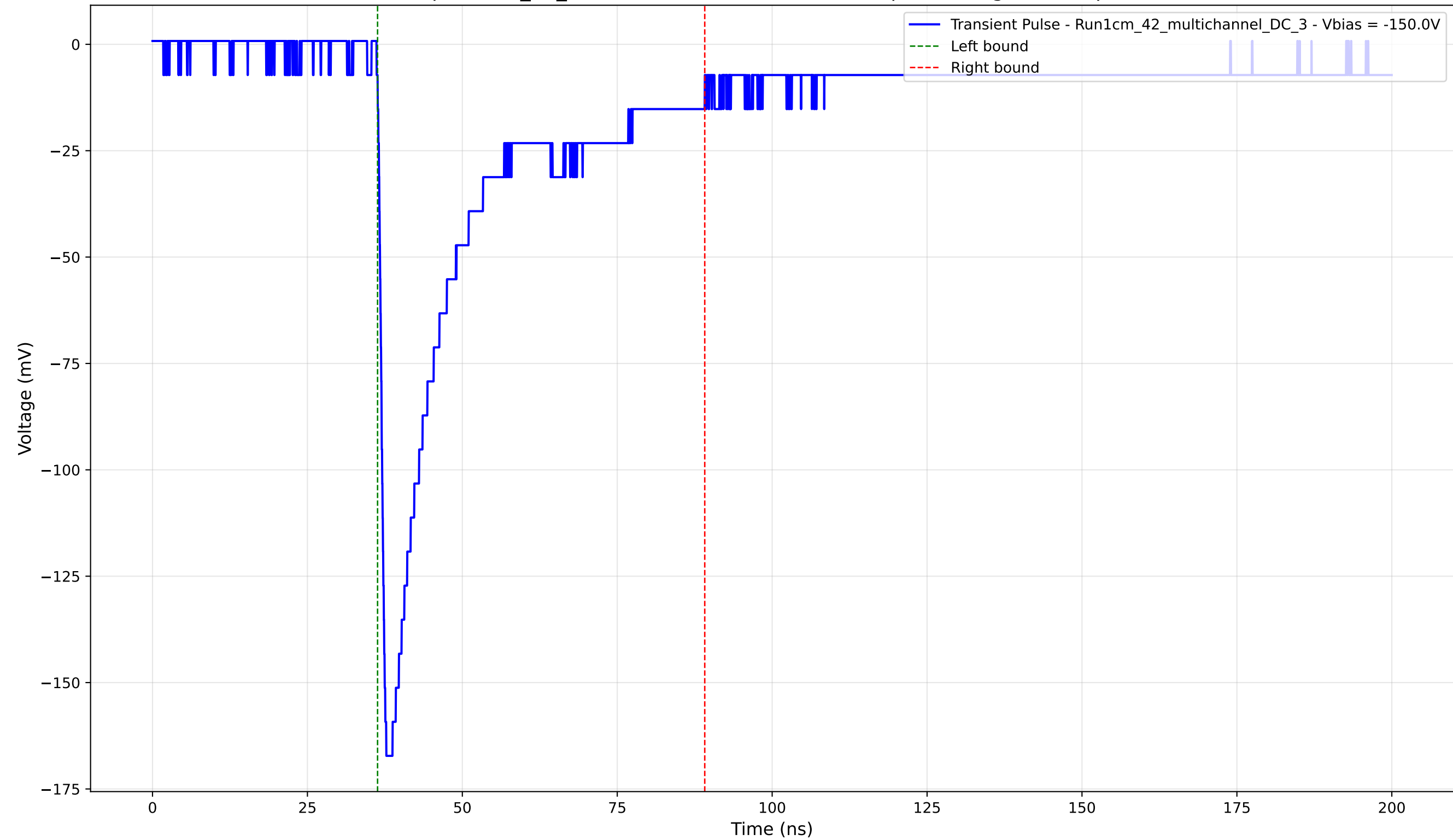
Transient Pulse - Sample: 1cm_42_multichannel - Position: 1045.0 \mu\text{m} - Charge: 44.97 pC - Rise Time: 1.04 ns
