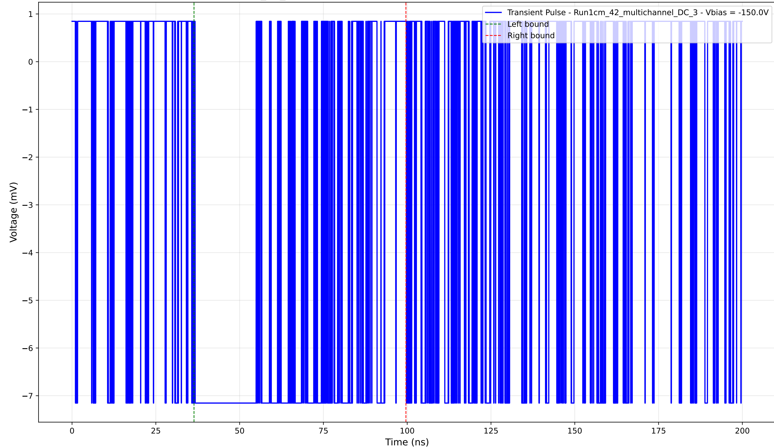
Transient Pulse - Sample: 1cm_42_multichannel - Position: 1865.0 \mu\text{m} - Charge: 5.77 pC - Rise Time: 0.00 ns (N/A)
