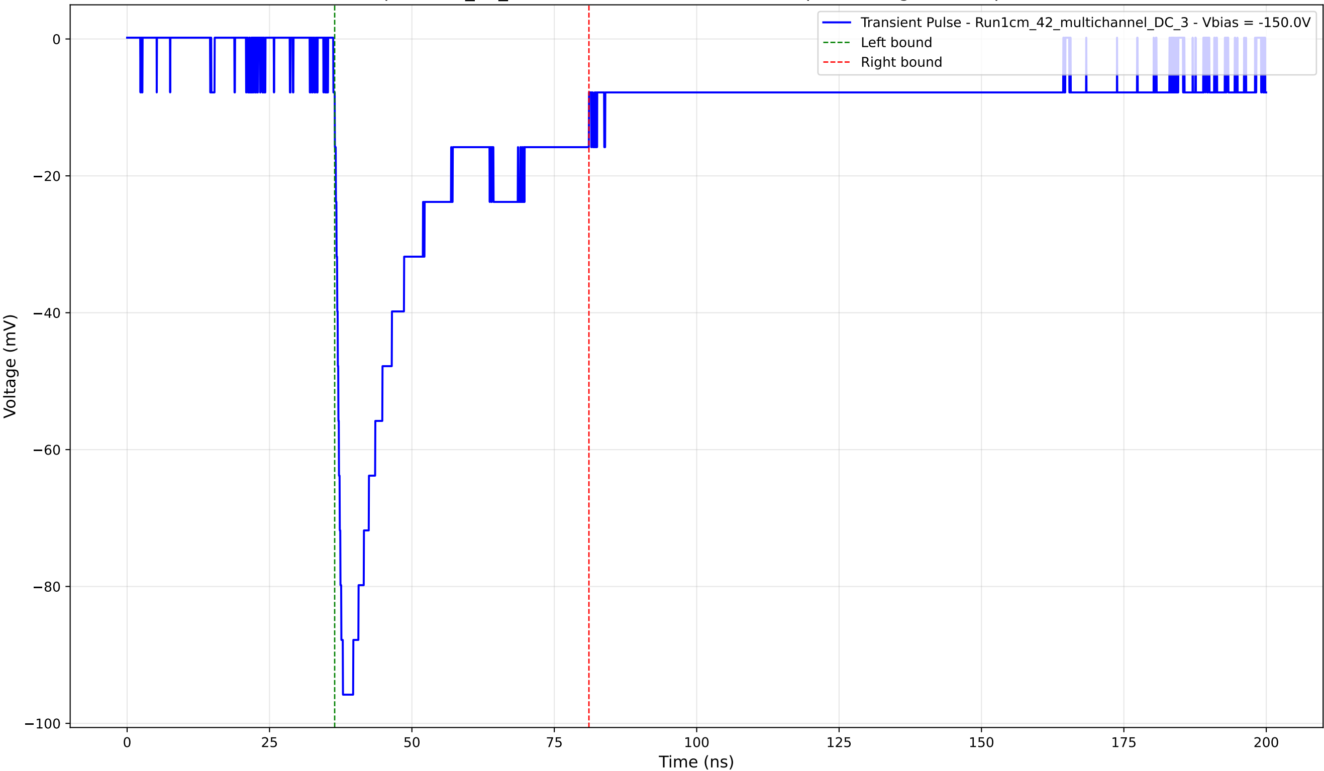
Transient Pulse - Sample: 1cm_42_multichannel - Position: 1305.0 \mu\text{m} - Charge: 28.60 pC - Rise Time: 1.16 ns
