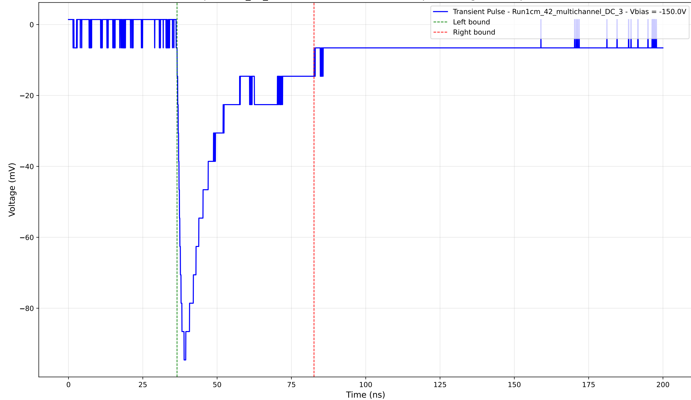
Transient Pulse - Sample: 1cm_42_multichannel - Position: 3320.0 \mu\text{m} - Charge: 28.48 pC - Rise Time: 1.63 ns
