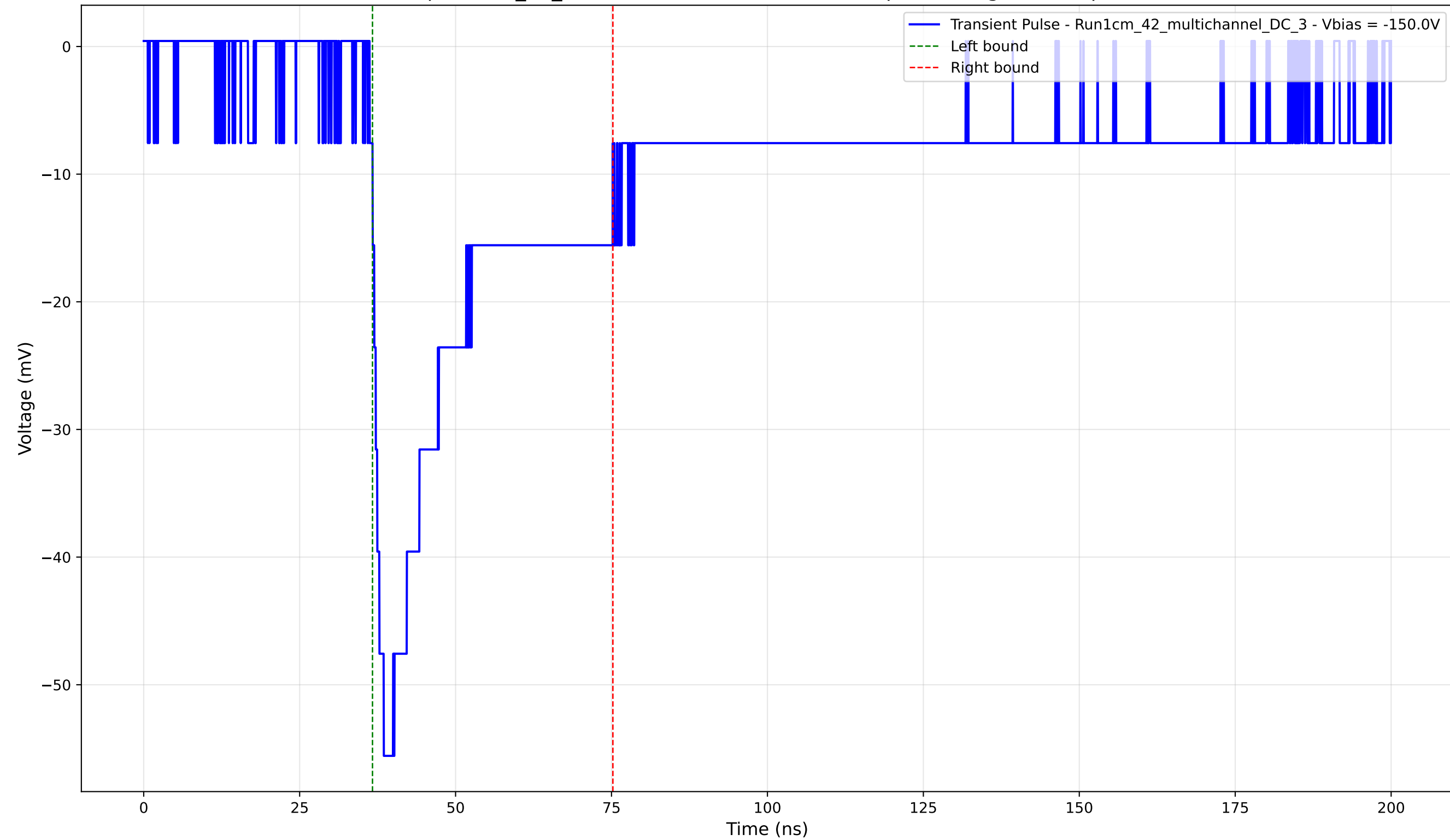
Transient Pulse - Sample: 1cm_42_multichannel - Position: 1820.0 \mu\text{m} - Charge: 18.12 pC - Rise Time: 2.27 ns
