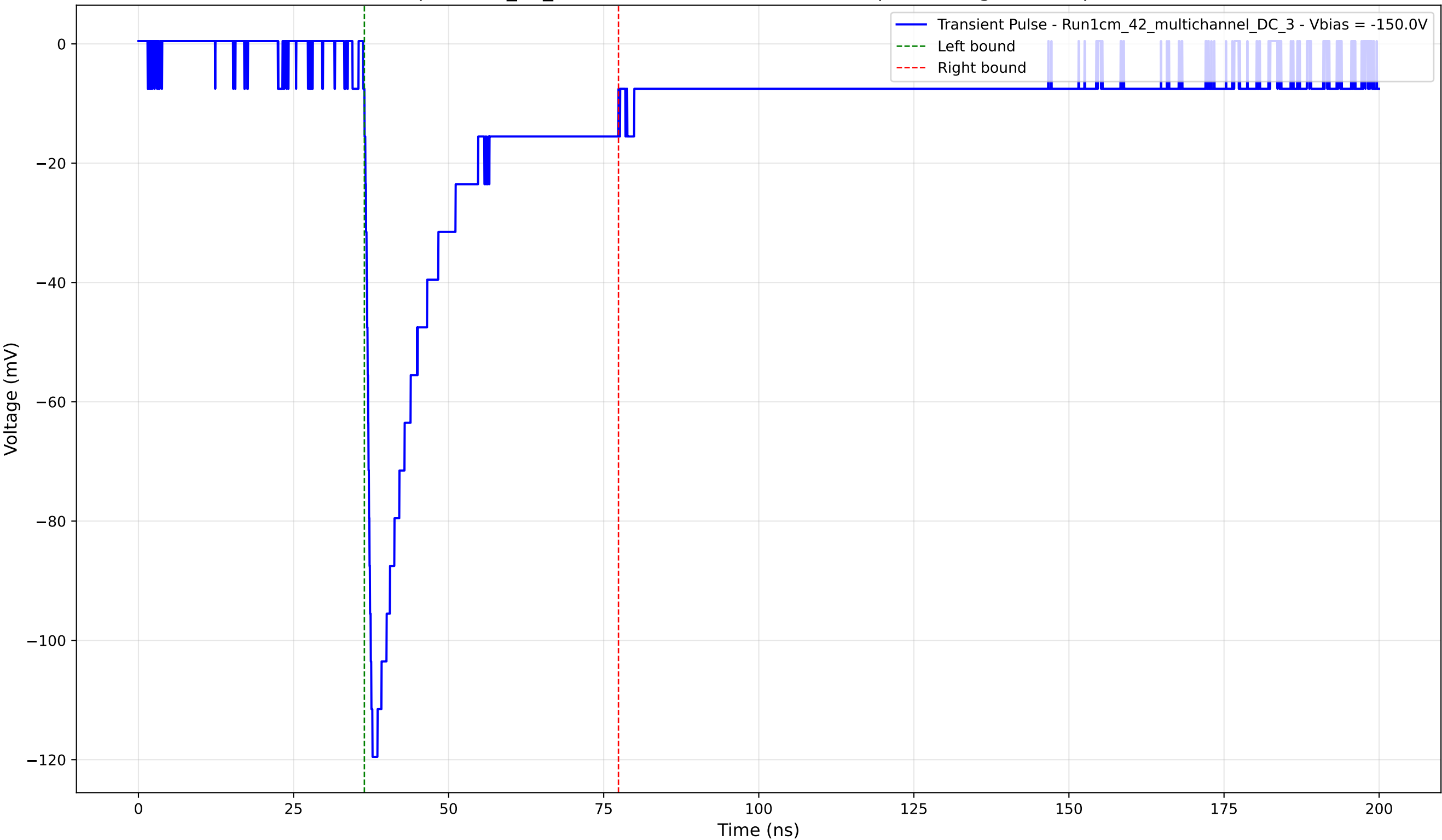
Transient Pulse - Sample: 1cm_42_multichannel - Position: 3950.0 \mu\text{m} - Charge: 27.46 pC - Rise Time: 1.11 ns
