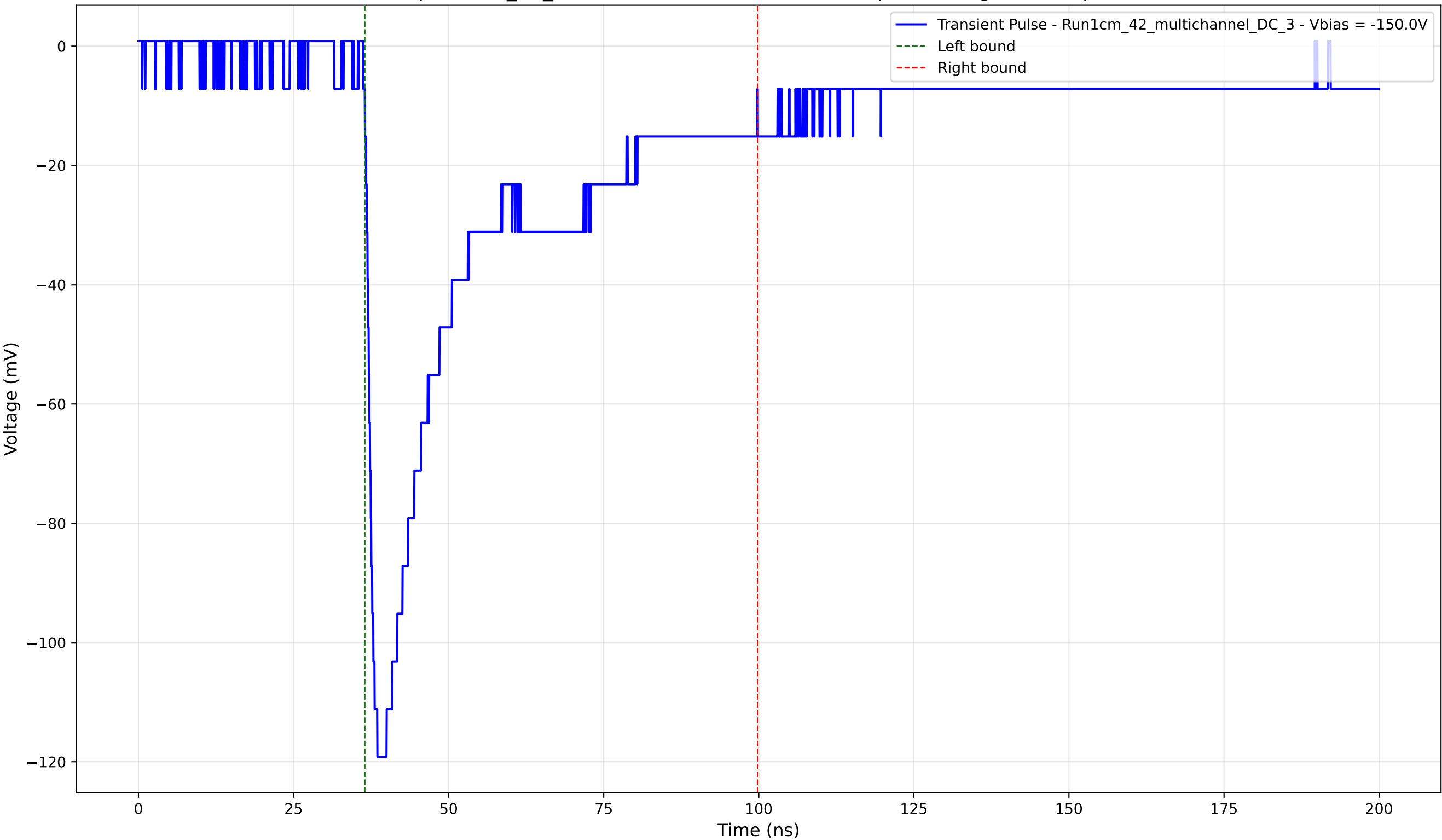
Transient Pulse - Sample: 1cm_42_multichannel - Position: 1695.0 \mu\text{m} - Charge: 44.90 pC - Rise Time: 1.57 ns
