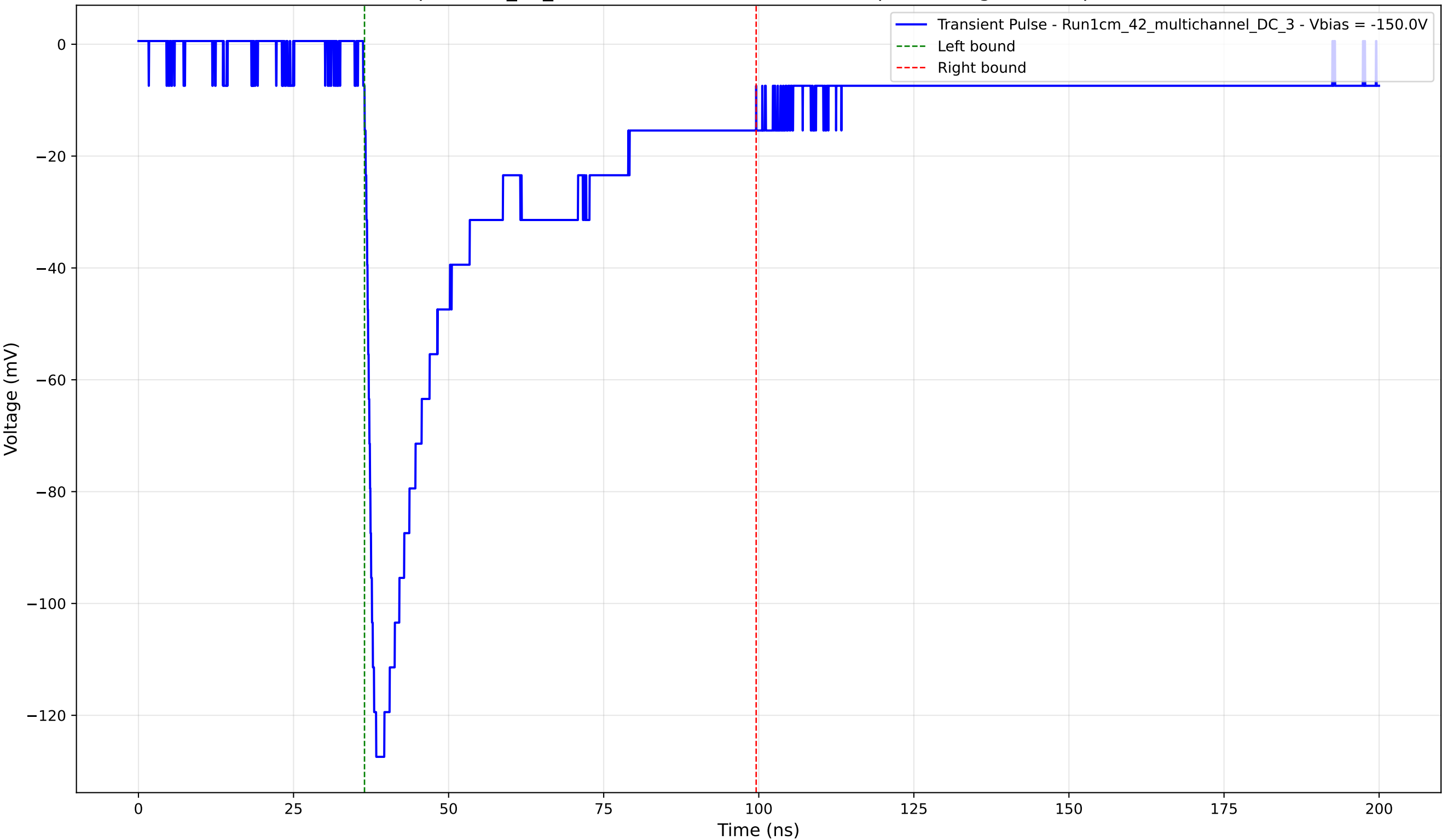
Transient Pulse - Sample: 1cm_42_multichannel - Position: 1555.0 \mu\text{m} - Charge: 45.82 pC - Rise Time: 1.53 ns
