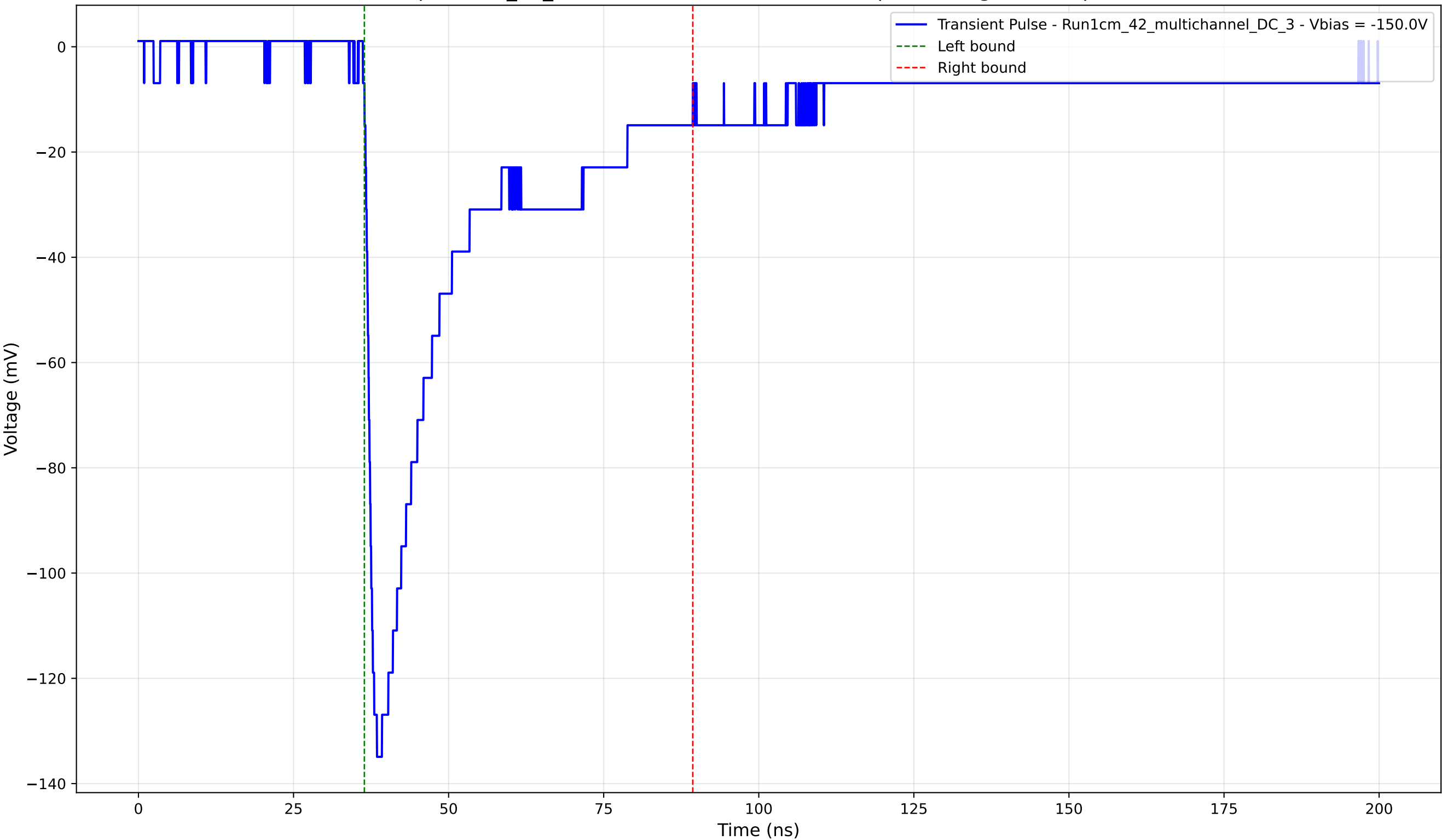
Transient Pulse - Sample: 1cm_42_multichannel - Position: 1500.0 \mu\text{m} - Charge: 43.09 pC - Rise Time: 1.56 ns
