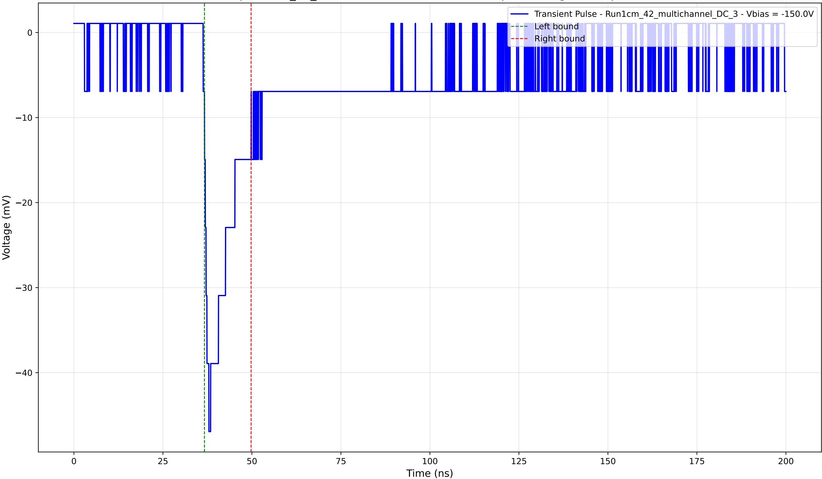
Transient Pulse - Sample: 1cm_42_multichannel - Position: 3930.0 \mu\text{m} - Charge: 6.71 pC - Rise Time: 1.61 ns
