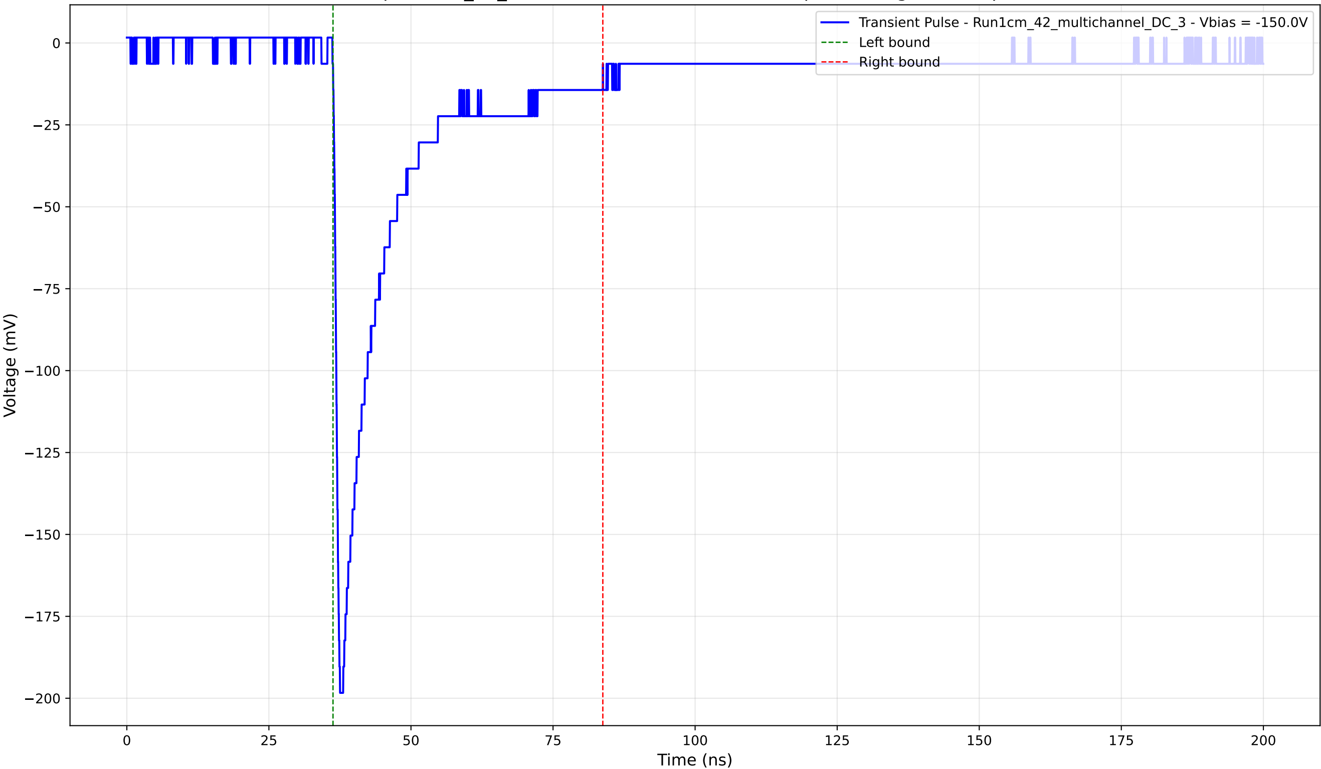
Transient Pulse - Sample: 1cm_42_multichannel - Position: 4200.0 \mu\text{m} - Charge: 40.18 pC - Rise Time: 0.95 ns
