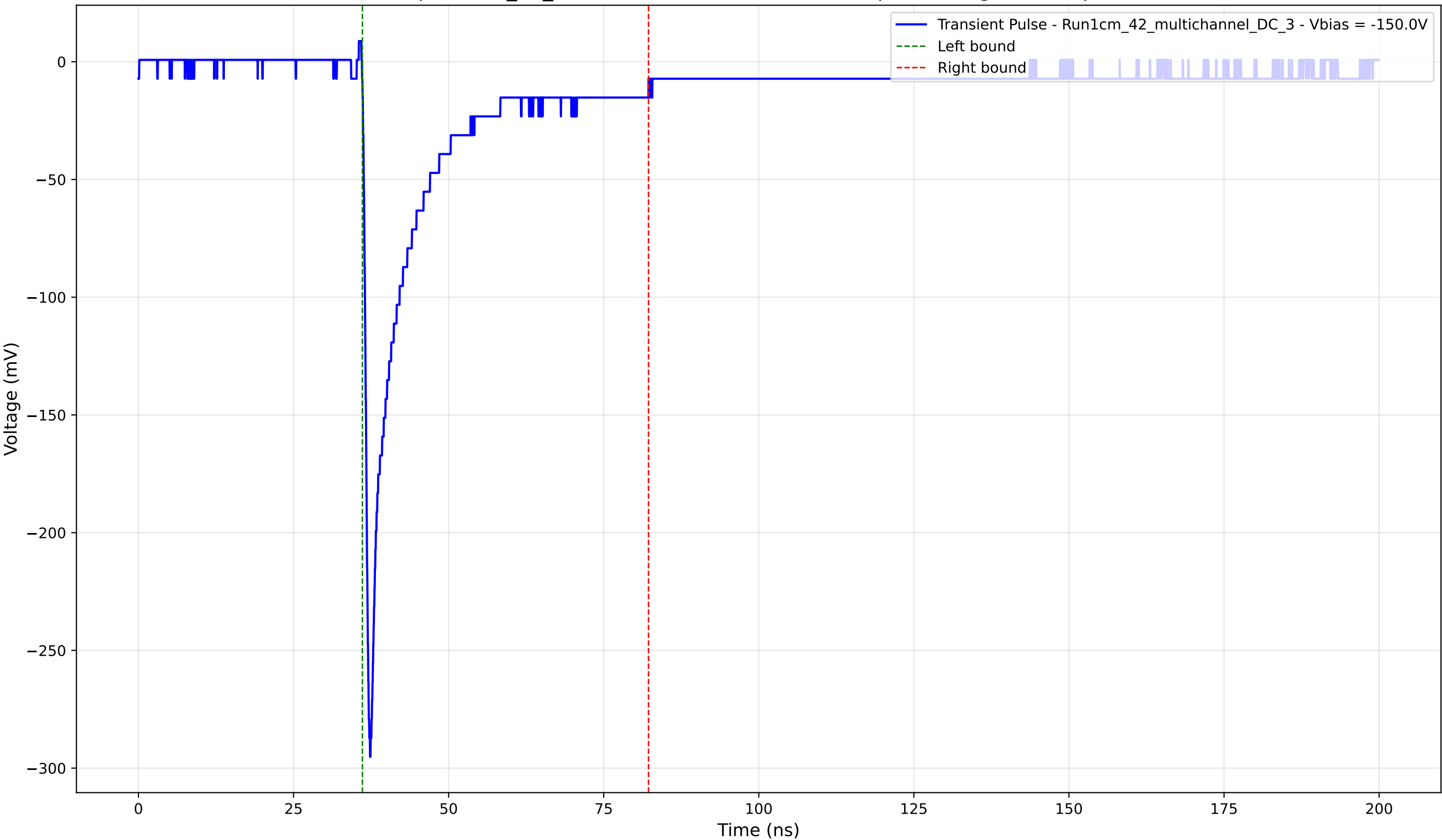
Transient Pulse - Sample: 1cm_42_multichannel - Position: 4580.0 \mu\text{m} - Charge: 41.12 pC - Rise Time: 0.88 ns
