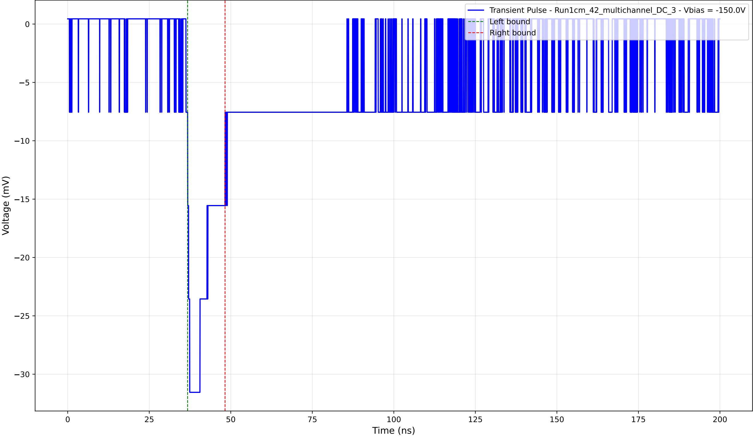
Transient Pulse - Sample: 1cm_42_multichannel - Position: 3925.0 \mu\text{m} - Charge: 5.00 pC - Rise Time: 1.15 ns
