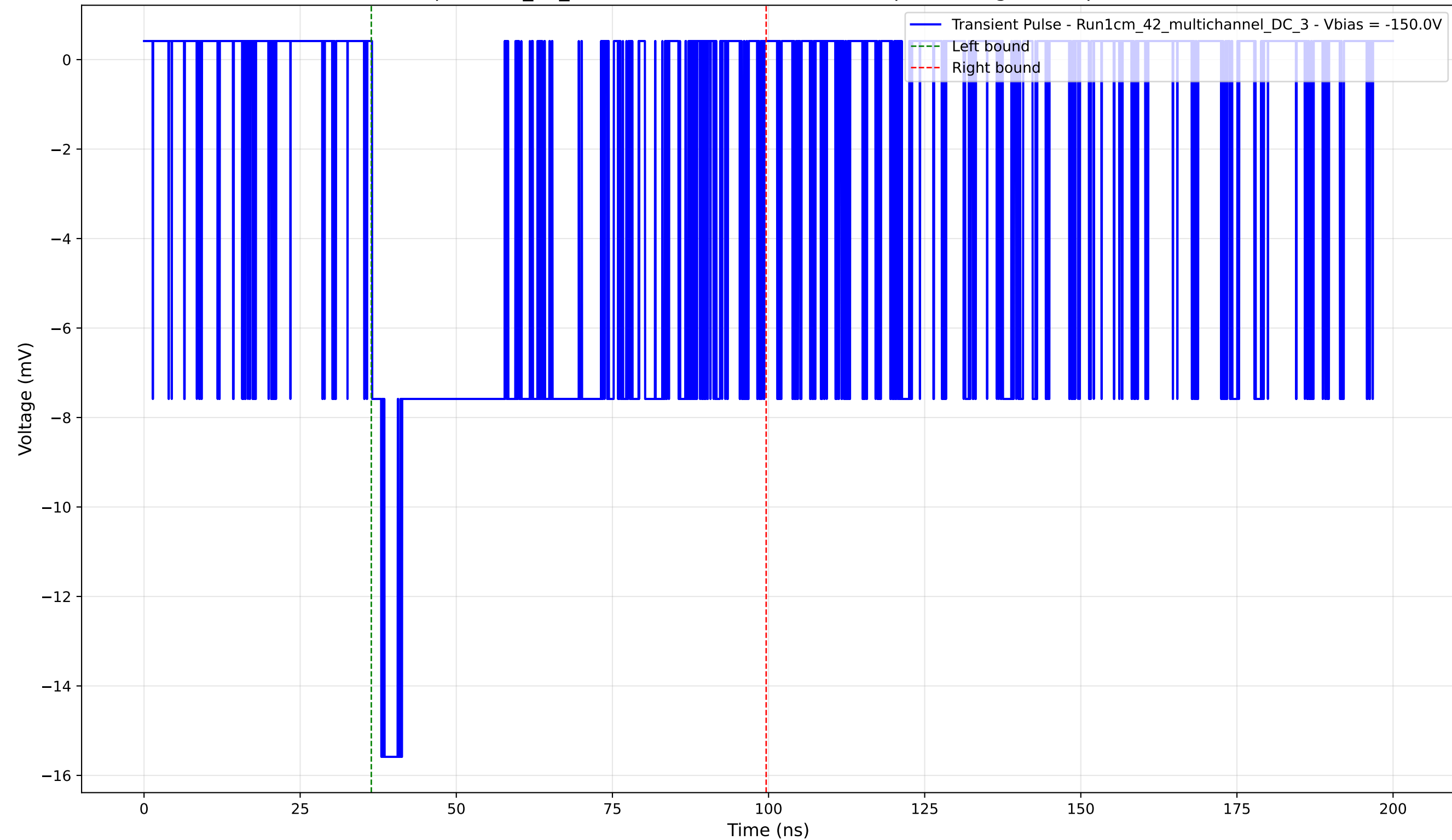
Transient Pulse - Sample: 1cm_42_multichannel - Position: 1380.0 \mu\text{m} - Charge: 7.43 pC - Rise Time: 1.48 ns
