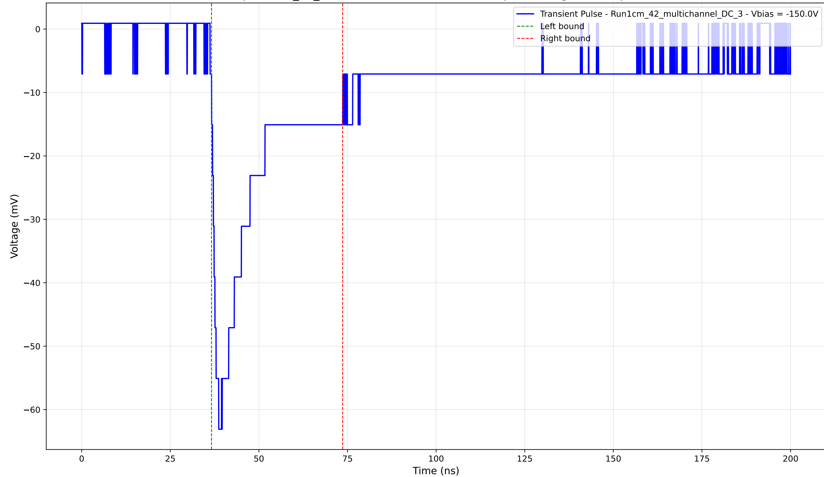
Transient Pulse - Sample: 1cm_42_multichannel - Position: 3335.0 \mu\text{m} - Charge: 18.01 pC - Rise Time: 2.44 ns
