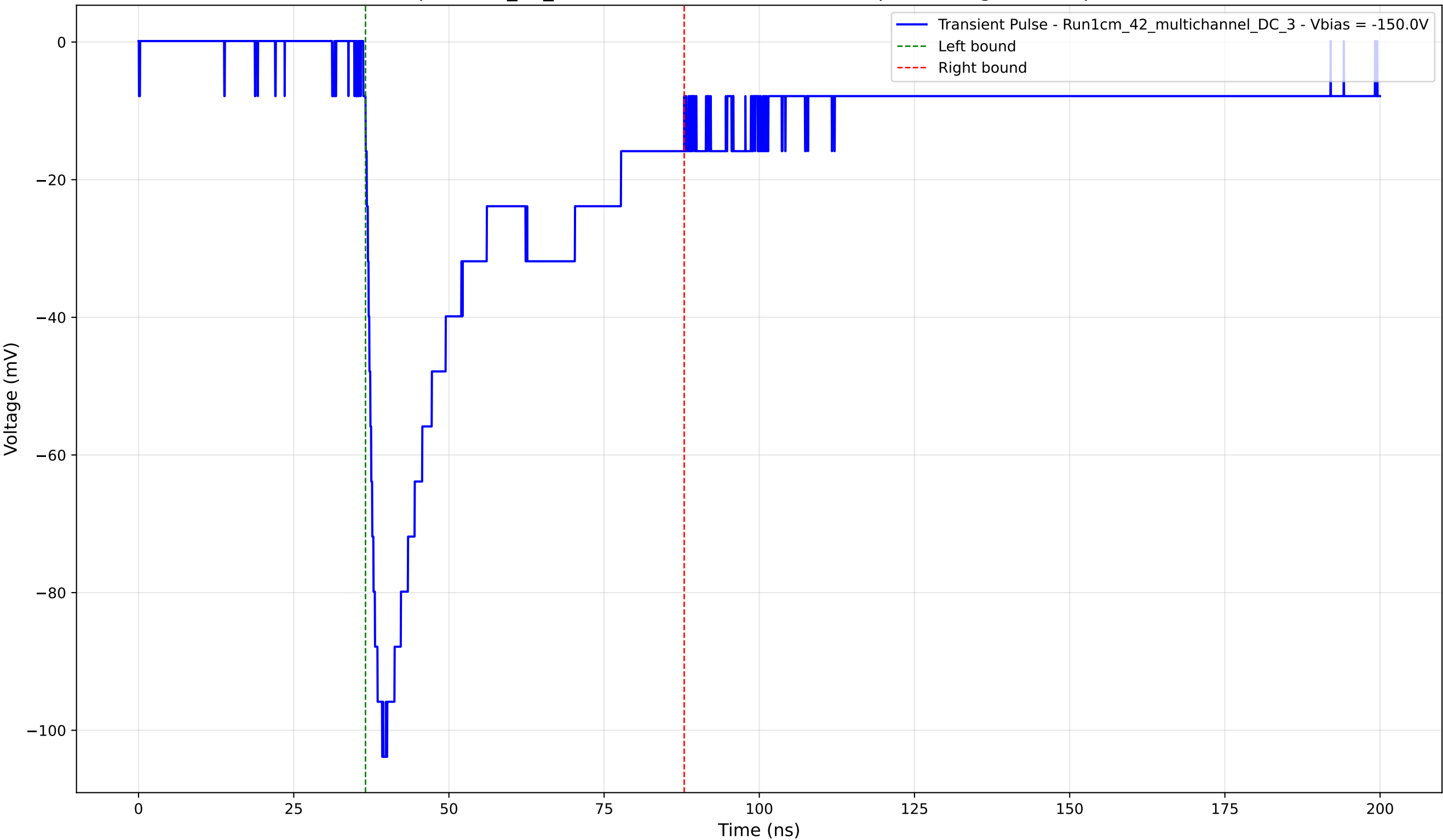
Transient Pulse - Sample: 1cm_42_multichannel - Position: 2985.0 \mu\text{m} - Charge: 37.63 pC - Rise Time: 1.93 ns
