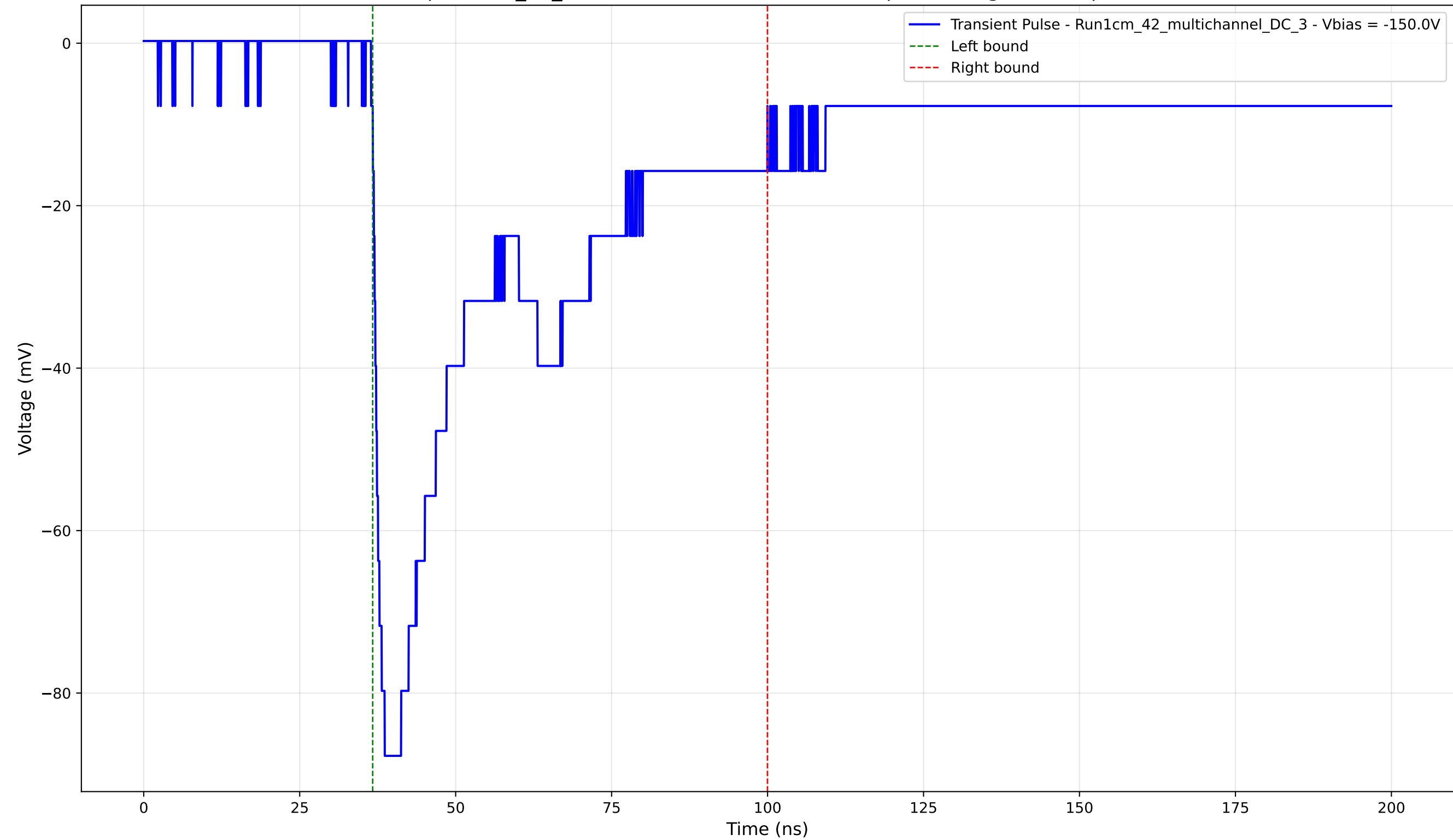
Transient Pulse - Sample: 1cm_42_multichannel - Position: 2085.0 \mu\text{m} - Charge: 41.04 pC - Rise Time: 1.44 ns
