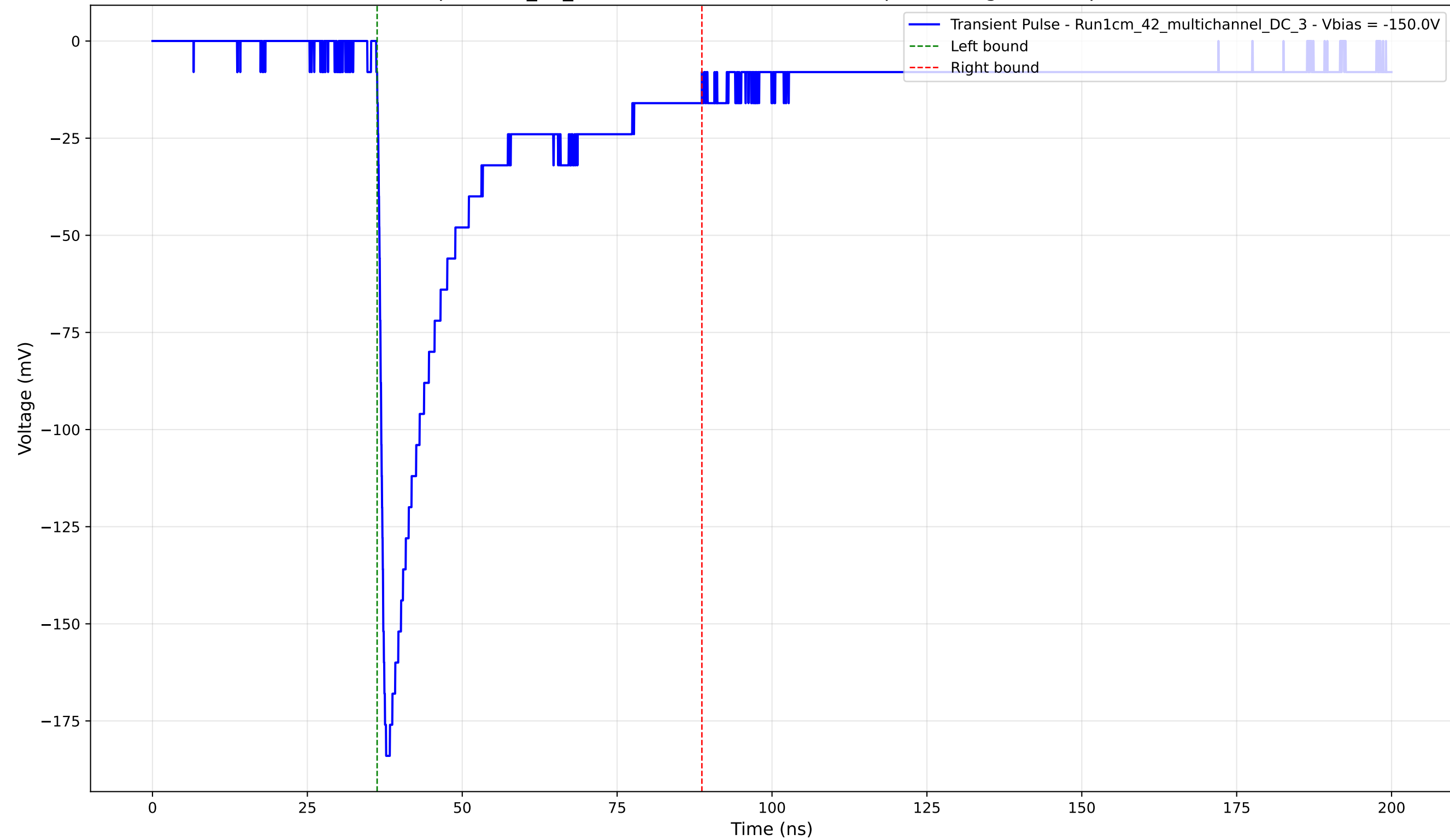
Transient Pulse - Sample: 1cm_42_multichannel - Position: 955.0 \mu\text{m} - Charge: 46.92 pC - Rise Time: 1.05 ns
