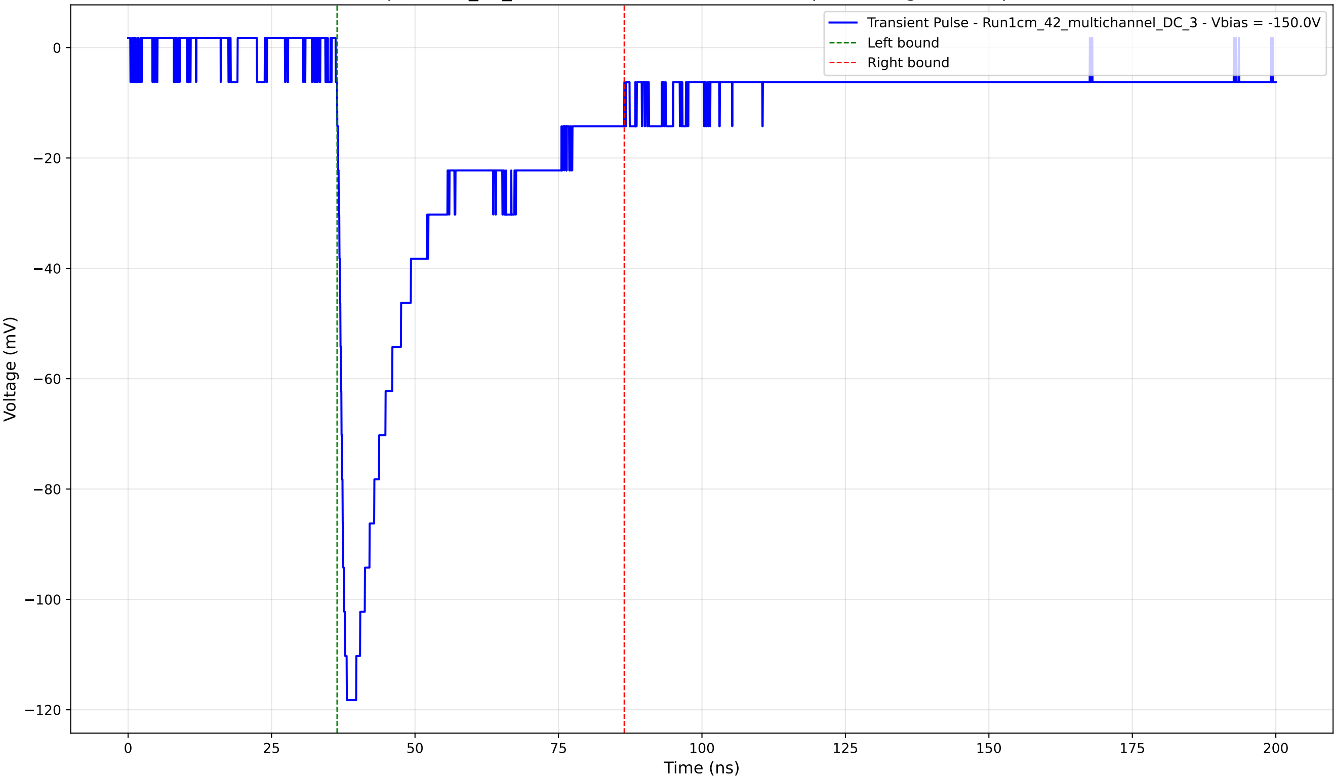
Transient Pulse - Sample: 1cm_42_multichannel - Position: 1435.0 \mu\text{m} - Charge: 36.71 pC - Rise Time: 1.37 ns
