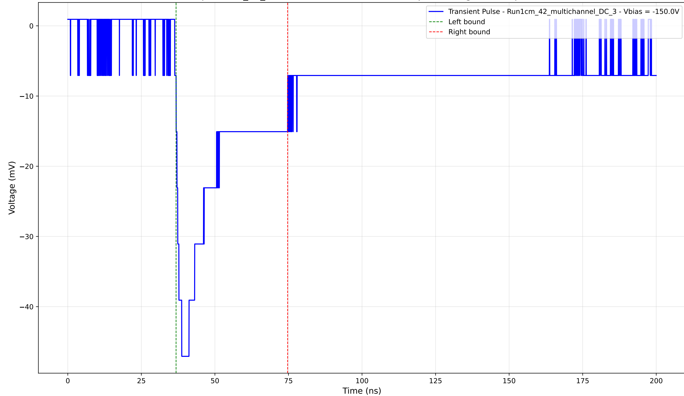
Transient Pulse - Sample: 1cm_42_multichannel - Position: 2830.0 \mu\text{m} - Charge: 16.34 pC - Rise Time: 2.39 ns
