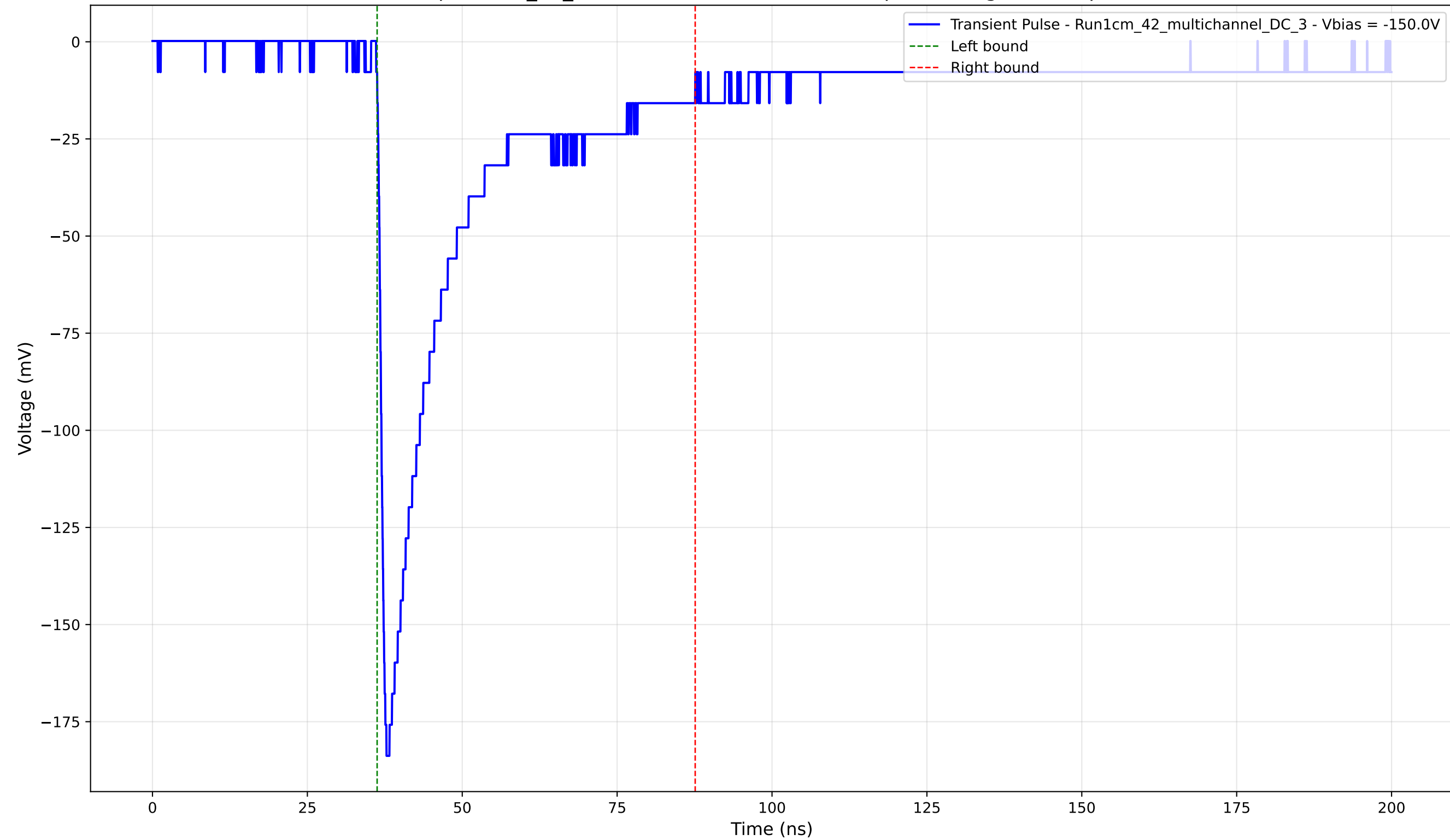
Transient Pulse - Sample: 1cm_42_multichannel - Position: 975.0 \mu\text{m} - Charge: 46.22 pC - Rise Time: 1.09 ns
