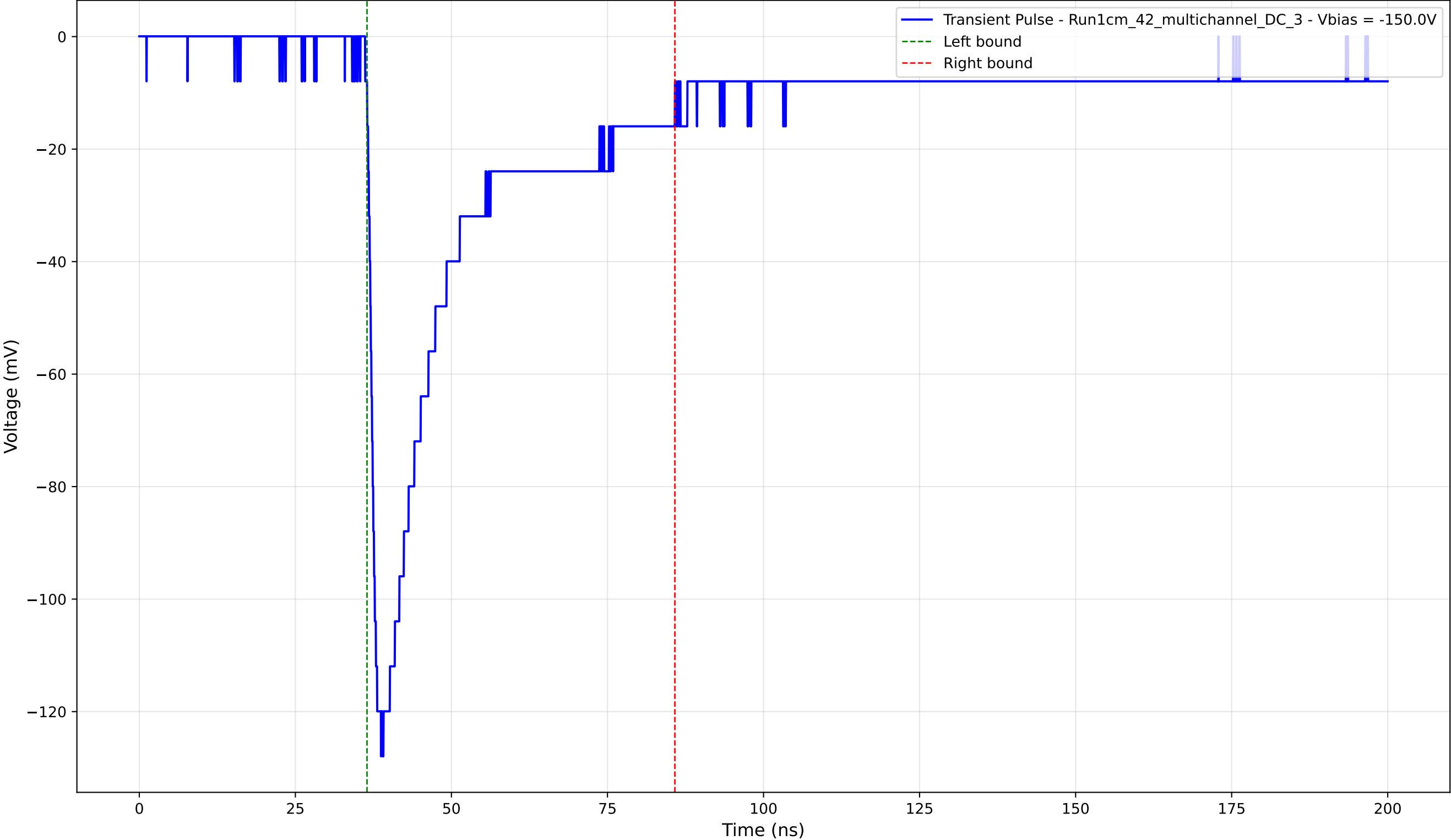
Transient Pulse - Sample: 1cm_42_multichannel - Position: 3490.0 \mu\text{m} - Charge: 37.77 pC - Rise Time: 1.61 ns
