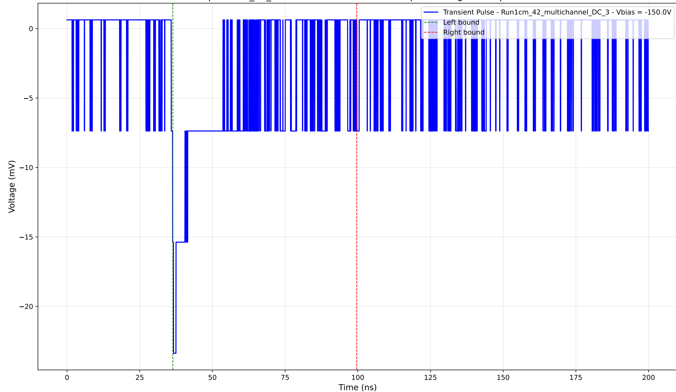
Transient Pulse - Sample: 1cm_42_multichannel - Position: 45.0 \mu\text{m} - Charge: 6.04 pC - Rise Time: 0.79 ns
