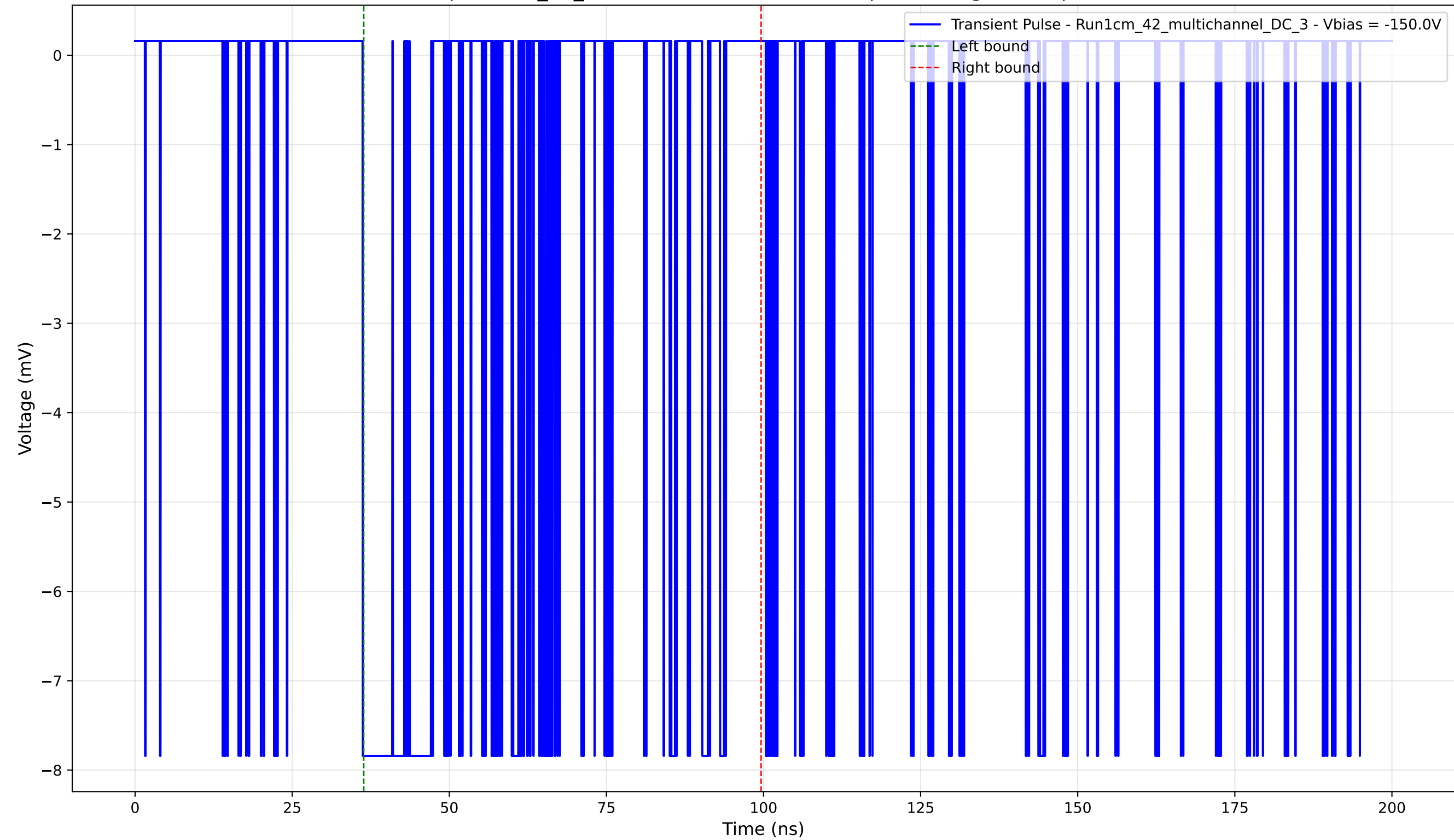
Transient Pulse - Sample: 1cm_42_multichannel - Position: 0.0 \mu\text{m} - Charge: 2.98 pC - Rise Time: 0.02 ns
