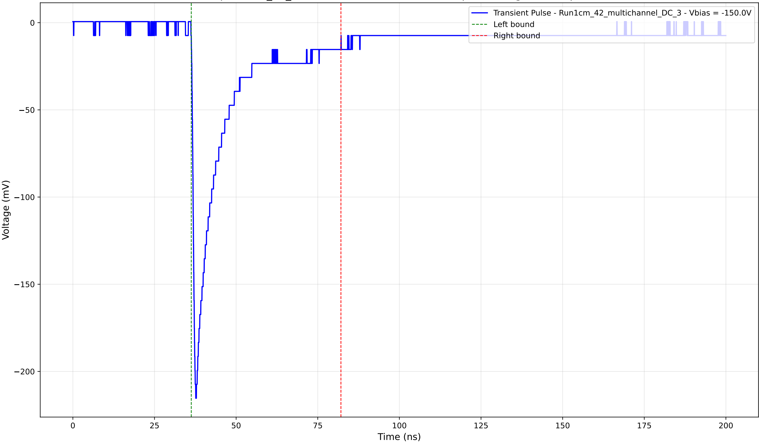
Transient Pulse - Sample: 1cm_42_multichannel - Position: 4225.0 \mu\text{m} - Charge: 41.66 pC - Rise Time: 1.02 ns
