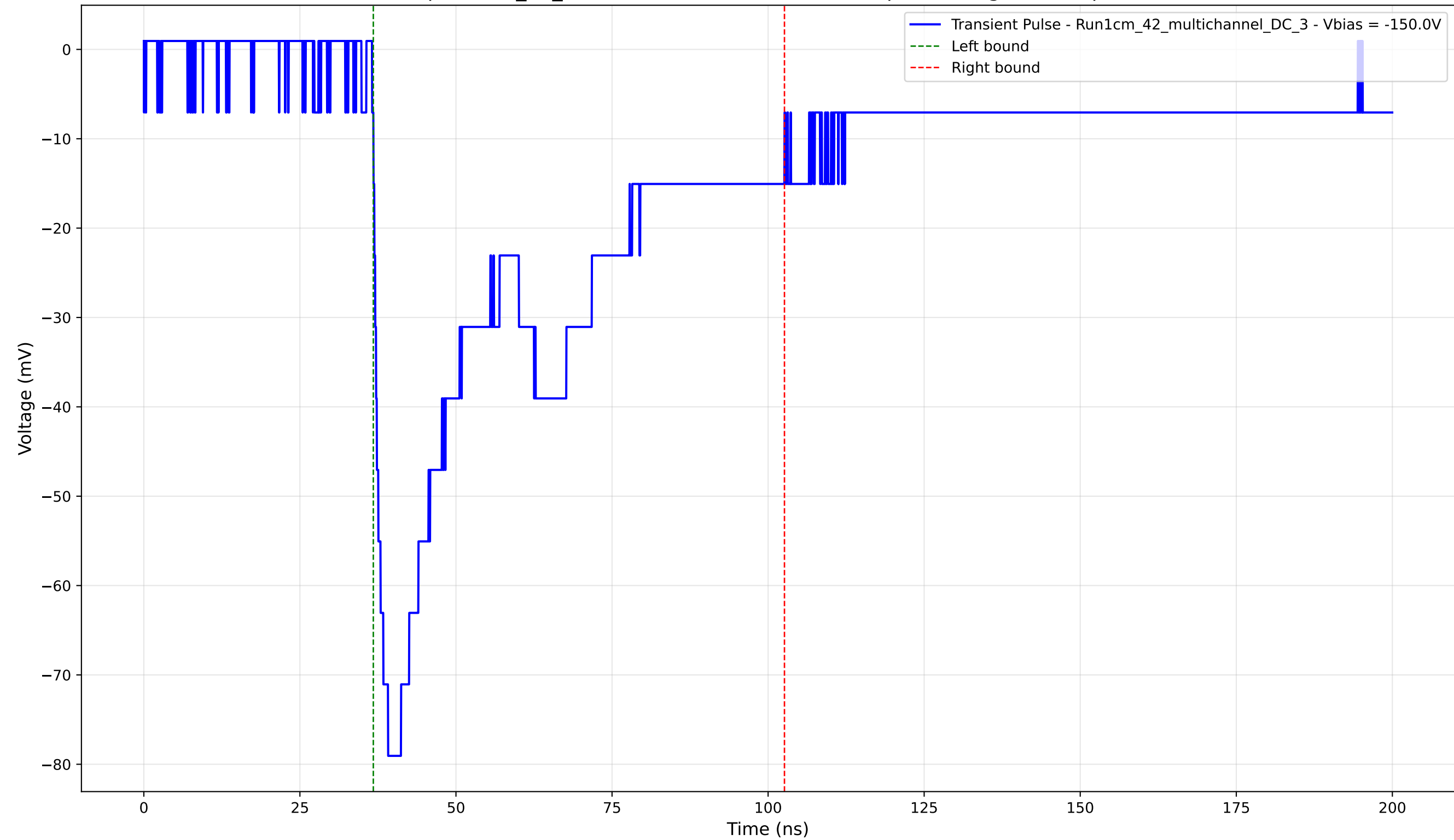
Transient Pulse - Sample: 1cm_42_multichannel - Position: 2460.0 \mu\text{m} - Charge: 39.40 pC - Rise Time: 2.36 ns
