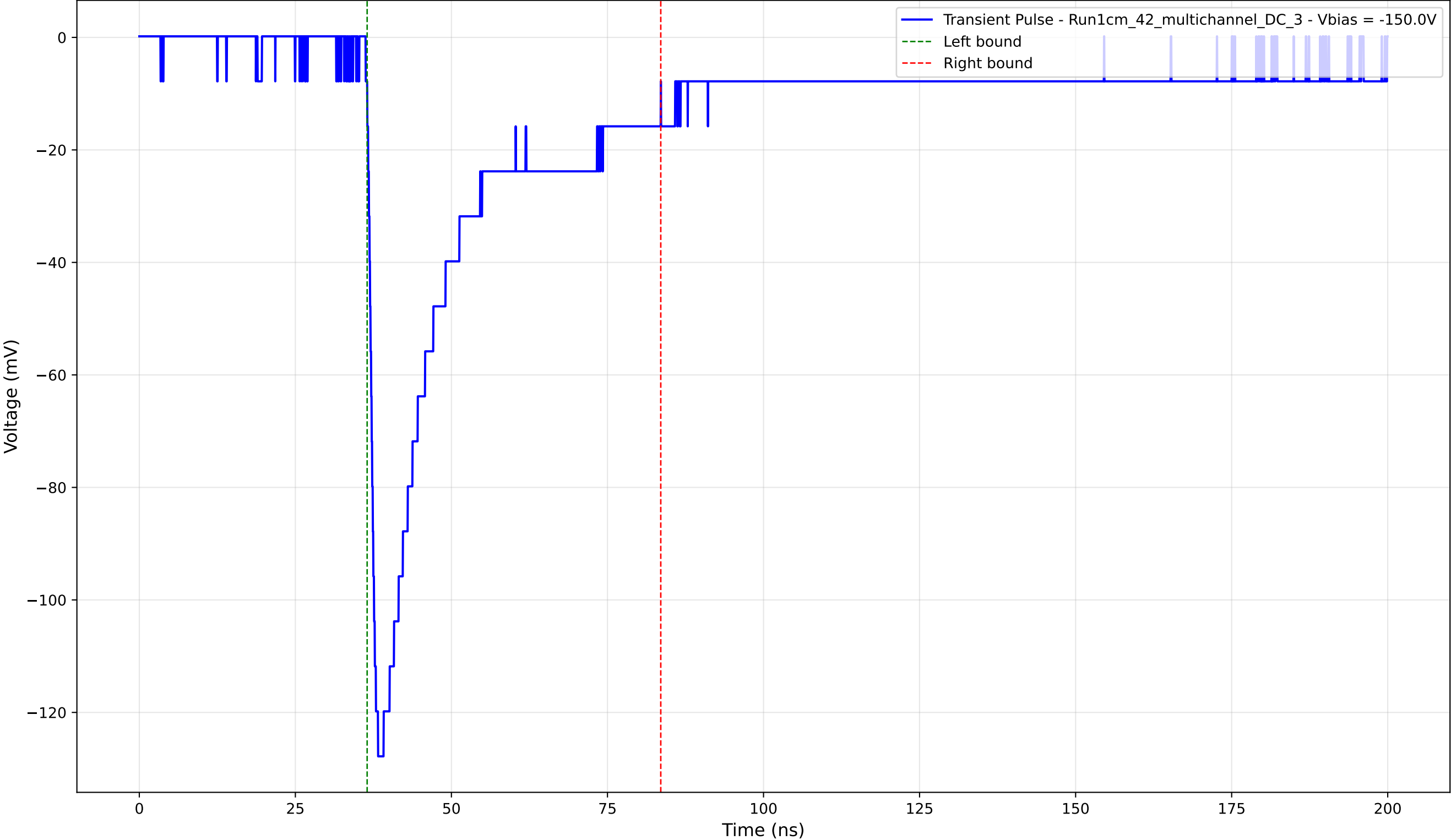
Transient Pulse - Sample: 1cm_42_multichannel - Position: 3610.0 \mu\text{m} - Charge: 36.38 pC - Rise Time: 1.39 ns
