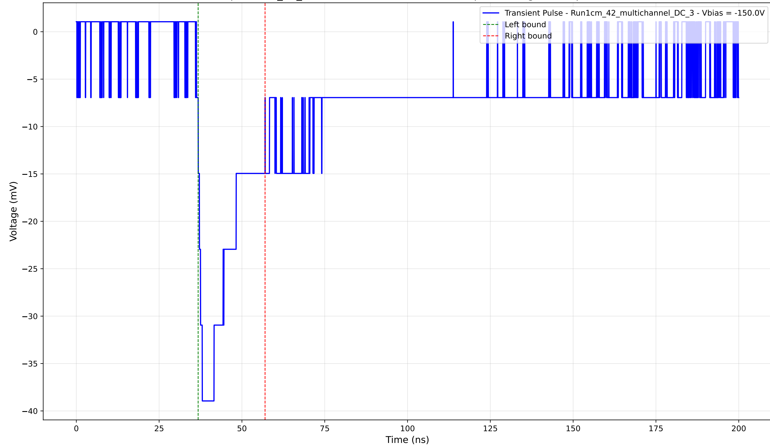
Transient Pulse - Sample: 1cm_42_multichannel - Position: 1825.0 \mu\text{m} - Charge: 9.49 pC - Rise Time: 1.75 ns
