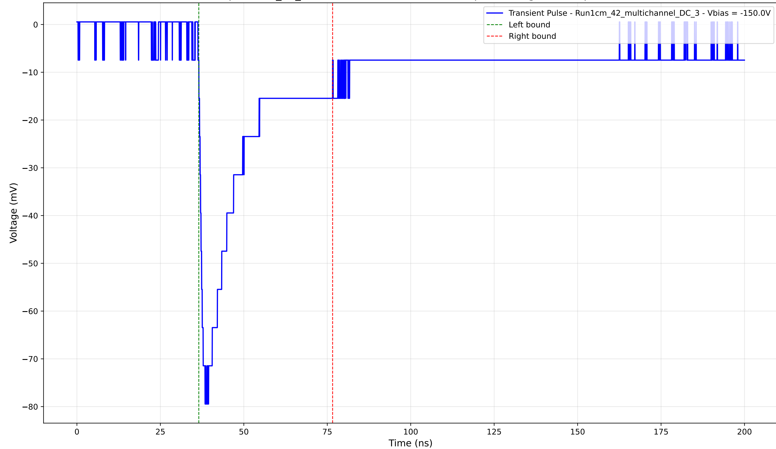
Transient Pulse - Sample: 1cm_42_multichannel - Position: 1415.0 \mu\text{m} - Charge: 22.36 pC - Rise Time: 1.86 ns
