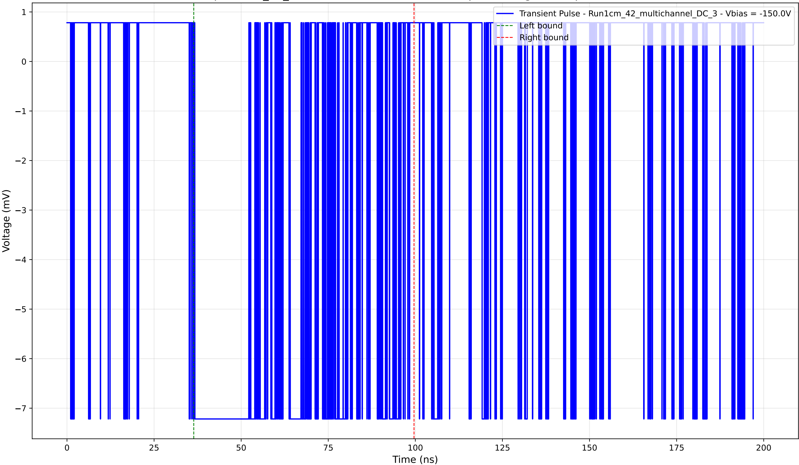
Transient Pulse - Sample: 1cm_42_multichannel - Position: 2870.0 \mu\text{m} - Charge: 5.20 pC - Rise Time: 0.00 ns (N/A)
