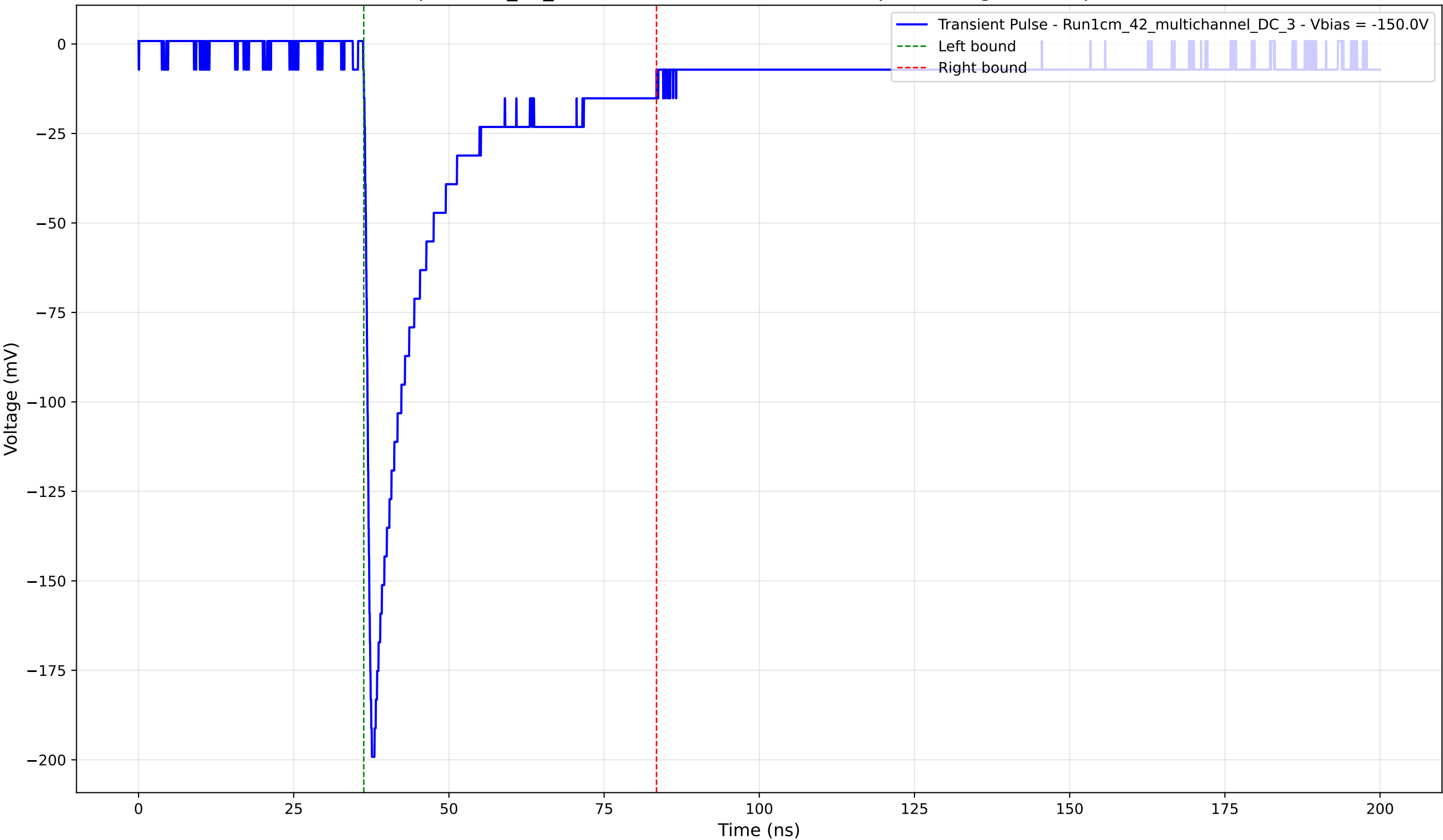
Transient Pulse - Sample: 1cm_42_multichannel - Position: 4180.0 \mu\text{m} - Charge: 40.61 pC - Rise Time: 0.99 ns
