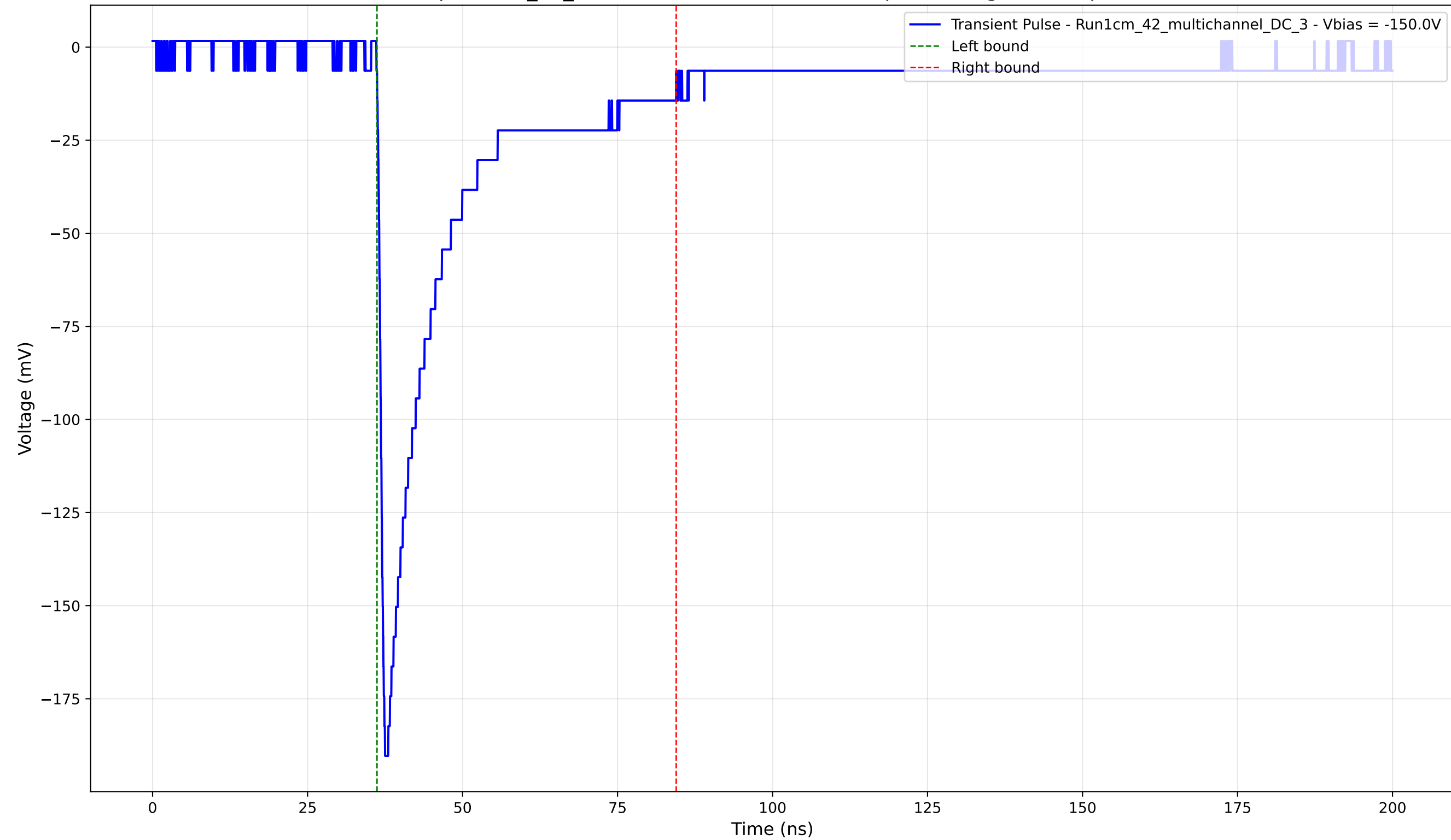
Transient Pulse - Sample: 1cm_42_multichannel - Position: 775.0 \mu\text{m} - Charge: 41.55 pC - Rise Time: 0.99 ns
