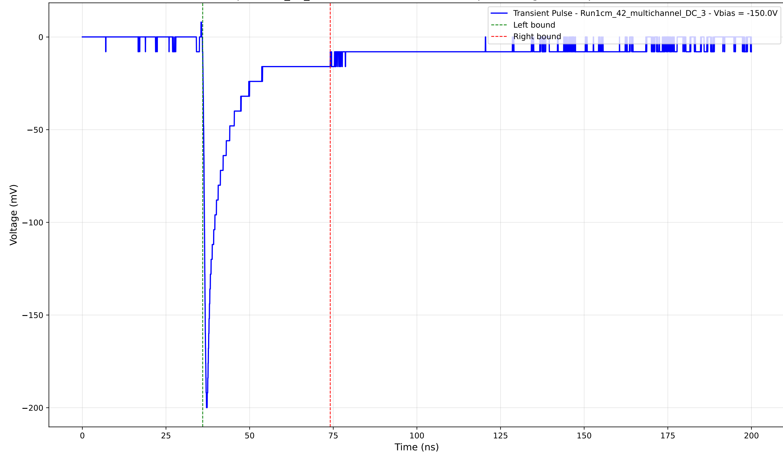
Transient Pulse - Sample: 1cm_42_multichannel - Position: 295.0 \mu\text{m} - Charge: 28.71 pC - Rise Time: 0.87 ns
