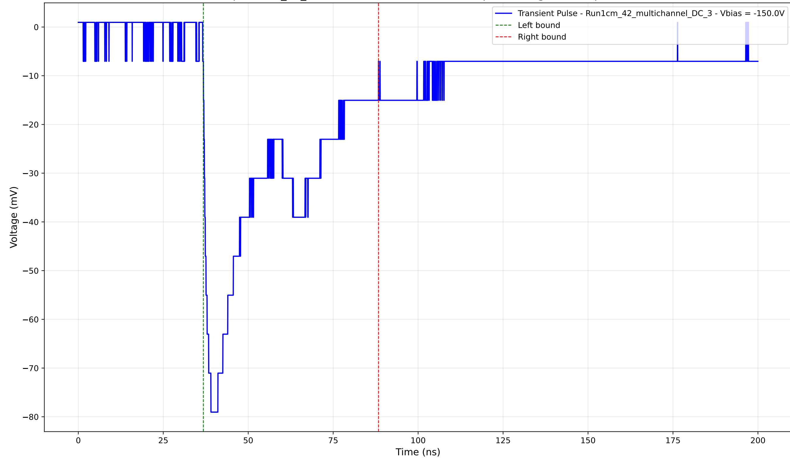
Transient Pulse - Sample: 1cm_42_multichannel - Position: 2530.0 \mu\text{m} - Charge: 34.53 pC - Rise Time: 2.22 ns
