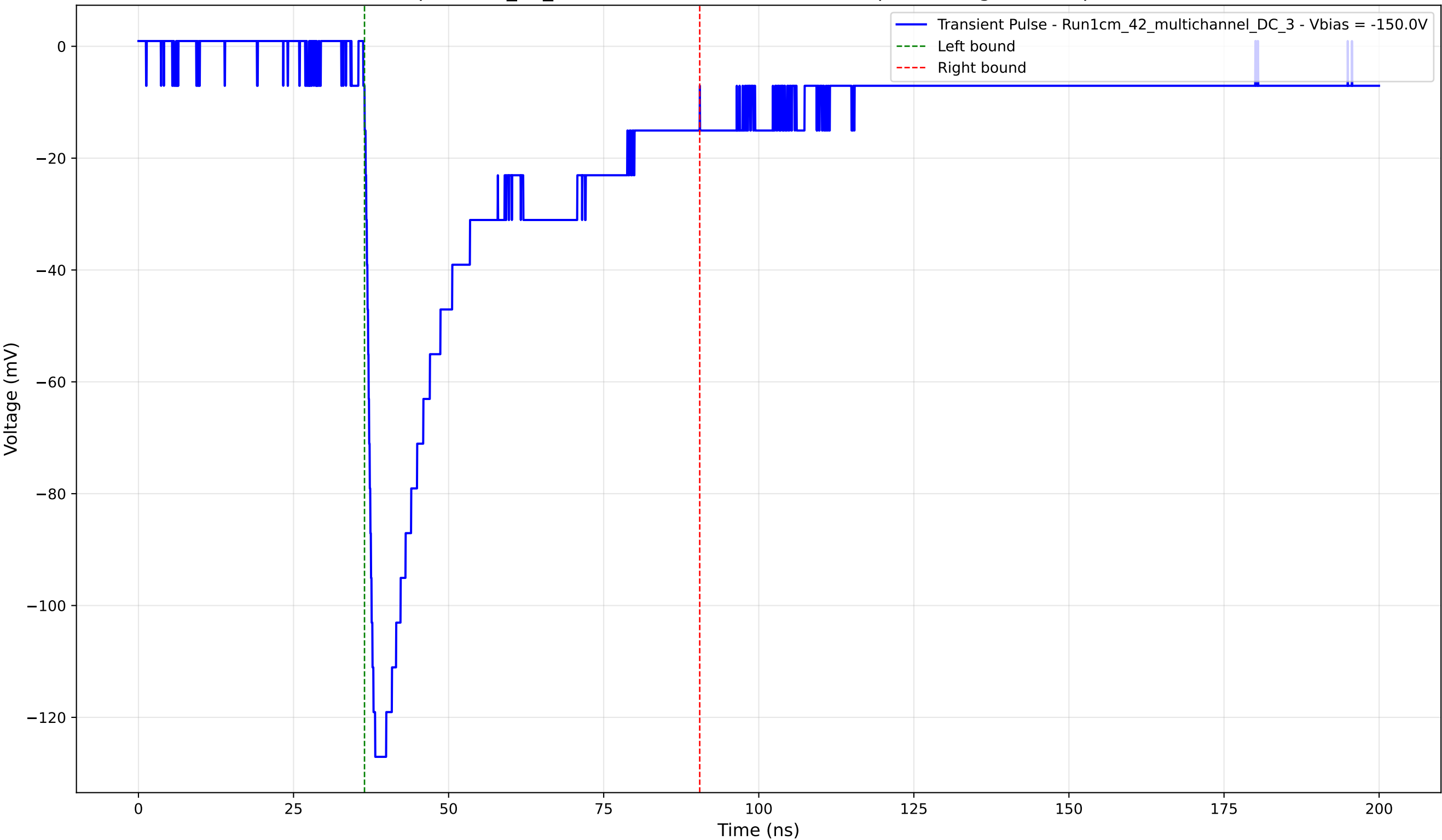
Transient Pulse - Sample: 1cm_42_multichannel - Position: 1530.0 \mu\text{m} - Charge: 43.11 pC - Rise Time: 1.43 ns
