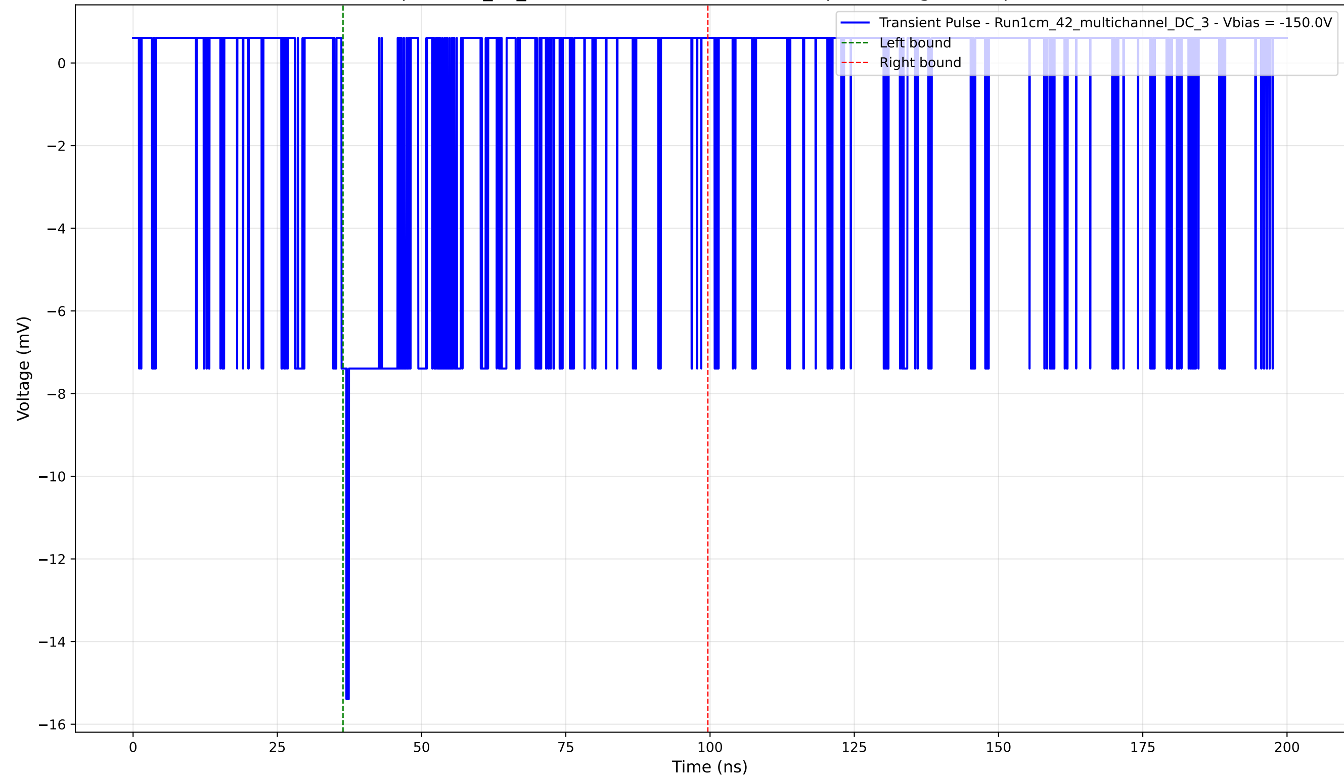
Transient Pulse - Sample: 1cm_42_multichannel - Position: 4905.0 \mu\text{m} - Charge: 2.70 pC - Rise Time: 0.88 ns
