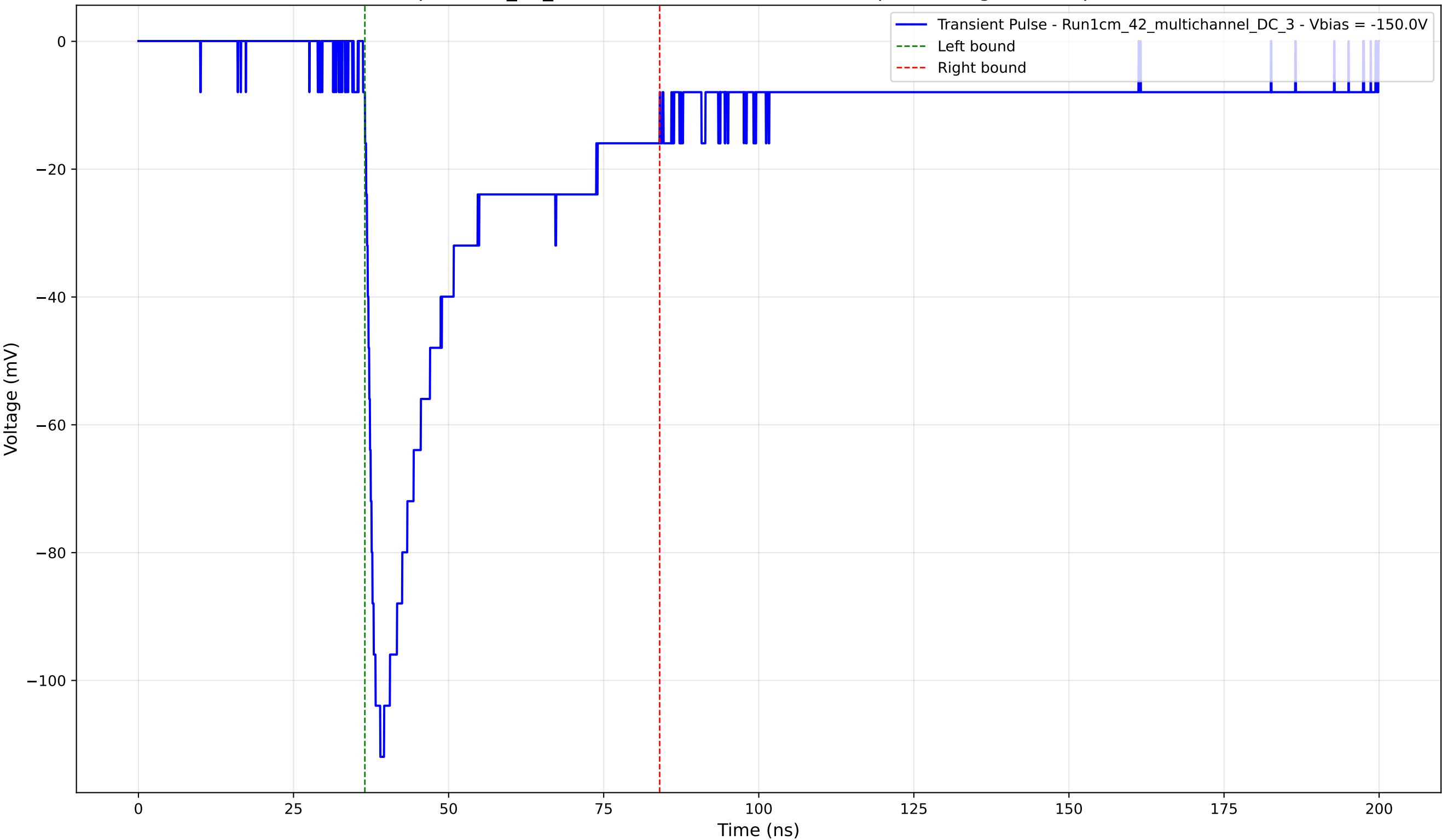
Transient Pulse - Sample: 1cm_42_multichannel - Position: 3305.0 \mu\text{m} - Charge: 34.87 pC - Rise Time: 1.71 ns
