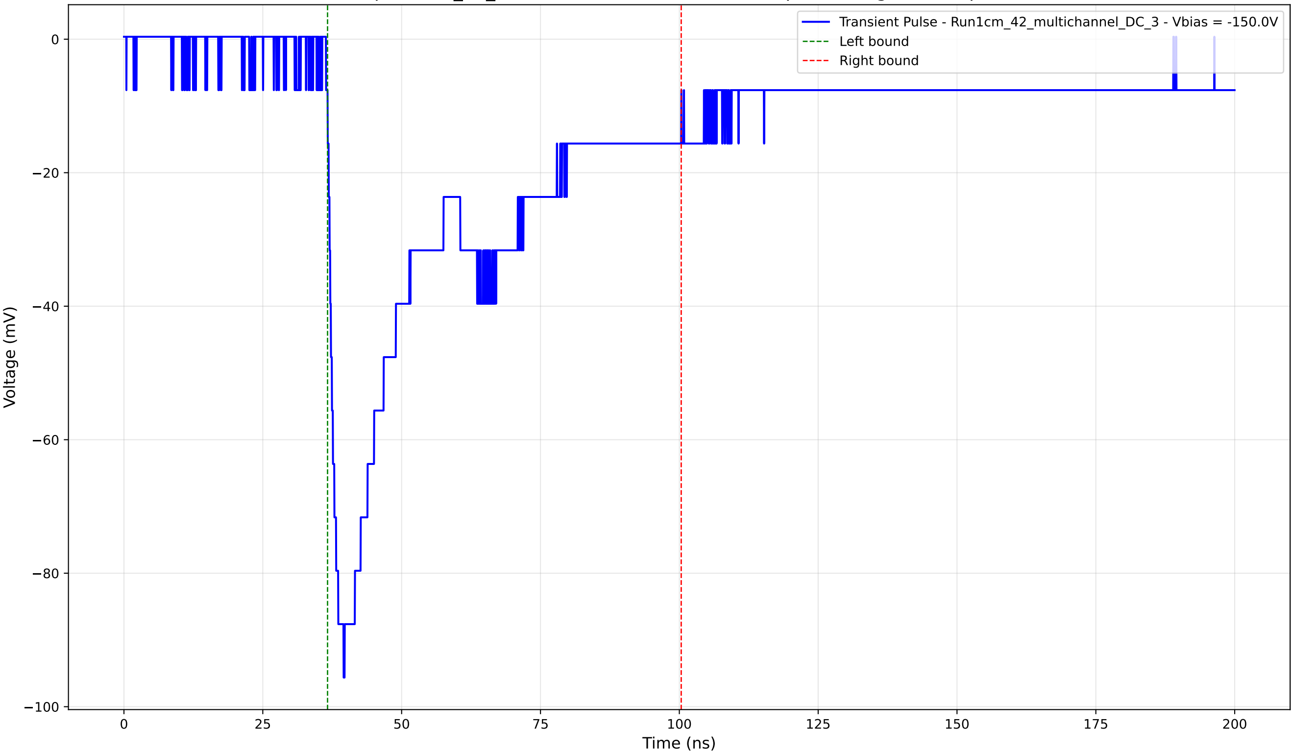
Transient Pulse - Sample: 1cm_42_multichannel - Position: 2715.0 \mu\text{m} - Charge: 41.00 pC - Rise Time: 1.92 ns
