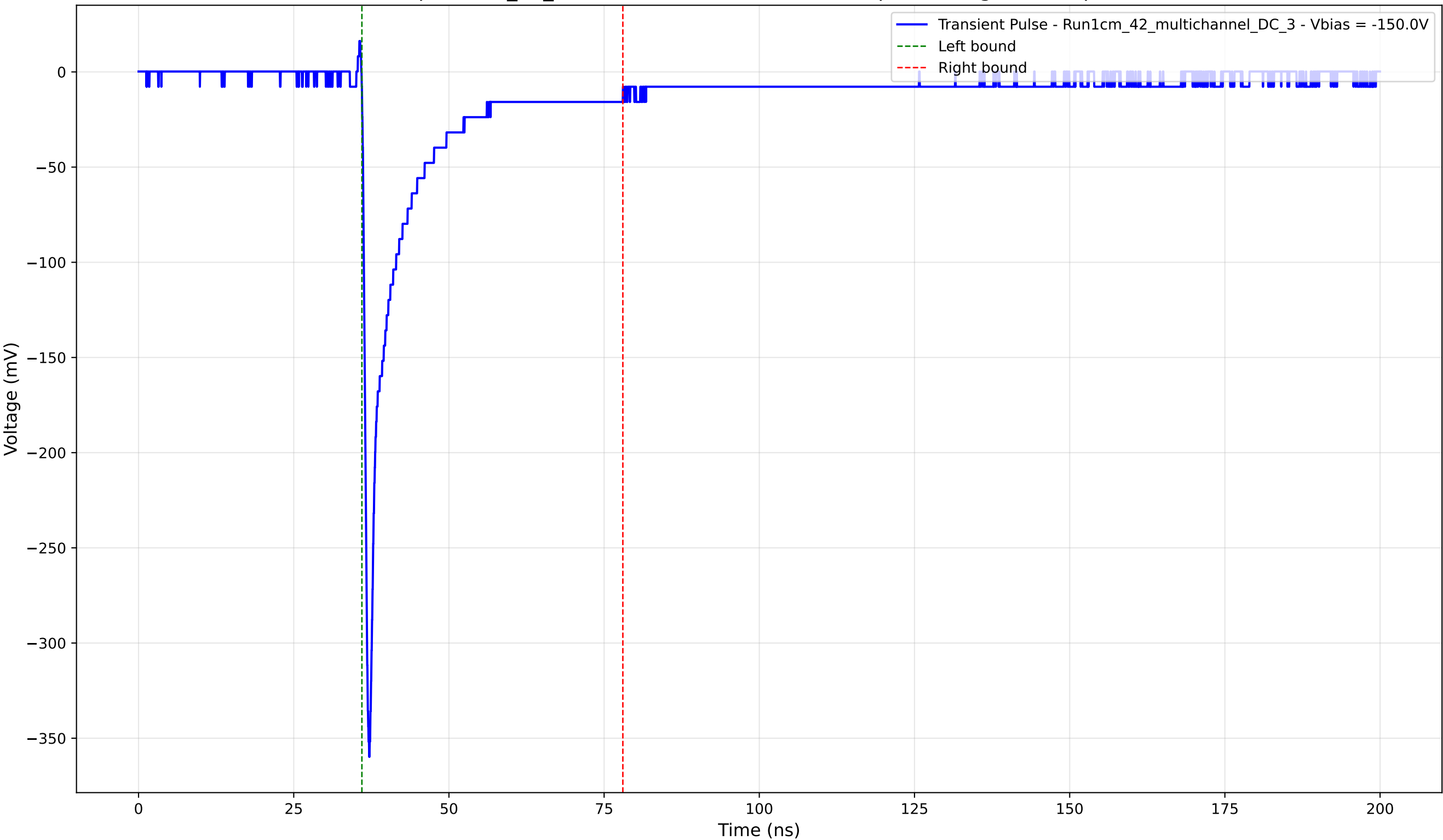
Transient Pulse - Sample: 1cm_42_multichannel - Position: 4800.0 \mu\text{m} - Charge: 39.62 pC - Rise Time: 0.79 ns
