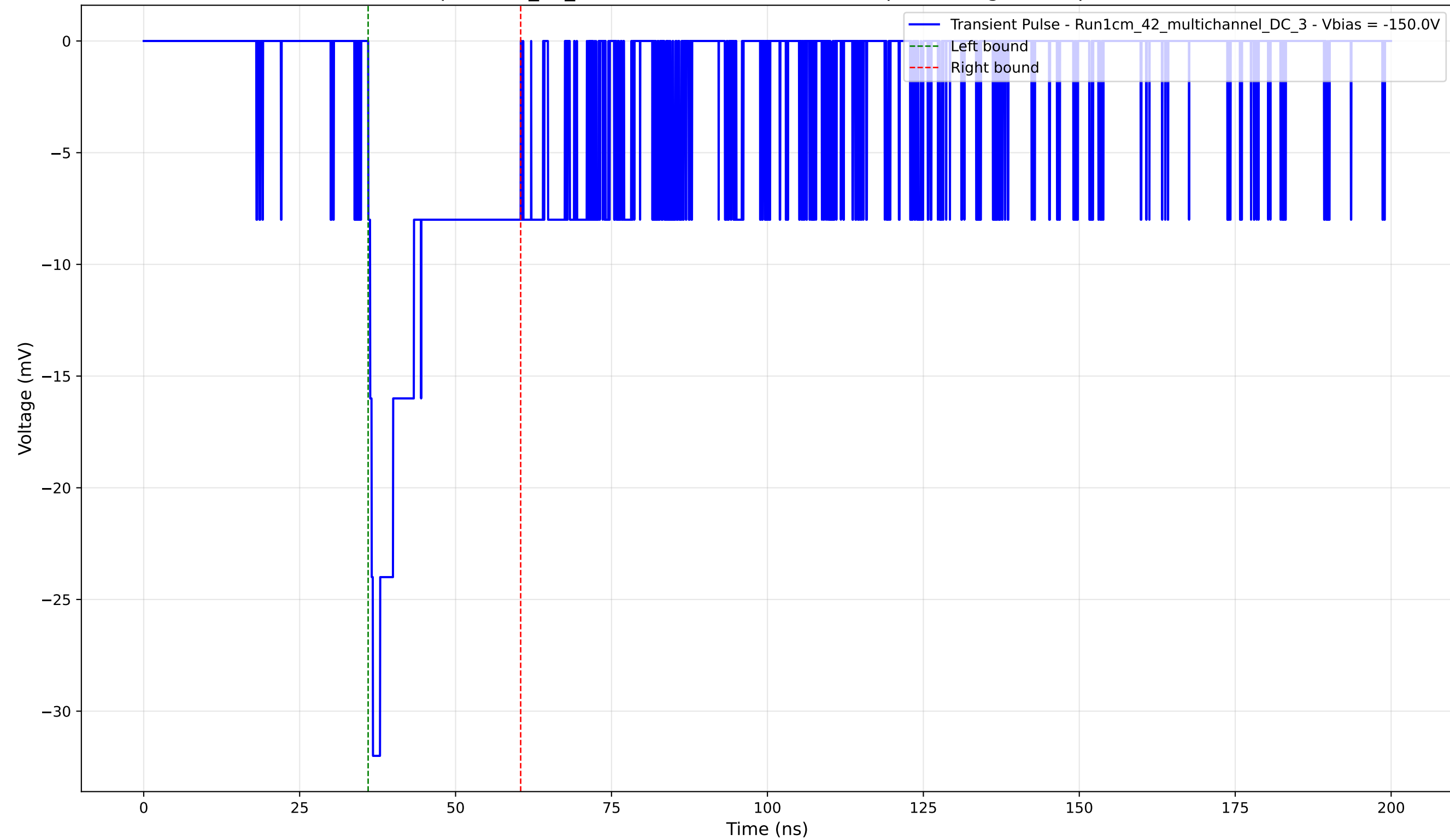
Transient Pulse - Sample: 1cm_42_multichannel - Position: 325.0 \mu\text{m} - Charge: 5.78 pC - Rise Time: 0.75 ns
