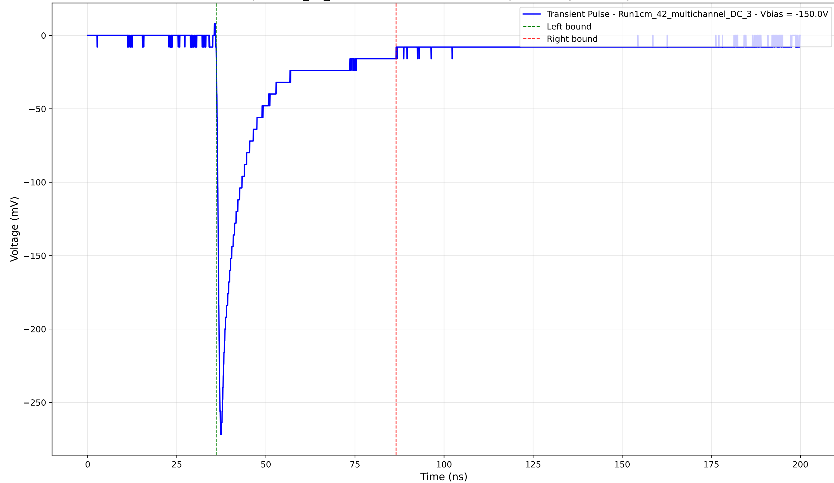
Transient Pulse - Sample: 1cm_42_multichannel - Position: 510.0 \mu\text{m} - Charge: 49.57 pC - Rise Time: 0.91 ns
