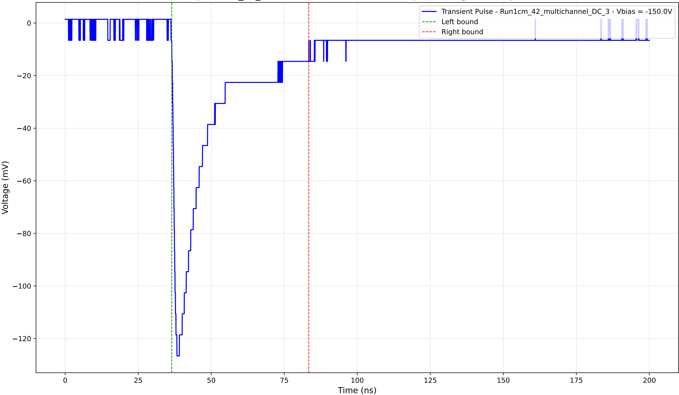
Transient Pulse - Sample: 1cm_42_multichannel - Position: 3615.0 \mu\text{m} - Charge: 35.14 pC - Rise Time: 1.42 ns
