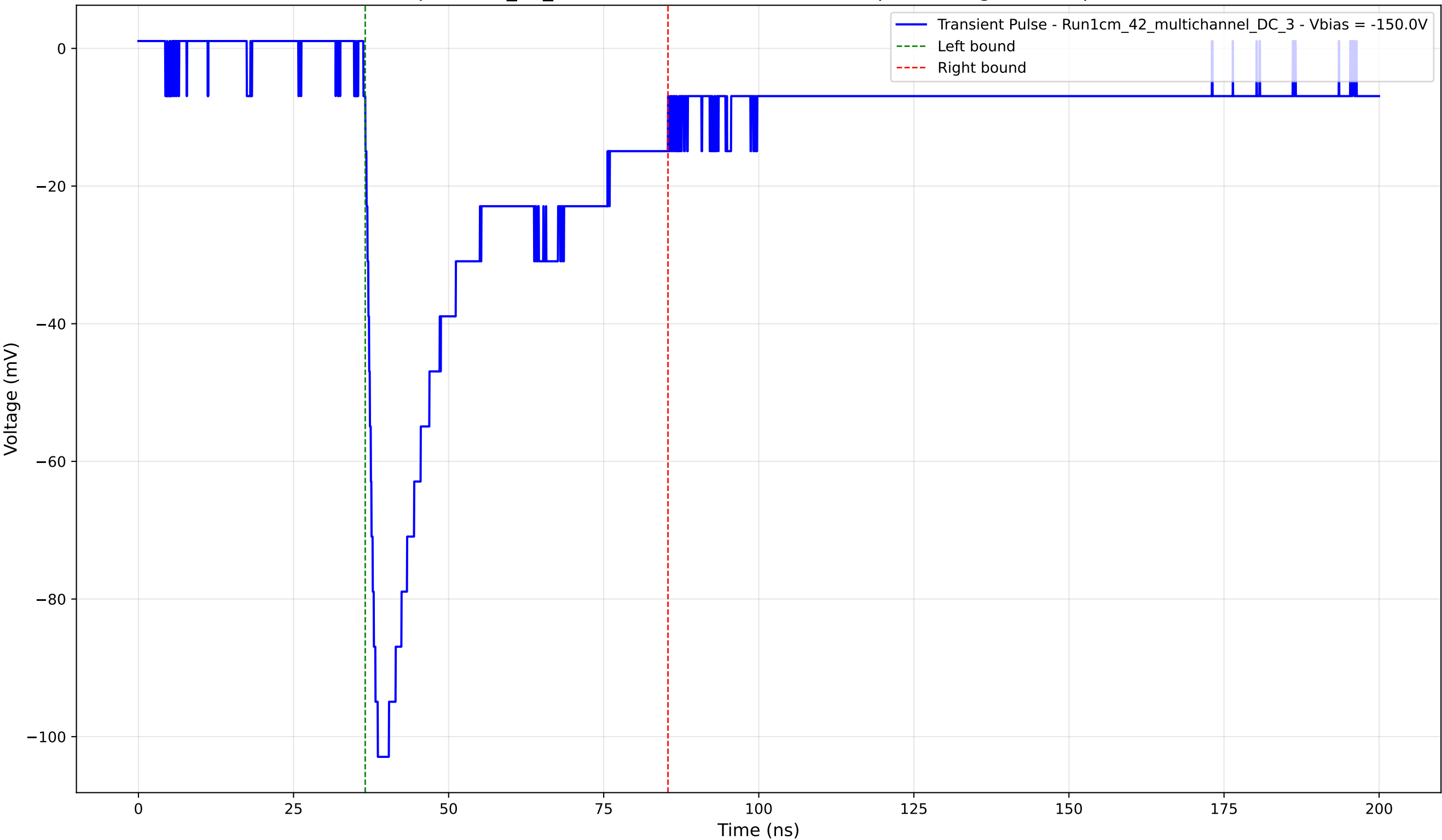
Transient Pulse - Sample: 1cm_42_multichannel - Position: 3145.0 \mu\text{m} - Charge: 34.73 pC - Rise Time: 1.63 ns
