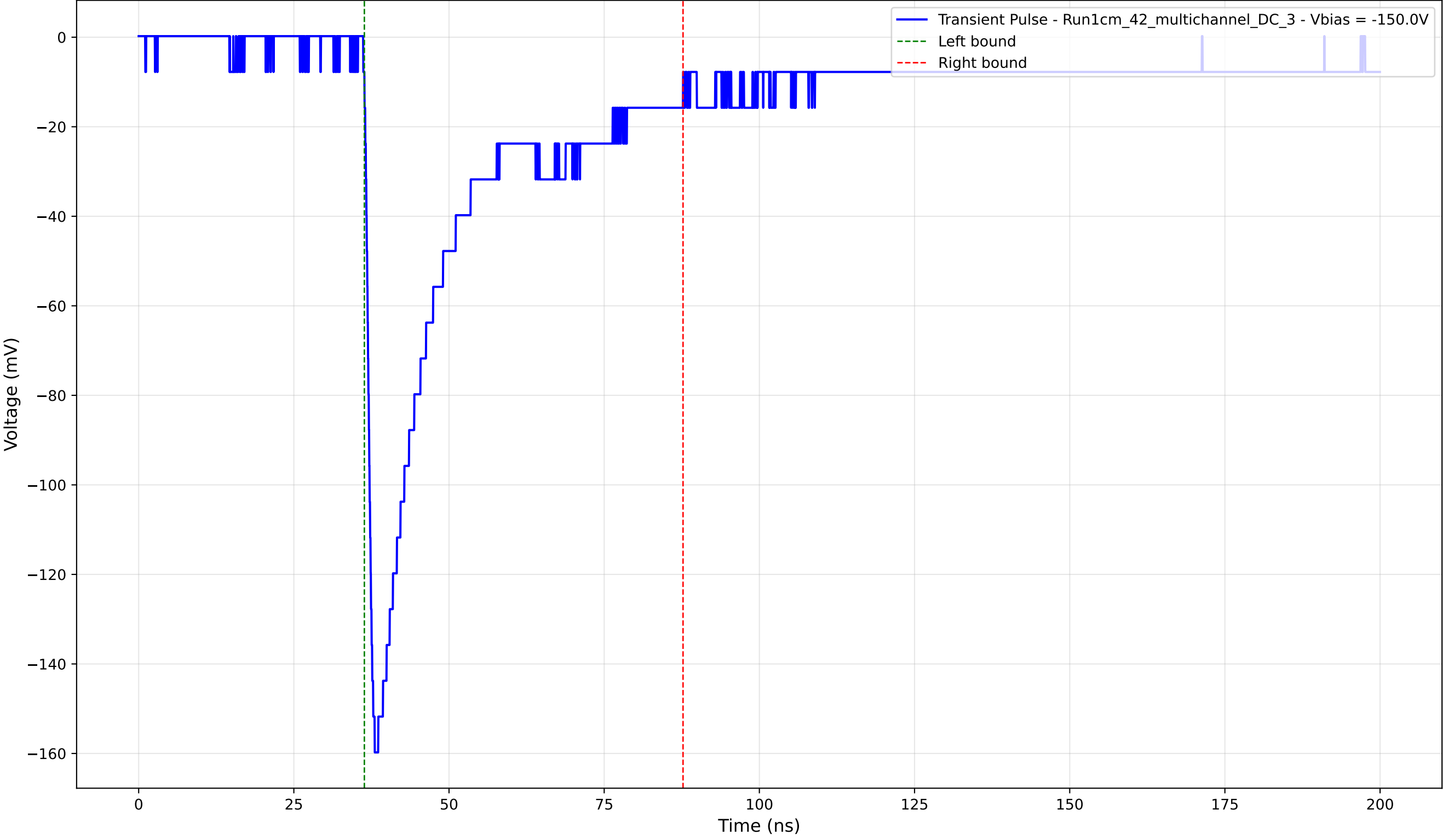
Transient Pulse - Sample: 1cm_42_multichannel - Position: 1190.0 \mu\text{m} - Charge: 44.61 pC - Rise Time: 1.30 ns
