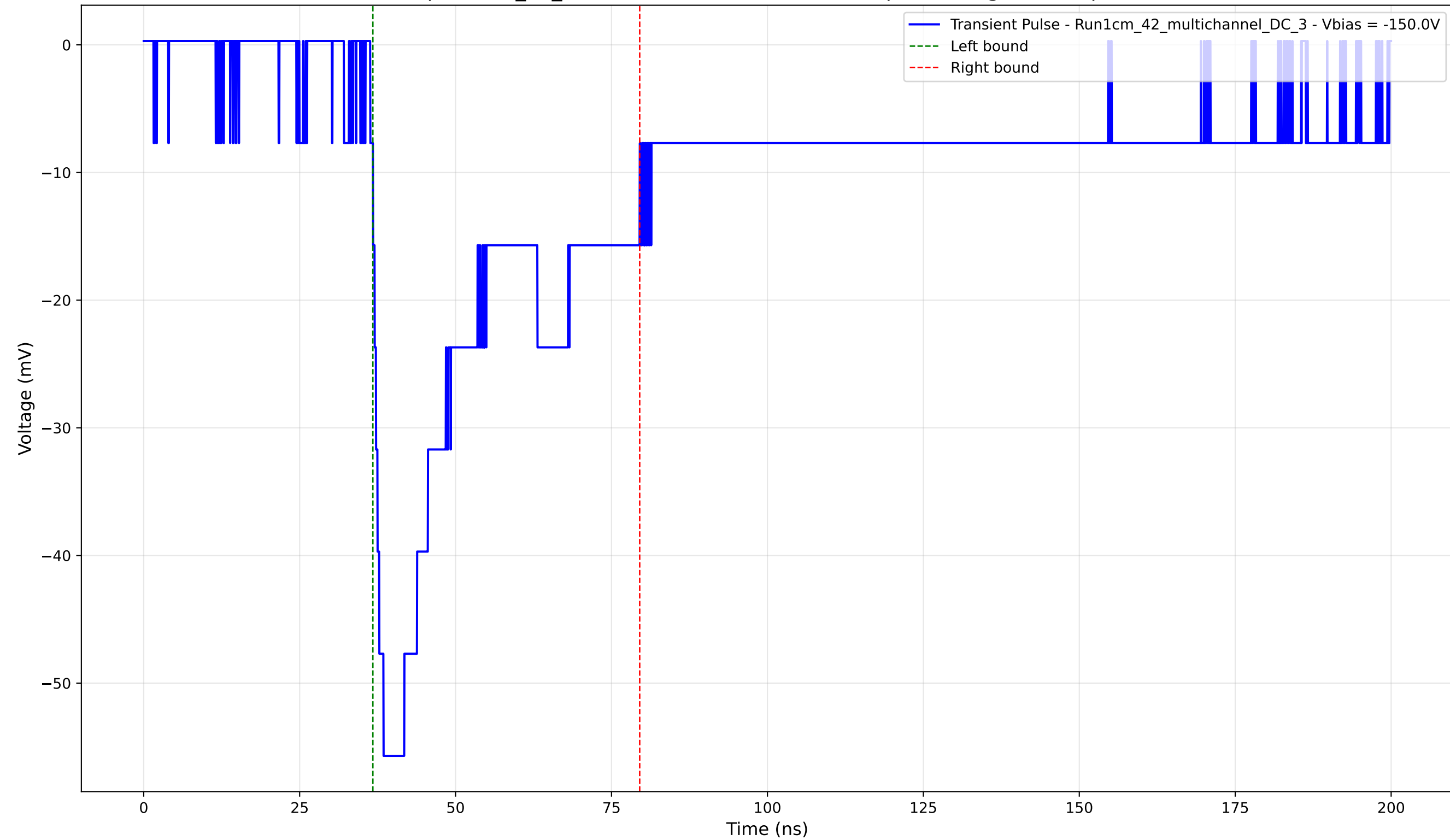
Transient Pulse - Sample: 1cm_42_multichannel - Position: 2825.0 \mu\text{m} - Charge: 21.64 pC - Rise Time: 2.13 ns
