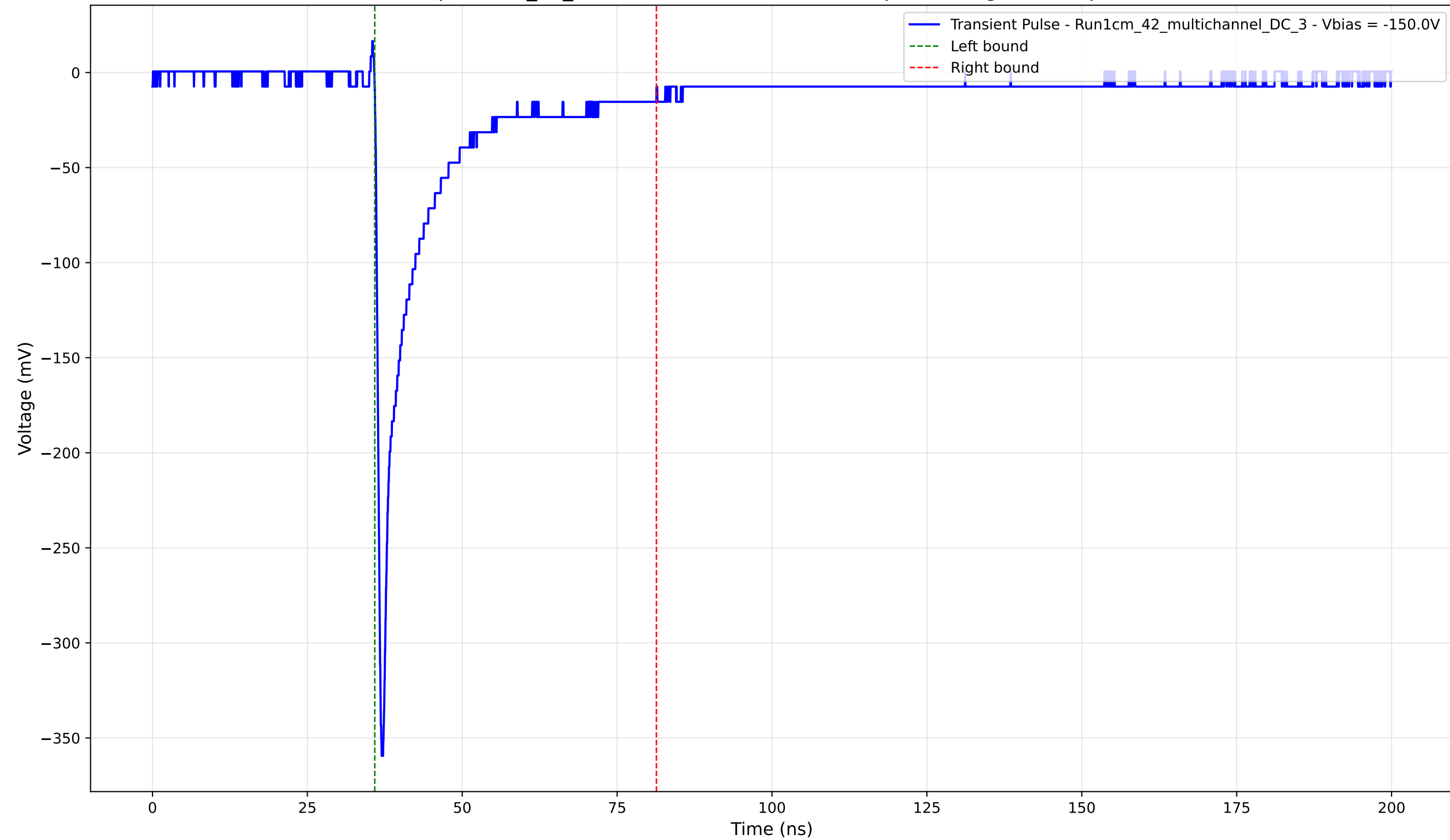
Transient Pulse - Sample: 1cm_42_multichannel - Position: 180.0 \mu\text{m} - Charge: 47.12 pC - Rise Time: 0.79 ns
