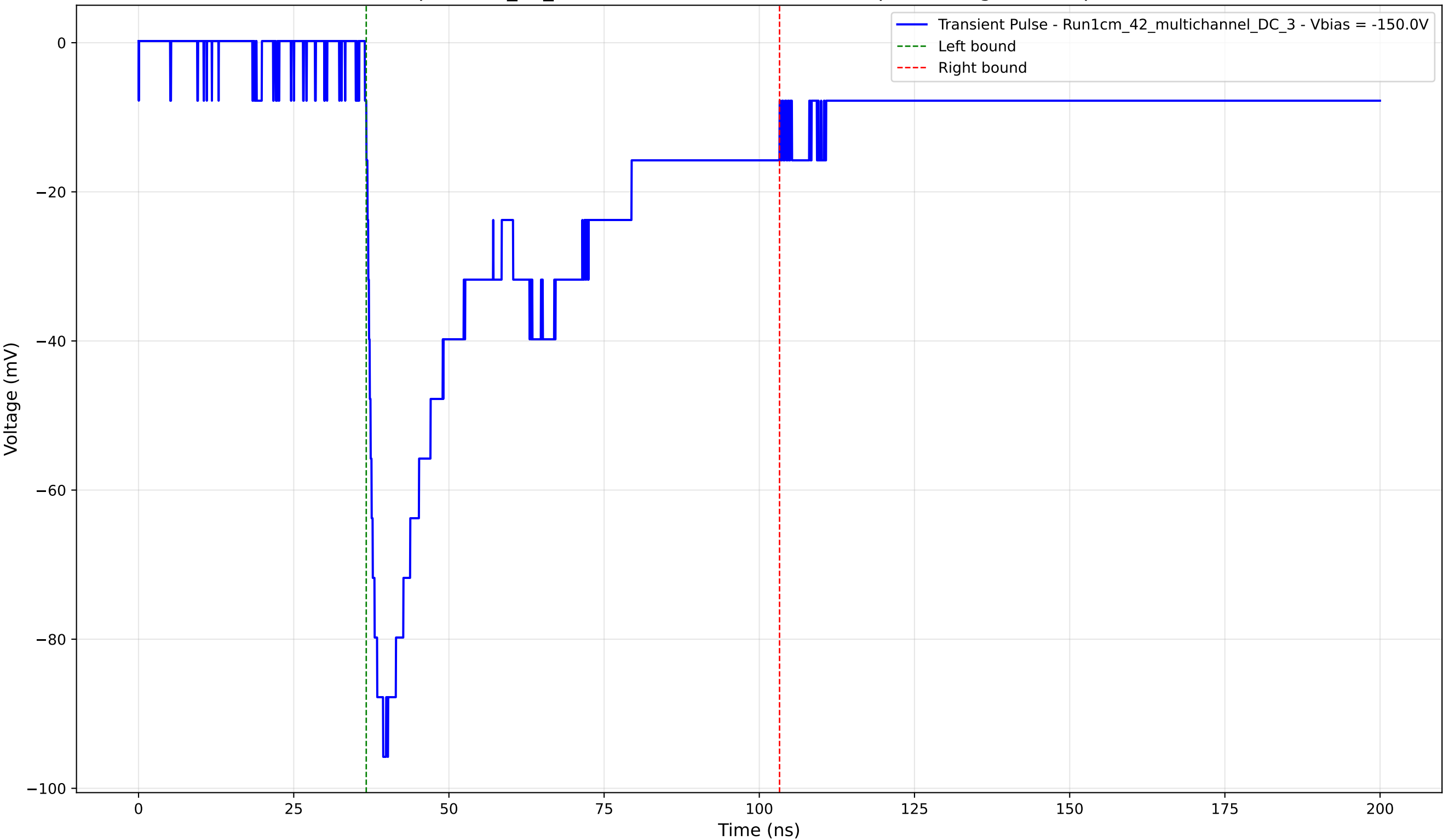
Transient Pulse - Sample: 1cm_42_multichannel - Position: 2070.0 \mu\text{m} - Charge: 43.08 pC - Rise Time: 1.76 ns
