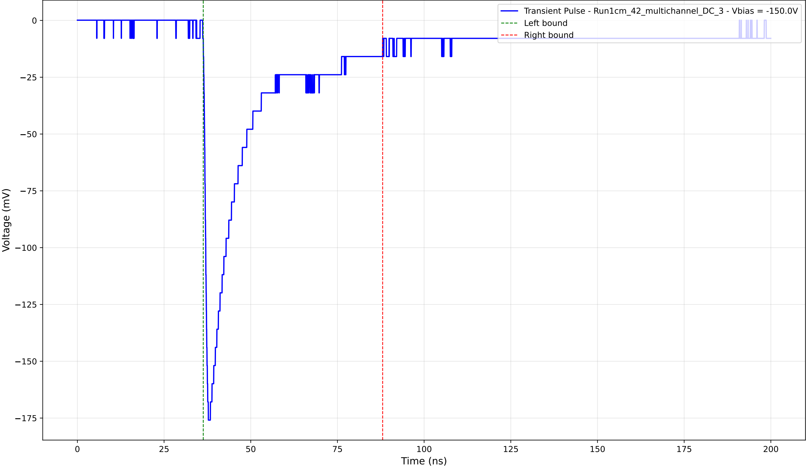
Transient Pulse - Sample: 1cm_42_multichannel - Position: 1005.0 \mu\text{m} - Charge: 45.25 pC - Rise Time: 1.08 ns
