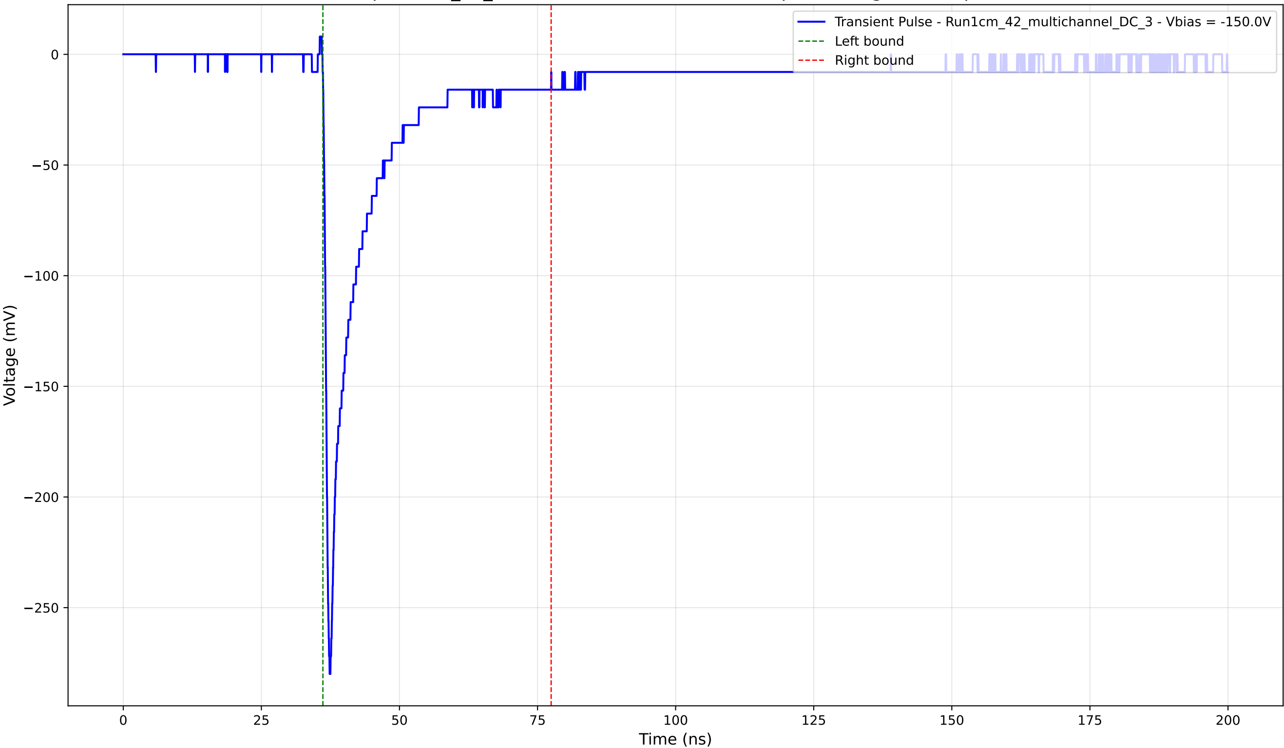
Transient Pulse - Sample: 1cm_42_multichannel - Position: 4535.0 \mu\text{m} - Charge: 39.86 pC - Rise Time: 0.87 ns
