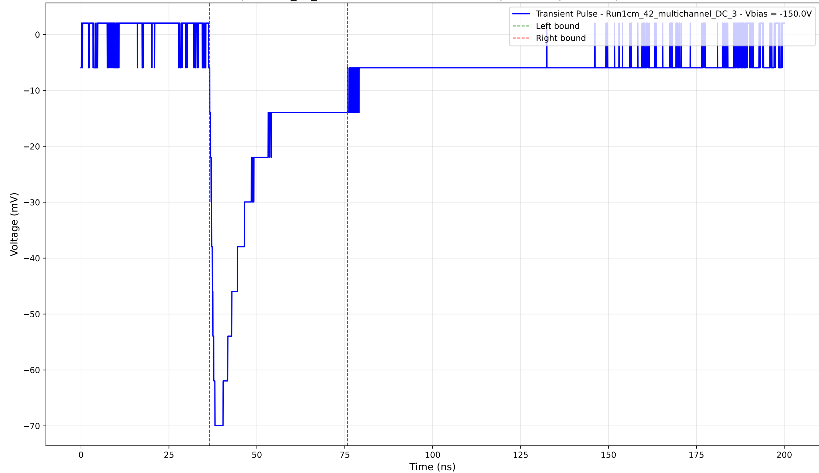
Transient Pulse - Sample: 1cm_42_multichannel - Position: 3440.0 \mu\text{m} - Charge: 19.96 pC - Rise Time: 1.50 ns
