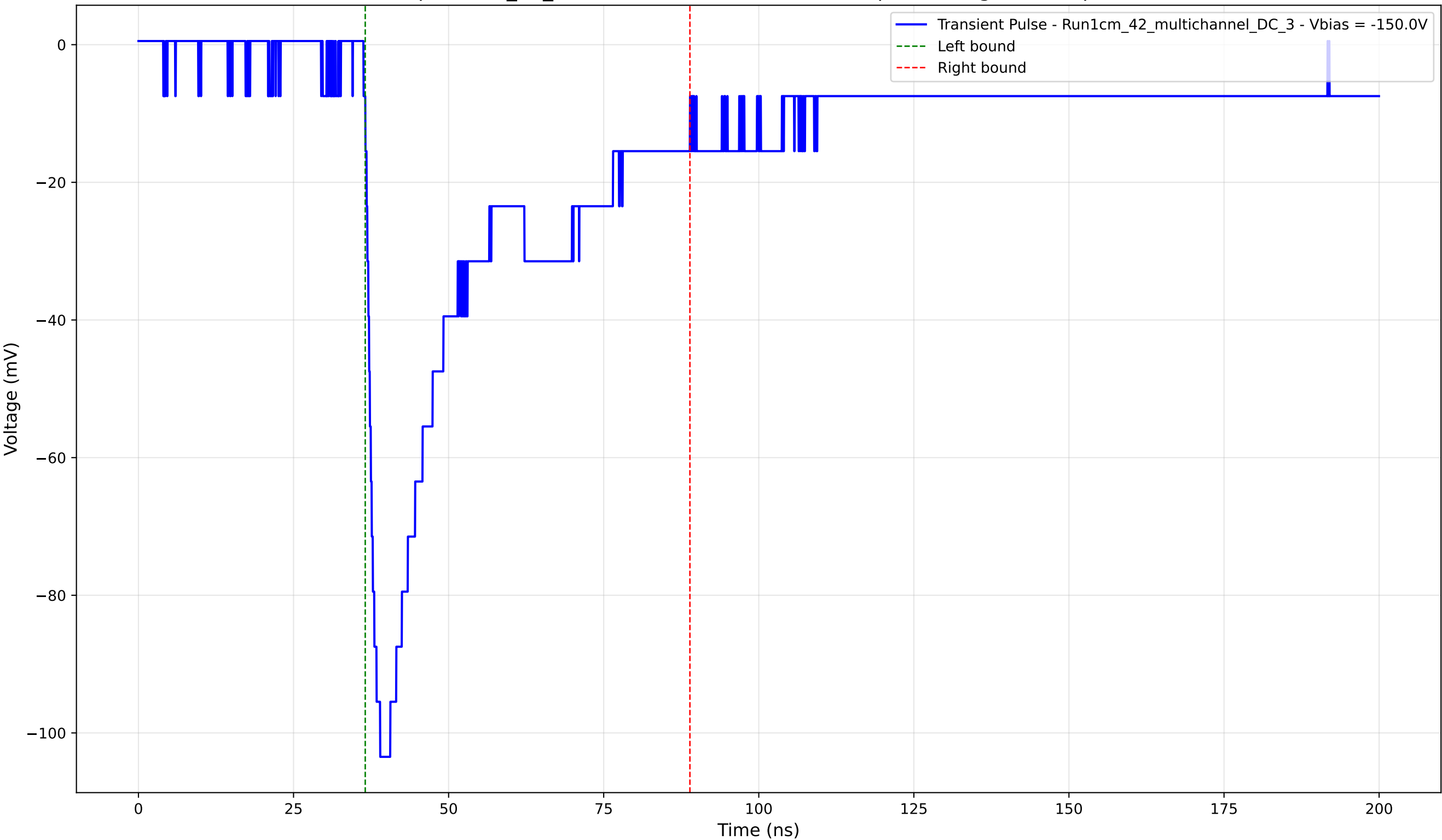
Transient Pulse - Sample: 1cm_42_multichannel - Position: 3010.0 \mu\text{m} - Charge: 37.77 pC - Rise Time: 1.81 ns
