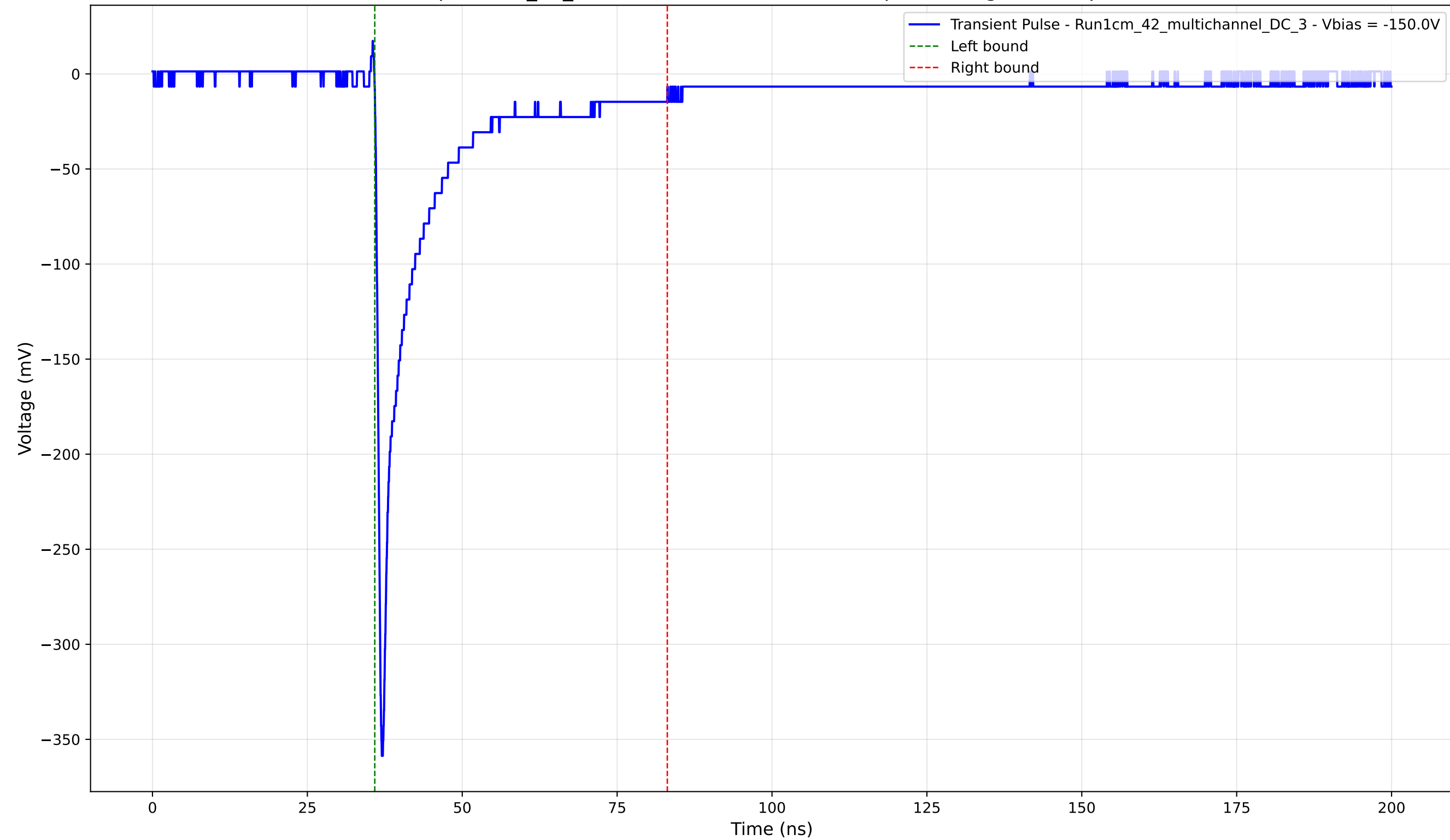
Transient Pulse - Sample: 1cm_42_multichannel - Position: 185.0 \mu\text{m} - Charge: 47.05 pC - Rise Time: 0.81 ns
