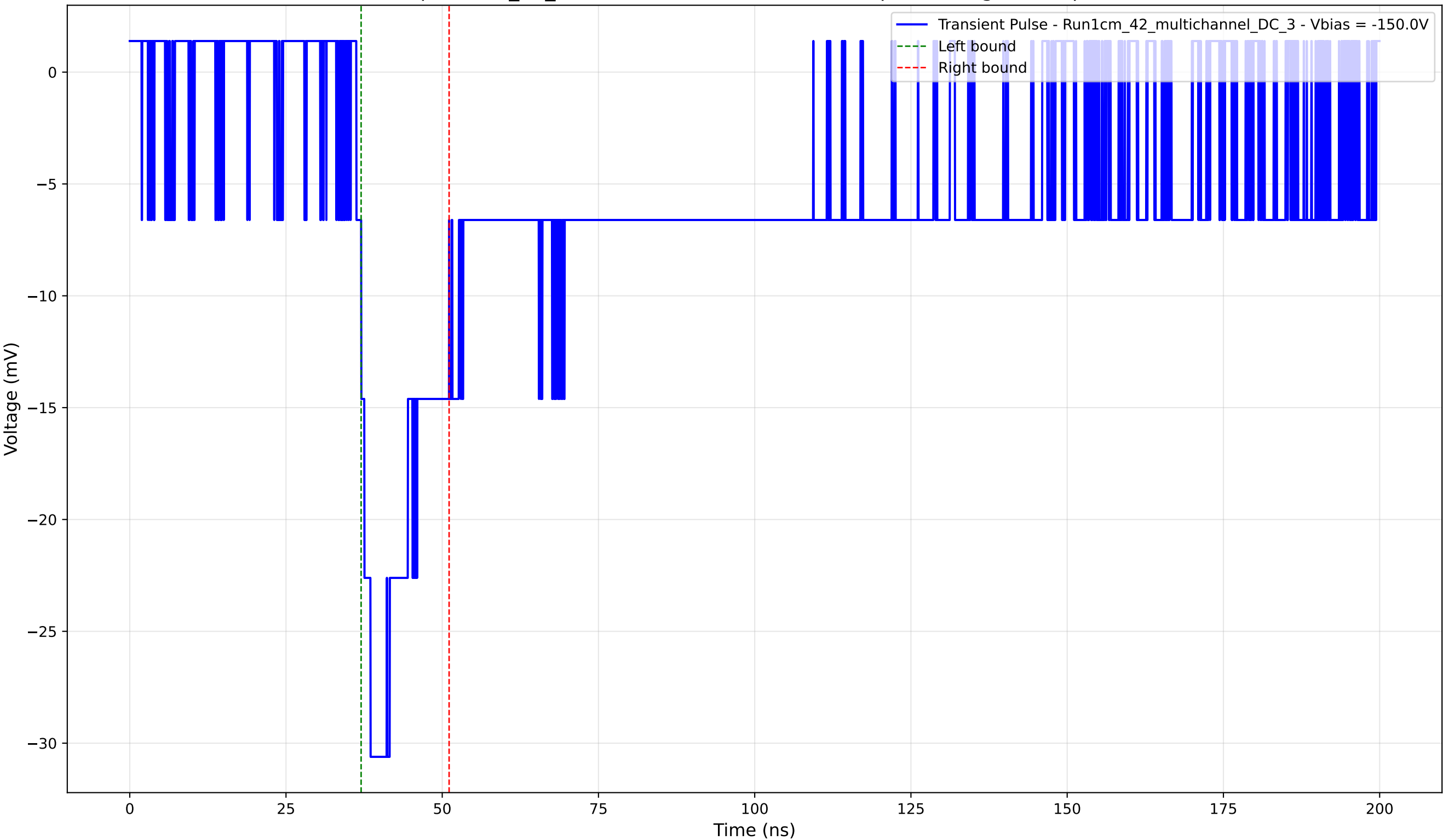
Transient Pulse - Sample: 1cm_42_multichannel - Position: 2840.0 \mu\text{m} - Charge: 5.76 pC - Rise Time: 2.27 ns
