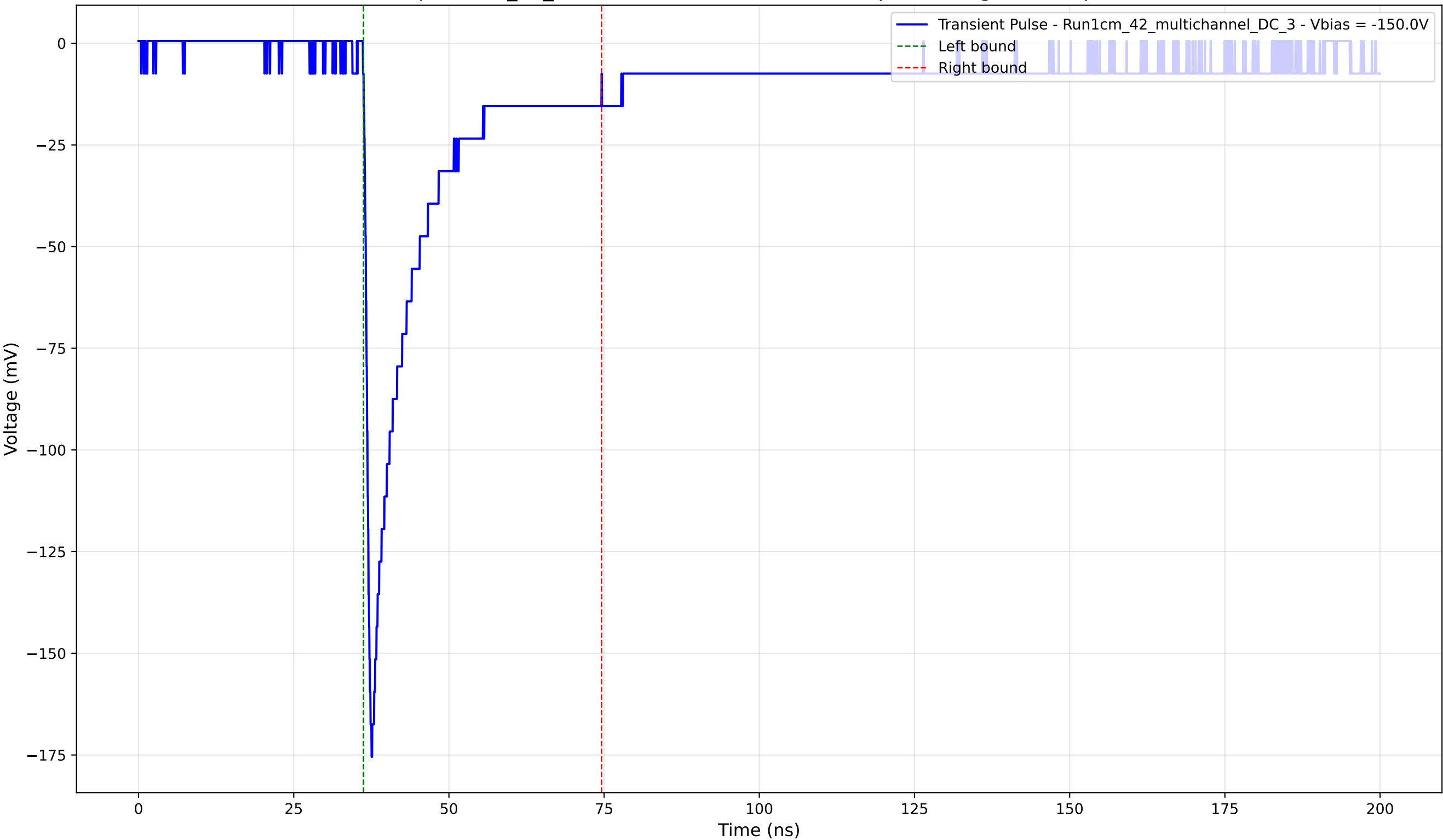
Transient Pulse - Sample: 1cm_42_multichannel - Position: 4320.0 \mu\text{m} - Charge: 29.52 pC - Rise Time: 0.91 ns
