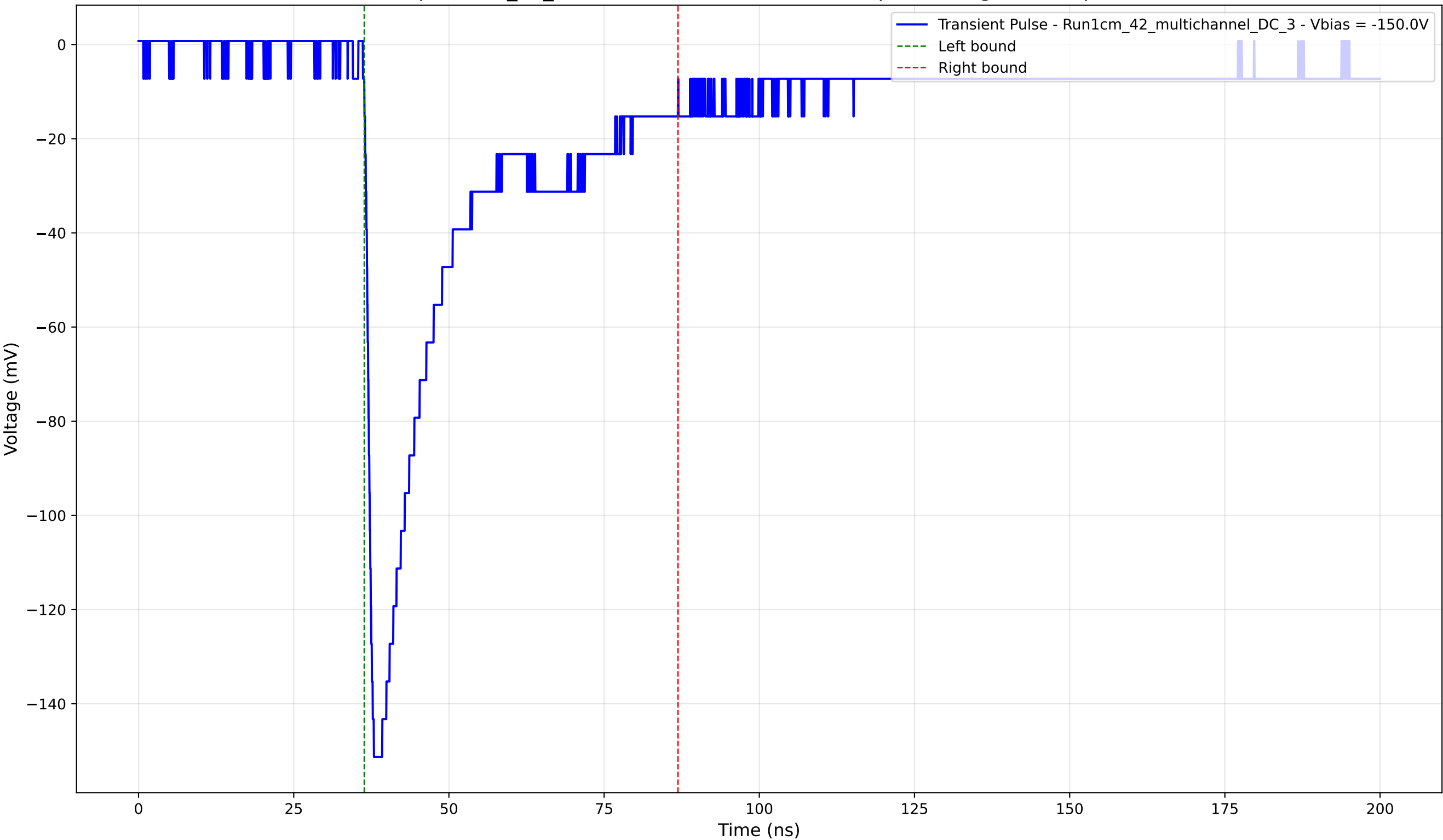
Transient Pulse - Sample: 1cm_42_multichannel - Position: 1245.0 \mu\text{m} - Charge: 44.30 pC - Rise Time: 1.34 ns
