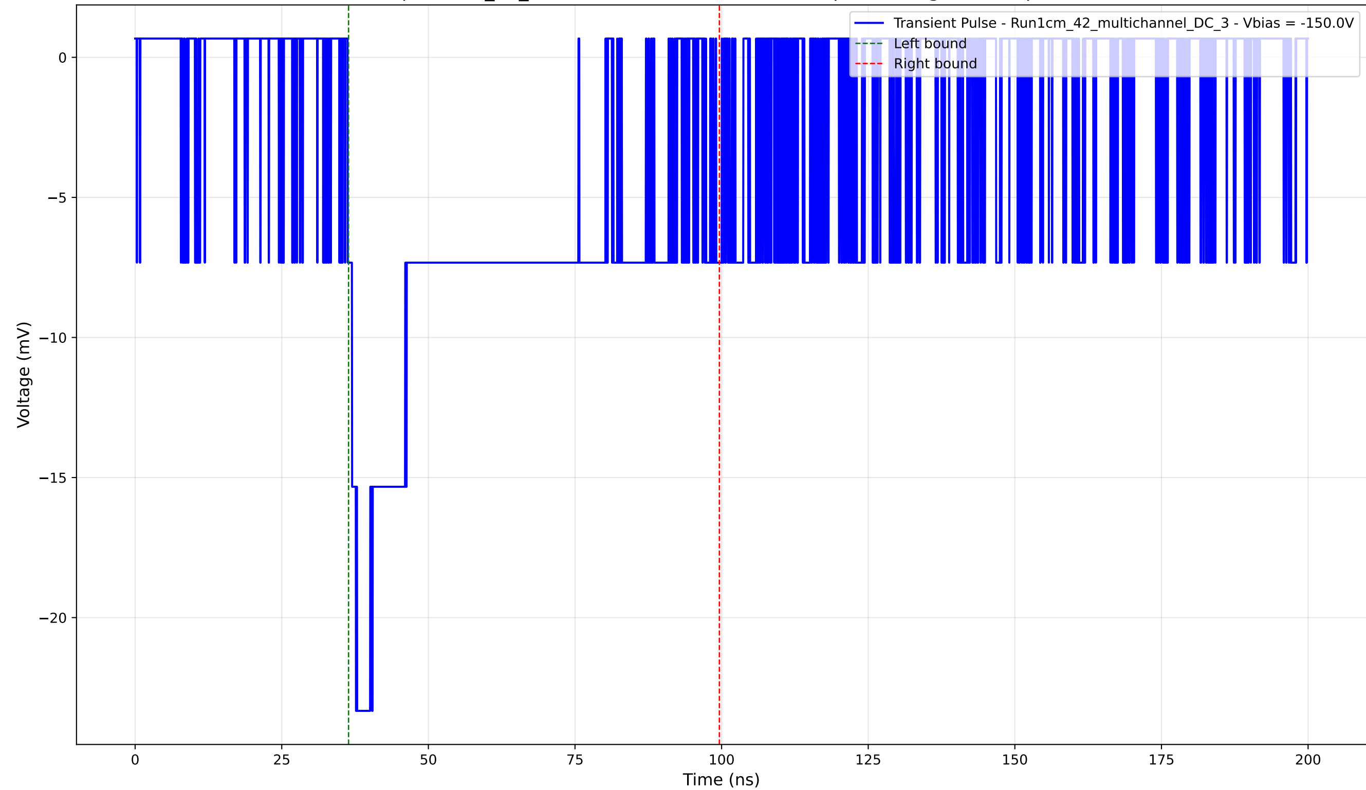
Transient Pulse - Sample: 1cm_42_multichannel - Position: 1335.0 \mu\text{m} - Charge: 10.14 pC - Rise Time: 1.42 ns
