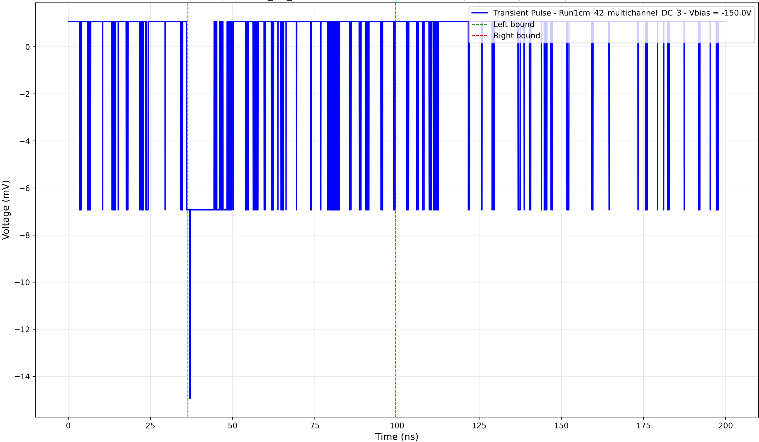
Transient Pulse - Sample: 1cm_42_multichannel - Position: 4915.0 \mu\text{m} - Charge: 1.58 pC - Rise Time: 0.90 ns
