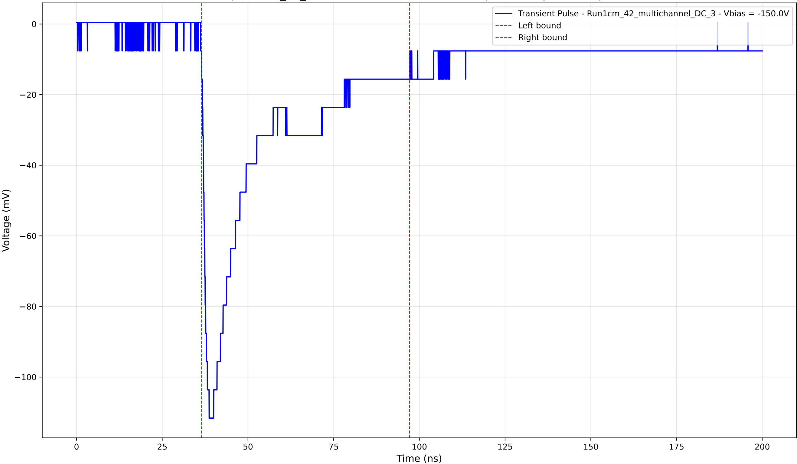
Transient Pulse - Sample: 1cm_42_multichannel - Position: 1770.0 \mu\text{m} - Charge: 42.54 pC - Rise Time: 1.67 ns
