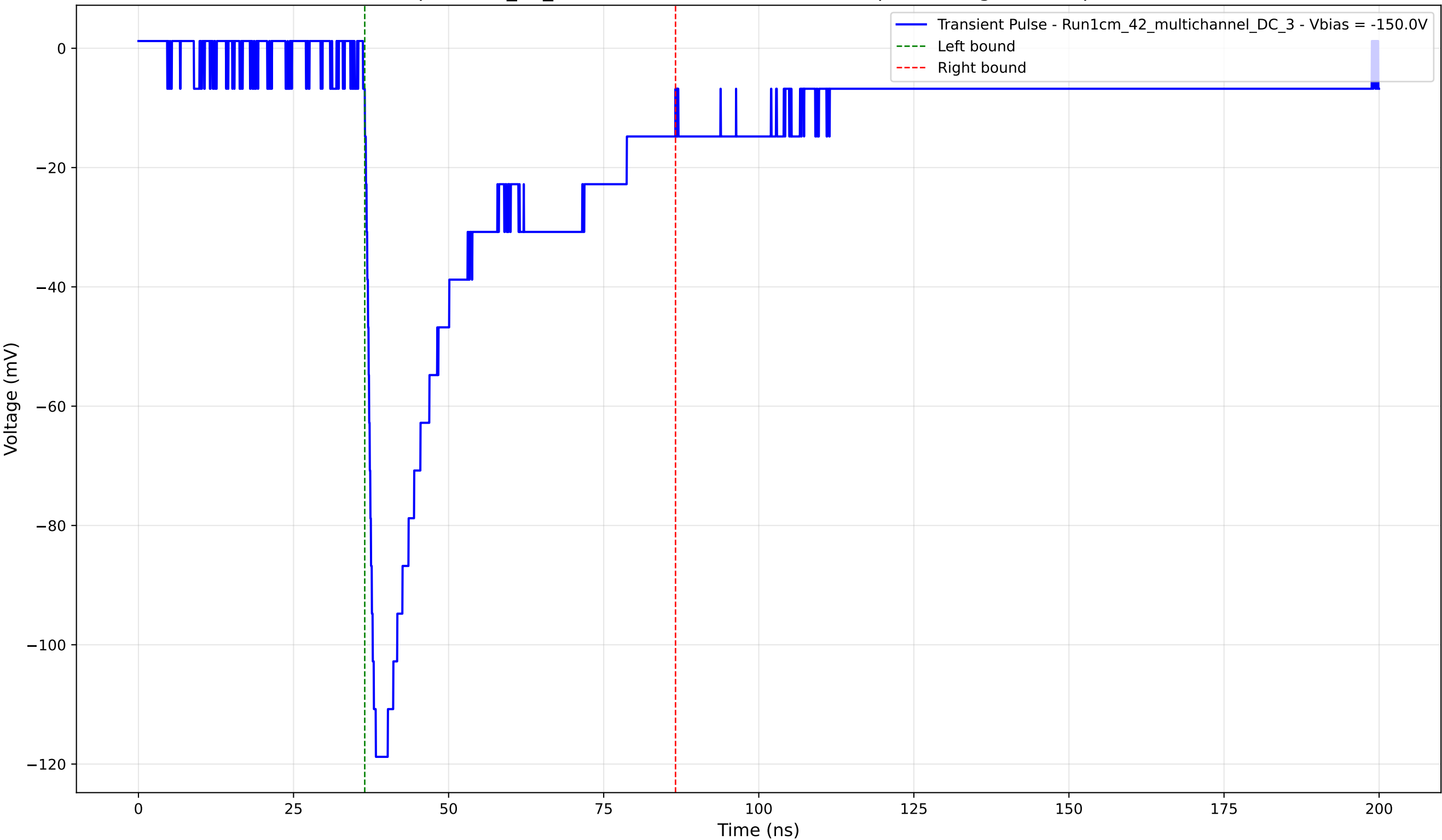
Transient Pulse - Sample: 1cm_42_multichannel - Position: 1615.0 \mu\text{m} - Charge: 40.40 pC - Rise Time: 1.45 ns
