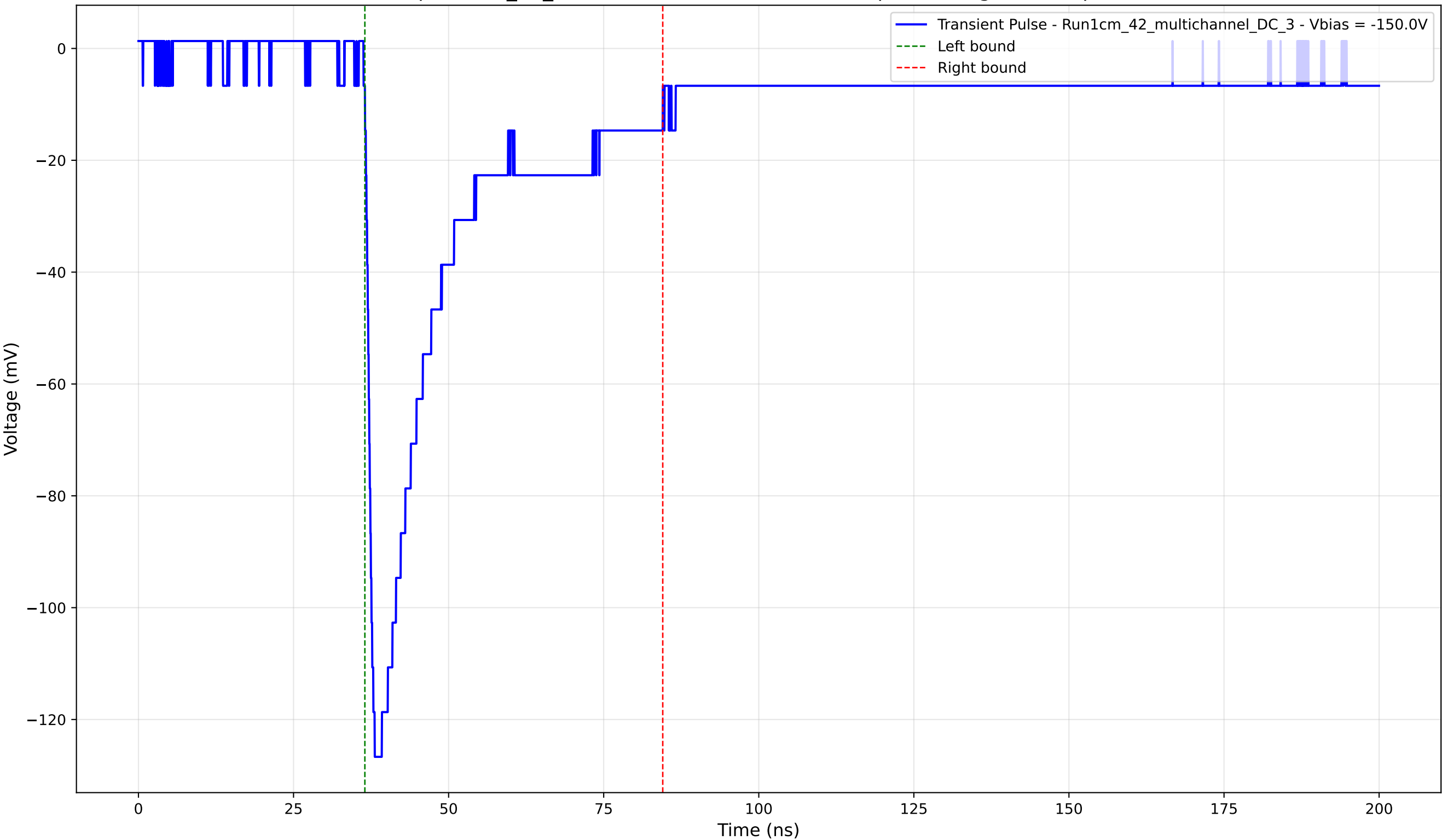
Transient Pulse - Sample: 1cm_42_multichannel - Position: 3635.0 \mu\text{m} - Charge: 35.47 pC - Rise Time: 1.35 ns
