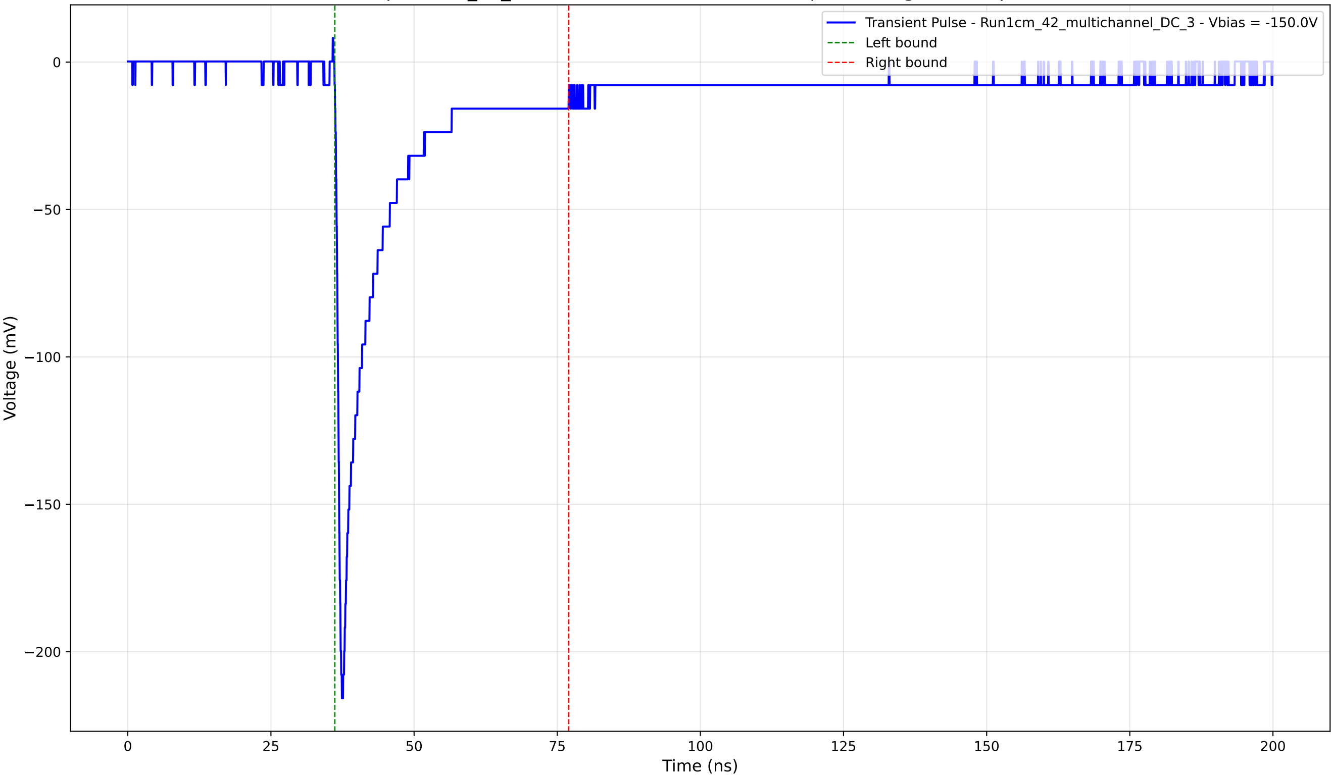
Transient Pulse - Sample: 1cm_42_multichannel - Position: 4465.0 \mu\text{m} - Charge: 33.36 pC - Rise Time: 0.93 ns
