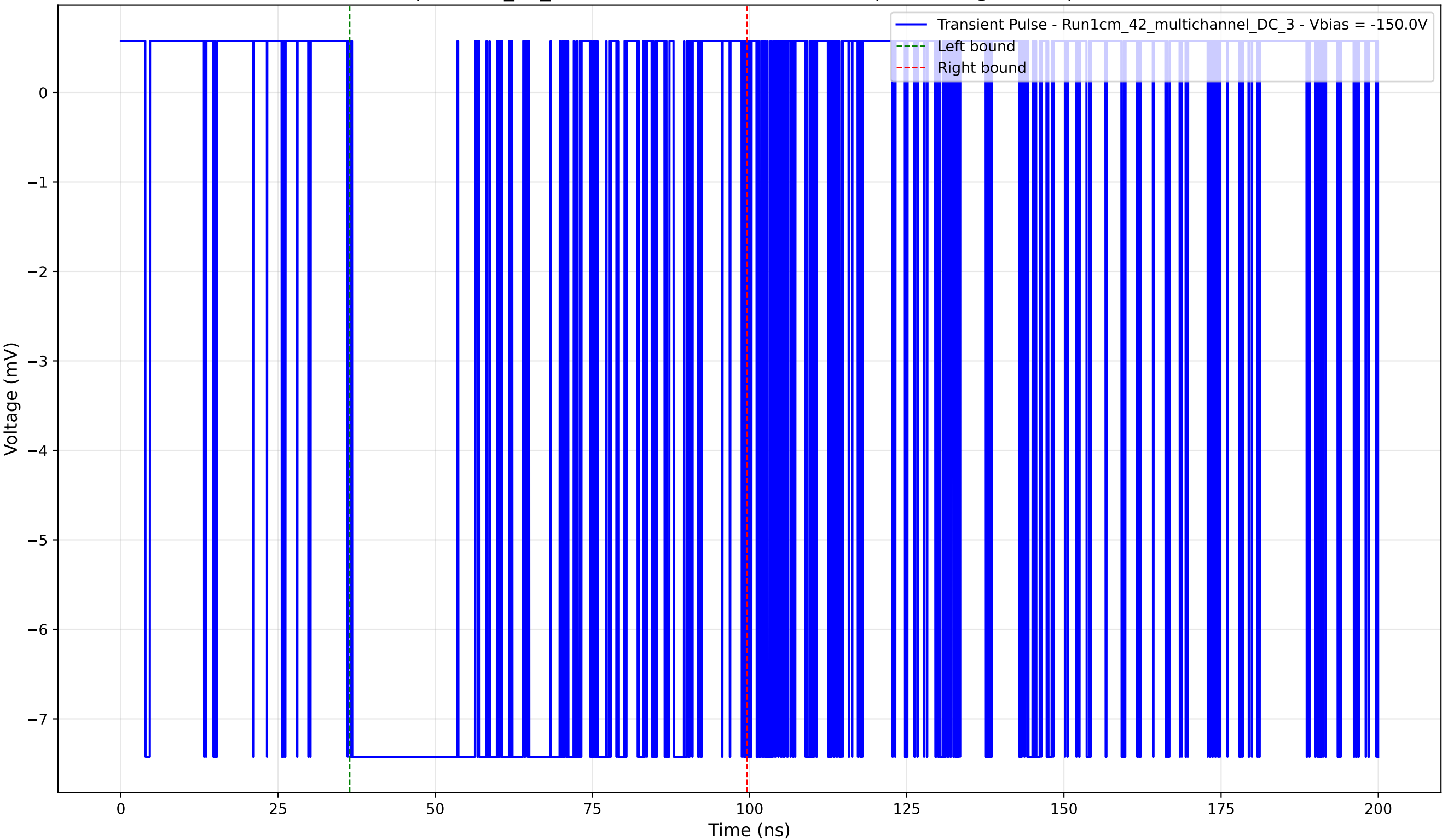
Transient Pulse - Sample: 1cm_42_multichannel - Position: 2375.0 \mu\text{m} - Charge: 6.15 pC - Rise Time: 0.02 ns
