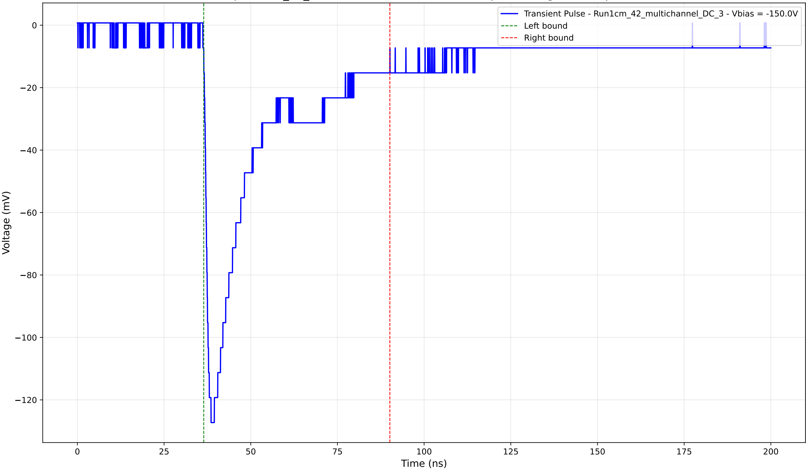
Transient Pulse - Sample: 1cm_42_multichannel - Position: 1570.0 \mu\text{m} - Charge: 42.29 pC - Rise Time: 1.59 ns
