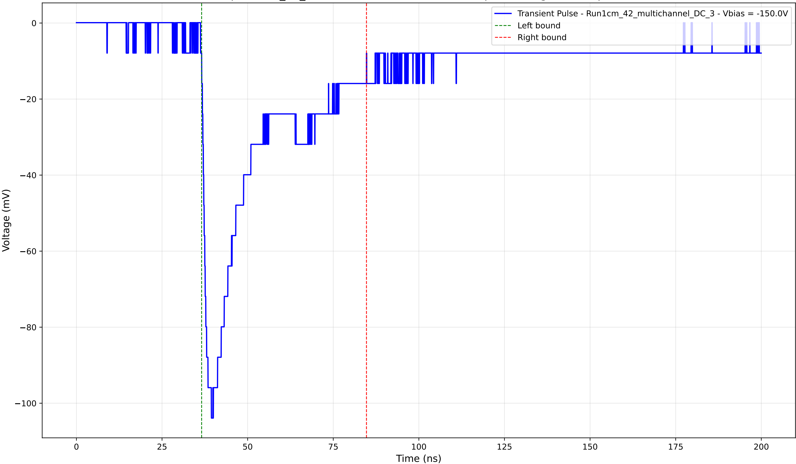
Transient Pulse - Sample: 1cm_42_multichannel - Position: 3100.0 \mu\text{m} - Charge: 35.21 pC - Rise Time: 1.85 ns
