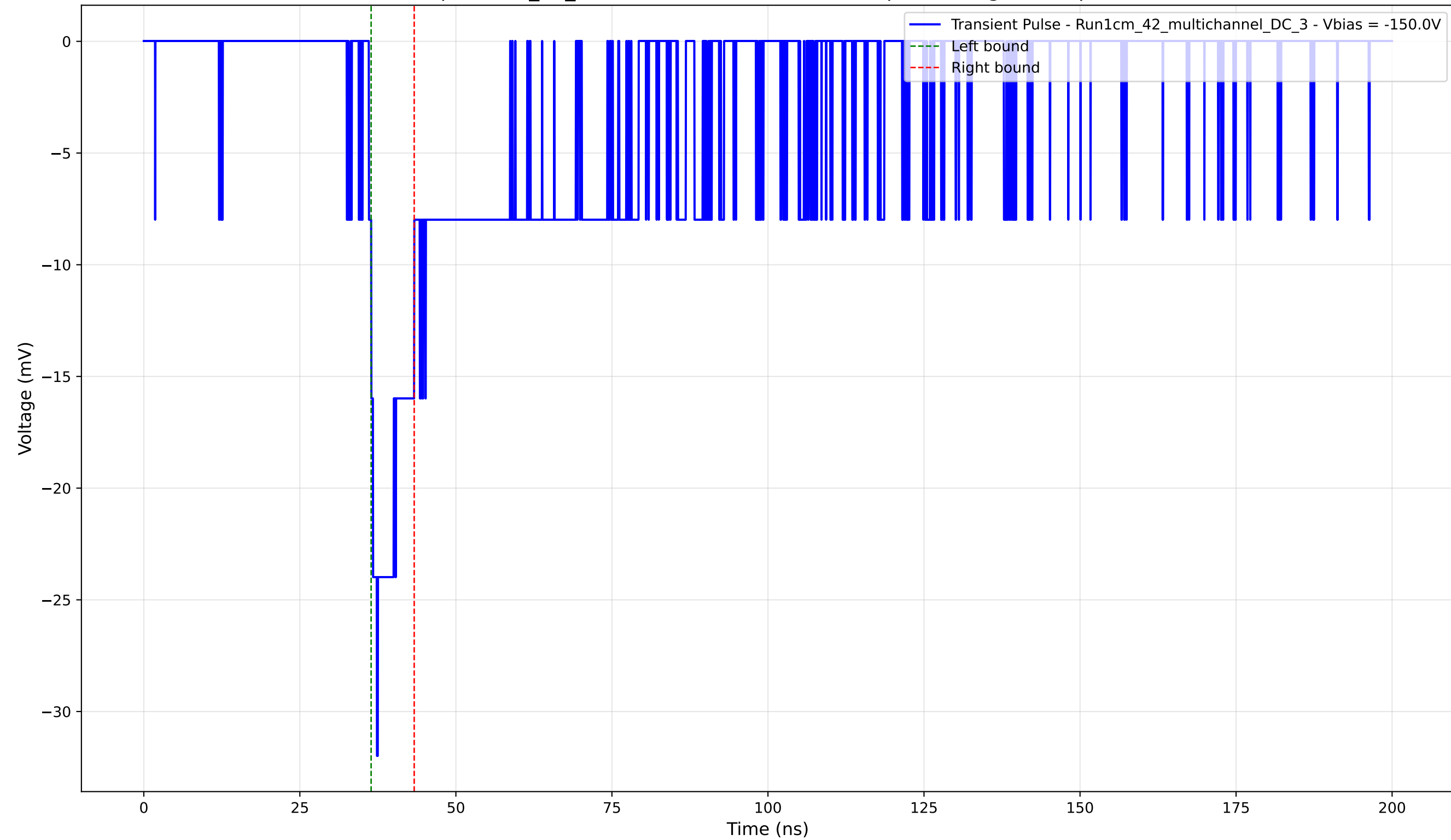
Transient Pulse - Sample: 1cm_42_multichannel - Position: 375.0 \mu\text{m} - Charge: 2.77 pC - Rise Time: 1.29 ns
