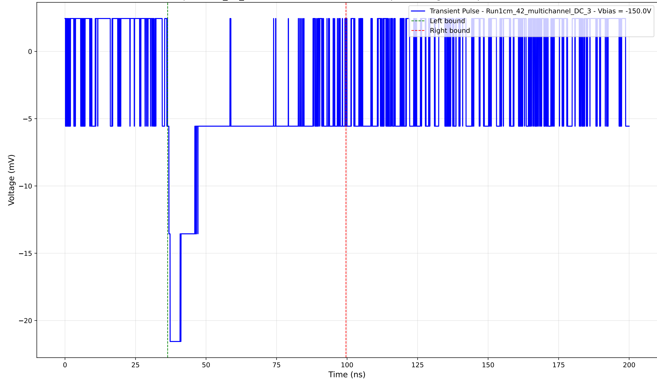
Transient Pulse - Sample: 1cm_42_multichannel - Position: 3920.0 \mu\text{m} - Charge: 8.51 pC - Rise Time: 0.00 ns (N/A)
