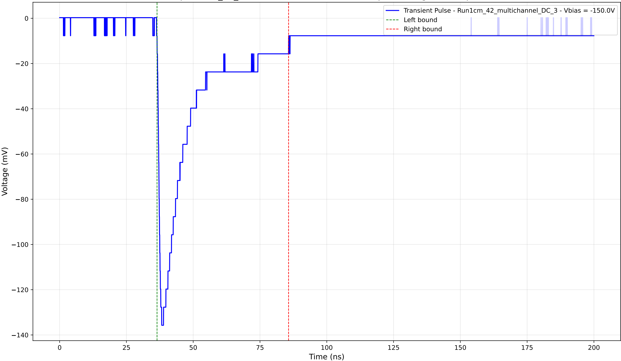
Transient Pulse - Sample: 1cm_42_multichannel - Position: 3670.0 \mu\text{m} - Charge: 38.00 pC - Rise Time: 1.39 ns
