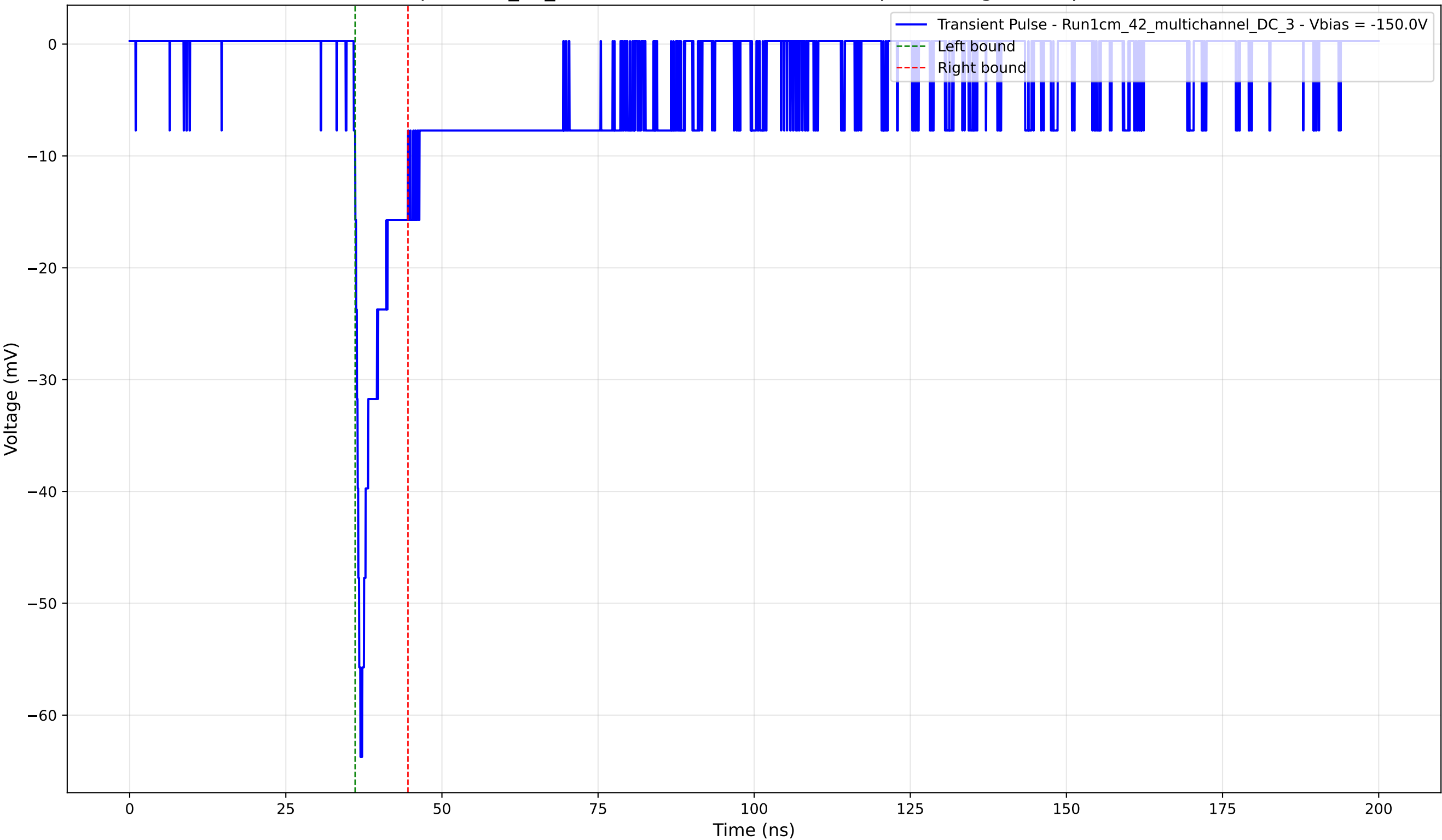
Transient Pulse - Sample: 1cm_42_multichannel - Position: 4870.0 \mu\text{m} - Charge: 4.62 pC - Rise Time: 1.06 ns
