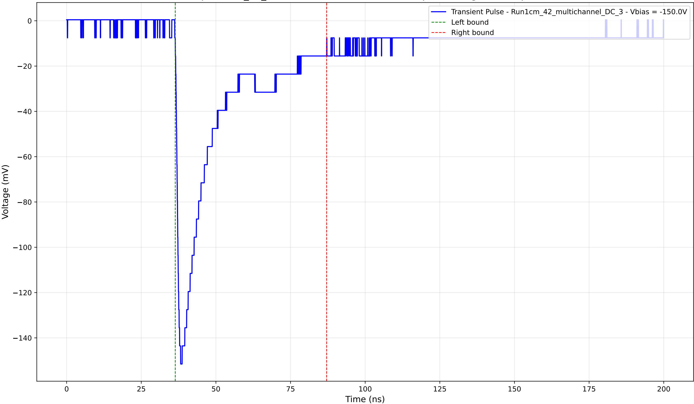
Transient Pulse - Sample: 1cm_42_multichannel - Position: 1265.0 \mu\text{m} - Charge: 43.62 pC - Rise Time: 1.44 ns
