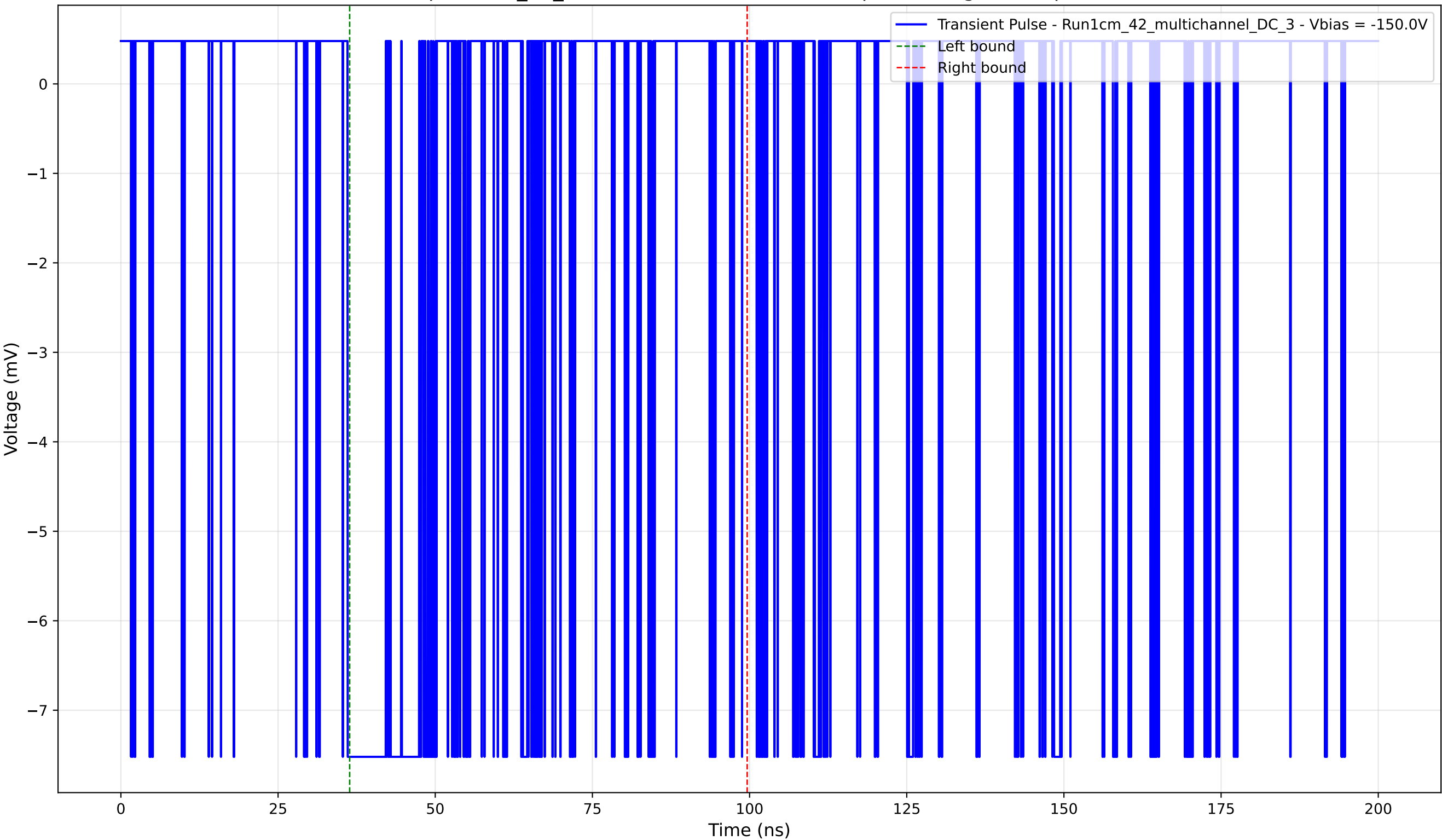
Transient Pulse - Sample: 1cm_42_multichannel - Position: 10.0 \mu\text{m} - Charge: 2.39 pC - Rise Time: 0.02 ns
