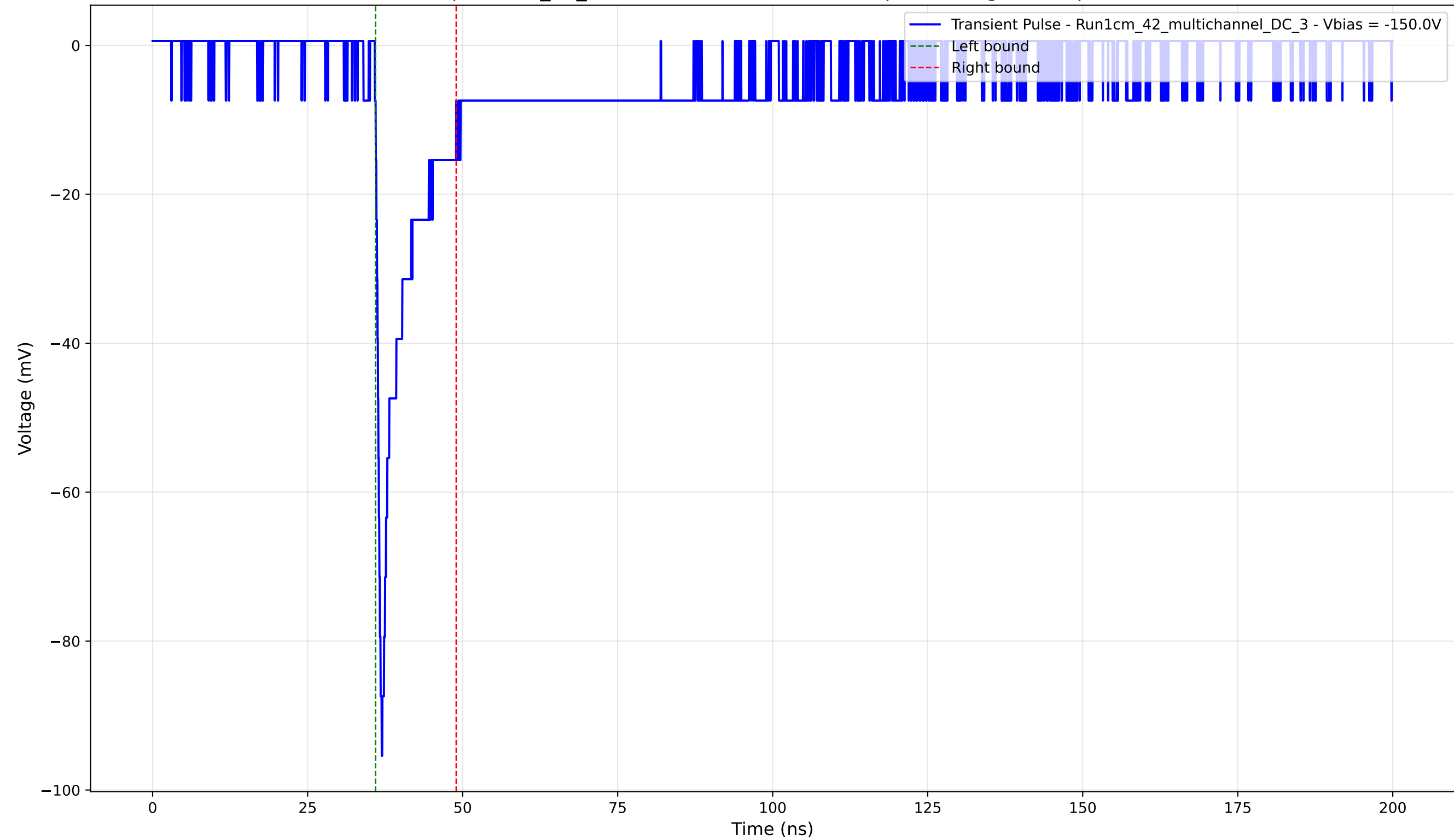
Transient Pulse - Sample: 1cm_42_multichannel - Position: 65.0 \mu\text{m} - Charge: 8.30 pC - Rise Time: 0.79 ns
