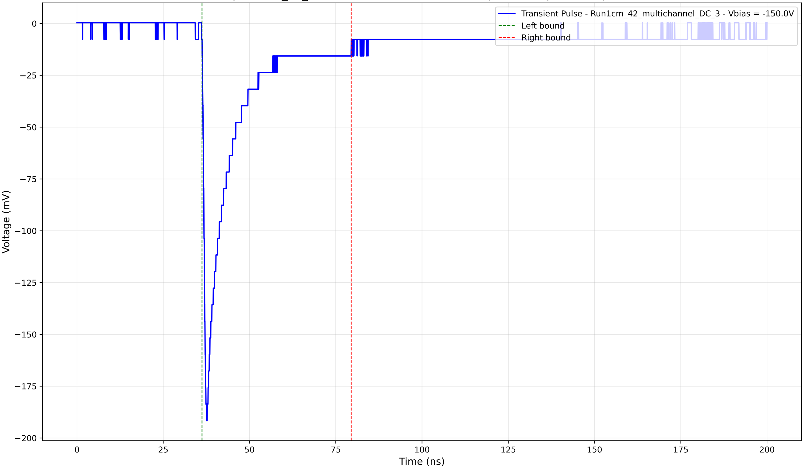
Transient Pulse - Sample: 1cm_42_multichannel - Position: 4305.0 \mu\text{m} - Charge: 34.21 pC - Rise Time: 0.95 ns
