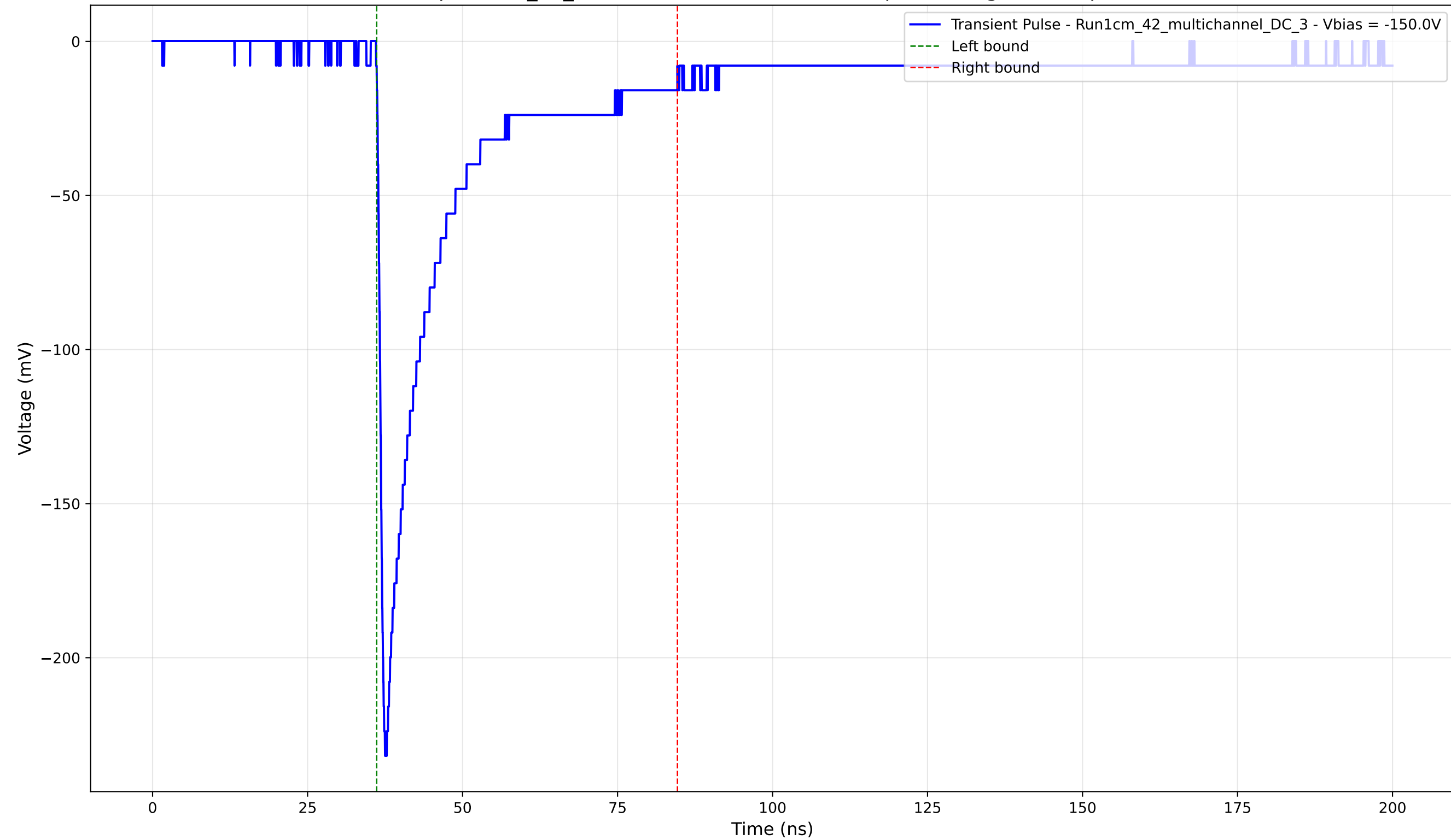
Transient Pulse - Sample: 1cm_42_multichannel - Position: 670.0 \mu\text{m} - Charge: 47.01 pC - Rise Time: 1.02 ns
