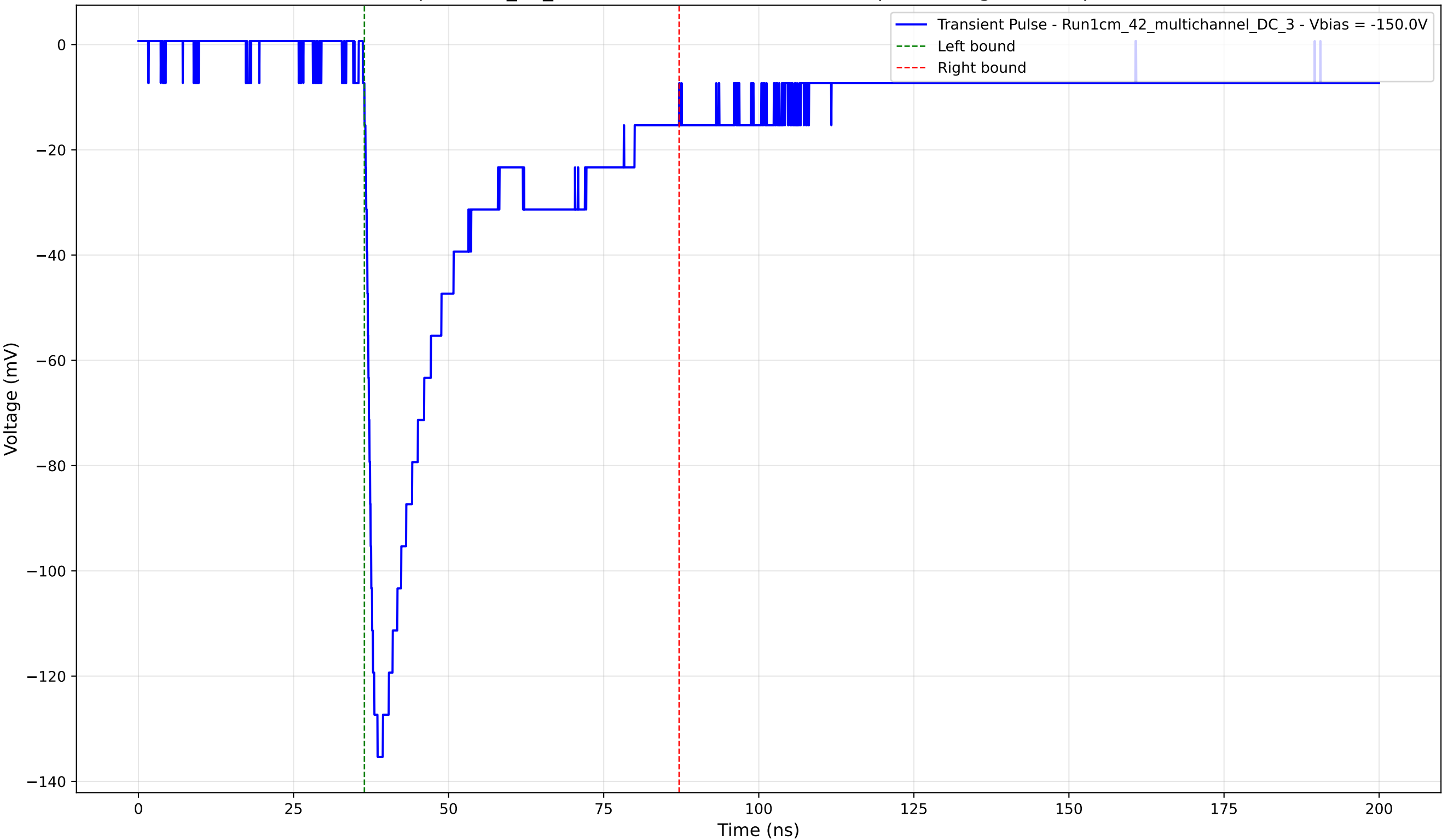
Transient Pulse - Sample: 1cm_42_multichannel - Position: 1490.0 \mu\text{m} - Charge: 43.02 pC - Rise Time: 1.58 ns
