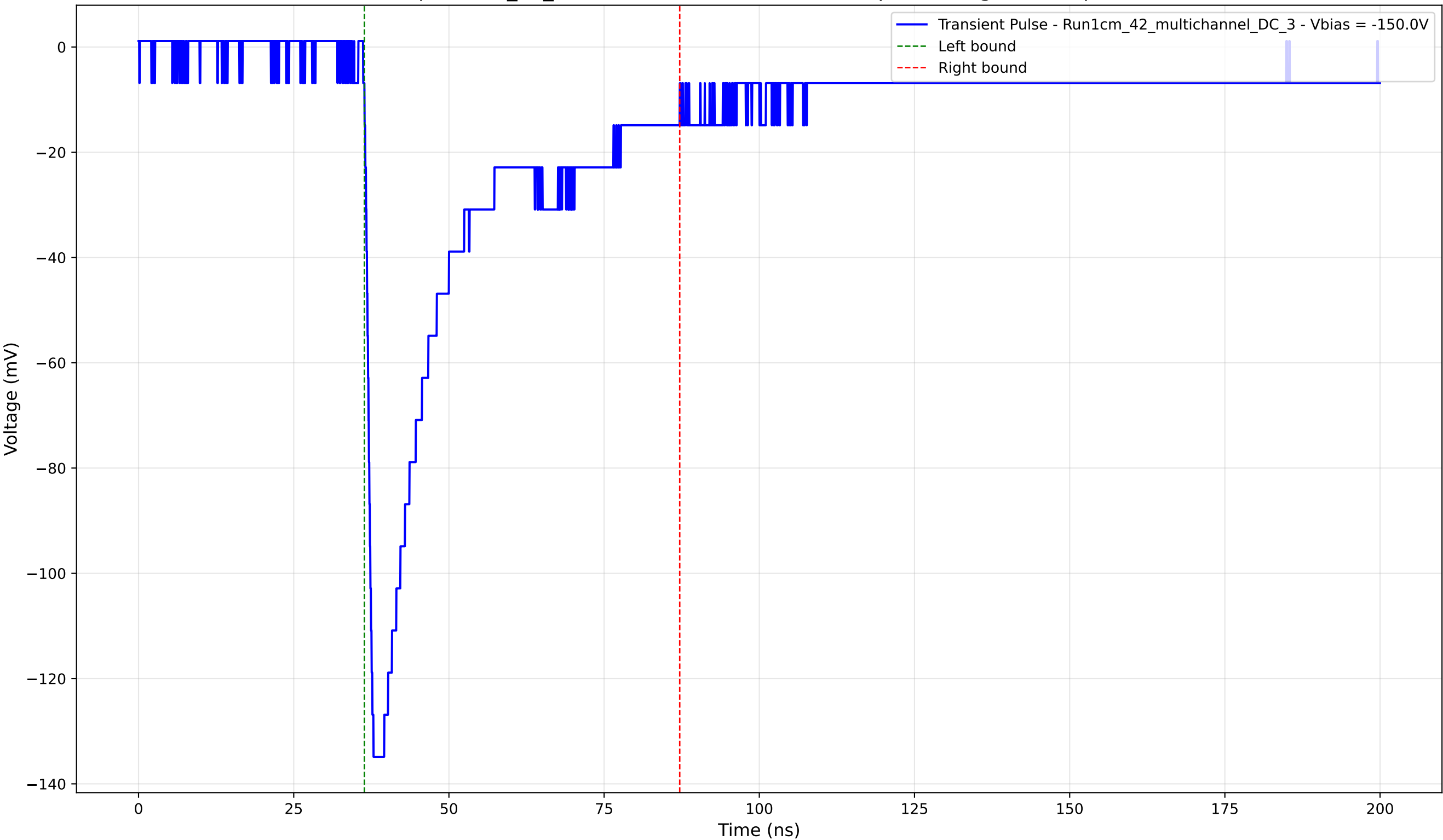
Transient Pulse - Sample: 1cm_42_multichannel - Position: 1280.0 \mu\text{m} - Charge: 40.75 pC - Rise Time: 1.26 ns
