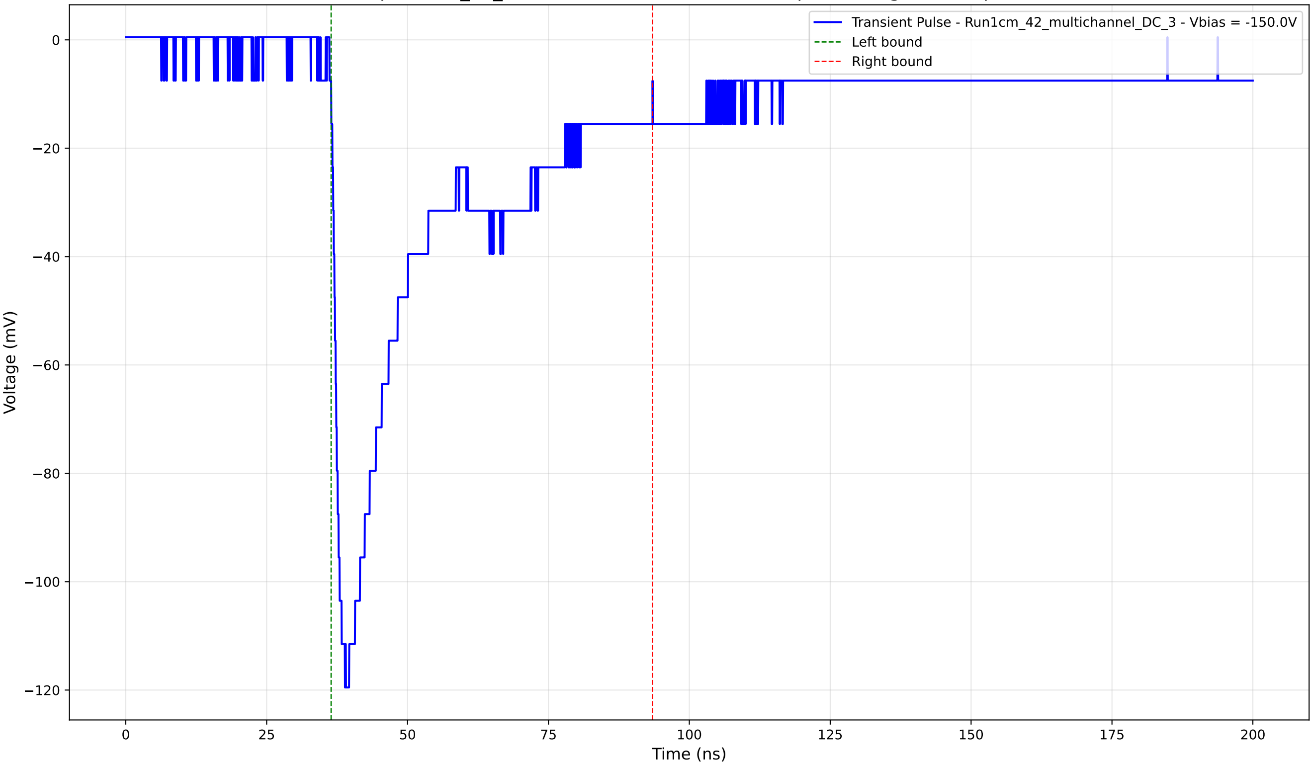
Transient Pulse - Sample: 1cm_42_multichannel - Position: 1735.0 \mu\text{m} - Charge: 43.04 pC - Rise Time: 1.85 ns
