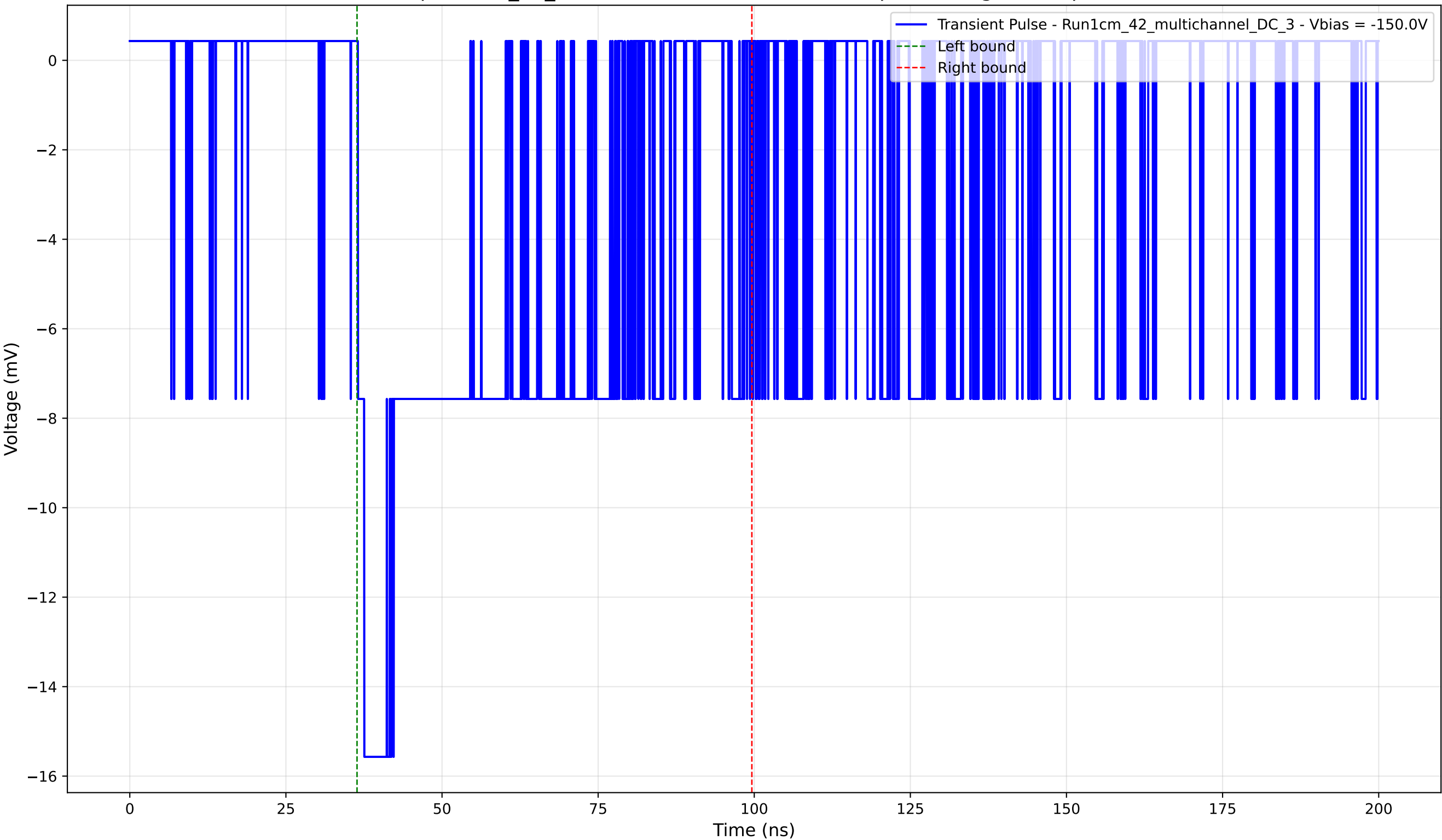
Transient Pulse - Sample: 1cm_42_multichannel - Position: 3870.0 \mu\text{m} - Charge: 7.37 pC - Rise Time: 1.02 ns
