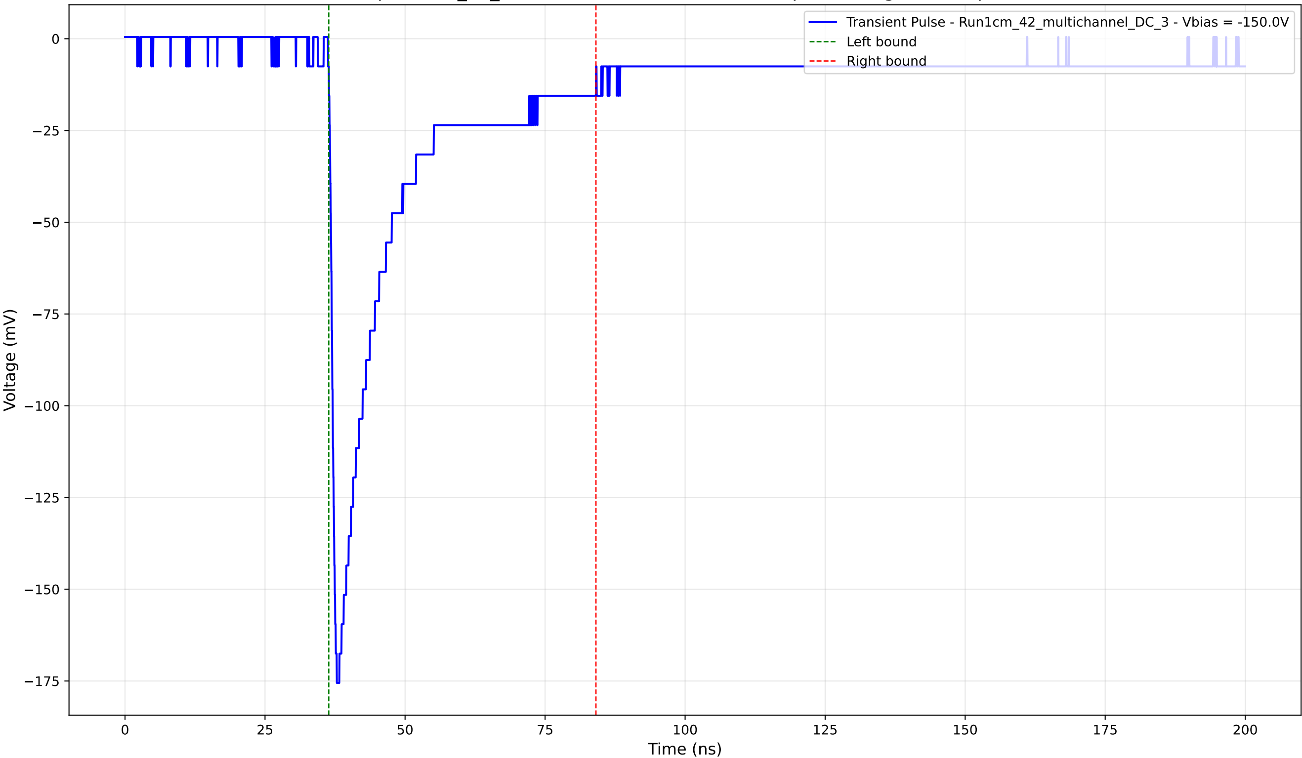
Transient Pulse - Sample: 1cm_42_multichannel - Position: 4000.0 \mu\text{m} - Charge: 40.56 pC - Rise Time: 1.03 ns
