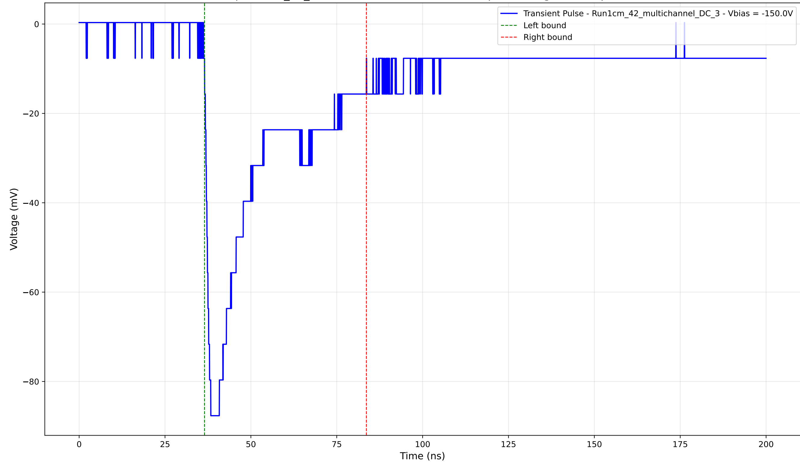
Transient Pulse - Sample: 1cm_42_multichannel - Position: 1800.0 \mu\text{m} - Charge: 32.17 pC - Rise Time: 1.46 ns
