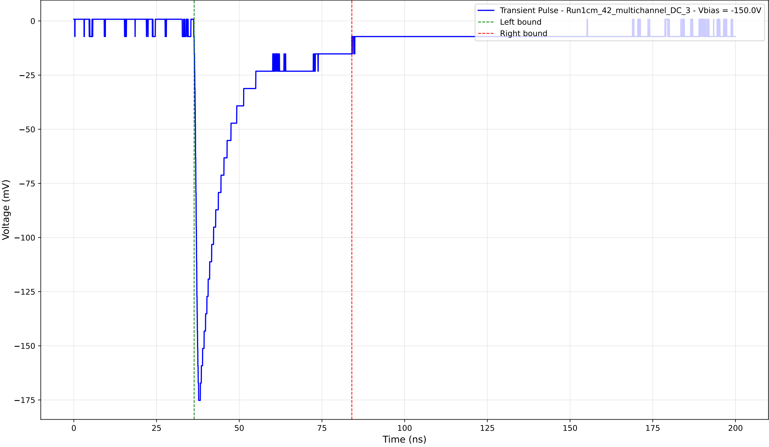
Transient Pulse - Sample: 1cm_42_multichannel - Position: 4040.0 \mu\text{m} - Charge: 39.64 pC - Rise Time: 1.01 ns
