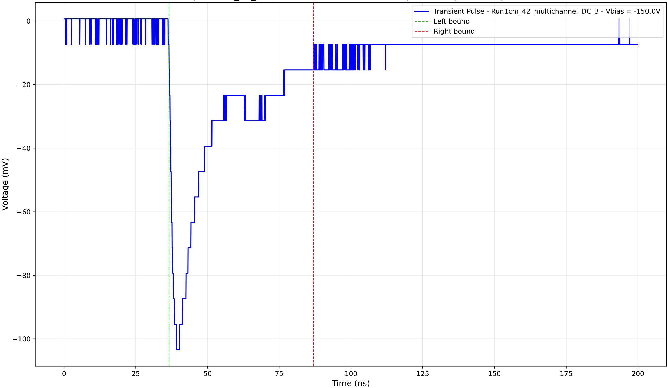
Transient Pulse - Sample: 1cm_42_multichannel - Position: 3025.0 \mu\text{m} - Charge: 36.18 pC - Rise Time: 1.87 ns
