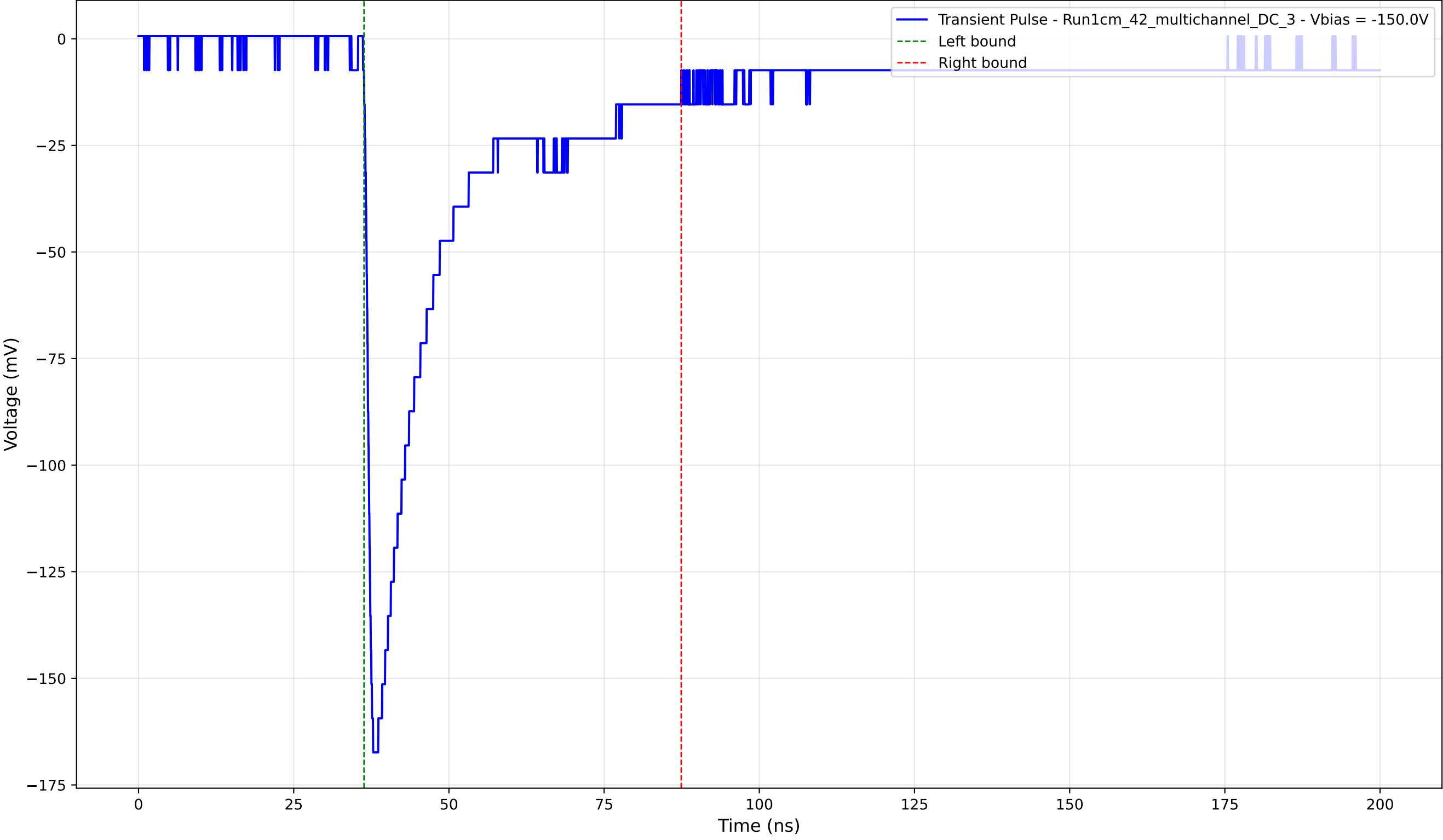
Transient Pulse - Sample: 1cm_42_multichannel - Position: 1060.0 \mu\text{m} - Charge: 44.45 pC - Rise Time: 1.08 ns
