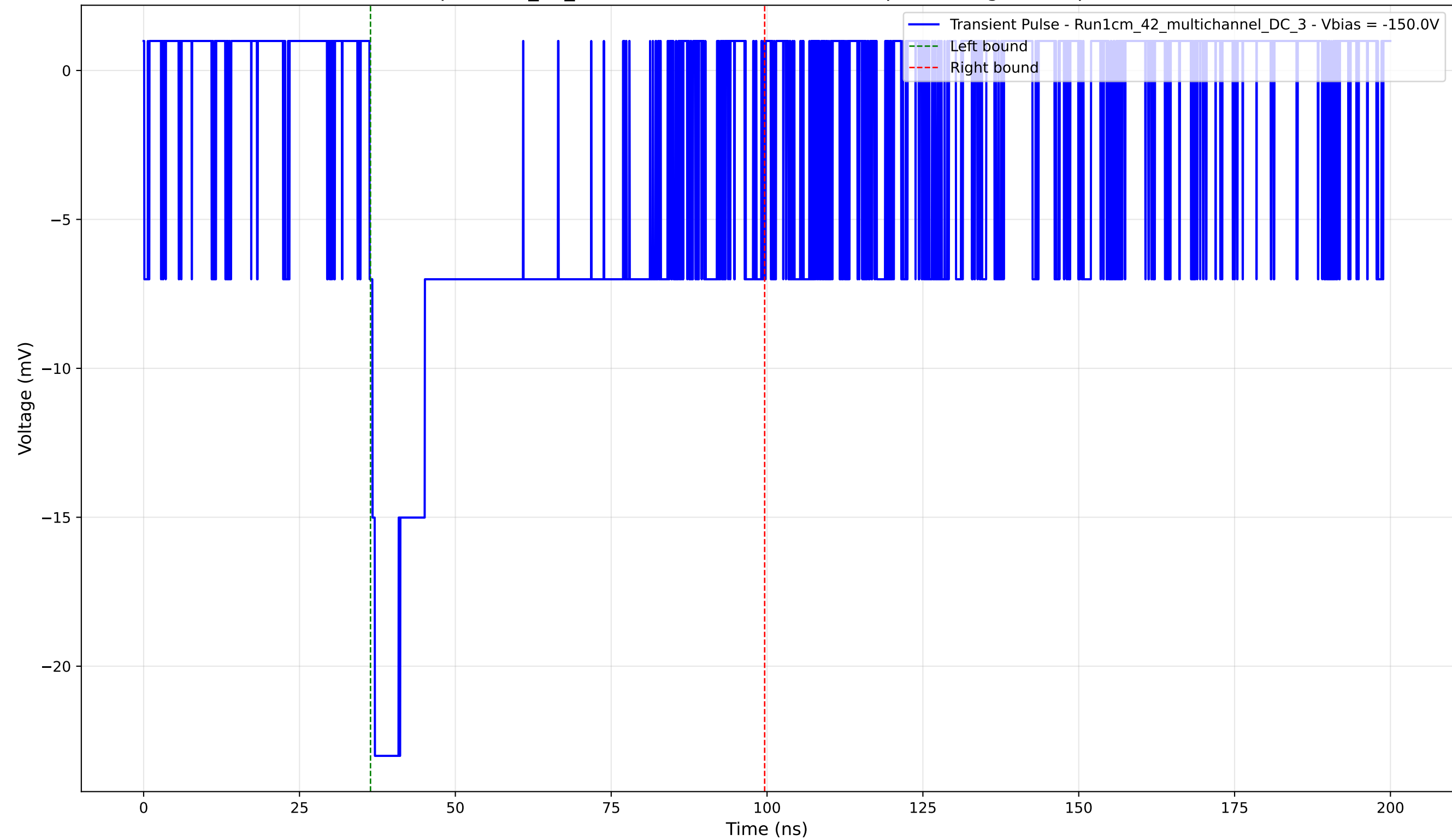
Transient Pulse - Sample: 1cm_42_multichannel - Position: 830.0 \mu\text{m} - Charge: 9.42 pC - Rise Time: 0.86 ns
