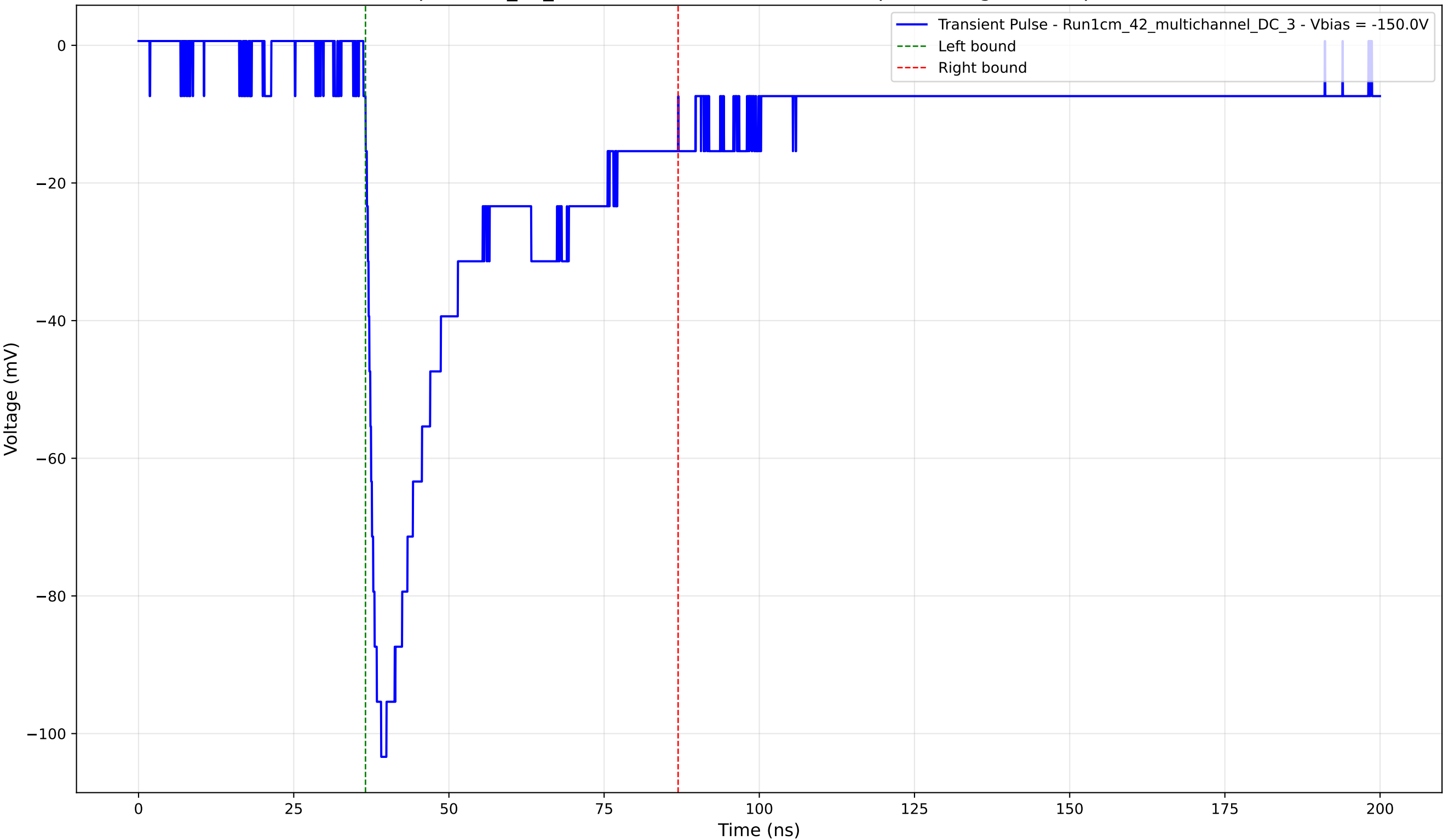
Transient Pulse - Sample: 1cm_42_multichannel - Position: 3060.0 \mu\text{m} - Charge: 35.94 pC - Rise Time: 1.81 ns
