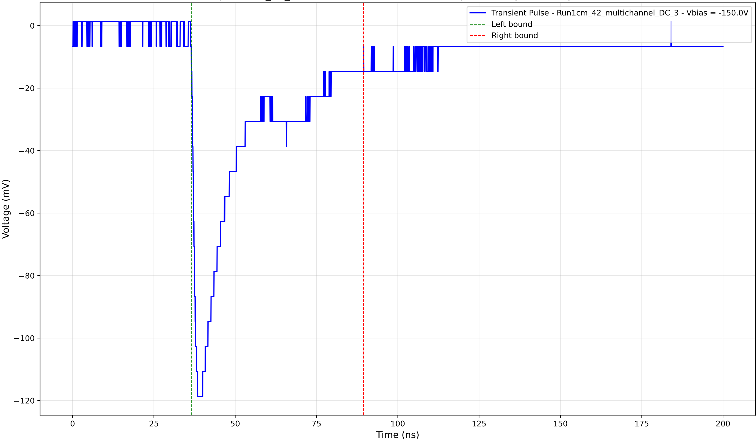
Transient Pulse - Sample: 1cm_42_multichannel - Position: 1665.0 \mu\text{m} - Charge: 41.08 pC - Rise Time: 1.57 ns
