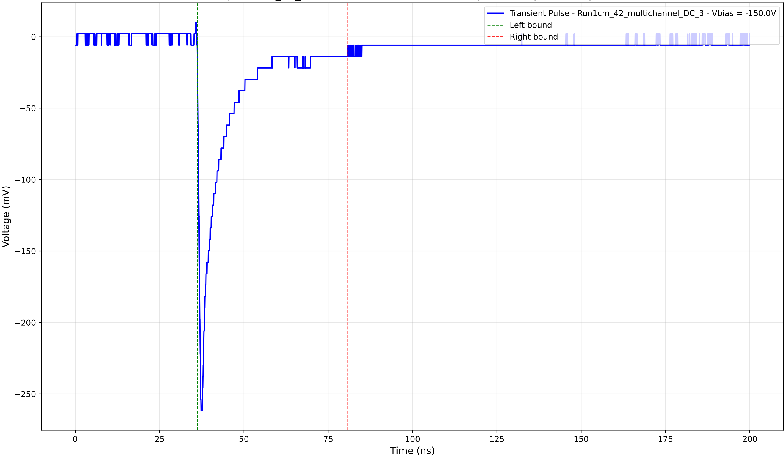
Transient Pulse - Sample: 1cm_42_multichannel - Position: 4515.0 \mu\text{m} - Charge: 38.84 pC - Rise Time: 0.83 ns
