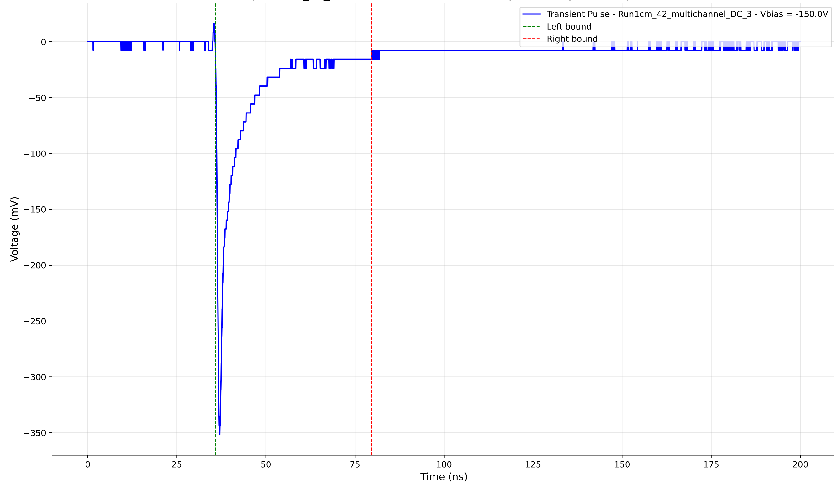
Transient Pulse - Sample: 1cm_42_multichannel - Position: 115.0 \mu\text{m} - Charge: 42.23 pC - Rise Time: 0.79 ns
