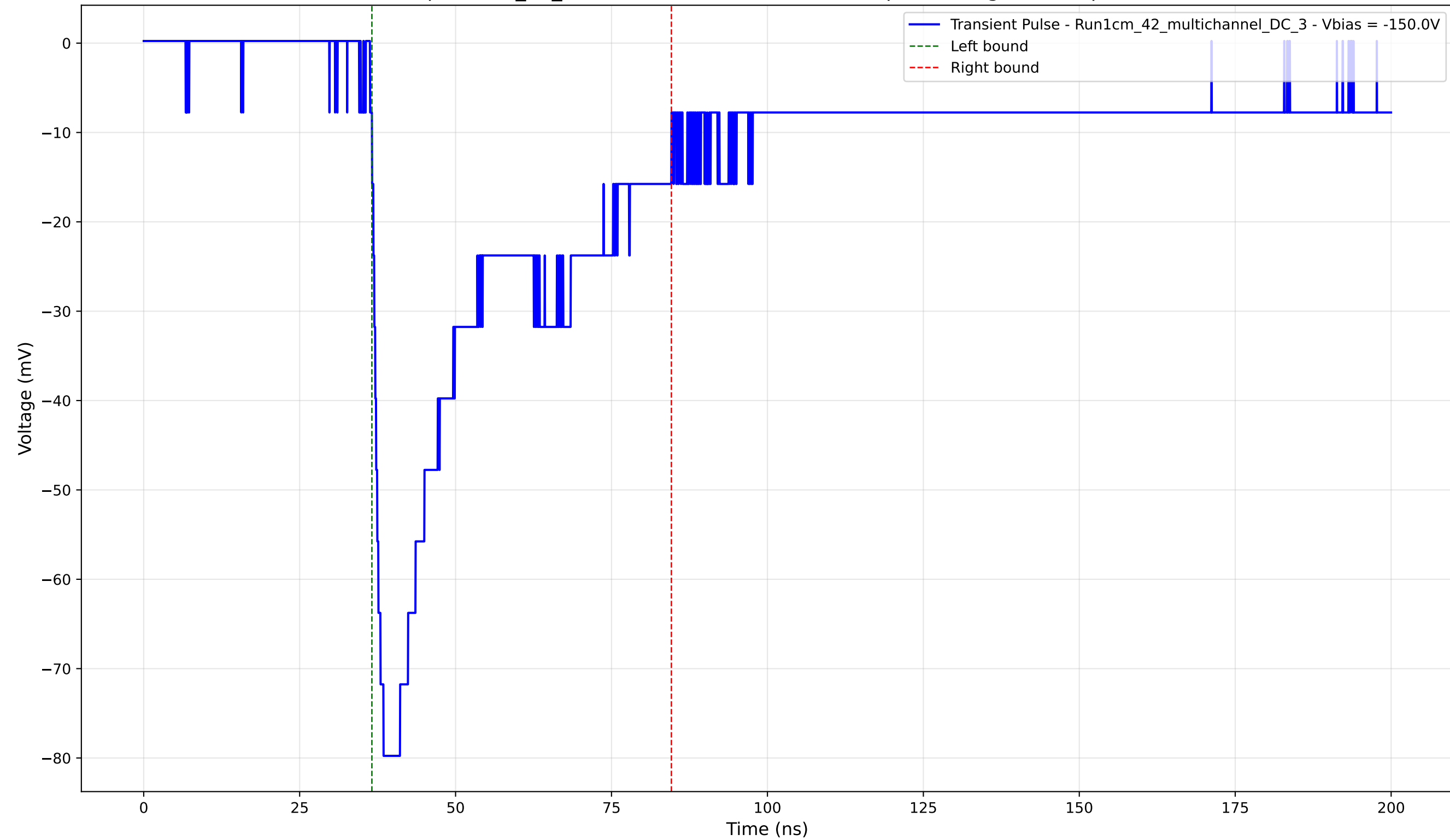
Transient Pulse - Sample: 1cm_42_multichannel - Position: 1935.0 \mu\text{m} - Charge: 31.71 pC - Rise Time: 1.86 ns
