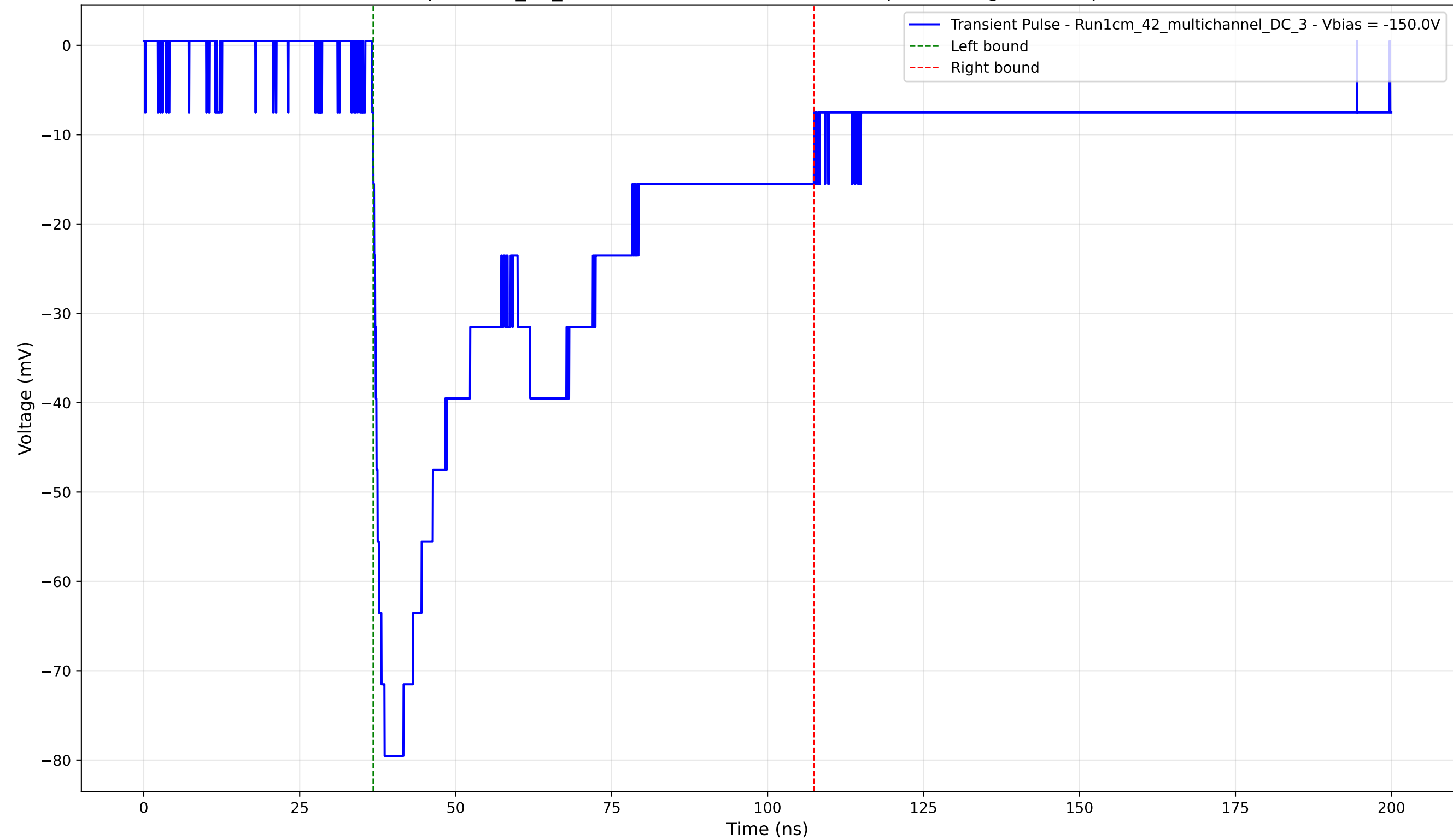
Transient Pulse - Sample: 1cm_42_multichannel - Position: 2275.0 \mu\text{m} - Charge: 43.01 pC - Rise Time: 1.82 ns
