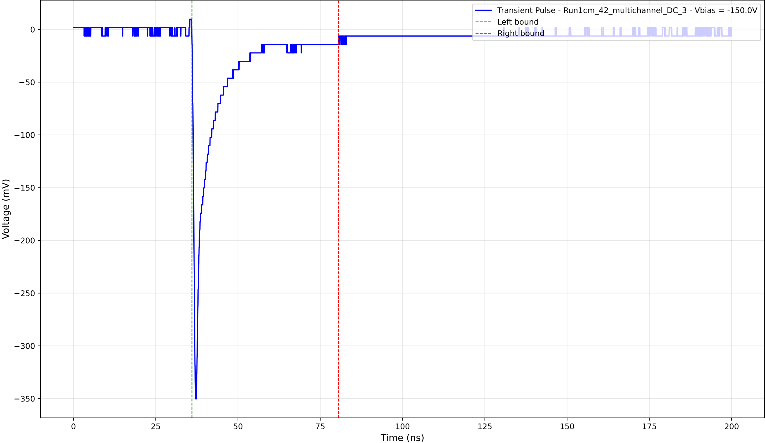
Transient Pulse - Sample: 1cm_42_multichannel - Position: 4745.0 \mu\text{m} - Charge: 41.26 pC - Rise Time: 0.79 ns
