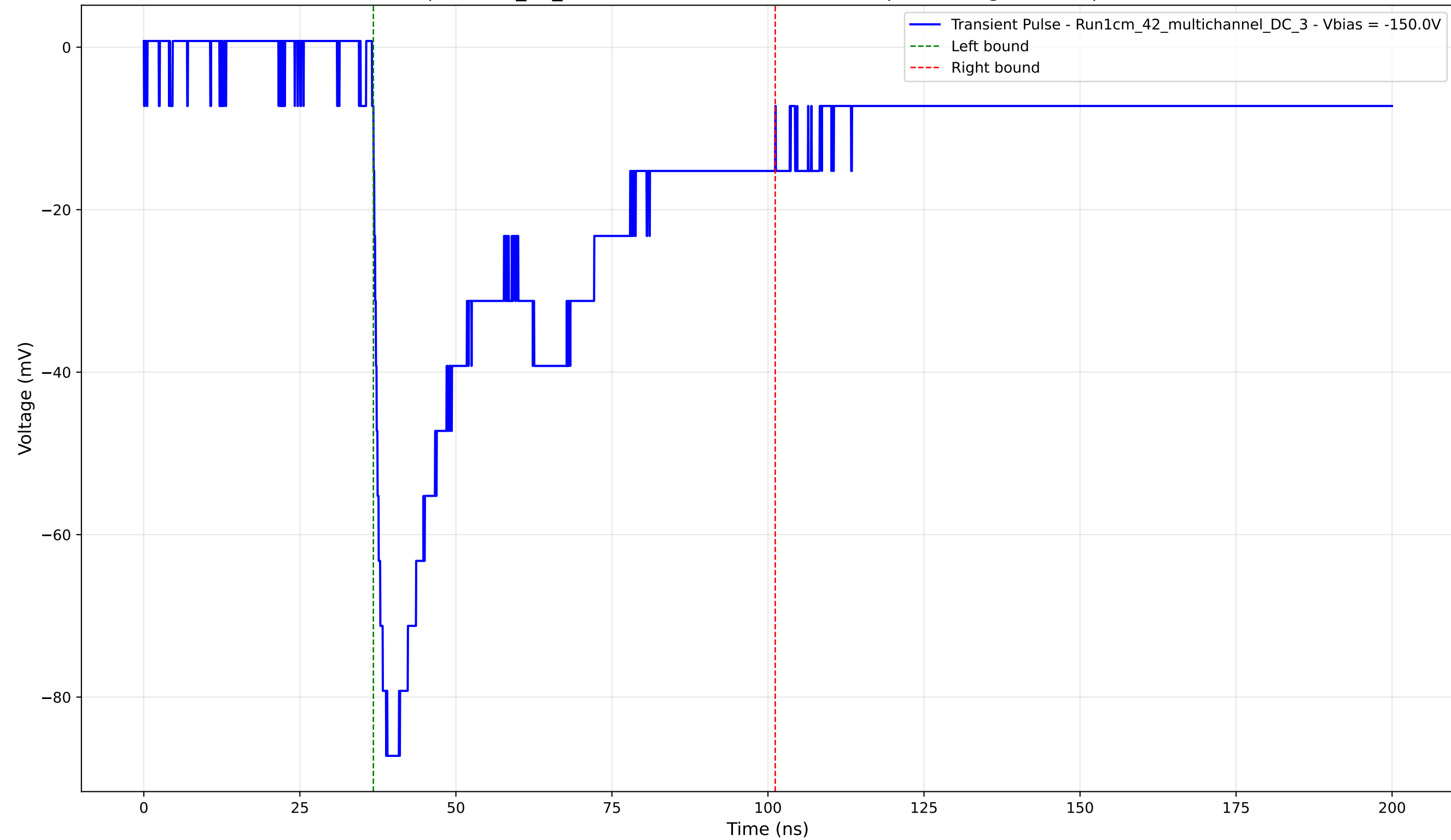
Transient Pulse - Sample: 1cm_42_multichannel - Position: 2190.0 \mu\text{m} - Charge: 41.32 pC - Rise Time: 1.50 ns
