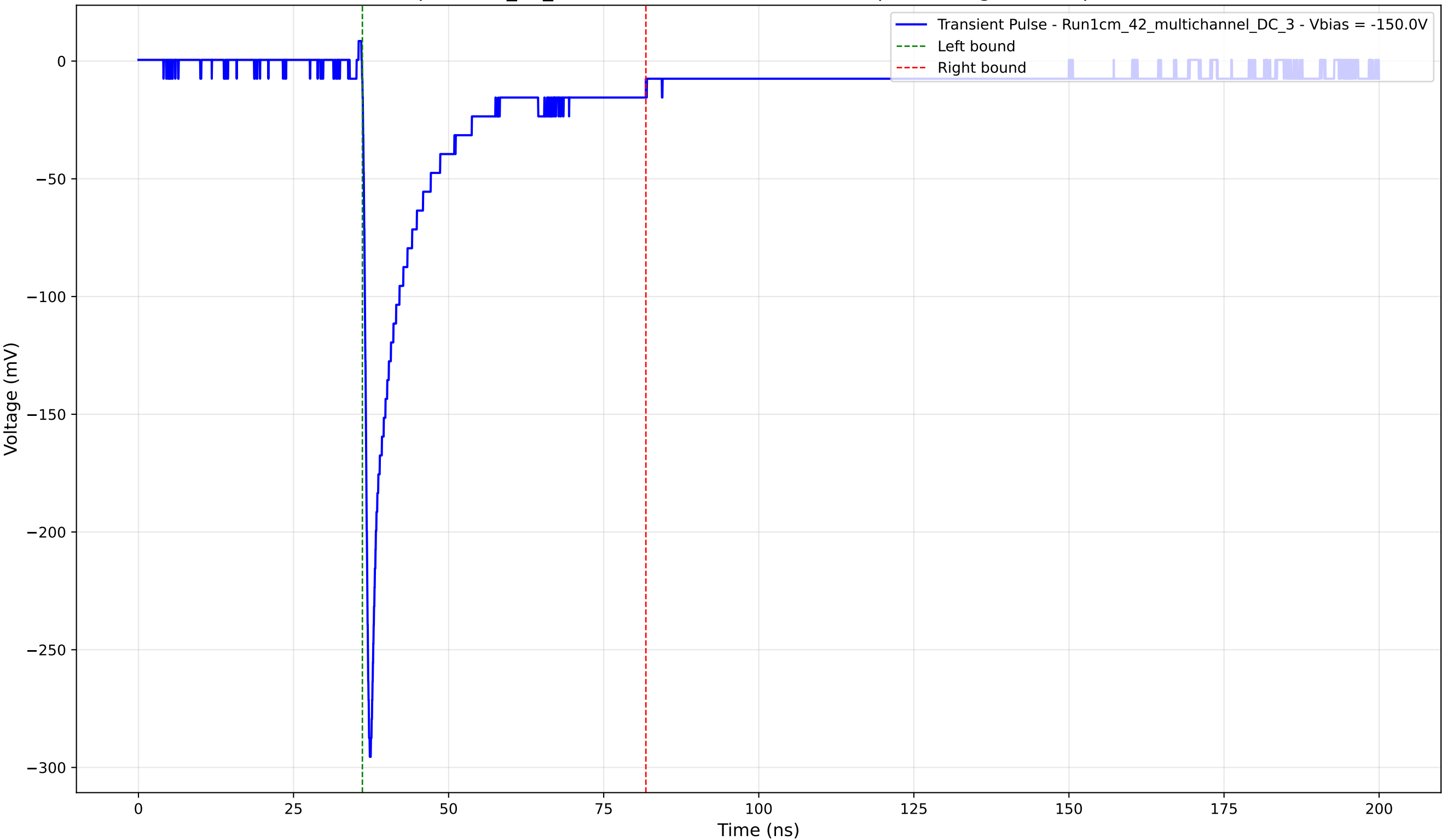
Transient Pulse - Sample: 1cm_42_multichannel - Position: 4585.0 \mu\text{m} - Charge: 41.55 pC - Rise Time: 0.86 ns
