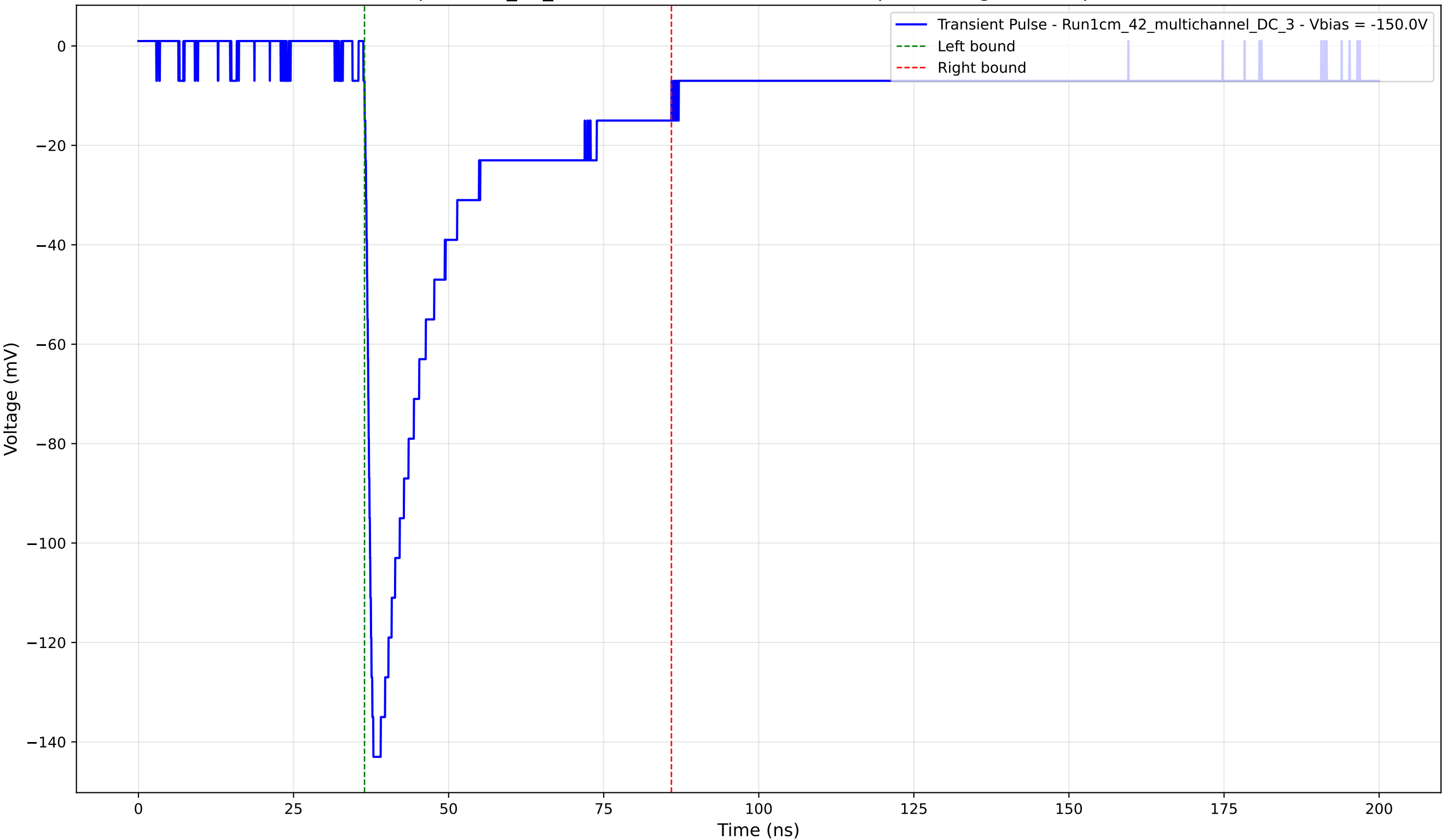
Transient Pulse - Sample: 1cm_42_multichannel - Position: 3790.0 \mu\text{m} - Charge: 38.56 pC - Rise Time: 1.24 ns
