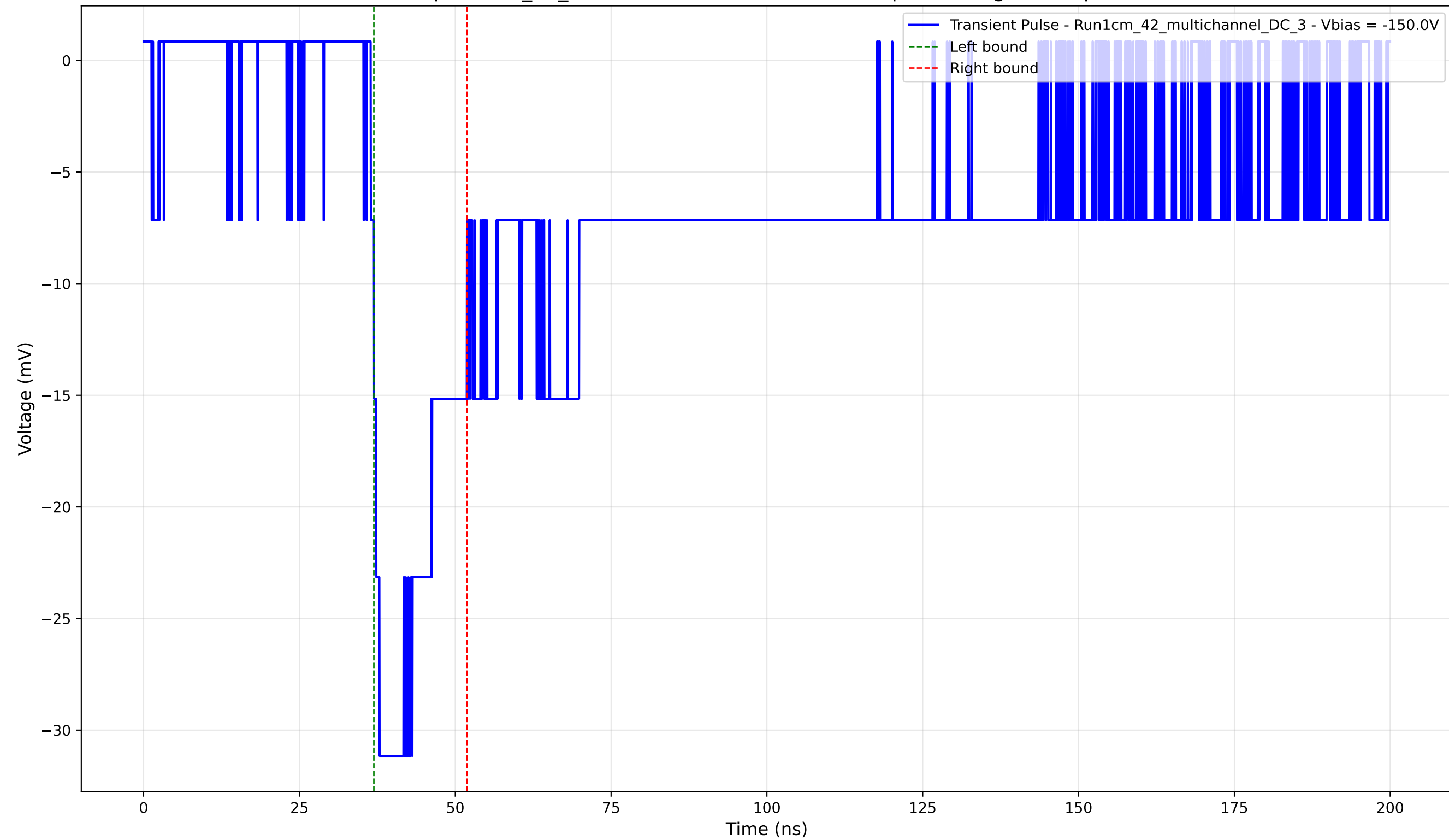
Transient Pulse - Sample: 1cm_42_multichannel - Position: 1910.0 \mu\text{m} - Charge: 6.72 pC - Rise Time: 1.41 ns
