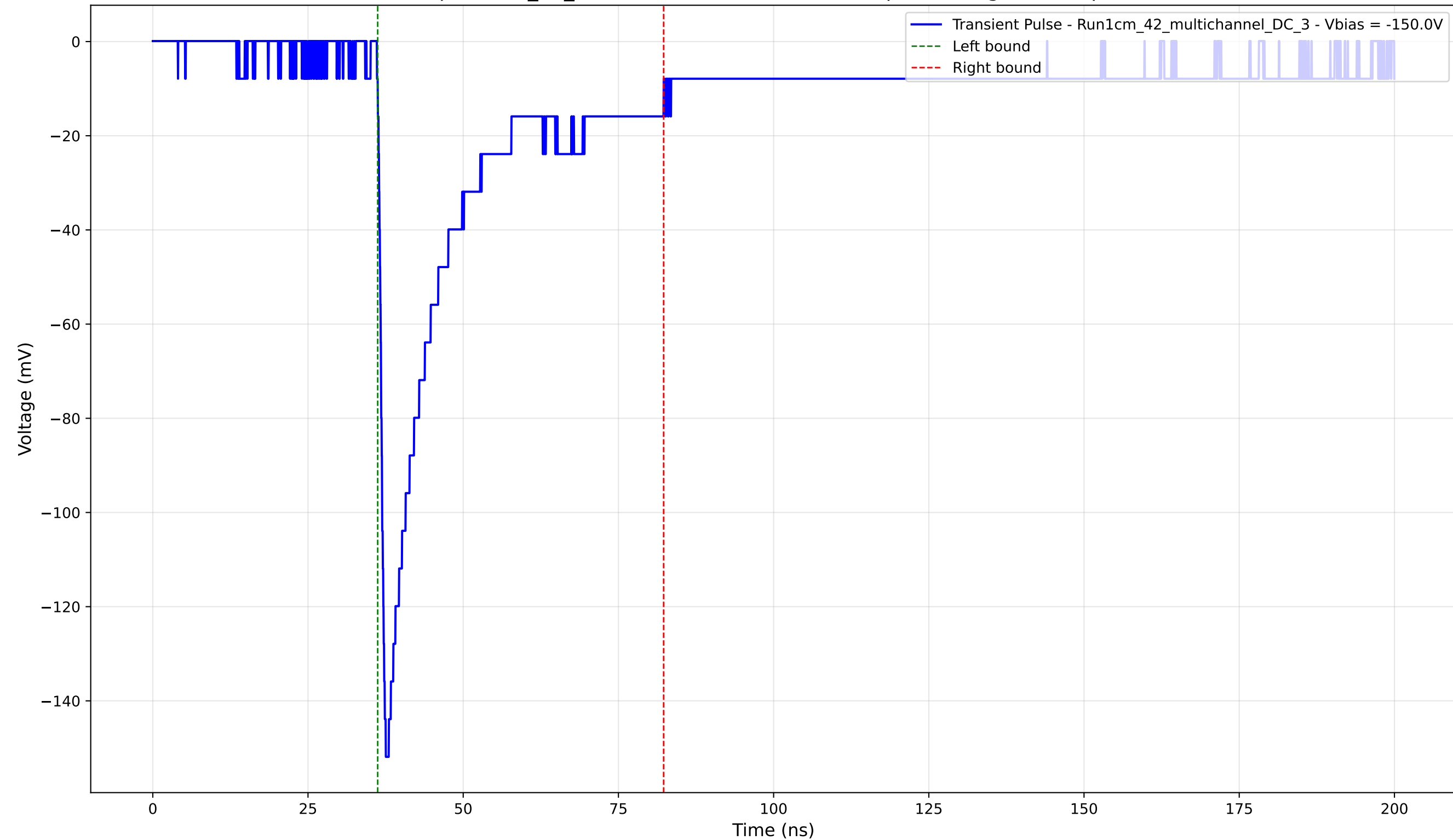
Transient Pulse - Sample: 1cm_42_multichannel - Position: 795.0 \mu\text{m} - Charge: 34.03 pC - Rise Time: 1.12 ns
