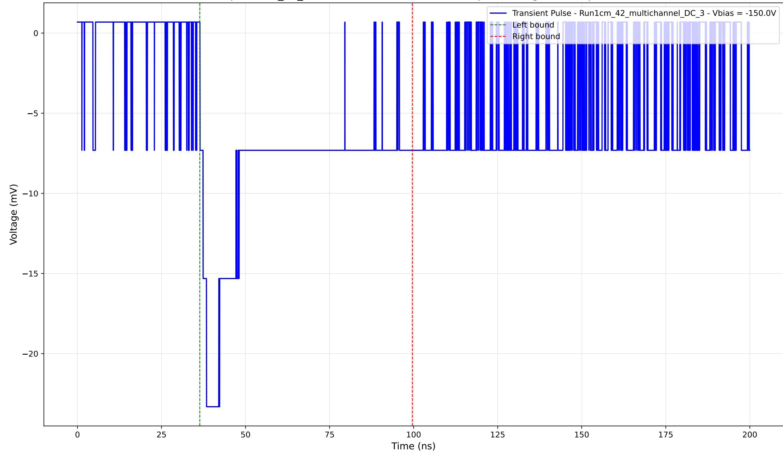
Transient Pulse - Sample: 1cm_42_multichannel - Position: 2845.0 \mu\text{m} - Charge: 11.40 pC - Rise Time: 1.96 ns
