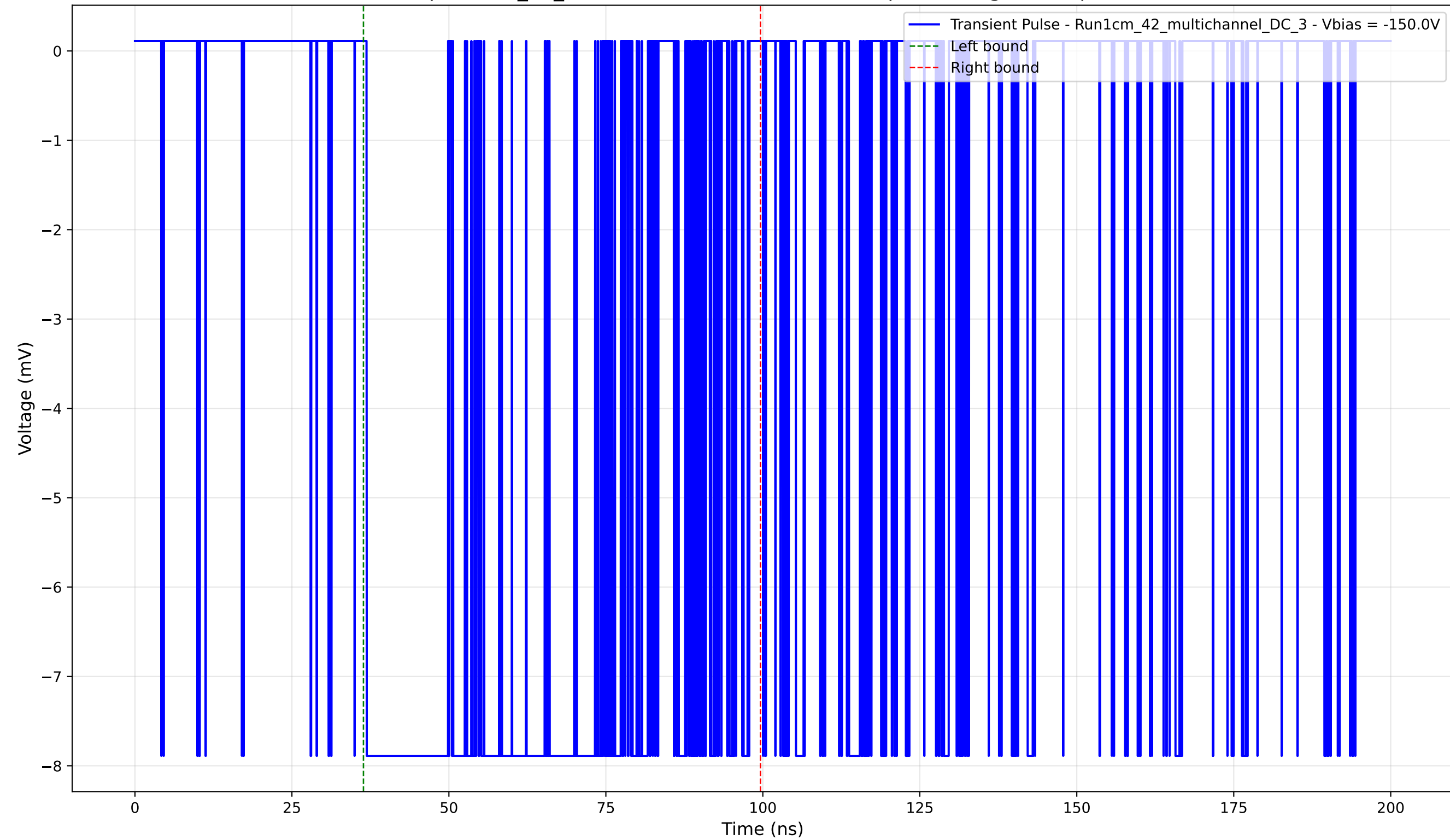
Transient Pulse - Sample: 1cm_42_multichannel - Position: 2380.0 \mu\text{m} - Charge: 7.23 pC - Rise Time: 0.02 ns
