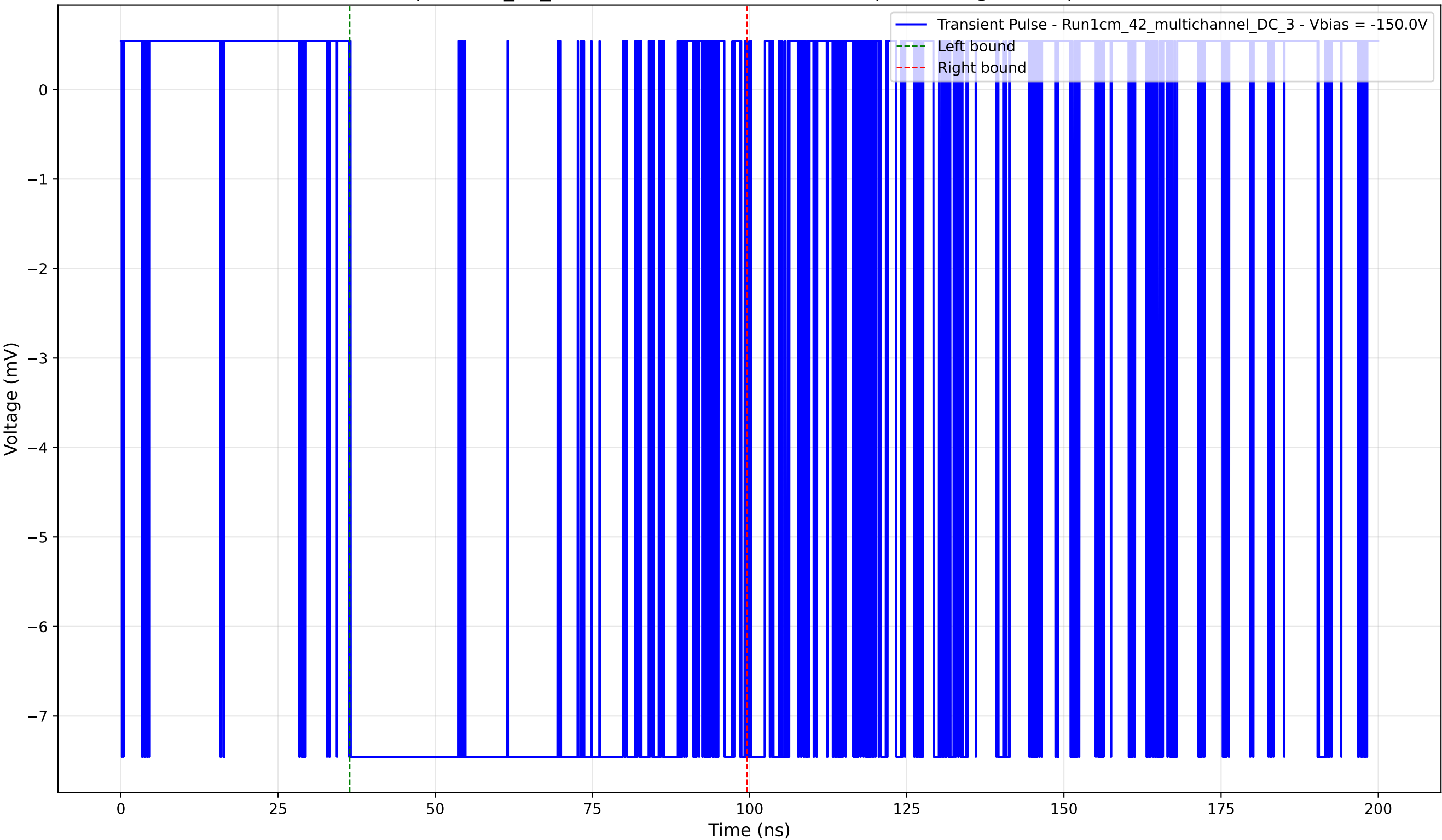
Transient Pulse - Sample: 1cm_42_multichannel - Position: 2395.0 \mu\text{m} - Charge: 7.89 pC - Rise Time: 0.02 ns
