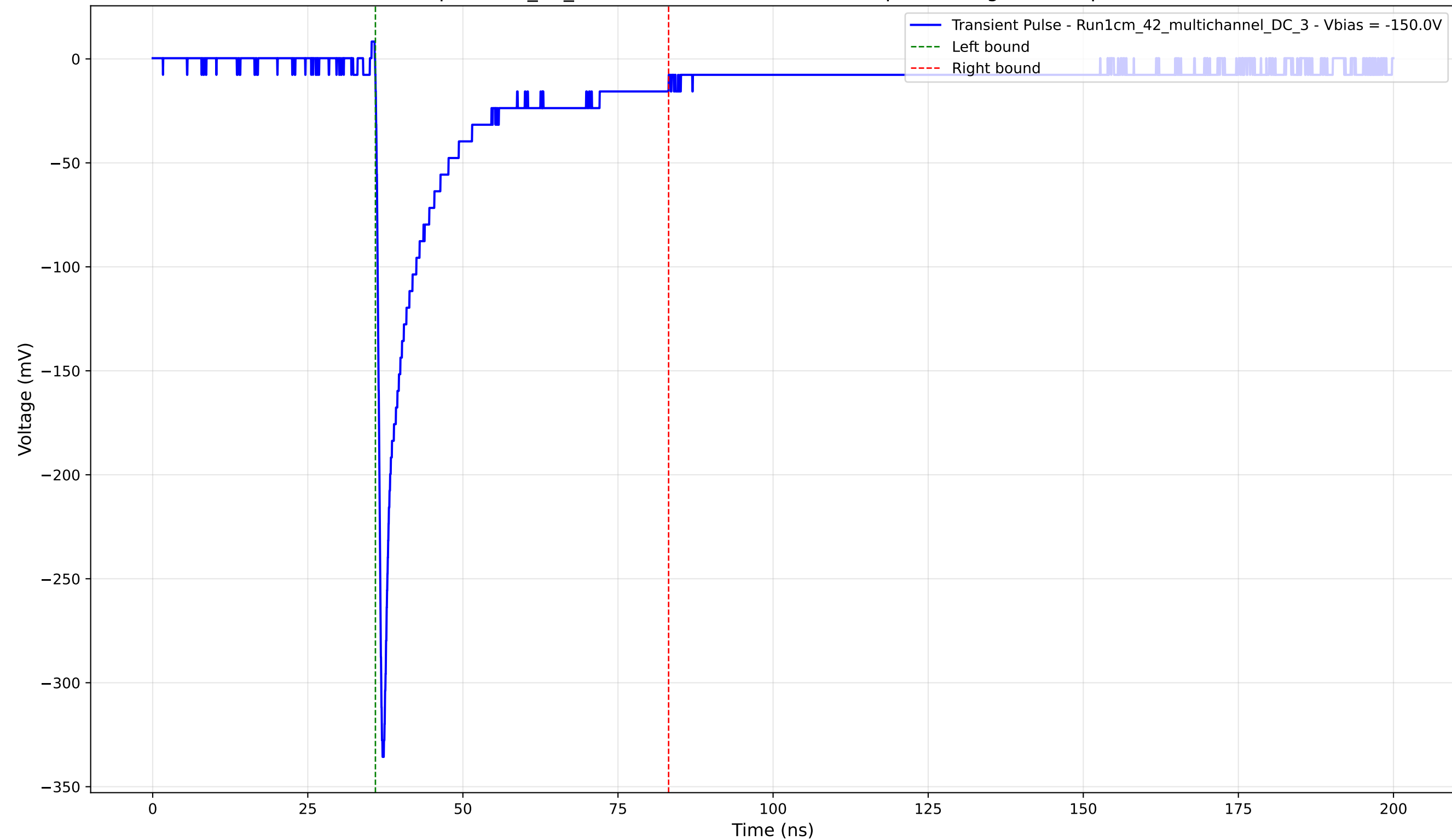
Transient Pulse - Sample: 1cm_42_multichannel - Position: 230.0 \mu\text{m} - Charge: 46.99 pC - Rise Time: 0.80 ns
