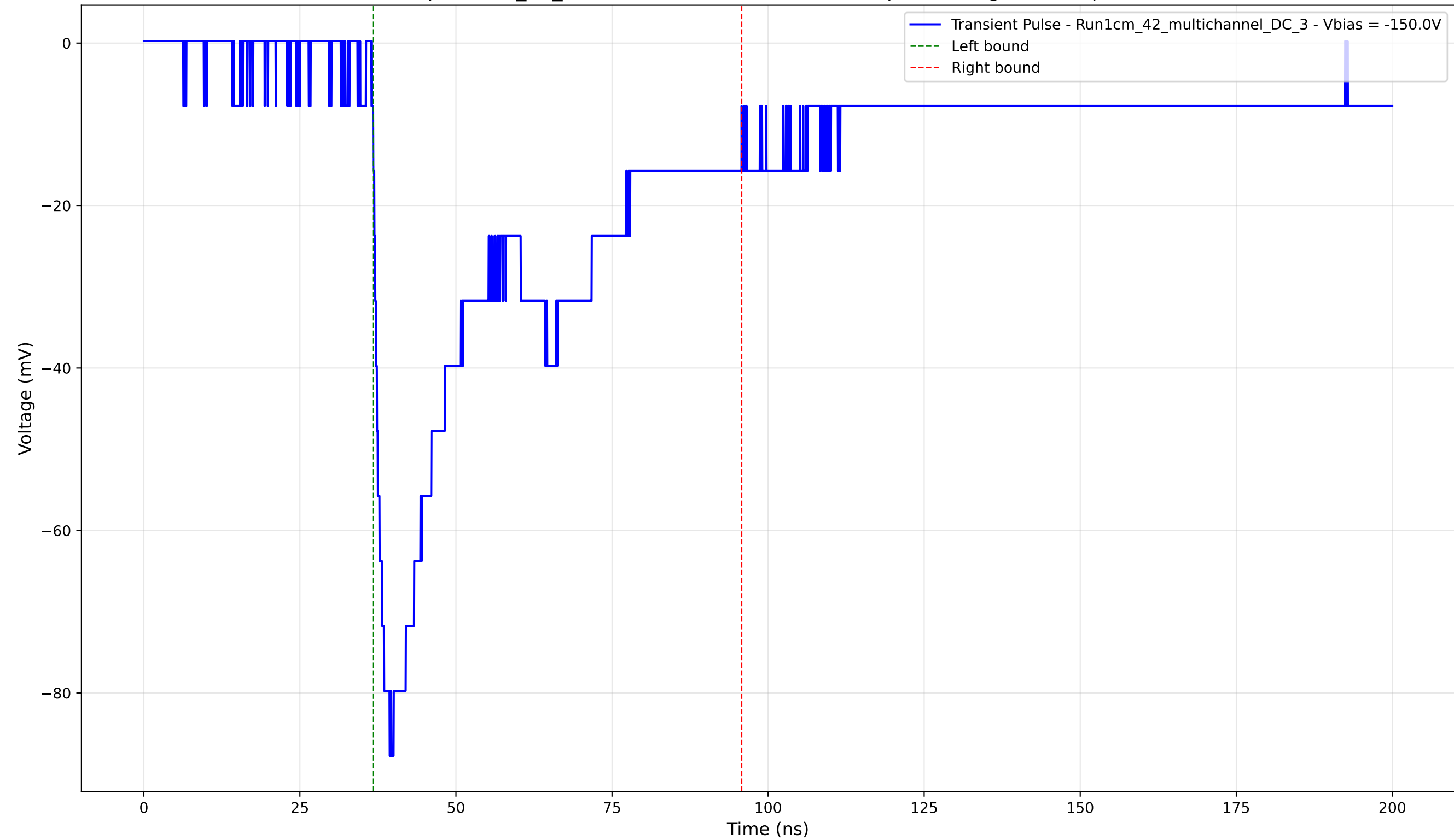
Transient Pulse - Sample: 1cm_42_multichannel - Position: 2635.0 \mu\text{m} - Charge: 38.14 pC - Rise Time: 1.76 ns
