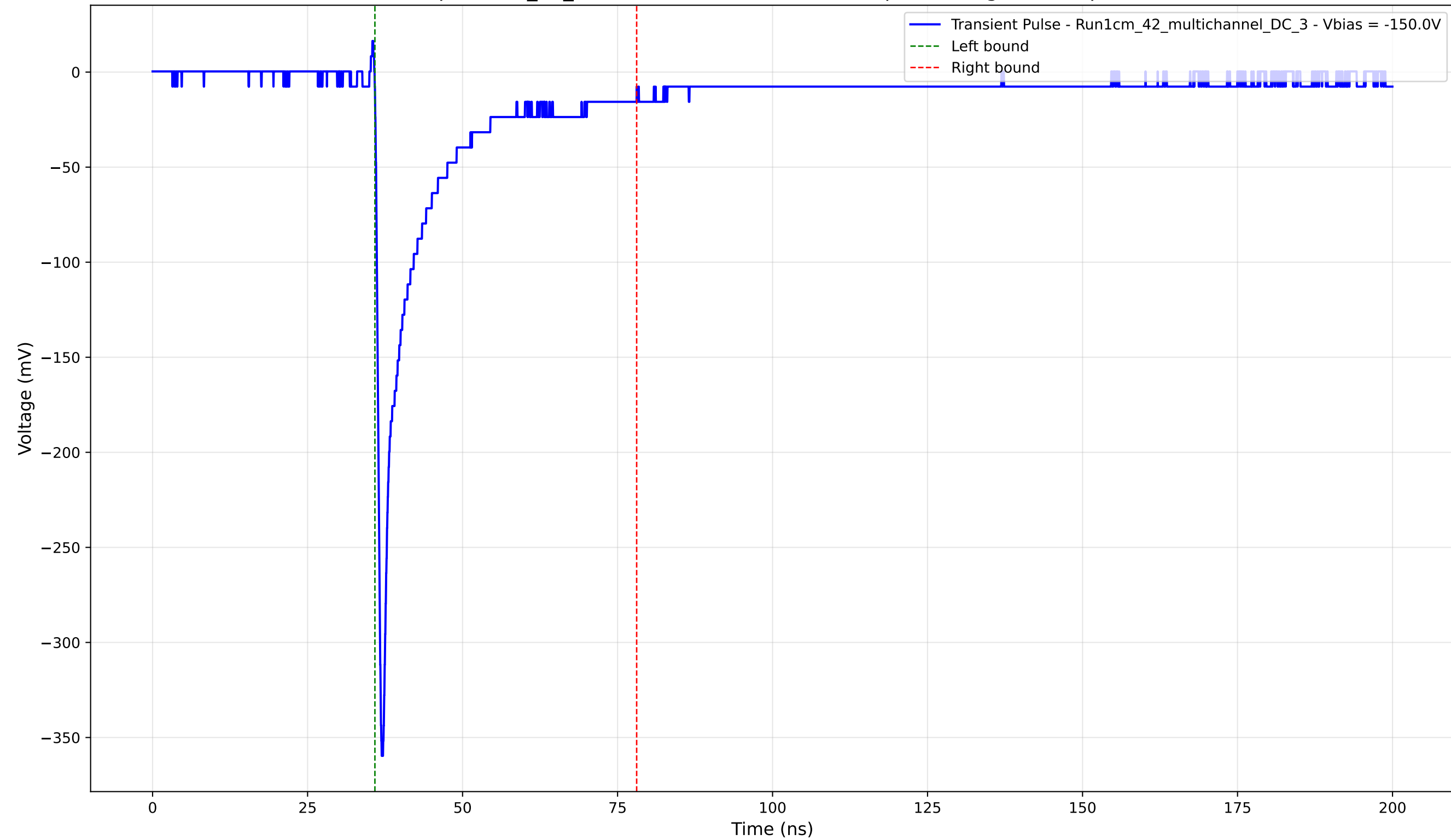
Transient Pulse - Sample: 1cm_42_multichannel - Position: 145.0 \mu\text{m} - Charge: 44.75 pC - Rise Time: 0.78 ns
