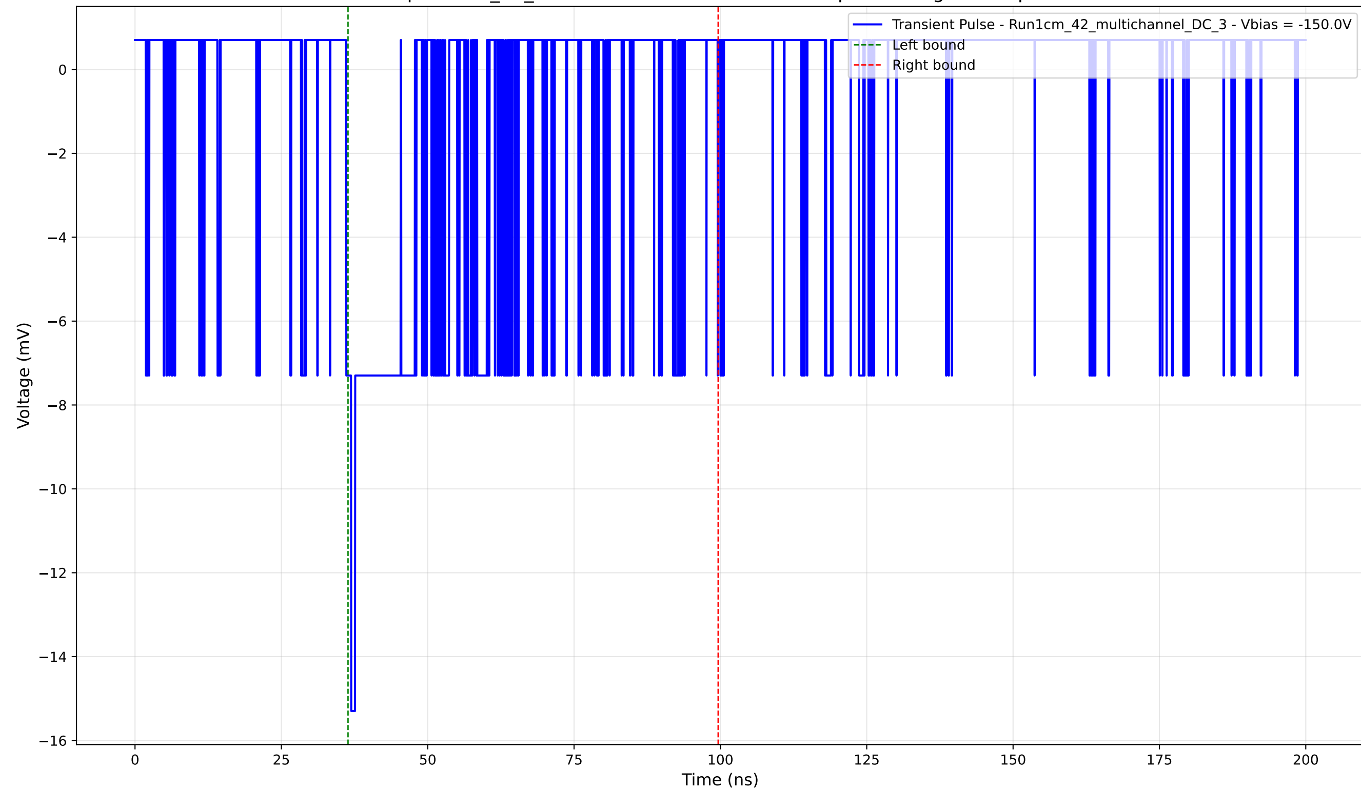
Transient Pulse - Sample: 1cm_42_multichannel - Position: 4920.0 \mu\text{m} - Charge: 2.85 pC - Rise Time: 0.86 ns
