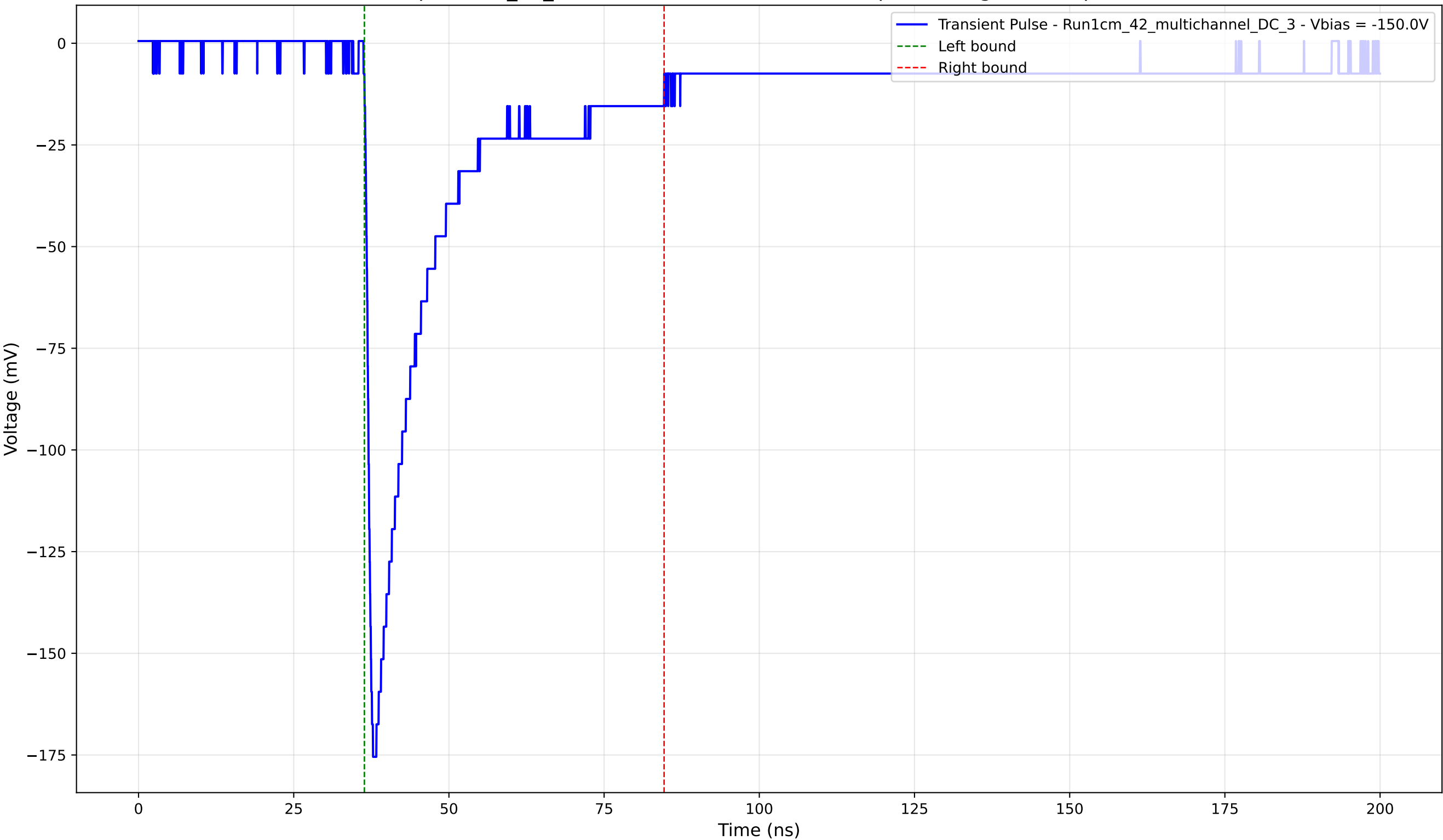
Transient Pulse - Sample: 1cm_42_multichannel - Position: 4015.0 \mu\text{m} - Charge: 40.50 pC - Rise Time: 0.99 ns
