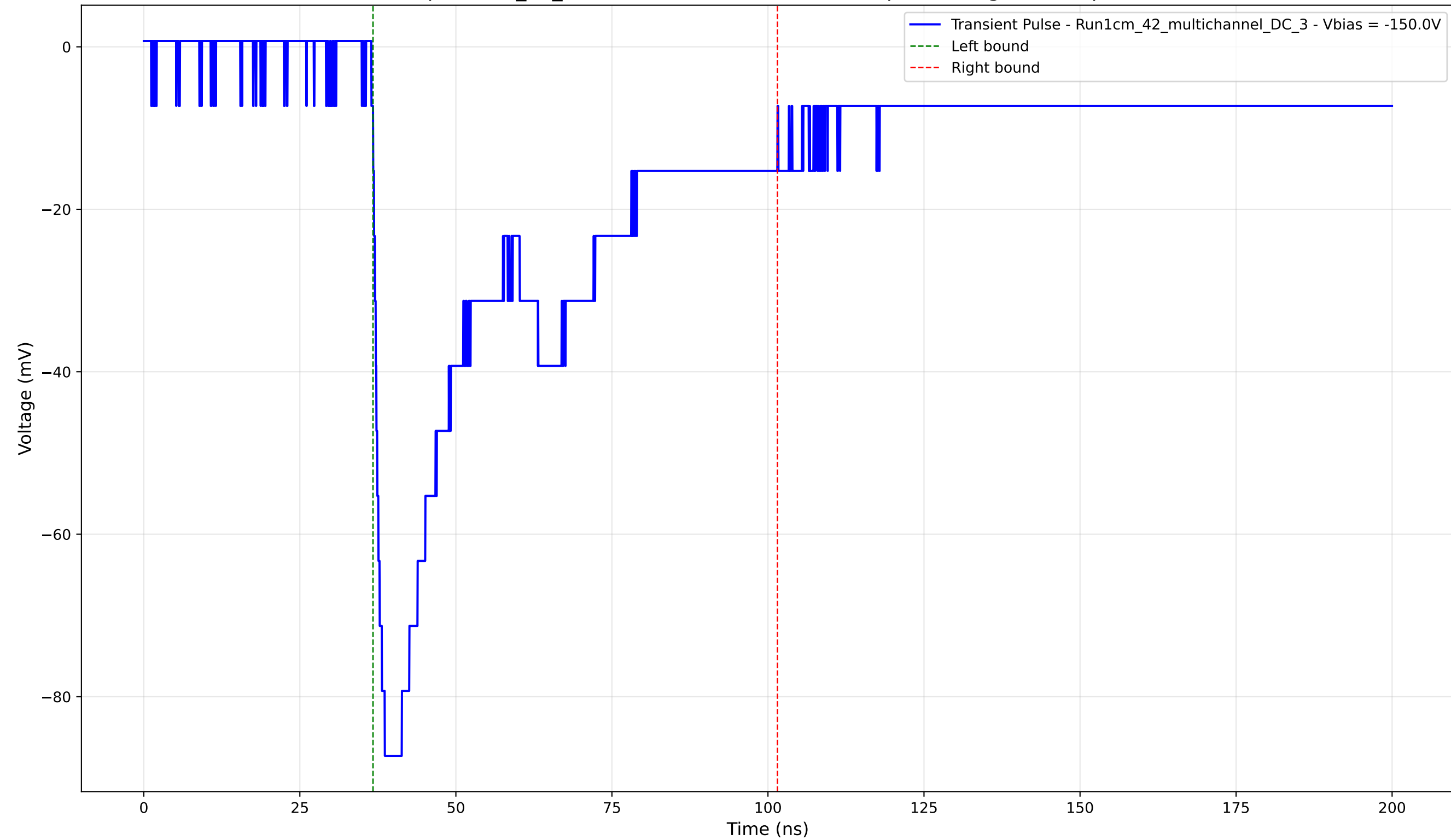
Transient Pulse - Sample: 1cm_42_multichannel - Position: 2095.0 \mu\text{m} - Charge: 41.52 pC - Rise Time: 1.42 ns
