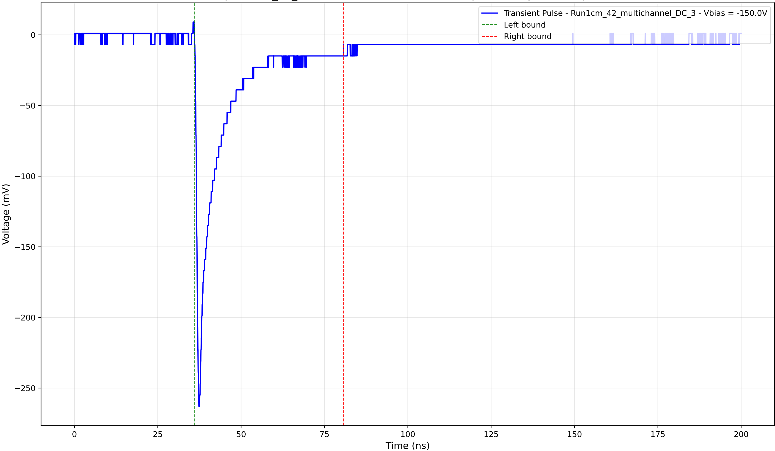
Transient Pulse - Sample: 1cm_42_multichannel - Position: 4510.0 \mu\text{m} - Charge: 39.32 pC - Rise Time: 0.87 ns
