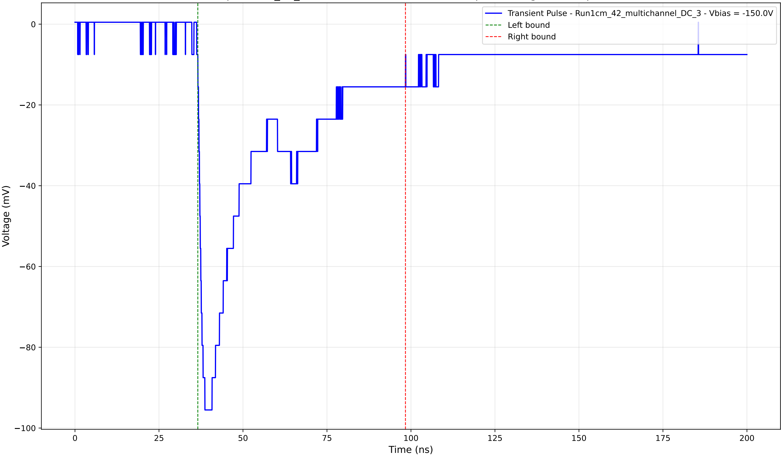
Transient Pulse - Sample: 1cm_42_multichannel - Position: 1965.0 \mu\text{m} - Charge: 41.30 pC - Rise Time: 1.55 ns
