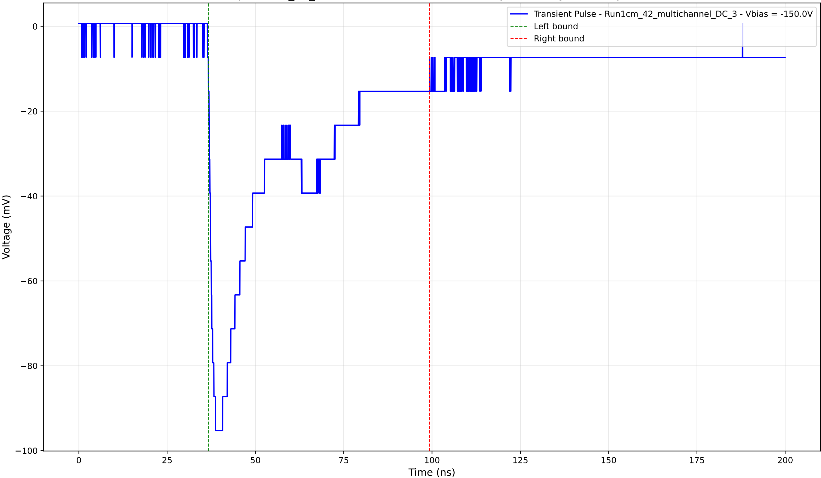
Transient Pulse - Sample: 1cm_42_multichannel - Position: 2040.0 \mu\text{m} - Charge: 42.35 pC - Rise Time: 1.57 ns
