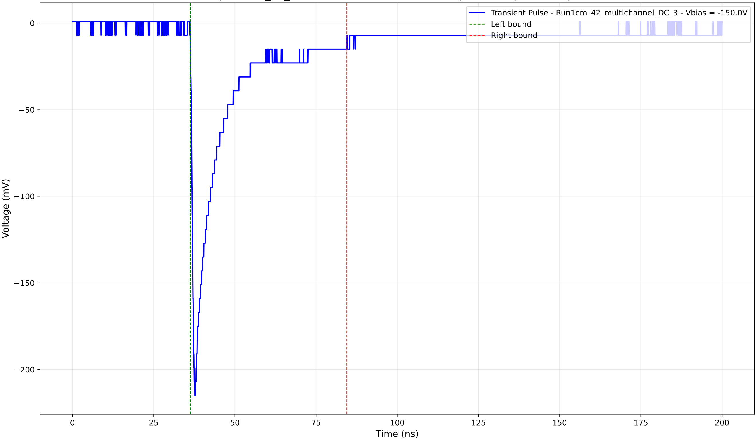
Transient Pulse - Sample: 1cm_42_multichannel - Position: 4230.0 \mu\text{m} - Charge: 41.56 pC - Rise Time: 1.02 ns
