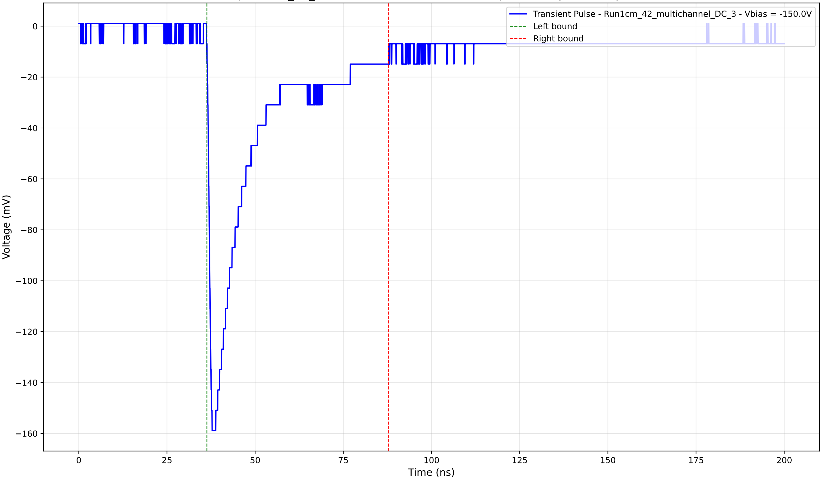
Transient Pulse - Sample: 1cm_42_multichannel - Position: 1115.0 \mu\text{m} - Charge: 43.38 pC - Rise Time: 1.18 ns
