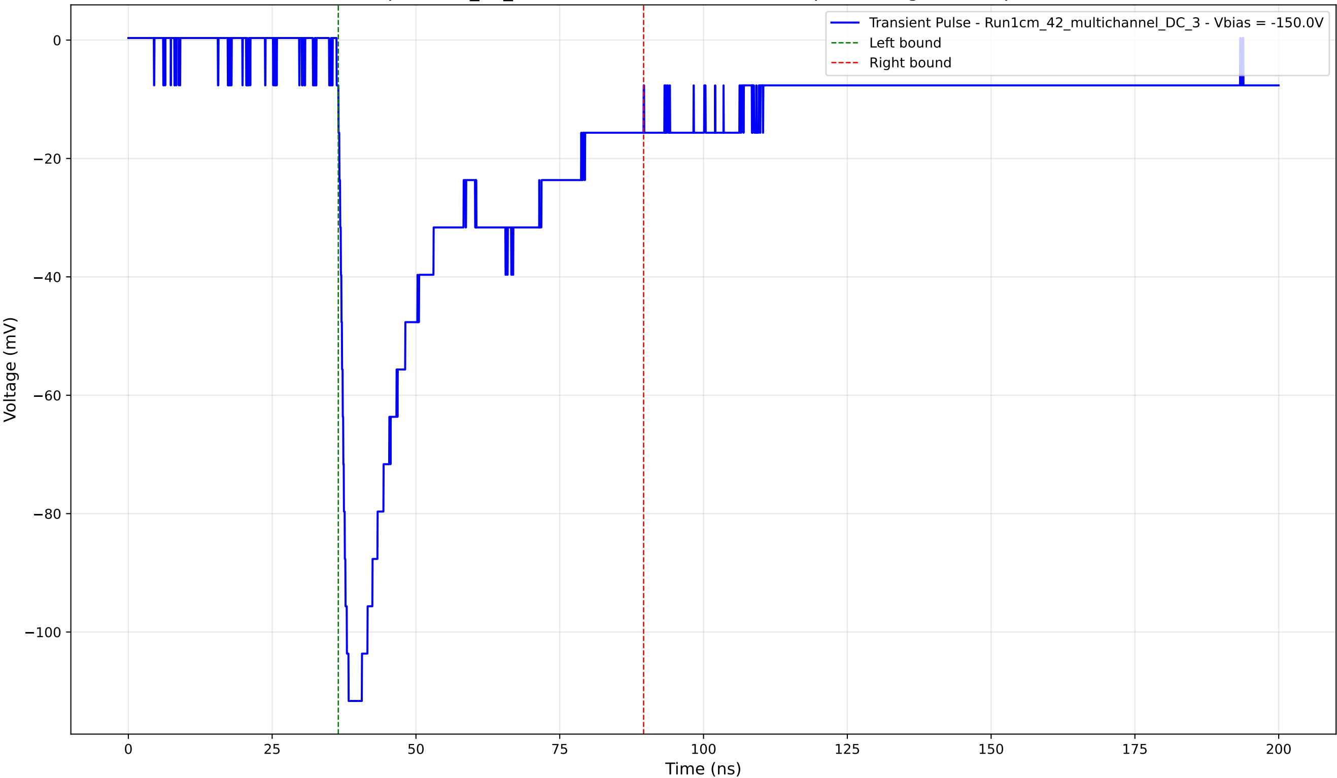
Transient Pulse - Sample: 1cm_42_multichannel - Position: 1740.0 \mu\text{m} - Charge: 41.73 pC - Rise Time: 1.47 ns
