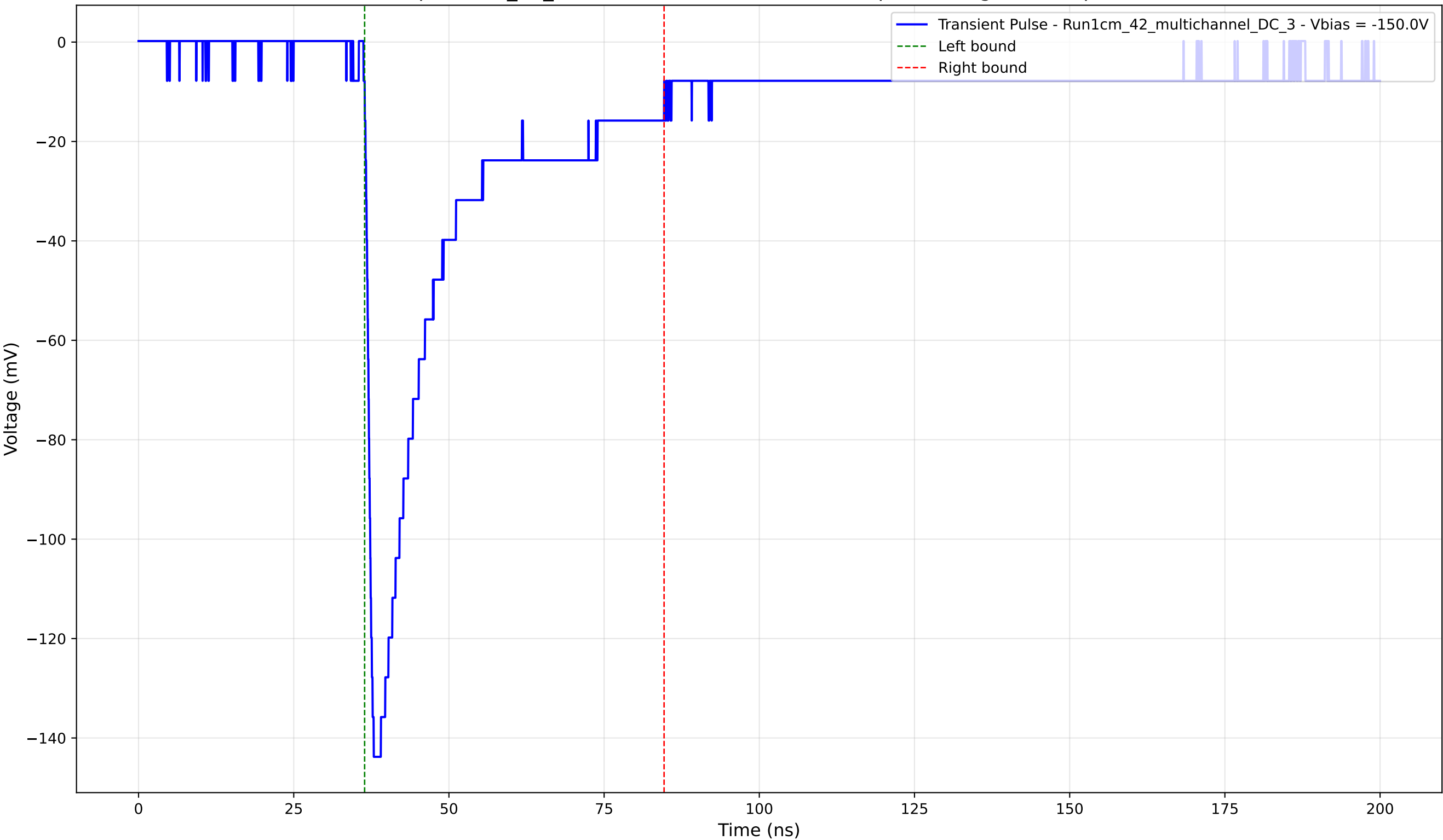
Transient Pulse - Sample: 1cm_42_multichannel - Position: 3795.0 \mu\text{m} - Charge: 38.79 pC - Rise Time: 1.26 ns
