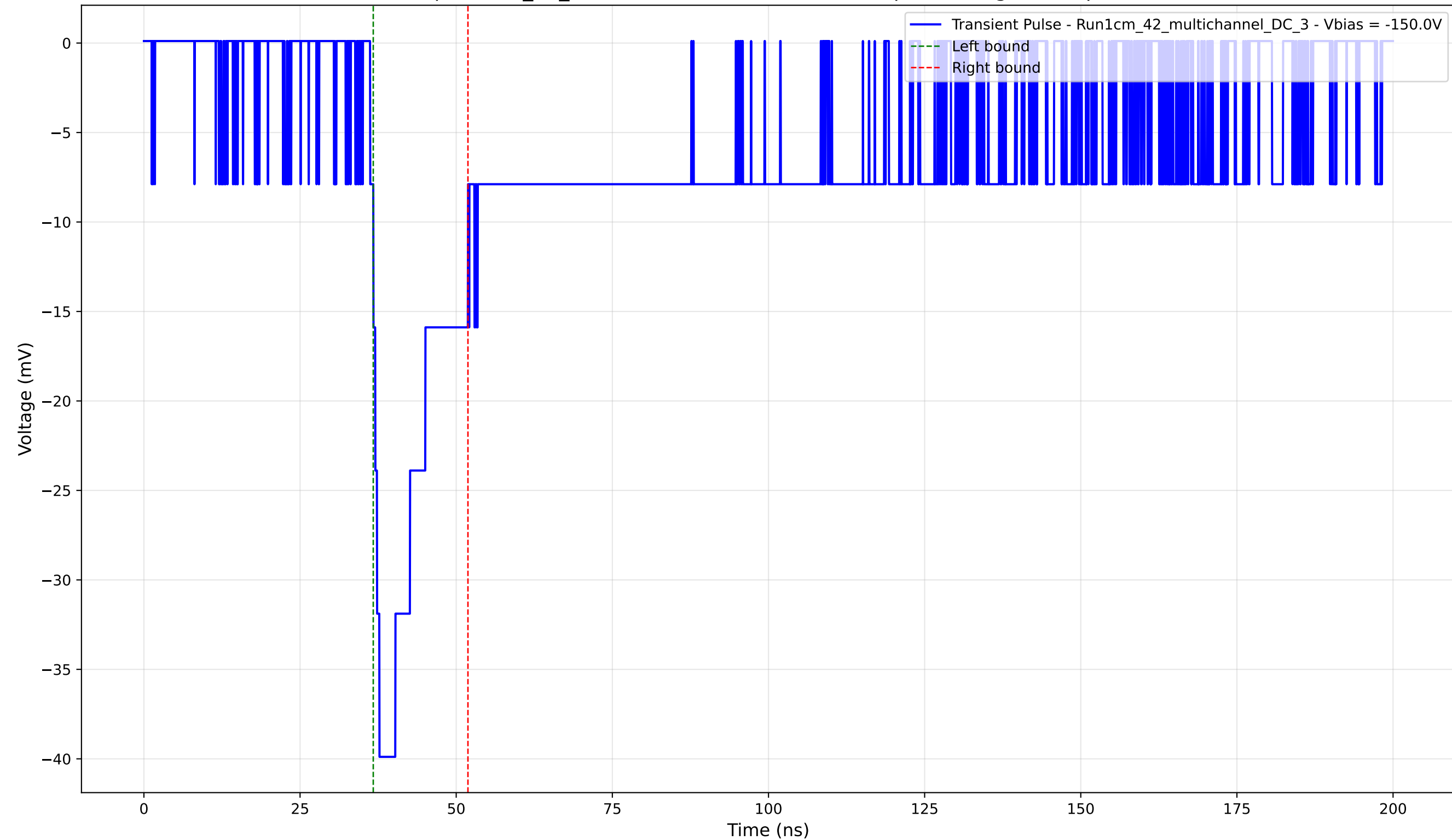
Transient Pulse - Sample: 1cm_42_multichannel - Position: 1325.0 \mu\text{m} - Charge: 7.35 pC - Rise Time: 1.49 ns
