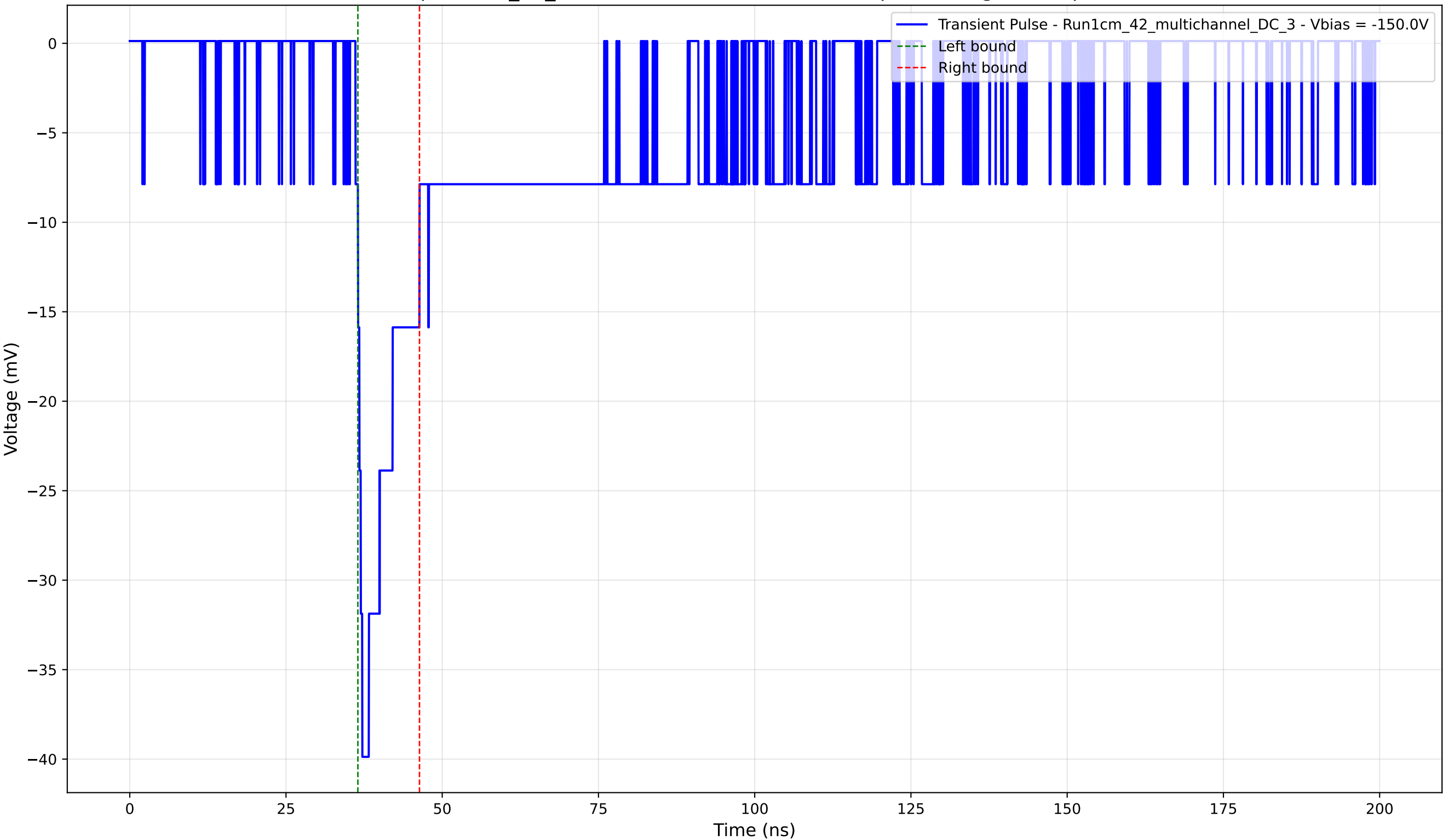
Transient Pulse - Sample: 1cm_42_multichannel - Position: 4355.0 \mu\text{m} - Charge: 4.63 pC - Rise Time: 1.09 ns
