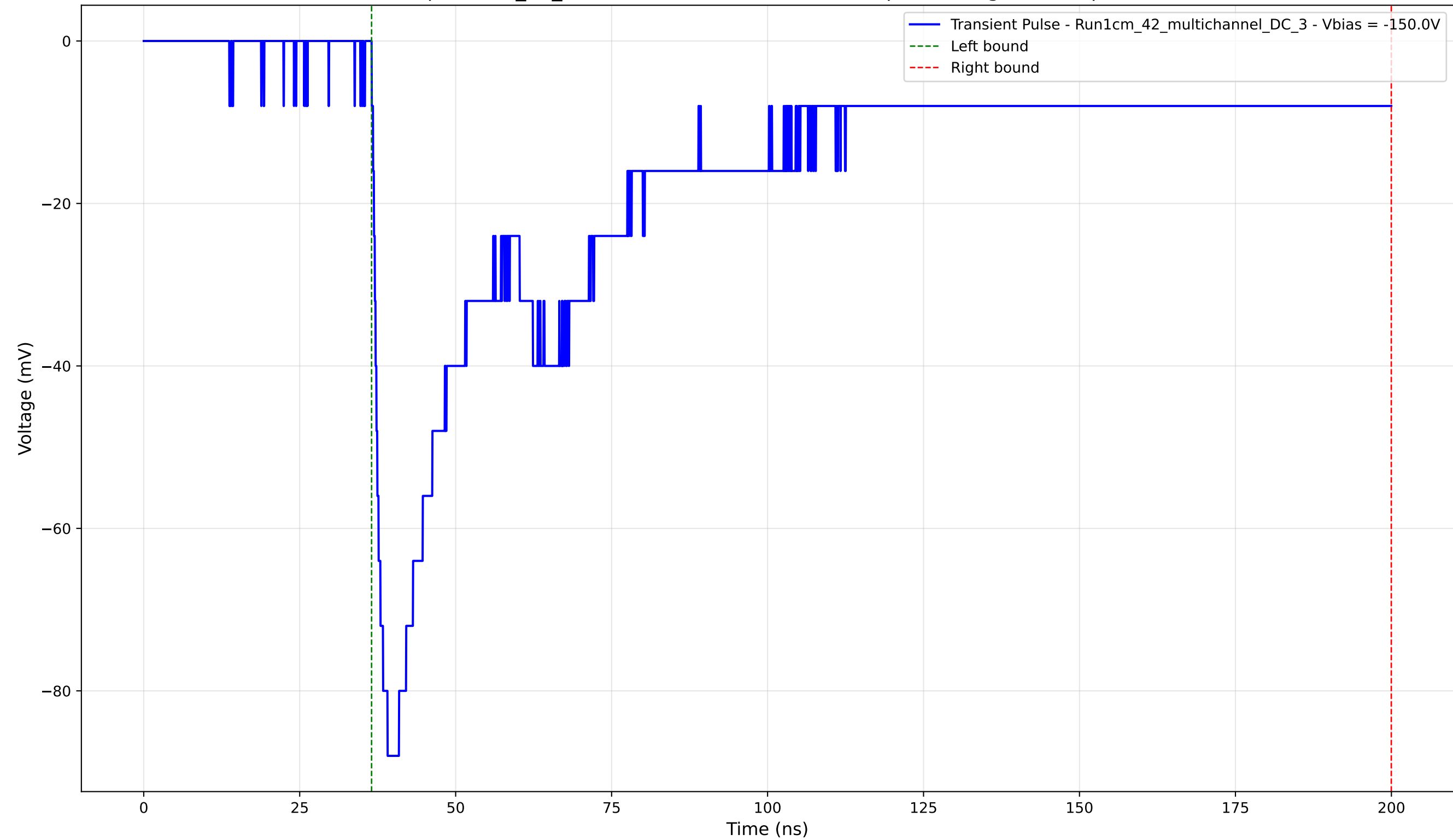
Transient Pulse - Sample: 1cm_42_multichannel - Position: 2155.0 \mu\text{m} - Charge: 57.87 pC - Rise Time: 1.62 ns
