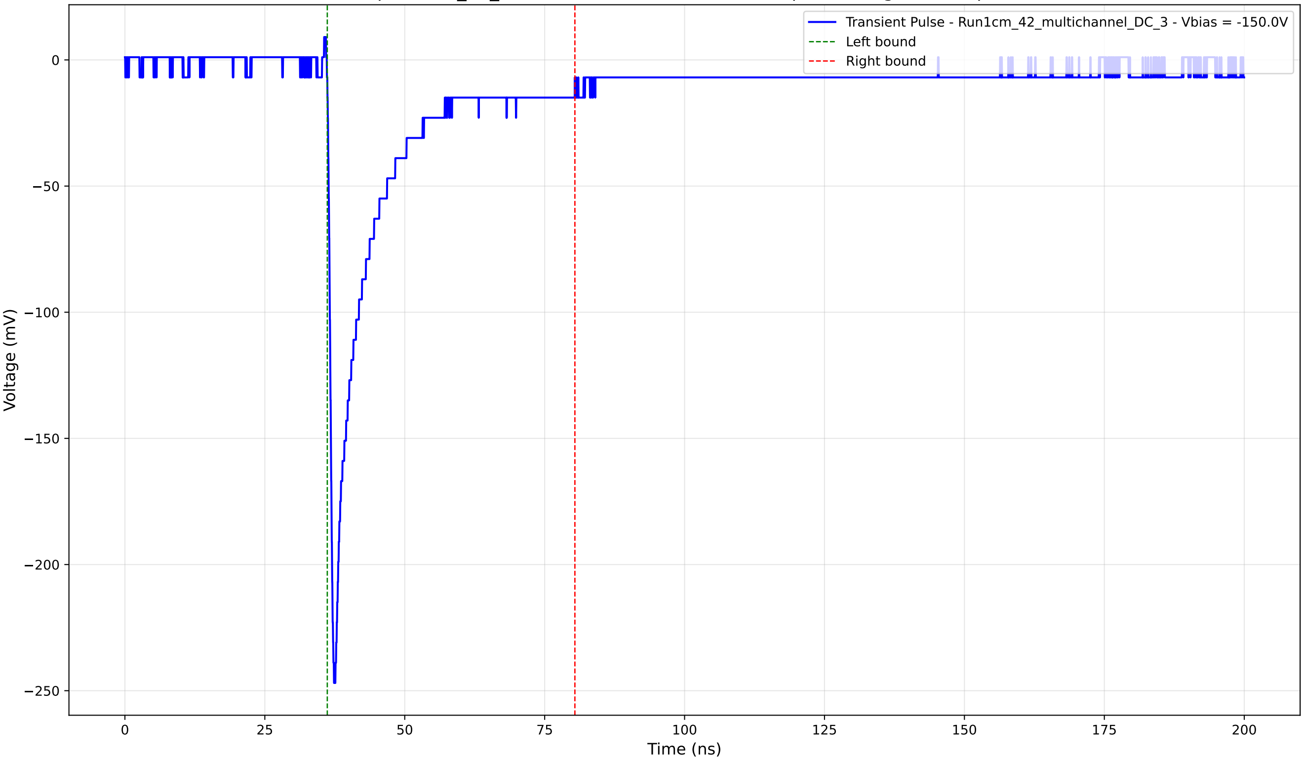
Transient Pulse - Sample: 1cm_42_multichannel - Position: 4485.0 \mu\text{m} - Charge: 37.57 pC - Rise Time: 0.84 ns
