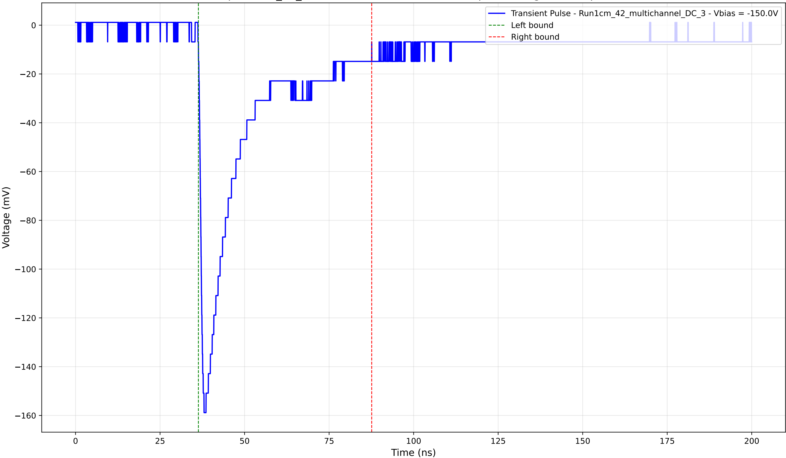
Transient Pulse - Sample: 1cm_42_multichannel - Position: 1160.0 \mu\text{m} - Charge: 43.30 pC - Rise Time: 1.30 ns
