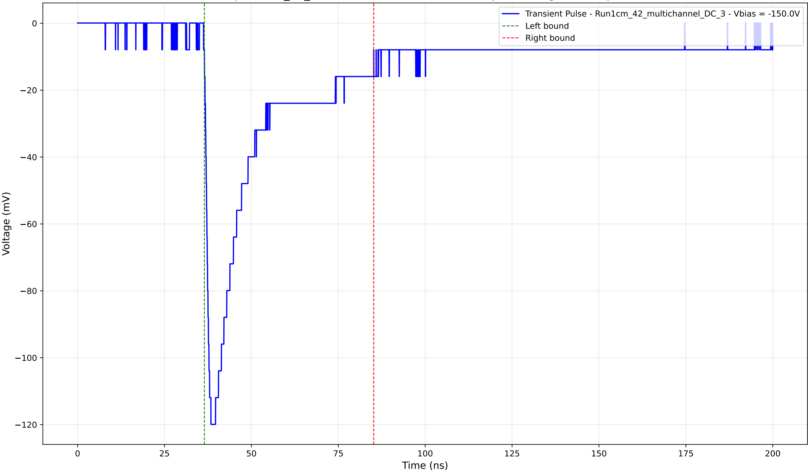
Transient Pulse - Sample: 1cm_42_multichannel - Position: 3470.0 \mu\text{m} - Charge: 36.51 pC - Rise Time: 1.49 ns
