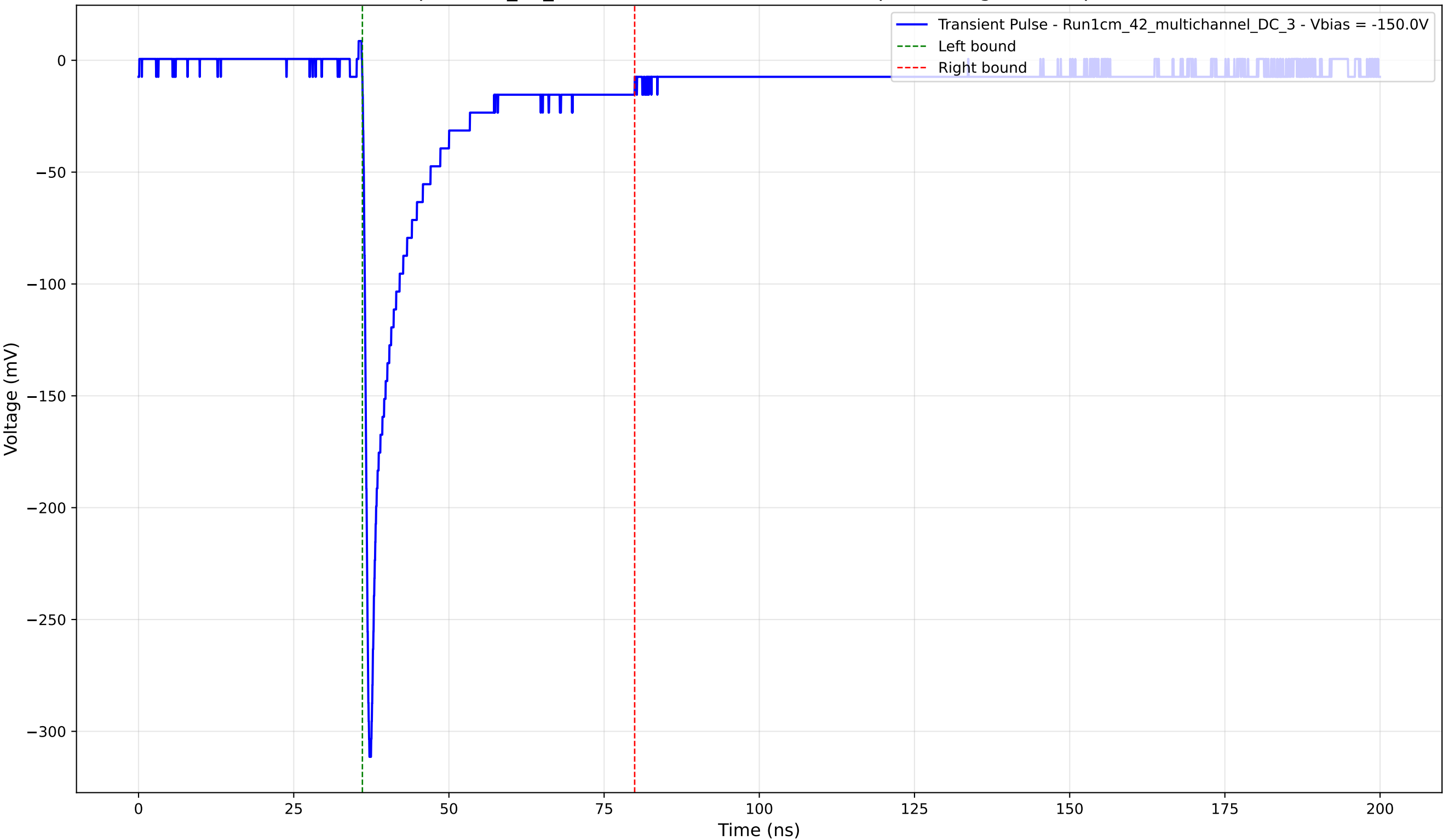
Transient Pulse - Sample: 1cm_42_multichannel - Position: 4640.0 \mu\text{m} - Charge: 40.81 pC - Rise Time: 0.84 ns
