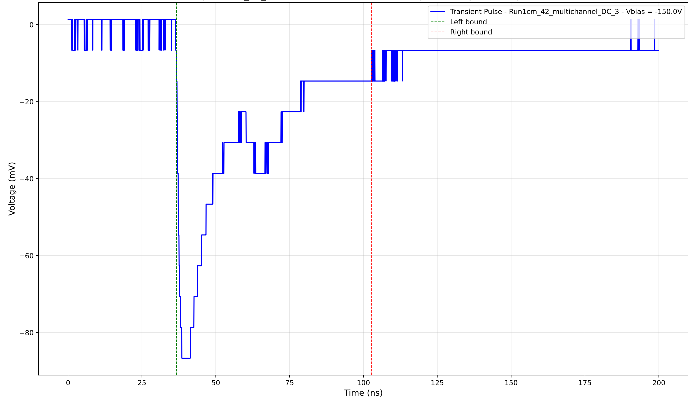
Transient Pulse - Sample: 1cm_42_multichannel - Position: 2090.0 \mu\text{m} - Charge: 41.22 pC - Rise Time: 1.39 ns
