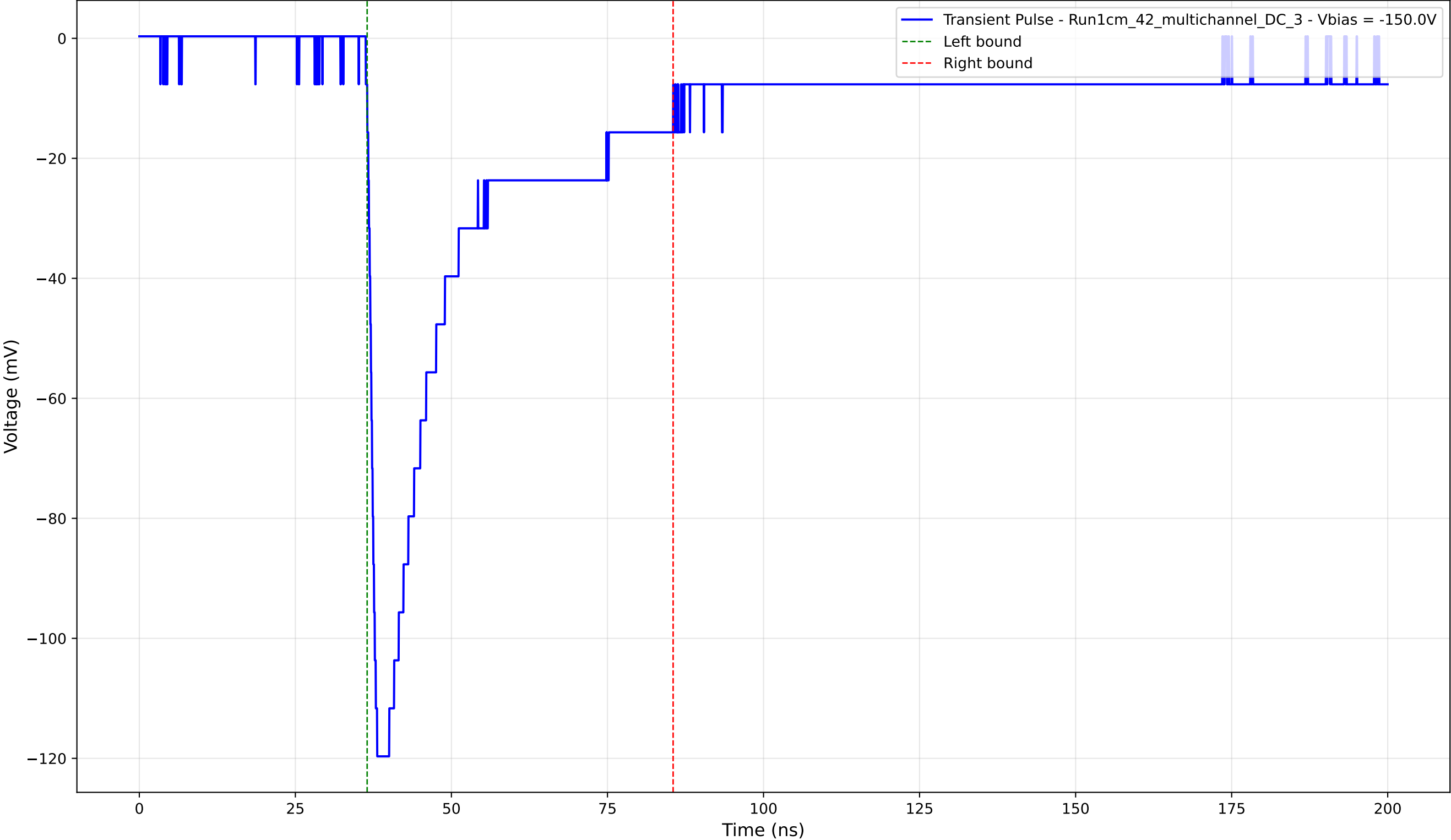
Transient Pulse - Sample: 1cm_42_multichannel - Position: 3485.0 \mu\text{m} - Charge: 37.14 pC - Rise Time: 1.37 ns
