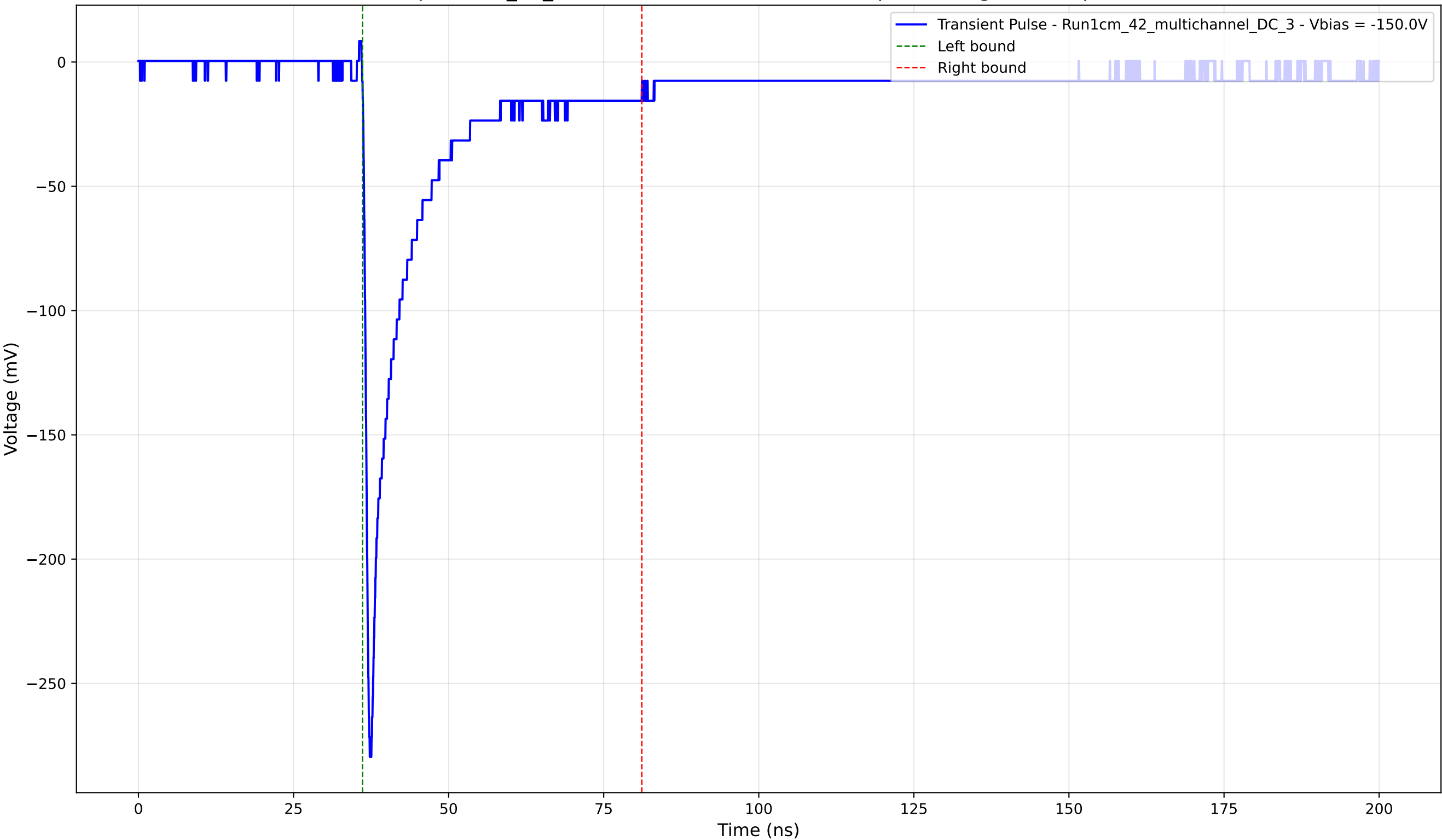
Transient Pulse - Sample: 1cm_42_multichannel - Position: 4545.0 \mu\text{m} - Charge: 40.72 pC - Rise Time: 0.85 ns
