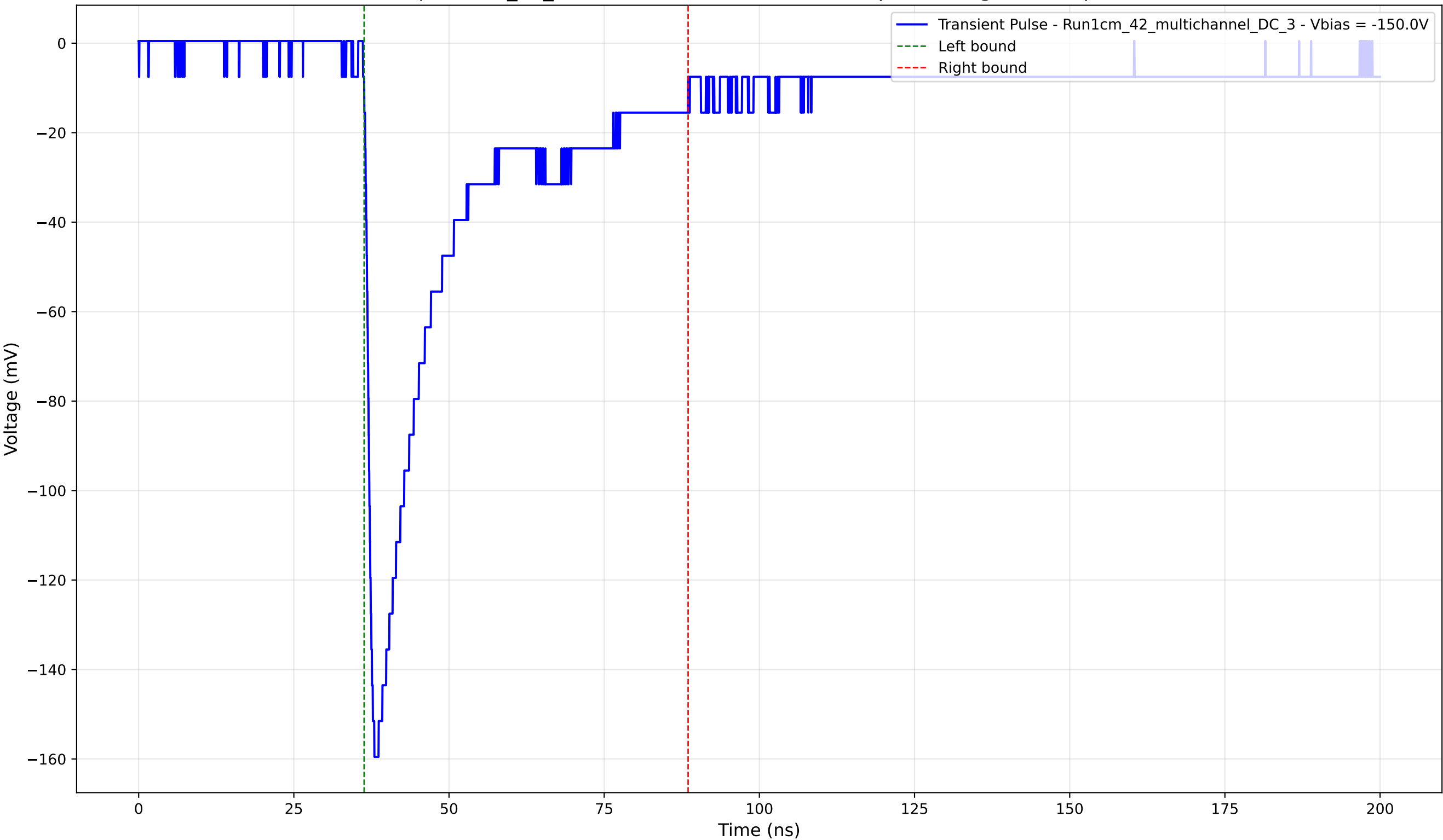
Transient Pulse - Sample: 1cm_42_multichannel - Position: 1150.0 \mu\text{m} - Charge: 44.26 pC - Rise Time: 1.26 ns
