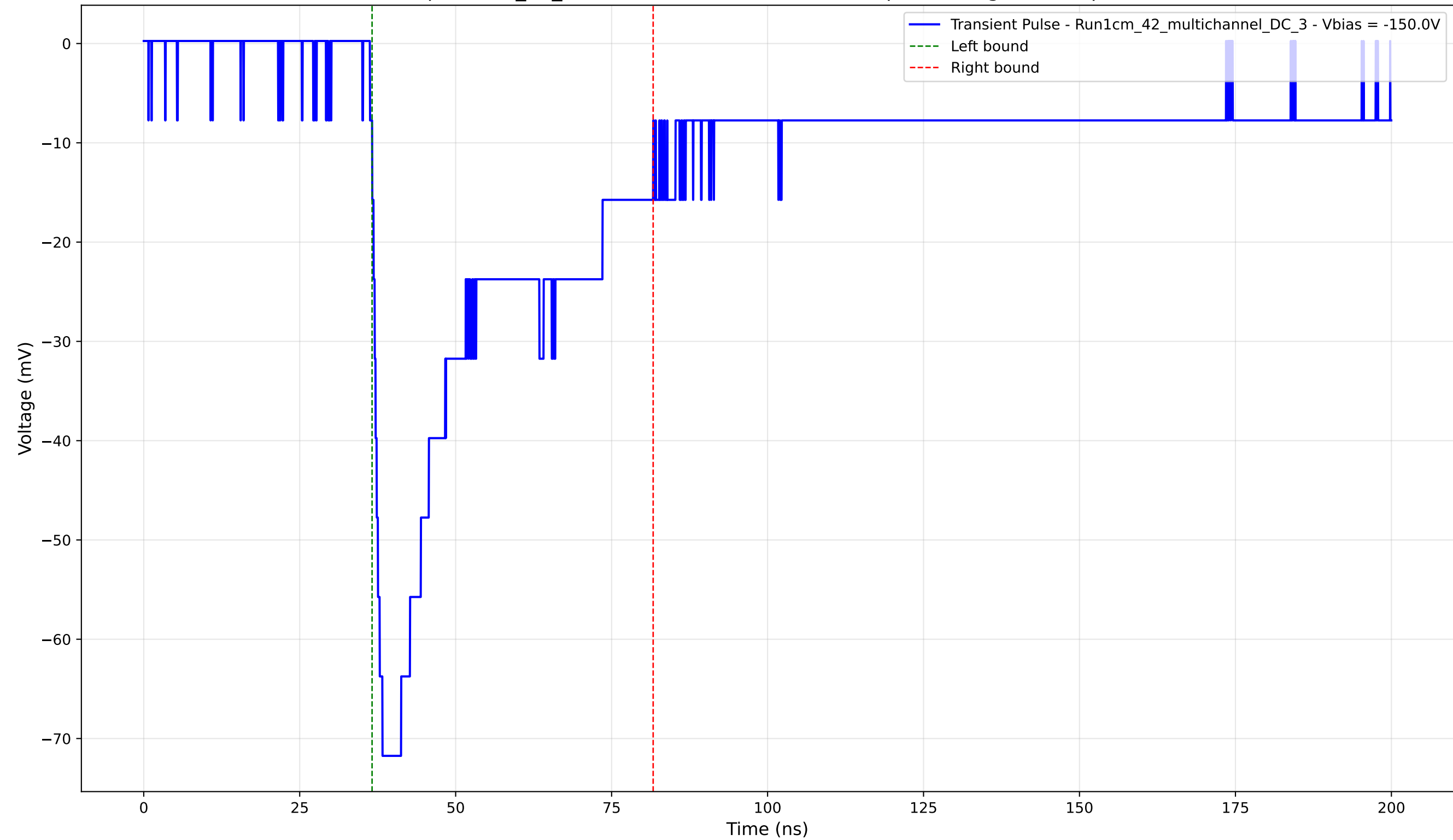
Transient Pulse - Sample: 1cm_42_multichannel - Position: 1930.0 \mu\text{m} - Charge: 28.16 pC - Rise Time: 2.00 ns
