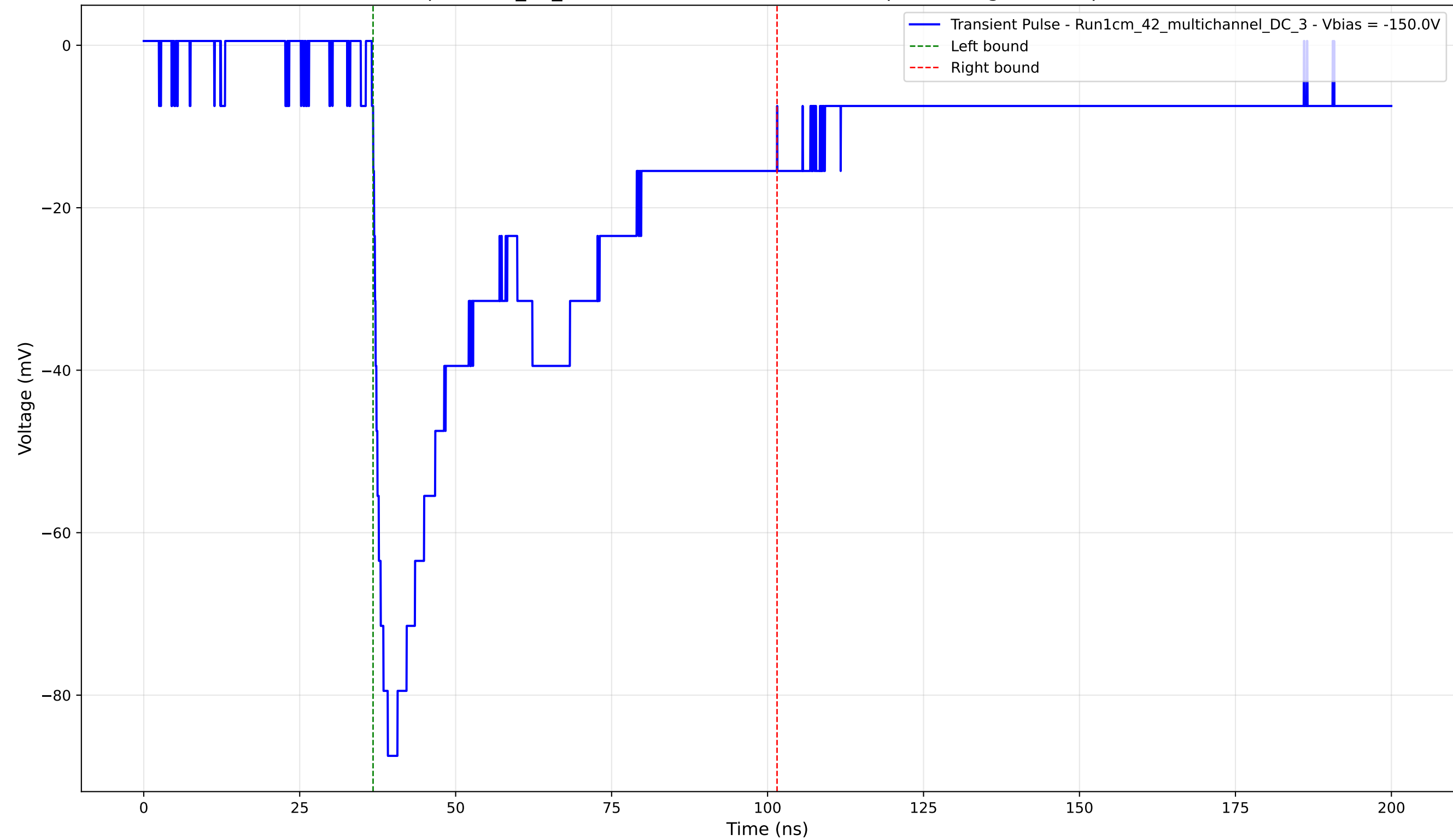
Transient Pulse - Sample: 1cm_42_multichannel - Position: 2225.0 \mu\text{m} - Charge: 41.77 pC - Rise Time: 1.66 ns
