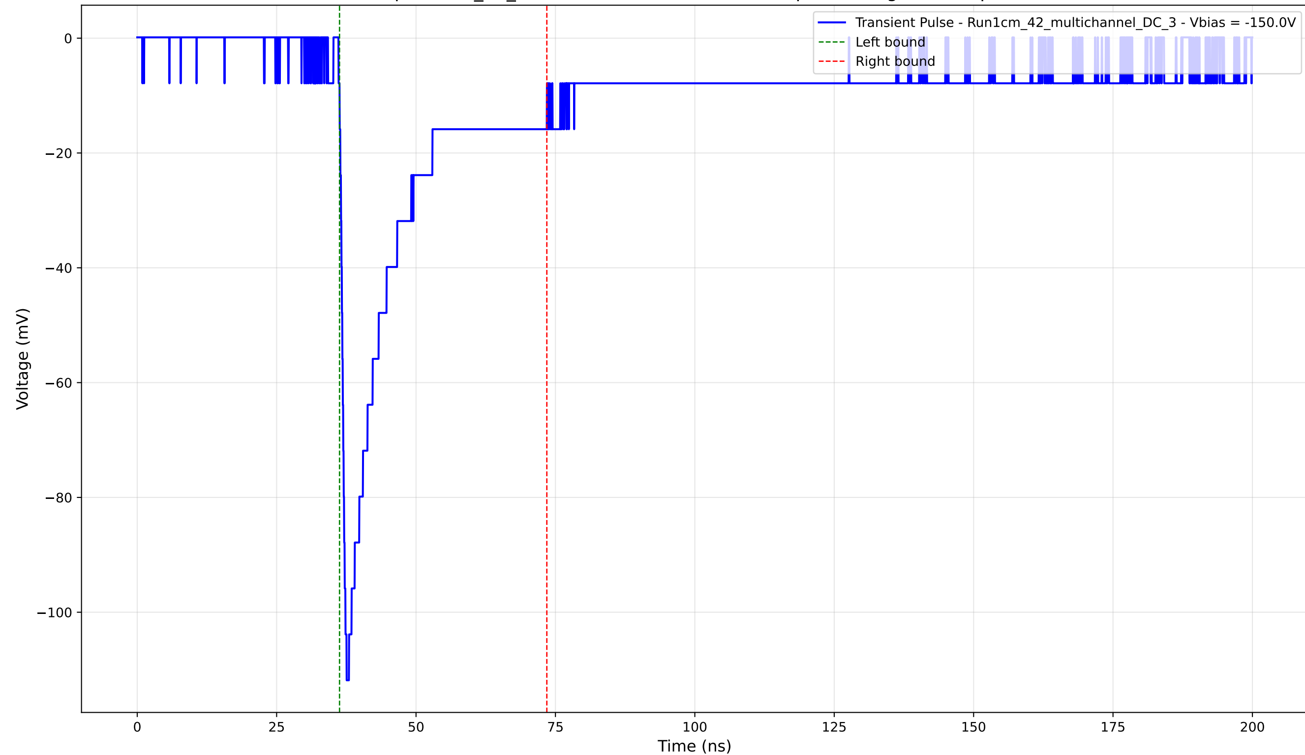
Transient Pulse - Sample: 1cm_42_multichannel - Position: 805.0 \mu\text{m} - Charge: 23.48 pC - Rise Time: 1.05 ns
