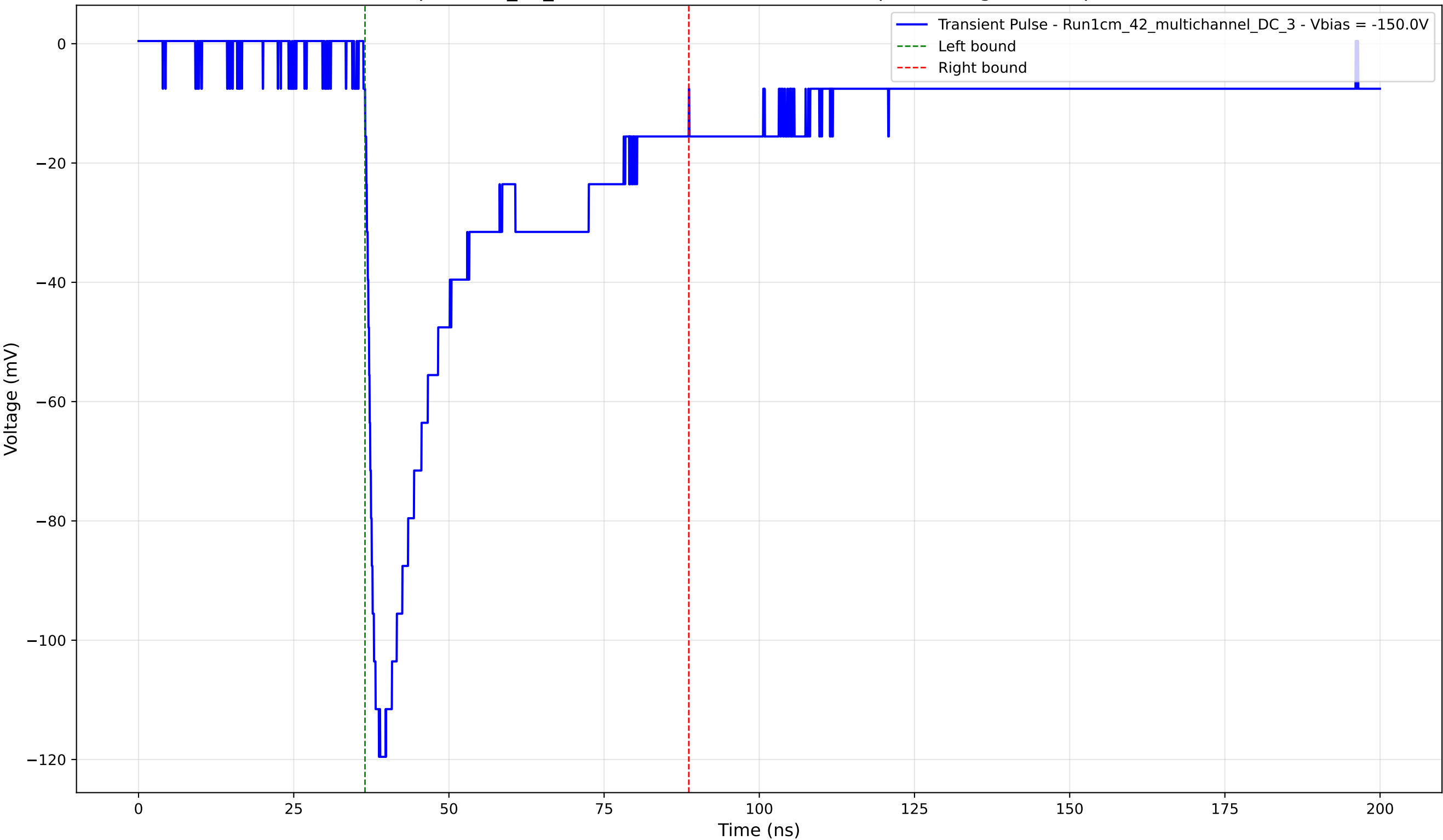
Transient Pulse - Sample: 1cm_42_multichannel - Position: 1715.0 \mu\text{m} - Charge: 41.65 pC - Rise Time: 1.69 ns
