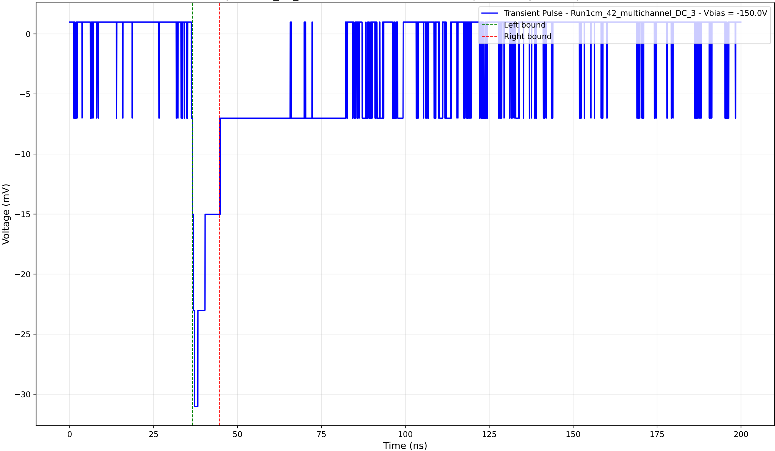
Transient Pulse - Sample: 1cm_42_multichannel - Position: 4360.0 \mu\text{m} - Charge: 3.14 pC - Rise Time: 0.97 ns
