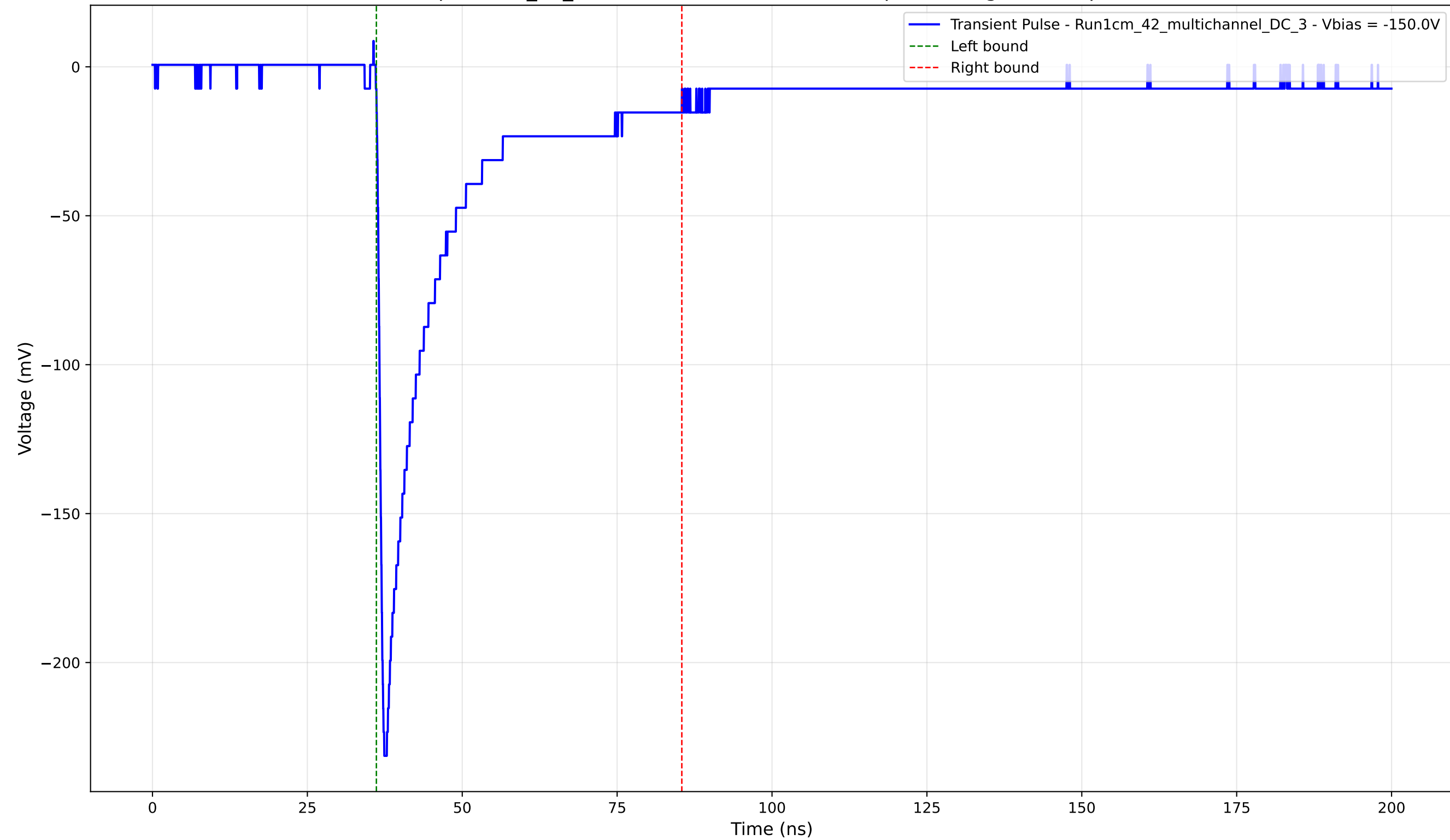
Transient Pulse - Sample: 1cm_42_multichannel - Position: 640.0 \mu\text{m} - Charge: 46.83 pC - Rise Time: 1.00 ns
