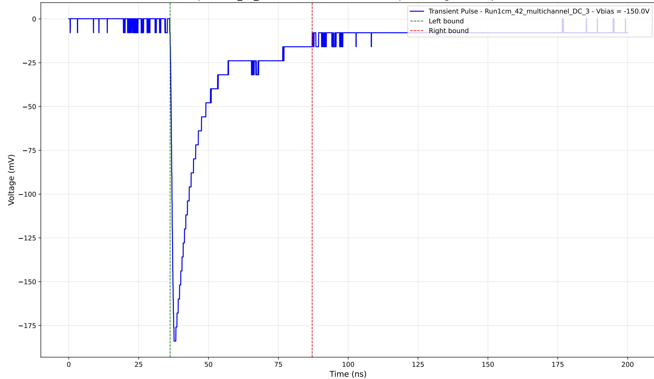
Transient Pulse - Sample: 1cm_42_multichannel - Position: 950.0 \mu\text{m} - Charge: 45.90 pC - Rise Time: 1.05 ns
