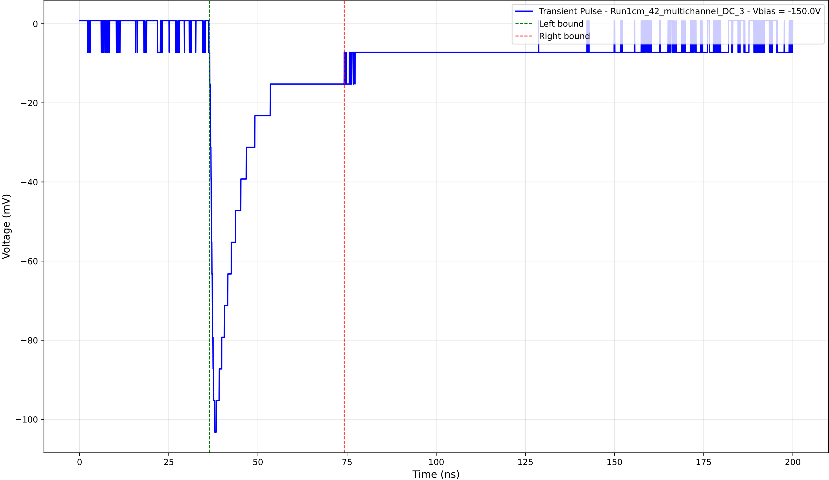
Transient Pulse - Sample: 1cm_42_multichannel - Position: 3945.0 \mu\text{m} - Charge: 22.97 pC - Rise Time: 1.11 ns
