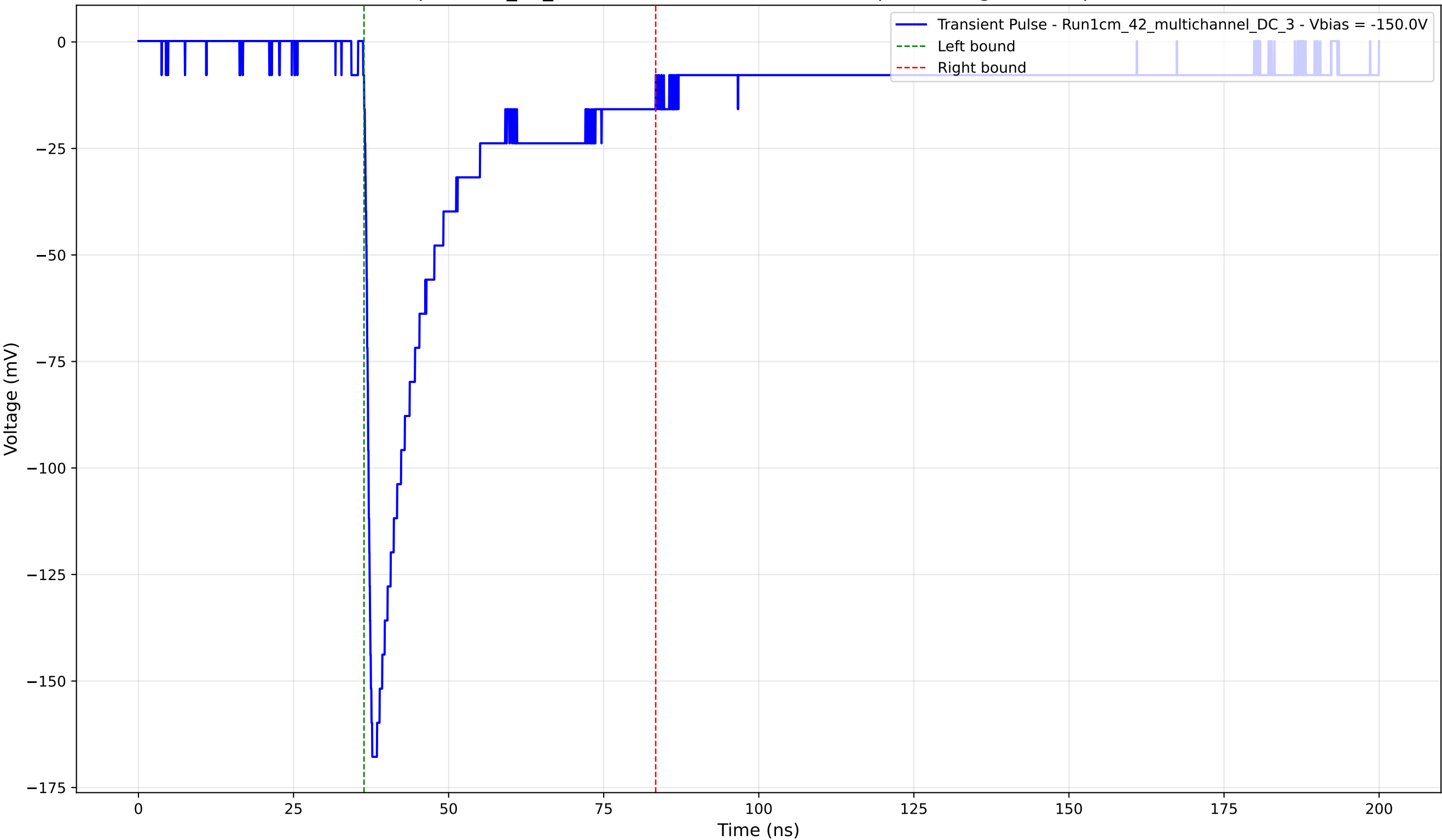
Transient Pulse - Sample: 1cm_42_multichannel - Position: 3985.0 \mu\text{m} - Charge: 39.86 pC - Rise Time: 0.98 ns
