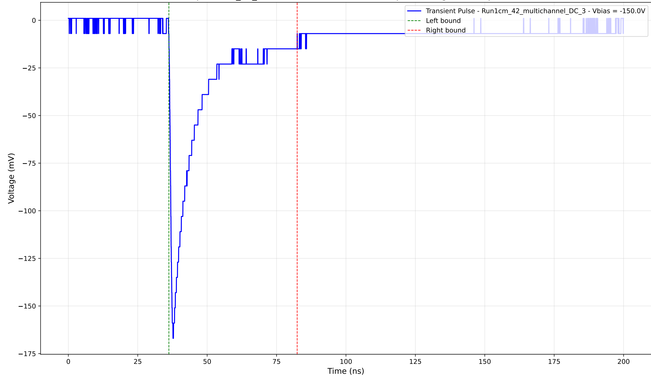
Transient Pulse - Sample: 1cm_42_multichannel - Position: 790.0 \mu\text{m} - Charge: 35.94 pC - Rise Time: 1.00 ns
