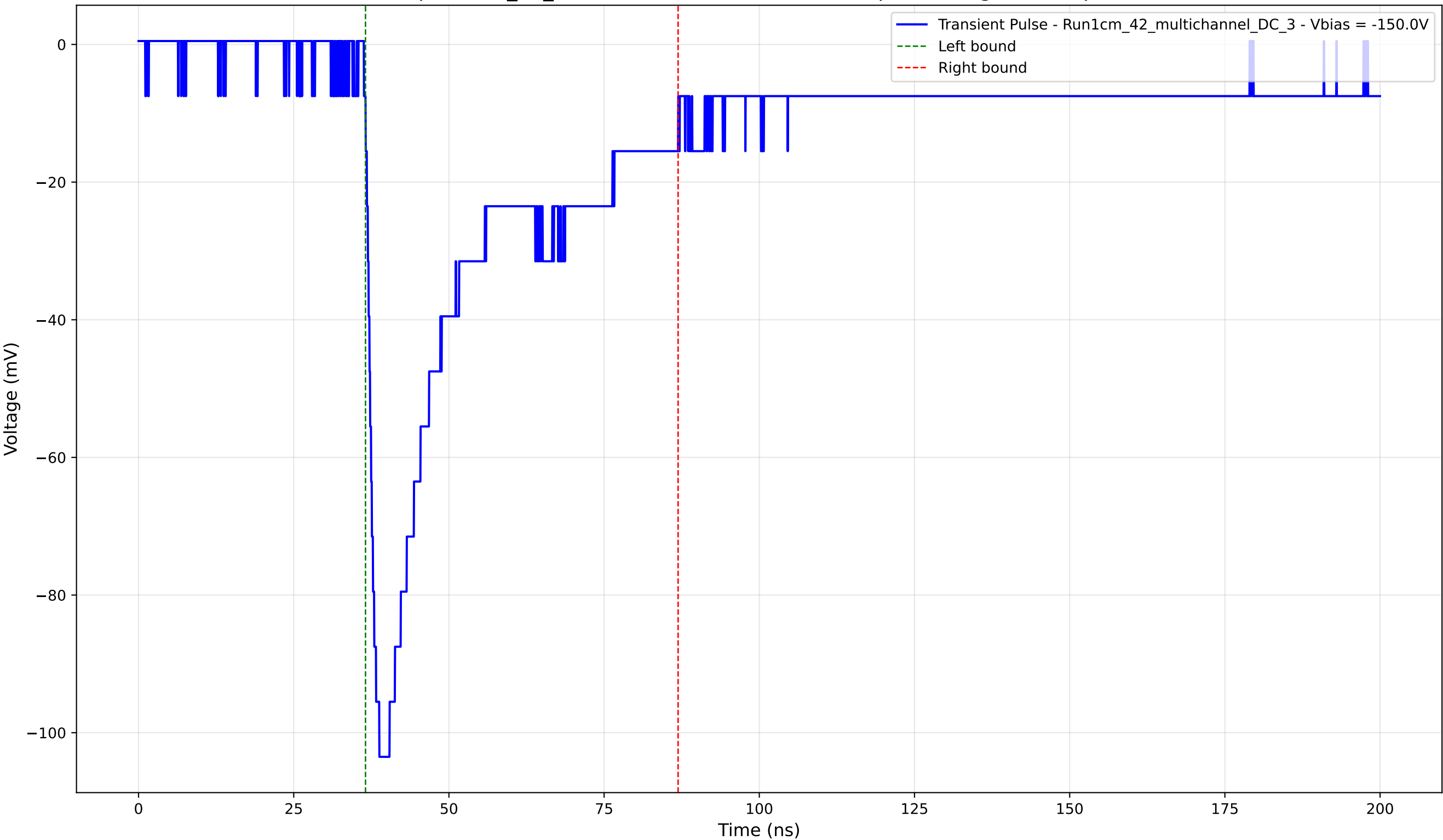
Transient Pulse - Sample: 1cm_42_multichannel - Position: 3135.0 \mu\text{m} - Charge: 35.84 pC - Rise Time: 1.69 ns
