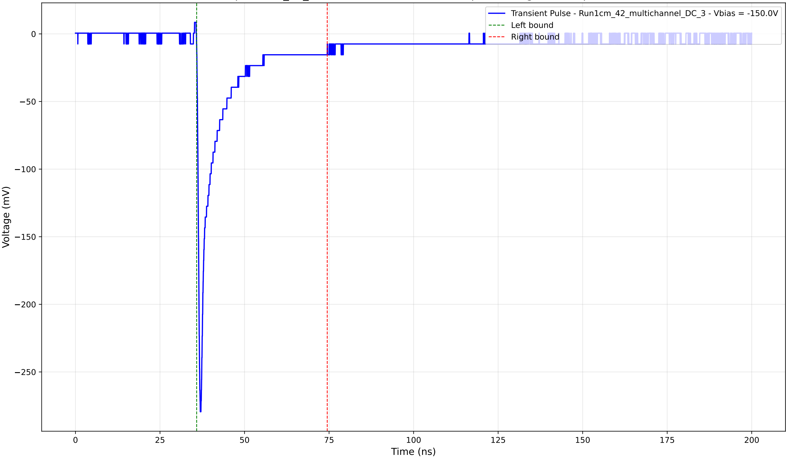
Transient Pulse - Sample: 1cm_42_multichannel - Position: 90.0 \mu\text{m} - Charge: 32.63 pC - Rise Time: 0.79 ns
