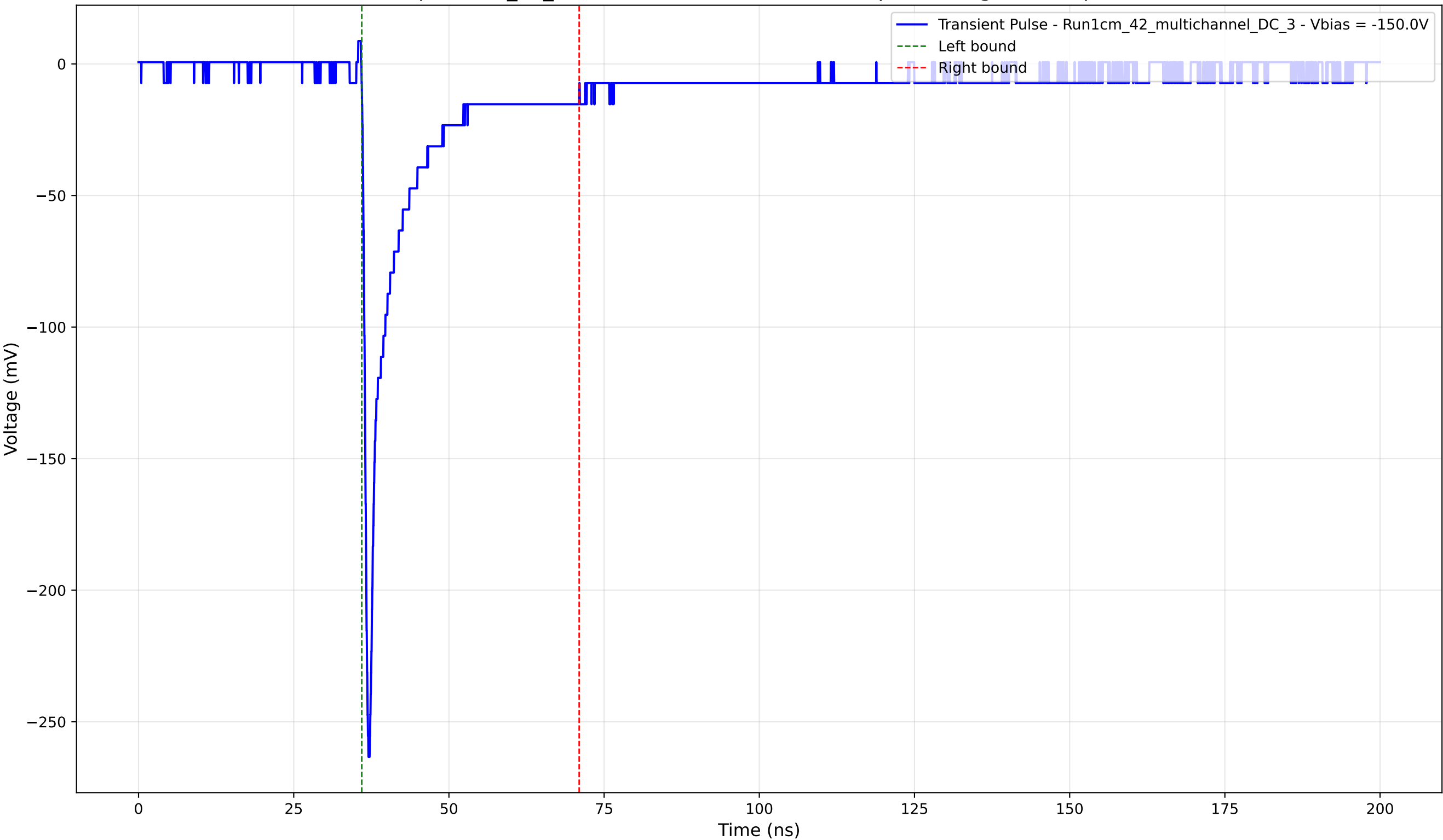
Transient Pulse - Sample: 1cm_42_multichannel - Position: 4840.0 \mu\text{m} - Charge: 28.14 pC - Rise Time: 0.77 ns
