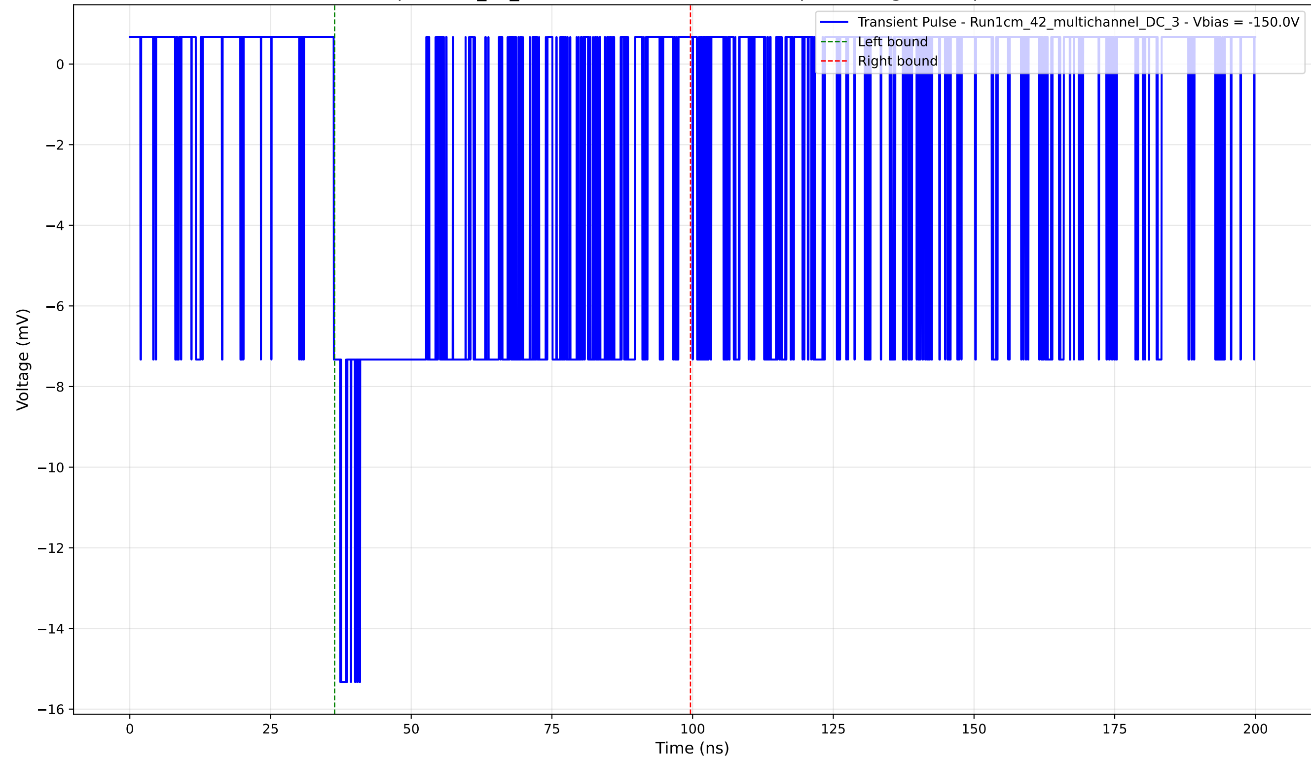
Transient Pulse - Sample: 1cm_42_multichannel - Position: 860.0 \mu\text{m} - Charge: 6.61 pC - Rise Time: 1.16 ns
