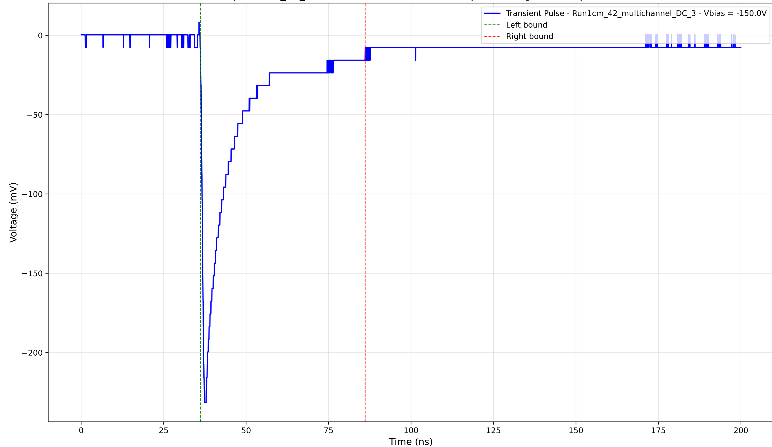
Transient Pulse - Sample: 1cm_42_multichannel - Position: 645.0 \mu\text{m} - Charge: 47.68 pC - Rise Time: 0.98 ns
