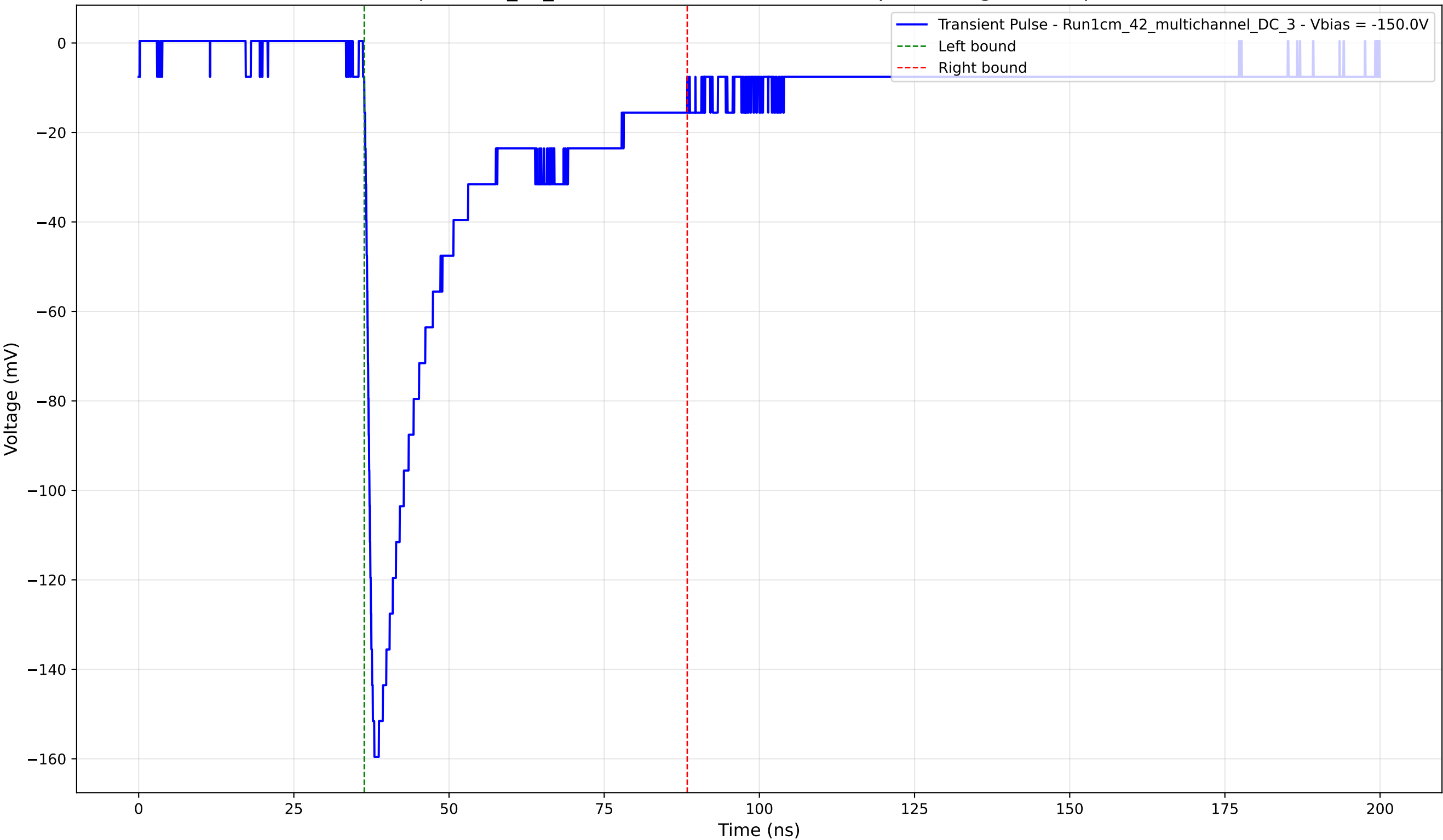
Transient Pulse - Sample: 1cm_42_multichannel - Position: 1155.0 \mu\text{m} - Charge: 44.42 pC - Rise Time: 1.26 ns
