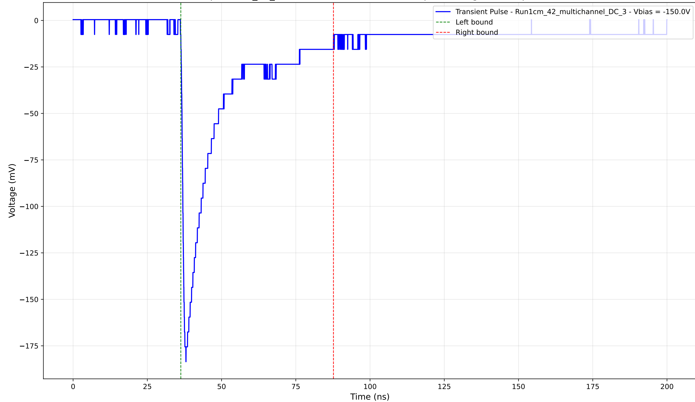
Transient Pulse - Sample: 1cm_42_multichannel - Position: 990.0 \mu\text{m} - Charge: 45.46 pC - Rise Time: 1.11 ns
