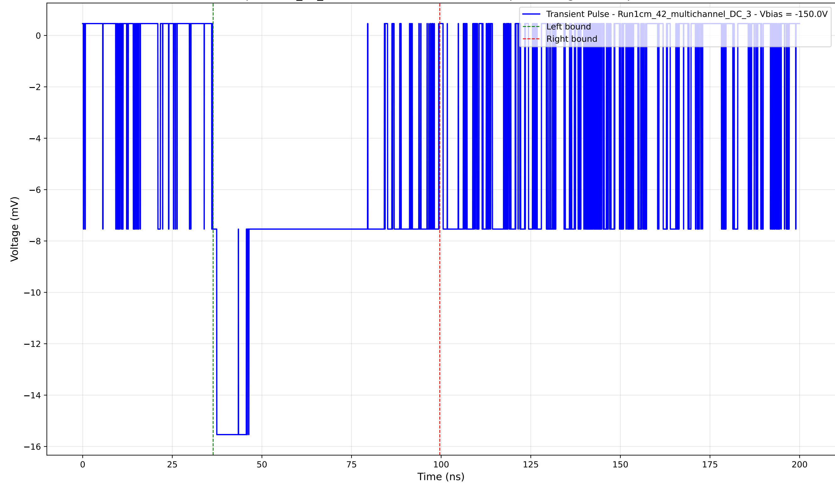
Transient Pulse - Sample: 1cm_42_multichannel - Position: 1840.0 \mu\text{m} - Charge: 10.41 pC - Rise Time: 1.16 ns
