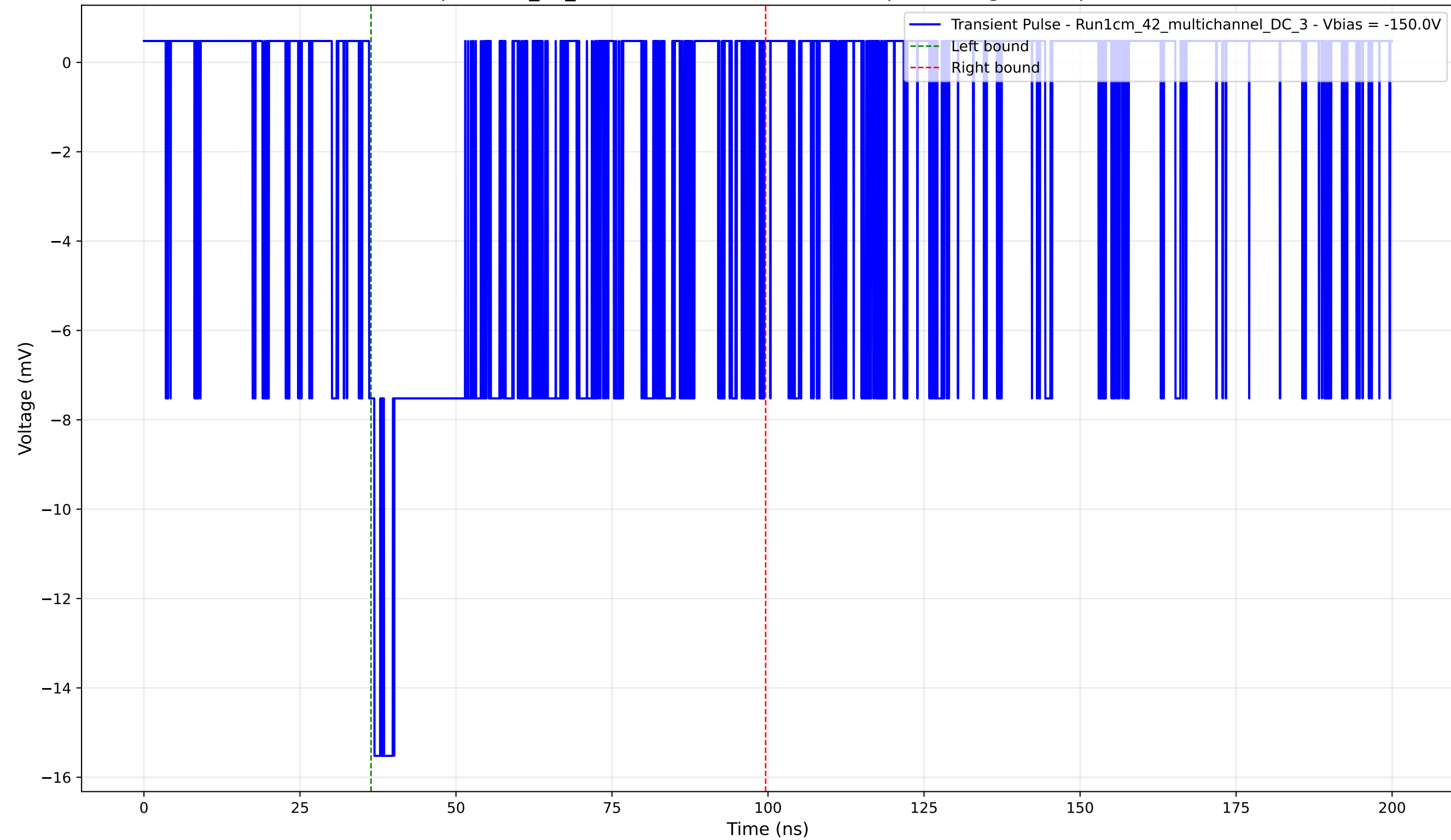
Transient Pulse - Sample: 1cm_42_multichannel - Position: 350.0 \mu\text{m} - Charge: 5.98 pC - Rise Time: 0.86 ns
