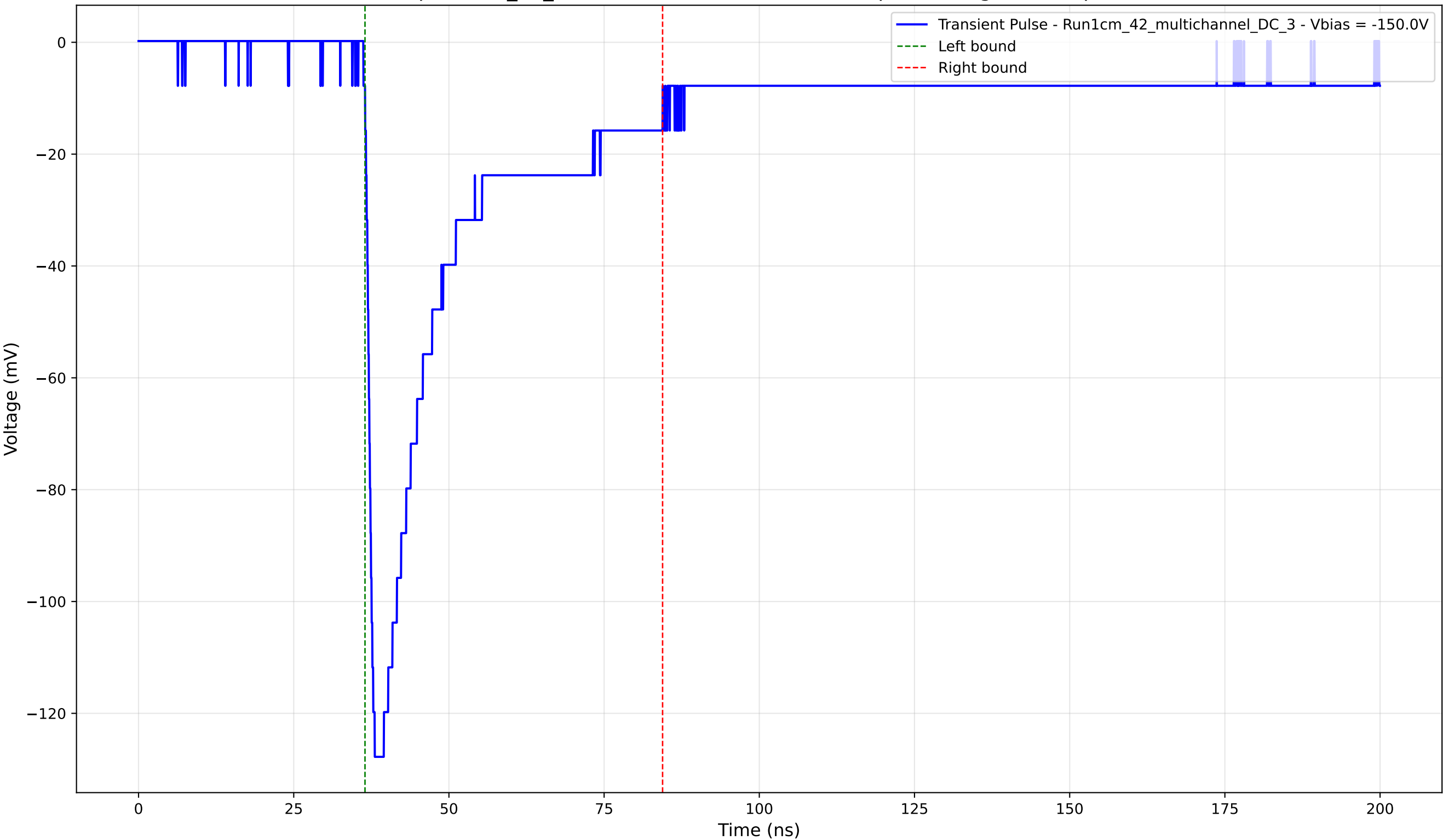
Transient Pulse - Sample: 1cm_42_multichannel - Position: 3645.0 \mu\text{m} - Charge: 37.02 pC - Rise Time: 1.31 ns
