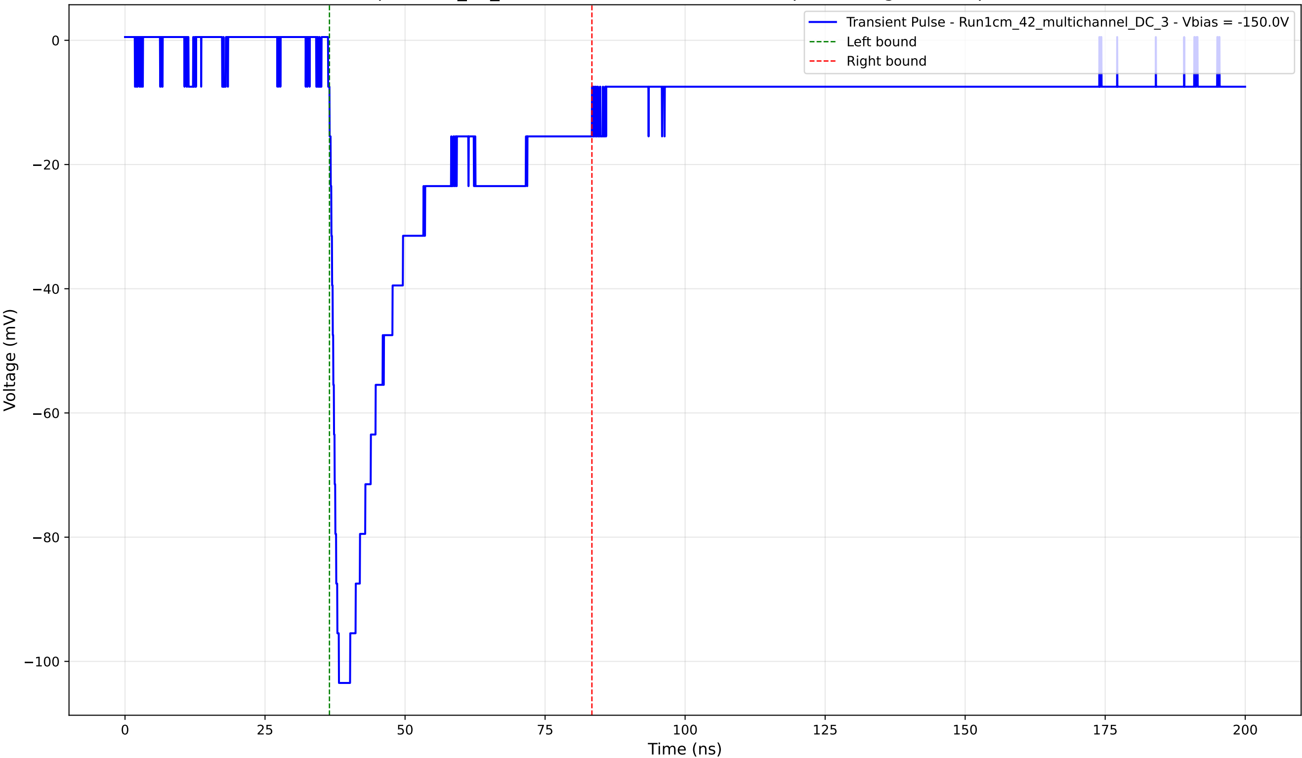
Transient Pulse - Sample: 1cm_42_multichannel - Position: 3455.0 \mu\text{m} - Charge: 31.95 pC - Rise Time: 1.39 ns
