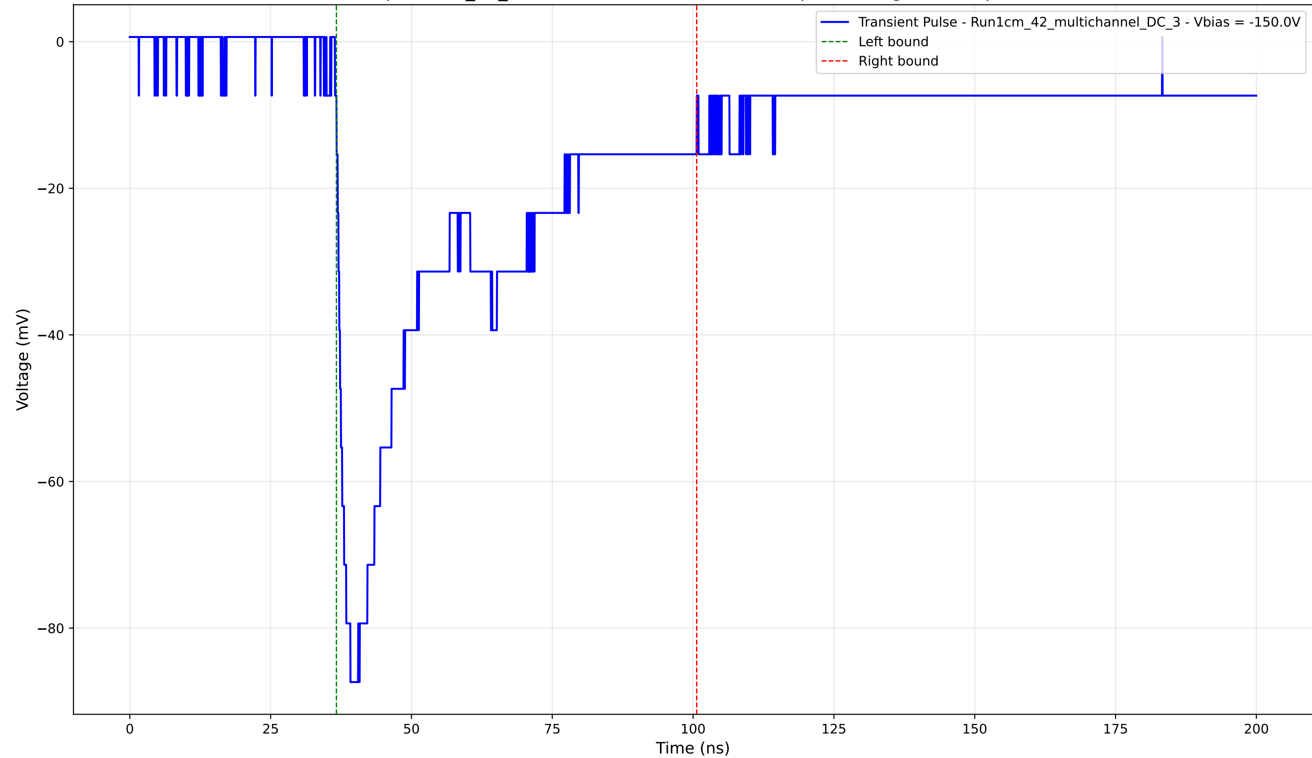
Transient Pulse - Sample: 1cm_42_multichannel - Position: 2665.0 \mu\text{m} - Charge: 39.62 pC - Rise Time: 1.74 ns
