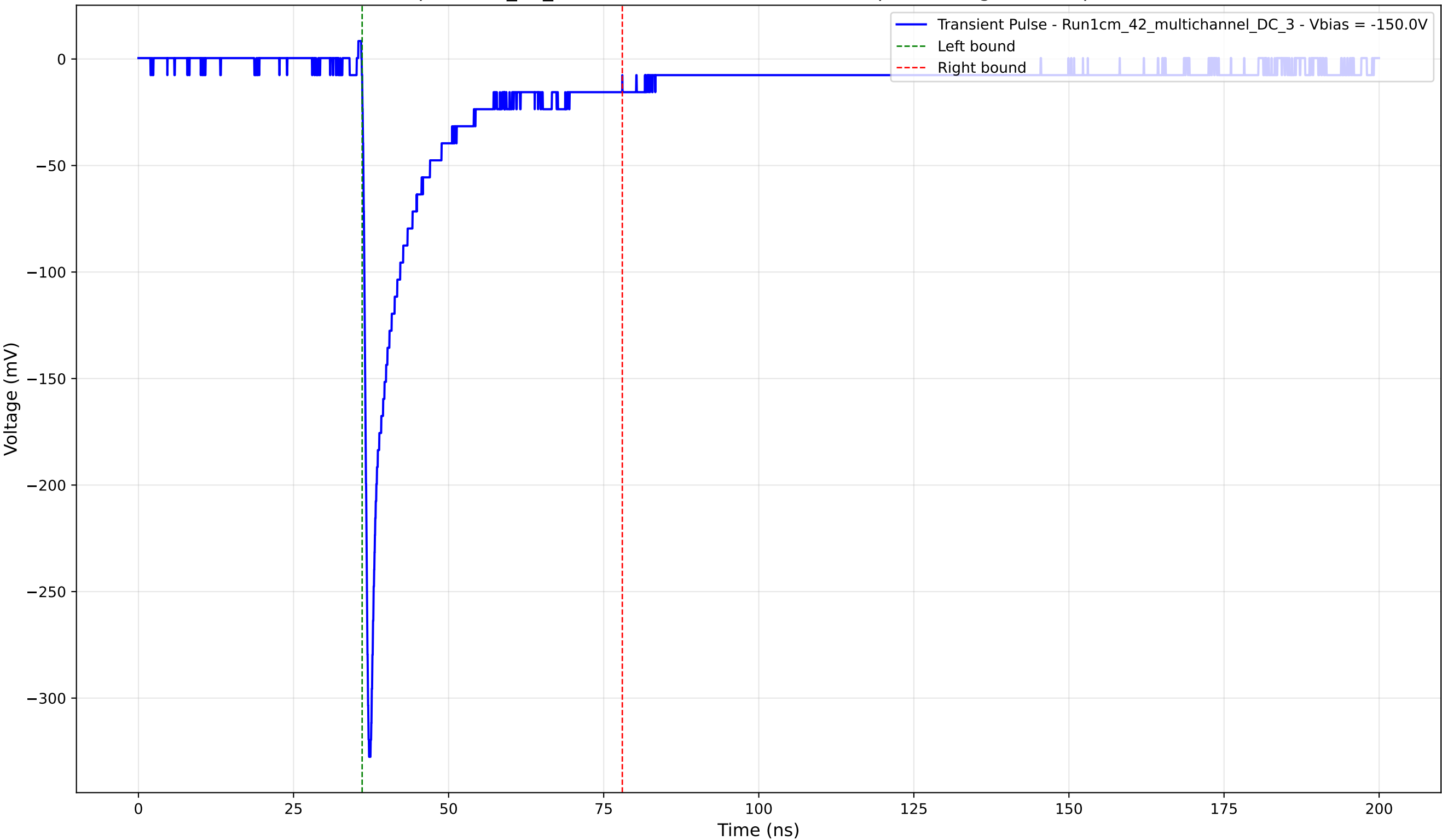
Transient Pulse - Sample: 1cm_42_multichannel - Position: 4665.0 \mu\text{m} - Charge: 42.26 pC - Rise Time: 0.80 ns
