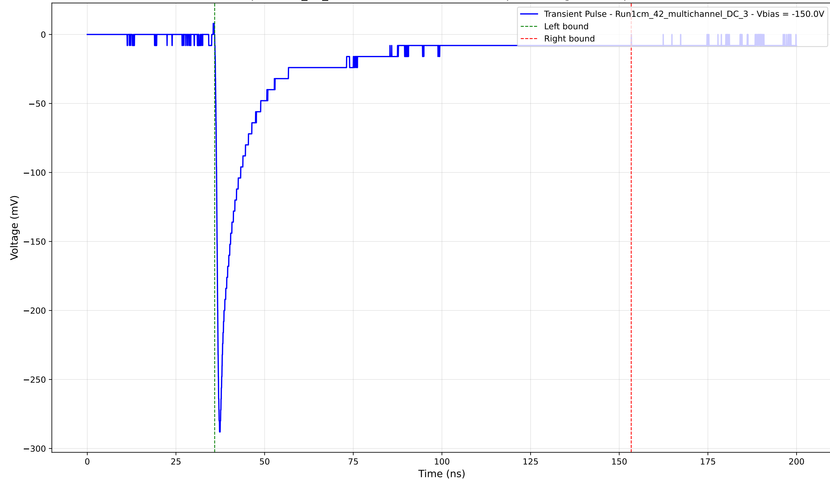
Transient Pulse - Sample: 1cm_42_multichannel - Position: 455.0 \mu\text{m} - Charge: 61.20 pC - Rise Time: 0.91 ns
