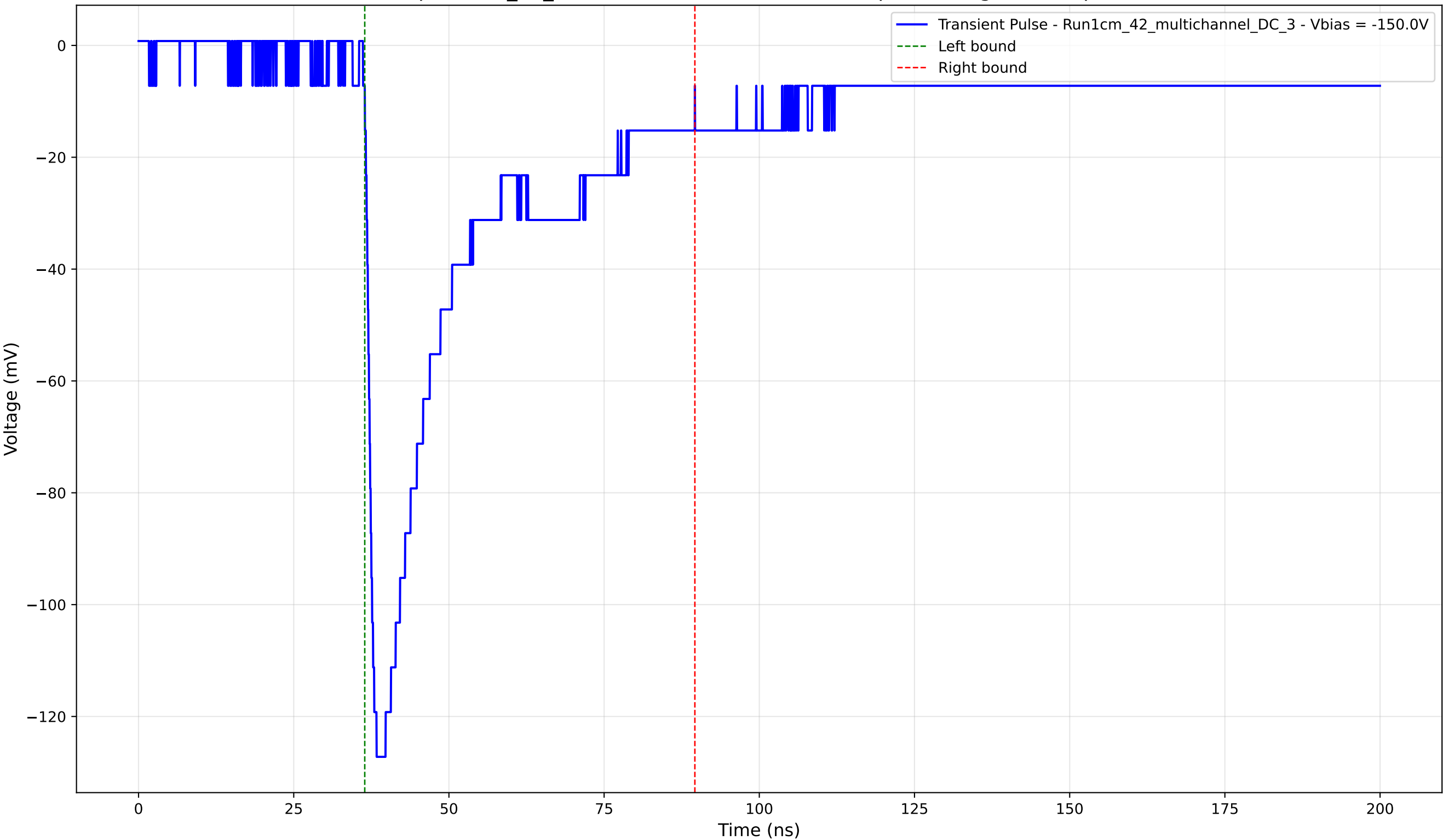
Transient Pulse - Sample: 1cm_42_multichannel - Position: 1545.0 \mu\text{m} - Charge: 42.53 pC - Rise Time: 1.51 ns
