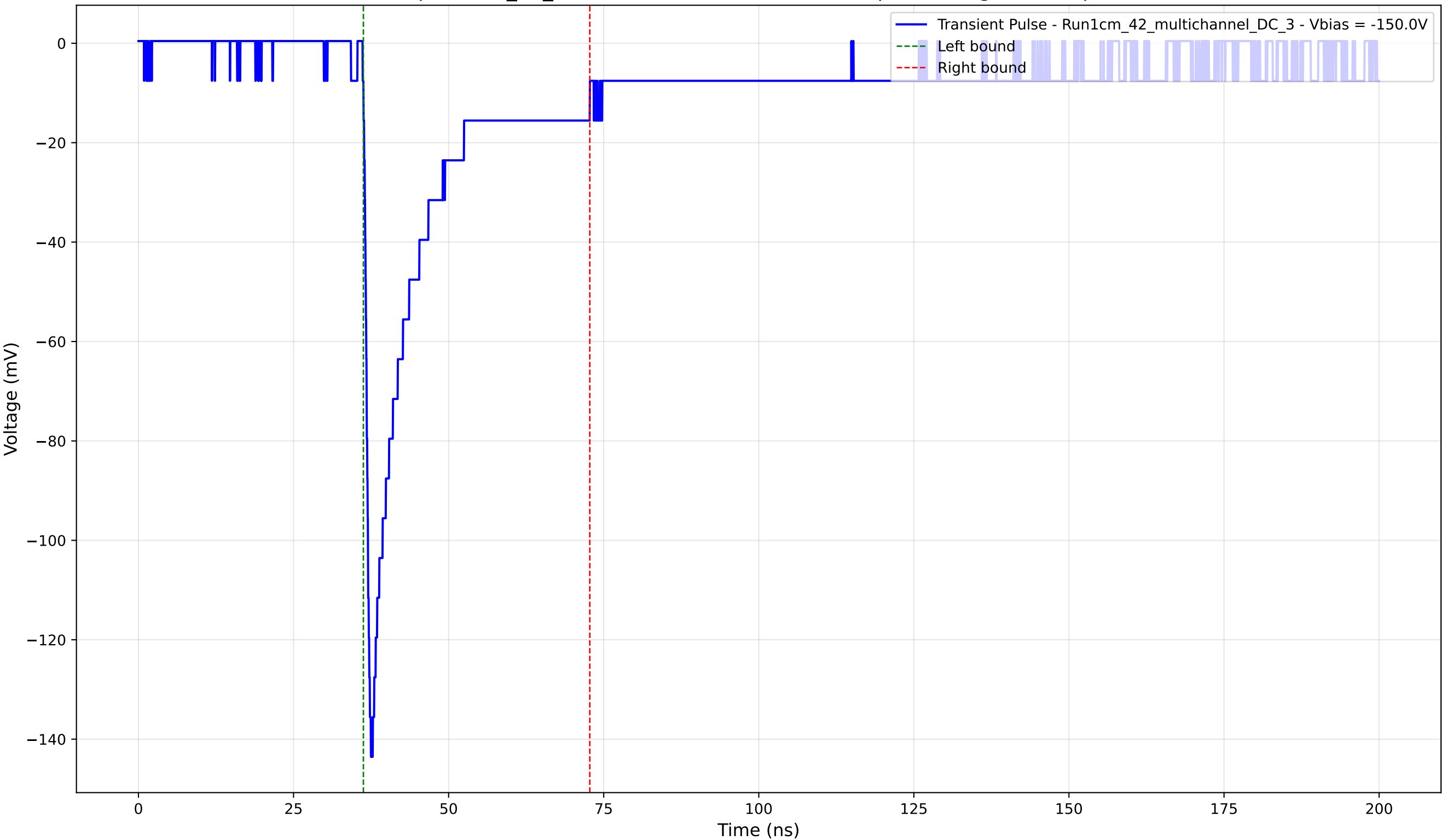
Transient Pulse - Sample: 1cm_42_multichannel - Position: 4330.0 \mu\text{m} - Charge: 24.76 pC - Rise Time: 1.02 ns
