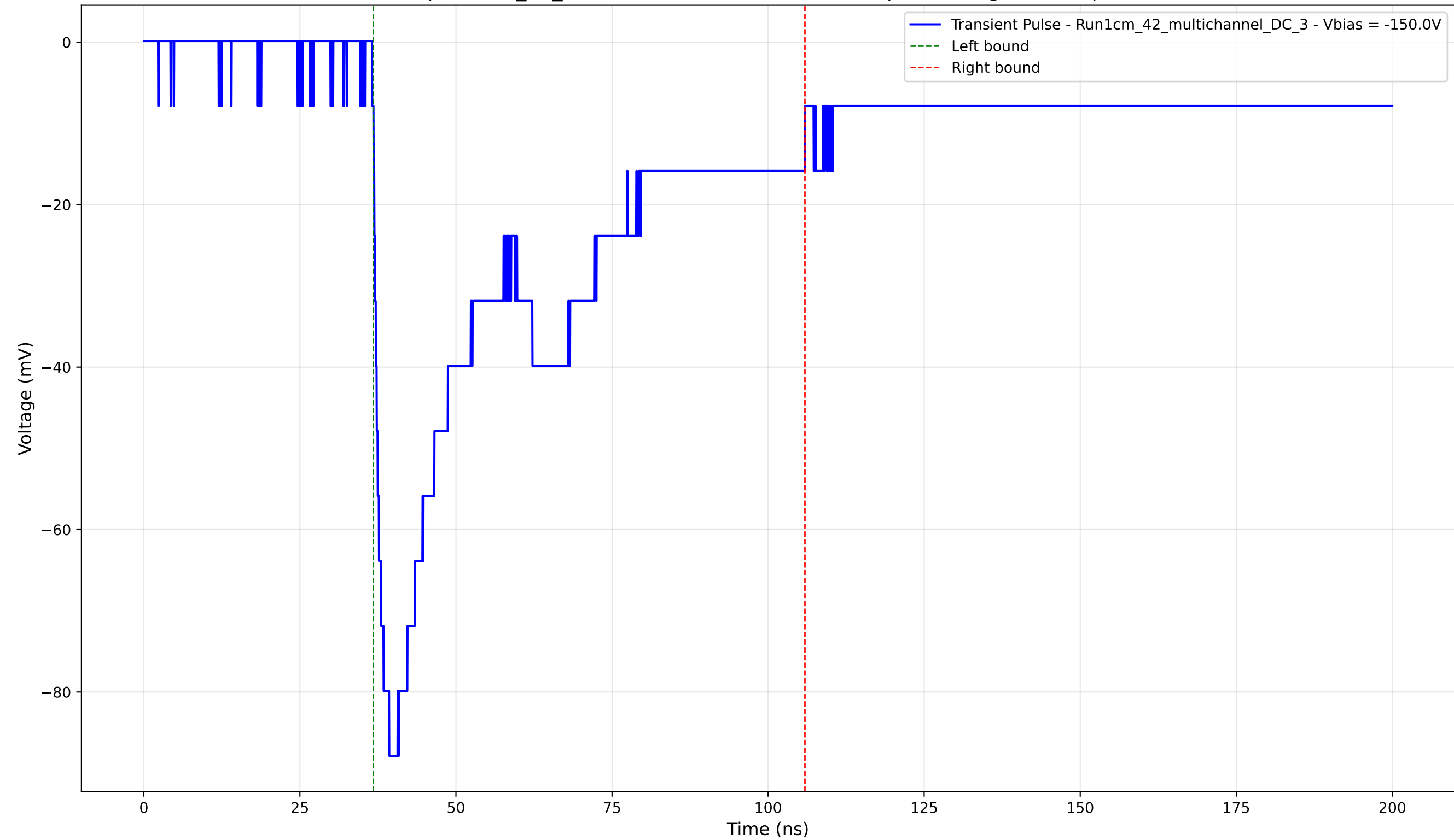
Transient Pulse - Sample: 1cm_42_multichannel - Position: 2235.0 \mu\text{m} - Charge: 43.58 pC - Rise Time: 1.62 ns
