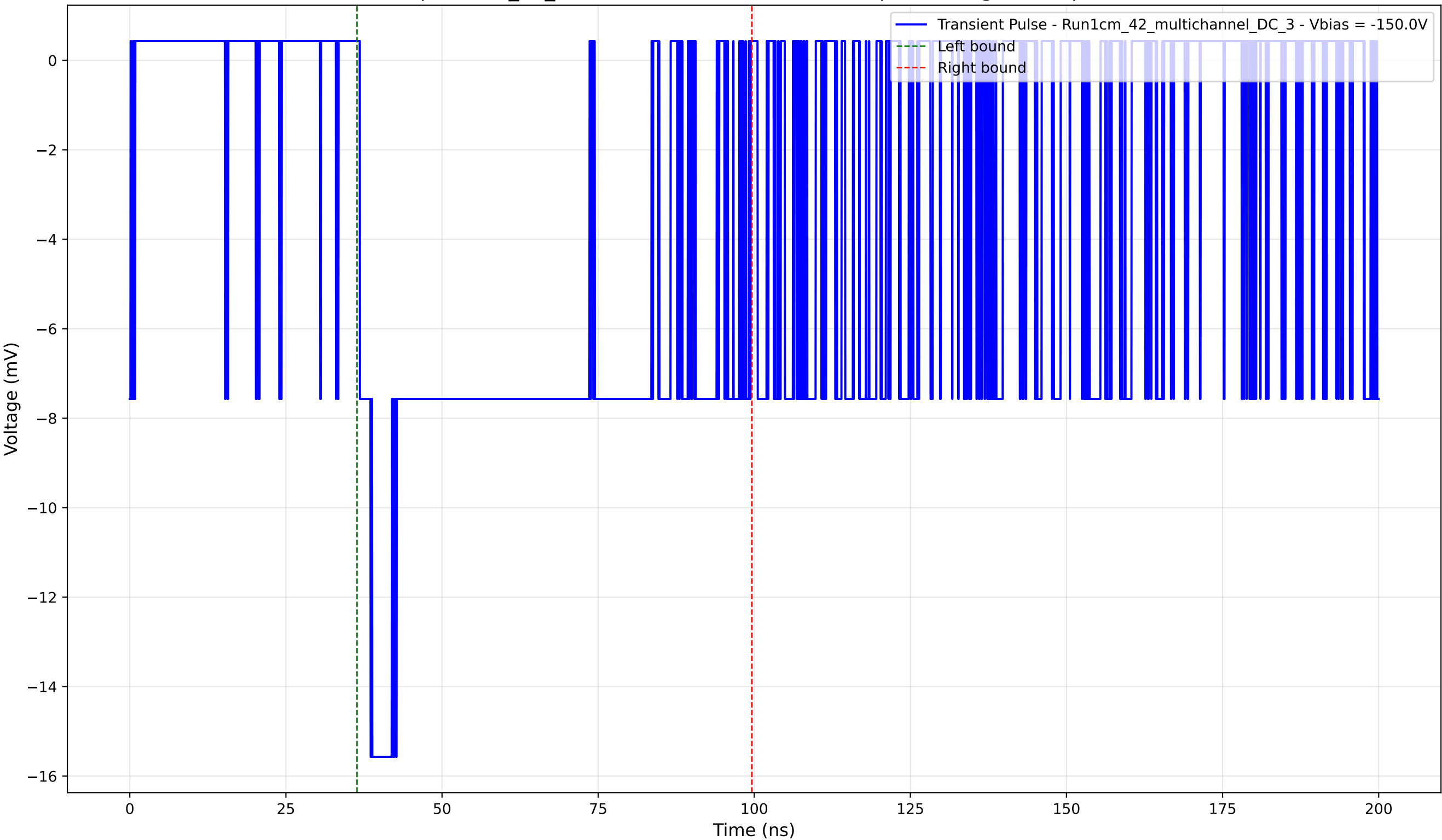
Transient Pulse - Sample: 1cm_42_multichannel - Position: 2400.0 \mu\text{m} - Charge: 9.08 pC - Rise Time: 1.74 ns
