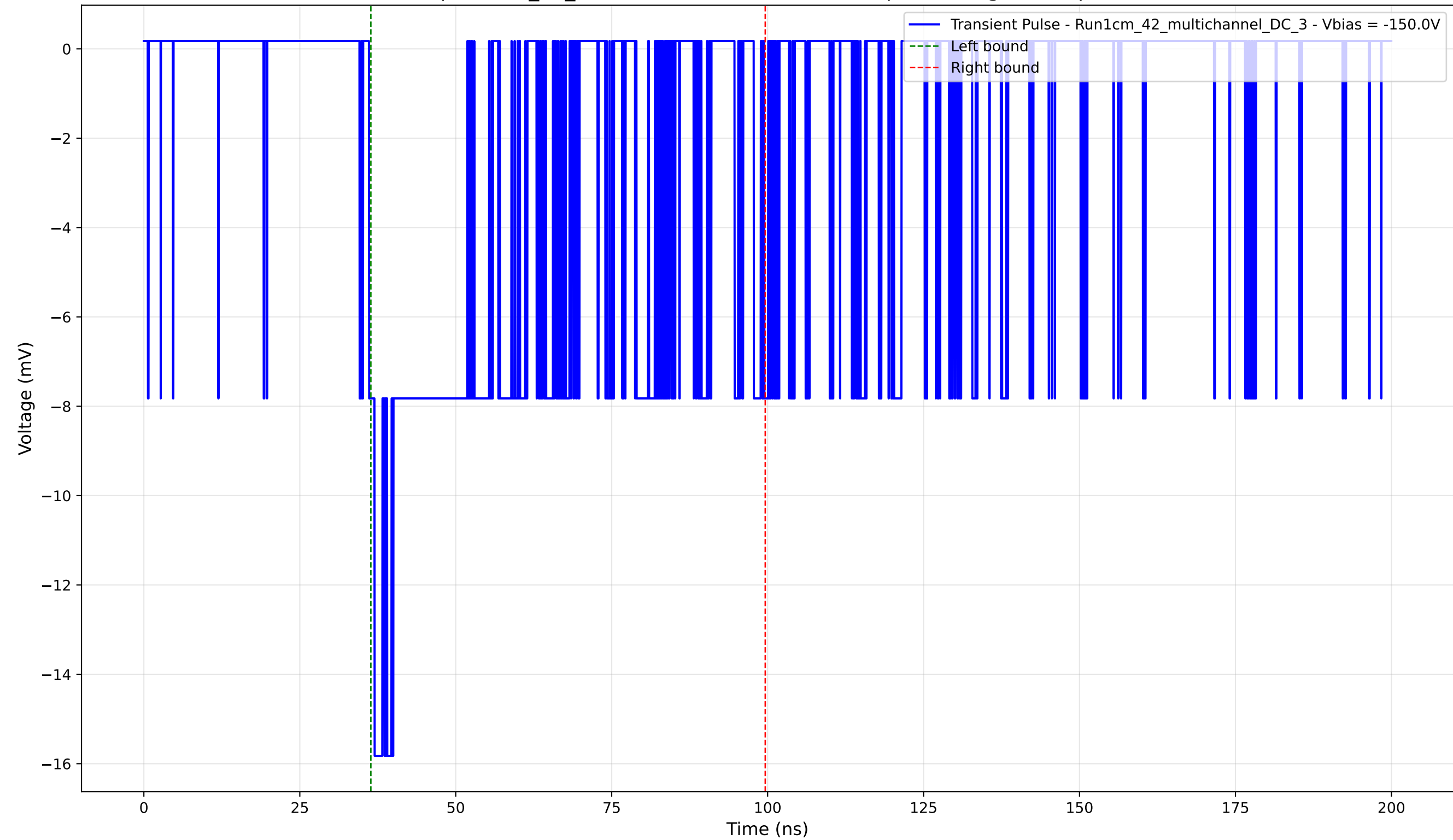
Transient Pulse - Sample: 1cm_42_multichannel - Position: 355.0 \mu\text{m} - Charge: 6.11 pC - Rise Time: 0.90 ns
