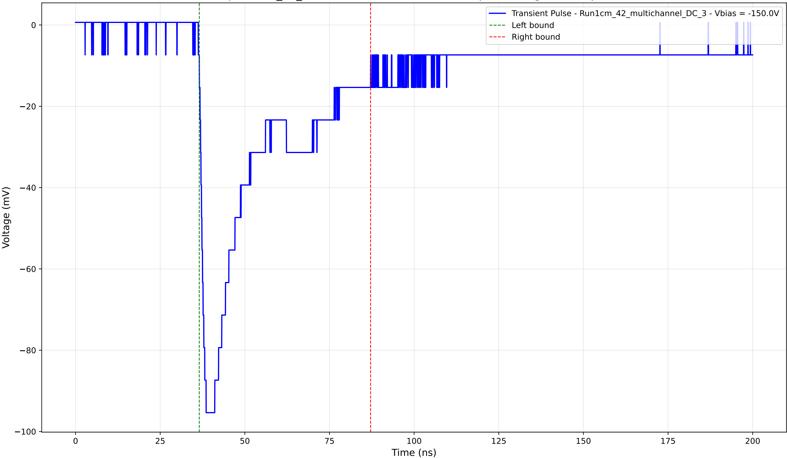
Transient Pulse - Sample: 1cm_42_multichannel - Position: 2970.0 \mu\text{m} - Charge: 36.33 pC - Rise Time: 1.61 ns
