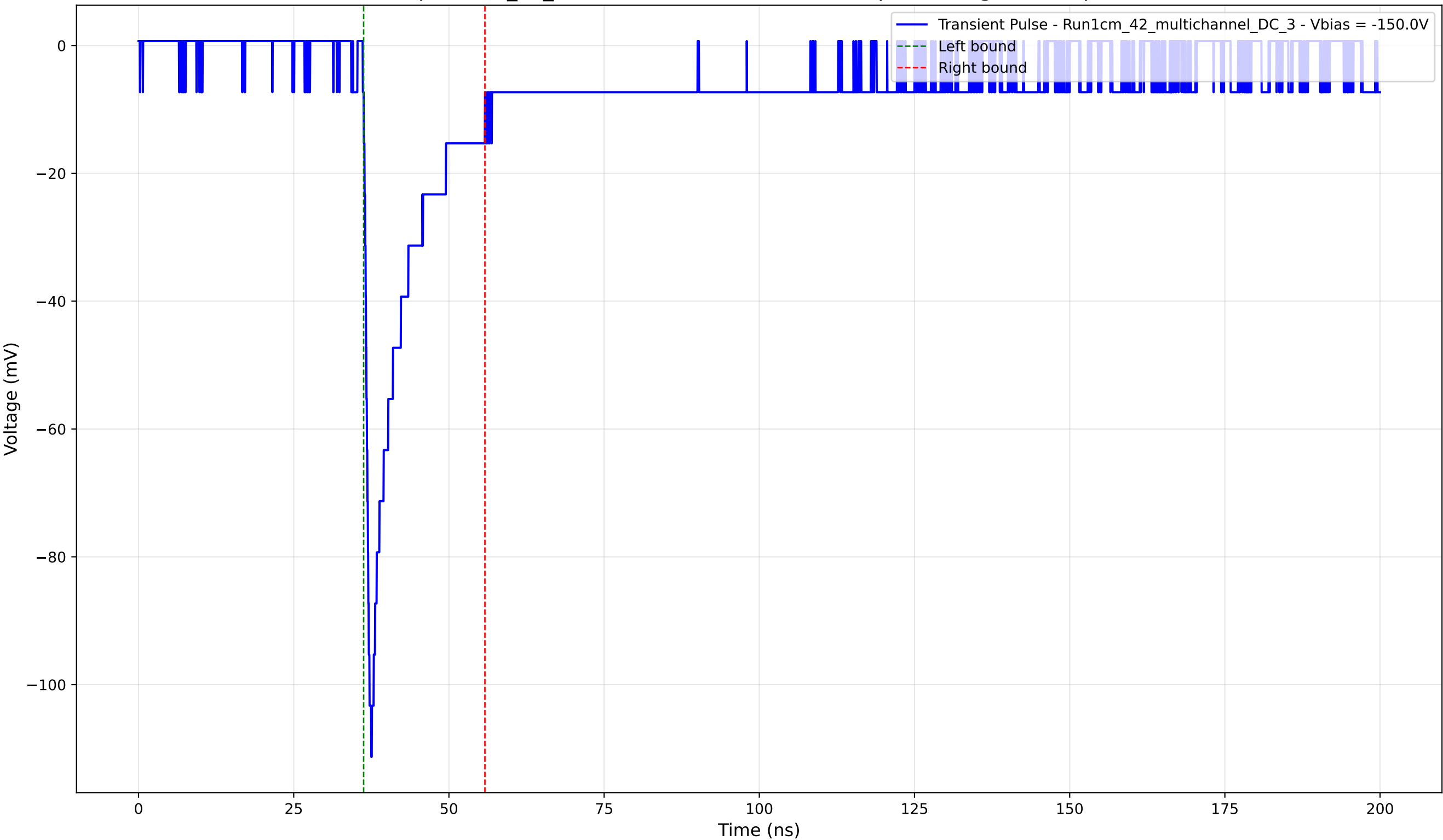
Transient Pulse - Sample: 1cm_42_multichannel - Position: 4440.0 \mu\text{m} - Charge: 14.02 pC - Rise Time: 0.93 ns
