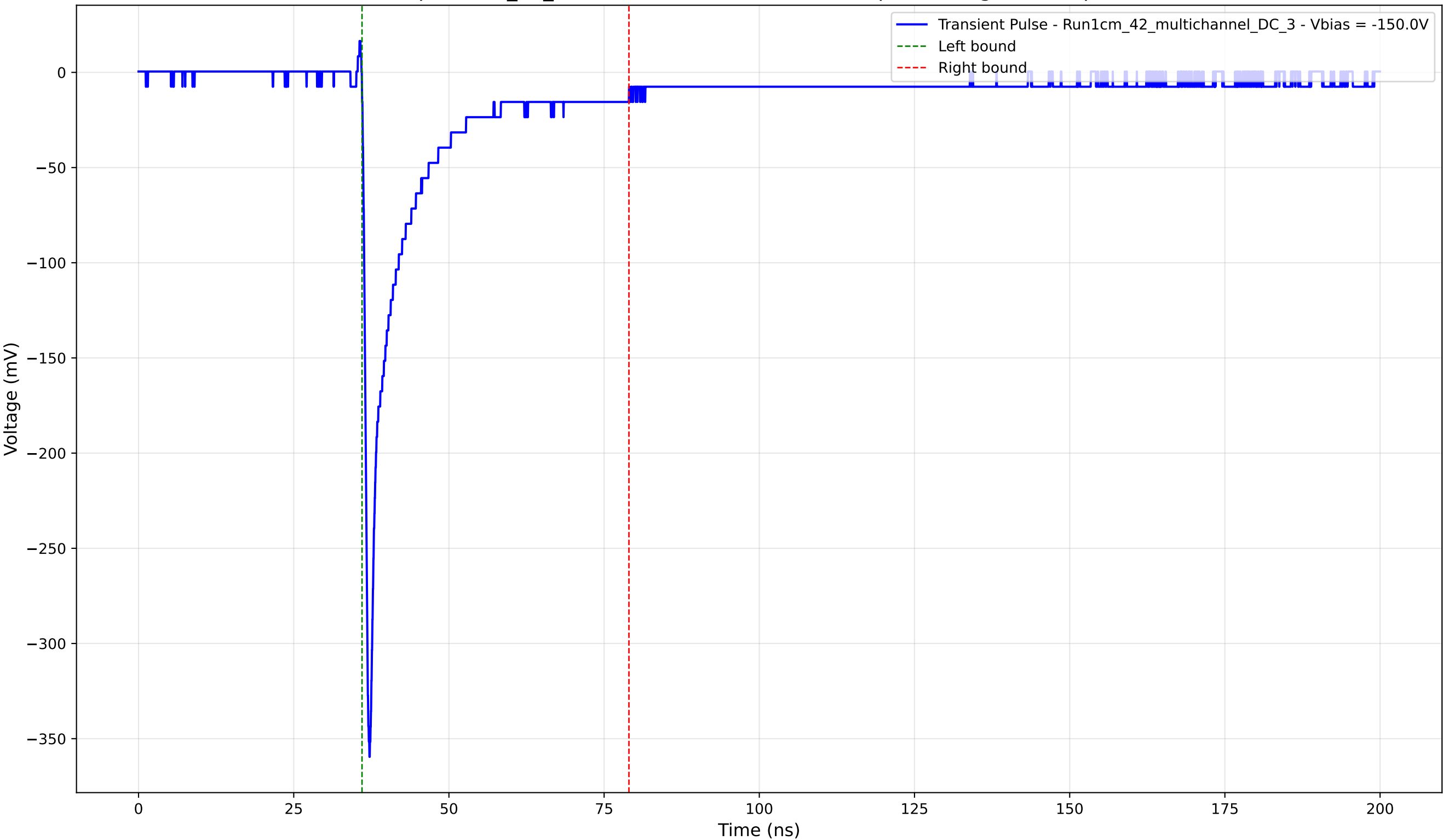
Transient Pulse - Sample: 1cm_42_multichannel - Position: 4750.0 \mu\text{m} - Charge: 41.65 pC - Rise Time: 0.81 ns
