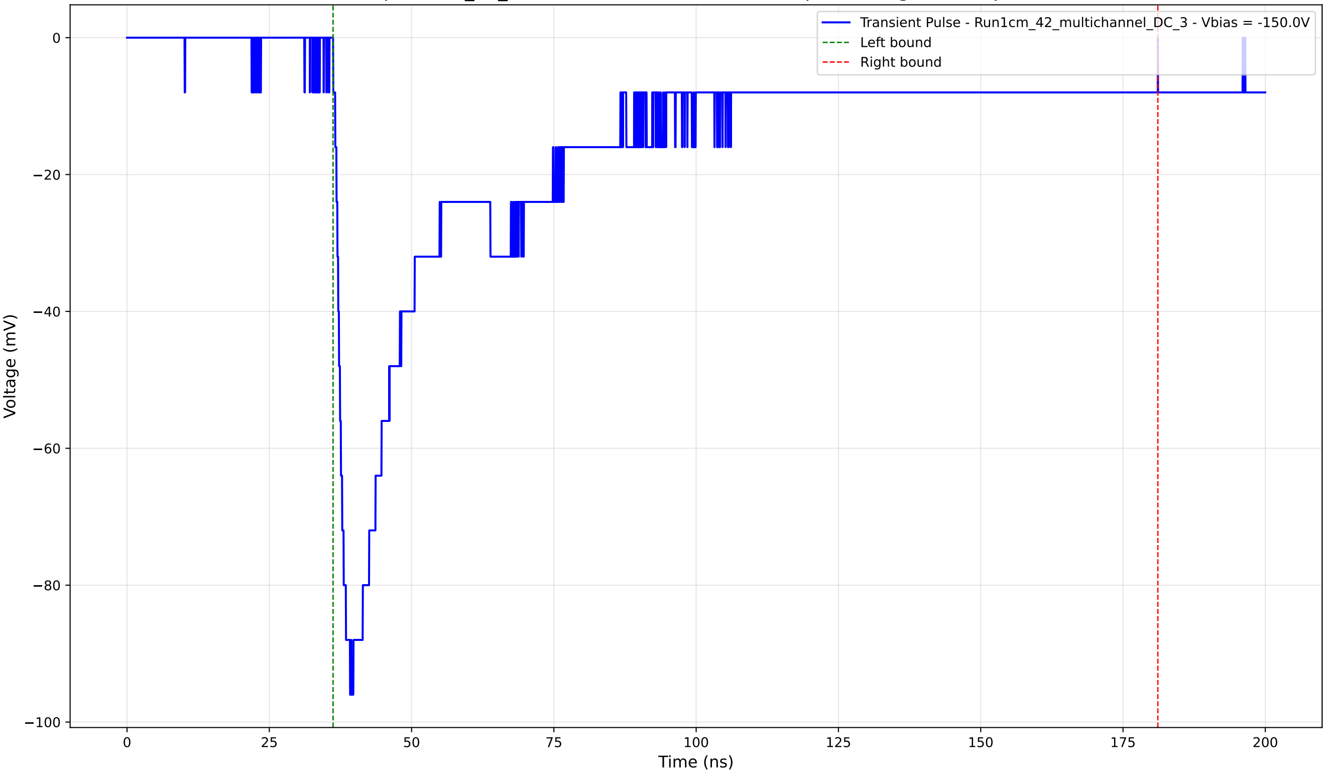
Transient Pulse - Sample: 1cm_42_multichannel - Position: 2955.0 \mu\text{m} - Charge: 50.67 pC - Rise Time: 1.90 ns
