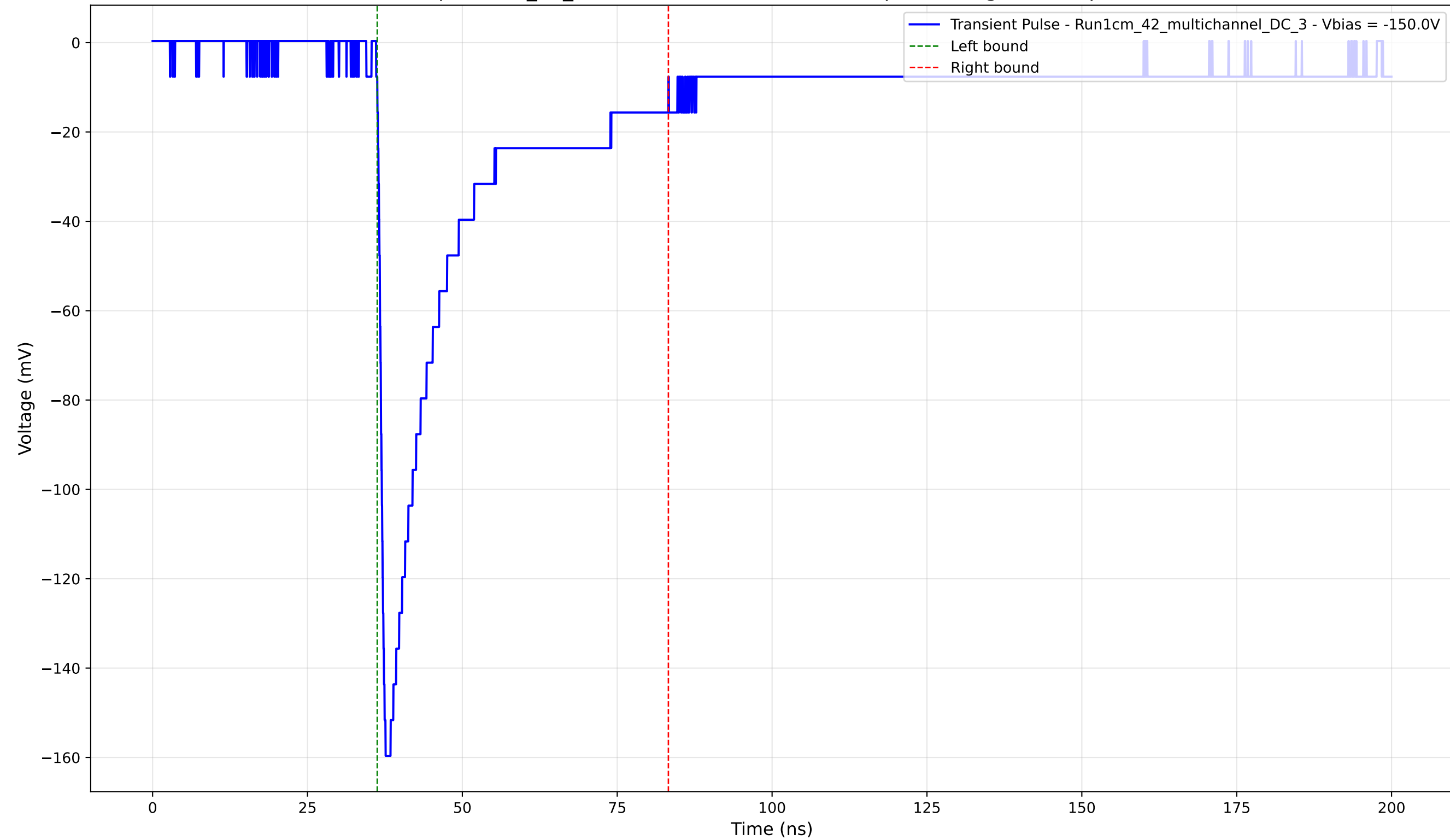
Transient Pulse - Sample: 1cm_42_multichannel - Position: 925.0 \mu\text{m} - Charge: 39.56 pC - Rise Time: 1.08 ns
