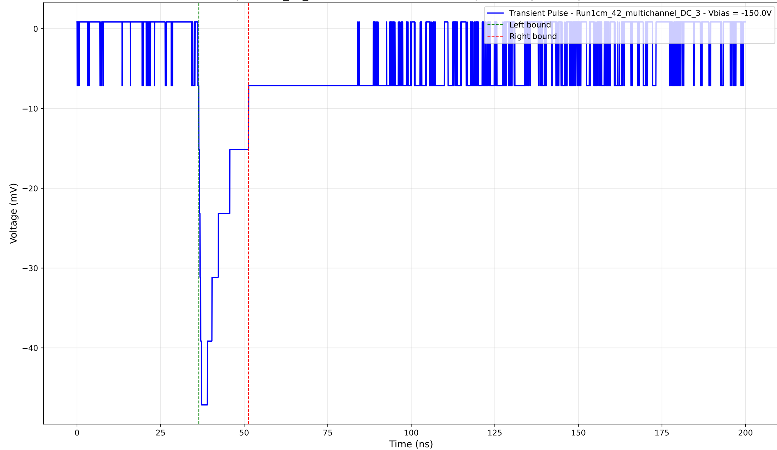
Transient Pulse - Sample: 1cm_42_multichannel - Position: 820.0 \mu\text{m} - Charge: 7.66 pC - Rise Time: 1.09 ns
