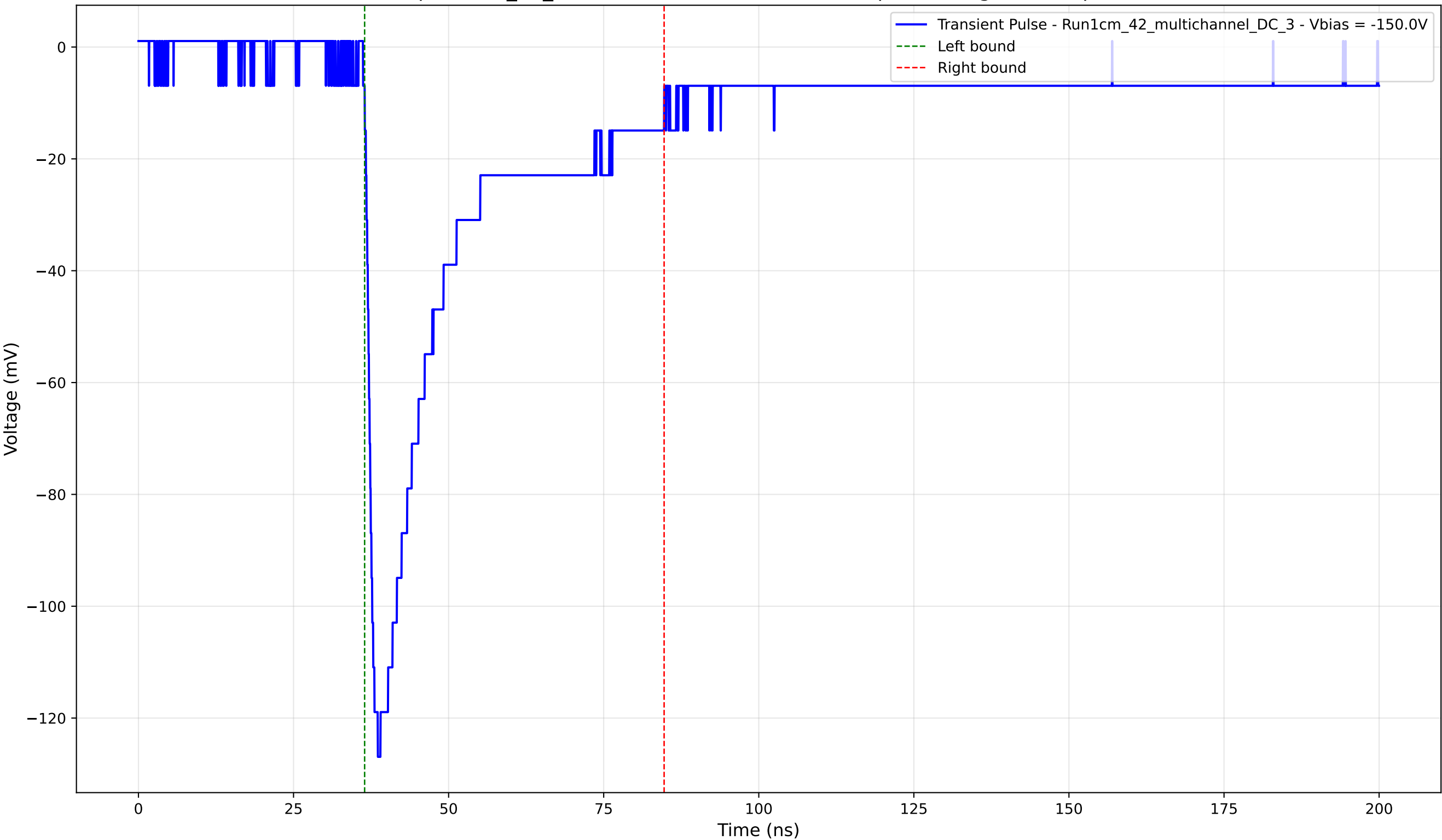
Transient Pulse - Sample: 1cm_42_multichannel - Position: 3510.0 \mu\text{m} - Charge: 36.45 pC - Rise Time: 1.57 ns
