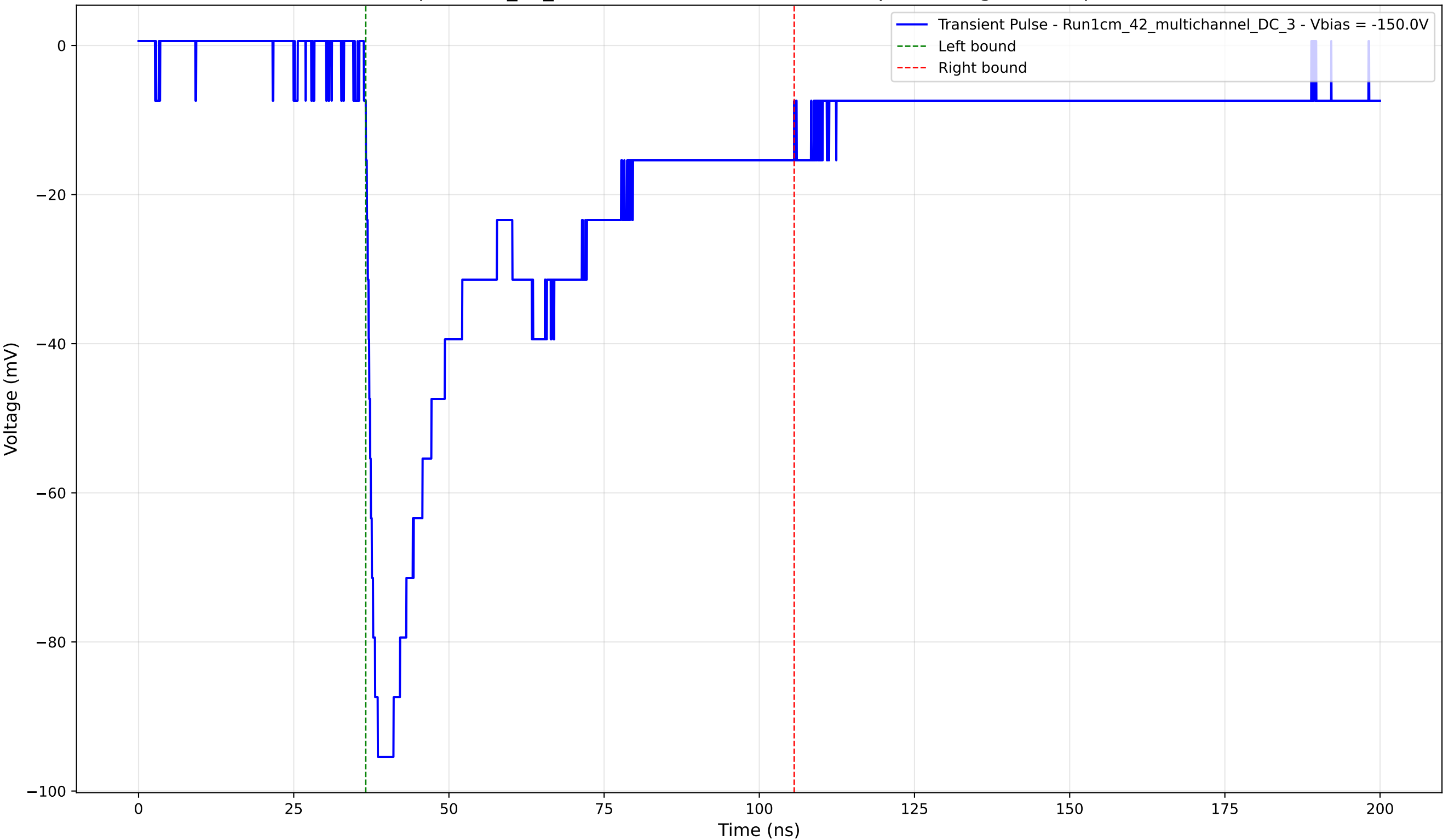
Transient Pulse - Sample: 1cm_42_multichannel - Position: 1975.0 \mu\text{m} - Charge: 43.85 pC - Rise Time: 1.49 ns
