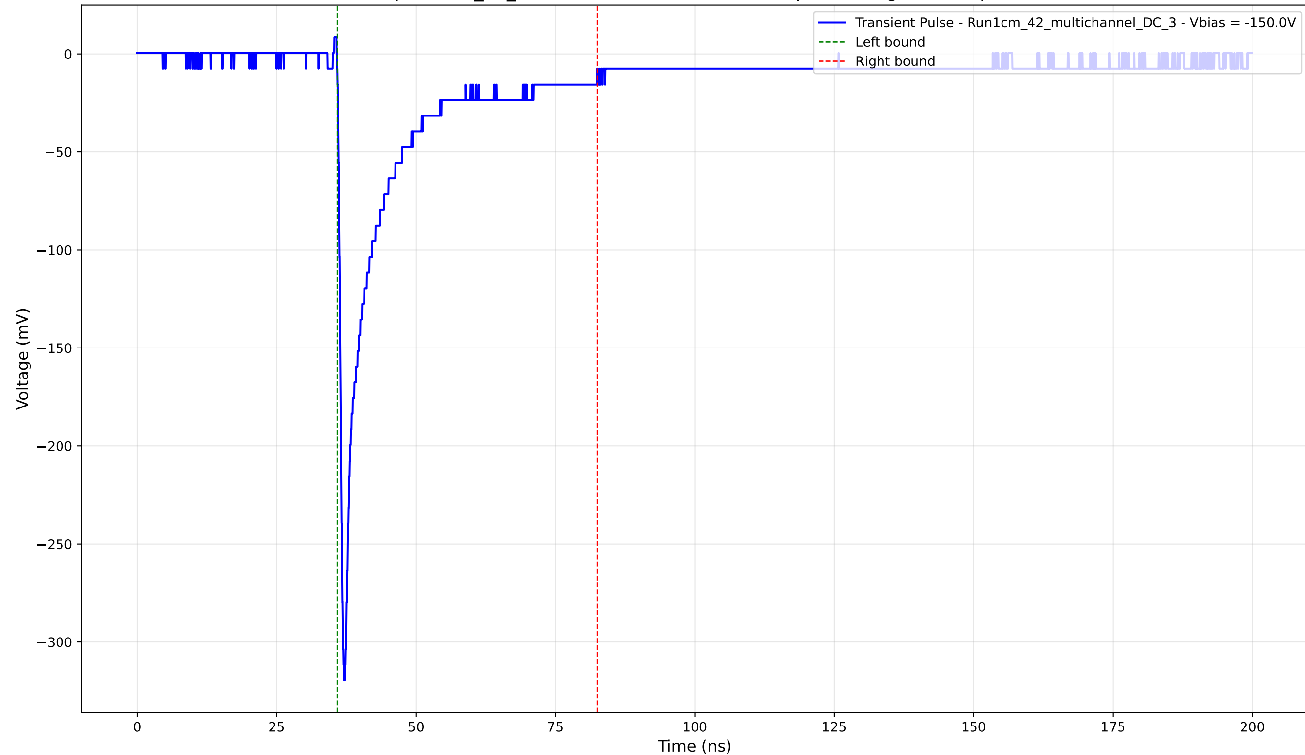
Transient Pulse - Sample: 1cm_42_multichannel - Position: 250.0 \mu\text{m} - Charge: 45.03 pC - Rise Time: 0.84 ns
