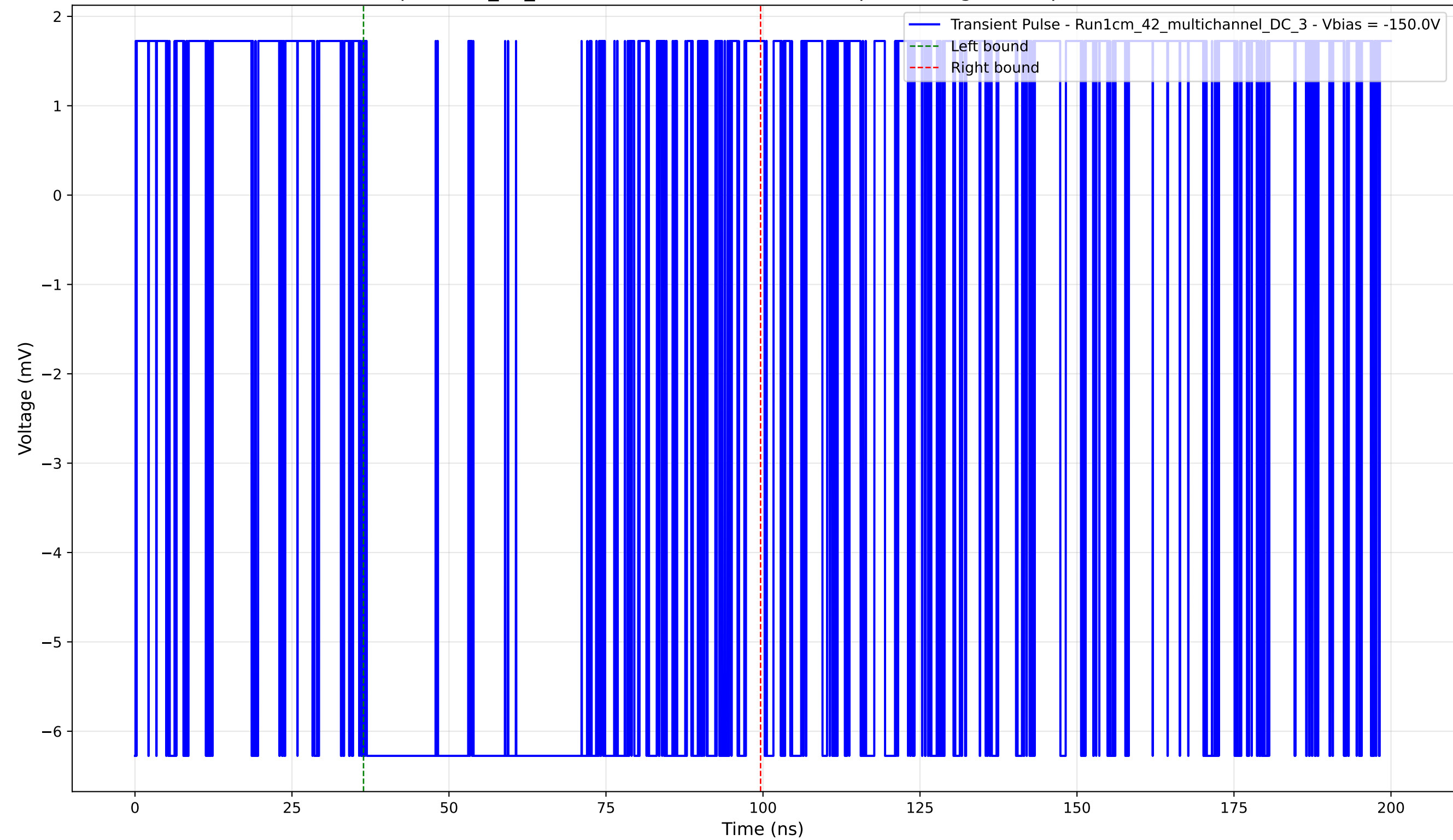
Transient Pulse - Sample: 1cm_42_multichannel - Position: 2360.0 \mu\text{m} - Charge: 5.88 pC - Rise Time: 0.00 ns (N/A)
