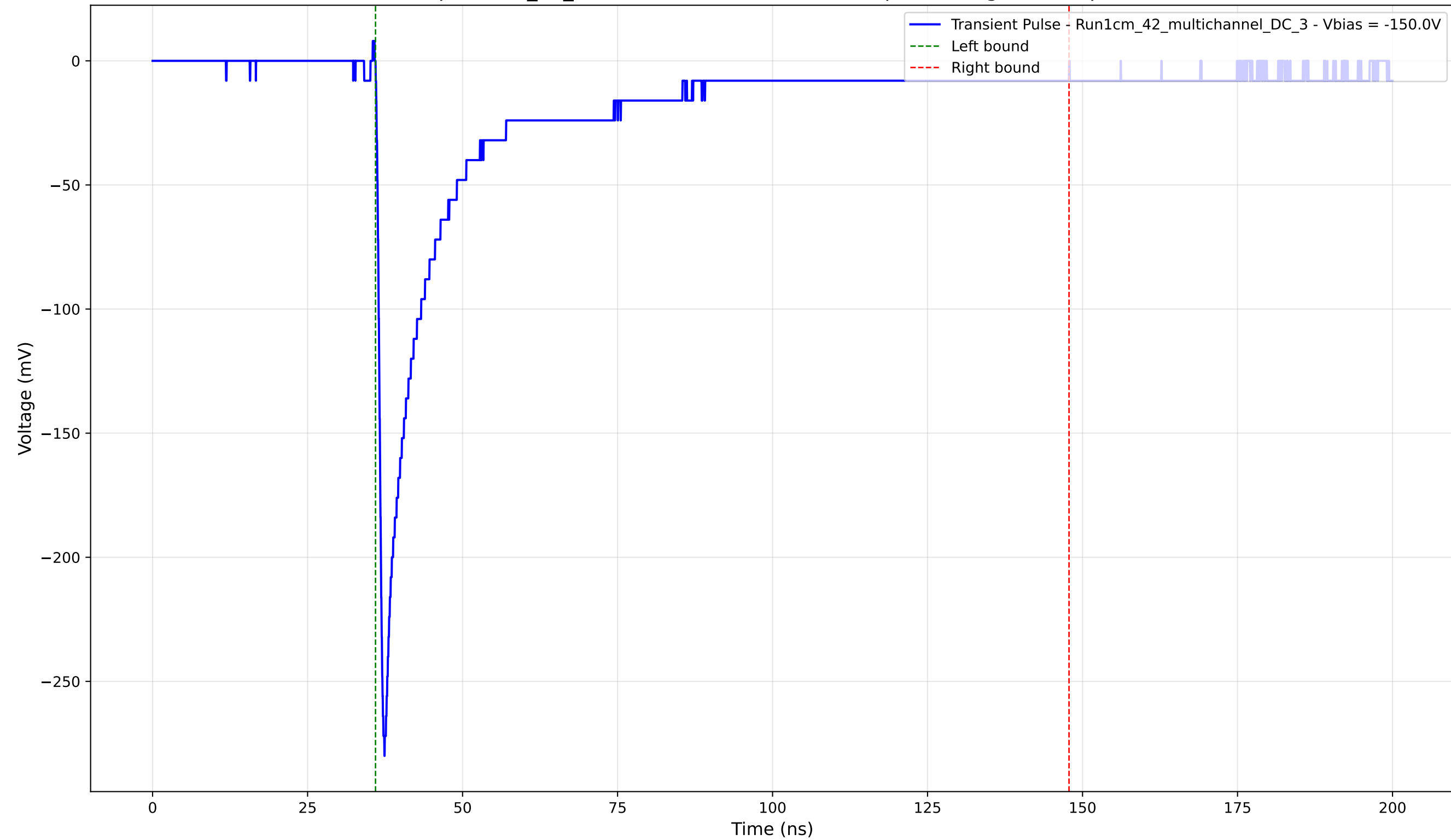
Transient Pulse - Sample: 1cm_42_multichannel - Position: 495.0 \mu\text{m} - Charge: 59.93 pC - Rise Time: 0.93 ns
