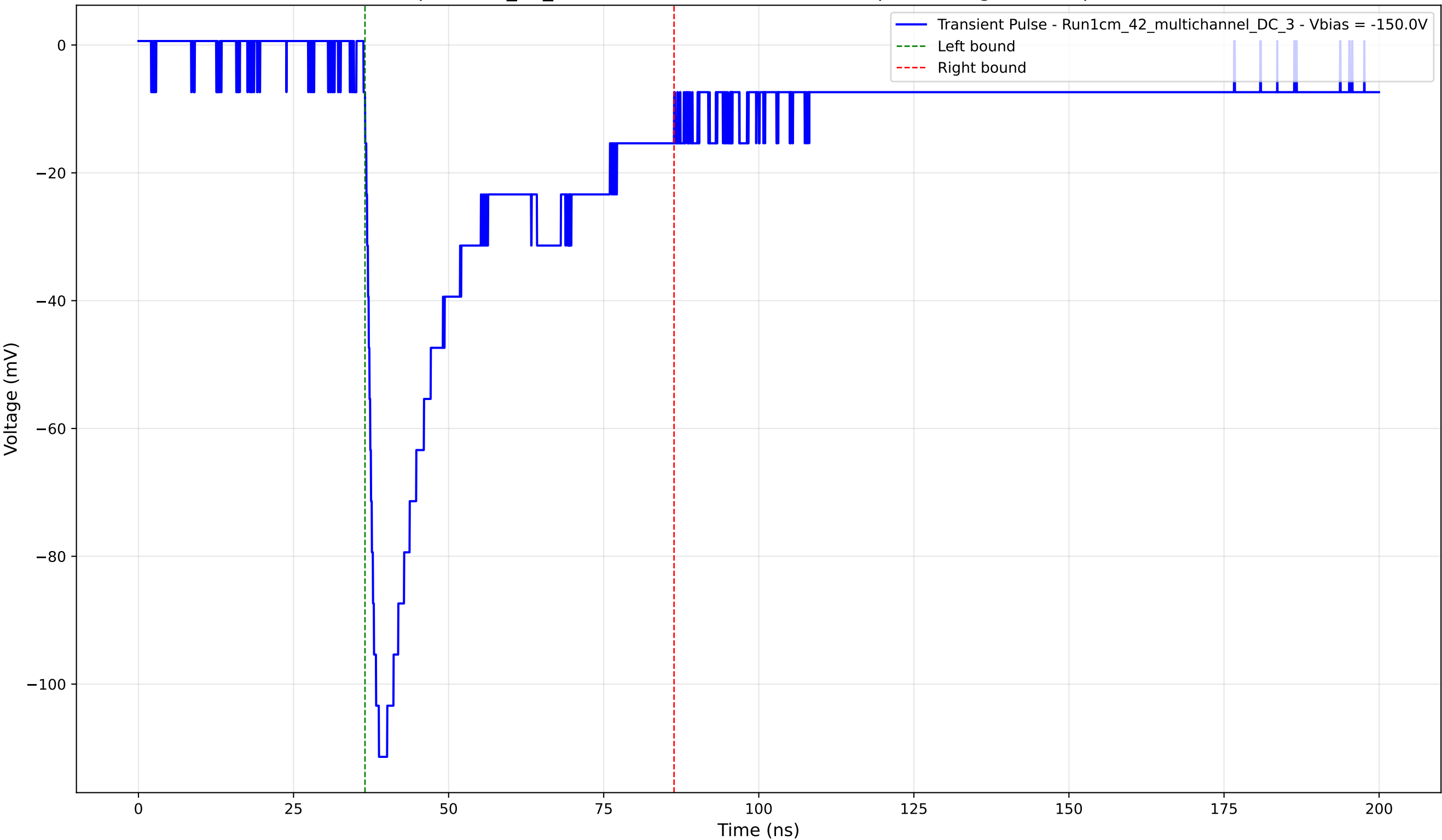
Transient Pulse - Sample: 1cm_42_multichannel - Position: 3195.0 \mu\text{m} - Charge: 36.97 pC - Rise Time: 1.77 ns
