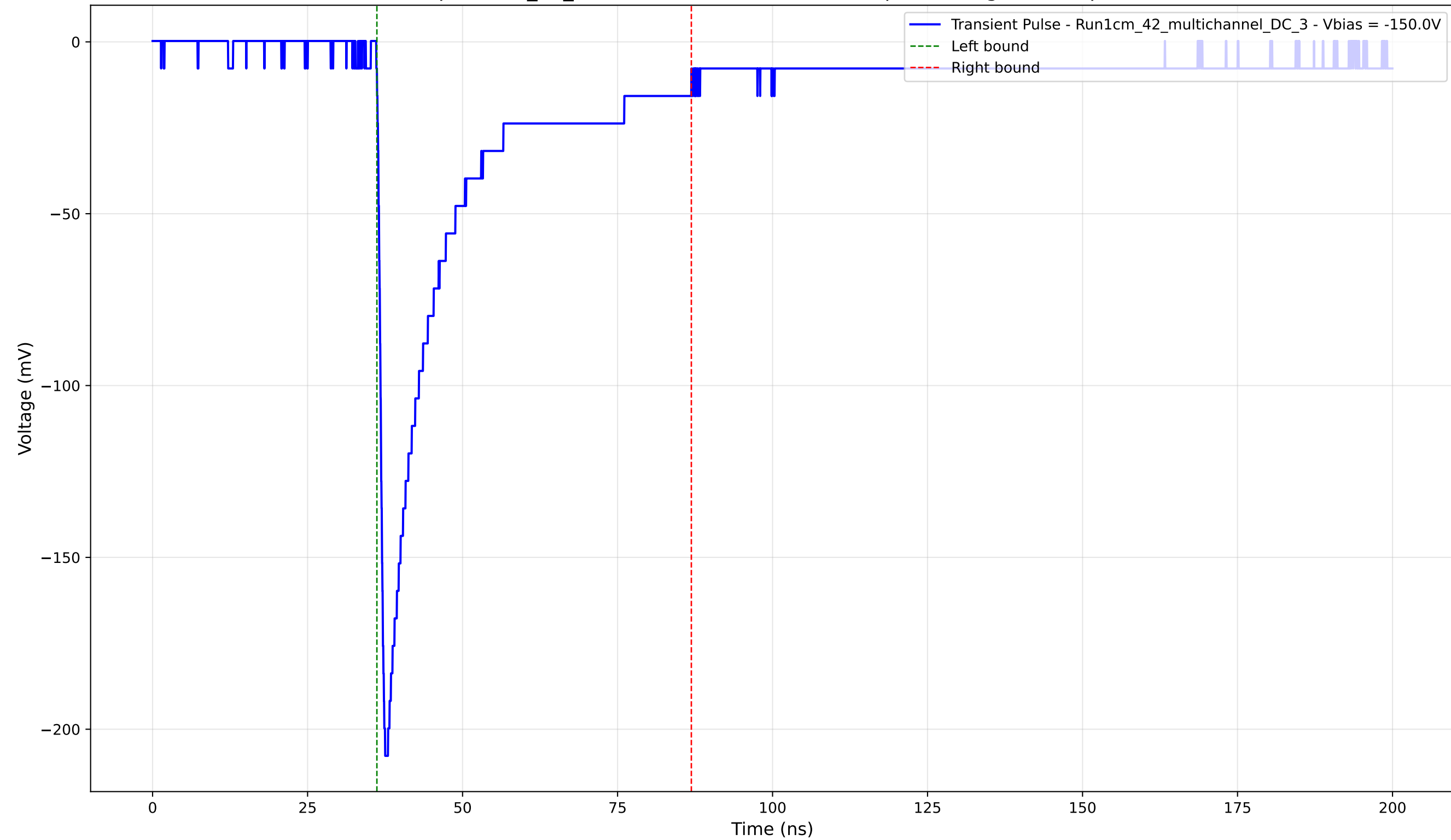
Transient Pulse - Sample: 1cm_42_multichannel - Position: 755.0 \mu\text{m} - Charge: 46.18 pC - Rise Time: 1.03 ns
