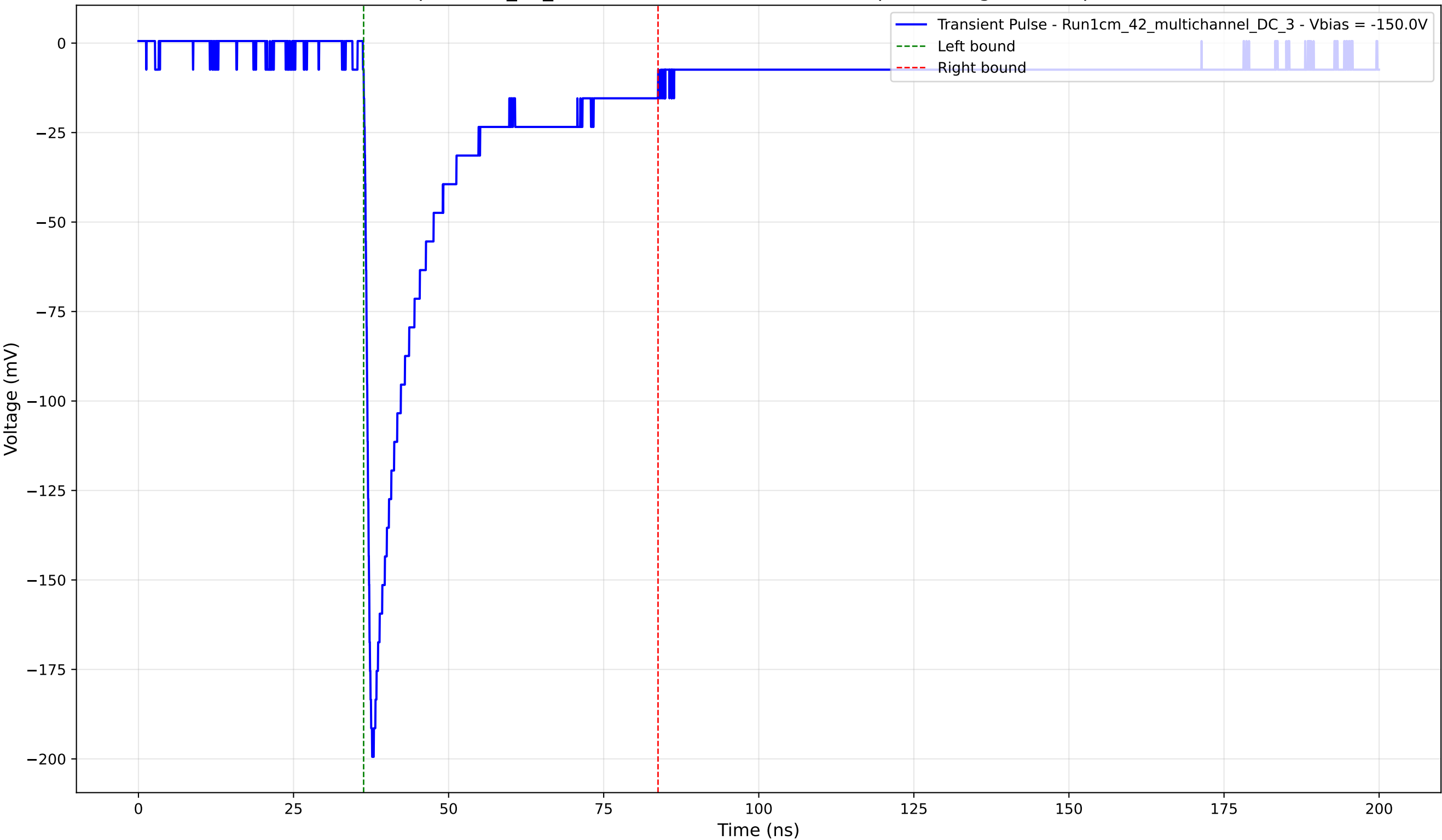
Transient Pulse - Sample: 1cm_42_multichannel - Position: 4170.0 \mu\text{m} - Charge: 40.91 pC - Rise Time: 1.01 ns
