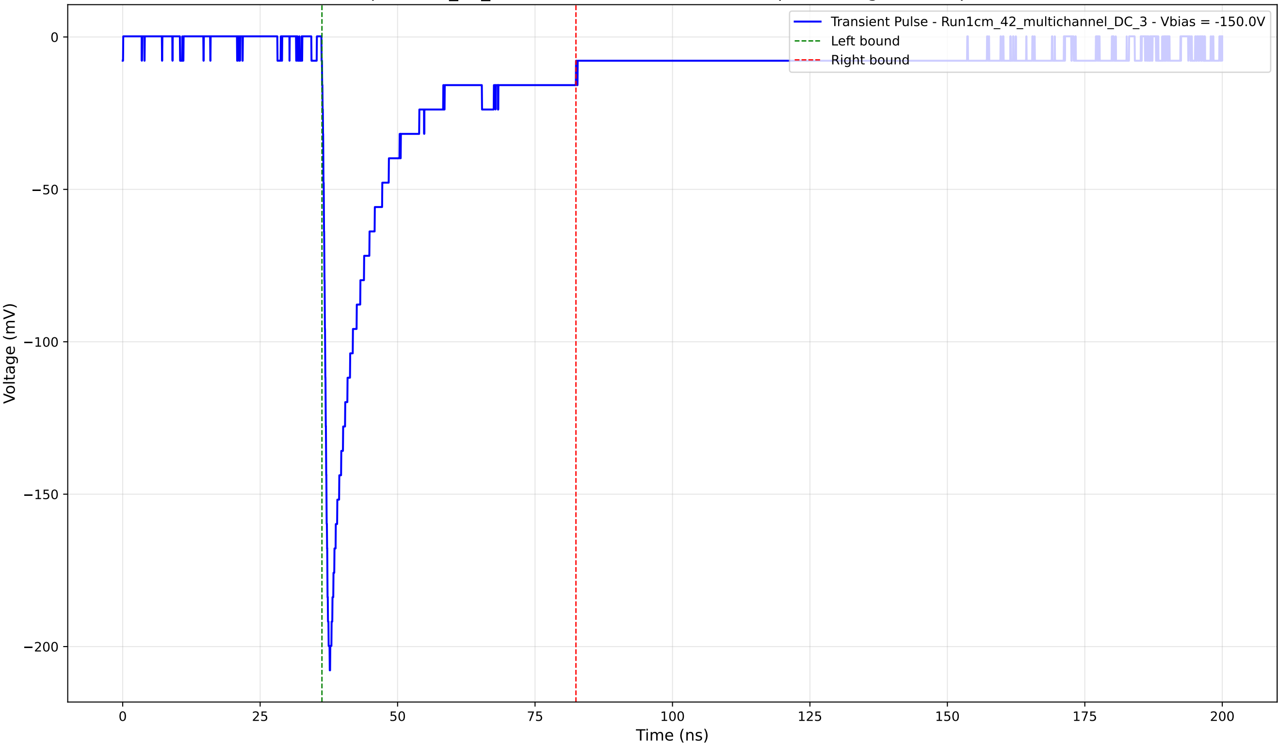
Transient Pulse - Sample: 1cm_42_multichannel - Position: 4265.0 \mu\text{m} - Charge: 38.22 pC - Rise Time: 0.99 ns
