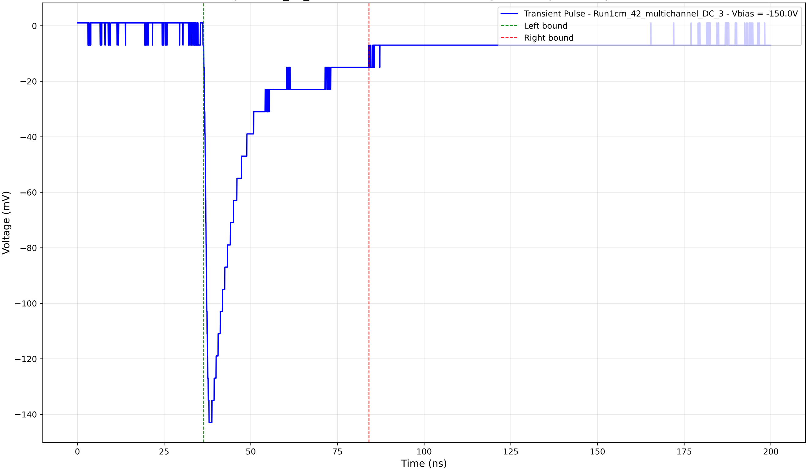
Transient Pulse - Sample: 1cm_42_multichannel - Position: 3805.0 \mu\text{m} - Charge: 36.84 pC - Rise Time: 1.26 ns
