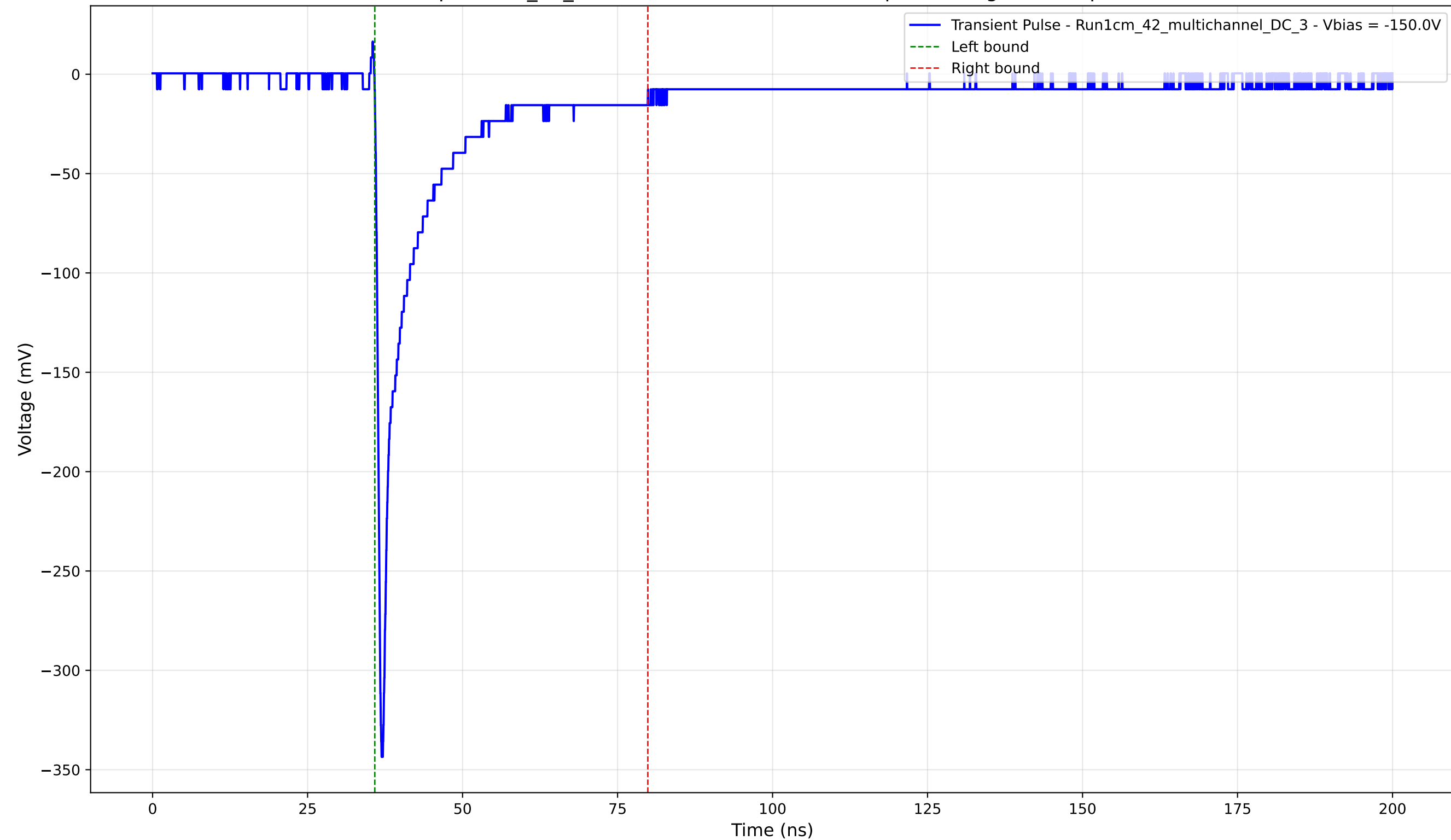
Transient Pulse - Sample: 1cm_42_multichannel - Position: 110.0 \mu\text{m} - Charge: 41.18 pC - Rise Time: 0.77 ns
