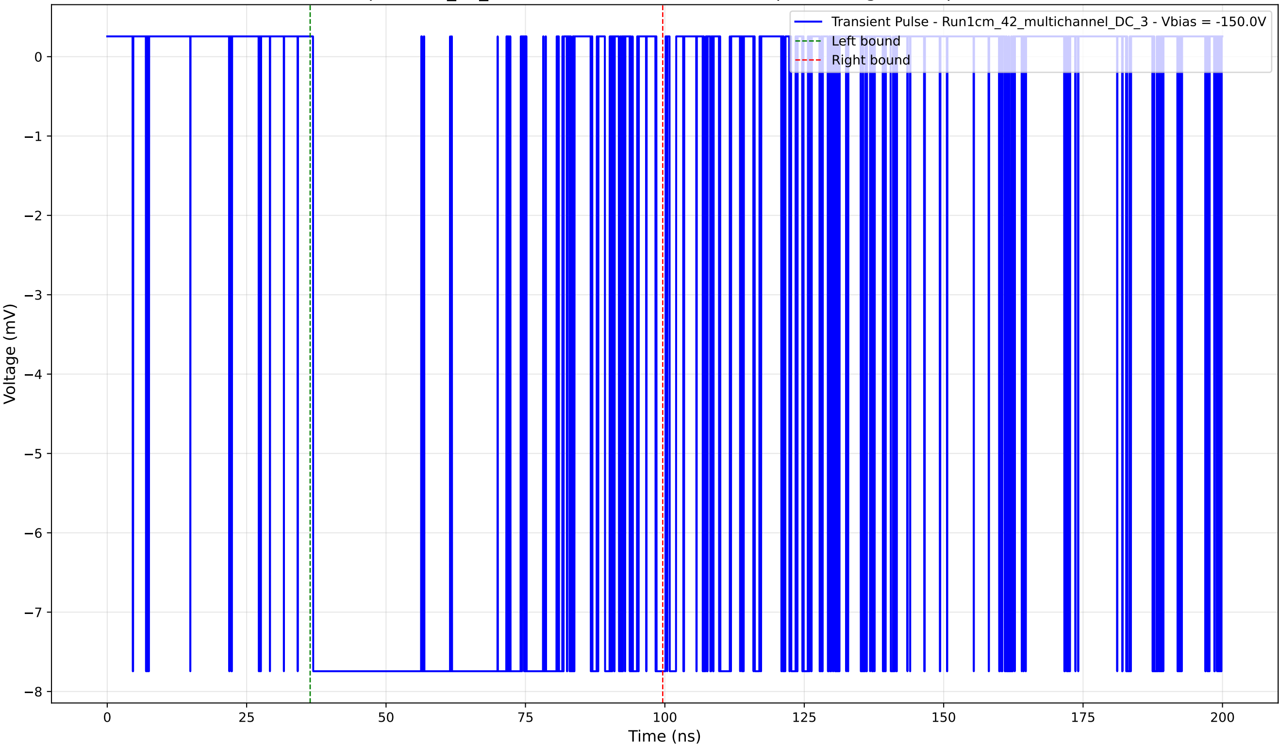
Transient Pulse - Sample: 1cm_42_multichannel - Position: 2390.0 \mu\text{m} - Charge: 7.57 pC - Rise Time: 0.02 ns
