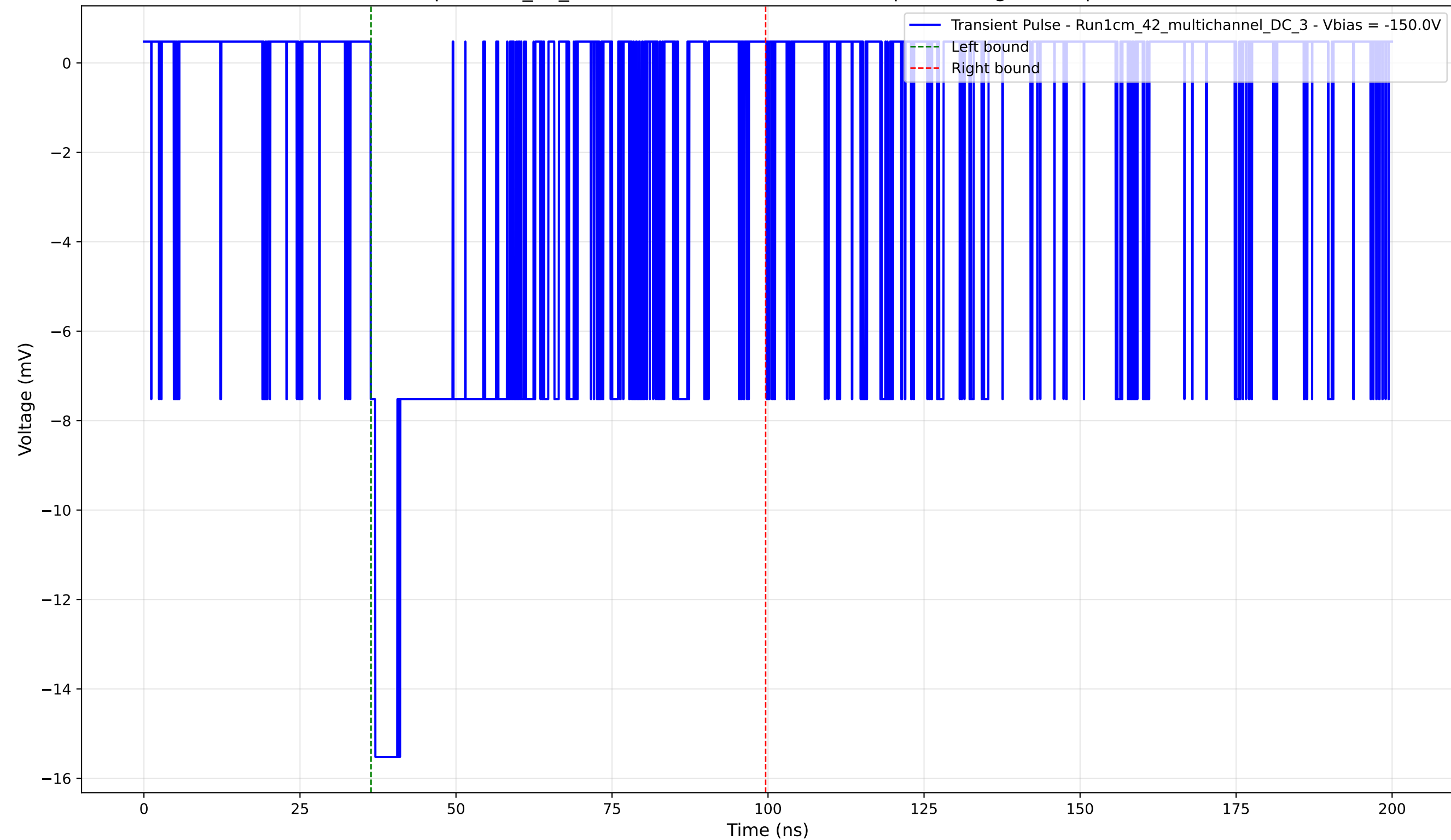
Transient Pulse - Sample: 1cm_42_multichannel - Position: 4405.0 \mu\text{m} - Charge: 5.72 pC - Rise Time: 0.76 ns
