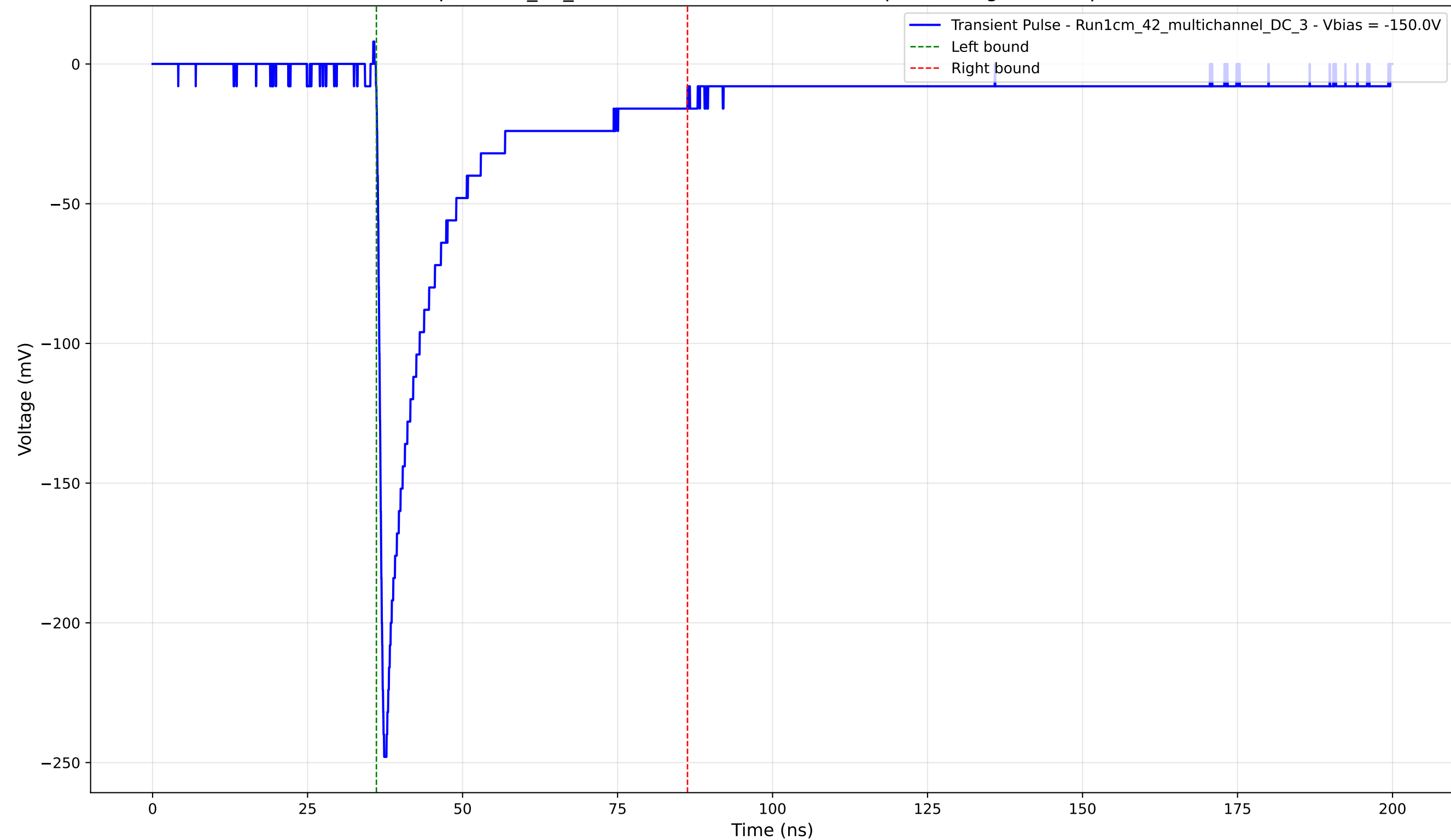
Transient Pulse - Sample: 1cm_42_multichannel - Position: 580.0 \mu\text{m} - Charge: 48.44 pC - Rise Time: 0.90 ns
