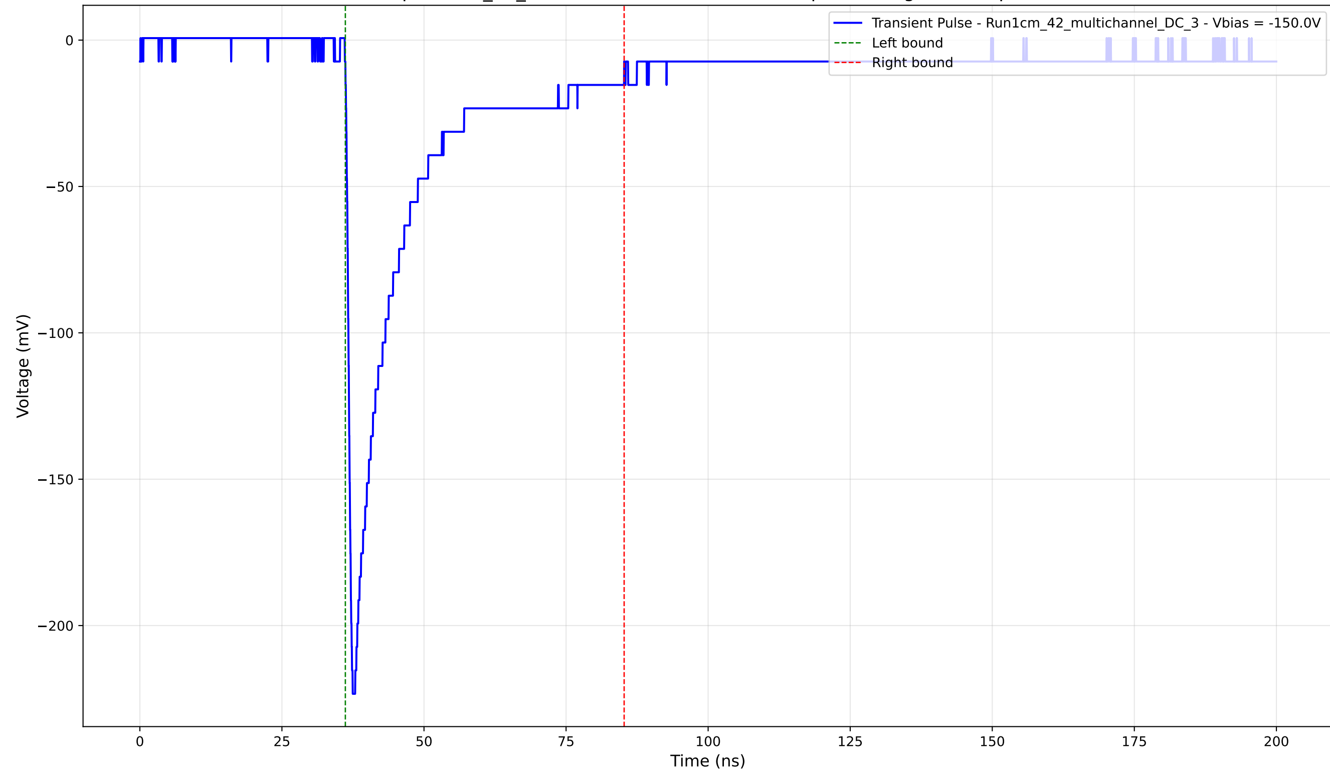
Transient Pulse - Sample: 1cm_42_multichannel - Position: 695.0 \mu\text{m} - Charge: 46.51 pC - Rise Time: 1.00 ns
