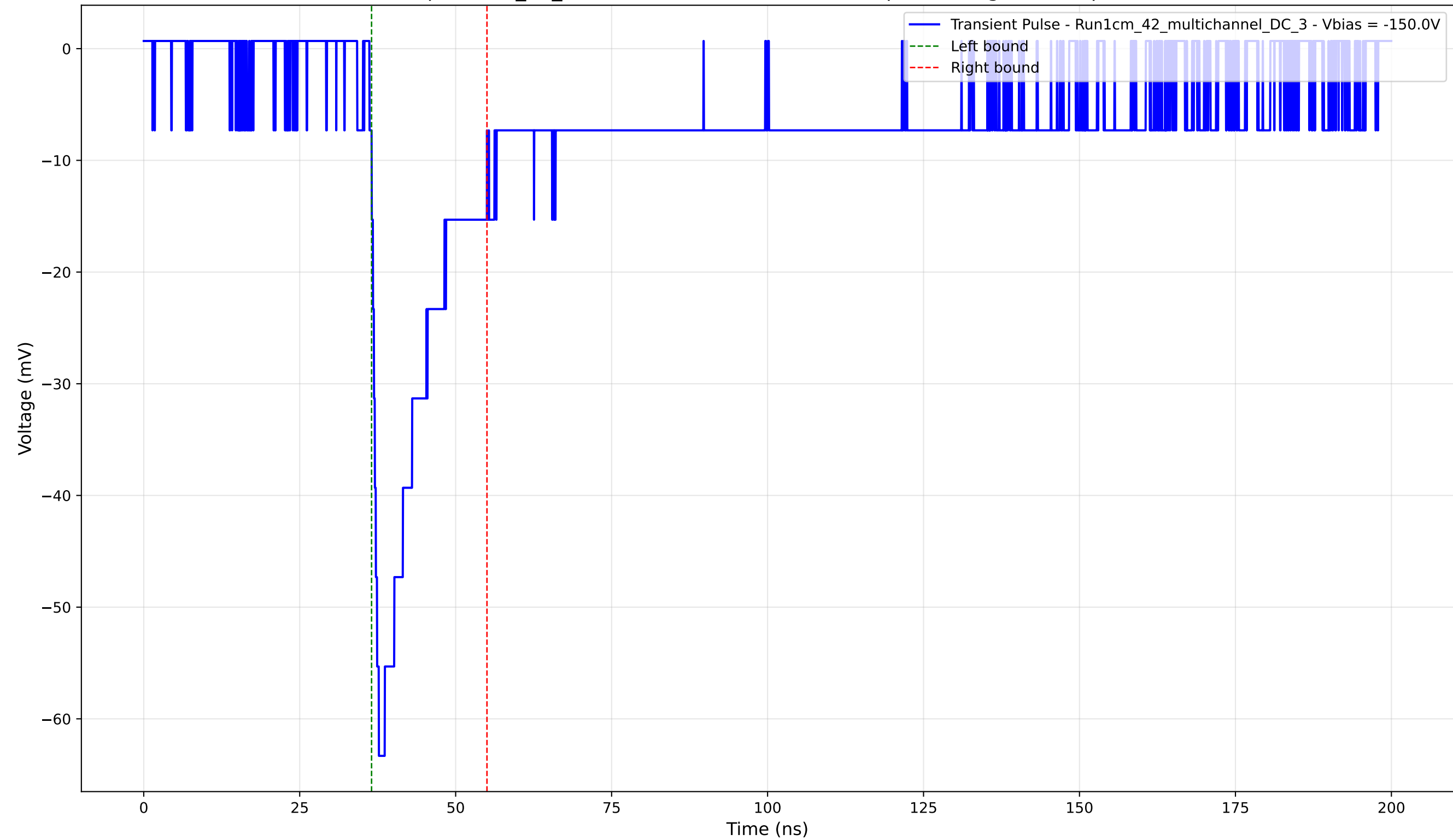
Transient Pulse - Sample: 1cm_42_multichannel - Position: 3935.0 \mu\text{m} - Charge: 11.13 pC - Rise Time: 1.50 ns
