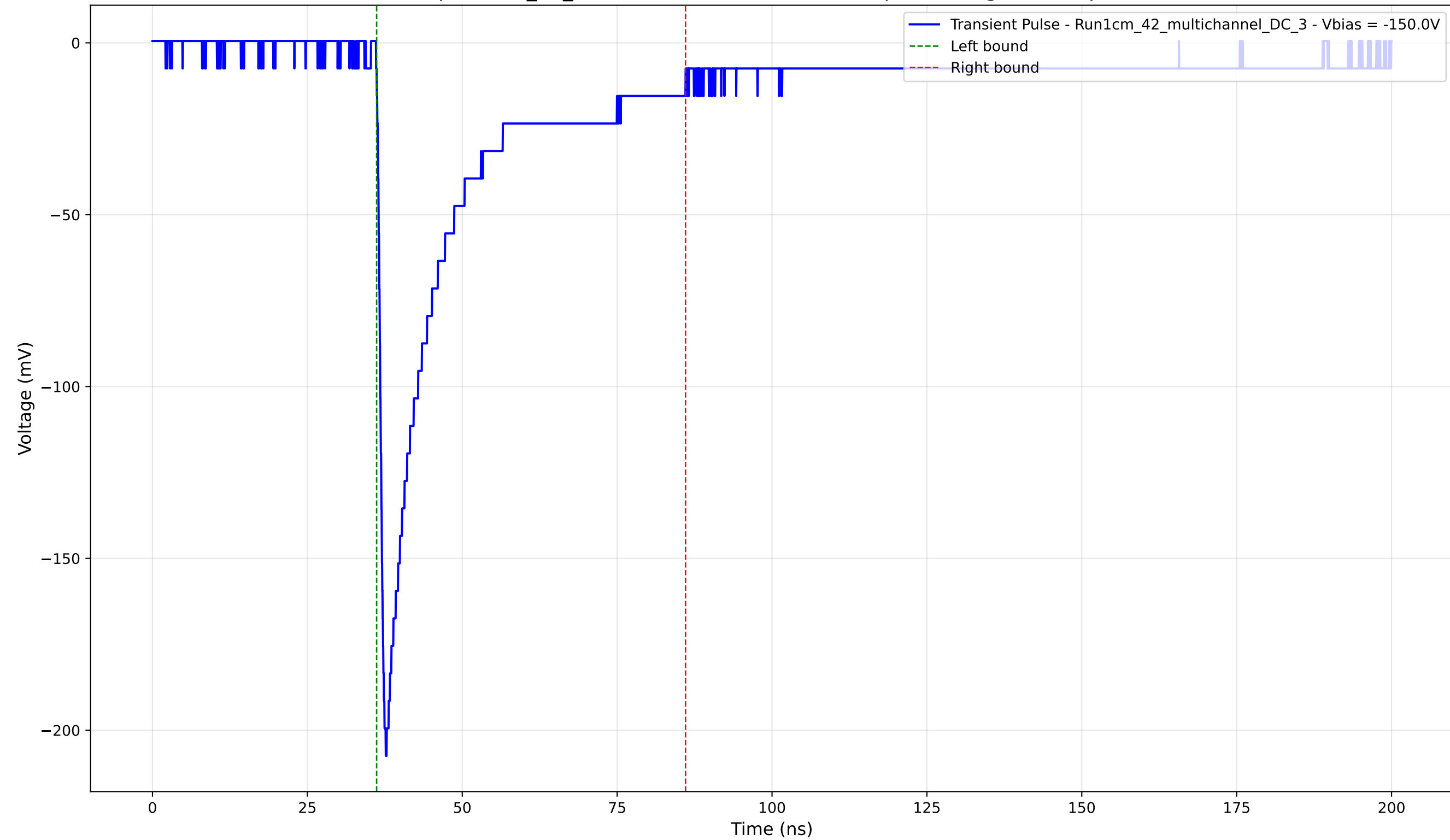
Transient Pulse - Sample: 1cm_42_multichannel - Position: 760.0 \mu\text{m} - Charge: 44.96 pC - Rise Time: 1.07 ns
