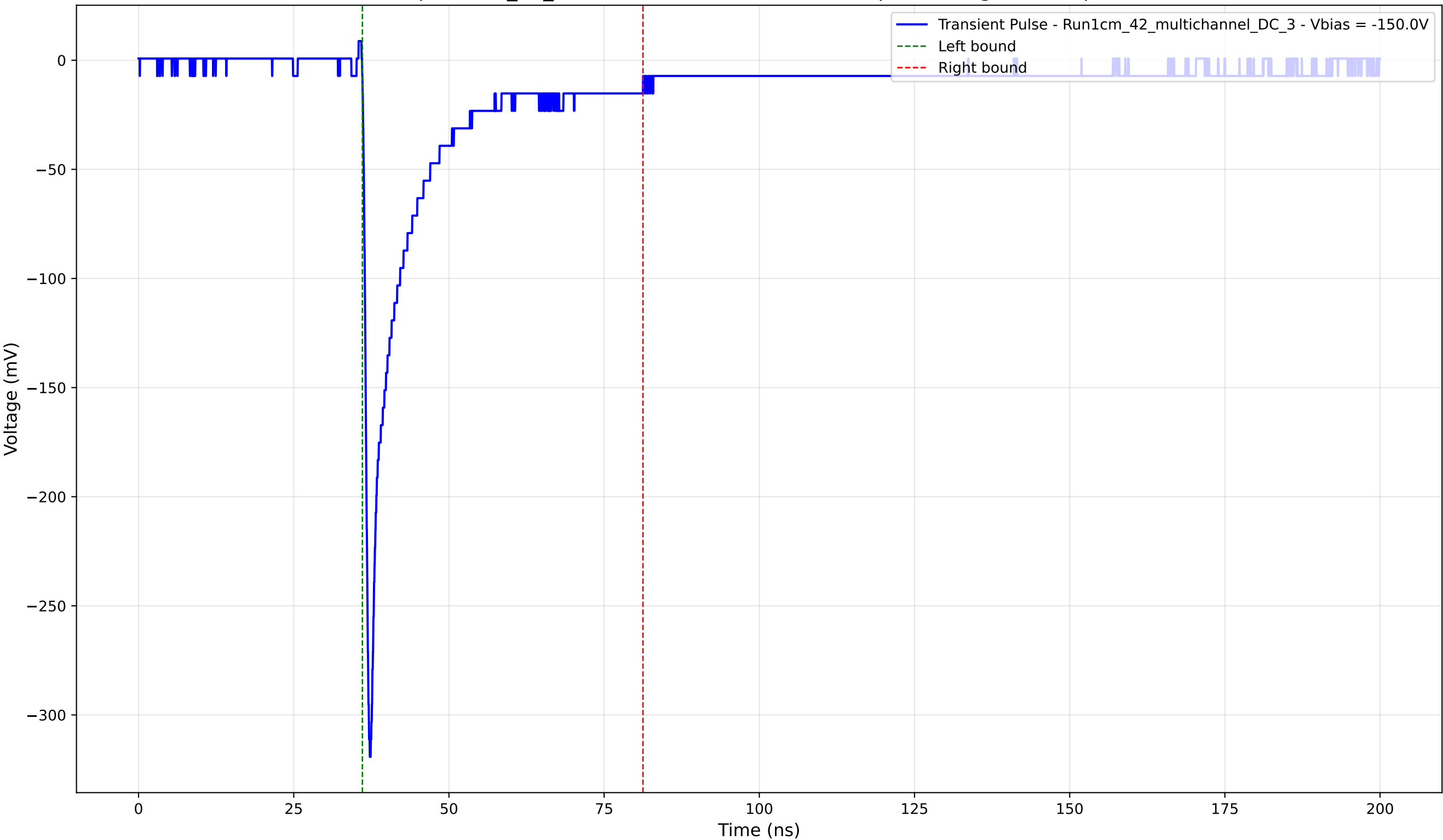
Transient Pulse - Sample: 1cm_42_multichannel - Position: 4645.0 \mu\text{m} - Charge: 41.92 pC - Rise Time: 0.84 ns
