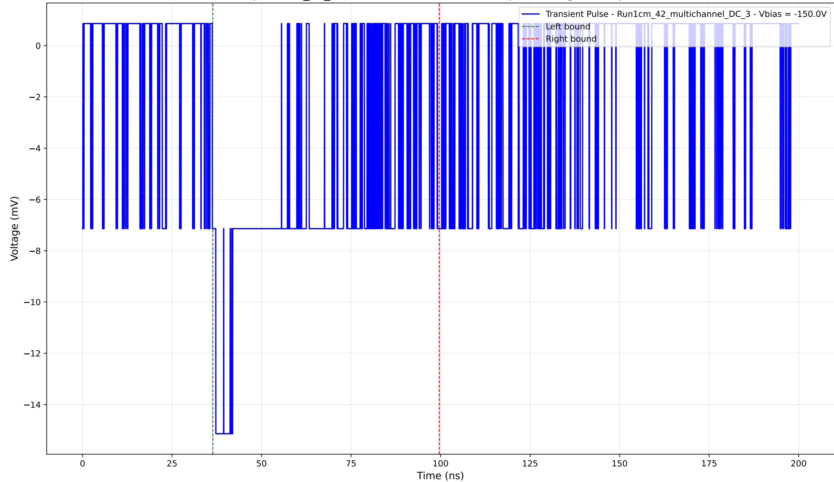
Transient Pulse - Sample: 1cm_42_multichannel - Position: 870.0 \mu\text{m} - Charge: 6.90 pC - Rise Time: 1.00 ns
