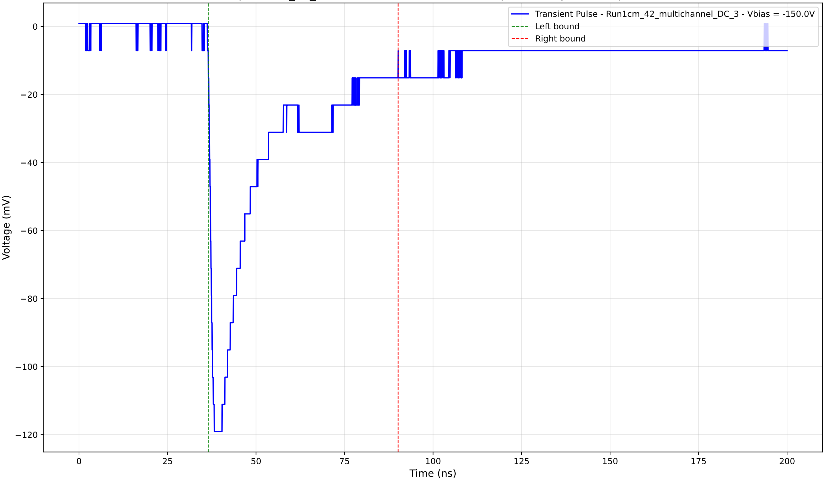
Transient Pulse - Sample: 1cm_42_multichannel - Position: 1585.0 \mu\text{m} - Charge: 41.78 pC - Rise Time: 1.41 ns
