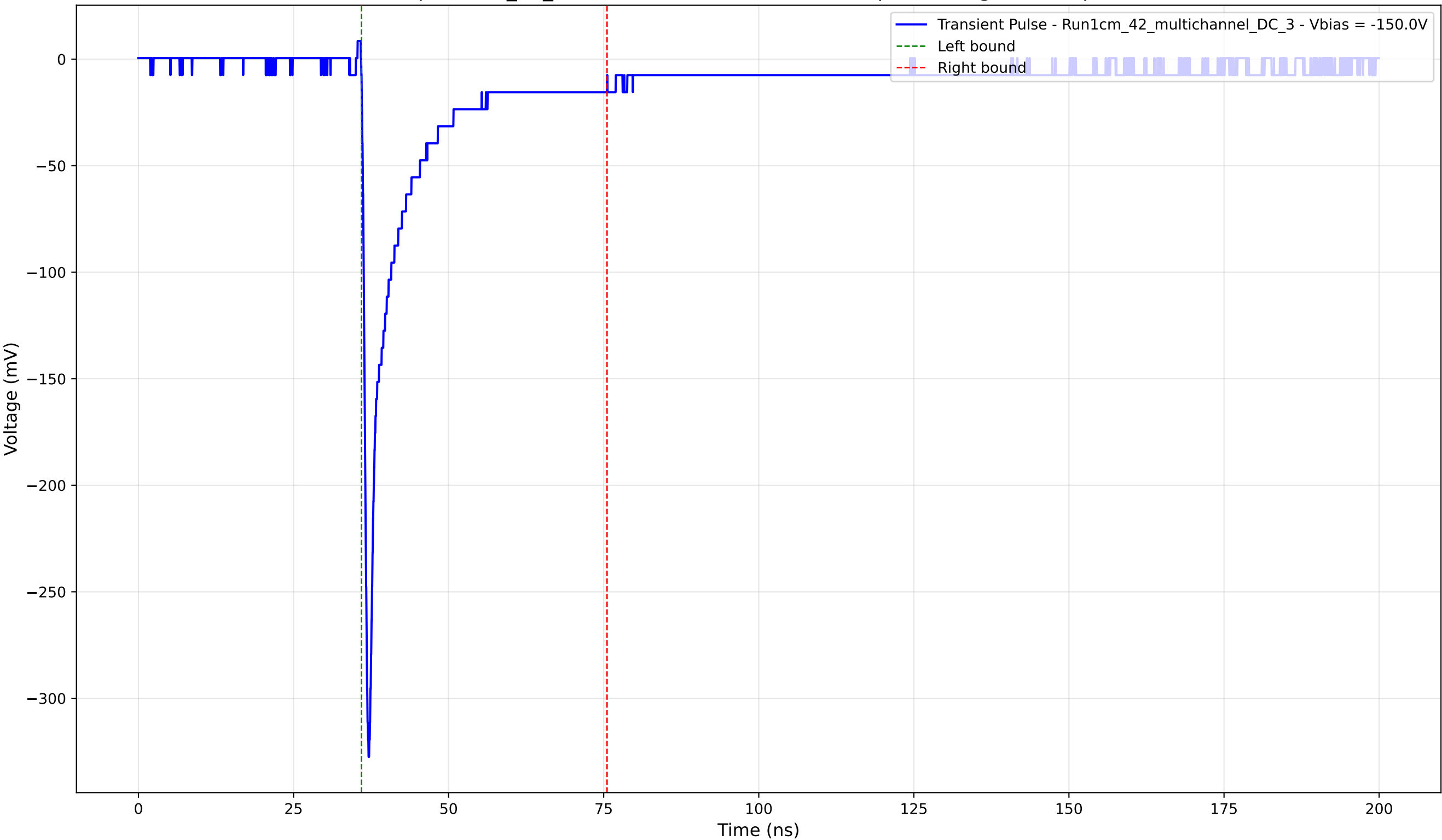
Transient Pulse - Sample: 1cm_42_multichannel - Position: 4825.0 \mu\text{m} - Charge: 35.32 pC - Rise Time: 0.78 ns
