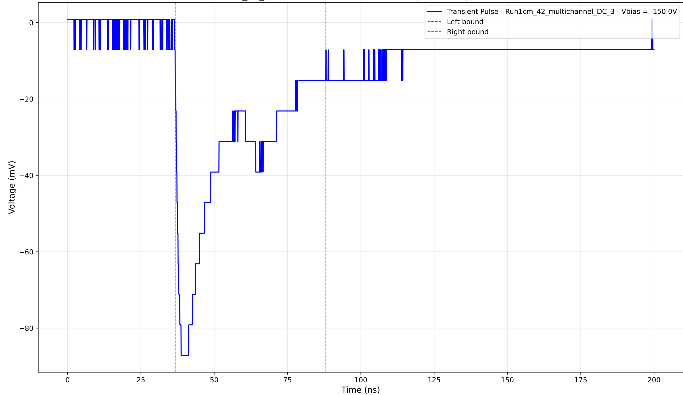
Transient Pulse - Sample: 1cm_42_multichannel - Position: 2695.0 \mu\text{m} - Charge: 36.12 pC - Rise Time: 1.62 ns
