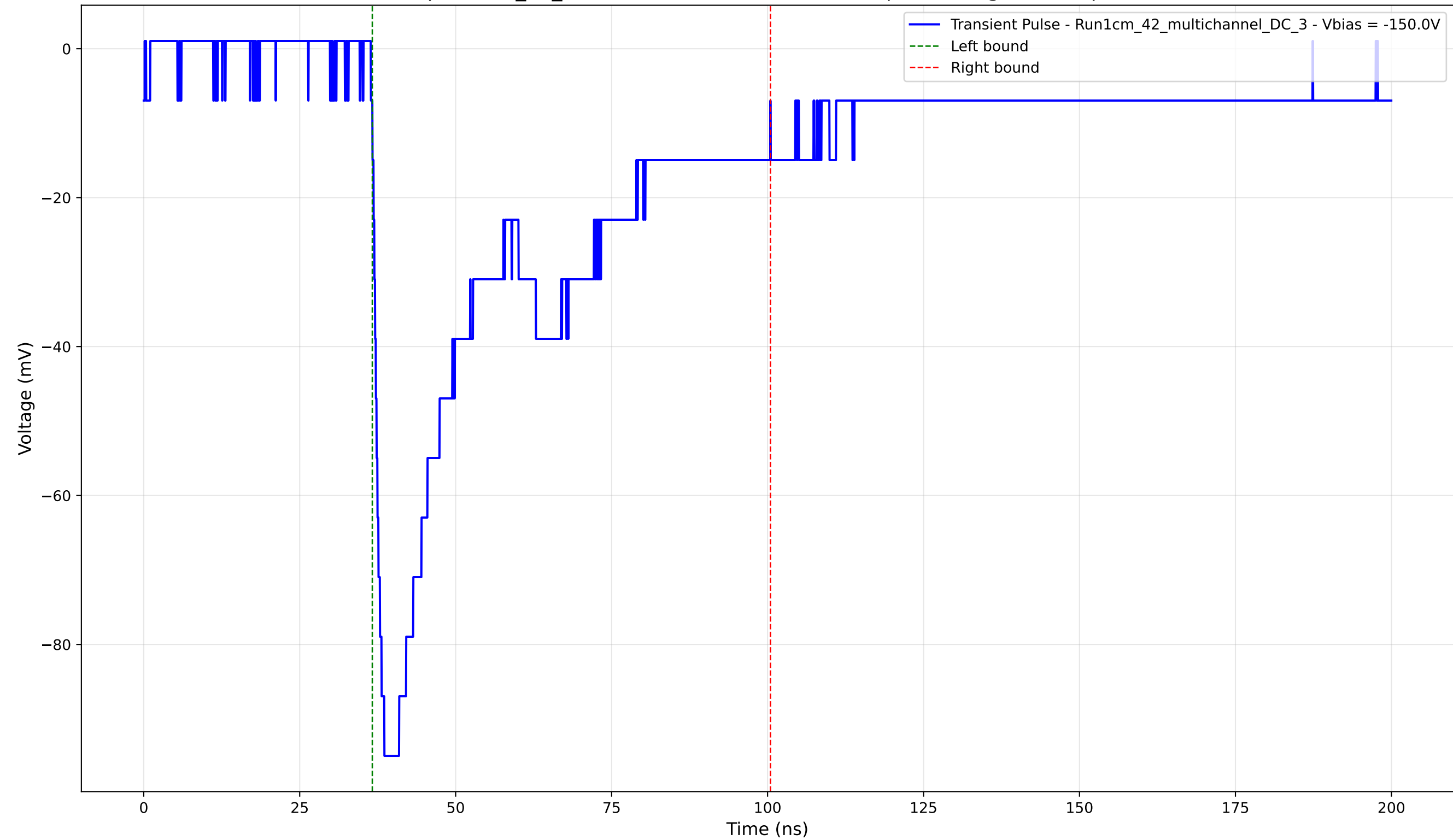
Transient Pulse - Sample: 1cm_42_multichannel - Position: 2020.0 \mu\text{m} - Charge: 42.29 pC - Rise Time: 1.47 ns
