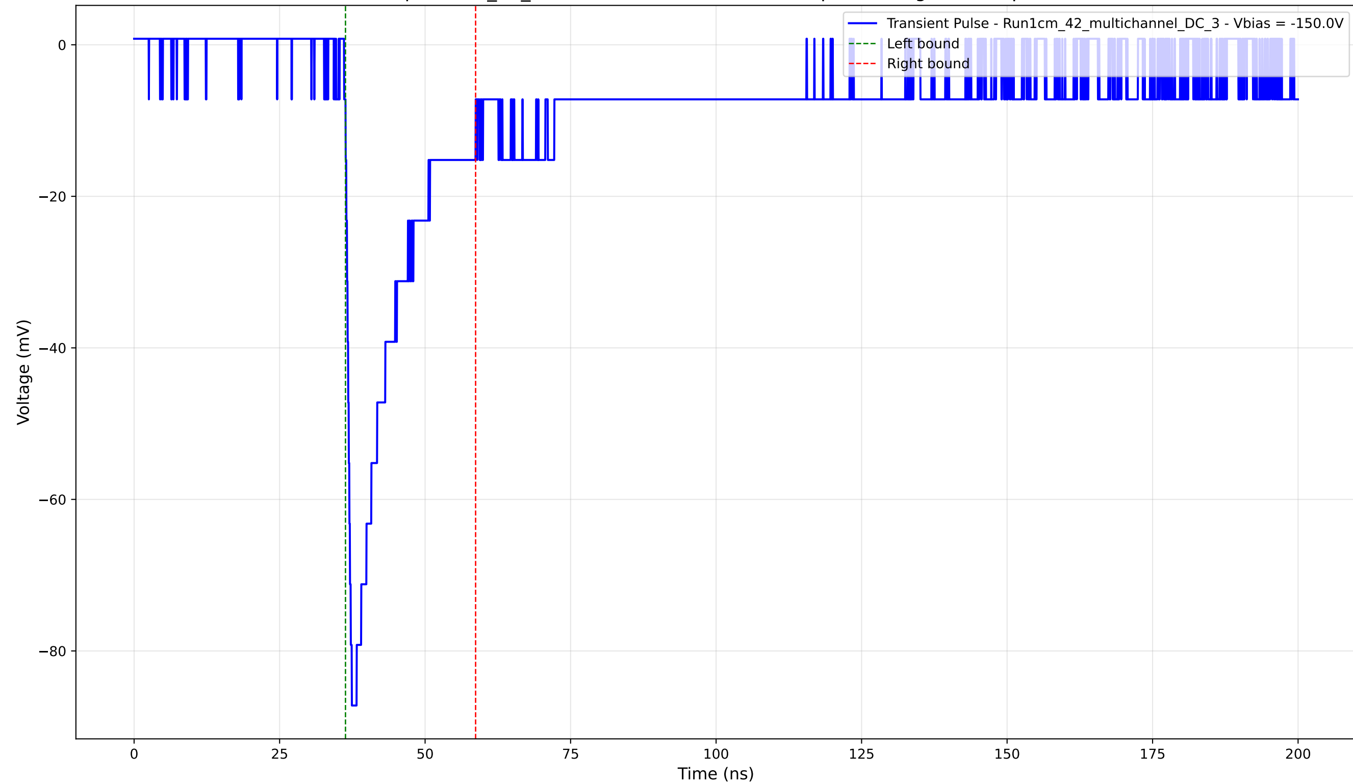
Transient Pulse - Sample: 1cm_42_multichannel - Position: 810.0 \mu\text{m} - Charge: 15.45 pC - Rise Time: 0.90 ns
