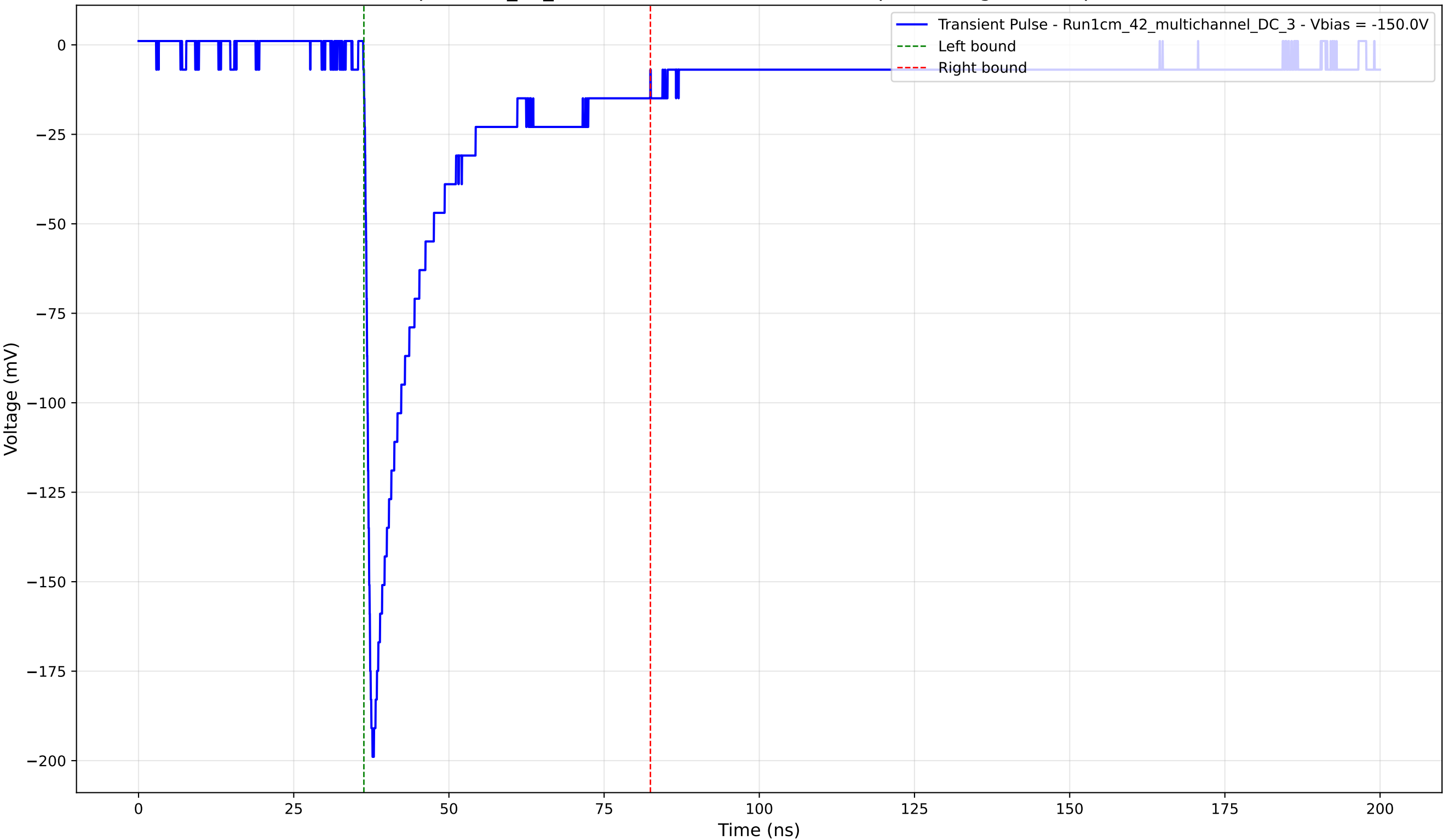
Transient Pulse - Sample: 1cm_42_multichannel - Position: 4175.0 \mu\text{m} - Charge: 39.74 pC - Rise Time: 1.01 ns
