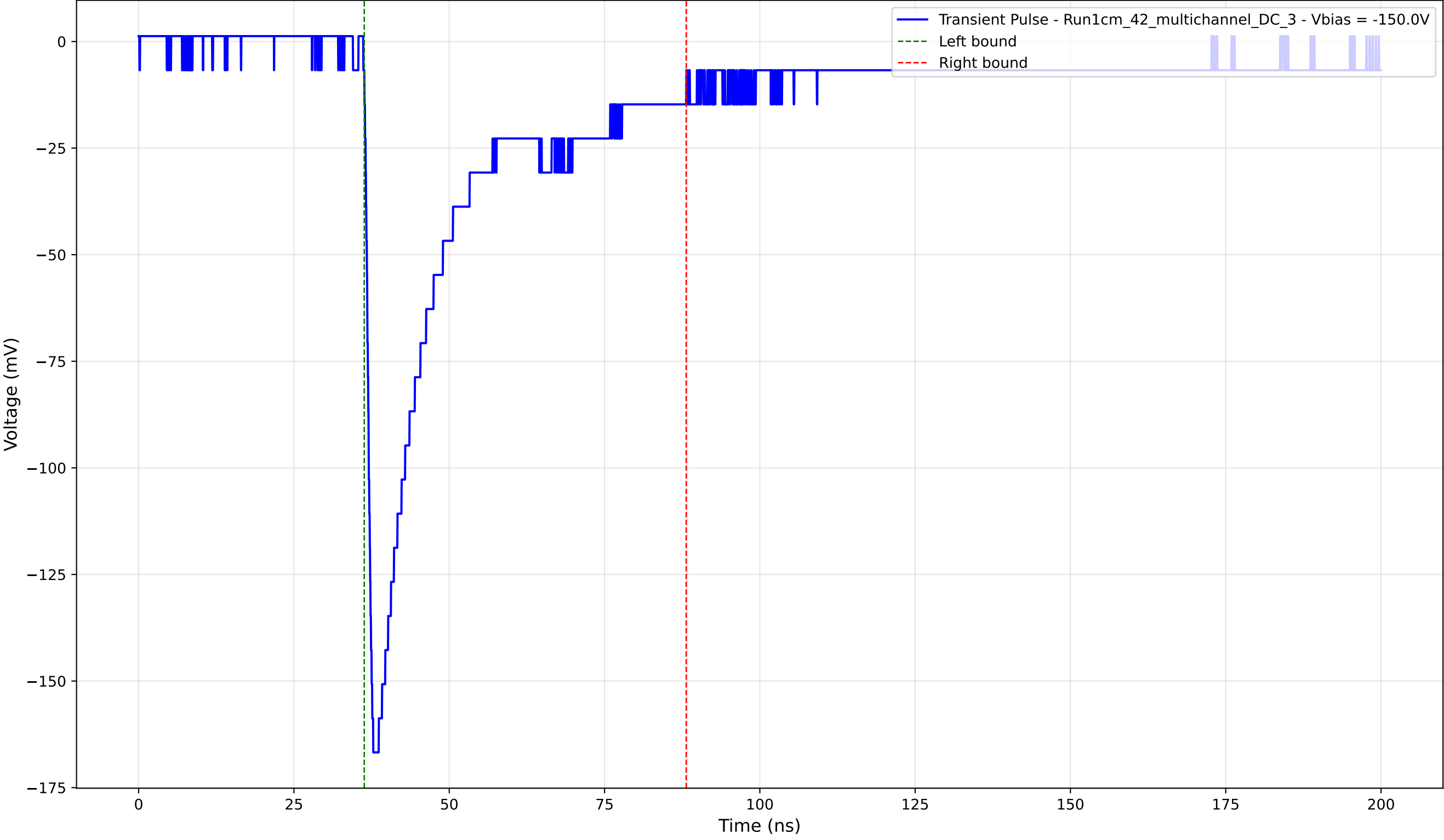
Transient Pulse - Sample: 1cm_42_multichannel - Position: 1065.0 \mu\text{m} - Charge: 44.17 pC - Rise Time: 1.08 ns
