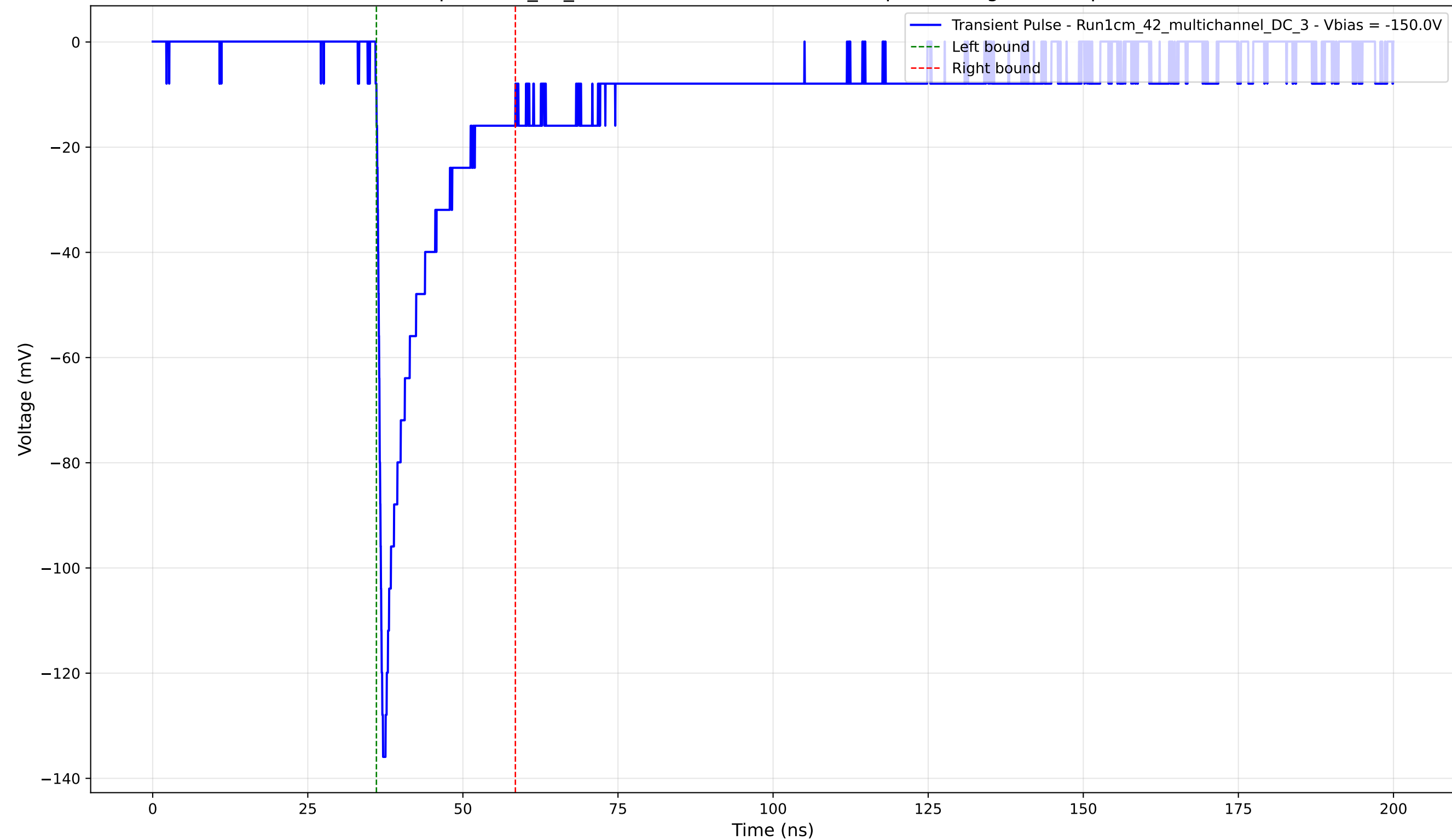
Transient Pulse - Sample: 1cm_42_multichannel - Position: 400.0 \mu\text{m} - Charge: 18.70 pC - Rise Time: 0.93 ns
