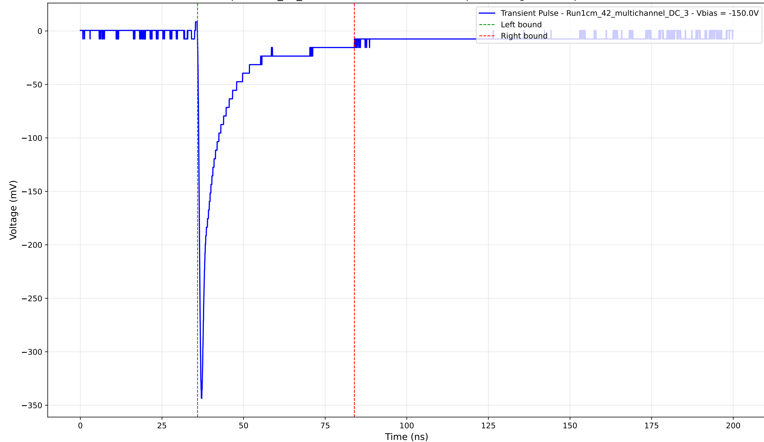
Transient Pulse - Sample: 1cm_42_multichannel - Position: 225.0 \mu\text{m} - Charge: 47.55 pC - Rise Time: 0.81 ns
