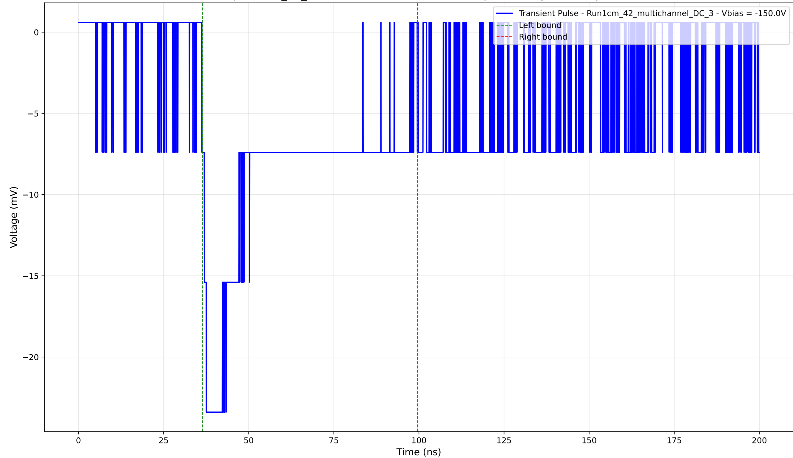
Transient Pulse - Sample: 1cm_42_multichannel - Position: 1395.0 \mu\text{m} - Charge: 11.59 pC - Rise Time: 1.29 ns
