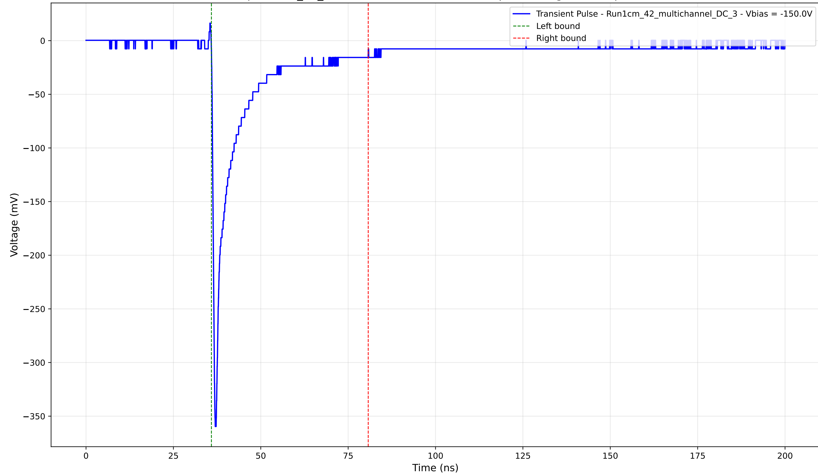
Transient Pulse - Sample: 1cm_42_multichannel - Position: 170.0 \mu\text{m} - Charge: 47.01 pC - Rise Time: 0.78 ns
