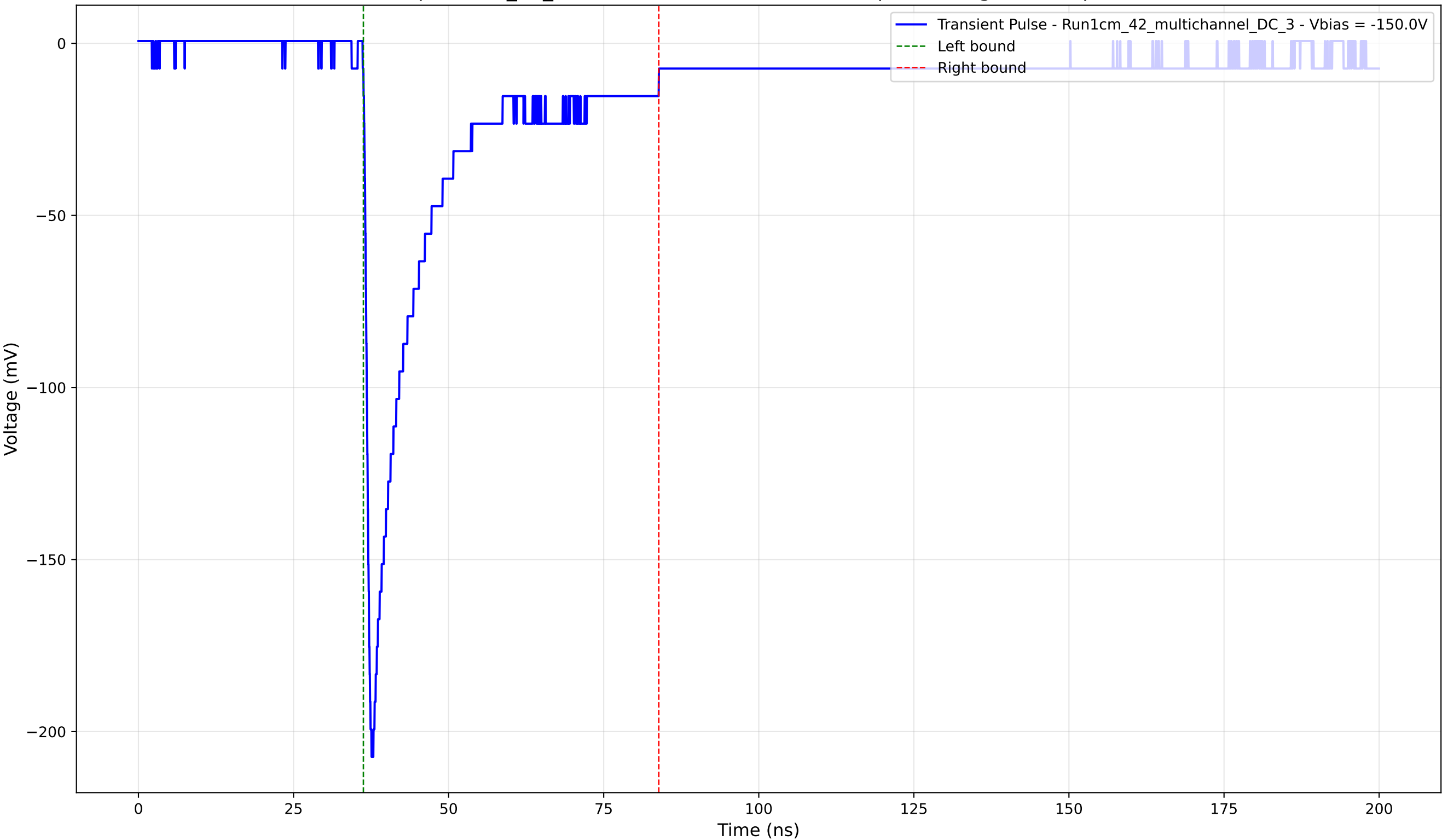
Transient Pulse - Sample: 1cm_42_multichannel - Position: 4250.0 \mu\text{m} - Charge: 39.86 pC - Rise Time: 0.97 ns
