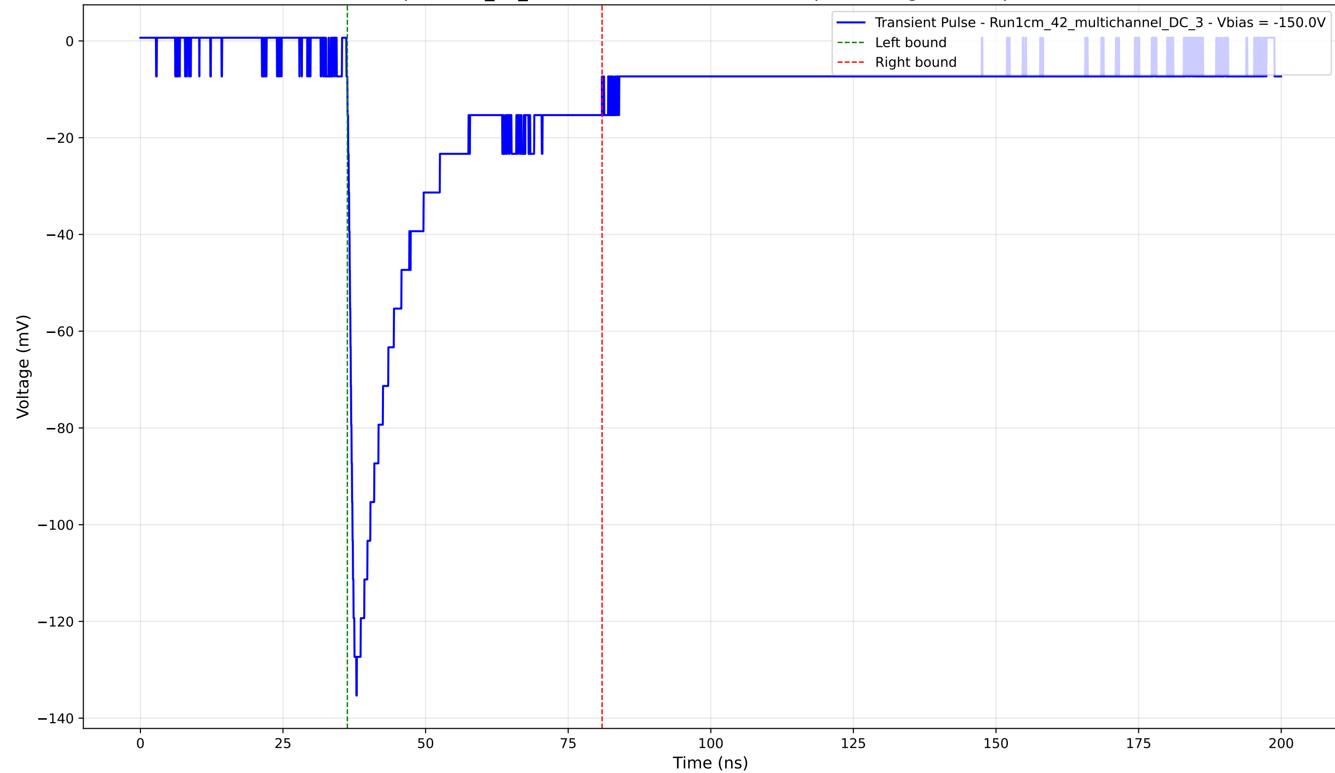
Transient Pulse - Sample: 1cm_42_multichannel - Position: 915.0 \mu\text{m} - Charge: 31.34 pC - Rise Time: 1.22 ns
