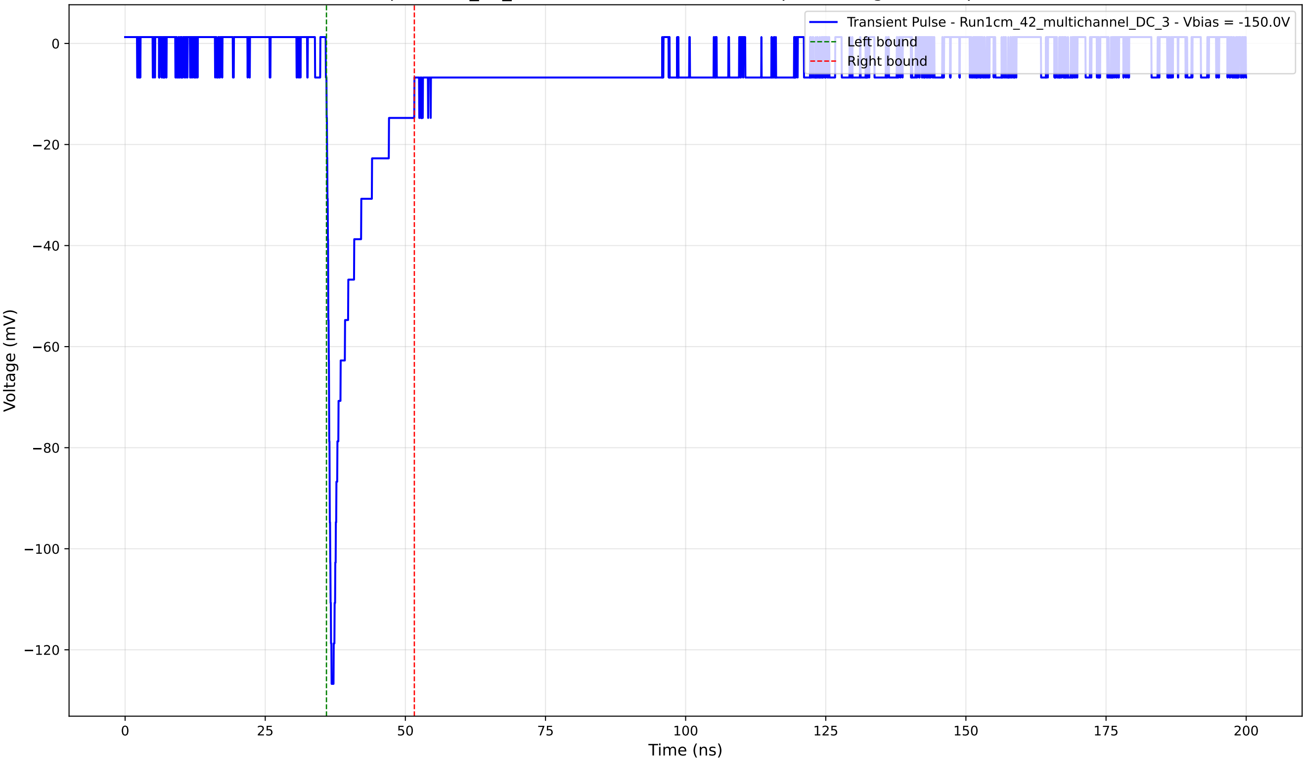
Transient Pulse - Sample: 1cm_42_multichannel - Position: 70.0 \mu\text{m} - Charge: 11.84 pC - Rise Time: 0.79 ns
