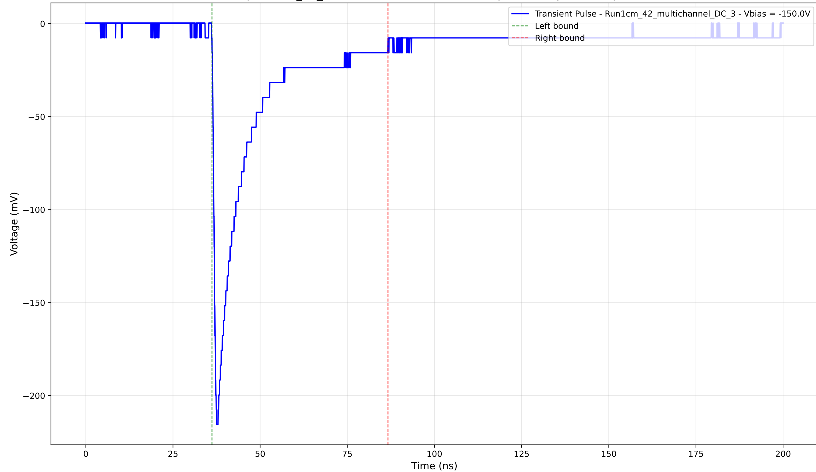
Transient Pulse - Sample: 1cm_42_multichannel - Position: 730.0 \mu\text{m} - Charge: 46.51 pC - Rise Time: 1.01 ns
