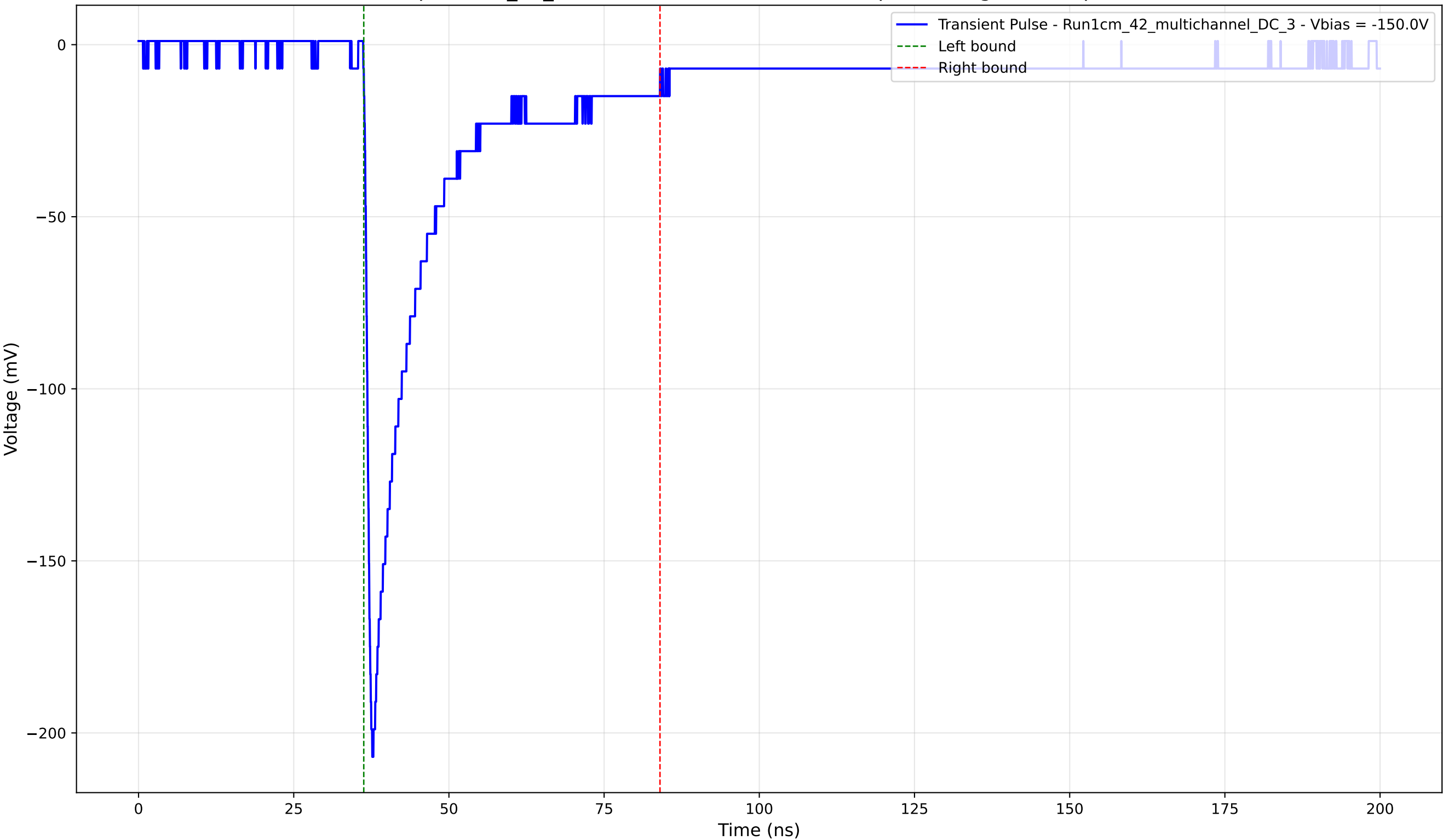
Transient Pulse - Sample: 1cm_42_multichannel - Position: 4195.0 \mu\text{m} - Charge: 40.85 pC - Rise Time: 1.03 ns
