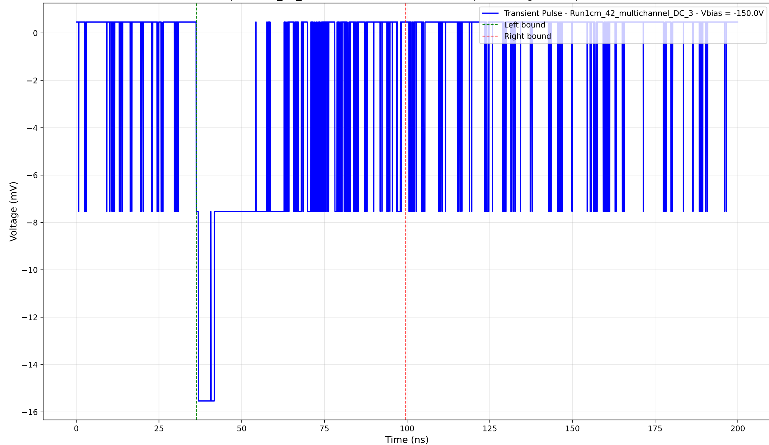
Transient Pulse - Sample: 1cm_42_multichannel - Position: 4410.0 \mu\text{m} - Charge: 6.30 pC - Rise Time: 0.66 ns
