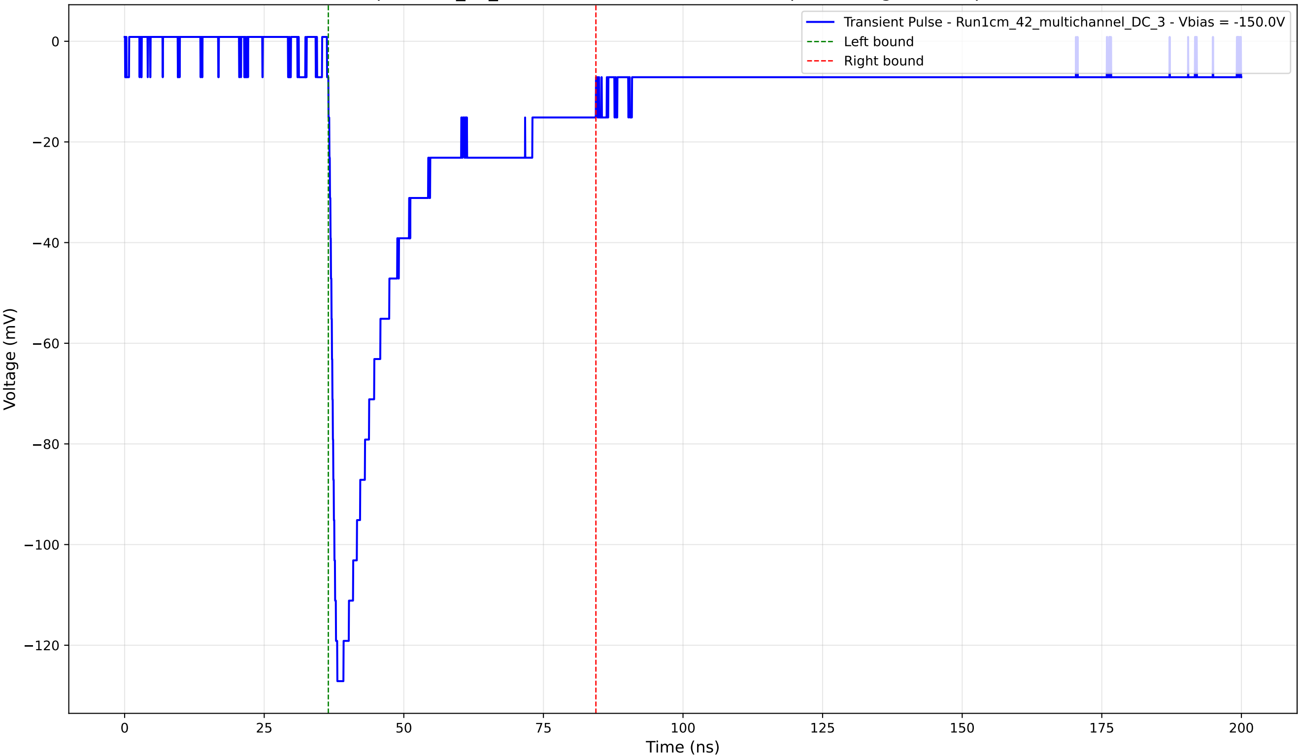
Transient Pulse - Sample: 1cm_42_multichannel - Position: 3625.0 \mu\text{m} - Charge: 35.90 pC - Rise Time: 1.35 ns
