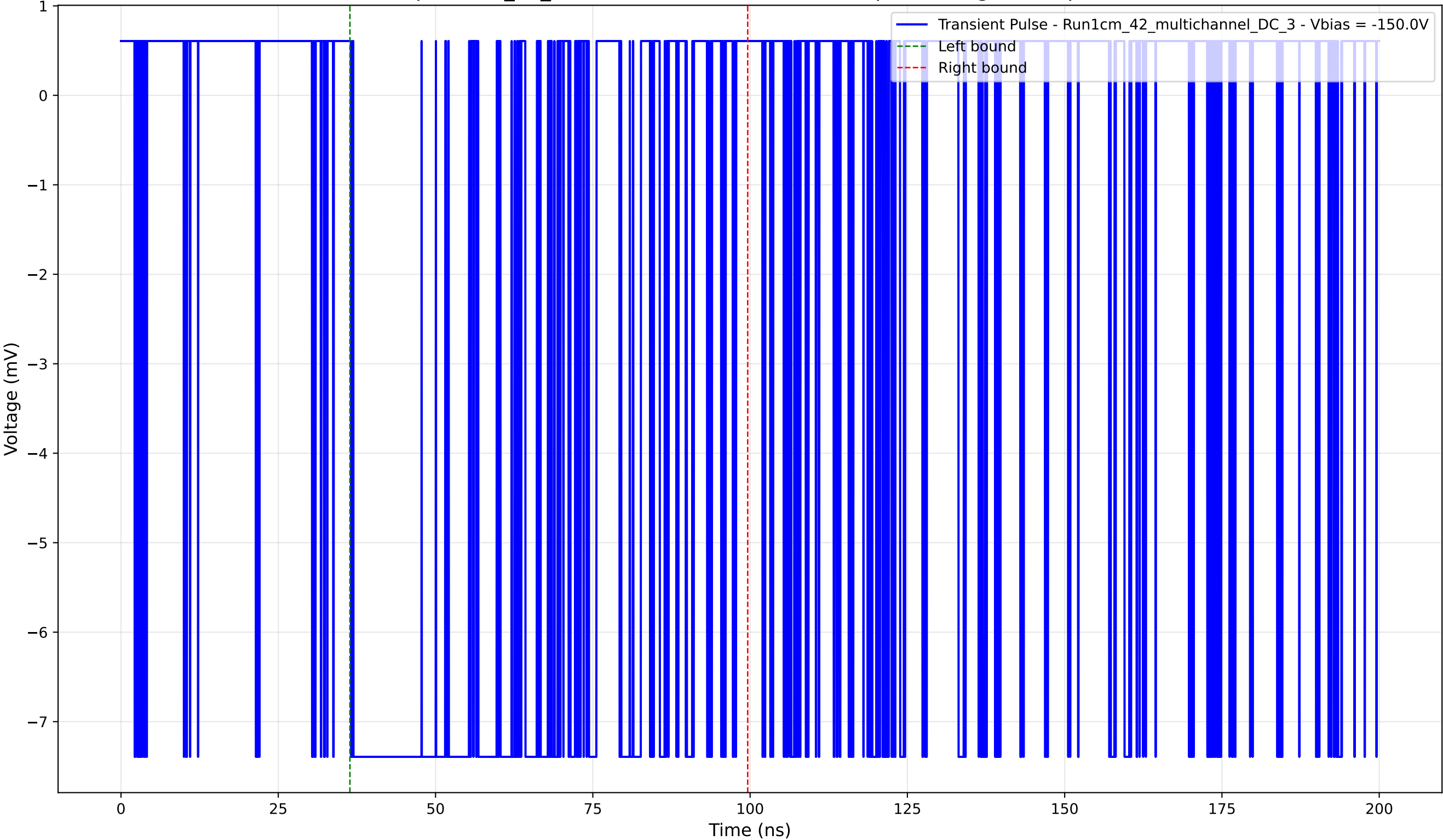
Transient Pulse - Sample: 1cm_42_multichannel - Position: 3385.0 \mu\text{m} - Charge: 5.44 pC - Rise Time: 0.02 ns
