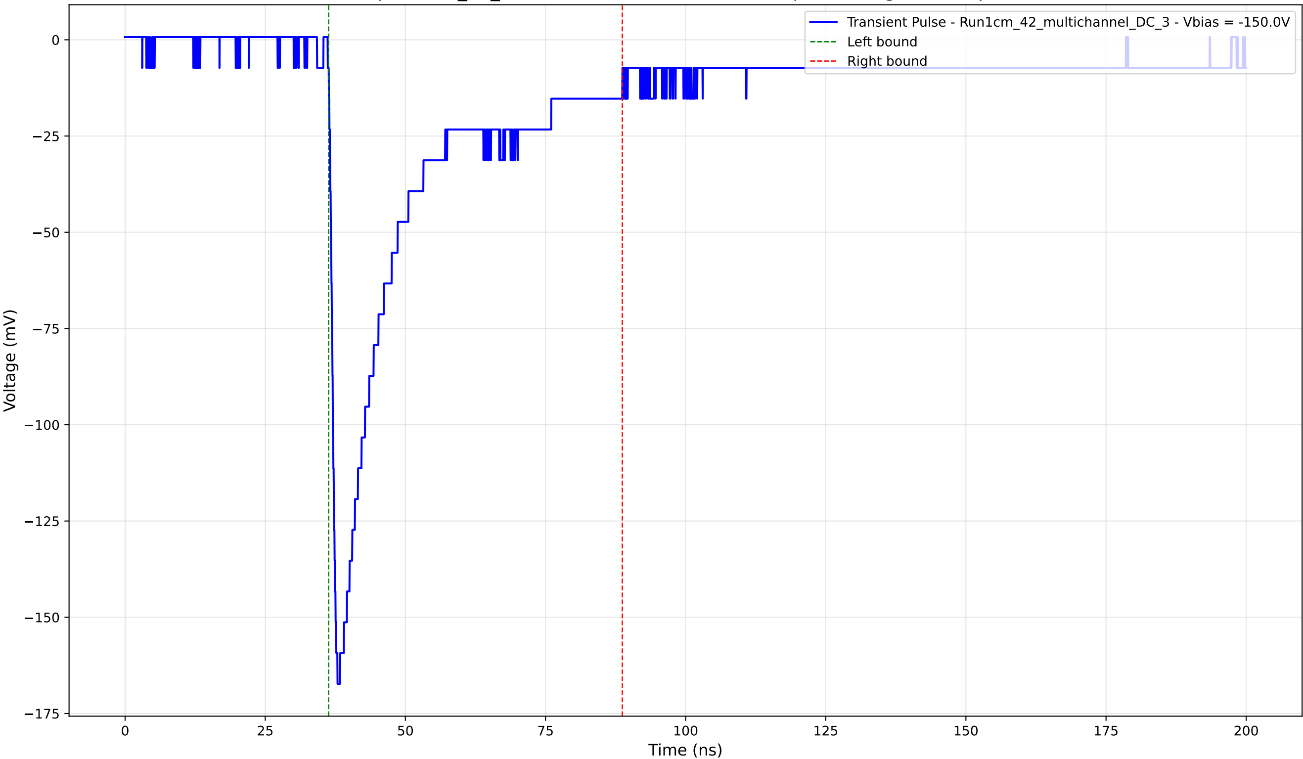
Transient Pulse - Sample: 1cm_42_multichannel - Position: 1075.0 \mu\text{m} - Charge: 44.04 pC - Rise Time: 1.12 ns
