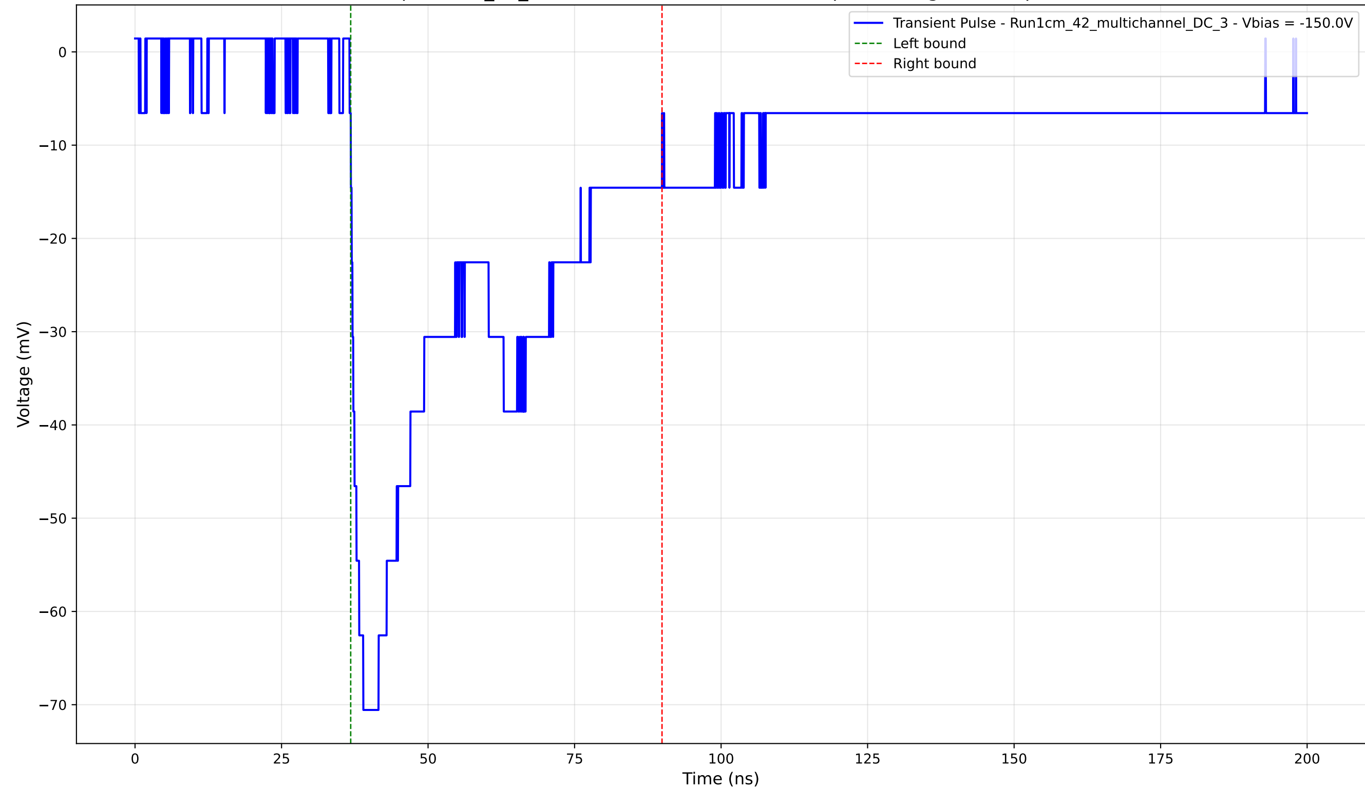
Transient Pulse - Sample: 1cm_42_multichannel - Position: 2445.0 \mu\text{m} - Charge: 32.81 pC - Rise Time: 2.14 ns
