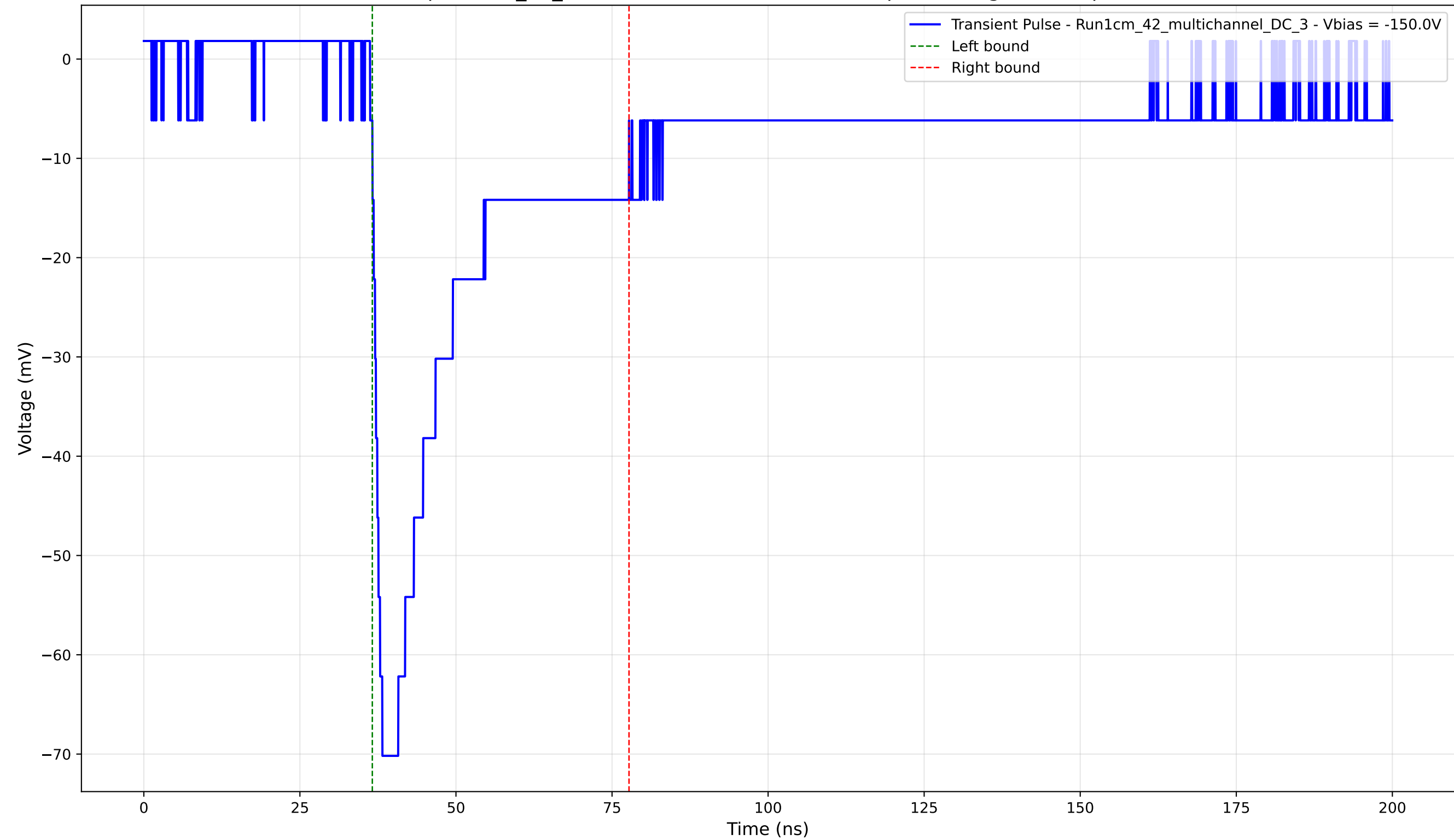
Transient Pulse - Sample: 1cm_42_multichannel - Position: 3330.0 \mu\text{m} - Charge: 21.15 pC - Rise Time: 1.60 ns
