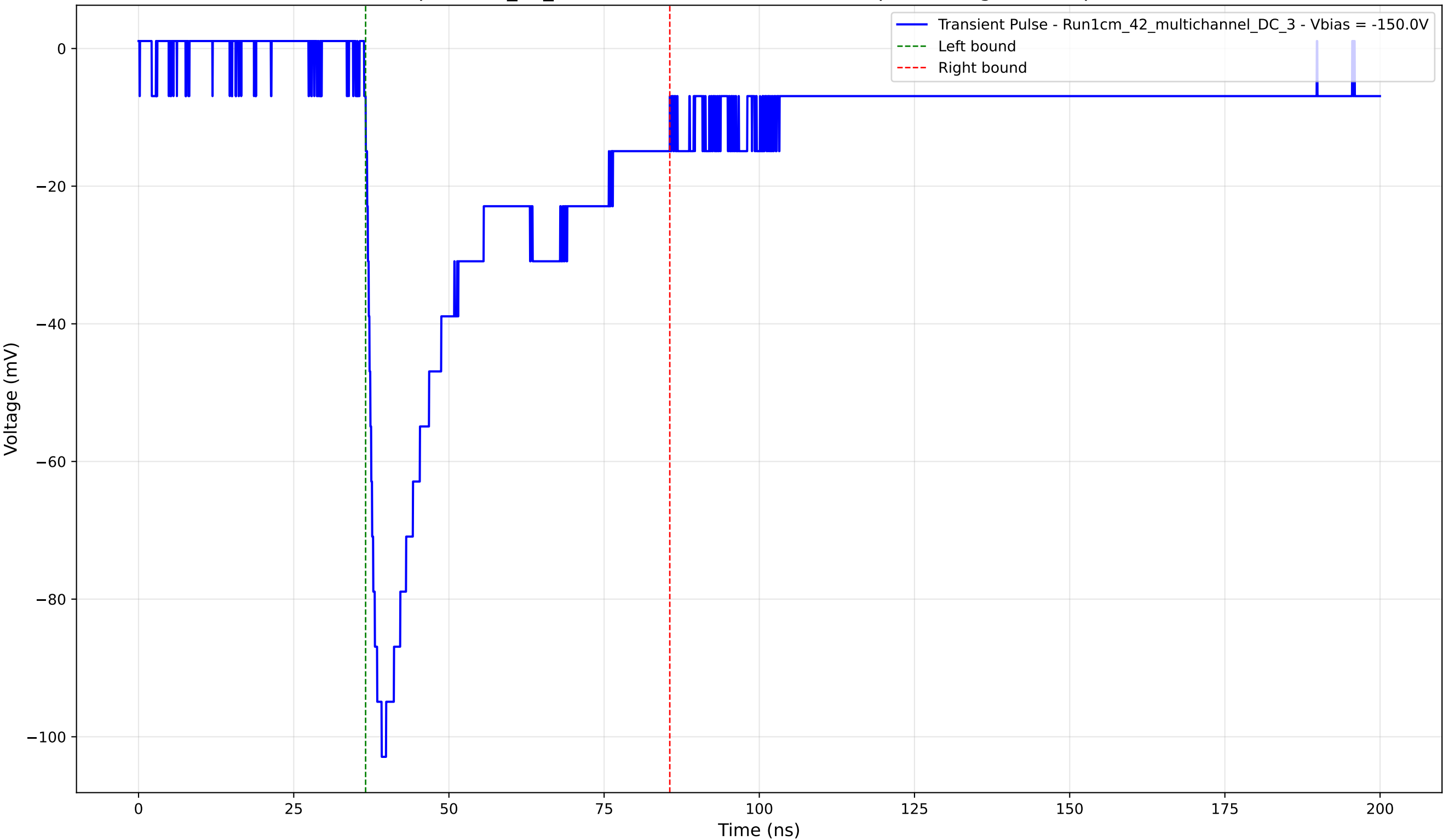
Transient Pulse - Sample: 1cm_42_multichannel - Position: 3055.0 \mu\text{m} - Charge: 34.72 pC - Rise Time: 1.85 ns
