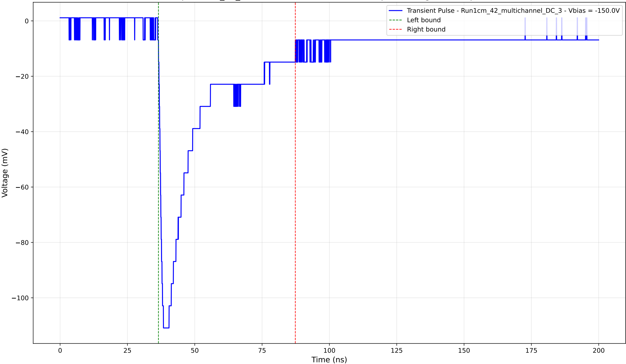
Transient Pulse - Sample: 1cm_42_multichannel - Position: 3285.0 \mu\text{m} - Charge: 36.61 pC - Rise Time: 1.49 ns
