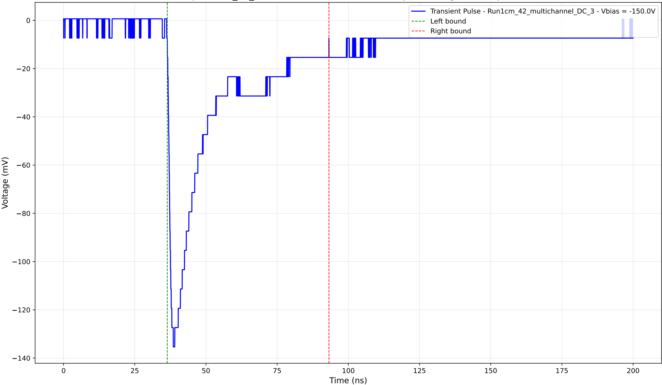
Transient Pulse - Sample: 1cm_42_multichannel - Position: 1510.0 \mu\text{m} - Charge: 44.51 pC - Rise Time: 1.58 ns
