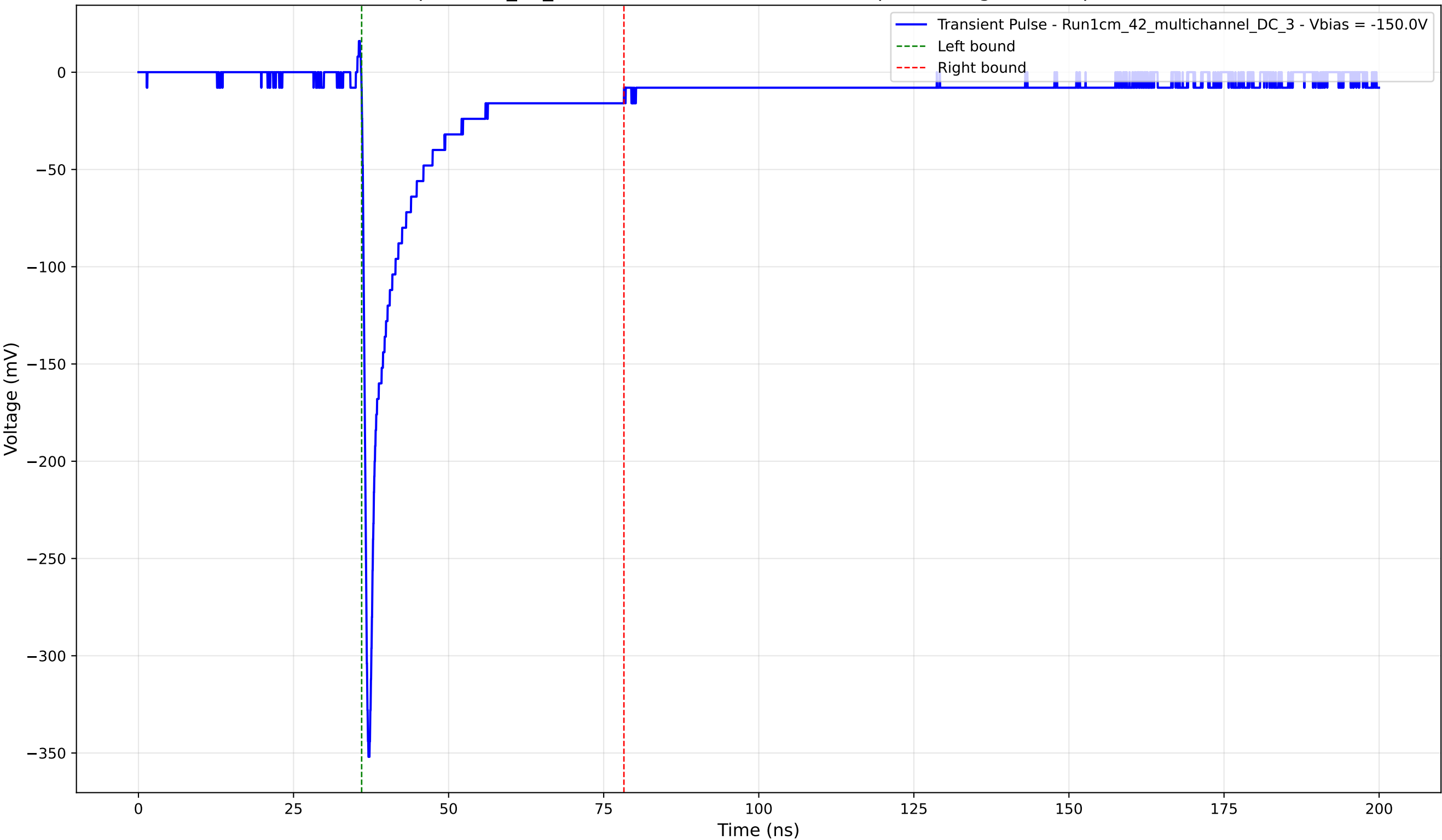
Transient Pulse - Sample: 1cm_42_multichannel - Position: 4805.0 \mu\text{m} - Charge: 39.42 pC - Rise Time: 0.77 ns
