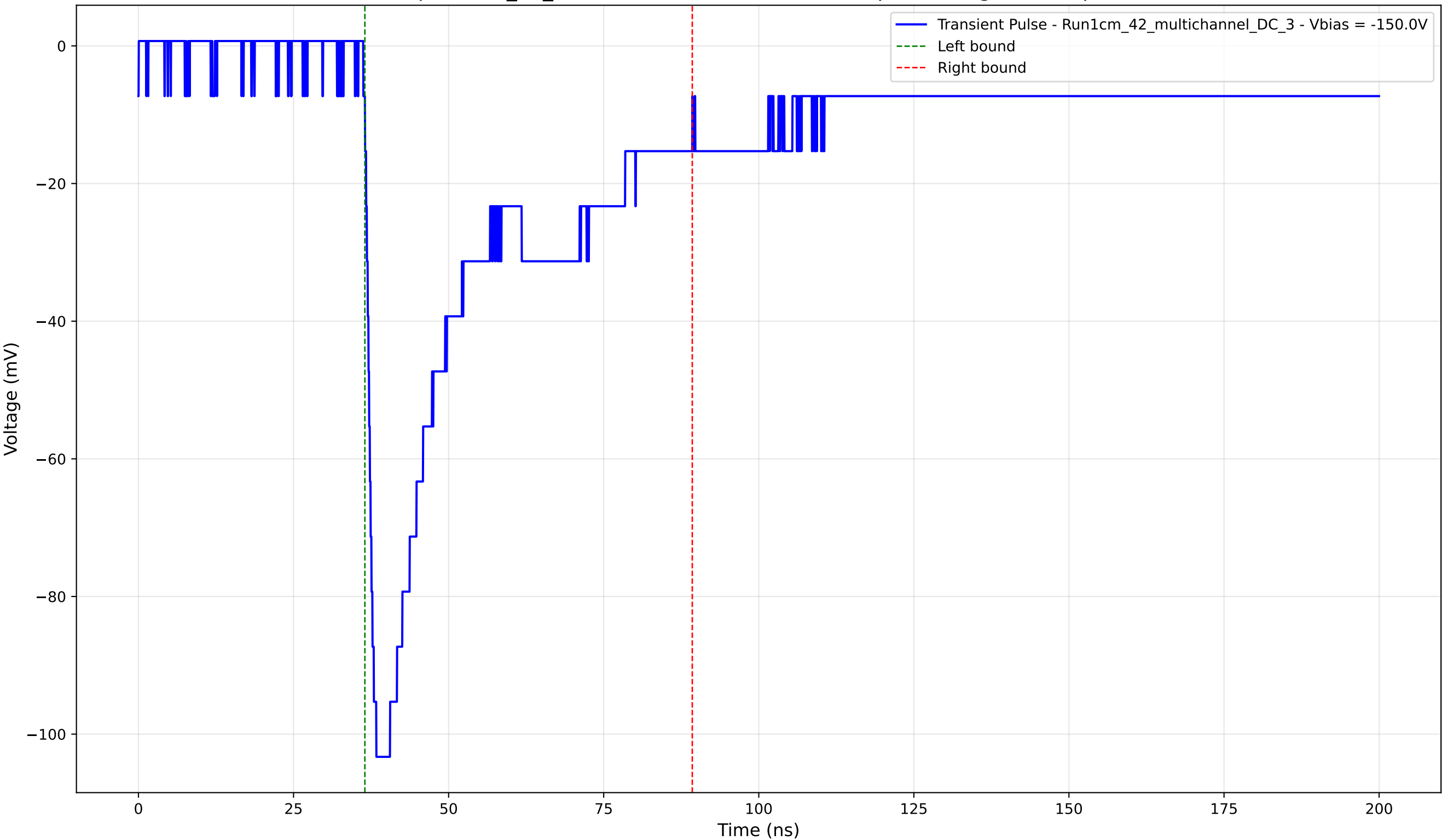
Transient Pulse - Sample: 1cm_42_multichannel - Position: 1780.0 \mu\text{m} - Charge: 39.02 pC - Rise Time: 1.43 ns
