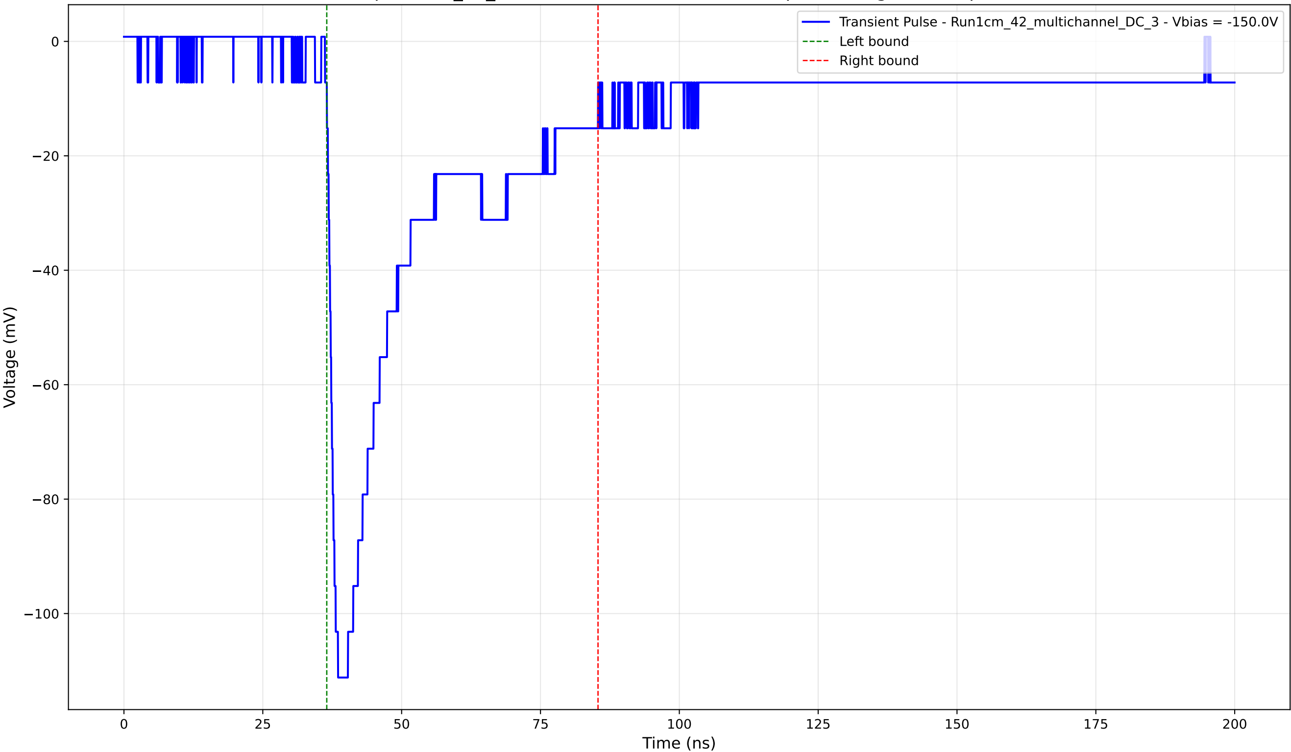
Transient Pulse - Sample: 1cm_42_multichannel - Position: 3225.0 \mu\text{m} - Charge: 36.89 pC - Rise Time: 1.59 ns
