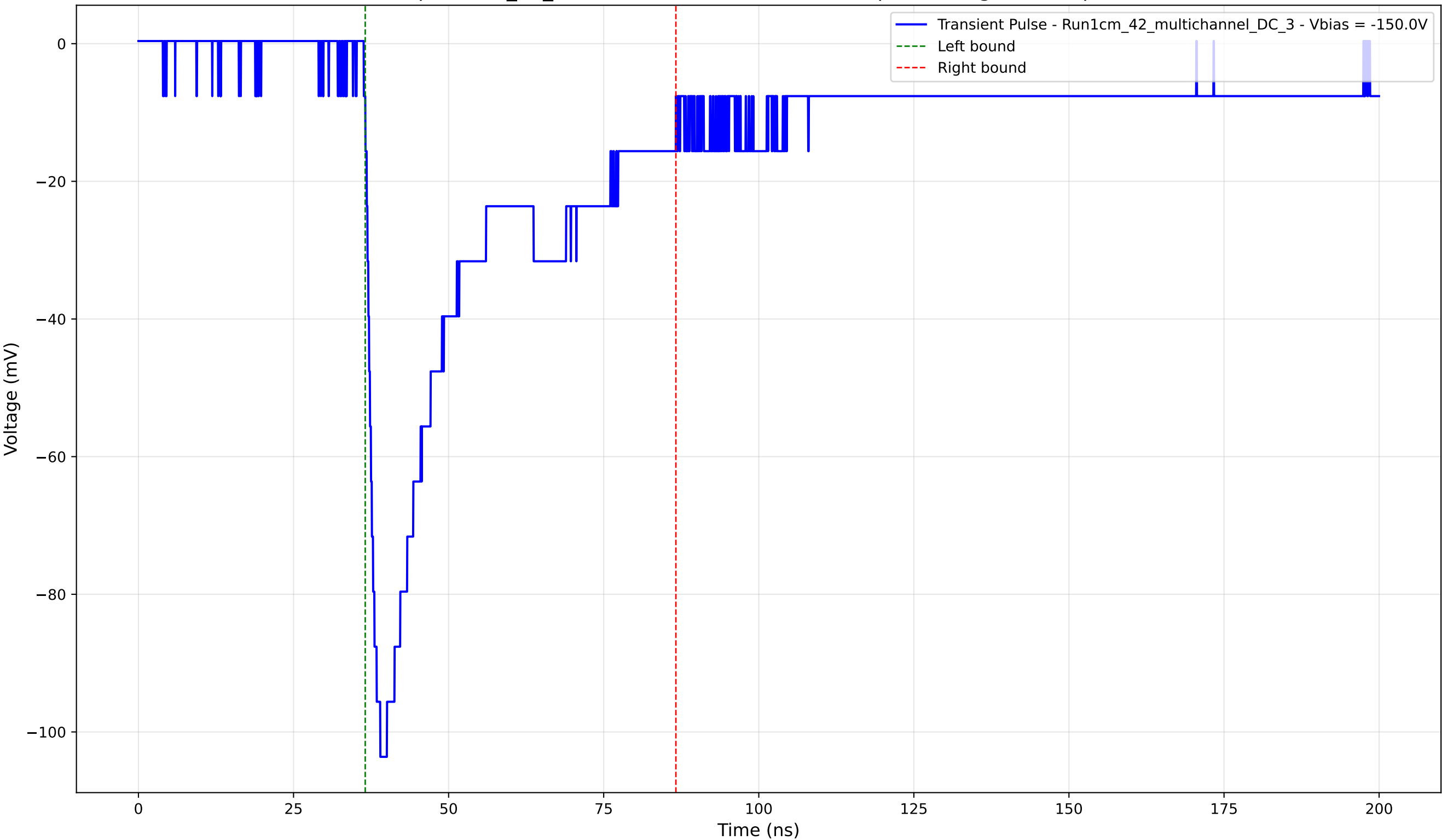
Transient Pulse - Sample: 1cm_42_multichannel - Position: 3035.0 \mu\text{m} - Charge: 36.29 pC - Rise Time: 1.83 ns
