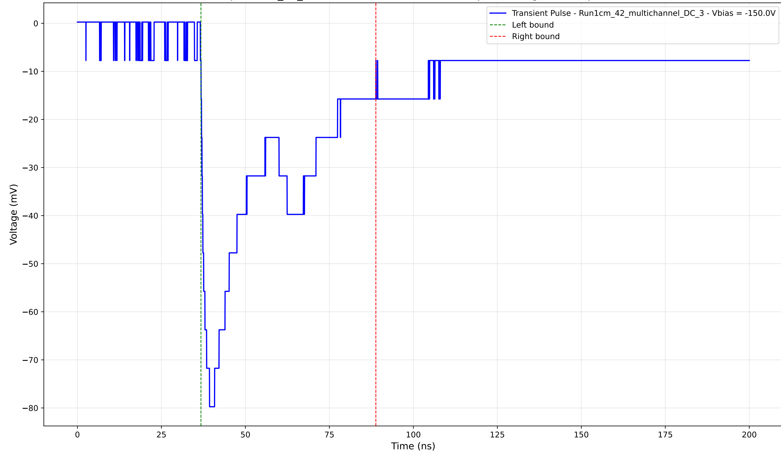
Transient Pulse - Sample: 1cm_42_multichannel - Position: 2455.0 \mu\text{m} - Charge: 35.18 pC - Rise Time: 2.54 ns
