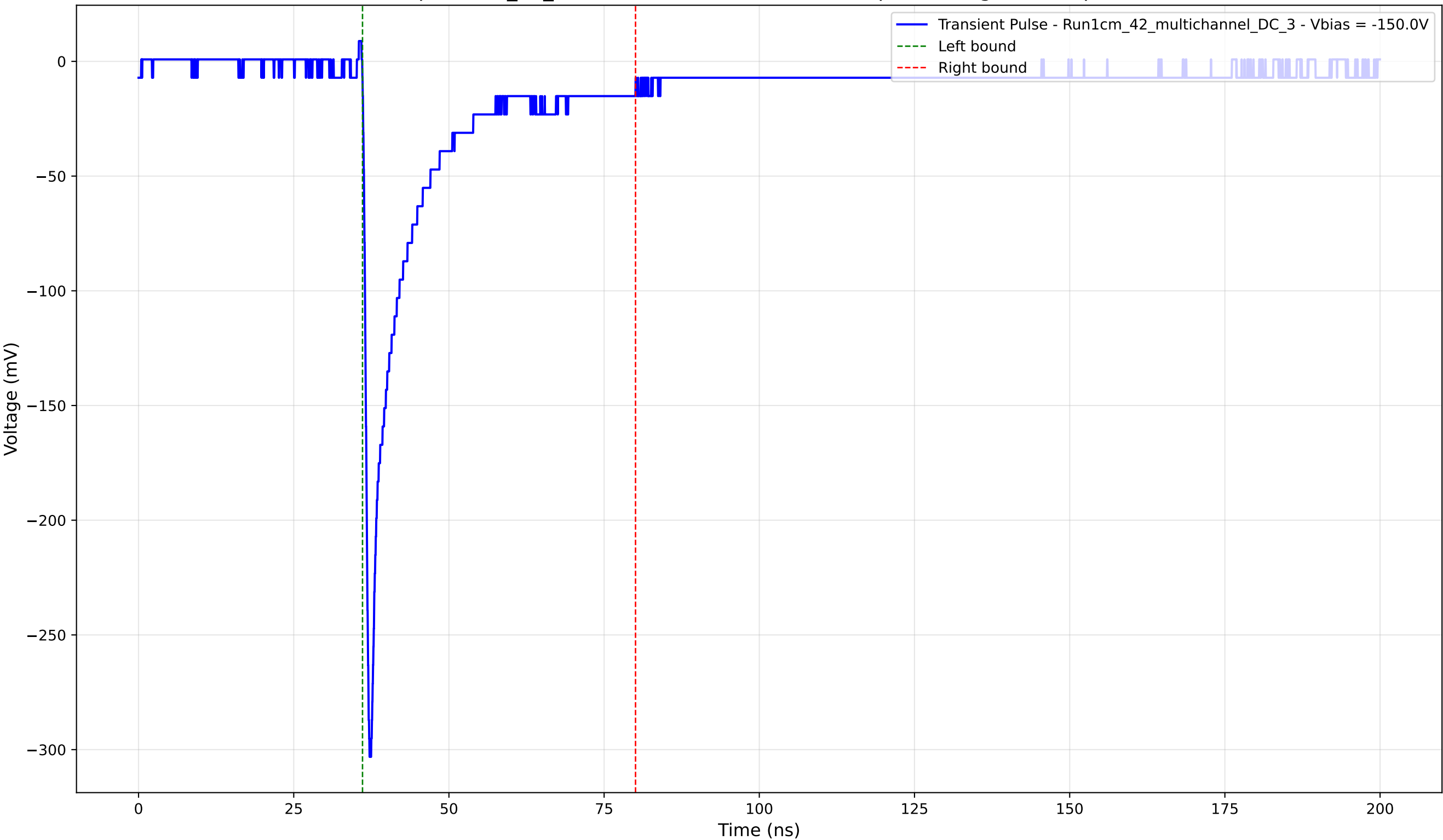
Transient Pulse - Sample: 1cm_42_multichannel - Position: 4615.0 \mu\text{m} - Charge: 41.24 pC - Rise Time: 0.84 ns
