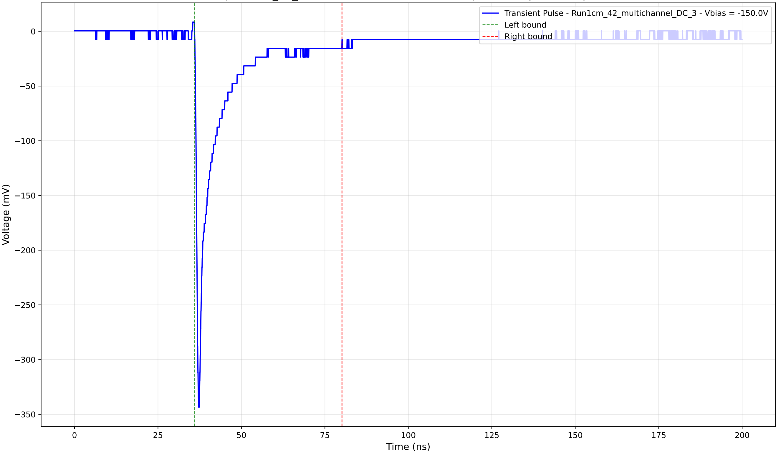
Transient Pulse - Sample: 1cm_42_multichannel - Position: 4690.0 \mu\text{m} - Charge: 43.11 pC - Rise Time: 0.81 ns
