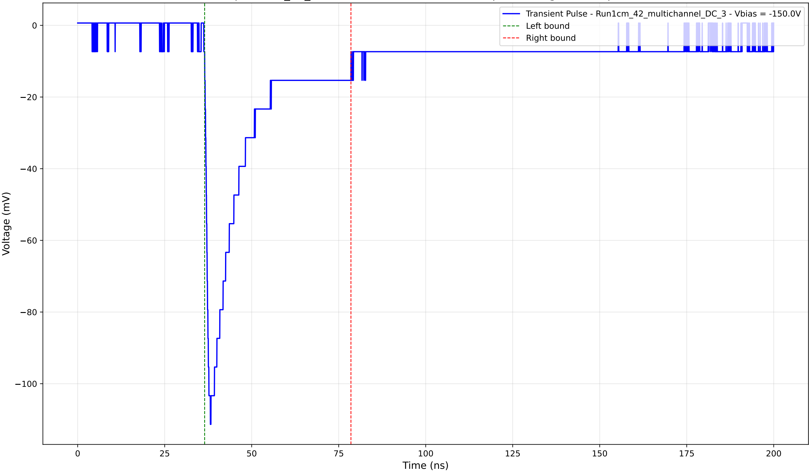
Transient Pulse - Sample: 1cm_42_multichannel - Position: 3830.0 \mu\text{m} - Charge: 26.57 pC - Rise Time: 1.21 ns
