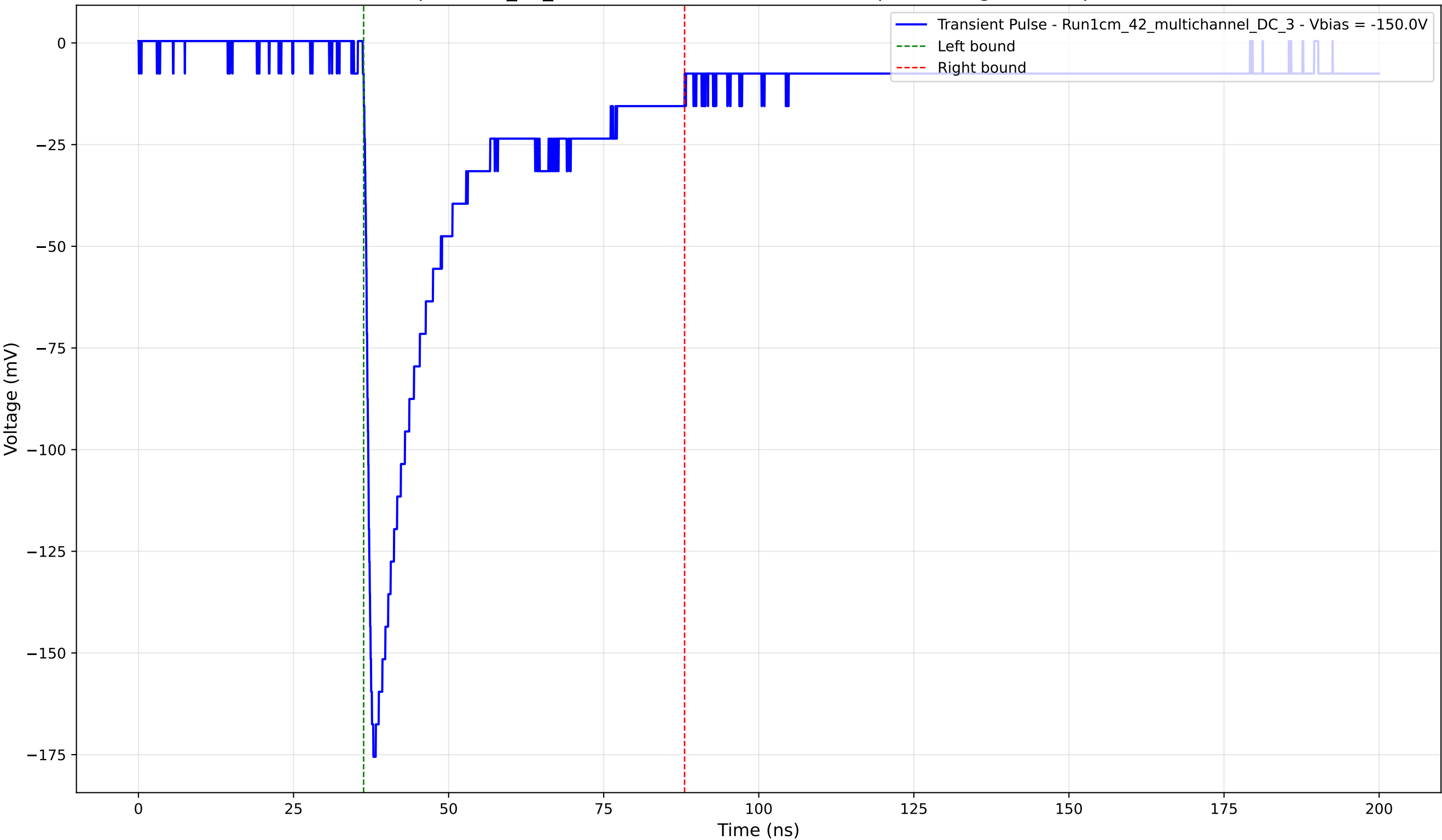
Transient Pulse - Sample: 1cm_42_multichannel - Position: 1025.0 \mu\text{m} - Charge: 44.98 pC - Rise Time: 1.09 ns
