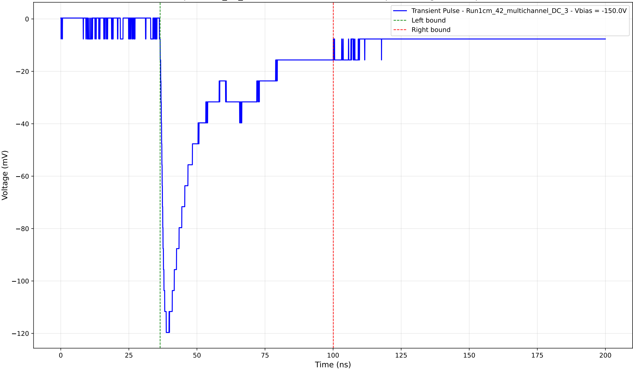
Transient Pulse - Sample: 1cm_42_multichannel - Position: 1700.0 \mu\text{m} - Charge: 45.57 pC - Rise Time: 1.67 ns
