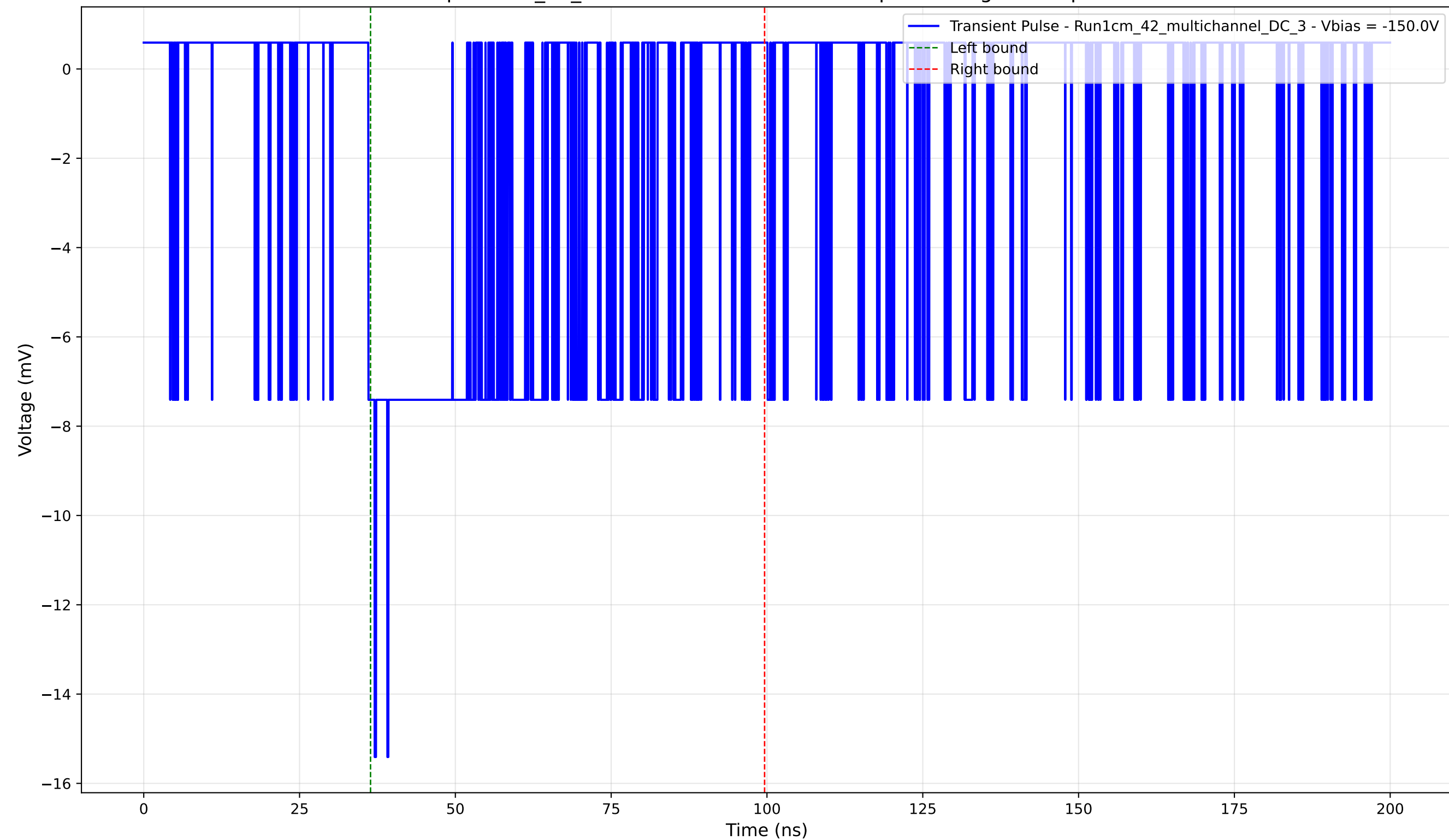
Transient Pulse - Sample: 1cm_42_multichannel - Position: 30.0 \mu\text{m} - Charge: 4.93 pC - Rise Time: 1.02 ns
