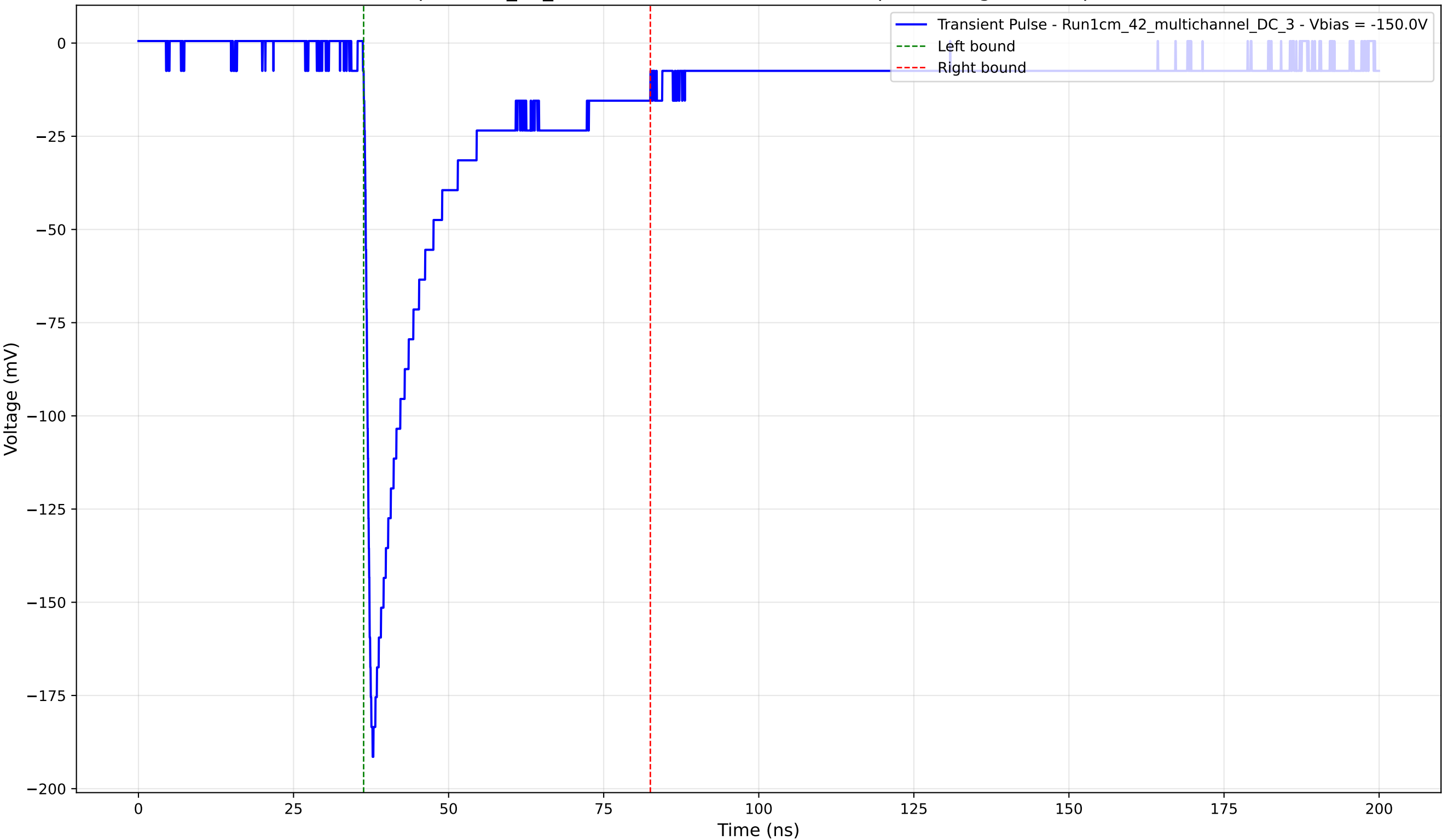
Transient Pulse - Sample: 1cm_42_multichannel - Position: 4140.0 \mu\text{m} - Charge: 39.73 pC - Rise Time: 1.03 ns
