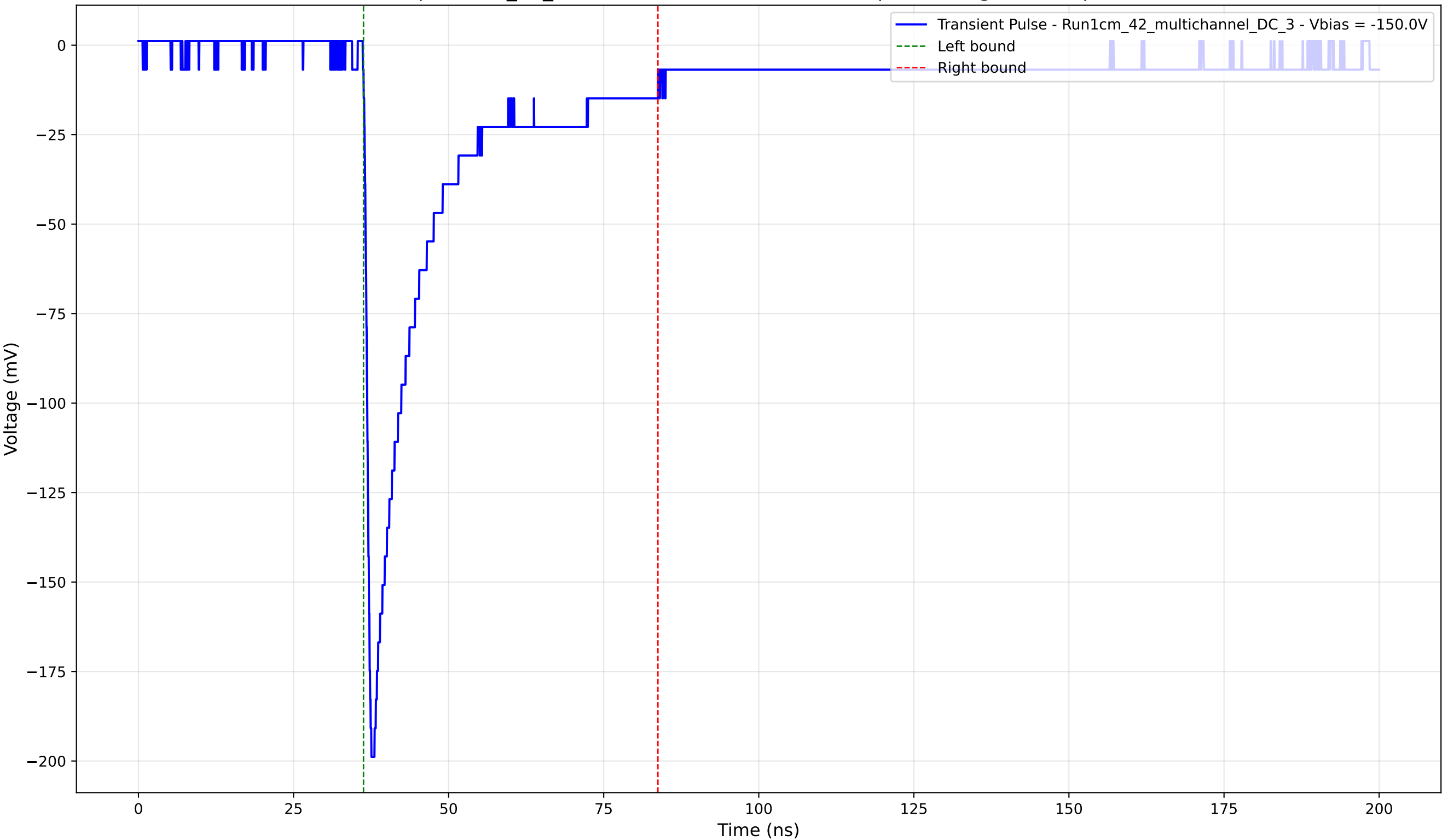
Transient Pulse - Sample: 1cm_42_multichannel - Position: 4190.0 \mu\text{m} - Charge: 40.78 pC - Rise Time: 0.95 ns
