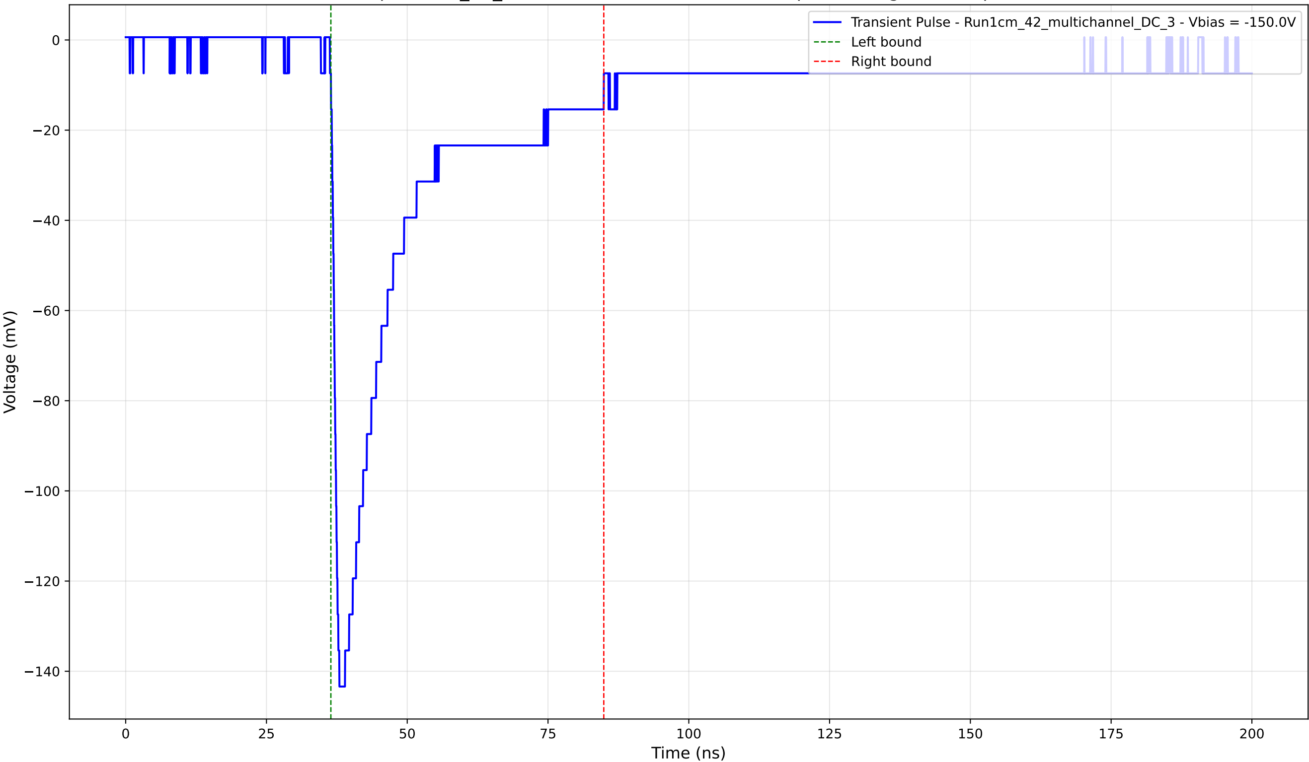
Transient Pulse - Sample: 1cm_42_multichannel - Position: 3745.0 \mu\text{m} - Charge: 38.88 pC - Rise Time: 1.30 ns
