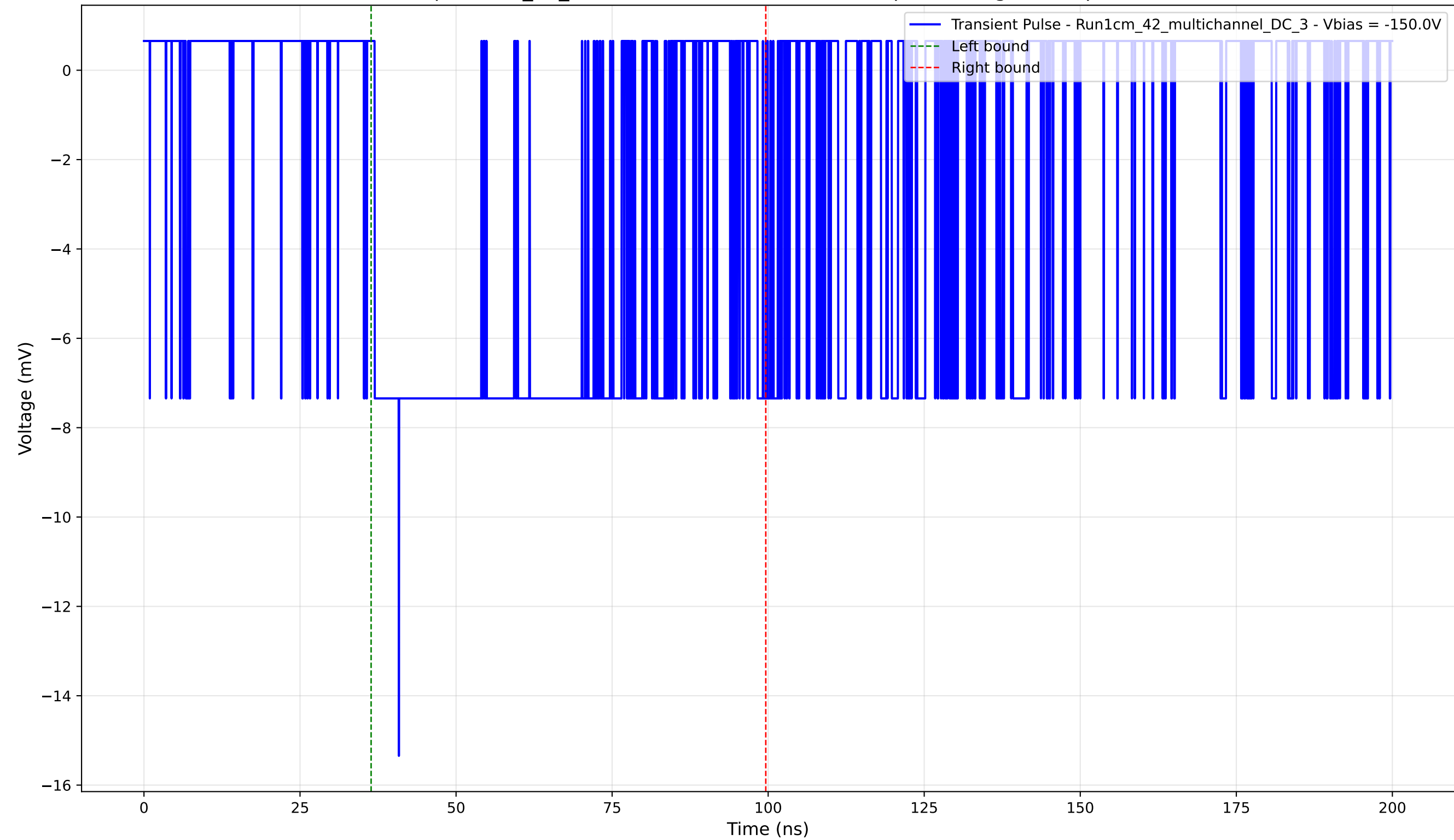
Transient Pulse - Sample: 1cm_42_multichannel - Position: 2860.0 \mu\text{m} - Charge: 6.55 pC - Rise Time: 3.88 ns
