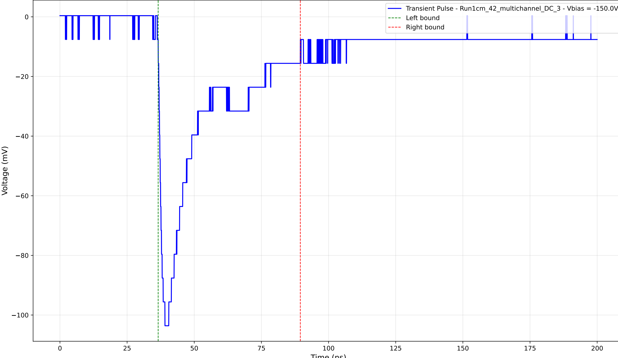
Transient Pulse - Sample: 1cm 42 multichannel - Position: 3000.0 \mu\text{m} - Charge: 37.79 pC - Rise Time: 1.85 ns
