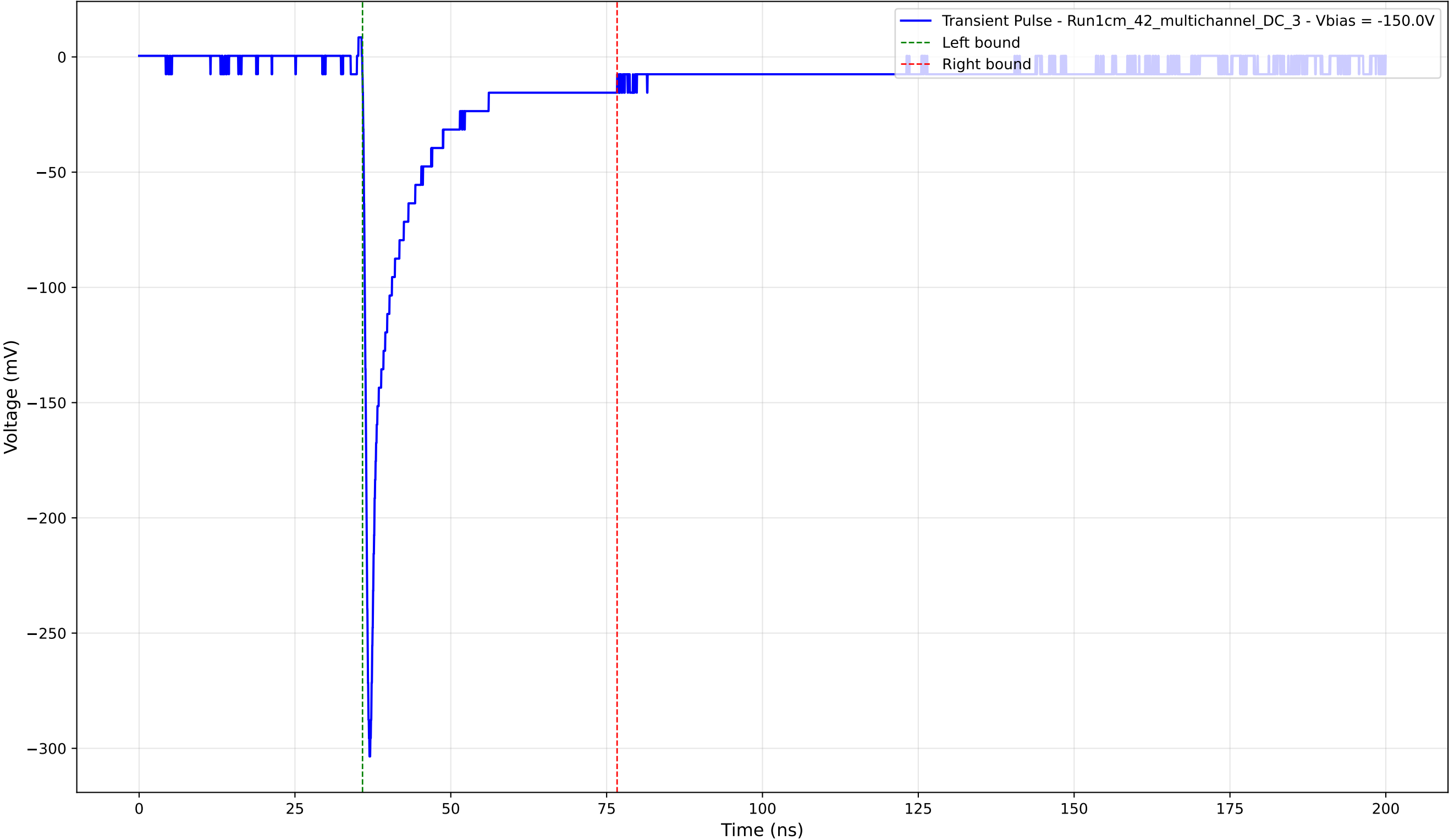
Transient Pulse - Sample: 1cm_42_multichannel - Position: 95.0 \mu\text{m} - Charge: 35.48 pC - Rise Time: 0.80 ns
