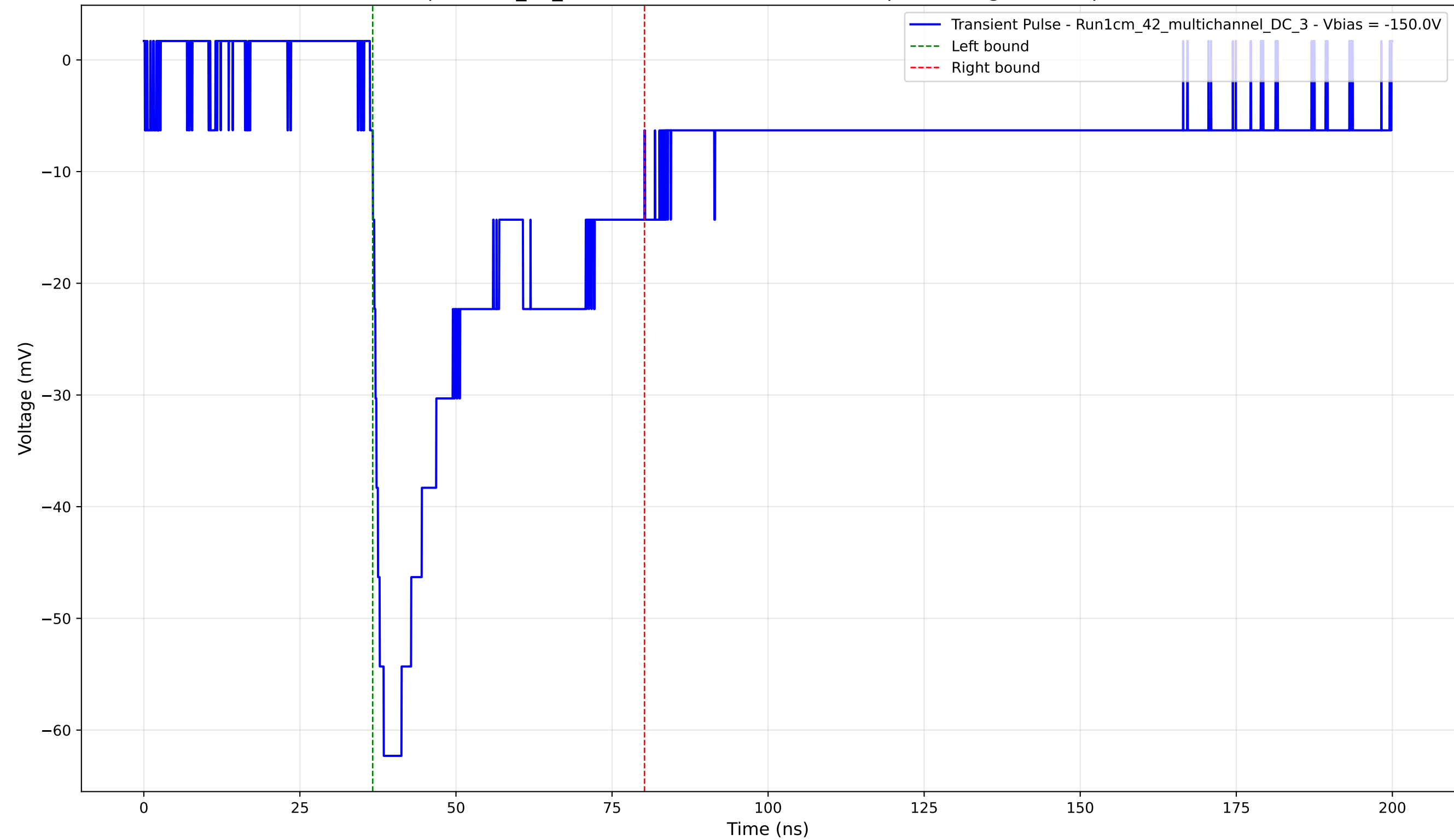
Transient Pulse - Sample: 1cm_42_multichannel - Position: 1925.0 \mu\text{m} - Charge: 23.23 pC - Rise Time: 2.20 ns
