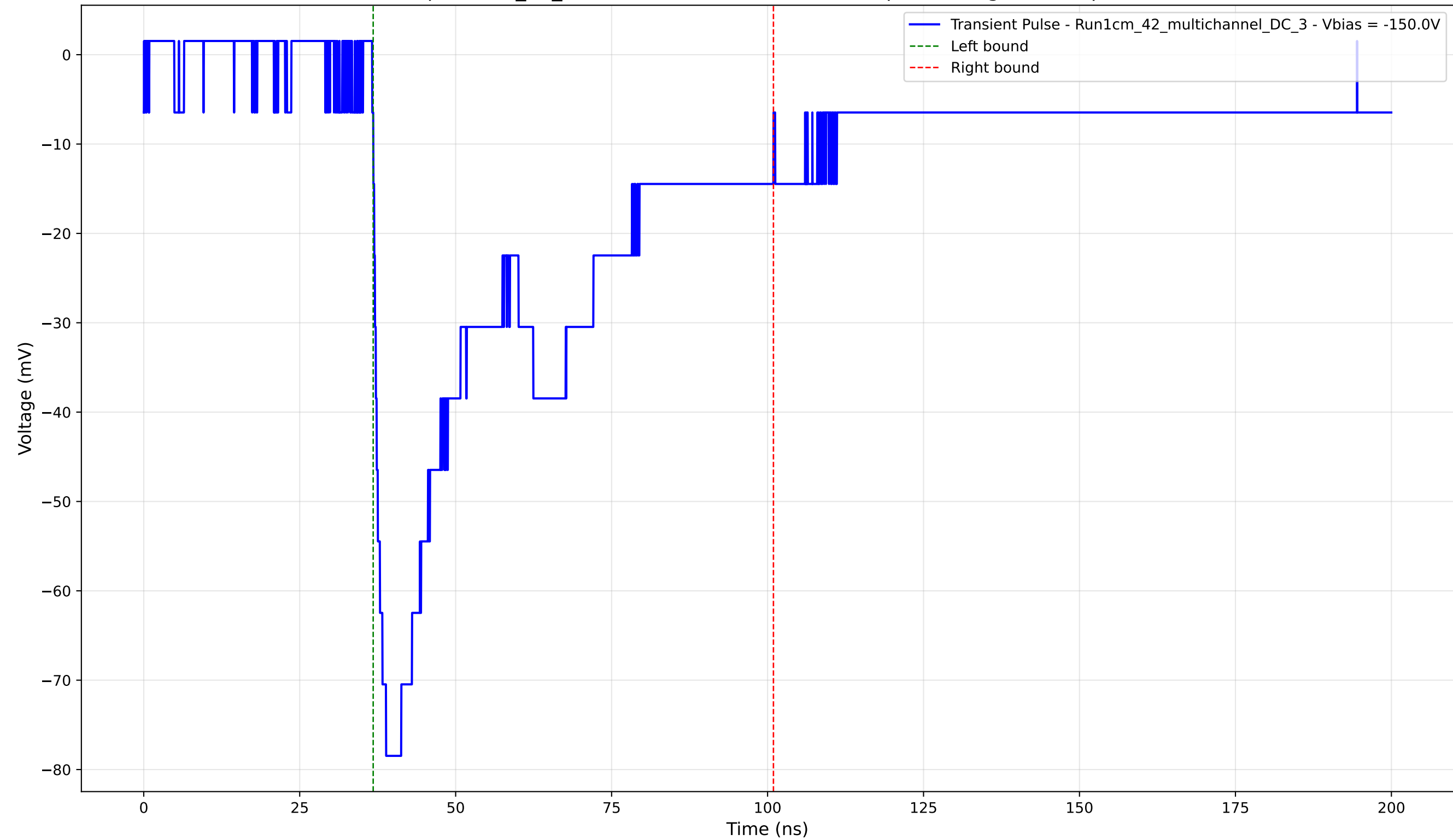
Transient Pulse - Sample: 1cm_42_multichannel - Position: 2490.0 \mu\text{m} - Charge: 38.81 pC - Rise Time: 2.06 ns
