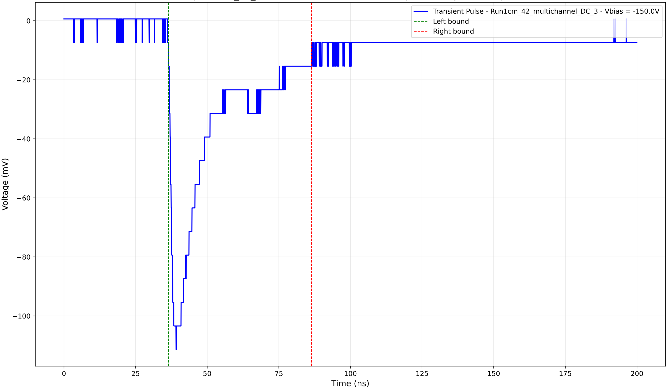
Transient Pulse - Sample: 1cm_42_multichannel - Position: 3190.0 \mu\text{m} - Charge: 36.30 pC - Rise Time: 1.79 ns
