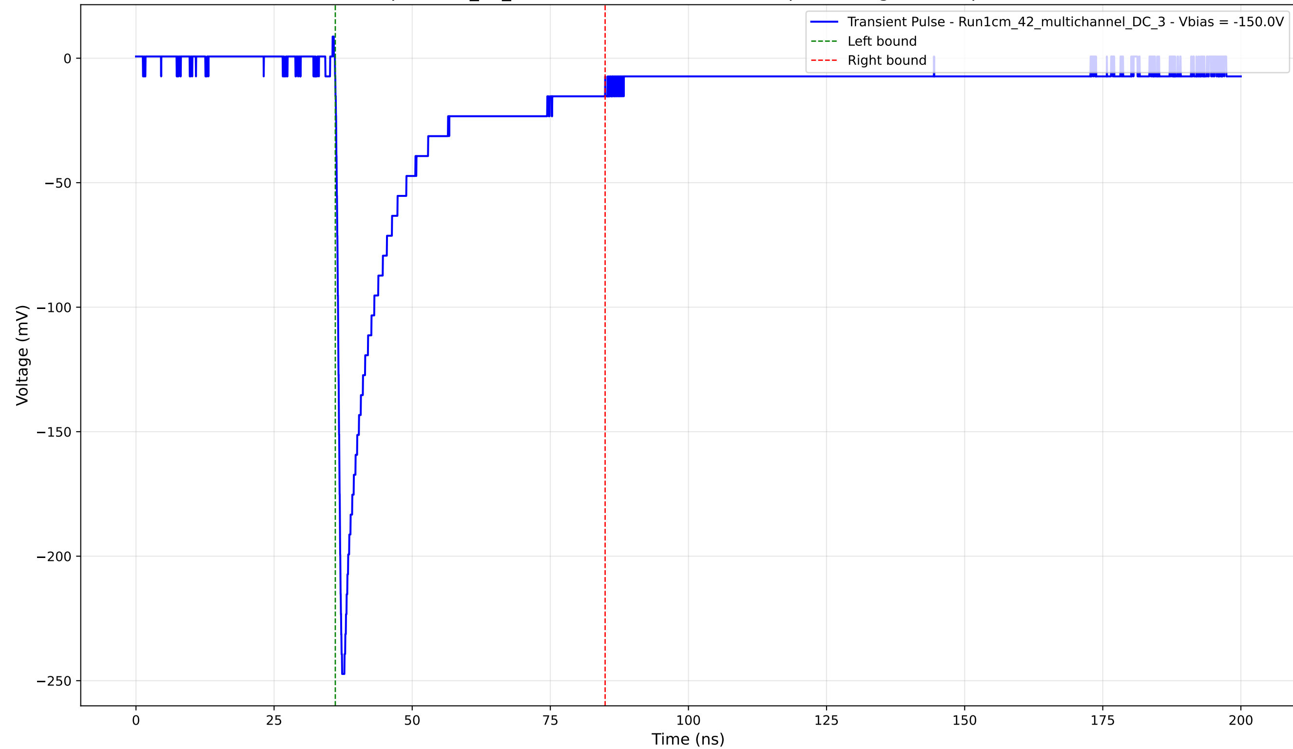
Transient Pulse - Sample: 1cm_42_multichannel - Position: 570.0 \mu\text{m} - Charge: 47.32 pC - Rise Time: 0.86 ns
