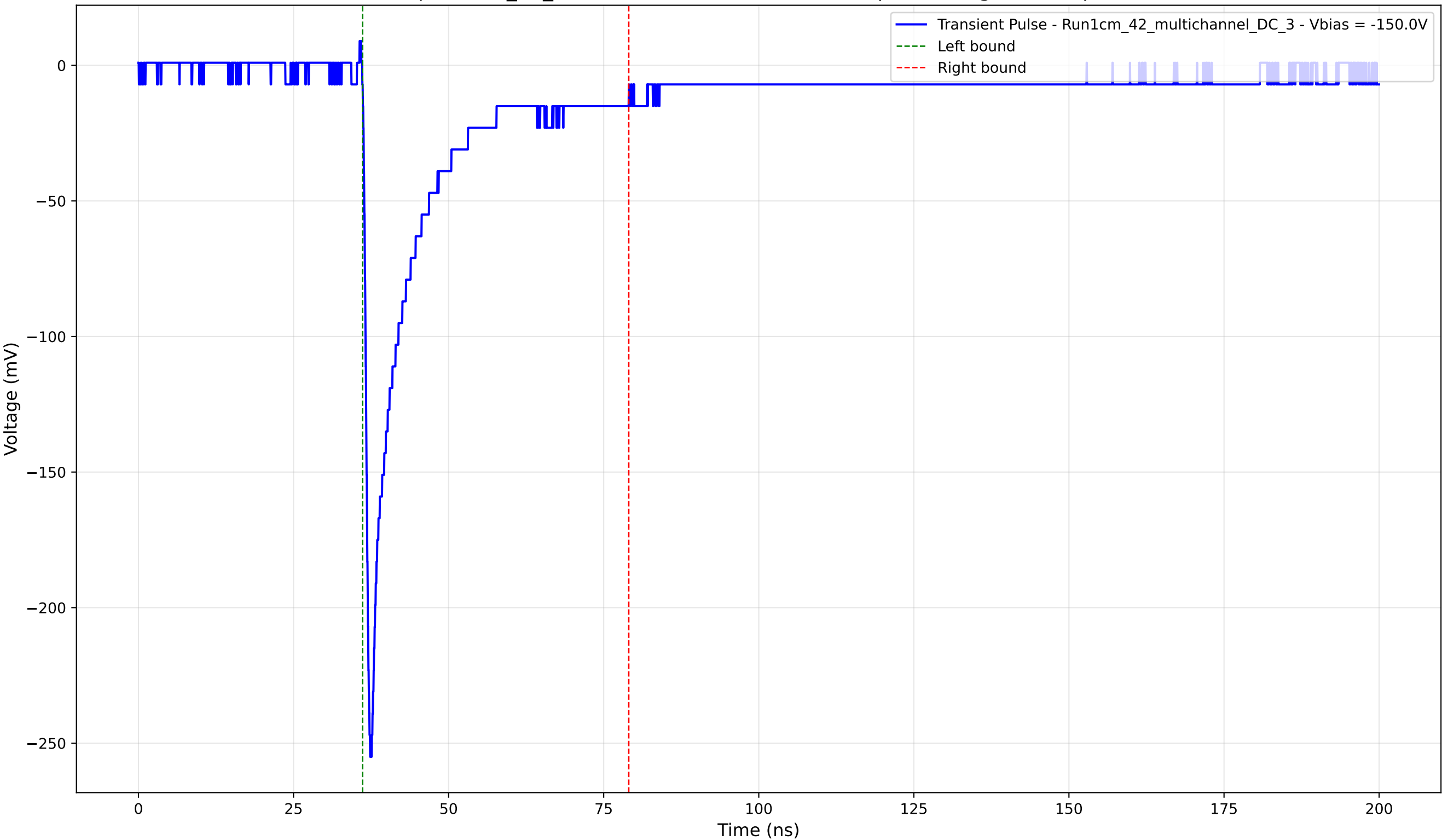
Transient Pulse - Sample: 1cm_42_multichannel - Position: 4495.0 \mu\text{m} - Charge: 38.04 pC - Rise Time: 0.83 ns
