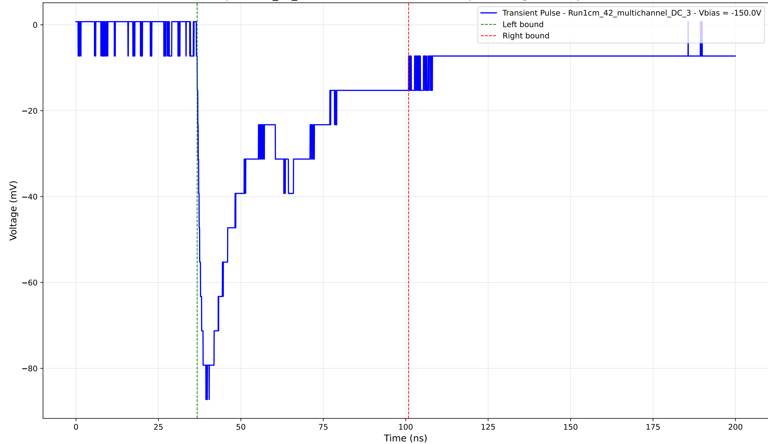
Transient Pulse - Sample: 1cm_42_multichannel - Position: 2630.0 \mu\text{m} - Charge: 38.94 pC - Rise Time: 1.80 ns
