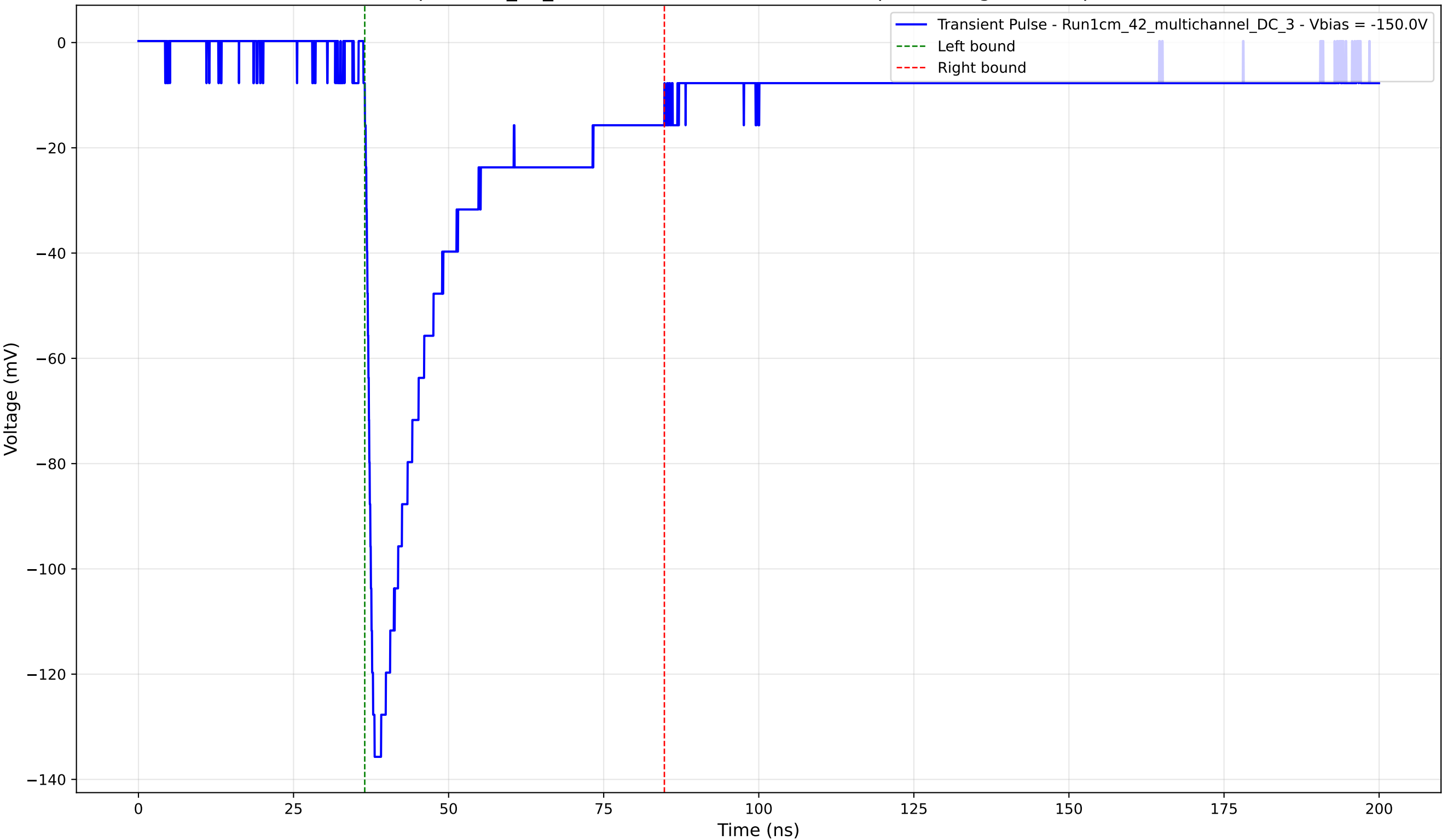
Transient Pulse - Sample: 1cm_42_multichannel - Position: 3690.0 \mu\text{m} - Charge: 37.79 pC - Rise Time: 1.33 ns
