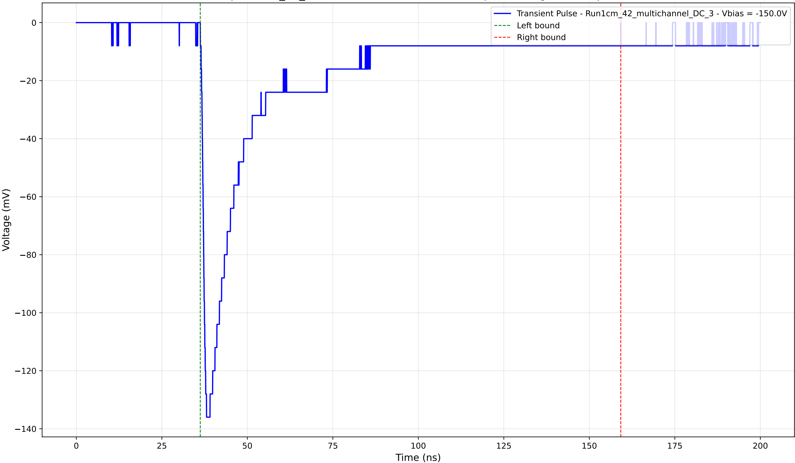
Transient Pulse - Sample: 1cm_42_multichannel - Position: 3700.0 \mu\text{m} - Charge: 49.92 pC - Rise Time: 1.35 ns
