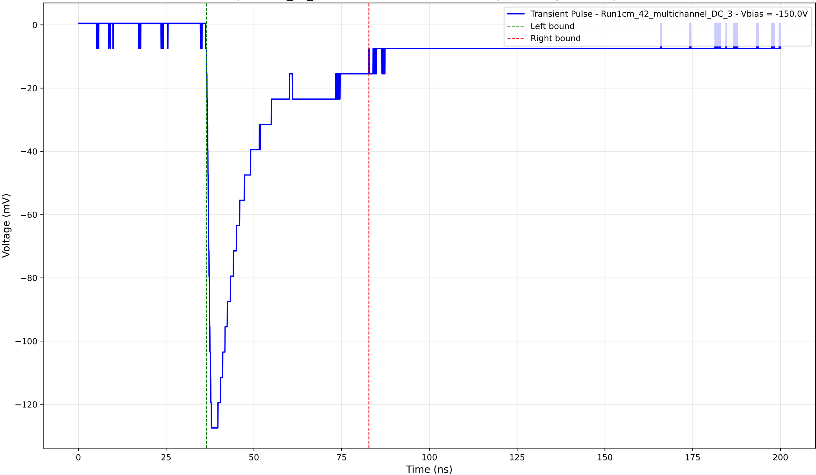
Transient Pulse - Sample: 1cm_42_multichannel - Position: 3660.0 \mu\text{m} - Charge: 36.53 pC - Rise Time: 1.21 ns
