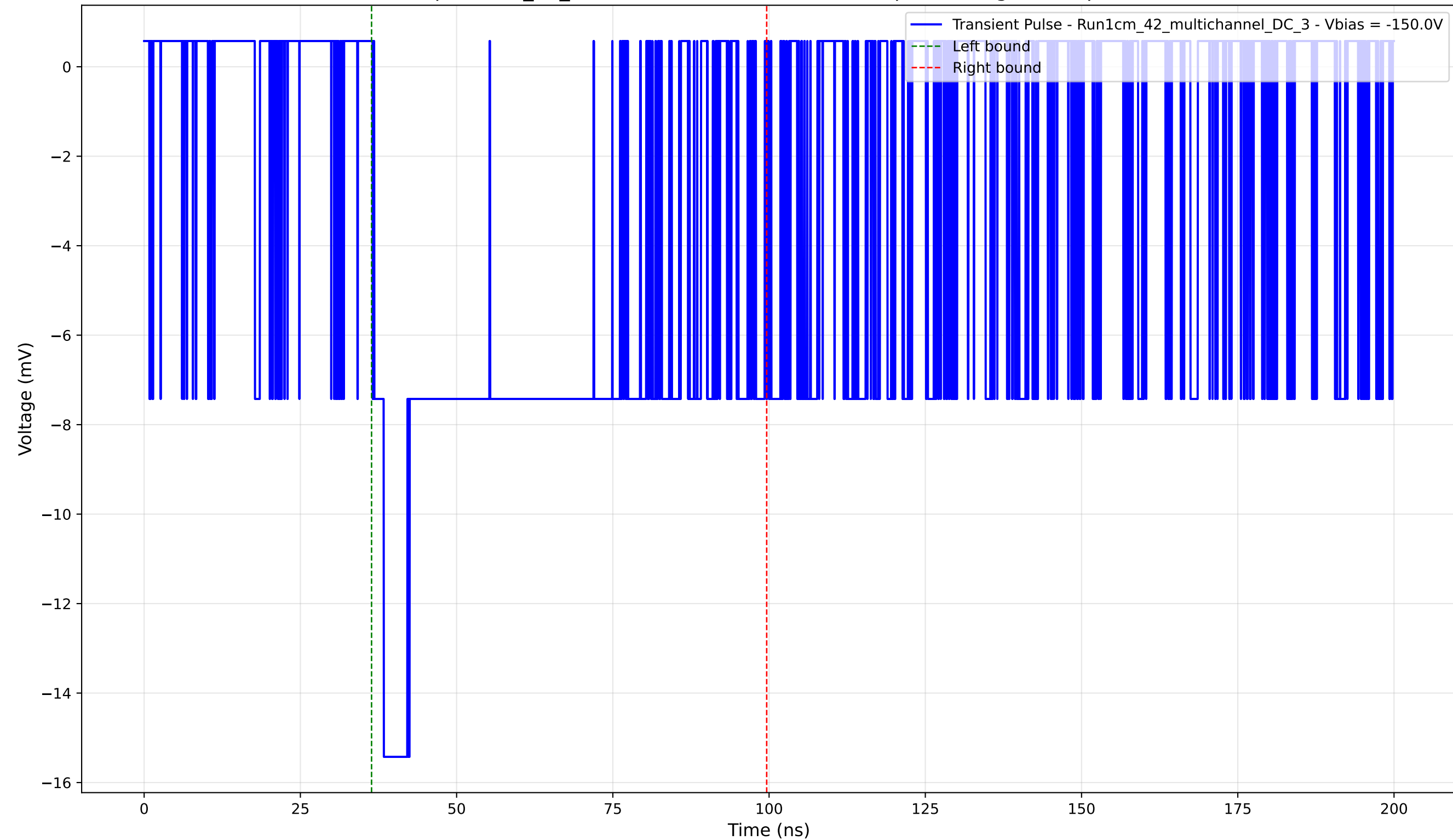
Transient Pulse - Sample: 1cm_42_multichannel - Position: 2855.0 \mu\text{m} - Charge: 8.54 pC - Rise Time: 1.54 ns
