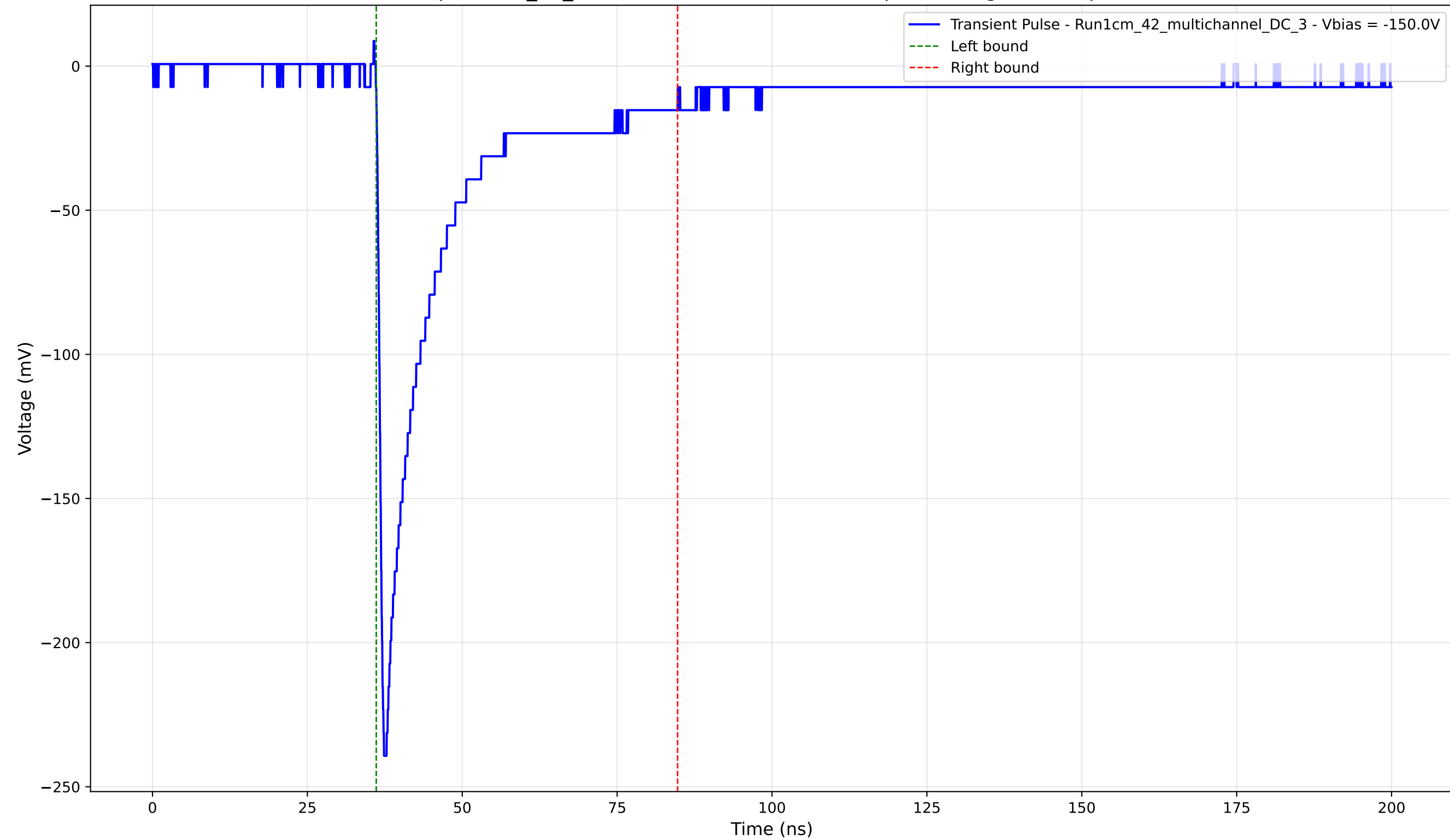
Transient Pulse - Sample: 1cm_42_multichannel - Position: 620.0 \mu\text{m} - Charge: 47.24 pC - Rise Time: 0.96 ns
