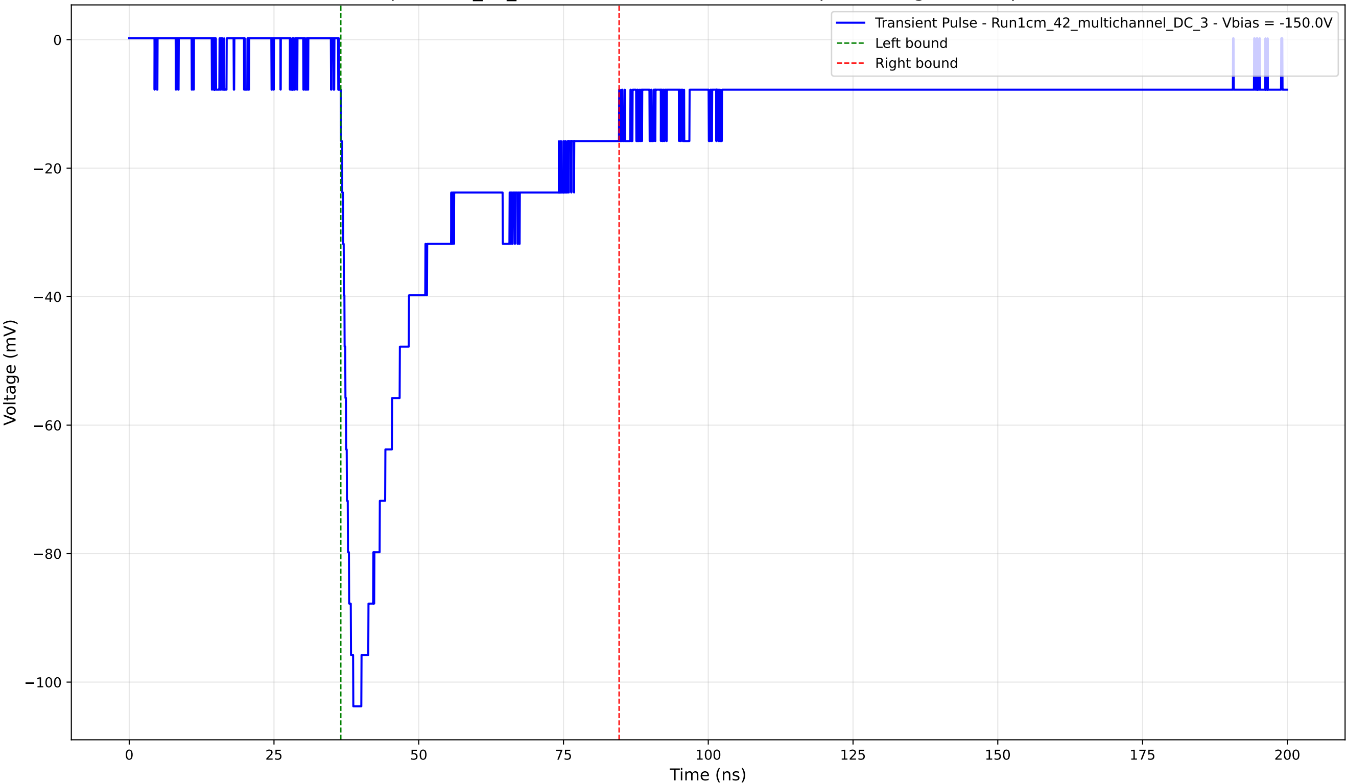
Transient Pulse - Sample: 1cm_42_multichannel - Position: 3150.0 \mu\text{m} - Charge: 34.80 pC - Rise Time: 1.73 ns
