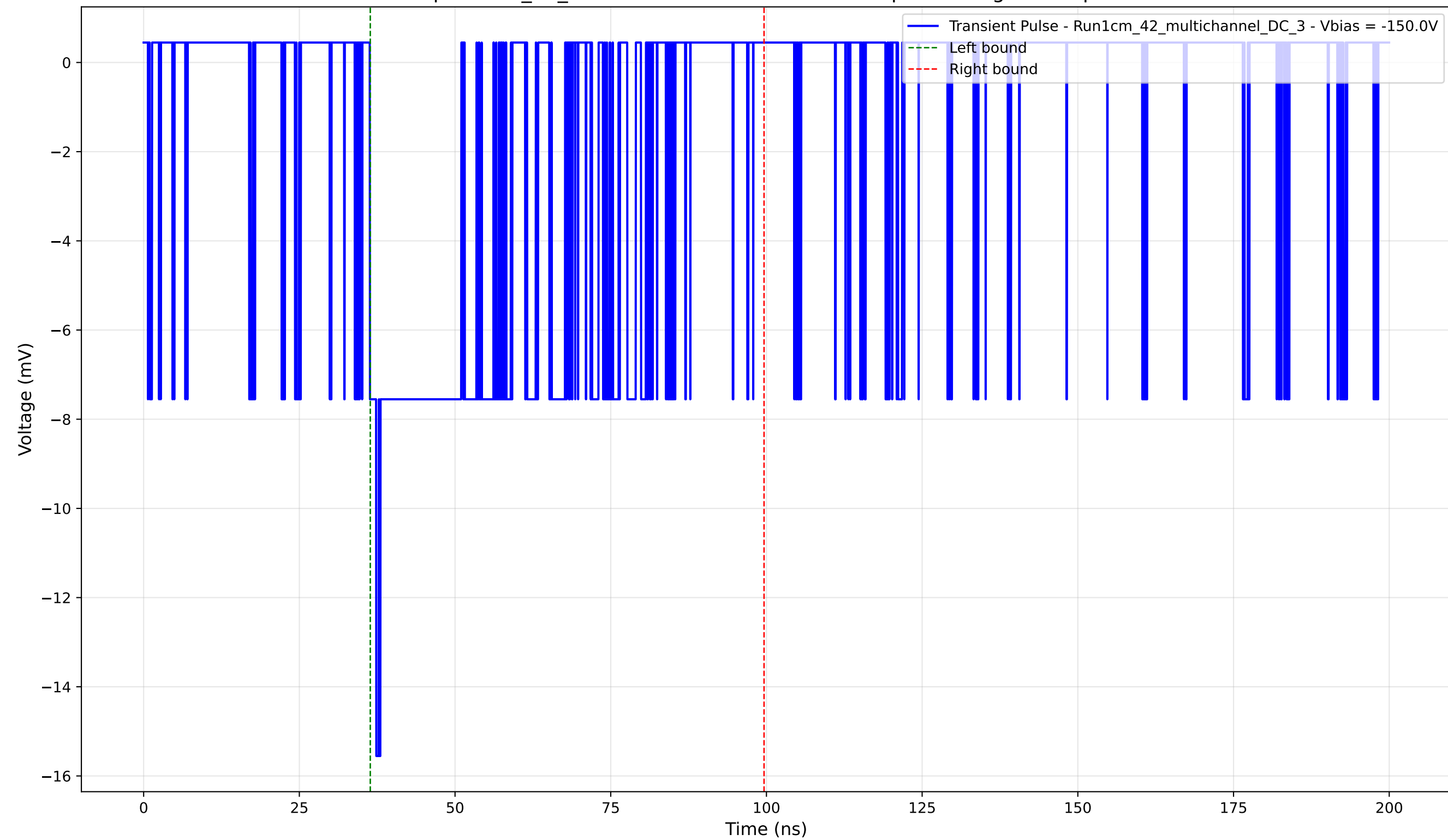
Transient Pulse - Sample: 1cm_42_multichannel - Position: 4385.0 \mu\text{m} - Charge: 4.83 pC - Rise Time: 1.04 ns
