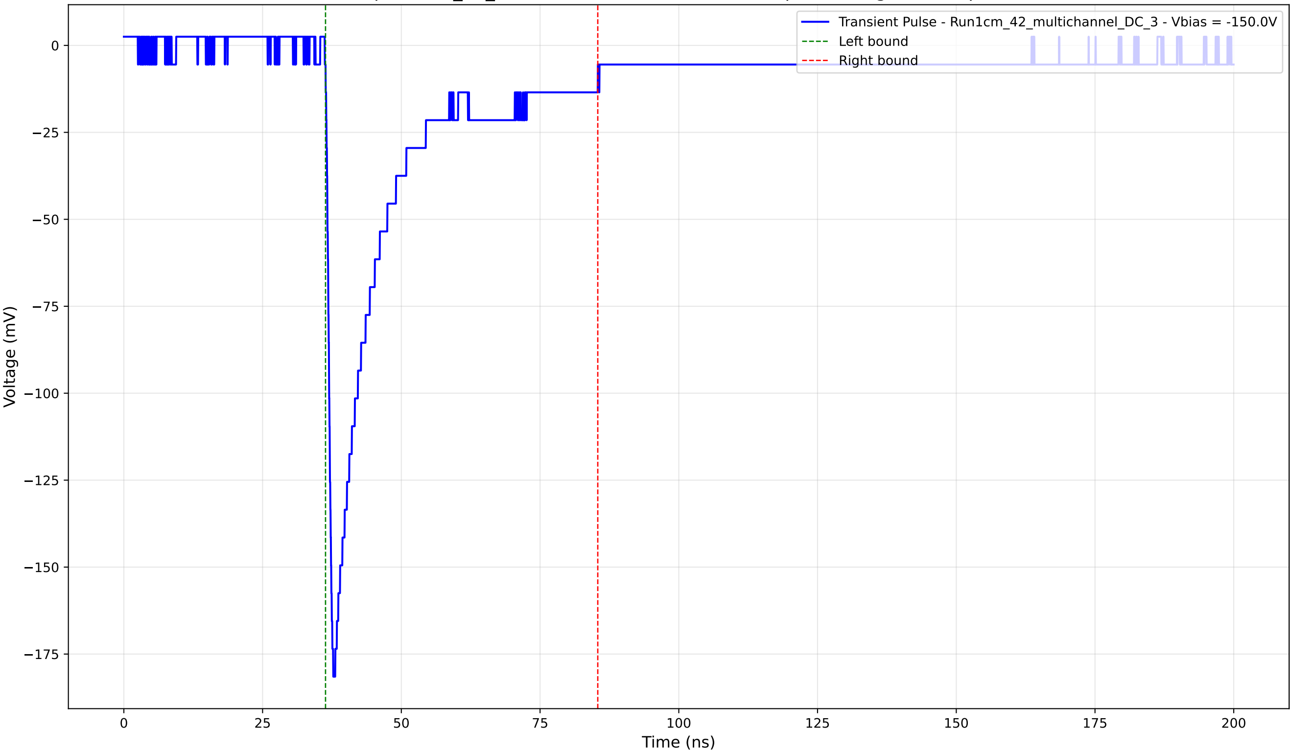
Transient Pulse - Sample: 1cm_42_multichannel - Position: 4100.0 \mu\text{m} - Charge: 37.98 pC - Rise Time: 1.01 ns
