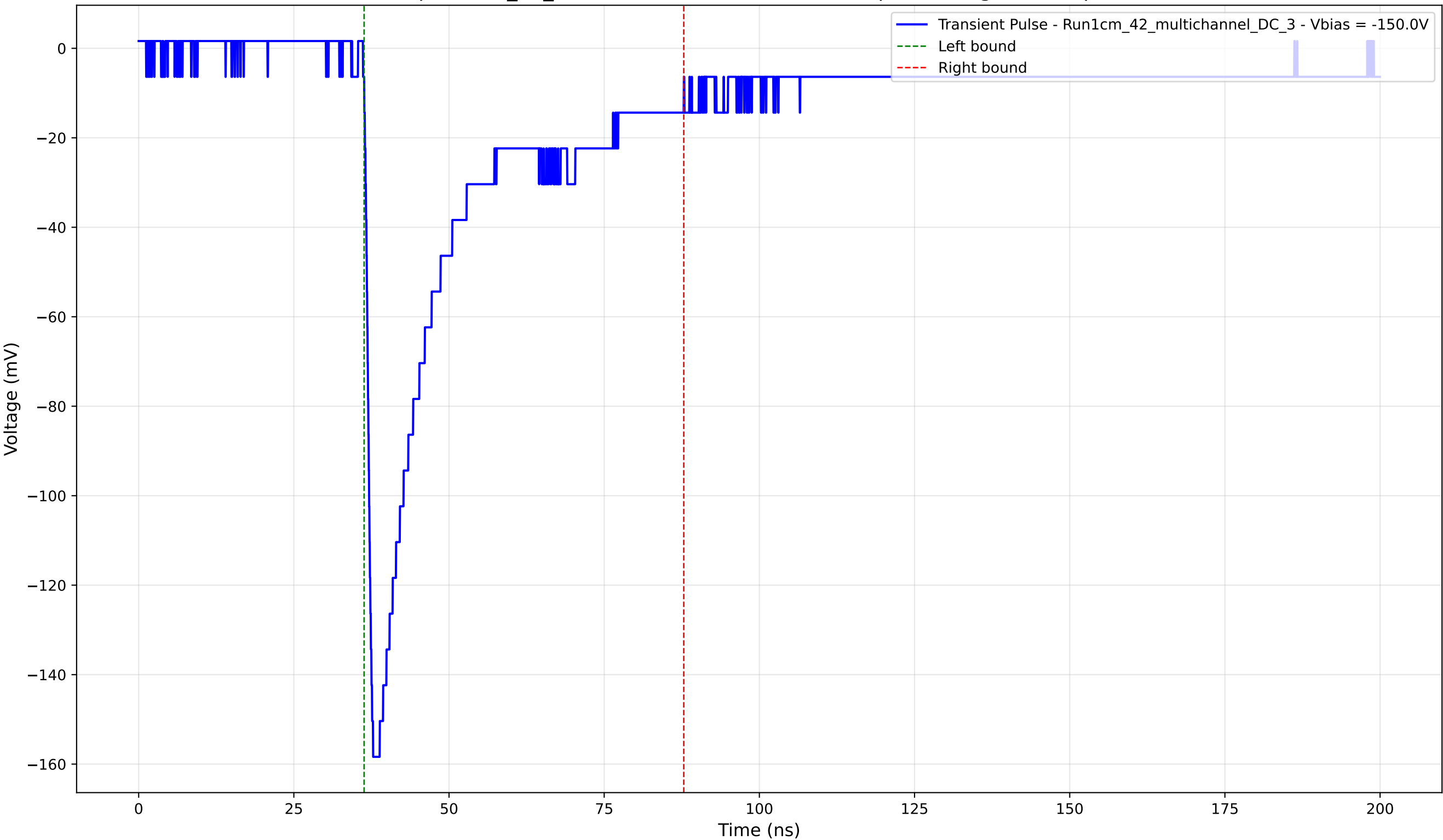
Transient Pulse - Sample: 1cm_42_multichannel - Position: 1095.0 \mu\text{m} - Charge: 42.79 pC - Rise Time: 1.18 ns
