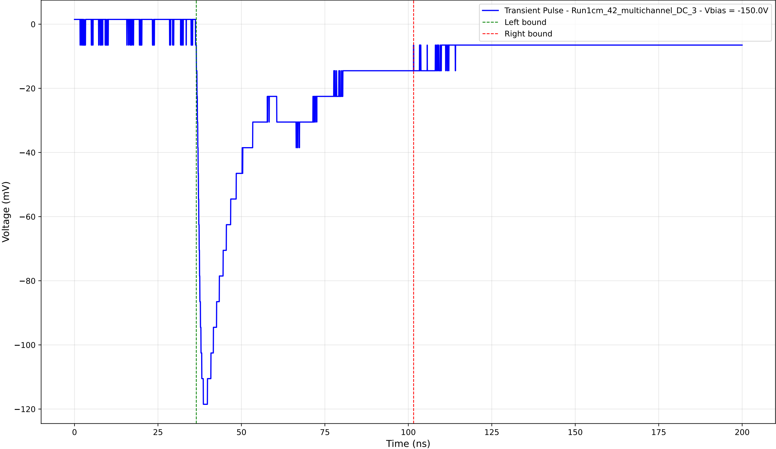
Transient Pulse - Sample: 1cm_42_multichannel - Position: 1705.0 \mu\text{m} - Charge: 44.50 pC - Rise Time: 1.63 ns
