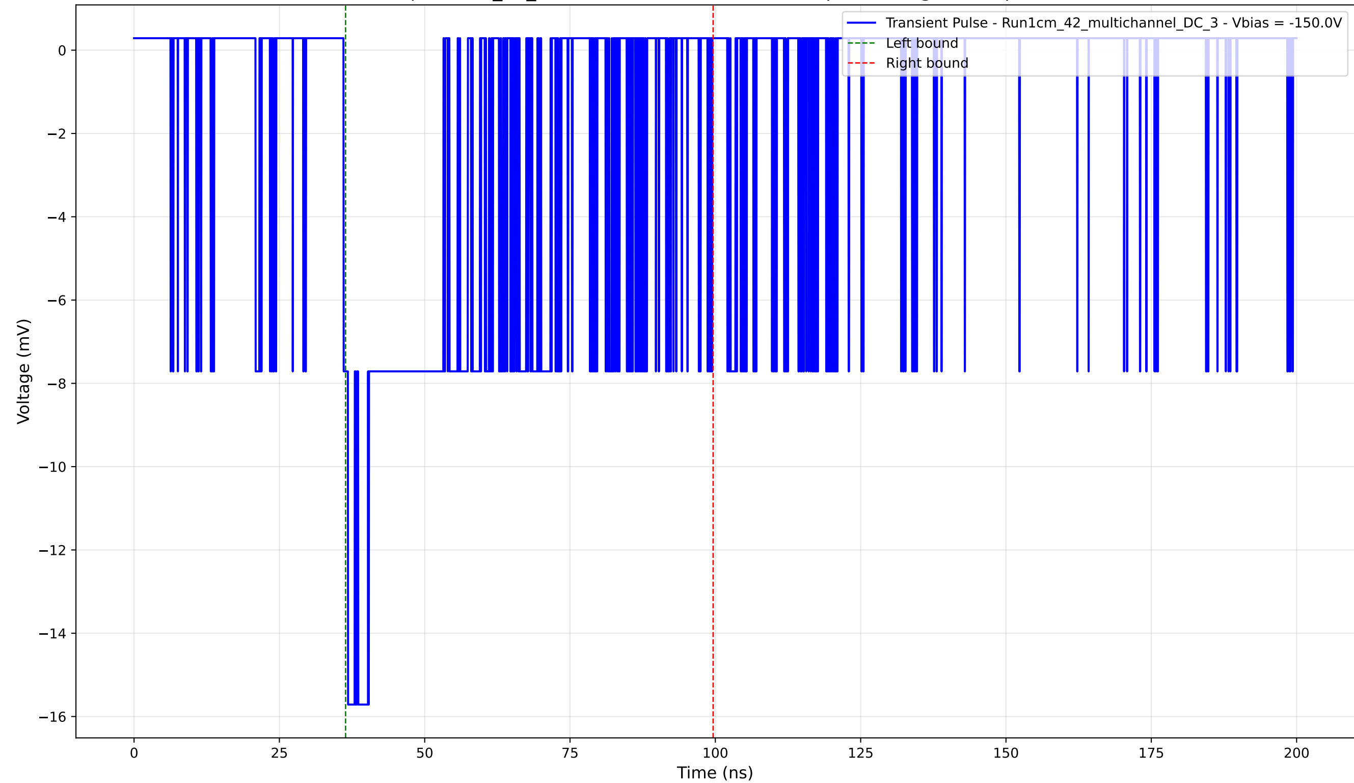
Transient Pulse - Sample: 1cm_42_multichannel - Position: 360.0 \mu\text{m} - Charge: 5.71 pC - Rise Time: 0.78 ns
