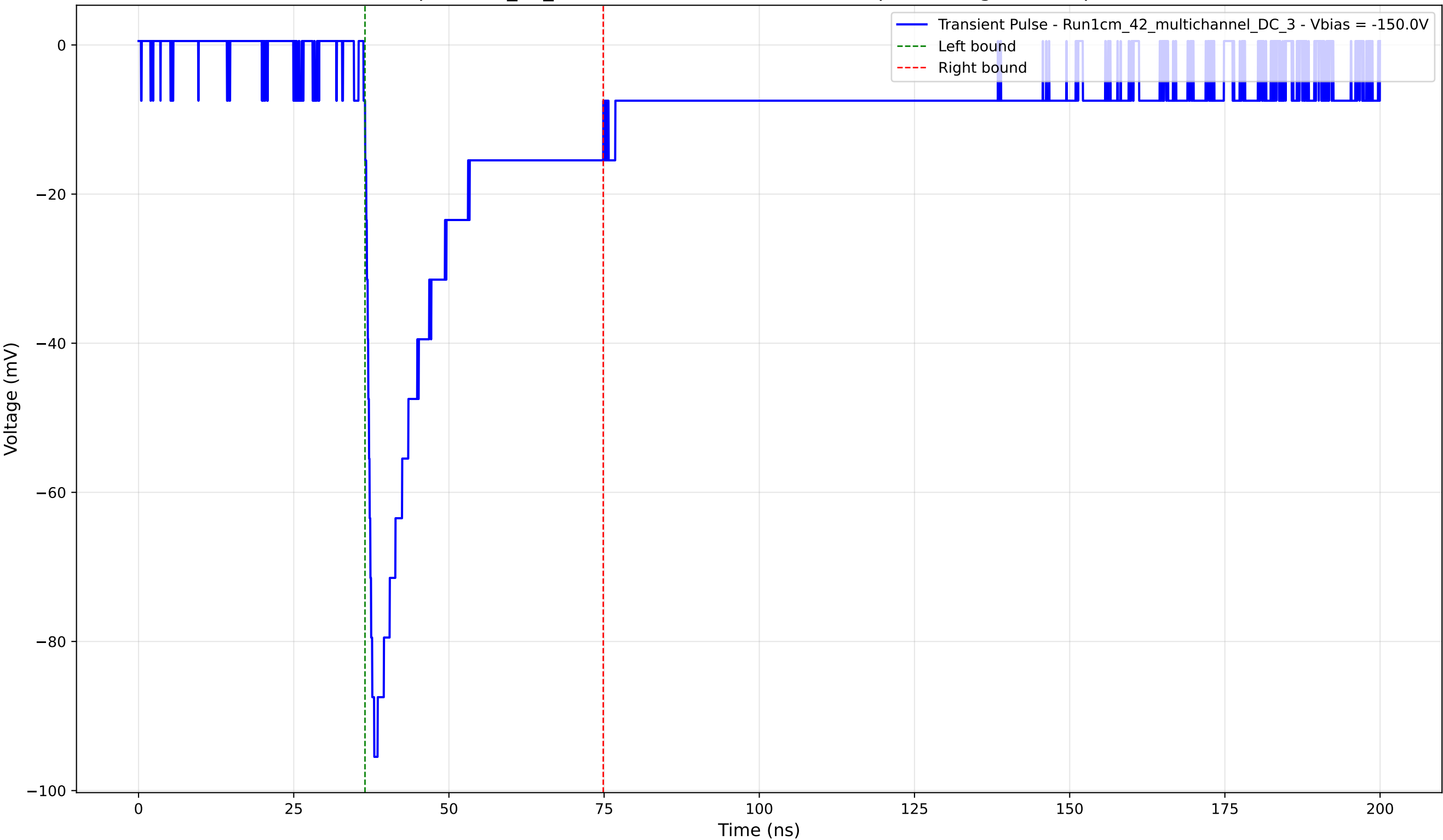
Transient Pulse - Sample: 1cm_42_multichannel - Position: 3835.0 \mu\text{m} - Charge: 22.80 pC - Rise Time: 1.15 ns
