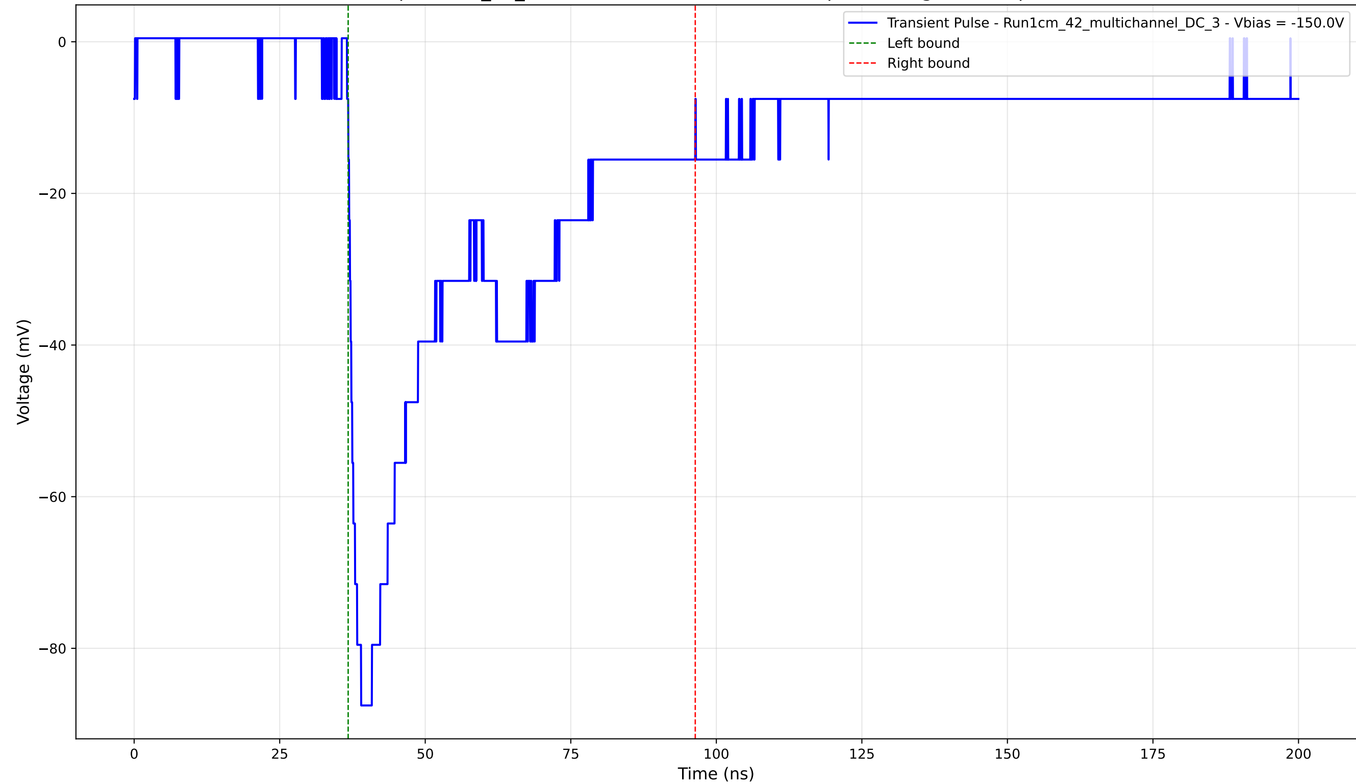
Transient Pulse - Sample: 1cm_42_multichannel - Position: 2175.0 \mu\text{m} - Charge: 40.07 pC - Rise Time: 1.54 ns
