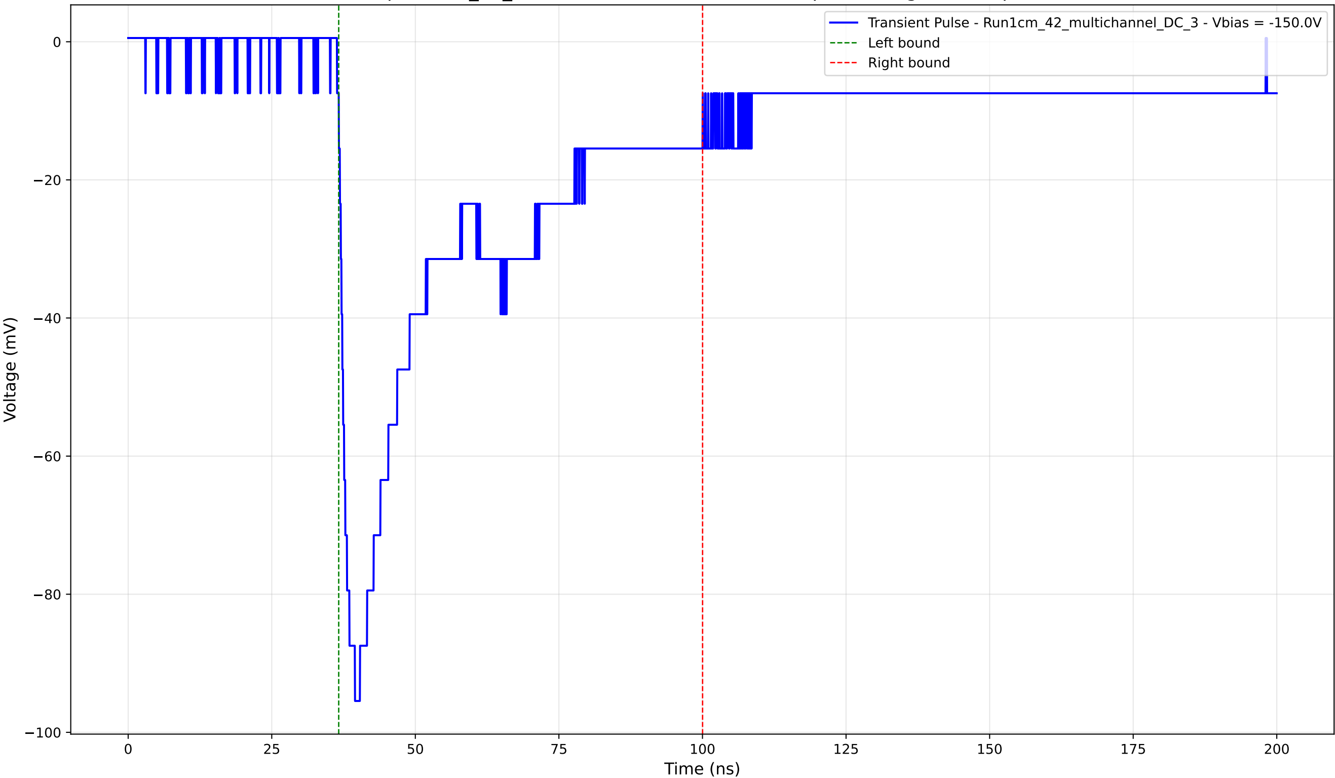
Transient Pulse - Sample: 1cm_42_multichannel - Position: 2750.0 \mu\text{m} - Charge: 40.61 pC - Rise Time: 1.85 ns
