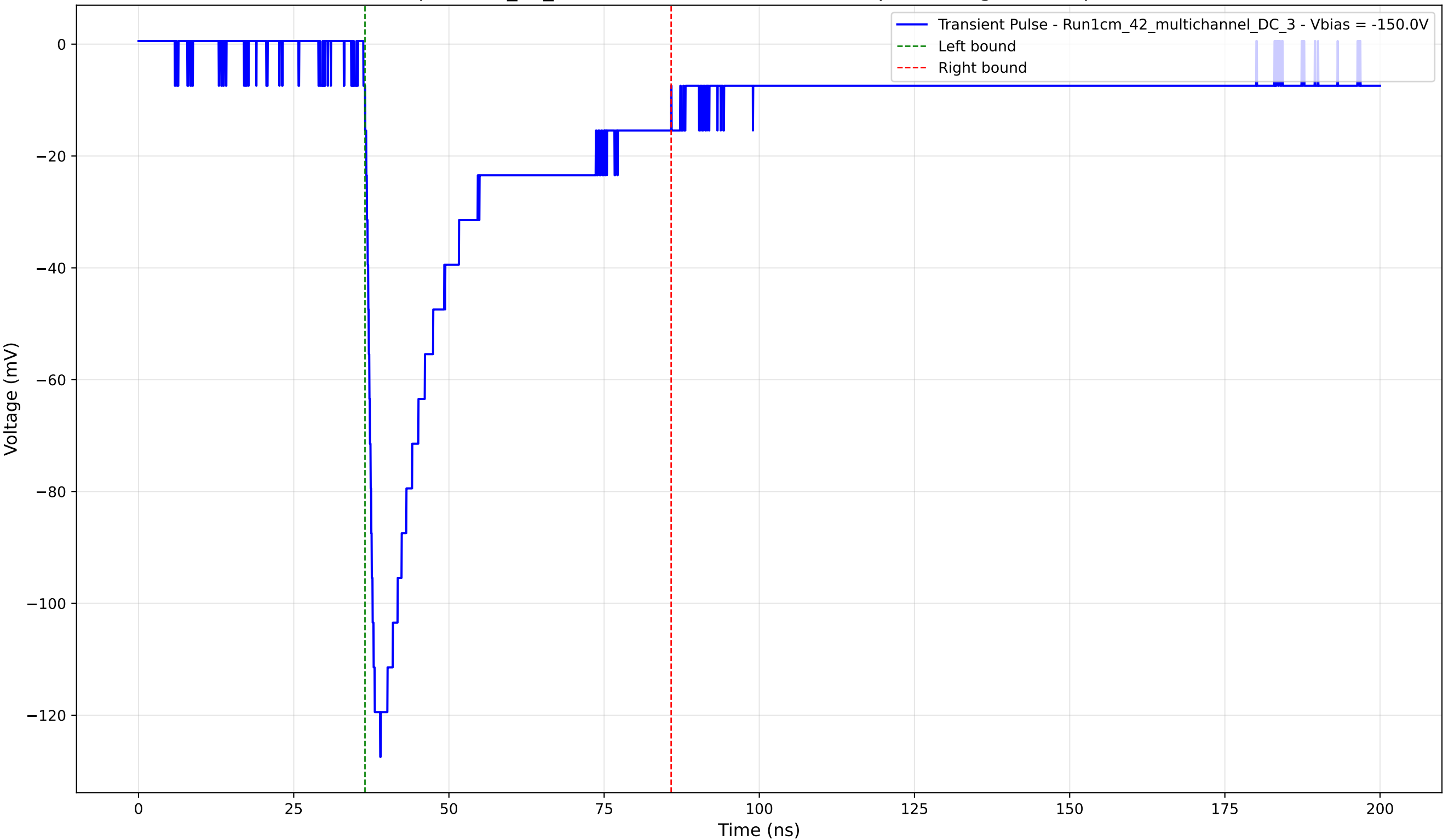
Transient Pulse - Sample: 1cm_42_multichannel - Position: 3495.0 \mu\text{m} - Charge: 37.07 pC - Rise Time: 1.55 ns
