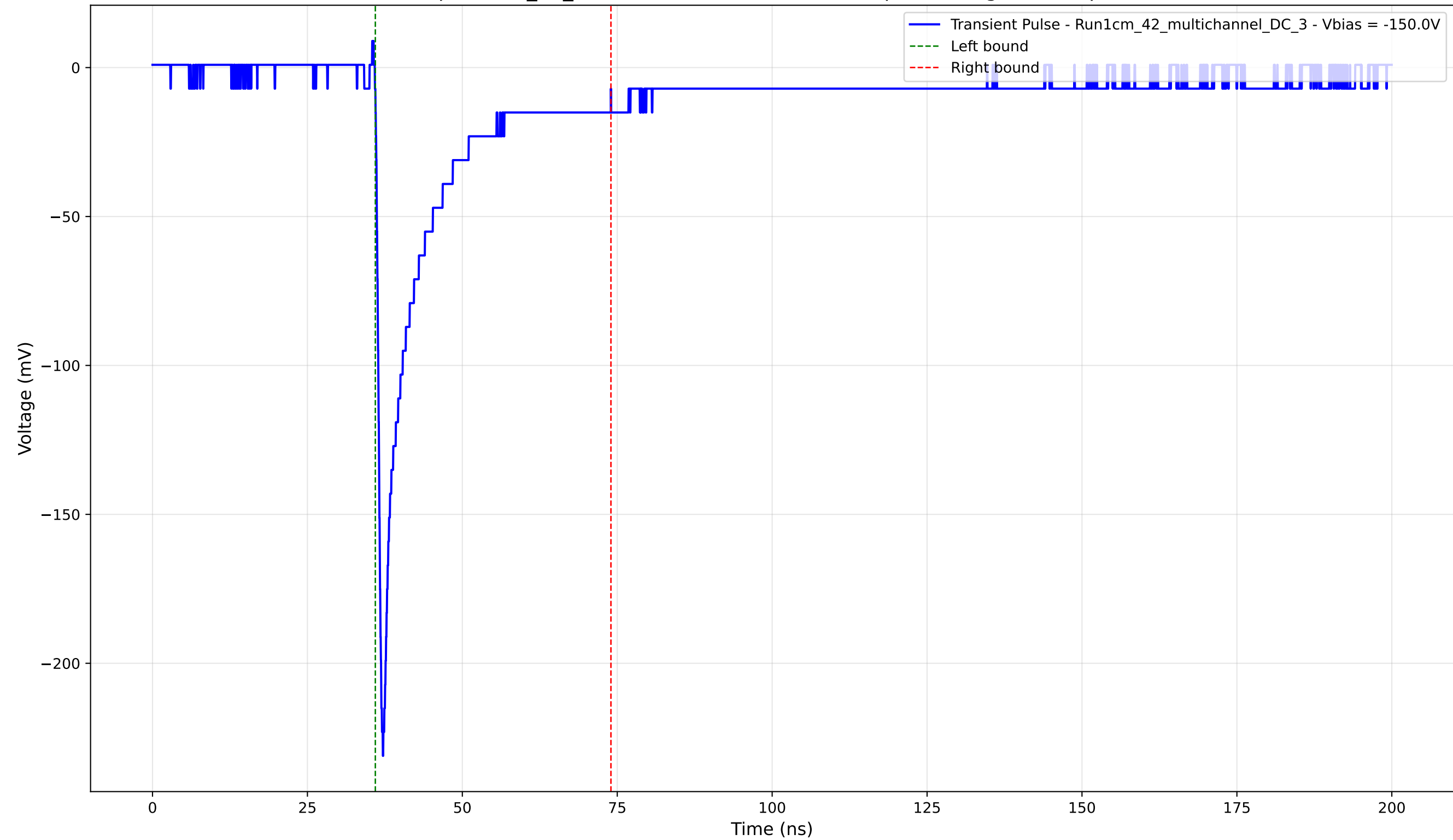
Transient Pulse - Sample: 1cm_42_multichannel - Position: 290.0 \mu\text{m} - Charge: 31.45 pC - Rise Time: 0.86 ns
