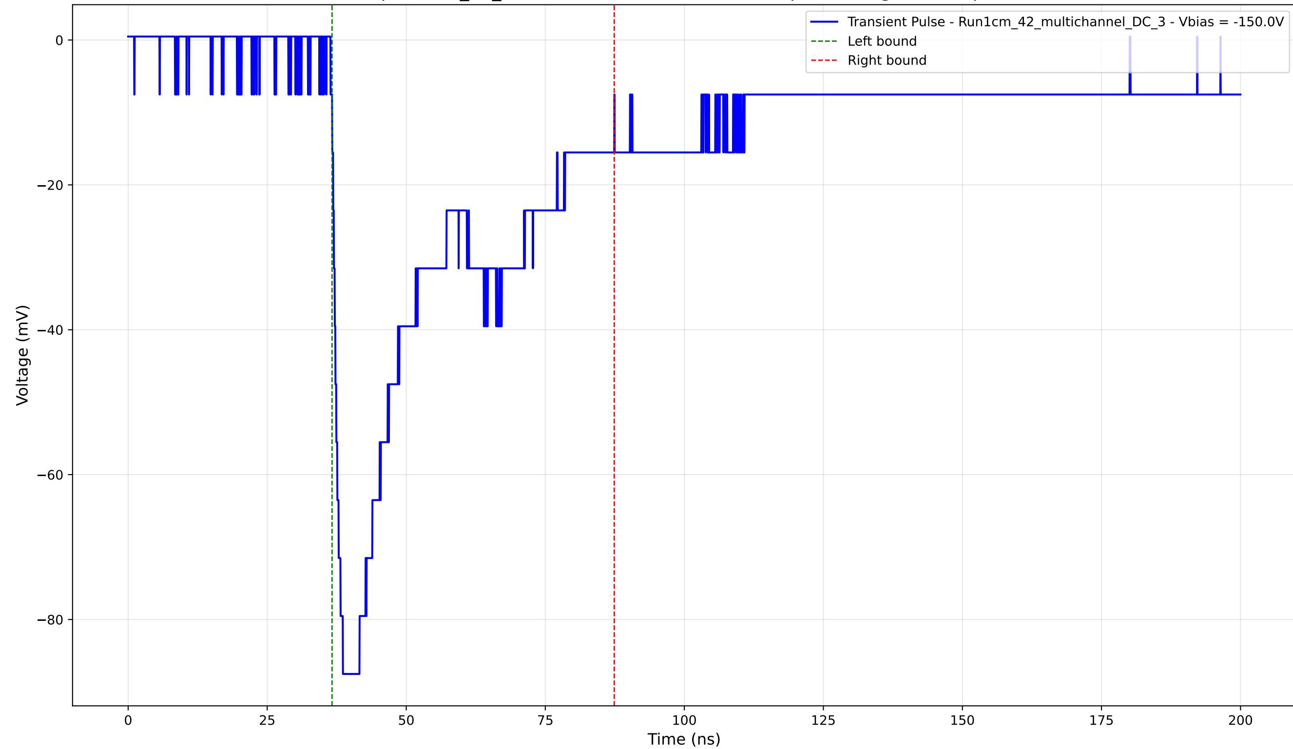
Transient Pulse - Sample: 1cm_42_multichannel - Position: 2735.0 \mu\text{m} - Charge: 36.55 pC - Rise Time: 1.52 ns
