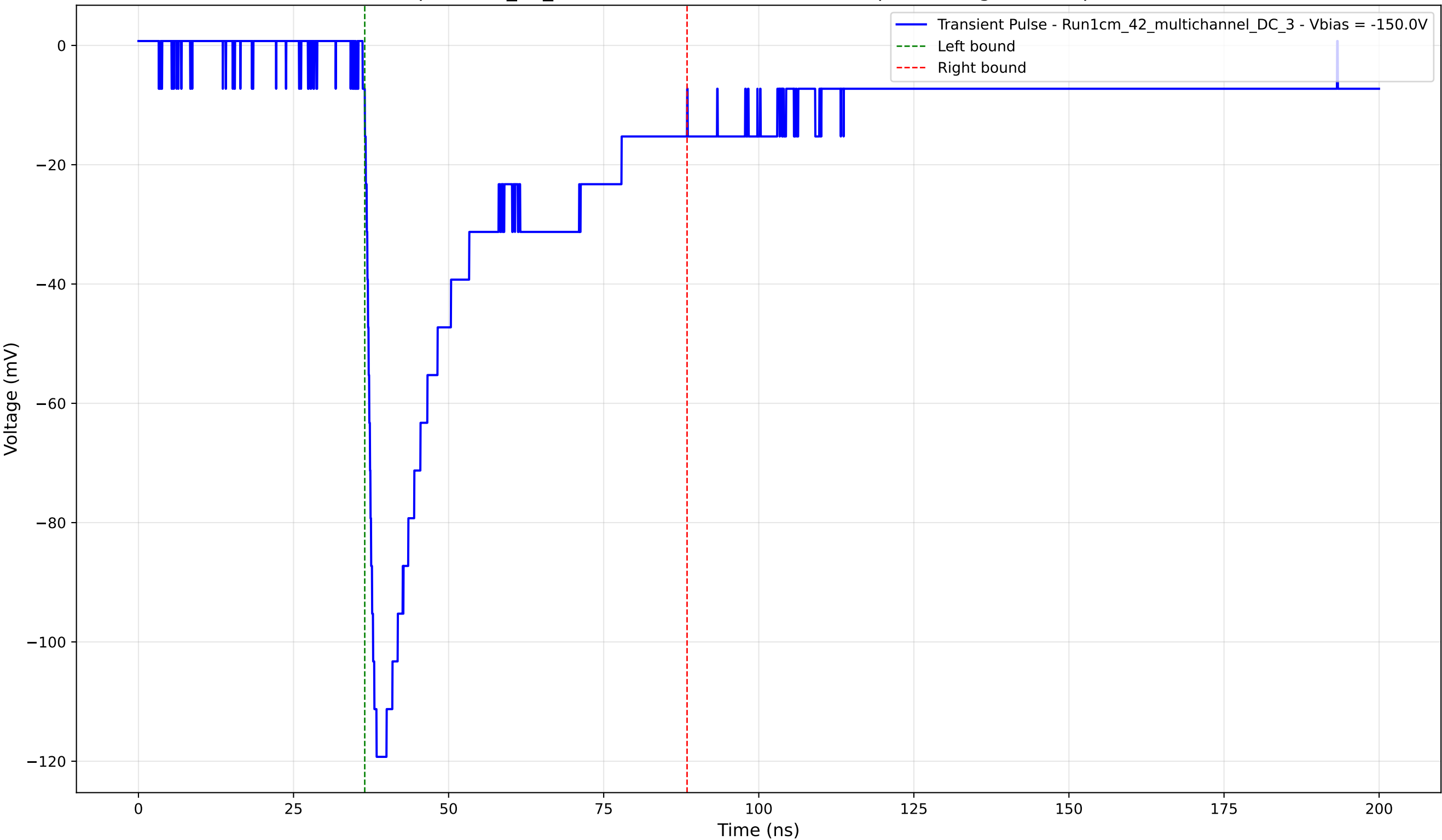
Transient Pulse - Sample: 1cm_42_multichannel - Position: 1650.0 \mu\text{m} - Charge: 41.11 pC - Rise Time: 1.53 ns
