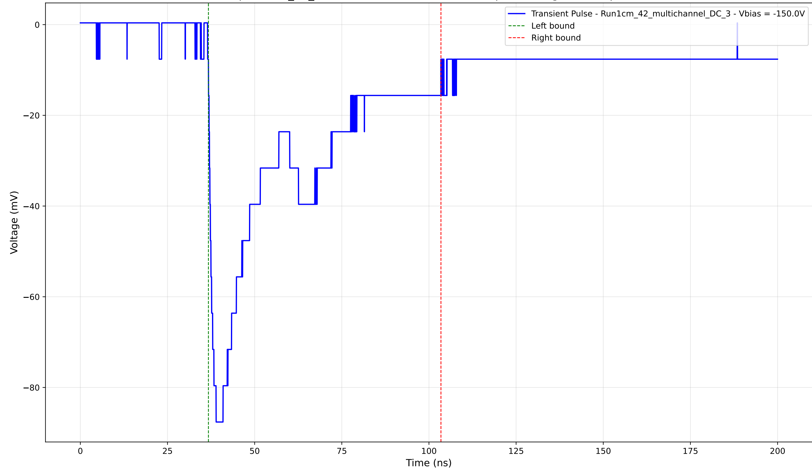
Transient Pulse - Sample: 1cm_42_multichannel - Position: 2170.0 \mu\text{m} - Charge: 41.94 pC - Rise Time: 1.58 ns
