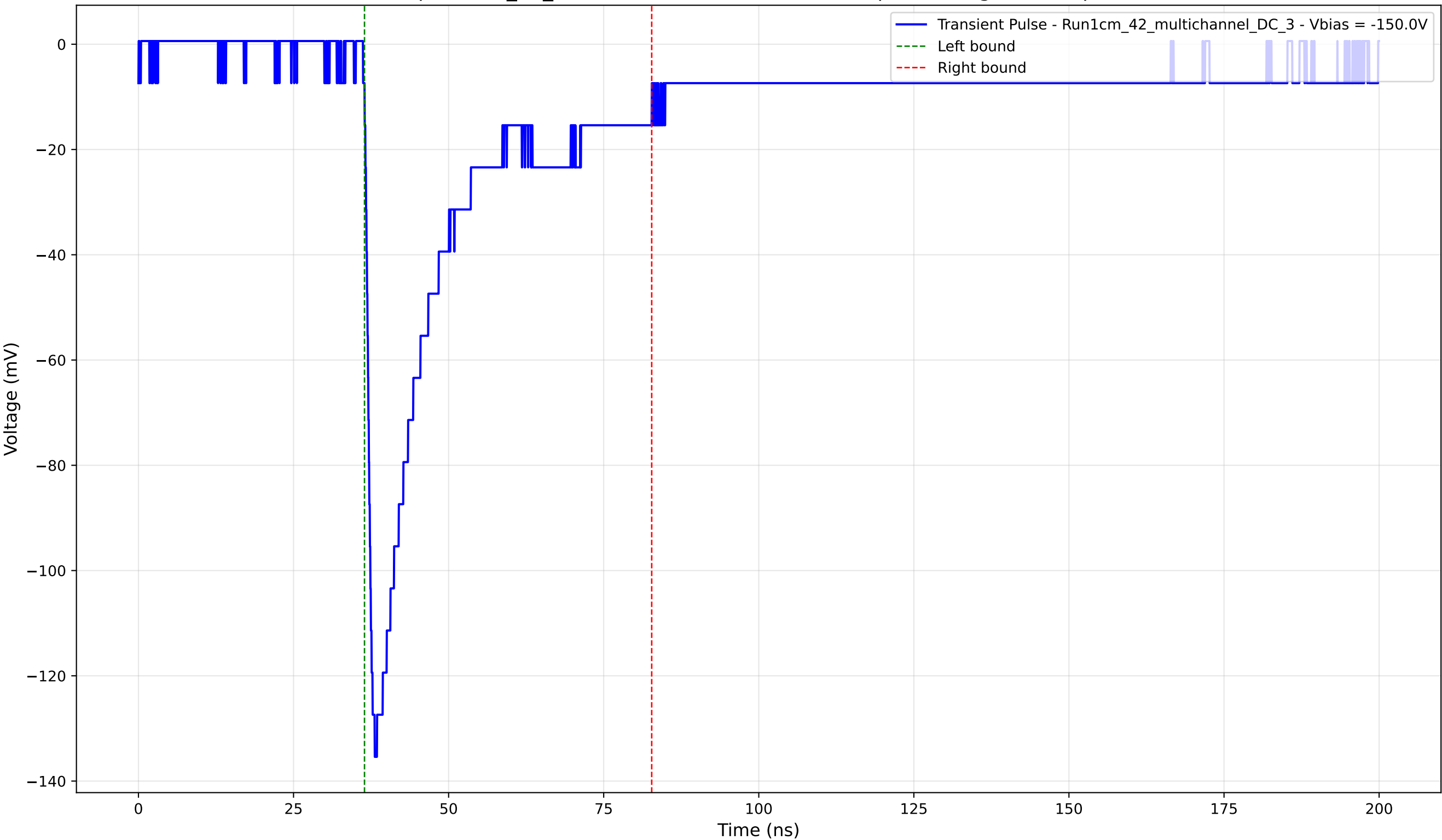
Transient Pulse - Sample: 1cm_42_multichannel - Position: 3815.0 \mu\text{m} - Charge: 34.28 pC - Rise Time: 1.28 ns
