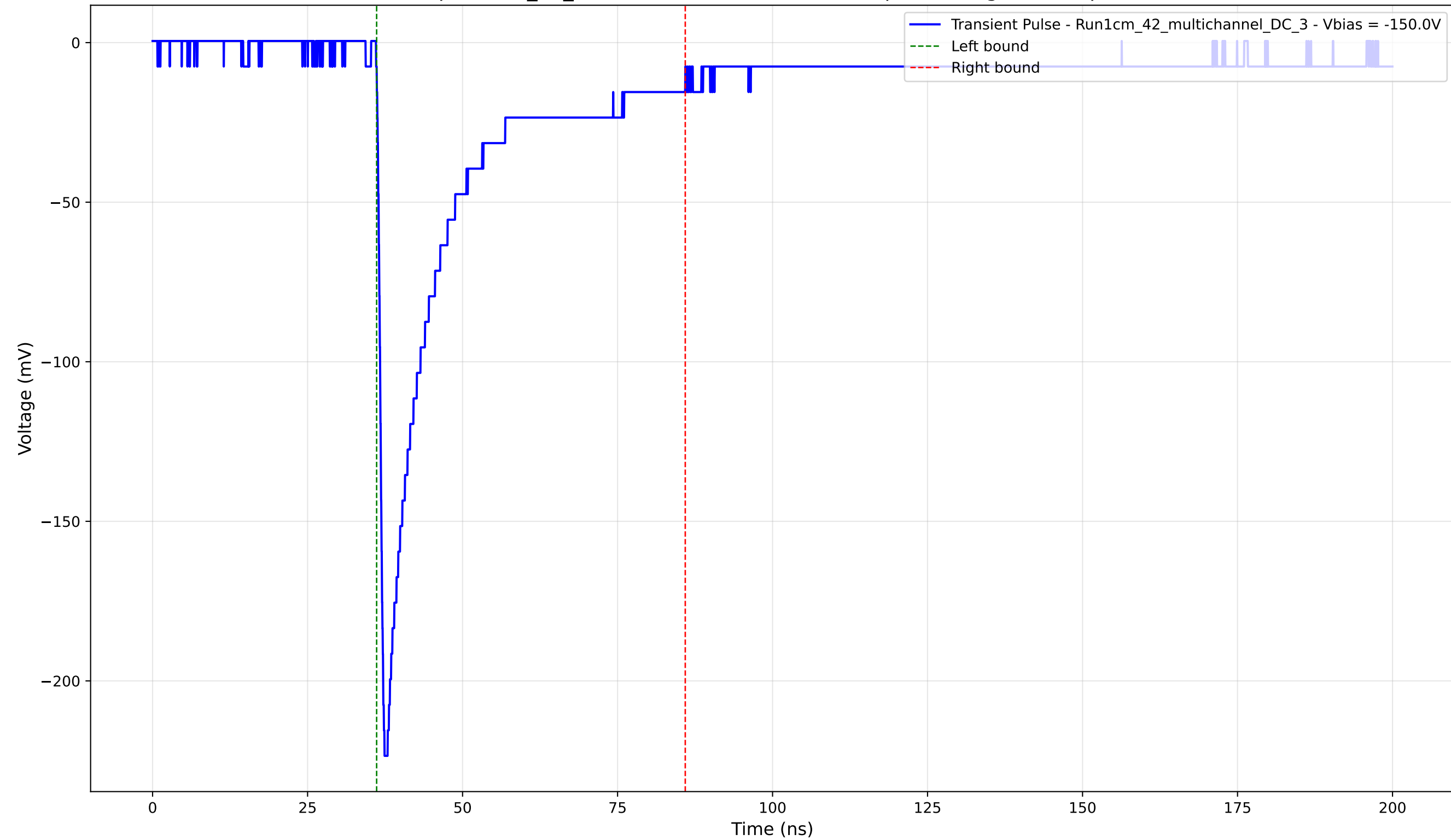
Transient Pulse - Sample: 1cm_42_multichannel - Position: 685.0 \mu\text{m} - Charge: 47.10 pC - Rise Time: 0.98 ns
