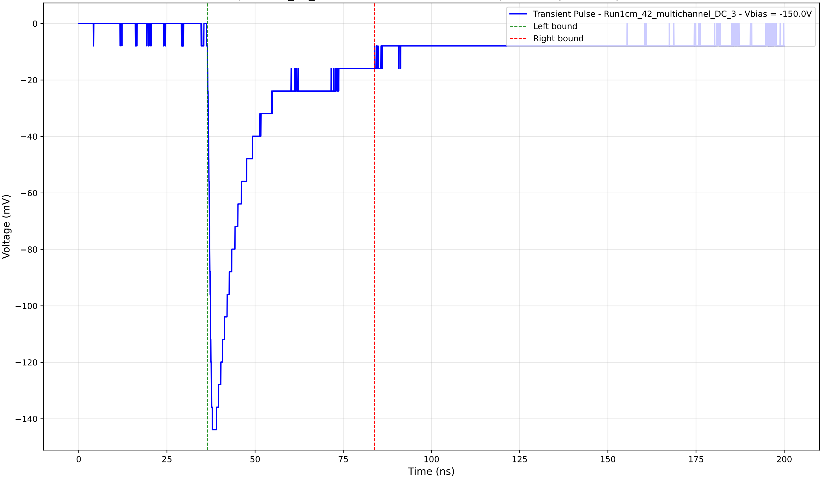
Transient Pulse - Sample: 1cm_42_multichannel - Position: 3800.0 \mu\text{m} - Charge: 38.39 pC - Rise Time: 1.22 ns
