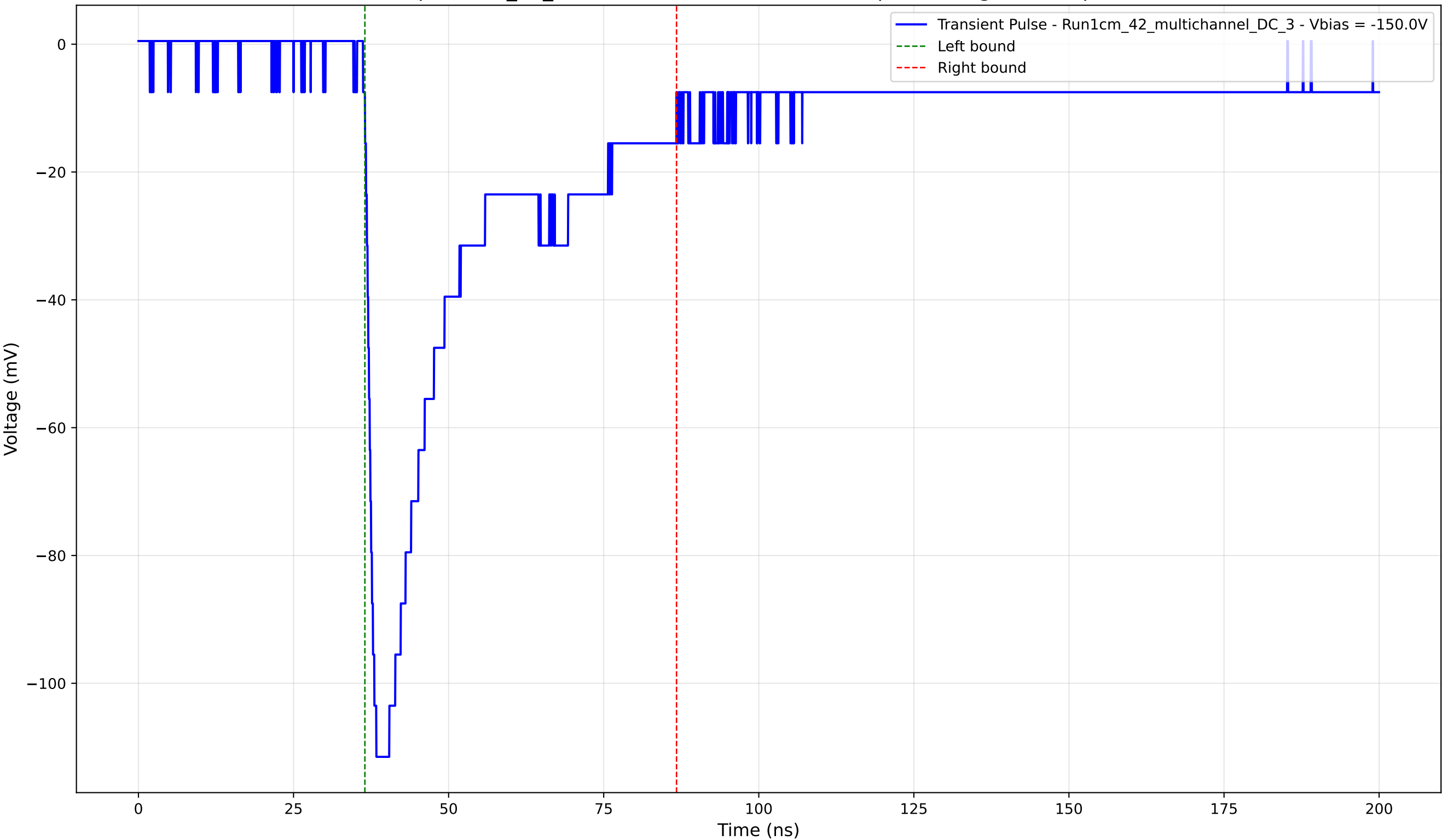
Transient Pulse - Sample: 1cm_42_multichannel - Position: 3280.0 \mu\text{m} - Charge: 37.75 pC - Rise Time: 1.51 ns
