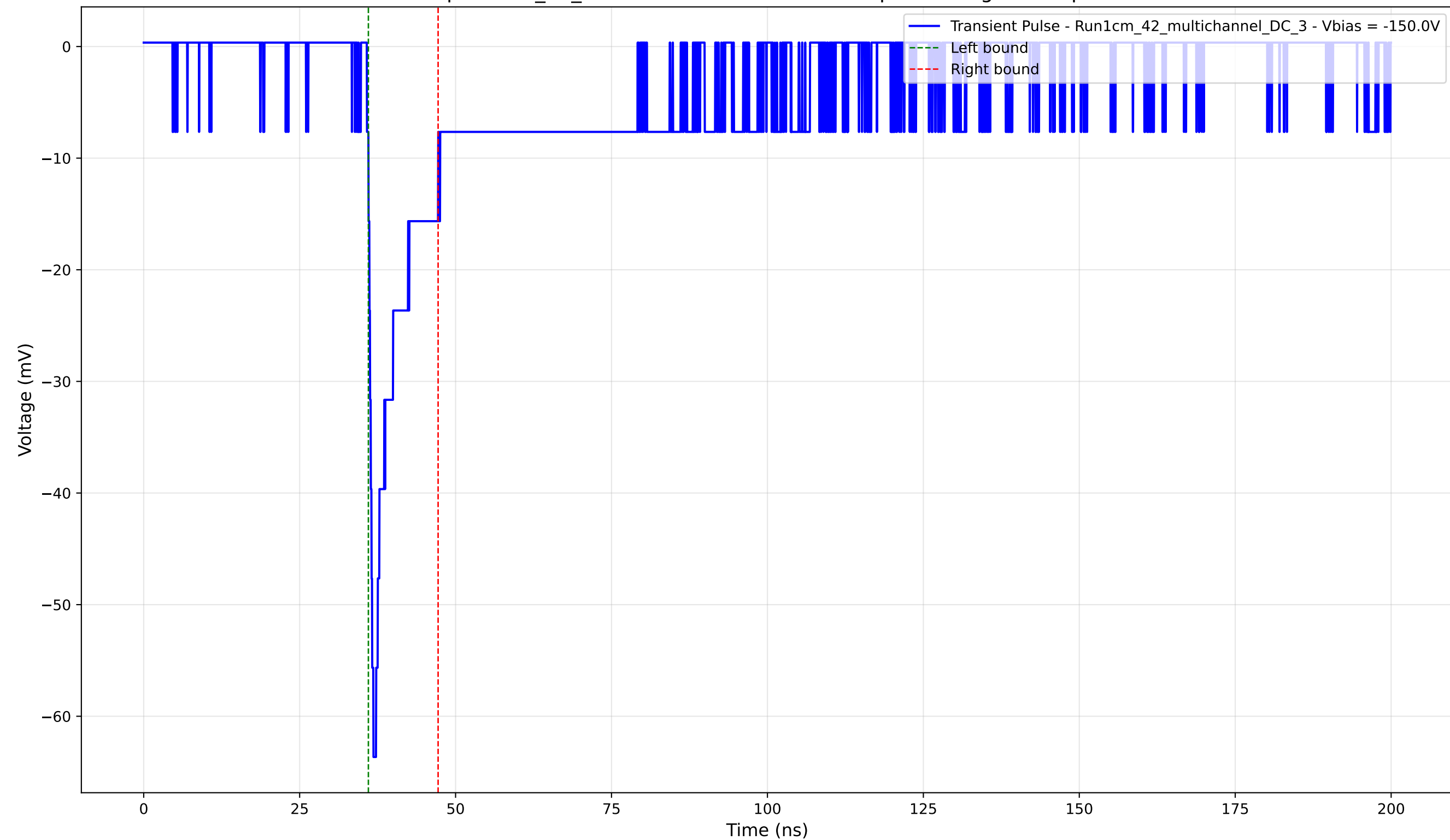
Transient Pulse - Sample: 1cm_42_multichannel - Position: 60.0 \mu\text{m} - Charge: 5.87 pC - Rise Time: 1.04 ns
