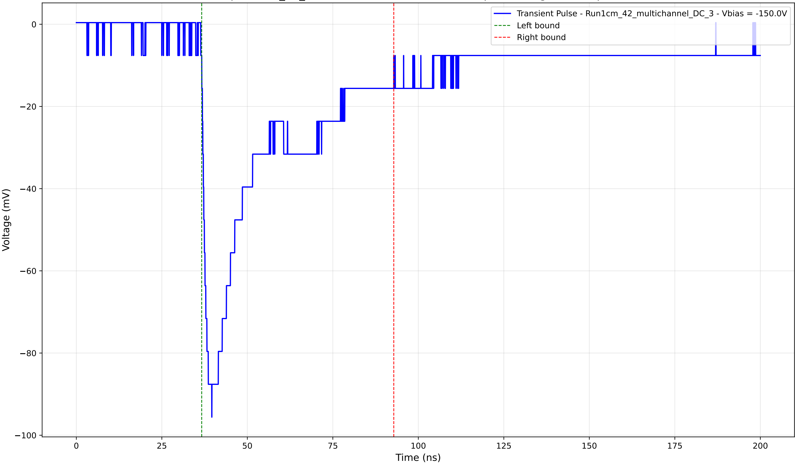
Transient Pulse - Sample: 1cm_42_multichannel - Position: 2775.0 \mu\text{m} - Charge: 37.76 pC - Rise Time: 1.92 ns
