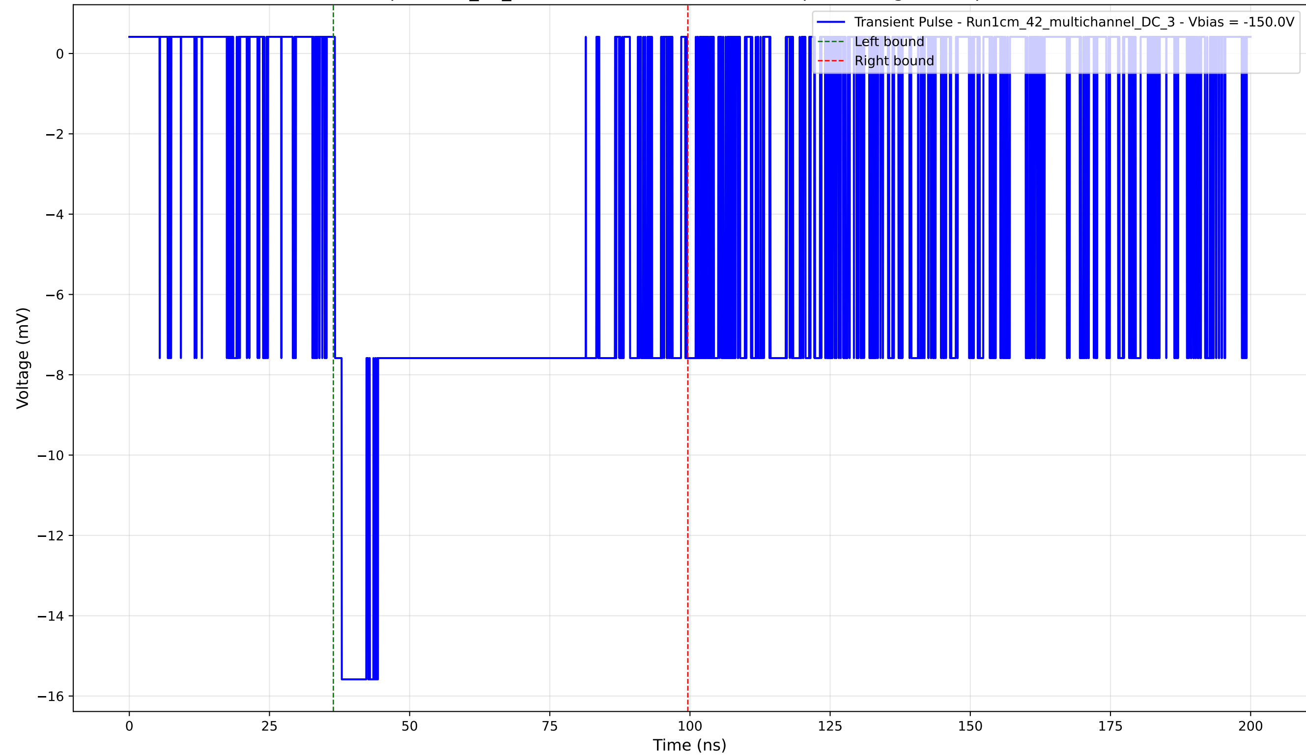
Transient Pulse - Sample: 1cm_42_multichannel - Position: 1895.0 \mu\text{m} - Charge: 9.59 pC - Rise Time: 1.22 ns
