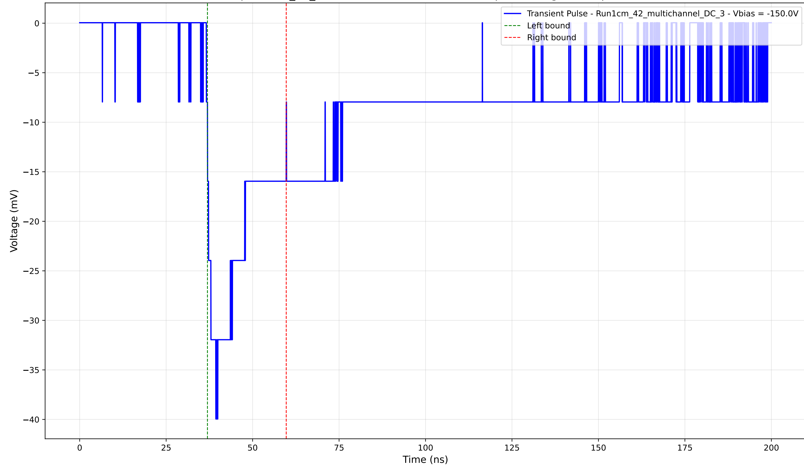
Transient Pulse - Sample: 1cm_42_multichannel - Position: 2420.0 \mu\text{m} - Charge: 9.99 pC - Rise Time: 2.75 ns
