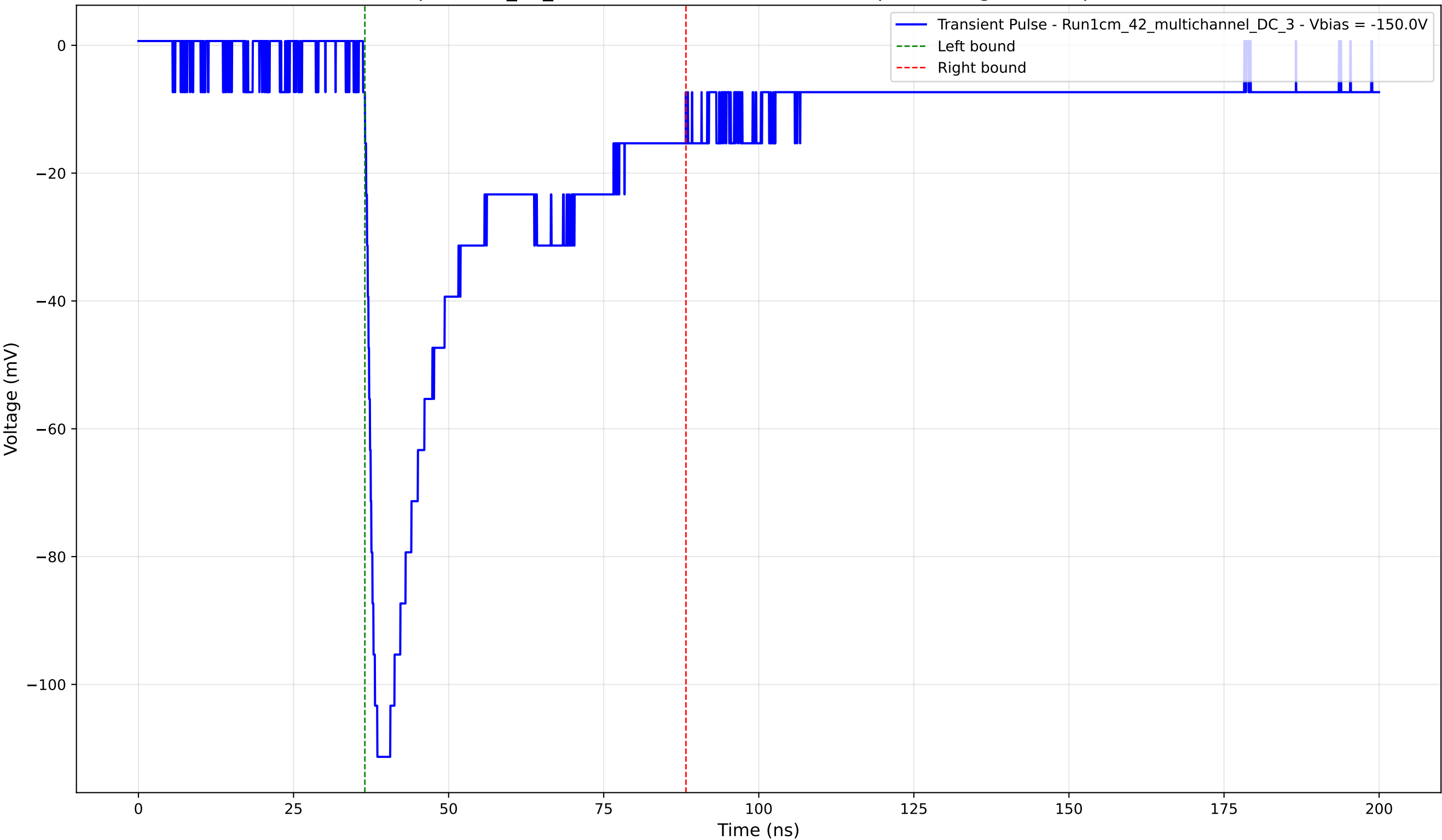
Transient Pulse - Sample: 1cm_42_multichannel - Position: 3235.0 \mu\text{m} - Charge: 38.24 pC - Rise Time: 1.61 ns
