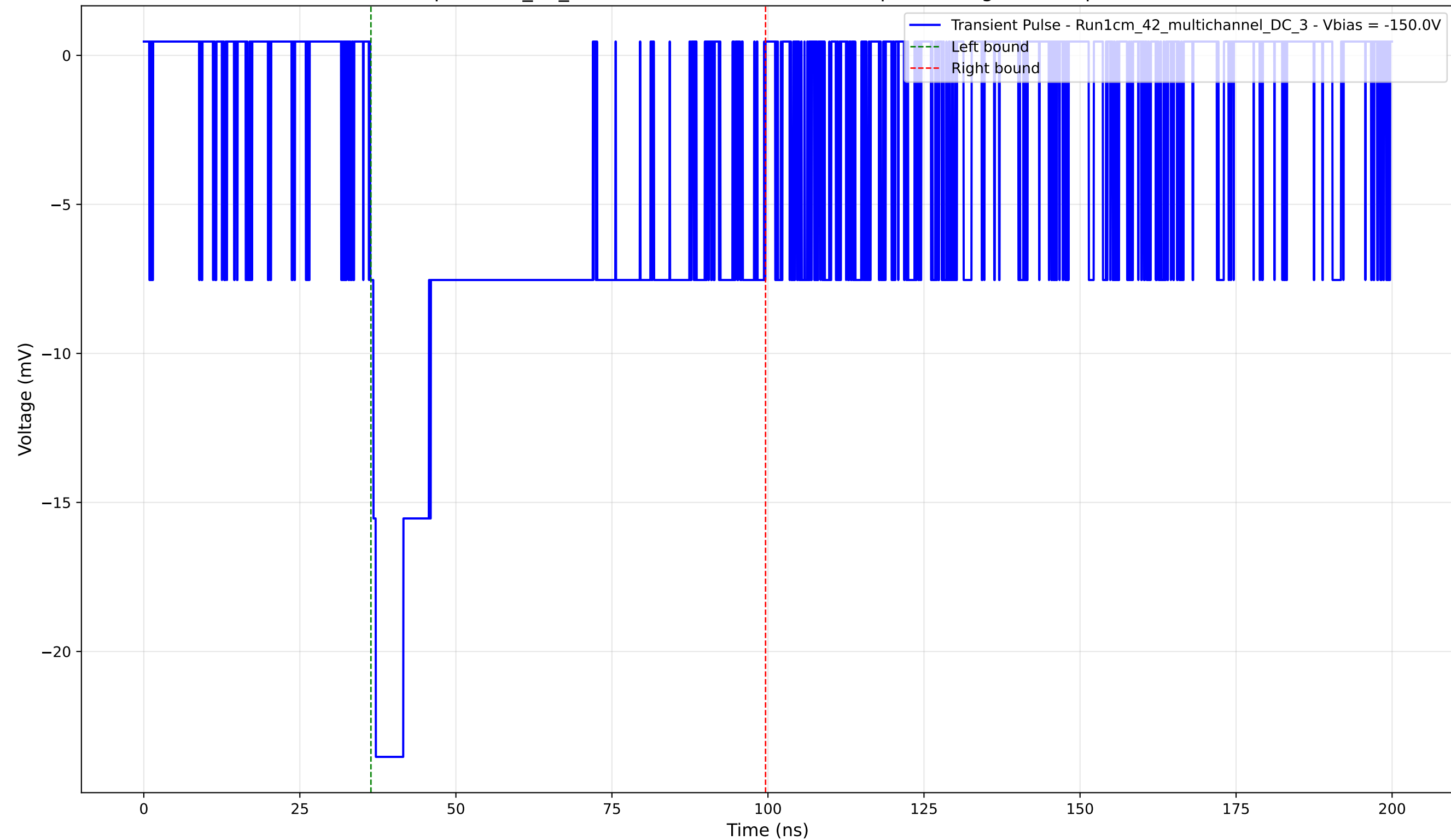
Transient Pulse - Sample: 1cm_42_multichannel - Position: 885.0 \mu\text{m} - Charge: 10.90 pC - Rise Time: 0.89 ns
