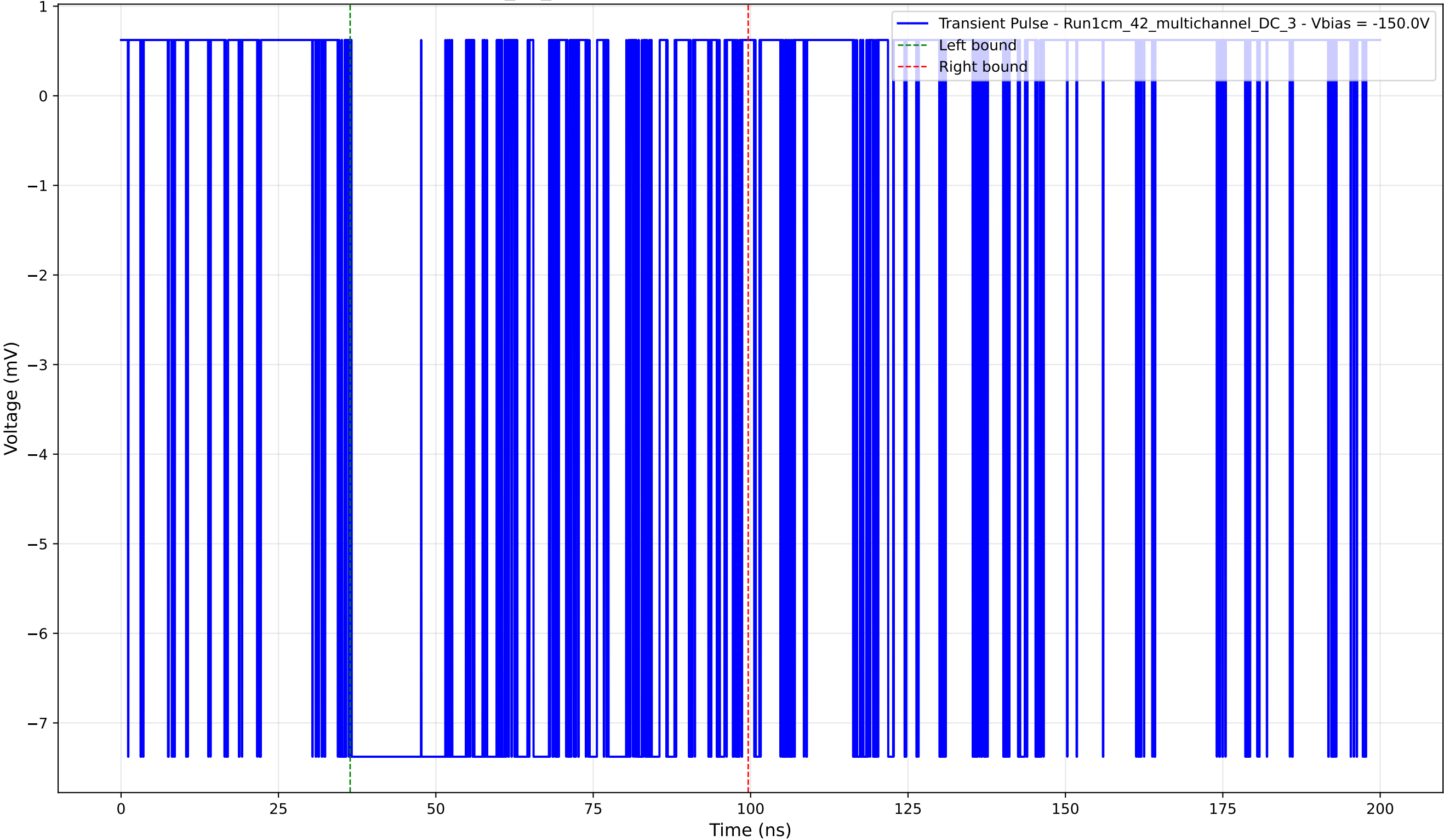
Transient Pulse - Sample: 1cm_42_multichannel - Position: 3885.0 \mu\text{m} - Charge: 5.74 pC - Rise Time: 0.02 ns
