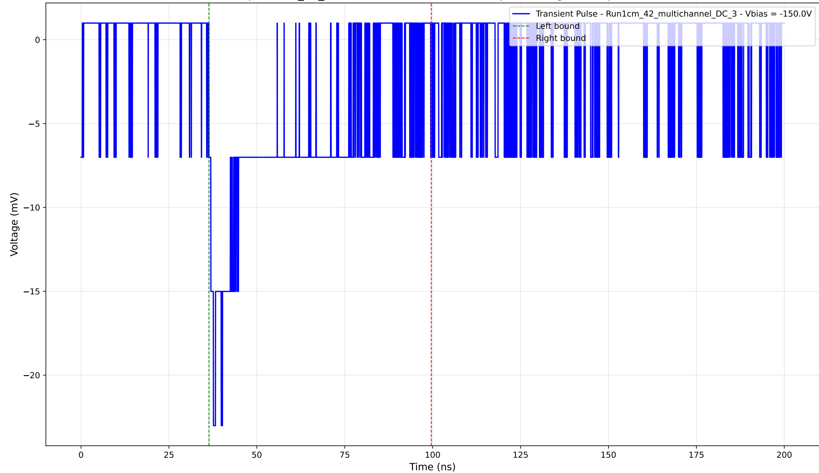
Transient Pulse - Sample: 1cm_42_multichannel - Position: 880.0 \mu\text{m} - Charge: 7.58 pC - Rise Time: 1.28 ns
