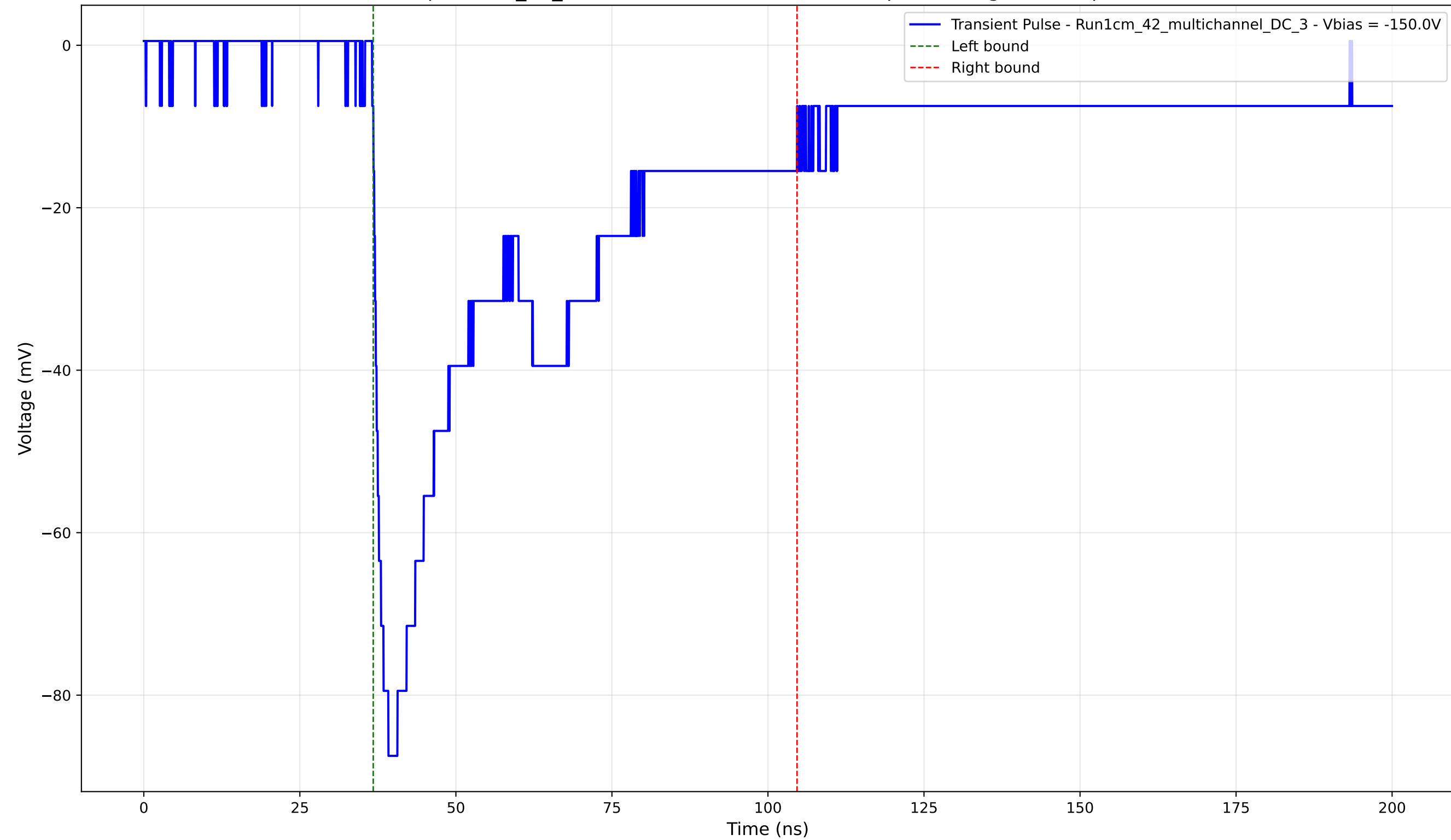
Transient Pulse - Sample: 1cm_42_multichannel - Position: 2230.0 \mu\text{m} - Charge: 42.60 pC - Rise Time: 1.64 ns
