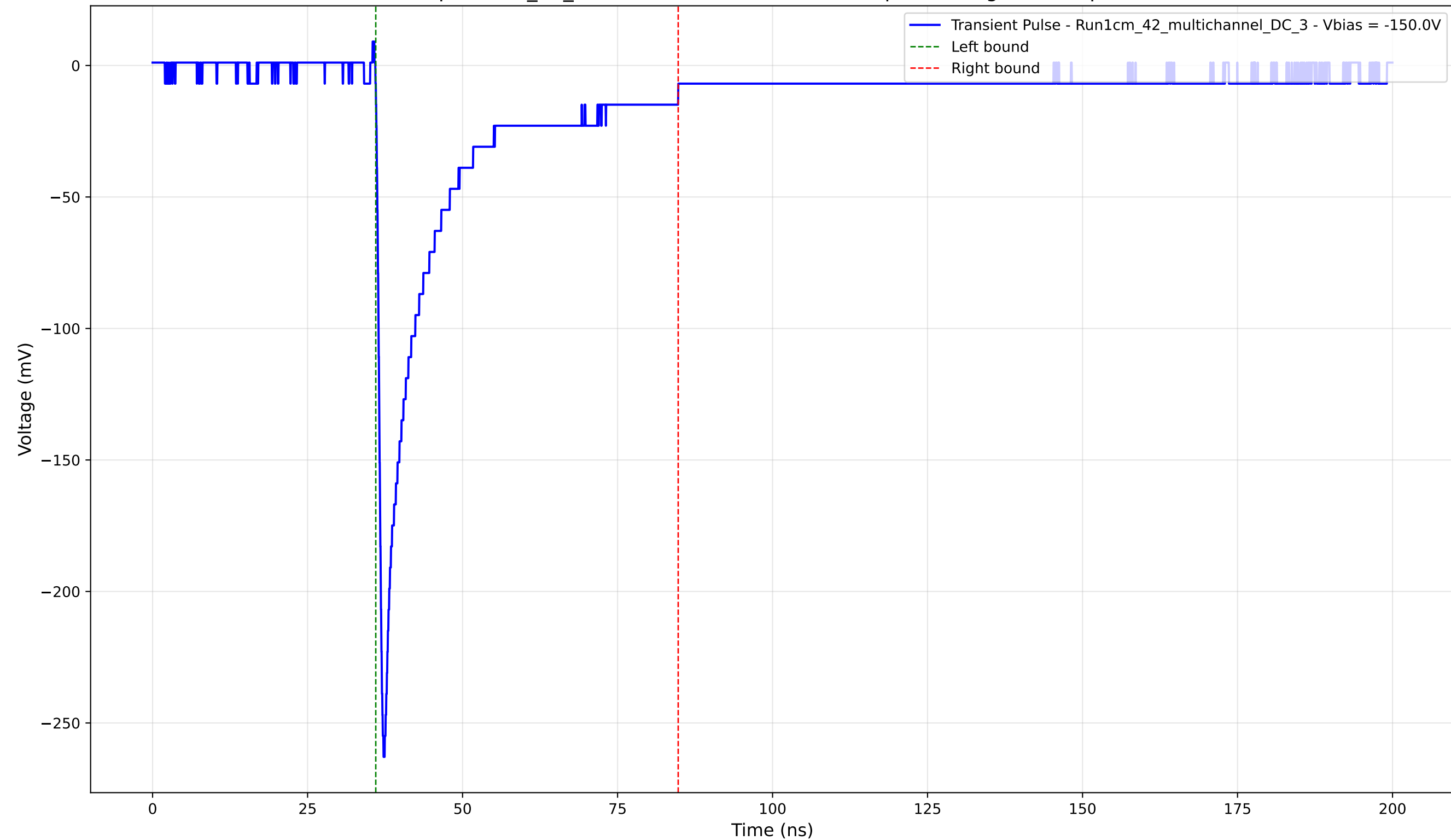
Transient Pulse - Sample: 1cm_42_multichannel - Position: 425.0 \mu\text{m} - Charge: 44.39 pC - Rise Time: 0.87 ns
