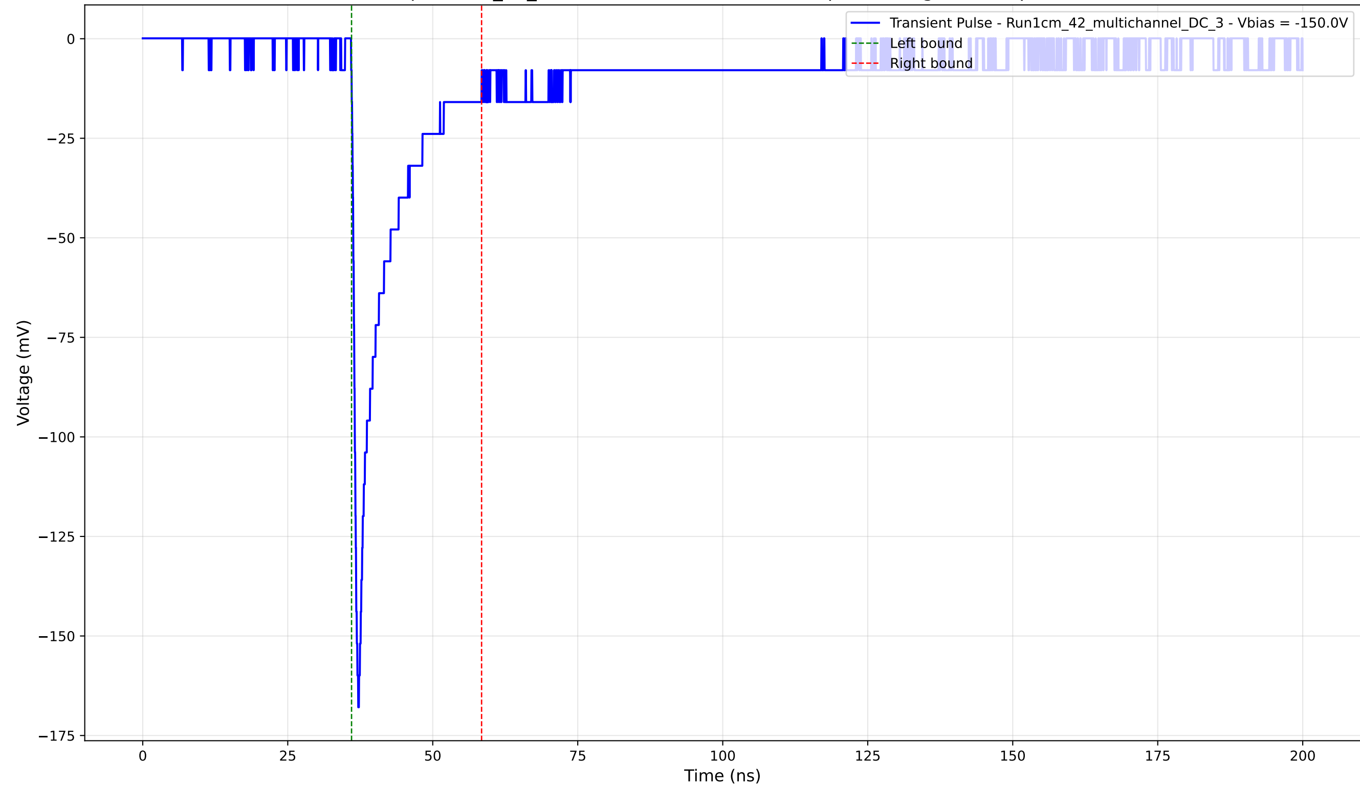
Transient Pulse - Sample: 1cm_42_multichannel - Position: 300.0 \mu\text{m} - Charge: 19.94 pC - Rise Time: 0.82 ns
