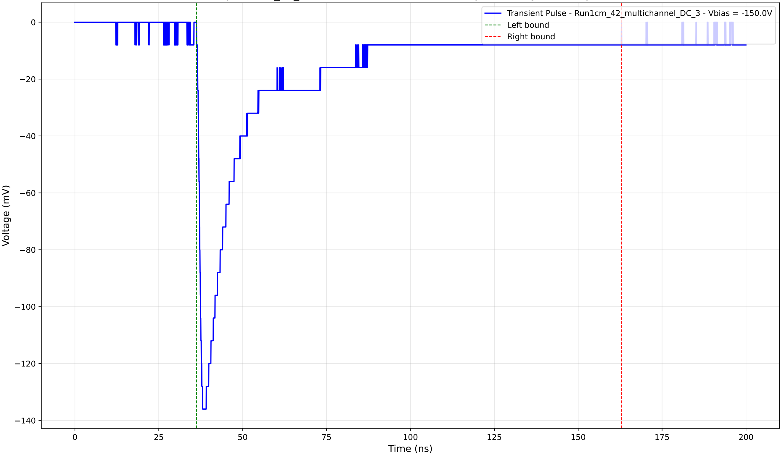
Transient Pulse - Sample: 1cm_42_multichannel - Position: 3695.0 \mu\text{m} - Charge: 50.60 pC - Rise Time: 1.33 ns
