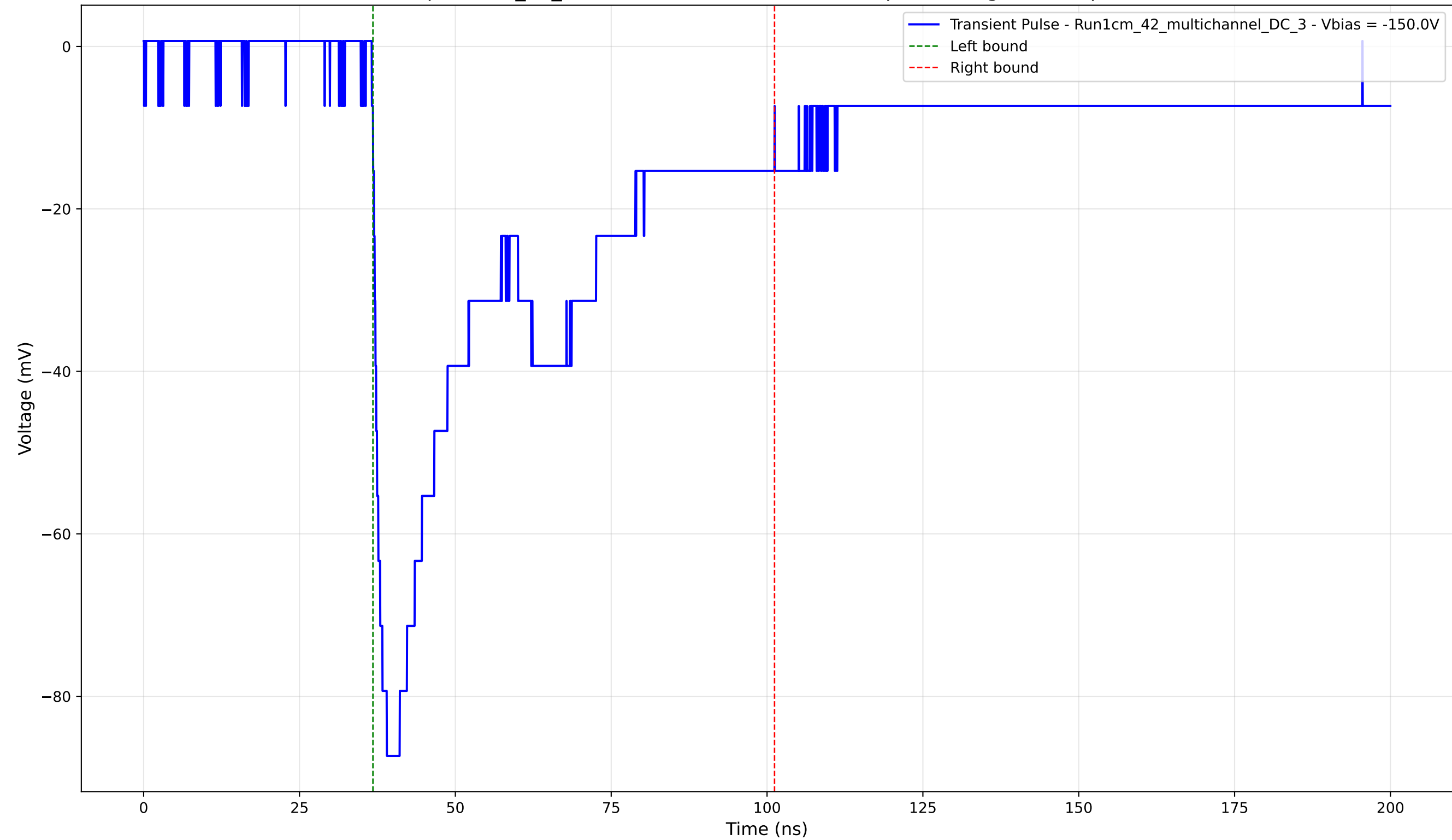
Transient Pulse - Sample: 1cm_42_multichannel - Position: 2200.0 \mu\text{m} - Charge: 41.48 pC - Rise Time: 1.52 ns
