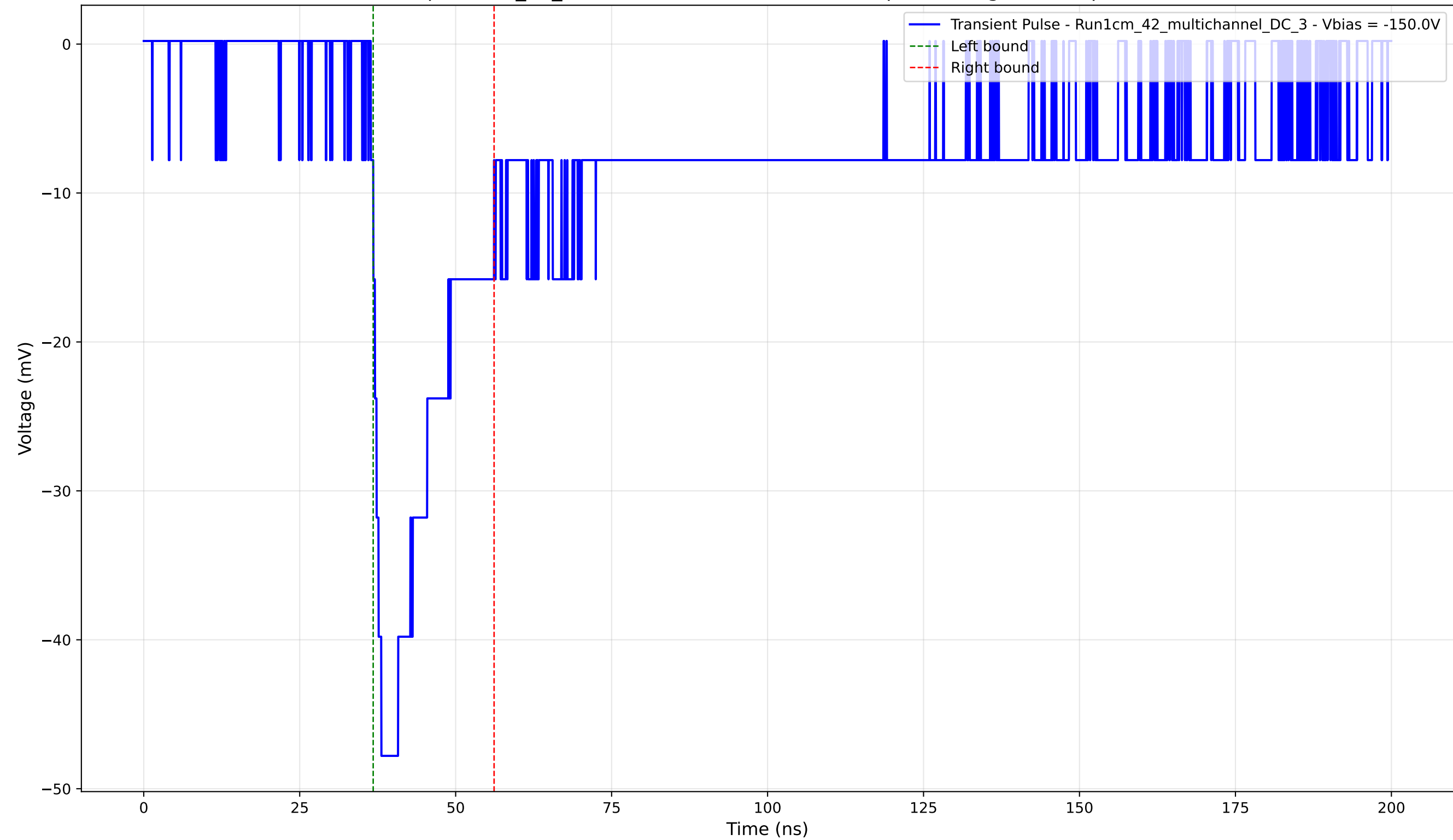
Transient Pulse - Sample: 1cm_42_multichannel - Position: 3340.0 \mu\text{m} - Charge: 10.62 pC - Rise Time: 1.69 ns
