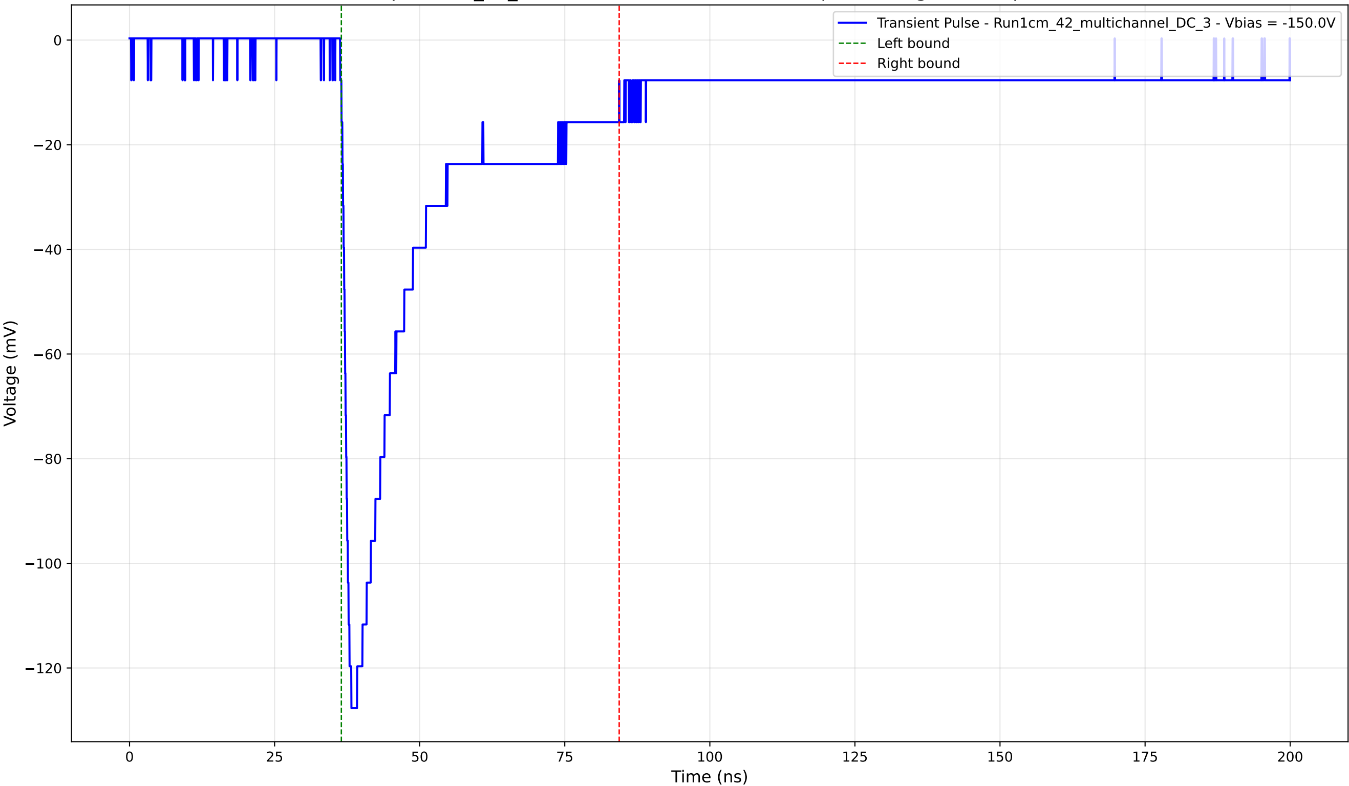
Transient Pulse - Sample: 1cm_42_multichannel - Position: 3595.0 \mu\text{m} - Charge: 36.75 pC - Rise Time: 1.39 ns
