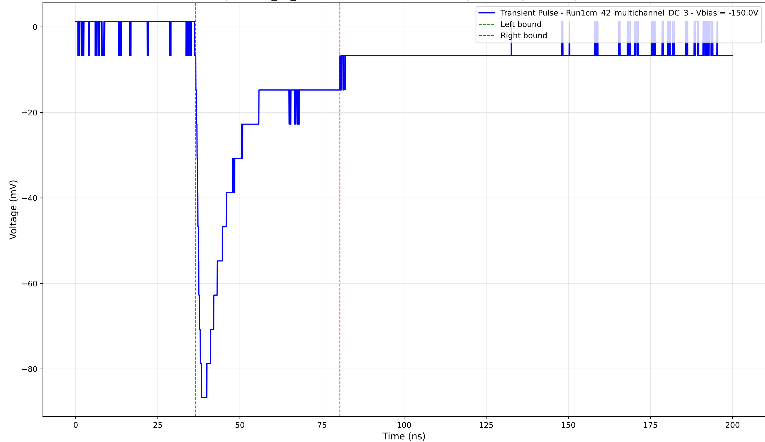
Transient Pulse - Sample: 1cm_42_multichannel - Position: 3445.0 \mu\text{m} - Charge: 24.94 pC - Rise Time: 1.36 ns
