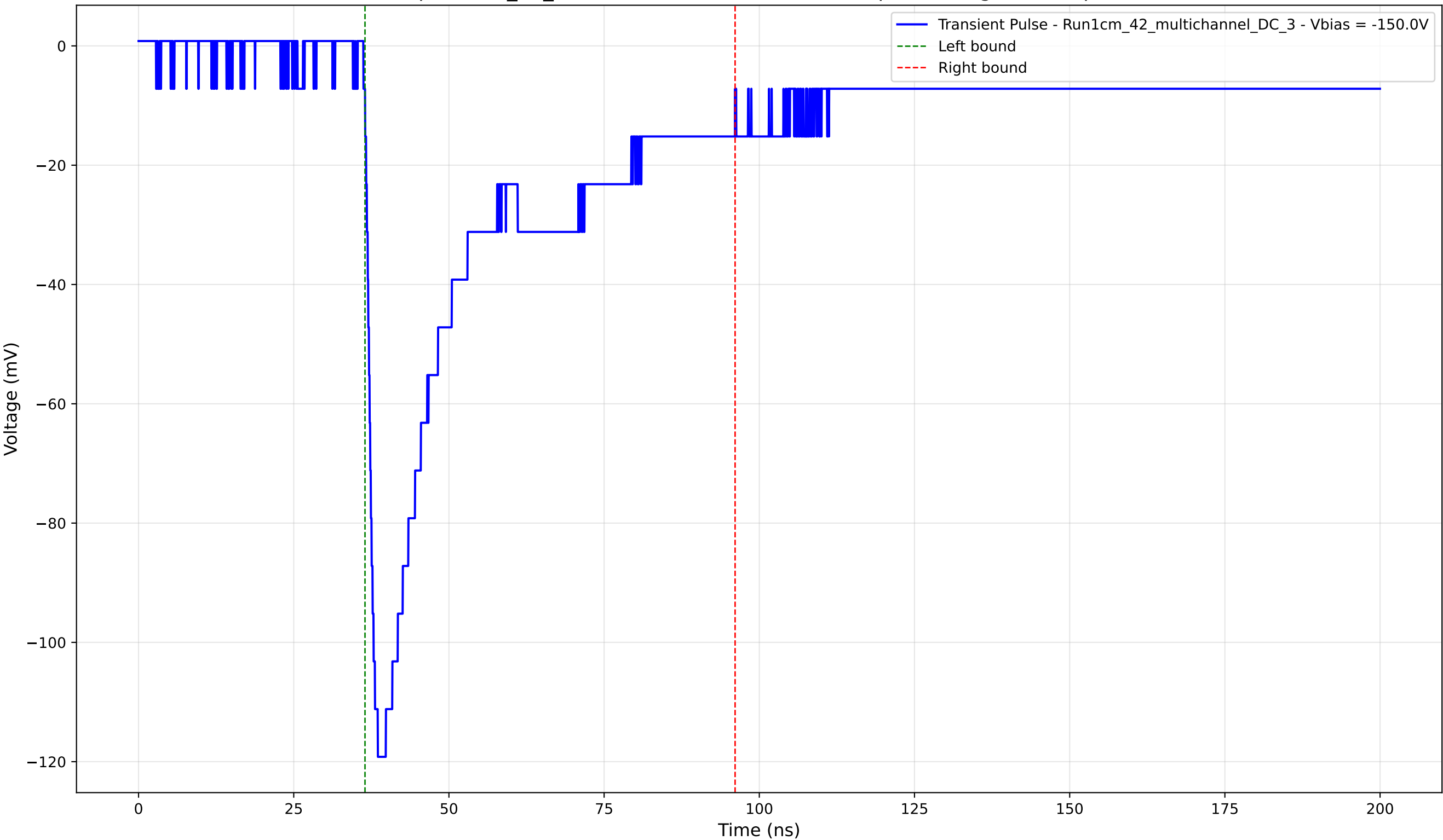
Transient Pulse - Sample: 1cm_42_multichannel - Position: 1675.0 \mu\text{m} - Charge: 43.53 pC - Rise Time: 1.59 ns
