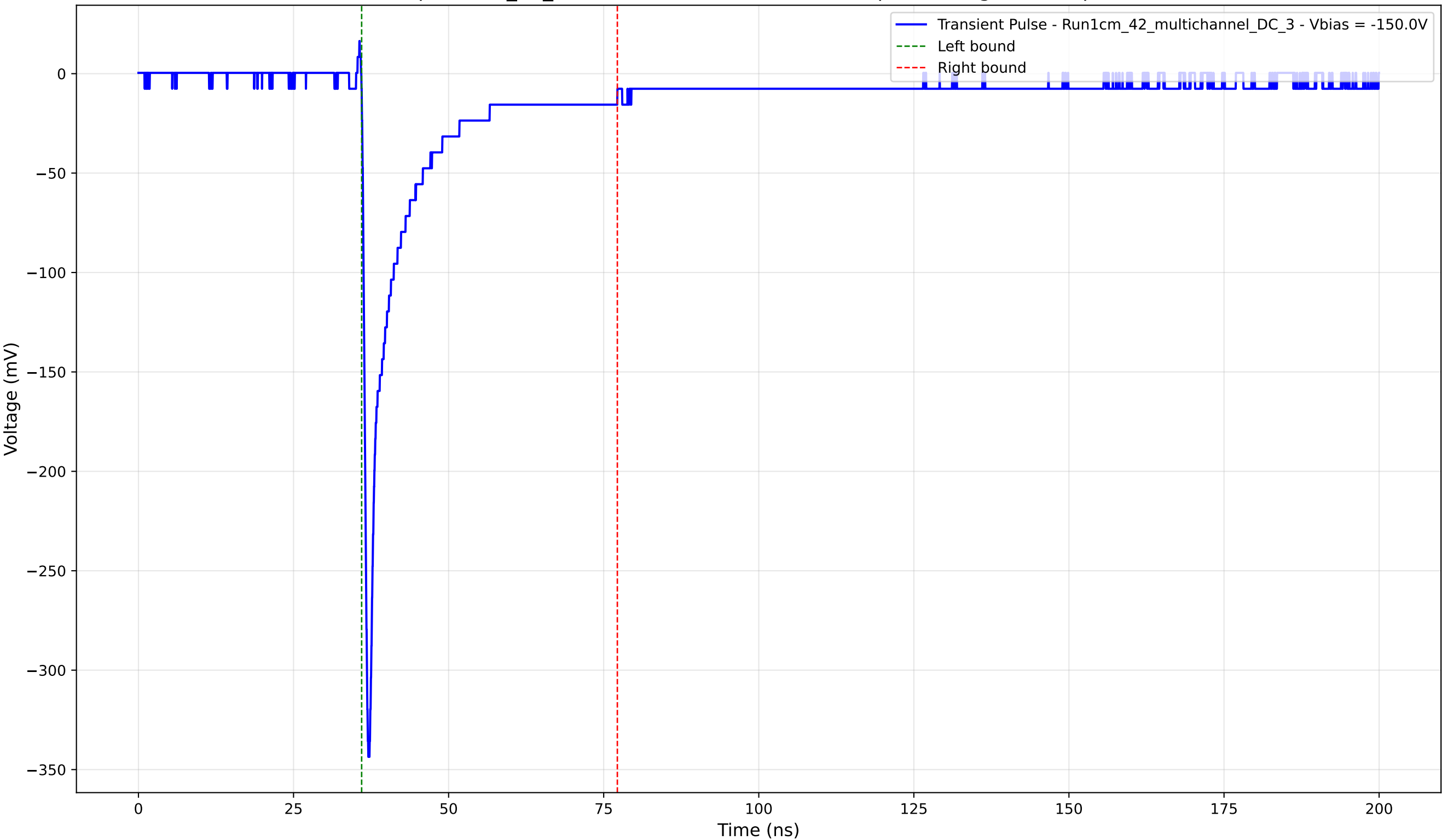
Transient Pulse - Sample: 1cm_42_multichannel - Position: 4810.0 \mu\text{m} - Charge: 38.01 pC - Rise Time: 0.77 ns
