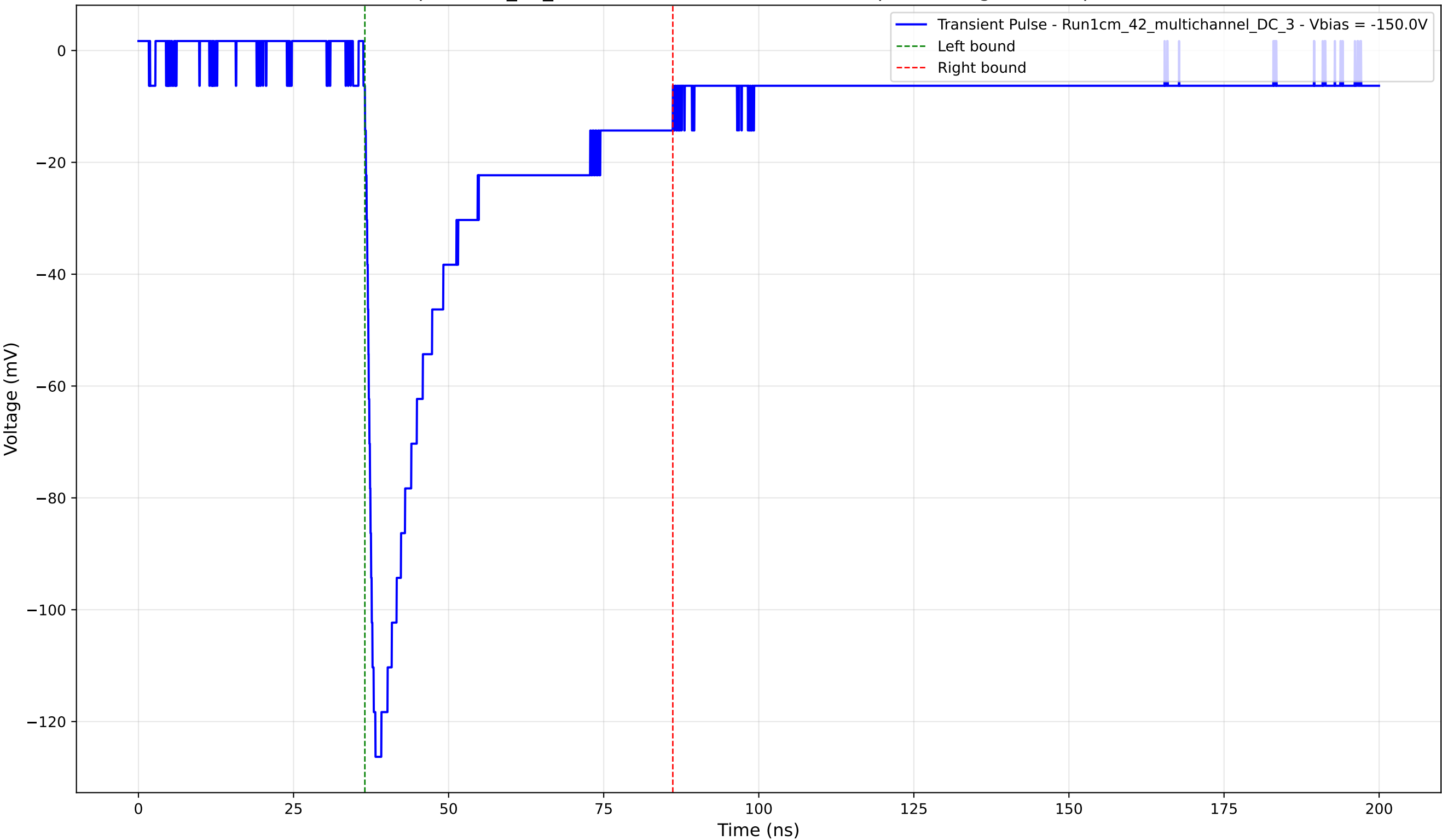
Transient Pulse - Sample: 1cm_42_multichannel - Position: 3585.0 \mu\text{m} - Charge: 35.92 pC - Rise Time: 1.40 ns
