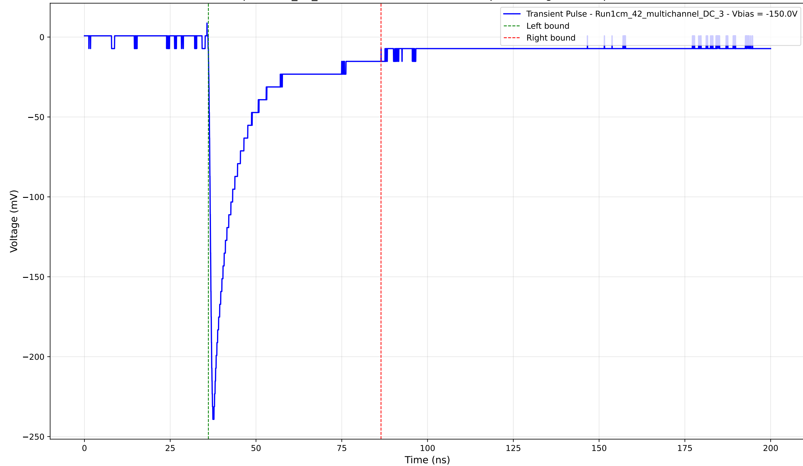
Transient Pulse - Sample: 1cm_42_multichannel - Position: 625.0 \mu\text{m} - Charge: 47.67 pC - Rise Time: 0.98 ns
