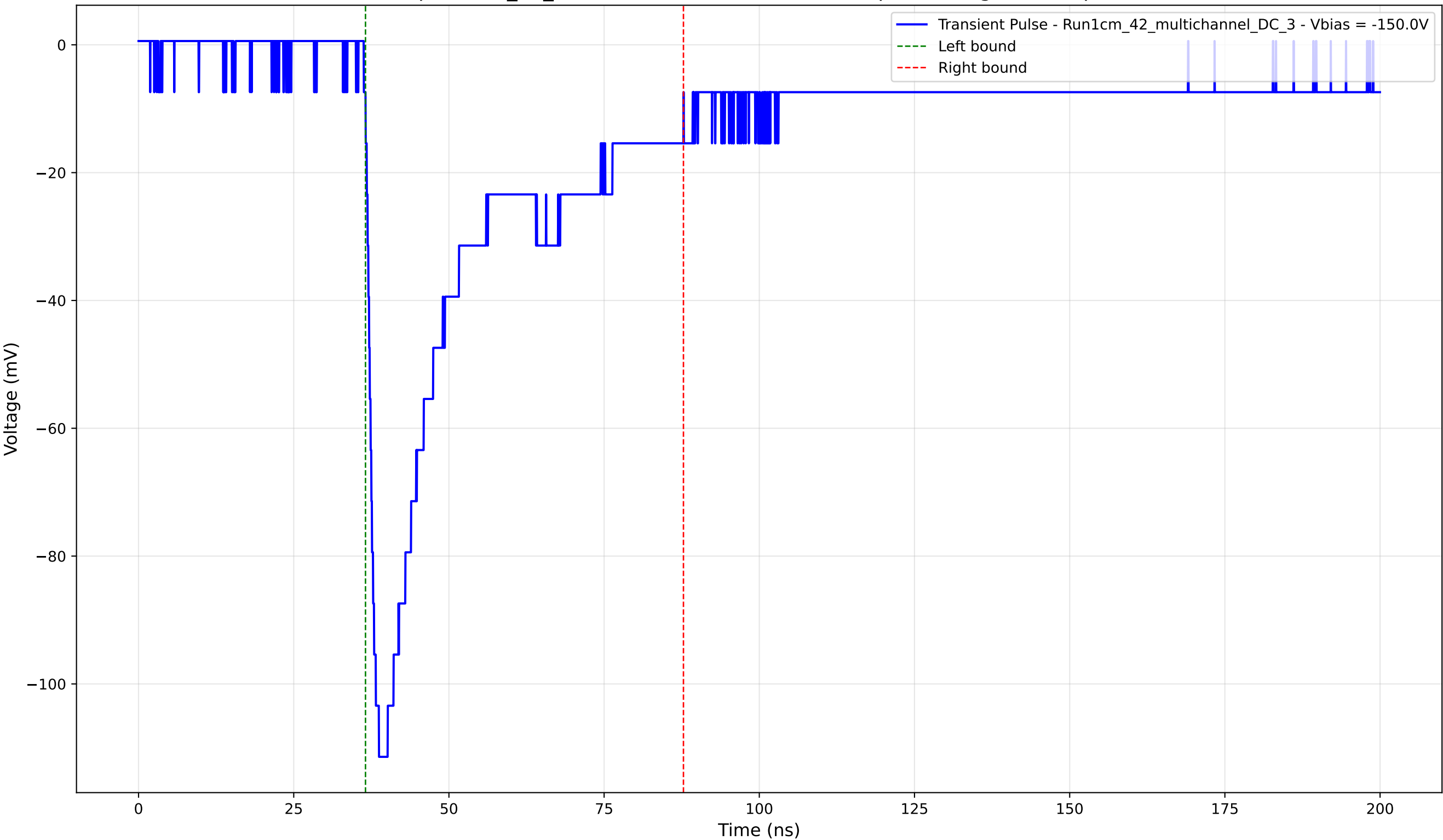
Transient Pulse - Sample: 1cm_42_multichannel - Position: 3215.0 \mu\text{m} - Charge: 37.30 pC - Rise Time: 1.65 ns
