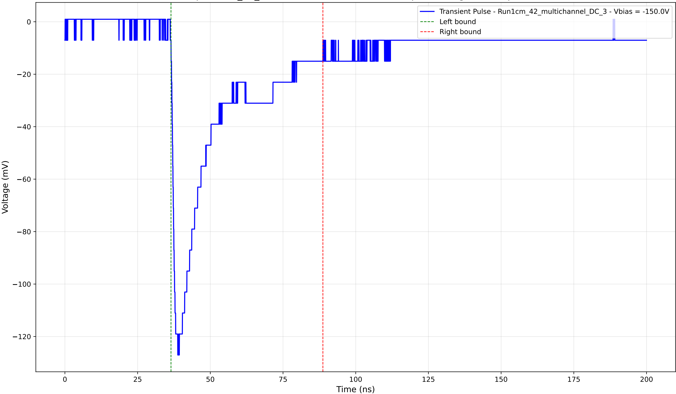
Transient Pulse - Sample: 1cm_42_multichannel - Position: 1580.0 \mu\text{m} - Charge: 41.57 pC - Rise Time: 1.59 ns
