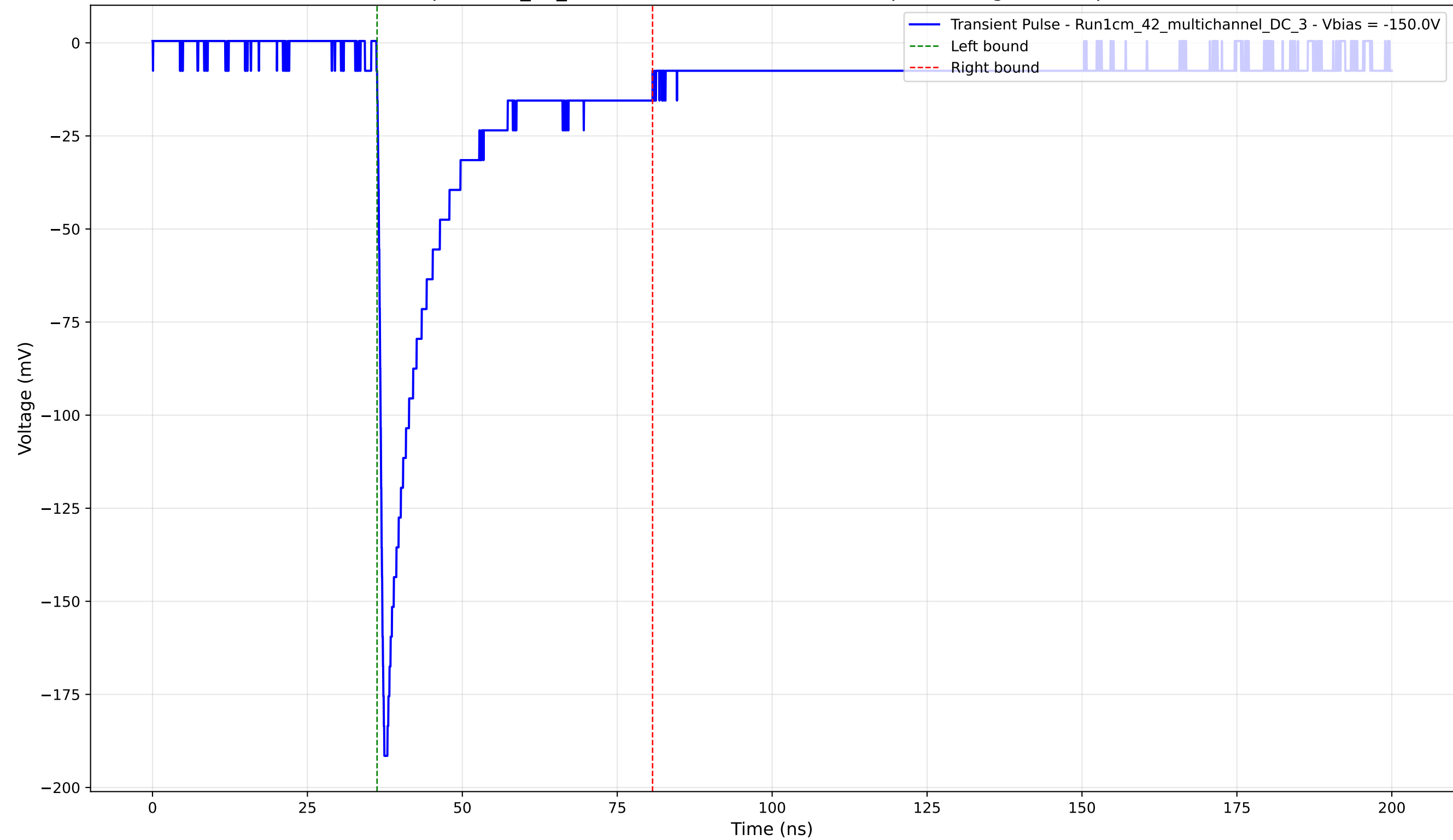
Transient Pulse - Sample: 1cm_42_multichannel - Position: 4300.0 \mu\text{m} - Charge: 35.30 pC - Rise Time: 0.91 ns
