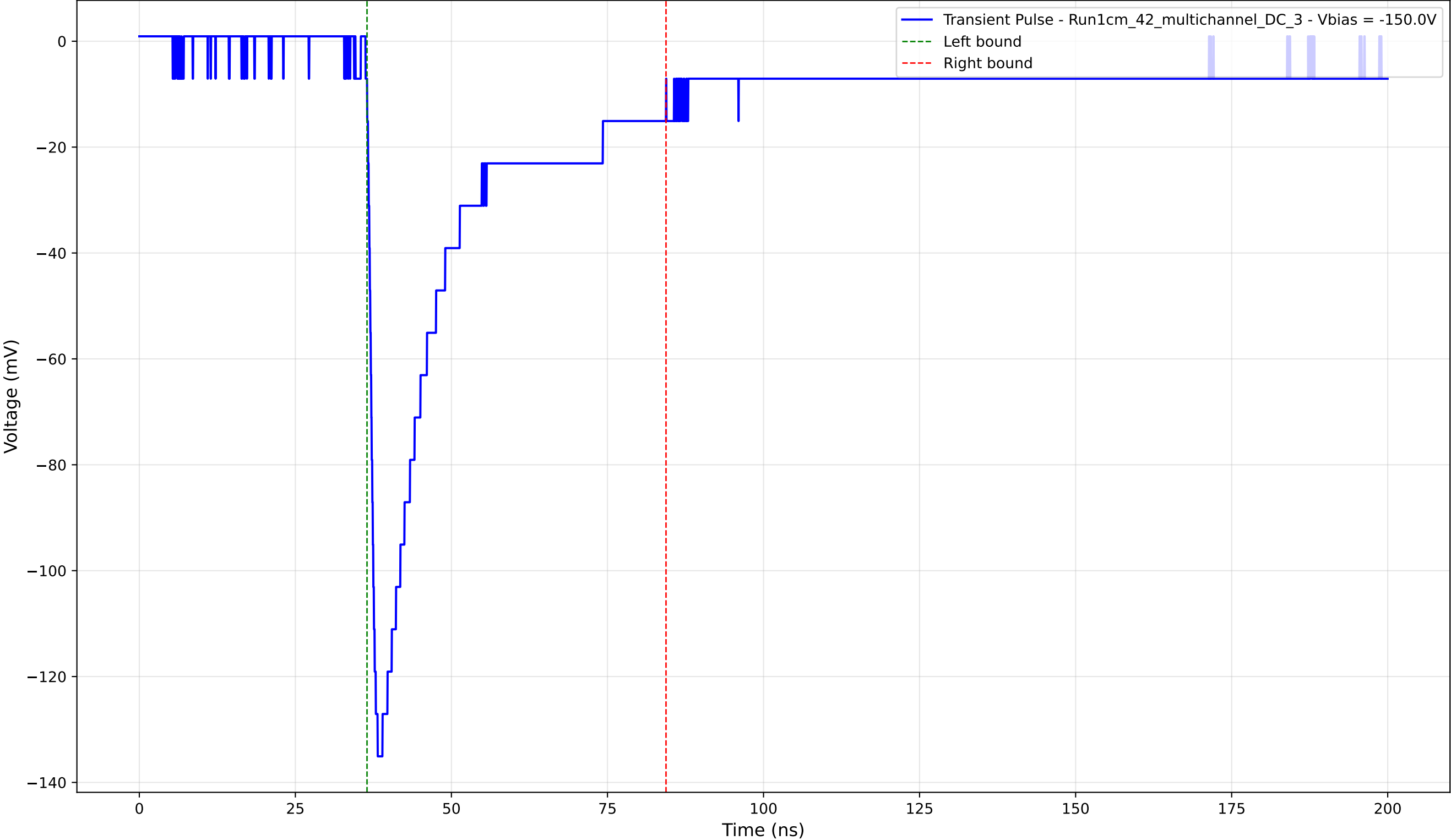
Transient Pulse - Sample: 1cm_42_multichannel - Position: 3665.0 \mu\text{m} - Charge: 37.05 pC - Rise Time: 1.38 ns
