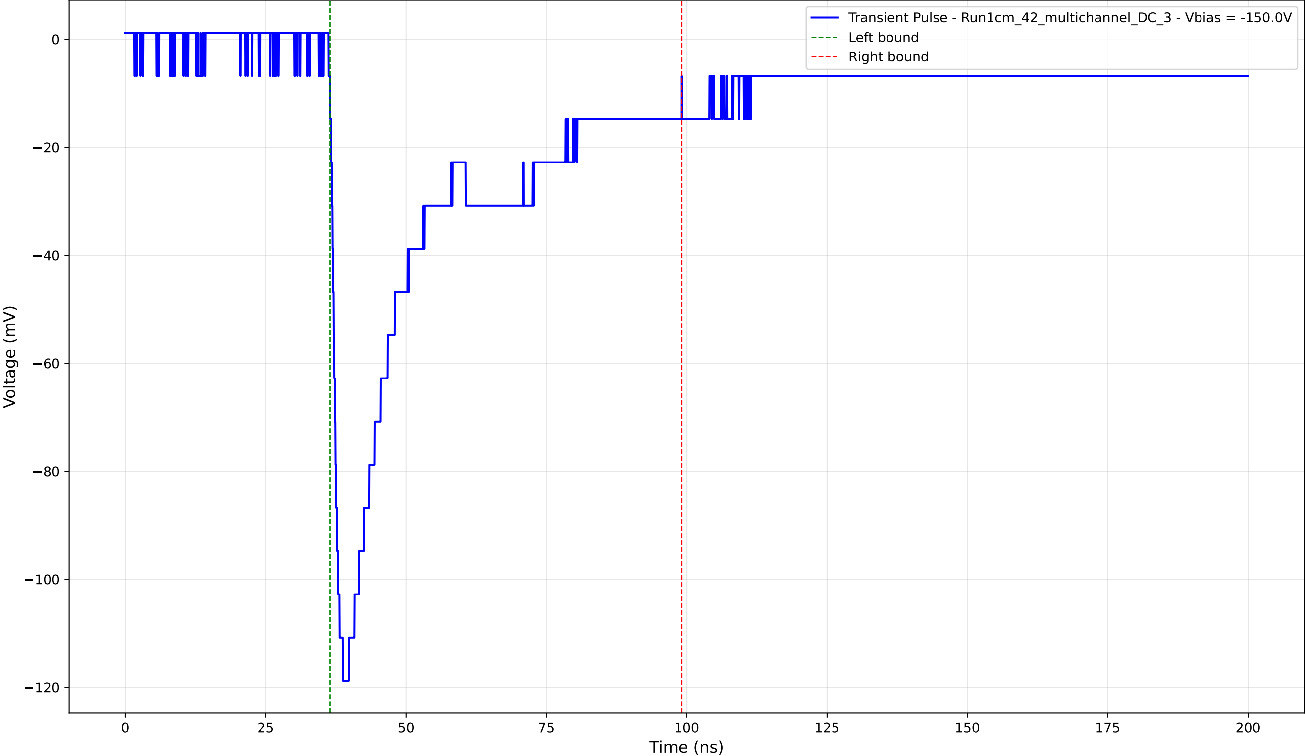
Transient Pulse - Sample: 1cm_42_multichannel - Position: 1720.0 \mu\text{m} - Charge: 44.13 pC - Rise Time: 1.67 ns
