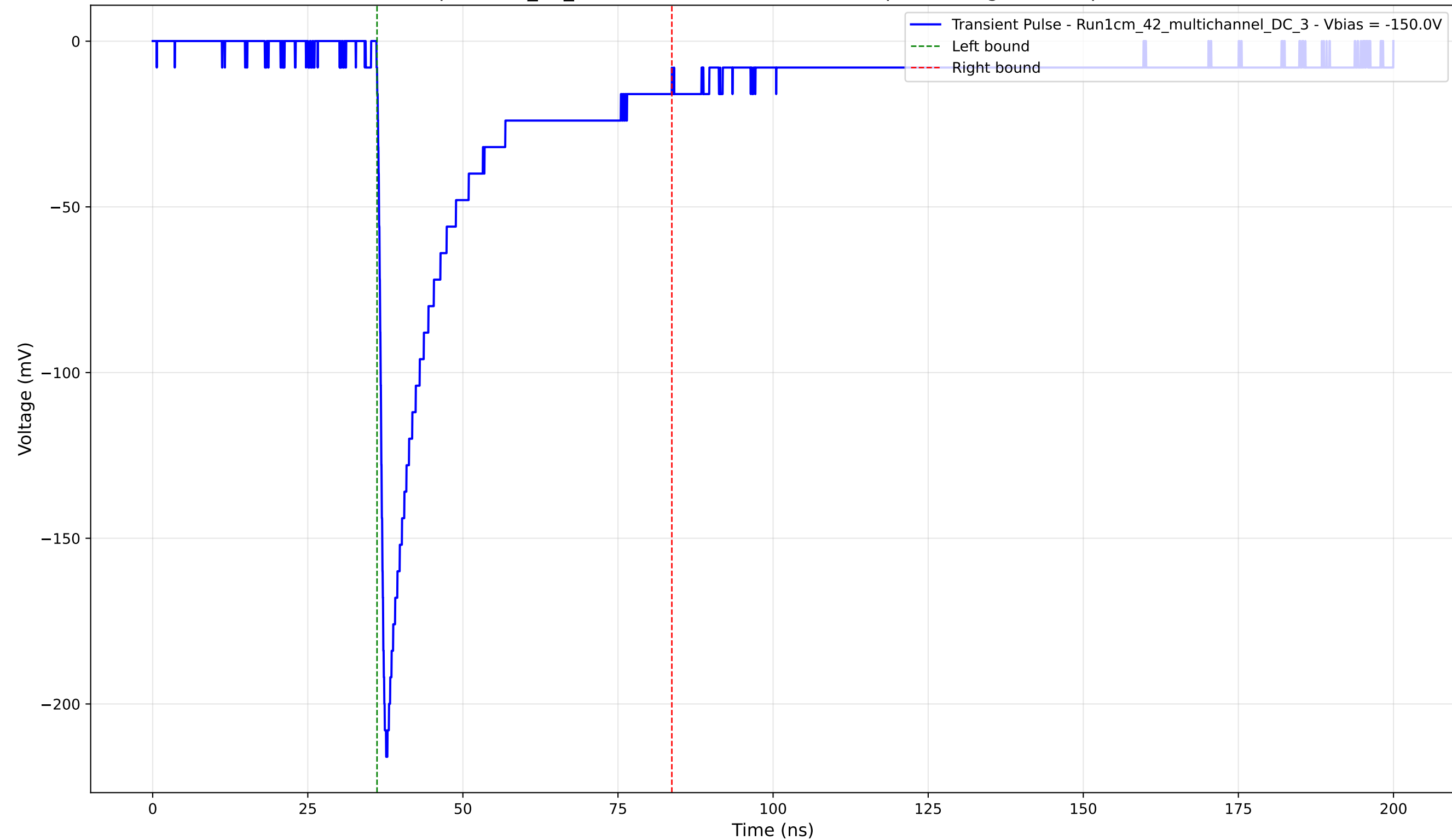
Transient Pulse - Sample: 1cm_42_multichannel - Position: 740.0 \mu\text{m} - Charge: 45.86 pC - Rise Time: 1.05 ns
