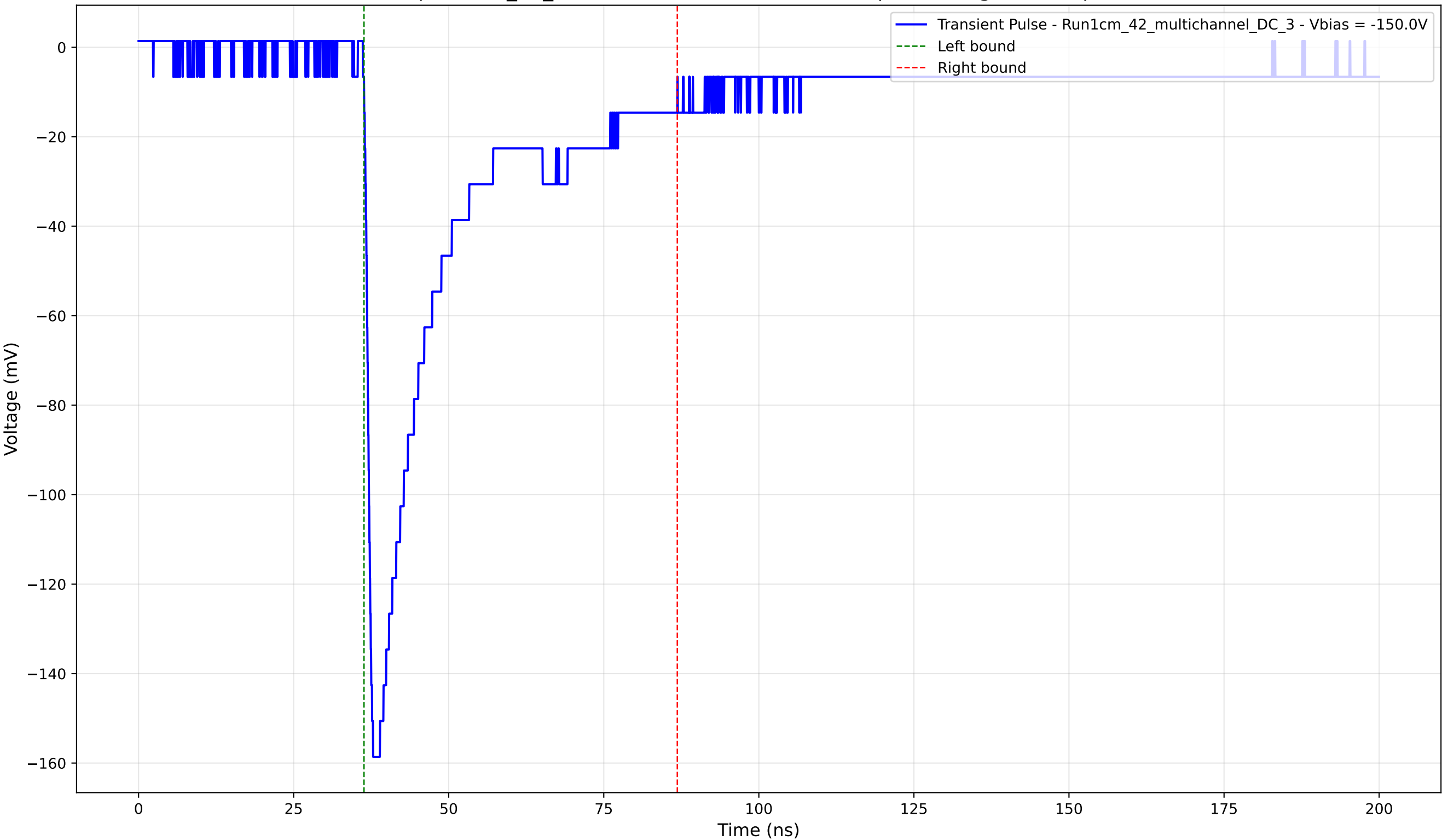
Transient Pulse - Sample: 1cm_42_multichannel - Position: 1110.0 \mu\text{m} - Charge: 42.78 pC - Rise Time: 1.20 ns
