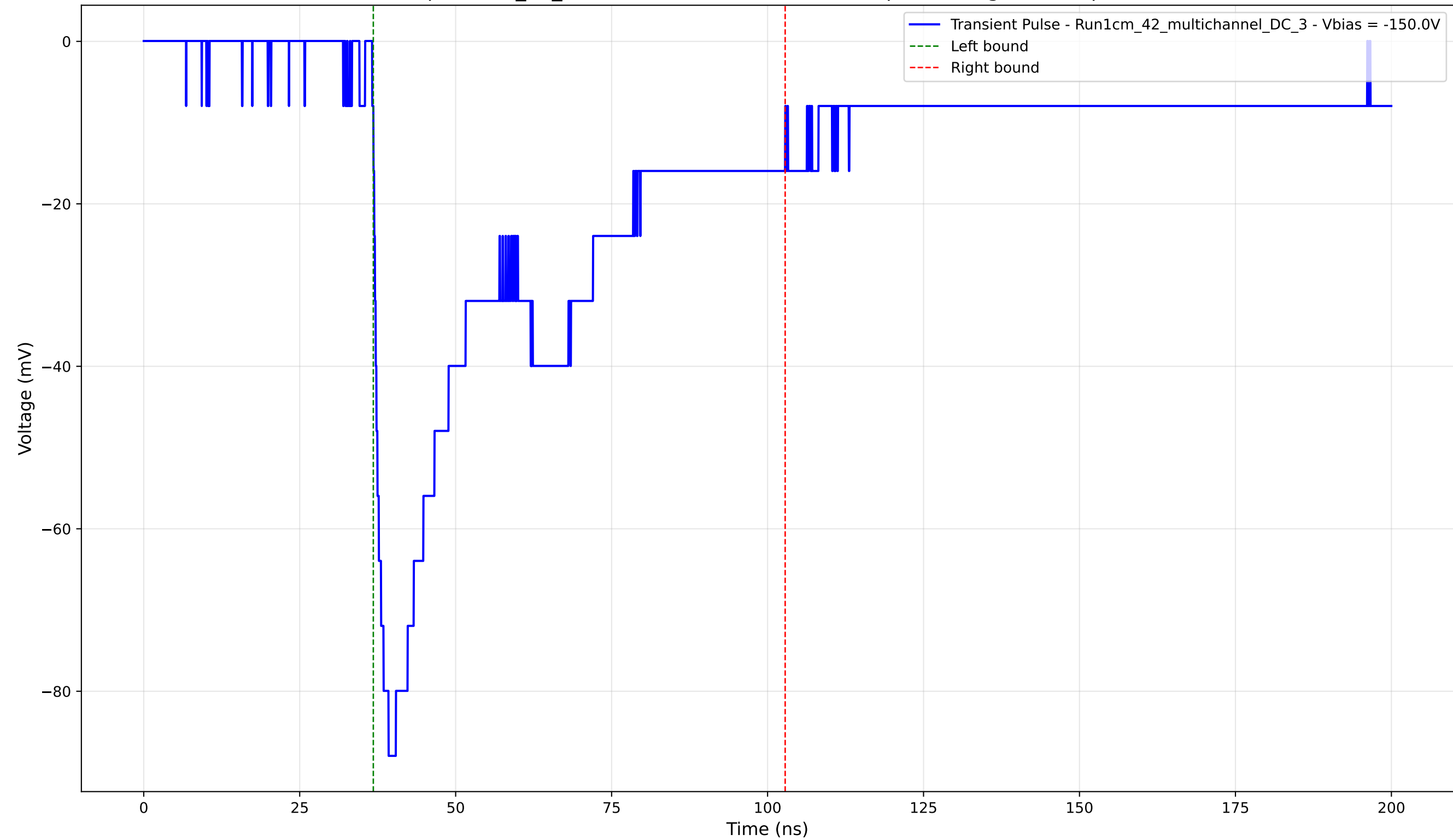
Transient Pulse - Sample: 1cm_42_multichannel - Position: 2250.0 \mu\text{m} - Charge: 42.55 pC - Rise Time: 1.64 ns
