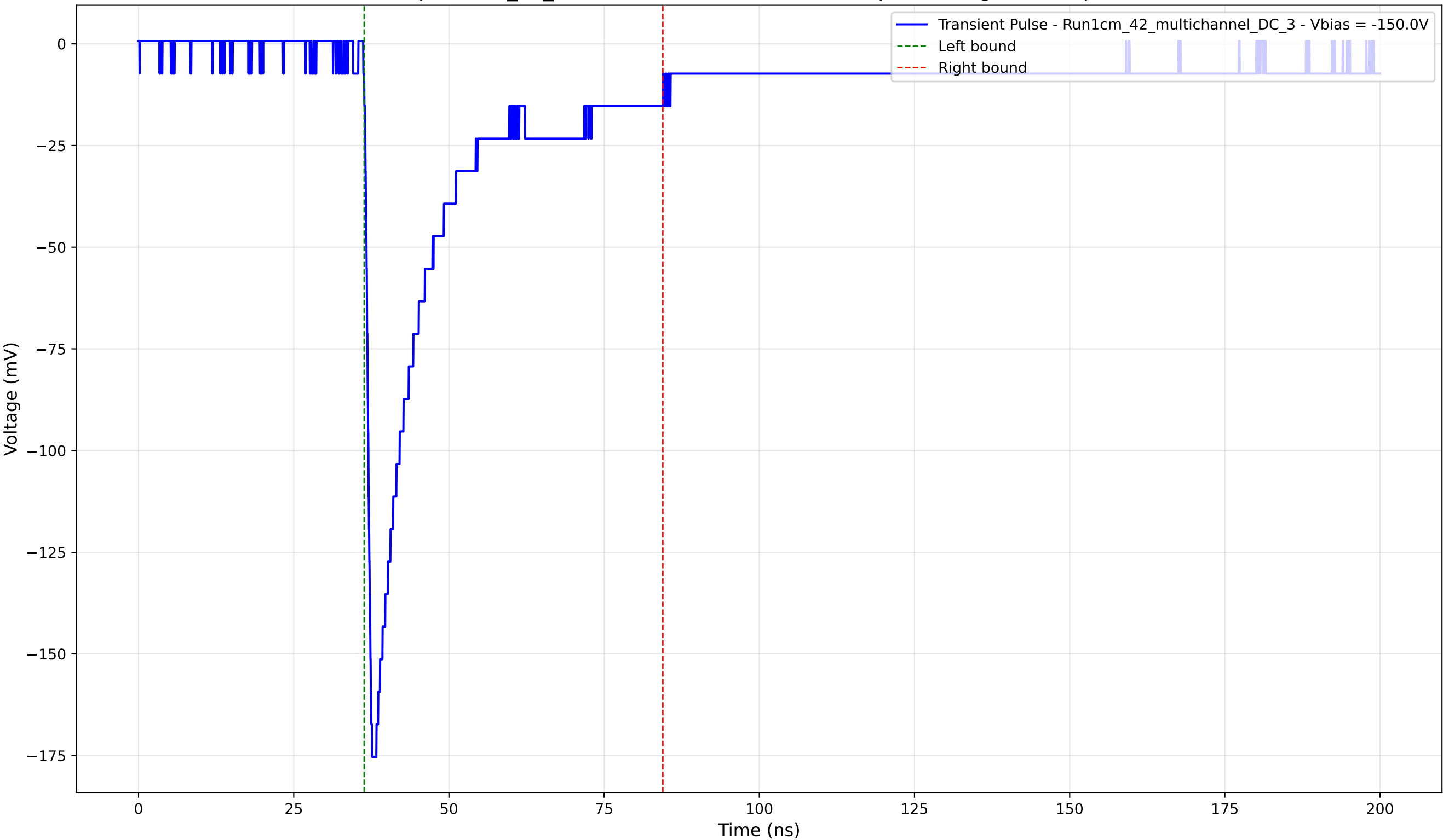
Transient Pulse - Sample: 1cm_42_multichannel - Position: 4085.0 \mu\text{m} - Charge: 39.40 pC - Rise Time: 0.95 ns
