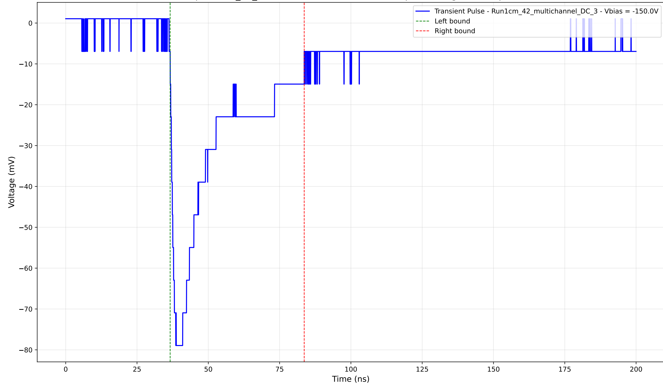
Transient Pulse - Sample: 1cm_42_multichannel - Position: 2945.0 \mu\text{m} - Charge: 28.76 pC - Rise Time: 1.96 ns
