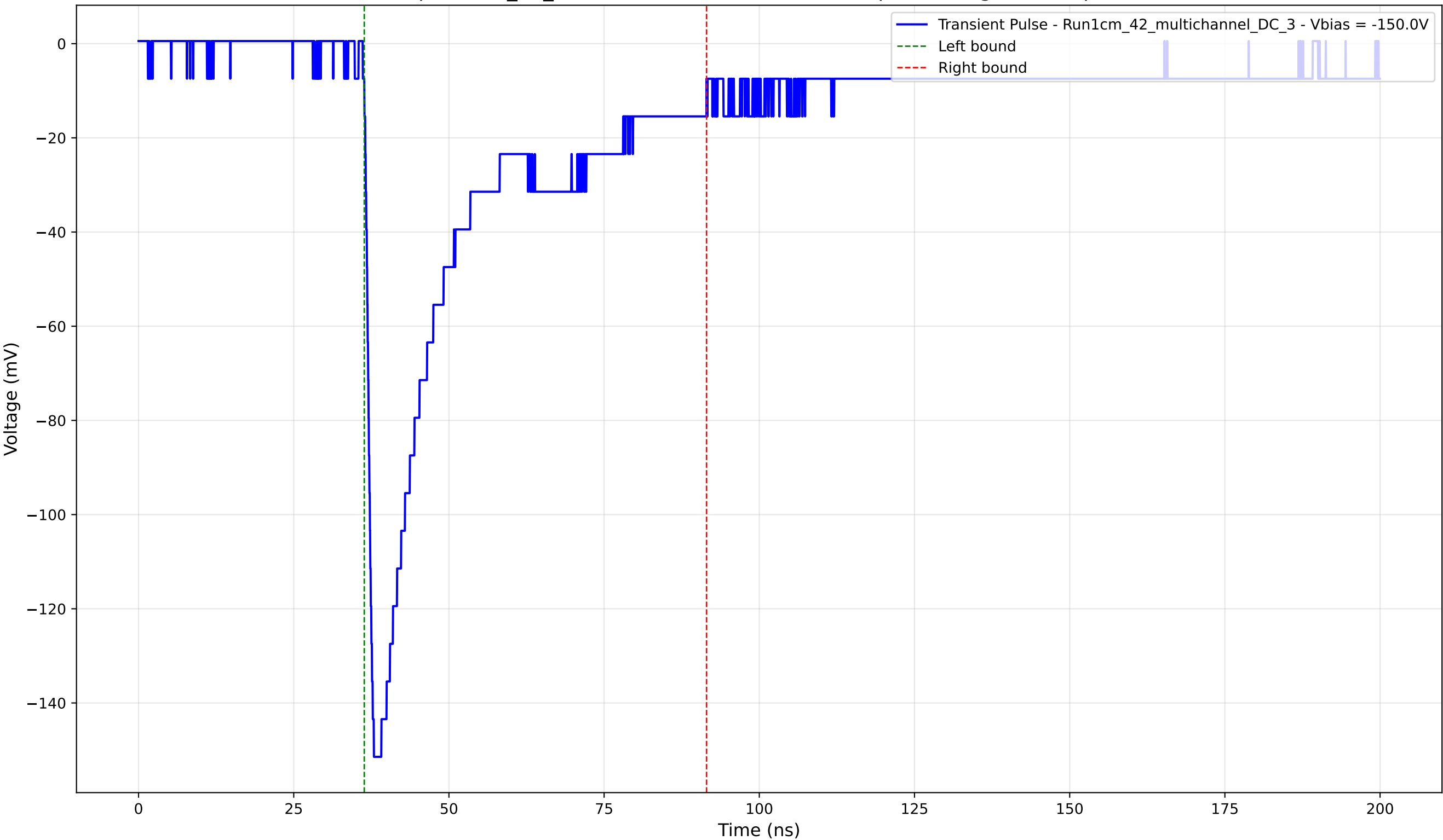
Transient Pulse - Sample: 1cm_42_multichannel - Position: 1250.0 \mu\text{m} - Charge: 46.09 pC - Rise Time: 1.34 ns
