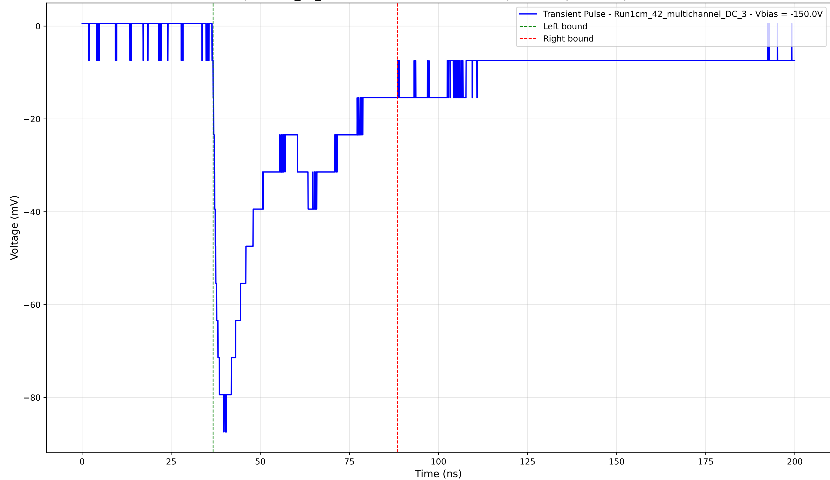
Transient Pulse - Sample: 1cm_42_multichannel - Position: 2620.0 \mu\text{m} - Charge: 35.38 pC - Rise Time: 1.76 ns
