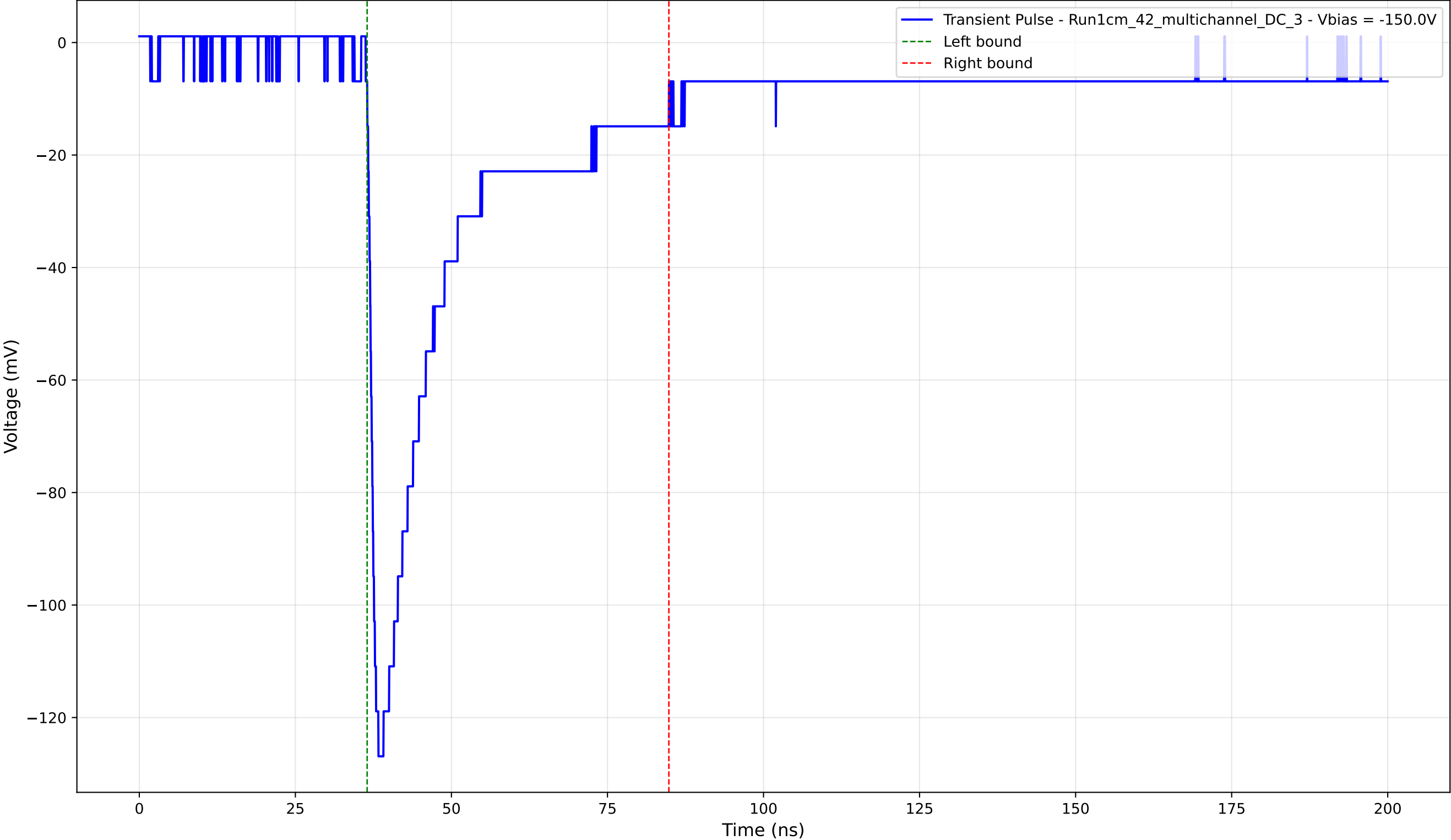
Transient Pulse - Sample: 1cm_42_multichannel - Position: 3605.0 \mu\text{m} - Charge: 35.72 pC - Rise Time: 1.41 ns
