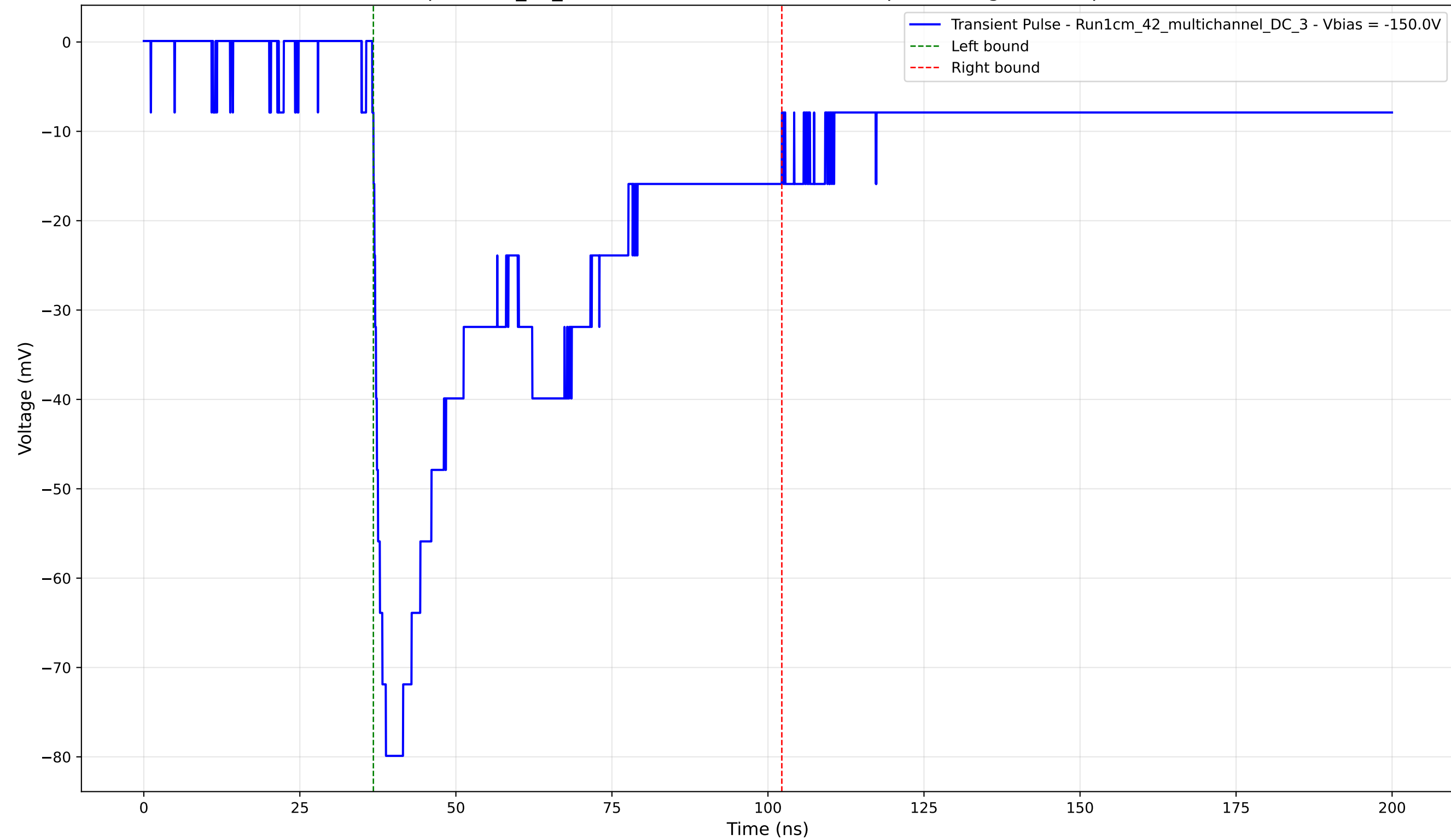
Transient Pulse - Sample: 1cm_42_multichannel - Position: 2485.0 \mu\text{m} - Charge: 41.11 pC - Rise Time: 2.00 ns
