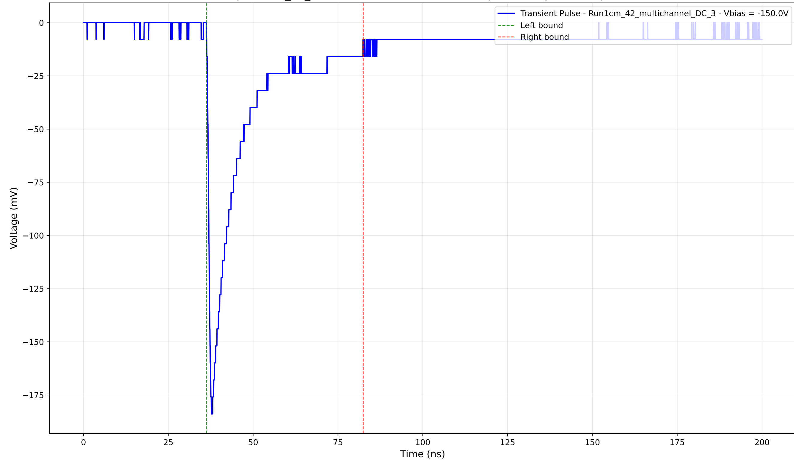
Transient Pulse - Sample: 1cm_42_multichannel - Position: 4120.0 \mu\text{m} - Charge: 39.54 pC - Rise Time: 0.99 ns
