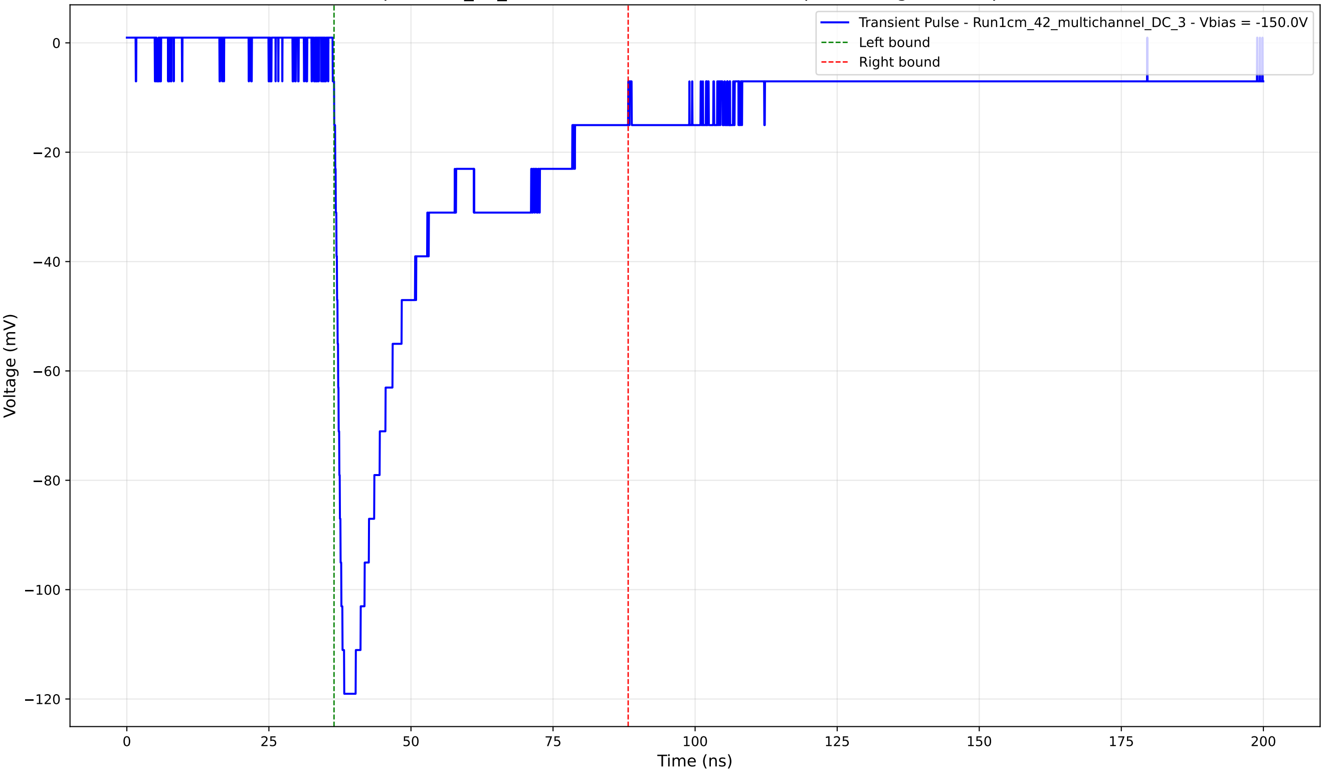
Transient Pulse - Sample: 1cm_42_multichannel - Position: 1620.0 \mu\text{m} - Charge: 41.21 pC - Rise Time: 1.47 ns
