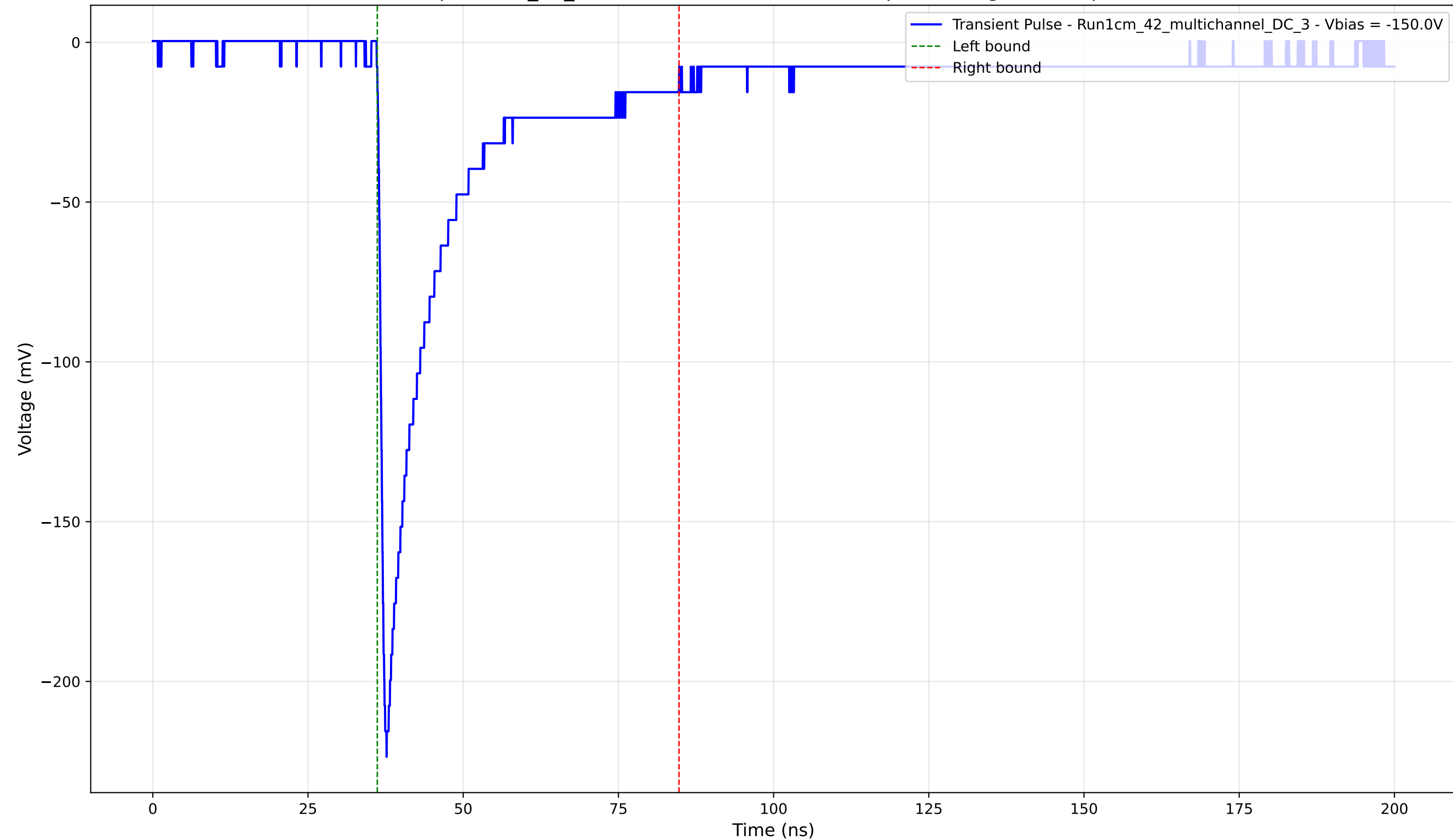
Transient Pulse - Sample: 1cm_42_multichannel - Position: 715.0 \mu\text{m} - Charge: 46.10 pC - Rise Time: 1.06 ns
