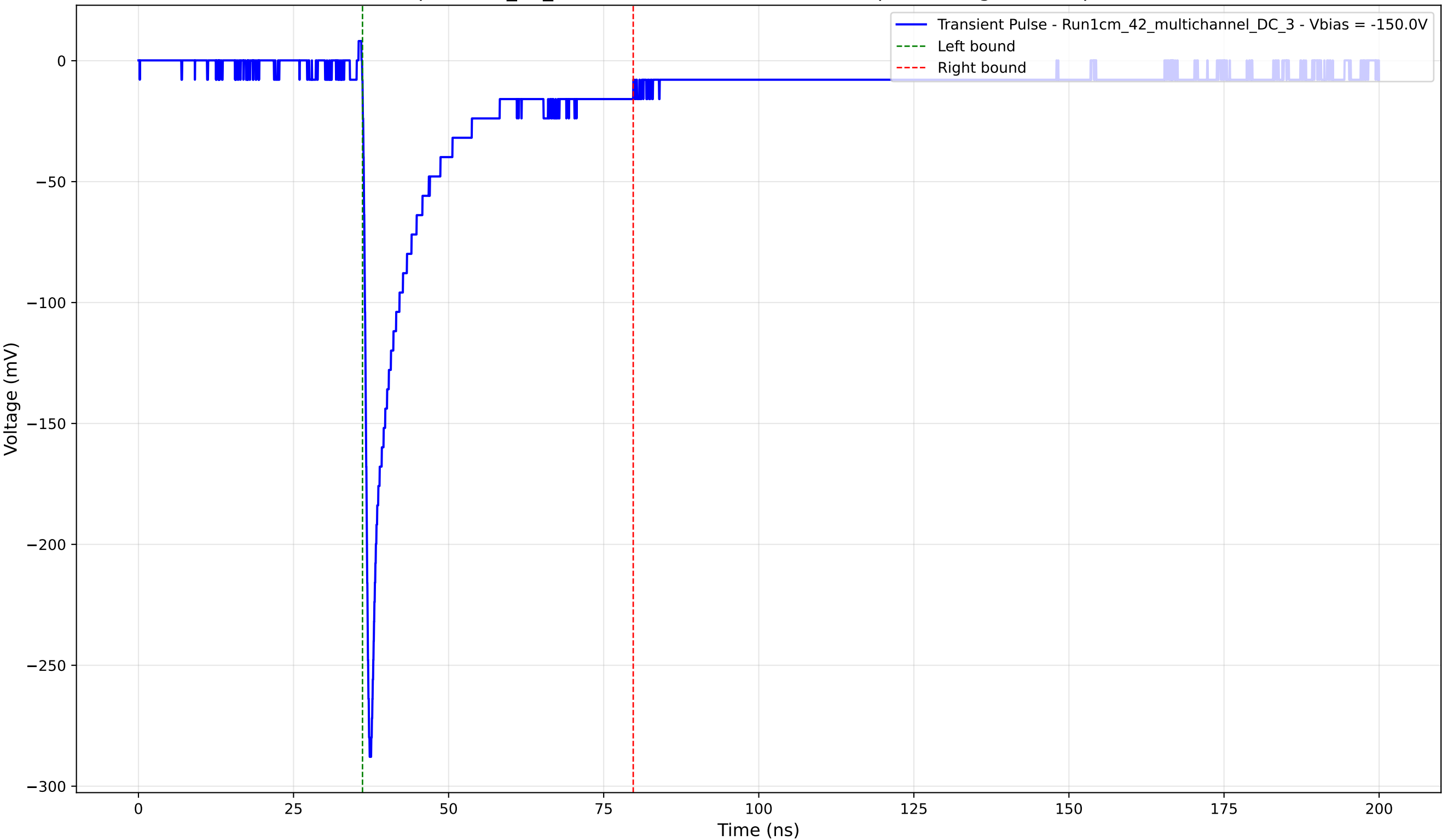
Transient Pulse - Sample: 1cm_42_multichannel - Position: 4570.0 \mu\text{m} - Charge: 40.85 pC - Rise Time: 0.85 ns
