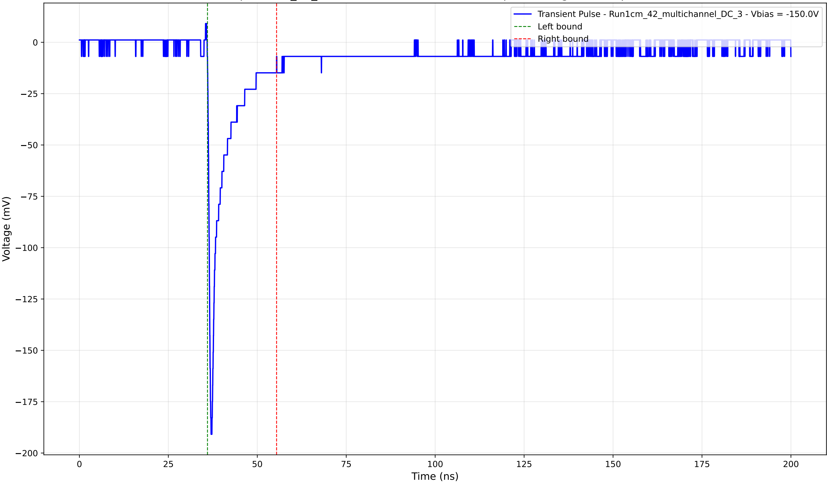
Transient Pulse - Sample: 1cm_42_multichannel - Position: 4850.0 \mu\text{m} - Charge: 17.26 pC - Rise Time: 0.77 ns
