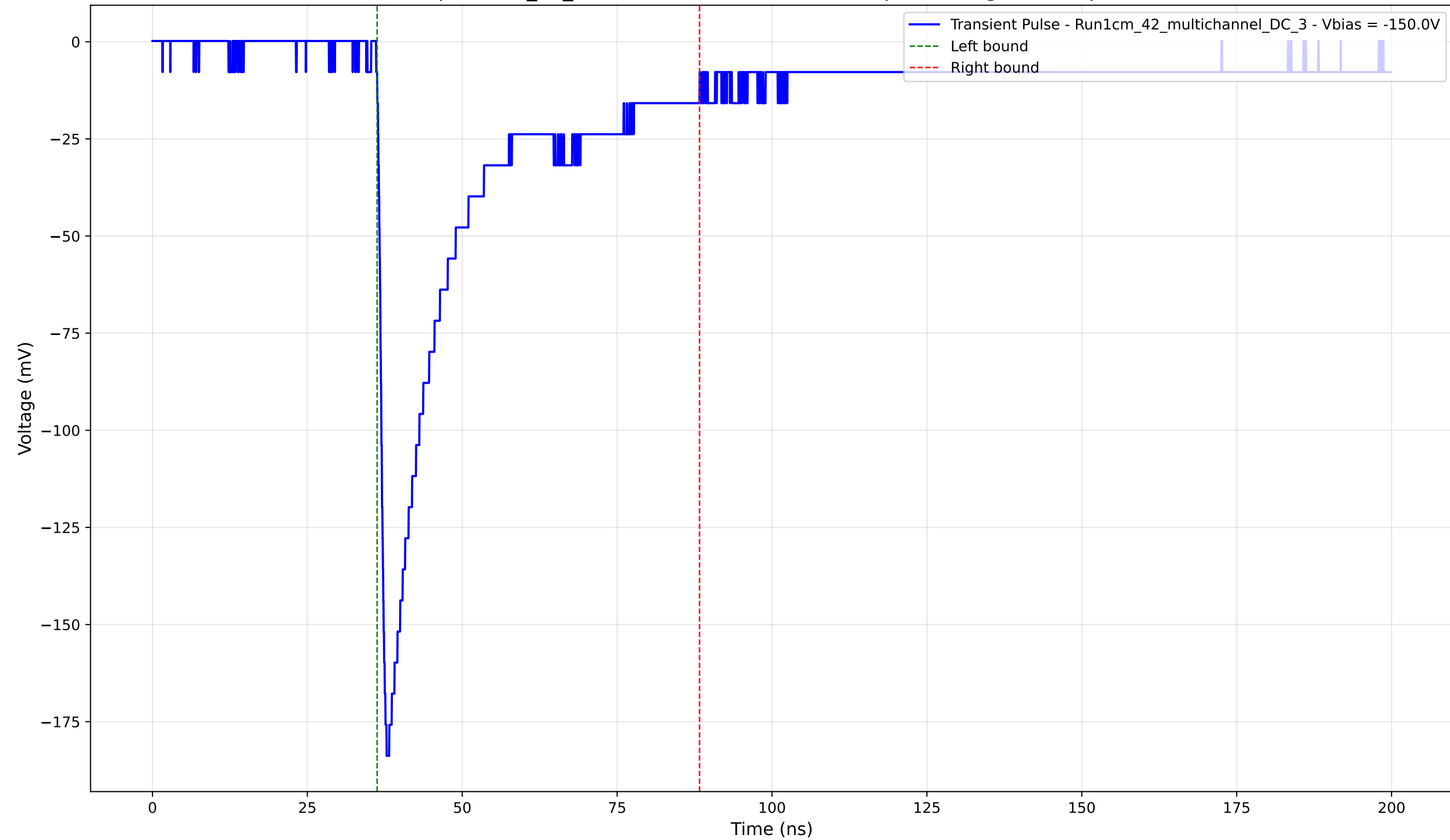
Transient Pulse - Sample: 1cm_42_multichannel - Position: 980.0 \mu\text{m} - Charge: 46.46 pC - Rise Time: 1.09 ns
