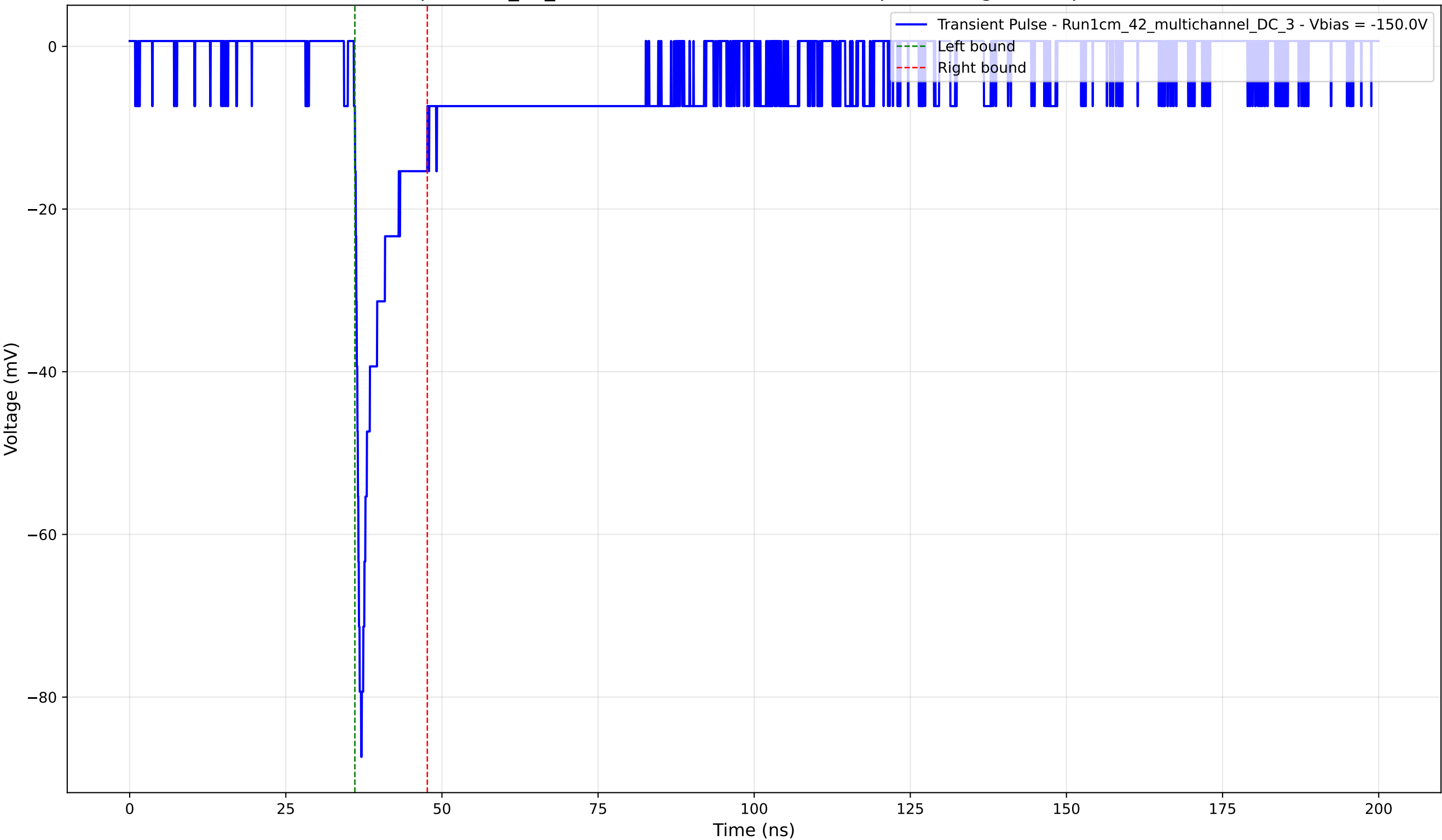
Transient Pulse - Sample: 1cm_42_multichannel - Position: 4865.0 \mu\text{m} - Charge: 6.92 pC - Rise Time: 0.76 ns
