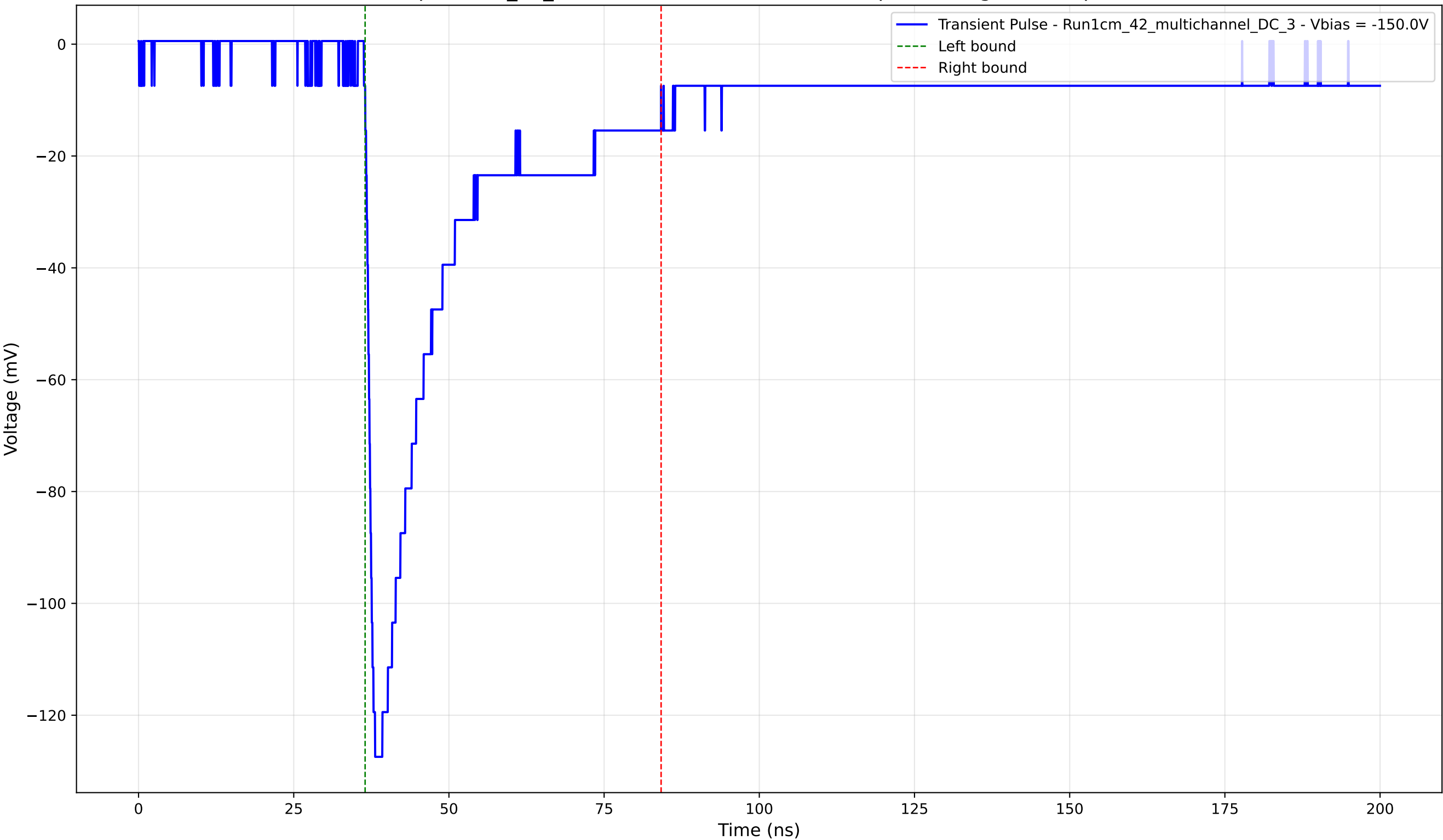
Transient Pulse - Sample: 1cm_42_multichannel - Position: 3630.0 \mu\text{m} - Charge: 36.13 pC - Rise Time: 1.33 ns
