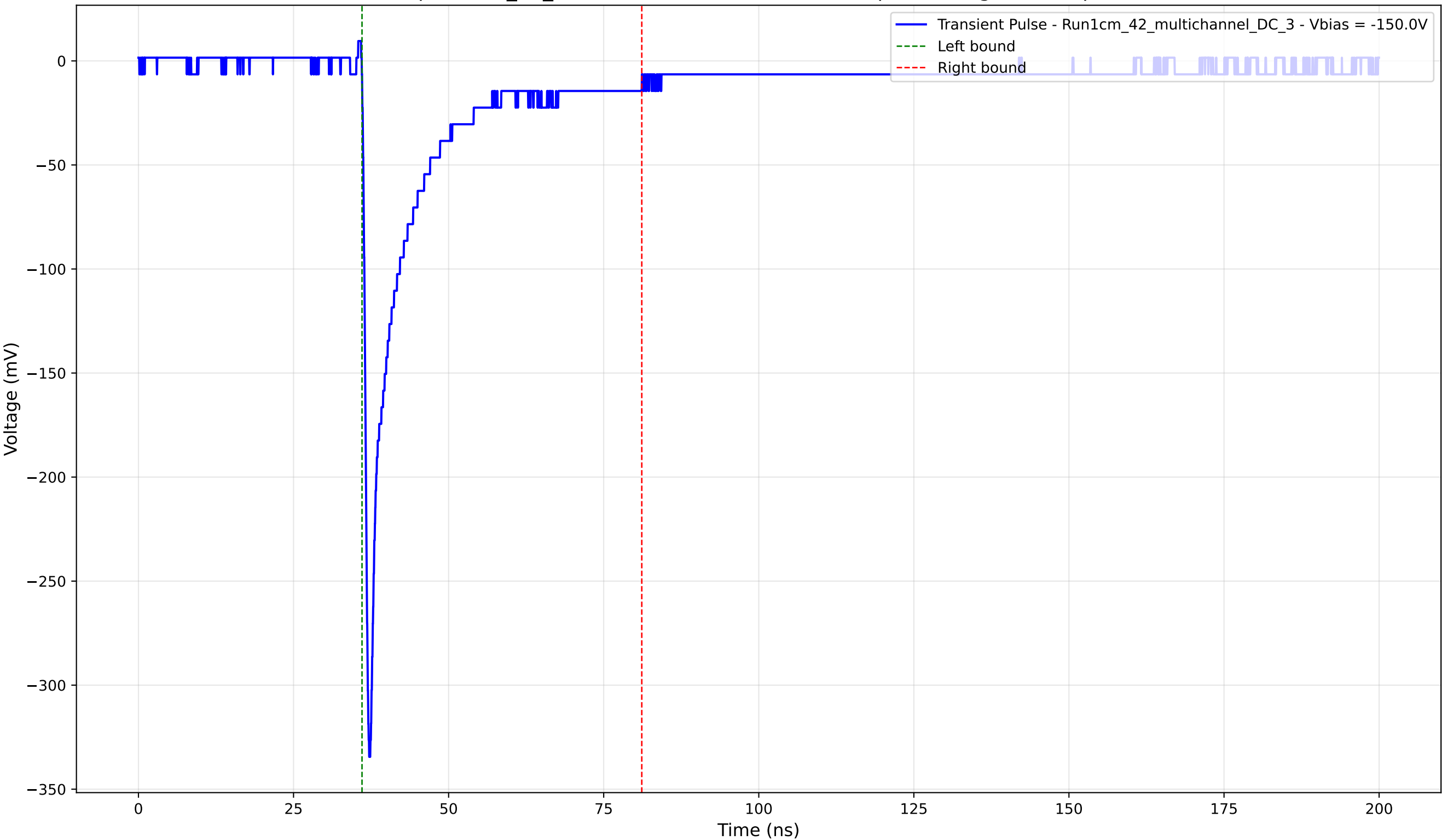
Transient Pulse - Sample: 1cm_42_multichannel - Position: 4675.0 \mu\text{m} - Charge: 42.12 pC - Rise Time: 0.81 ns
