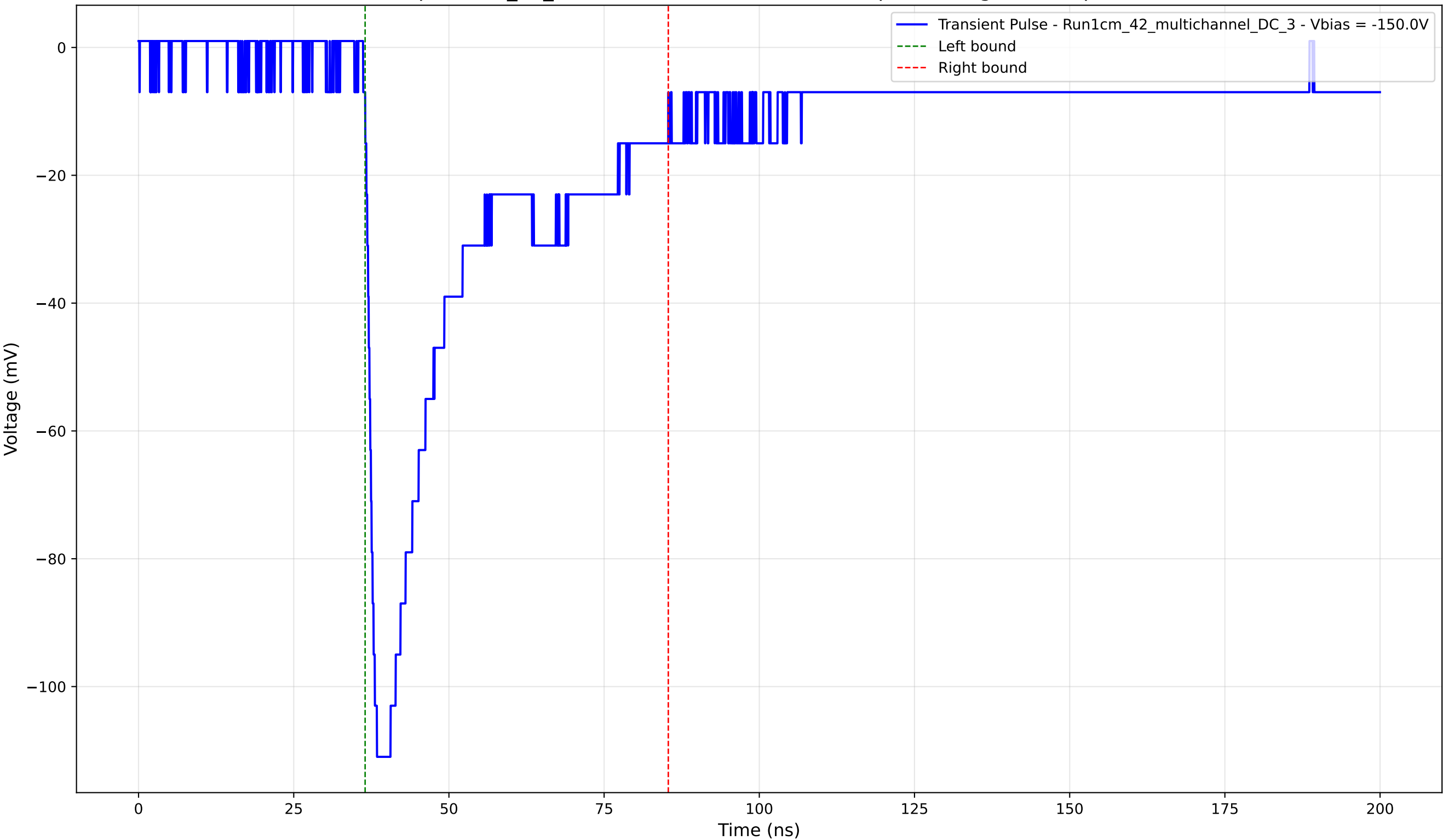
Transient Pulse - Sample: 1cm_42_multichannel - Position: 3250.0 \mu\text{m} - Charge: 37.31 pC - Rise Time: 1.55 ns
