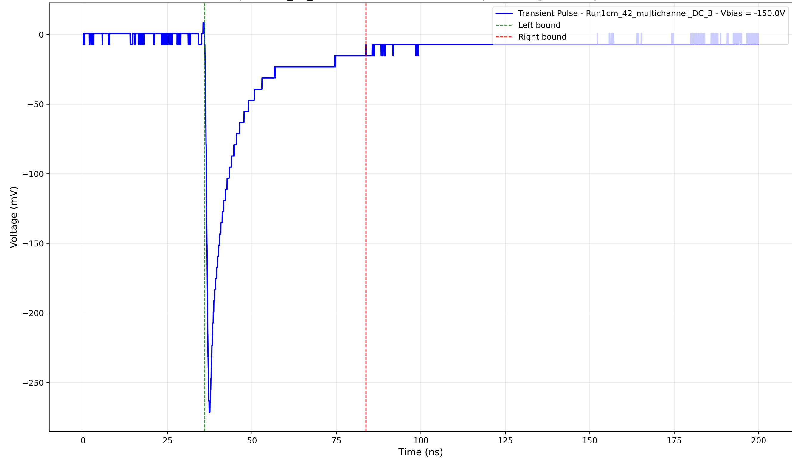
Transient Pulse - Sample: 1cm_42_multichannel - Position: 505.0 \mu\text{m} - Charge: 47.96 pC - Rise Time: 0.91 ns
