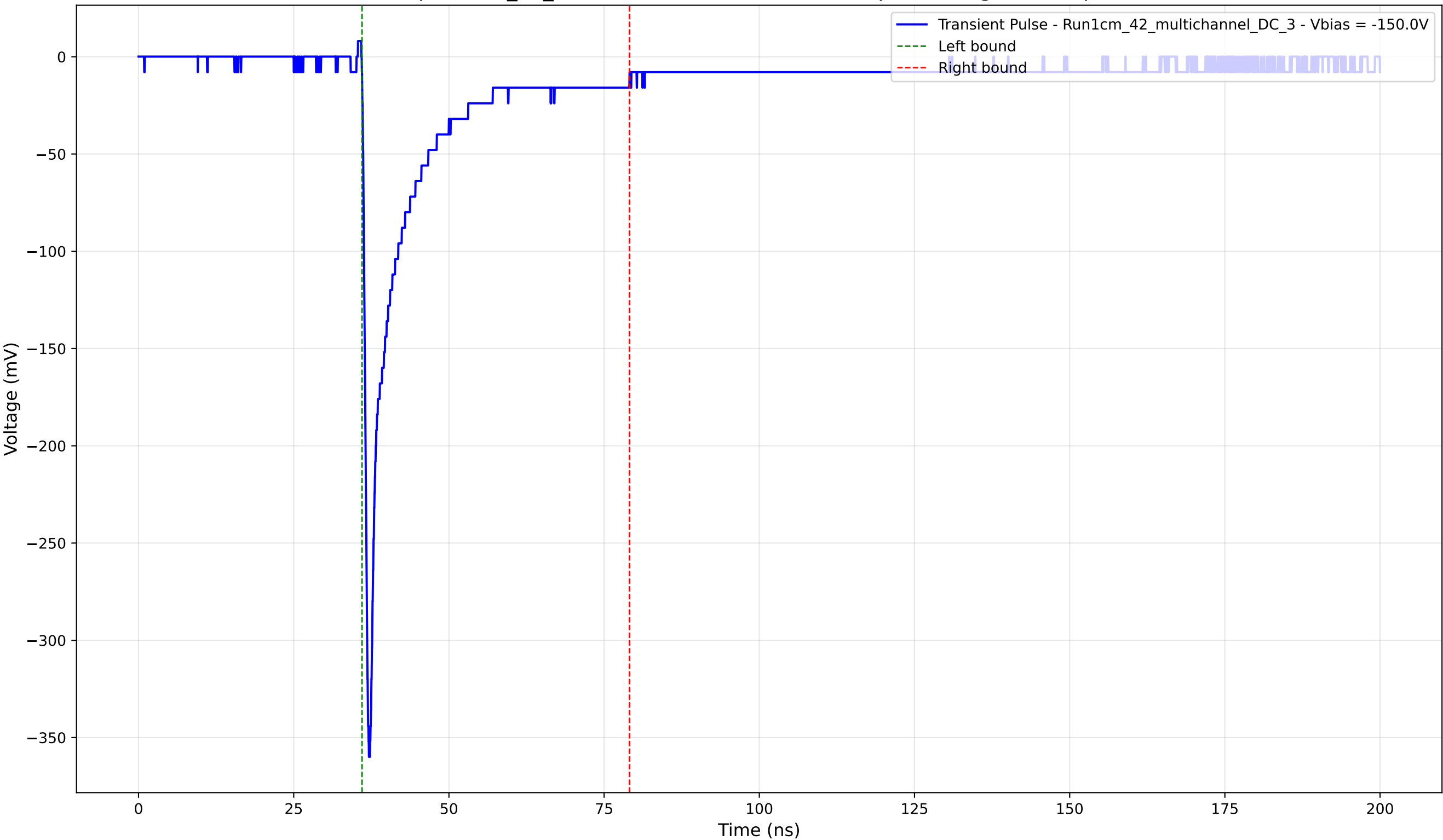
Transient Pulse - Sample: 1cm_42_multichannel - Position: 4770.0 \mu\text{m} - Charge: 41.63 pC - Rise Time: 0.80 ns
