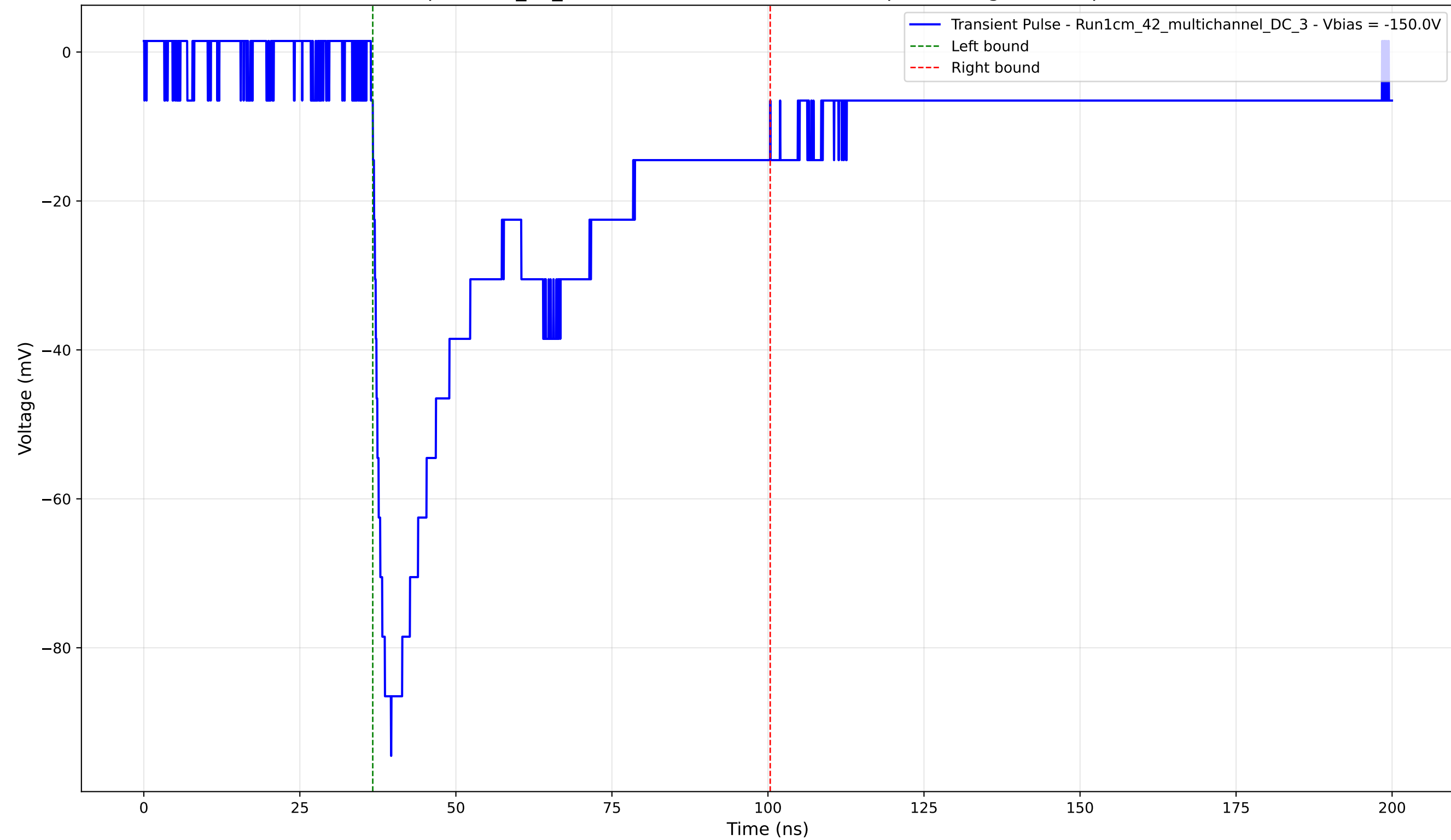
Transient Pulse - Sample: 1cm_42_multichannel - Position: 2710.0 \mu\text{m} - Charge: 39.71 pC - Rise Time: 1.93 ns
