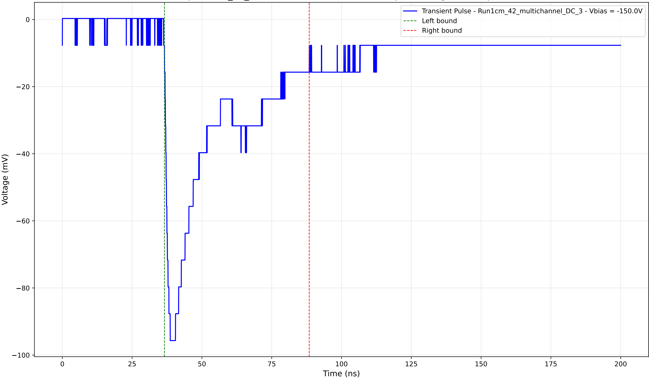
Transient Pulse - Sample: 1cm_42_multichannel - Position: 1955.0 \mu\text{m} - Charge: 37.60 pC - Rise Time: 1.60 ns
