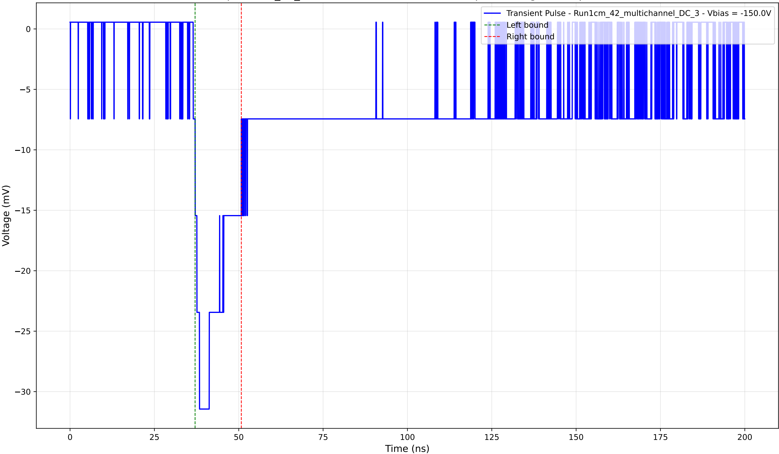
Transient Pulse - Sample: 1cm_42_multichannel - Position: 2920.0 \mu\text{m} - Charge: 5.94 pC - Rise Time: 1.87 ns
