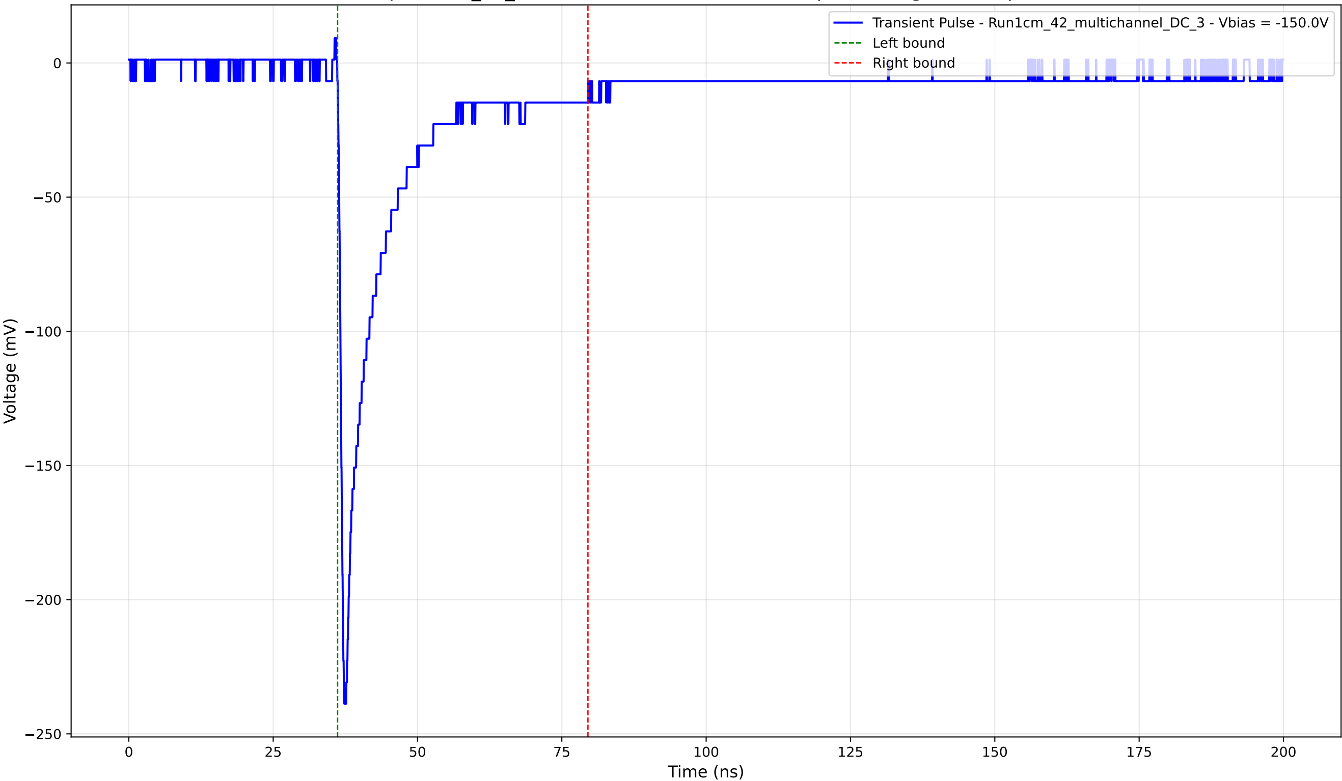
Transient Pulse - Sample: 1cm_42_multichannel - Position: 4480.0 \mu\text{m} - Charge: 36.59 pC - Rise Time: 0.88 ns
