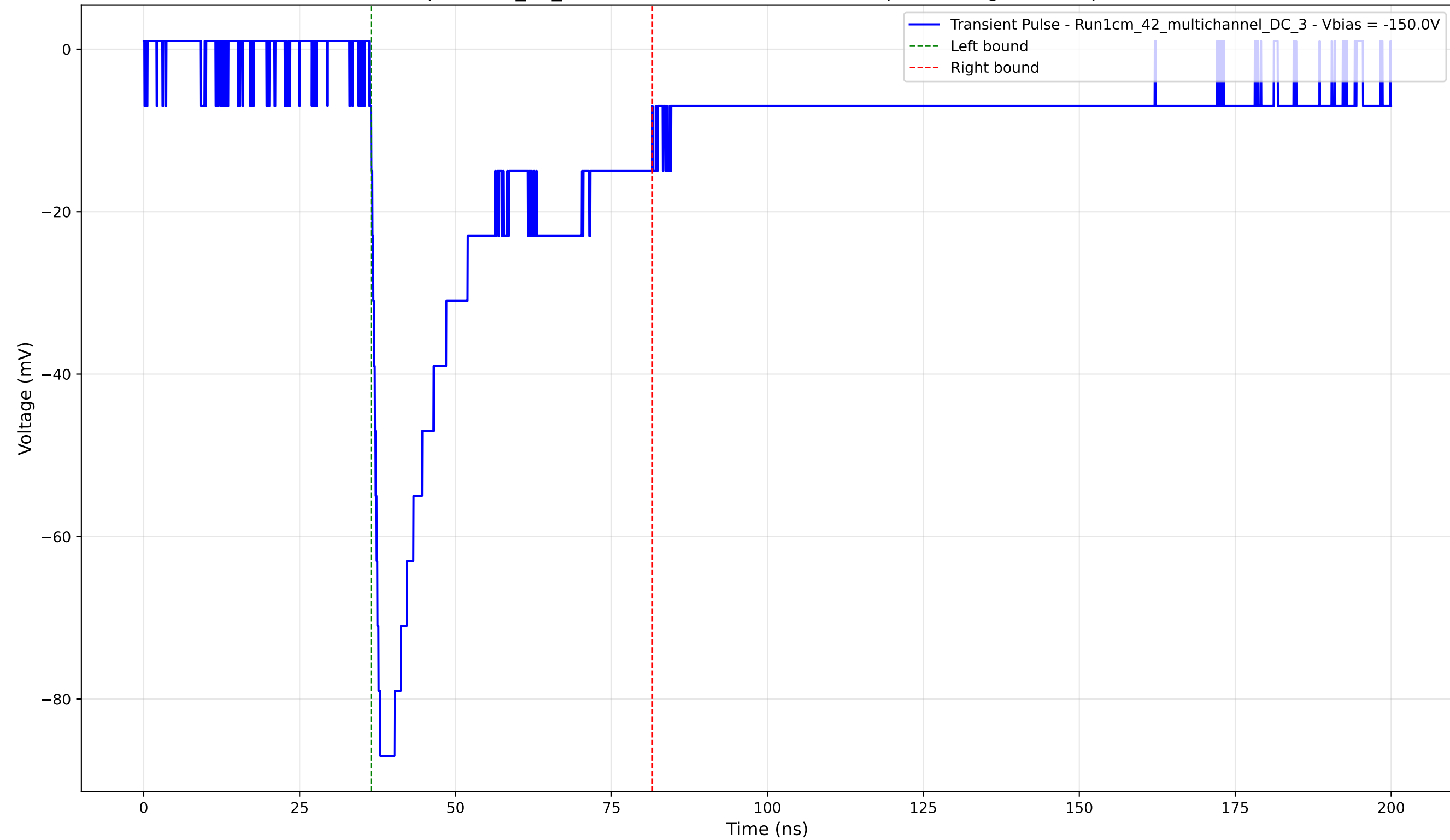
Transient Pulse - Sample: 1cm_42_multichannel - Position: 1420.0 \mu\text{m} - Charge: 27.75 pC - Rise Time: 1.18 ns
