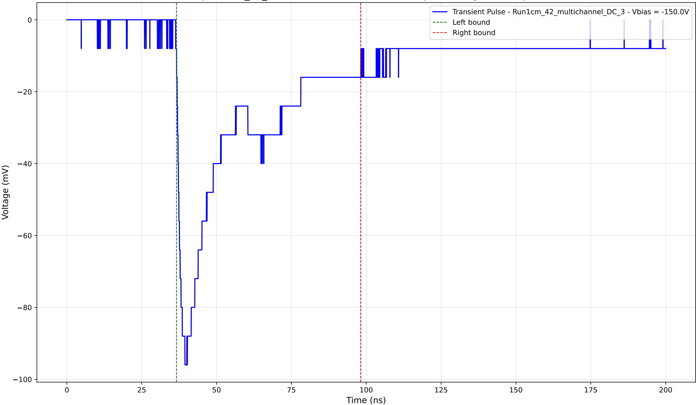
Transient Pulse - Sample: 1cm_42_multichannel - Position: 2755.0 \mu\text{m} - Charge: 40.31 pC - Rise Time: 1.92 ns
