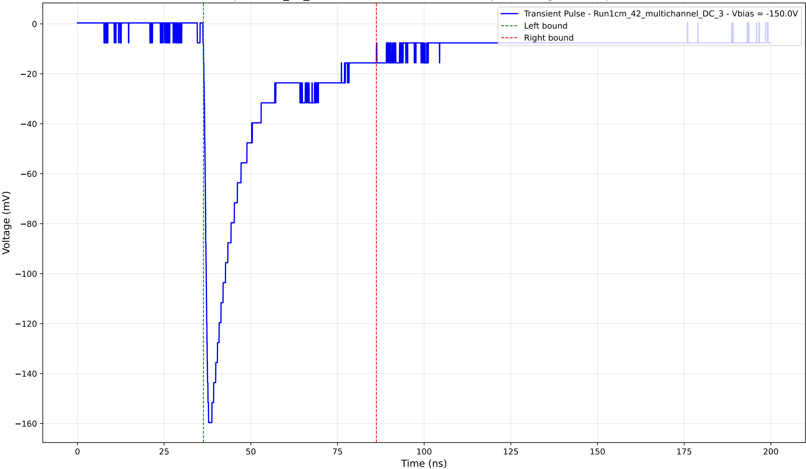
Transient Pulse - Sample: 1cm_42_multichannel - Position: 1100.0 \mu\text{m} - Charge: 43.45 pC - Rise Time: 1.20 ns
