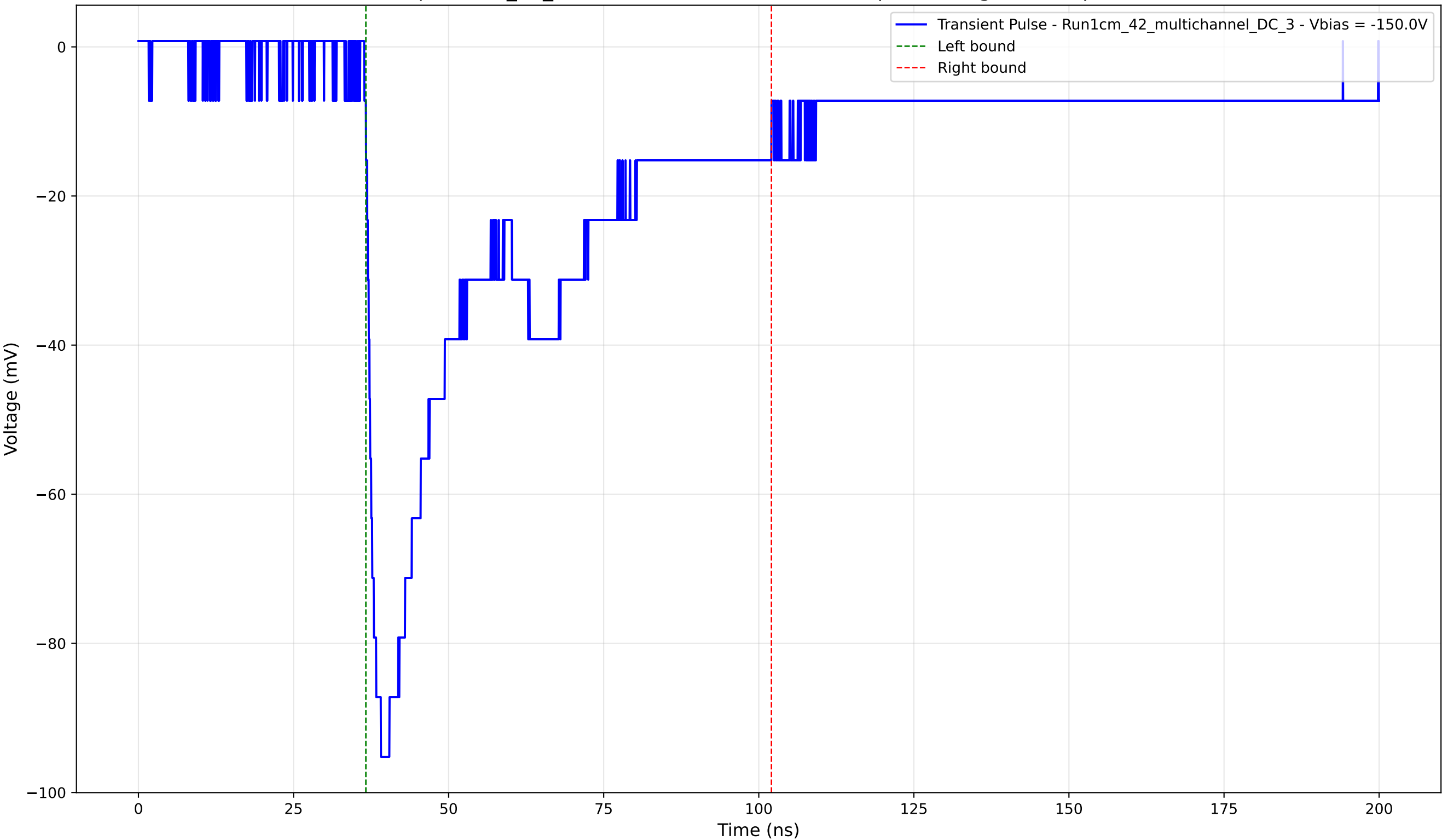
Transient Pulse - Sample: 1cm_42_multichannel - Position: 2055.0 \mu\text{m} - Charge: 42.69 pC - Rise Time: 1.65 ns
