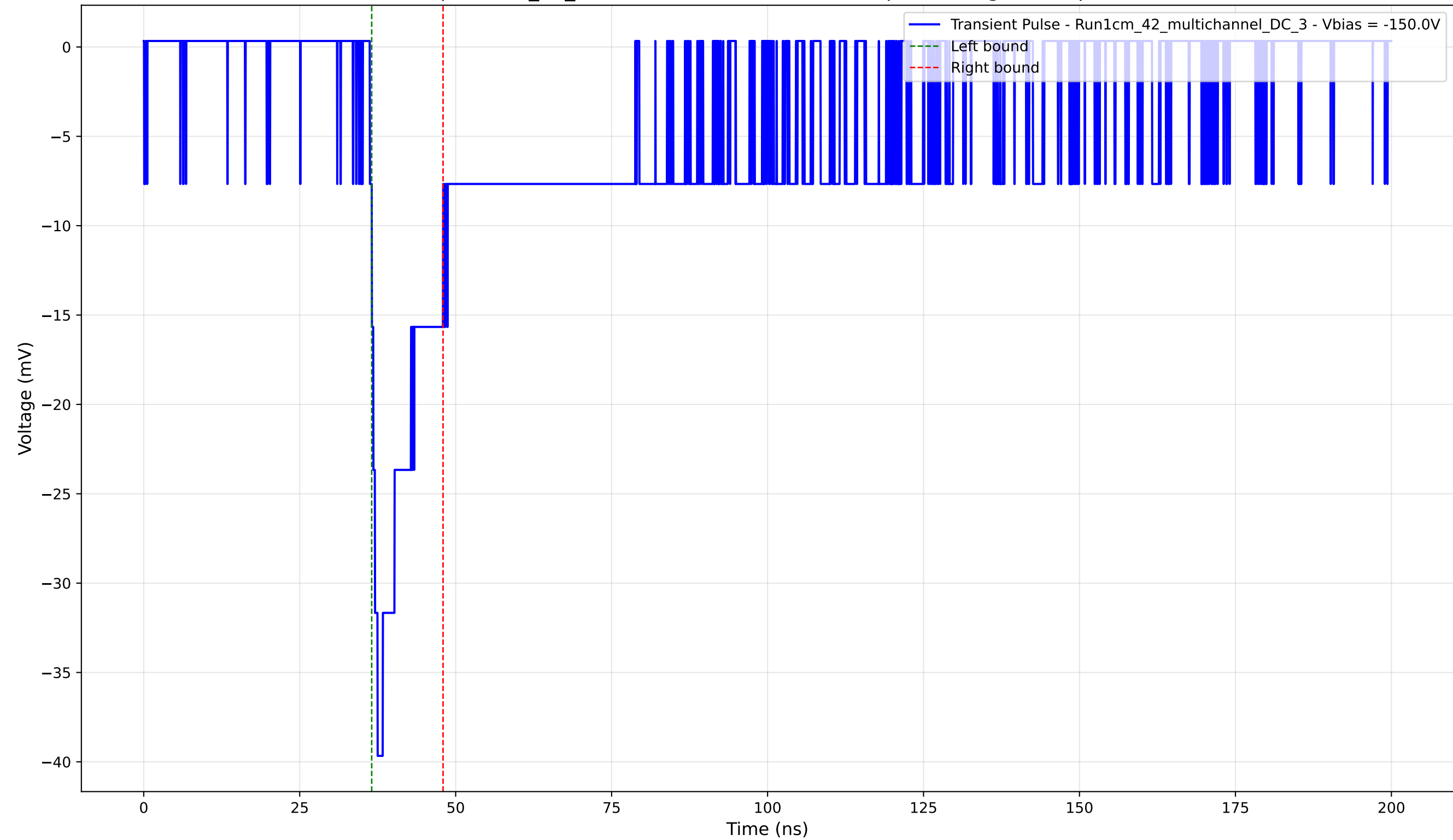
Transient Pulse - Sample: 1cm_42_multichannel - Position: 825.0 \mu\text{m} - Charge: 5.21 pC - Rise Time: 1.25 ns
