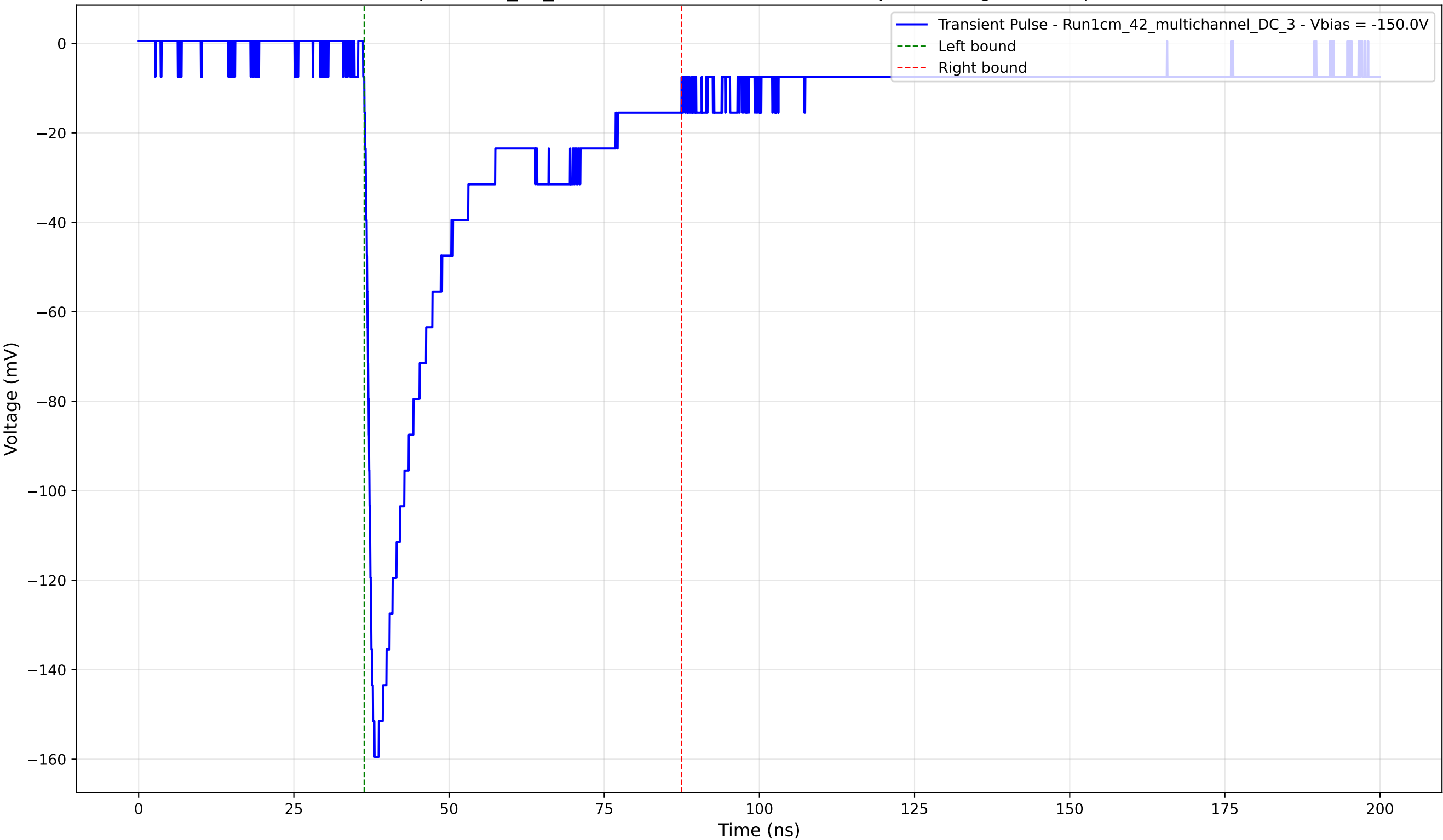
Transient Pulse - Sample: 1cm_42_multichannel - Position: 1165.0 \mu\text{m} - Charge: 44.15 pC - Rise Time: 1.28 ns
