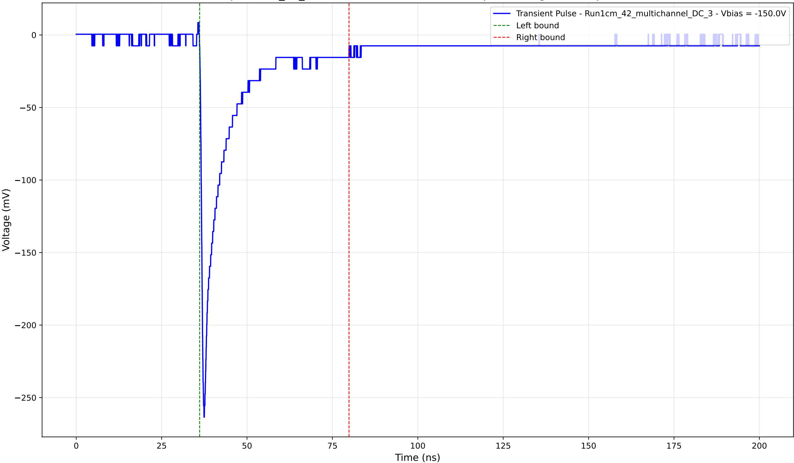
Transient Pulse - Sample: 1cm_42_multichannel - Position: 4500.0 \mu\text{m} - Charge: 39.55 pC - Rise Time: 0.87 ns
