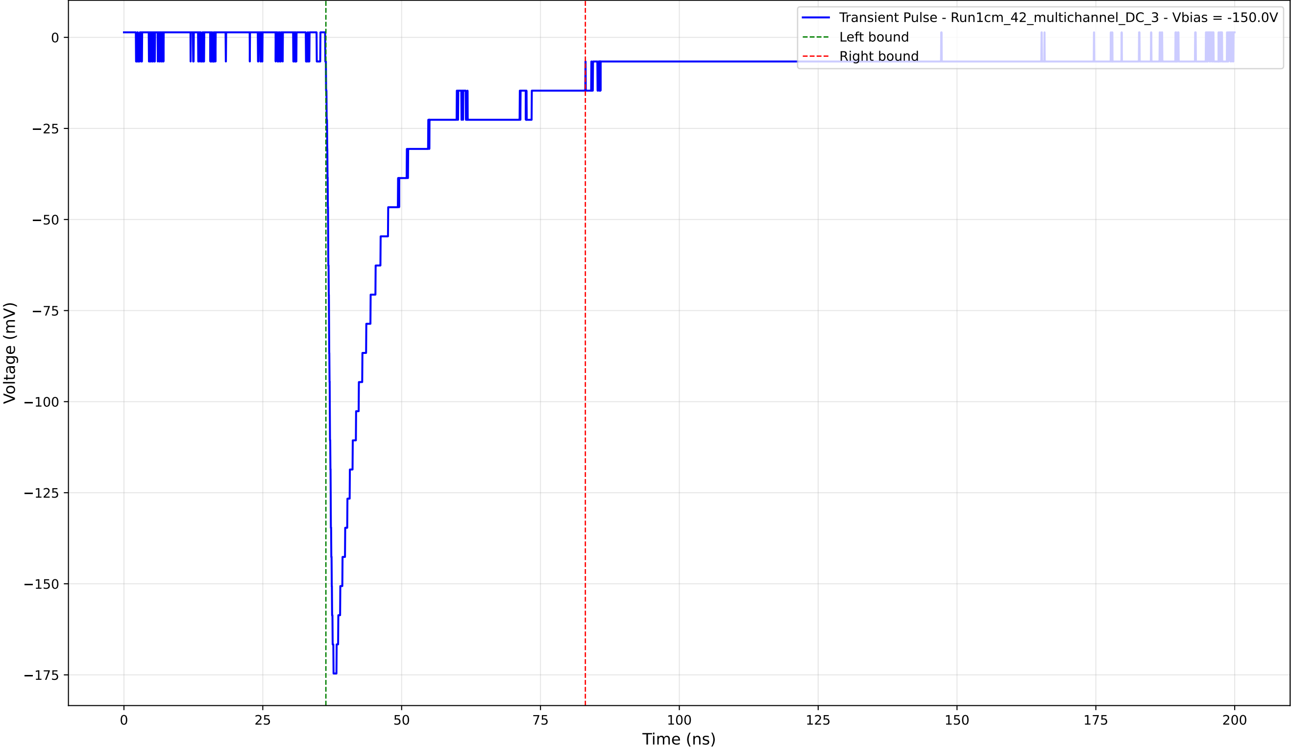
Transient Pulse - Sample: 1cm_42_multichannel - Position: 4035.0 \mu\text{m} - Charge: 38.65 pC - Rise Time: 0.99 ns
