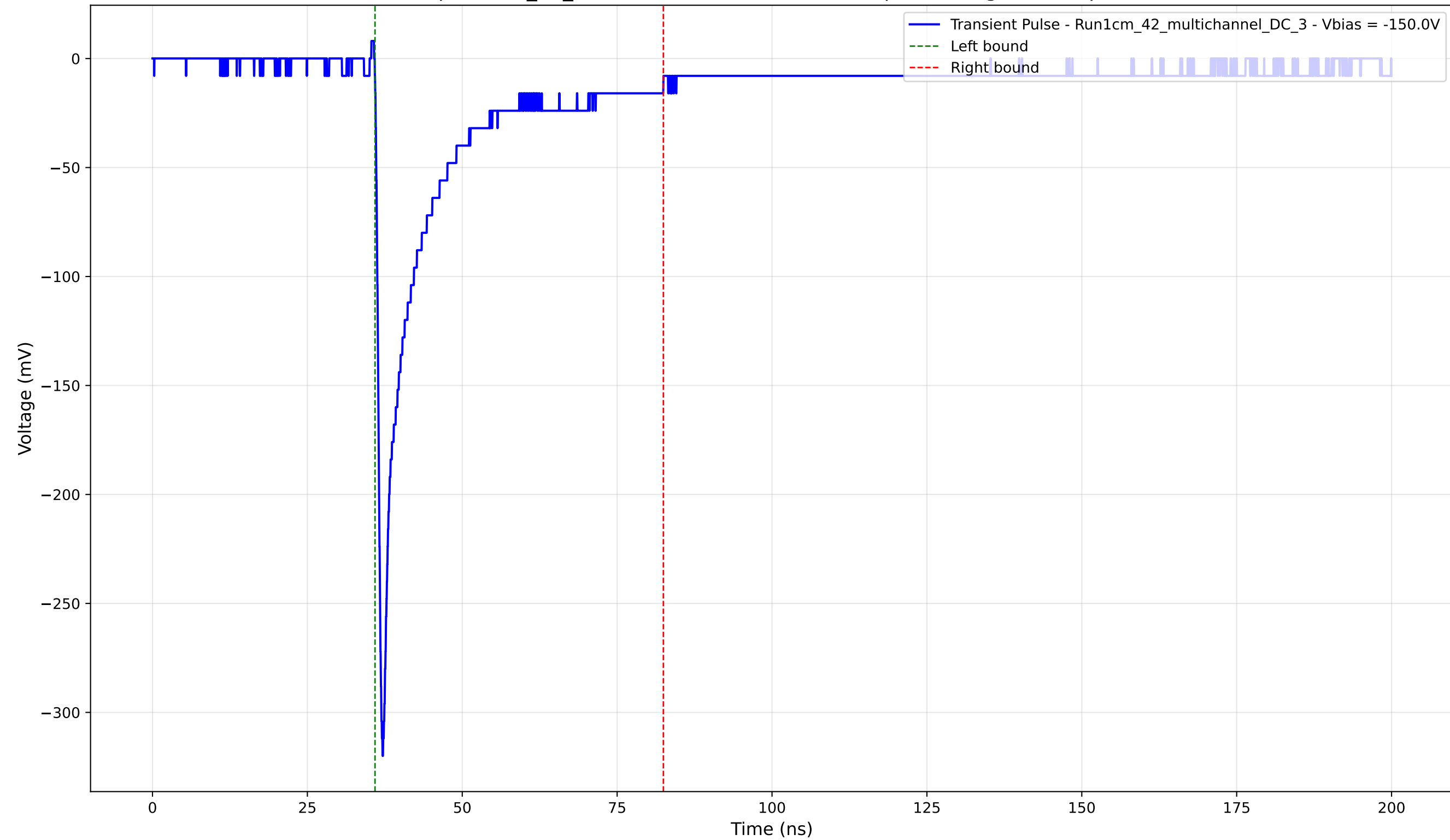
Transient Pulse - Sample: 1cm_42_multichannel - Position: 255.0 \mu\text{m} - Charge: 45.30 pC - Rise Time: 0.86 ns
