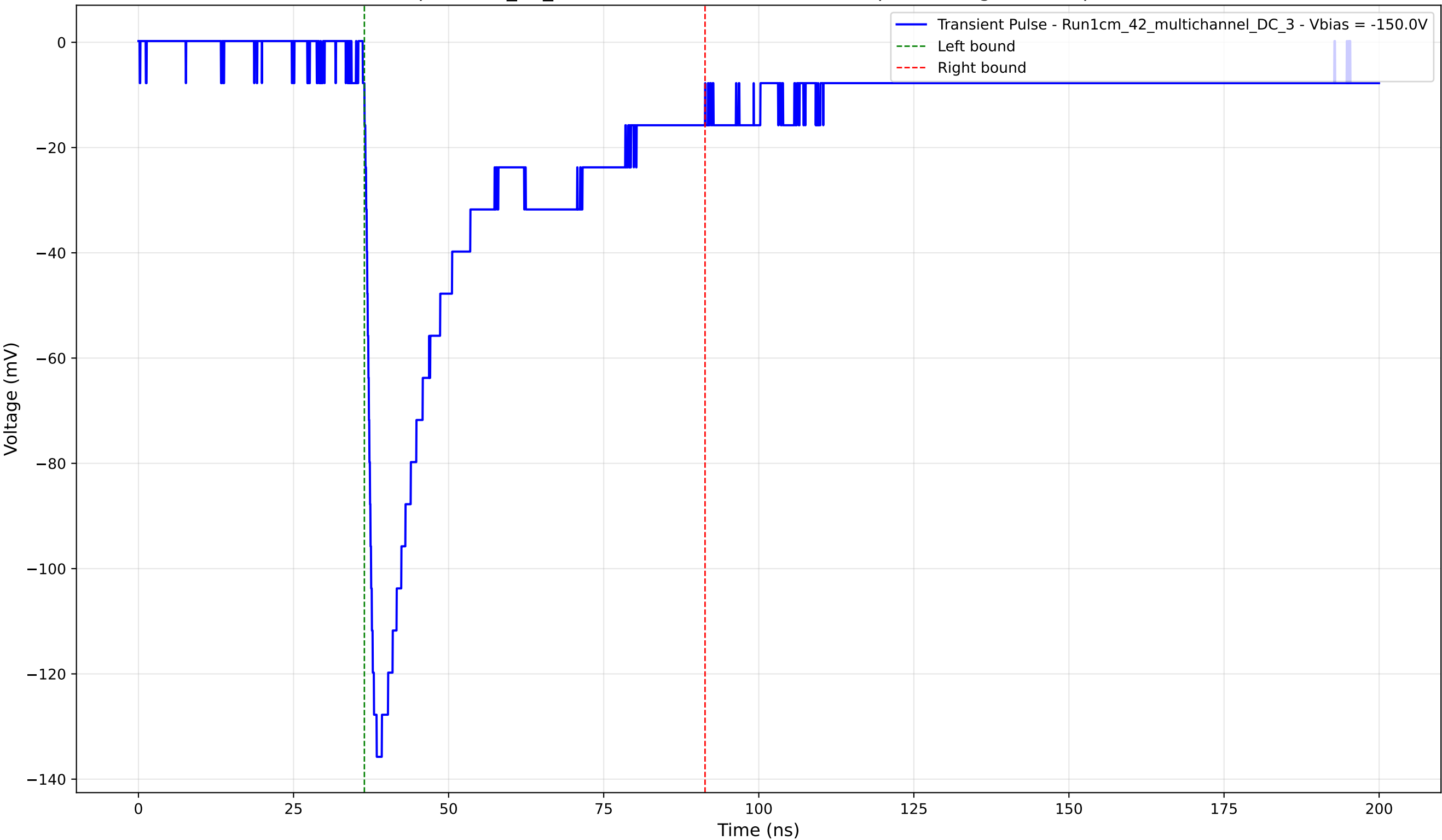
Transient Pulse - Sample: 1cm_42_multichannel - Position: 1465.0 \mu\text{m} - Charge: 44.24 pC - Rise Time: 1.53 ns
