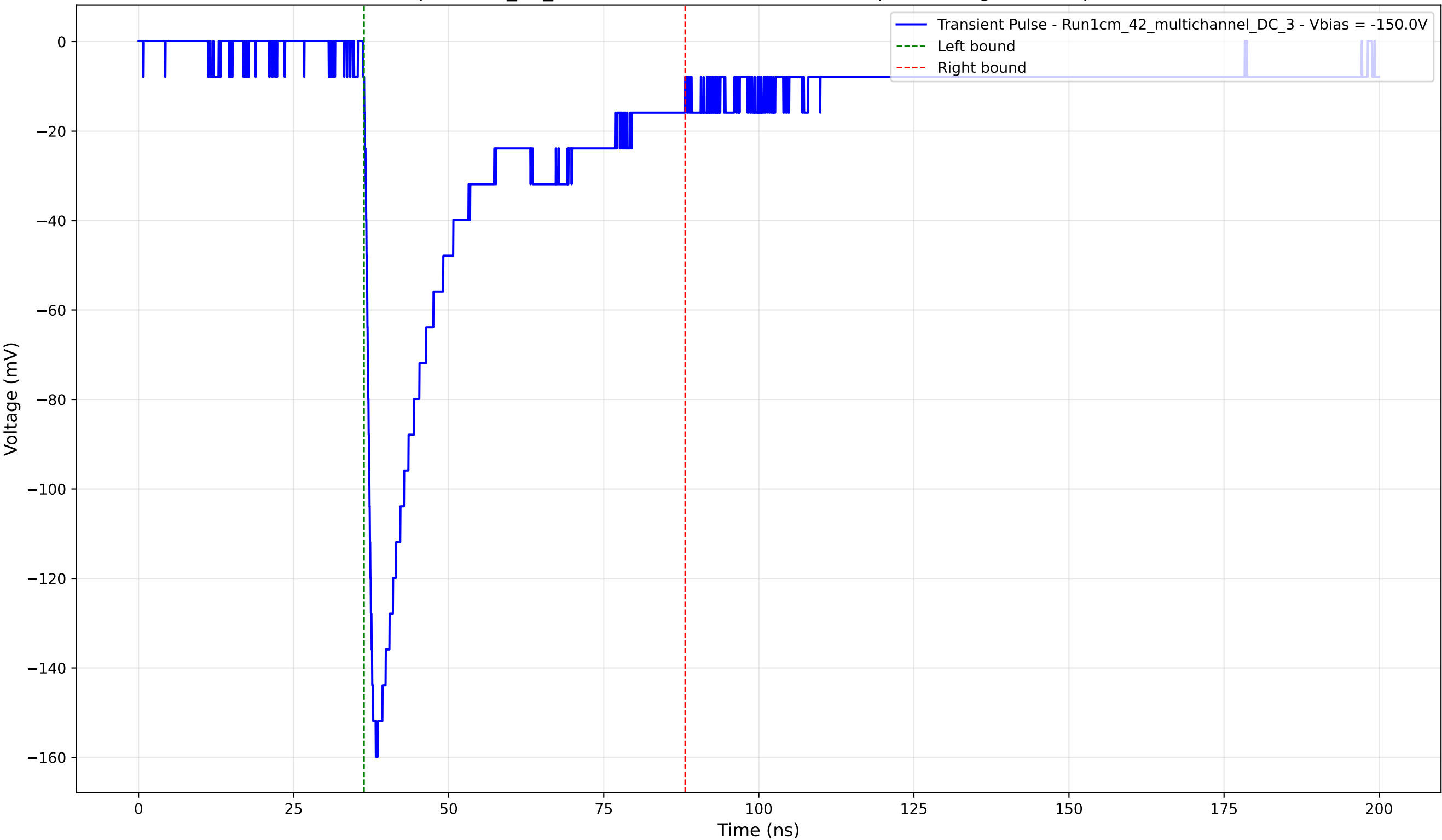
Transient Pulse - Sample: 1cm_42_multichannel - Position: 1210.0 \mu\text{m} - Charge: 44.95 pC - Rise Time: 1.36 ns
