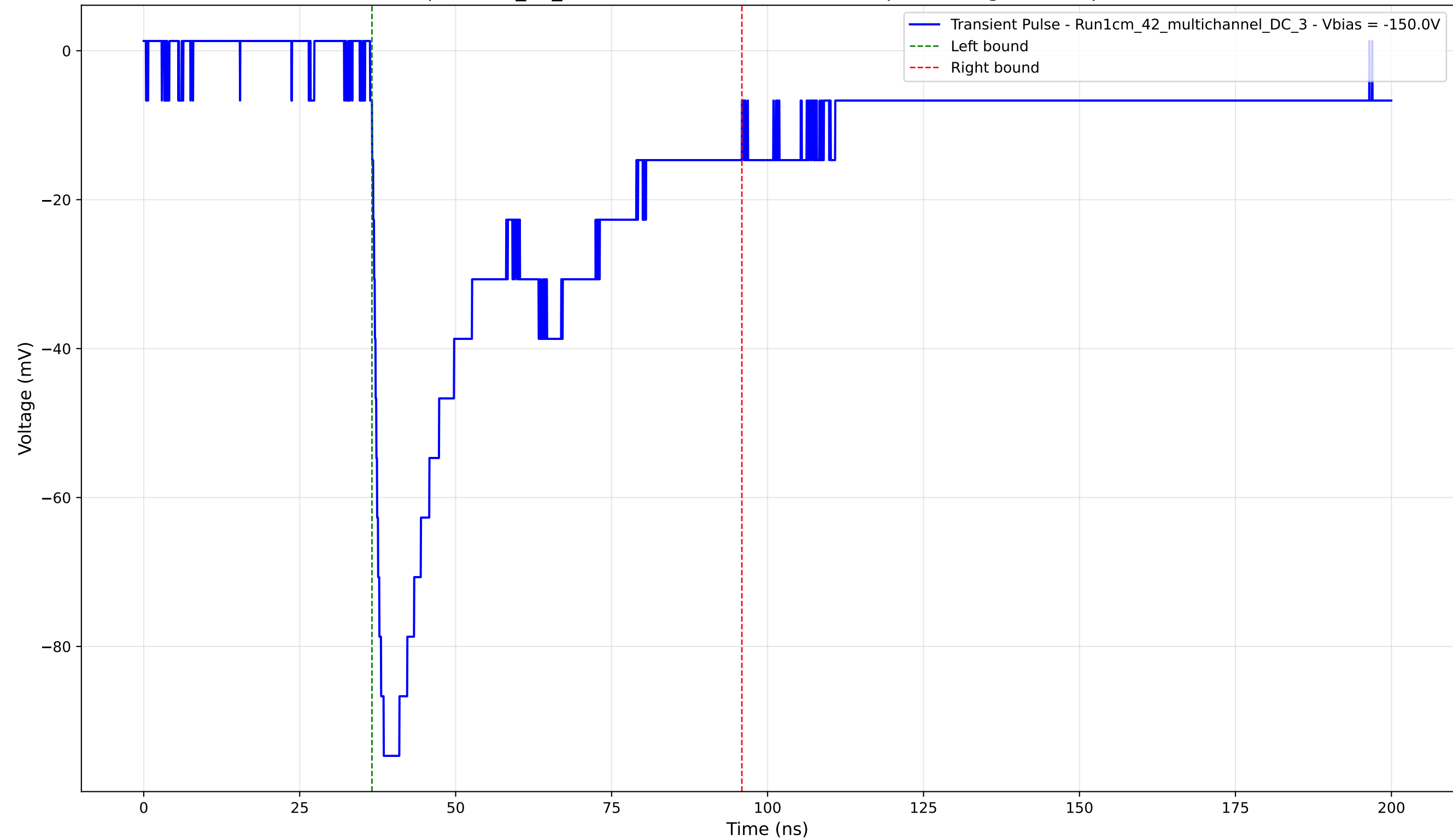
Transient Pulse - Sample: 1cm_42_multichannel - Position: 1980.0 \mu\text{m} - Charge: 40.74 pC - Rise Time: 1.45 ns
