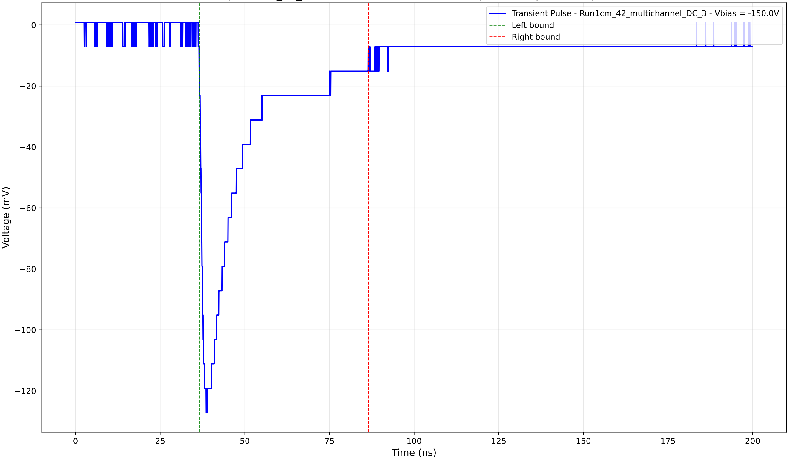
Transient Pulse - Sample: 1cm_42_multichannel - Position: 3515.0 \mu\text{m} - Charge: 37.20 pC - Rise Time: 1.55 ns
