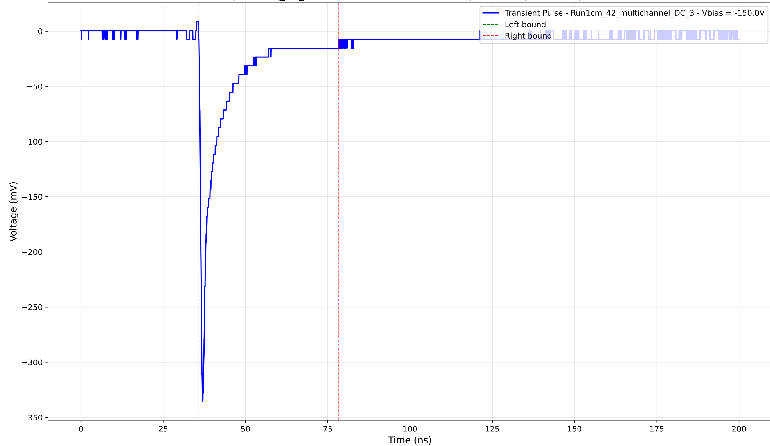
Transient Pulse - Sample: 1cm_42_multichannel - Position: 105.0 \mu\text{m} - Charge: 39.18 pC - Rise Time: 0.79 ns
