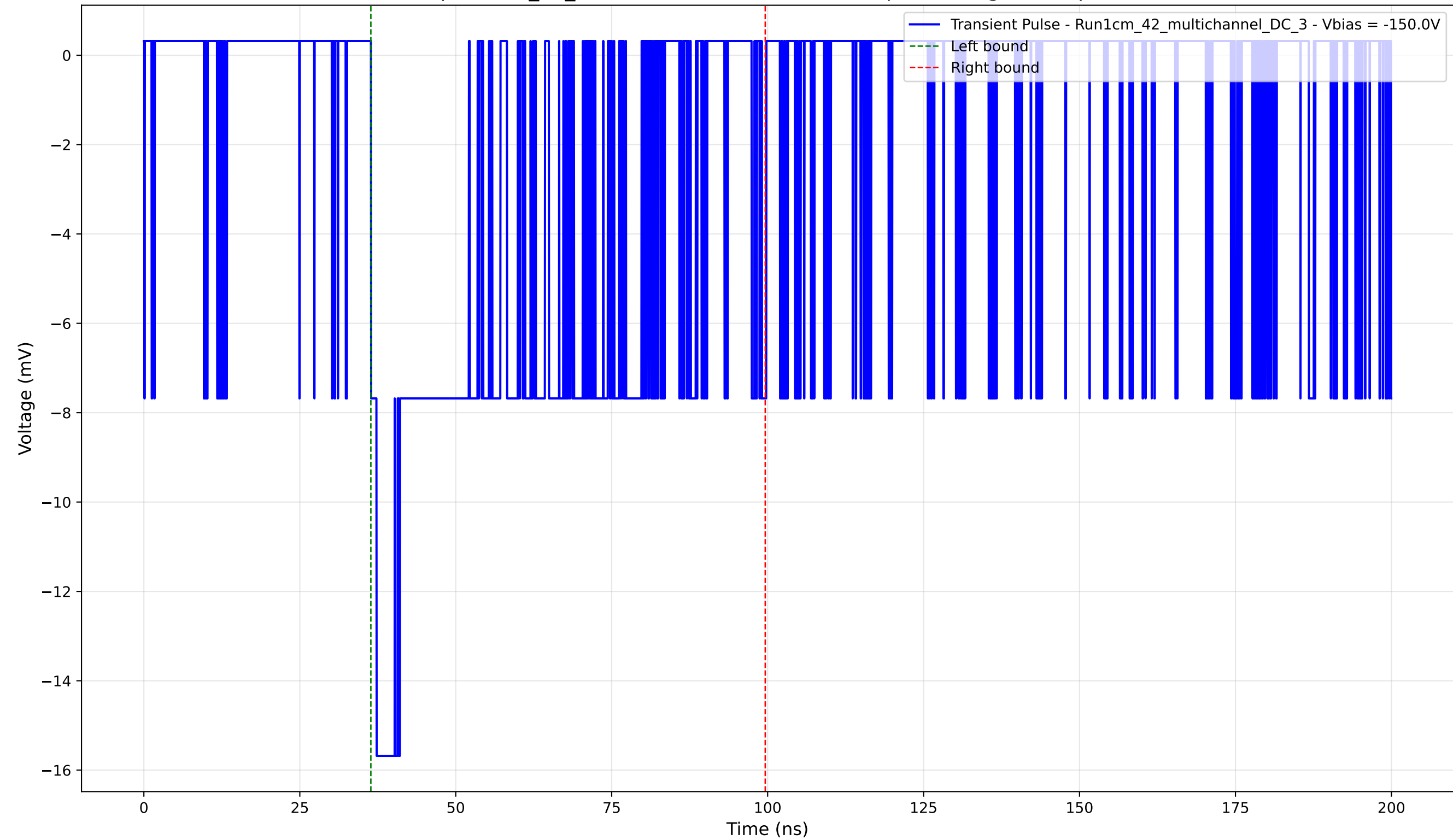
Transient Pulse - Sample: 1cm_42_multichannel - Position: 845.0 \mu\text{m} - Charge: 6.72 pC - Rise Time: 0.90 ns
