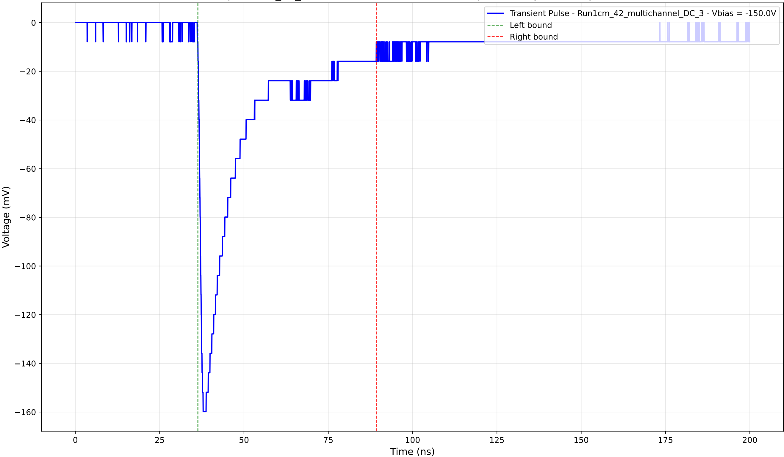
Transient Pulse - Sample: 1cm_42_multichannel - Position: 1145.0 \mu\text{m} - Charge: 45.06 pC - Rise Time: 1.22 ns
