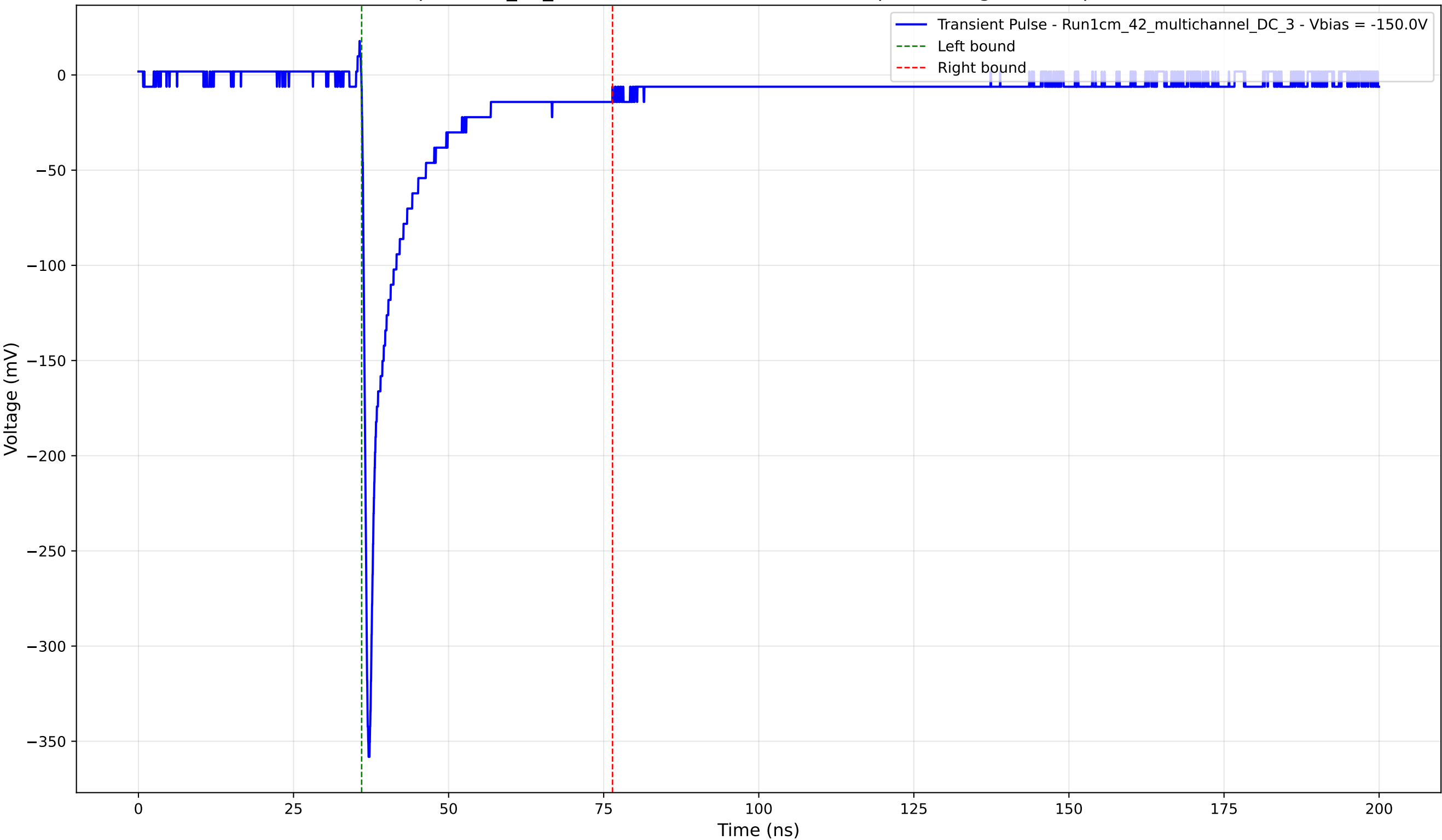
Transient Pulse - Sample: 1cm_42_multichannel - Position: 4795.0 \mu\text{m} - Charge: 38.40 pC - Rise Time: 0.78 ns
