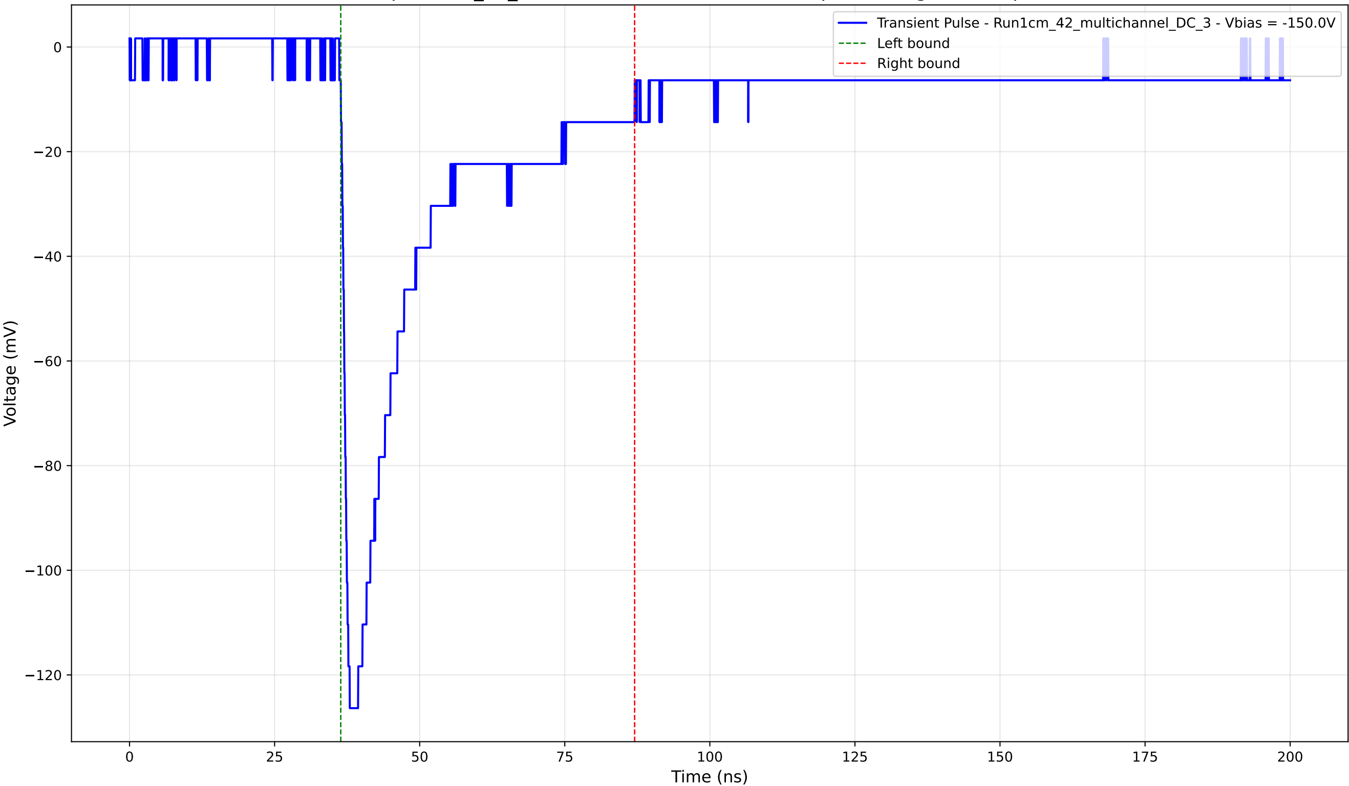
Transient Pulse - Sample: 1cm_42_multichannel - Position: 1290.0 \mu\text{m} - Charge: 37.15 pC - Rise Time: 1.28 ns
