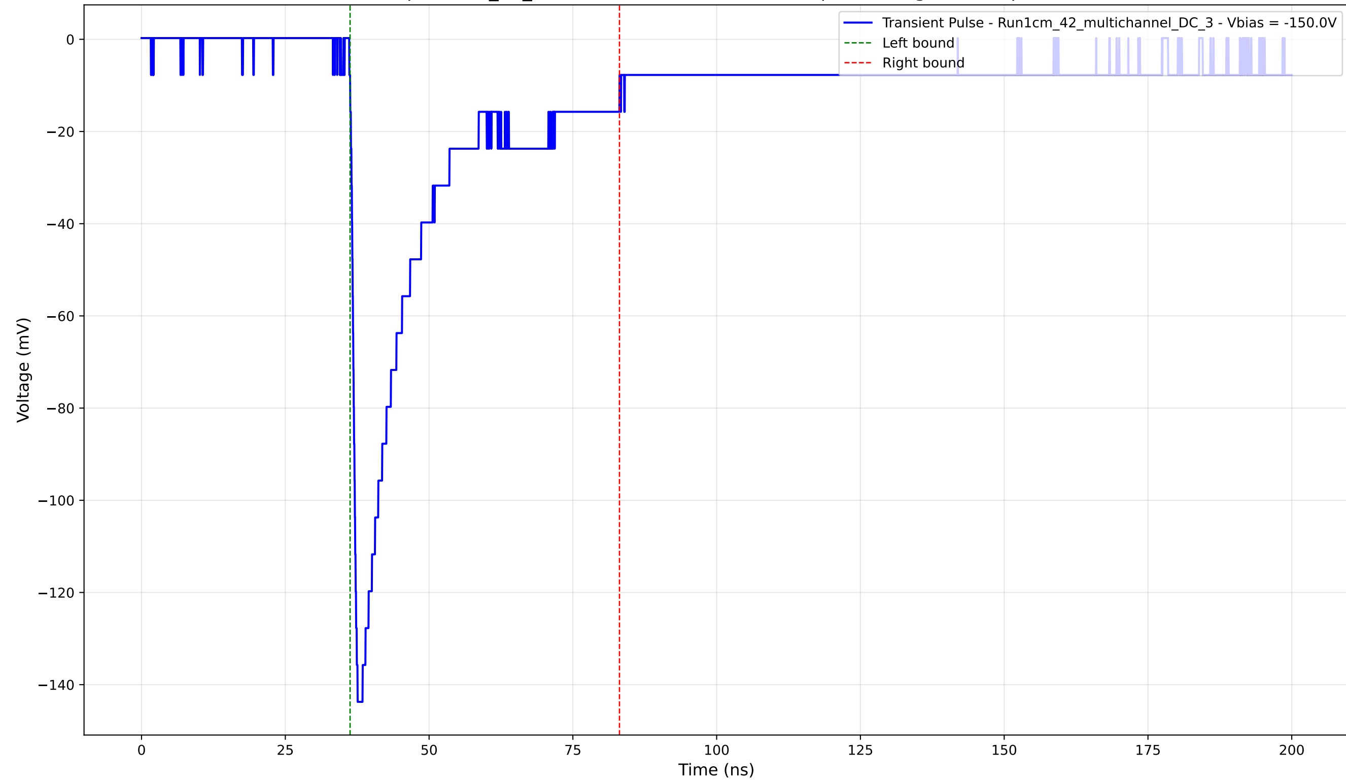
Transient Pulse - Sample: 1cm_42_multichannel - Position: 920.0 \mu\text{m} - Charge: 35.92 pC - Rise Time: 1.14 ns
