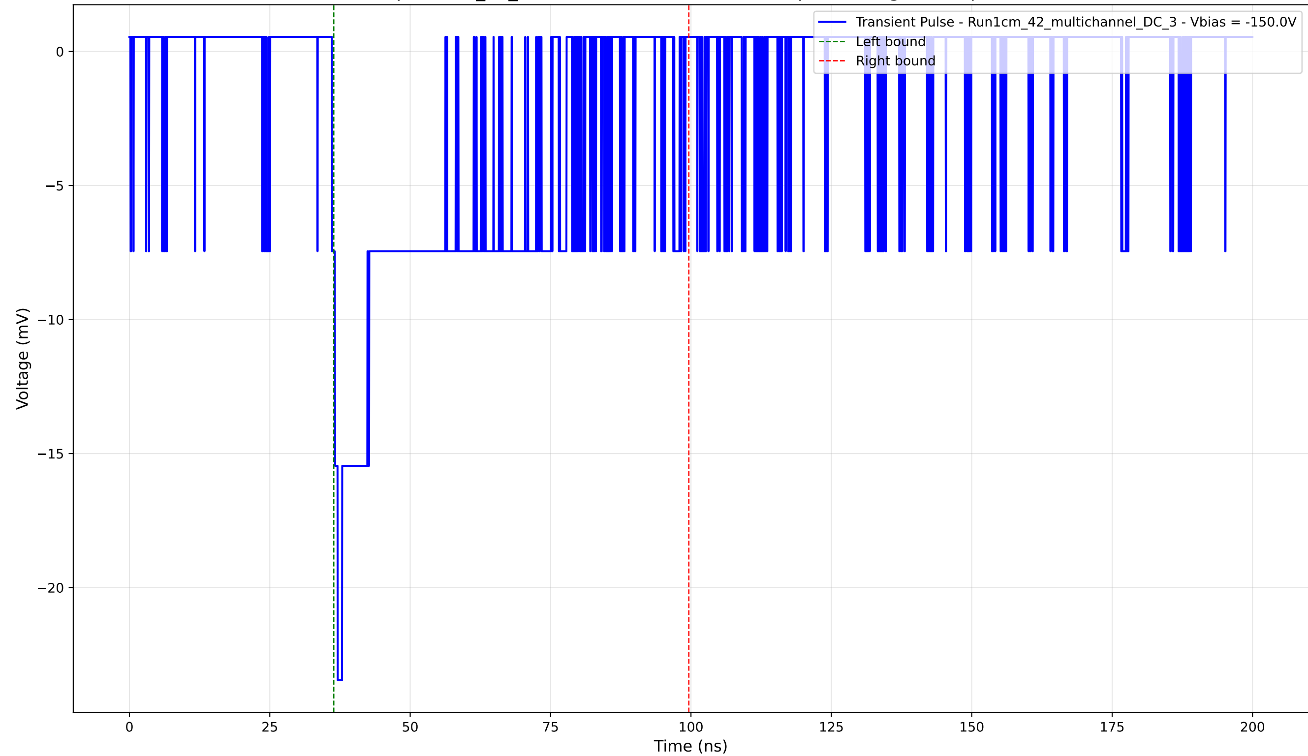
Transient Pulse - Sample: 1cm_42_multichannel - Position: 370.0 \mu\text{m} - Charge: 7.21 pC - Rise Time: 1.01 ns
