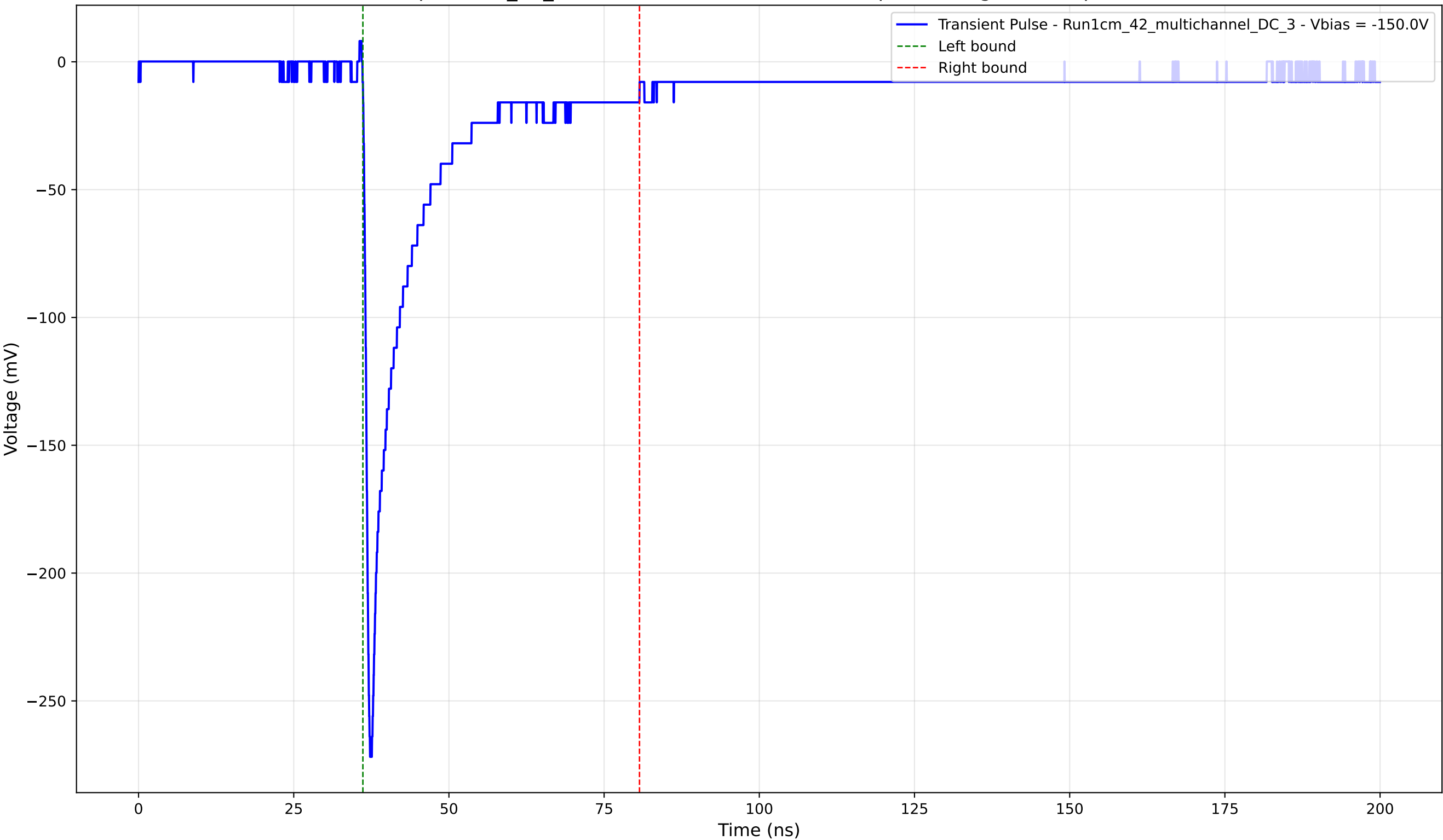
Transient Pulse - Sample: 1cm_42_multichannel - Position: 4530.0 \mu\text{m} - Charge: 40.68 pC - Rise Time: 0.85 ns
