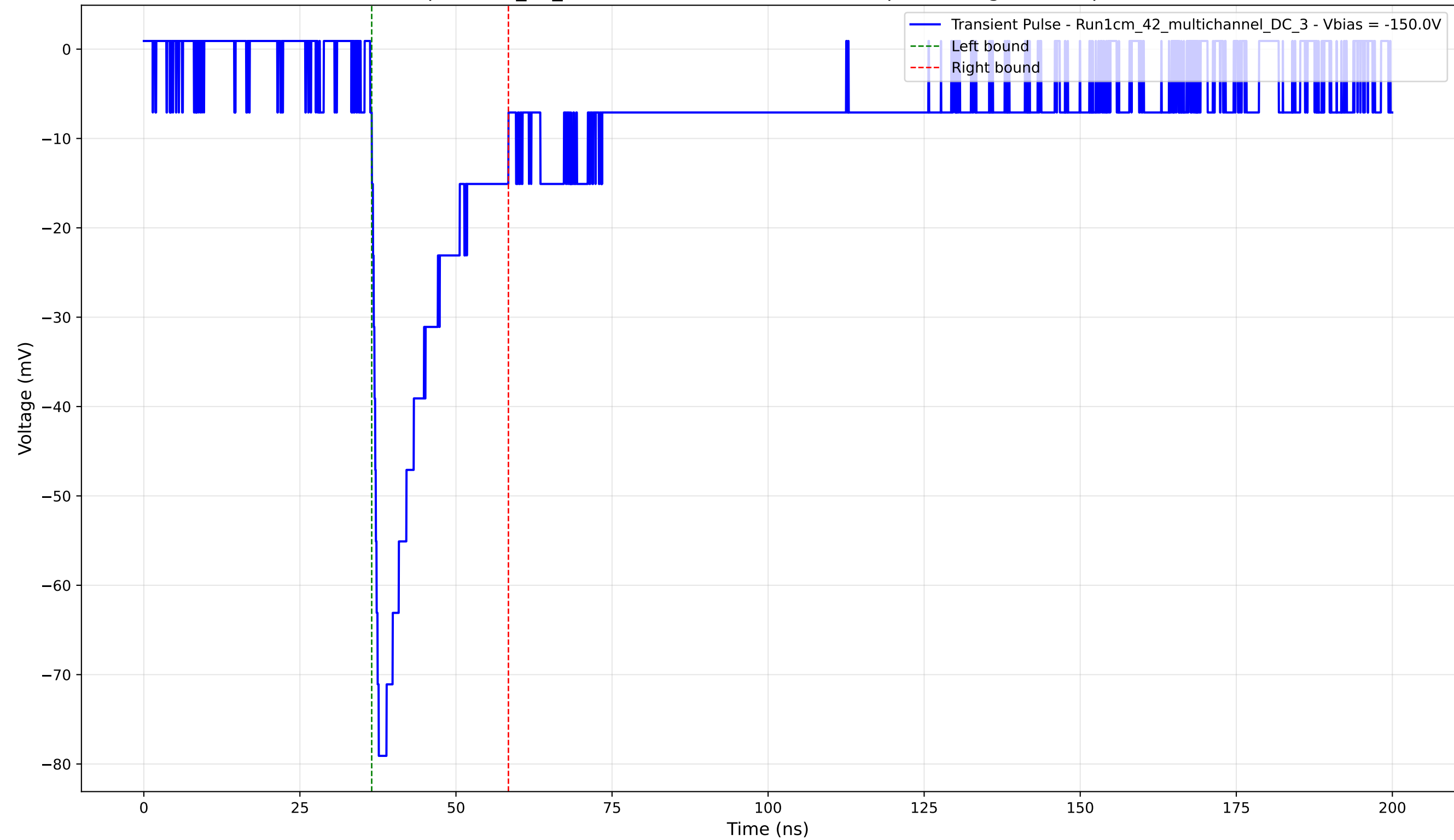
Transient Pulse - Sample: 1cm_42_multichannel - Position: 3940.0 \mu\text{m} - Charge: 14.74 pC - Rise Time: 1.12 ns
