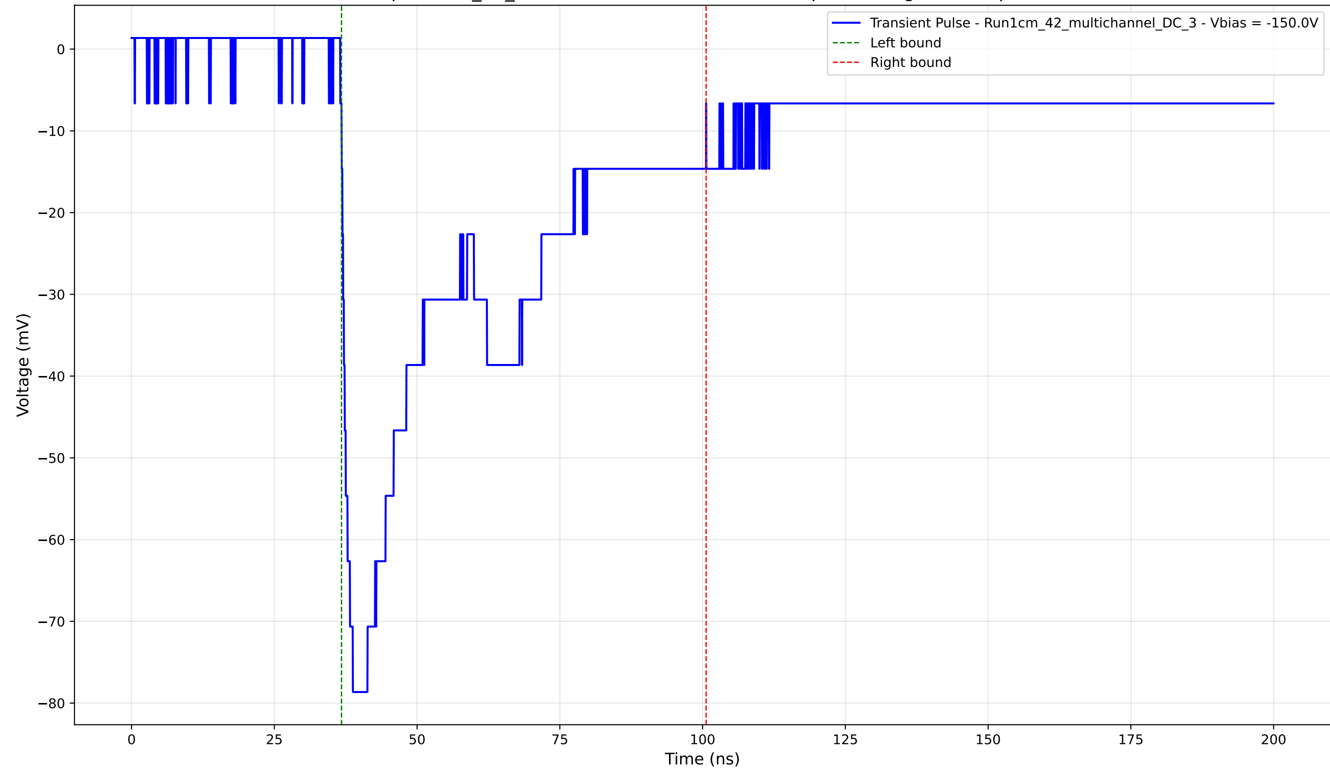
Transient Pulse - Sample: 1cm_42_multichannel - Position: 2285.0 \mu\text{m} - Charge: 38.98 pC - Rise Time: 1.98 ns
