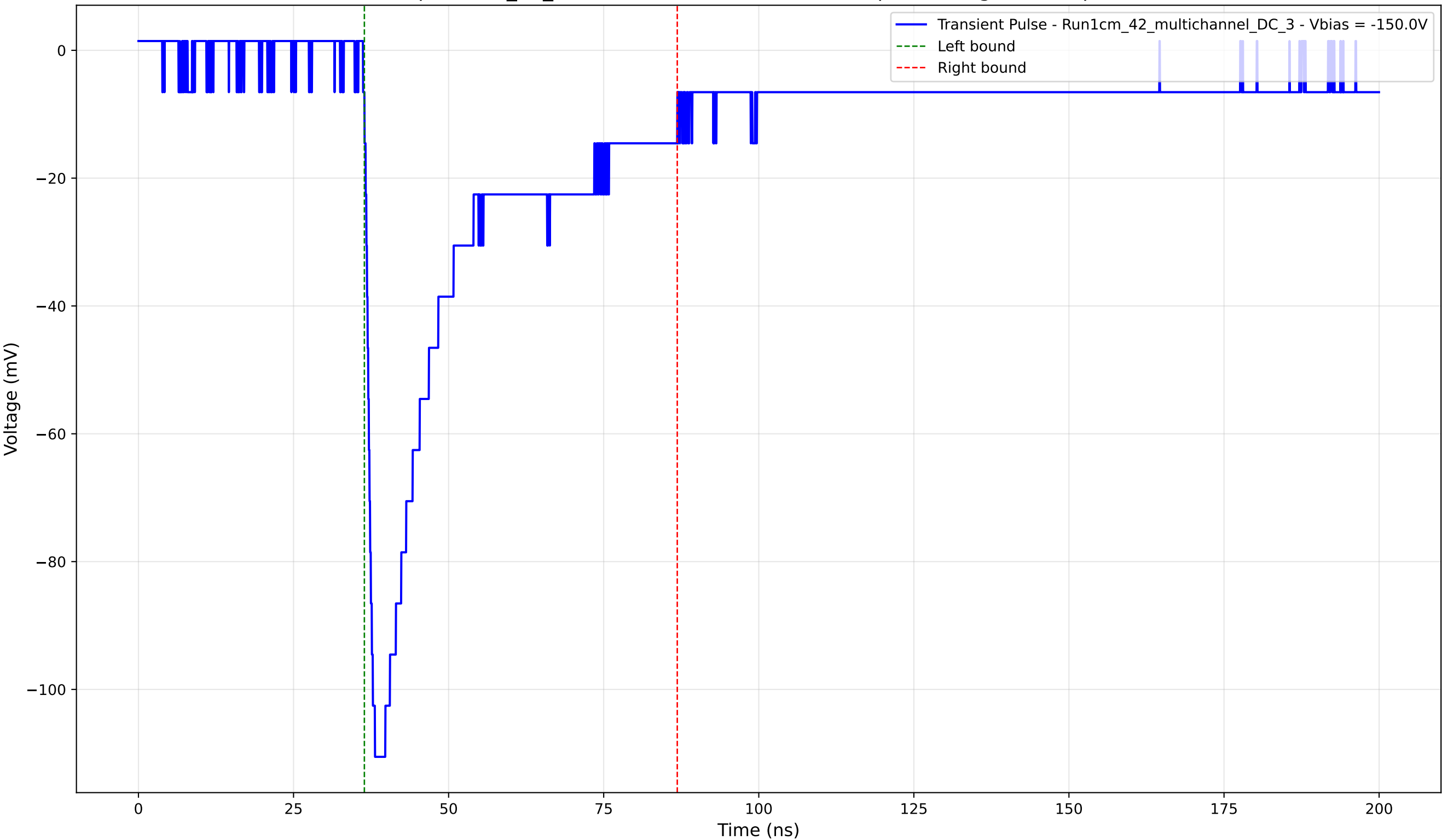
Transient Pulse - Sample: 1cm_42_multichannel - Position: 1430.0 \mu\text{m} - Charge: 34.73 pC - Rise Time: 1.35 ns
