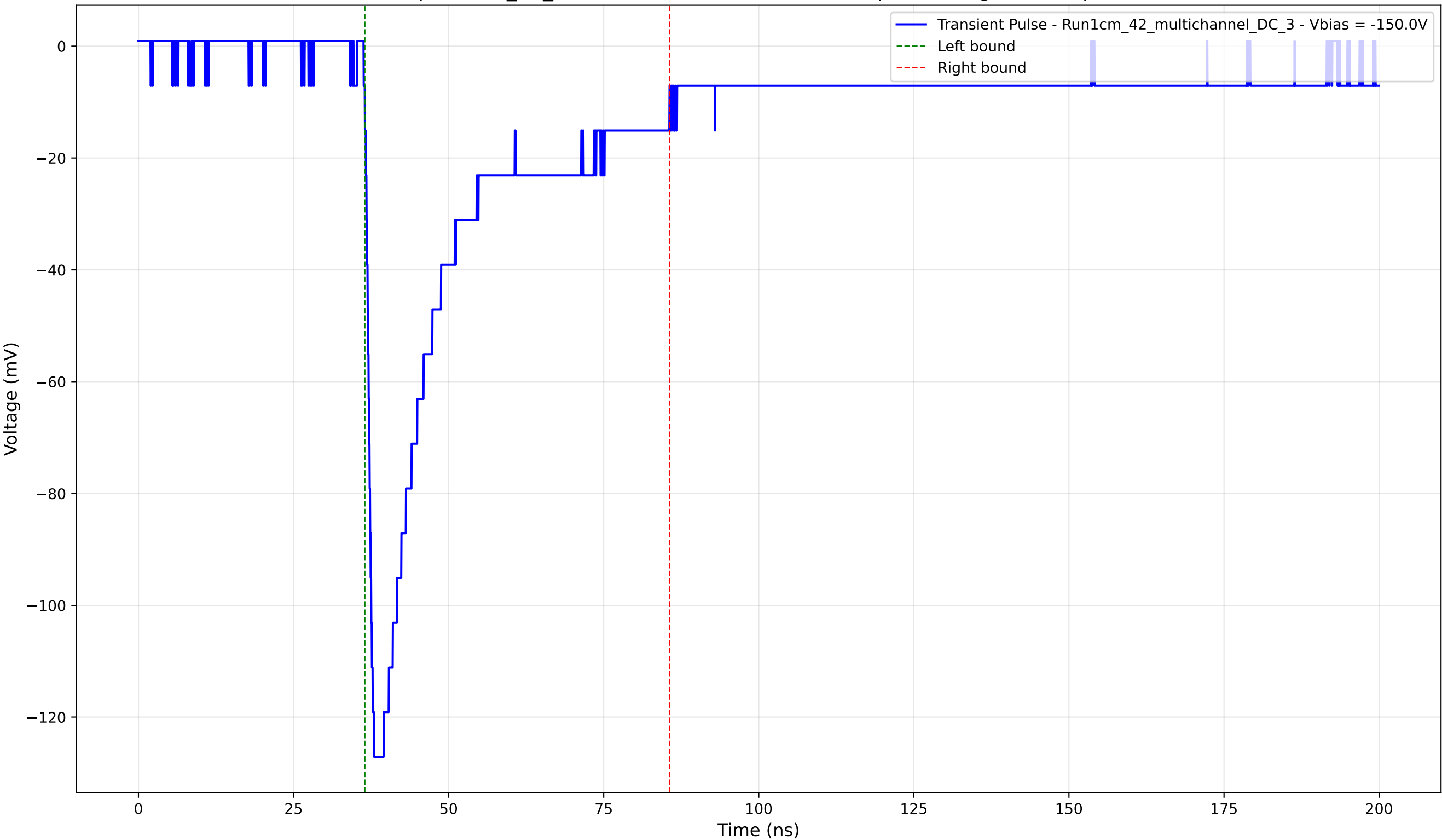
Transient Pulse - Sample: 1cm_42_multichannel - Position: 3655.0 \mu\text{m} - Charge: 36.75 pC - Rise Time: 1.27 ns
