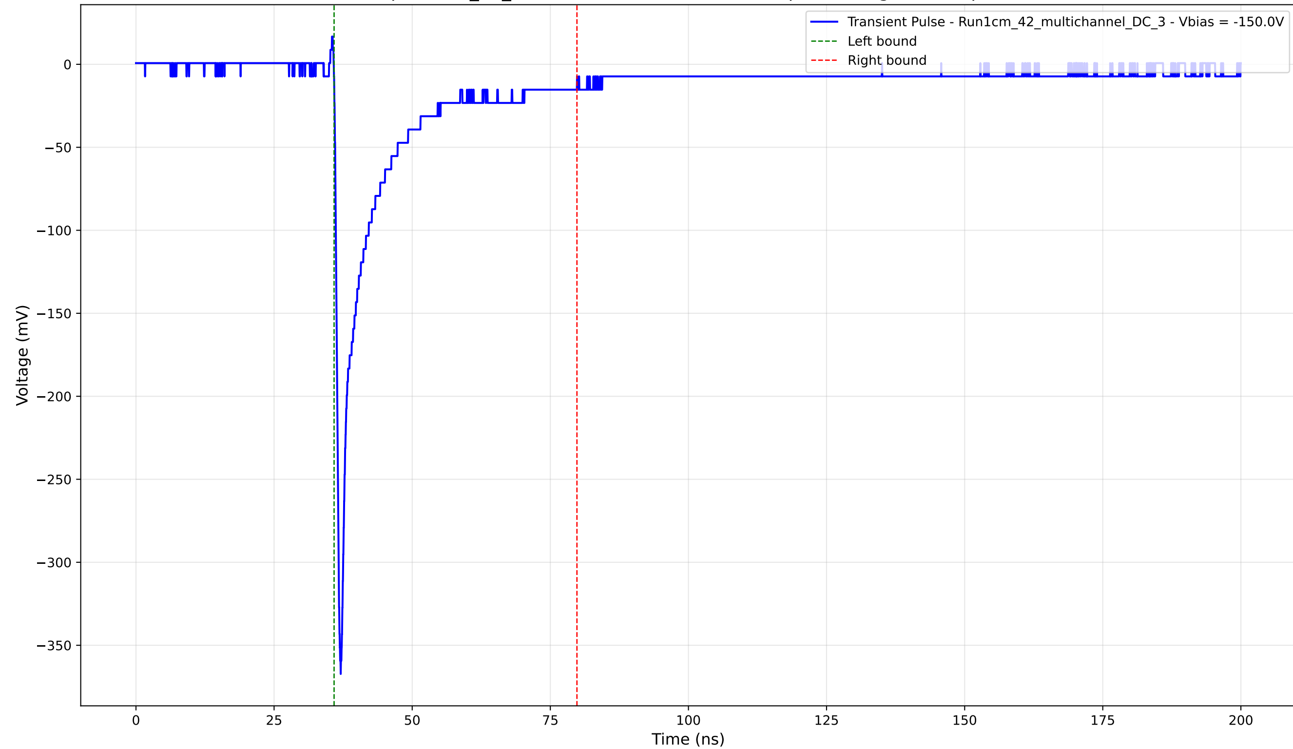
Transient Pulse - Sample: 1cm_42_multichannel - Position: 140.0 \mu\text{m} - Charge: 45.23 pC - Rise Time: 0.81 ns
