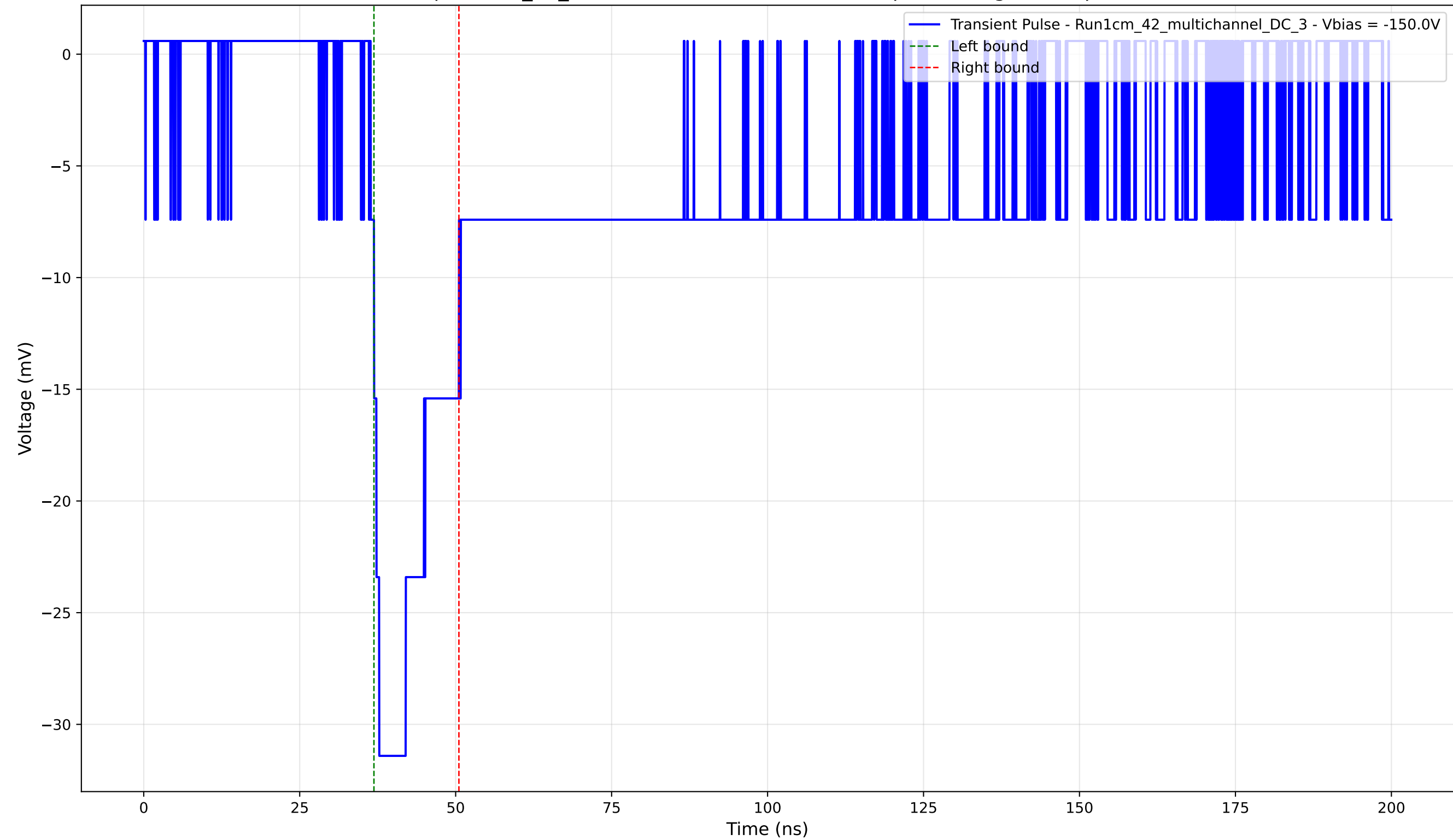
Transient Pulse - Sample: 1cm_42_multichannel - Position: 3425.0 \mu\text{m} - Charge: 6.11 pC - Rise Time: 1.37 ns
