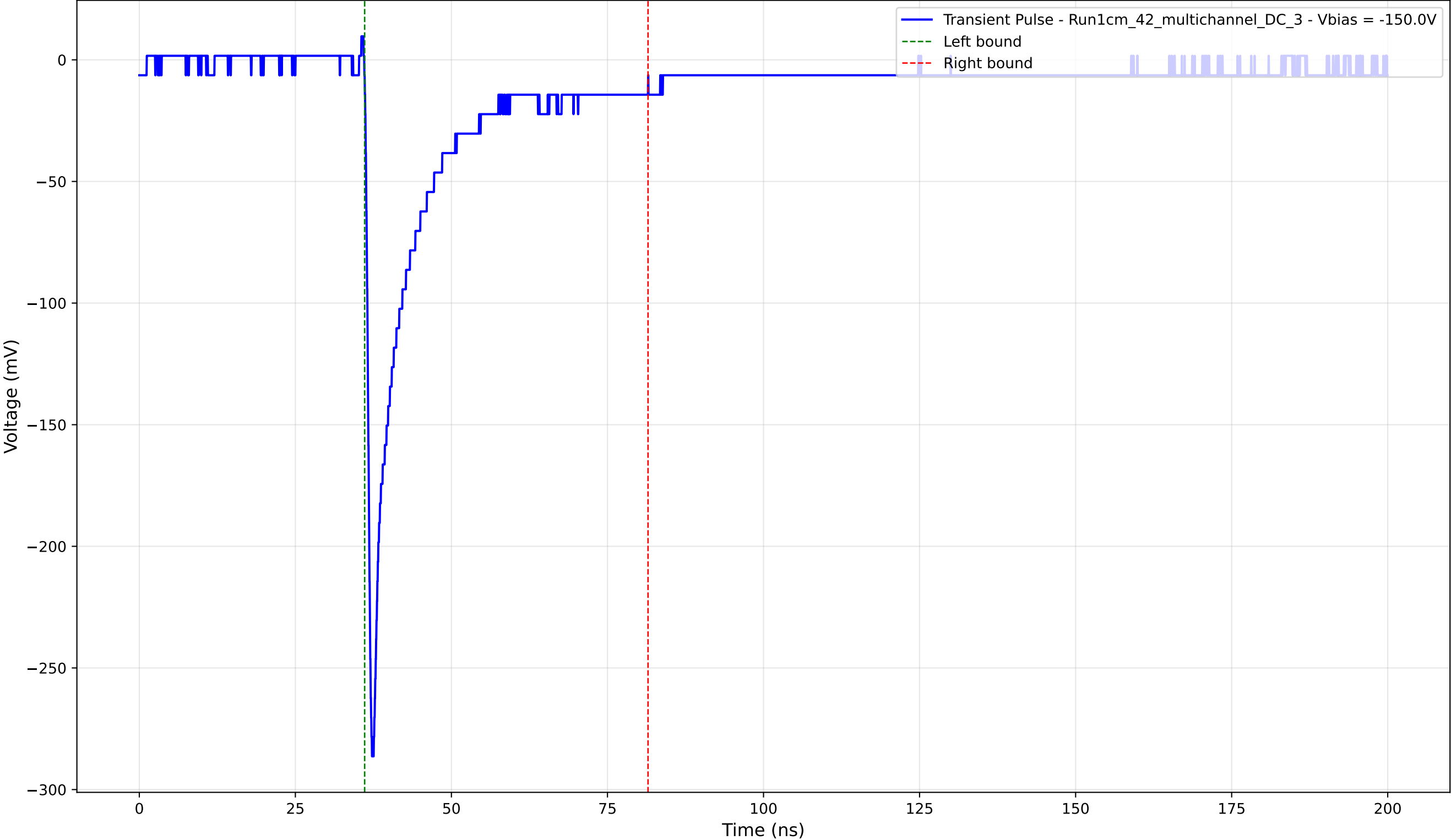
Transient Pulse - Sample: 1cm_42_multichannel - Position: 4565.0 \mu\text{m} - Charge: 40.59 pC - Rise Time: 0.84 ns
