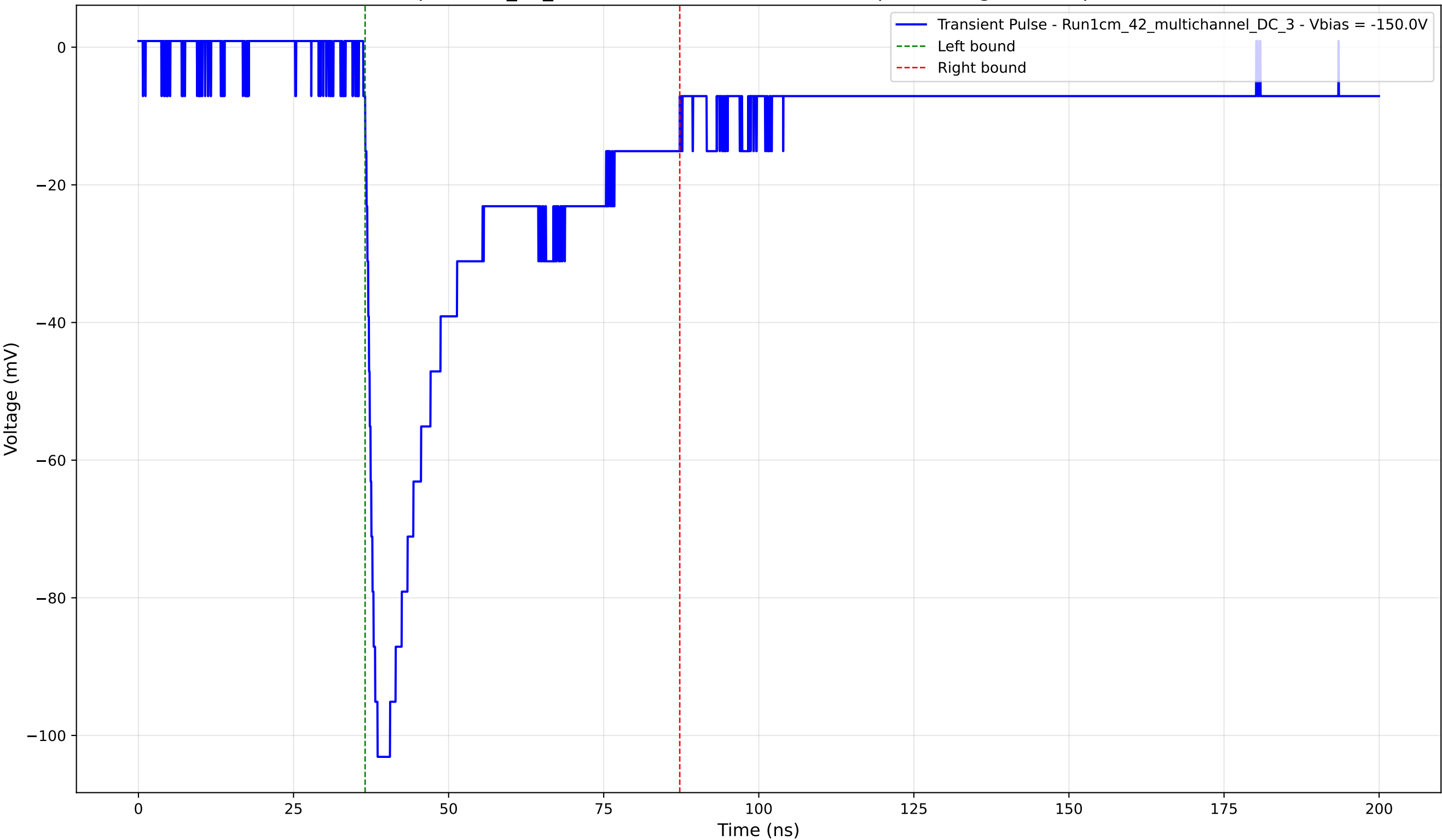
Transient Pulse - Sample: 1cm_42_multichannel - Position: 3170.0 \mu\text{m} - Charge: 35.65 pC - Rise Time: 1.61 ns
