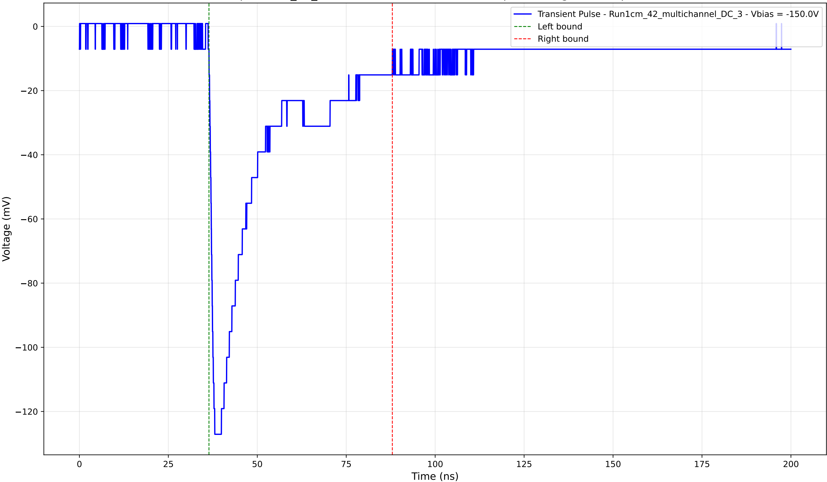
Transient Pulse - Sample: 1cm_42_multichannel - Position: 1450.0 \mu\text{m} - Charge: 41.26 pC - Rise Time: 1.39 ns
