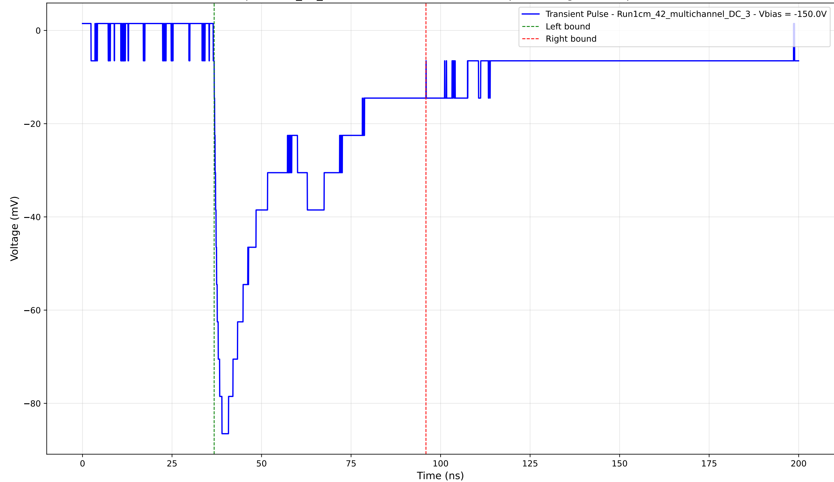
Transient Pulse - Sample: 1cm_42_multichannel - Position: 2150.0 \mu\text{m} - Charge: 38.30 pC - Rise Time: 1.53 ns
