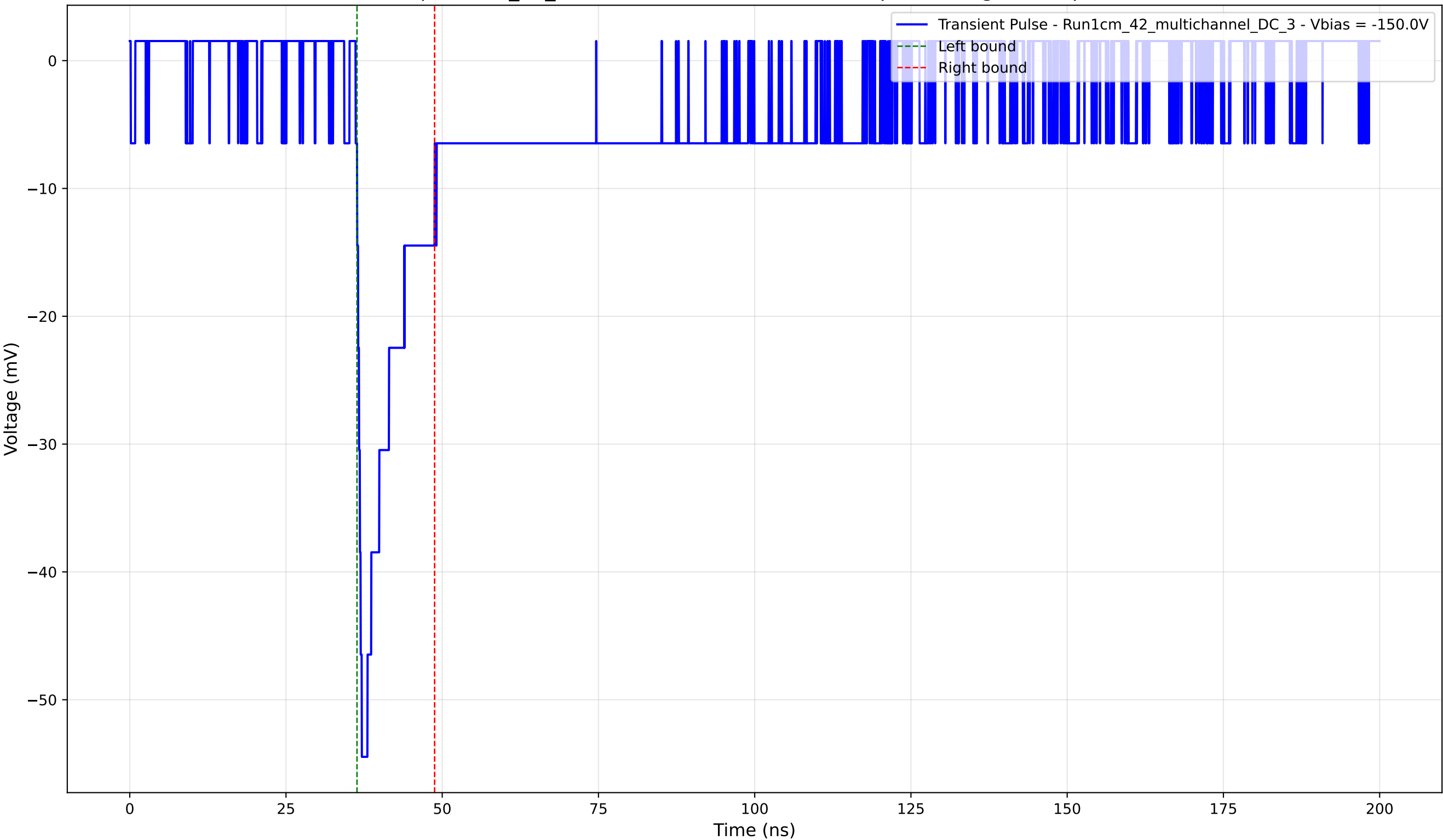
Transient Pulse - Sample: 1cm_42_multichannel - Position: 4430.0 \mu\text{m} - Charge: 6.46 pC - Rise Time: 0.98 ns
