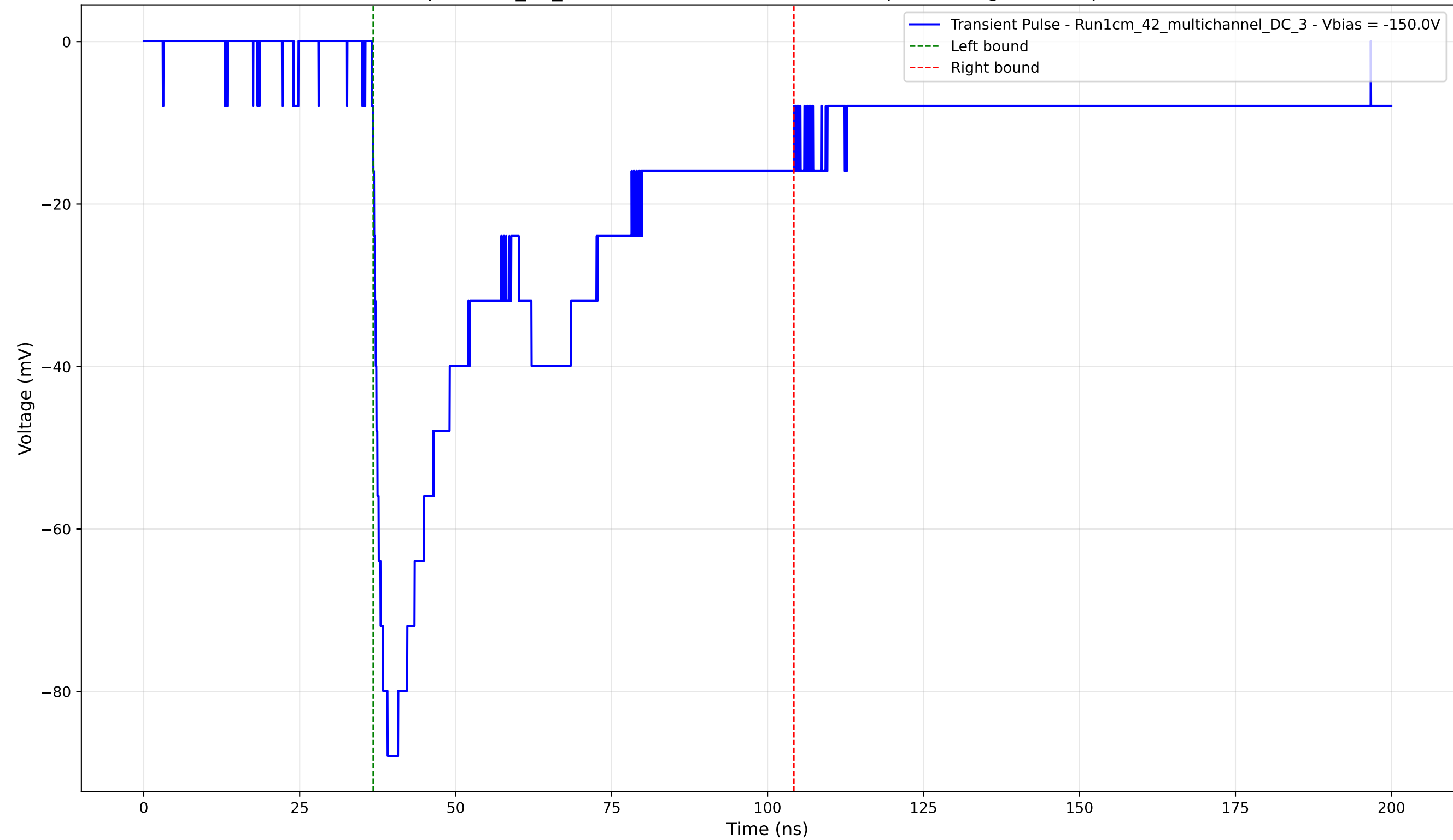
Transient Pulse - Sample: 1cm_42_multichannel - Position: 2210.0 \mu\text{m} - Charge: 43.32 pC - Rise Time: 1.56 ns
