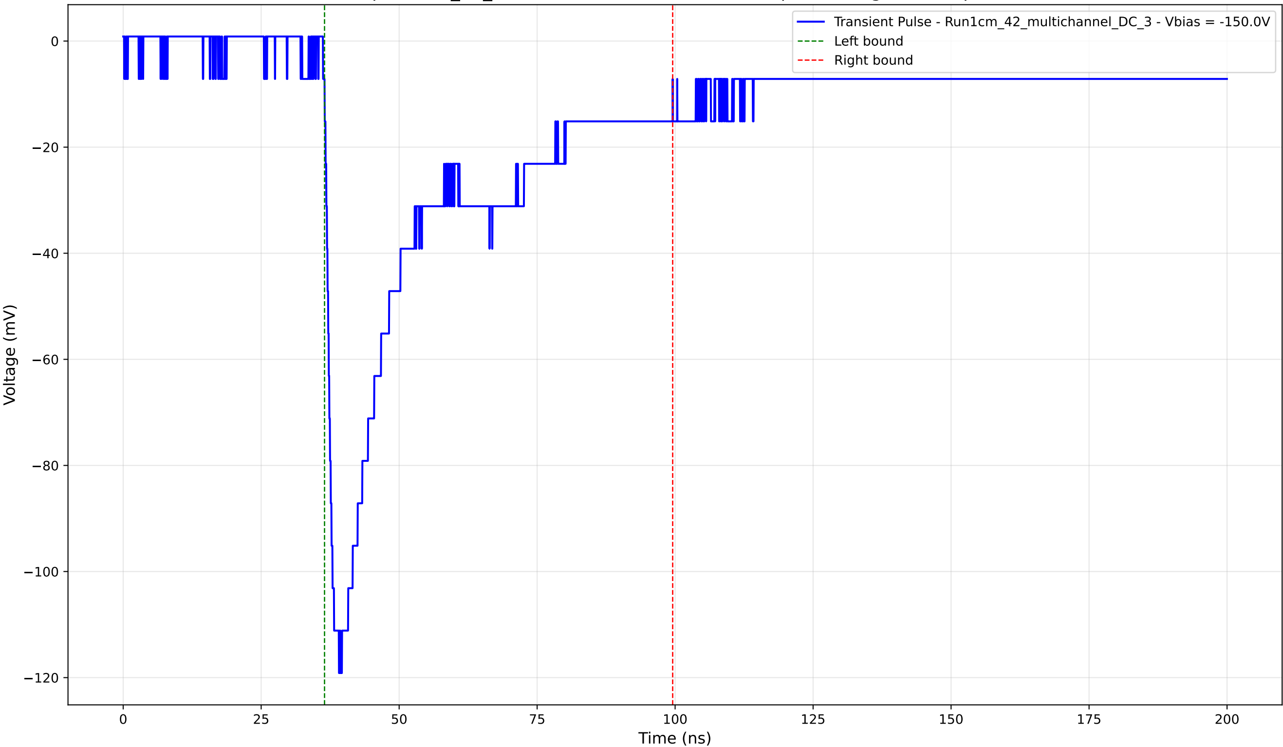
Transient Pulse - Sample: 1cm_42_multichannel - Position: 1725.0 \mu\text{m} - Charge: 44.52 pC - Rise Time: 1.71 ns
