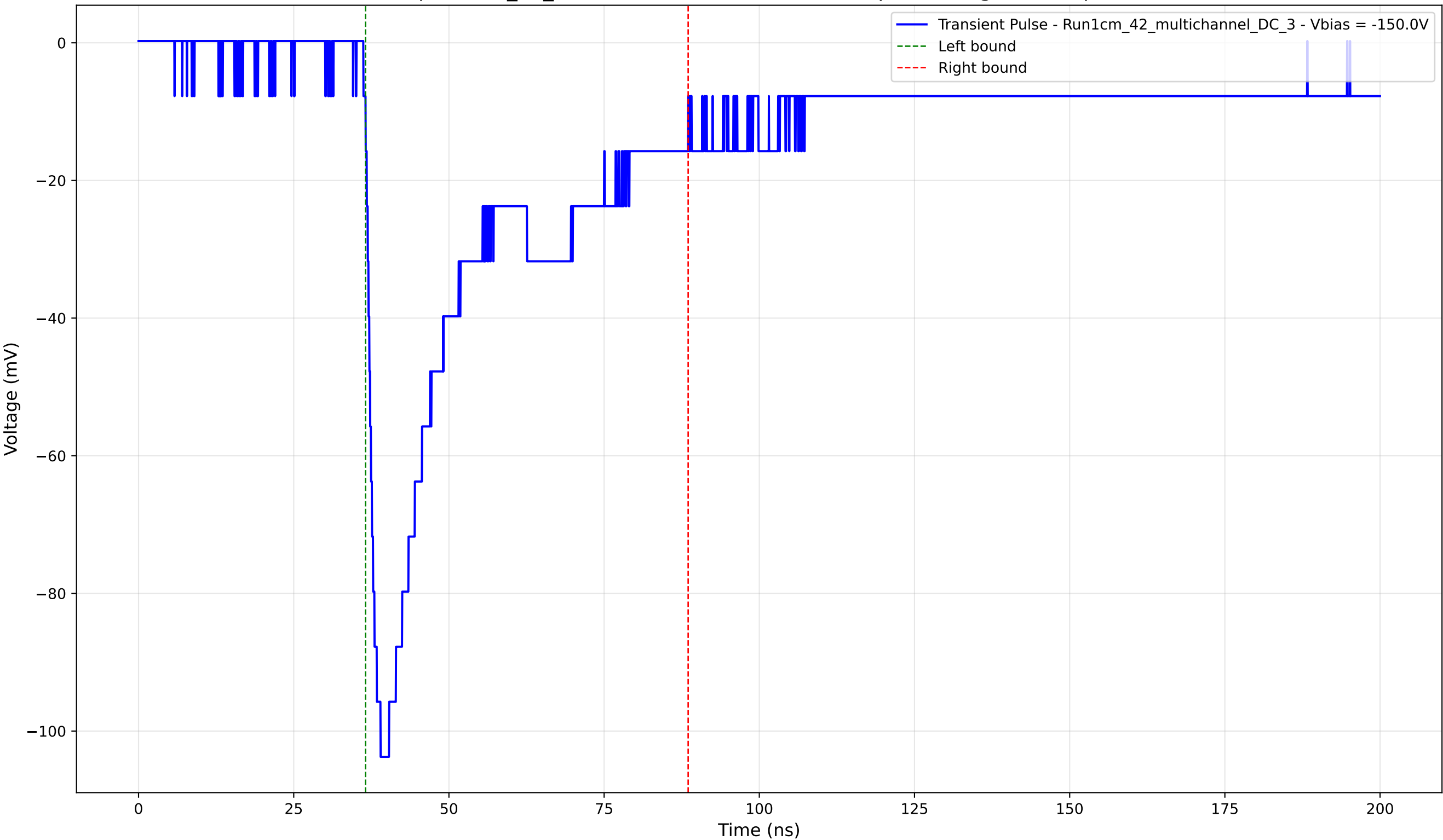
Transient Pulse - Sample: 1cm_42_multichannel - Position: 3015.0 \mu\text{m} - Charge: 37.76 pC - Rise Time: 1.81 ns
