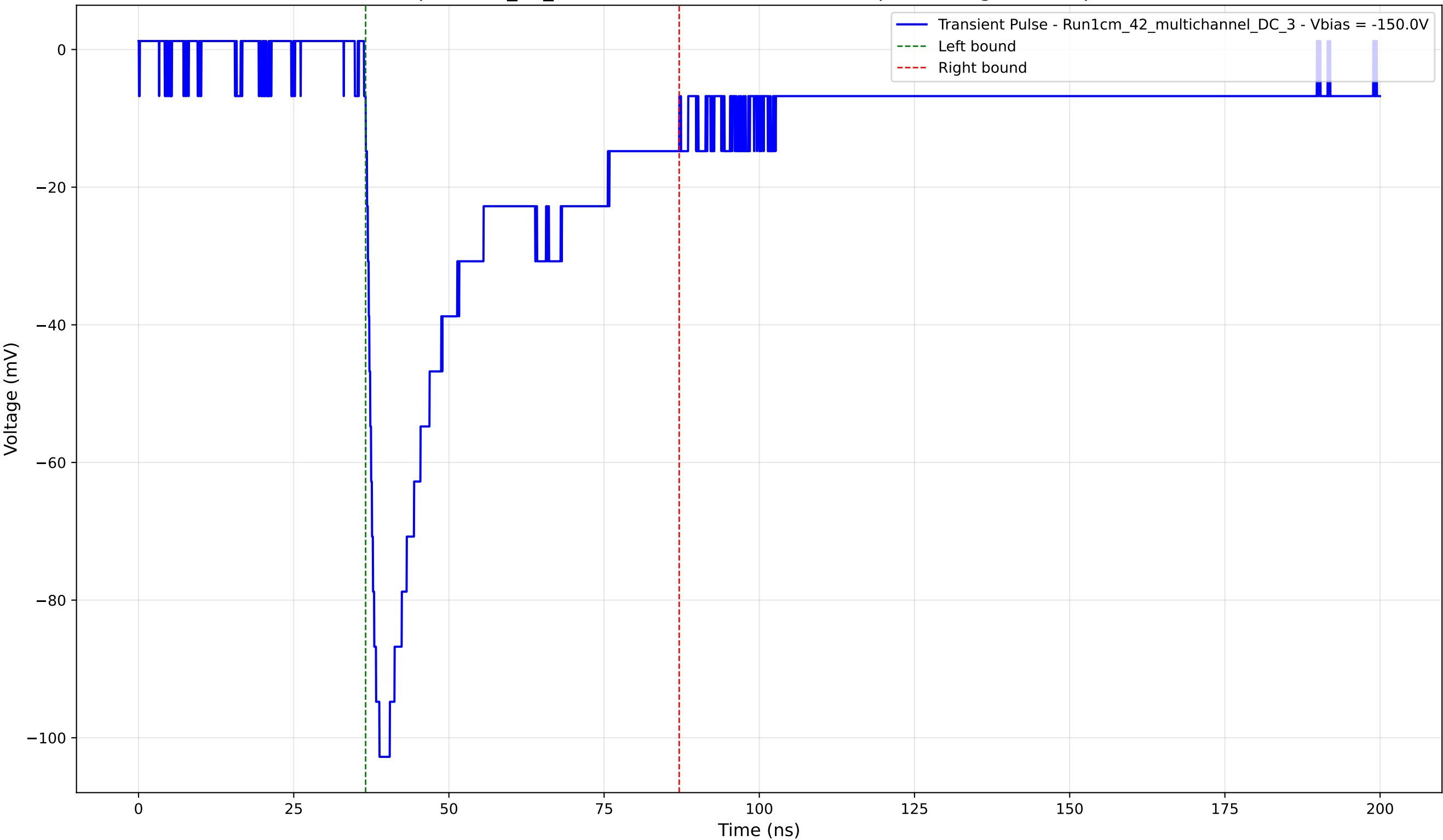
Transient Pulse - Sample: 1cm_42_multichannel - Position: 3115.0 \mu\text{m} - Charge: 35.08 pC - Rise Time: 1.67 ns
