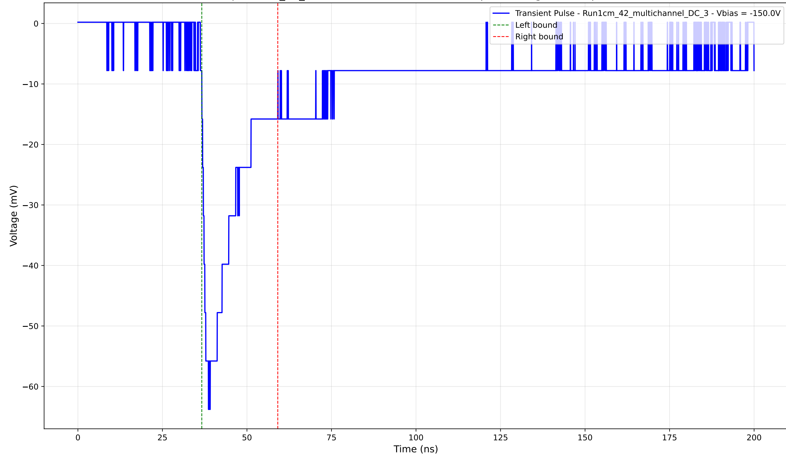
Transient Pulse - Sample: 1cm_42_multichannel - Position: 3435.0 \mu\text{m} - Charge: 13.51 pC - Rise Time: 2.38 ns
