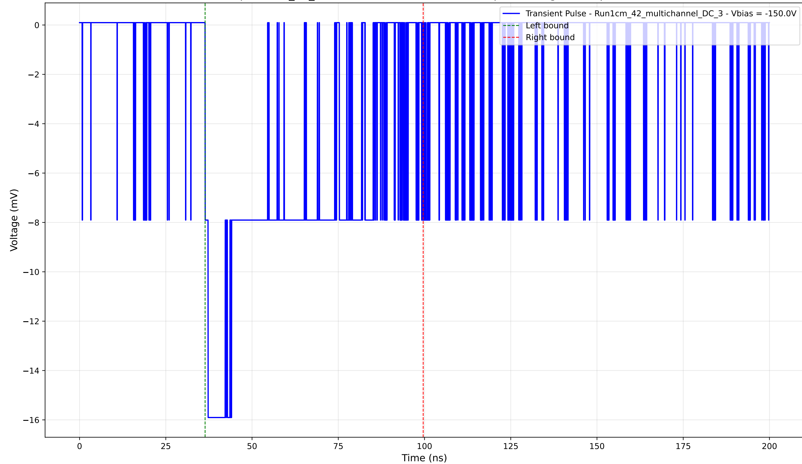
Transient Pulse - Sample: 1cm_42_multichannel - Position: 3865.0 \mu\text{m} - Charge: 8.63 pC - Rise Time: 0.88 ns
