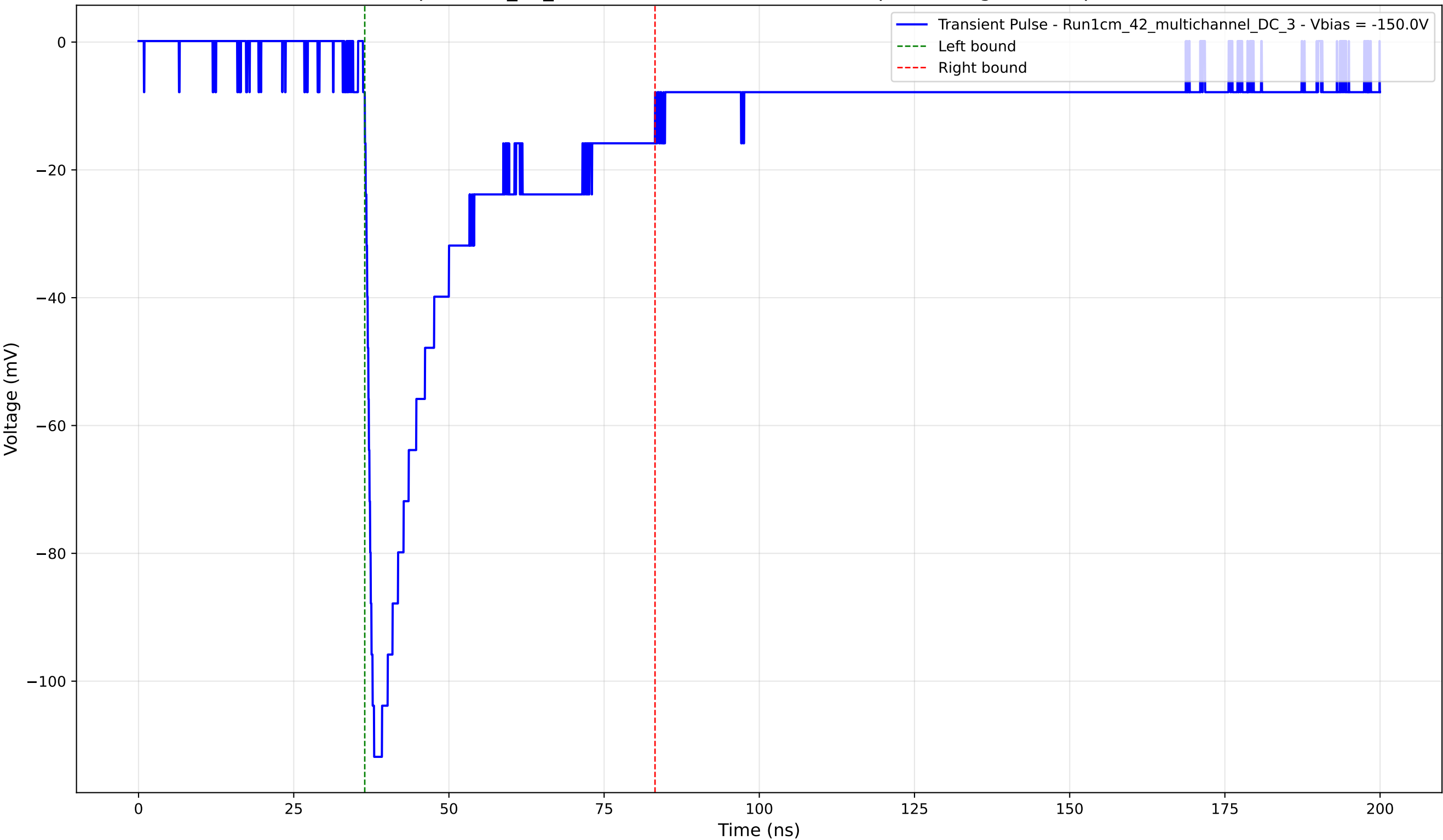
Transient Pulse - Sample: 1cm_42_multichannel - Position: 1300.0 \mu\text{m} - Charge: 33.23 pC - Rise Time: 1.25 ns
