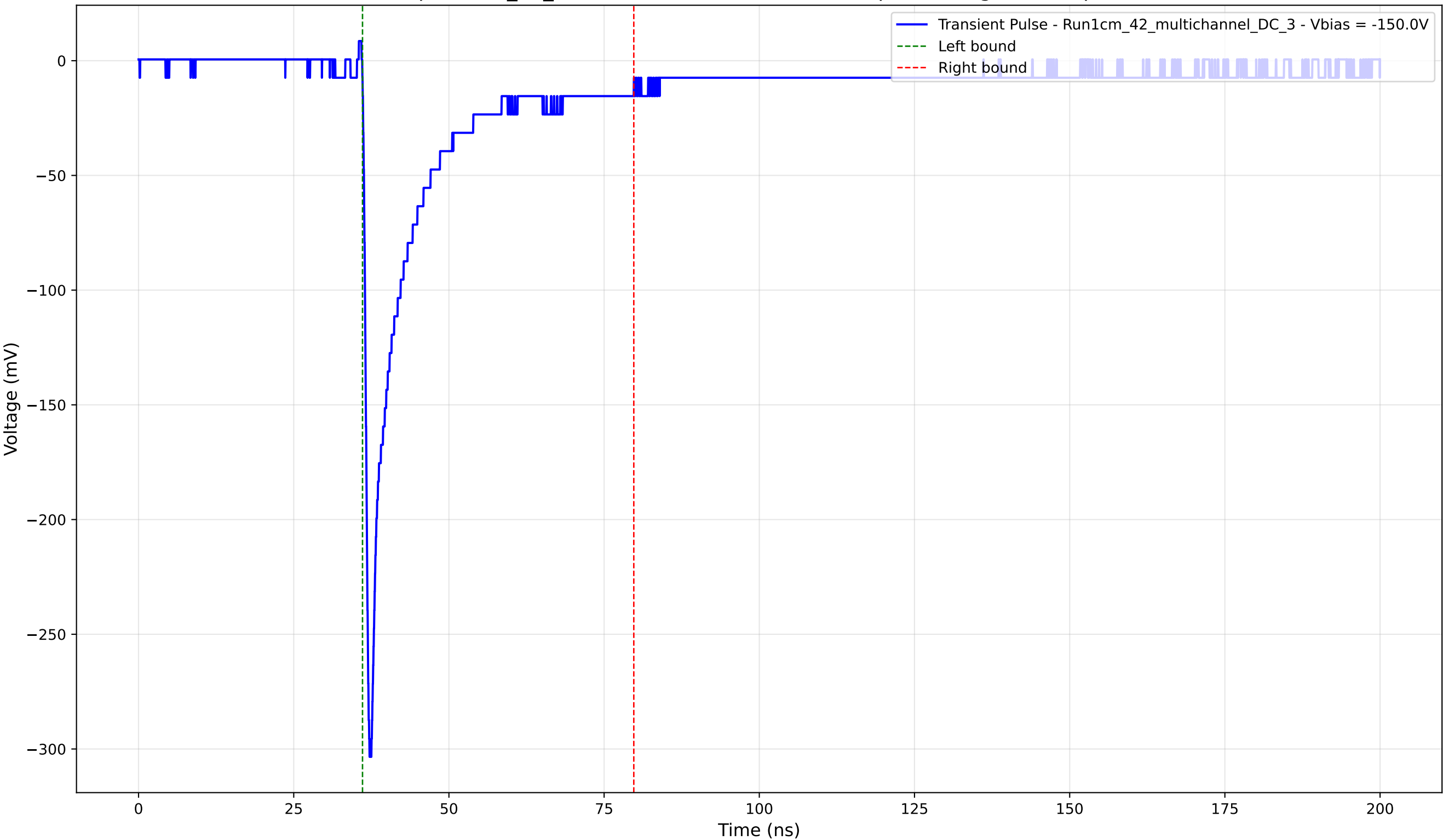
Transient Pulse - Sample: 1cm_42_multichannel - Position: 4610.0 \mu\text{m} - Charge: 41.69 pC - Rise Time: 0.84 ns
