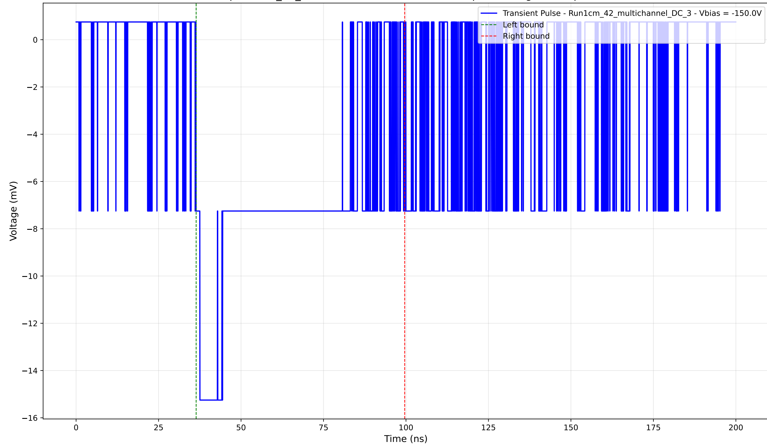
Transient Pulse - Sample: 1cm_42_multichannel - Position: 3360.0 \mu\text{m} - Charge: 8.91 pC - Rise Time: 1.18 ns
