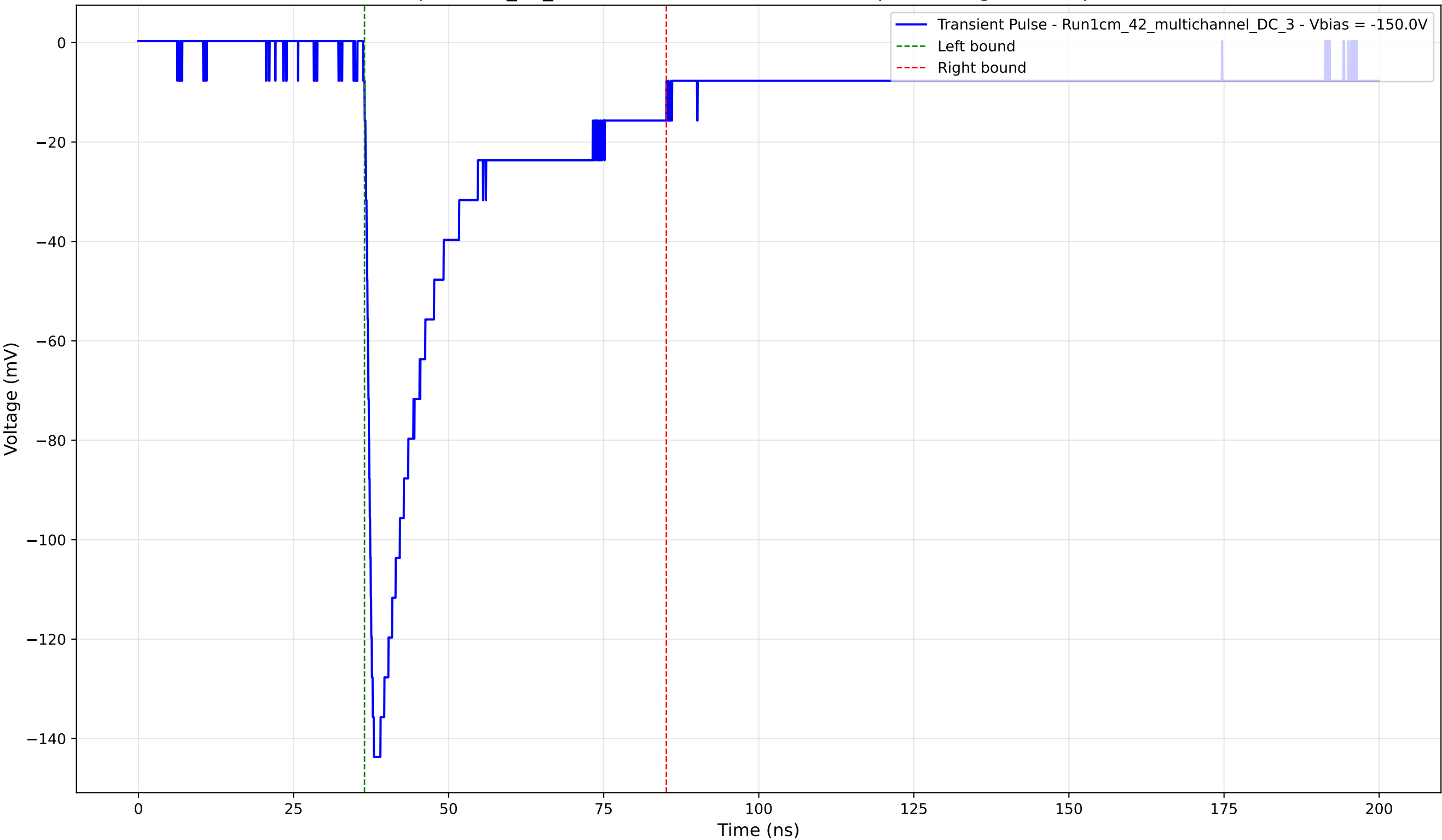
Transient Pulse - Sample: 1cm_42_multichannel - Position: 3750.0 \mu\text{m} - Charge: 38.92 pC - Rise Time: 1.30 ns
