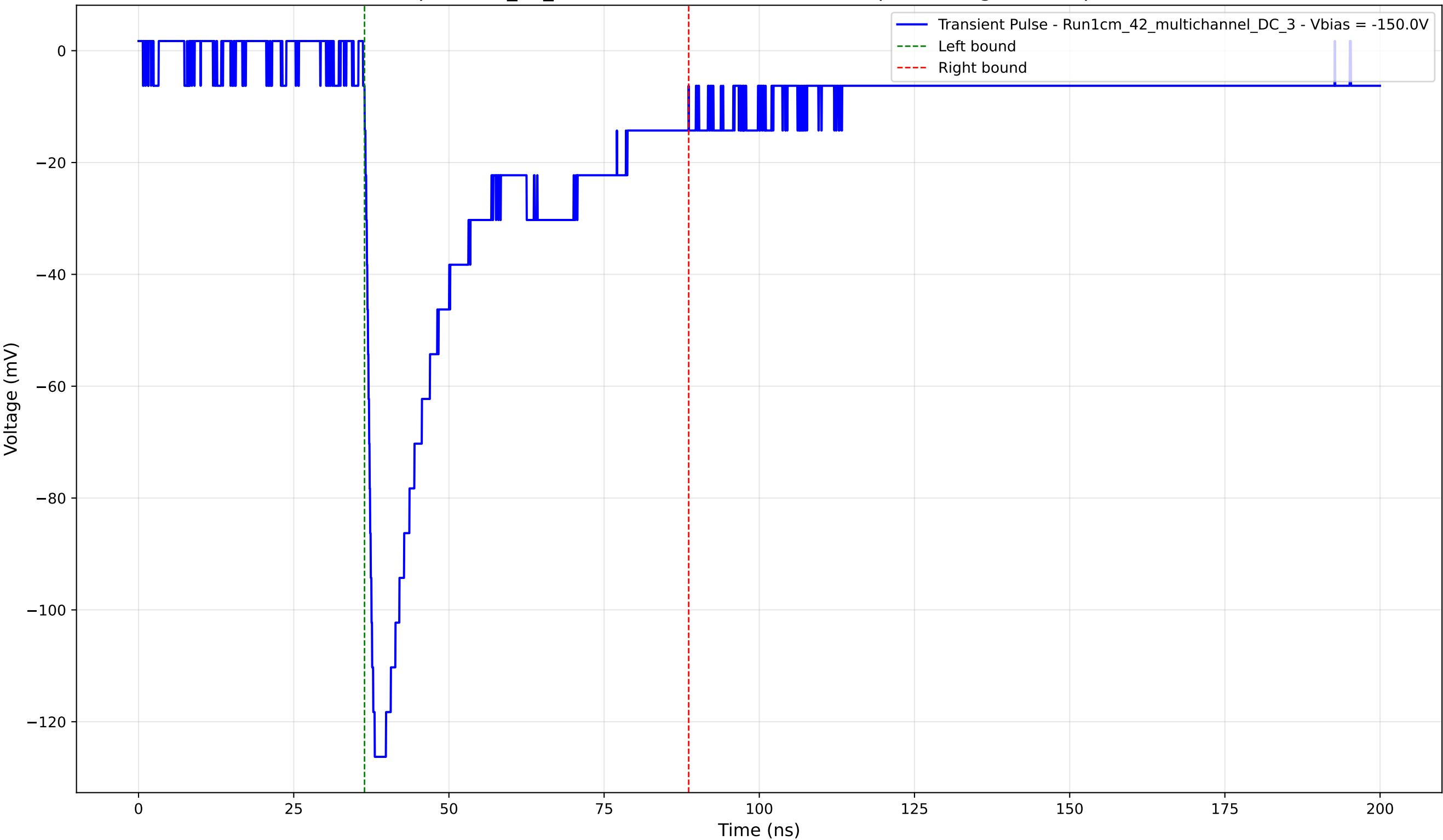
Transient Pulse - Sample: 1cm_42_multichannel - Position: 1445.0 \mu\text{m} - Charge: 40.75 pC - Rise Time: 1.38 ns
