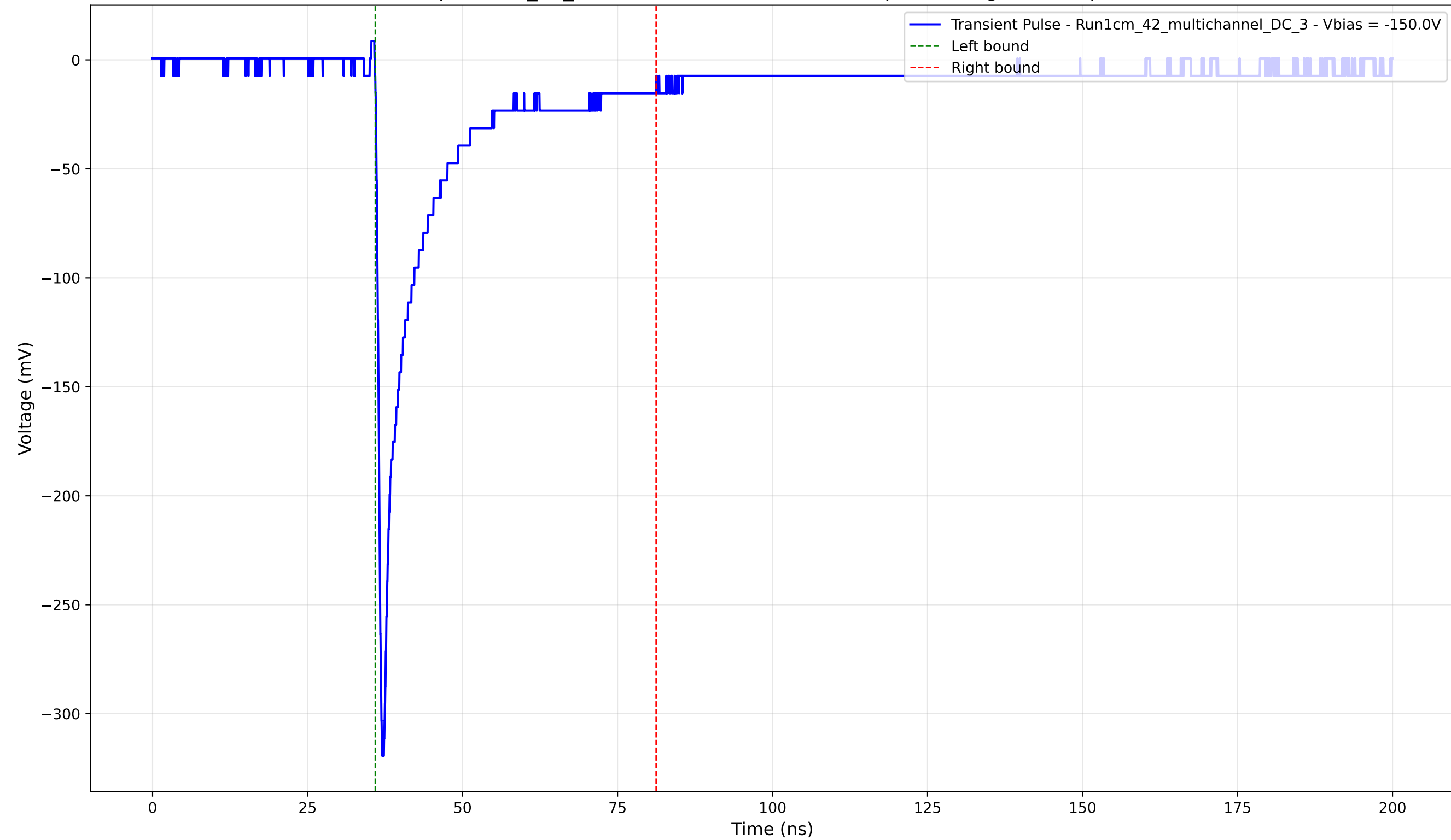
Transient Pulse - Sample: 1cm_42_multichannel - Position: 245.0 \mu\text{m} - Charge: 45.12 pC - Rise Time: 0.82 ns
