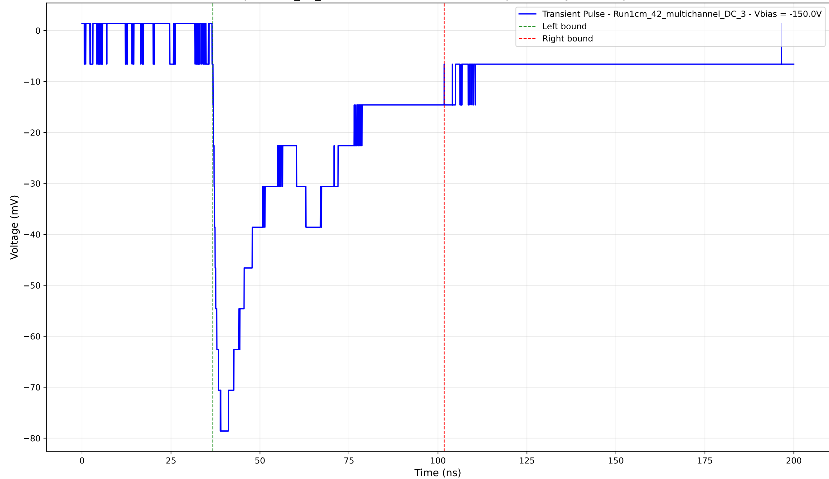
Transient Pulse - Sample: 1cm_42_multichannel - Position: 2560.0 \mu\text{m} - Charge: 38.14 pC - Rise Time: 2.10 ns
