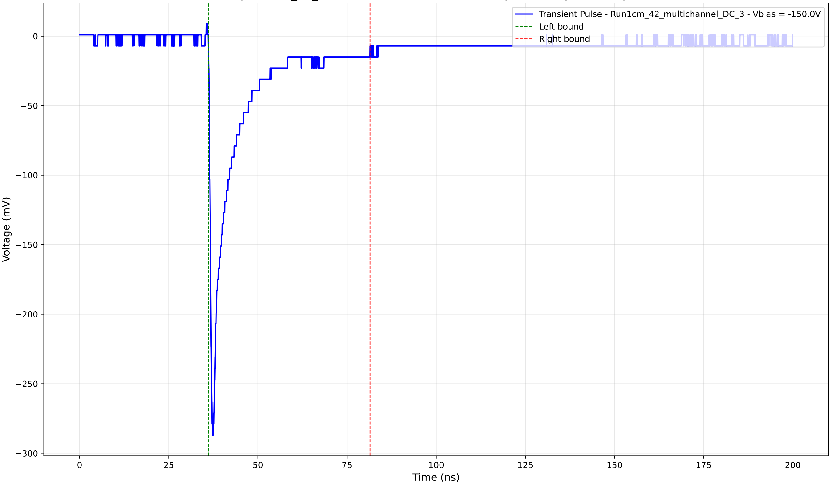
Transient Pulse - Sample: 1cm_42_multichannel - Position: 4575.0 \mu\text{m} - Charge: 40.66 pC - Rise Time: 0.85 ns
