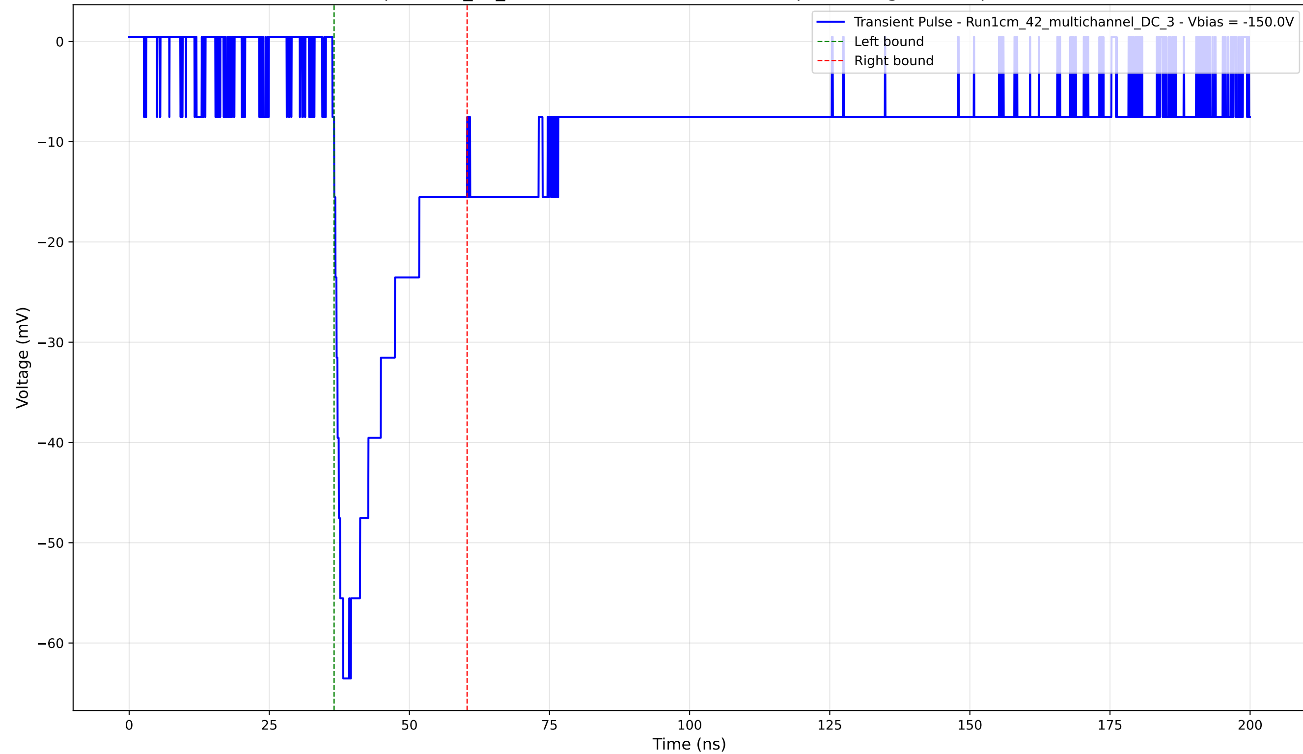
Transient Pulse - Sample: 1cm_42_multichannel - Position: 1410.0 \mu\text{m} - Charge: 14.29 pC - Rise Time: 1.92 ns
