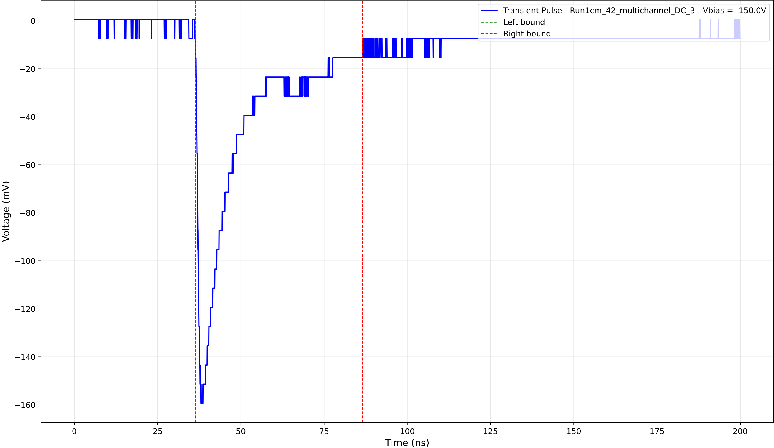
Transient Pulse - Sample: 1cm_42_multichannel - Position: 1170.0 \mu\text{m} - Charge: 43.82 pC - Rise Time: 1.30 ns
