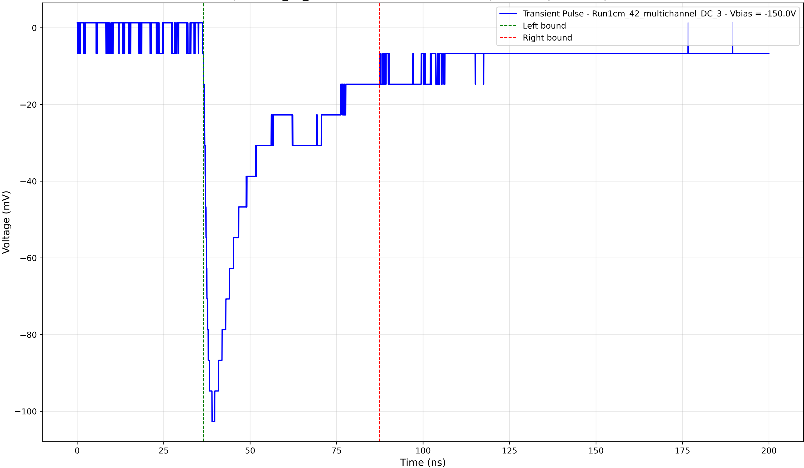
Transient Pulse - Sample: 1cm_42_multichannel - Position: 1790.0 \mu\text{m} - Charge: 35.93 pC - Rise Time: 1.73 ns
