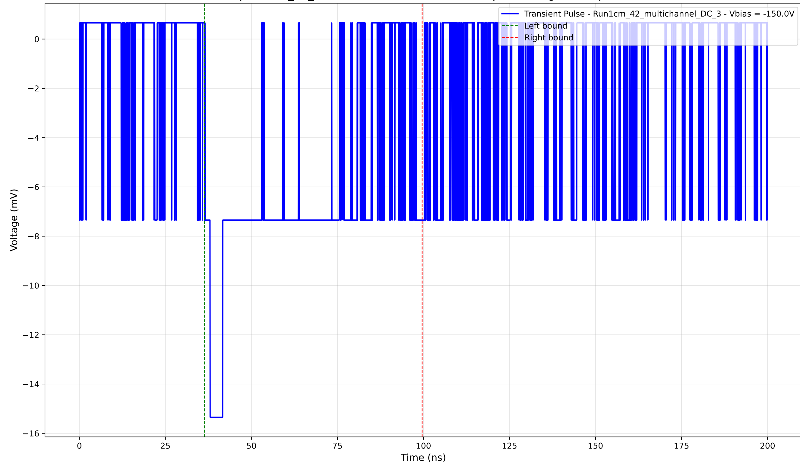
Transient Pulse - Sample: 1cm_42_multichannel - Position: 3365.0 \mu\text{m} - Charge: 7.74 pC - Rise Time: 1.46 ns
