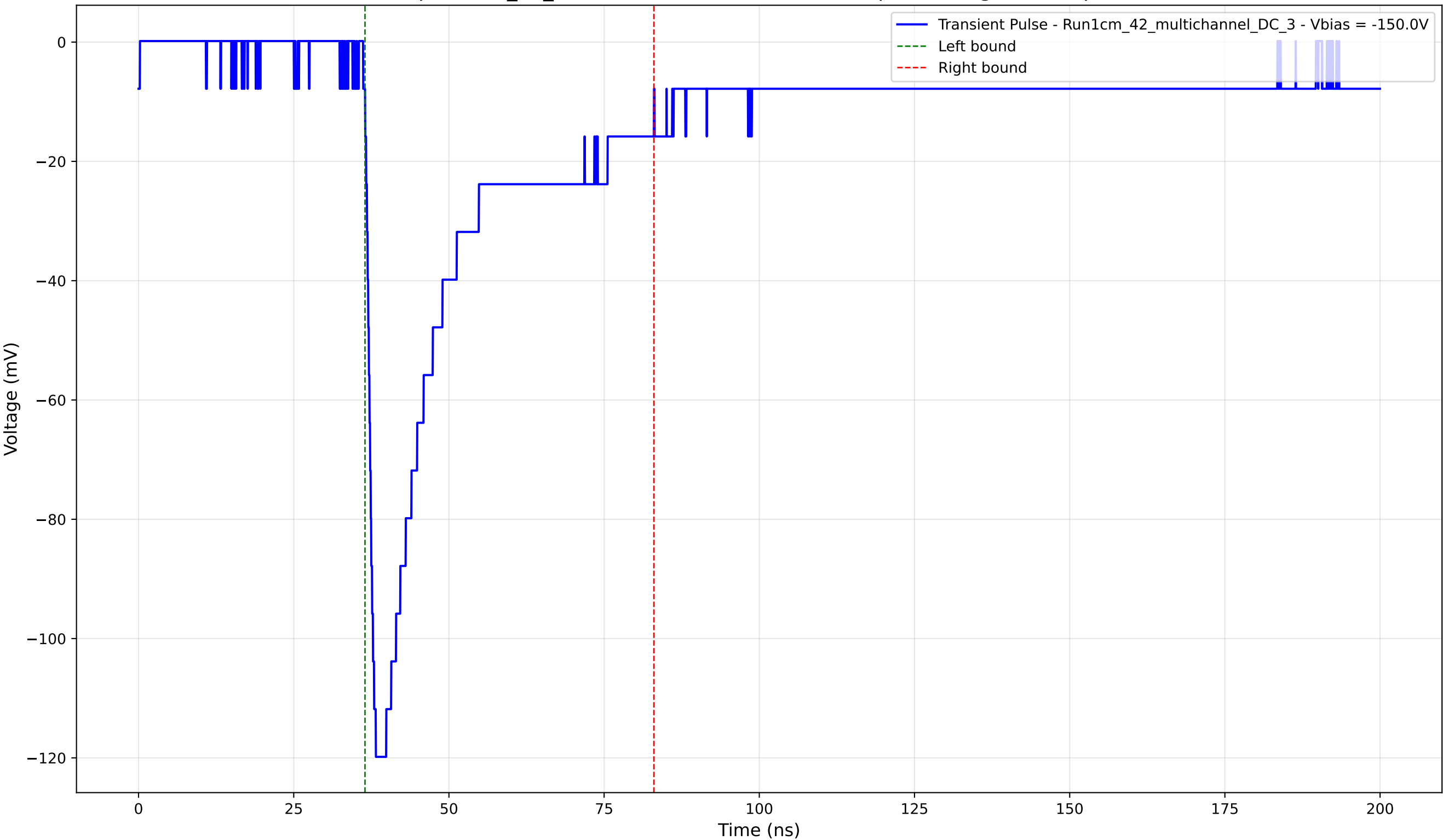
Transient Pulse - Sample: 1cm_42_multichannel - Position: 3475.0 \mu\text{m} - Charge: 36.21 pC - Rise Time: 1.45 ns
