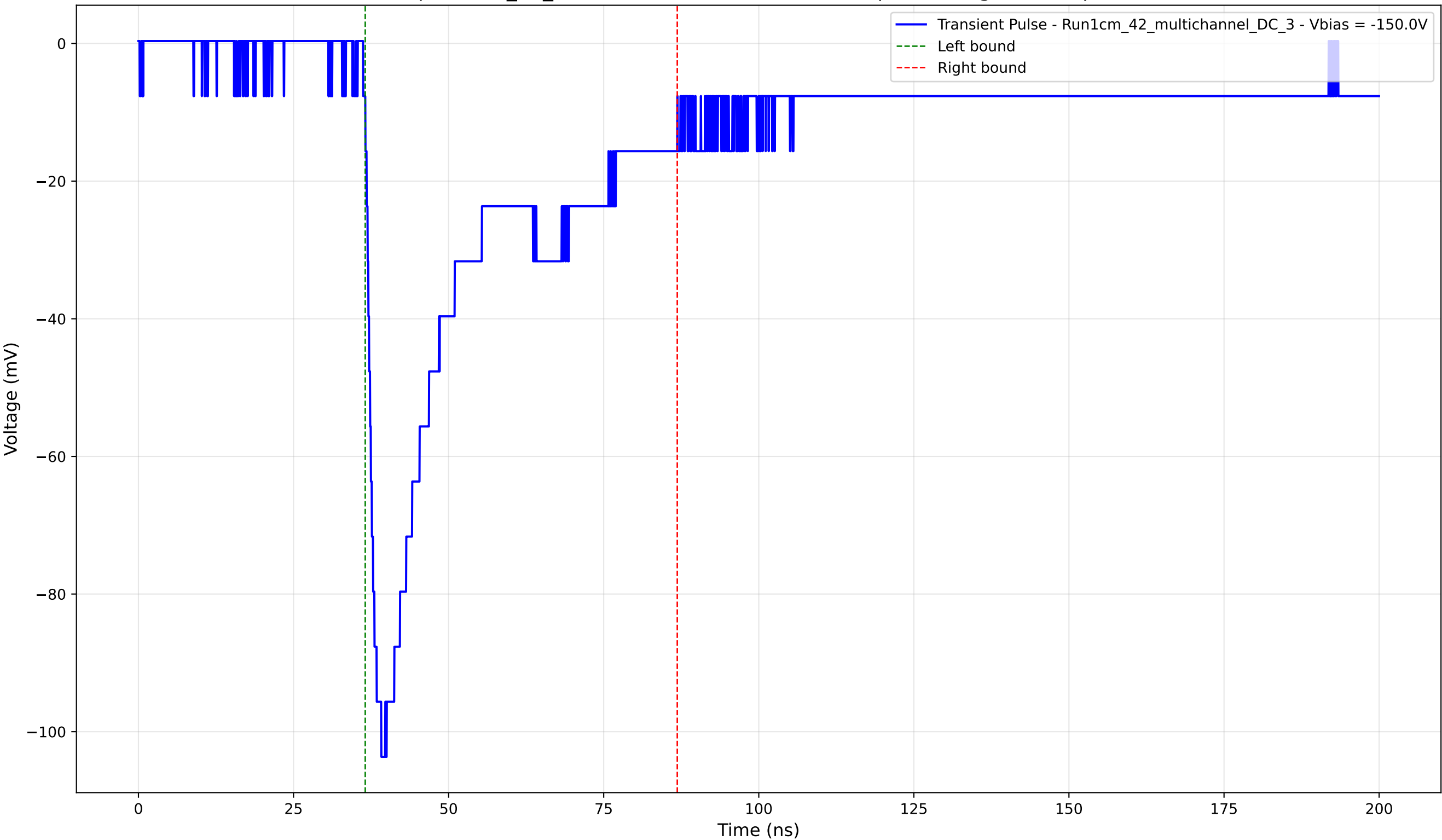
Transient Pulse - Sample: 1cm_42_multichannel - Position: 3085.0 \mu\text{m} - Charge: 35.79 pC - Rise Time: 1.83 ns
