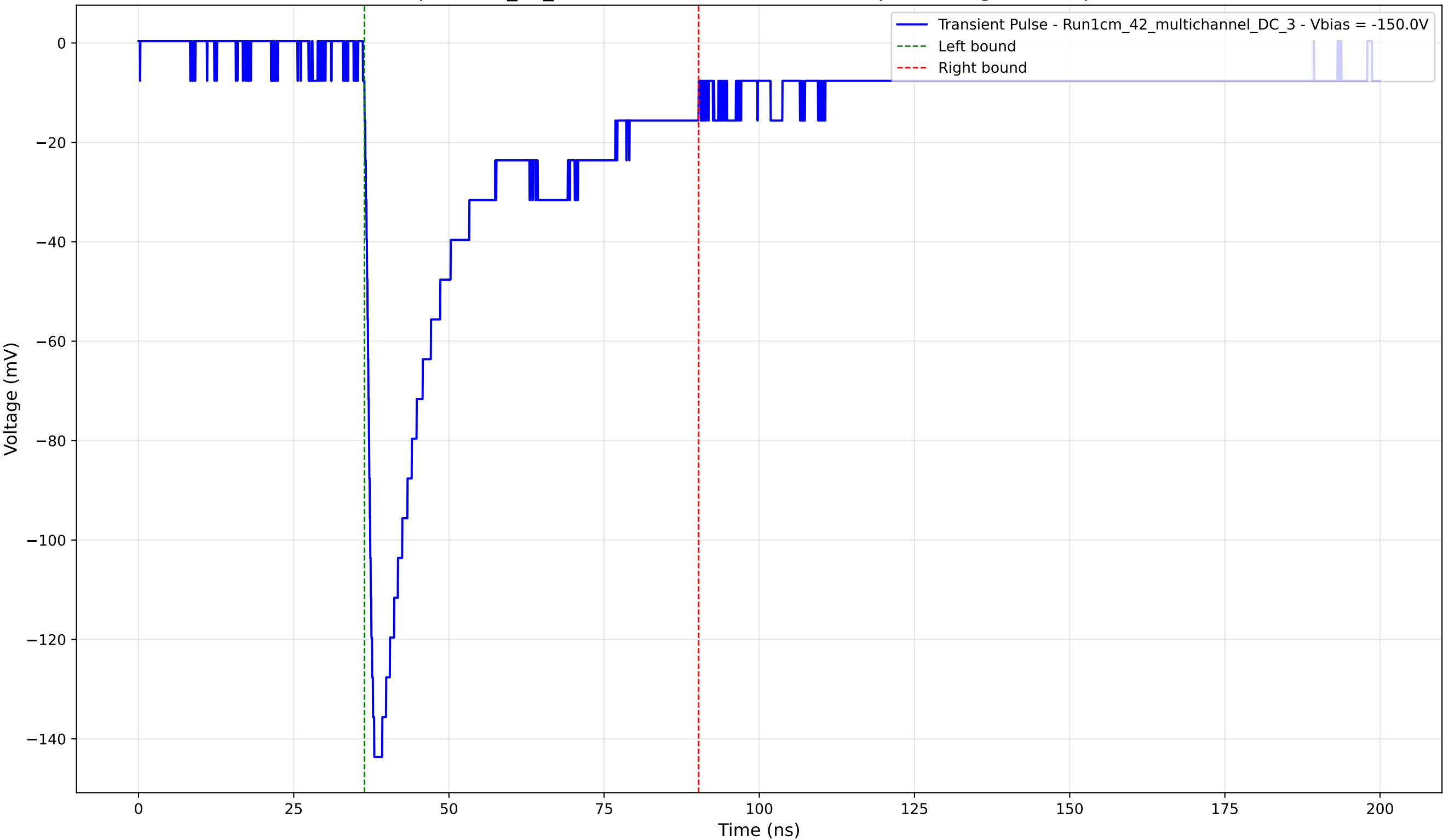
Transient Pulse - Sample: 1cm_42_multichannel - Position: 1275.0 \mu\text{m} - Charge: 43.69 pC - Rise Time: 1.36 ns
