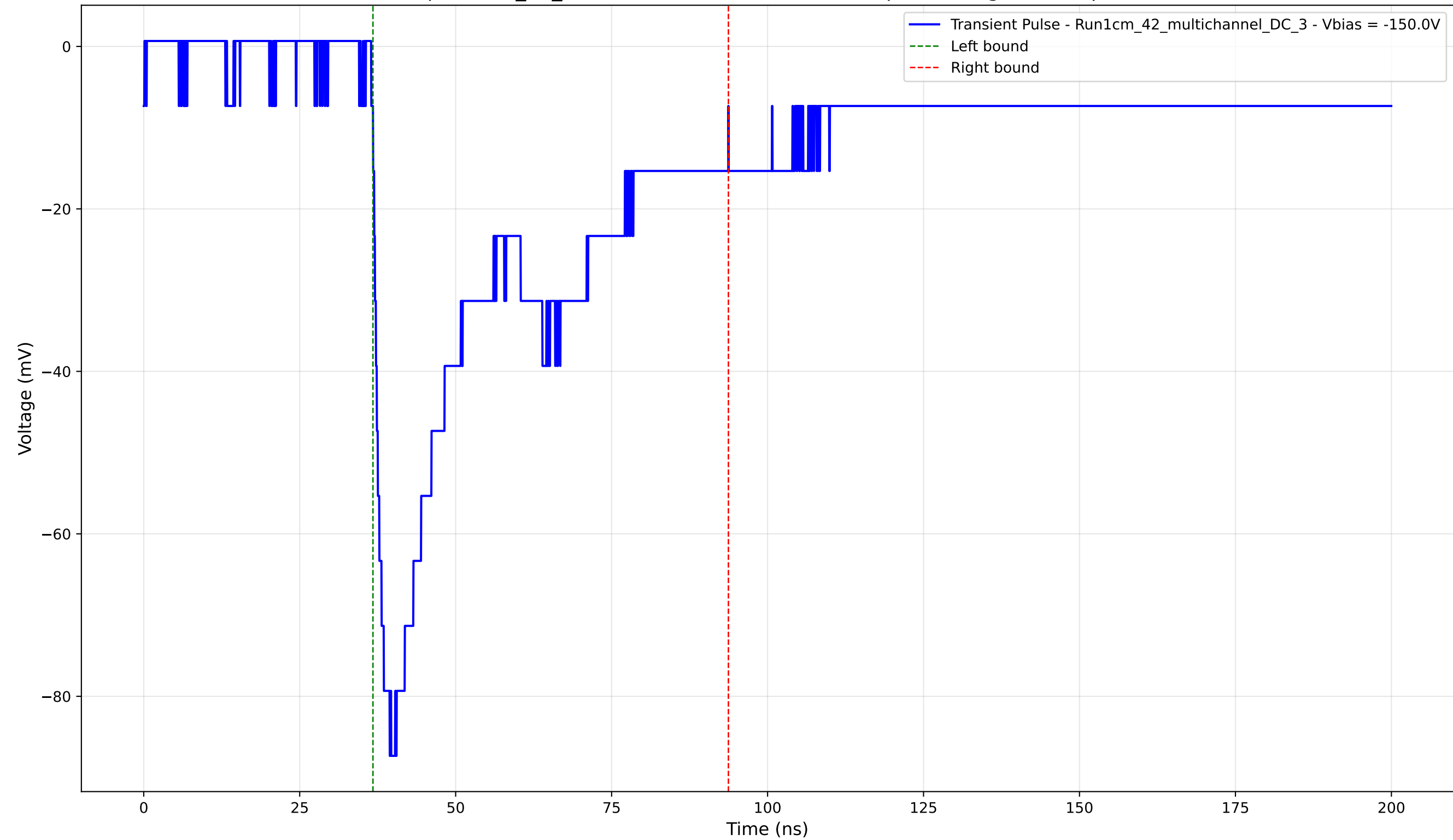
Transient Pulse - Sample: 1cm_42_multichannel - Position: 2650.0 \mu\text{m} - Charge: 36.88 pC - Rise Time: 1.74 ns
