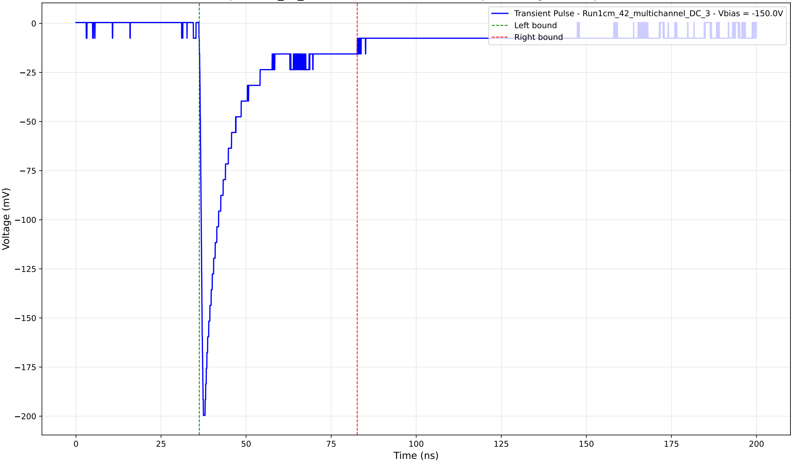
Transient Pulse - Sample: 1cm_42_multichannel - Position: 4260.0 \mu\text{m} - Charge: 38.27 pC - Rise Time: 0.93 ns
