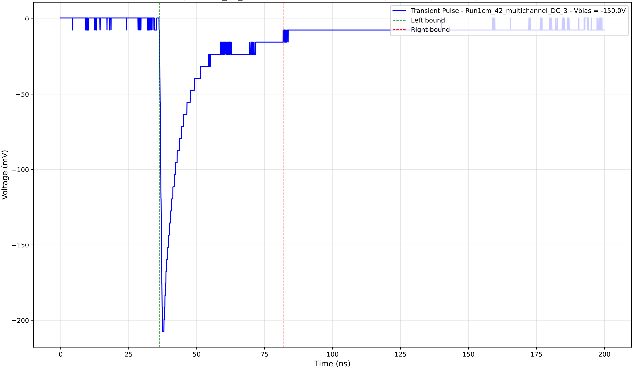
Transient Pulse - Sample: 1cm_42_multichannel - Position: 4240.0 \mu\text{m} - Charge: 40.59 pC - Rise Time: 0.95 ns
