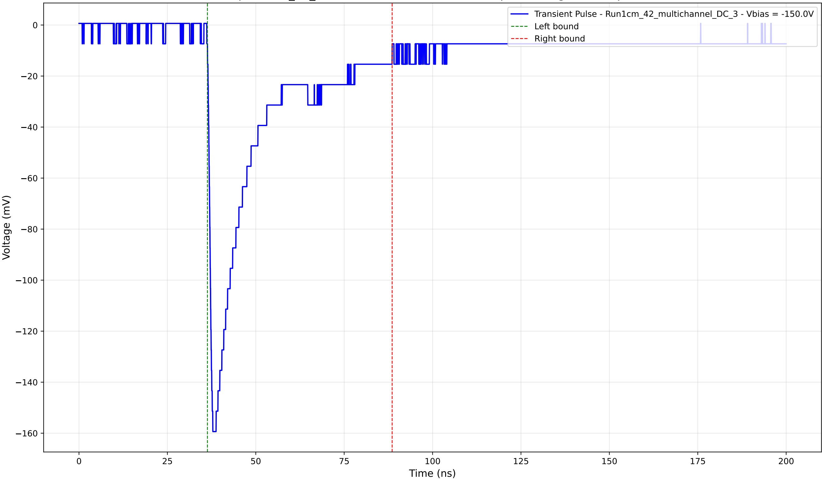
Transient Pulse - Sample: 1cm_42_multichannel - Position: 1130.0 \mu\text{m} - Charge: 44.08 pC - Rise Time: 1.22 ns
