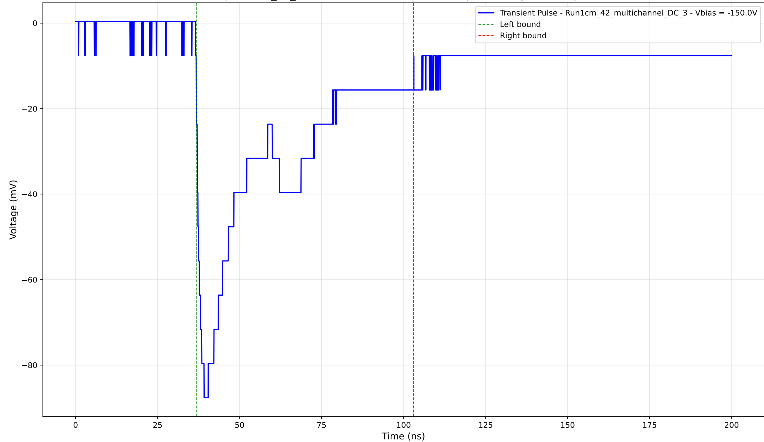
Transient Pulse - Sample: 1cm_42_multichannel - Position: 2245.0 \mu\text{m} - Charge: 42.37 pC - Rise Time: 1.72 ns
