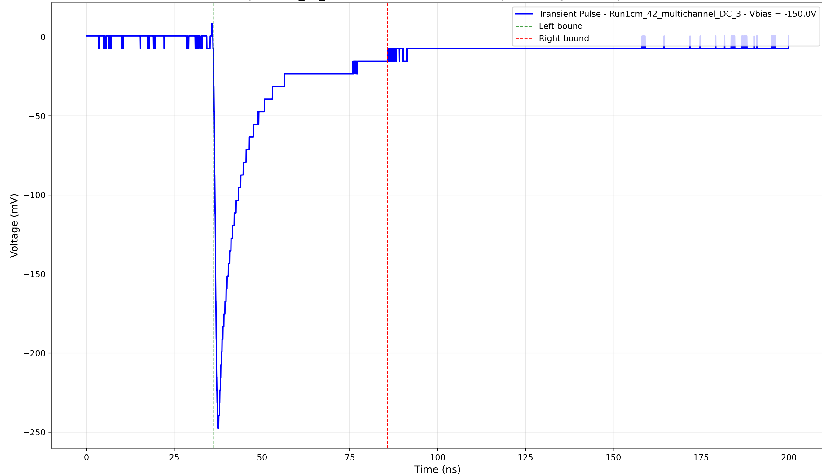
Transient Pulse - Sample: 1cm_42_multichannel - Position: 585.0 \mu\text{m} - Charge: 47.91 pC - Rise Time: 0.90 ns
