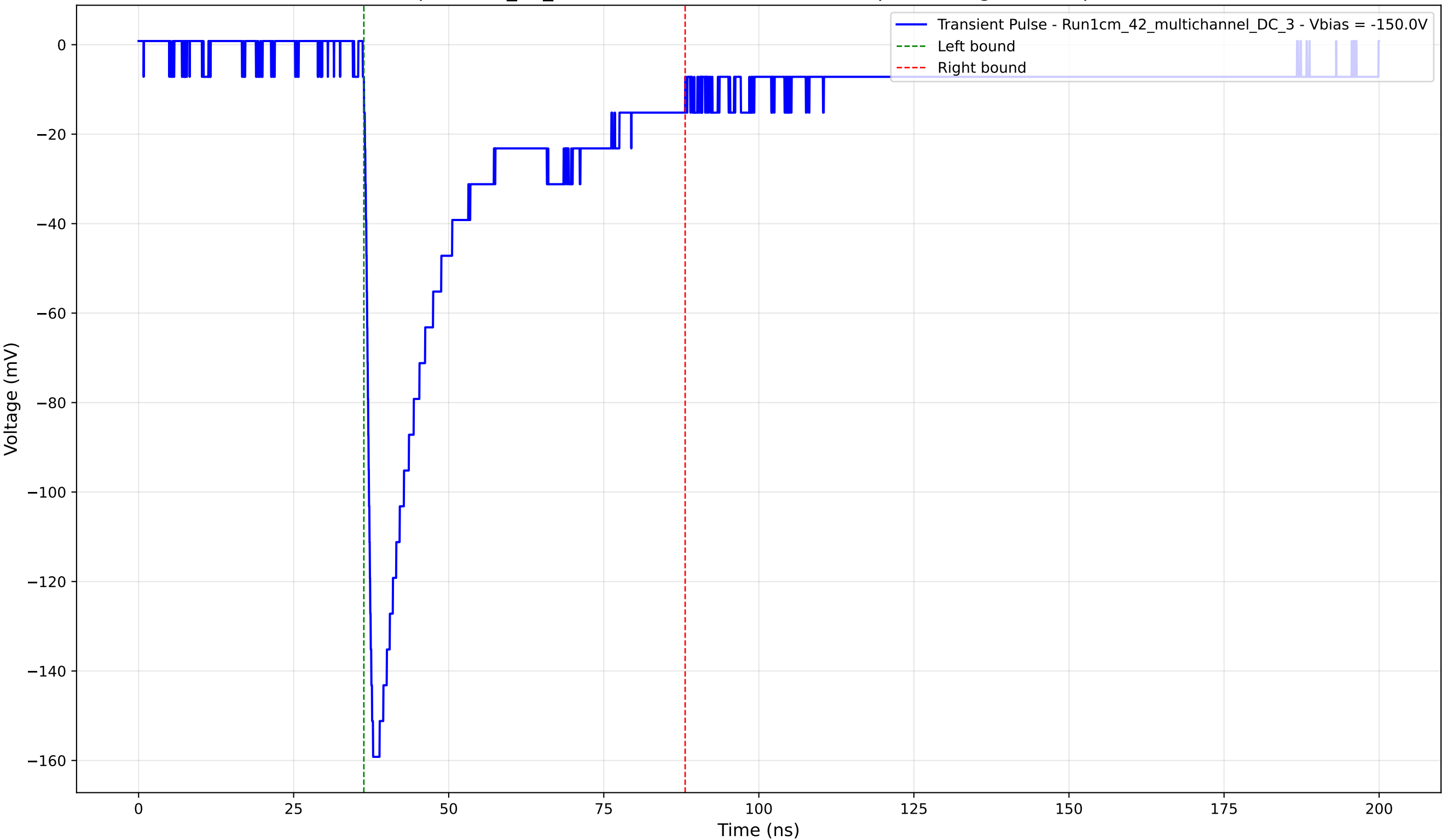
Transient Pulse - Sample: 1cm_42_multichannel - Position: 1125.0 \mu\text{m} - Charge: 44.03 pC - Rise Time: 1.18 ns
