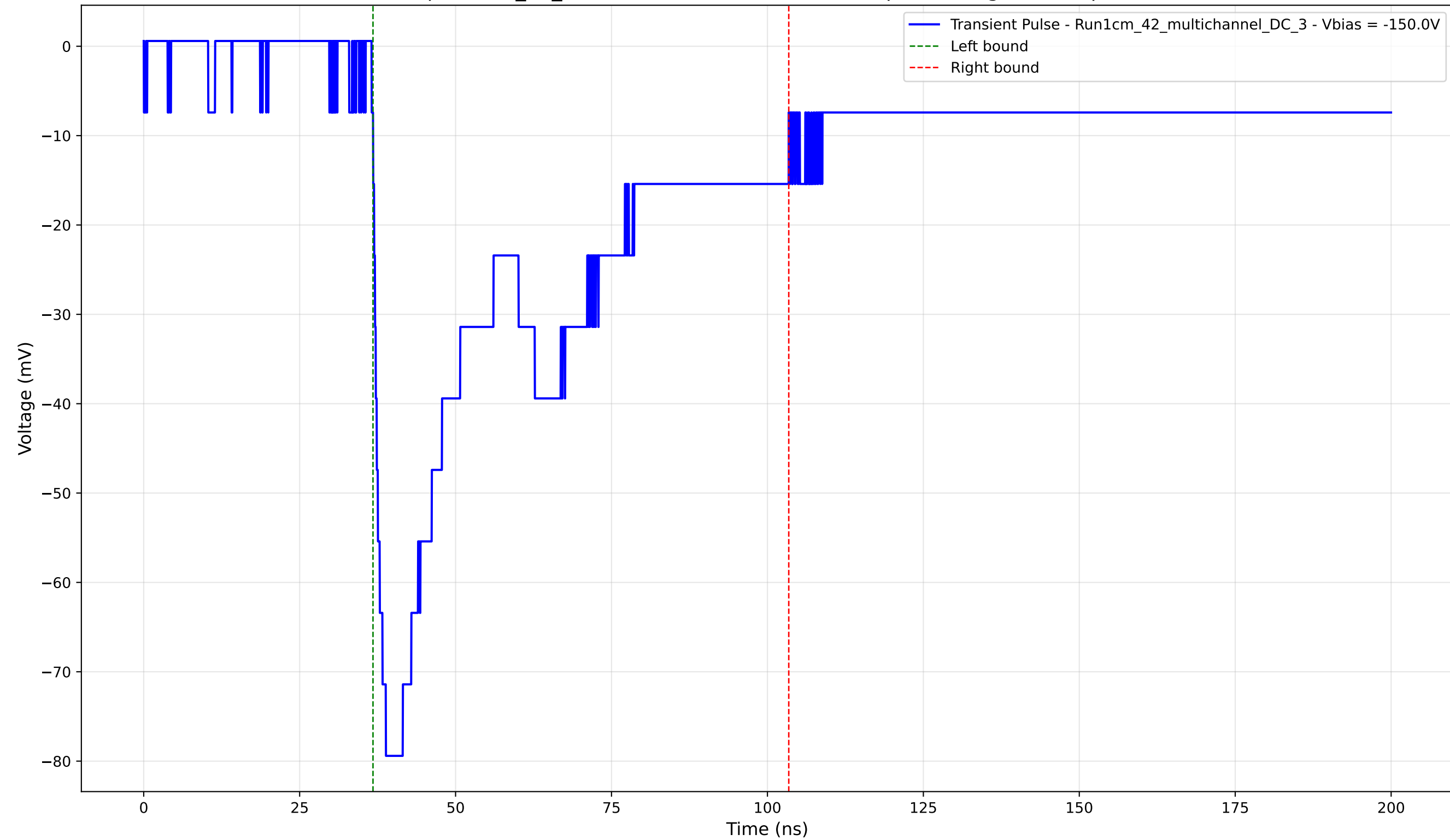
Transient Pulse - Sample: 1cm_42_multichannel - Position: 2515.0 \mu\text{m} - Charge: 40.10 pC - Rise Time: 2.06 ns
