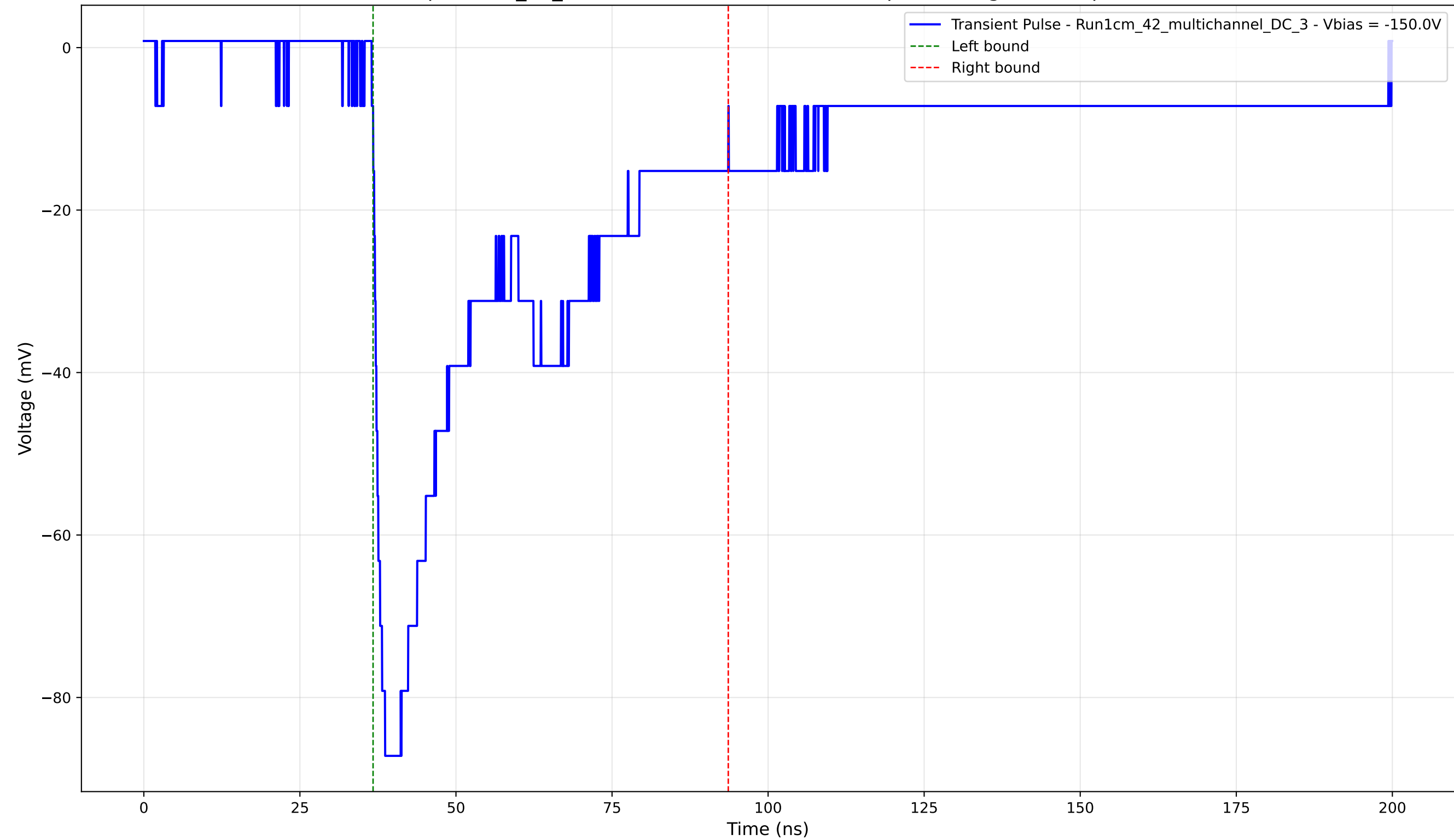
Transient Pulse - Sample: 1cm_42_multichannel - Position: 2120.0 \mu\text{m} - Charge: 39.19 pC - Rise Time: 1.44 ns
