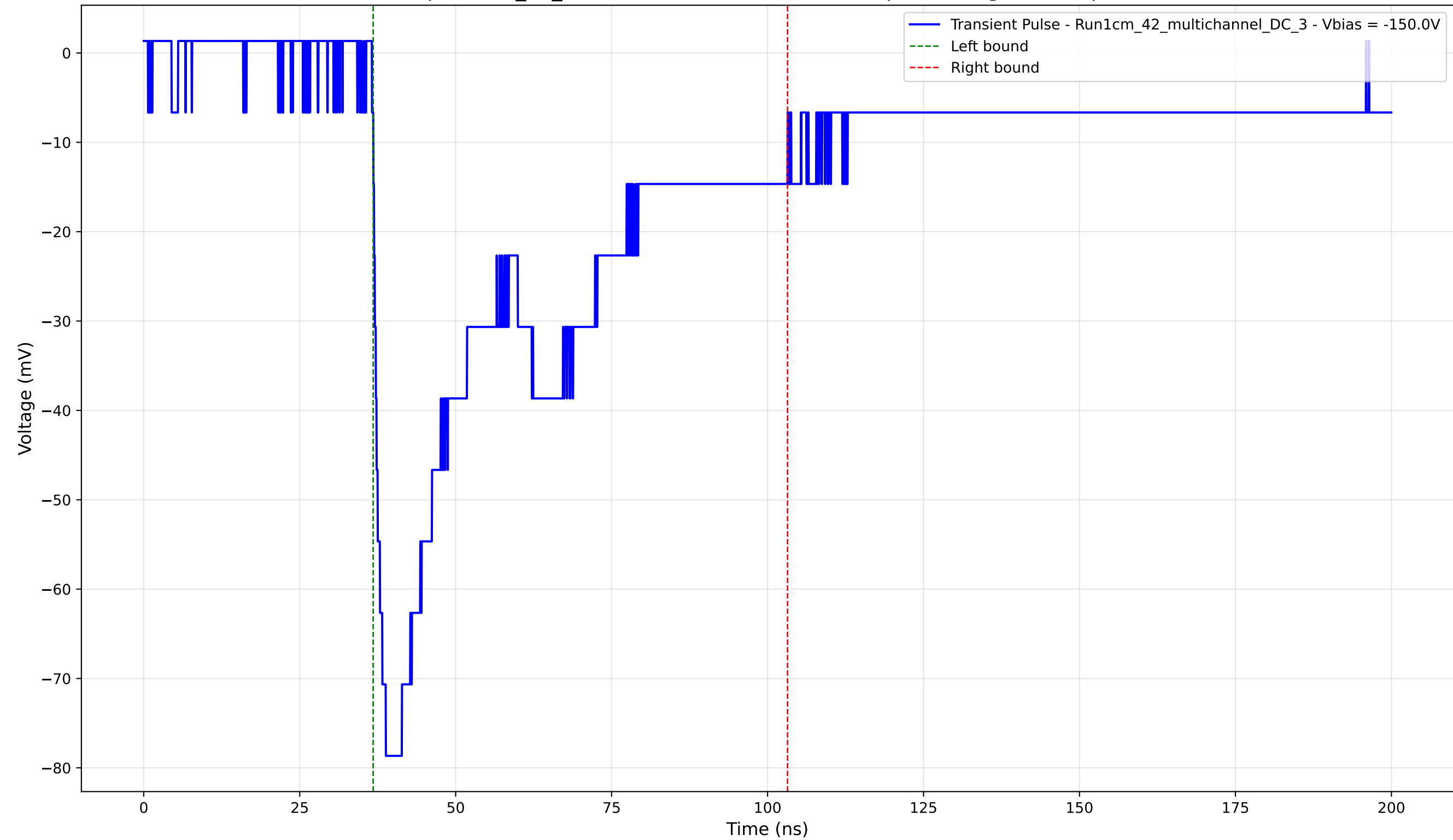
Transient Pulse - Sample: 1cm_42_multichannel - Position: 2470.0 \mu\text{m} - Charge: 40.04 pC - Rise Time: 2.02 ns
