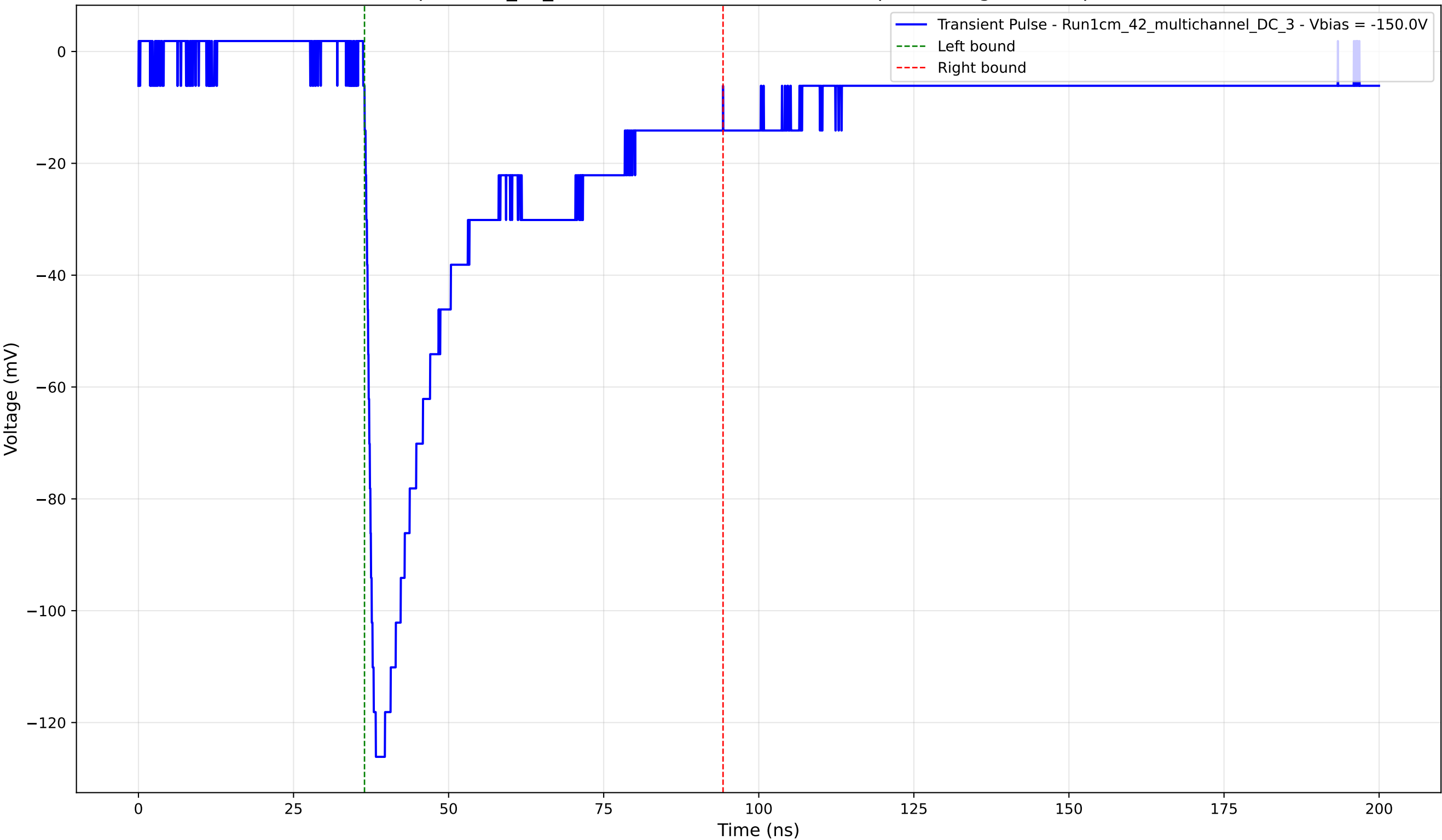
Transient Pulse - Sample: 1cm_42_multichannel - Position: 1535.0 \mu\text{m} - Charge: 42.75 pC - Rise Time: 1.46 ns
