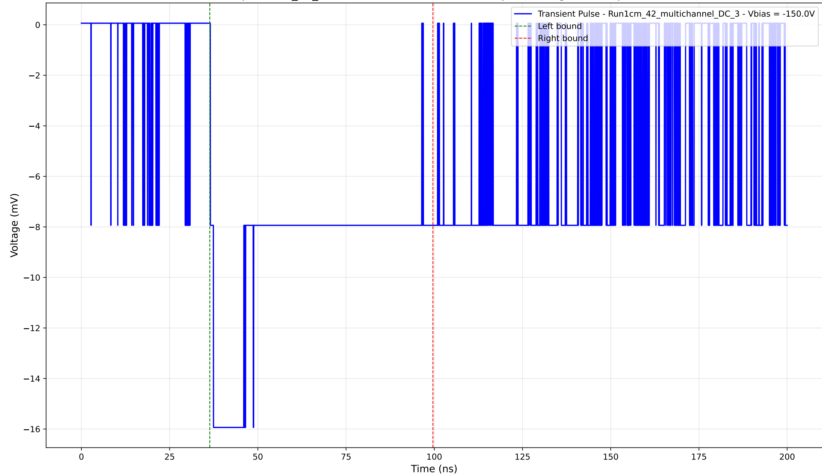
Transient Pulse - Sample: 1cm_42_multichannel - Position: 2340.0 \mu\text{m} - Charge: 11.41 pC - Rise Time: 0.90 ns
