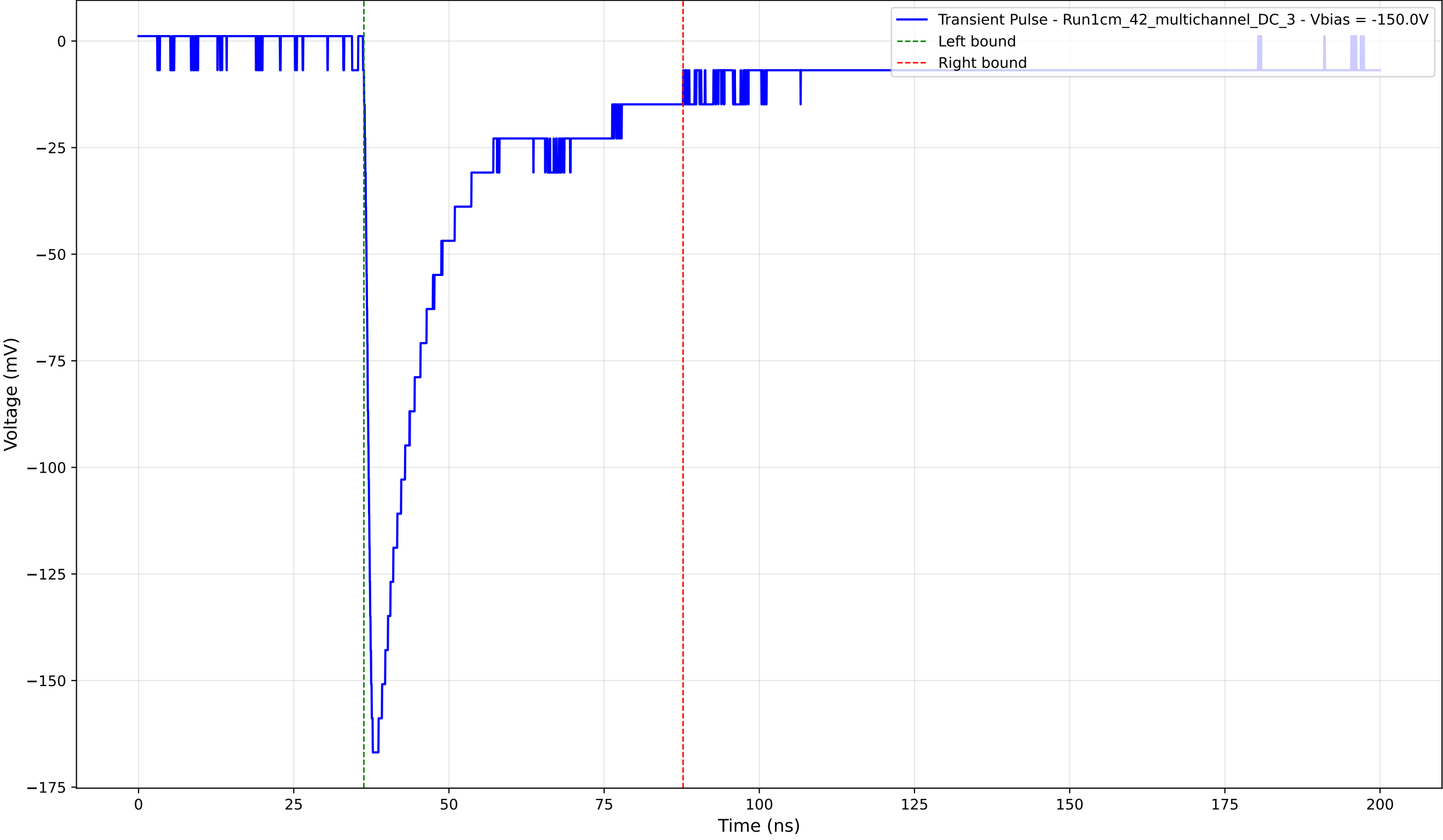
Transient Pulse - Sample: 1cm_42_multichannel - Position: 1055.0 \mu\text{m} - Charge: 44.11 pC - Rise Time: 1.04 ns
