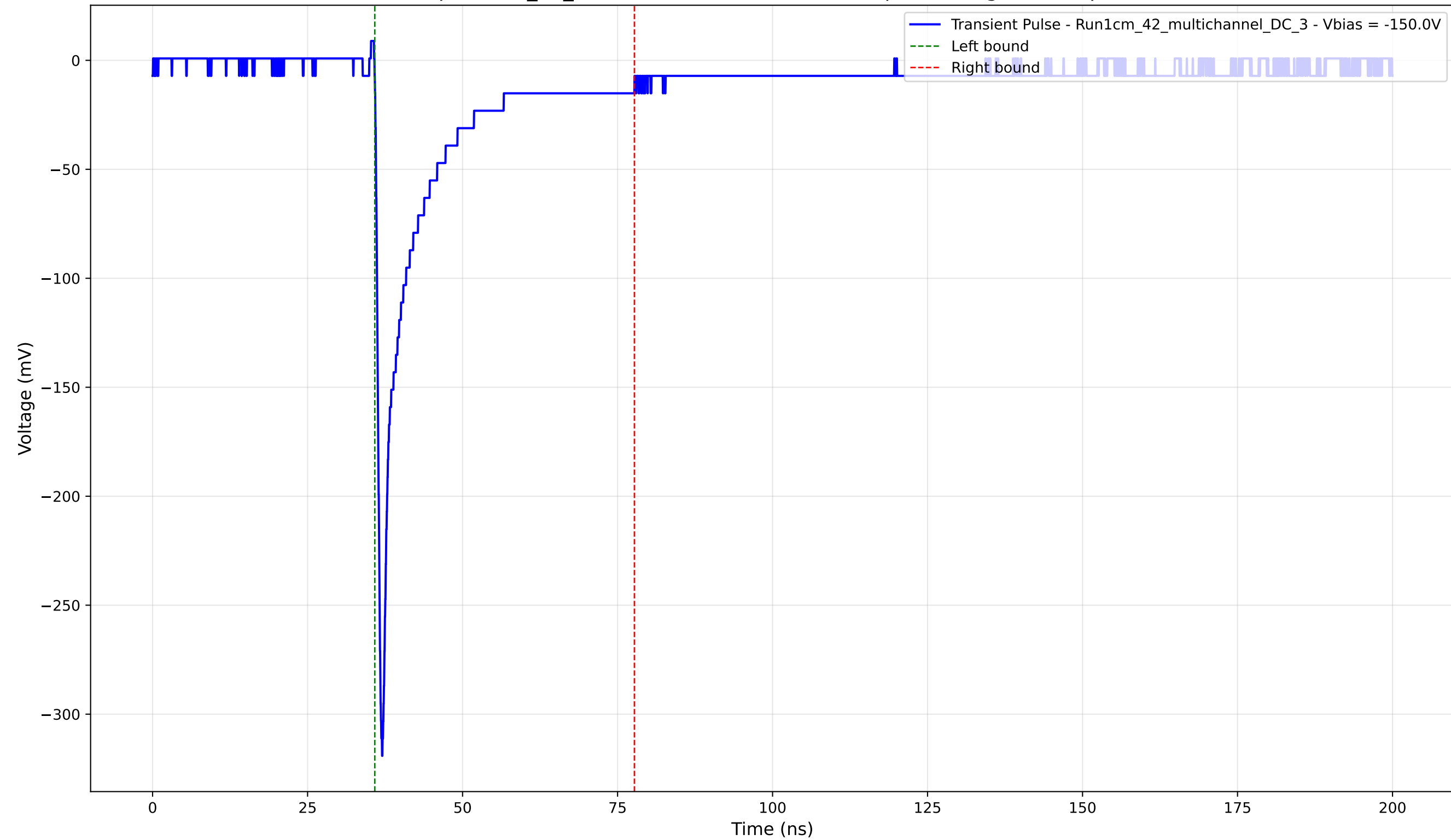
Transient Pulse - Sample: 1cm_42_multichannel - Position: 100.0 \mu\text{m} - Charge: 36.98 pC - Rise Time: 0.80 ns
