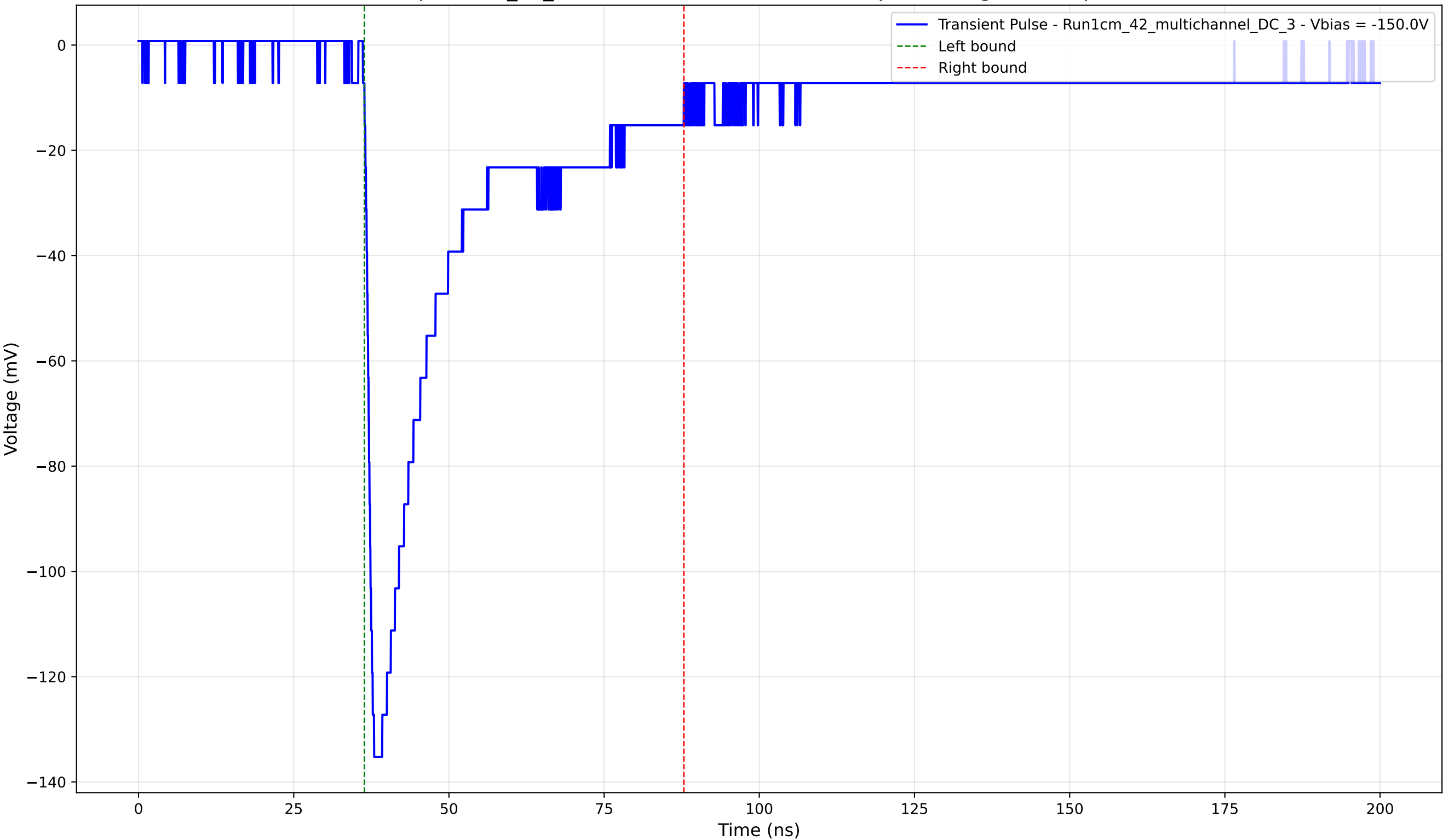
Transient Pulse - Sample: 1cm_42_multichannel - Position: 1285.0 \mu\text{m} - Charge: 40.16 pC - Rise Time: 1.32 ns
