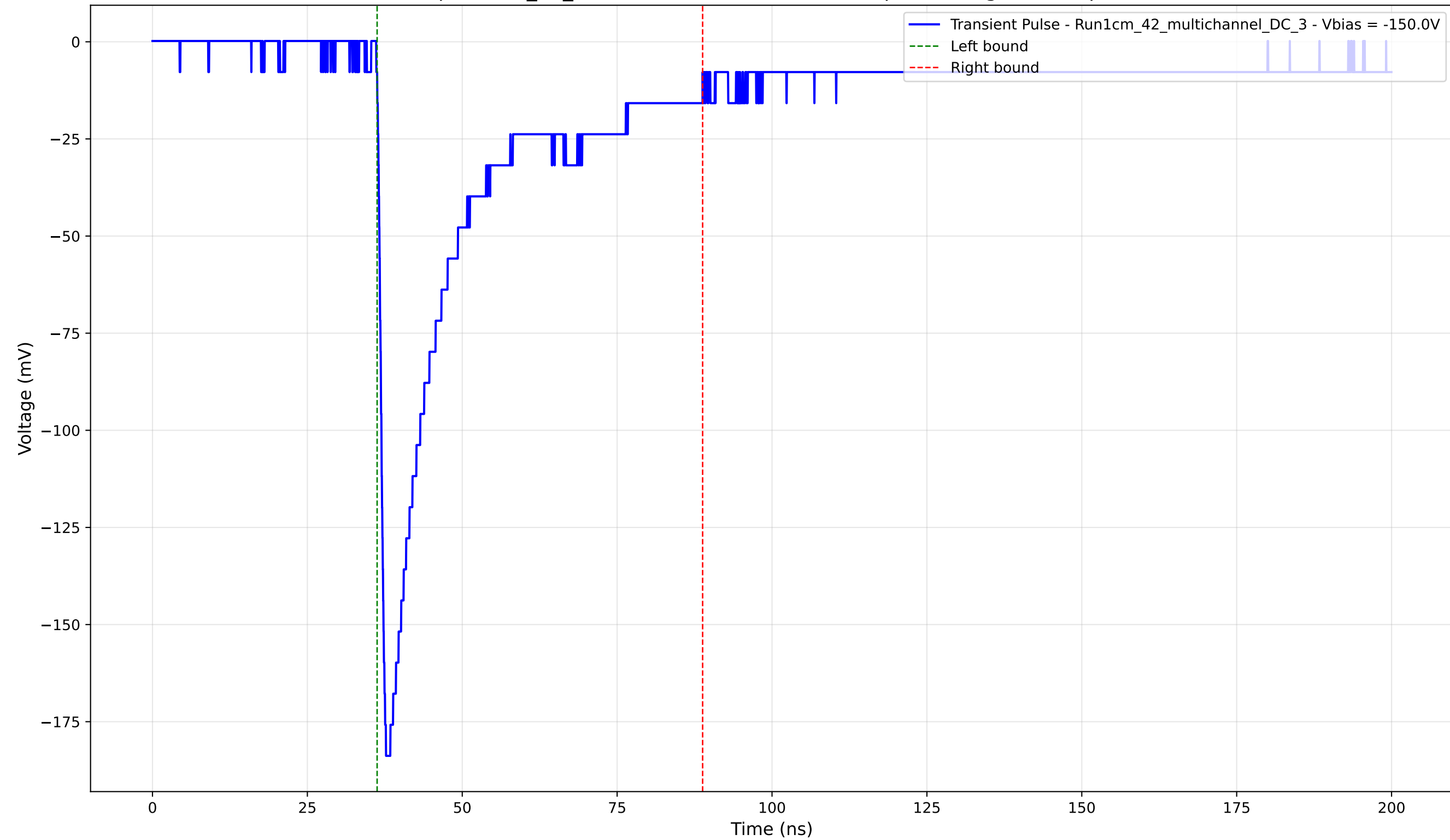
Transient Pulse - Sample: 1cm_42_multichannel - Position: 970.0 \mu\text{m} - Charge: 47.15 pC - Rise Time: 1.07 ns
