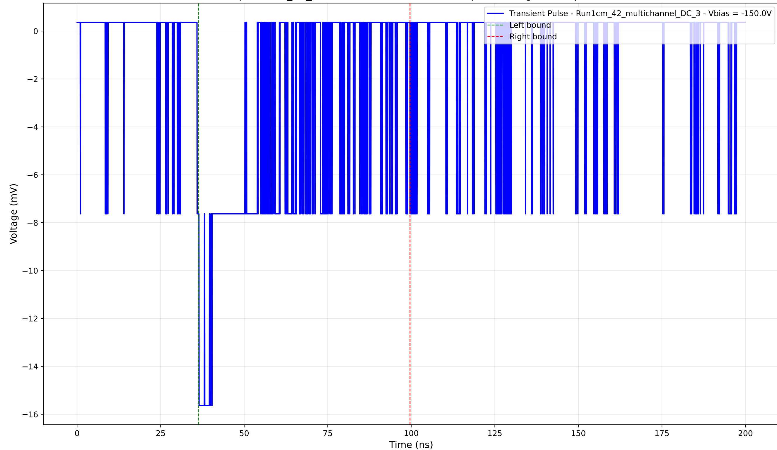
Transient Pulse - Sample: 1cm_42_multichannel - Position: 40.0 \mu\text{m} - Charge: 4.95 pC - Rise Time: 0.60 ns
