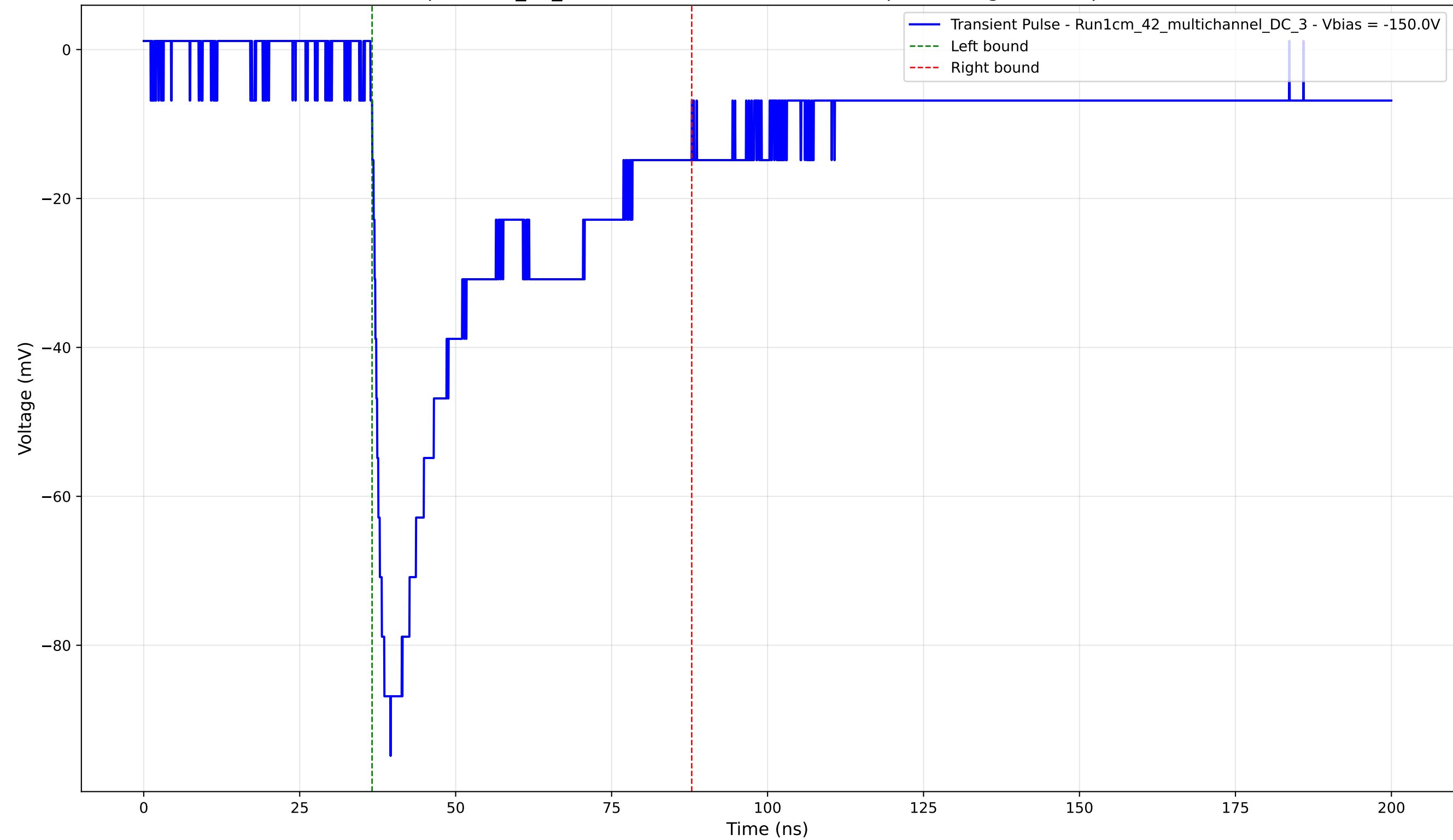
Transient Pulse - Sample: 1cm_42_multichannel - Position: 2780.0 \mu\text{m} - Charge: 35.21 pC - Rise Time: 1.95 ns
