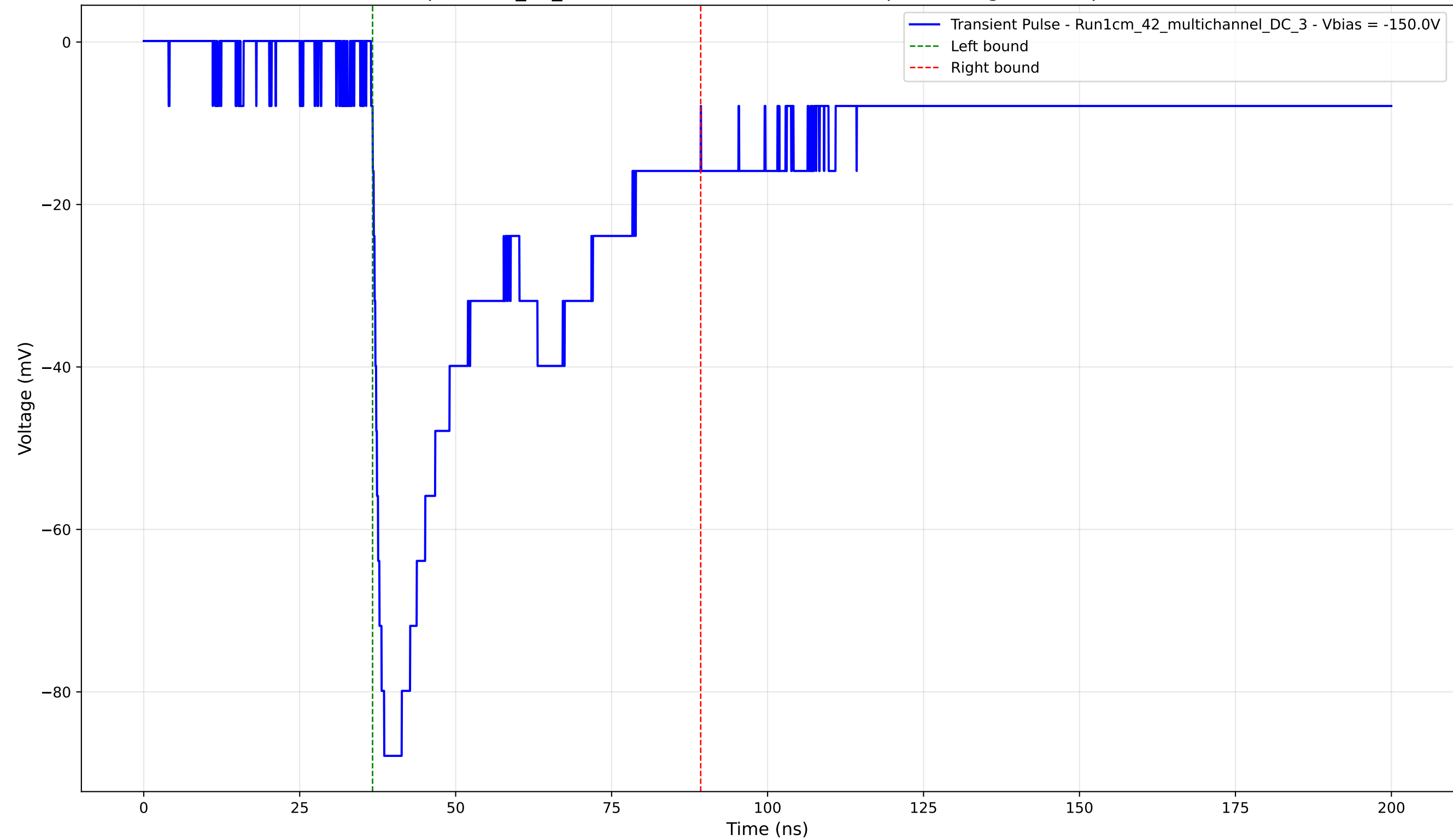
Transient Pulse - Sample: 1cm_42_multichannel - Position: 2080.0 \mu\text{m} - Charge: 38.45 pC - Rise Time: 1.44 ns
