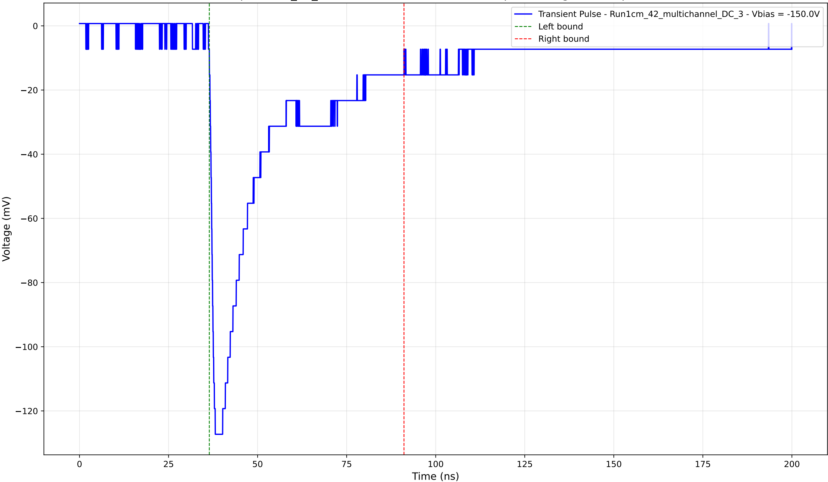
Transient Pulse - Sample: 1cm_42_multichannel - Position: 1515.0 \mu\text{m} - Charge: 43.69 pC - Rise Time: 1.41 ns
