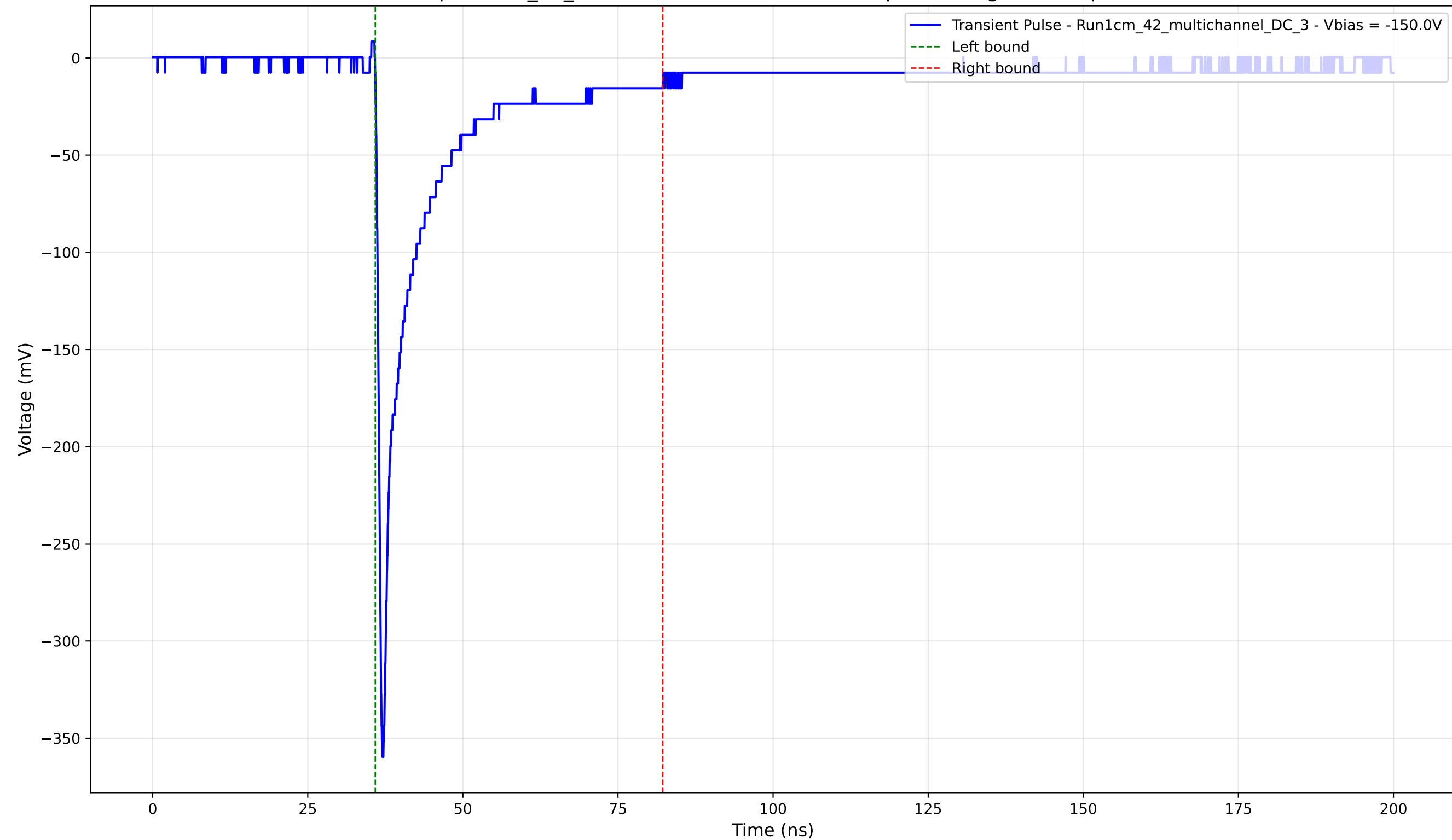
Transient Pulse - Sample: 1cm_42_multichannel - Position: 190.0 \mu\text{m} - Charge: 47.73 pC - Rise Time: 0.81 ns
