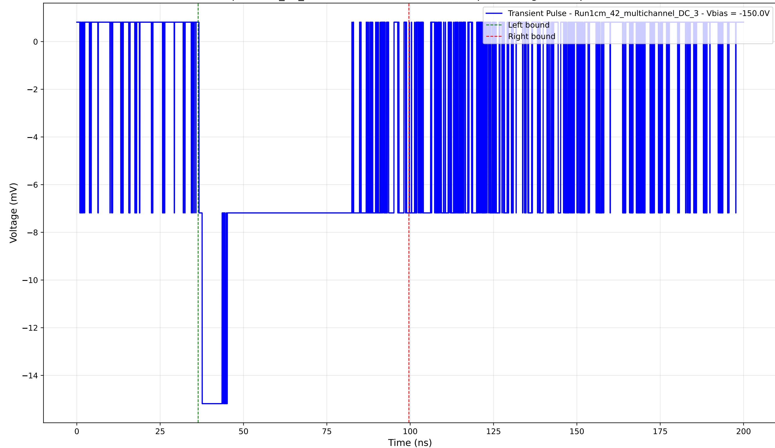
Transient Pulse - Sample: 1cm_42_multichannel - Position: 2850.0 \mu\text{m} - Charge: 9.38 pC - Rise Time: 0.98 ns
