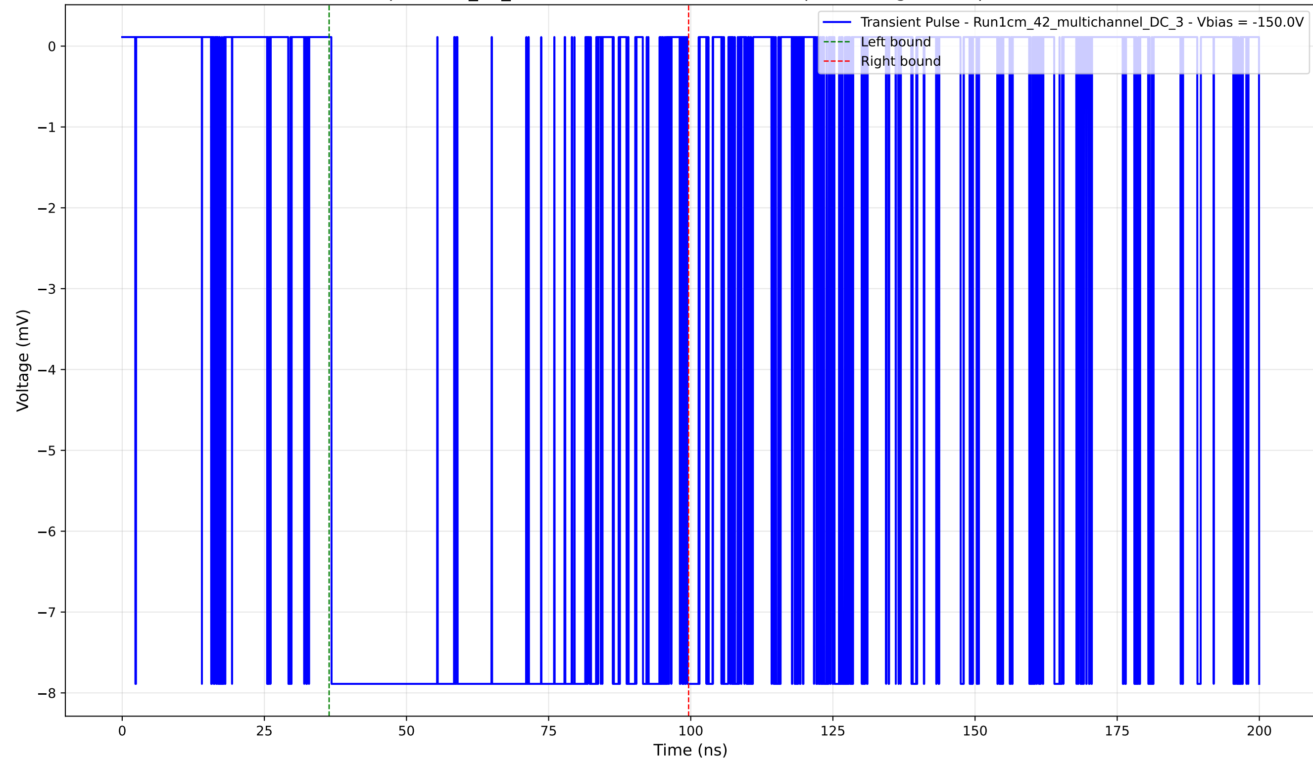
Transient Pulse - Sample: 1cm_42_multichannel - Position: 1885.0 \mu\text{m} - Charge: 8.23 pC - Rise Time: 0.02 ns
