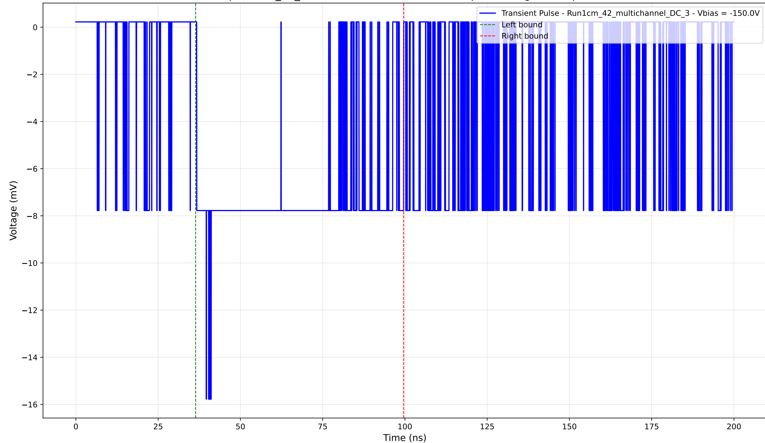
Transient Pulse - Sample: 1cm_42_multichannel - Position: 2900.0 \mu\text{m} - Charge: 8.82 pC - Rise Time: 2.94 ns
