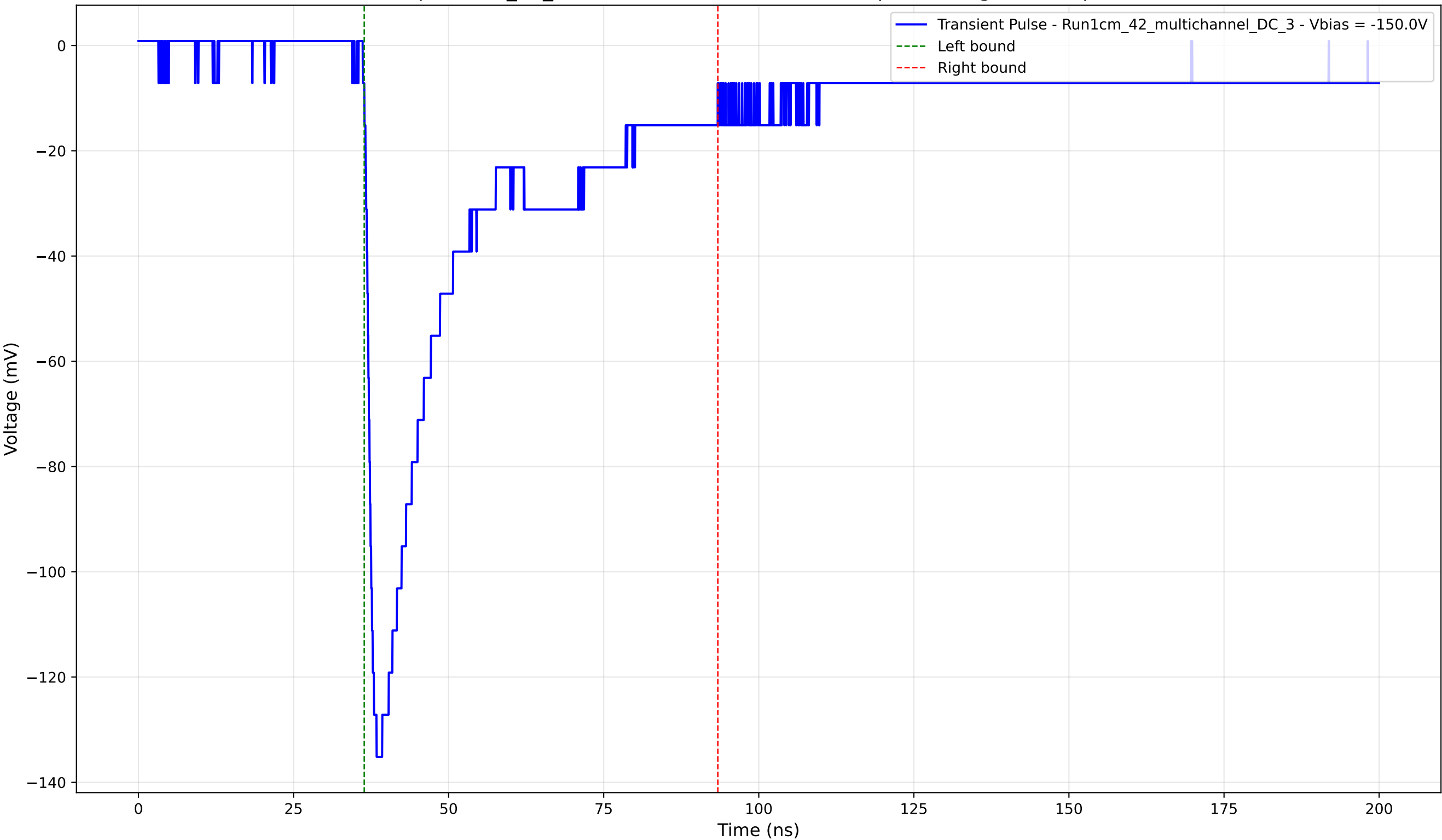
Transient Pulse - Sample: 1cm_42_multichannel - Position: 1475.0 \mu\text{m} - Charge: 44.36 pC - Rise Time: 1.54 ns
