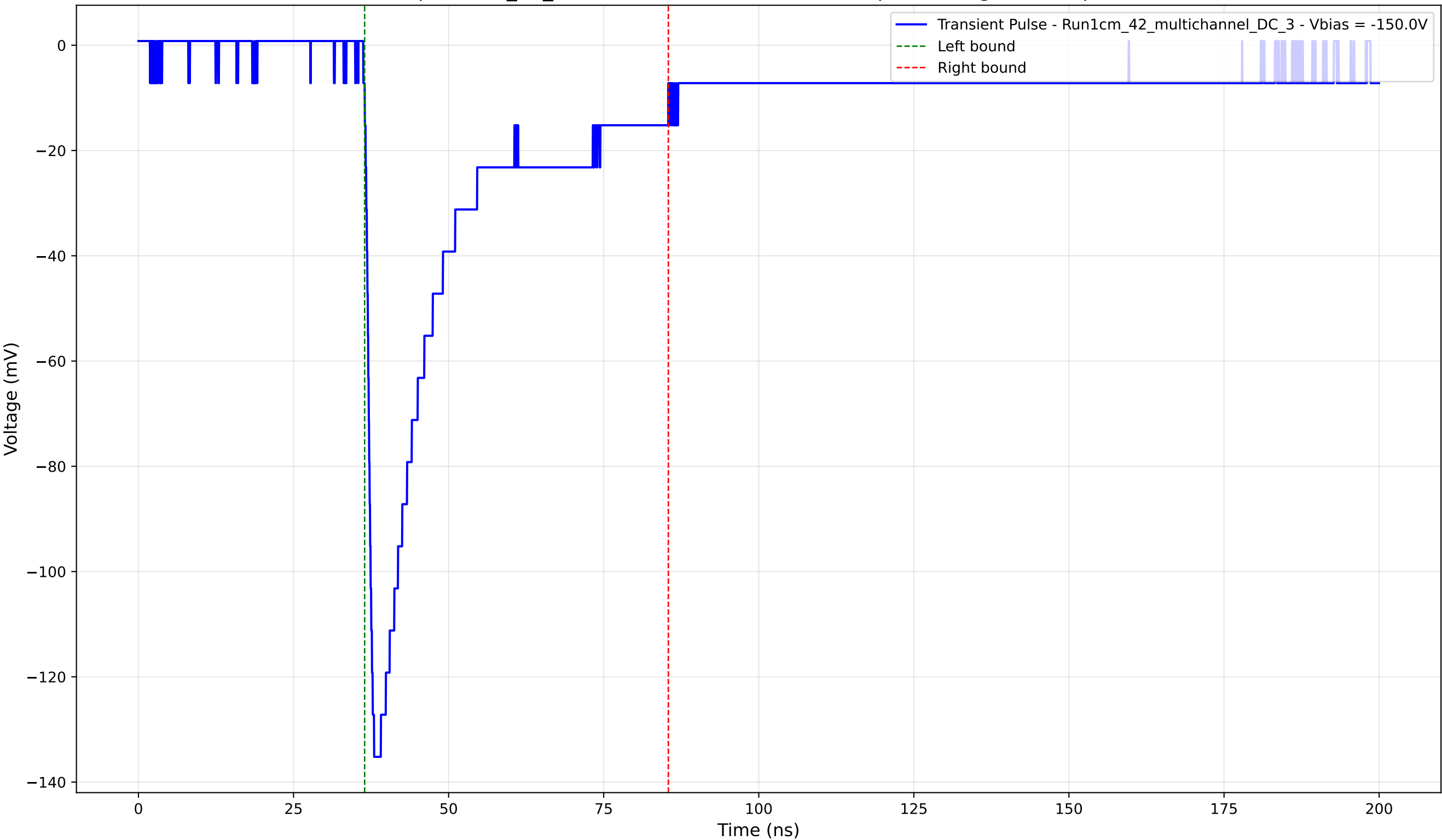
Transient Pulse - Sample: 1cm_42_multichannel - Position: 3710.0 \mu\text{m} - Charge: 37.40 pC - Rise Time: 1.28 ns
