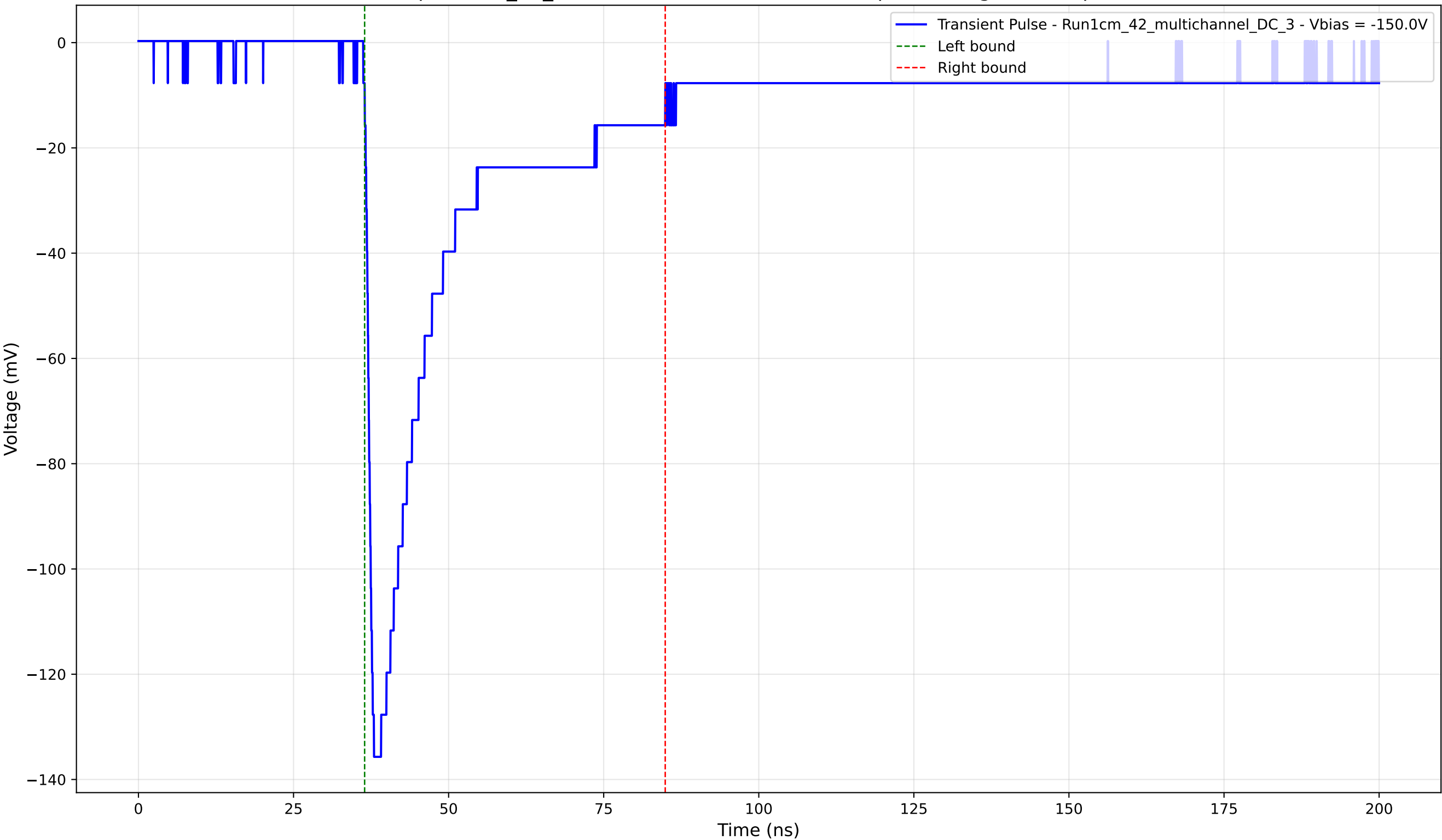
Transient Pulse - Sample: 1cm_42_multichannel - Position: 3705.0 \mu\text{m} - Charge: 37.83 pC - Rise Time: 1.29 ns
