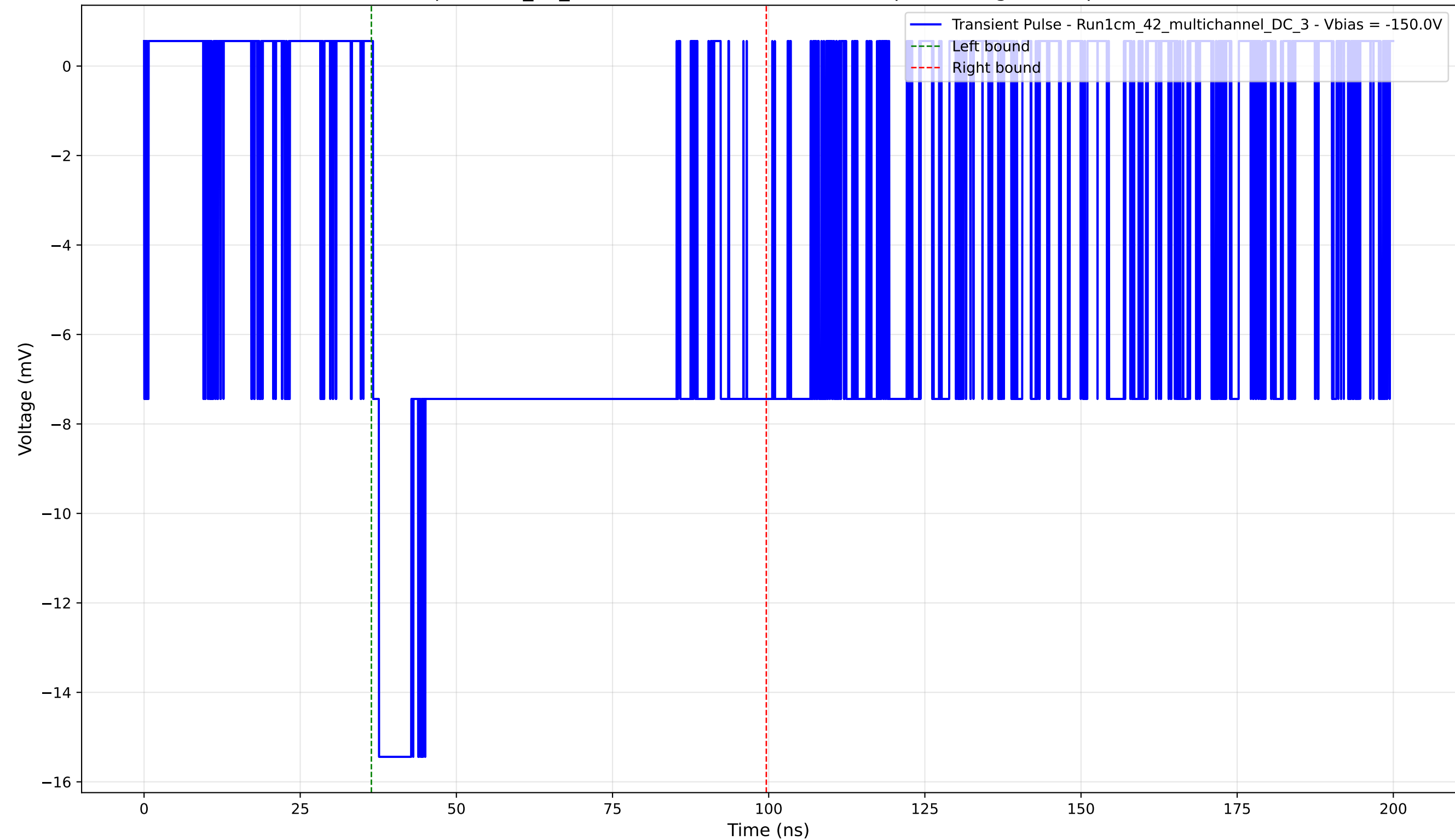
Transient Pulse - Sample: 1cm_42_multichannel - Position: 2345.0 \mu\text{m} - Charge: 9.86 pC - Rise Time: 0.96 ns
