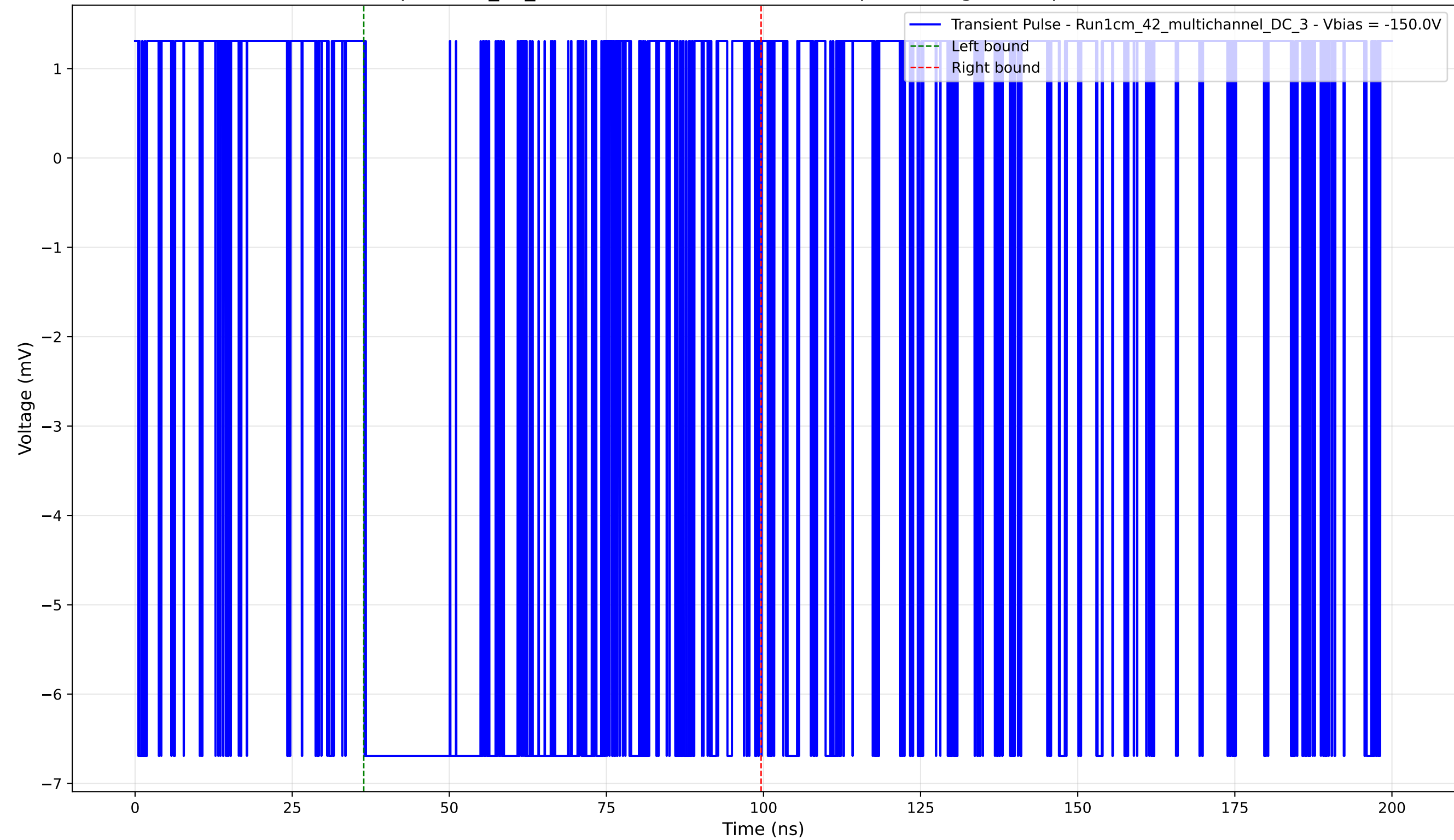
Transient Pulse - Sample: 1cm_42_multichannel - Position: 1870.0 \mu\text{m} - Charge: 5.22 pC - Rise Time: 0.00 ns (N/A)
