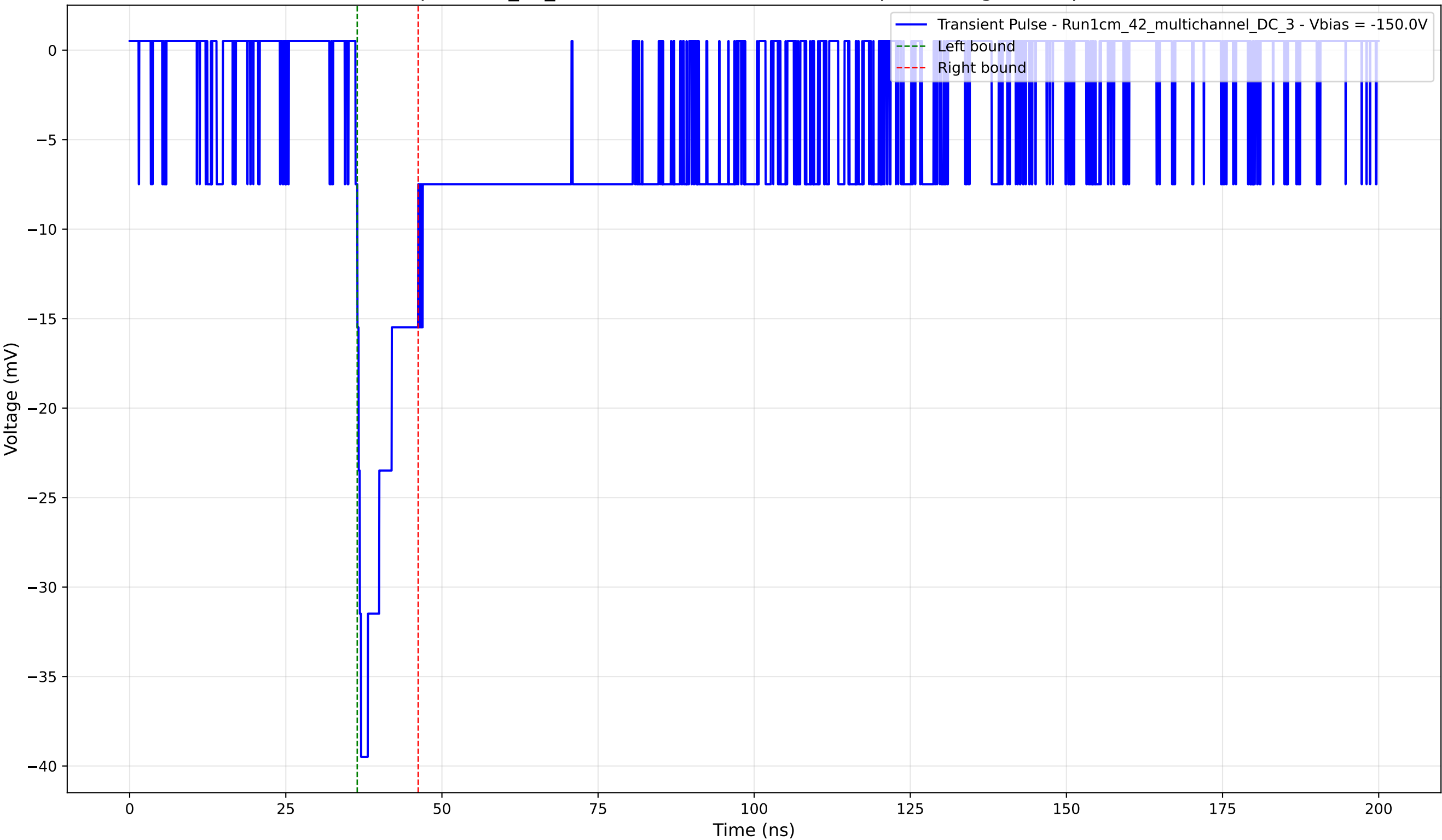
Transient Pulse - Sample: 1cm_42_multichannel - Position: 4425.0 \mu\text{m} - Charge: 4.54 pC - Rise Time: 0.89 ns
