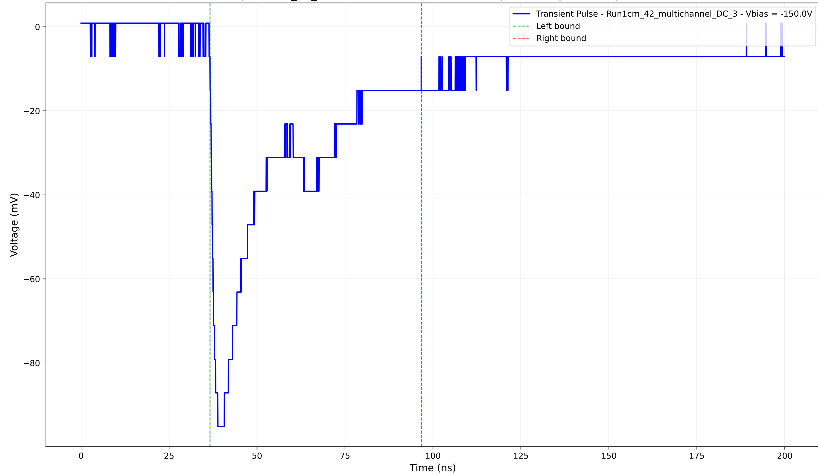
Transient Pulse - Sample: 1cm_42_multichannel - Position: 2045.0 \mu\text{m} - Charge: 40.99 pC - Rise Time: 1.59 ns
