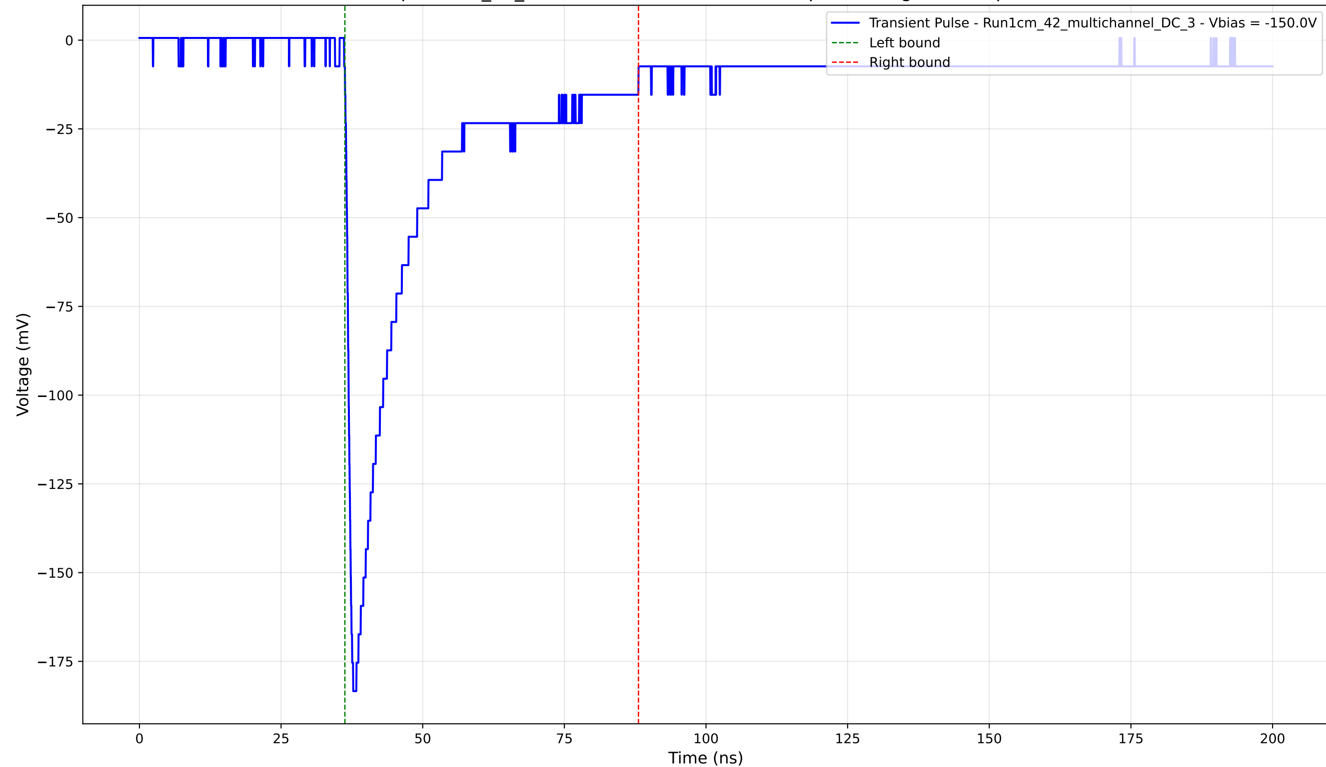
Transient Pulse - Sample: 1cm_42_multichannel - Position: 945.0 \mu\text{m} - Charge: 45.34 pC - Rise Time: 1.07 ns
