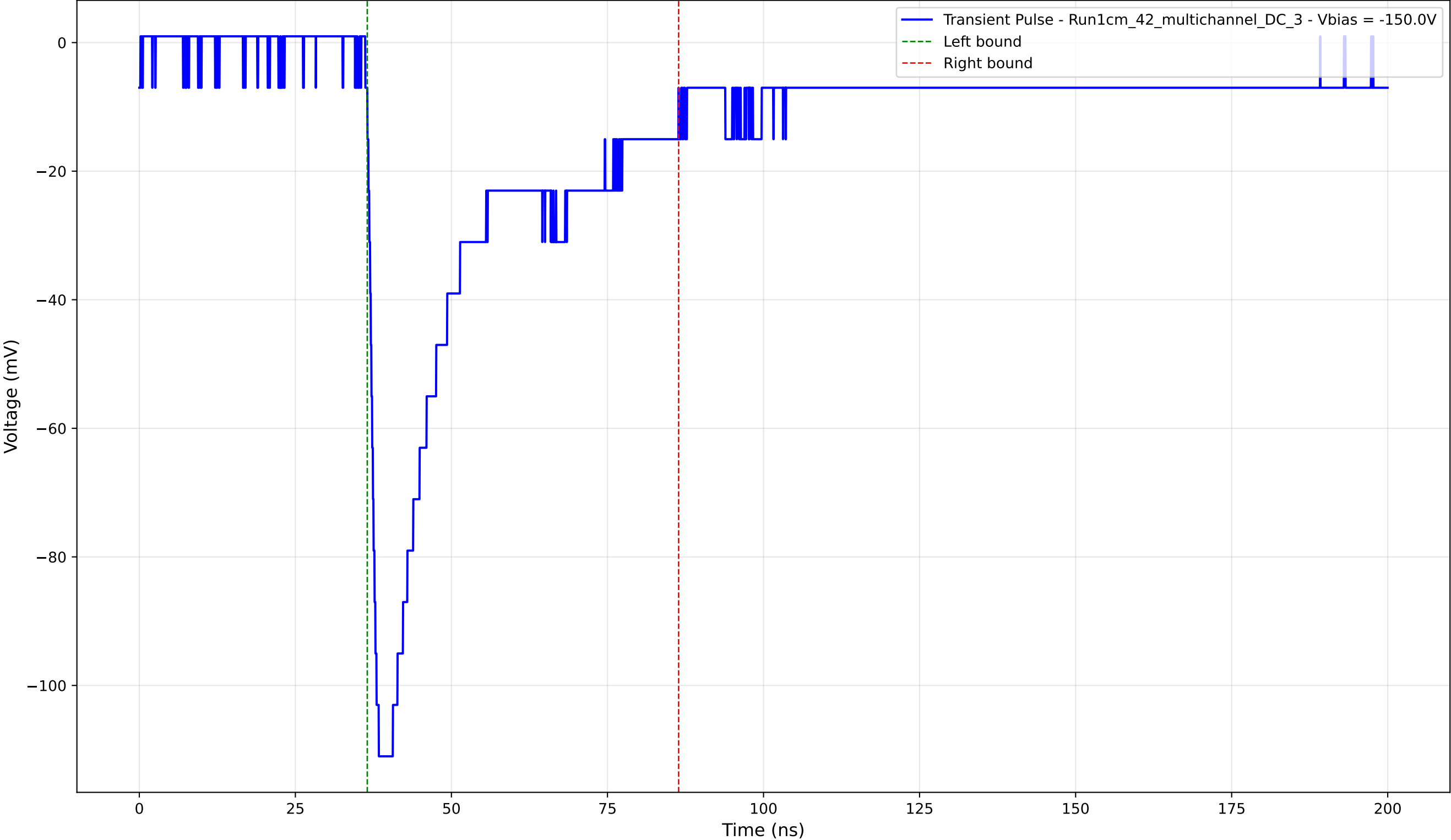
Transient Pulse - Sample: 1cm_42_multichannel - Position: 3290.0 \mu\text{m} - Charge: 36.73 pC - Rise Time: 1.47 ns
