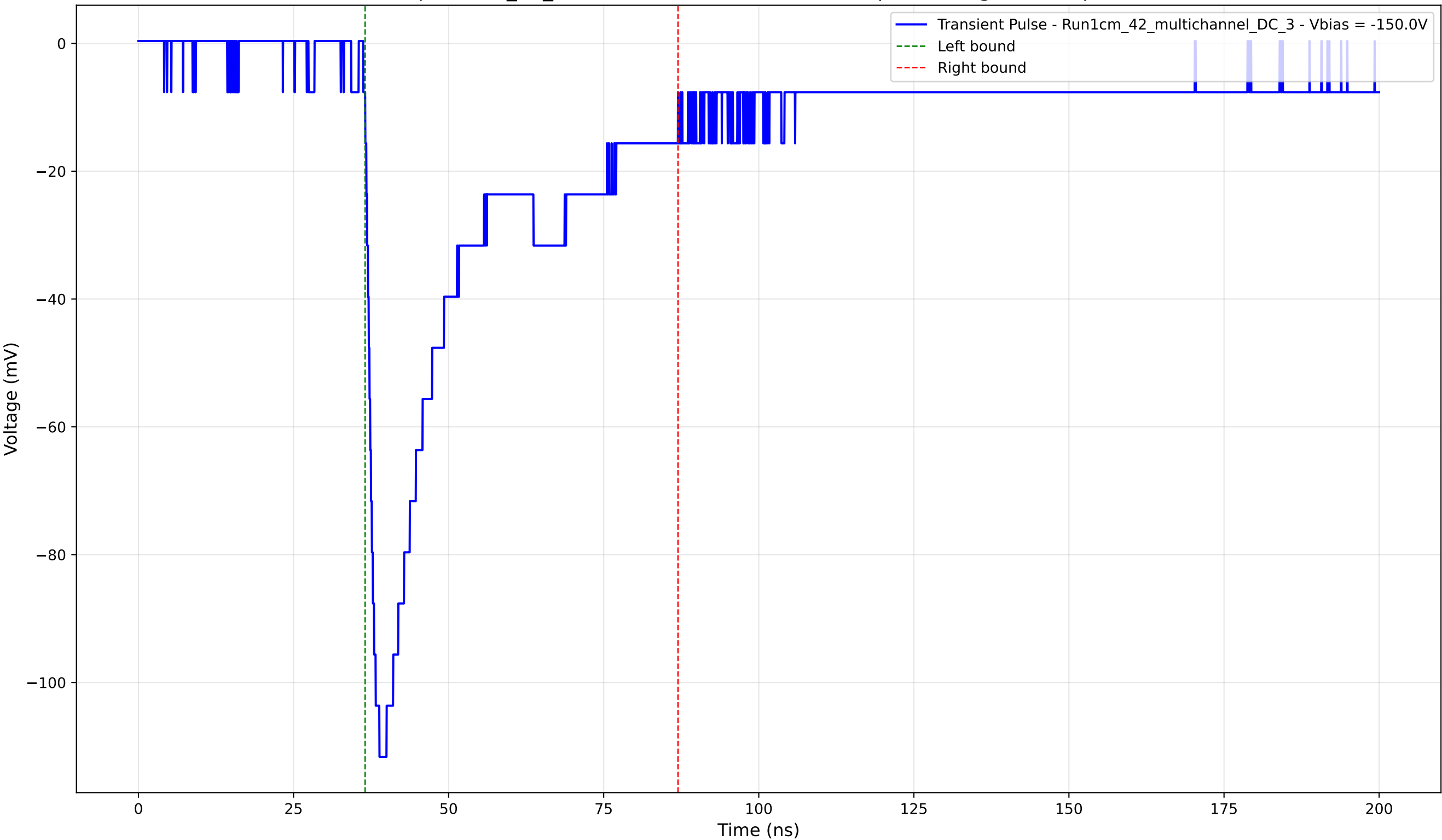
Transient Pulse - Sample: 1cm_42_multichannel - Position: 3200.0 \mu\text{m} - Charge: 37.46 pC - Rise Time: 1.69 ns
