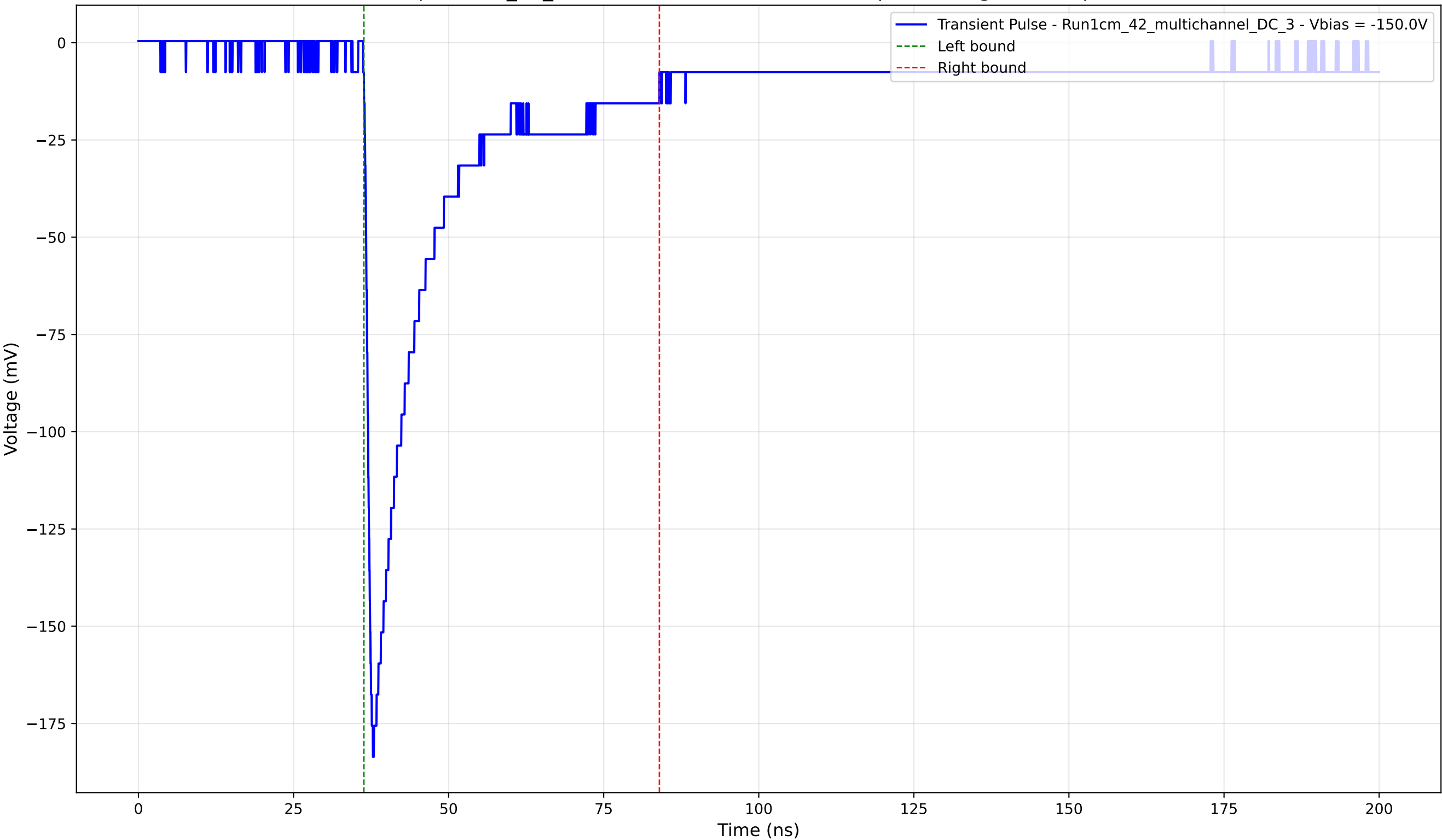
Transient Pulse - Sample: 1cm_42_multichannel - Position: 4070.0 \mu\text{m} - Charge: 40.37 pC - Rise Time: 1.03 ns
