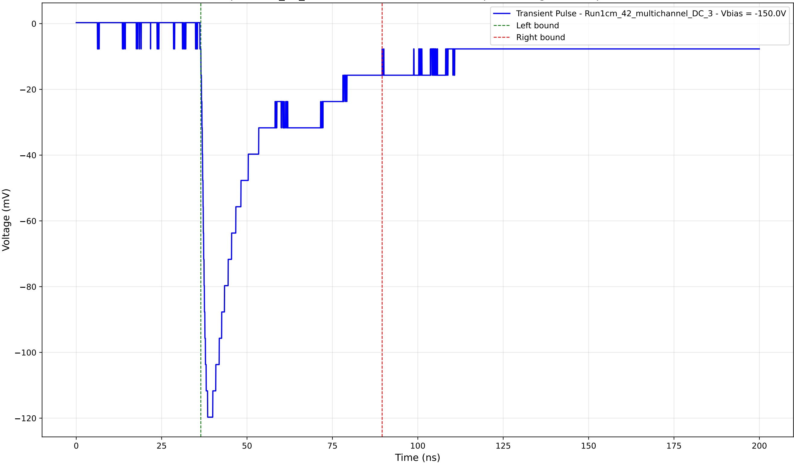
Transient Pulse - Sample: 1cm_42_multichannel - Position: 1670.0 \mu\text{m} - Charge: 42.19 pC - Rise Time: 1.55 ns
