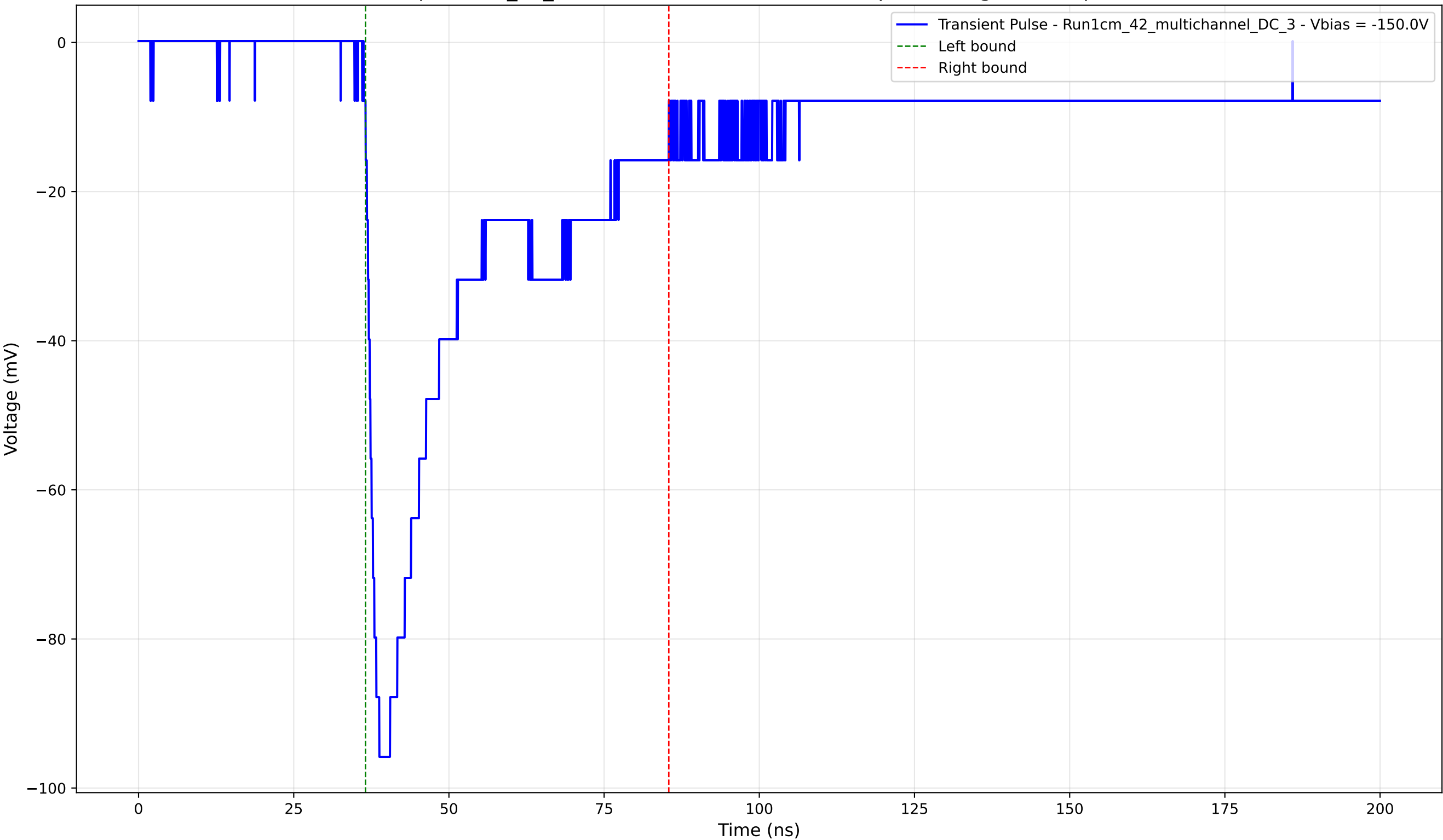
Transient Pulse - Sample: 1cm_42_multichannel - Position: 2960.0 \mu\text{m} - Charge: 35.06 pC - Rise Time: 1.74 ns
