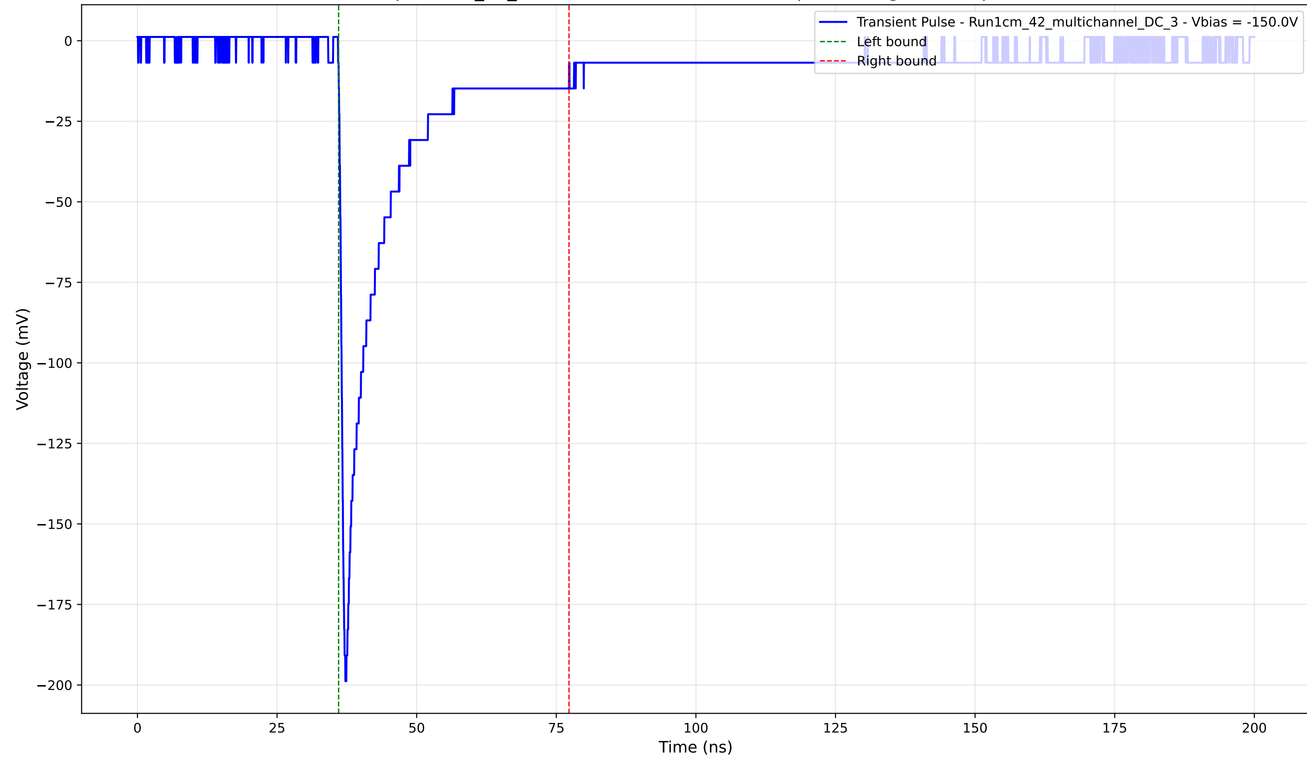
Transient Pulse - Sample: 1cm_42_multichannel - Position: 410.0 \mu\text{m} - Charge: 31.69 pC - Rise Time: 0.91 ns
