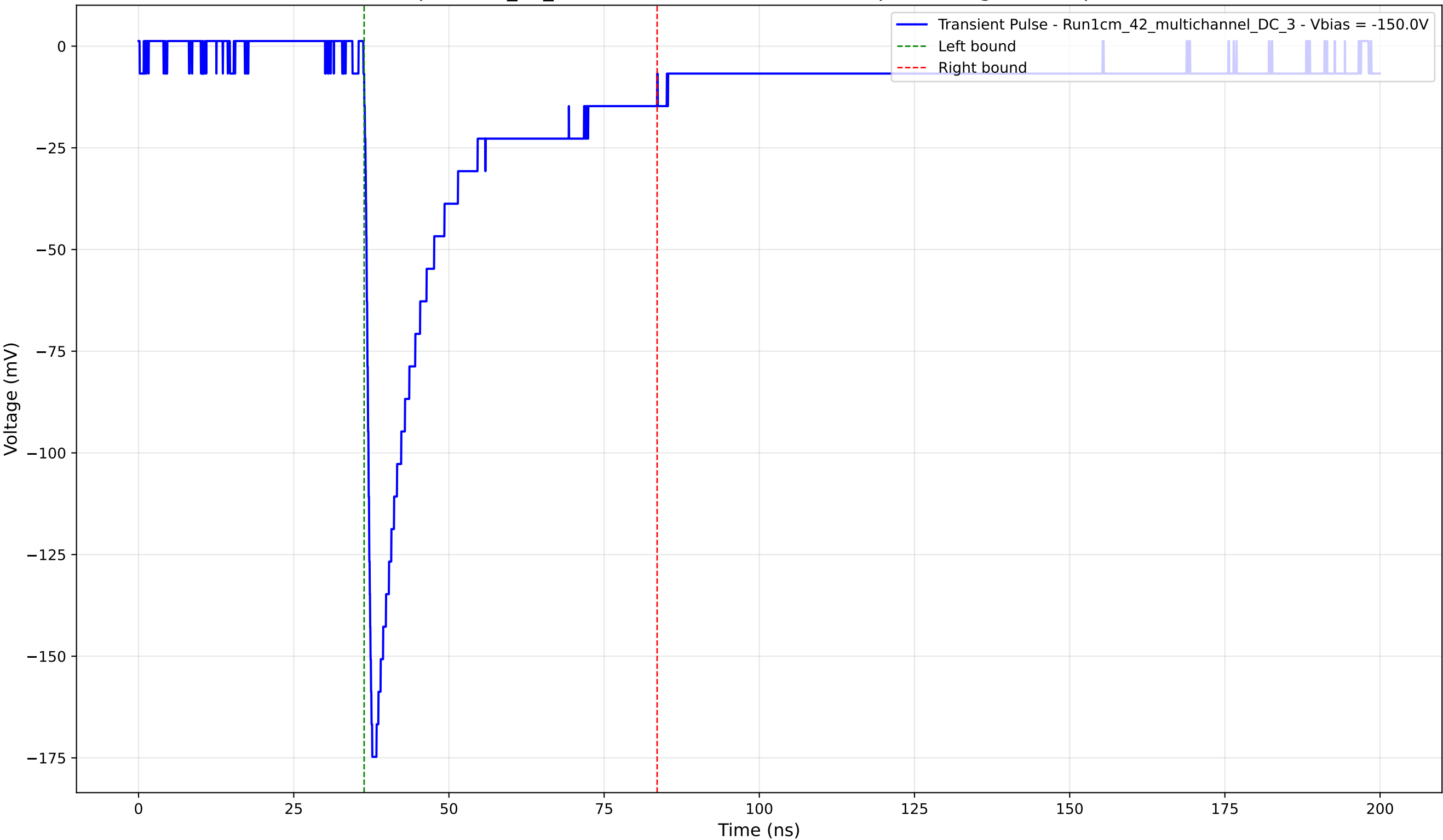
Transient Pulse - Sample: 1cm_42_multichannel - Position: 4050.0 \mu\text{m} - Charge: 39.32 pC - Rise Time: 0.99 ns
