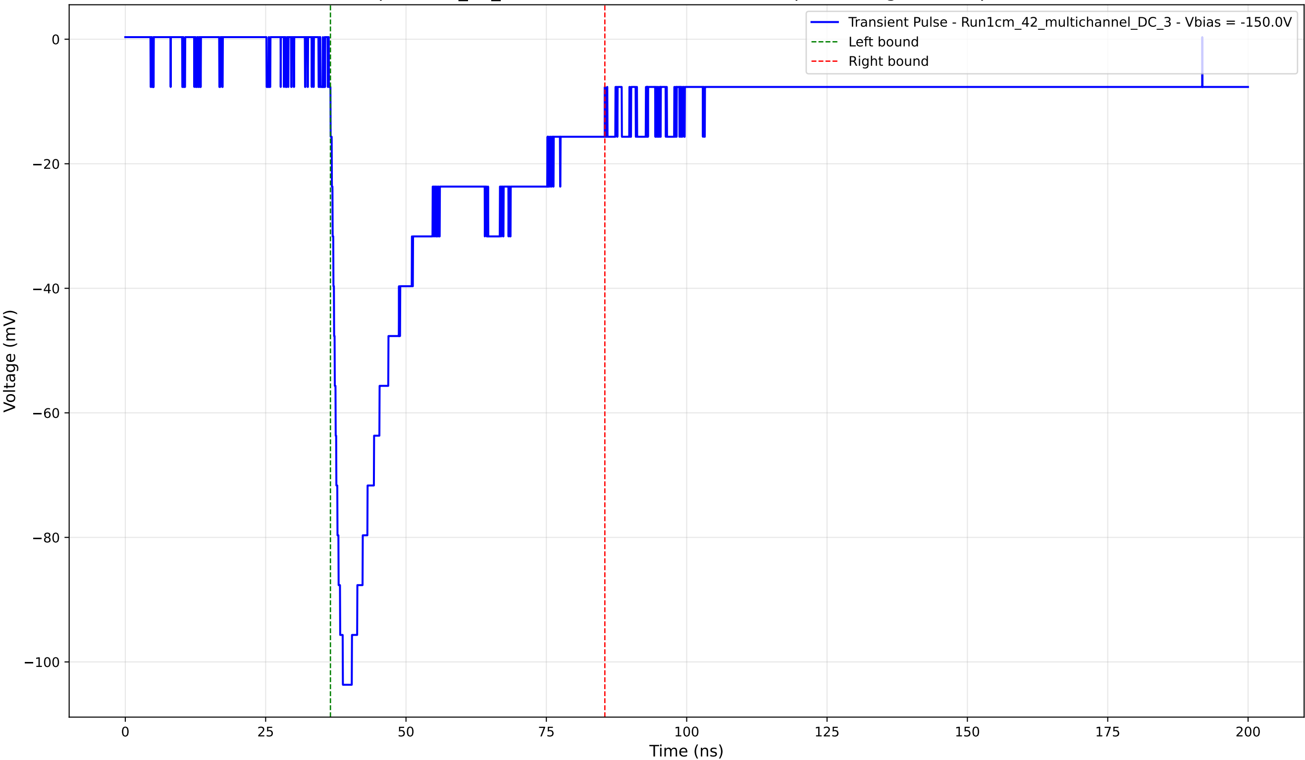
Transient Pulse - Sample: 1cm_42_multichannel - Position: 3130.0 \mu\text{m} - Charge: 35.20 pC - Rise Time: 1.71 ns
