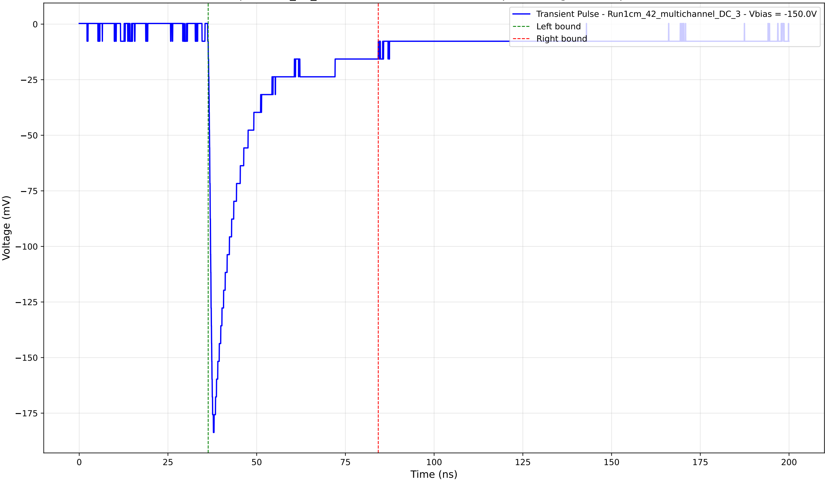
Transient Pulse - Sample: 1cm_42_multichannel - Position: 4065.0 \mu\text{m} - Charge: 40.23 pC - Rise Time: 1.03 ns
