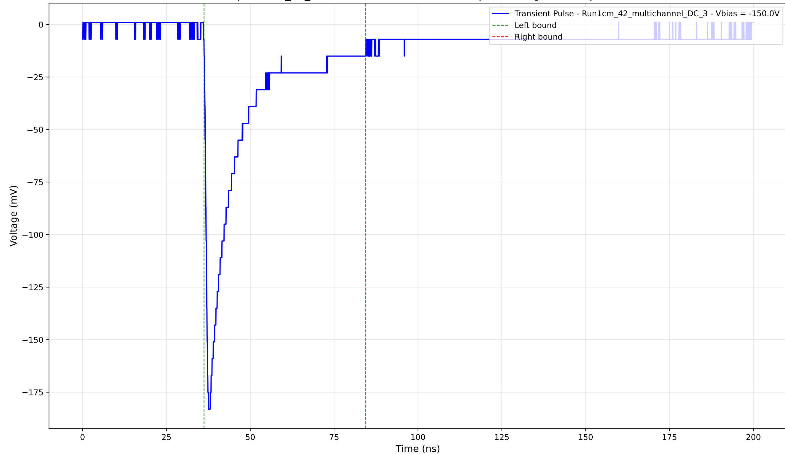
Transient Pulse - Sample: 1cm_42_multichannel - Position: 780.0 \mu\text{m} - Charge: 40.68 pC - Rise Time: 0.97 ns
