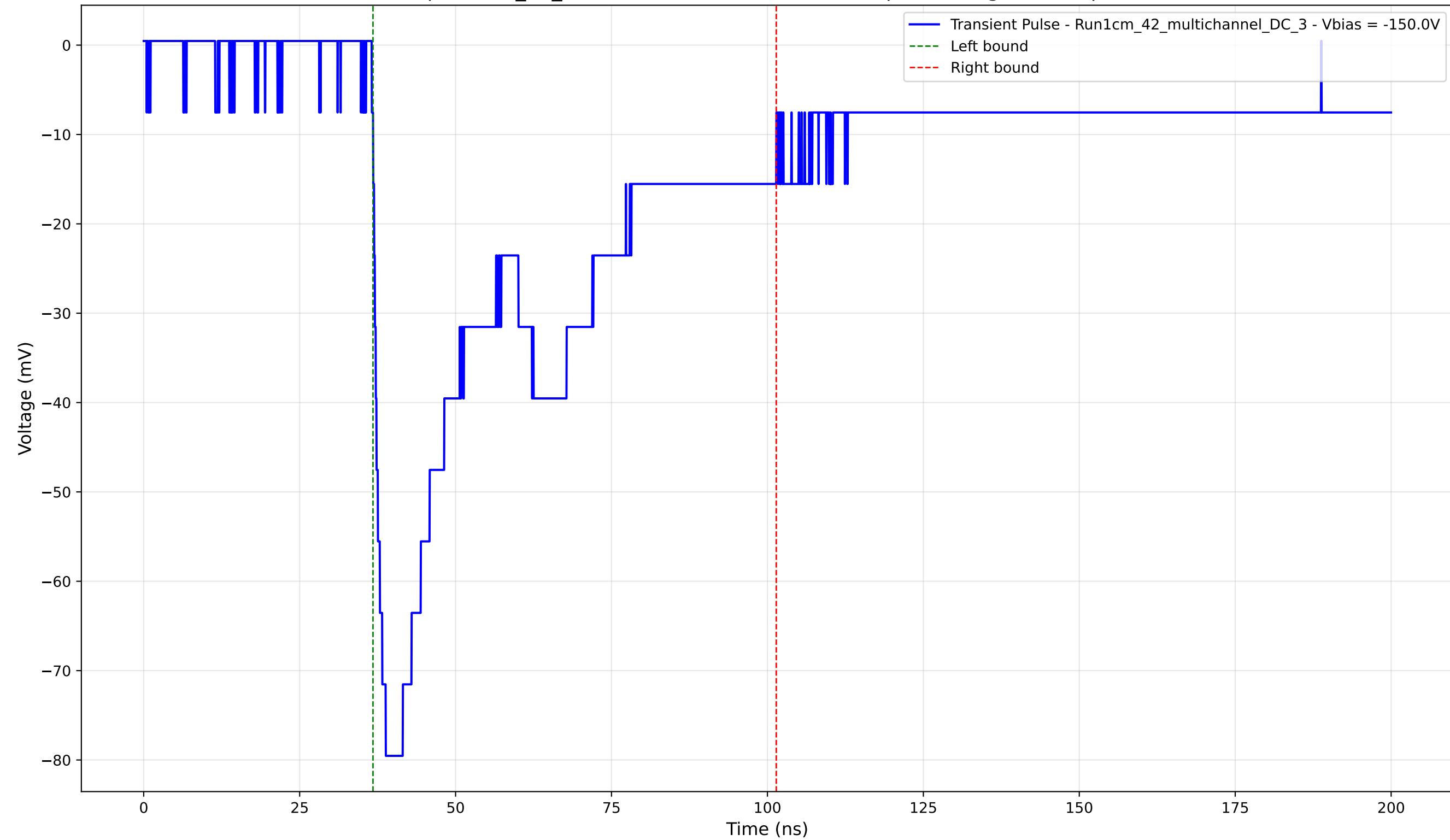
Transient Pulse - Sample: 1cm_42_multichannel - Position: 2500.0 \mu\text{m} - Charge: 40.13 pC - Rise Time: 2.04 ns
