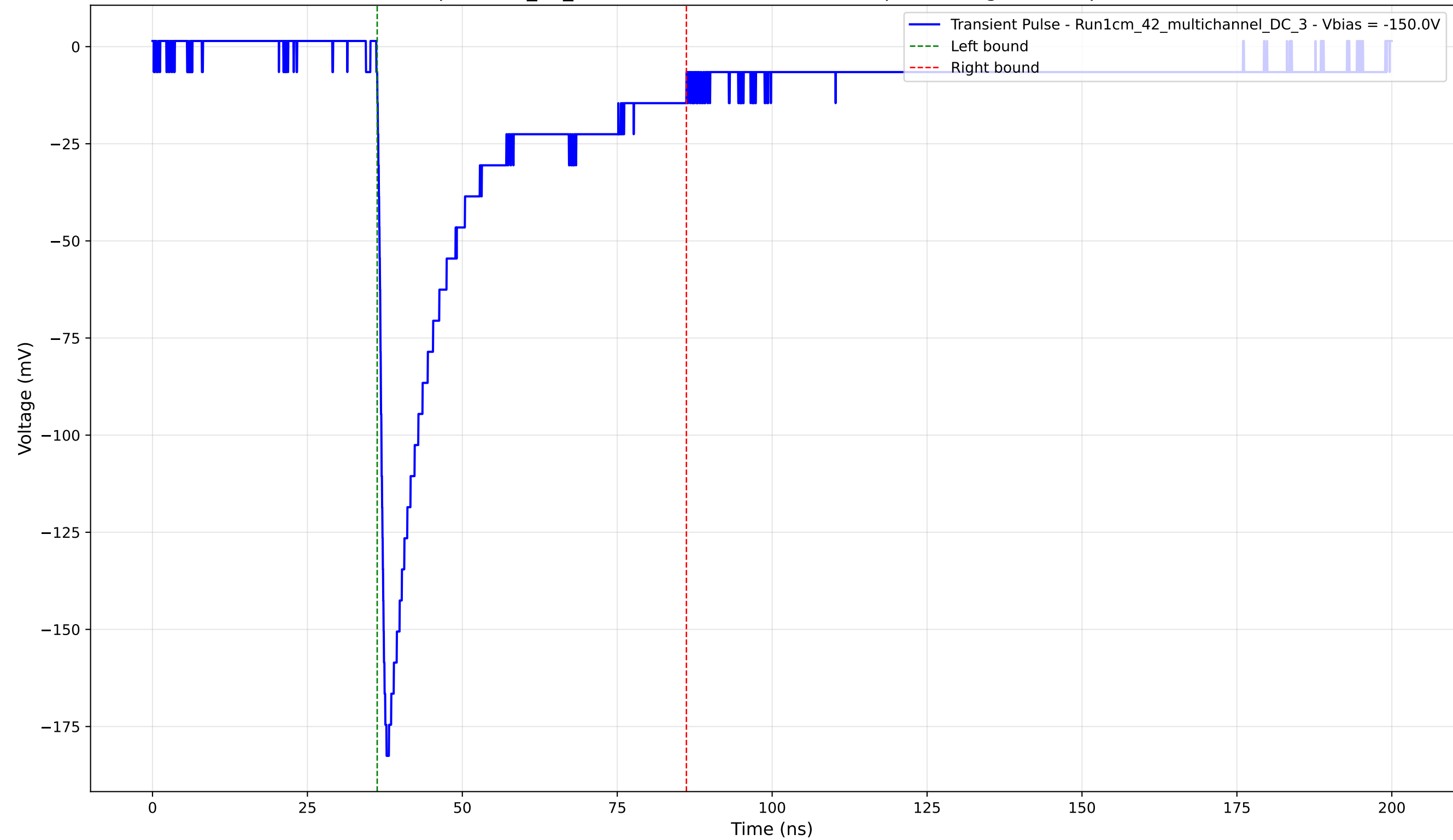
Transient Pulse - Sample: 1cm_42_multichannel - Position: 940.0 \mu\text{m} - Charge: 43.42 pC - Rise Time: 1.09 ns
