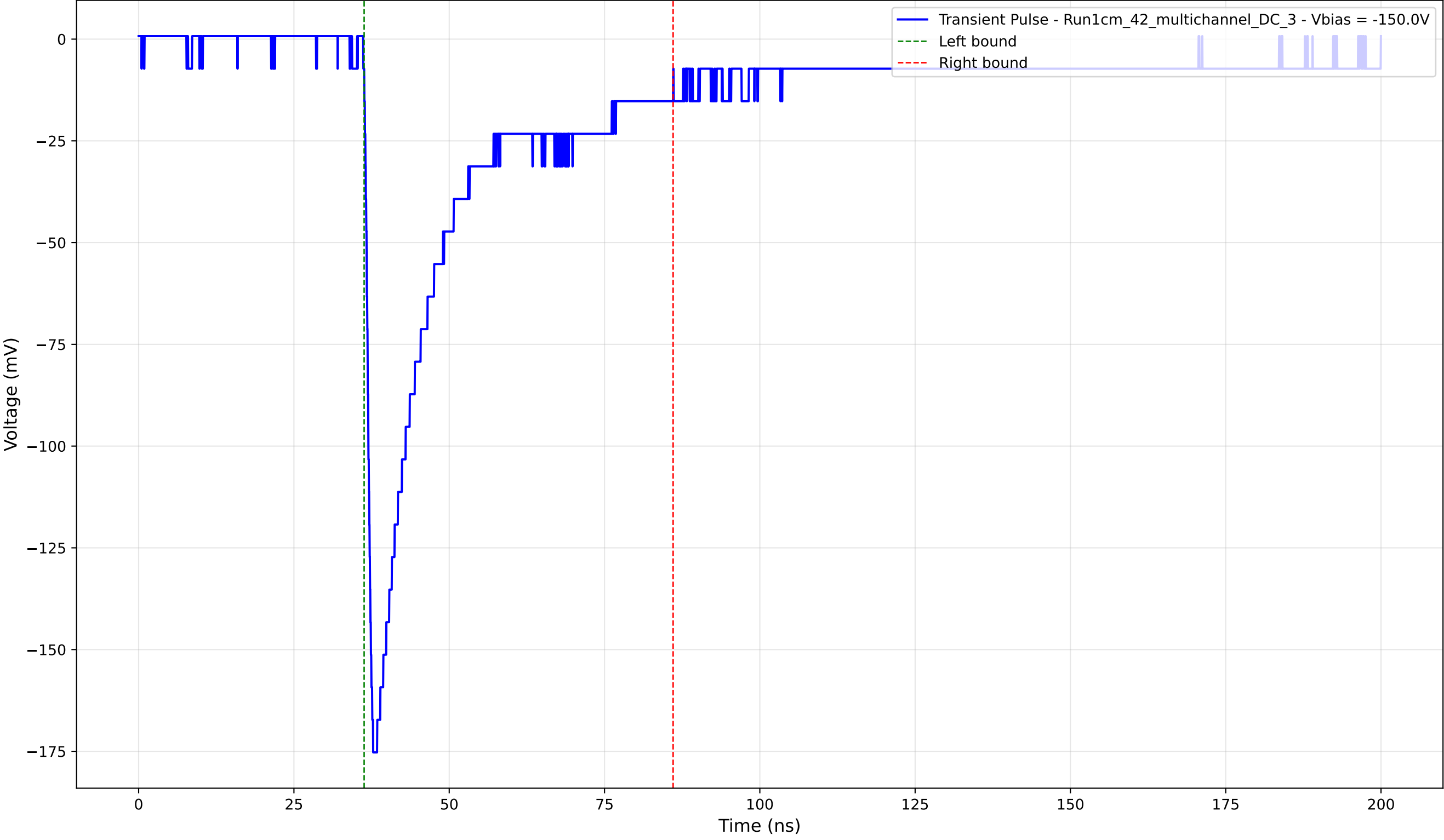
Transient Pulse - Sample: 1cm_42_multichannel - Position: 1010.0 \mu\text{m} - Charge: 44.25 pC - Rise Time: 1.05 ns
