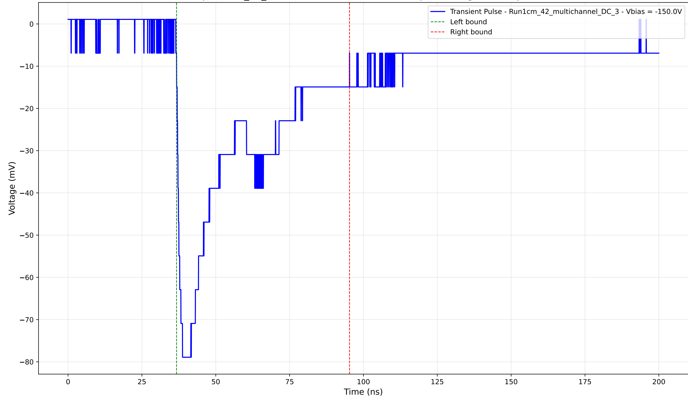
Transient Pulse - Sample: 1cm_42_multichannel - Position: 2600.0 \mu\text{m} - Charge: 36.59 pC - Rise Time: 2.02 ns
