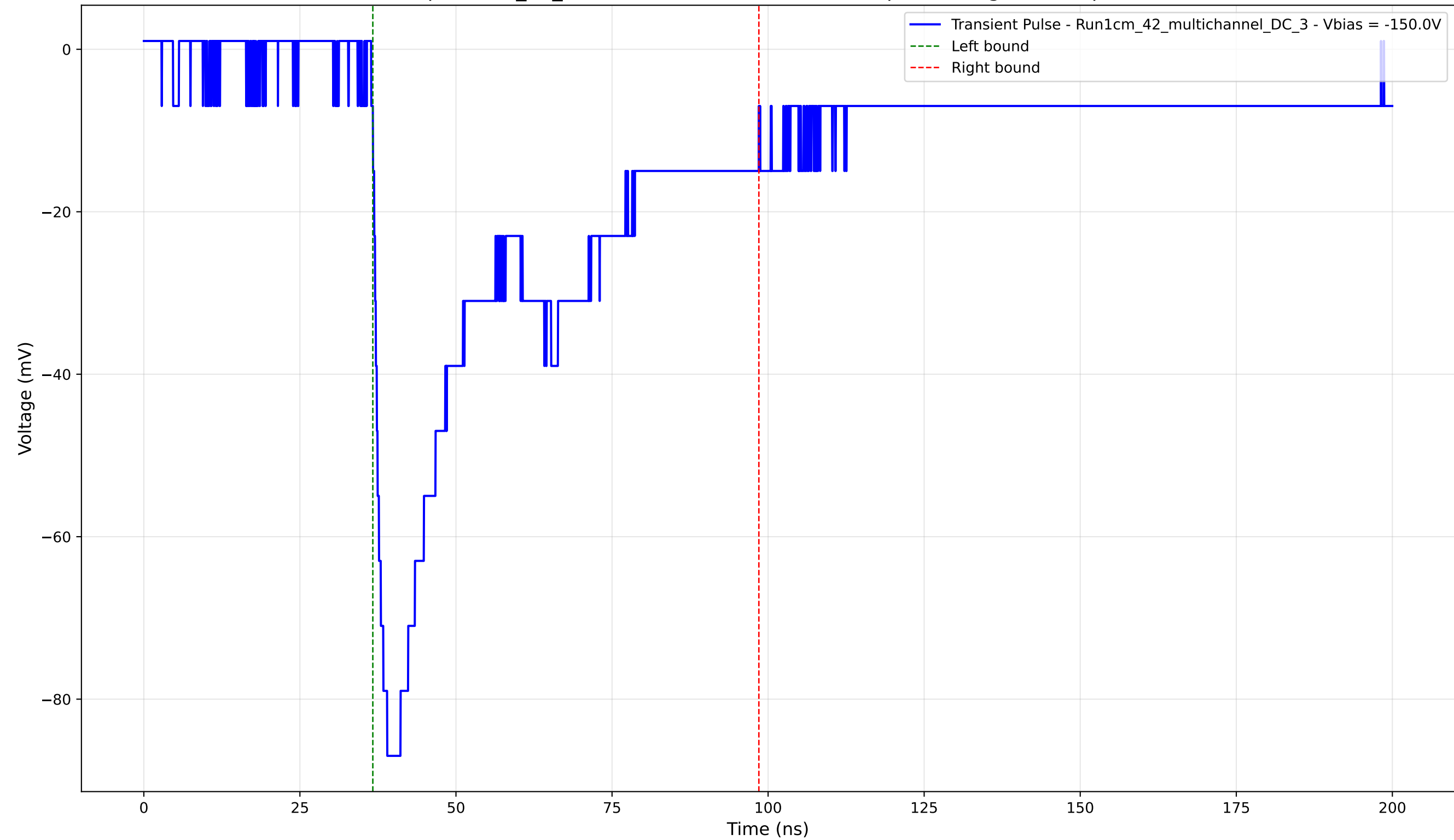
Transient Pulse - Sample: 1cm_42_multichannel - Position: 2685.0 \mu\text{m} - Charge: 38.86 pC - Rise Time: 1.68 ns
