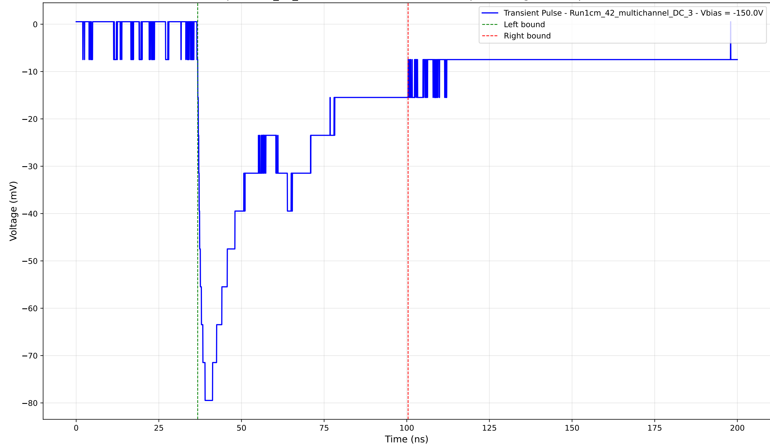
Transient Pulse - Sample: 1cm_42_multichannel - Position: 2575.0 \mu\text{m} - Charge: 38.42 pC - Rise Time: 2.22 ns
