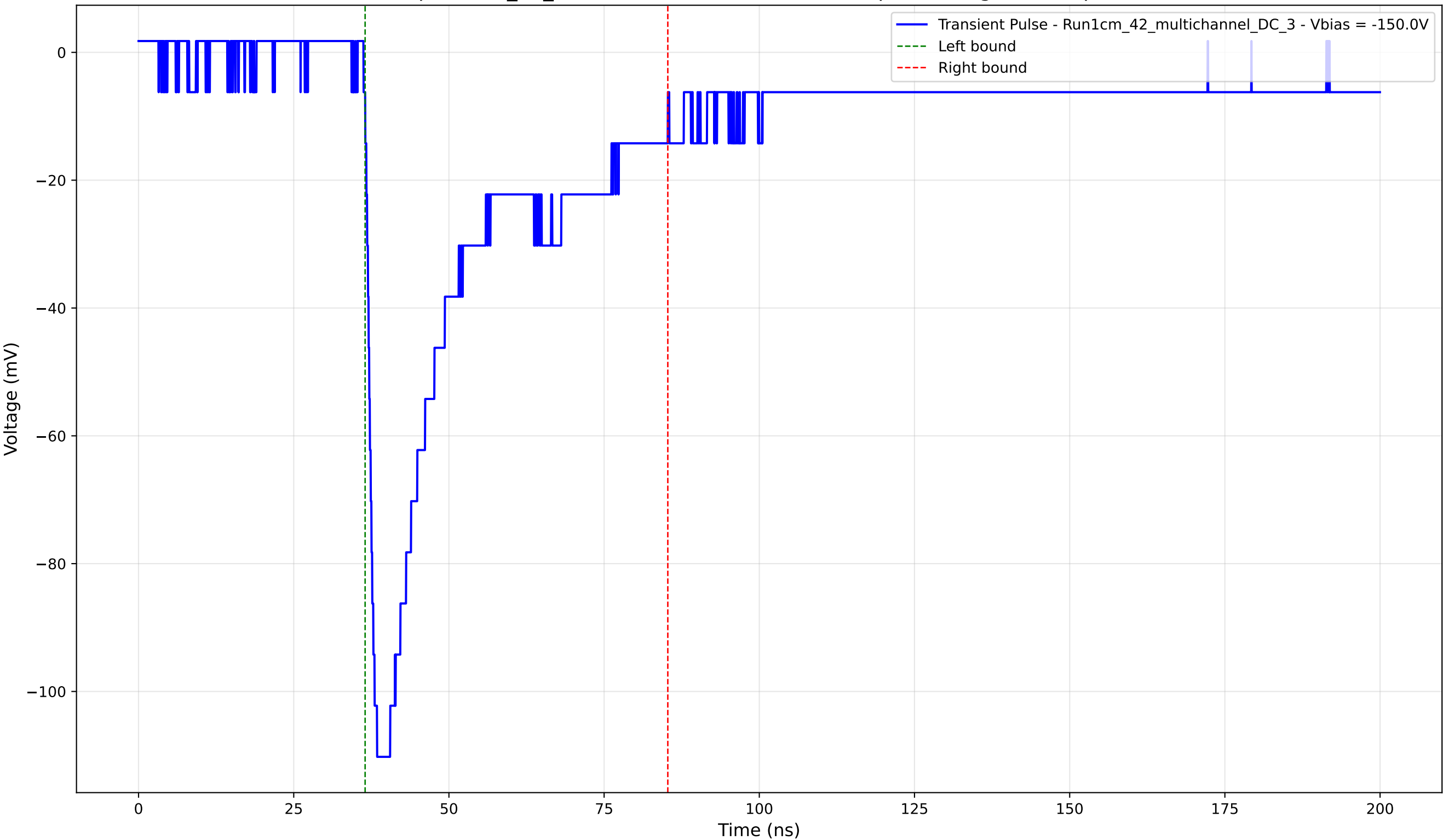
Transient Pulse - Sample: 1cm_42_multichannel - Position: 3265.0 \mu\text{m} - Charge: 36.01 pC - Rise Time: 1.51 ns
