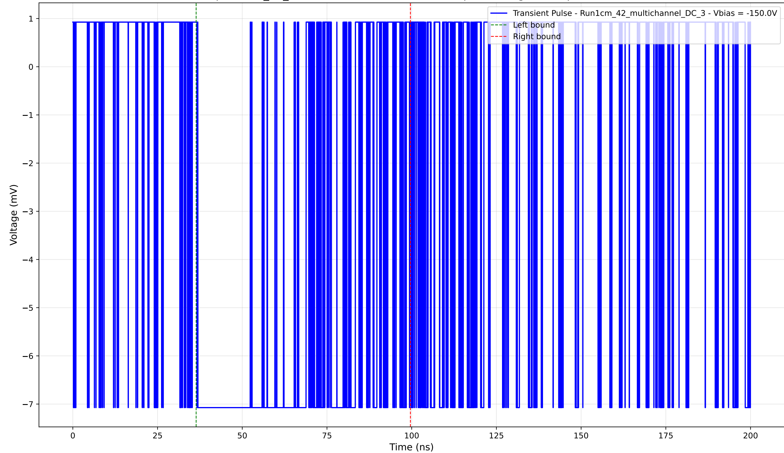
Transient Pulse - Sample: 1cm_42_multichannel - Position: 3380.0 \mu\text{m} - Charge: 5.98 pC - Rise Time: 0.00 ns (N/A)
