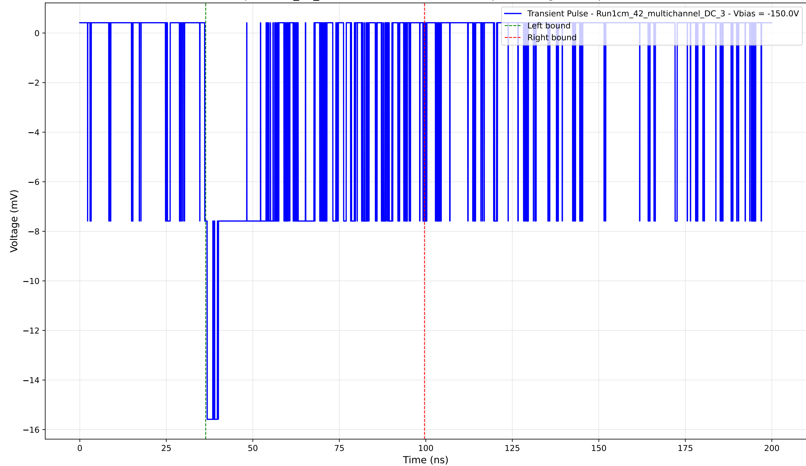
Transient Pulse - Sample: 1cm_42_multichannel - Position: 345.0 \mu\text{m} - Charge: 5.73 pC - Rise Time: 0.72 ns
