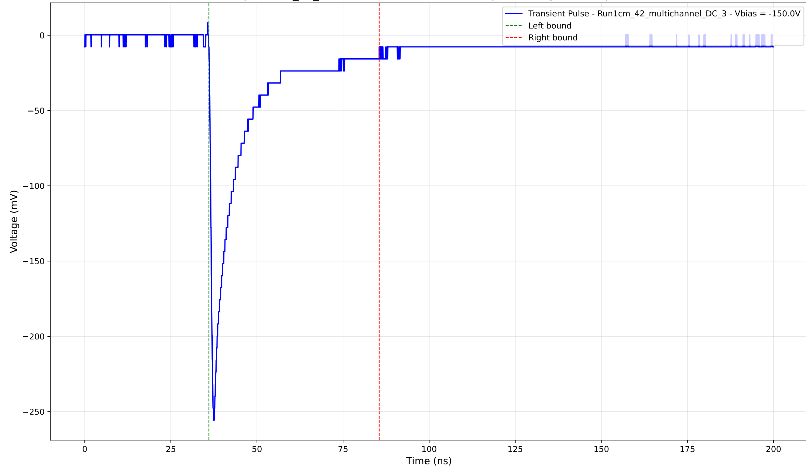
Transient Pulse - Sample: 1cm_42_multichannel - Position: 555.0 \mu\text{m} - Charge: 48.10 pC - Rise Time: 0.92 ns
