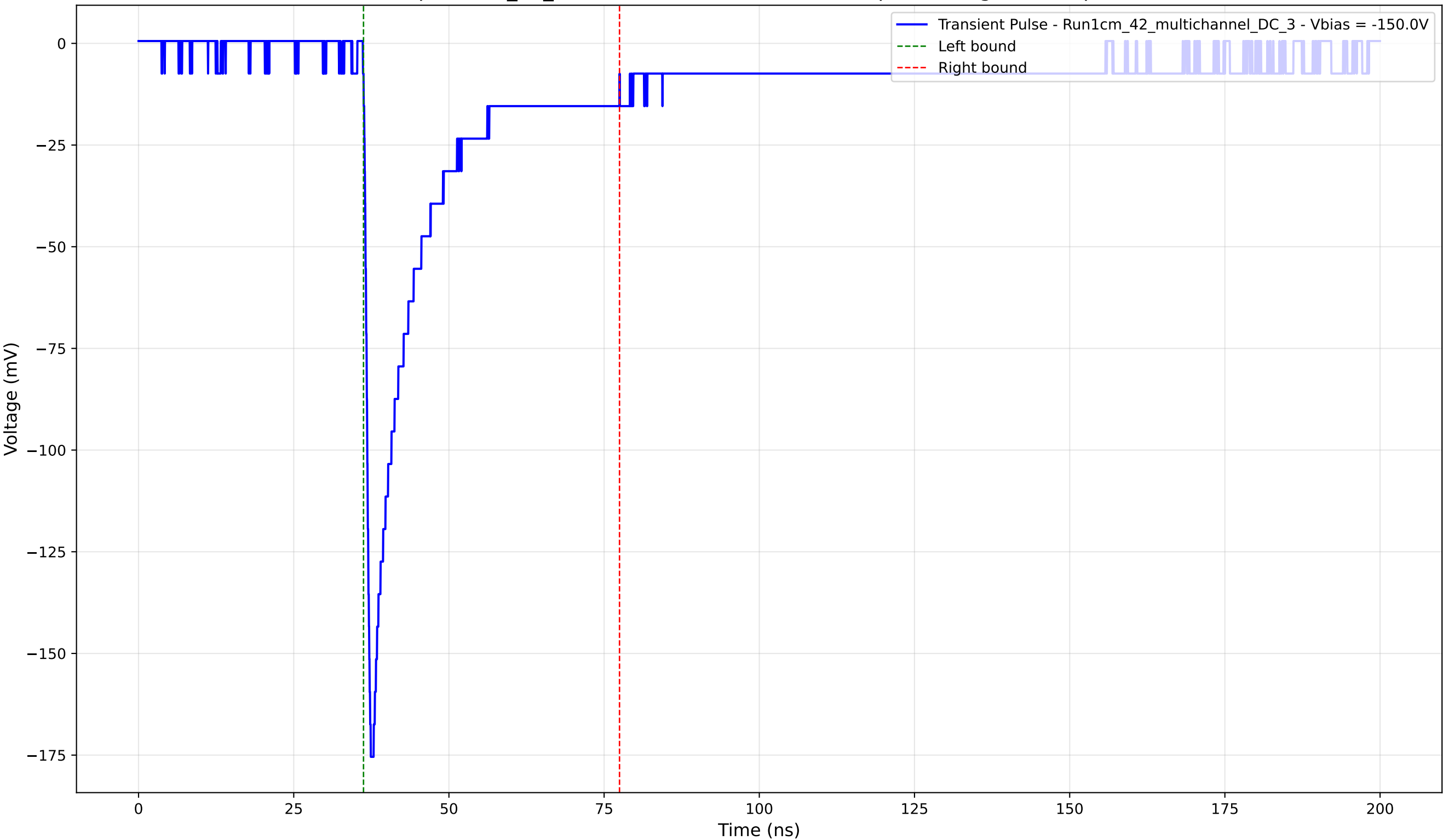
Transient Pulse - Sample: 1cm_42_multichannel - Position: 4315.0 \mu\text{m} - Charge: 31.36 pC - Rise Time: 0.87 ns
