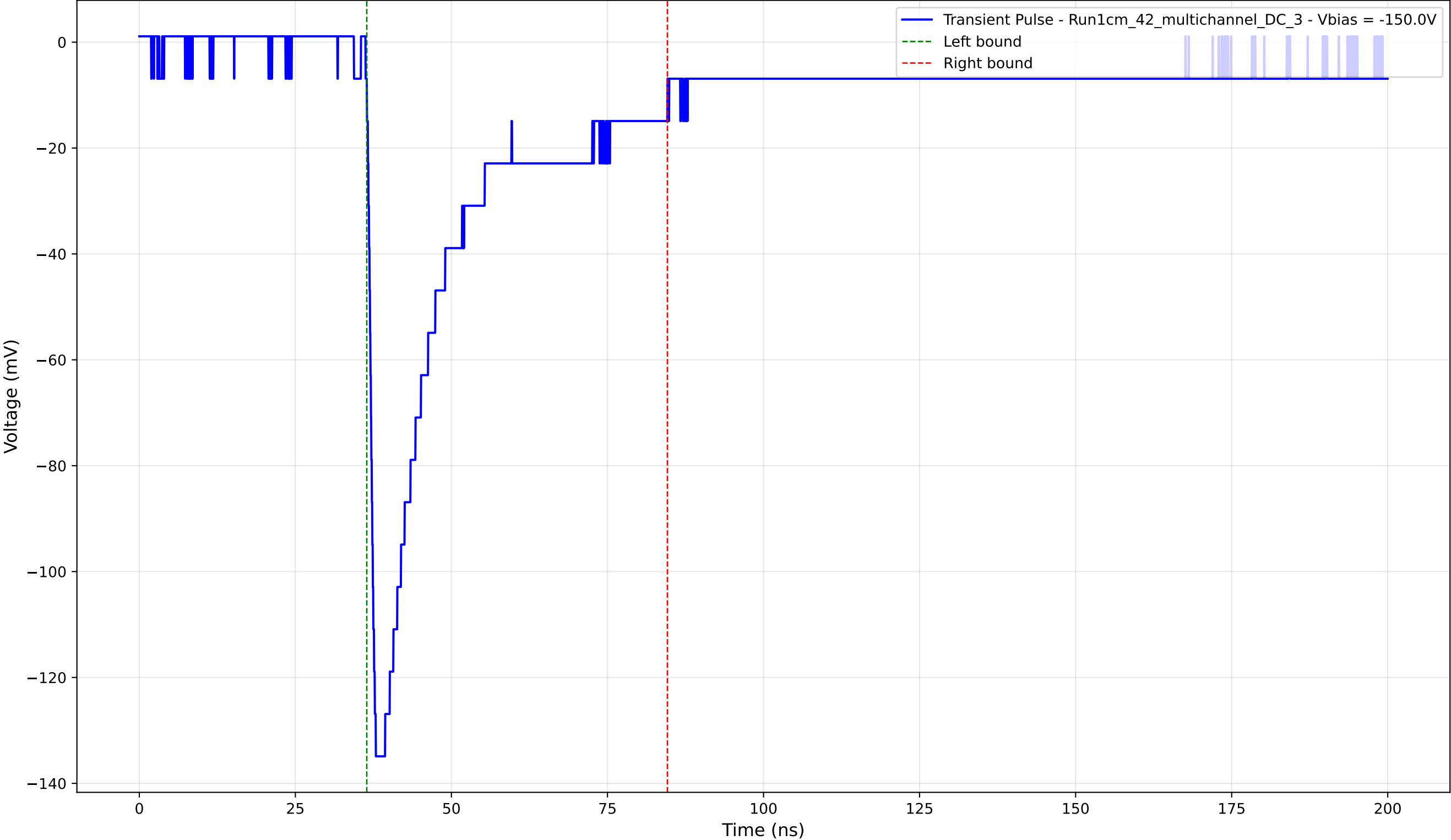
Transient Pulse - Sample: 1cm_42_multichannel - Position: 3725.0 \mu\text{m} - Charge: 37.41 pC - Rise Time: 1.26 ns
