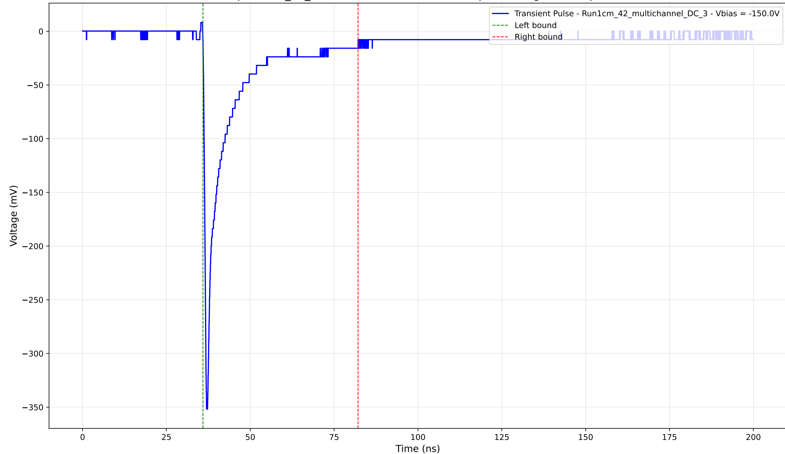
Transient Pulse - Sample: 1cm_42_multichannel - Position: 200.0 \mu\text{m} - Charge: 47.88 pC - Rise Time: 0.79 ns
