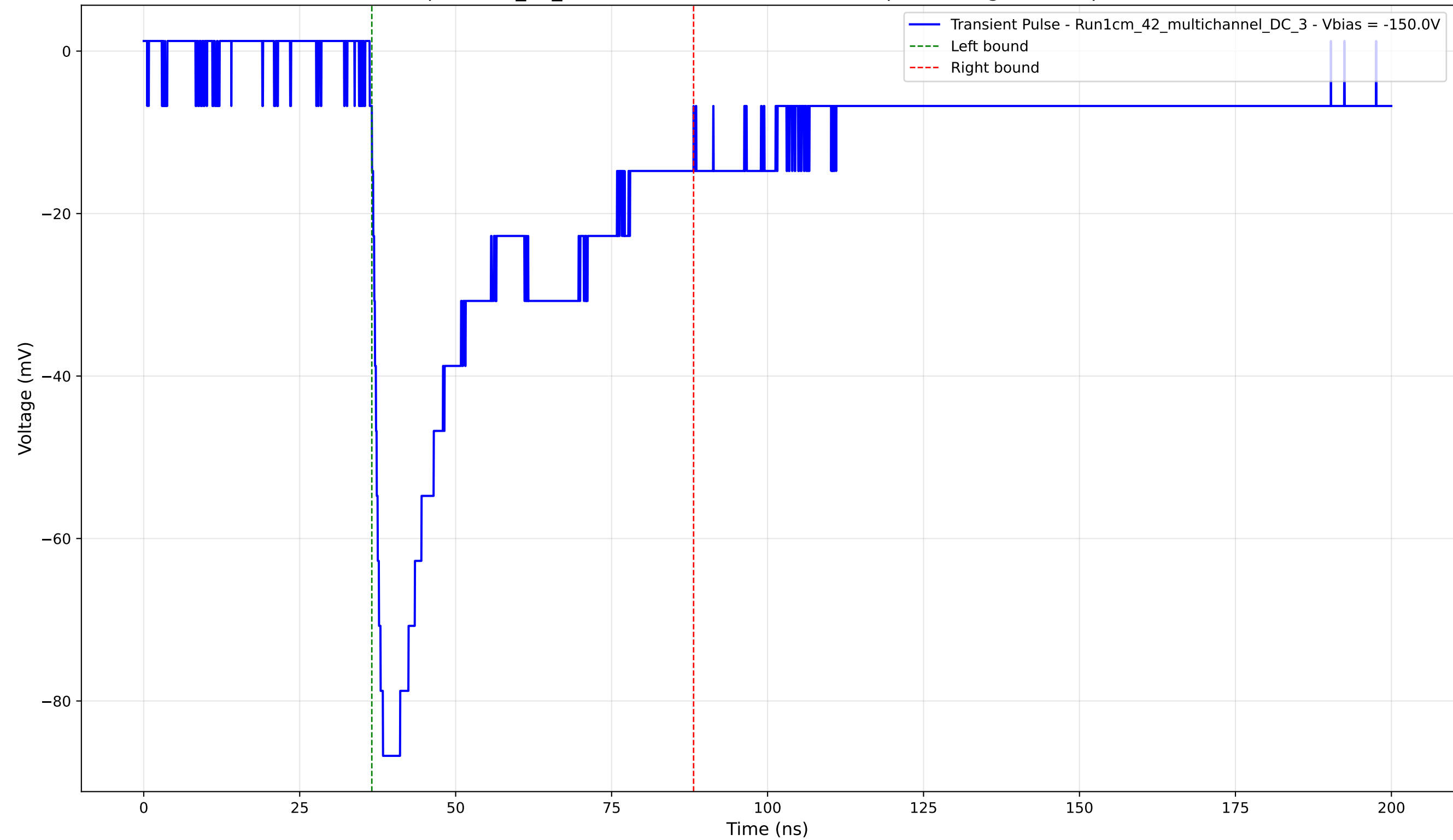
Transient Pulse - Sample: 1cm_42_multichannel - Position: 1945.0 \mu\text{m} - Charge: 34.86 pC - Rise Time: 1.40 ns
