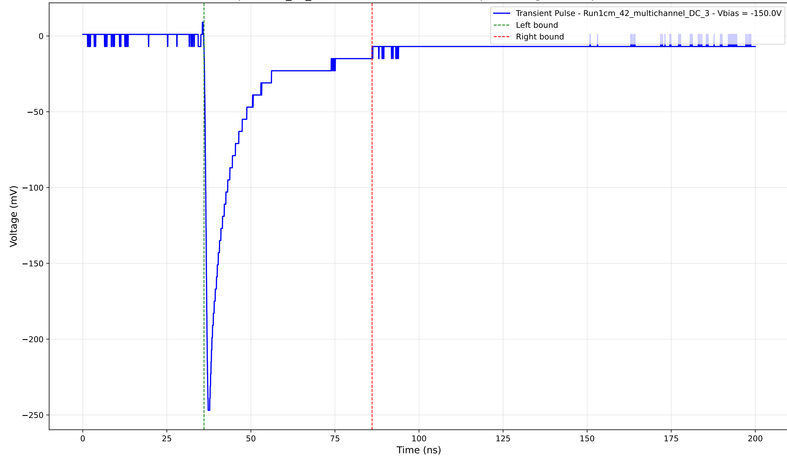
Transient Pulse - Sample: 1cm_42_multichannel - Position: 565.0 \mu\text{m} - Charge: 47.18 pC - Rise Time: 0.88 ns
