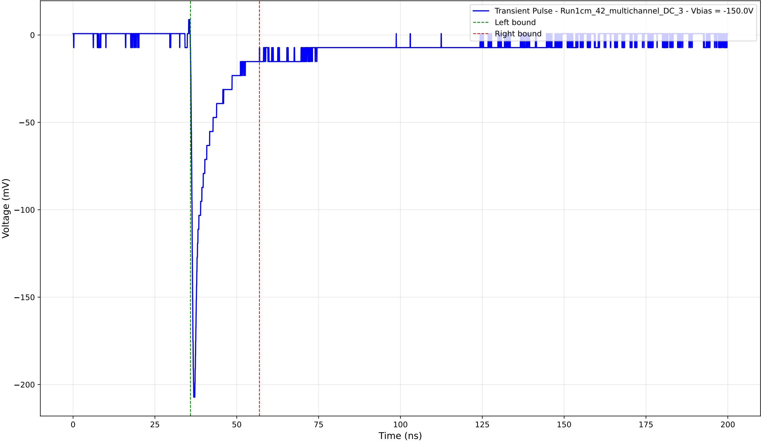
Transient Pulse - Sample: 1cm_42_multichannel - Position: 80.0 \mu\text{m} - Charge: 20.83 pC - Rise Time: 0.79 ns
