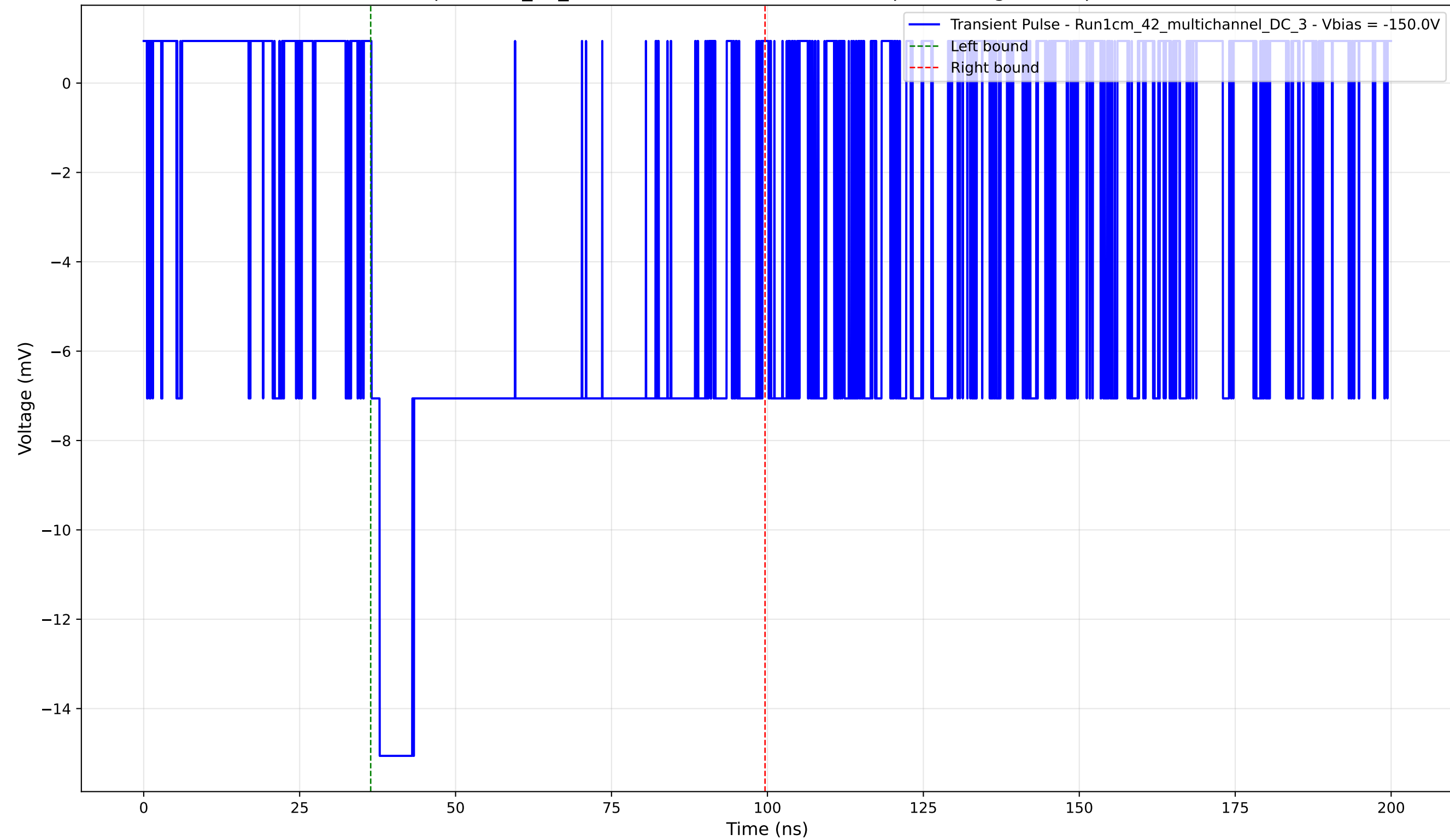
Transient Pulse - Sample: 1cm_42_multichannel - Position: 2905.0 \mu\text{m} - Charge: 9.11 pC - Rise Time: 1.32 ns
