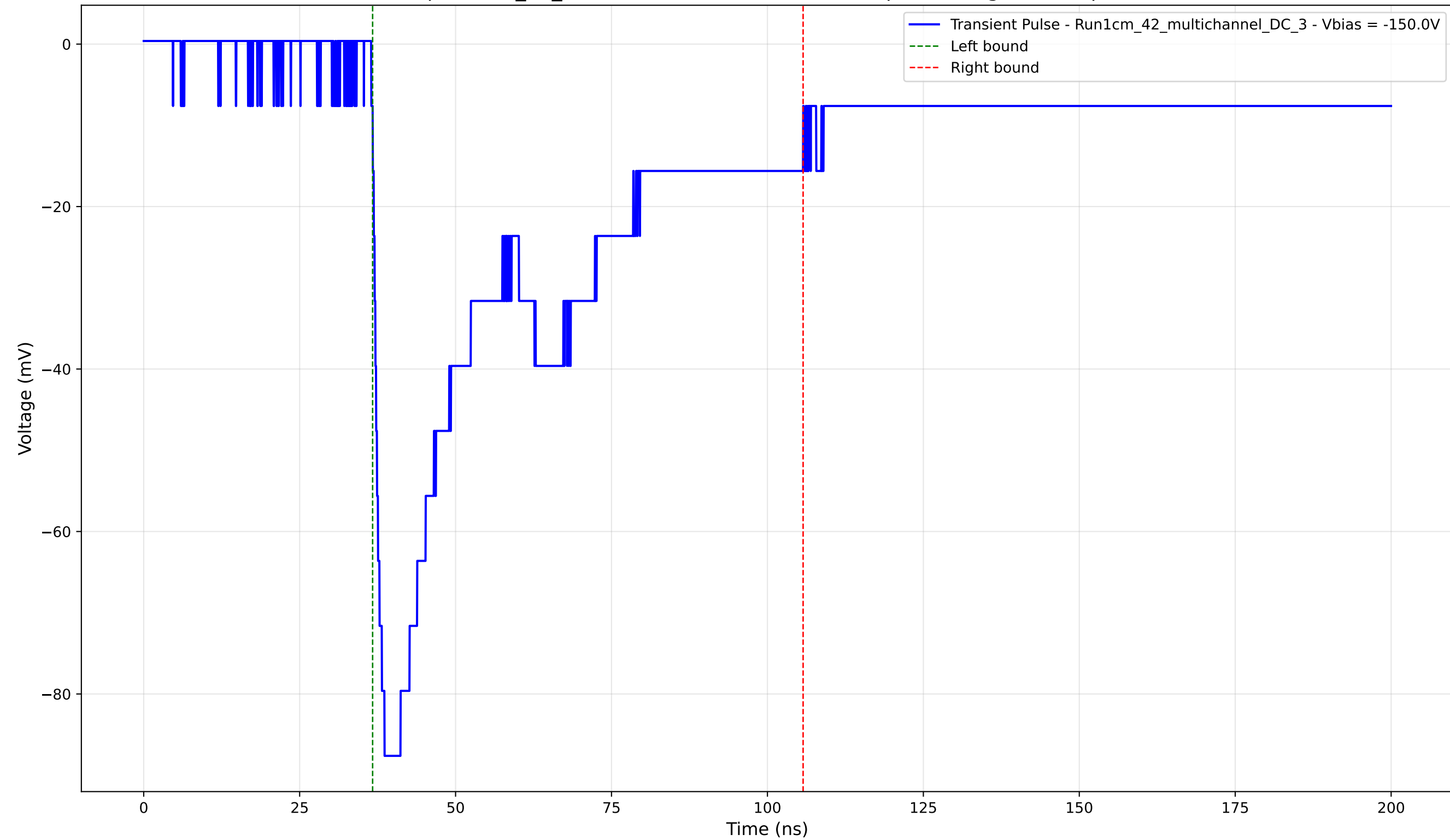
Transient Pulse - Sample: 1cm_42_multichannel - Position: 2130.0 \mu\text{m} - Charge: 43.59 pC - Rise Time: 1.48 ns
