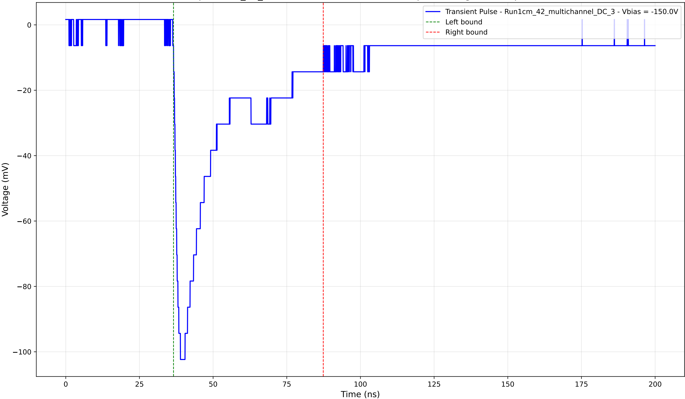
Transient Pulse - Sample: 1cm_42_multichannel - Position: 3030.0 \mu\text{m} - Charge: 35.40 pC - Rise Time: 1.79 ns
