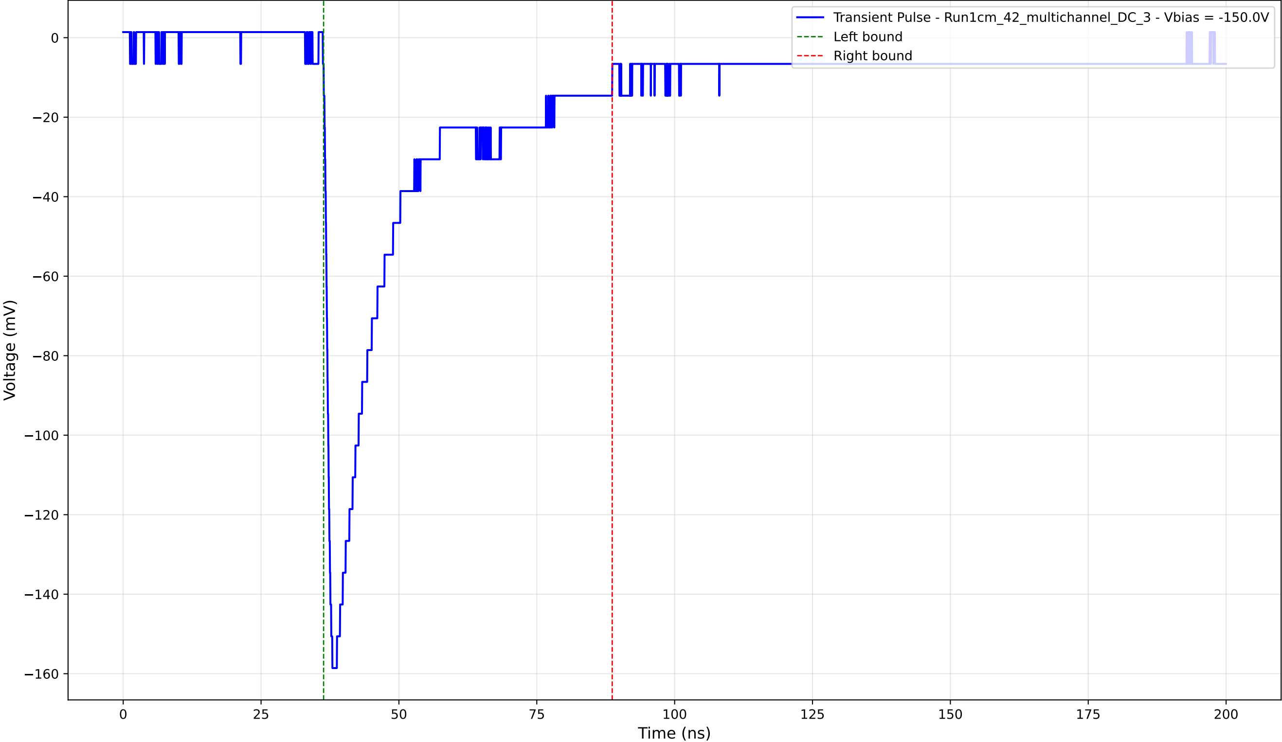
Transient Pulse - Sample: 1cm_42_multichannel - Position: 1135.0 \mu\text{m} - Charge: 43.21 pC - Rise Time: 1.24 ns
