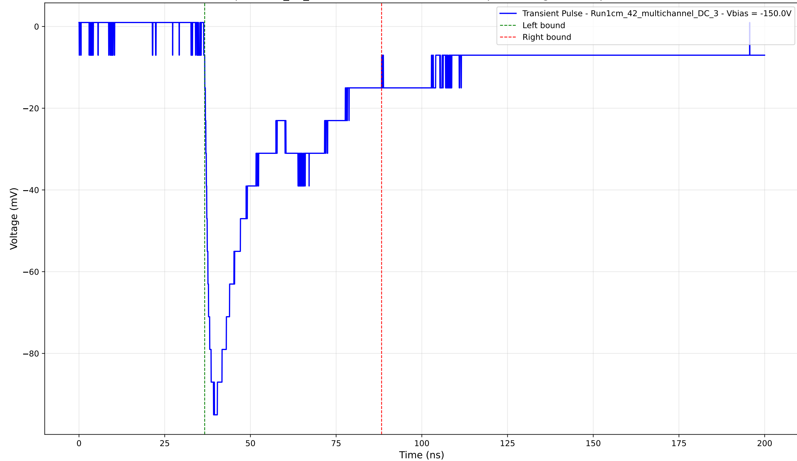
Transient Pulse - Sample: 1cm_42_multichannel - Position: 2740.0 \mu\text{m} - Charge: 36.95 pC - Rise Time: 1.87 ns
