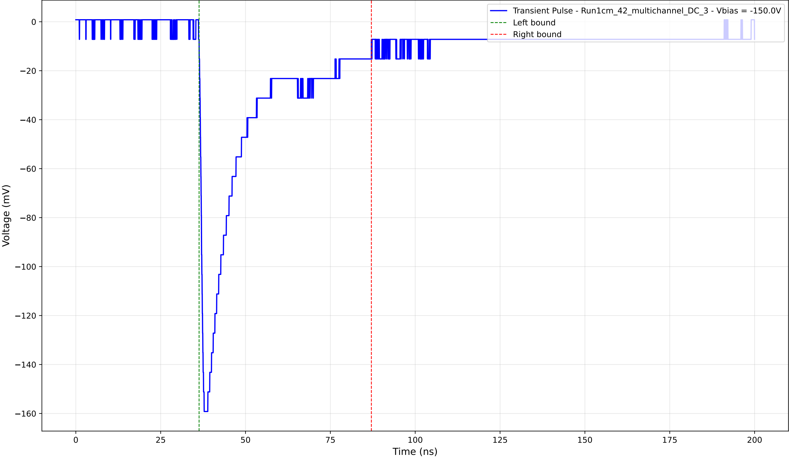
Transient Pulse - Sample: 1cm_42_multichannel - Position: 1105.0 \mu\text{m} - Charge: 43.57 pC - Rise Time: 1.18 ns
