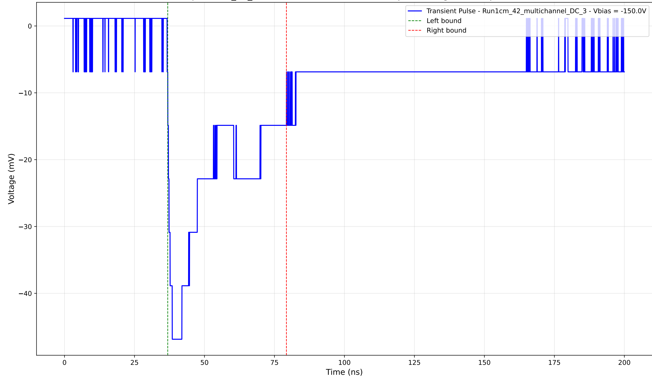
Transient Pulse - Sample: 1cm_42_multichannel - Position: 2320.0 \mu\text{m} - Charge: 20.08 pC - Rise Time: 1.83 ns
