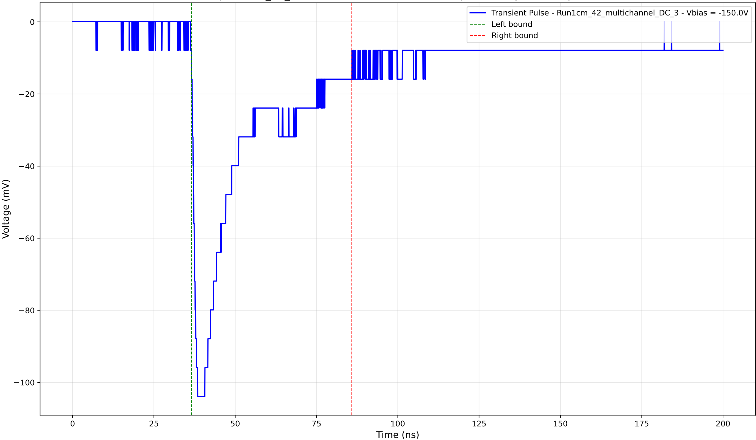
Transient Pulse - Sample: 1cm_42_multichannel - Position: 3175.0 \mu\text{m} - Charge: 36.37 pC - Rise Time: 1.51 ns
