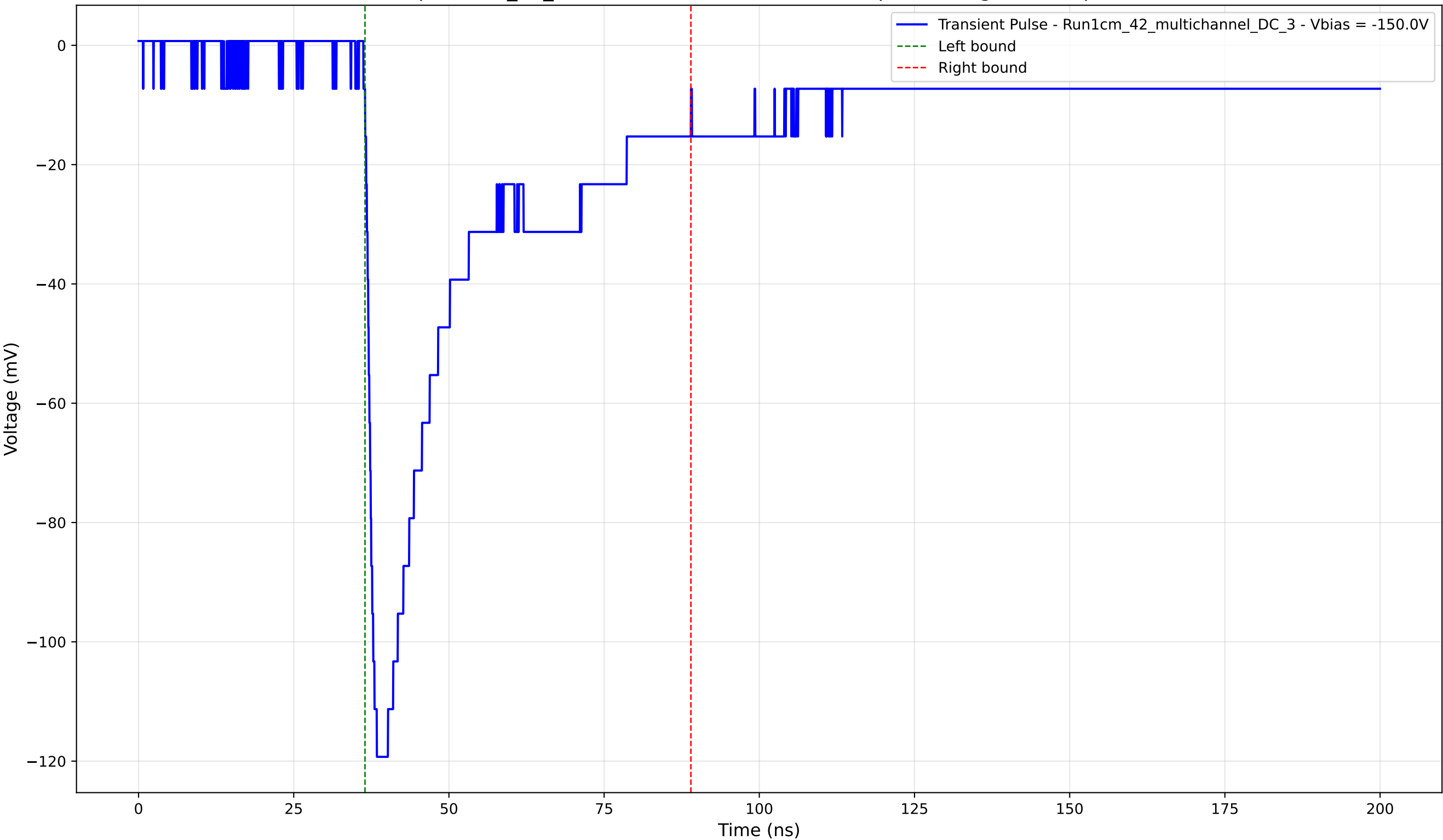
Transient Pulse - Sample: 1cm_42_multichannel - Position: 1630.0 \mu\text{m} - Charge: 41.52 pC - Rise Time: 1.51 ns
