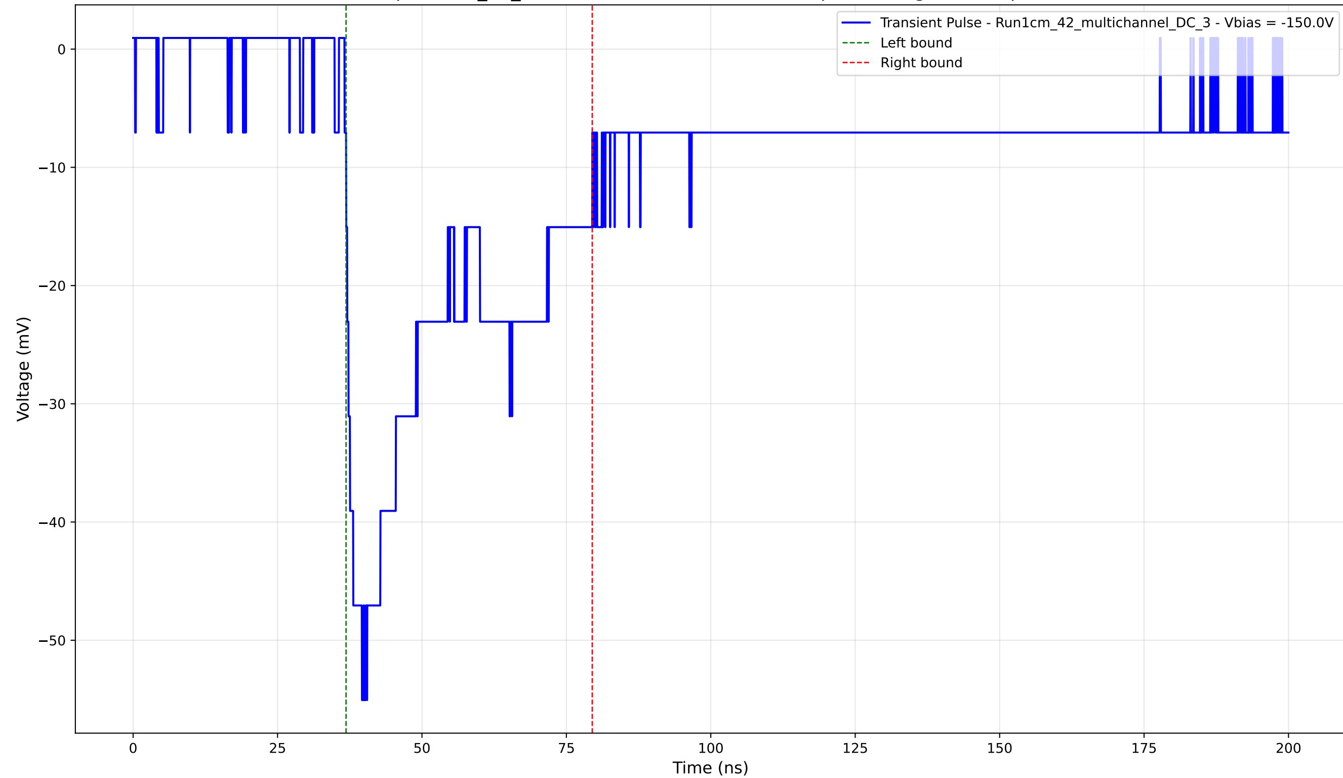
Transient Pulse - Sample: 1cm_42_multichannel - Position: 2430.0 \mu\text{m} - Charge: 21.83 pC - Rise Time: 3.01 ns
