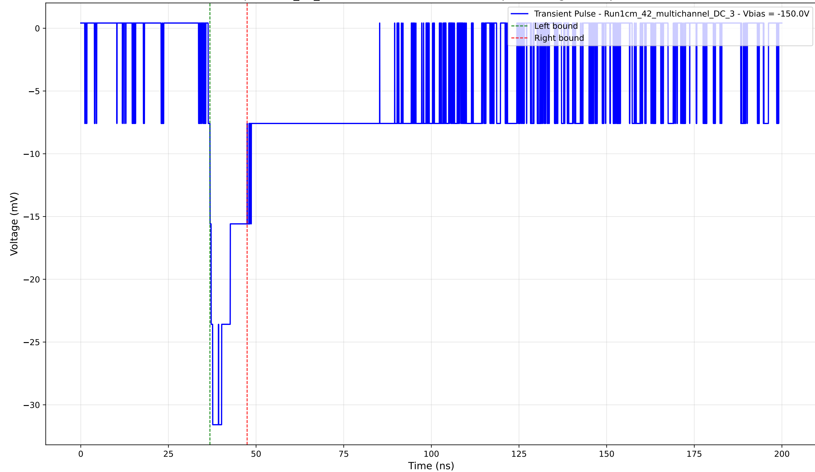
Transient Pulse - Sample: 1cm_42_multichannel - Position: 3855.0 \mu\text{m} - Charge: 4.58 pC - Rise Time: 1.29 ns
