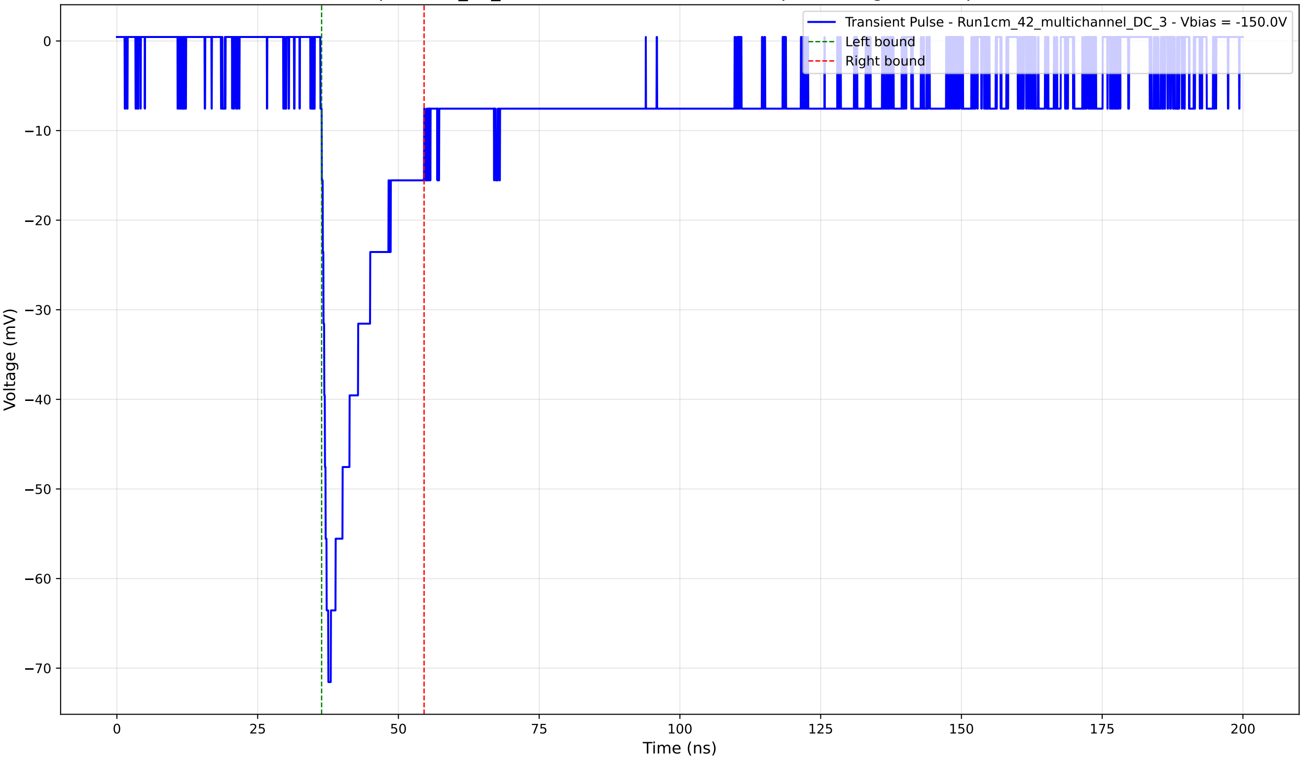
Transient Pulse - Sample: 1cm_42_multichannel - Position: 815.0 \mu\text{m} - Charge: 11.37 pC - Rise Time: 1.40 ns
