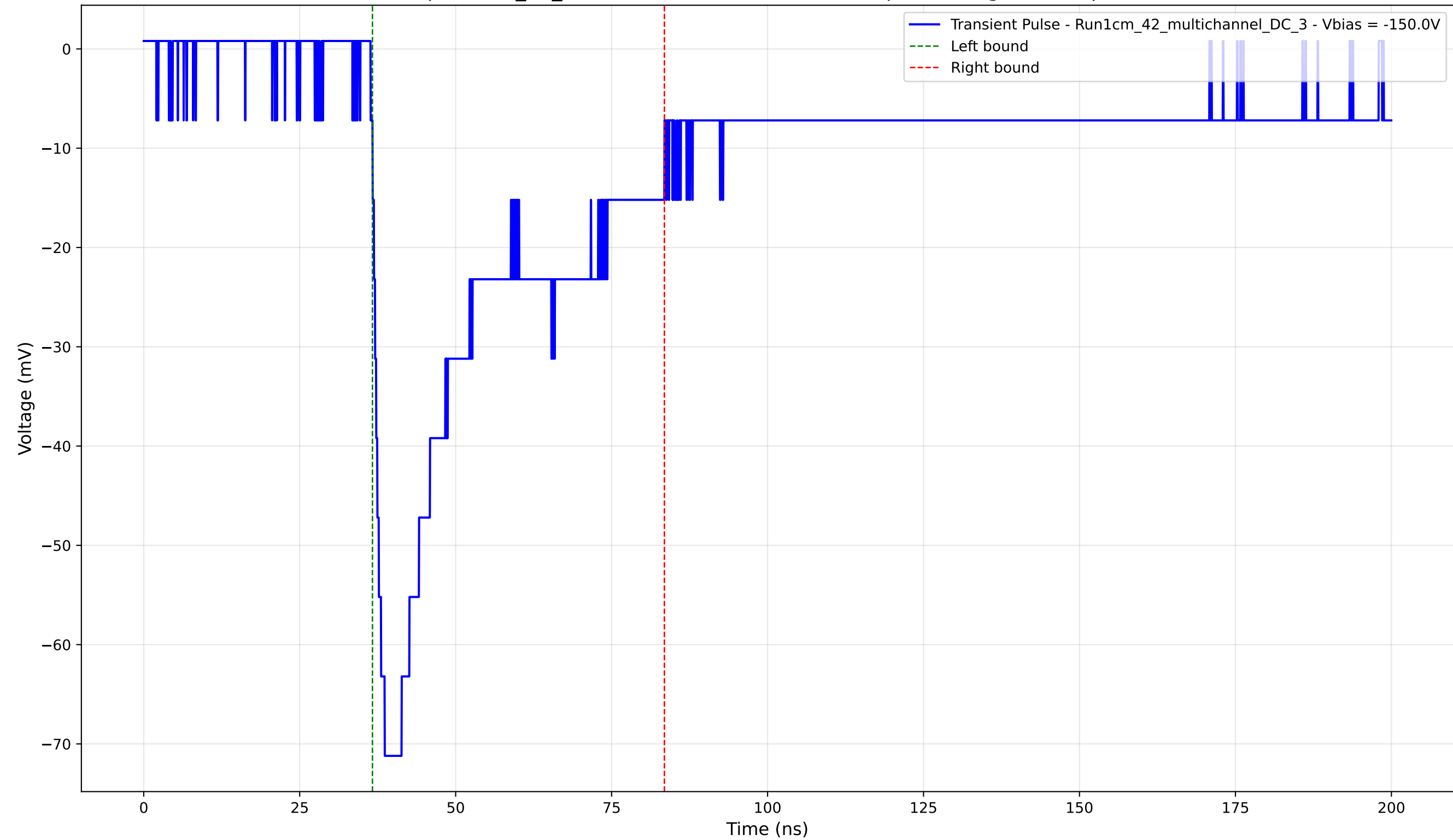
Transient Pulse - Sample: 1cm_42_multichannel - Position: 2815.0 \mu\text{m} - Charge: 27.84 pC - Rise Time: 2.26 ns
