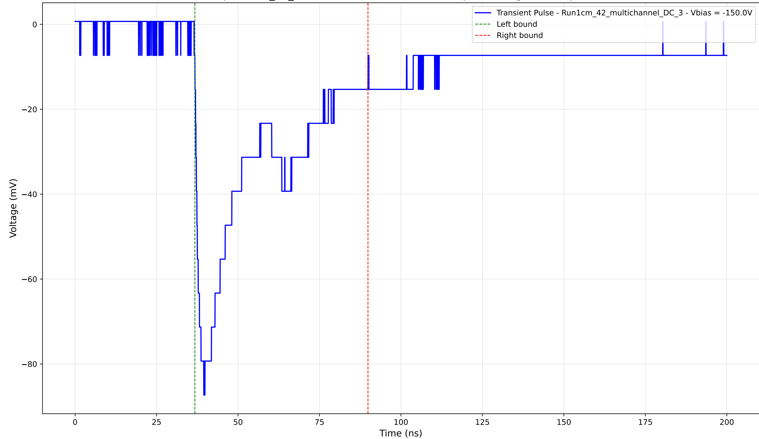
Transient Pulse - Sample: 1cm_42_multichannel - Position: 2605.0 \mu\text{m} - Charge: 36.02 pC - Rise Time: 1.88 ns
