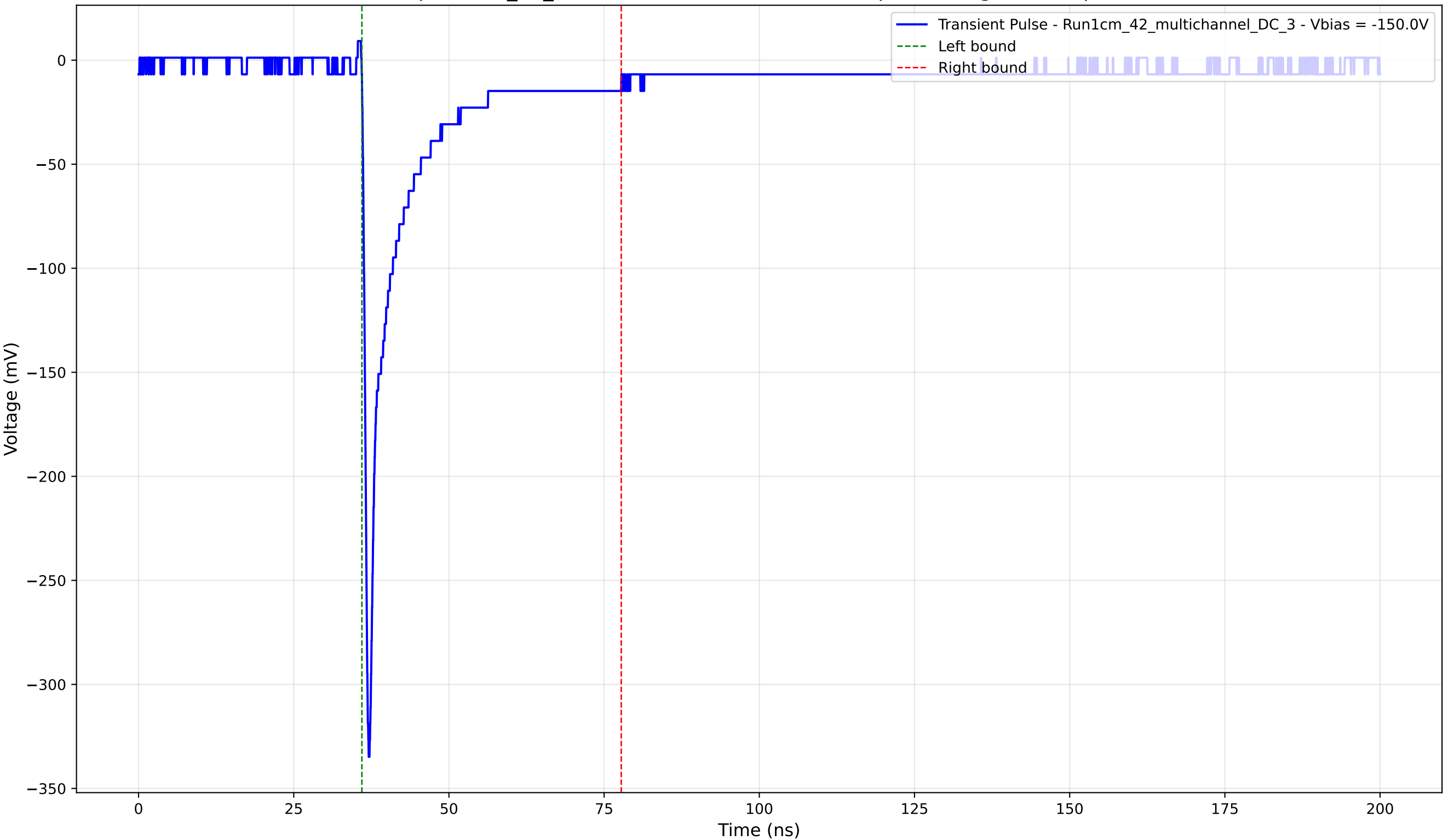
Transient Pulse - Sample: 1cm_42_multichannel - Position: 4820.0 \mu\text{m} - Charge: 36.50 pC - Rise Time: 0.77 ns
