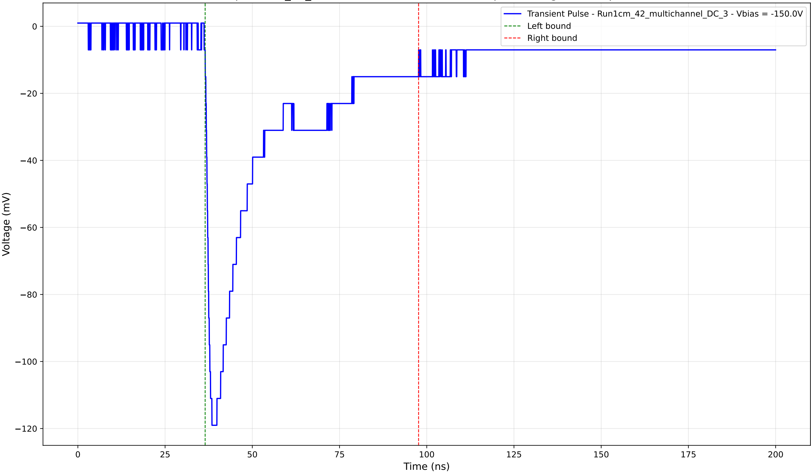
Transient Pulse - Sample: 1cm_42_multichannel - Position: 1660.0 \mu\text{m} - Charge: 43.84 pC - Rise Time: 1.53 ns
