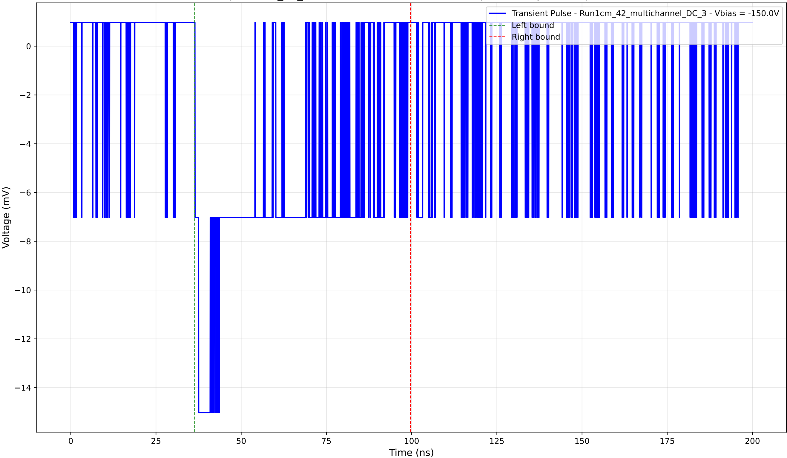
Transient Pulse - Sample: 1cm_42_multichannel - Position: 1345.0 \mu\text{m} - Charge: 7.12 pC - Rise Time: 1.10 ns
