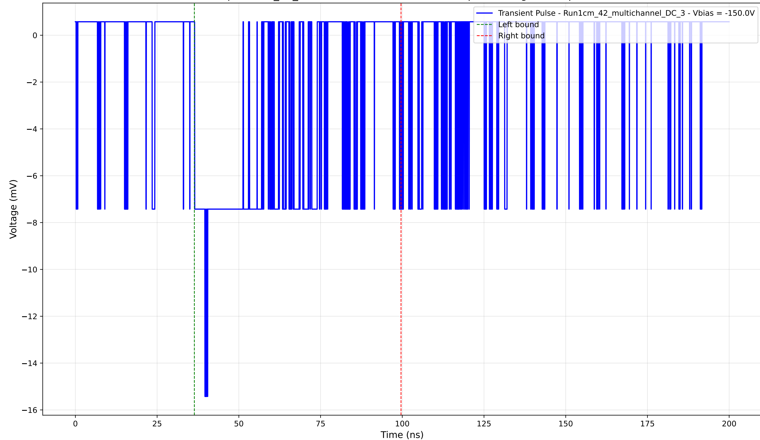
Transient Pulse - Sample: 1cm_42_multichannel - Position: 3900.0 \mu\text{m} - Charge: 4.78 pC - Rise Time: 3.16 ns
