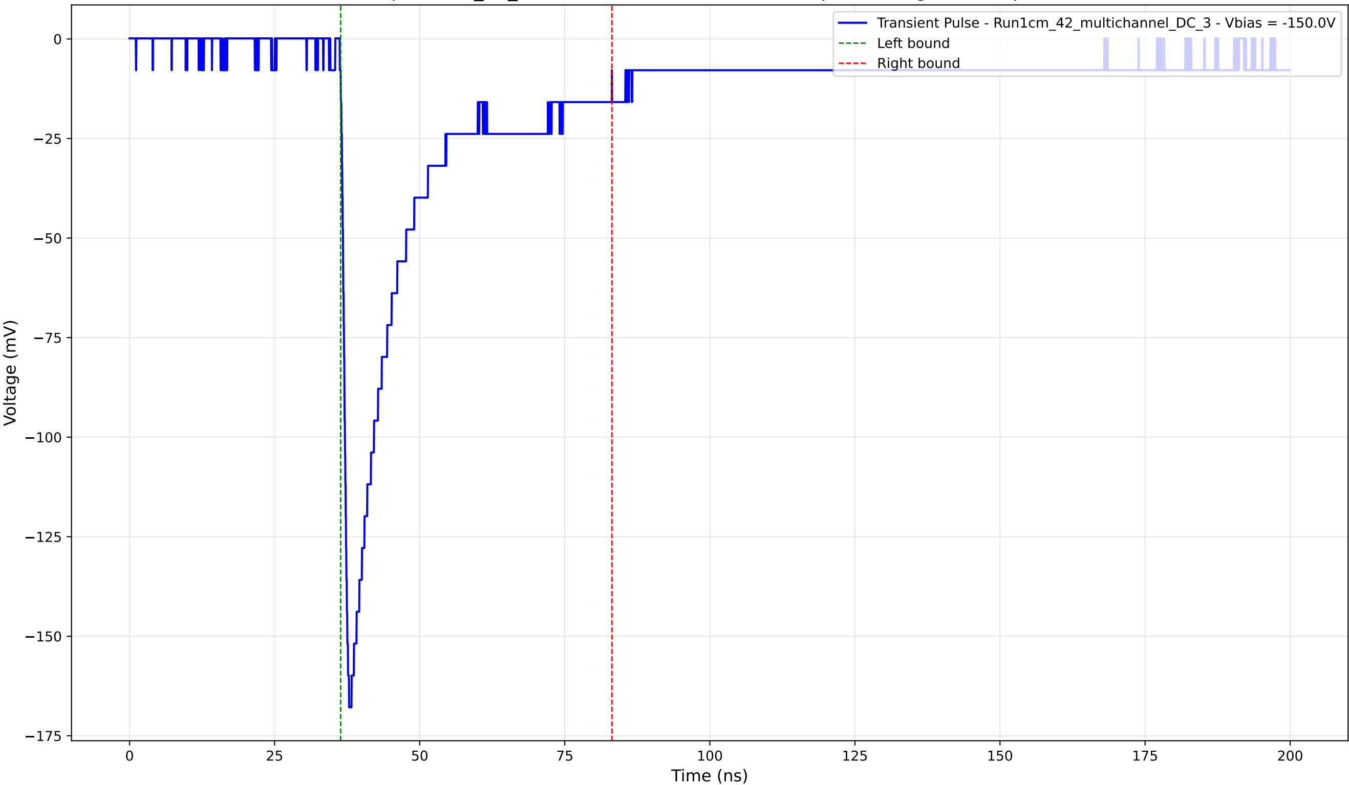
Transient Pulse - Sample: 1cm_42_multichannel - Position: 3975.0 \mu\text{m} - Charge: 39.19 pC - Rise Time: 1.04 ns
