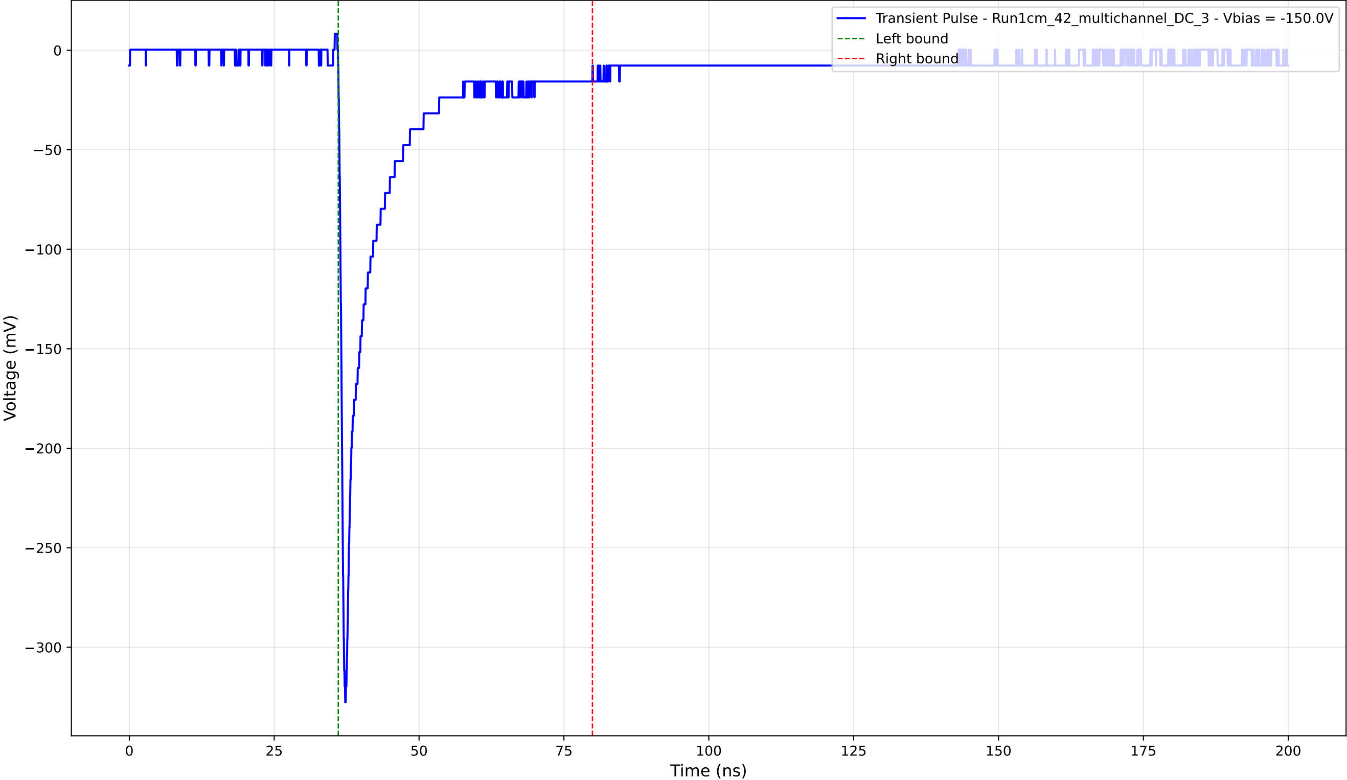
Transient Pulse - Sample: 1cm_42_multichannel - Position: 4660.0 \mu\text{m} - Charge: 42.48 pC - Rise Time: 0.82 ns
