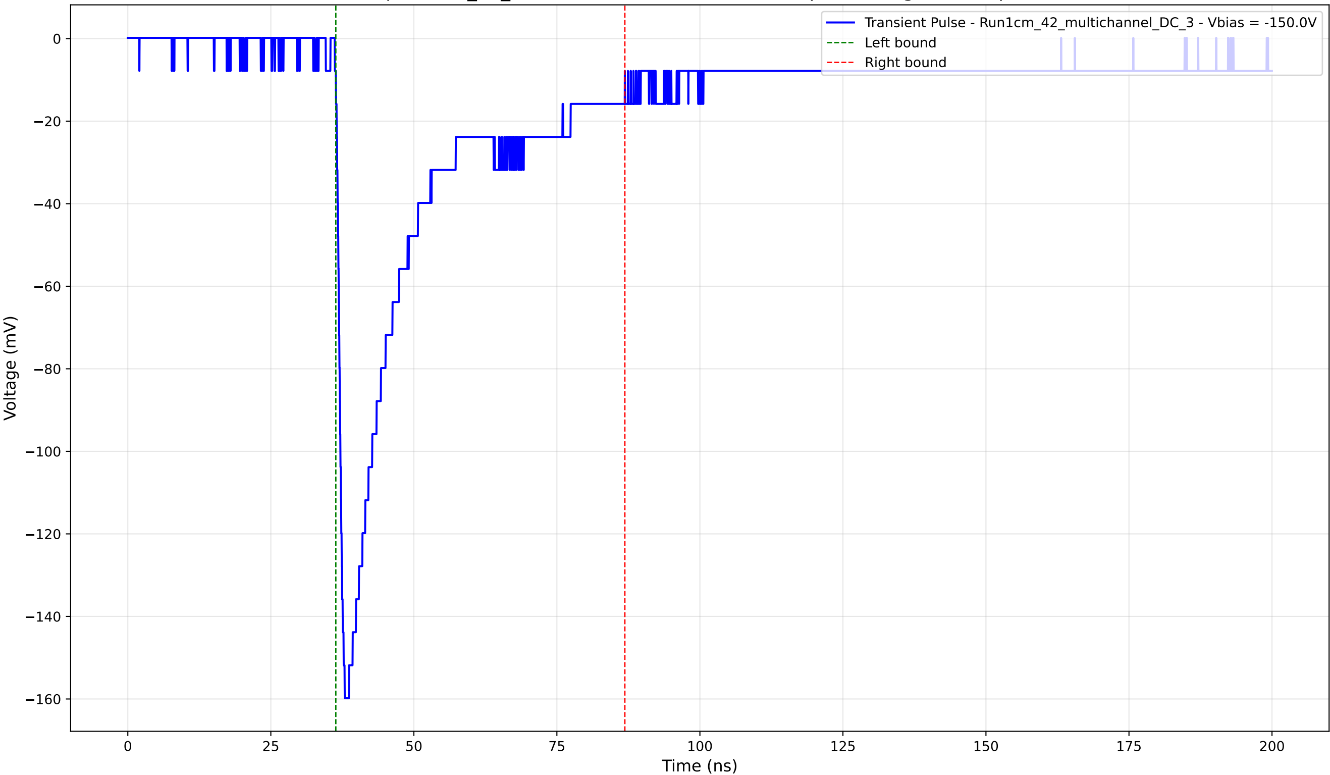
Transient Pulse - Sample: 1cm_42_multichannel - Position: 1140.0 \mu\text{m} - Charge: 43.85 pC - Rise Time: 1.24 ns
