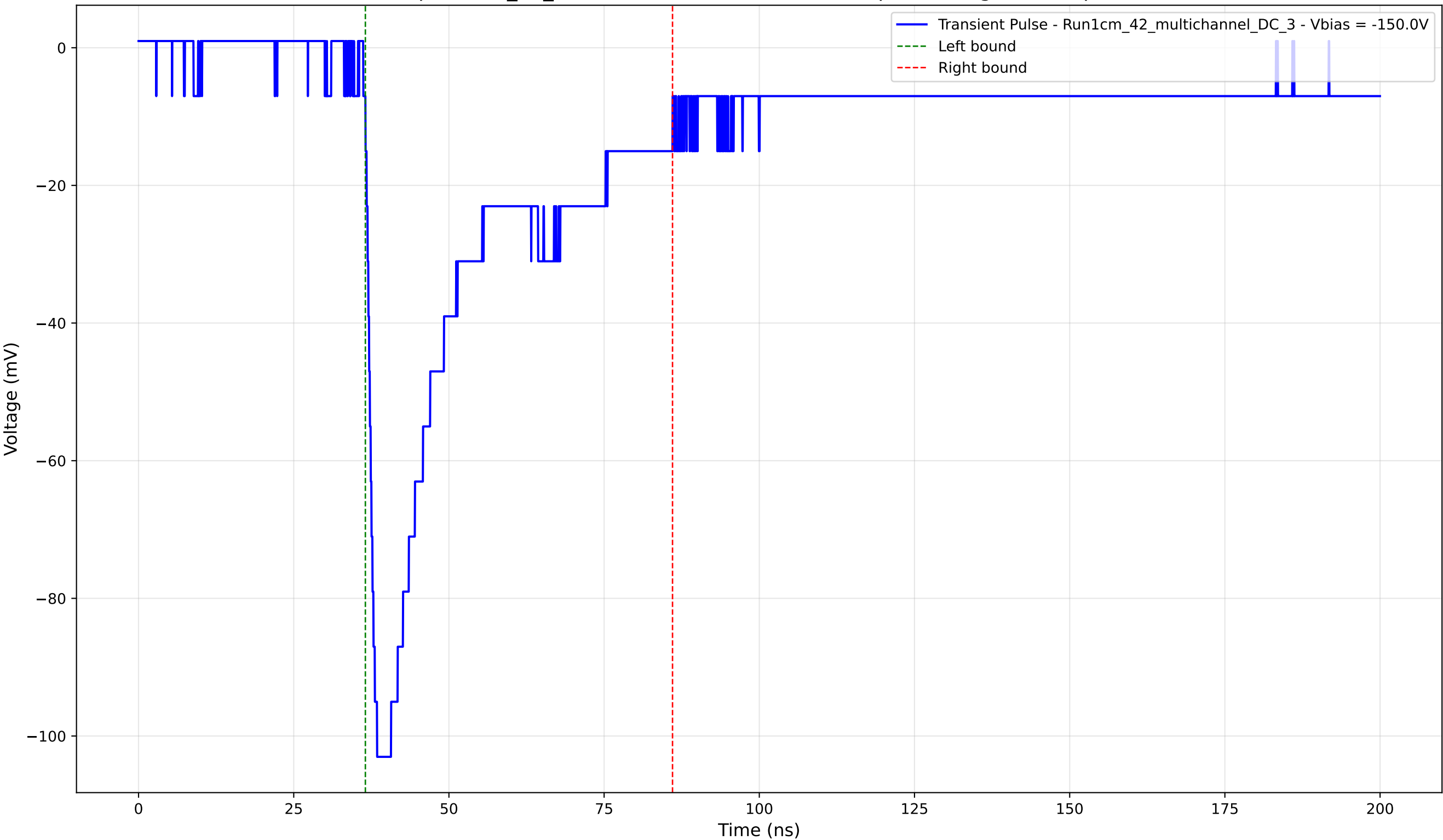
Transient Pulse - Sample: 1cm_42_multichannel - Position: 3180.0 \mu\text{m} - Charge: 35.44 pC - Rise Time: 1.51 ns
