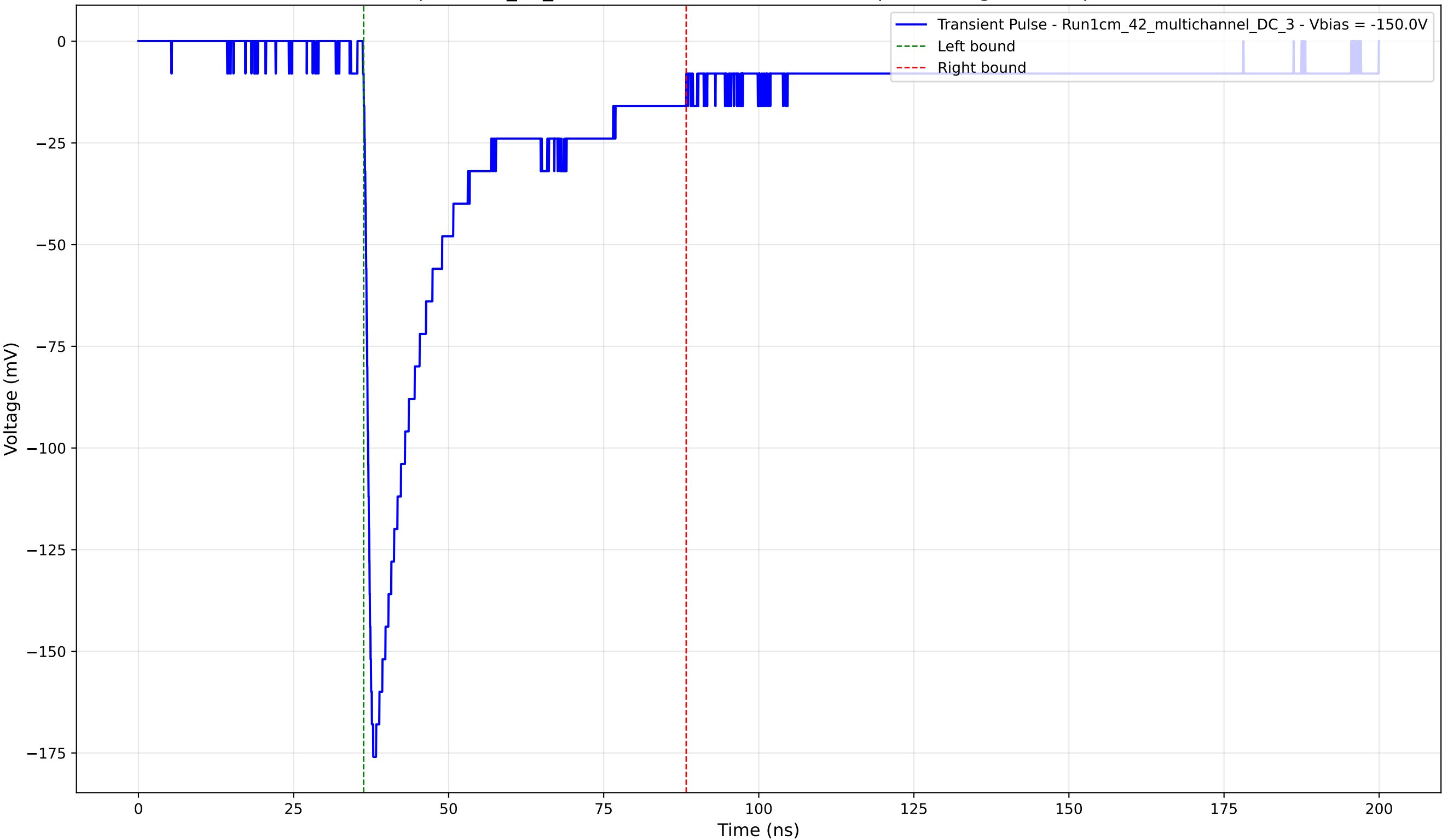
Transient Pulse - Sample: 1cm_42_multichannel - Position: 1015.0 \mu\text{m} - Charge: 45.56 pC - Rise Time: 1.10 ns
