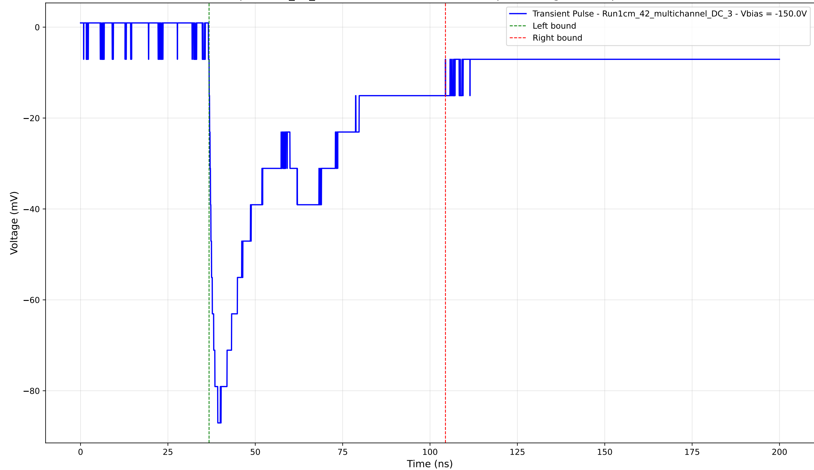
Transient Pulse - Sample: 1cm_42_multichannel - Position: 2270.0 \mu\text{m} - Charge: 42.09 pC - Rise Time: 1.66 ns
