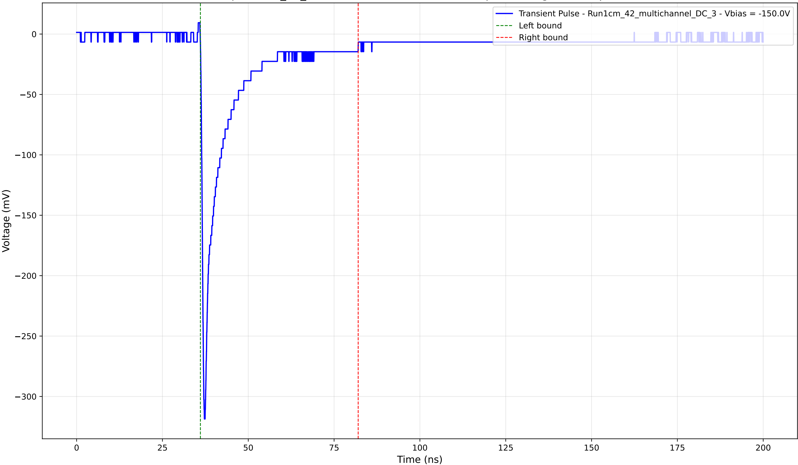
Transient Pulse - Sample: 1cm_42_multichannel - Position: 4650.0 \mu\text{m} - Charge: 41.94 pC - Rise Time: 0.82 ns
