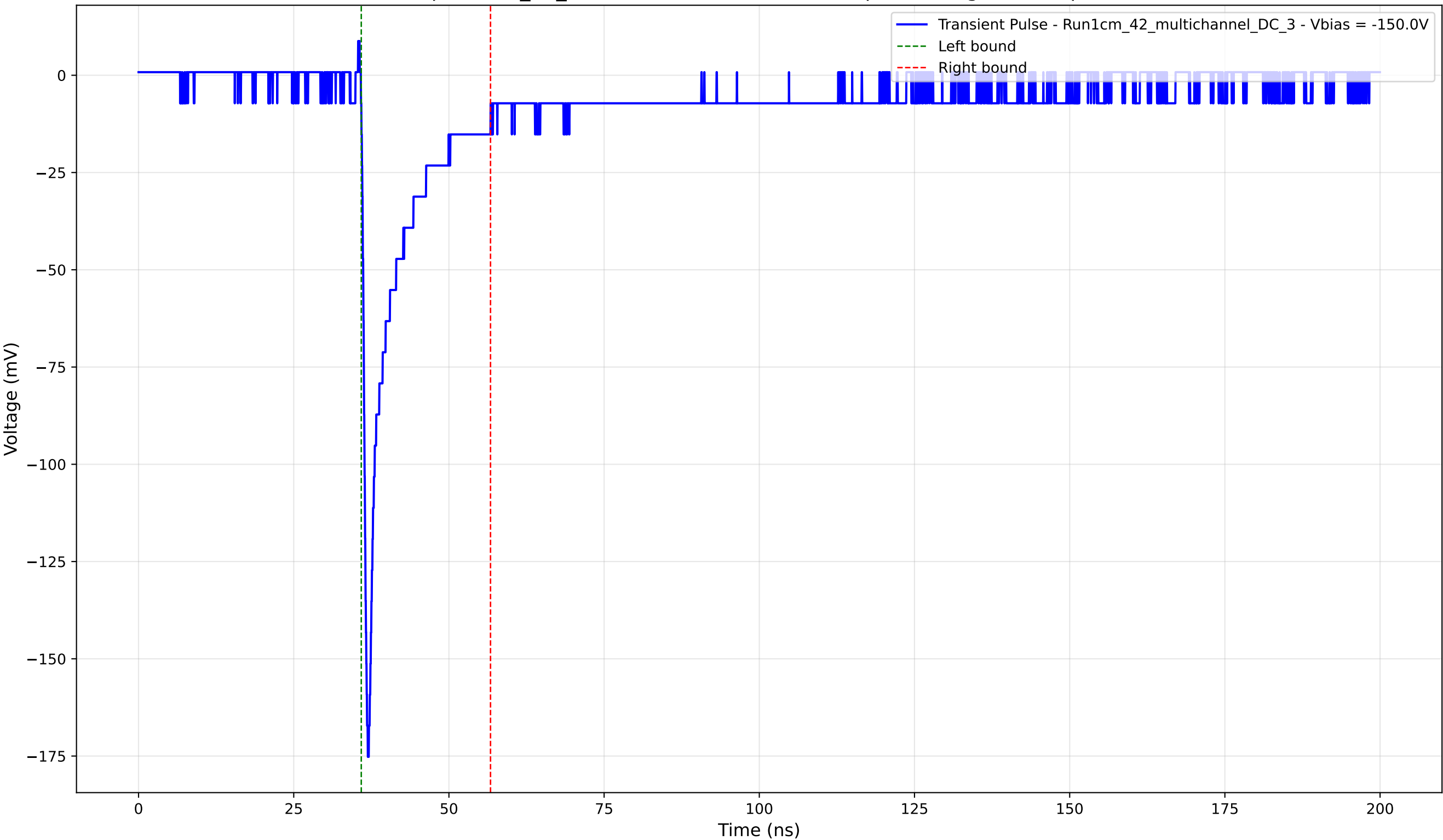
Transient Pulse - Sample: 1cm_42_multichannel - Position: 75.0 \mu\text{m} - Charge: 17.35 pC - Rise Time: 0.77 ns
