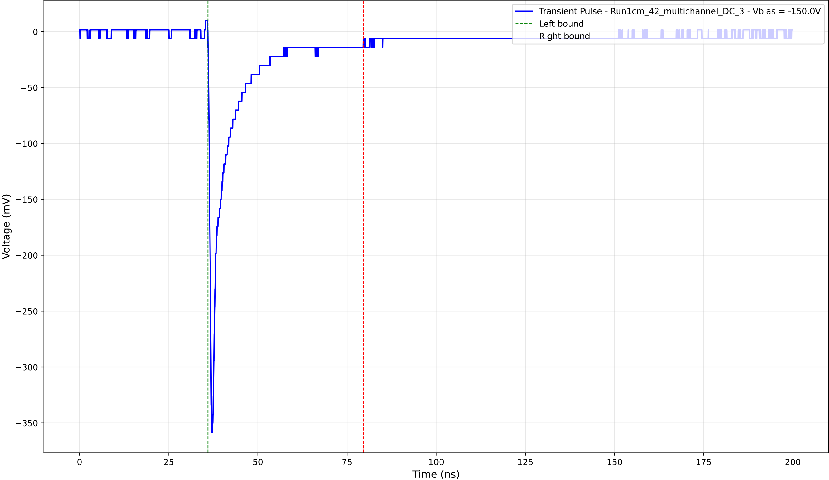
Transient Pulse - Sample: 1cm_42_multichannel - Position: 4775.0 \mu\text{m} - Charge: 40.52 pC - Rise Time: 0.78 ns
