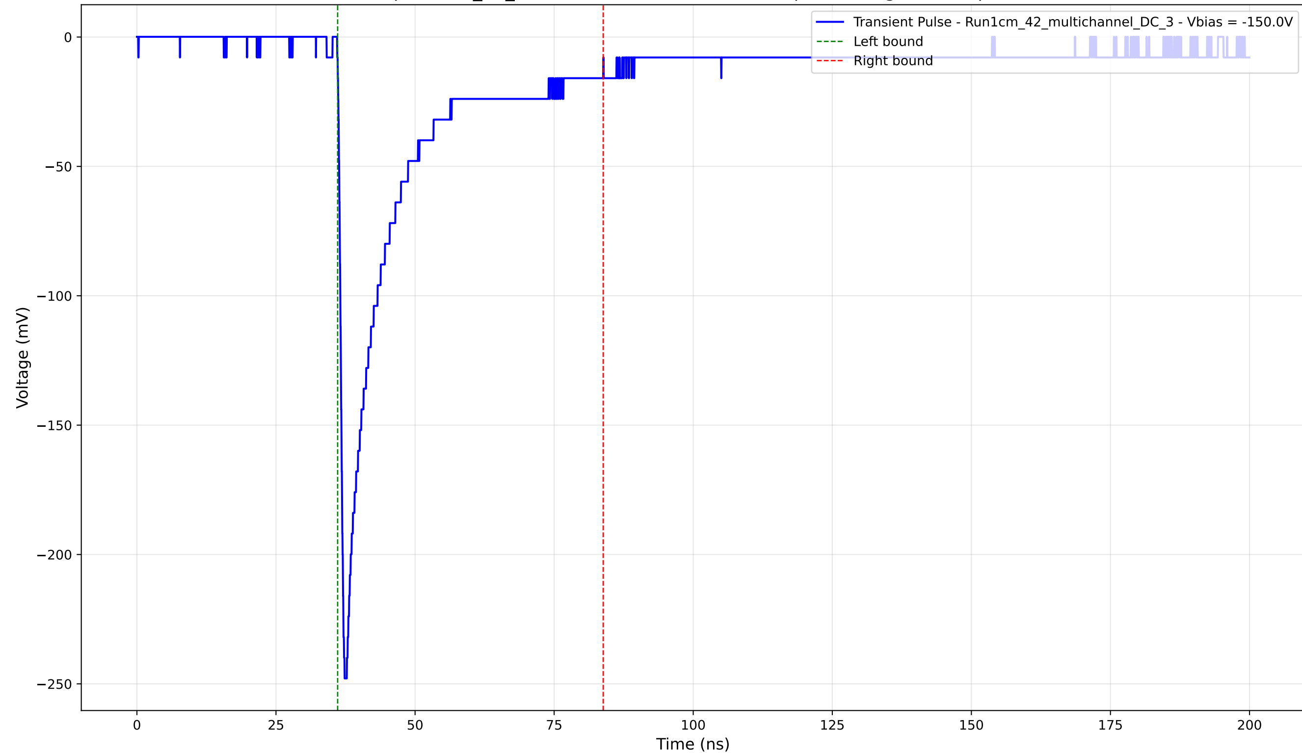
Transient Pulse - Sample: 1cm_42_multichannel - Position: 575.0 \mu\text{m} - Charge: 47.75 pC - Rise Time: 0.90 ns
