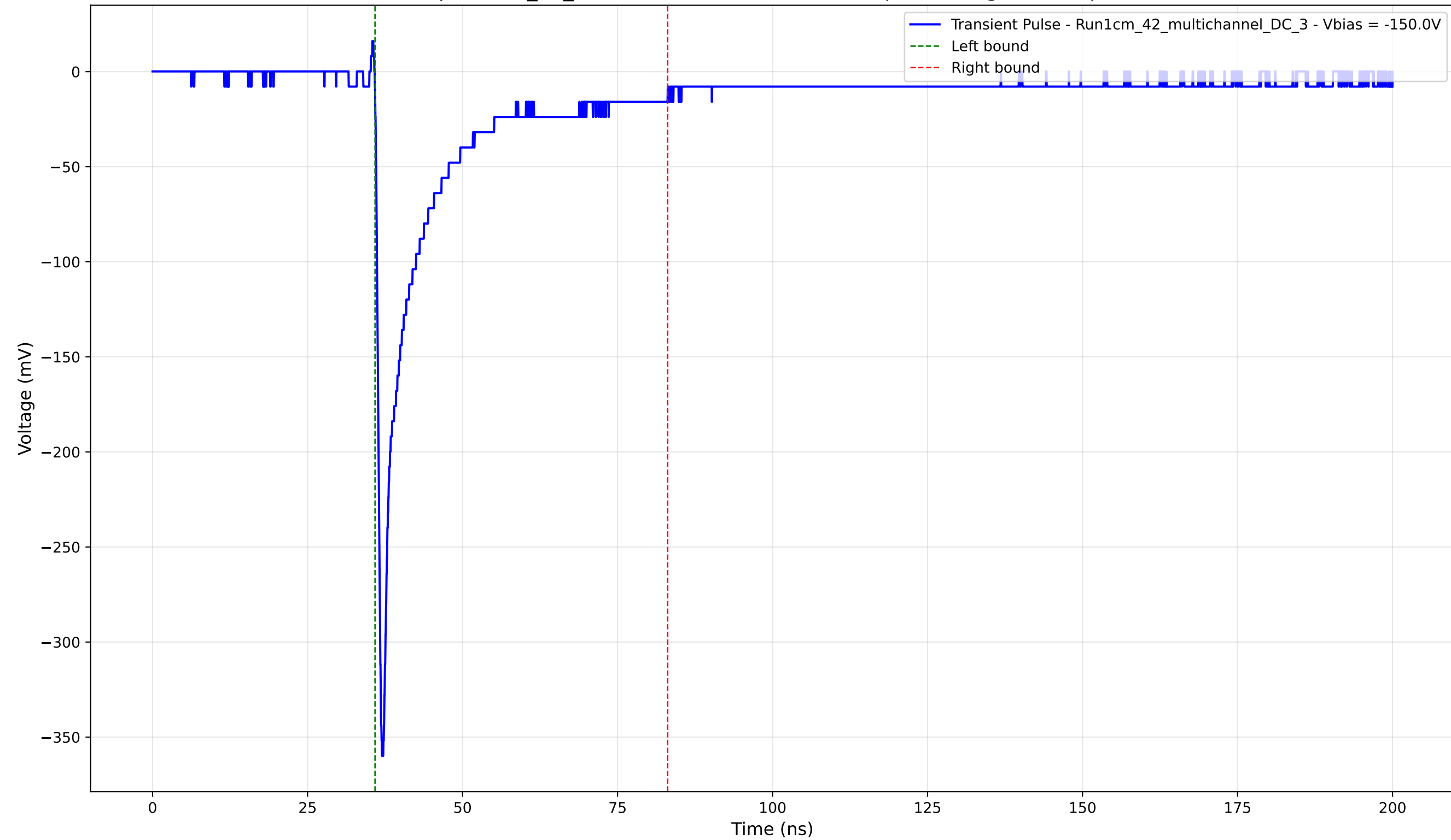
Transient Pulse - Sample: 1cm_42_multichannel - Position: 175.0 \mu\text{m} - Charge: 47.87 pC - Rise Time: 0.79 ns
