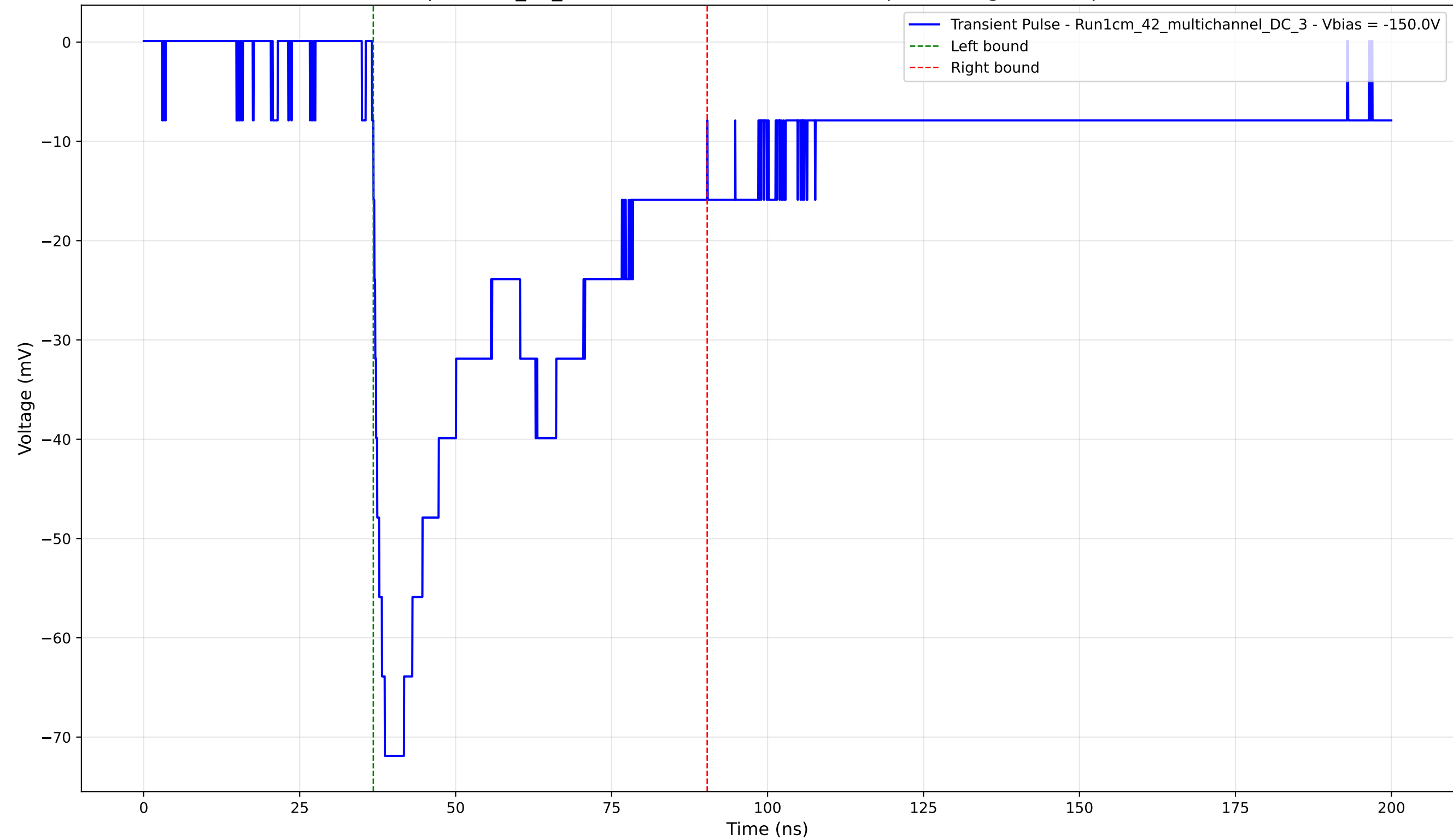
Transient Pulse - Sample: 1cm_42_multichannel - Position: 2300.0 \mu\text{m} - Charge: 34.67 pC - Rise Time: 2.04 ns
