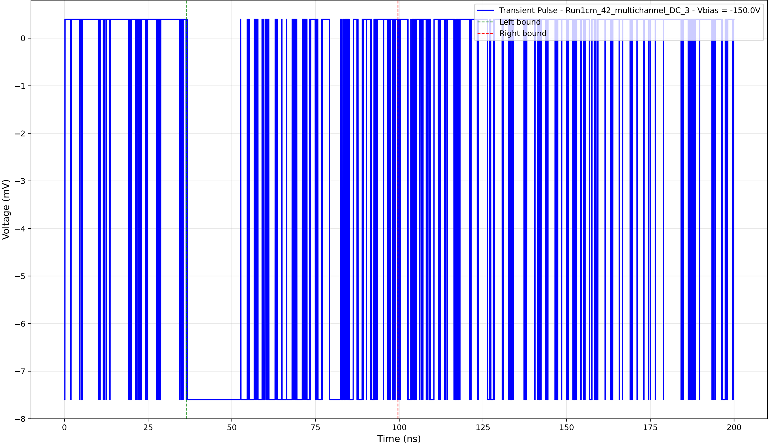
Transient Pulse - Sample: 1cm_42_multichannel - Position: 2880.0 \mu\text{m} - Charge: 6.53 pC - Rise Time: 0.00 ns (N/A)
