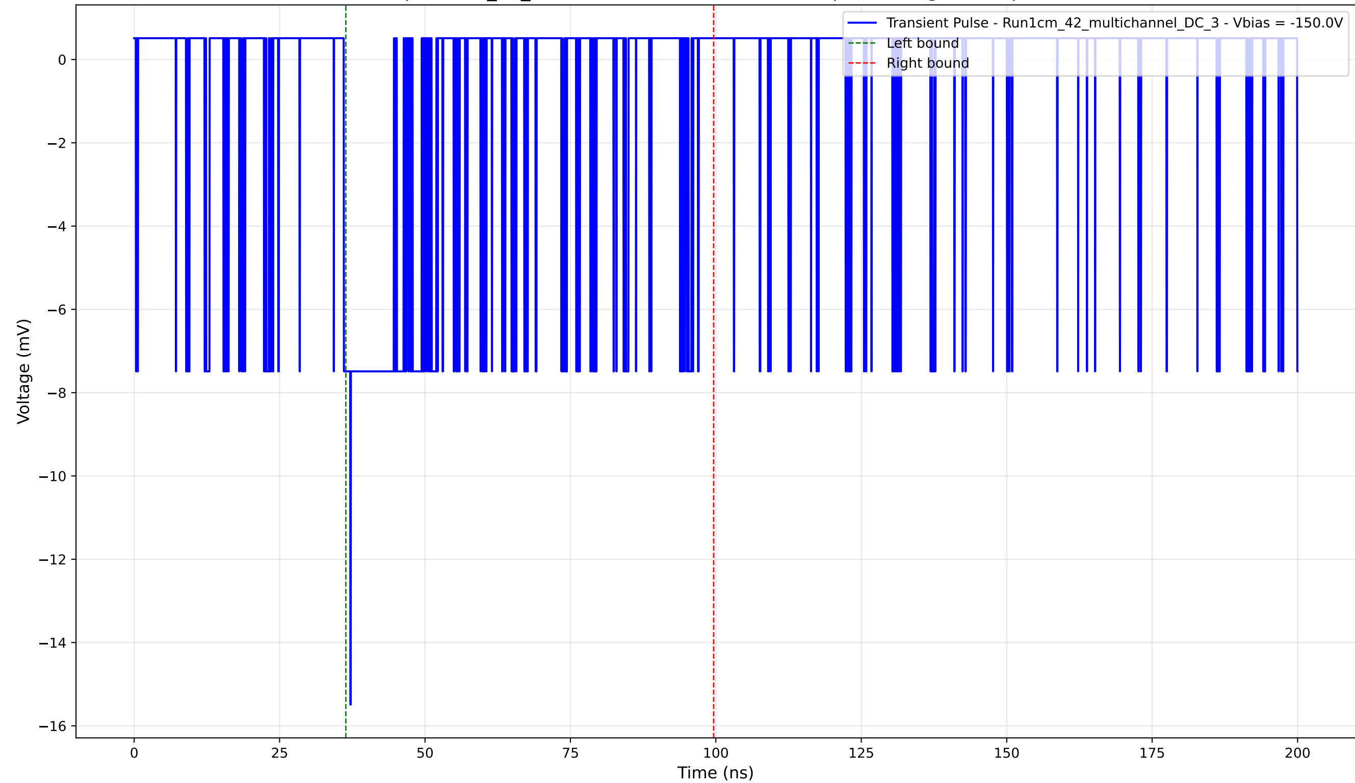
Transient Pulse - Sample: 1cm_42_multichannel - Position: 4910.0 \mu\text{m} - Charge: 2.50 pC - Rise Time: 1.14 ns
