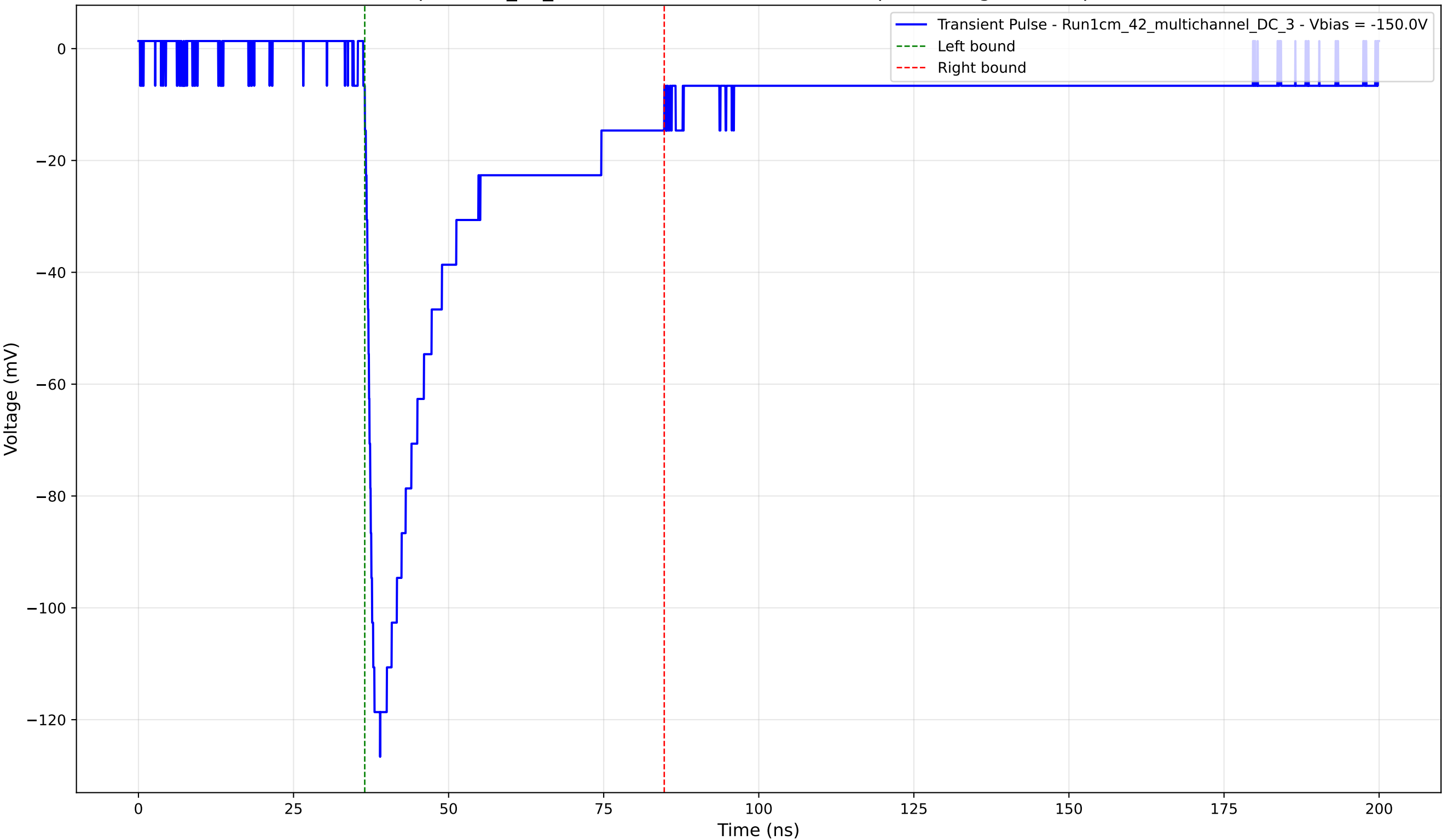
Transient Pulse - Sample: 1cm_42_multichannel - Position: 3530.0 \mu\text{m} - Charge: 35.79 pC - Rise Time: 1.54 ns
