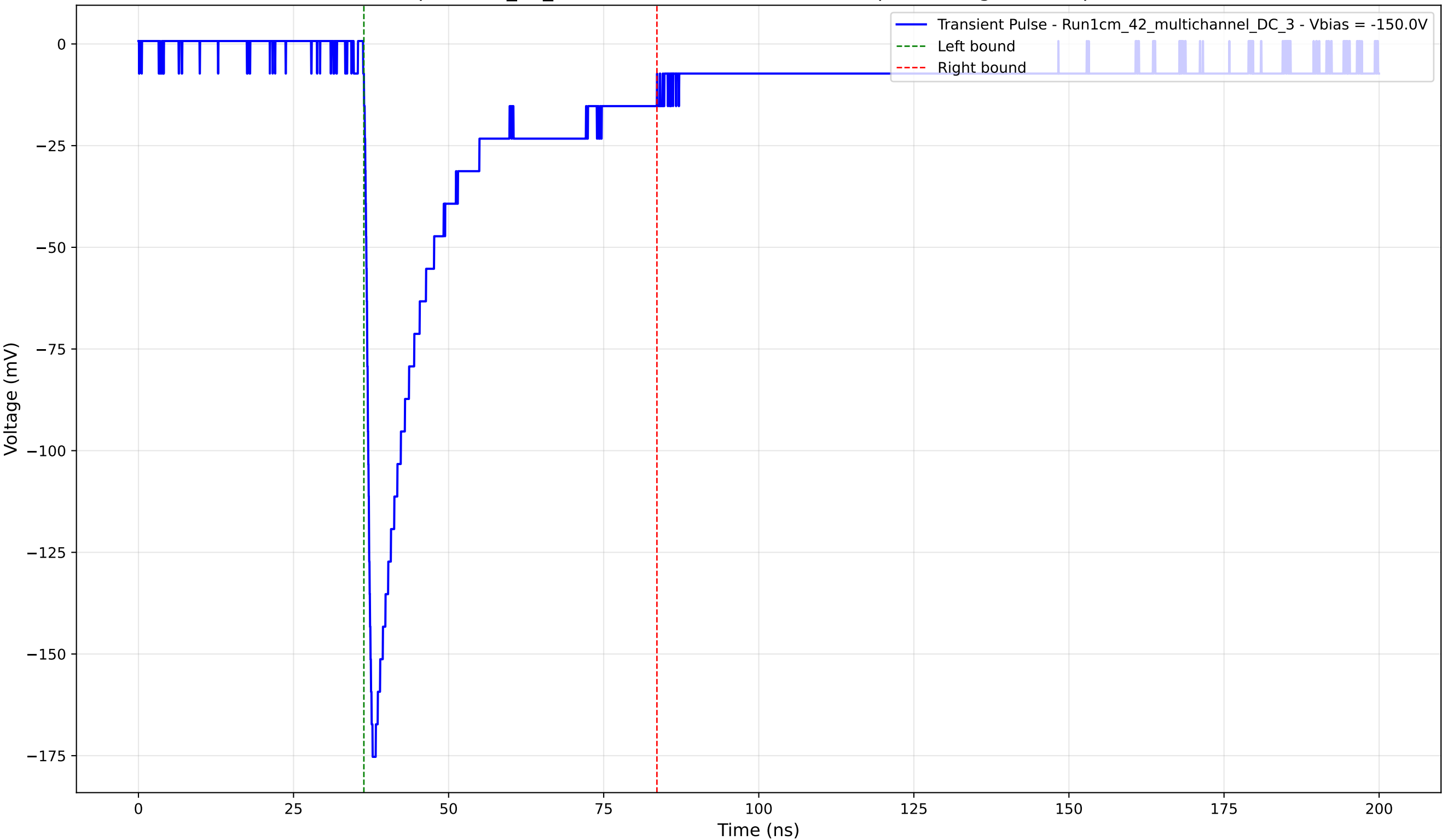
Transient Pulse - Sample: 1cm_42_multichannel - Position: 4030.0 \mu\text{m} - Charge: 39.81 pC - Rise Time: 1.01 ns
