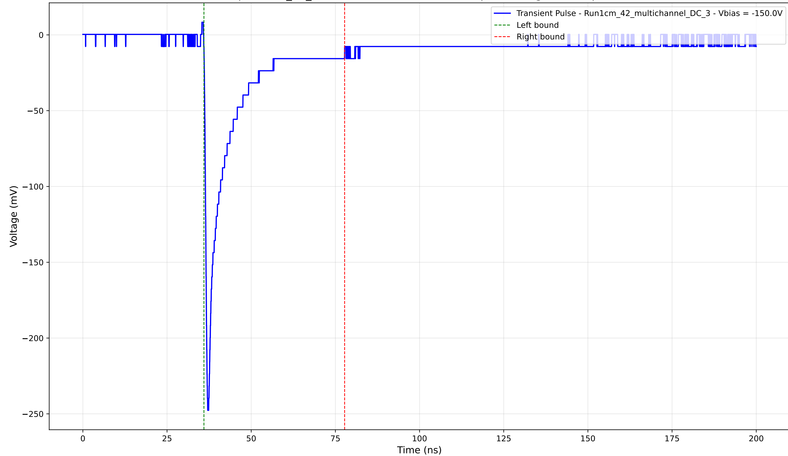
Transient Pulse - Sample: 1cm_42_multichannel - Position: 285.0 \mu\text{m} - Charge: 35.32 pC - Rise Time: 0.80 ns
