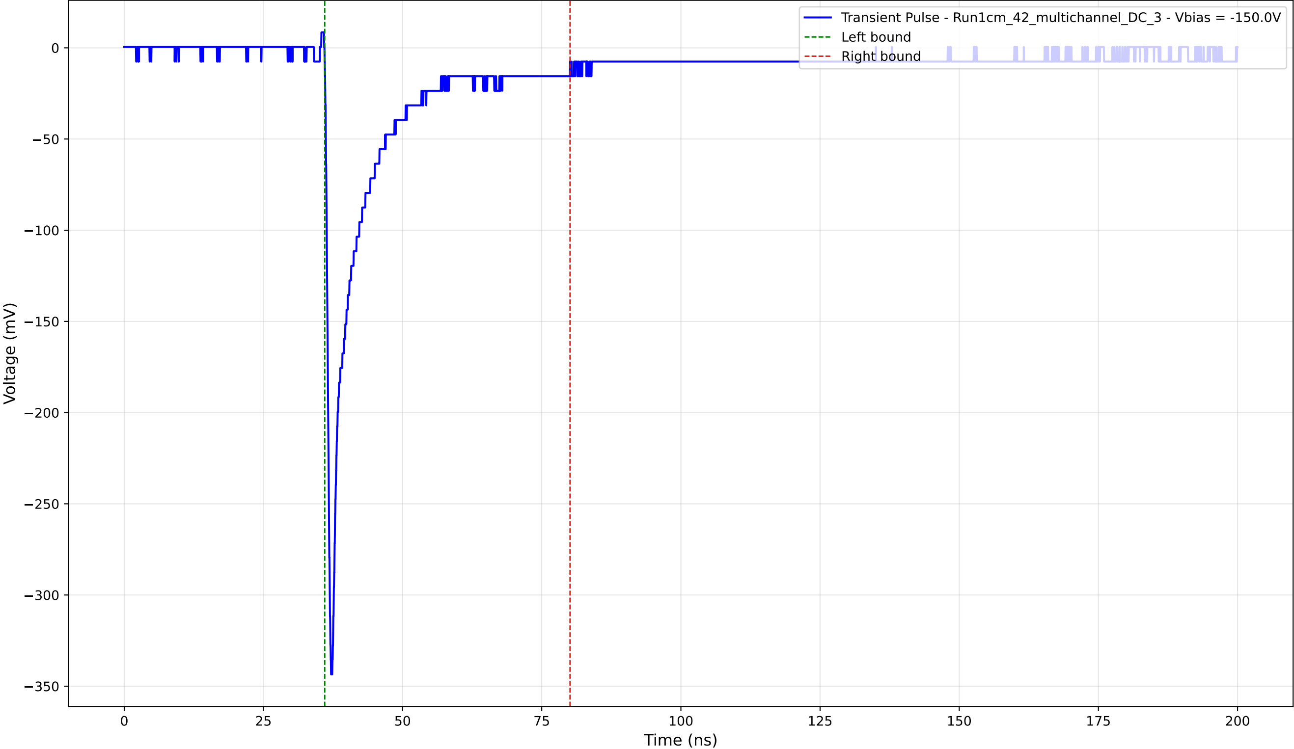
Transient Pulse - Sample: 1cm_42_multichannel - Position: 4700.0 \mu\text{m} - Charge: 42.61 pC - Rise Time: 0.79 ns
