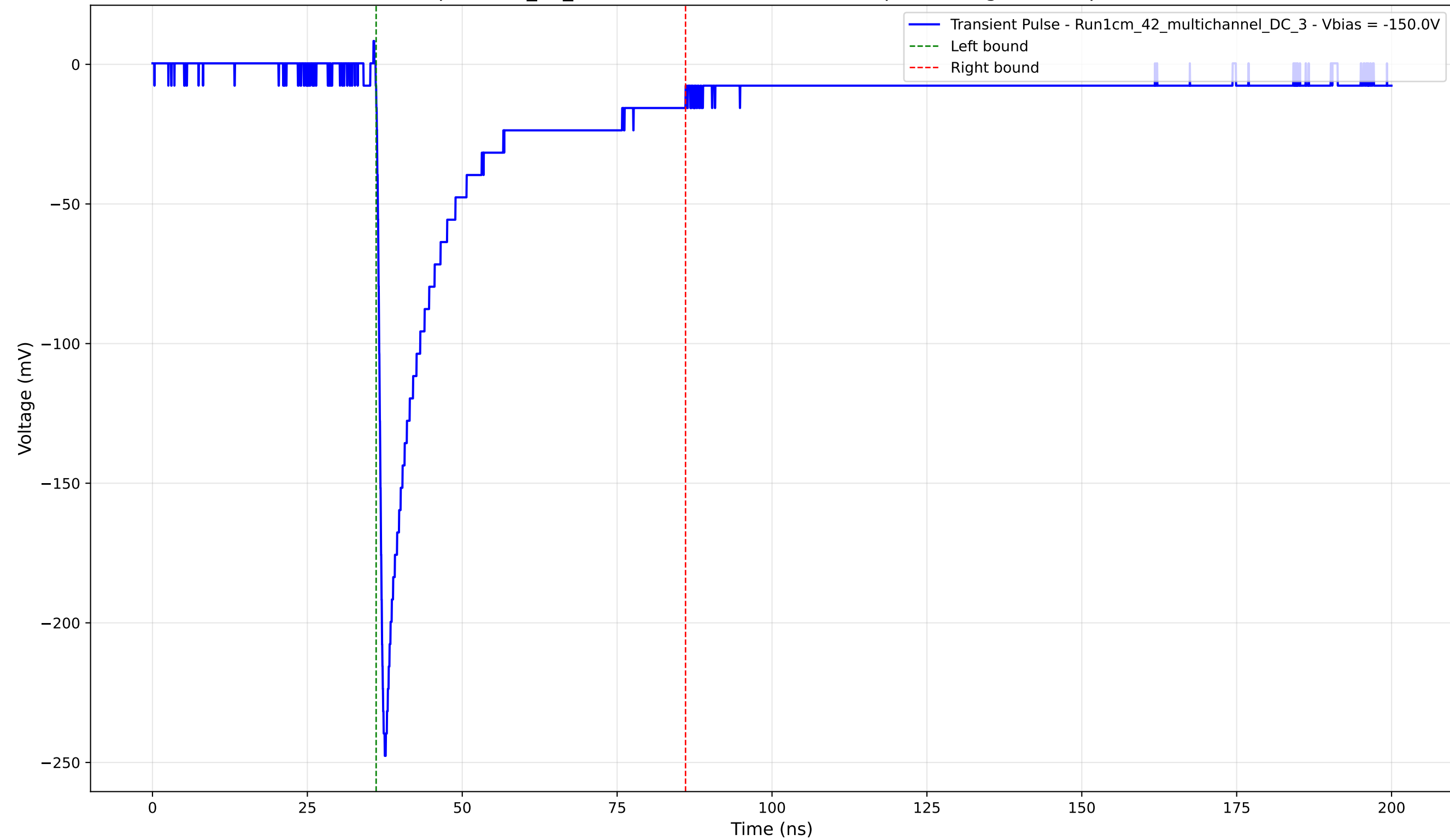
Transient Pulse - Sample: 1cm_42_multichannel - Position: 605.0 \mu\text{m} - Charge: 48.17 pC - Rise Time: 0.92 ns
