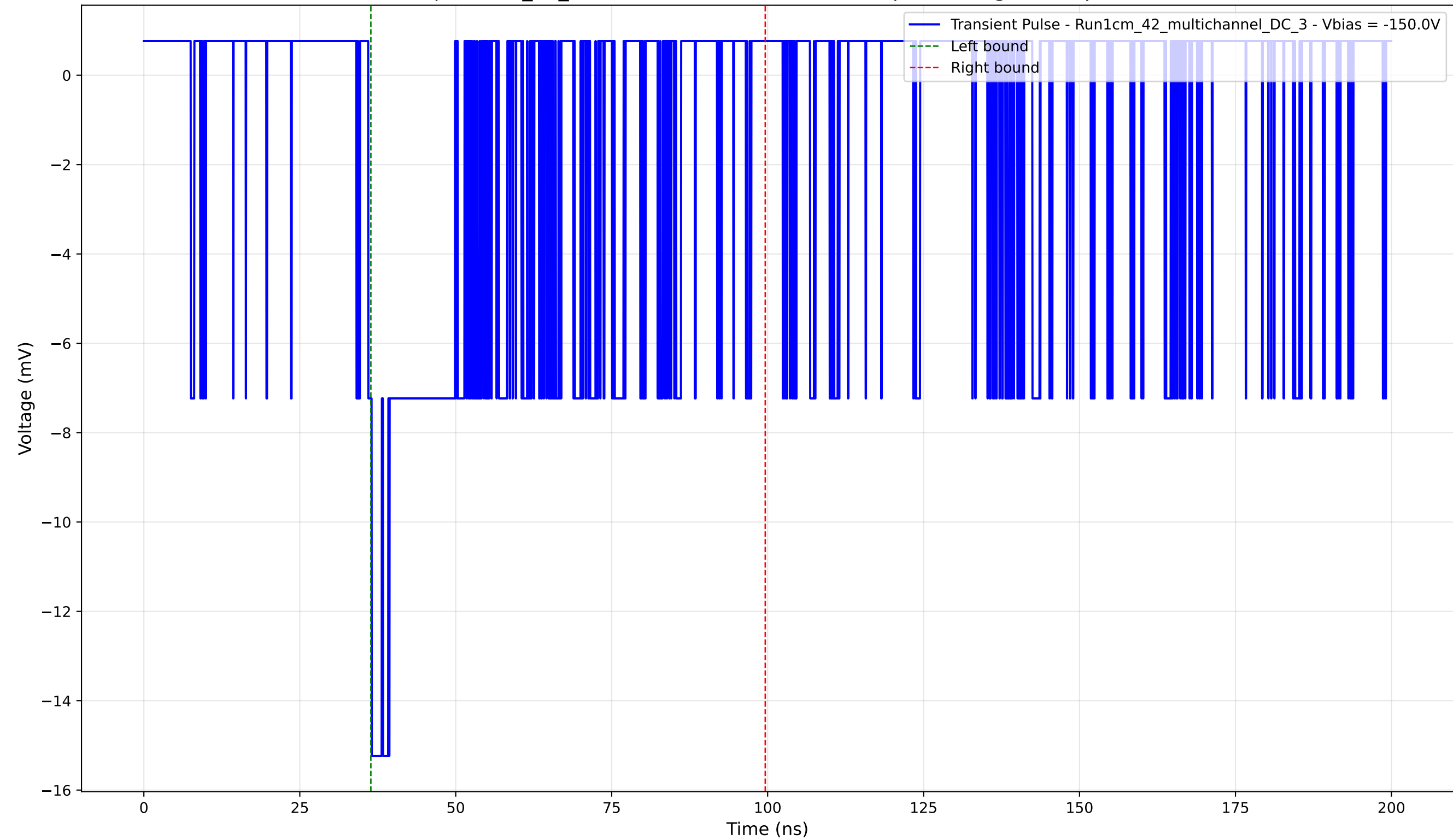
Transient Pulse - Sample: 1cm_42_multichannel - Position: 4890.0 \mu\text{m} - Charge: 4.18 pC - Rise Time: 0.56 ns
