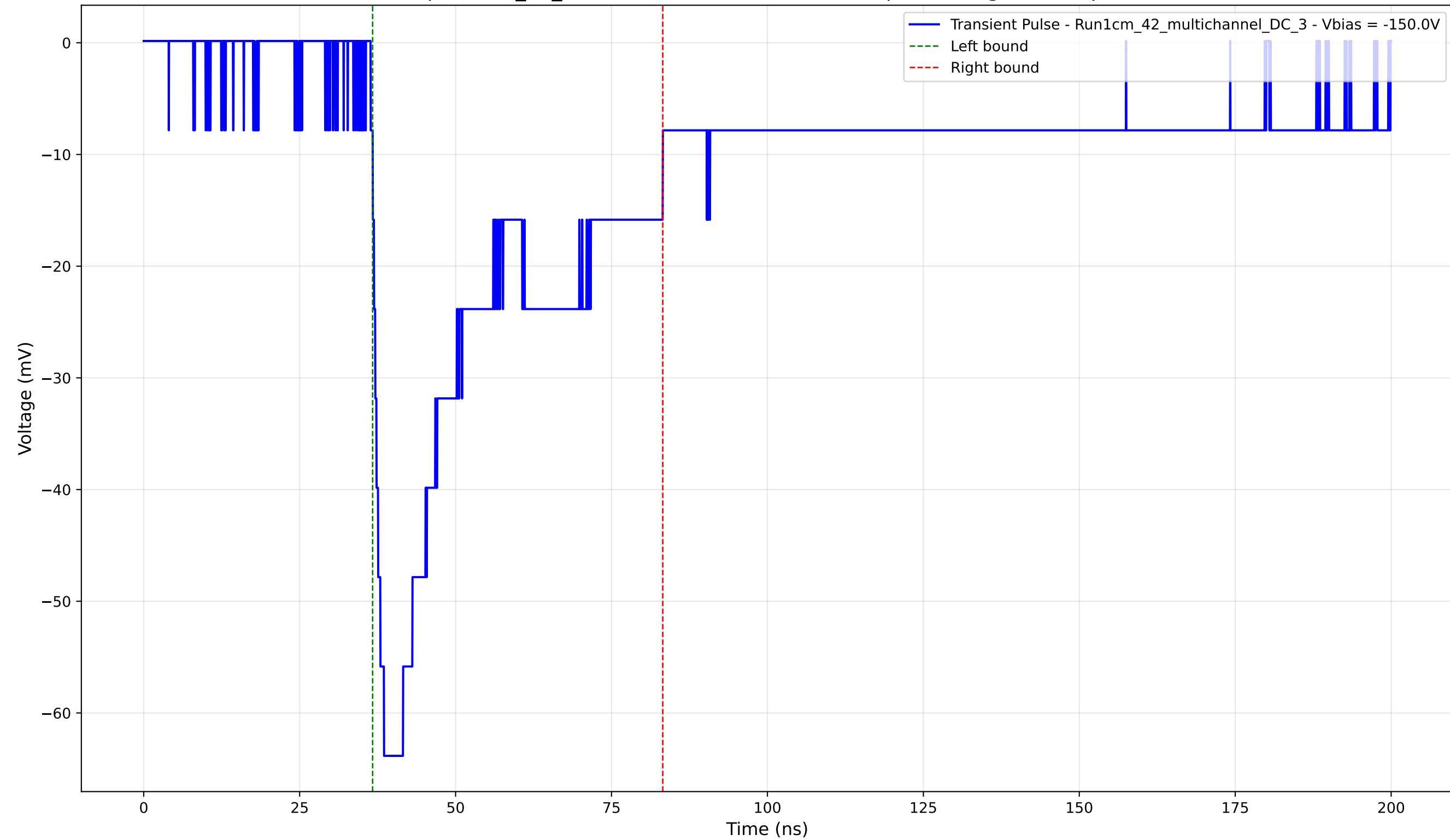
Transient Pulse - Sample: 1cm_42_multichannel - Position: 2820.0 \mu\text{m} - Charge: 25.82 pC - Rise Time: 2.14 ns
