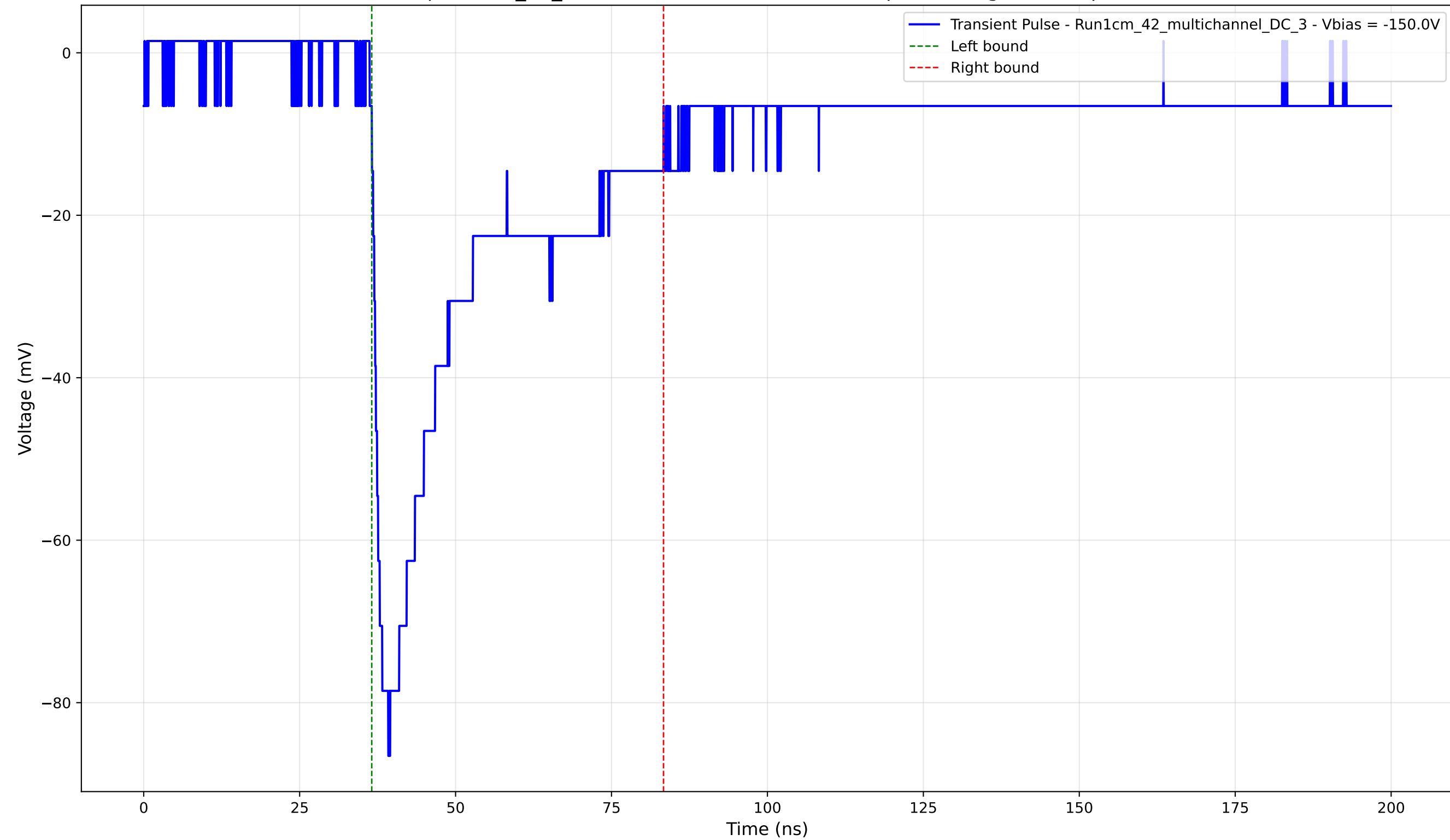
Transient Pulse - Sample: 1cm_42_multichannel - Position: 1805.0 \mu\text{m} - Charge: 28.81 pC - Rise Time: 1.67 ns
