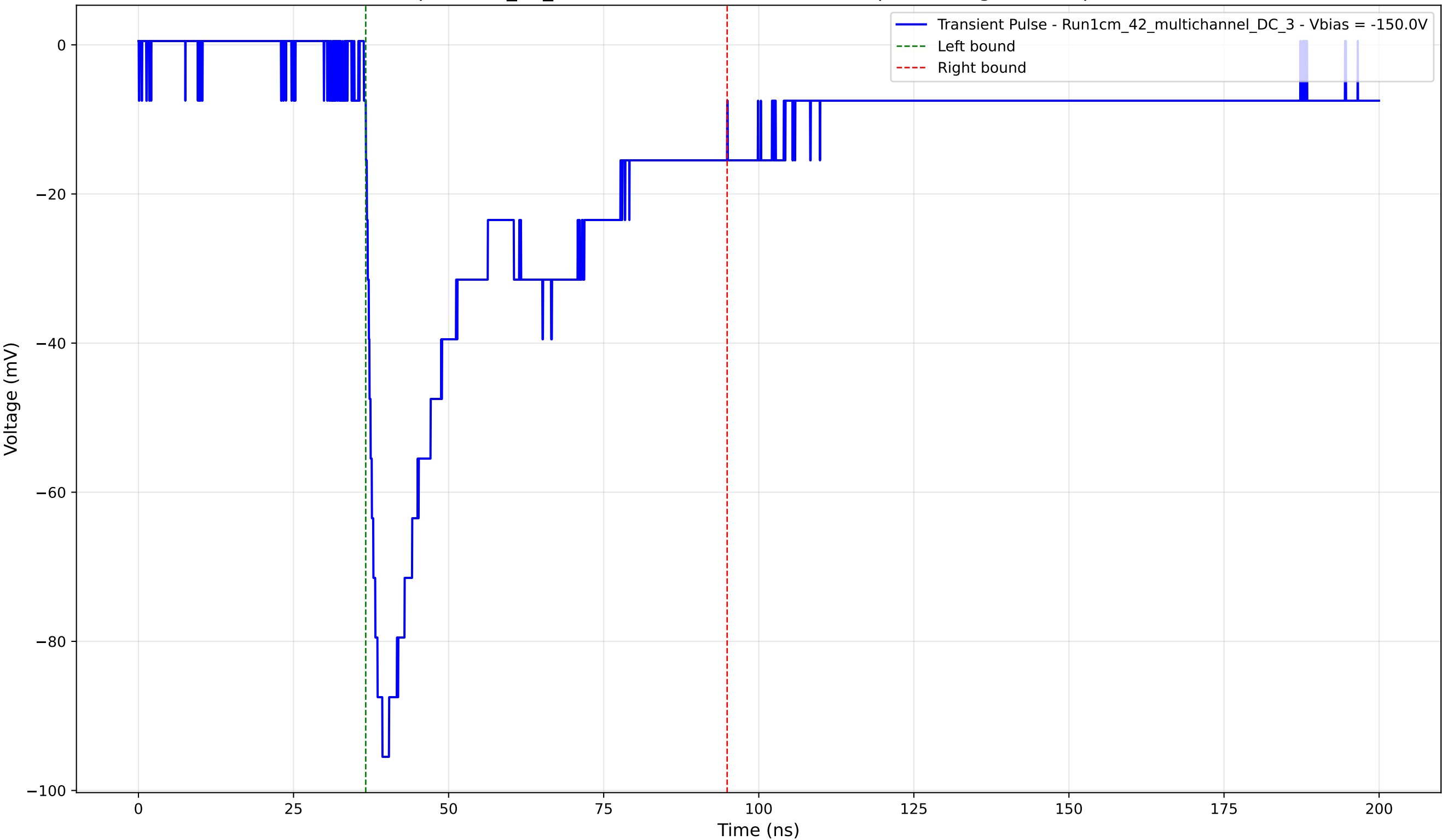
Transient Pulse - Sample: 1cm_42_multichannel - Position: 2765.0 \mu\text{m} - Charge: 38.83 pC - Rise Time: 1.89 ns
