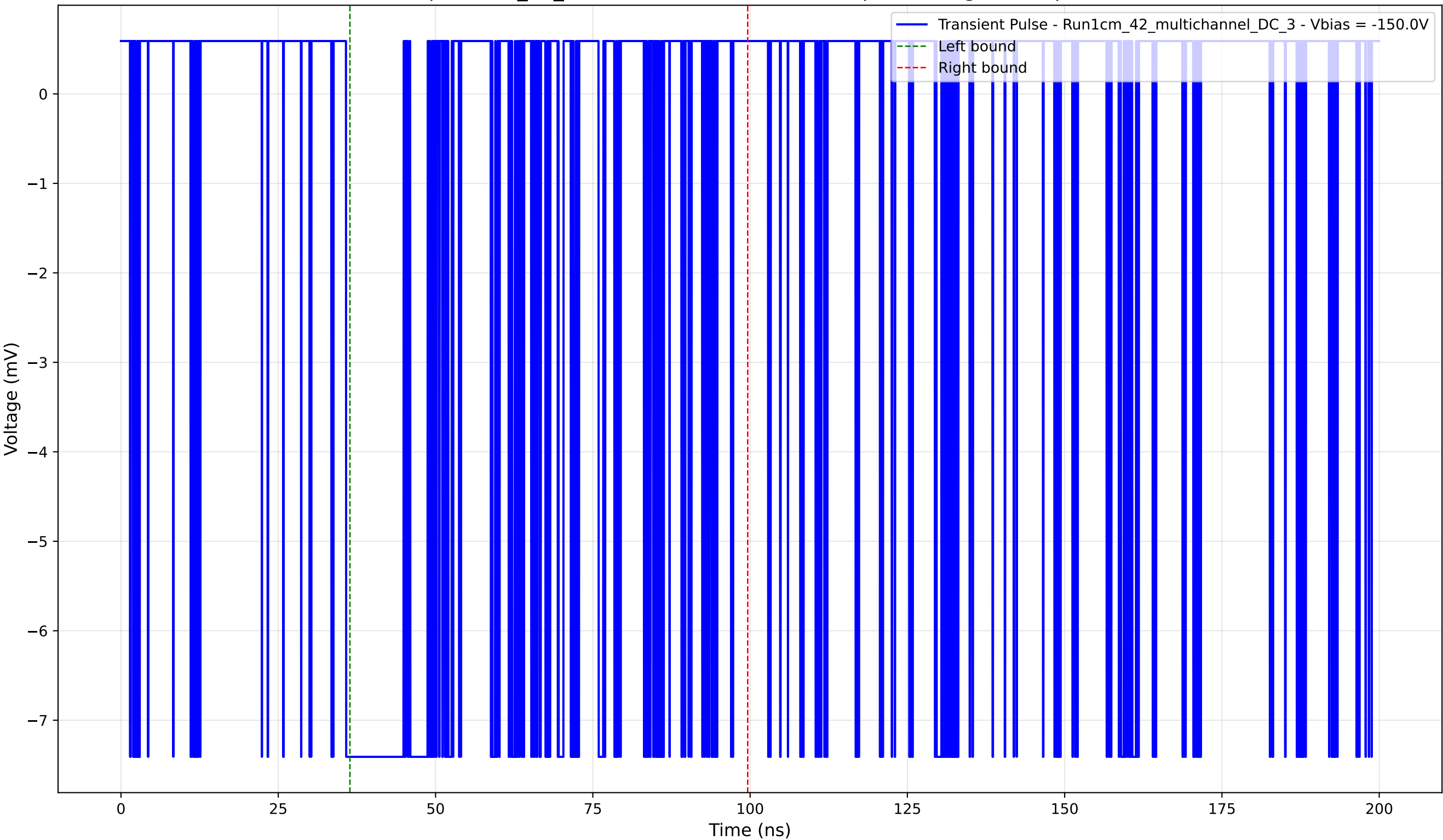
Transient Pulse - Sample: 1cm_42_multichannel - Position: 15.0 \mu\text{m} - Charge: 3.03 pC - Rise Time: 0.02 ns
