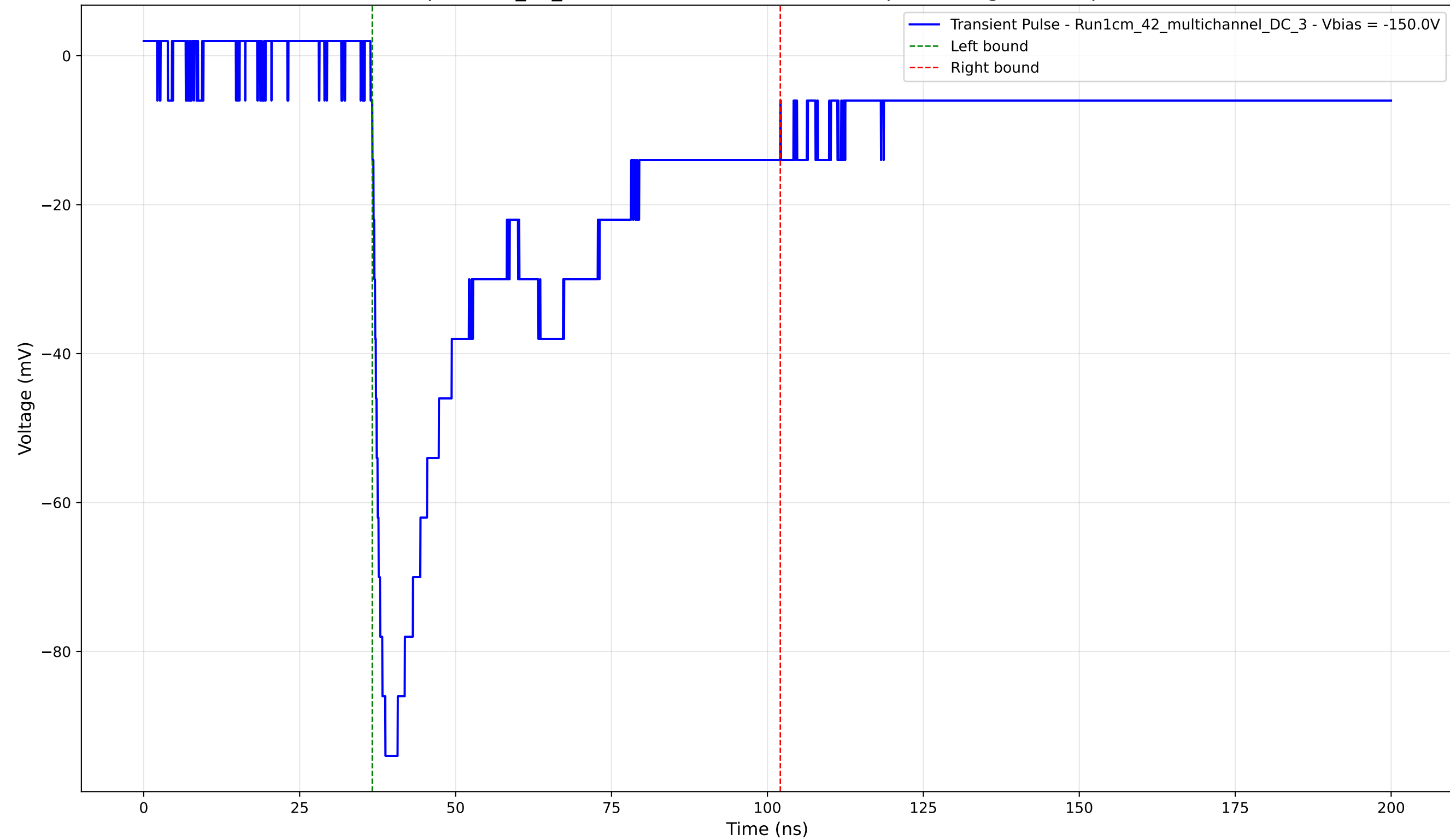
Transient Pulse - Sample: 1cm_42_multichannel - Position: 2035.0 \mu\text{m} - Charge: 41.24 pC - Rise Time: 1.61 ns
