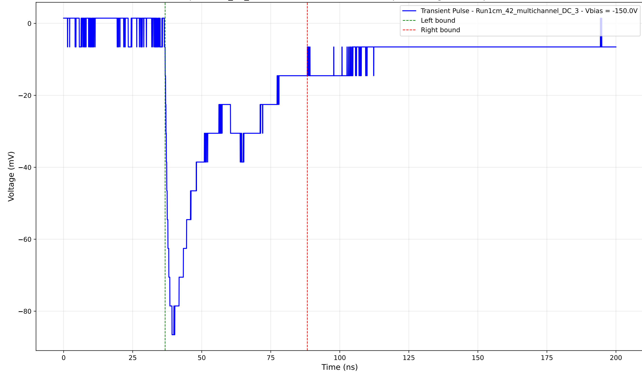
Transient Pulse - Sample: 1cm_42_multichannel - Position: 2645.0 \mu\text{m} - Charge: 34.49 pC - Rise Time: 1.71 ns
