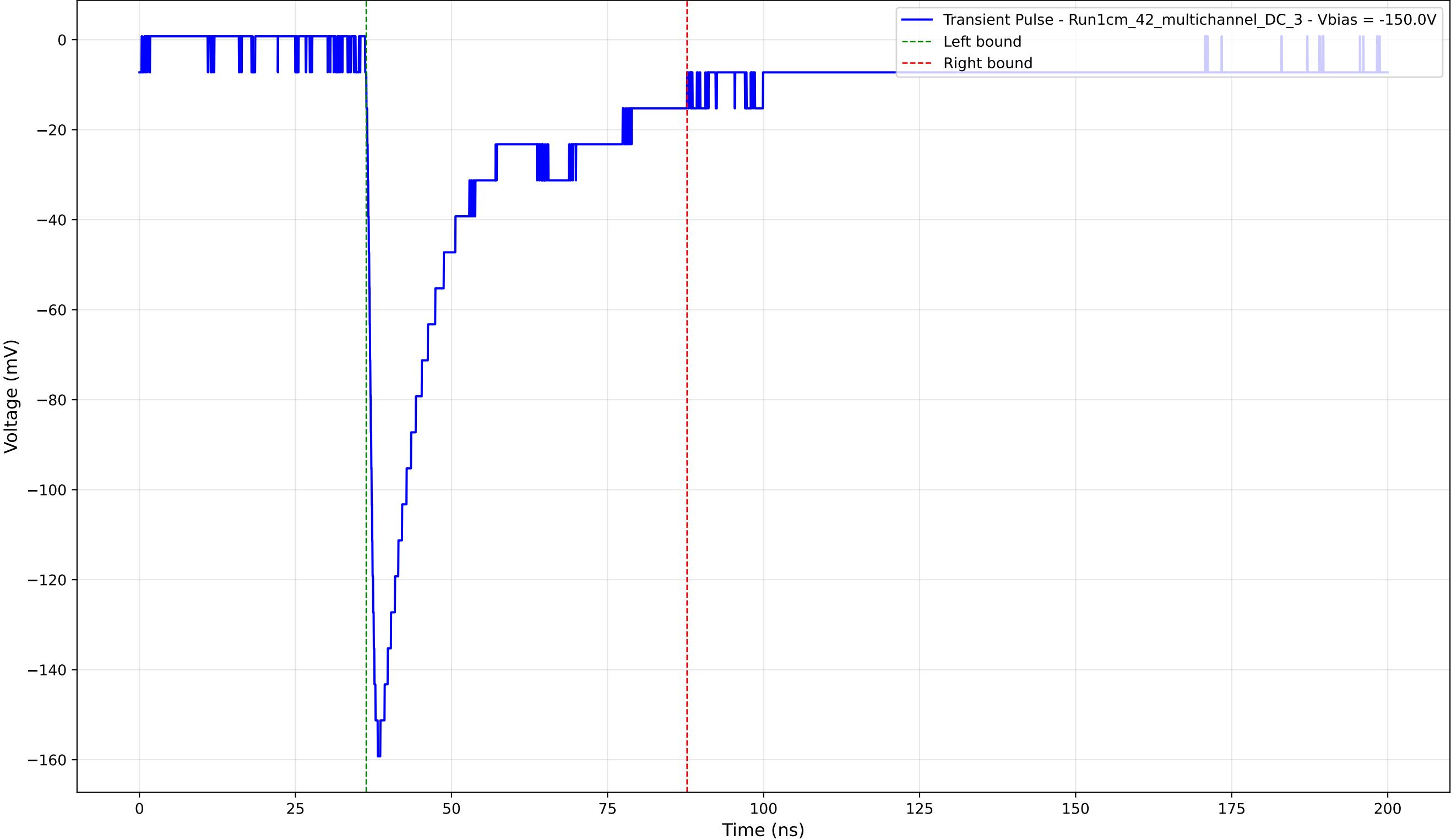
Transient Pulse - Sample: 1cm_42_multichannel - Position: 1180.0 \mu\text{m} - Charge: 43.80 pC - Rise Time: 1.34 ns
