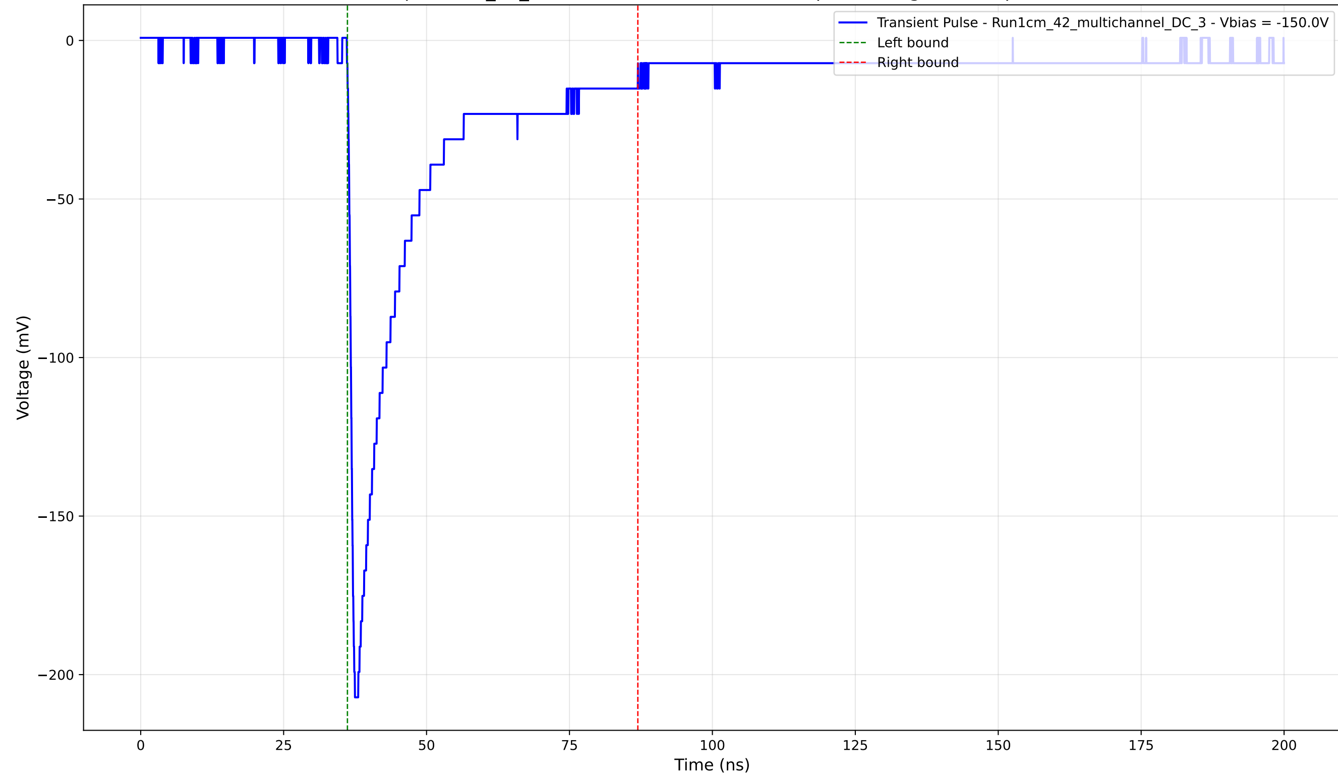
Transient Pulse - Sample: 1cm_42_multichannel - Position: 745.0 \mu\text{m} - Charge: 45.64 pC - Rise Time: 0.99 ns
