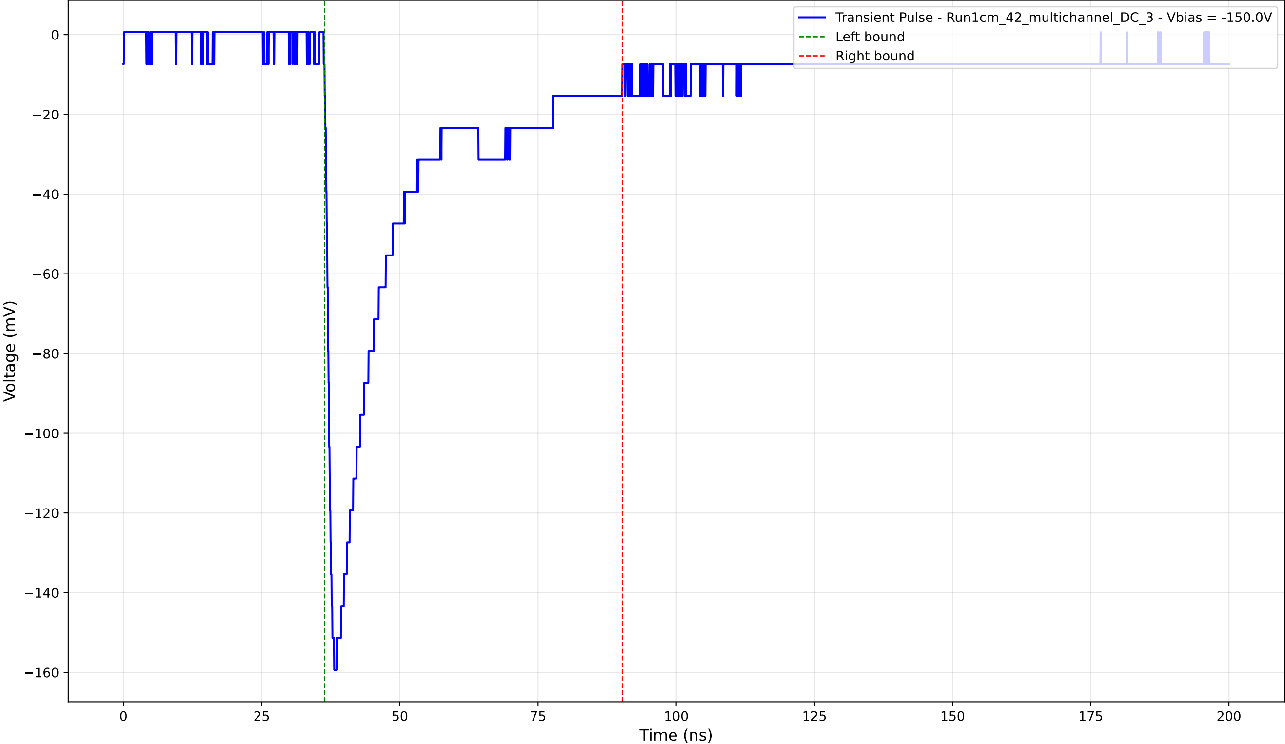
Transient Pulse - Sample: 1cm_42_multichannel - Position: 1195.0 \mu\text{m} - Charge: 44.84 pC - Rise Time: 1.30 ns
