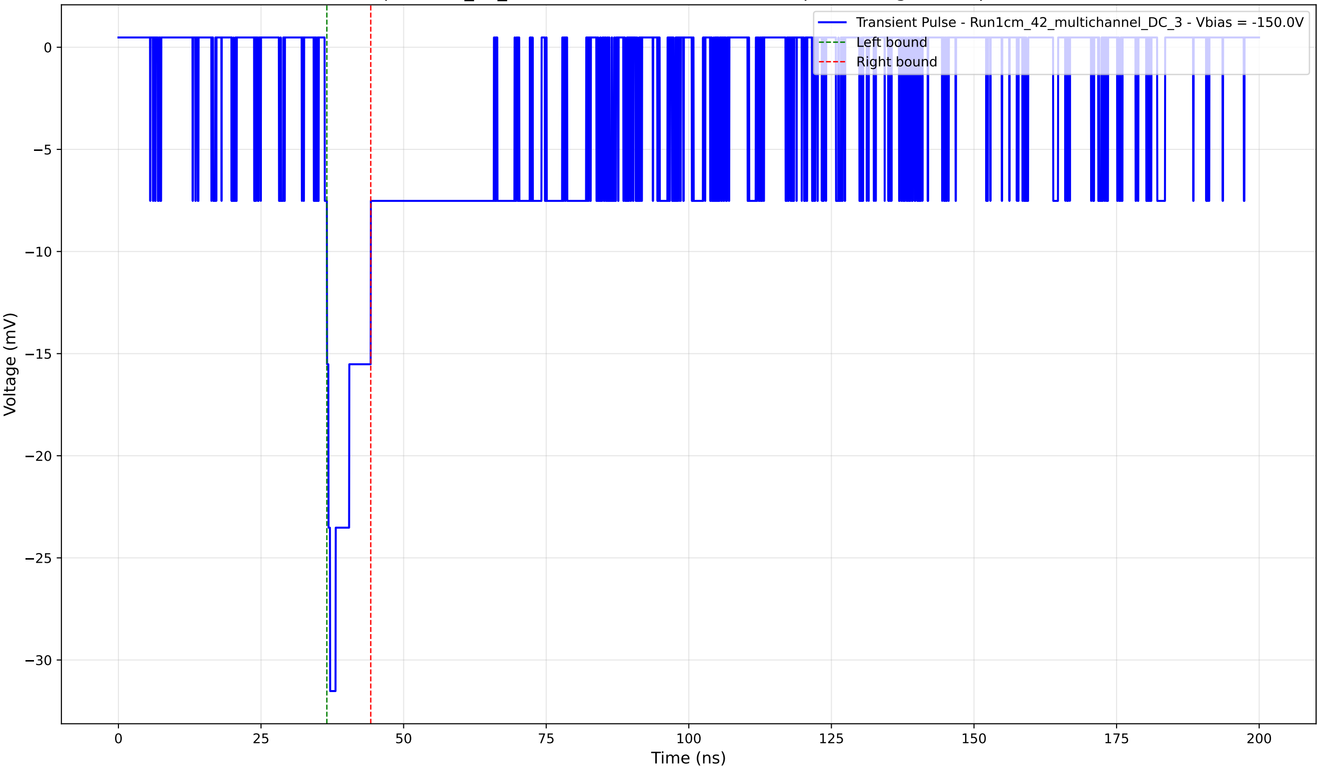
Transient Pulse - Sample: 1cm_42_multichannel - Position: 4420.0 \mu\text{m} - Charge: 3.13 pC - Rise Time: 0.95 ns
