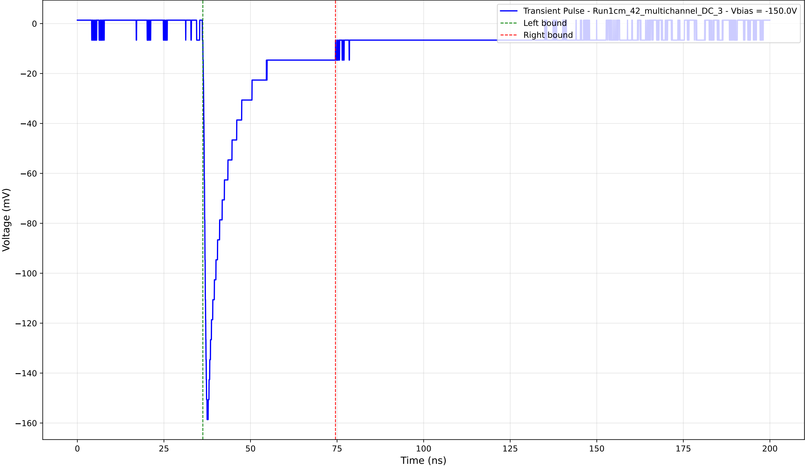
Transient Pulse - Sample: 1cm_42_multichannel - Position: 4325.0 \mu\text{m} - Charge: 27.06 pC - Rise Time: 0.96 ns
