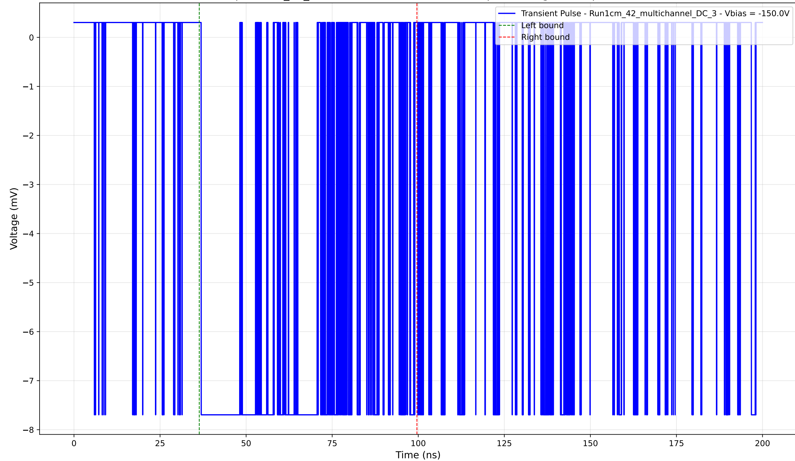
Transient Pulse - Sample: 1cm_42_multichannel - Position: 2370.0 \mu\text{m} - Charge: 6.02 pC - Rise Time: 0.02 ns
