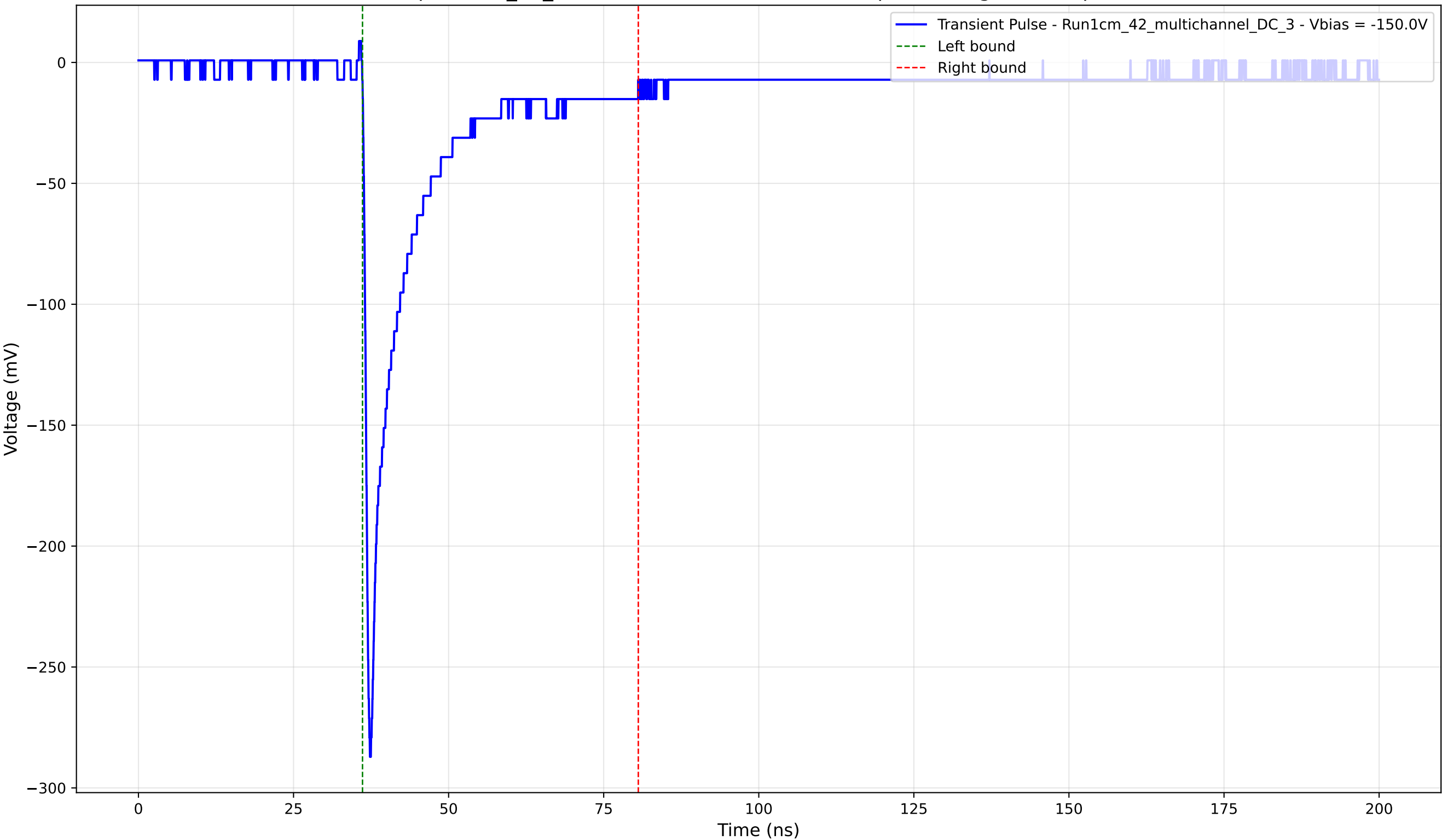
Transient Pulse - Sample: 1cm_42_multichannel - Position: 4555.0 \mu\text{m} - Charge: 40.72 pC - Rise Time: 0.87 ns
