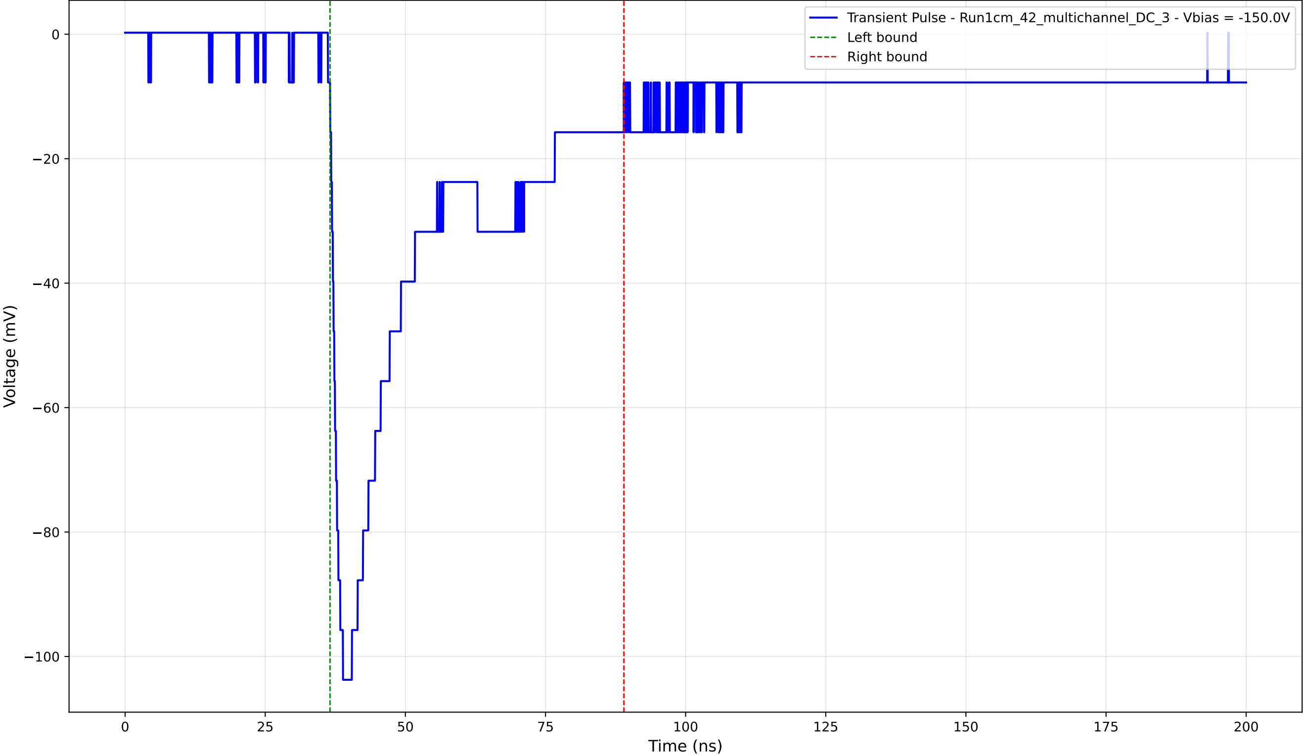
Transient Pulse - Sample: 1cm_42_multichannel - Position: 3005.0 \mu\text{m} - Charge: 37.83 pC - Rise Time: 1.81 ns
