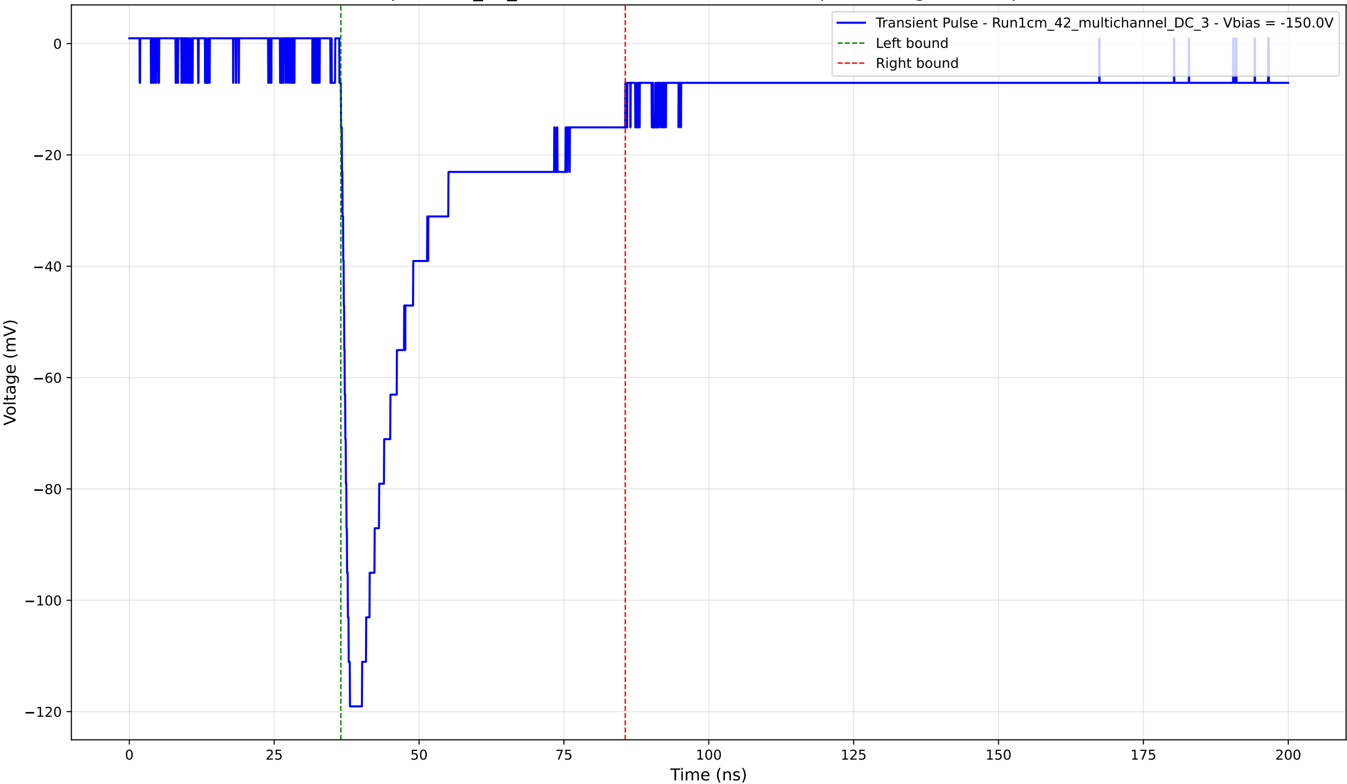
Transient Pulse - Sample: 1cm_42_multichannel - Position: 3525.0 \mu\text{m} - Charge: 36.62 pC - Rise Time: 1.33 ns
