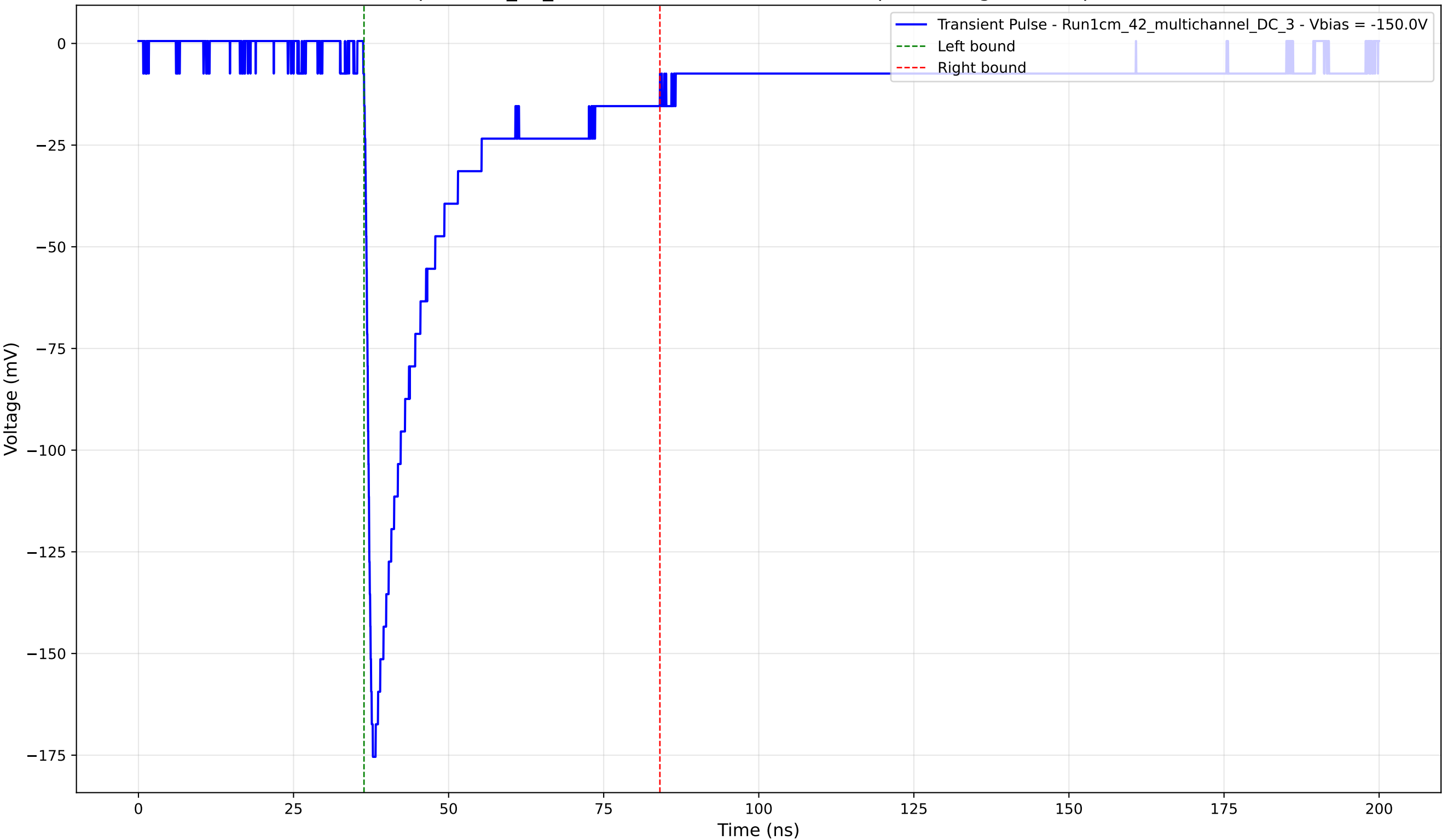
Transient Pulse - Sample: 1cm_42_multichannel - Position: 4010.0 \mu\text{m} - Charge: 40.36 pC - Rise Time: 1.03 ns
