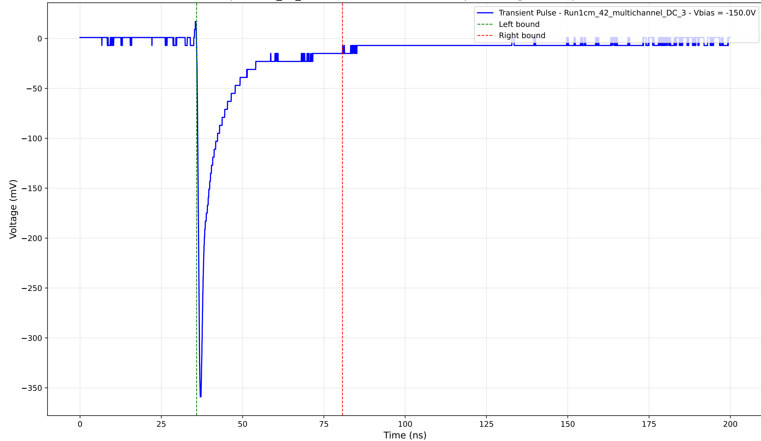
Transient Pulse - Sample: 1cm_42_multichannel - Position: 160.0 \mu\text{m} - Charge: 45.86 pC - Rise Time: 0.79 ns
