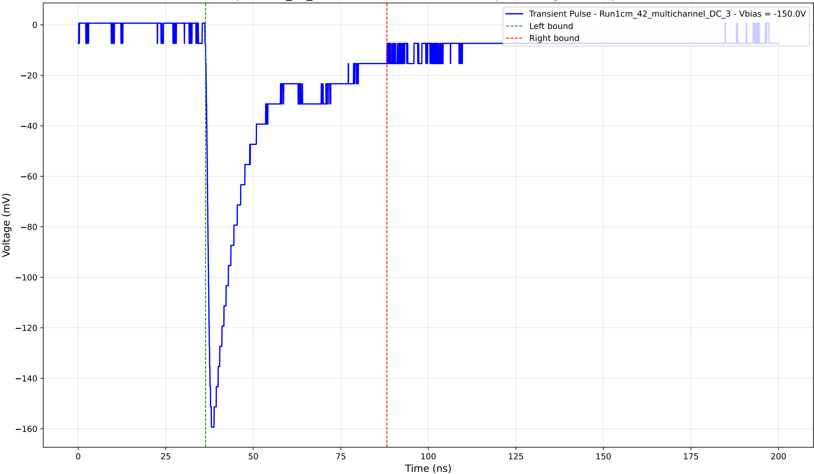
Transient Pulse - Sample: 1cm_42_multichannel - Position: 1205.0 \mu\text{m} - Charge: 45.22 pC - Rise Time: 1.30 ns
