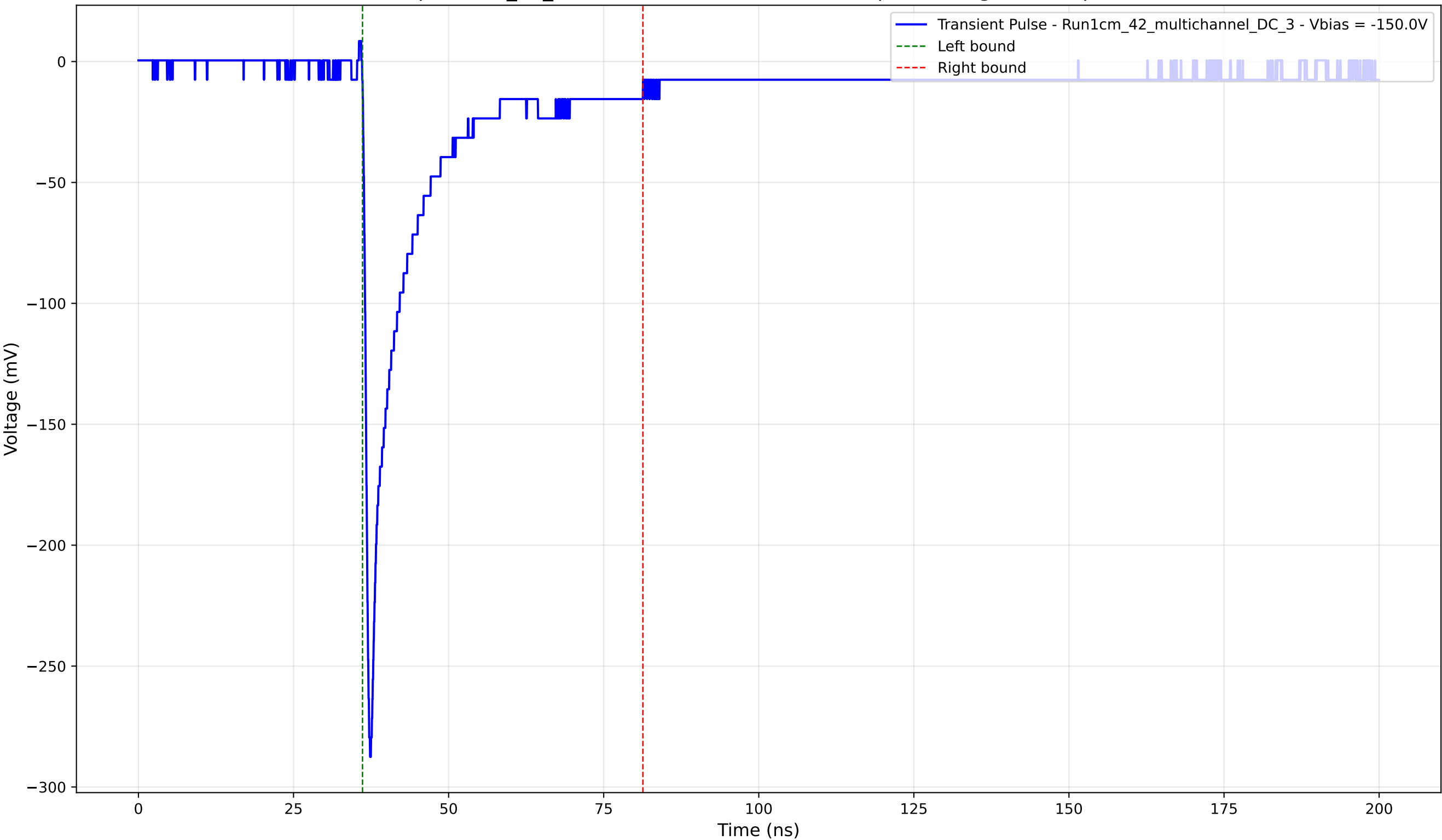
Transient Pulse - Sample: 1cm_42_multichannel - Position: 4560.0 \mu\text{m} - Charge: 41.62 pC - Rise Time: 0.87 ns
