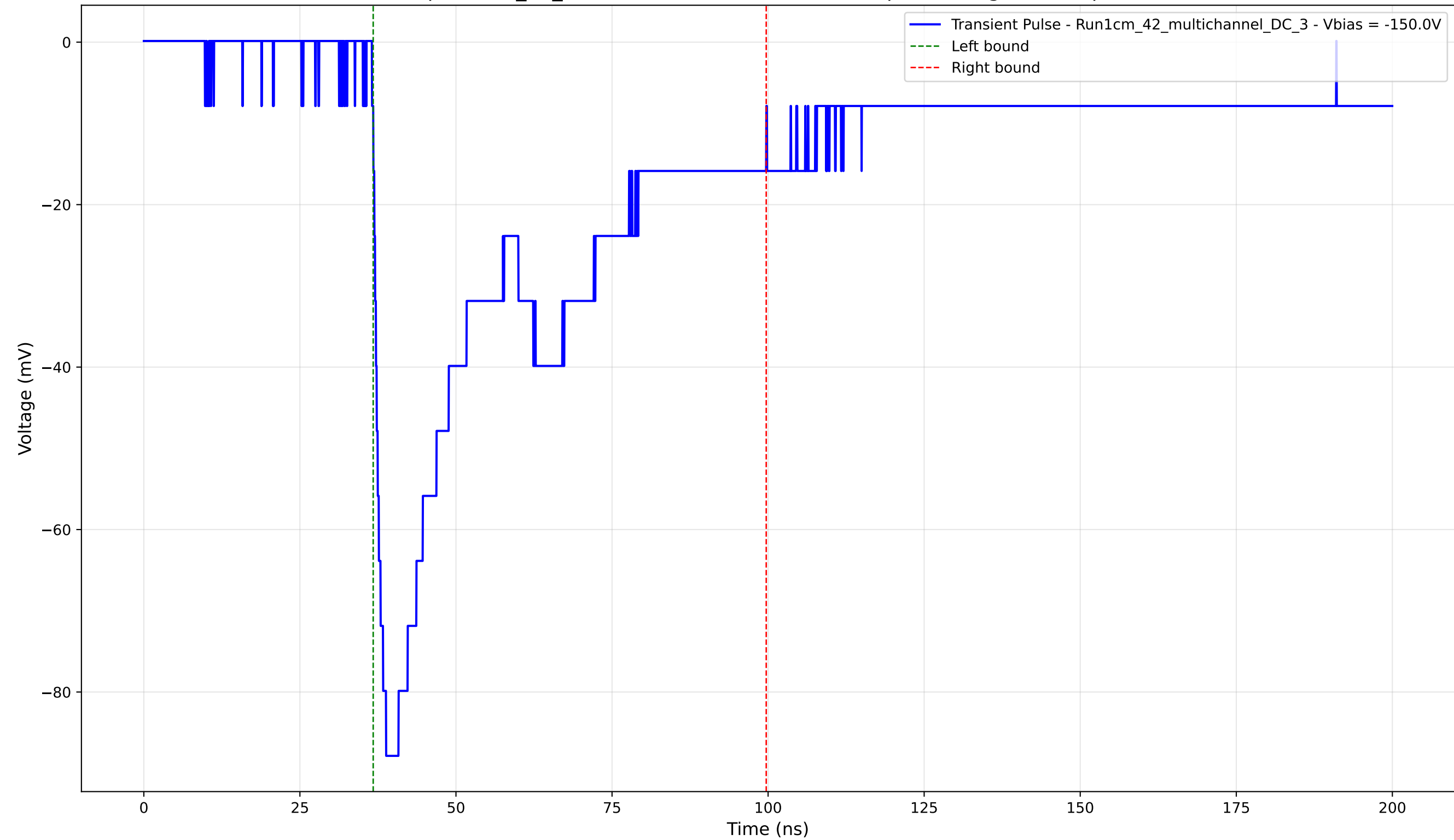
Transient Pulse - Sample: 1cm_42_multichannel - Position: 2180.0 \mu\text{m} - Charge: 41.34 pC - Rise Time: 1.58 ns
