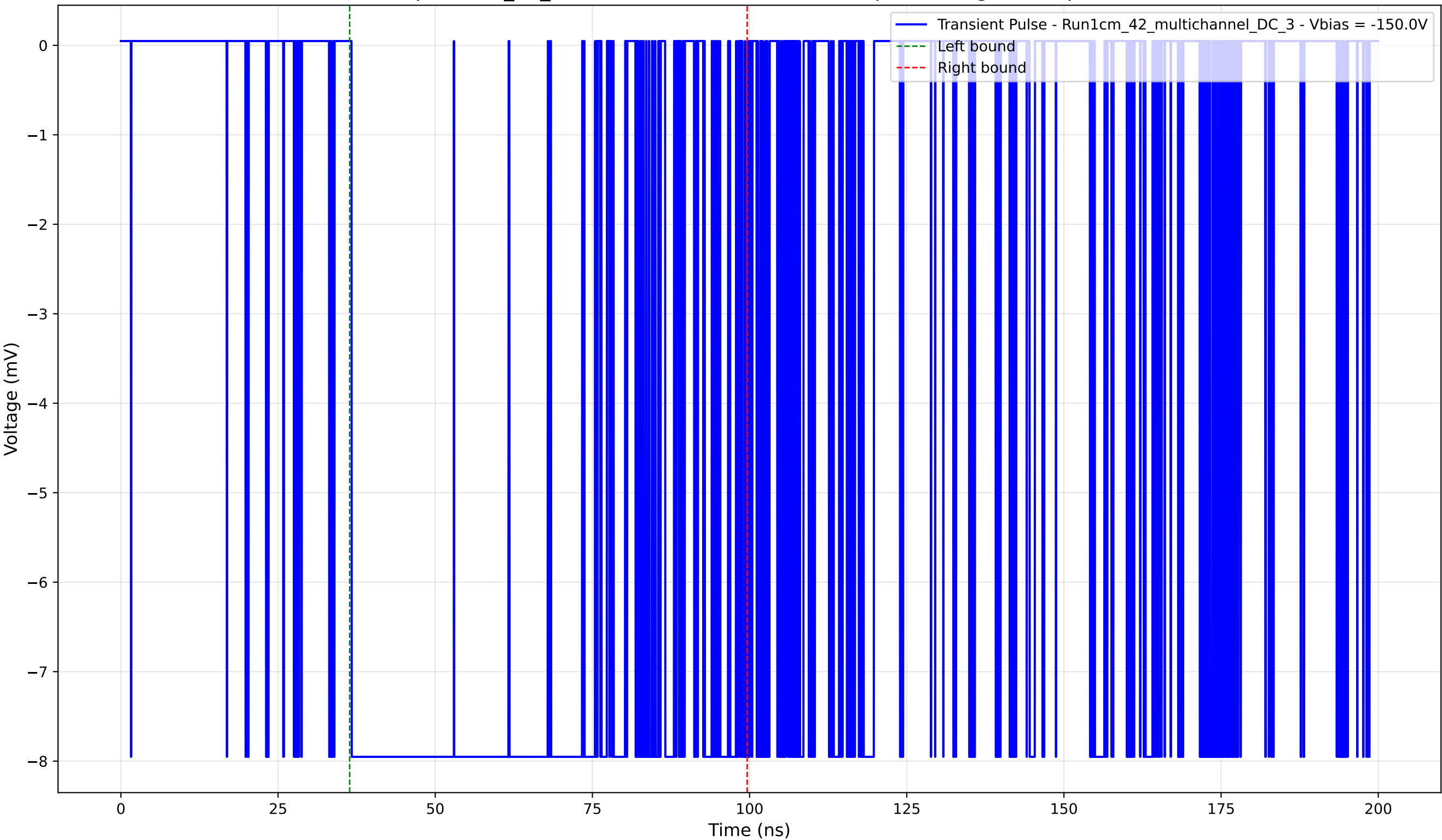
Transient Pulse - Sample: 1cm_42_multichannel - Position: 2355.0 \mu\text{m} - Charge: 8.30 pC - Rise Time: 0.02 ns
