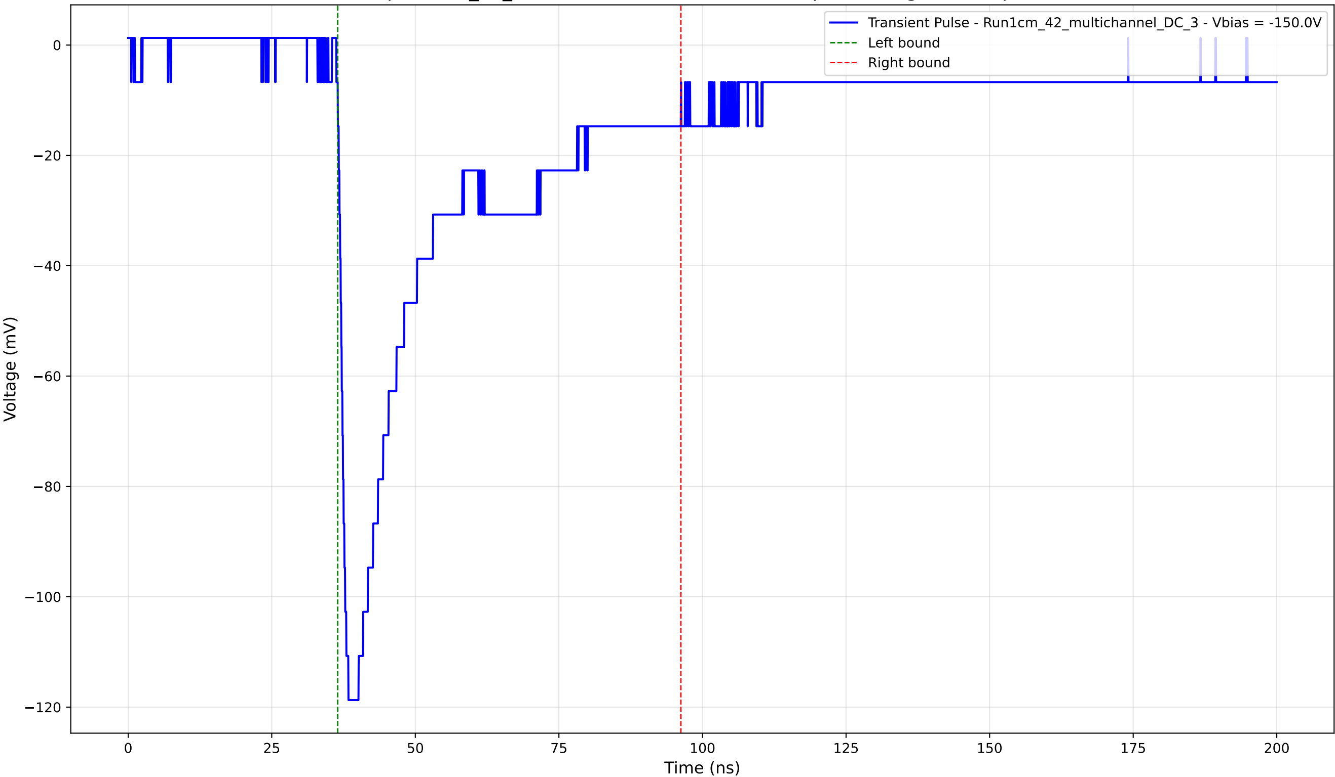
Transient Pulse - Sample: 1cm_42_multichannel - Position: 1640.0 \mu\text{m} - Charge: 42.85 pC - Rise Time: 1.49 ns
