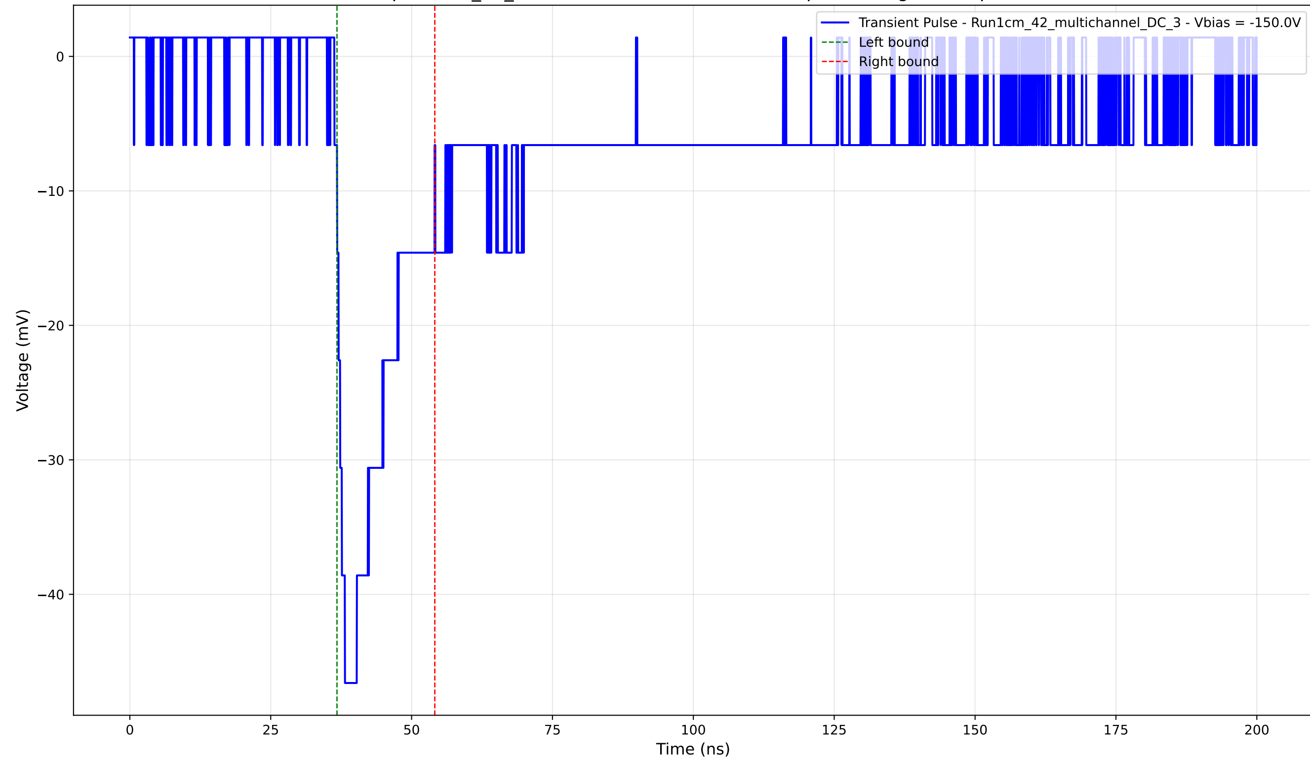
Transient Pulse - Sample: 1cm_42_multichannel - Position: 3430.0 \mu\text{m} - Charge: 9.08 pC - Rise Time: 1.87 ns
