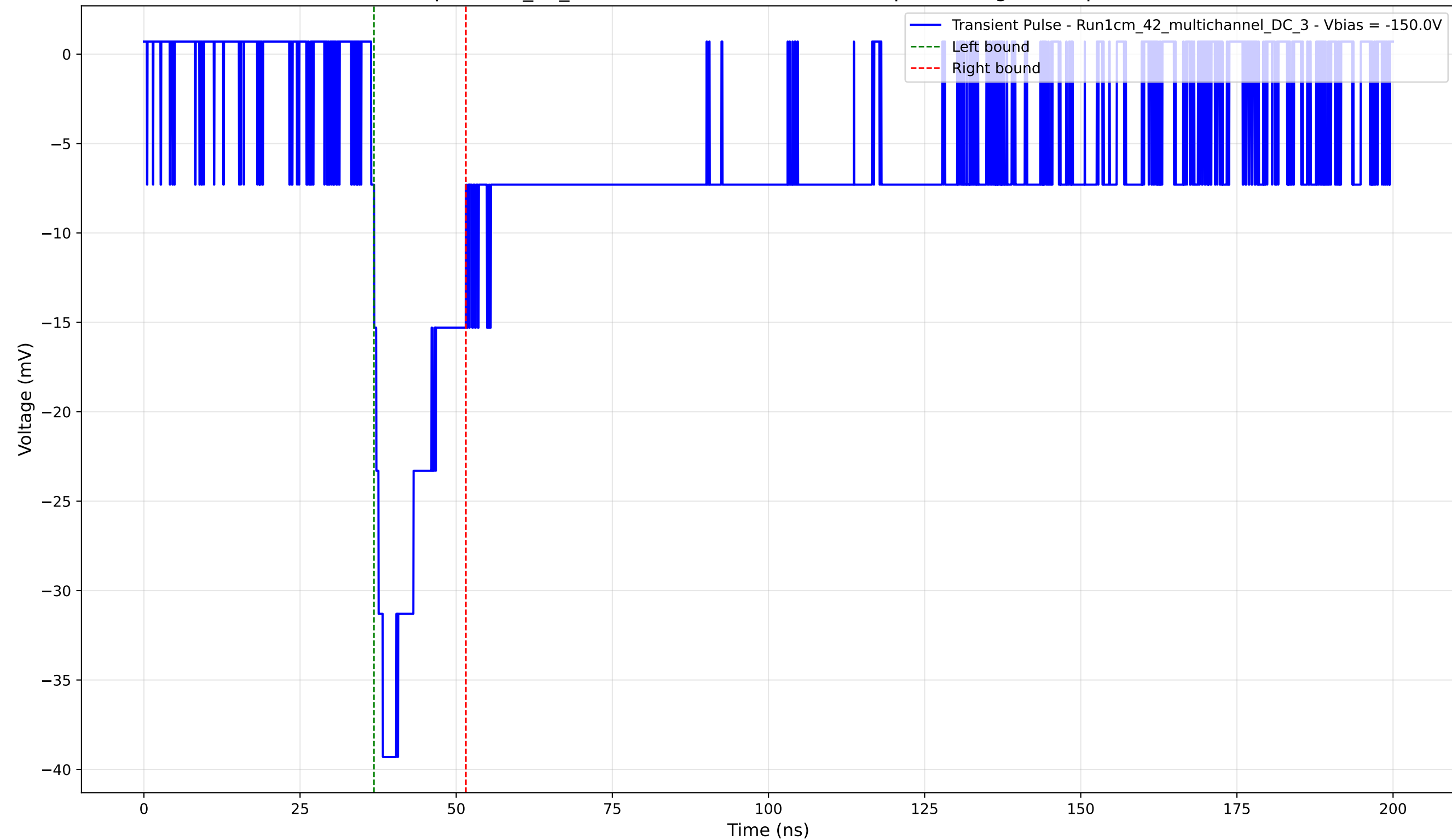
Transient Pulse - Sample: 1cm_42_multichannel - Position: 3345.0 \mu\text{m} - Charge: 7.23 pC - Rise Time: 1.87 ns
