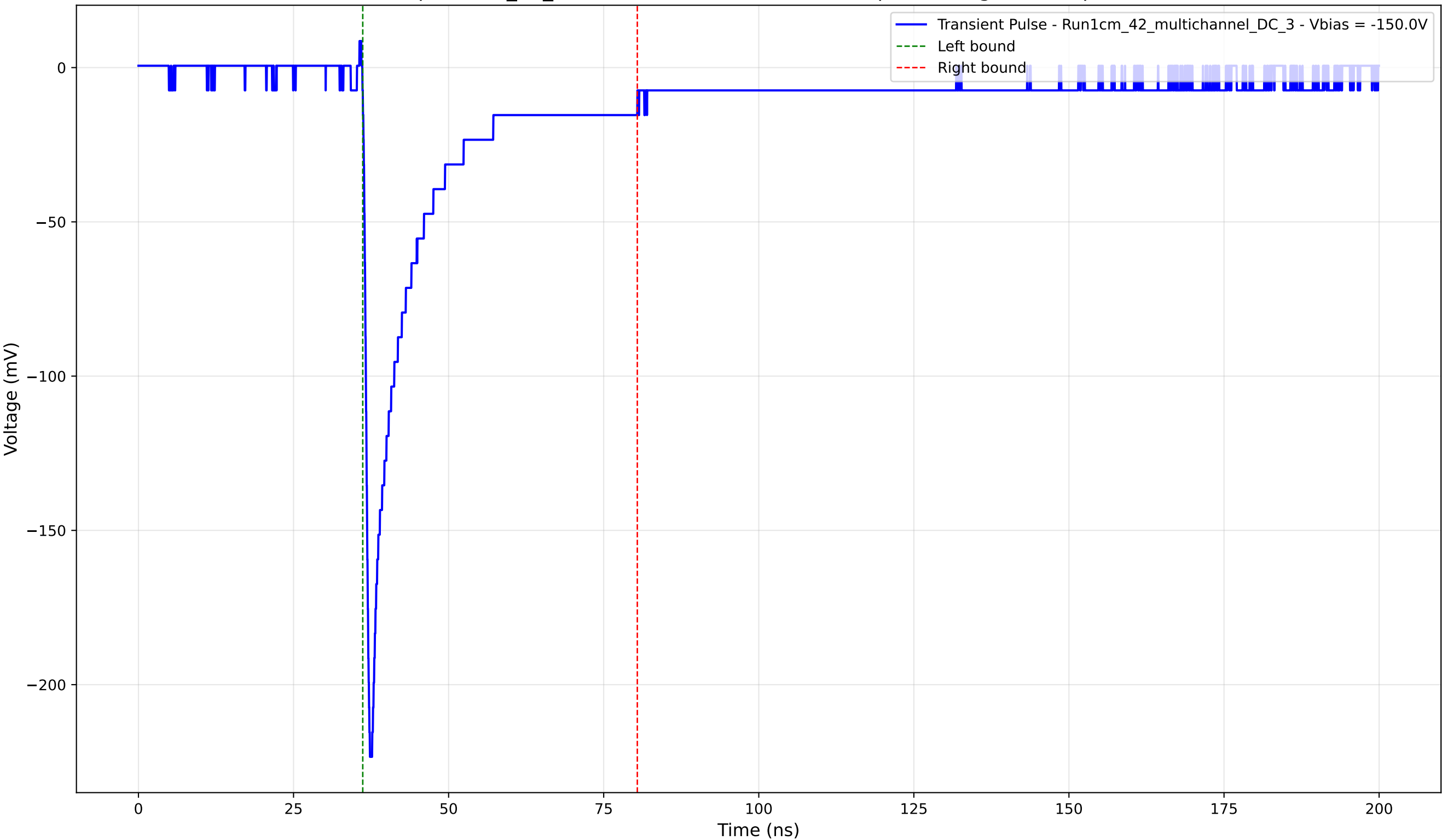
Transient Pulse - Sample: 1cm_42_multichannel - Position: 4470.0 \mu\text{m} - Charge: 35.45 pC - Rise Time: 0.90 ns
