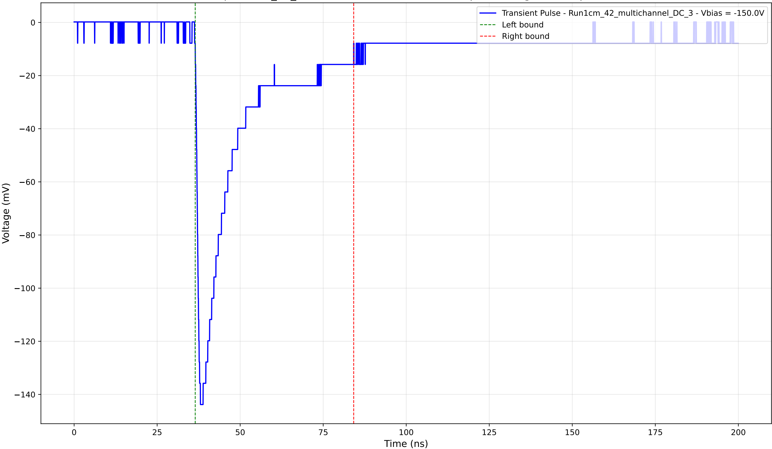
Transient Pulse - Sample: 1cm_42_multichannel - Position: 3735.0 \mu\text{m} - Charge: 38.74 pC - Rise Time: 1.30 ns
