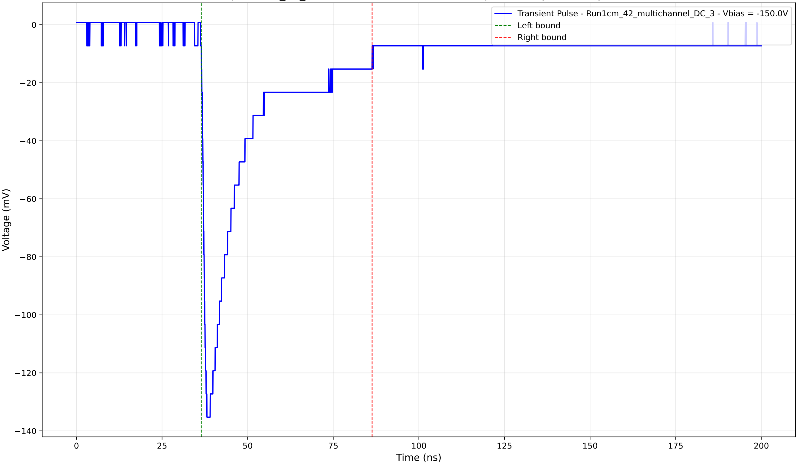
Transient Pulse - Sample: 1cm_42_multichannel - Position: 3685.0 \mu\text{m} - Charge: 37.92 pC - Rise Time: 1.38 ns
