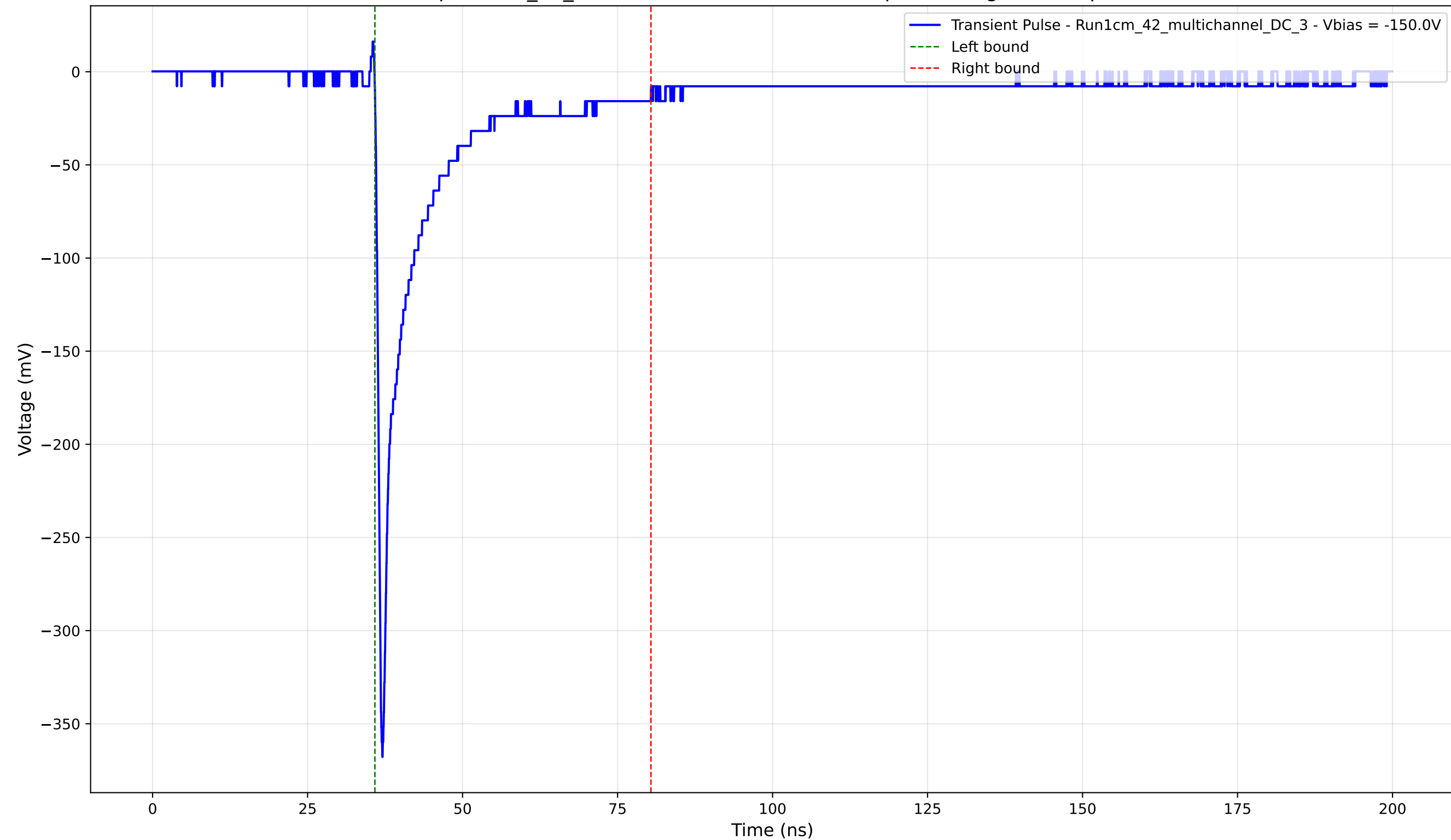
Transient Pulse - Sample: 1cm_42_multichannel - Position: 155.0 \mu\text{m} - Charge: 46.33 pC - Rise Time: 0.82 ns
