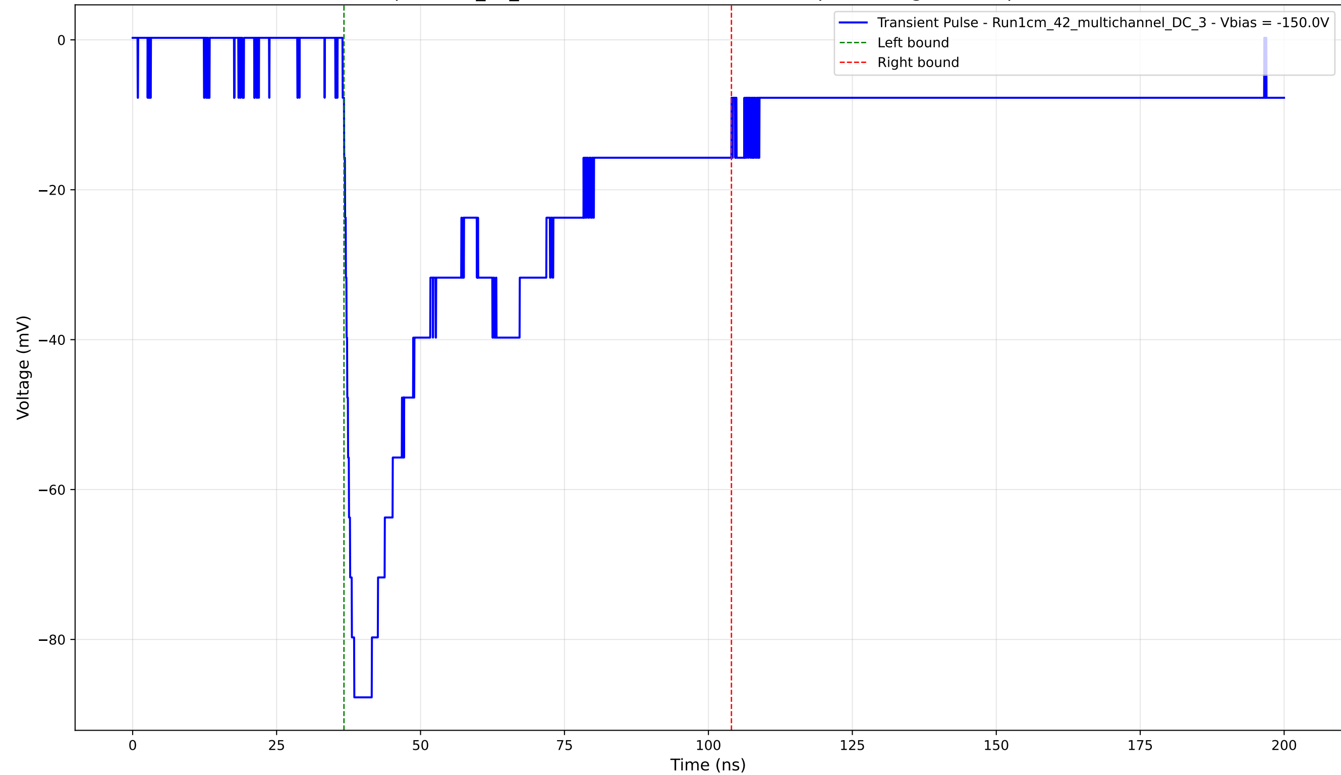
Transient Pulse - Sample: 1cm_42_multichannel - Position: 2105.0 \mu\text{m} - Charge: 43.00 pC - Rise Time: 1.36 ns
