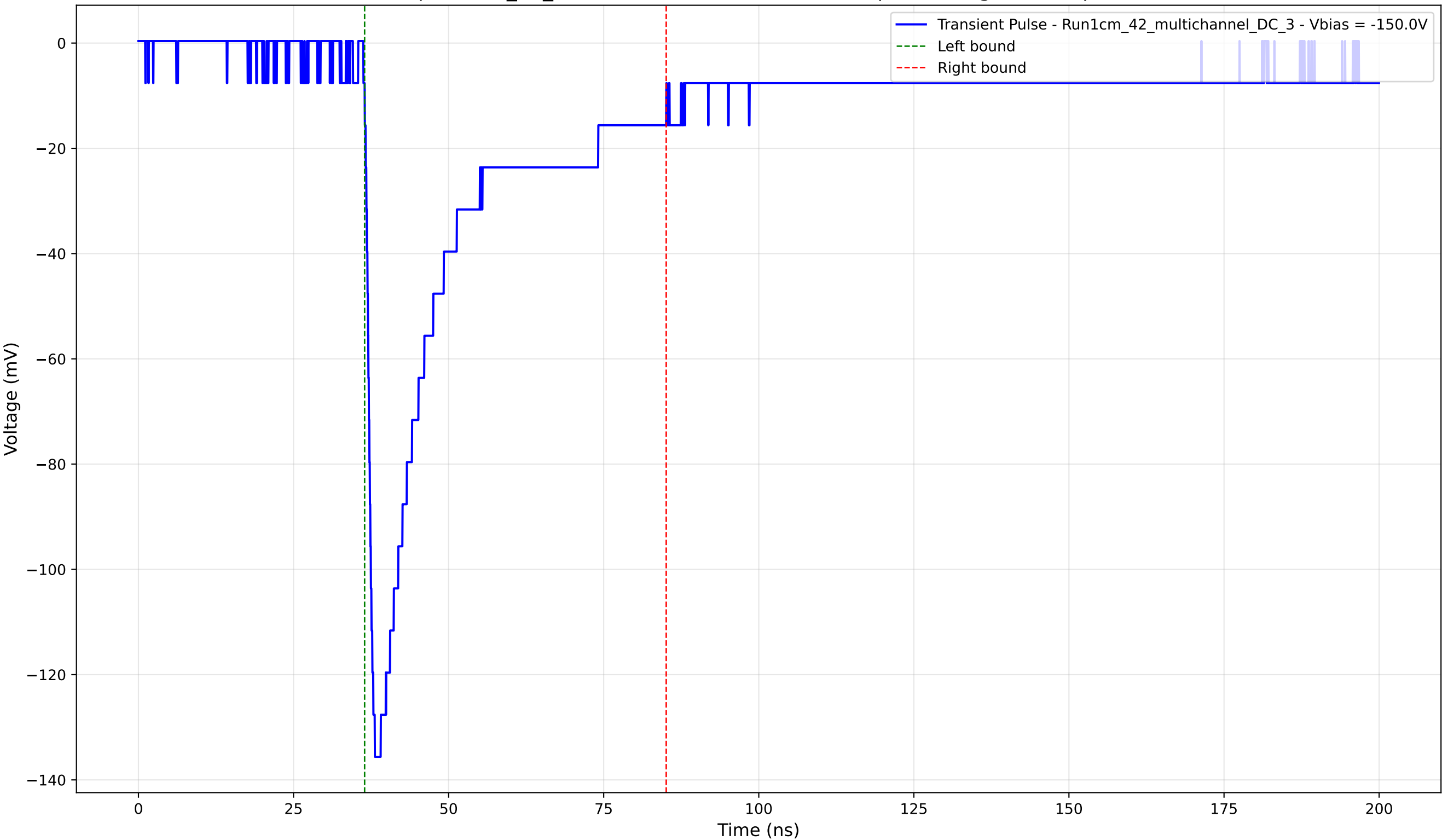
Transient Pulse - Sample: 1cm_42_multichannel - Position: 3680.0 \mu\text{m} - Charge: 37.94 pC - Rise Time: 1.39 ns
