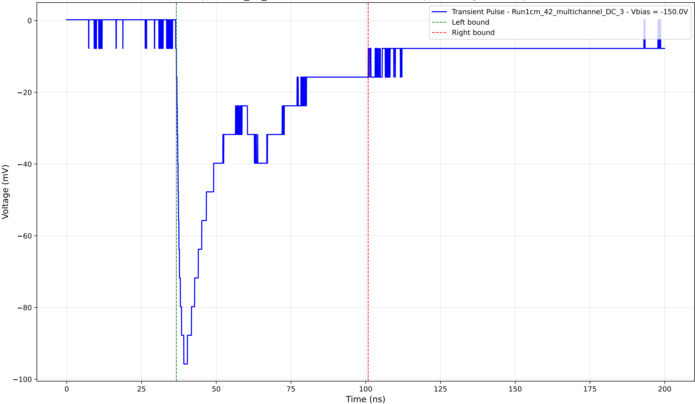
Transient Pulse - Sample: 1cm_42_multichannel - Position: 2060.0 \mu\text{m} - Charge: 42.38 pC - Rise Time: 1.74 ns
