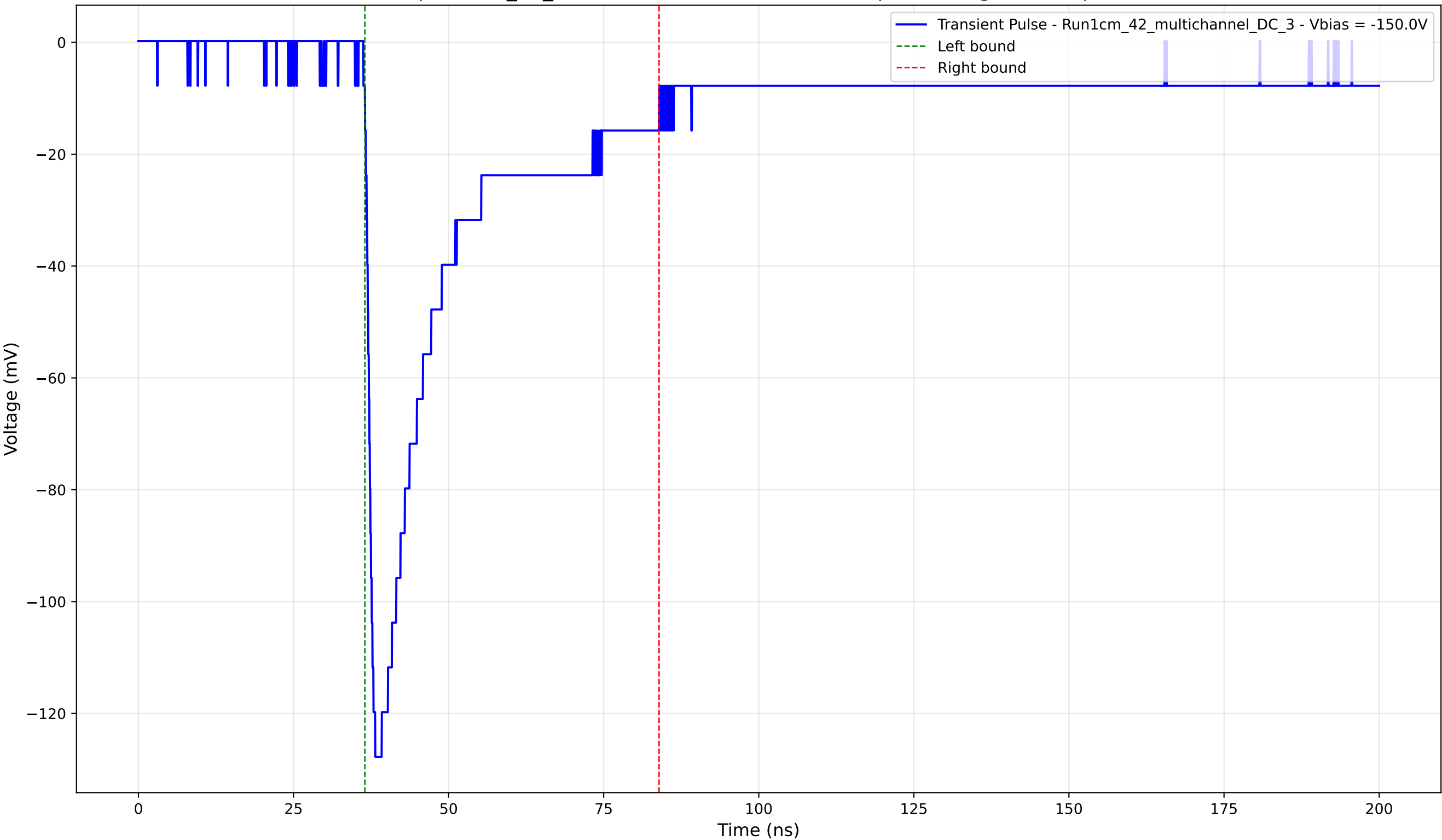
Transient Pulse - Sample: 1cm_42_multichannel - Position: 3620.0 \mu\text{m} - Charge: 36.67 pC - Rise Time: 1.37 ns
