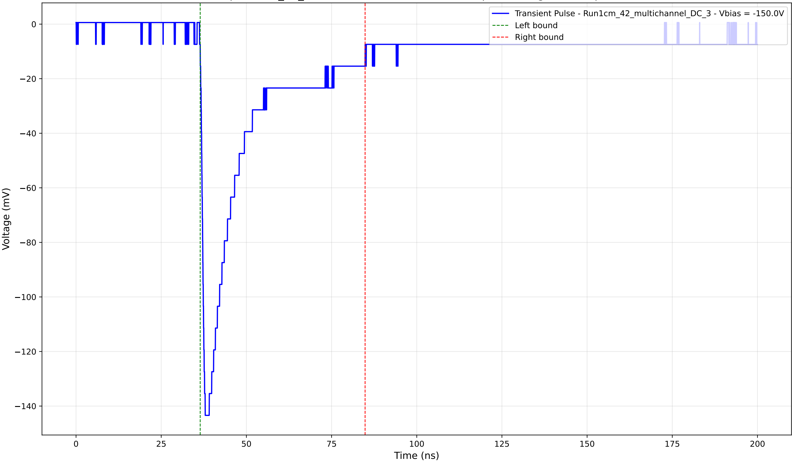
Transient Pulse - Sample: 1cm_42_multichannel - Position: 3755.0 \mu\text{m} - Charge: 39.04 pC - Rise Time: 1.26 ns
