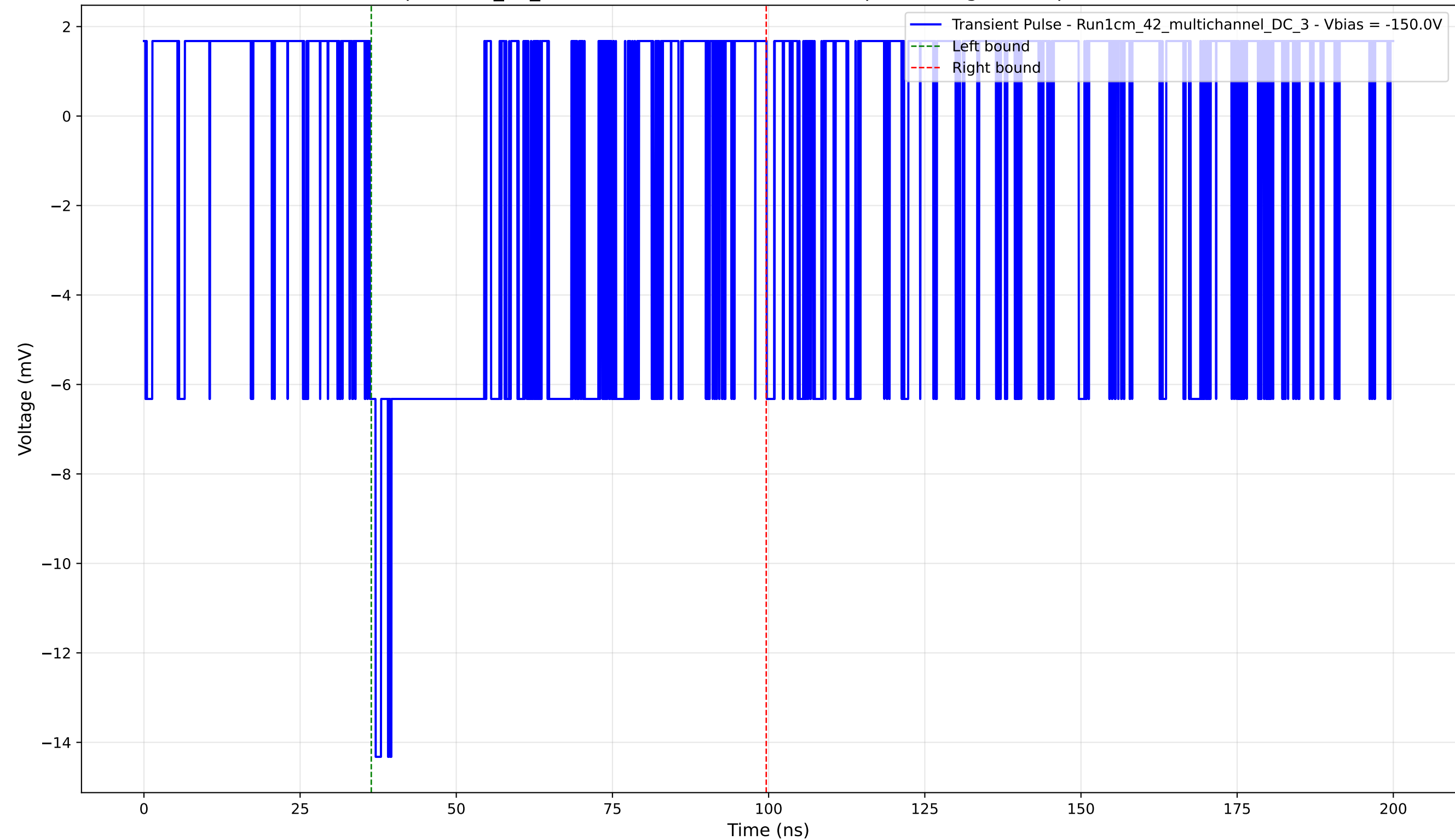
Transient Pulse - Sample: 1cm_42_multichannel - Position: 4395.0 \mu\text{m} - Charge: 3.99 pC - Rise Time: 0.00 ns (N/A)
