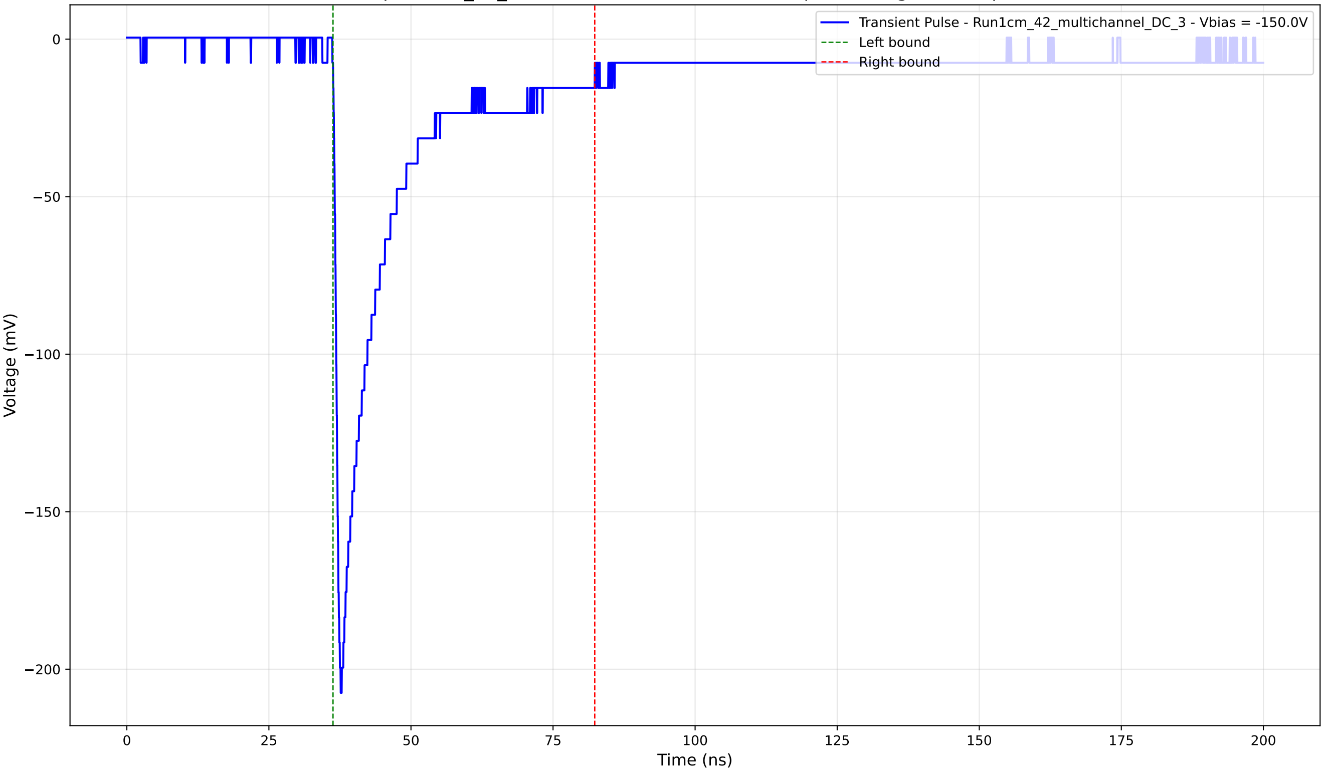
Transient Pulse - Sample: 1cm_42_multichannel - Position: 4205.0 \mu\text{m} - Charge: 40.60 pC - Rise Time: 1.01 ns
