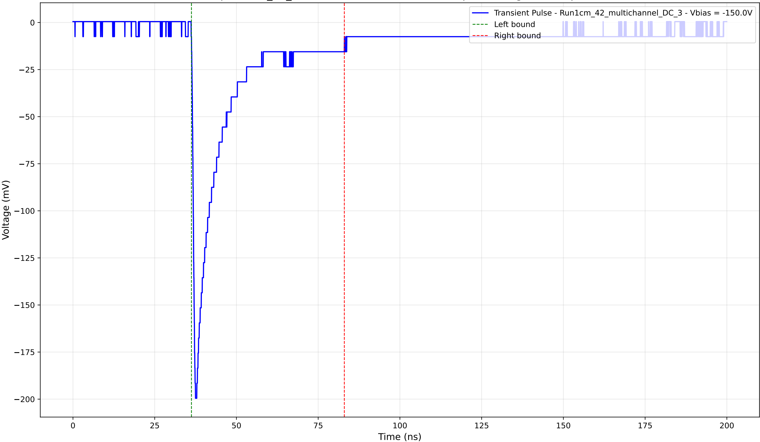
Transient Pulse - Sample: 1cm_42_multichannel - Position: 4280.0 \mu\text{m} - Charge: 37.46 pC - Rise Time: 0.93 ns
