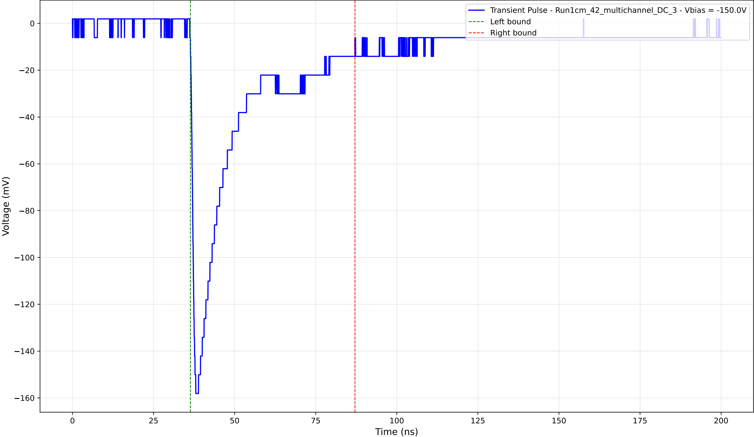
Transient Pulse - Sample: 1cm_42_multichannel - Position: 1220.0 \mu\text{m} - Charge: 43.99 pC - Rise Time: 1.30 ns
