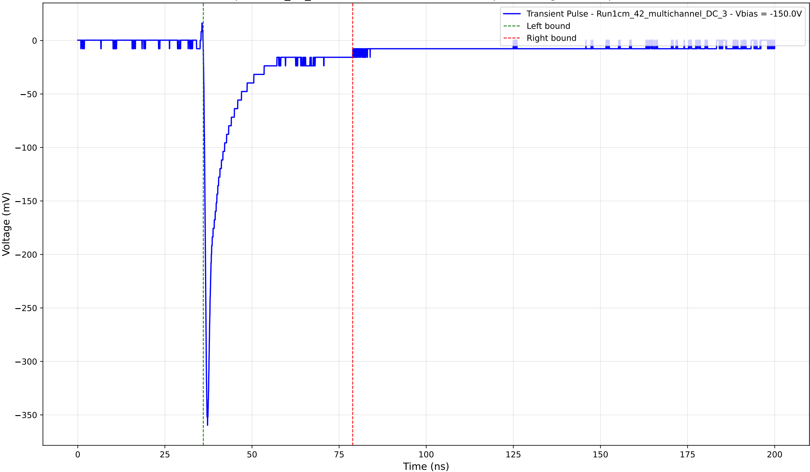
Transient Pulse - Sample: 1cm_42_multichannel - Position: 4725.0 \mu\text{m} - Charge: 42.91 pC - Rise Time: 0.82 ns
