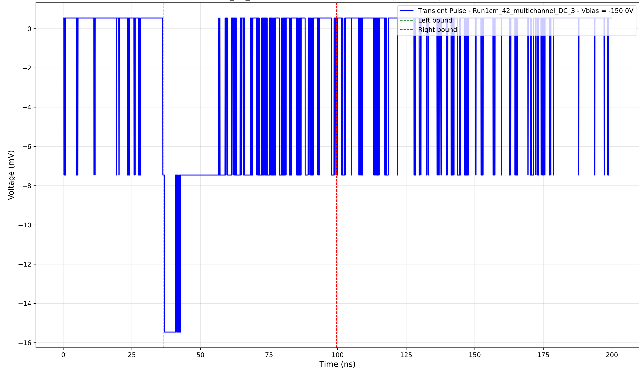
Transient Pulse - Sample: 1cm_42_multichannel - Position: 4370.0 \mu\text{m} - Charge: 6.48 pC - Rise Time: 0.62 ns
