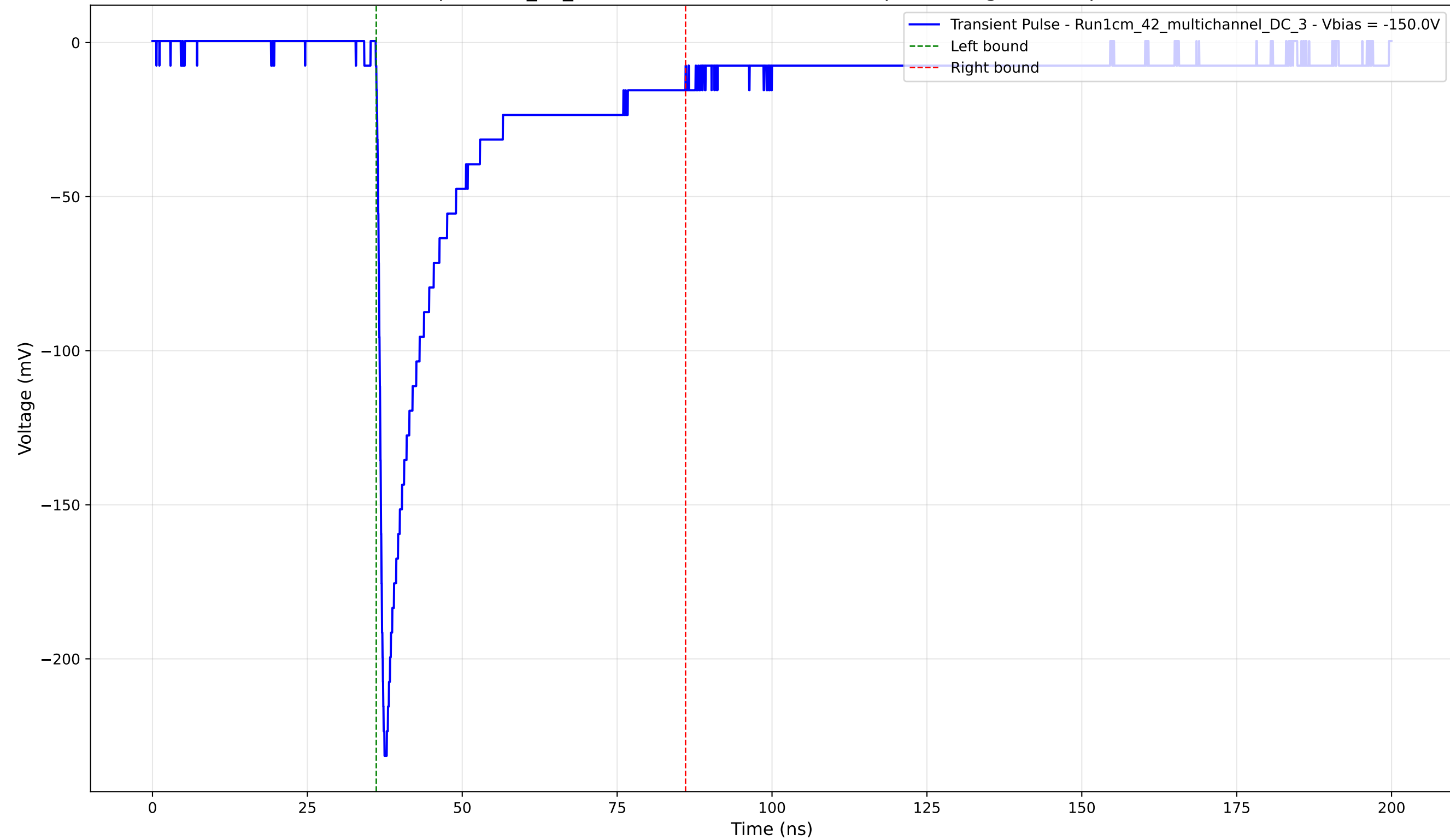
Transient Pulse - Sample: 1cm_42_multichannel - Position: 650.0 \mu\text{m} - Charge: 47.28 pC - Rise Time: 1.02 ns
