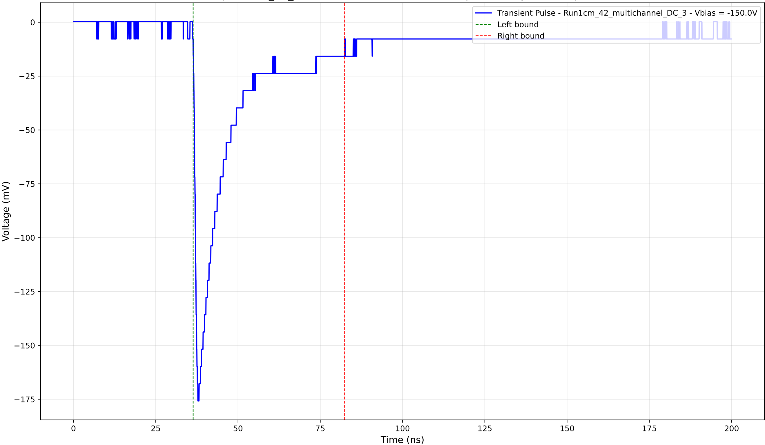
Transient Pulse - Sample: 1cm_42_multichannel - Position: 4005.0 \mu\text{m} - Charge: 40.04 pC - Rise Time: 1.06 ns
