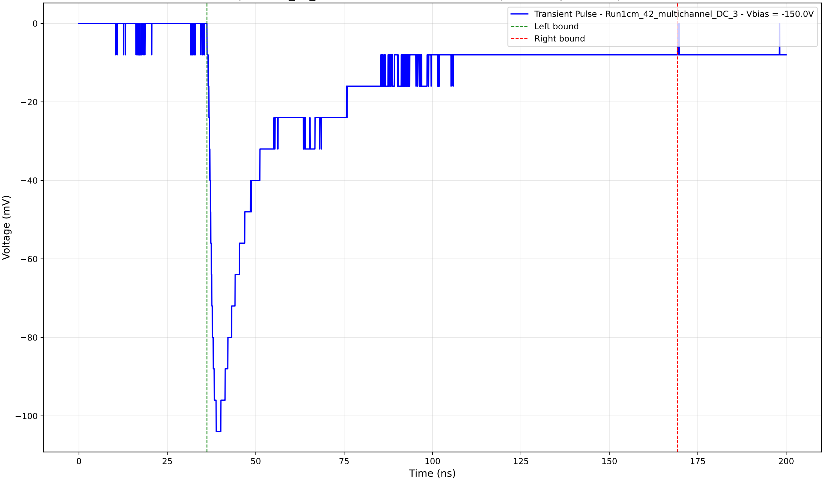
Transient Pulse - Sample: 1cm_42_multichannel - Position: 3140.0 \mu\text{m} - Charge: 50.15 pC - Rise Time: 1.73 ns
