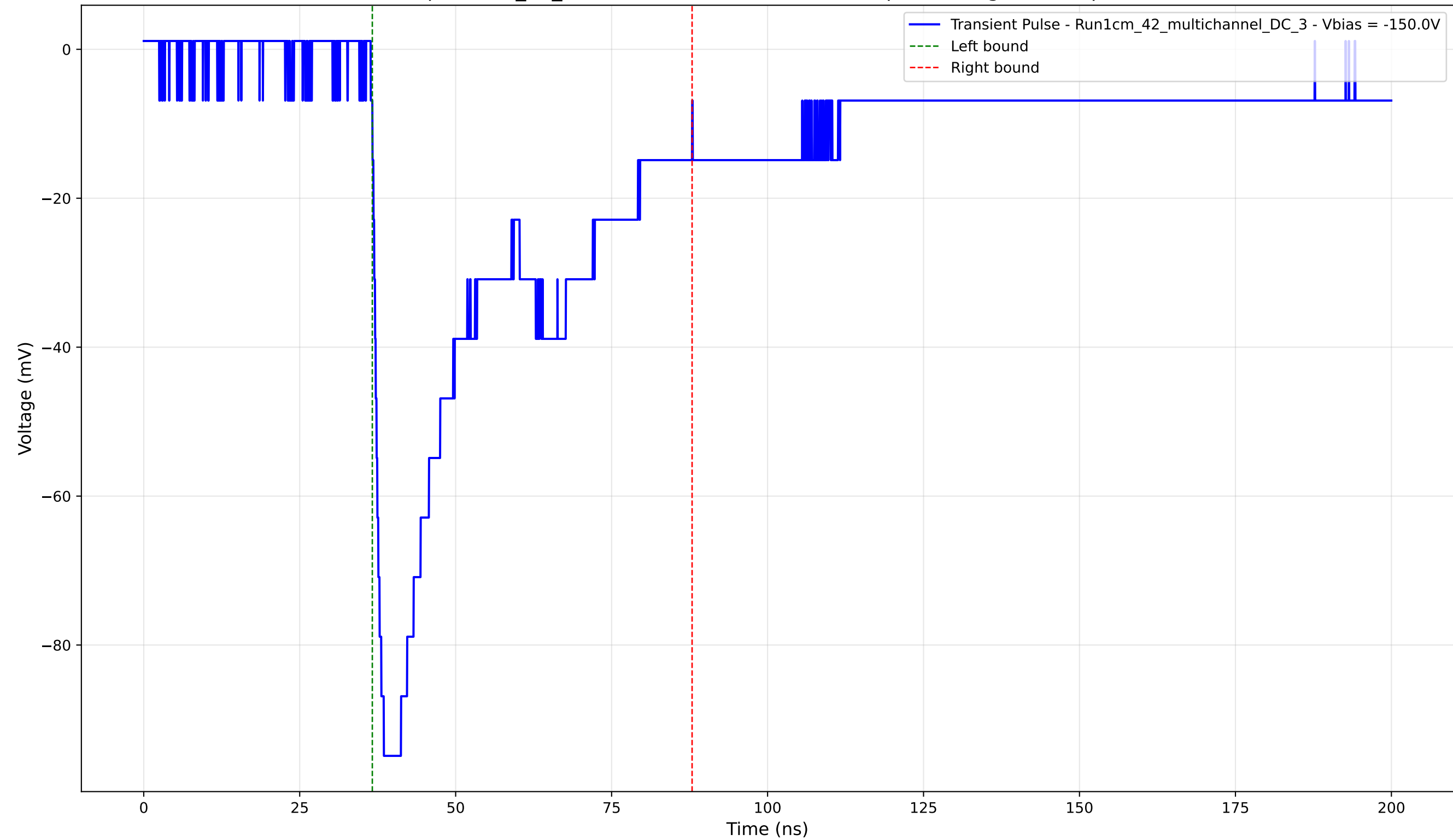
Transient Pulse - Sample: 1cm_42_multichannel - Position: 2010.0 \mu\text{m} - Charge: 38.78 pC - Rise Time: 1.43 ns
