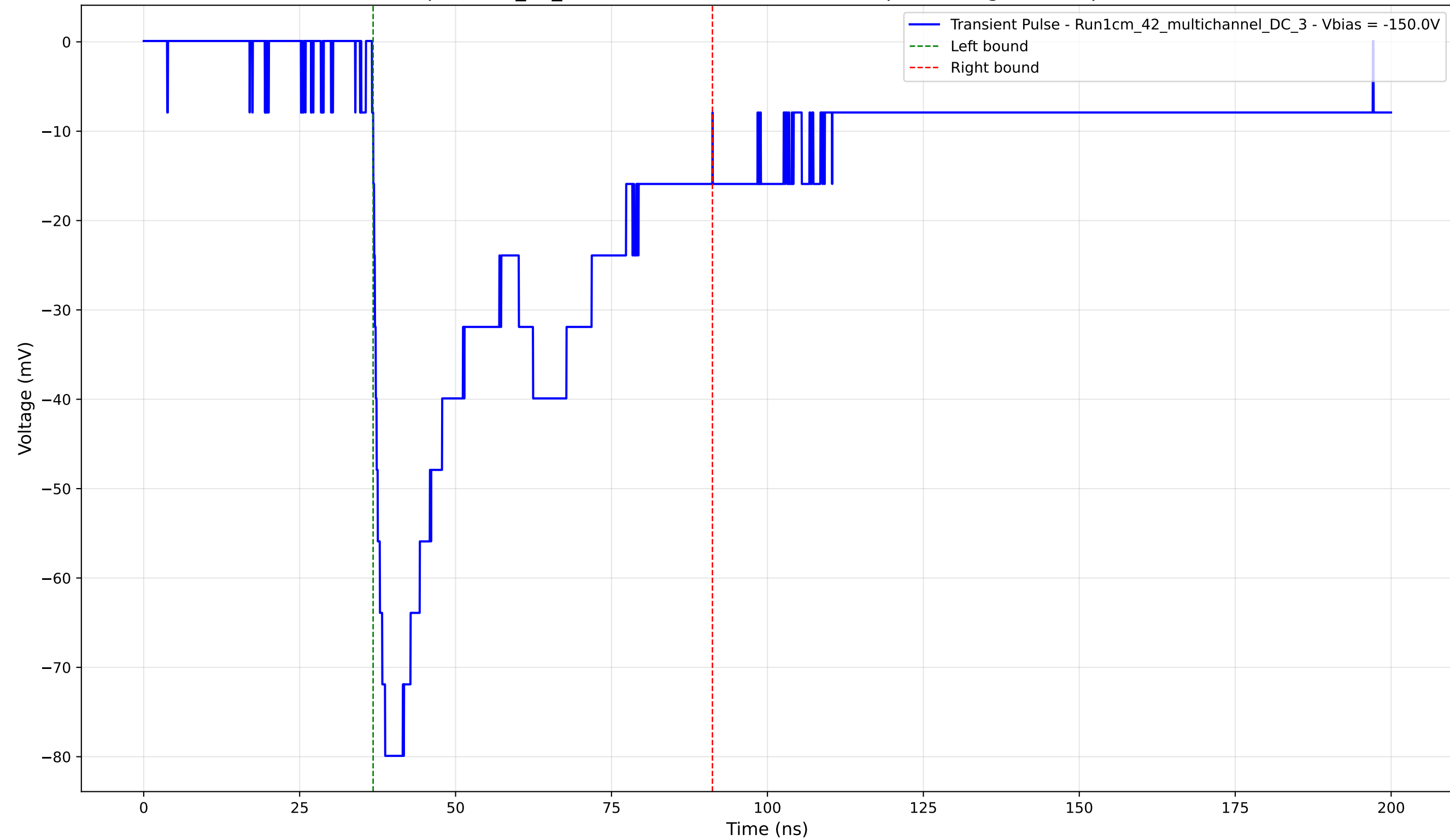
Transient Pulse - Sample: 1cm_42_multichannel - Position: 2495.0 \mu\text{m} - Charge: 37.27 pC - Rise Time: 1.92 ns
