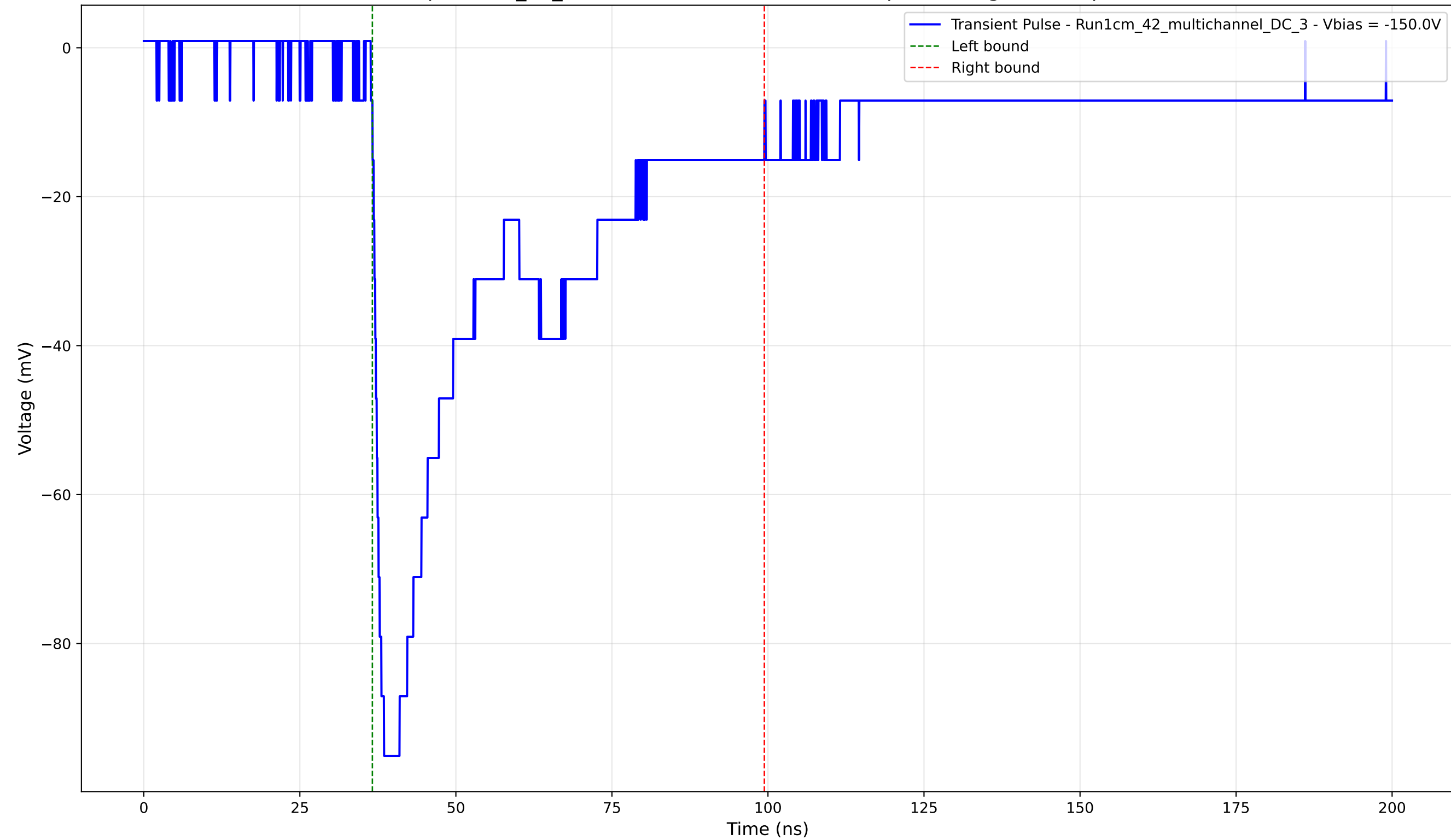
Transient Pulse - Sample: 1cm_42_multichannel - Position: 2005.0 \mu\text{m} - Charge: 42.11 pC - Rise Time: 1.43 ns
