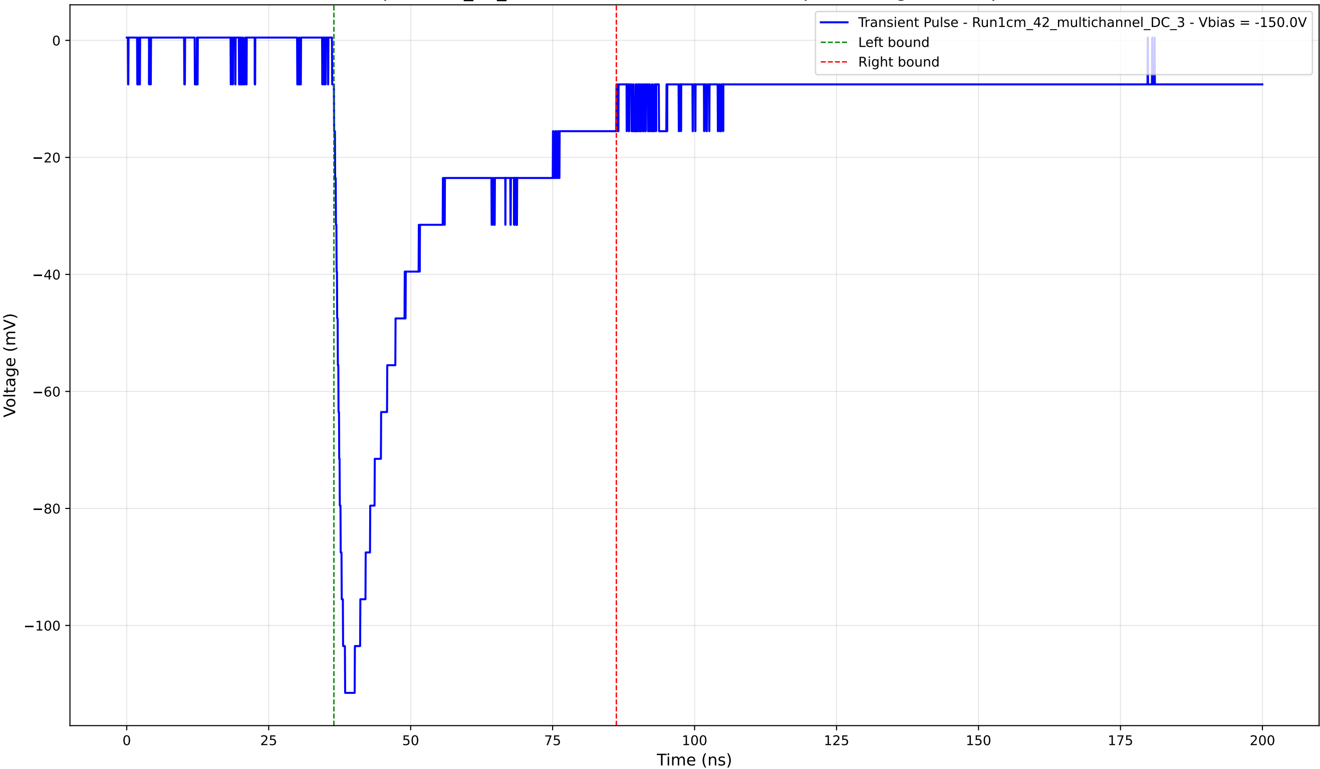
Transient Pulse - Sample: 1cm_42_multichannel - Position: 3295.0 \mu\text{m} - Charge: 36.50 pC - Rise Time: 1.59 ns
