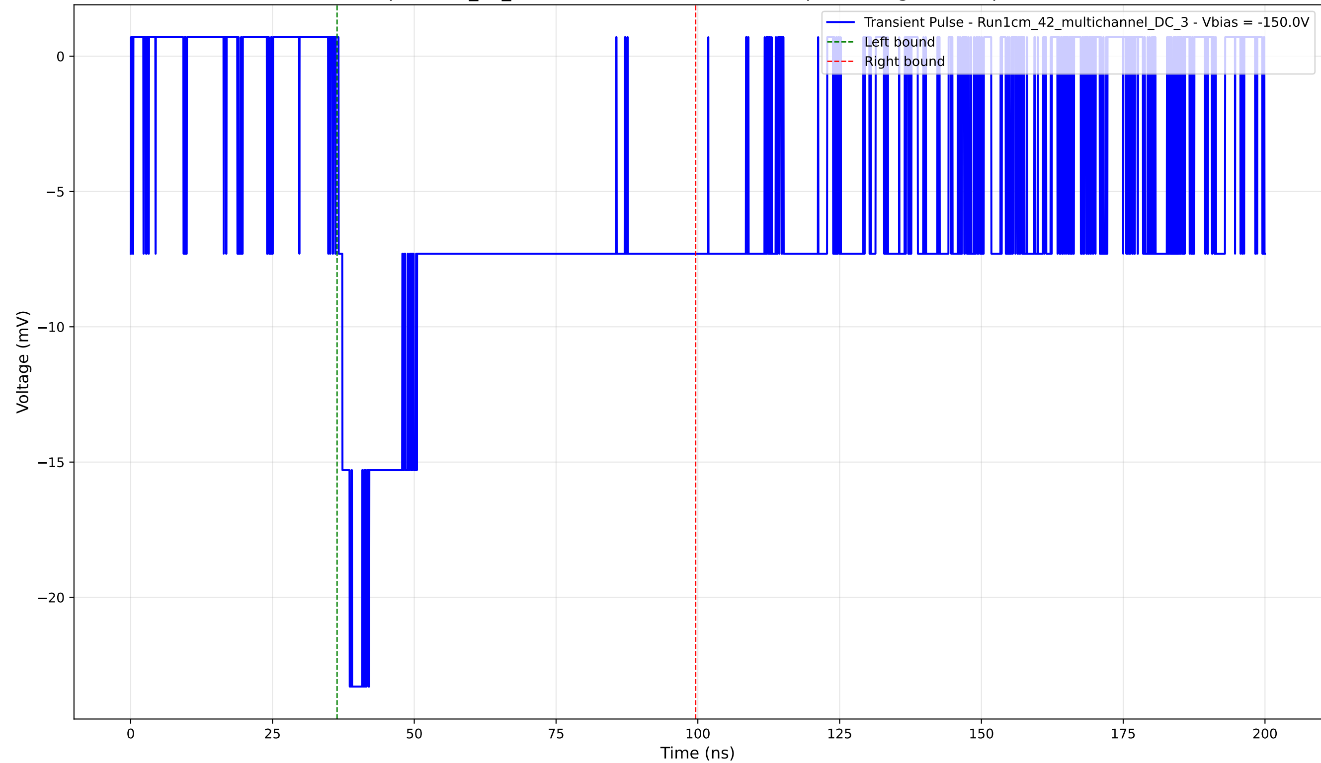
Transient Pulse - Sample: 1cm_42_multichannel - Position: 2410.0 \mu\text{m} - Charge: 11.50 pC - Rise Time: 1.96 ns
