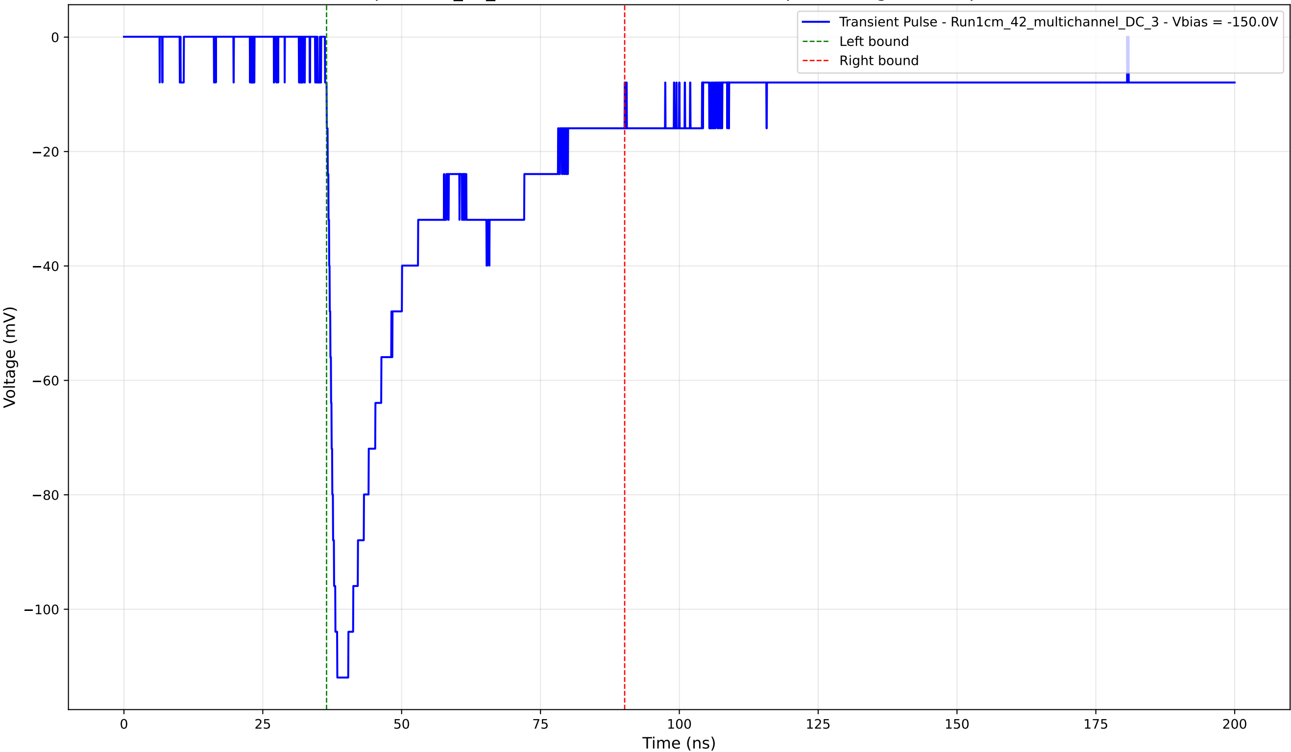
Transient Pulse - Sample: 1cm_42_multichannel - Position: 1750.0 \mu\text{m} - Charge: 41.61 pC - Rise Time: 1.57 ns
