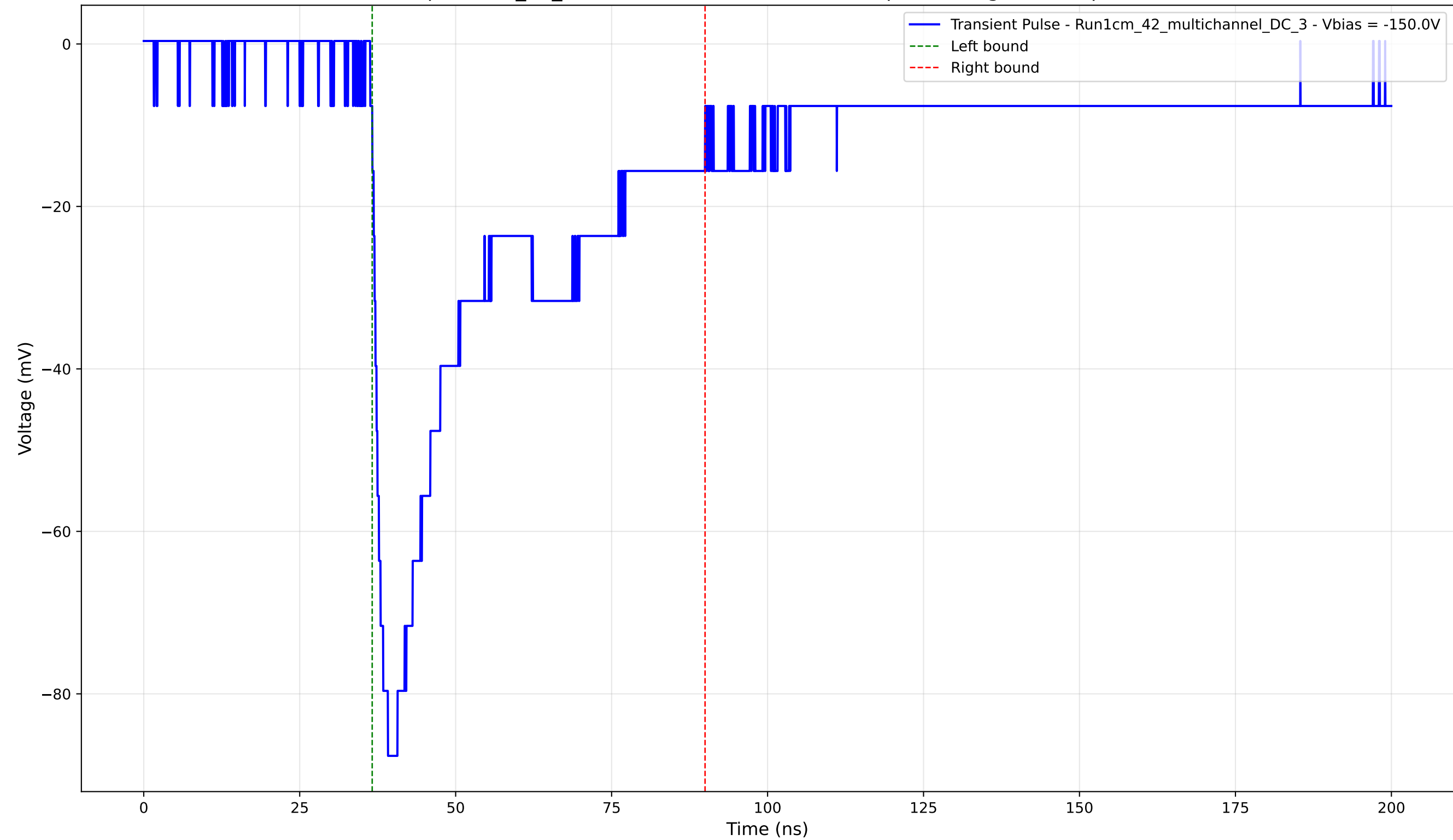
Transient Pulse - Sample: 1cm_42_multichannel - Position: 2800.0 \mu\text{m} - Charge: 35.03 pC - Rise Time: 1.76 ns
