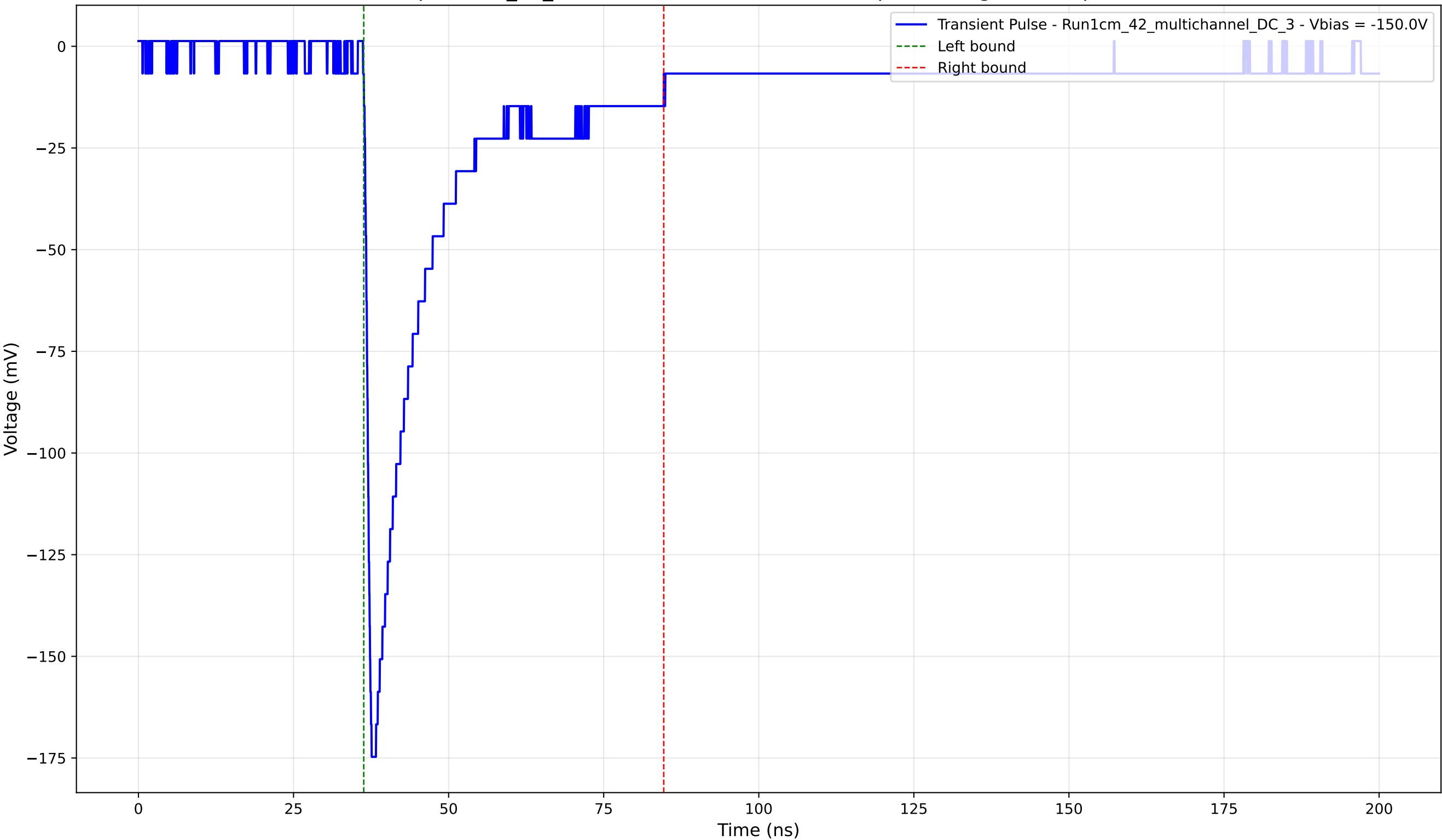
Transient Pulse - Sample: 1cm_42_multichannel - Position: 4090.0 \mu\text{m} - Charge: 38.69 pC - Rise Time: 0.93 ns
