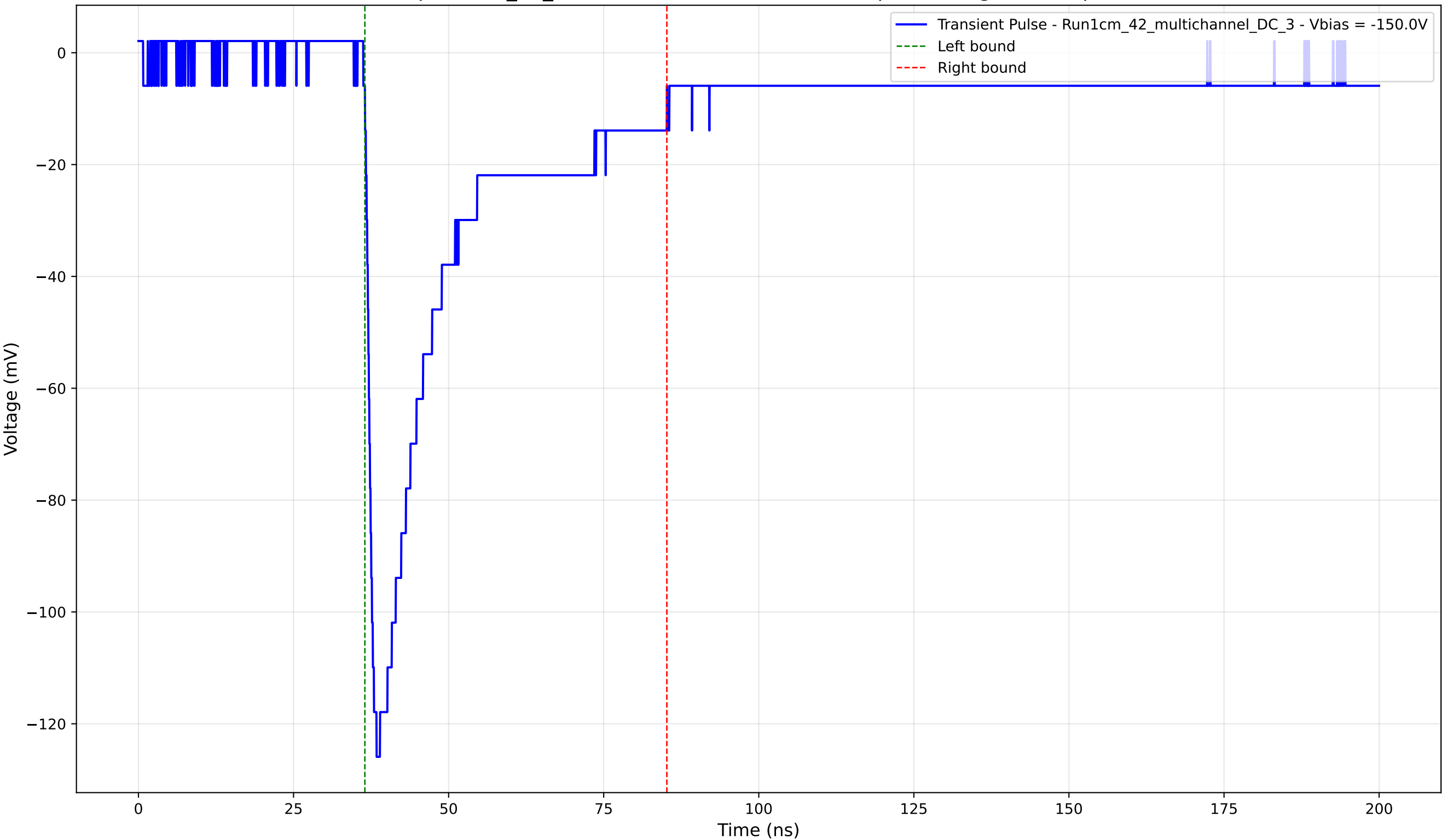
Transient Pulse - Sample: 1cm_42_multichannel - Position: 3575.0 \mu\text{m} - Charge: 35.03 pC - Rise Time: 1.44 ns
