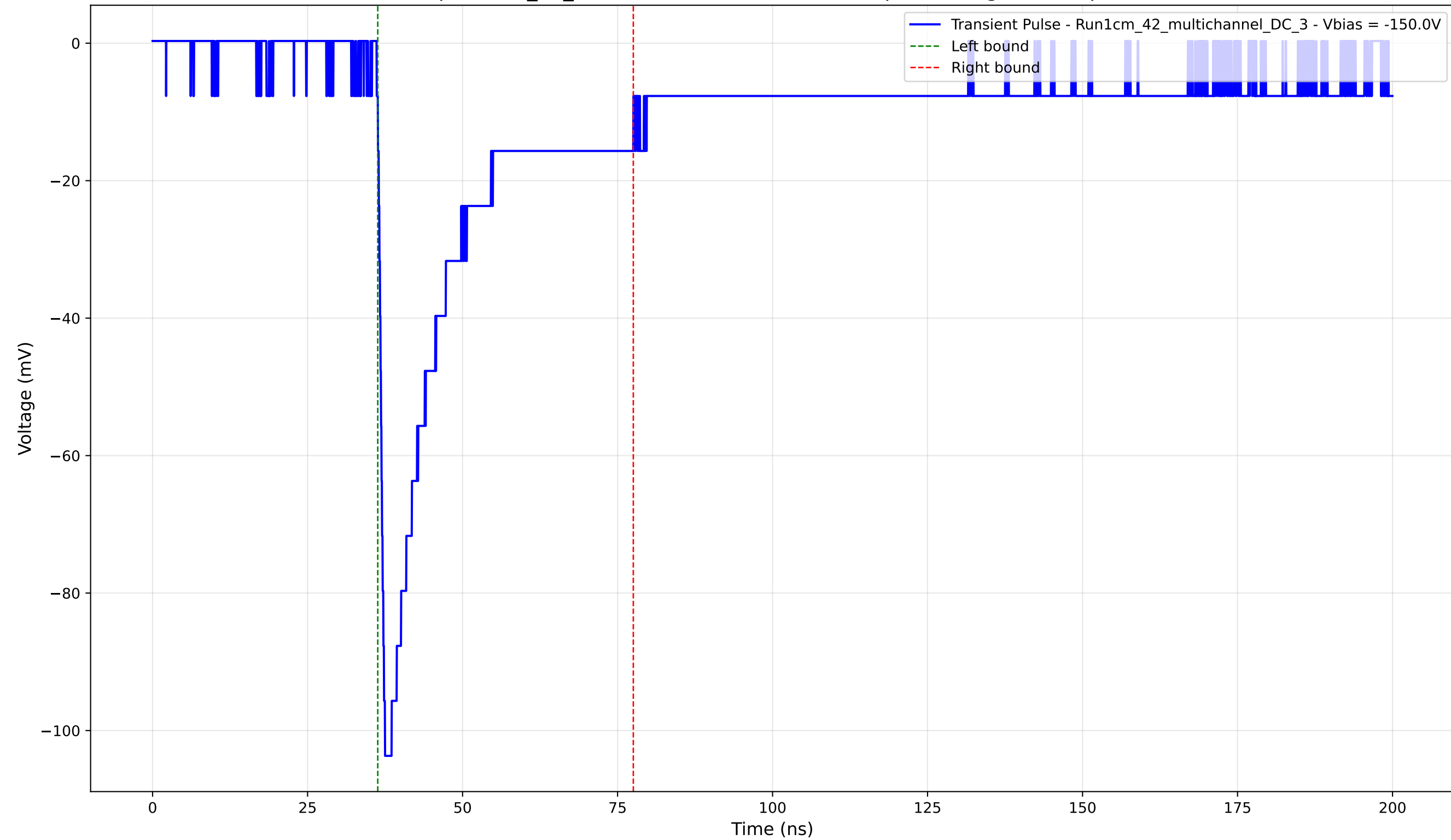
Transient Pulse - Sample: 1cm_42_multichannel - Position: 910.0 \mu\text{m} - Charge: 25.56 pC - Rise Time: 0.99 ns
