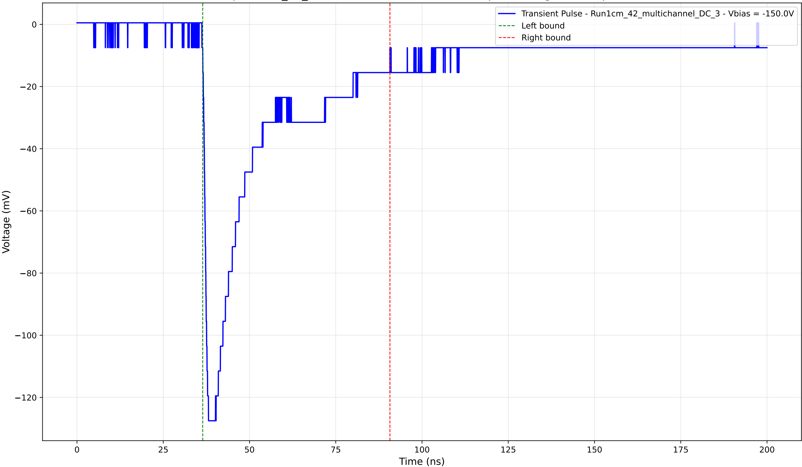
Transient Pulse - Sample: 1cm_42_multichannel - Position: 1520.0 \mu\text{m} - Charge: 44.09 pC - Rise Time: 1.39 ns
