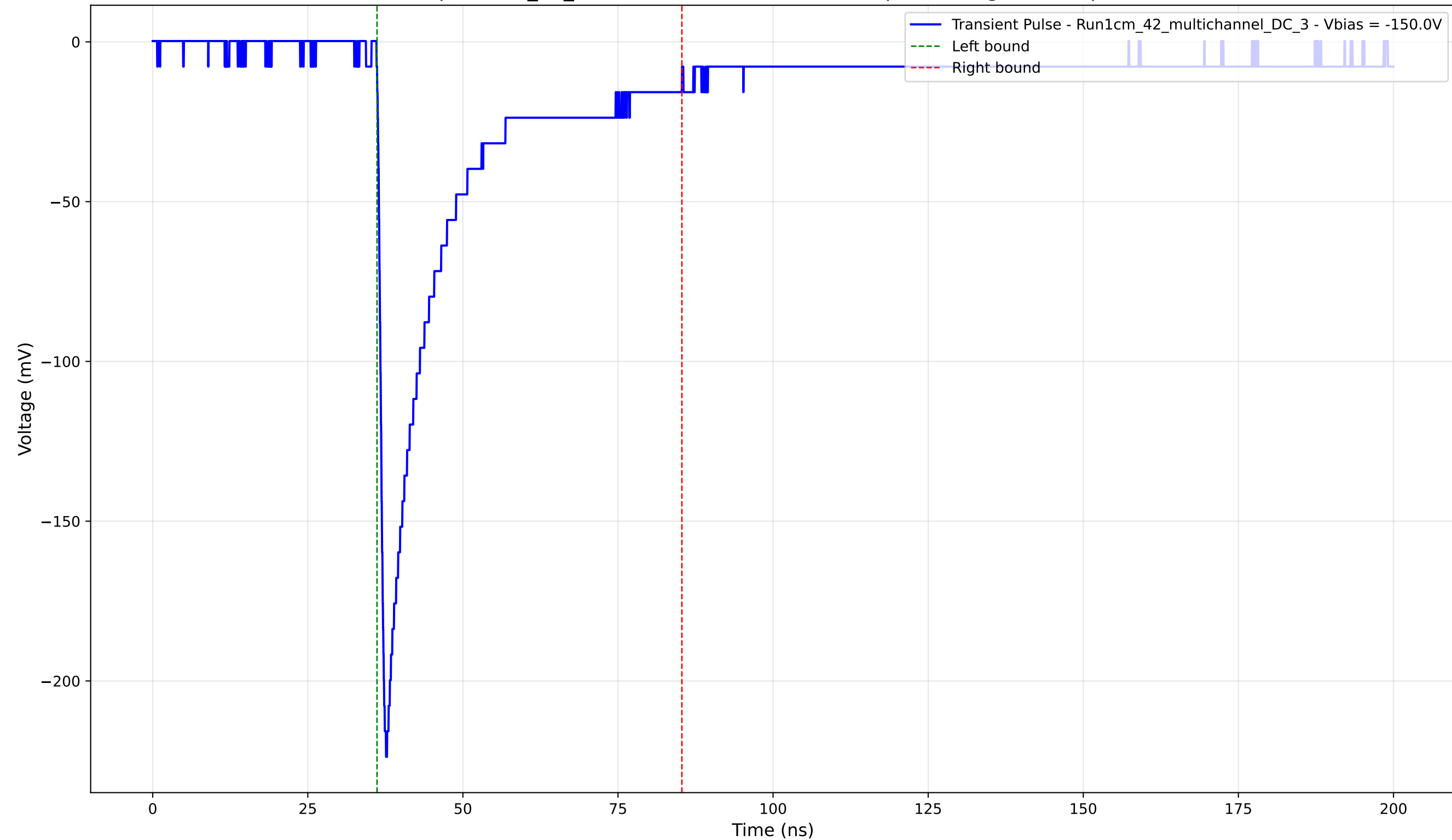
Transient Pulse - Sample: 1cm_42_multichannel - Position: 710.0 \mu\text{m} - Charge: 46.61 pC - Rise Time: 1.04 ns
