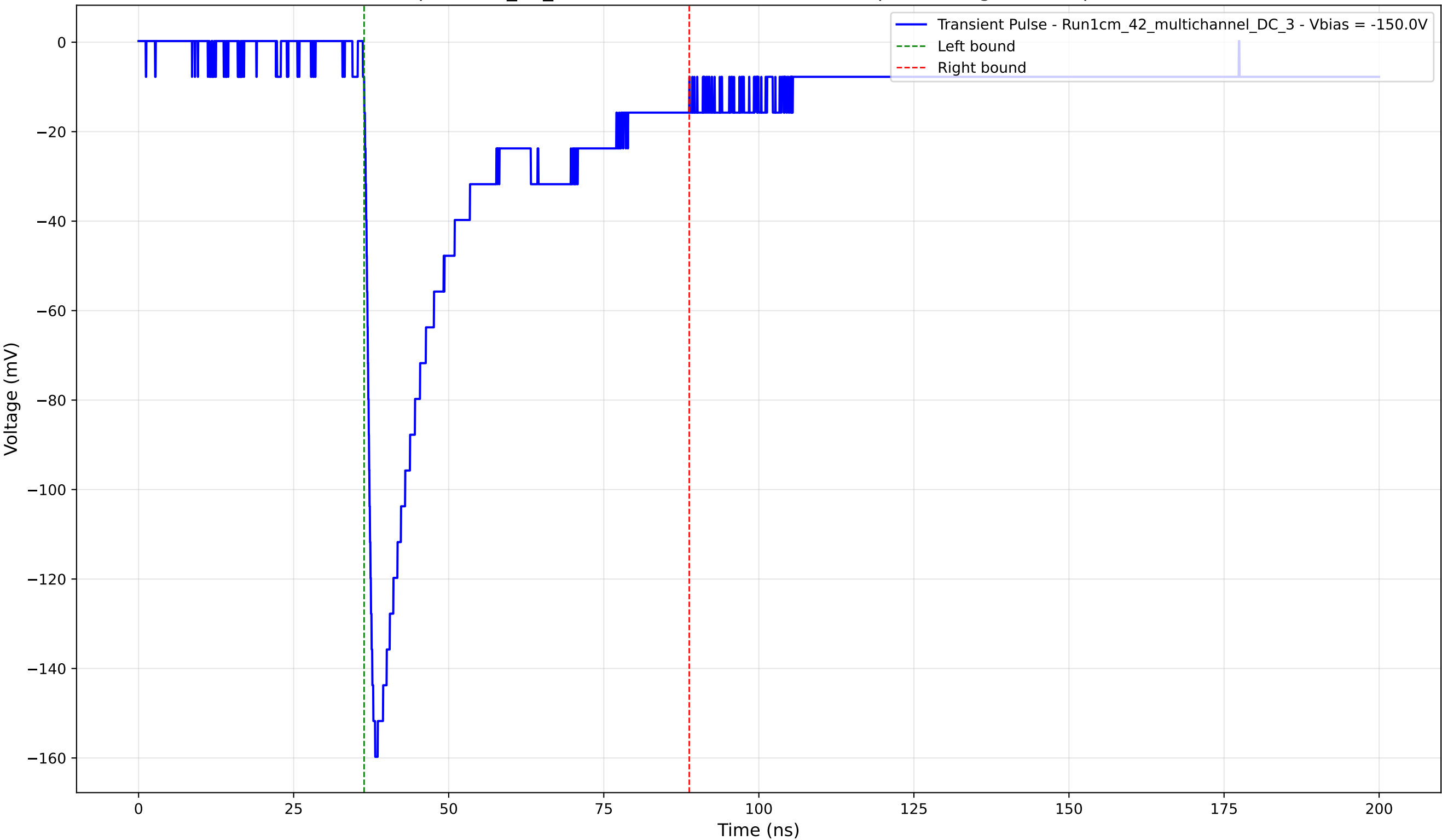
Transient Pulse - Sample: 1cm_42_multichannel - Position: 1230.0 \mu\text{m} - Charge: 45.51 pC - Rise Time: 1.36 ns
