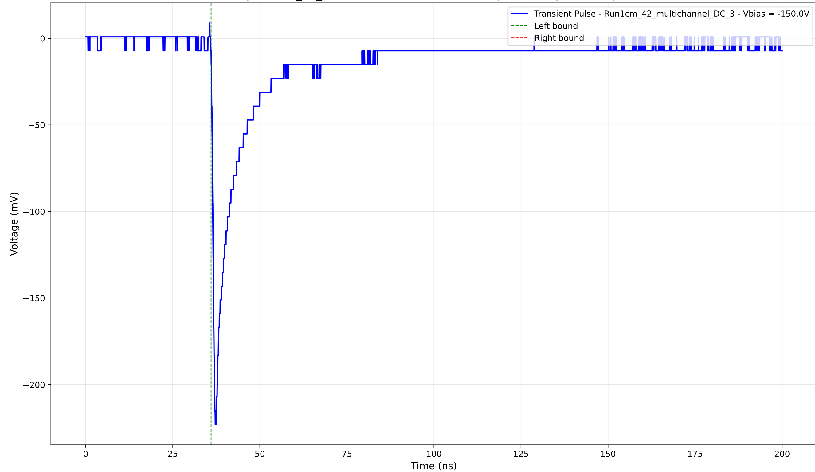
Transient Pulse - Sample: 1cm_42_multichannel - Position: 415.0 \mu\text{m} - Charge: 36.01 pC - Rise Time: 0.90 ns
