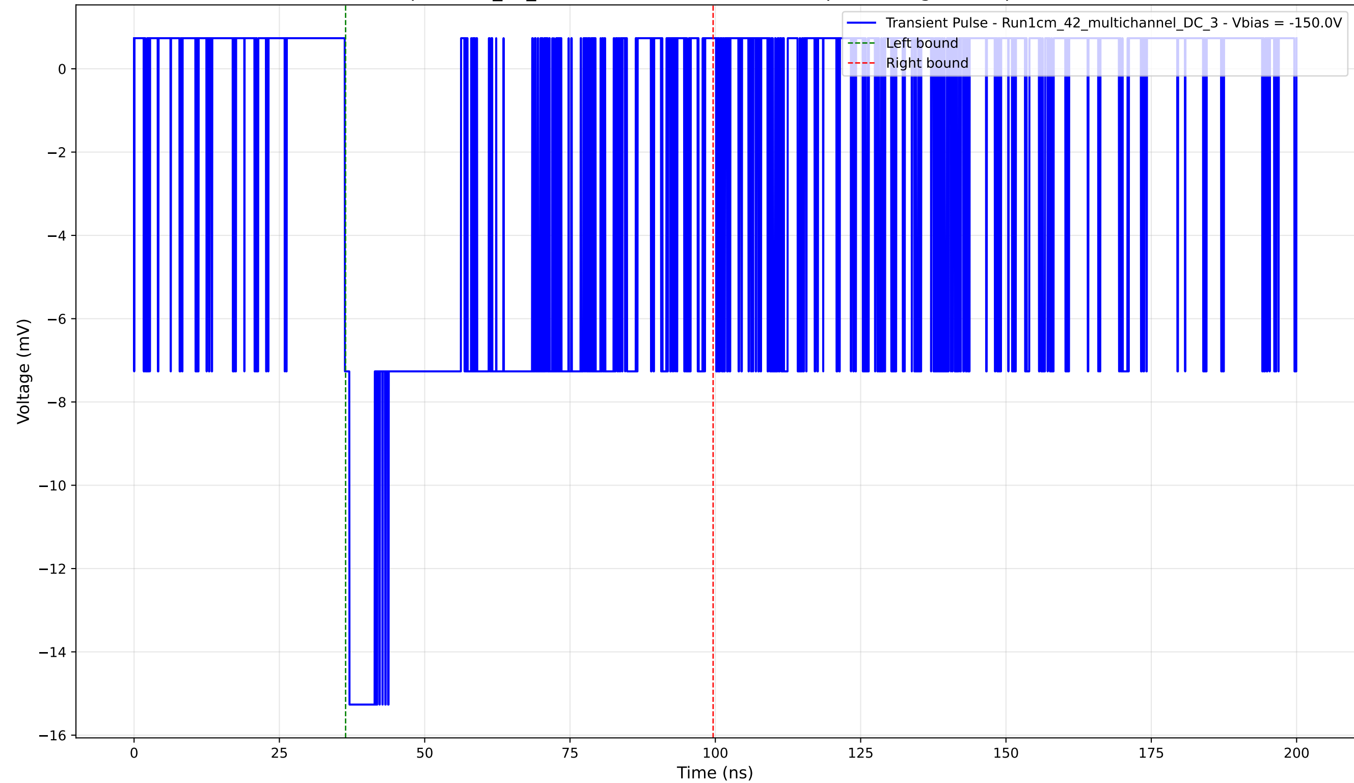
Transient Pulse - Sample: 1cm_42_multichannel - Position: 840.0 \mu\text{m} - Charge: 7.31 pC - Rise Time: 0.80 ns
