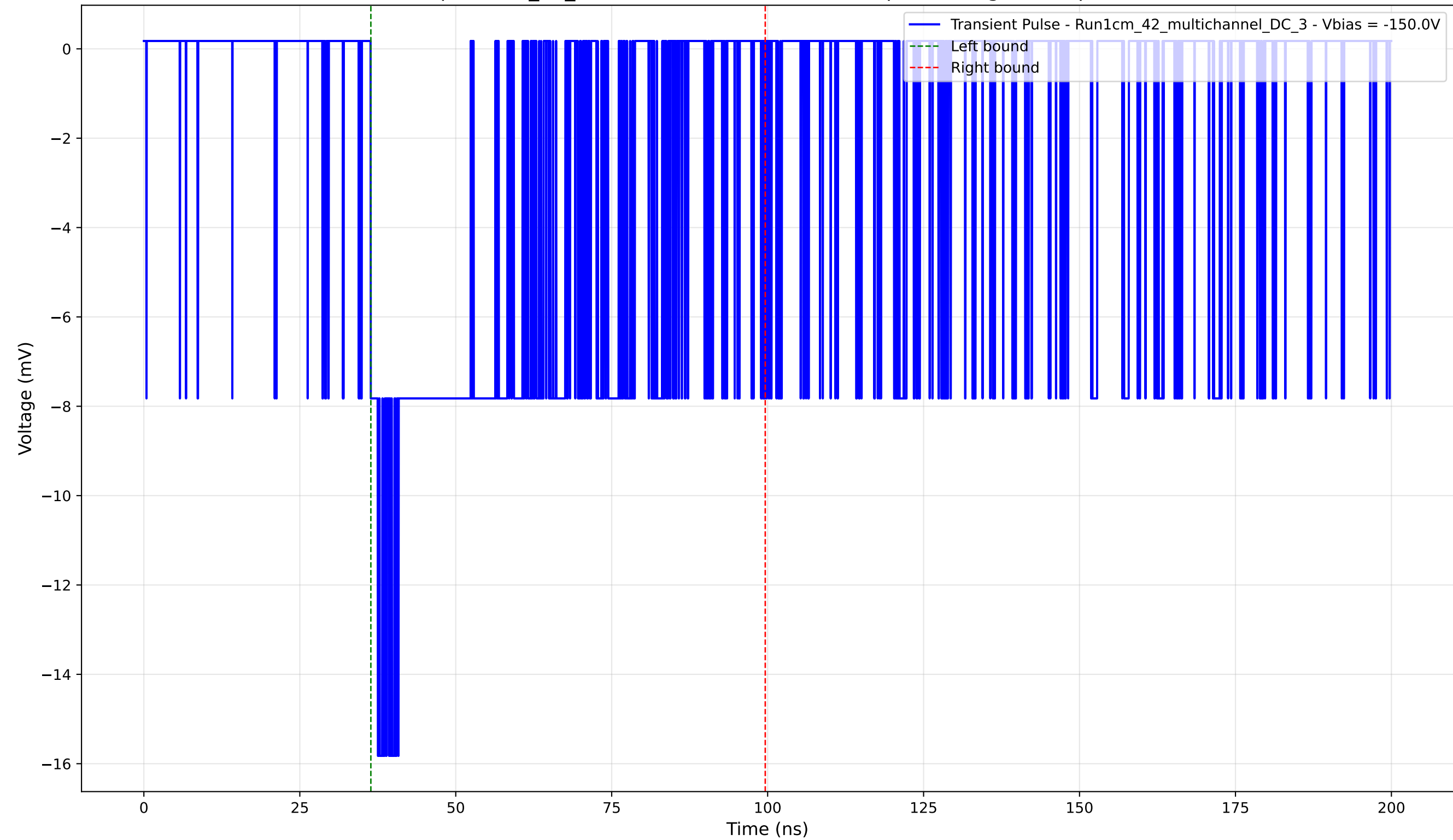
Transient Pulse - Sample: 1cm_42_multichannel - Position: 855.0 \mu\text{m} - Charge: 6.16 pC - Rise Time: 1.16 ns
