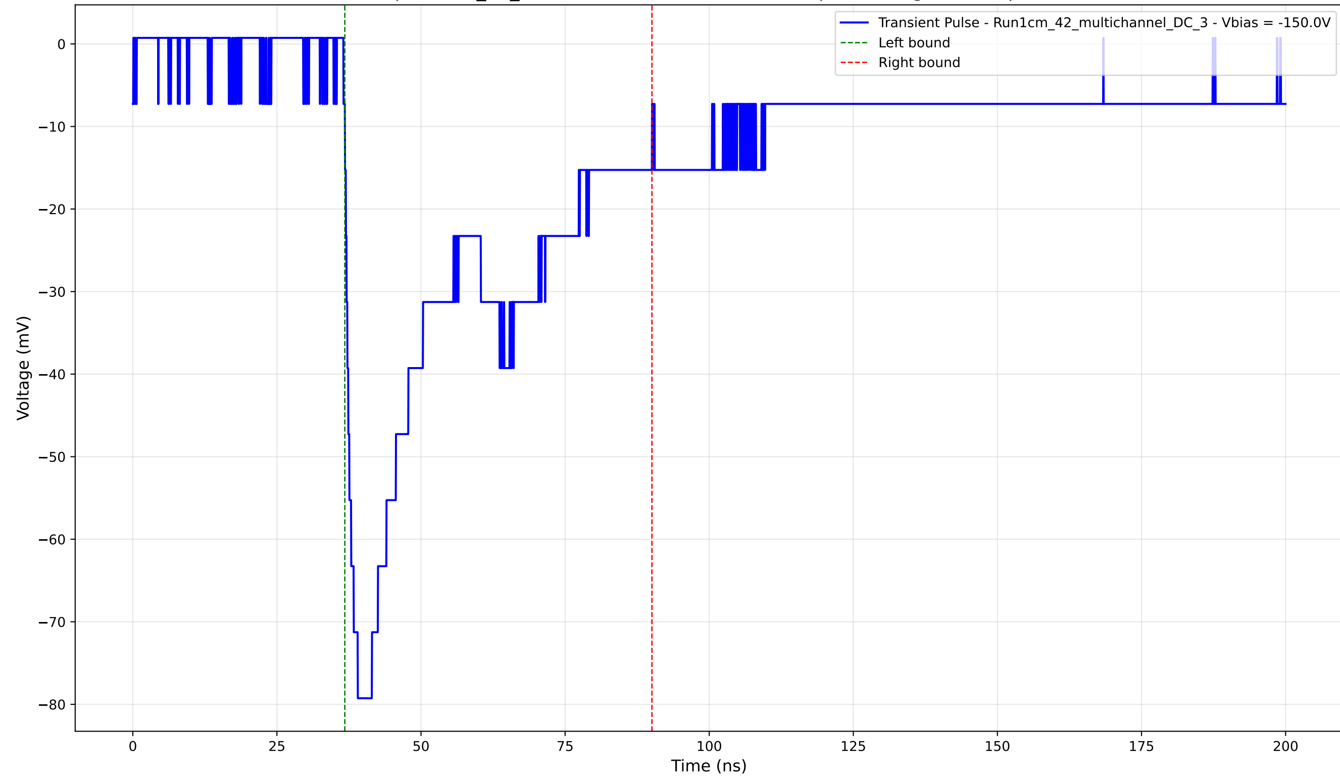
Transient Pulse - Sample: 1cm_42_multichannel - Position: 2565.0 \mu\text{m} - Charge: 34.82 pC - Rise Time: 2.24 ns
