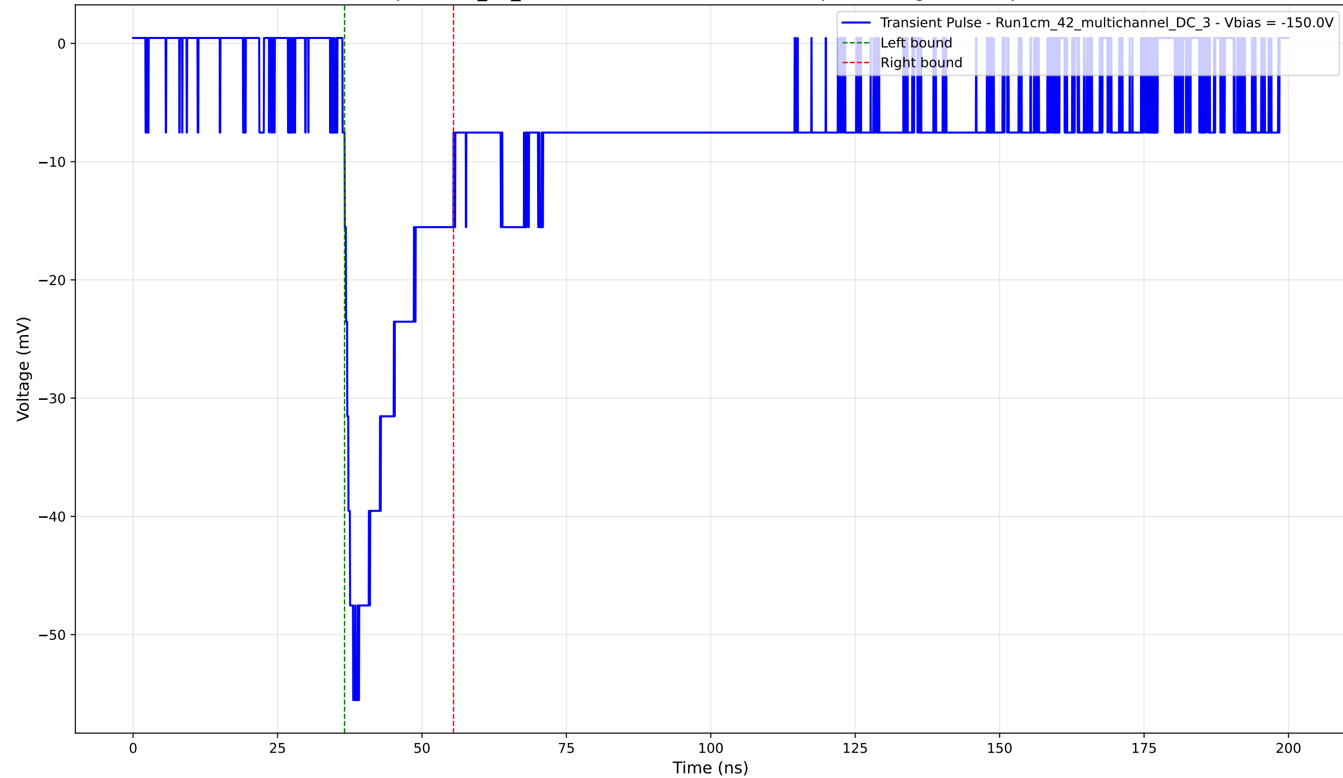
Transient Pulse - Sample: 1cm_42_multichannel - Position: 1320.0 \mu\text{m} - Charge: 10.61 pC - Rise Time: 1.85 ns
