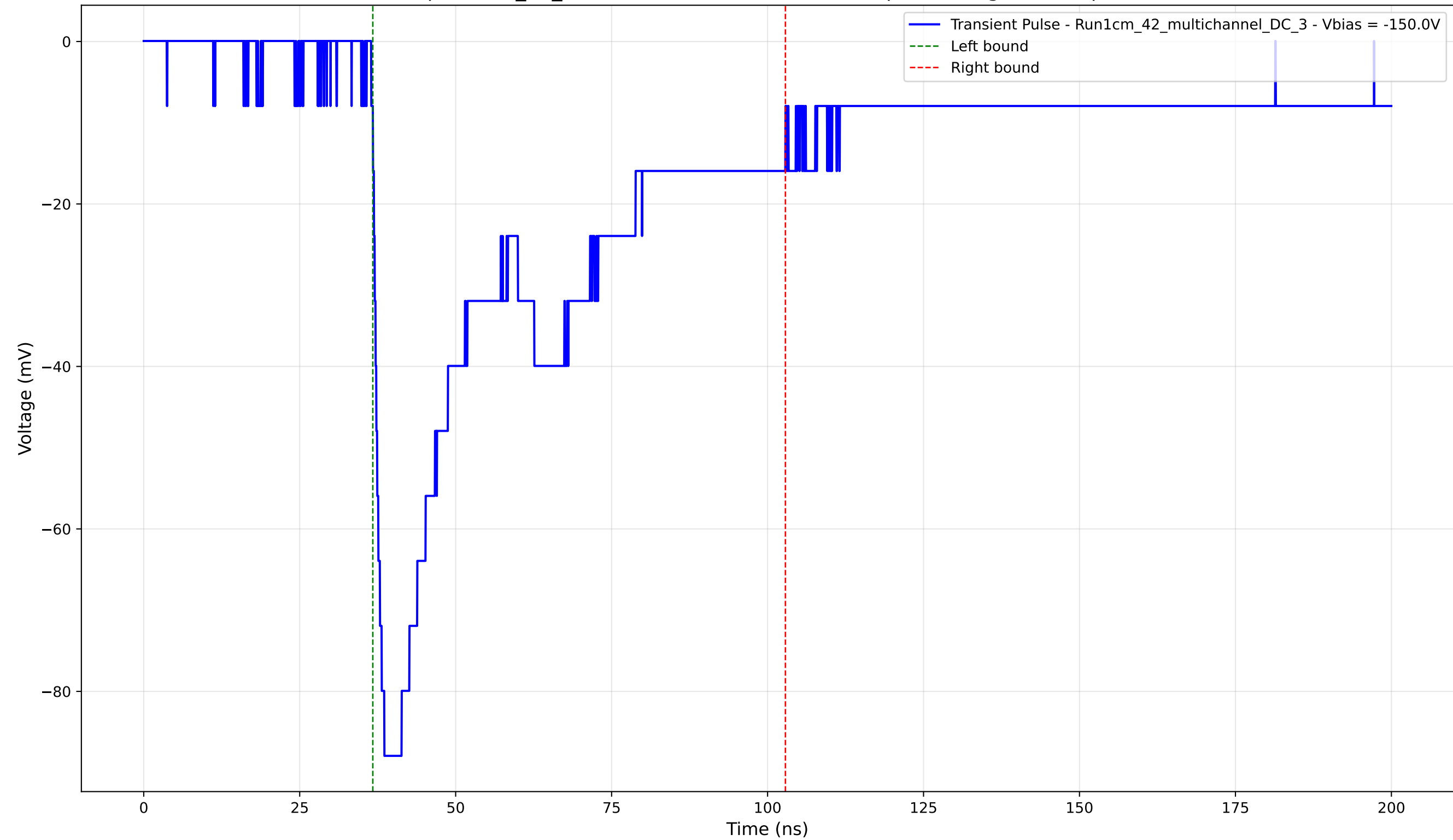
Transient Pulse - Sample: 1cm_42_multichannel - Position: 2110.0 \mu\text{m} - Charge: 42.95 pC - Rise Time: 1.42 ns
