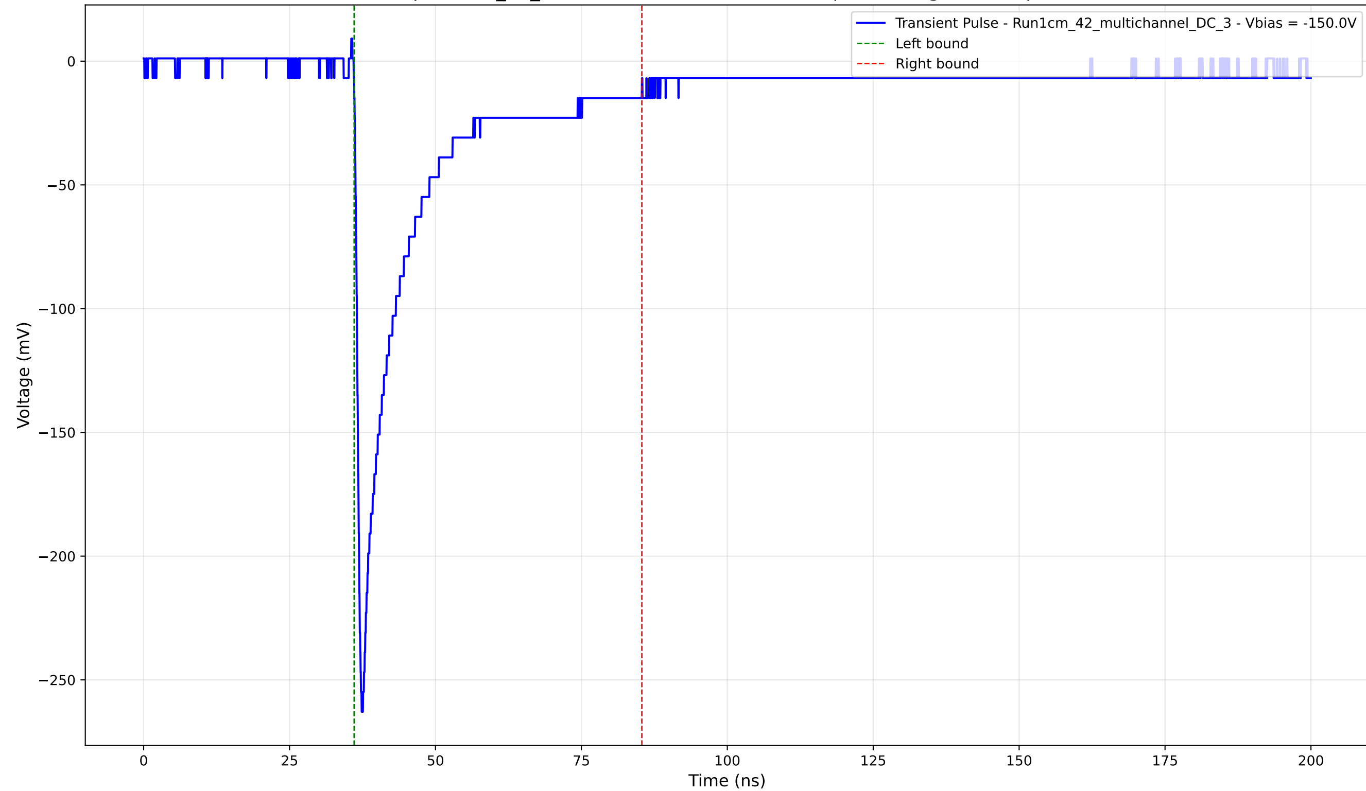
Transient Pulse - Sample: 1cm_42_multichannel - Position: 535.0 \mu\text{m} - Charge: 47.78 pC - Rise Time: 0.91 ns
