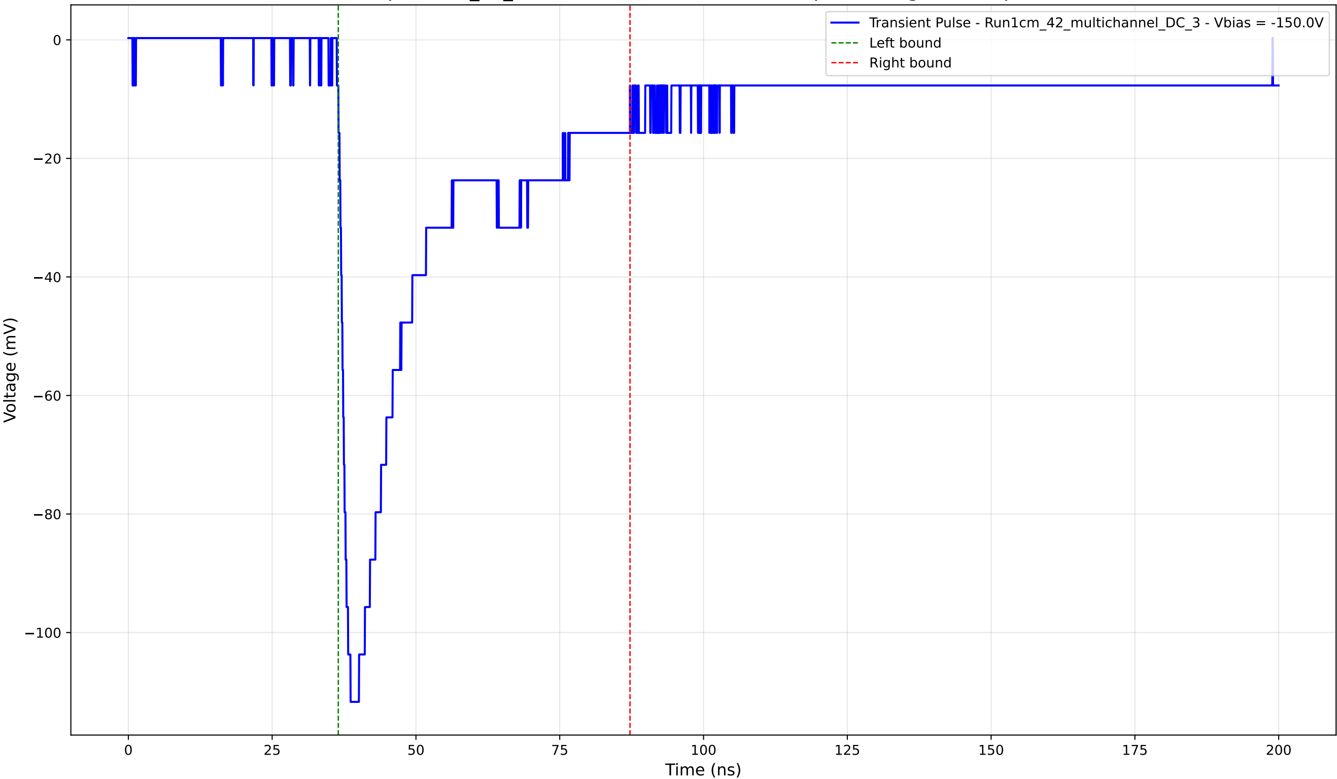
Transient Pulse - Sample: 1cm_42_multichannel - Position: 3210.0 \mu\text{m} - Charge: 37.76 pC - Rise Time: 1.69 ns
