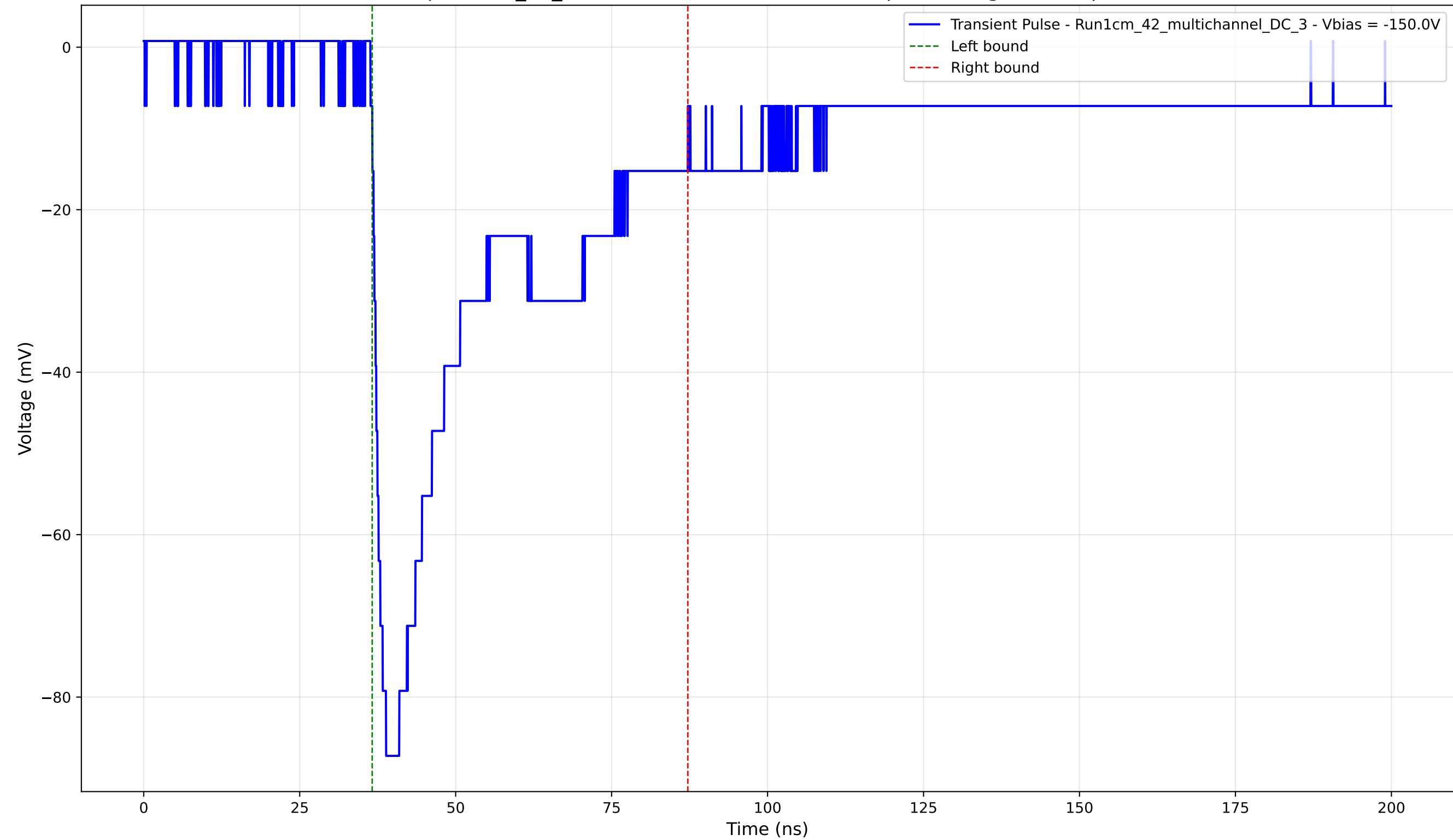
Transient Pulse - Sample: 1cm_42_multichannel - Position: 2795.0 \mu\text{m} - Charge: 34.33 pC - Rise Time: 1.68 ns
