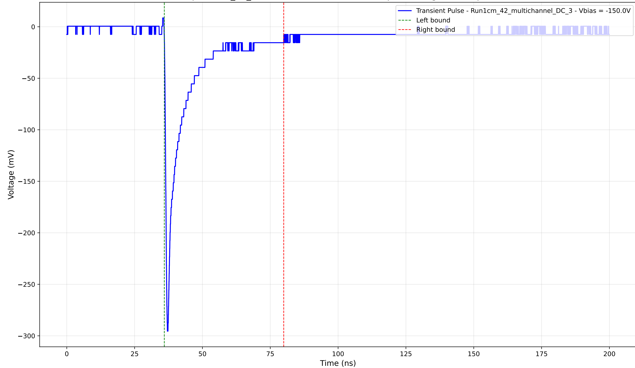
Transient Pulse - Sample: 1cm_42_multichannel - Position: 270.0 \mu\text{m} - Charge: 41.56 pC - Rise Time: 0.84 ns
