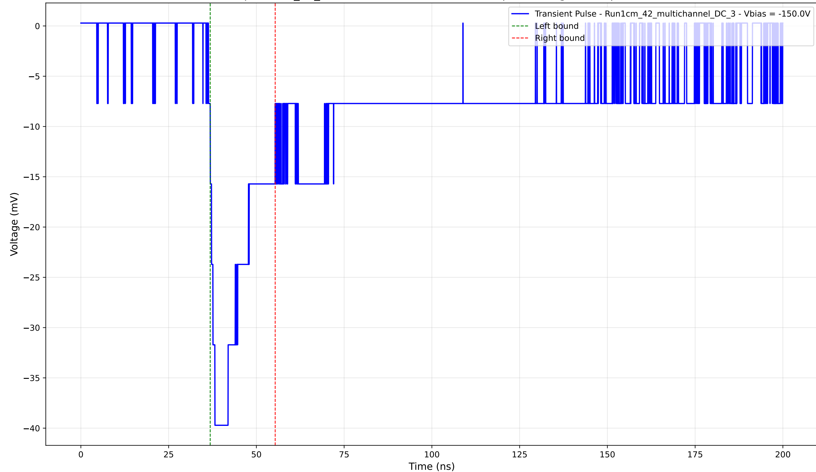
Transient Pulse - Sample: 1cm_42_multichannel - Position: 2925.0 \mu\text{m} - Charge: 9.19 pC - Rise Time: 1.83 ns
