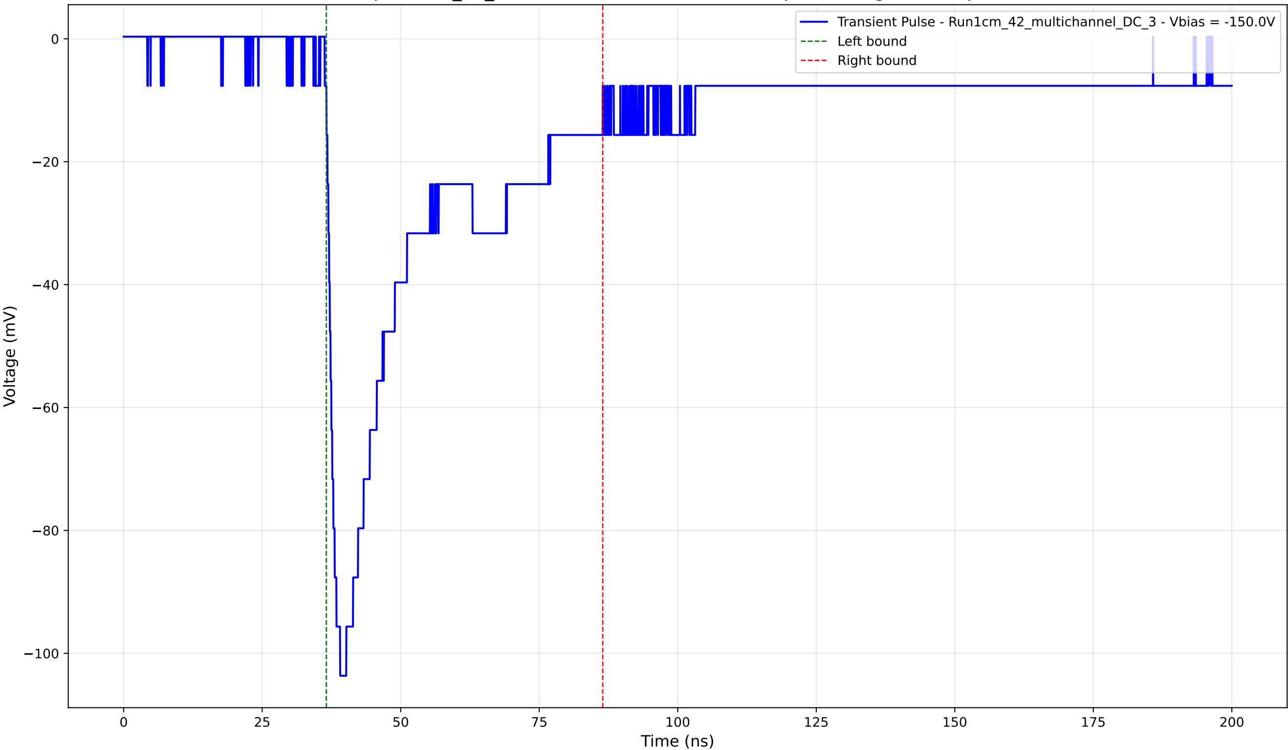
Transient Pulse - Sample: 1cm_42_multichannel - Position: 3045.0 \mu\text{m} - Charge: 36.33 pC - Rise Time: 1.81 ns
