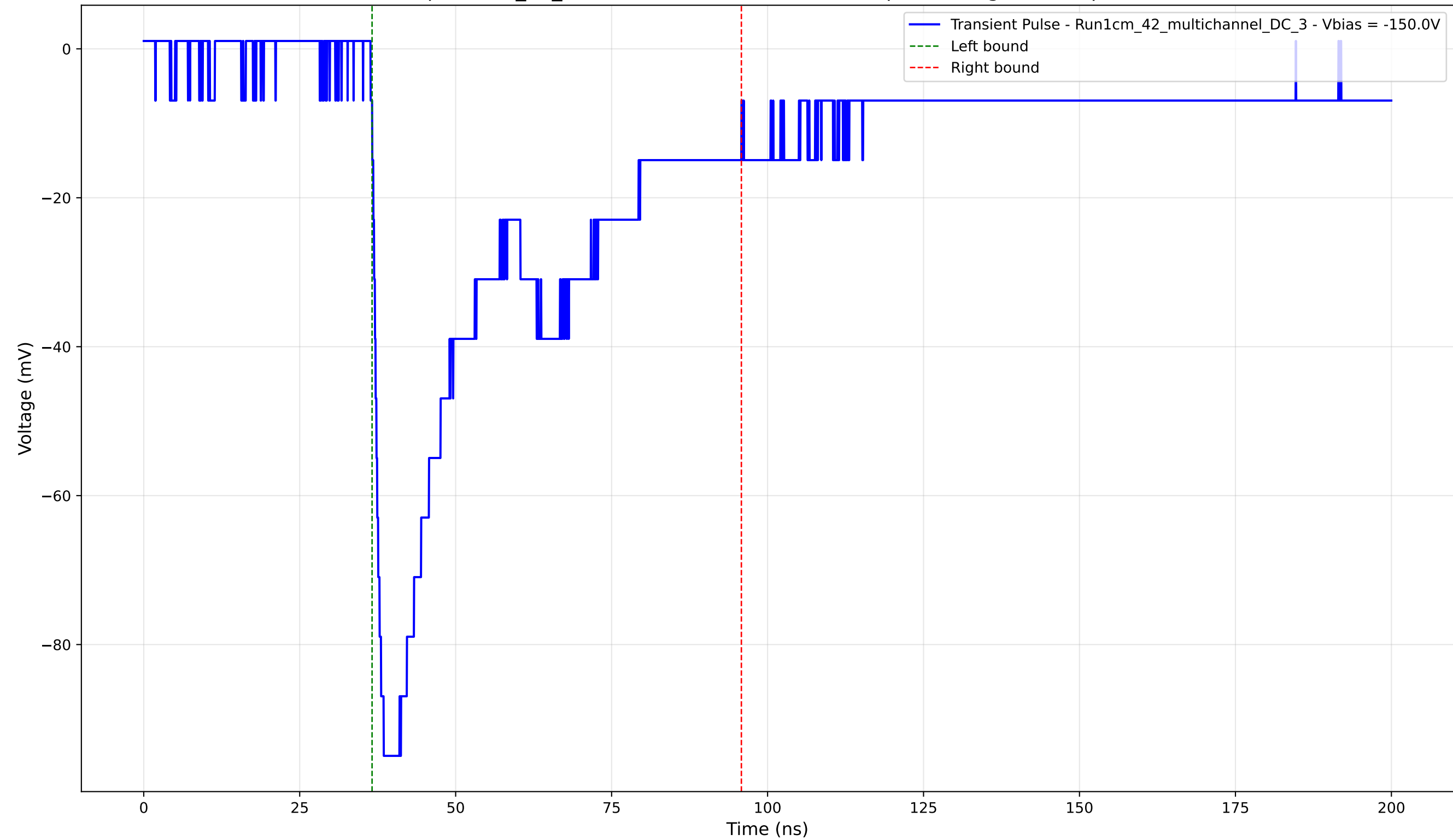
Transient Pulse - Sample: 1cm_42_multichannel - Position: 1985.0 \mu\text{m} - Charge: 40.94 pC - Rise Time: 1.43 ns
