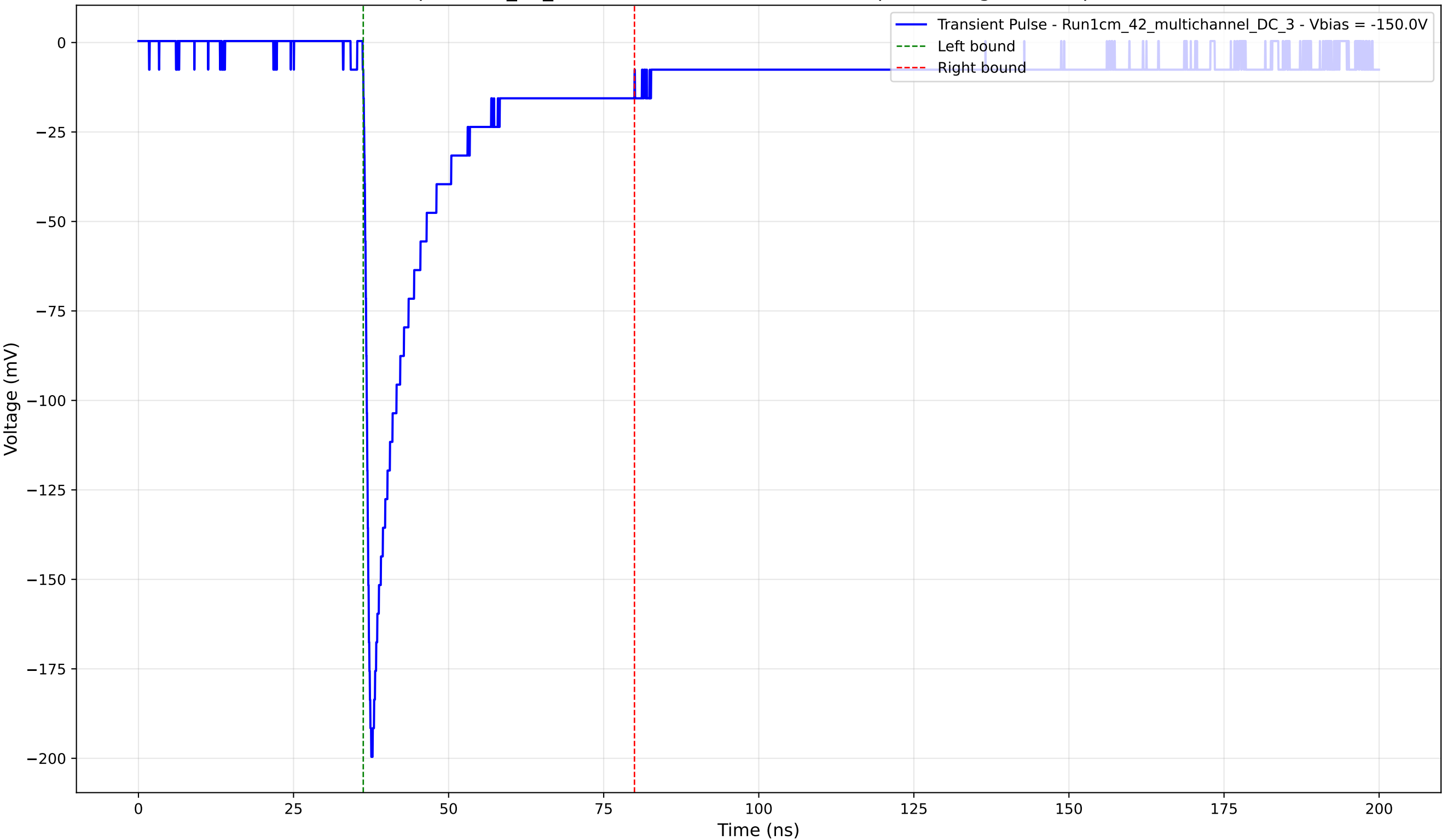
Transient Pulse - Sample: 1cm_42_multichannel - Position: 4295.0 \mu\text{m} - Charge: 35.62 pC - Rise Time: 0.97 ns
