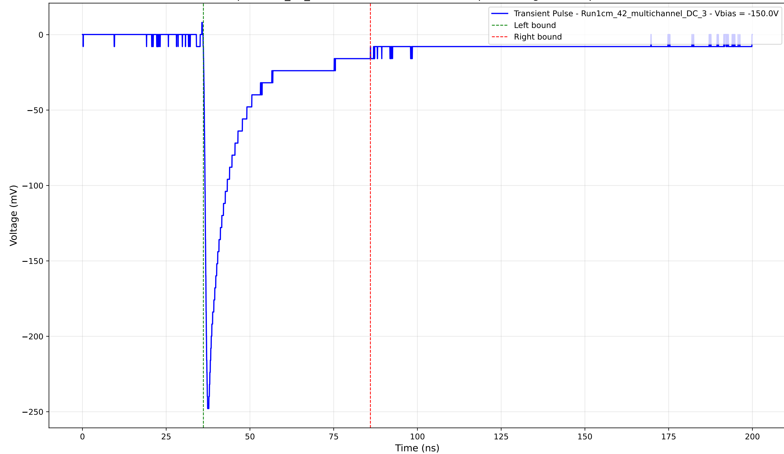
Transient Pulse - Sample: 1cm_42_multichannel - Position: 595.0 \mu\text{m} - Charge: 48.53 pC - Rise Time: 0.92 ns
