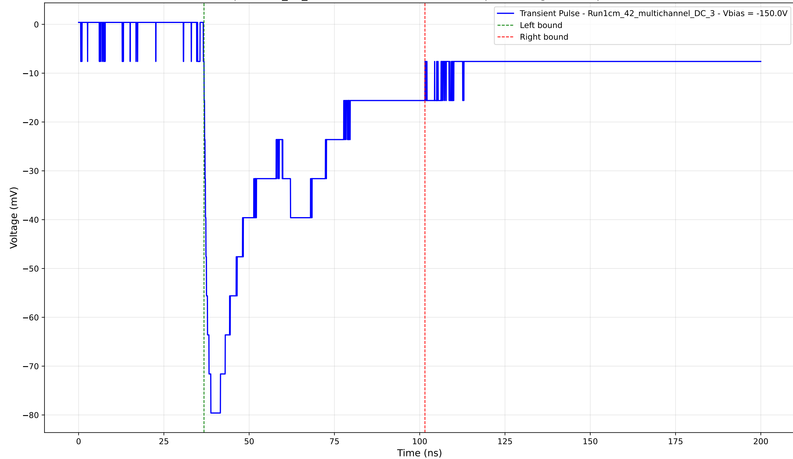
Transient Pulse - Sample: 1cm_42_multichannel - Position: 2280.0 \mu\text{m} - Charge: 40.97 pC - Rise Time: 2.00 ns
