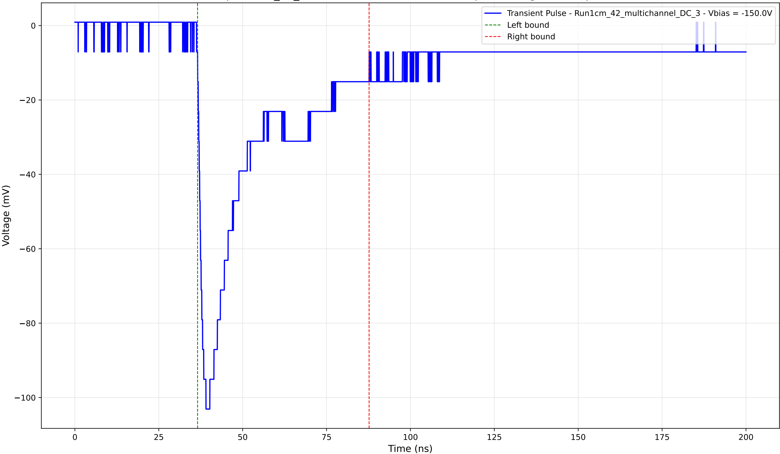
Transient Pulse - Sample: 1cm_42_multichannel - Position: 2990.0 \mu\text{m} - Charge: 36.60 pC - Rise Time: 1.83 ns
