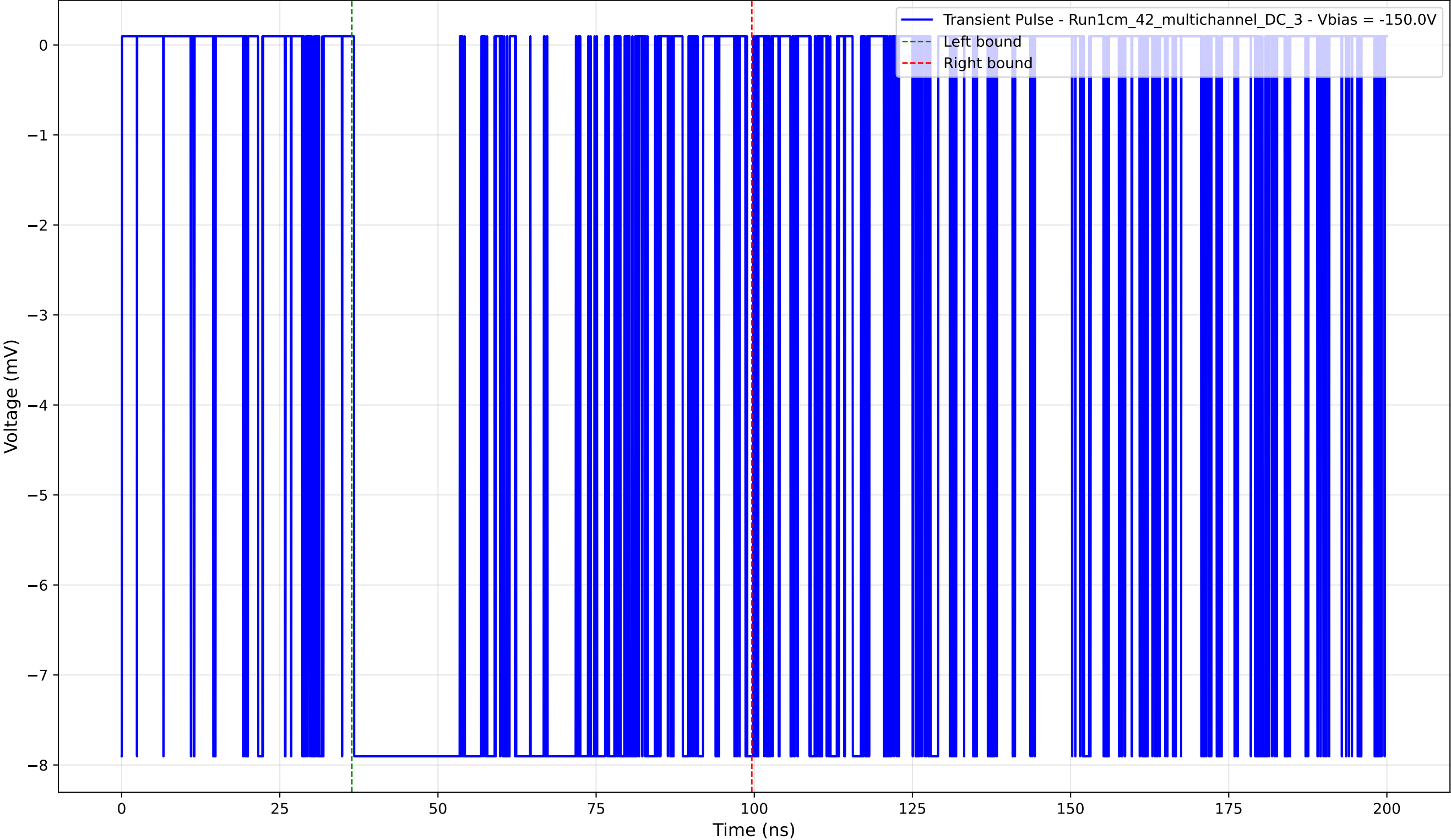
Transient Pulse - Sample: 1cm_42_multichannel - Position: 1875.0 \mu\text{m} - Charge: 6.99 pC - Rise Time: 0.00 ns (N/A)
