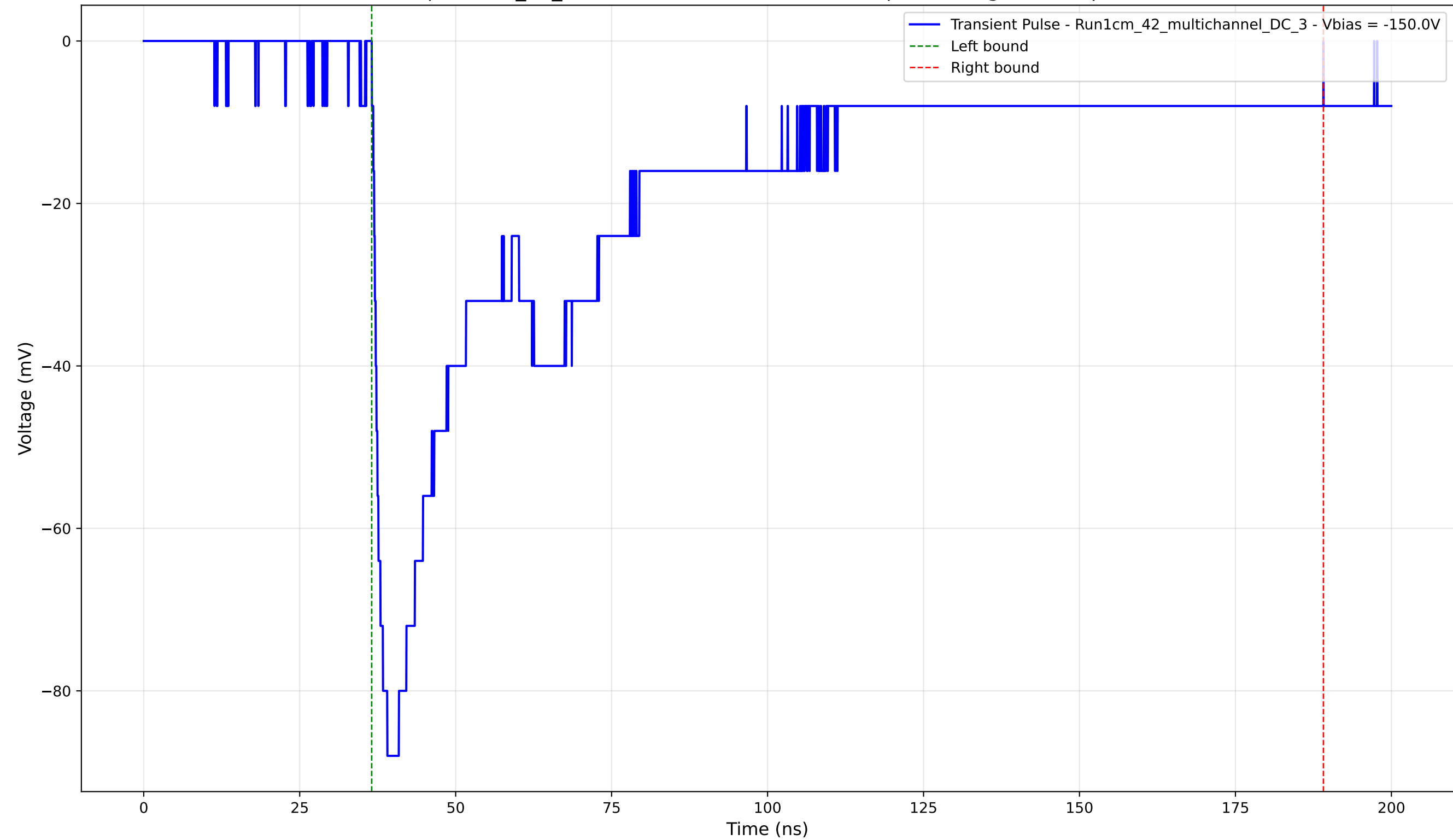
Transient Pulse - Sample: 1cm_42_multichannel - Position: 2195.0 \mu\text{m} - Charge: 57.13 pC - Rise Time: 1.56 ns
