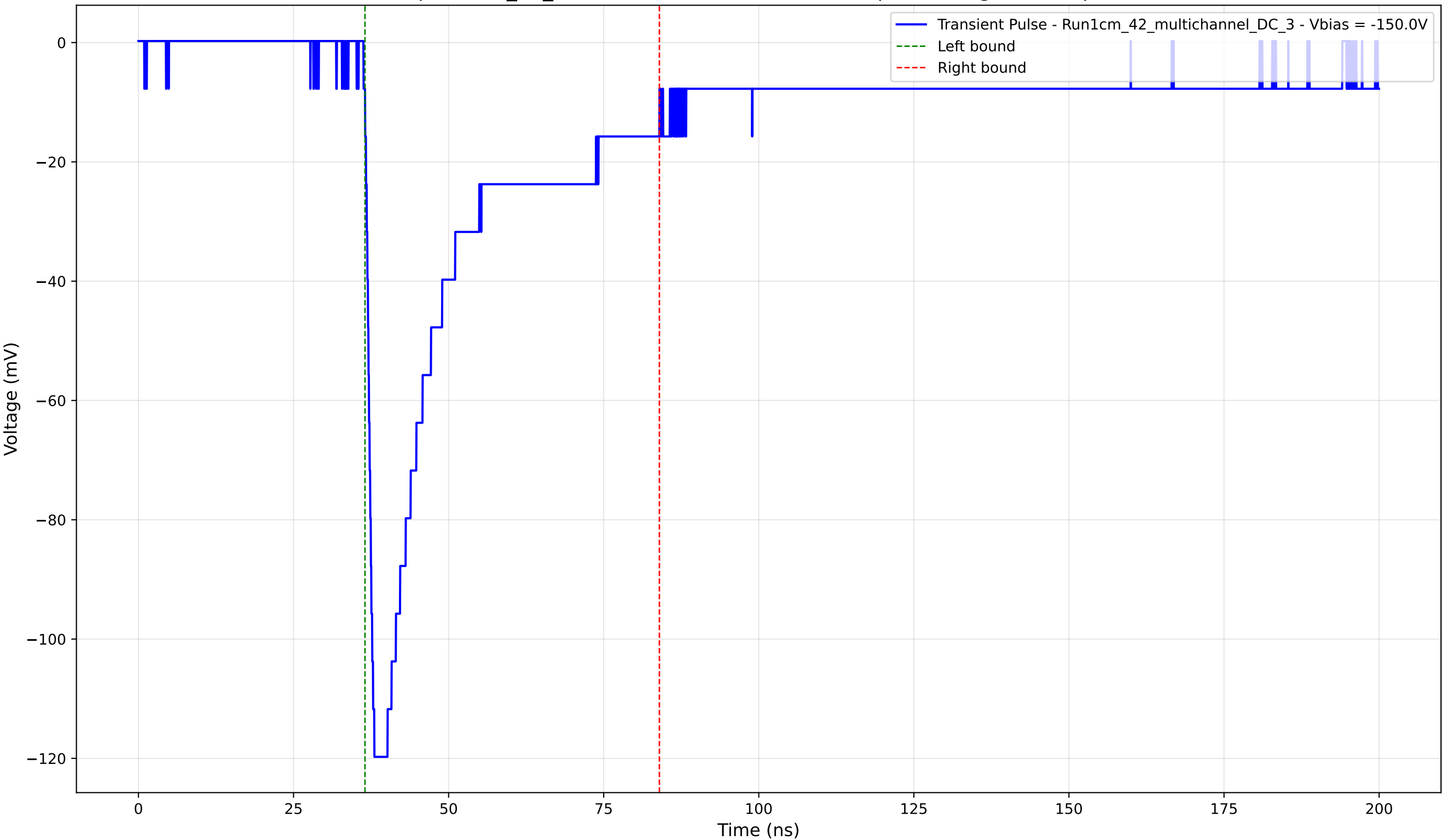
Transient Pulse - Sample: 1cm_42_multichannel - Position: 3545.0 \mu\text{m} - Charge: 36.31 pC - Rise Time: 1.29 ns
