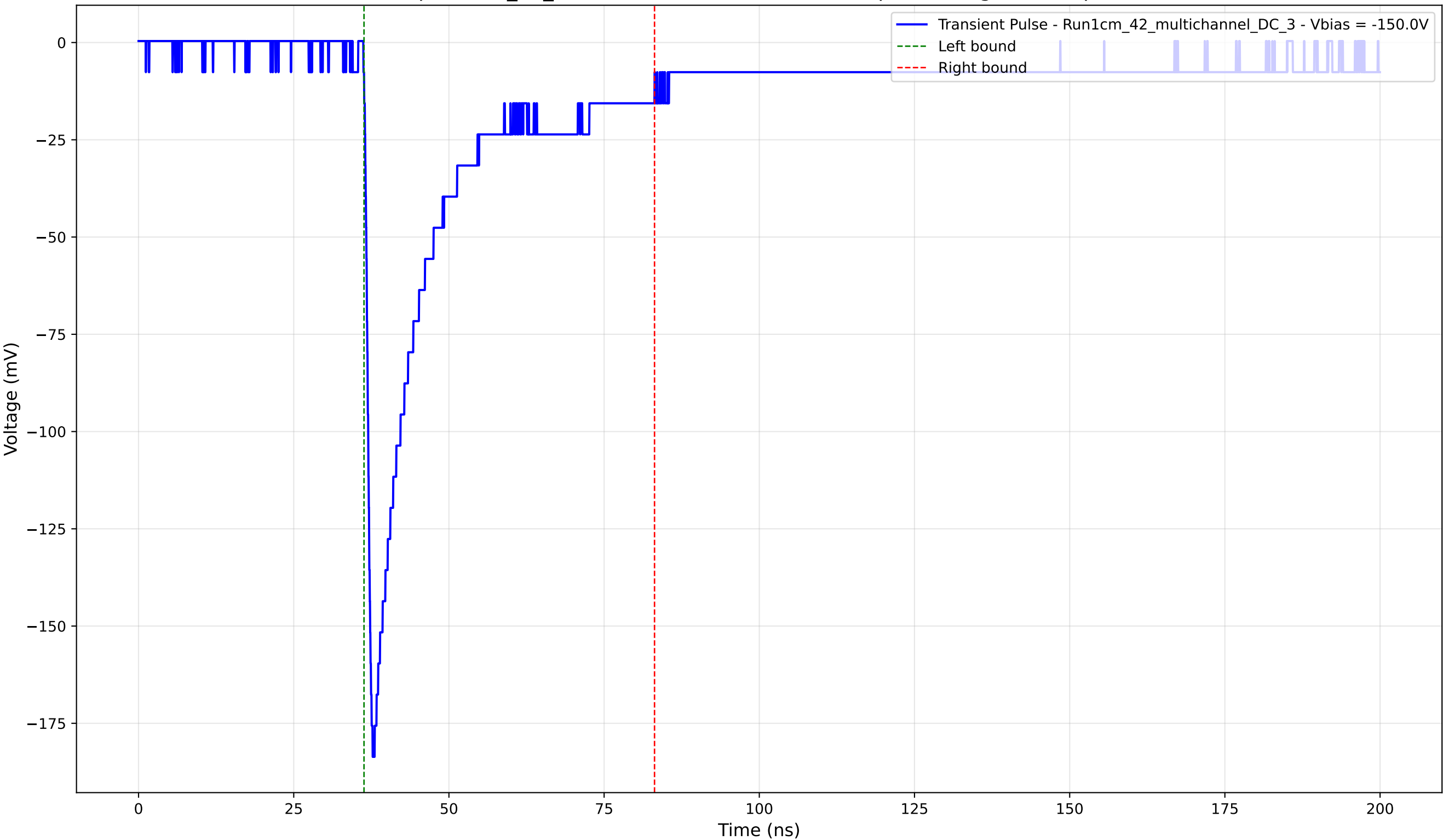
Transient Pulse - Sample: 1cm_42_multichannel - Position: 4110.0 \mu\text{m} - Charge: 39.48 pC - Rise Time: 0.99 ns
