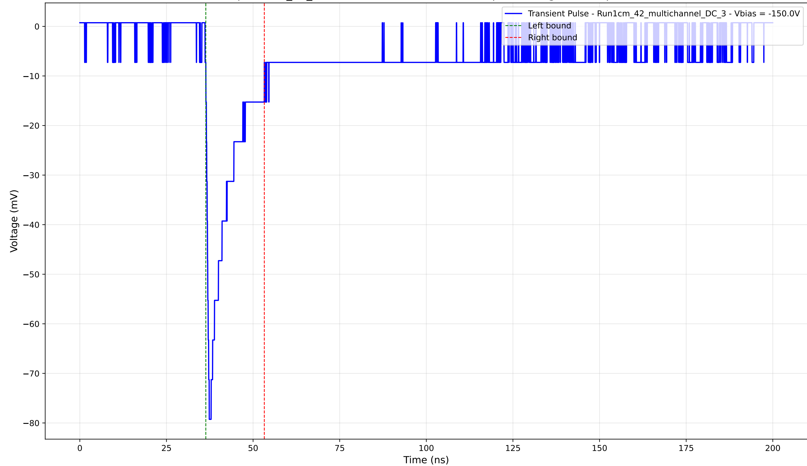
Transient Pulse - Sample: 1cm_42_multichannel - Position: 4345.0 \mu\text{m} - Charge: 10.80 pC - Rise Time: 0.98 ns
