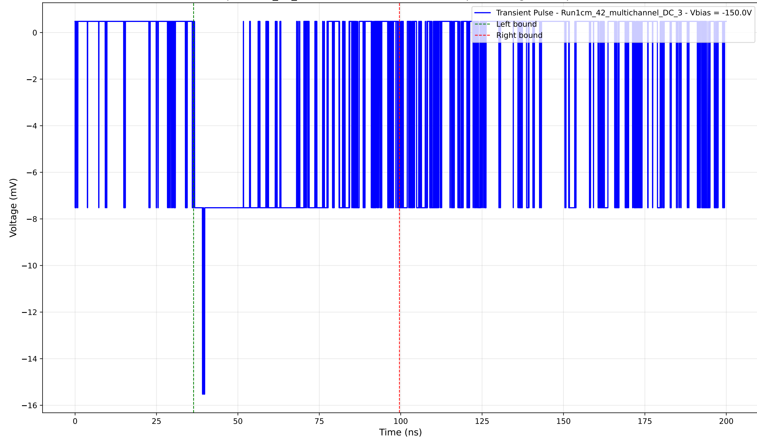
Transient Pulse - Sample: 1cm_42_multichannel - Position: 3370.0 \mu\text{m} - Charge: 6.64 pC - Rise Time: 2.44 ns
