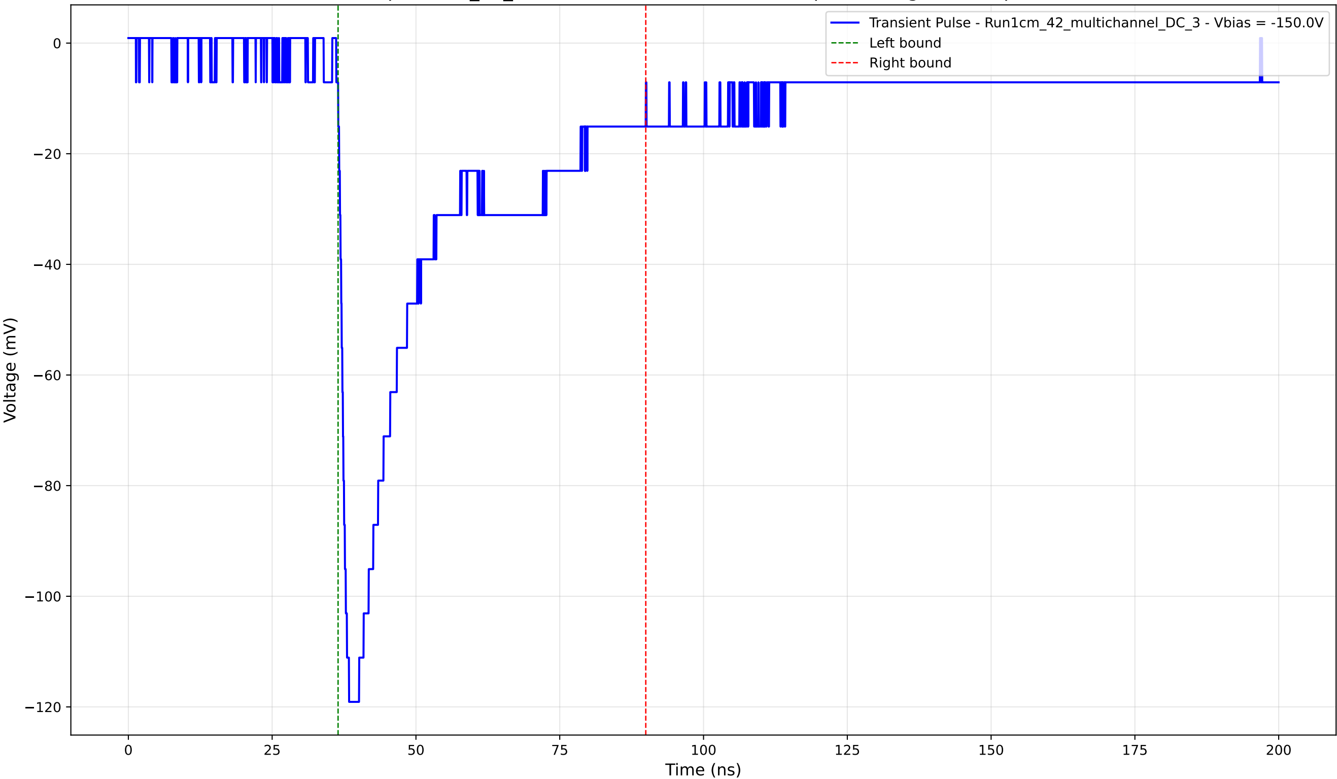
Transient Pulse - Sample: 1cm_42_multichannel - Position: 1655.0 \mu\text{m} - Charge: 41.80 pC - Rise Time: 1.53 ns
