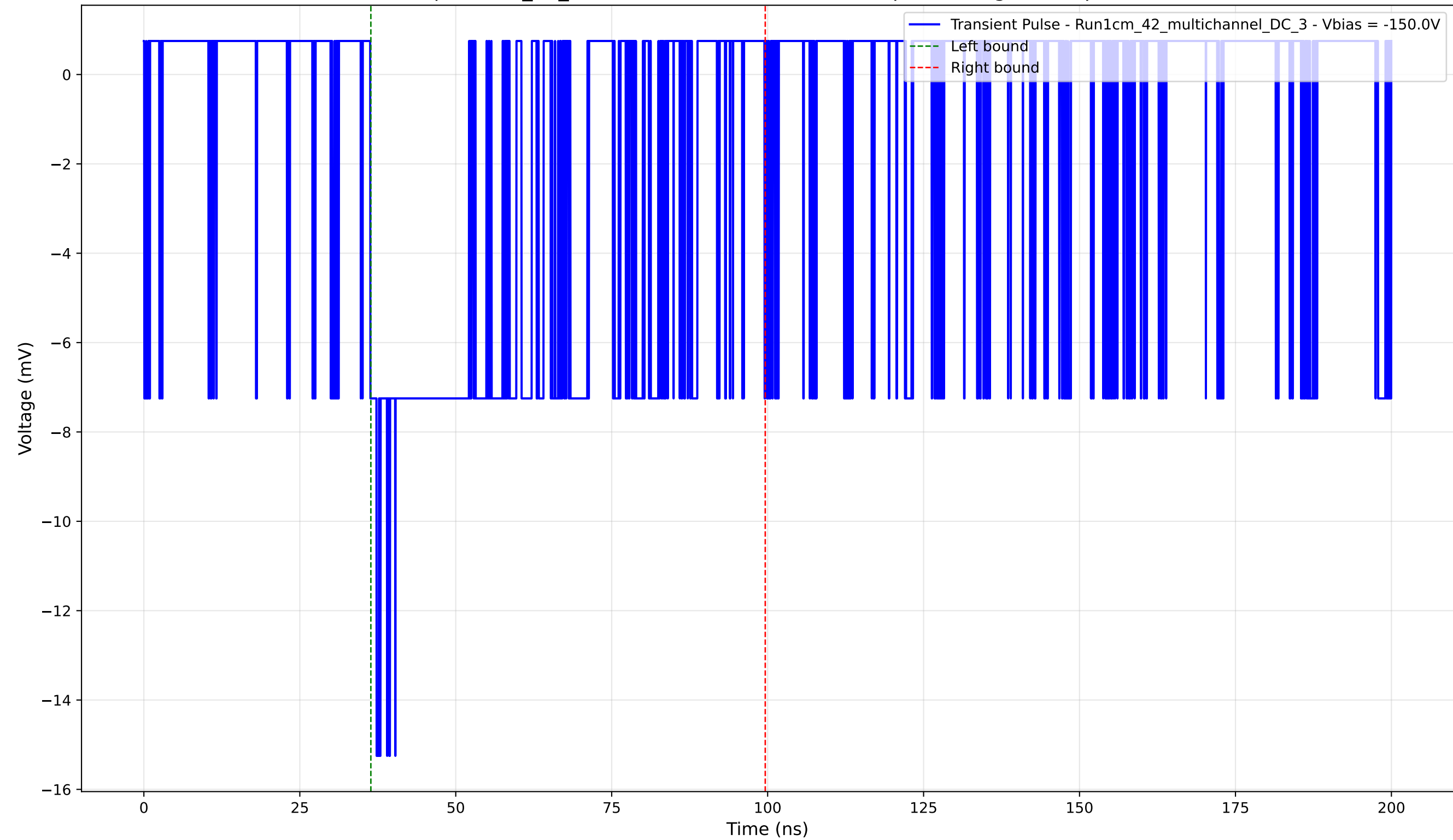
Transient Pulse - Sample: 1cm_42_multichannel - Position: 4390.0 \mu\text{m} - Charge: 4.88 pC - Rise Time: 1.02 ns
