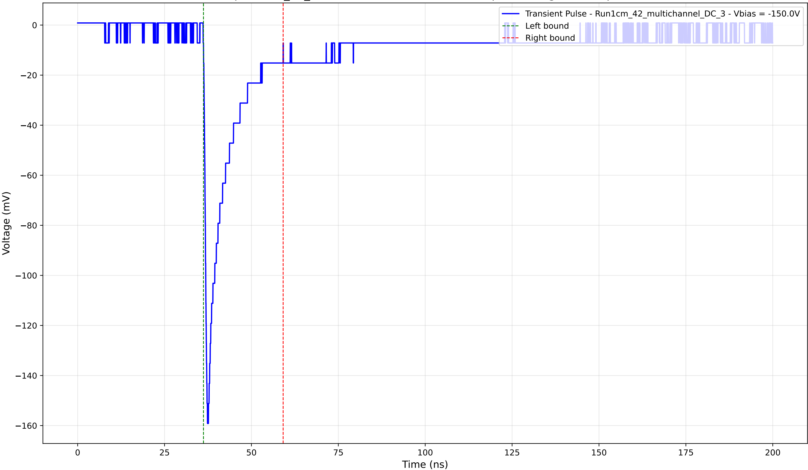
Transient Pulse - Sample: 1cm_42_multichannel - Position: 4450.0 \mu\text{m} - Charge: 20.87 pC - Rise Time: 0.92 ns
