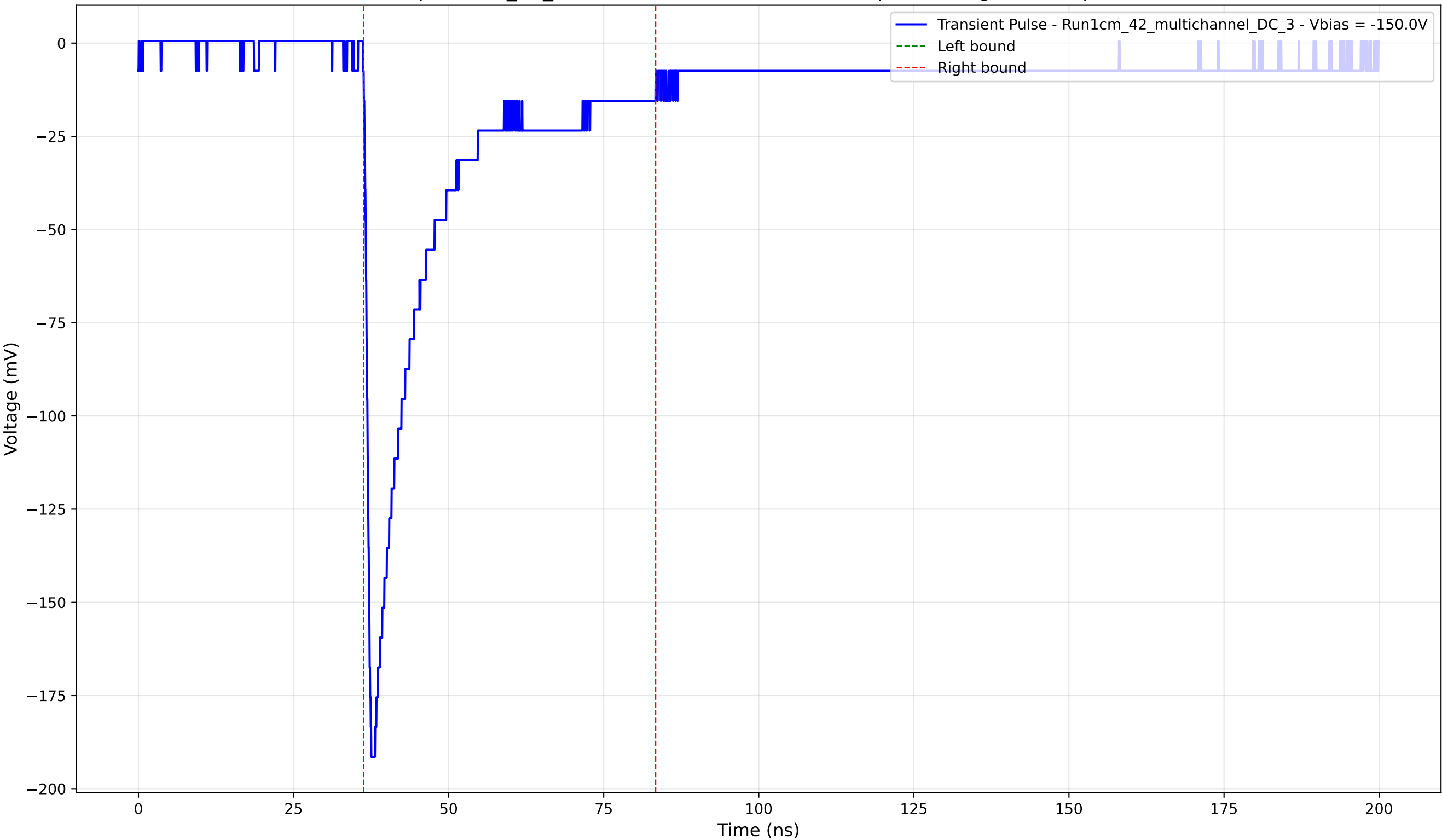
Transient Pulse - Sample: 1cm_42_multichannel - Position: 4160.0 \mu\text{m} - Charge: 40.74 pC - Rise Time: 0.93 ns
