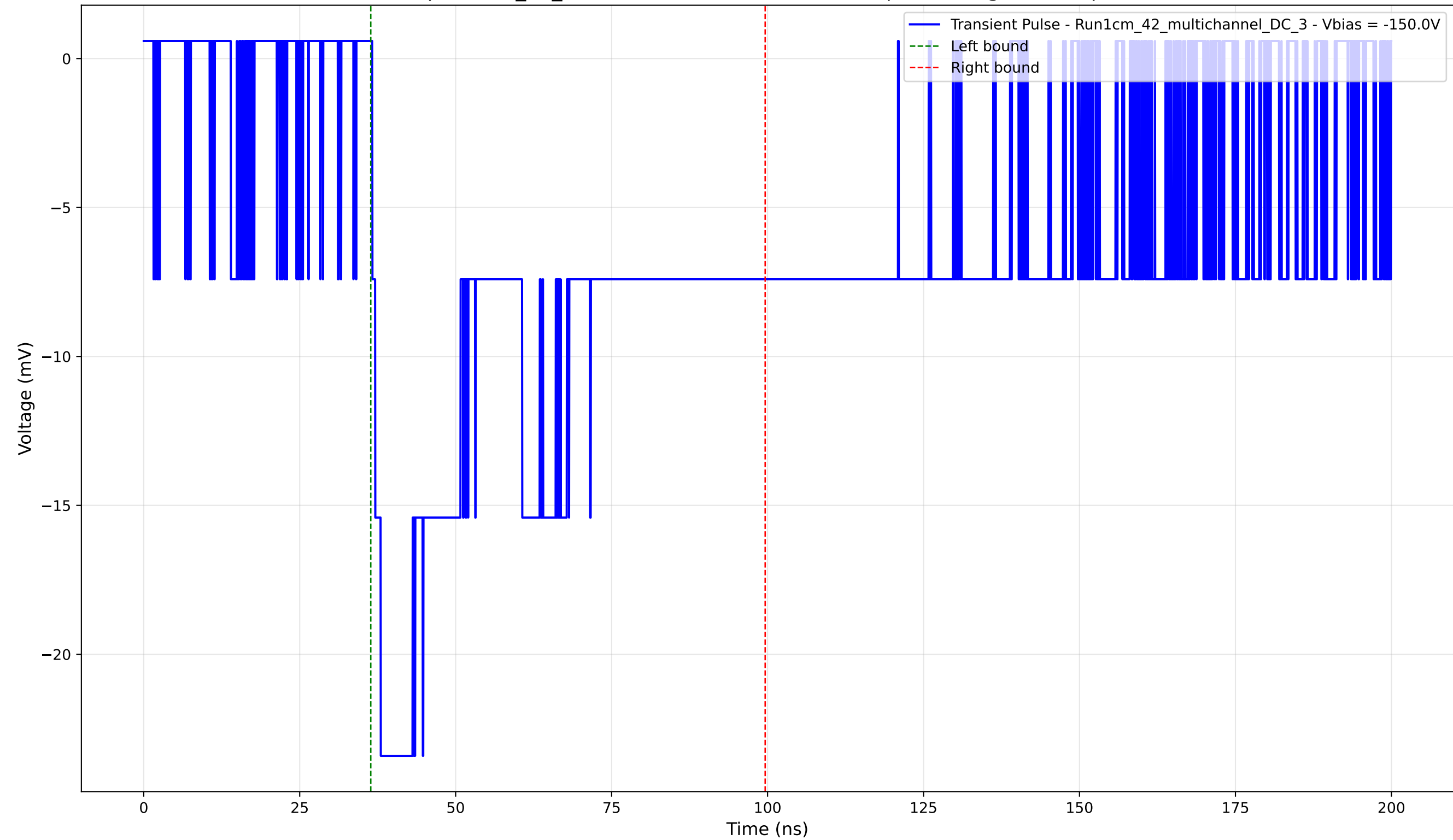
Transient Pulse - Sample: 1cm_42_multichannel - Position: 2335.0 \mu\text{m} - Charge: 13.49 pC - Rise Time: 1.35 ns
