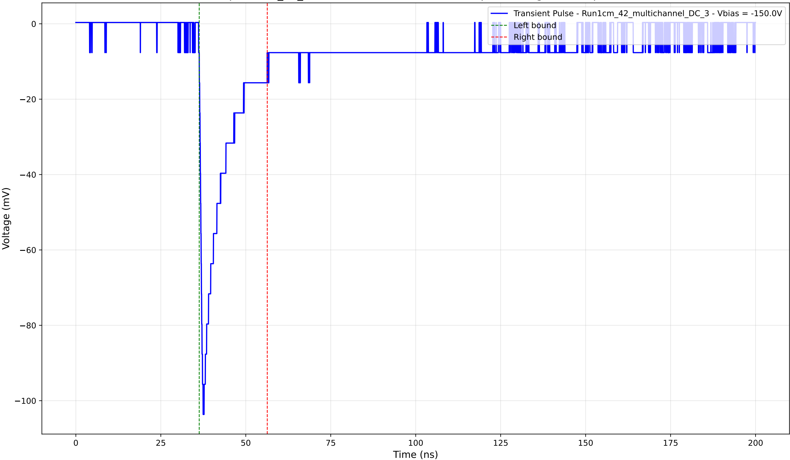
Transient Pulse - Sample: 1cm_42_multichannel - Position: 4340.0 \mu\text{m} - Charge: 14.60 pC - Rise Time: 0.95 ns
