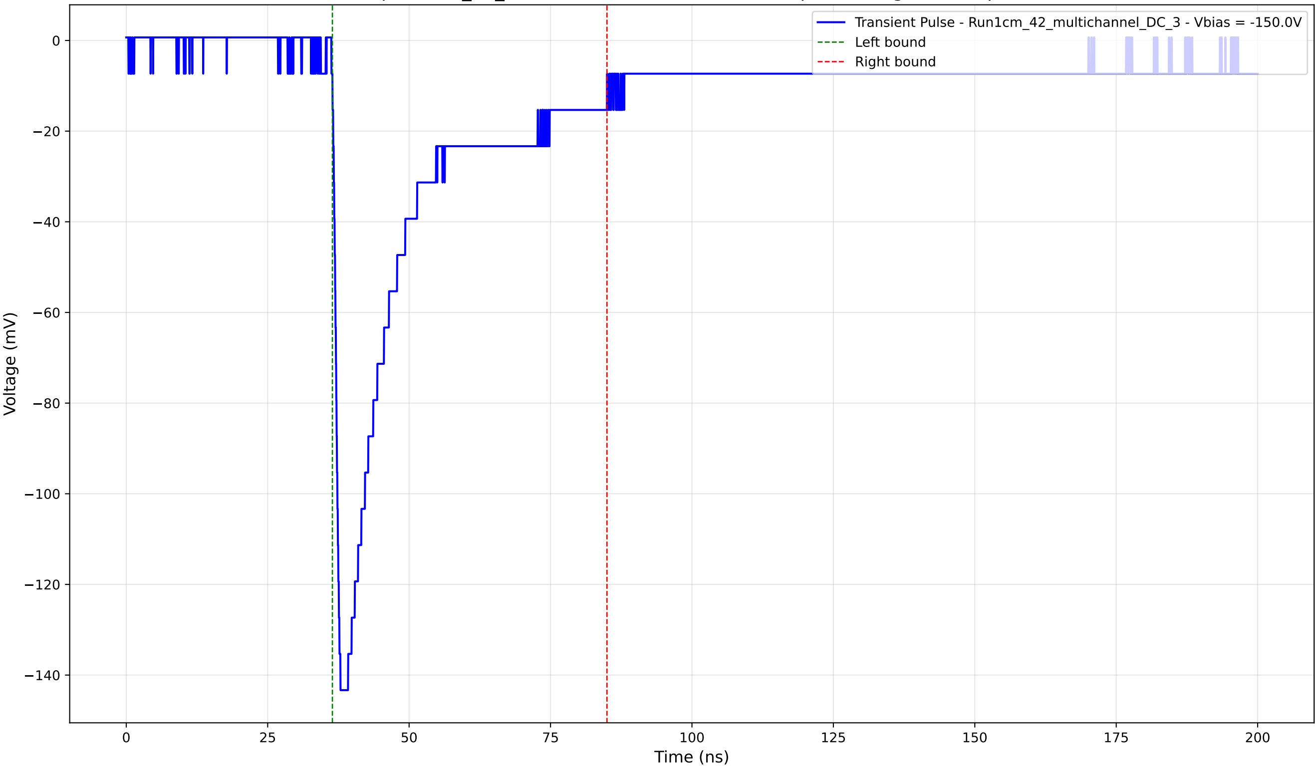
Transient Pulse - Sample: 1cm_42_multichannel - Position: 3765.0 \mu\text{m} - Charge: 38.88 pC - Rise Time: 1.22 ns
