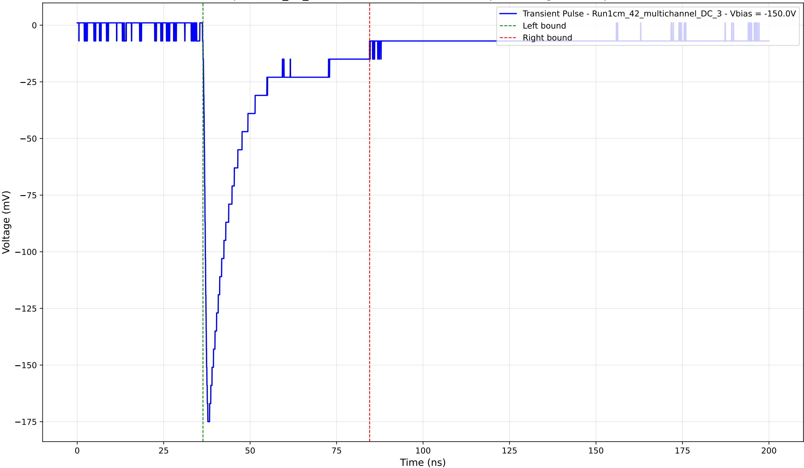
Transient Pulse - Sample: 1cm_42_multichannel - Position: 4020.0 \mu\text{m} - Charge: 39.99 pC - Rise Time: 1.01 ns
