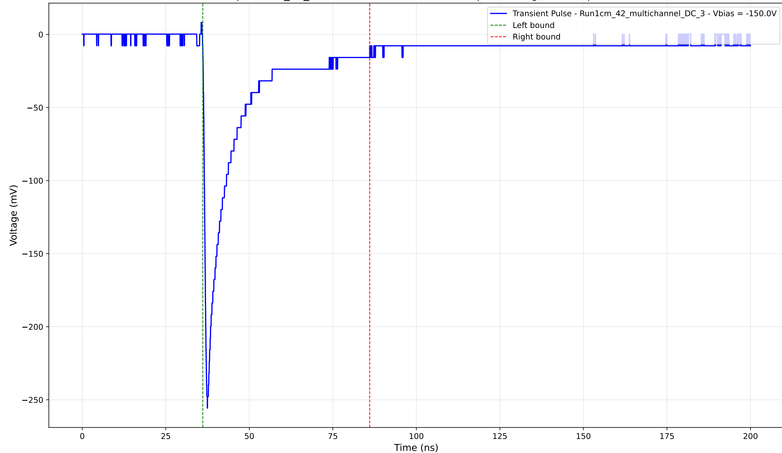
Transient Pulse - Sample: 1cm_42_multichannel - Position: 560.0 \mu\text{m} - Charge: 48.17 pC - Rise Time: 0.94 ns
