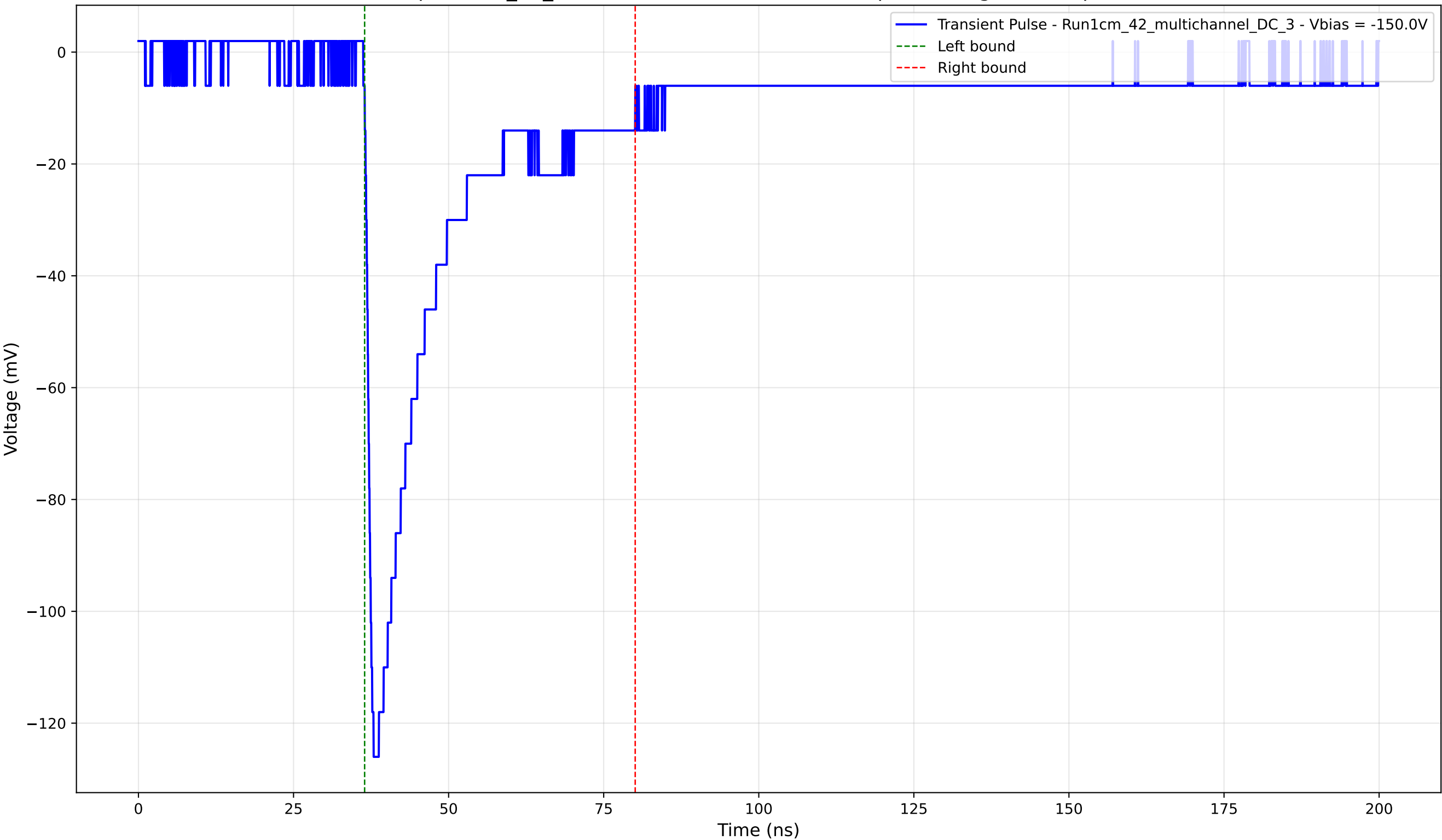
Transient Pulse - Sample: 1cm_42_multichannel - Position: 3820.0 \mu\text{m} - Charge: 30.68 pC - Rise Time: 1.20 ns
