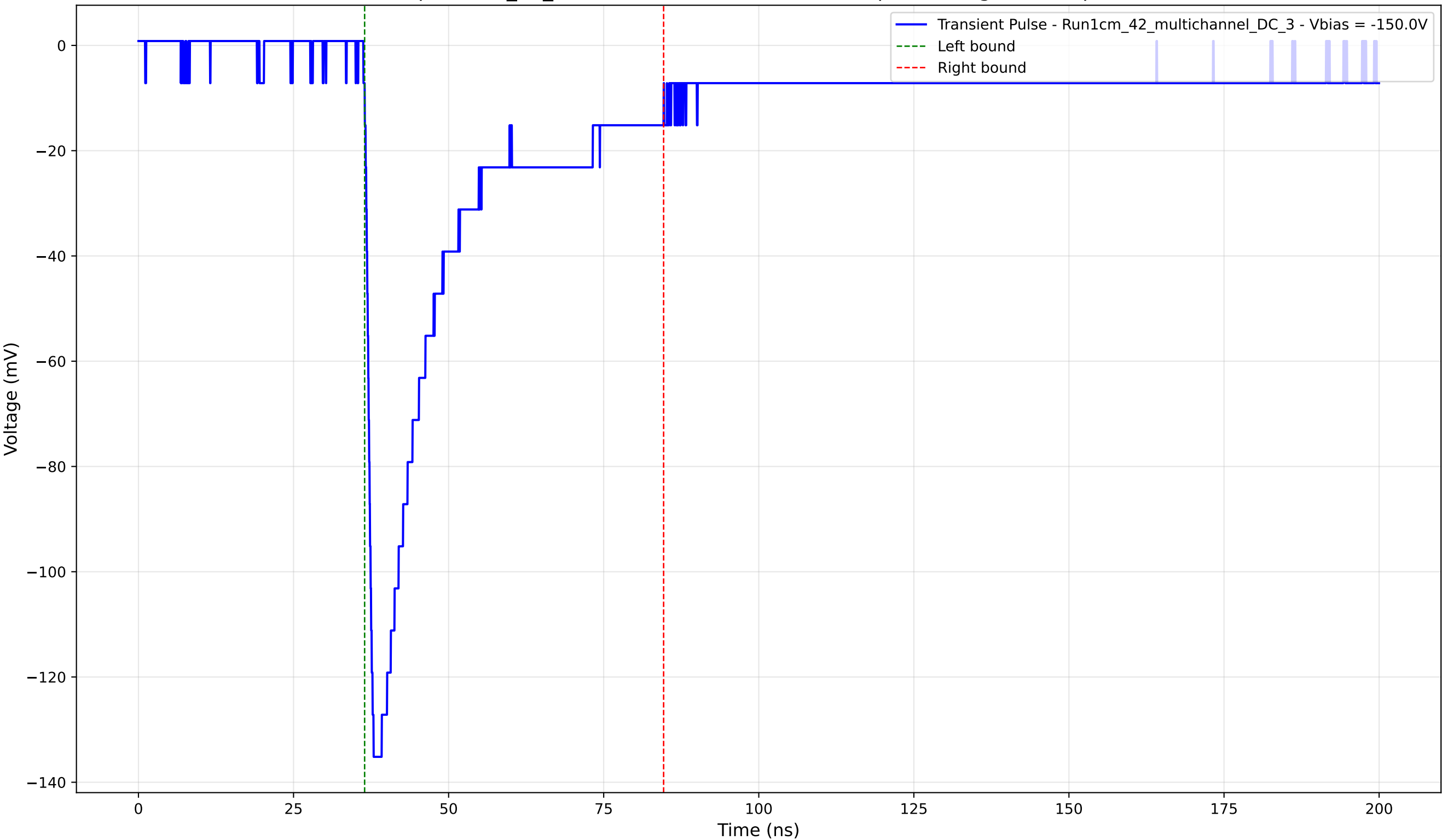
Transient Pulse - Sample: 1cm_42_multichannel - Position: 3715.0 \mu\text{m} - Charge: 37.58 pC - Rise Time: 1.26 ns
