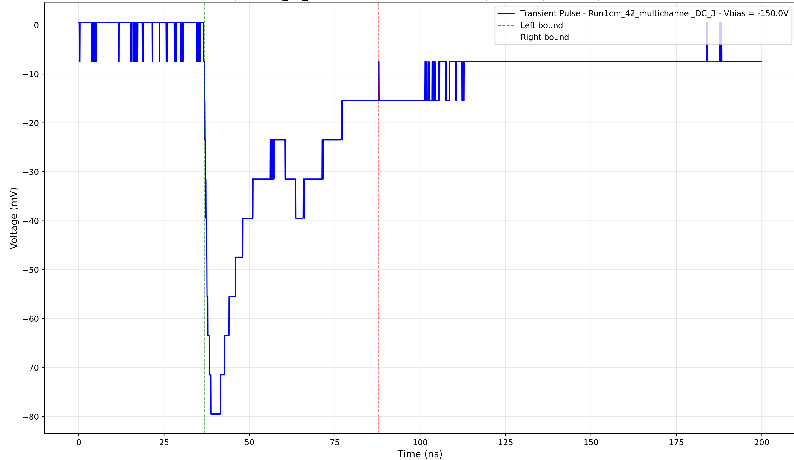
Transient Pulse - Sample: 1cm_42_multichannel - Position: 2585.0 \mu\text{m} - Charge: 34.84 pC - Rise Time: 1.96 ns
