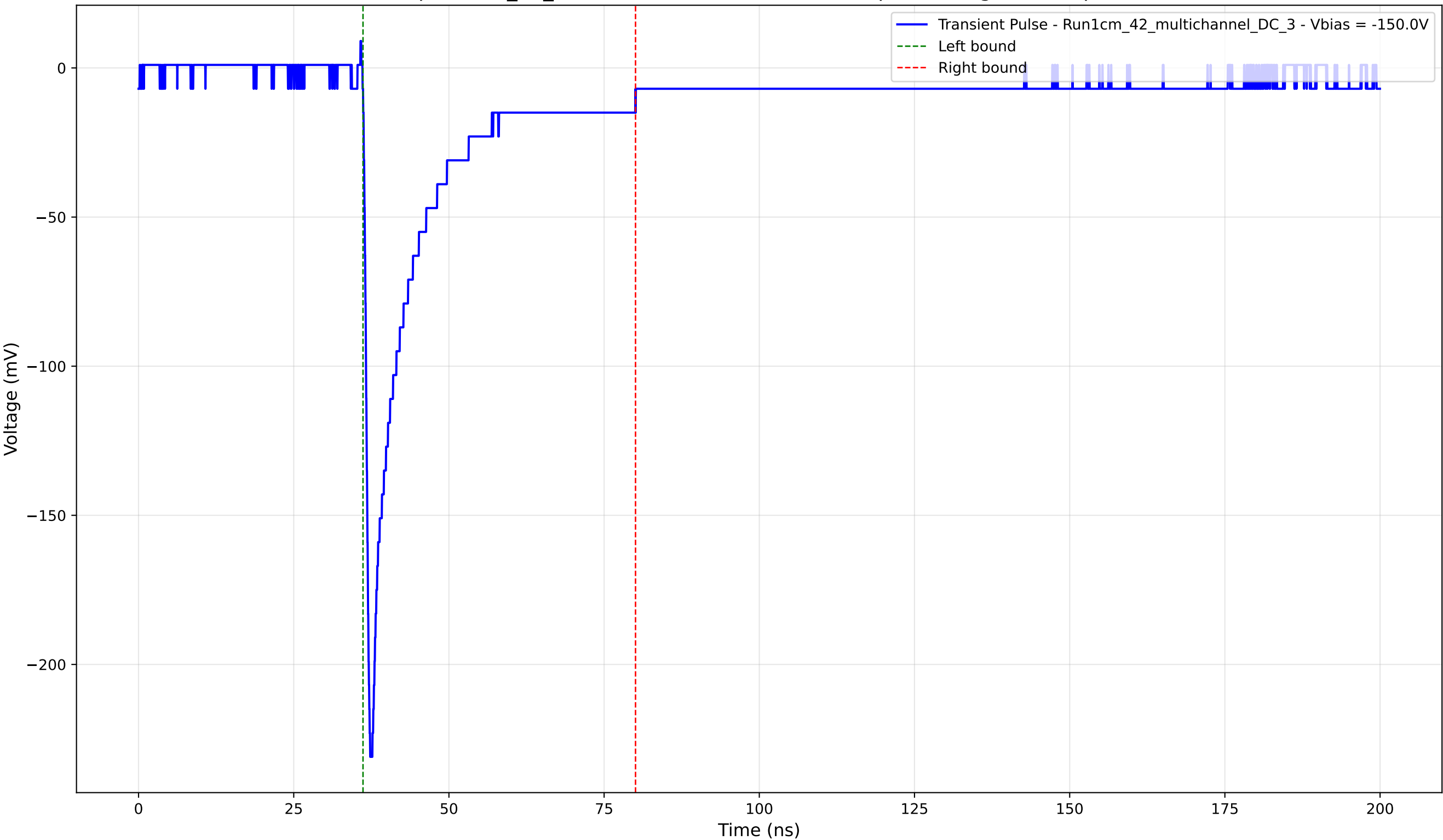
Transient Pulse - Sample: 1cm_42_multichannel - Position: 4475.0 \mu\text{m} - Charge: 36.06 pC - Rise Time: 0.88 ns
