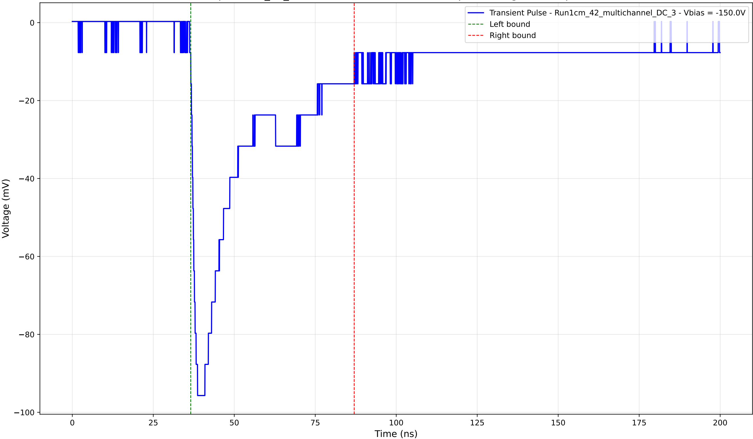
Transient Pulse - Sample: 1cm_42_multichannel - Position: 2965.0 \mu\text{m} - Charge: 35.97 pC - Rise Time: 1.66 ns
