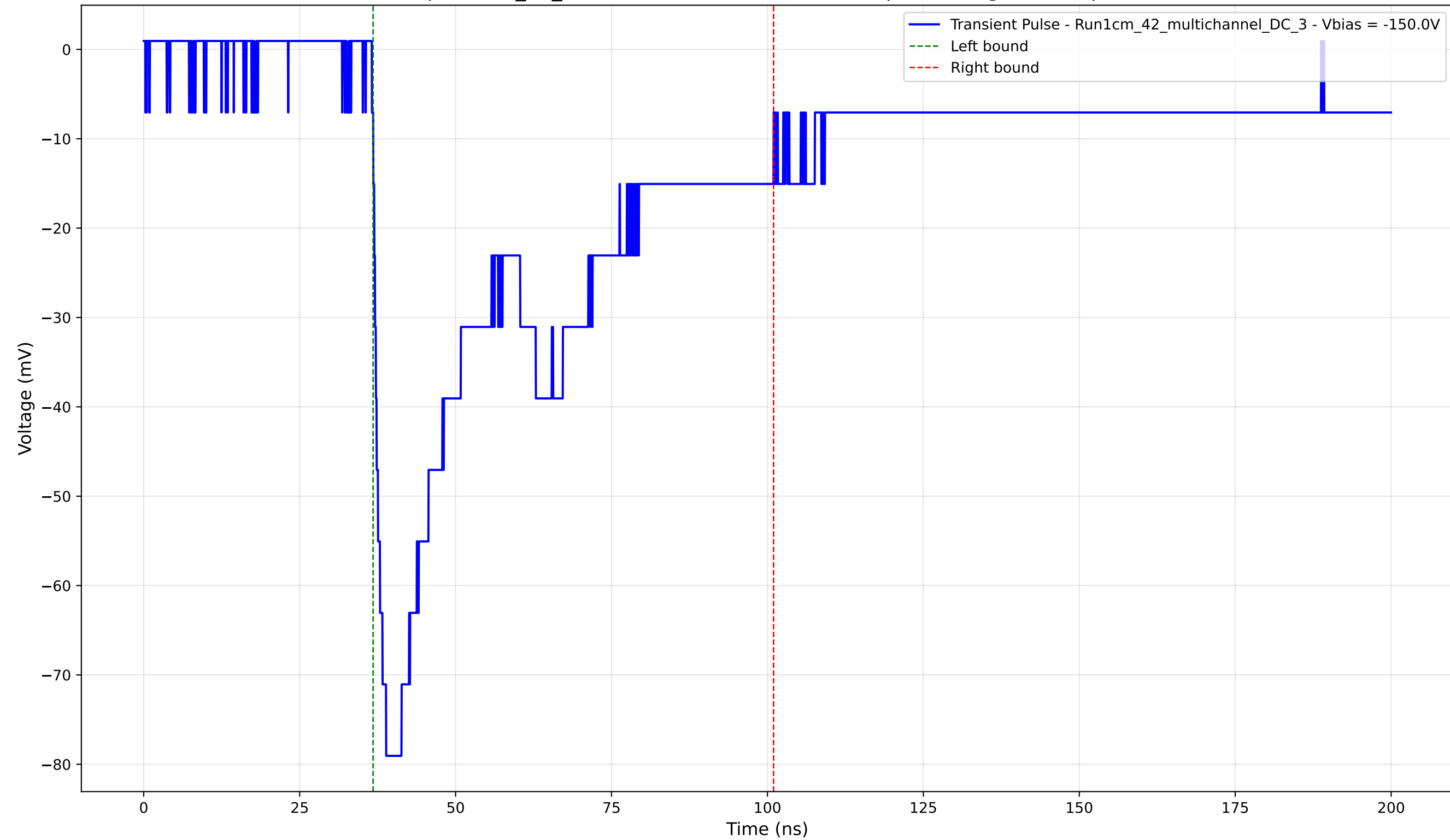
Transient Pulse - Sample: 1cm_42_multichannel - Position: 2520.0 \mu\text{m} - Charge: 38.71 pC - Rise Time: 2.08 ns
