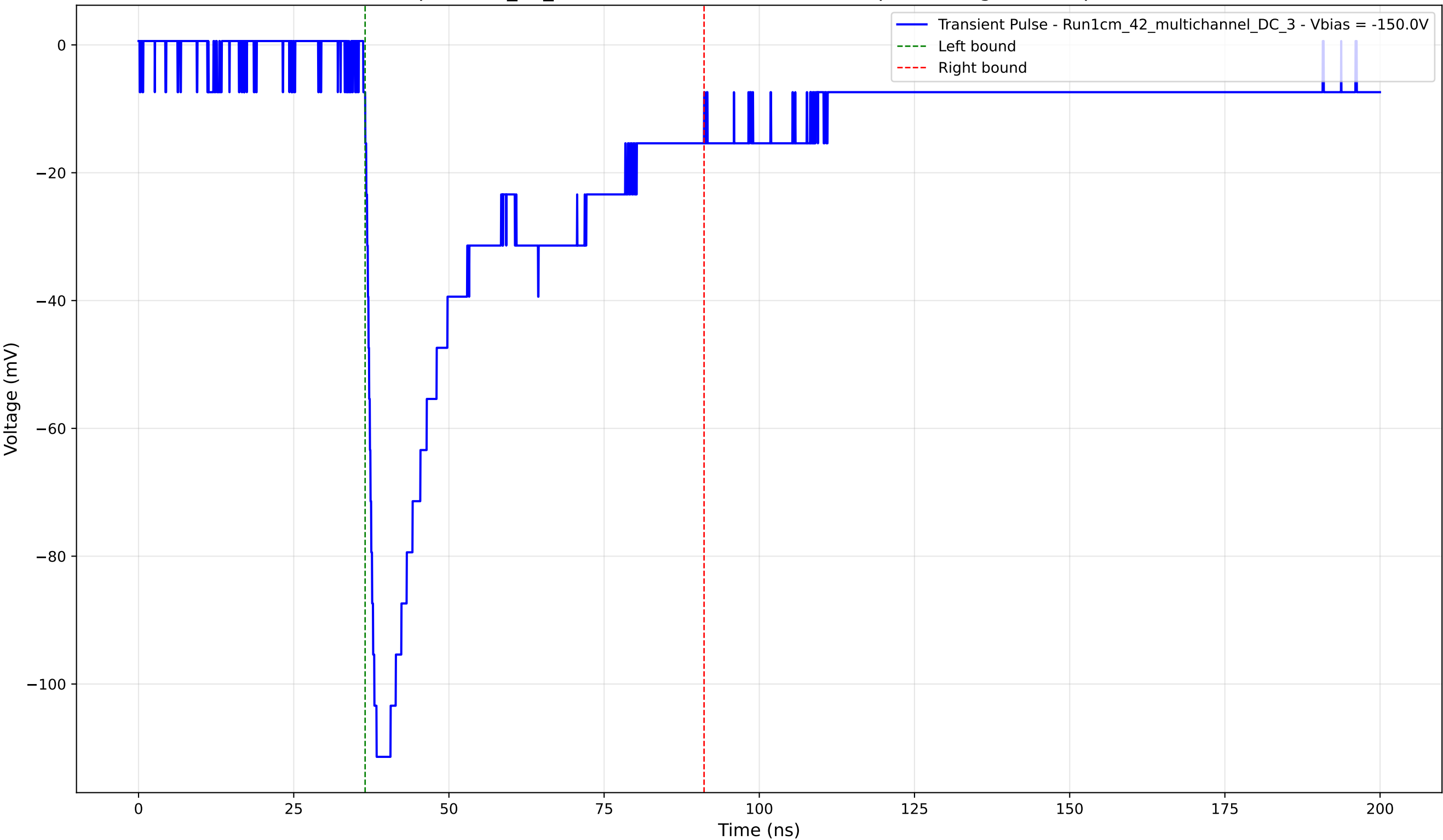
Transient Pulse - Sample: 1cm_42_multichannel - Position: 1745.0 \mu\text{m} - Charge: 41.64 pC - Rise Time: 1.47 ns
