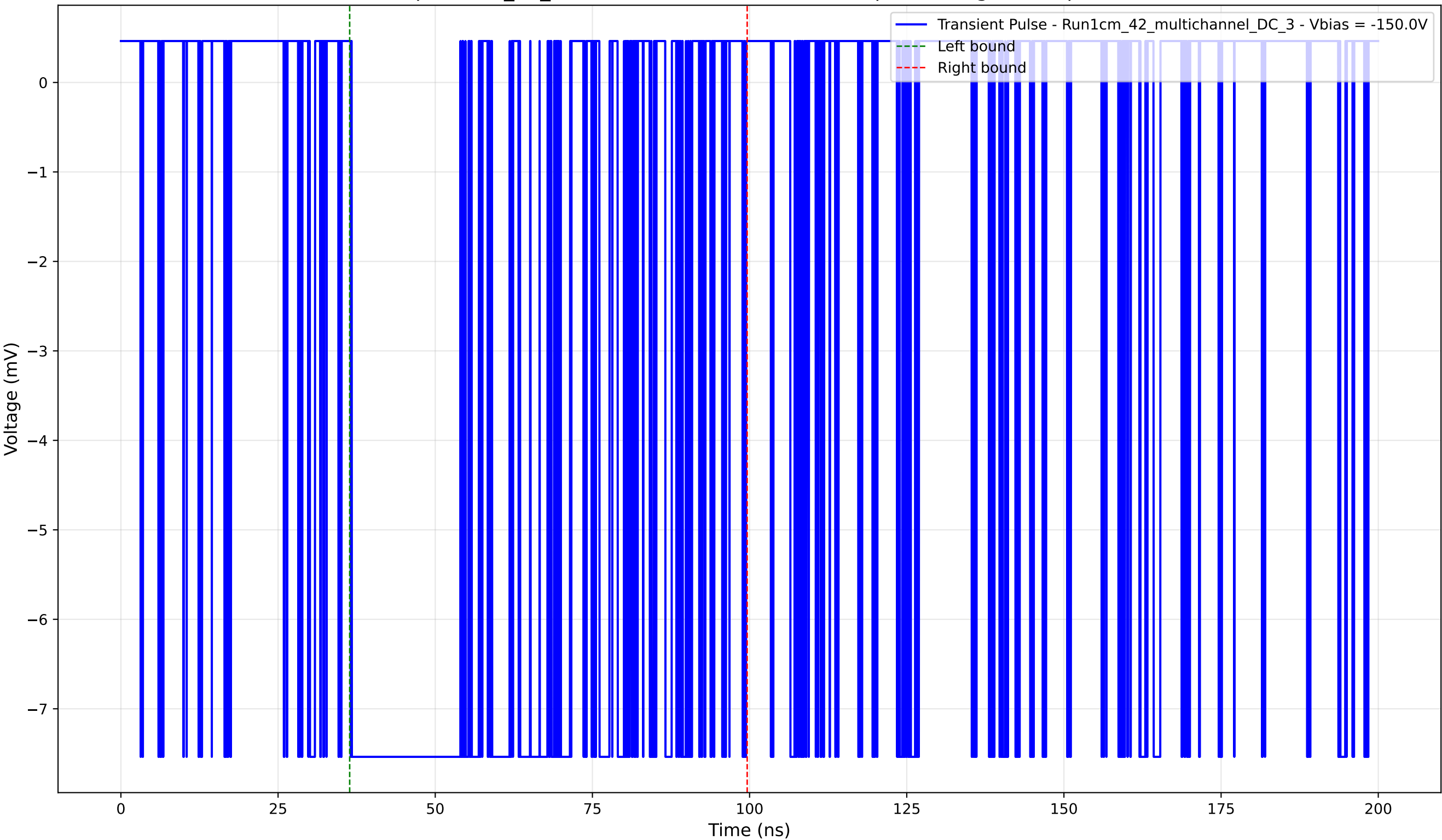
Transient Pulse - Sample: 1cm_42_multichannel - Position: 3895.0 \mu\text{m} - Charge: 5.84 pC - Rise Time: 0.02 ns
