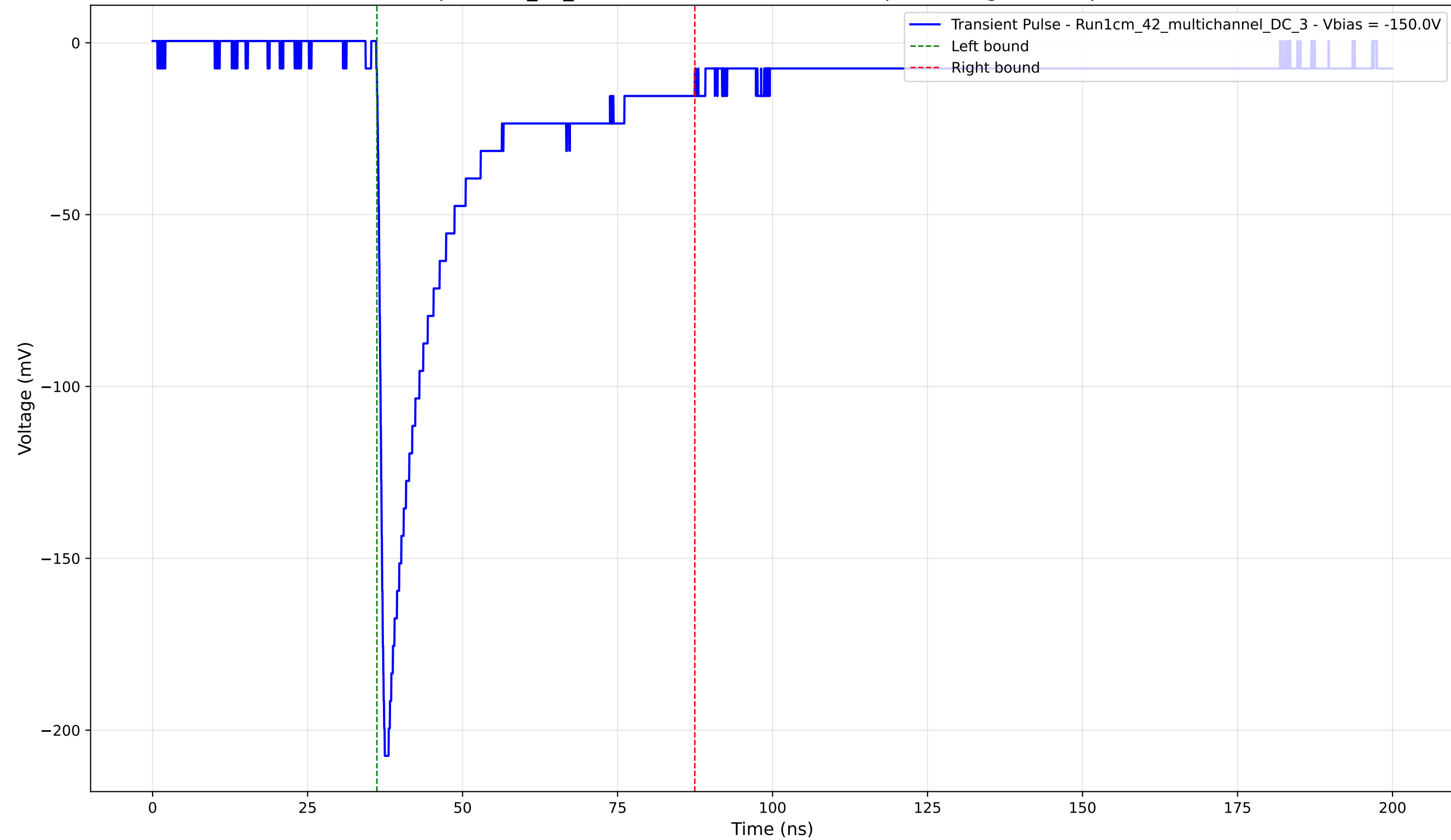
Transient Pulse - Sample: 1cm_42_multichannel - Position: 750.0 \mu\text{m} - Charge: 46.24 pC - Rise Time: 0.99 ns
