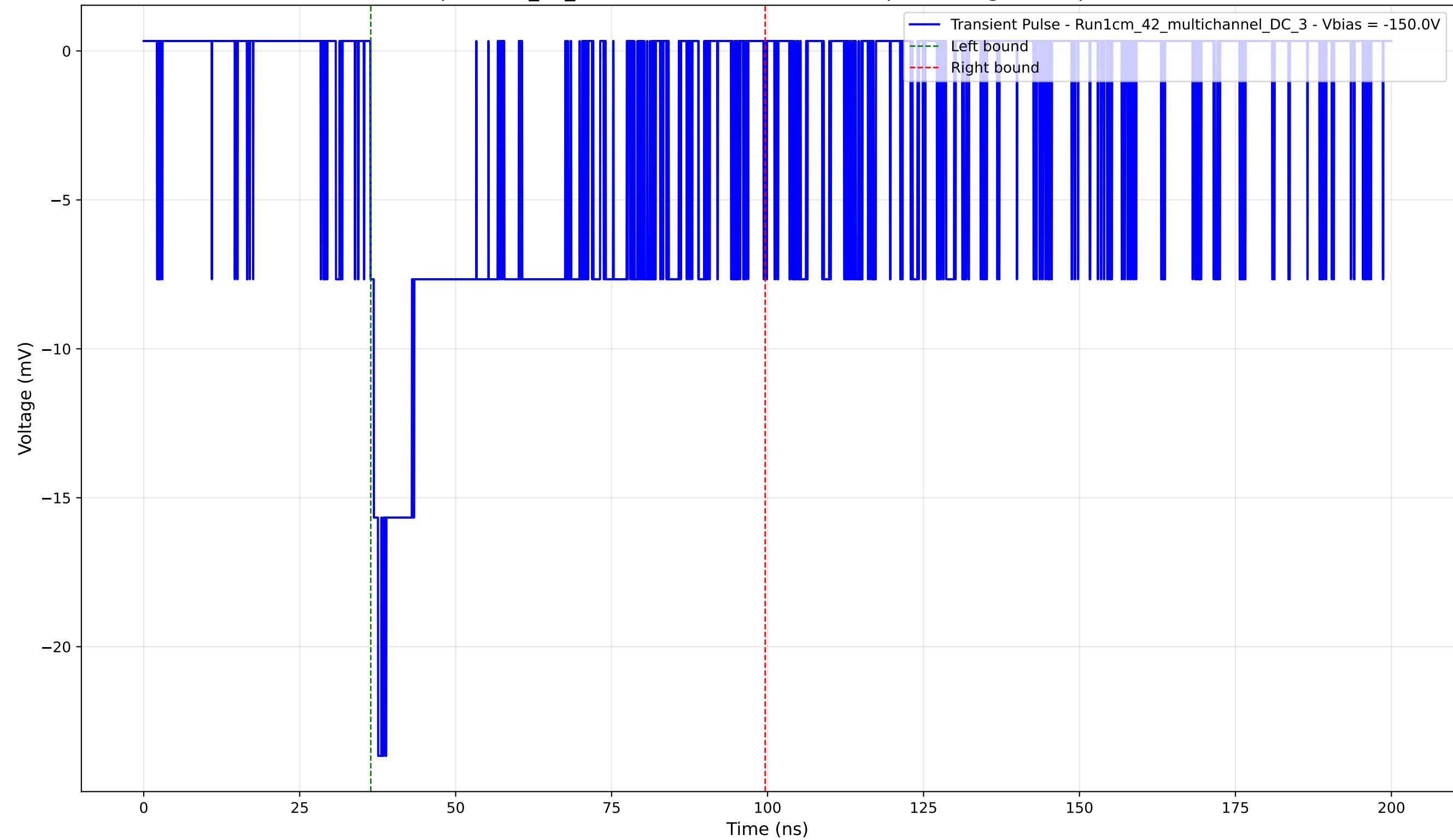
Transient Pulse - Sample: 1cm_42_multichannel - Position: 835.0 \mu\text{m} - Charge: 8.00 pC - Rise Time: 1.23 ns
