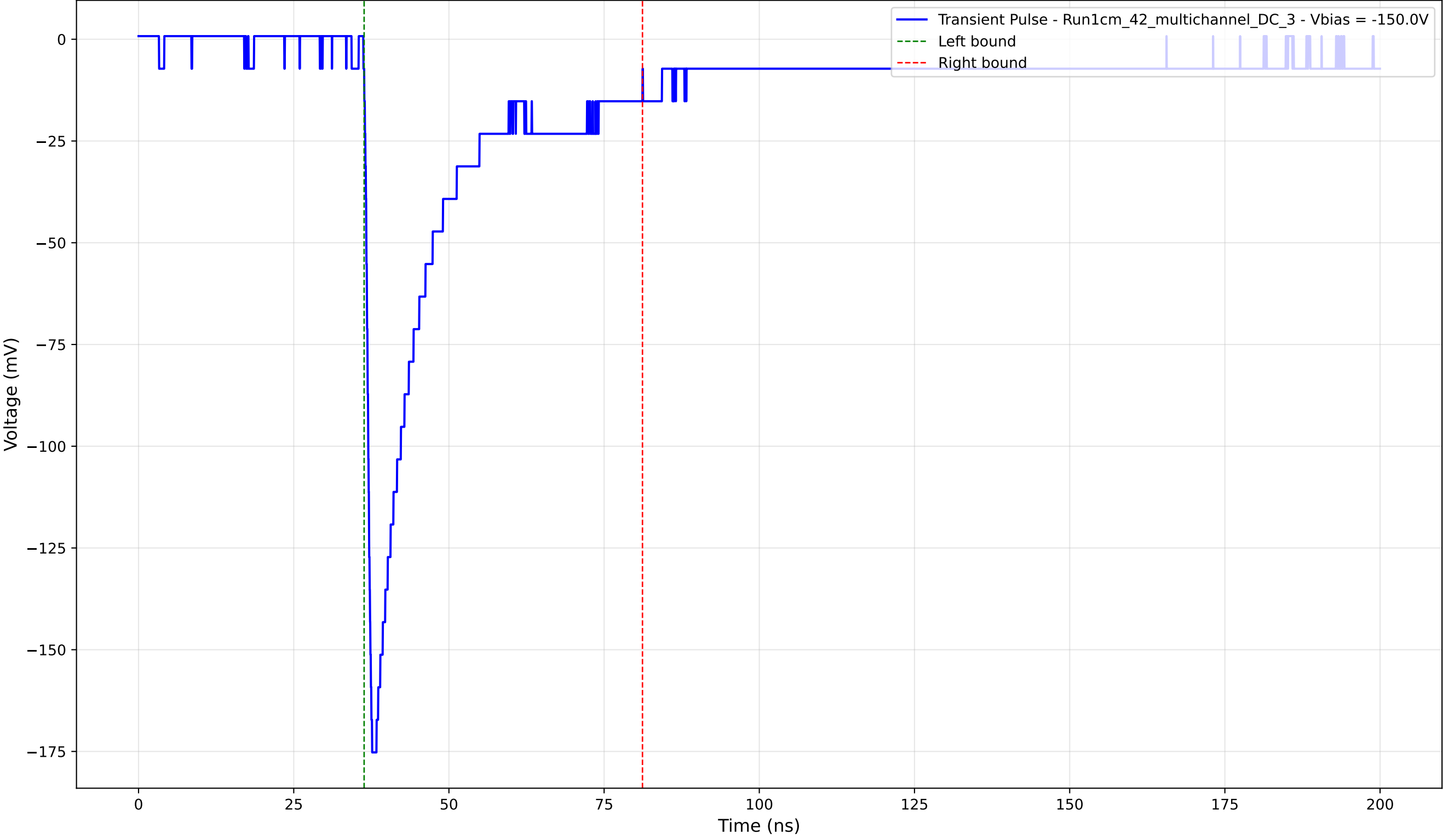
Transient Pulse - Sample: 1cm_42_multichannel - Position: 4080.0 \mu\text{m} - Charge: 38.68 pC - Rise Time: 0.97 ns
