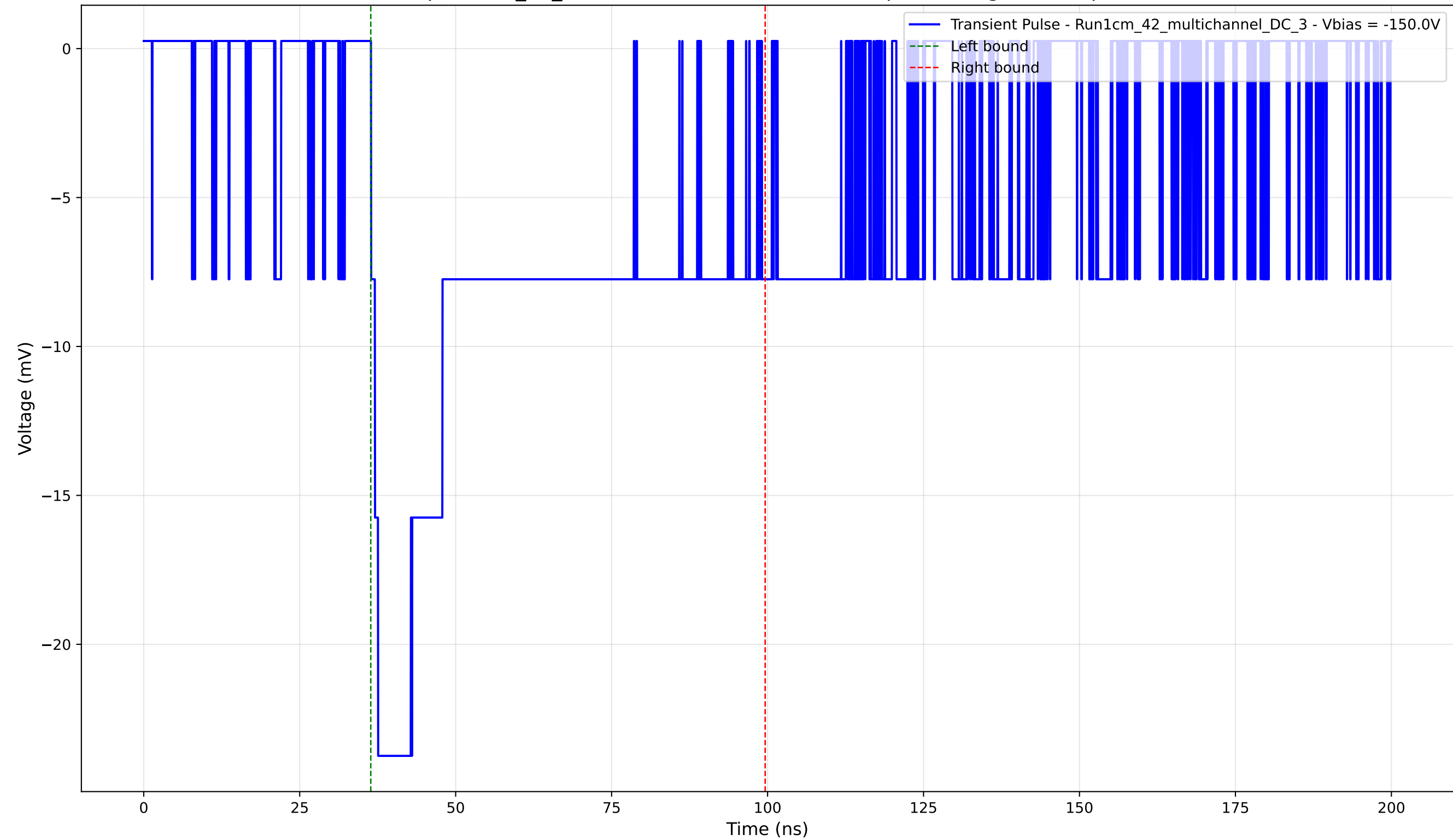
Transient Pulse - Sample: 1cm_42_multichannel - Position: 3420.0 \mu\text{m} - Charge: 12.08 pC - Rise Time: 1.13 ns
