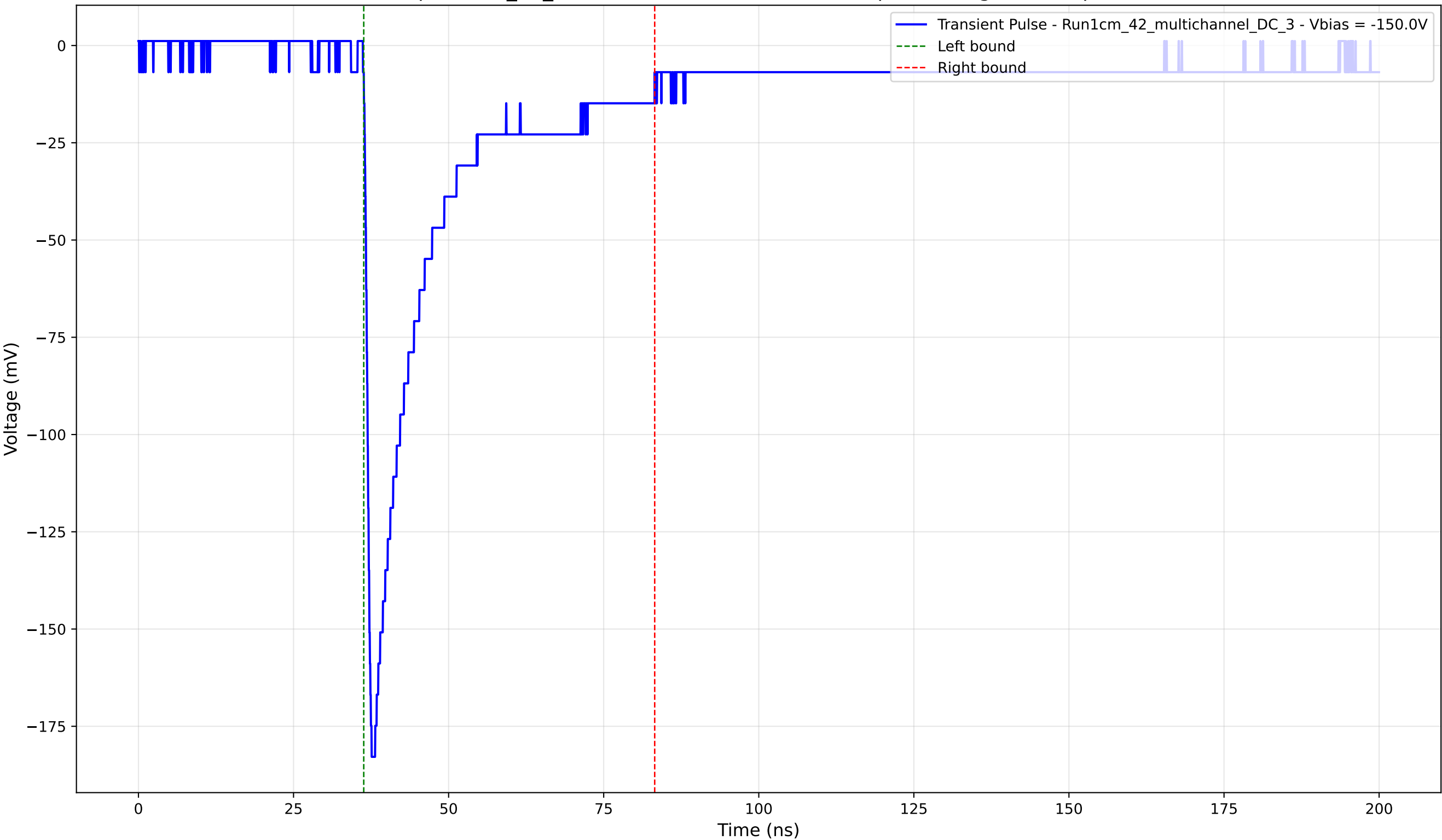
Transient Pulse - Sample: 1cm_42_multichannel - Position: 4130.0 \mu\text{m} - Charge: 39.34 pC - Rise Time: 0.95 ns
