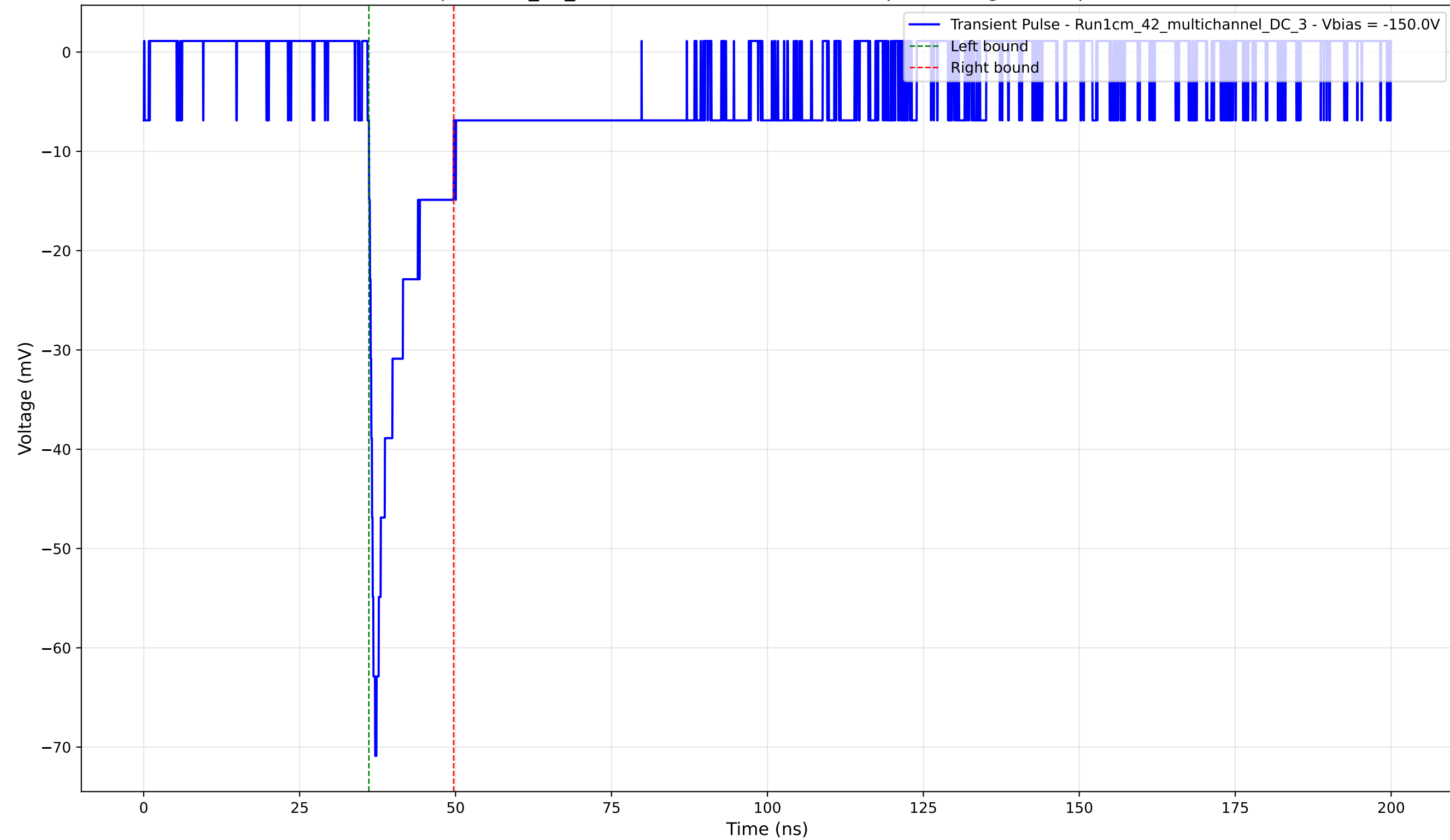
Transient Pulse - Sample: 1cm_42_multichannel - Position: 315.0 \mu\text{m} - Charge: 7.38 pC - Rise Time: 1.00 ns
