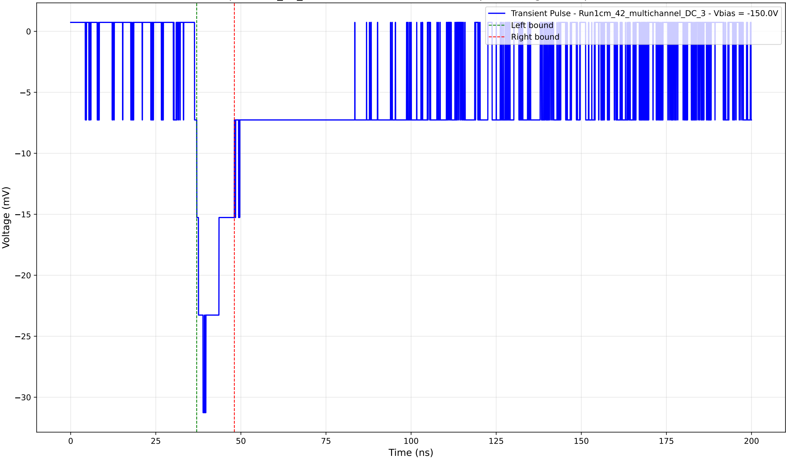
Transient Pulse - Sample: 1cm_42_multichannel - Position: 3350.0 \mu\text{m} - Charge: 4.45 pC - Rise Time: 2.51 ns
