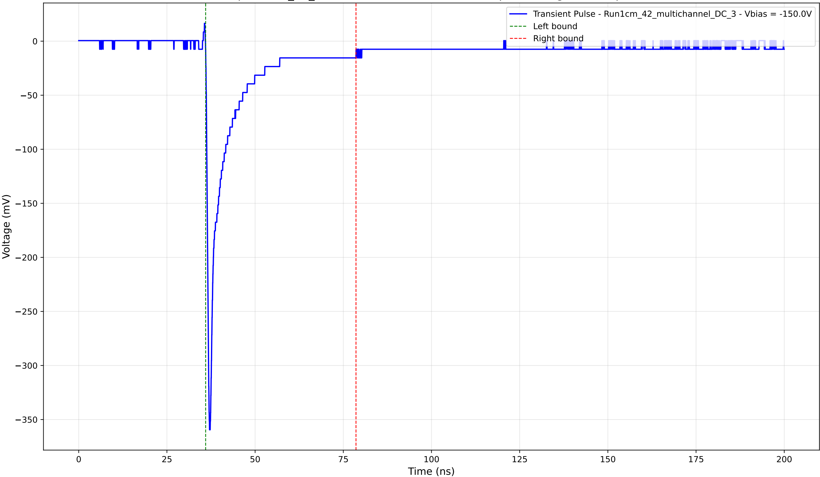
Transient Pulse - Sample: 1cm_42_multichannel - Position: 4785.0 \mu\text{m} - Charge: 40.68 pC - Rise Time: 0.78 ns
