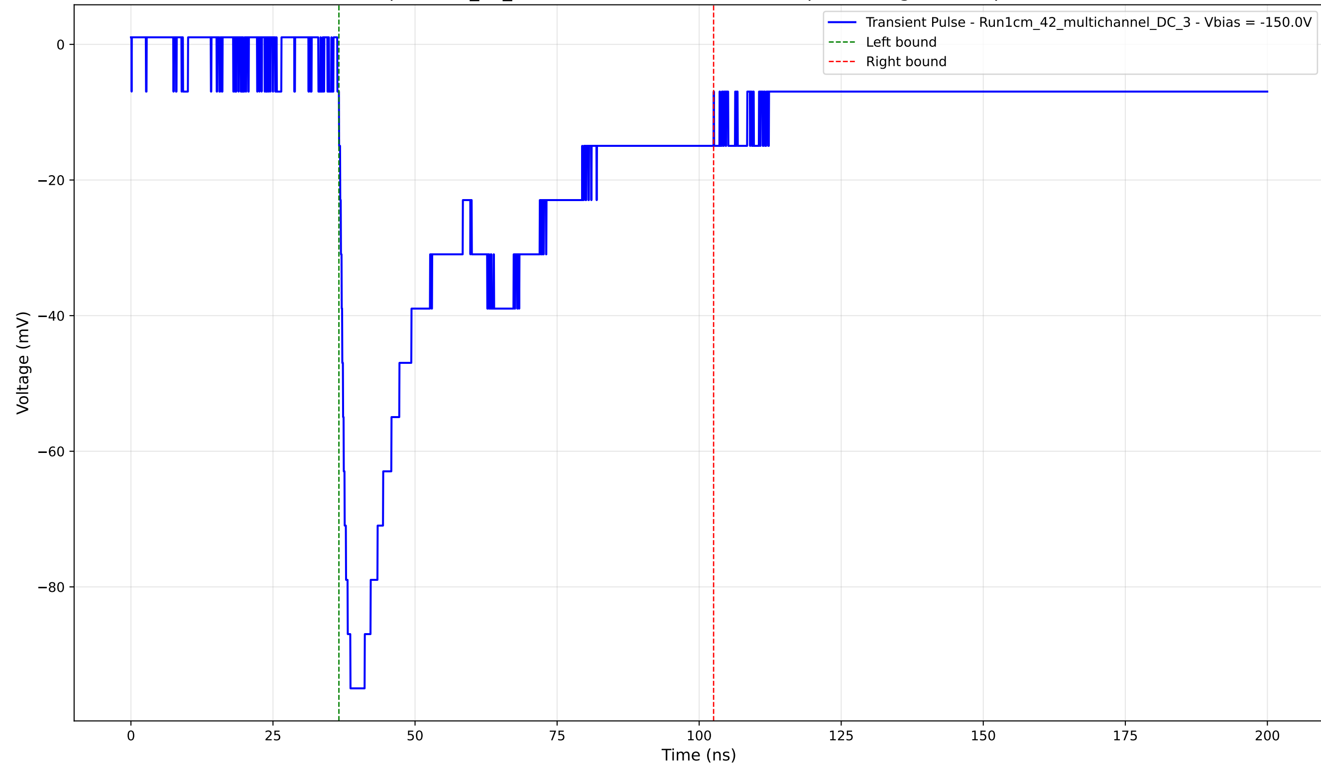
Transient Pulse - Sample: 1cm_42_multichannel - Position: 2015.0 \mu\text{m} - Charge: 43.18 pC - Rise Time: 1.53 ns
