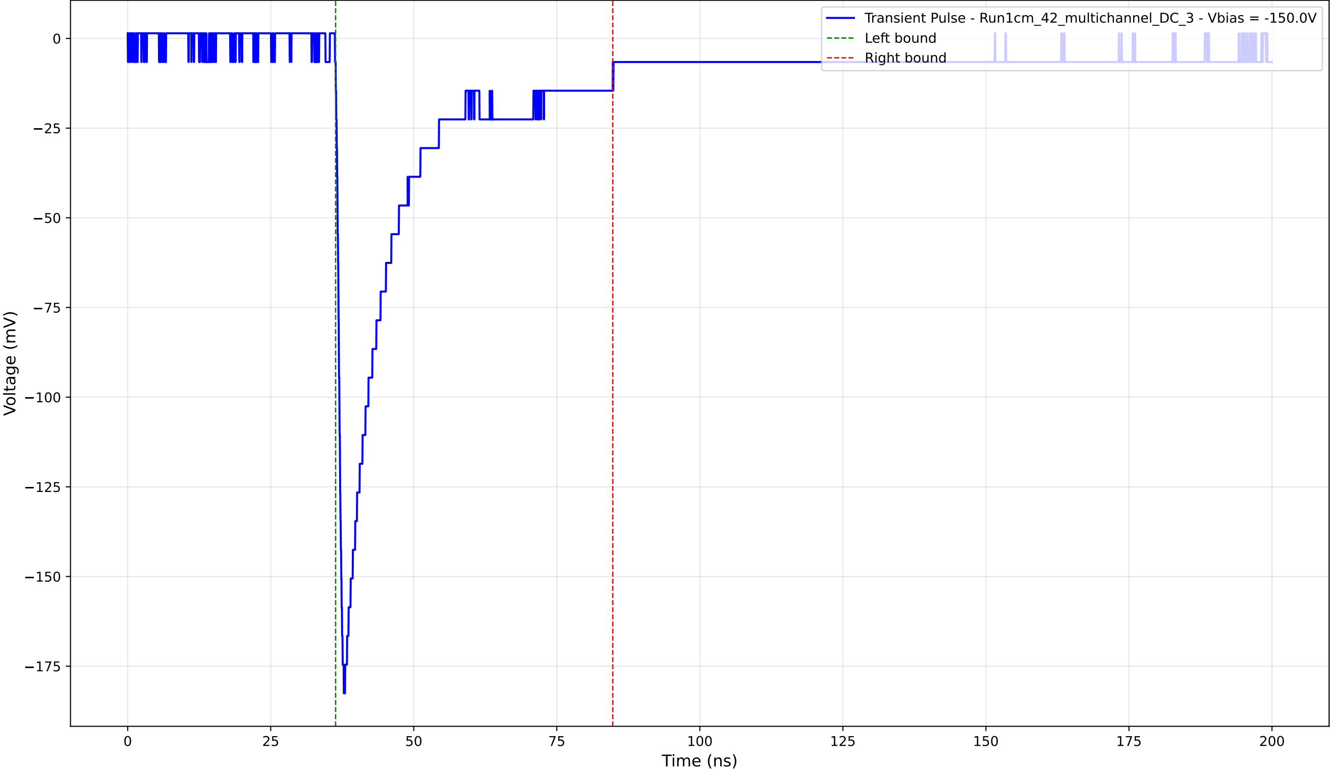
Transient Pulse - Sample: 1cm_42_multichannel - Position: 4105.0 \mu\text{m} - Charge: 38.71 pC - Rise Time: 1.03 ns
