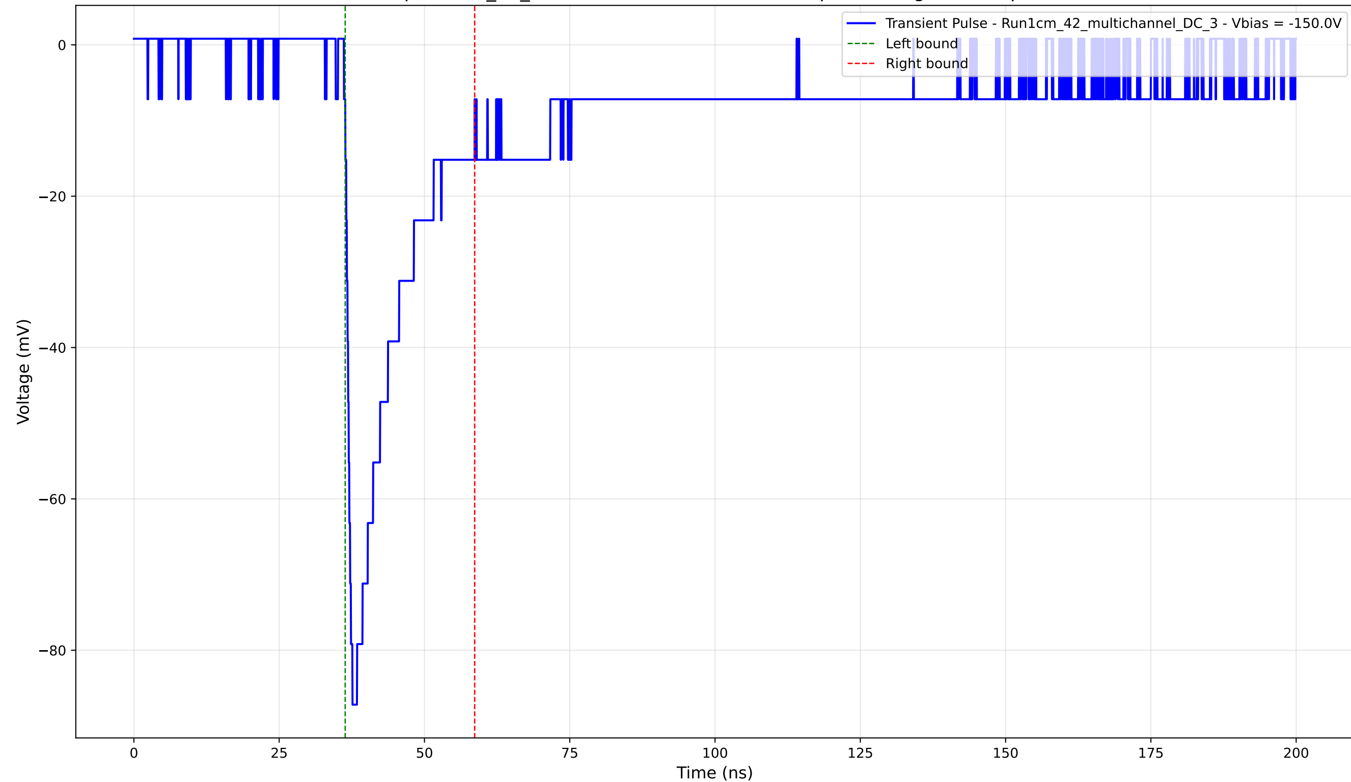
Transient Pulse - Sample: 1cm_42_multichannel - Position: 905.0 \mu\text{m} - Charge: 16.01 pC - Rise Time: 0.98 ns
