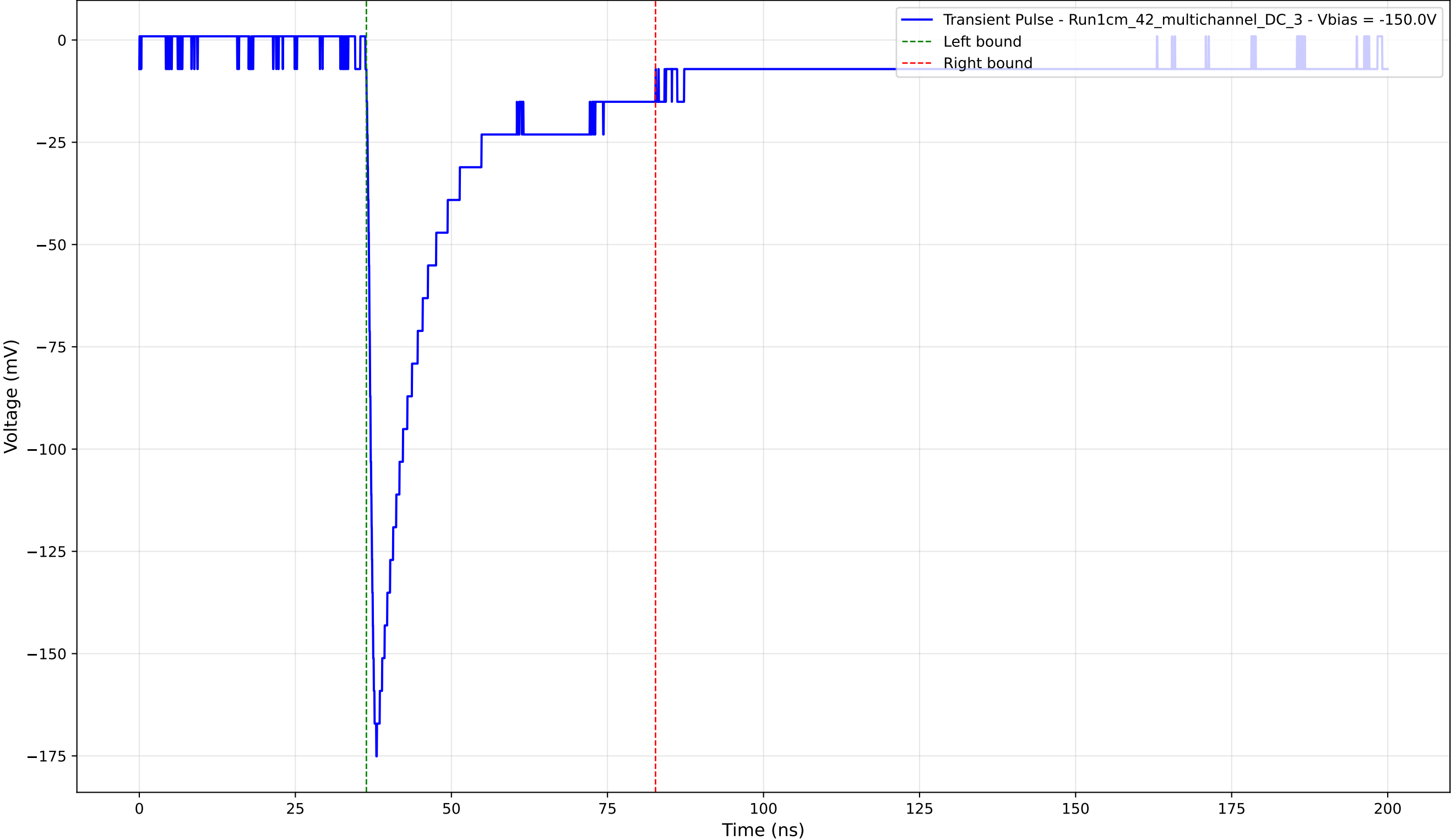
Transient Pulse - Sample: 1cm_42_multichannel - Position: 3995.0 \mu\text{m} - Charge: 39.03 pC - Rise Time: 1.07 ns
