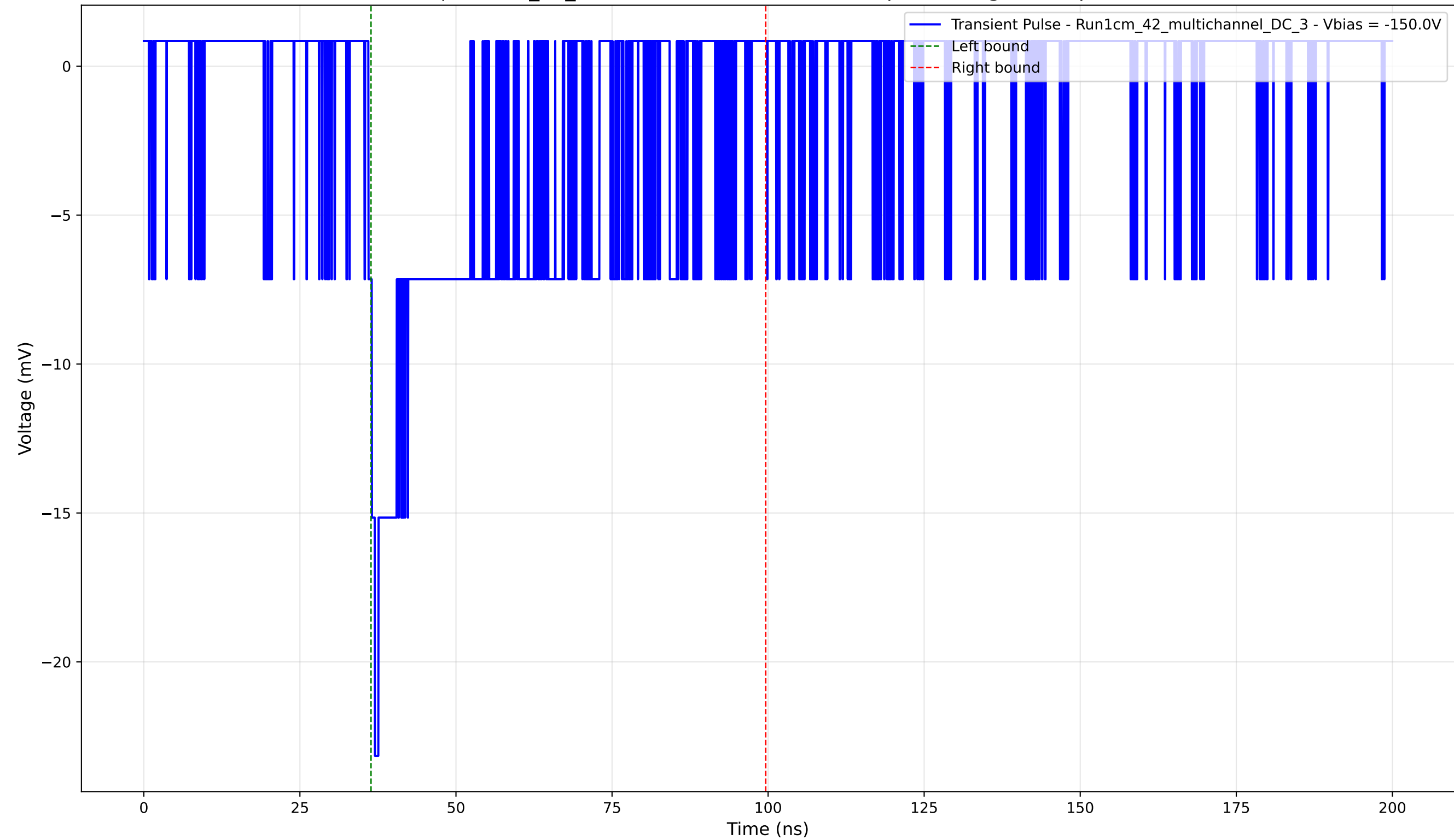
Transient Pulse - Sample: 1cm_42_multichannel - Position: 335.0 \mu\text{m} - Charge: 5.69 pC - Rise Time: 1.04 ns
