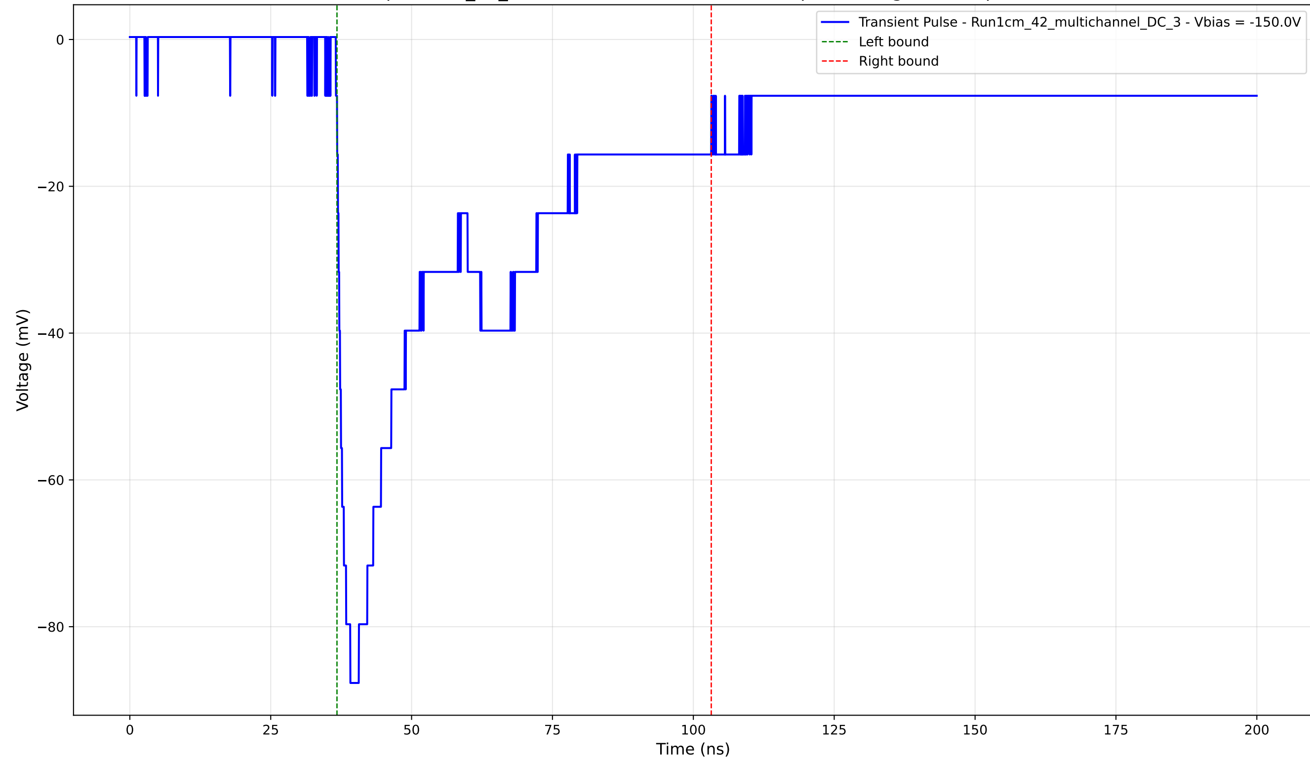
Transient Pulse - Sample: 1cm_42_multichannel - Position: 2205.0 \mu\text{m} - Charge: 42.26 pC - Rise Time: 1.62 ns
