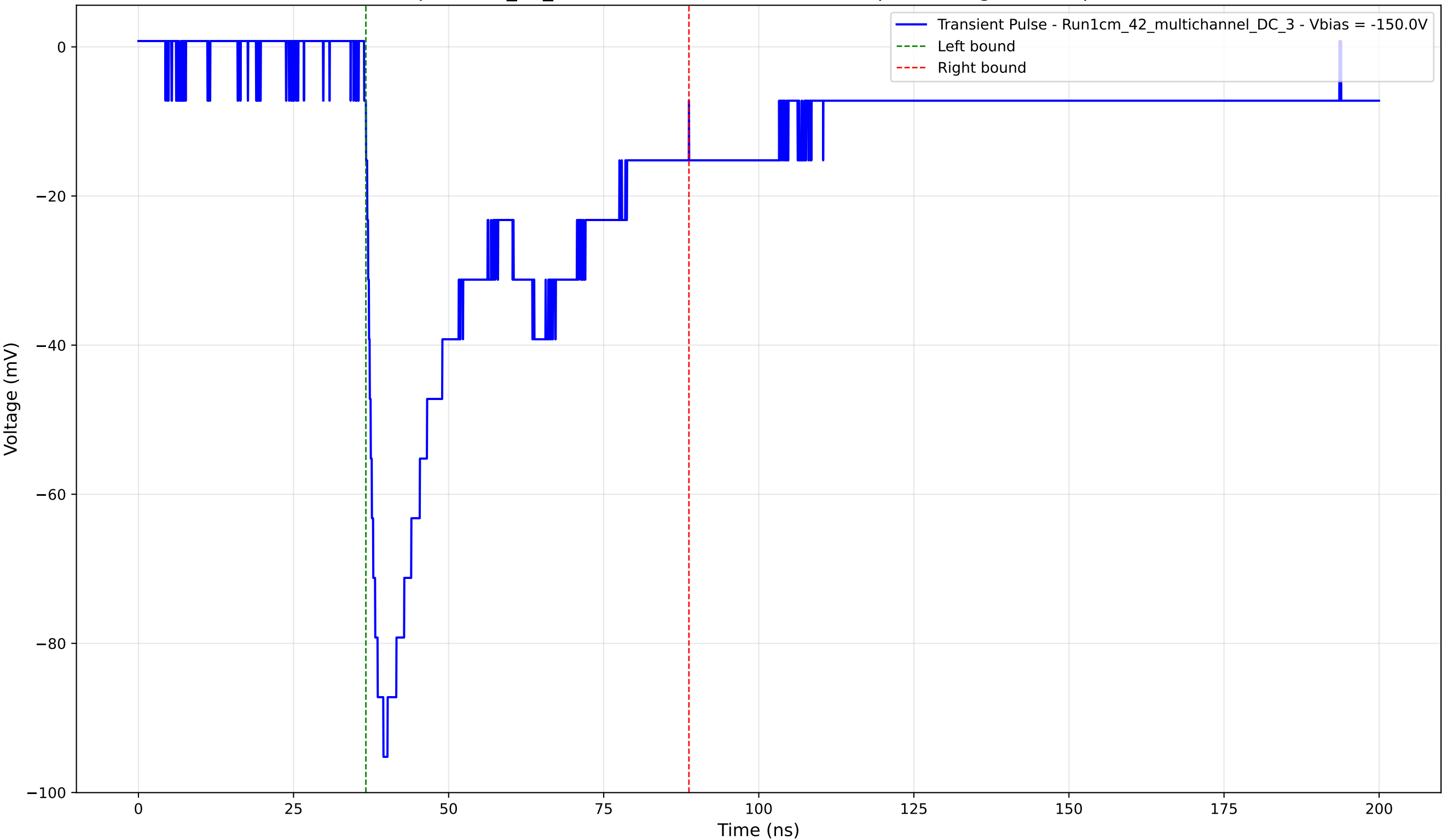
Transient Pulse - Sample: 1cm_42_multichannel - Position: 2720.0 \mu\text{m} - Charge: 37.18 pC - Rise Time: 1.89 ns
