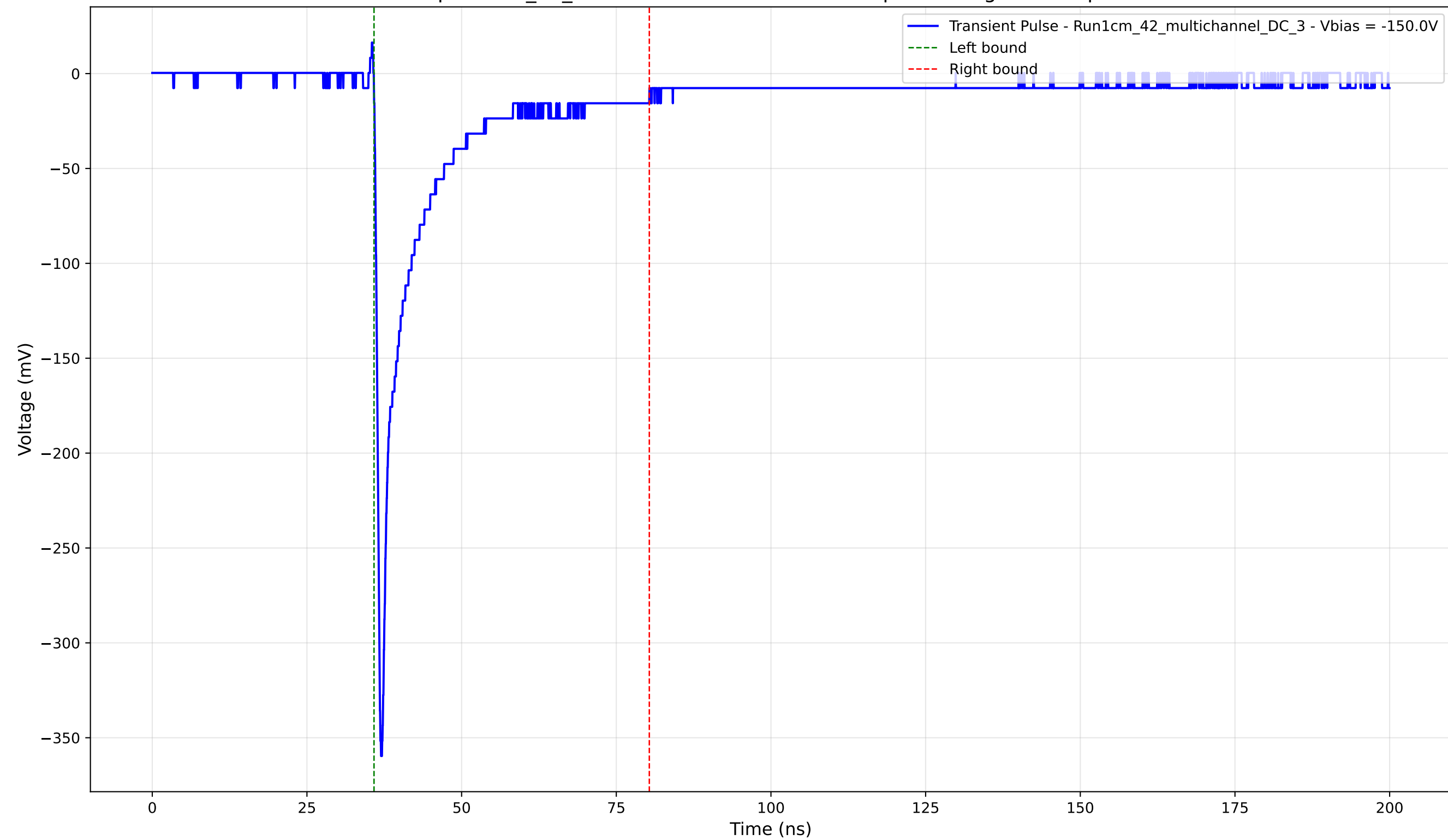
Transient Pulse - Sample: 1cm_42_multichannel - Position: 125.0 \mu\text{m} - Charge: 43.93 pC - Rise Time: 0.80 ns
