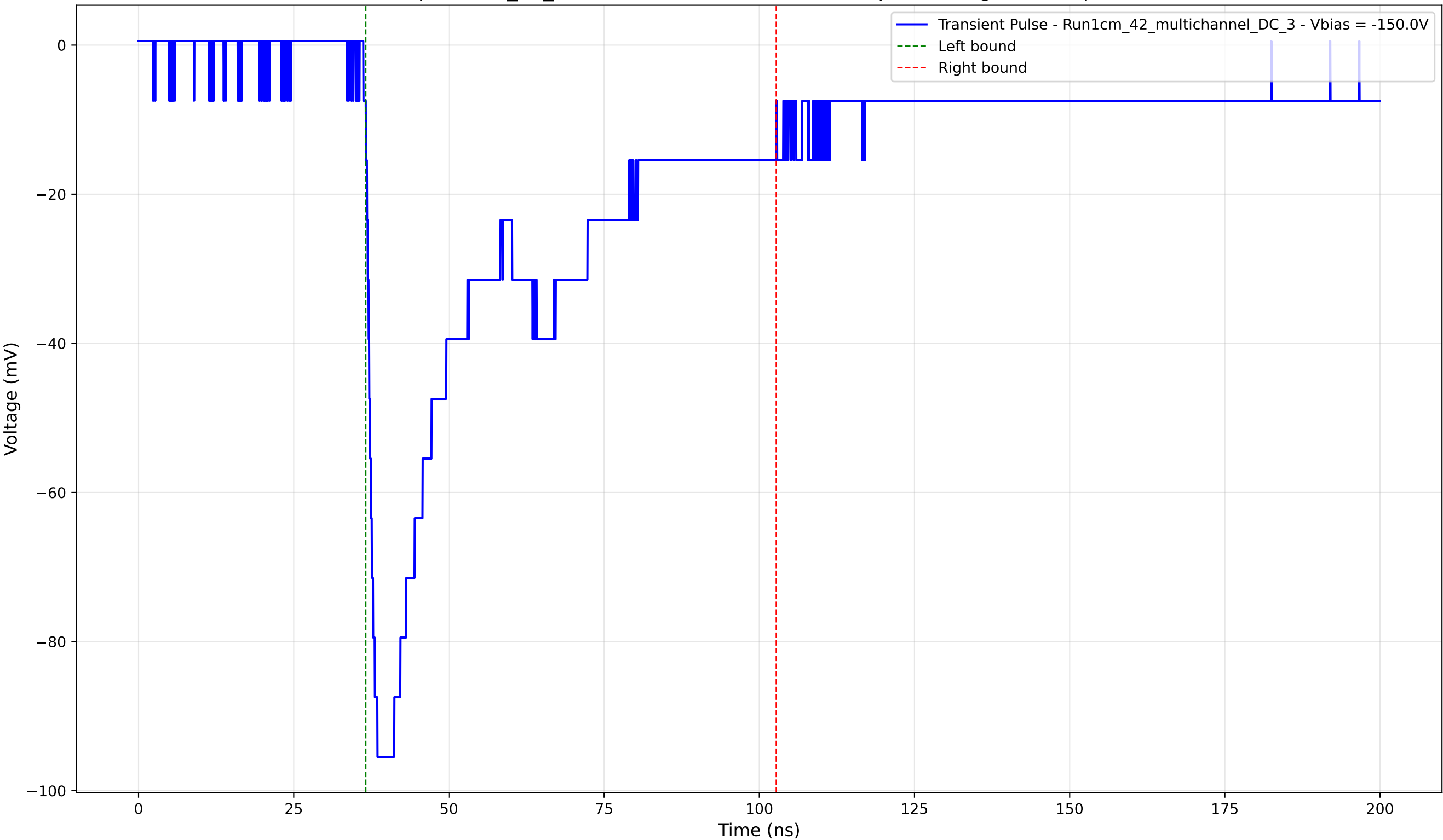
Transient Pulse - Sample: 1cm_42_multichannel - Position: 1995.0 \mu\text{m} - Charge: 43.73 pC - Rise Time: 1.45 ns
