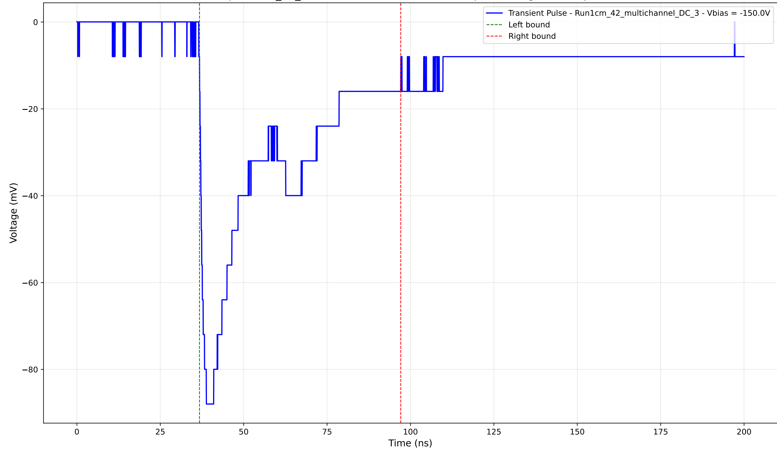
Transient Pulse - Sample: 1cm_42_multichannel - Position: 2165.0 \mu\text{m} - Charge: 40.52 pC - Rise Time: 1.50 ns
