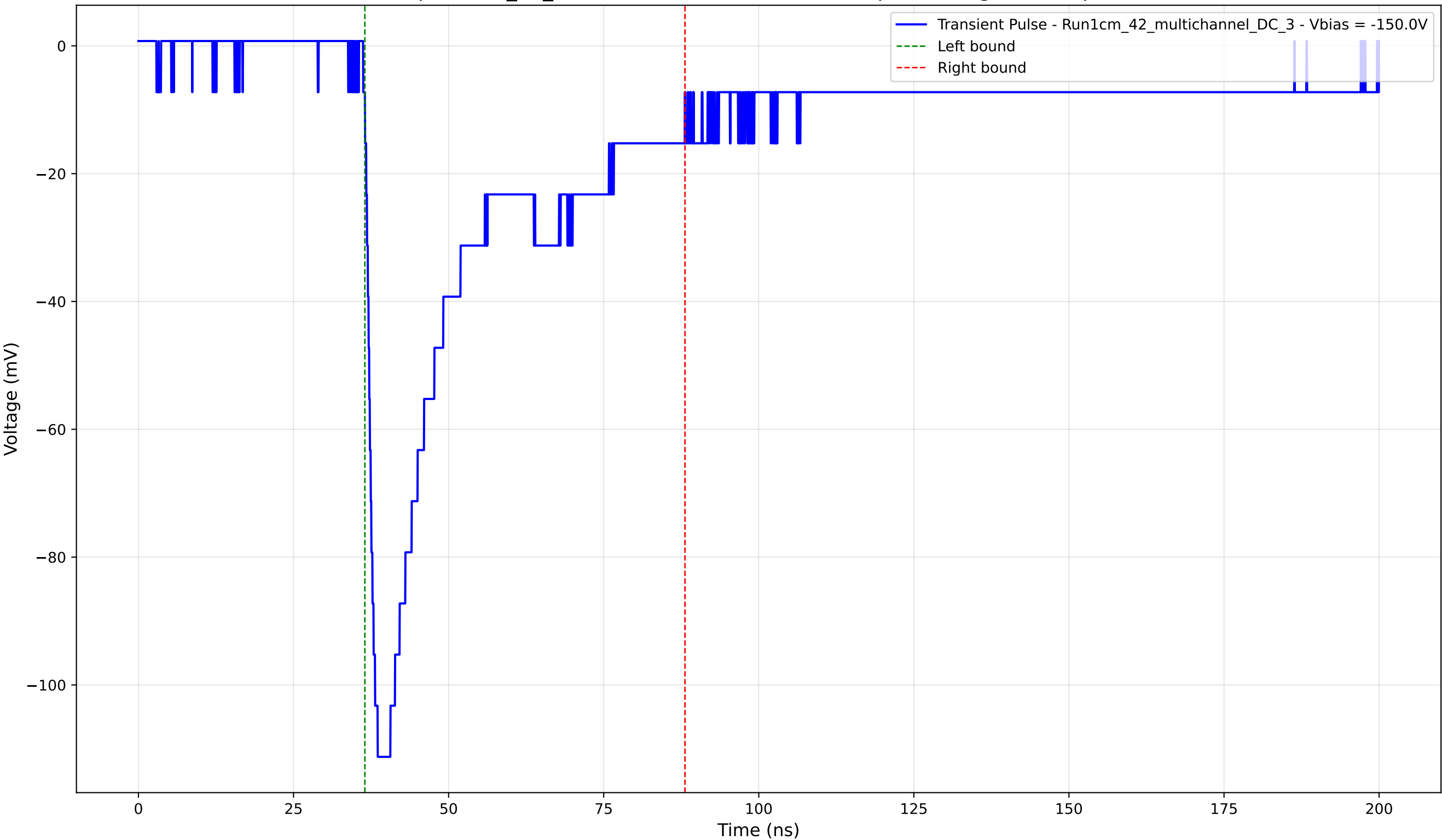
Transient Pulse - Sample: 1cm_42_multichannel - Position: 3240.0 \mu\text{m} - Charge: 37.95 pC - Rise Time: 1.63 ns
