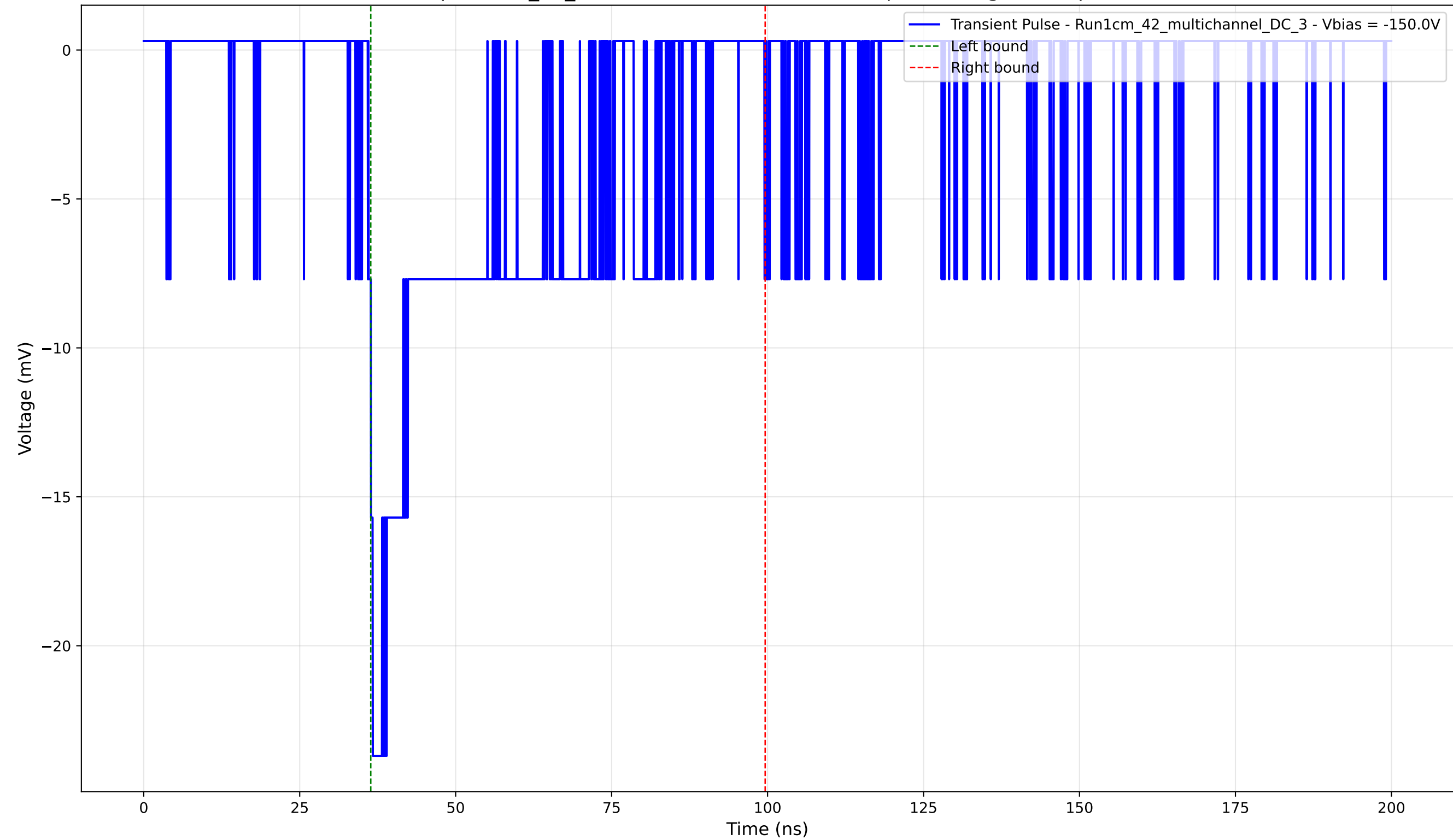
Transient Pulse - Sample: 1cm_42_multichannel - Position: 330.0 \mu\text{m} - Charge: 7.22 pC - Rise Time: 0.67 ns
