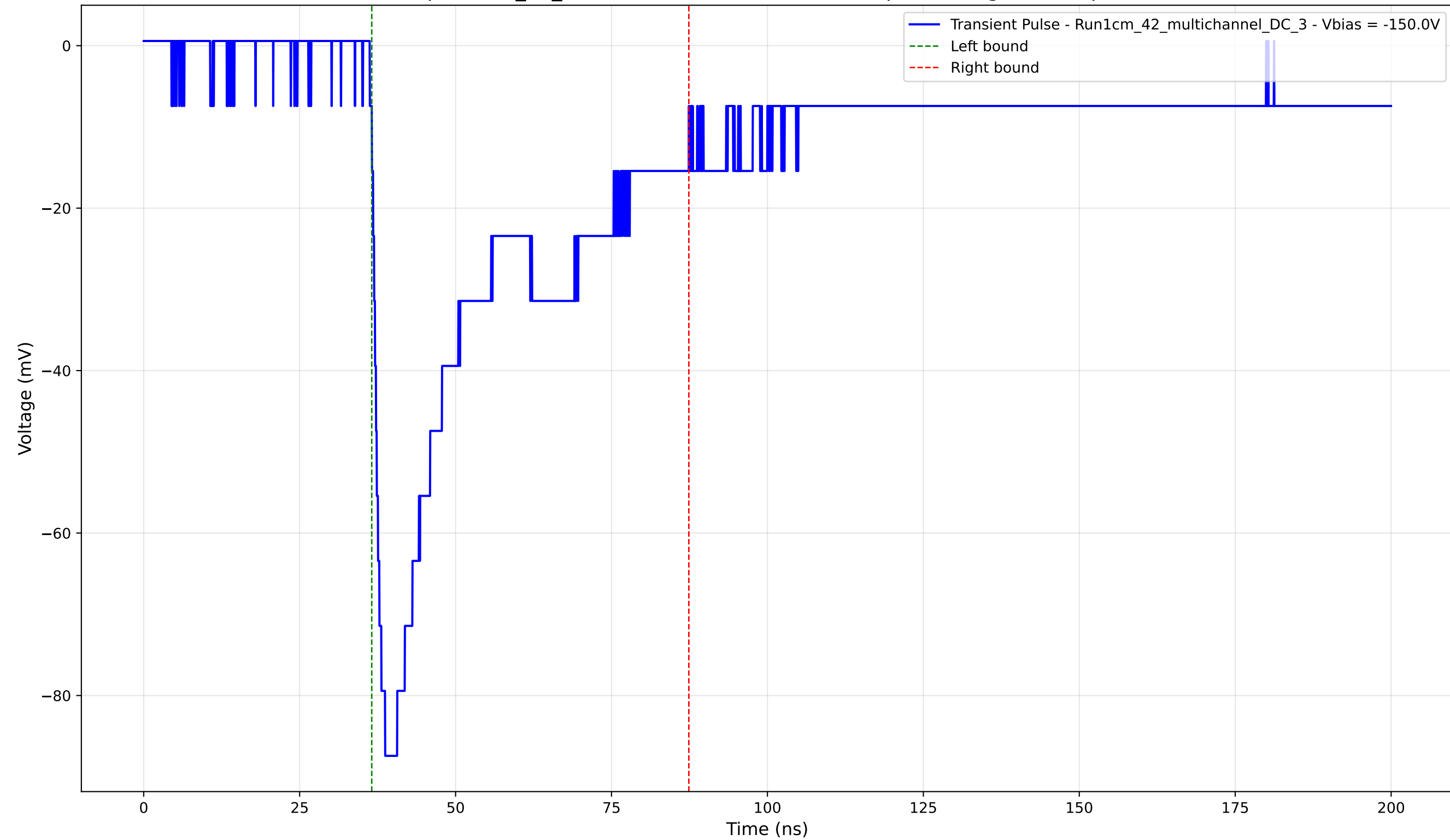
Transient Pulse - Sample: 1cm_42_multichannel - Position: 1940.0 \mu\text{m} - Charge: 34.28 pC - Rise Time: 1.54 ns
