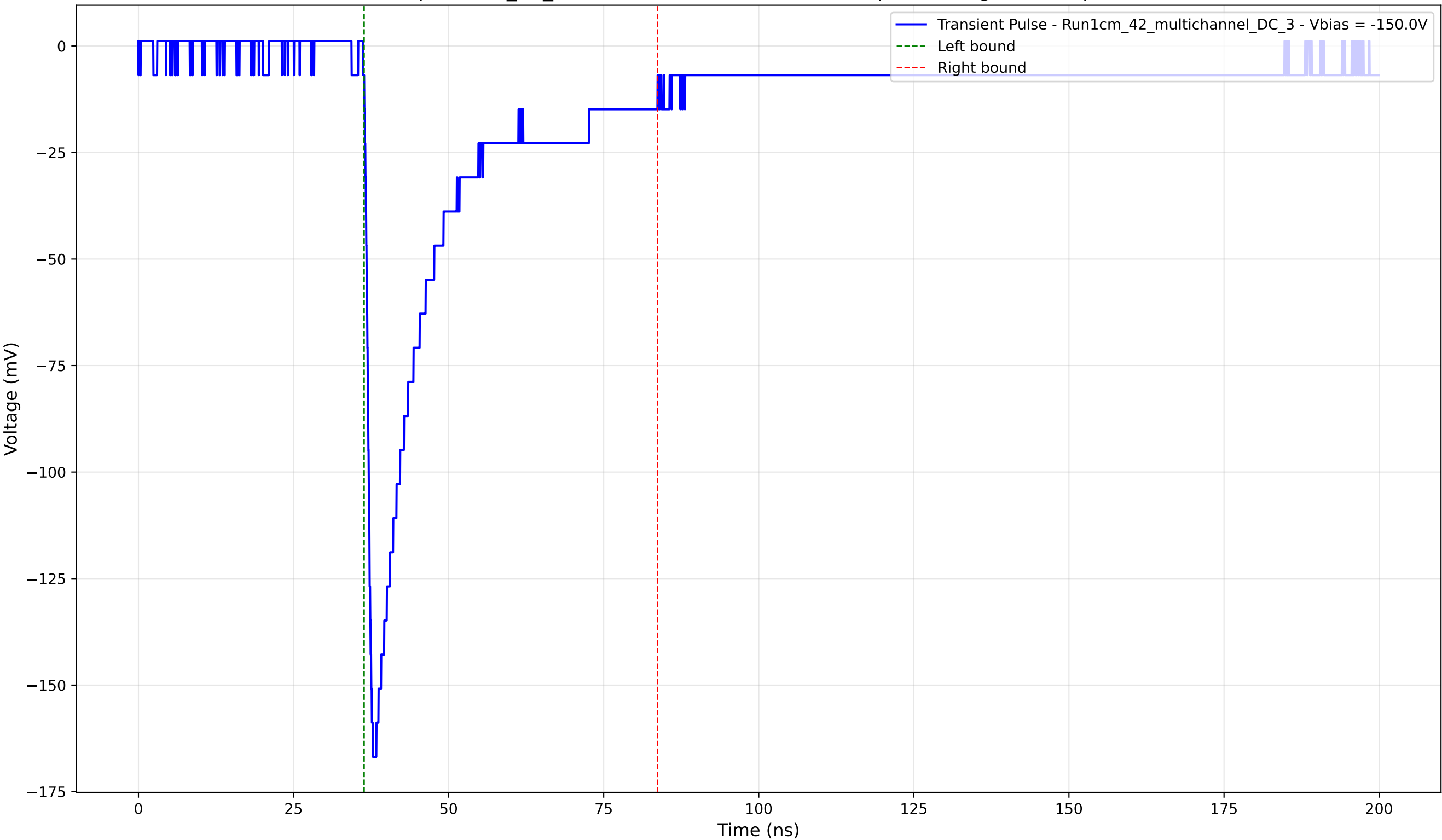
Transient Pulse - Sample: 1cm_42_multichannel - Position: 3980.0 \mu\text{m} - Charge: 38.80 pC - Rise Time: 1.04 ns
