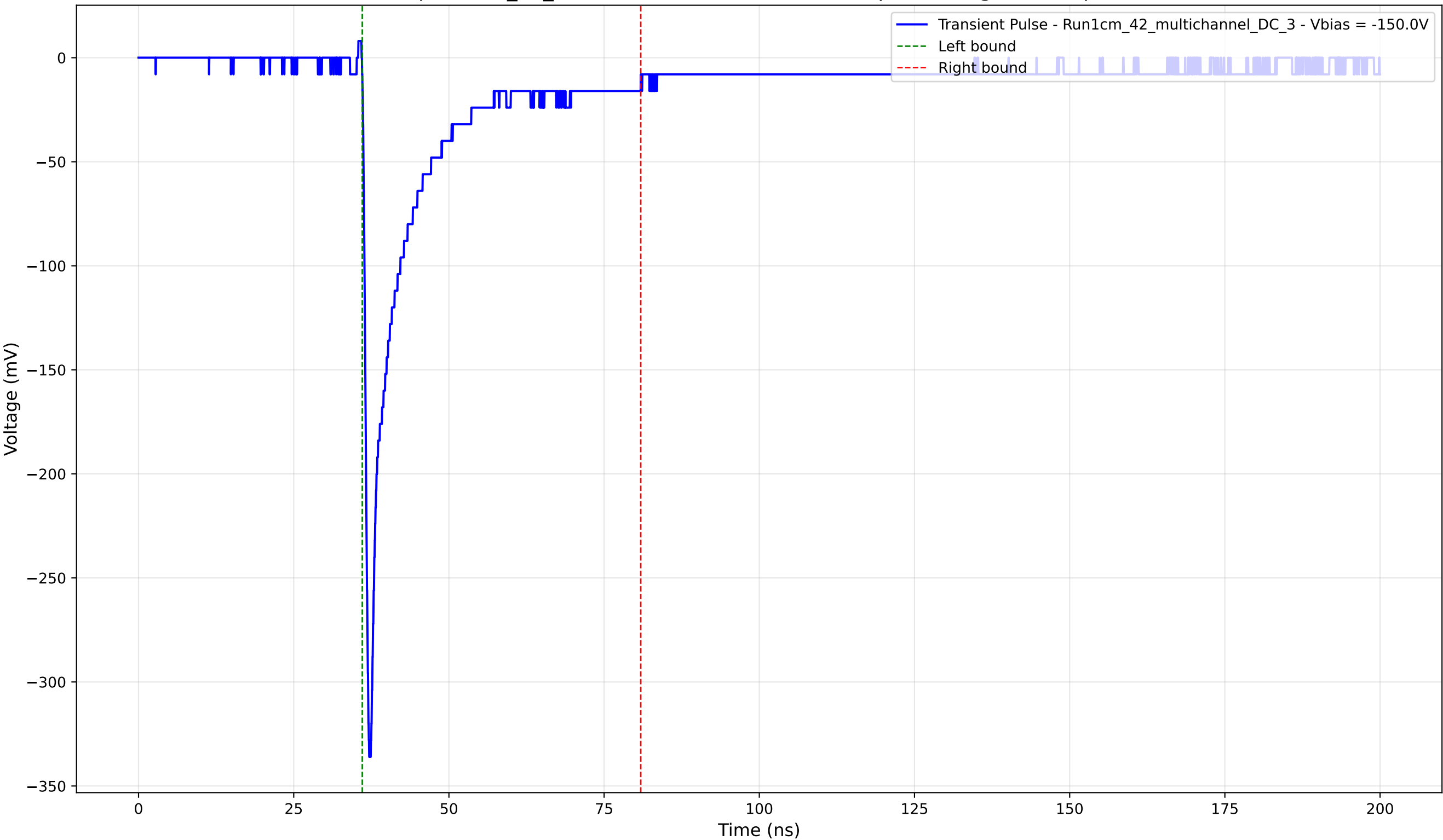
Transient Pulse - Sample: 1cm_42_multichannel - Position: 4685.0 \mu\text{m} - Charge: 43.34 pC - Rise Time: 0.79 ns
