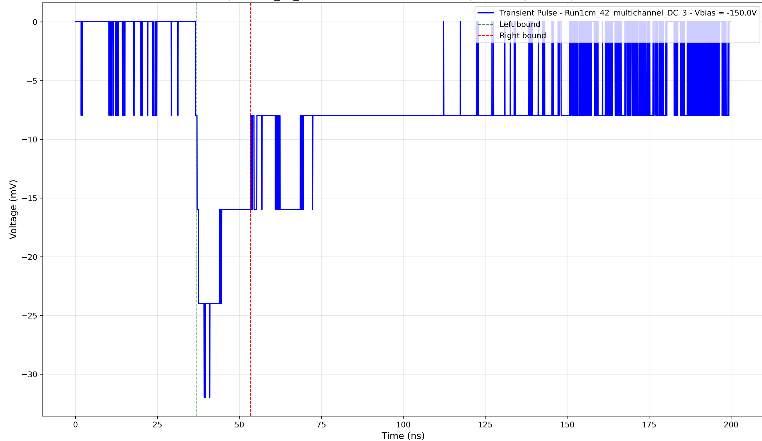
Transient Pulse - Sample: 1cm_42_multichannel - Position: 2415.0 \mu\text{m} - Charge: 6.33 pC - Rise Time: 2.63 ns
