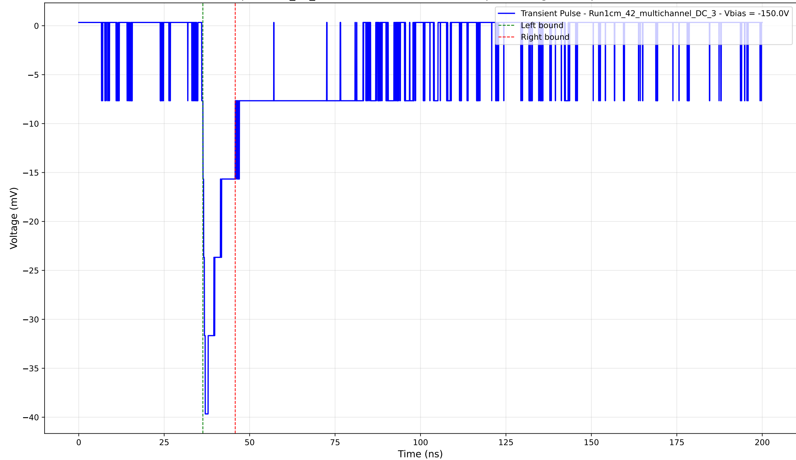
Transient Pulse - Sample: 1cm_42_multichannel - Position: 380.0 \mu\text{m} - Charge: 4.38 pC - Rise Time: 1.03 ns
