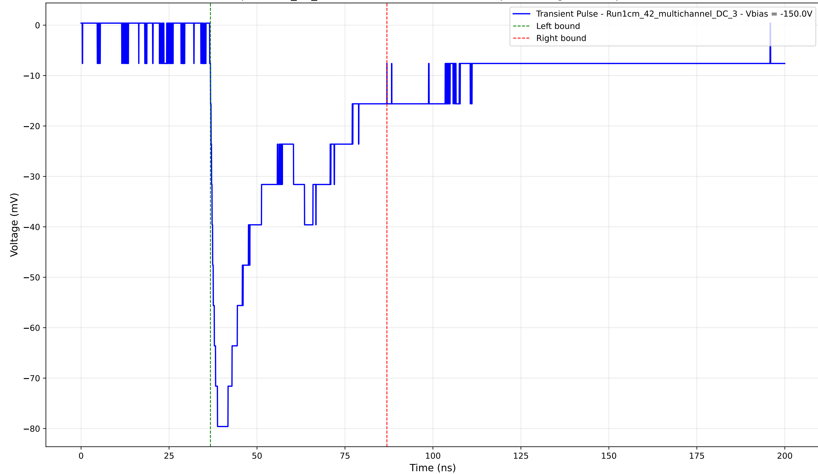
Transient Pulse - Sample: 1cm_42_multichannel - Position: 2590.0 \mu\text{m} - Charge: 34.80 pC - Rise Time: 2.00 ns
