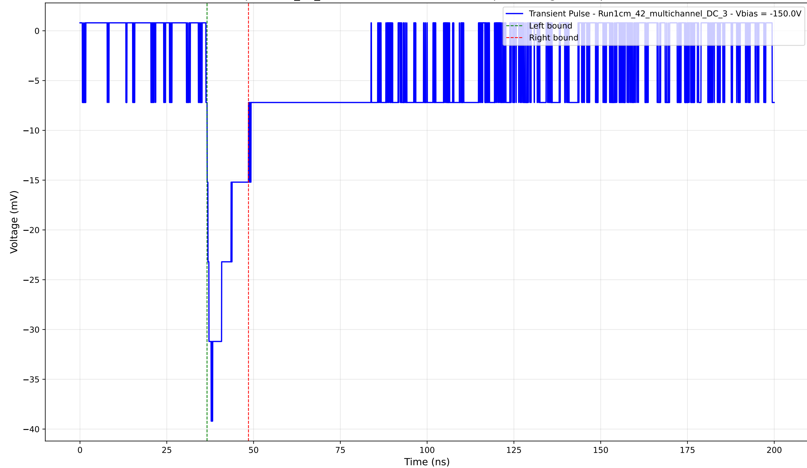
Transient Pulse - Sample: 1cm_42_multichannel - Position: 890.0 \mu\text{m} - Charge: 5.36 pC - Rise Time: 1.51 ns
