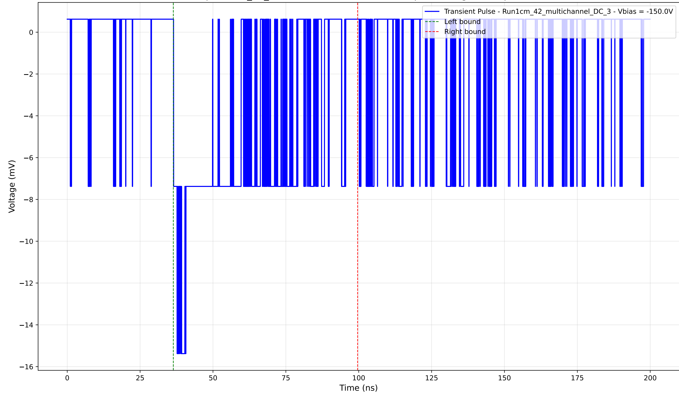
Transient Pulse - Sample: 1cm_42_multichannel - Position: 865.0 \mu\text{m} - Charge: 5.92 pC - Rise Time: 1.22 ns
