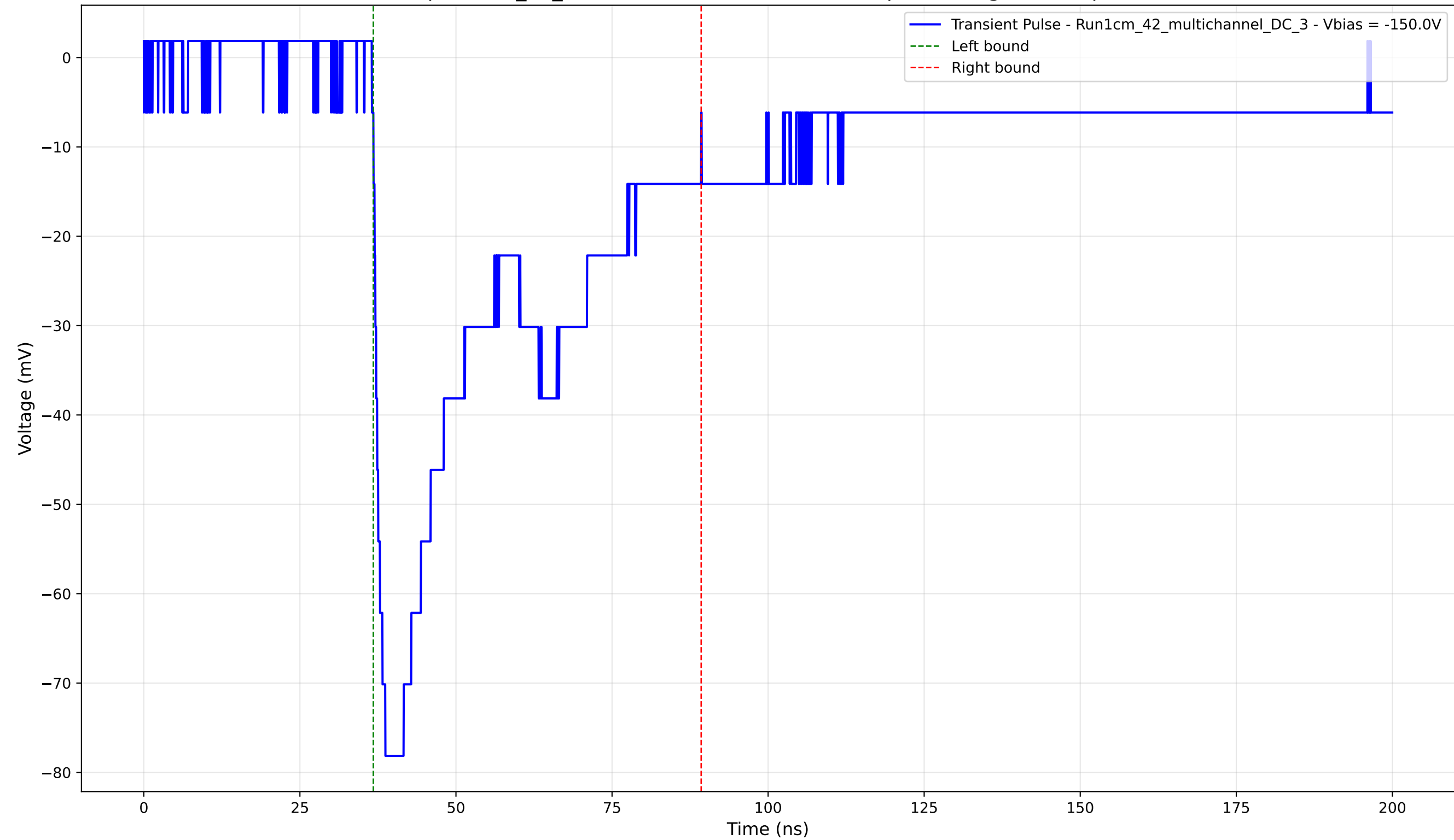
Transient Pulse - Sample: 1cm_42_multichannel - Position: 2595.0 \mu\text{m} - Charge: 34.24 pC - Rise Time: 1.92 ns
