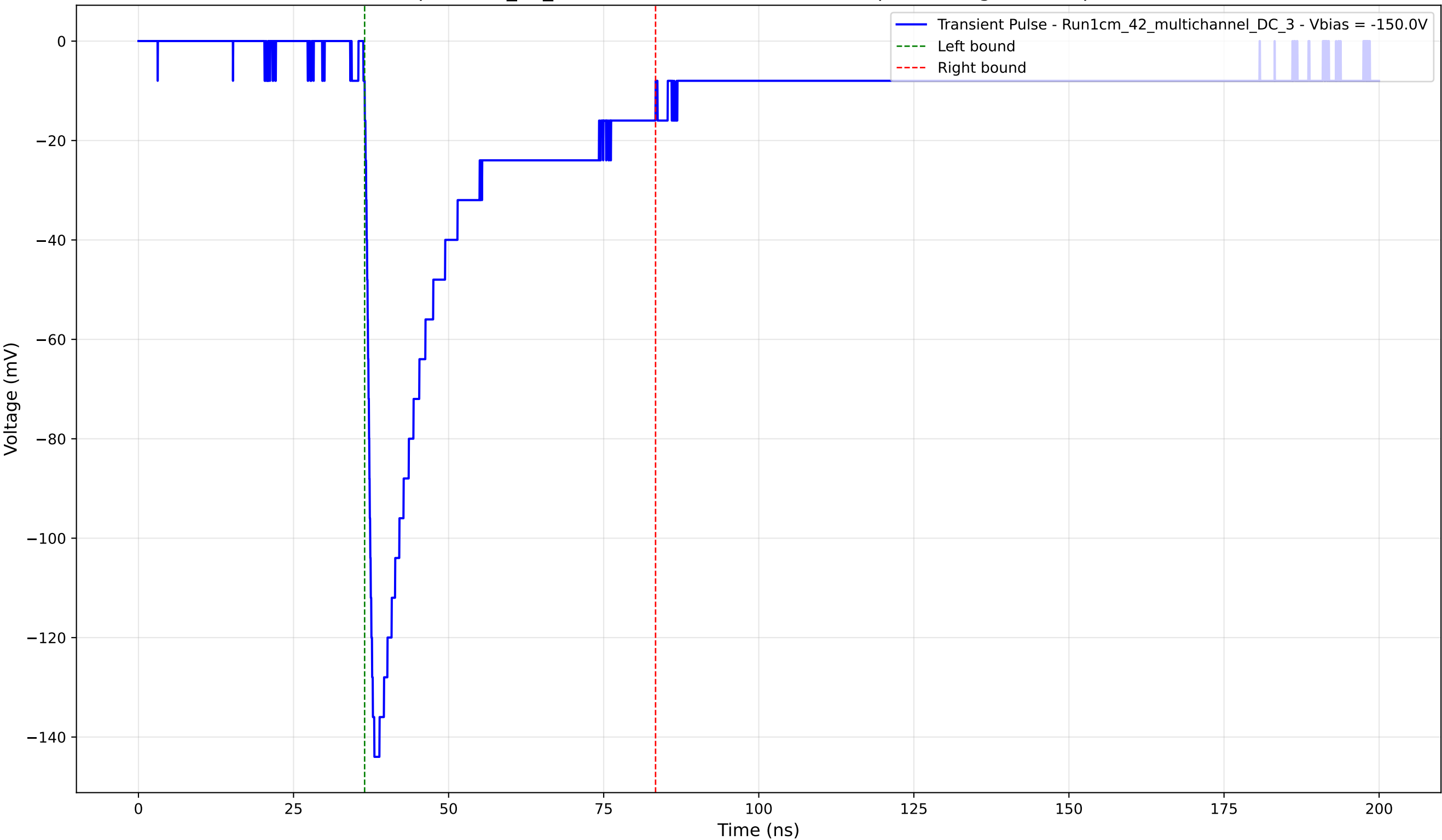
Transient Pulse - Sample: 1cm_42_multichannel - Position: 3740.0 \mu\text{m} - Charge: 38.65 pC - Rise Time: 1.30 ns
