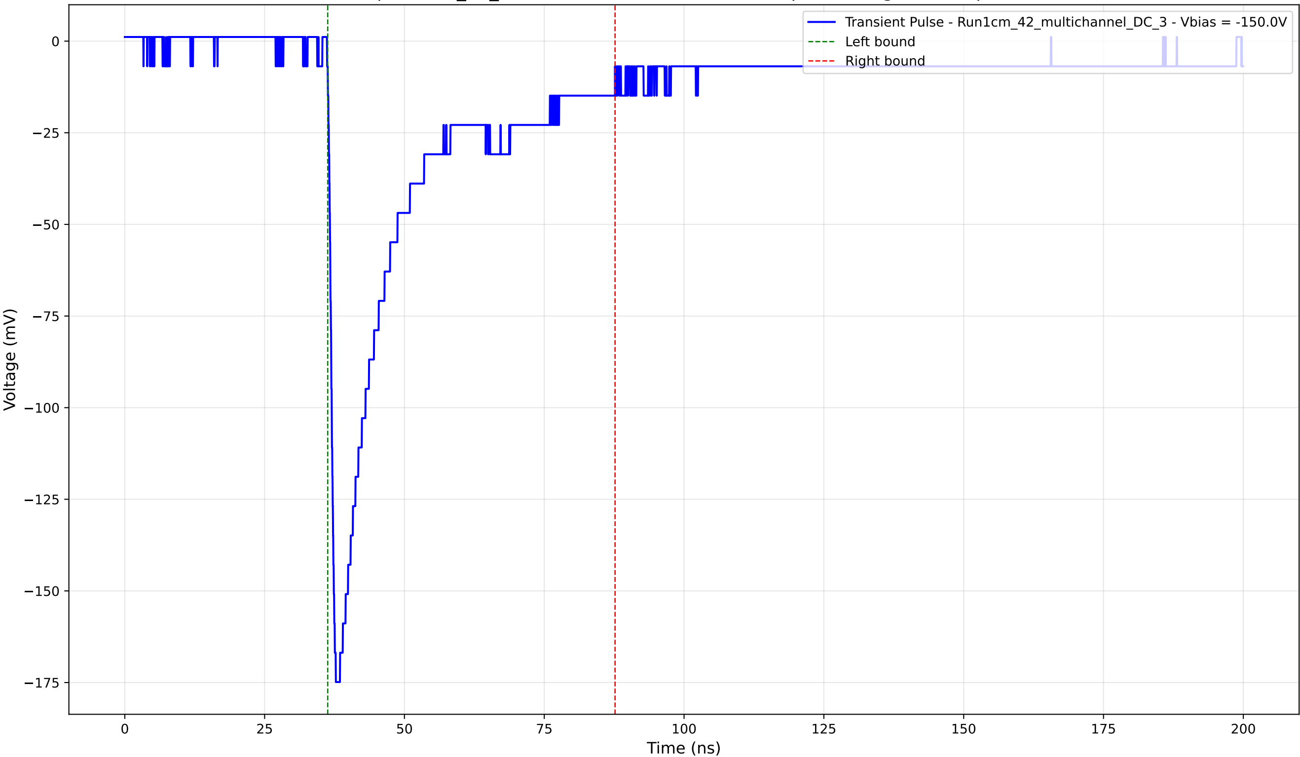
Transient Pulse - Sample: 1cm_42_multichannel - Position: 1000.0 \mu\text{m} - Charge: 45.04 pC - Rise Time: 1.05 ns
