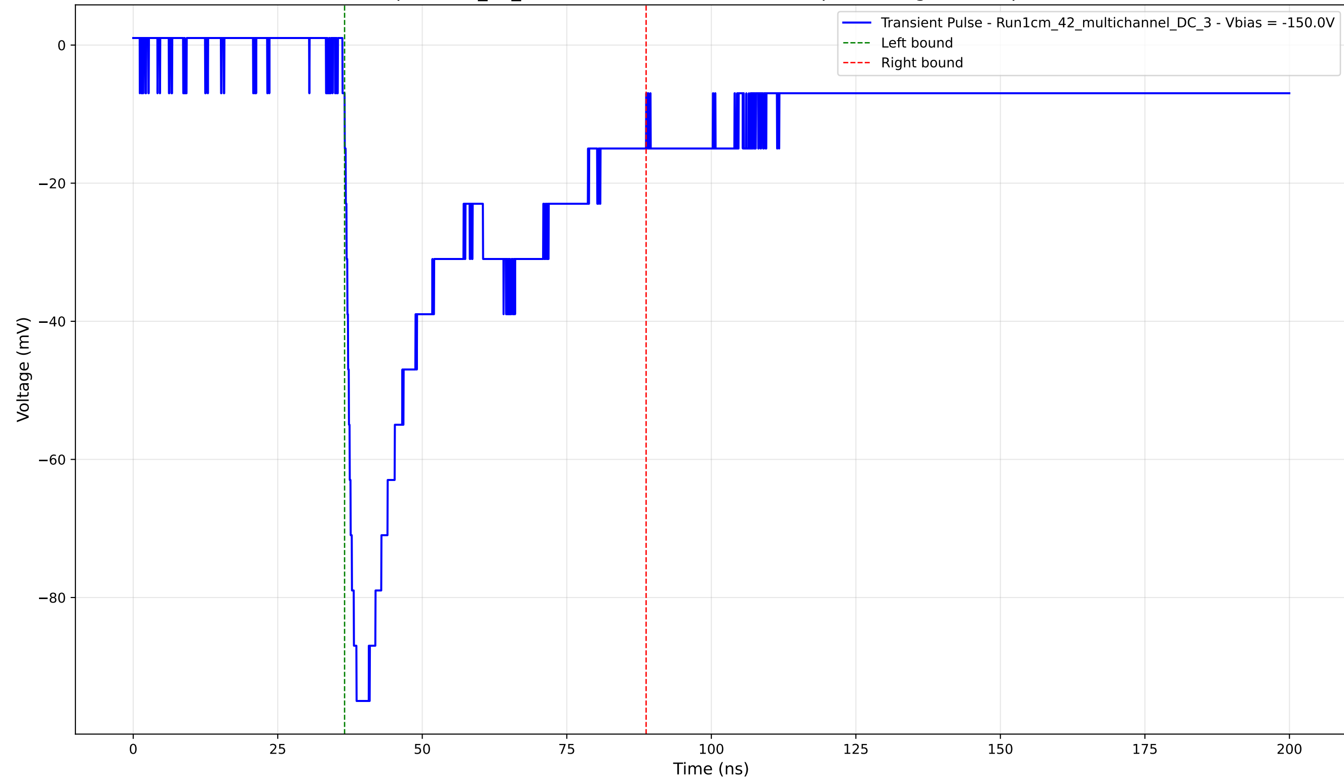
Transient Pulse - Sample: 1cm_42_multichannel - Position: 1960.0 \mu\text{m} - Charge: 37.43 pC - Rise Time: 1.59 ns
