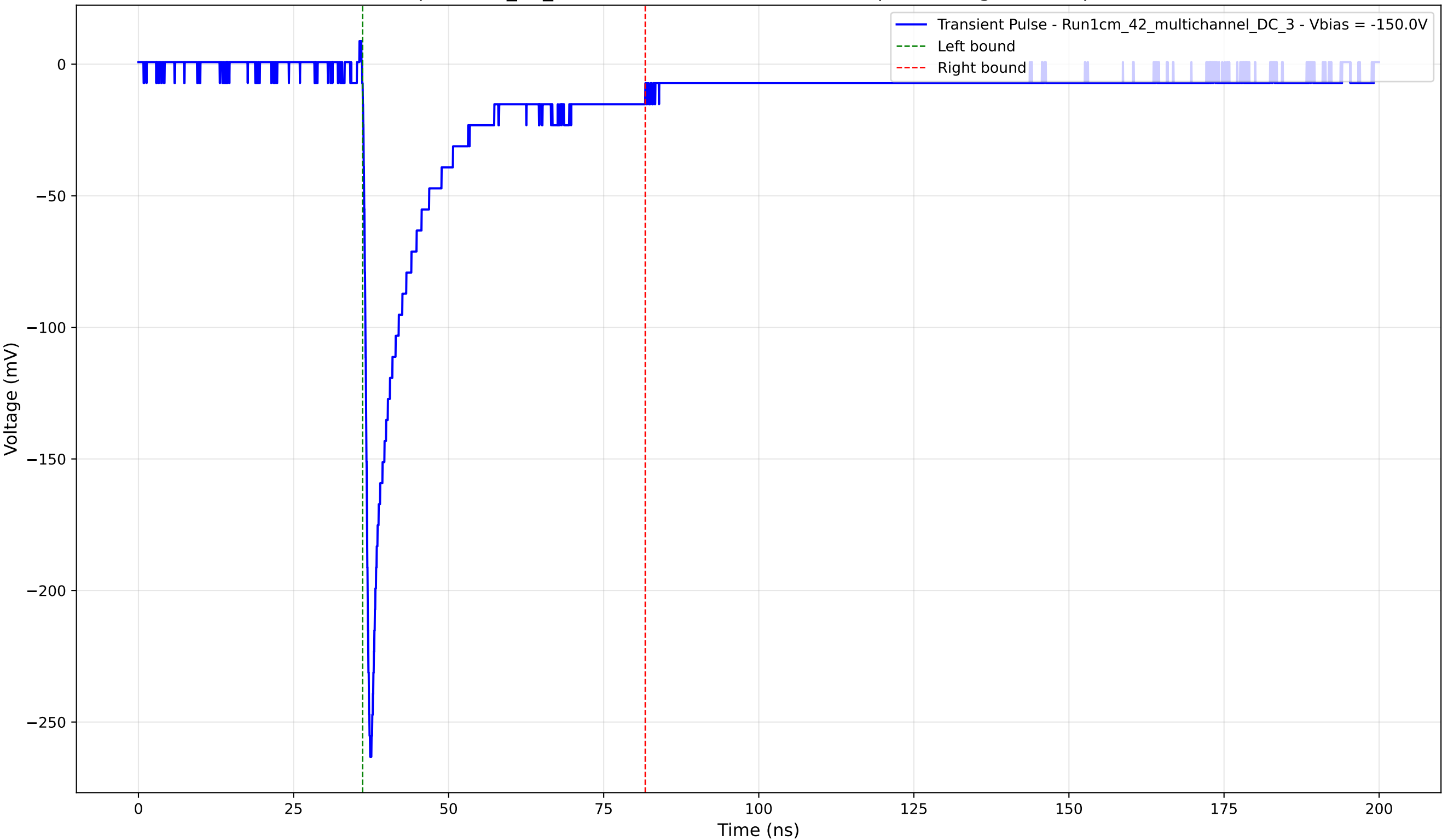
Transient Pulse - Sample: 1cm_42_multichannel - Position: 4505.0 \mu\text{m} - Charge: 39.55 pC - Rise Time: 0.87 ns
