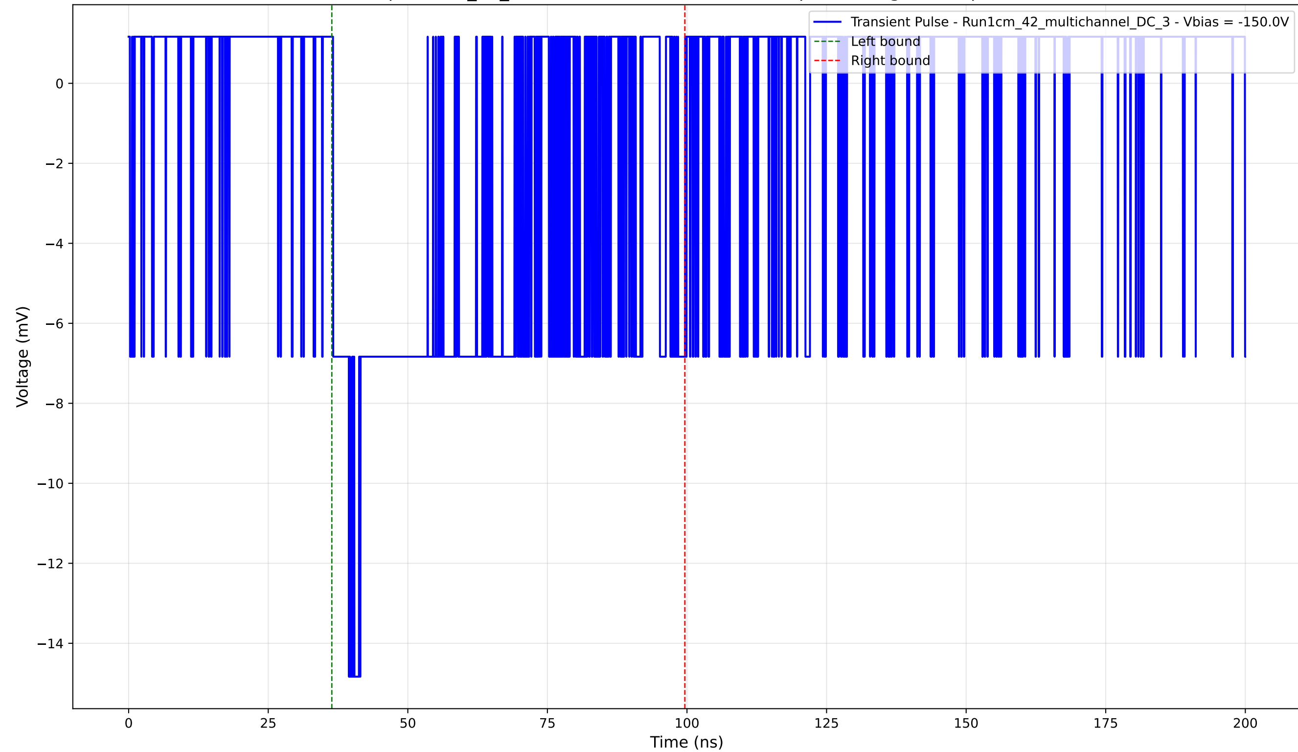
Transient Pulse - Sample: 1cm_42_multichannel - Position: 3405.0 \mu\text{m} - Charge: 5.72 pC - Rise Time: 2.86 ns
