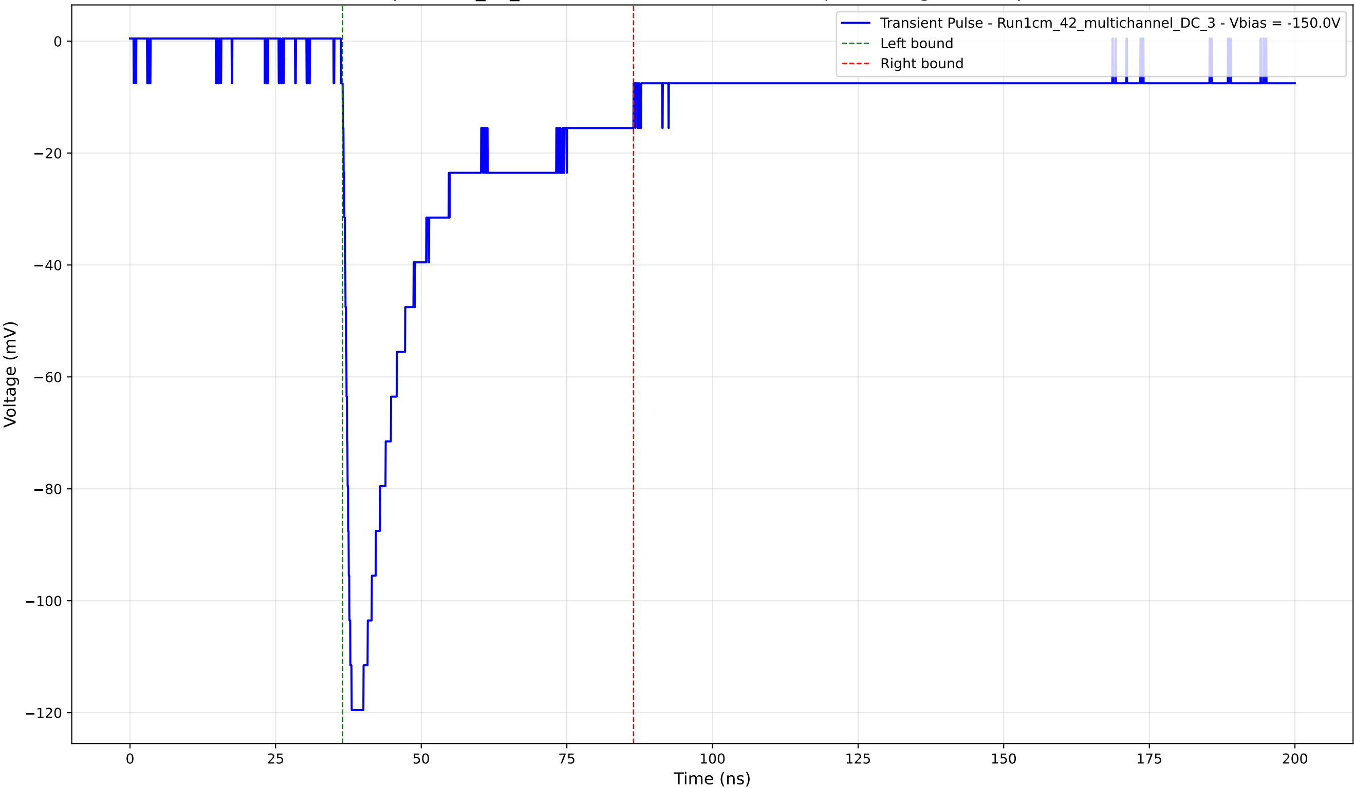
Transient Pulse - Sample: 1cm_42_multichannel - Position: 3565.0 \mu\text{m} - Charge: 36.72 pC - Rise Time: 1.31 ns
