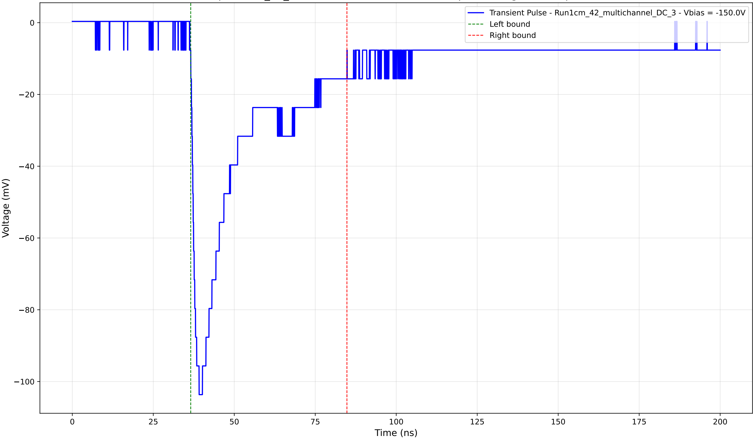
Transient Pulse - Sample: 1cm_42_multichannel - Position: 3080.0 \mu\text{m} - Charge: 35.14 pC - Rise Time: 1.83 ns
