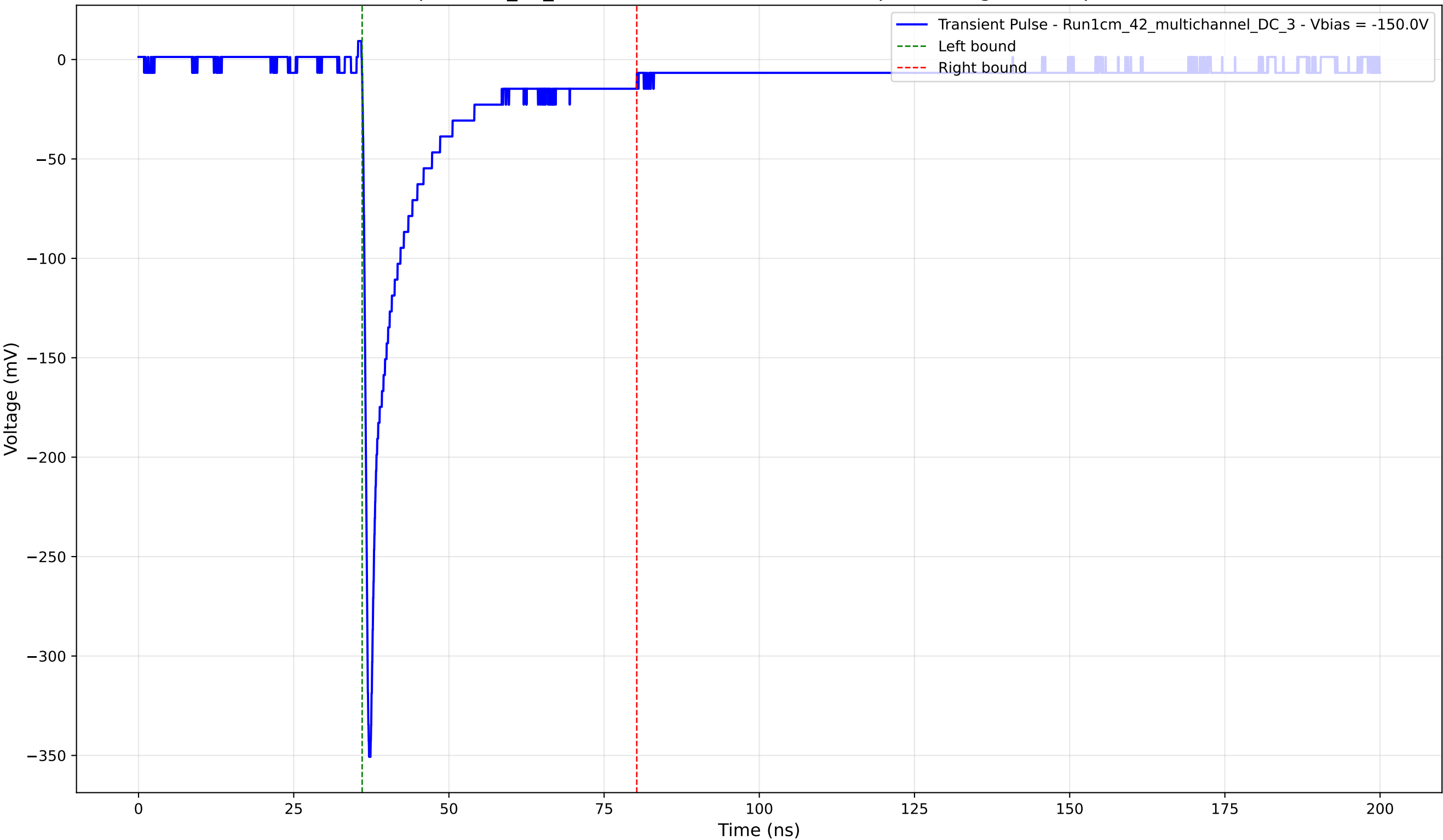
Transient Pulse - Sample: 1cm_42_multichannel - Position: 4720.0 \mu\text{m} - Charge: 42.49 pC - Rise Time: 0.79 ns
