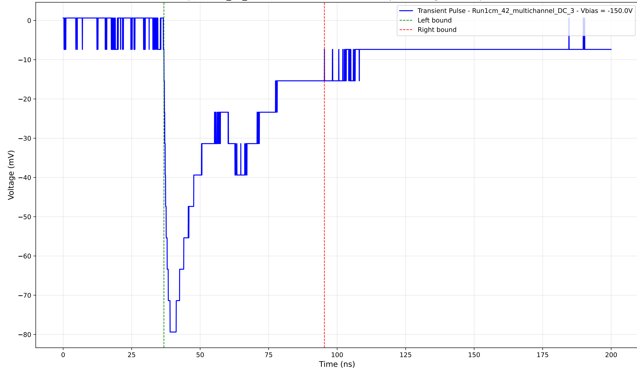
Transient Pulse - Sample: 1cm_42_multichannel - Position: 2535.0 \mu\text{m} - Charge: 37.02 pC - Rise Time: 2.24 ns
