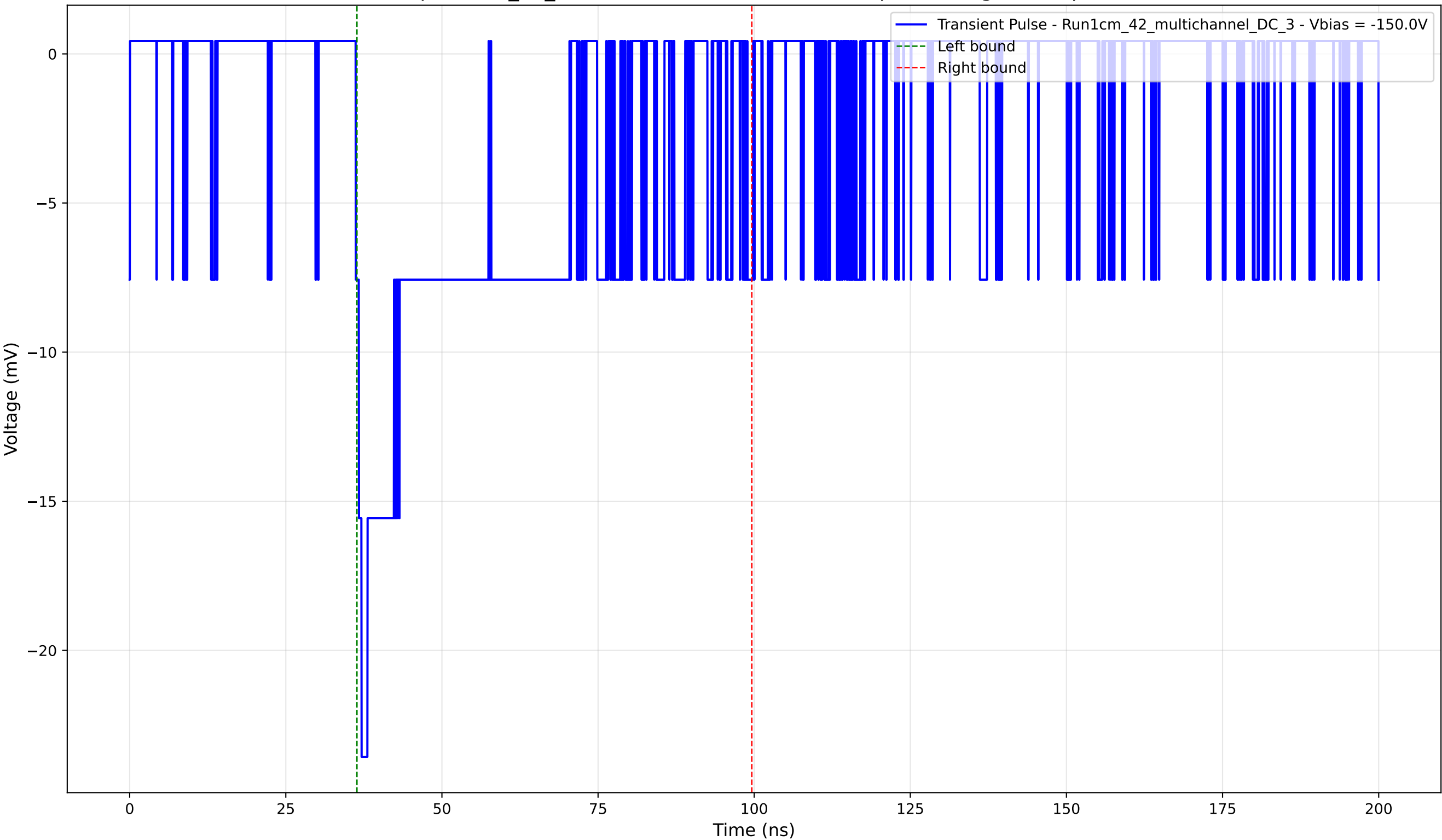
Transient Pulse - Sample: 1cm_42_multichannel - Position: 4415.0 \mu\text{m} - Charge: 7.94 pC - Rise Time: 0.93 ns
