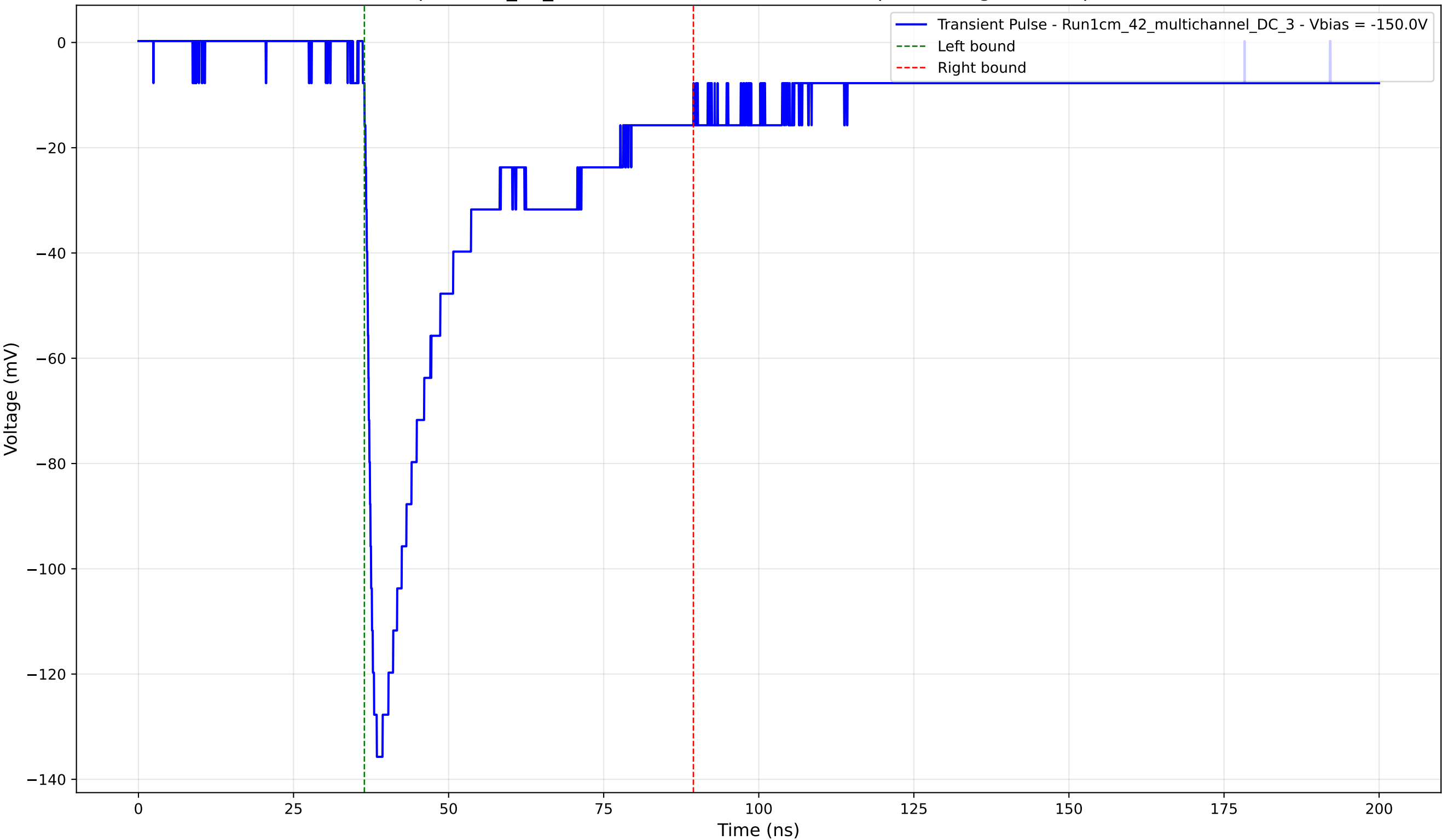
Transient Pulse - Sample: 1cm_42_multichannel - Position: 1485.0 \mu\text{m} - Charge: 43.77 pC - Rise Time: 1.55 ns
