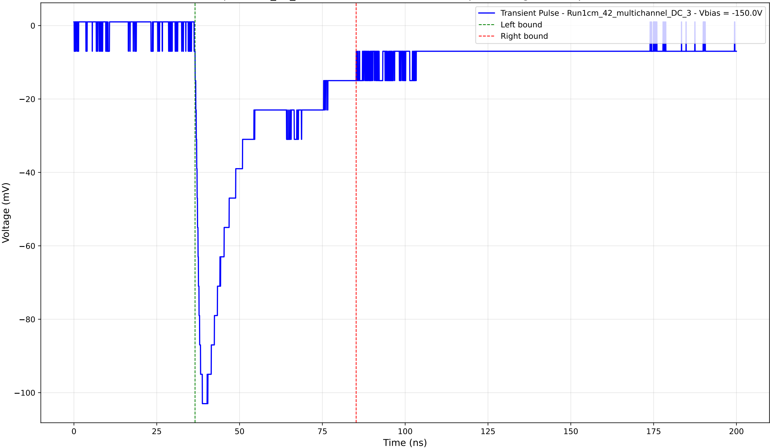
Transient Pulse - Sample: 1cm_42_multichannel - Position: 3155.0 \mu\text{m} - Charge: 34.30 pC - Rise Time: 1.65 ns
