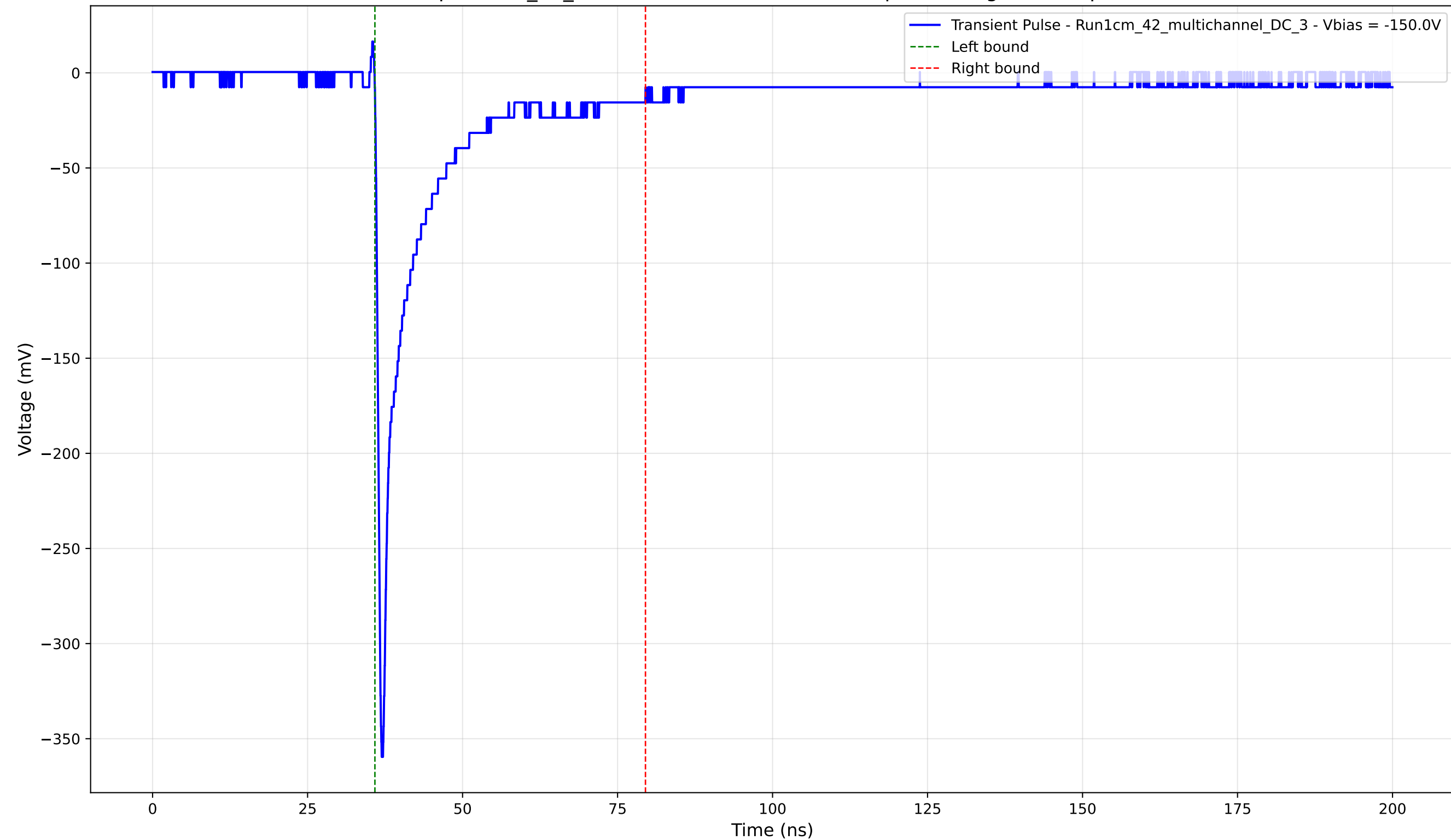
Transient Pulse - Sample: 1cm_42_multichannel - Position: 135.0 \mu\text{m} - Charge: 44.57 pC - Rise Time: 0.79 ns
