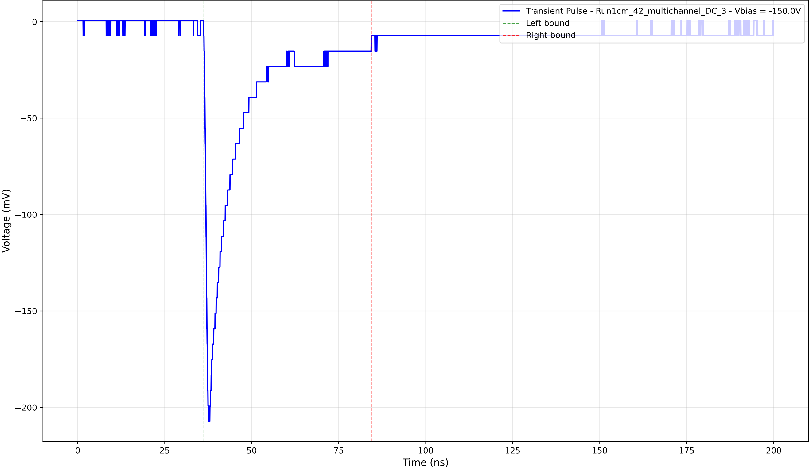
Transient Pulse - Sample: 1cm_42_multichannel - Position: 4210.0 \mu\text{m} - Charge: 41.22 pC - Rise Time: 0.99 ns
