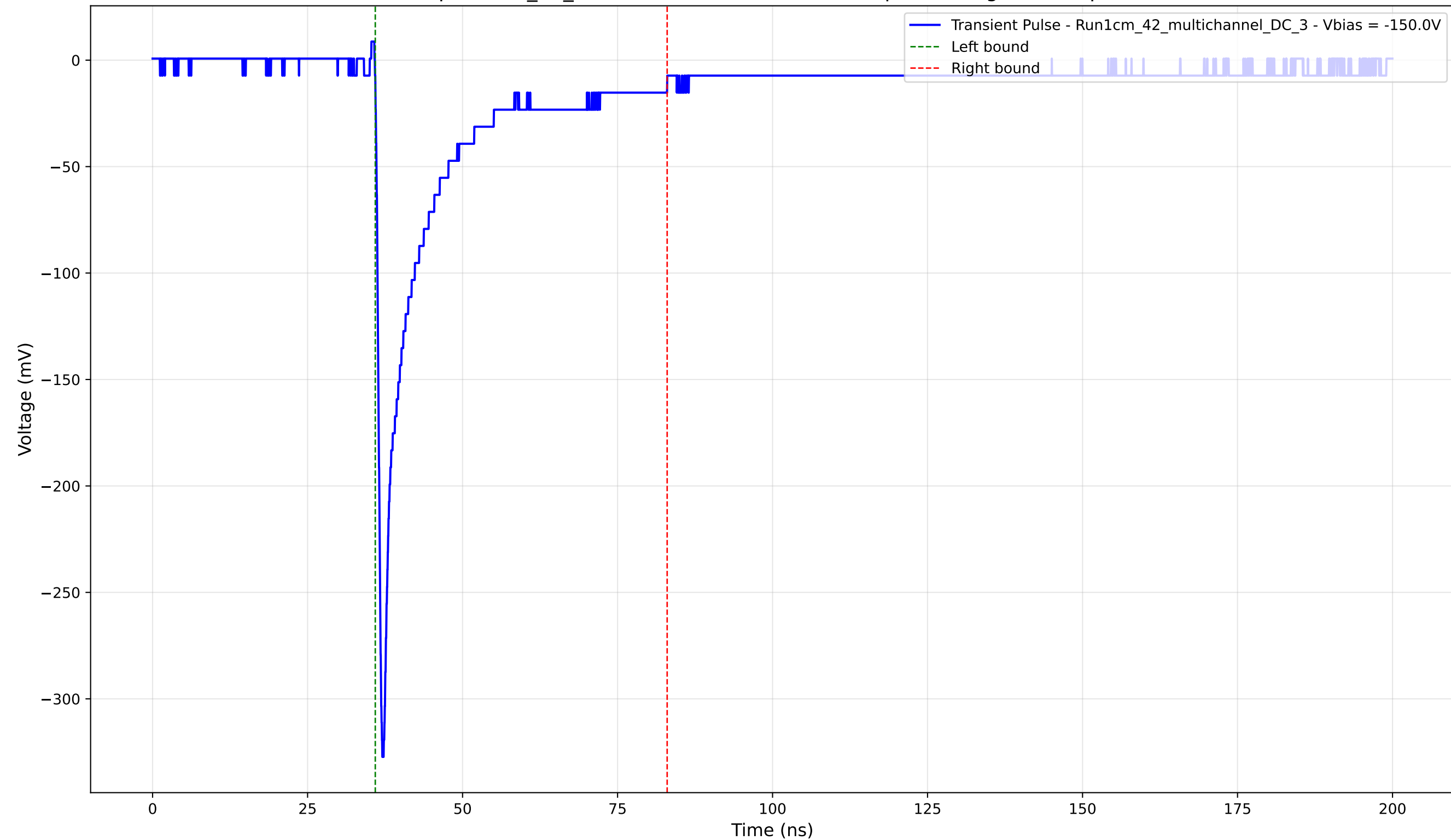
Transient Pulse - Sample: 1cm_42_multichannel - Position: 240.0 \mu\text{m} - Charge: 46.12 pC - Rise Time: 0.80 ns
