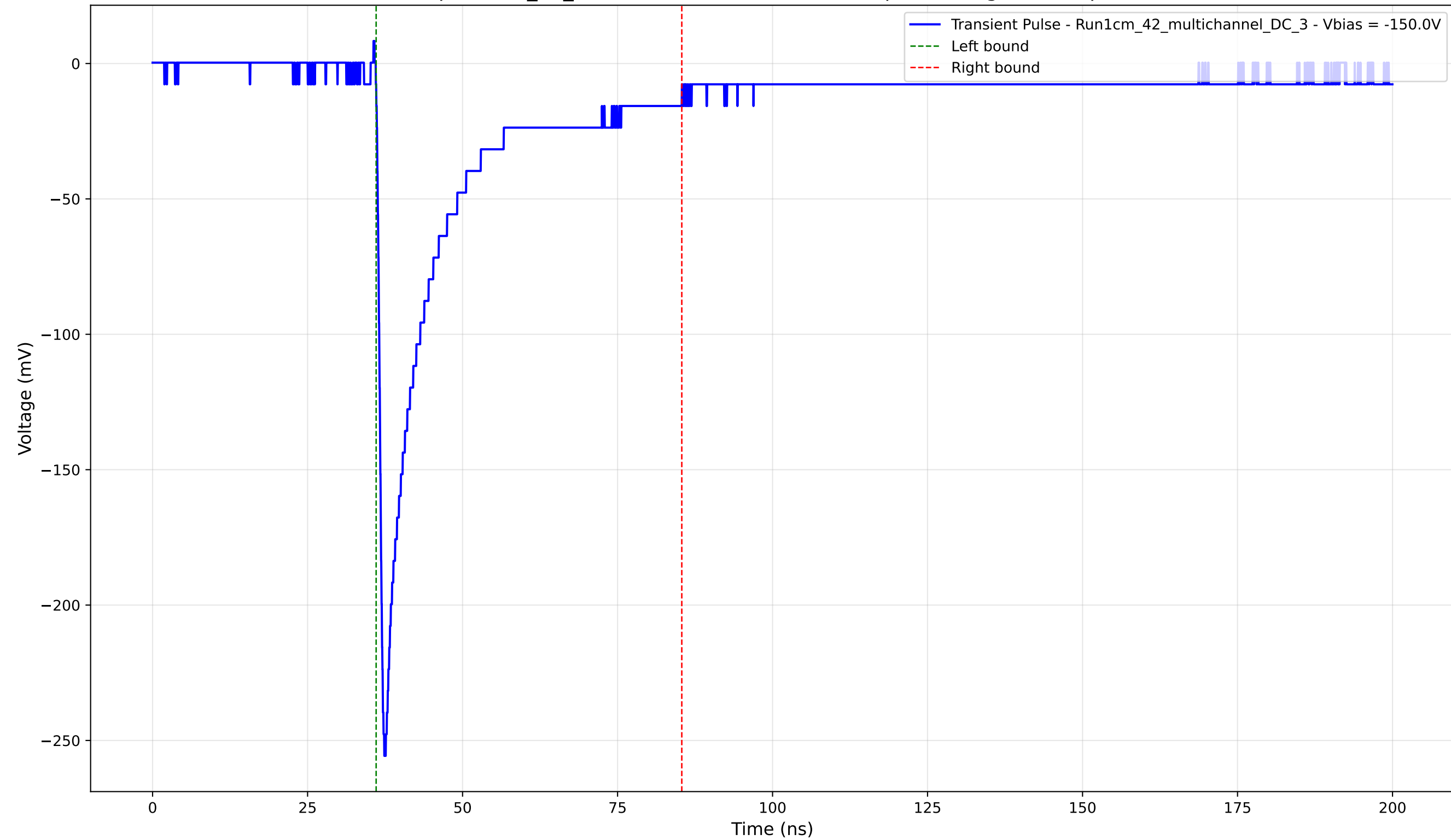
Transient Pulse - Sample: 1cm_42_multichannel - Position: 550.0 \mu\text{m} - Charge: 48.05 pC - Rise Time: 0.92 ns
