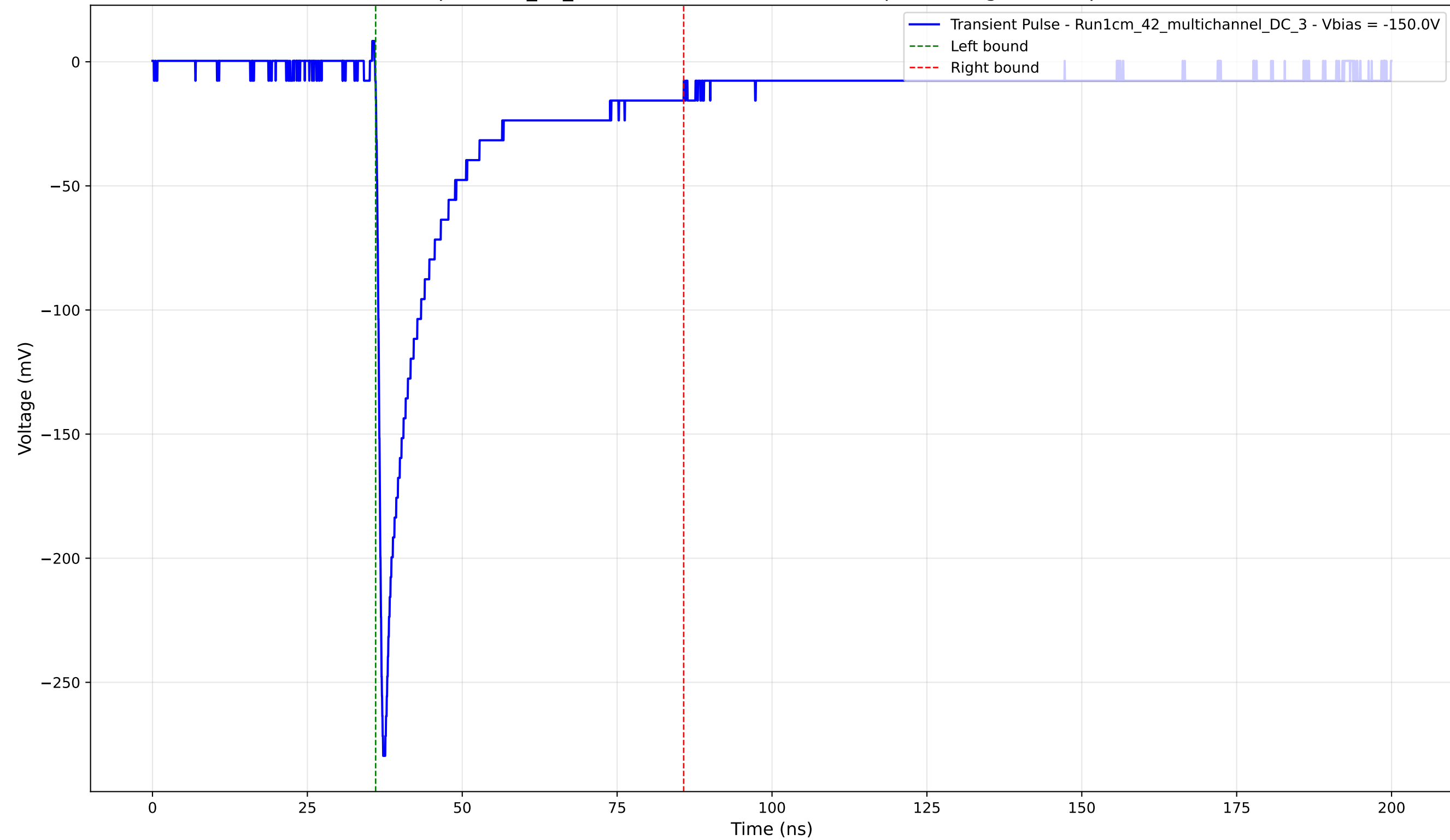
Transient Pulse - Sample: 1cm_42_multichannel - Position: 475.0 \mu\text{m} - Charge: 49.58 pC - Rise Time: 0.89 ns
