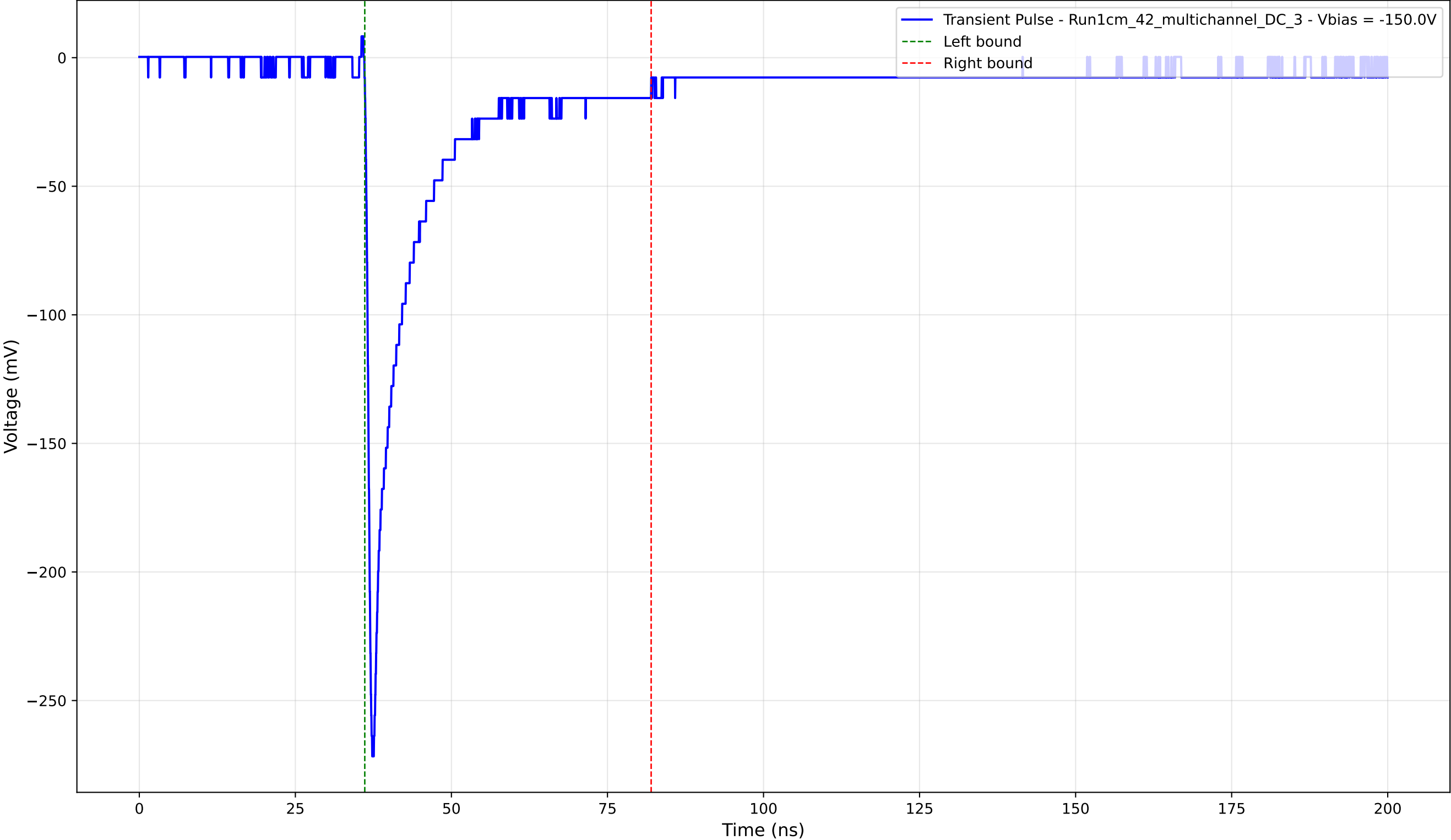
Transient Pulse - Sample: 1cm_42_multichannel - Position: 4525.0 \mu\text{m} - Charge: 41.05 pC - Rise Time: 0.85 ns
