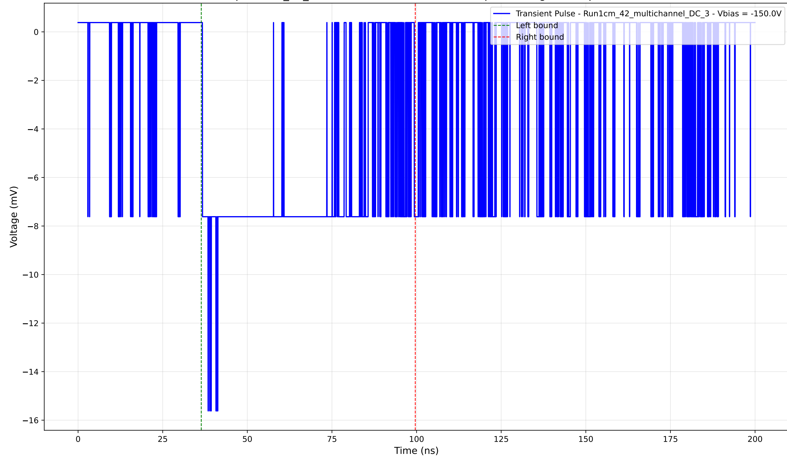
Transient Pulse - Sample: 1cm_42_multichannel - Position: 1850.0 \mu\text{m} - Charge: 7.63 pC - Rise Time: 1.68 ns
