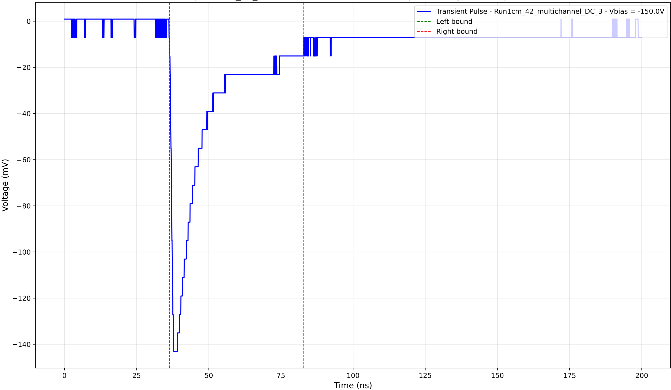
Transient Pulse - Sample: 1cm_42_multichannel - Position: 3785.0 \mu\text{m} - Charge: 37.97 pC - Rise Time: 1.22 ns
