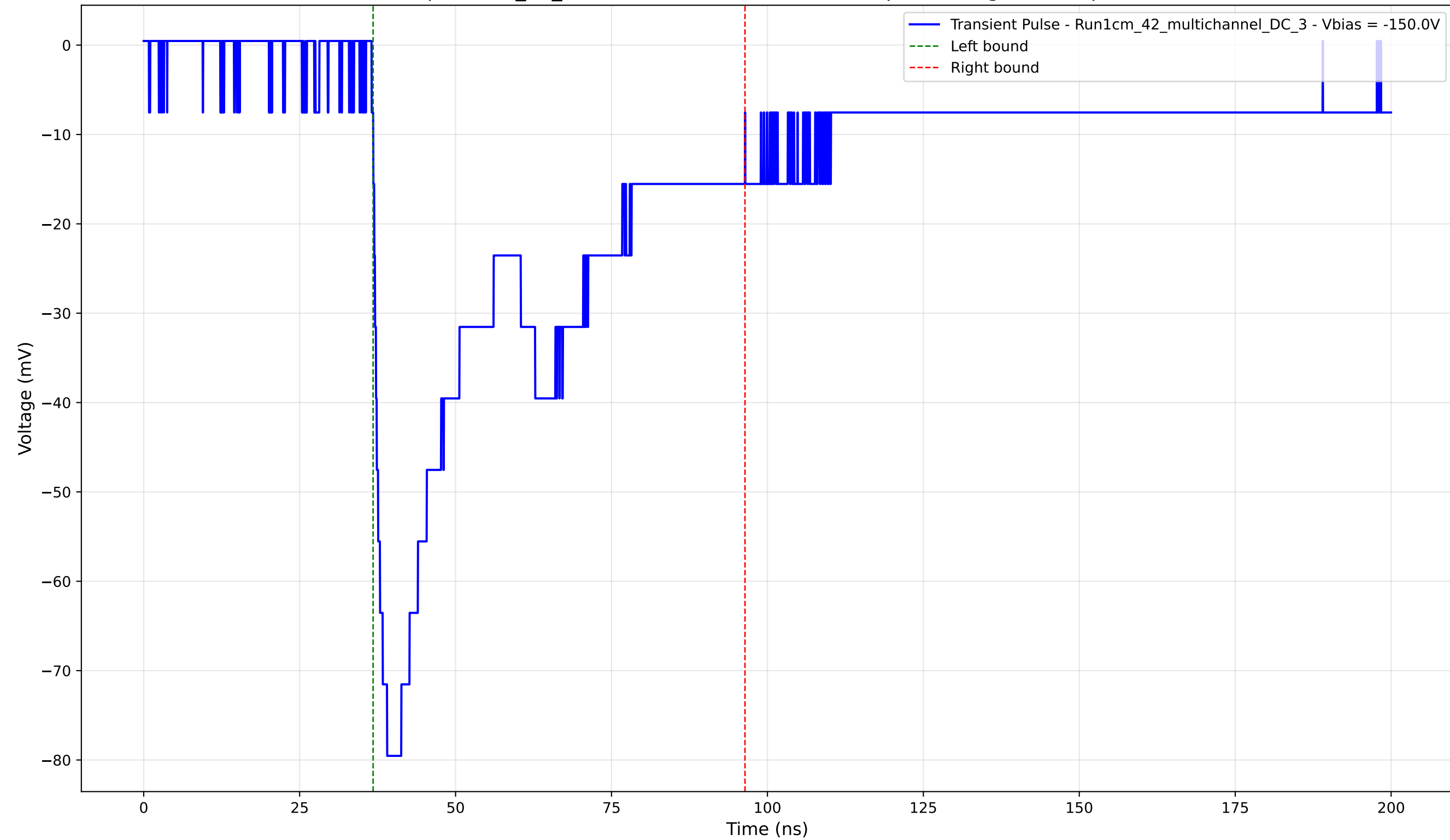
Transient Pulse - Sample: 1cm_42_multichannel - Position: 2540.0 \mu\text{m} - Charge: 37.35 pC - Rise Time: 2.24 ns
