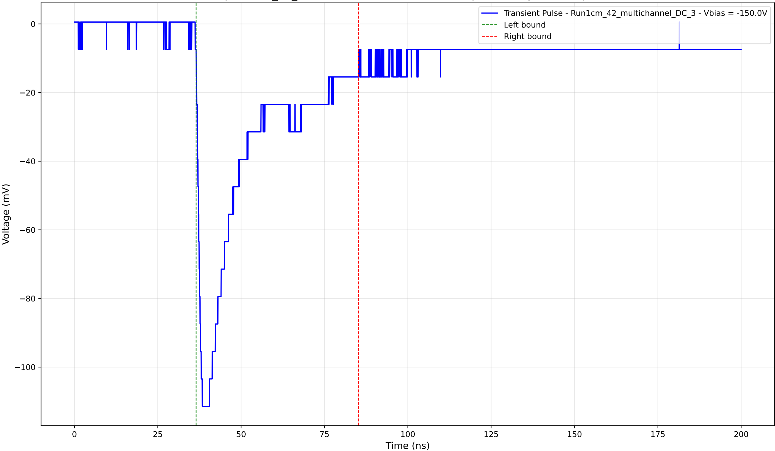
Transient Pulse - Sample: 1cm_42_multichannel - Position: 3275.0 \mu\text{m} - Charge: 37.23 pC - Rise Time: 1.51 ns
