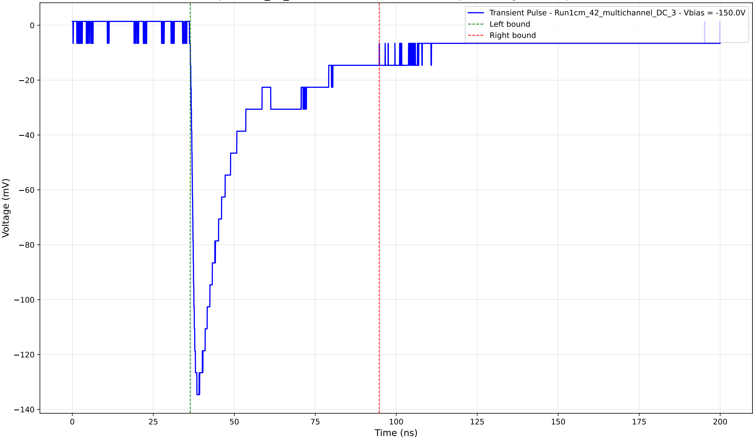
Transient Pulse - Sample: 1cm_42_multichannel - Position: 1505.0 \mu\text{m} - Charge: 44.51 pC - Rise Time: 1.56 ns
