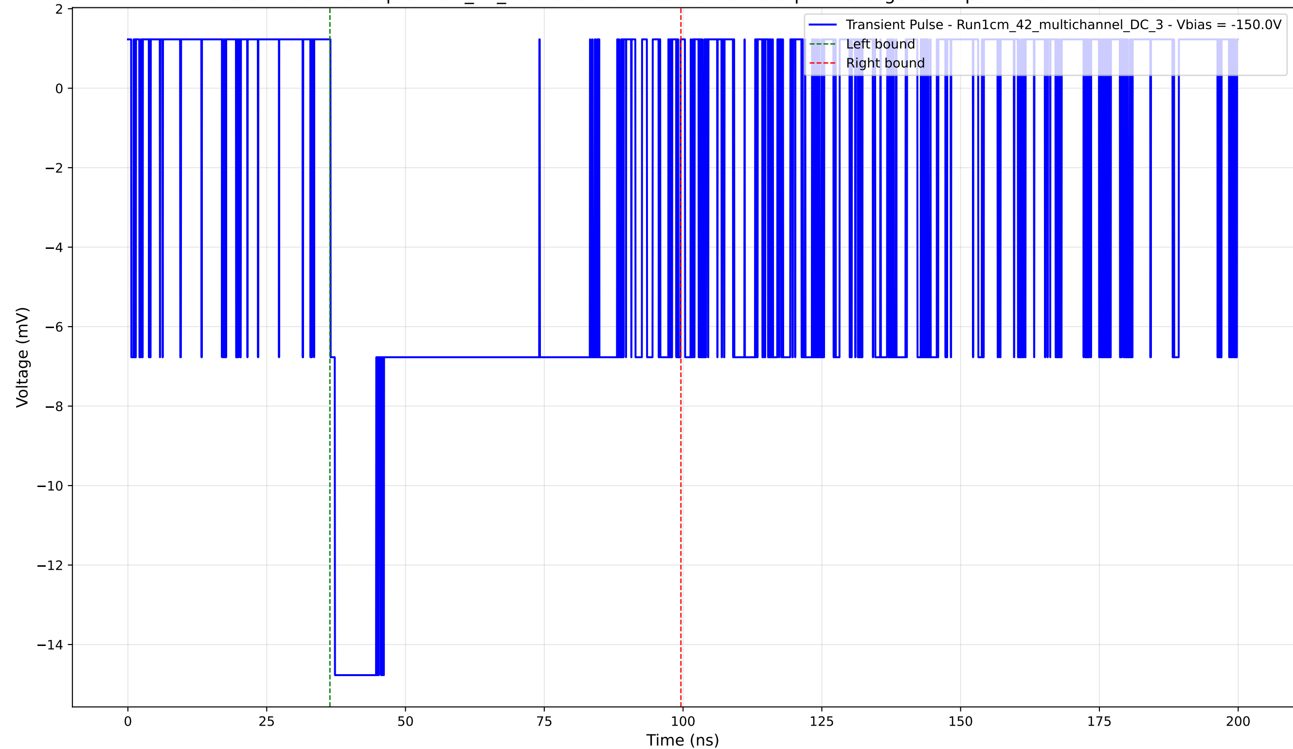
Transient Pulse - Sample: 1cm_42_multichannel - Position: 3415.0 \mu\text{m} - Charge: 8.74 pC - Rise Time: 0.80 ns
