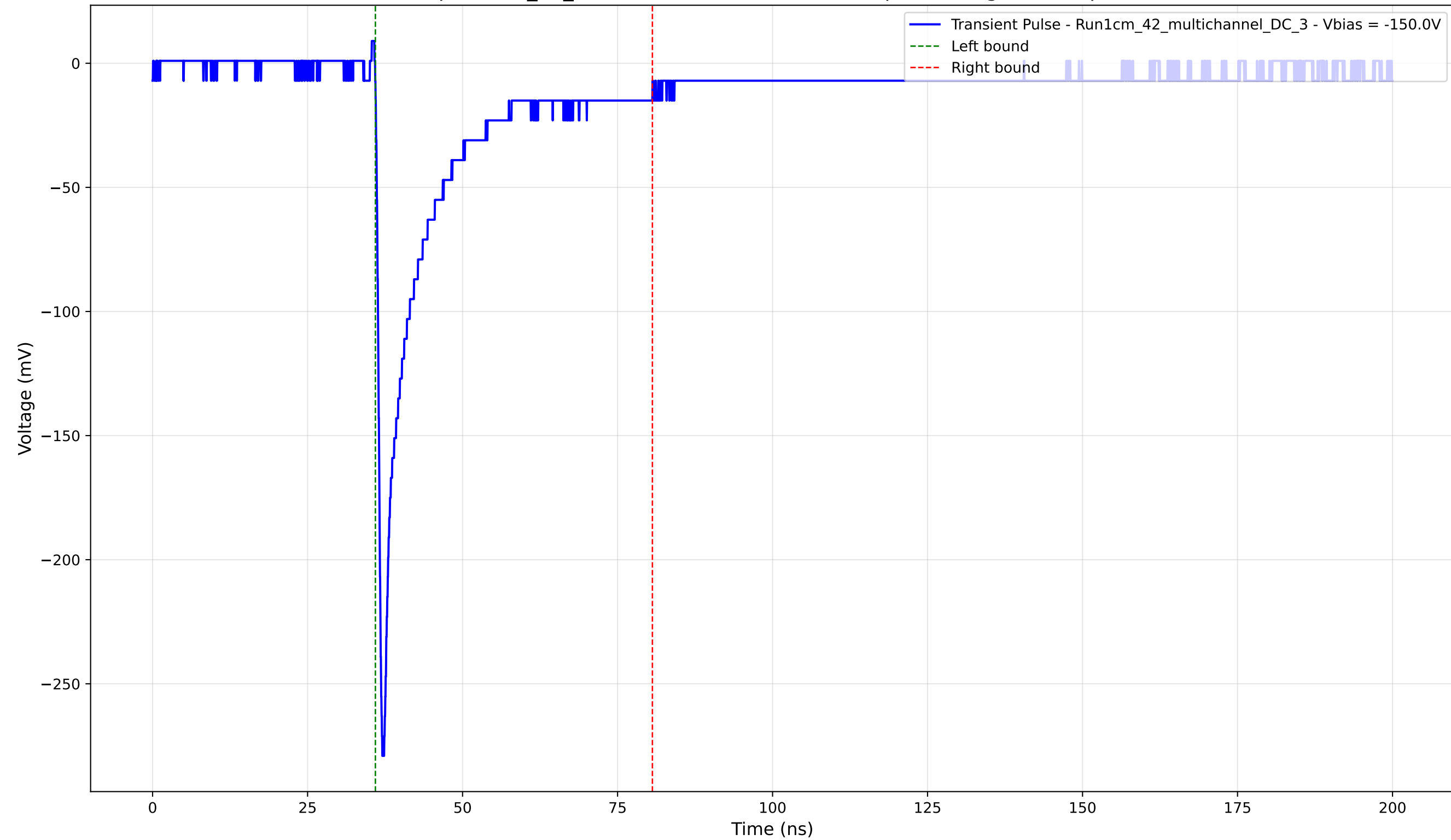
Transient Pulse - Sample: 1cm_42_multichannel - Position: 275.0 \mu\text{m} - Charge: 39.31 pC - Rise Time: 0.83 ns
