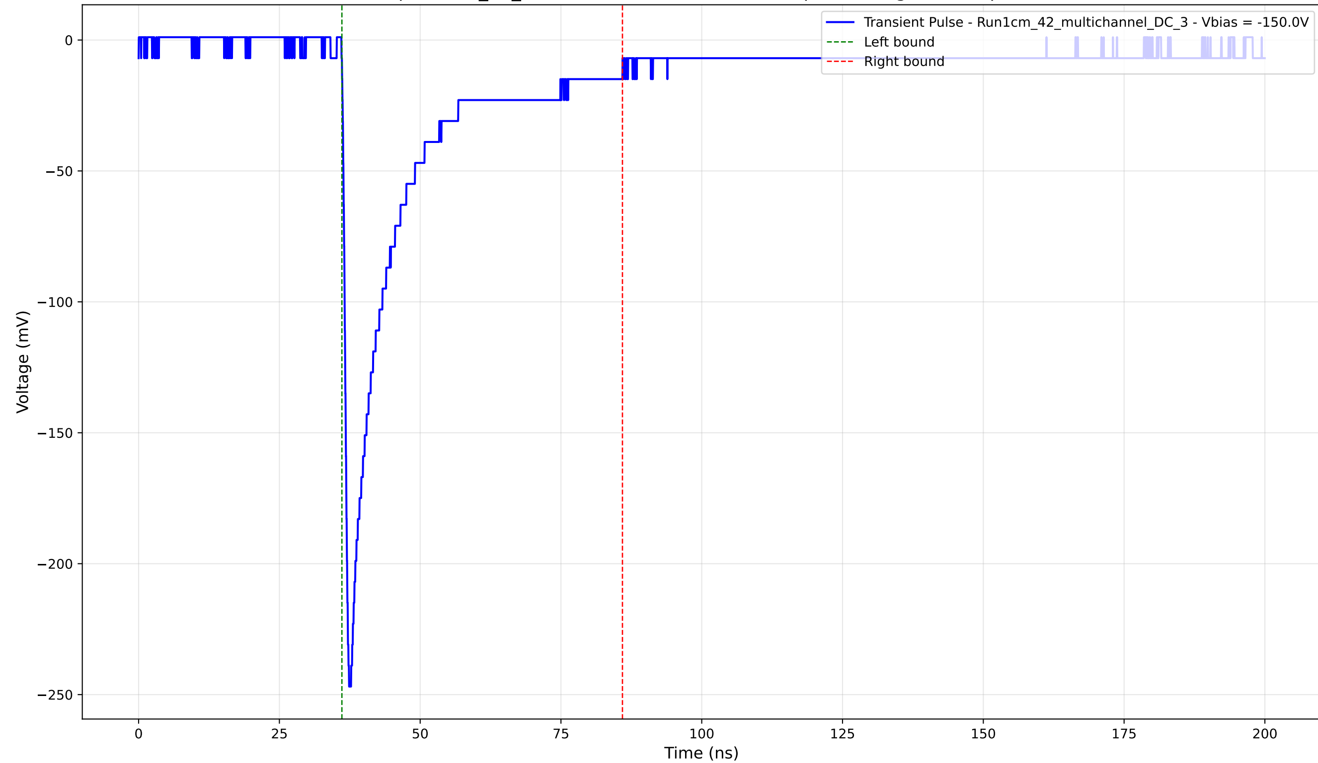
Transient Pulse - Sample: 1cm_42_multichannel - Position: 600.0 \mu\text{m} - Charge: 47.80 pC - Rise Time: 0.92 ns
