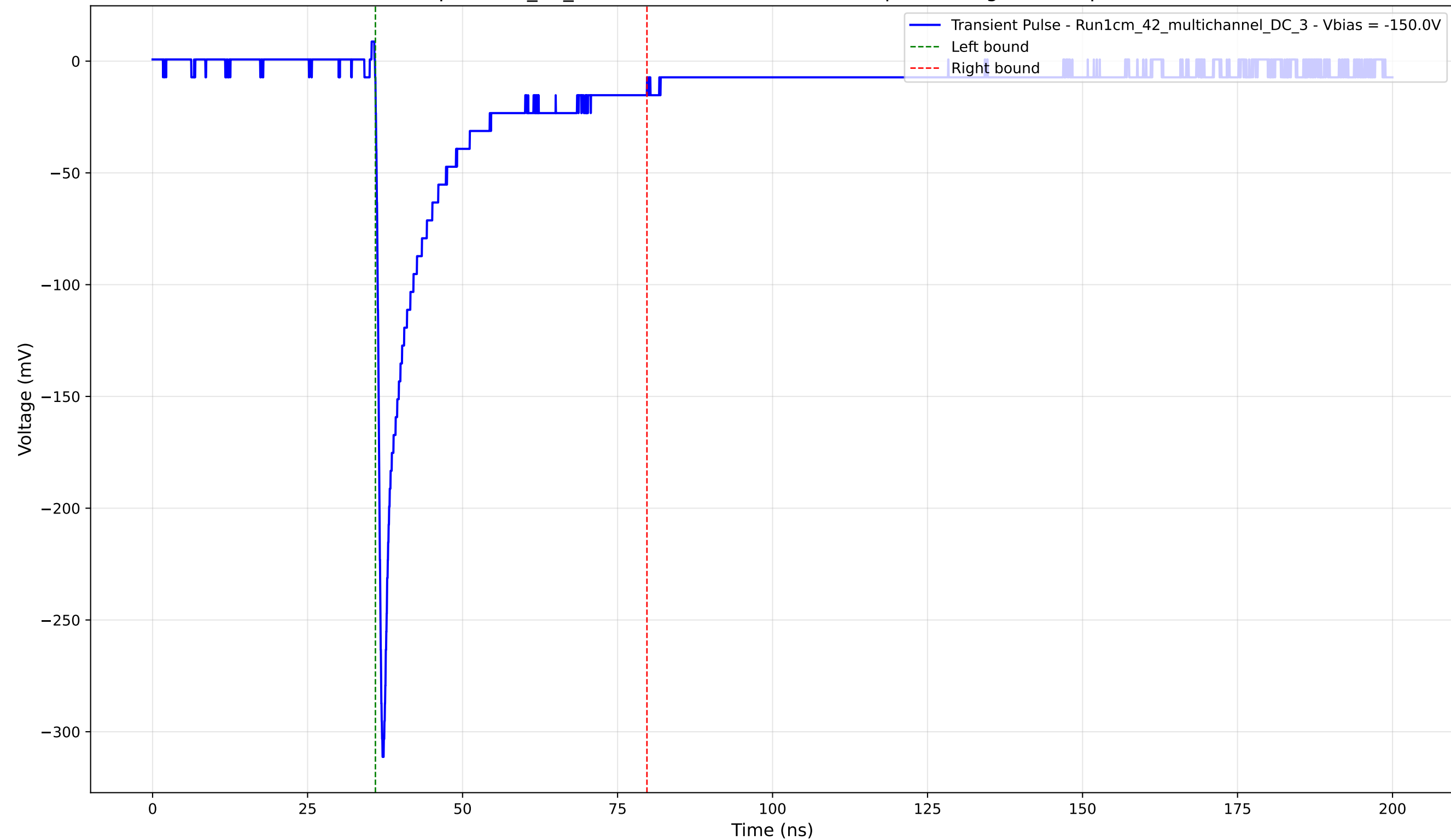
Transient Pulse - Sample: 1cm_42_multichannel - Position: 260.0 \mu\text{m} - Charge: 43.28 pC - Rise Time: 0.86 ns
