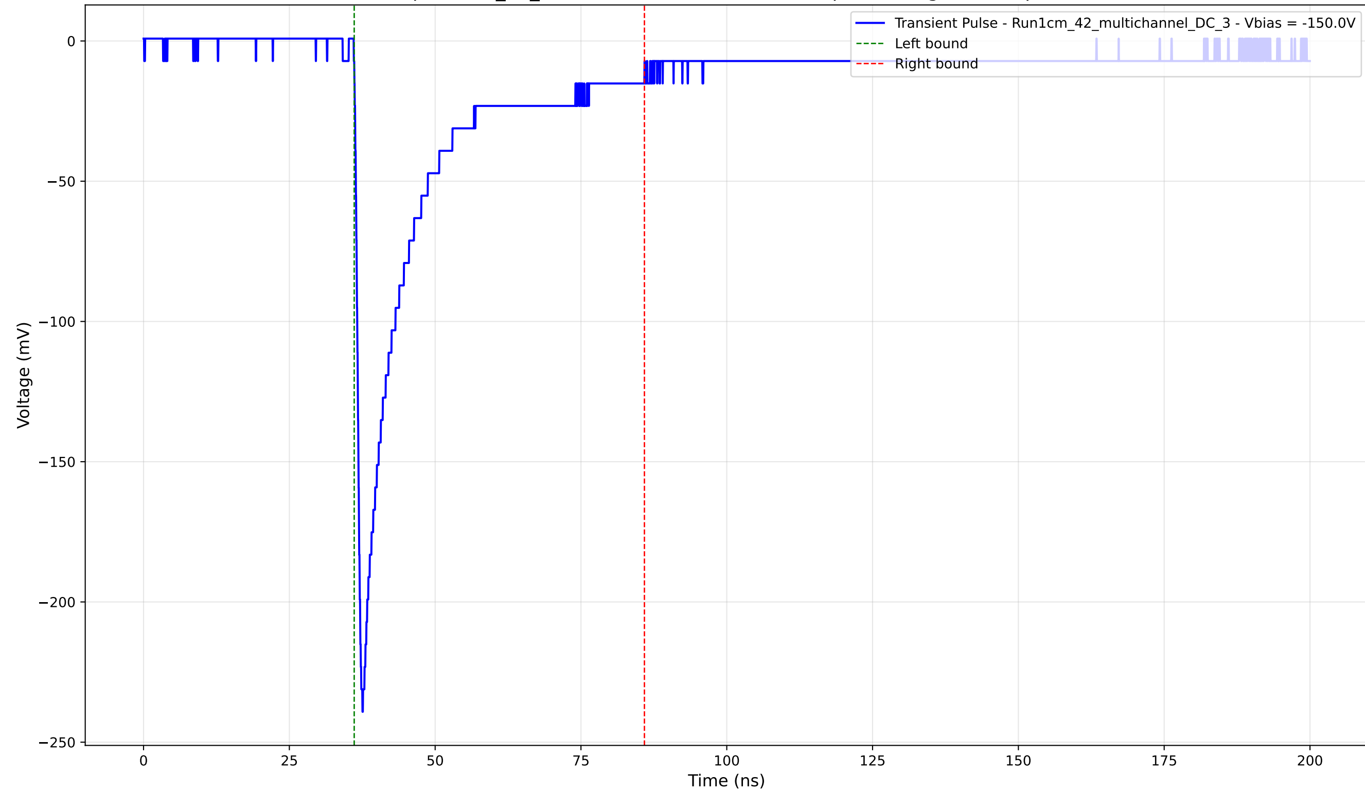
Transient Pulse - Sample: 1cm_42_multichannel - Position: 635.0 \mu\text{m} - Charge: 47.00 pC - Rise Time: 0.98 ns
