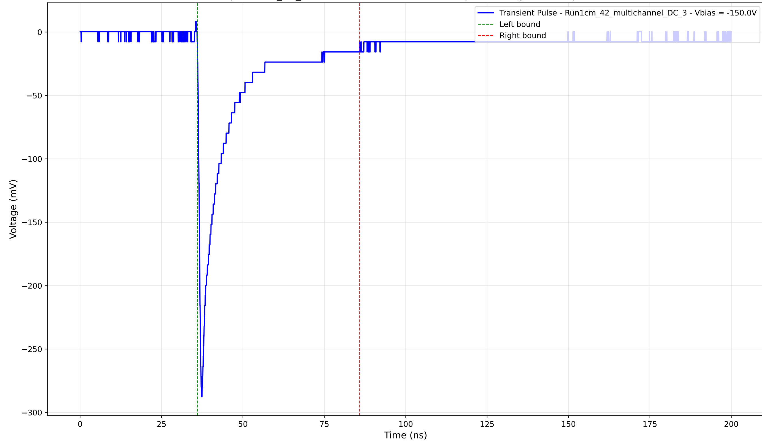
Transient Pulse - Sample: 1cm_42_multichannel - Position: 460.0 \mu\text{m} - Charge: 49.91 pC - Rise Time: 0.91 ns
