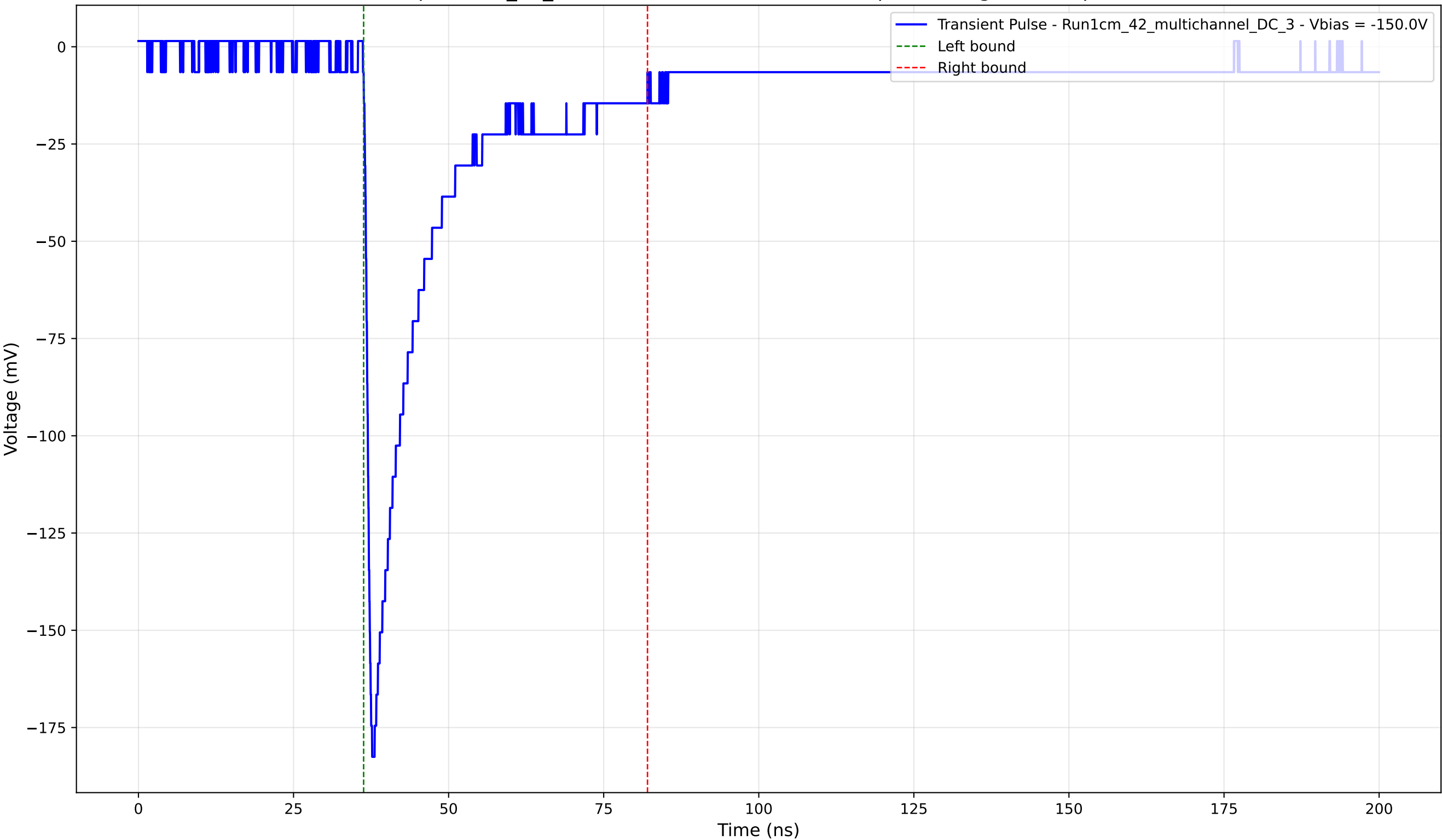
Transient Pulse - Sample: 1cm_42_multichannel - Position: 4125.0 \mu\text{m} - Charge: 38.06 pC - Rise Time: 0.99 ns
