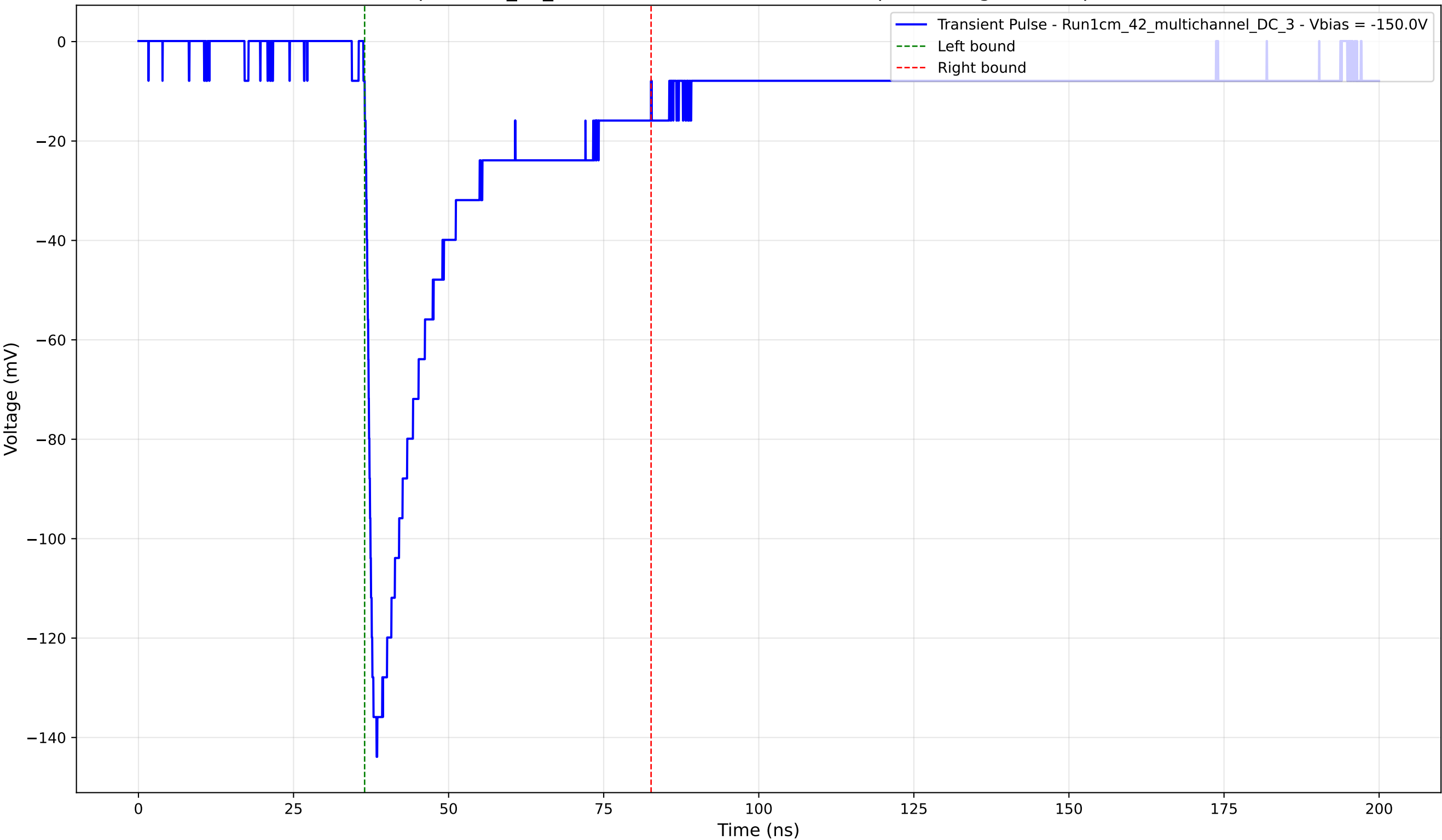
Transient Pulse - Sample: 1cm_42_multichannel - Position: 3720.0 \mu\text{m} - Charge: 37.68 pC - Rise Time: 1.40 ns
