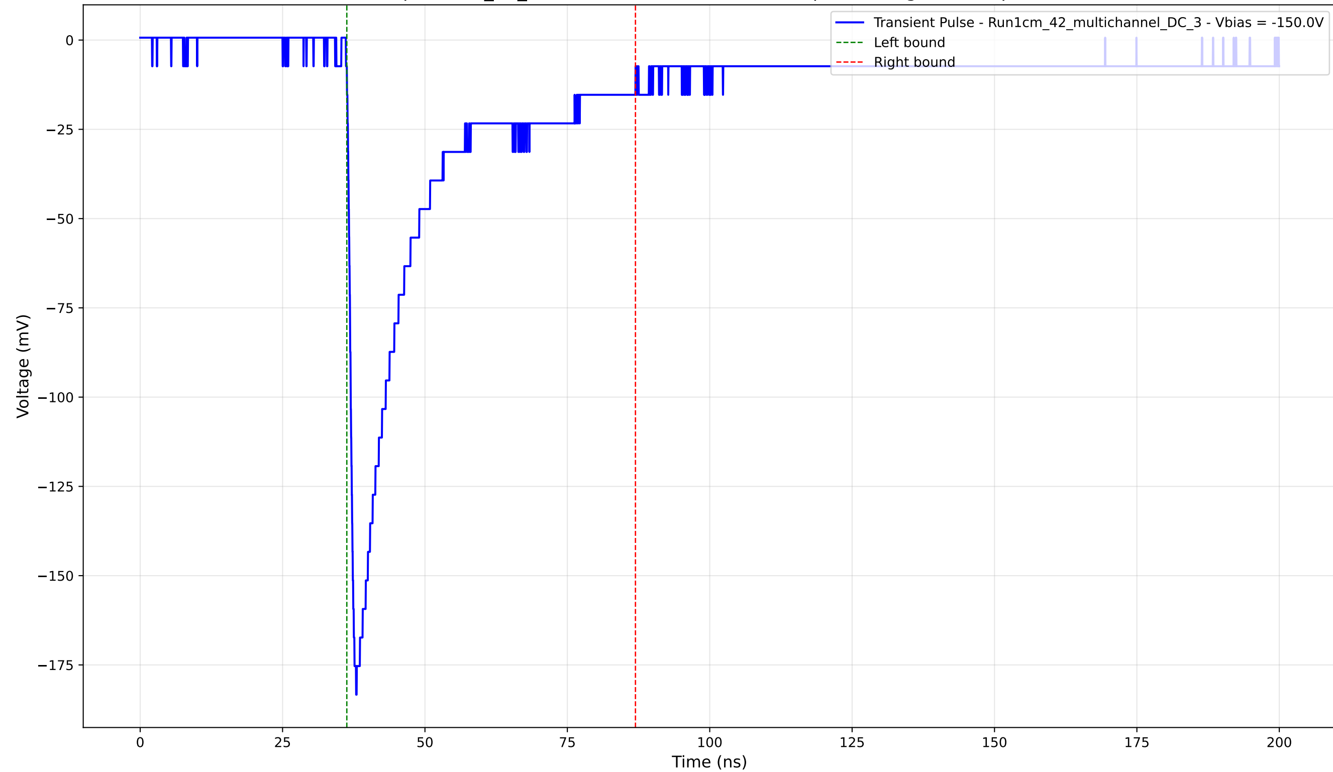
Transient Pulse - Sample: 1cm_42_multichannel - Position: 985.0 \mu\text{m} - Charge: 44.97 pC - Rise Time: 1.11 ns
