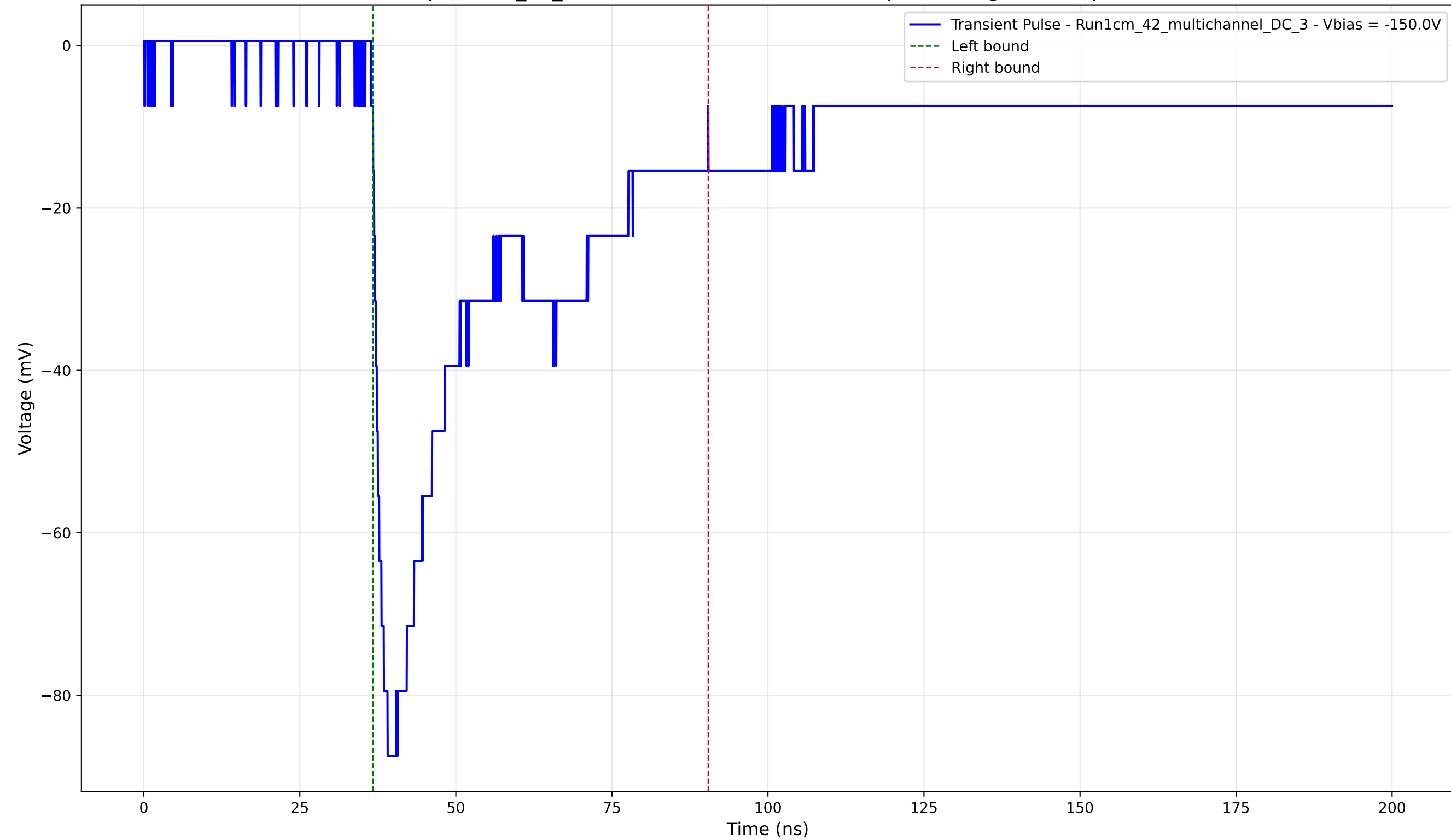
Transient Pulse - Sample: 1cm_42_multichannel - Position: 2670.0 \mu\text{m} - Charge: 36.02 pC - Rise Time: 1.74 ns
