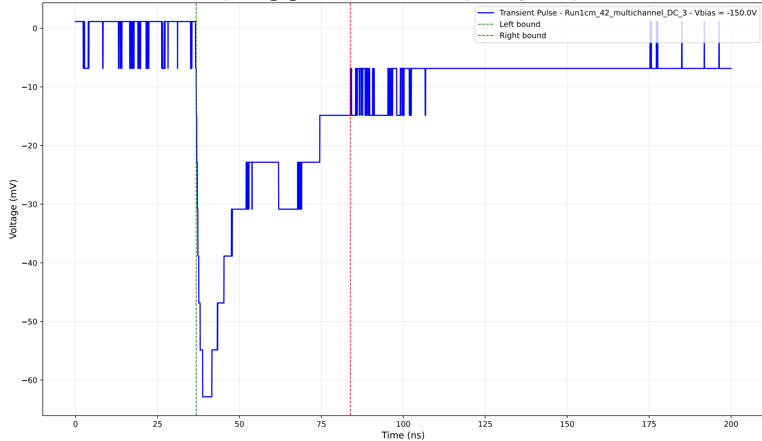
Transient Pulse - Sample: 1cm_42_multichannel - Position: 2310.0 \mu\text{m} - Charge: 27.62 pC - Rise Time: 2.16 ns
