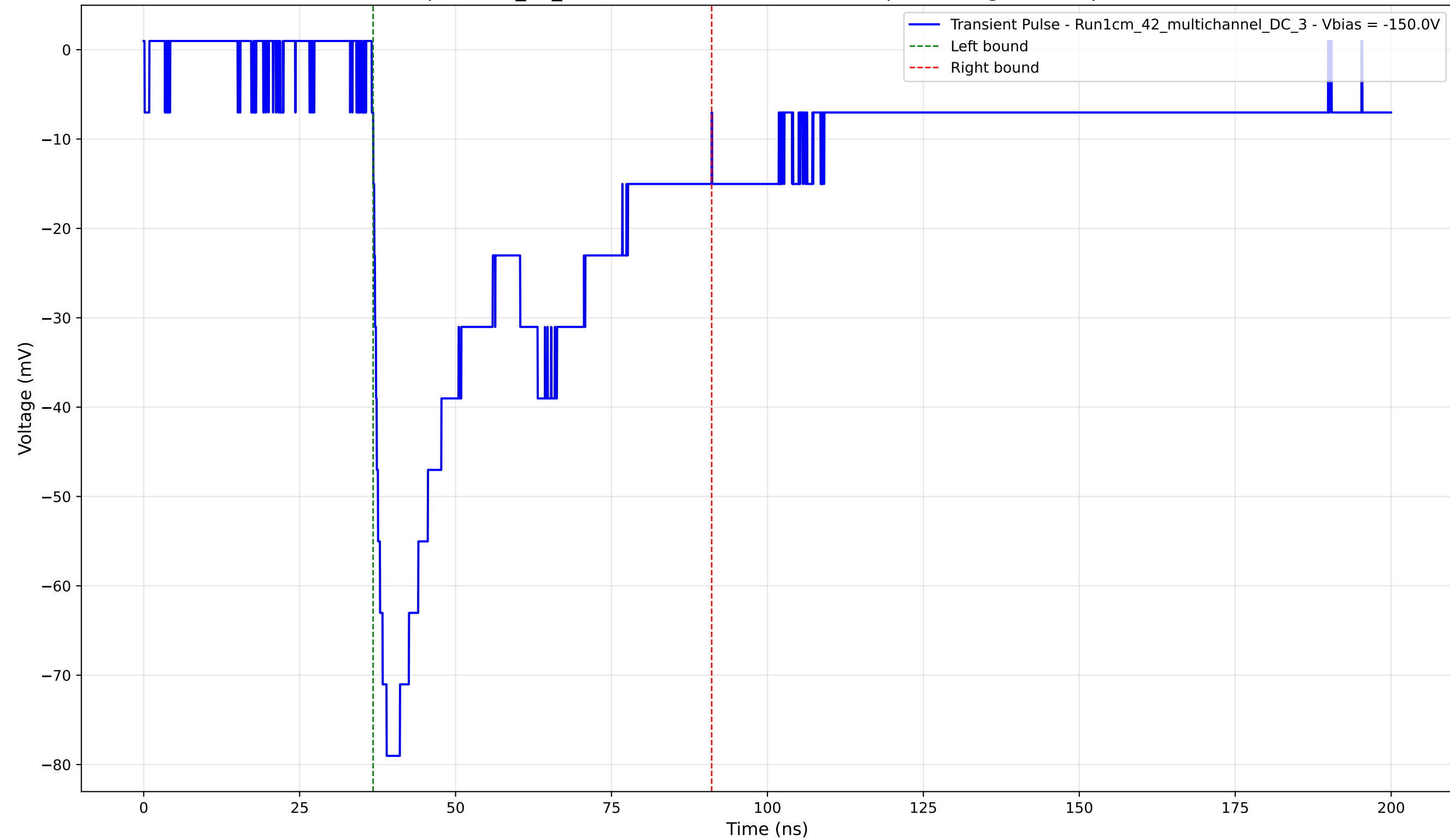
Transient Pulse - Sample: 1cm_42_multichannel - Position: 2570.0 \mu\text{m} - Charge: 35.06 pC - Rise Time: 2.16 ns
