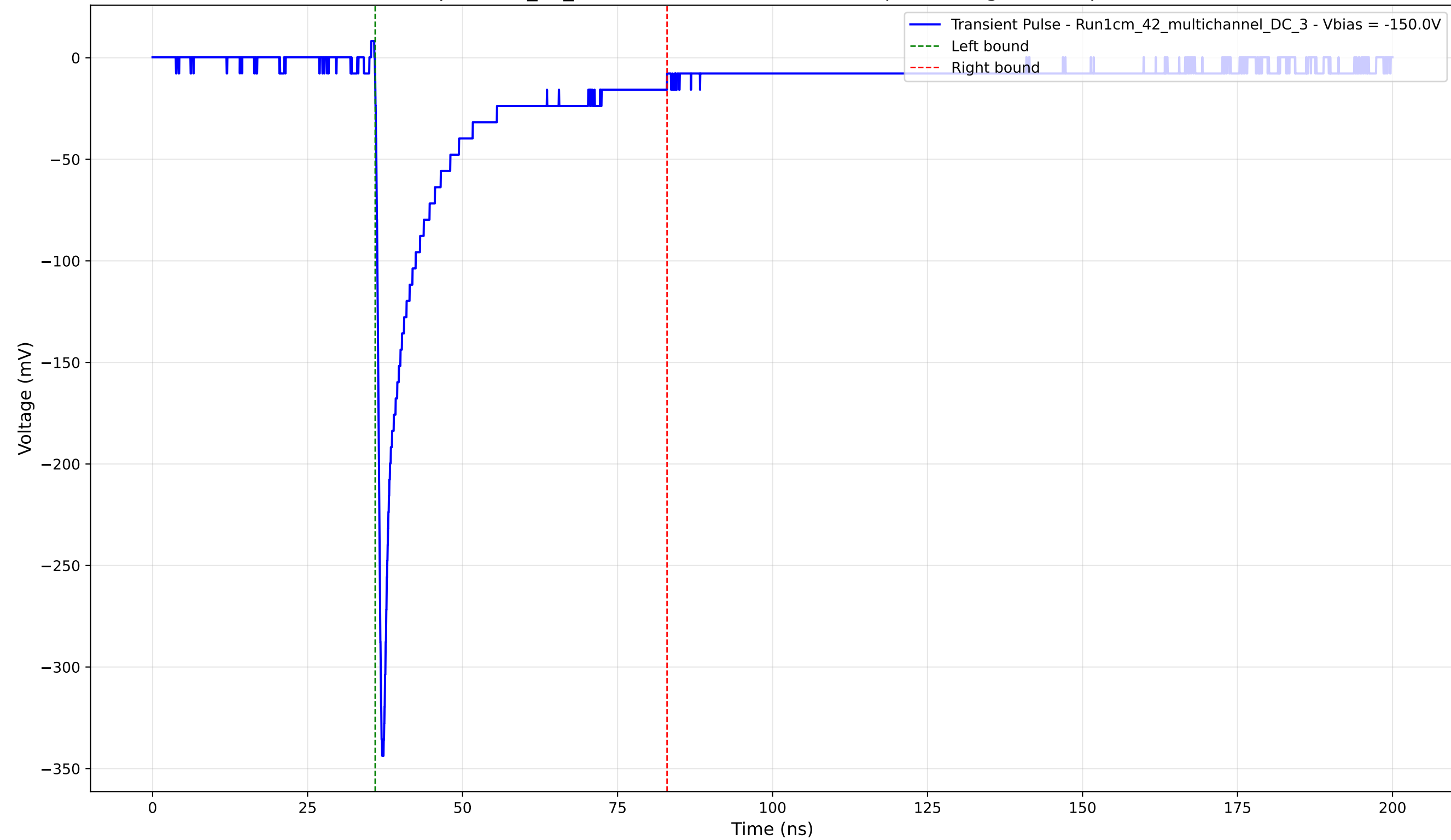
Transient Pulse - Sample: 1cm_42_multichannel - Position: 215.0 \mu\text{m} - Charge: 47.75 pC - Rise Time: 0.79 ns
