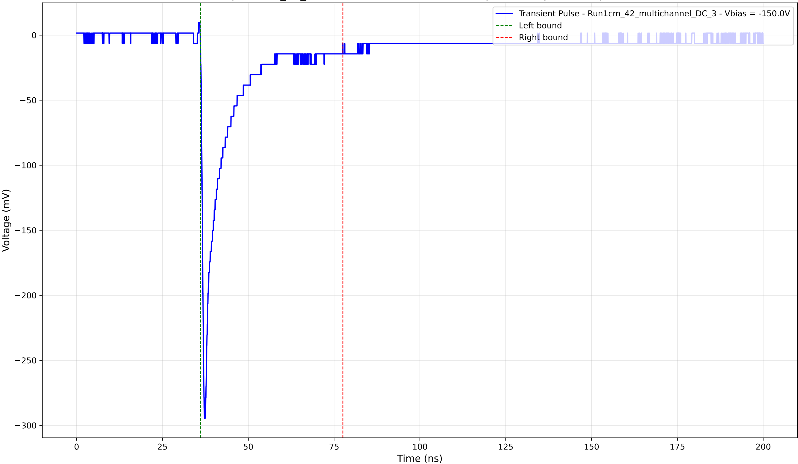
Transient Pulse - Sample: 1cm_42_multichannel - Position: 4600.0 \mu\text{m} - Charge: 39.44 pC - Rise Time: 0.84 ns
