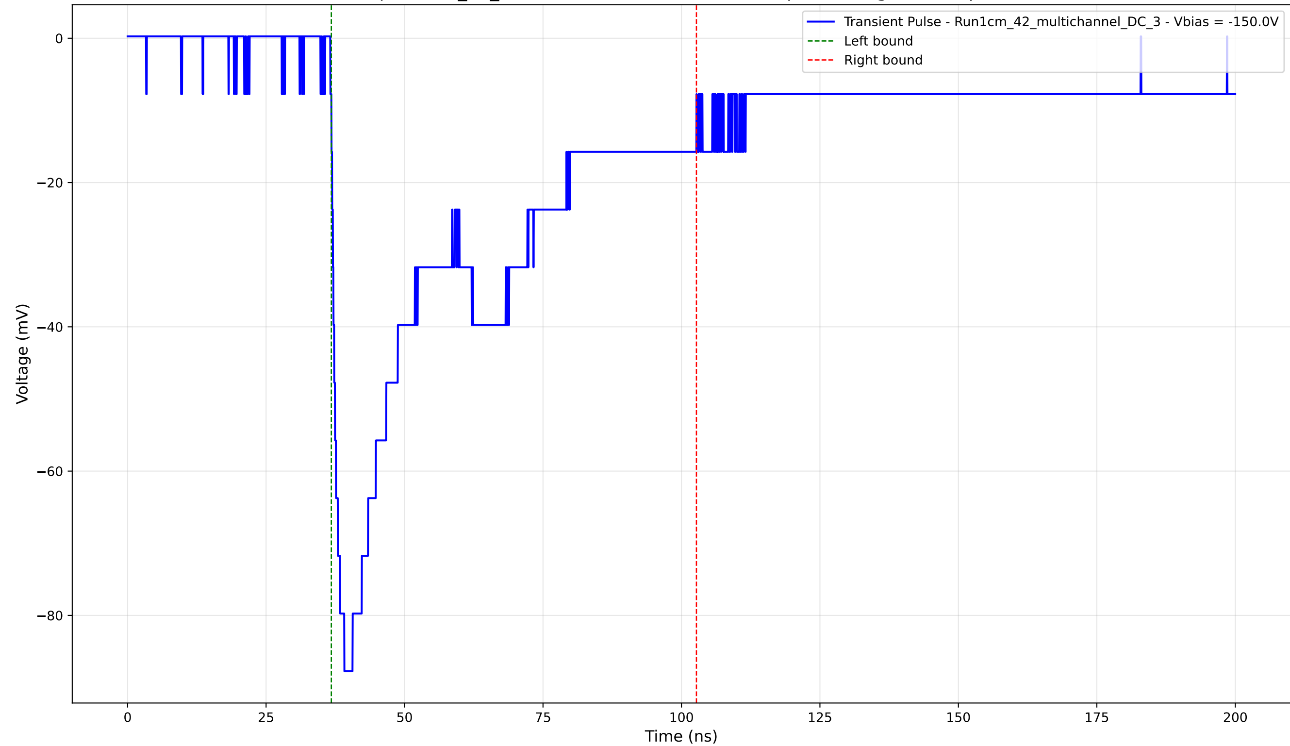
Transient Pulse - Sample: 1cm_42_multichannel - Position: 2240.0 \mu\text{m} - Charge: 42.70 pC - Rise Time: 1.58 ns
