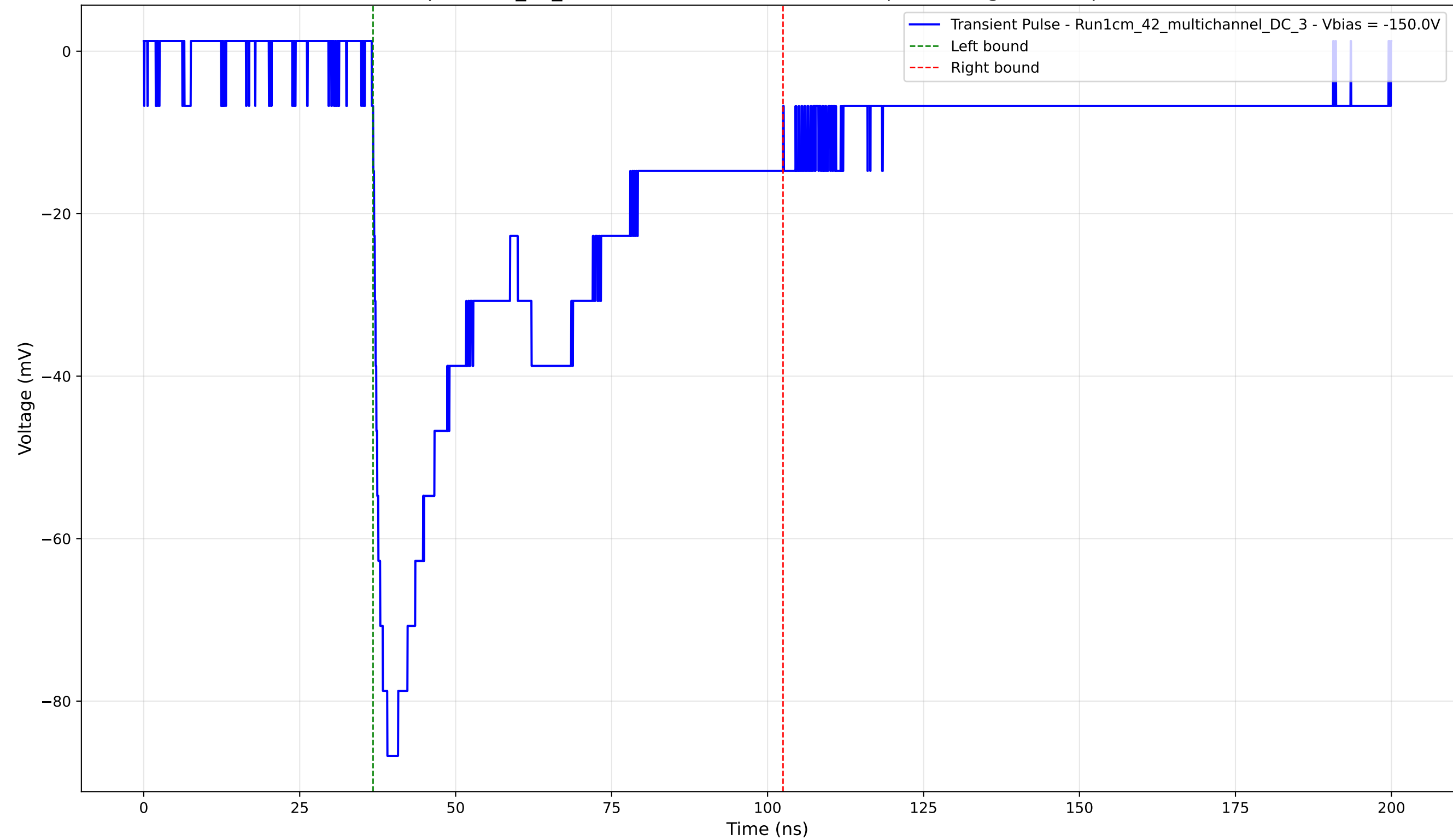
Transient Pulse - Sample: 1cm_42_multichannel - Position: 2220.0 \mu\text{m} - Charge: 41.26 pC - Rise Time: 1.56 ns
