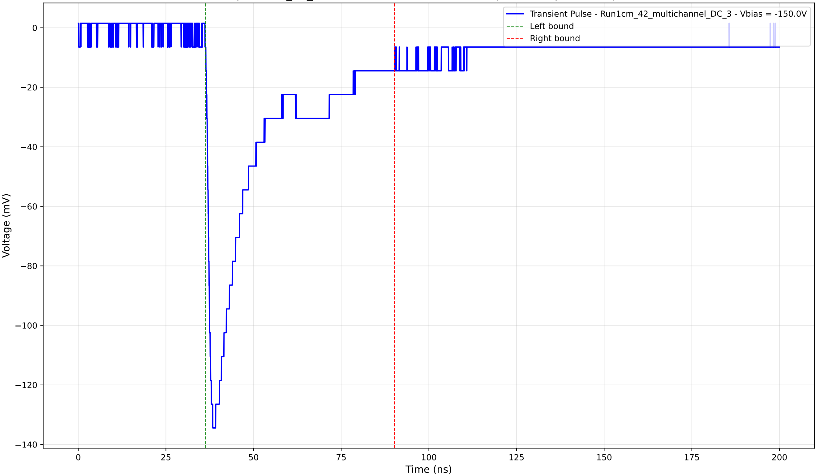
Transient Pulse - Sample: 1cm_42_multichannel - Position: 1455.0 \mu\text{m} - Charge: 42.55 pC - Rise Time: 1.54 ns
