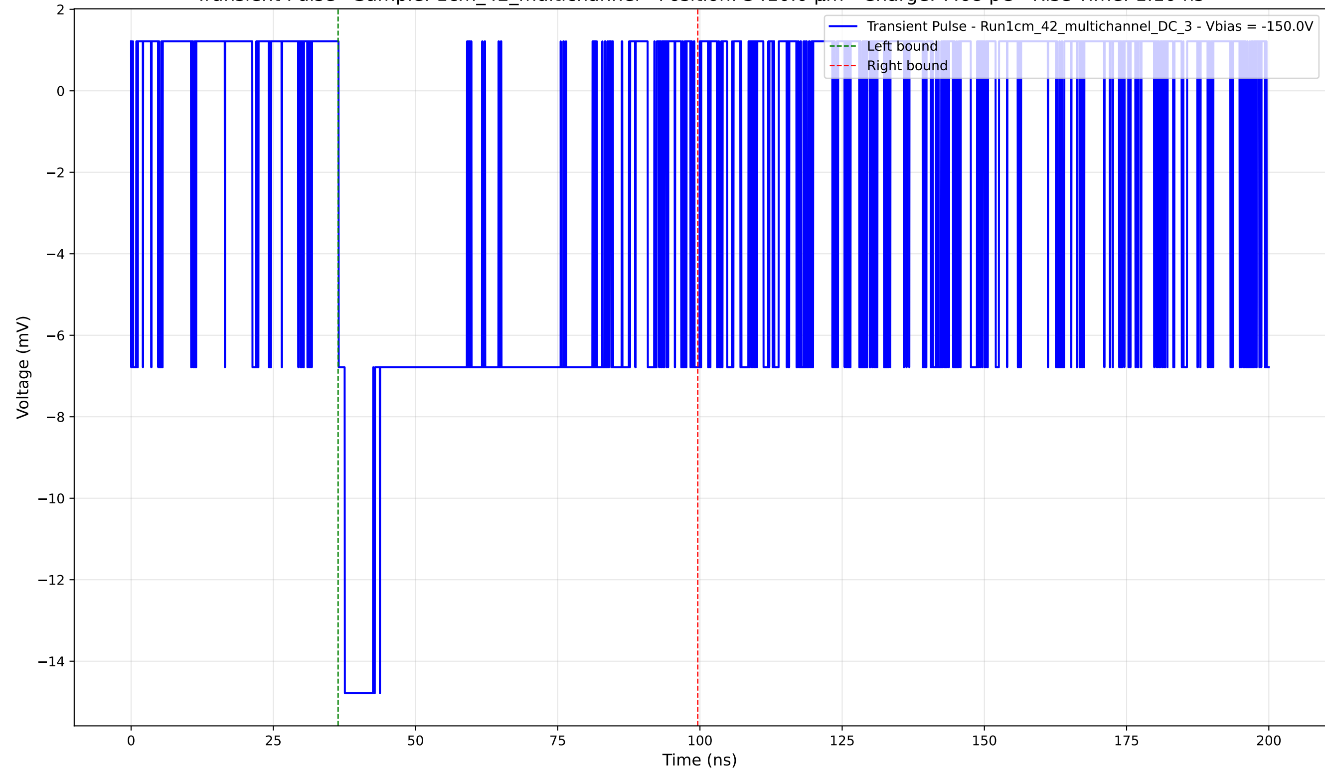
Transient Pulse - Sample: 1cm_42_multichannel - Position: 3410.0 \mu\text{m} - Charge: 7.68 pC - Rise Time: 1.10 ns
