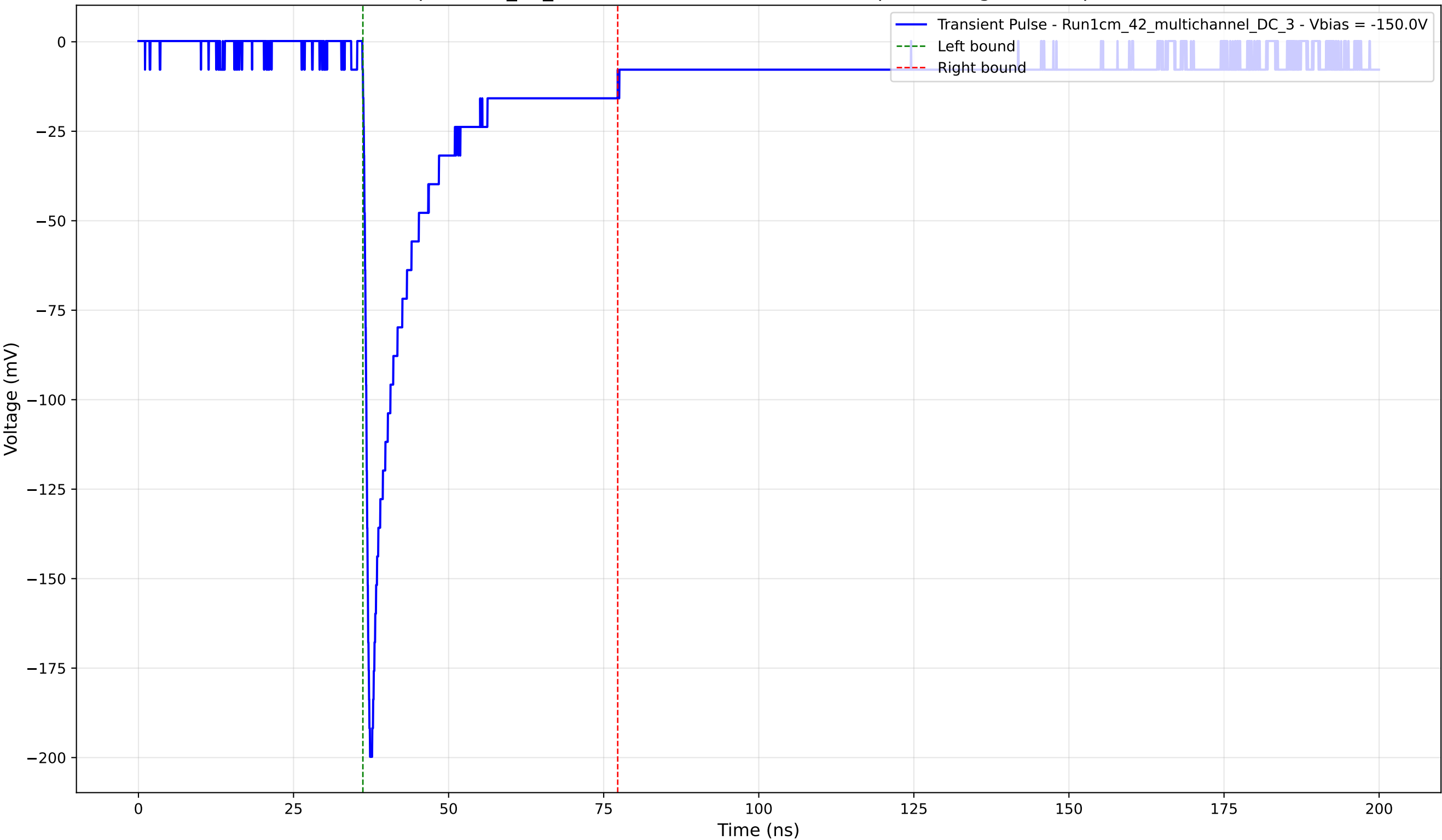
Transient Pulse - Sample: 1cm_42_multichannel - Position: 4460.0 \mu\text{m} - Charge: 31.97 pC - Rise Time: 0.89 ns
