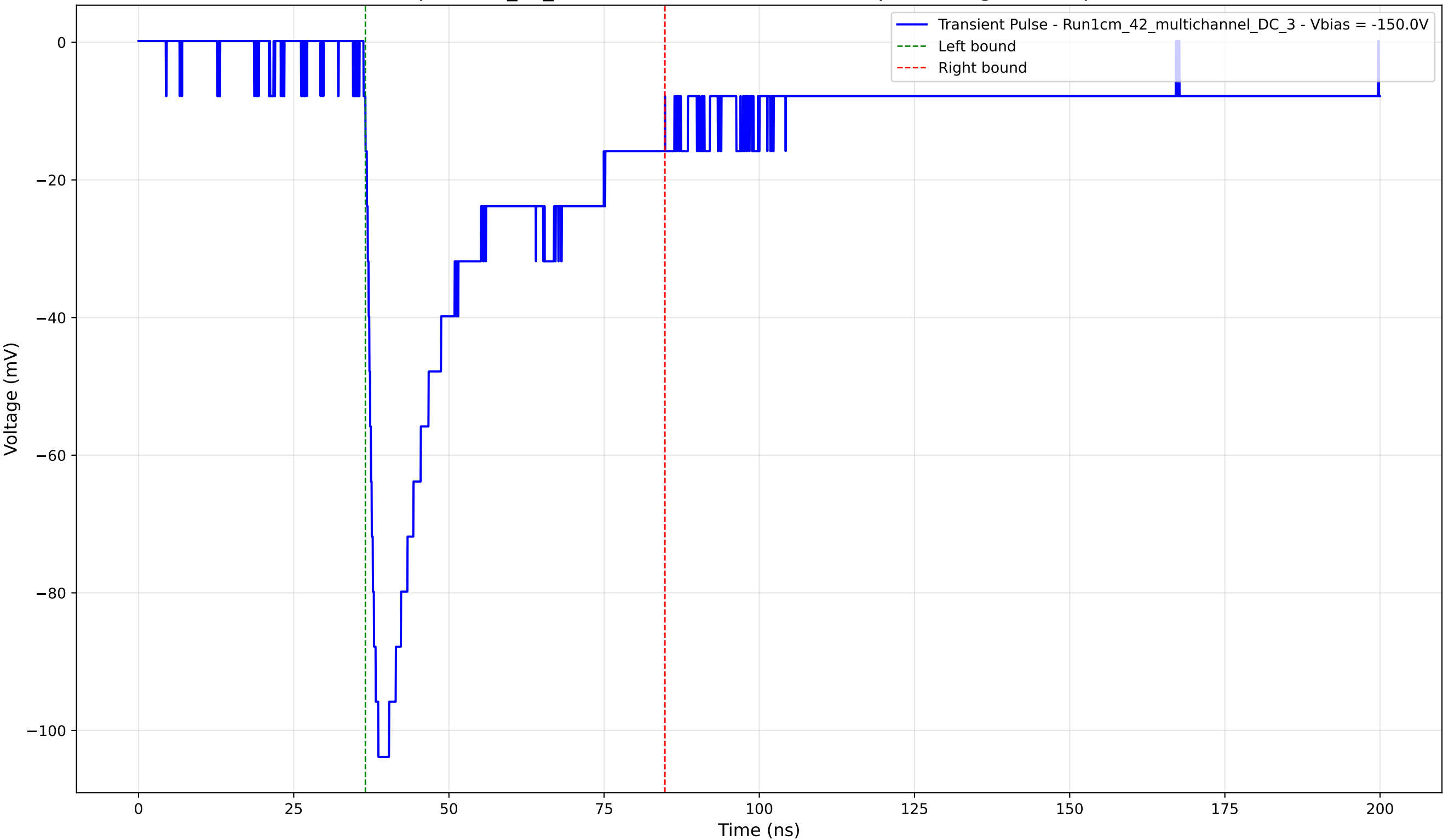
Transient Pulse - Sample: 1cm_42_multichannel - Position: 3160.0 \mu\text{m} - Charge: 35.06 pC - Rise Time: 1.65 ns
