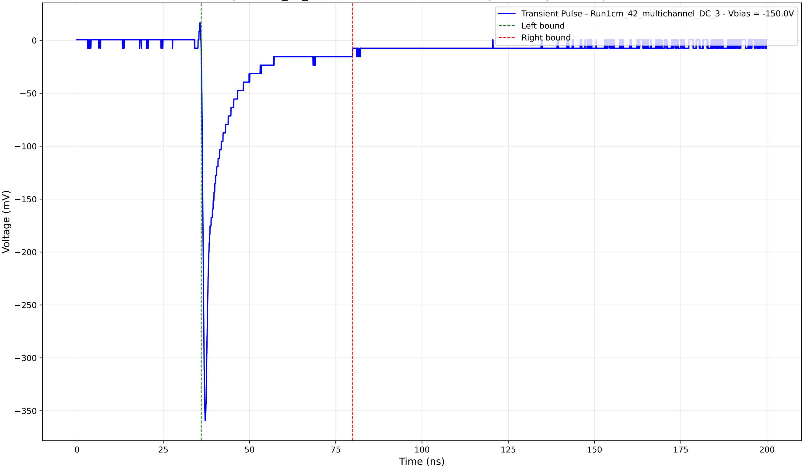
Transient Pulse - Sample: 1cm_42_multichannel - Position: 4765.0 \mu\text{m} - Charge: 41.42 pC - Rise Time: 0.79 ns
