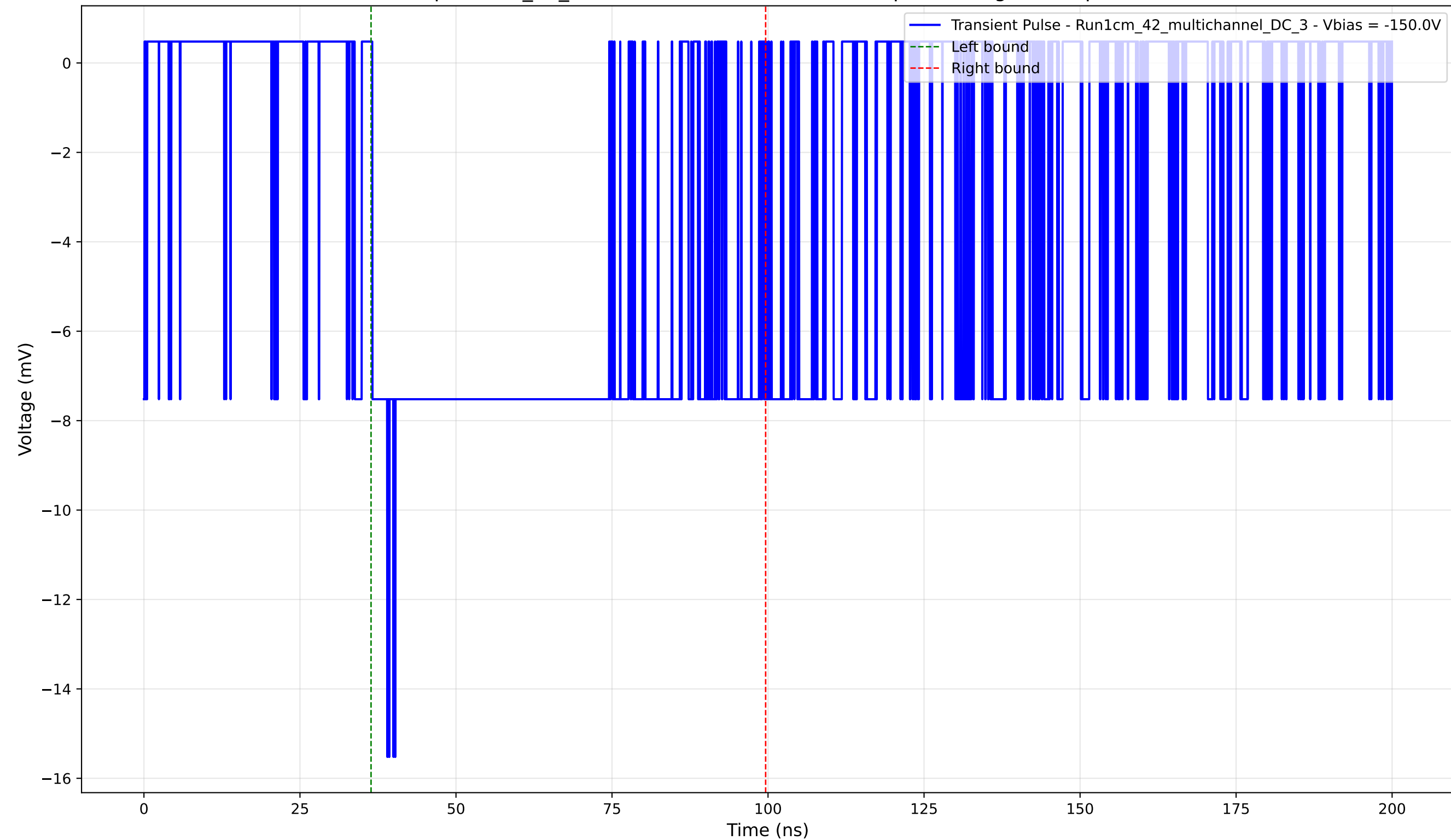
Transient Pulse - Sample: 1cm_42_multichannel - Position: 2350.0 \mu\text{m} - Charge: 8.53 pC - Rise Time: 2.40 ns
