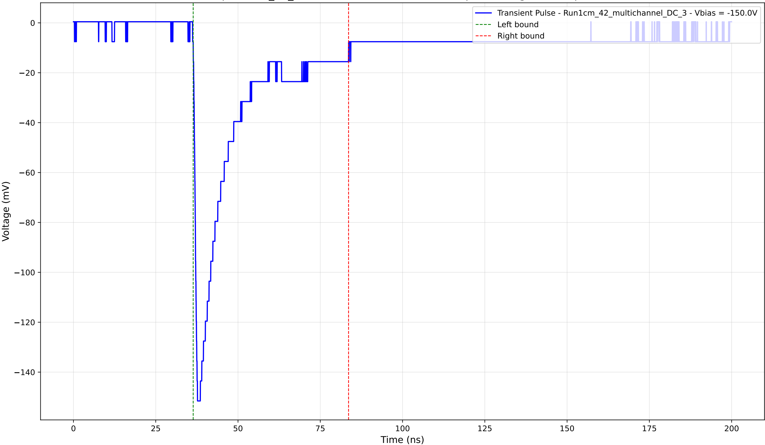
Transient Pulse - Sample: 1cm_42_multichannel - Position: 3965.0 \mu\text{m} - Charge: 36.83 pC - Rise Time: 1.16 ns
