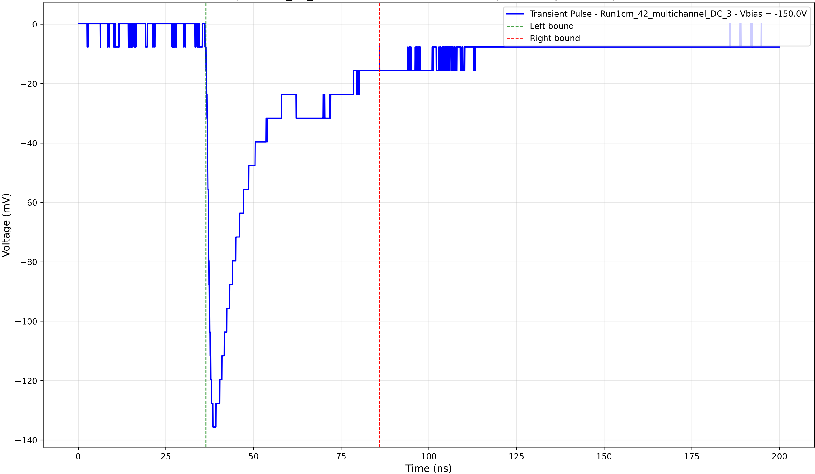
Transient Pulse - Sample: 1cm_42_multichannel - Position: 1480.0 \mu\text{m} - Charge: 42.59 pC - Rise Time: 1.53 ns
