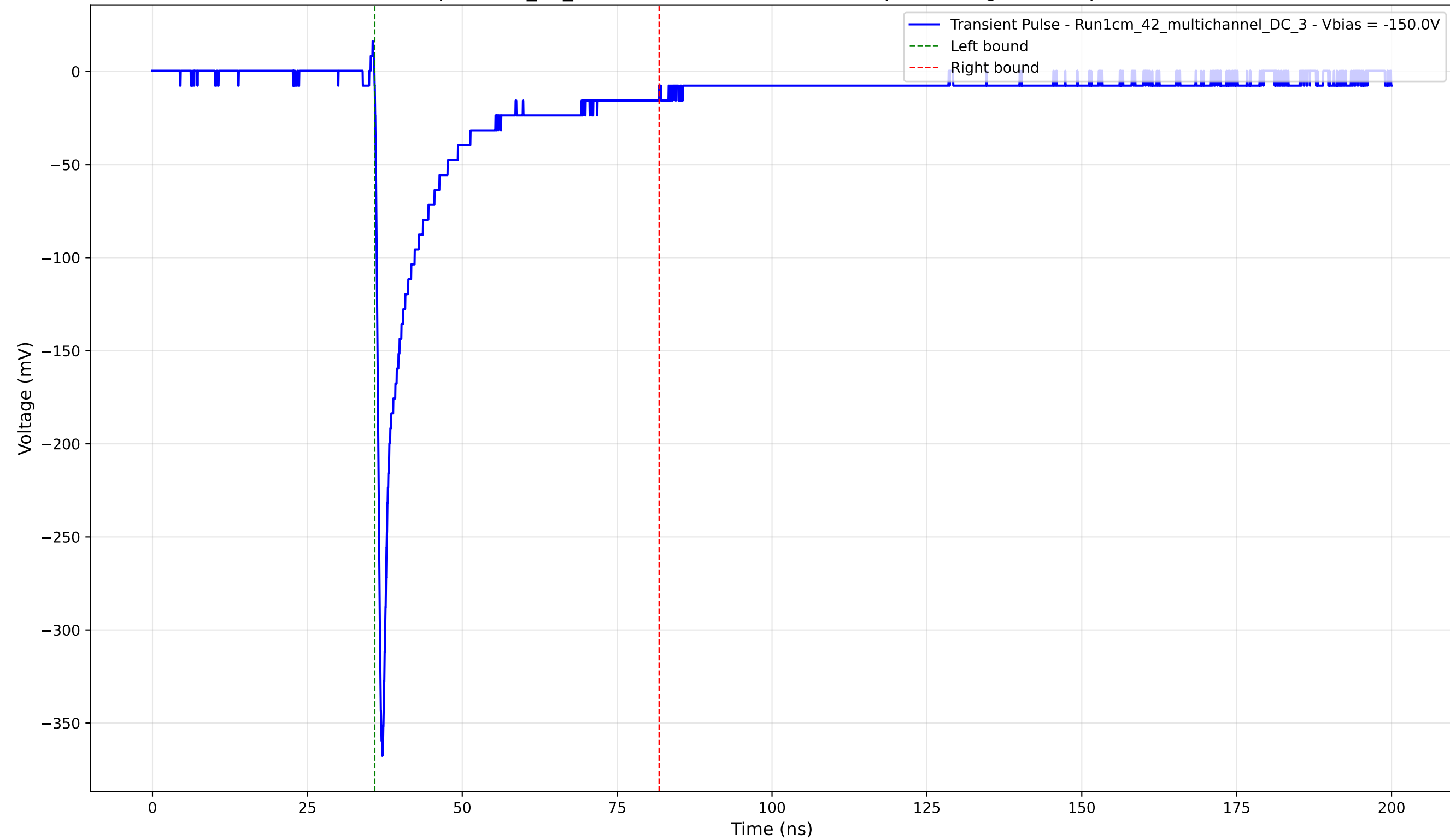
Transient Pulse - Sample: 1cm_42_multichannel - Position: 165.0 \mu\text{m} - Charge: 47.02 pC - Rise Time: 0.83 ns
