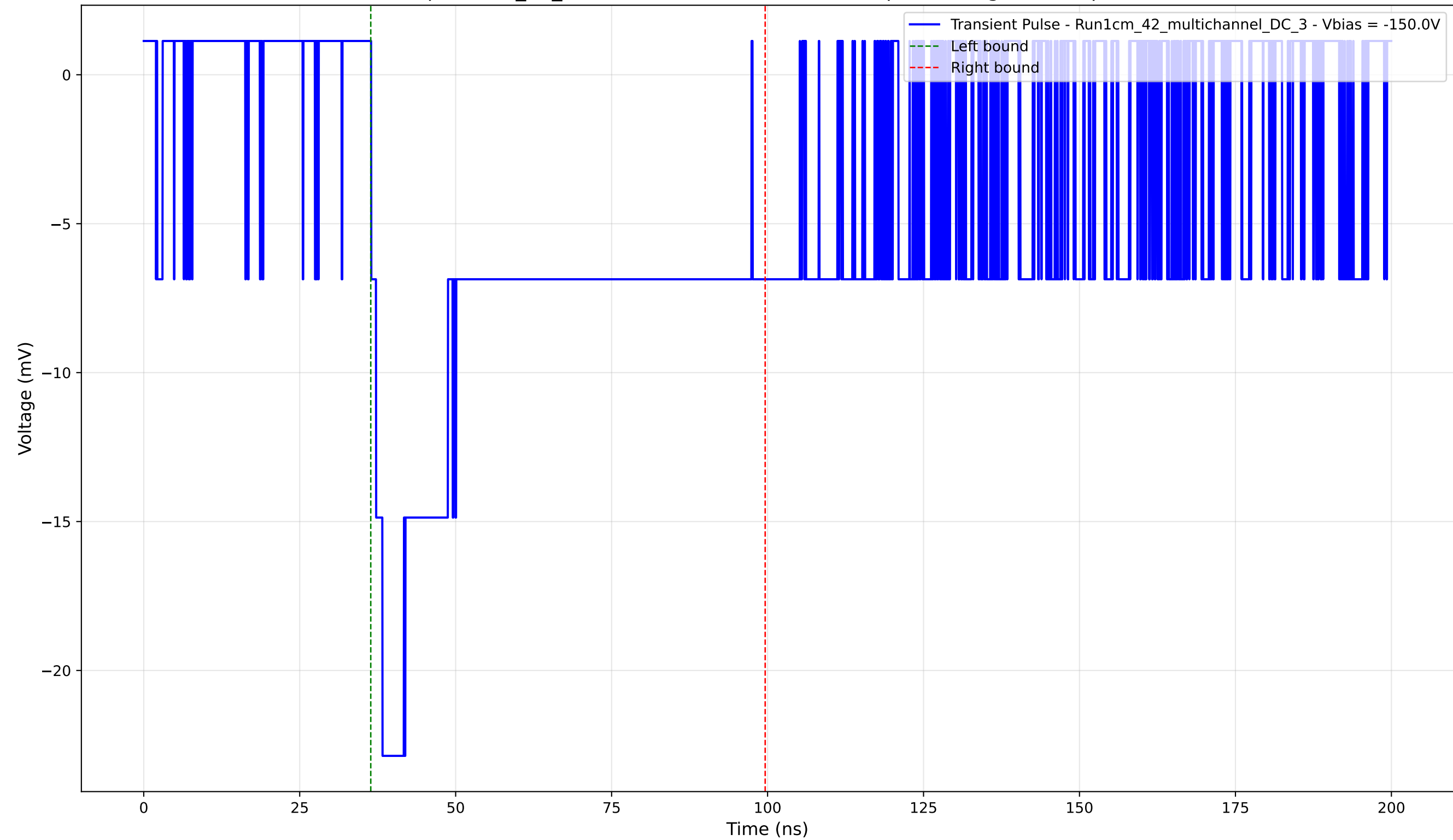
Transient Pulse - Sample: 1cm_42_multichannel - Position: 2915.0 \mu\text{m} - Charge: 11.09 pC - Rise Time: 1.82 ns
