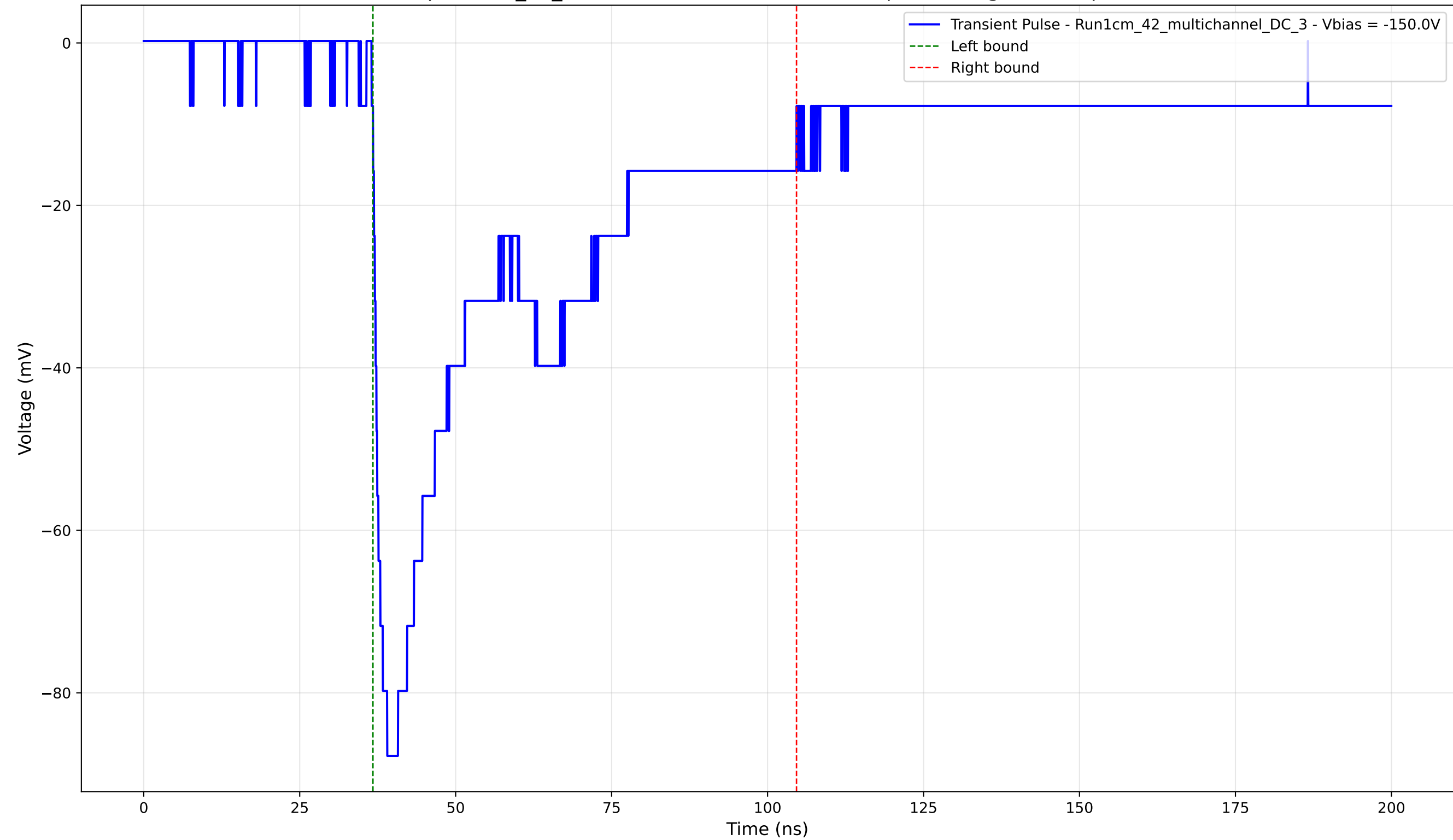
Transient Pulse - Sample: 1cm_42_multichannel - Position: 2160.0 \mu\text{m} - Charge: 42.22 pC - Rise Time: 1.58 ns
