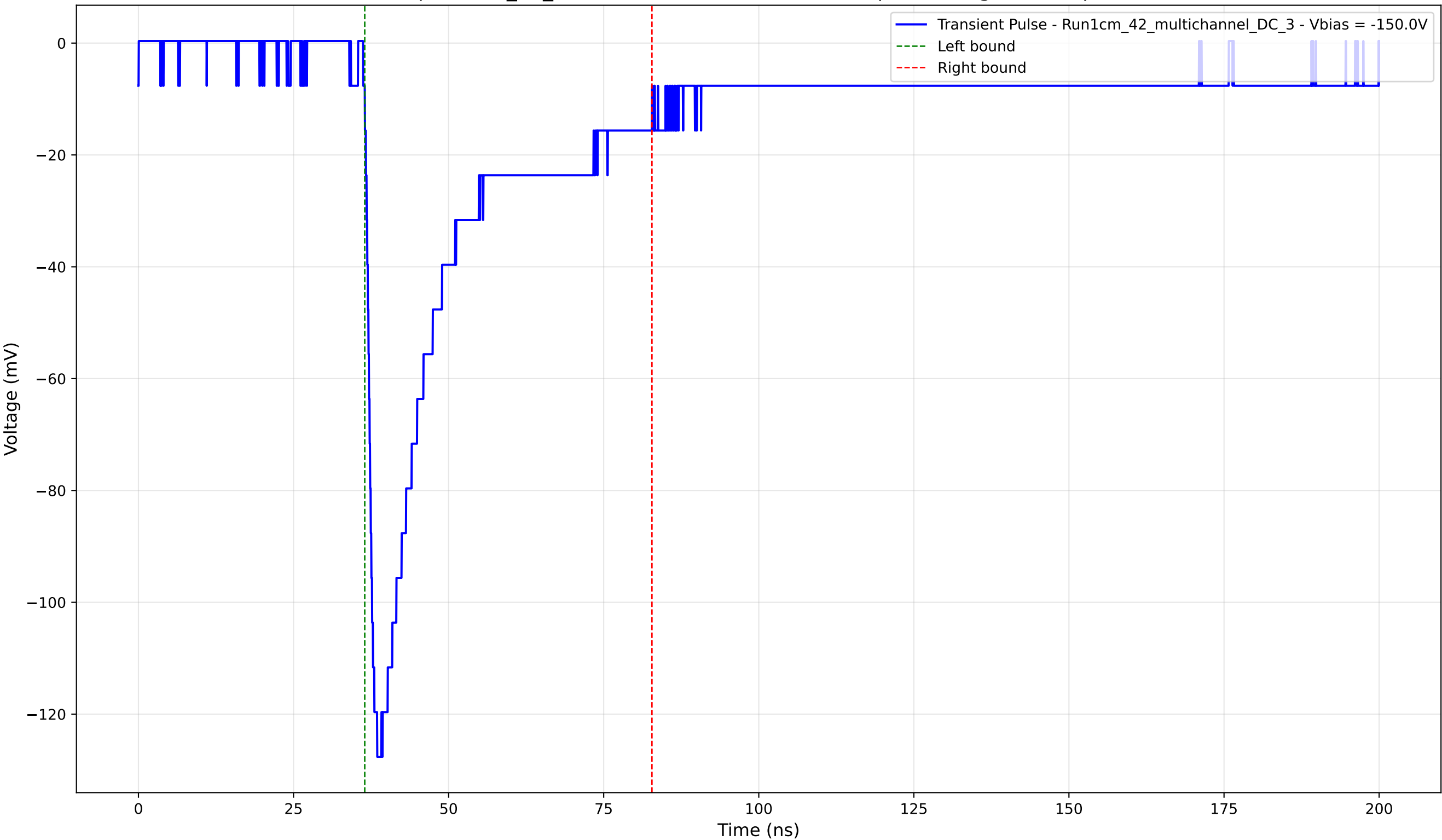
Transient Pulse - Sample: 1cm_42_multichannel - Position: 3550.0 \mu\text{m} - Charge: 36.17 pC - Rise Time: 1.53 ns
