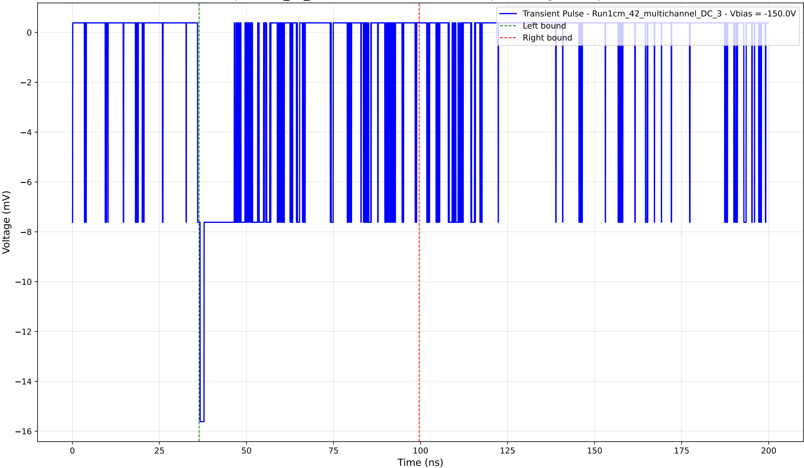
Transient Pulse - Sample: 1cm_42_multichannel - Position: 4895.0 \mu\text{m} - Charge: 3.67 pC - Rise Time: 0.72 ns
