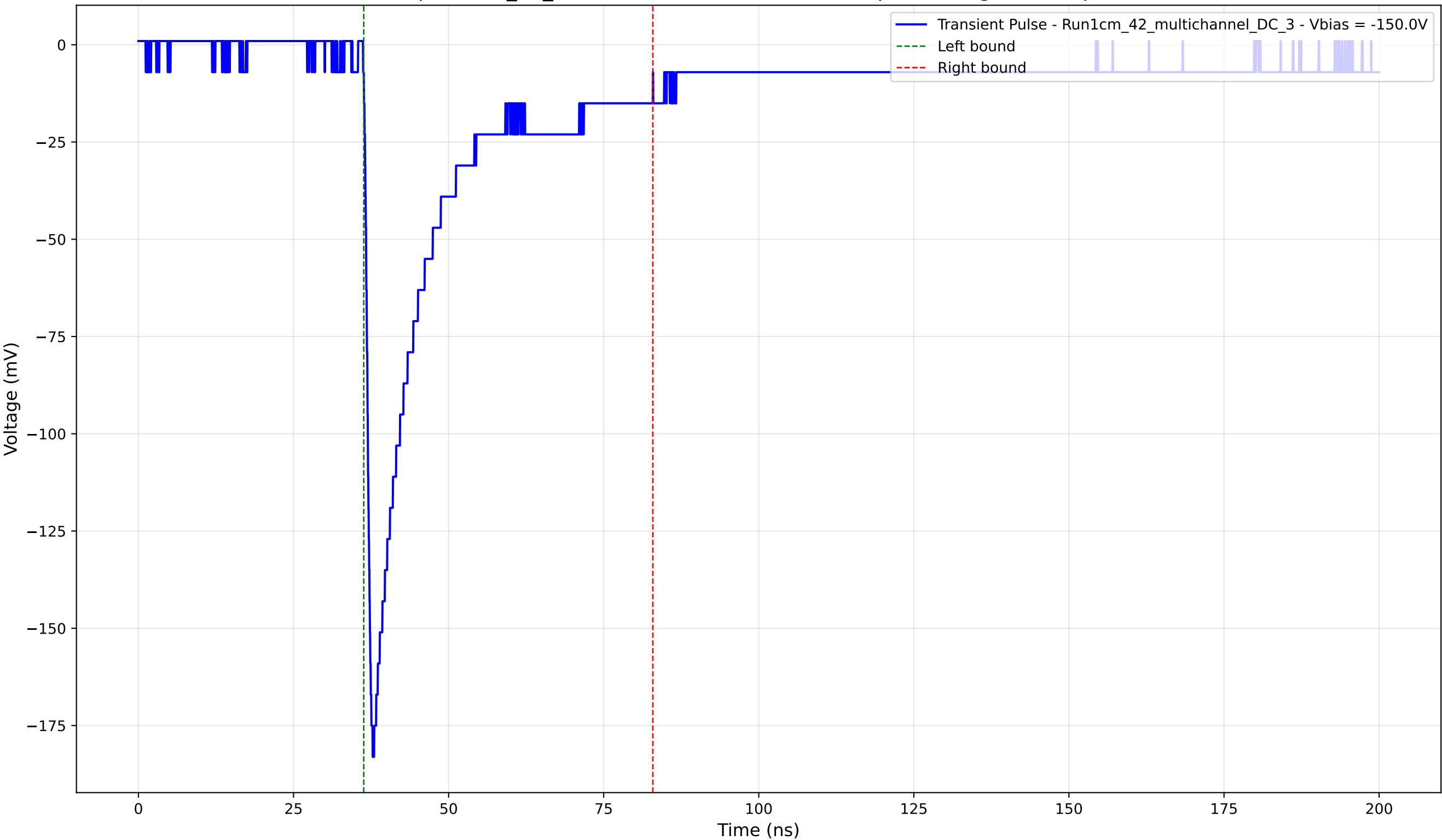
Transient Pulse - Sample: 1cm_42_multichannel - Position: 4115.0 \mu\text{m} - Charge: 38.62 pC - Rise Time: 1.01 ns
