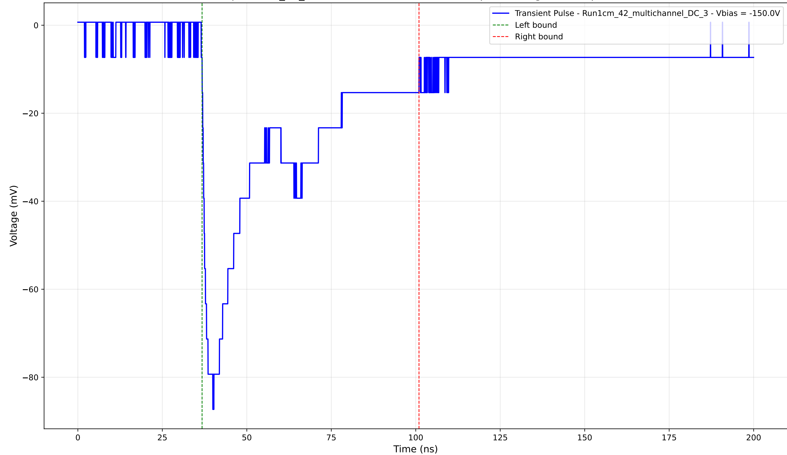
Transient Pulse - Sample: 1cm_42_multichannel - Position: 2625.0 \mu\text{m} - Charge: 39.01 pC - Rise Time: 1.76 ns
