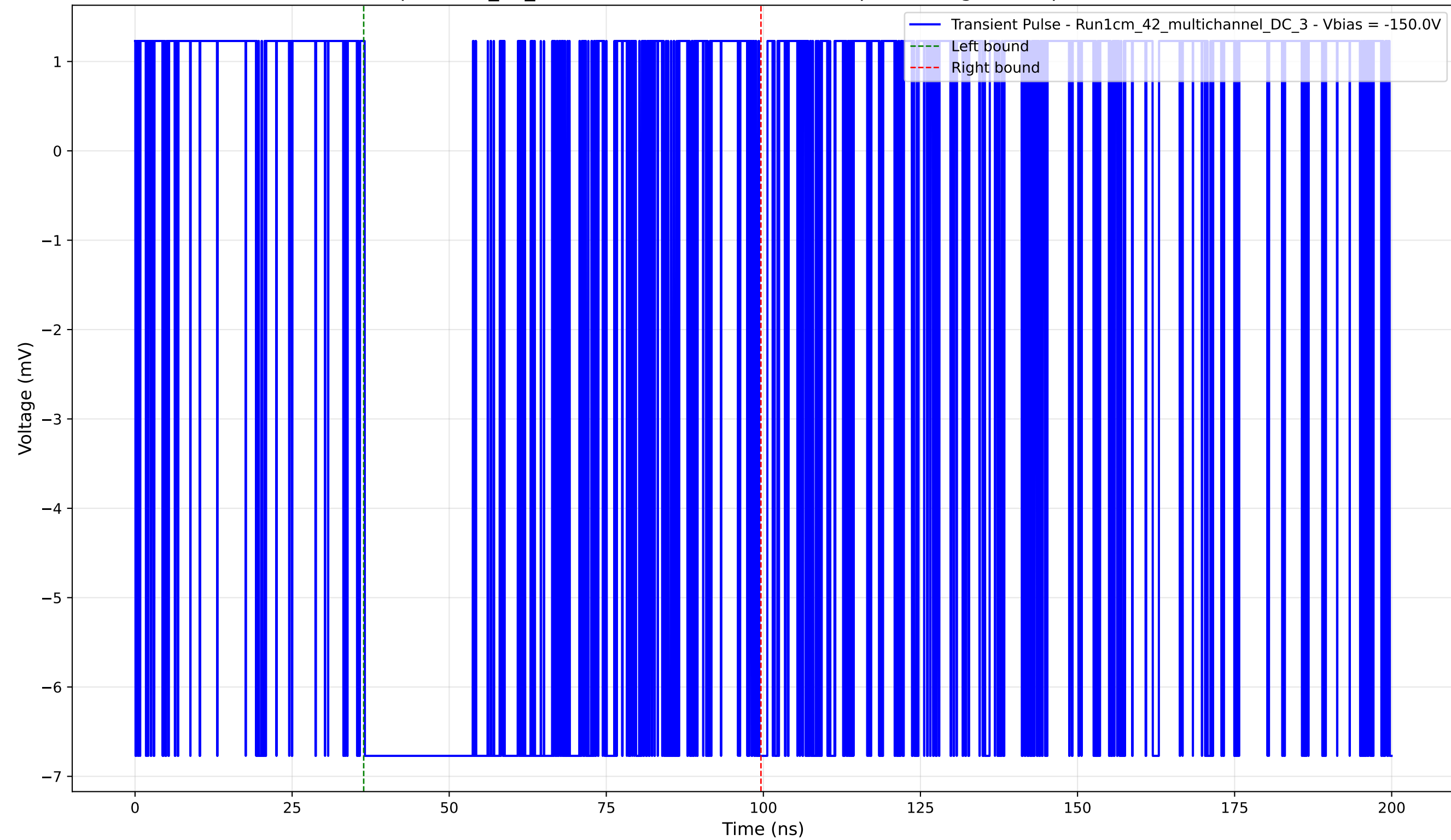
Transient Pulse - Sample: 1cm_42_multichannel - Position: 3375.0 \mu\text{m} - Charge: 5.01 pC - Rise Time: 0.00 ns (N/A)
