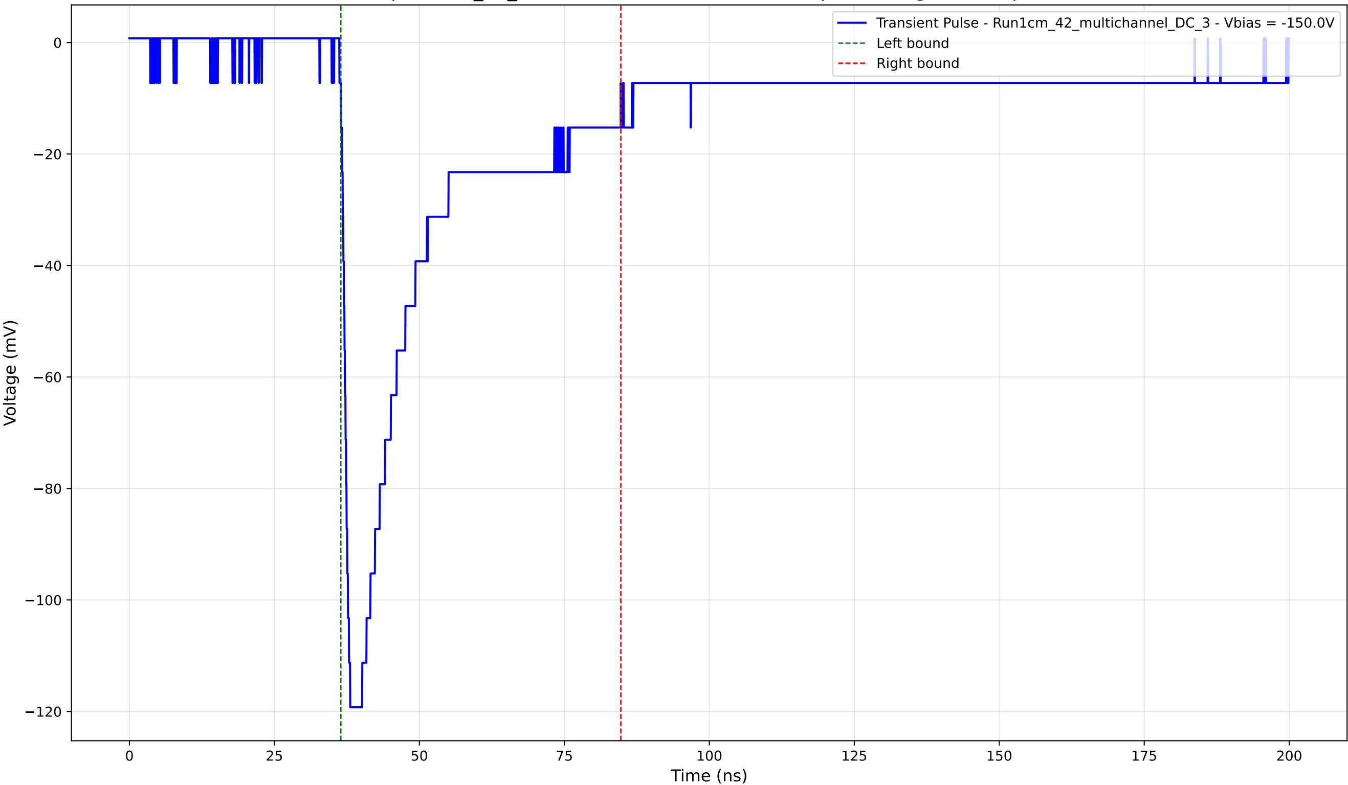
Transient Pulse - Sample: 1cm_42_multichannel - Position: 3500.0 \mu\text{m} - Charge: 36.60 pC - Rise Time: 1.39 ns
