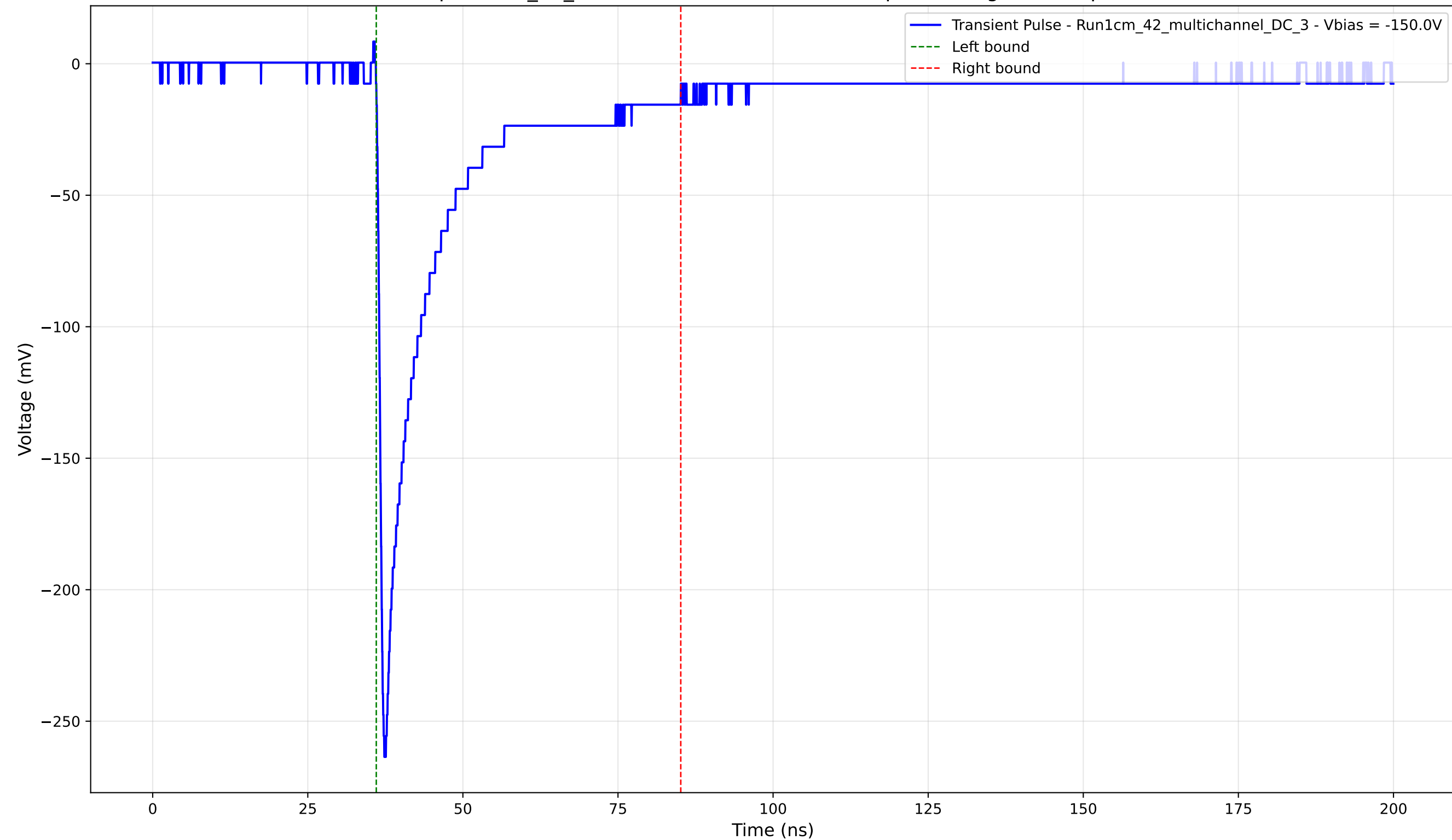
Transient Pulse - Sample: 1cm_42_multichannel - Position: 530.0 \mu\text{m} - Charge: 48.62 pC - Rise Time: 0.91 ns
