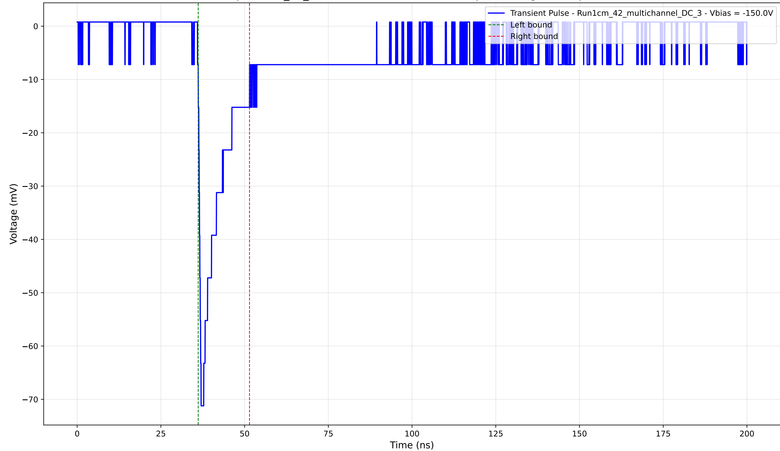
Transient Pulse - Sample: 1cm_42_multichannel - Position: 390.0 \mu\text{m} - Charge: 9.45 pC - Rise Time: 1.06 ns
