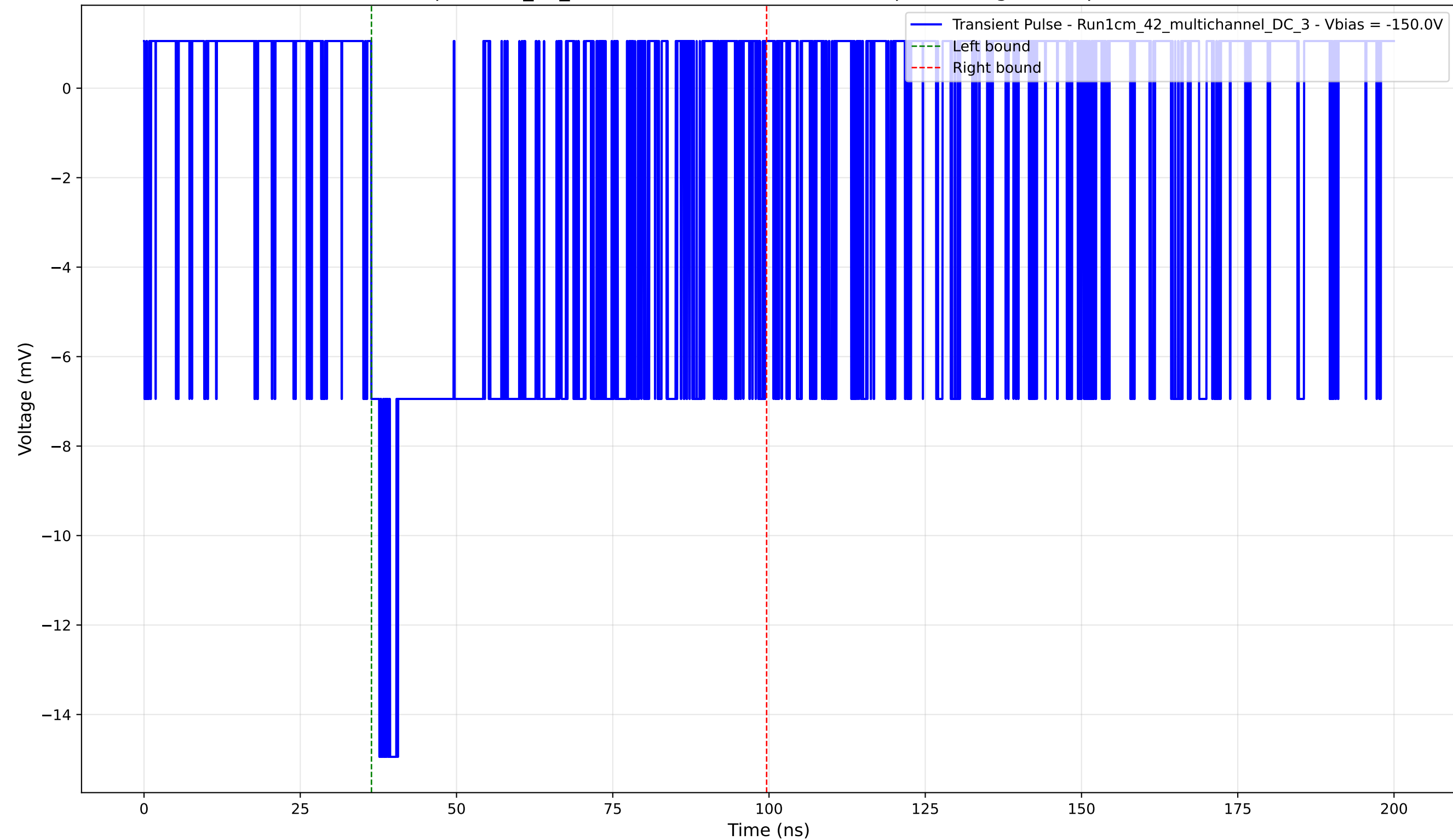
Transient Pulse - Sample: 1cm_42_multichannel - Position: 3875.0 \mu\text{m} - Charge: 5.98 pC - Rise Time: 1.30 ns
