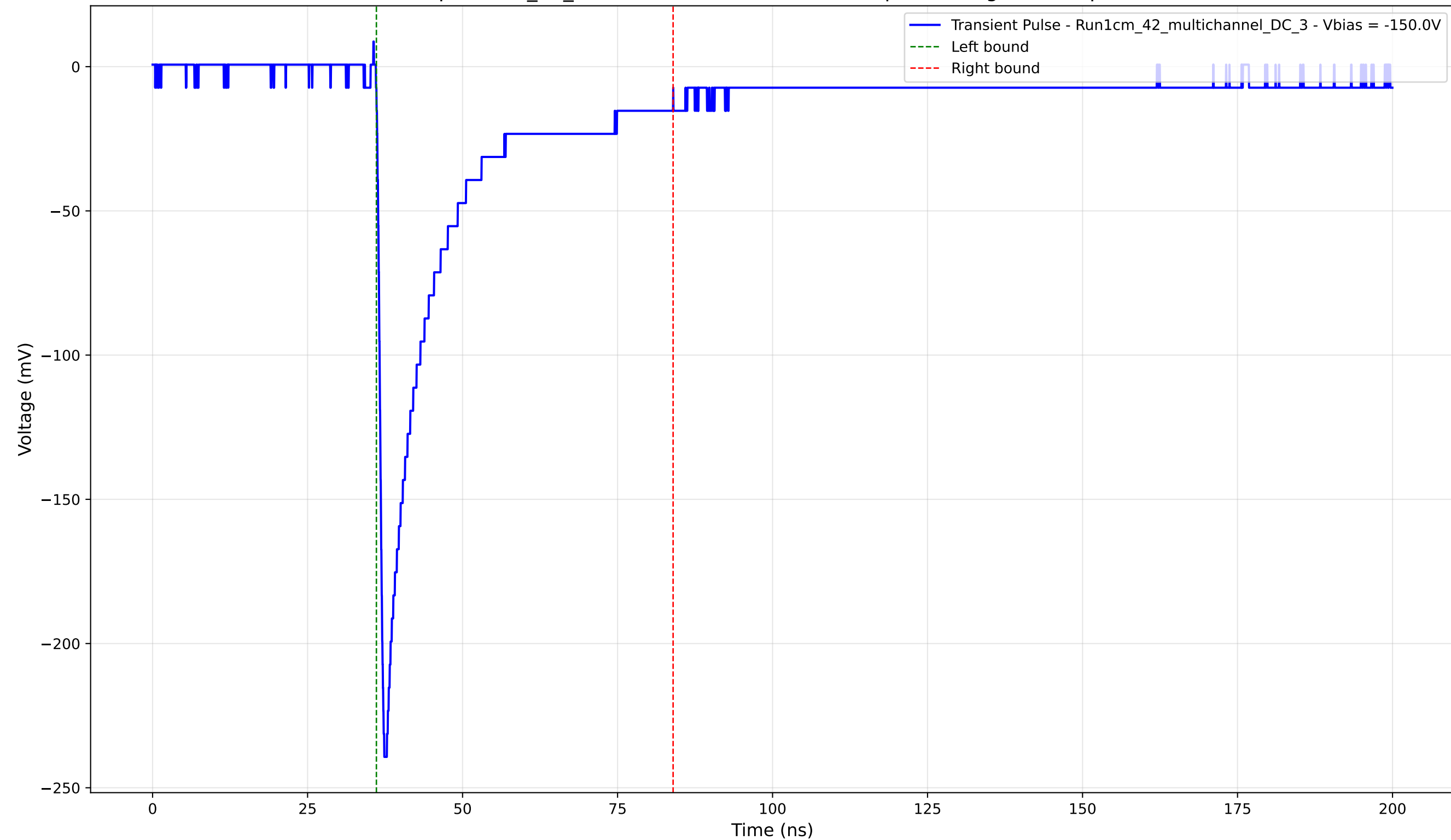
Transient Pulse - Sample: 1cm_42_multichannel - Position: 615.0 \mu\text{m} - Charge: 46.85 pC - Rise Time: 0.96 ns
