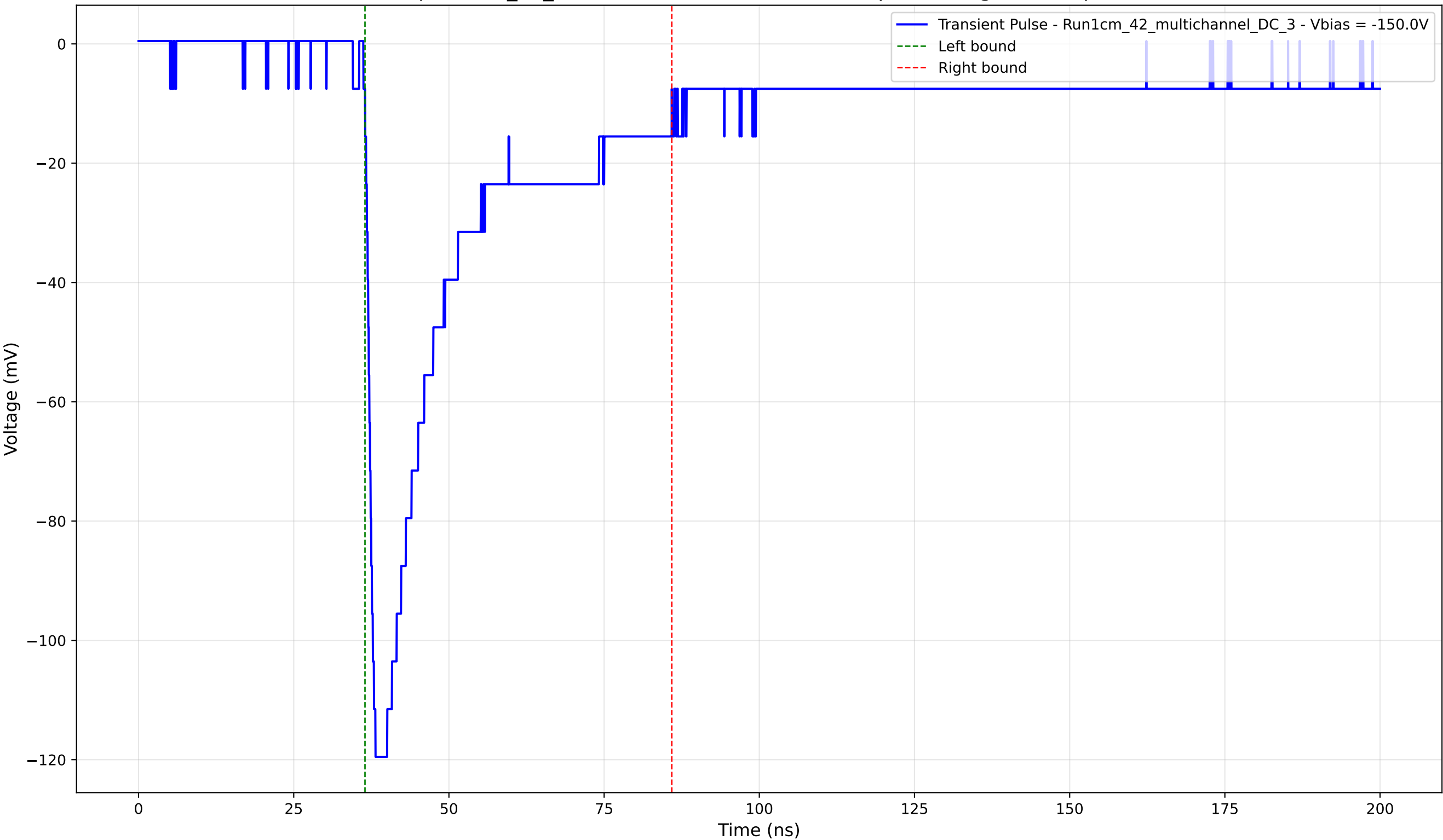
Transient Pulse - Sample: 1cm_42_multichannel - Position: 3480.0 \mu\text{m} - Charge: 37.04 pC - Rise Time: 1.43 ns
