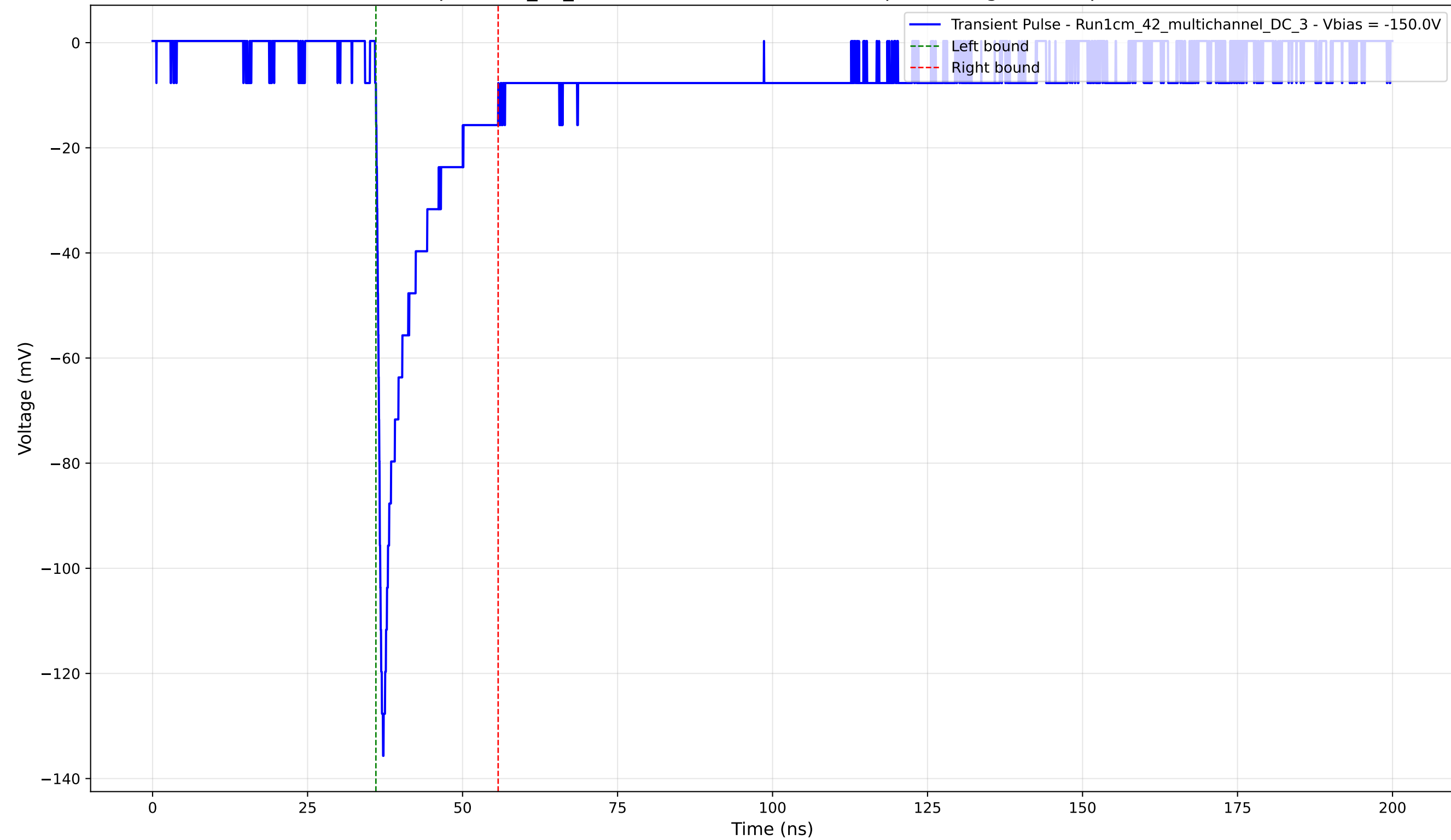
Transient Pulse - Sample: 1cm_42_multichannel - Position: 305.0 \mu\text{m} - Charge: 15.73 pC - Rise Time: 0.95 ns
