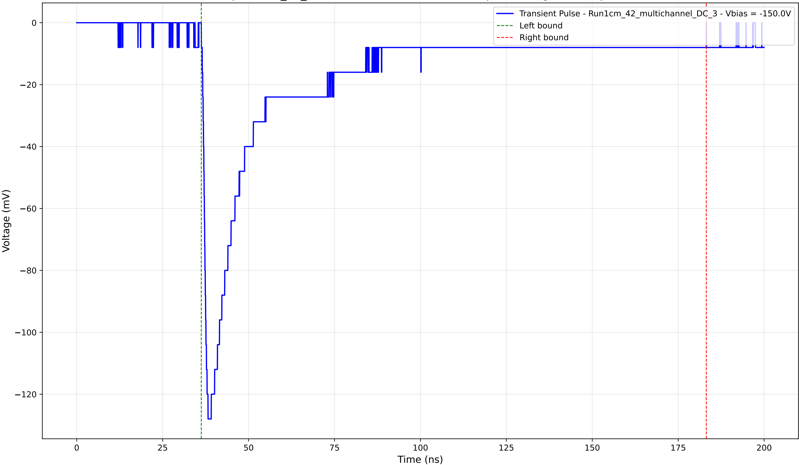
Transient Pulse - Sample: 1cm_42_multichannel - Position: 3590.0 \mu\text{m} - Charge: 53.16 pC - Rise Time: 1.41 ns
