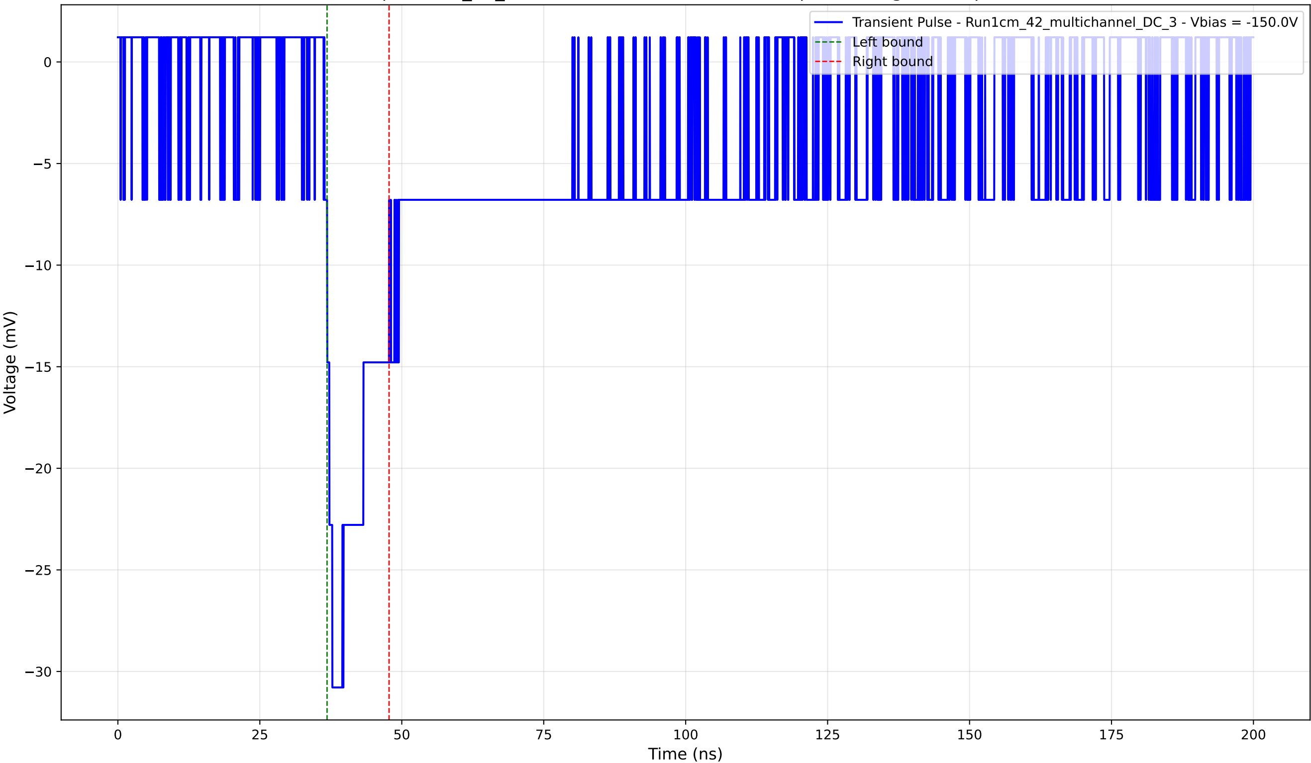
Transient Pulse - Sample: 1cm_42_multichannel - Position: 1330.0 \mu\text{m} - Charge: 4.49 pC - Rise Time: 1.37 ns
