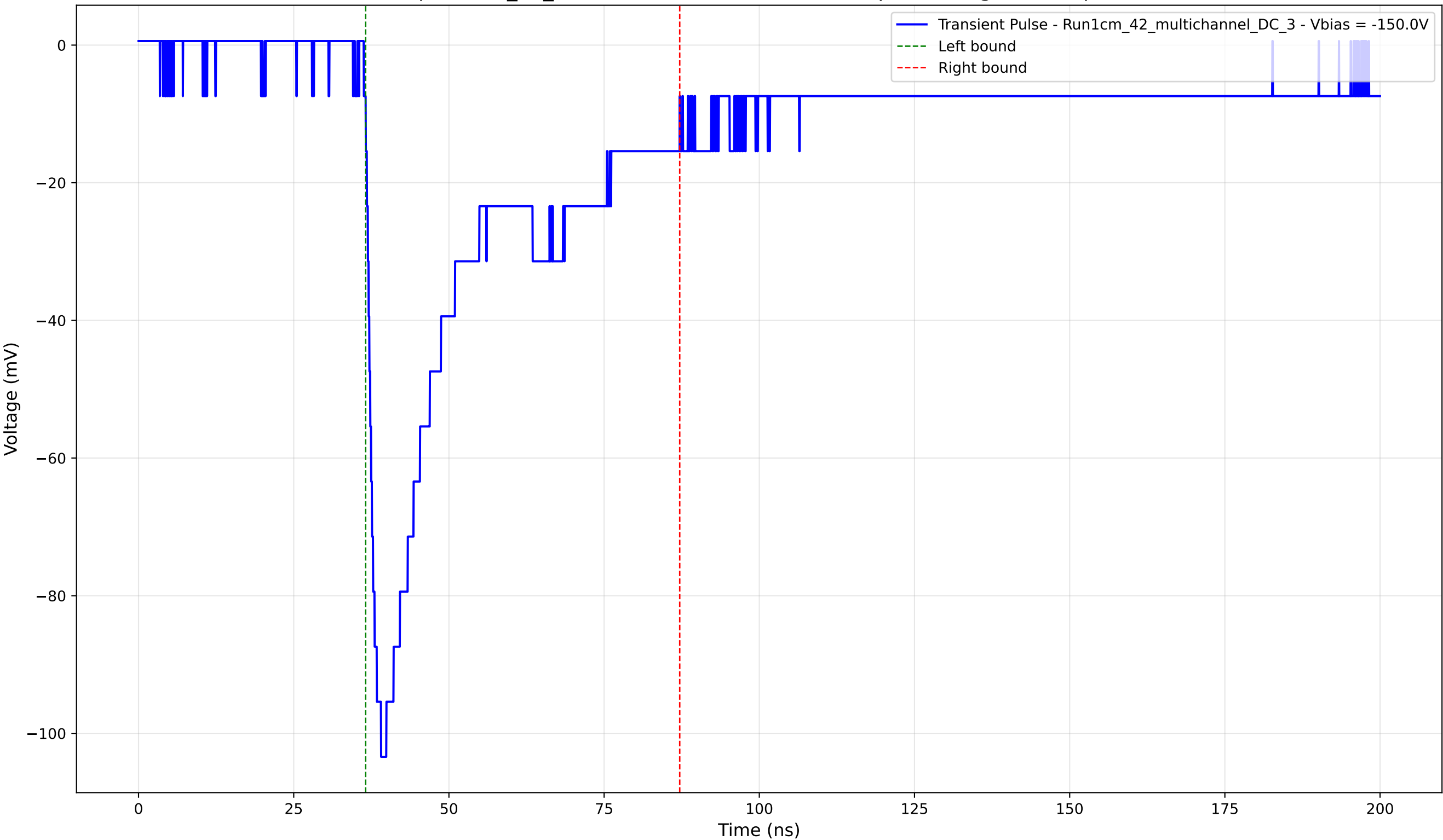
Transient Pulse - Sample: 1cm_42_multichannel - Position: 3090.0 \mu\text{m} - Charge: 35.55 pC - Rise Time: 1.79 ns
