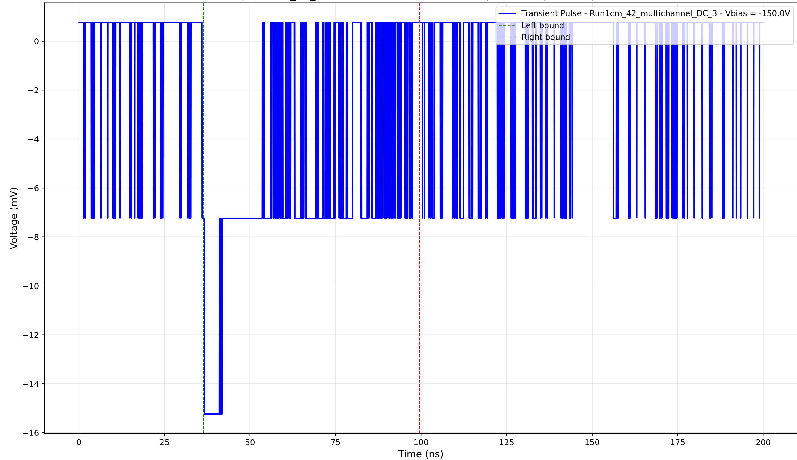
Transient Pulse - Sample: 1cm_42_multichannel - Position: 365.0 \mu\text{m} - Charge: 6.55 pC - Rise Time: 0.70 ns
