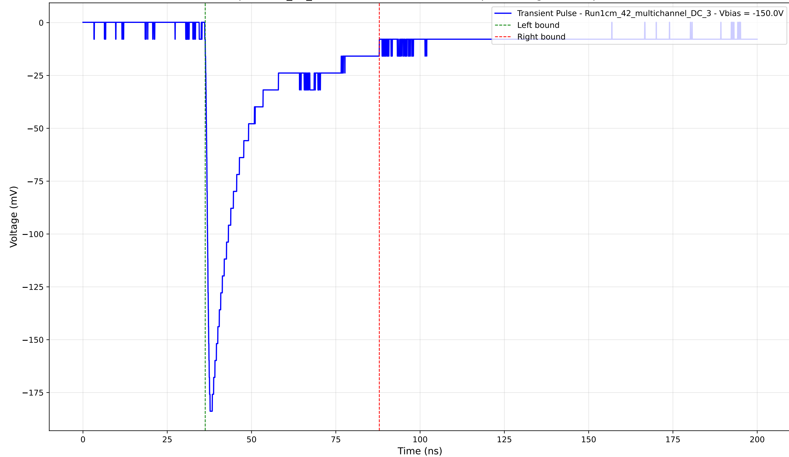
Transient Pulse - Sample: 1cm_42_multichannel - Position: 965.0 \mu\text{m} - Charge: 46.57 pC - Rise Time: 1.07 ns
