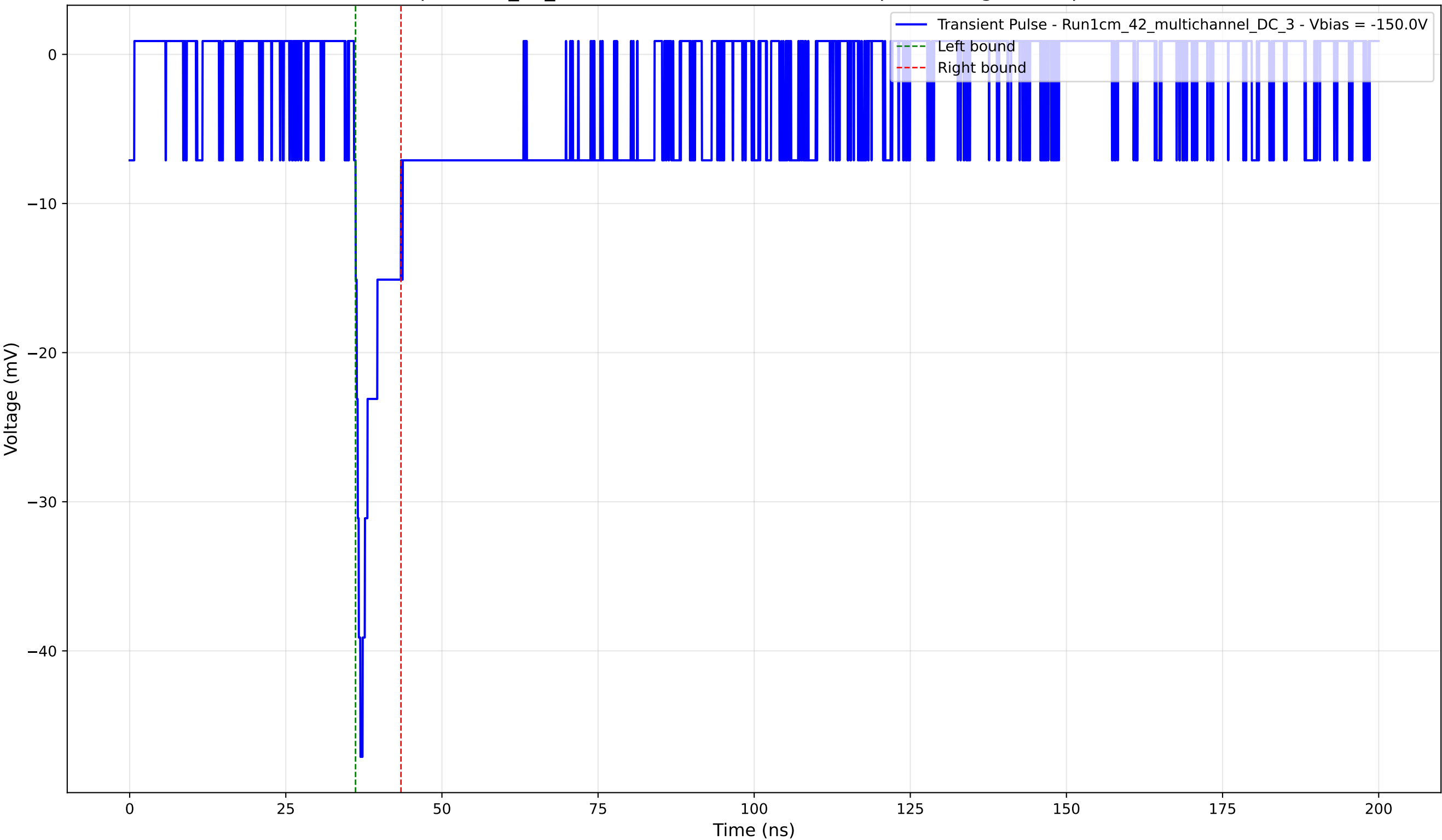
Transient Pulse - Sample: 1cm_42_multichannel - Position: 4875.0 \mu\text{m} - Charge: 3.19 pC - Rise Time: 1.03 ns
