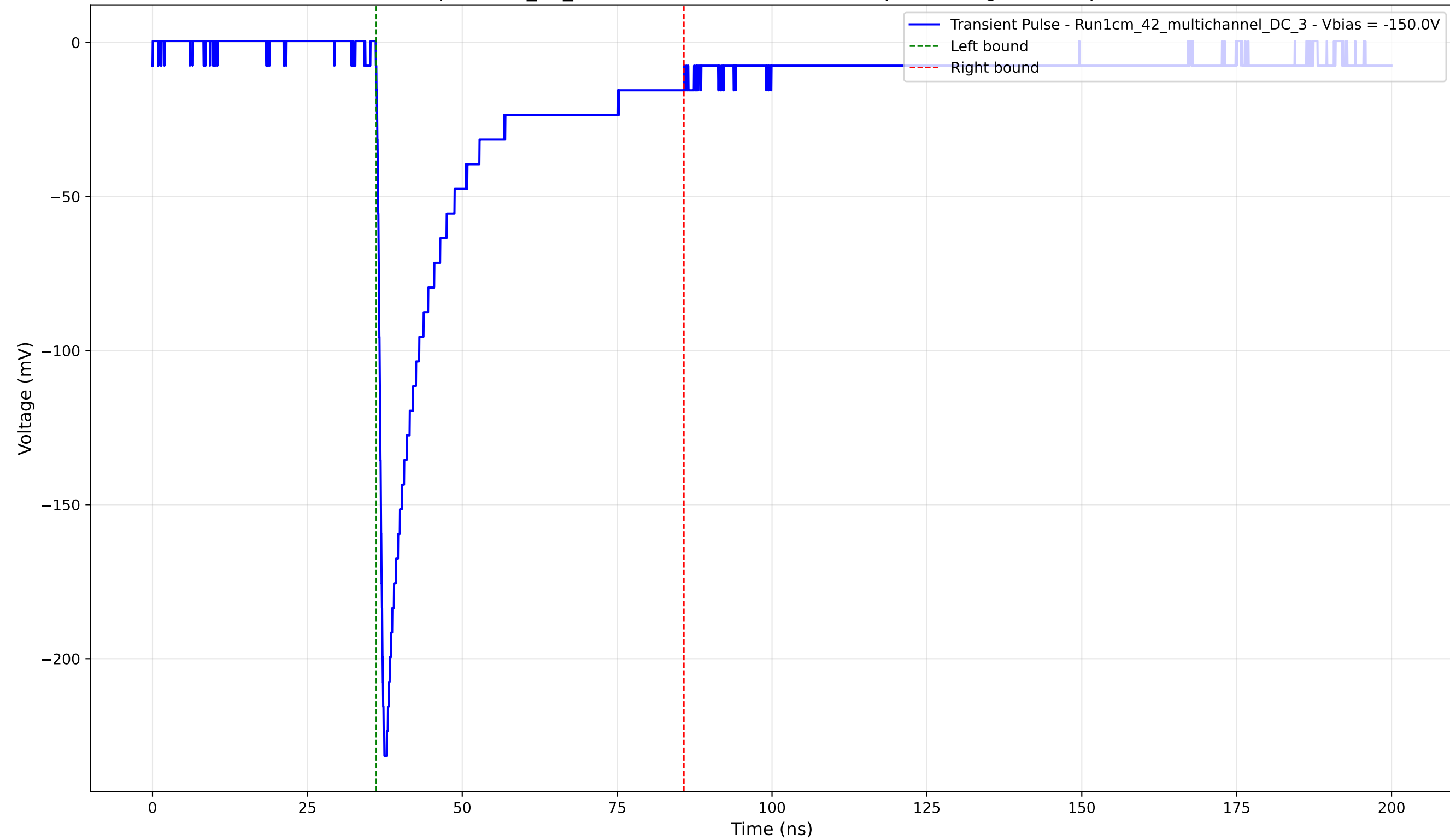
Transient Pulse - Sample: 1cm_42_multichannel - Position: 655.0 \mu\text{m} - Charge: 46.98 pC - Rise Time: 1.00 ns
