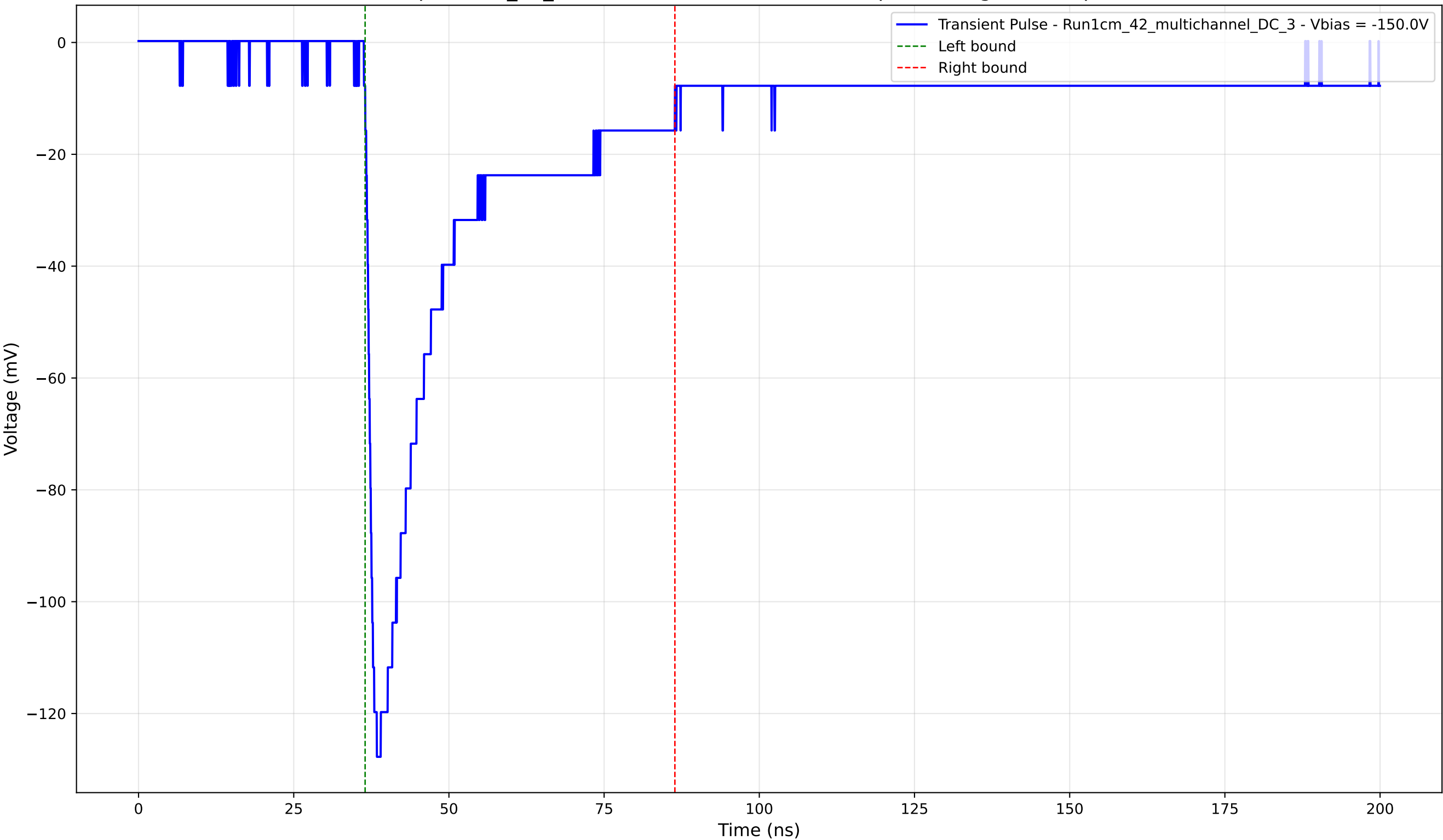
Transient Pulse - Sample: 1cm_42_multichannel - Position: 3570.0 \mu\text{m} - Charge: 37.23 pC - Rise Time: 1.45 ns
