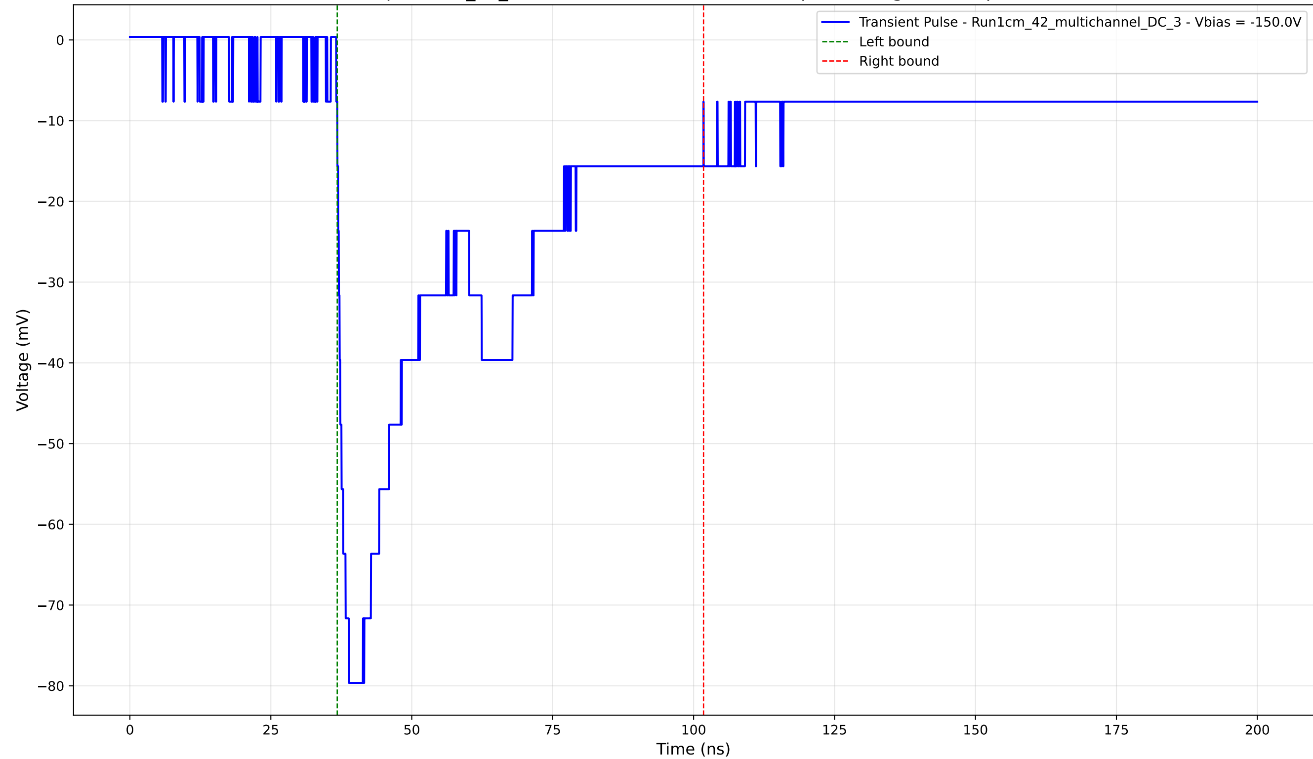
Transient Pulse - Sample: 1cm_42_multichannel - Position: 2505.0 \mu\text{m} - Charge: 40.29 pC - Rise Time: 2.06 ns
