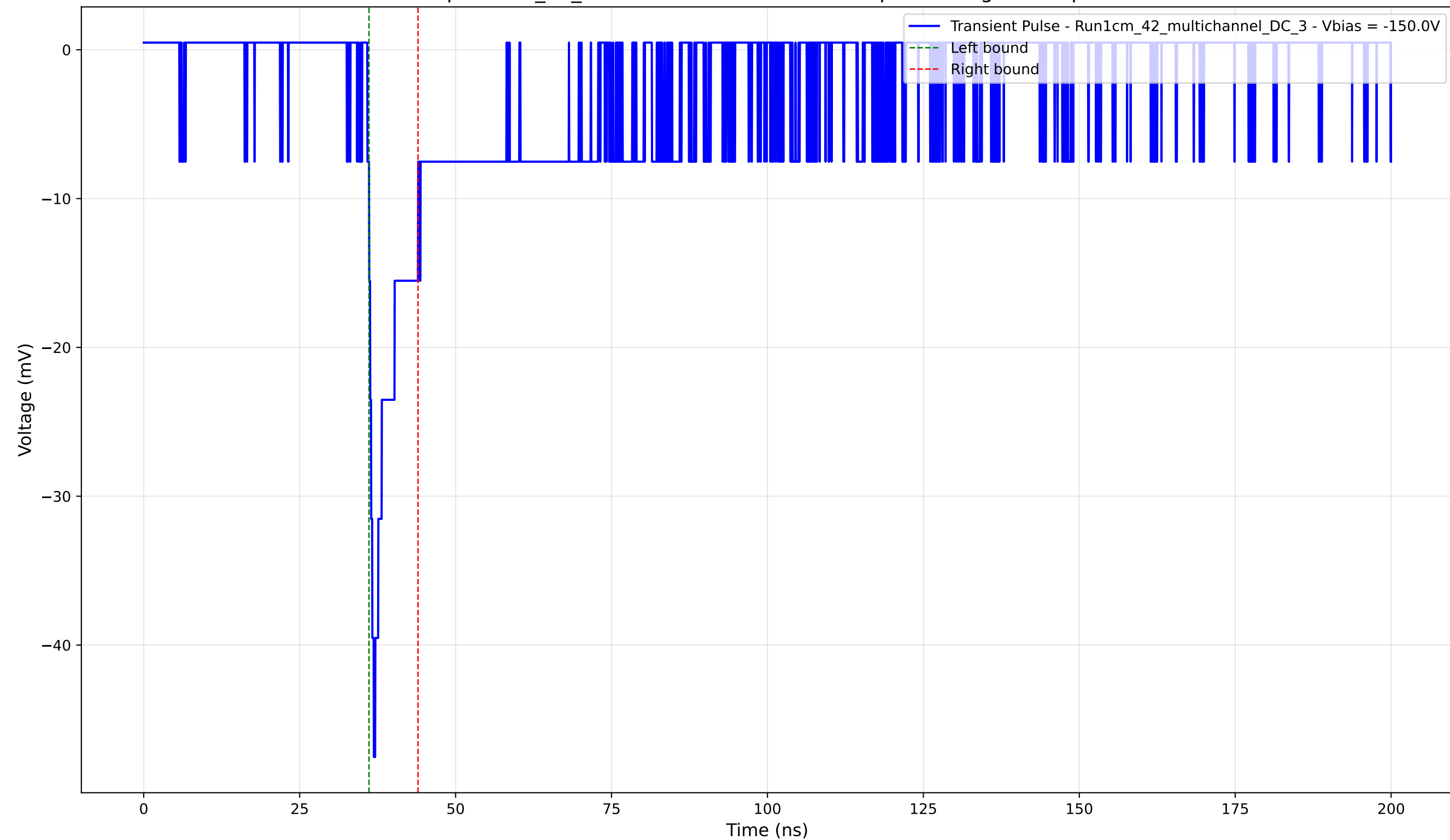
Transient Pulse - Sample: 1cm_42_multichannel - Position: 55.0 \mu\text{m} - Charge: 3.53 pC - Rise Time: 1.03 ns
