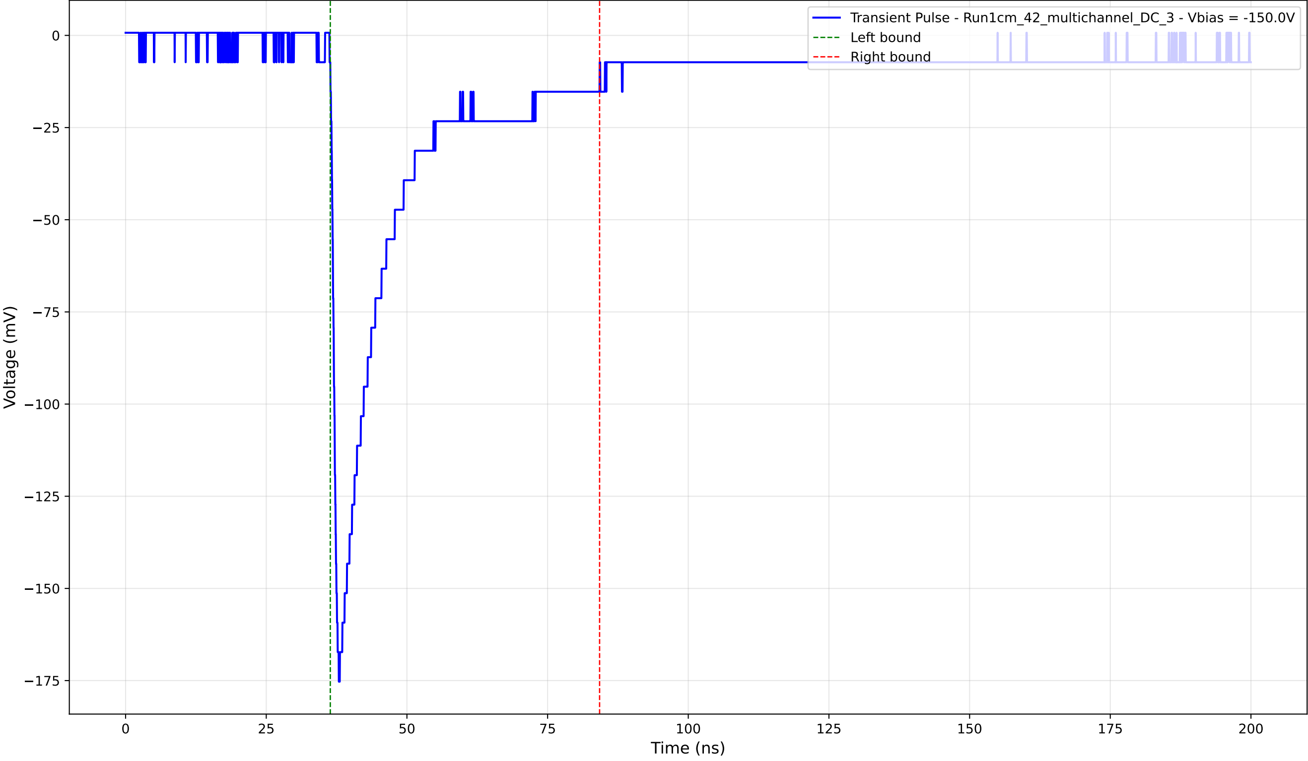
Transient Pulse - Sample: 1cm_42_multichannel - Position: 3990.0 \mu\text{m} - Charge: 39.80 pC - Rise Time: 1.07 ns
