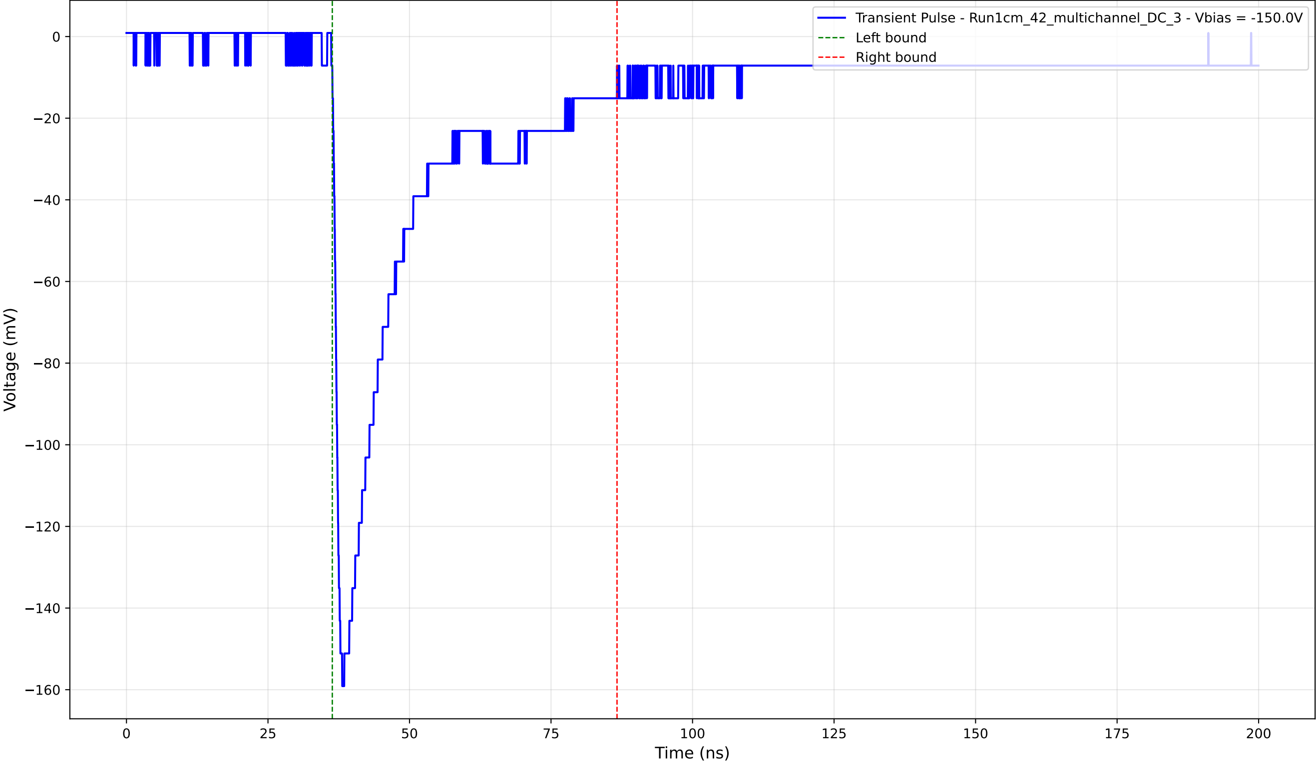
Transient Pulse - Sample: 1cm_42_multichannel - Position: 1200.0 \mu\text{m} - Charge: 43.94 pC - Rise Time: 1.30 ns
