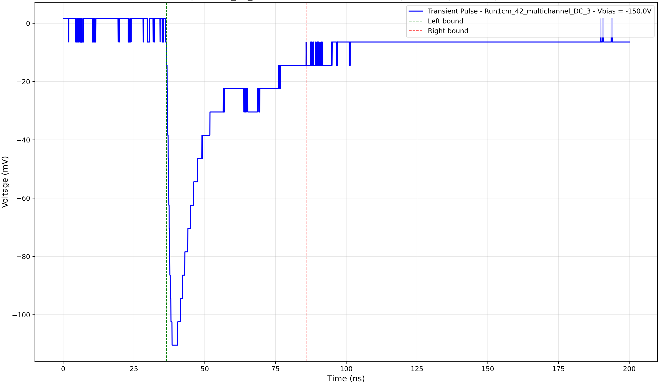
Transient Pulse - Sample: 1cm_42_multichannel - Position: 3245.0 \mu\text{m} - Charge: 36.47 pC - Rise Time: 1.55 ns
