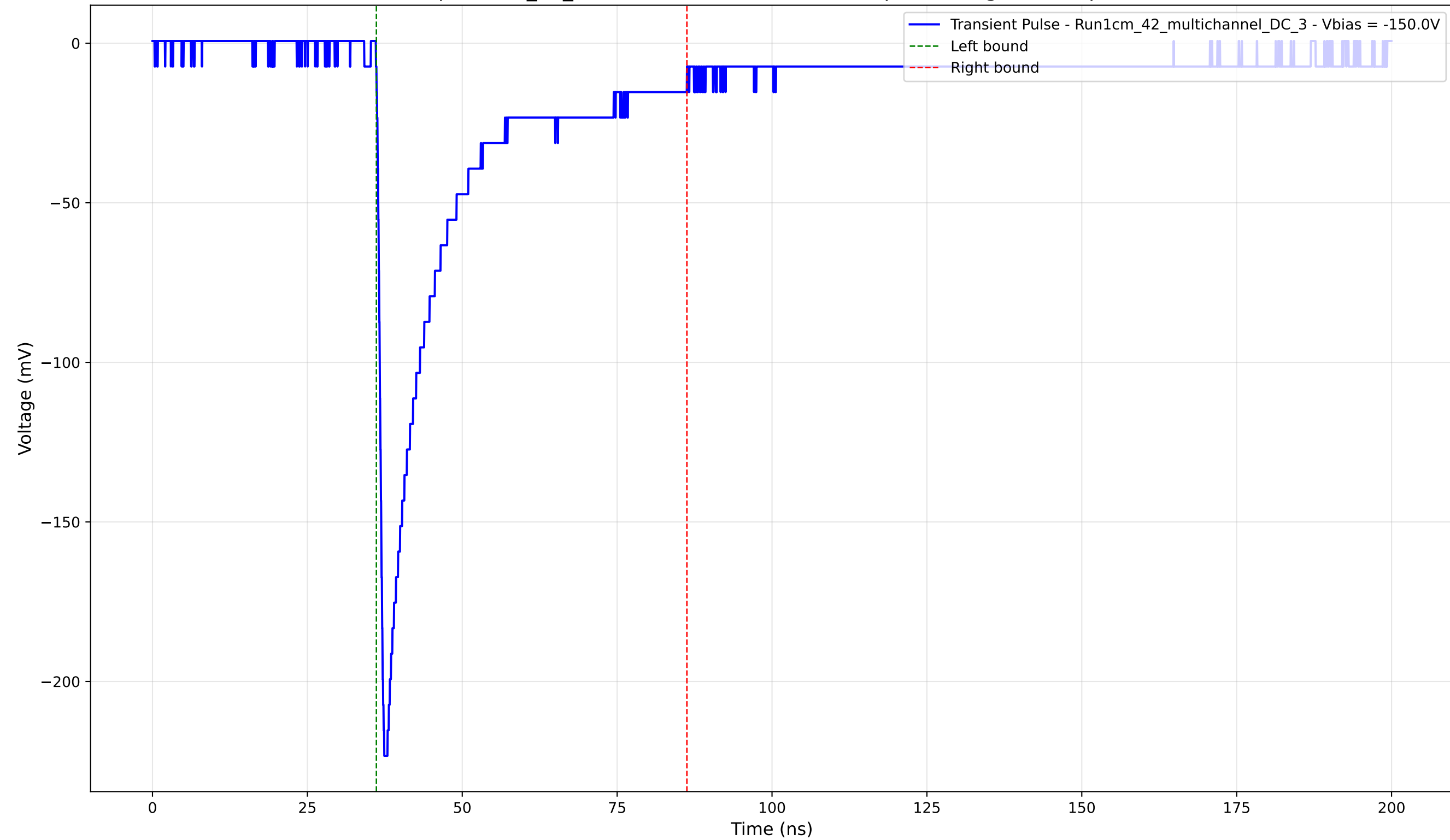
Transient Pulse - Sample: 1cm_42_multichannel - Position: 690.0 \mu\text{m} - Charge: 47.05 pC - Rise Time: 0.98 ns
