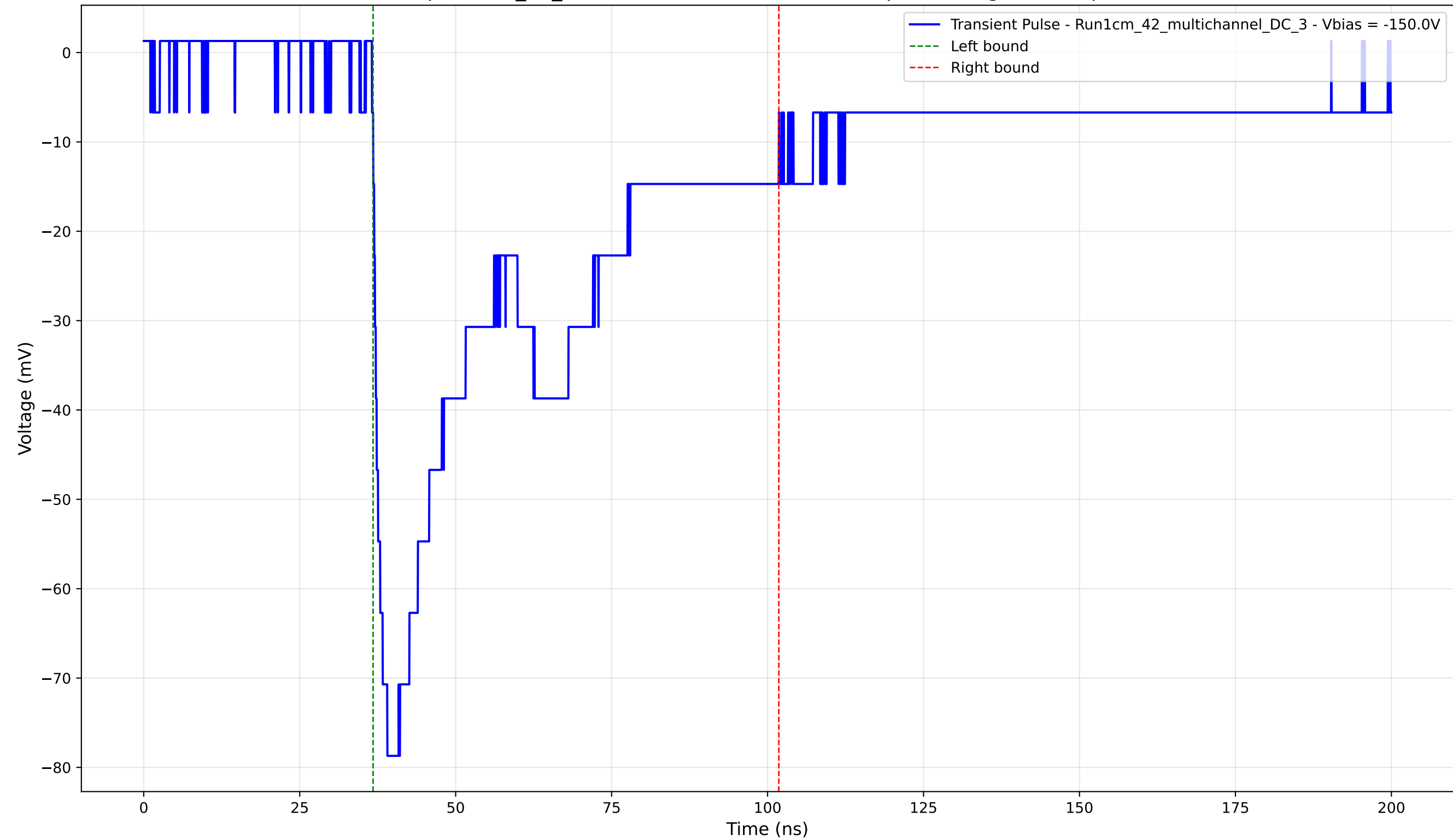
Transient Pulse - Sample: 1cm_42_multichannel - Position: 2465.0 \mu\text{m} - Charge: 38.87 pC - Rise Time: 2.28 ns
