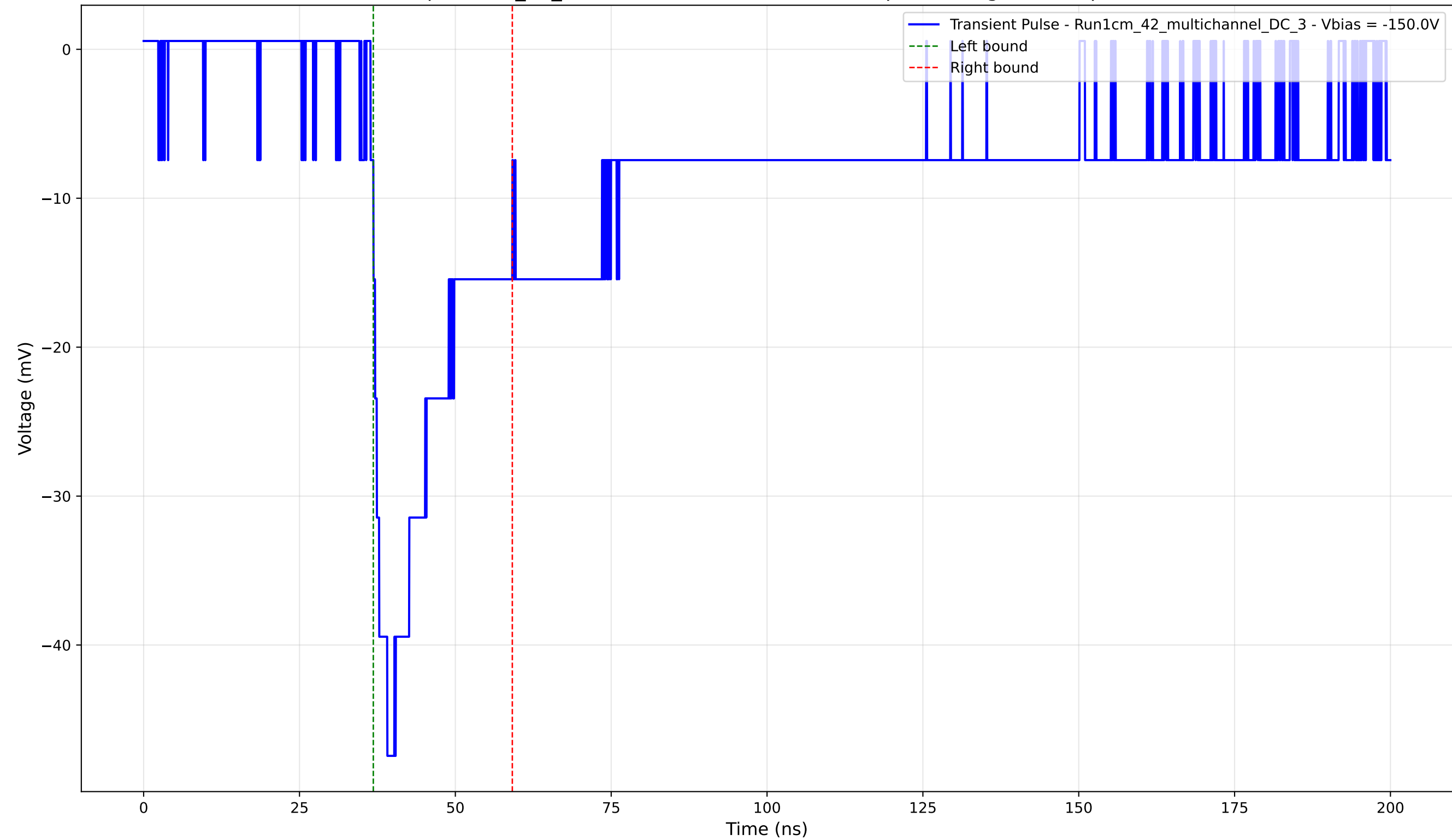
Transient Pulse - Sample: 1cm_42_multichannel - Position: 1915.0 \mu\text{m} - Charge: 11.07 pC - Rise Time: 2.69 ns
