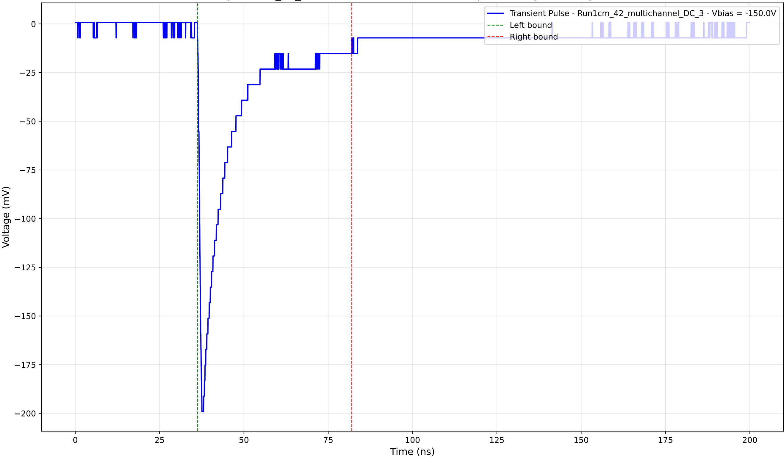
Transient Pulse - Sample: 1cm_42_multichannel - Position: 4185.0 \mu\text{m} - Charge: 40.11 pC - Rise Time: 0.97 ns
