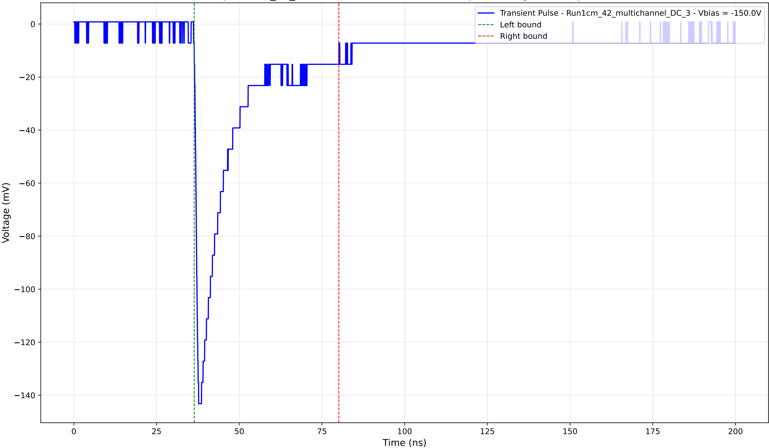
Transient Pulse - Sample: 1cm_42_multichannel - Position: 3960.0 \mu\text{m} - Charge: 33.25 pC - Rise Time: 1.16 ns
