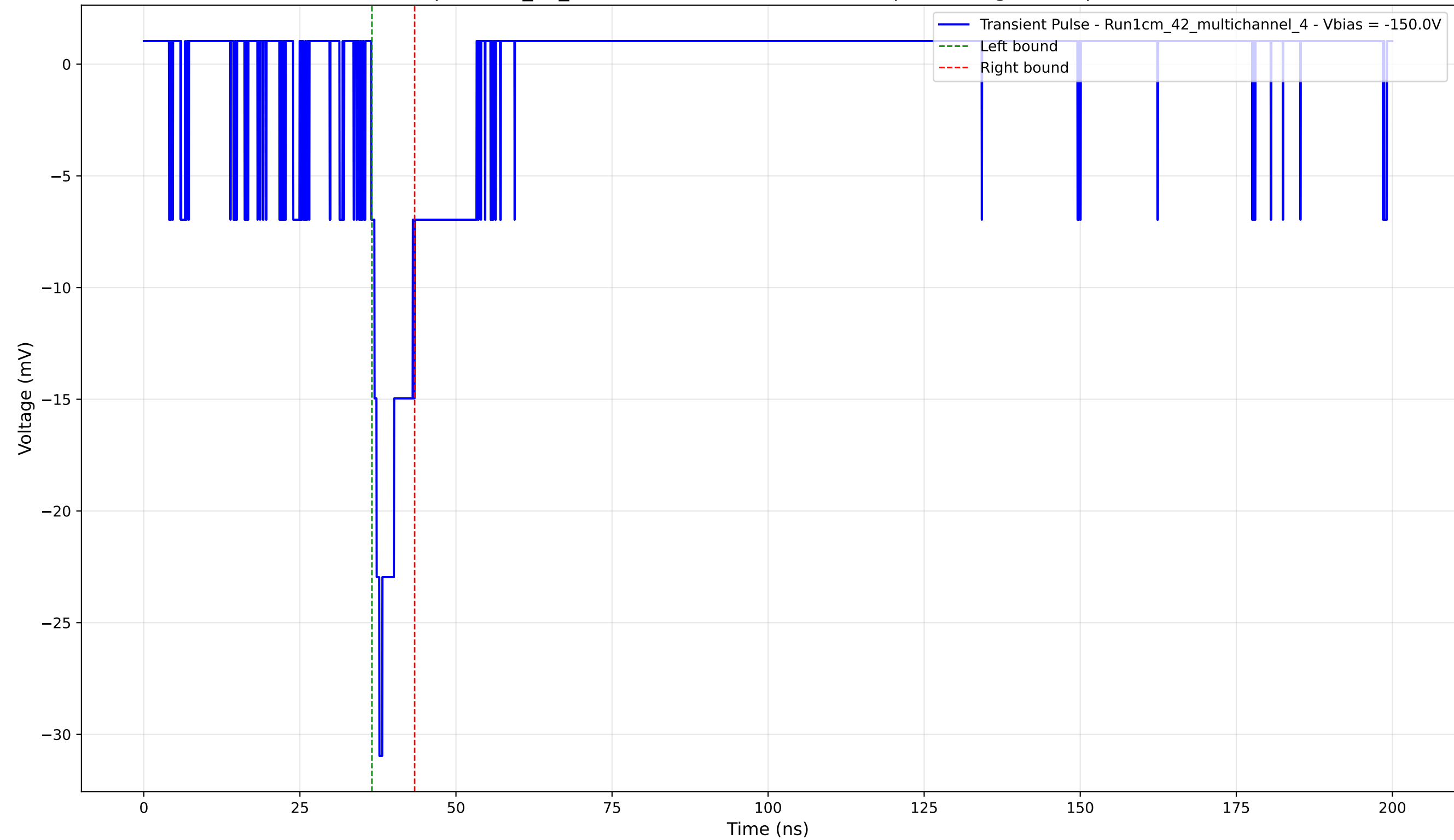
Transient Pulse - Sample: 1cm_42_multichannel - Position: 3290.0 \mu\text{m} - Charge: 2.48 pC - Rise Time: 1.29 ns
