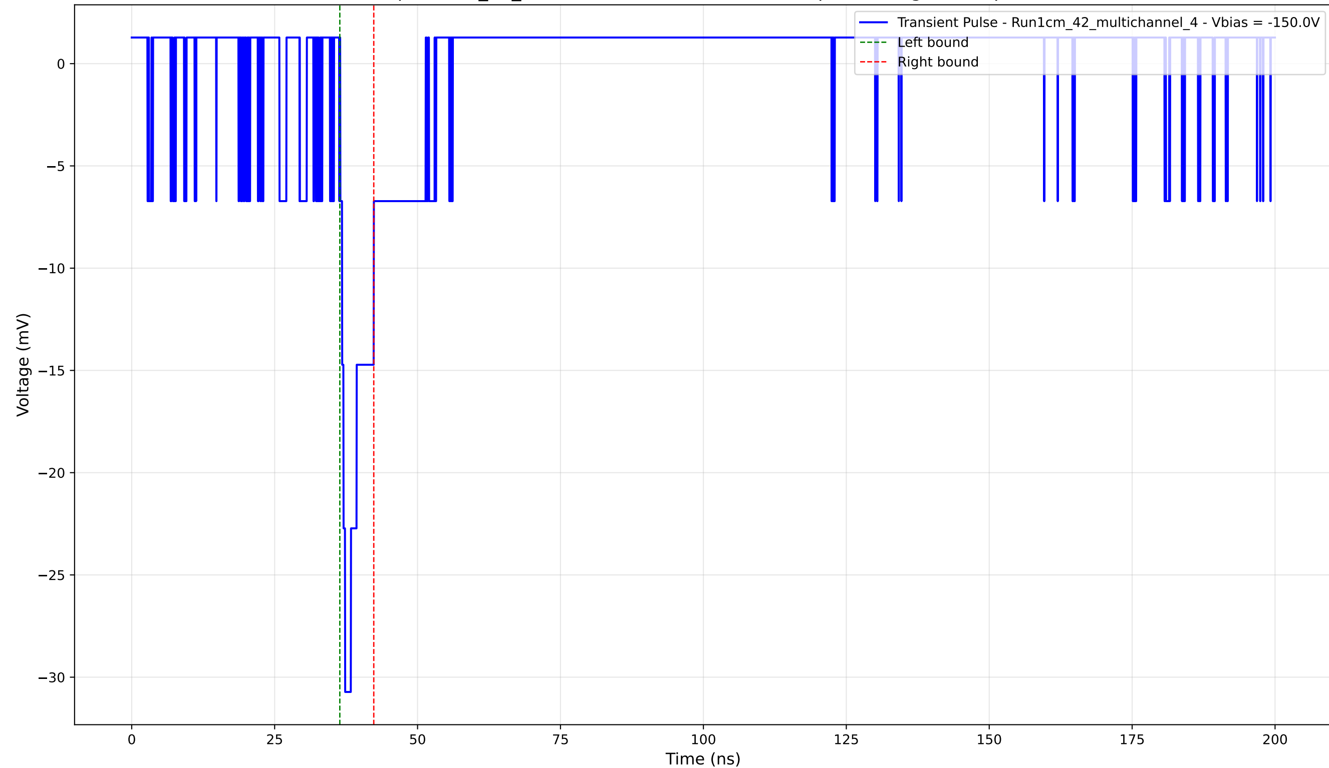
Transient Pulse - Sample: 1cm_42_multichannel - Position: 3110.0 \mu\text{m} - Charge: 2.21 pC - Rise Time: 0.85 ns
