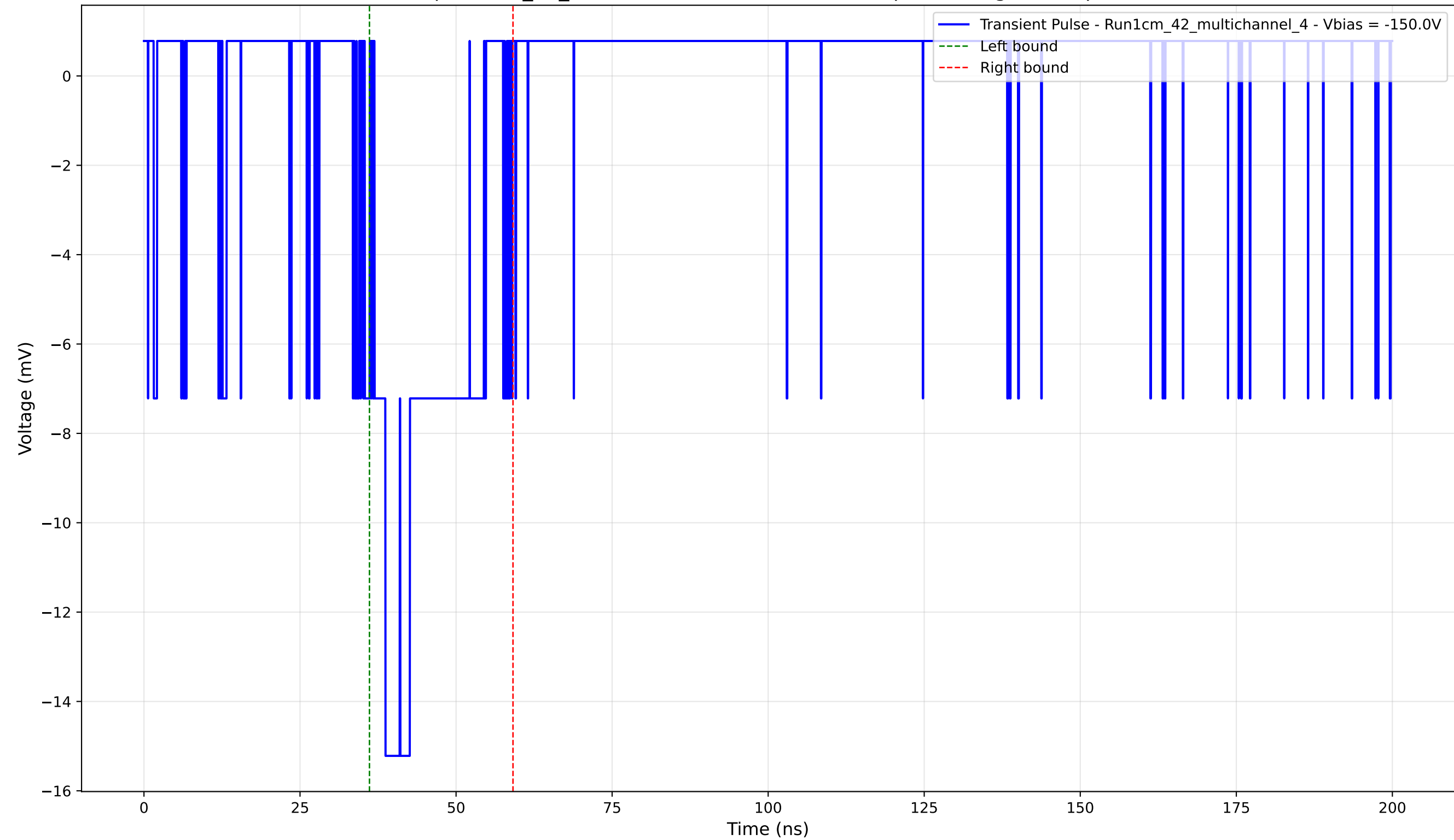
Transient Pulse - Sample: 1cm_42_multichannel - Position: 4640.0 \mu\text{m} - Charge: 3.24 pC - Rise Time: 1.76 ns
