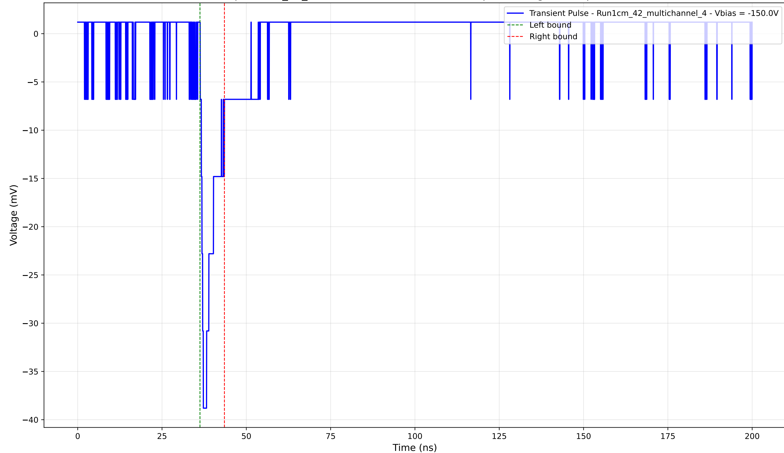
Transient Pulse - Sample: 1cm_42_multichannel - Position: 1760.0 \mu\text{m} - Charge: 3.04 pC - Rise Time: 0.93 ns
