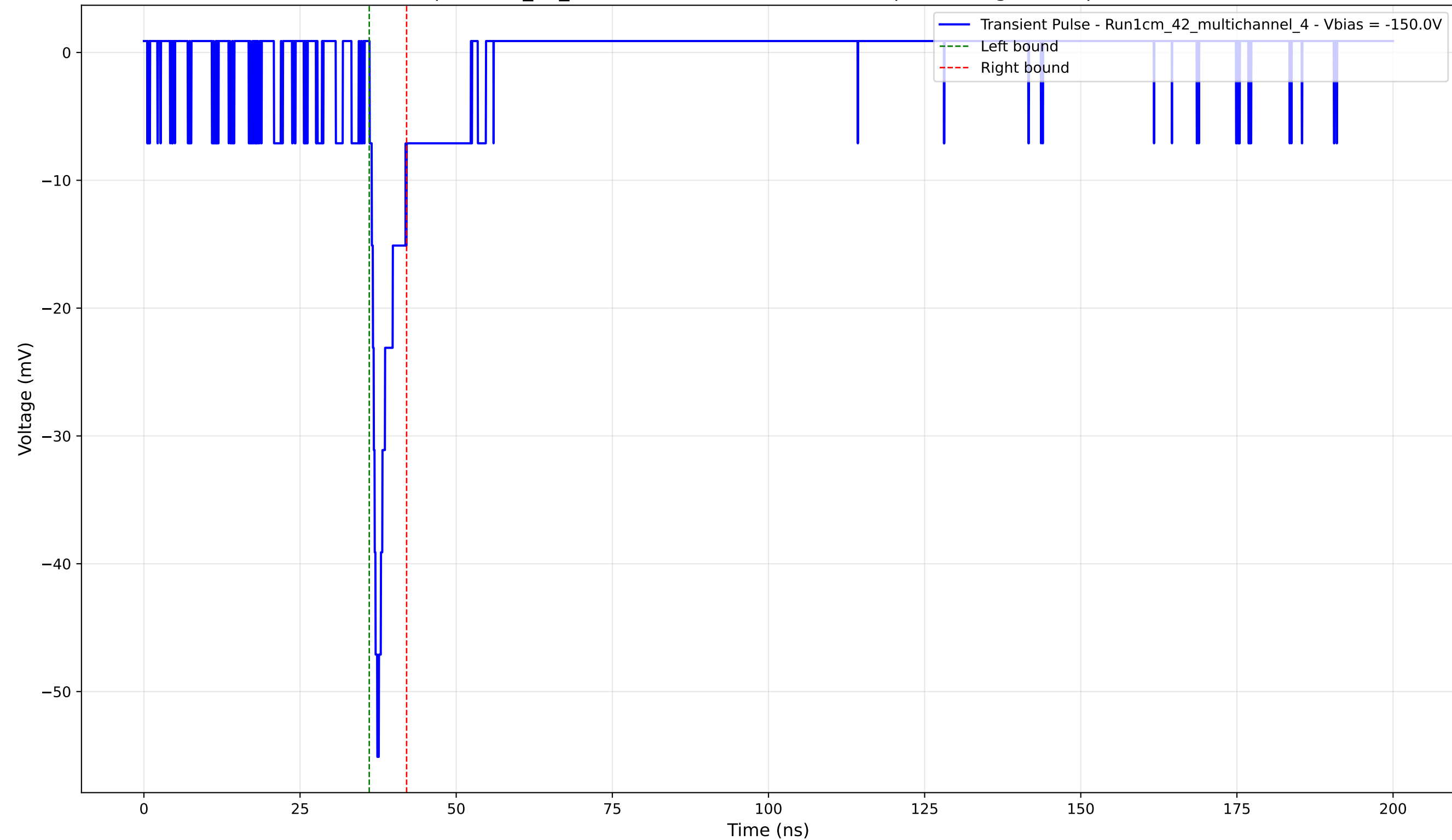
Transient Pulse - Sample: 1cm_42_multichannel - Position: 2780.0 \mu\text{m} - Charge: 2.90 pC - Rise Time: 1.23 ns
