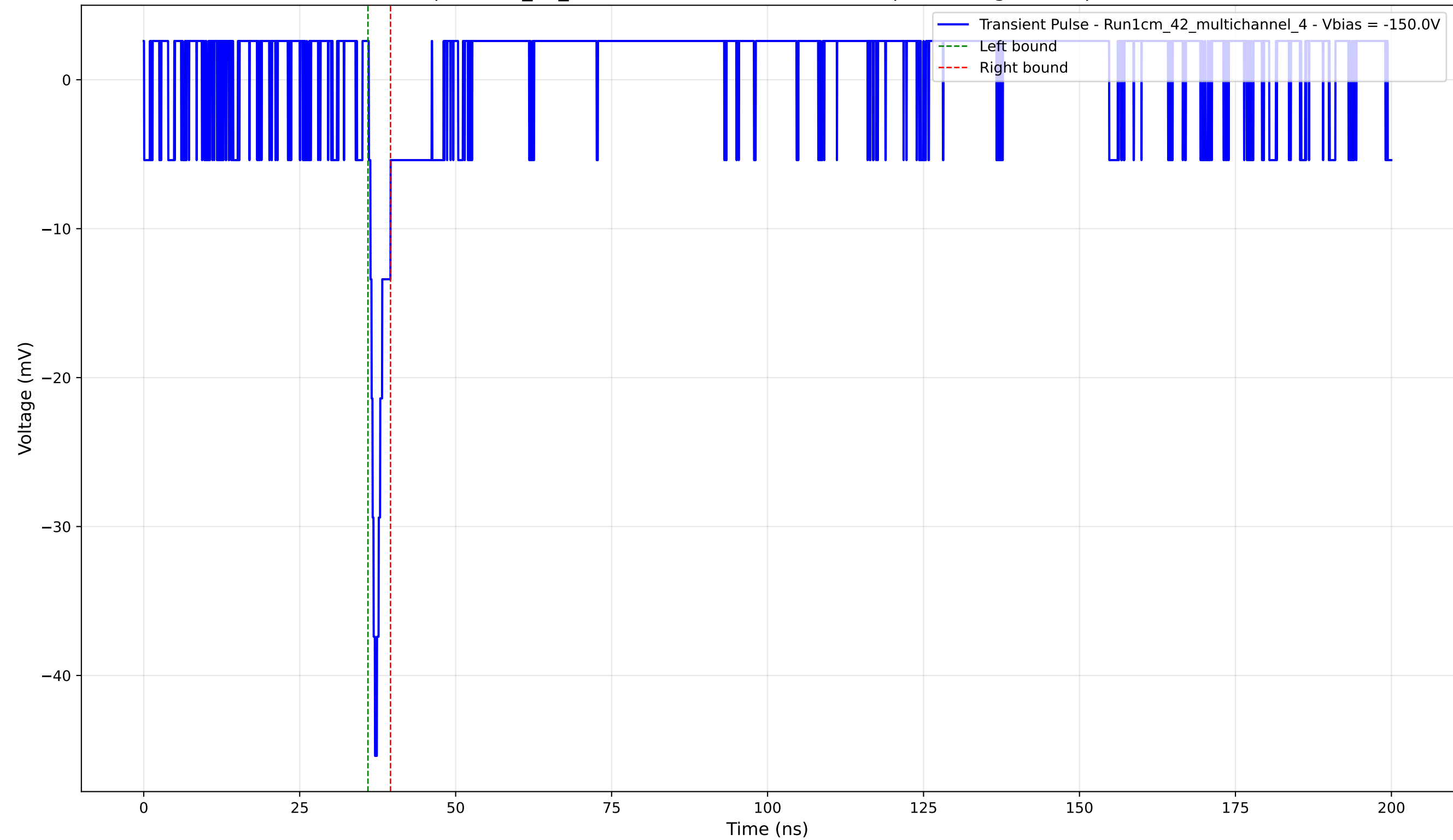
Transient Pulse - Sample: 1cm_42_multichannel - Position: 2335.0 \mu\text{m} - Charge: 1.53 pC - Rise Time: 0.99 ns
