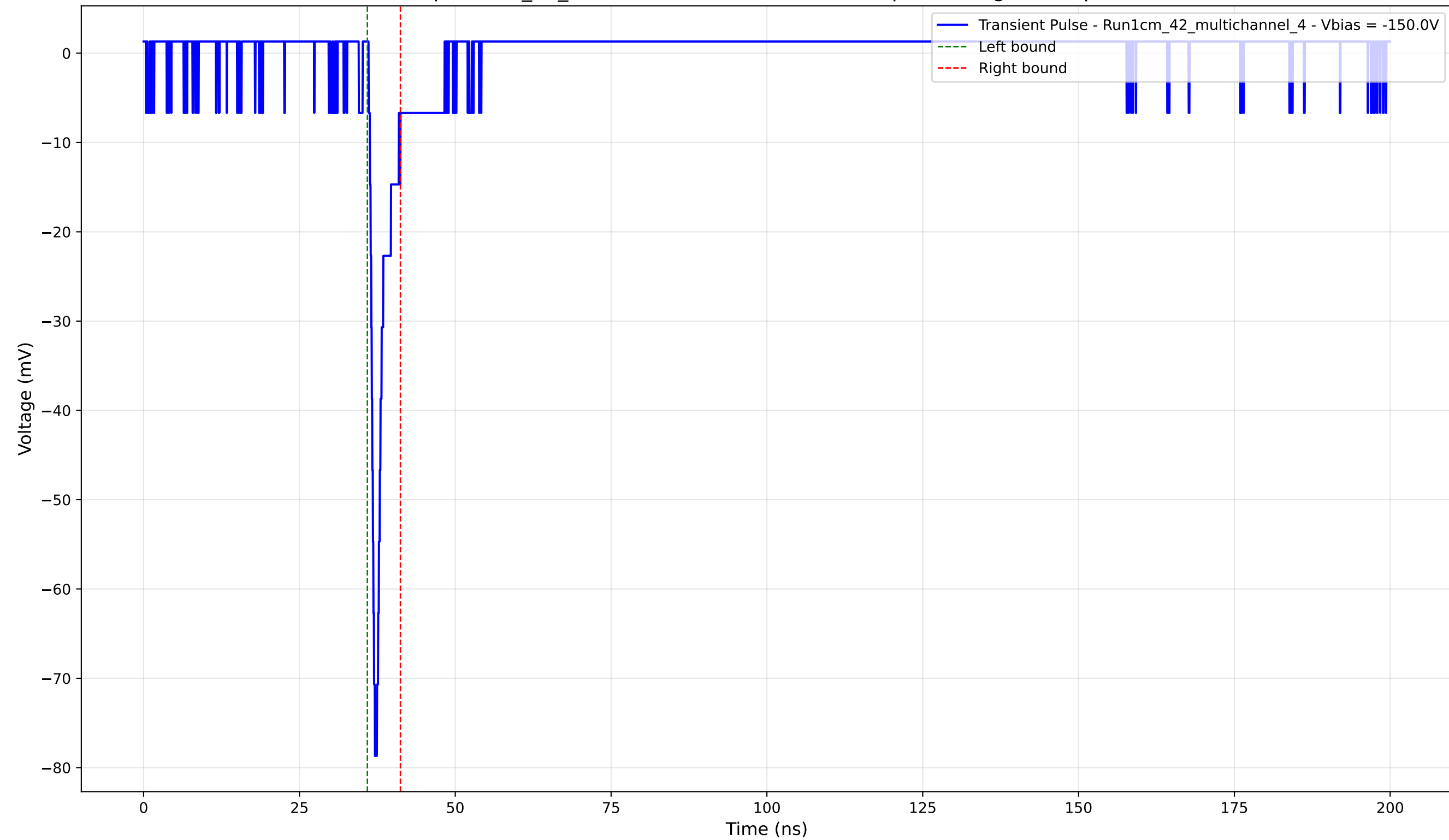
Transient Pulse - Sample: 1cm_42_multichannel - Position: 2520.0 \mu\text{m} - Charge: 3.21 pC - Rise Time: 0.82 ns
