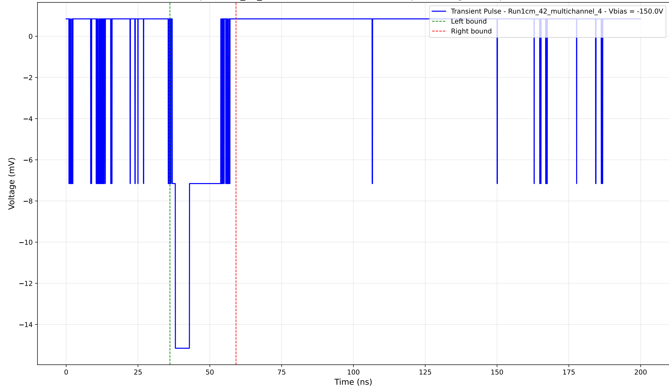
Transient Pulse - Sample: 1cm_42_multichannel - Position: 4065.0 \mu\text{m} - Charge: 3.37 pC - Rise Time: 1.08 ns
