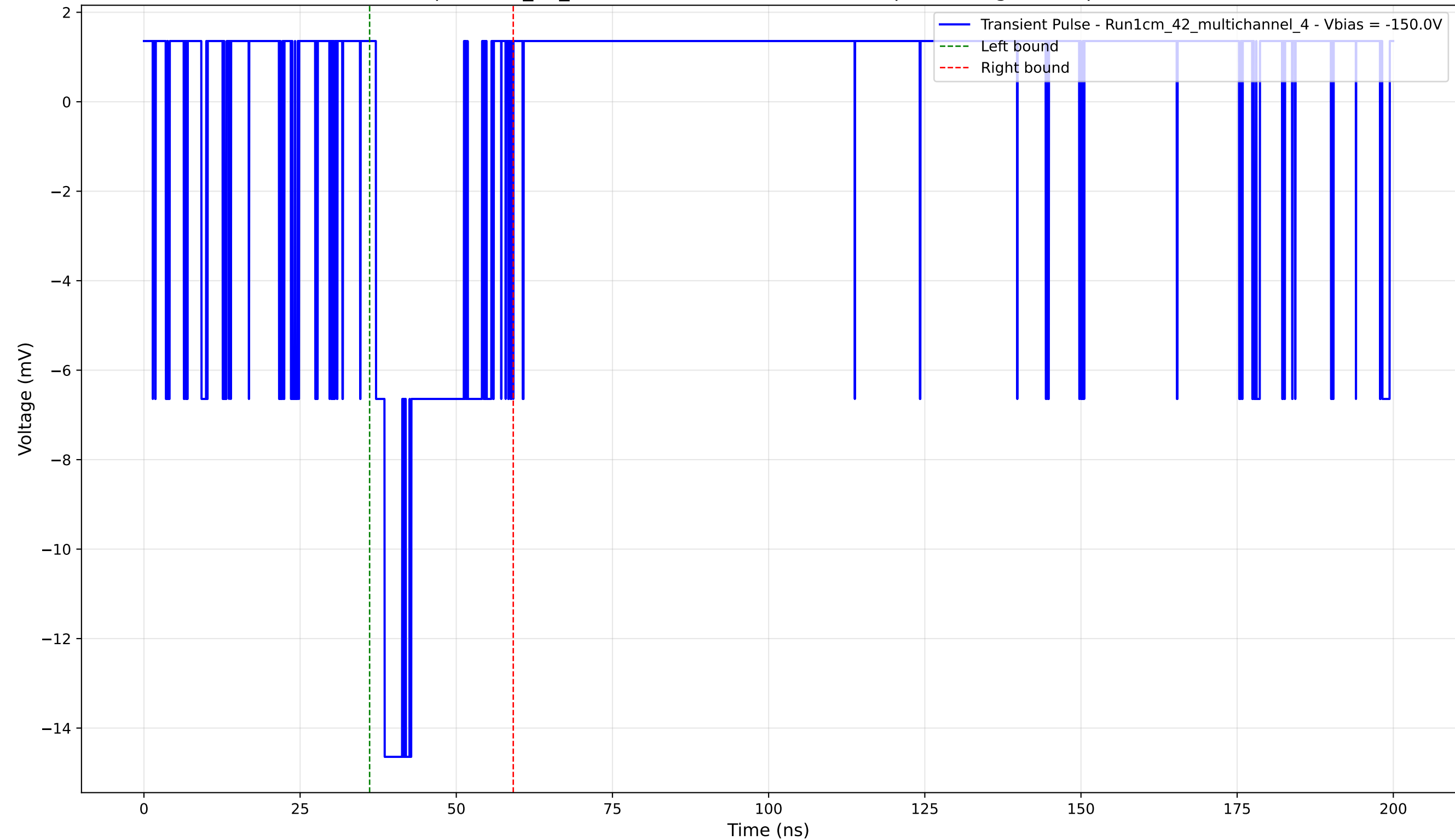
Transient Pulse - Sample: 1cm_42_multichannel - Position: 4730.0 \mu\text{m} - Charge: 2.90 pC - Rise Time: 1.40 ns
