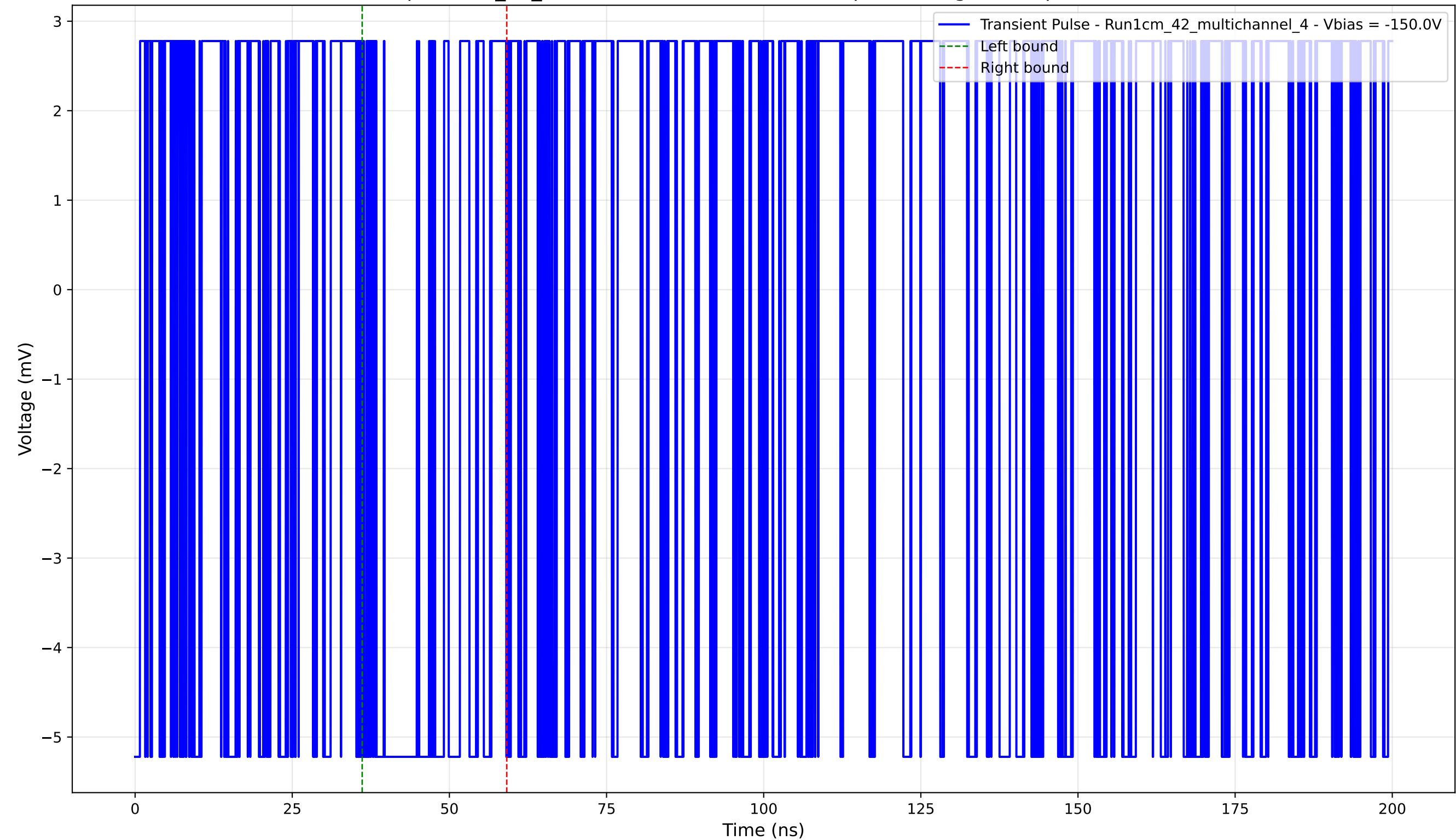
Transient Pulse - Sample: 1cm_42_multichannel - Position: 395.0 \mu\text{m} - Charge: 1.20 pC - Rise Time: 0.00 ns (N/A)
