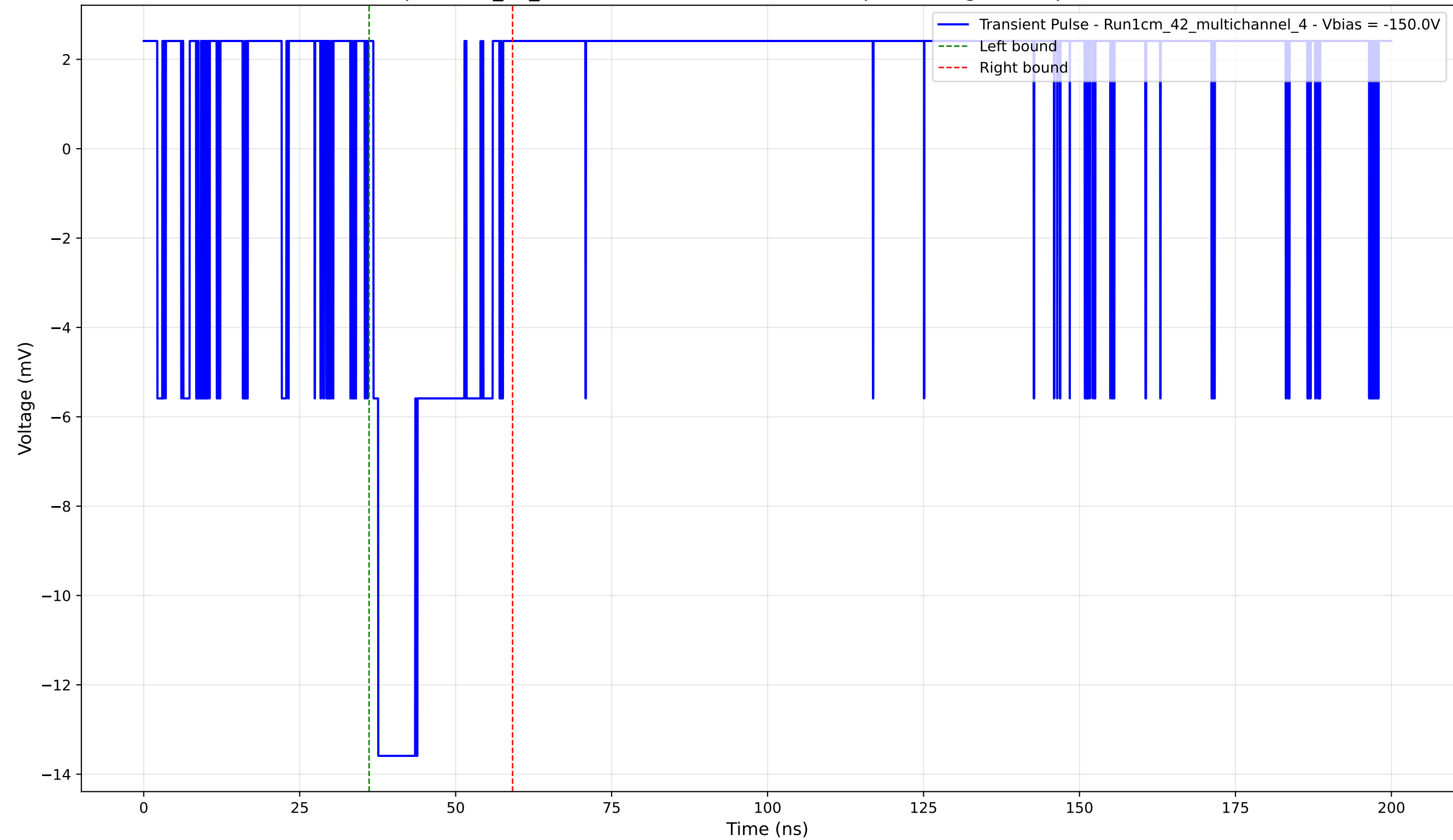
Transient Pulse - Sample: 1cm_42_multichannel - Position: 3770.0 \mu\text{m} - Charge: 2.94 pC - Rise Time: 0.00 ns (N/A)
