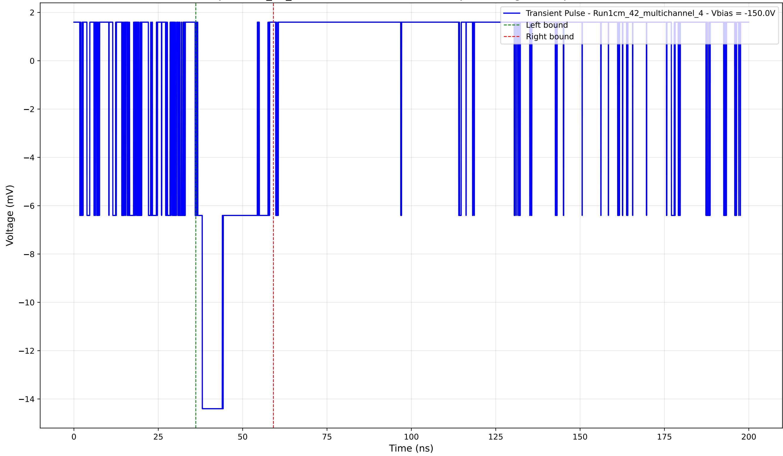
Transient Pulse - Sample: 1cm_42_multichannel - Position: 530.0 \mu\text{m} - Charge: 3.60 pC - Rise Time: 0.00 ns (N/A)
