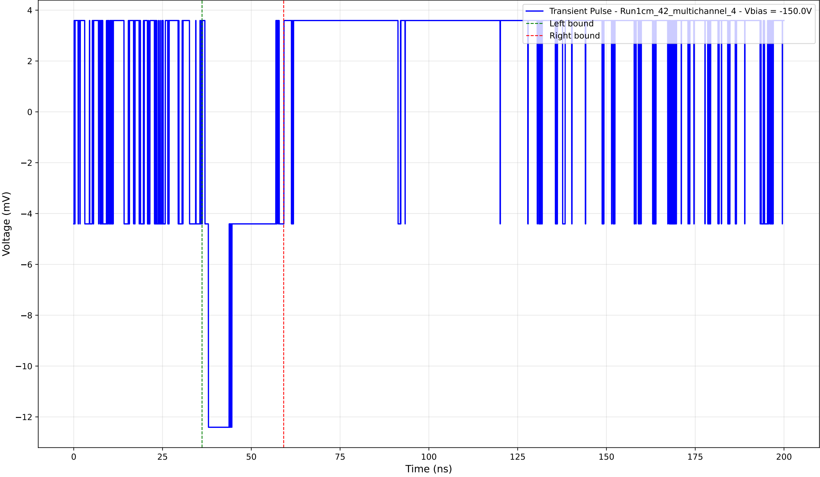
Transient Pulse - Sample: 1cm_42_multichannel - Position: 560.0 \mu\text{m} - Charge: 2.79 pC - Rise Time: 0.00 ns (N/A)
