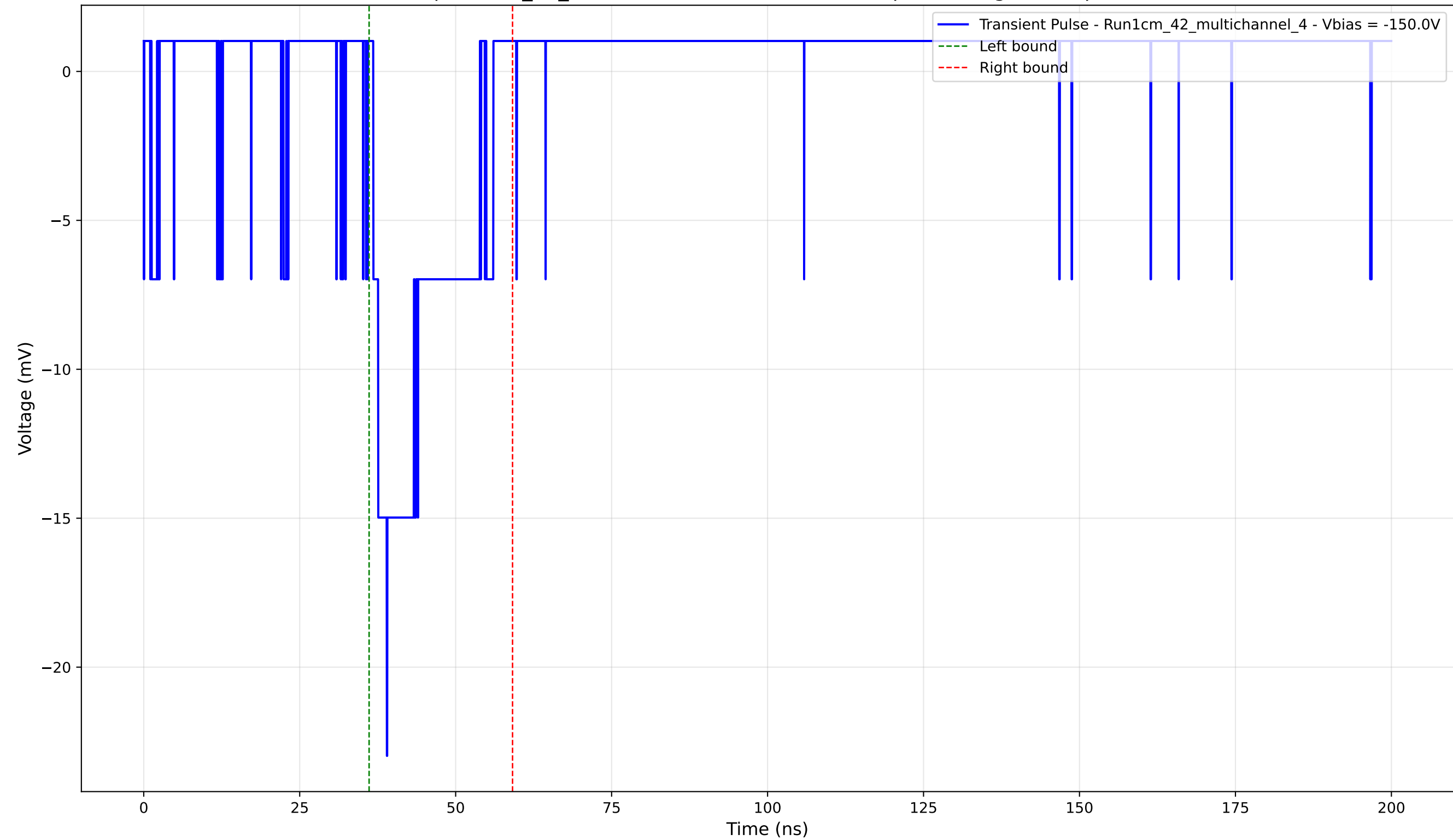
Transient Pulse - Sample: 1cm_42_multichannel - Position: 3790.0 \mu\text{m} - Charge: 3.44 pC - Rise Time: 2.18 ns
