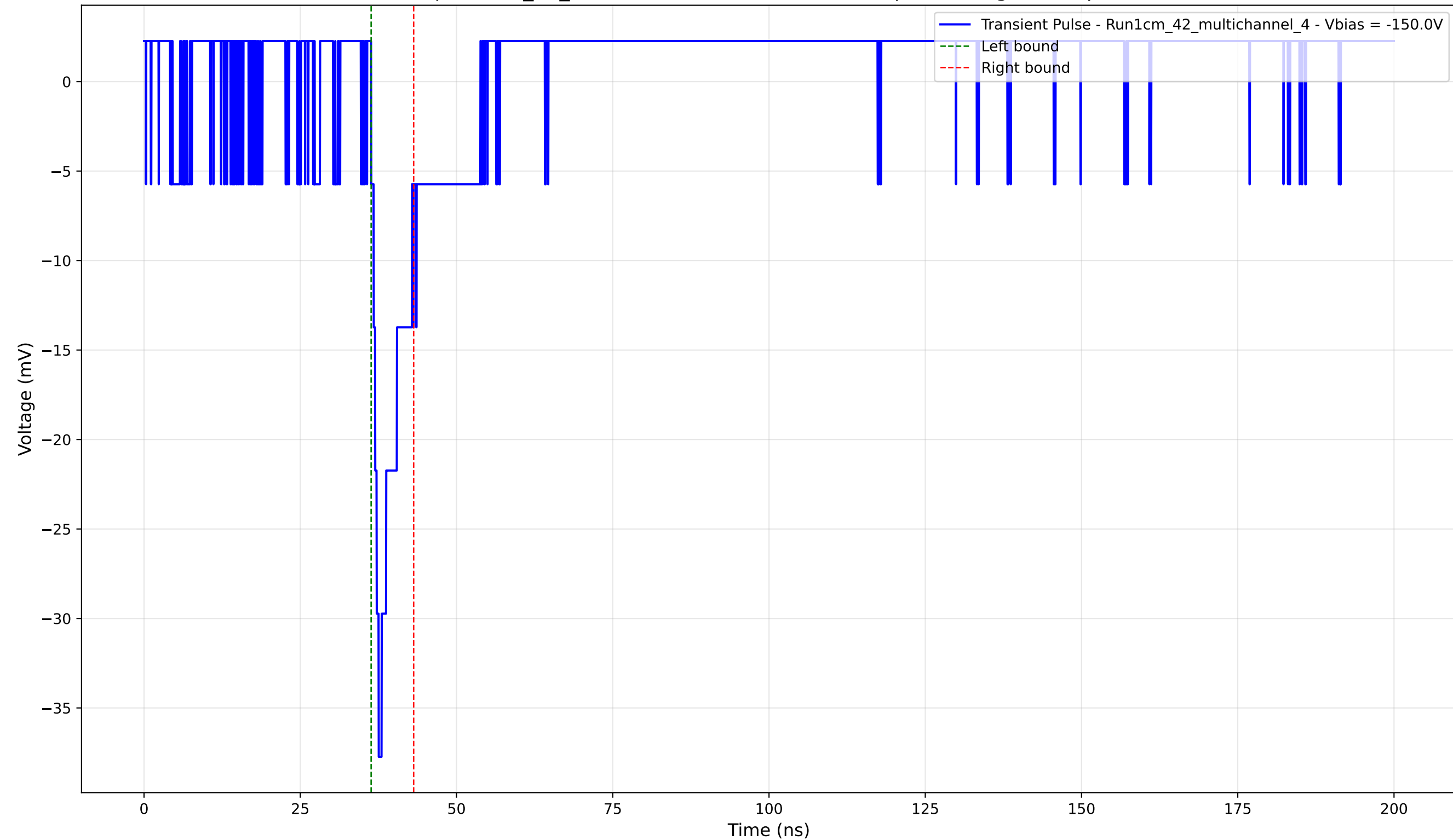
Transient Pulse - Sample: 1cm_42_multichannel - Position: 1670.0 \mu\text{m} - Charge: 2.65 pC - Rise Time: 1.21 ns
