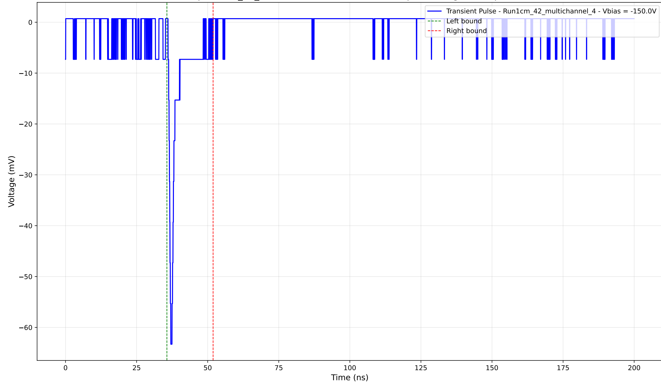
Transient Pulse - Sample: 1cm_42_multichannel - Position: 2325.0 \mu\text{m} - Charge: 3.84 pC - Rise Time: 0.96 ns
