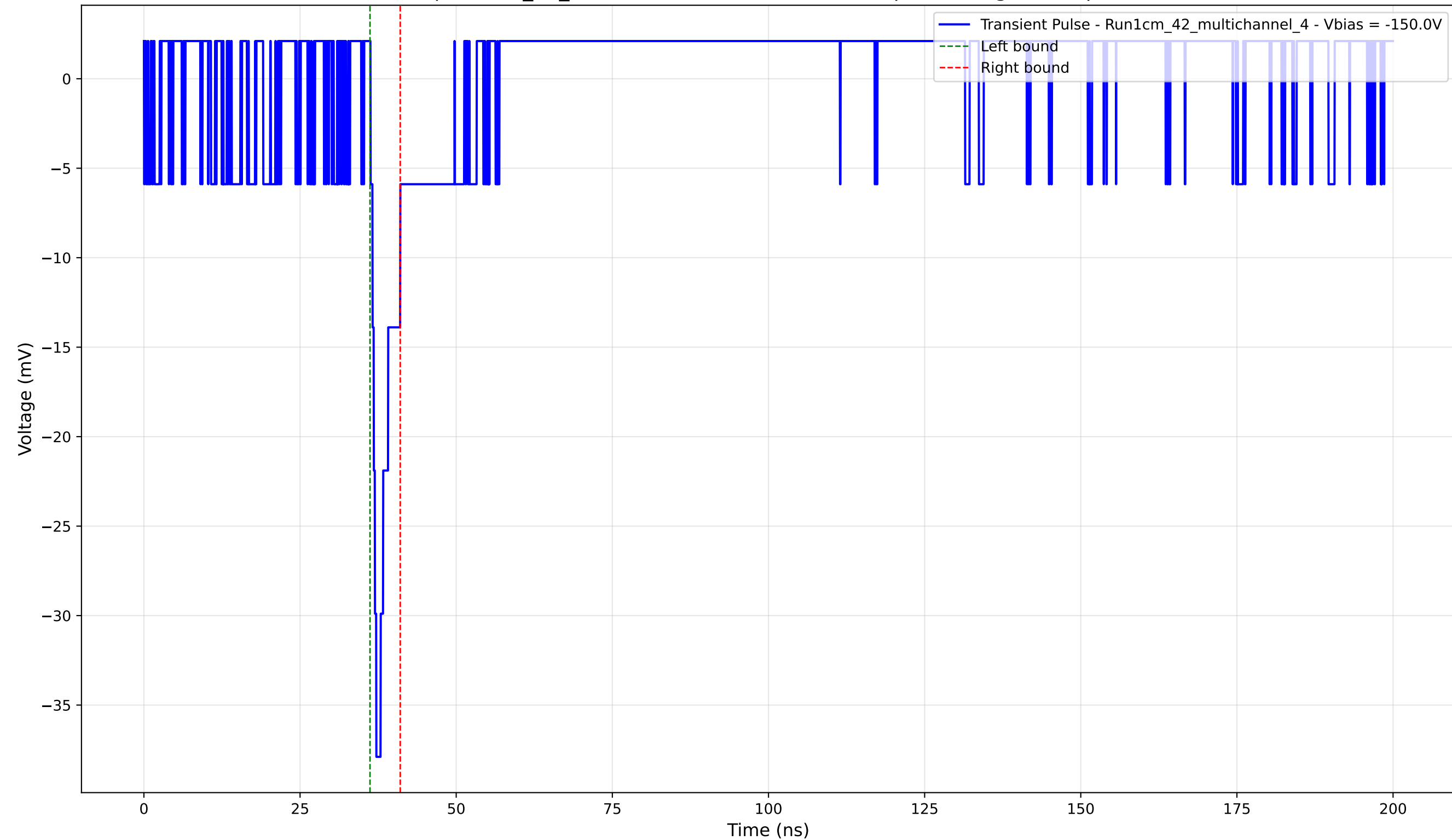
Transient Pulse - Sample: 1cm_42_multichannel - Position: 1940.0 \mu\text{m} - Charge: 1.96 pC - Rise Time: 0.93 ns
