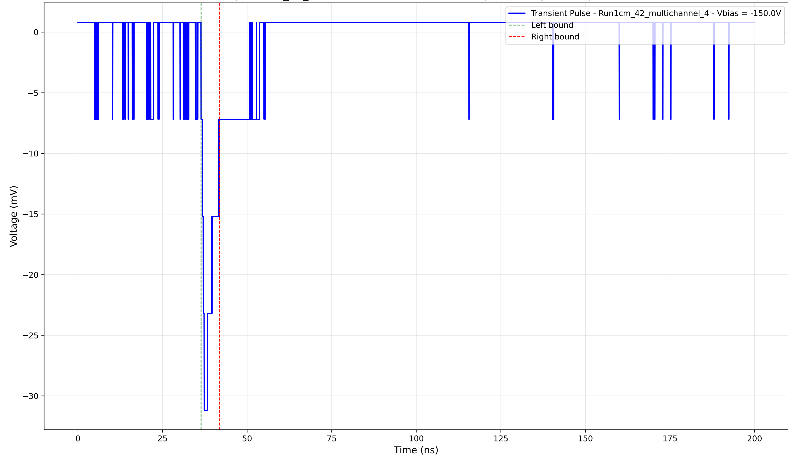
Transient Pulse - Sample: 1cm_42_multichannel - Position: 3100.0 \mu\text{m} - Charge: 2.14 pC - Rise Time: 0.93 ns
