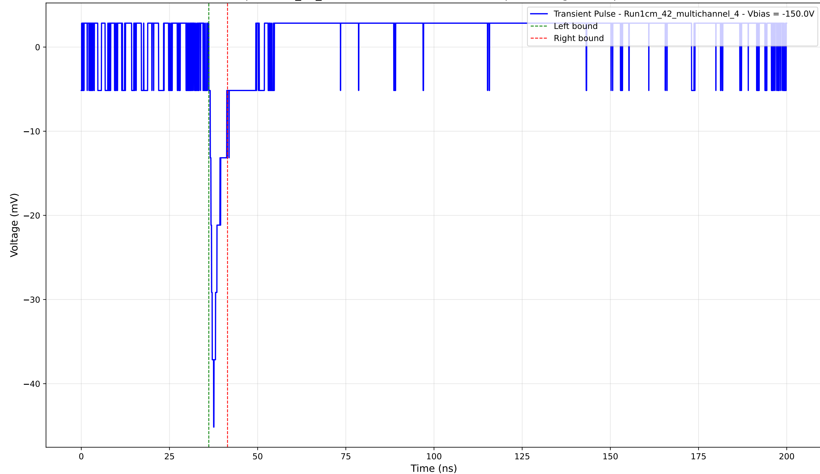
Transient Pulse - Sample: 1cm_42_multichannel - Position: 1945.0 \mu\text{m} - Charge: 2.15 pC - Rise Time: 1.37 ns
