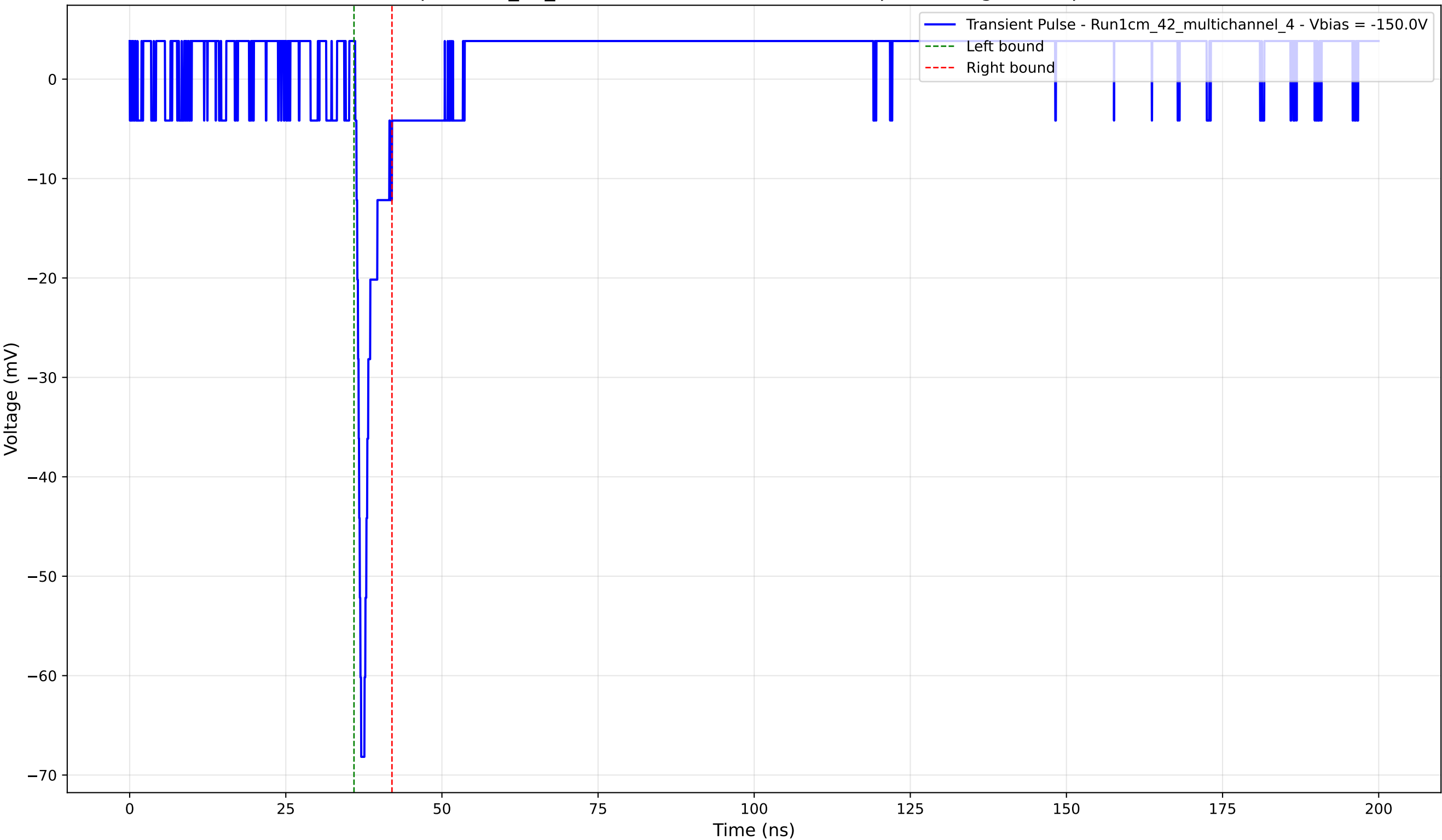
Transient Pulse - Sample: 1cm_42_multichannel - Position: 2200.0 \mu\text{m} - Charge: 3.03 pC - Rise Time: 0.75 ns
