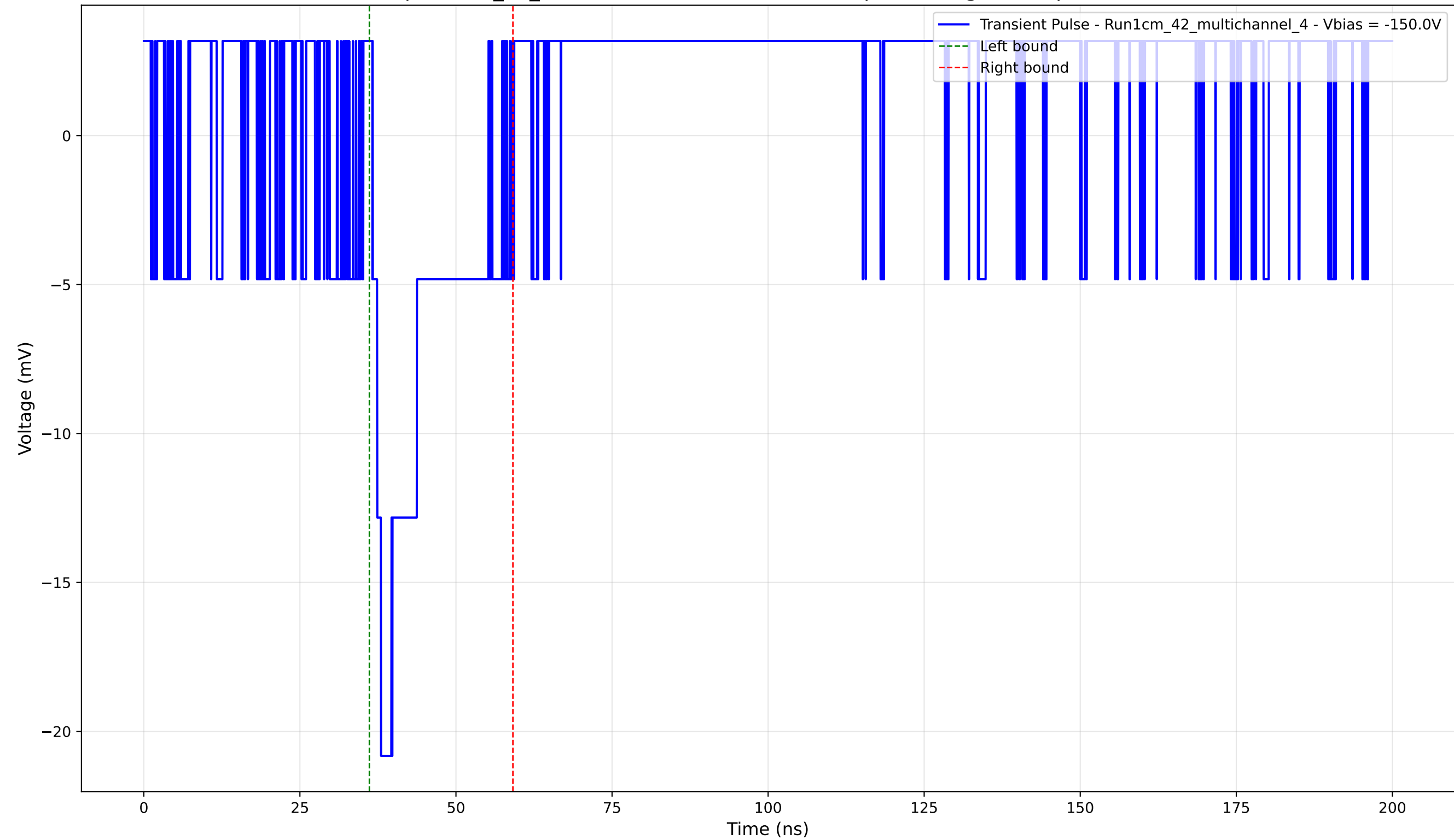
Transient Pulse - Sample: 1cm_42_multichannel - Position: 1075.0 \mu\text{m} - Charge: 3.27 pC - Rise Time: 0.00 ns (N/A)
