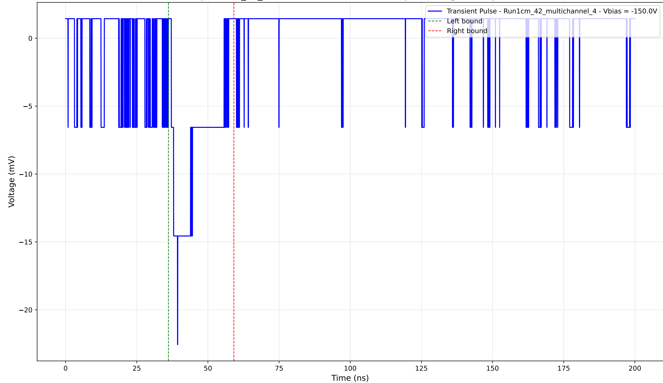
Transient Pulse - Sample: 1cm_42_multichannel - Position: 675.0 \mu\text{m} - Charge: 3.41 pC - Rise Time: 2.20 ns
