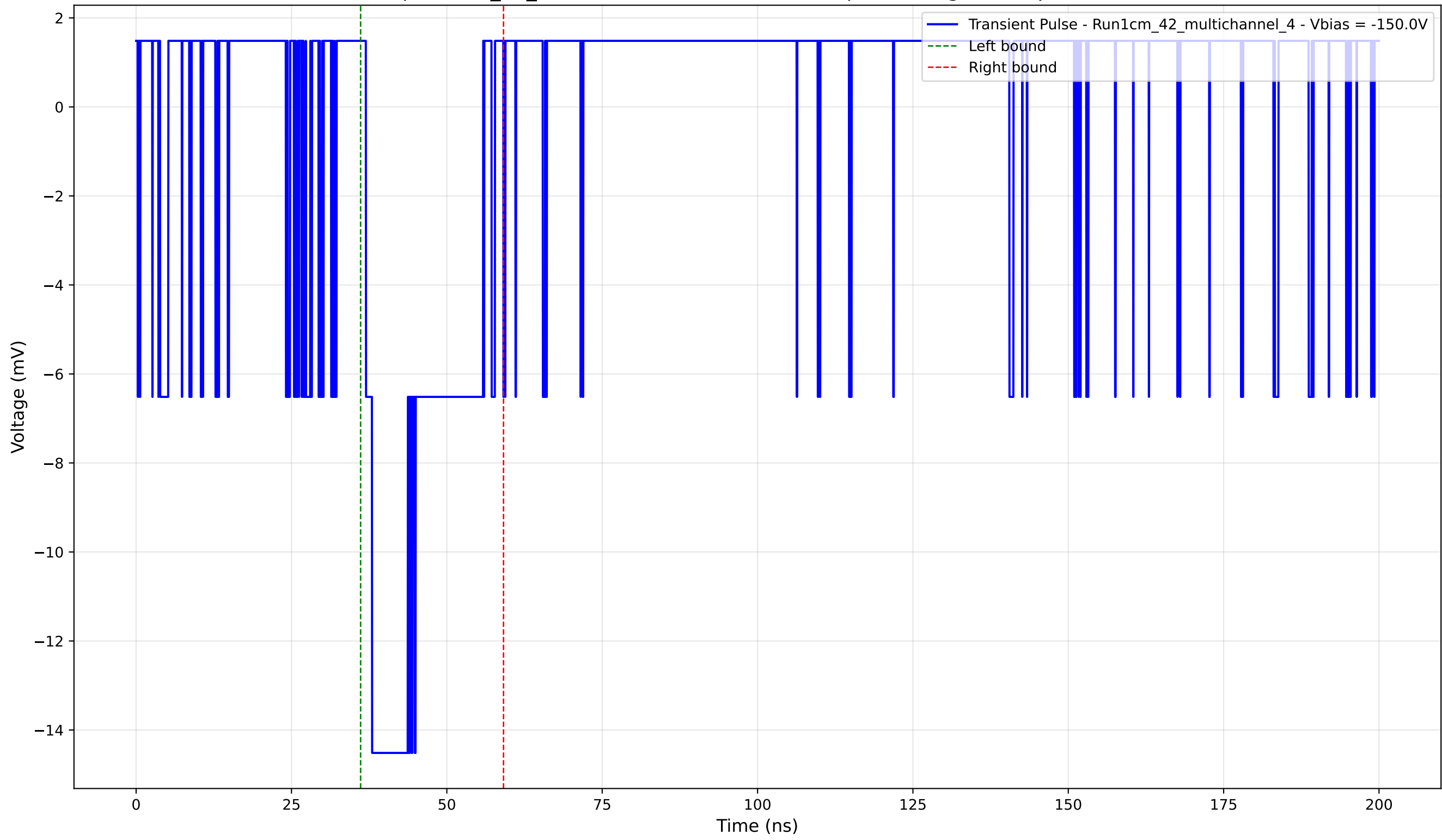
Transient Pulse - Sample: 1cm_42_multichannel - Position: 595.0 \mu\text{m} - Charge: 3.43 pC - Rise Time: 0.00 ns (N/A)
