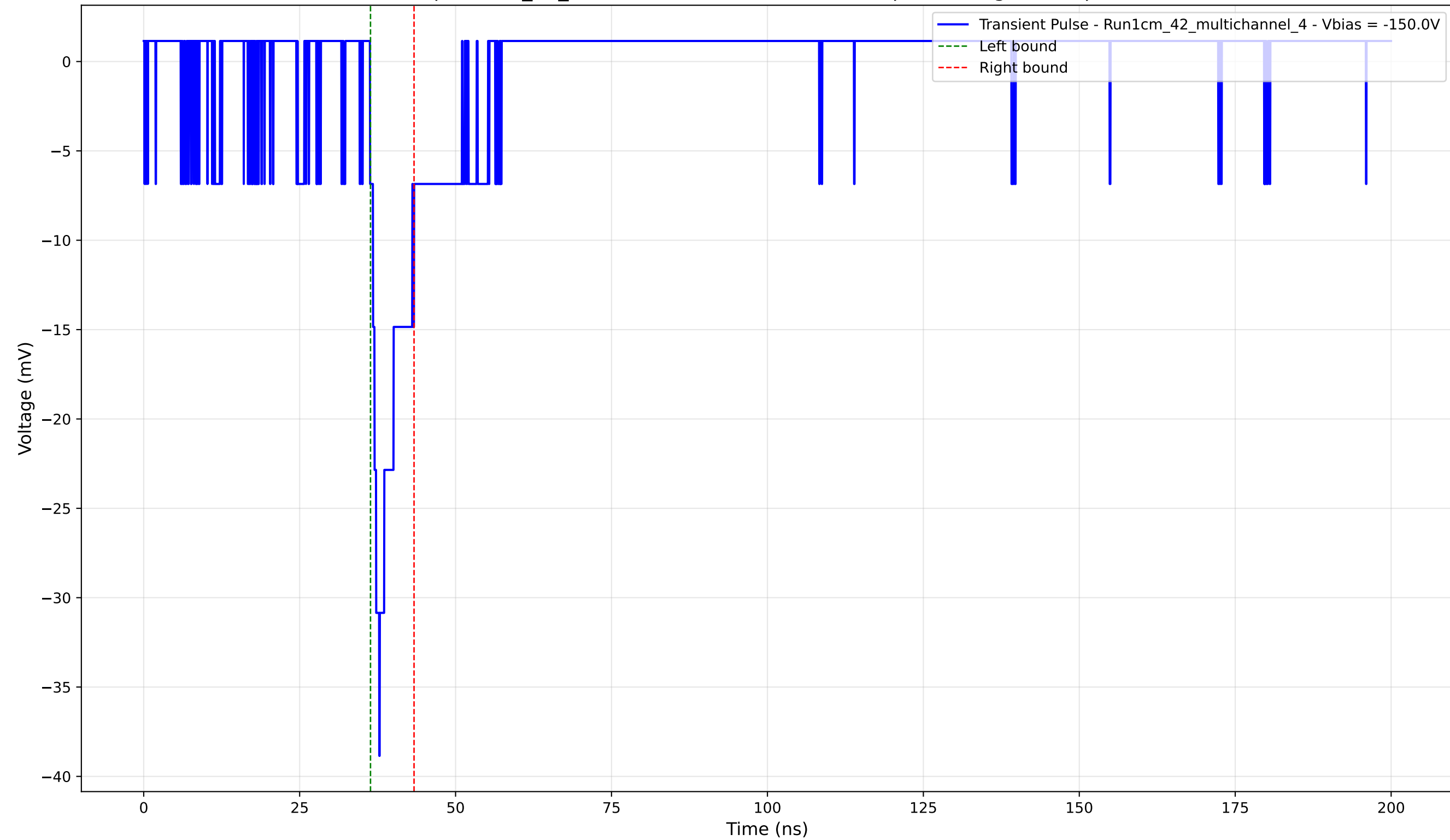
Transient Pulse - Sample: 1cm_42_multichannel - Position: 1650.0 \mu\text{m} - Charge: 2.70 pC - Rise Time: 1.49 ns
