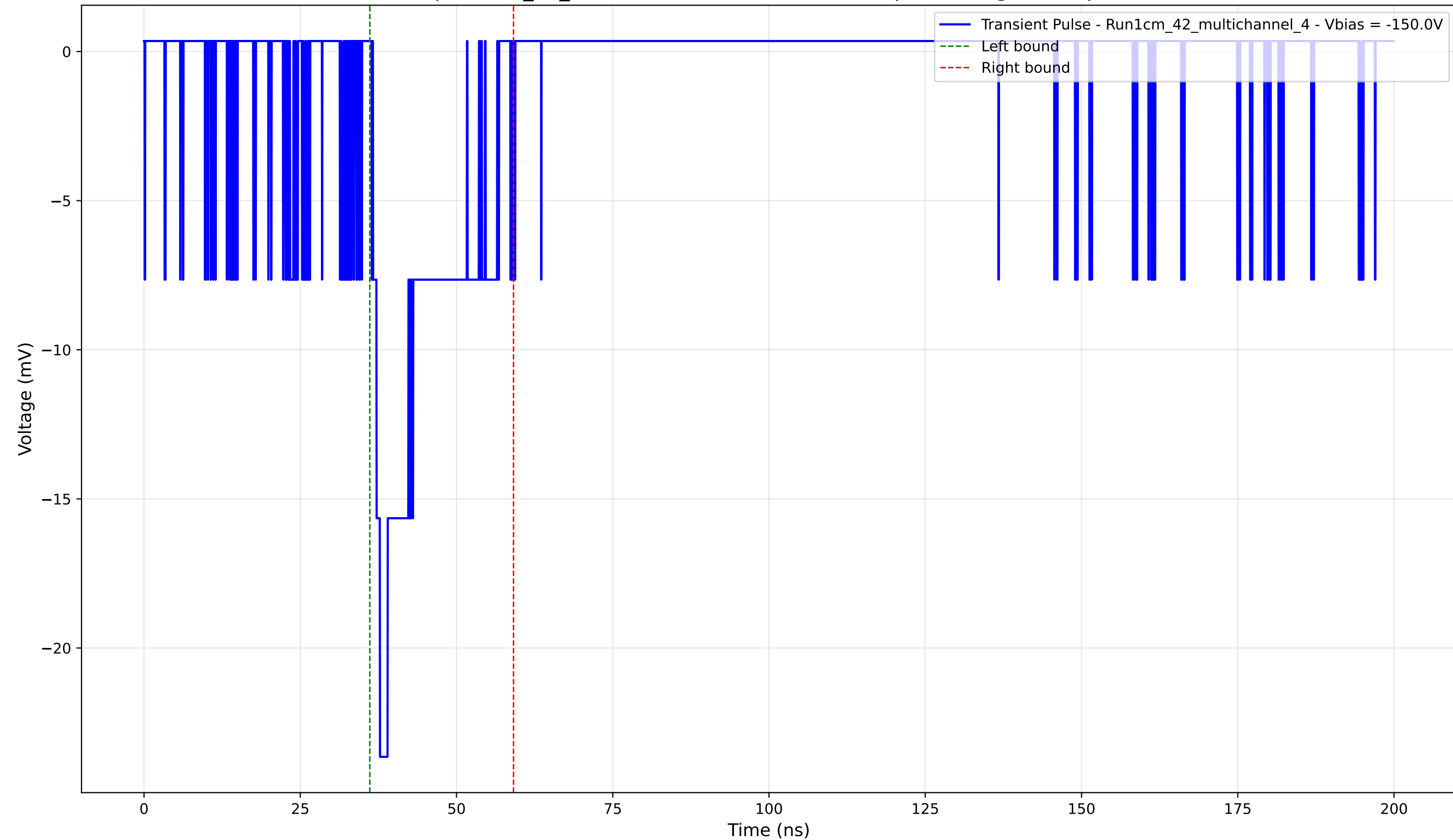
Transient Pulse - Sample: 1cm_42_multichannel - Position: 3475.0 \mu\text{m} - Charge: 4.13 pC - Rise Time: 1.11 ns
