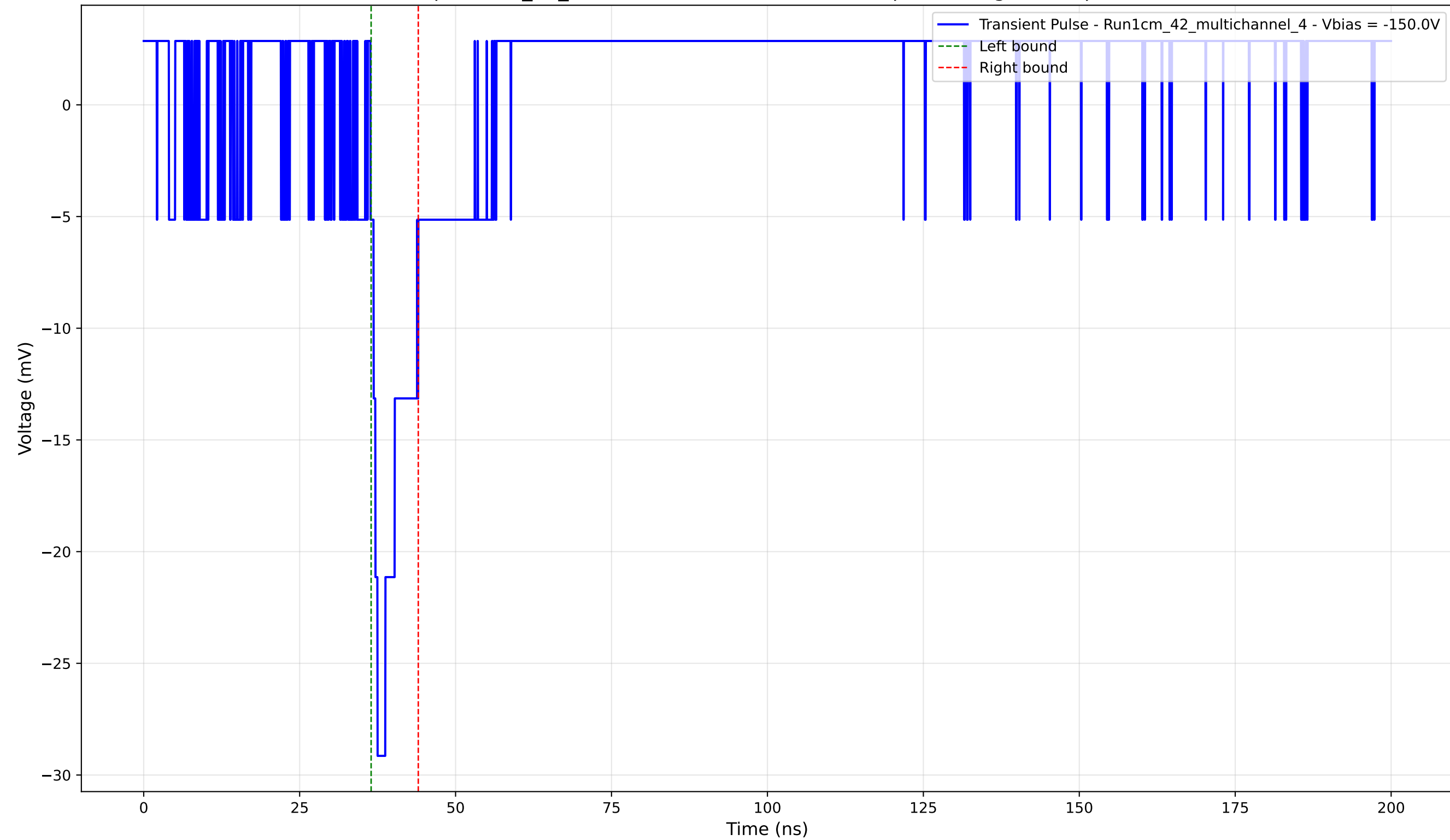
Transient Pulse - Sample: 1cm_42_multichannel - Position: 1525.0 \mu\text{m} - Charge: 2.61 pC - Rise Time: 1.14 ns
