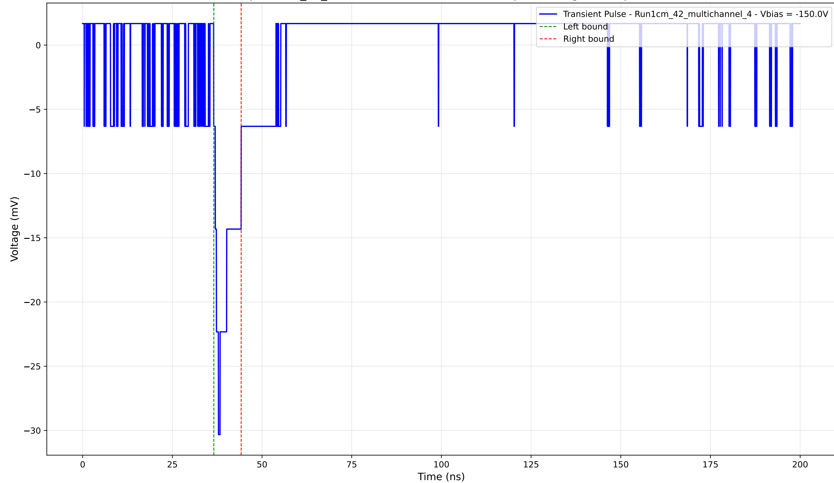
Transient Pulse - Sample: 1cm_42_multichannel - Position: 1455.0 \mu\text{m} - Charge: 2.65 pC - Rise Time: 1.33 ns
