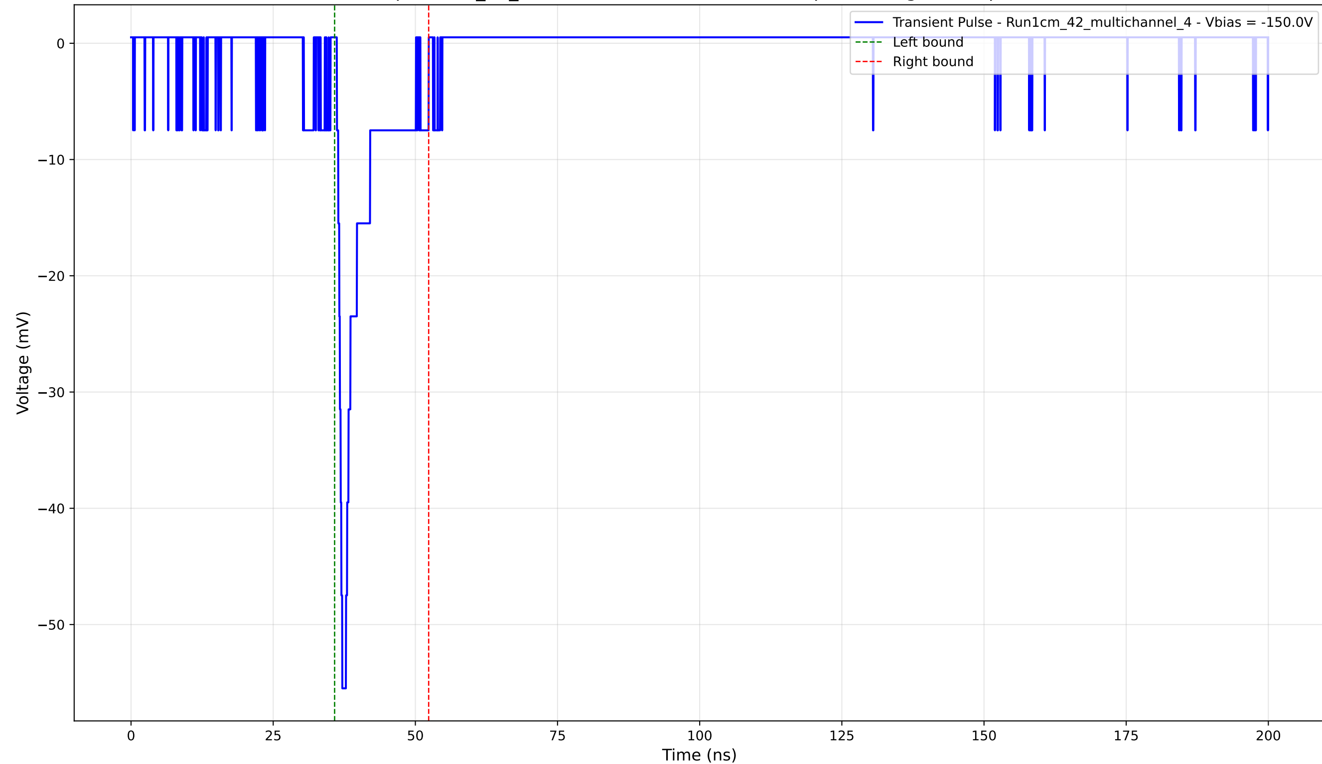
Transient Pulse - Sample: 1cm_42_multichannel - Position: 2055.0 \mu\text{m} - Charge: 4.51 pC - Rise Time: 0.95 ns
