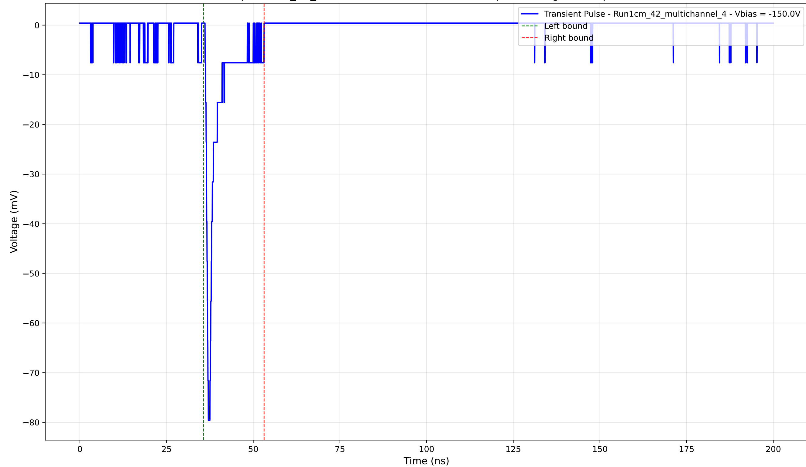
Transient Pulse - Sample: 1cm_42_multichannel - Position: 2280.0 \mu\text{m} - Charge: 4.99 pC - Rise Time: 0.78 ns
