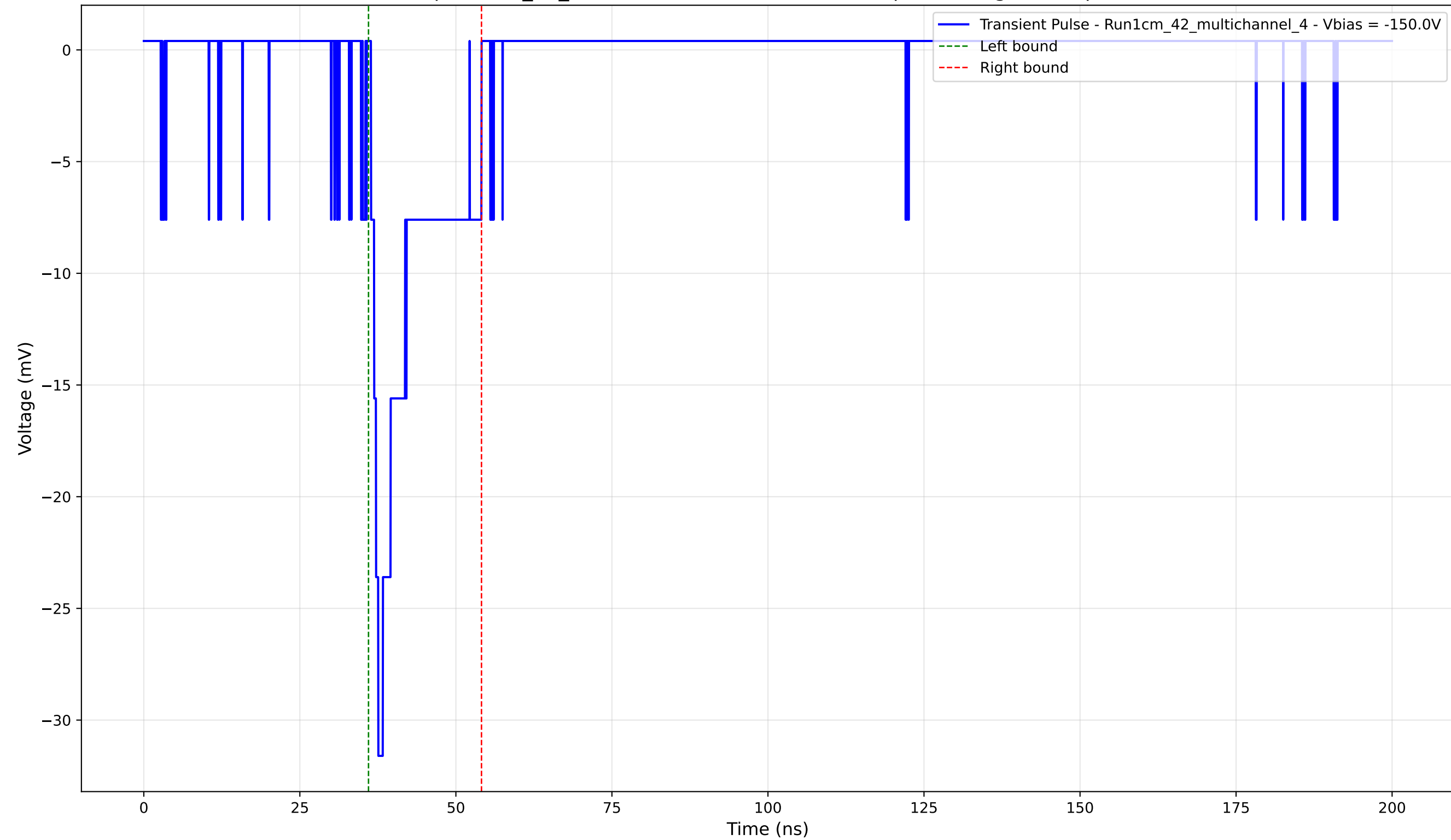
Transient Pulse - Sample: 1cm_42_multichannel - Position: 3190.0 \mu\text{m} - Charge: 3.99 pC - Rise Time: 1.17 ns
