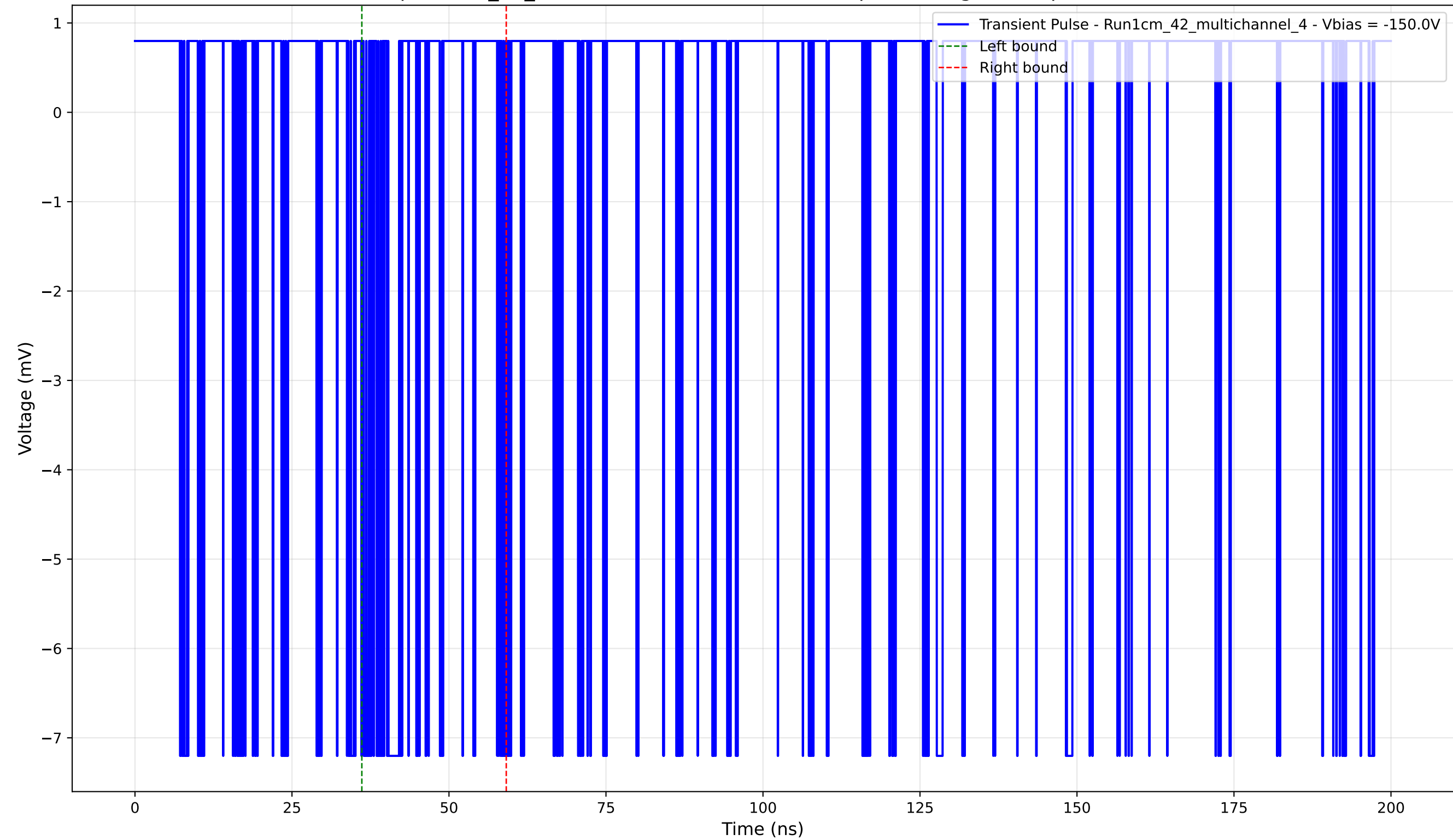
Transient Pulse - Sample: 1cm_42_multichannel - Position: 3380.0 \mu\text{m} - Charge: 0.61 pC - Rise Time: 0.00 ns (N/A)
