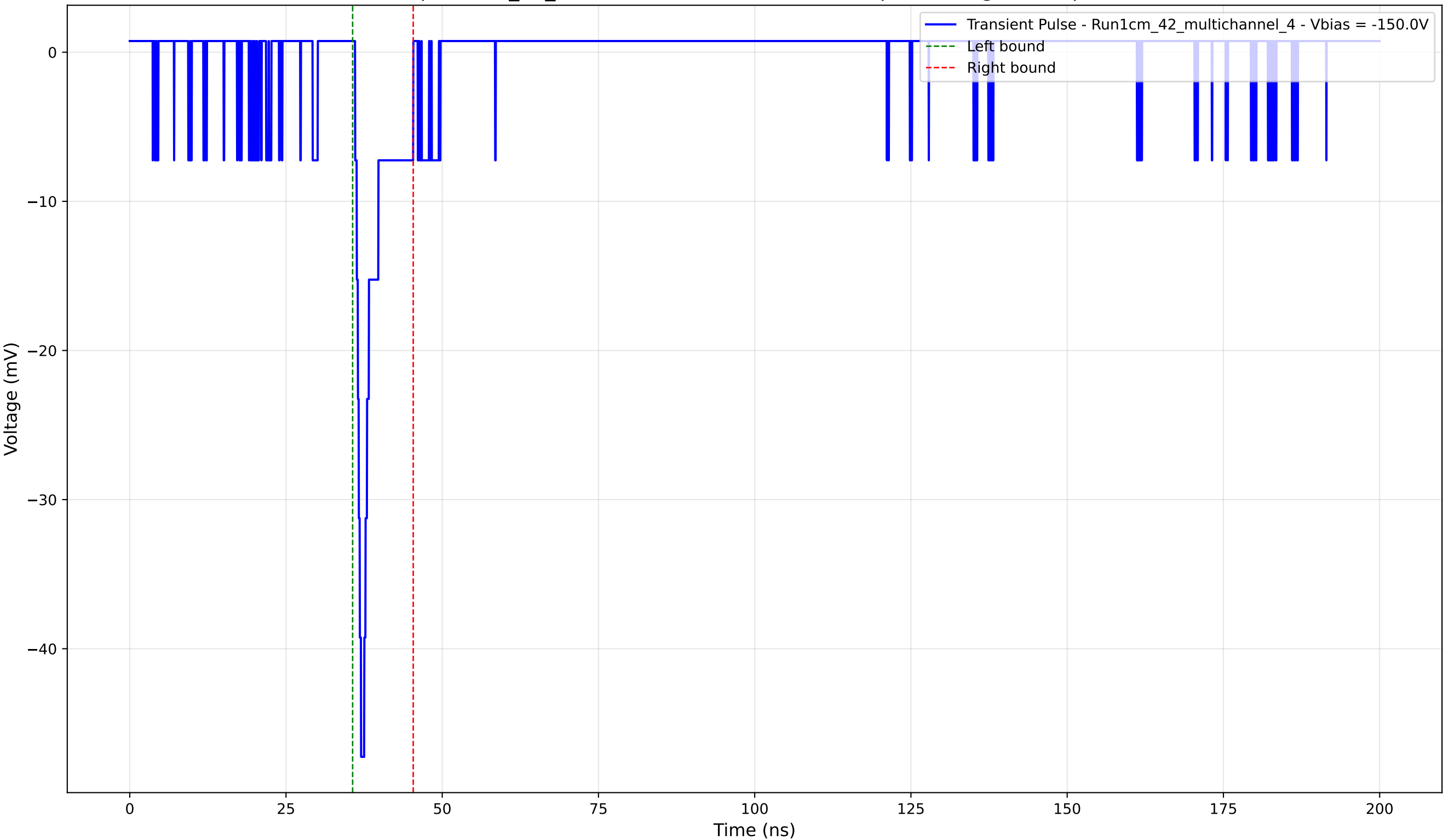
Transient Pulse - Sample: 1cm_42_multichannel - Position: 2440.0 \mu\text{m} - Charge: 2.62 pC - Rise Time: 0.95 ns
