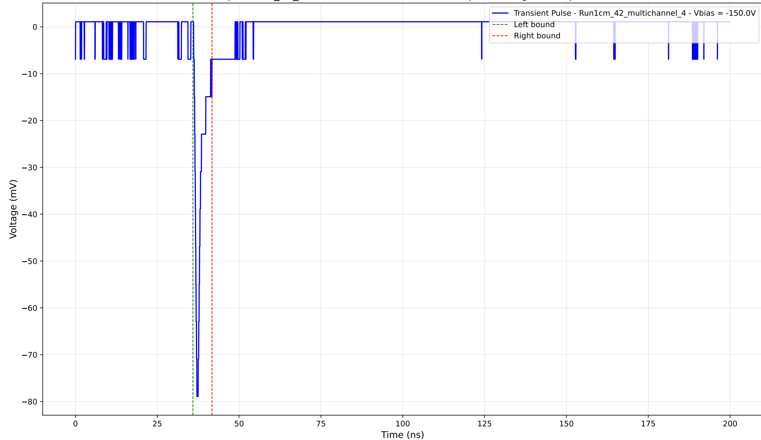
Transient Pulse - Sample: 1cm_42_multichannel - Position: 2230.0 \mu\text{m} - Charge: 3.45 pC - Rise Time: 0.82 ns
