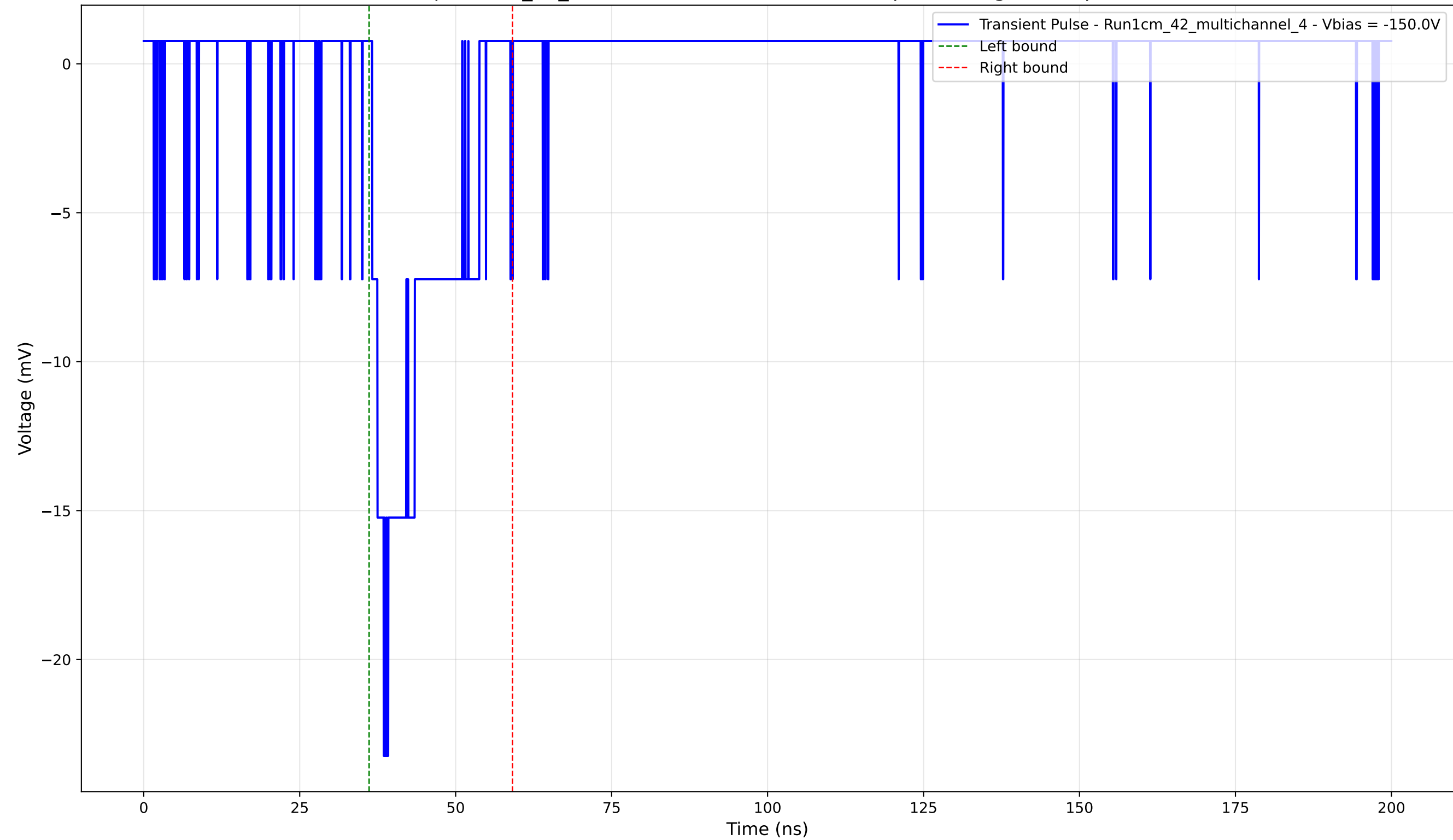
Transient Pulse - Sample: 1cm_42_multichannel - Position: 3615.0 \mu\text{m} - Charge: 3.42 pC - Rise Time: 1.86 ns
