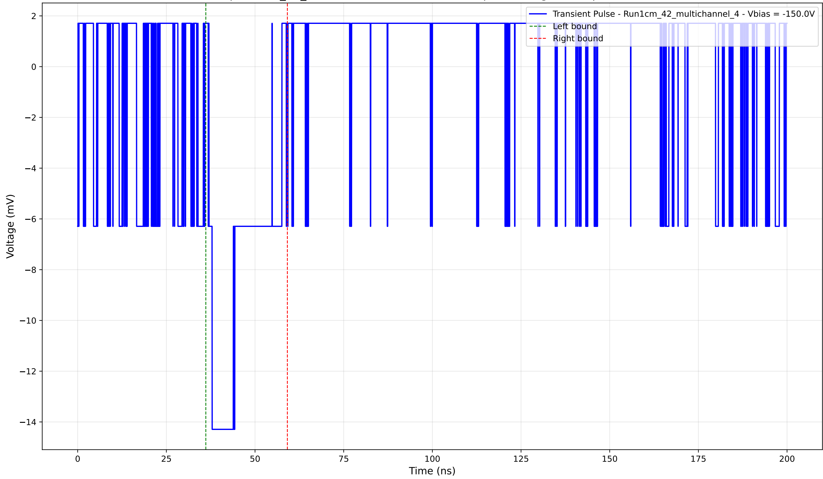
Transient Pulse - Sample: 1cm_42_multichannel - Position: 665.0 \mu\text{m} - Charge: 3.52 pC - Rise Time: 0.00 ns (N/A)
