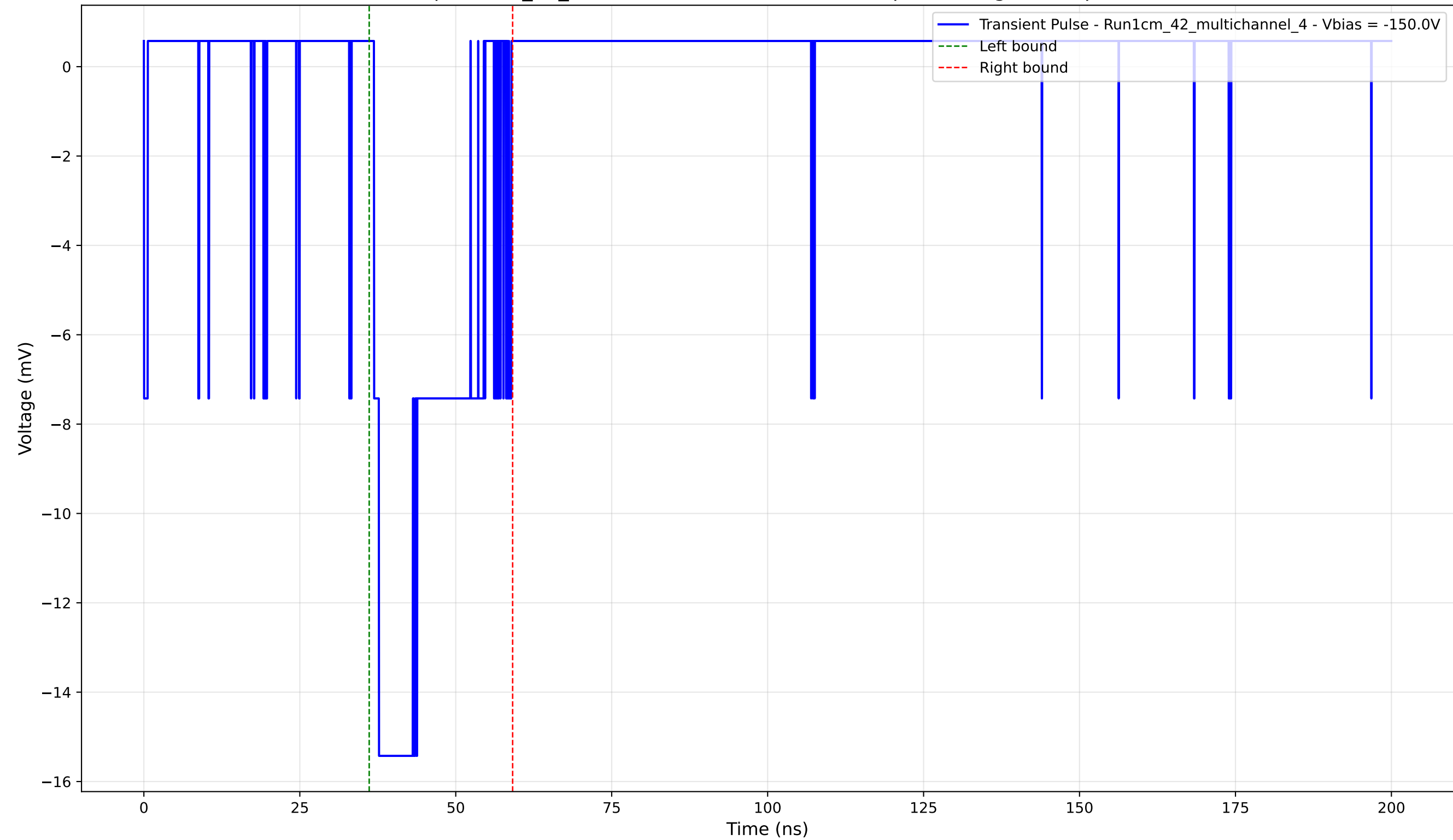
Transient Pulse - Sample: 1cm_42_multichannel - Position: 3805.0 \mu\text{m} - Charge: 3.65 pC - Rise Time: 0.80 ns
