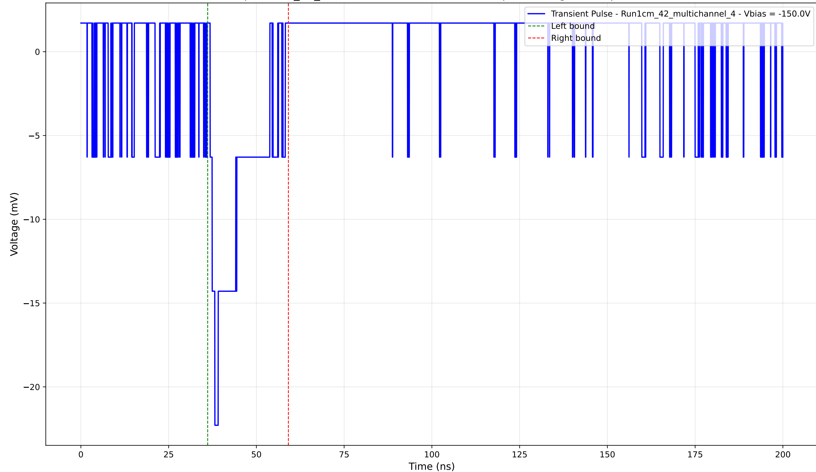
Transient Pulse - Sample: 1cm_42_multichannel - Position: 1085.0 \mu\text{m} - Charge: 3.60 pC - Rise Time: 1.36 ns
