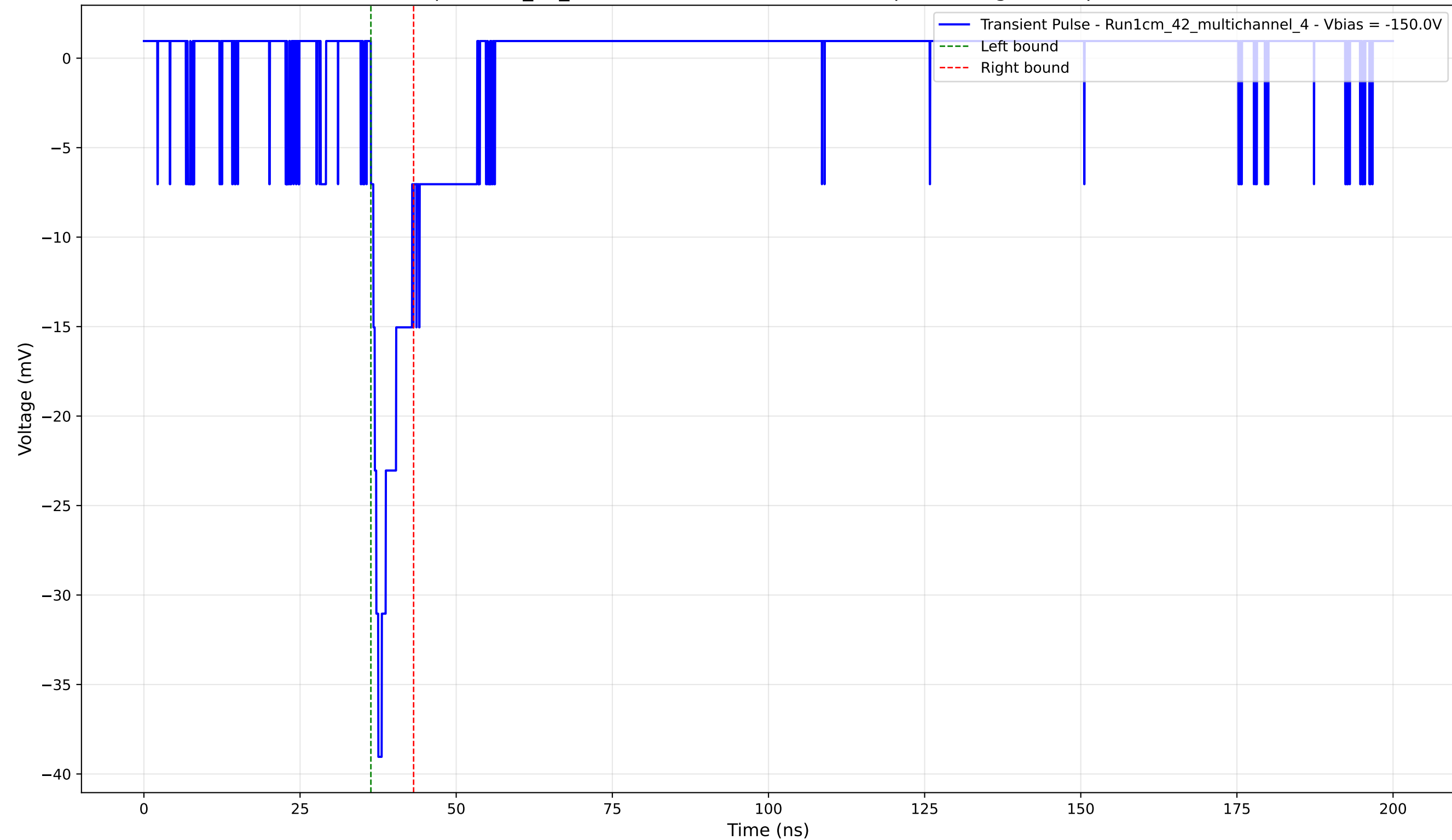
Transient Pulse - Sample: 1cm_42_multichannel - Position: 1660.0 \mu\text{m} - Charge: 2.86 pC - Rise Time: 1.19 ns
