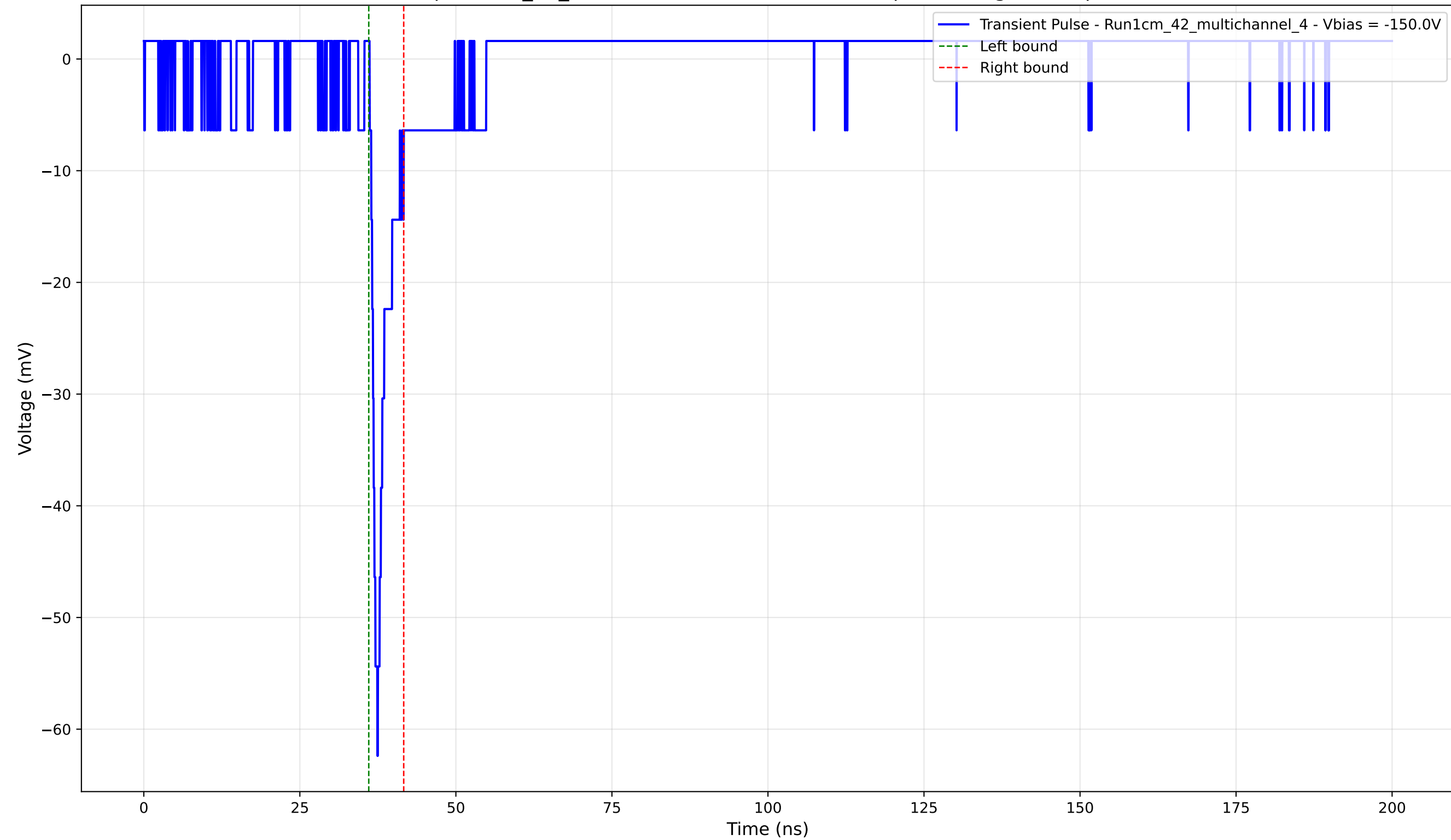
Transient Pulse - Sample: 1cm_42_multichannel - Position: 2075.0 \mu\text{m} - Charge: 2.79 pC - Rise Time: 1.24 ns
