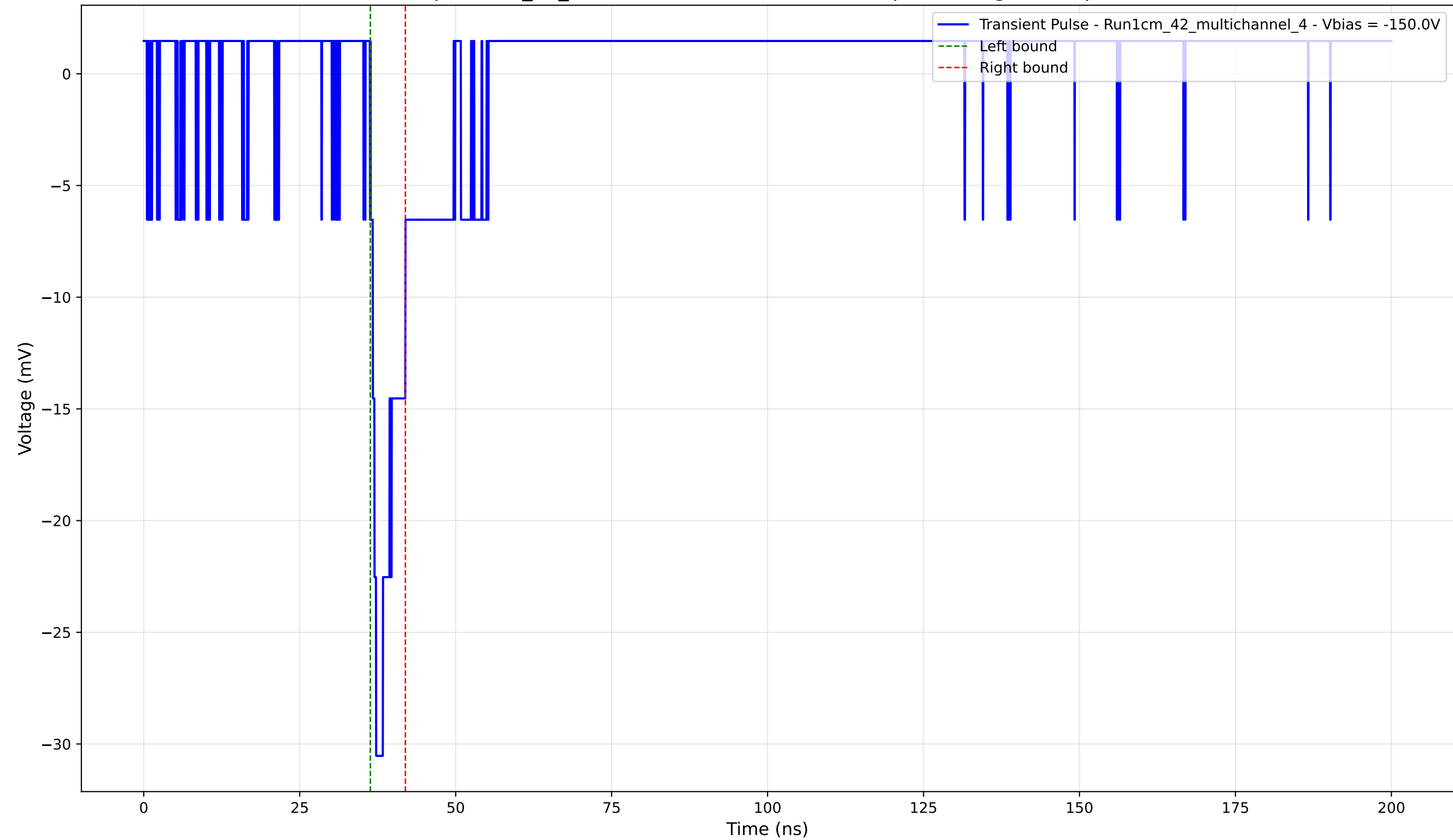
Transient Pulse - Sample: 1cm_42_multichannel - Position: 3070.0 \mu\text{m} - Charge: 2.15 pC - Rise Time: 0.89 ns
