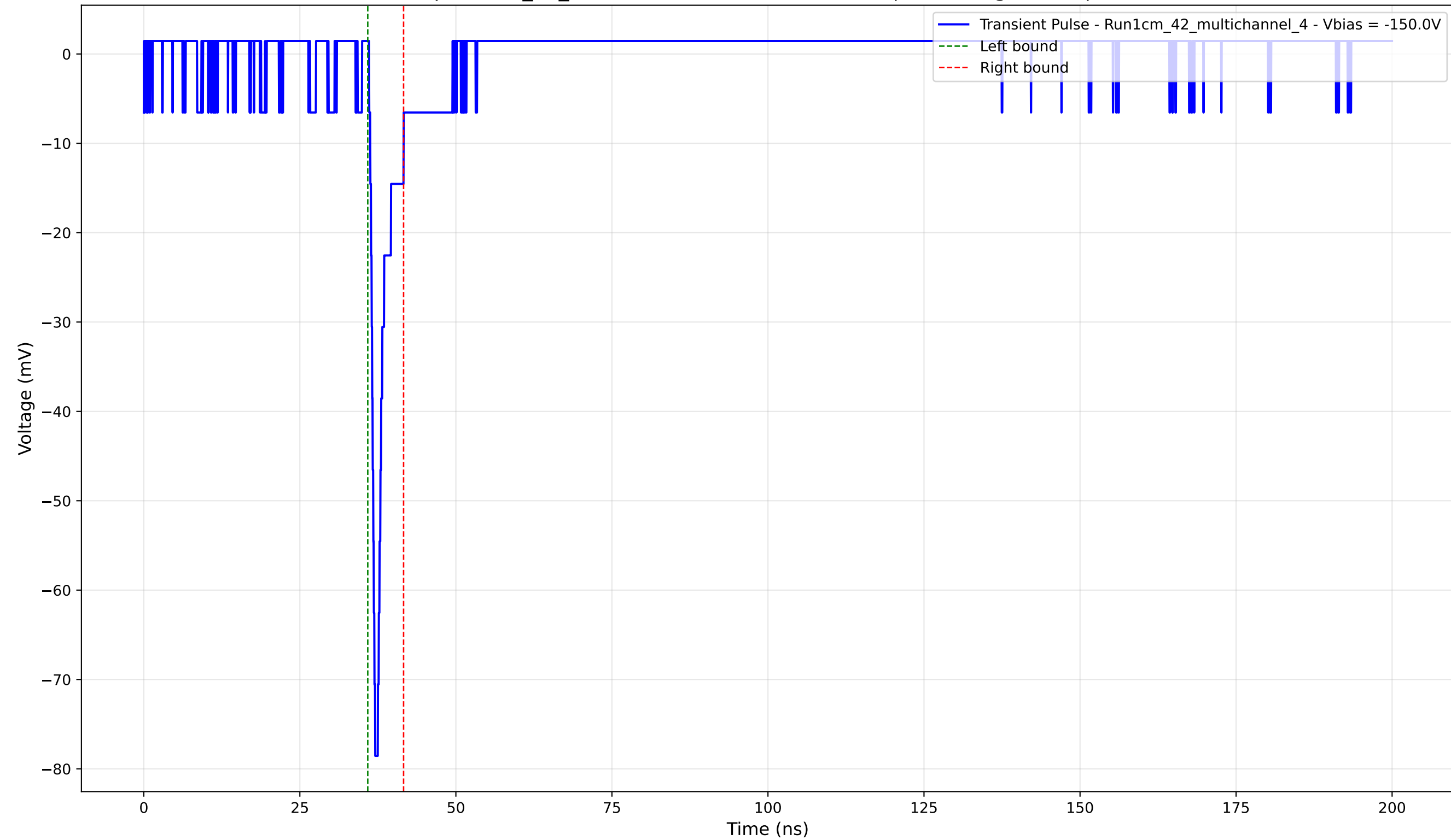
Transient Pulse - Sample: 1cm_42_multichannel - Position: 2505.0 \mu\text{m} - Charge: 3.39 pC - Rise Time: 0.80 ns
