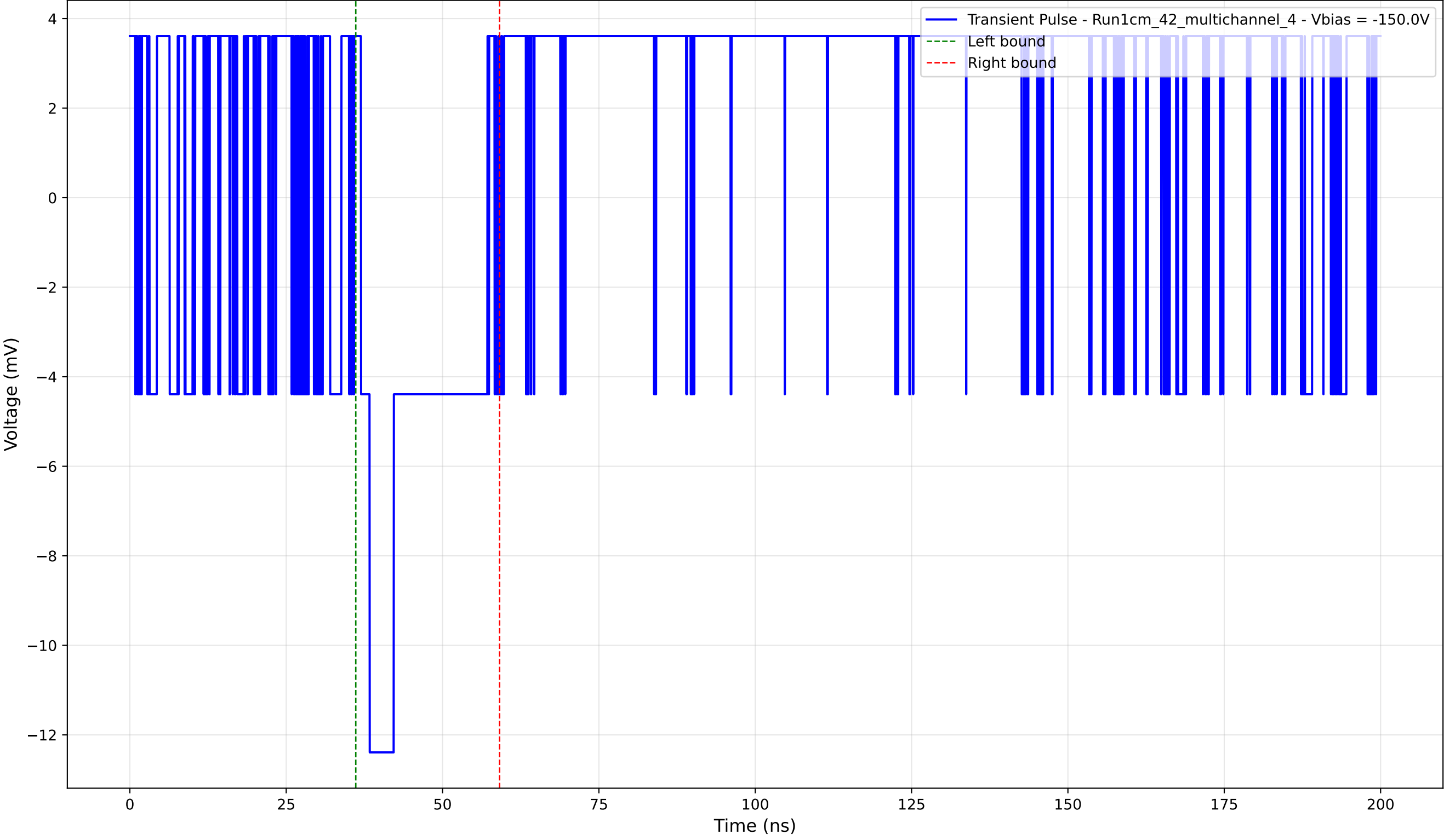
Transient Pulse - Sample: 1cm_42_multichannel - Position: 230.0 \mu\text{m} - Charge: 2.28 pC - Rise Time: 0.00 ns (N/A)
