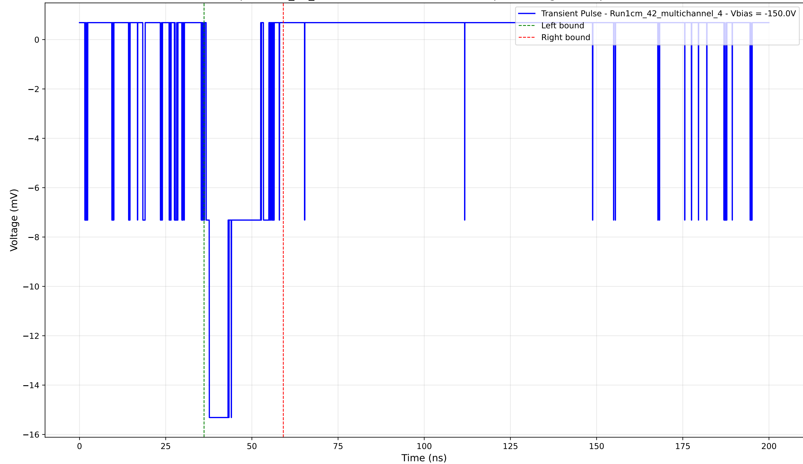
Transient Pulse - Sample: 1cm_42_multichannel - Position: 3765.0 \mu\text{m} - Charge: 3.55 pC - Rise Time: 0.92 ns
