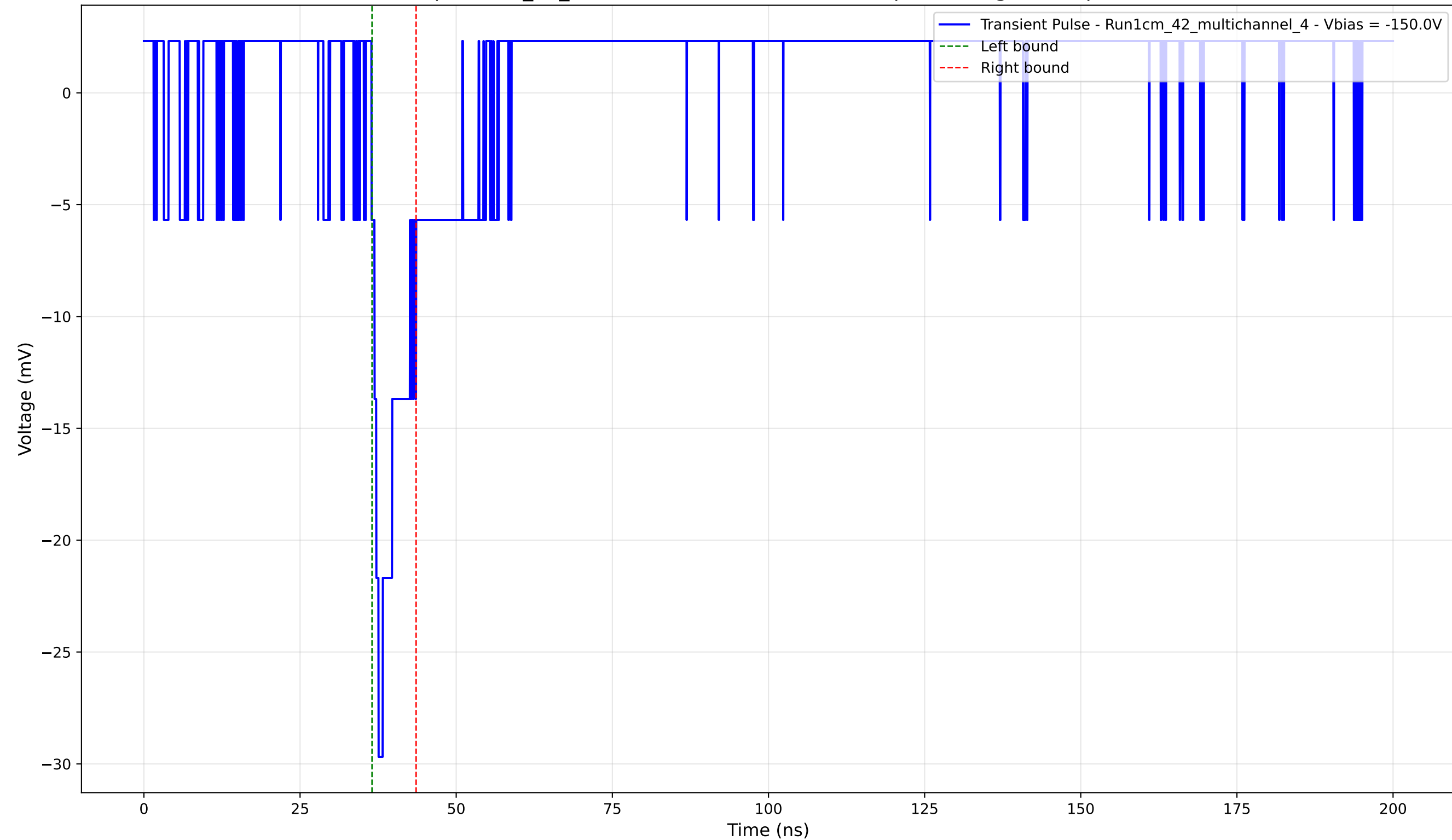
Transient Pulse - Sample: 1cm_42_multichannel - Position: 3225.0 \mu\text{m} - Charge: 2.30 pC - Rise Time: 1.14 ns
