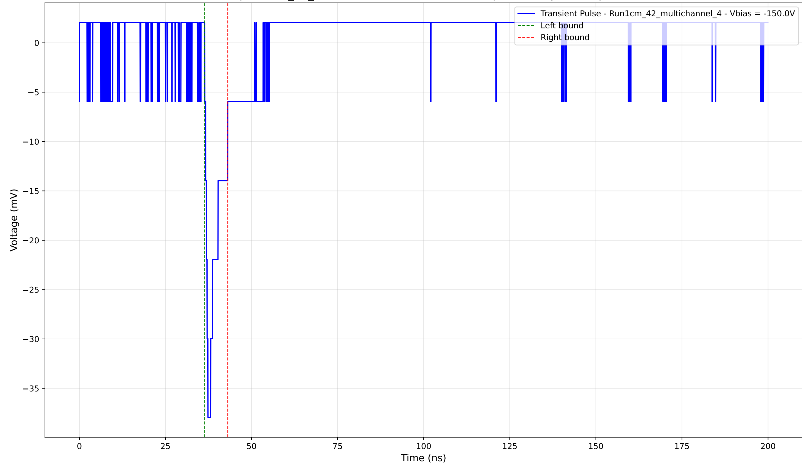
Transient Pulse - Sample: 1cm_42_multichannel - Position: 1735.0 \mu\text{m} - Charge: 2.75 pC - Rise Time: 0.95 ns
