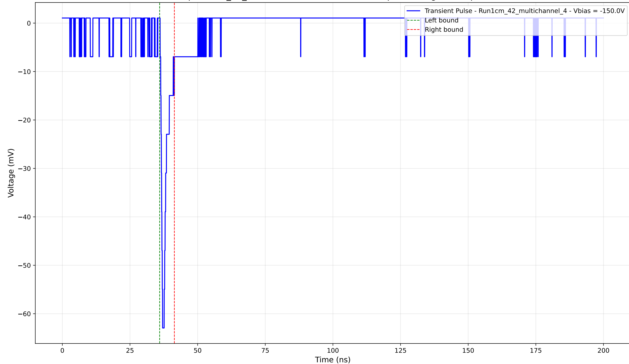
Transient Pulse - Sample: 1cm_42_multichannel - Position: 2590.0 \mu\text{m} - Charge: 2.93 pC - Rise Time: 0.90 ns
