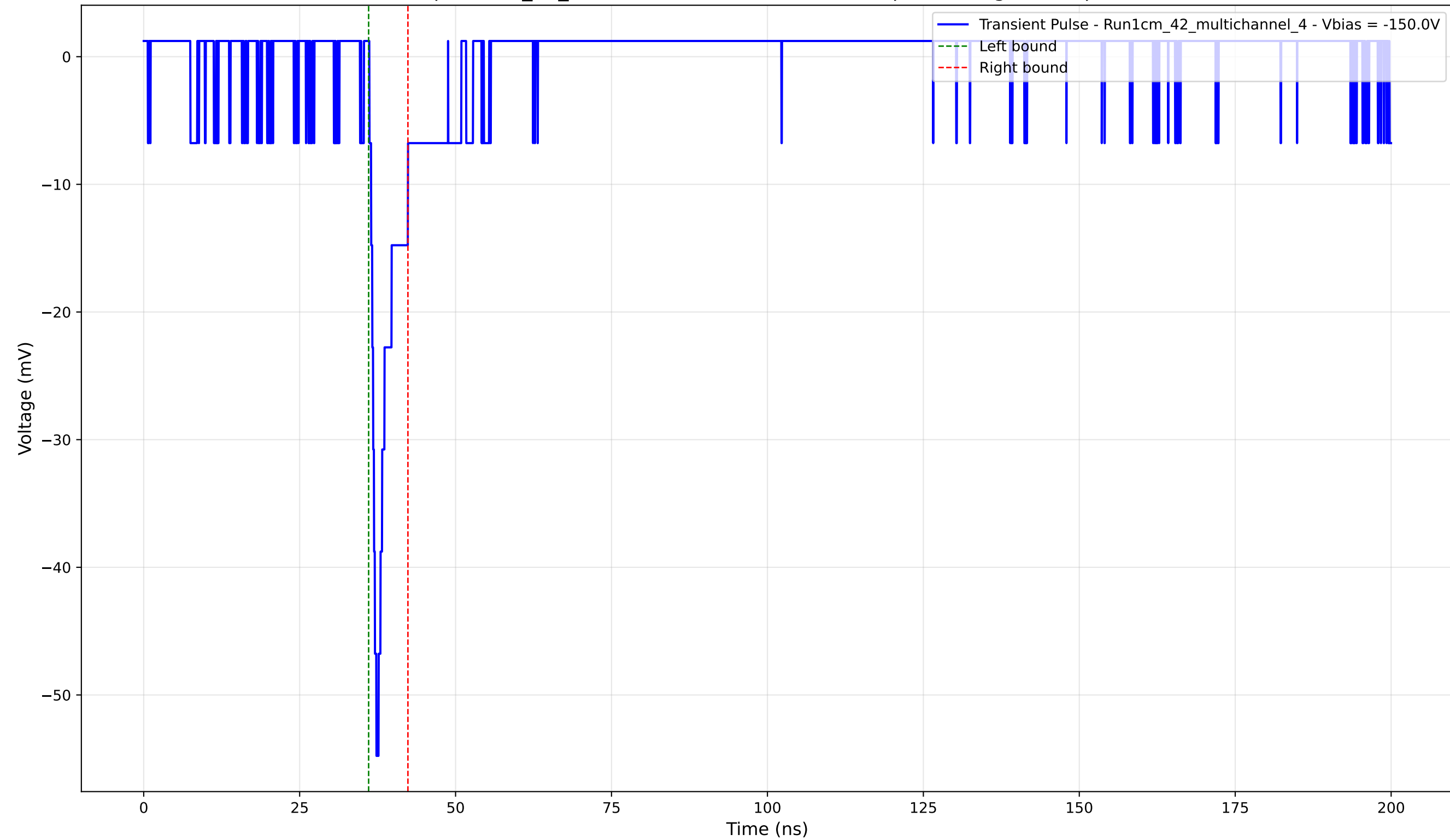
Transient Pulse - Sample: 1cm_42_multichannel - Position: 2765.0 \mu\text{m} - Charge: 2.98 pC - Rise Time: 1.12 ns
