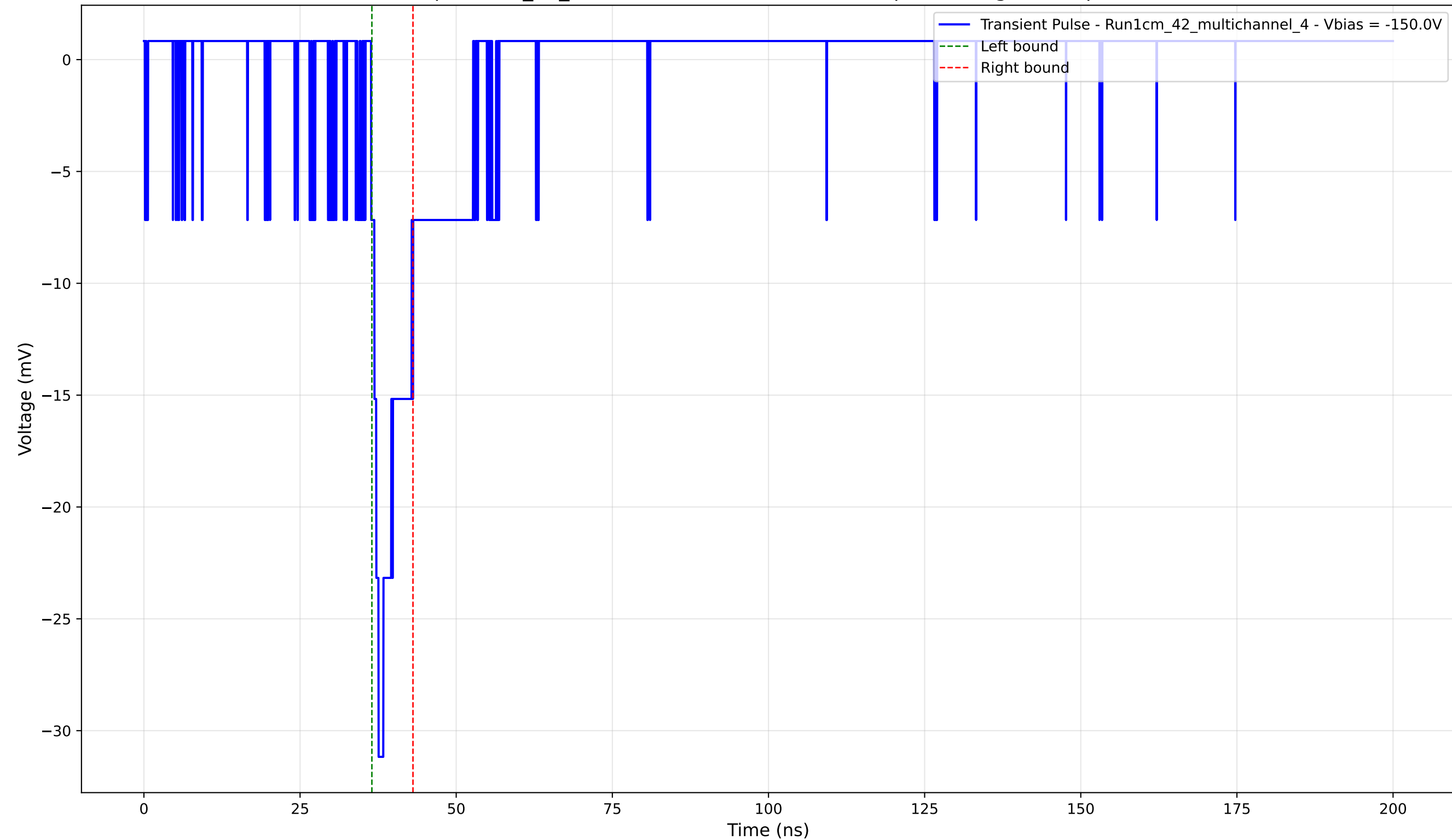
Transient Pulse - Sample: 1cm_42_multichannel - Position: 3220.0 \mu\text{m} - Charge: 2.43 pC - Rise Time: 1.19 ns
