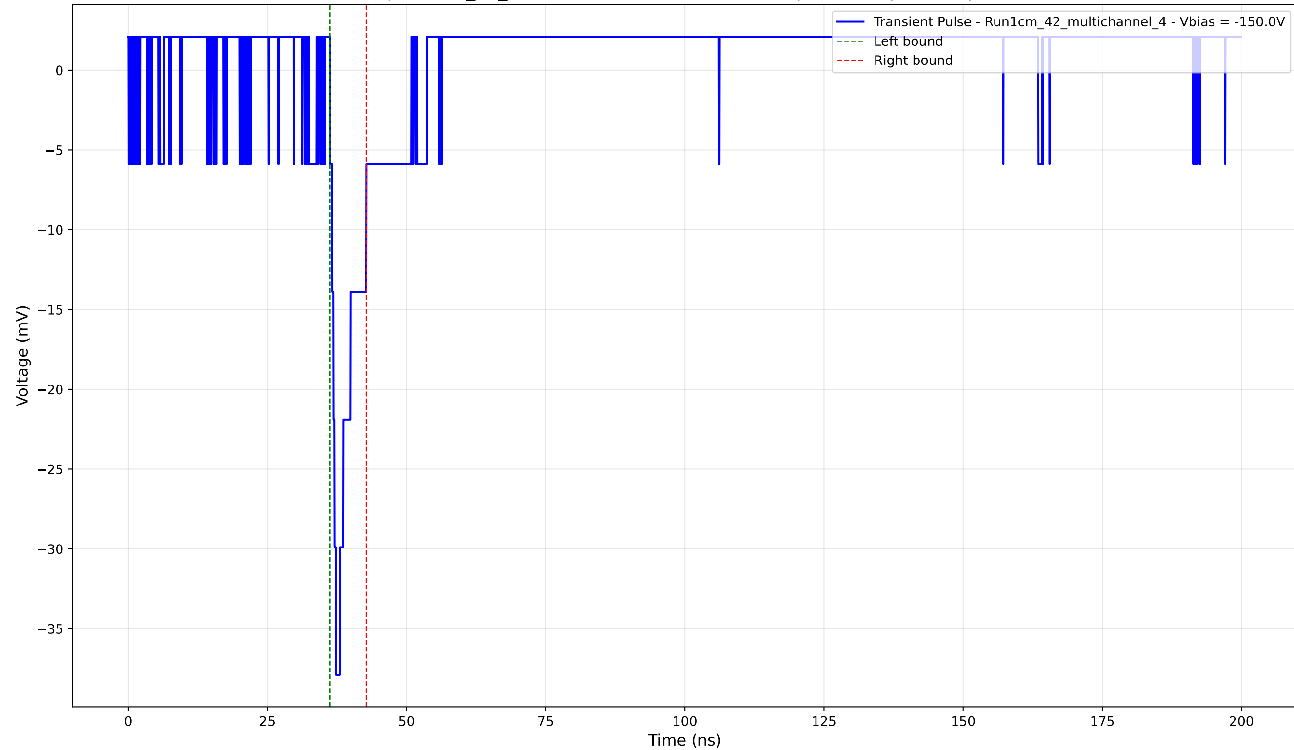
Transient Pulse - Sample: 1cm_42_multichannel - Position: 2980.0 \mu\text{m} - Charge: 2.64 pC - Rise Time: 1.07 ns
