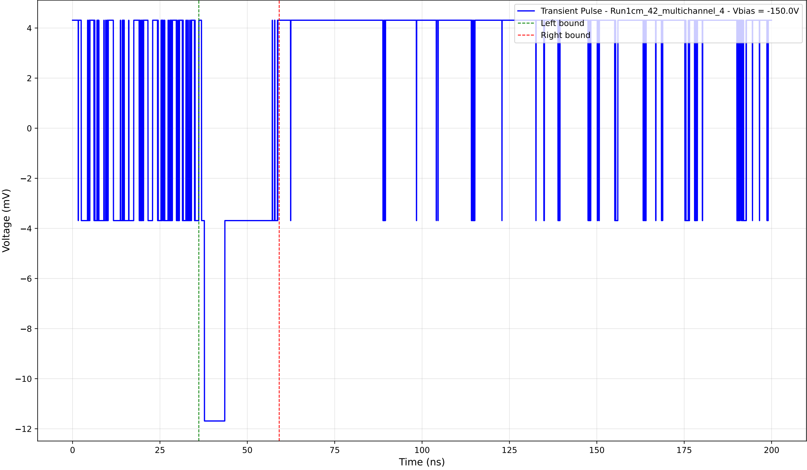
Transient Pulse - Sample: 1cm_42_multichannel - Position: 790.0 \mu\text{m} - Charge: 2.42 pC - Rise Time: 0.00 ns (N/A)
