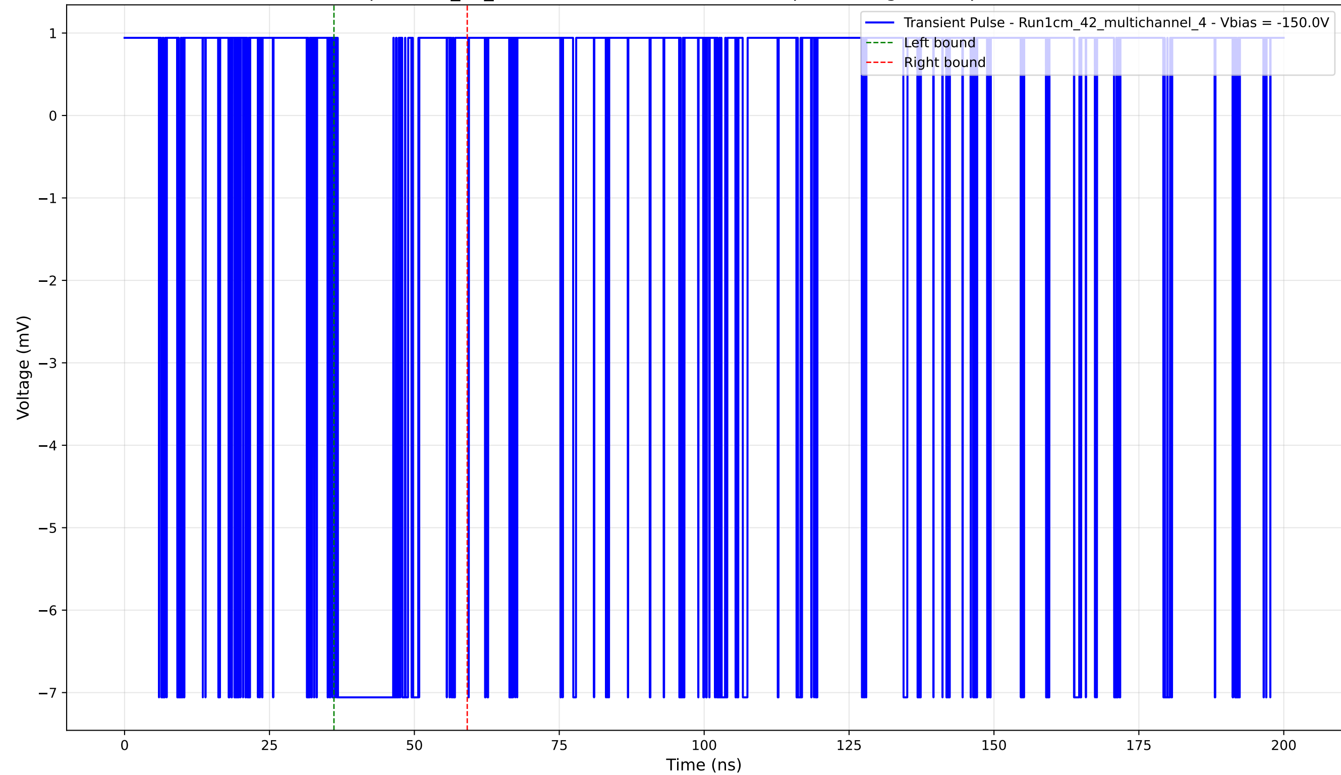
Transient Pulse - Sample: 1cm_42_multichannel - Position: 3435.0 \mu\text{m} - Charge: 1.67 pC - Rise Time: 0.00 ns (N/A)
