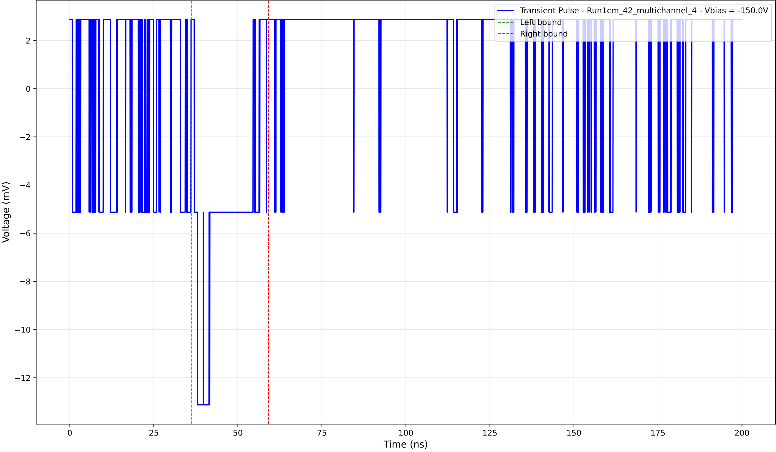
Transient Pulse - Sample: 1cm_42_multichannel - Position: 810.0 \mu\text{m} - Charge: 2.27 pC - Rise Time: 0.00 ns (N/A)
