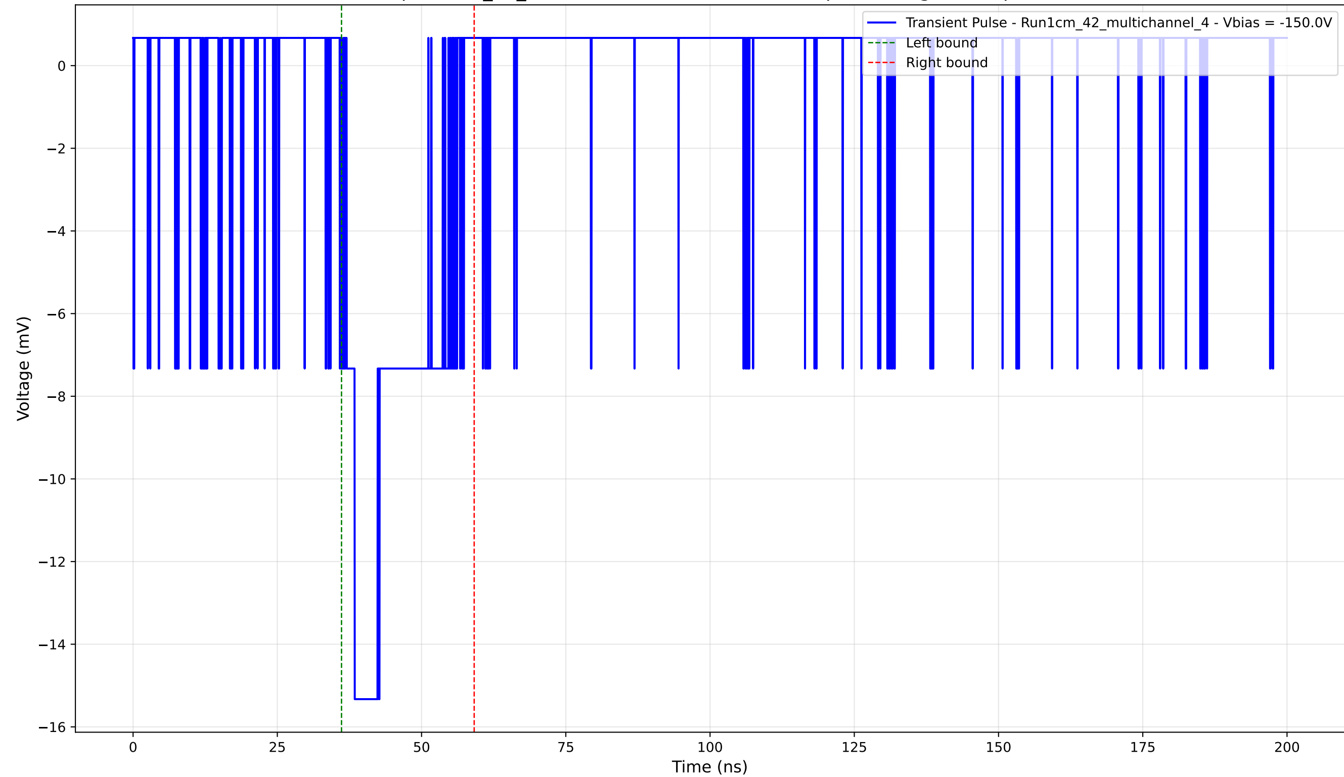
Transient Pulse - Sample: 1cm_42_multichannel - Position: 4605.0 \mu\text{m} - Charge: 3.39 pC - Rise Time: 1.40 ns
