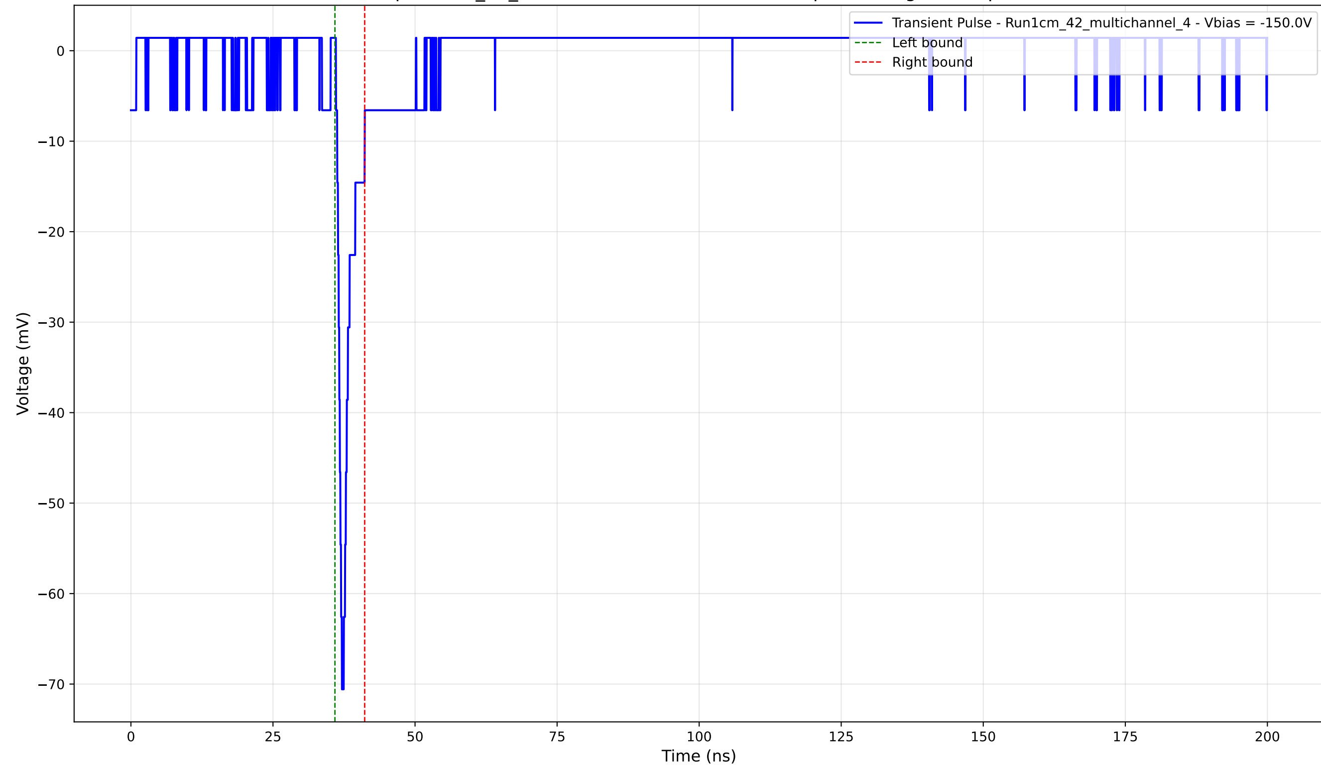
Transient Pulse - Sample: 1cm_42_multichannel - Position: 2555.0 \mu\text{m} - Charge: 2.99 pC - Rise Time: 0.84 ns
