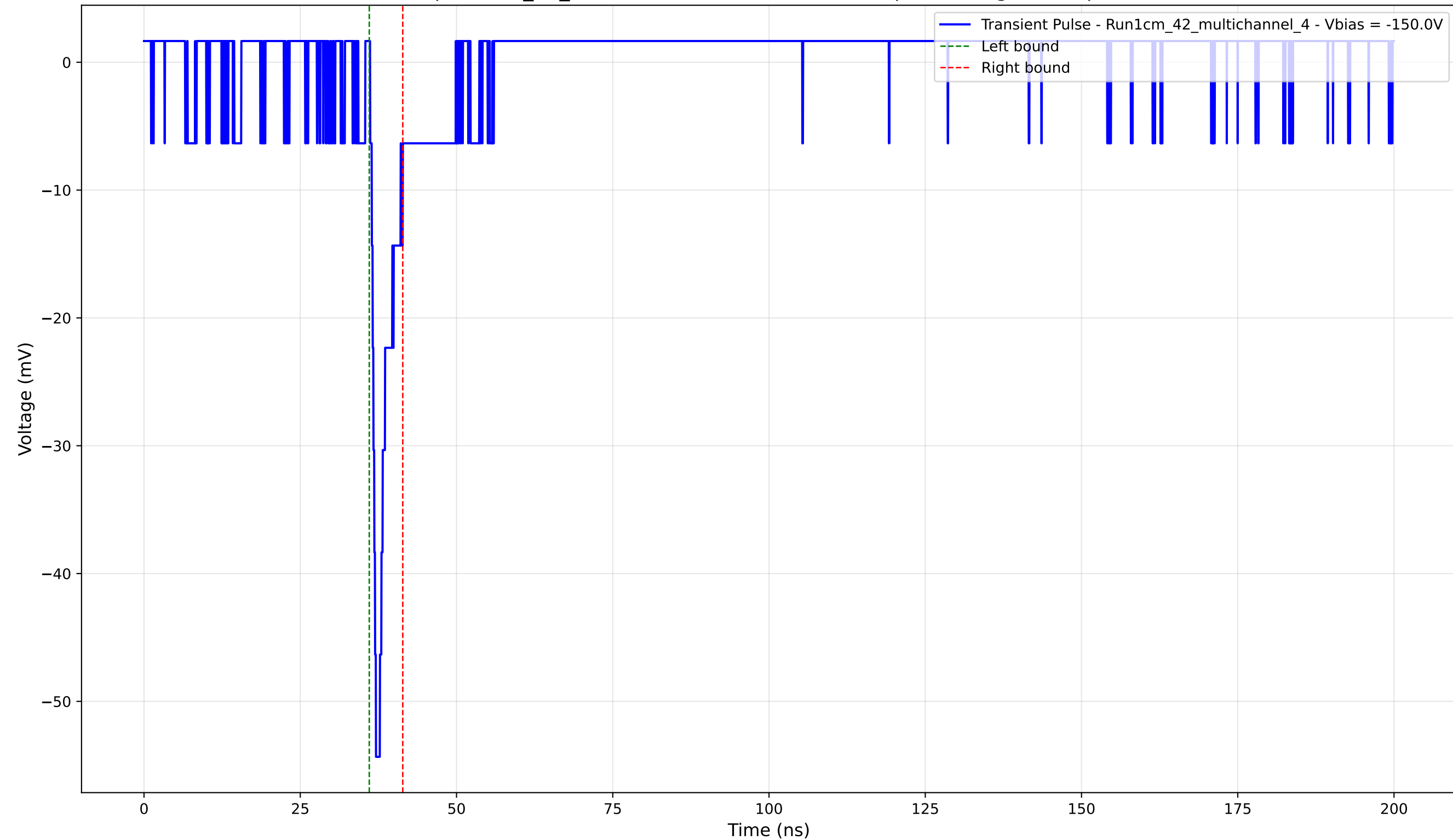
Transient Pulse - Sample: 1cm_42_multichannel - Position: 2705.0 \mu\text{m} - Charge: 2.74 pC - Rise Time: 0.92 ns
