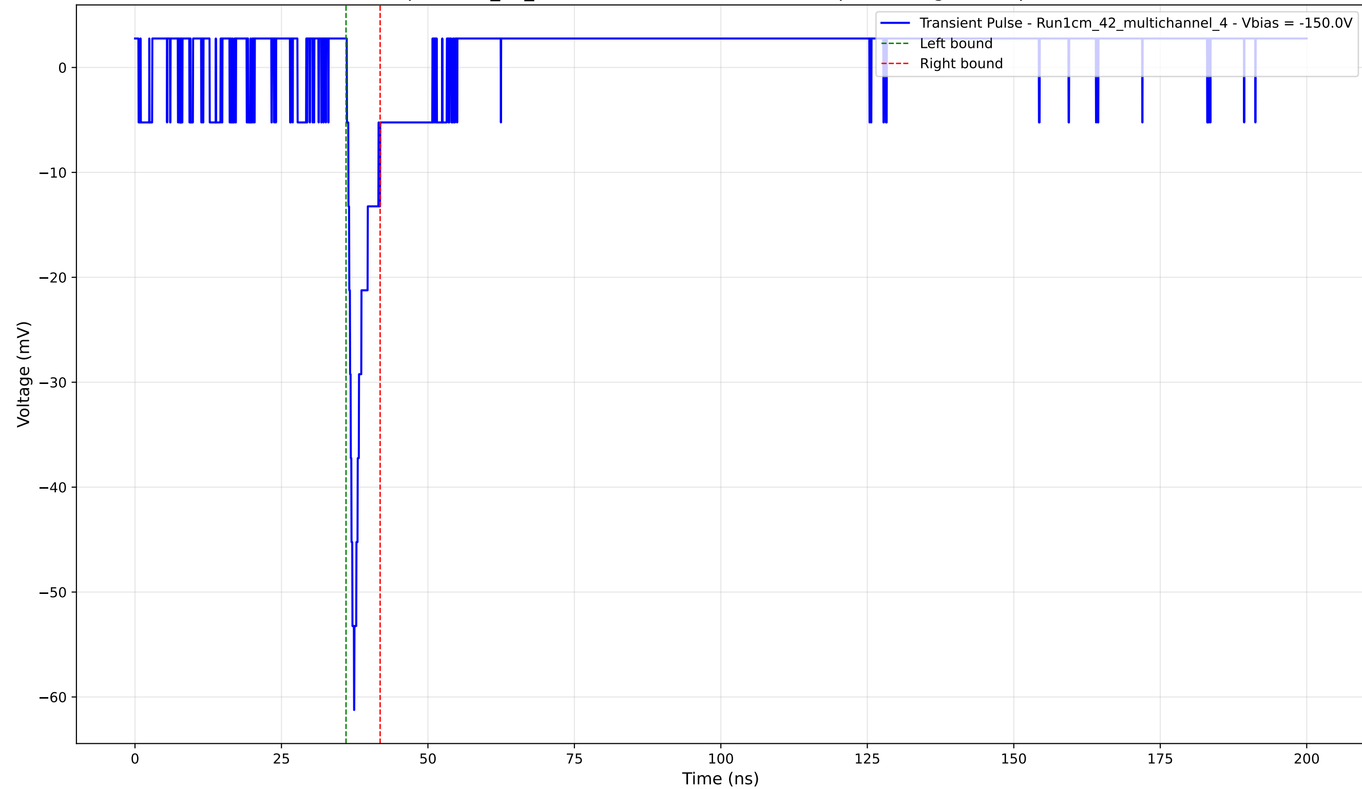
Transient Pulse - Sample: 1cm_42_multichannel - Position: 2065.0 \mu\text{m} - Charge: 2.77 pC - Rise Time: 0.98 ns
