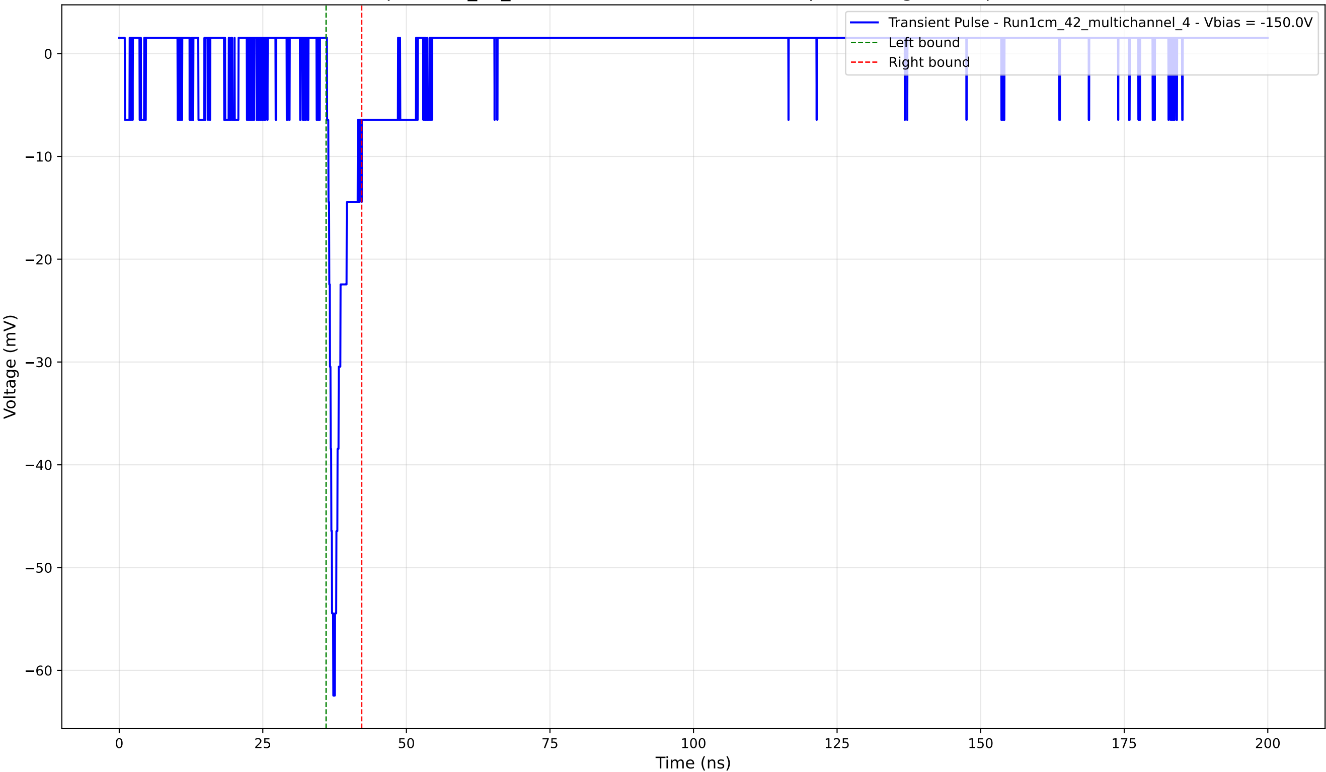
Transient Pulse - Sample: 1cm_42_multichannel - Position: 2675.0 \mu\text{m} - Charge: 2.98 pC - Rise Time: 1.08 ns
