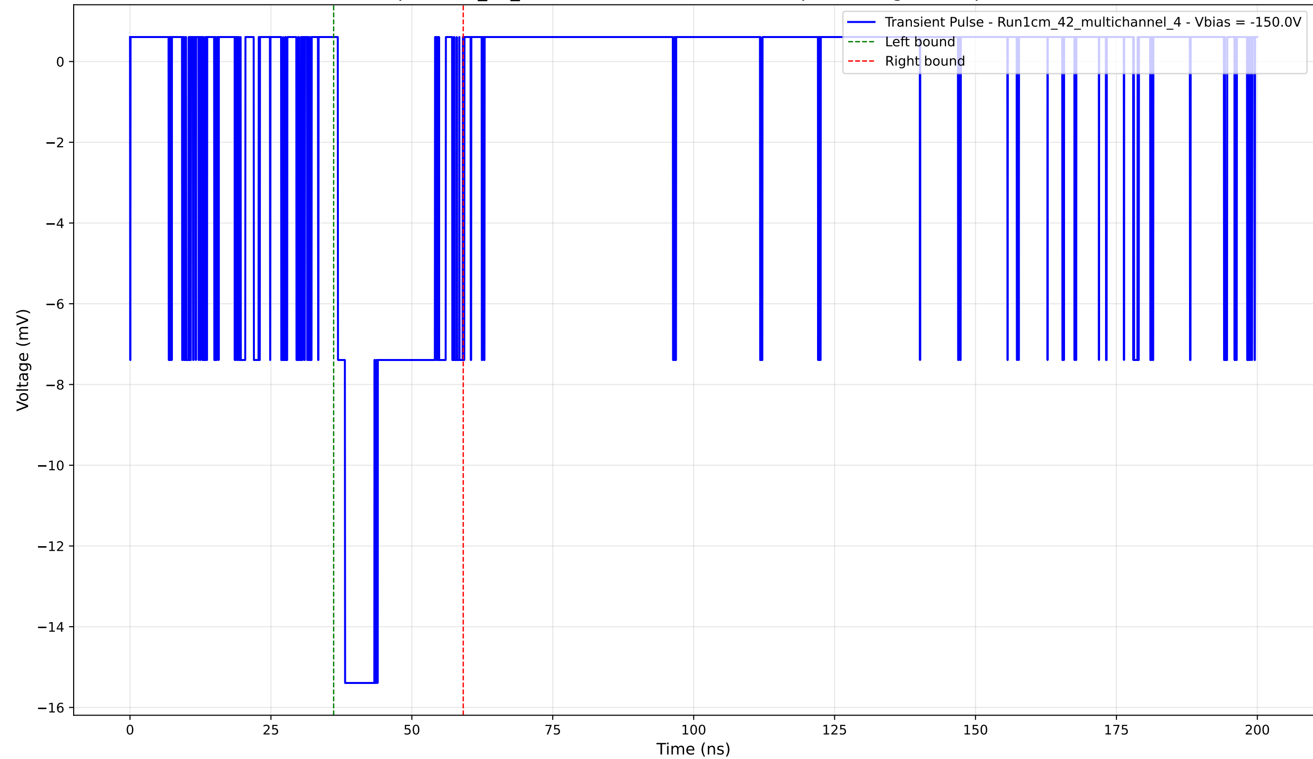
Transient Pulse - Sample: 1cm_42_multichannel - Position: 455.0 \mu\text{m} - Charge: 3.87 pC - Rise Time: 1.28 ns
