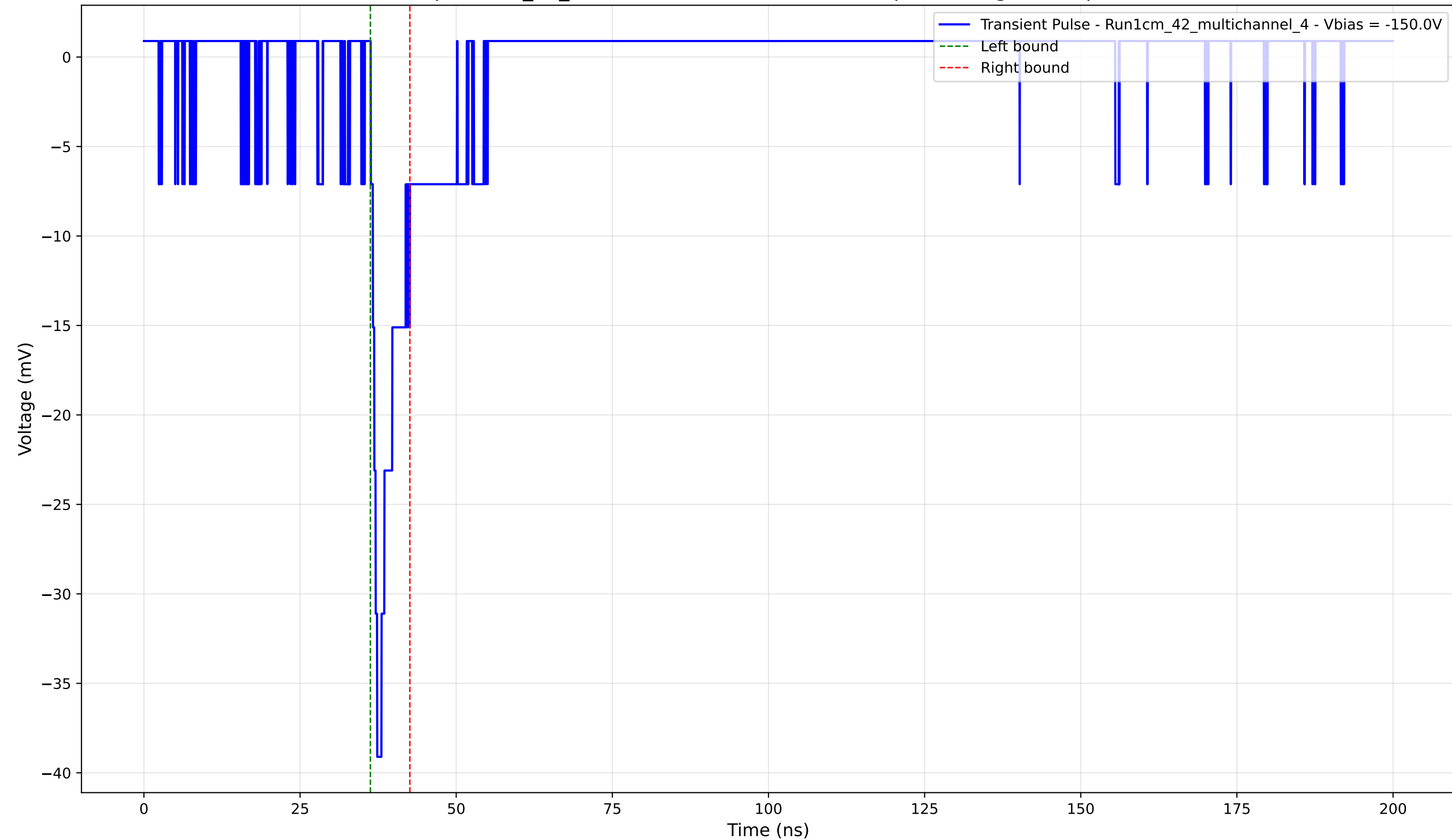
Transient Pulse - Sample: 1cm_42_multichannel - Position: 3010.0 \mu\text{m} - Charge: 2.58 pC - Rise Time: 1.03 ns
