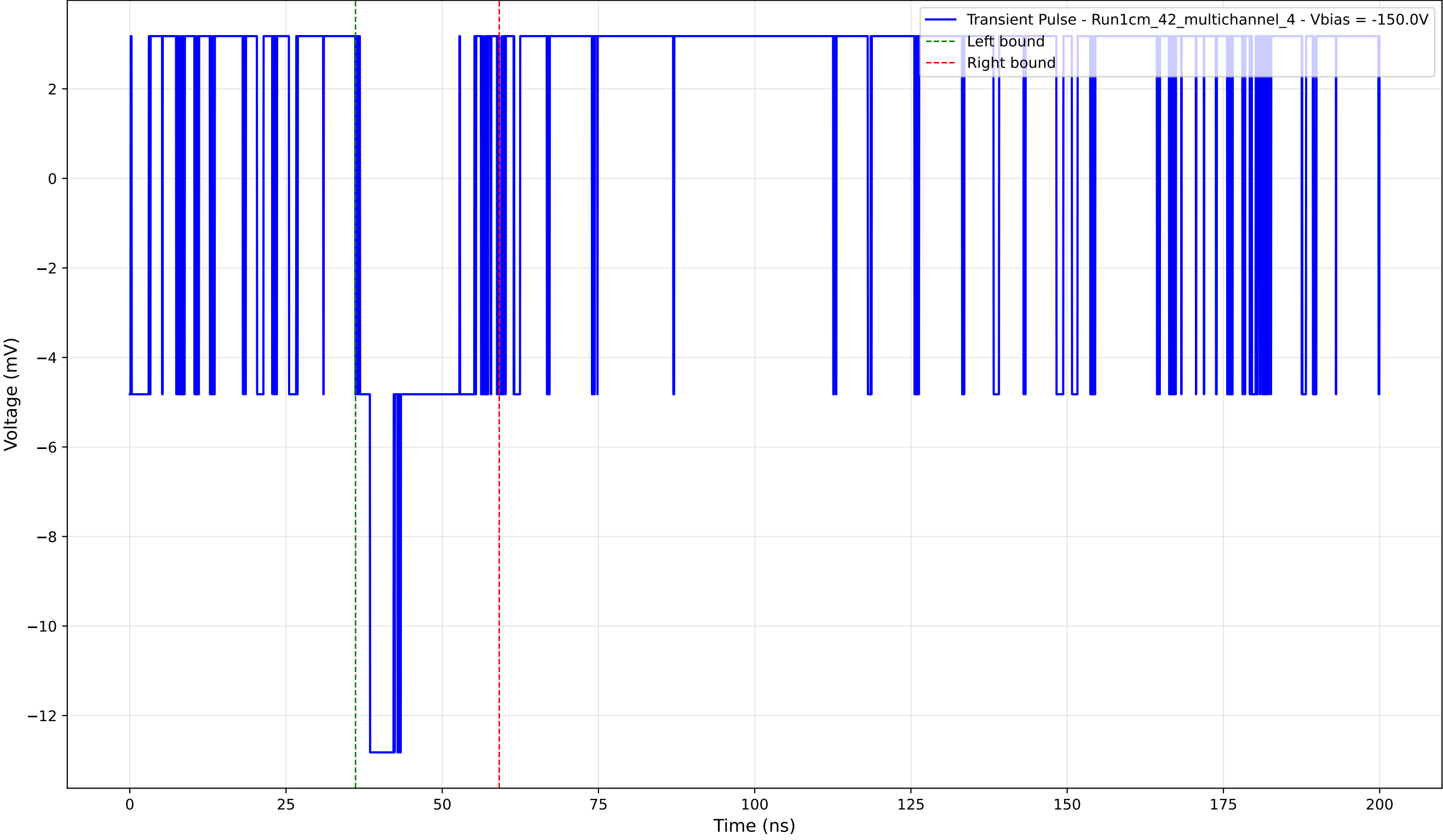
Transient Pulse - Sample: 1cm_42_multichannel - Position: 155.0 \mu\text{m} - Charge: 2.36 pC - Rise Time: 0.00 ns (N/A)
