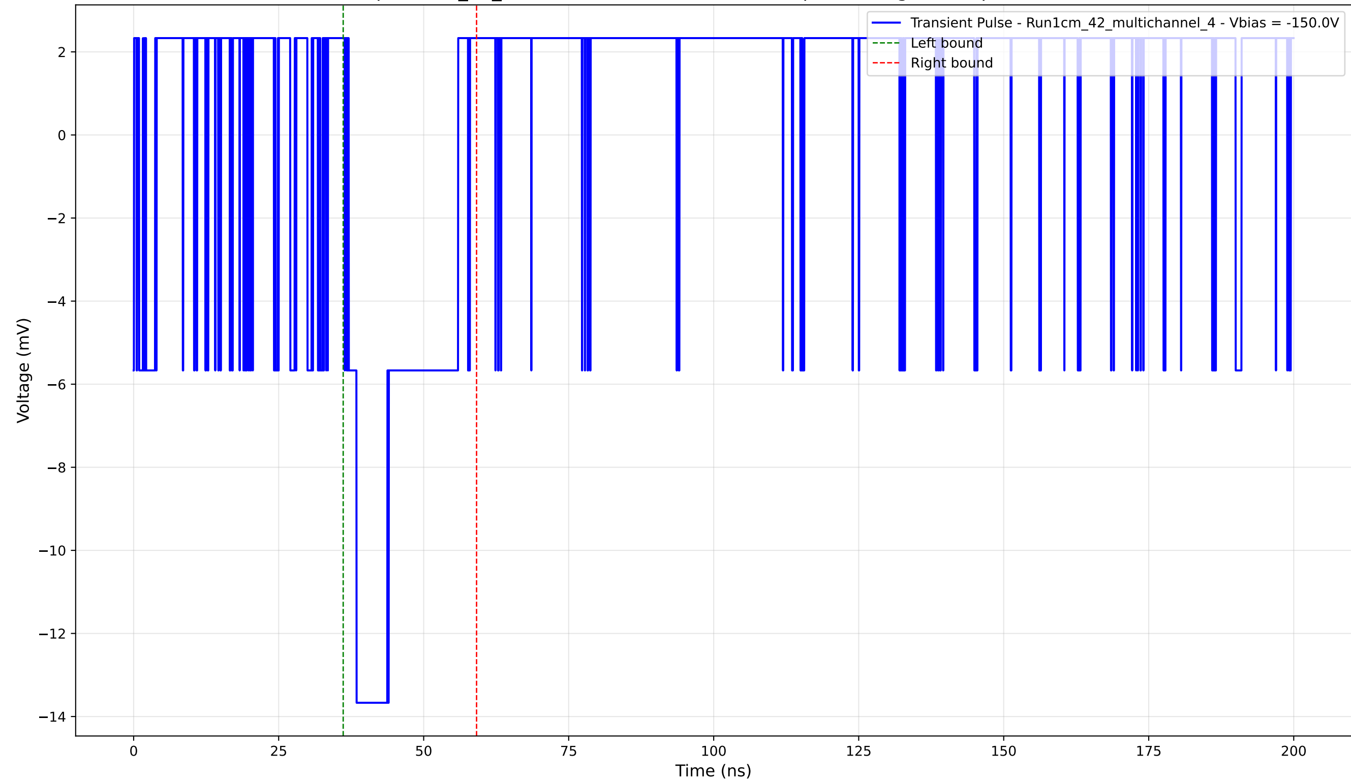
Transient Pulse - Sample: 1cm_42_multichannel - Position: 4495.0 \mu\text{m} - Charge: 2.86 pC - Rise Time: 0.00 ns (N/A)
