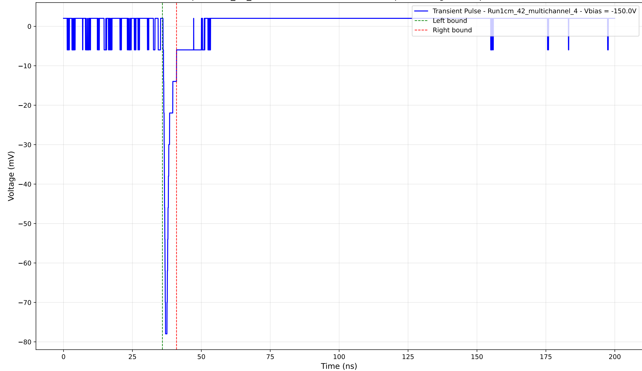
Transient Pulse - Sample: 1cm_42_multichannel - Position: 2490.0 \mu\text{m} - Charge: 3.20 pC - Rise Time: 0.74 ns
