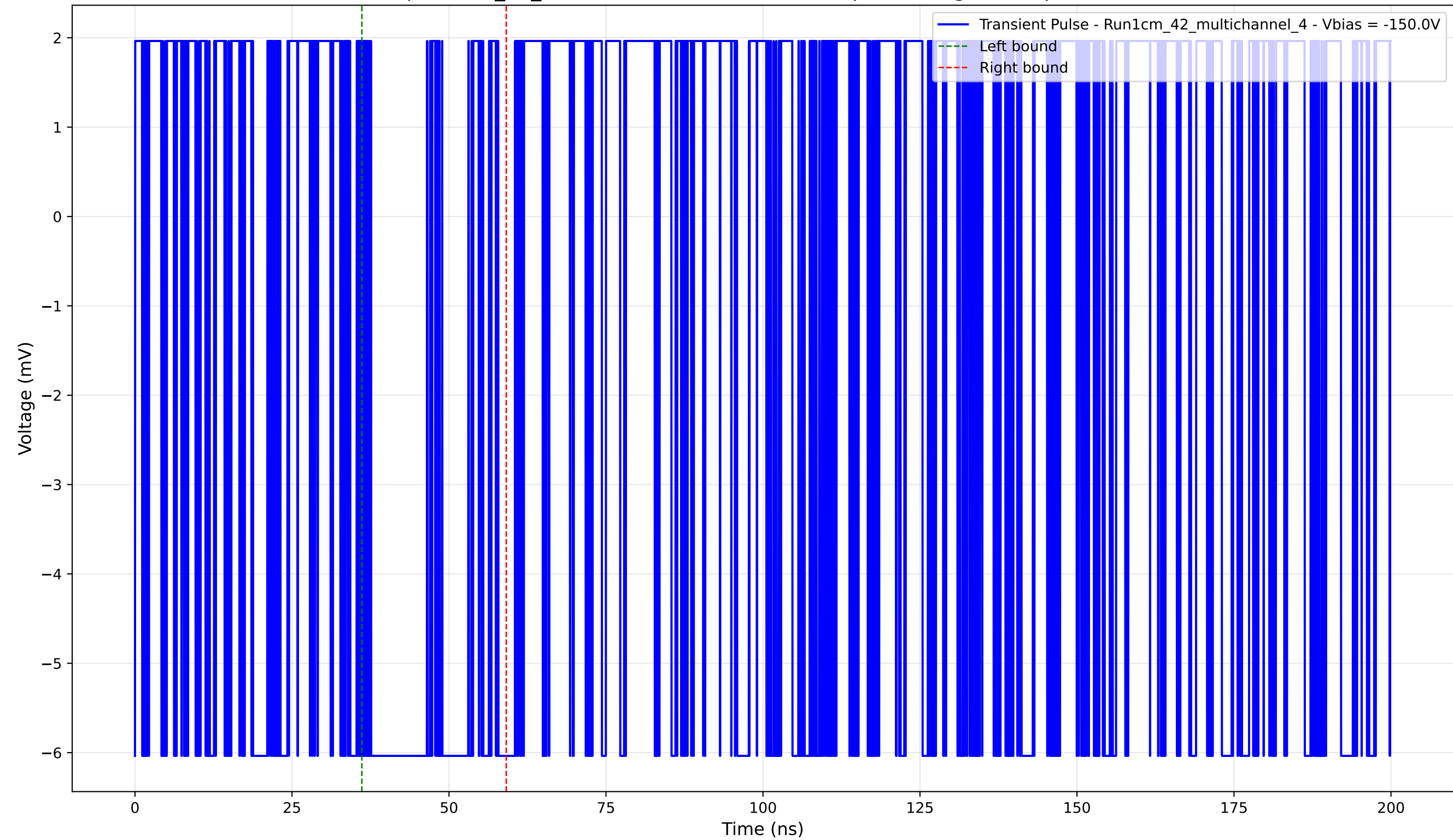
Transient Pulse - Sample: 1cm_42_multichannel - Position: 835.0 \mu\text{m} - Charge: 2.08 pC - Rise Time: 0.00 ns (N/A)
