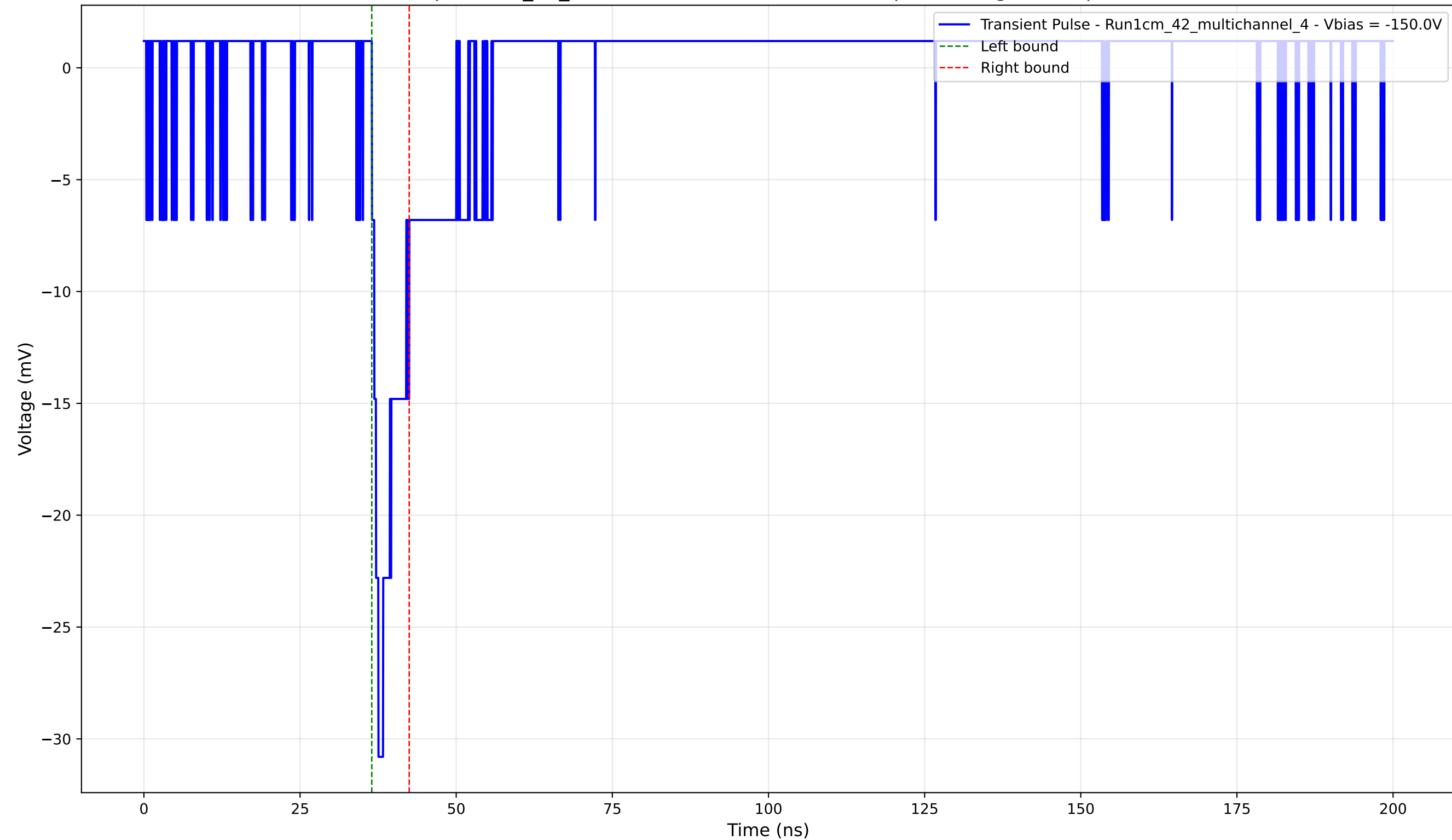
Transient Pulse - Sample: 1cm_42_multichannel - Position: 3185.0 \mu\text{m} - Charge: 2.16 pC - Rise Time: 1.05 ns
