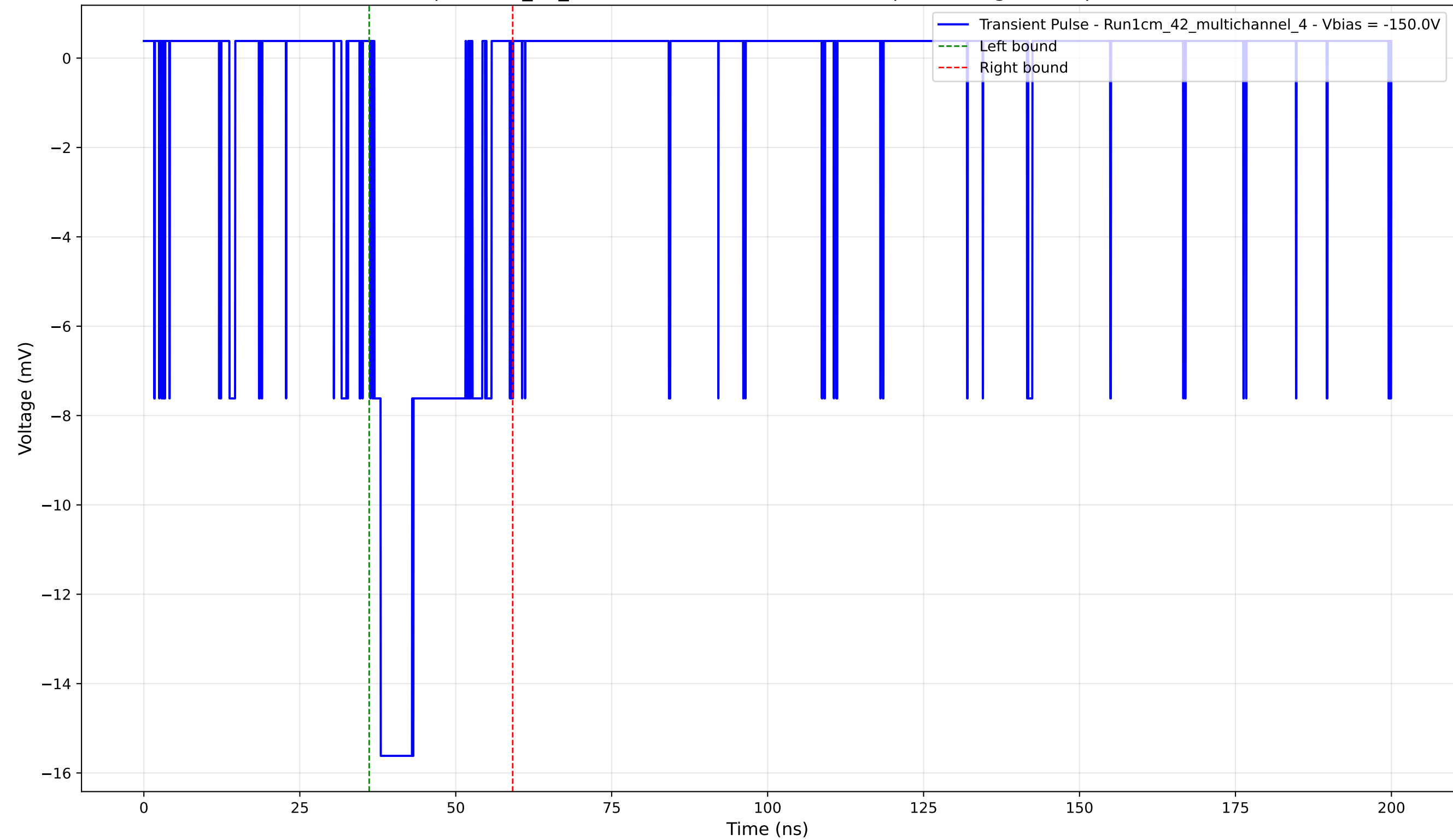
Transient Pulse - Sample: 1cm_42_multichannel - Position: 3980.0 \mu\text{m} - Charge: 3.53 pC - Rise Time: 1.02 ns
