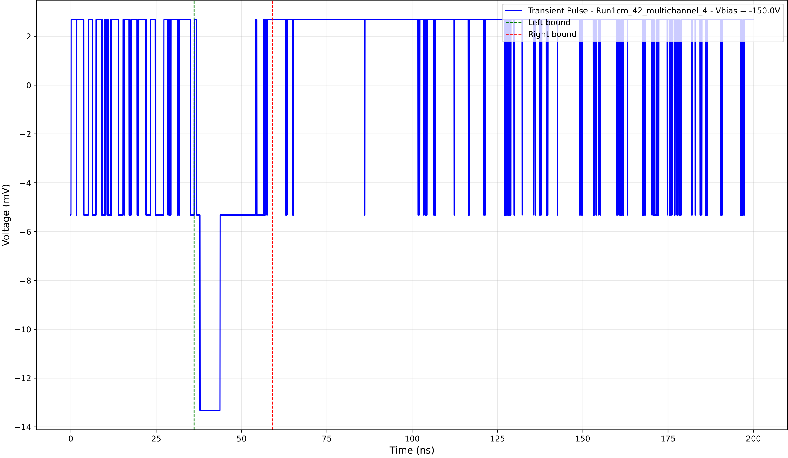
Transient Pulse - Sample: 1cm_42_multichannel - Position: 705.0 \mu\text{m} - Charge: 2.87 pC - Rise Time: 0.00 ns (N/A)
