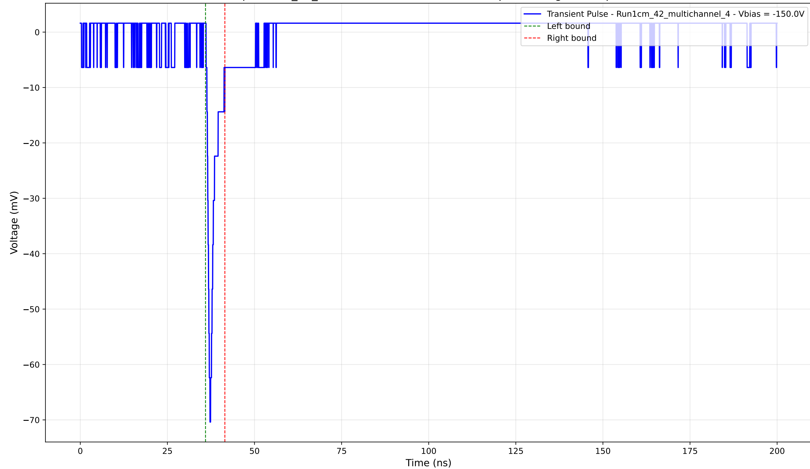
Transient Pulse - Sample: 1cm_42_multichannel - Position: 2575.0 \mu\text{m} - Charge: 3.01 pC - Rise Time: 0.90 ns
