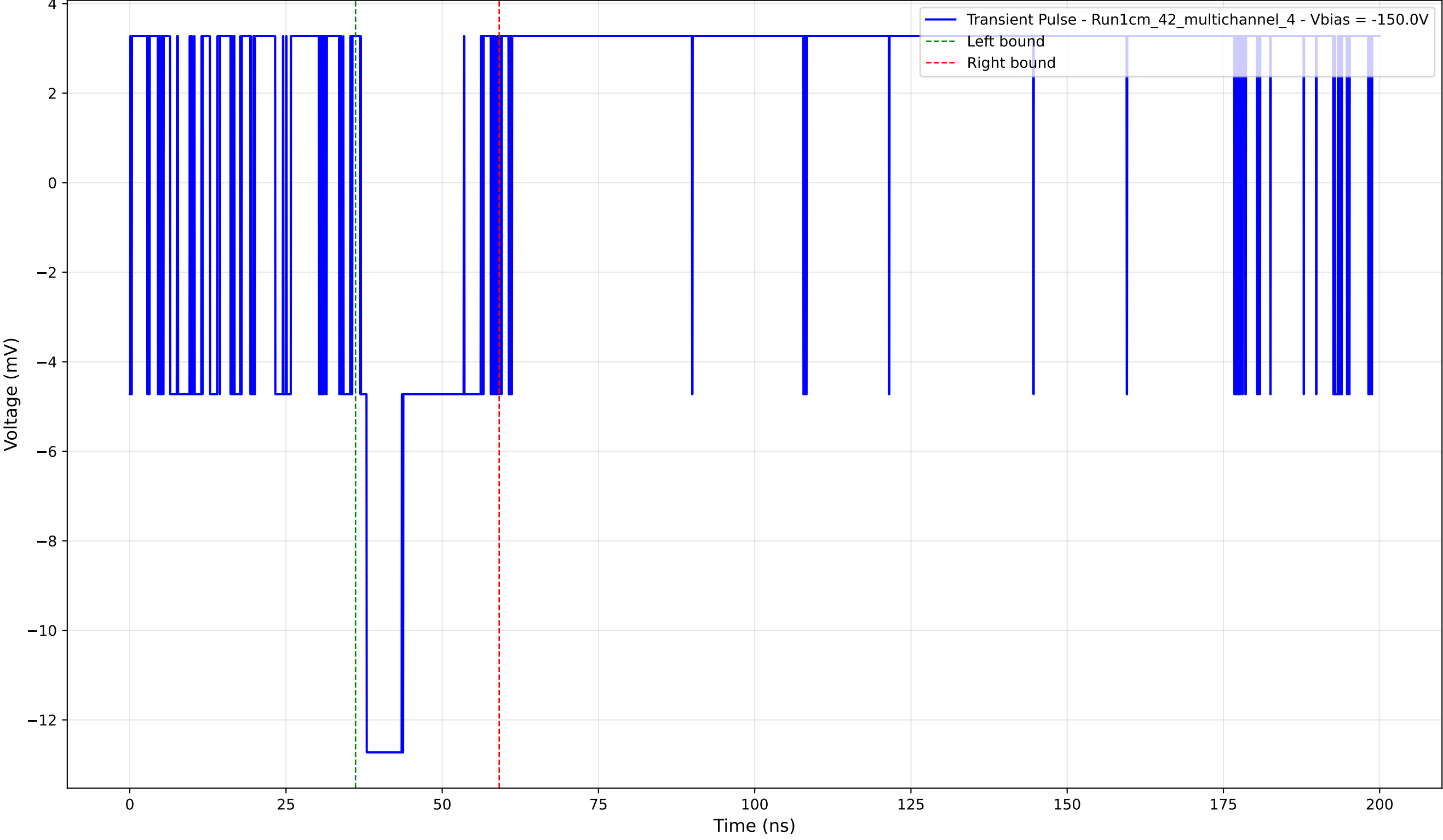
Transient Pulse - Sample: 1cm_42_multichannel - Position: 655.0 \mu\text{m} - Charge: 2.59 pC - Rise Time: 0.00 ns (N/A)
