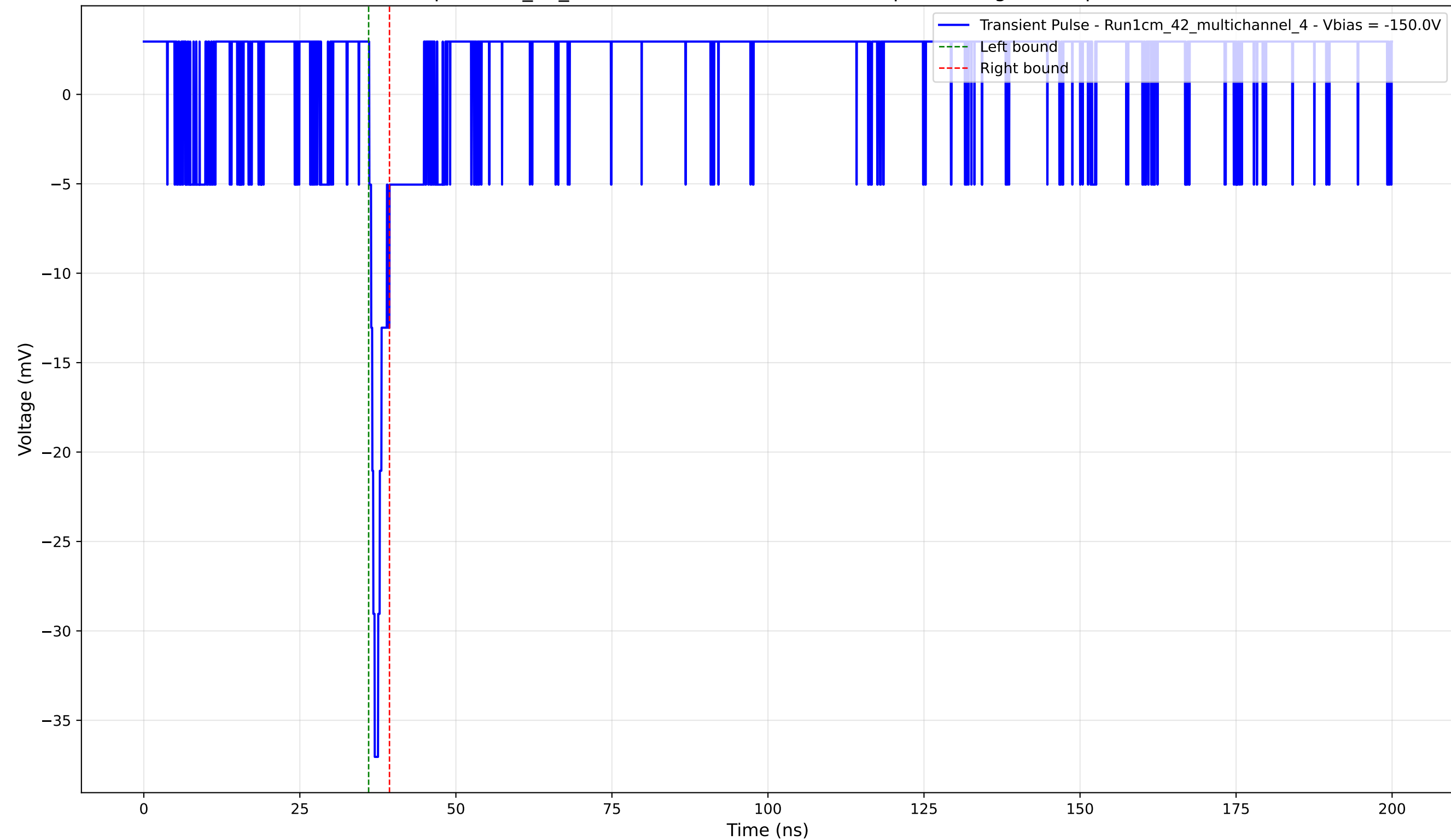
Transient Pulse - Sample: 1cm_42_multichannel - Position: 2435.0 \mu\text{m} - Charge: 1.27 pC - Rise Time: 0.87 ns
