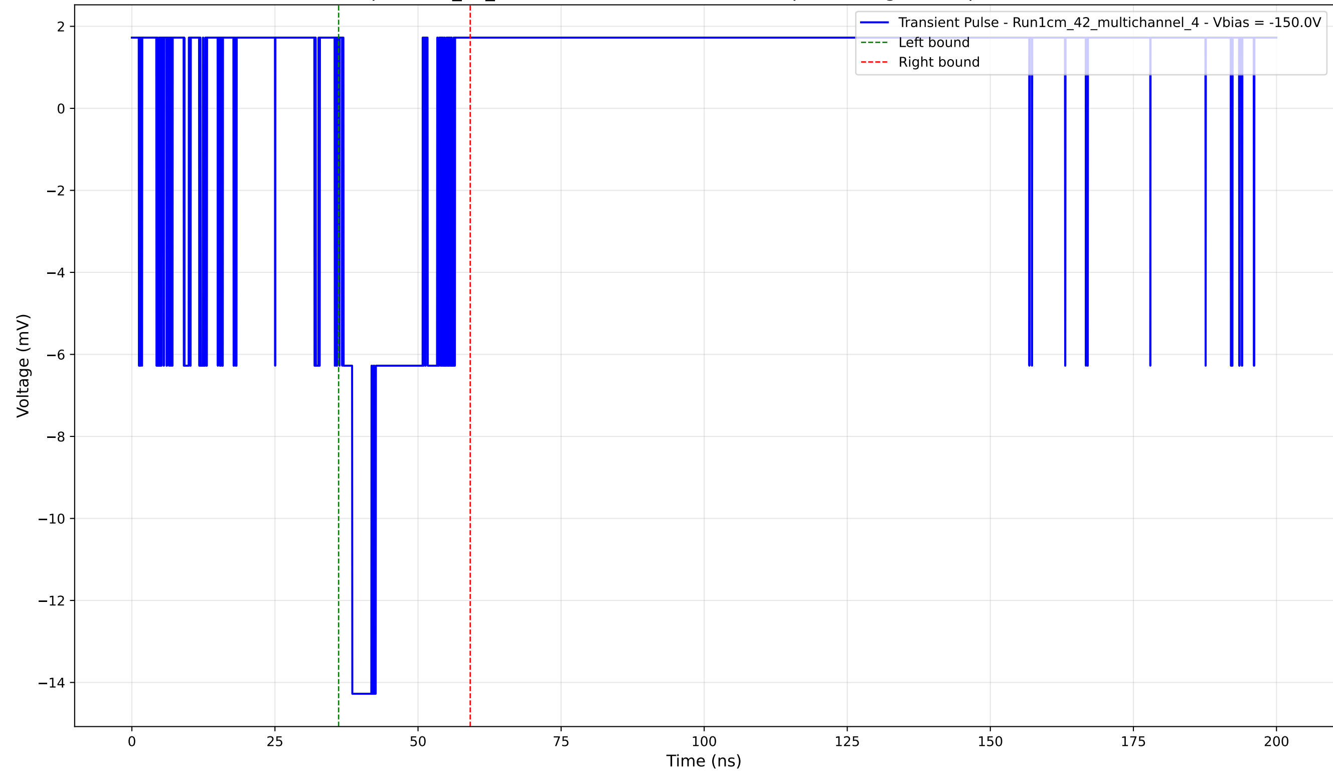
Transient Pulse - Sample: 1cm_42_multichannel - Position: 4175.0 \mu\text{m} - Charge: 2.60 pC - Rise Time: 0.00 ns (N/A)
