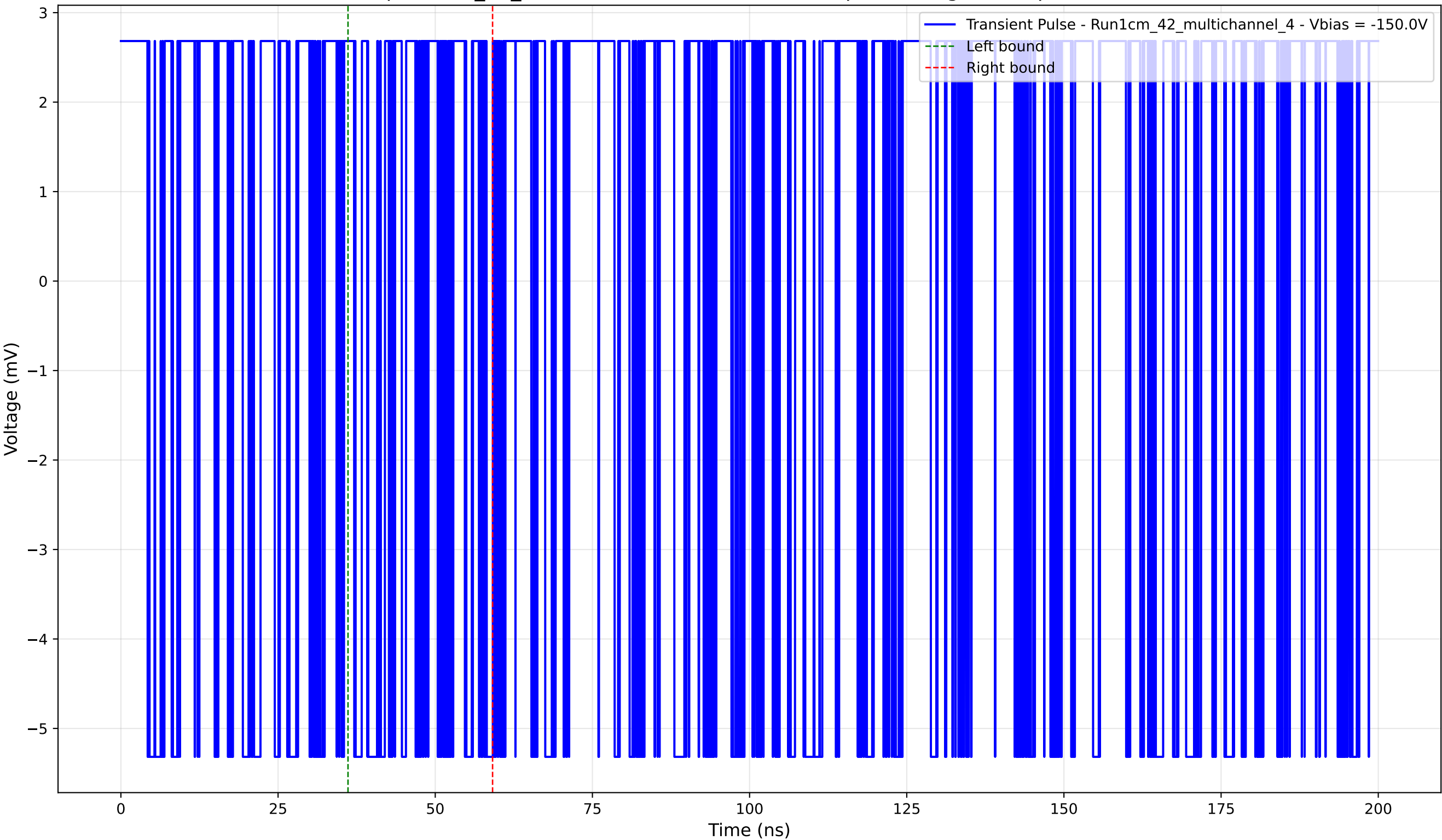
Transient Pulse - Sample: 1cm_42_multichannel - Position: 1375.0 \mu\text{m} - Charge: 0.25 pC - Rise Time: 0.00 ns (N/A)
