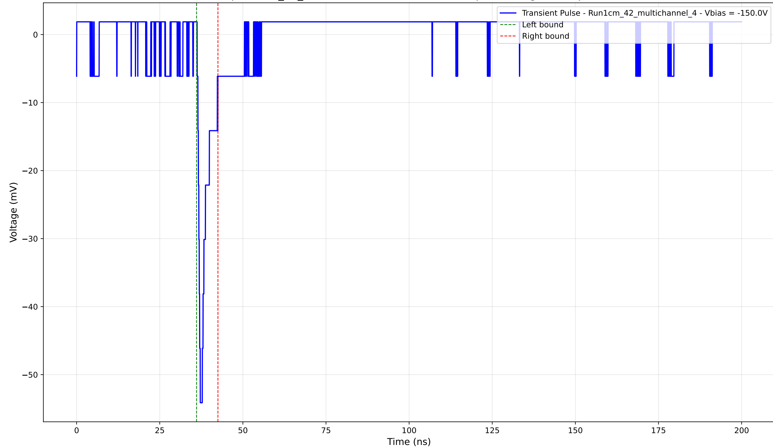
Transient Pulse - Sample: 1cm_42_multichannel - Position: 2005.0 \mu\text{m} - Charge: 3.05 pC - Rise Time: 0.94 ns
