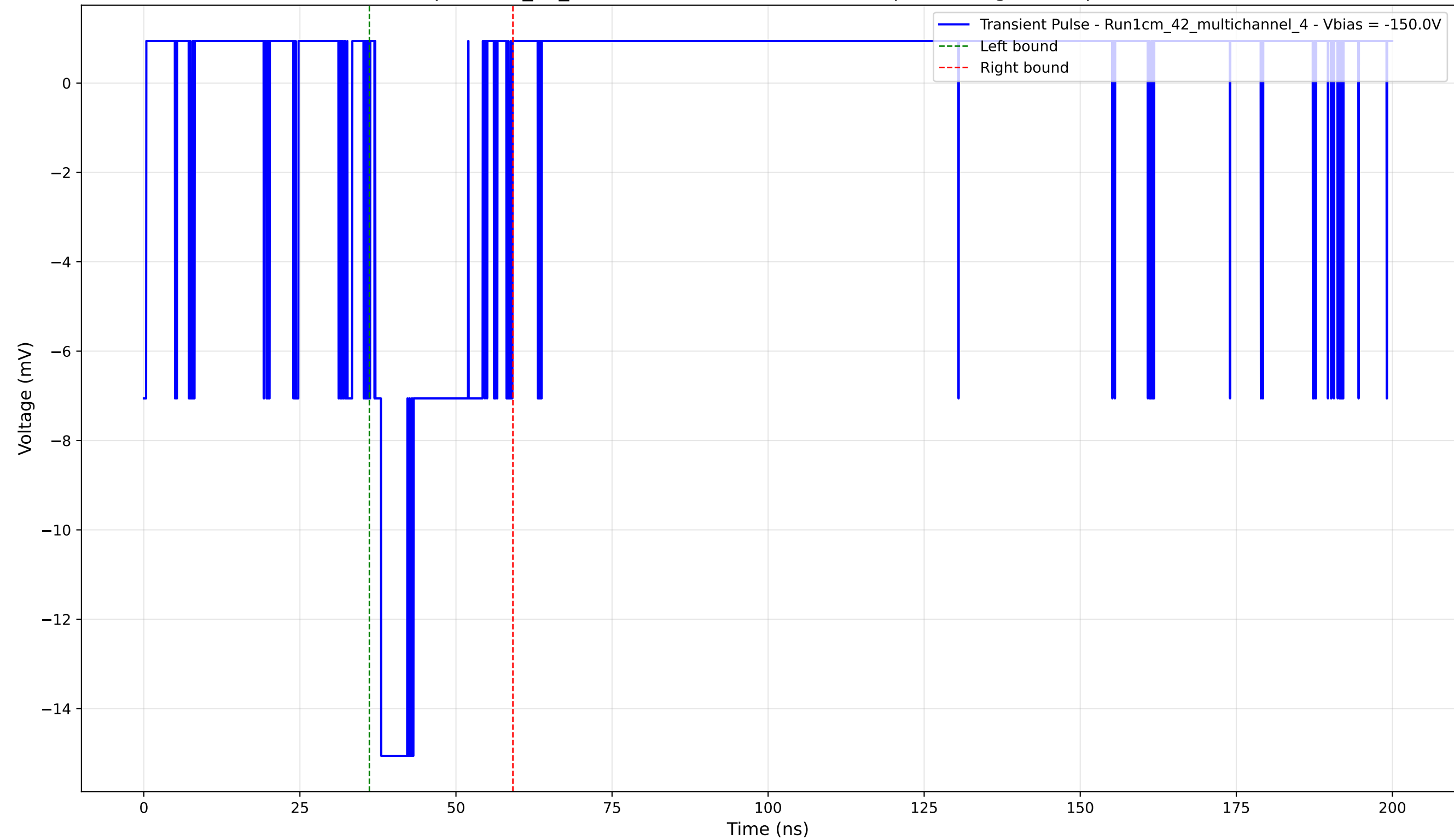
Transient Pulse - Sample: 1cm_42_multichannel - Position: 4085.0 \mu\text{m} - Charge: 3.29 pC - Rise Time: 0.94 ns
