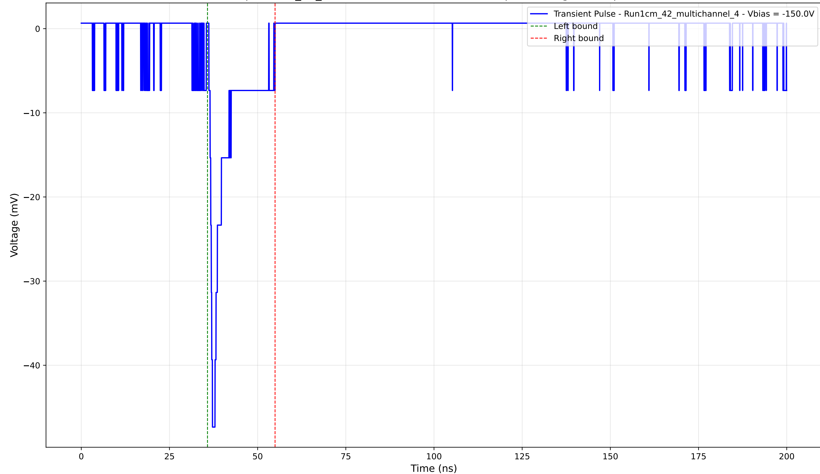
Transient Pulse - Sample: 1cm_42_multichannel - Position: 2795.0 \mu\text{m} - Charge: 4.67 pC - Rise Time: 1.01 ns
