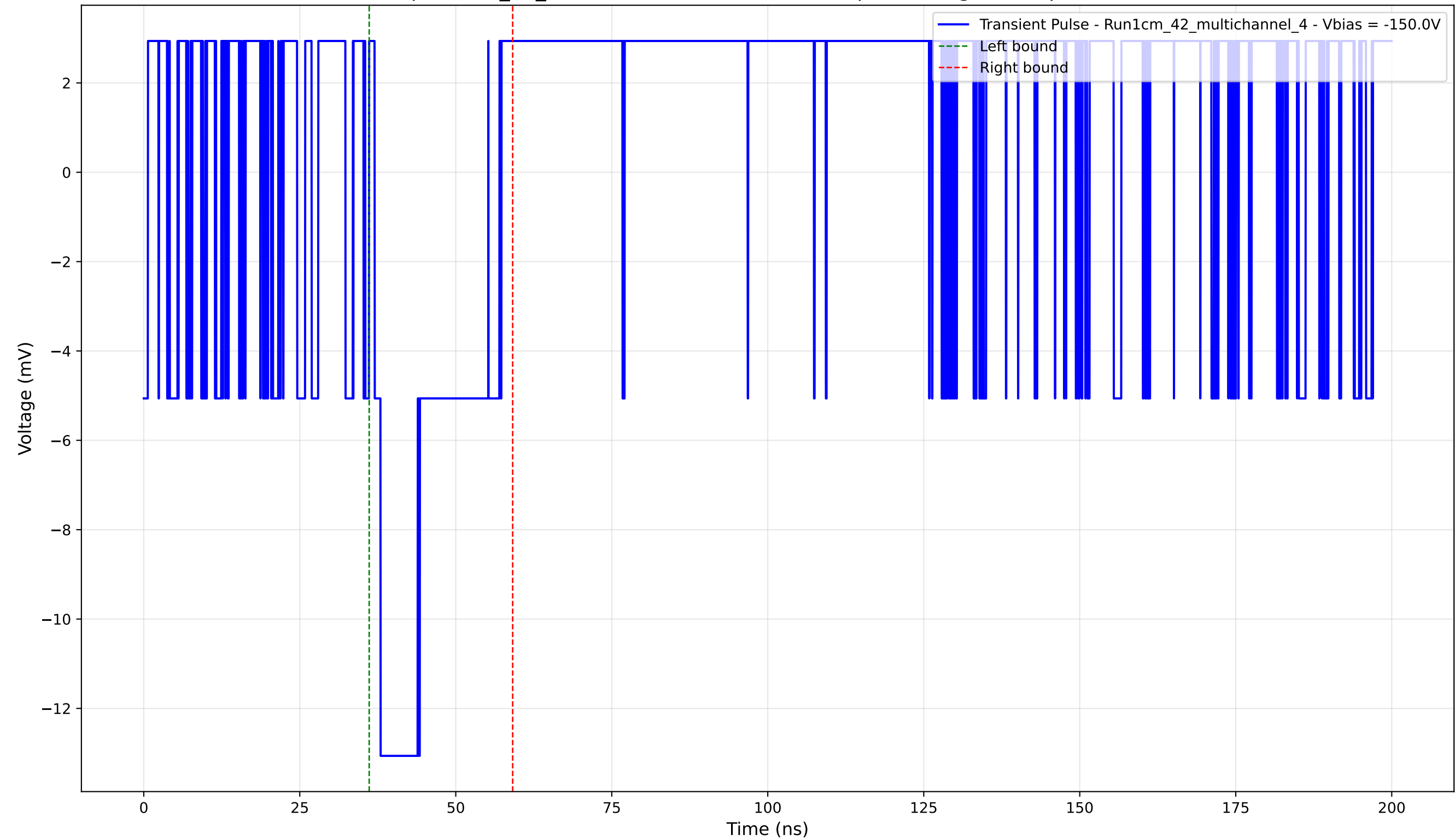
Transient Pulse - Sample: 1cm_42_multichannel - Position: 525.0 \mu\text{m} - Charge: 2.84 pC - Rise Time: 0.00 ns (N/A)
