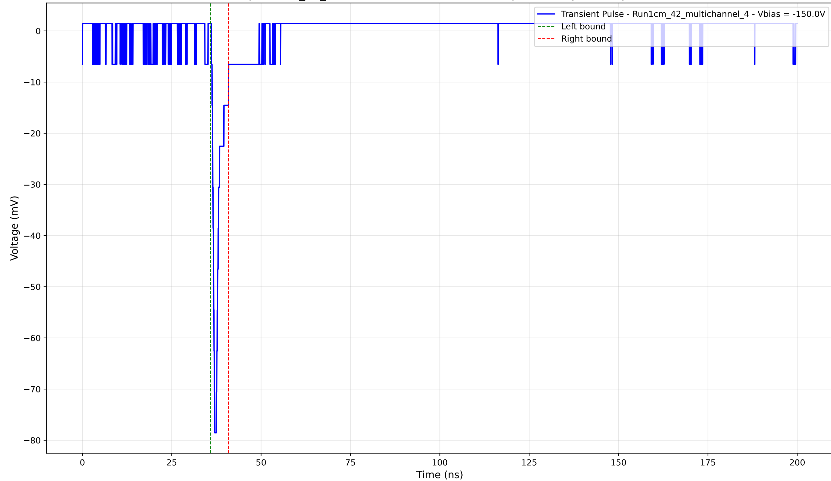
Transient Pulse - Sample: 1cm_42_multichannel - Position: 2470.0 \mu\text{m} - Charge: 3.17 pC - Rise Time: 0.76 ns
