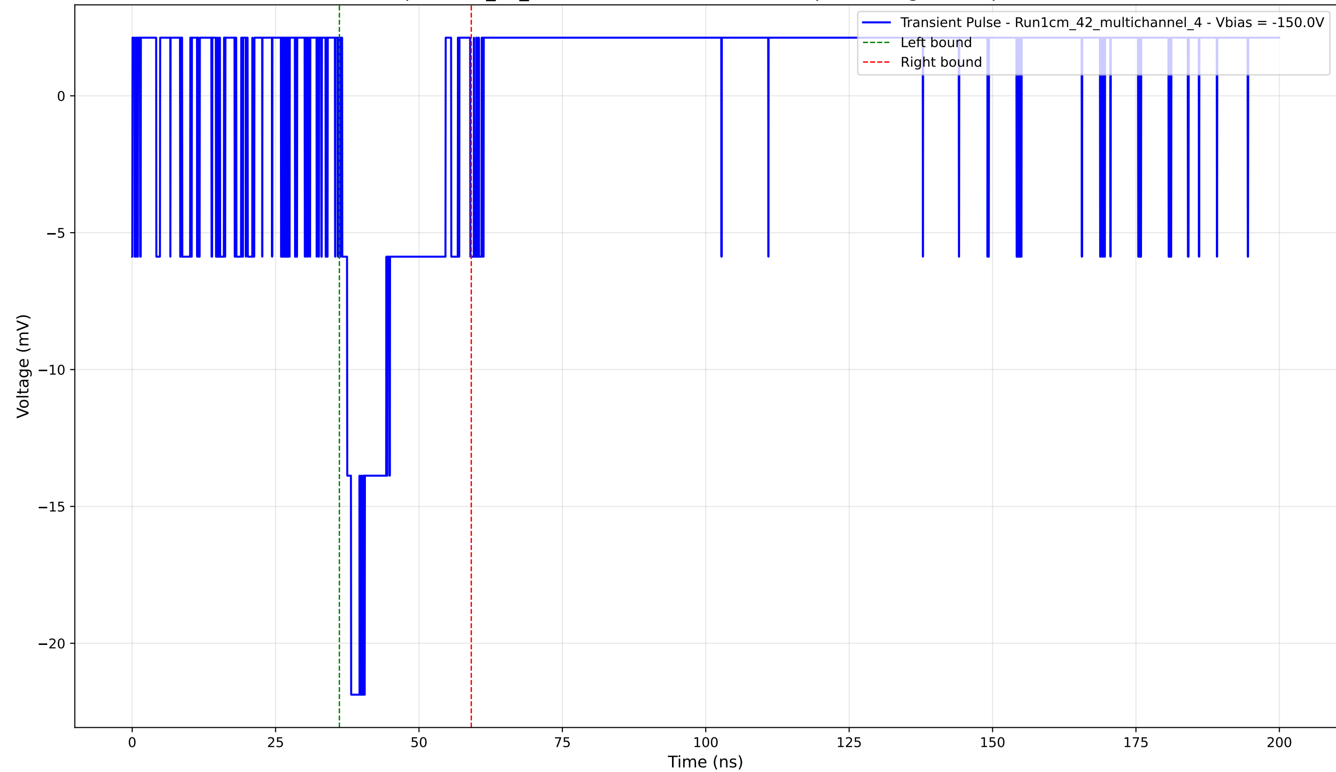
Transient Pulse - Sample: 1cm_42_multichannel - Position: 990.0 \mu\text{m} - Charge: 3.63 pC - Rise Time: 1.56 ns
