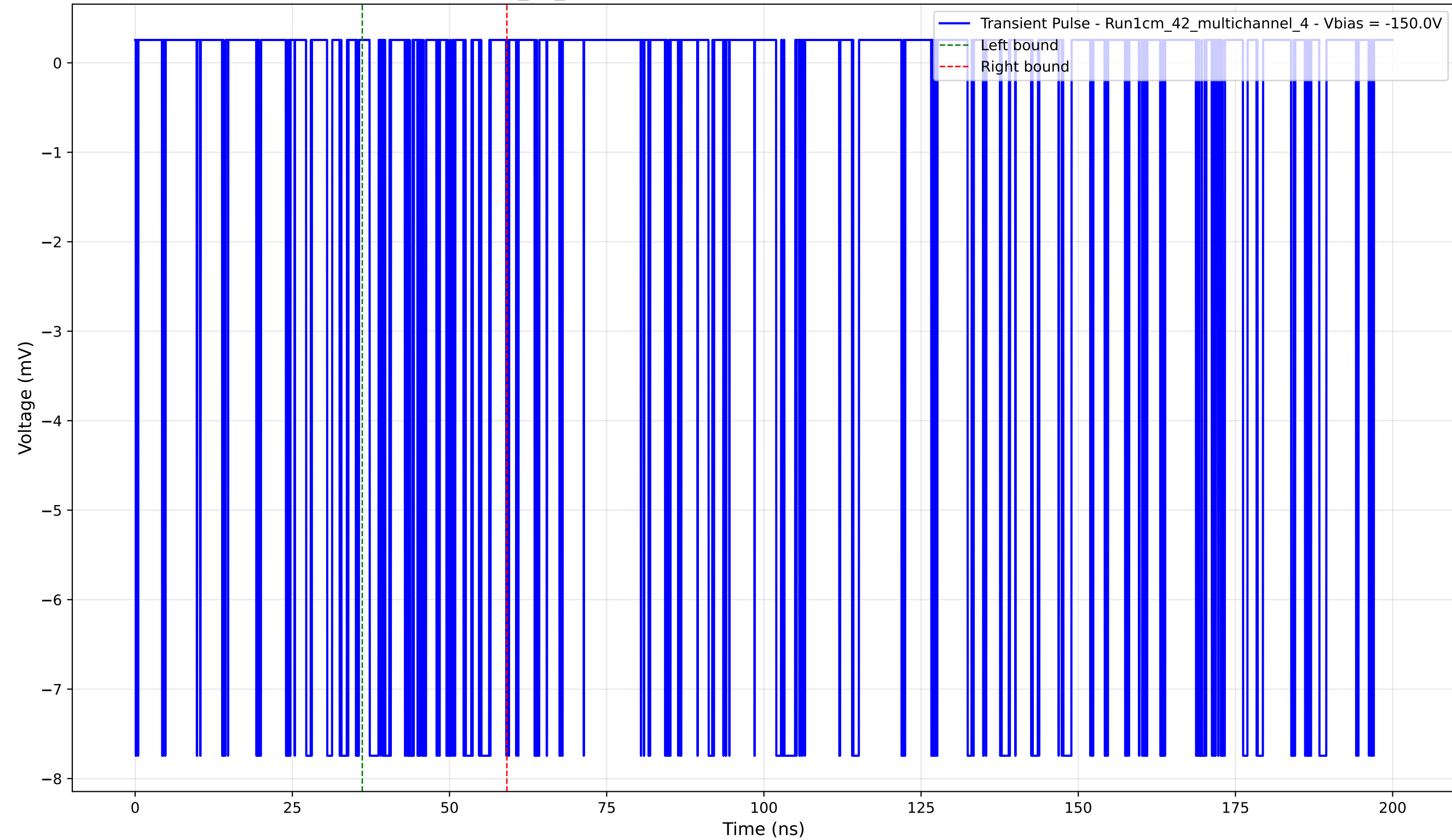
Transient Pulse - Sample: 1cm_42_multichannel - Position: 1875.0 \mu\text{m} - Charge: 1.21 pC - Rise Time: 0.02 ns
