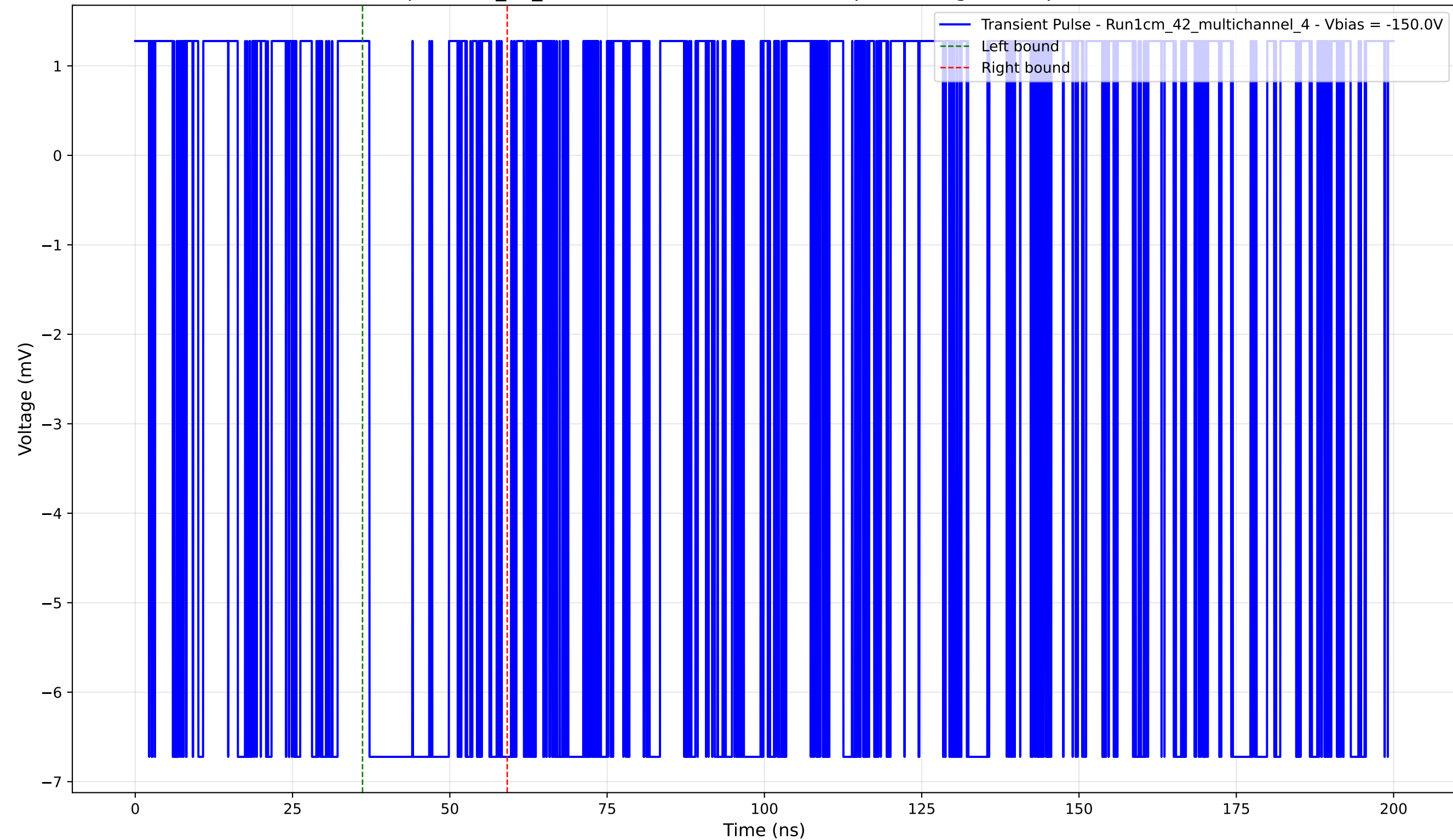
Transient Pulse - Sample: 1cm_42_multichannel - Position: 330.0 \mu\text{m} - Charge: 2.11 pC - Rise Time: 0.00 ns (N/A)
