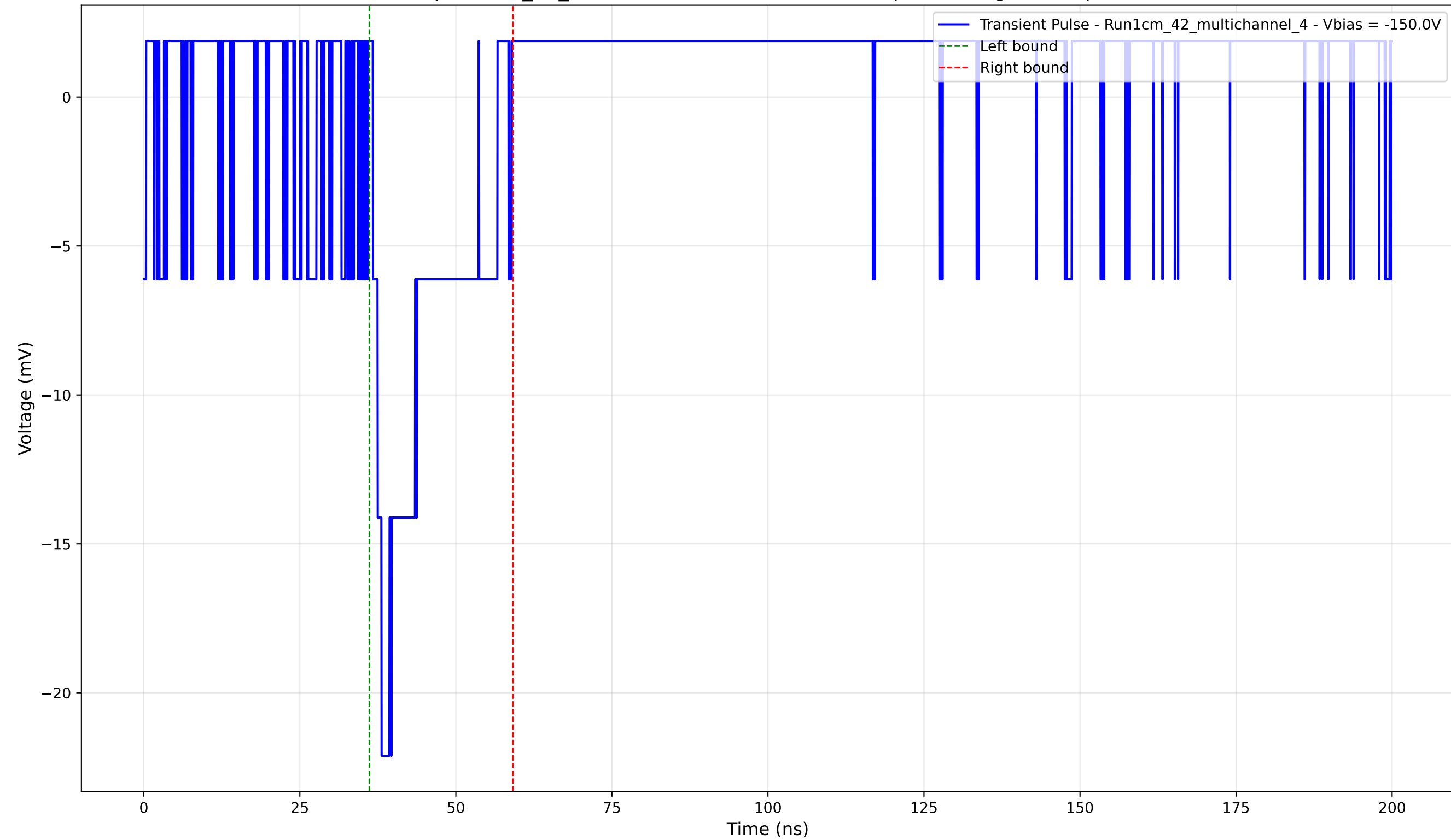
Transient Pulse - Sample: 1cm_42_multichannel - Position: 1115.0 \mu\text{m} - Charge: 3.59 pC - Rise Time: 1.40 ns
