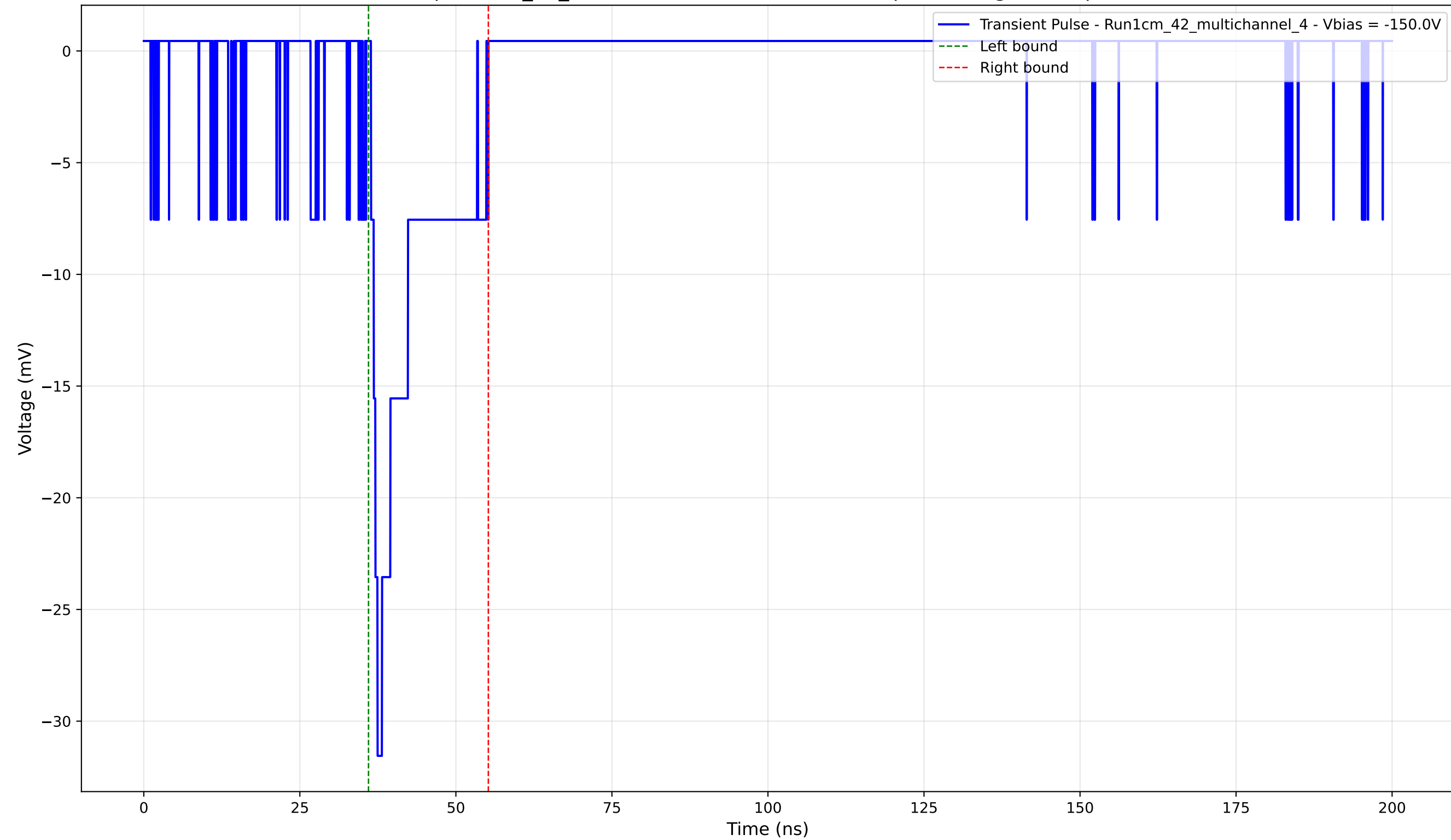
Transient Pulse - Sample: 1cm_42_multichannel - Position: 3160.0 \mu\text{m} - Charge: 4.15 pC - Rise Time: 1.05 ns
