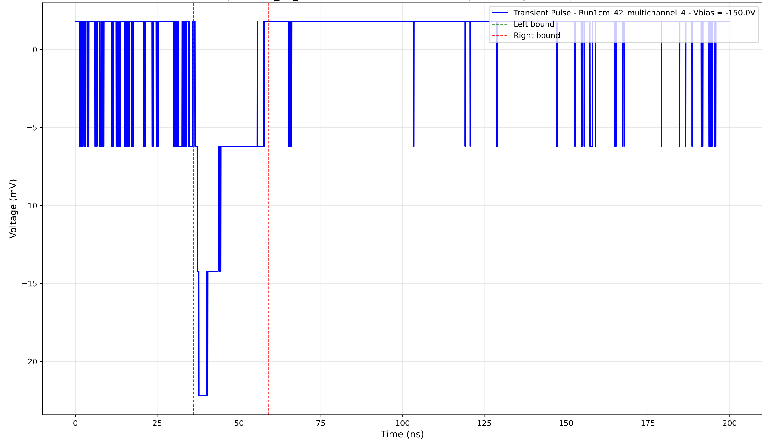
Transient Pulse - Sample: 1cm_42_multichannel - Position: 1220.0 \mu\text{m} - Charge: 4.04 pC - Rise Time: 1.20 ns
