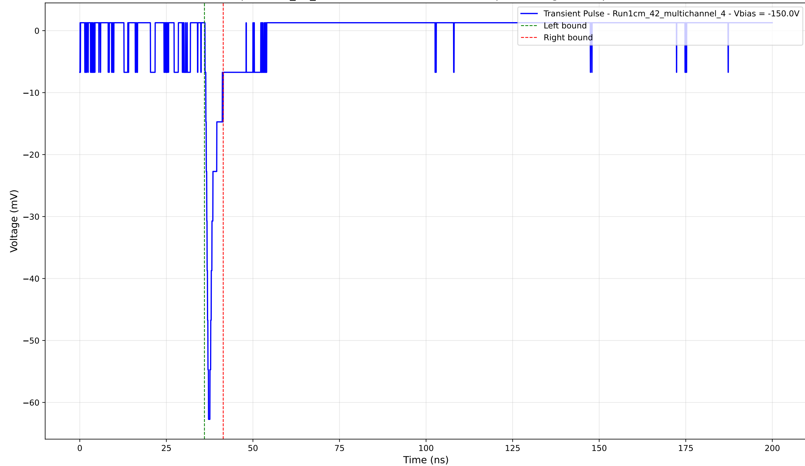
Transient Pulse - Sample: 1cm_42_multichannel - Position: 2635.0 \mu\text{m} - Charge: 2.86 pC - Rise Time: 1.00 ns
