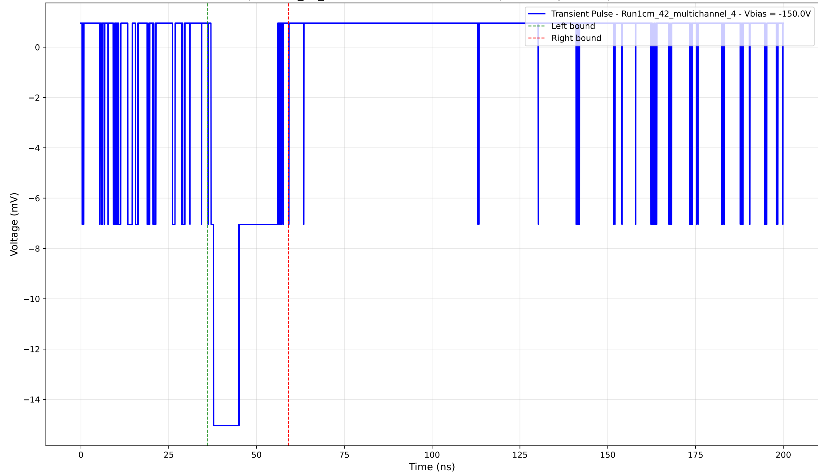
Transient Pulse - Sample: 1cm_42_multichannel - Position: 710.0 \mu\text{m} - Charge: 3.83 pC - Rise Time: 0.76 ns
