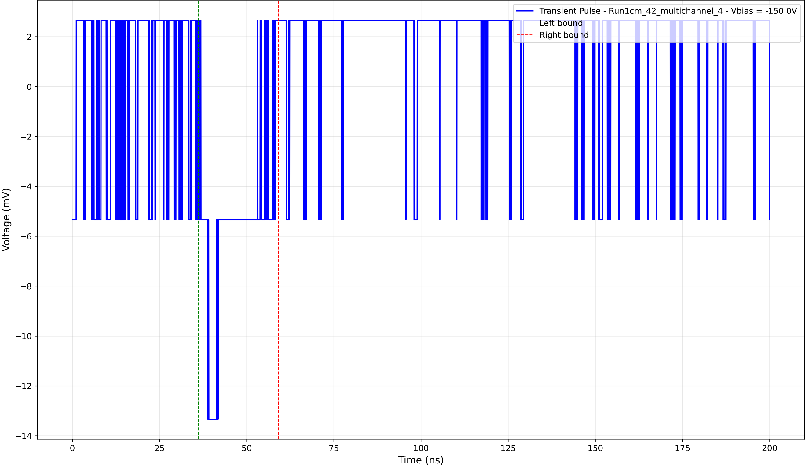
Transient Pulse - Sample: 1cm_42_multichannel - Position: 425.0 \mu\text{m} - Charge: 2.47 pC - Rise Time: 0.00 ns (N/A)
