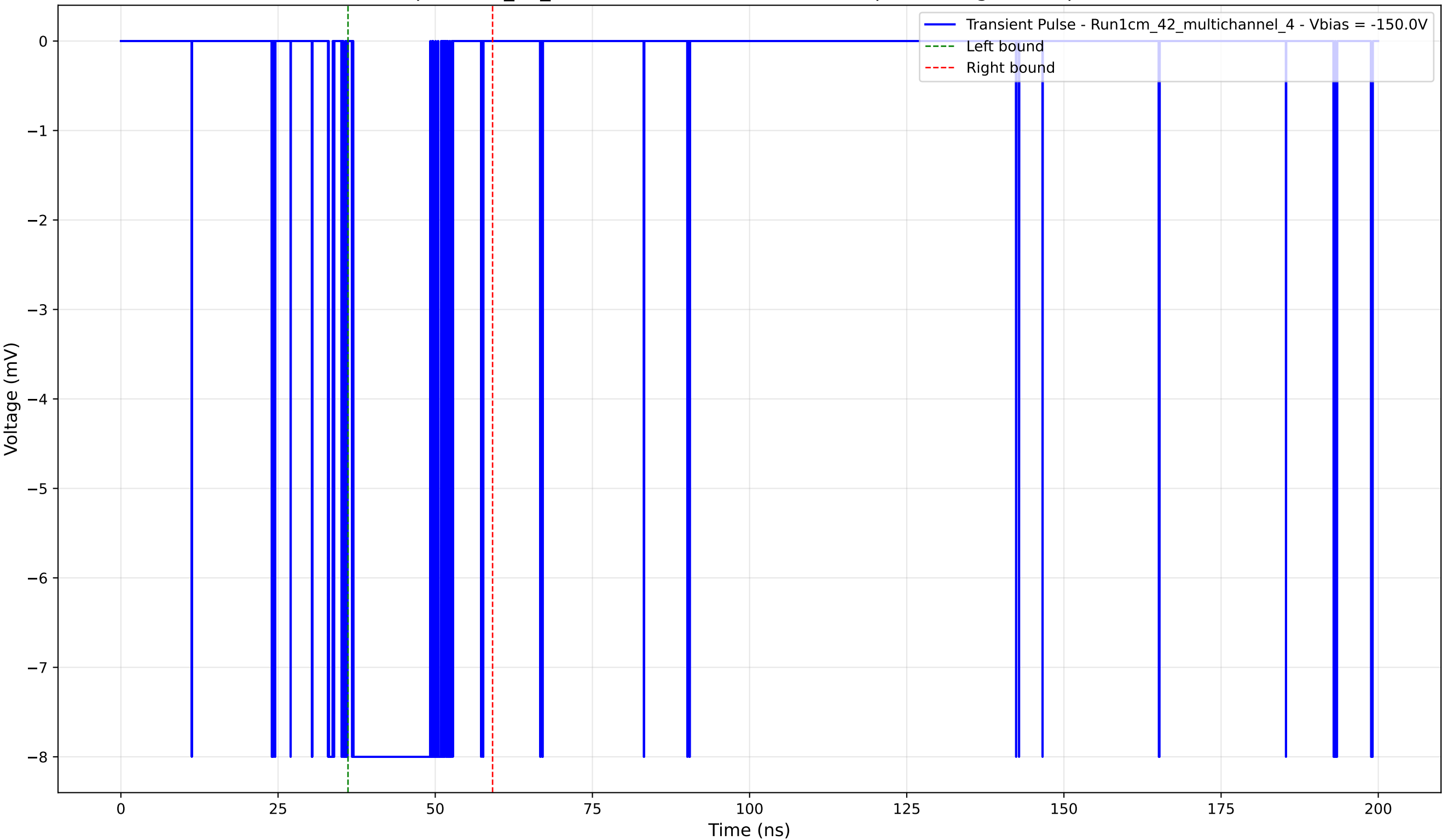
Transient Pulse - Sample: 1cm_42_multichannel - Position: 3955.0 \mu\text{m} - Charge: 2.35 pC - Rise Time: 0.02 ns
