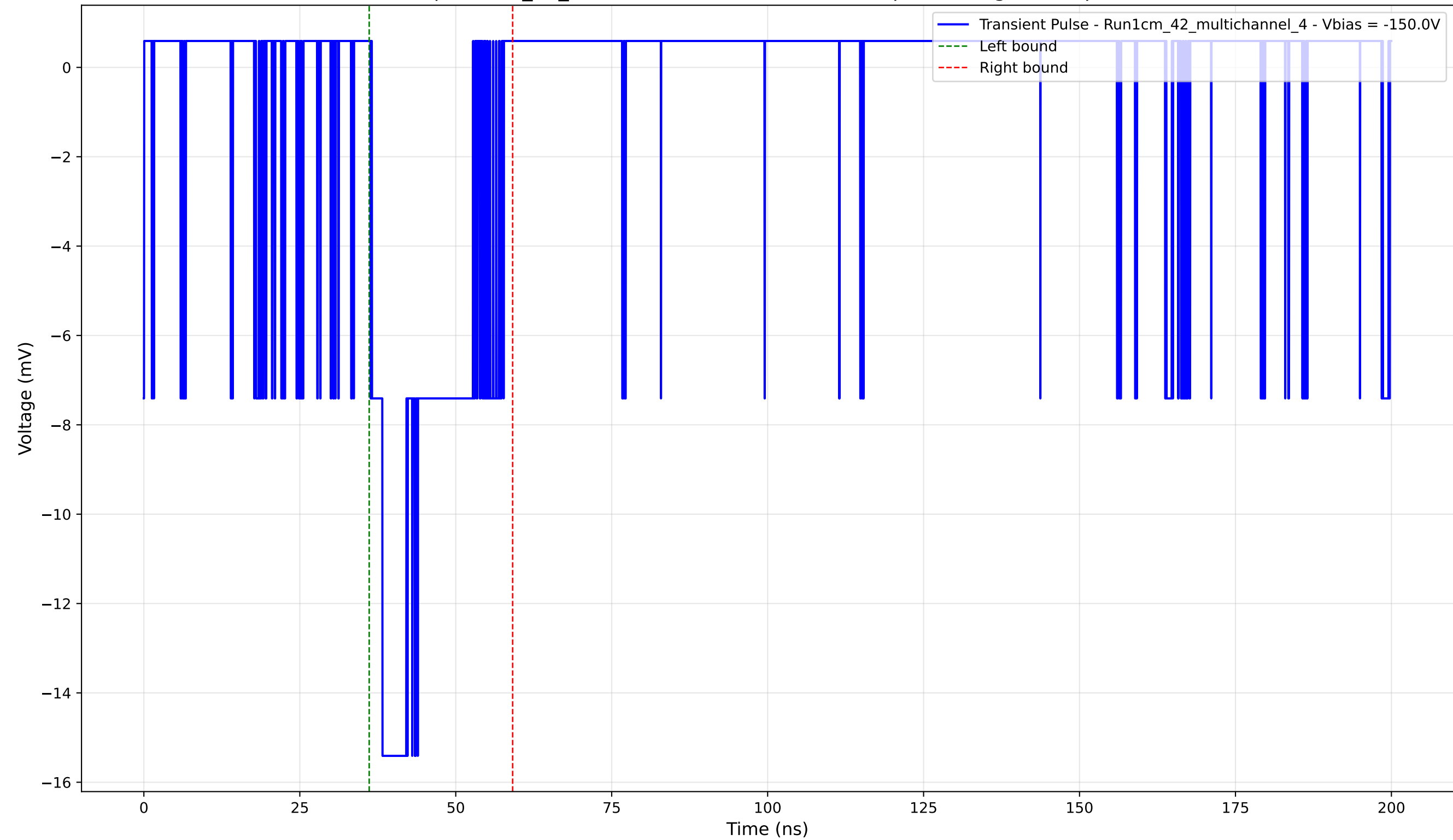
Transient Pulse - Sample: 1cm_42_multichannel - Position: 4320.0 \mu\text{m} - Charge: 3.49 pC - Rise Time: 1.70 ns
