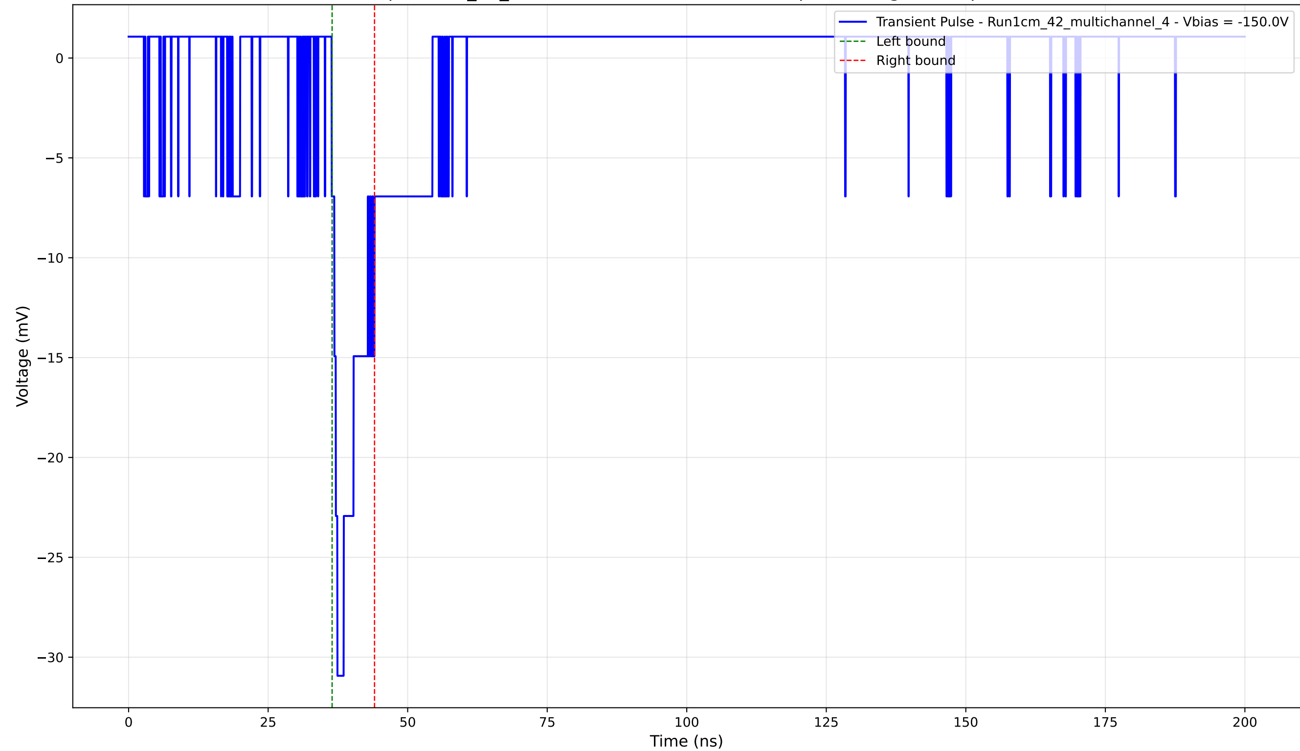
Transient Pulse - Sample: 1cm_42_multichannel - Position: 1565.0 \mu\text{m} - Charge: 2.83 pC - Rise Time: 1.03 ns
