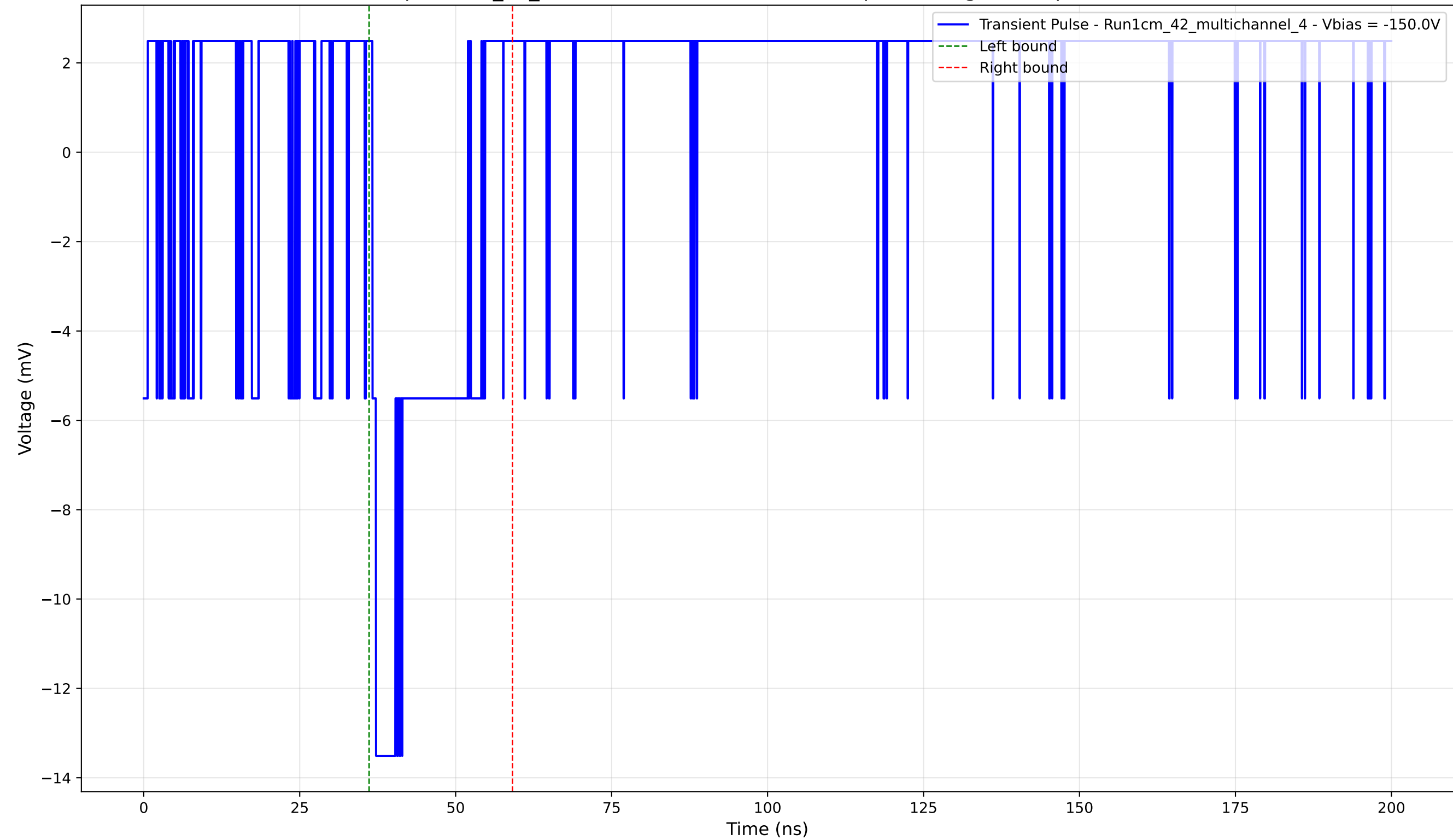
Transient Pulse - Sample: 1cm_42_multichannel - Position: 3340.0 \mu\text{m} - Charge: 2.22 pC - Rise Time: 0.00 ns (N/A)
