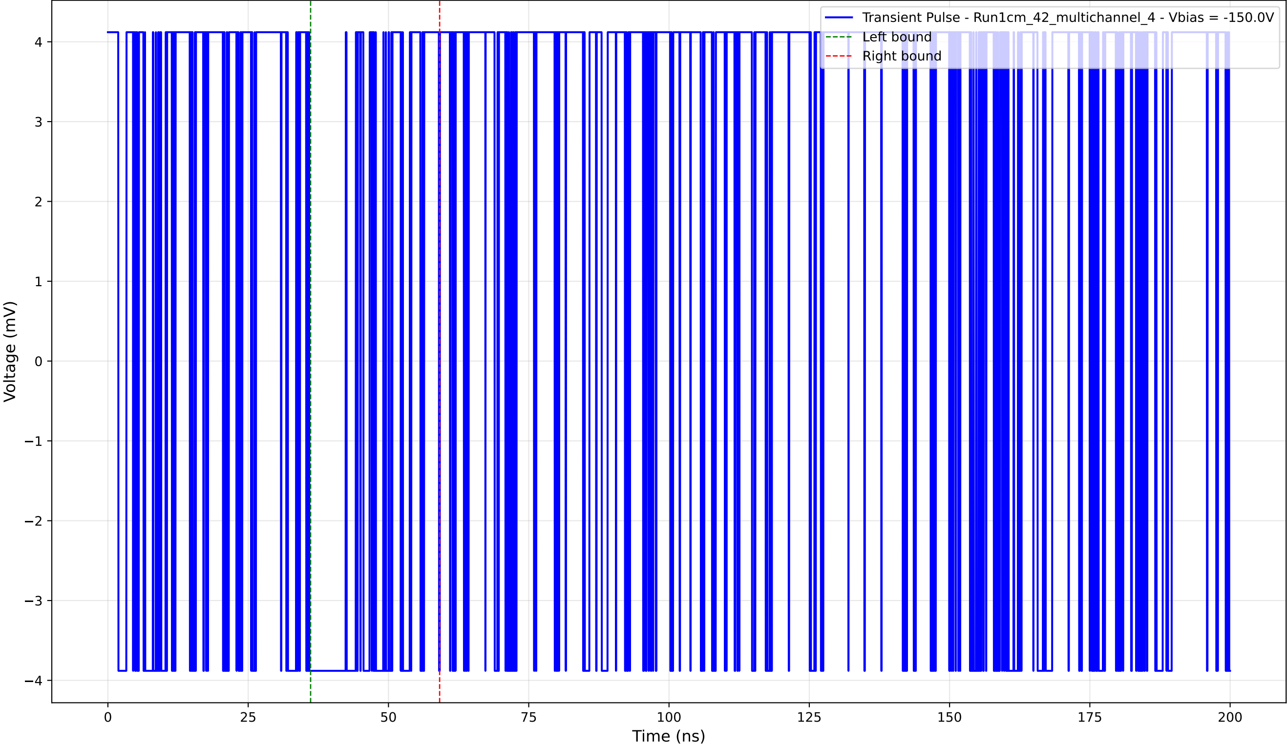
Transient Pulse - Sample: 1cm_42_multichannel - Position: 1845.0 \mu\text{m} - Charge: 0.41 pC - Rise Time: 0.00 ns (N/A)
