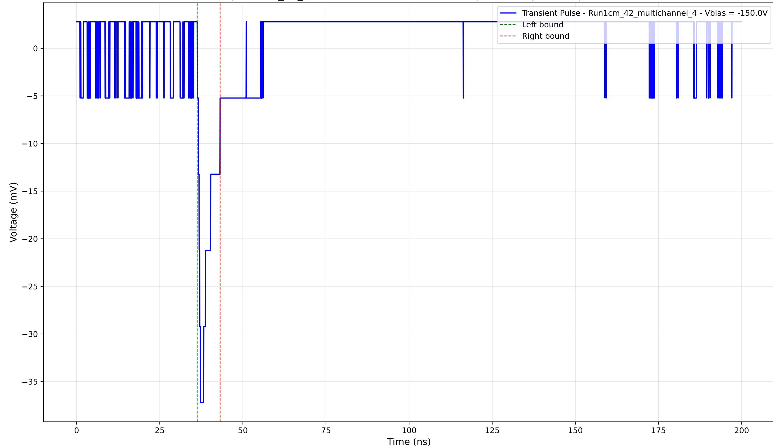
Transient Pulse - Sample: 1cm_42_multichannel - Position: 1755.0 \mu\text{m} - Charge: 2.74 pC - Rise Time: 0.97 ns
