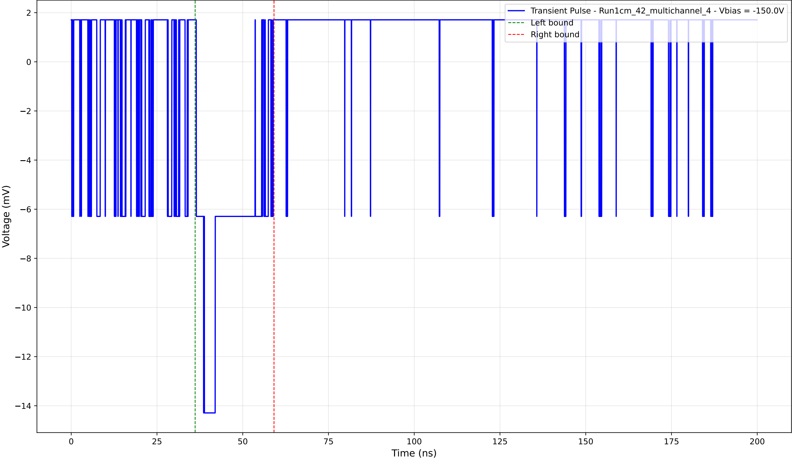
Transient Pulse - Sample: 1cm_42_multichannel - Position: 140.0 \mu\text{m} - Charge: 3.08 pC - Rise Time: 0.00 ns (N/A)
