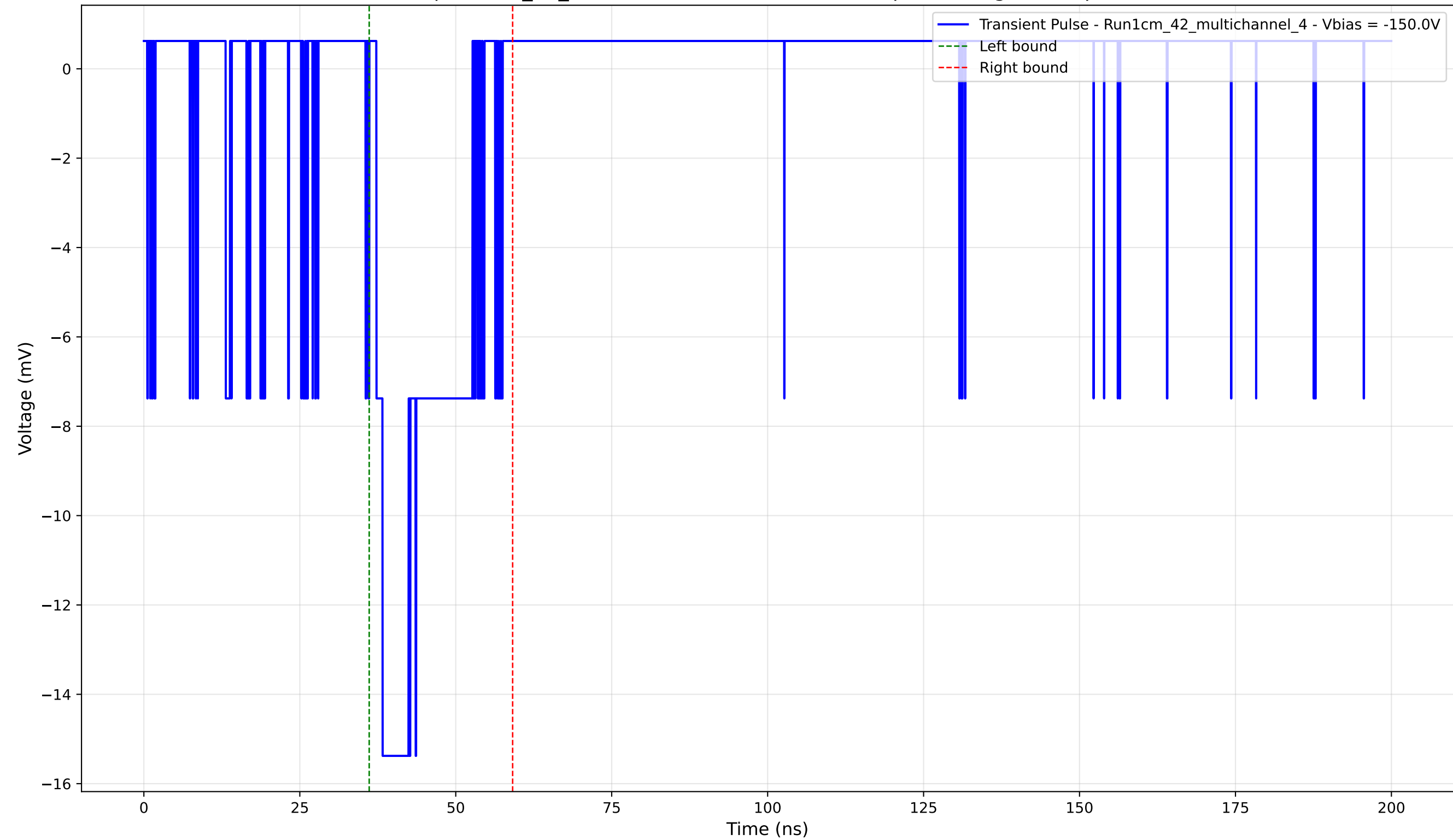
Transient Pulse - Sample: 1cm_42_multichannel - Position: 4165.0 \mu\text{m} - Charge: 3.17 pC - Rise Time: 1.00 ns
