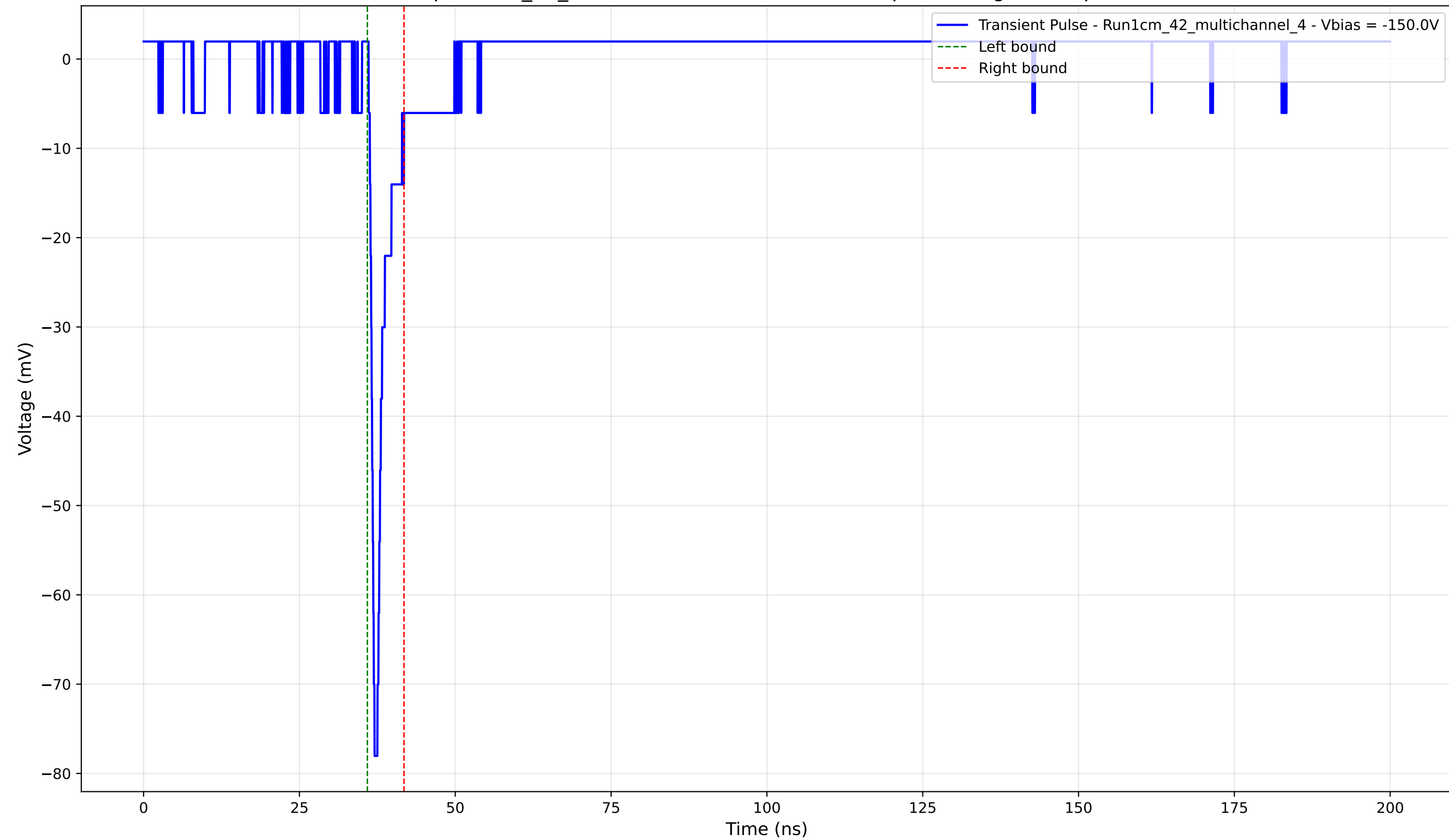
Transient Pulse - Sample: 1cm_42_multichannel - Position: 2245.0 \mu\text{m} - Charge: 3.46 pC - Rise Time: 0.76 ns
