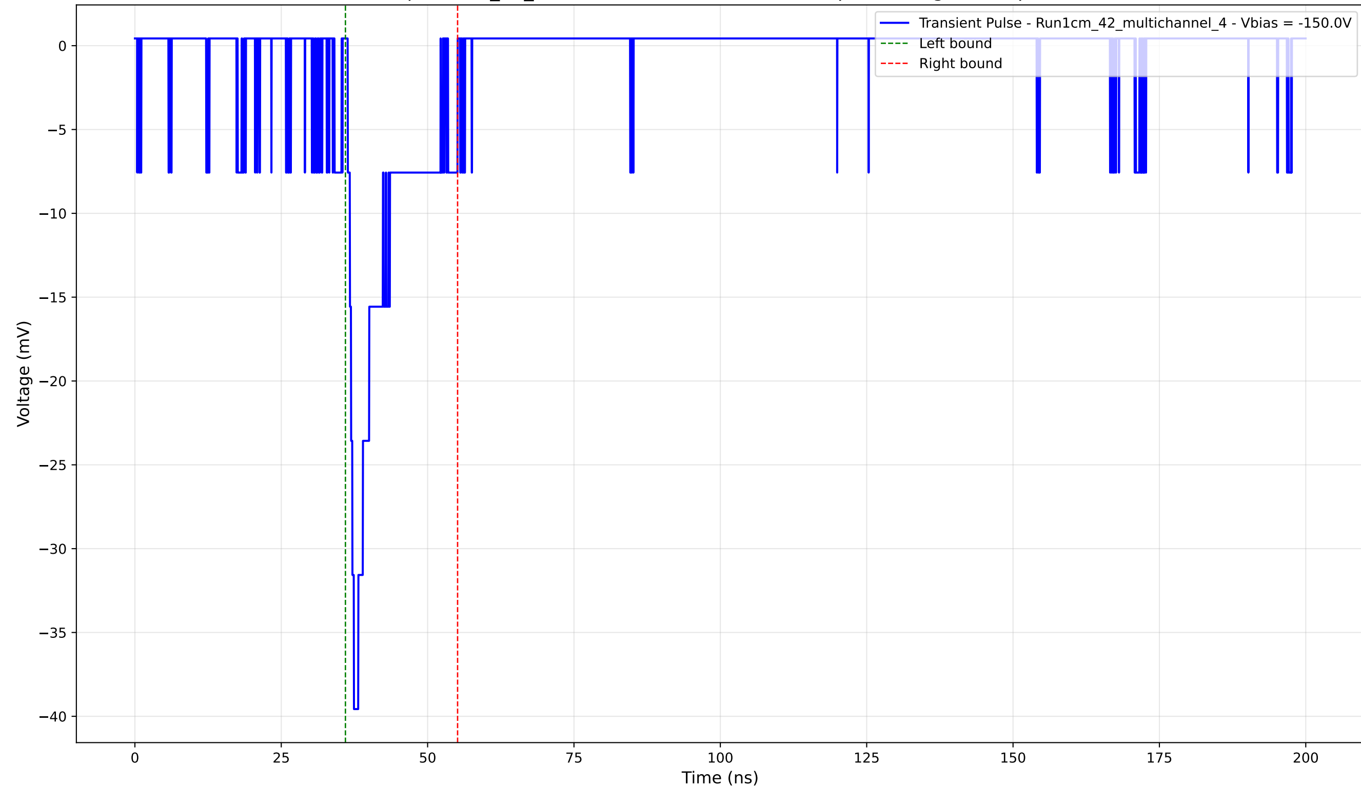
Transient Pulse - Sample: 1cm_42_multichannel - Position: 1720.0 \mu\text{m} - Charge: 4.69 pC - Rise Time: 1.05 ns
