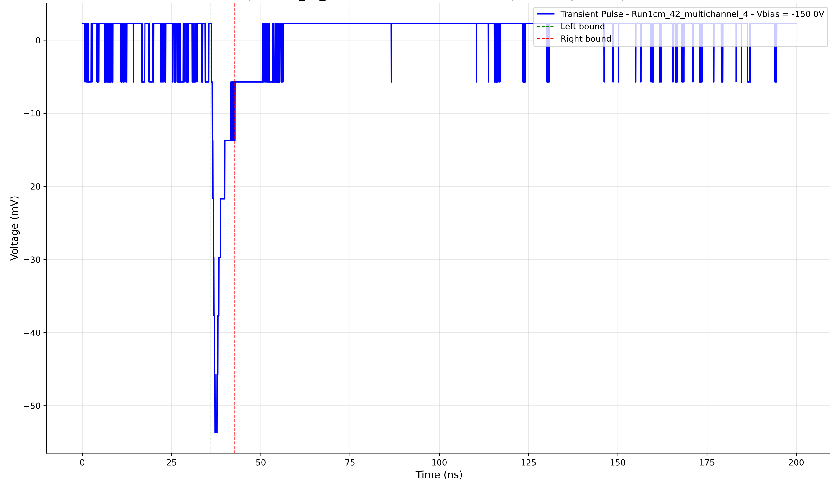
Transient Pulse - Sample: 1cm_42_multichannel - Position: 2730.0 \mu\text{m} - Charge: 3.00 pC - Rise Time: 1.02 ns
