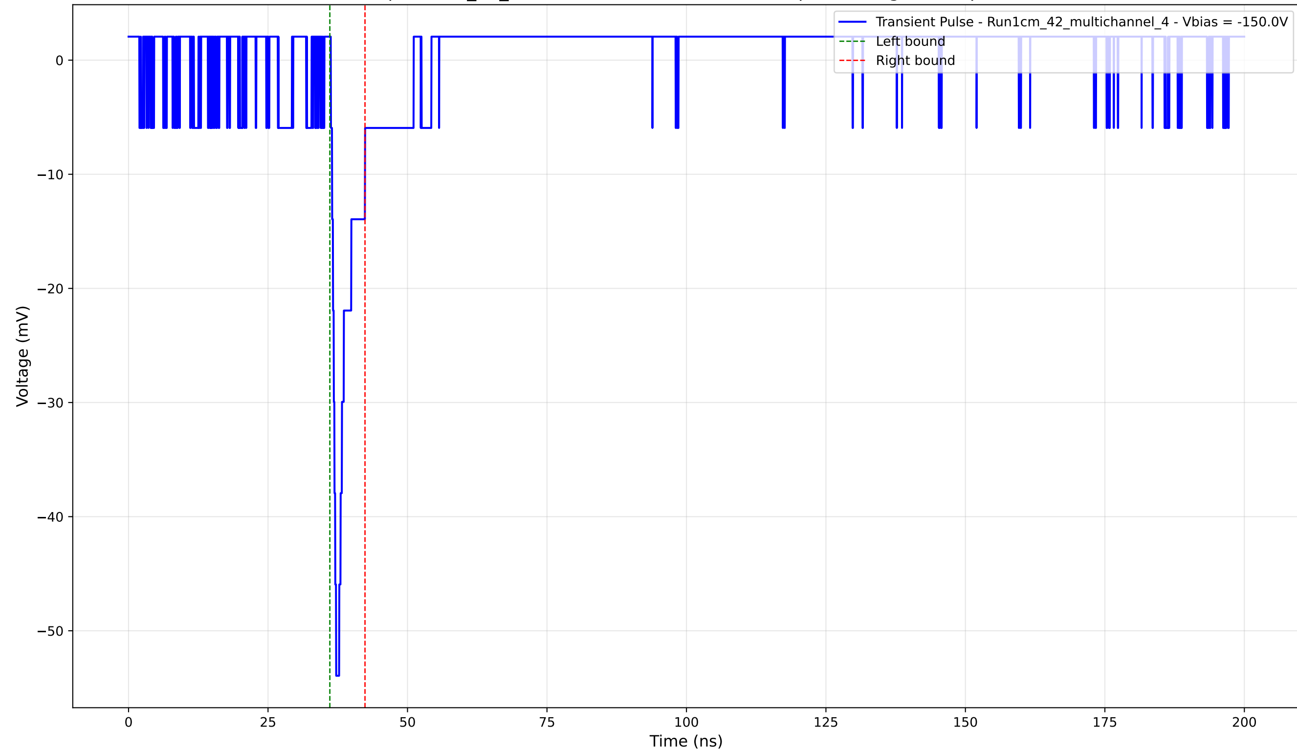
Transient Pulse - Sample: 1cm_42_multichannel - Position: 2760.0 \mu\text{m} - Charge: 2.94 pC - Rise Time: 0.94 ns
