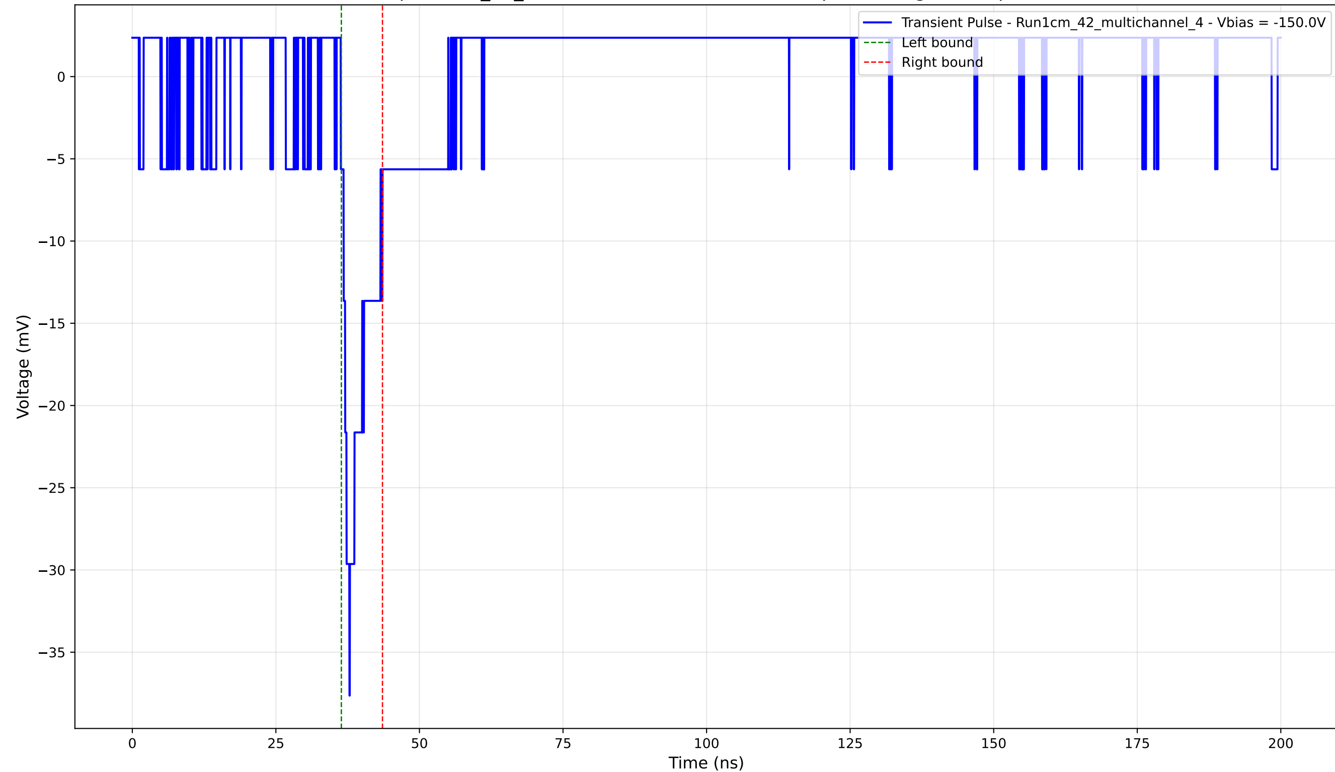
Transient Pulse - Sample: 1cm_42_multichannel - Position: 1625.0 \mu\text{m} - Charge: 2.60 pC - Rise Time: 1.51 ns
