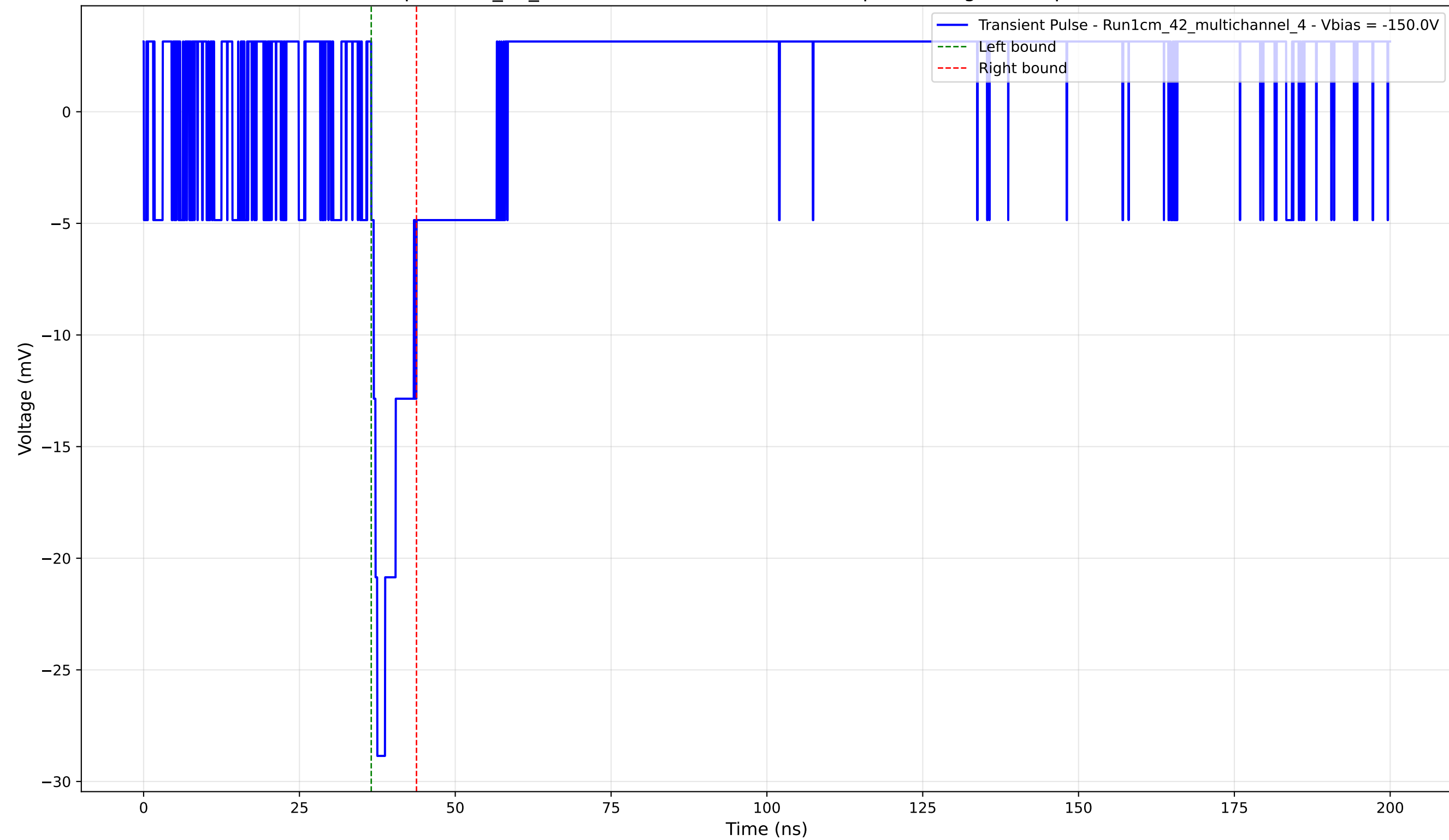
Transient Pulse - Sample: 1cm_42_multichannel - Position: 1505.0 \mu\text{m} - Charge: 2.48 pC - Rise Time: 0.00 ns (N/A)
