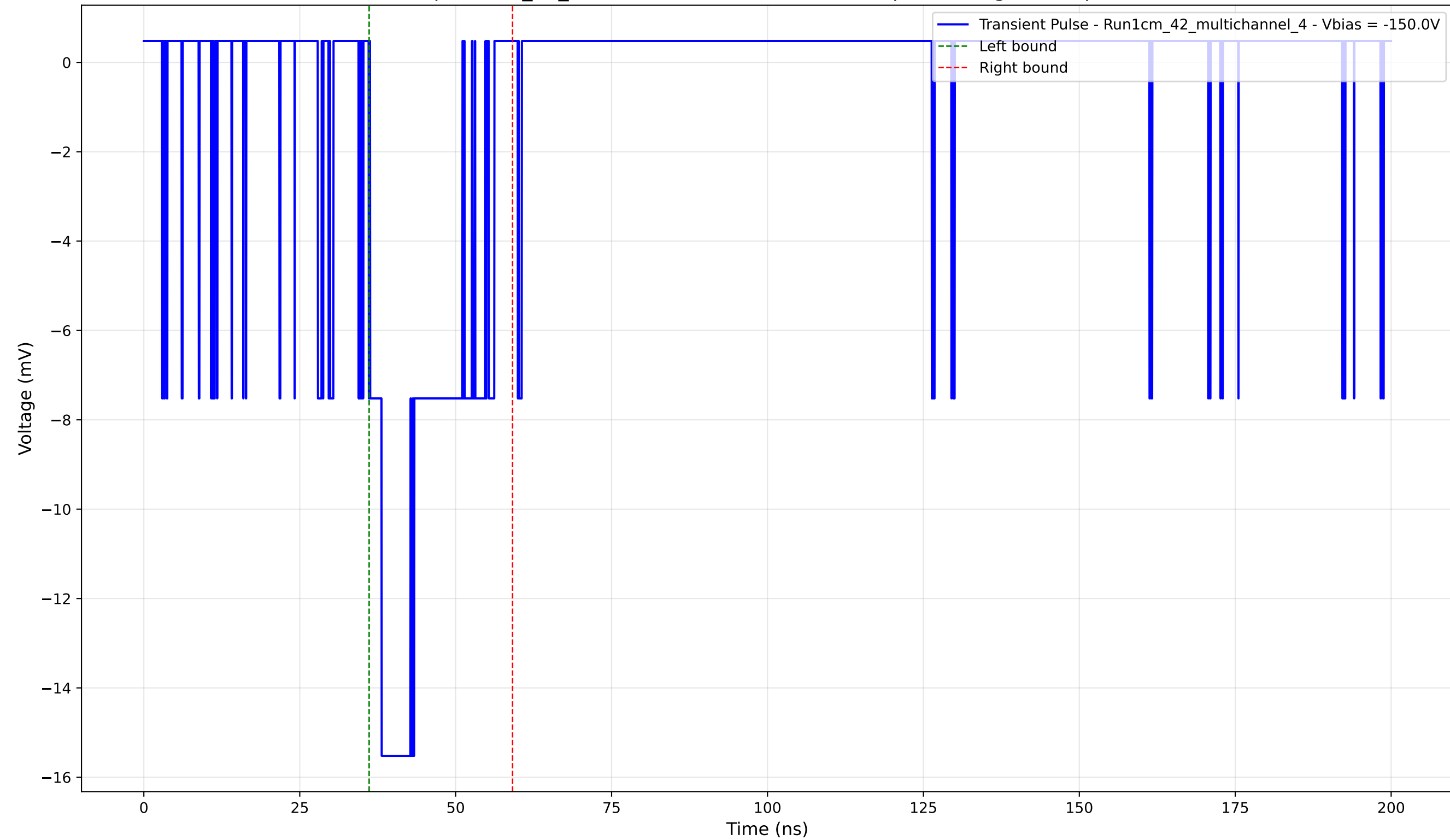
Transient Pulse - Sample: 1cm_42_multichannel - Position: 4080.0 \mu\text{m} - Charge: 3.66 pC - Rise Time: 1.86 ns
