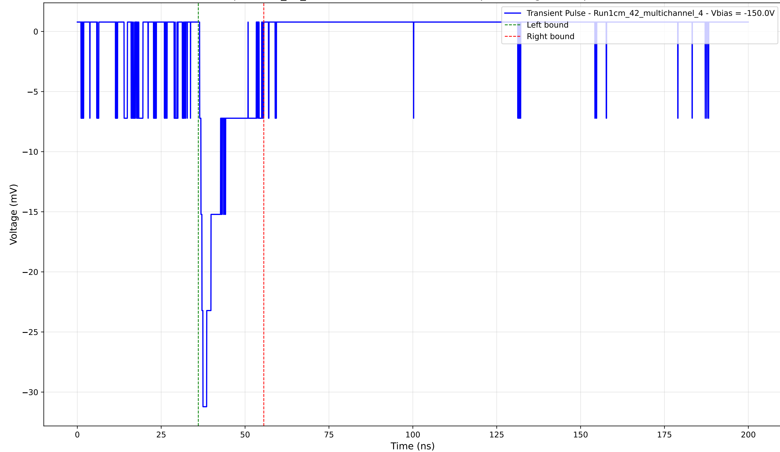
Transient Pulse - Sample: 1cm_42_multichannel - Position: 1560.0 \mu\text{m} - Charge: 4.23 pC - Rise Time: 0.99 ns
