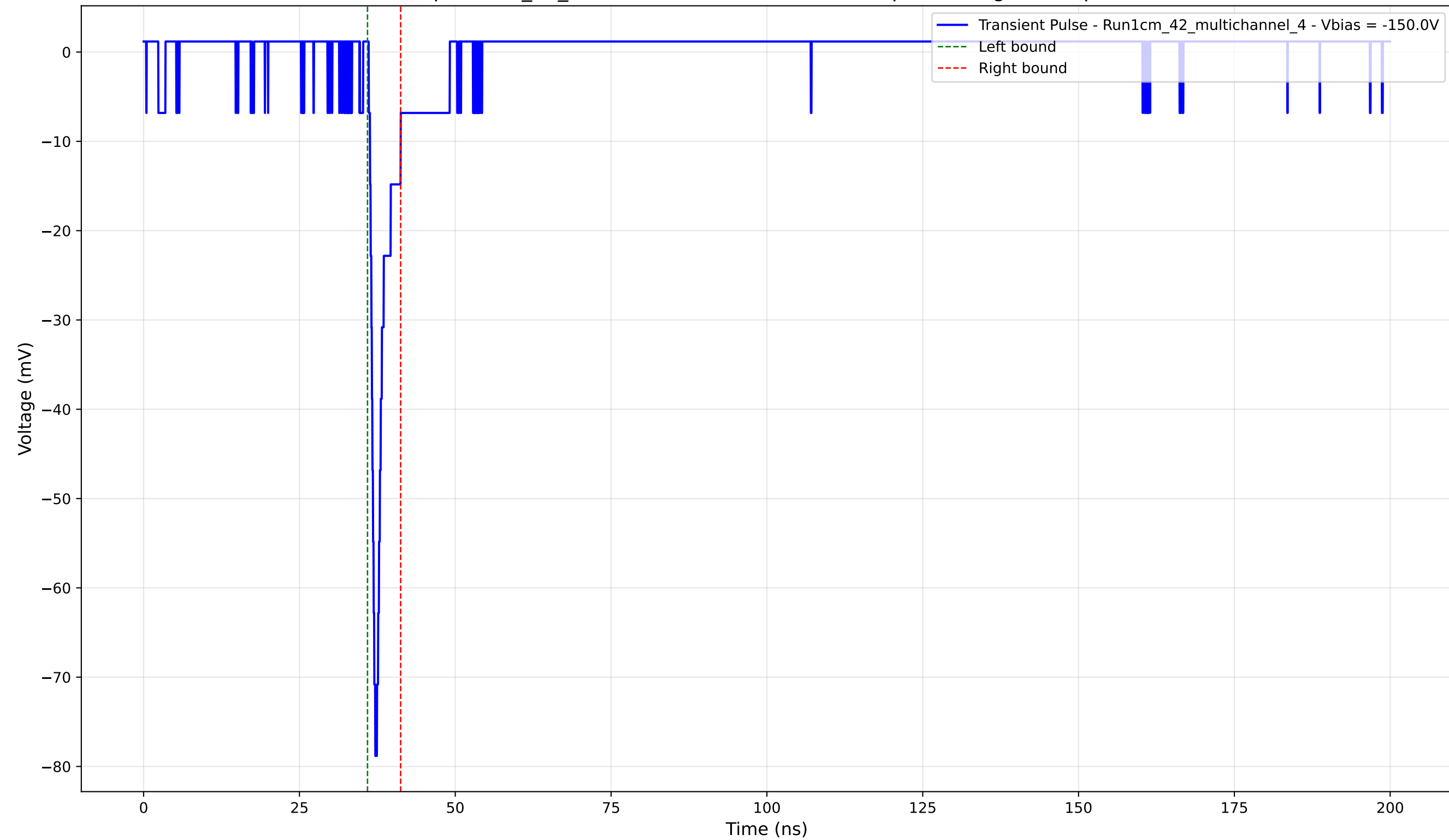
Transient Pulse - Sample: 1cm_42_multichannel - Position: 2225.0 \mu\text{m} - Charge: 3.24 pC - Rise Time: 0.86 ns
