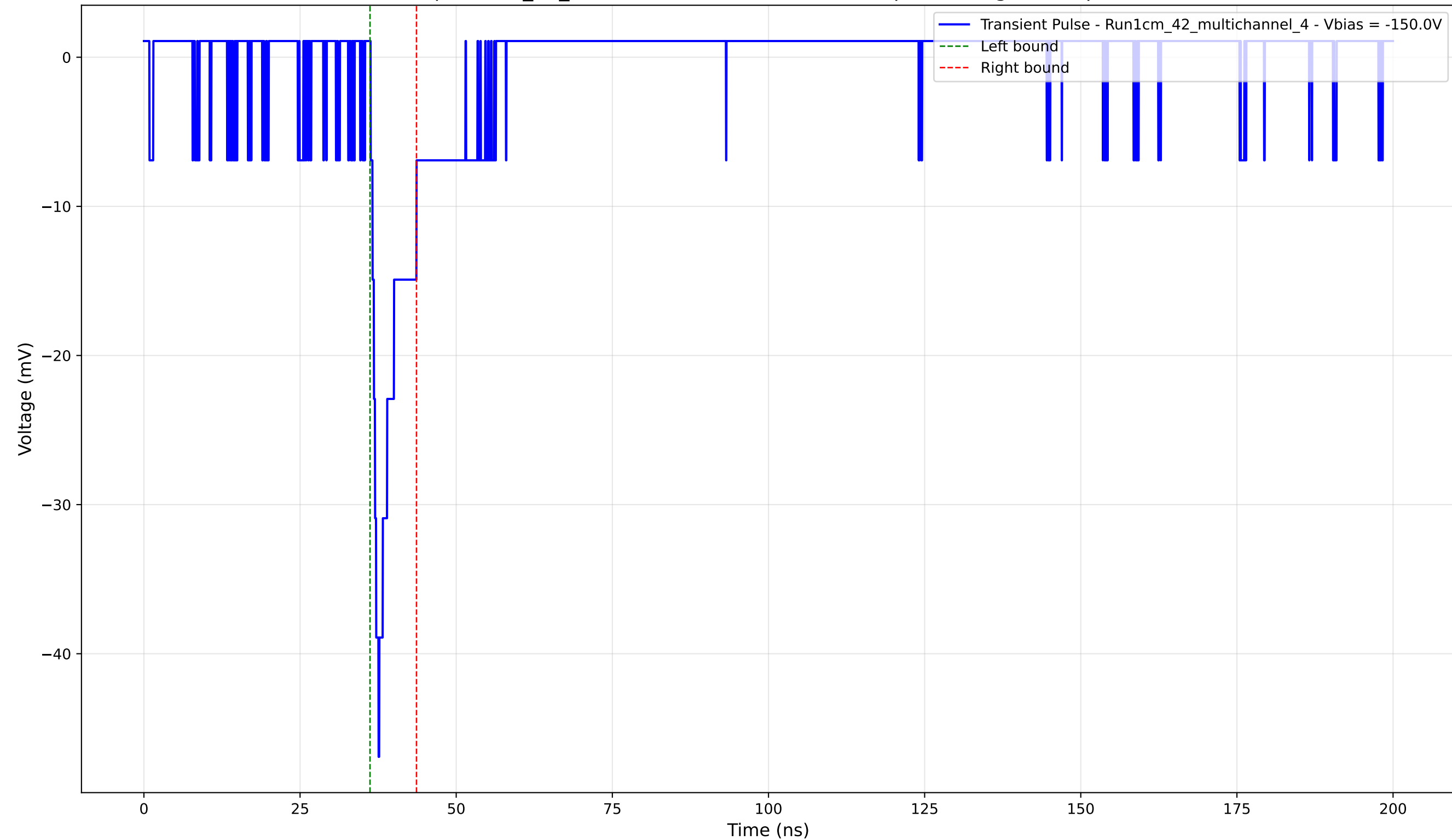
Transient Pulse - Sample: 1cm_42_multichannel - Position: 1785.0 \mu\text{m} - Charge: 3.16 pC - Rise Time: 1.27 ns
