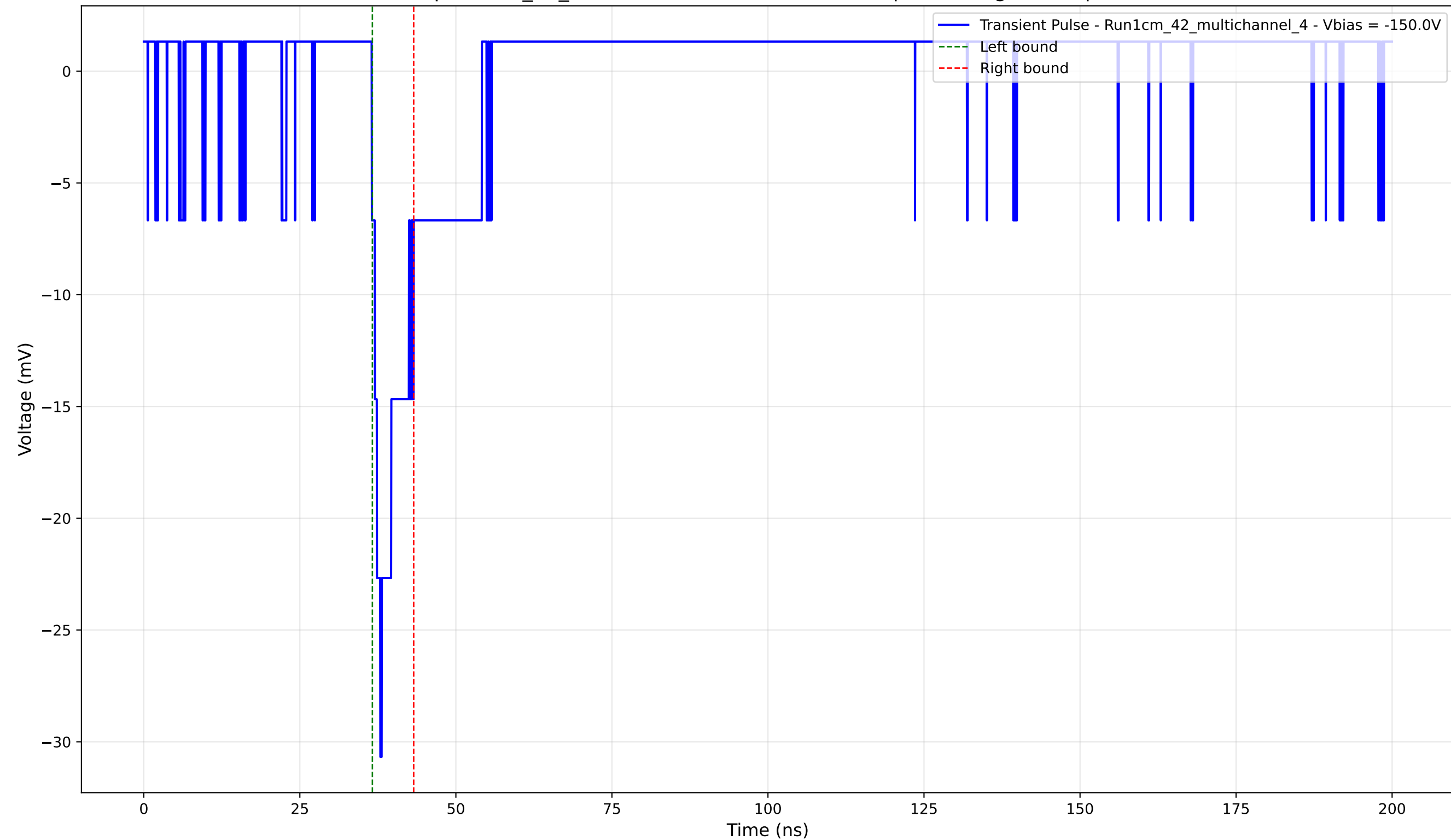
Transient Pulse - Sample: 1cm_42_multichannel - Position: 3305.0 \mu\text{m} - Charge: 2.22 pC - Rise Time: 1.37 ns
