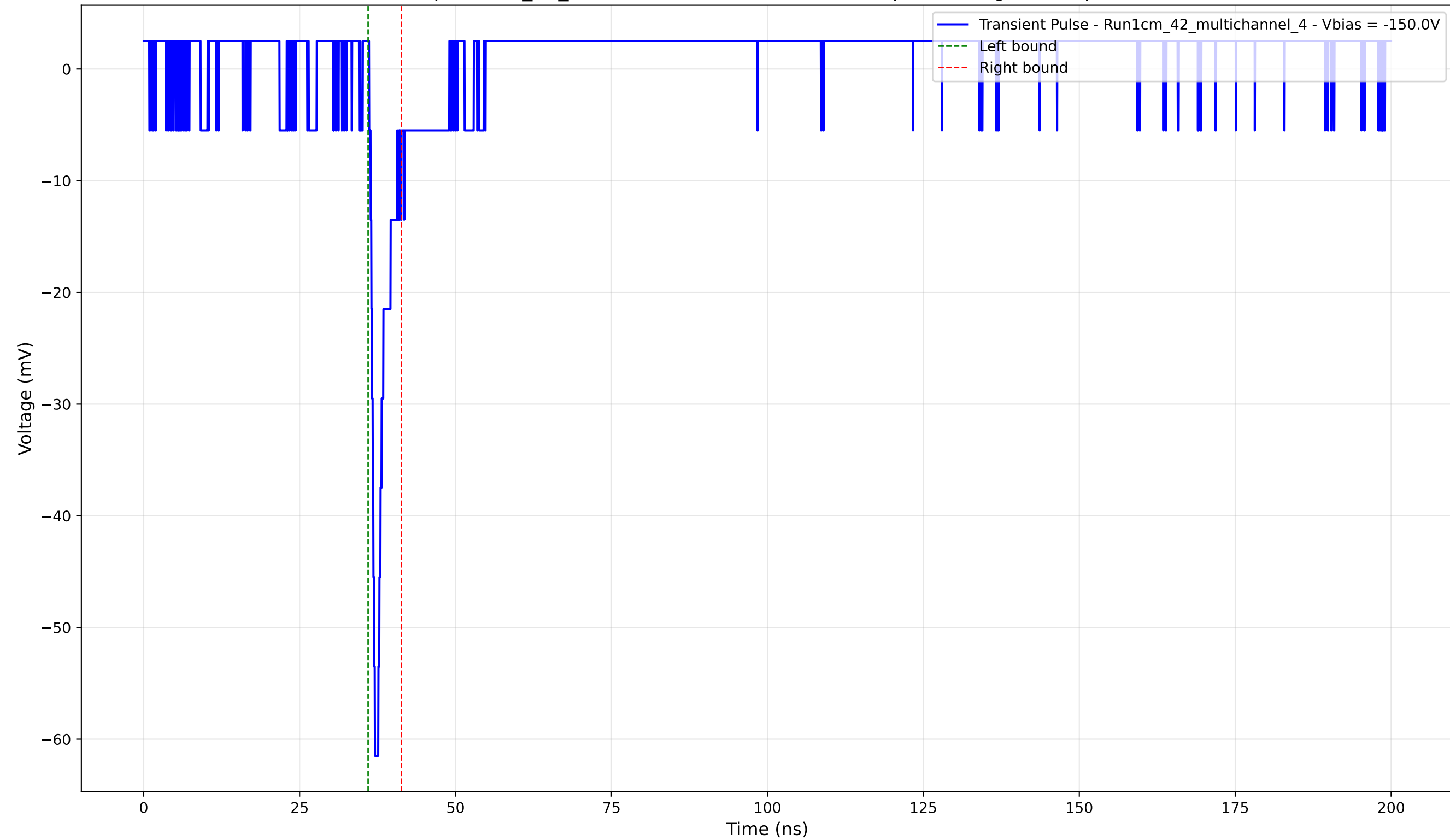
Transient Pulse - Sample: 1cm_42_multichannel - Position: 2595.0 \mu\text{m} - Charge: 2.72 pC - Rise Time: 0.70 ns
