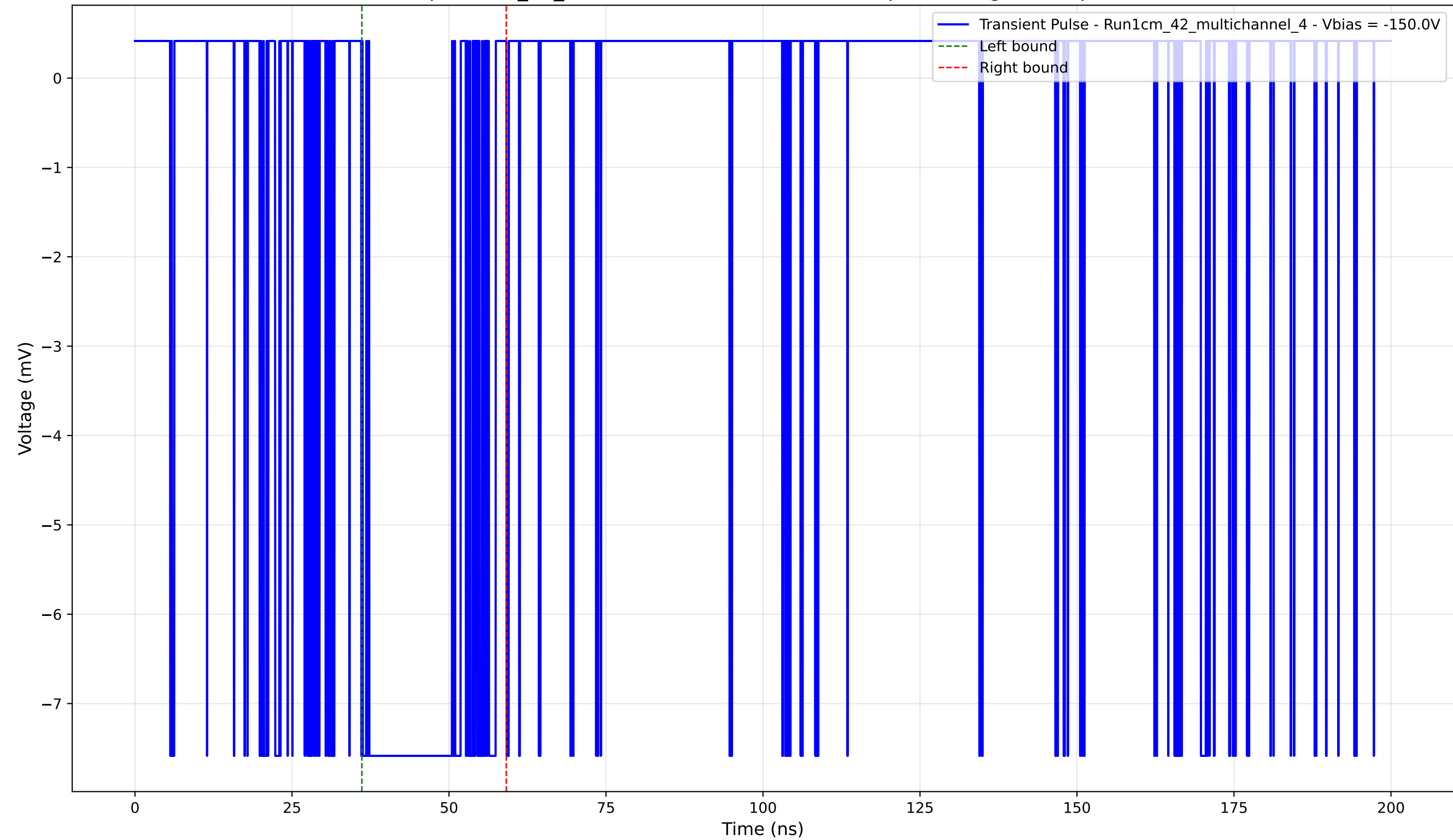
Transient Pulse - Sample: 1cm_42_multichannel - Position: 4850.0 \mu\text{m} - Charge: 2.72 pC - Rise Time: 0.02 ns
