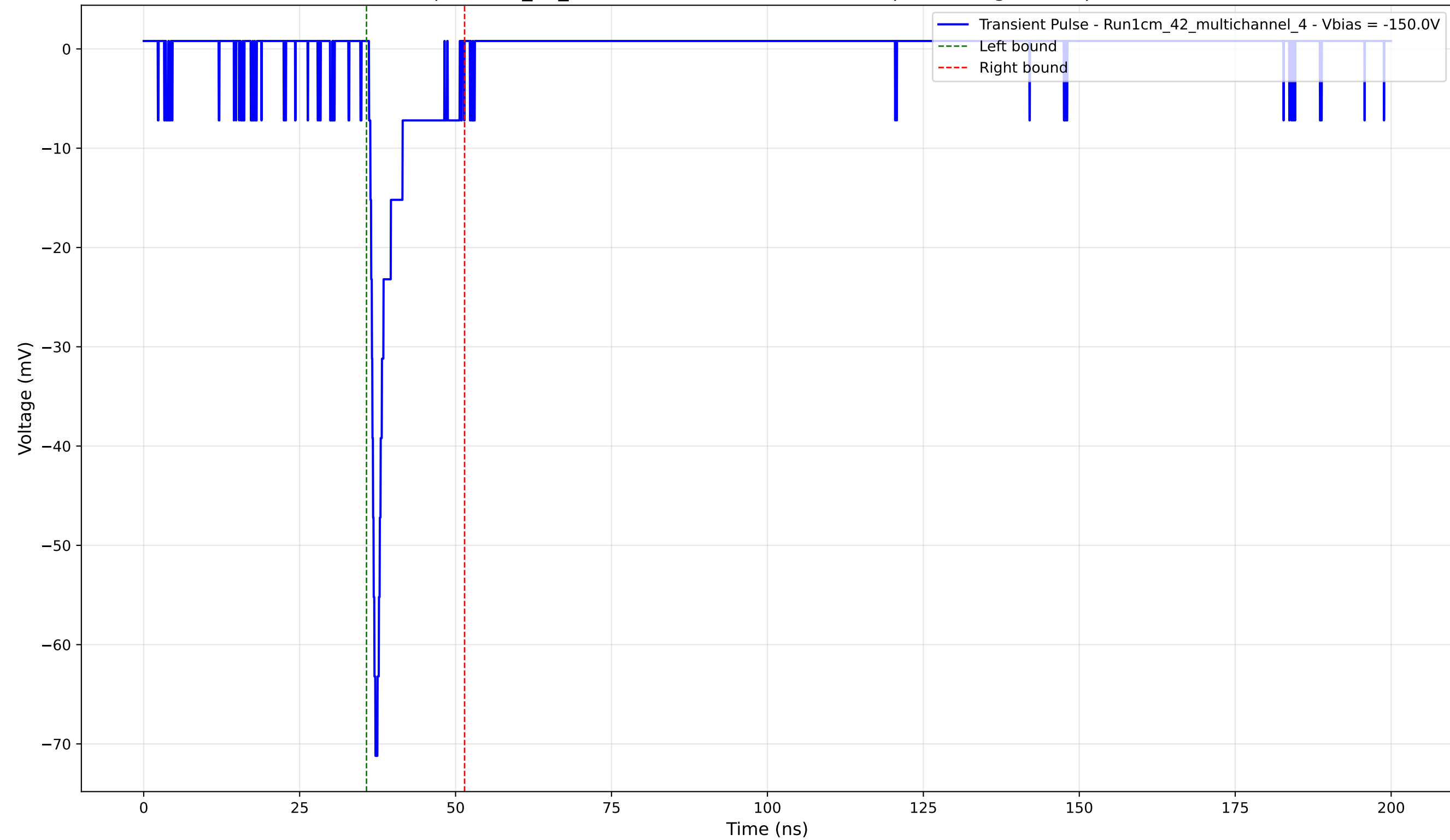
Transient Pulse - Sample: 1cm_42_multichannel - Position: 2570.0 \mu\text{m} - Charge: 4.47 pC - Rise Time: 1.02 ns
