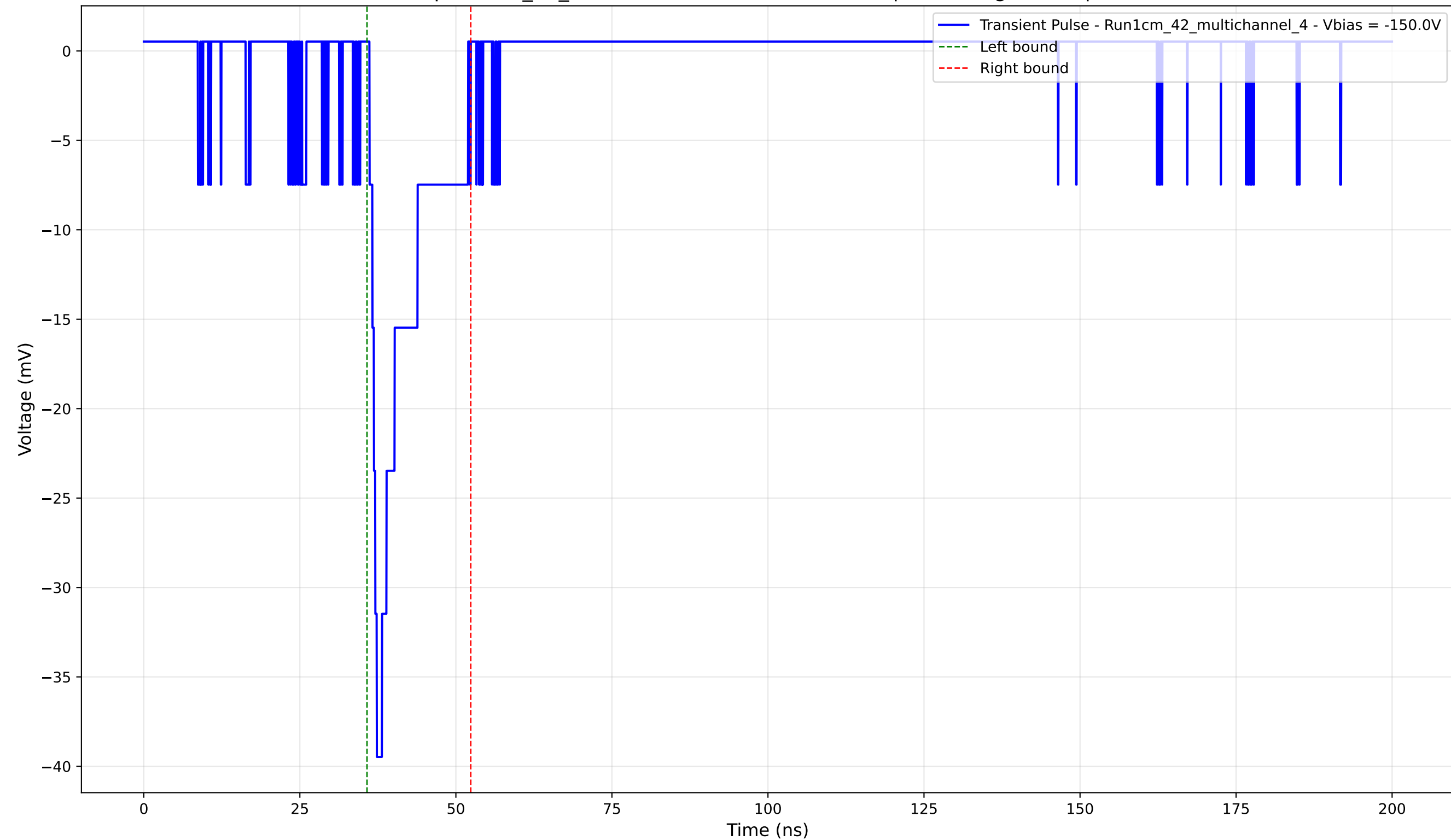
Transient Pulse - Sample: 1cm_42_multichannel - Position: 1730.0 \mu\text{m} - Charge: 4.49 pC - Rise Time: 1.17 ns
