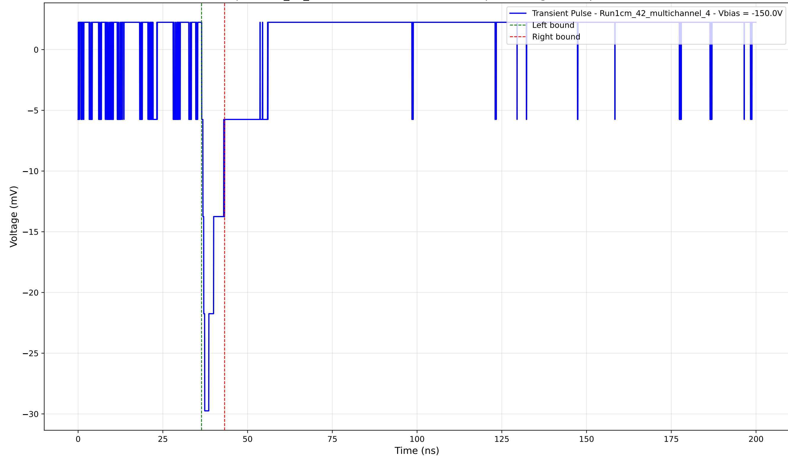
Transient Pulse - Sample: 1cm_42_multichannel - Position: 1630.0 \mu\text{m} - Charge: 2.45 pC - Rise Time: 0.90 ns
