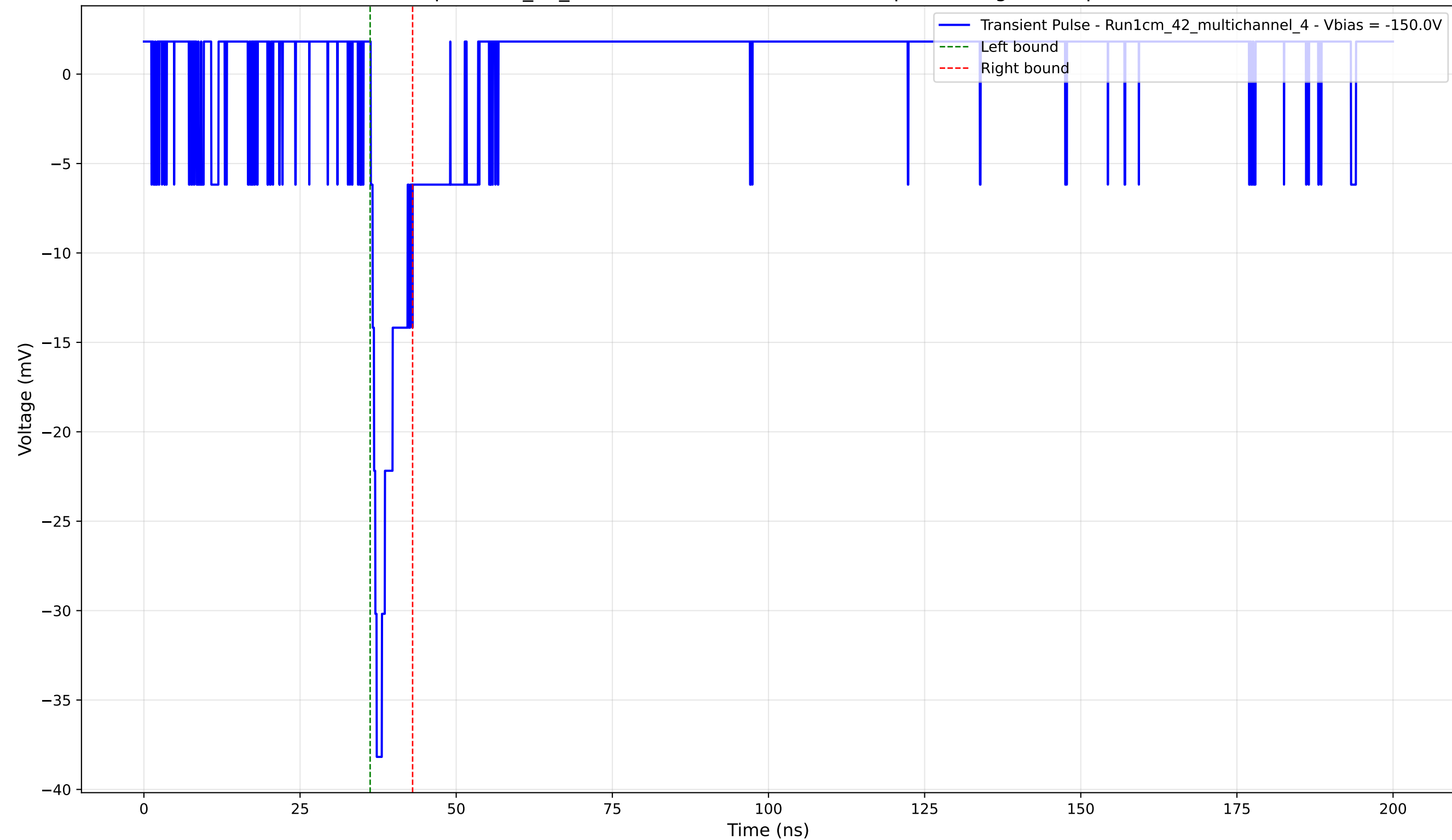
Transient Pulse - Sample: 1cm_42_multichannel - Position: 2985.0 \mu\text{m} - Charge: 2.62 pC - Rise Time: 0.95 ns
