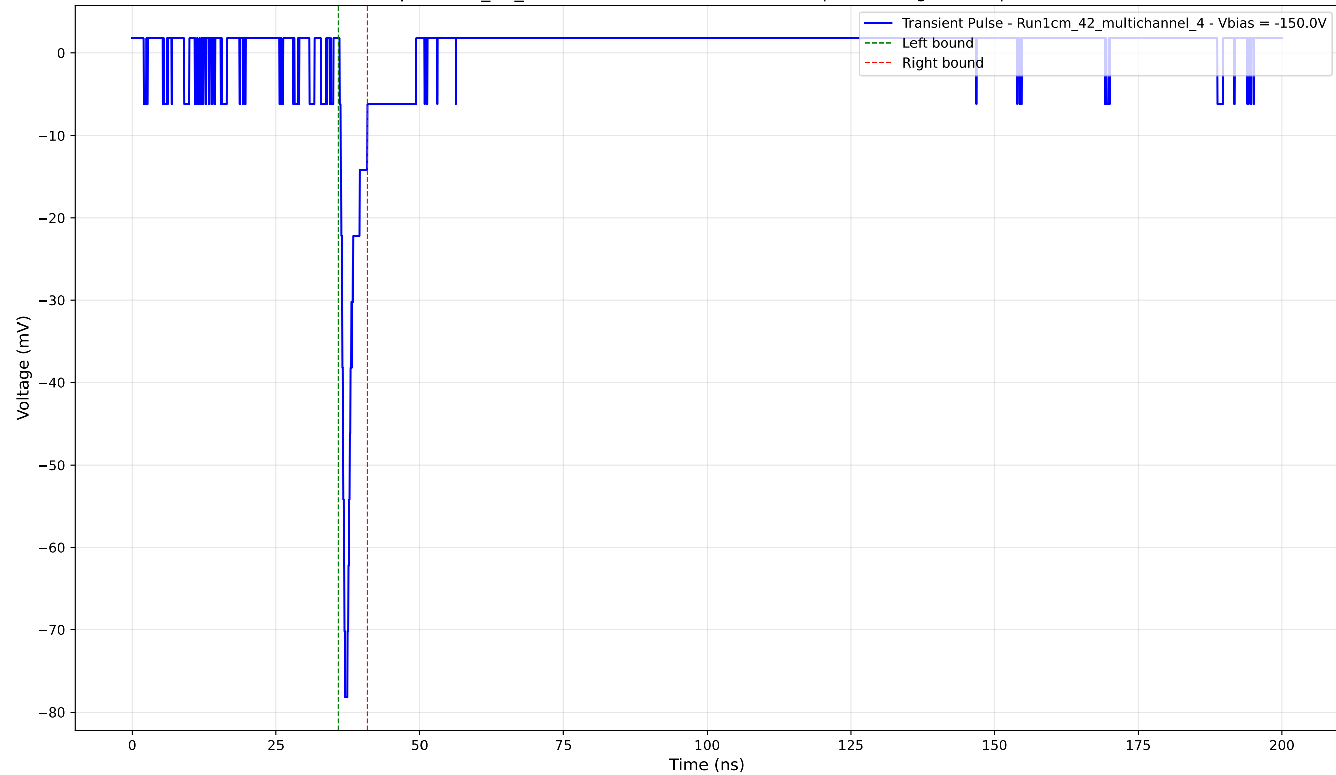
Transient Pulse - Sample: 1cm_42_multichannel - Position: 2300.0 \mu\text{m} - Charge: 3.10 pC - Rise Time: 0.80 ns
