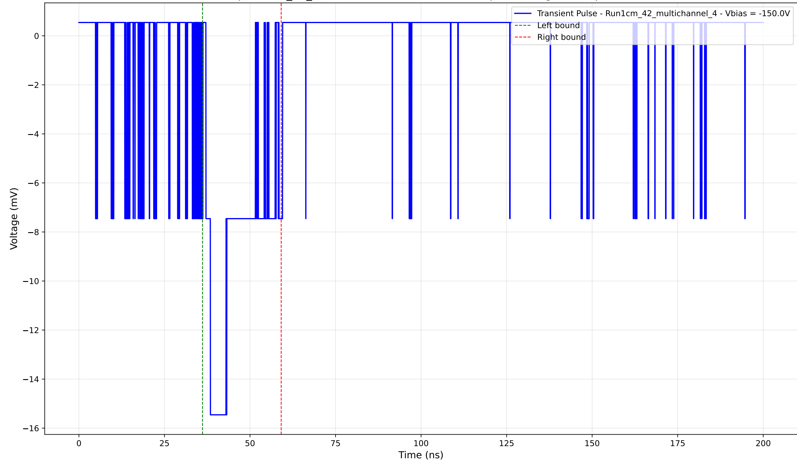
Transient Pulse - Sample: 1cm_42_multichannel - Position: 4325.0 \mu\text{m} - Charge: 3.72 pC - Rise Time: 1.32 ns
