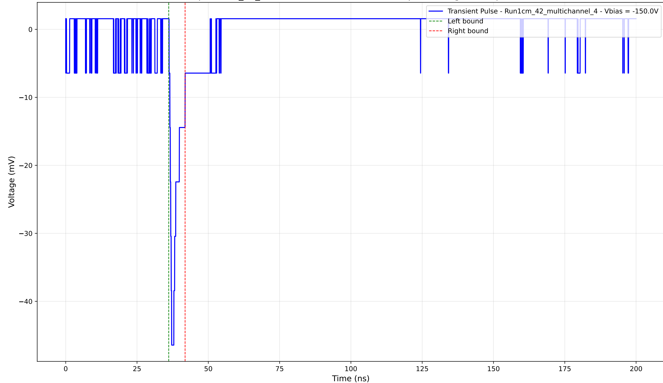
Transient Pulse - Sample: 1cm_42_multichannel - Position: 2805.0 \mu\text{m} - Charge: 2.68 pC - Rise Time: 0.91 ns
