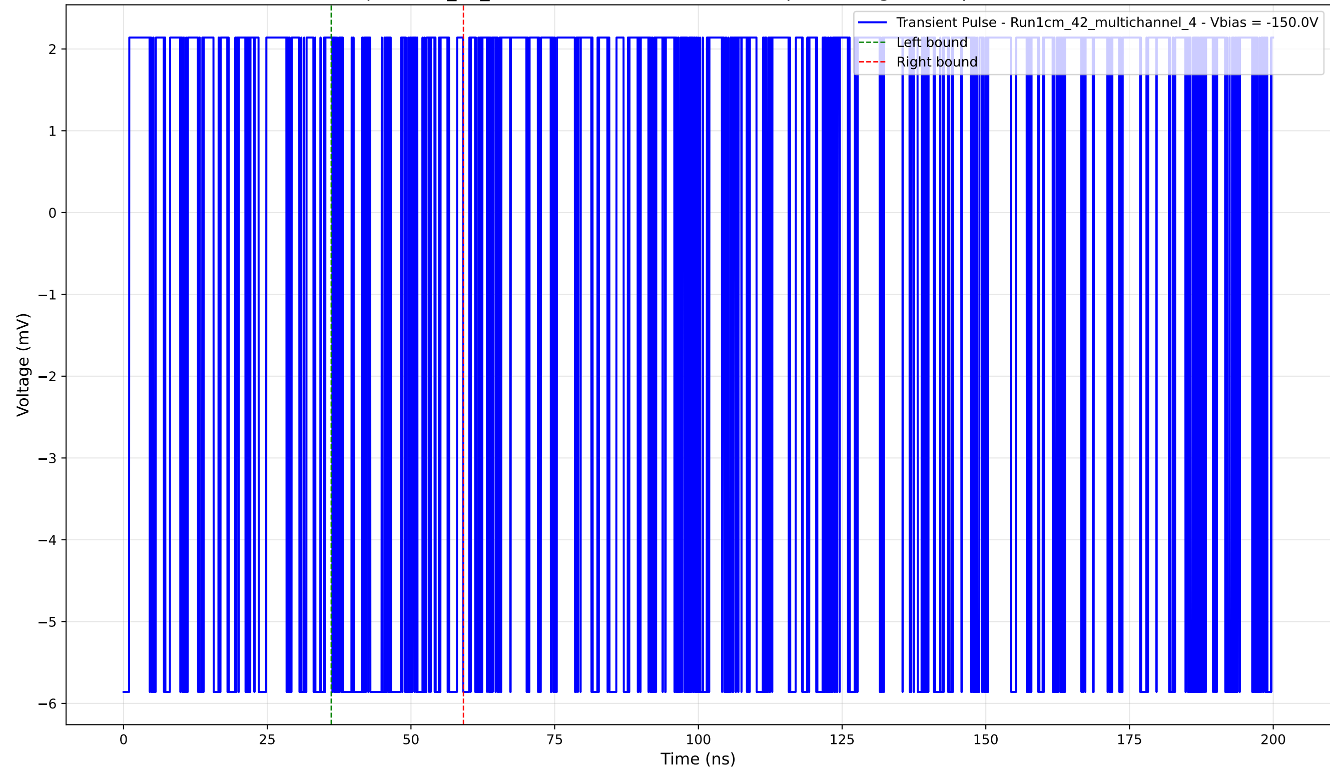
Transient Pulse - Sample: 1cm_42_multichannel - Position: 1355.0 \mu\text{m} - Charge: 1.28 pC - Rise Time: 0.00 ns (N/A)
