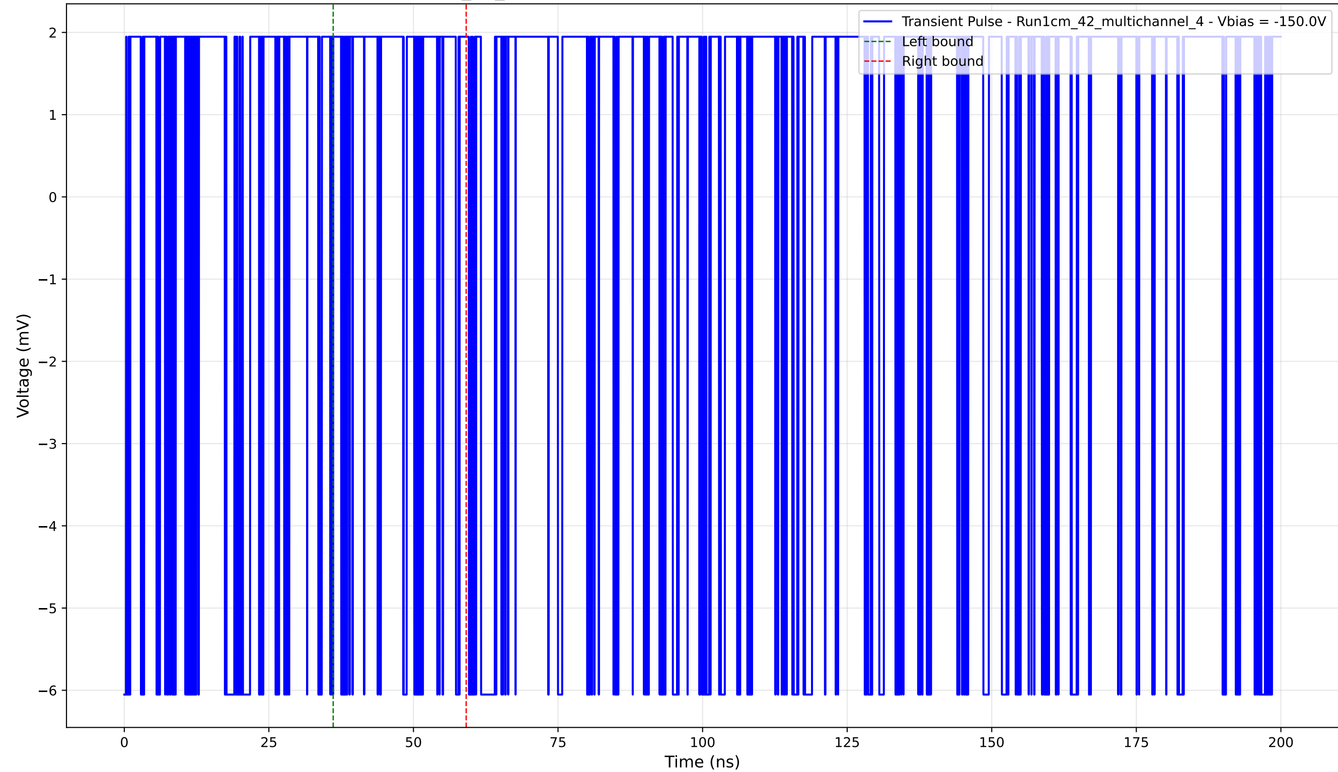
Transient Pulse - Sample: 1cm_42_multichannel - Position: 40.0 \mu\text{m} - Charge: 0.37 pC - Rise Time: 0.00 ns (N/A)
