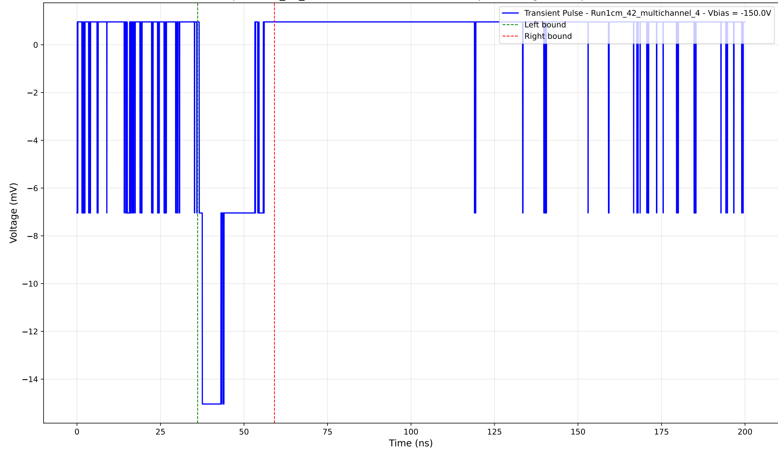
Transient Pulse - Sample: 1cm_42_multichannel - Position: 3750.0 \mu\text{m} - Charge: 3.44 pC - Rise Time: 0.94 ns
