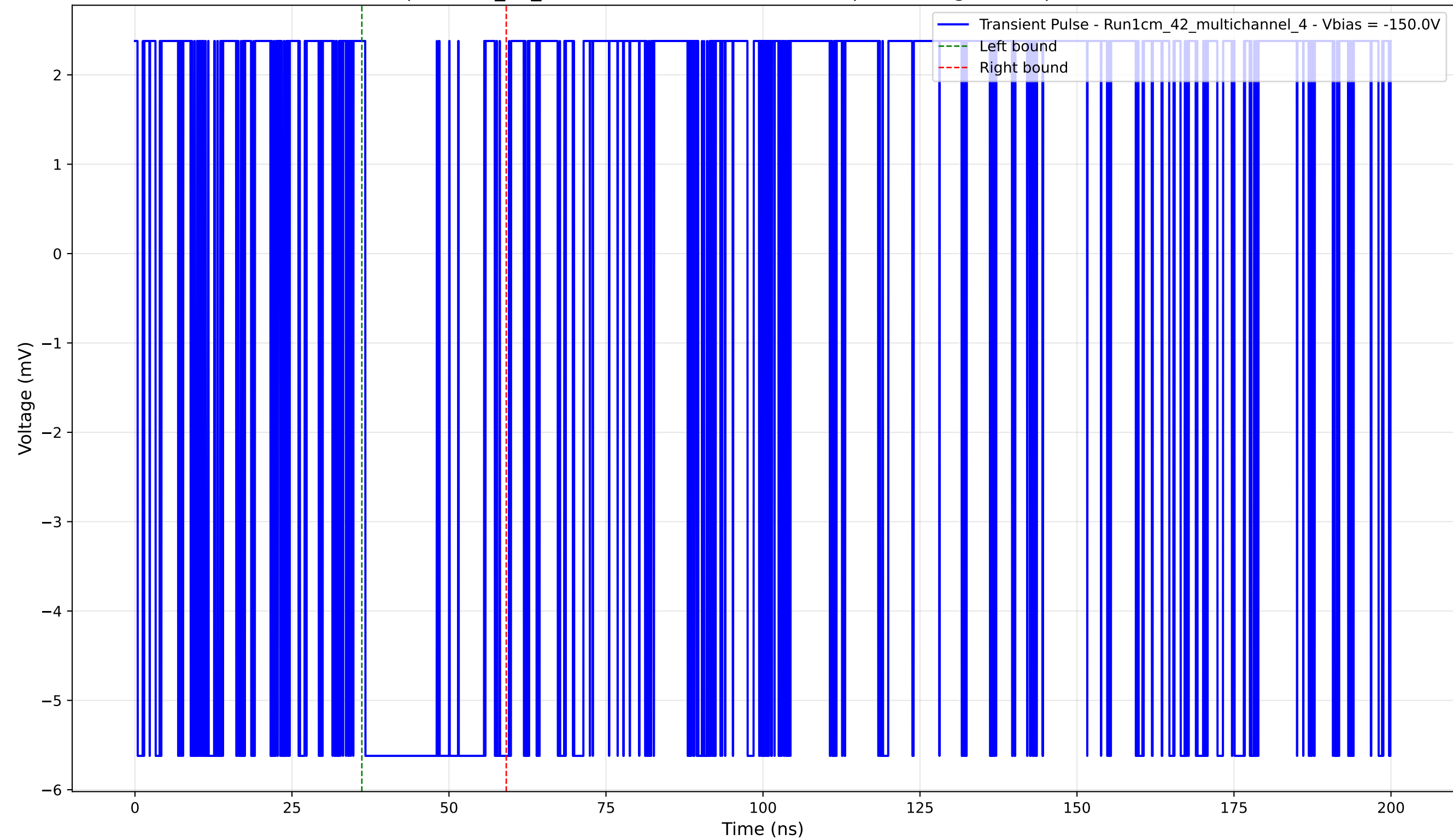
Transient Pulse - Sample: 1cm_42_multichannel - Position: 825.0 \mu\text{m} - Charge: 2.15 pC - Rise Time: 0.00 ns (N/A)
