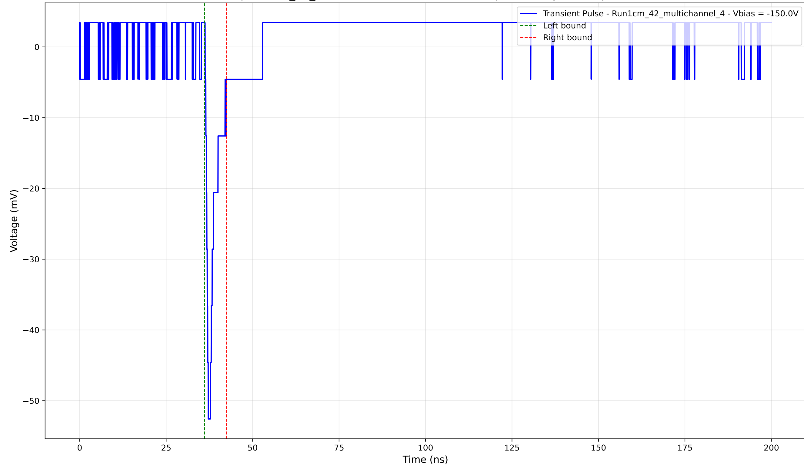
Transient Pulse - Sample: 1cm_42_multichannel - Position: 2015.0 \mu\text{m} - Charge: 2.83 pC - Rise Time: 0.70 ns
