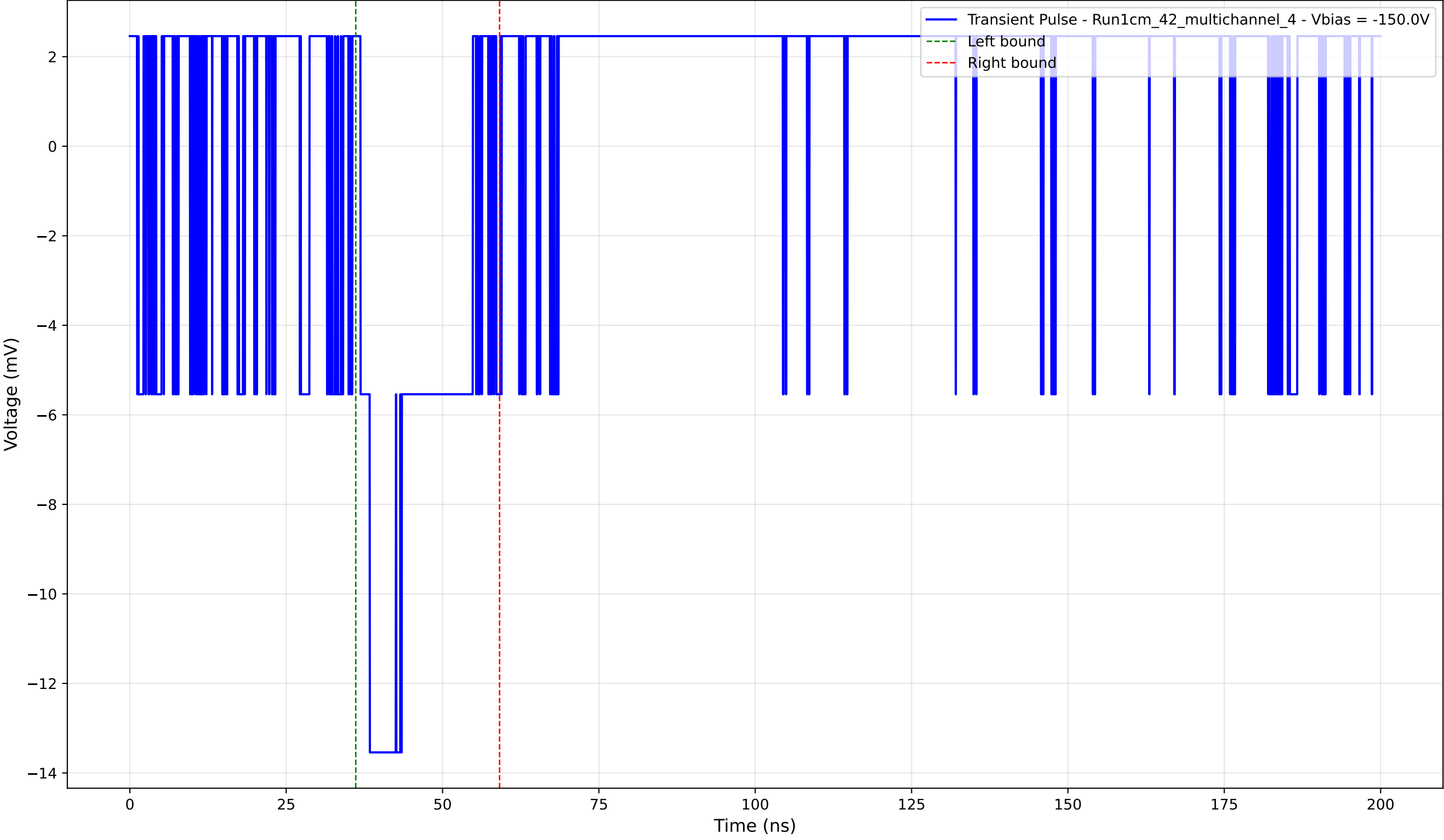
Transient Pulse - Sample: 1cm_42_multichannel - Position: 220.0 \mu\text{m} - Charge: 2.77 pC - Rise Time: 0.00 ns (N/A)
