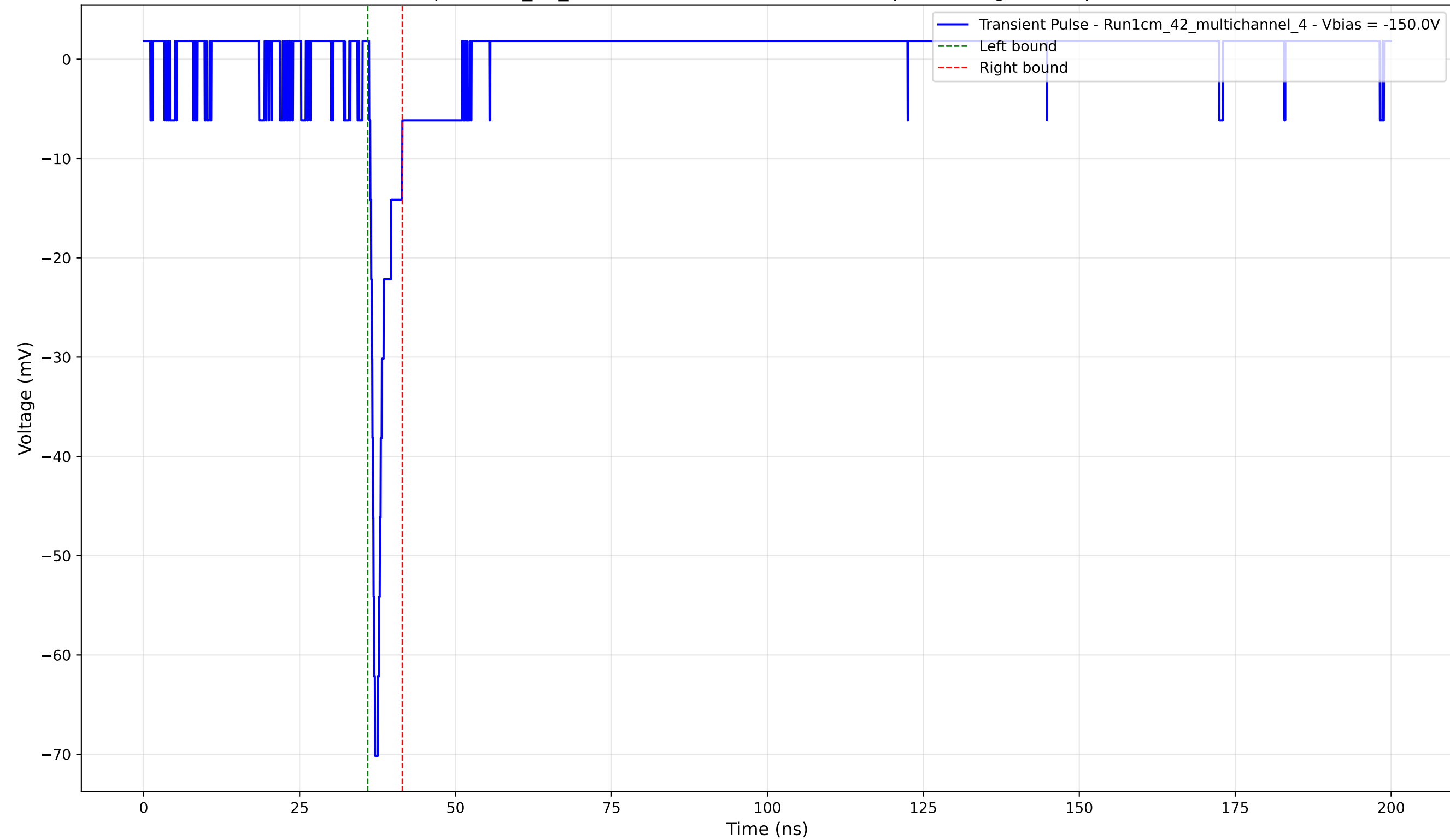
Transient Pulse - Sample: 1cm_42_multichannel - Position: 2565.0 \mu\text{m} - Charge: 3.10 pC - Rise Time: 0.78 ns
