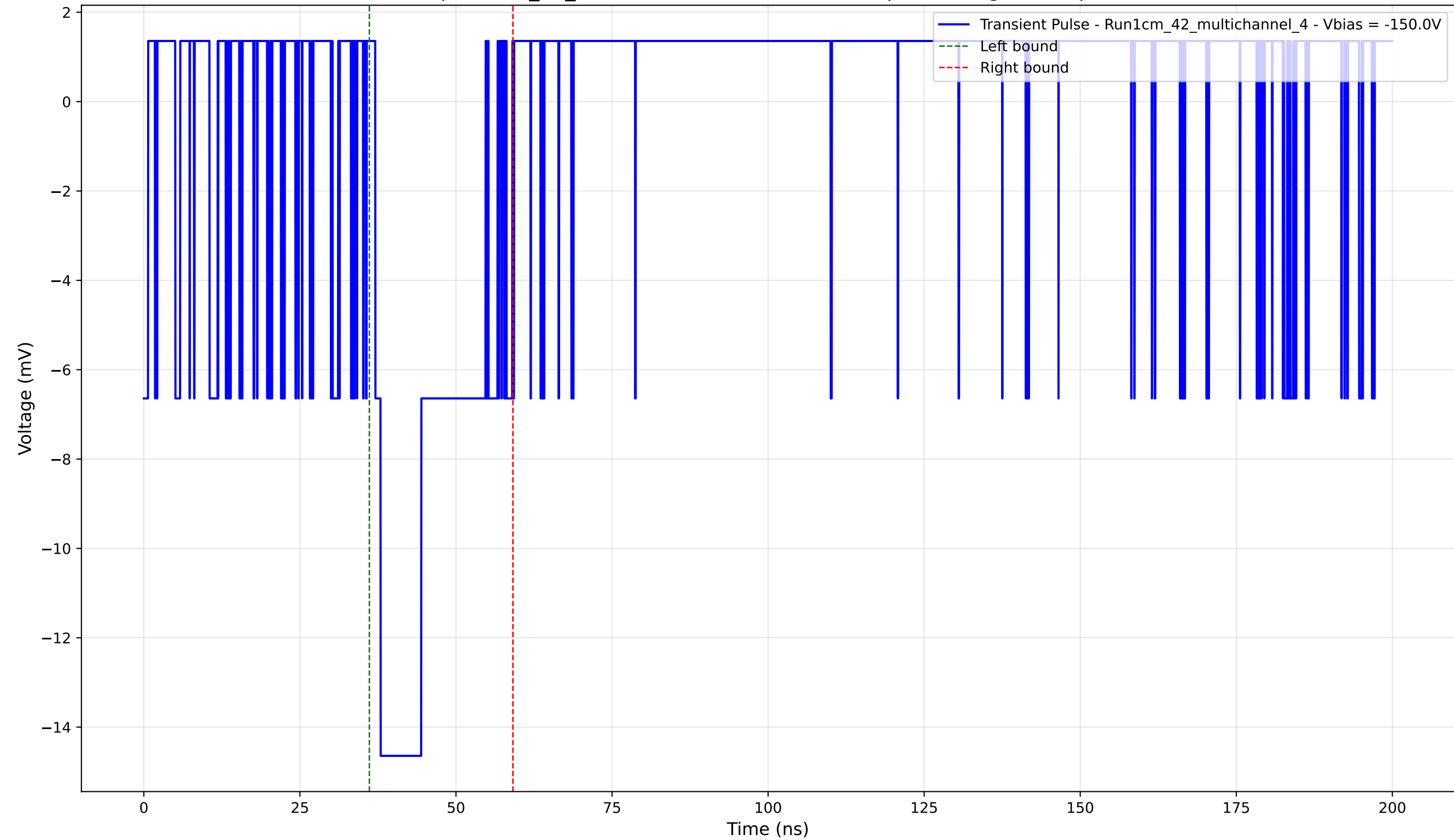
Transient Pulse - Sample: 1cm_42_multichannel - Position: 640.0 \mu\text{m} - Charge: 3.76 pC - Rise Time: 0.86 ns
