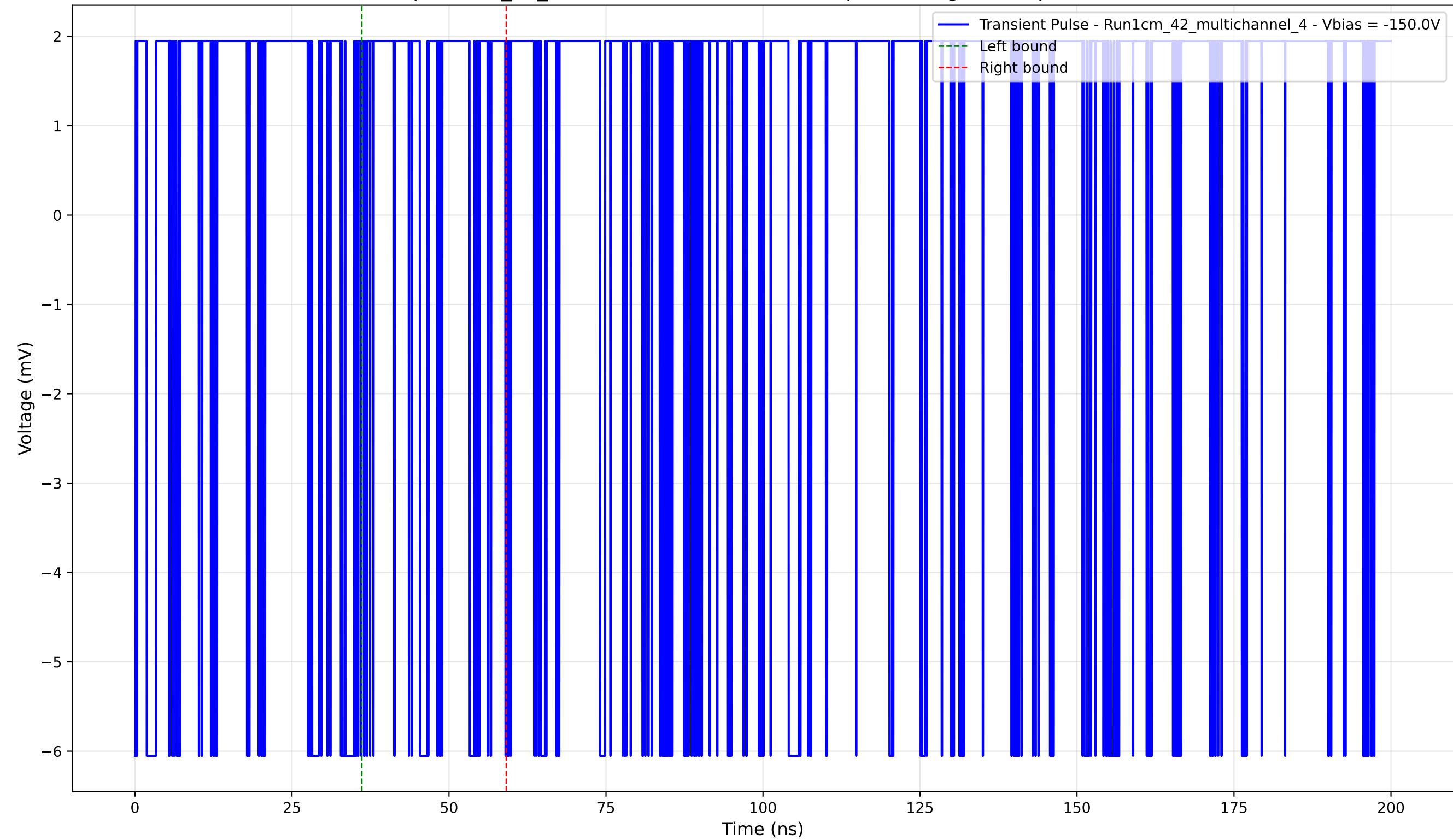
Transient Pulse - Sample: 1cm_42_multichannel - Position: 30.0 \mu\text{m} - Charge: 0.29 pC - Rise Time: 0.00 ns (N/A)
