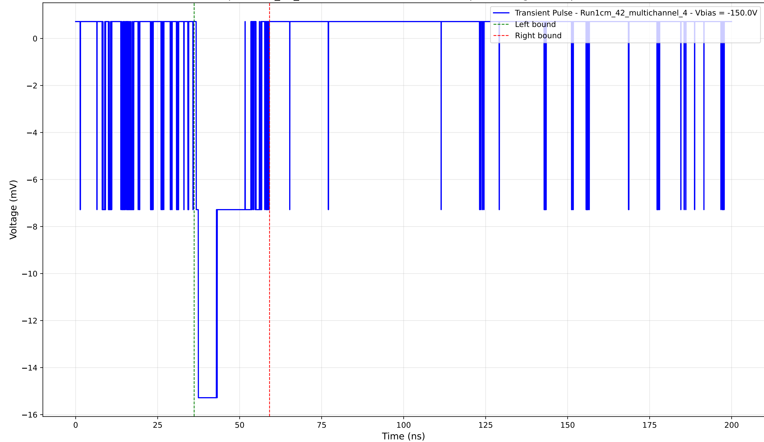
Transient Pulse - Sample: 1cm_42_multichannel - Position: 3610.0 \mu\text{m} - Charge: 3.60 pC - Rise Time: 0.66 ns
