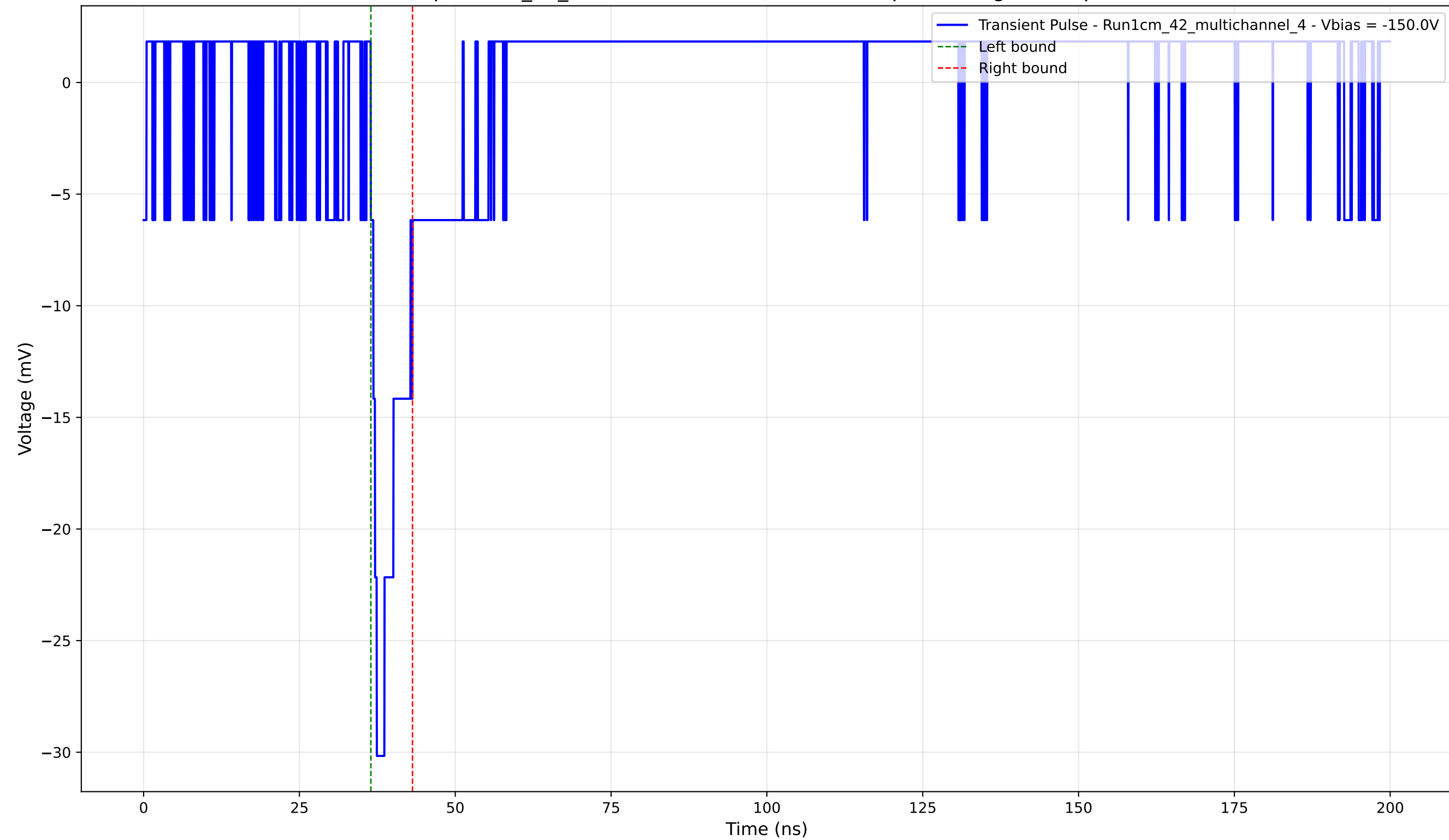
Transient Pulse - Sample: 1cm_42_multichannel - Position: 1580.0 \mu\text{m} - Charge: 2.47 pC - Rise Time: 0.97 ns
