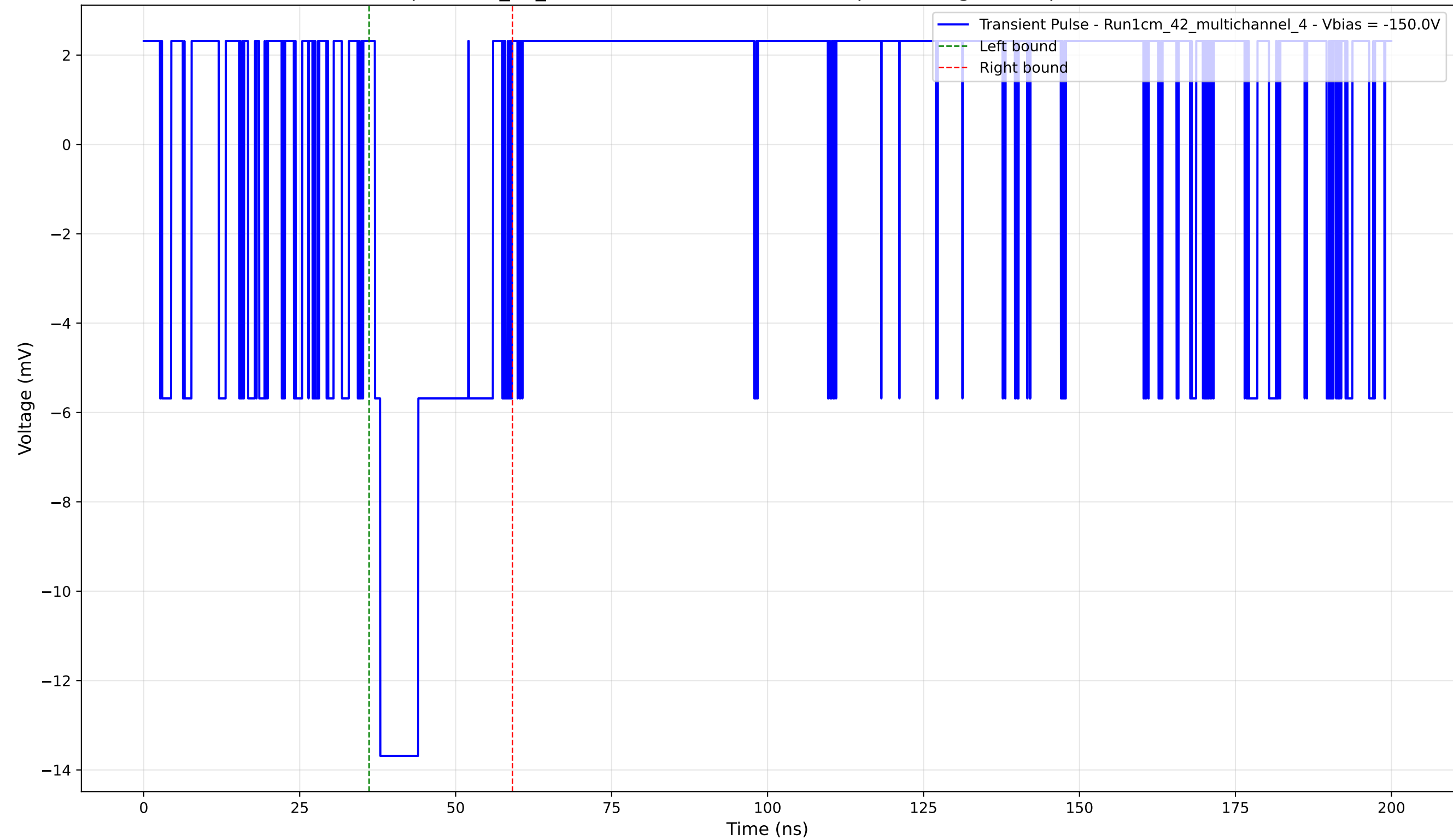
Transient Pulse - Sample: 1cm_42_multichannel - Position: 590.0 \mu\text{m} - Charge: 3.11 pC - Rise Time: 0.00 ns (N/A)
