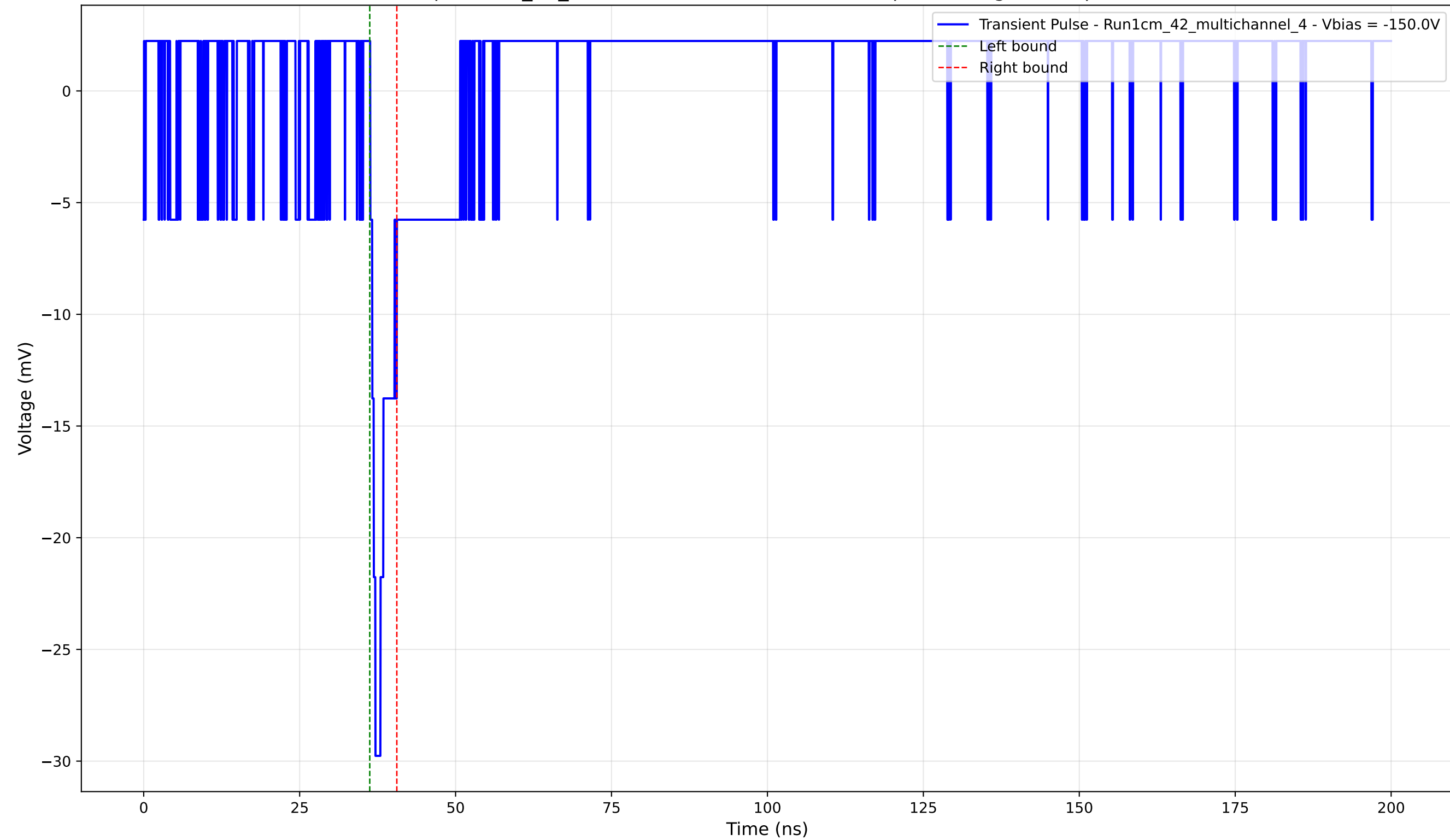
Transient Pulse - Sample: 1cm_42_multichannel - Position: 2835.0 \mu\text{m} - Charge: 1.47 pC - Rise Time: 0.84 ns
