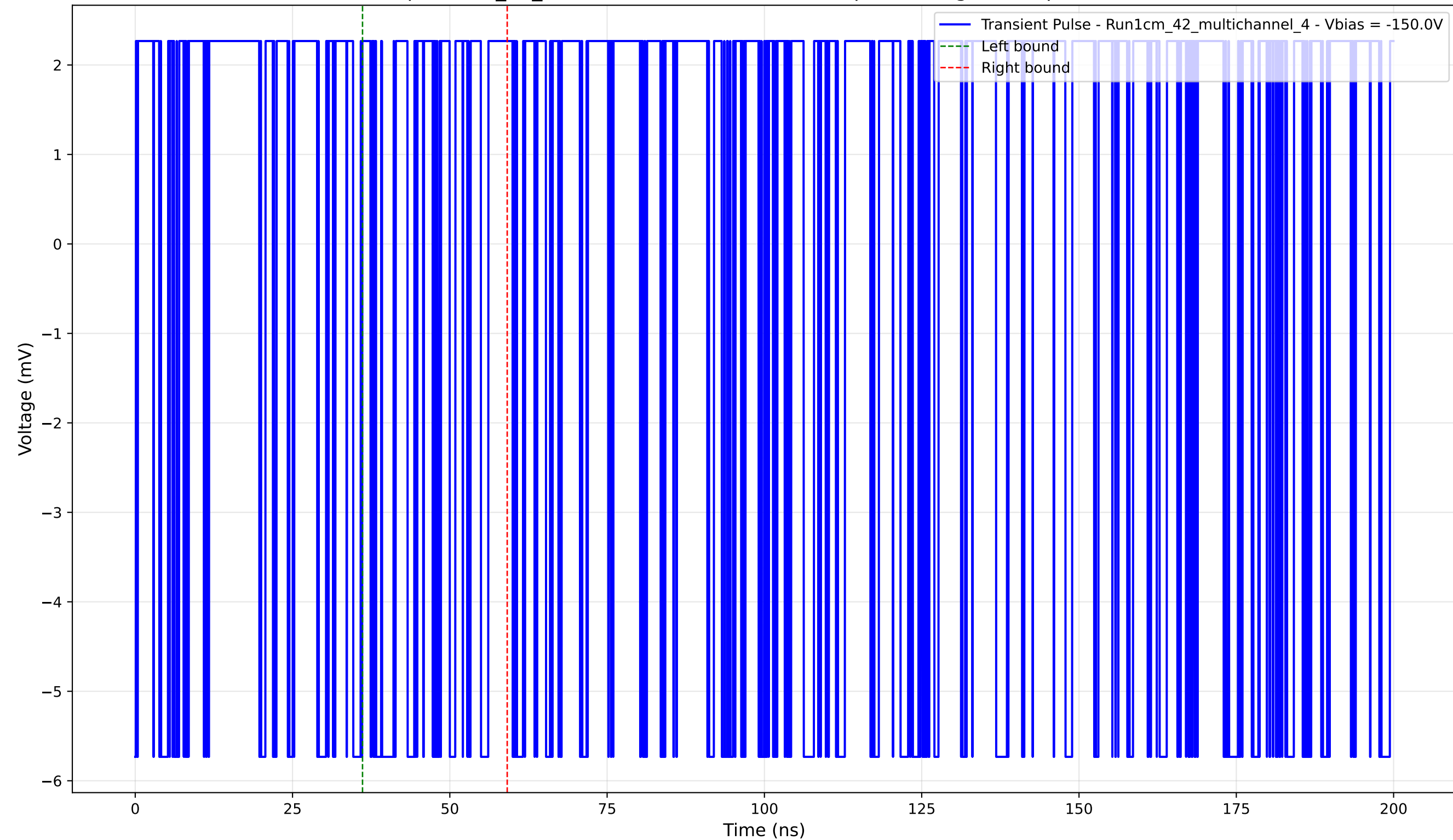
Transient Pulse - Sample: 1cm_42_multichannel - Position: 885.0 \mu\text{m} - Charge: 0.23 pC - Rise Time: 0.00 ns (N/A)
