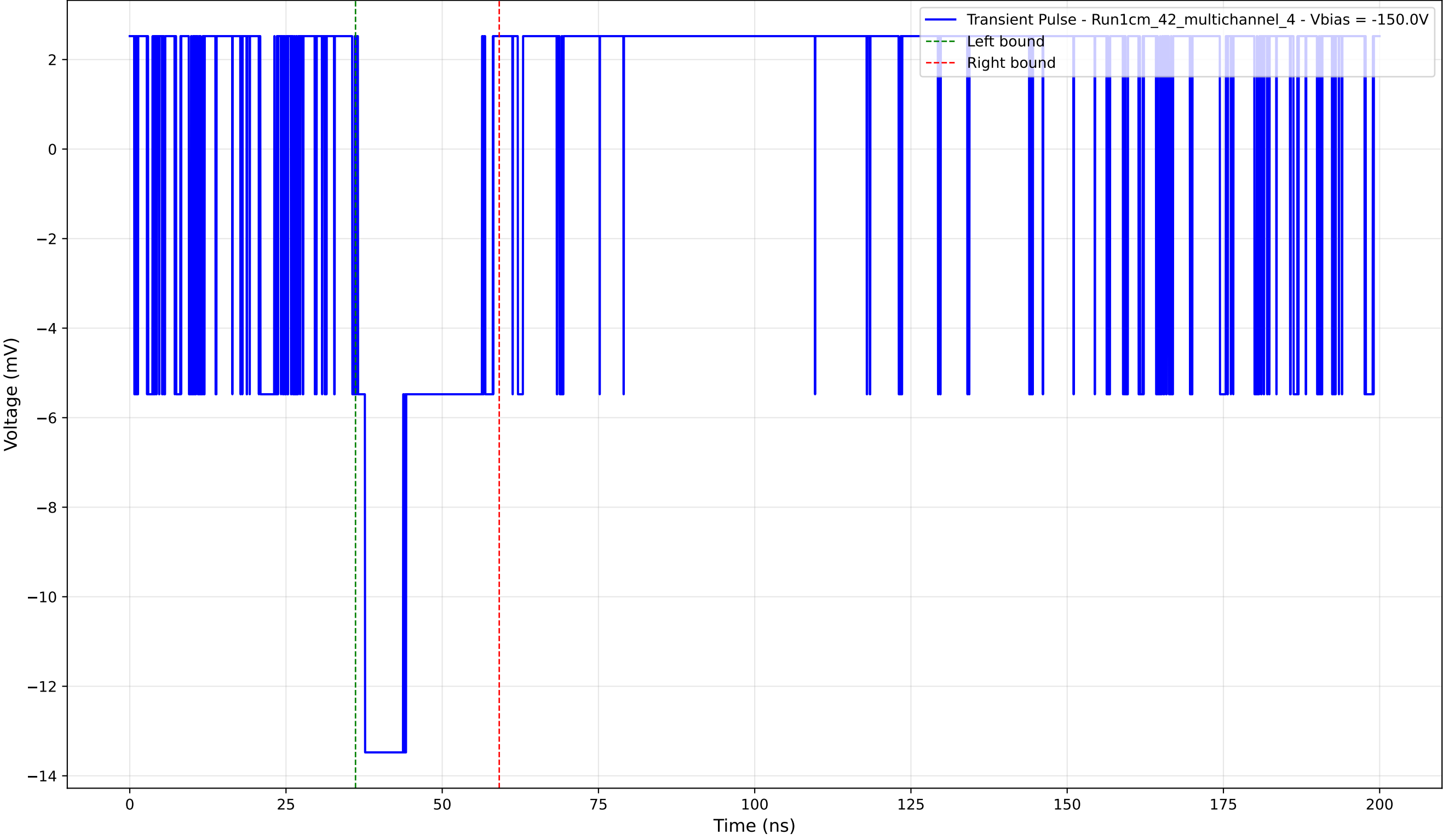
Transient Pulse - Sample: 1cm_42_multichannel - Position: 940.0 \mu\text{m} - Charge: 3.30 pC - Rise Time: 0.00 ns (N/A)
