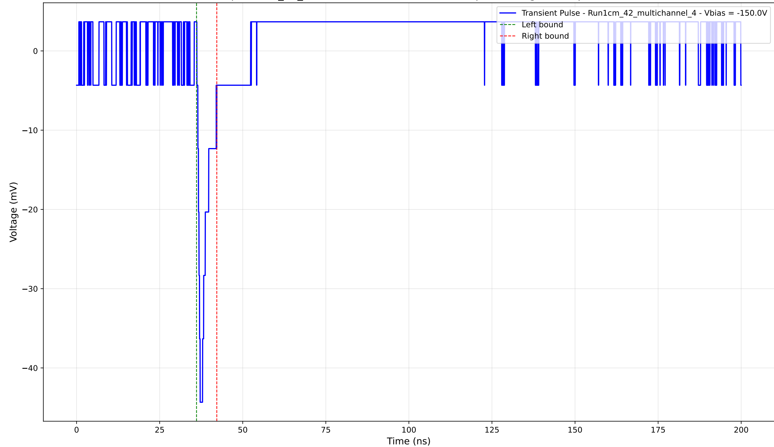
Transient Pulse - Sample: 1cm_42_multichannel - Position: 1955.0 \mu\text{m} - Charge: 2.53 pC - Rise Time: 0.70 ns
