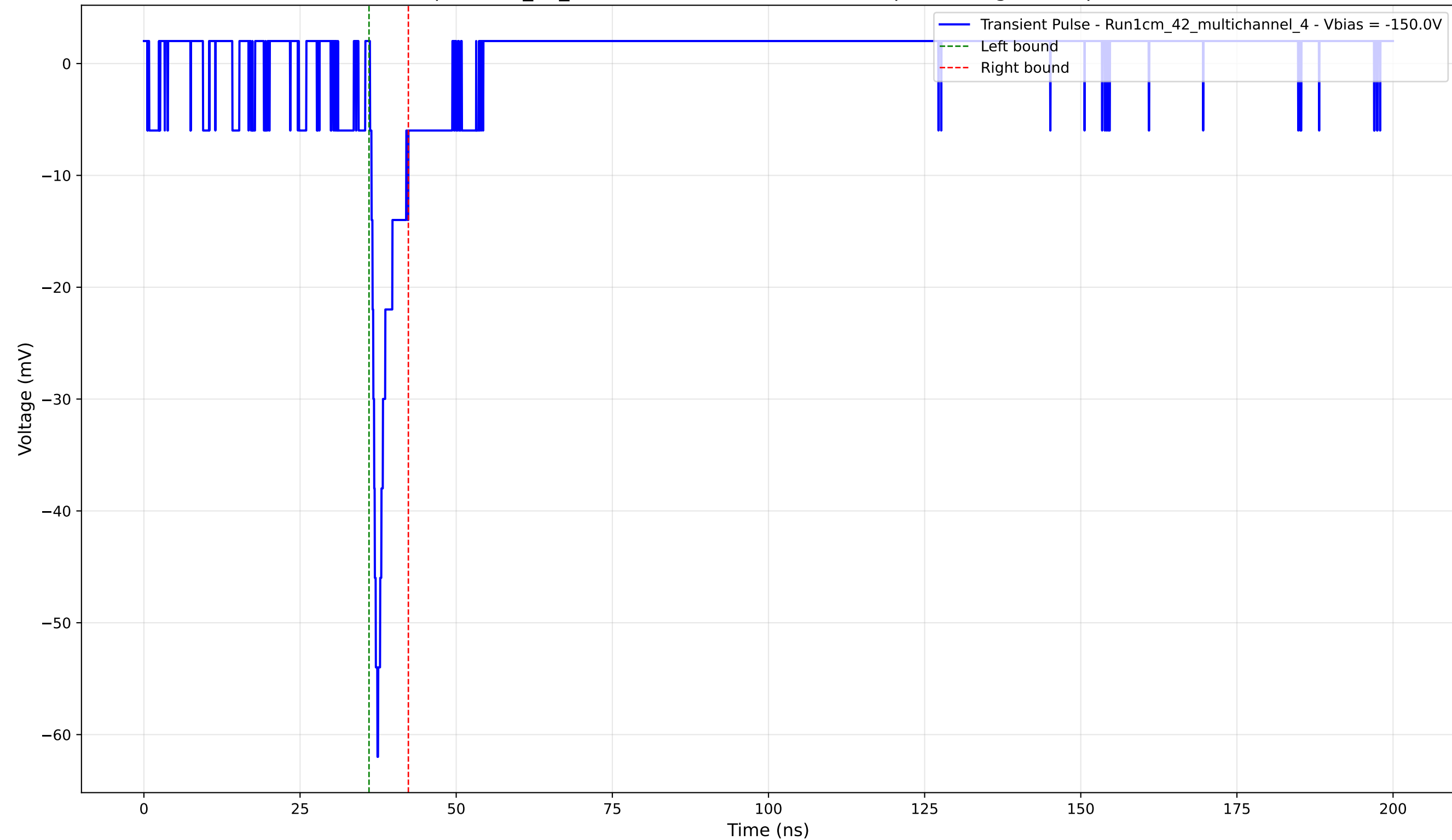
Transient Pulse - Sample: 1cm_42_multichannel - Position: 2040.0 \mu\text{m} - Charge: 2.98 pC - Rise Time: 0.96 ns
