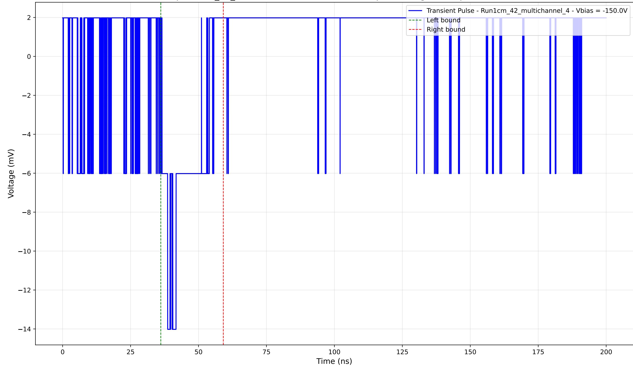
Transient Pulse - Sample: 1cm_42_multichannel - Position: 4820.0 \mu\text{m} - Charge: 2.30 pC - Rise Time: 0.00 ns (N/A)
