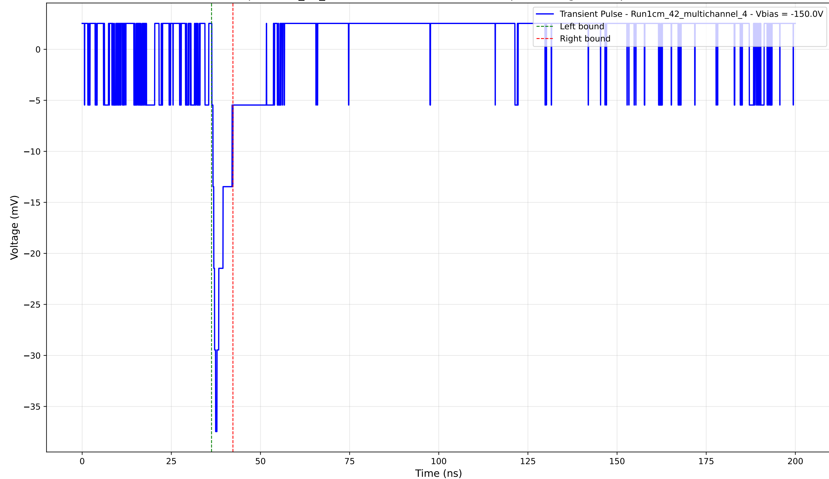
Transient Pulse - Sample: 1cm_42_multichannel - Position: 1815.0 \mu\text{m} - Charge: 2.19 pC - Rise Time: 1.07 ns
