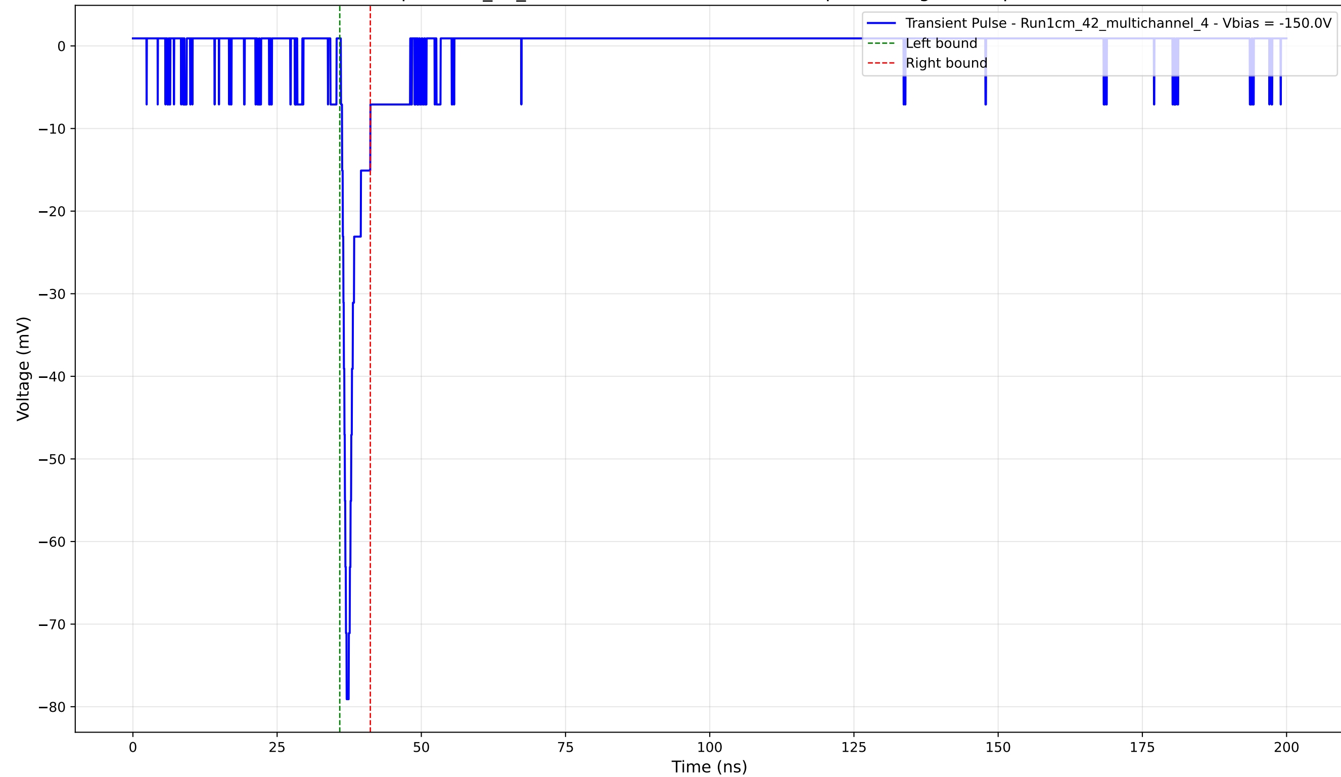
Transient Pulse - Sample: 1cm_42_multichannel - Position: 2305.0 \mu\text{m} - Charge: 3.25 pC - Rise Time: 0.80 ns
