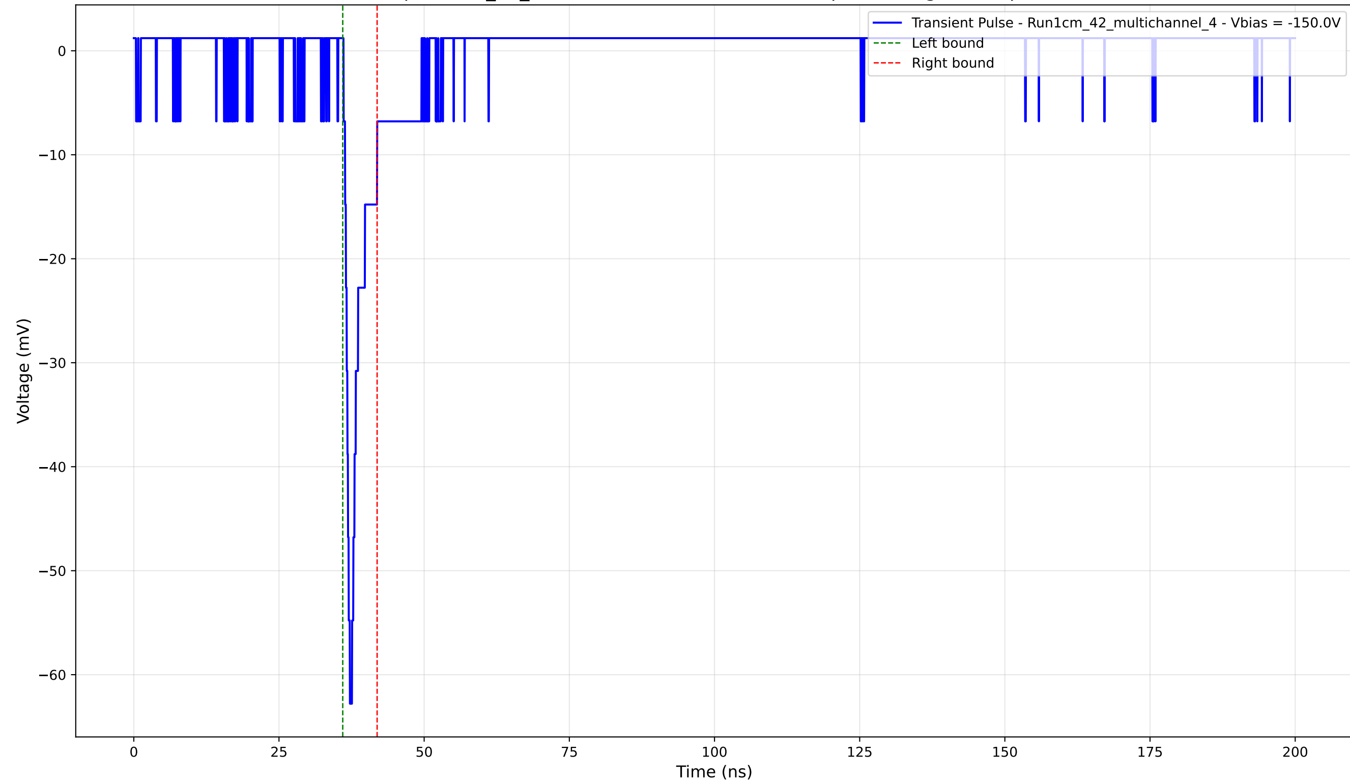
Transient Pulse - Sample: 1cm_42_multichannel - Position: 2115.0 \mu\text{m} - Charge: 3.10 pC - Rise Time: 1.08 ns
