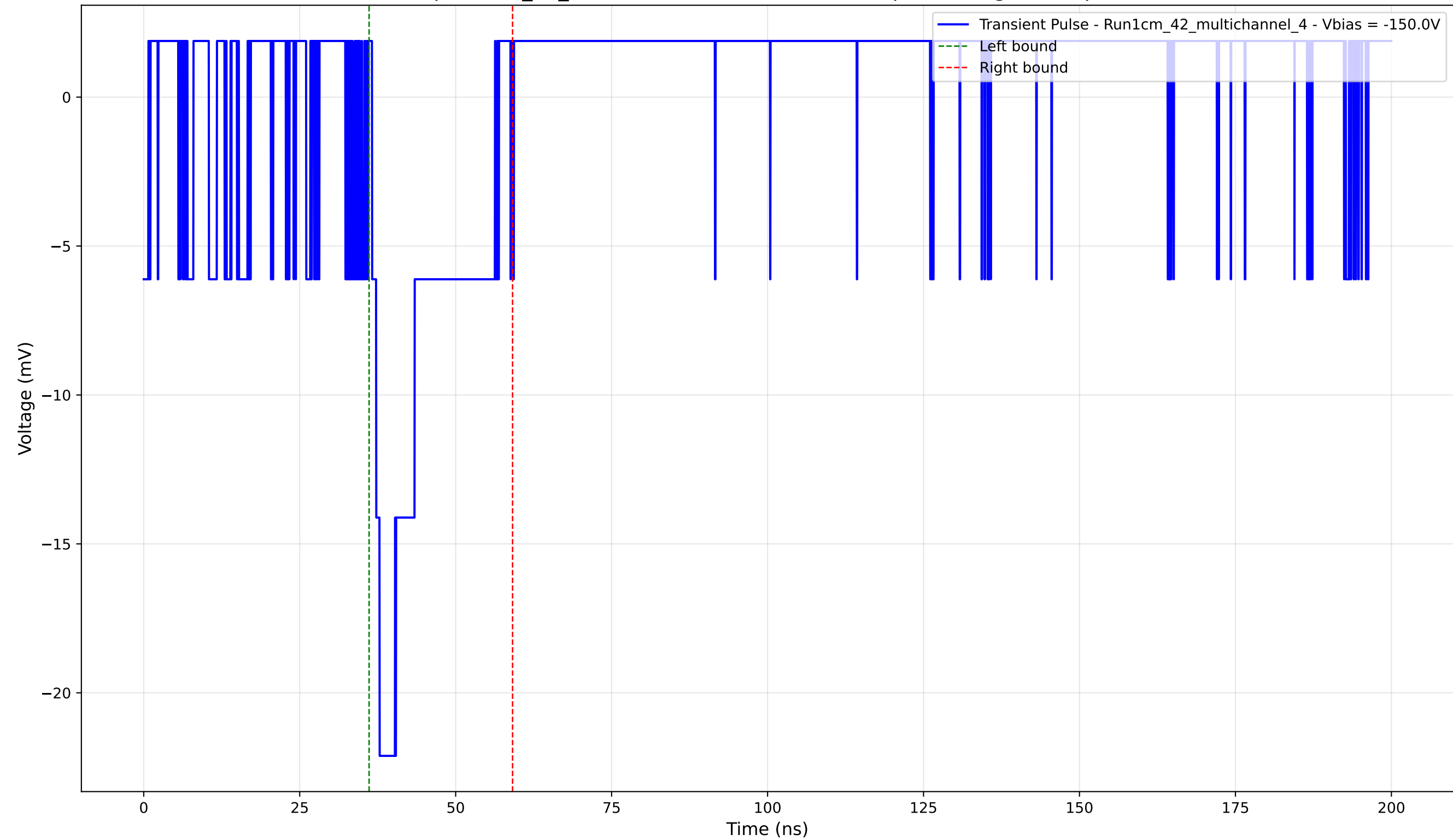
Transient Pulse - Sample: 1cm_42_multichannel - Position: 1185.0 \mu\text{m} - Charge: 3.76 pC - Rise Time: 1.22 ns
