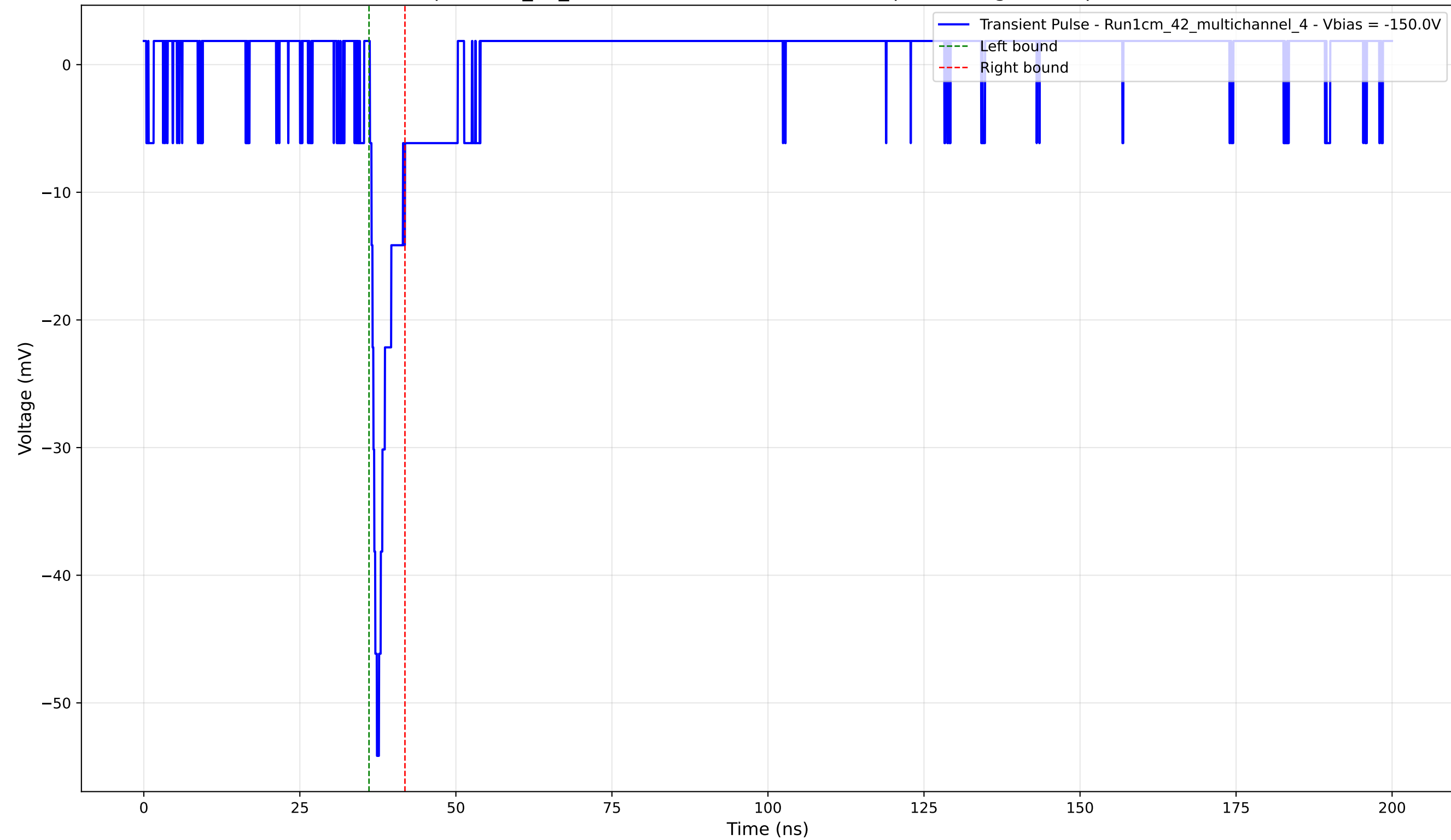
Transient Pulse - Sample: 1cm_42_multichannel - Position: 2770.0 \mu\text{m} - Charge: 2.70 pC - Rise Time: 1.12 ns
