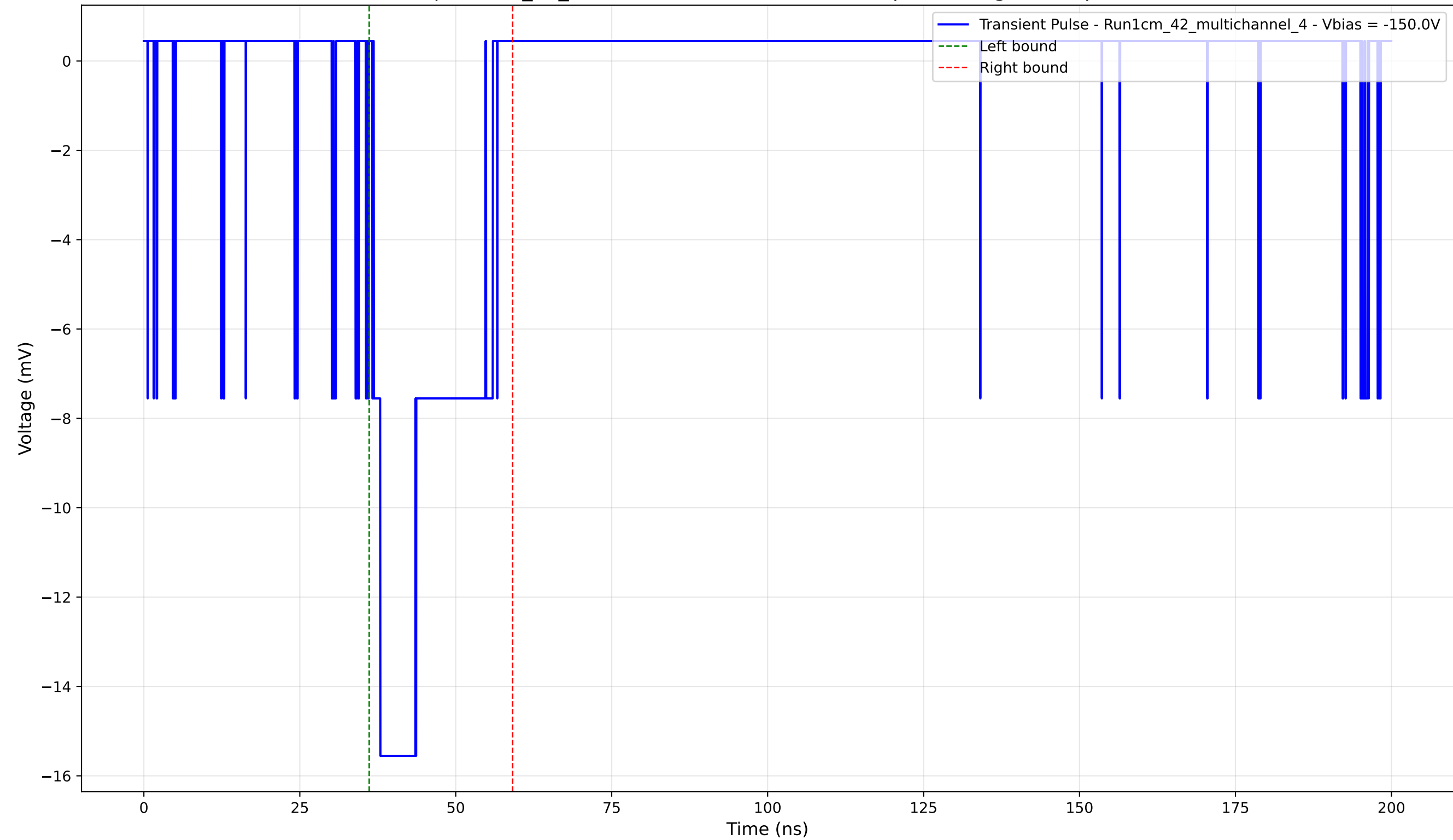
Transient Pulse - Sample: 1cm_42_multichannel - Position: 4000.0 \mu\text{m} - Charge: 3.78 pC - Rise Time: 1.06 ns
