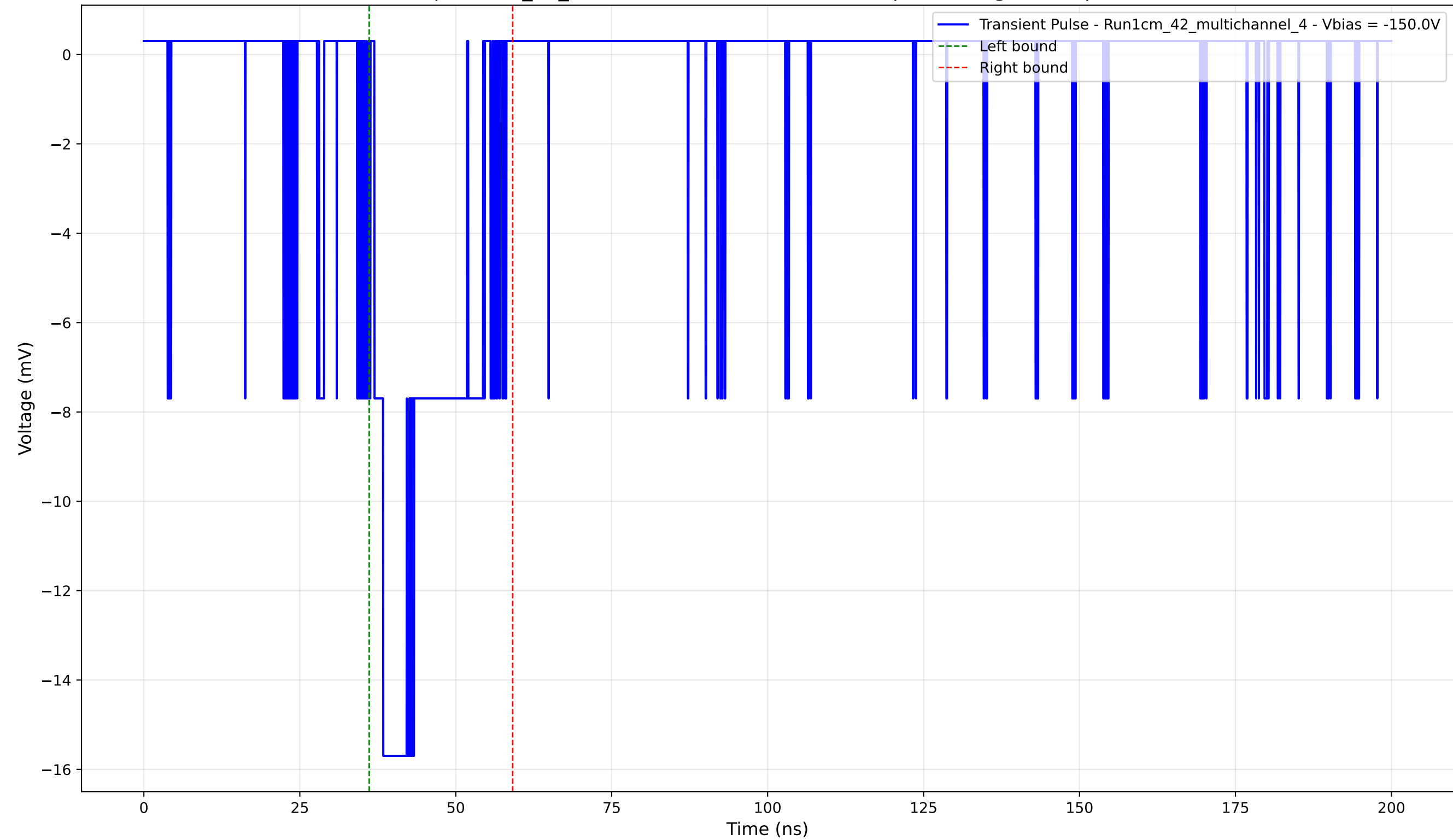
Transient Pulse - Sample: 1cm_42_multichannel - Position: 4755.0 \mu\text{m} - Charge: 3.57 pC - Rise Time: 1.42 ns
