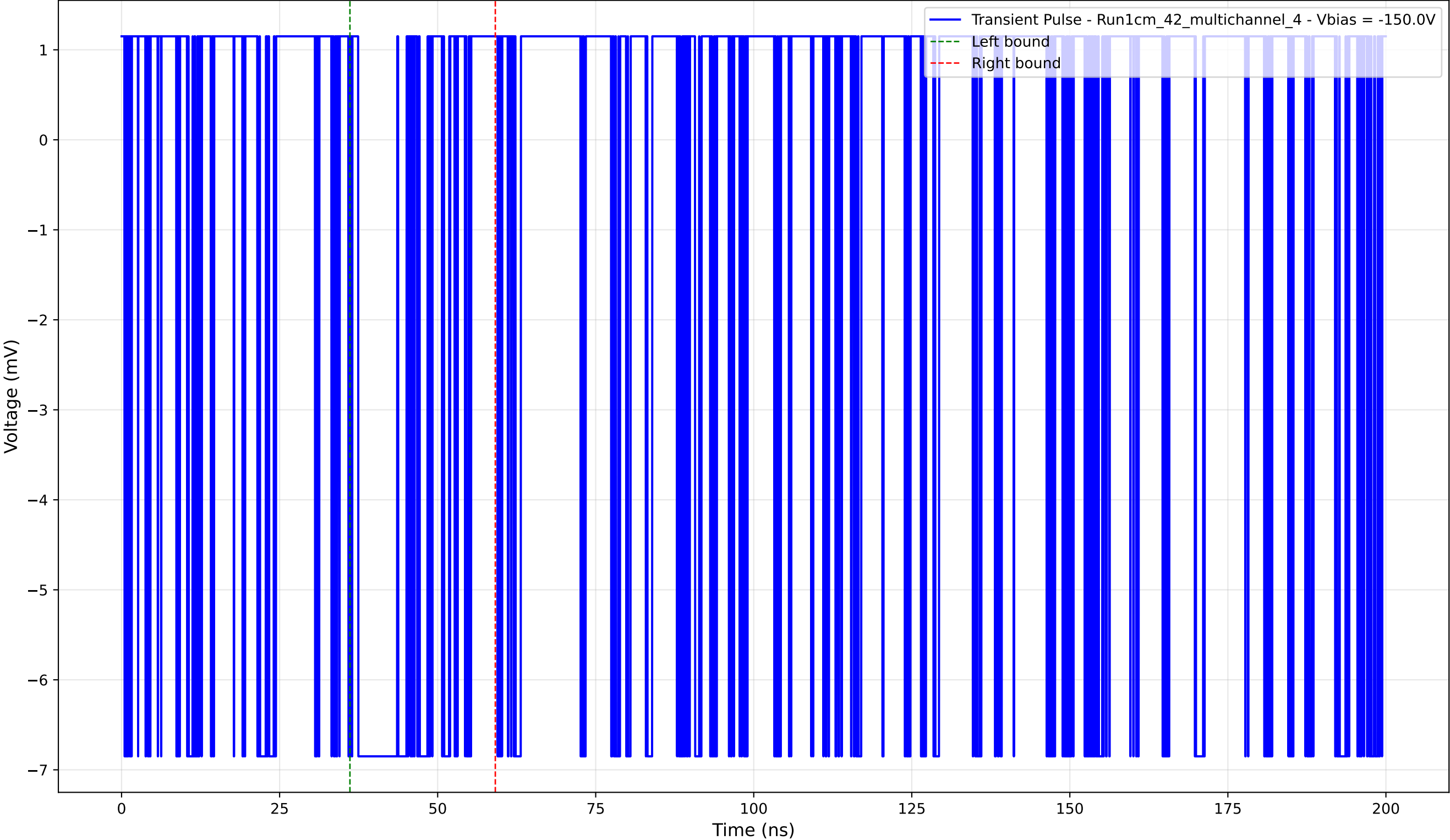
Transient Pulse - Sample: 1cm_42_multichannel - Position: 4435.0 \mu\text{m} - Charge: 1.32 pC - Rise Time: 0.00 ns (N/A)
