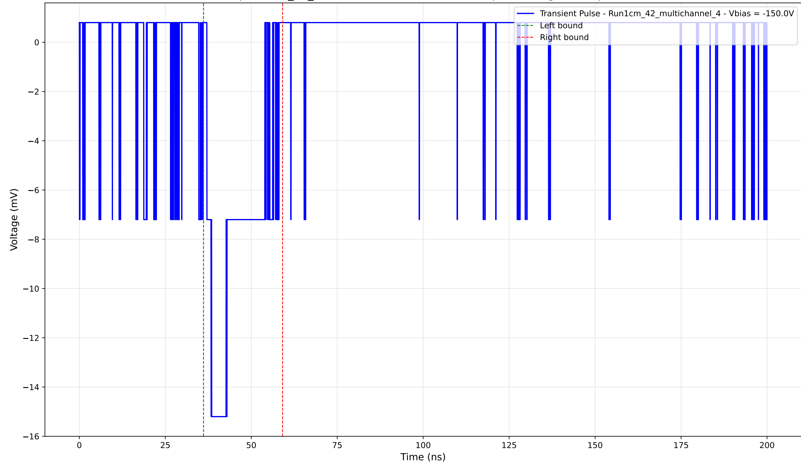
Transient Pulse - Sample: 1cm_42_multichannel - Position: 4505.0 \mu\text{m} - Charge: 3.38 pC - Rise Time: 1.24 ns
