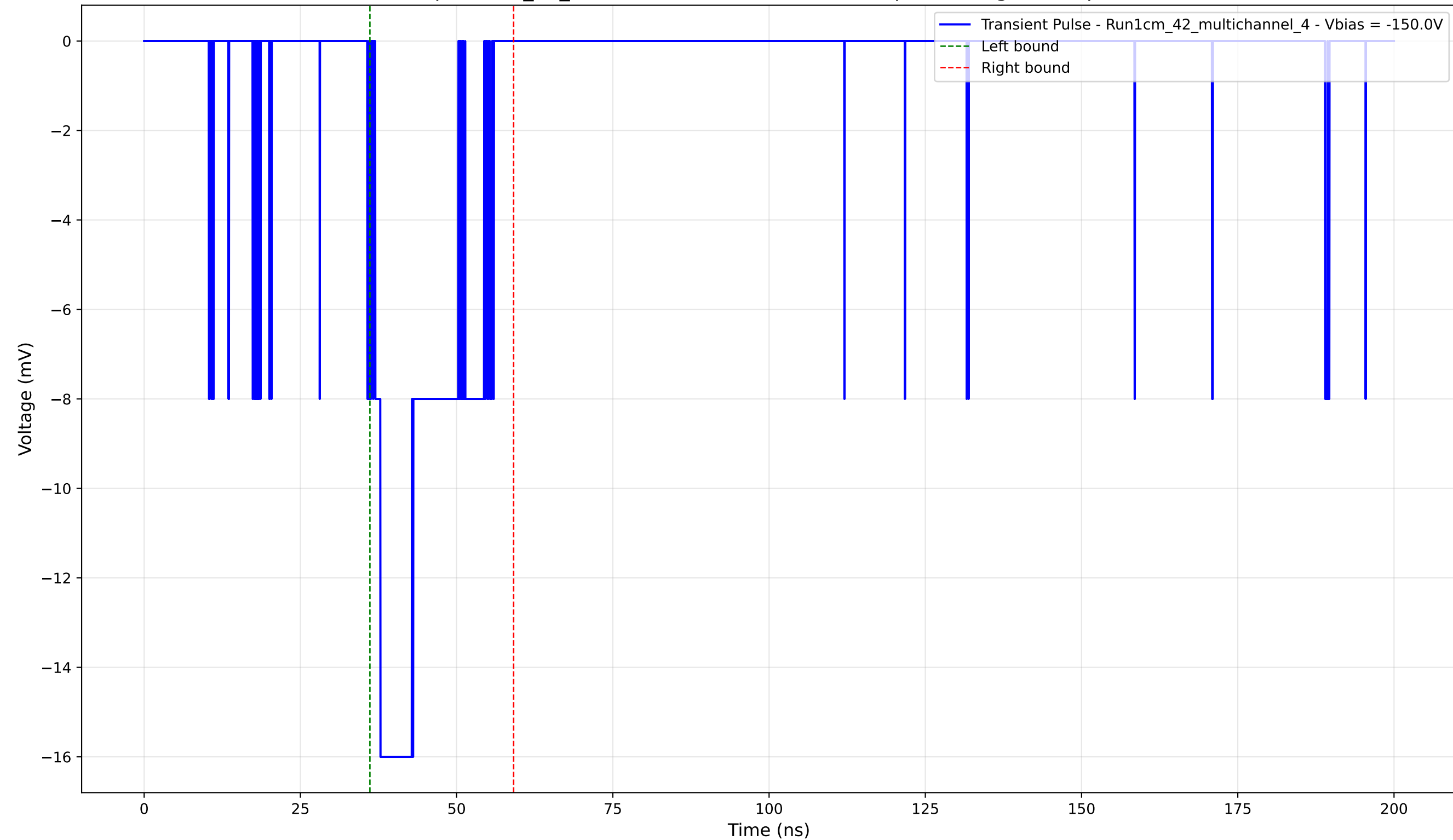
Transient Pulse - Sample: 1cm_42_multichannel - Position: 3825.0 \mu\text{m} - Charge: 3.71 pC - Rise Time: 0.84 ns
