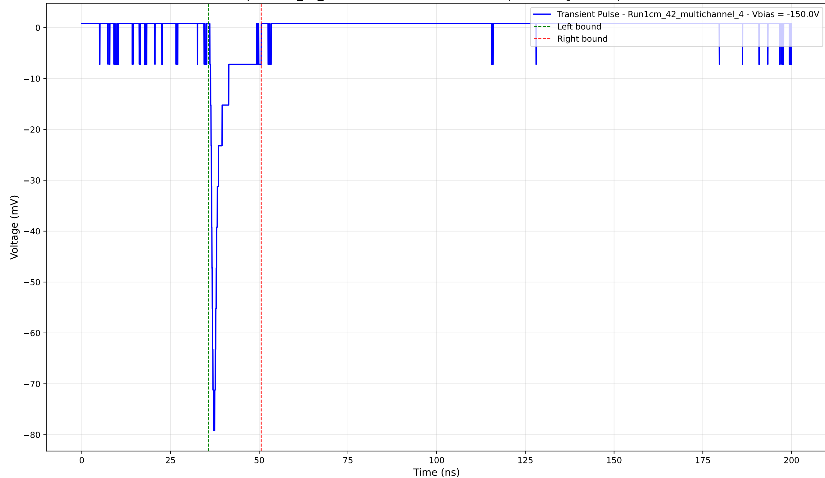
Transient Pulse - Sample: 1cm_42_multichannel - Position: 2510.0 \mu\text{m} - Charge: 4.62 pC - Rise Time: 0.82 ns
