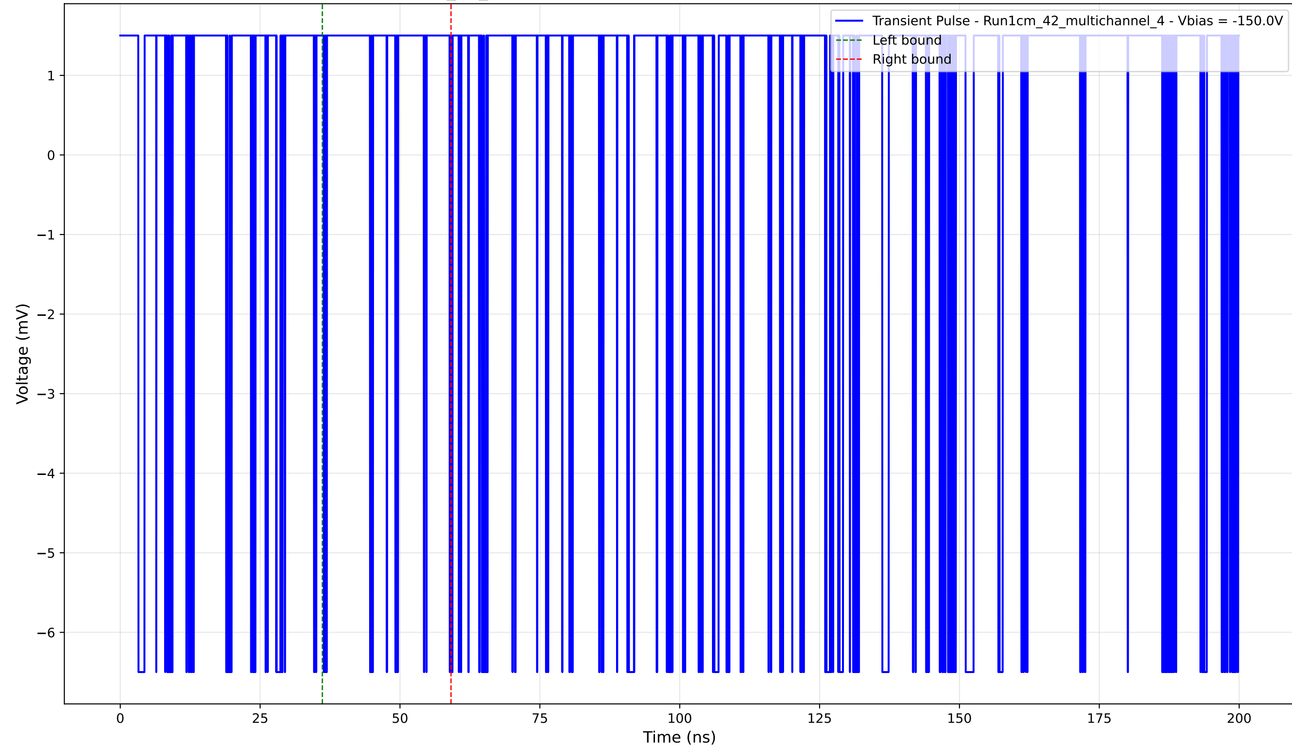
Transient Pulse - Sample: 1cm_42_multichannel - Position: 45.0 \mu\text{m} - Charge: 0.42 pC - Rise Time: 0.00 ns (N/A)
