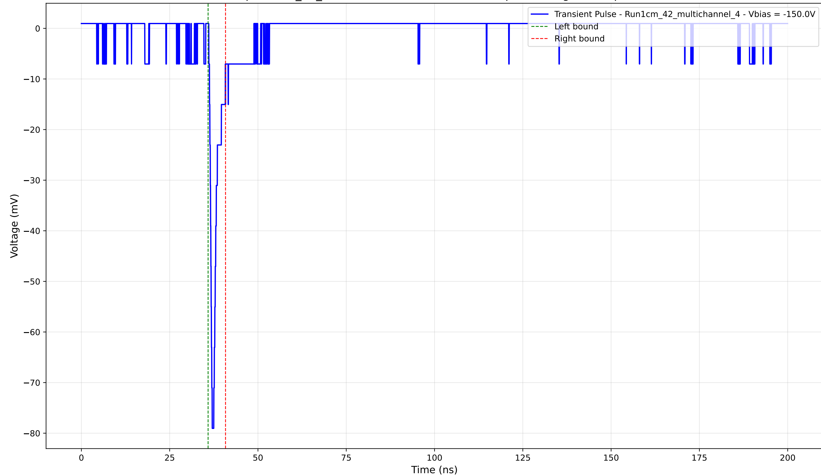
Transient Pulse - Sample: 1cm_42_multichannel - Position: 2495.0 \mu\text{m} - Charge: 3.23 pC - Rise Time: 0.78 ns
