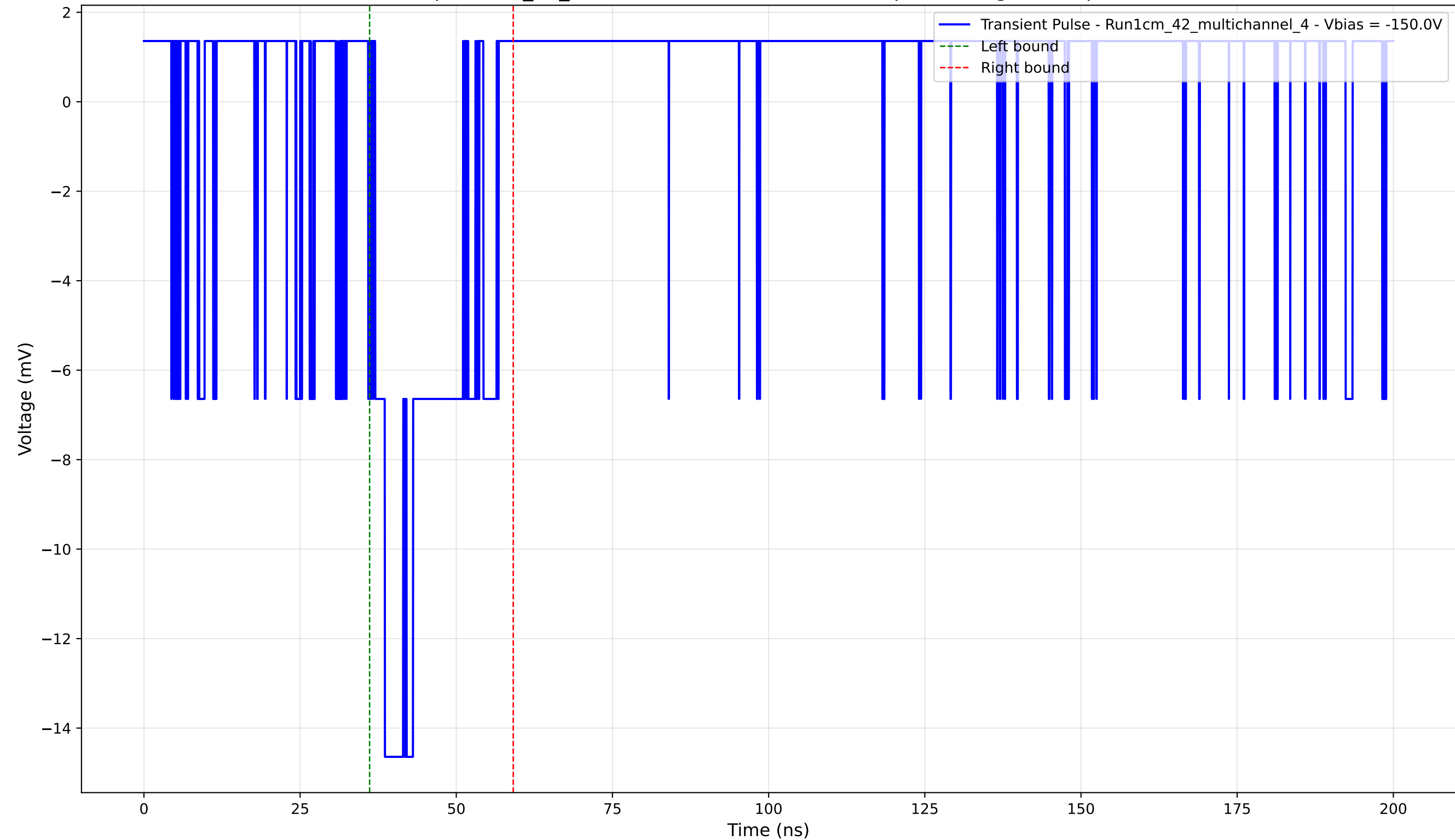
Transient Pulse - Sample: 1cm_42_multichannel - Position: 4485.0 \mu\text{m} - Charge: 2.97 pC - Rise Time: 1.56 ns
