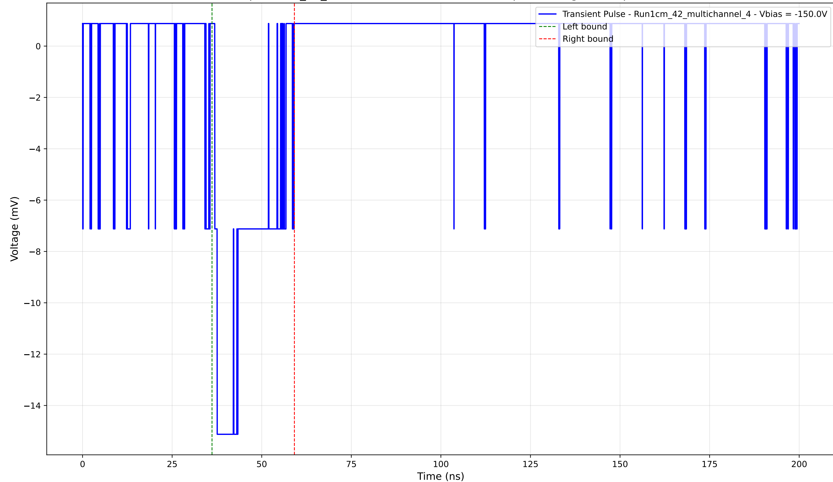
Transient Pulse - Sample: 1cm_42_multichannel - Position: 3725.0 \mu\text{m} - Charge: 3.61 pC - Rise Time: 0.68 ns
