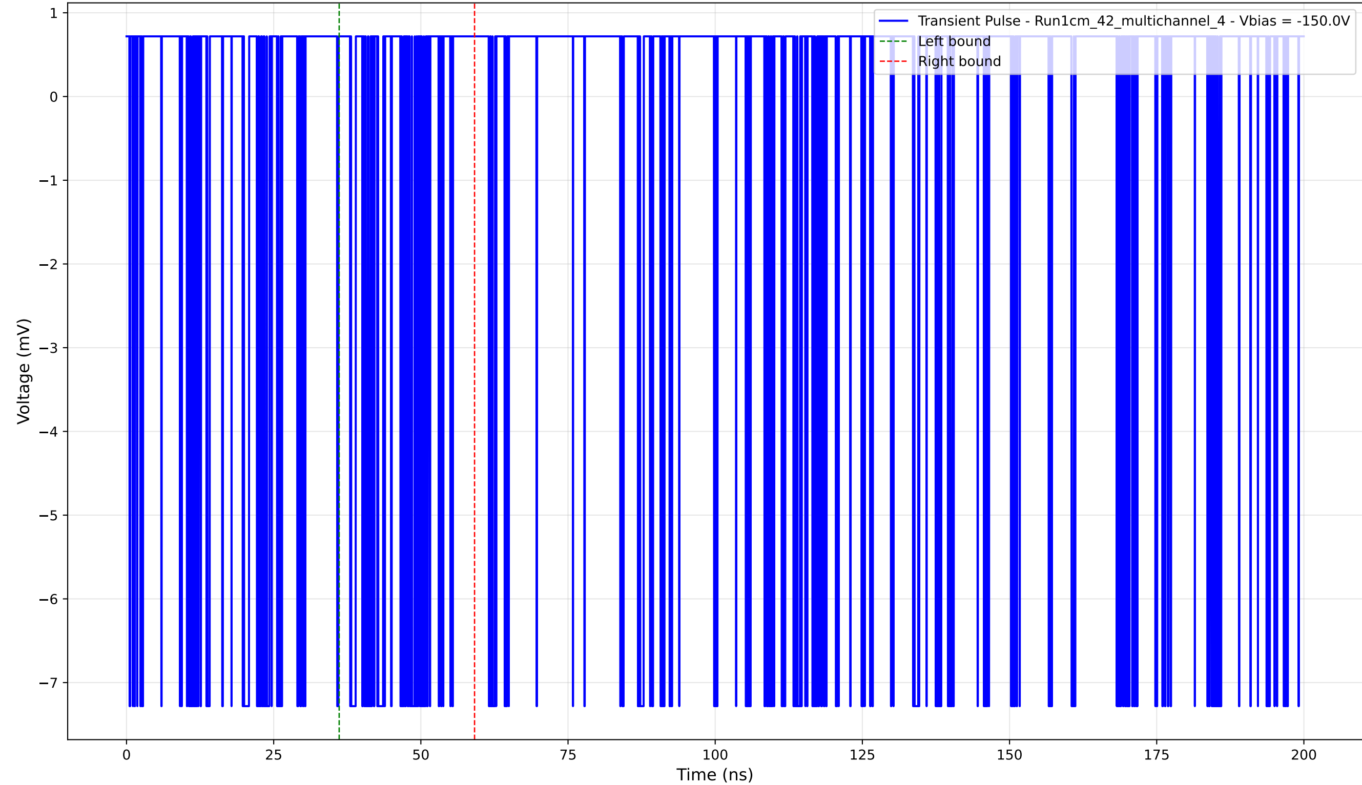
Transient Pulse - Sample: 1cm_42_multichannel - Position: 4395.0 \mu\text{m} - Charge: 0.78 pC - Rise Time: 0.02 ns
