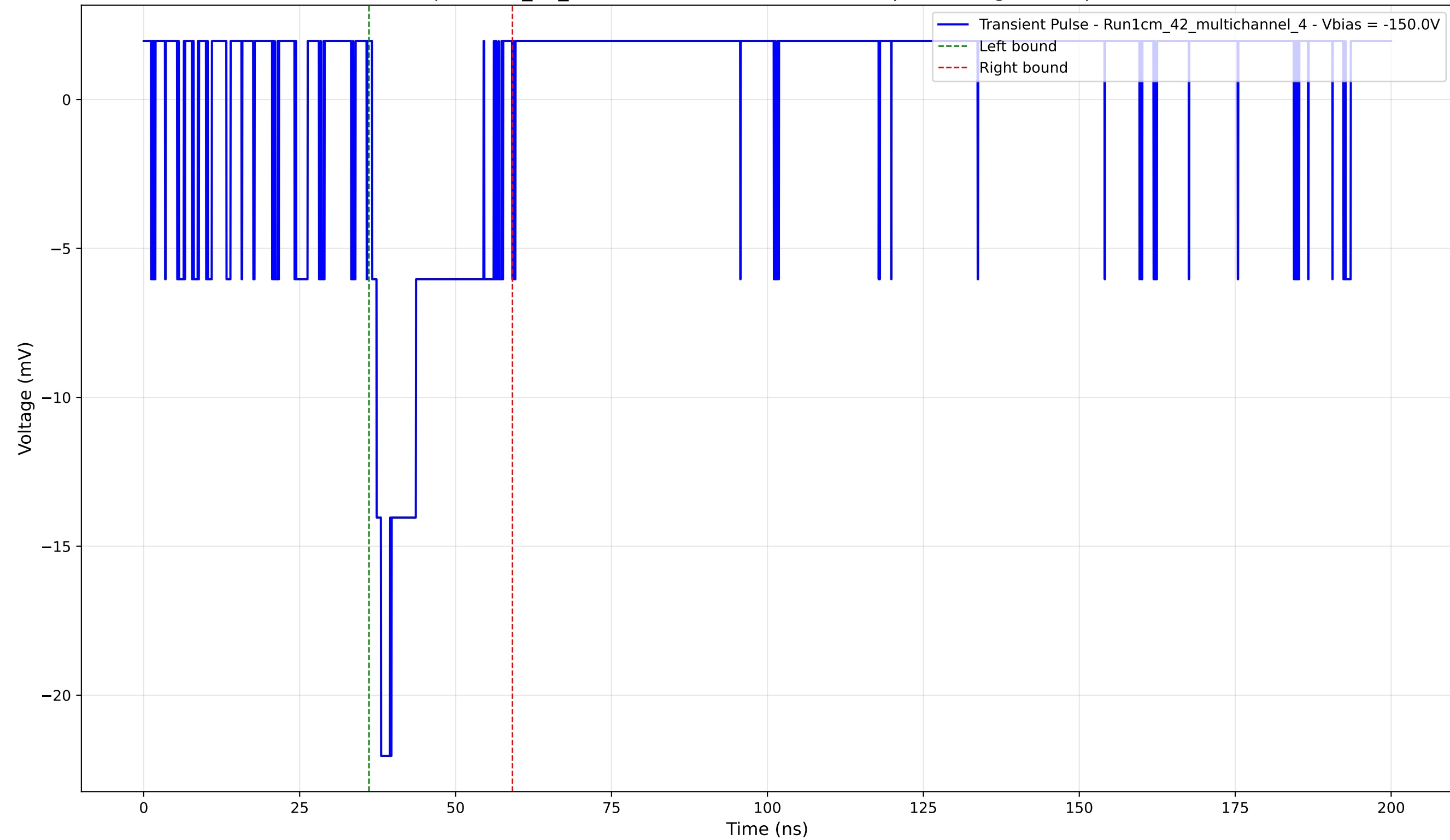
Transient Pulse - Sample: 1cm_42_multichannel - Position: 1130.0 \mu\text{m} - Charge: 3.65 pC - Rise Time: 1.44 ns
