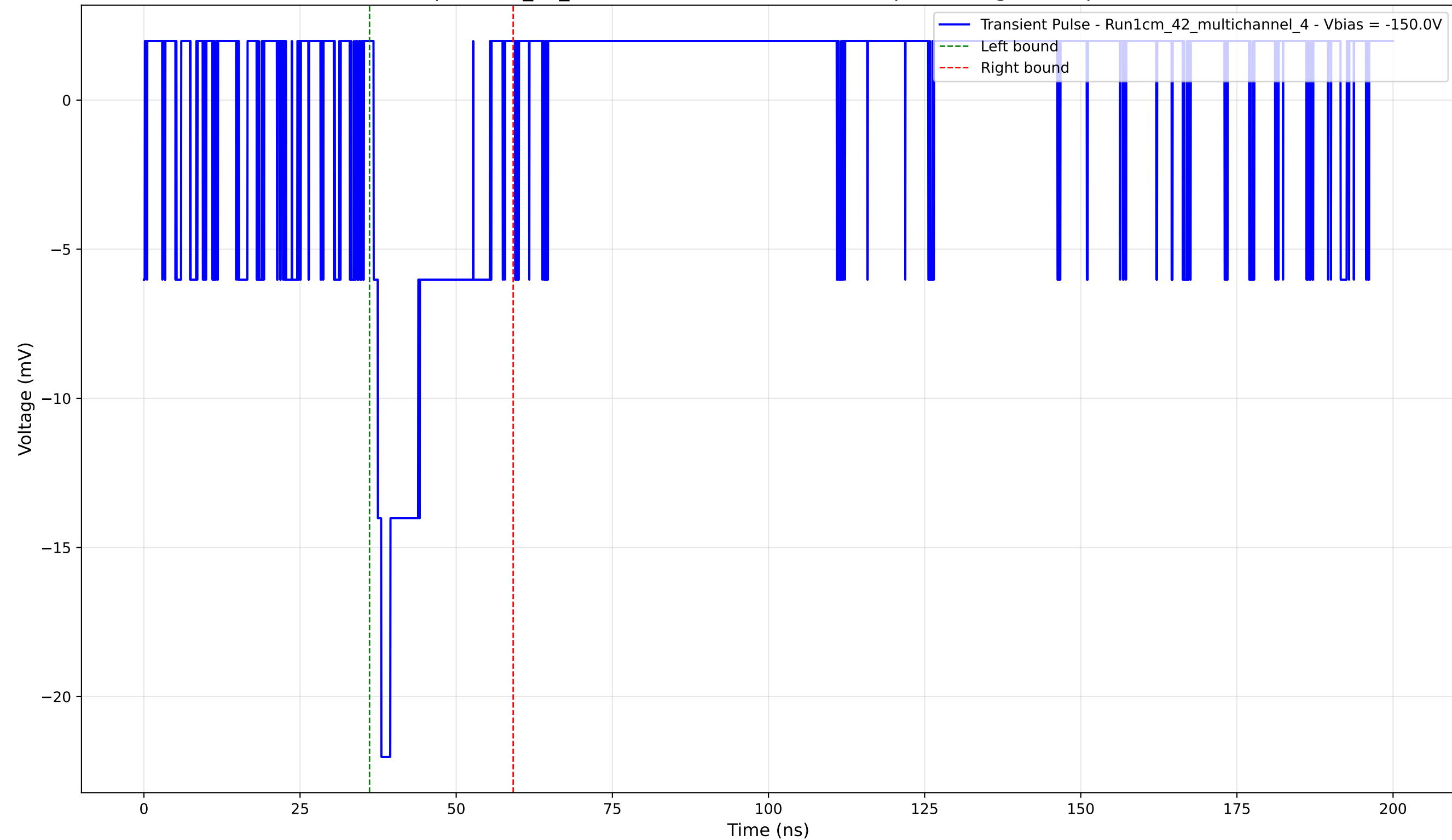
Transient Pulse - Sample: 1cm_42_multichannel - Position: 1100.0 \mu\text{m} - Charge: 3.38 pC - Rise Time: 1.24 ns
