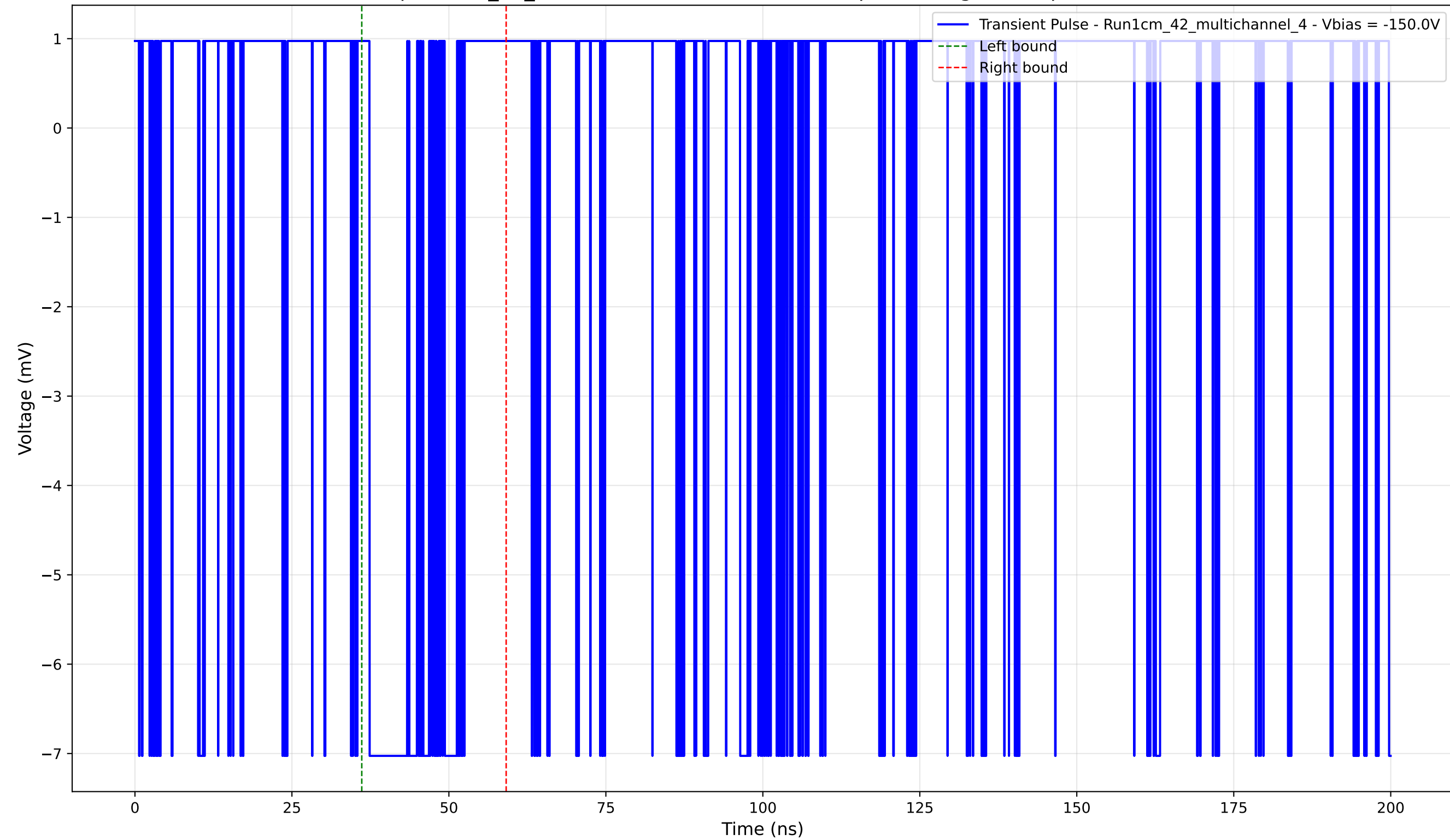
Transient Pulse - Sample: 1cm_42_multichannel - Position: 4870.0 \mu\text{m} - Charge: 1.50 pC - Rise Time: 0.00 ns (N/A)
