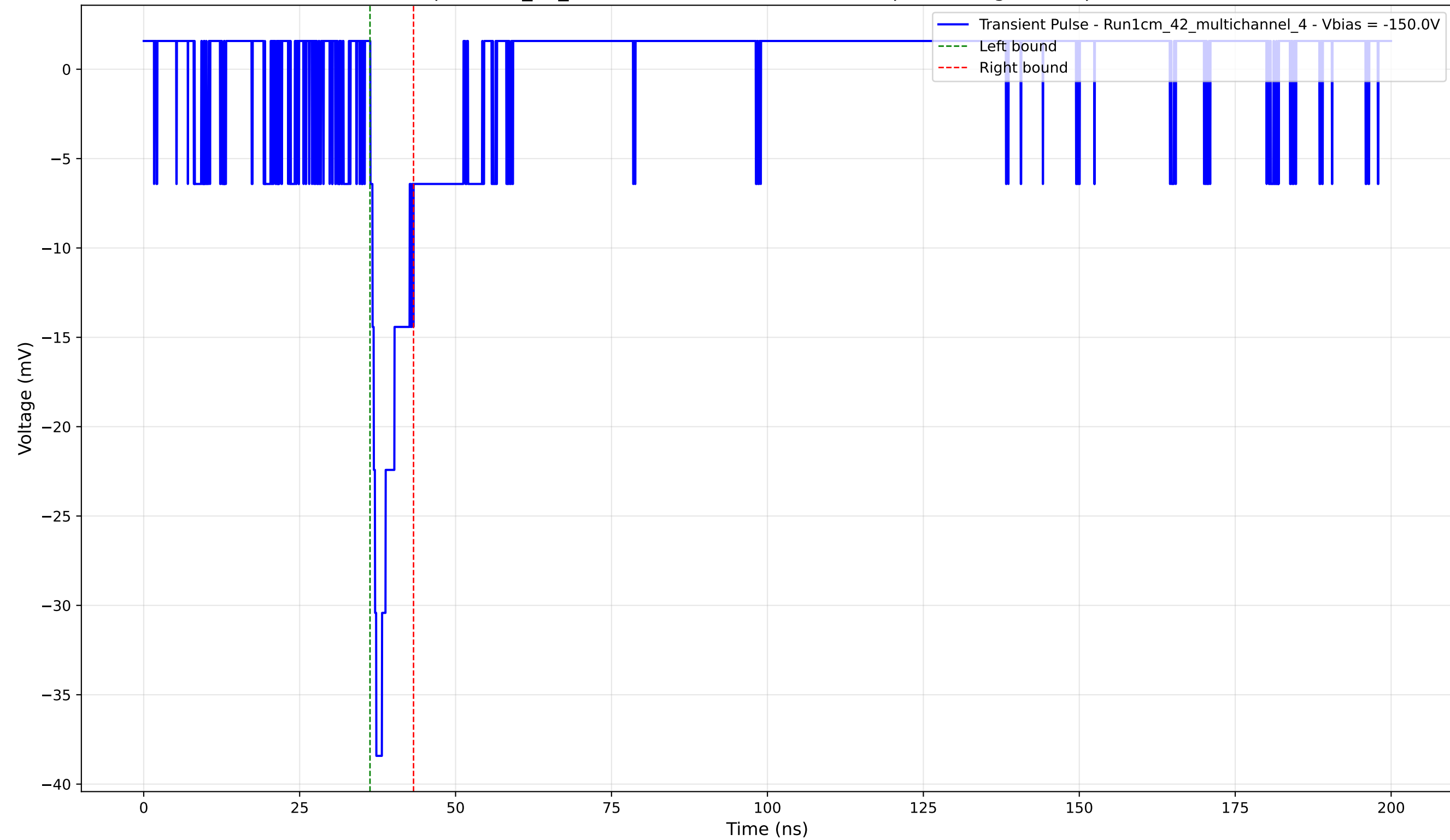
Transient Pulse - Sample: 1cm_42_multichannel - Position: 1745.0 \mu\text{m} - Charge: 2.83 pC - Rise Time: 0.95 ns
