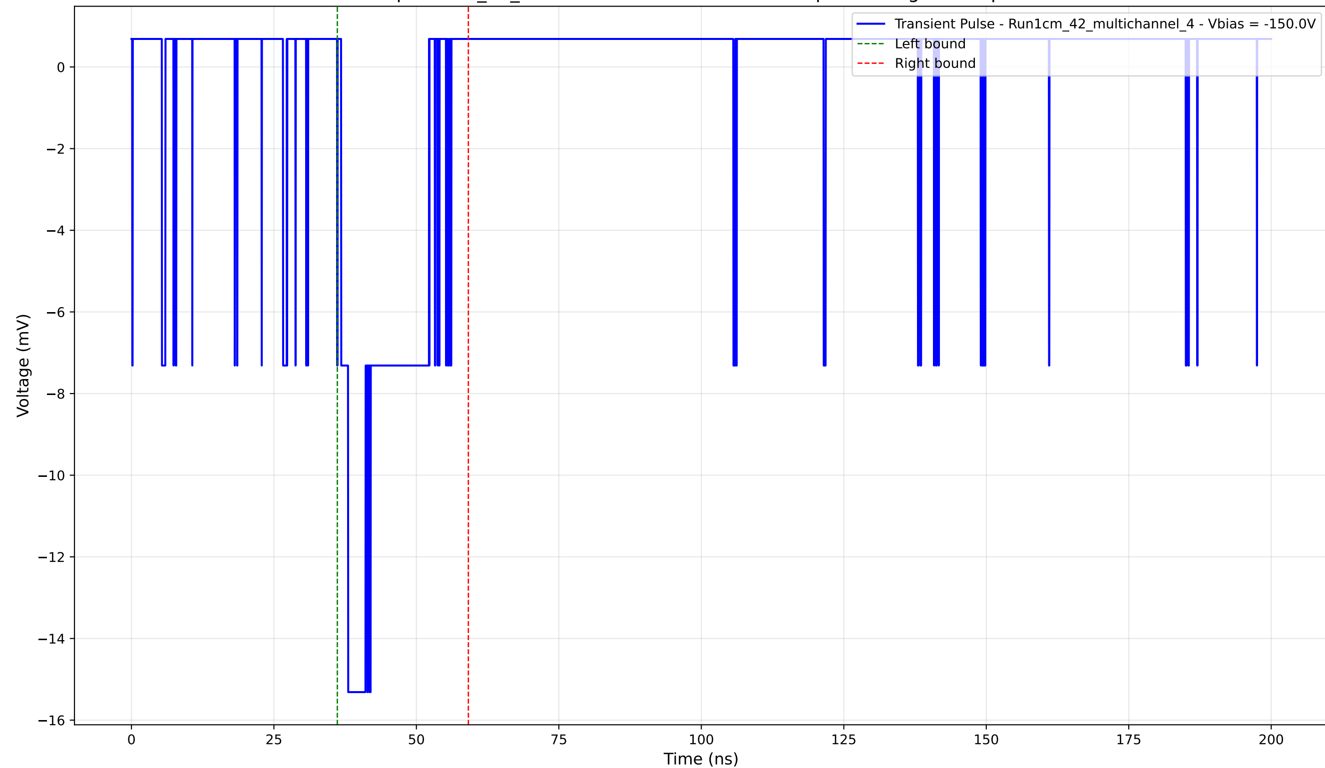
Transient Pulse - Sample: 1cm_42_multichannel - Position: 3840.0 \mu\text{m} - Charge: 2.77 pC - Rise Time: 1.24 ns
