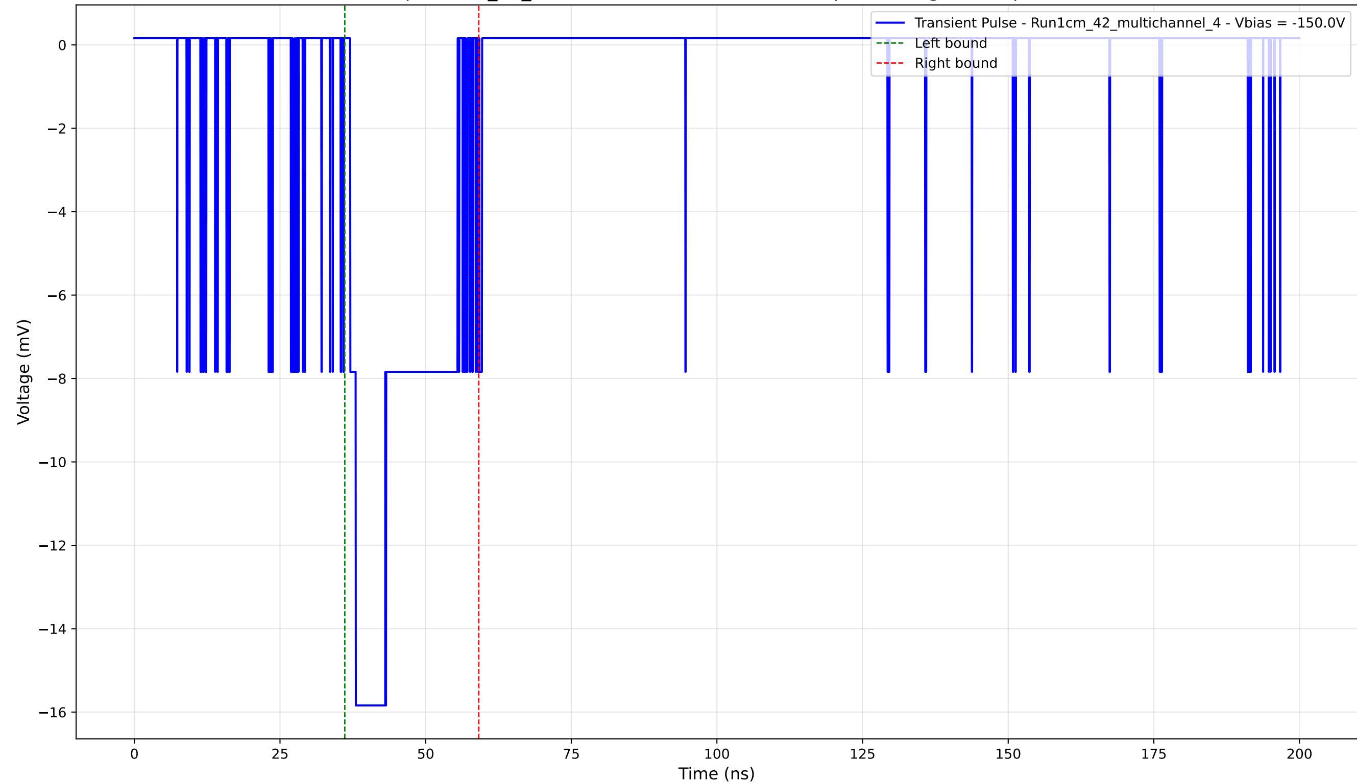
Transient Pulse - Sample: 1cm_42_multichannel - Position: 3995.0 \mu\text{m} - Charge: 3.89 pC - Rise Time: 0.96 ns
