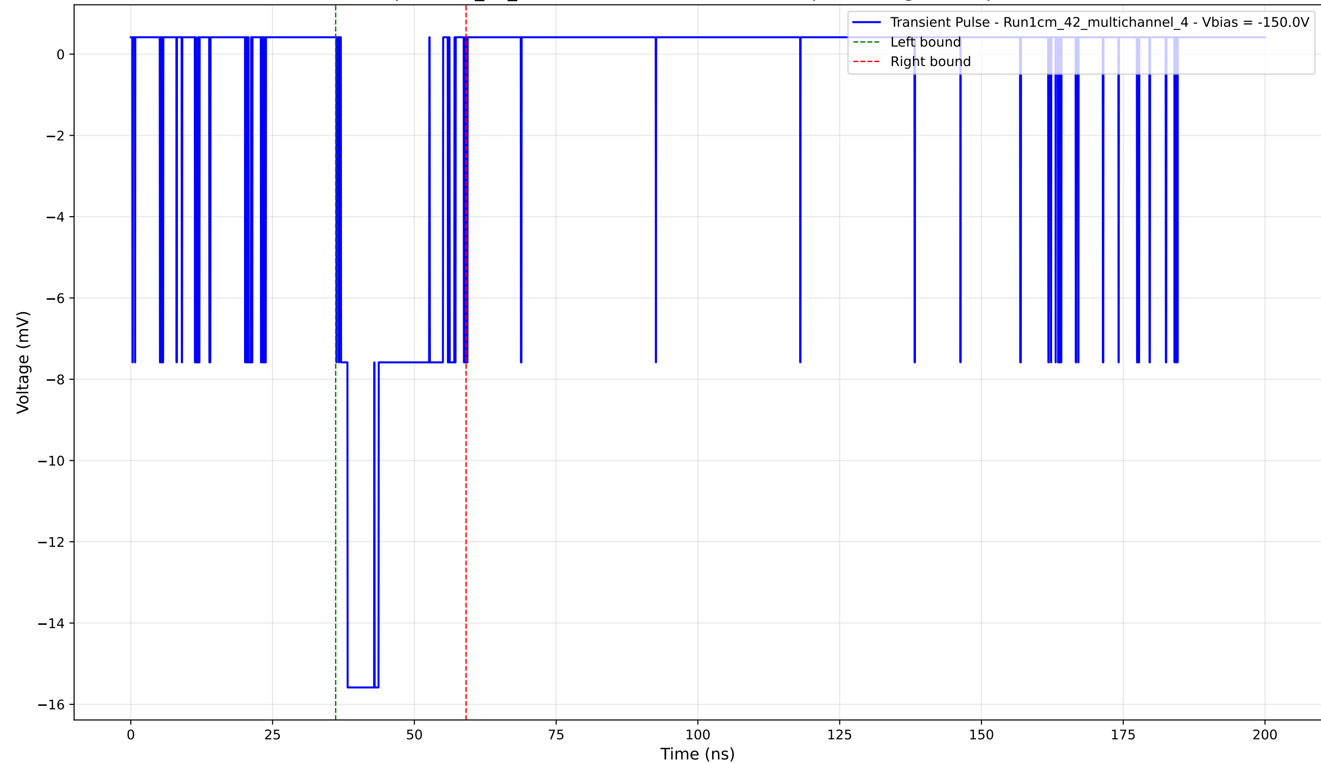
Transient Pulse - Sample: 1cm_42_multichannel - Position: 4095.0 \mu\text{m} - Charge: 3.79 pC - Rise Time: 1.18 ns
