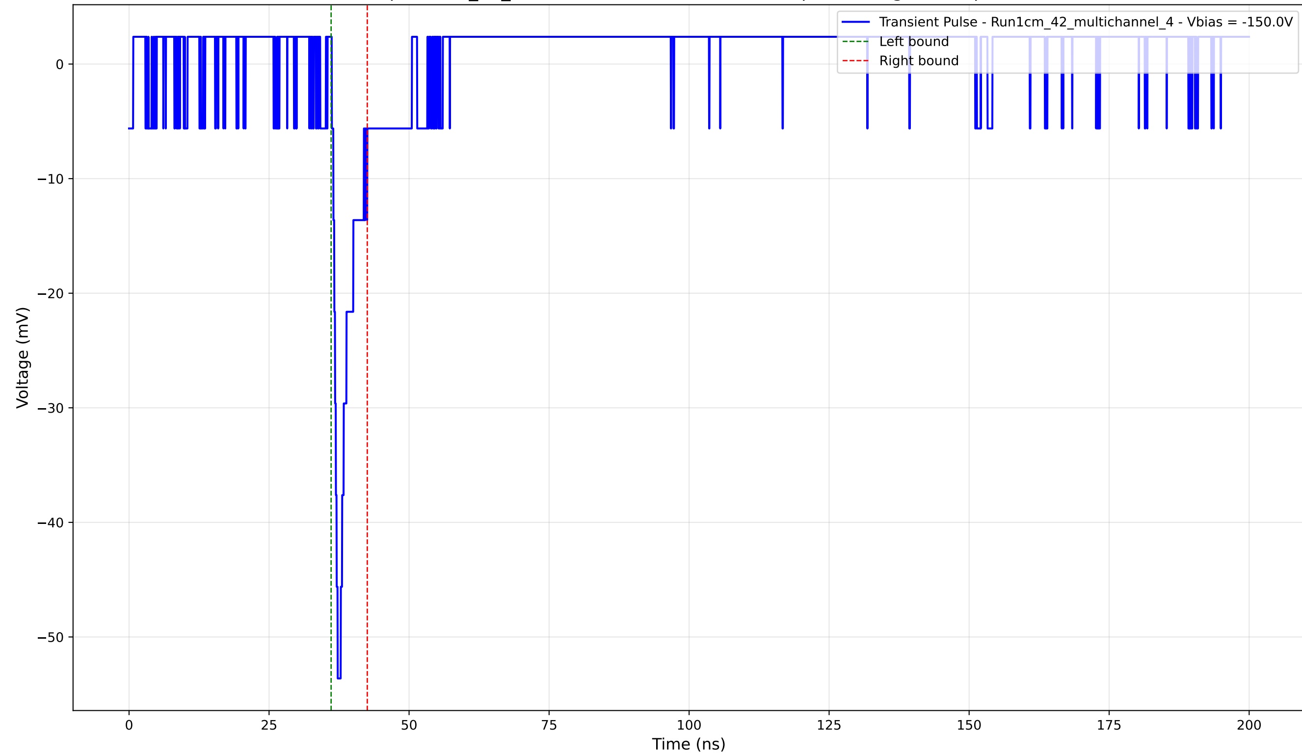
Transient Pulse - Sample: 1cm_42_multichannel - Position: 1980.0 \mu\text{m} - Charge: 2.96 pC - Rise Time: 1.04 ns
