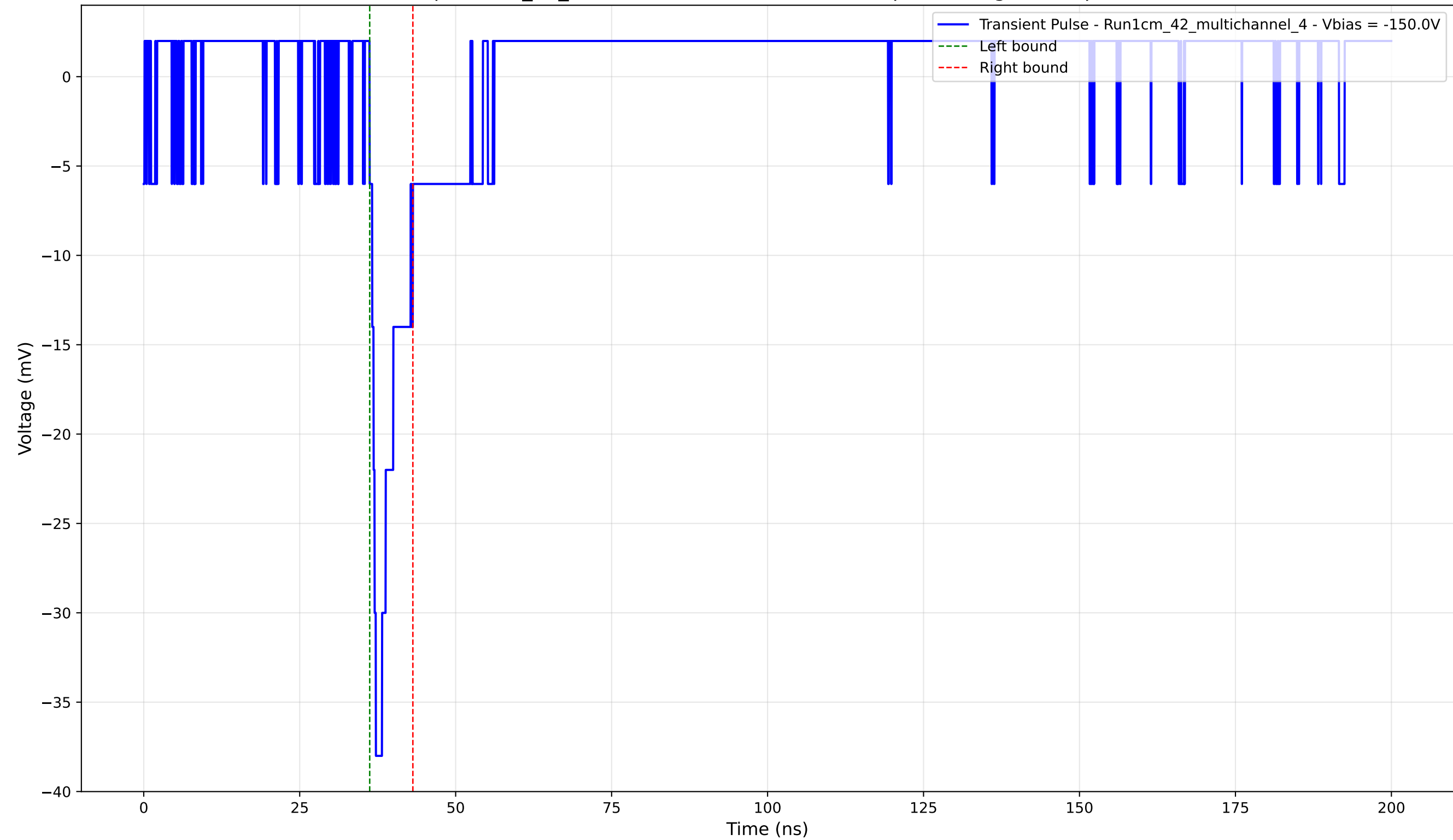
Transient Pulse - Sample: 1cm_42_multichannel - Position: 1800.0 \mu\text{m} - Charge: 2.81 pC - Rise Time: 1.01 ns
