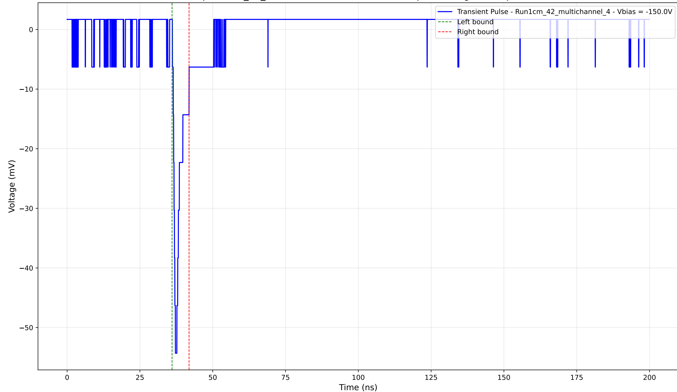
Transient Pulse - Sample: 1cm_42_multichannel - Position: 2720.0 \mu\text{m} - Charge: 2.84 pC - Rise Time: 1.02 ns
