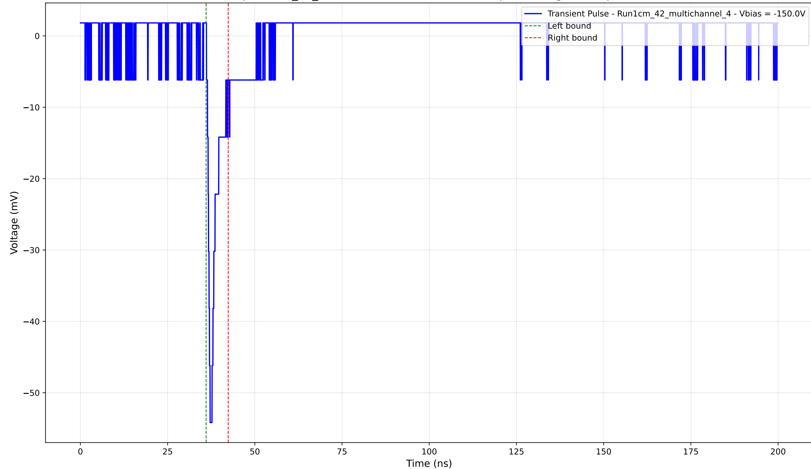
Transient Pulse - Sample: 1cm_42_multichannel - Position: 2750.0 \mu\text{m} - Charge: 2.91 pC - Rise Time: 1.02 ns
