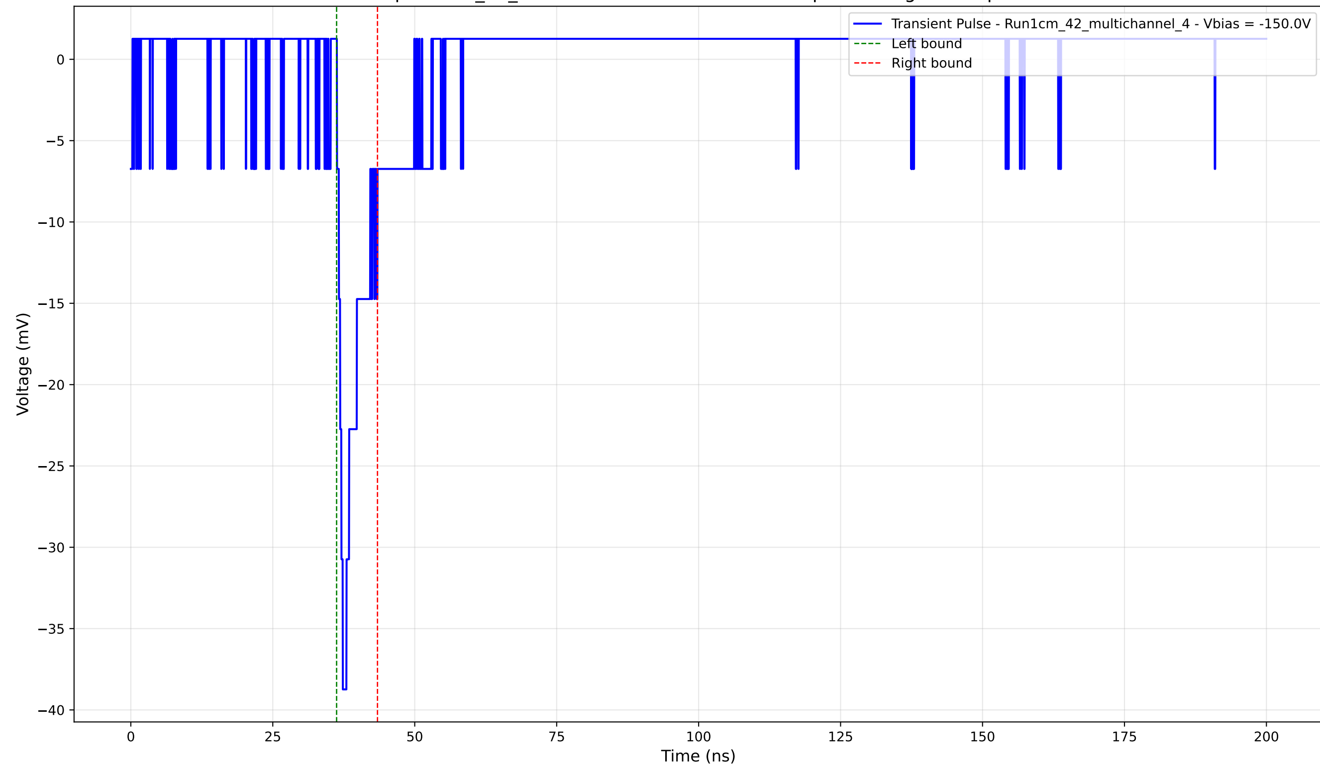
Transient Pulse - Sample: 1cm_42_multichannel - Position: 2995.0 \mu\text{m} - Charge: 2.71 pC - Rise Time: 1.03 ns
