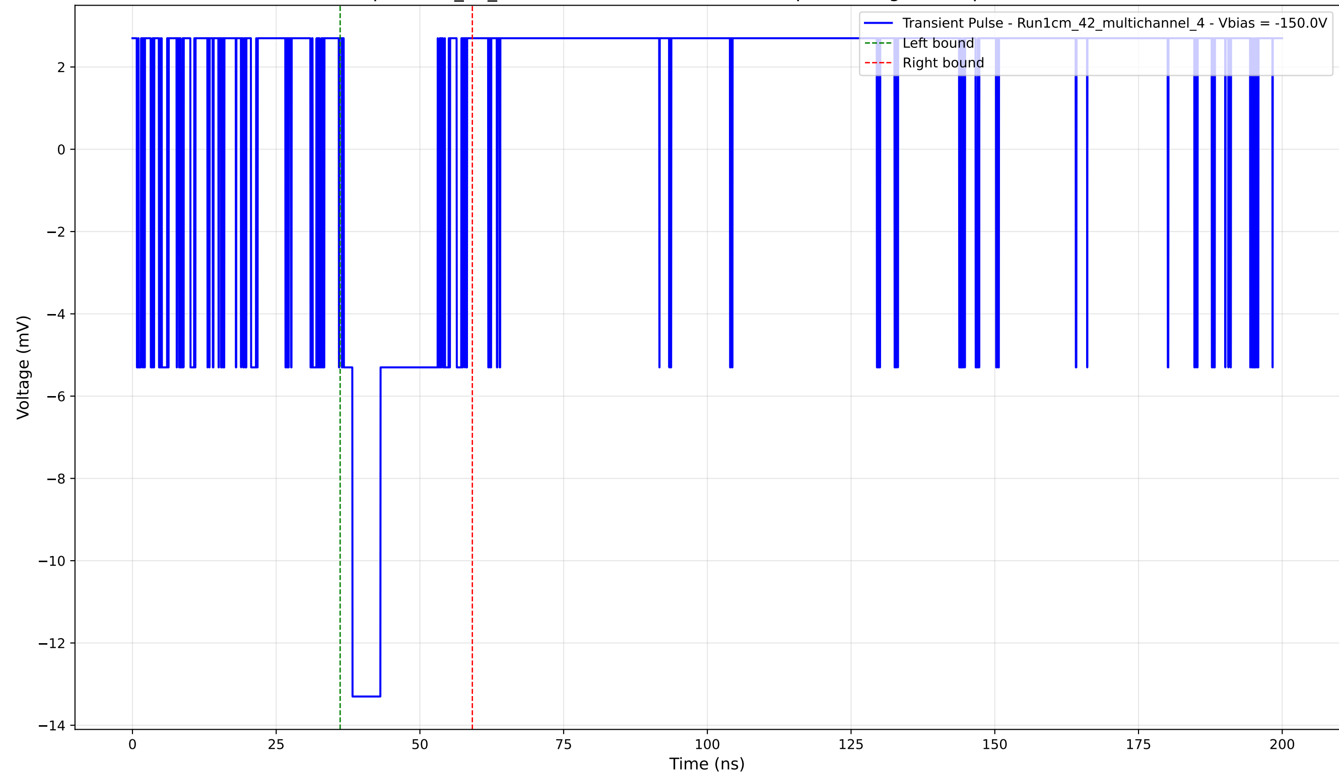
Transient Pulse - Sample: 1cm_42_multichannel - Position: 4190.0 \mu\text{m} - Charge: 2.57 pC - Rise Time: 0.00 ns (N/A)
