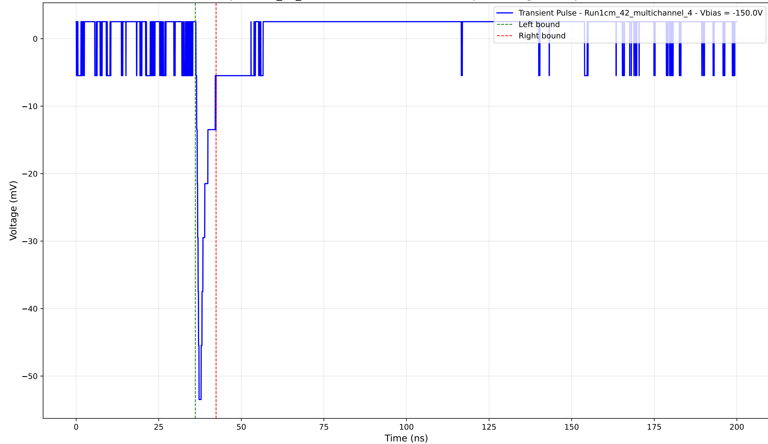
Transient Pulse - Sample: 1cm_42_multichannel - Position: 1985.0 \mu\text{m} - Charge: 2.96 pC - Rise Time: 0.94 ns
