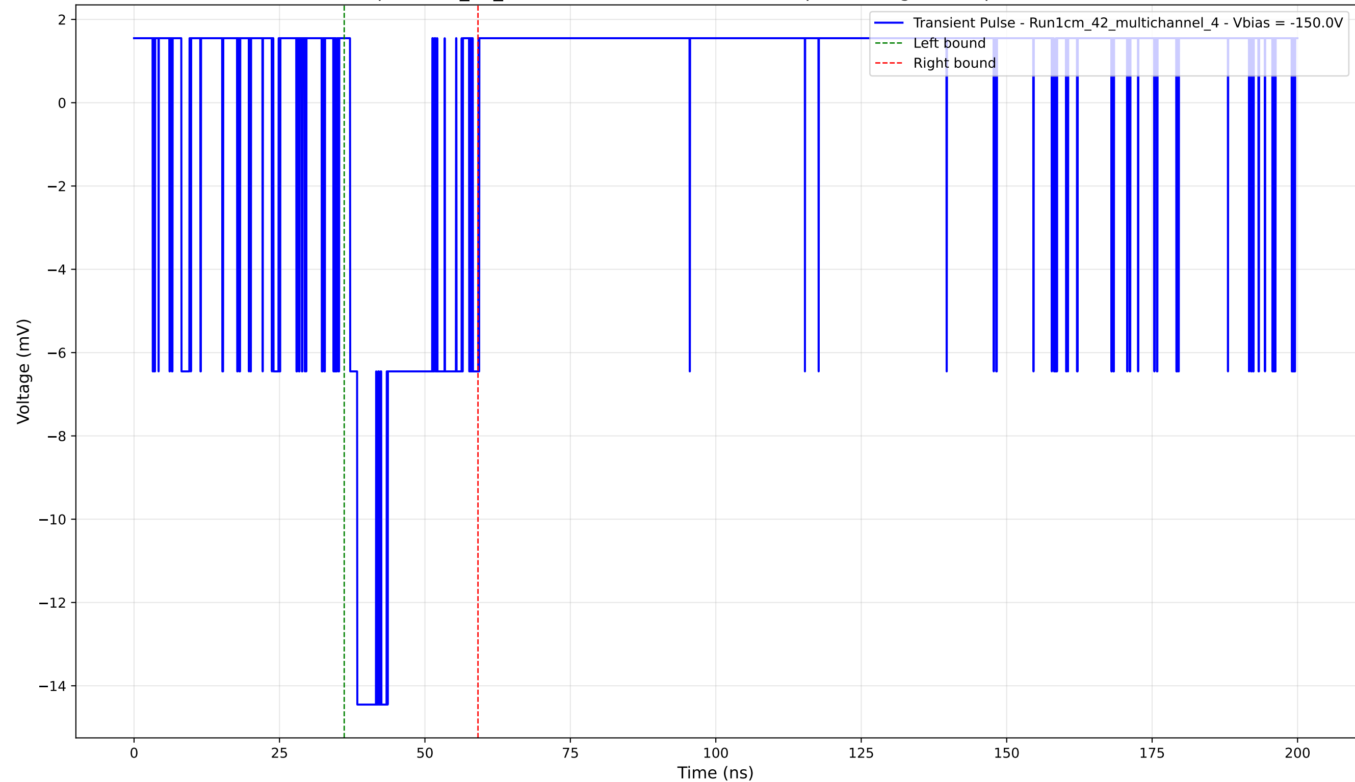
Transient Pulse - Sample: 1cm_42_multichannel - Position: 4565.0 \mu\text{m} - Charge: 3.27 pC - Rise Time: 0.00 ns (N/A)
