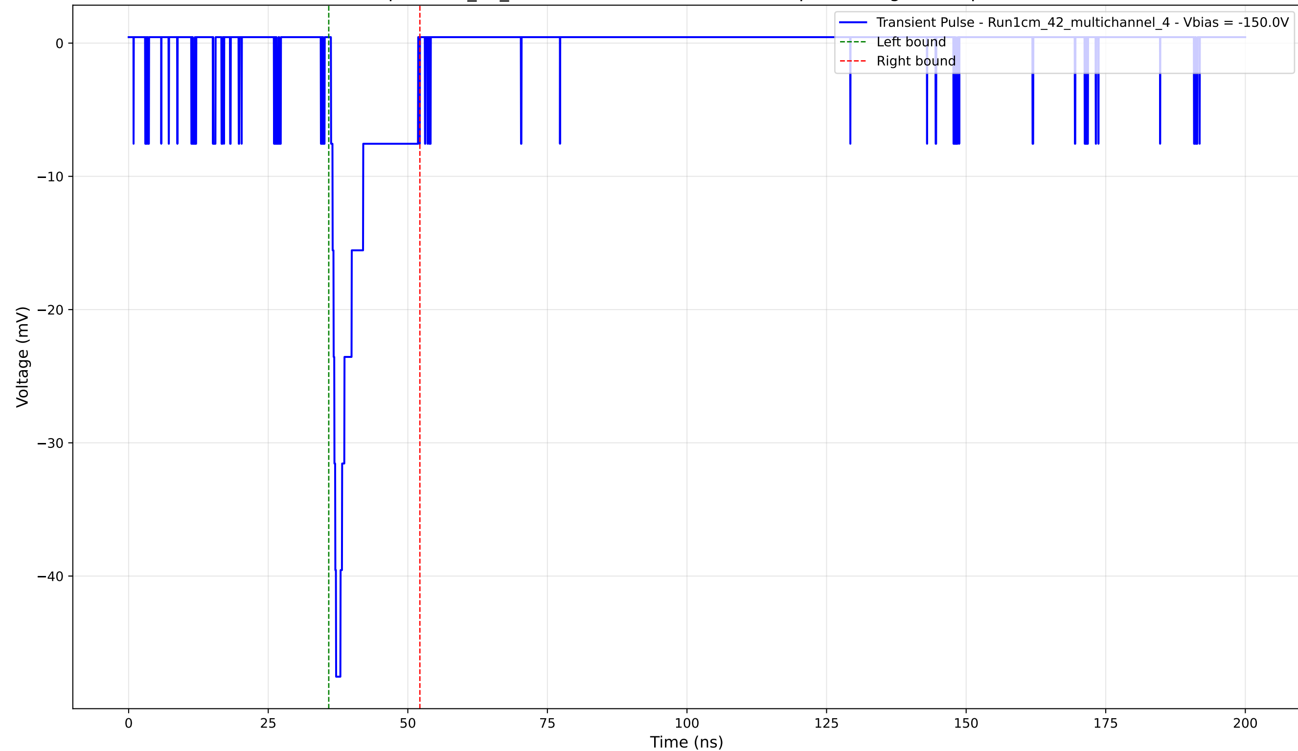
Transient Pulse - Sample: 1cm_42_multichannel - Position: 2810.0 \mu\text{m} - Charge: 4.37 pC - Rise Time: 0.91 ns
