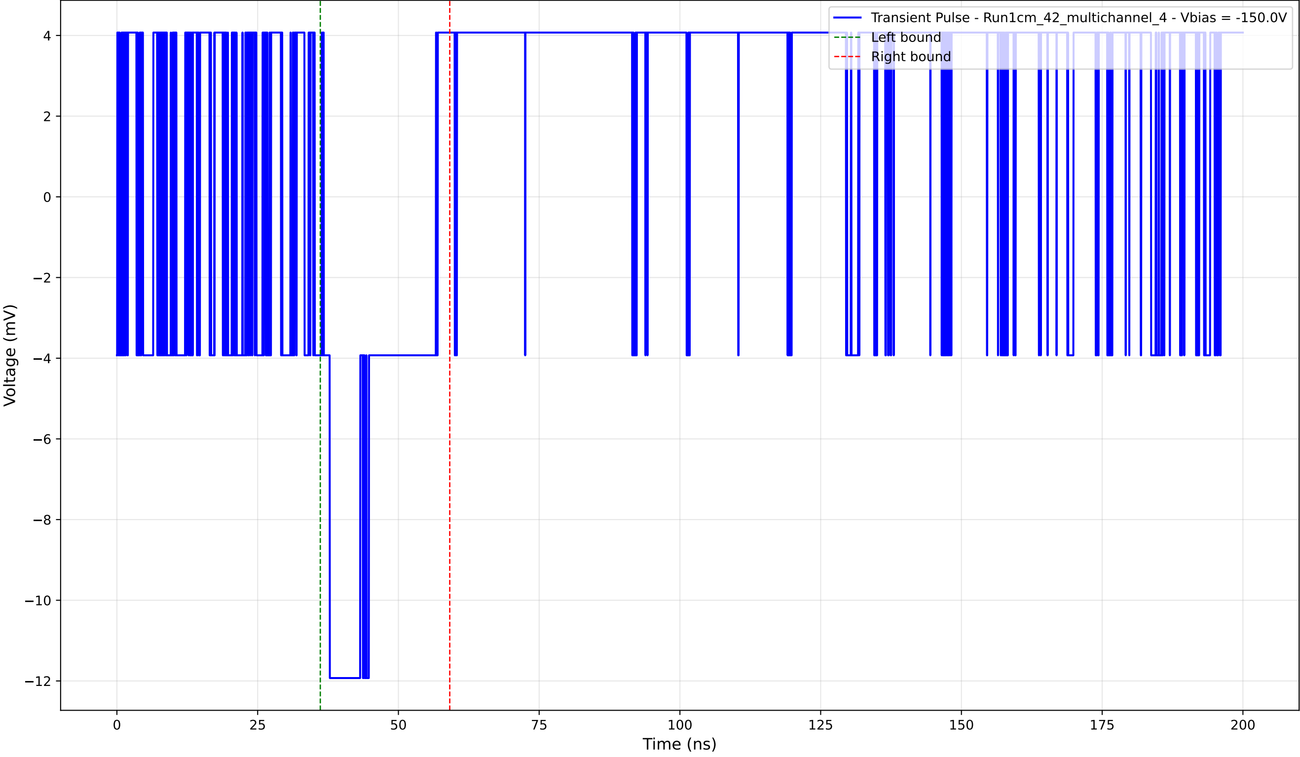
Transient Pulse - Sample: 1cm_42_multichannel - Position: 785.0 \mu\text{m} - Charge: 2.42 pC - Rise Time: 0.00 ns (N/A)
