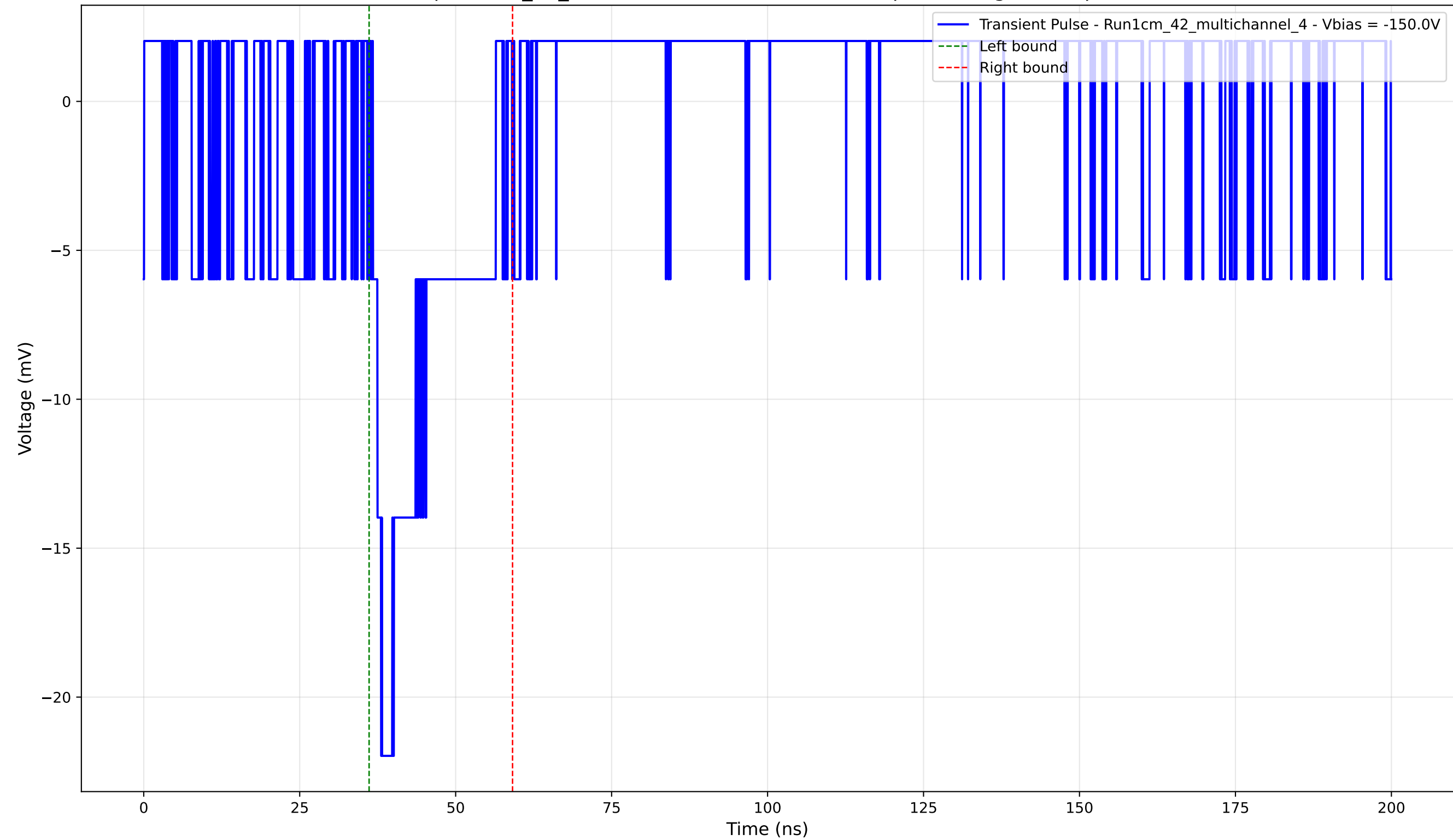
Transient Pulse - Sample: 1cm_42_multichannel - Position: 1045.0 \mu\text{m} - Charge: 3.77 pC - Rise Time: 1.32 ns
