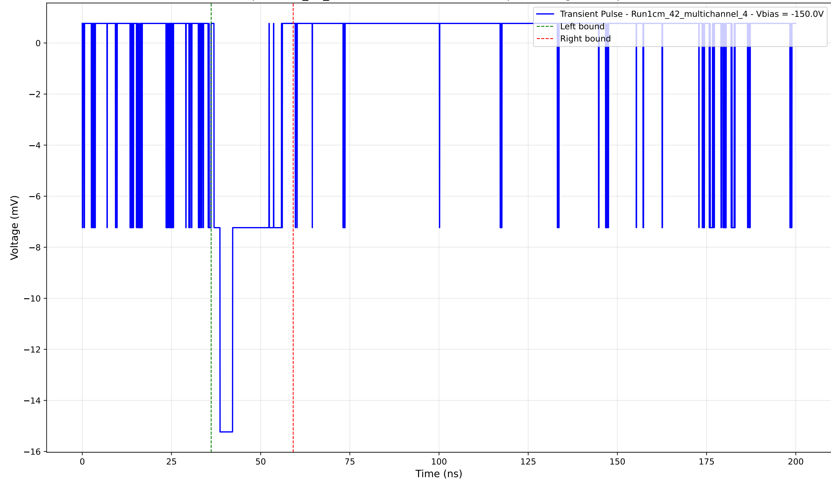
Transient Pulse - Sample: 1cm_42_multichannel - Position: 150.0 \mu\text{m} - Charge: 3.25 pC - Rise Time: 1.70 ns
