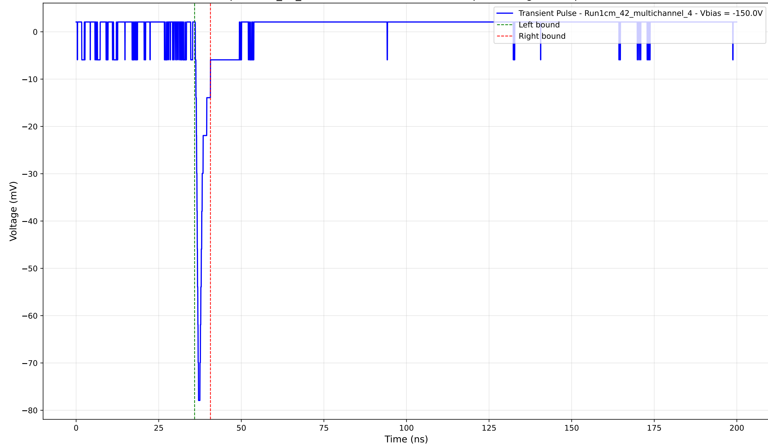
Transient Pulse - Sample: 1cm_42_multichannel - Position: 2285.0 \mu\text{m} - Charge: 3.03 pC - Rise Time: 0.80 ns
