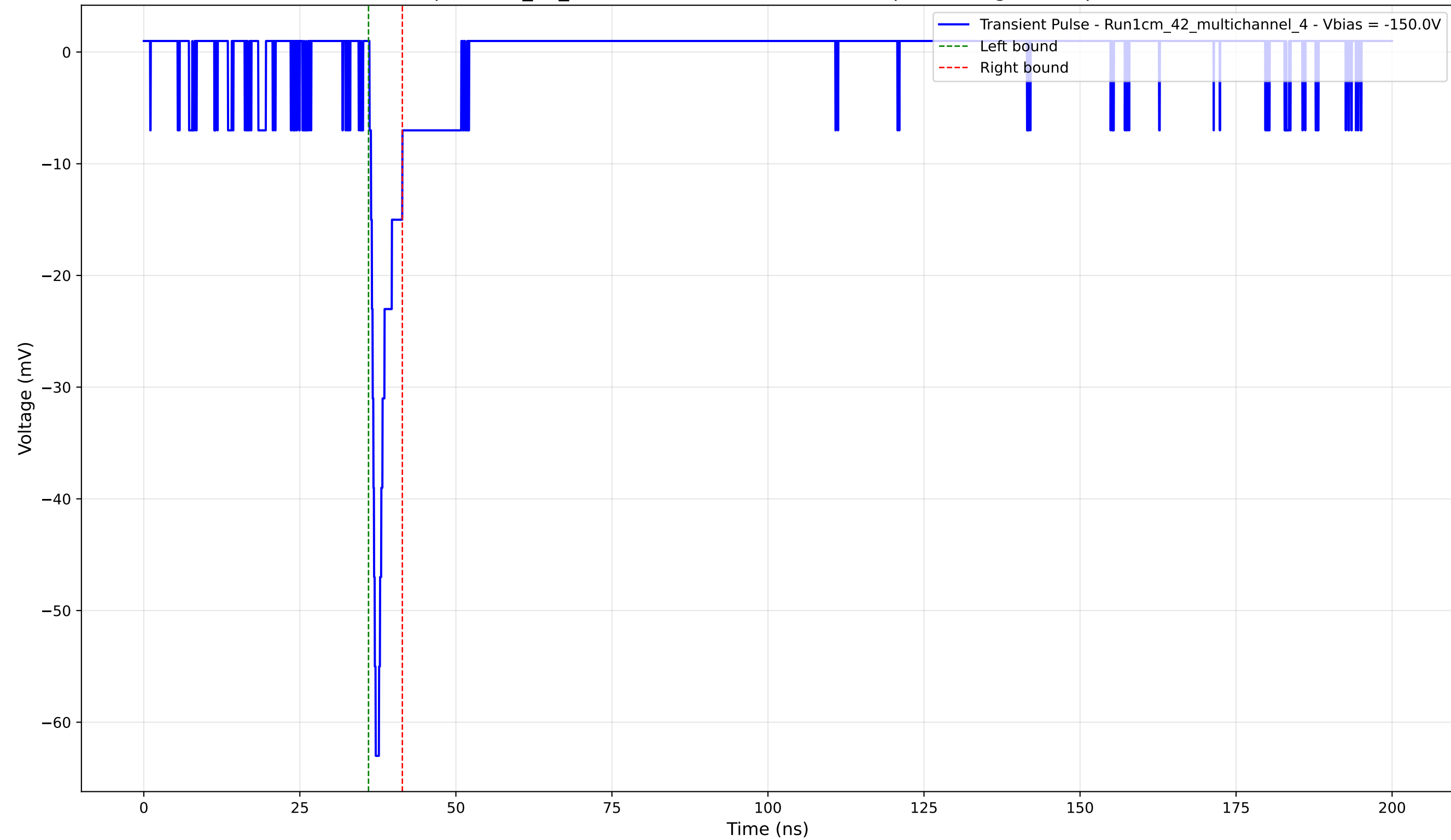
Transient Pulse - Sample: 1cm_42_multichannel - Position: 2125.0 \mu\text{m} - Charge: 3.00 pC - Rise Time: 0.98 ns
