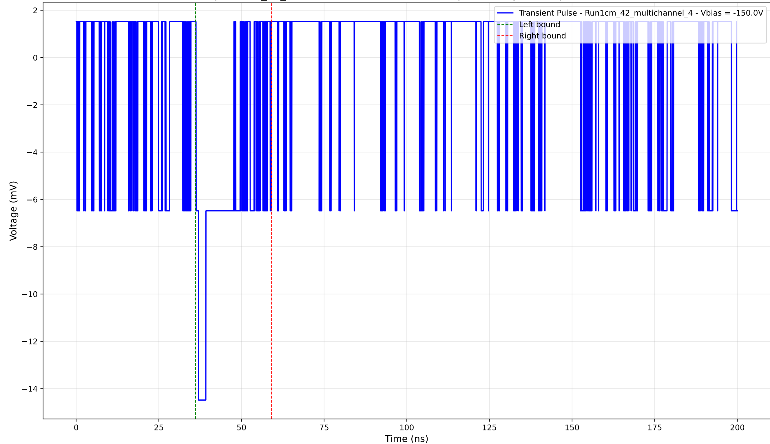
Transient Pulse - Sample: 1cm_42_multichannel - Position: 1835.0 \mu\text{m} - Charge: 2.43 pC - Rise Time: 0.00 ns (N/A)
