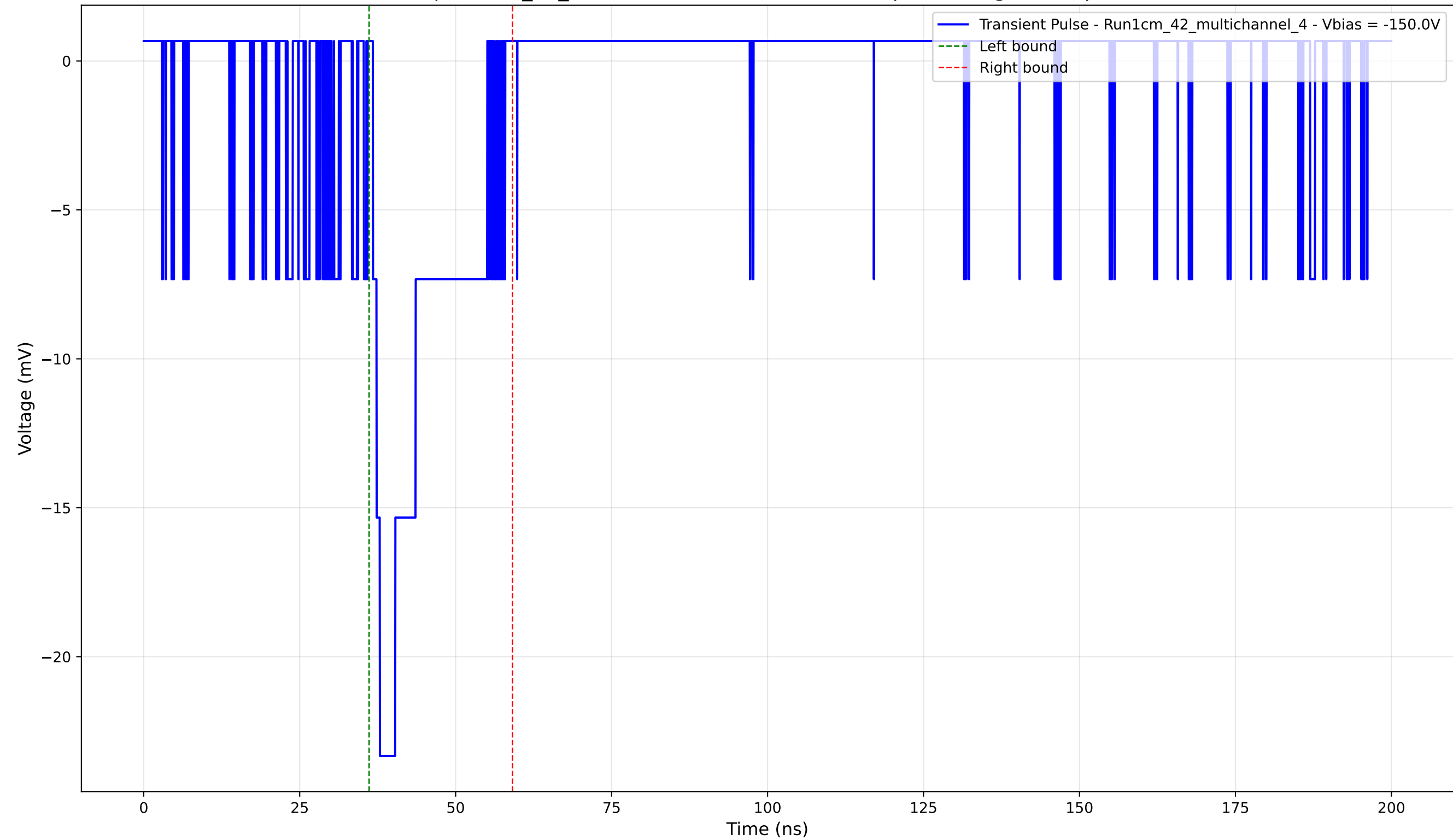
Transient Pulse - Sample: 1cm_42_multichannel - Position: 1170.0 \mu\text{m} - Charge: 4.27 pC - Rise Time: 1.12 ns
