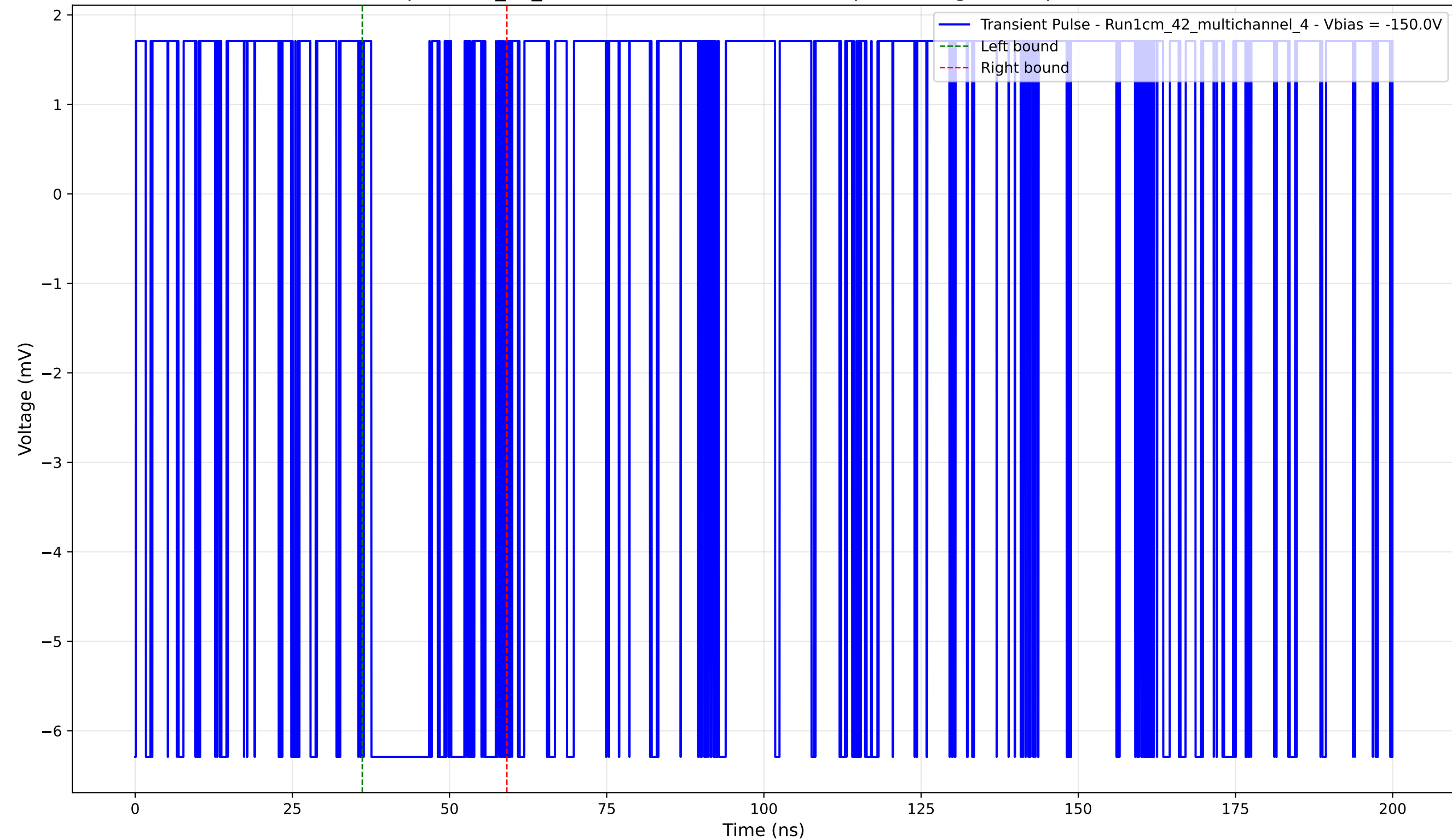
Transient Pulse - Sample: 1cm_42_multichannel - Position: 905.0 \mu\text{m} - Charge: 1.88 pC - Rise Time: 0.00 ns (N/A)
