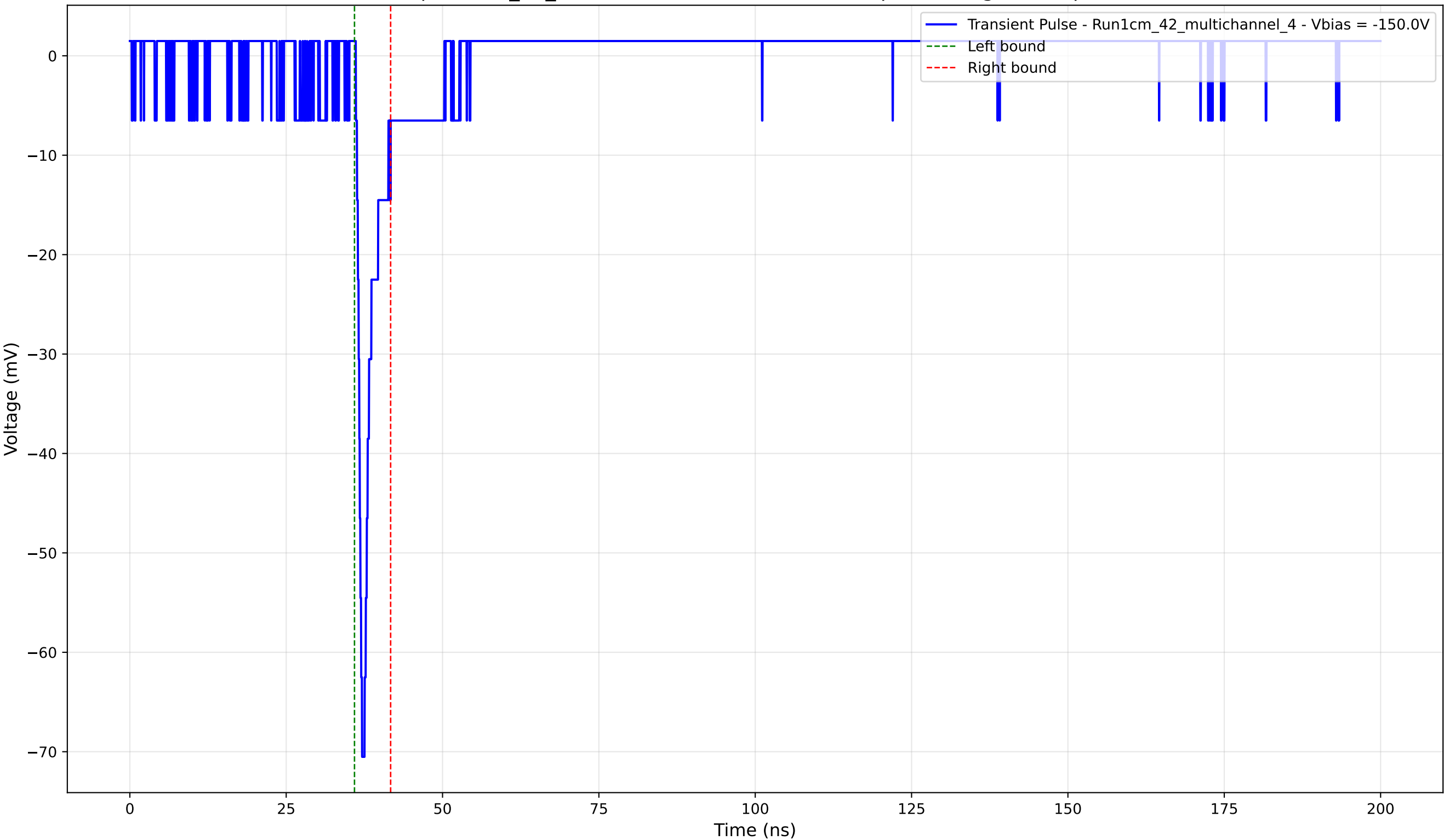
Transient Pulse - Sample: 1cm_42_multichannel - Position: 2180.0 \mu\text{m} - Charge: 3.19 pC - Rise Time: 0.82 ns
