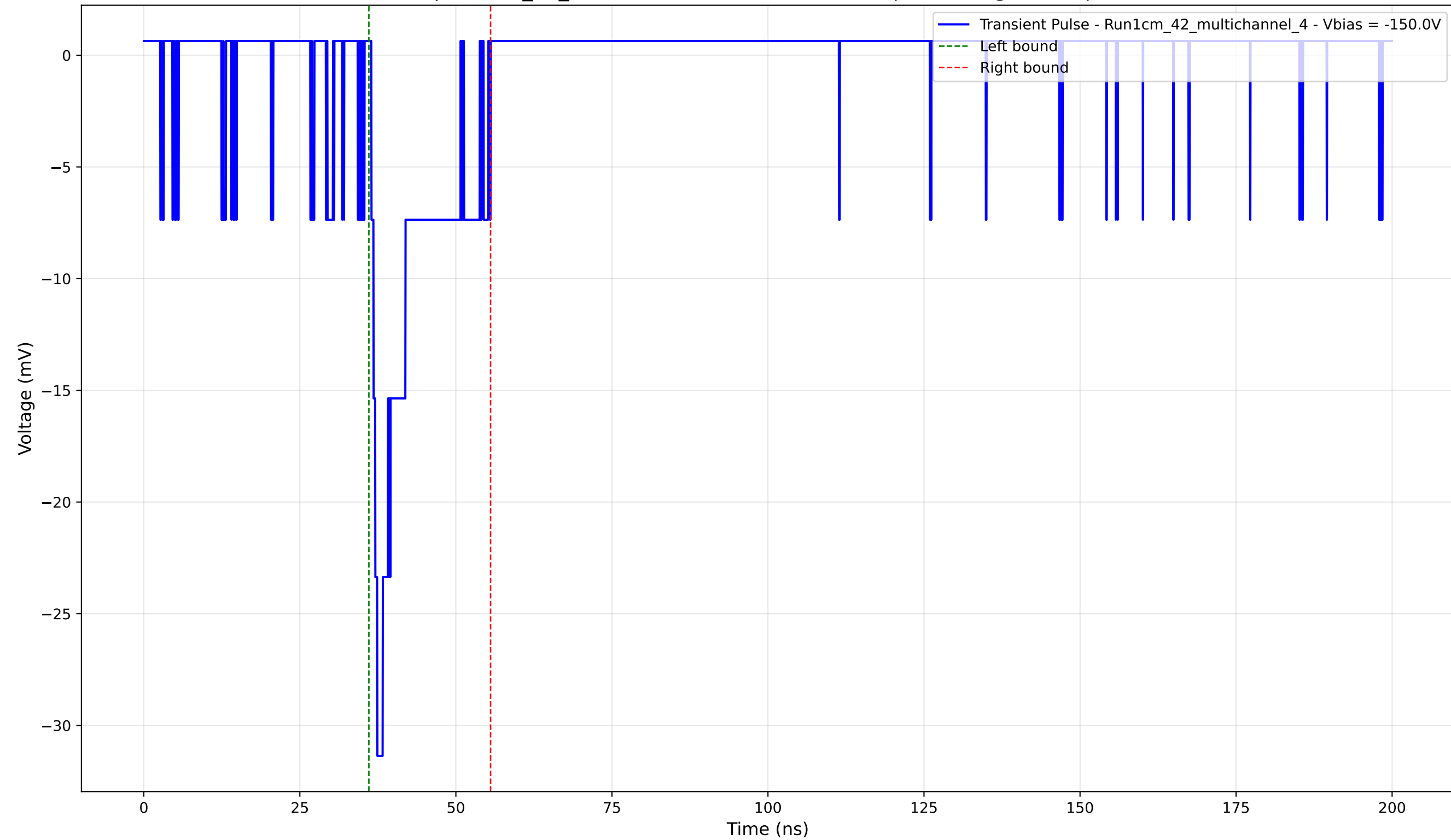
Transient Pulse - Sample: 1cm_42_multichannel - Position: 3120.0 \mu\text{m} - Charge: 3.96 pC - Rise Time: 0.95 ns
