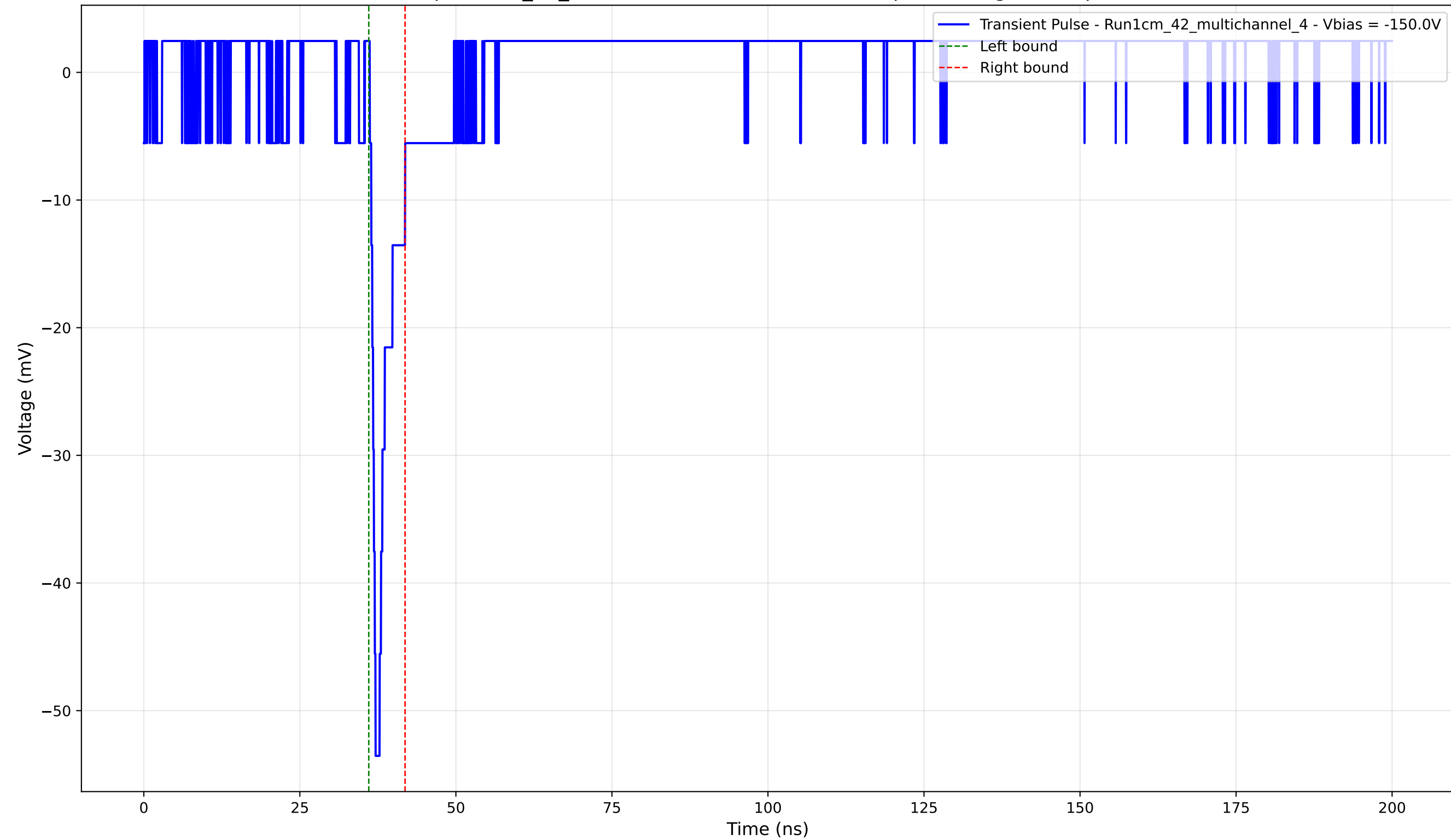
Transient Pulse - Sample: 1cm_42_multichannel - Position: 2725.0 \mu\text{m} - Charge: 2.79 pC - Rise Time: 0.92 ns
