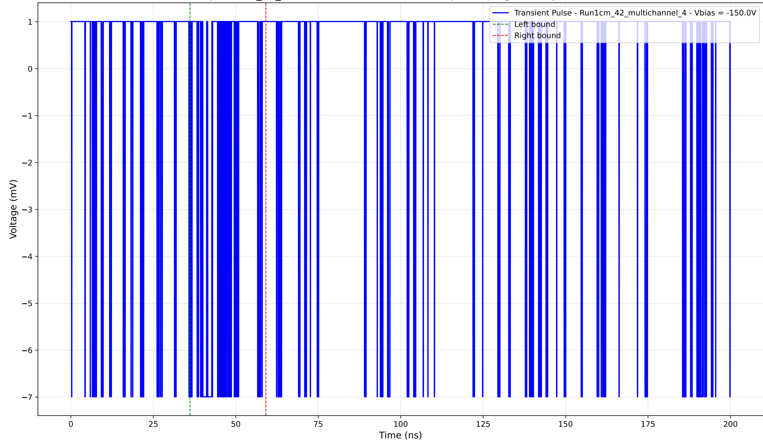
Transient Pulse - Sample: 1cm_42_multichannel - Position: 3895.0 \mu\text{m} - Charge: 0.60 pC - Rise Time: 0.00 ns (N/A)
