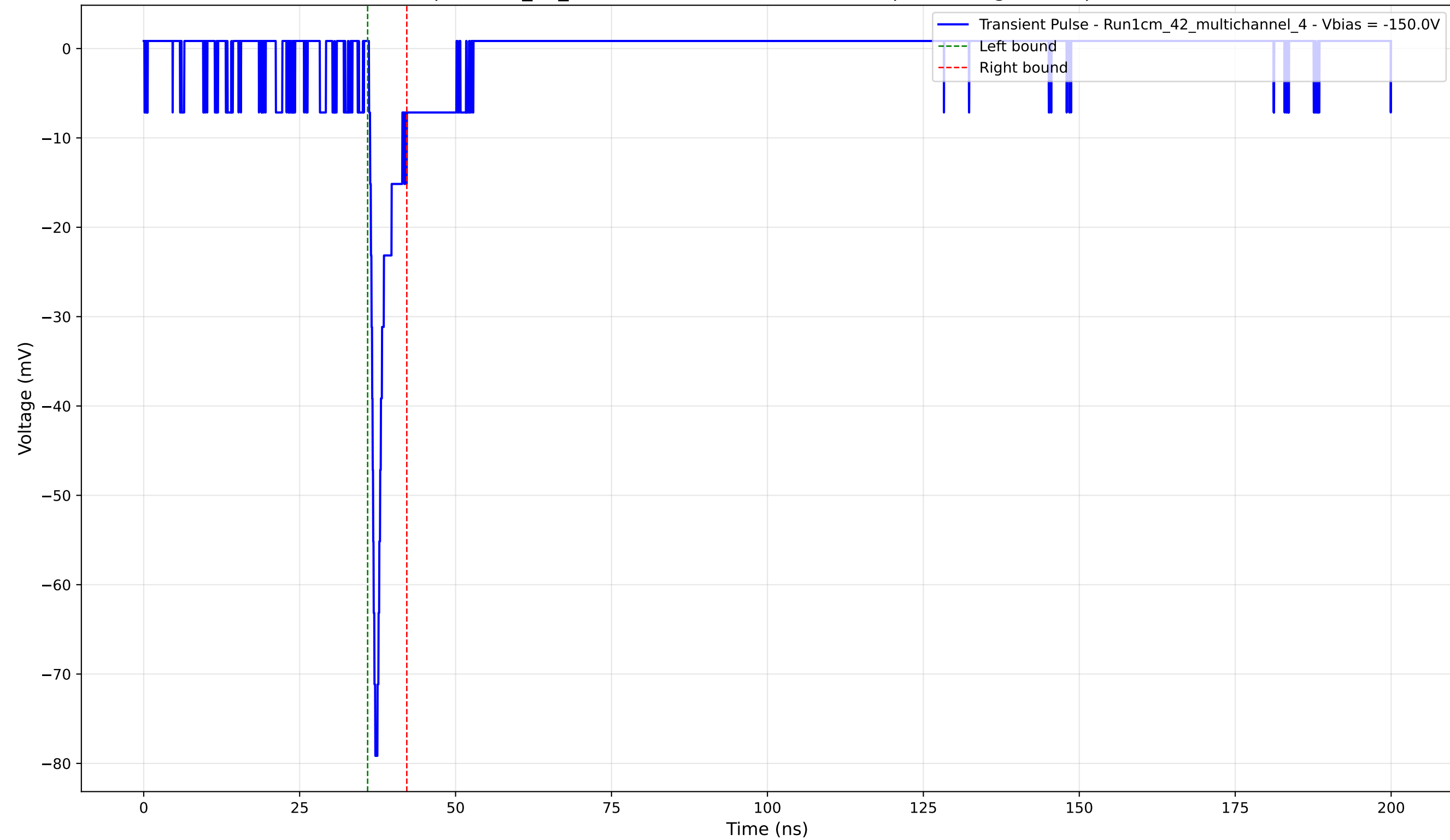
Transient Pulse - Sample: 1cm_42_multichannel - Position: 2240.0 \mu\text{m} - Charge: 3.52 pC - Rise Time: 0.84 ns
