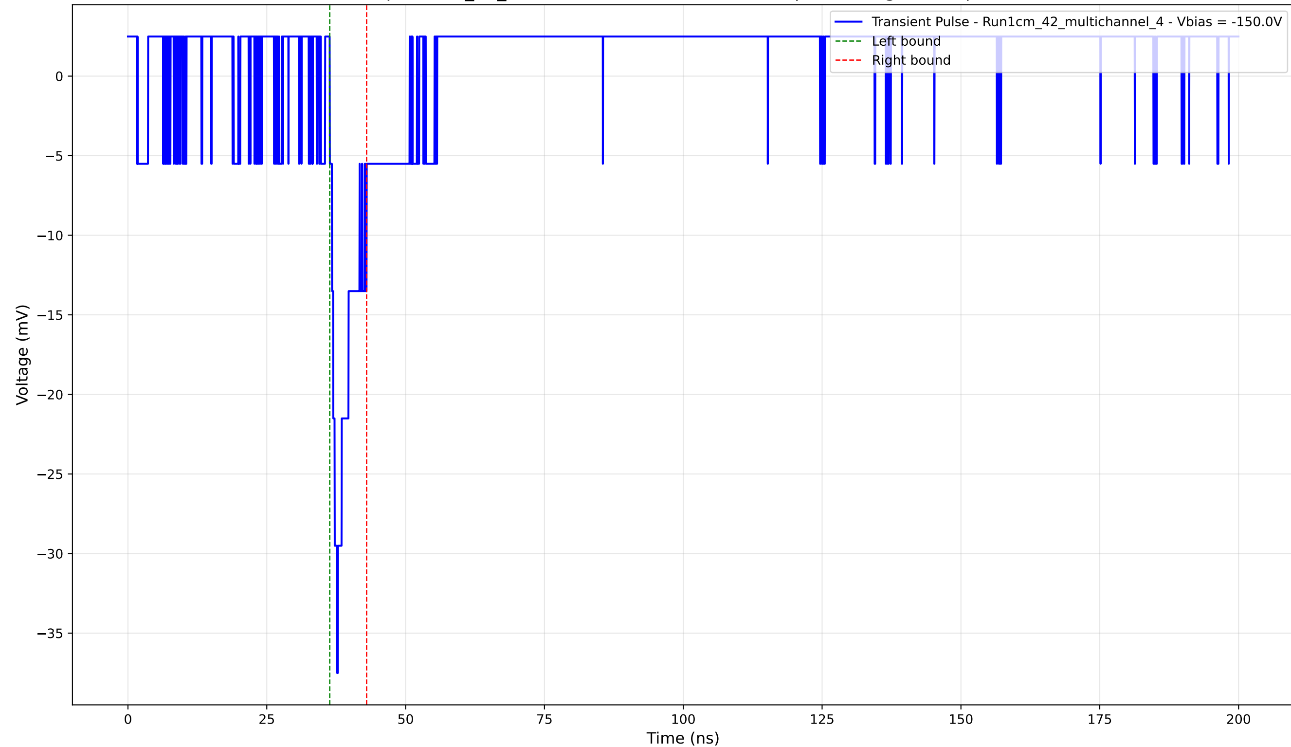
Transient Pulse - Sample: 1cm_42_multichannel - Position: 3065.0 \mu\text{m} - Charge: 2.37 pC - Rise Time: 1.33 ns
