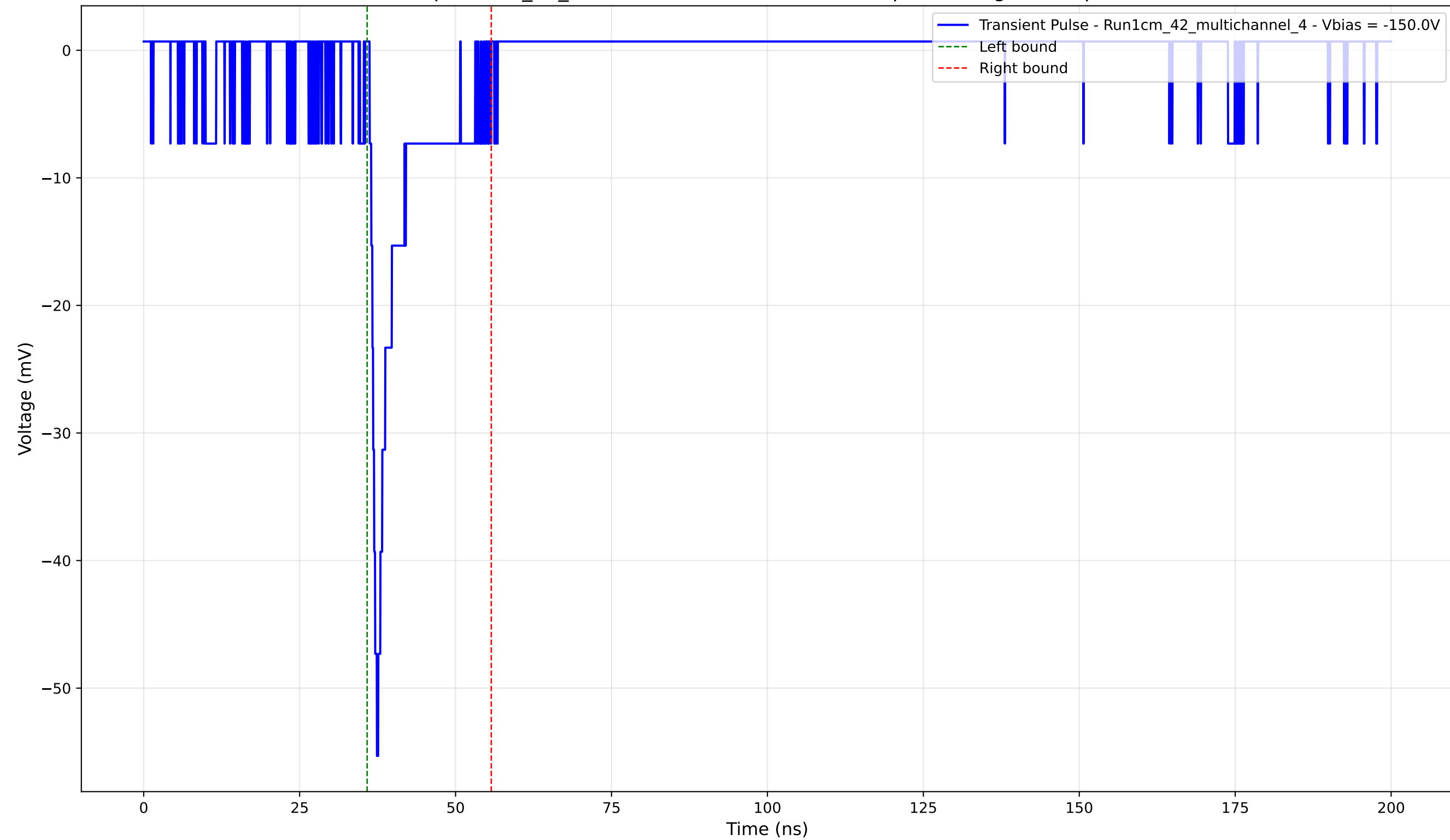
Transient Pulse - Sample: 1cm_42_multichannel - Position: 2785.0 \mu\text{m} - Charge: 4.72 pC - Rise Time: 1.17 ns
