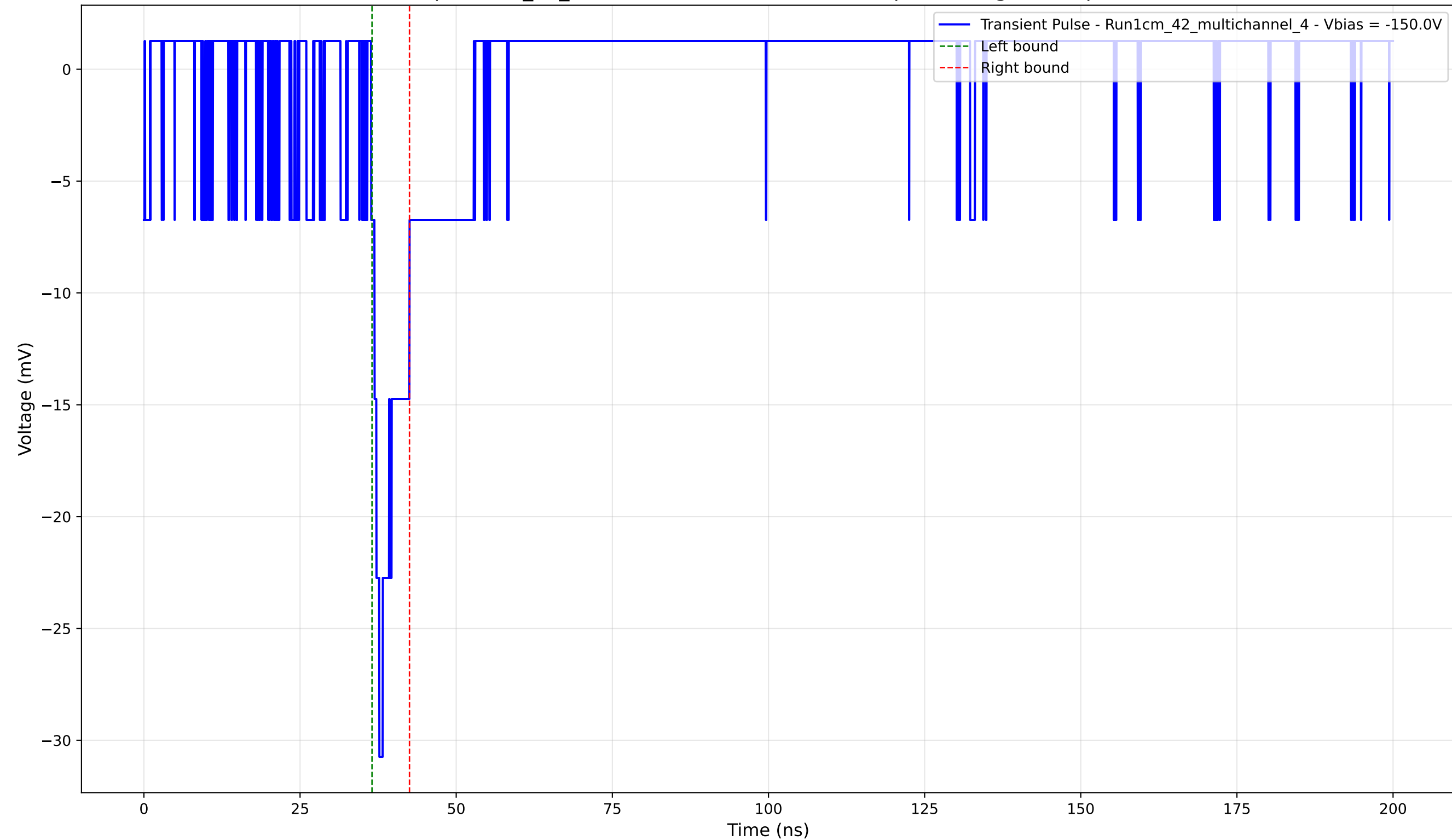
Transient Pulse - Sample: 1cm_42_multichannel - Position: 3230.0 \mu\text{m} - Charge: 2.17 pC - Rise Time: 1.31 ns
