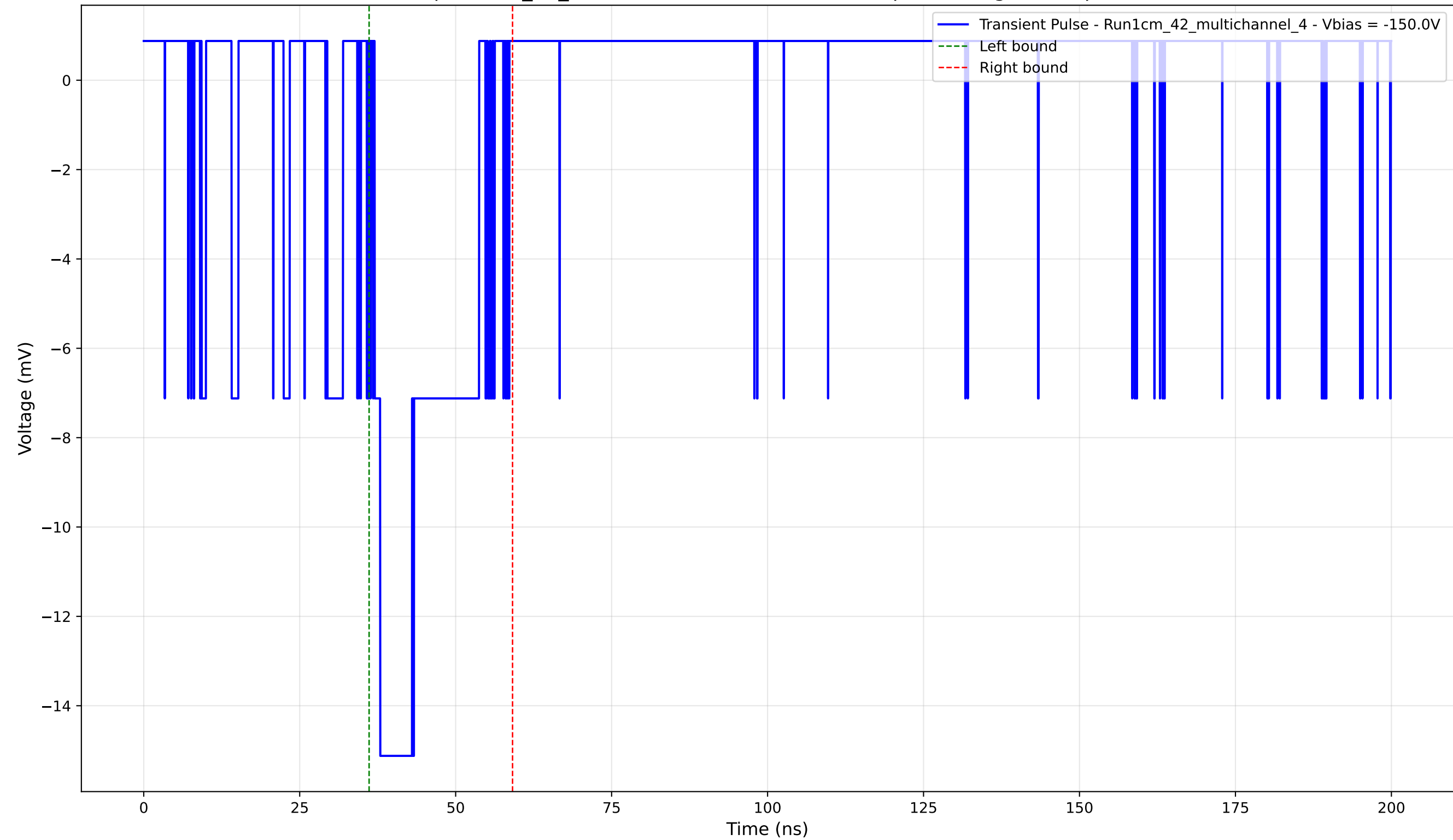
Transient Pulse - Sample: 1cm_42_multichannel - Position: 4015.0 \mu\text{m} - Charge: 3.32 pC - Rise Time: 0.90 ns
