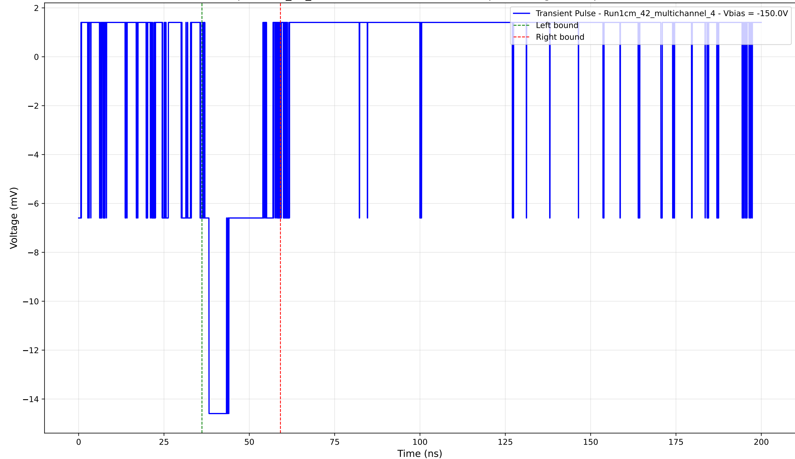
Transient Pulse - Sample: 1cm_42_multichannel - Position: 4300.0 \mu\text{m} - Charge: 3.53 pC - Rise Time: 1.24 ns
