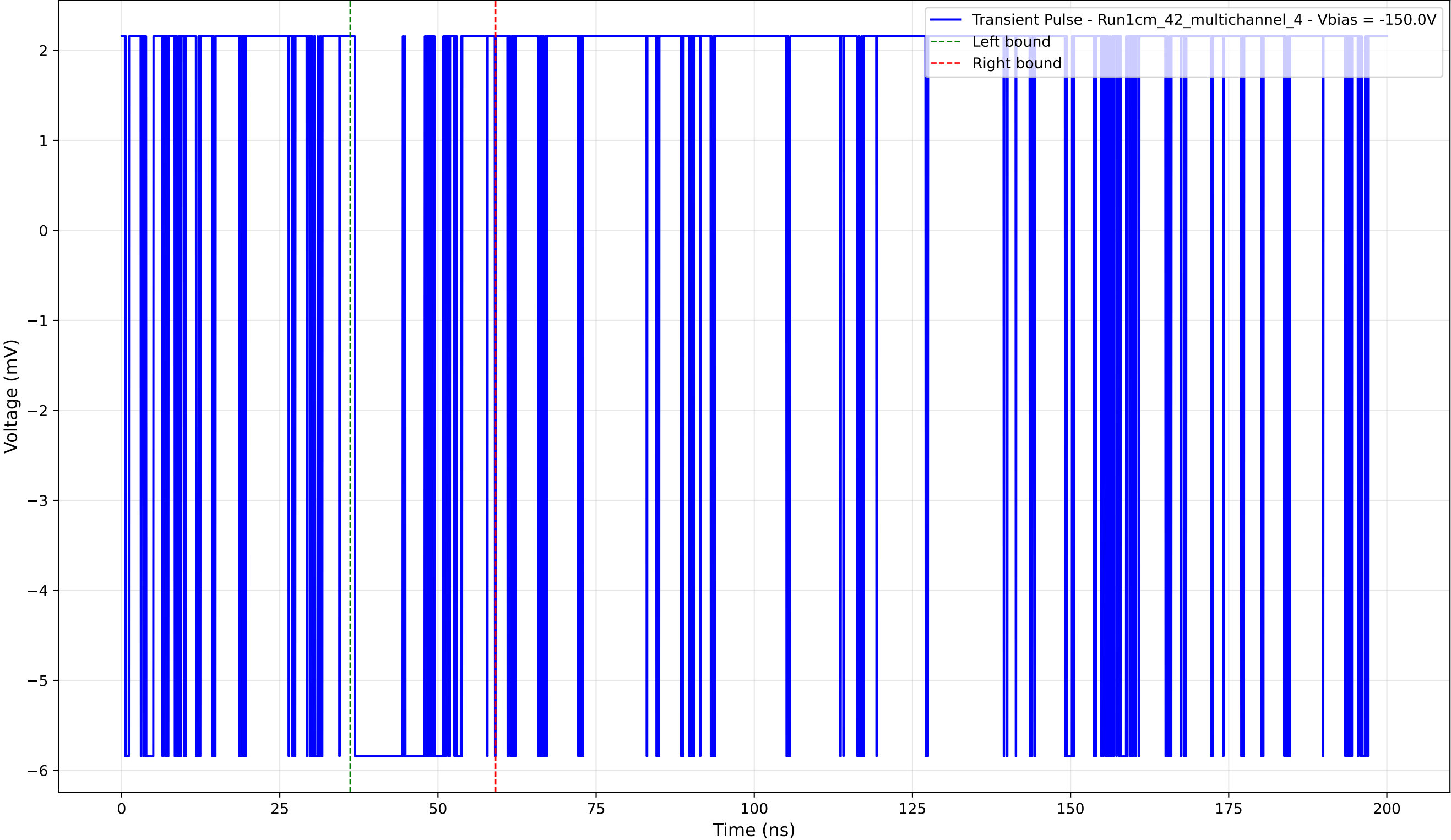
Transient Pulse - Sample: 1cm_42_multichannel - Position: 3440.0 \mu\text{m} - Charge: 1.28 pC - Rise Time: 0.00 ns (N/A)
