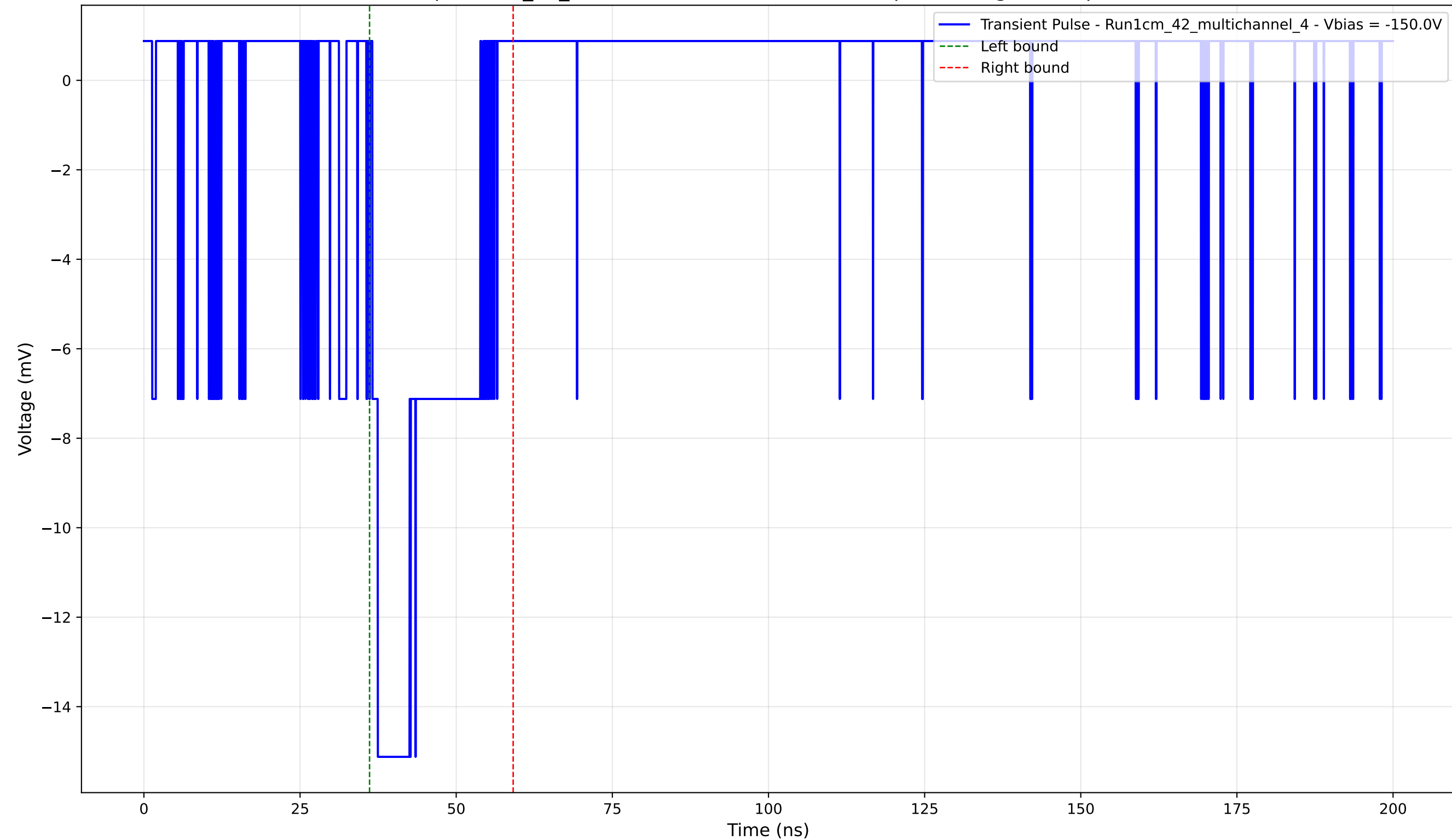
Transient Pulse - Sample: 1cm_42_multichannel - Position: 3700.0 \mu\text{m} - Charge: 3.34 pC - Rise Time: 0.88 ns
