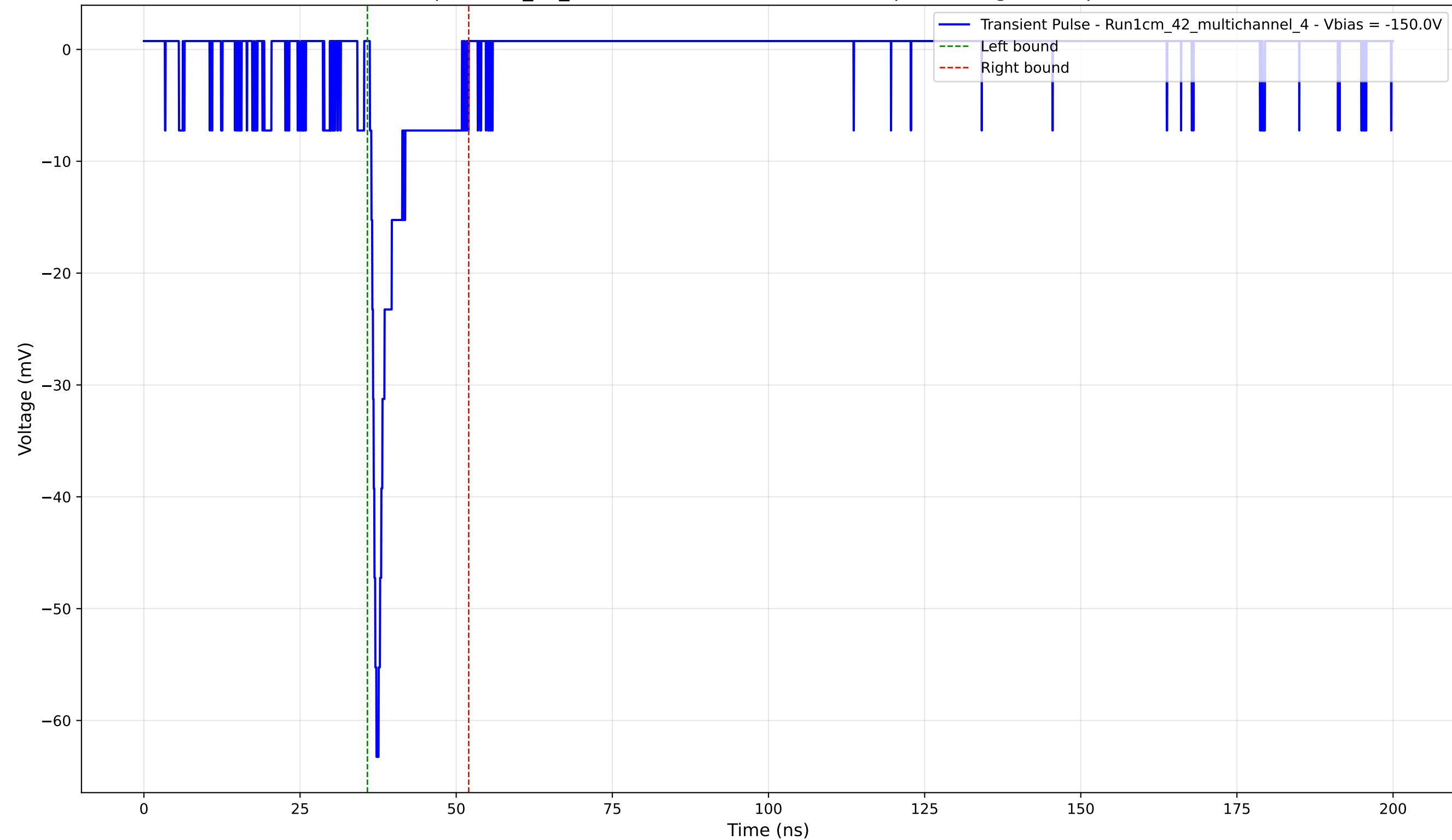
Transient Pulse - Sample: 1cm_42_multichannel - Position: 2105.0 \mu\text{m} - Charge: 4.41 pC - Rise Time: 1.04 ns
