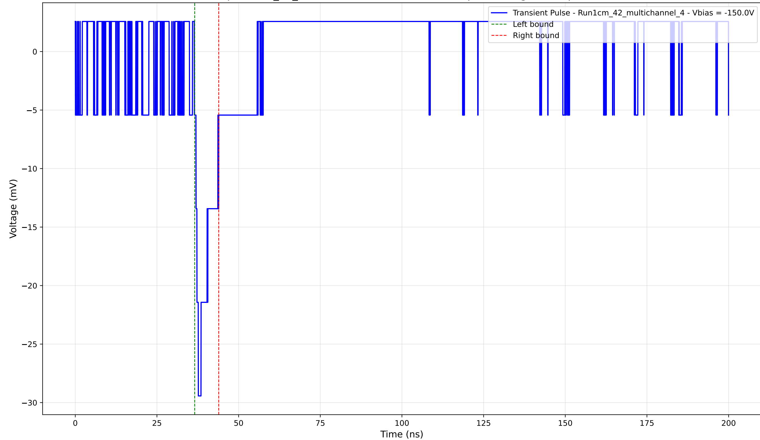
Transient Pulse - Sample: 1cm_42_multichannel - Position: 1460.0 \mu\text{m} - Charge: 2.52 pC - Rise Time: 1.22 ns
