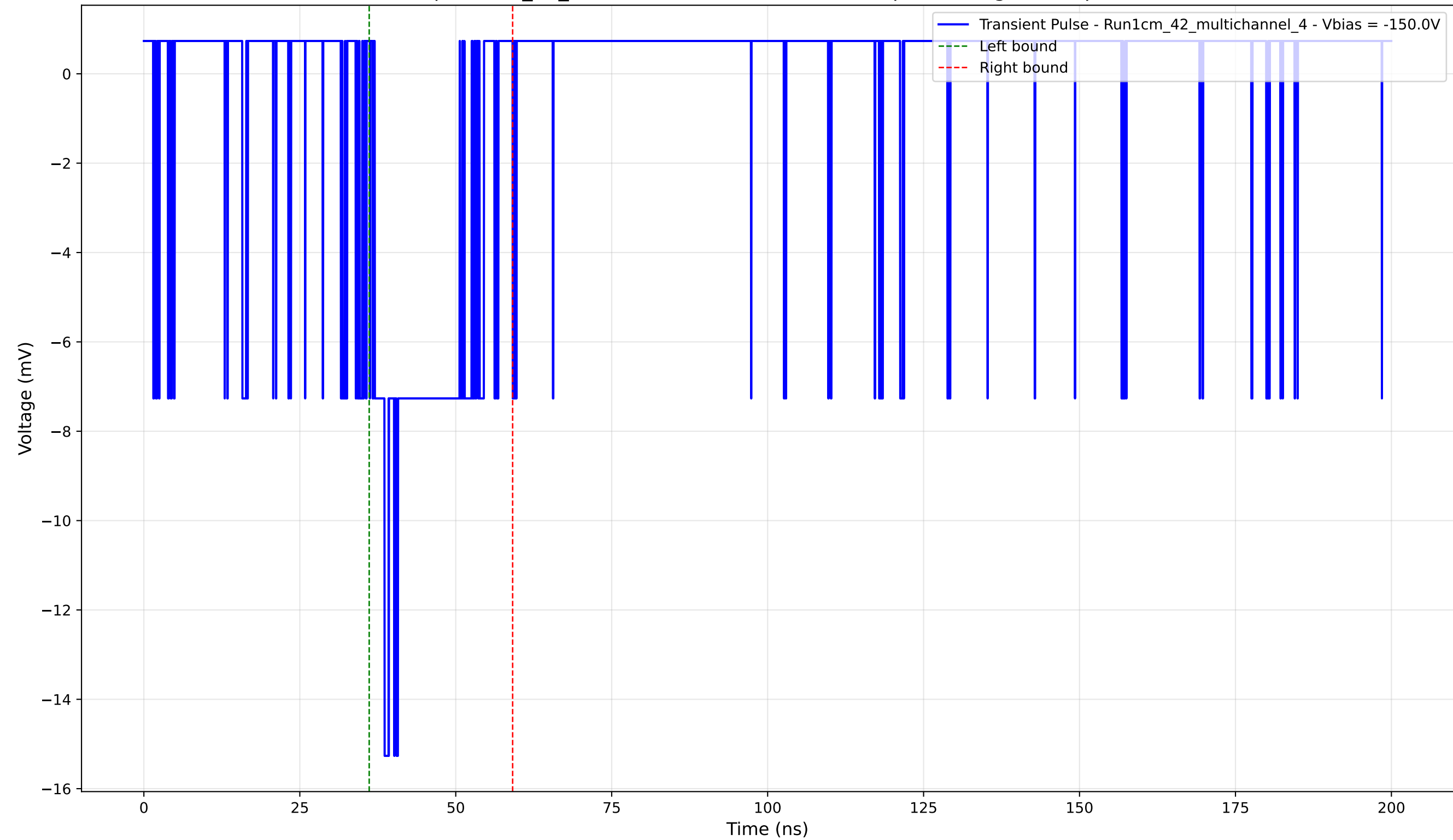
Transient Pulse - Sample: 1cm_42_multichannel - Position: 4825.0 \mu\text{m} - Charge: 2.58 pC - Rise Time: 1.58 ns
