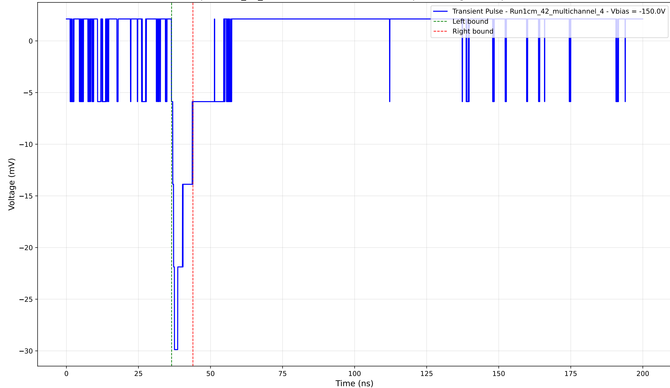
Transient Pulse - Sample: 1cm_42_multichannel - Position: 1510.0 \mu\text{m} - Charge: 2.66 pC - Rise Time: 1.06 ns
