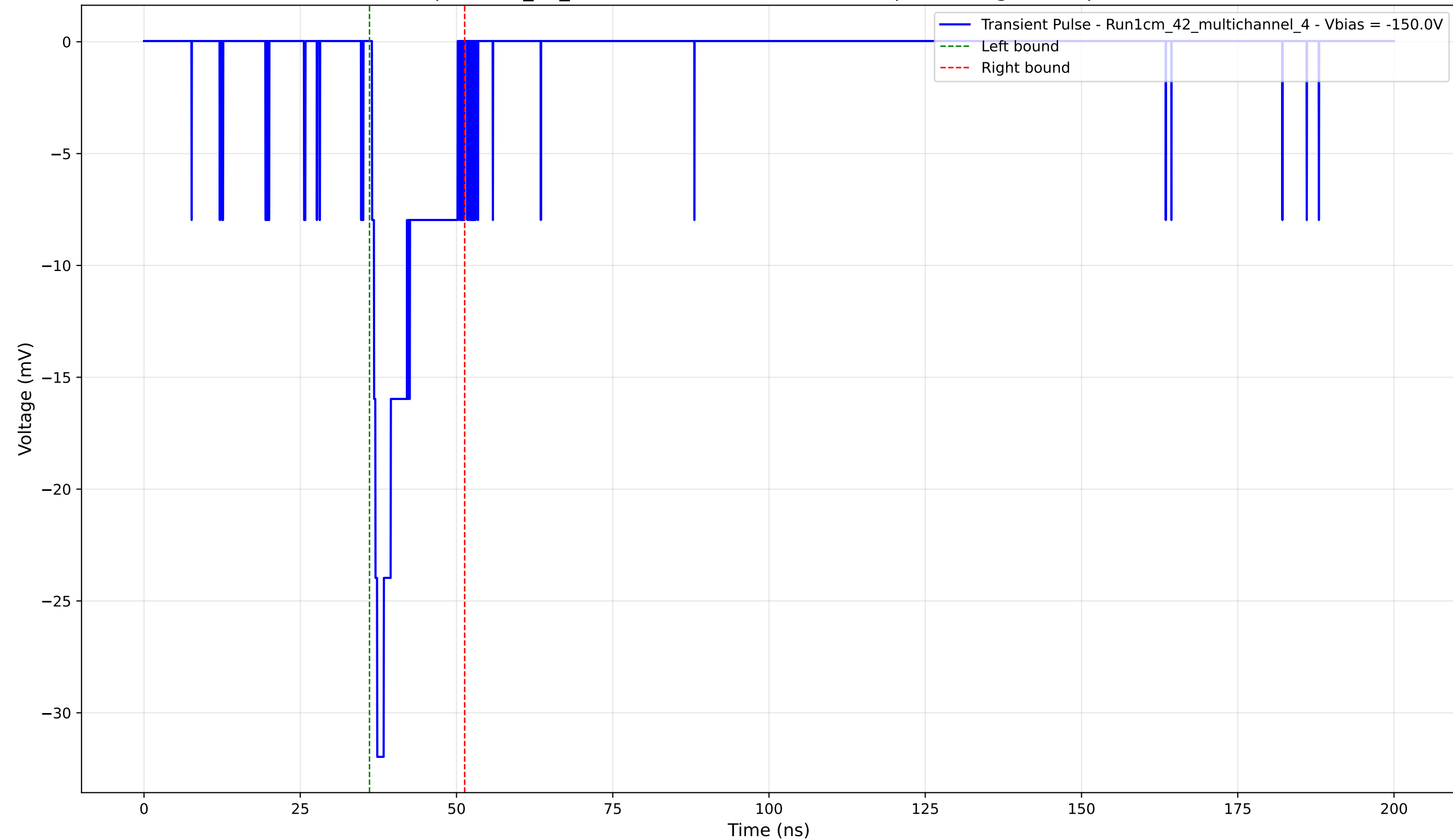
Transient Pulse - Sample: 1cm_42_multichannel - Position: 3085.0 \mu\text{m} - Charge: 3.68 pC - Rise Time: 0.83 ns
