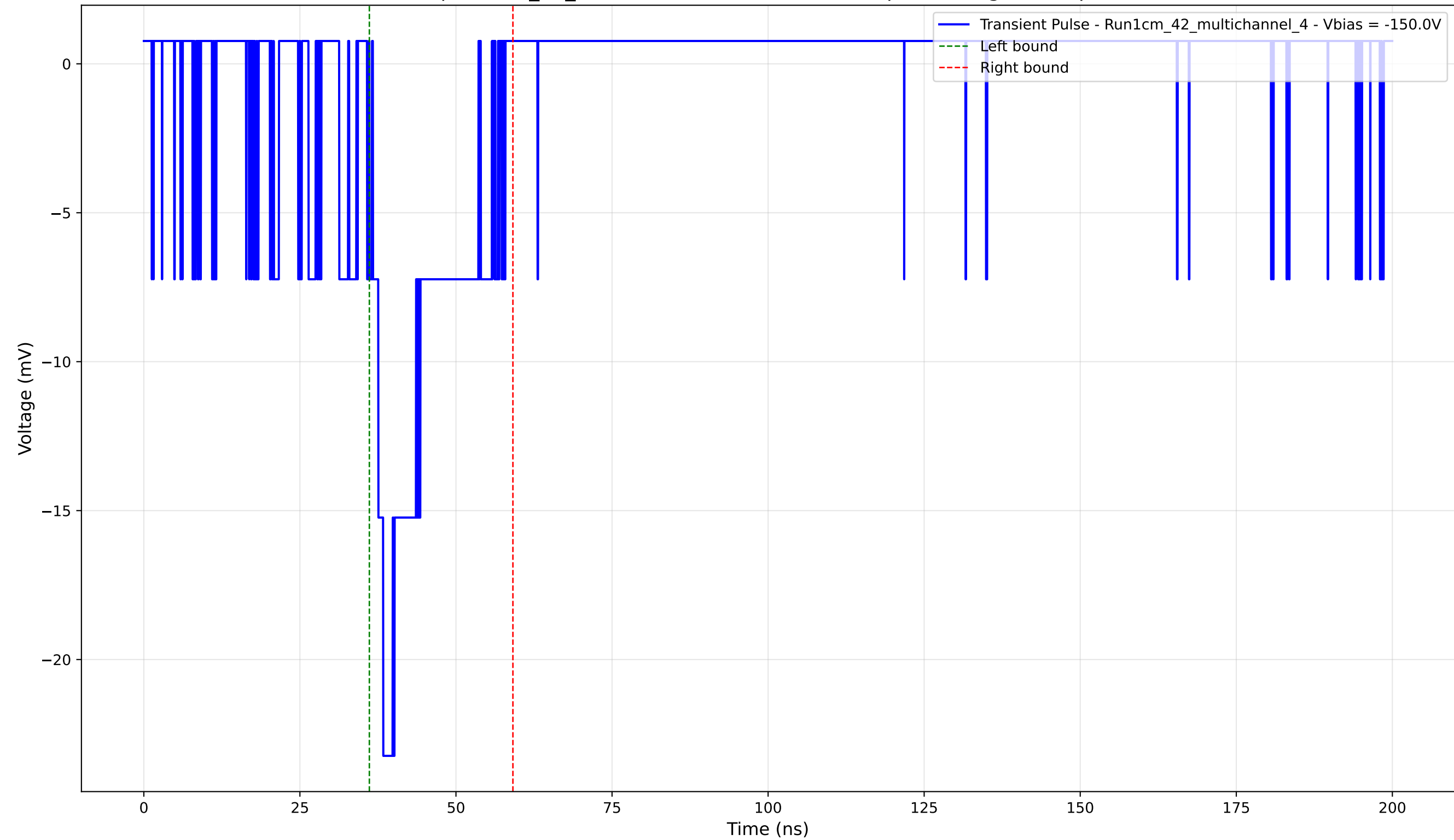
Transient Pulse - Sample: 1cm_42_multichannel - Position: 980.0 \mu\text{m} - Charge: 4.16 pC - Rise Time: 1.66 ns
