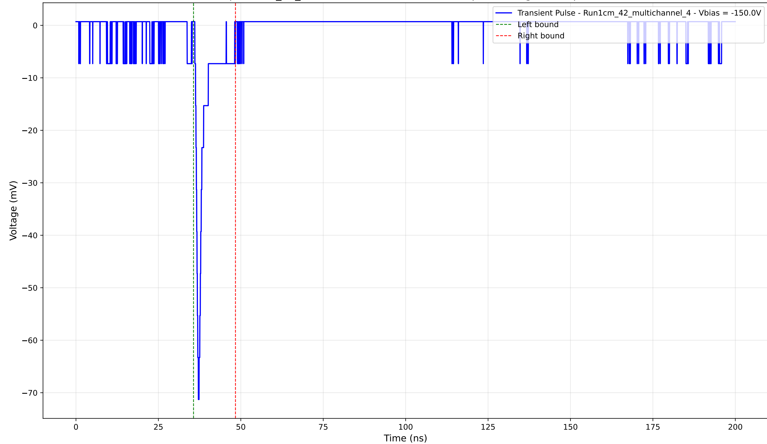
Transient Pulse - Sample: 1cm_42_multichannel - Position: 2320.0 \mu\text{m} - Charge: 3.70 pC - Rise Time: 1.06 ns
