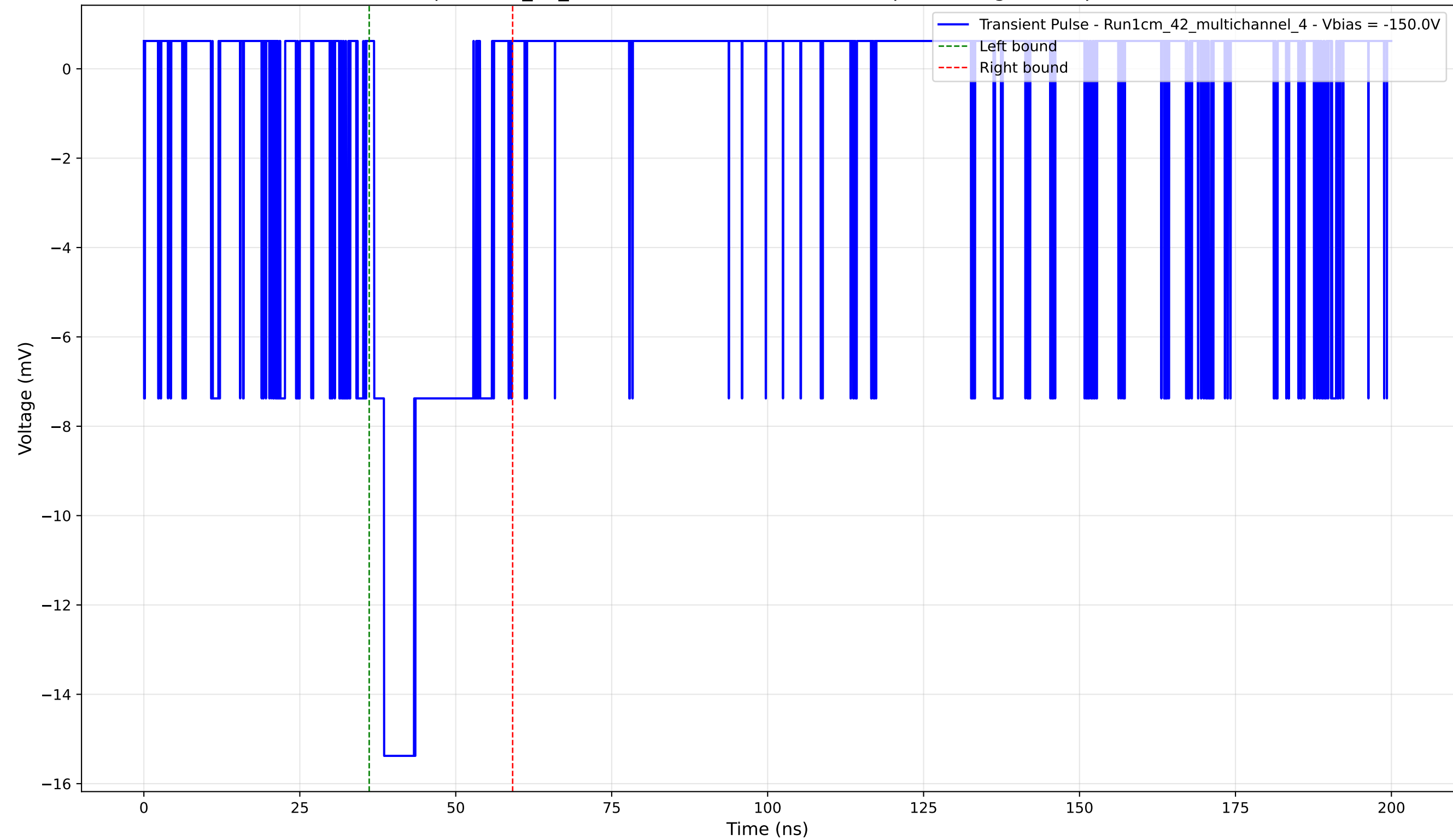
Transient Pulse - Sample: 1cm_42_multichannel - Position: 4555.0 \mu\text{m} - Charge: 3.51 pC - Rise Time: 1.60 ns
