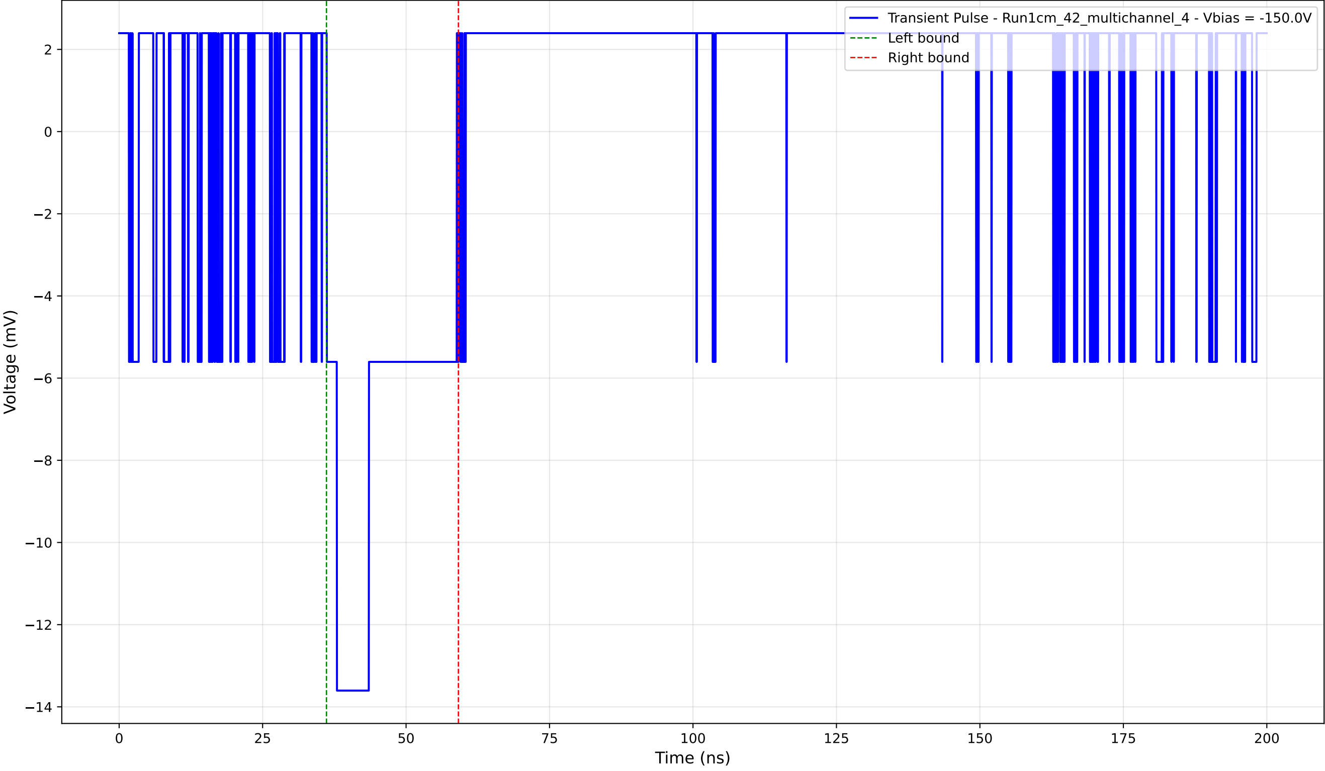
Transient Pulse - Sample: 1cm_42_multichannel - Position: 600.0 \mu\text{m} - Charge: 3.44 pC - Rise Time: 0.00 ns (N/A)
