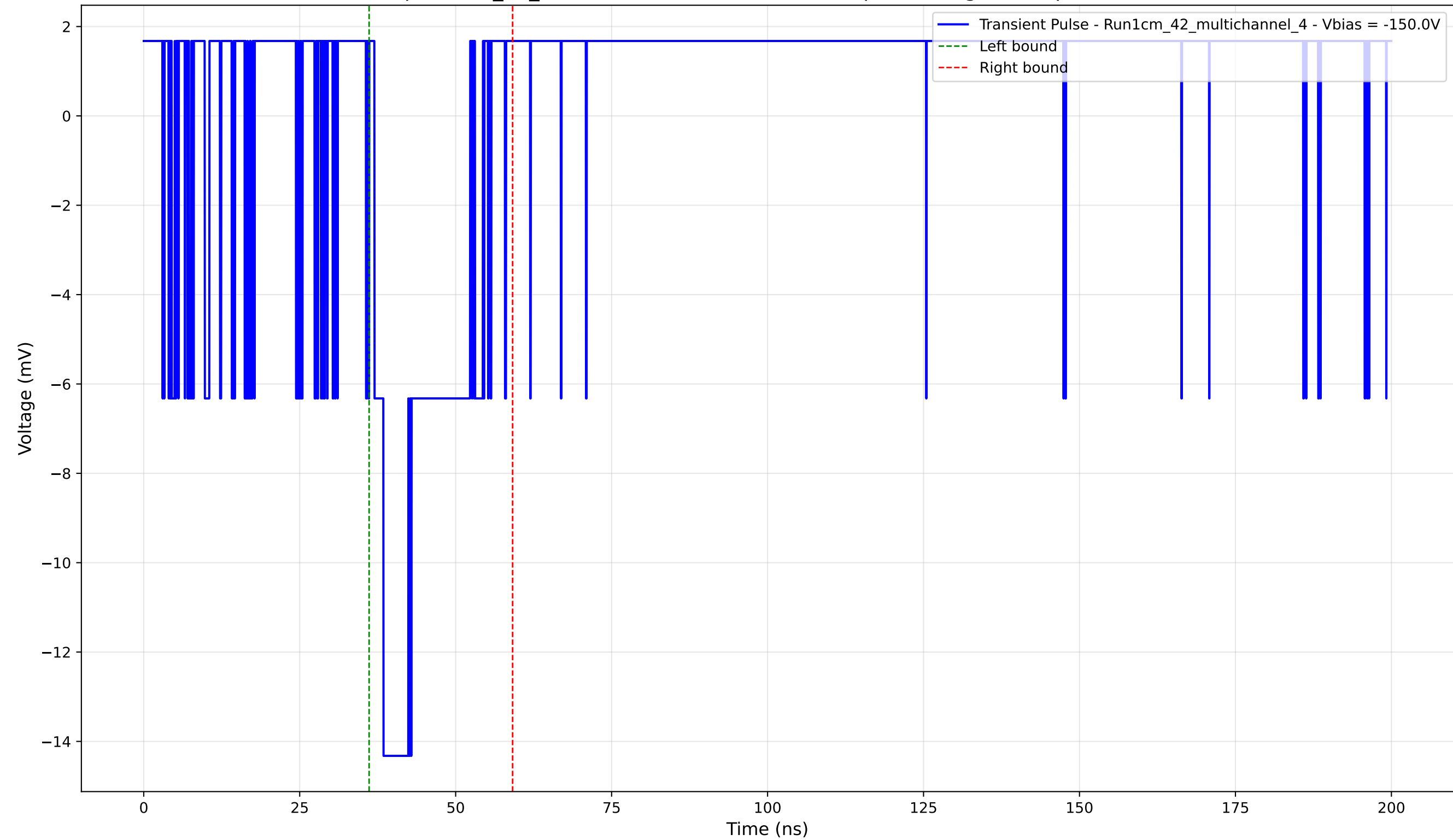
Transient Pulse - Sample: 1cm_42_multichannel - Position: 4675.0 \mu\text{m} - Charge: 2.67 pC - Rise Time: 0.00 ns (N/A)
