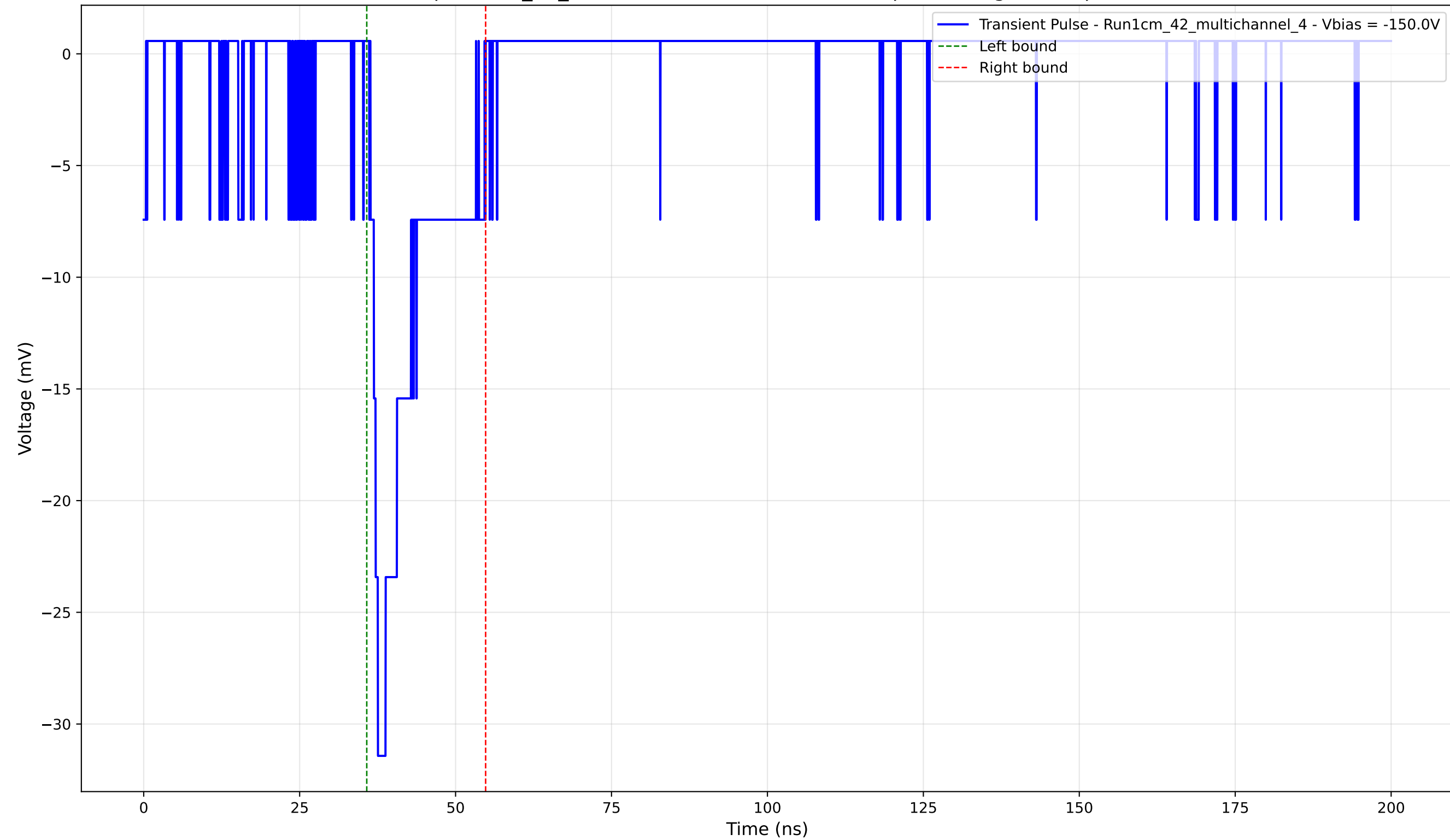
Transient Pulse - Sample: 1cm_42_multichannel - Position: 1515.0 \mu\text{m} - Charge: 4.47 pC - Rise Time: 1.19 ns
