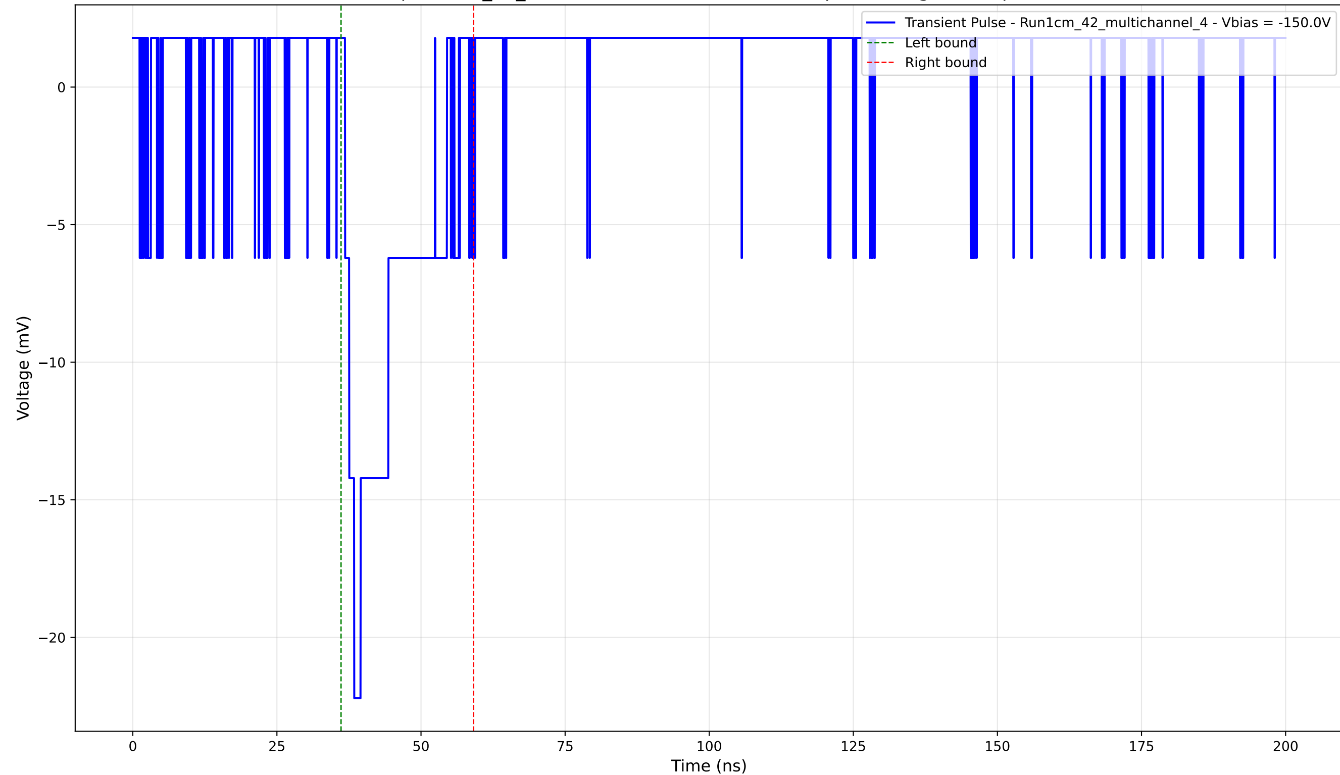
Transient Pulse - Sample: 1cm_42_multichannel - Position: 3680.0 \mu\text{m} - Charge: 3.48 pC - Rise Time: 1.60 ns
