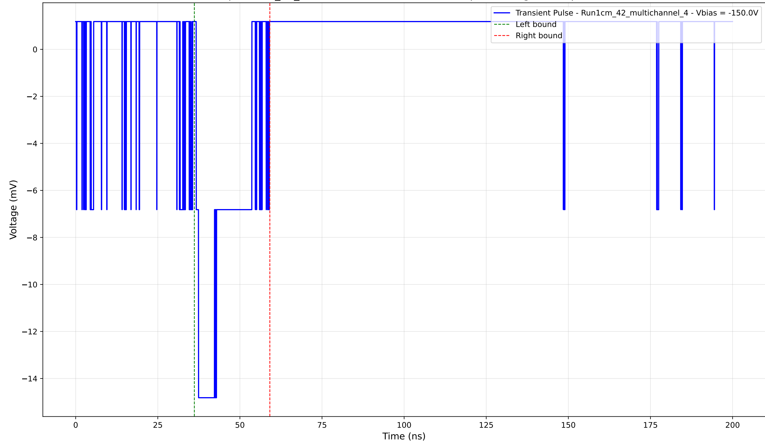
Transient Pulse - Sample: 1cm_42_multichannel - Position: 3605.0 \mu\text{m} - Charge: 3.18 pC - Rise Time: 0.72 ns
