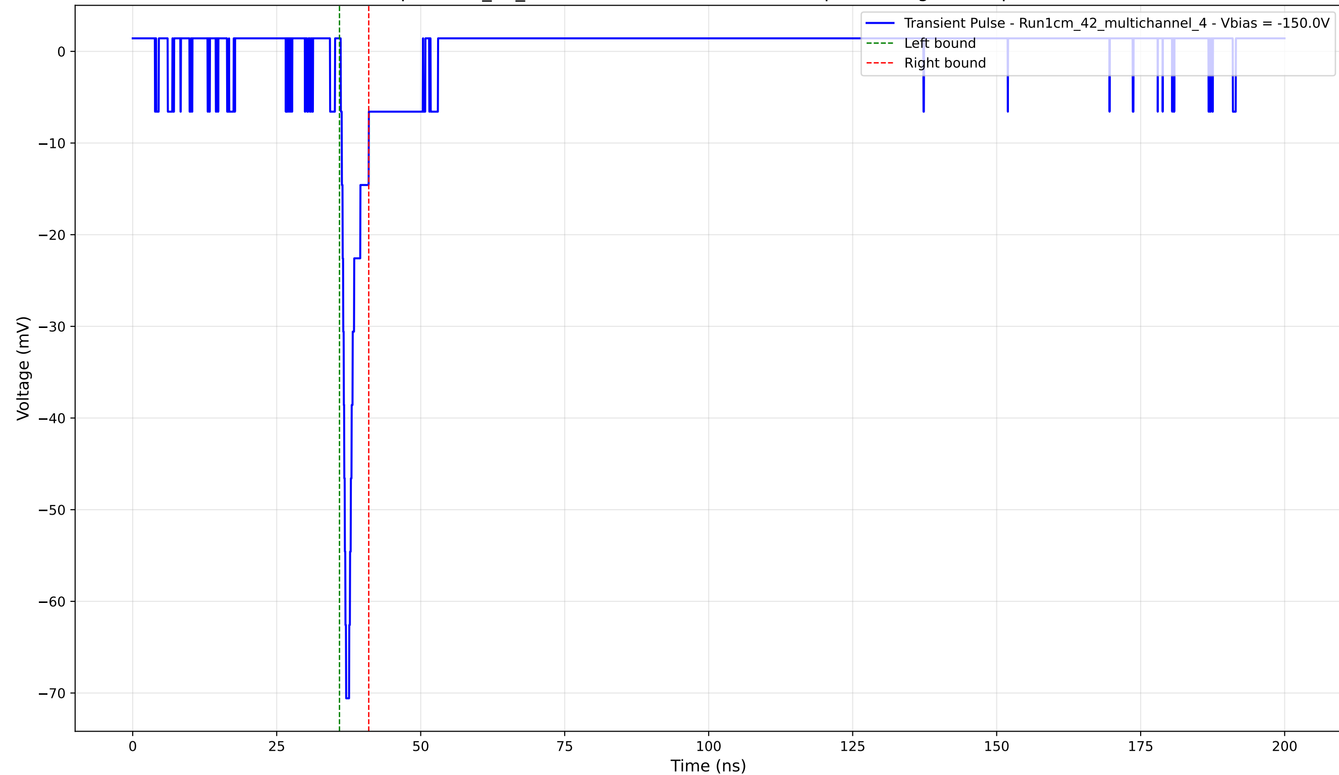
Transient Pulse - Sample: 1cm_42_multichannel - Position: 2545.0 \mu\text{m} - Charge: 3.01 pC - Rise Time: 0.76 ns
