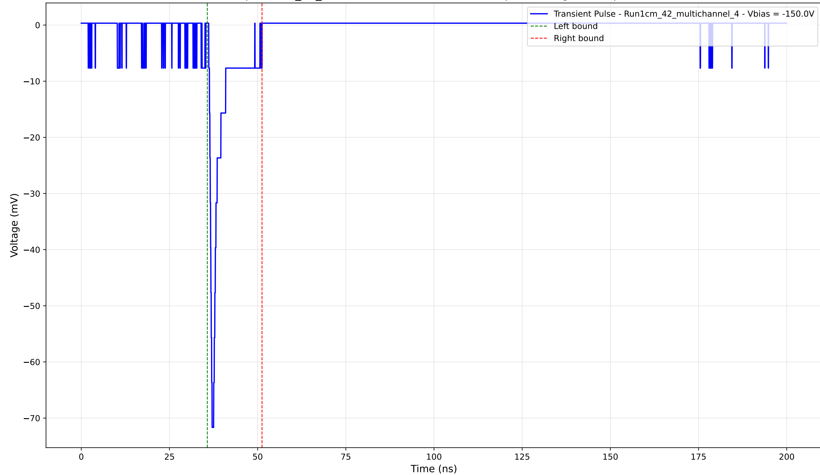
Transient Pulse - Sample: 1cm_42_multichannel - Position: 2560.0 \mu\text{m} - Charge: 4.58 pC - Rise Time: 0.94 ns
