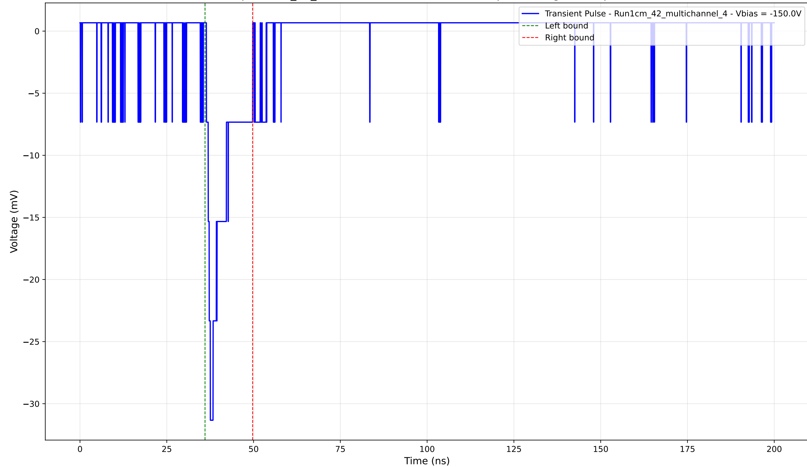
Transient Pulse - Sample: 1cm_42_multichannel - Position: 3215.0 \mu\text{m} - Charge: 3.26 pC - Rise Time: 1.13 ns
