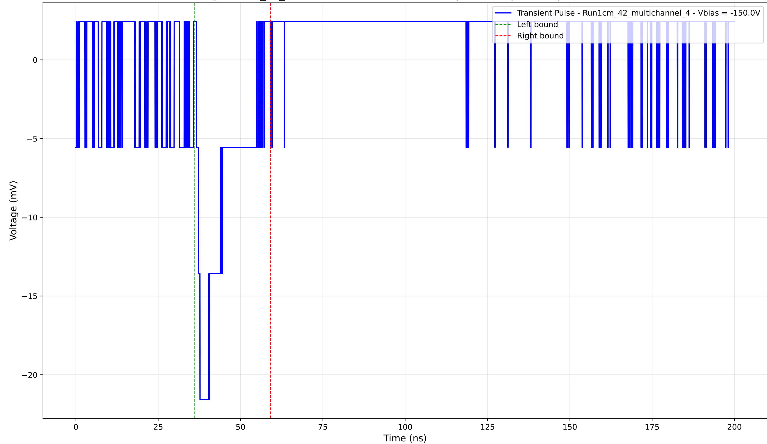
Transient Pulse - Sample: 1cm_42_multichannel - Position: 1210.0 \mu\text{m} - Charge: 3.63 pC - Rise Time: 0.00 ns (N/A)
