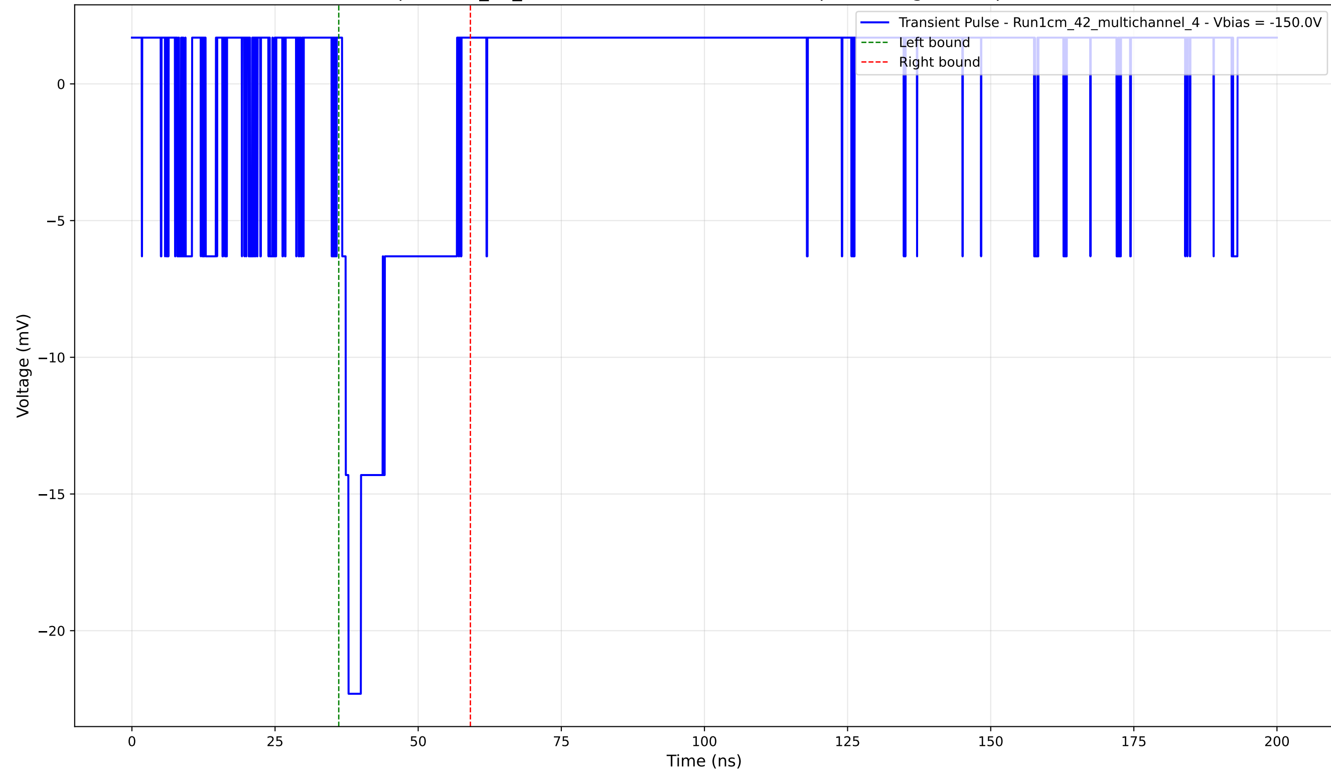
Transient Pulse - Sample: 1cm_42_multichannel - Position: 1155.0 \mu\text{m} - Charge: 3.88 pC - Rise Time: 1.12 ns
