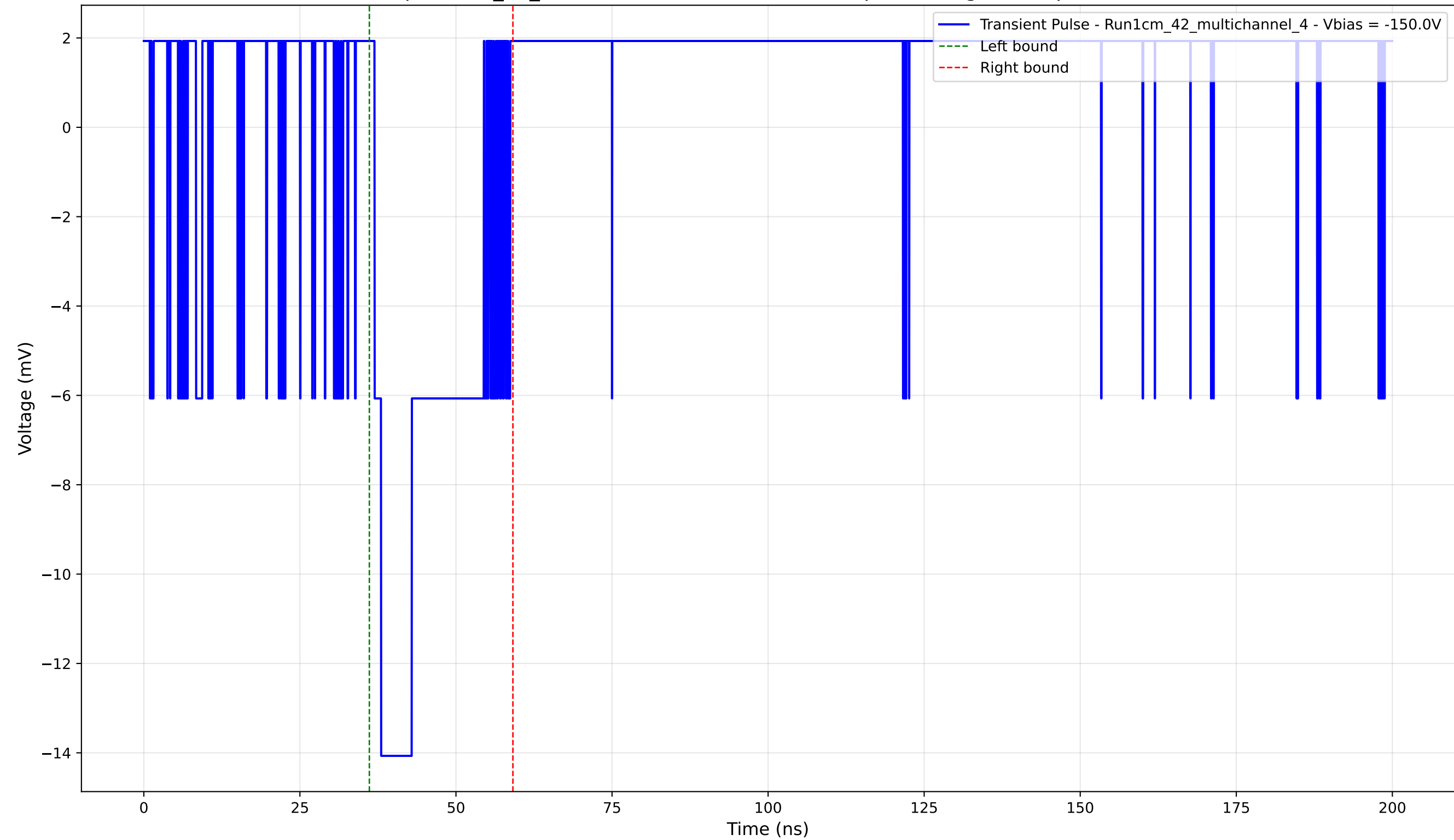
Transient Pulse - Sample: 1cm_42_multichannel - Position: 3975.0 \mu\text{m} - Charge: 3.04 pC - Rise Time: 0.00 ns (N/A)
