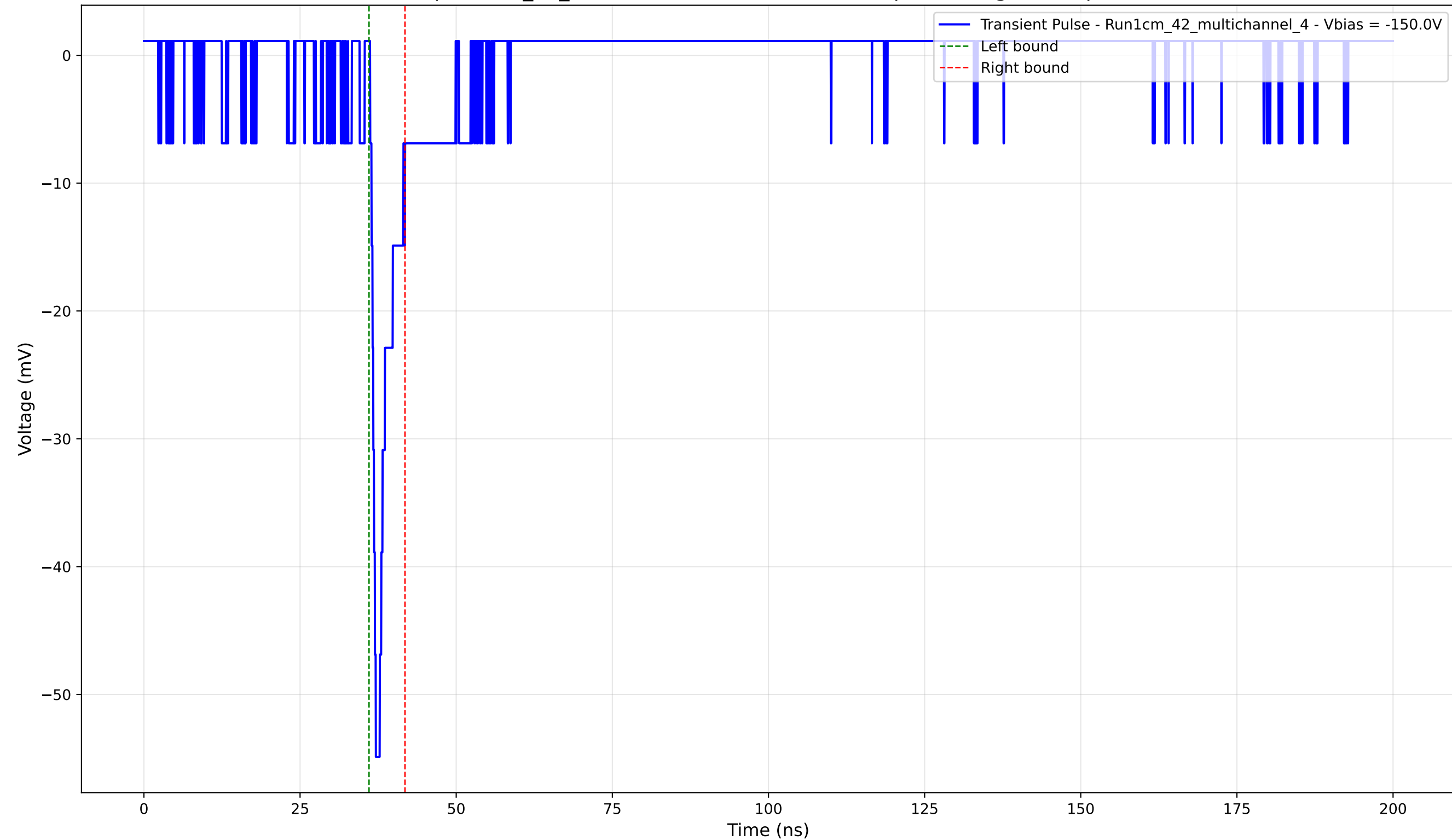
Transient Pulse - Sample: 1cm_42_multichannel - Position: 2700.0 \mu\text{m} - Charge: 2.90 pC - Rise Time: 0.90 ns
