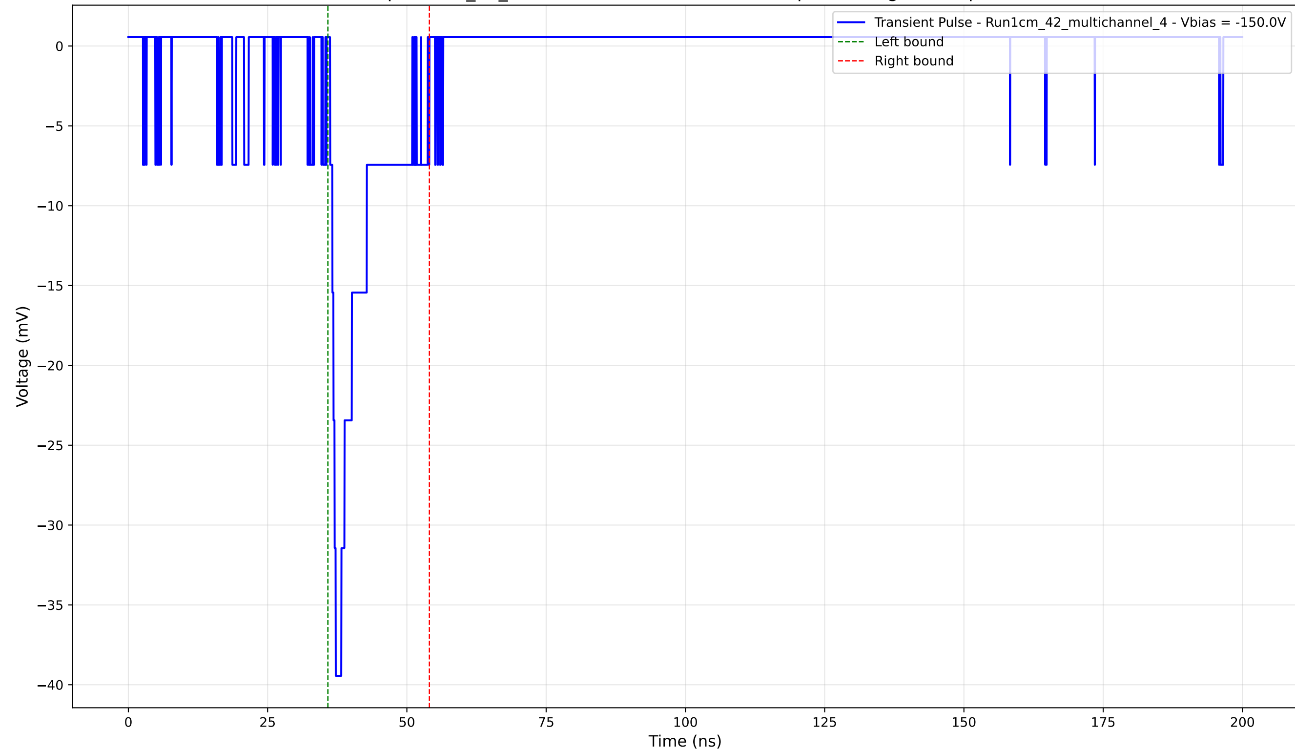
Transient Pulse - Sample: 1cm_42_multichannel - Position: 1775.0 \mu\text{m} - Charge: 4.53 pC - Rise Time: 1.01 ns
