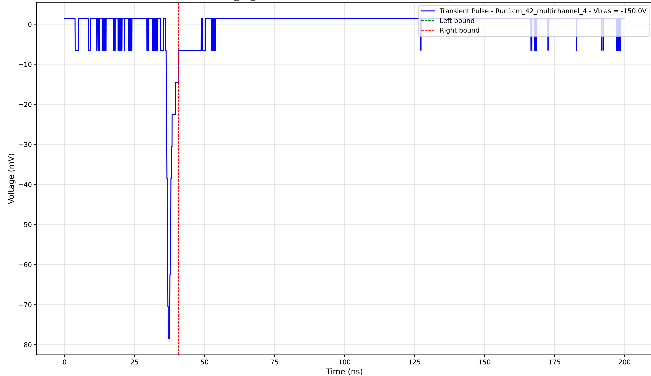
Transient Pulse - Sample: 1cm_42_multichannel - Position: 2290.0 \mu\text{m} - Charge: 3.10 pC - Rise Time: 0.76 ns
