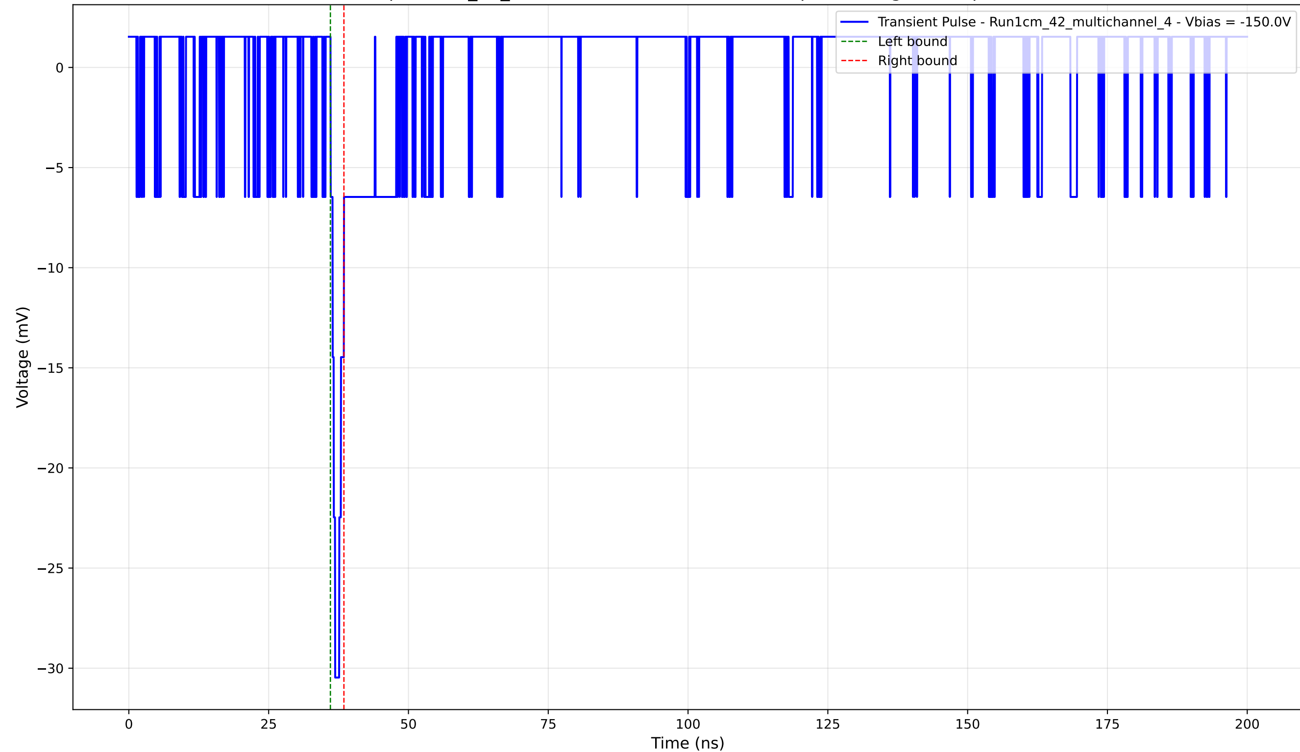
Transient Pulse - Sample: 1cm_42_multichannel - Position: 2340.0 \mu\text{m} - Charge: 0.95 pC - Rise Time: 0.81 ns
