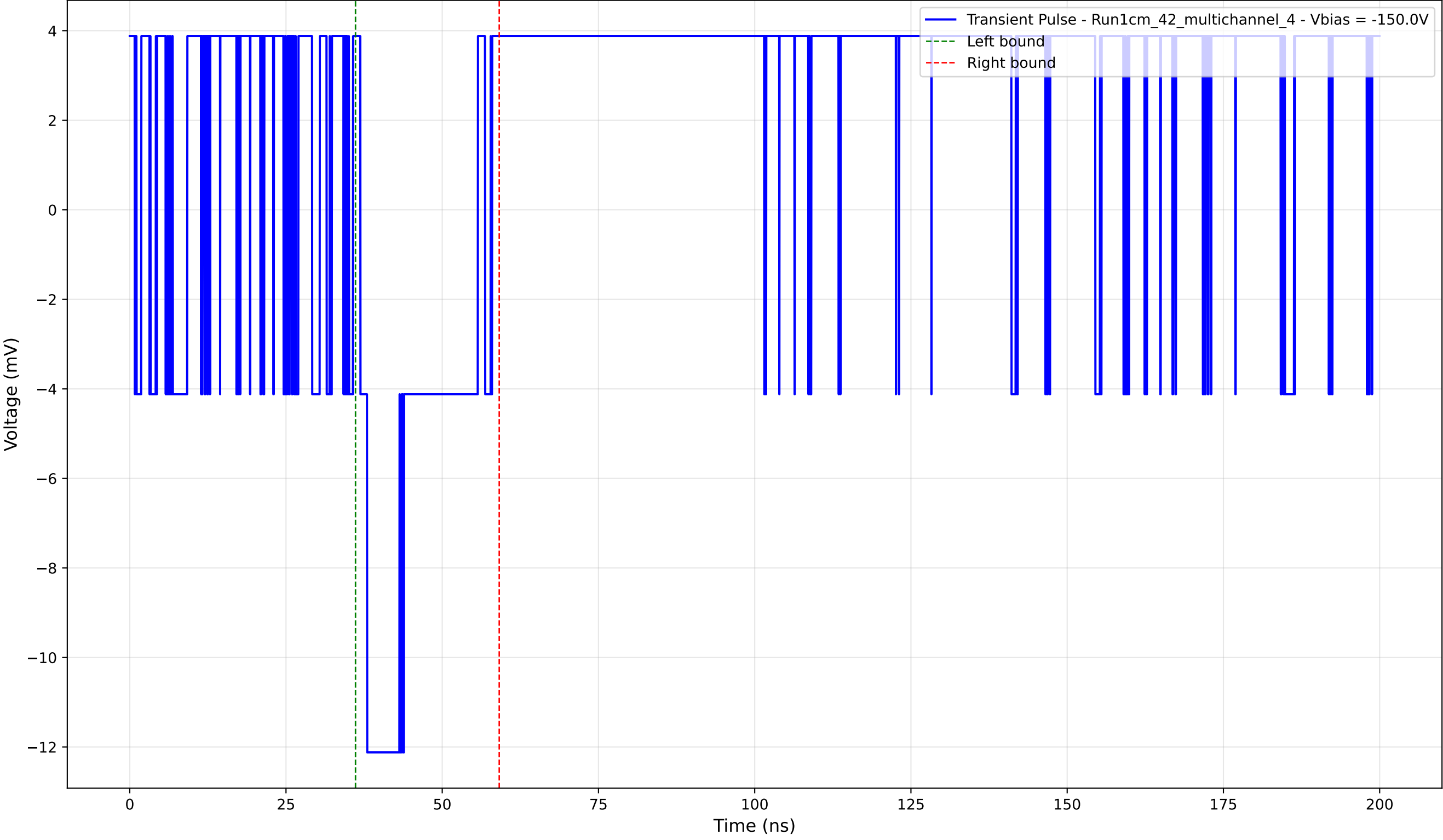
Transient Pulse - Sample: 1cm_42_multichannel - Position: 535.0 \mu\text{m} - Charge: 2.30 pC - Rise Time: 0.00 ns (N/A)
