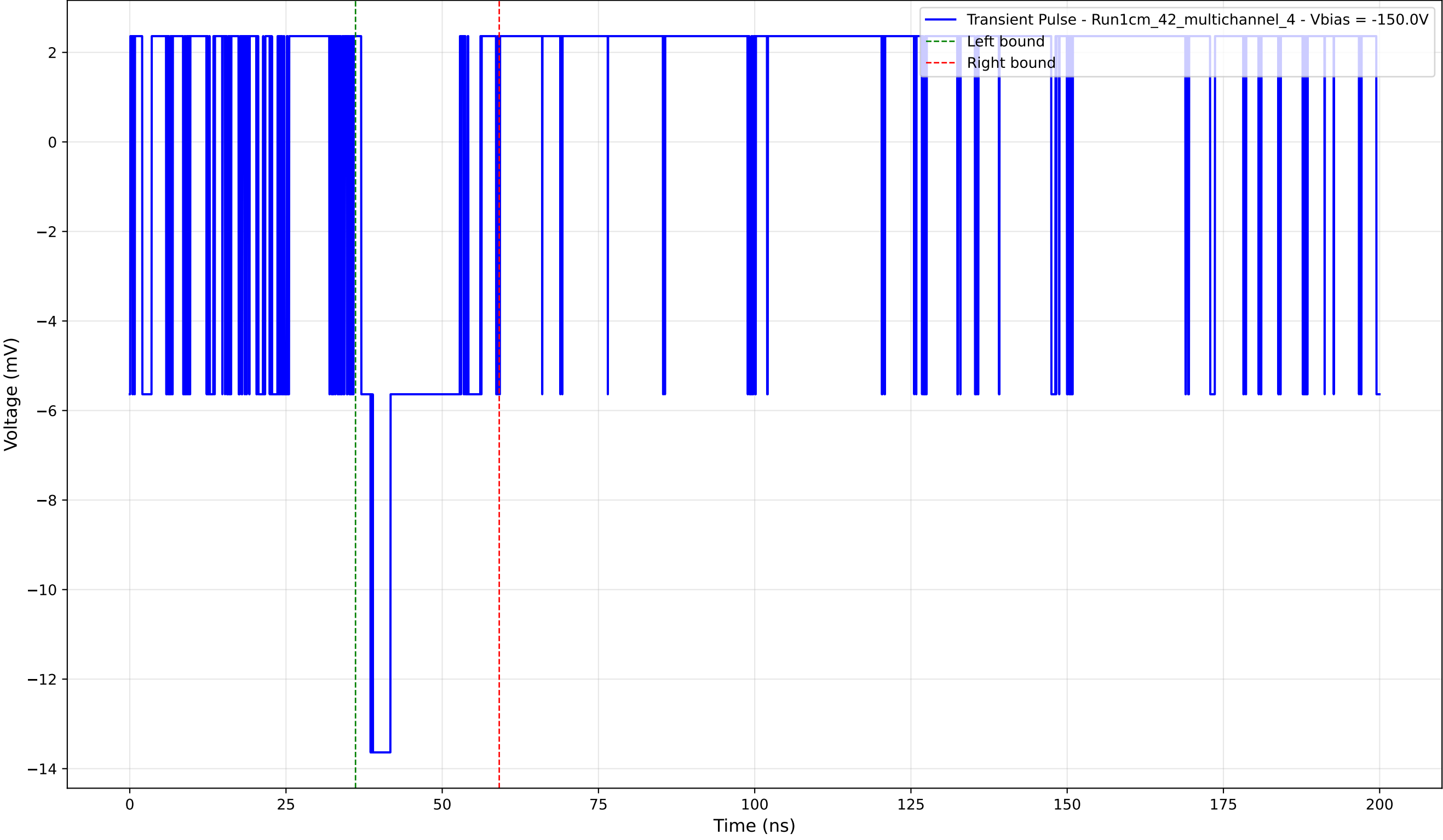
Transient Pulse - Sample: 1cm_42_multichannel - Position: 195.0 \mu\text{m} - Charge: 2.38 pC - Rise Time: 0.00 ns (N/A)
