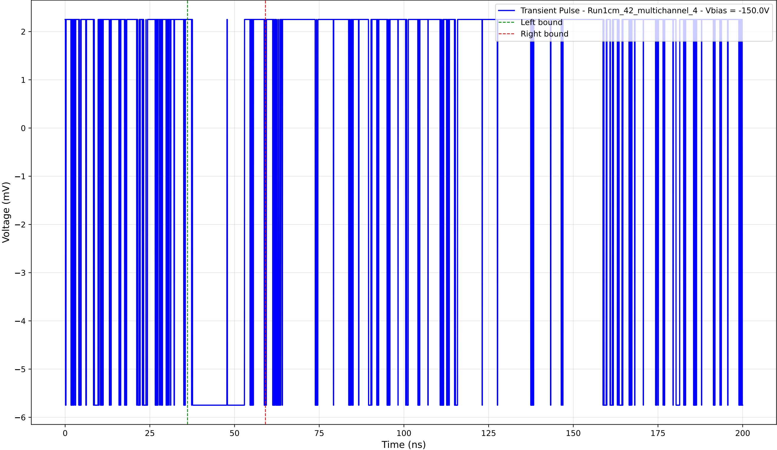
Transient Pulse - Sample: 1cm_42_multichannel - Position: 4360.0 \mu\text{m} - Charge: 1.52 pC - Rise Time: 0.00 ns (N/A)
