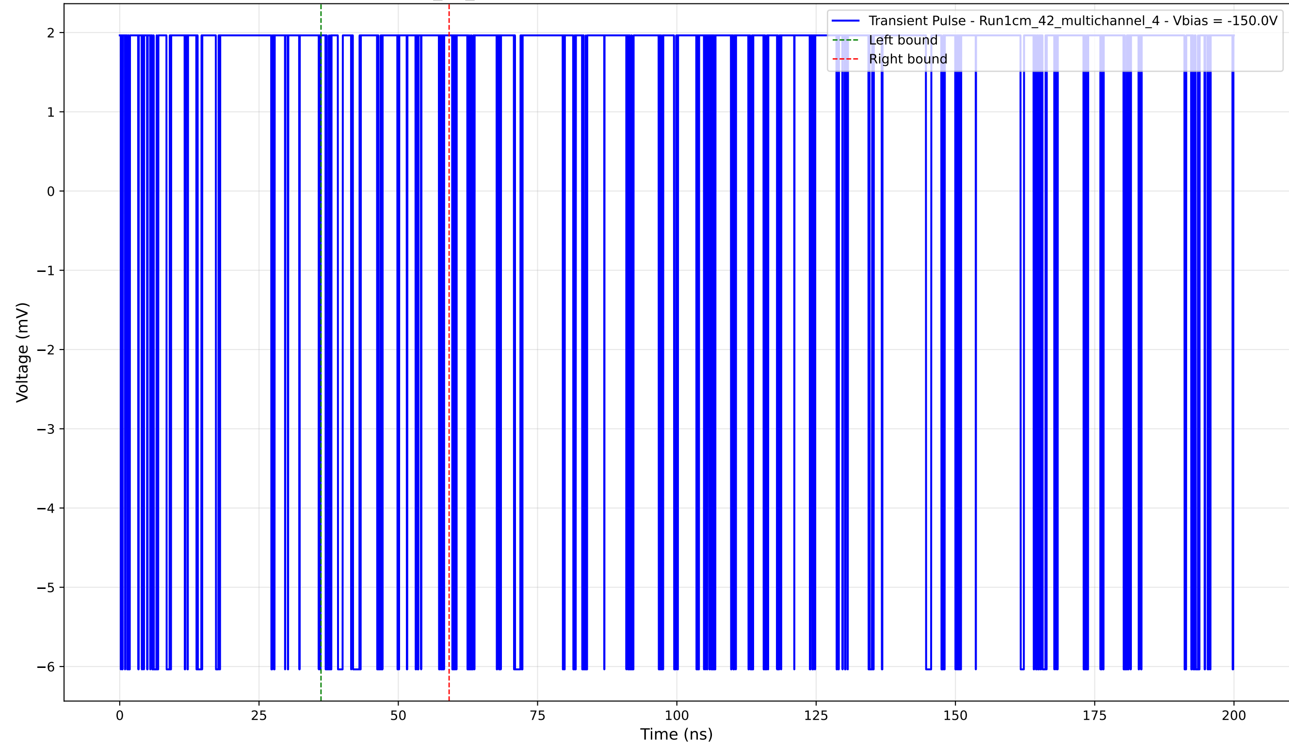
Transient Pulse - Sample: 1cm_42_multichannel - Position: 4410.0 \mu\text{m} - Charge: 0.16 pC - Rise Time: 0.00 ns (N/A)
