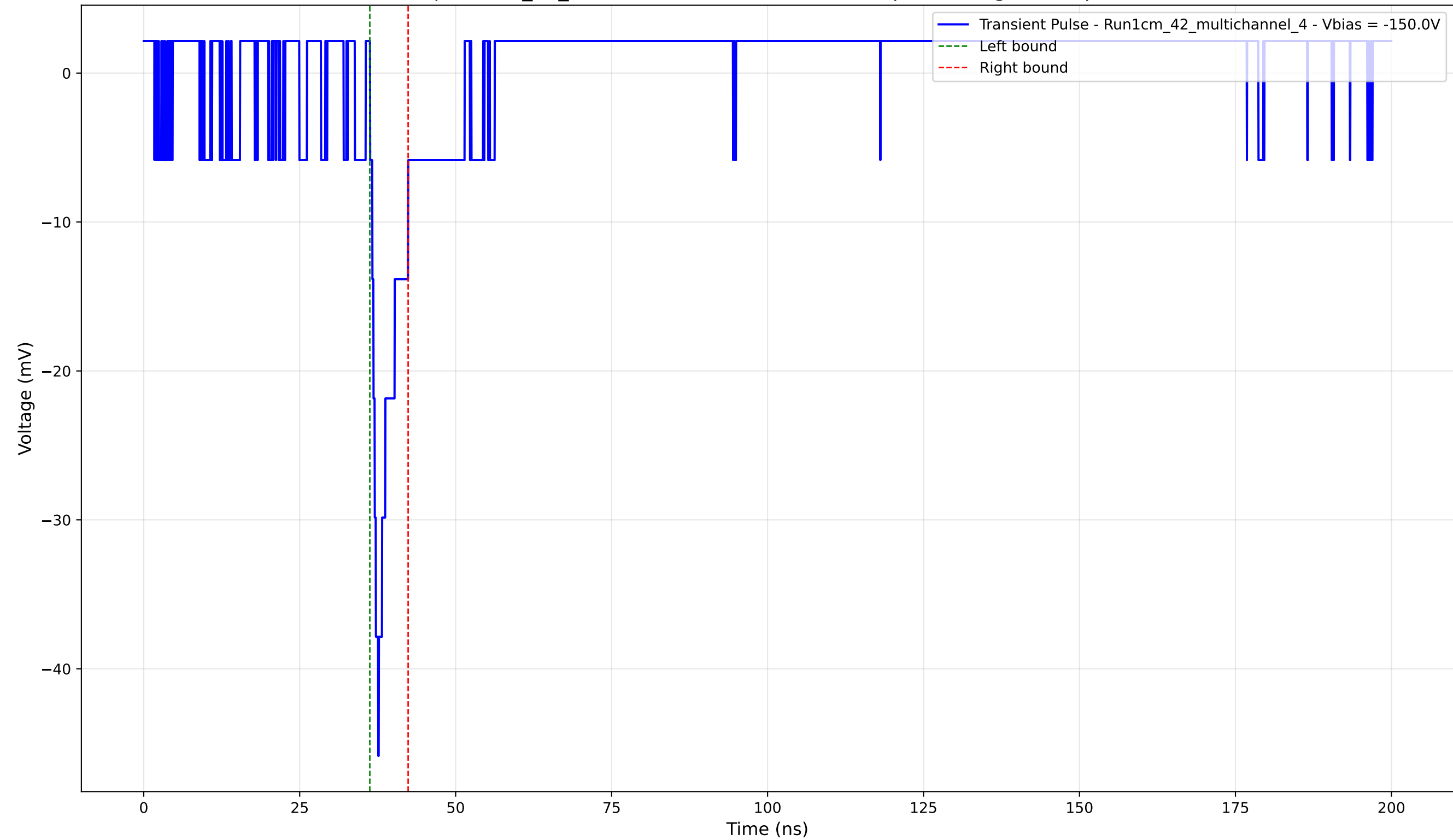
Transient Pulse - Sample: 1cm_42_multichannel - Position: 1795.0 \mu\text{m} - Charge: 2.62 pC - Rise Time: 1.31 ns
