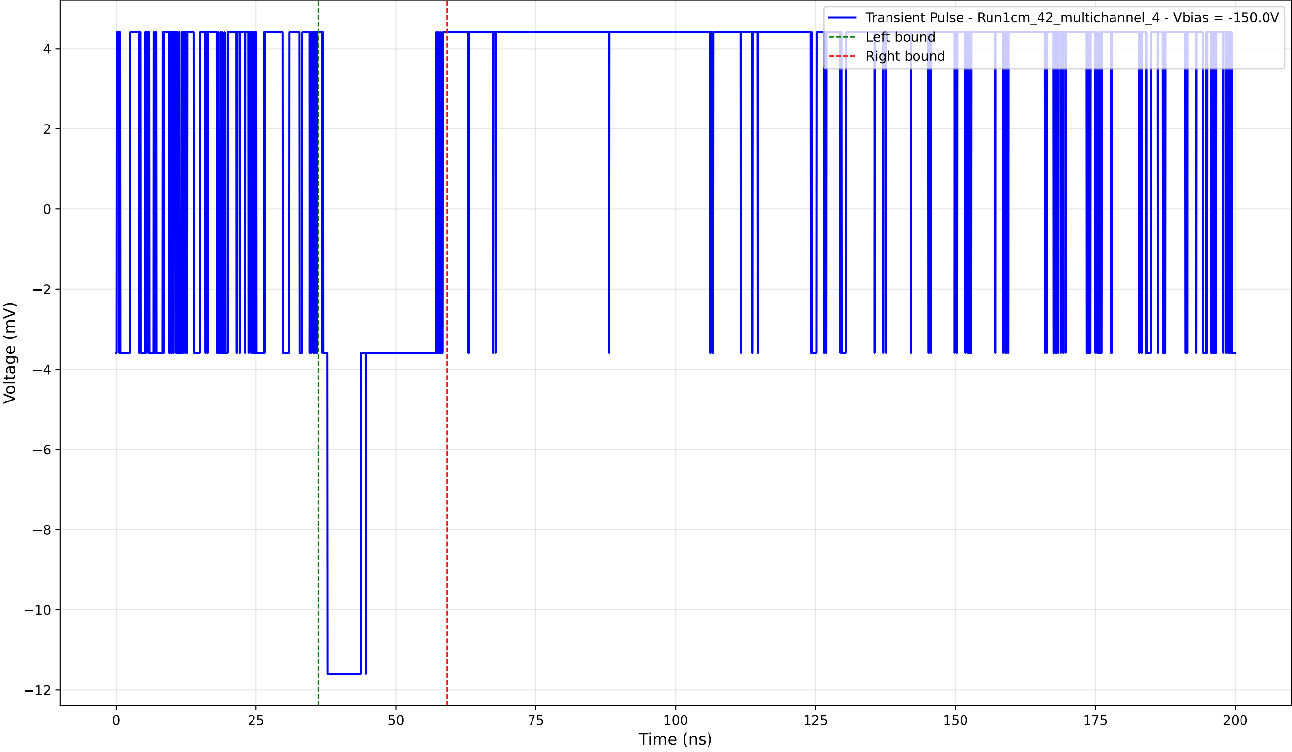
Transient Pulse - Sample: 1cm_42_multichannel - Position: 715.0 \mu\text{m} - Charge: 2.32 pC - Rise Time: 0.00 ns (N/A)
