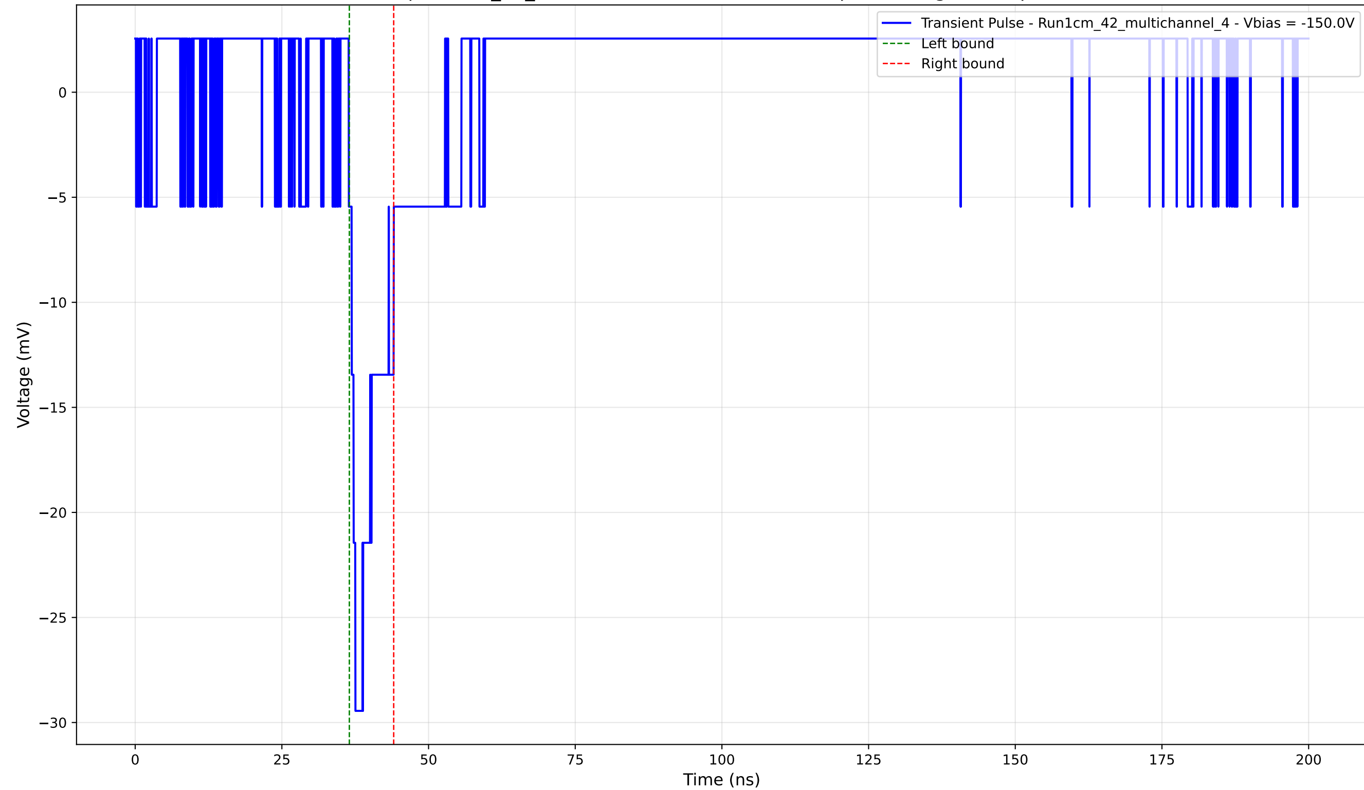
Transient Pulse - Sample: 1cm_42_multichannel - Position: 1500.0 \mu\text{m} - Charge: 2.65 pC - Rise Time: 1.14 ns
