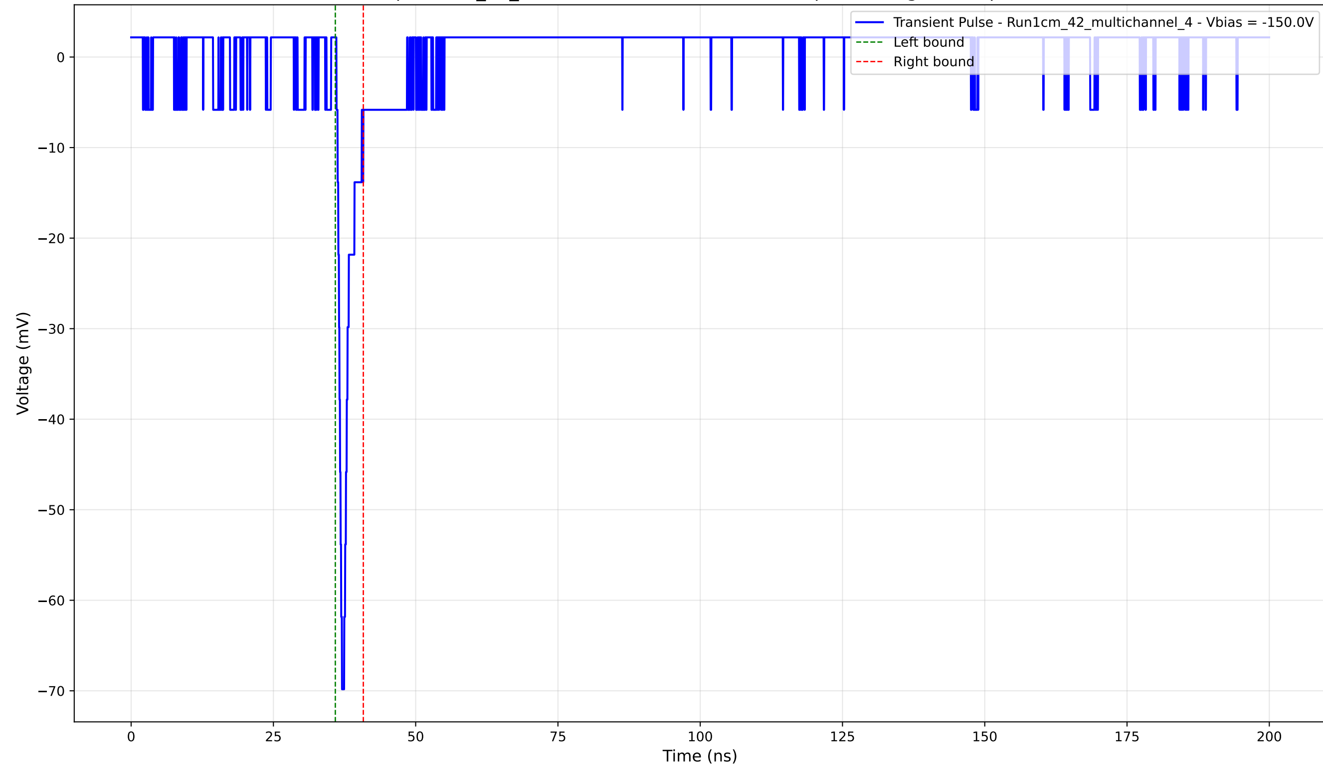
Transient Pulse - Sample: 1cm_42_multichannel - Position: 2315.0 \mu\text{m} - Charge: 2.71 pC - Rise Time: 0.78 ns
