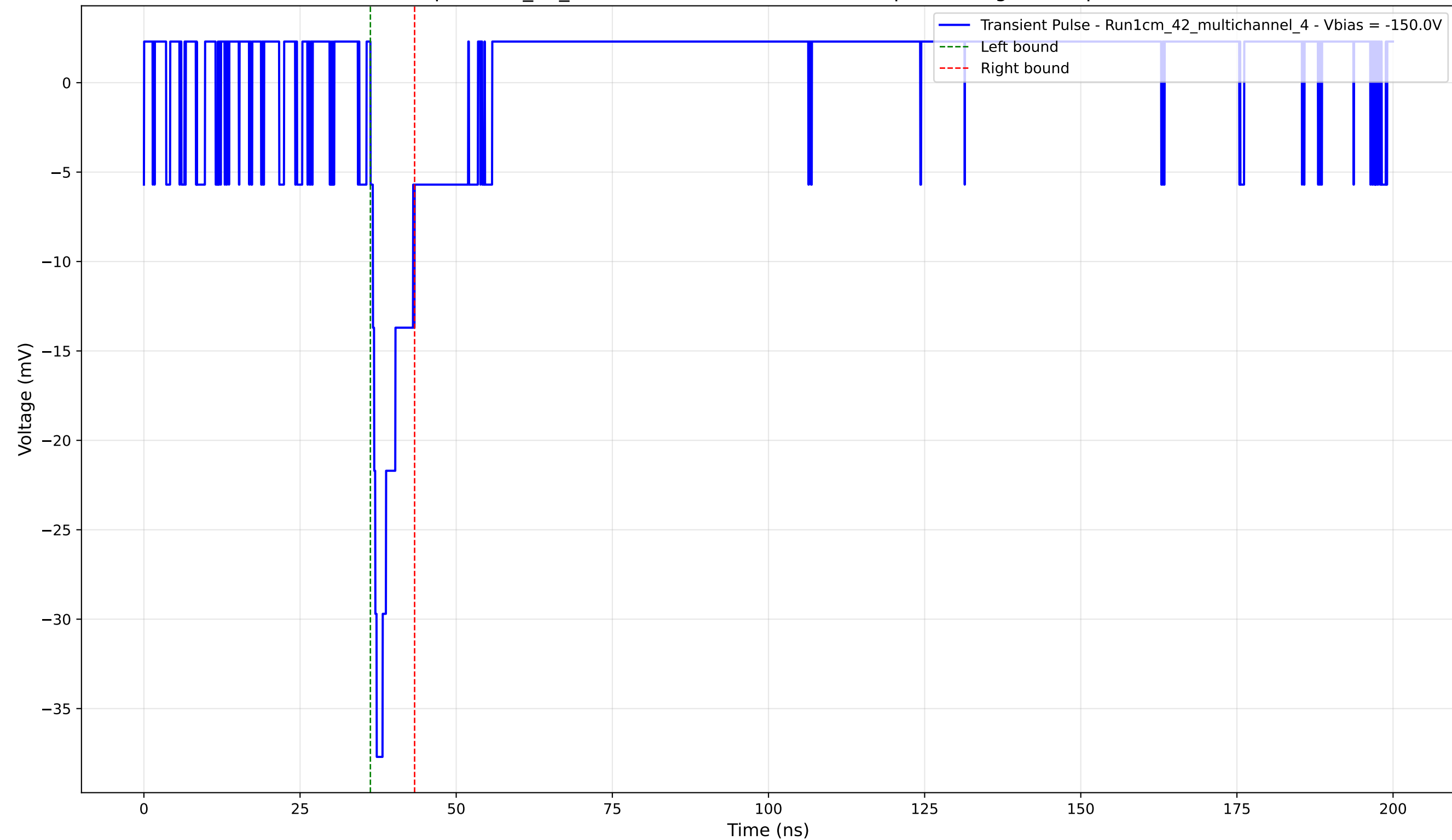
Transient Pulse - Sample: 1cm_42_multichannel - Position: 1750.0 \mu\text{m} - Charge: 2.82 pC - Rise Time: 0.99 ns
