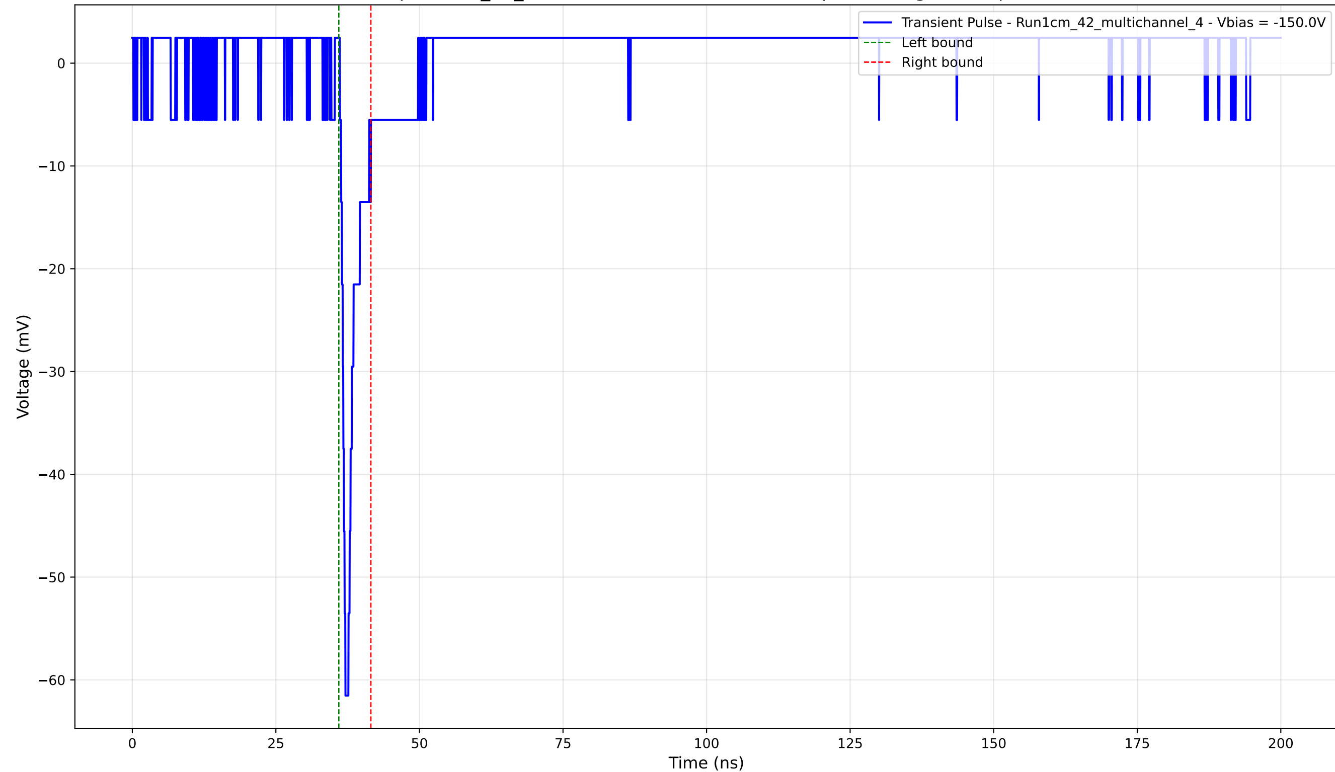
Transient Pulse - Sample: 1cm_42_multichannel - Position: 2625.0 \mu\text{m} - Charge: 2.86 pC - Rise Time: 0.76 ns
