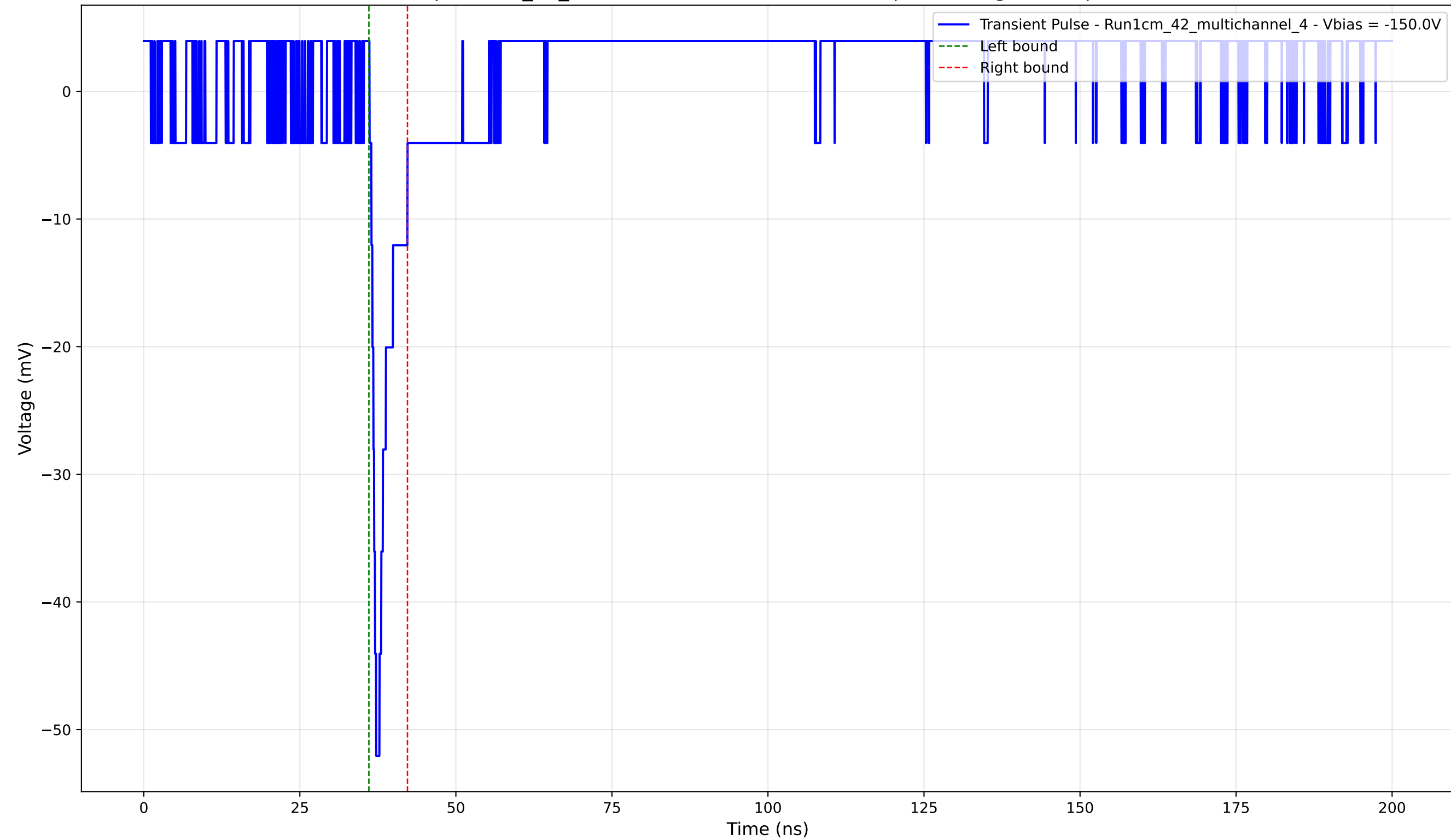
Transient Pulse - Sample: 1cm_42_multichannel - Position: 1990.0 \mu\text{m} - Charge: 2.73 pC - Rise Time: 0.78 ns
