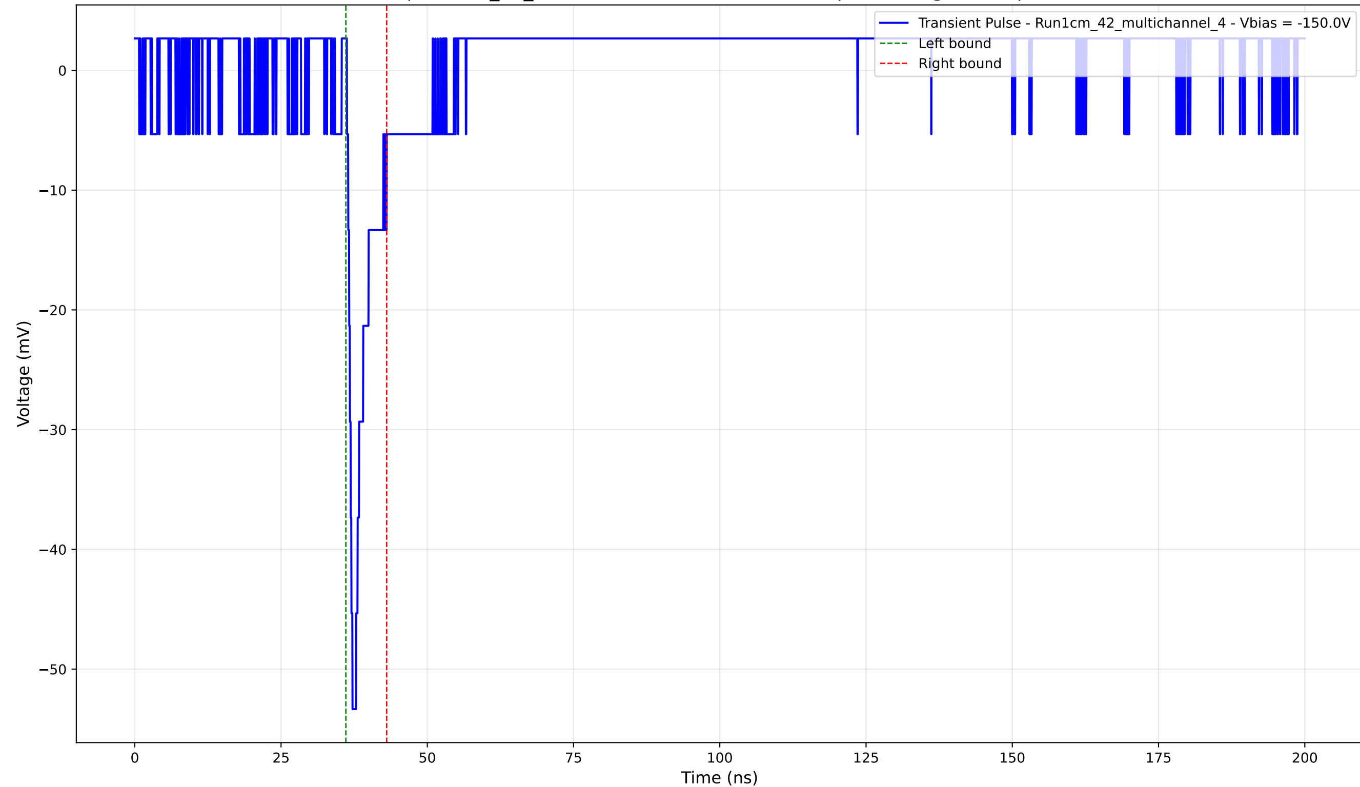
Transient Pulse - Sample: 1cm_42_multichannel - Position: 2000.0 \mu\text{m} - Charge: 3.13 pC - Rise Time: 0.74 ns
