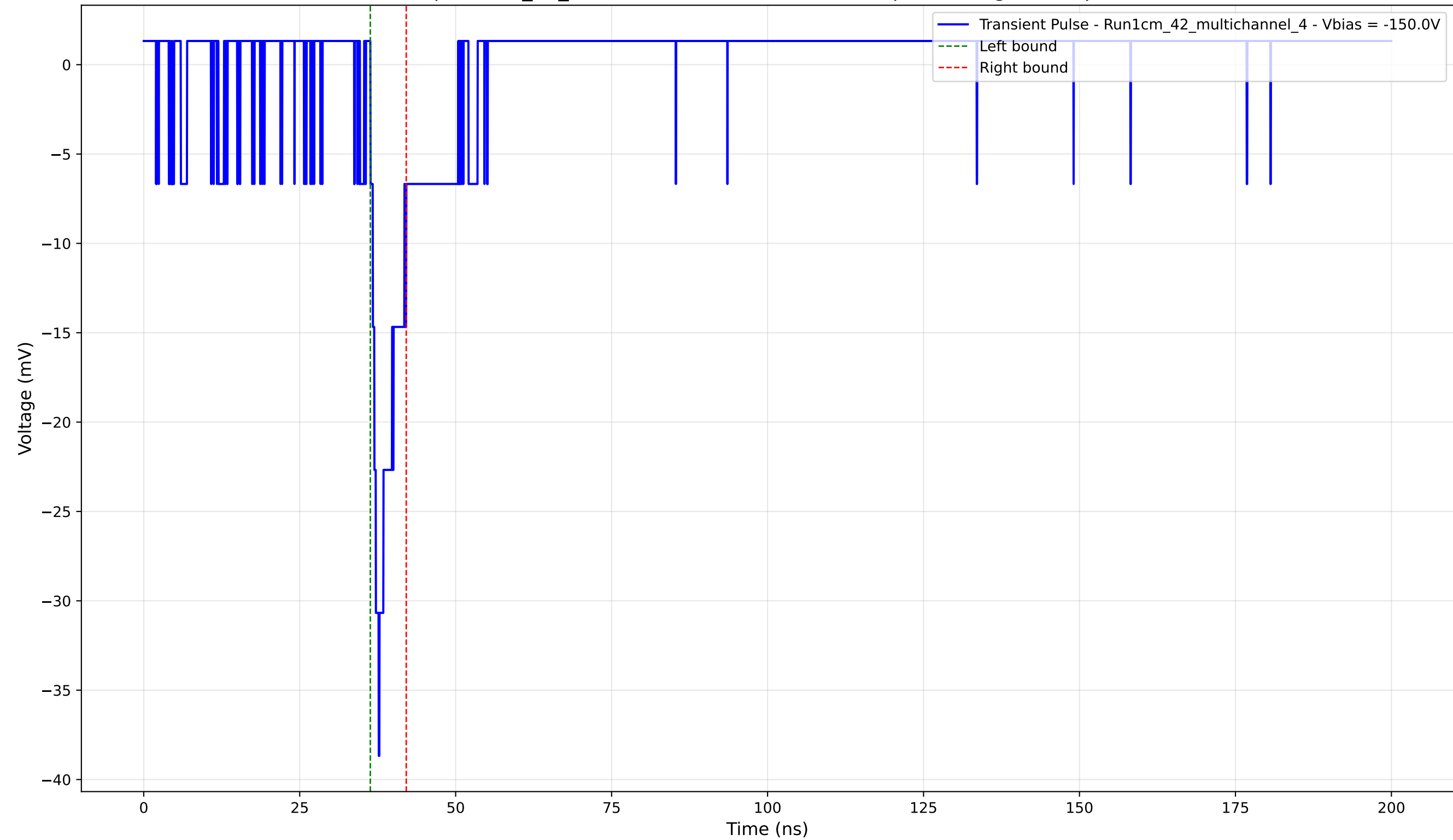
Transient Pulse - Sample: 1cm_42_multichannel - Position: 3055.0 \mu\text{m} - Charge: 2.30 pC - Rise Time: 1.33 ns
