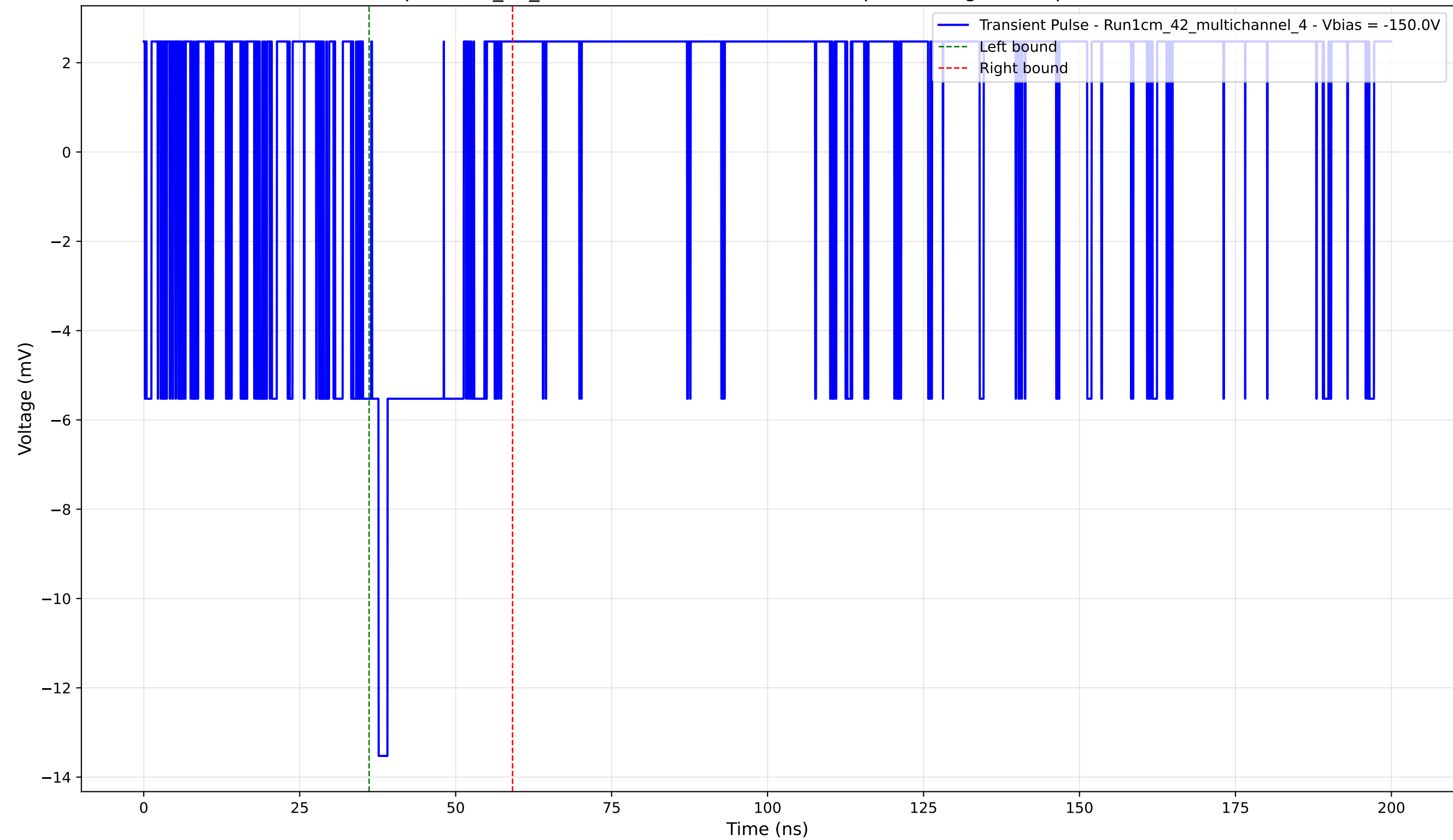
Transient Pulse - Sample: 1cm_42_multichannel - Position: 1420.0 \mu\text{m} - Charge: 1.94 pC - Rise Time: 0.00 ns (N/A)
