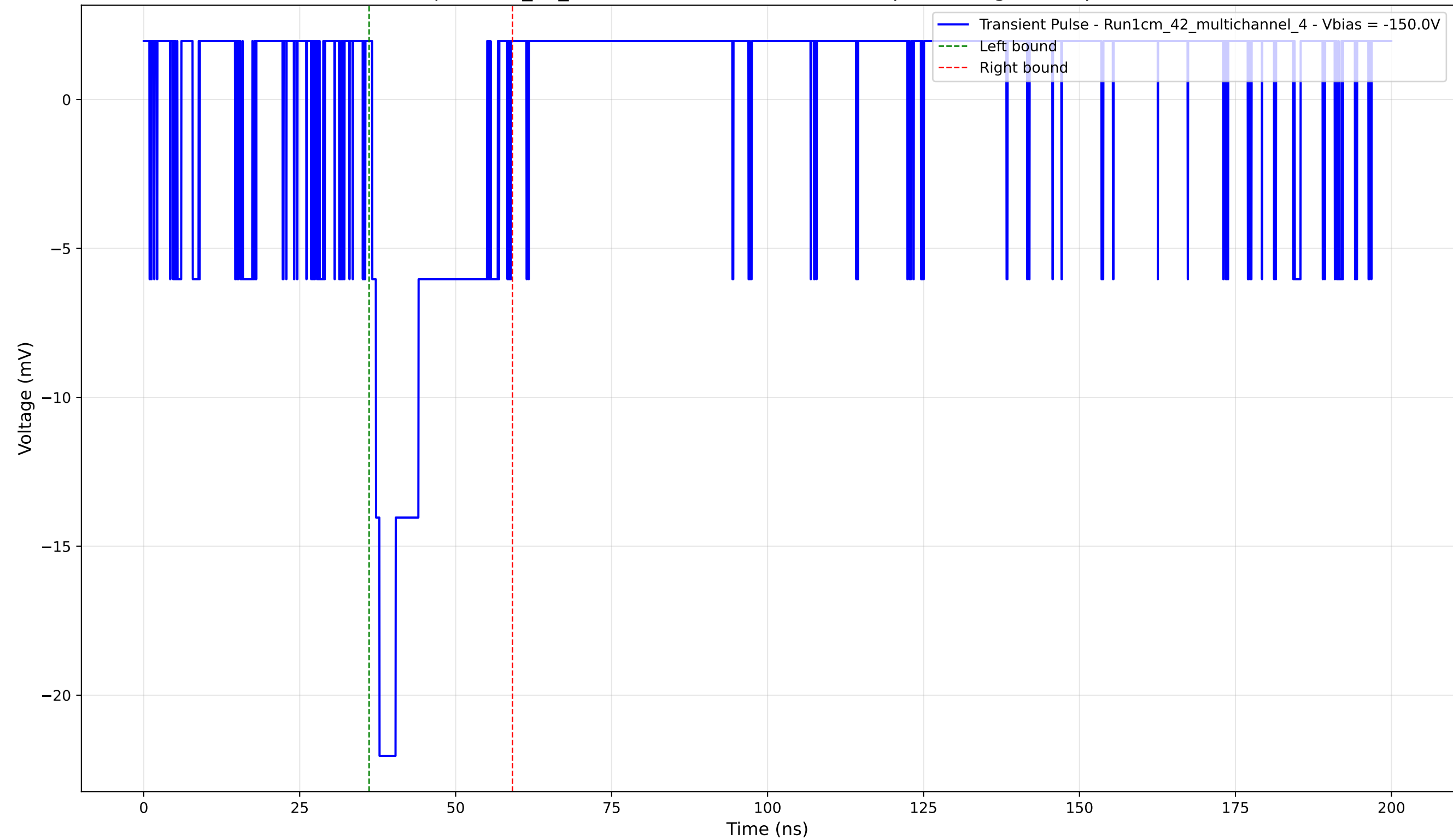
Transient Pulse - Sample: 1cm_42_multichannel - Position: 1190.0 \mu\text{m} - Charge: 3.85 pC - Rise Time: 1.18 ns
