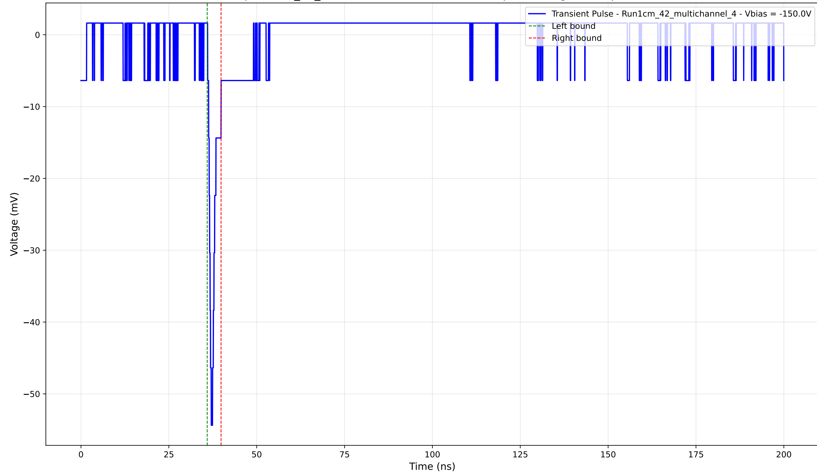
Transient Pulse - Sample: 1cm_42_multichannel - Position: 2330.0 \mu\text{m} - Charge: 1.95 pC - Rise Time: 1.02 ns
