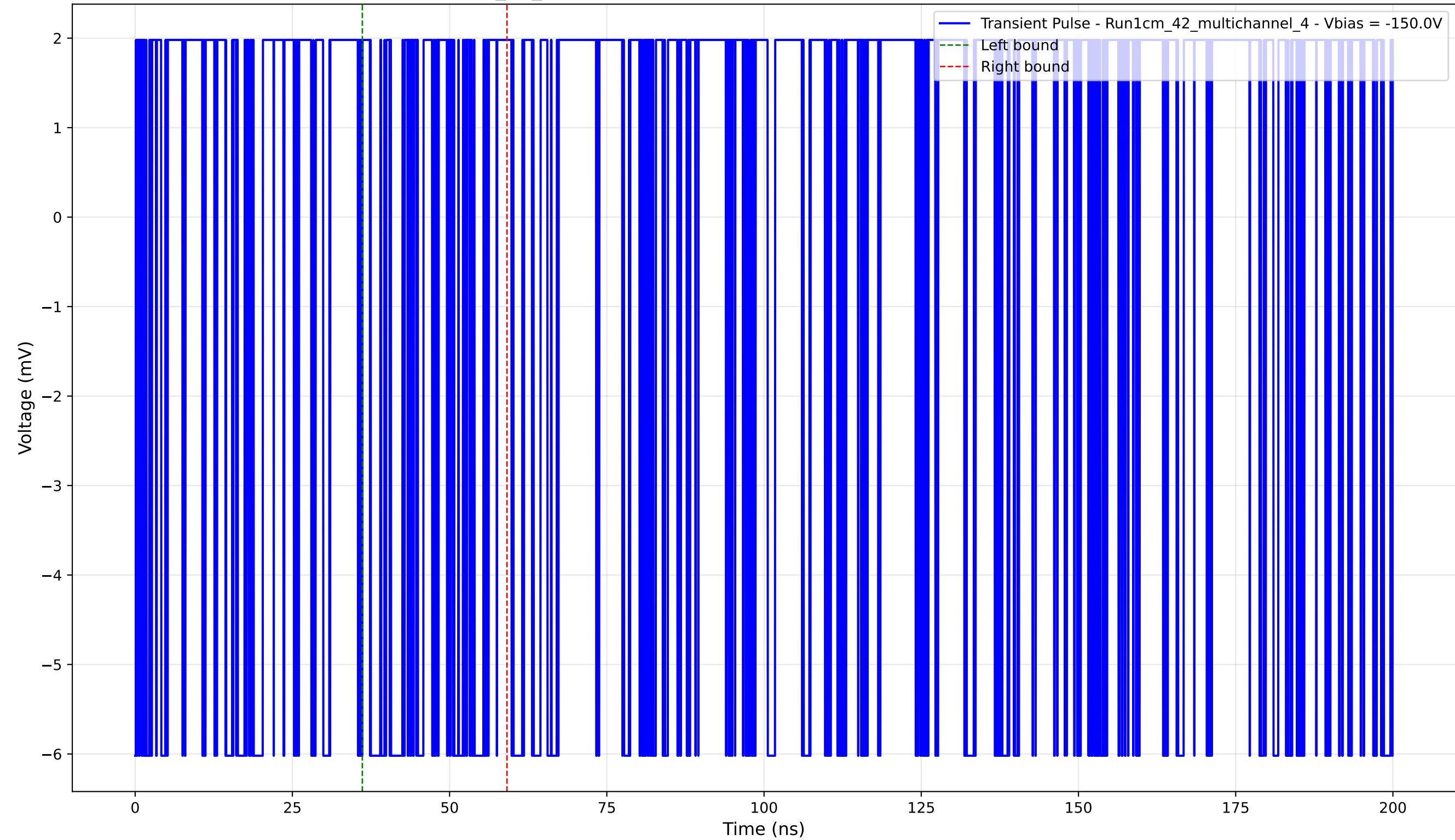
Transient Pulse - Sample: 1cm_42_multichannel - Position: 360.0 \mu\text{m} - Charge: 0.86 pC - Rise Time: 0.00 ns (N/A)
