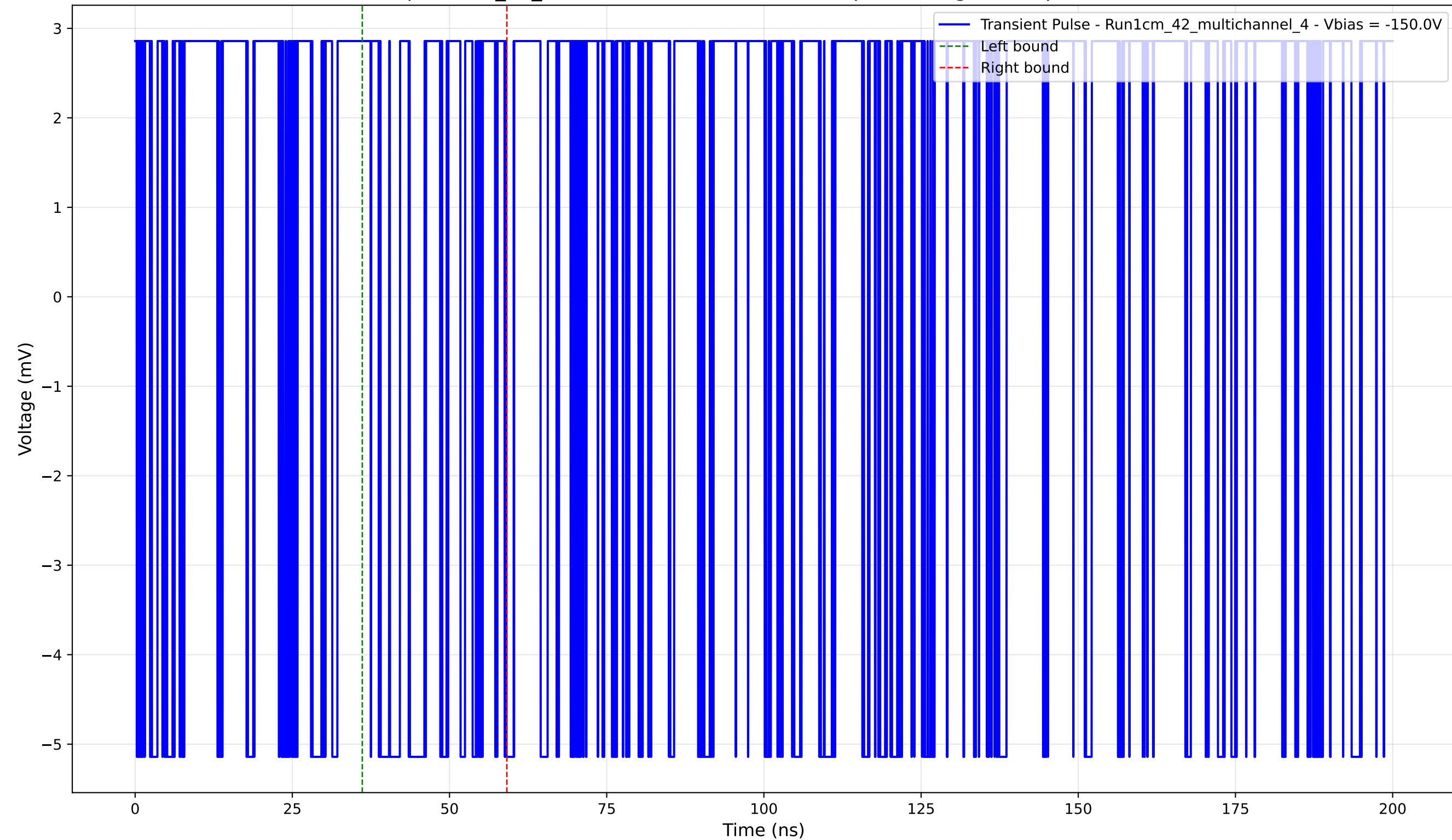
Transient Pulse - Sample: 1cm_42_multichannel - Position: 365.0 \mu\text{m} - Charge: 0.11 pC - Rise Time: 0.00 ns (N/A)
