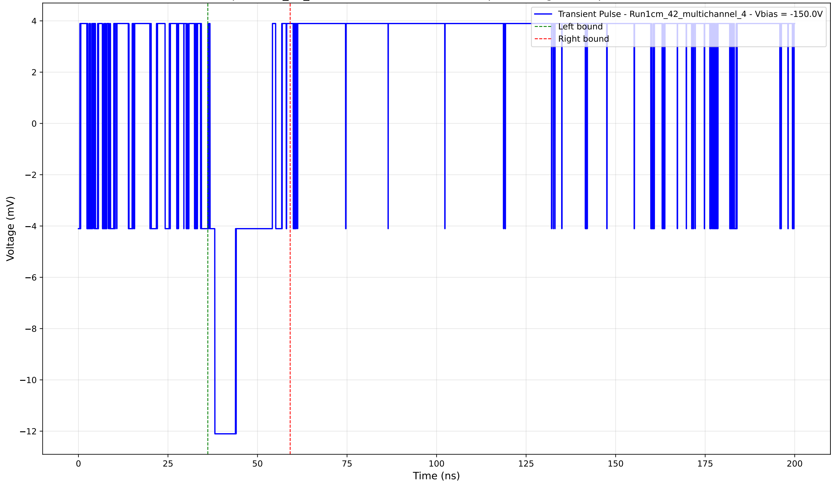
Transient Pulse - Sample: 1cm_42_multichannel - Position: 520.0 \mu\text{m} - Charge: 2.27 pC - Rise Time: 0.00 ns (N/A)
