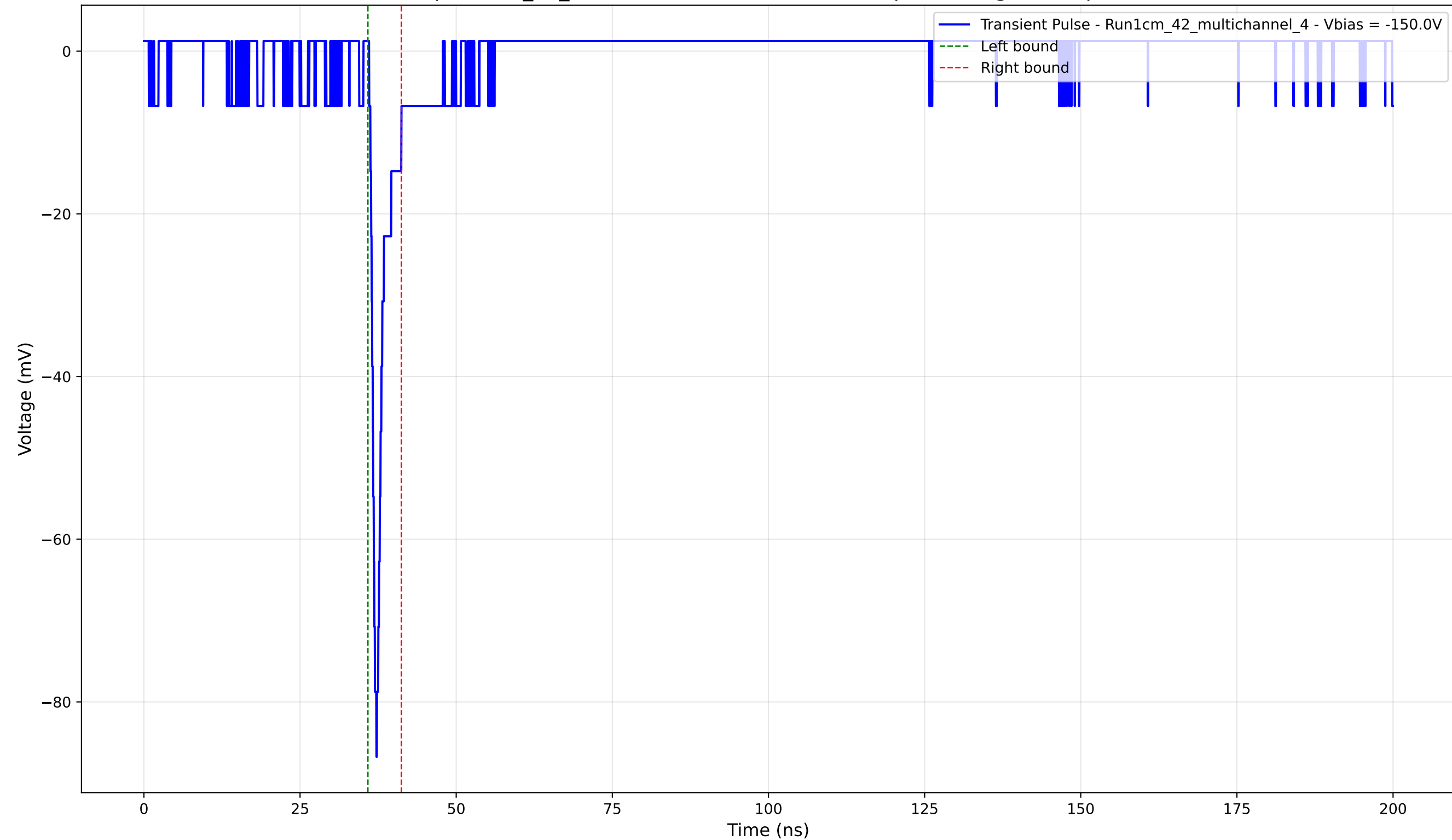
Transient Pulse - Sample: 1cm_42_multichannel - Position: 2475.0 \mu\text{m} - Charge: 3.36 pC - Rise Time: 0.74 ns
