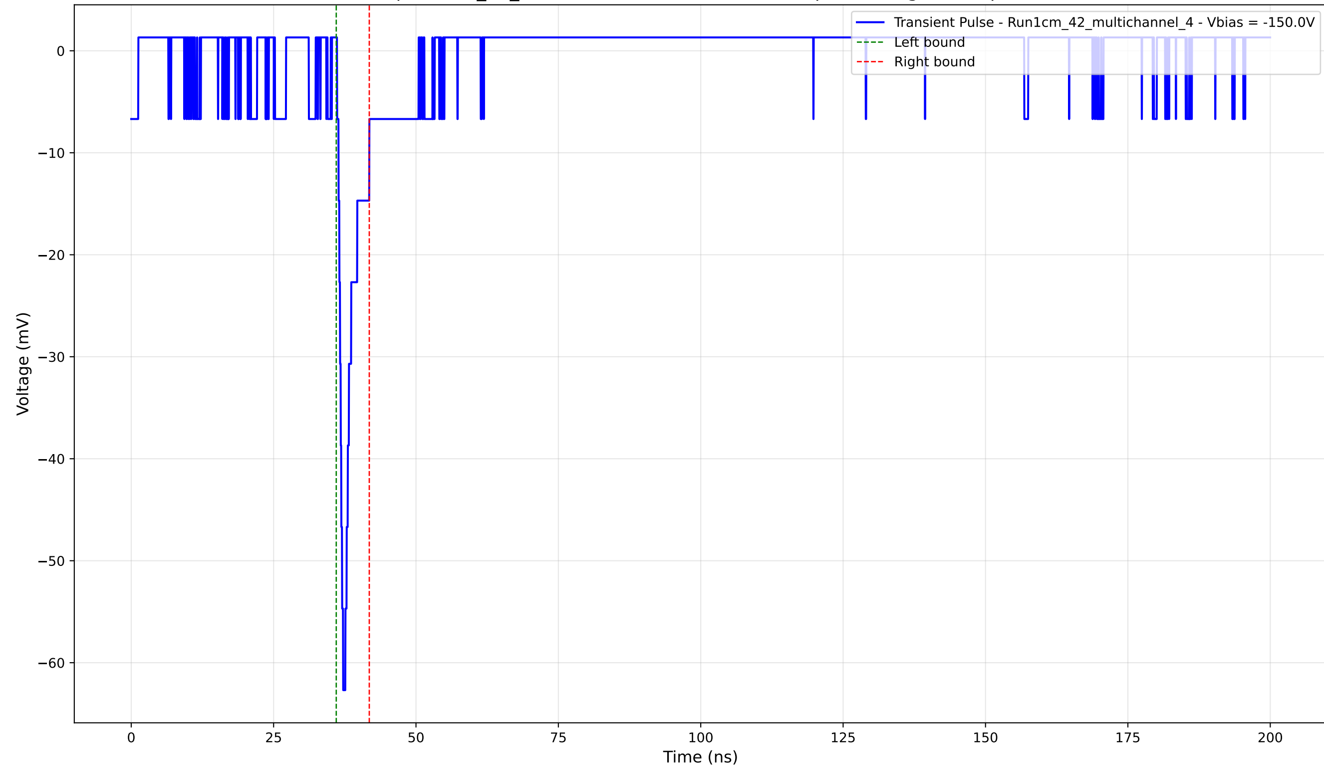
Transient Pulse - Sample: 1cm_42_multichannel - Position: 2100.0 \mu\text{m} - Charge: 3.04 pC - Rise Time: 1.06 ns
