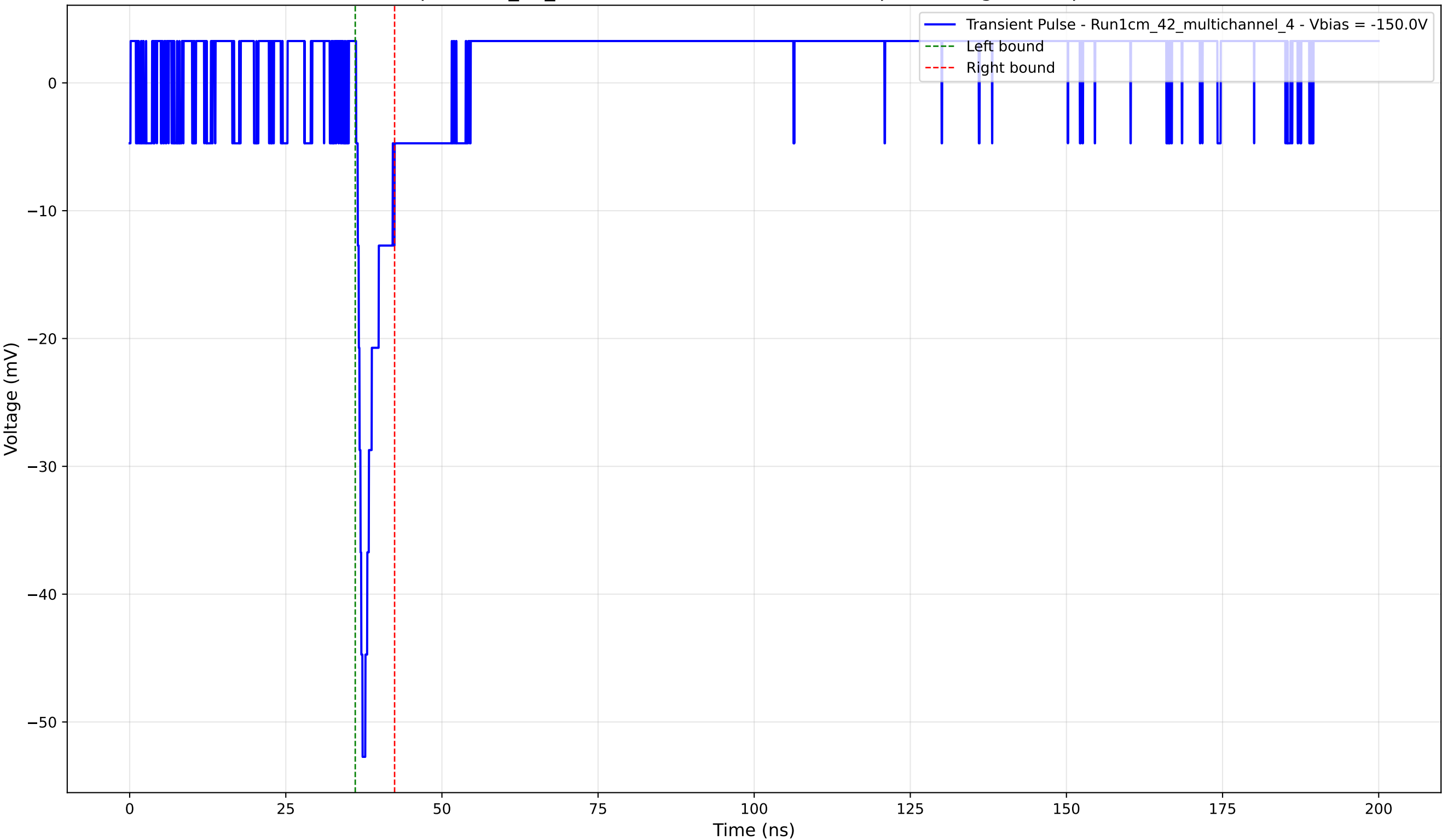
Transient Pulse - Sample: 1cm_42_multichannel - Position: 1970.0 \mu\text{m} - Charge: 2.76 pC - Rise Time: 0.78 ns
