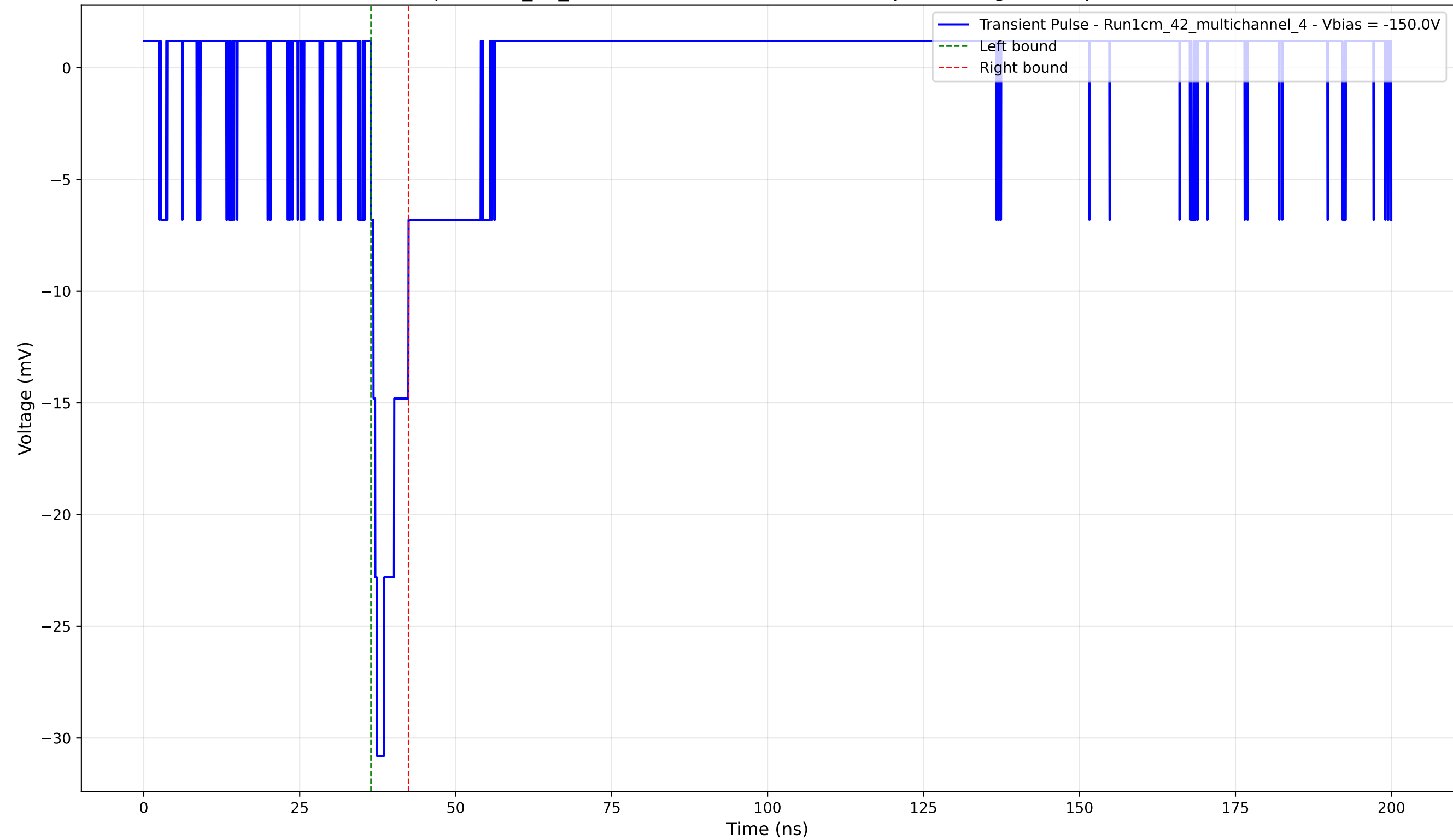
Transient Pulse - Sample: 1cm_42_multichannel - Position: 1575.0 \mu\text{m} - Charge: 2.39 pC - Rise Time: 0.95 ns
