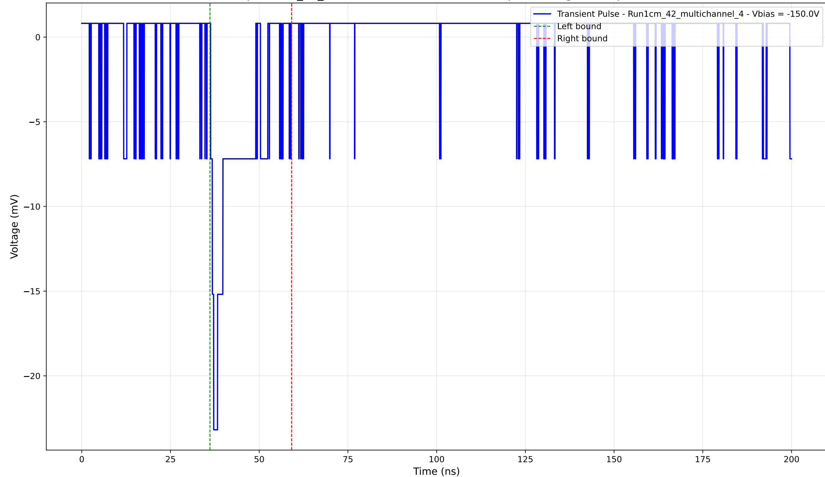
Transient Pulse - Sample: 1cm_42_multichannel - Position: 1830.0 \mu\text{m} - Charge: 2.80 pC - Rise Time: 0.88 ns
