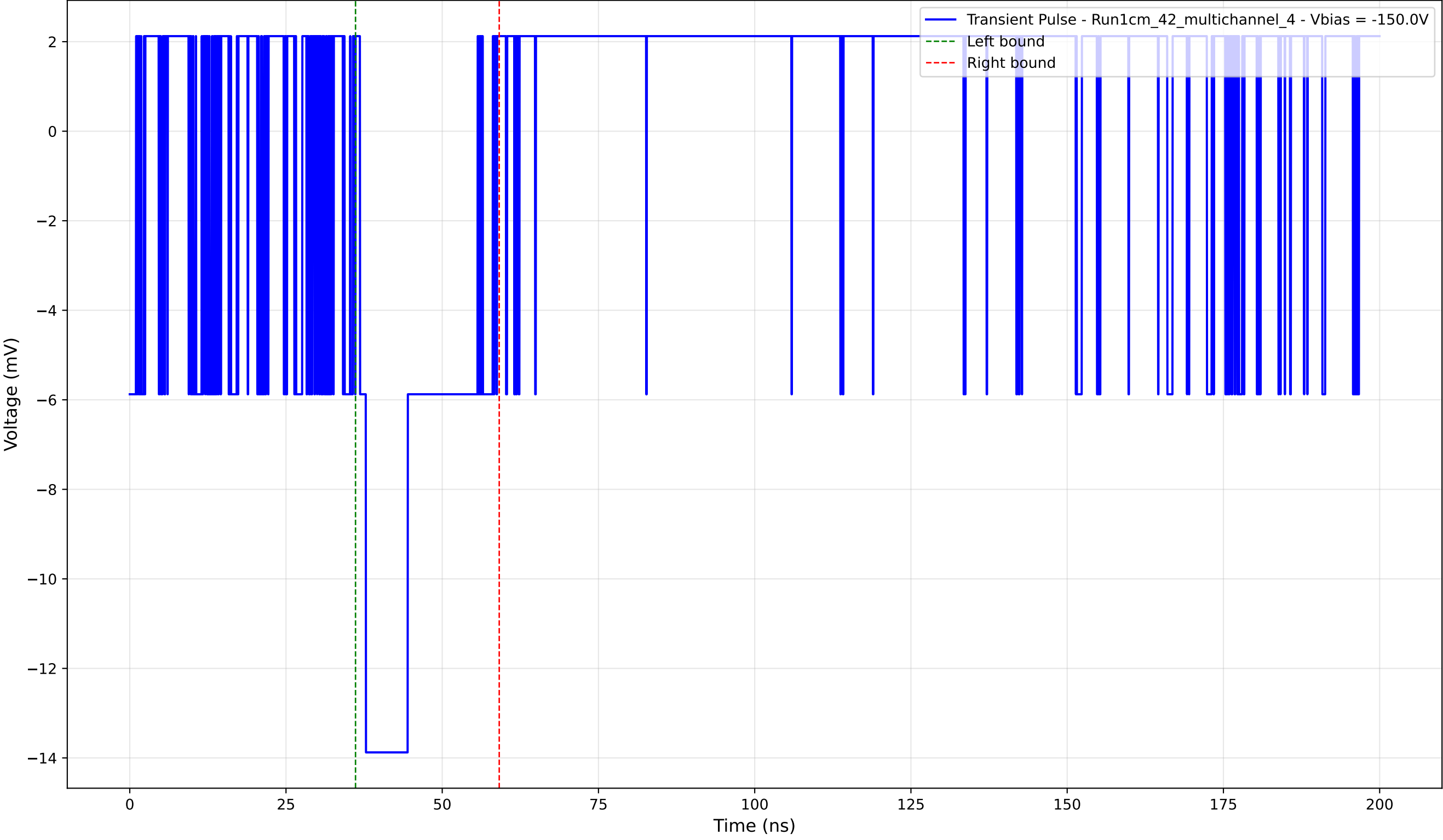
Transient Pulse - Sample: 1cm_42_multichannel - Position: 770.0 \mu\text{m} - Charge: 3.47 pC - Rise Time: 0.00 ns (N/A)
