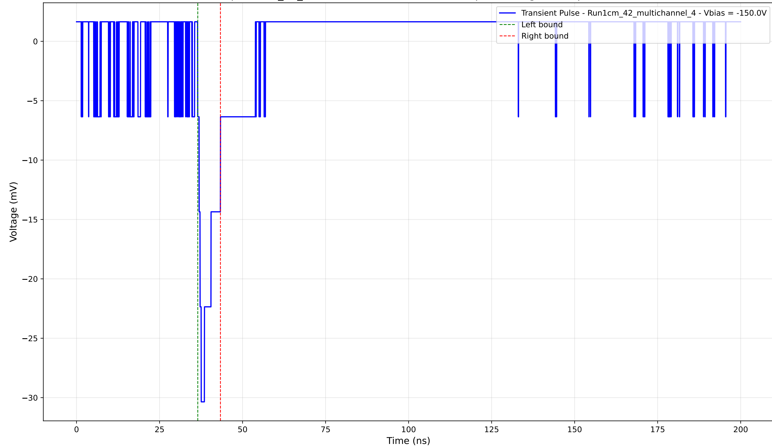
Transient Pulse - Sample: 1cm_42_multichannel - Position: 1490.0 \mu\text{m} - Charge: 2.58 pC - Rise Time: 1.07 ns
