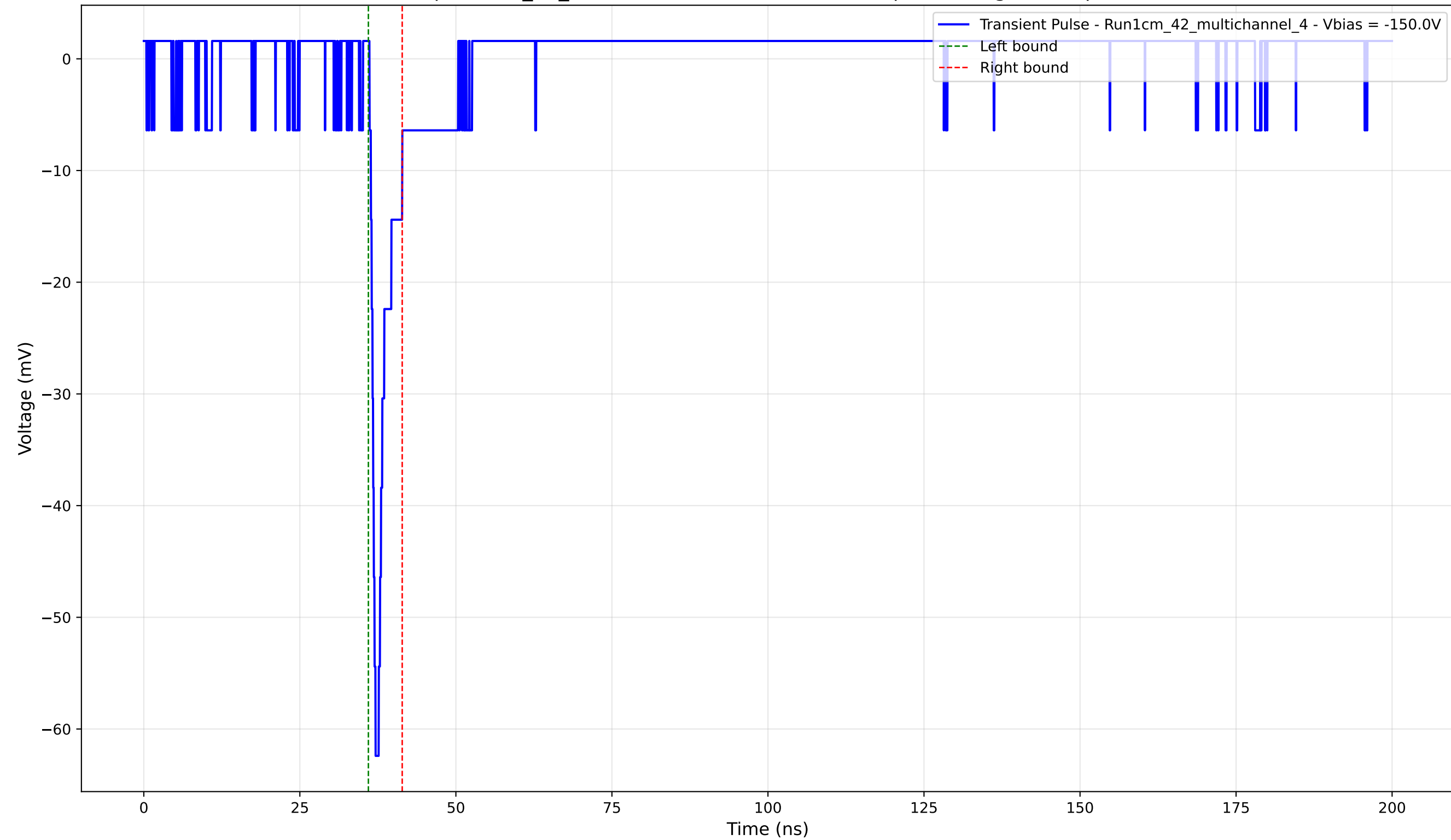
Transient Pulse - Sample: 1cm_42_multichannel - Position: 2145.0 \mu\text{m} - Charge: 2.92 pC - Rise Time: 0.96 ns
