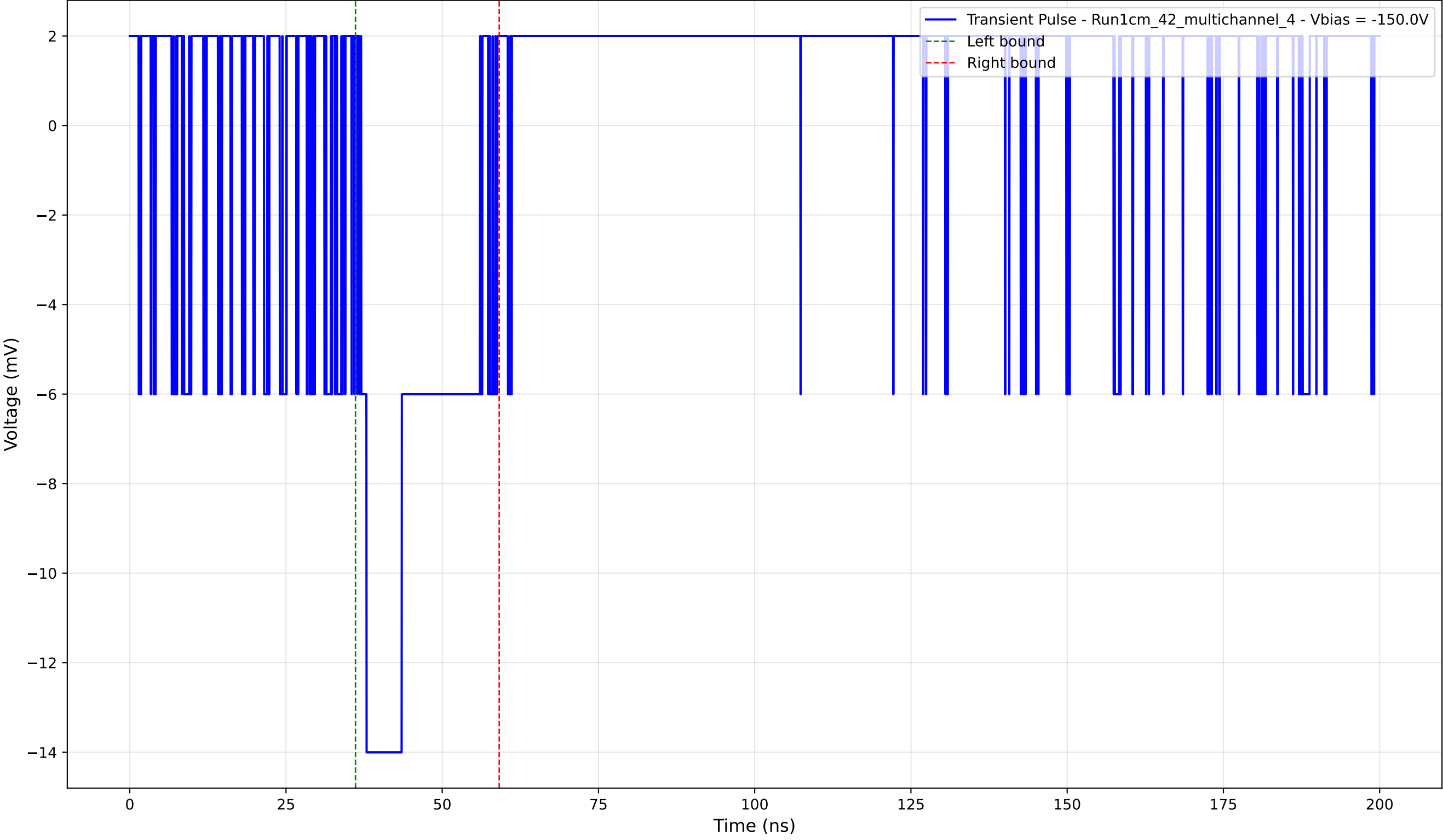
Transient Pulse - Sample: 1cm_42_multichannel - Position: 645.0 \mu\text{m} - Charge: 3.24 pC - Rise Time: 0.00 ns (N/A)
