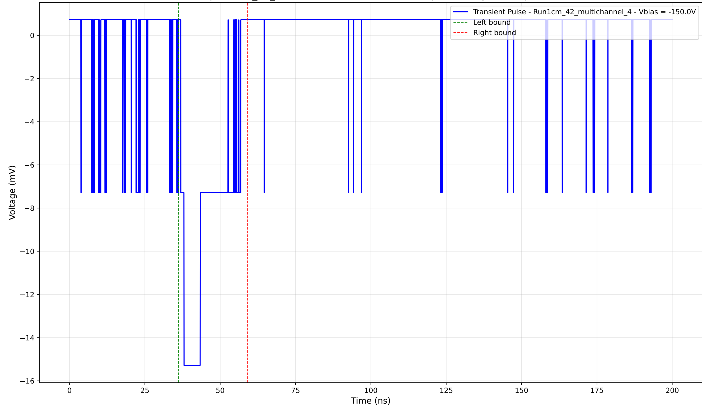
Transient Pulse - Sample: 1cm_42_multichannel - Position: 4075.0 \mu\text{m} - Charge: 3.60 pC - Rise Time: 1.08 ns
