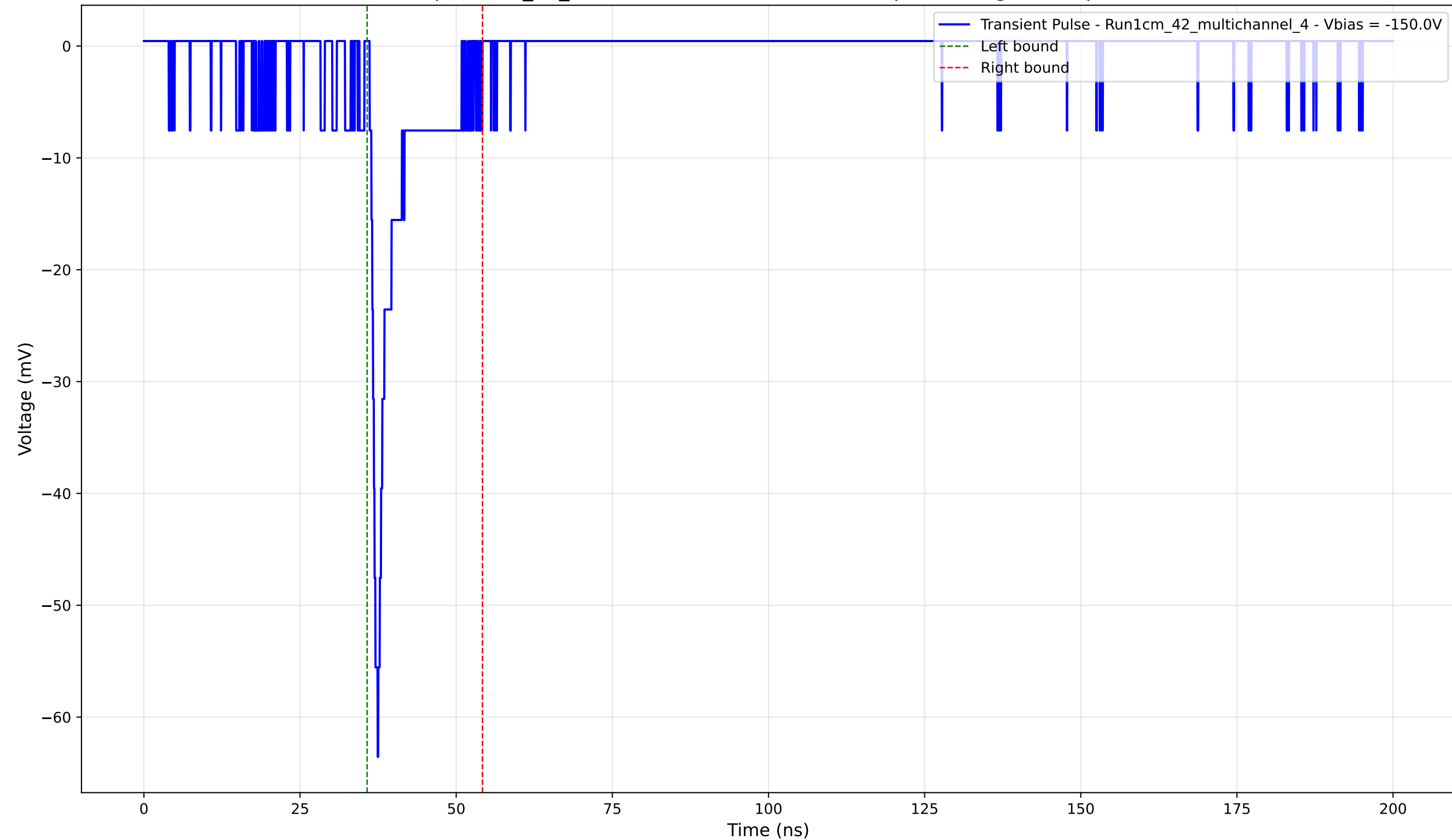
Transient Pulse - Sample: 1cm_42_multichannel - Position: 2670.0 \mu\text{m} - Charge: 4.61 pC - Rise Time: 1.28 ns
