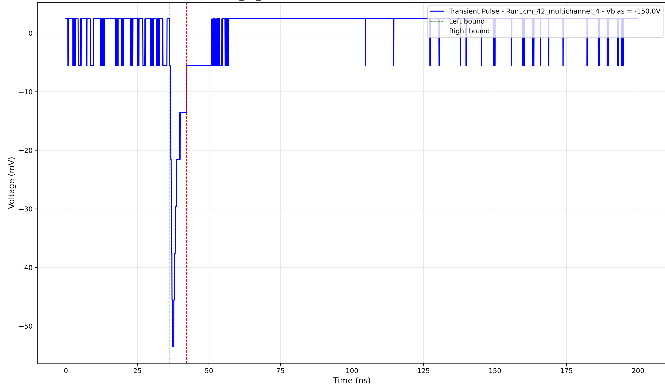
Transient Pulse - Sample: 1cm_42_multichannel - Position: 2775.0 \mu\text{m} - Charge: 2.81 pC - Rise Time: 1.06 ns
