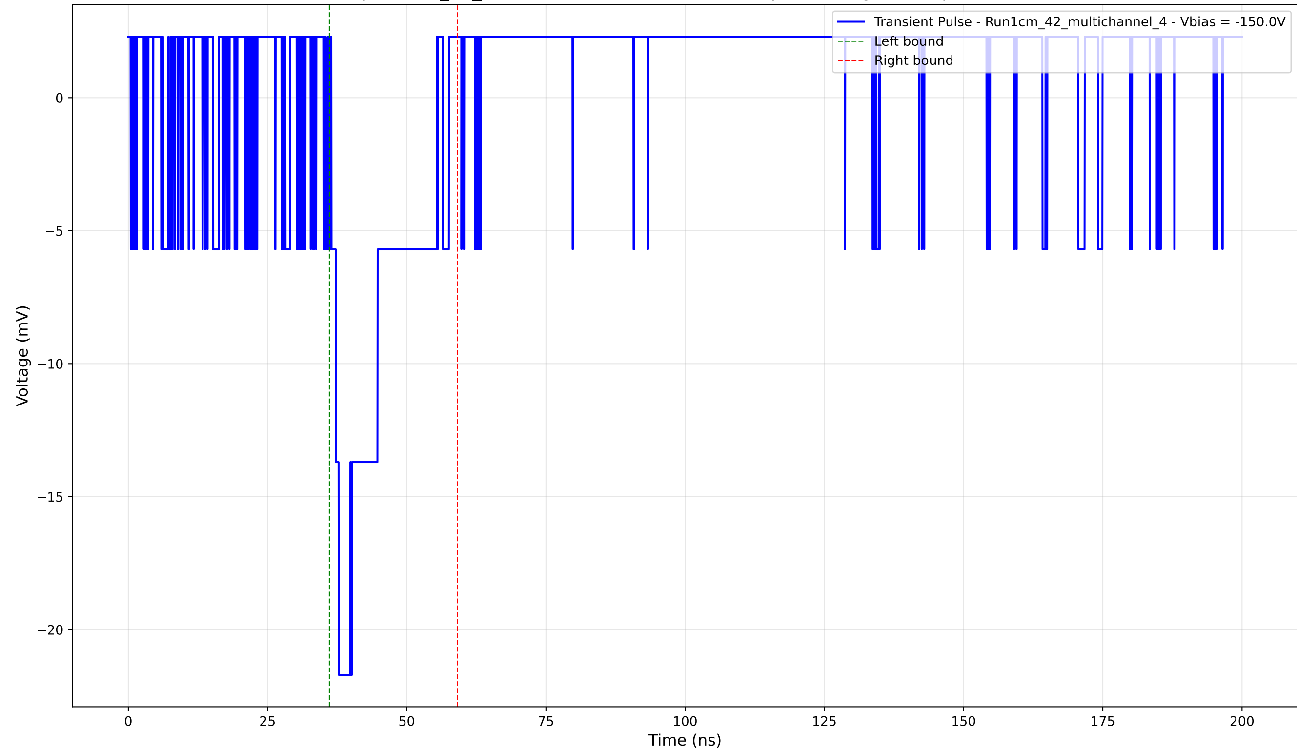
Transient Pulse - Sample: 1cm_42_multichannel - Position: 1160.0 \mu\text{m} - Charge: 3.73 pC - Rise Time: 0.00 ns (N/A)
