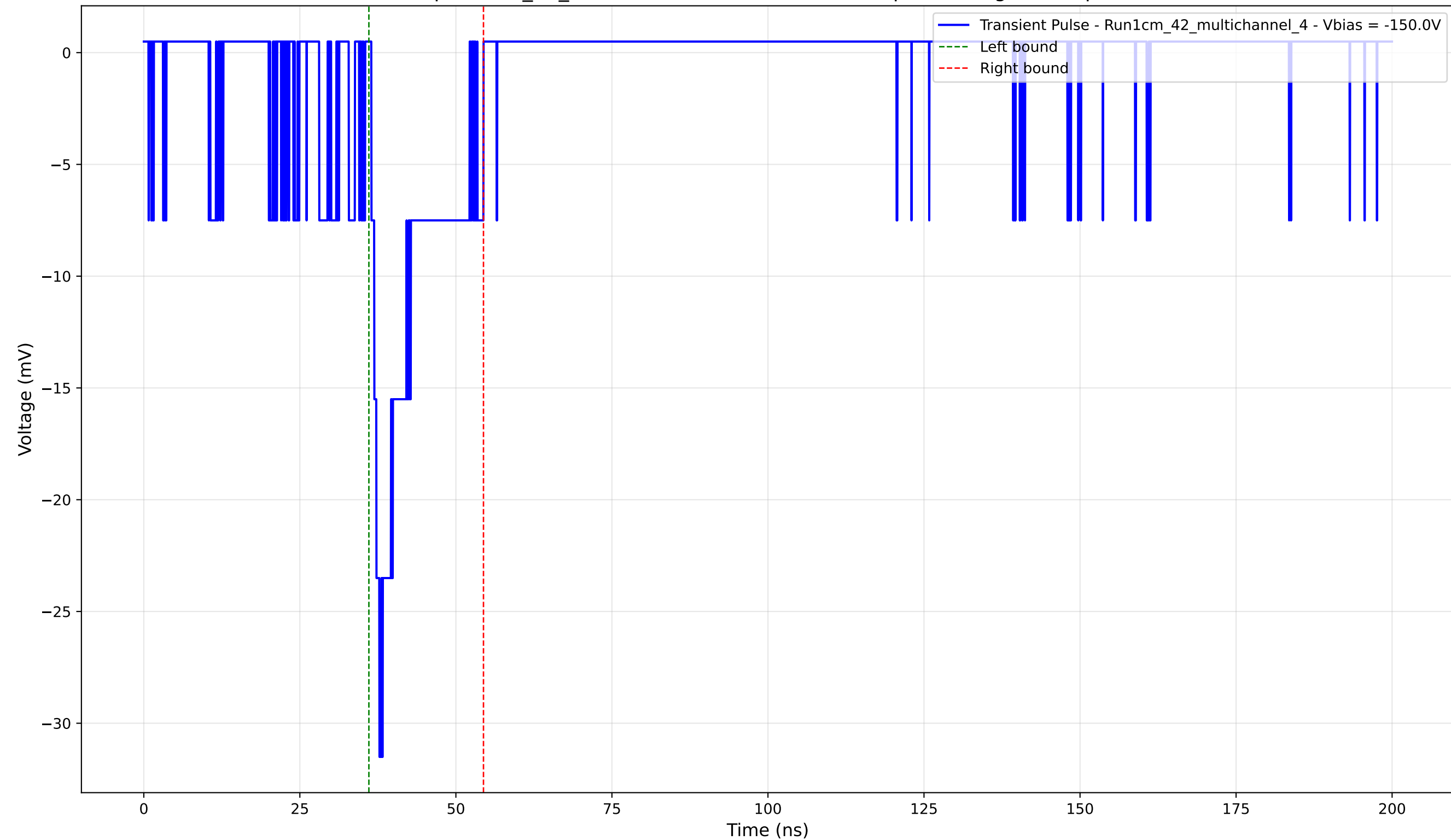
Transient Pulse - Sample: 1cm_42_multichannel - Position: 3270.0 \mu\text{m} - Charge: 3.99 pC - Rise Time: 1.29 ns
