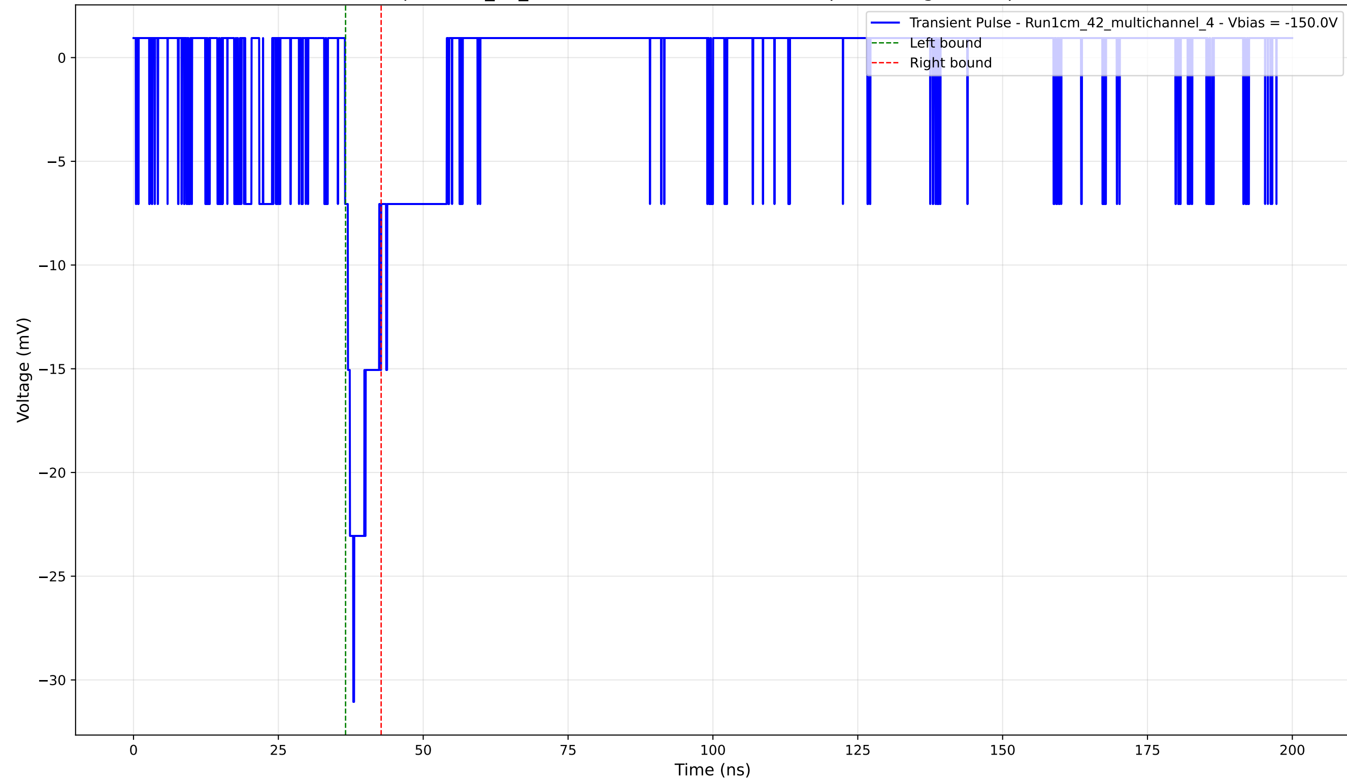
Transient Pulse - Sample: 1cm_42_multichannel - Position: 3280.0 \mu\text{m} - Charge: 2.21 pC - Rise Time: 1.43 ns
