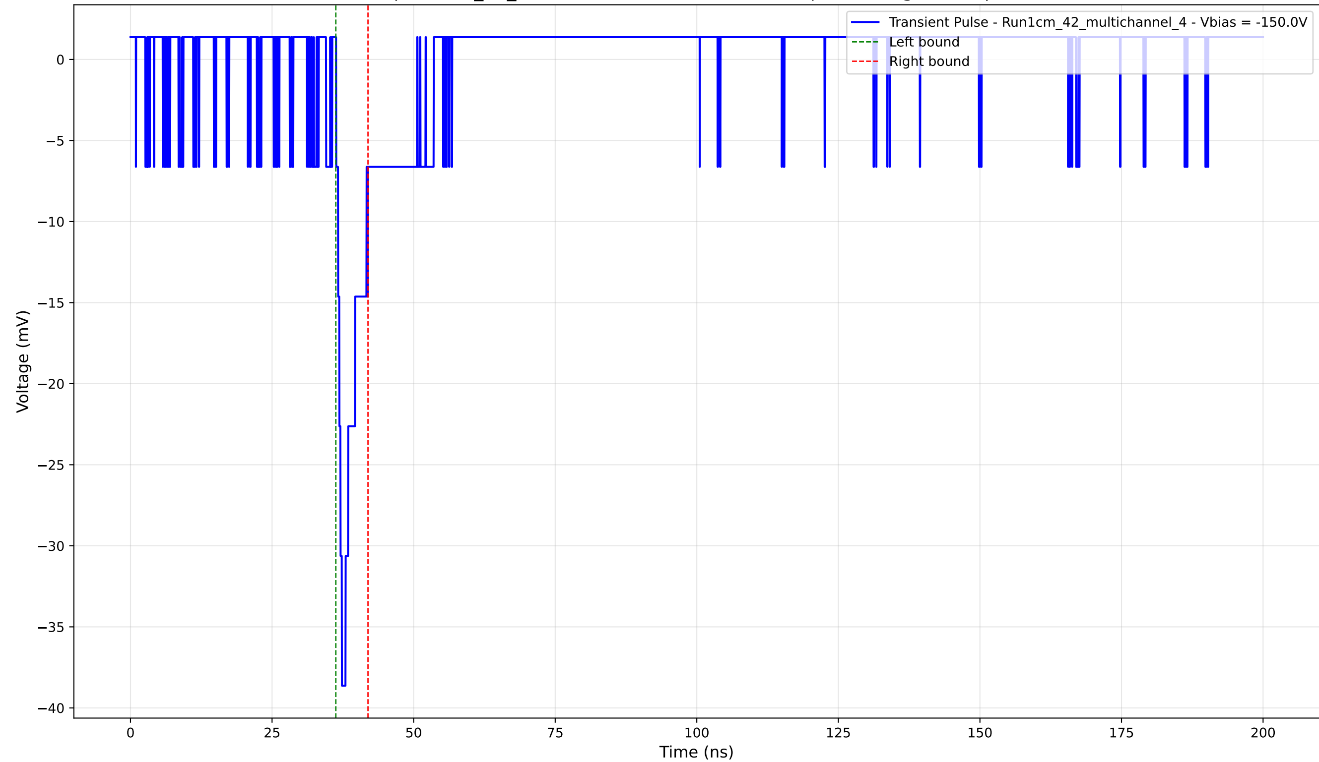
Transient Pulse - Sample: 1cm_42_multichannel - Position: 2970.0 \mu\text{m} - Charge: 2.33 pC - Rise Time: 1.01 ns
