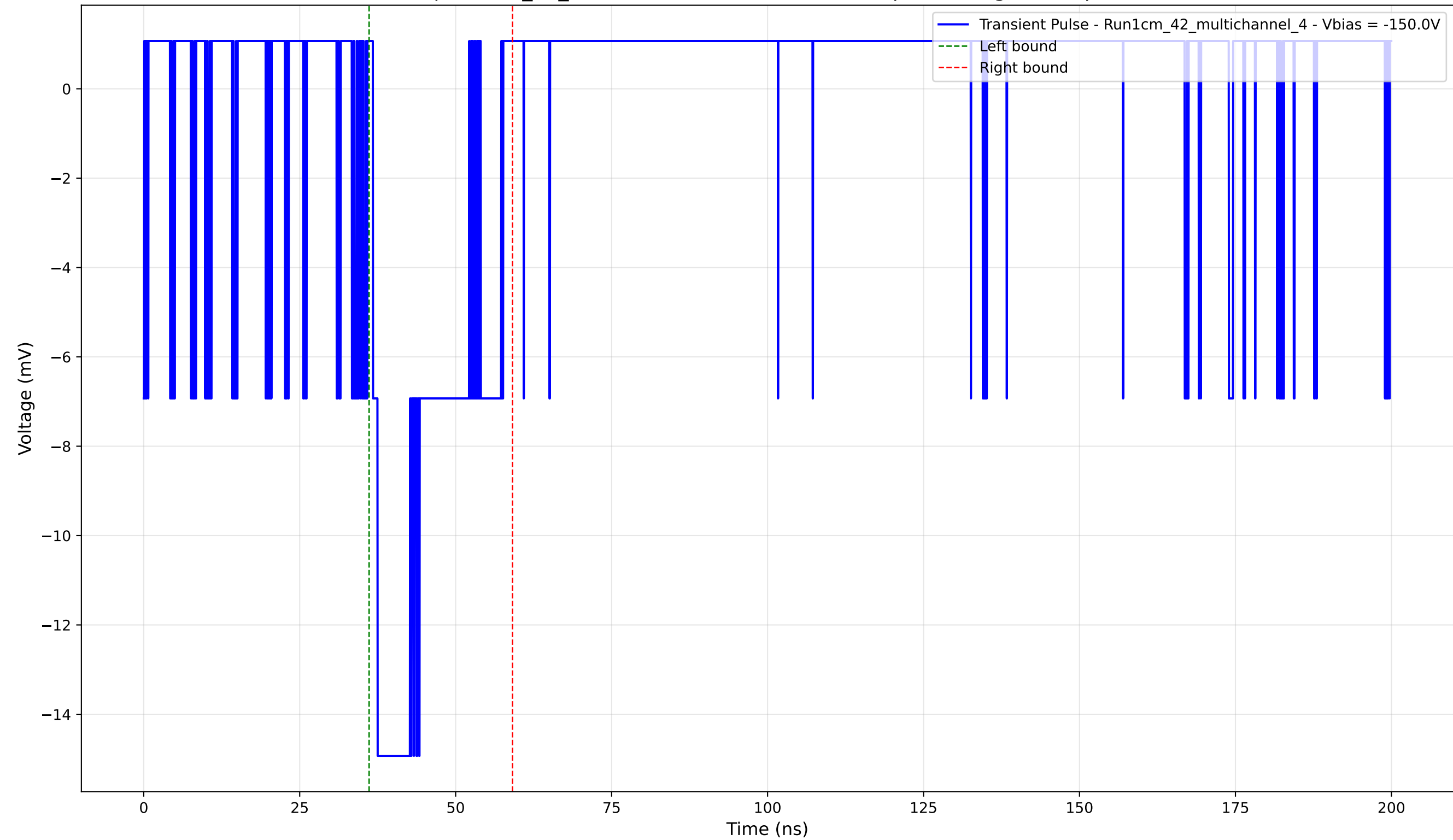
Transient Pulse - Sample: 1cm_42_multichannel - Position: 3655.0 \mu\text{m} - Charge: 3.60 pC - Rise Time: 0.76 ns
