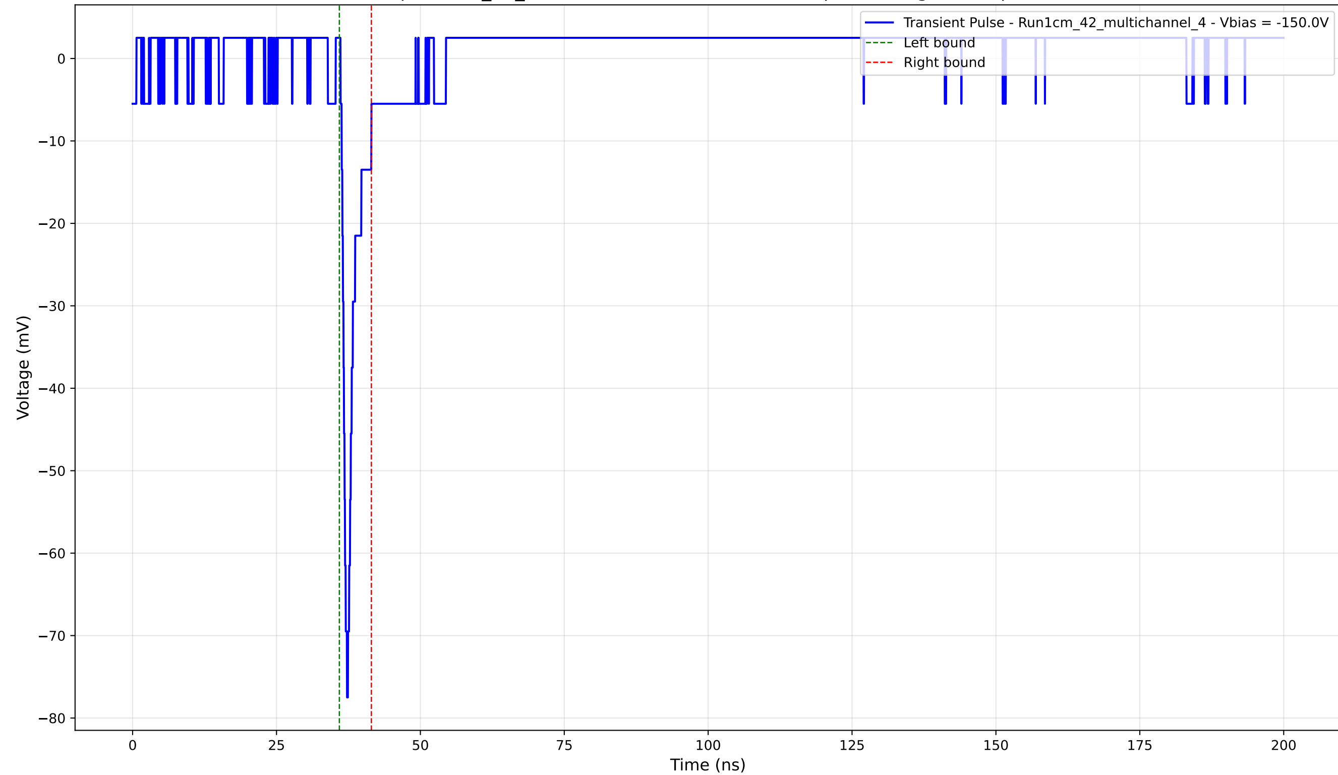
Transient Pulse - Sample: 1cm_42_multichannel - Position: 2210.0 \mu\text{m} - Charge: 3.19 pC - Rise Time: 0.93 ns
