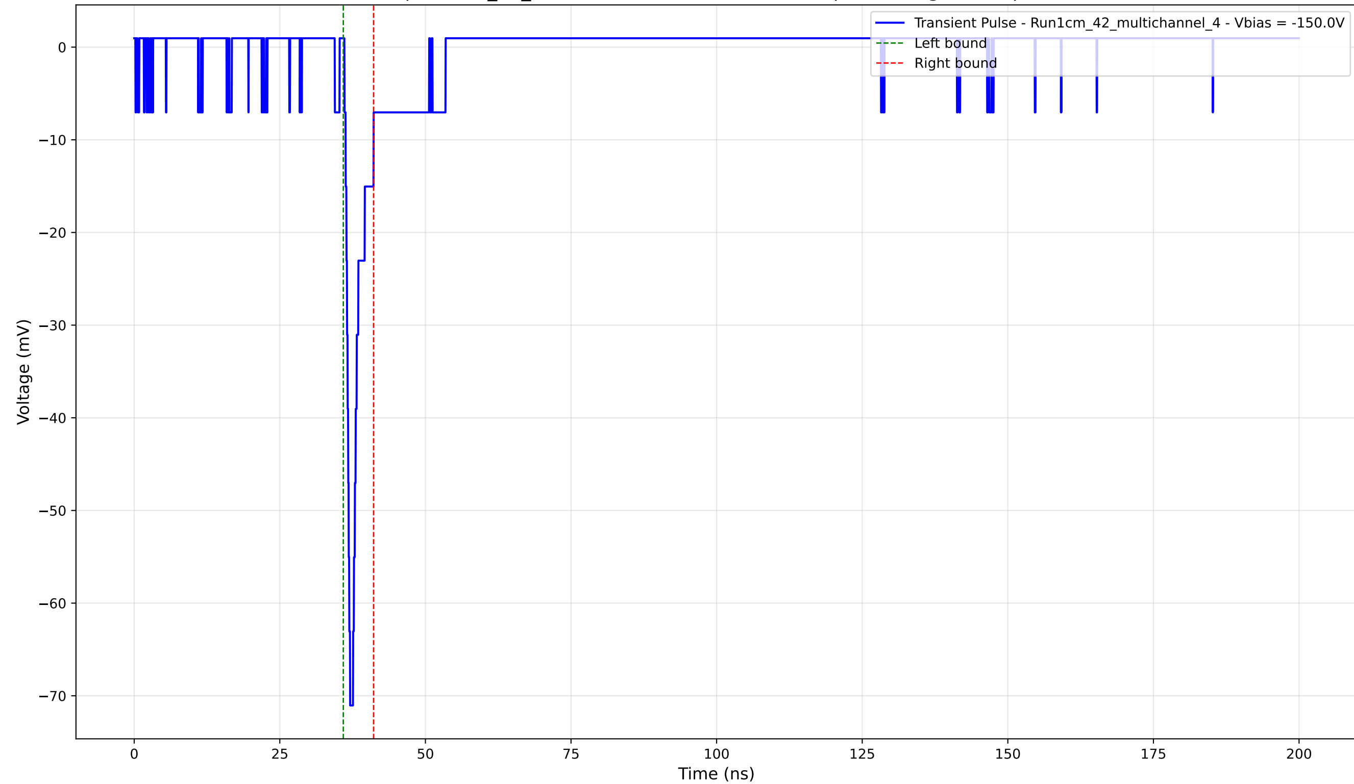
Transient Pulse - Sample: 1cm_42_multichannel - Position: 2220.0 \mu\text{m} - Charge: 3.12 pC - Rise Time: 0.78 ns
