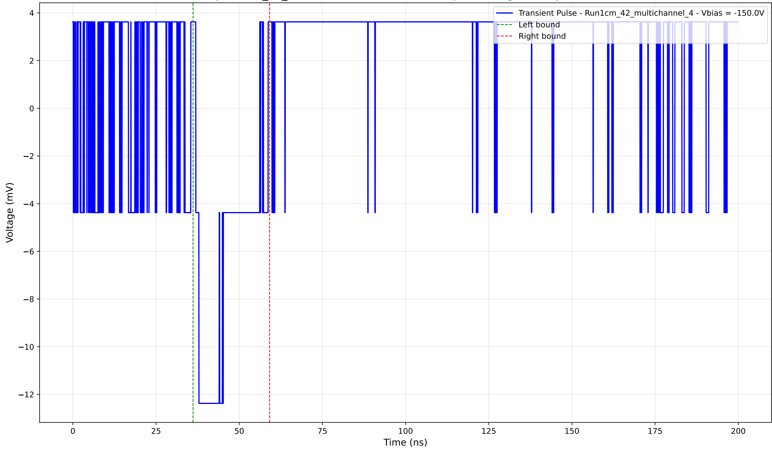
Transient Pulse - Sample: 1cm_42_multichannel - Position: 670.0 \mu\text{m} - Charge: 2.79 pC - Rise Time: 0.00 ns (N/A)
