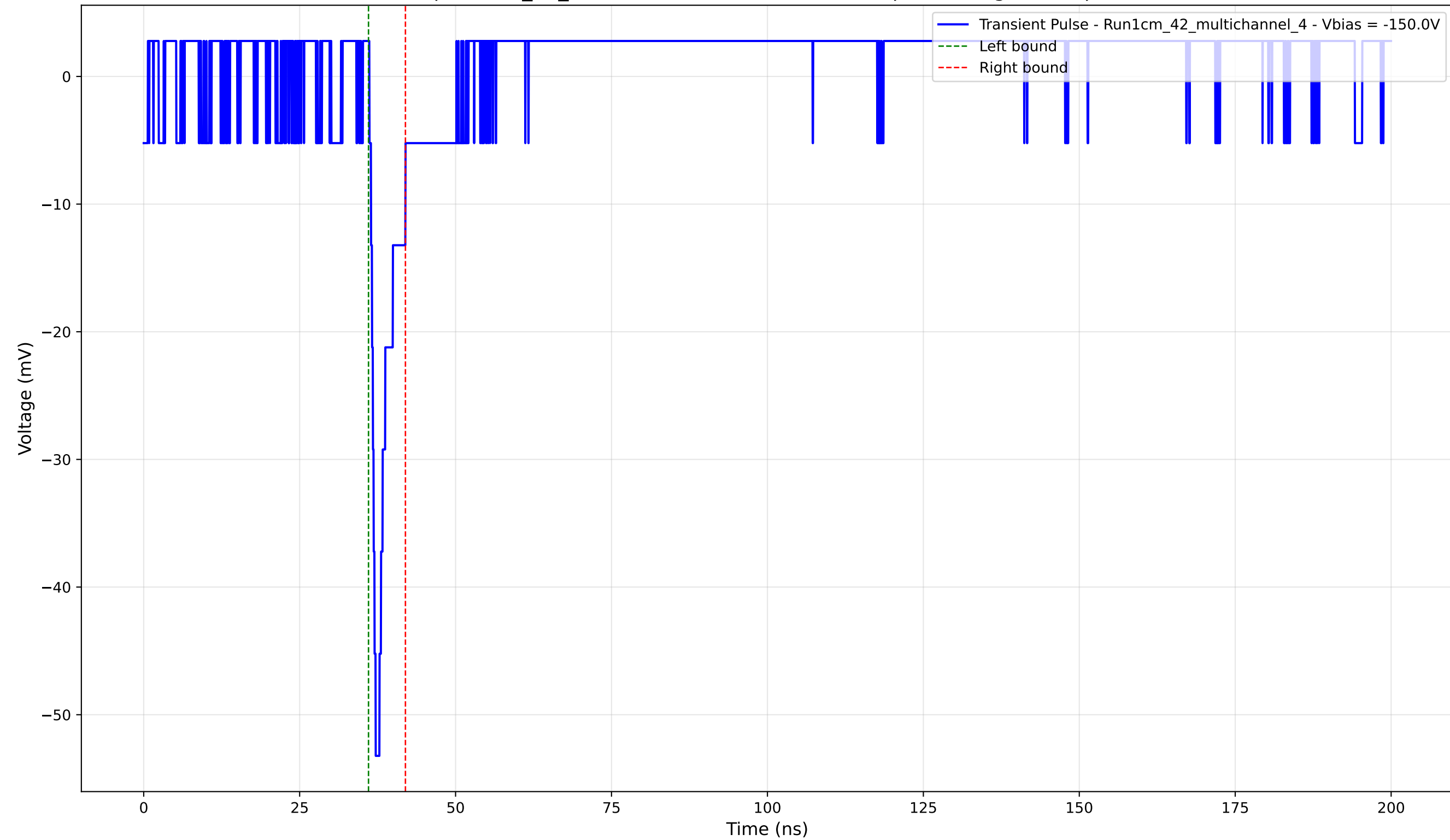
Transient Pulse - Sample: 1cm_42_multichannel - Position: 2020.0 \mu\text{m} - Charge: 2.83 pC - Rise Time: 0.76 ns
