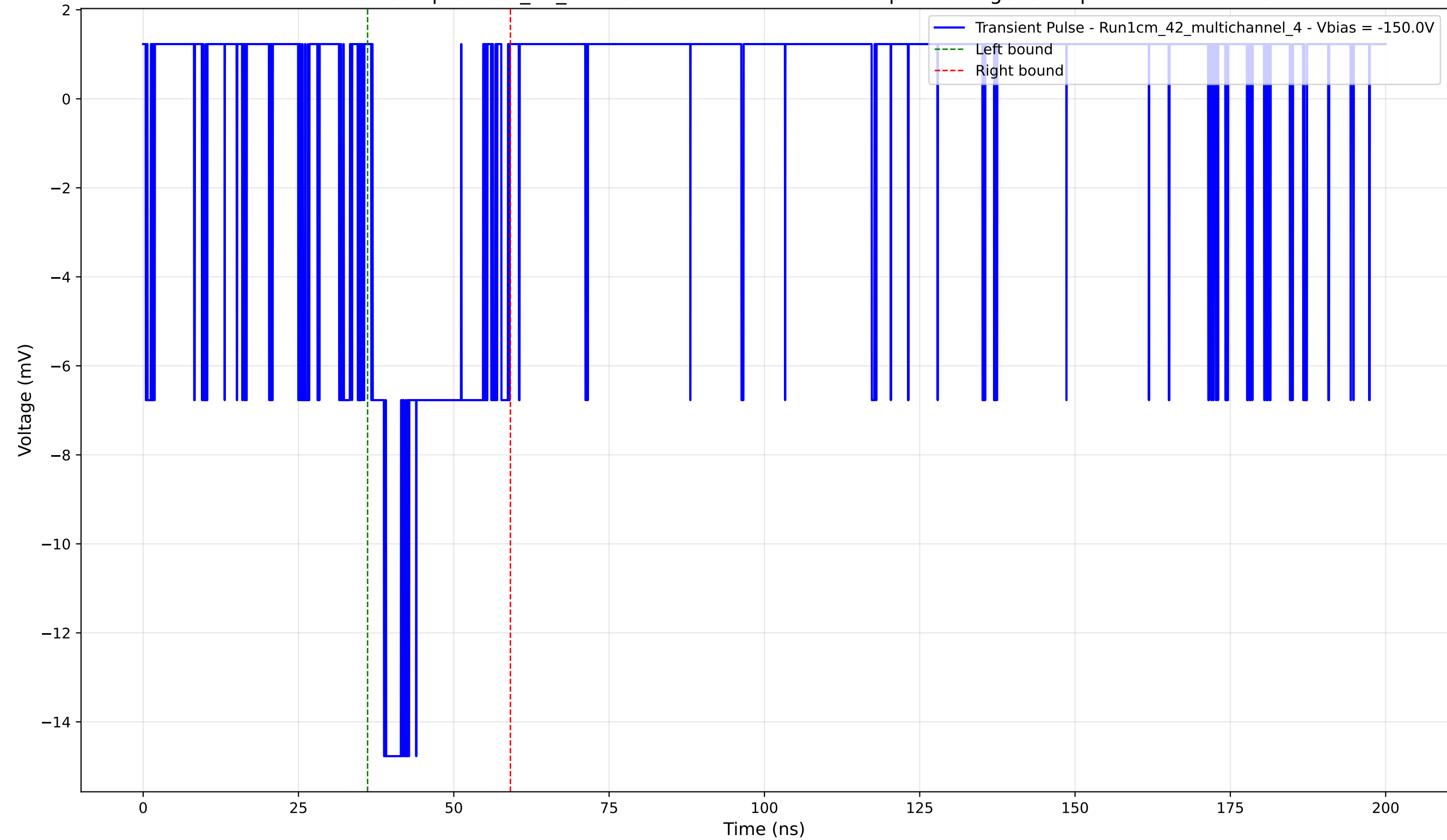
Transient Pulse - Sample: 1cm_42_multichannel - Position: 4480.0 \mu\text{m} - Charge: 3.20 pC - Rise Time: 1.84 ns
