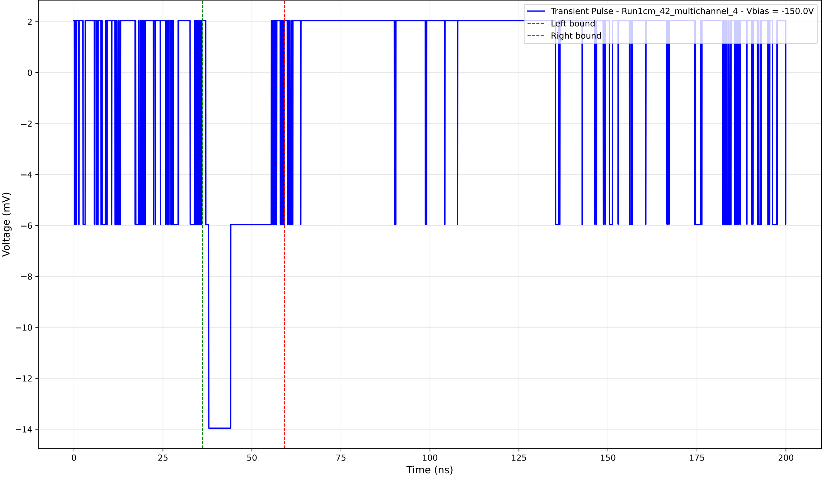
Transient Pulse - Sample: 1cm_42_multichannel - Position: 585.0 \mu\text{m} - Charge: 3.22 pC - Rise Time: 0.00 ns (N/A)
