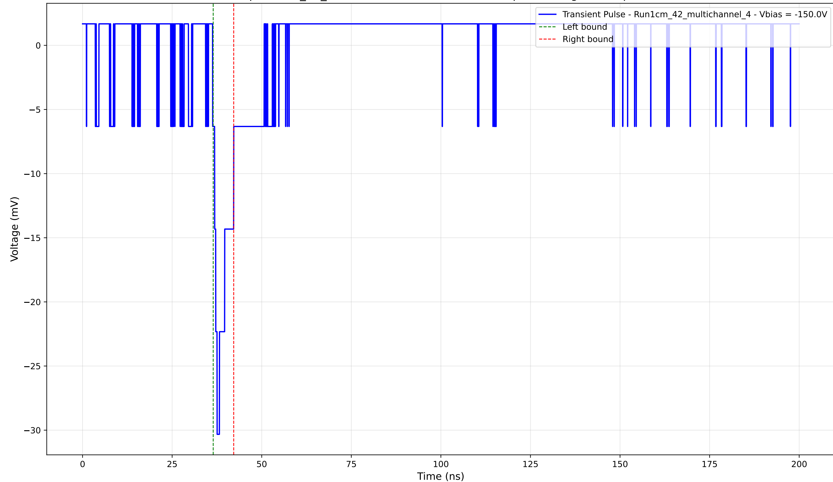
Transient Pulse - Sample: 1cm_42_multichannel - Position: 3170.0 \mu\text{m} - Charge: 2.08 pC - Rise Time: 1.25 ns
