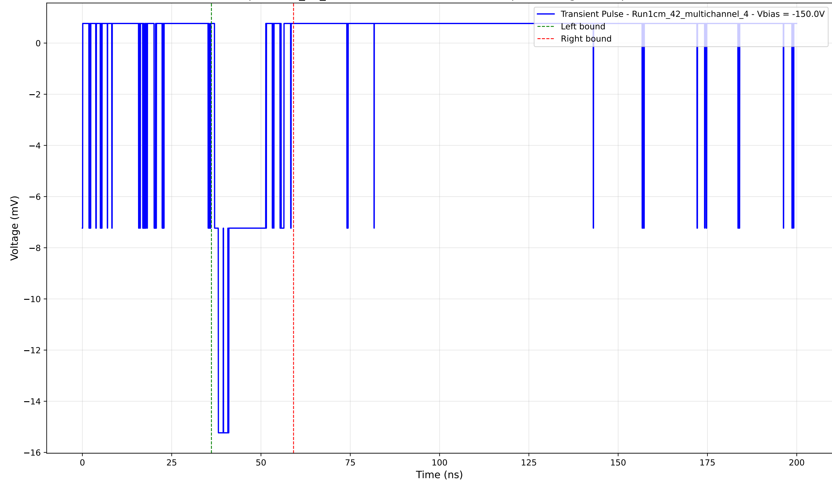
Transient Pulse - Sample: 1cm_42_multichannel - Position: 3845.0 \mu\text{m} - Charge: 2.60 pC - Rise Time: 1.08 ns
