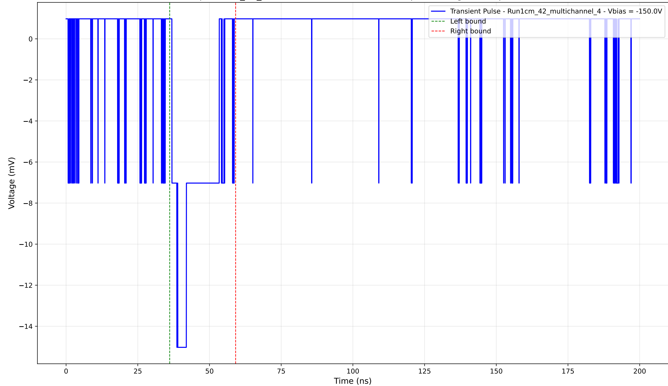
Transient Pulse - Sample: 1cm_42_multichannel - Position: 4765.0 \mu\text{m} - Charge: 2.94 pC - Rise Time: 1.74 ns
