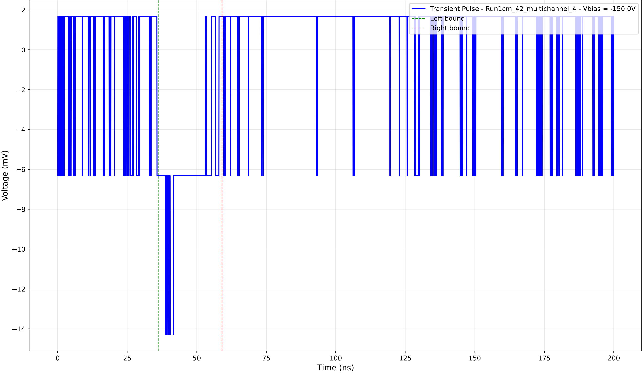
Transient Pulse - Sample: 1cm_42_multichannel - Position: 420.0 \mu\text{m} - Charge: 2.71 pC - Rise Time: 0.00 ns (N/A)
