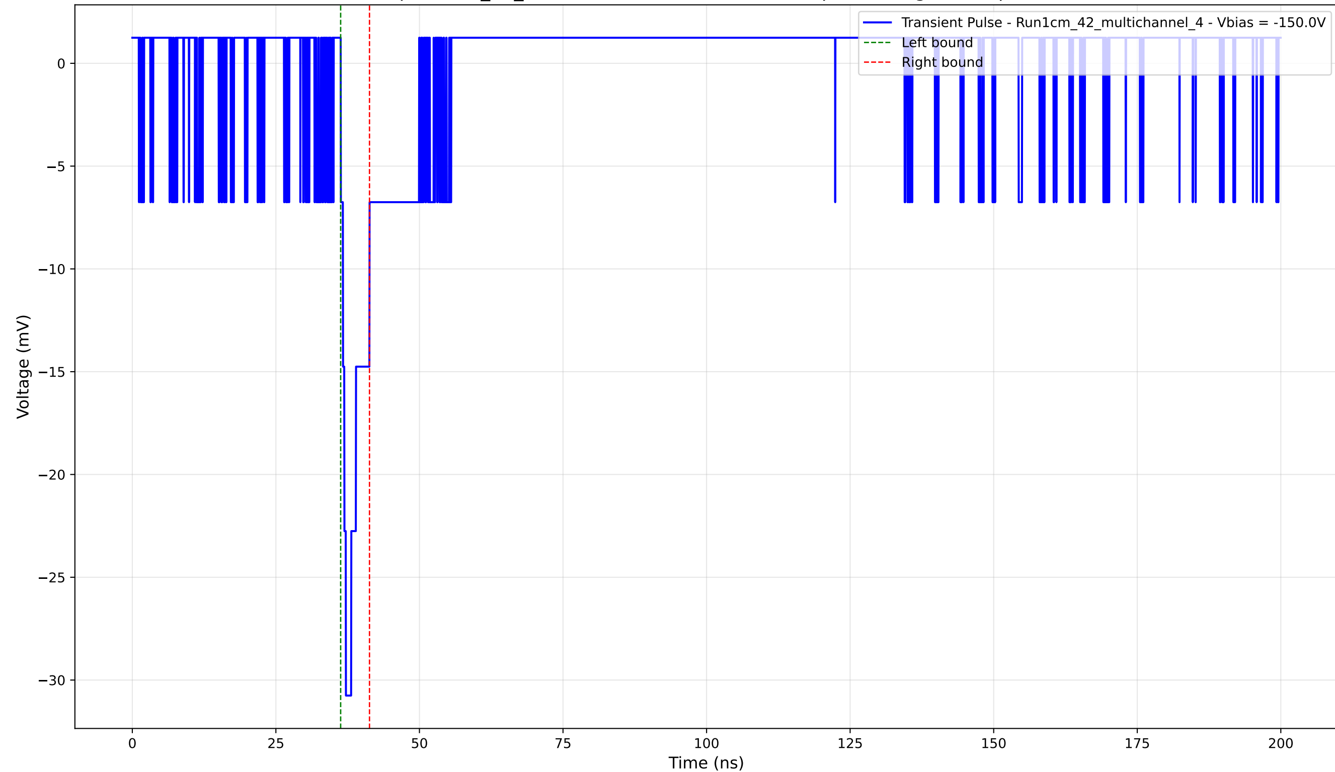
Transient Pulse - Sample: 1cm_42_multichannel - Position: 1820.0 \mu\text{m} - Charge: 1.89 pC - Rise Time: 0.89 ns
