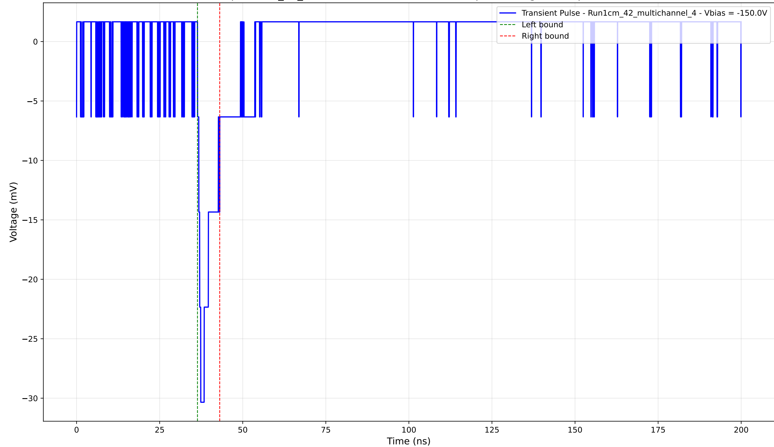
Transient Pulse - Sample: 1cm_42_multichannel - Position: 3140.0 \mu\text{m} - Charge: 2.39 pC - Rise Time: 0.97 ns
