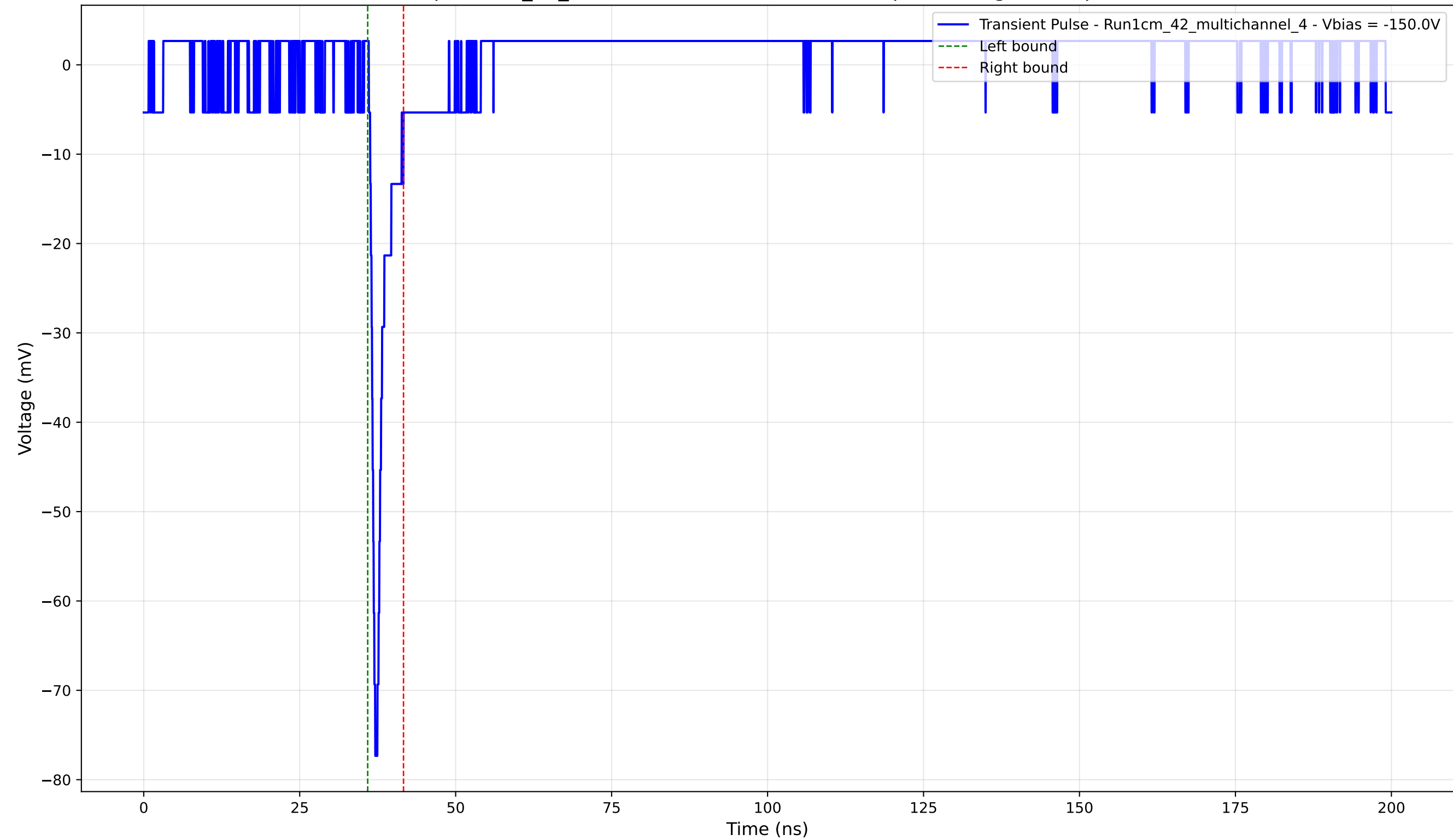
Transient Pulse - Sample: 1cm_42_multichannel - Position: 2525.0 \mu\text{m} - Charge: 3.23 pC - Rise Time: 0.81 ns
