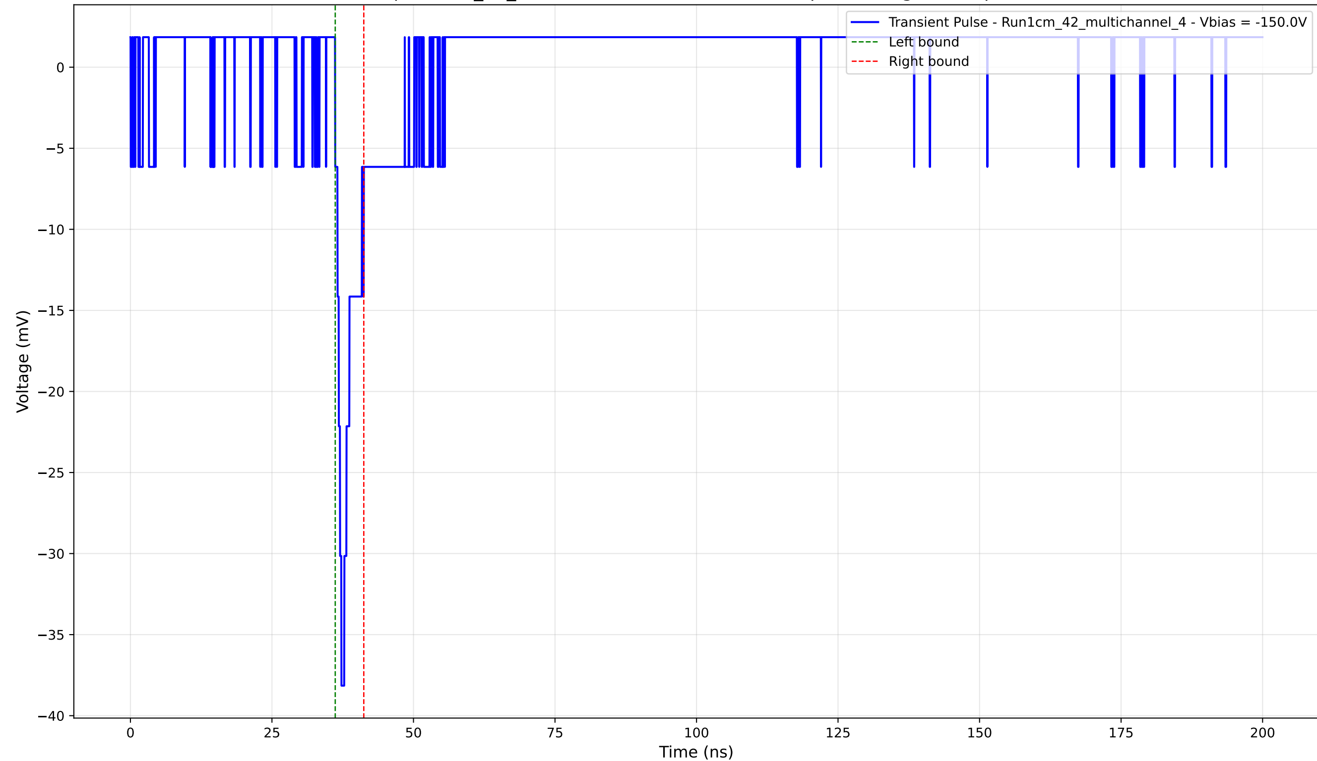
Transient Pulse - Sample: 1cm_42_multichannel - Position: 2830.0 \mu\text{m} - Charge: 1.89 pC - Rise Time: 1.11 ns
