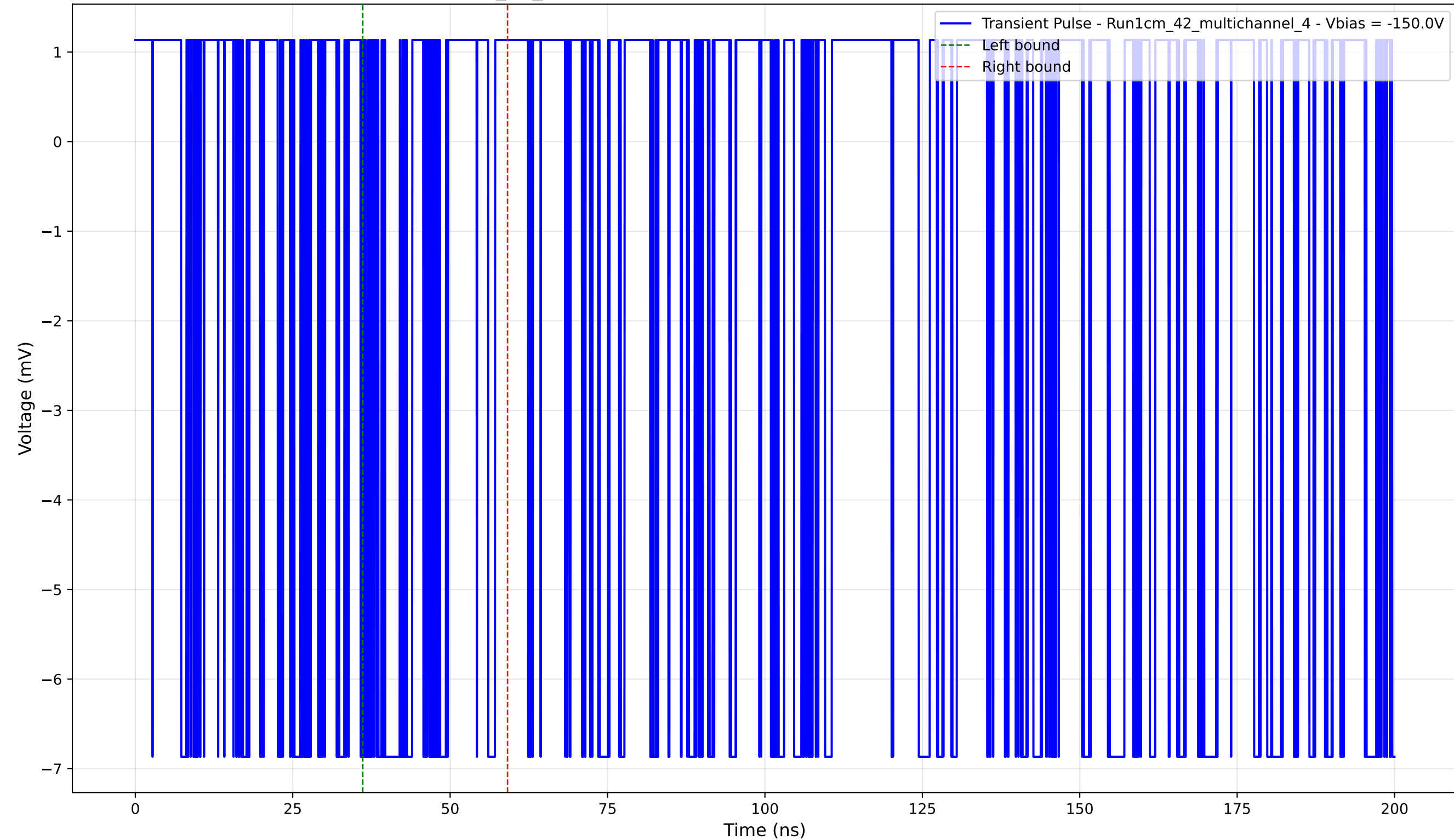
Transient Pulse - Sample: 1cm_42_multichannel - Position: 350.0 \mu\text{m} - Charge: 0.98 pC - Rise Time: 0.00 ns (N/A)
