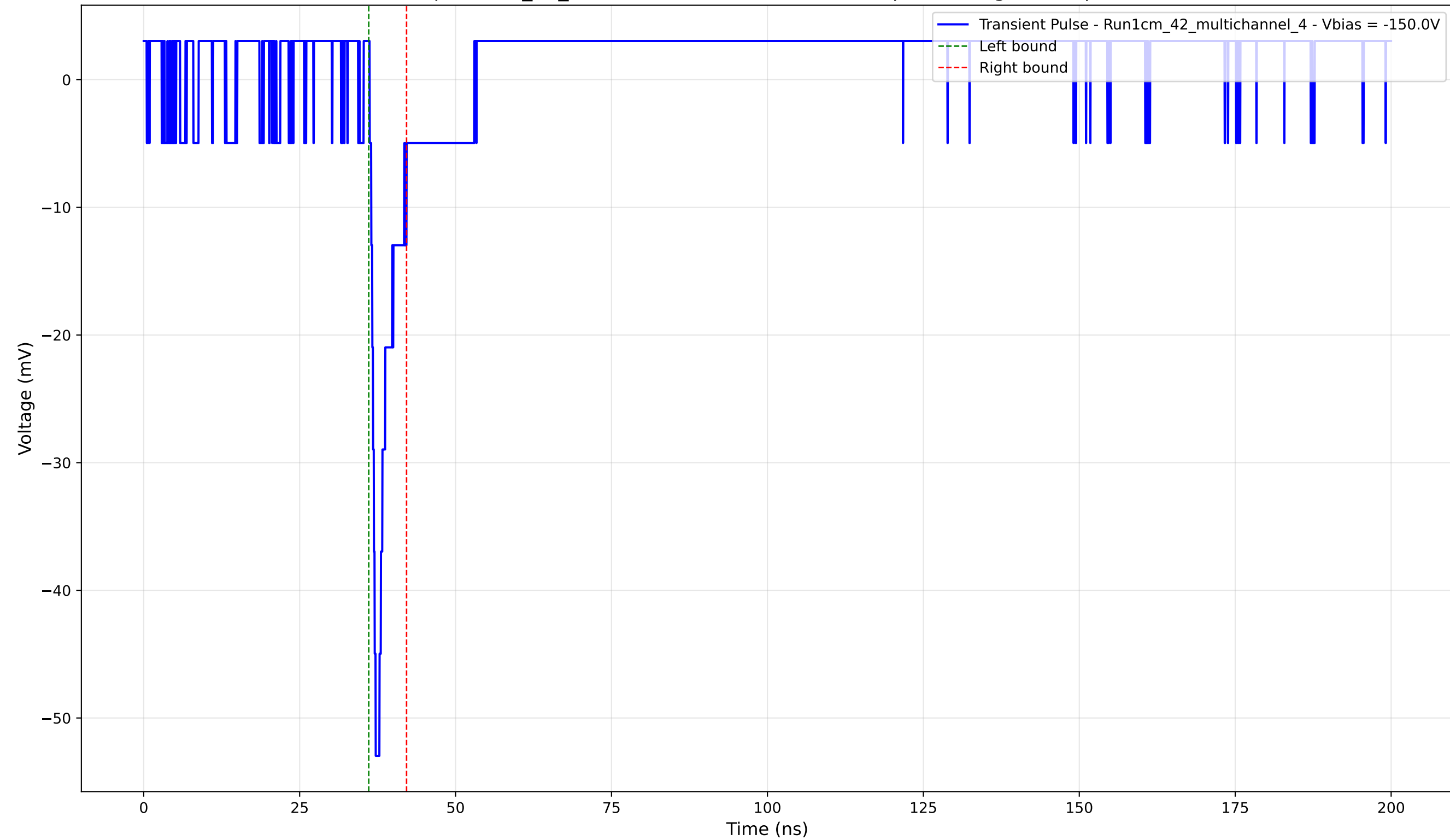
Transient Pulse - Sample: 1cm_42_multichannel - Position: 2010.0 \mu\text{m} - Charge: 2.79 pC - Rise Time: 0.72 ns
