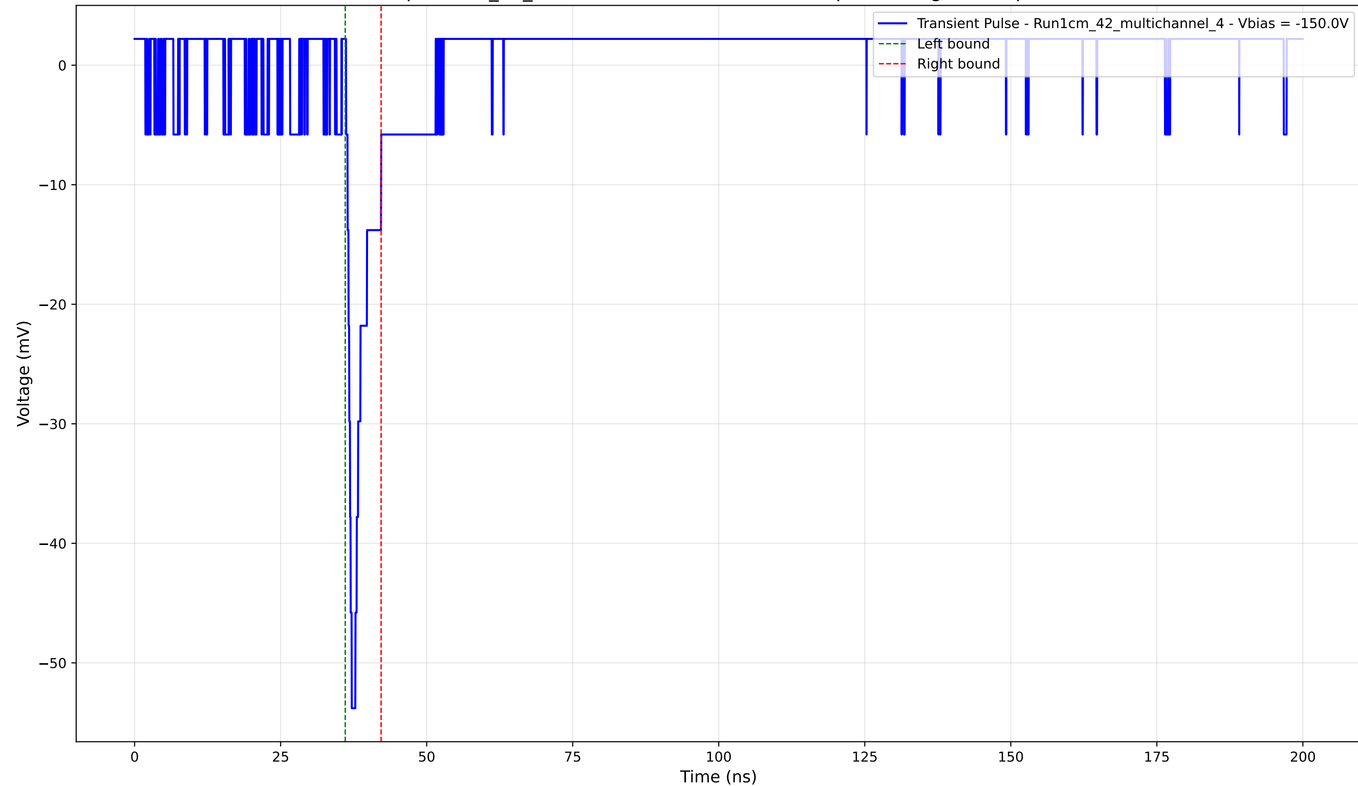
Transient Pulse - Sample: 1cm_42_multichannel - Position: 2035.0 \mu\text{m} - Charge: 2.91 pC - Rise Time: 0.96 ns
