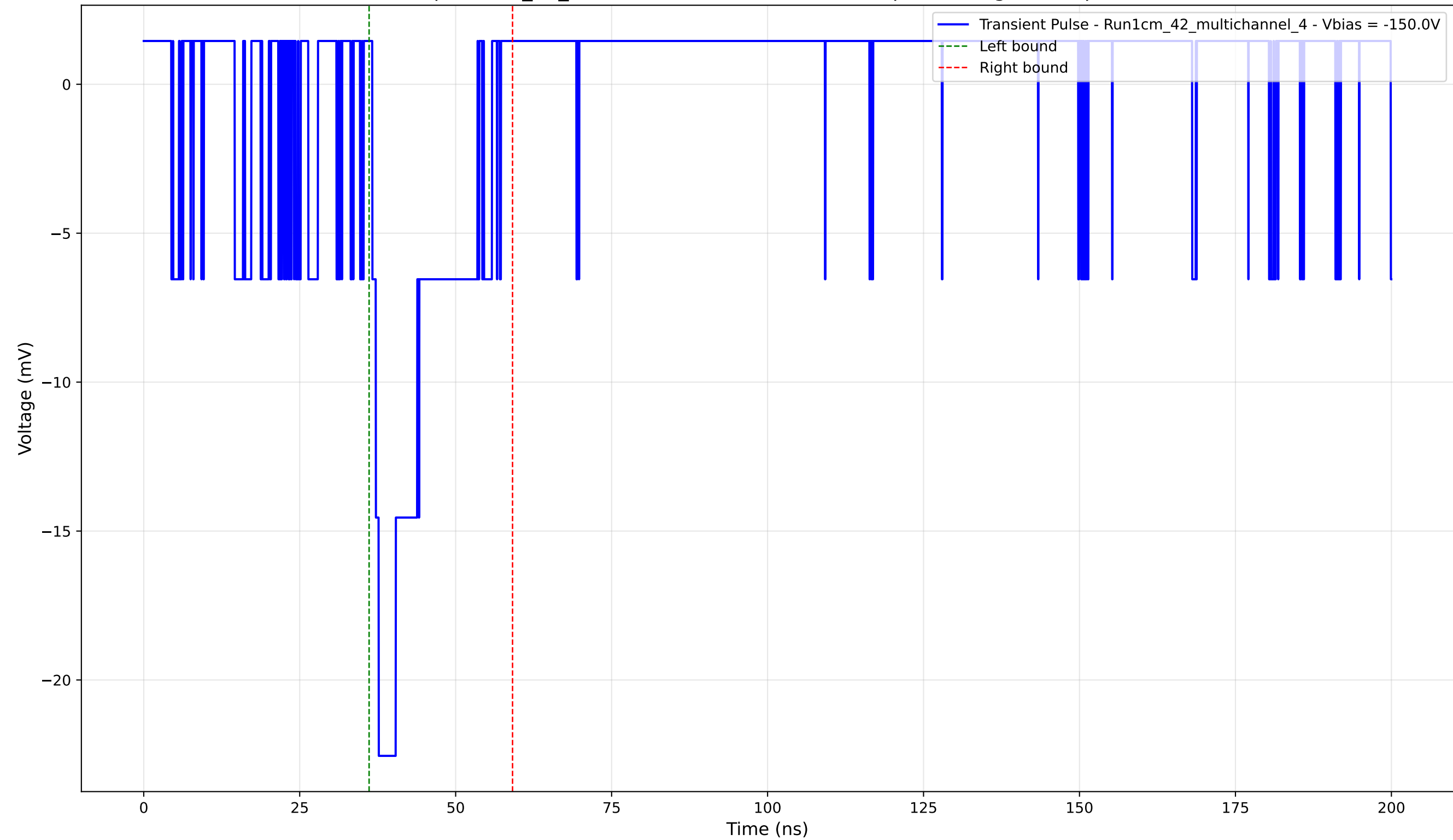
Transient Pulse - Sample: 1cm_42_multichannel - Position: 1240.0 \mu\text{m} - Charge: 3.84 pC - Rise Time: 1.04 ns
