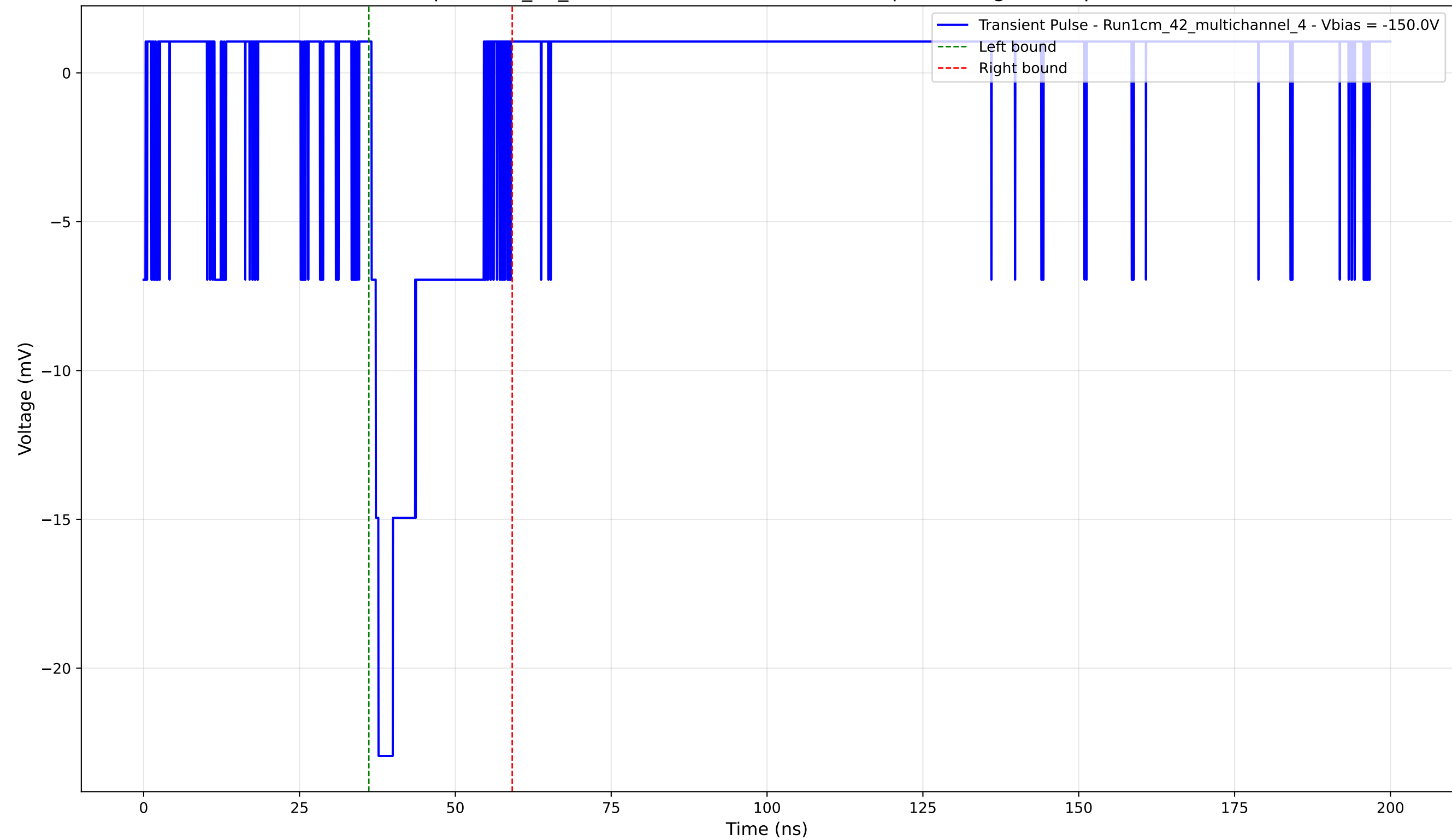
Transient Pulse - Sample: 1cm_42_multichannel - Position: 1230.0 \mu\text{m} - Charge: 4.03 pC - Rise Time: 1.12 ns
