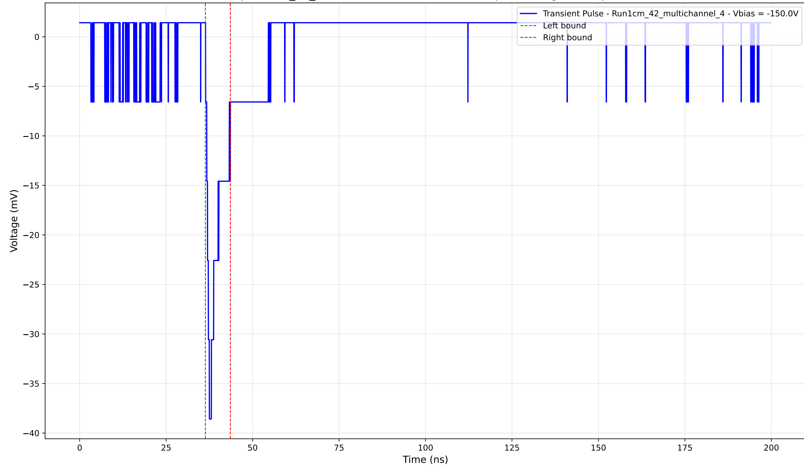
Transient Pulse - Sample: 1cm_42_multichannel - Position: 1690.0 \mu\text{m} - Charge: 2.86 pC - Rise Time: 1.09 ns
