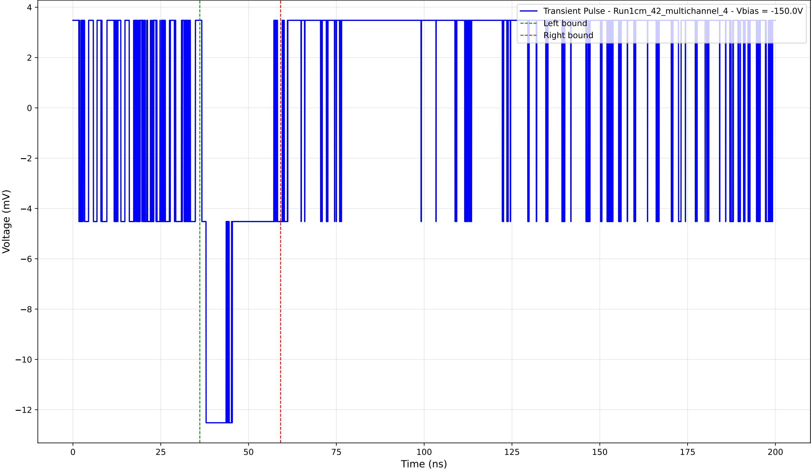
Transient Pulse - Sample: 1cm_42_multichannel - Position: 760.0 \mu\text{m} - Charge: 2.94 pC - Rise Time: 0.00 ns (N/A)
