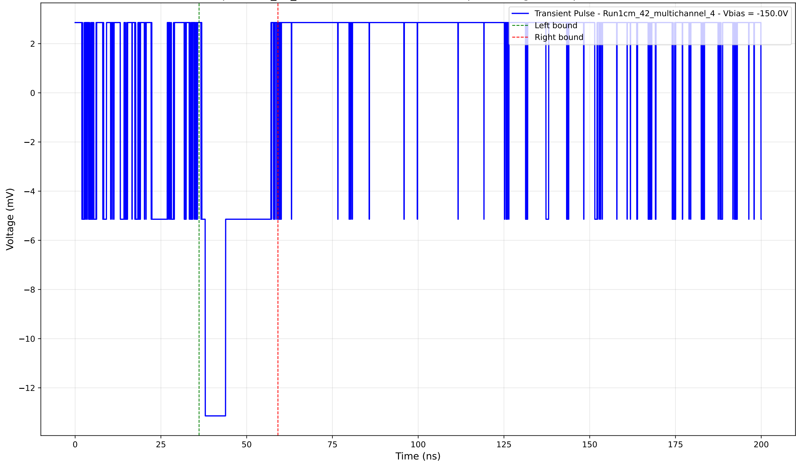
Transient Pulse - Sample: 1cm_42_multichannel - Position: 565.0 \mu\text{m} - Charge: 2.94 pC - Rise Time: 0.00 ns (N/A)
