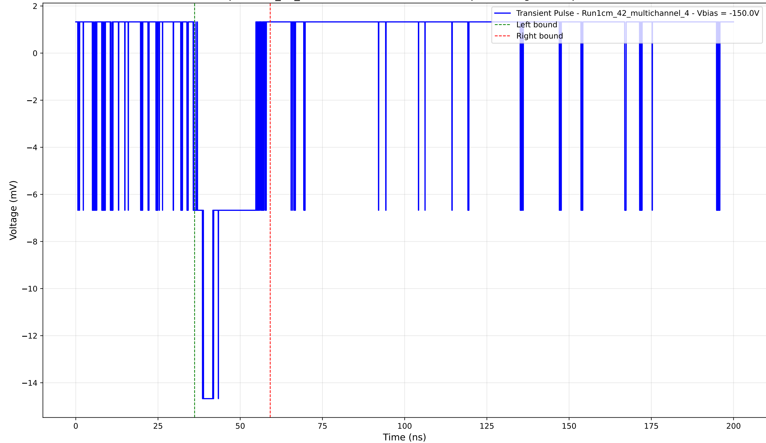
Transient Pulse - Sample: 1cm_42_multichannel - Position: 4725.0 \mu\text{m} - Charge: 3.08 pC - Rise Time: 1.54 ns
