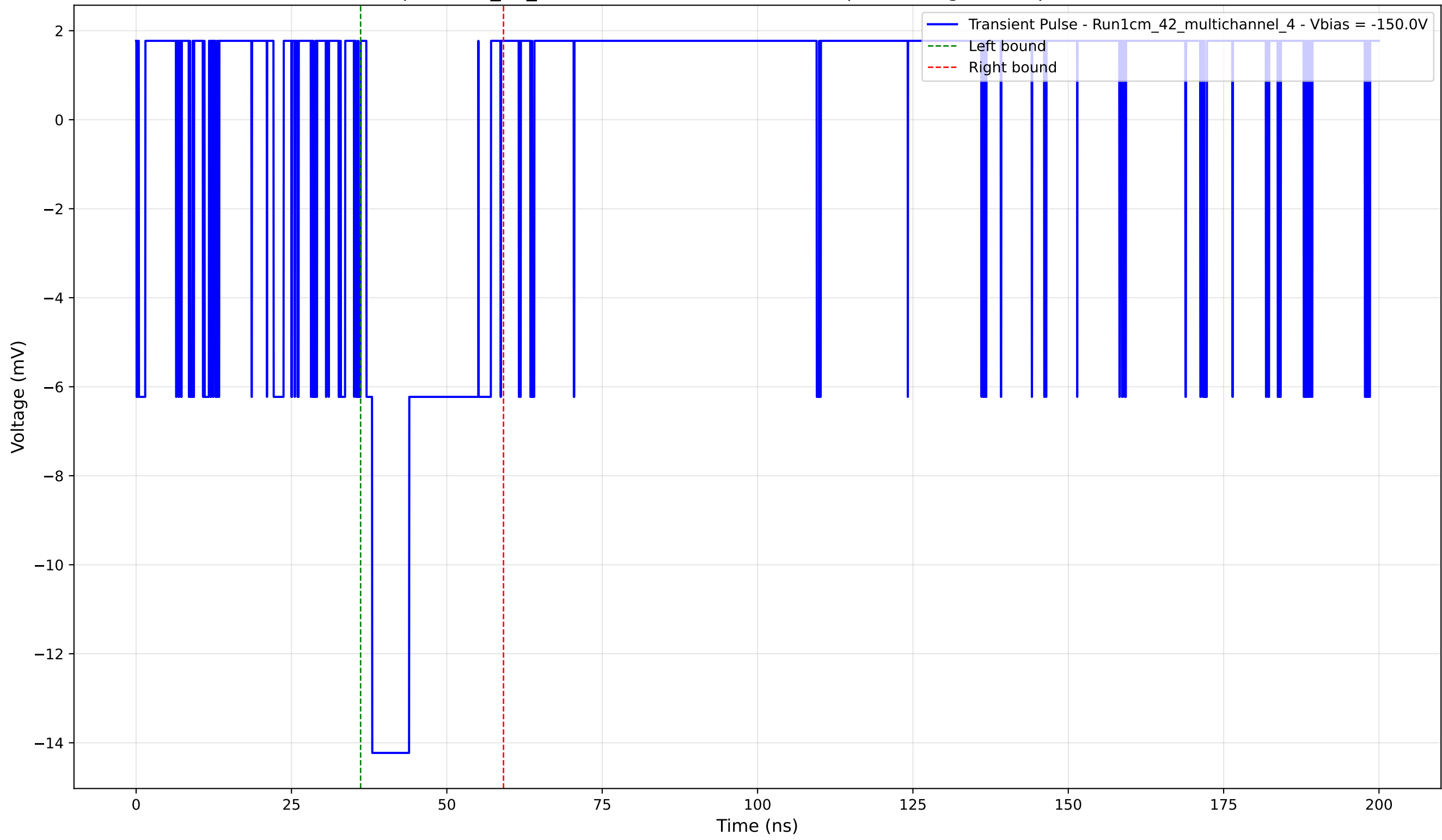
Transient Pulse - Sample: 1cm_42_multichannel - Position: 500.0 \mu\text{m} - Charge: 3.35 pC - Rise Time: 0.00 ns (N/A)
