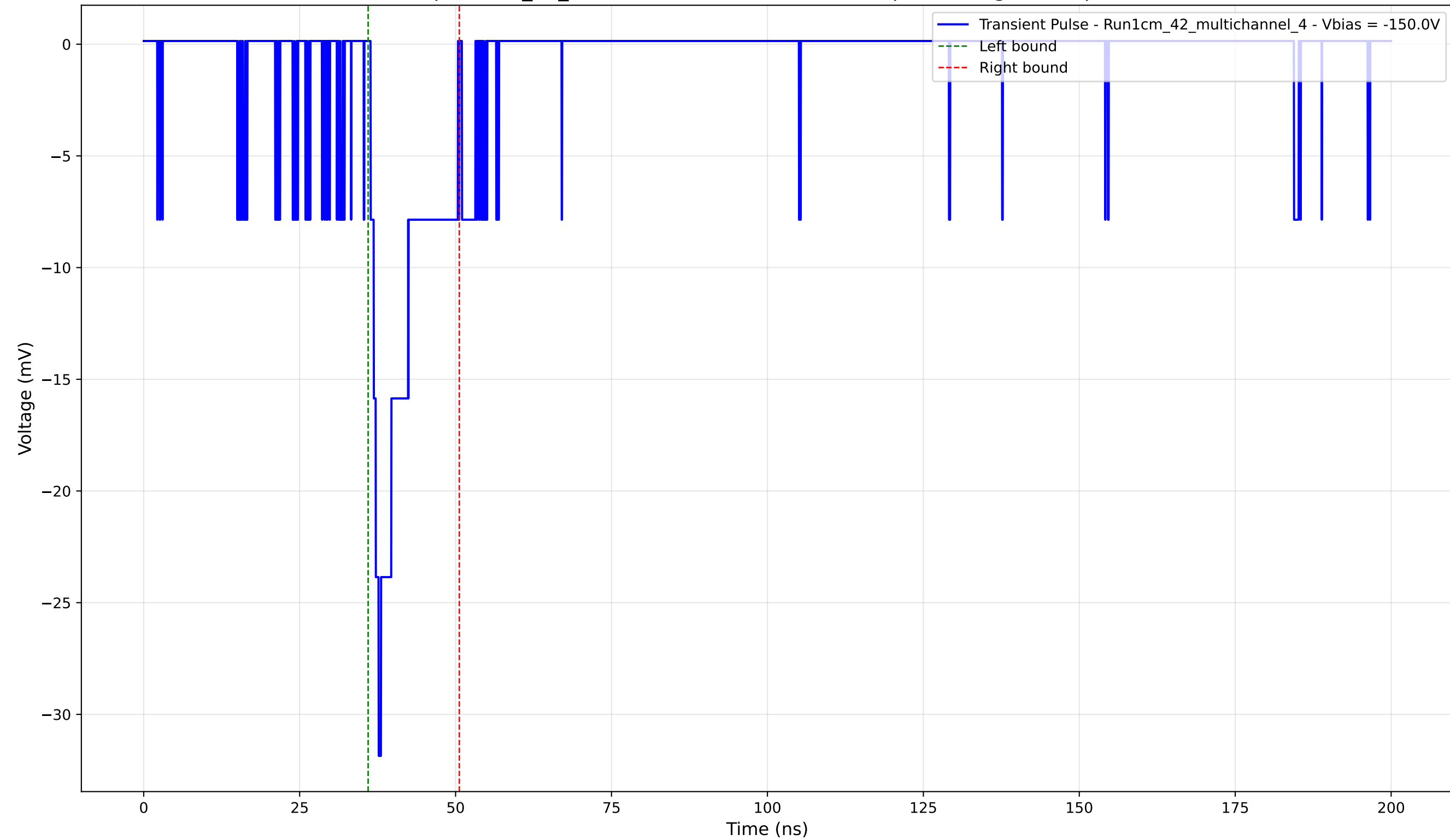
Transient Pulse - Sample: 1cm_42_multichannel - Position: 3210.0 \mu\text{m} - Charge: 3.56 pC - Rise Time: 1.29 ns
