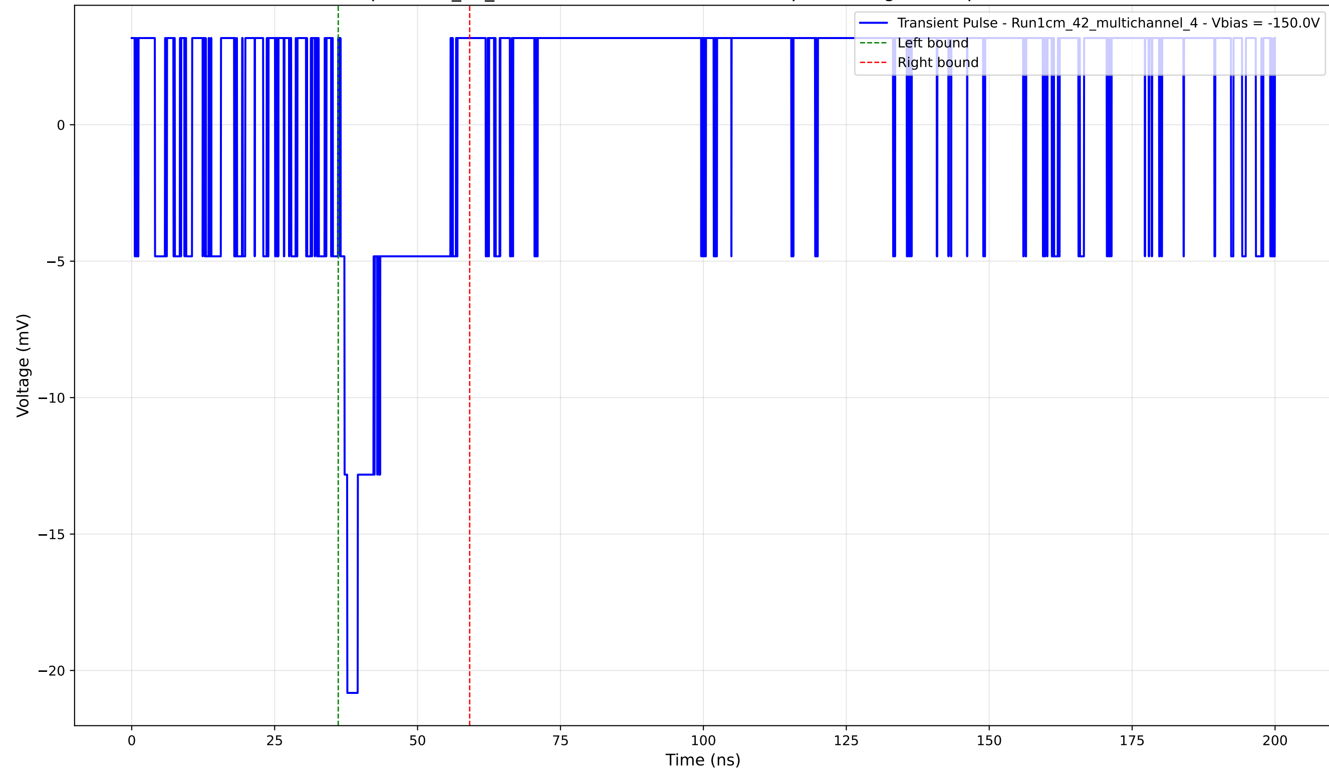
Transient Pulse - Sample: 1cm_42_multichannel - Position: 1305.0 \mu\text{m} - Charge: 2.91 pC - Rise Time: 0.00 ns (N/A)
