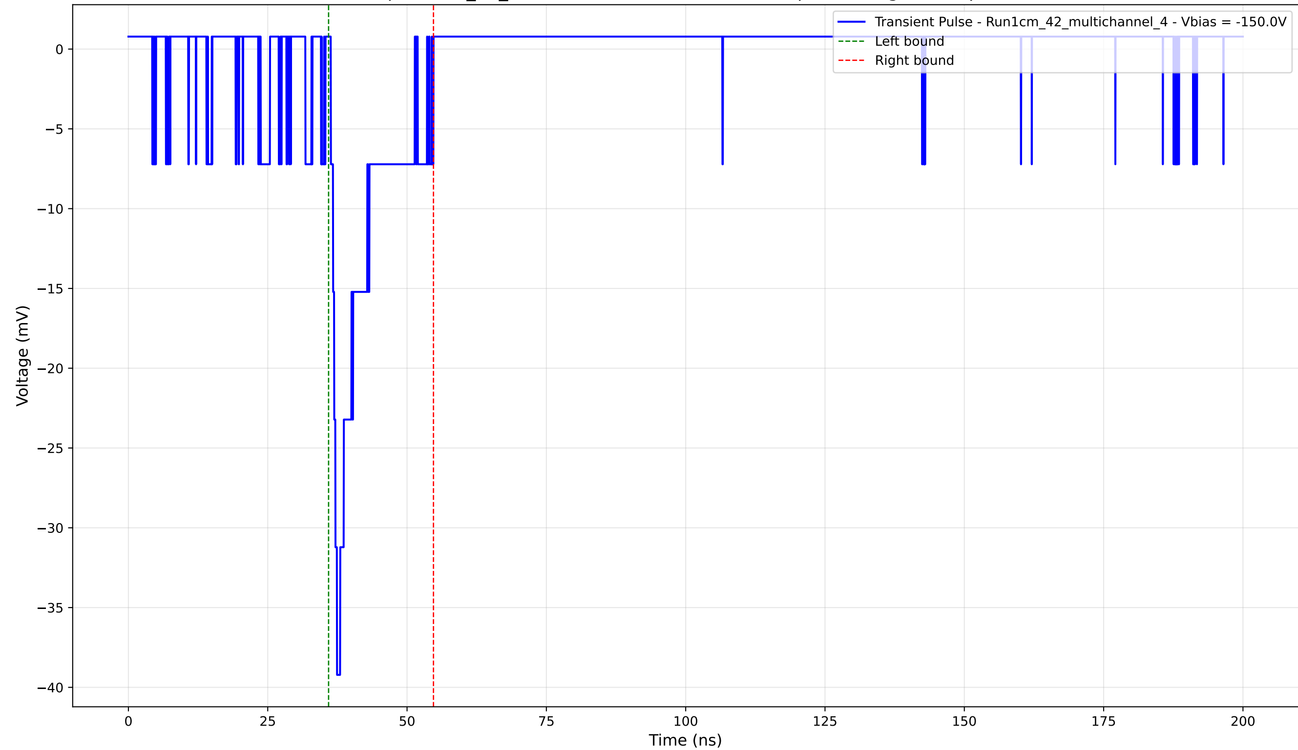
Transient Pulse - Sample: 1cm_42_multichannel - Position: 1700.0 \mu\text{m} - Charge: 4.43 pC - Rise Time: 1.11 ns
