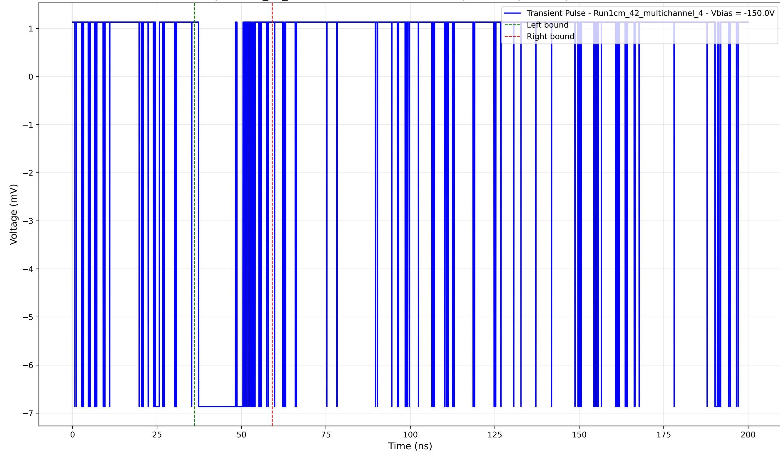
Transient Pulse - Sample: 1cm_42_multichannel - Position: 3945.0 \mu\text{m} - Charge: 1.83 pC - Rise Time: 0.00 ns (N/A)
