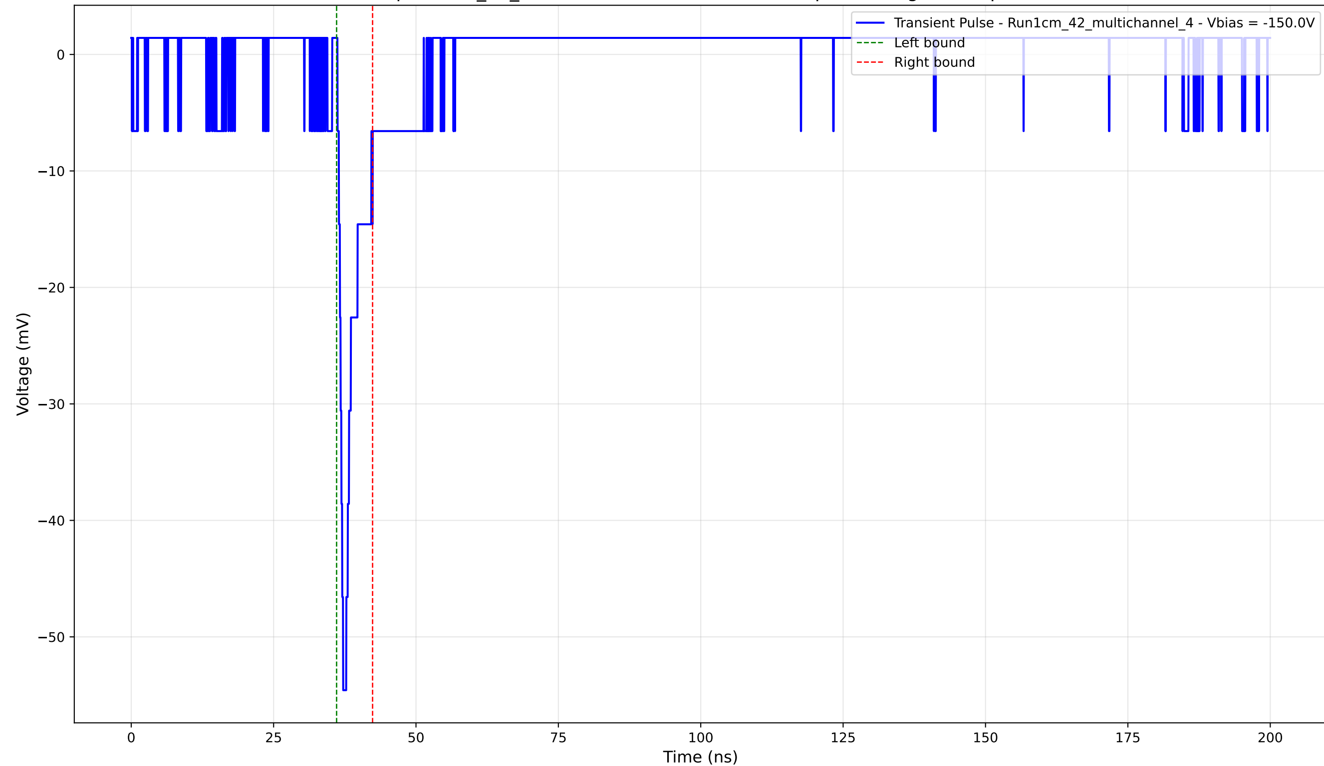
Transient Pulse - Sample: 1cm_42_multichannel - Position: 2755.0 \mu\text{m} - Charge: 2.97 pC - Rise Time: 0.98 ns
