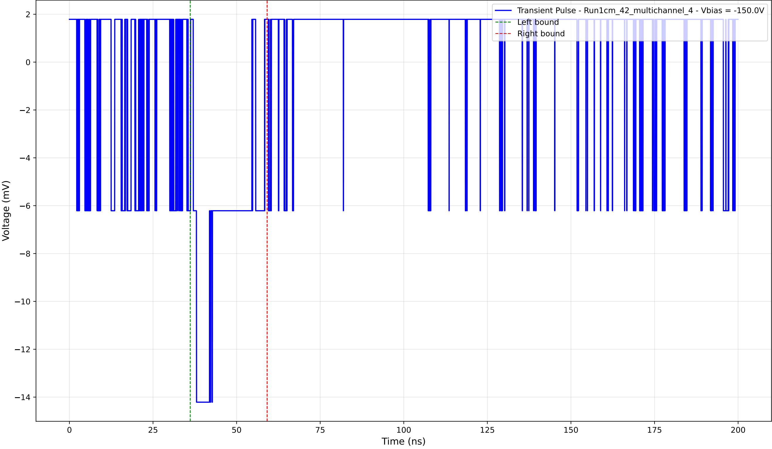
Transient Pulse - Sample: 1cm_42_multichannel - Position: 805.0 \mu\text{m} - Charge: 3.16 pC - Rise Time: 0.00 ns (N/A)
