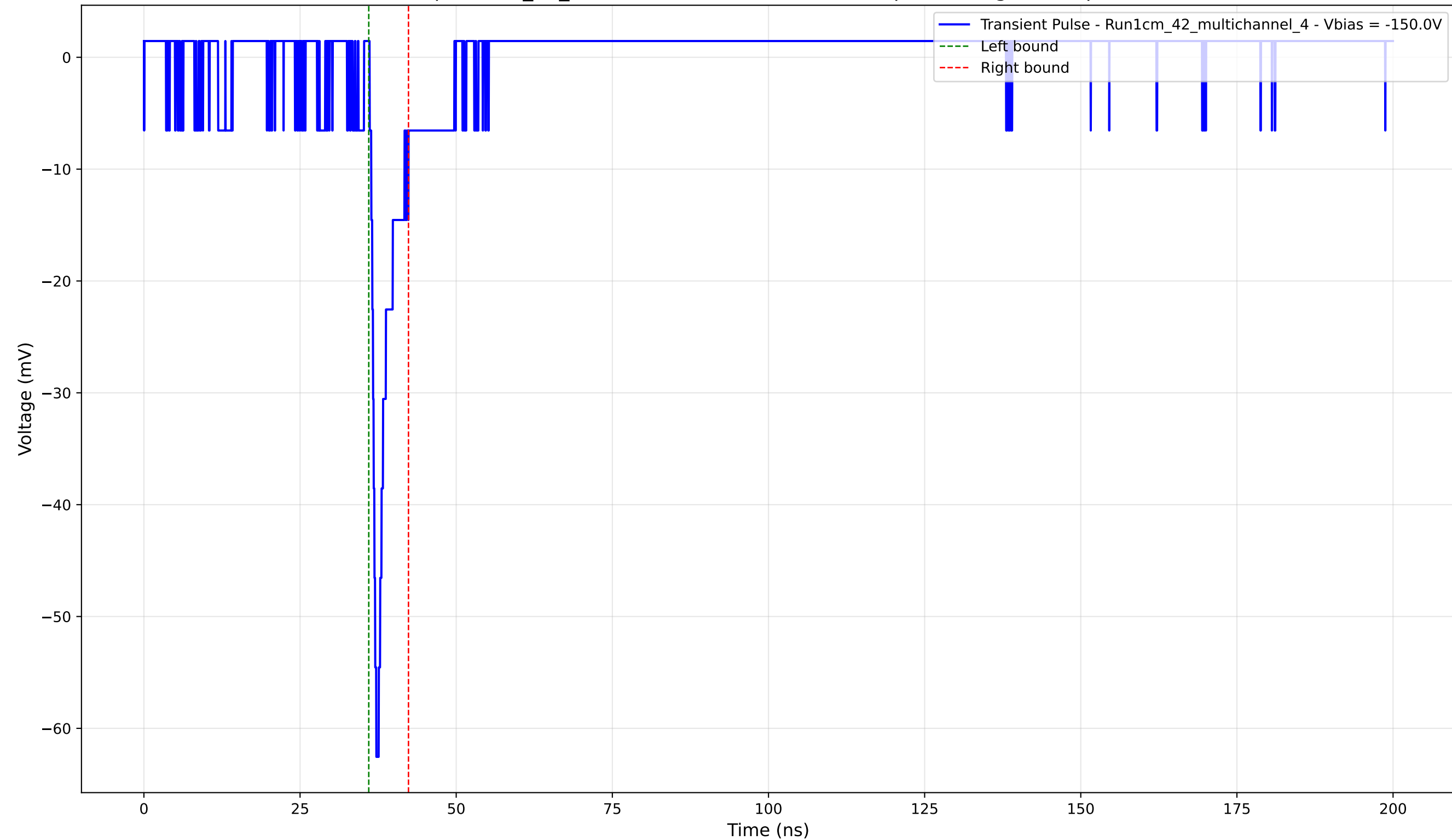
Transient Pulse - Sample: 1cm_42_multichannel - Position: 2095.0 \mu\text{m} - Charge: 3.16 pC - Rise Time: 1.06 ns
