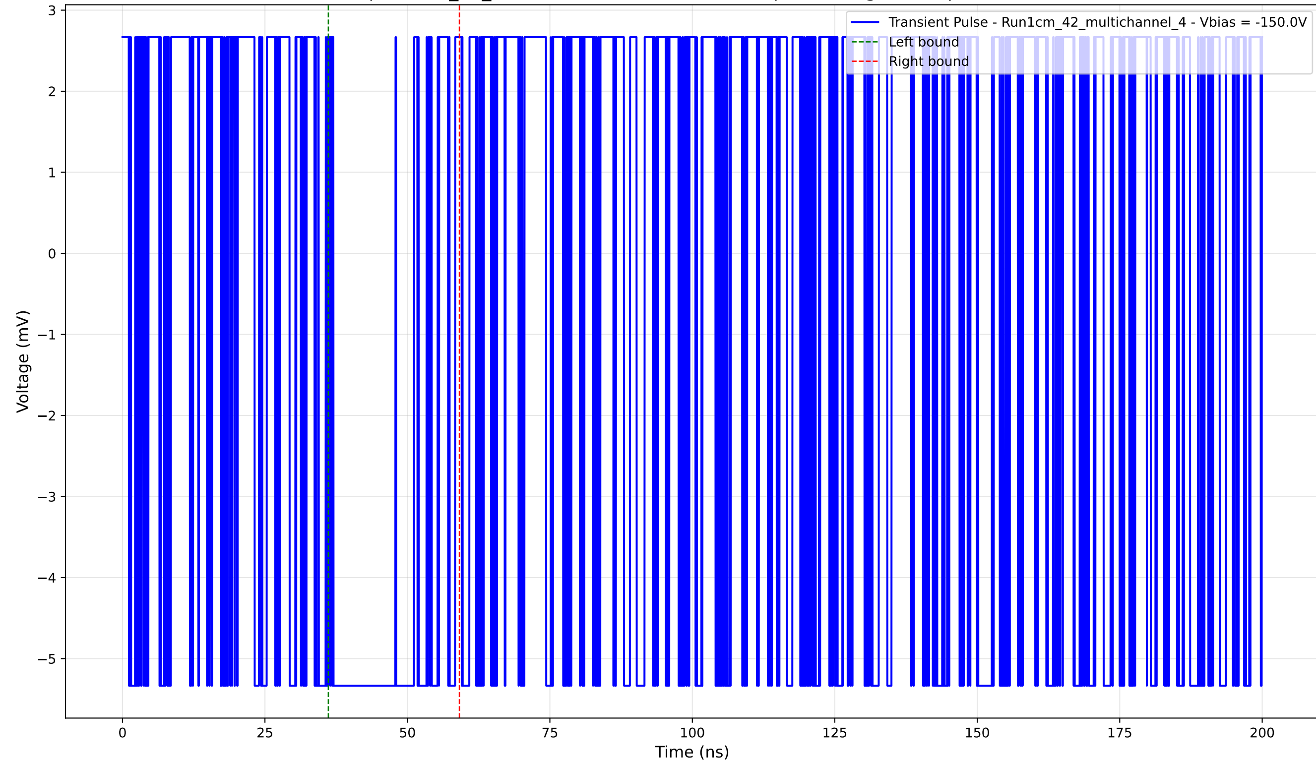
Transient Pulse - Sample: 1cm_42_multichannel - Position: 320.0 \mu\text{m} - Charge: 1.67 pC - Rise Time: 0.00 ns (N/A)
