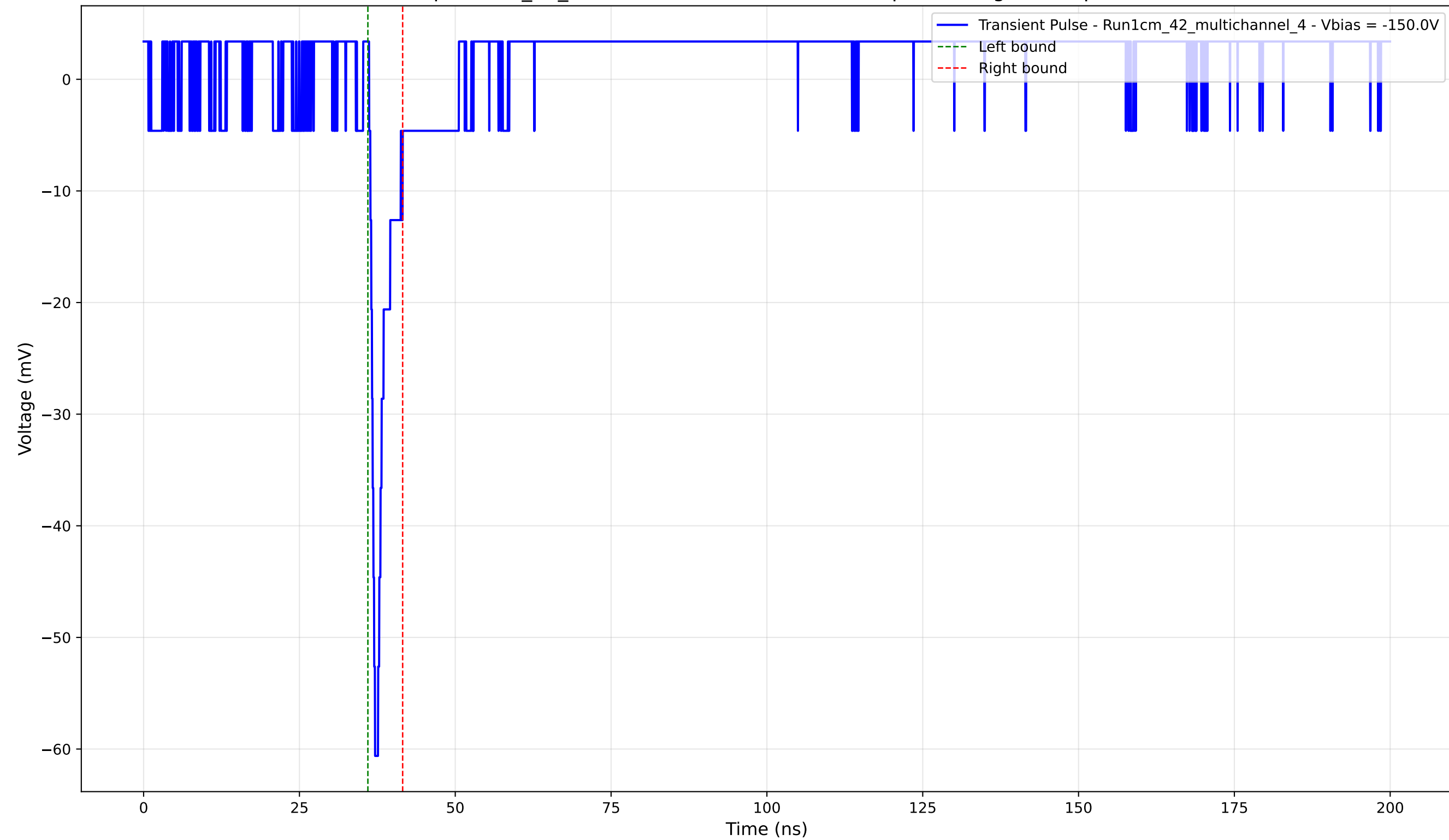
Transient Pulse - Sample: 1cm_42_multichannel - Position: 2620.0 \mu\text{m} - Charge: 2.70 pC - Rise Time: 0.76 ns
