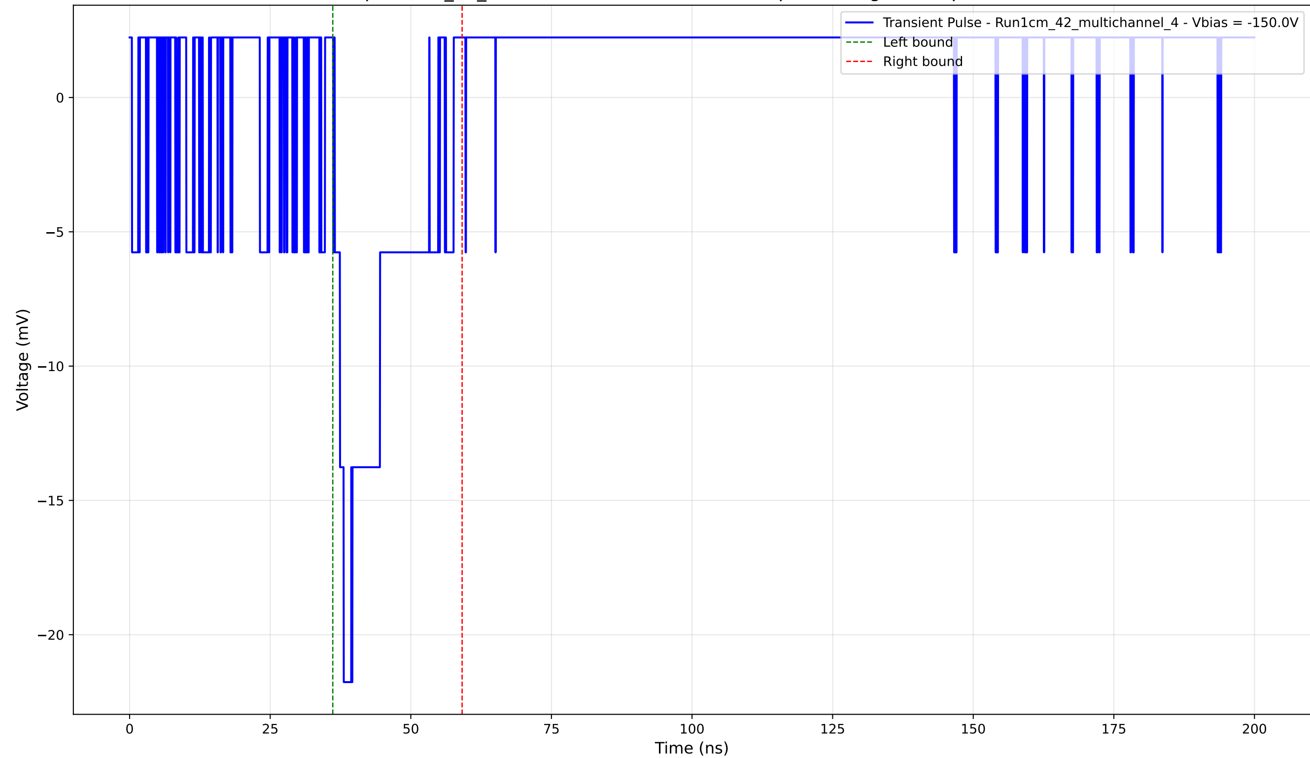
Transient Pulse - Sample: 1cm_42_multichannel - Position: 1125.0 \mu\text{m} - Charge: 3.56 pC - Rise Time: 0.00 ns (N/A)
