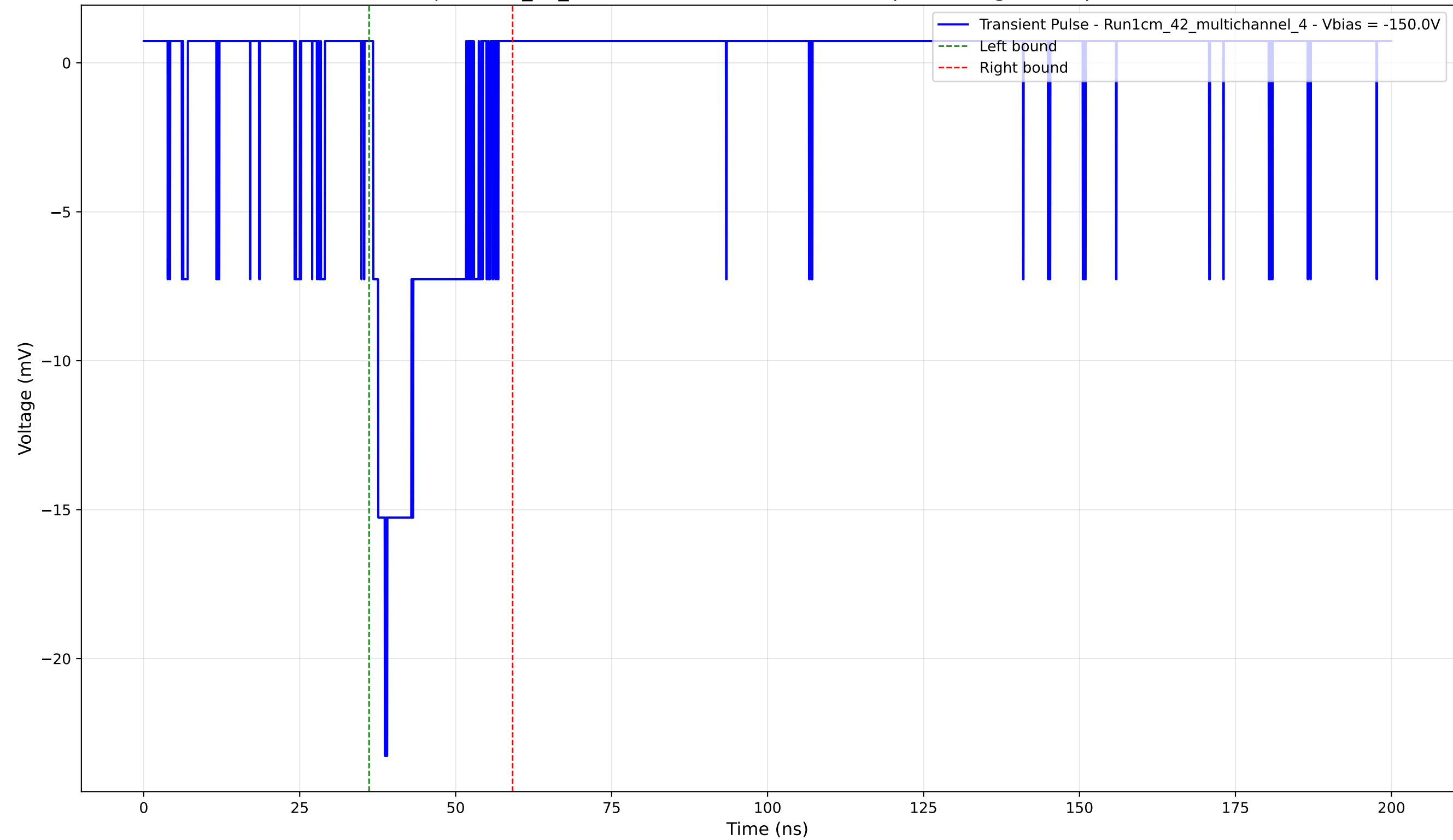
Transient Pulse - Sample: 1cm_42_multichannel - Position: 3735.0 \mu\text{m} - Charge: 3.36 pC - Rise Time: 1.88 ns
