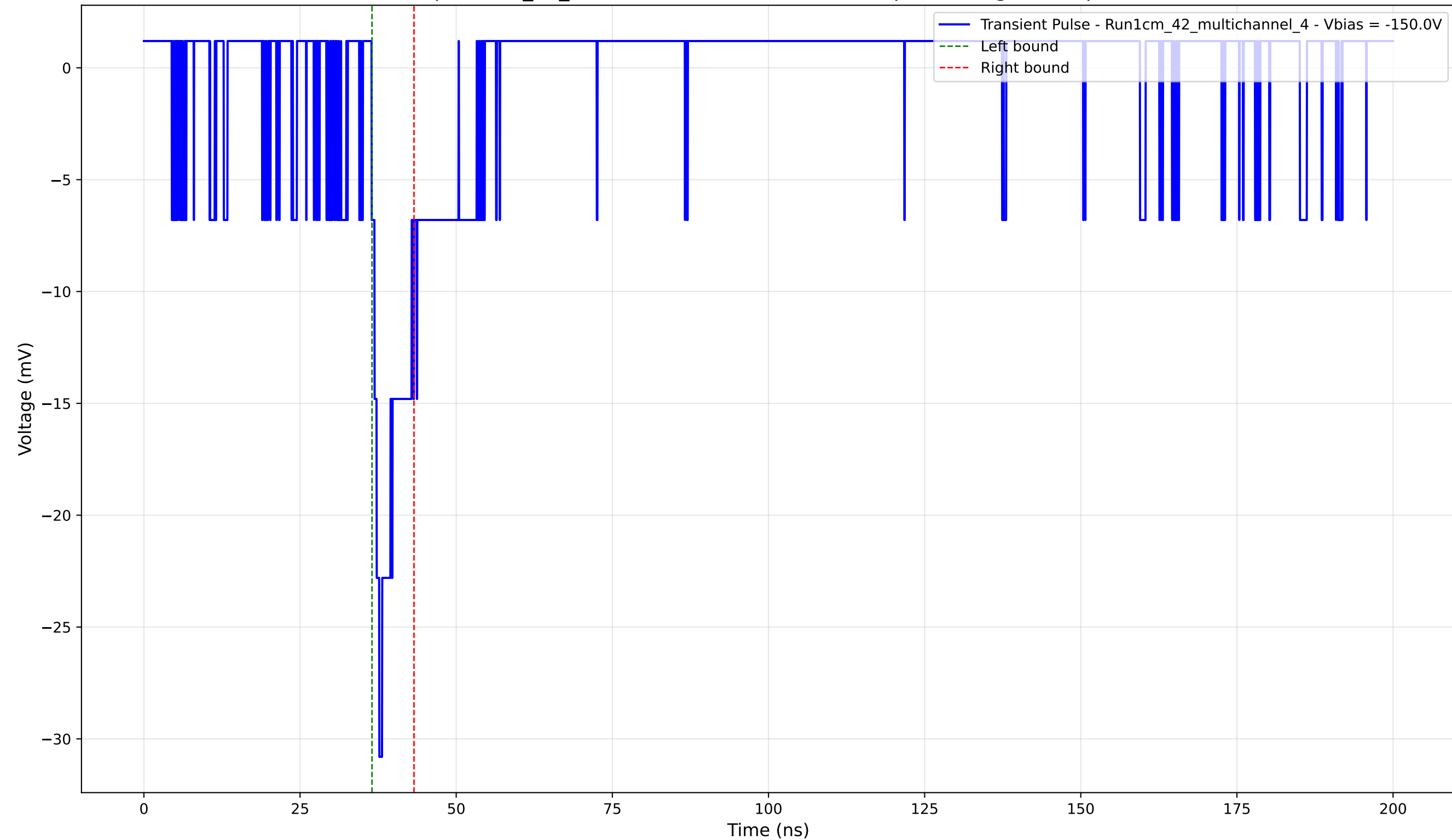
Transient Pulse - Sample: 1cm_42_multichannel - Position: 3265.0 \mu\text{m} - Charge: 2.33 pC - Rise Time: 1.23 ns
