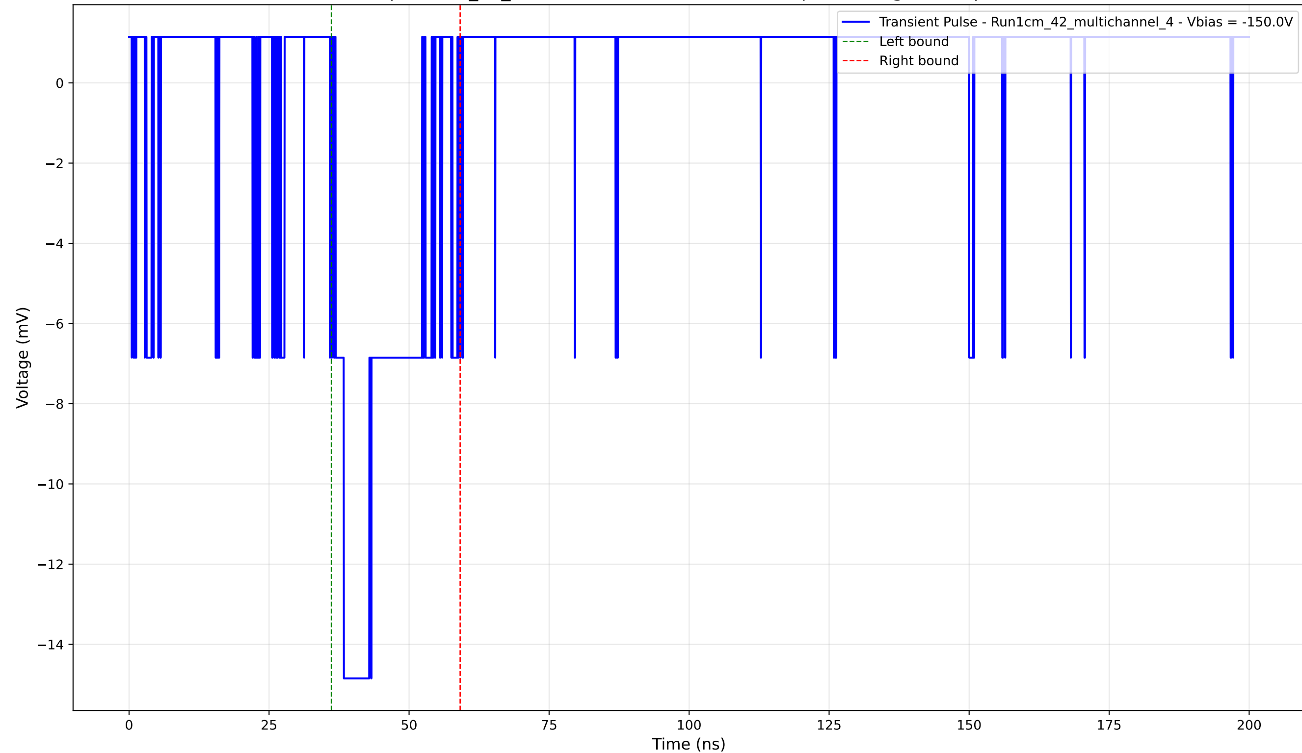
Transient Pulse - Sample: 1cm_42_multichannel - Position: 4240.0 \mu\text{m} - Charge: 3.18 pC - Rise Time: 1.48 ns
