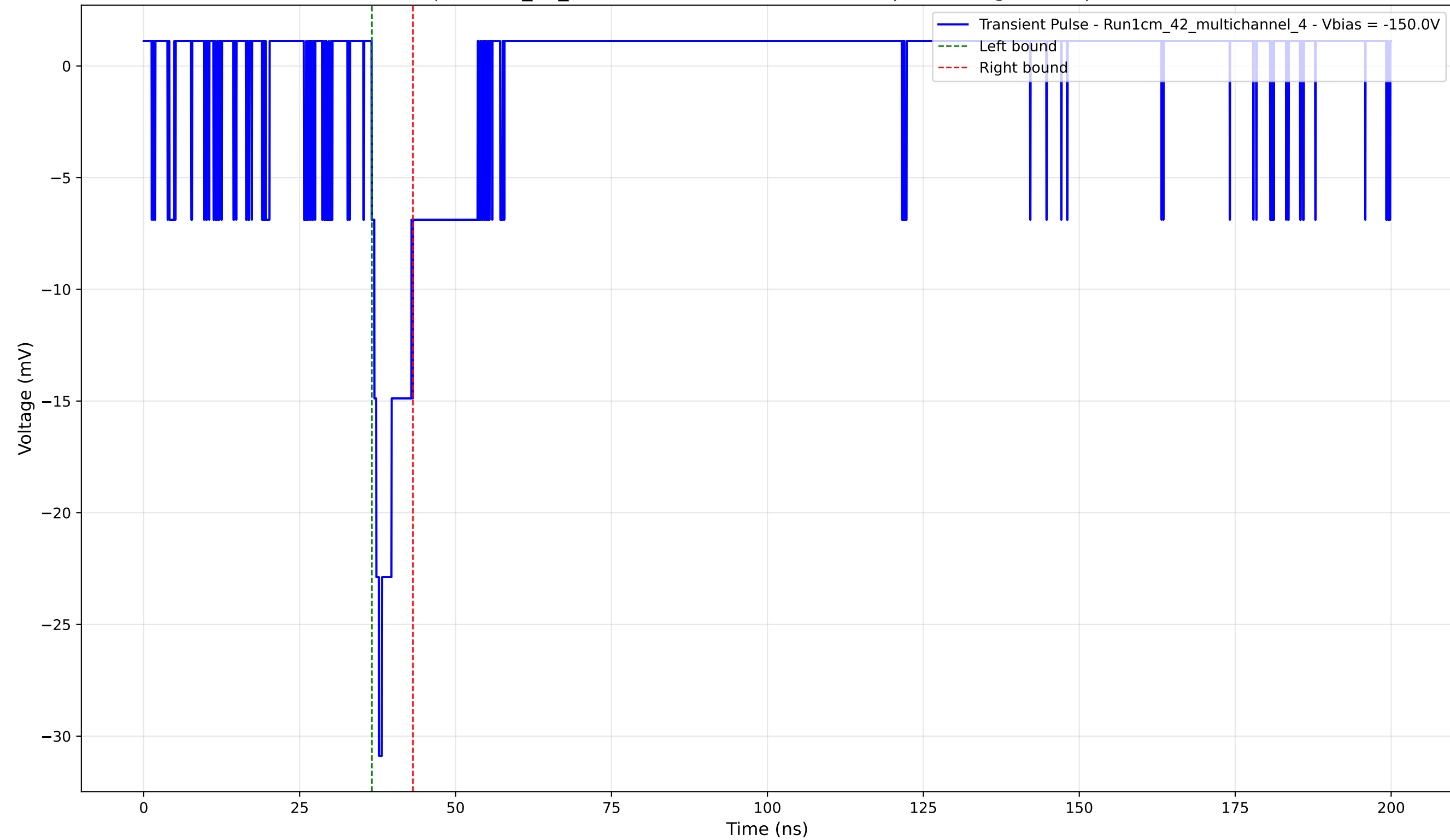
Transient Pulse - Sample: 1cm_42_multichannel - Position: 3255.0 \mu\text{m} - Charge: 2.35 pC - Rise Time: 1.19 ns
