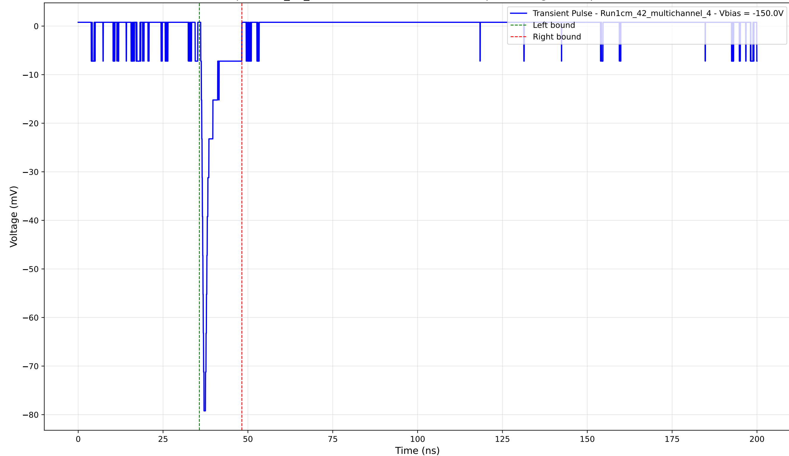
Transient Pulse - Sample: 1cm_42_multichannel - Position: 2515.0 \mu\text{m} - Charge: 4.35 pC - Rise Time: 0.80 ns
