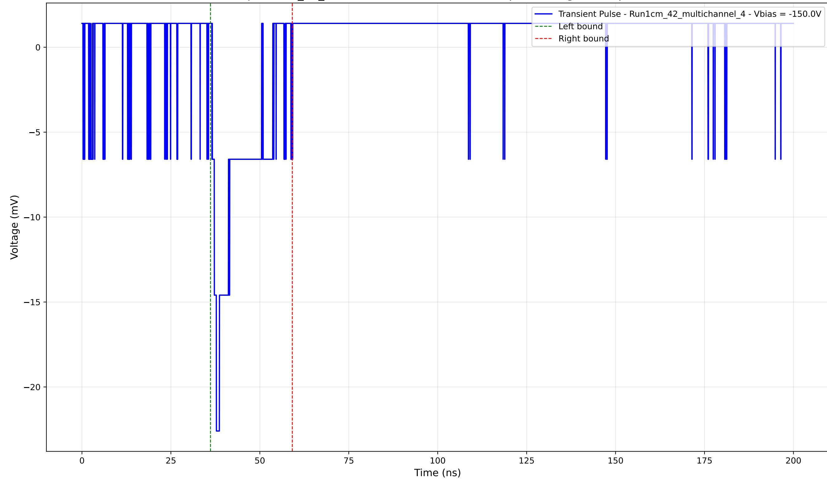
Transient Pulse - Sample: 1cm_42_multichannel - Position: 3335.0 \mu\text{m} - Charge: 2.94 pC - Rise Time: 1.16 ns
