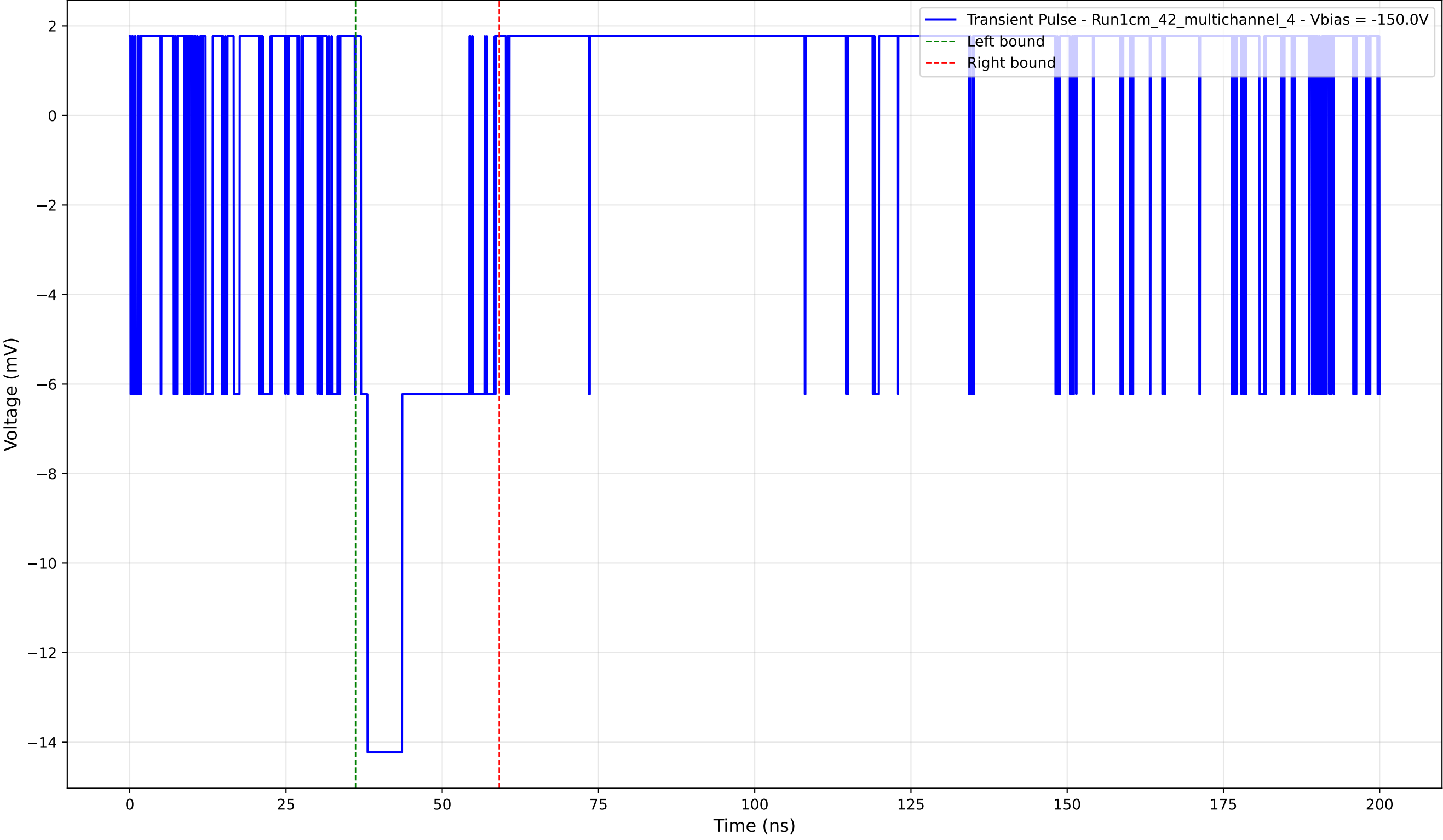
Transient Pulse - Sample: 1cm_42_multichannel - Position: 465.0 \mu\text{m} - Charge: 3.45 pC - Rise Time: 0.00 ns (N/A)
