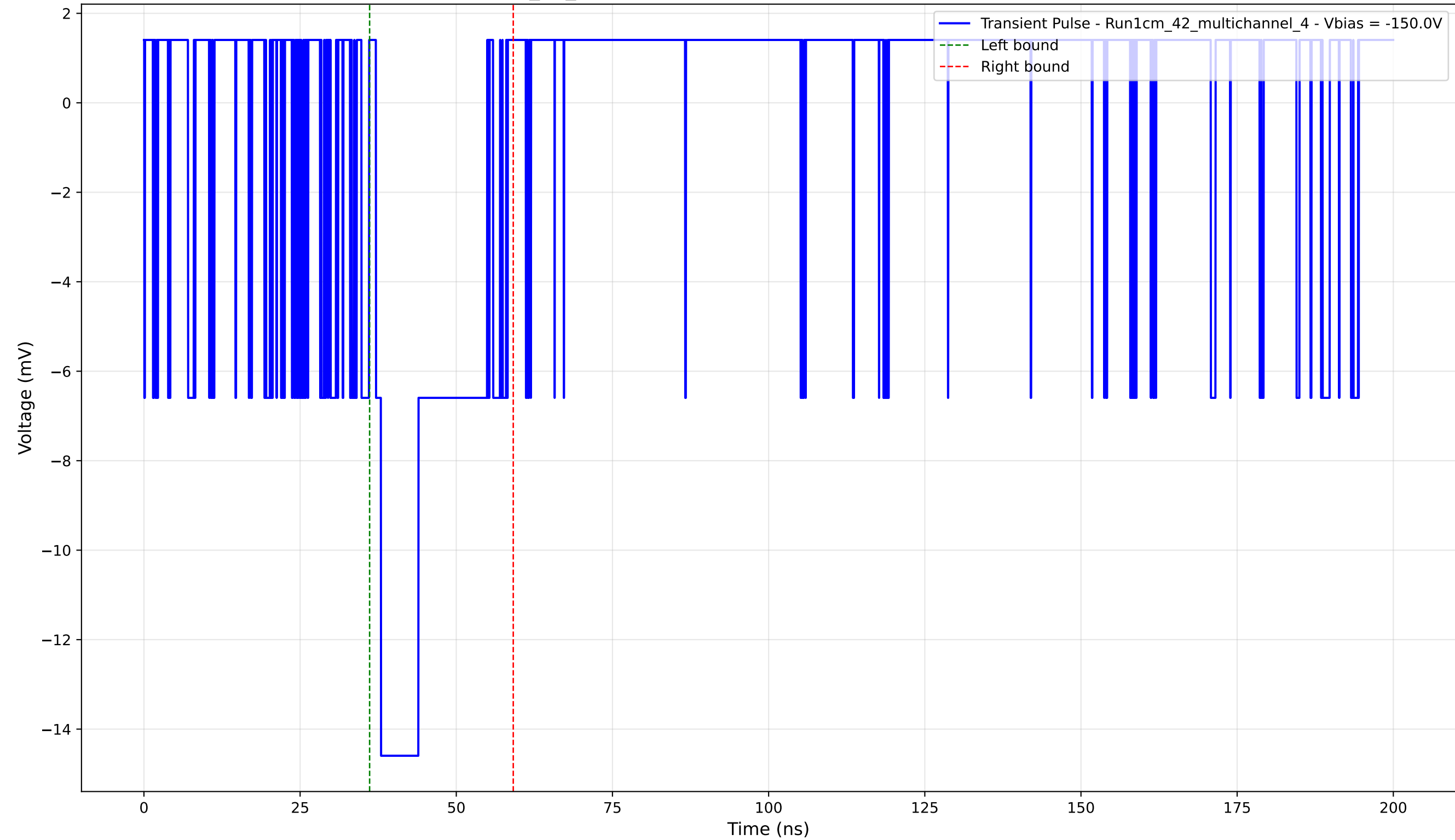
Transient Pulse - Sample: 1cm_42_multichannel - Position: 570.0 \mu\text{m} - Charge: 3.53 pC - Rise Time: 0.82 ns
