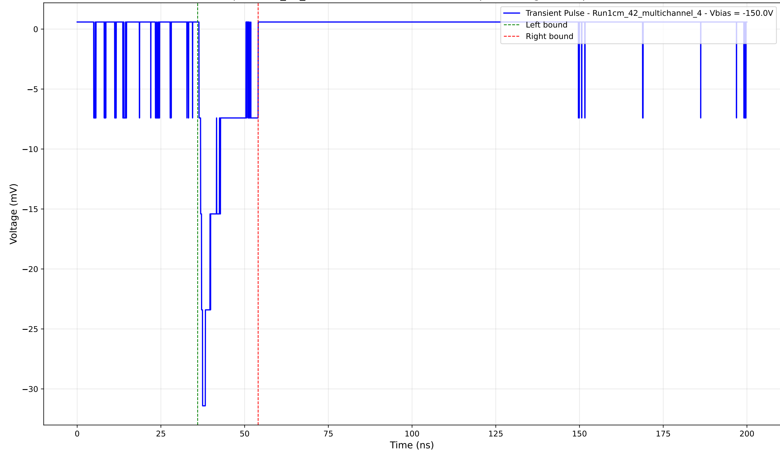
Transient Pulse - Sample: 1cm_42_multichannel - Position: 3180.0 \mu\text{m} - Charge: 3.94 pC - Rise Time: 1.07 ns
