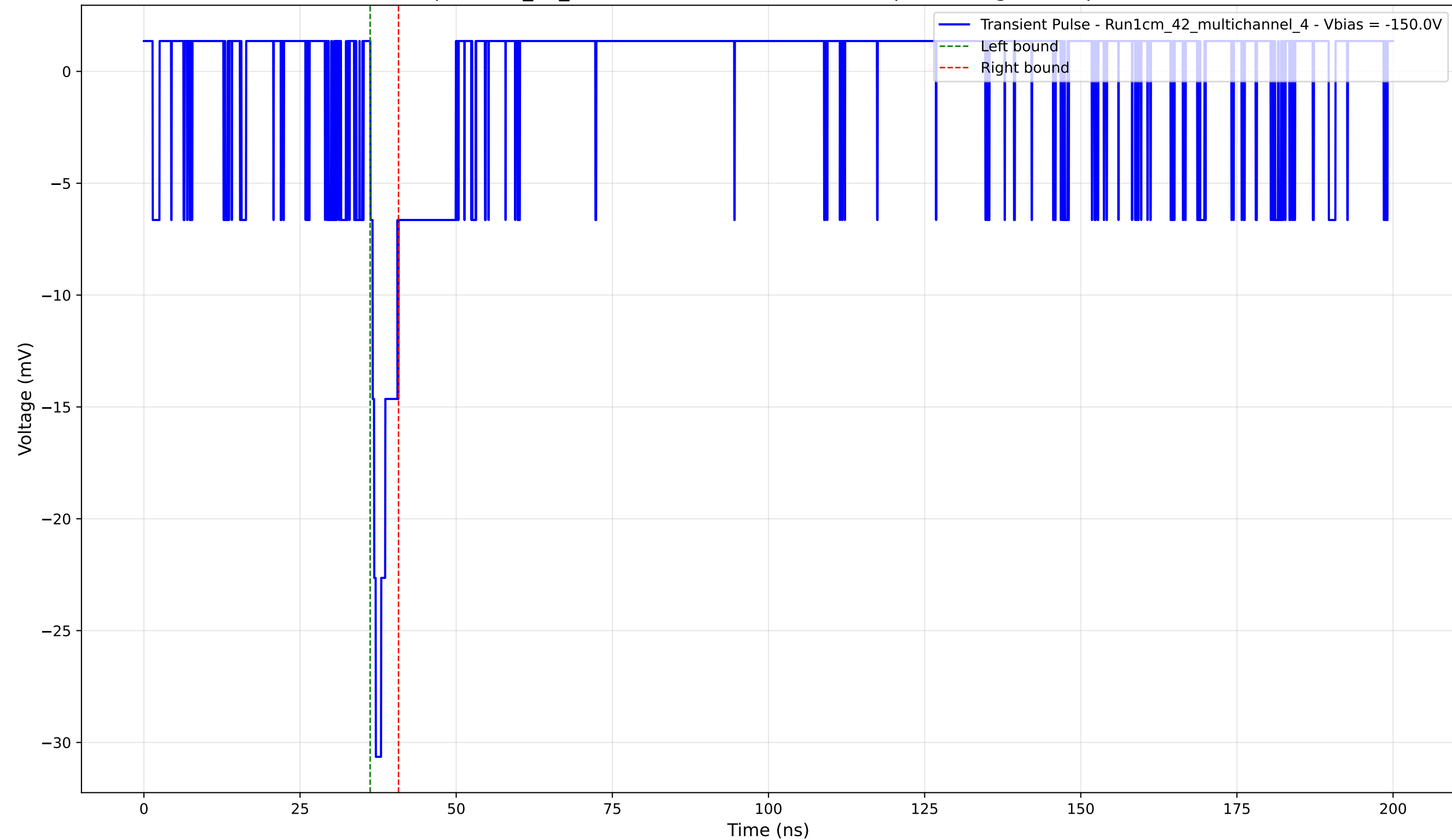
Transient Pulse - Sample: 1cm_42_multichannel - Position: 1935.0 \mu\text{m} - Charge: 1.68 pC - Rise Time: 0.87 ns
