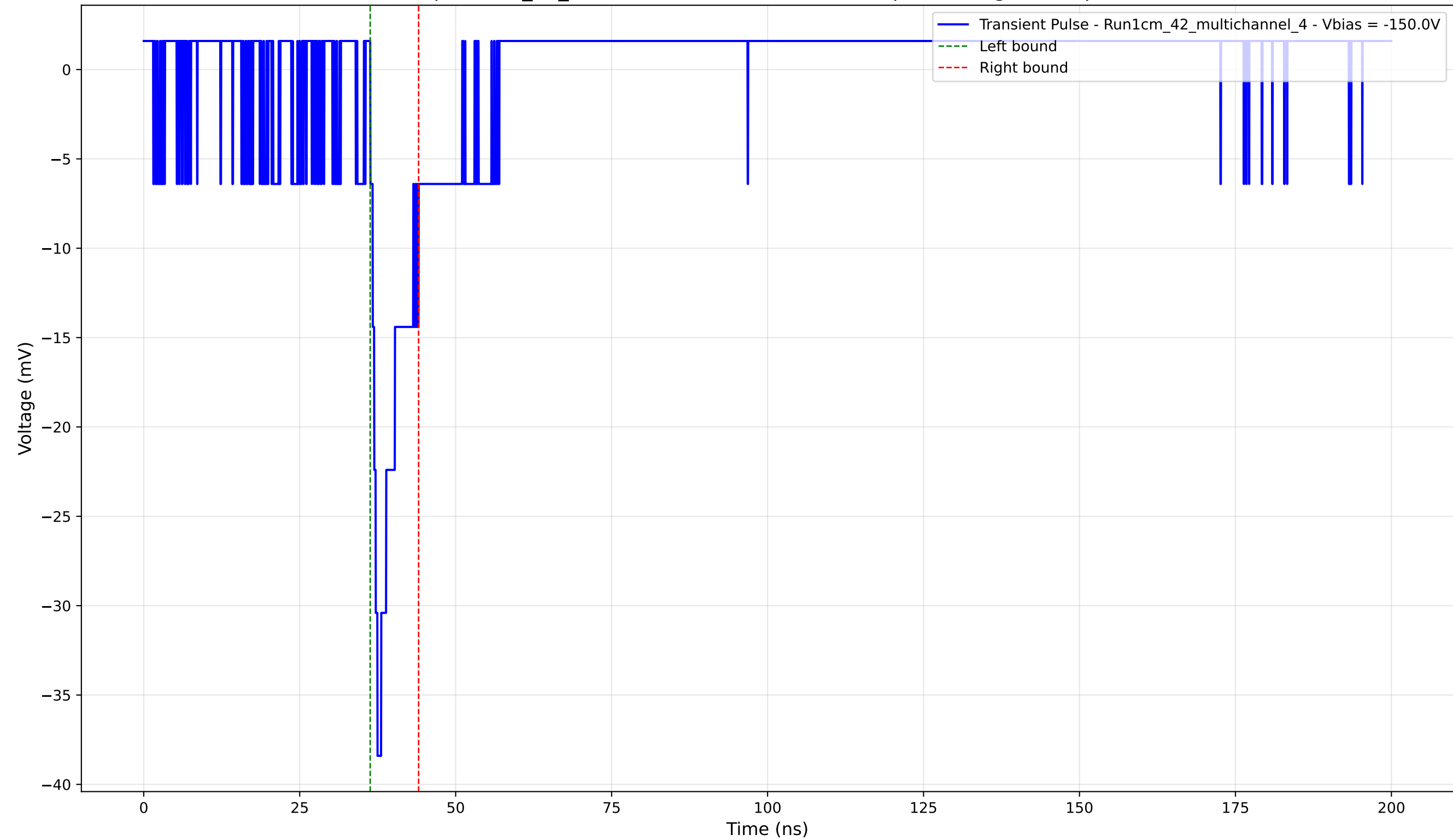
Transient Pulse - Sample: 1cm_42_multichannel - Position: 1685.0 \mu\text{m} - Charge: 3.01 pC - Rise Time: 1.15 ns
