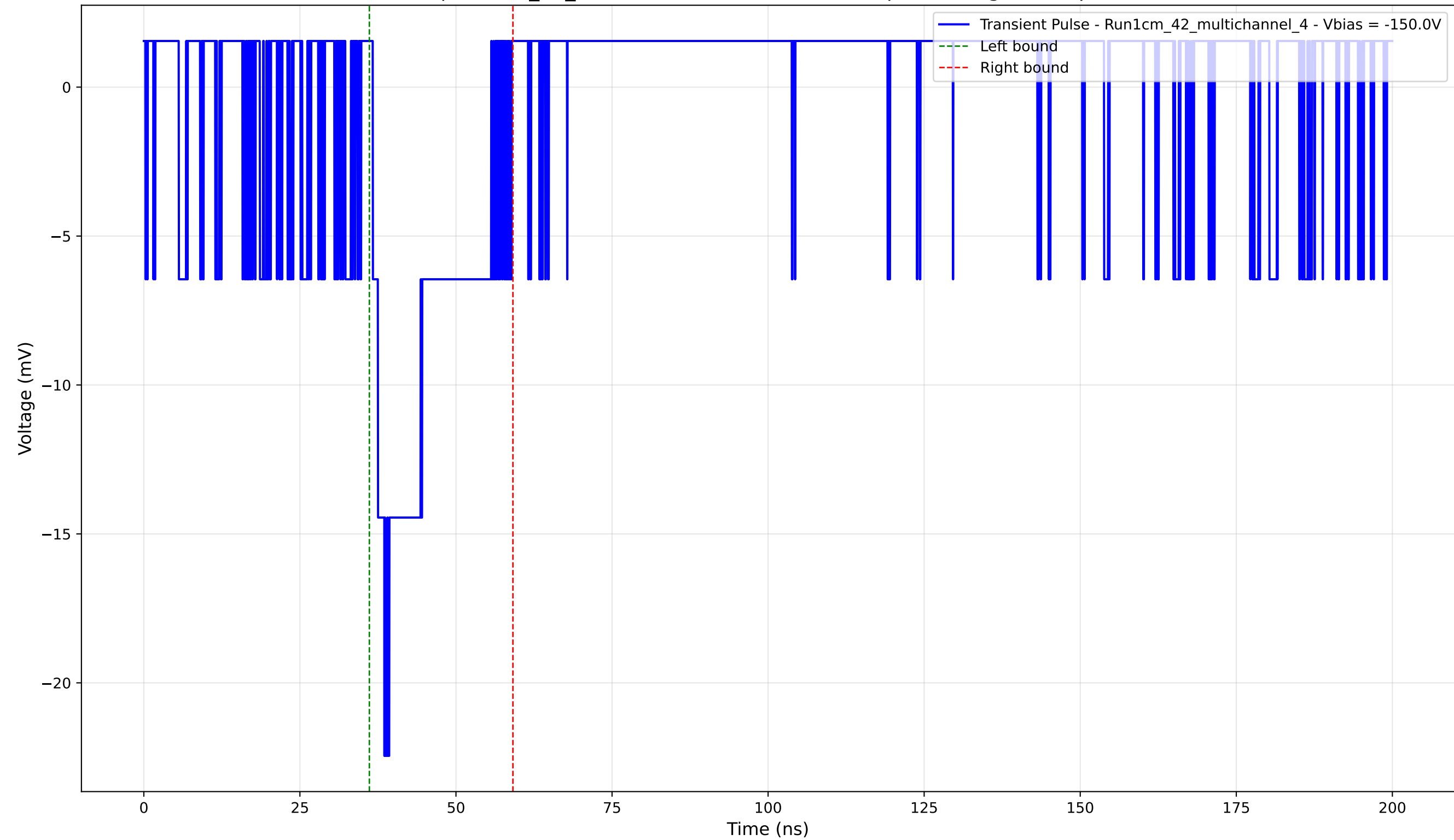
Transient Pulse - Sample: 1cm_42_multichannel - Position: 975.0 \mu\text{m} - Charge: 3.82 pC - Rise Time: 1.88 ns
