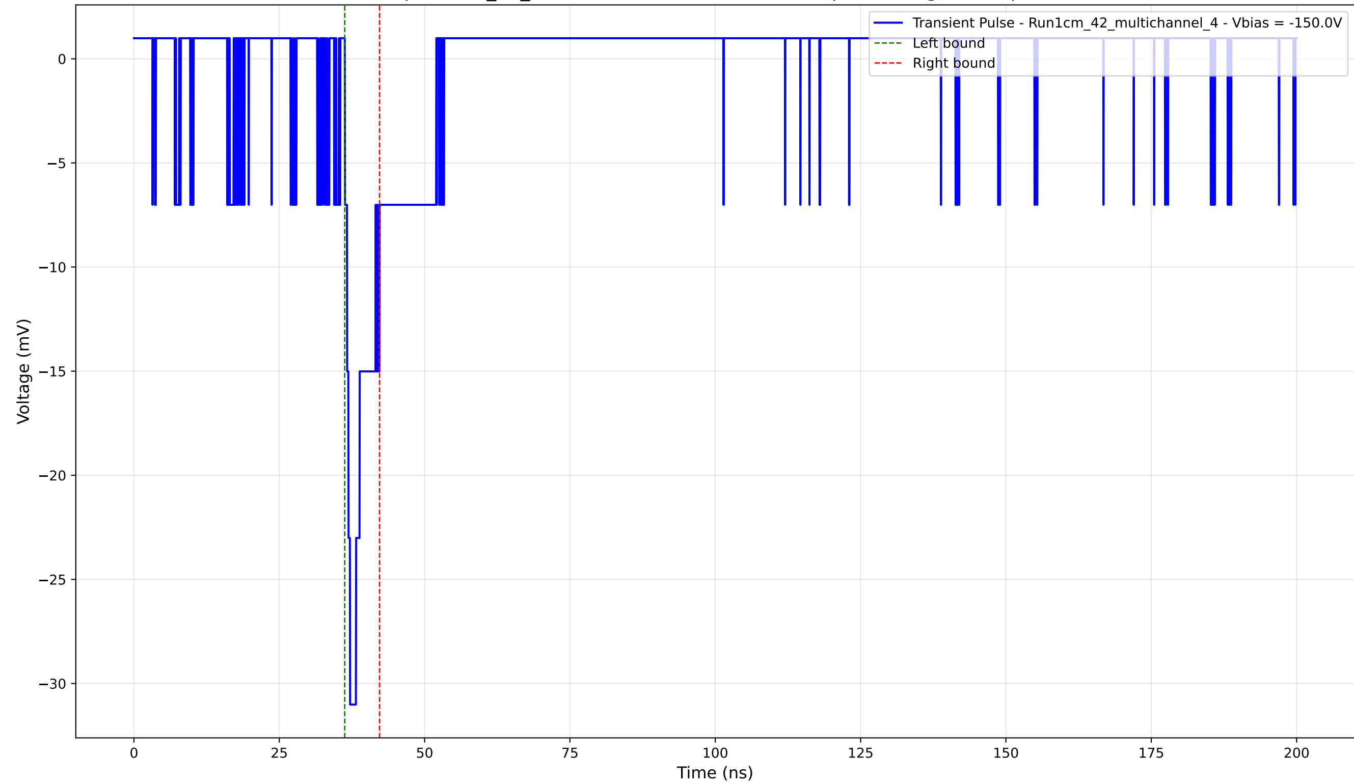
Transient Pulse - Sample: 1cm_42_multichannel - Position: 2955.0 \mu\text{m} - Charge: 2.17 pC - Rise Time: 0.89 ns
