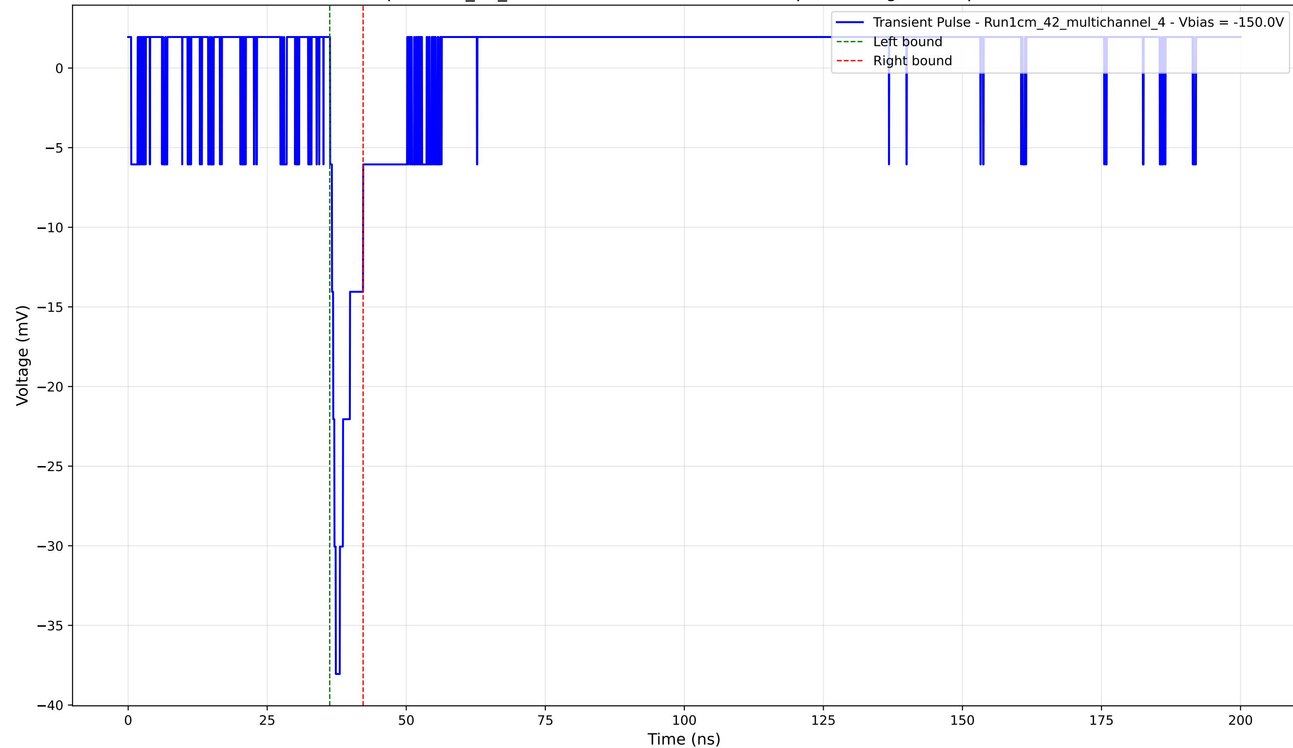
Transient Pulse - Sample: 1cm_42_multichannel - Position: 3005.0 \mu\text{m} - Charge: 2.46 pC - Rise Time: 1.03 ns
