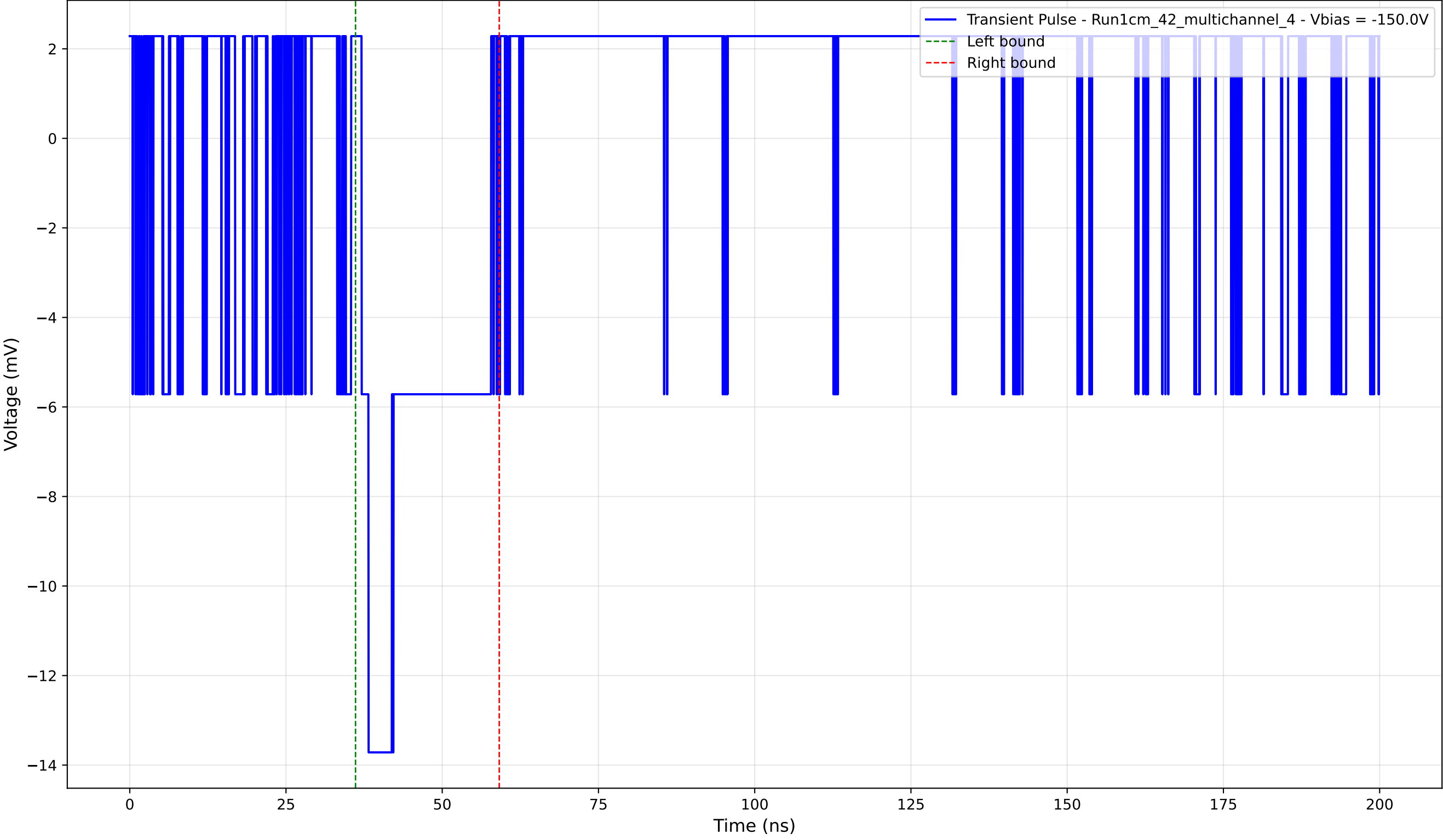
Transient Pulse - Sample: 1cm_42_multichannel - Position: 225.0 \mu\text{m} - Charge: 2.90 pC - Rise Time: 0.00 ns (N/A)
