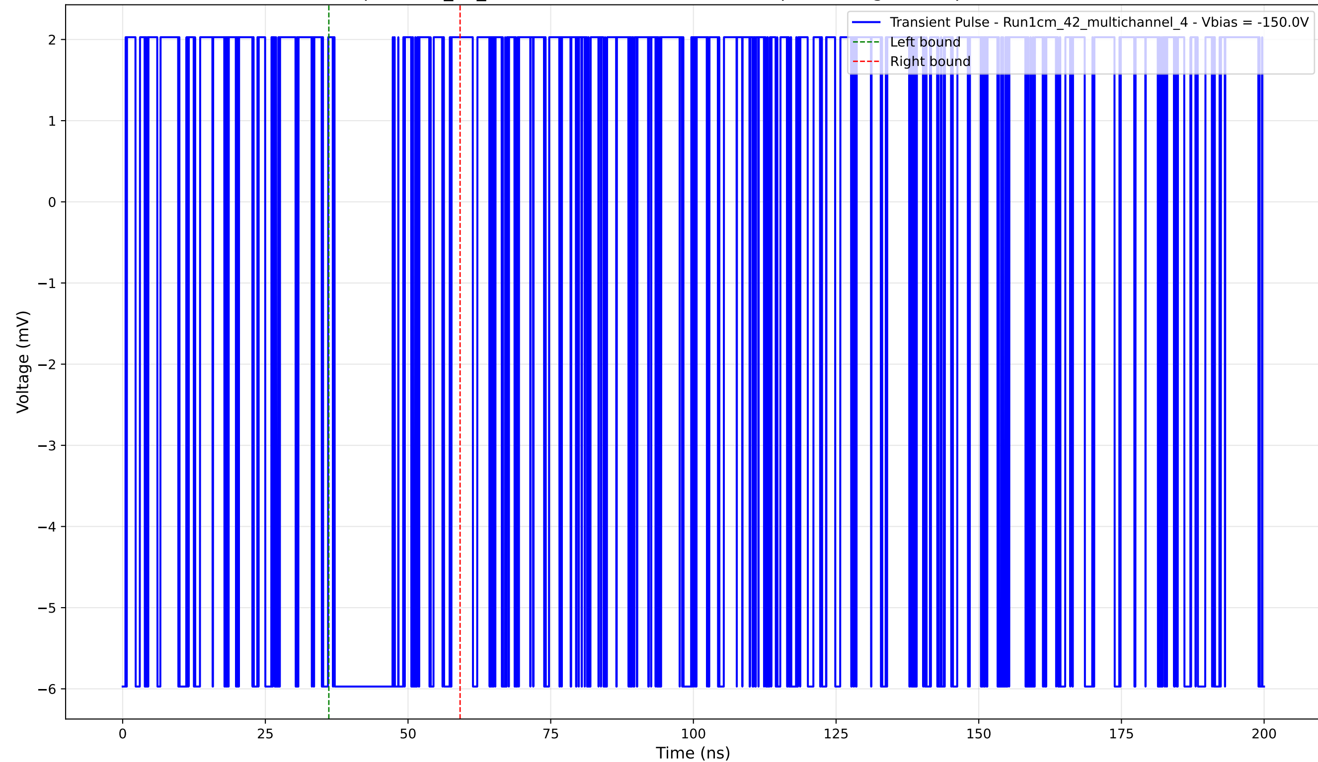
Transient Pulse - Sample: 1cm_42_multichannel - Position: 1340.0 \mu\text{m} - Charge: 1.45 pC - Rise Time: 0.00 ns (N/A)
