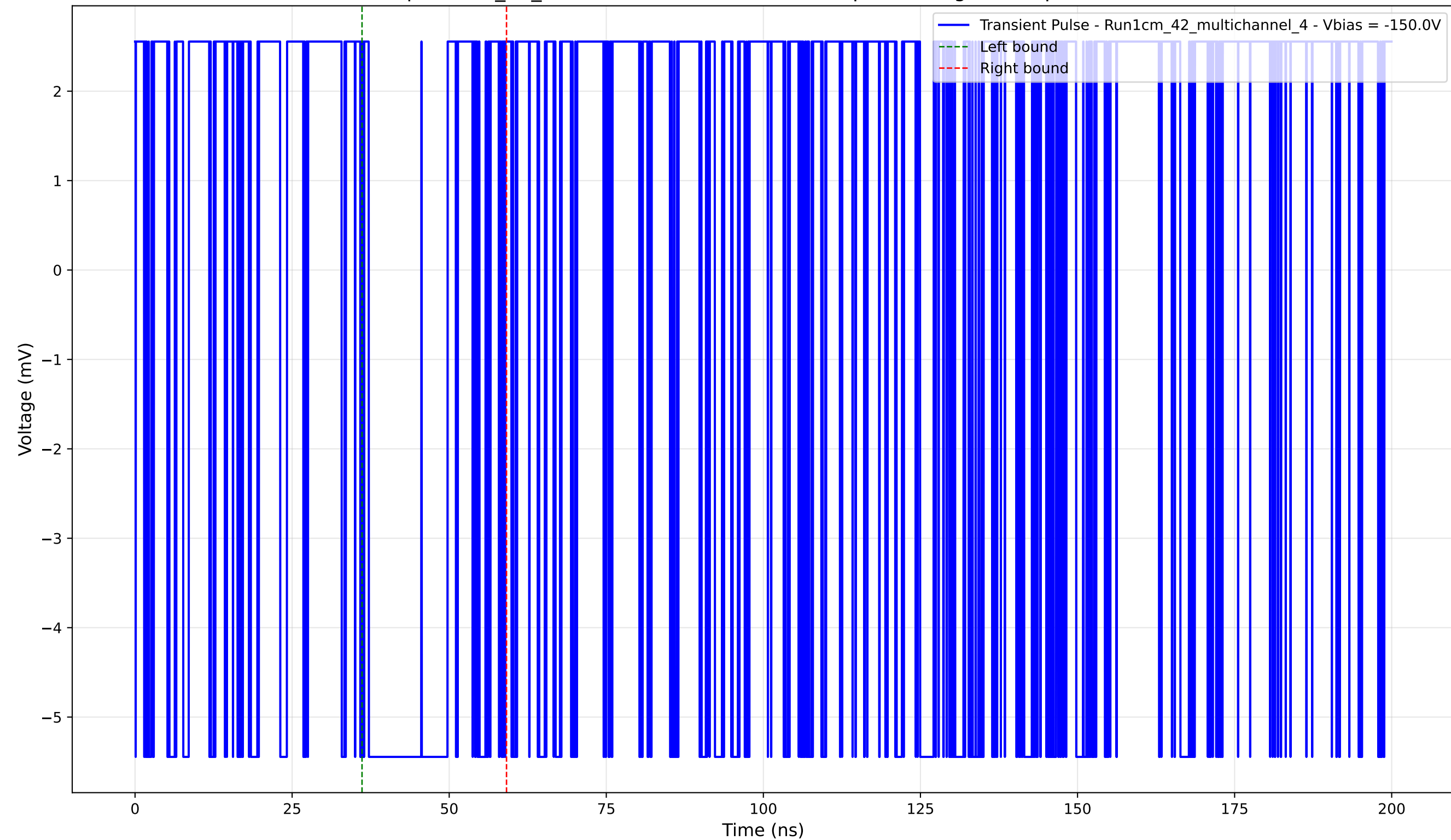
Transient Pulse - Sample: 1cm_42_multichannel - Position: 900.0 \mu\text{m} - Charge: 1.23 pC - Rise Time: 0.00 ns (N/A)
