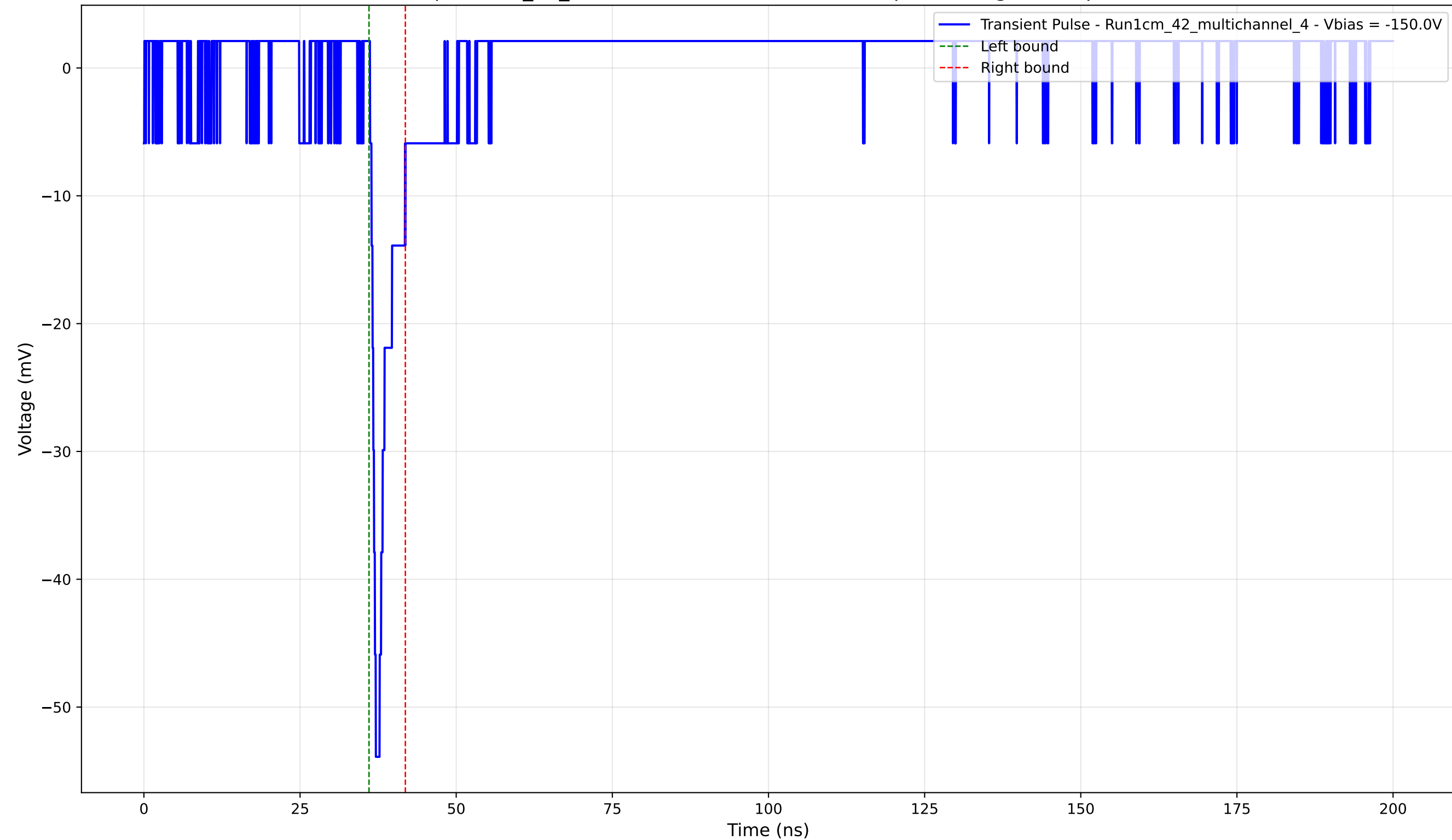
Transient Pulse - Sample: 1cm_42_multichannel - Position: 2710.0 \mu\text{m} - Charge: 2.79 pC - Rise Time: 0.92 ns
