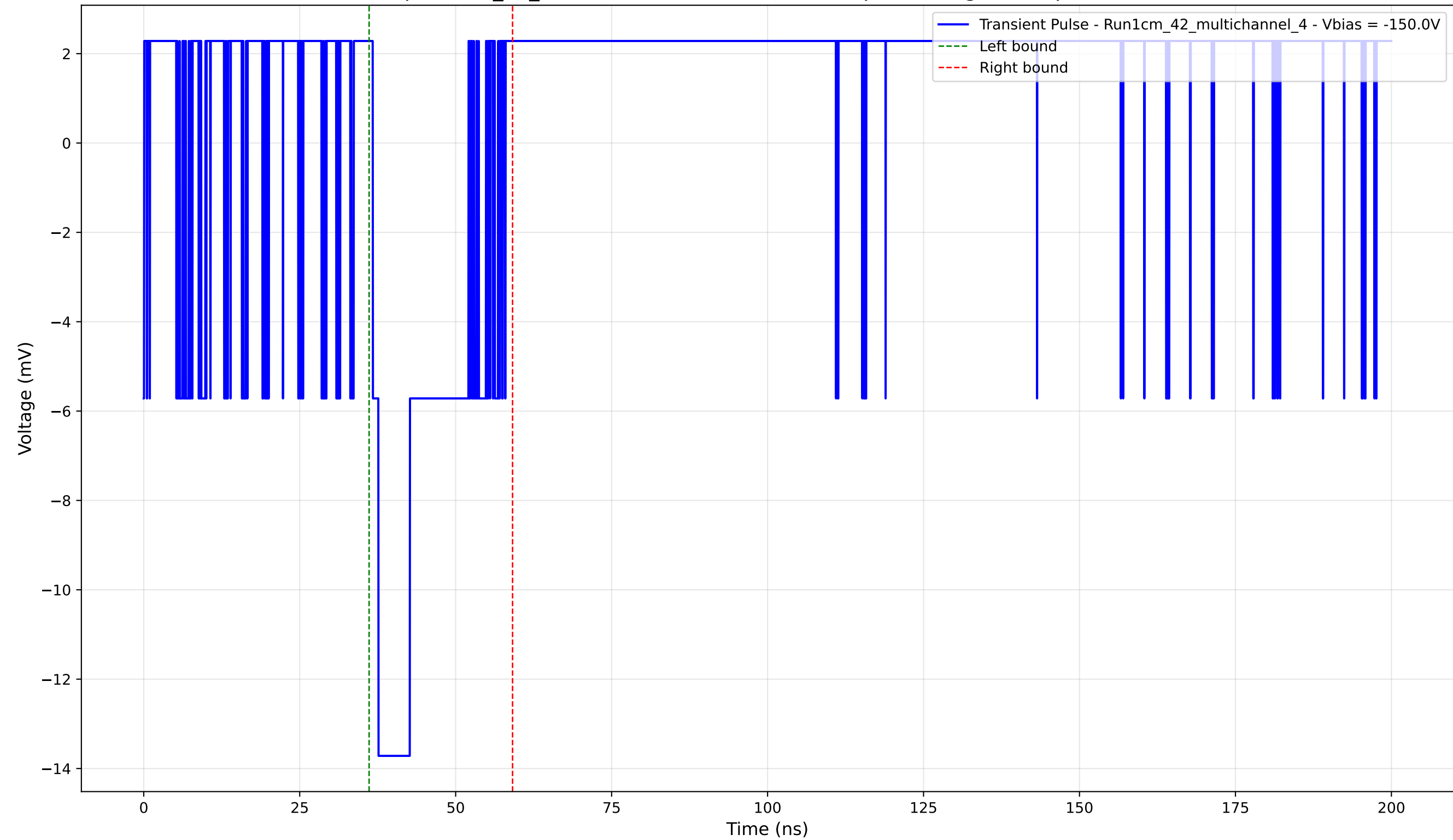
Transient Pulse - Sample: 1cm_42_multichannel - Position: 3720.0 \mu\text{m} - Charge: 2.77 pC - Rise Time: 0.00 ns (N/A)
