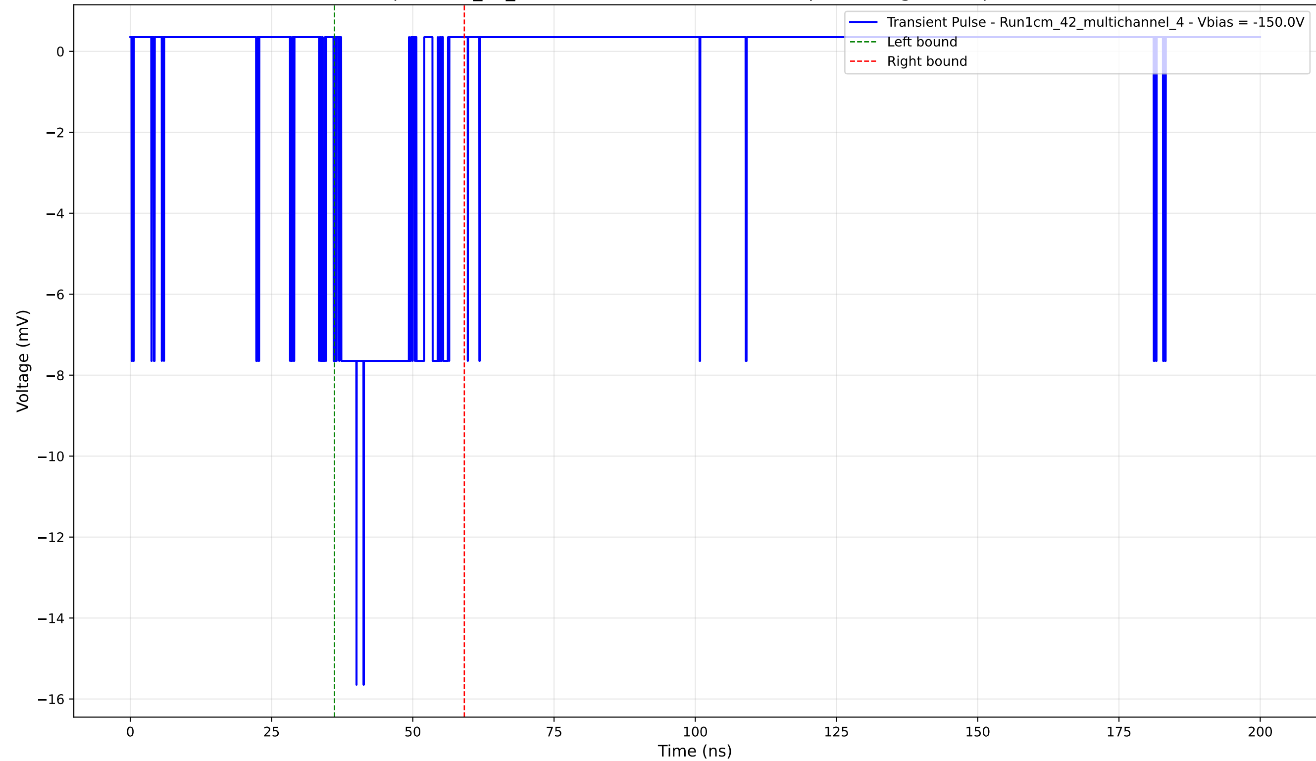
Transient Pulse - Sample: 1cm_42_multichannel - Position: 4830.0 \mu\text{m} - Charge: 2.47 pC - Rise Time: 2.70 ns
