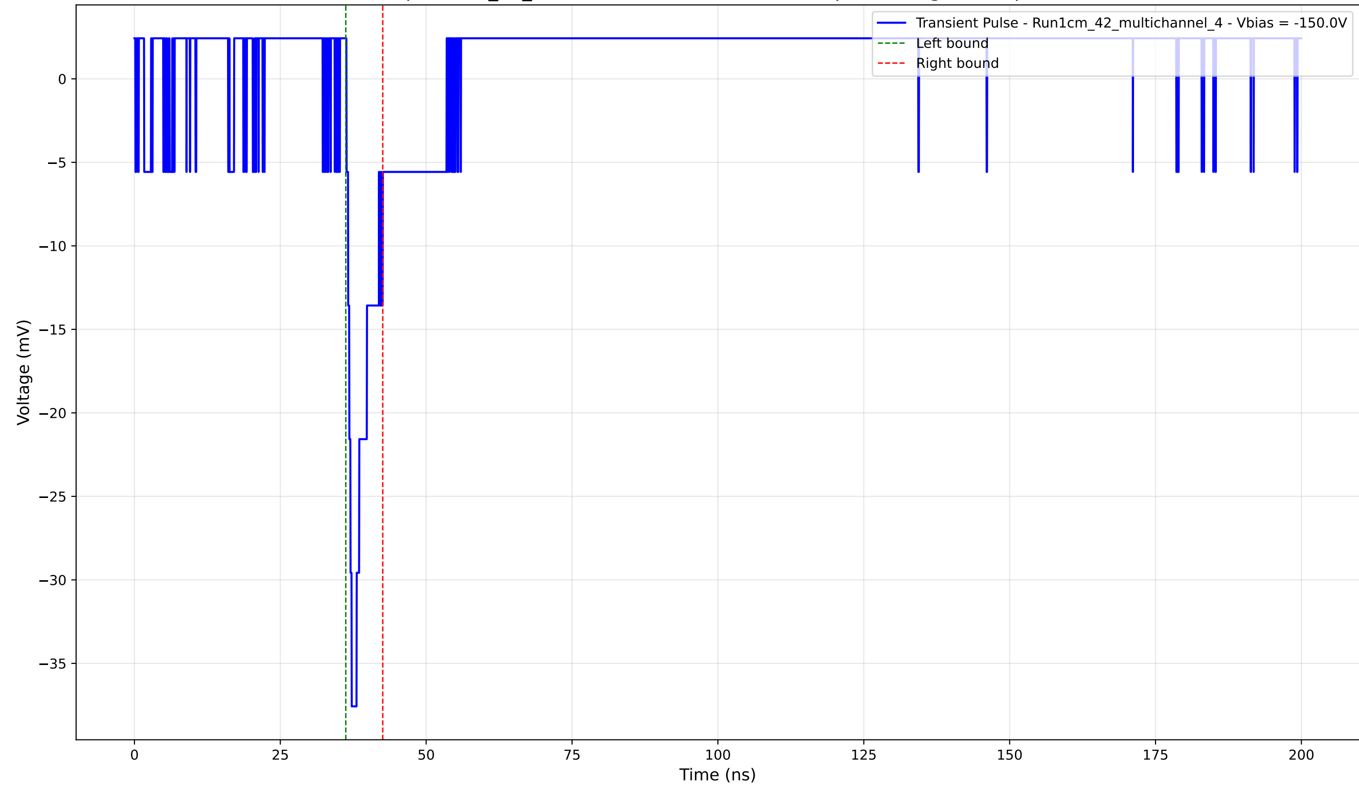
Transient Pulse - Sample: 1cm_42_multichannel - Position: 1805.0 \mu\text{m} - Charge: 2.47 pC - Rise Time: 0.89 ns
