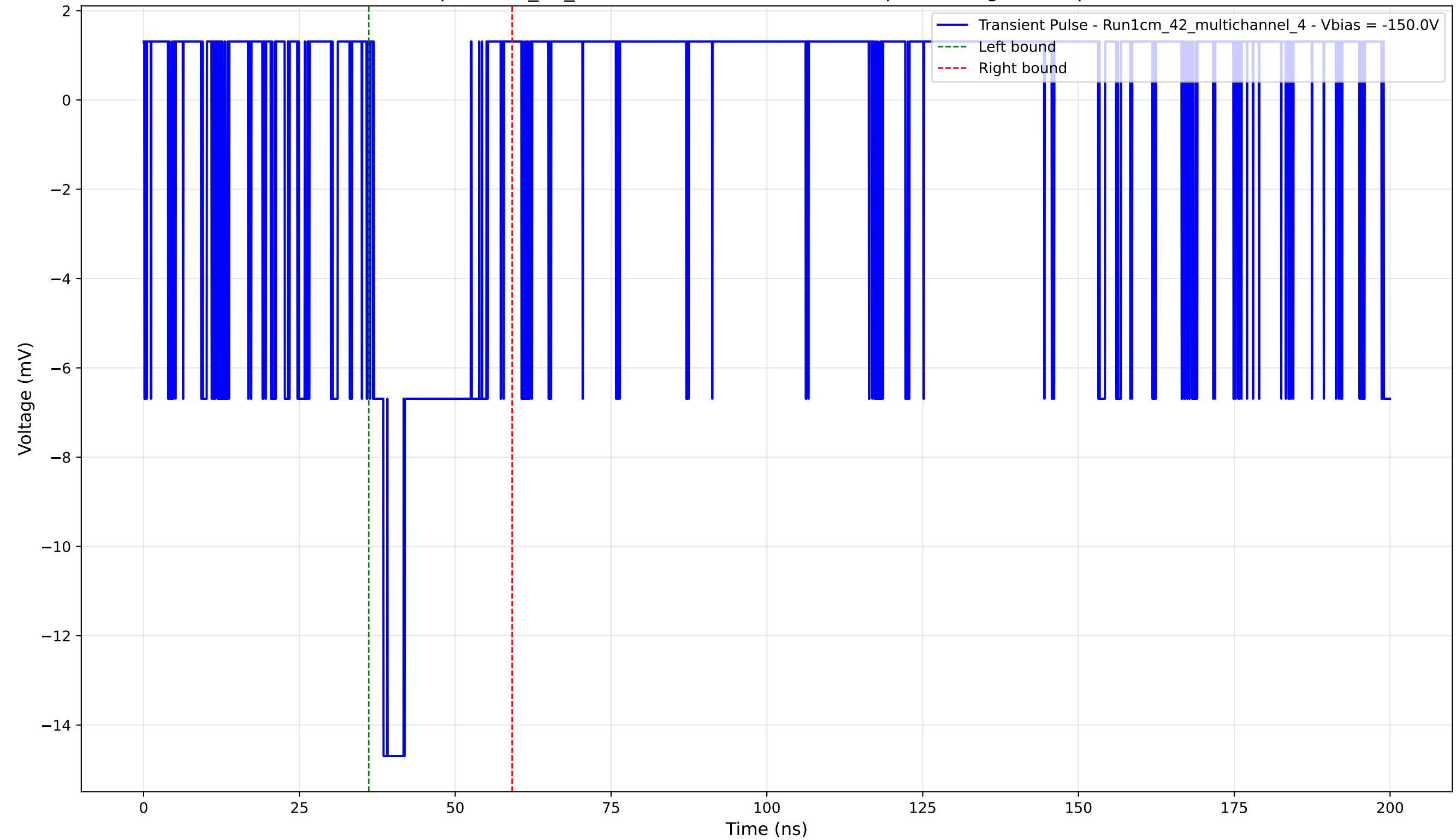
Transient Pulse - Sample: 1cm_42_multichannel - Position: 295.0 \mu\text{m} - Charge: 2.86 pC - Rise Time: 1.54 ns
