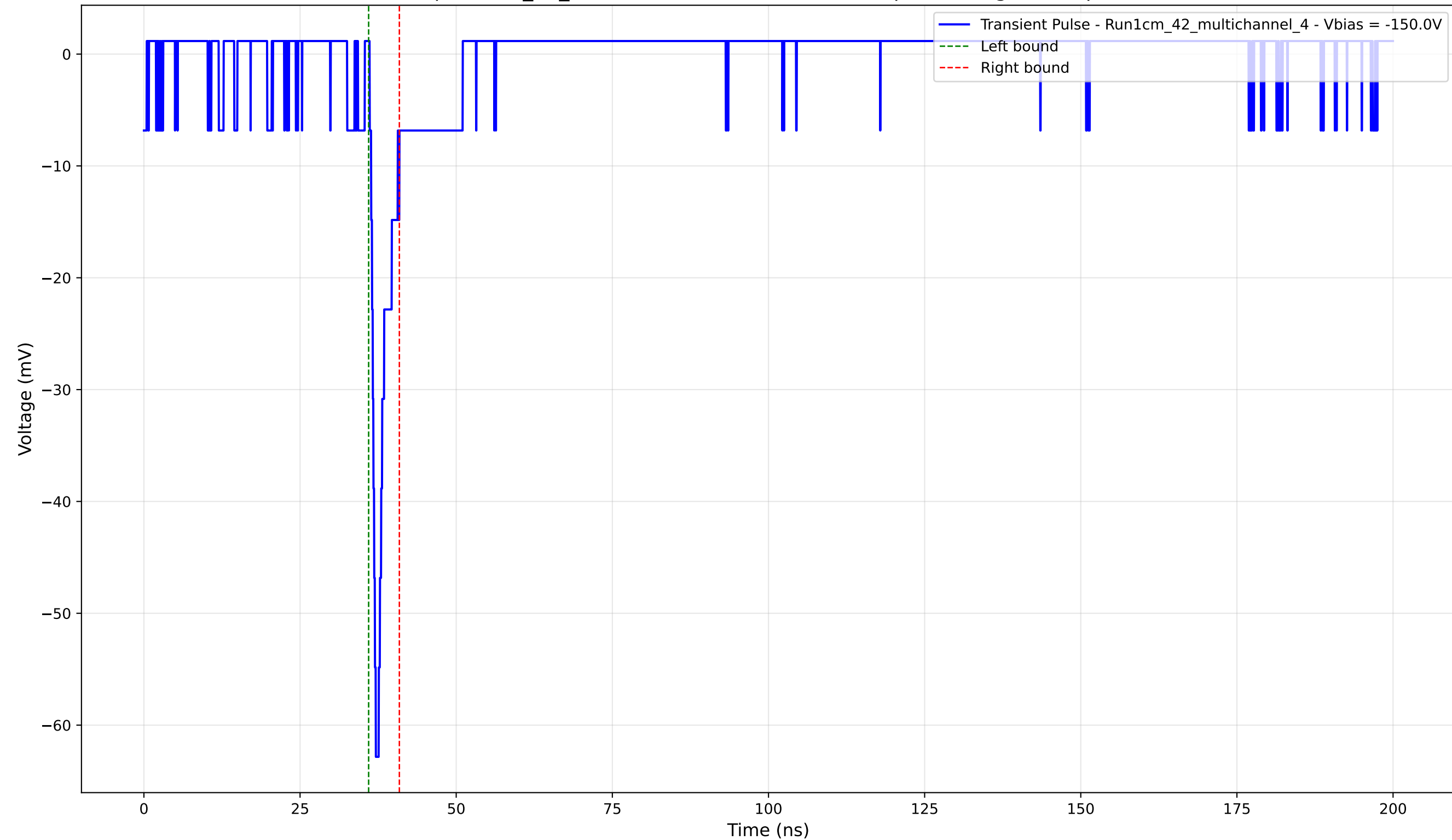
Transient Pulse - Sample: 1cm_42_multichannel - Position: 2615.0 \mu\text{m} - Charge: 2.75 pC - Rise Time: 0.98 ns
