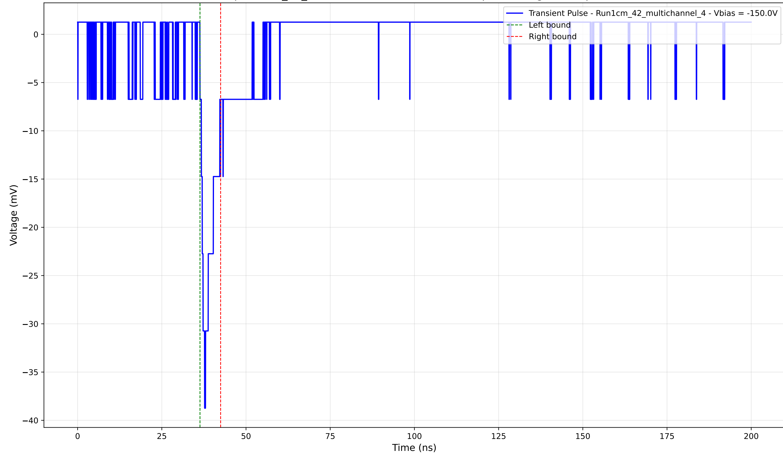
Transient Pulse - Sample: 1cm_42_multichannel - Position: 1645.0 \mu\text{m} - Charge: 2.54 pC - Rise Time: 1.39 ns
