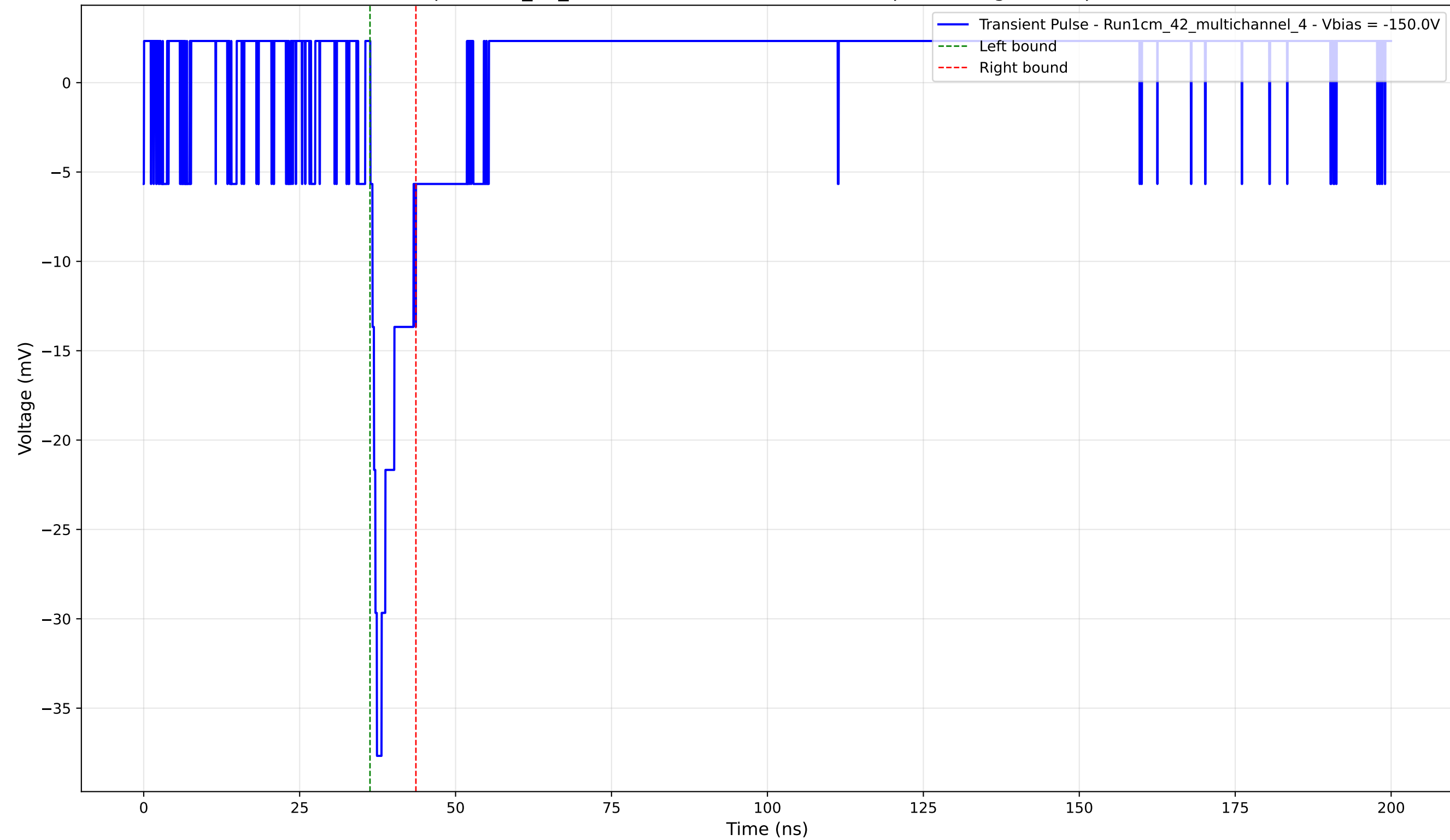
Transient Pulse - Sample: 1cm_42_multichannel - Position: 1715.0 \mu\text{m} - Charge: 2.78 pC - Rise Time: 1.05 ns
