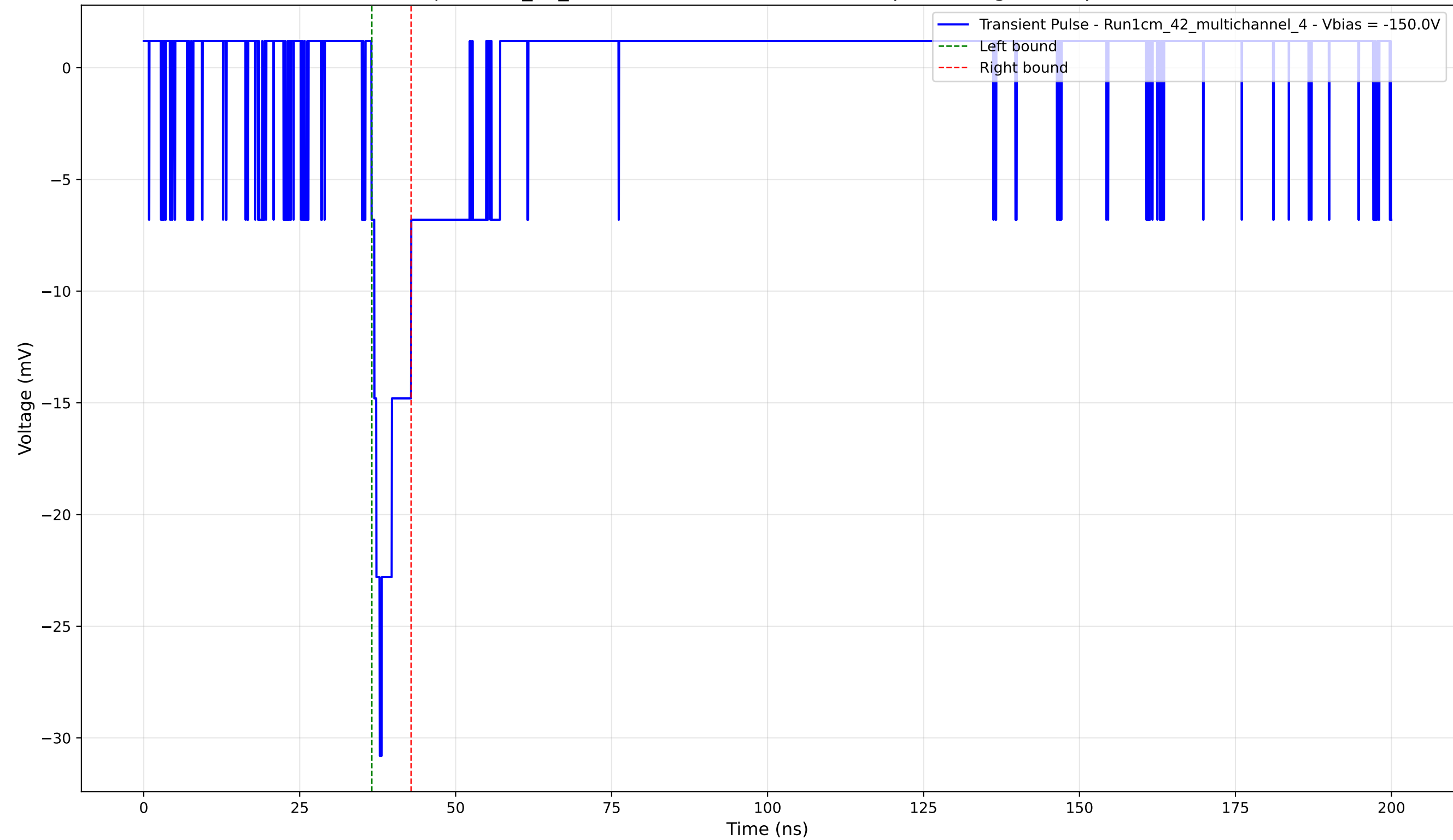
Transient Pulse - Sample: 1cm_42_multichannel - Position: 3285.0 \mu\text{m} - Charge: 2.25 pC - Rise Time: 1.33 ns
