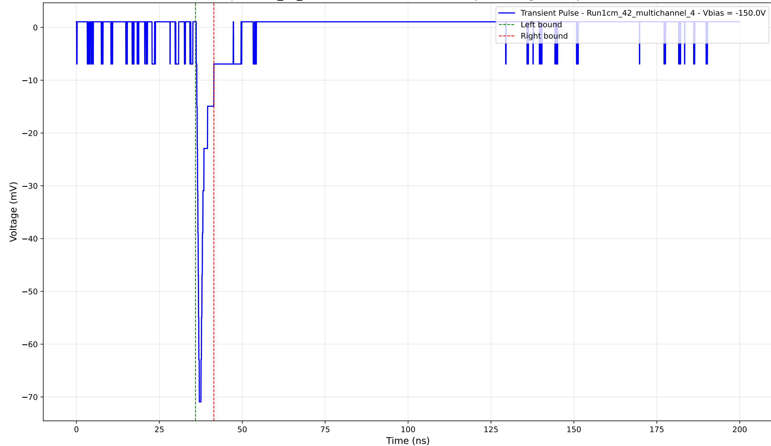
Transient Pulse - Sample: 1cm_42_multichannel - Position: 2530.0 \mu\text{m} - Charge: 3.19 pC - Rise Time: 0.76 ns
