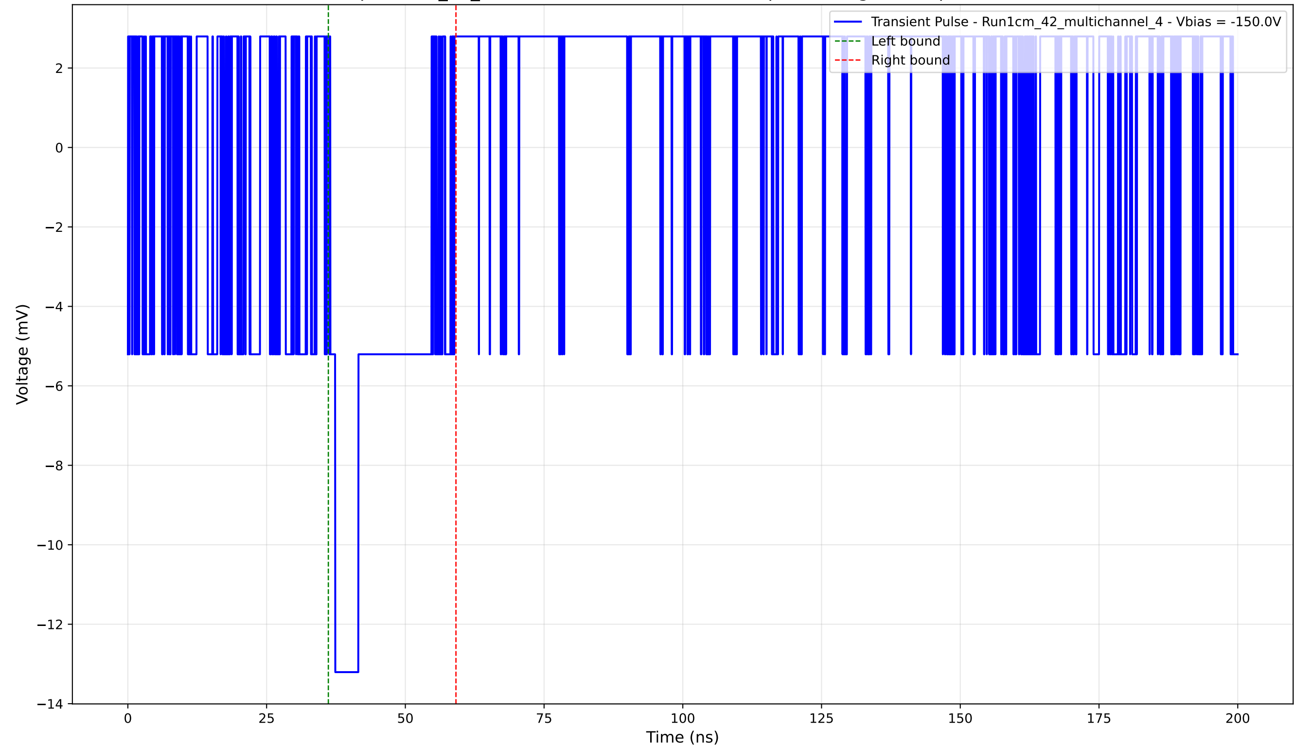
Transient Pulse - Sample: 1cm_42_multichannel - Position: 1320.0 \mu\text{m} - Charge: 2.72 pC - Rise Time: 0.00 ns (N/A)
