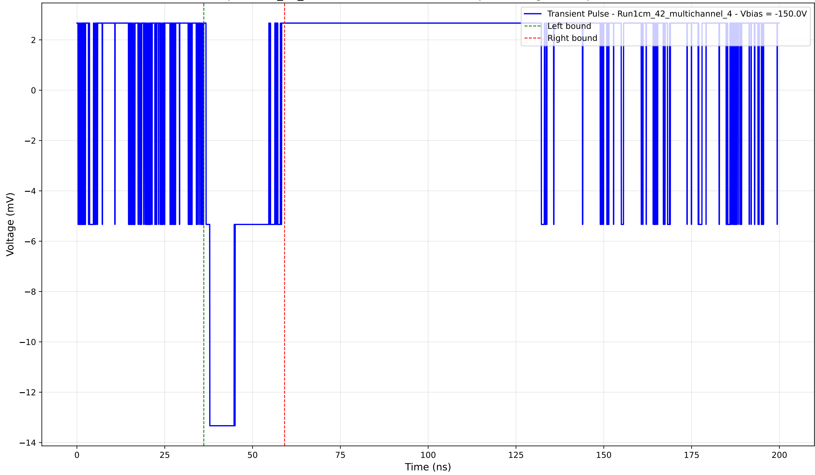
Transient Pulse - Sample: 1cm_42_multichannel - Position: 690.0 \mu\text{m} - Charge: 3.20 pC - Rise Time: 0.00 ns (N/A)
