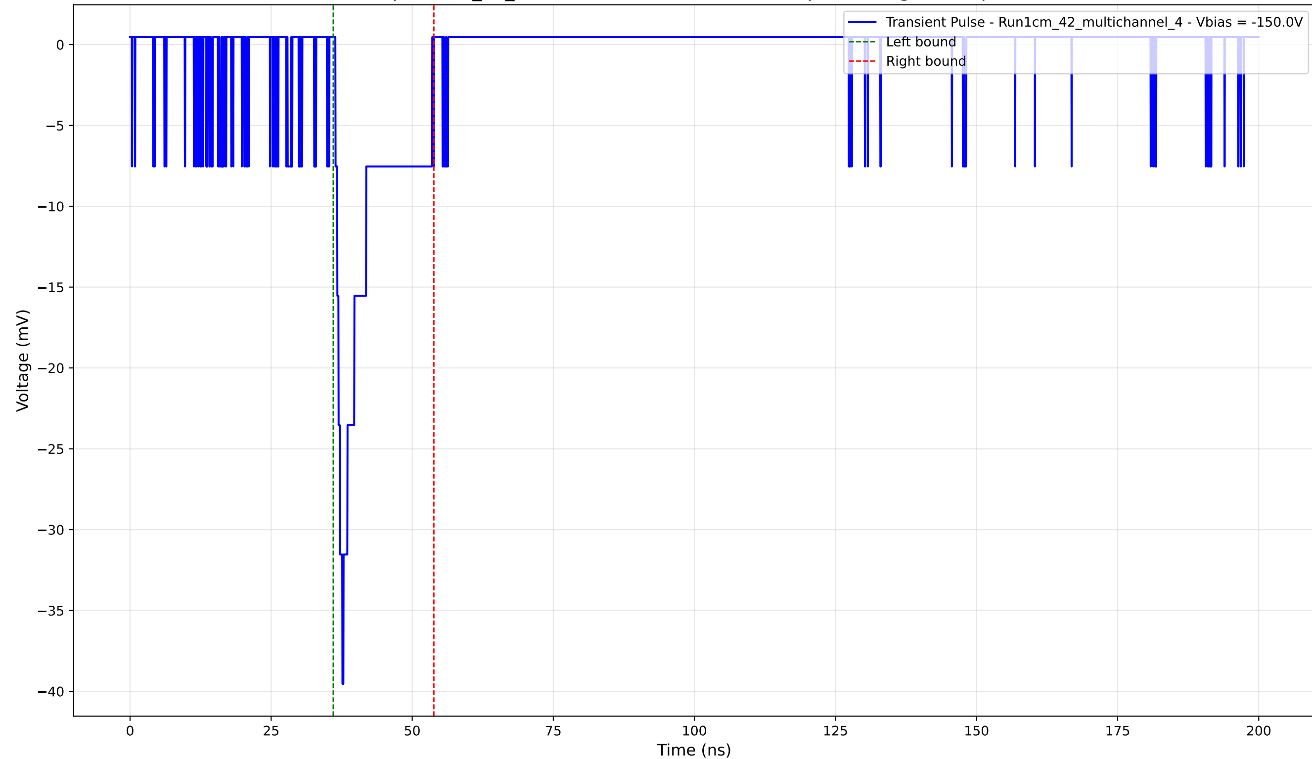
Transient Pulse - Sample: 1cm_42_multichannel - Position: 3035.0 \mu\text{m} - Charge: 4.11 pC - Rise Time: 1.23 ns
