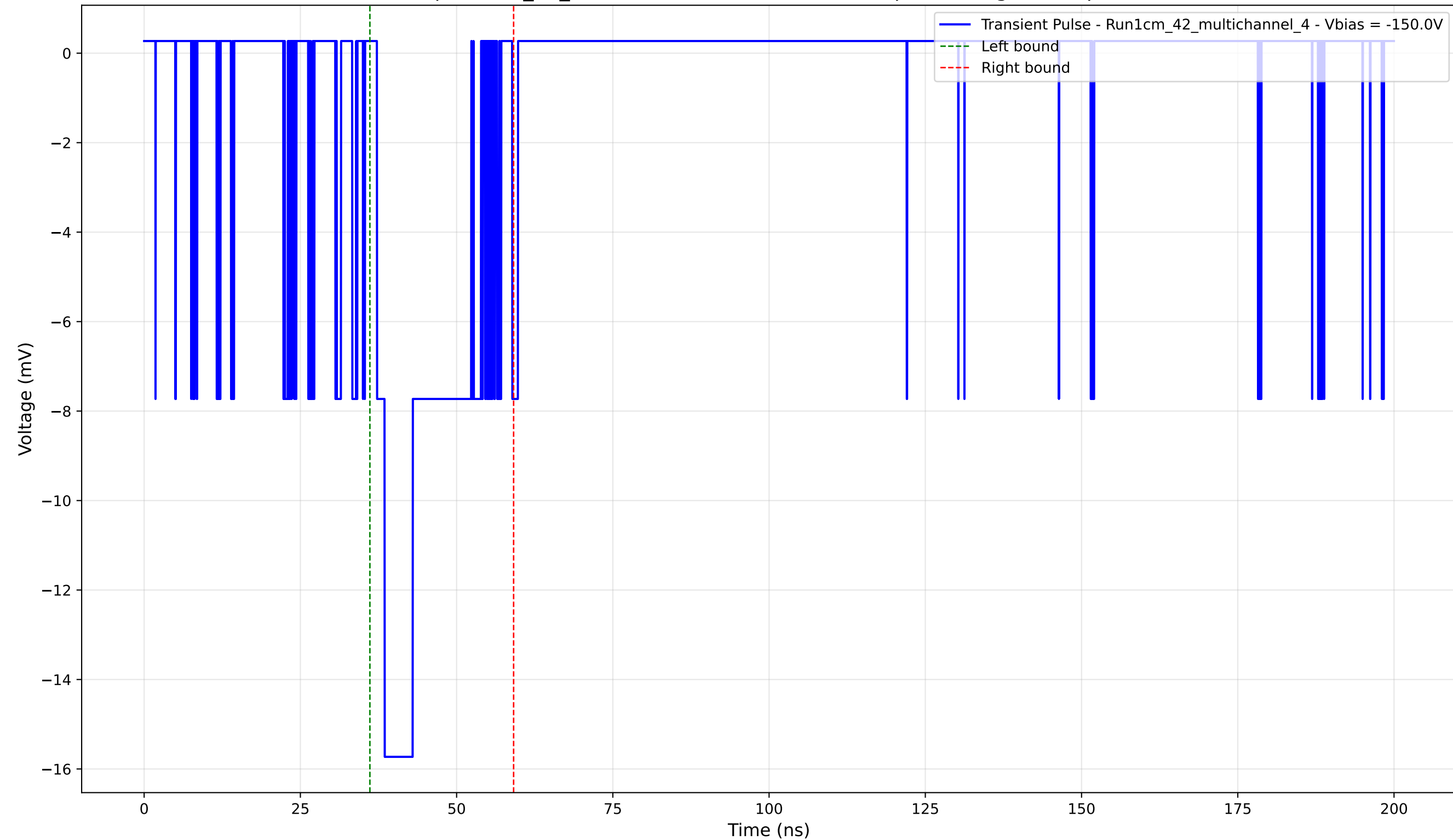
Transient Pulse - Sample: 1cm_42_multichannel - Position: 4280.0 \mu\text{m} - Charge: 3.49 pC - Rise Time: 1.24 ns
