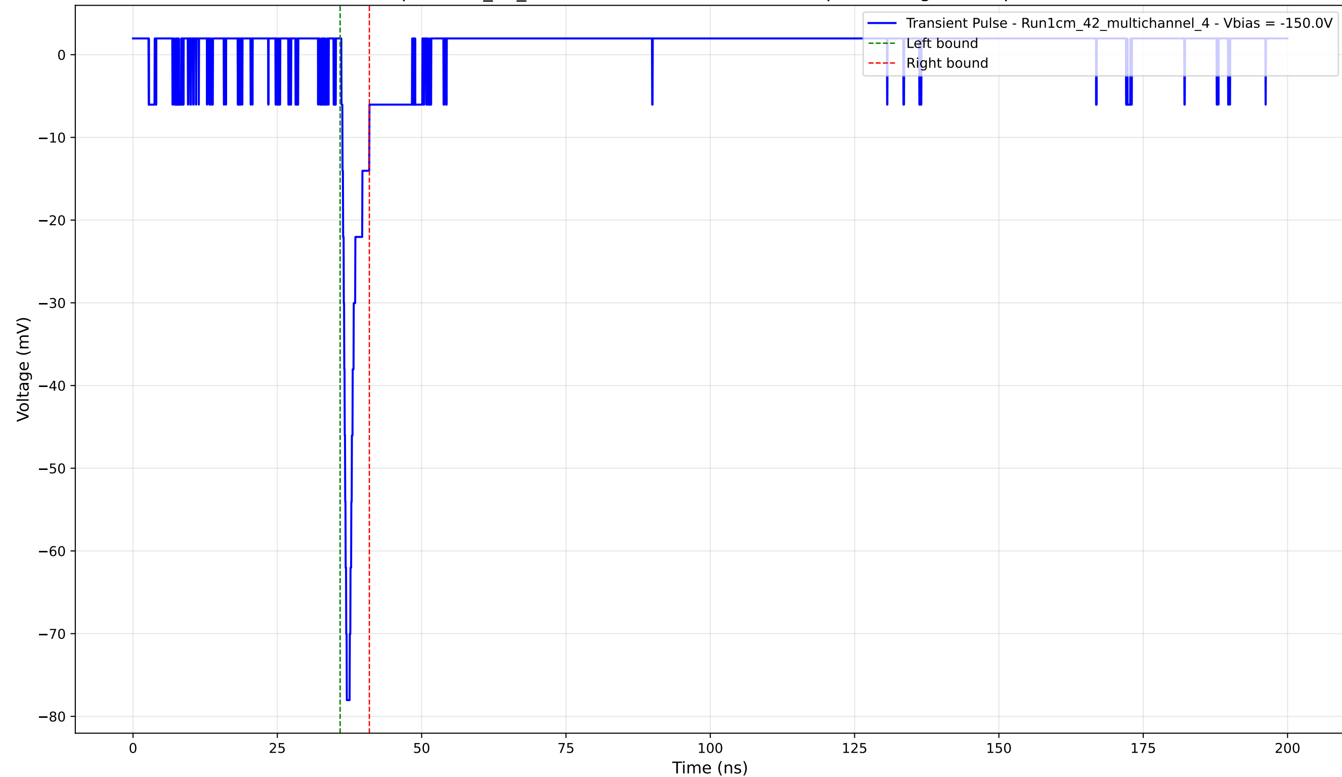
Transient Pulse - Sample: 1cm_42_multichannel - Position: 2265.0 \mu\text{m} - Charge: 3.20 pC - Rise Time: 0.76 ns
