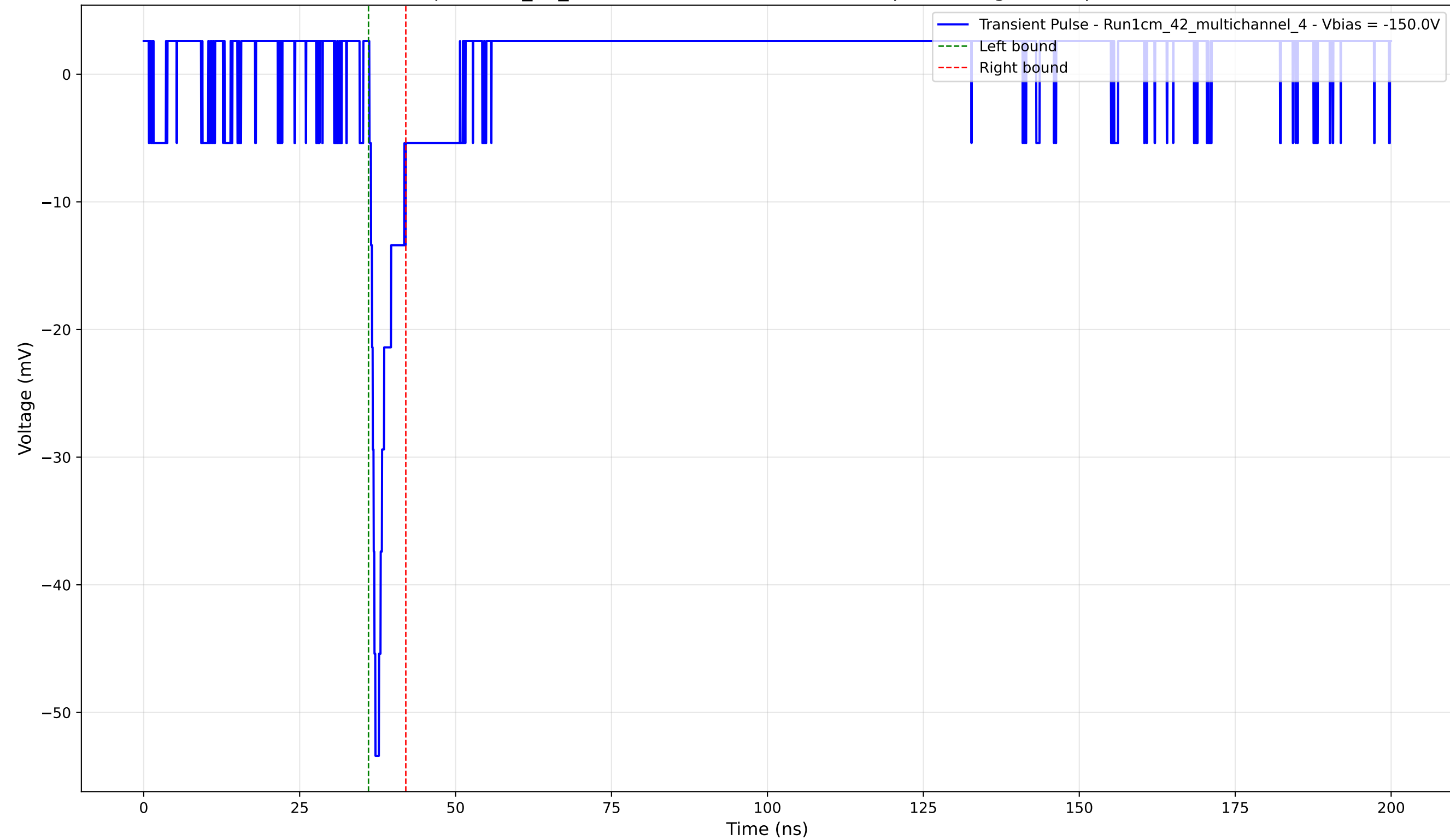
Transient Pulse - Sample: 1cm_42_multichannel - Position: 2715.0 \mu\text{m} - Charge: 2.75 pC - Rise Time: 0.96 ns
