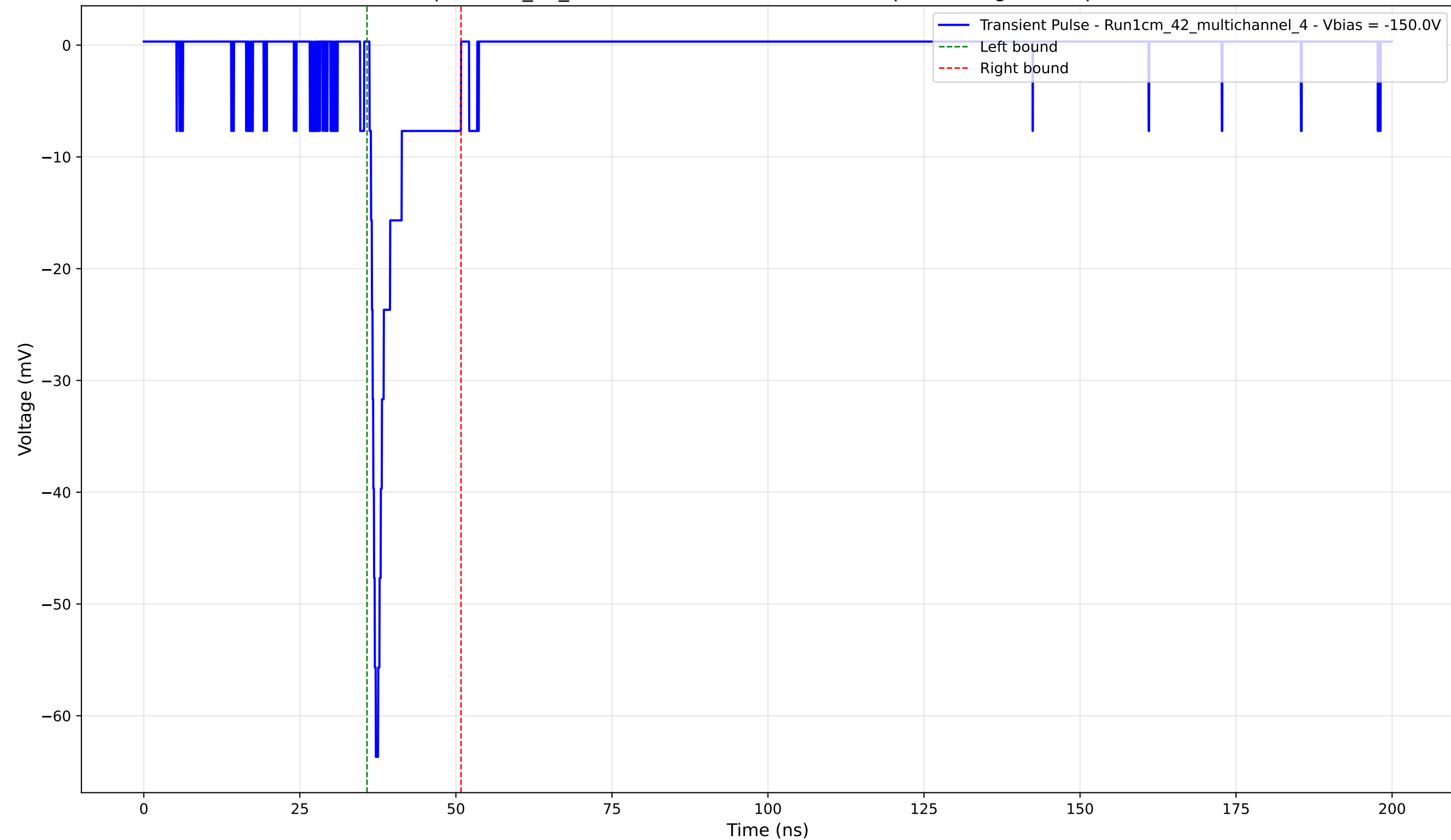
Transient Pulse - Sample: 1cm_42_multichannel - Position: 2630.0 \mu\text{m} - Charge: 4.36 pC - Rise Time: 1.00 ns
