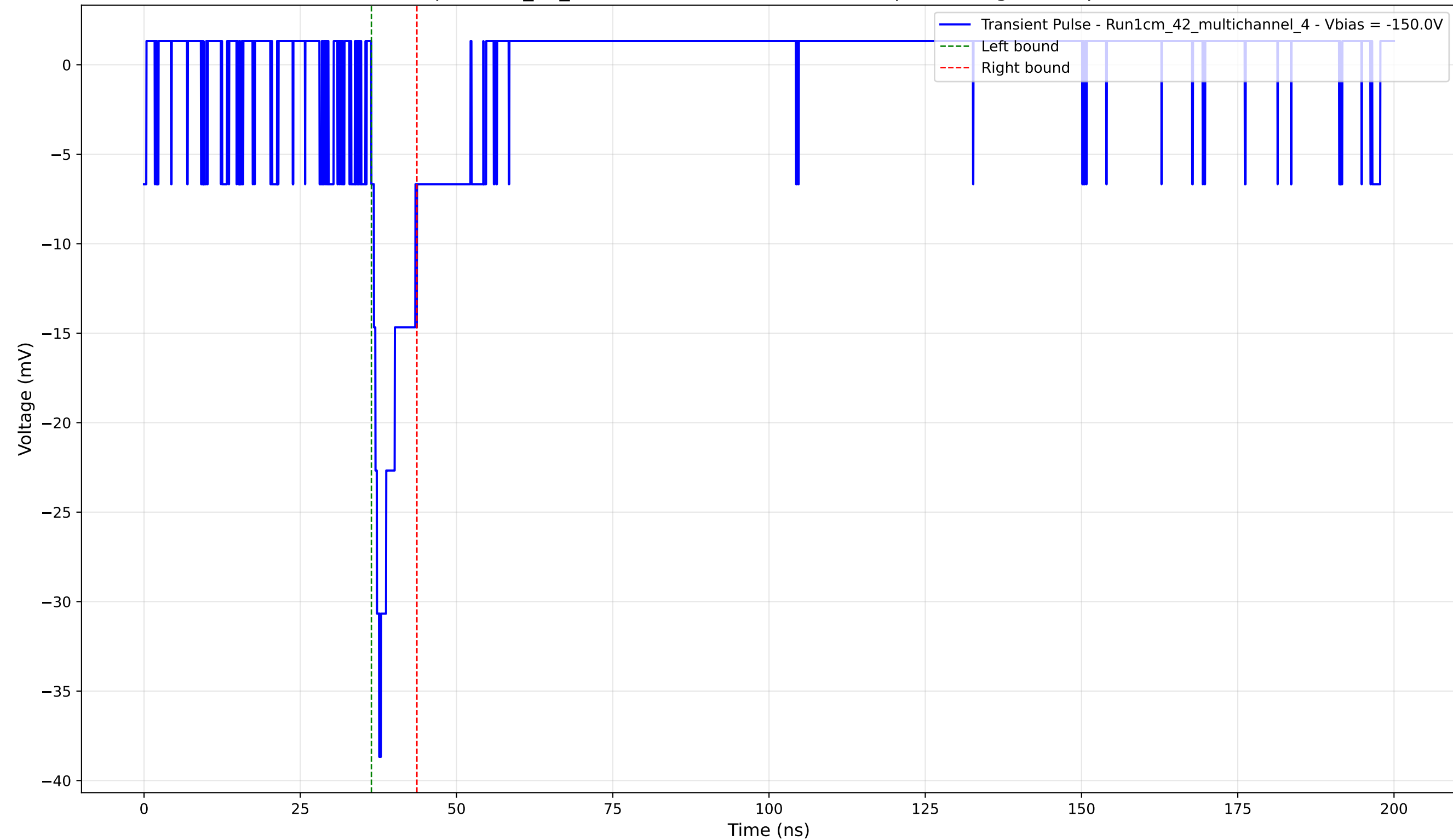
Transient Pulse - Sample: 1cm_42_multichannel - Position: 1655.0 \mu\text{m} - Charge: 2.81 pC - Rise Time: 1.27 ns
