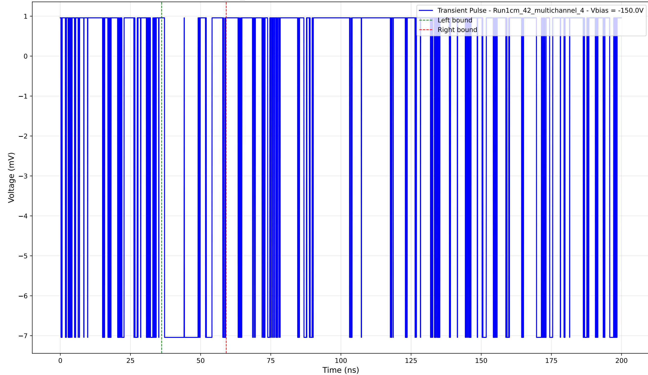
Transient Pulse - Sample: 1cm_42_multichannel - Position: 80.0 \mu\text{m} - Charge: 1.99 pC - Rise Time: 0.00 ns (N/A)
