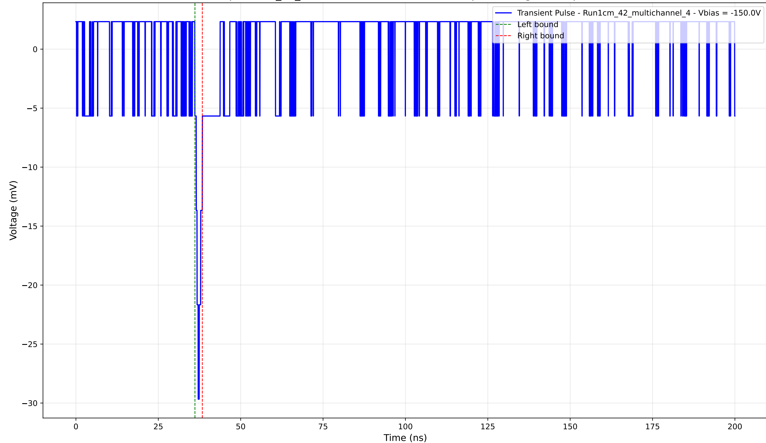
Transient Pulse - Sample: 1cm_42_multichannel - Position: 2430.0 \mu\text{m} - Charge: 0.78 pC - Rise Time: 1.04 ns
