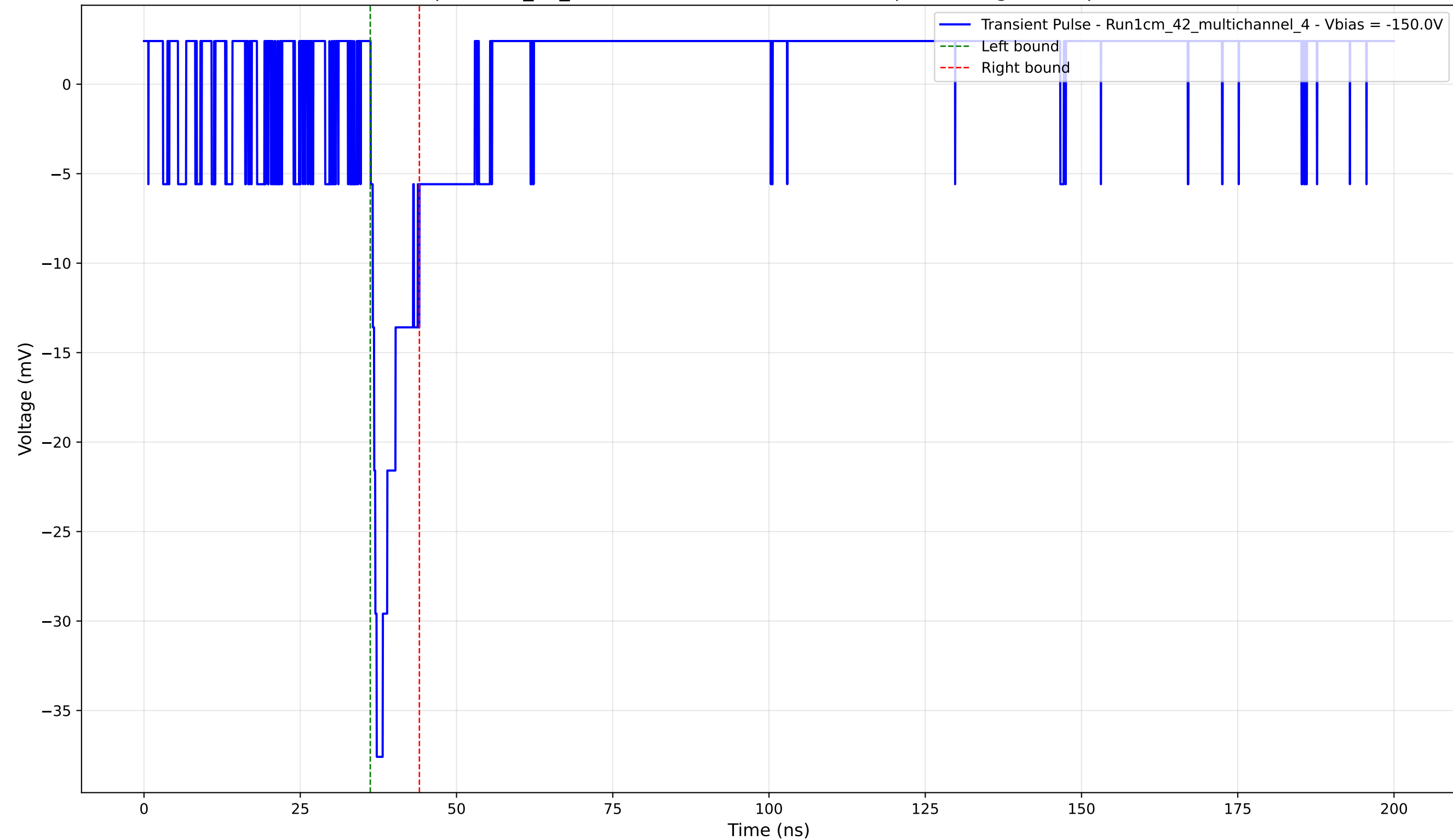
Transient Pulse - Sample: 1cm_42_multichannel - Position: 1765.0 \mu\text{m} - Charge: 3.04 pC - Rise Time: 0.97 ns
