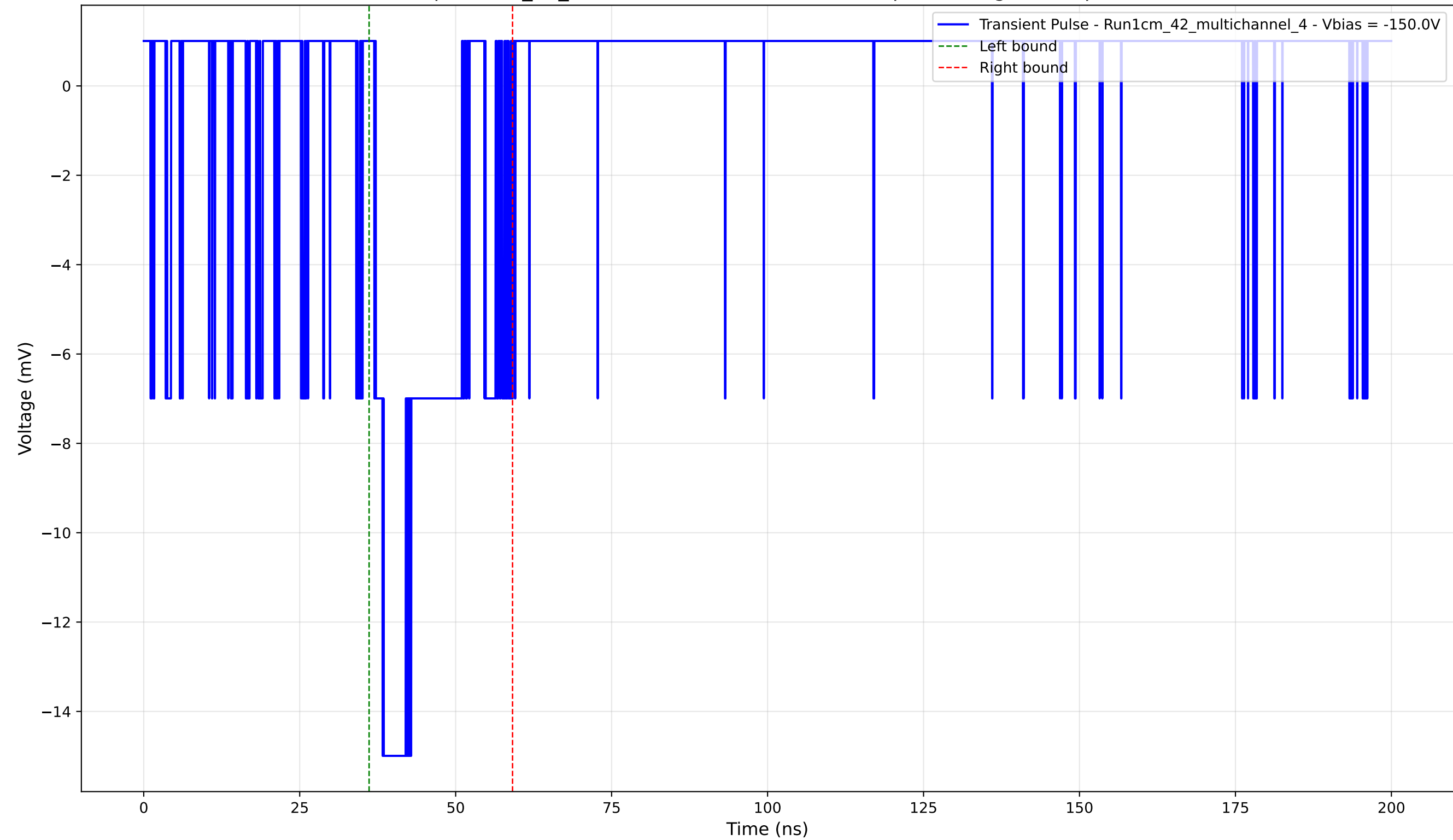
Transient Pulse - Sample: 1cm_42_multichannel - Position: 4635.0 \mu\text{m} - Charge: 2.99 pC - Rise Time: 1.10 ns
