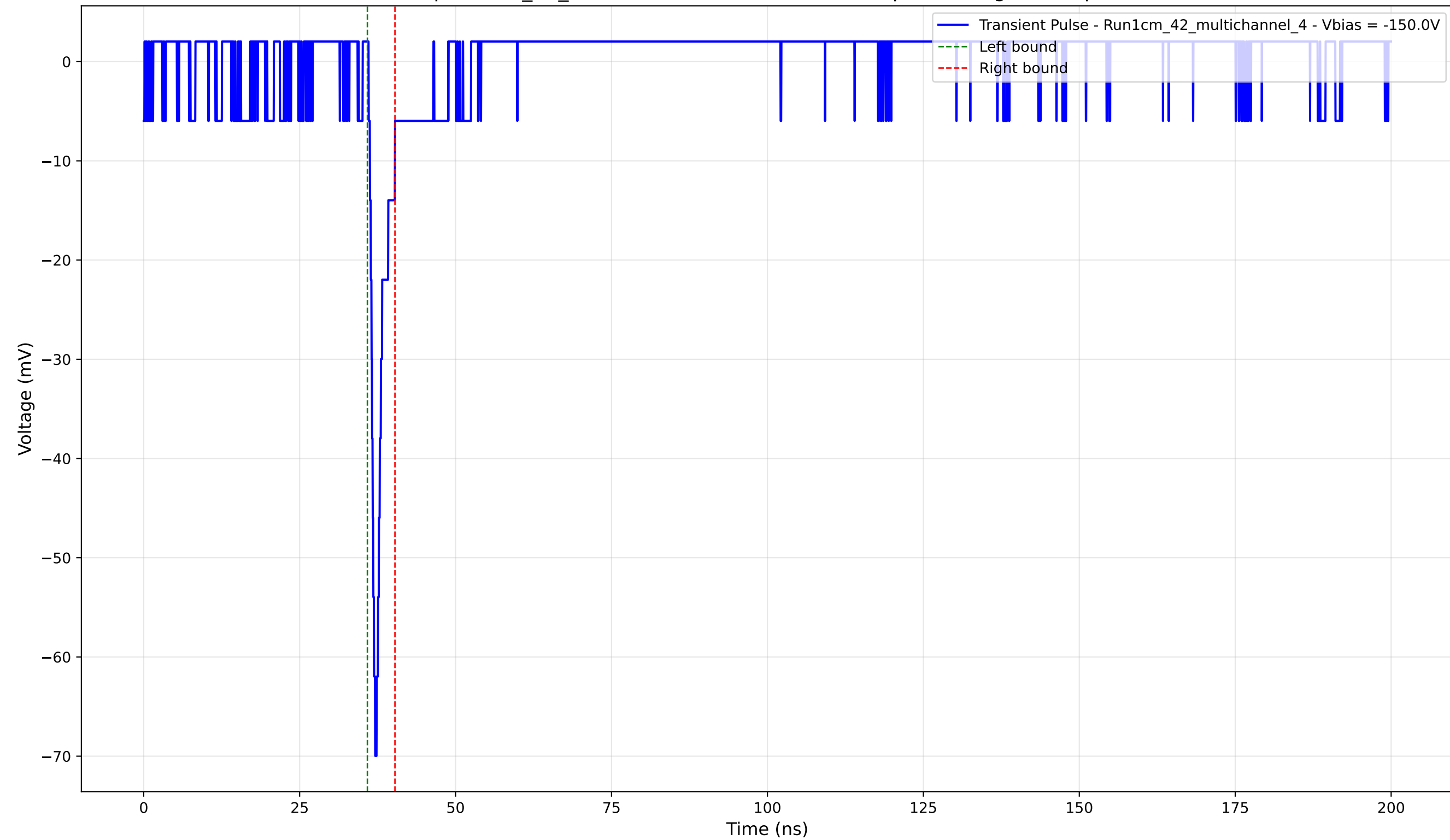
Transient Pulse - Sample: 1cm_42_multichannel - Position: 2450.0 \mu\text{m} - Charge: 2.56 pC - Rise Time: 0.86 ns
