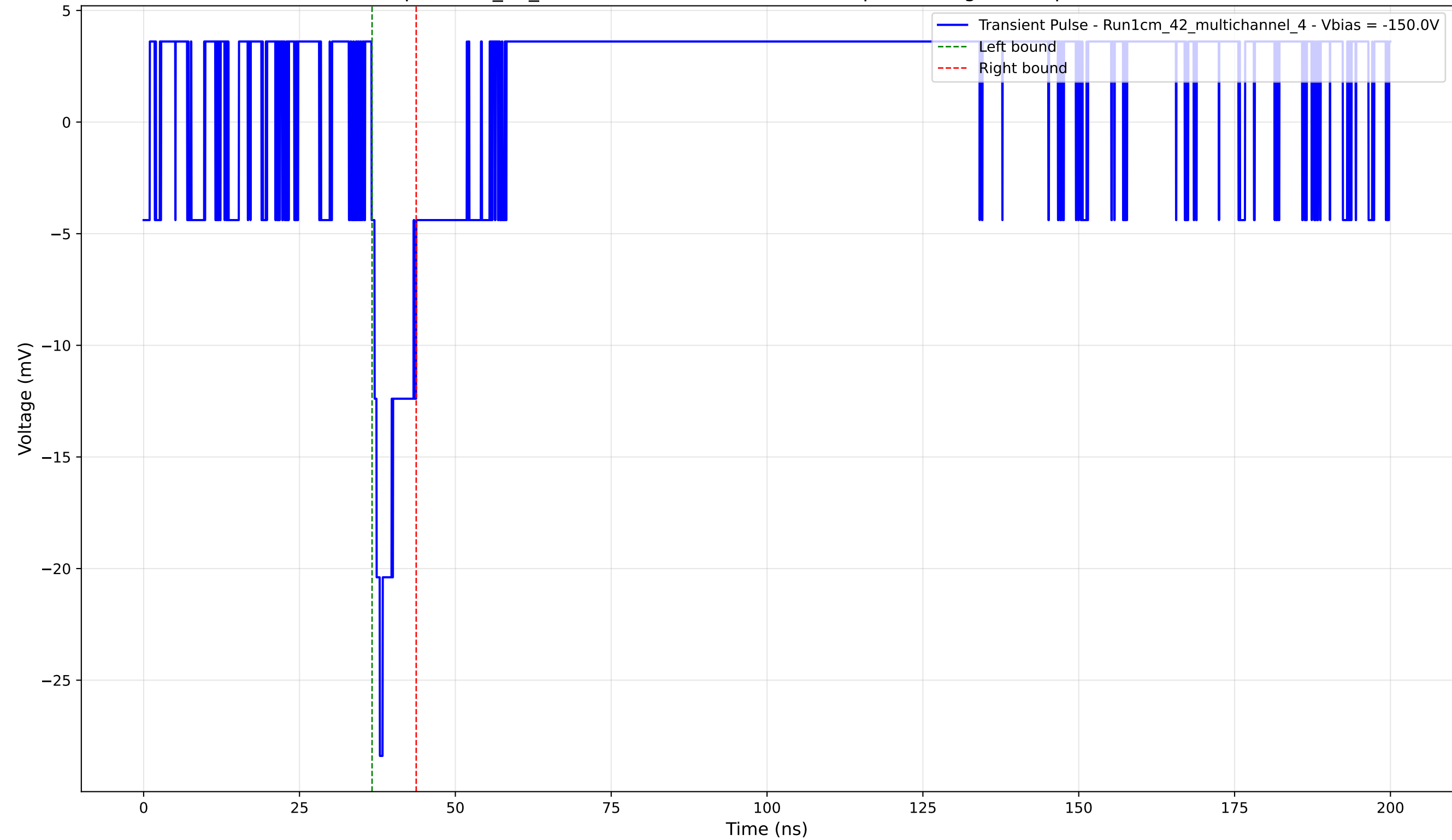
Transient Pulse - Sample: 1cm_42_multichannel - Position: 1445.0 \mu\text{m} - Charge: 2.16 pC - Rise Time: 0.00 ns (N/A)
