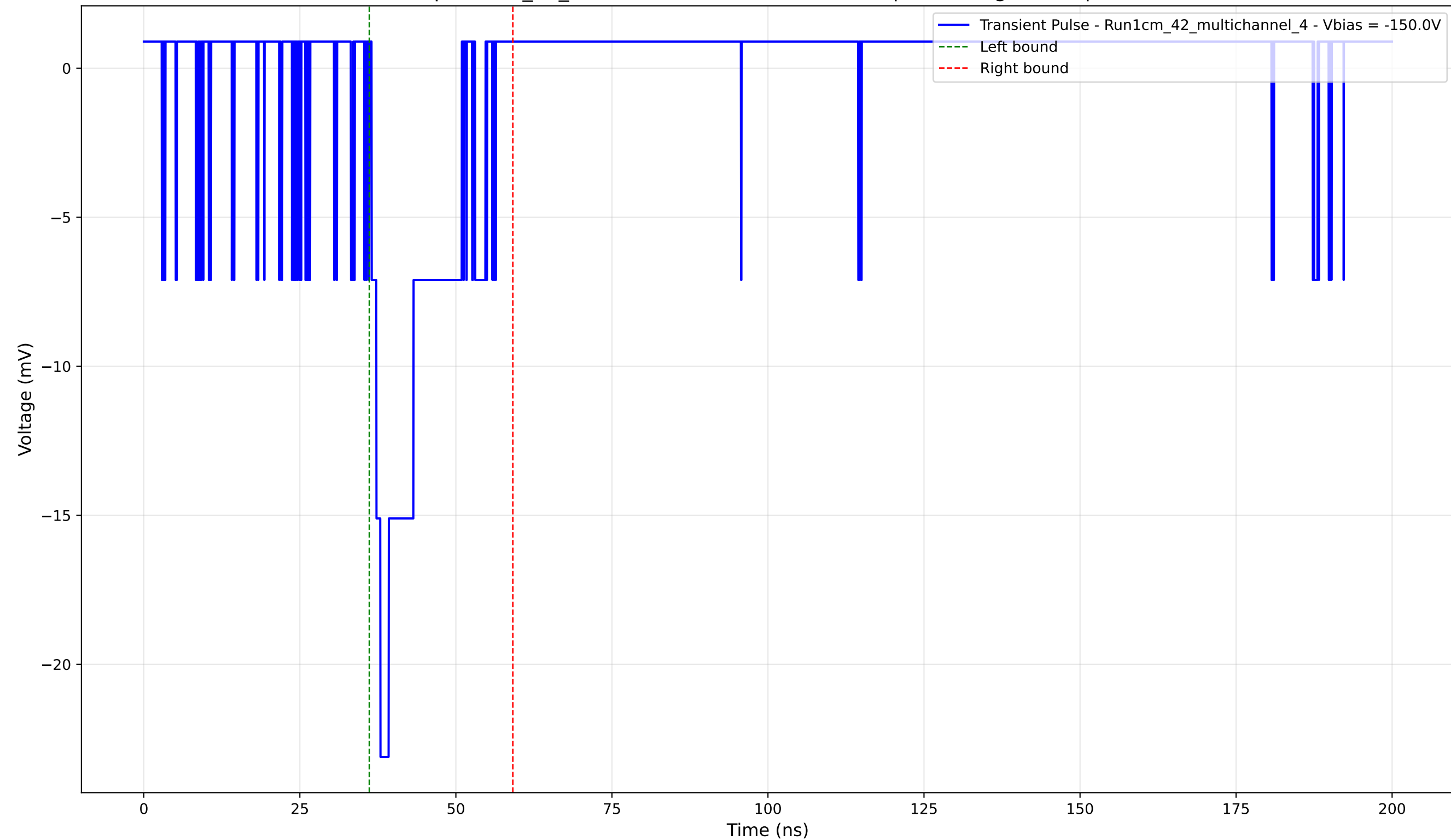
Transient Pulse - Sample: 1cm_42_multichannel - Position: 3525.0 \mu\text{m} - Charge: 3.42 pC - Rise Time: 1.42 ns
