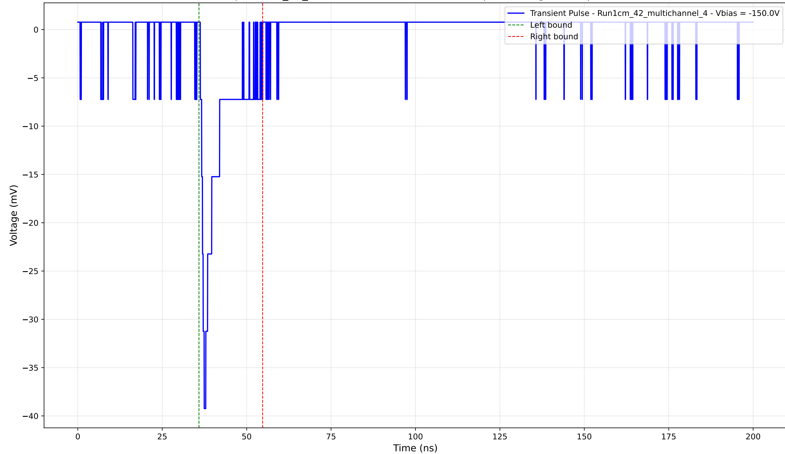
Transient Pulse - Sample: 1cm_42_multichannel - Position: 3020.0 \mu\text{m} - Charge: 4.08 pC - Rise Time: 1.15 ns
