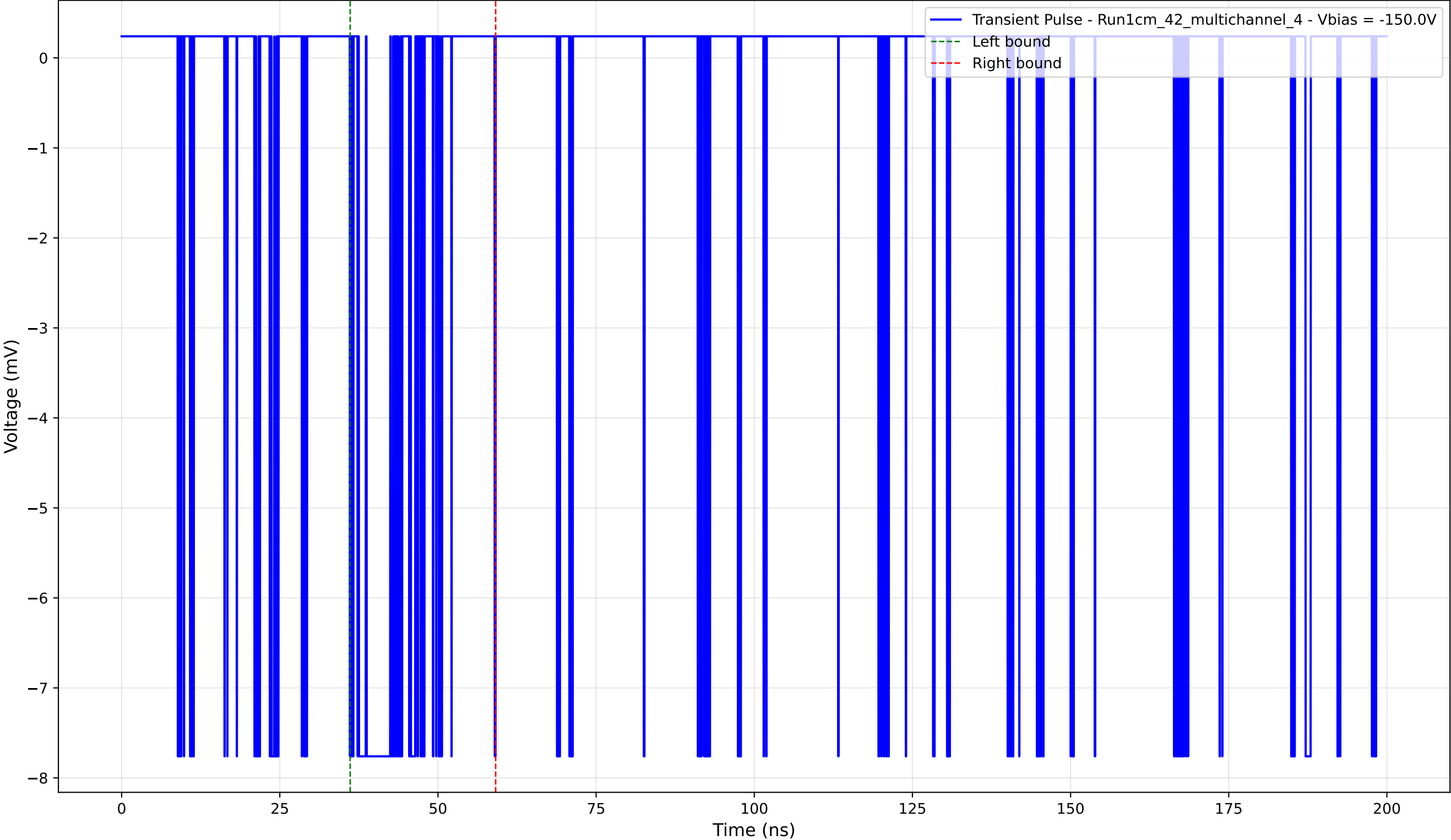
Transient Pulse - Sample: 1cm_42_multichannel - Position: 3875.0 \mu\text{m} - Charge: 1.21 pC - Rise Time: 0.02 ns
