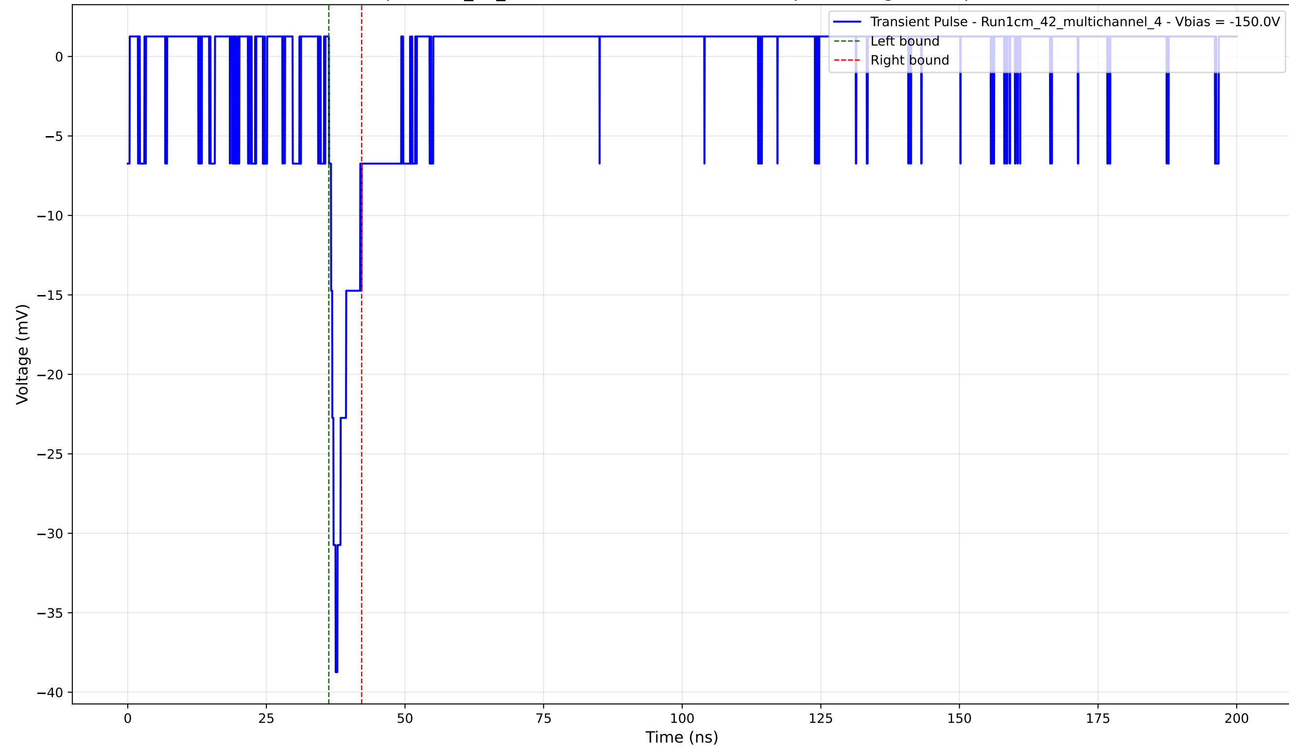
Transient Pulse - Sample: 1cm_42_multichannel - Position: 2965.0 \mu\text{m} - Charge: 2.31 pC - Rise Time: 1.21 ns
