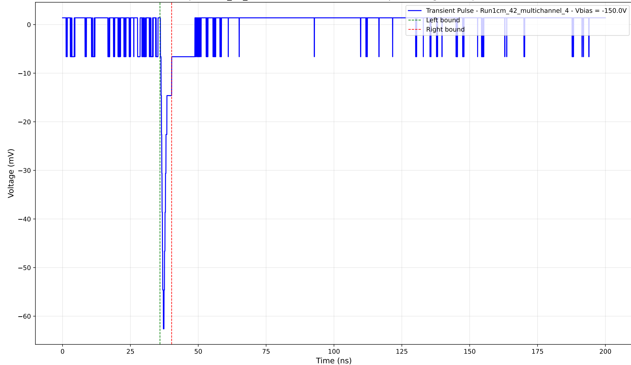
Transient Pulse - Sample: 1cm_42_multichannel - Position: 2445.0 \mu\text{m} - Charge: 2.23 pC - Rise Time: 1.08 ns
