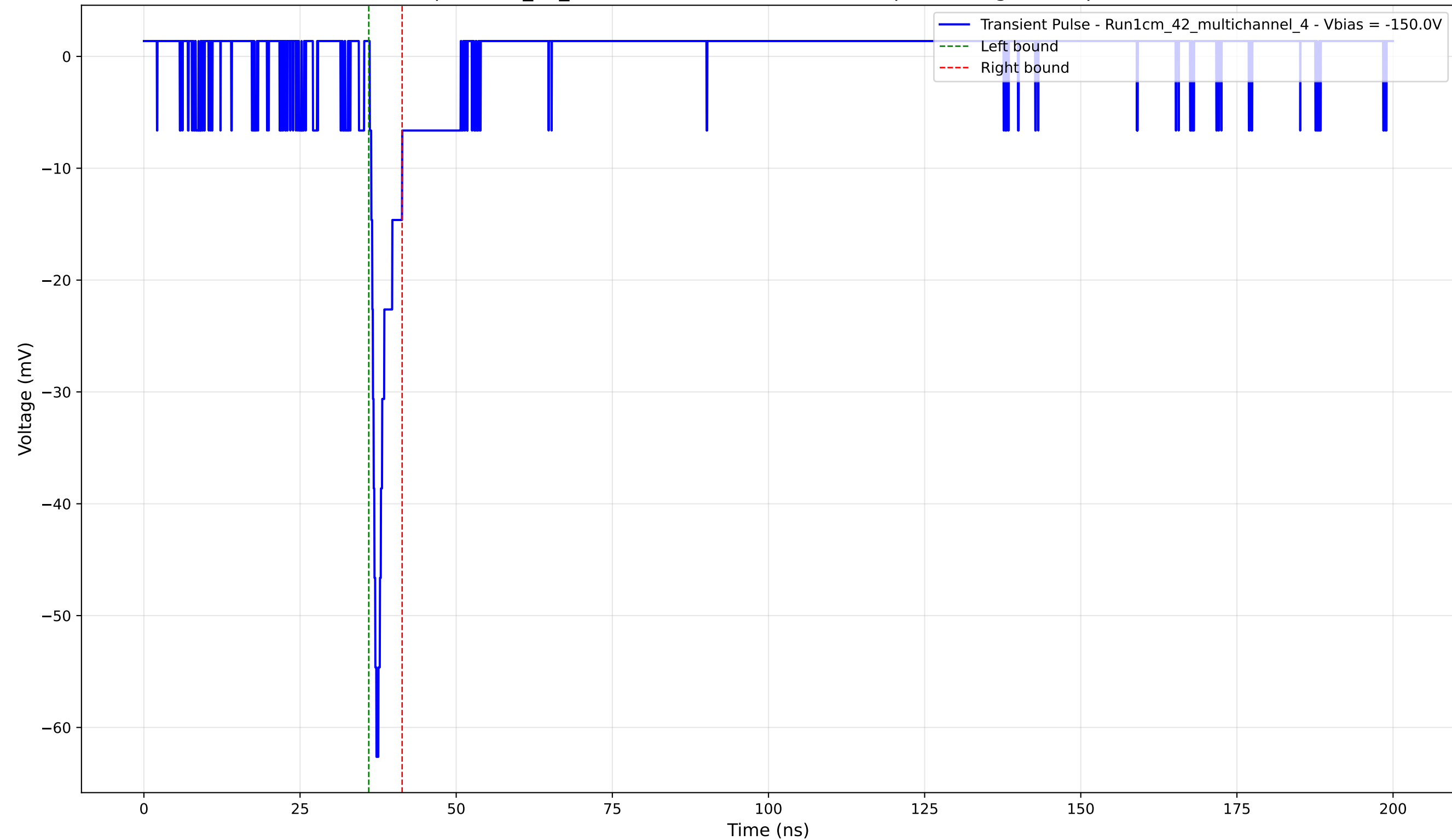
Transient Pulse - Sample: 1cm_42_multichannel - Position: 2650.0 \mu\text{m} - Charge: 2.83 pC - Rise Time: 1.06 ns
