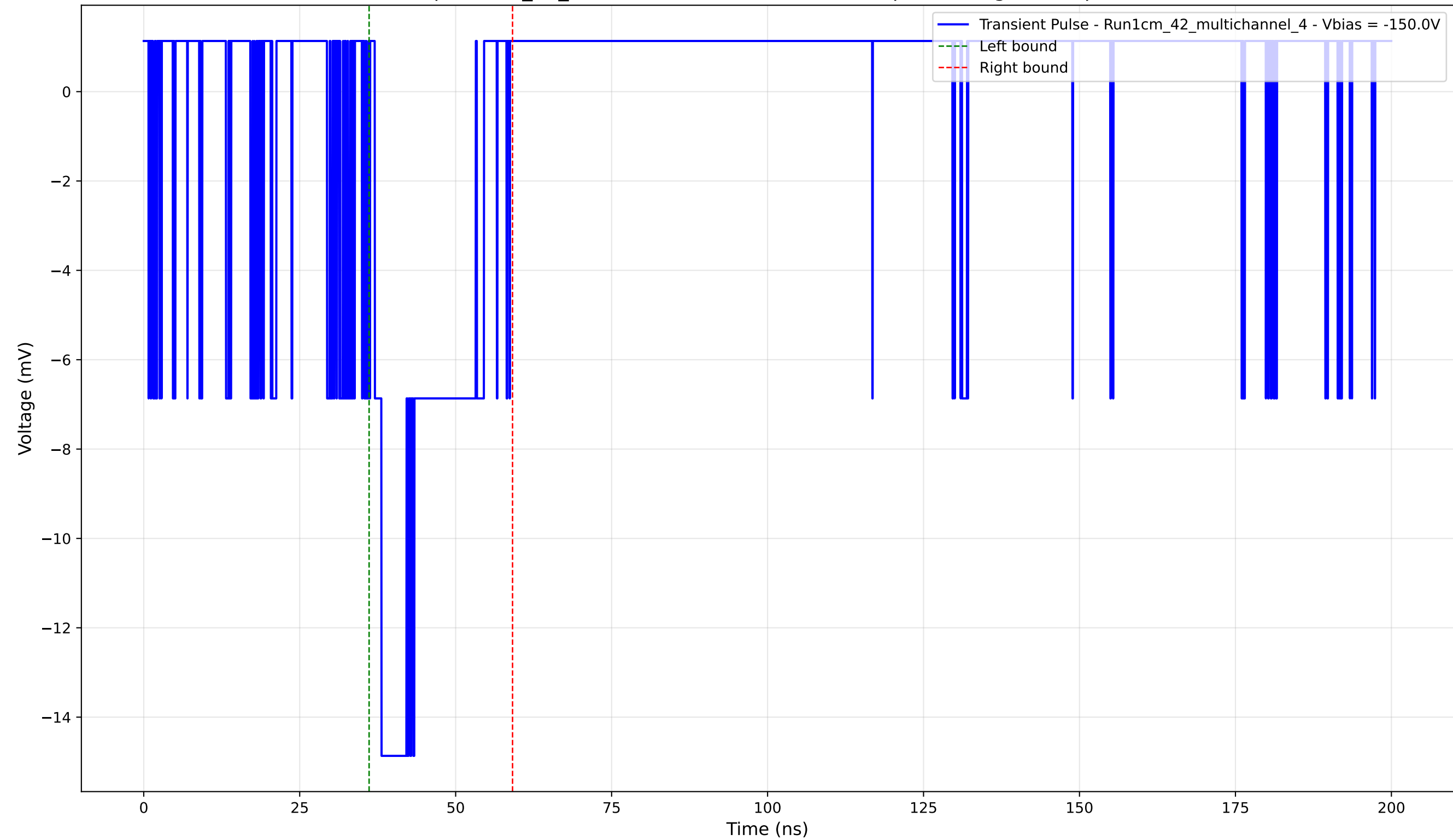
Transient Pulse - Sample: 1cm_42_multichannel - Position: 4070.0 \mu\text{m} - Charge: 3.03 pC - Rise Time: 1.08 ns
