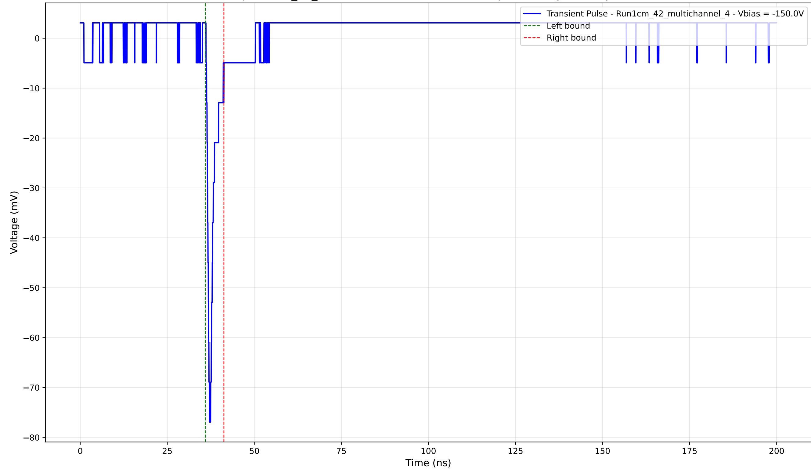
Transient Pulse - Sample: 1cm_42_multichannel - Position: 2235.0 \mu\text{m} - Charge: 3.09 pC - Rise Time: 0.81 ns
