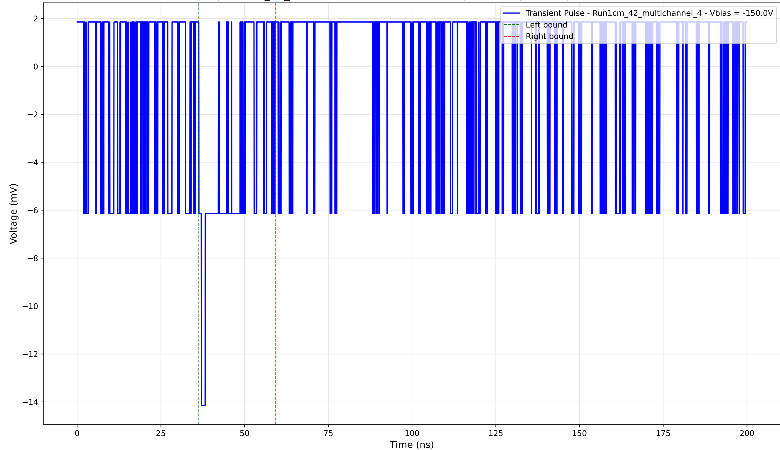
Transient Pulse - Sample: 1cm_42_multichannel - Position: 1920.0 \mu\text{m} - Charge: 1.69 pC - Rise Time: 0.00 ns (N/A)
