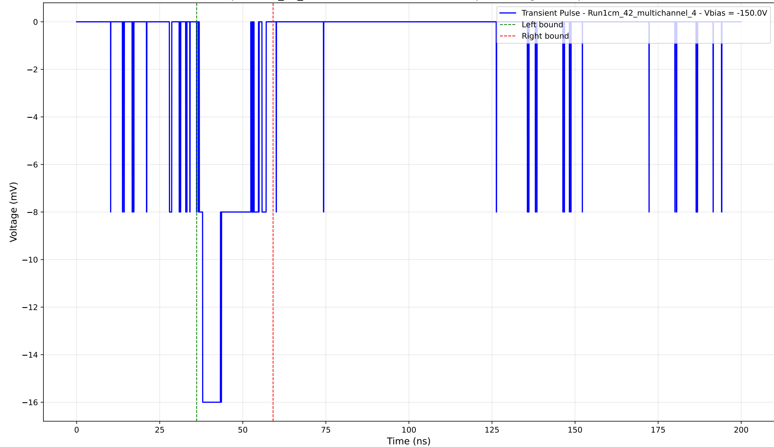
Transient Pulse - Sample: 1cm_42_multichannel - Position: 3985.0 \mu\text{m} - Charge: 3.90 pC - Rise Time: 1.02 ns
