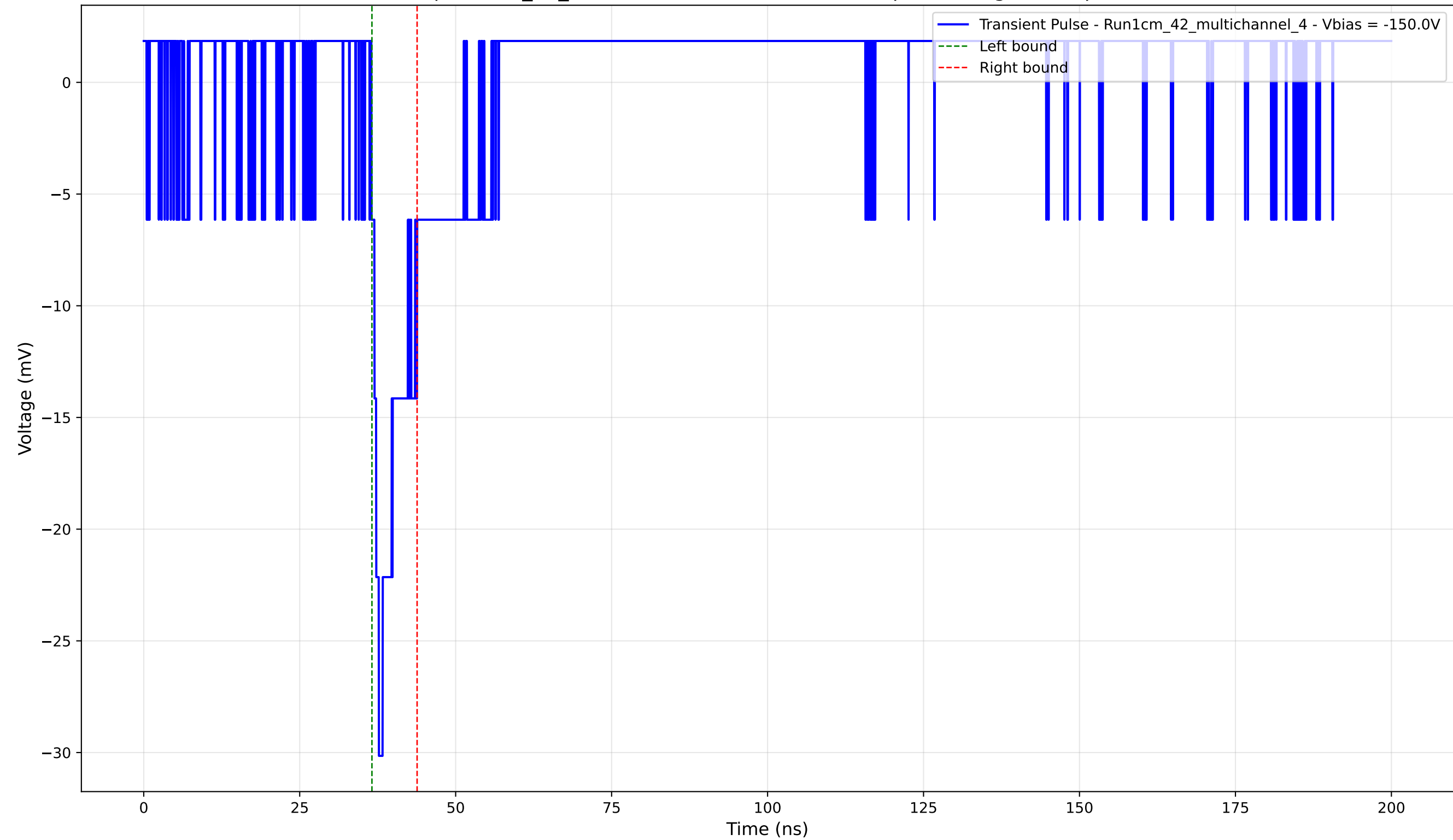
Transient Pulse - Sample: 1cm_42_multichannel - Position: 3275.0 \mu\text{m} - Charge: 2.44 pC - Rise Time: 1.19 ns
