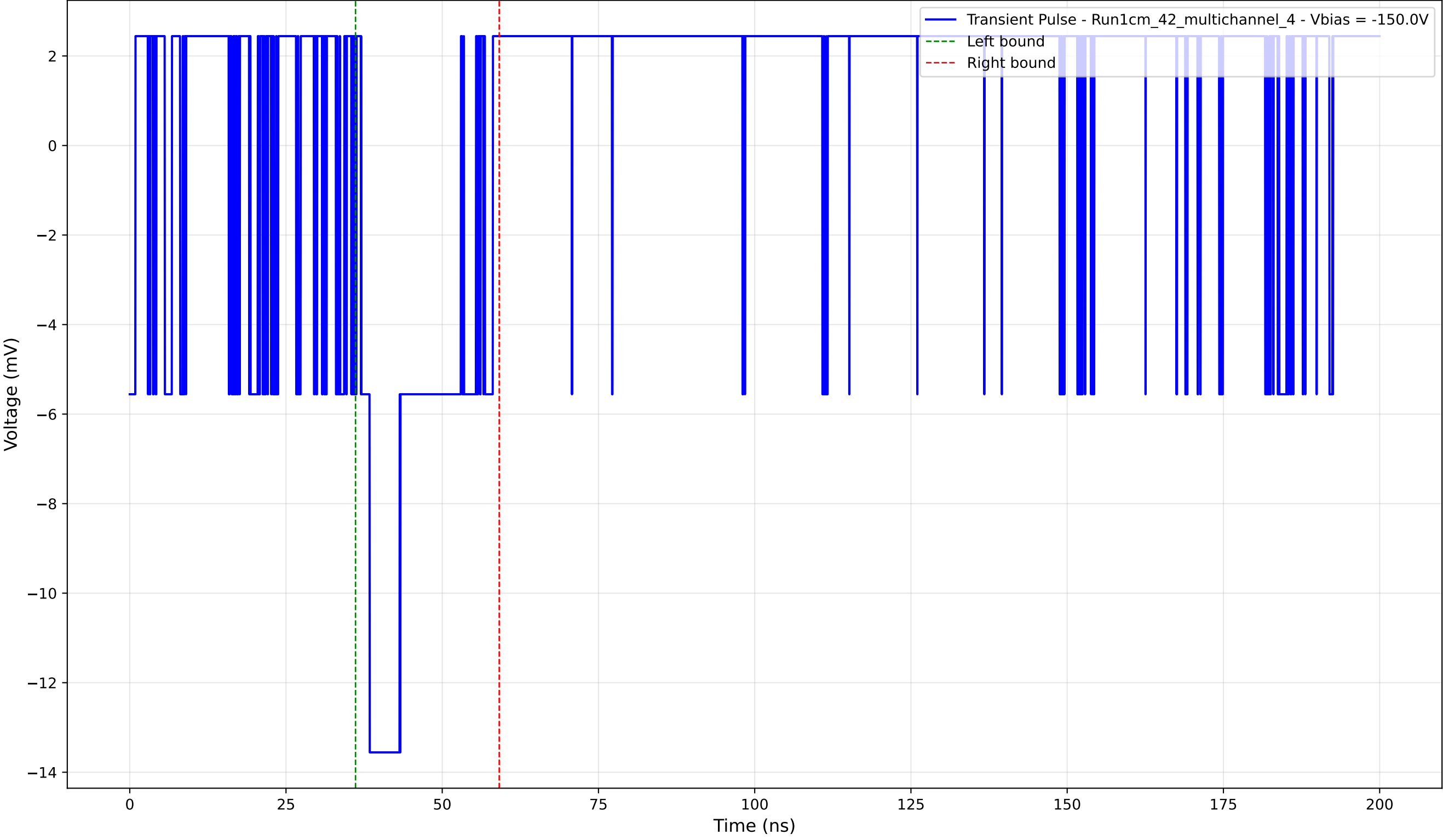
Transient Pulse - Sample: 1cm_42_multichannel - Position: 450.0 \mu\text{m} - Charge: 2.83 pC - Rise Time: 0.00 ns (N/A)
