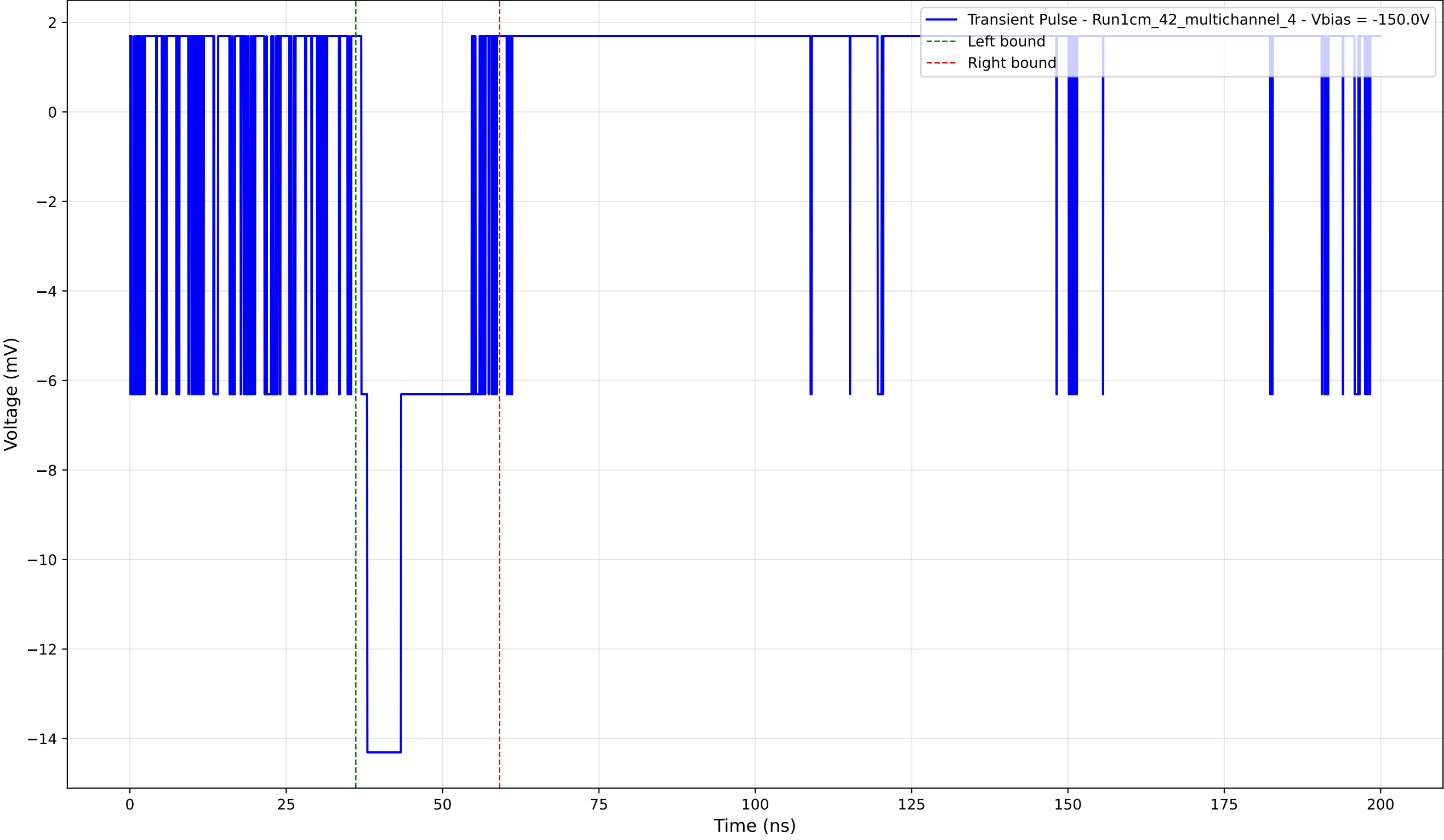
Transient Pulse - Sample: 1cm_42_multichannel - Position: 620.0 \mu\text{m} - Charge: 3.16 pC - Rise Time: 0.00 ns (N/A)
