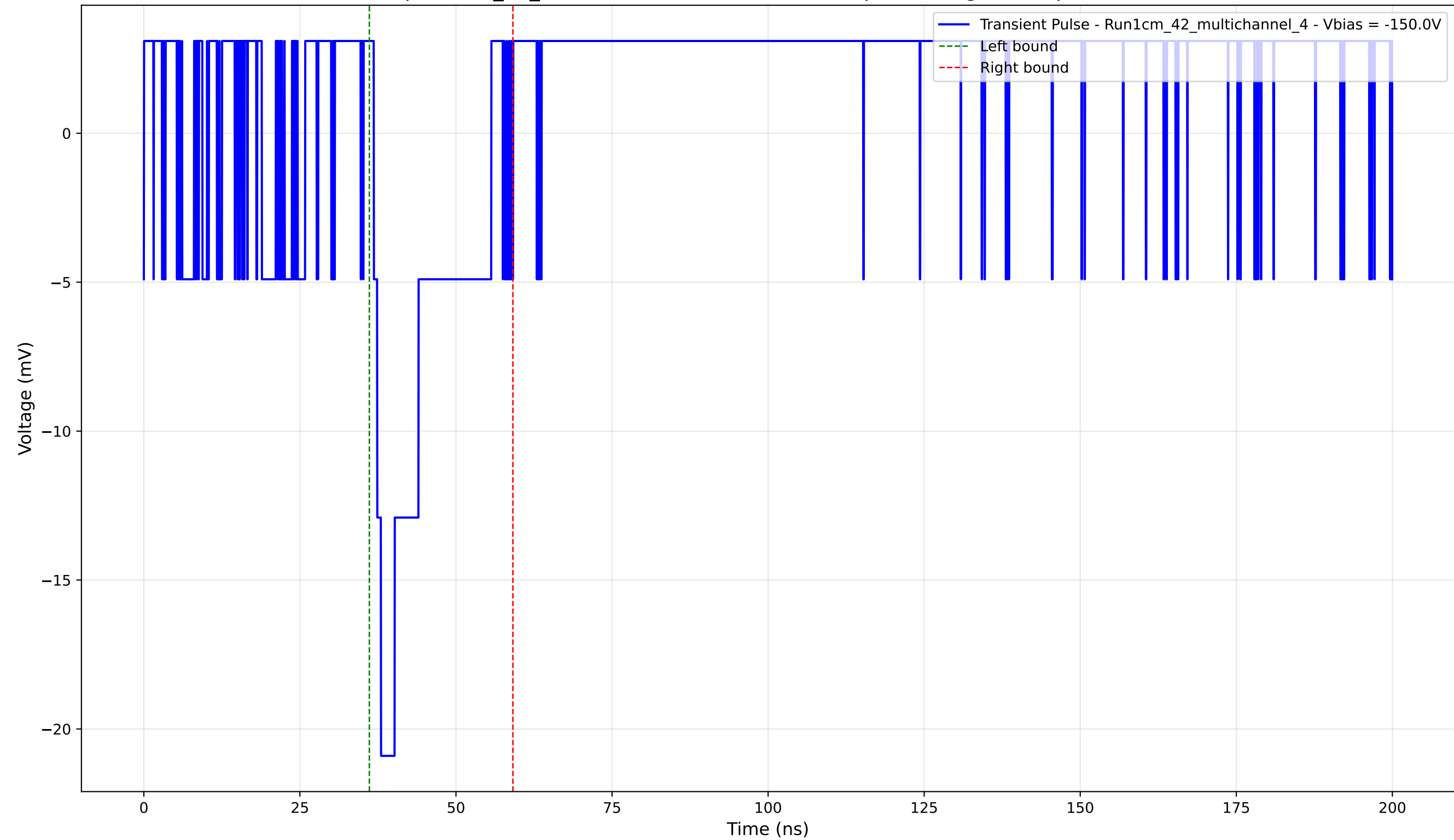
Transient Pulse - Sample: 1cm_42_multichannel - Position: 1090.0 \mu\text{m} - Charge: 3.17 pC - Rise Time: 0.00 ns (N/A)
