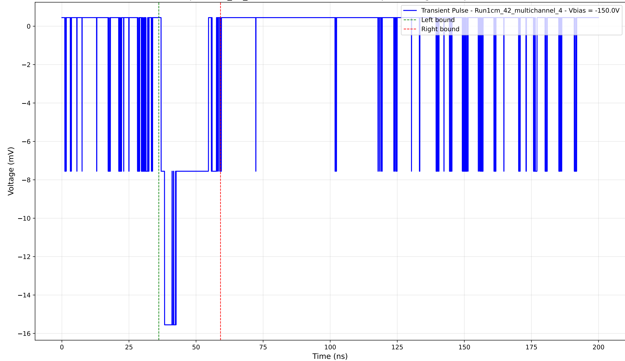
Transient Pulse - Sample: 1cm_42_multichannel - Position: 185.0 \mu\text{m} - Charge: 3.58 pC - Rise Time: 1.30 ns
