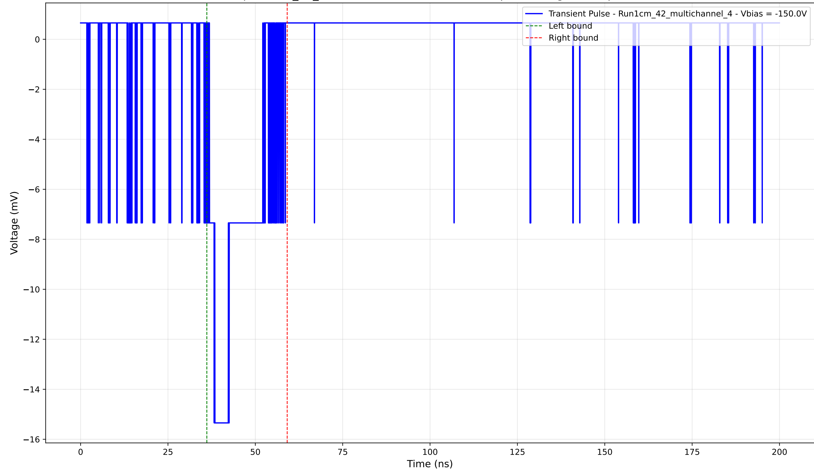
Transient Pulse - Sample: 1cm_42_multichannel - Position: 4160.0 \mu\text{m} - Charge: 3.19 pC - Rise Time: 1.36 ns
