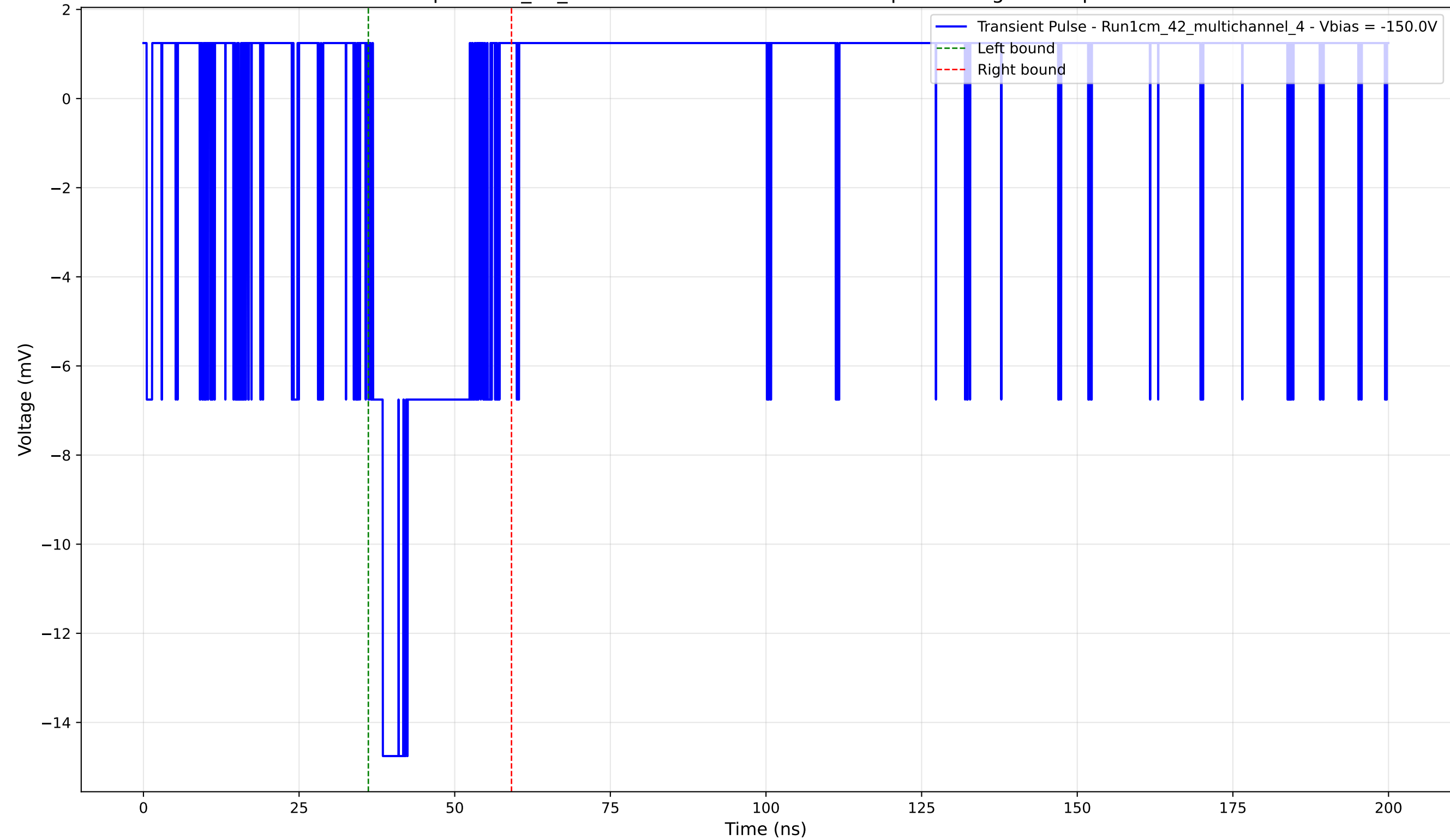
Transient Pulse - Sample: 1cm_42_multichannel - Position: 4775.0 \mu\text{m} - Charge: 2.92 pC - Rise Time: 1.58 ns
