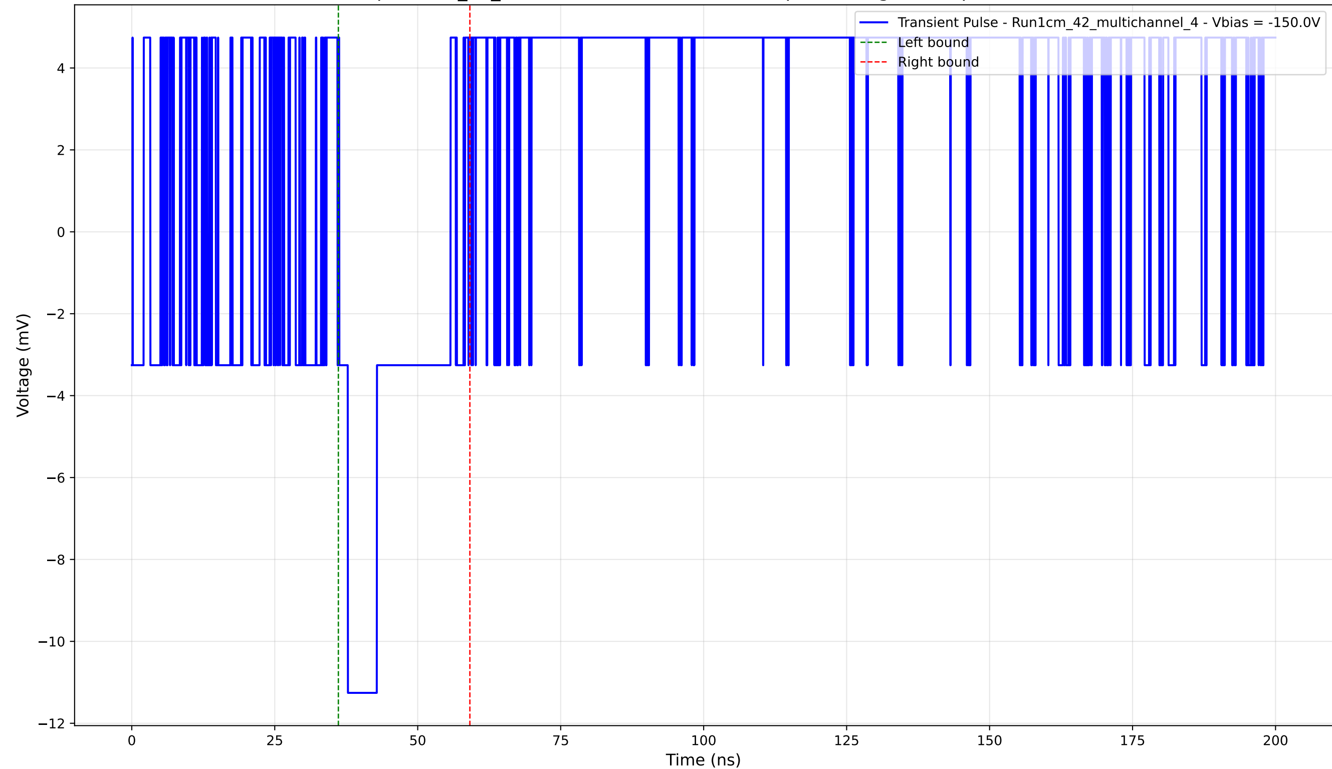
Transient Pulse - Sample: 1cm_42_multichannel - Position: 930.0 \mu\text{m} - Charge: 1.98 pC - Rise Time: 0.00 ns (N/A)
