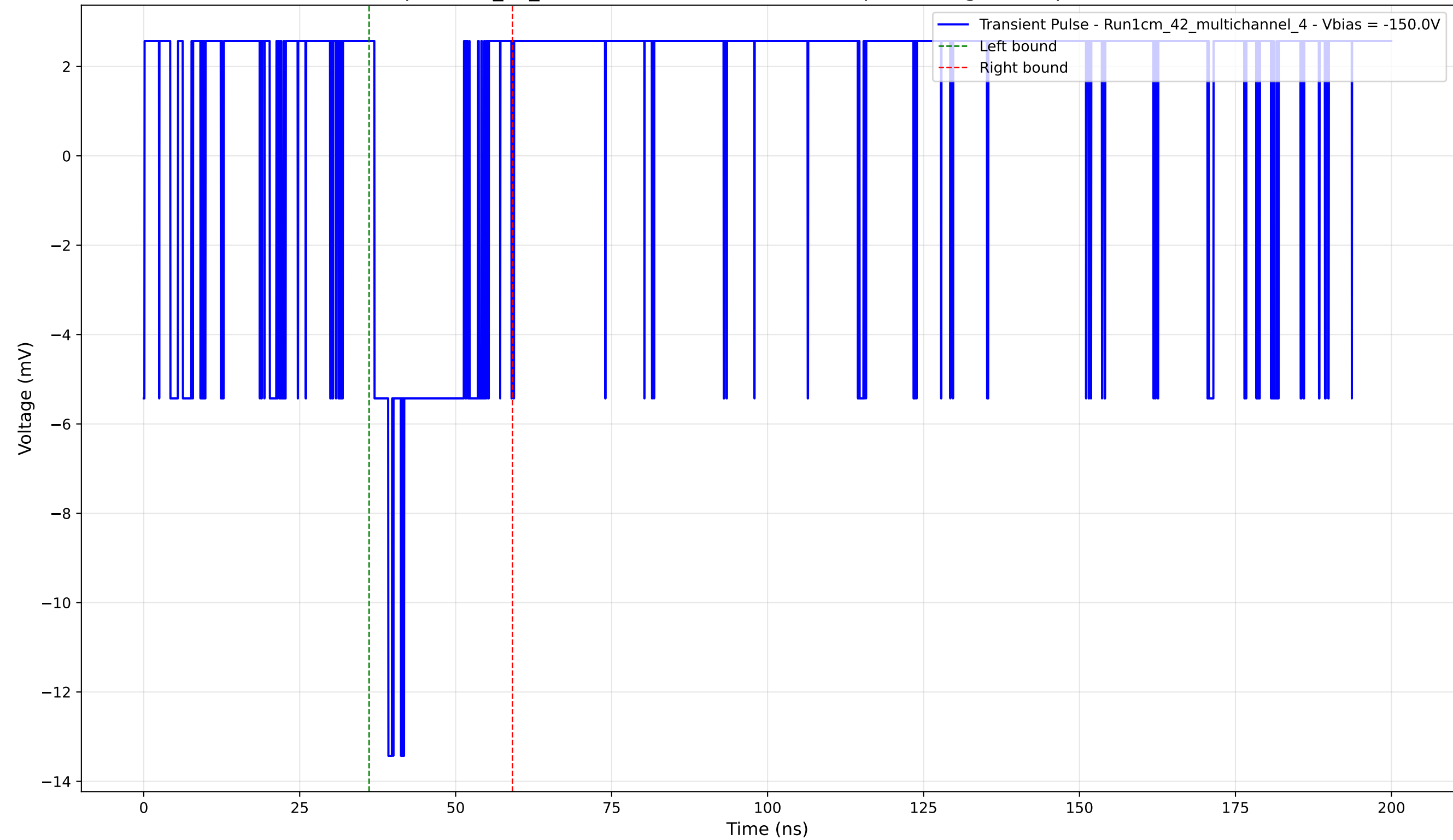
Transient Pulse - Sample: 1cm_42_multichannel - Position: 4835.0 \mu\text{m} - Charge: 1.71 pC - Rise Time: 0.00 ns (N/A)
