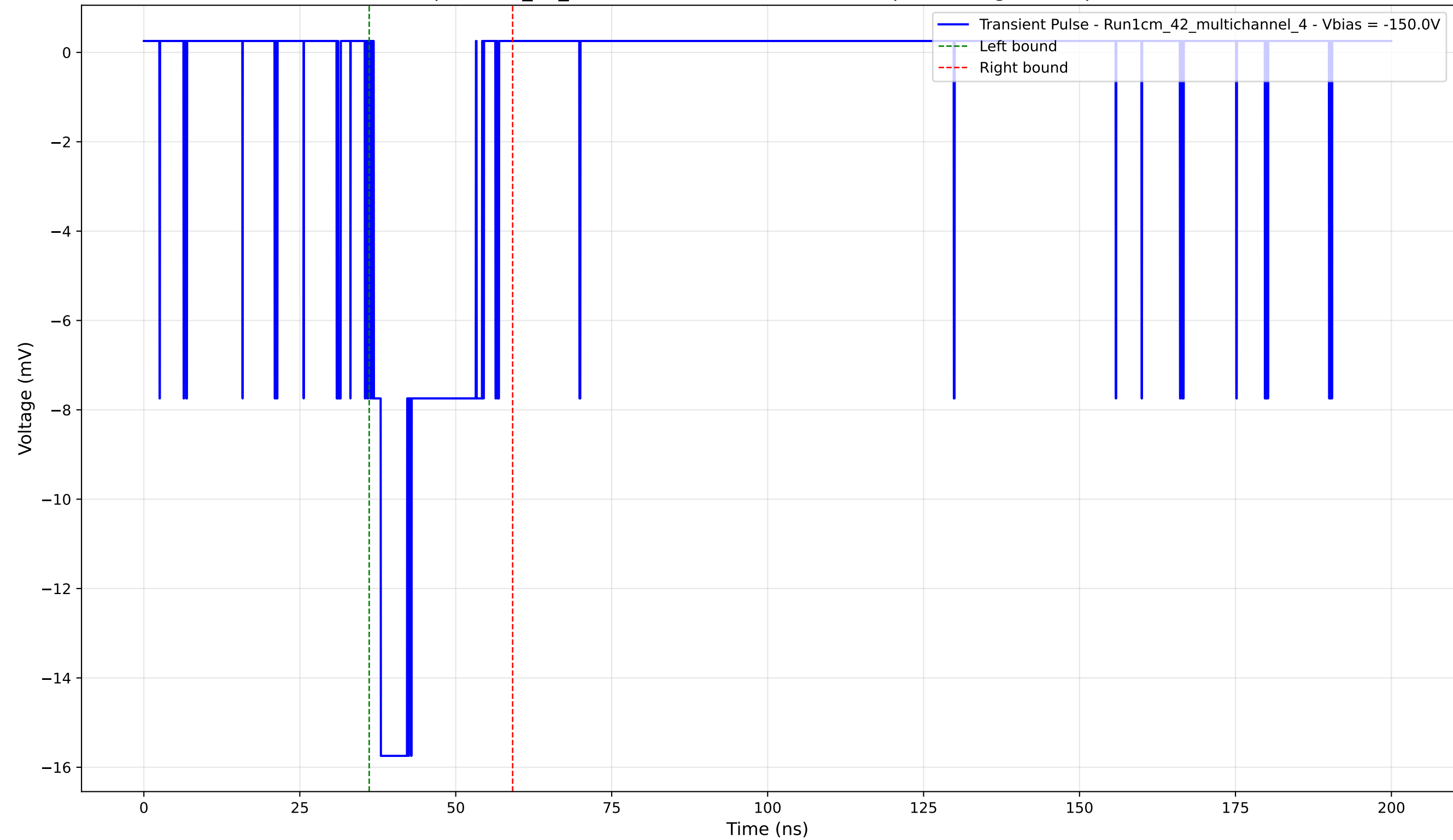
Transient Pulse - Sample: 1cm_42_multichannel - Position: 3830.0 \mu\text{m} - Charge: 3.46 pC - Rise Time: 1.14 ns
