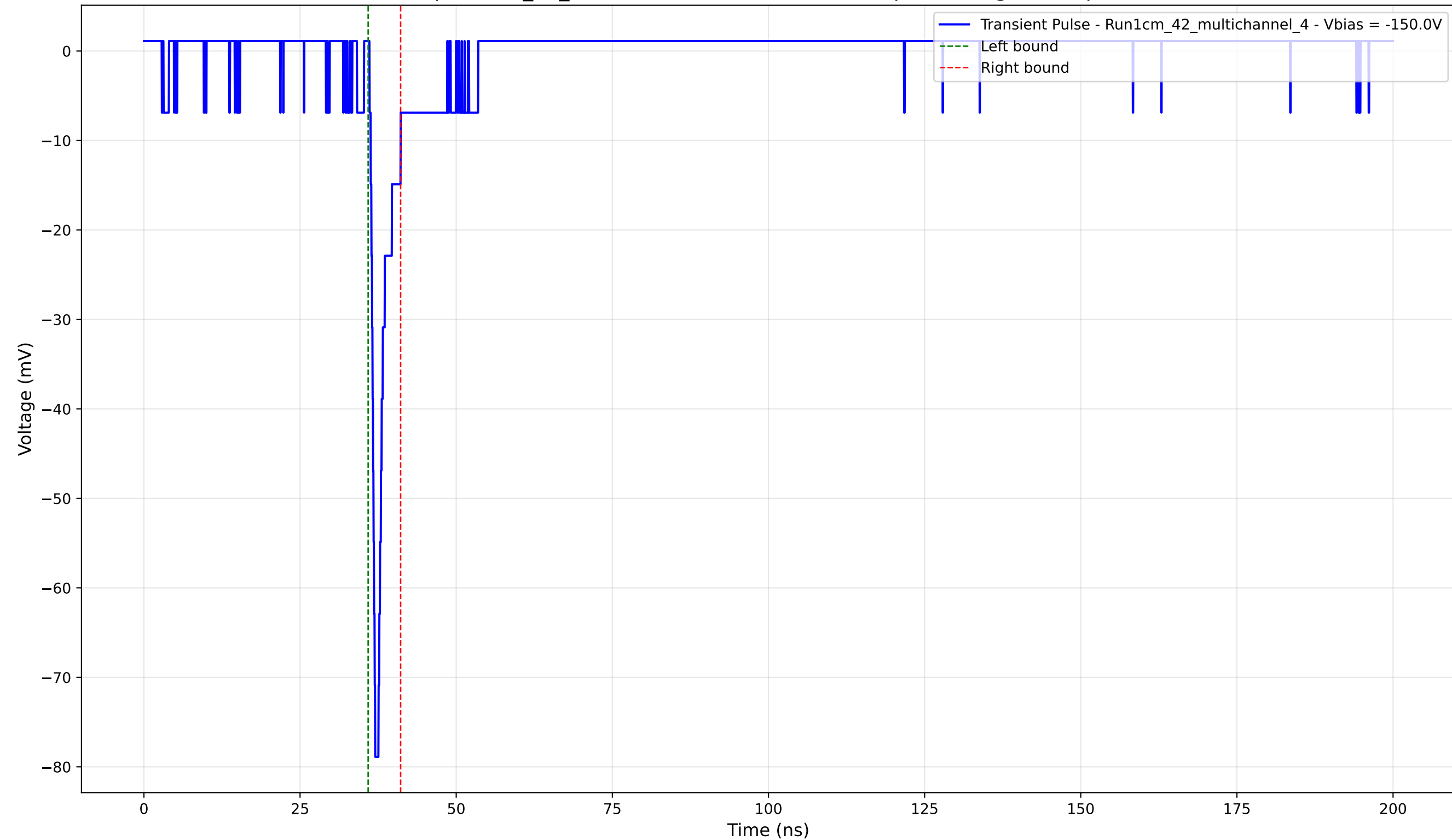
Transient Pulse - Sample: 1cm_42_multichannel - Position: 2250.0 \mu\text{m} - Charge: 3.33 pC - Rise Time: 0.74 ns
