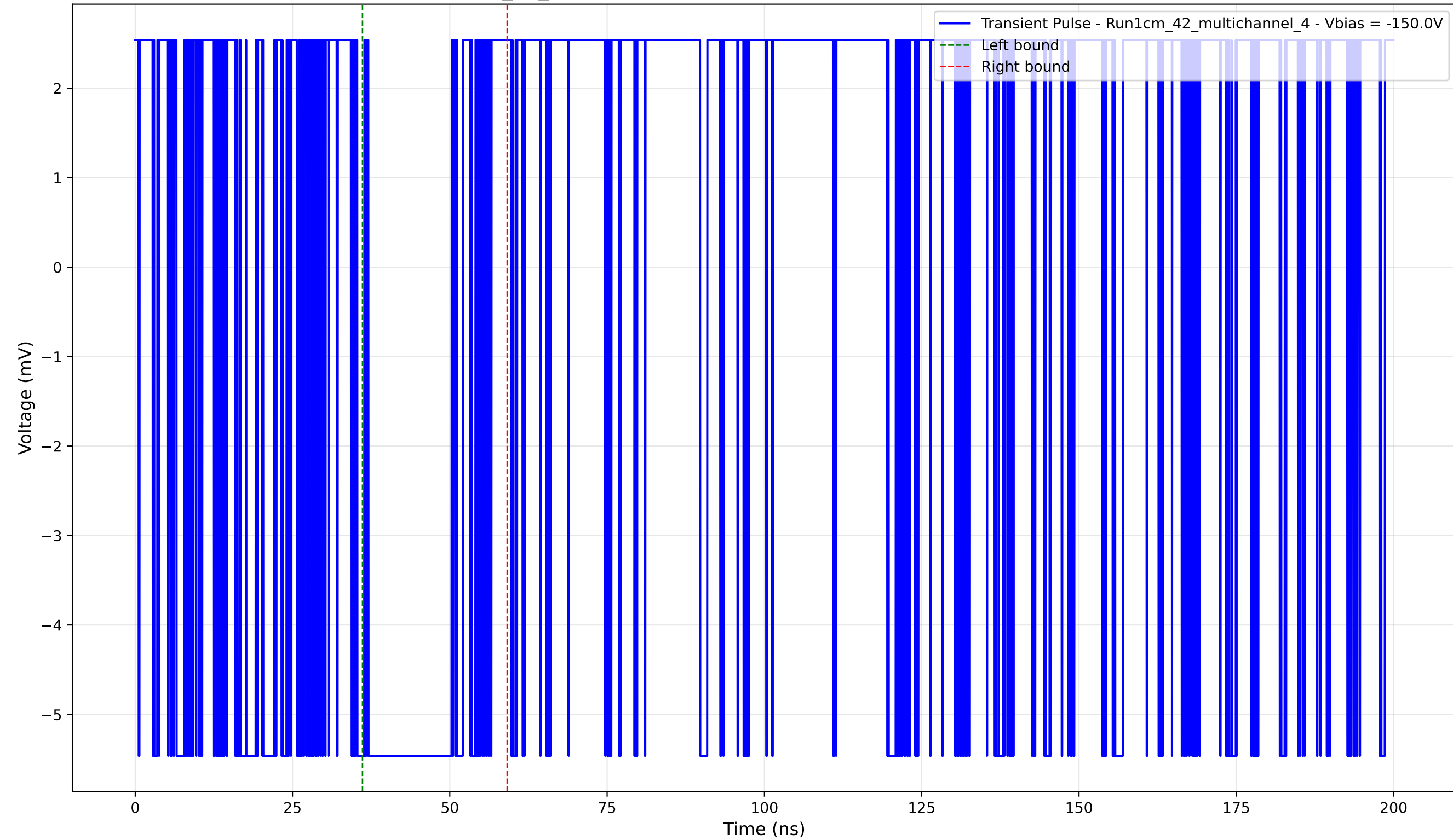
Transient Pulse - Sample: 1cm_42_multichannel - Position: 85.0 \mu\text{m} - Charge: 1.47 pC - Rise Time: 0.00 ns (N/A)
