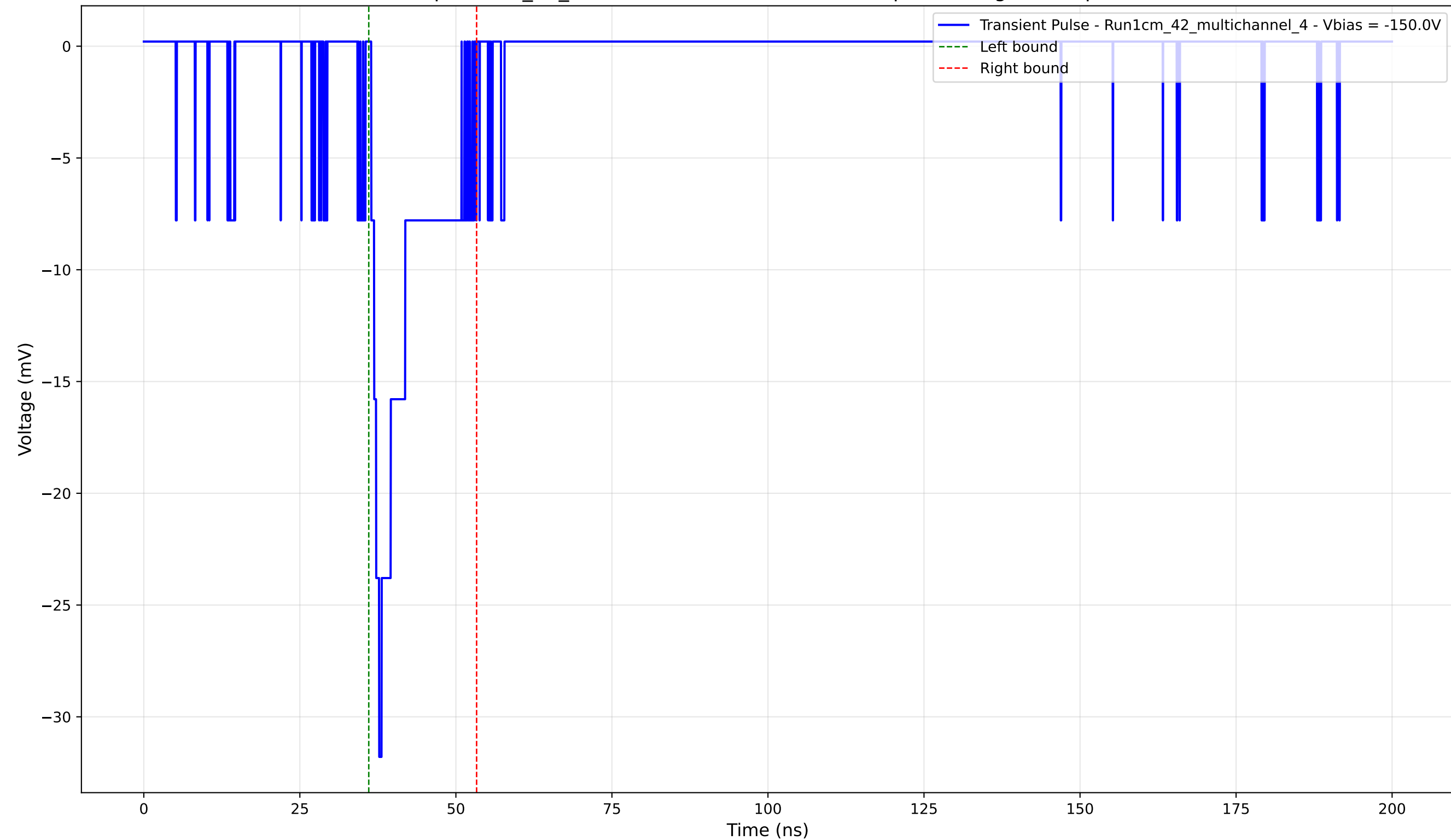
Transient Pulse - Sample: 1cm_42_multichannel - Position: 3175.0 \mu\text{m} - Charge: 3.73 pC - Rise Time: 1.27 ns
