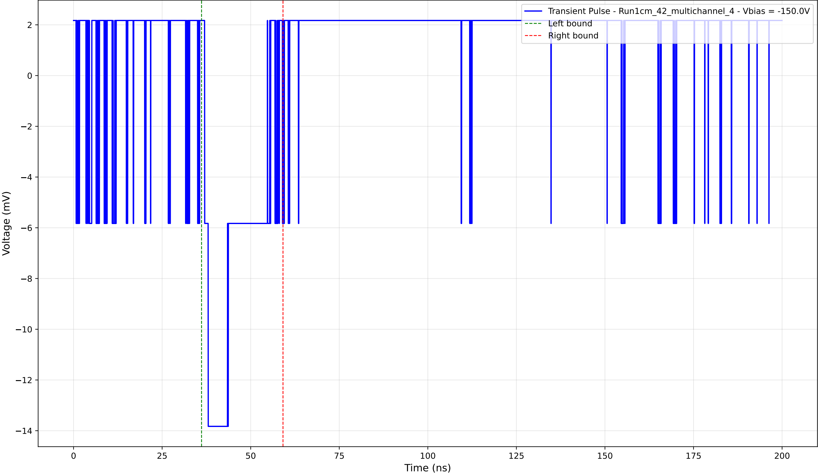
Transient Pulse - Sample: 1cm_42_multichannel - Position: 470.0 \mu\text{m} - Charge: 3.02 pC - Rise Time: 0.00 ns (N/A)
