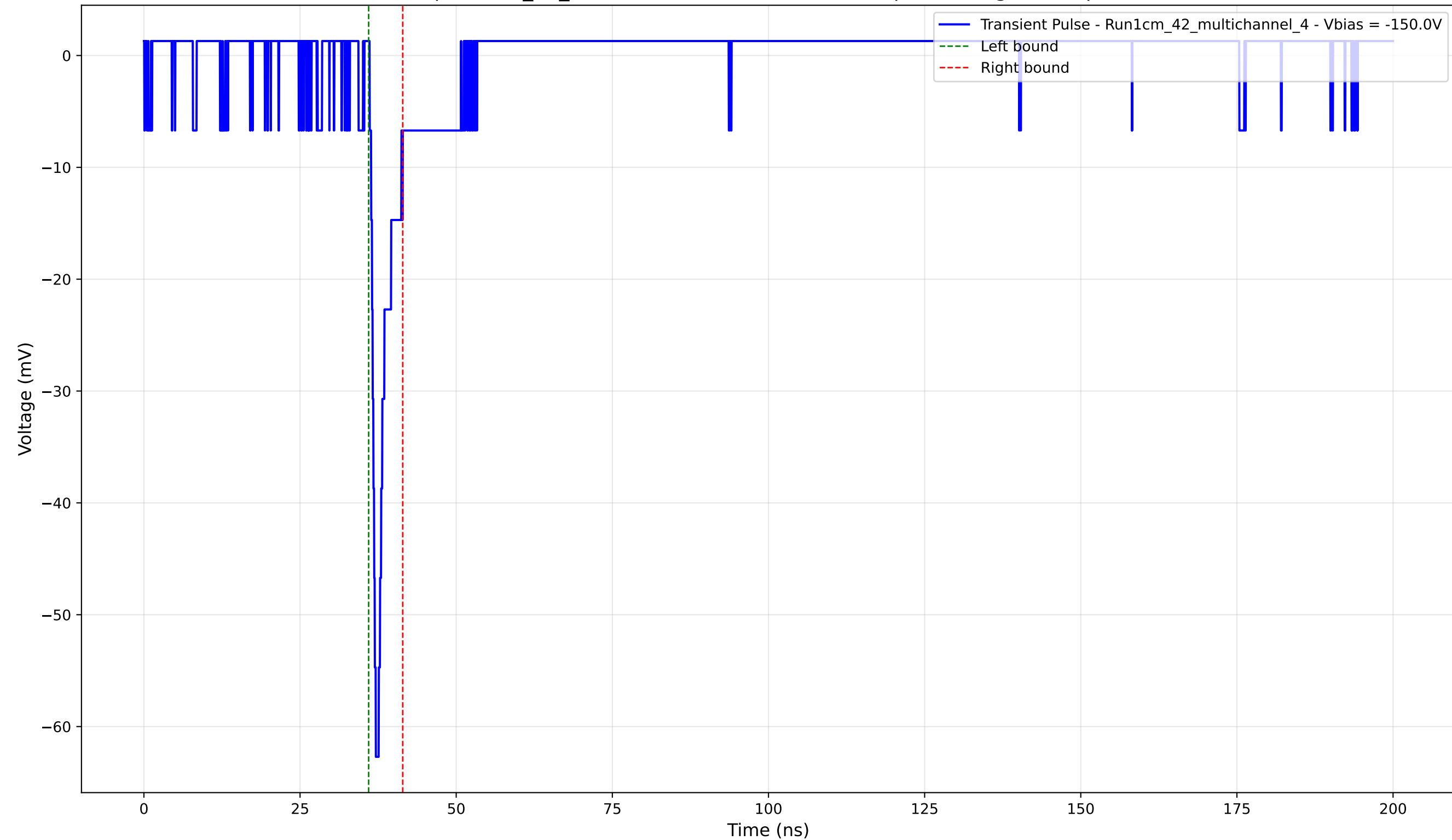
Transient Pulse - Sample: 1cm_42_multichannel - Position: 2610.0 \mu\text{m} - Charge: 2.90 pC - Rise Time: 0.98 ns
