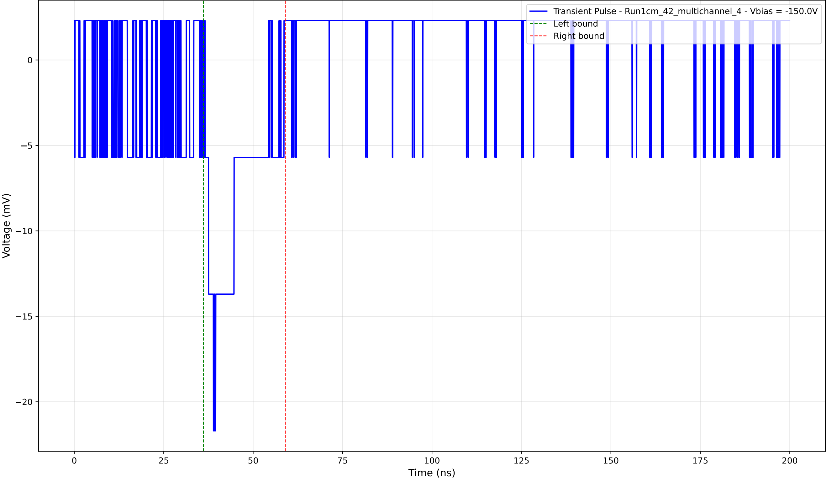
Transient Pulse - Sample: 1cm_42_multichannel - Position: 950.0 \mu\text{m} - Charge: 3.56 pC - Rise Time: 0.00 ns (N/A)
