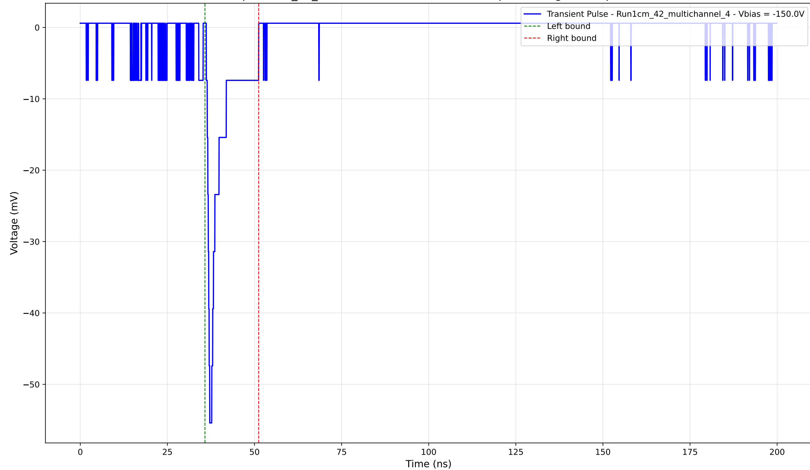
Transient Pulse - Sample: 1cm_42_multichannel - Position: 2050.0 \mu\text{m} - Charge: 4.39 pC - Rise Time: 0.97 ns
