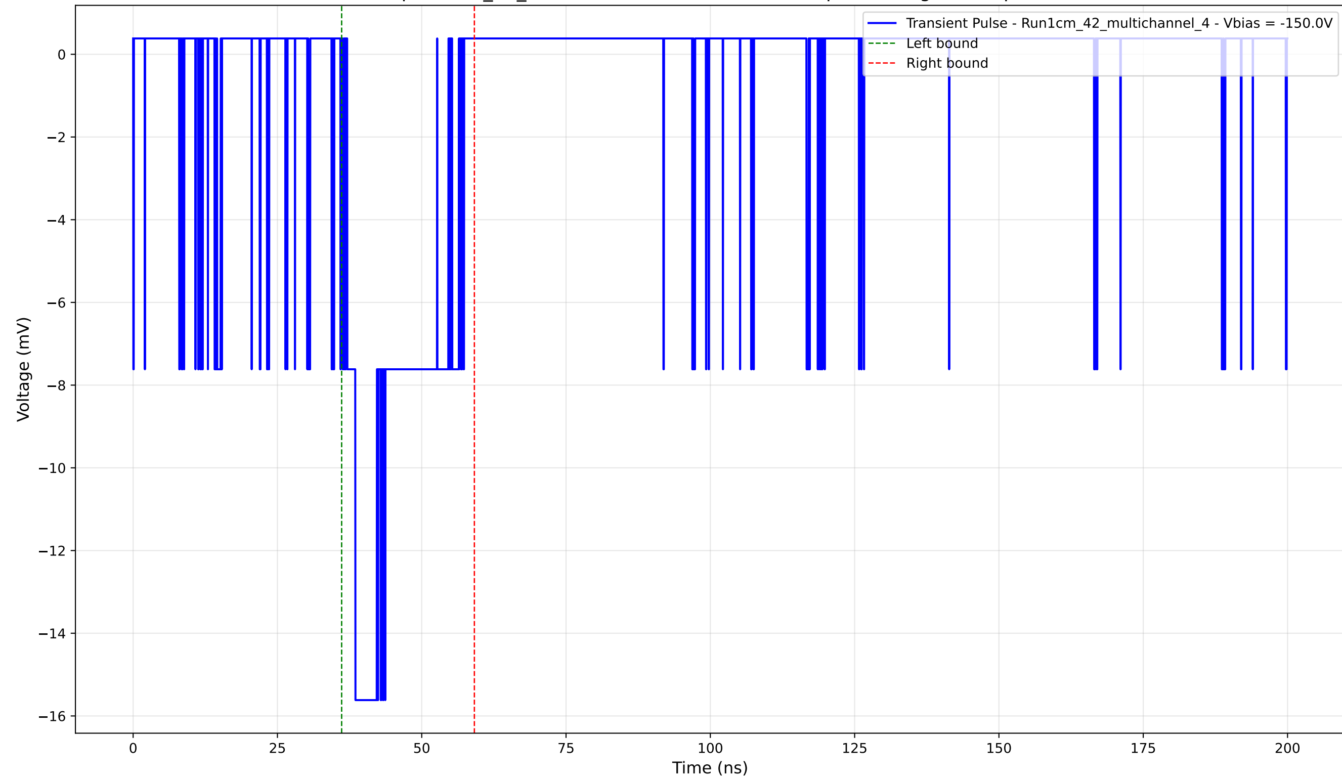
Transient Pulse - Sample: 1cm_42_multichannel - Position: 4590.0 \mu\text{m} - Charge: 3.59 pC - Rise Time: 1.42 ns
