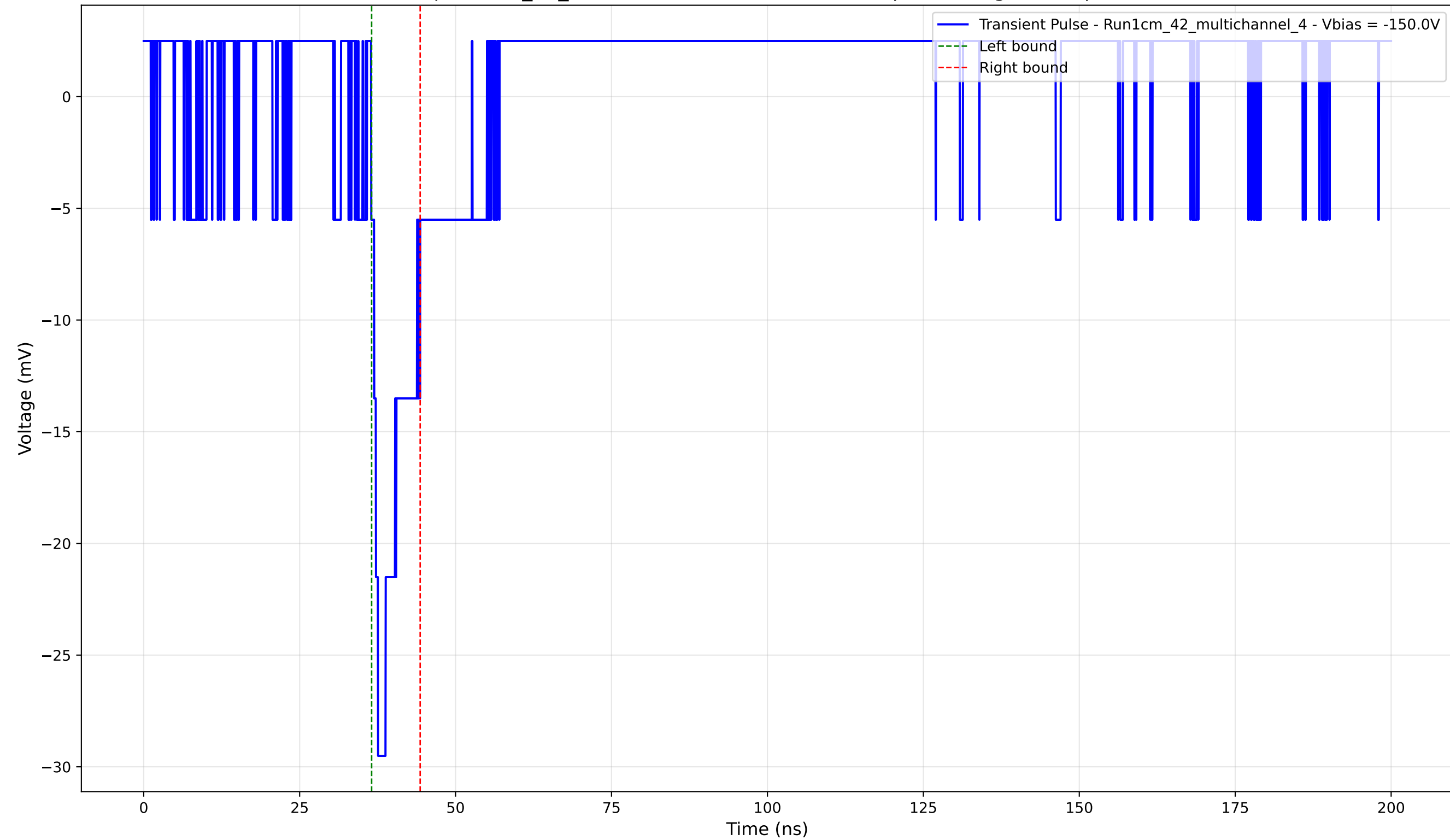
Transient Pulse - Sample: 1cm_42_multichannel - Position: 1485.0 \mu\text{m} - Charge: 2.69 pC - Rise Time: 1.12 ns
