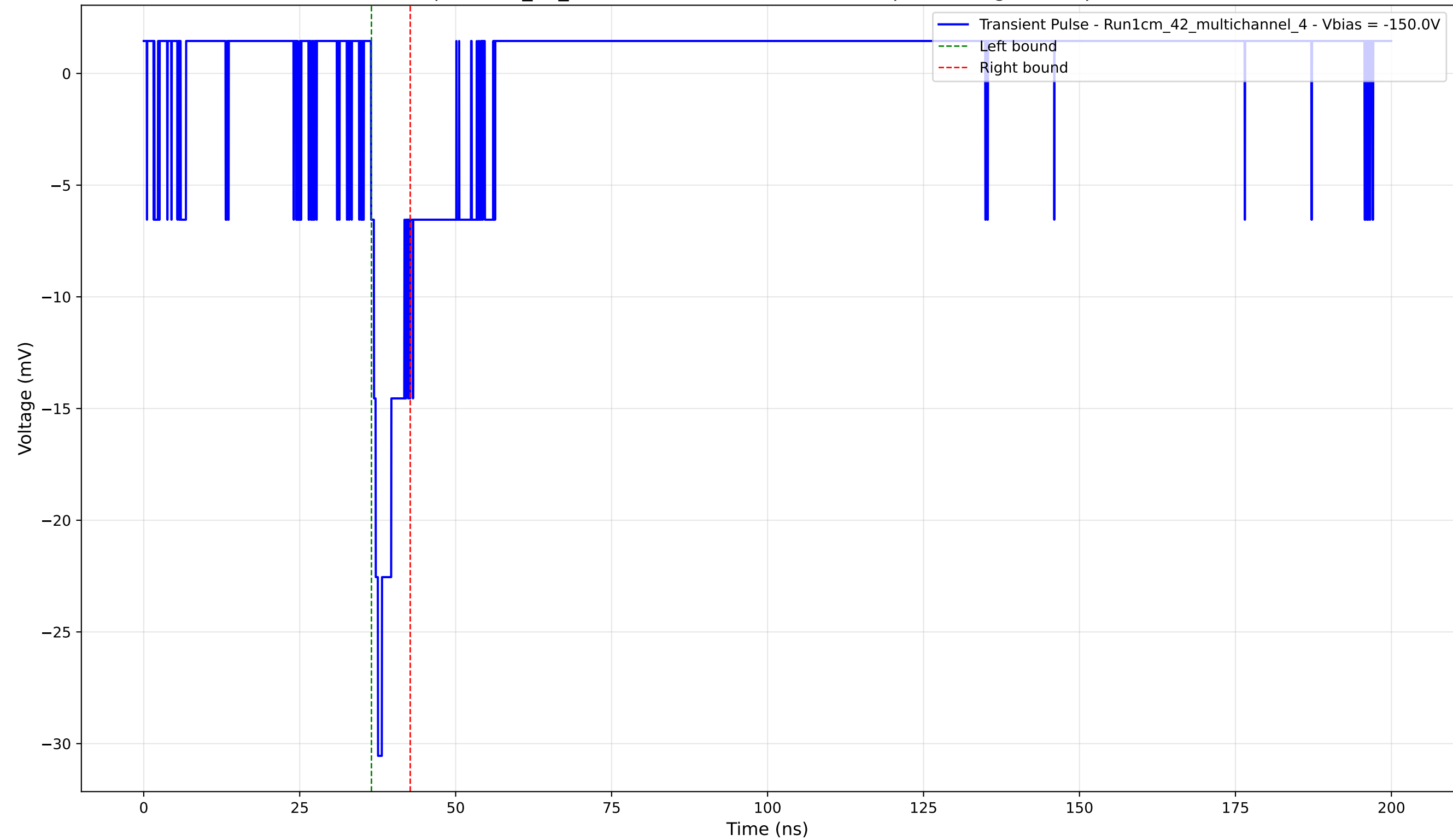
Transient Pulse - Sample: 1cm_42_multichannel - Position: 3195.0 \mu\text{m} - Charge: 2.15 pC - Rise Time: 1.11 ns
