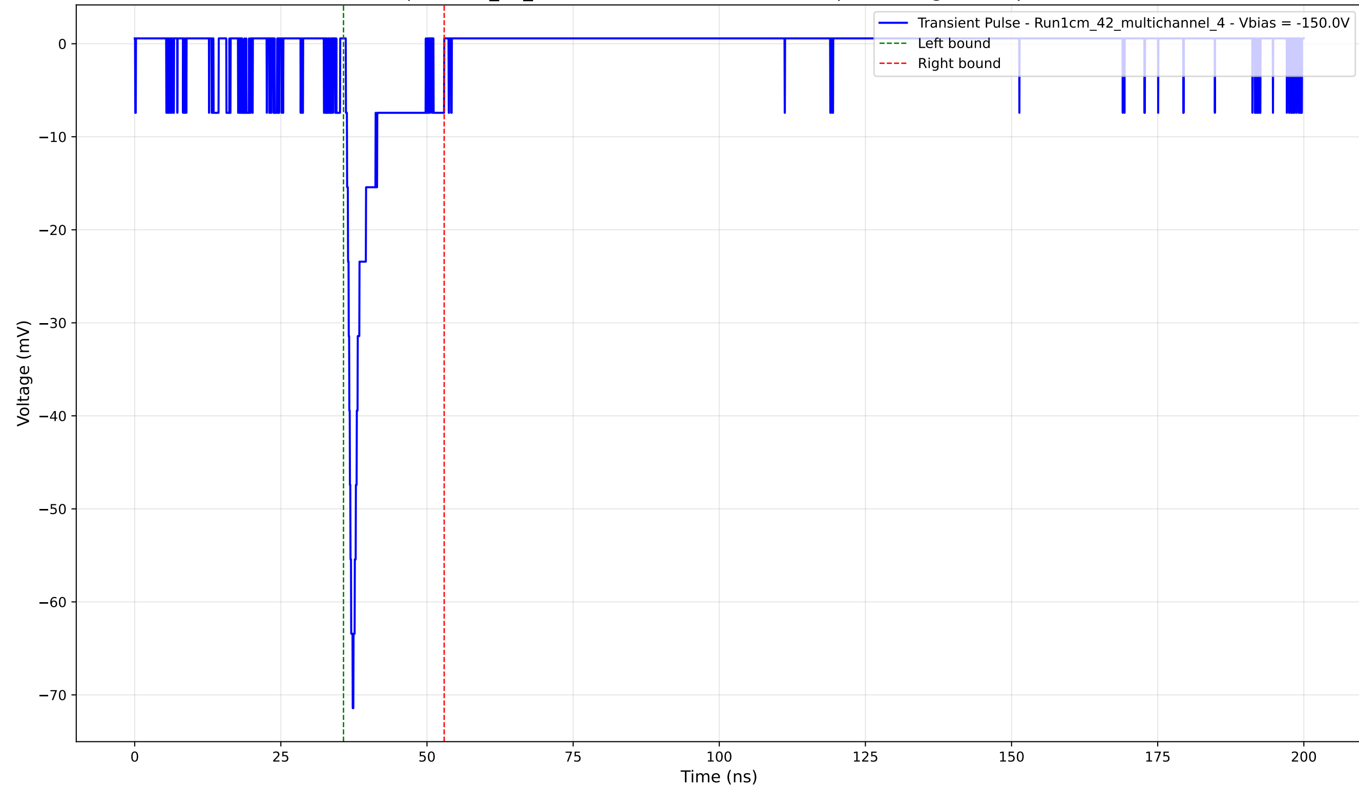
Transient Pulse - Sample: 1cm_42_multichannel - Position: 2585.0 \mu\text{m} - Charge: 4.65 pC - Rise Time: 1.16 ns
