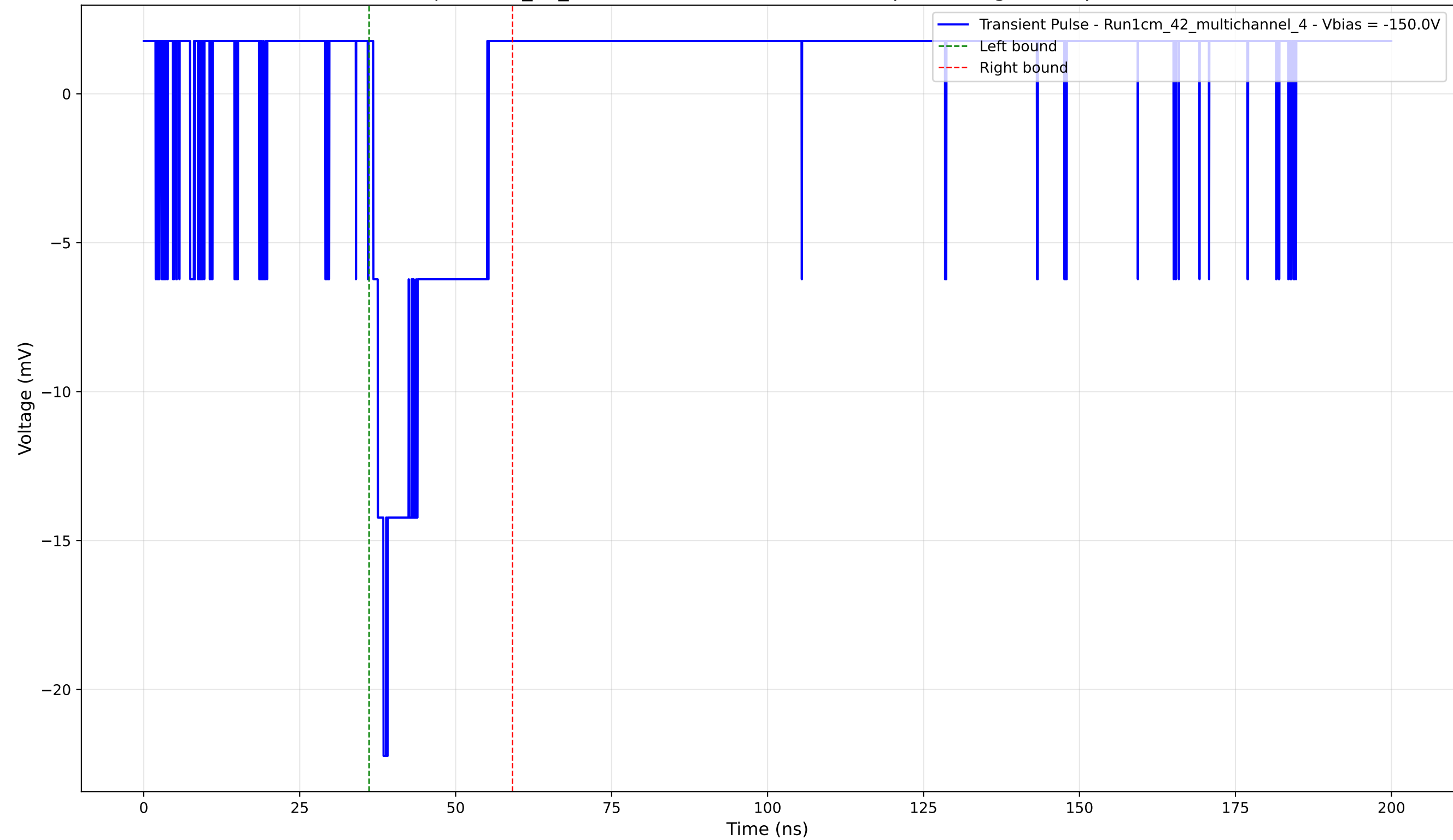
Transient Pulse - Sample: 1cm_42_multichannel - Position: 3715.0 \mu\text{m} - Charge: 3.20 pC - Rise Time: 1.64 ns
