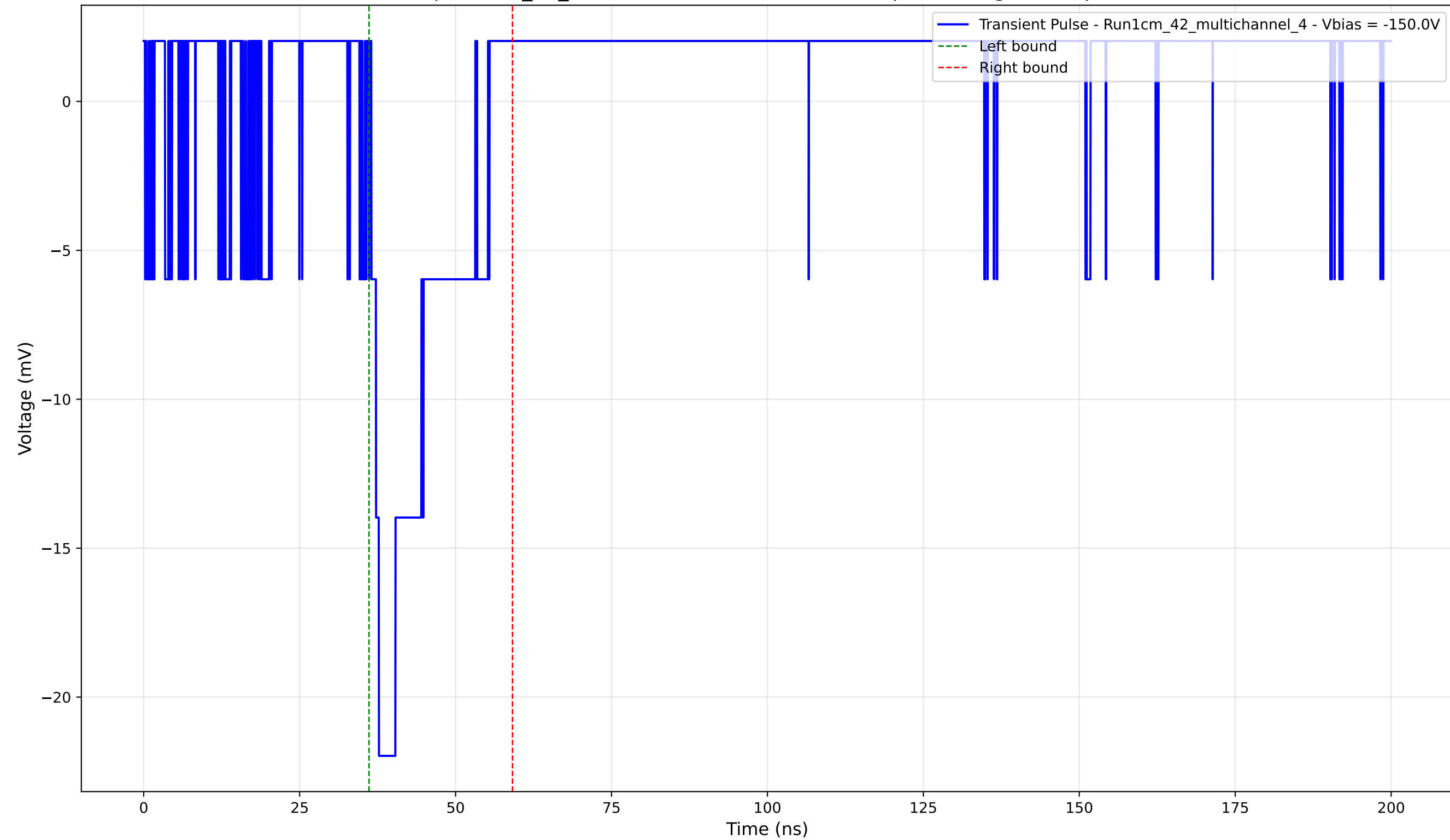
Transient Pulse - Sample: 1cm_42_multichannel - Position: 1225.0 \mu\text{m} - Charge: 3.67 pC - Rise Time: 1.22 ns
