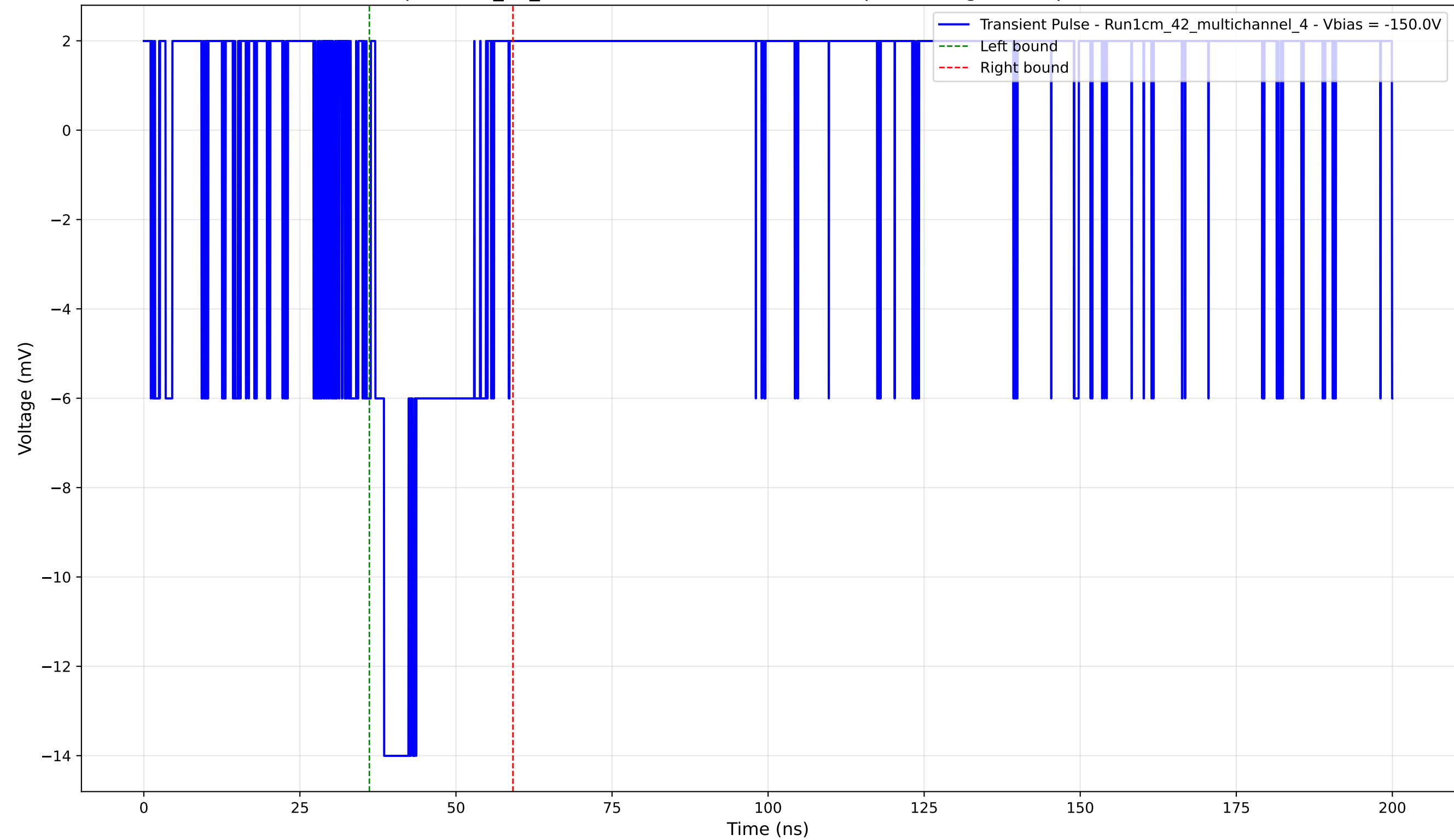
Transient Pulse - Sample: 1cm_42_multichannel - Position: 4550.0 \mu\text{m} - Charge: 2.74 pC - Rise Time: 0.00 ns (N/A)
