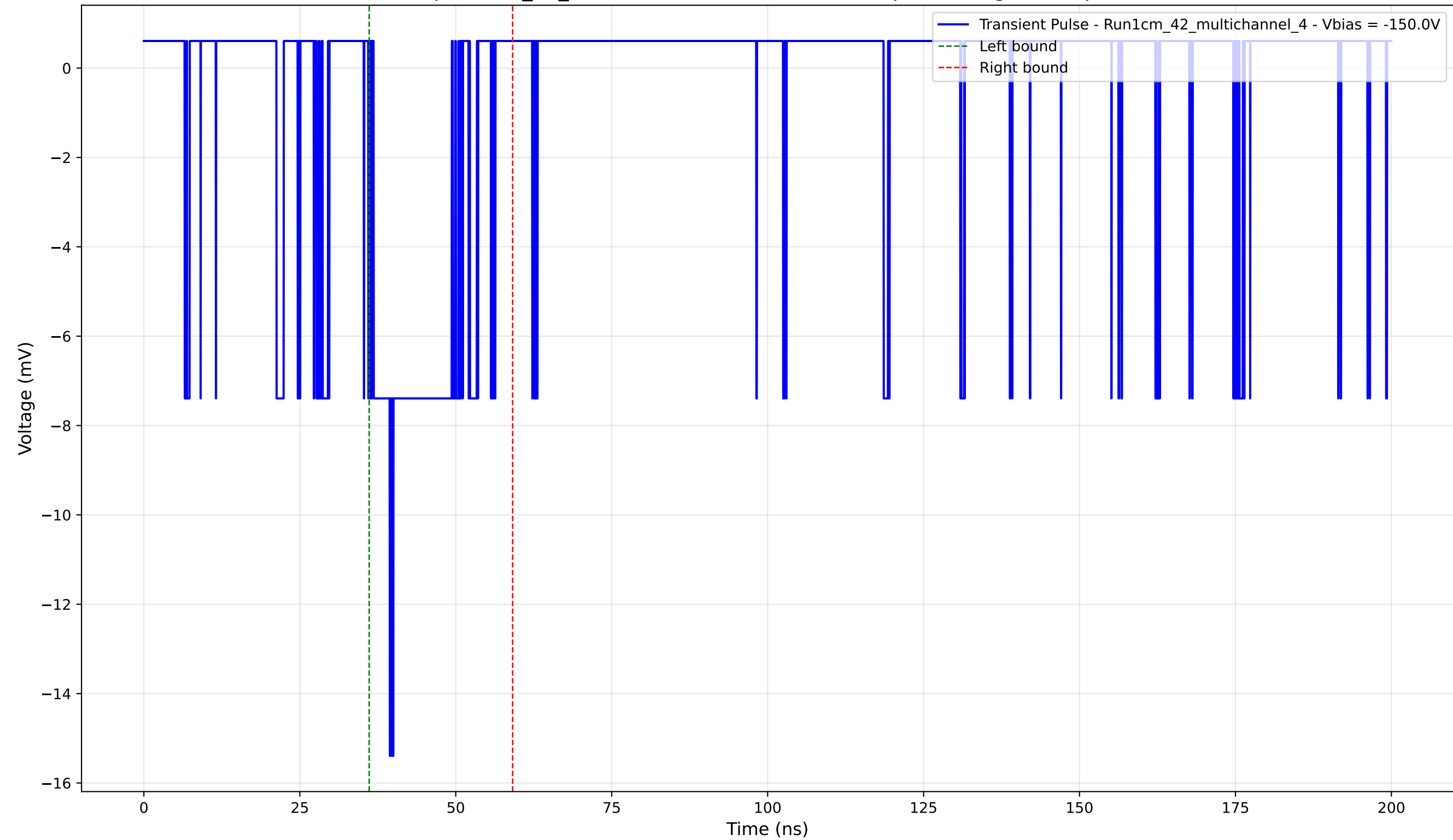
Transient Pulse - Sample: 1cm_42_multichannel - Position: 3850.0 \mu\text{m} - Charge: 2.23 pC - Rise Time: 2.60 ns
