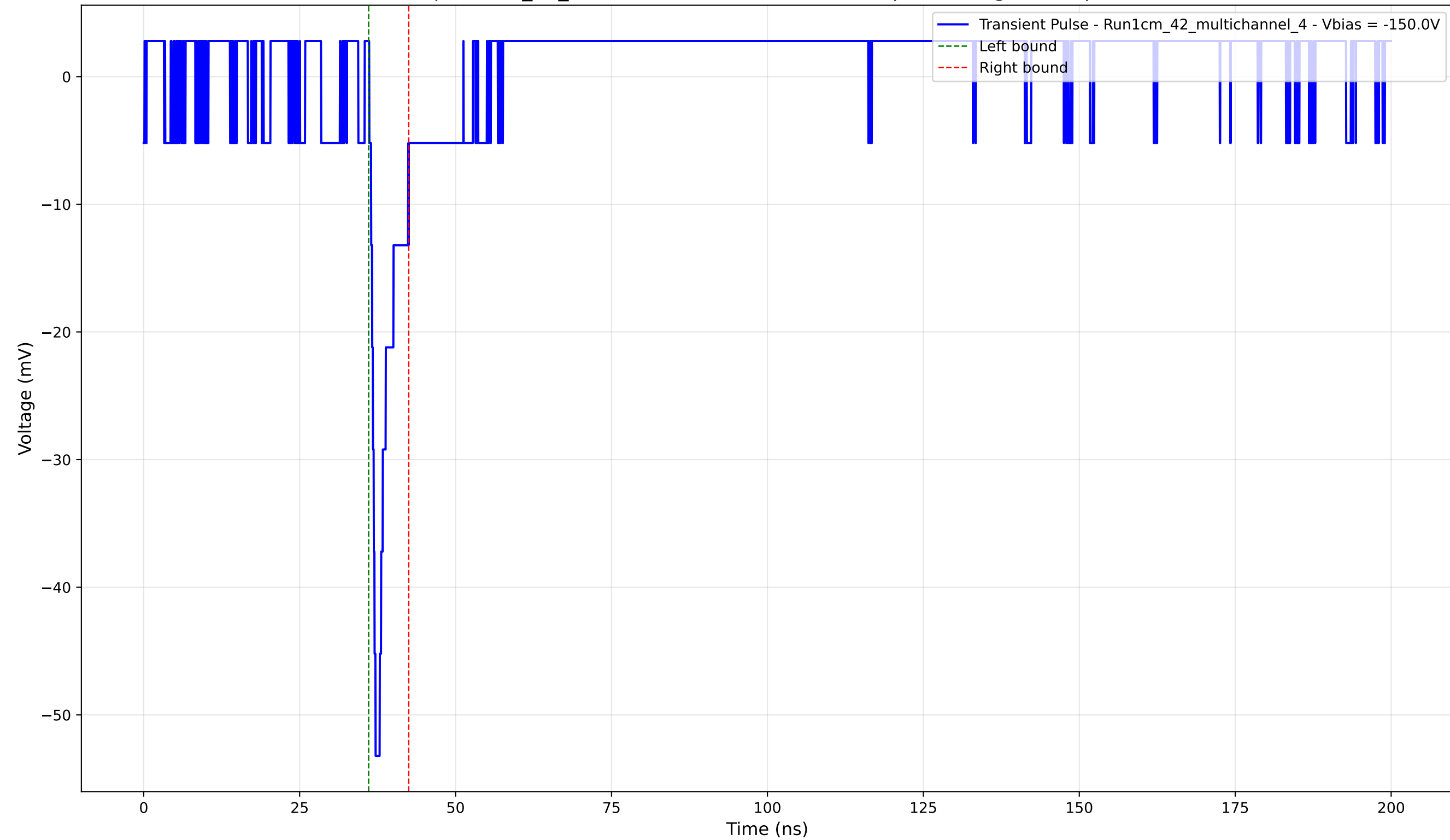
Transient Pulse - Sample: 1cm_42_multichannel - Position: 1995.0 \mu\text{m} - Charge: 2.99 pC - Rise Time: 0.72 ns
