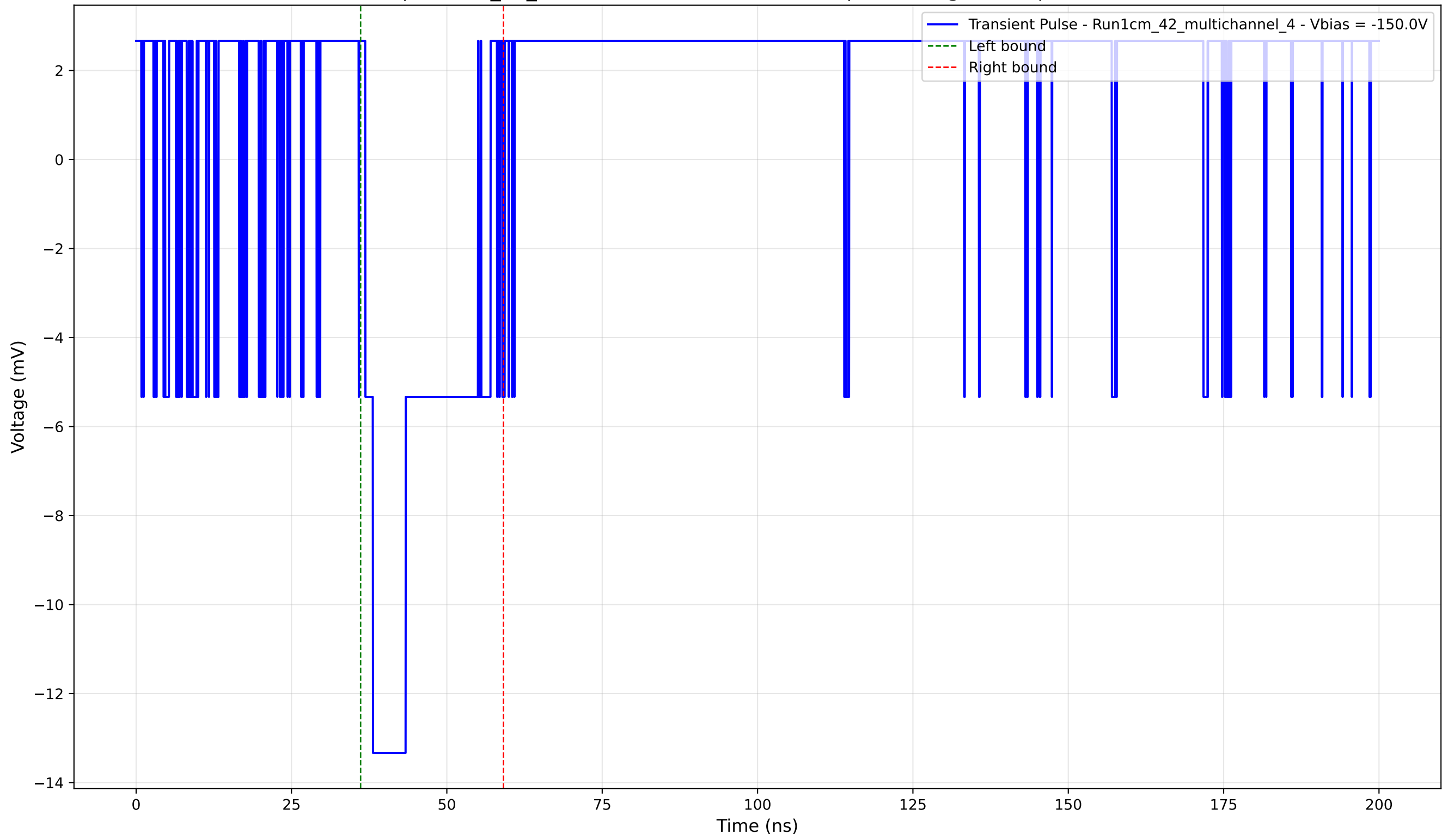
Transient Pulse - Sample: 1cm_42_multichannel - Position: 495.0 \mu\text{m} - Charge: 2.86 pC - Rise Time: 0.00 ns (N/A)
