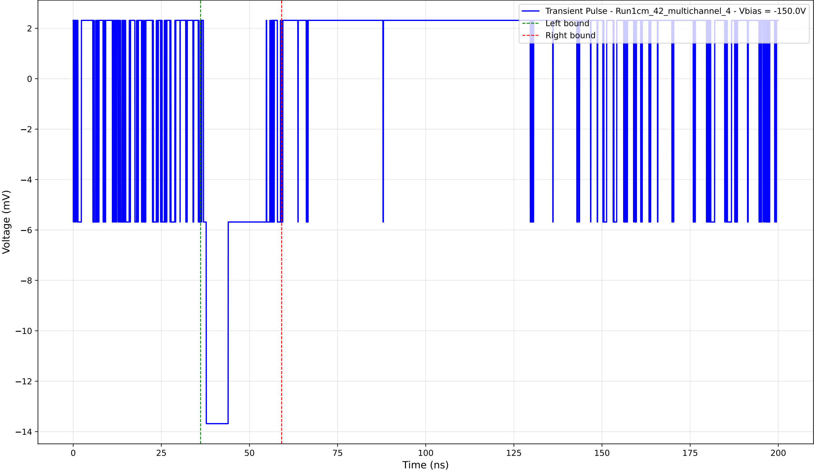
Transient Pulse - Sample: 1cm_42_multichannel - Position: 735.0 \mu\text{m} - Charge: 3.27 pC - Rise Time: 0.00 ns (N/A)
