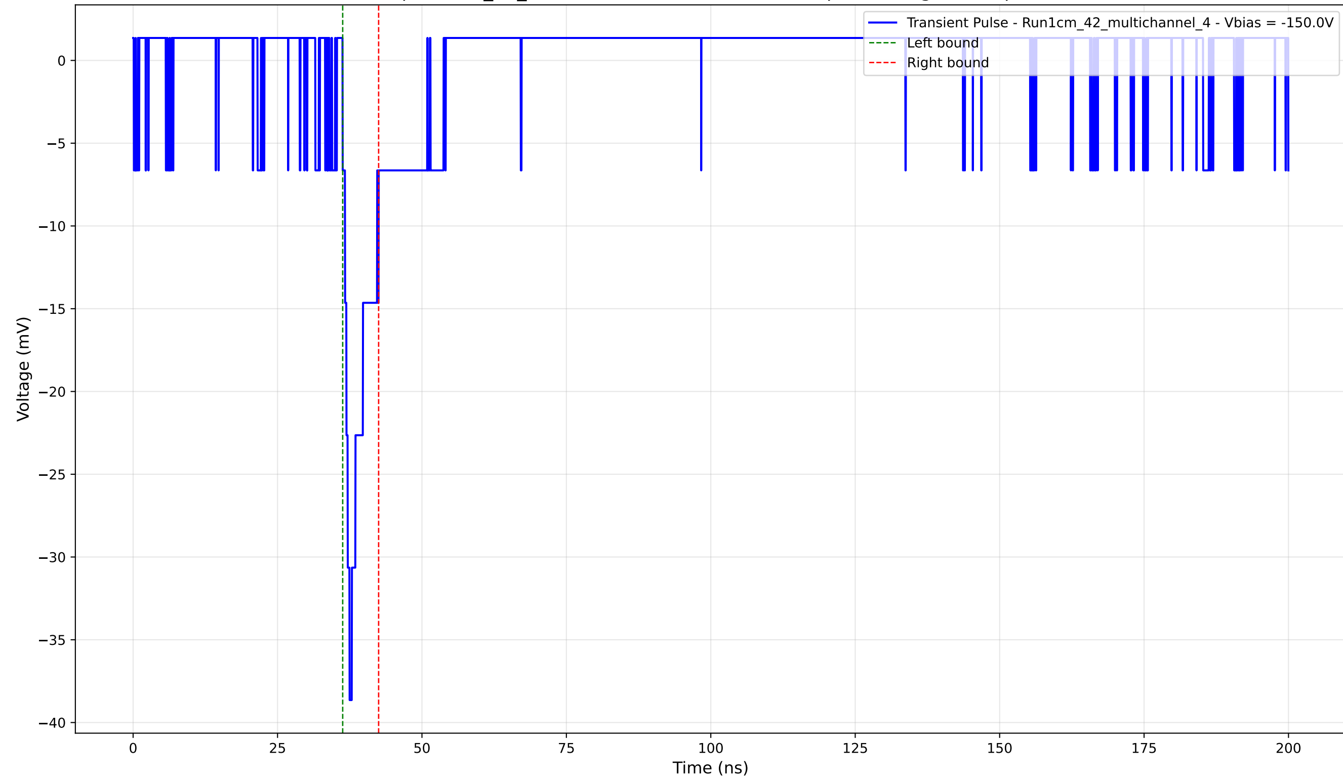
Transient Pulse - Sample: 1cm_42_multichannel - Position: 3030.0 \mu\text{m} - Charge: 2.47 pC - Rise Time: 1.21 ns
