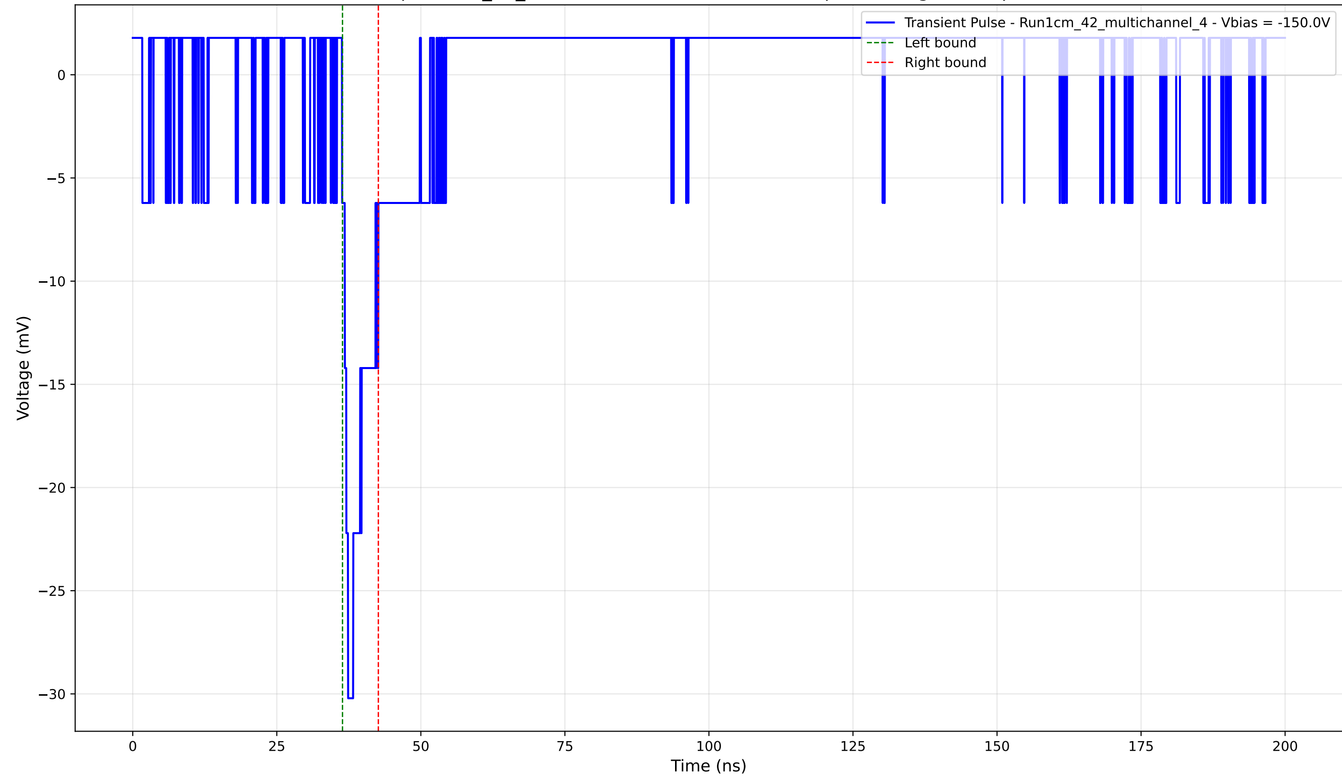
Transient Pulse - Sample: 1cm_42_multichannel - Position: 3090.0 \mu\text{m} - Charge: 2.20 pC - Rise Time: 1.05 ns
