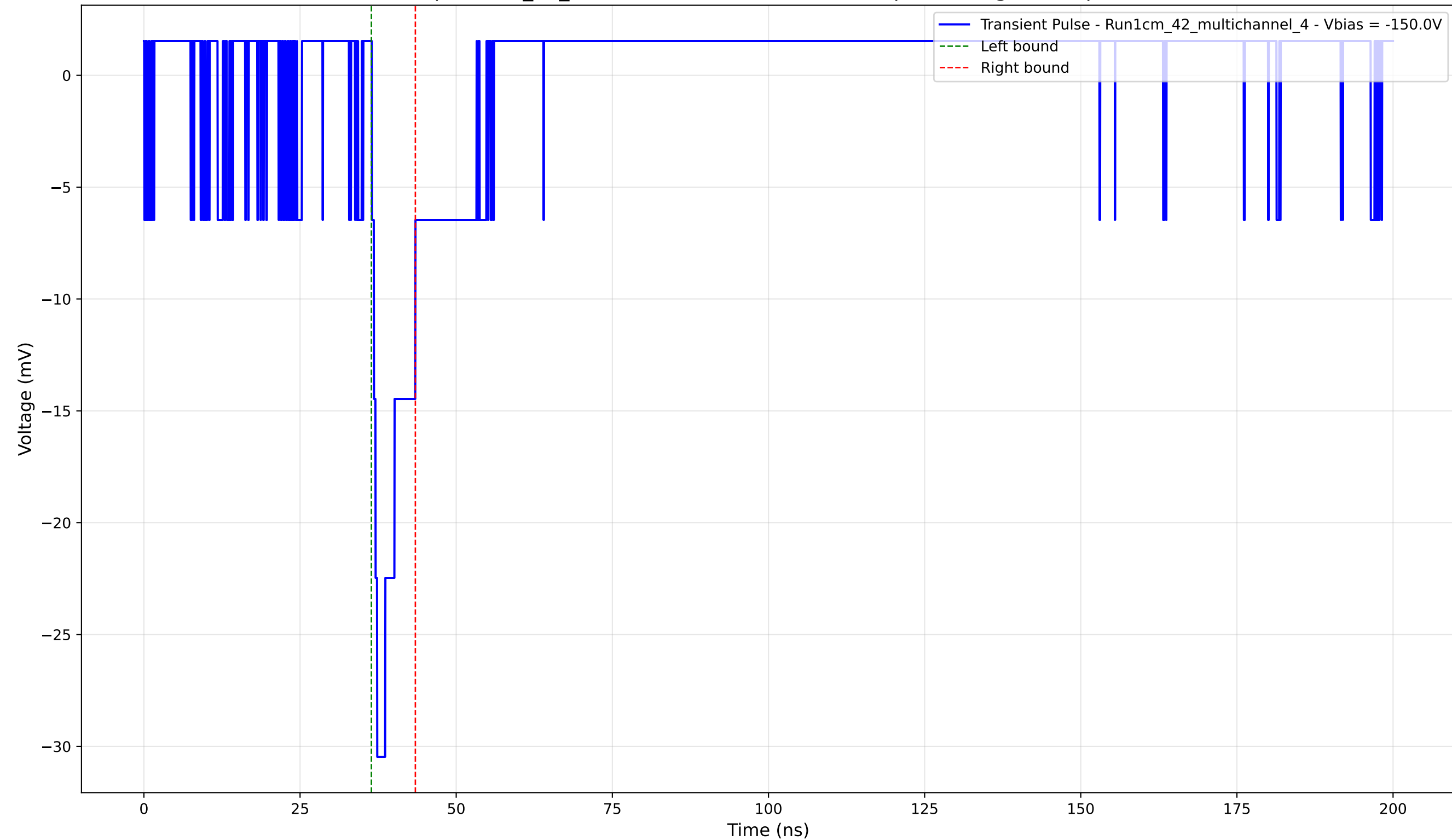
Transient Pulse - Sample: 1cm_42_multichannel - Position: 1615.0 \mu\text{m} - Charge: 2.66 pC - Rise Time: 0.85 ns
