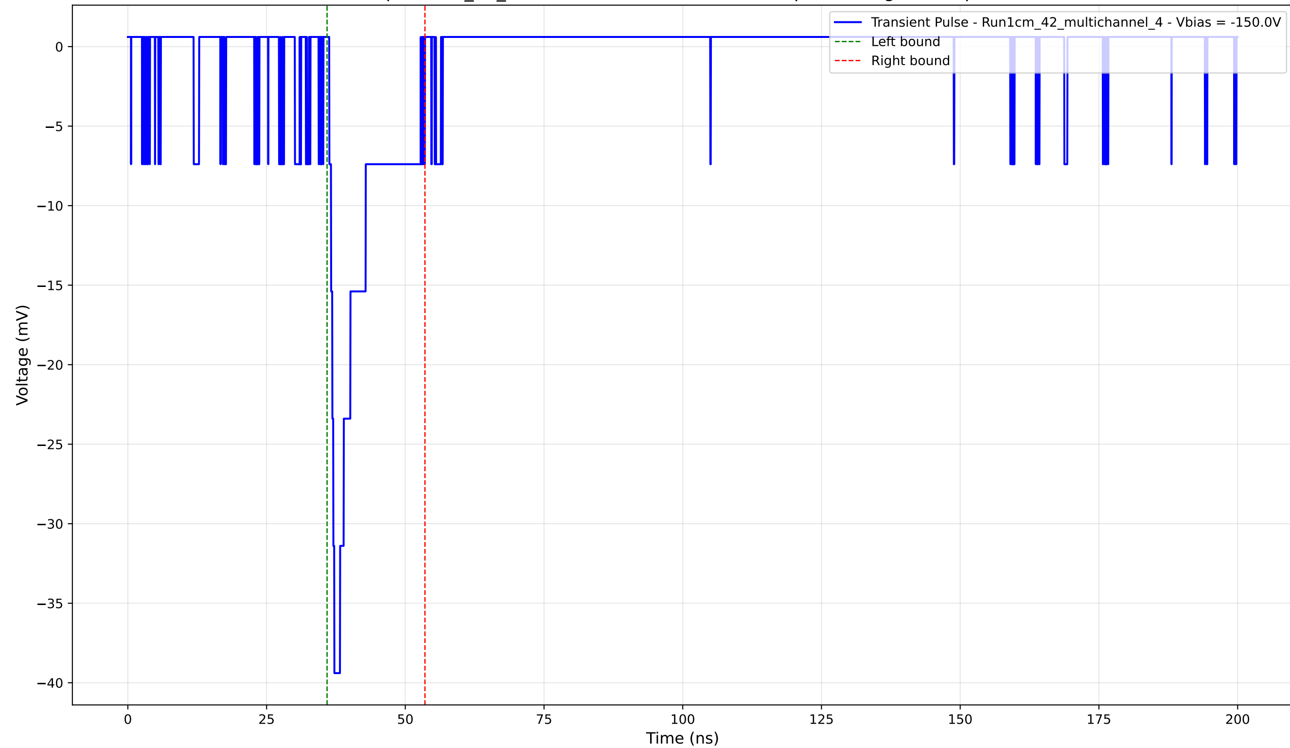
Transient Pulse - Sample: 1cm_42_multichannel - Position: 1770.0 \mu\text{m} - Charge: 4.49 pC - Rise Time: 0.91 ns
