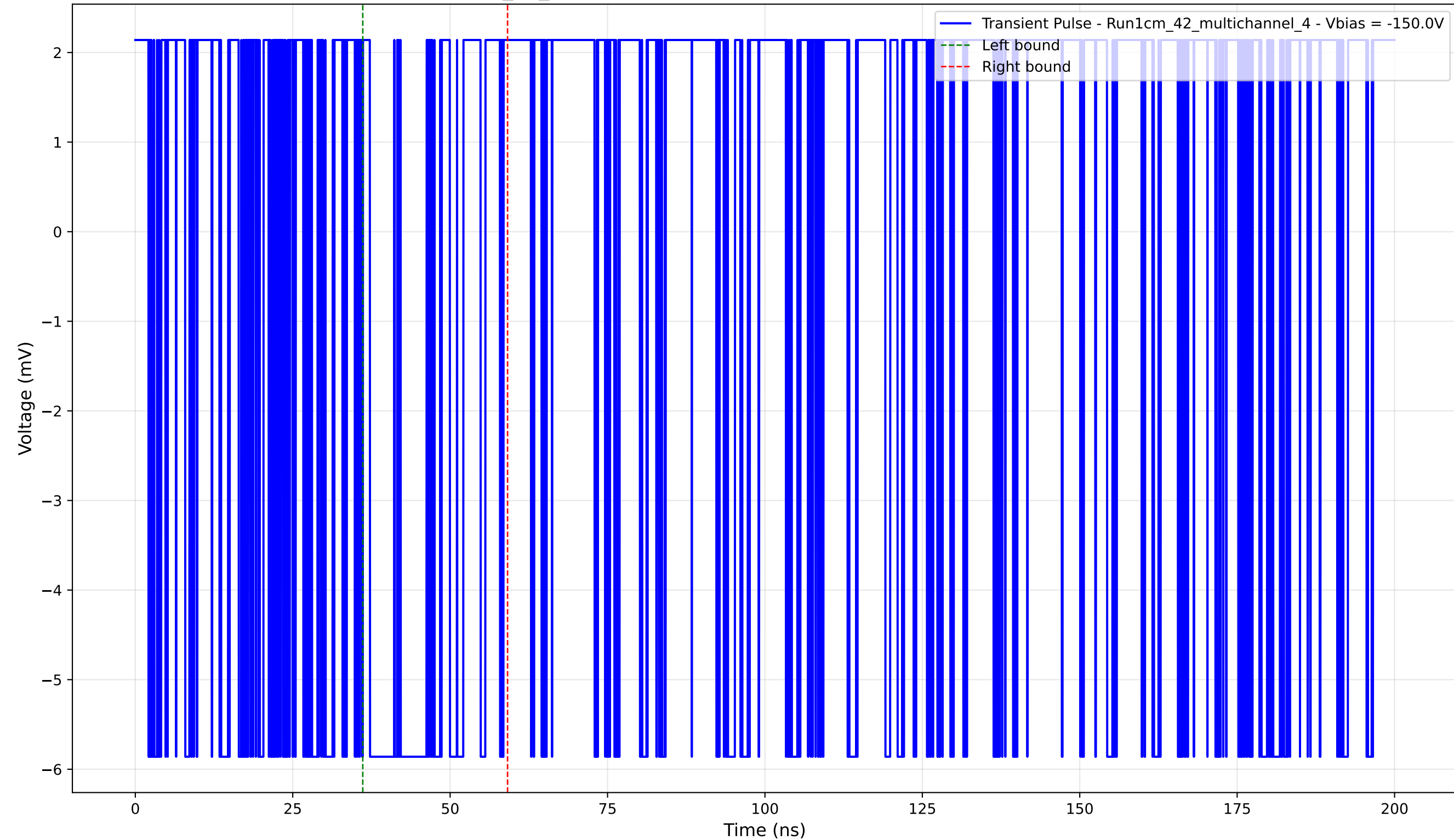
Transient Pulse - Sample: 1cm_42_multichannel - Position: 75.0 \mu\text{m} - Charge: 1.21 pC - Rise Time: 0.00 ns (N/A)
