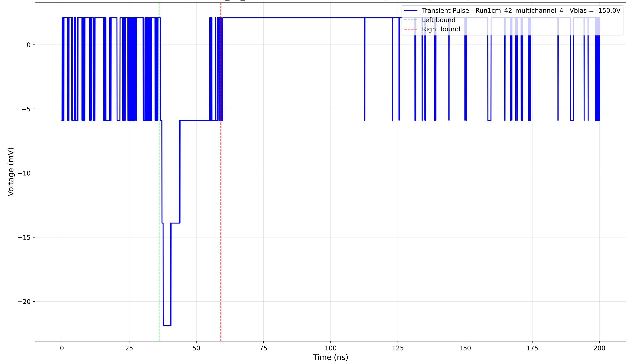
Transient Pulse - Sample: 1cm_42_multichannel - Position: 1205.0 \mu\text{m} - Charge: 3.96 pC - Rise Time: 1.10 ns
