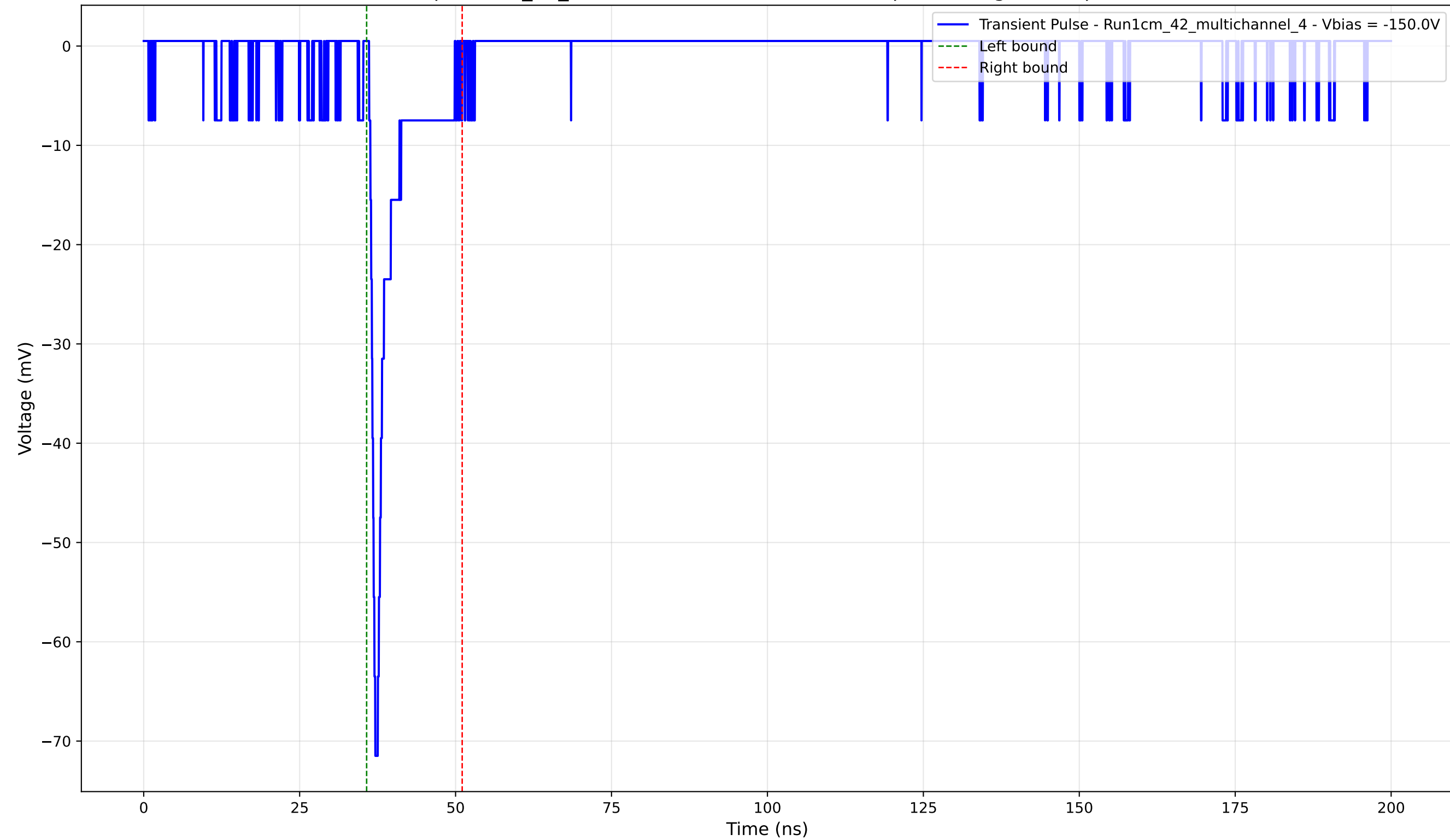
Transient Pulse - Sample: 1cm_42_multichannel - Position: 2195.0 \mu\text{m} - Charge: 4.53 pC - Rise Time: 0.98 ns
