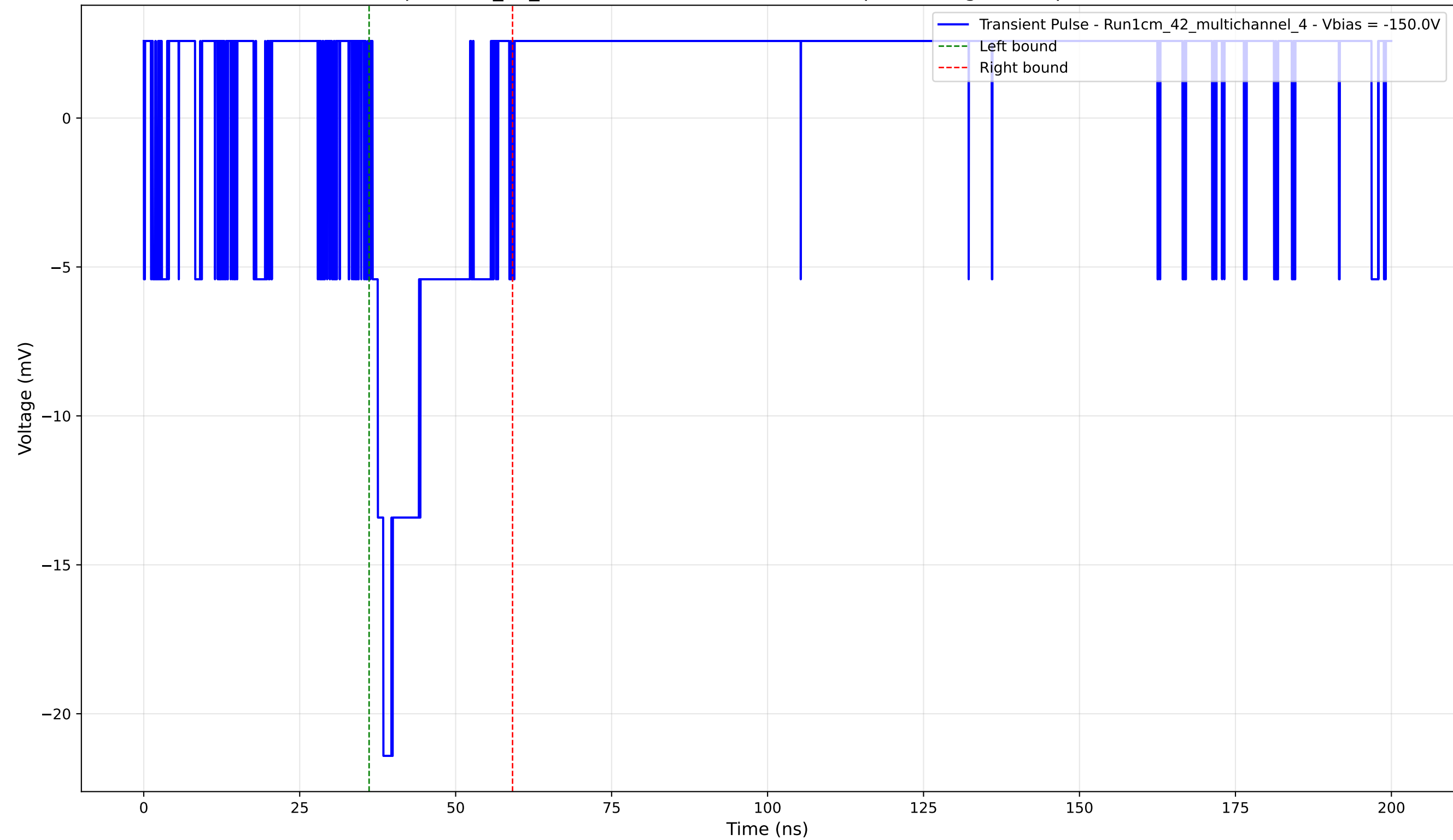
Transient Pulse - Sample: 1cm_42_multichannel - Position: 1060.0 \mu\text{m} - Charge: 3.28 pC - Rise Time: 0.00 ns (N/A)
