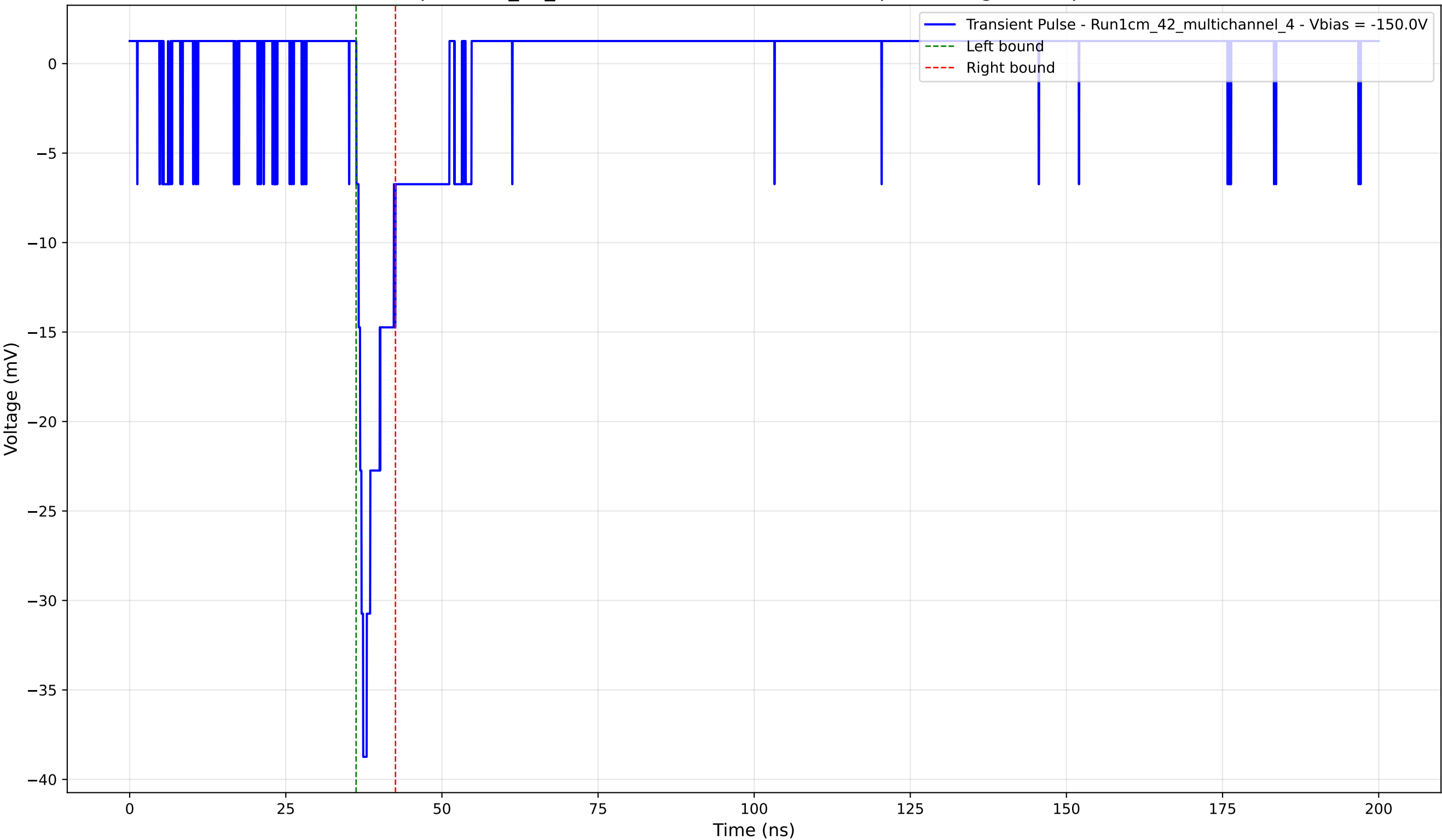
Transient Pulse - Sample: 1cm_42_multichannel - Position: 3025.0 \mu\text{m} - Charge: 2.60 pC - Rise Time: 1.09 ns
