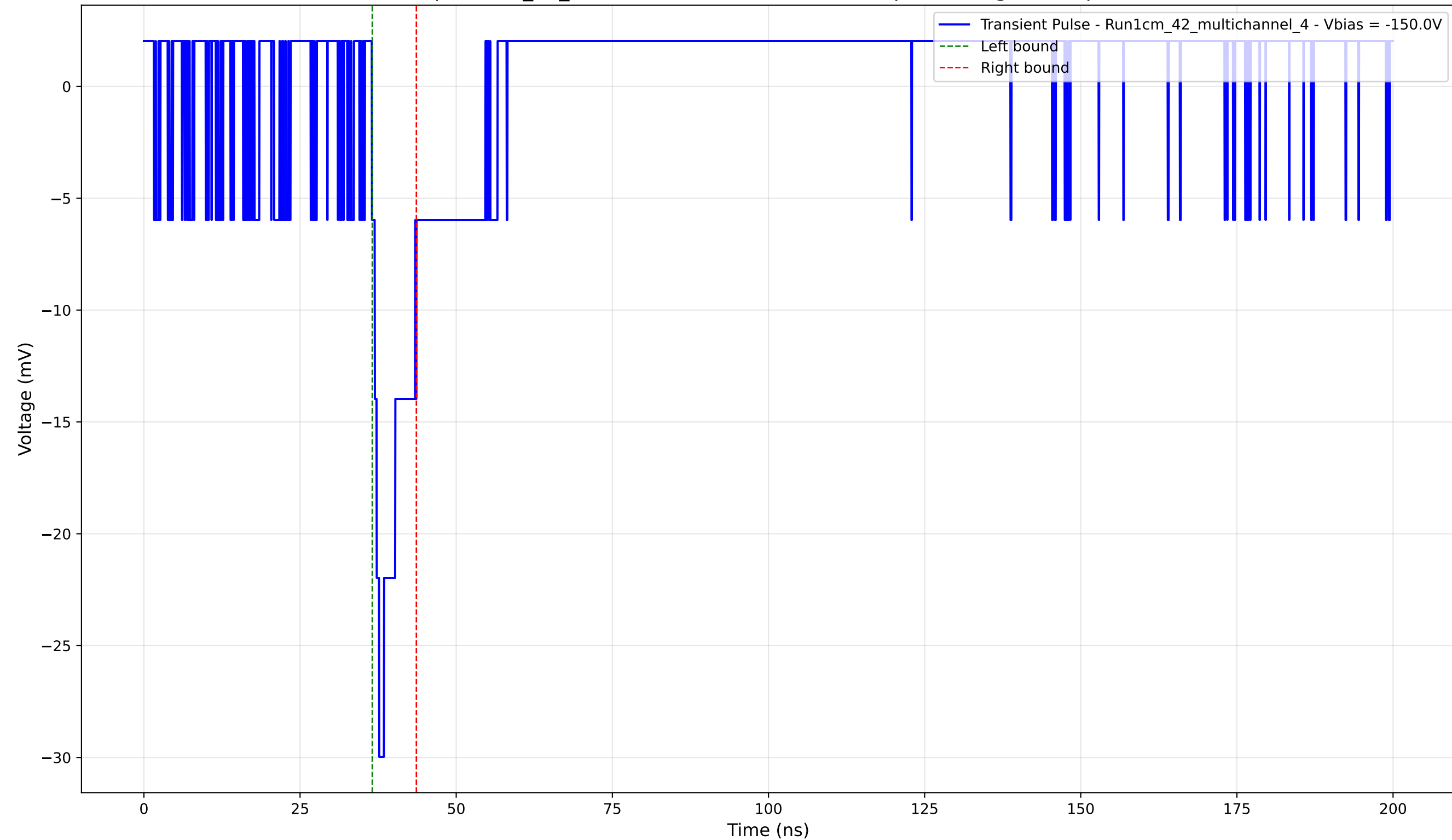
Transient Pulse - Sample: 1cm_42_multichannel - Position: 1475.0 \mu\text{m} - Charge: 2.49 pC - Rise Time: 1.18 ns
