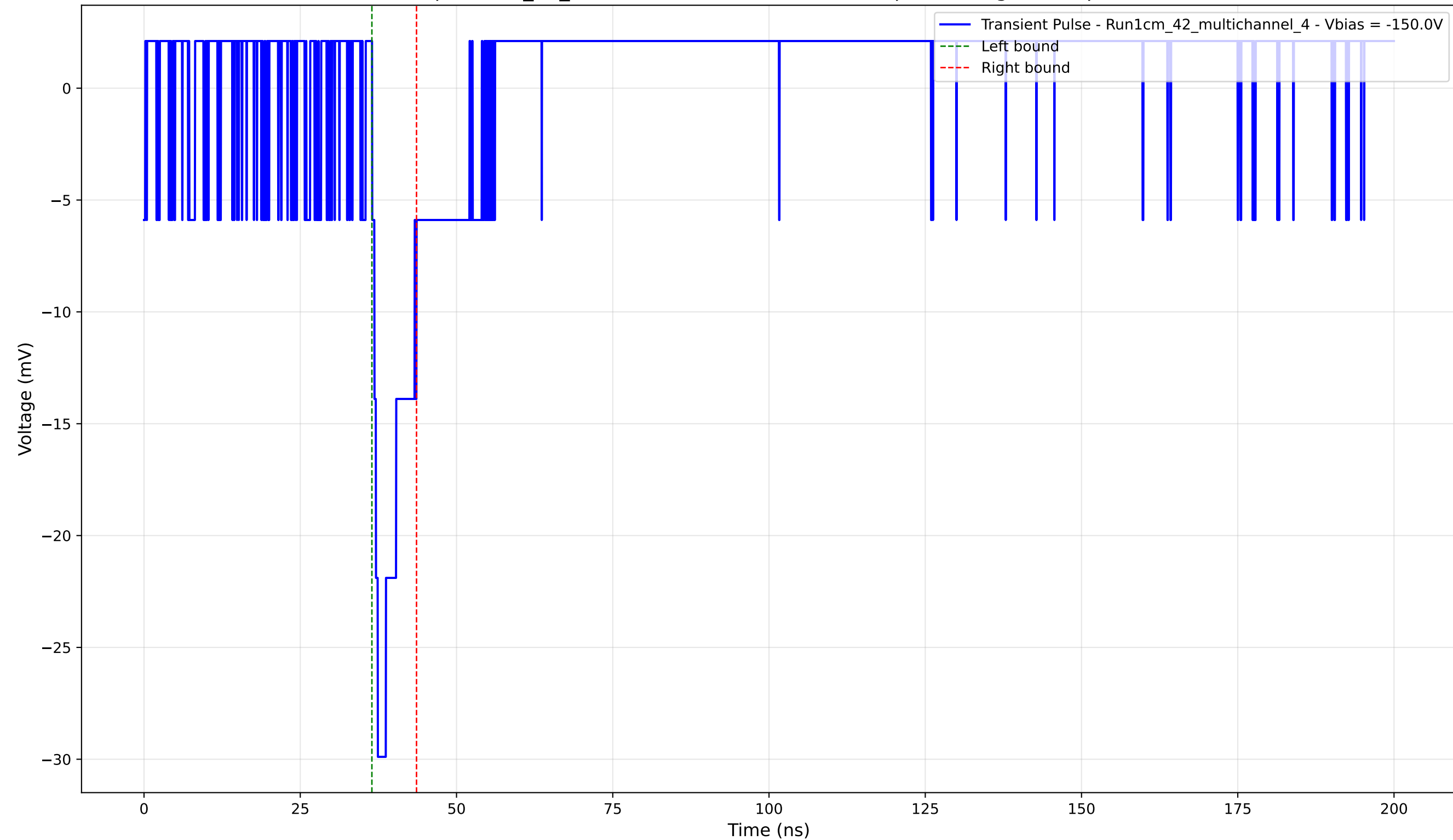
Transient Pulse - Sample: 1cm_42_multichannel - Position: 1570.0 \mu\text{m} - Charge: 2.62 pC - Rise Time: 0.92 ns
