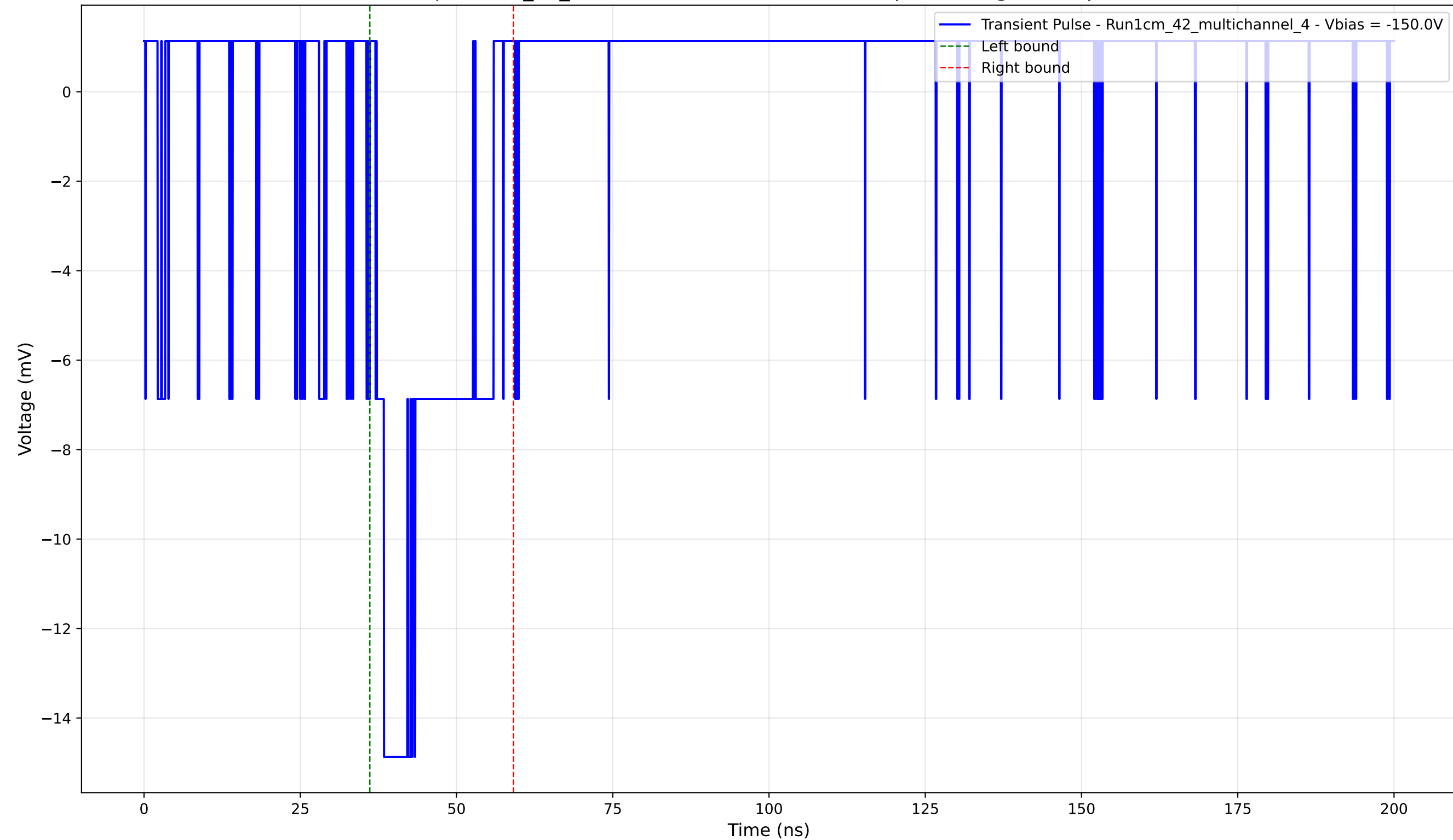
Transient Pulse - Sample: 1cm_42_multichannel - Position: 4185.0 \mu\text{m} - Charge: 3.19 pC - Rise Time: 1.16 ns
