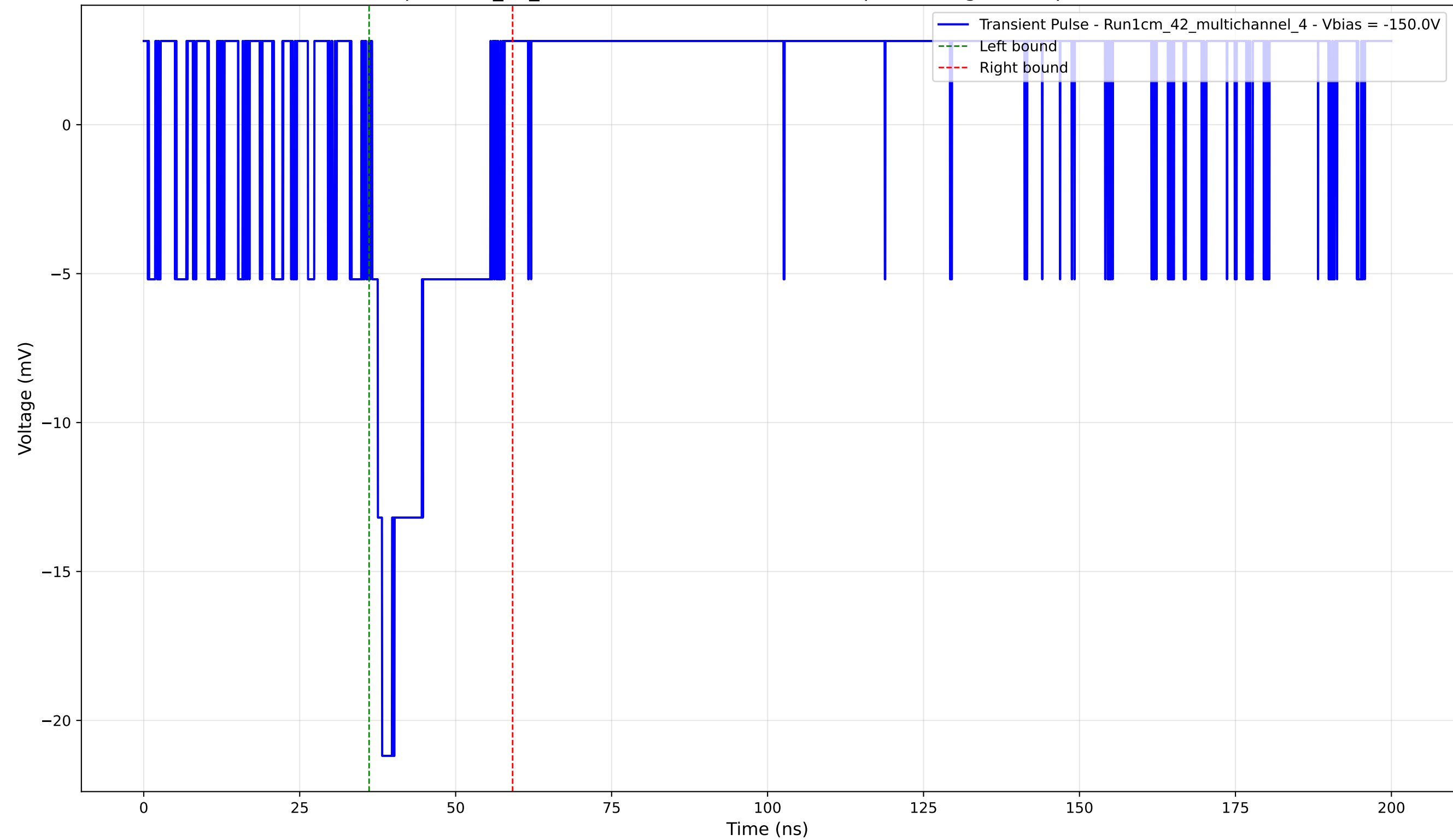
Transient Pulse - Sample: 1cm_42_multichannel - Position: 1020.0 \mu\text{m} - Charge: 3.39 pC - Rise Time: 0.00 ns (N/A)
