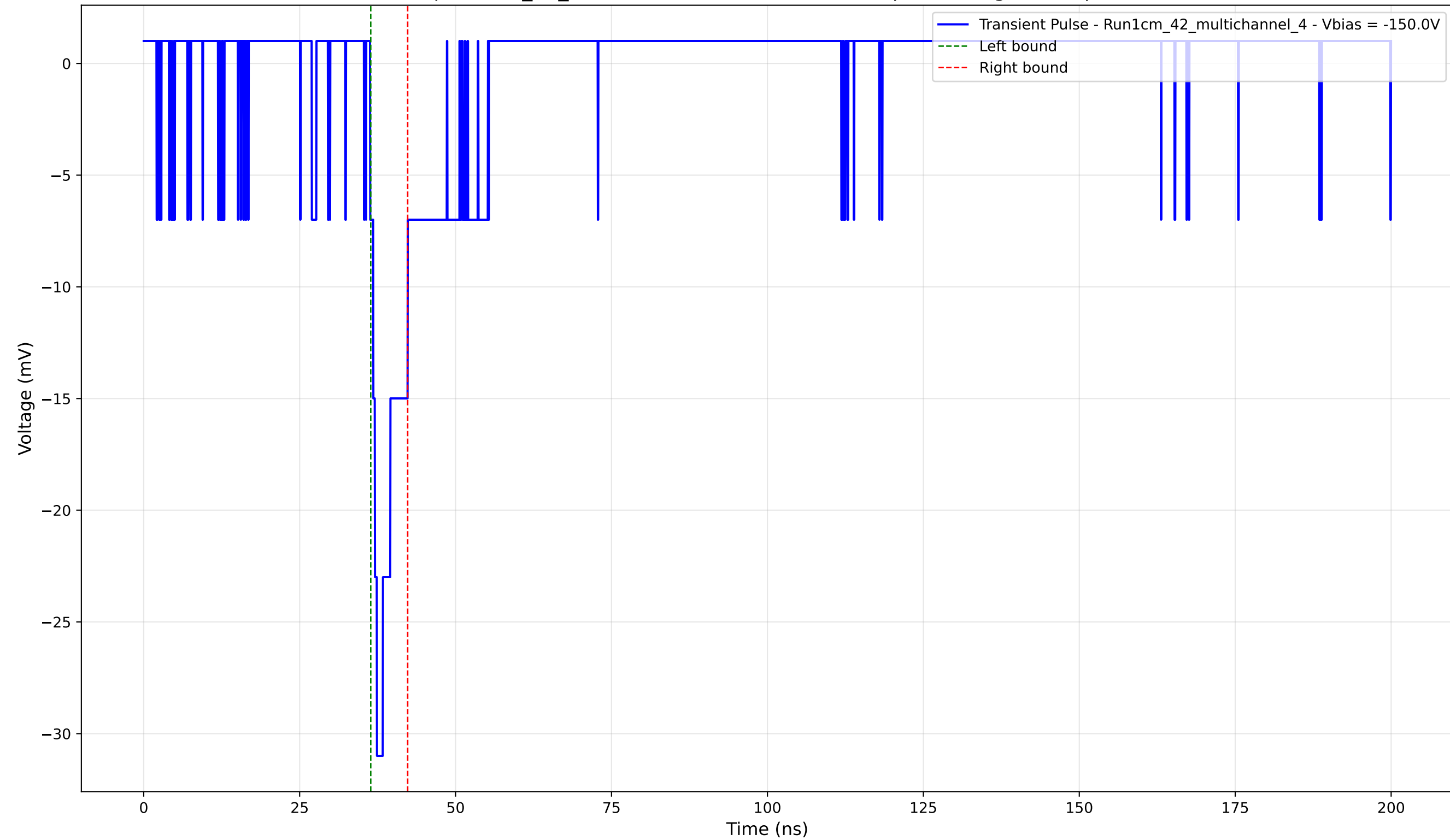
Transient Pulse - Sample: 1cm_42_multichannel - Position: 3135.0 \mu\text{m} - Charge: 2.26 pC - Rise Time: 1.09 ns
