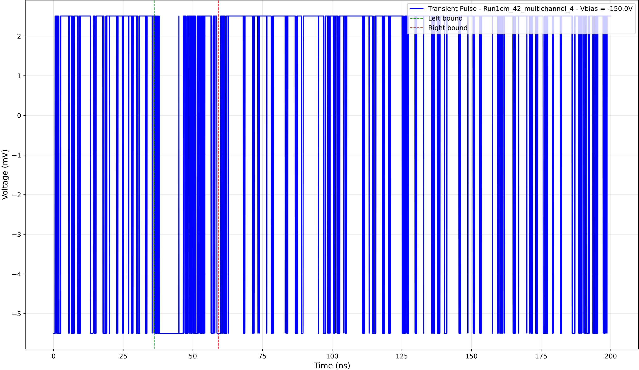
Transient Pulse - Sample: 1cm_42_multichannel - Position: 4370.0 \mu\text{m} - Charge: 1.07 pC - Rise Time: 0.00 ns (N/A)
