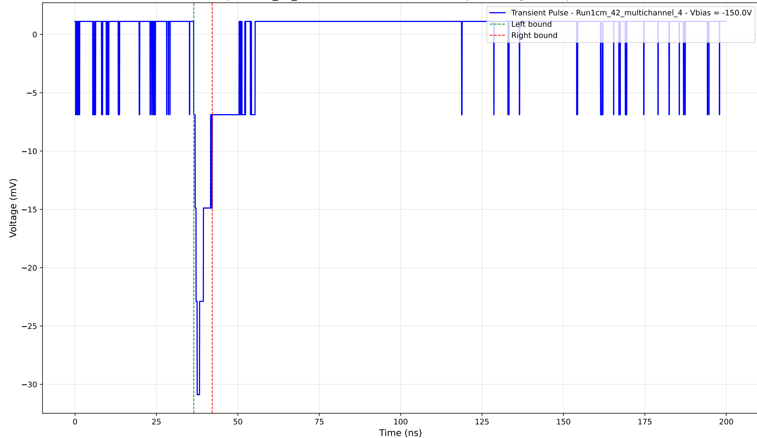
Transient Pulse - Sample: 1cm_42_multichannel - Position: 3150.0 \mu\text{m} - Charge: 2.06 pC - Rise Time: 1.07 ns
