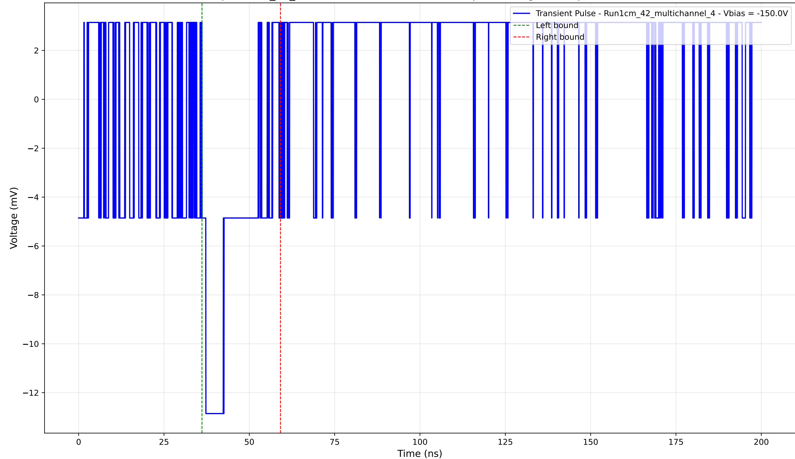
Transient Pulse - Sample: 1cm_42_multichannel - Position: 1315.0 \mu\text{m} - Charge: 2.56 pC - Rise Time: 0.00 ns (N/A)
