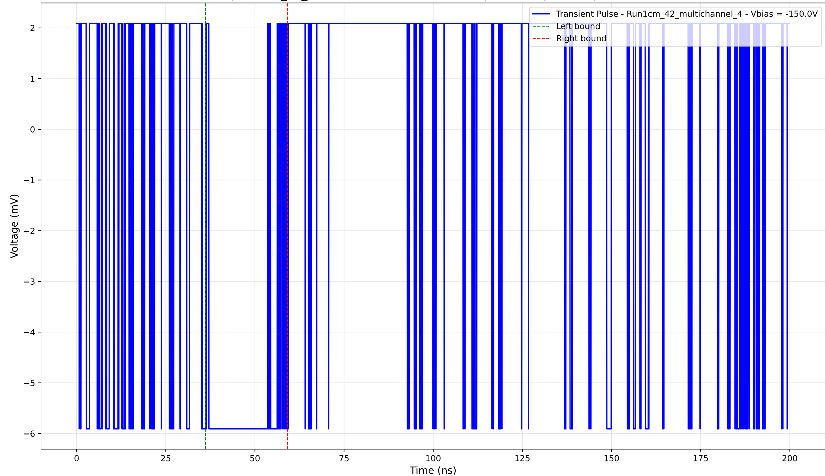
Transient Pulse - Sample: 1cm_42_multichannel - Position: 415.0 \mu\text{m} - Charge: 2.28 pC - Rise Time: 0.00 ns (N/A)
