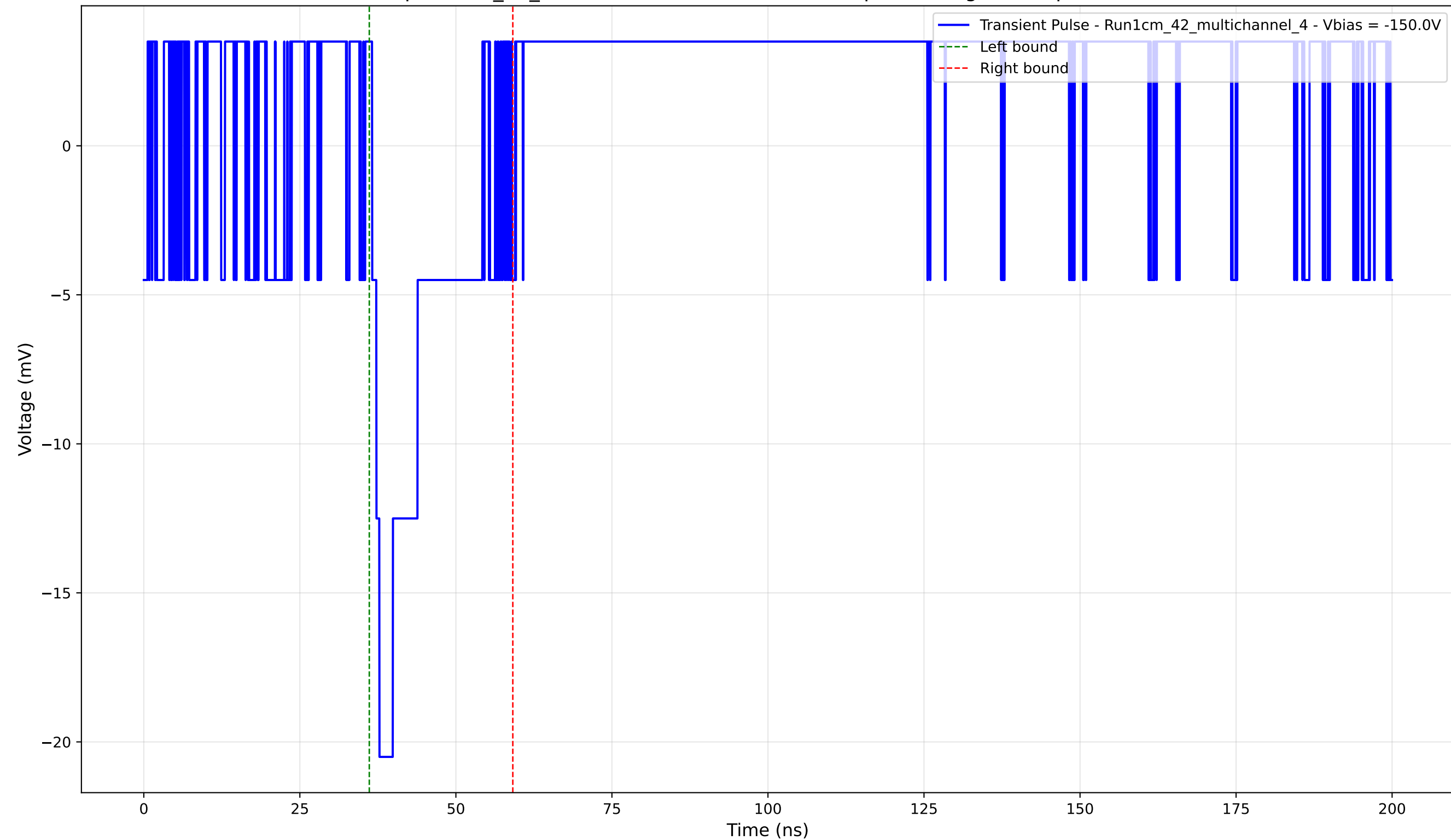
Transient Pulse - Sample: 1cm_42_multichannel - Position: 1195.0 \mu\text{m} - Charge: 3.02 pC - Rise Time: 0.00 ns (N/A)
