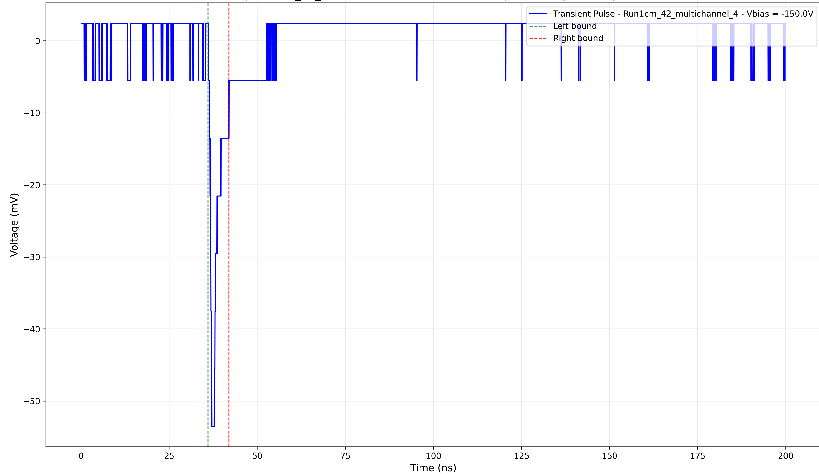
Transient Pulse - Sample: 1cm_42_multichannel - Position: 2685.0 \mu\text{m} - Charge: 2.80 pC - Rise Time: 0.90 ns
