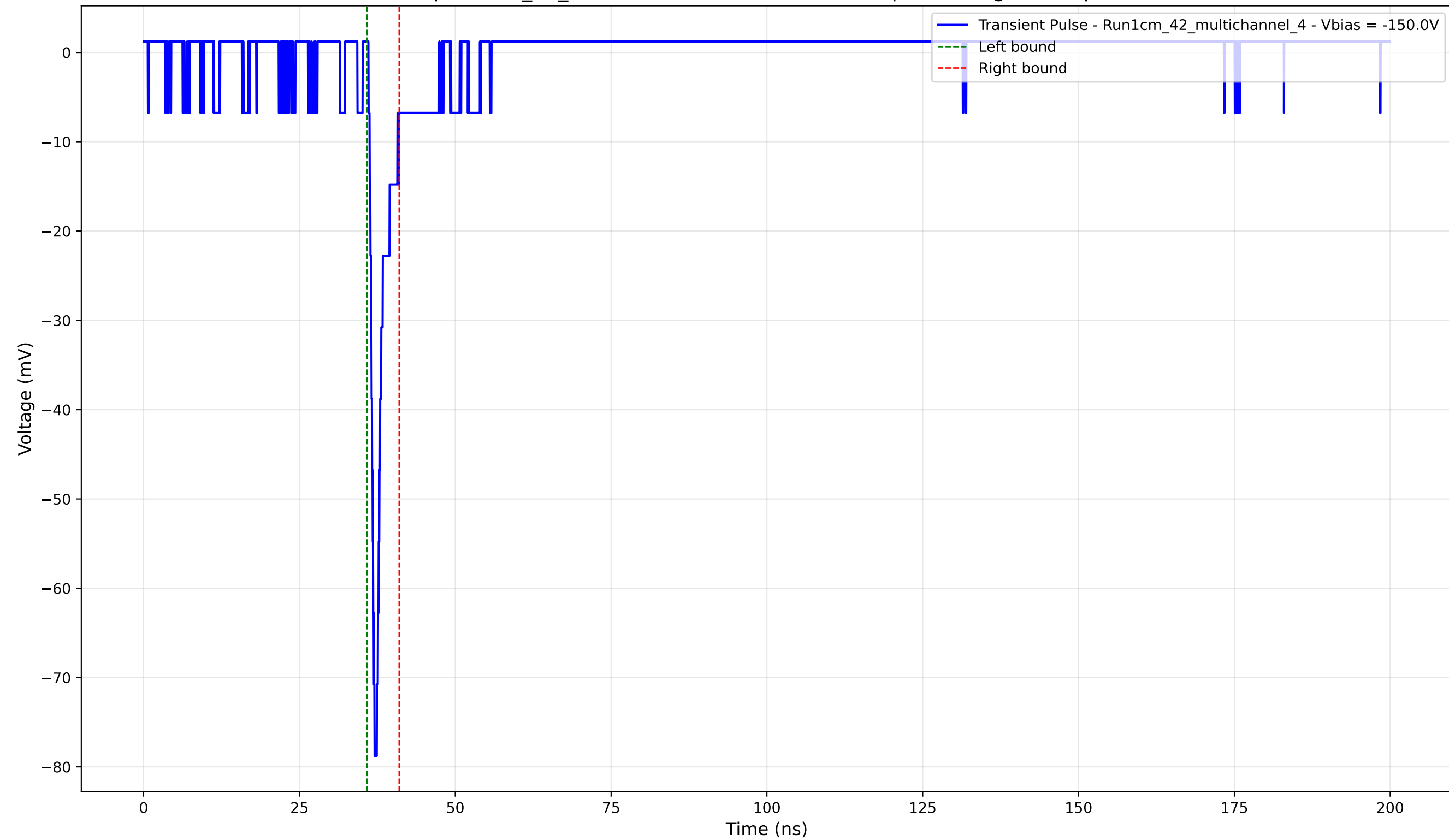
Transient Pulse - Sample: 1cm_42_multichannel - Position: 2460.0 \mu\text{m} - Charge: 3.13 pC - Rise Time: 0.80 ns
