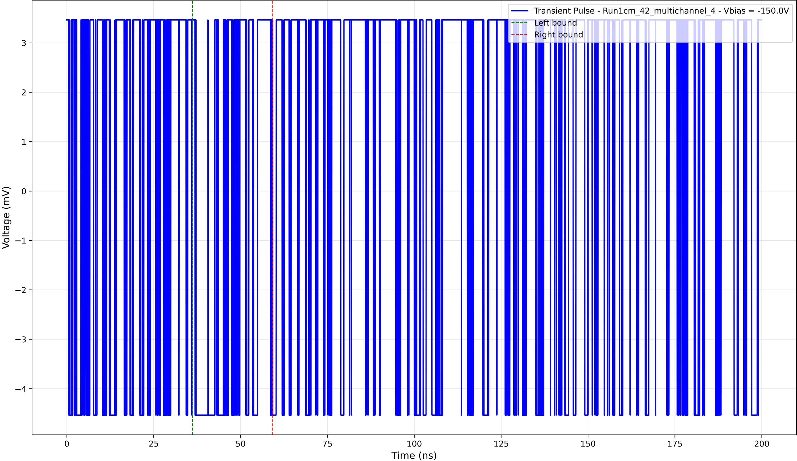
Transient Pulse - Sample: 1cm_42_multichannel - Position: 1345.0 \mu\text{m} - Charge: 0.17 pC - Rise Time: 0.00 ns (N/A)
