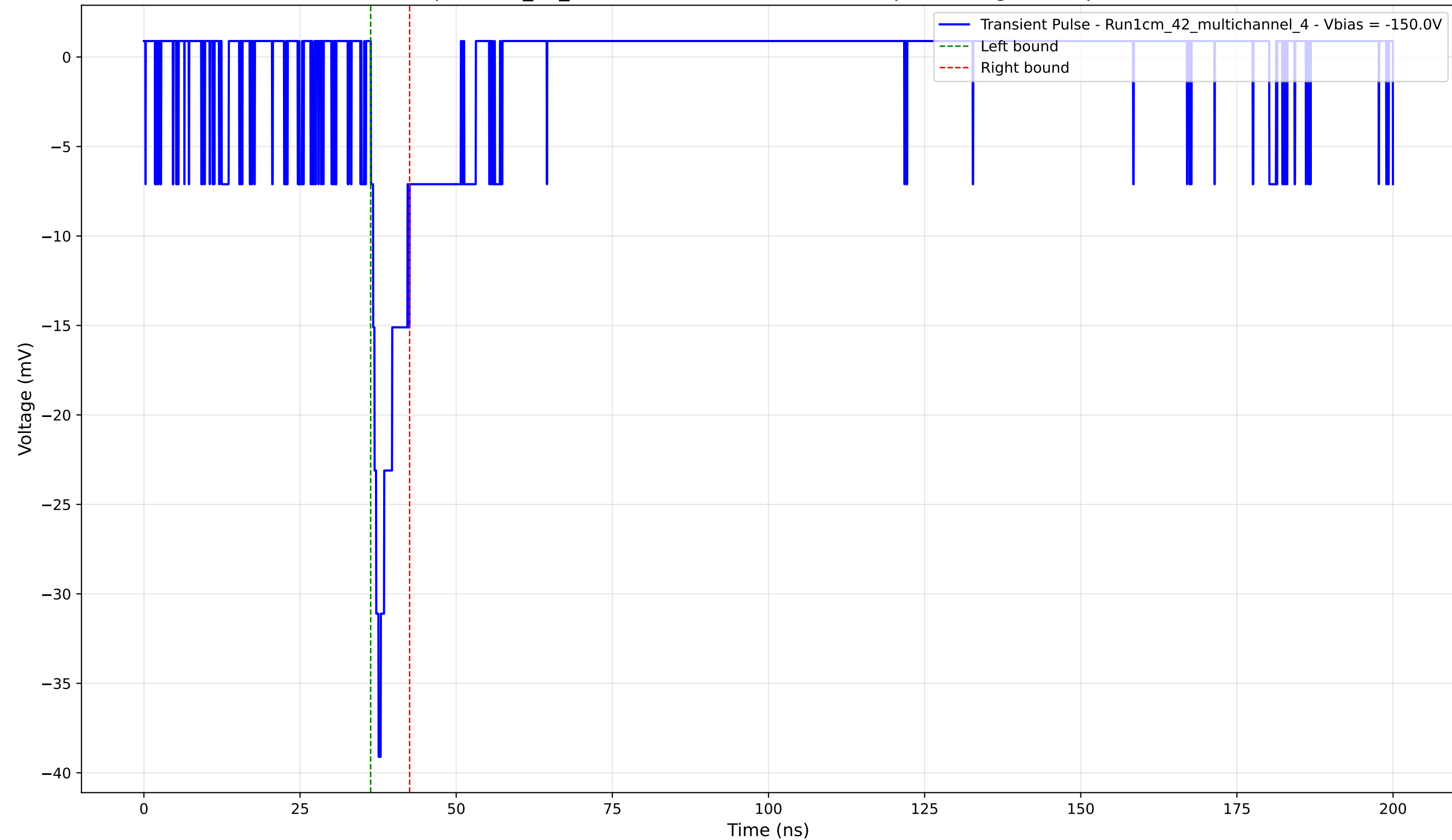
Transient Pulse - Sample: 1cm_42_multichannel - Position: 3045.0 \mu\text{m} - Charge: 2.51 pC - Rise Time: 1.23 ns
