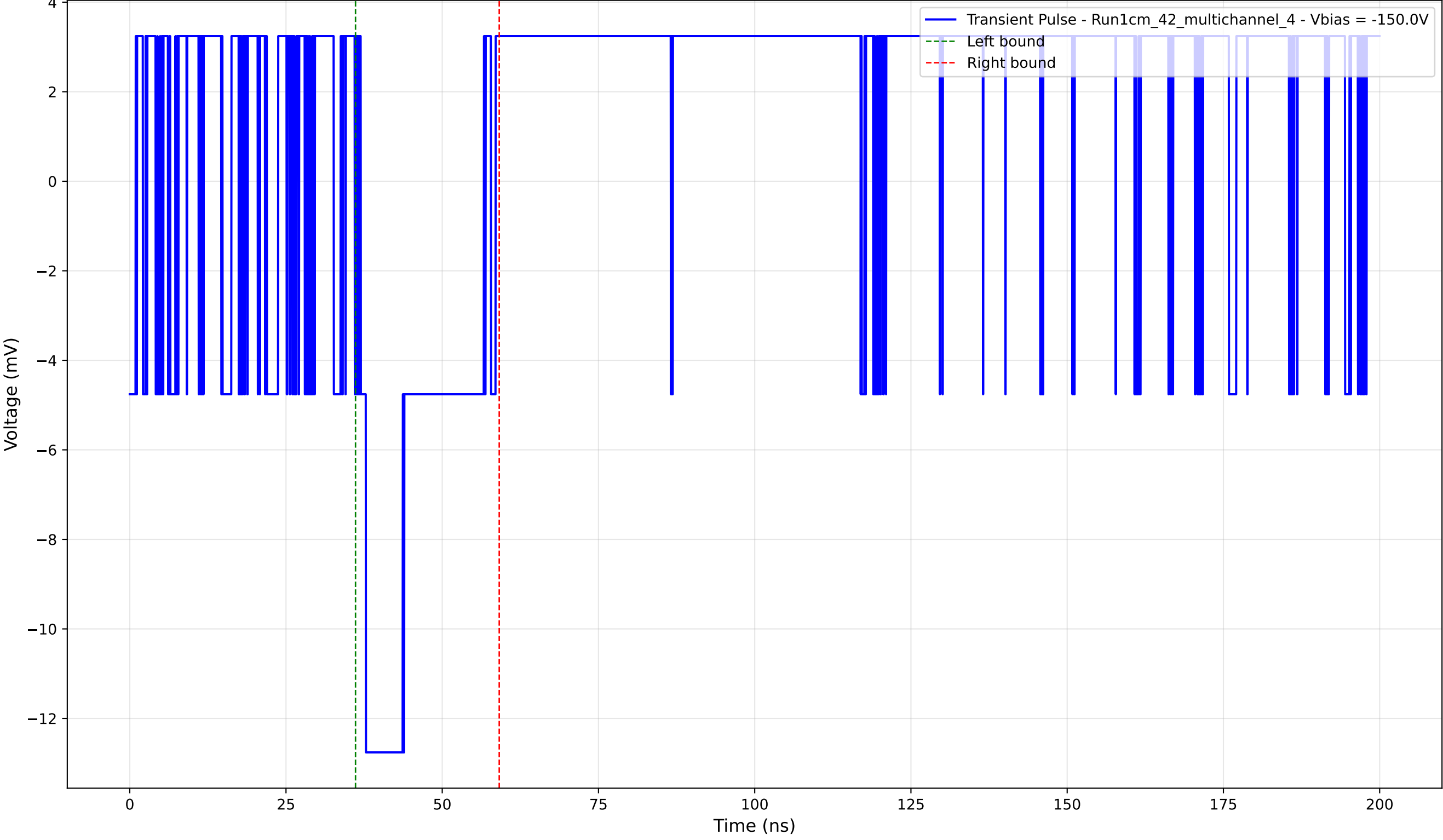
Transient Pulse - Sample: 1cm_42_multichannel - Position: 650.0 \mu\text{m} - Charge: 2.79 pC - Rise Time: 0.00 ns (N/A)
