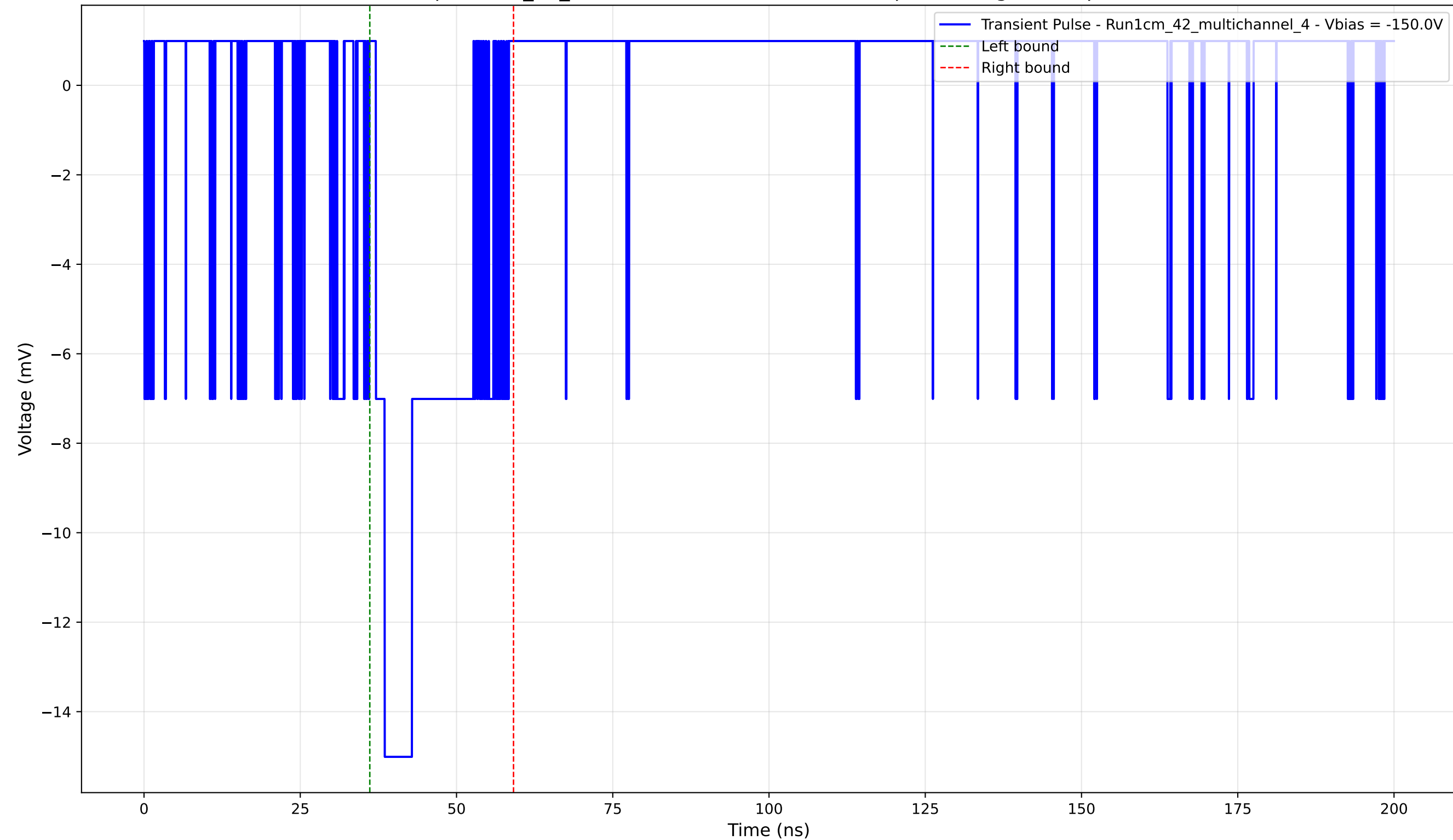
Transient Pulse - Sample: 1cm_42_multichannel - Position: 4315.0 \mu\text{m} - Charge: 3.32 pC - Rise Time: 1.42 ns
