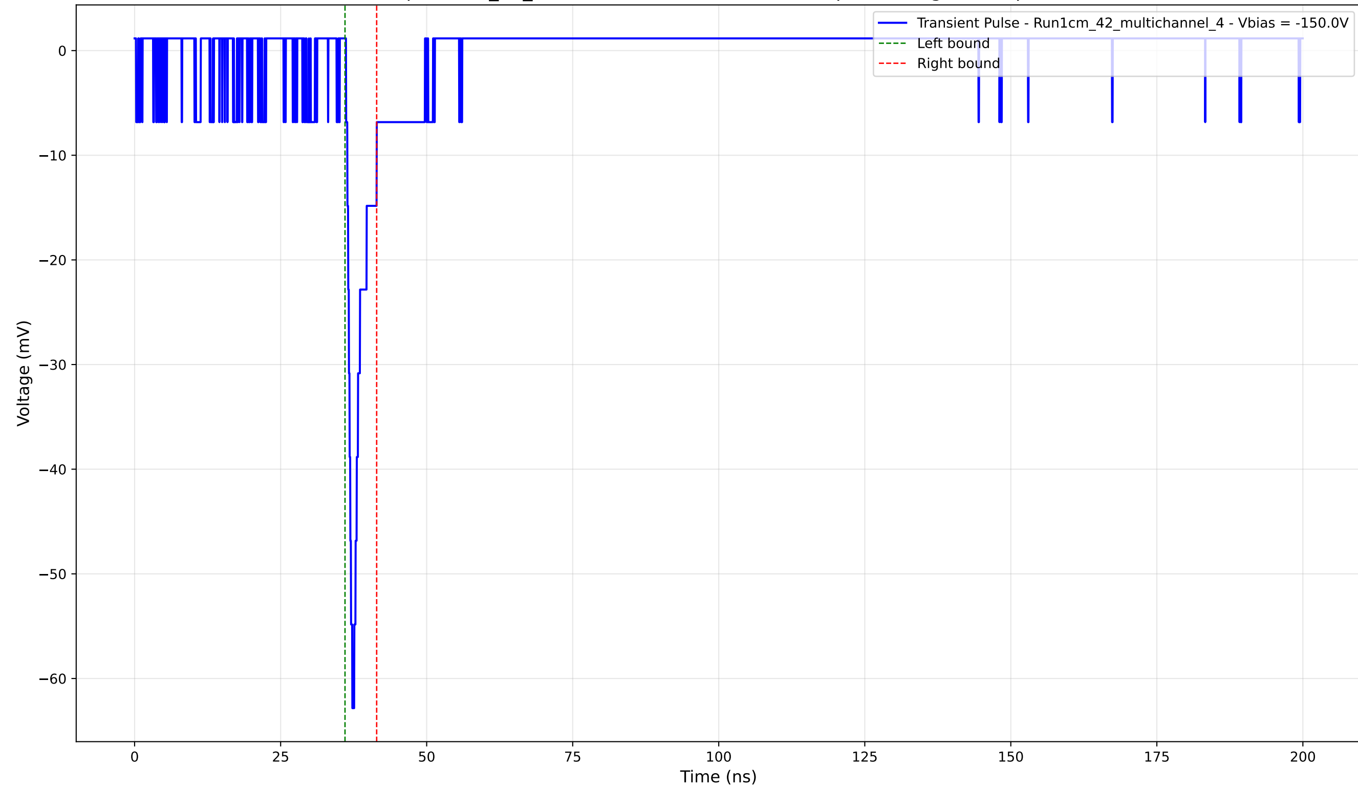
Transient Pulse - Sample: 1cm_42_multichannel - Position: 2090.0 \mu\text{m} - Charge: 2.91 pC - Rise Time: 1.06 ns
