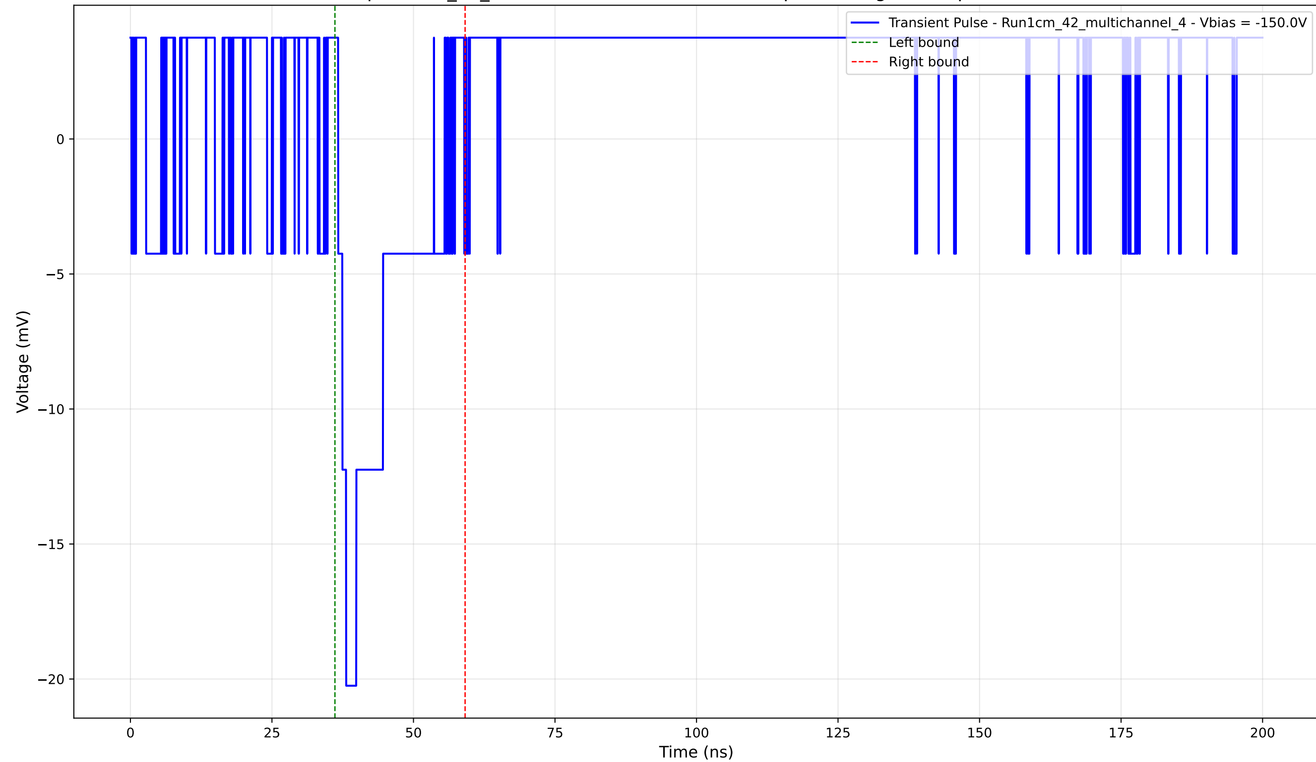
Transient Pulse - Sample: 1cm_42_multichannel - Position: 1030.0 \mu\text{m} - Charge: 2.87 pC - Rise Time: 0.00 ns (N/A)
