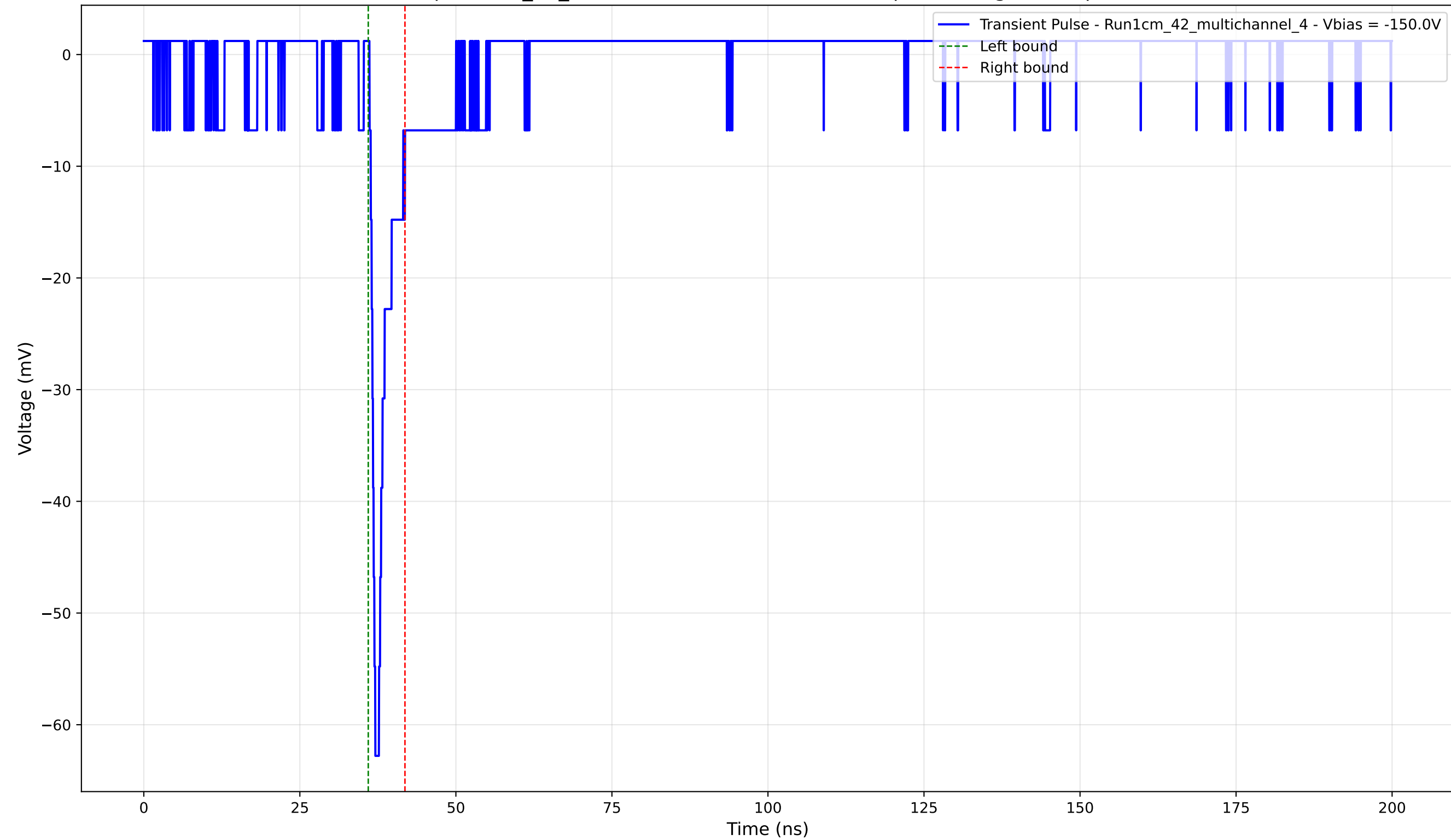
Transient Pulse - Sample: 1cm_42_multichannel - Position: 2160.0 \mu\text{m} - Charge: 3.13 pC - Rise Time: 0.92 ns
