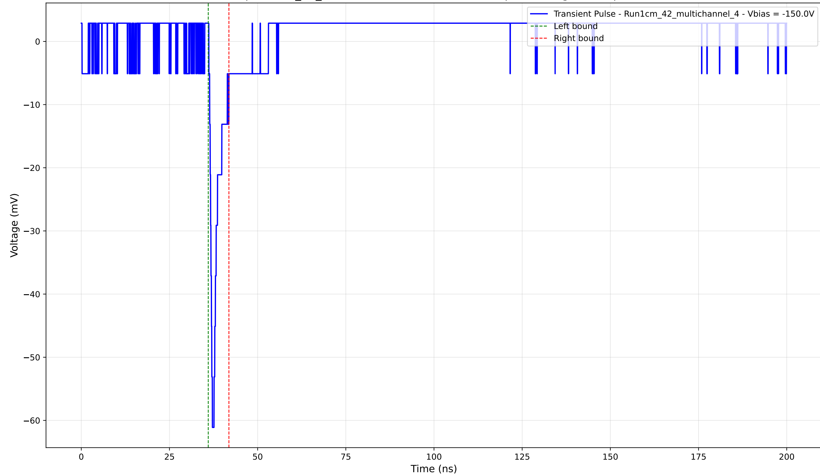
Transient Pulse - Sample: 1cm_42_multichannel - Position: 2110.0 \mu\text{m} - Charge: 2.89 pC - Rise Time: 0.78 ns
