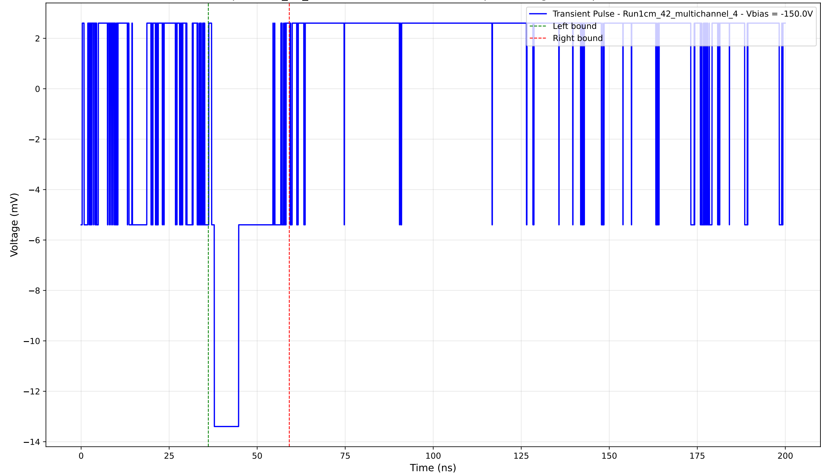
Transient Pulse - Sample: 1cm_42_multichannel - Position: 745.0 \mu\text{m} - Charge: 3.21 pC - Rise Time: 0.00 ns (N/A)
