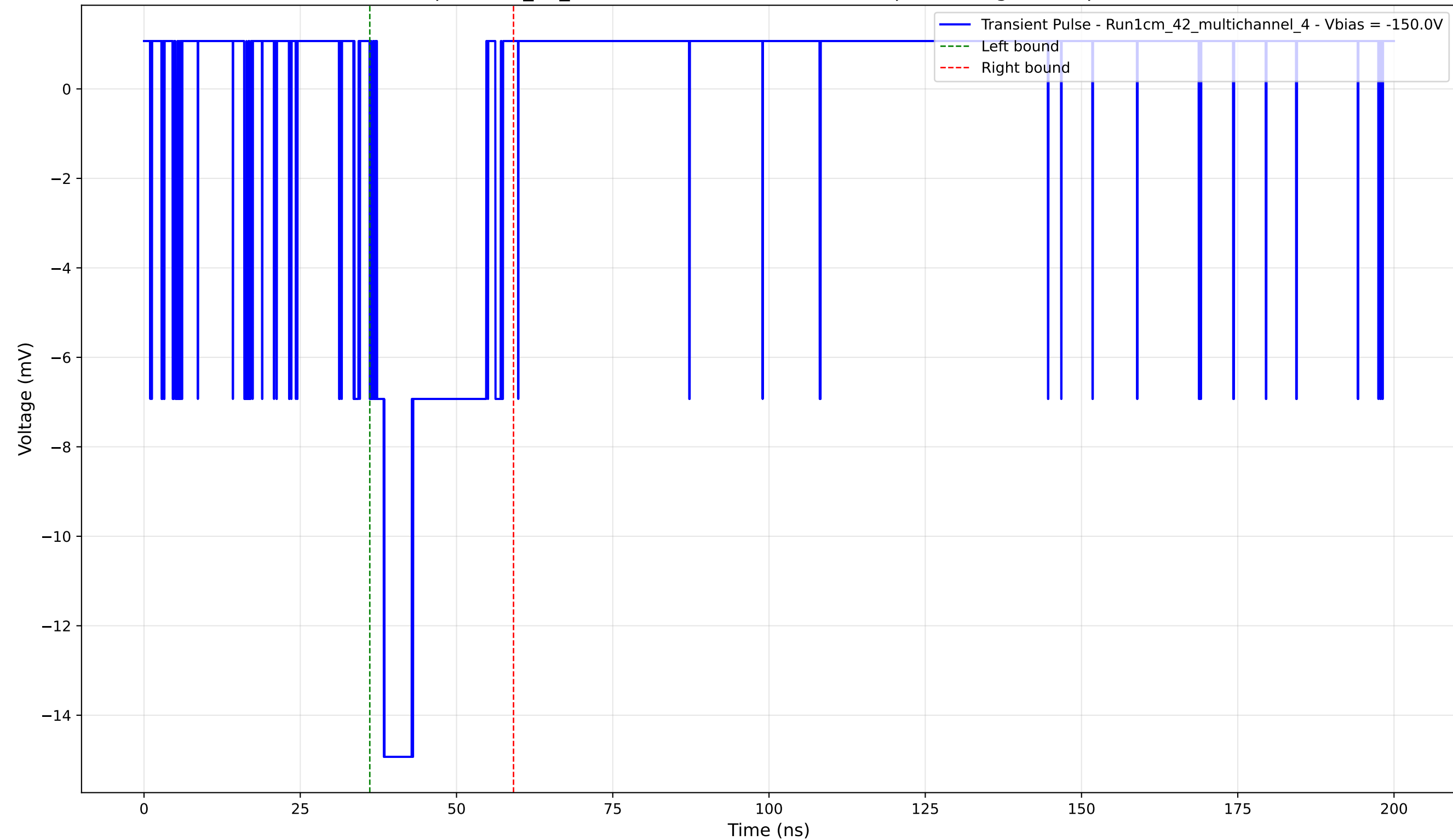
Transient Pulse - Sample: 1cm_42_multichannel - Position: 4245.0 \mu\text{m} - Charge: 3.32 pC - Rise Time: 1.10 ns
