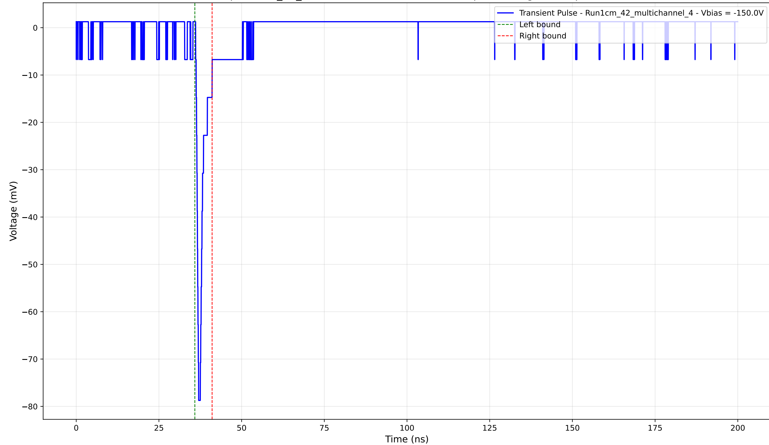
Transient Pulse - Sample: 1cm_42_multichannel - Position: 2485.0 \mu\text{m} - Charge: 3.30 pC - Rise Time: 0.76 ns
