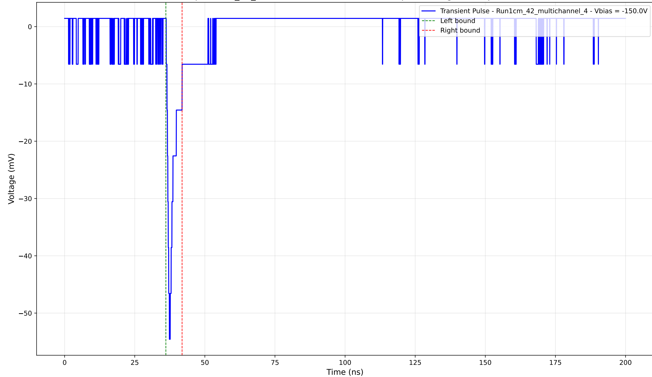
Transient Pulse - Sample: 1cm_42_multichannel - Position: 2790.0 \mu\text{m} - Charge: 2.80 pC - Rise Time: 1.12 ns
