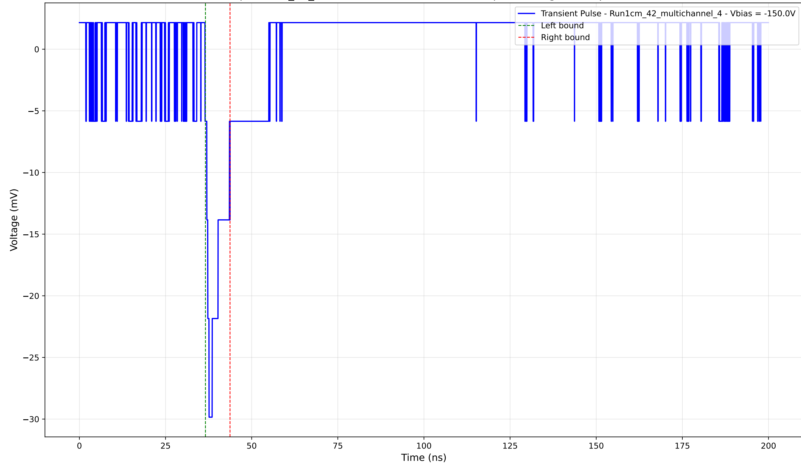
Transient Pulse - Sample: 1cm_42_multichannel - Position: 1465.0 \mu\text{m} - Charge: 2.51 pC - Rise Time: 1.18 ns
