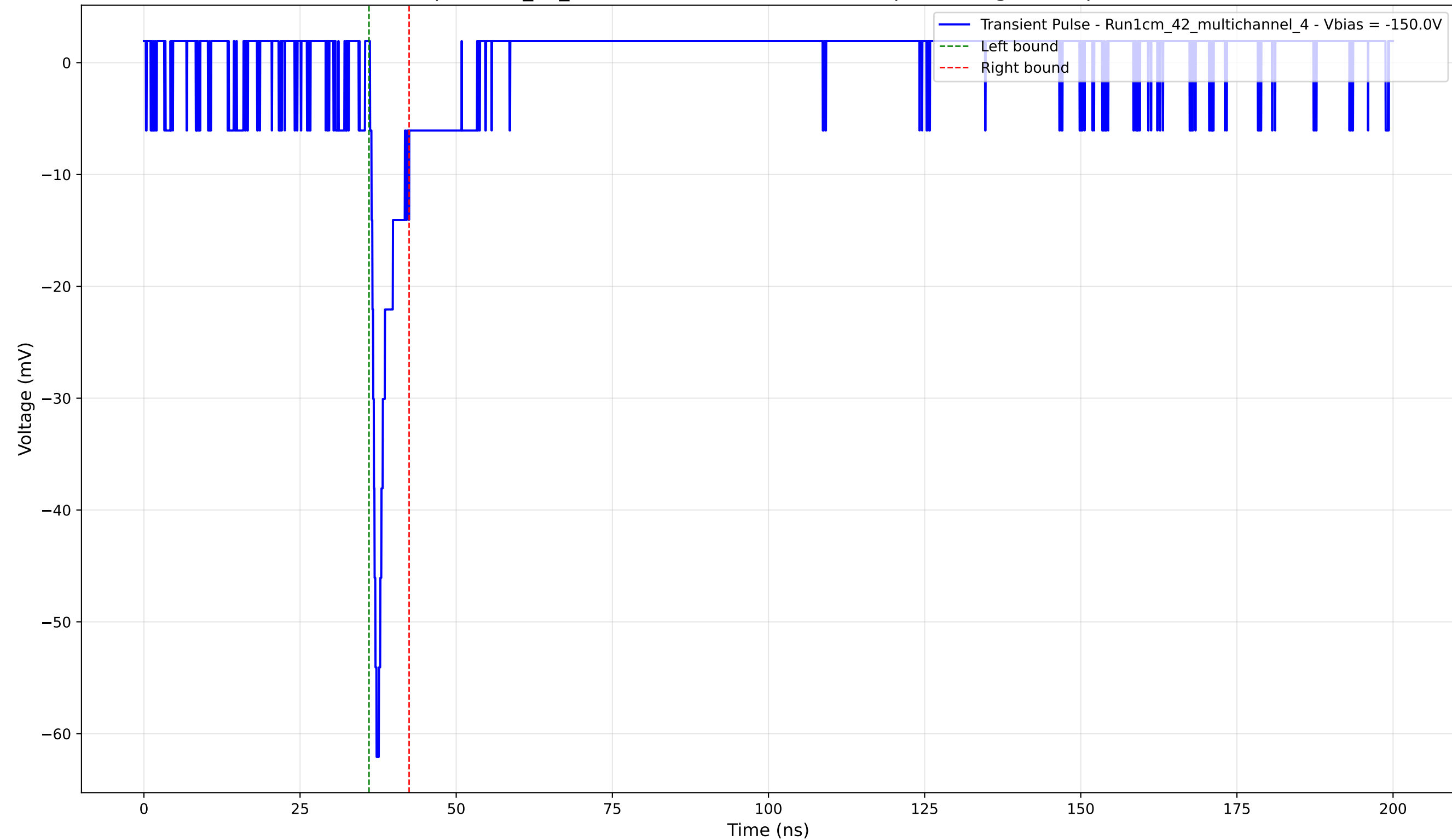
Transient Pulse - Sample: 1cm_42_multichannel - Position: 2080.0 \mu\text{m} - Charge: 3.05 pC - Rise Time: 0.82 ns
