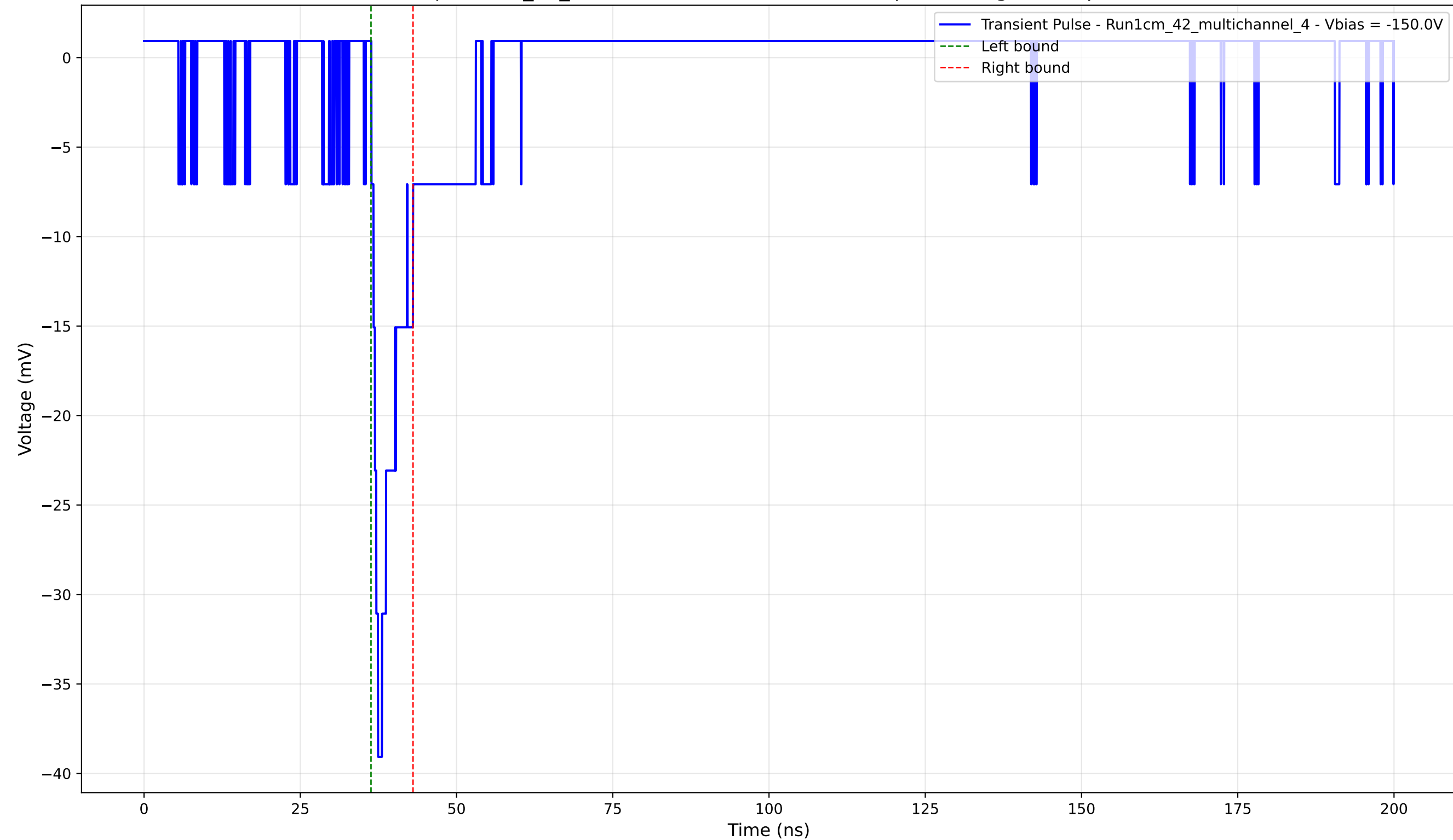
Transient Pulse - Sample: 1cm_42_multichannel - Position: 1710.0 \mu\text{m} - Charge: 2.83 pC - Rise Time: 1.07 ns
