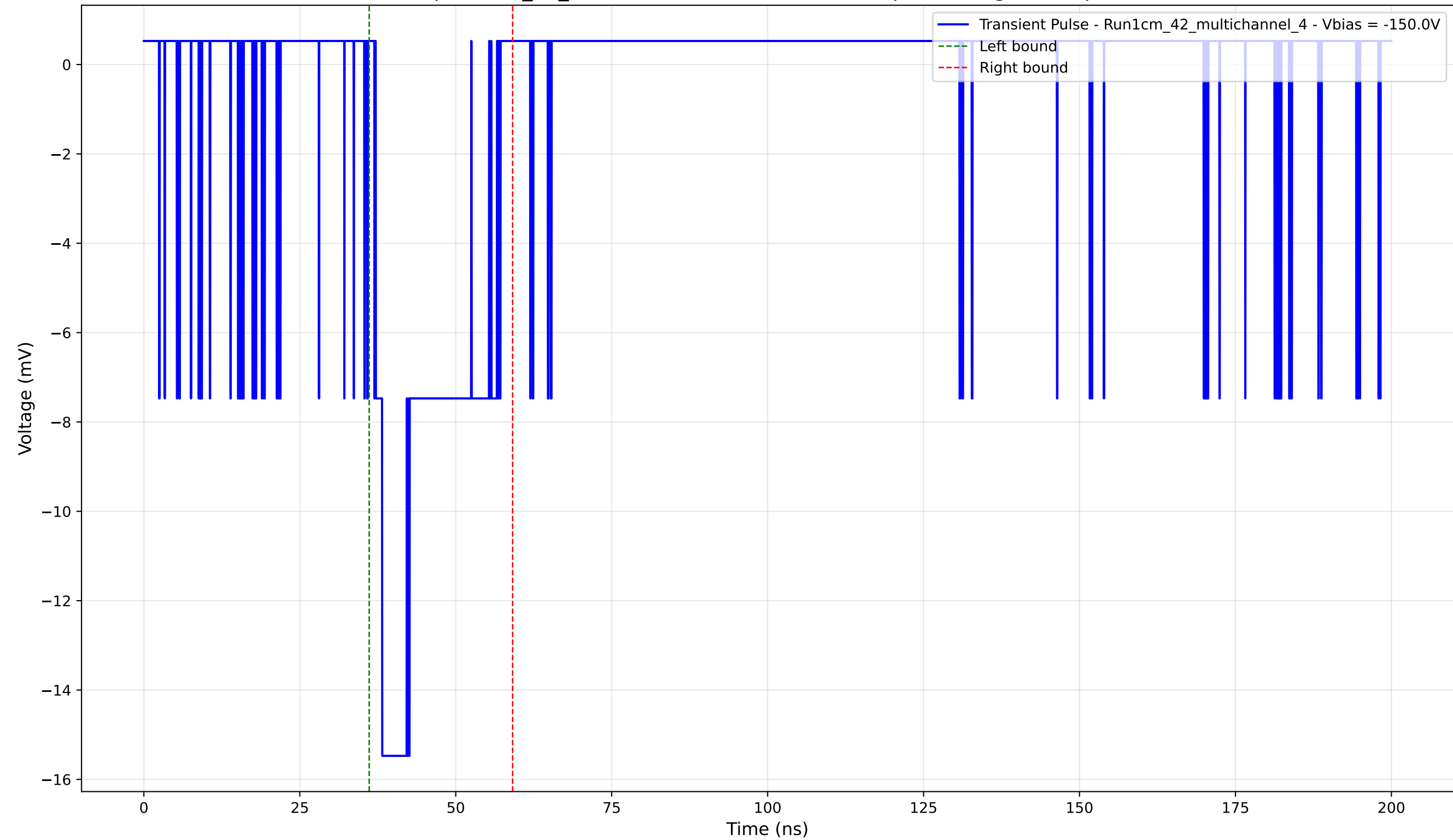
Transient Pulse - Sample: 1cm_42_multichannel - Position: 4105.0 \mu\text{m} - Charge: 3.55 pC - Rise Time: 1.04 ns
