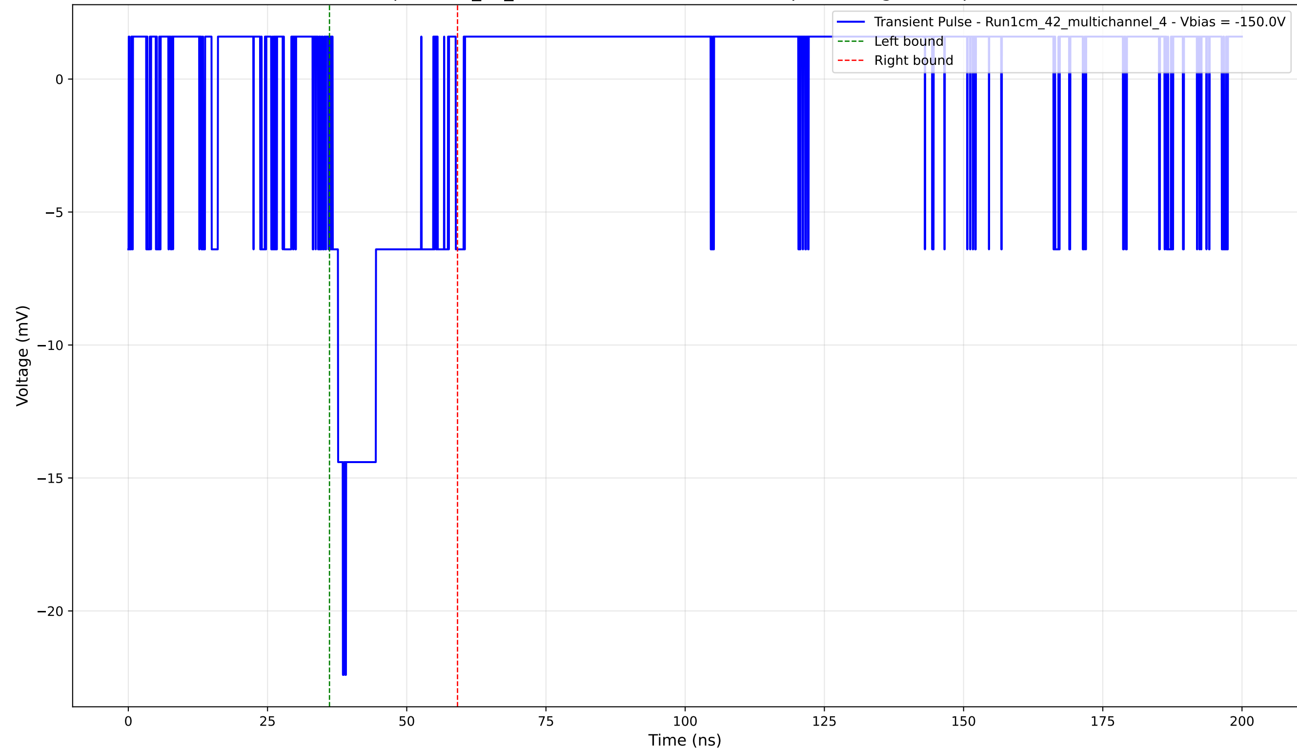
Transient Pulse - Sample: 1cm_42_multichannel - Position: 945.0 \mu\text{m} - Charge: 3.69 pC - Rise Time: 1.84 ns
