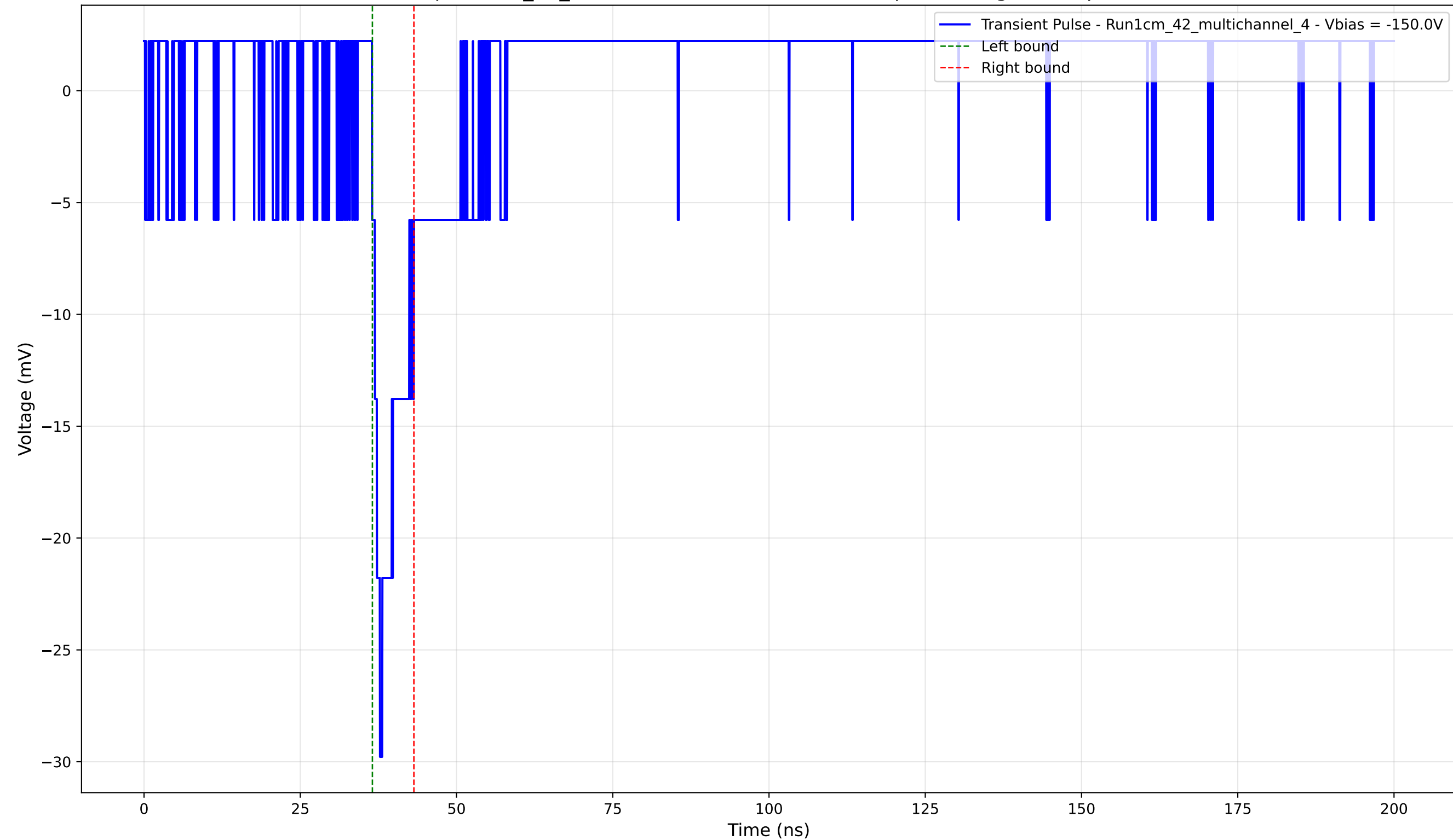
Transient Pulse - Sample: 1cm_42_multichannel - Position: 3240.0 \mu\text{m} - Charge: 2.16 pC - Rise Time: 1.28 ns
