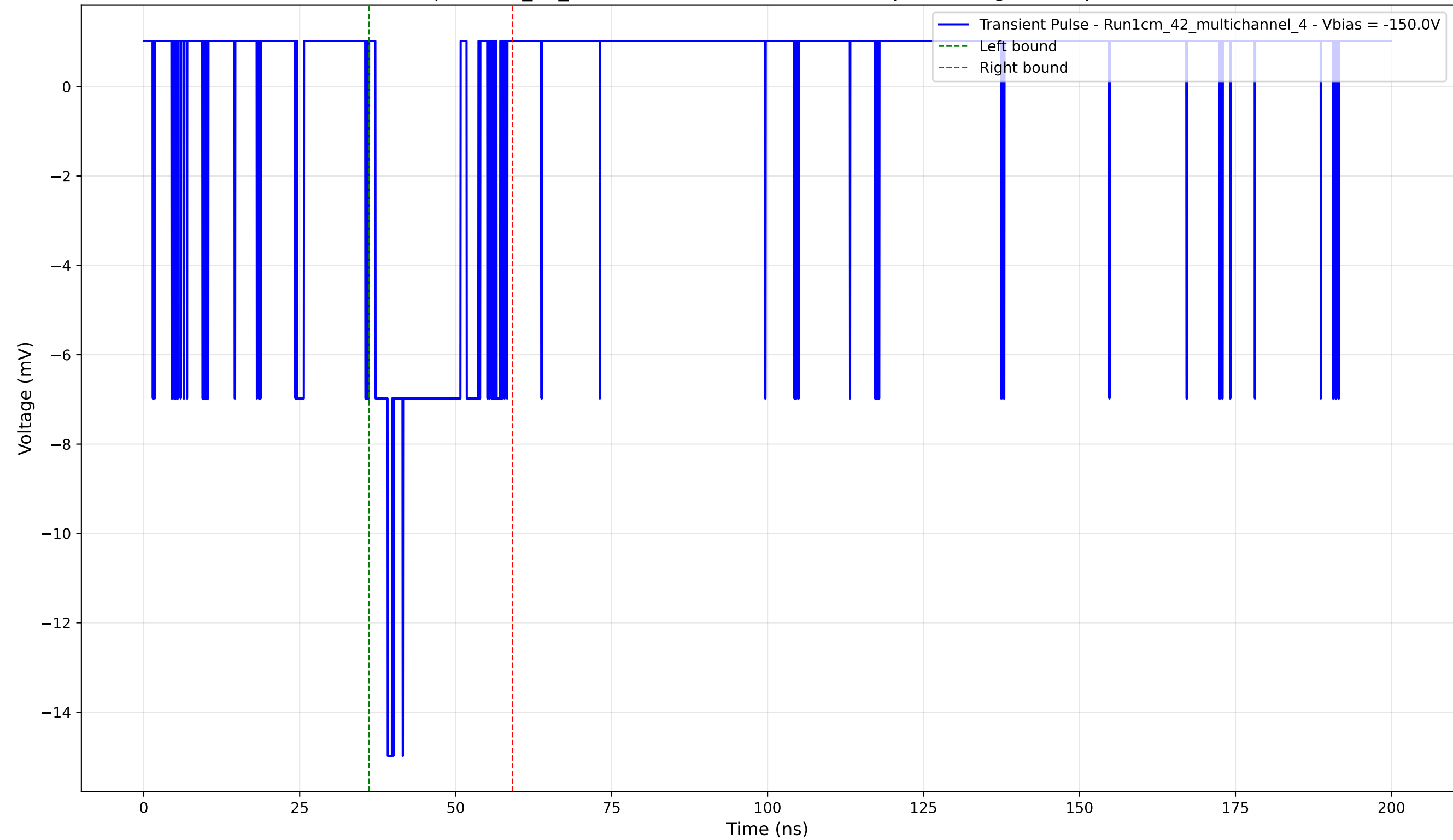
Transient Pulse - Sample: 1cm_42_multichannel - Position: 3960.0 \mu\text{m} - Charge: 2.43 pC - Rise Time: 1.98 ns
