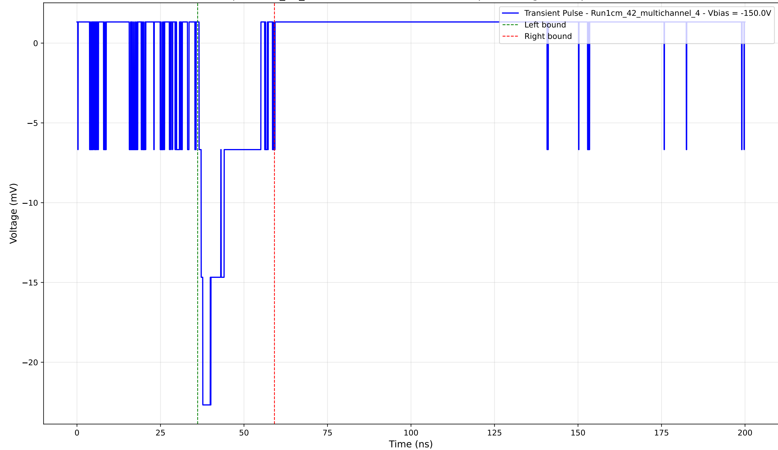
Transient Pulse - Sample: 1cm_42_multichannel - Position: 1295.0 \mu\text{m} - Charge: 4.01 pC - Rise Time: 1.12 ns
