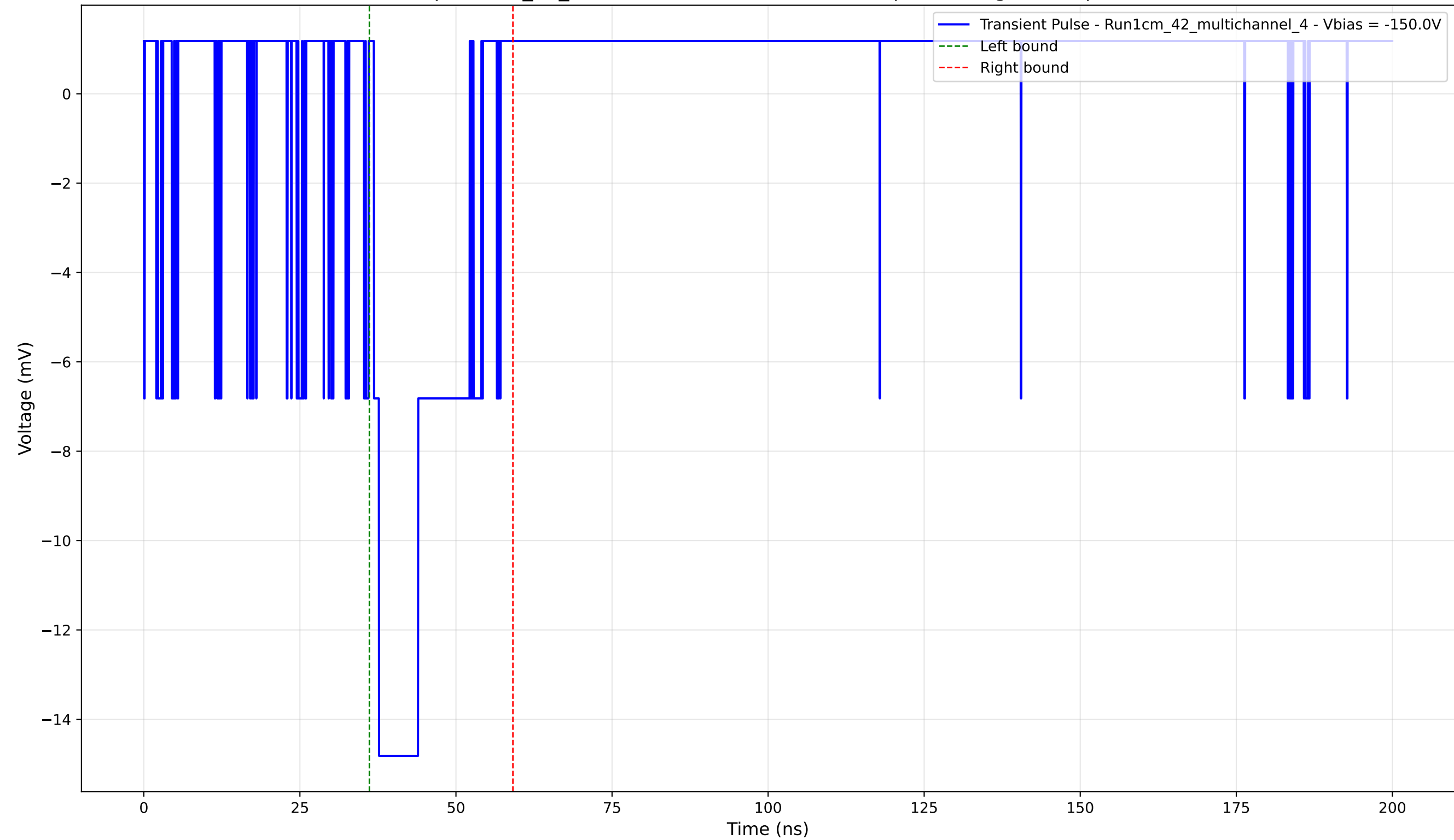
Transient Pulse - Sample: 1cm_42_multichannel - Position: 3800.0 \mu\text{m} - Charge: 3.24 pC - Rise Time: 0.82 ns
