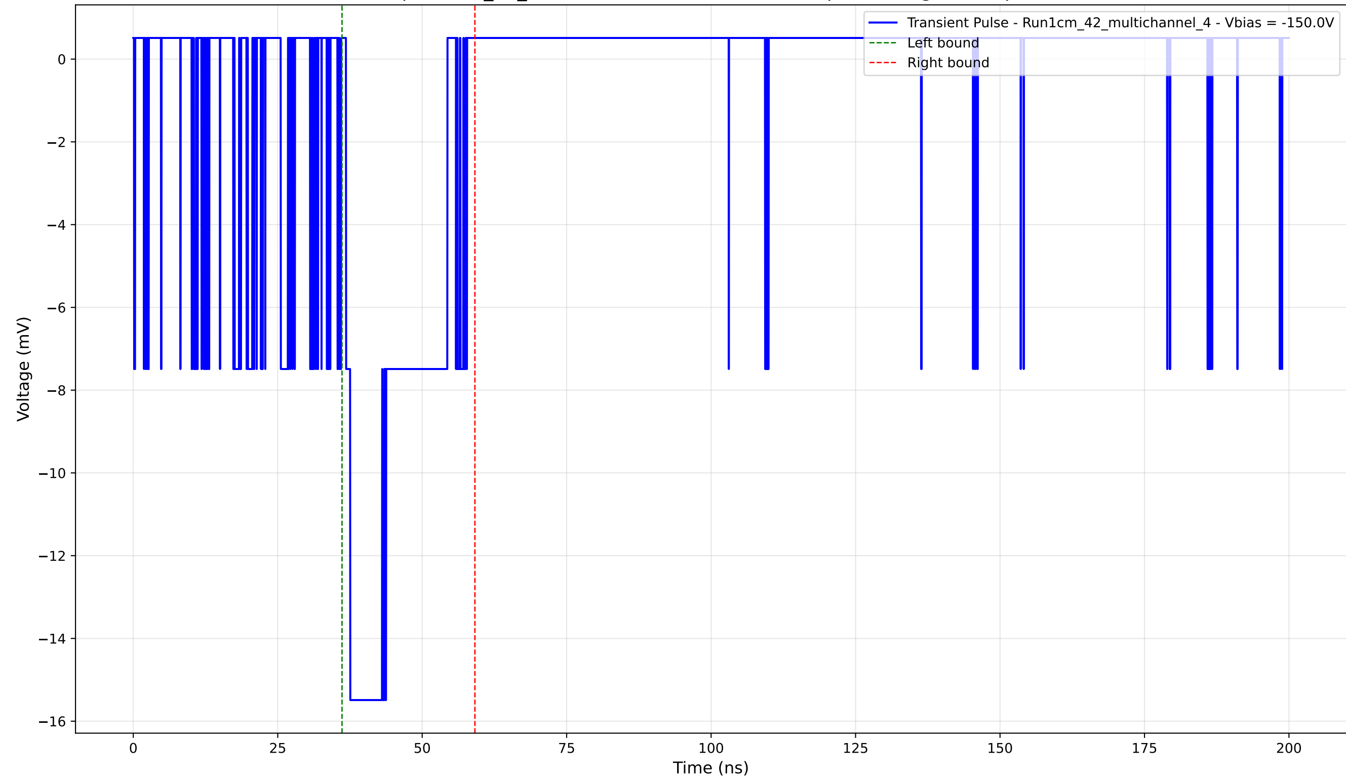
Transient Pulse - Sample: 1cm_42_multichannel - Position: 3755.0 \mu\text{m} - Charge: 3.74 pC - Rise Time: 0.74 ns
