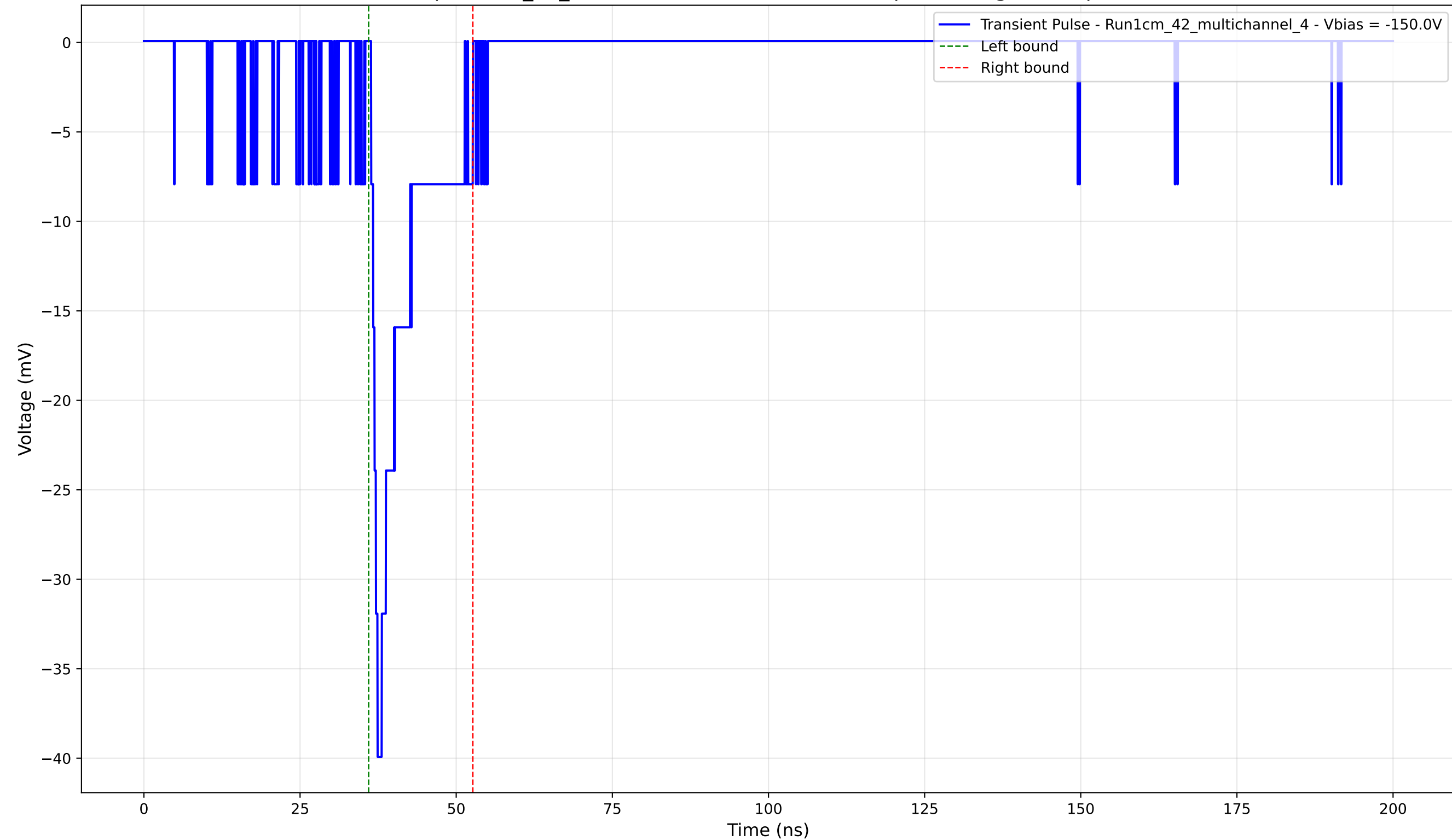
Transient Pulse - Sample: 1cm_42_multichannel - Position: 1705.0 \mu\text{m} - Charge: 4.39 pC - Rise Time: 1.03 ns
