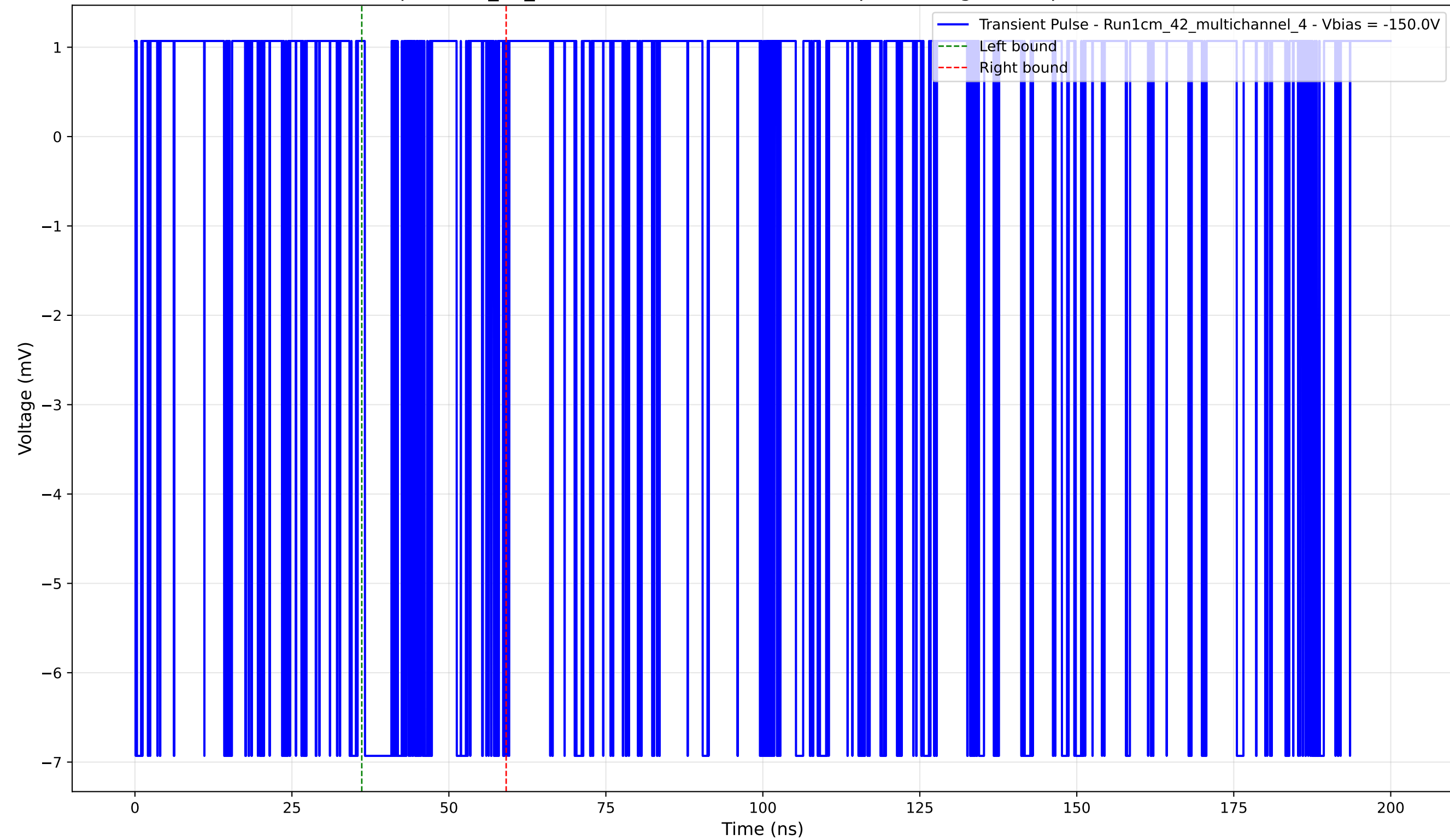
Transient Pulse - Sample: 1cm_42_multichannel - Position: 1905.0 \mu\text{m} - Charge: 1.26 pC - Rise Time: 0.00 ns (N/A)
