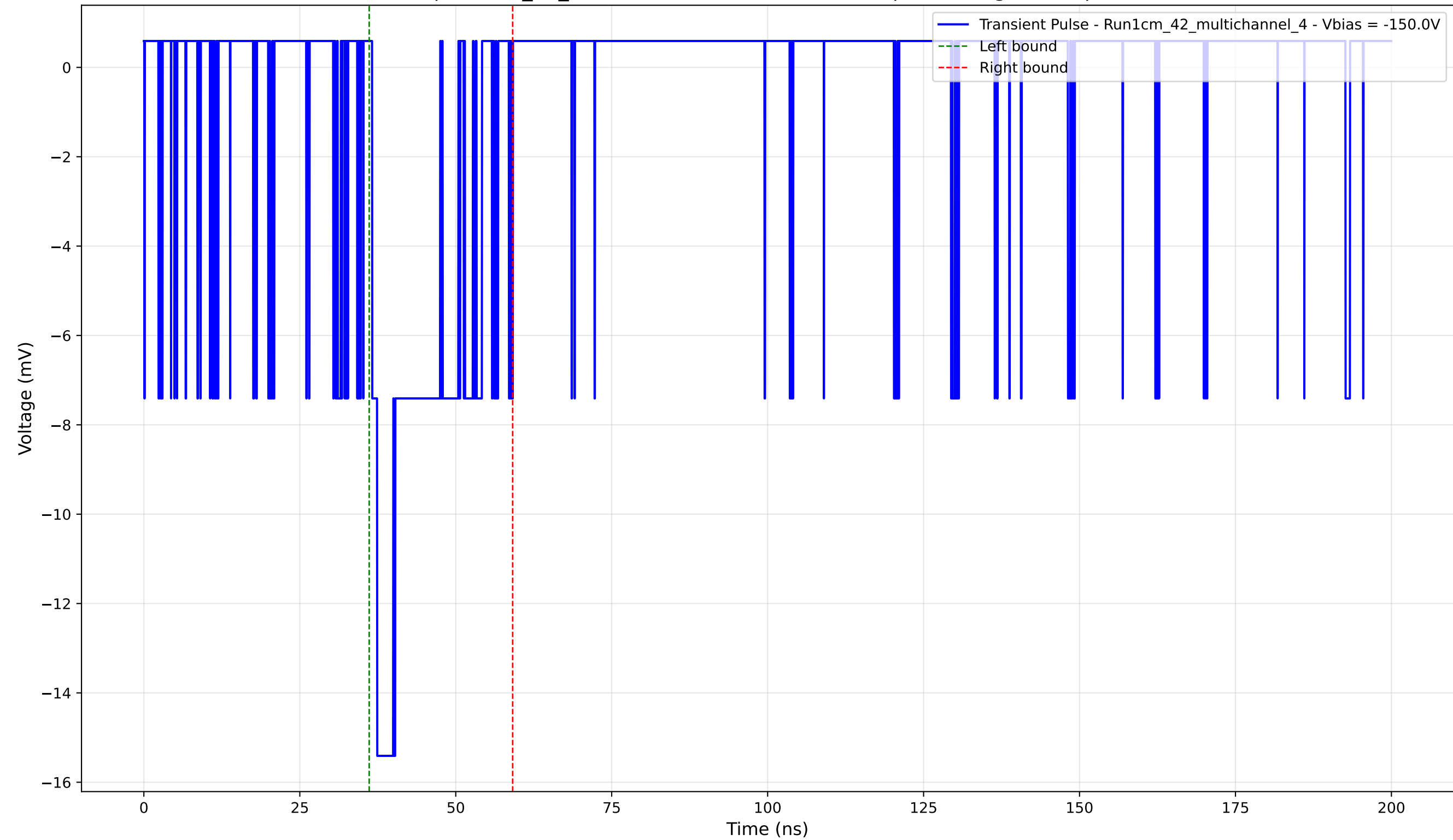
Transient Pulse - Sample: 1cm_42_multichannel - Position: 3345.0 \mu\text{m} - Charge: 2.97 pC - Rise Time: 0.82 ns
