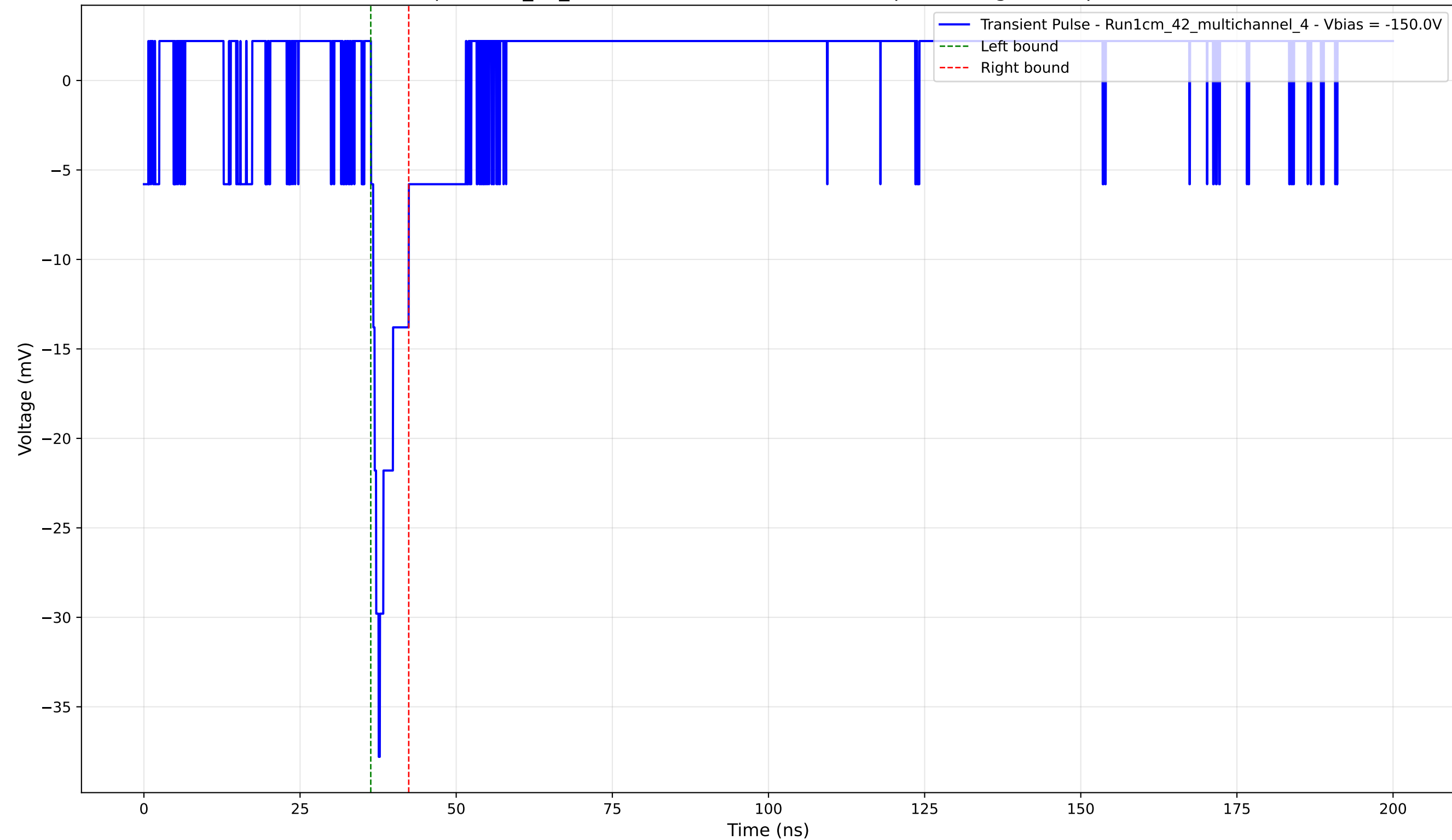
Transient Pulse - Sample: 1cm_42_multichannel - Position: 3040.0 \mu\text{m} - Charge: 2.30 pC - Rise Time: 1.23 ns
