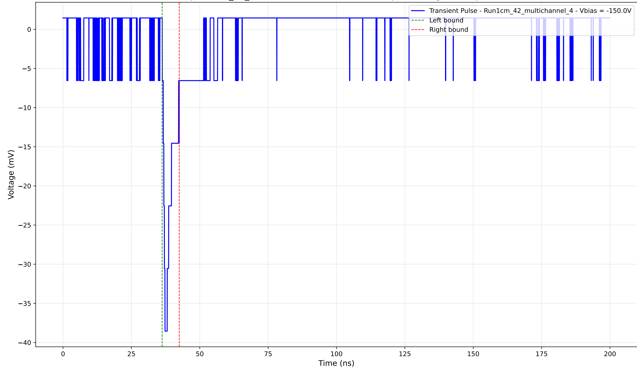
Transient Pulse - Sample: 1cm_42_multichannel - Position: 2990.0 \mu\text{m} - Charge: 2.55 pC - Rise Time: 1.01 ns
