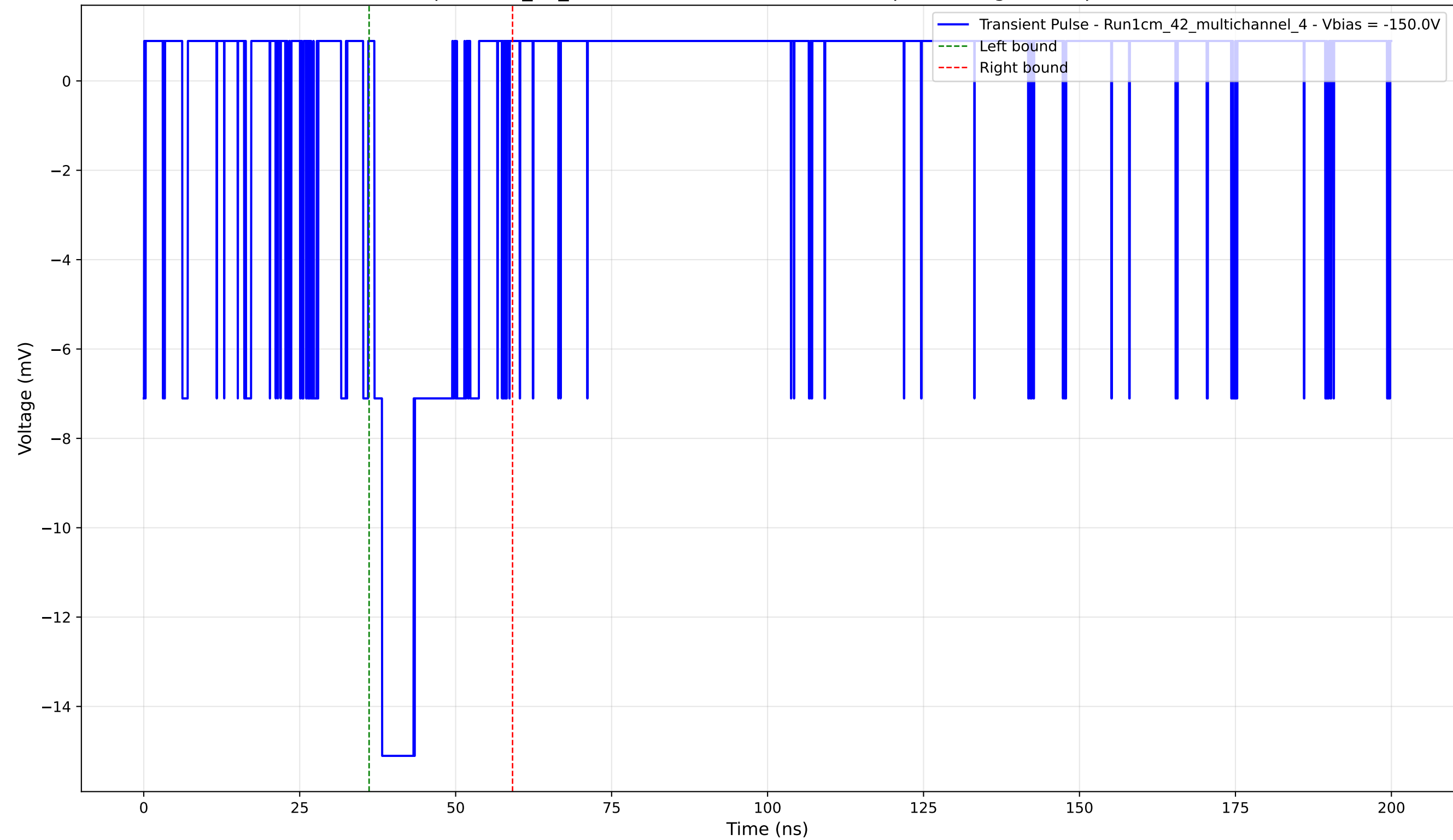
Transient Pulse - Sample: 1cm_42_multichannel - Position: 4530.0 \mu\text{m} - Charge: 3.03 pC - Rise Time: 1.24 ns
