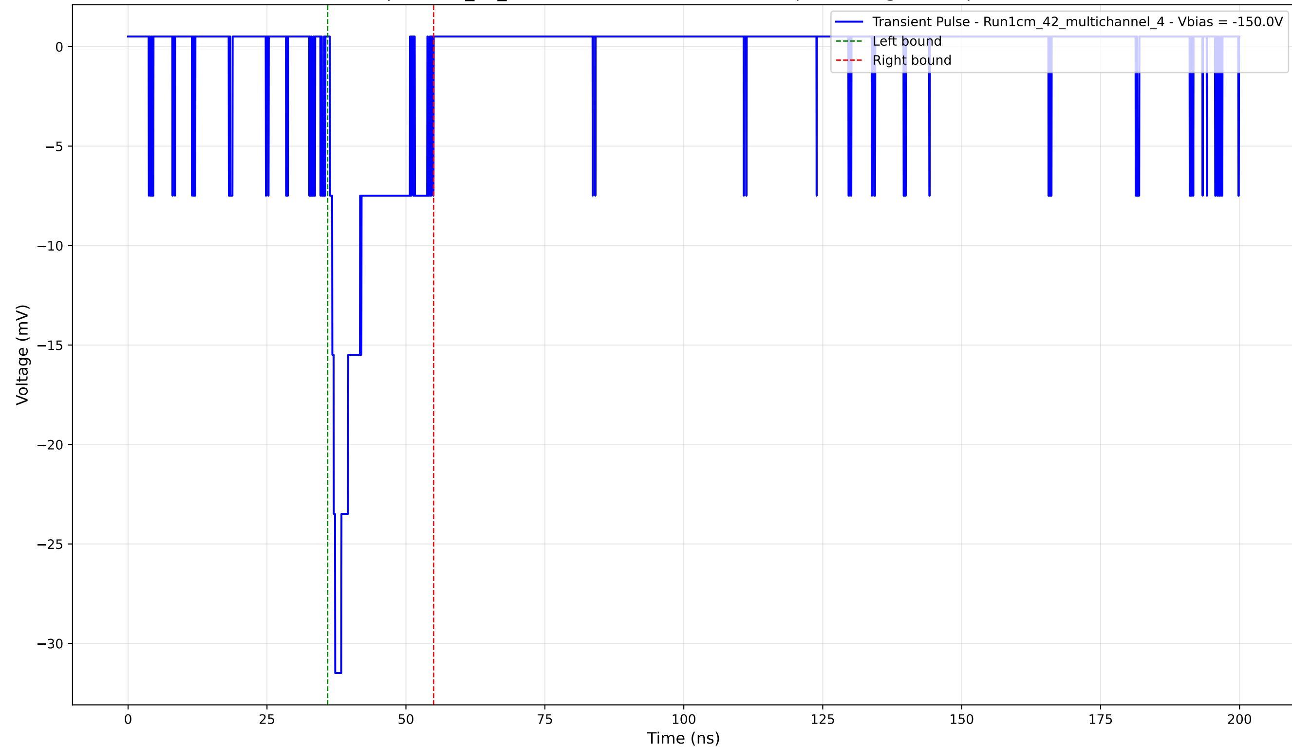
Transient Pulse - Sample: 1cm_42_multichannel - Position: 3075.0 \mu\text{m} - Charge: 4.02 pC - Rise Time: 0.95 ns
