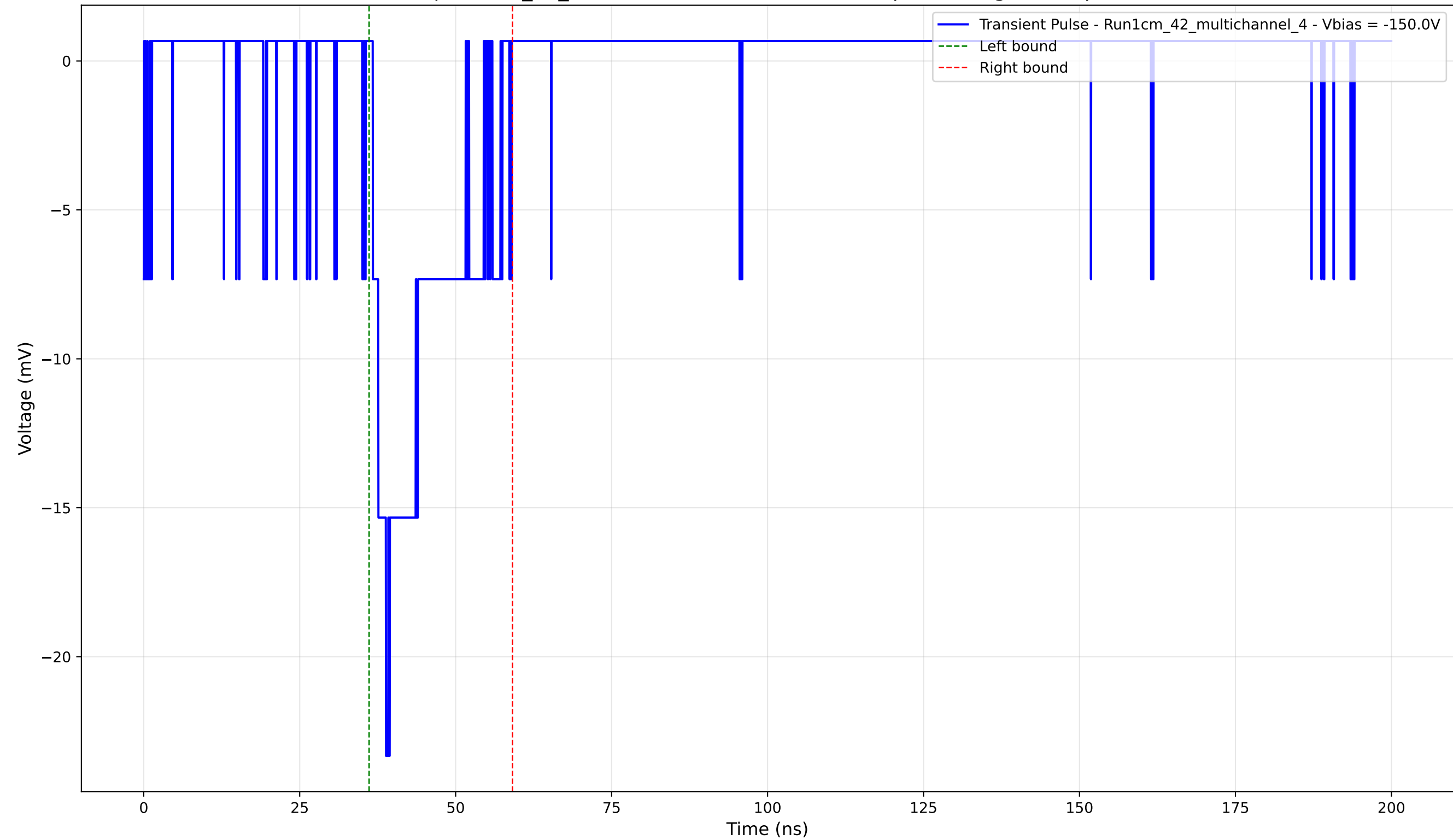
Transient Pulse - Sample: 1cm_42_multichannel - Position: 3740.0 \mu\text{m} - Charge: 3.88 pC - Rise Time: 2.12 ns
