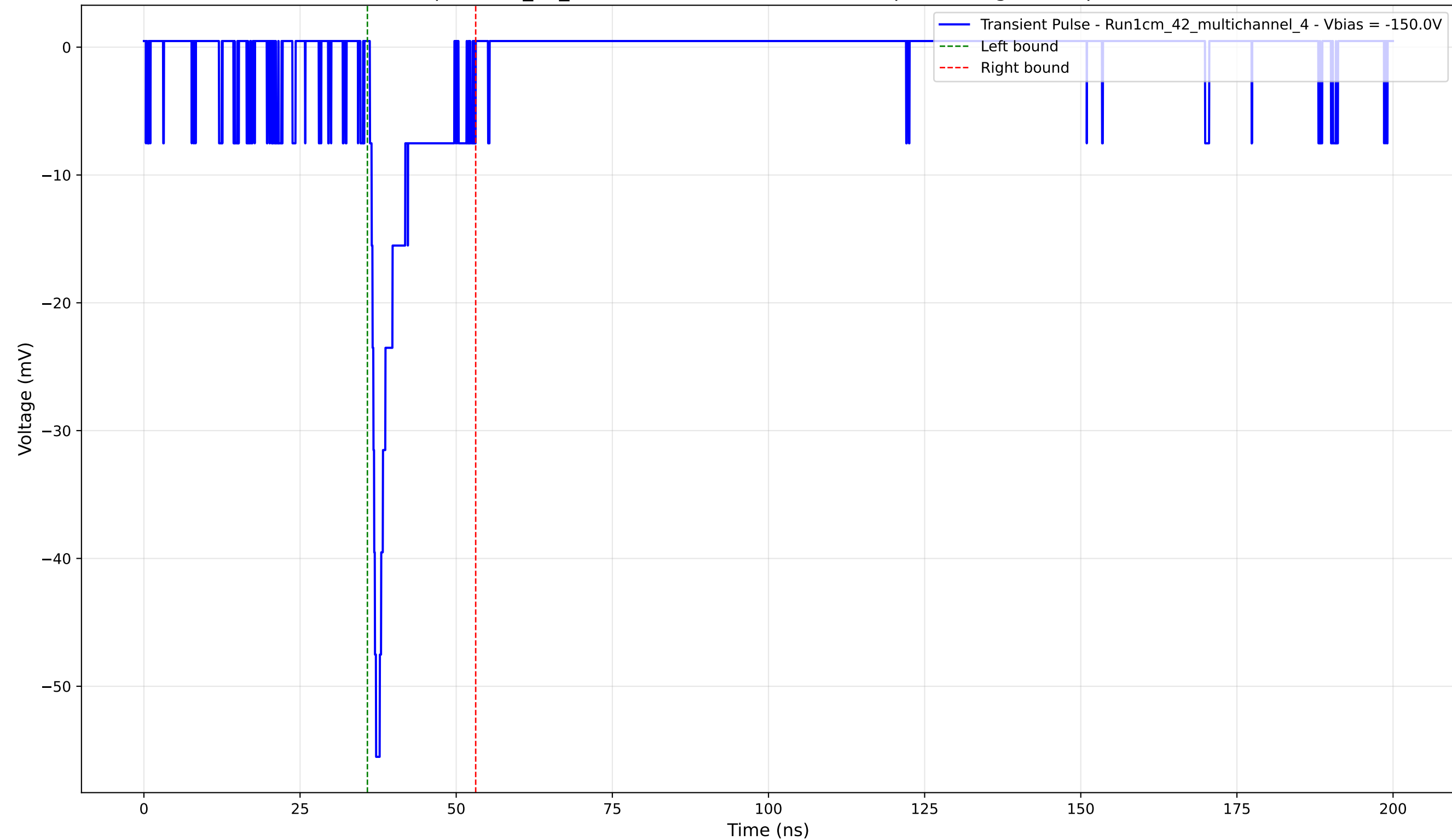
Transient Pulse - Sample: 1cm_42_multichannel - Position: 2735.0 \mu\text{m} - Charge: 4.54 pC - Rise Time: 0.99 ns
