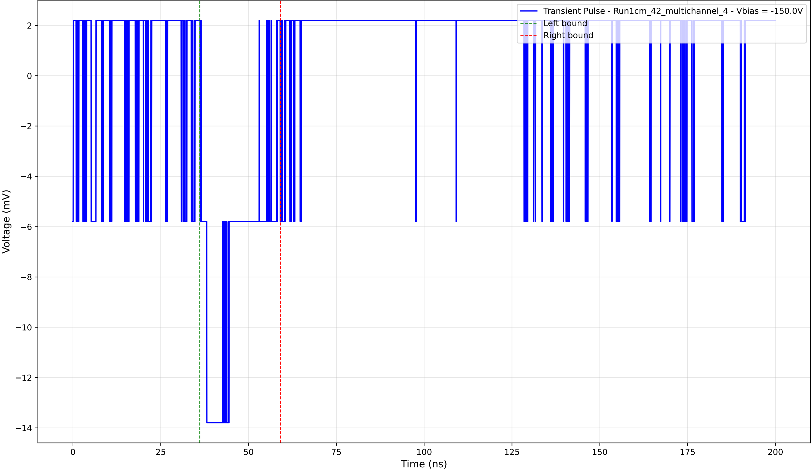
Transient Pulse - Sample: 1cm_42_multichannel - Position: 480.0 \mu\text{m} - Charge: 3.31 pC - Rise Time: 0.00 ns (N/A)
