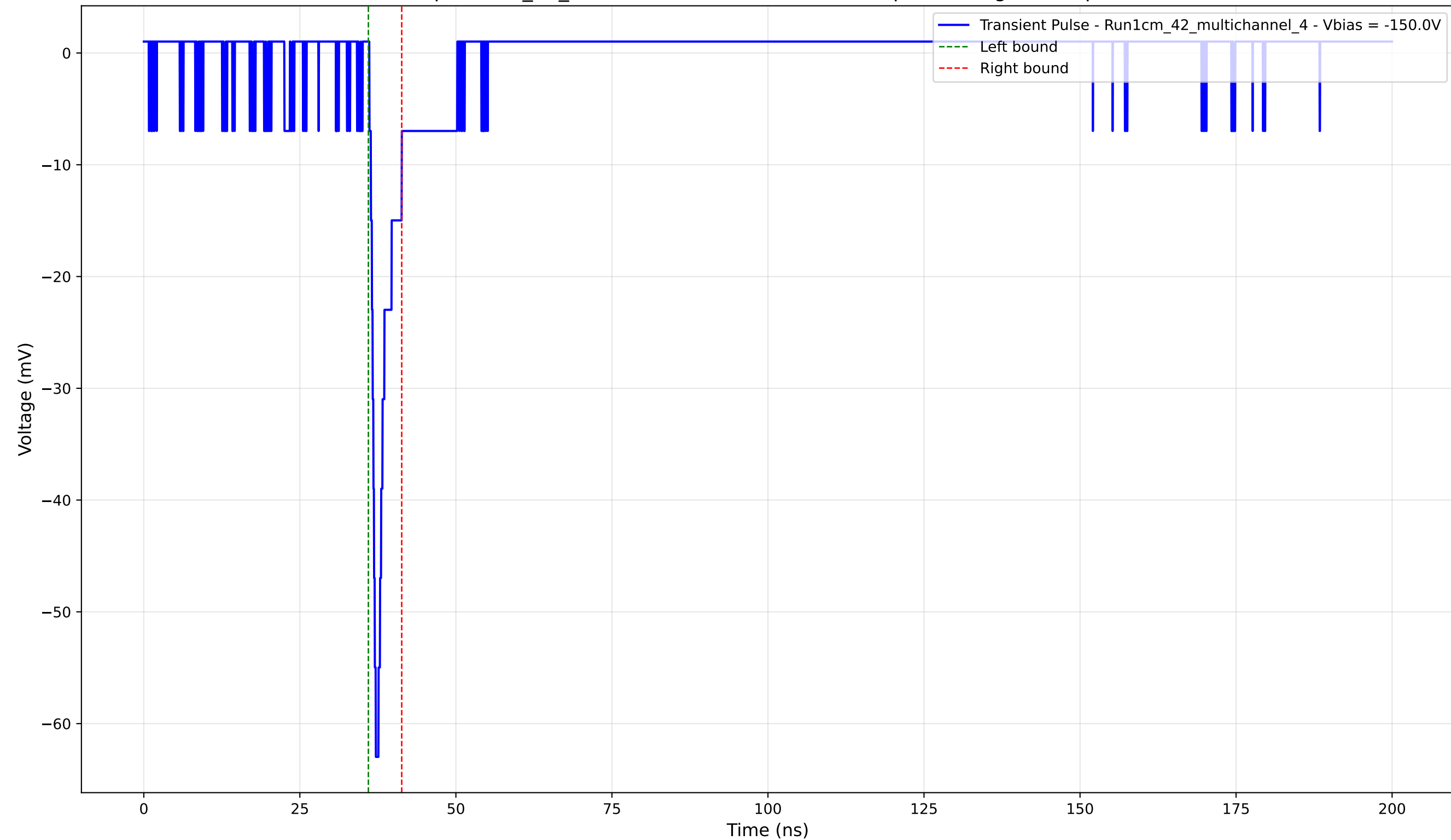
Transient Pulse - Sample: 1cm_42_multichannel - Position: 2120.0 \mu\text{m} - Charge: 2.94 pC - Rise Time: 1.02 ns
