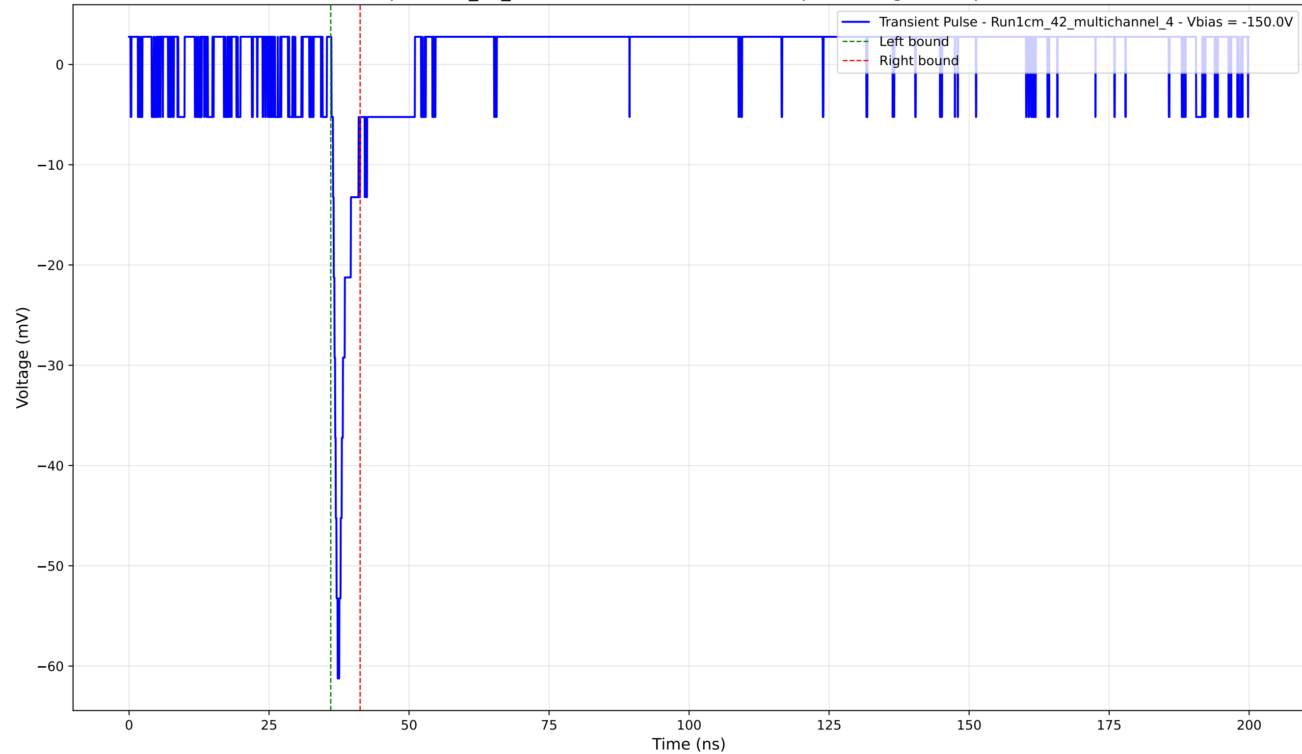
Transient Pulse - Sample: 1cm_42_multichannel - Position: 2655.0 \mu\text{m} - Charge: 2.63 pC - Rise Time: 0.84 ns
