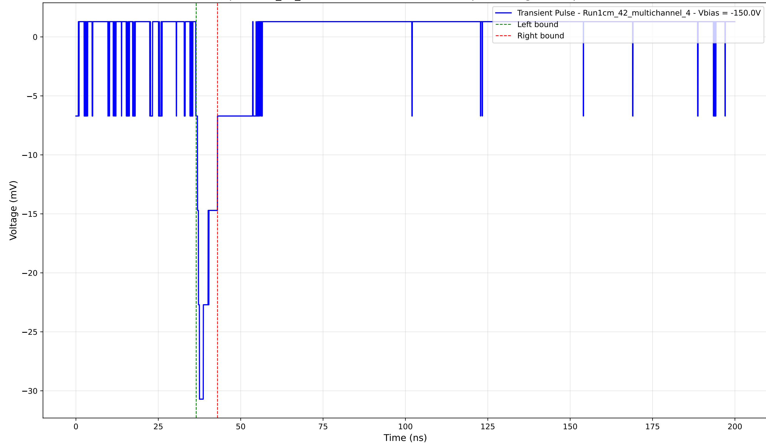
Transient Pulse - Sample: 1cm_42_multichannel - Position: 1530.0 \mu\text{m} - Charge: 2.51 pC - Rise Time: 1.11 ns
