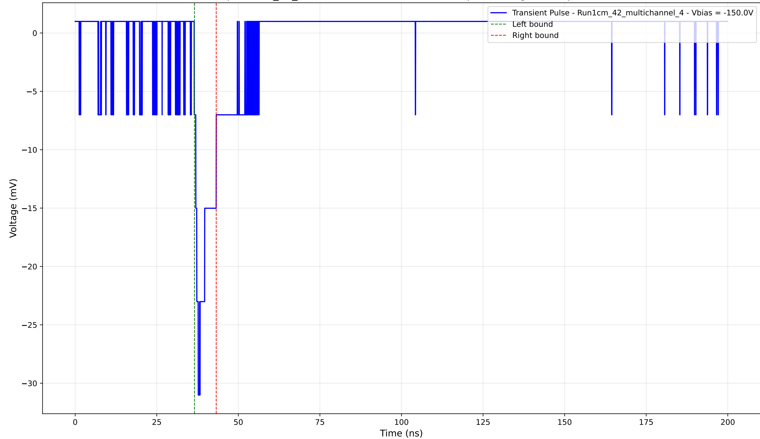
Transient Pulse - Sample: 1cm_42_multichannel - Position: 3250.0 \mu\text{m} - Charge: 2.39 pC - Rise Time: 1.23 ns
