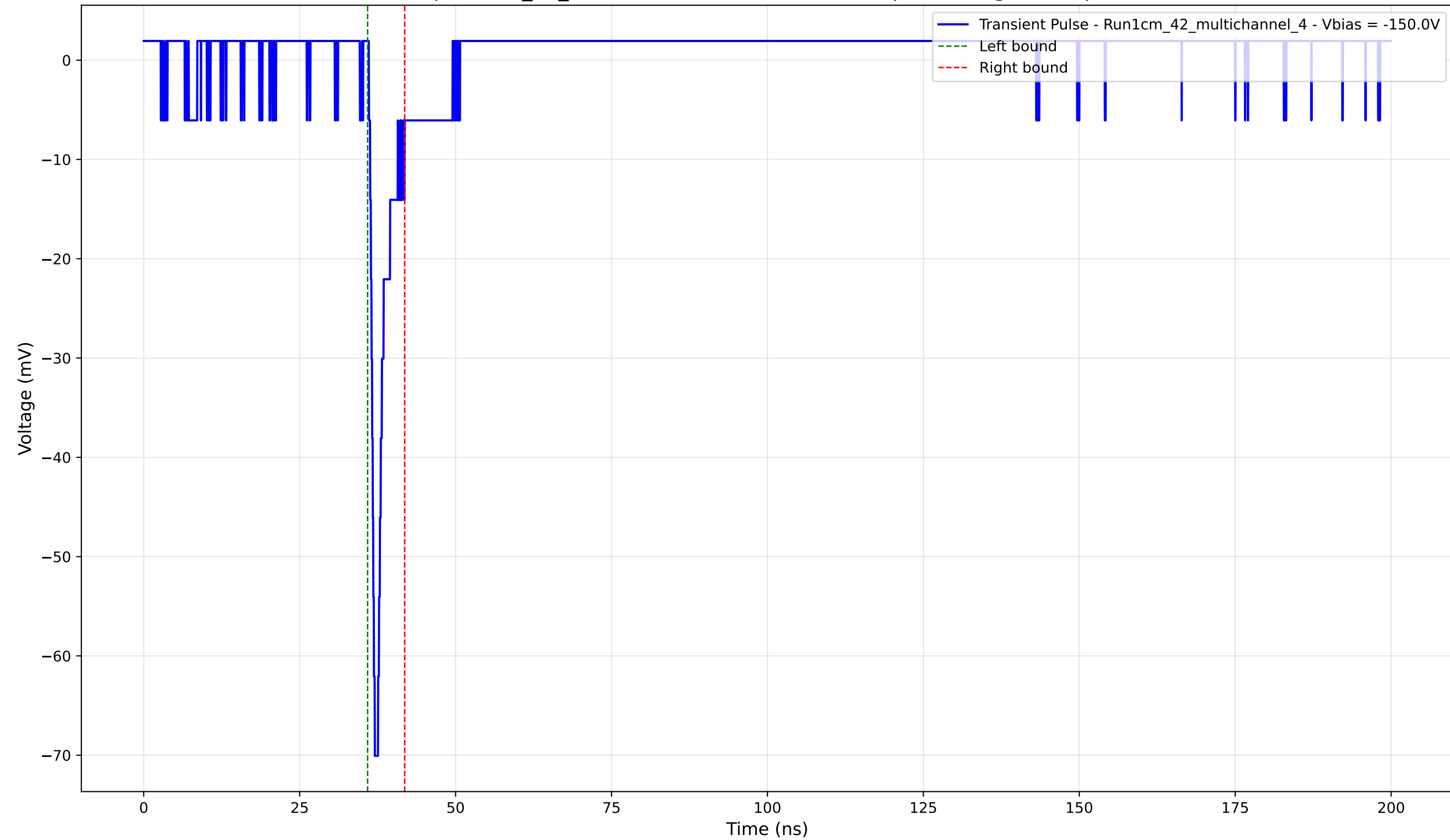
Transient Pulse - Sample: 1cm_42_multichannel - Position: 2540.0 \mu\text{m} - Charge: 3.17 pC - Rise Time: 0.76 ns
