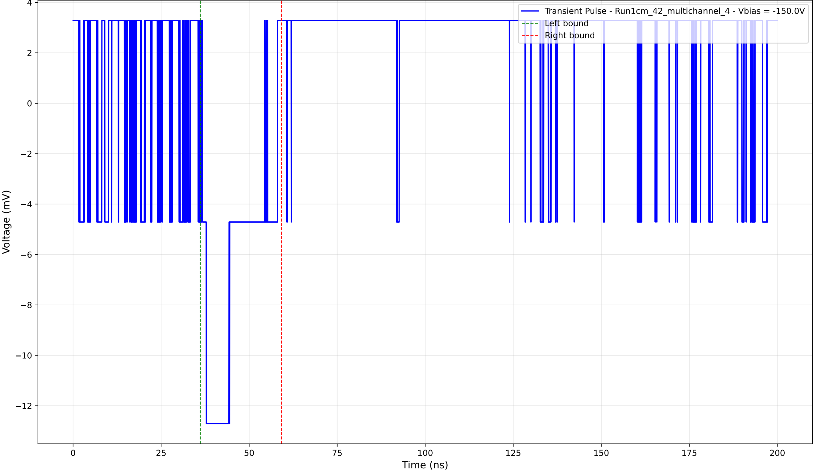
Transient Pulse - Sample: 1cm_42_multichannel - Position: 605.0 \mu\text{m} - Charge: 2.93 pC - Rise Time: 0.00 ns (N/A)
