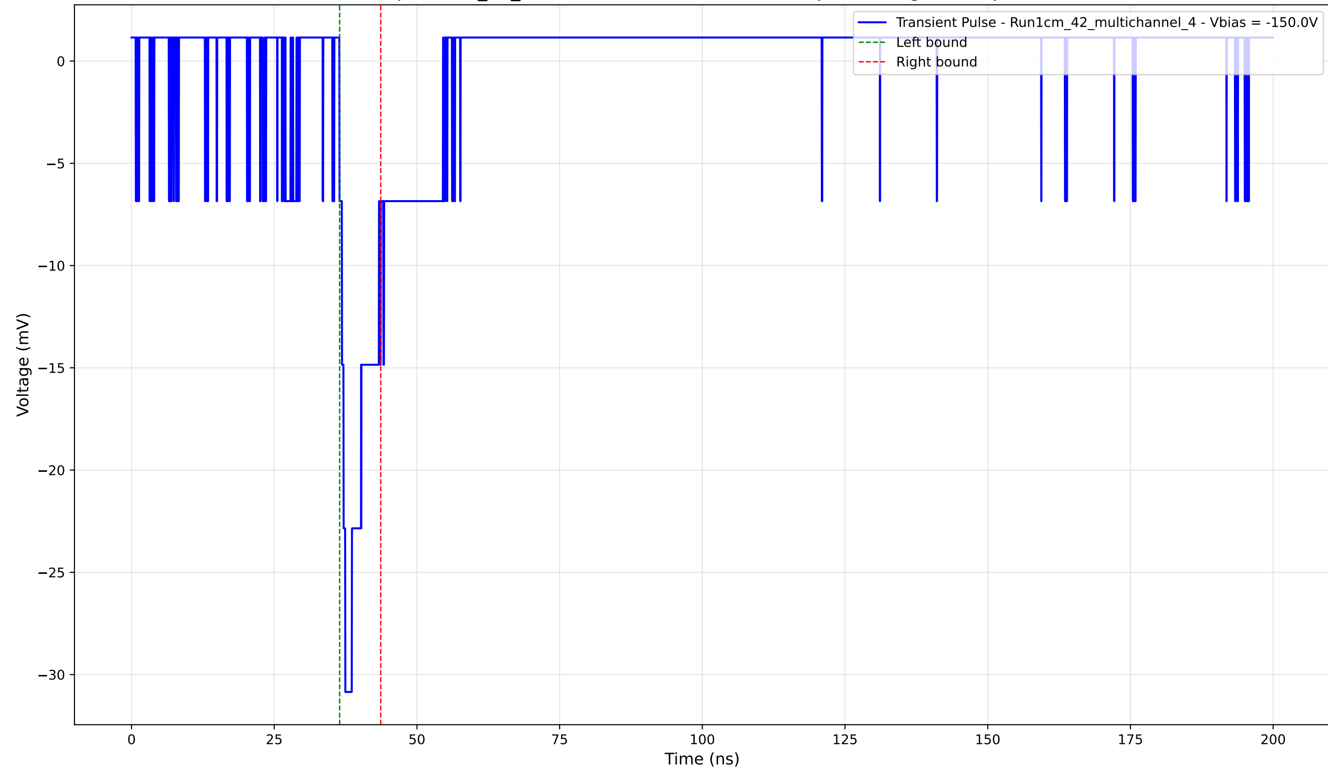
Transient Pulse - Sample: 1cm_42_multichannel - Position: 1555.0 \mu\text{m} - Charge: 2.71 pC - Rise Time: 1.03 ns
