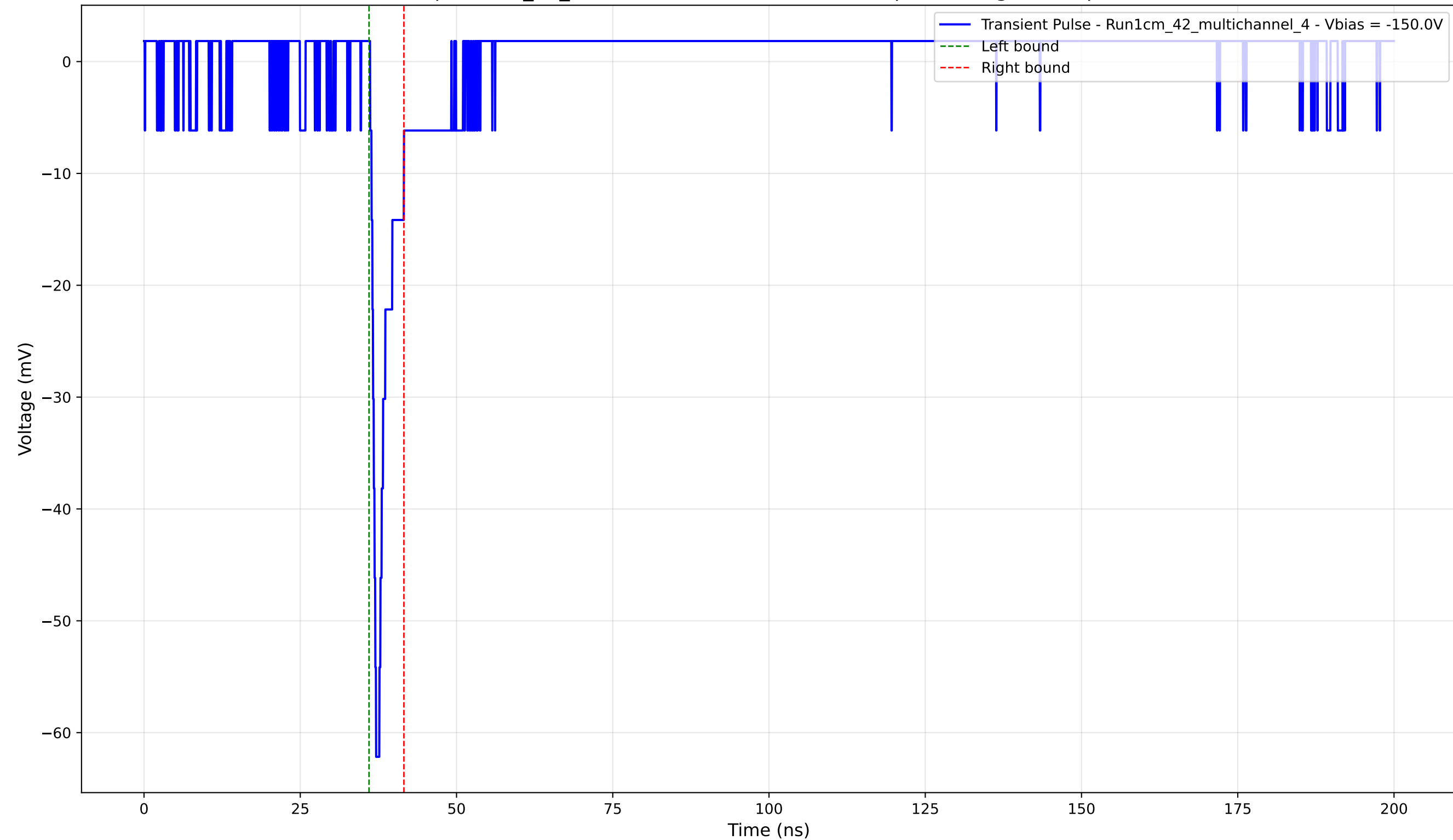
Transient Pulse - Sample: 1cm_42_multichannel - Position: 2130.0 \mu\text{m} - Charge: 2.95 pC - Rise Time: 0.74 ns
