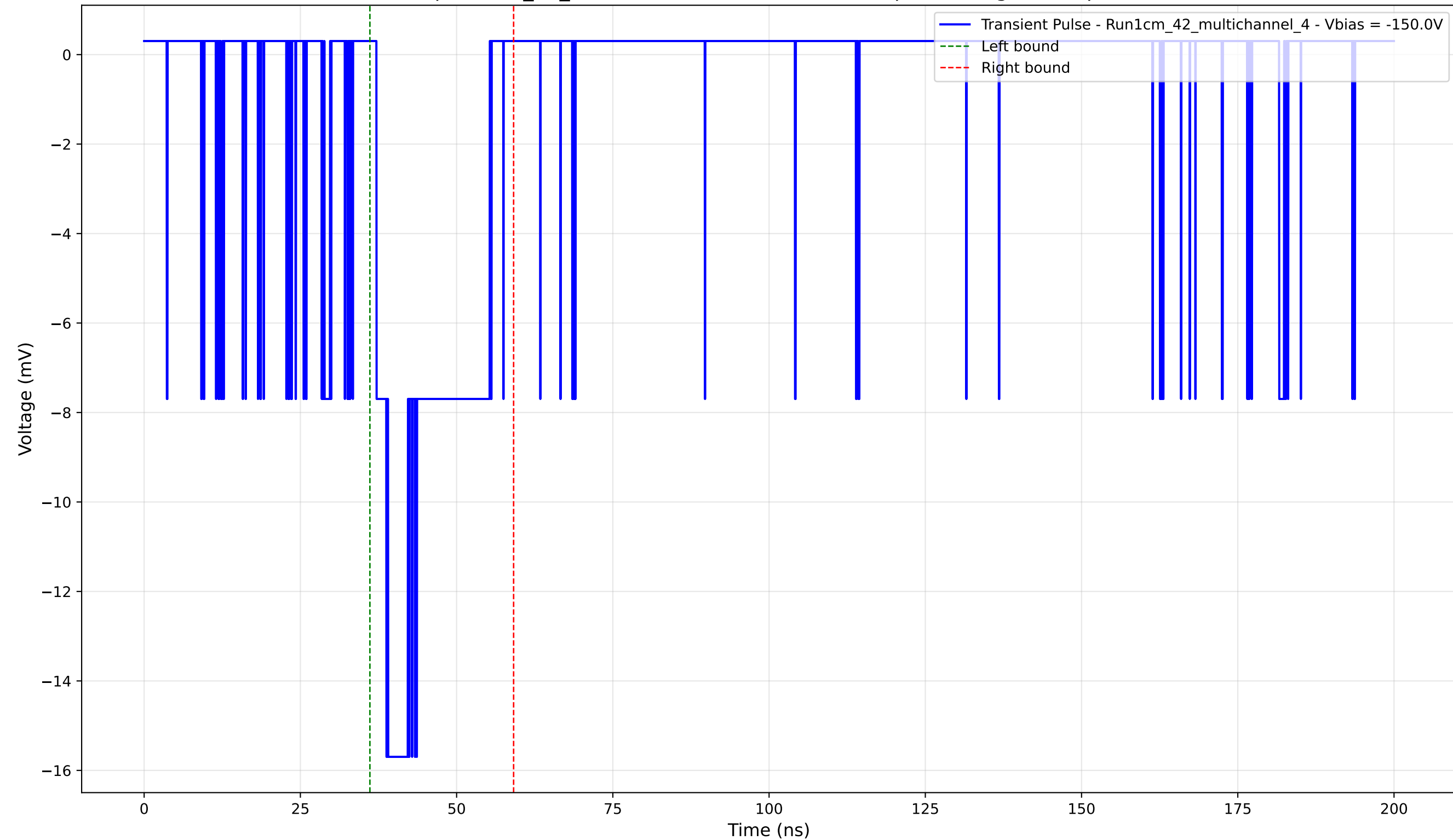
Transient Pulse - Sample: 1cm_42_multichannel - Position: 4620.0 \mu\text{m} - Charge: 3.35 pC - Rise Time: 1.60 ns
