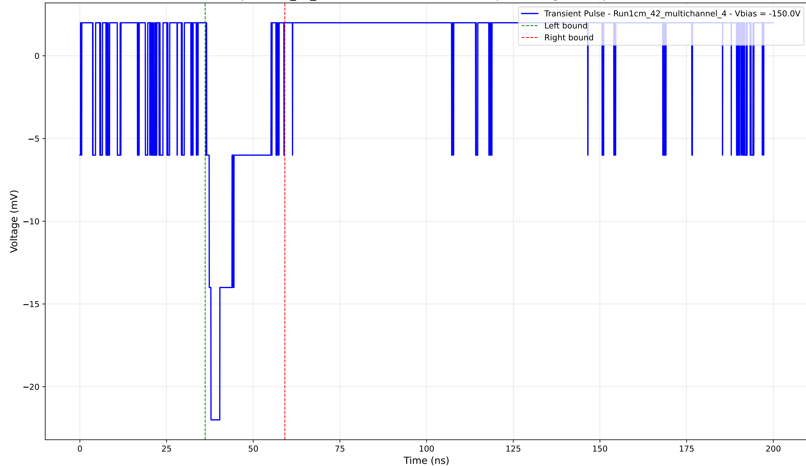
Transient Pulse - Sample: 1cm_42_multichannel - Position: 1175.0 \mu\text{m} - Charge: 3.63 pC - Rise Time: 1.26 ns
