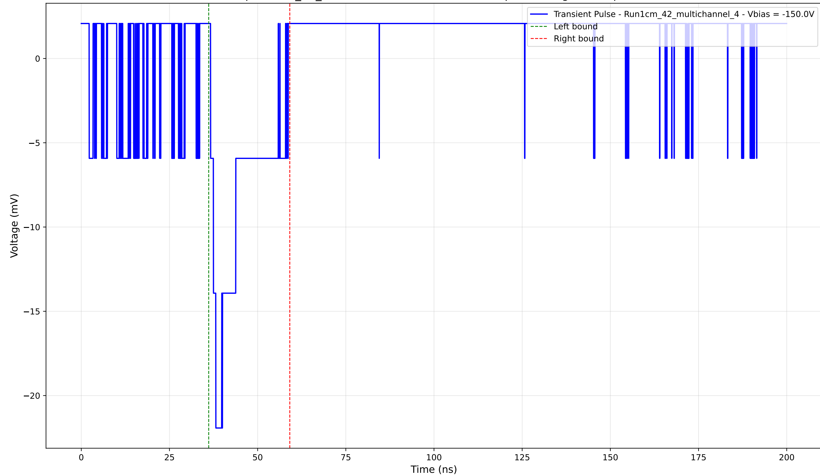
Transient Pulse - Sample: 1cm_42_multichannel - Position: 1105.0 \mu\text{m} - Charge: 3.80 pC - Rise Time: 1.50 ns
