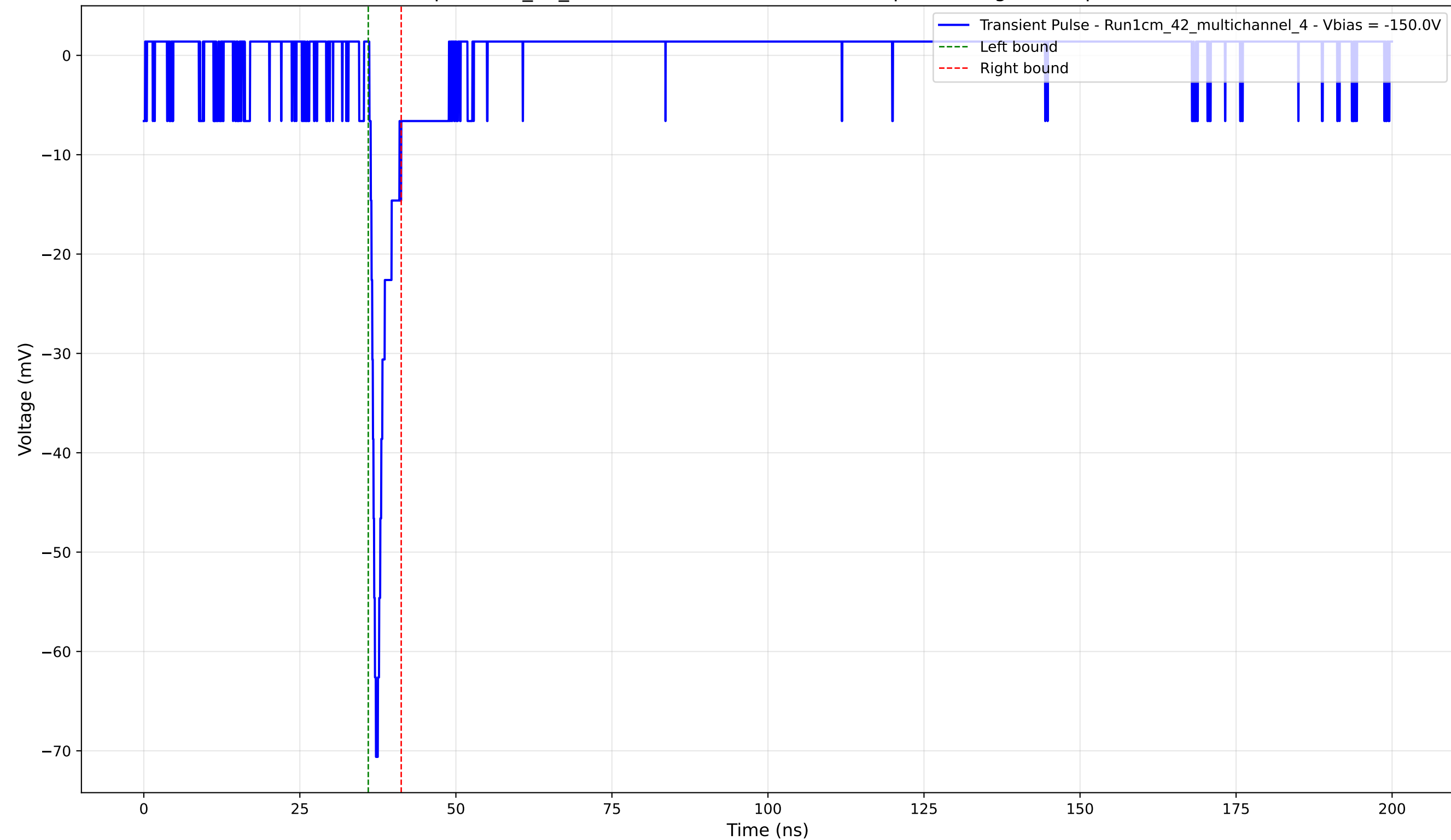
Transient Pulse - Sample: 1cm_42_multichannel - Position: 2175.0 \mu\text{m} - Charge: 3.03 pC - Rise Time: 0.84 ns
