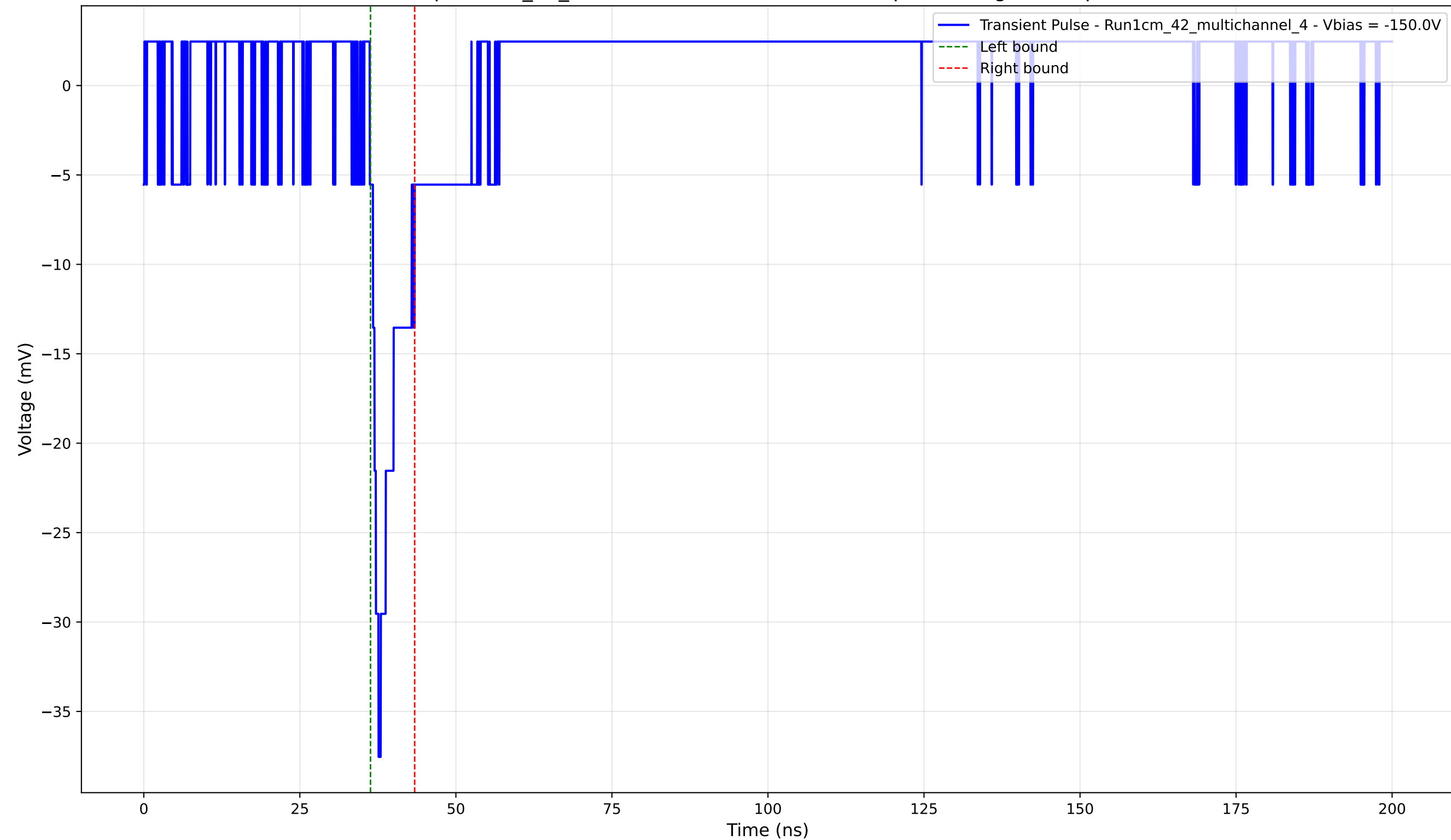
Transient Pulse - Sample: 1cm_42_multichannel - Position: 1675.0 \mu\text{m} - Charge: 2.59 pC - Rise Time: 1.41 ns
