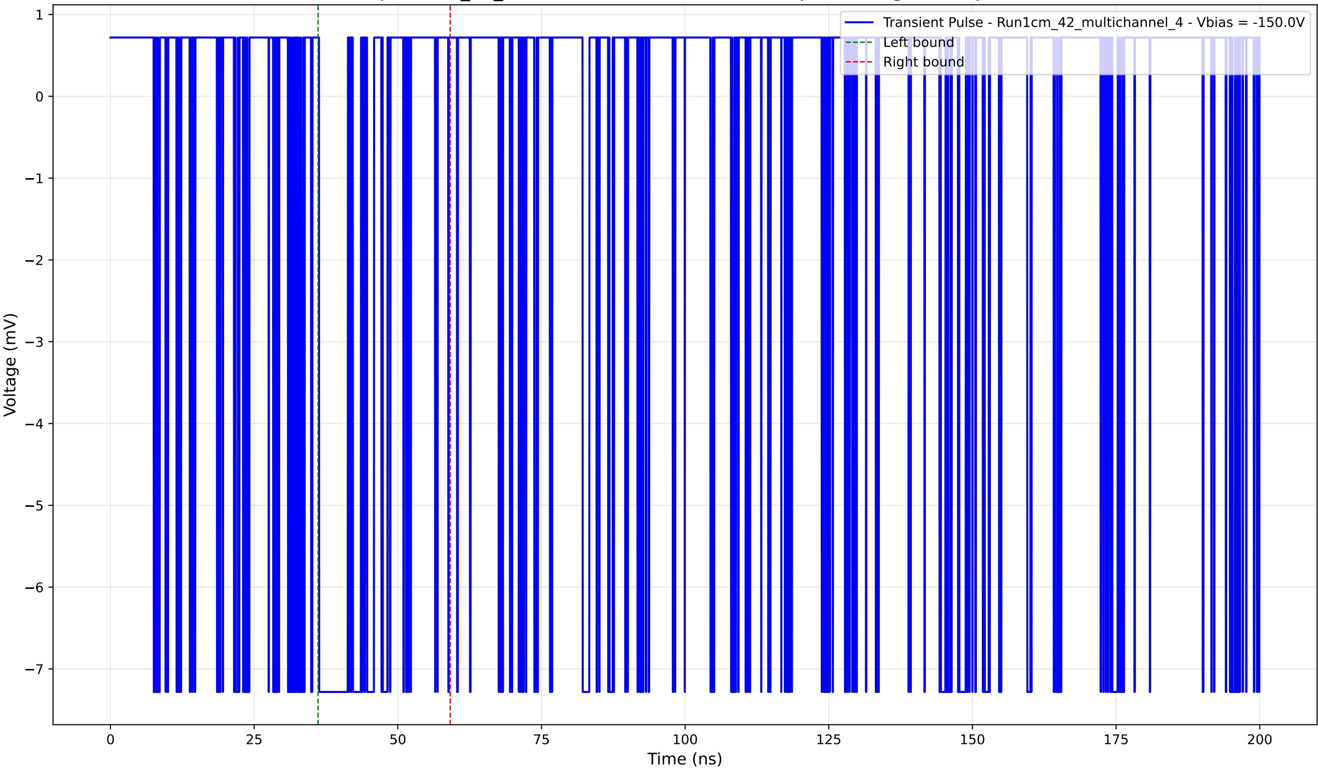
Transient Pulse - Sample: 1cm_42_multichannel - Position: 2415.0 \mu\text{m} - Charge: 1.27 pC - Rise Time: 0.02 ns
