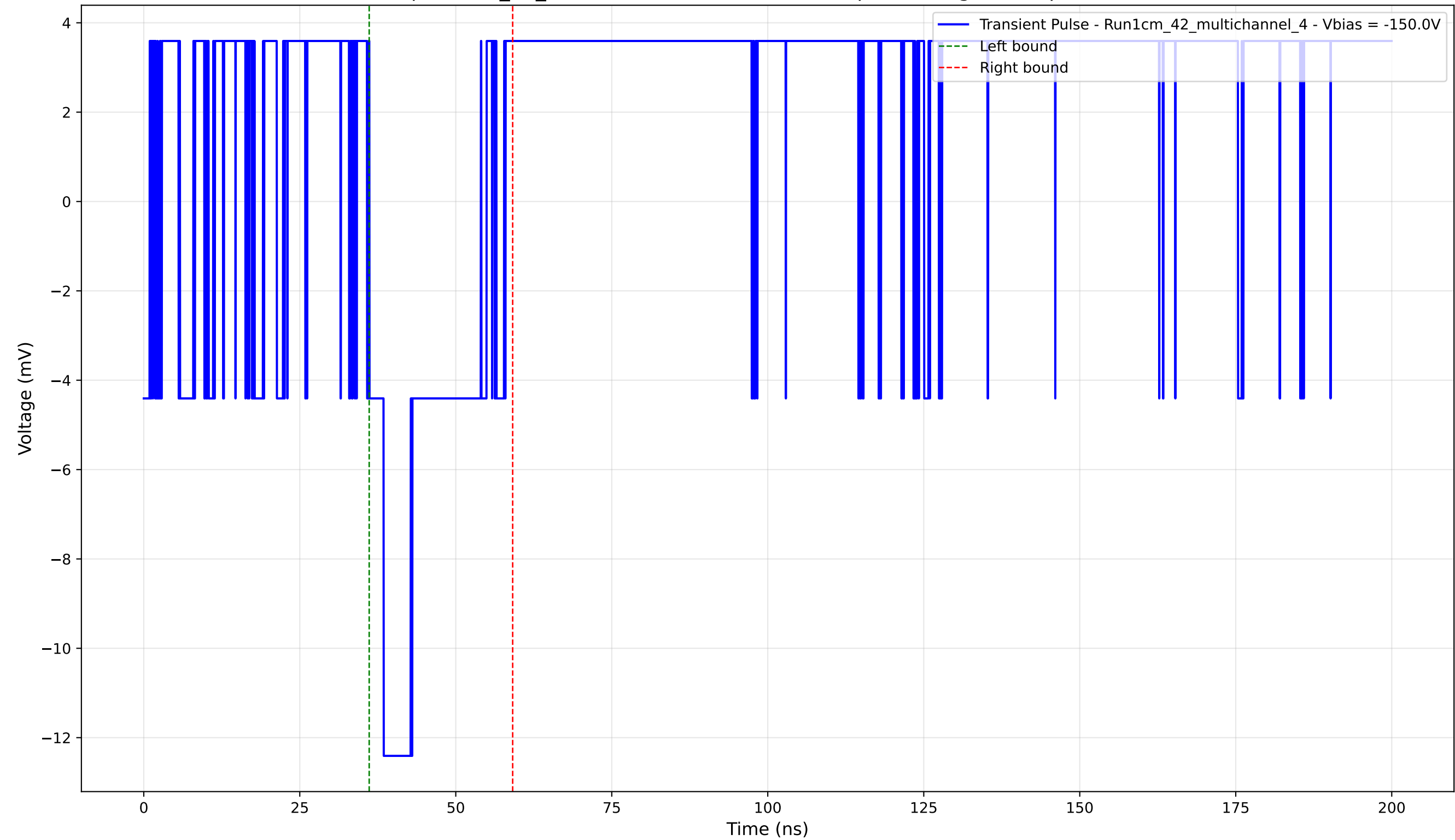
Transient Pulse - Sample: 1cm_42_multichannel - Position: 160.0 \mu\text{m} - Charge: 2.29 pC - Rise Time: 0.00 ns (N/A)
