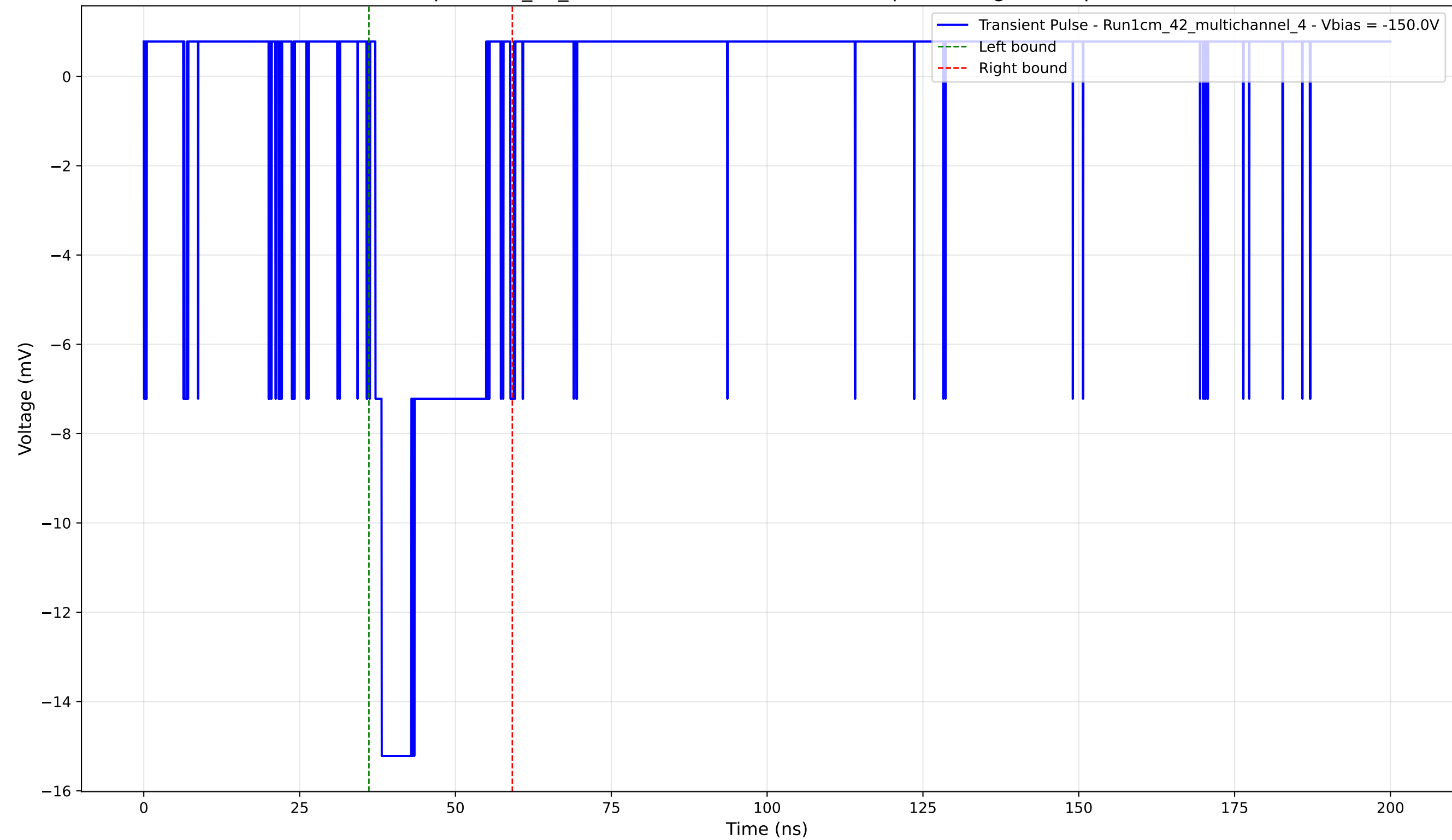
Transient Pulse - Sample: 1cm_42_multichannel - Position: 4130.0 \mu\text{m} - Charge: 3.42 pC - Rise Time: 1.02 ns
