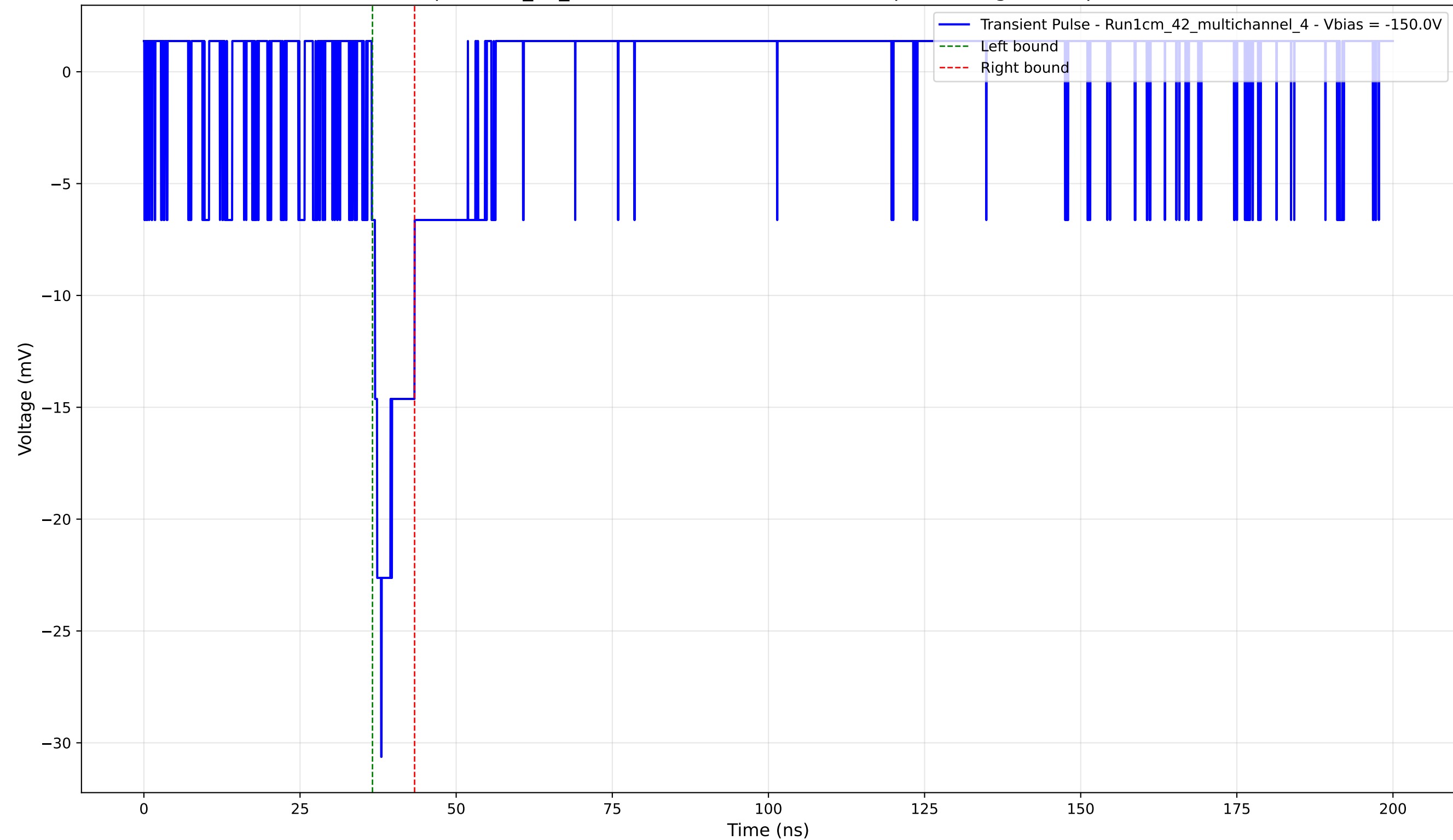
Transient Pulse - Sample: 1cm_42_multichannel - Position: 3300.0 \mu\text{m} - Charge: 2.28 pC - Rise Time: 1.51 ns
