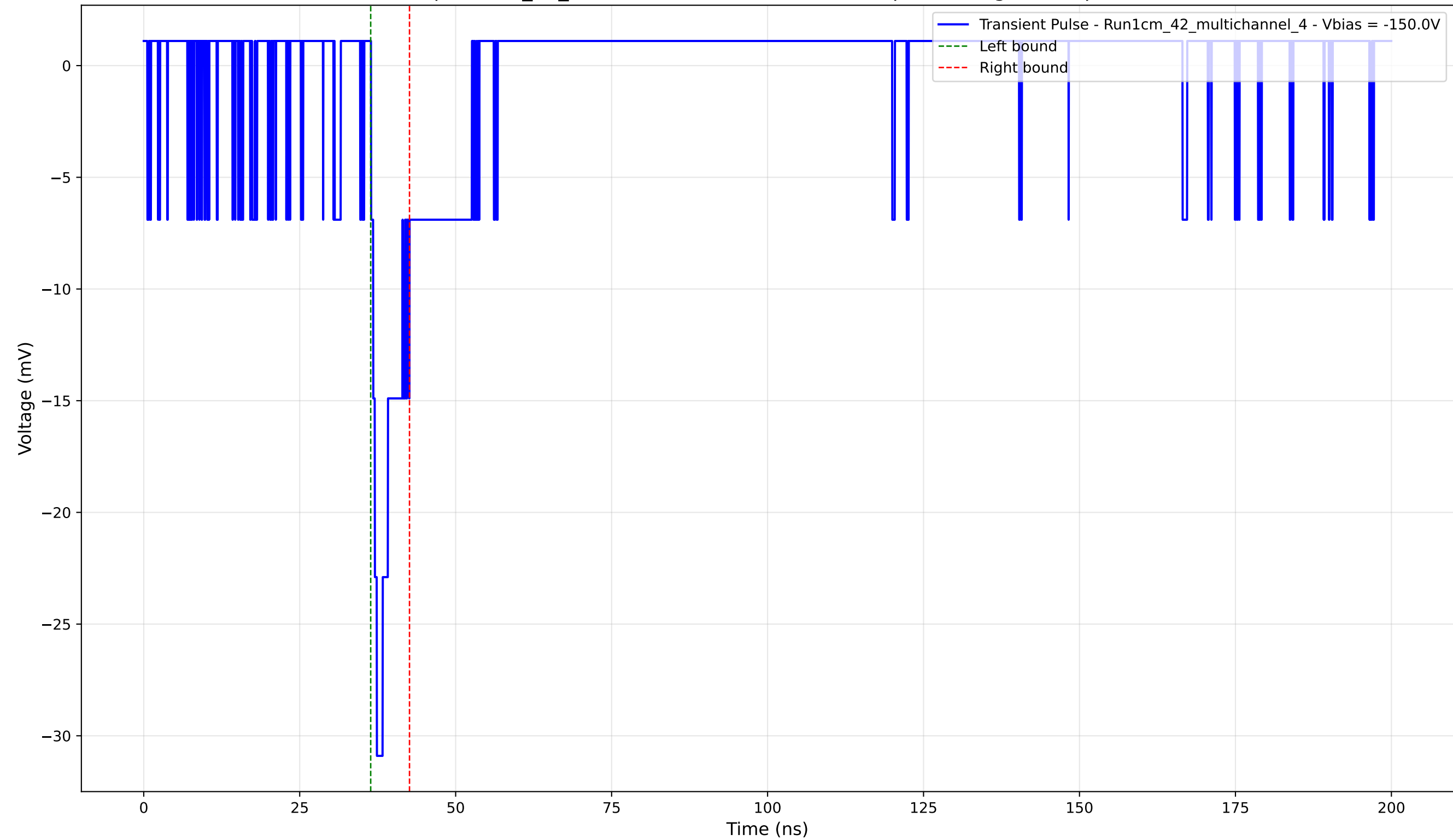
Transient Pulse - Sample: 1cm_42_multichannel - Position: 3105.0 \mu\text{m} - Charge: 2.18 pC - Rise Time: 0.93 ns
