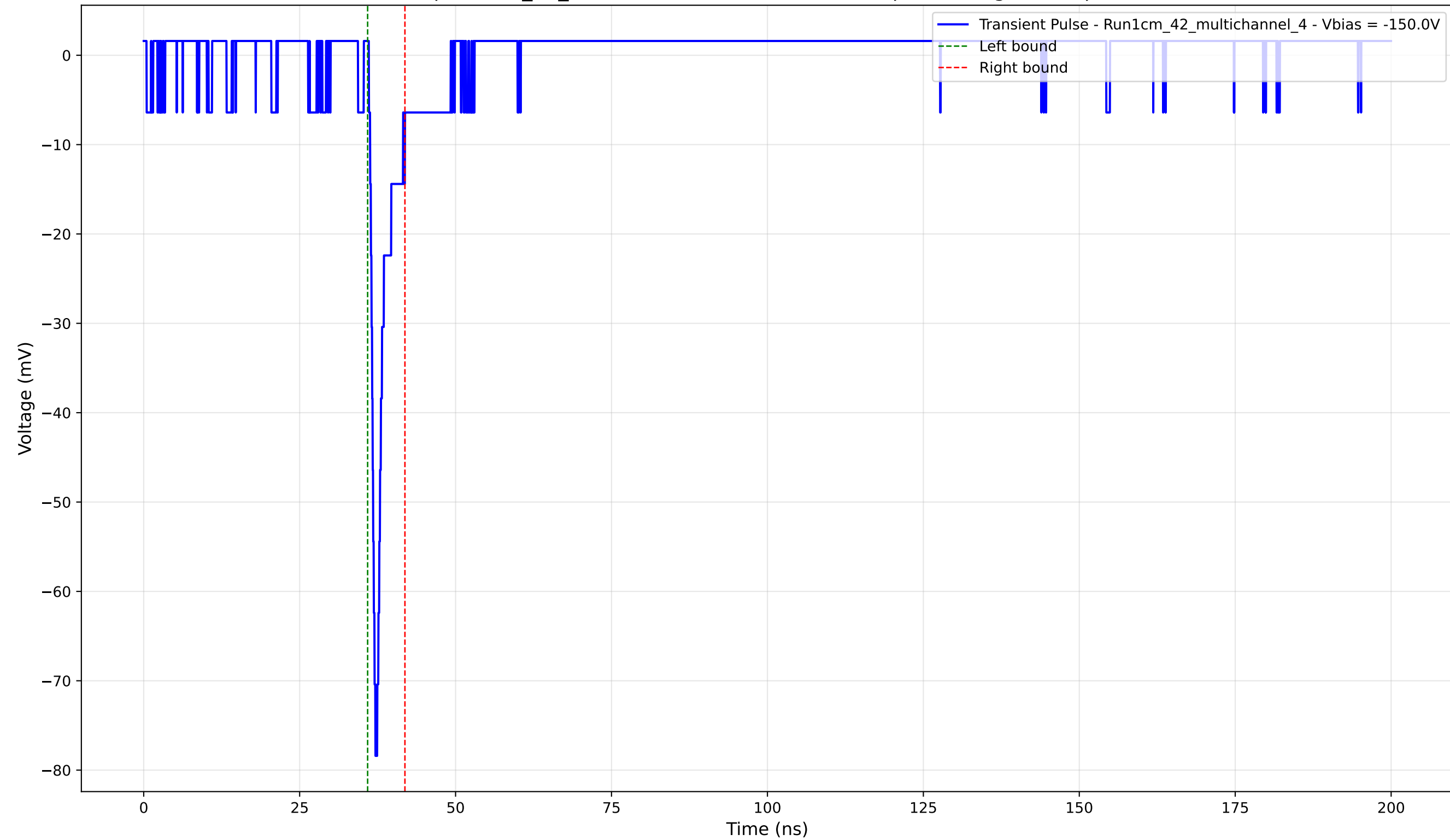
Transient Pulse - Sample: 1cm_42_multichannel - Position: 2535.0 \mu\text{m} - Charge: 3.38 pC - Rise Time: 0.86 ns
