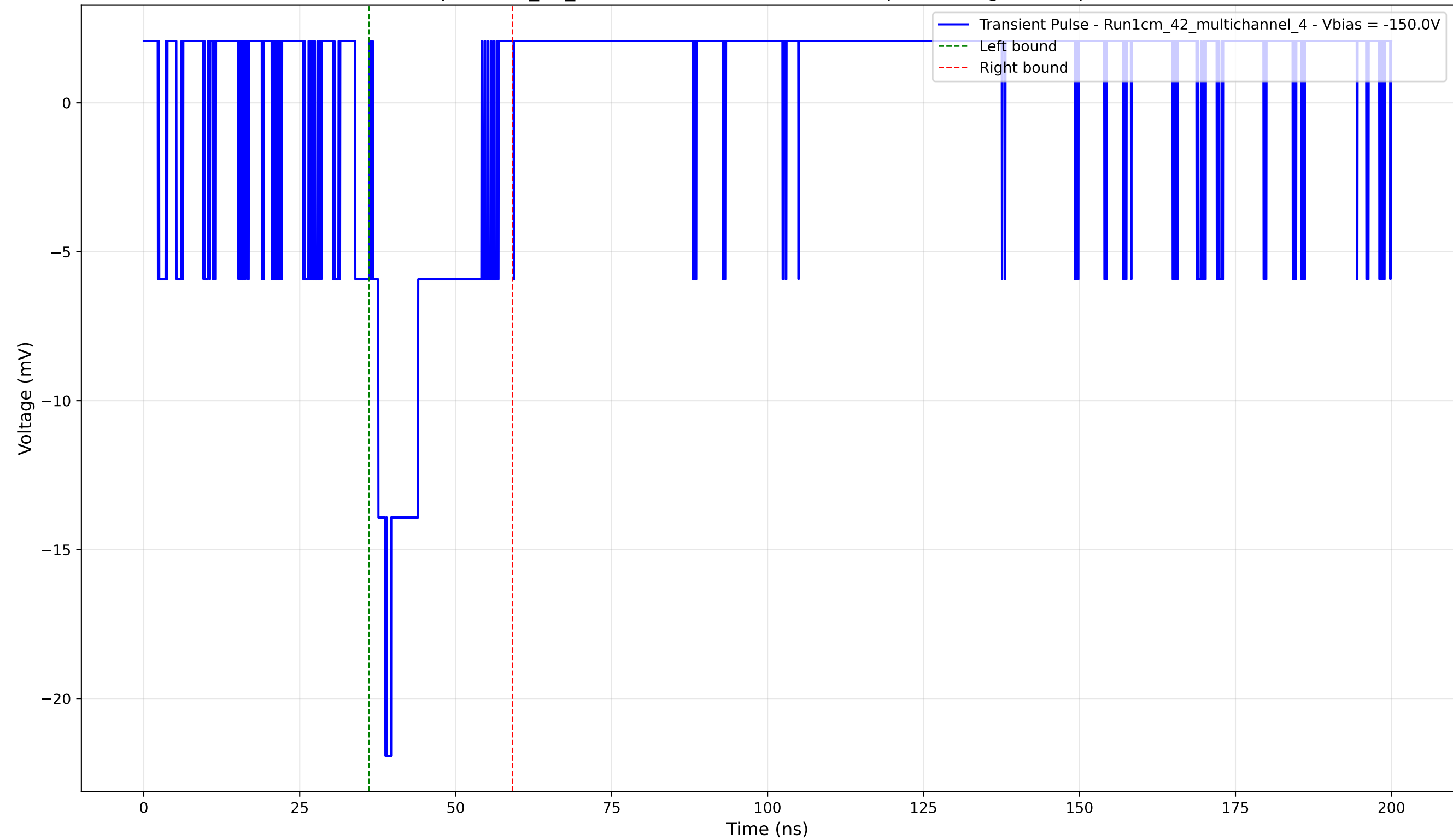
Transient Pulse - Sample: 1cm_42_multichannel - Position: 965.0 \mu\text{m} - Charge: 3.35 pC - Rise Time: 2.00 ns
