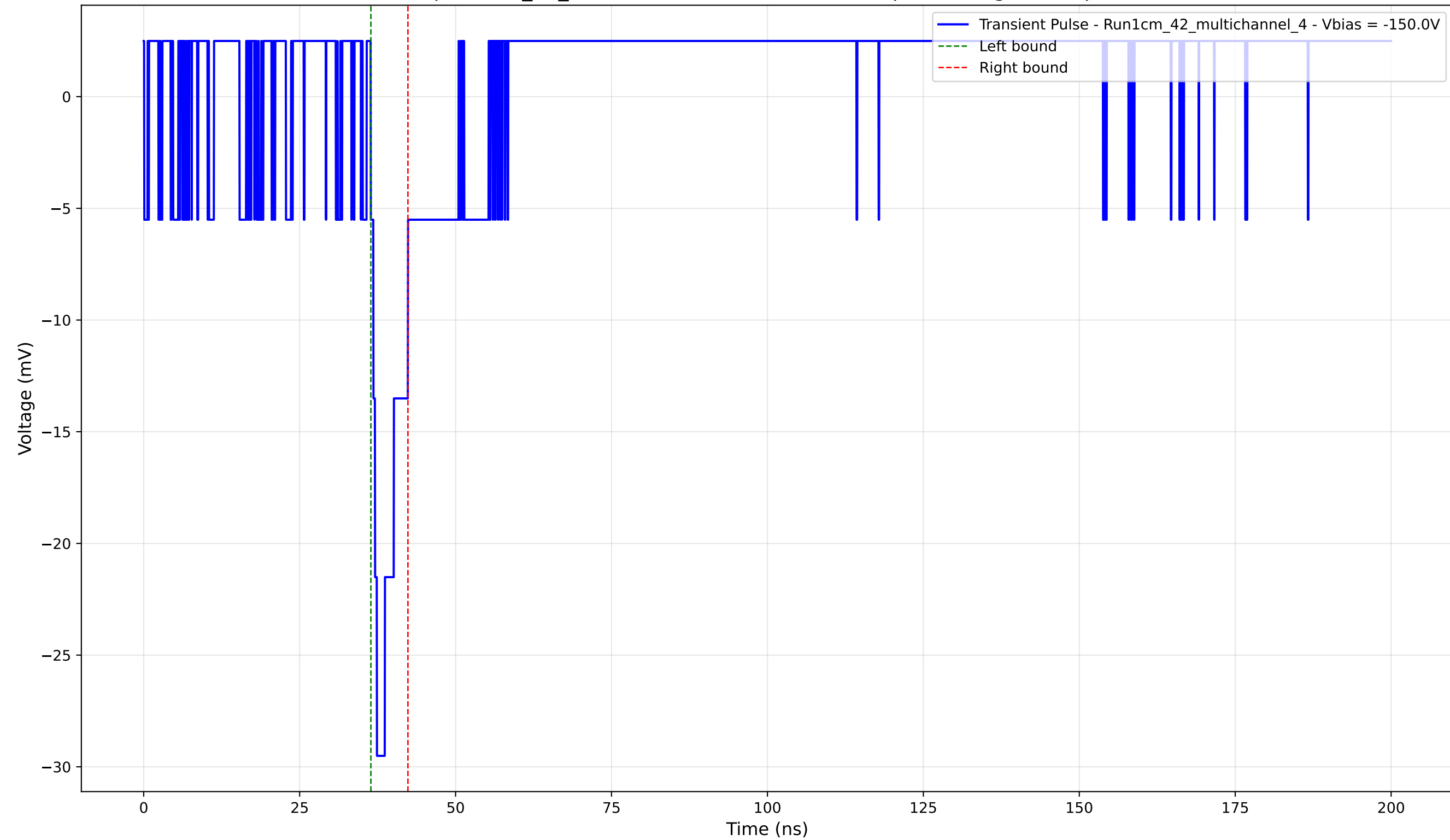
Transient Pulse - Sample: 1cm_42_multichannel - Position: 1585.0 \mu\text{m} - Charge: 2.23 pC - Rise Time: 1.00 ns
