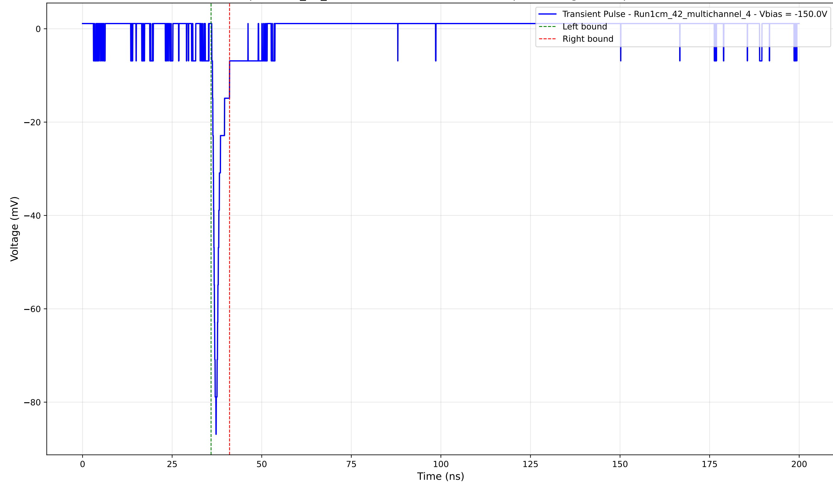
Transient Pulse - Sample: 1cm_42_multichannel - Position: 2480.0 \mu\text{m} - Charge: 3.33 pC - Rise Time: 0.76 ns
