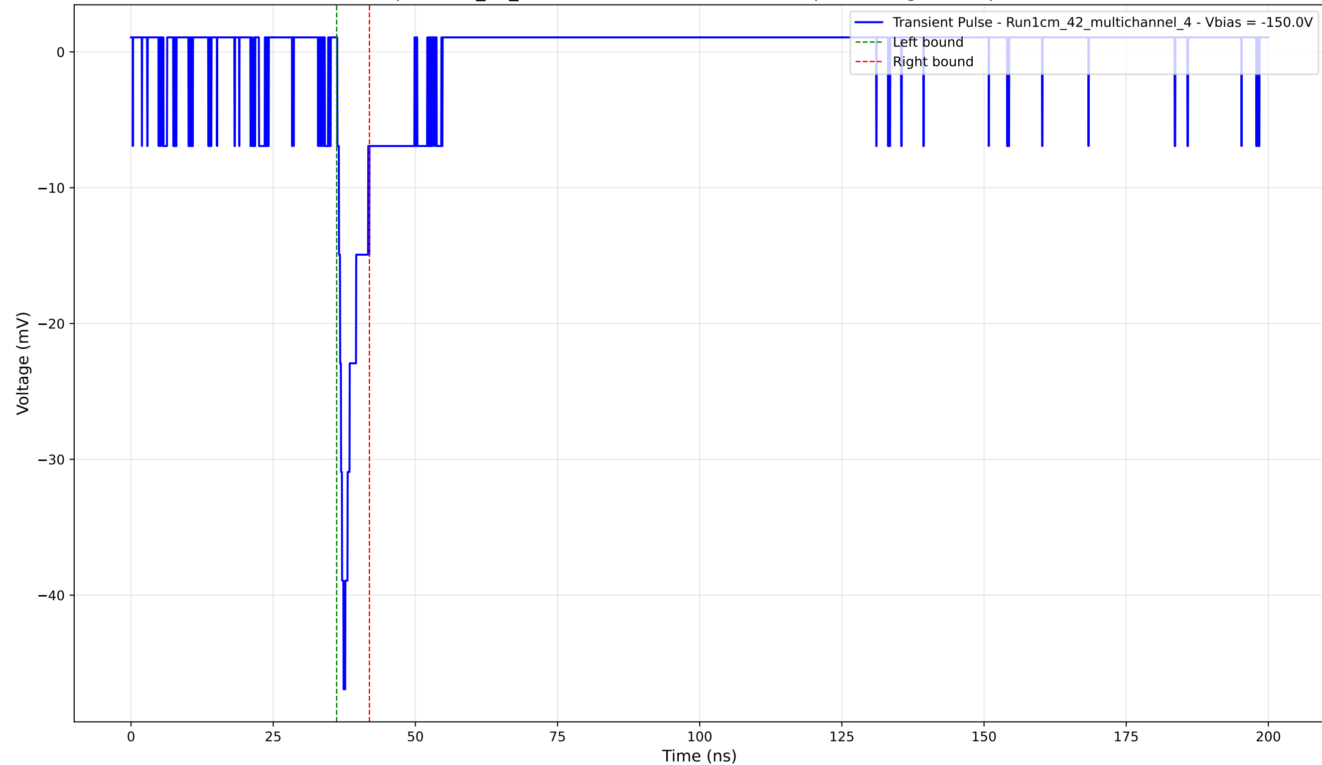
Transient Pulse - Sample: 1cm_42_multichannel - Position: 2820.0 \mu\text{m} - Charge: 2.51 pC - Rise Time: 1.09 ns
