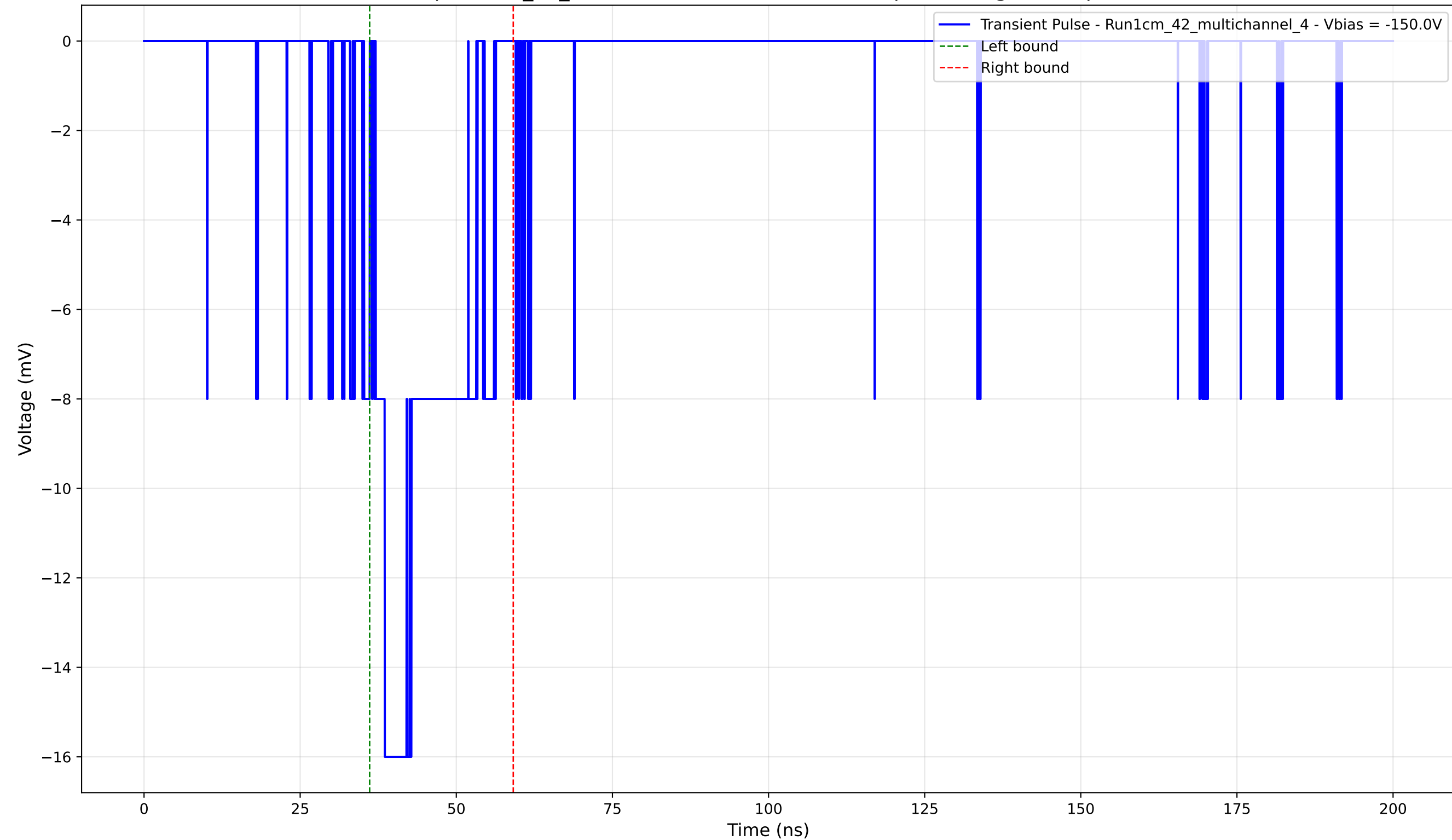
Transient Pulse - Sample: 1cm_42_multichannel - Position: 4770.0 \mu\text{m} - Charge: 3.56 pC - Rise Time: 1.46 ns
