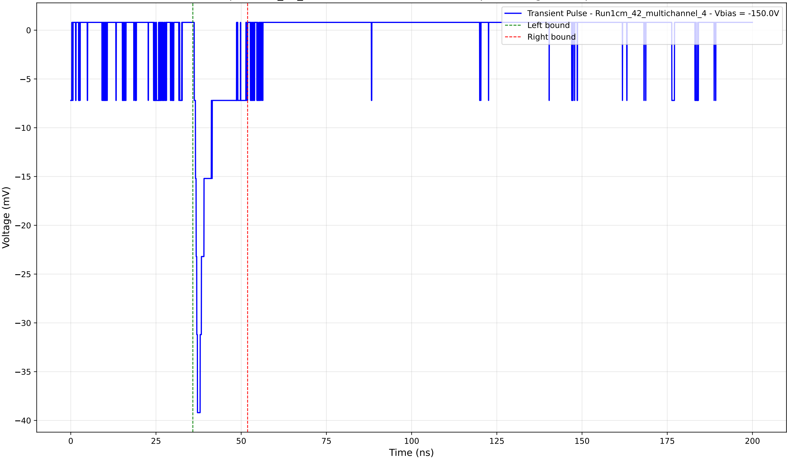
Transient Pulse - Sample: 1cm_42_multichannel - Position: 2825.0 \mu\text{m} - Charge: 3.64 pC - Rise Time: 0.95 ns
