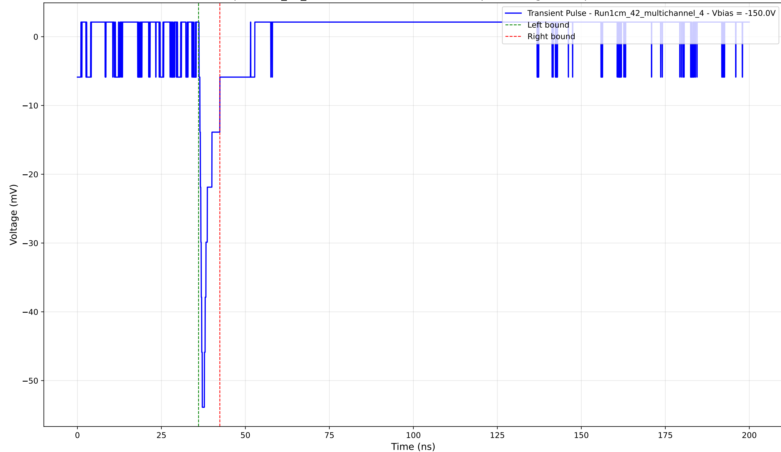
Transient Pulse - Sample: 1cm_42_multichannel - Position: 2030.0 \mu\text{m} - Charge: 3.02 pC - Rise Time: 0.96 ns
