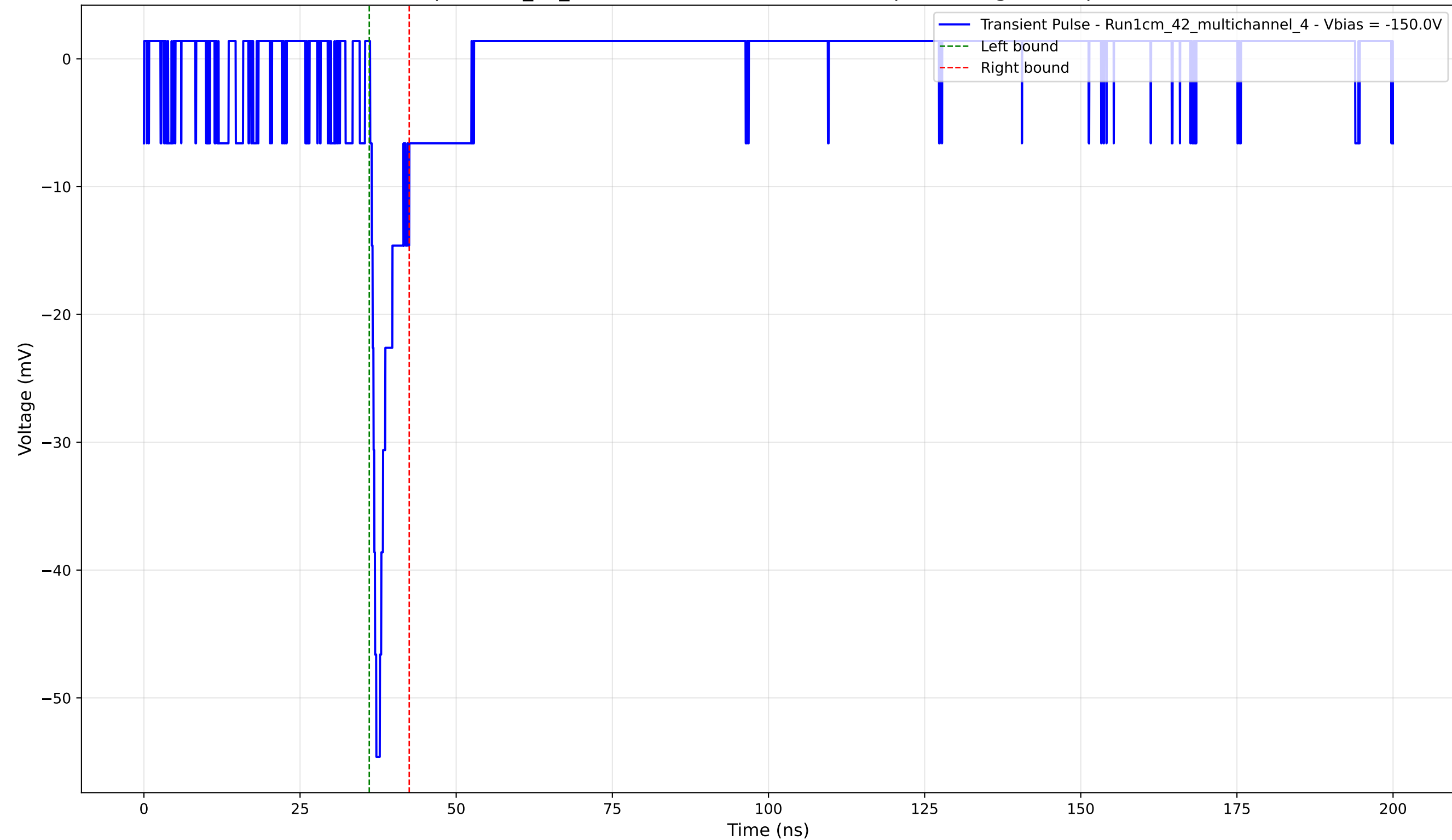
Transient Pulse - Sample: 1cm_42_multichannel - Position: 2740.0 \mu\text{m} - Charge: 3.01 pC - Rise Time: 0.98 ns
