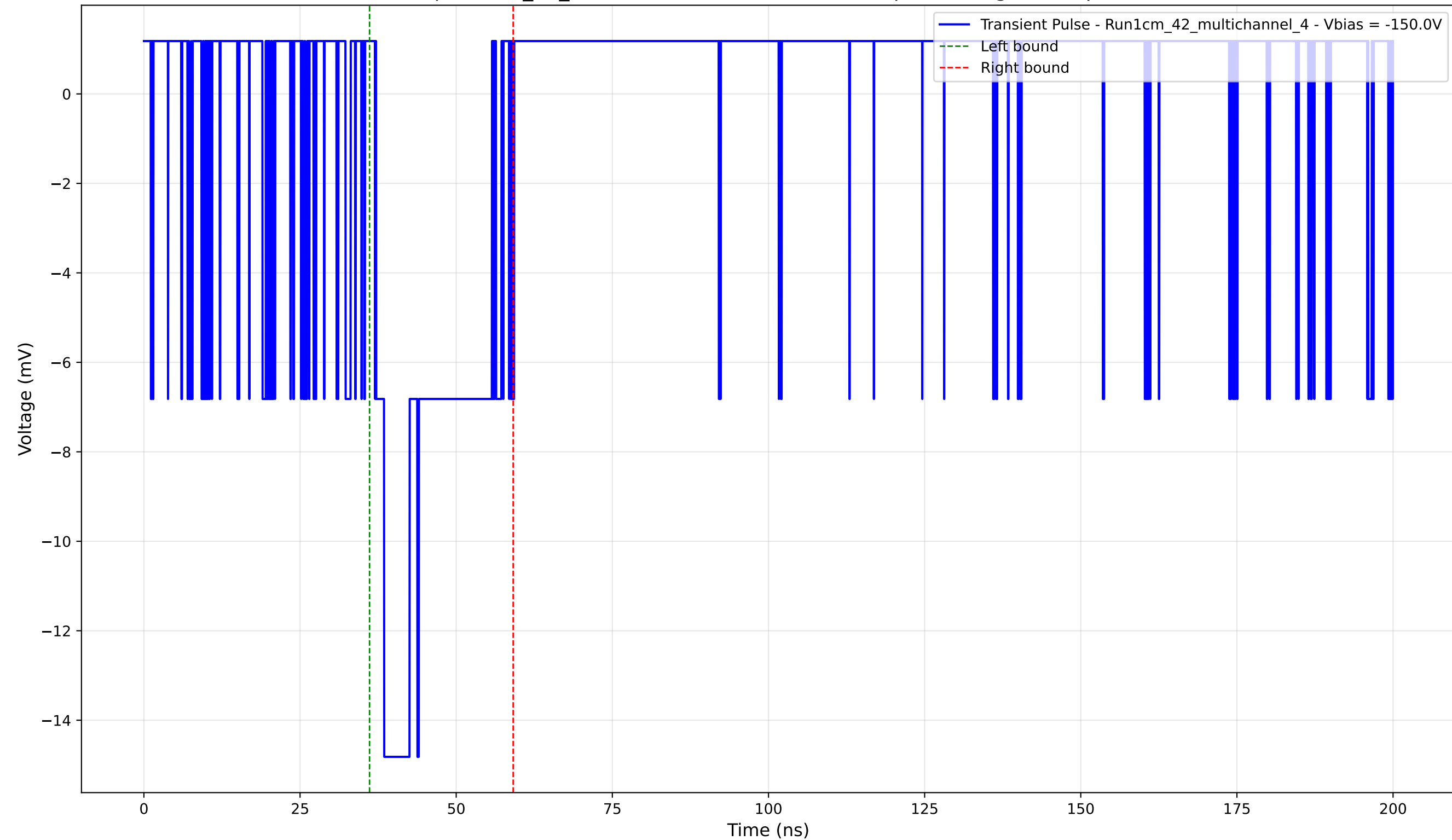
Transient Pulse - Sample: 1cm_42_multichannel - Position: 4585.0 \mu\text{m} - Charge: 3.34 pC - Rise Time: 1.30 ns
