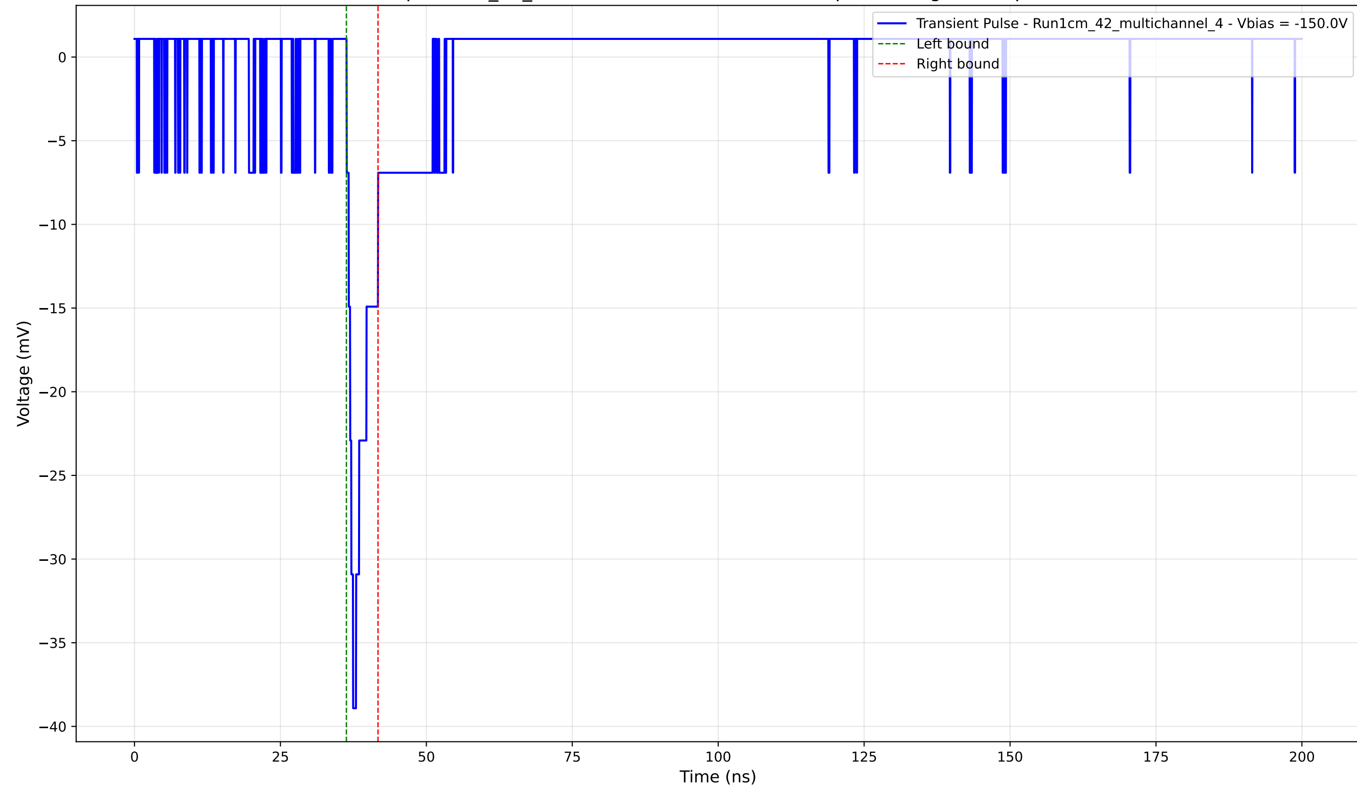
Transient Pulse - Sample: 1cm_42_multichannel - Position: 3015.0 \mu\text{m} - Charge: 2.29 pC - Rise Time: 1.11 ns
