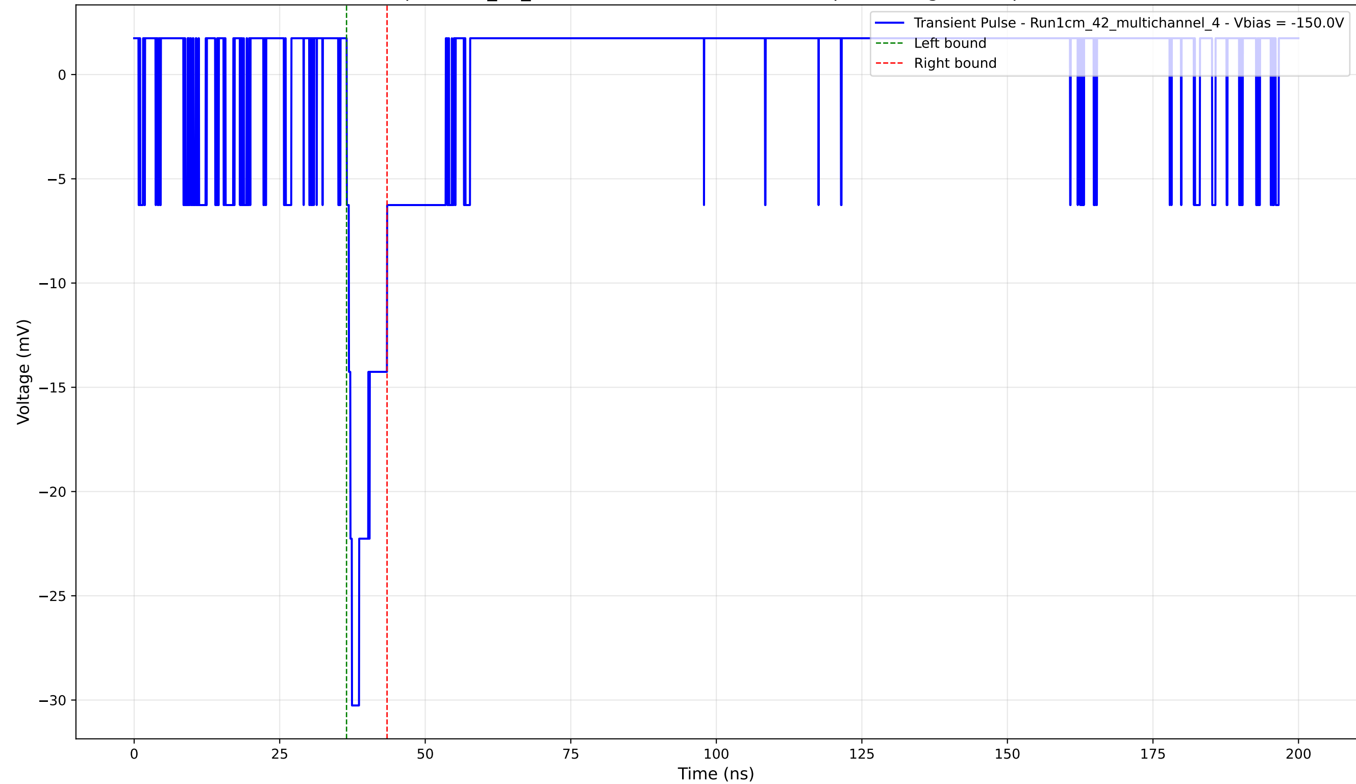
Transient Pulse - Sample: 1cm_42_multichannel - Position: 1545.0 \mu\text{m} - Charge: 2.63 pC - Rise Time: 0.89 ns
