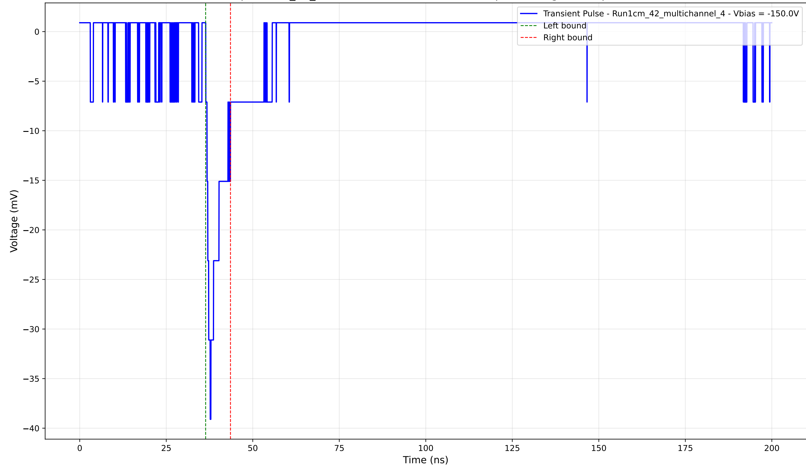
Transient Pulse - Sample: 1cm_42_multichannel - Position: 1640.0 \mu\text{m} - Charge: 2.82 pC - Rise Time: 1.29 ns
