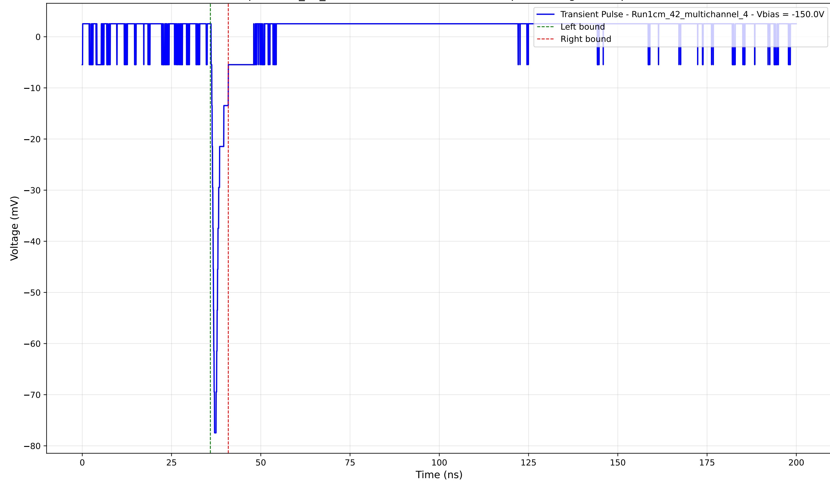
Transient Pulse - Sample: 1cm_42_multichannel - Position: 2500.0 \mu\text{m} - Charge: 3.09 pC - Rise Time: 0.77 ns
