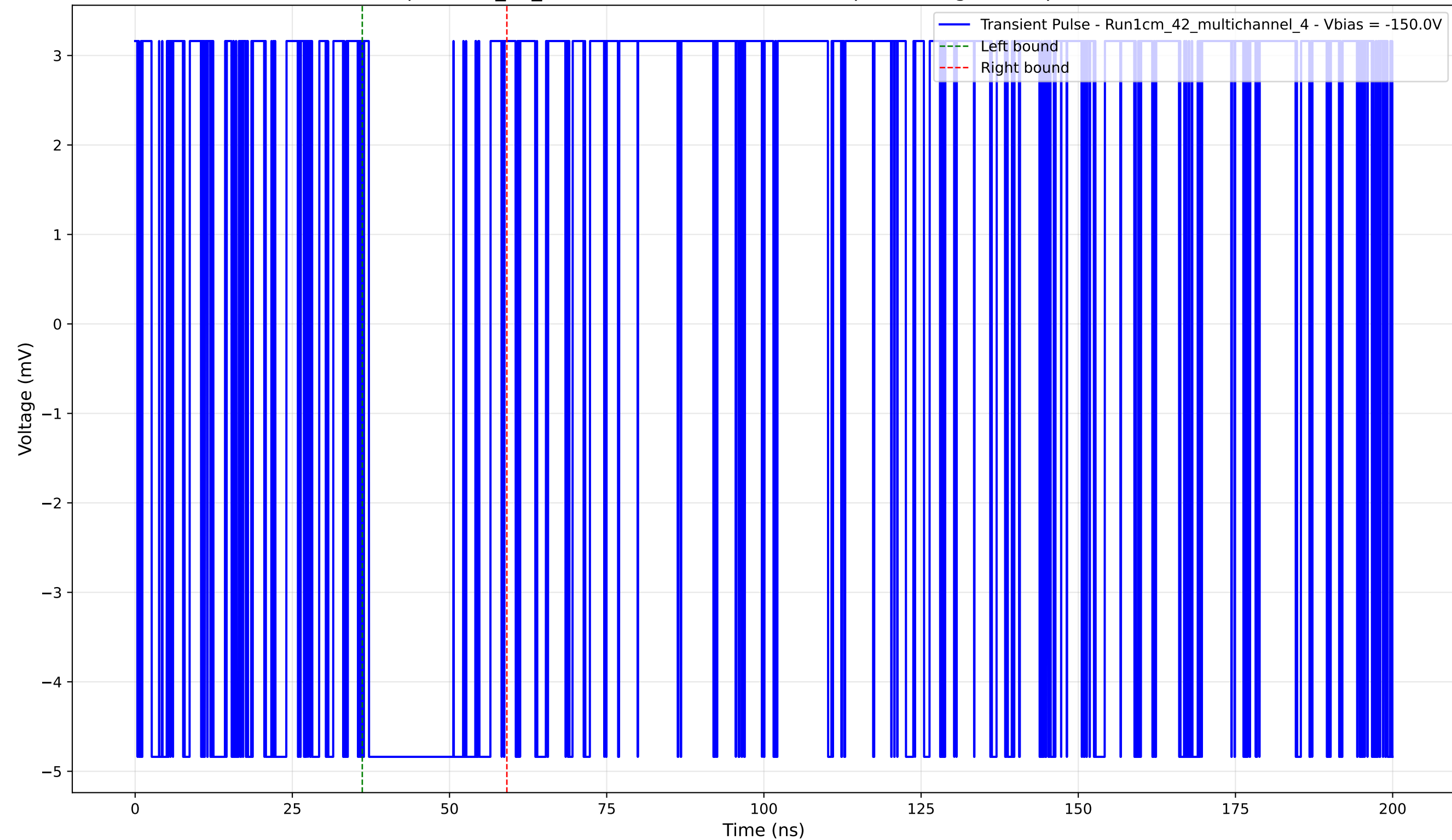
Transient Pulse - Sample: 1cm_42_multichannel - Position: 915.0 \mu\text{m} - Charge: 1.61 pC - Rise Time: 0.00 ns (N/A)
