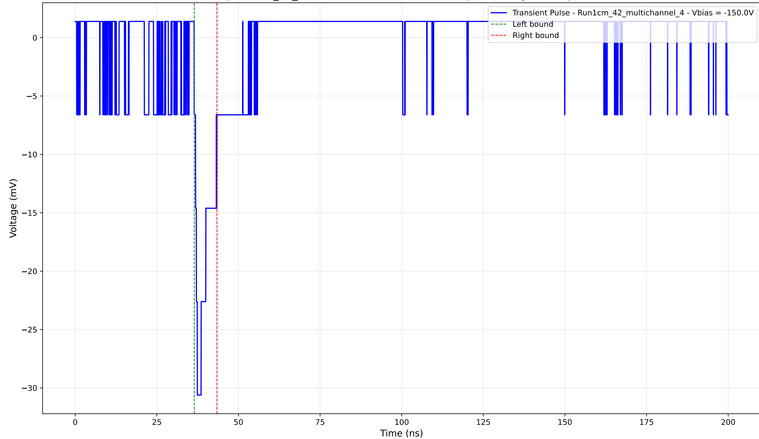
Transient Pulse - Sample: 1cm_42_multichannel - Position: 1595.0 \mu\text{m} - Charge: 2.62 pC - Rise Time: 0.97 ns
