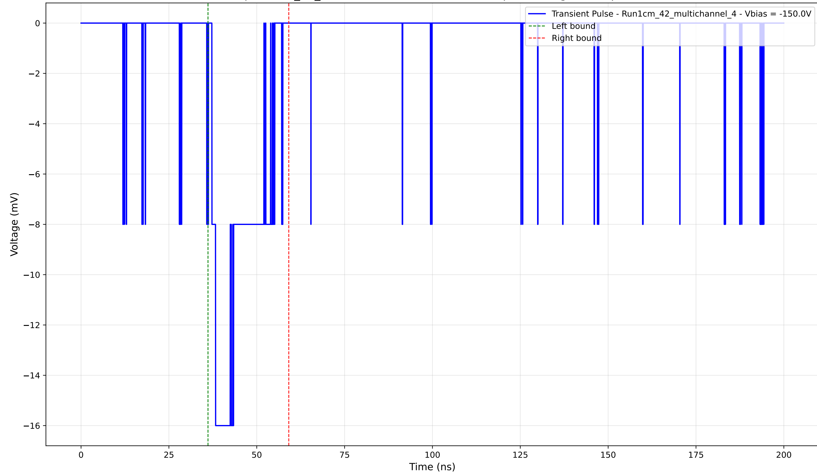
Transient Pulse - Sample: 1cm_42_multichannel - Position: 4250.0 \mu\text{m} - Charge: 3.59 pC - Rise Time: 1.06 ns
