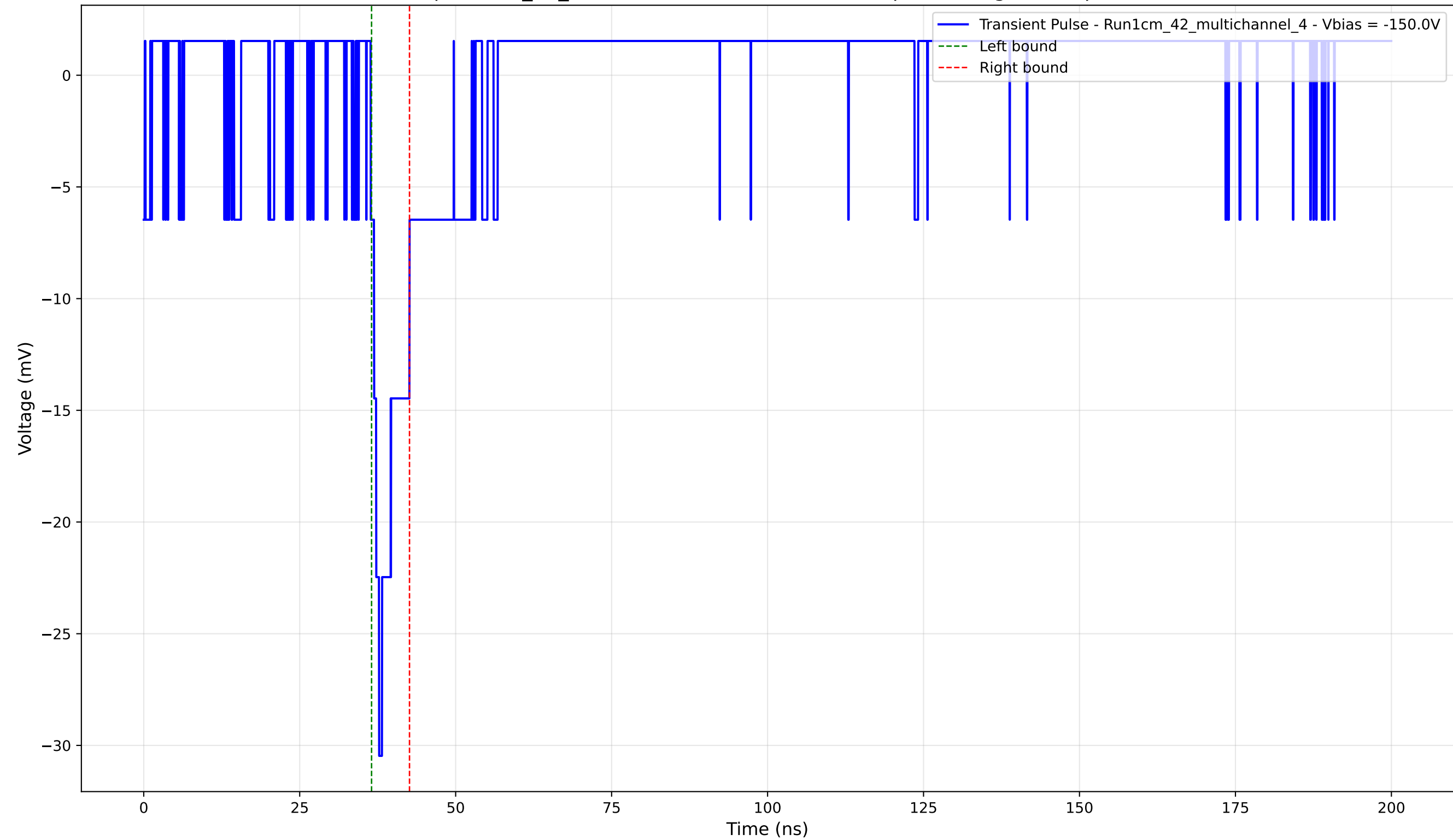
Transient Pulse - Sample: 1cm_42_multichannel - Position: 3245.0 \mu\text{m} - Charge: 2.15 pC - Rise Time: 1.35 ns
