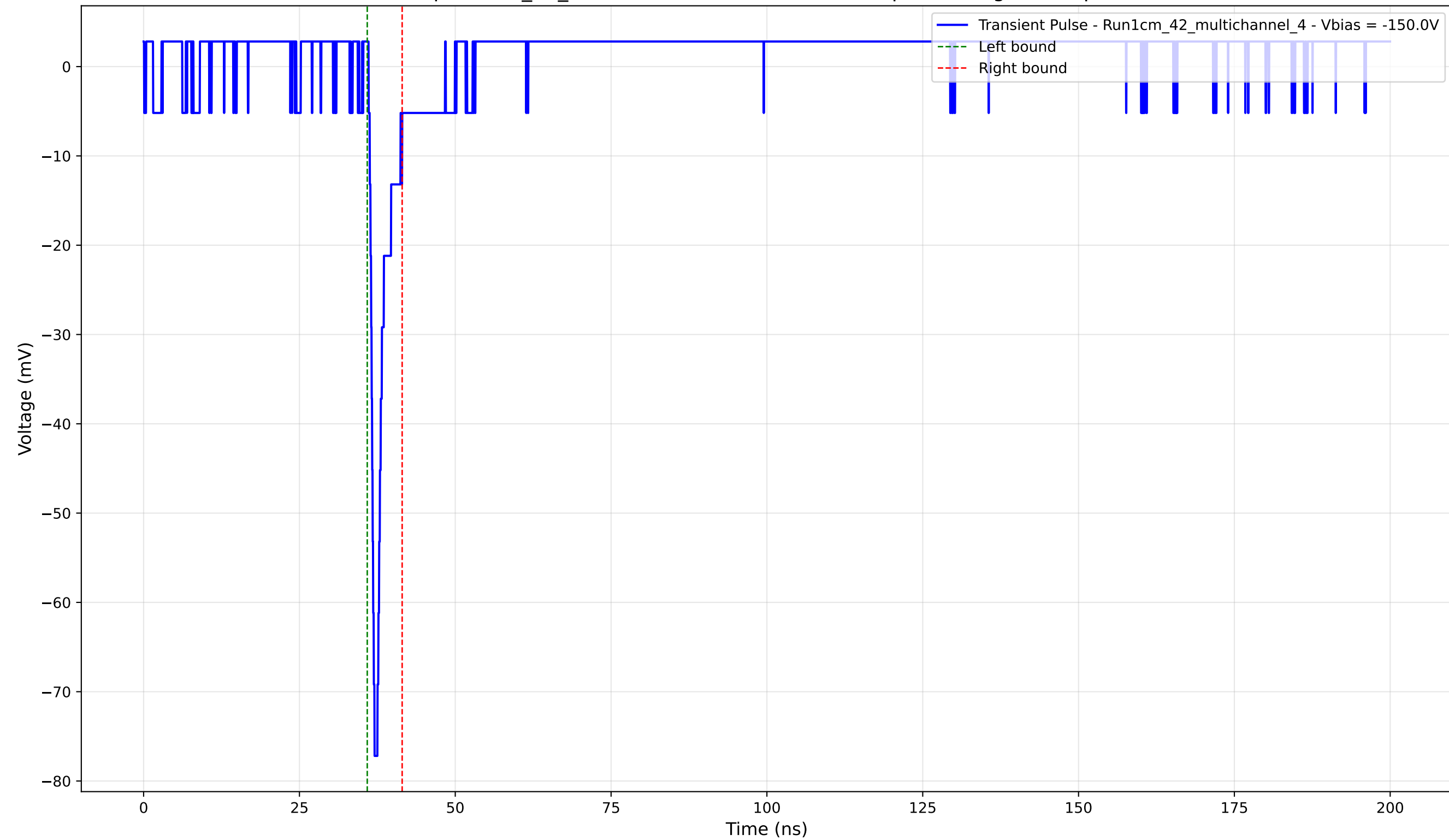
Transient Pulse - Sample: 1cm_42_multichannel - Position: 2270.0 \mu\text{m} - Charge: 3.23 pC - Rise Time: 0.77 ns
