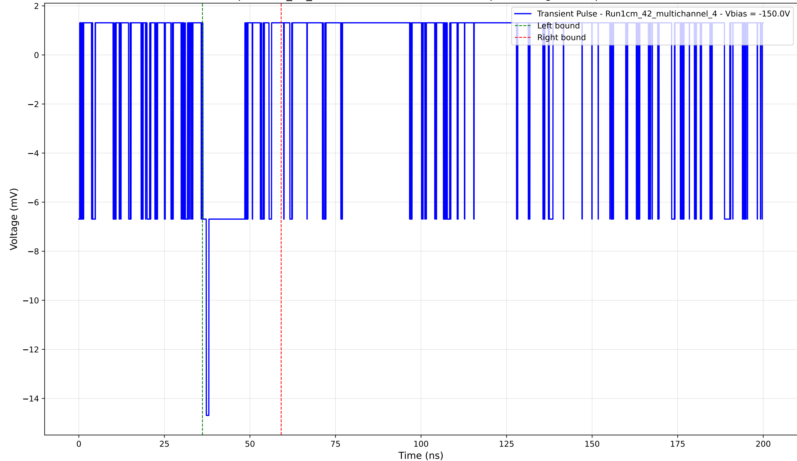
Transient Pulse - Sample: 1cm_42_multichannel - Position: 1840.0 \mu\text{m} - Charge: 1.84 pC - Rise Time: 1.02 ns
