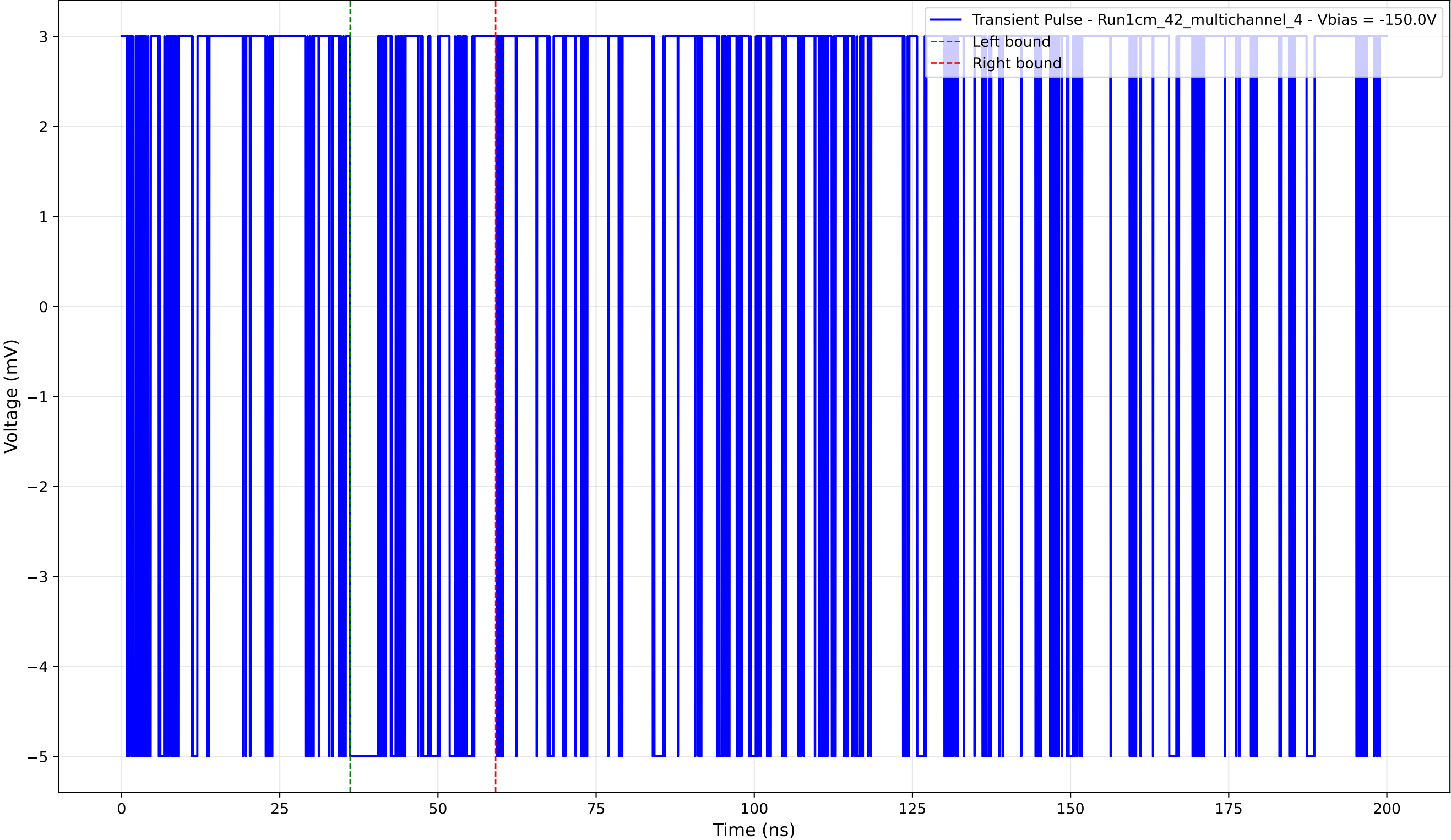
Transient Pulse - Sample: 1cm_42_multichannel - Position: 2410.0 \mu\text{m} - Charge: 0.55 pC - Rise Time: 0.00 ns (N/A)
