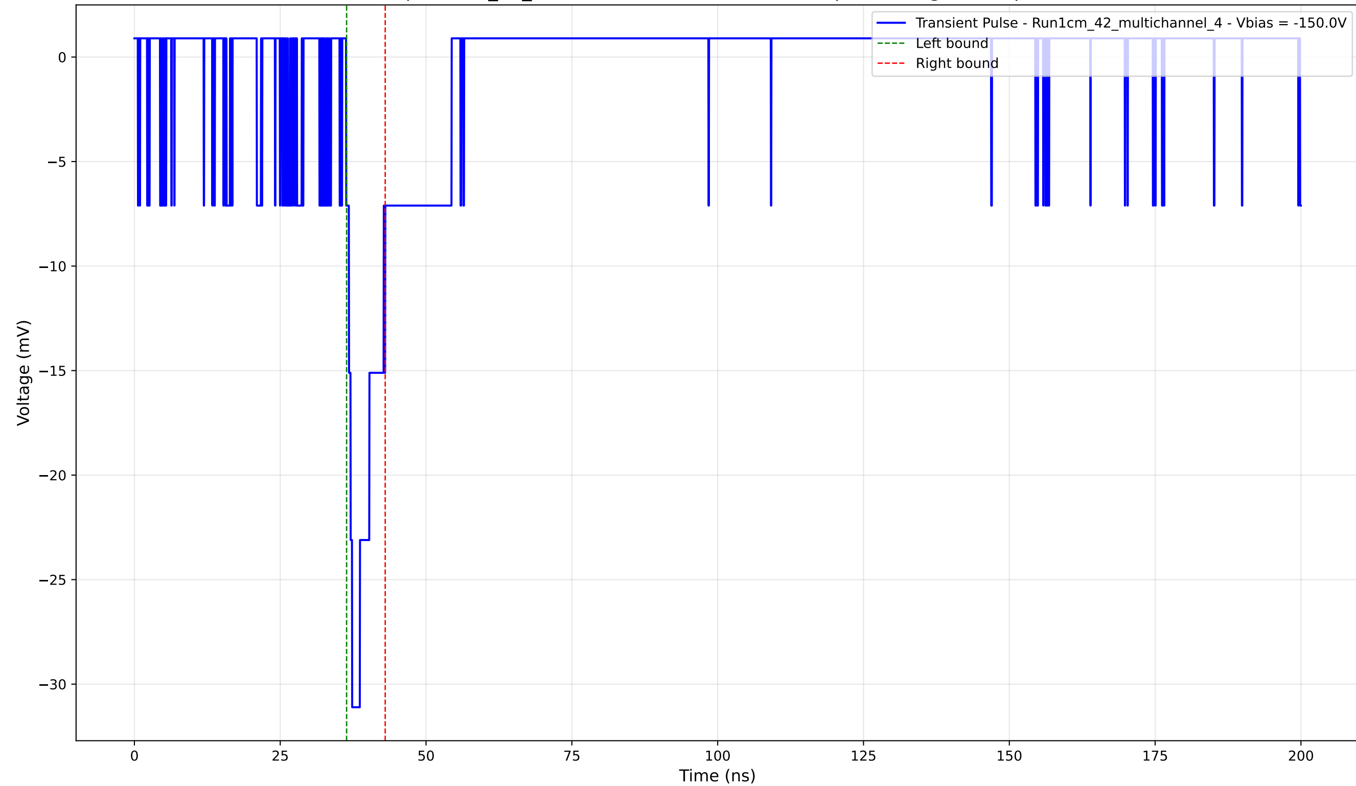
Transient Pulse - Sample: 1cm_42_multichannel - Position: 1620.0 \mu\text{m} - Charge: 2.64 pC - Rise Time: 1.03 ns
