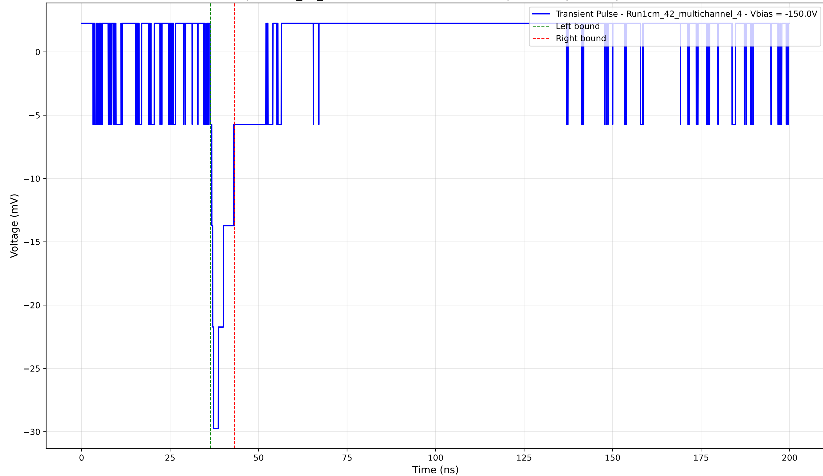
Transient Pulse - Sample: 1cm_42_multichannel - Position: 1635.0 \mu\text{m} - Charge: 2.49 pC - Rise Time: 1.04 ns
