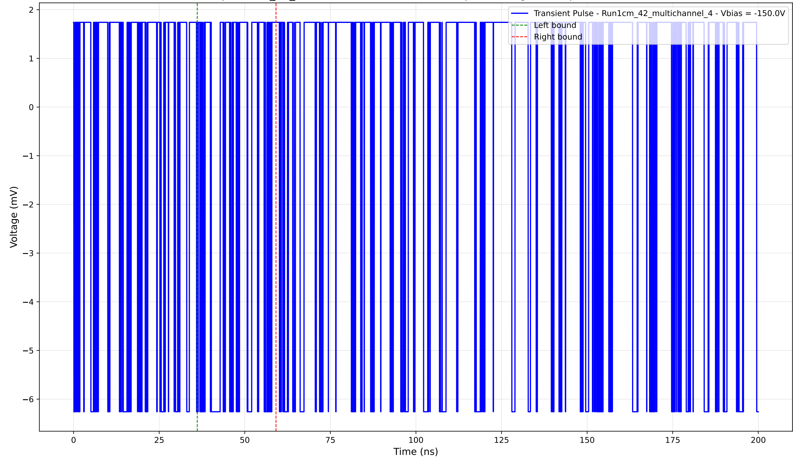
Transient Pulse - Sample: 1cm_42_multichannel - Position: 380.0 \mu\text{m} - Charge: 0.56 pC - Rise Time: 0.00 ns (N/A)
