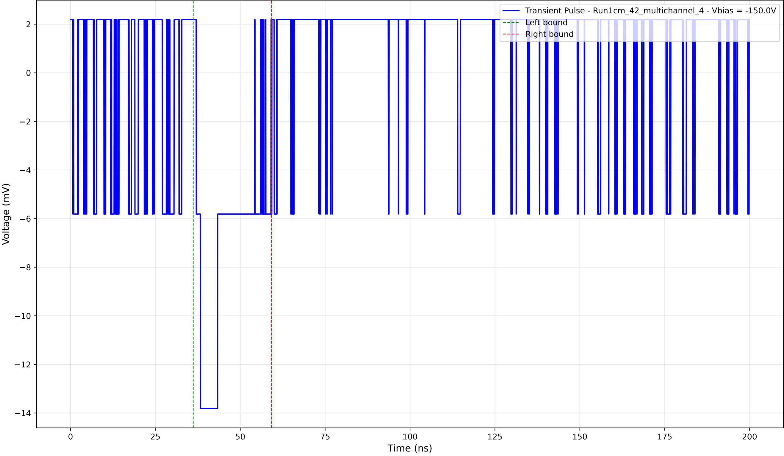
Transient Pulse - Sample: 1cm_42_multichannel - Position: 250.0 \mu\text{m} - Charge: 3.23 pC - Rise Time: 0.00 ns (N/A)
