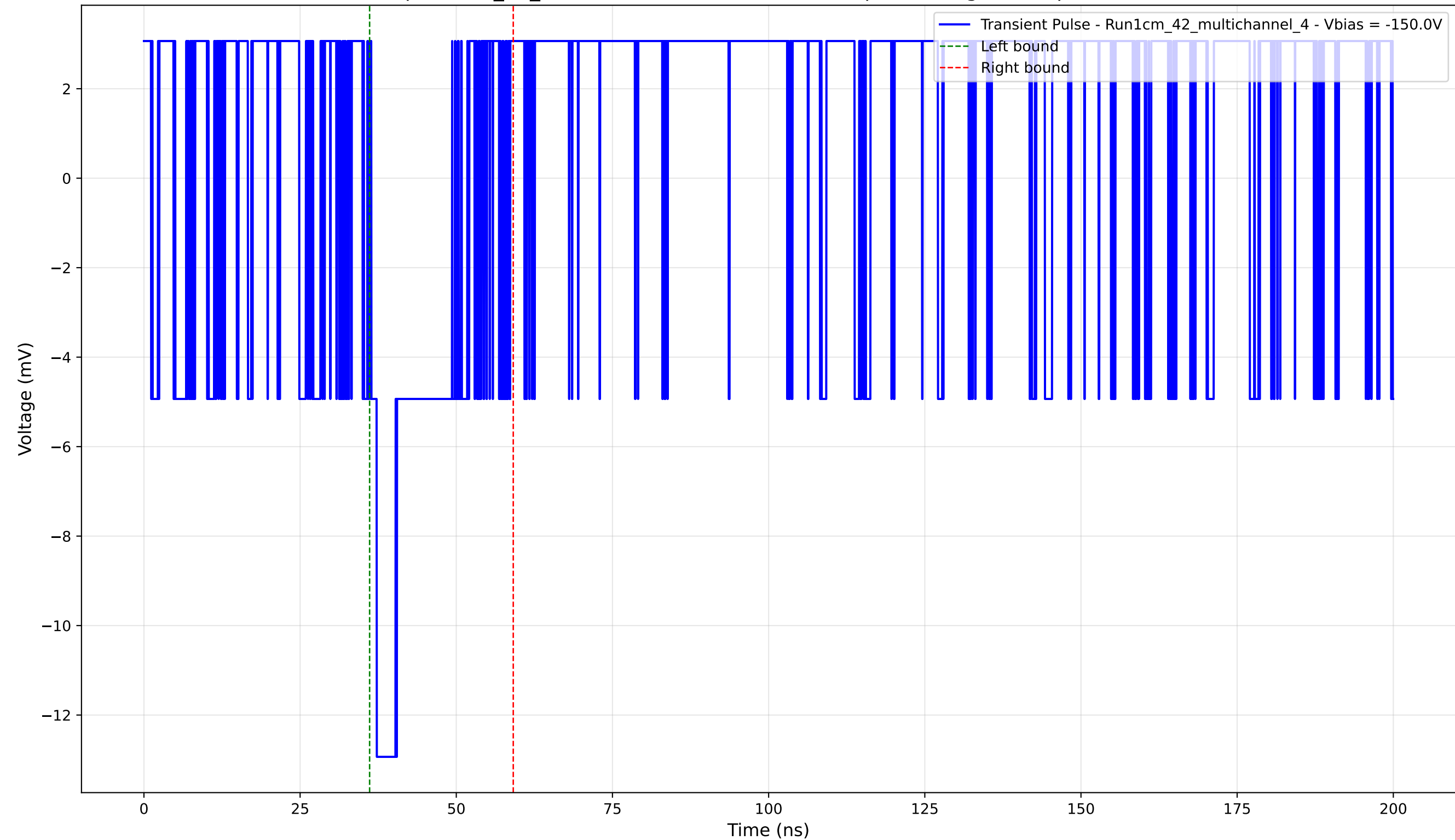
Transient Pulse - Sample: 1cm_42_multichannel - Position: 1425.0 \mu\text{m} - Charge: 1.84 pC - Rise Time: 0.00 ns (N/A)
