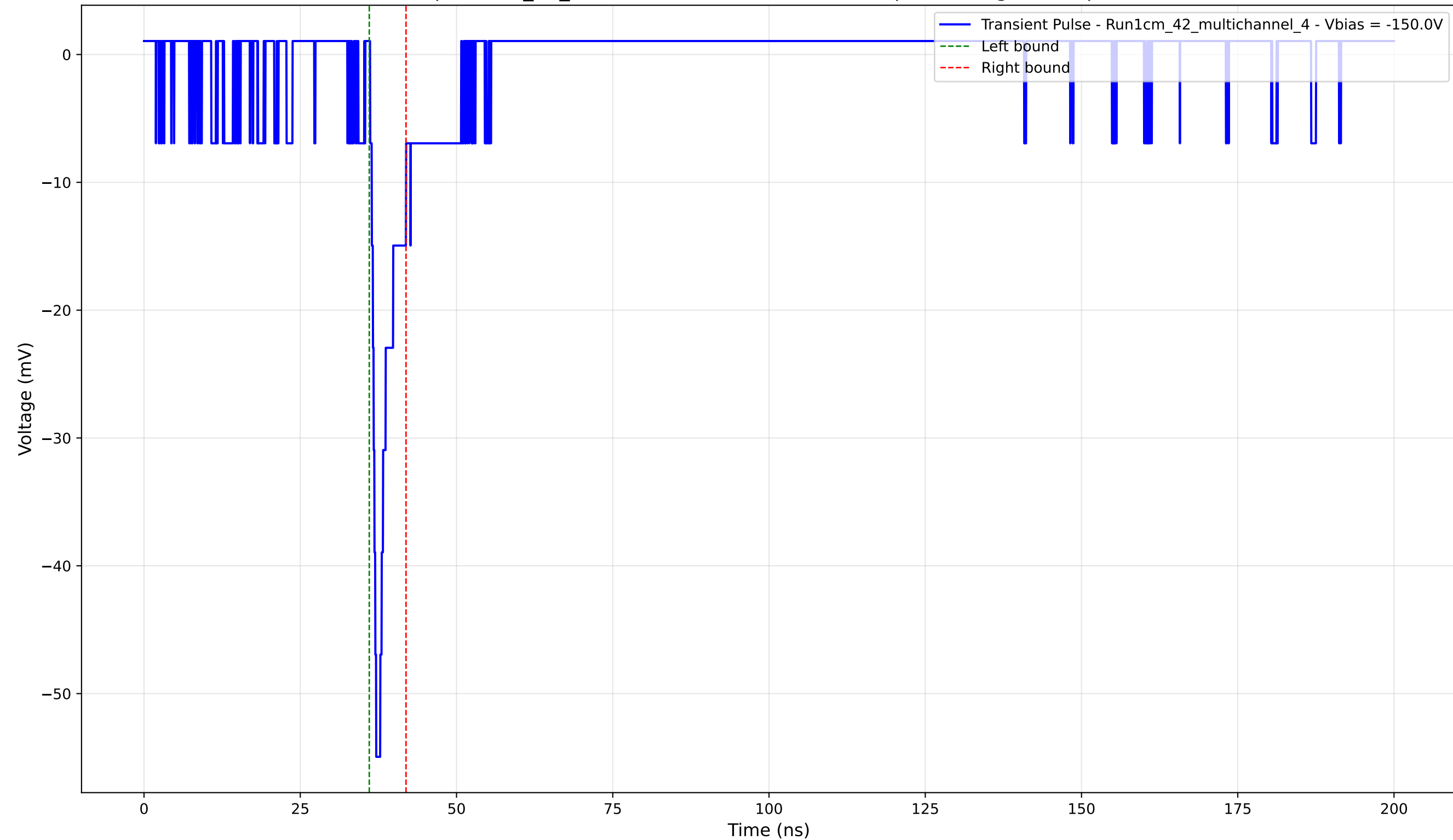
Transient Pulse - Sample: 1cm_42_multichannel - Position: 2045.0 \mu\text{m} - Charge: 2.99 pC - Rise Time: 0.96 ns
