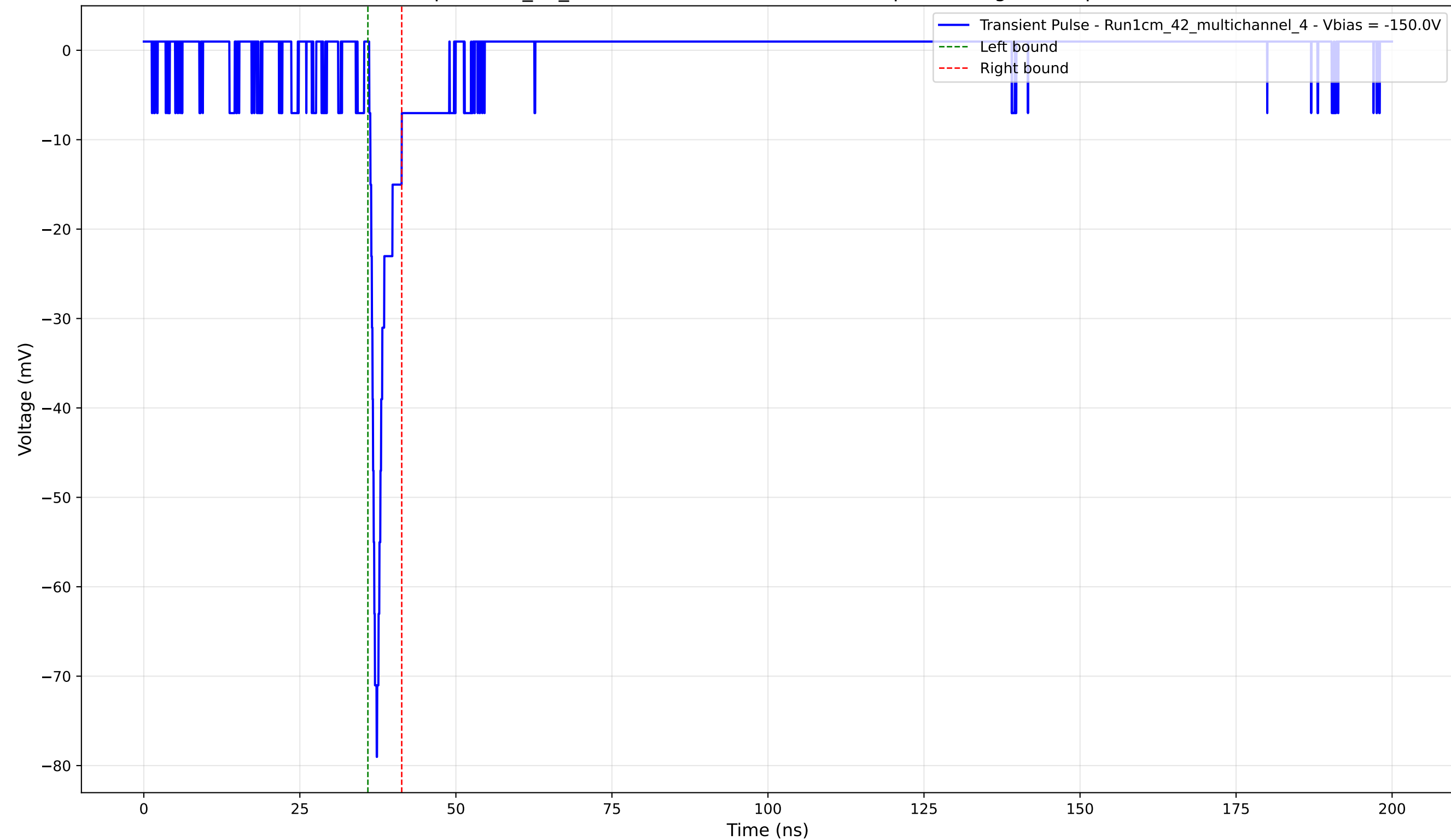
Transient Pulse - Sample: 1cm_42_multichannel - Position: 2215.0 \mu\text{m} - Charge: 3.26 pC - Rise Time: 1.02 ns
