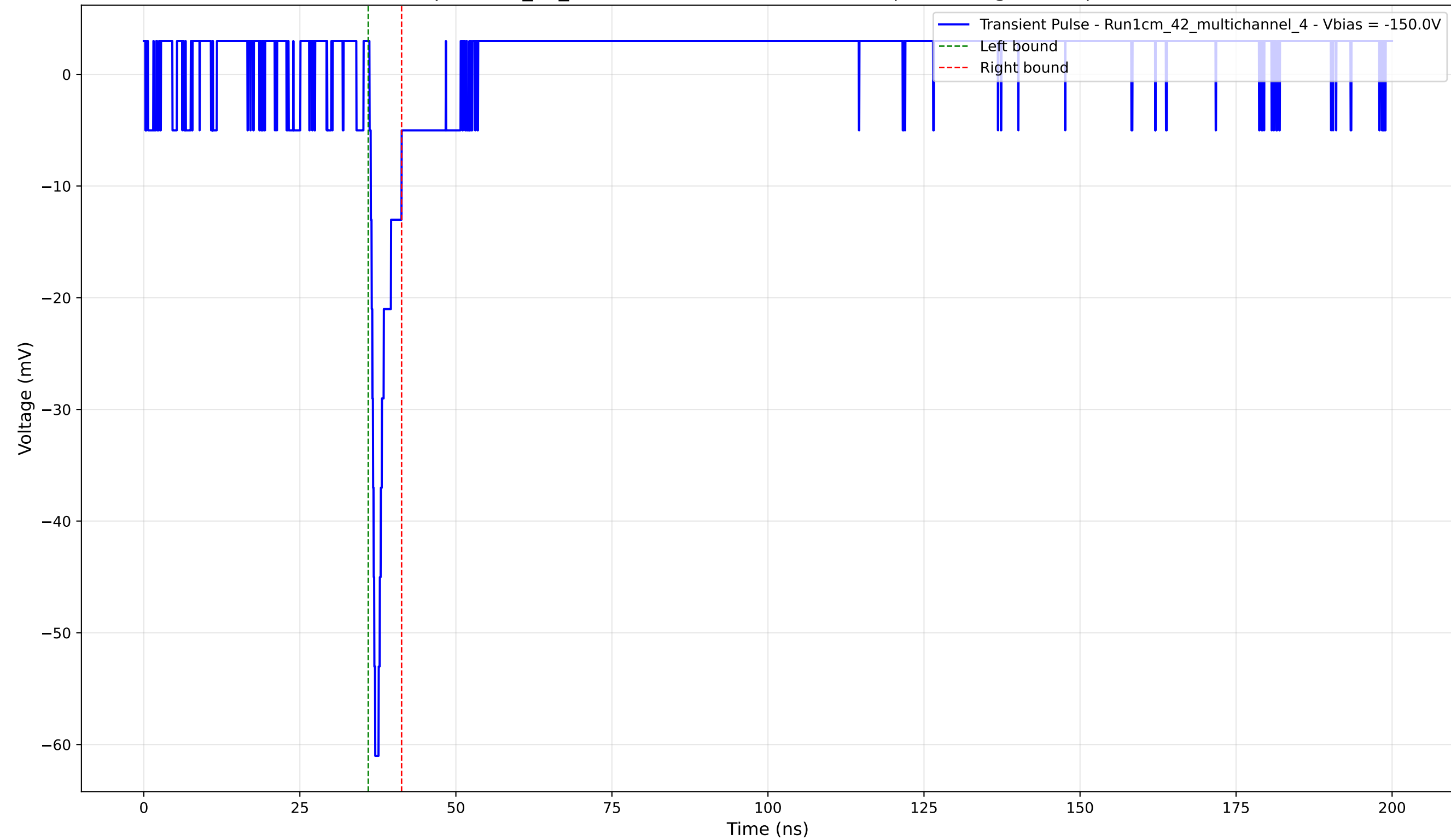
Transient Pulse - Sample: 1cm_42_multichannel - Position: 2600.0 \mu\text{m} - Charge: 2.72 pC - Rise Time: 0.72 ns
