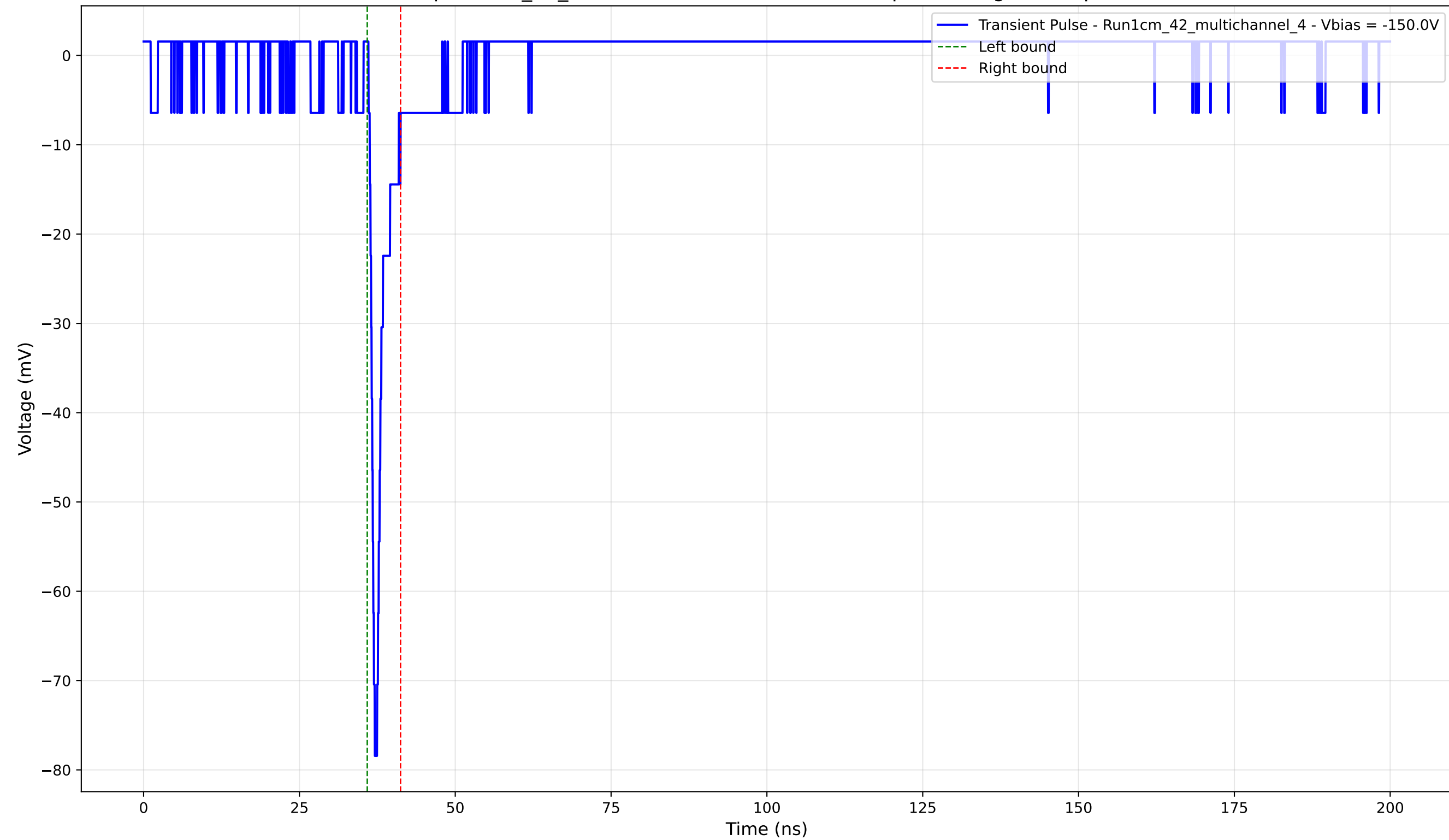
Transient Pulse - Sample: 1cm_42_multichannel - Position: 2275.0 \mu\text{m} - Charge: 3.17 pC - Rise Time: 0.82 ns
