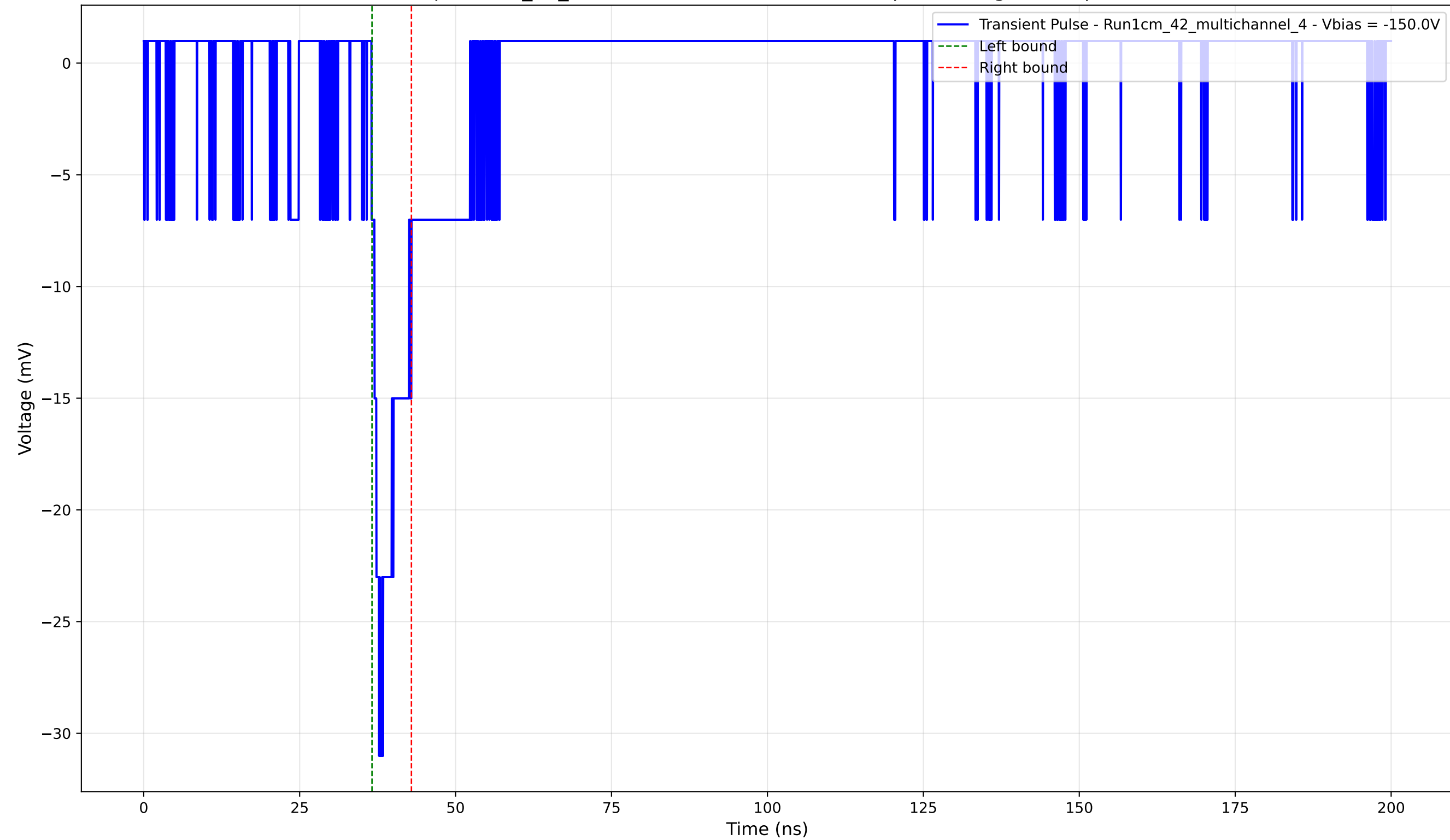
Transient Pulse - Sample: 1cm_42_multichannel - Position: 3295.0 \mu\text{m} - Charge: 2.28 pC - Rise Time: 1.21 ns
