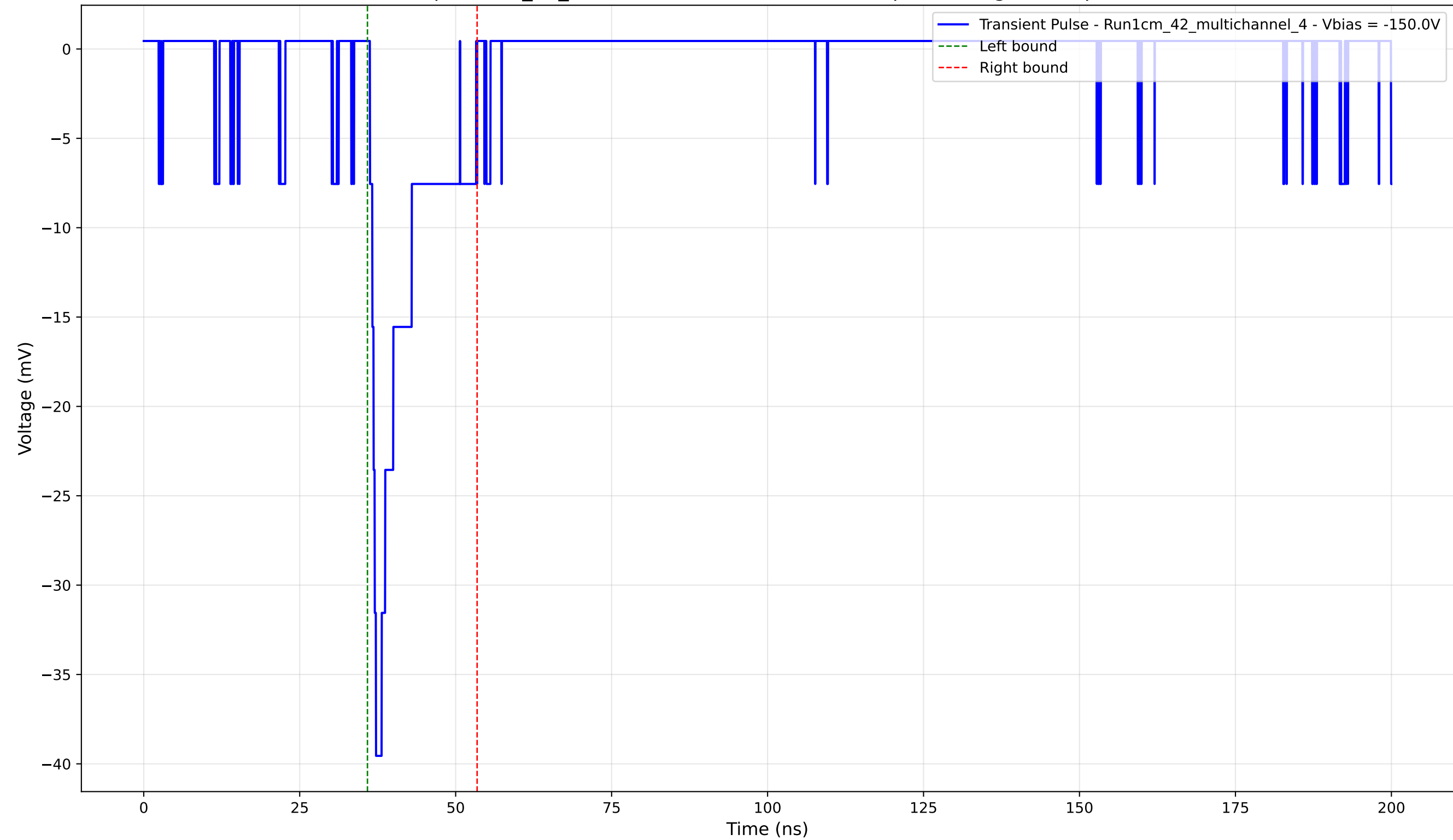
Transient Pulse - Sample: 1cm_42_multichannel - Position: 1790.0 \mu\text{m} - Charge: 4.51 pC - Rise Time: 0.97 ns
