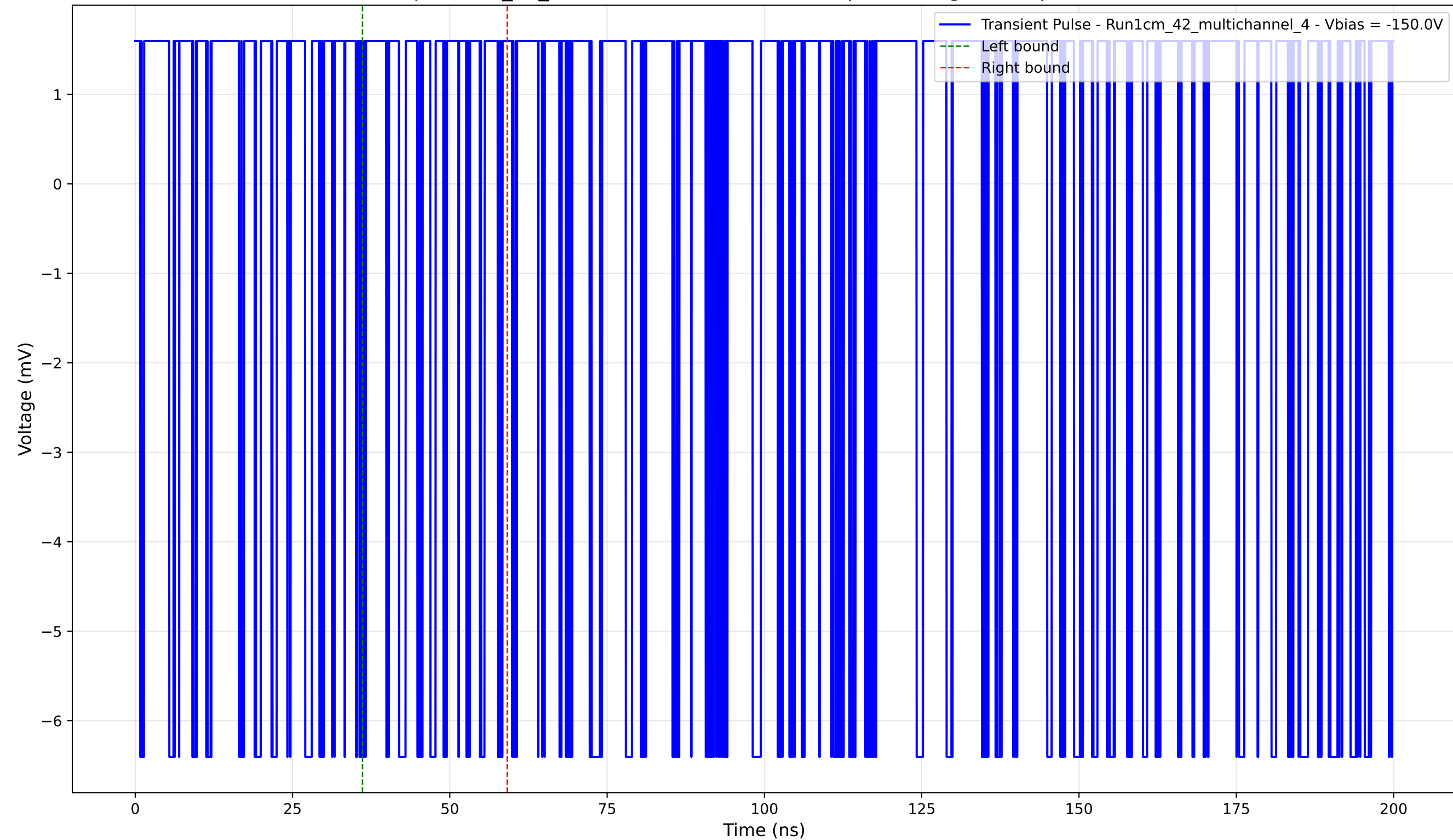
Transient Pulse - Sample: 1cm_42_multichannel - Position: 25.0 \mu\text{m} - Charge: 0.07 pC - Rise Time: 0.00 ns (N/A)
