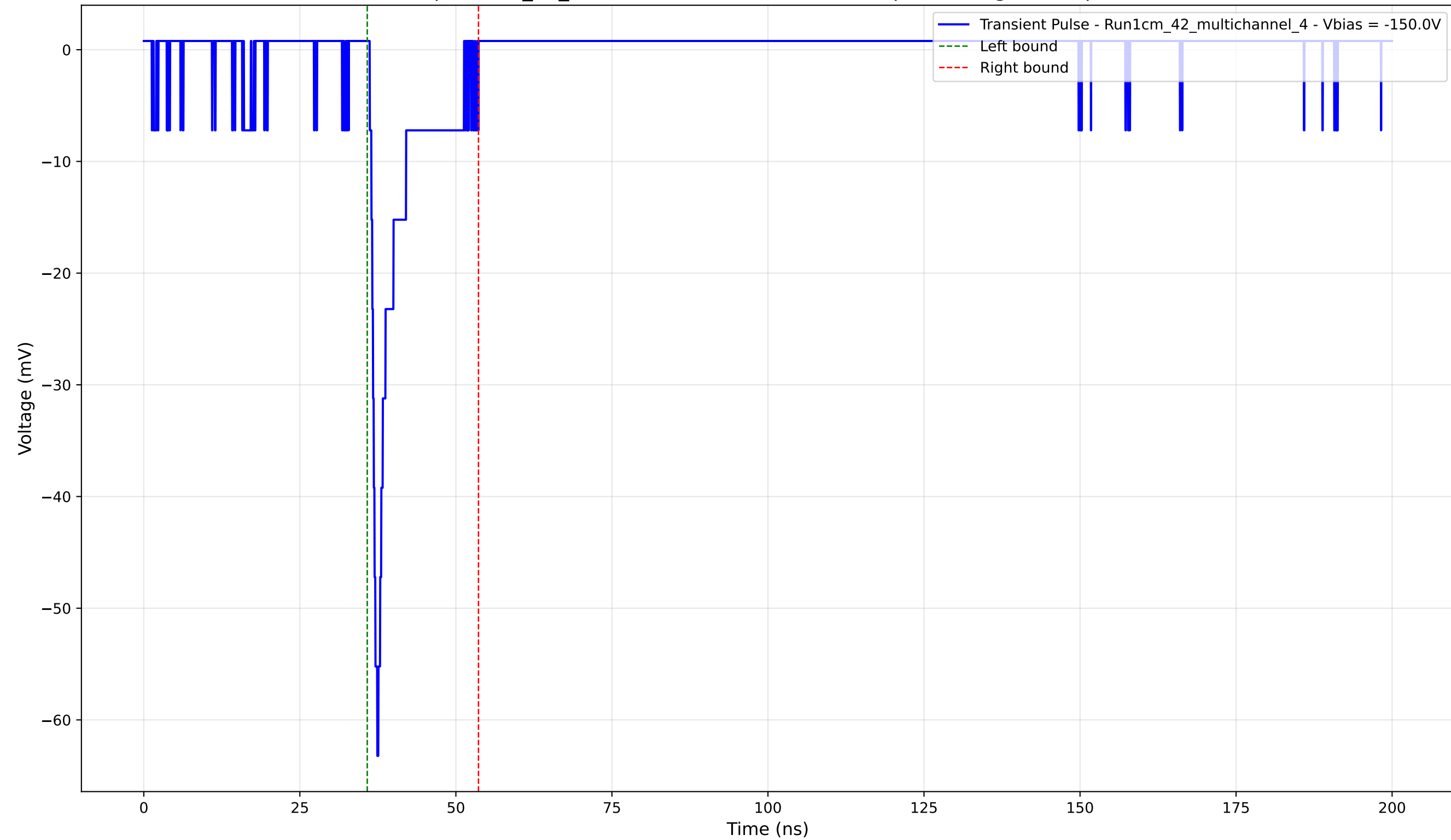
Transient Pulse - Sample: 1cm_42_multichannel - Position: 2060.0 \mu\text{m} - Charge: 4.62 pC - Rise Time: 1.20 ns
