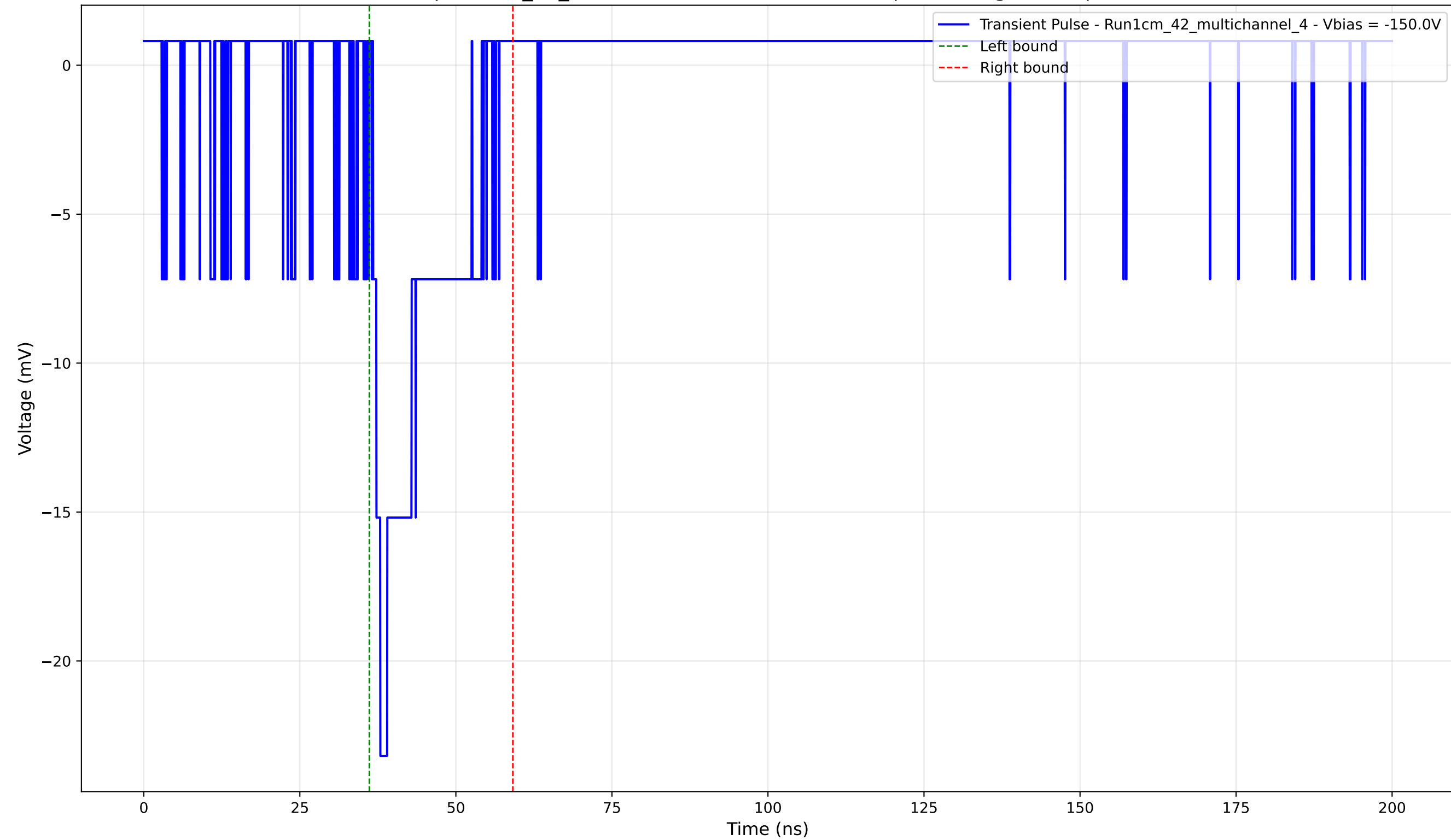
Transient Pulse - Sample: 1cm_42_multichannel - Position: 3535.0 \mu\text{m} - Charge: 3.59 pC - Rise Time: 1.16 ns
