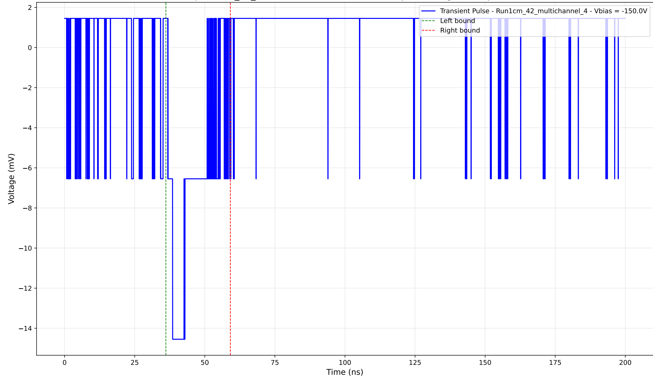
Transient Pulse - Sample: 1cm_42_multichannel - Position: 4655.0 \mu\text{m} - Charge: 2.93 pC - Rise Time: 1.64 ns
