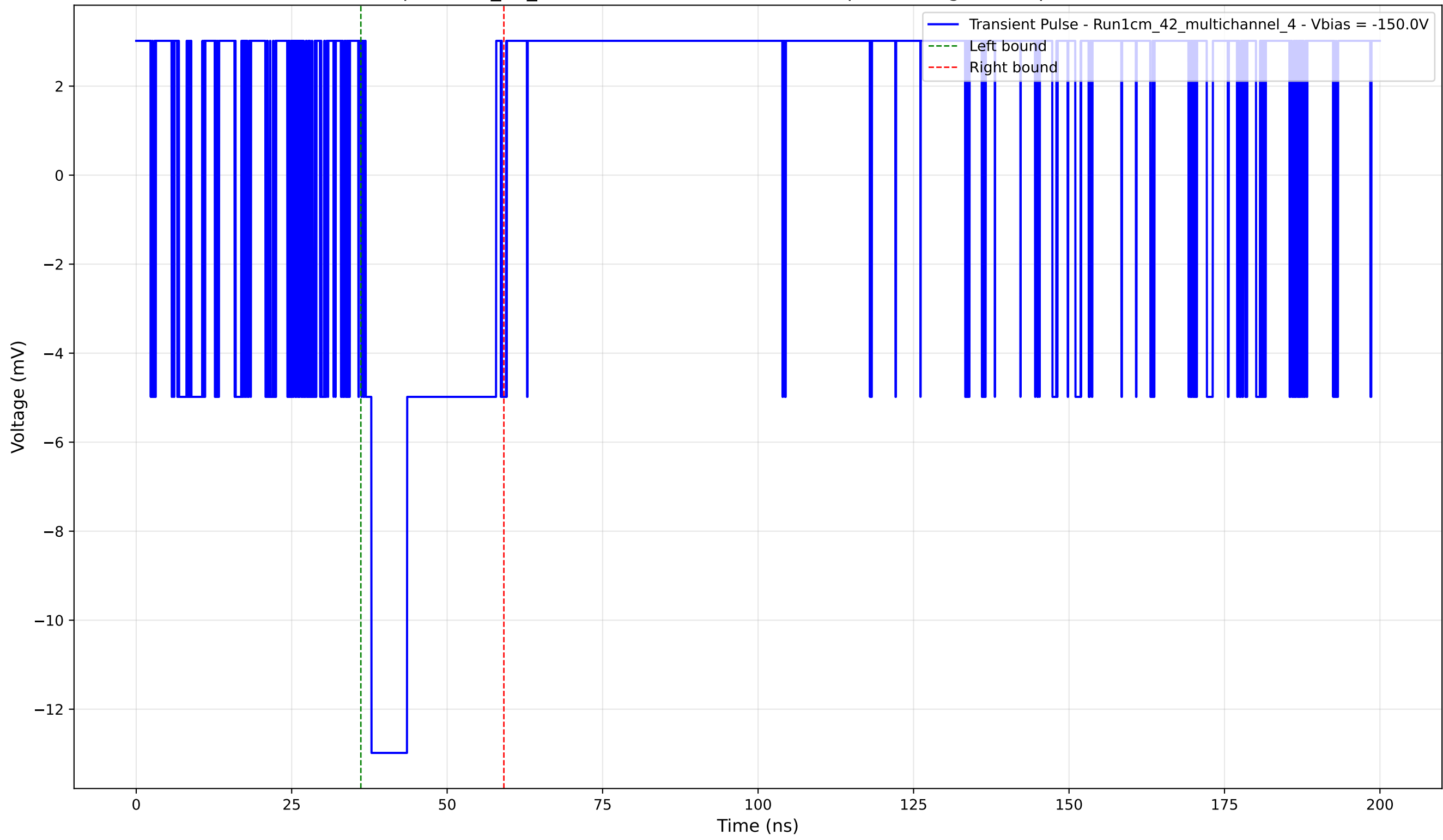
Transient Pulse - Sample: 1cm_42_multichannel - Position: 775.0 \mu\text{m} - Charge: 2.99 pC - Rise Time: 0.00 ns (N/A)
