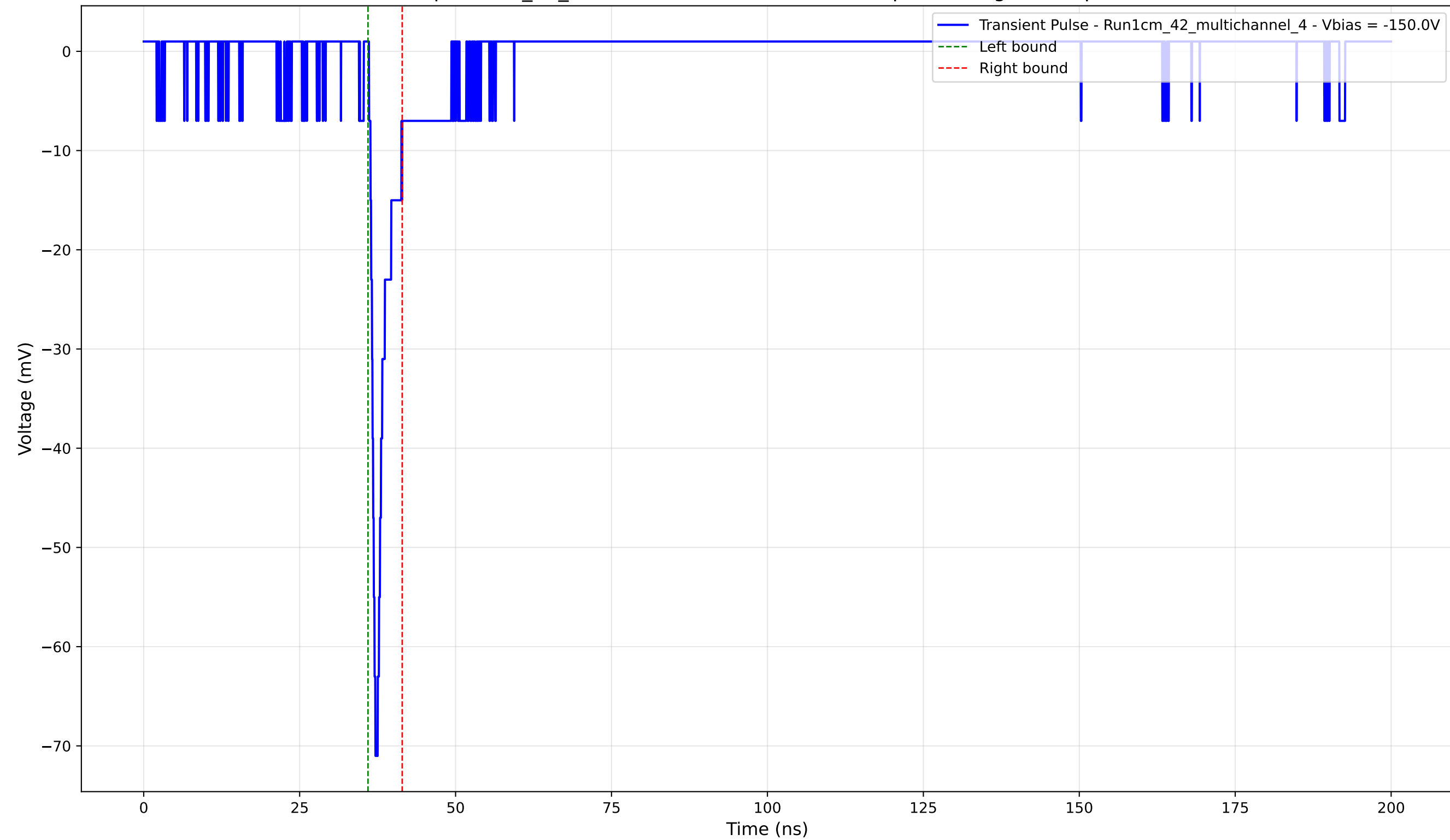
Transient Pulse - Sample: 1cm_42_multichannel - Position: 2170.0 \mu\text{m} - Charge: 3.18 pC - Rise Time: 0.80 ns
