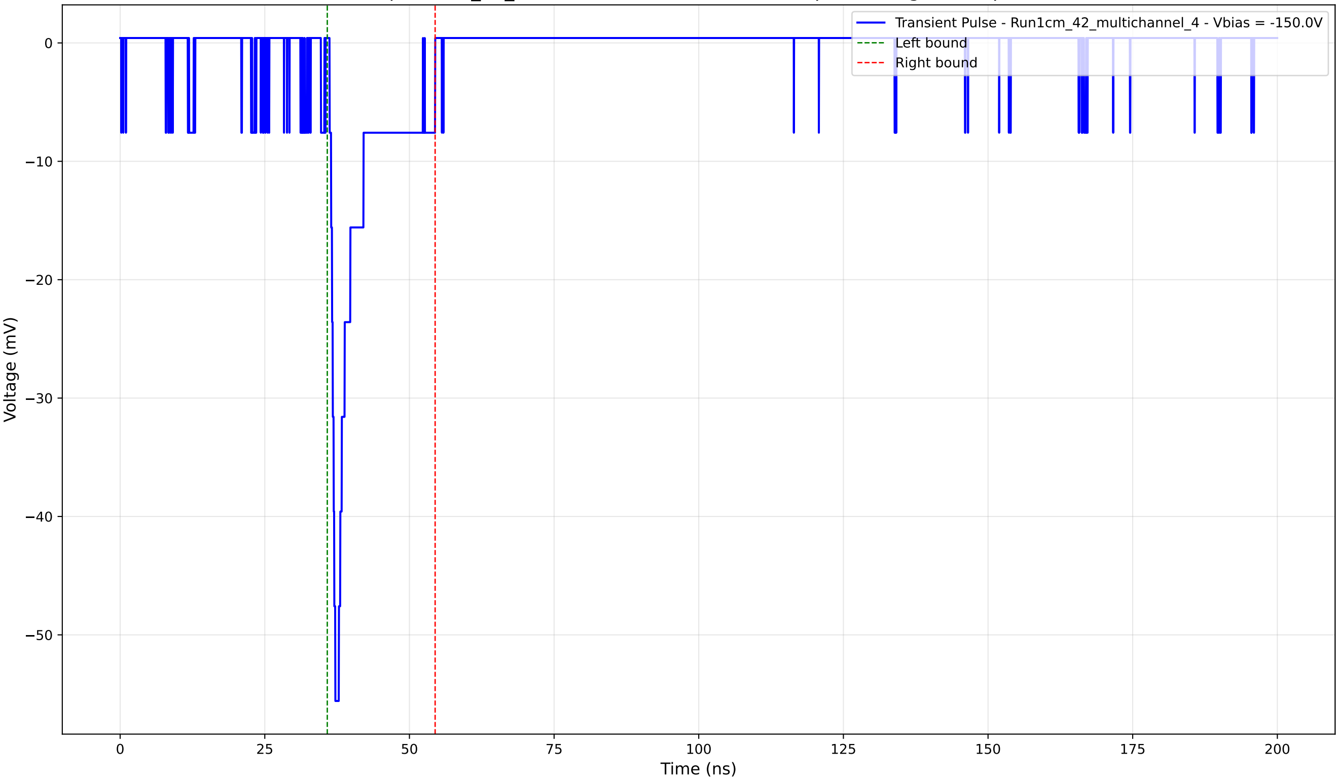
Transient Pulse - Sample: 1cm_42_multichannel - Position: 2025.0 \mu\text{m} - Charge: 4.97 pC - Rise Time: 0.99 ns
