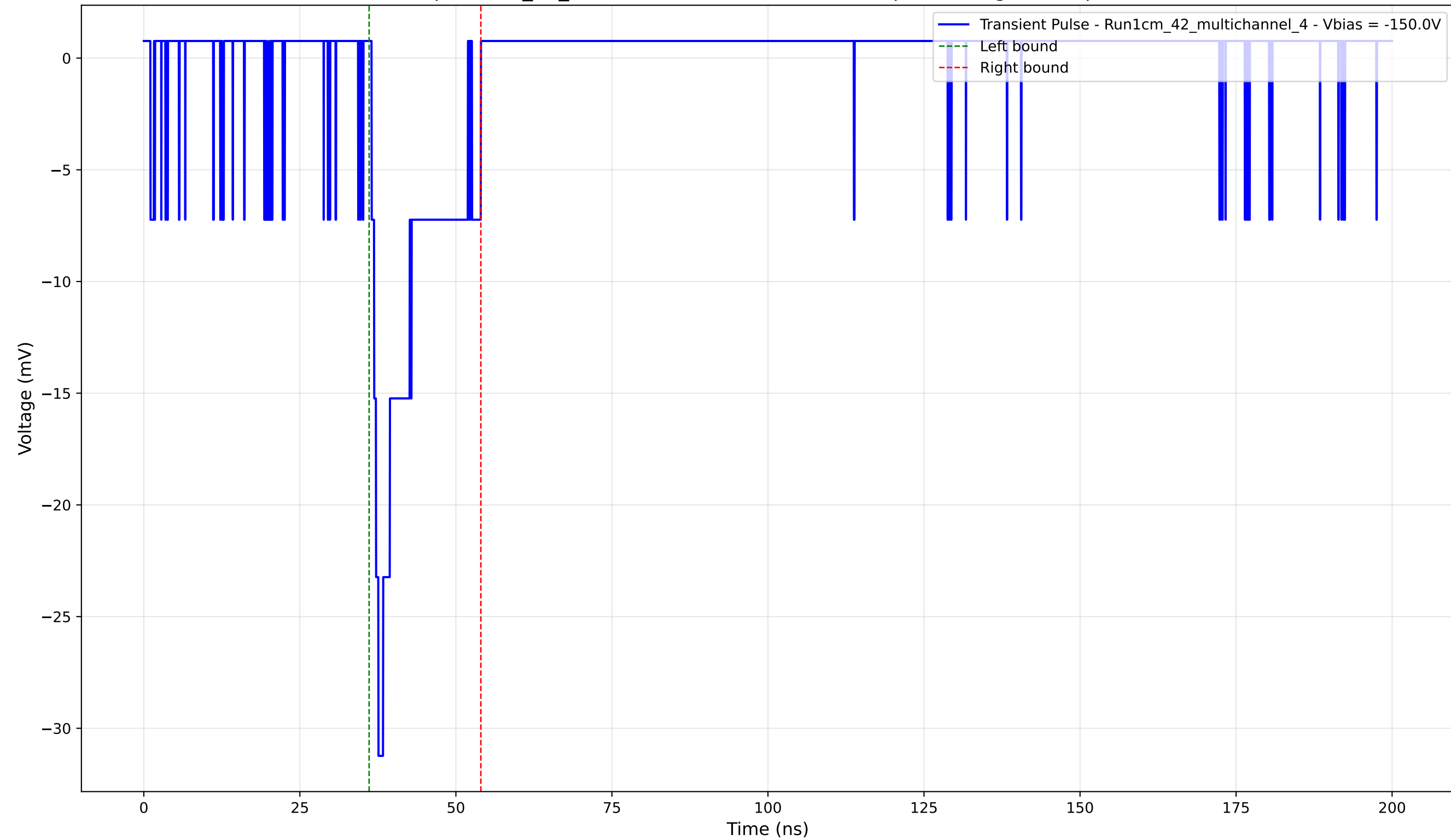
Transient Pulse - Sample: 1cm_42_multichannel - Position: 3200.0 \mu\text{m} - Charge: 3.83 pC - Rise Time: 1.09 ns
