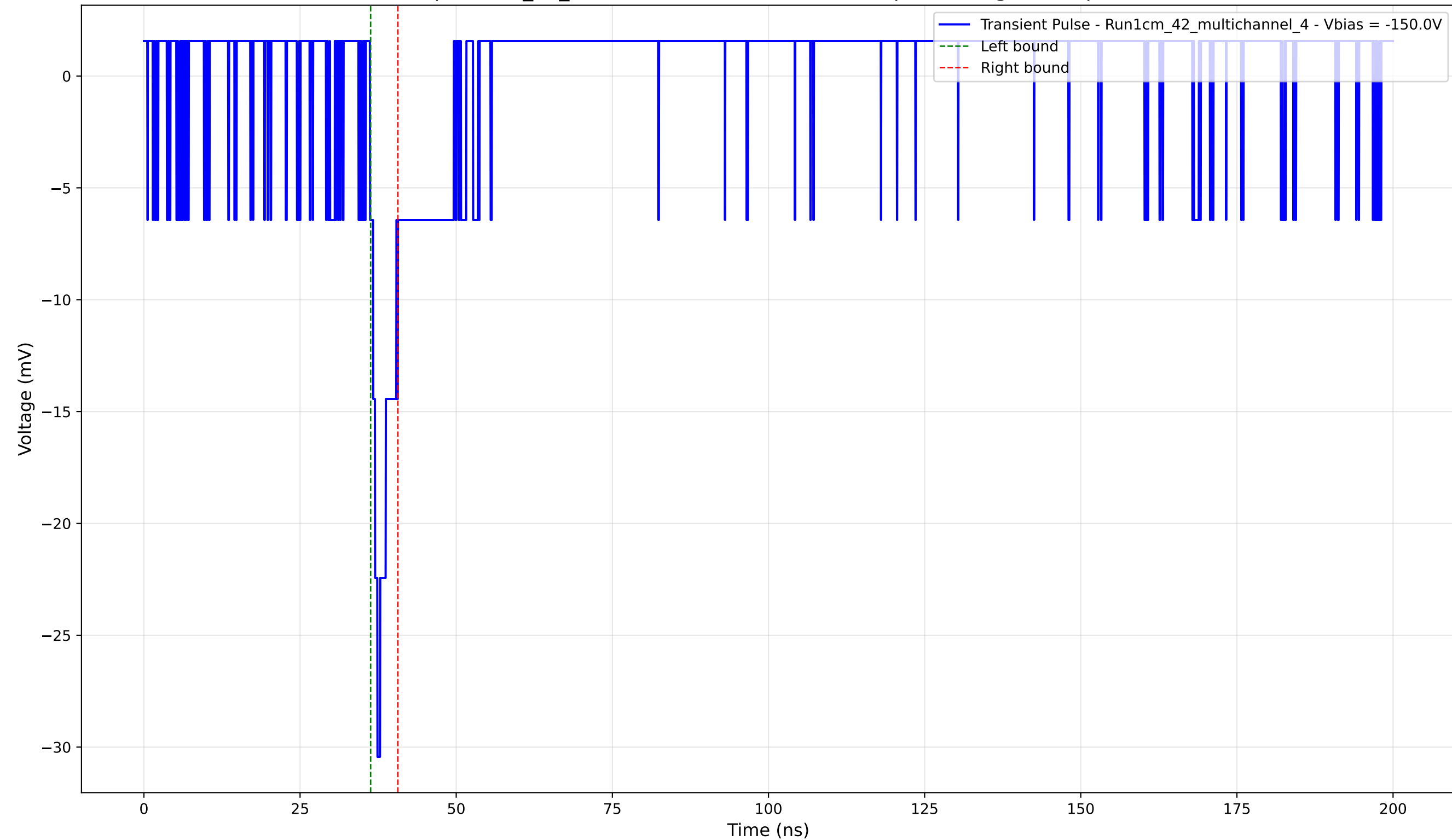
Transient Pulse - Sample: 1cm_42_multichannel - Position: 2950.0 \mu\text{m} - Charge: 1.53 pC - Rise Time: 1.19 ns
