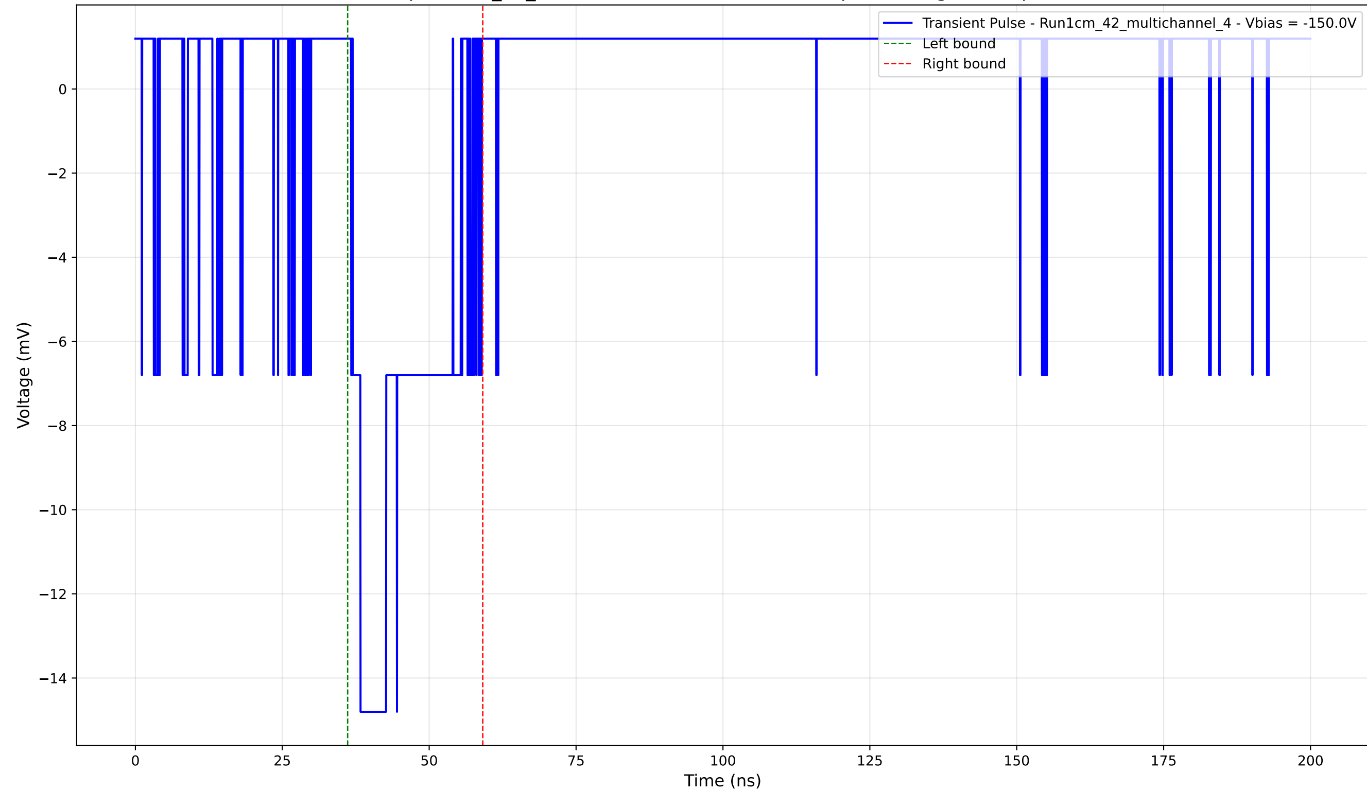
Transient Pulse - Sample: 1cm_42_multichannel - Position: 4210.0 \mu\text{m} - Charge: 3.32 pC - Rise Time: 1.32 ns
