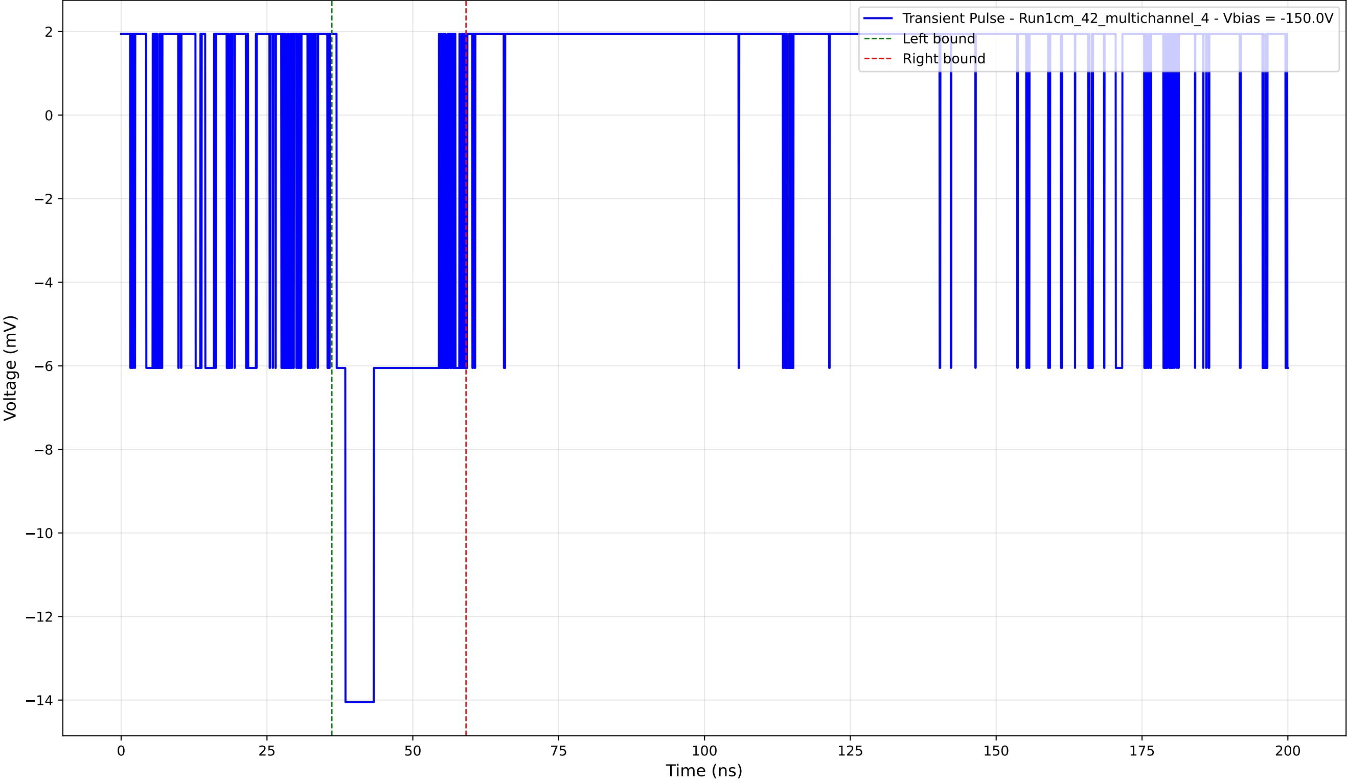
Transient Pulse - Sample: 1cm_42_multichannel - Position: 440.0 \mu\text{m} - Charge: 3.20 pC - Rise Time: 0.00 ns (N/A)
