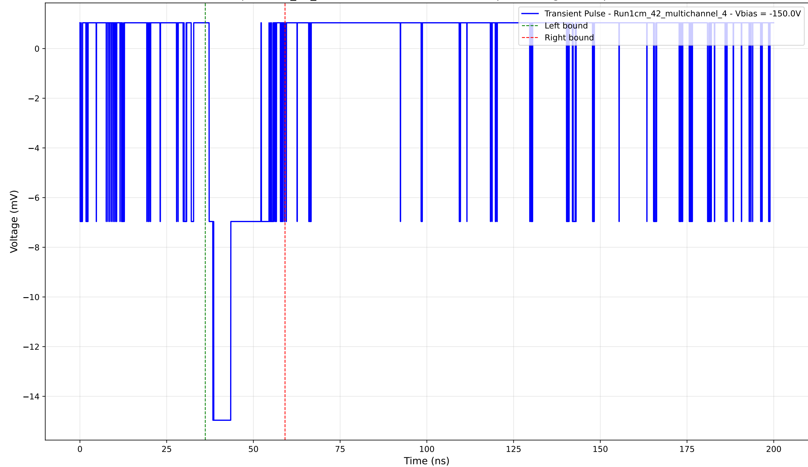
Transient Pulse - Sample: 1cm_42_multichannel - Position: 4580.0 \mu\text{m} - Charge: 3.39 pC - Rise Time: 1.10 ns
