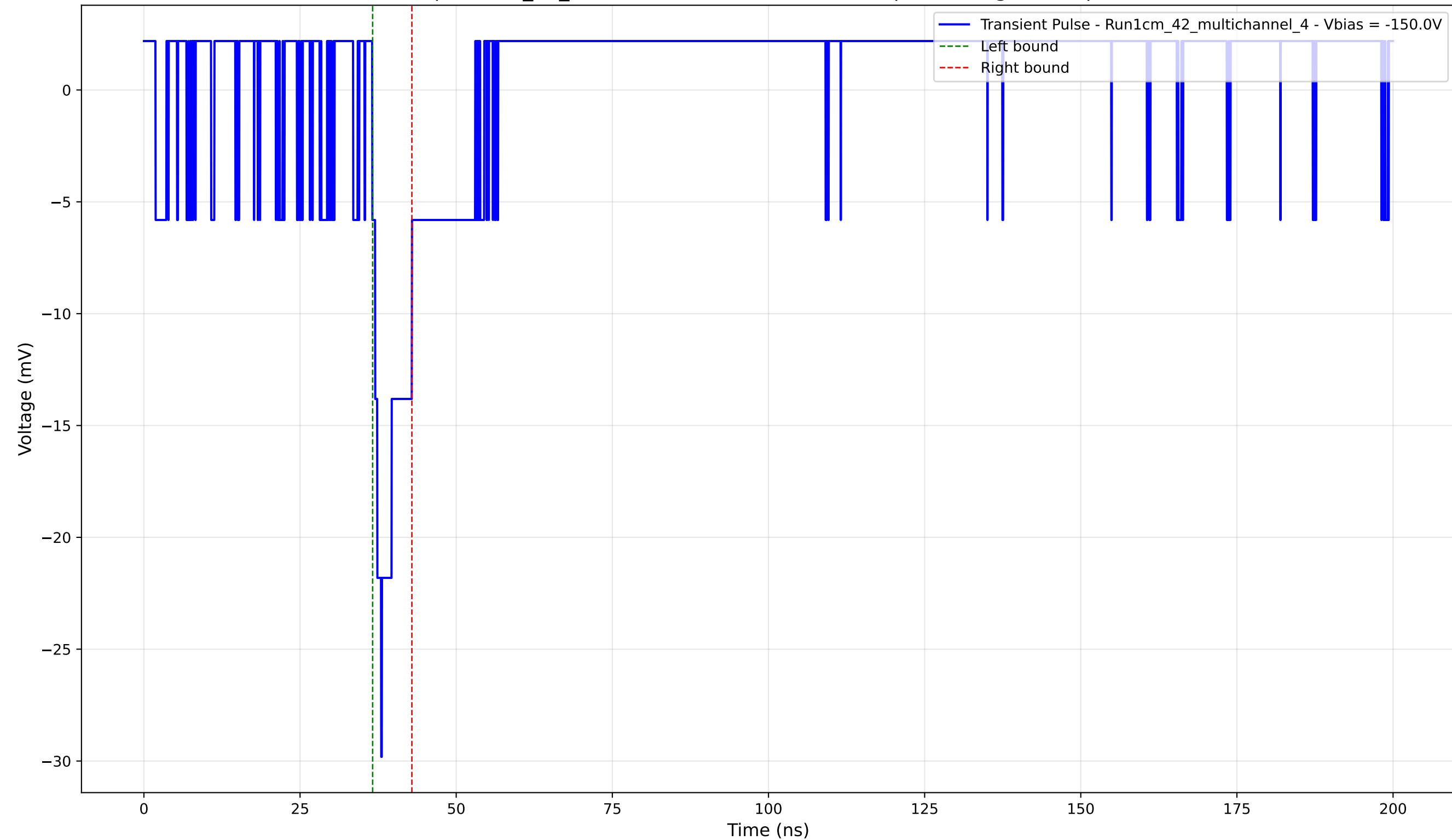
Transient Pulse - Sample: 1cm_42_multichannel - Position: 3310.0 \mu\text{m} - Charge: 2.06 pC - Rise Time: 1.44 ns
