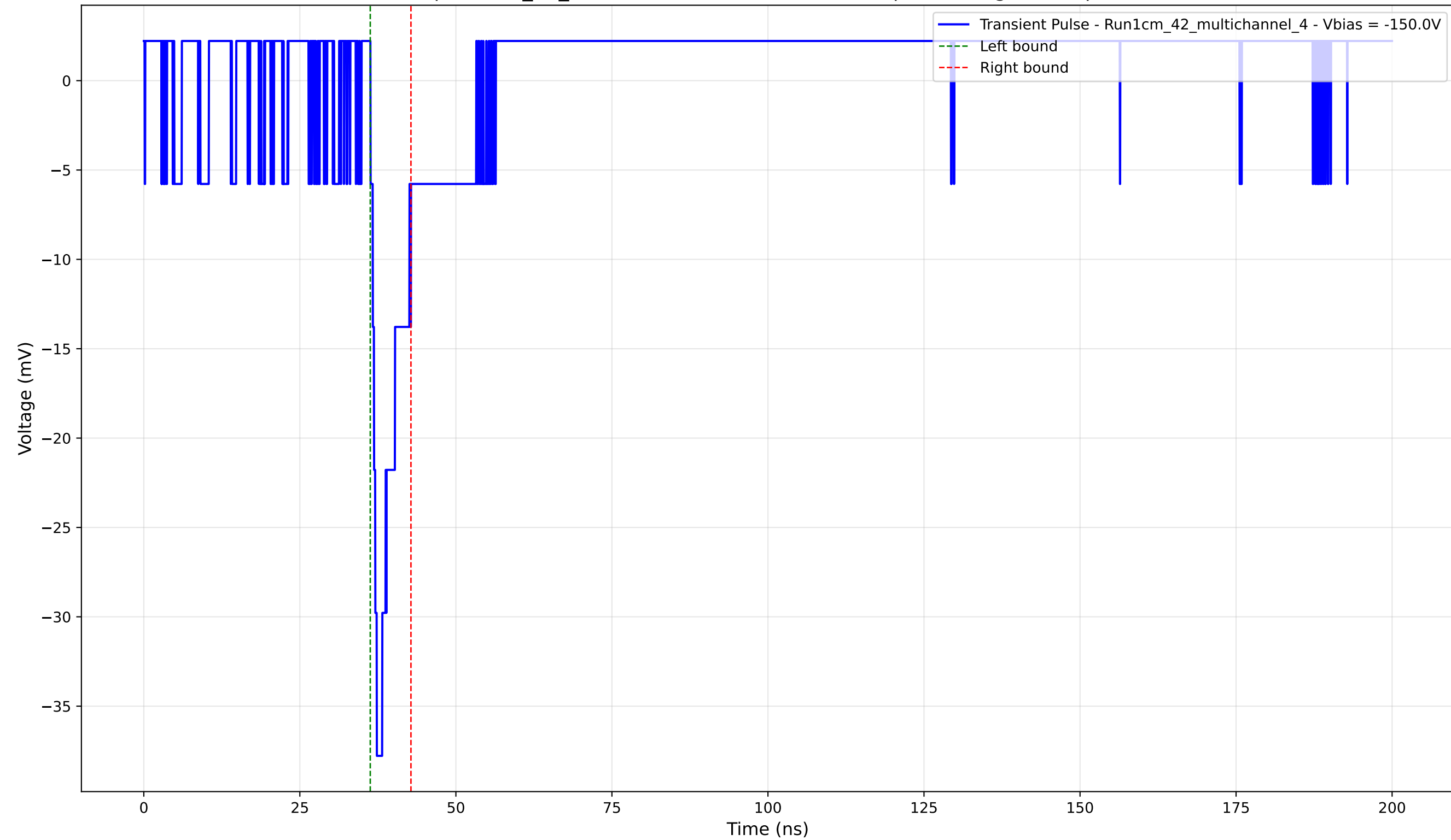
Transient Pulse - Sample: 1cm_42_multichannel - Position: 1740.0 \mu\text{m} - Charge: 2.65 pC - Rise Time: 1.01 ns
