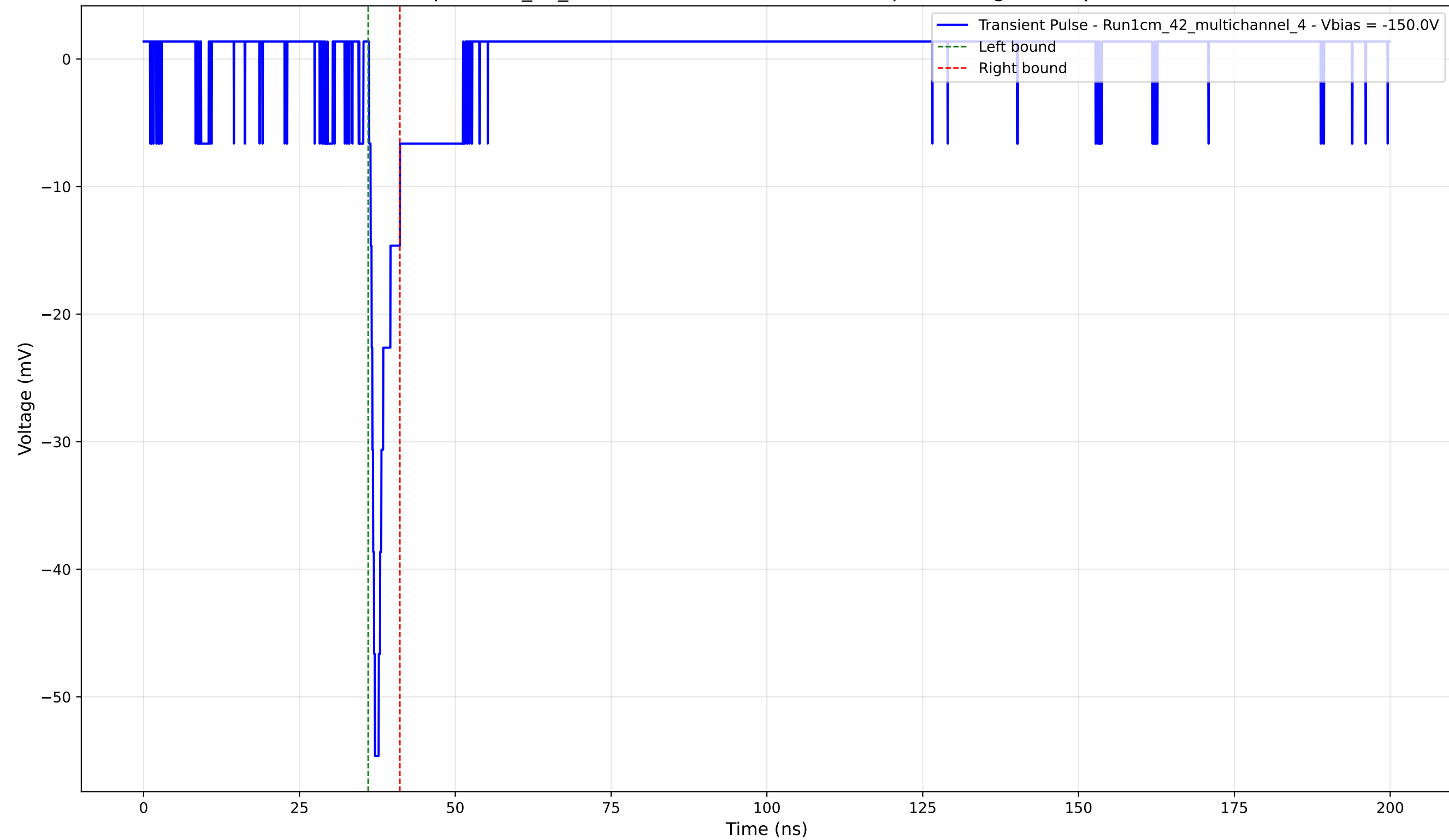
Transient Pulse - Sample: 1cm_42_multichannel - Position: 2680.0 \mu\text{m} - Charge: 2.63 pC - Rise Time: 0.92 ns
