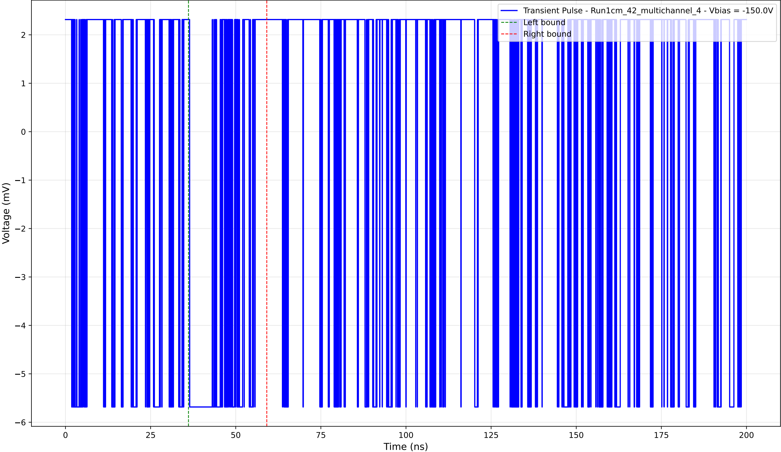
Transient Pulse - Sample: 1cm_42_multichannel - Position: 1910.0 \mu\text{m} - Charge: 1.12 pC - Rise Time: 0.00 ns (N/A)
