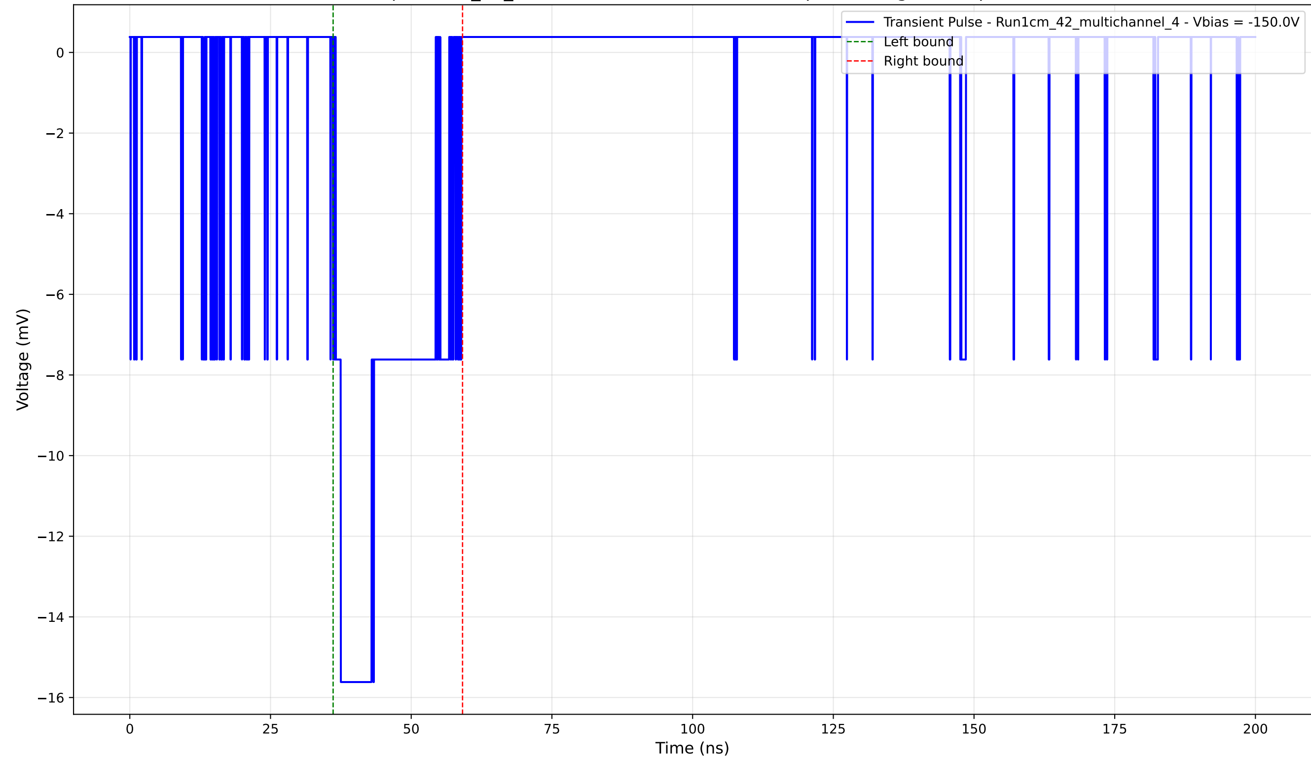
Transient Pulse - Sample: 1cm_42_multichannel - Position: 3620.0 \mu\text{m} - Charge: 4.02 pC - Rise Time: 0.90 ns
