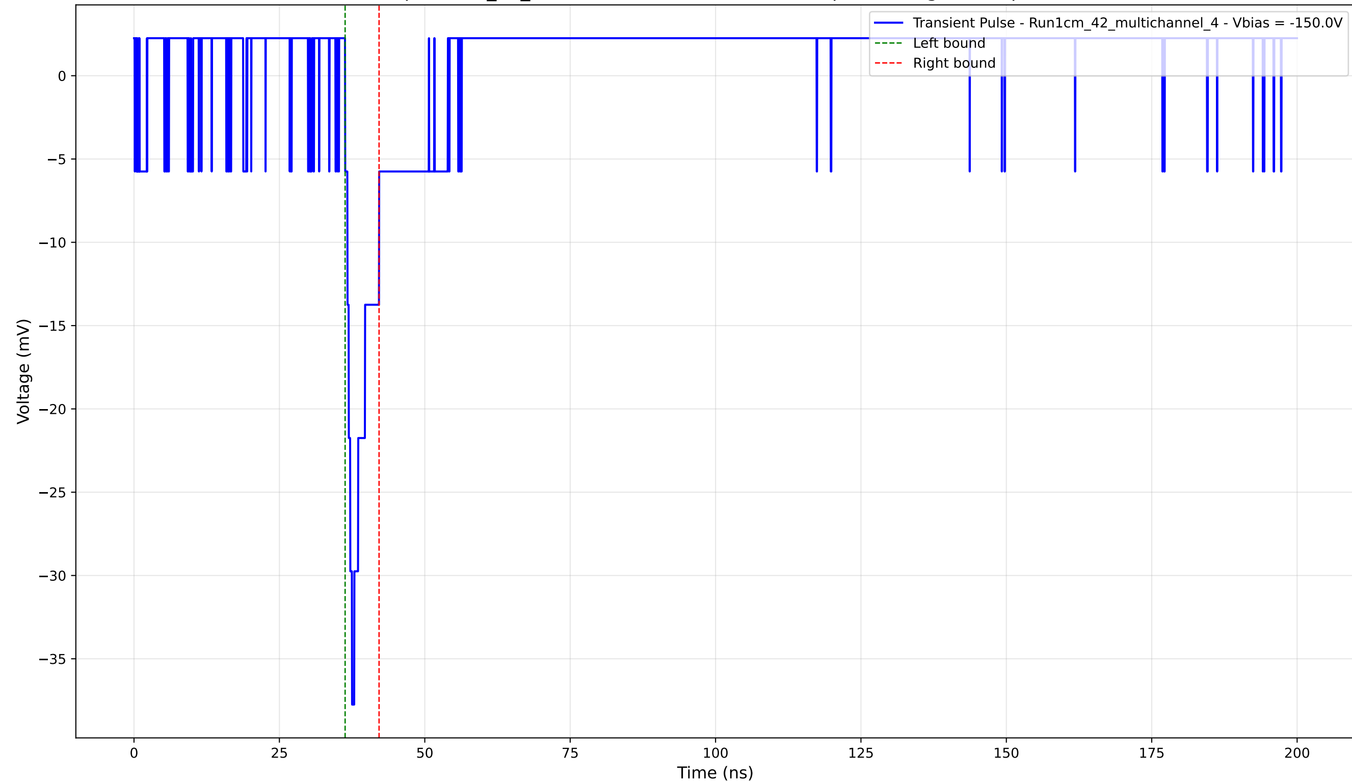
Transient Pulse - Sample: 1cm_42_multichannel - Position: 3050.0 \mu\text{m} - Charge: 2.27 pC - Rise Time: 1.19 ns
