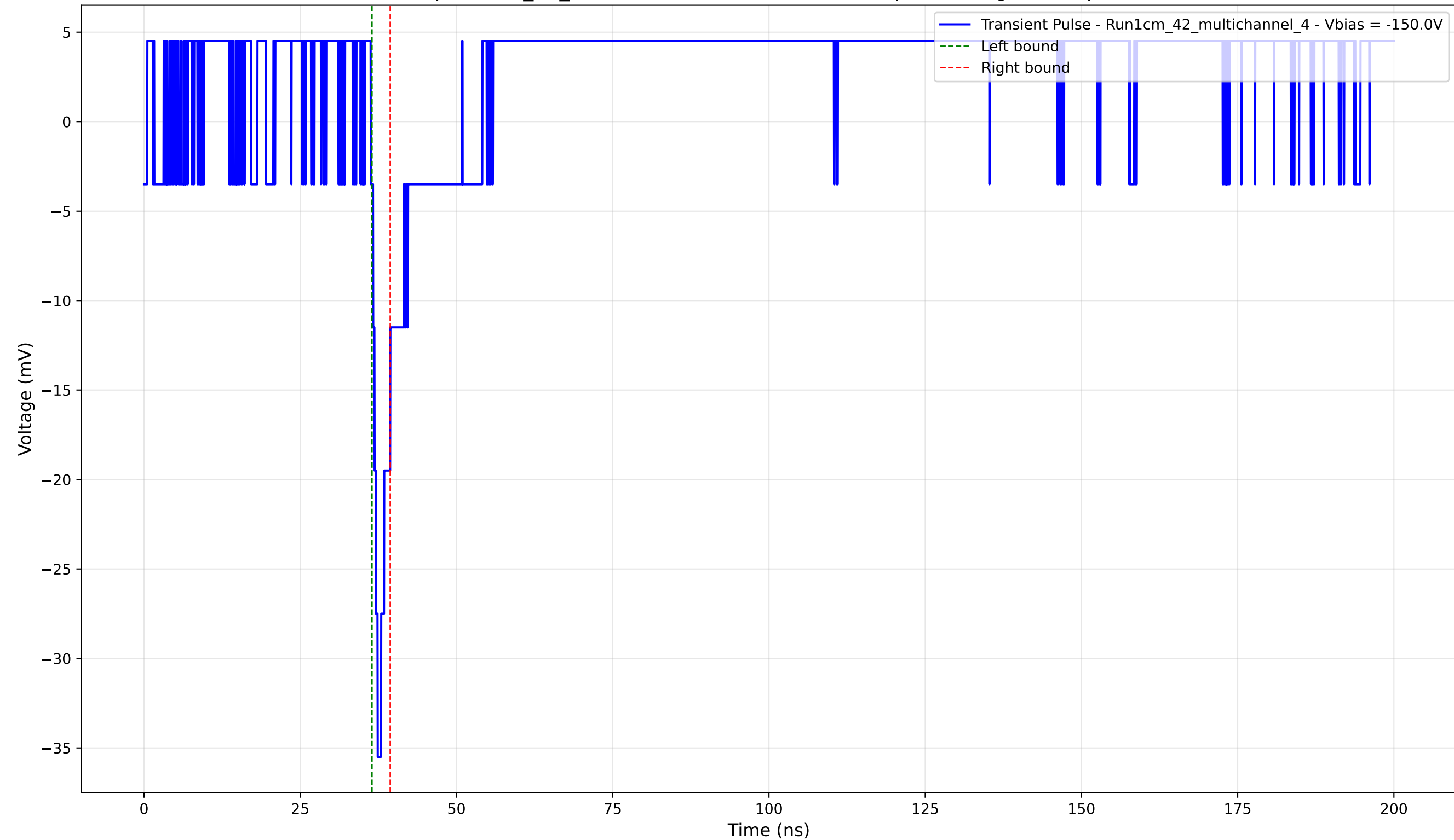
Transient Pulse - Sample: 1cm_42_multichannel - Position: 1810.0 \mu\text{m} - Charge: 1.35 pC - Rise Time: 0.74 ns
