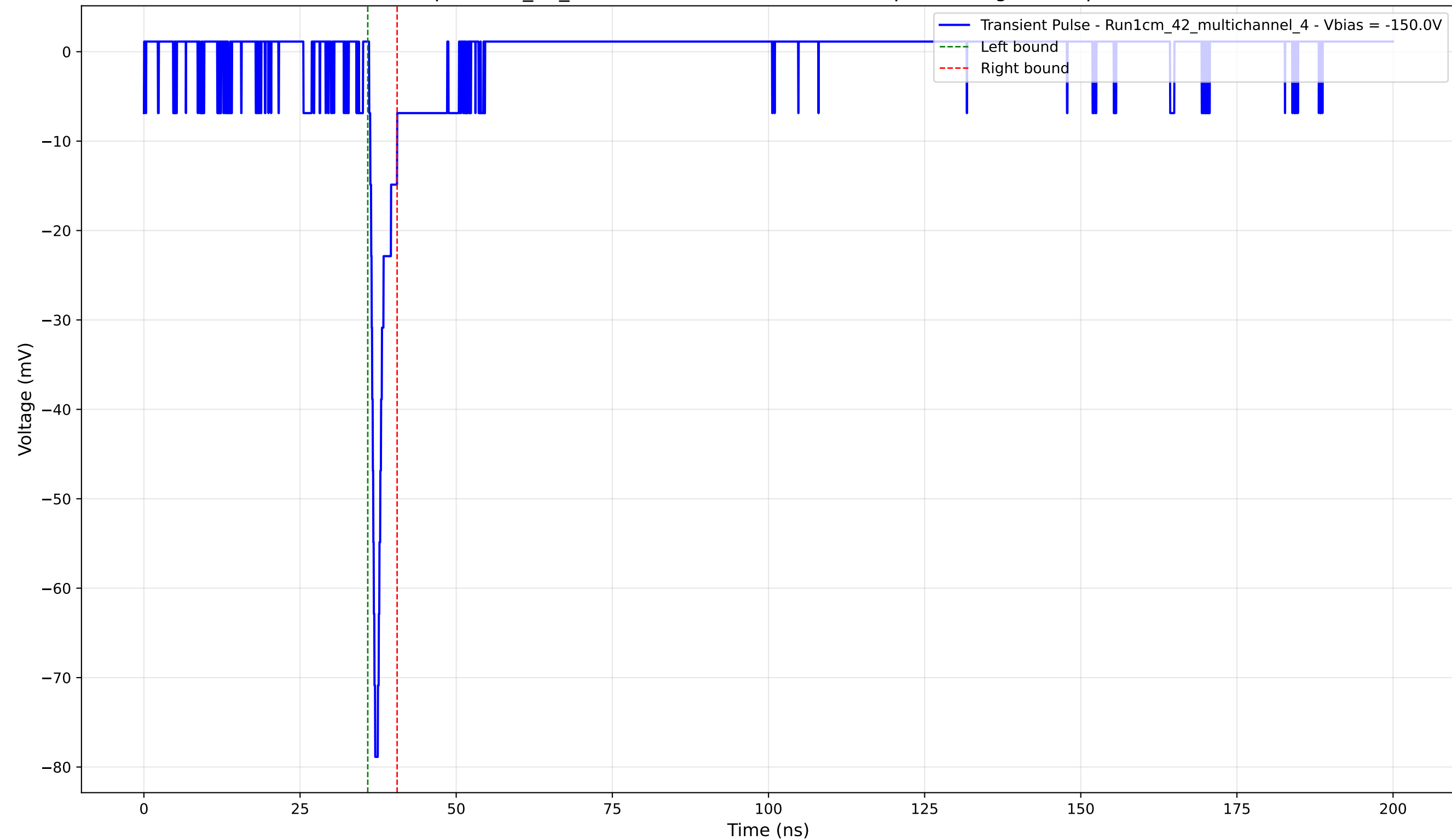
Transient Pulse - Sample: 1cm_42_multichannel - Position: 2465.0 \mu\text{m} - Charge: 3.08 pC - Rise Time: 0.80 ns
