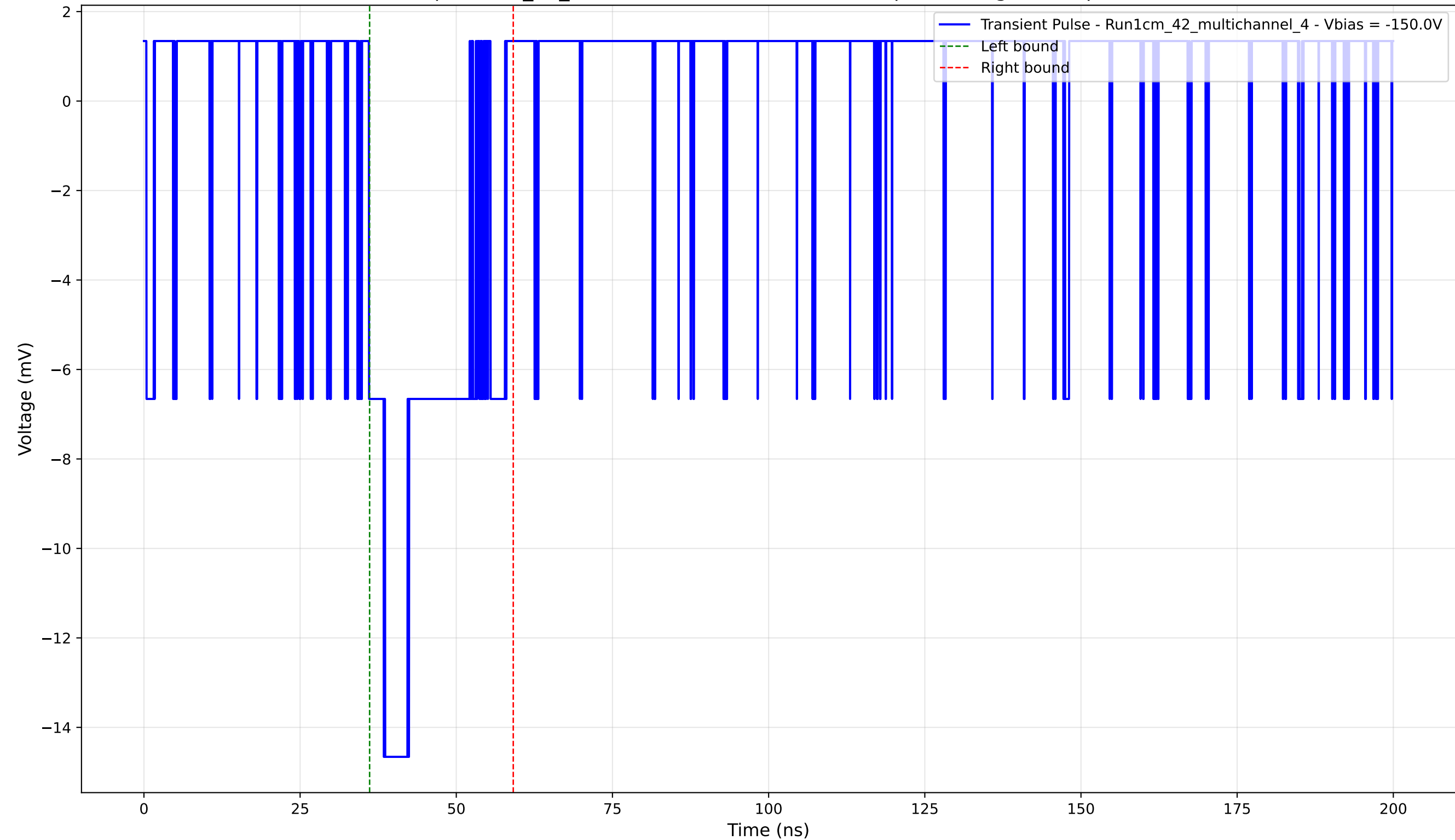
Transient Pulse - Sample: 1cm_42_multichannel - Position: 4795.0 \mu\text{m} - Charge: 3.20 pC - Rise Time: 2.38 ns
