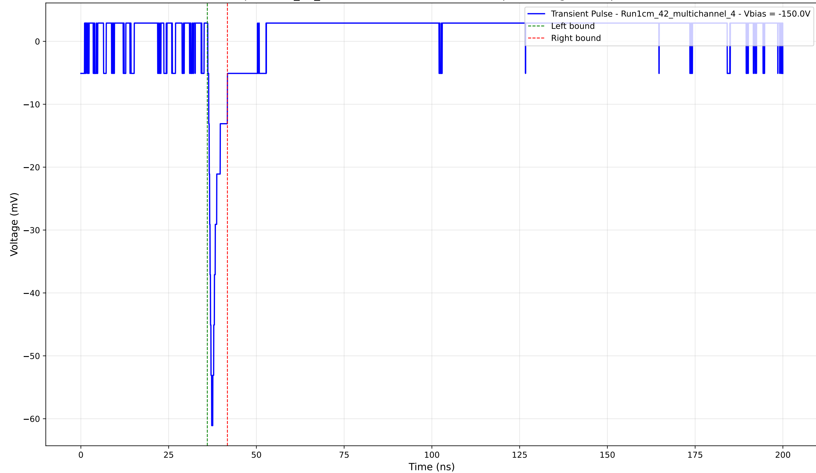
Transient Pulse - Sample: 1cm_42_multichannel - Position: 2085.0 \mu\text{m} - Charge: 2.83 pC - Rise Time: 0.86 ns
