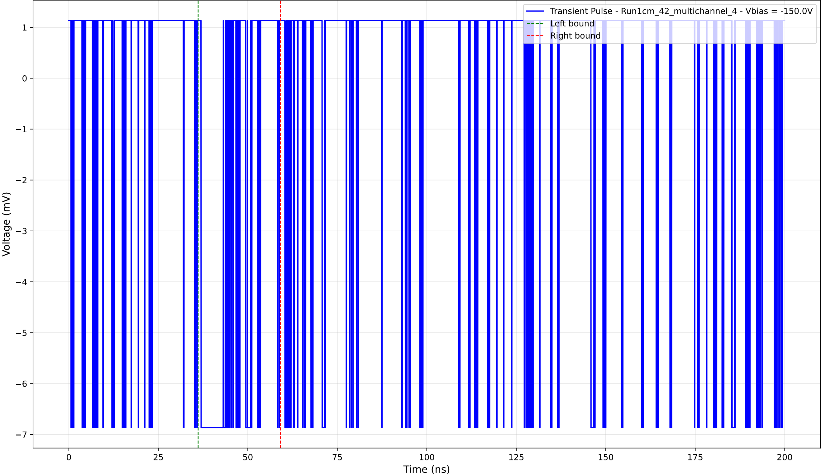
Transient Pulse - Sample: 1cm_42_multichannel - Position: 3430.0 \mu\text{m} - Charge: 1.11 pC - Rise Time: 0.00 ns (N/A)
