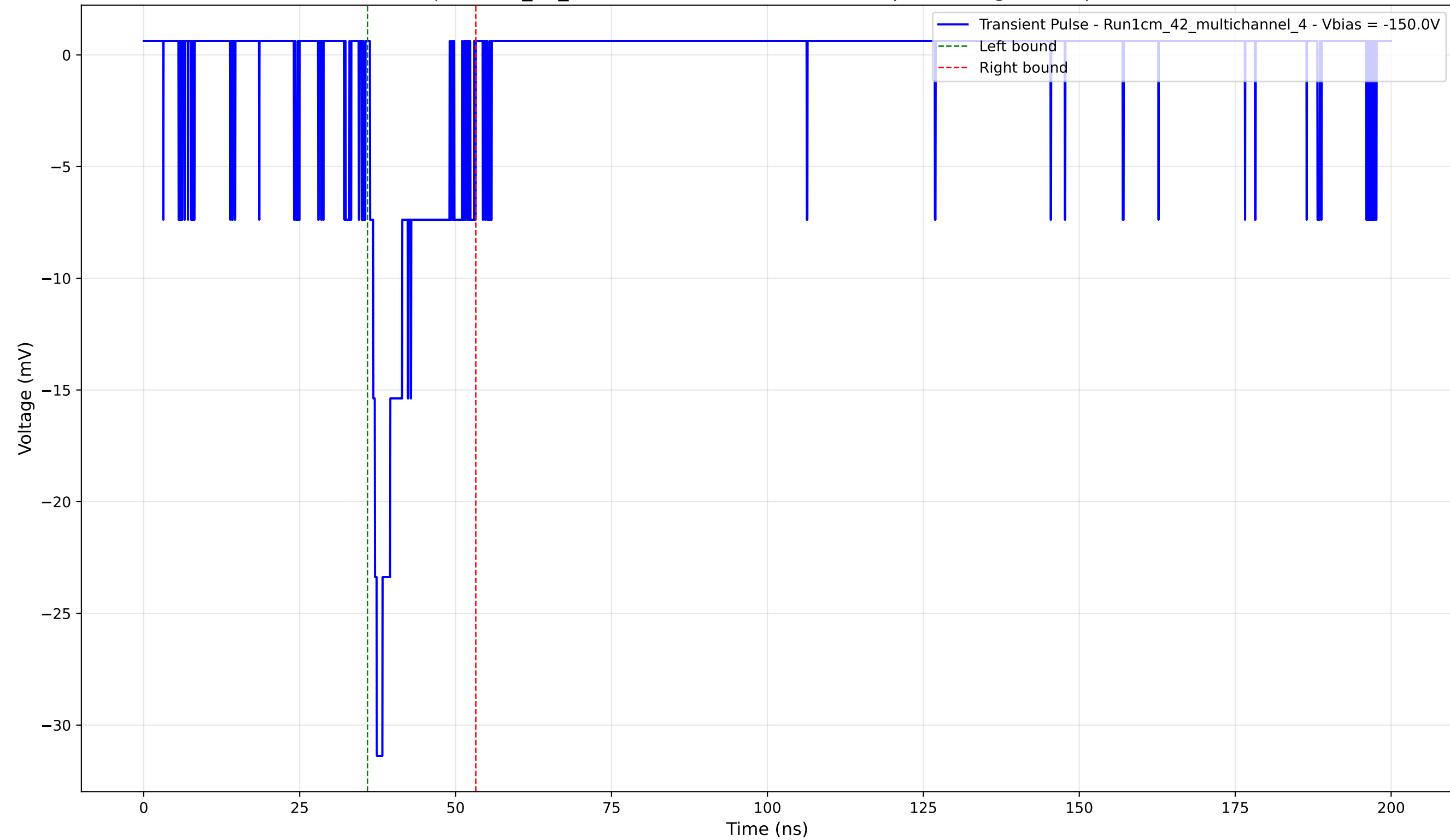
Transient Pulse - Sample: 1cm_42_multichannel - Position: 3095.0 \mu\text{m} - Charge: 3.60 pC - Rise Time: 1.09 ns
