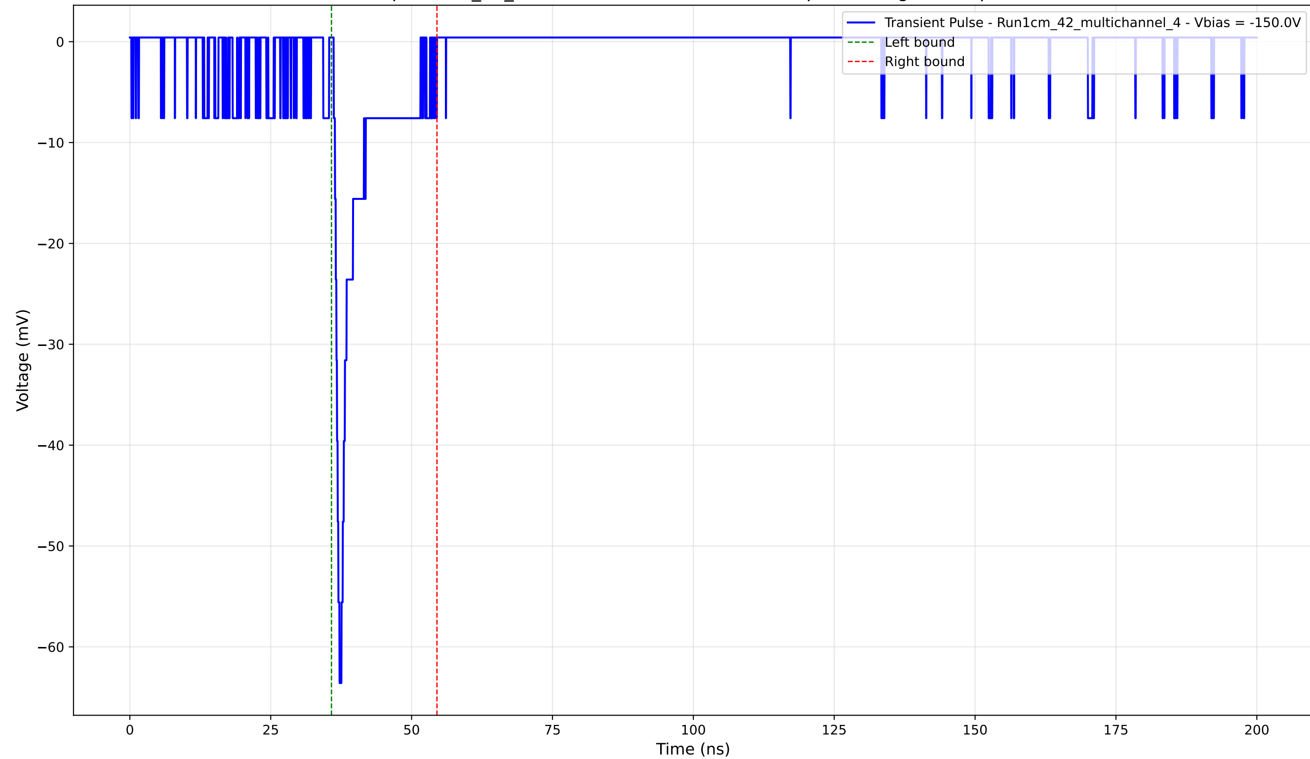
Transient Pulse - Sample: 1cm_42_multichannel - Position: 2645.0 \mu\text{m} - Charge: 4.77 pC - Rise Time: 1.02 ns
