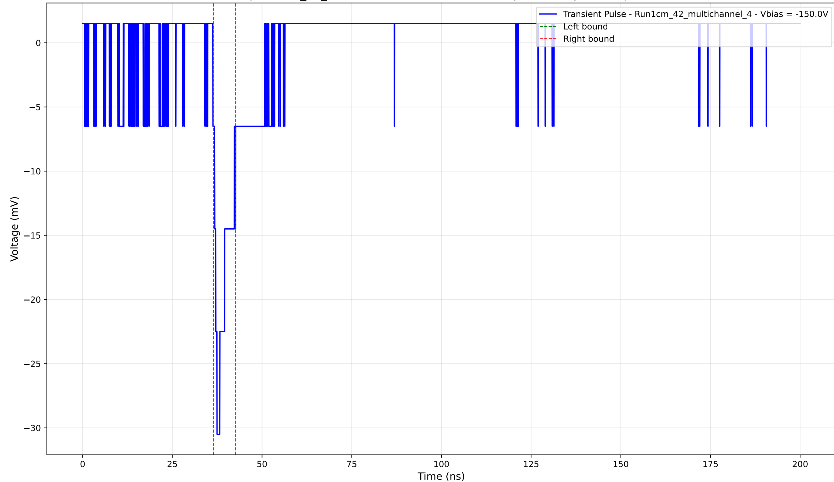
Transient Pulse - Sample: 1cm_42_multichannel - Position: 3145.0 \mu\text{m} - Charge: 2.22 pC - Rise Time: 1.15 ns
