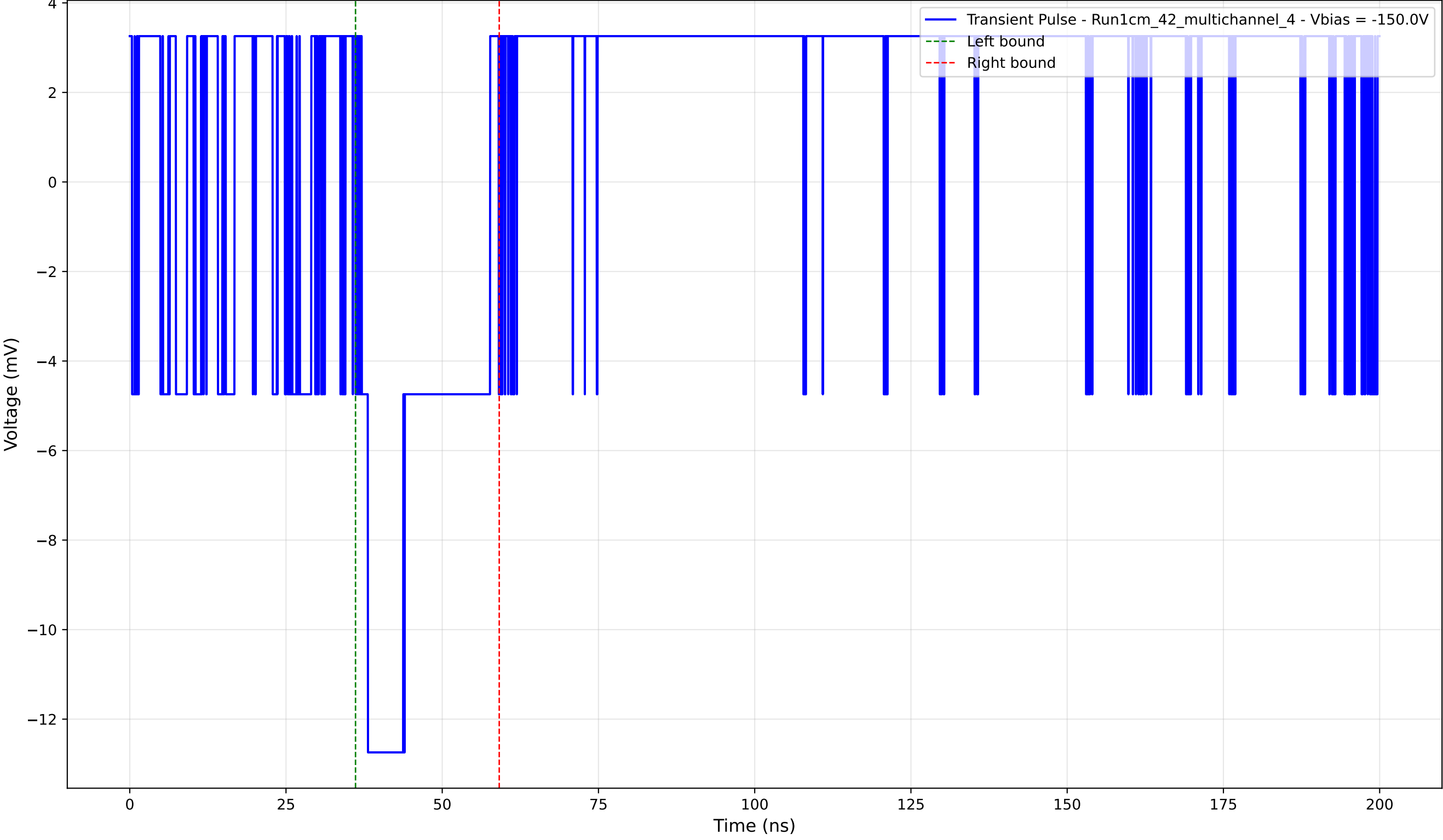
Transient Pulse - Sample: 1cm_42_multichannel - Position: 555.0 \mu\text{m} - Charge: 2.77 pC - Rise Time: 0.00 ns (N/A)
