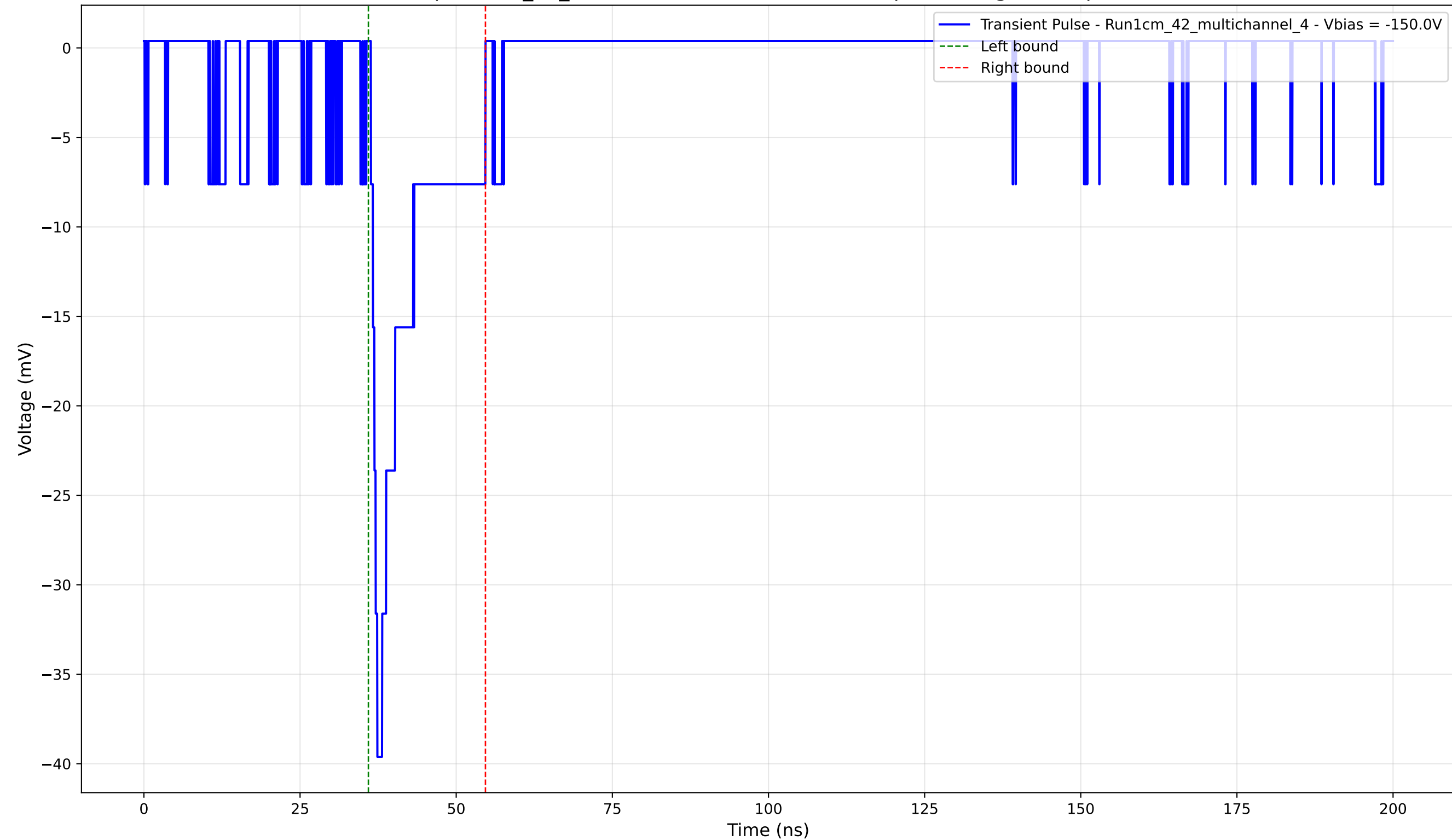
Transient Pulse - Sample: 1cm_42_multichannel - Position: 1725.0 \mu\text{m} - Charge: 4.77 pC - Rise Time: 1.03 ns
