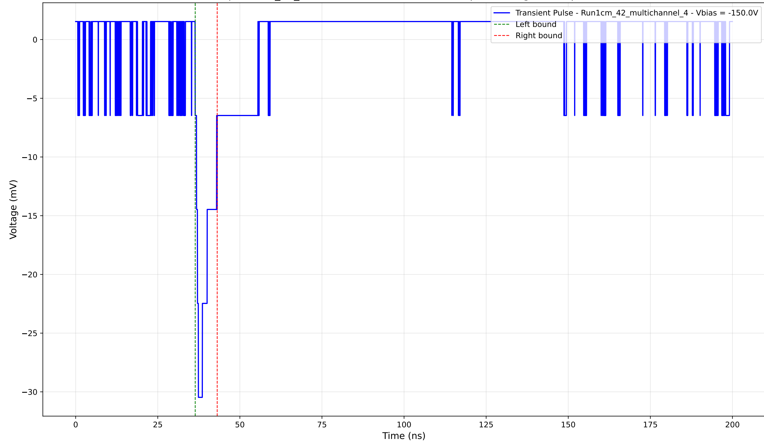
Transient Pulse - Sample: 1cm_42_multichannel - Position: 1590.0 \mu\text{m} - Charge: 2.53 pC - Rise Time: 0.99 ns
