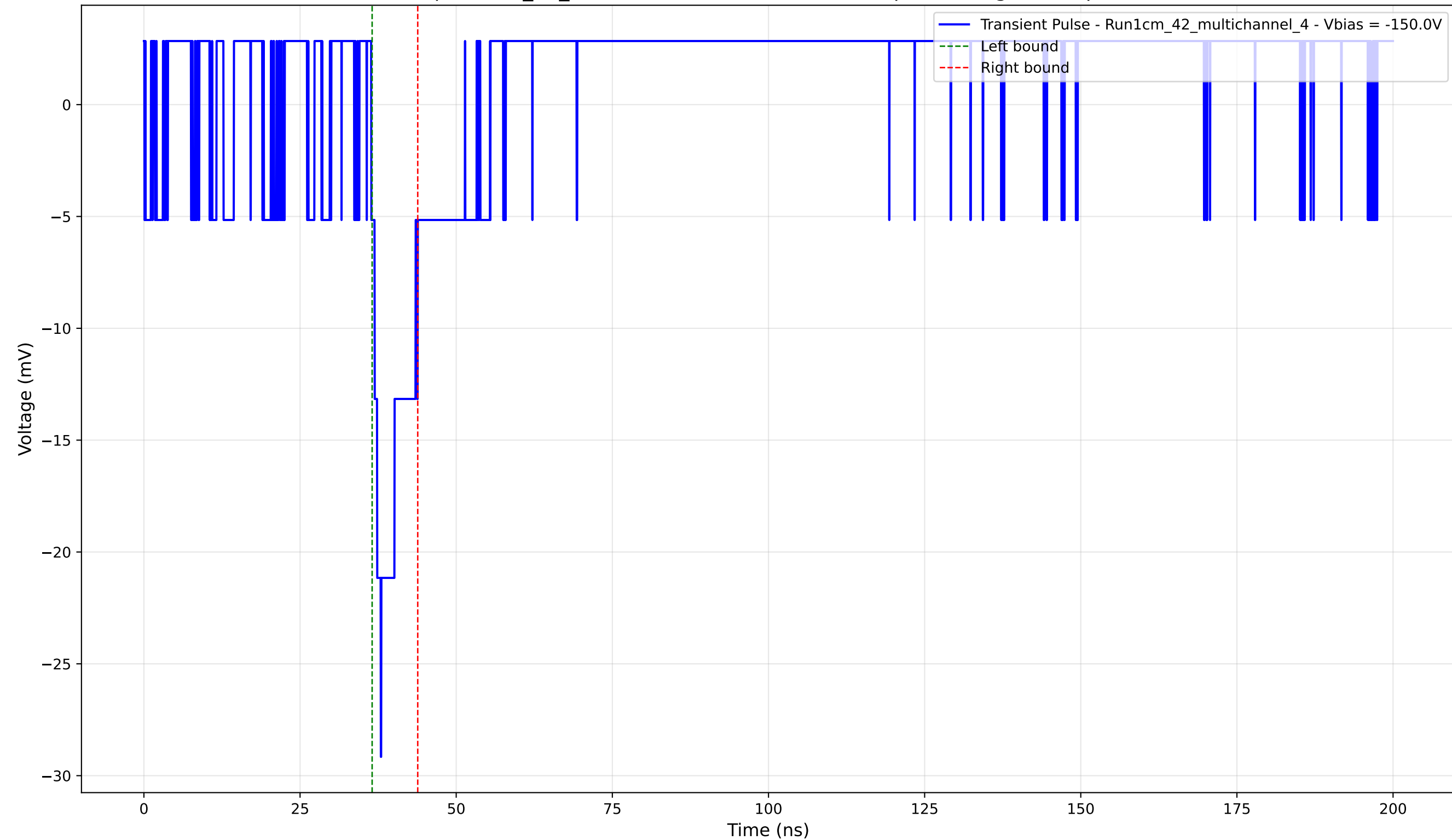
Transient Pulse - Sample: 1cm_42_multichannel - Position: 1450.0 \mu\text{m} - Charge: 2.28 pC - Rise Time: 1.54 ns
