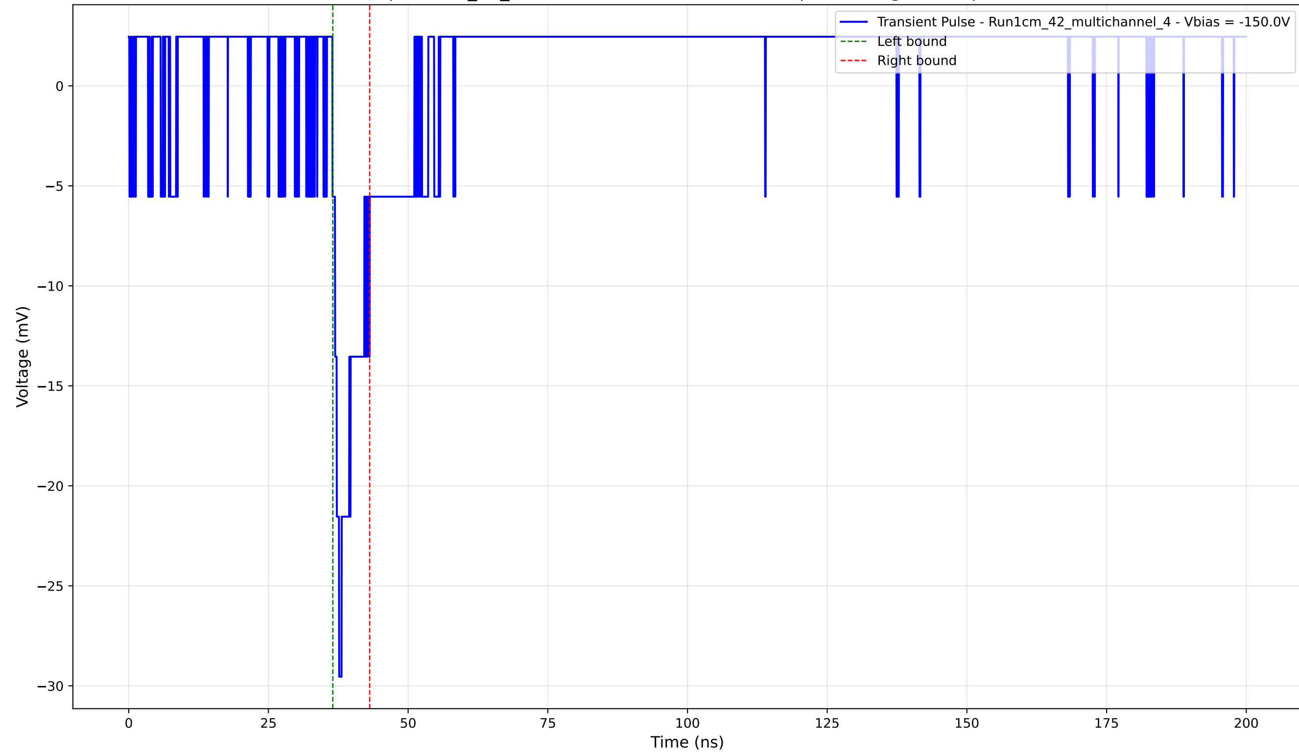
Transient Pulse - Sample: 1cm_42_multichannel - Position: 3235.0 \mu\text{m} - Charge: 2.10 pC - Rise Time: 1.20 ns
