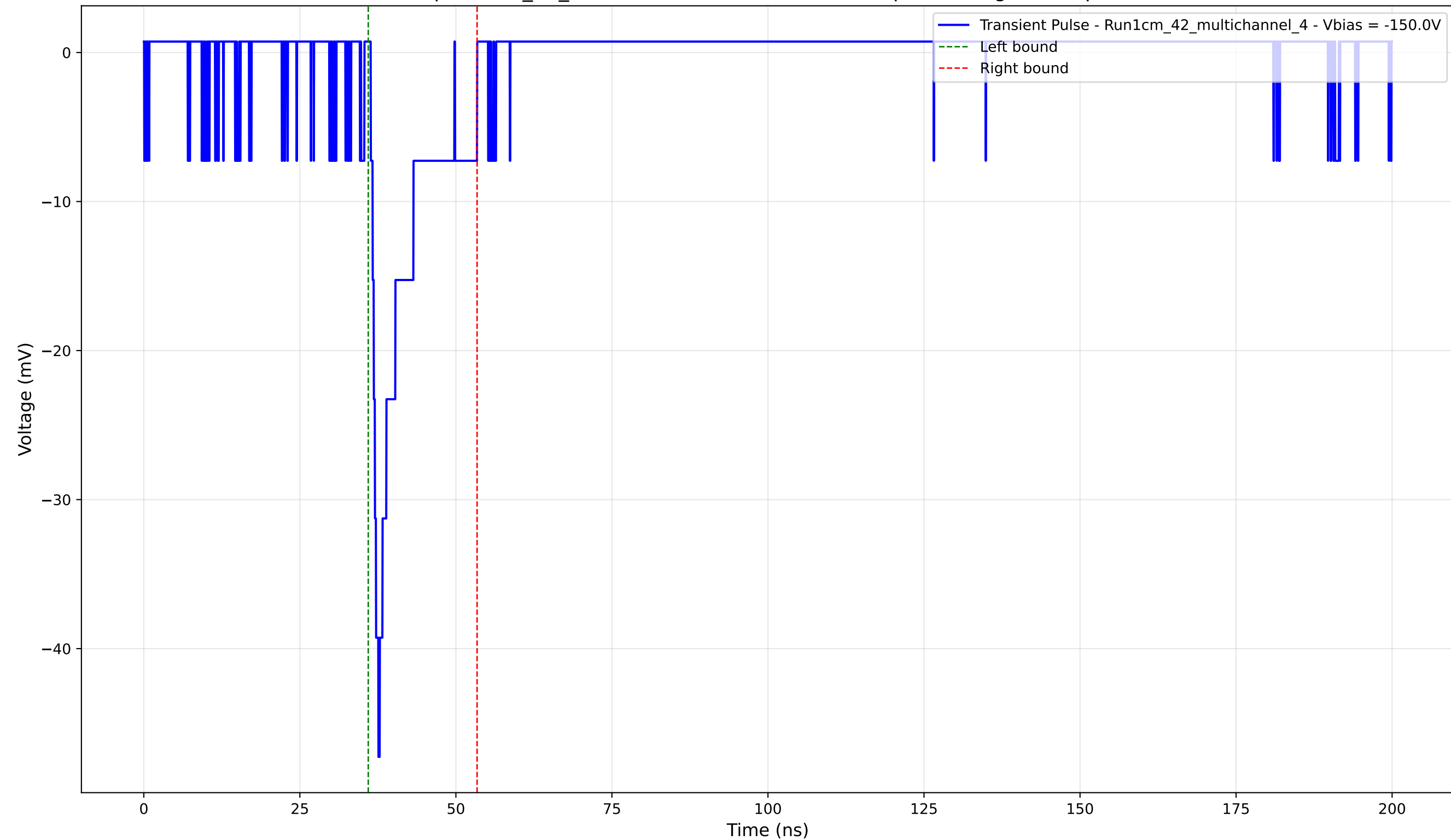
Transient Pulse - Sample: 1cm_42_multichannel - Position: 1780.0 \mu\text{m} - Charge: 4.55 pC - Rise Time: 1.23 ns
