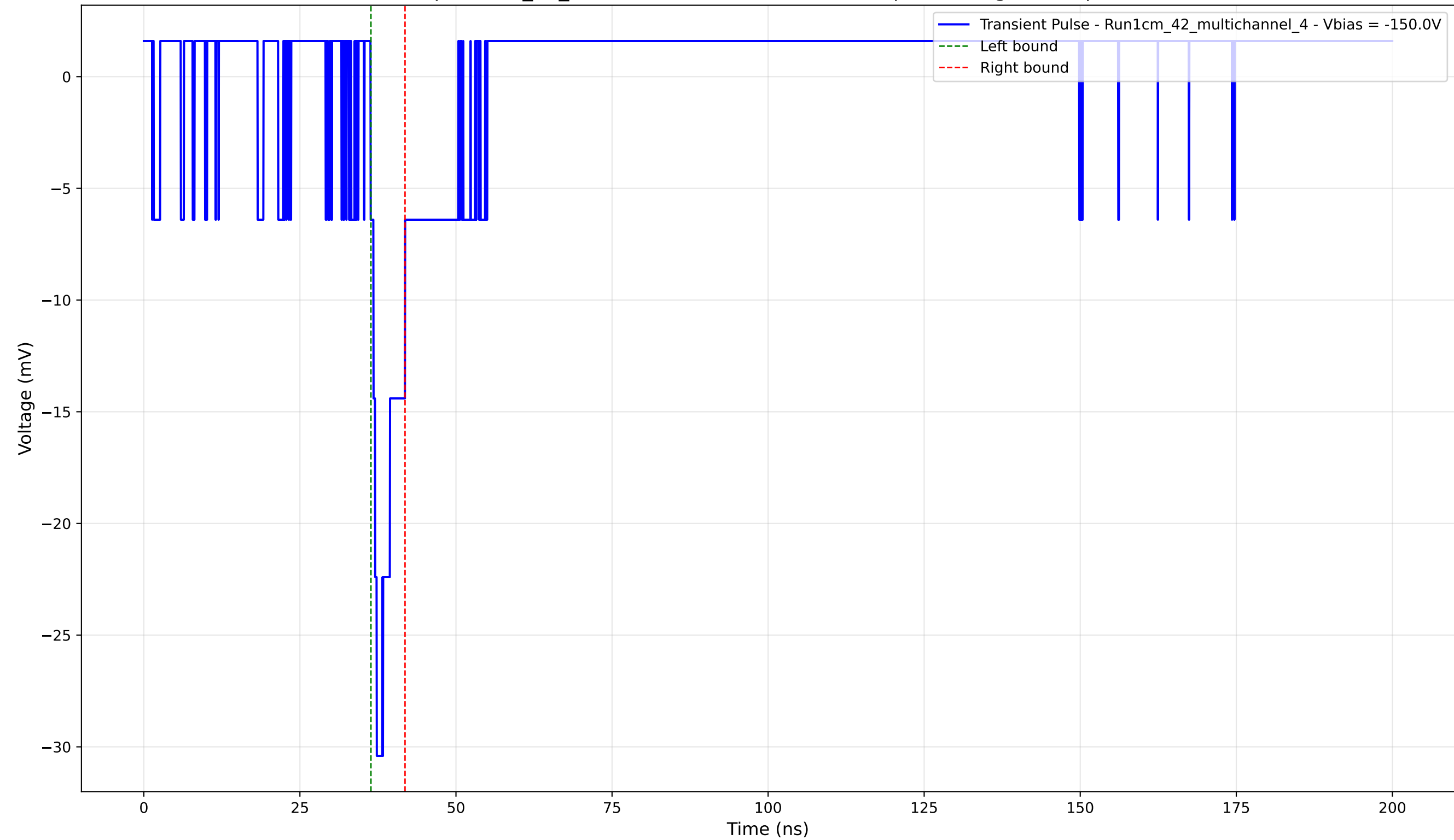
Transient Pulse - Sample: 1cm_42_multichannel - Position: 3080.0 \mu\text{m} - Charge: 2.05 pC - Rise Time: 0.99 ns
