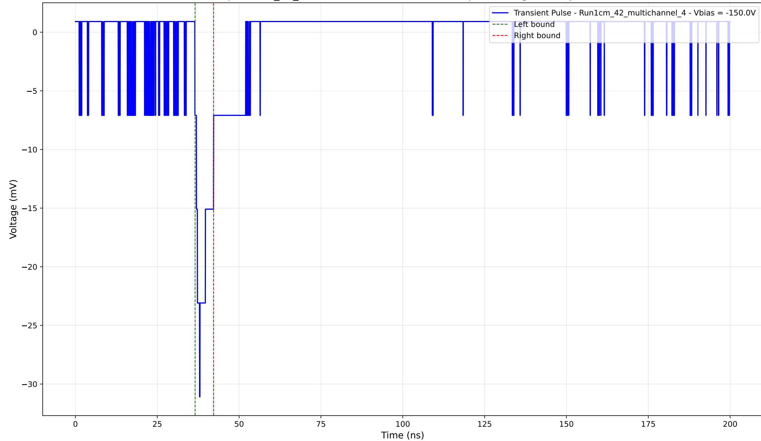
Transient Pulse - Sample: 1cm_42_multichannel - Position: 3260.0 \mu\text{m} - Charge: 2.05 pC - Rise Time: 1.45 ns
