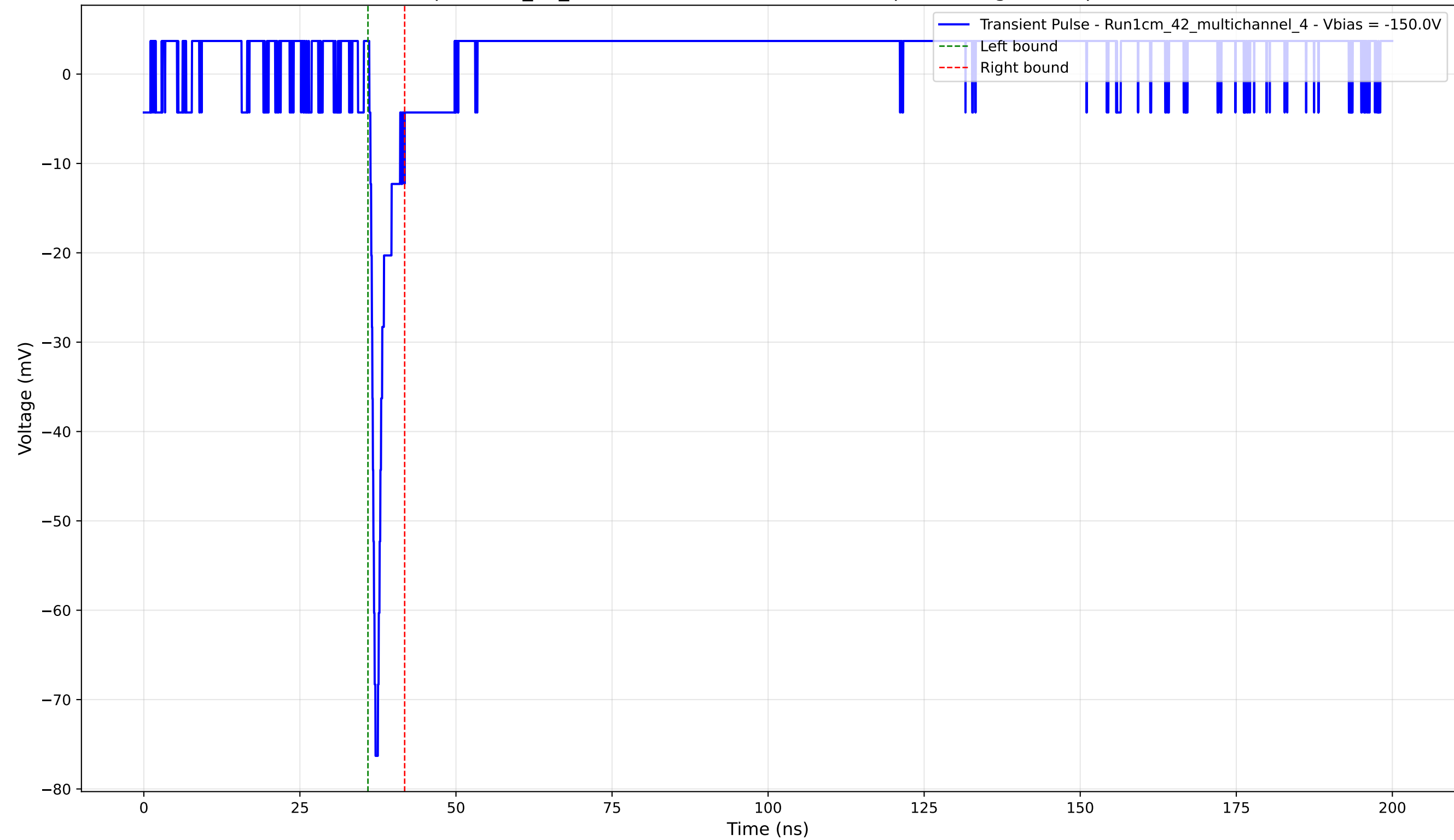
Transient Pulse - Sample: 1cm_42_multichannel - Position: 2255.0 \mu\text{m} - Charge: 3.05 pC - Rise Time: 0.81 ns
