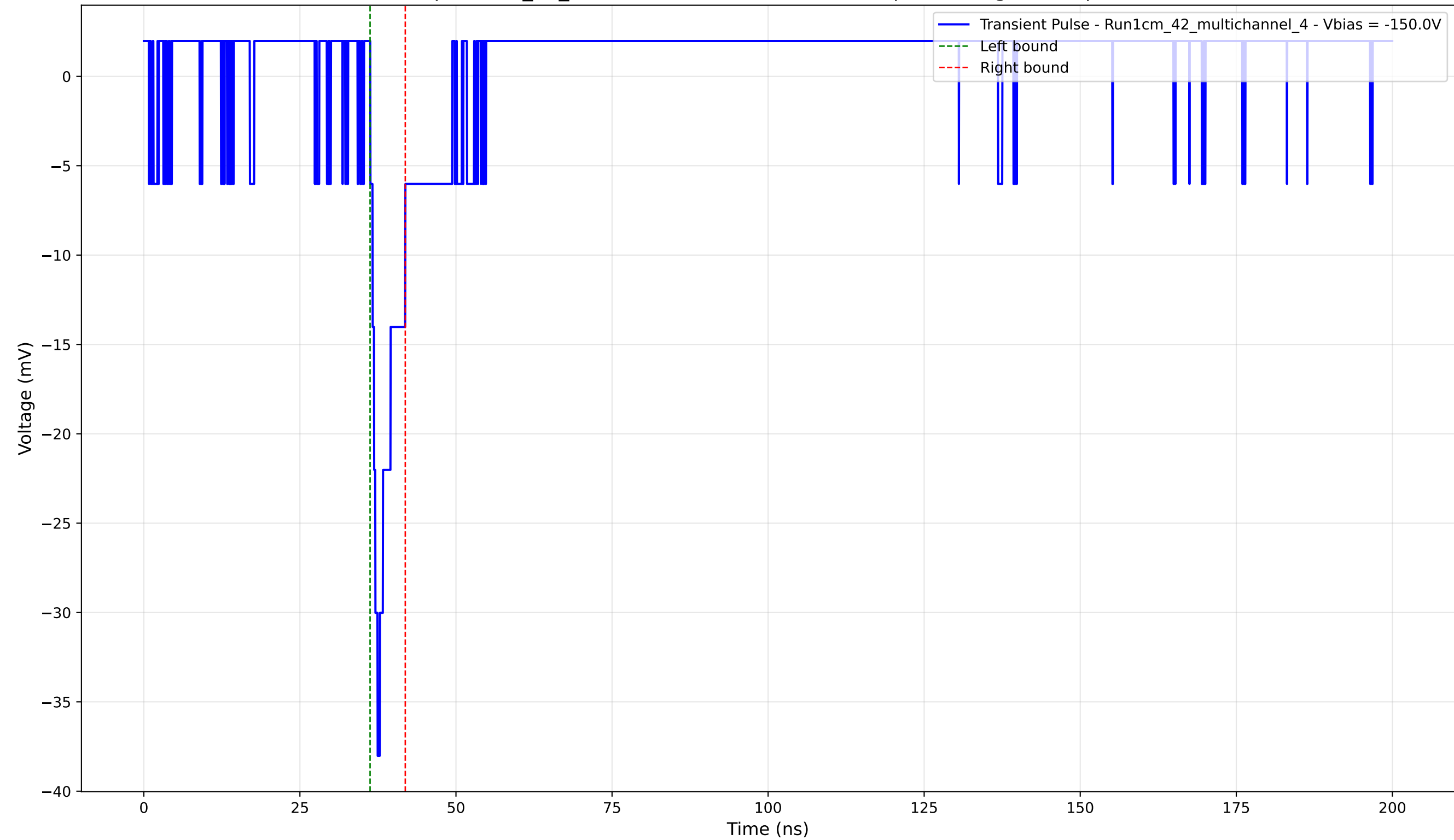
Transient Pulse - Sample: 1cm_42_multichannel - Position: 2960.0 \mu\text{m} - Charge: 2.19 pC - Rise Time: 1.17 ns
