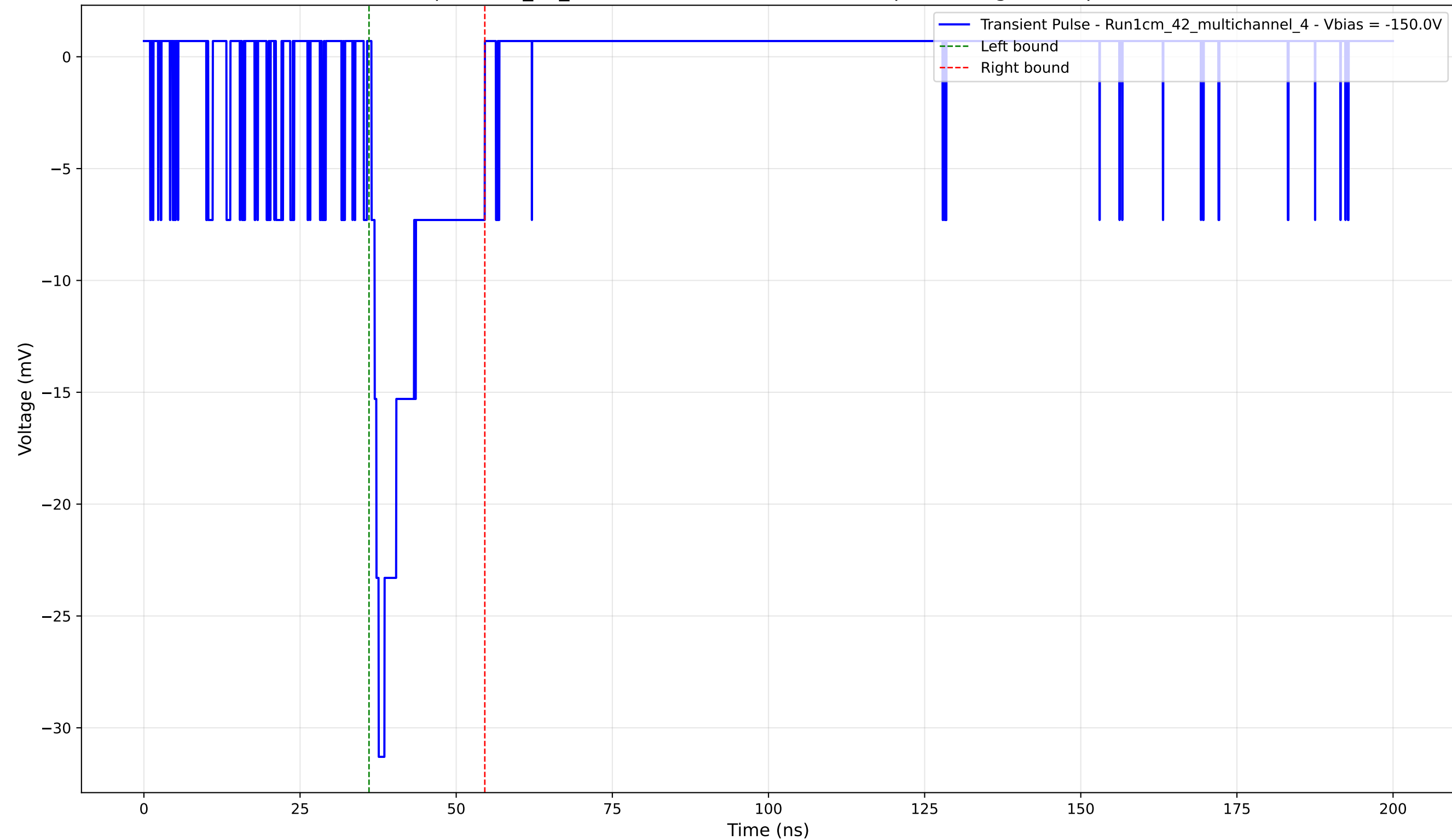
Transient Pulse - Sample: 1cm_42_multichannel - Position: 1495.0 \mu\text{m} - Charge: 4.33 pC - Rise Time: 1.15 ns
