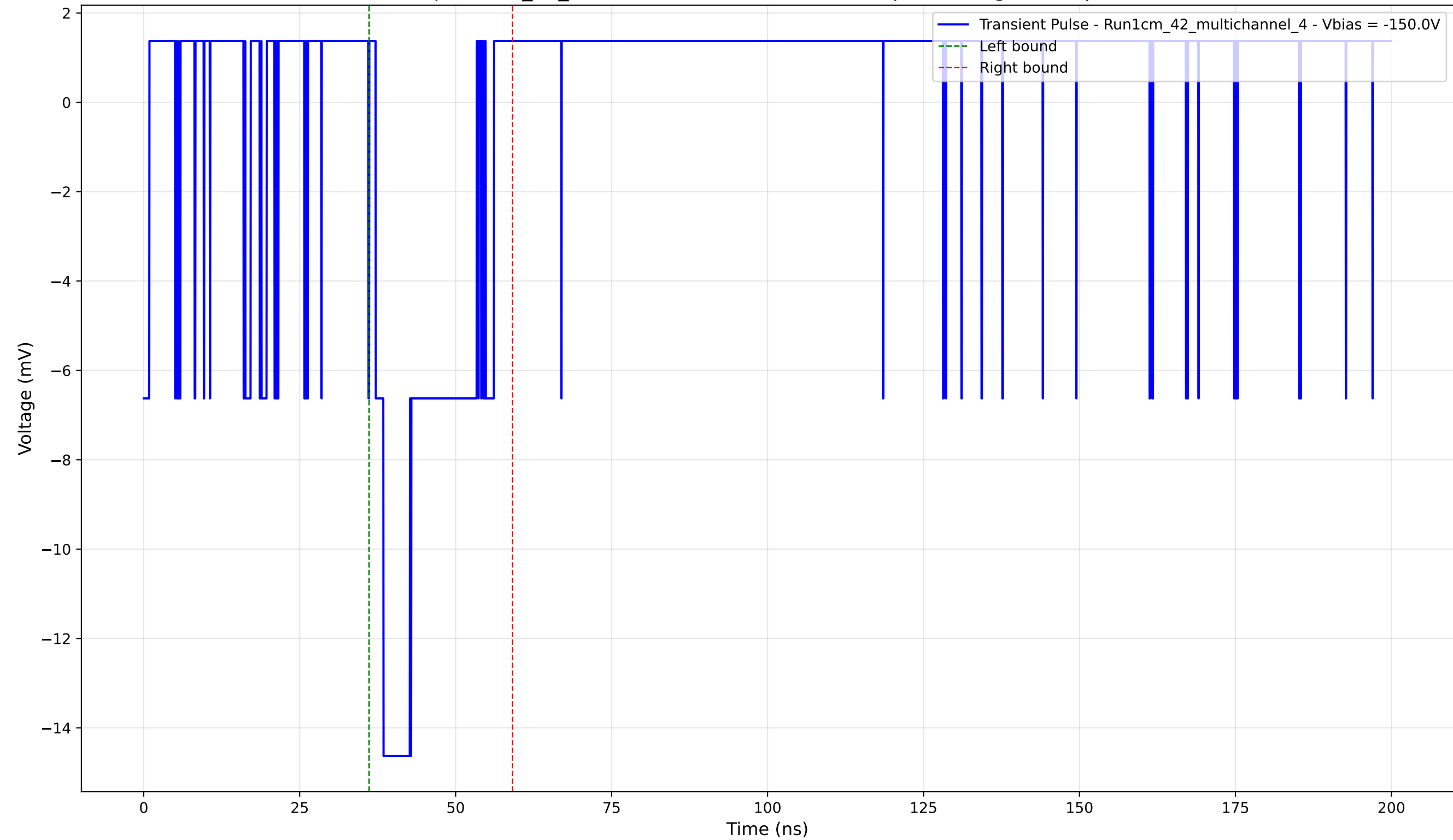
Transient Pulse - Sample: 1cm_42_multichannel - Position: 4230.0 \mu\text{m} - Charge: 2.94 pC - Rise Time: 1.26 ns
