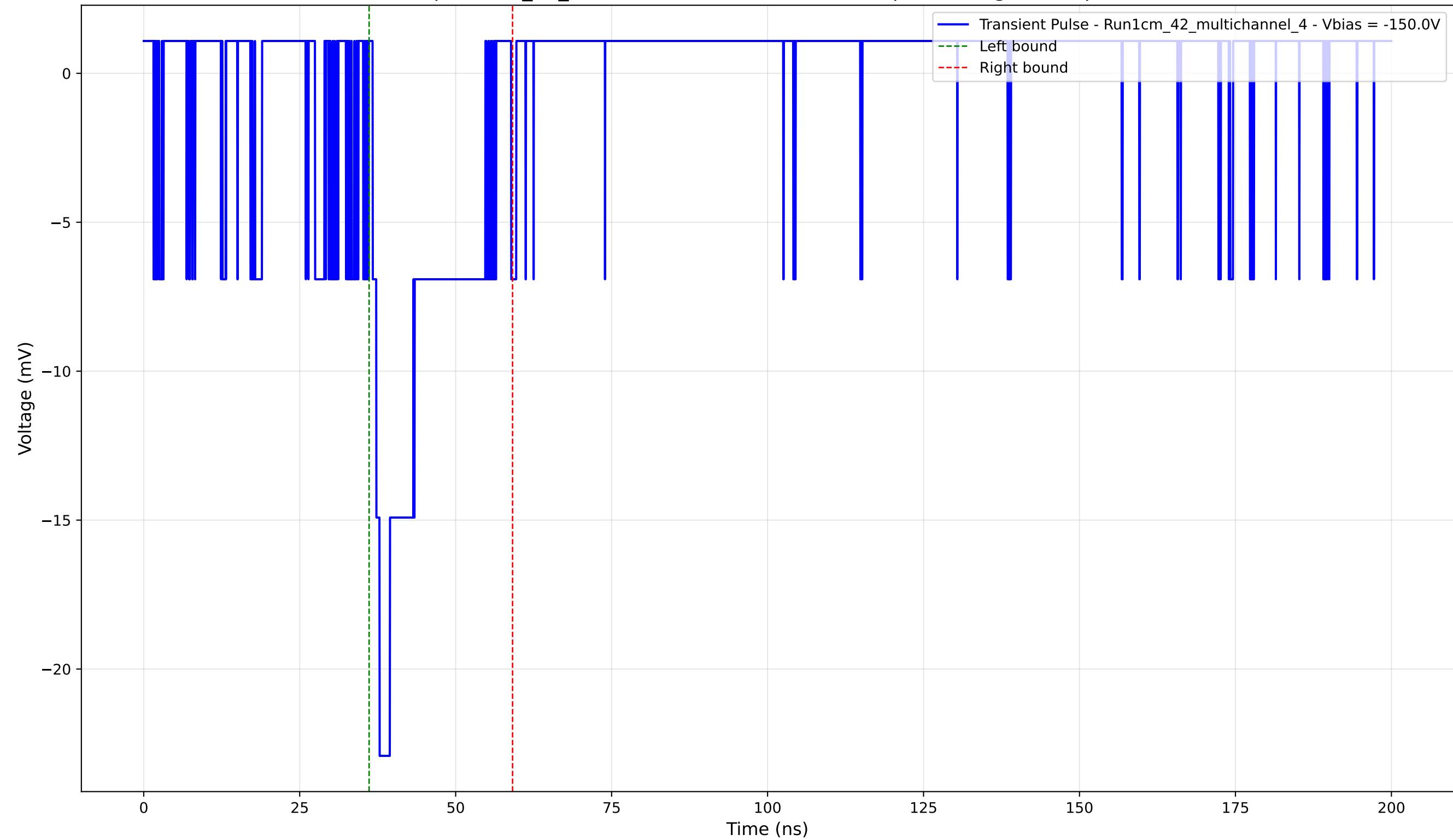
Transient Pulse - Sample: 1cm_42_multichannel - Position: 3515.0 \mu\text{m} - Charge: 3.84 pC - Rise Time: 1.12 ns
