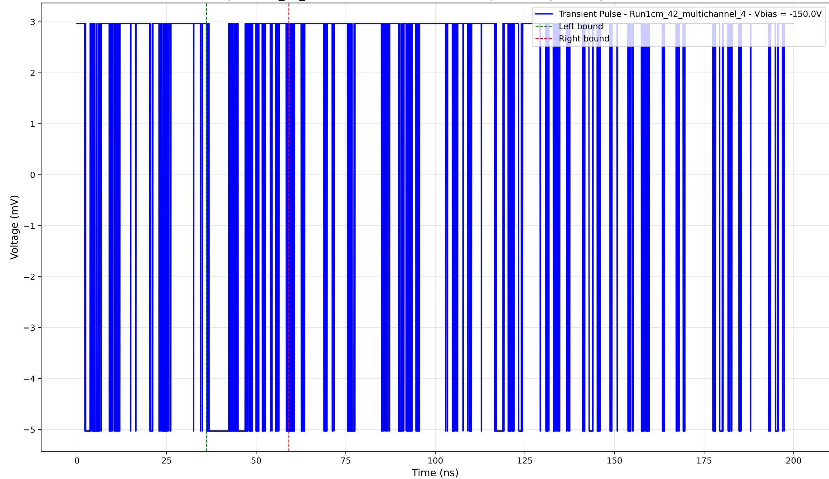
Transient Pulse - Sample: 1cm_42_multichannel - Position: 3425.0 \mu\text{m} - Charge: 0.61 pC - Rise Time: 0.00 ns (N/A)
