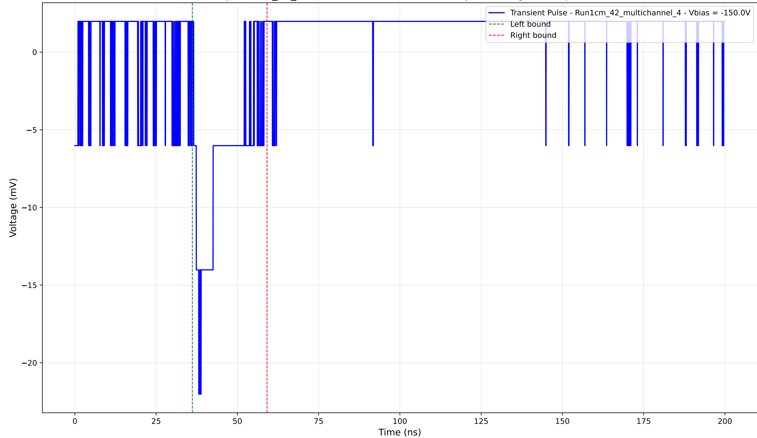
Transient Pulse - Sample: 1cm_42_multichannel - Position: 3585.0 \mu\text{m} - Charge: 3.14 pC - Rise Time: 1.56 ns
