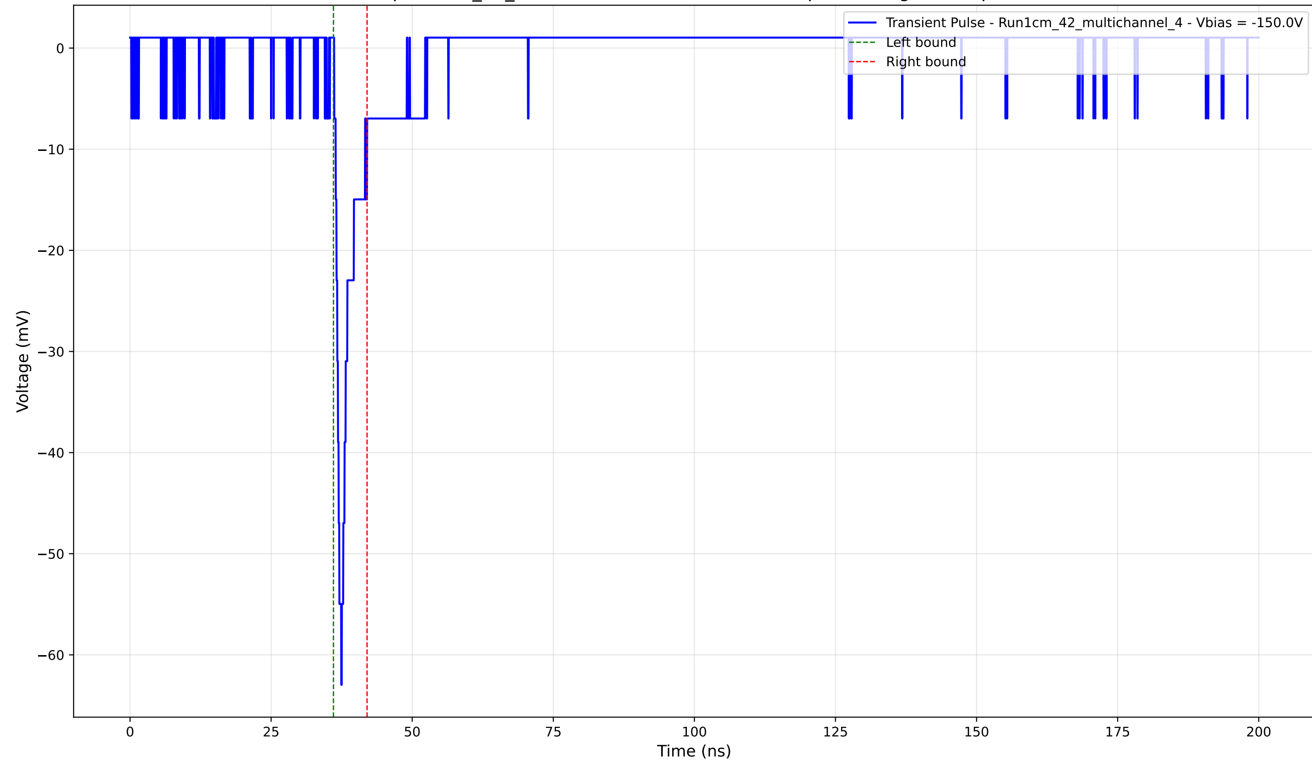
Transient Pulse - Sample: 1cm_42_multichannel - Position: 2690.0 \mu\text{m} - Charge: 2.97 pC - Rise Time: 1.24 ns
