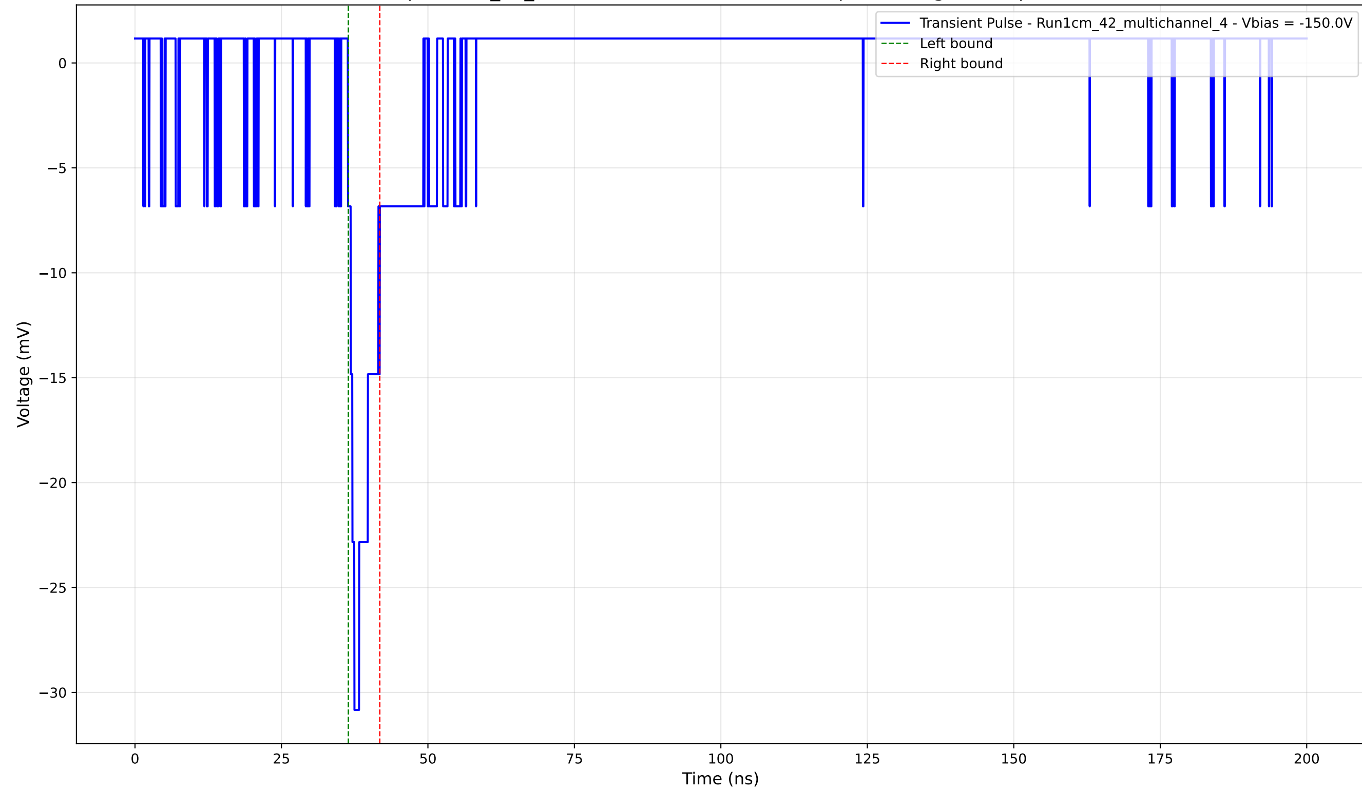
Transient Pulse - Sample: 1cm_42_multichannel - Position: 3125.0 \mu\text{m} - Charge: 2.06 pC - Rise Time: 1.11 ns
