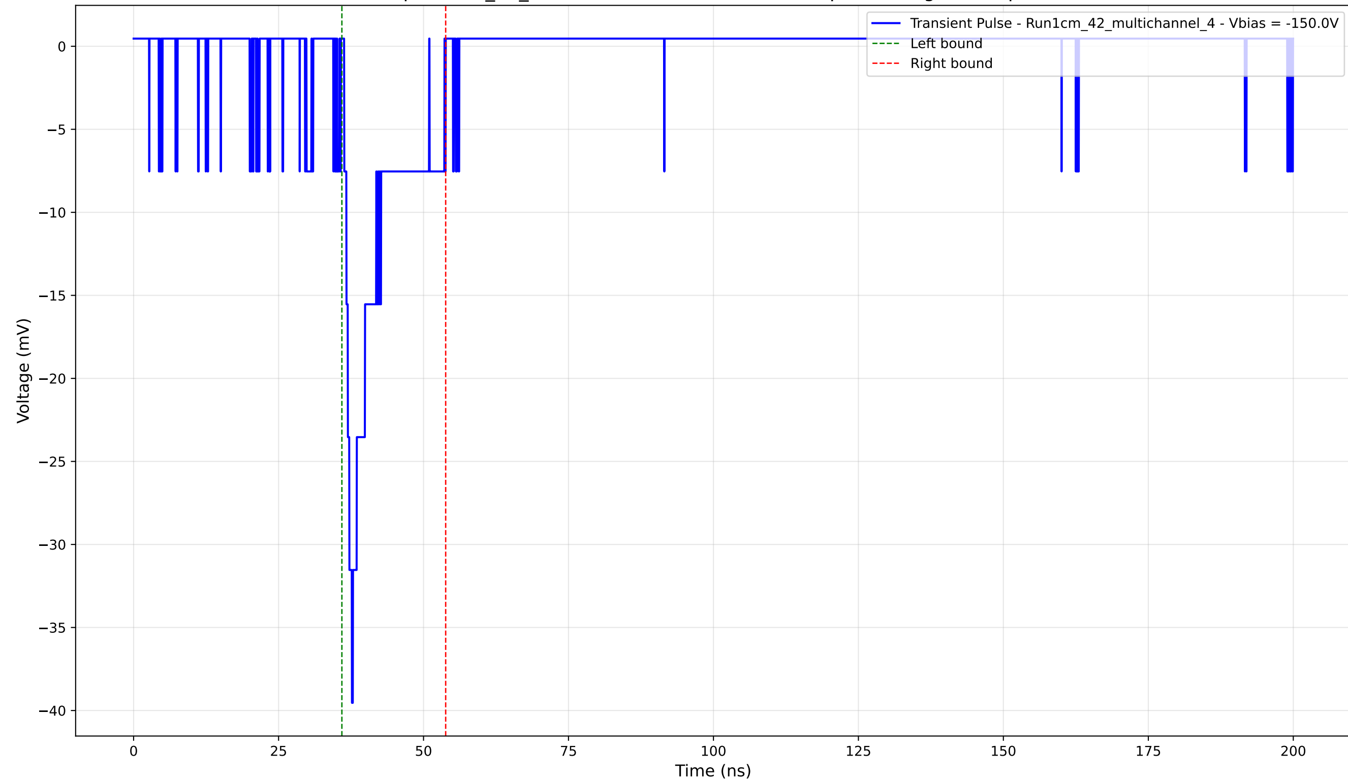
Transient Pulse - Sample: 1cm_42_multichannel - Position: 3060.0 \mu\text{m} - Charge: 4.22 pC - Rise Time: 1.33 ns
