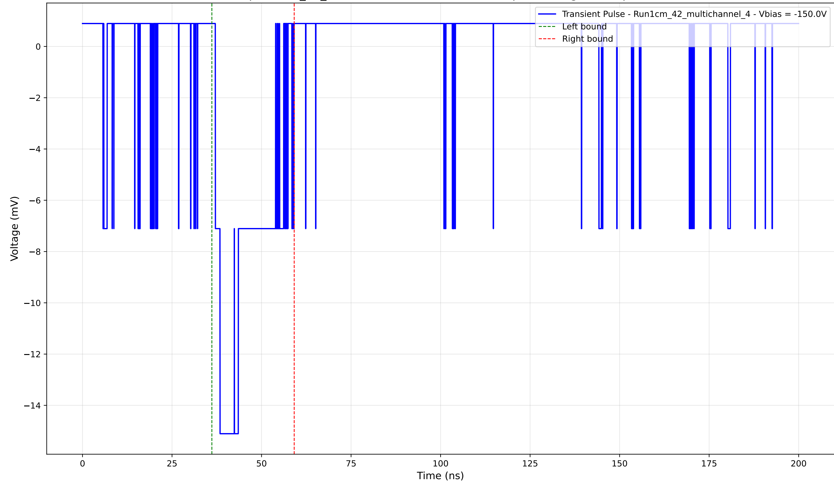
Transient Pulse - Sample: 1cm_42_multichannel - Position: 4255.0 \mu\text{m} - Charge: 3.55 pC - Rise Time: 1.32 ns
