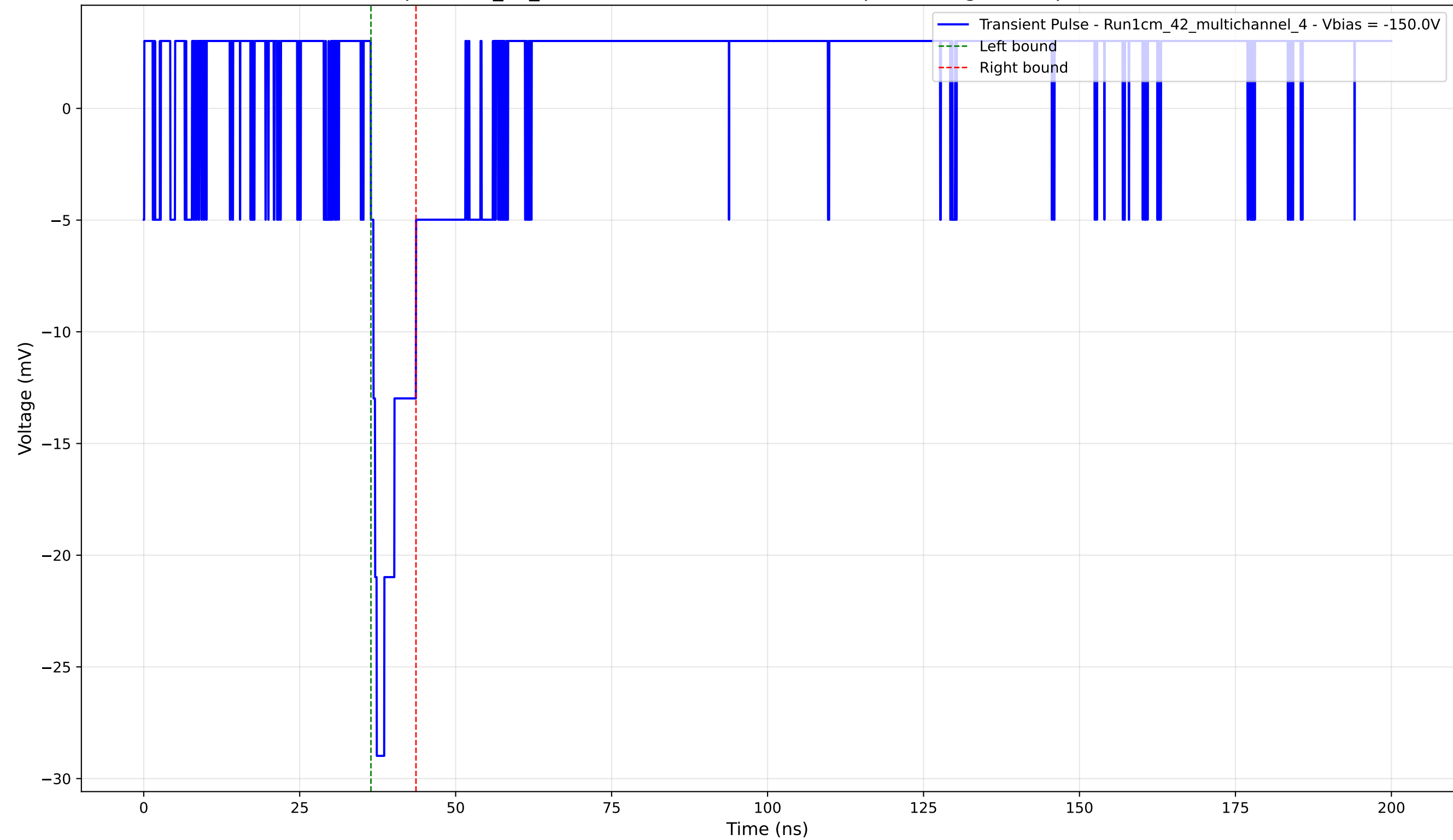
Transient Pulse - Sample: 1cm_42_multichannel - Position: 1605.0 \mu\text{m} - Charge: 2.50 pC - Rise Time: 0.00 ns (N/A)
