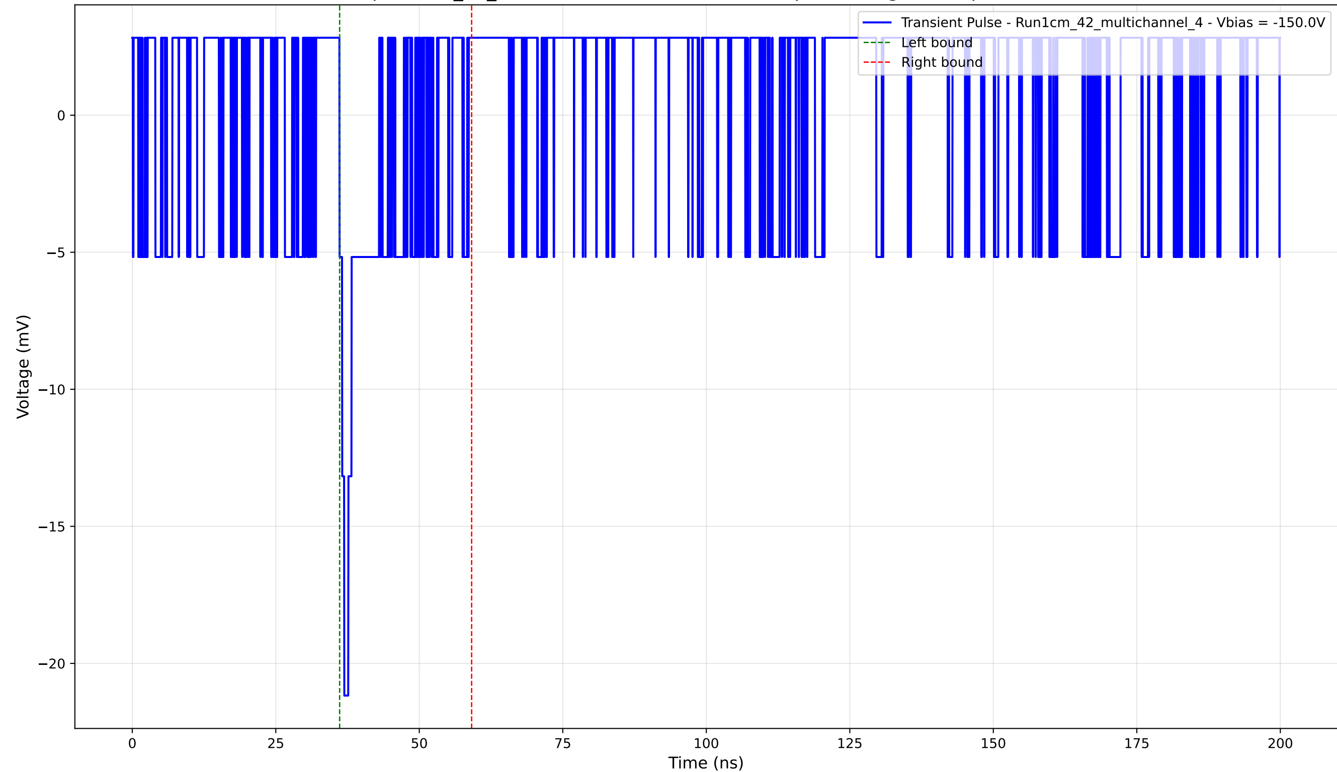
Transient Pulse - Sample: 1cm_42_multichannel - Position: 2345.0 \mu\text{m} - Charge: 1.36 pC - Rise Time: 0.00 ns (N/A)
