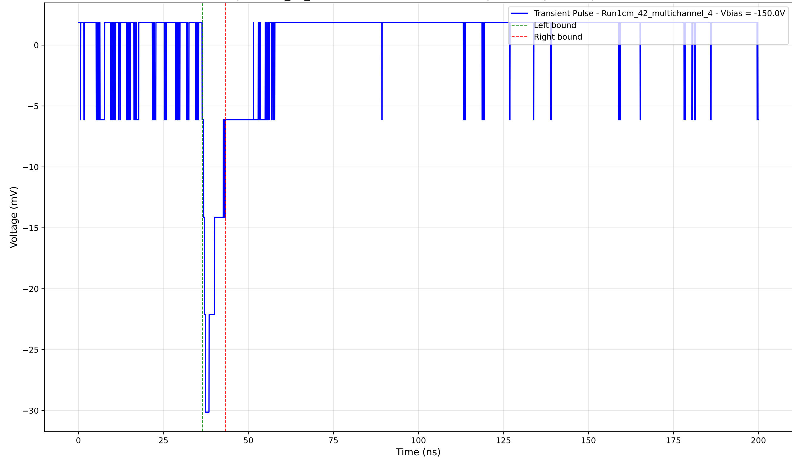
Transient Pulse - Sample: 1cm_42_multichannel - Position: 1600.0 \mu\text{m} - Charge: 2.46 pC - Rise Time: 0.97 ns
