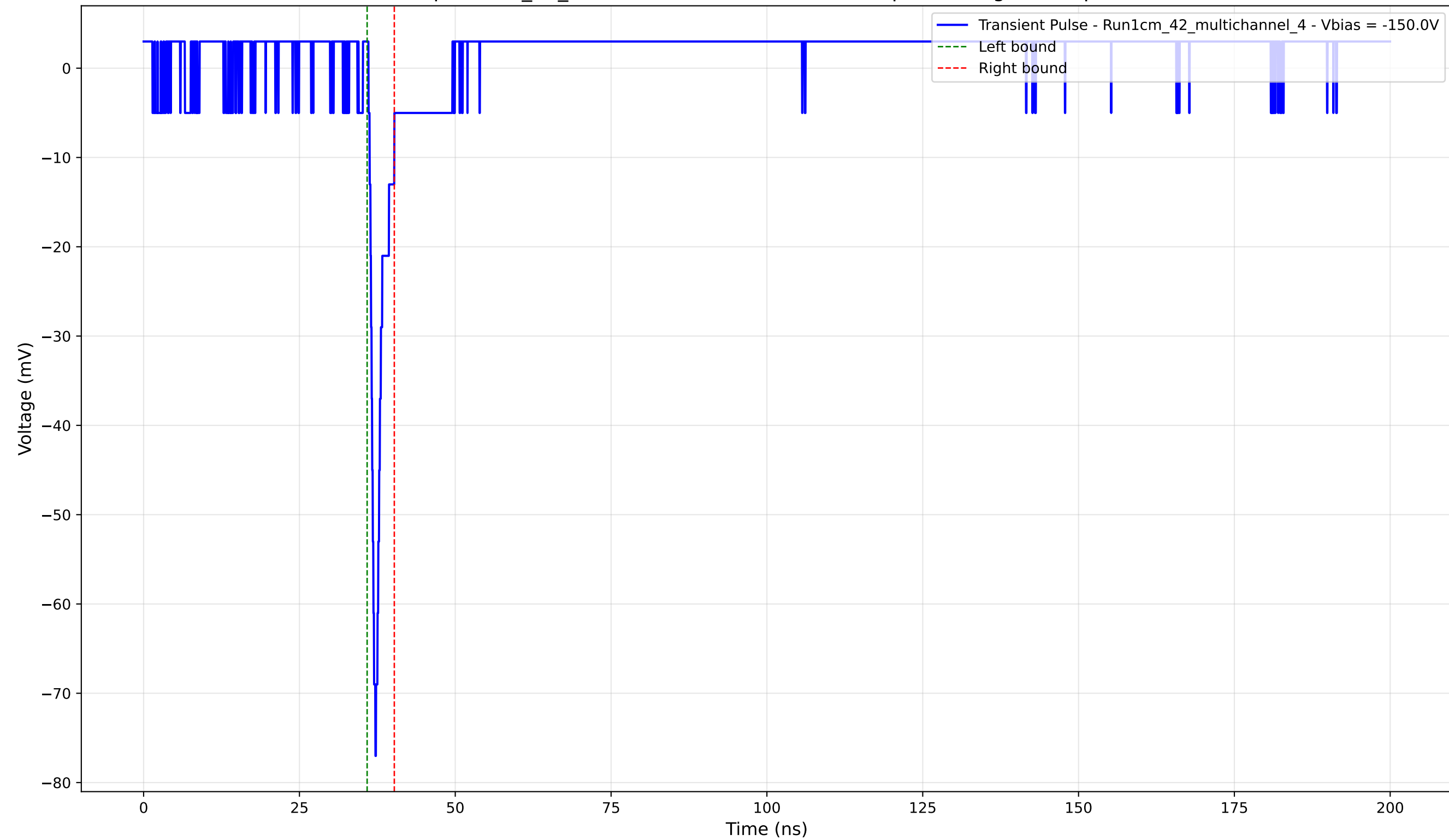
Transient Pulse - Sample: 1cm_42_multichannel - Position: 2455.0 \mu\text{m} - Charge: 2.63 pC - Rise Time: 0.93 ns
