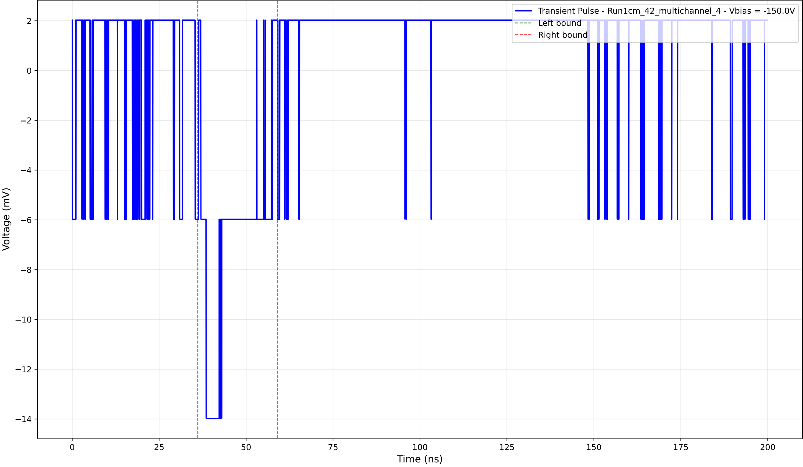
Transient Pulse - Sample: 1cm_42_multichannel - Position: 280.0 \mu\text{m} - Charge: 3.03 pC - Rise Time: 0.00 ns (N/A)
