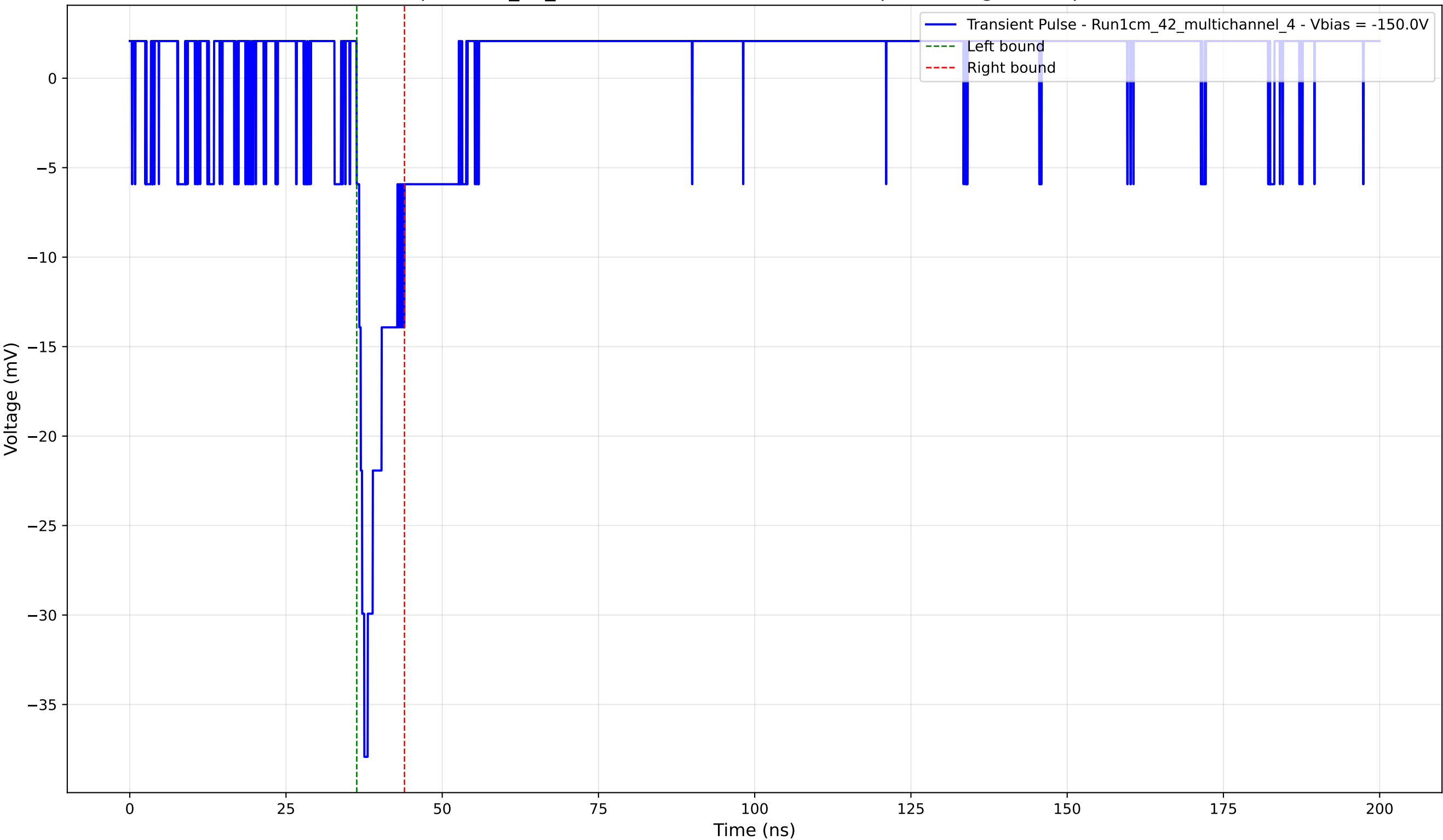
Transient Pulse - Sample: 1cm_42_multichannel - Position: 1680.0 \mu\text{m} - Charge: 2.88 pC - Rise Time: 1.23 ns
