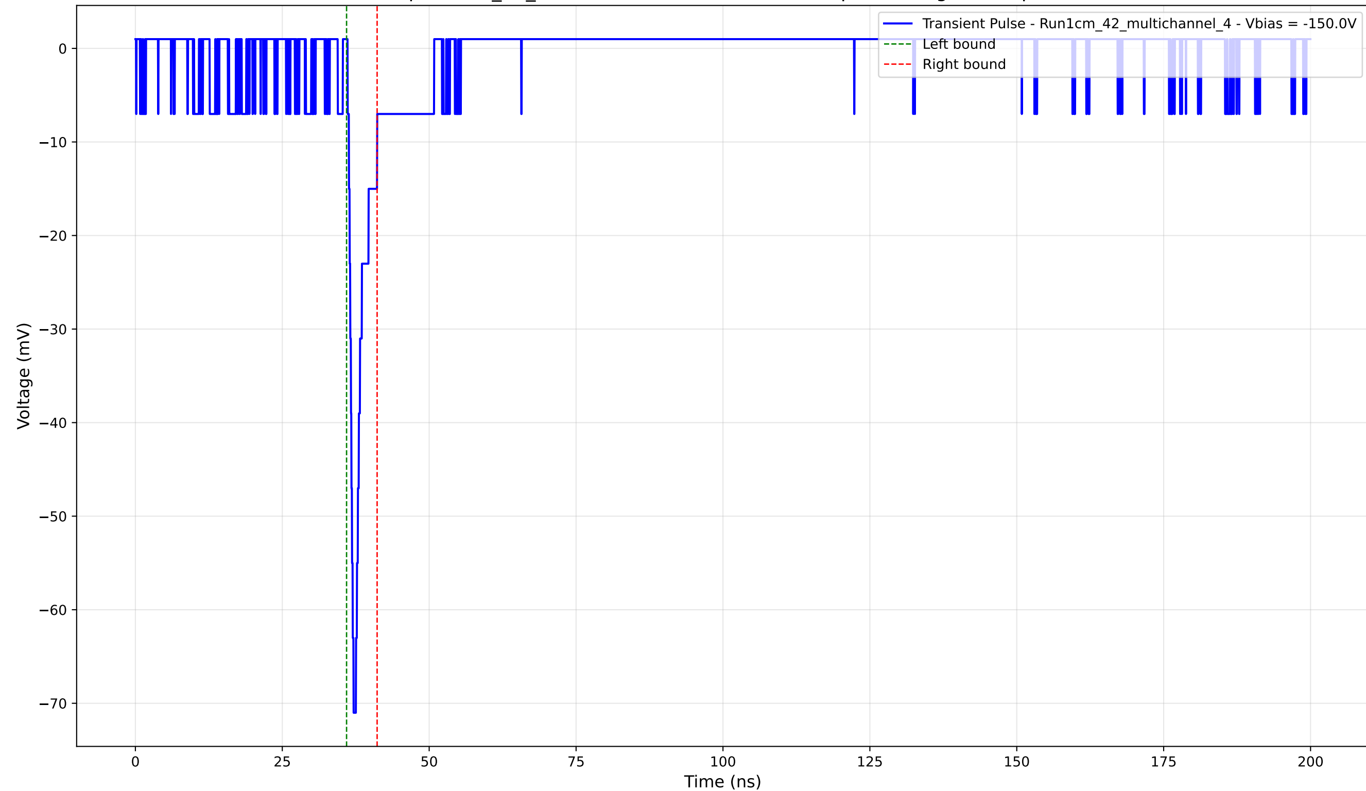
Transient Pulse - Sample: 1cm_42_multichannel - Position: 2190.0 \mu\text{m} - Charge: 3.09 pC - Rise Time: 0.80 ns
