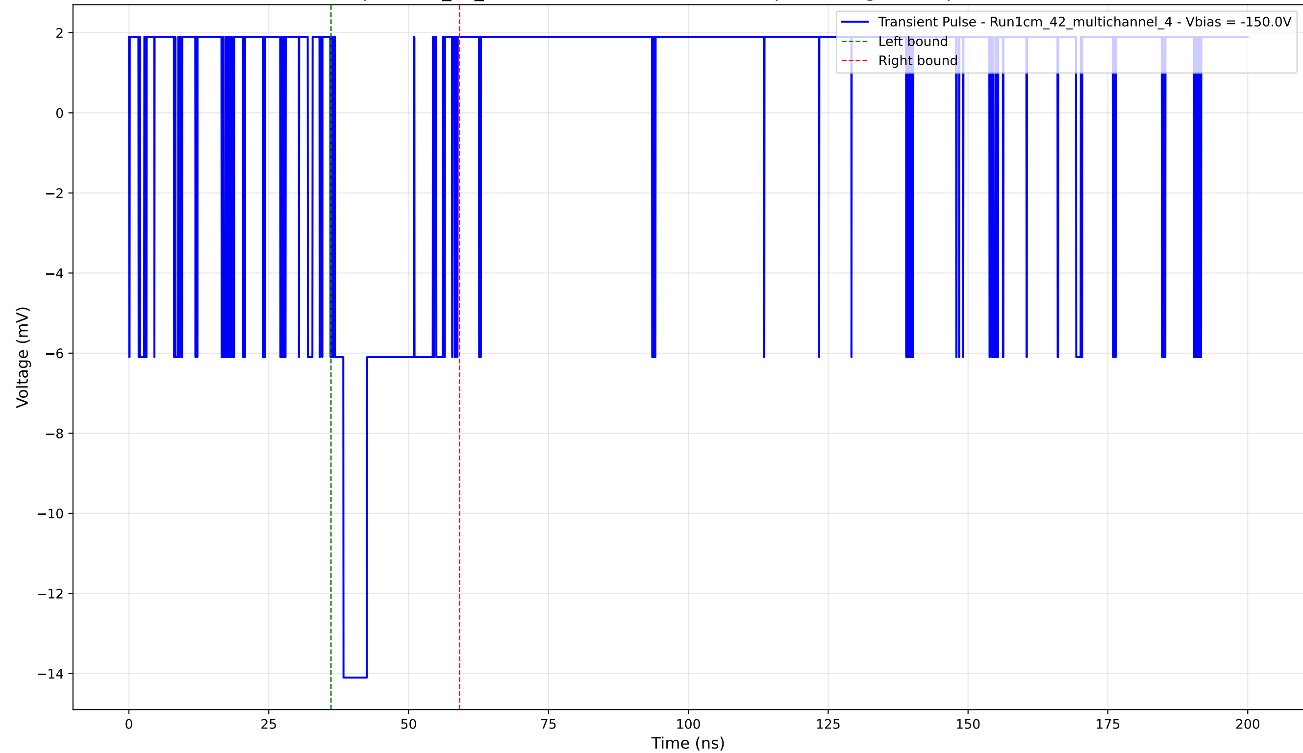
Transient Pulse - Sample: 1cm_42_multichannel - Position: 4760.0 \mu\text{m} - Charge: 2.89 pC - Rise Time: 0.00 ns (N/A)
