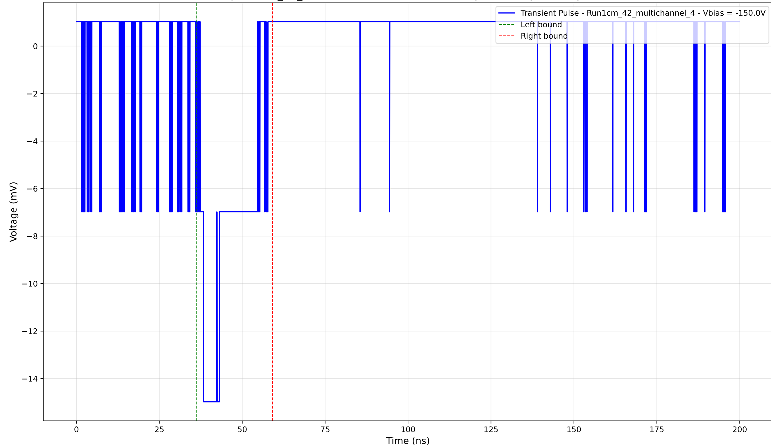
Transient Pulse - Sample: 1cm_42_multichannel - Position: 4520.0 \mu\text{m} - Charge: 3.35 pC - Rise Time: 1.04 ns
