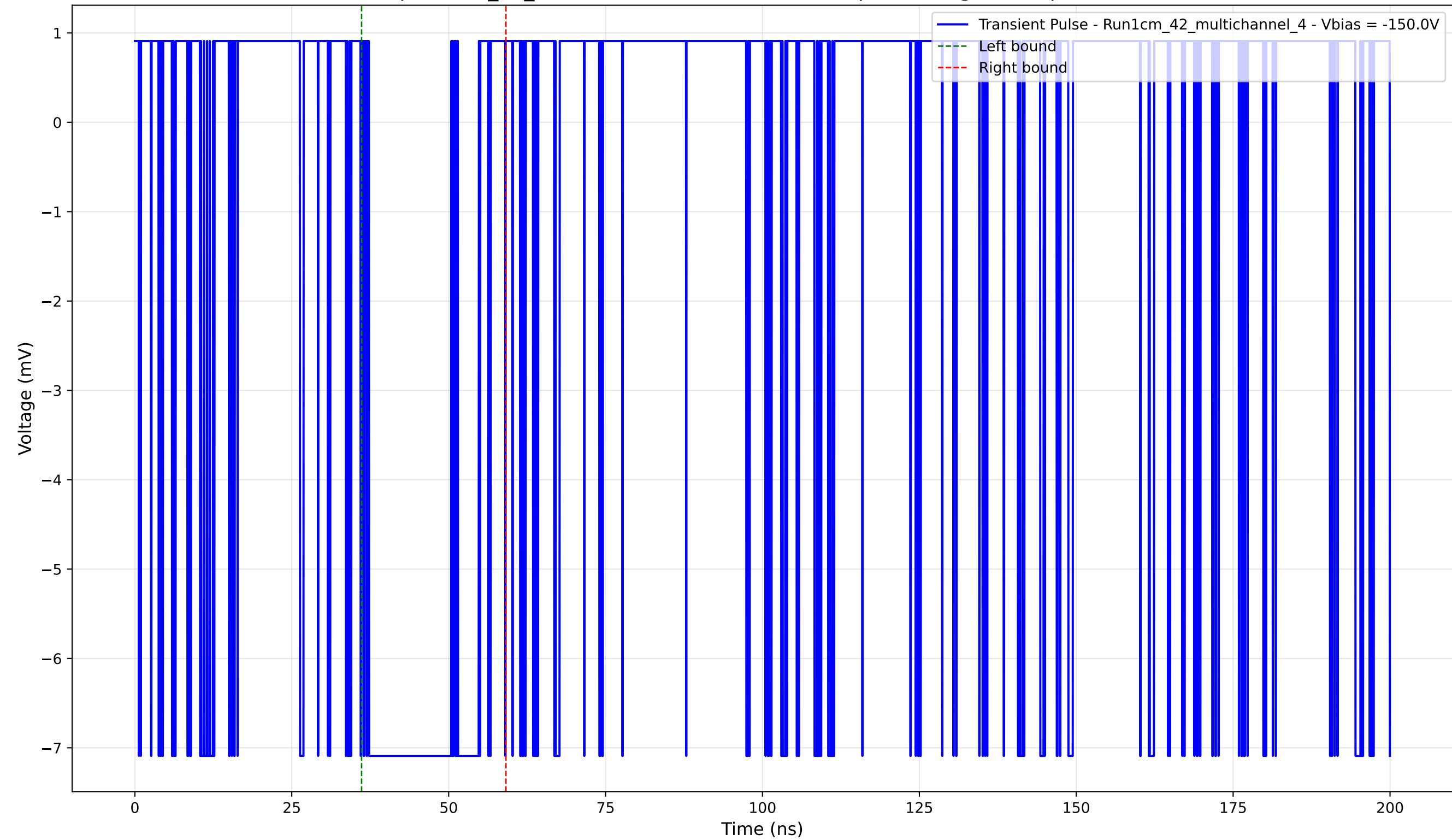
Transient Pulse - Sample: 1cm_42_multichannel - Position: 4355.0 \mu\text{m} - Charge: 2.36 pC - Rise Time: 0.00 ns (N/A)
