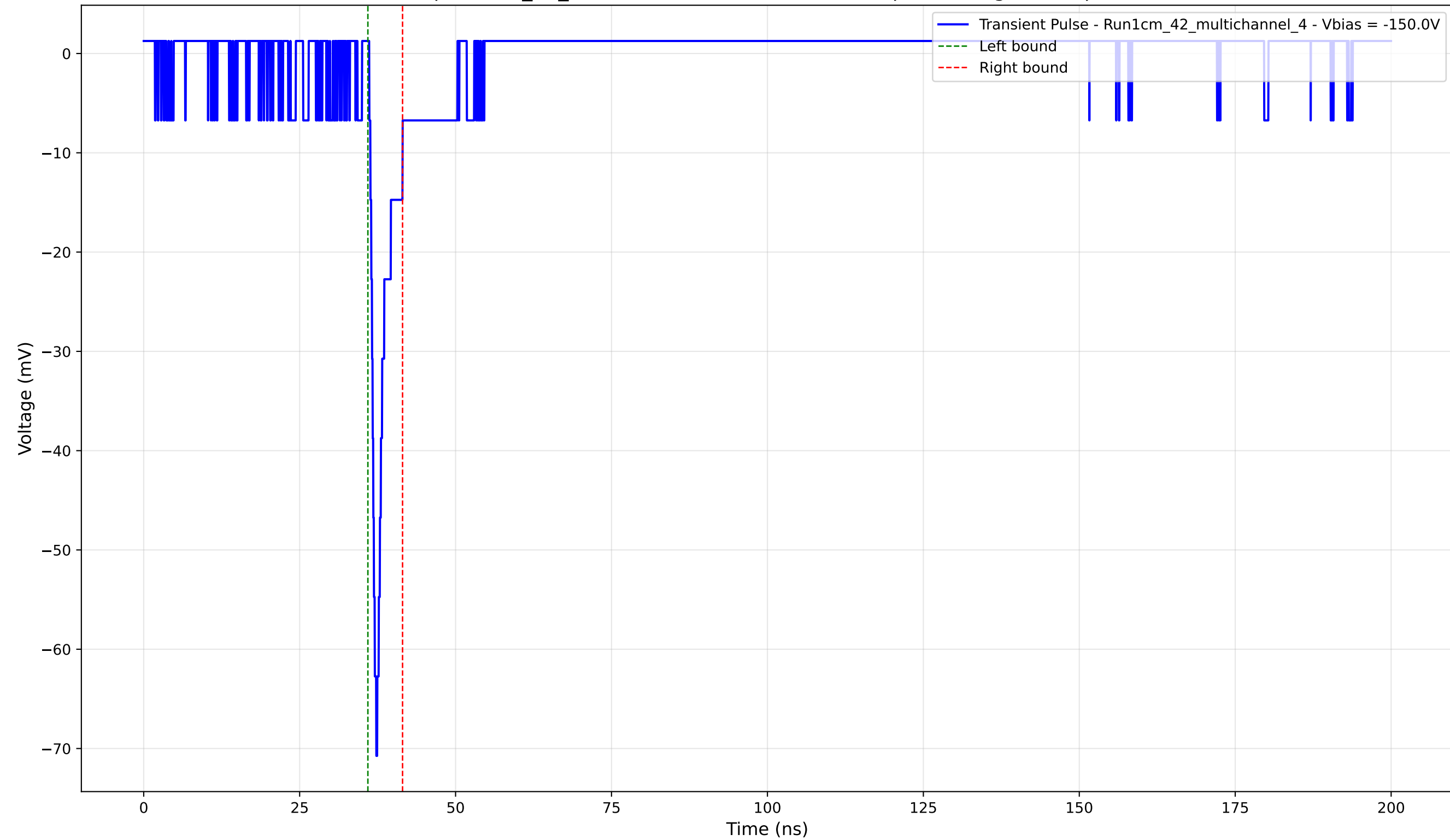
Transient Pulse - Sample: 1cm_42_multichannel - Position: 2165.0 \mu\text{m} - Charge: 3.08 pC - Rise Time: 0.96 ns
