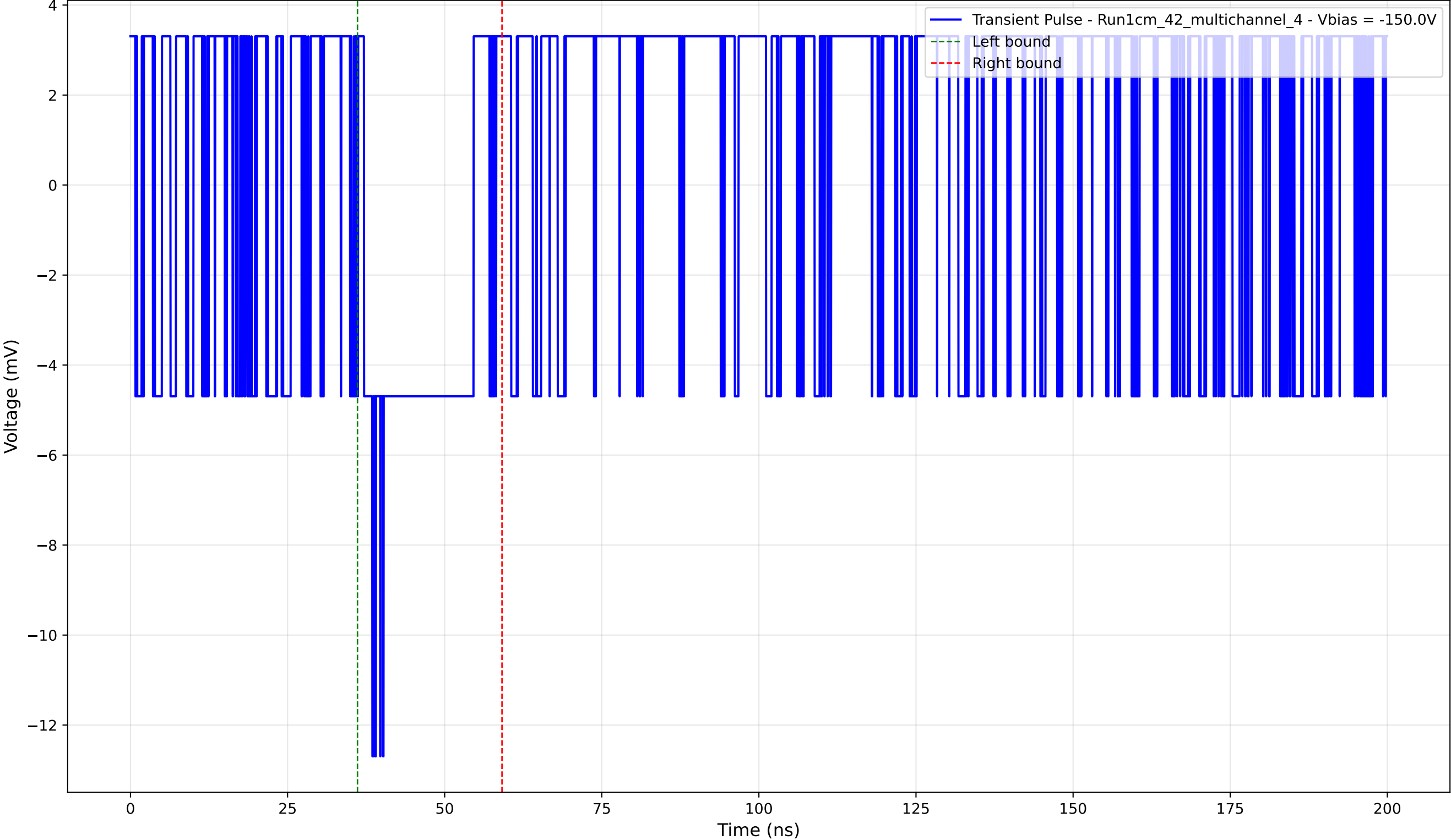
Transient Pulse - Sample: 1cm_42_multichannel - Position: 815.0 \mu\text{m} - Charge: 1.42 pC - Rise Time: 0.00 ns (N/A)
