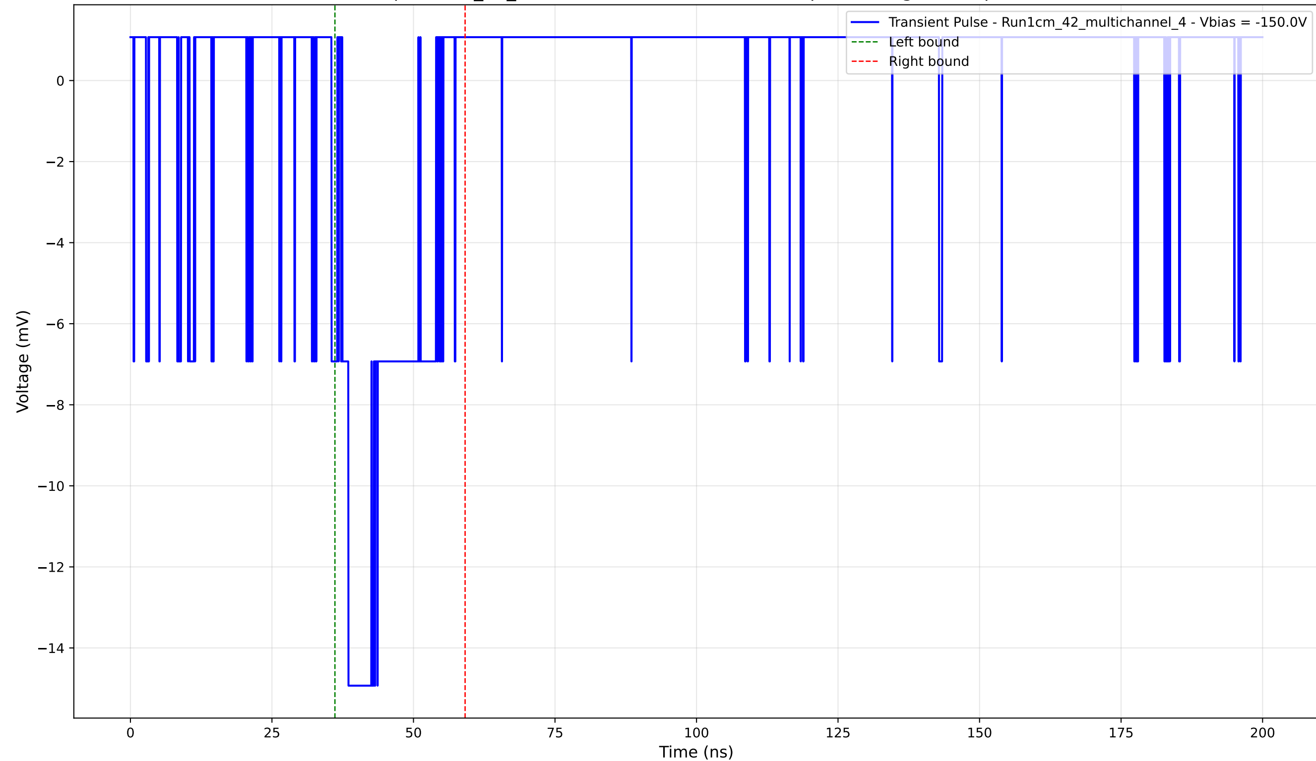
Transient Pulse - Sample: 1cm_42_multichannel - Position: 4525.0 \mu\text{m} - Charge: 3.06 pC - Rise Time: 1.08 ns
