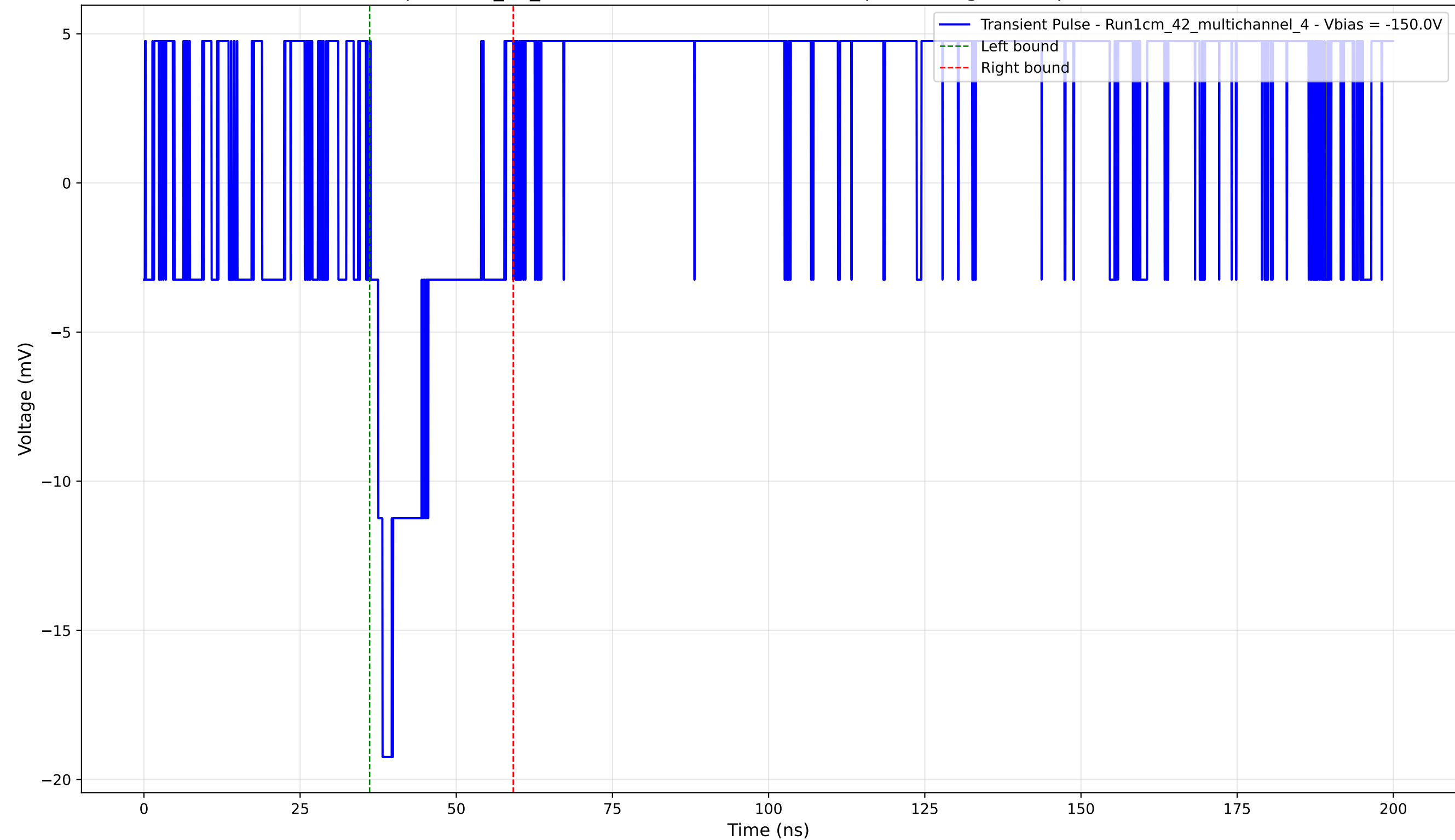
Transient Pulse - Sample: 1cm_42_multichannel - Position: 1010.0 \mu\text{m} - Charge: 2.69 pC - Rise Time: 0.00 ns (N/A)
