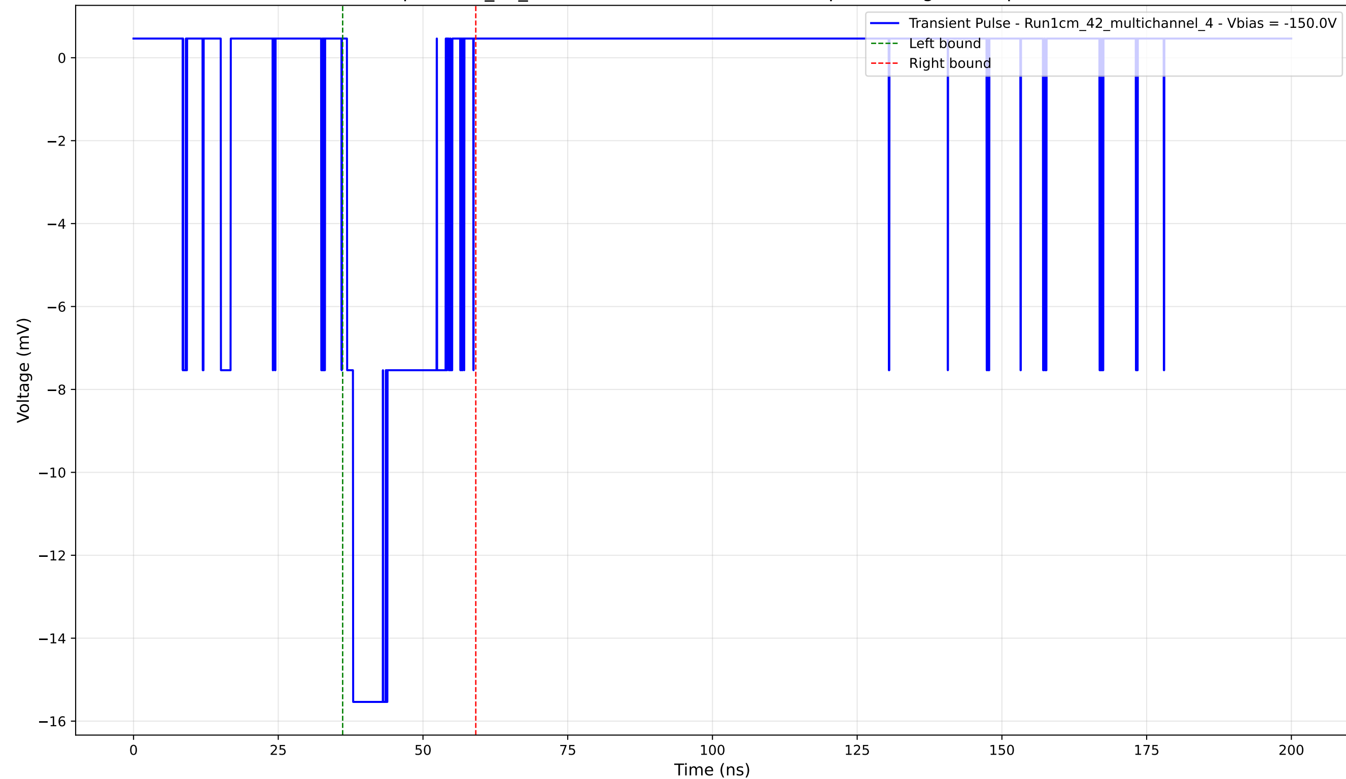
Transient Pulse - Sample: 1cm_42_multichannel - Position: 4005.0 \mu\text{m} - Charge: 3.58 pC - Rise Time: 1.06 ns
