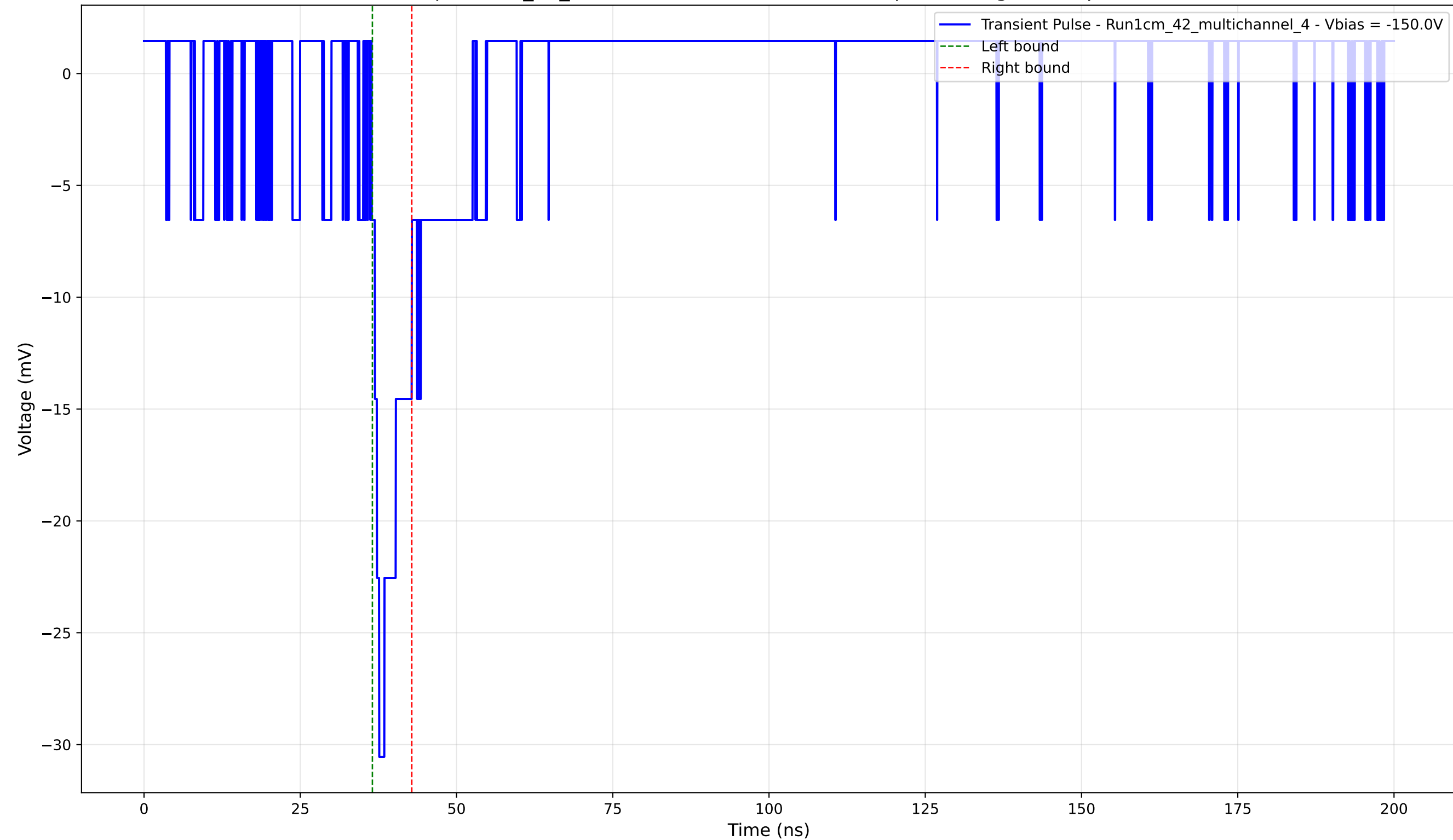
Transient Pulse - Sample: 1cm_42_multichannel - Position: 1470.0 \mu\text{m} - Charge: 2.39 pC - Rise Time: 1.21 ns
