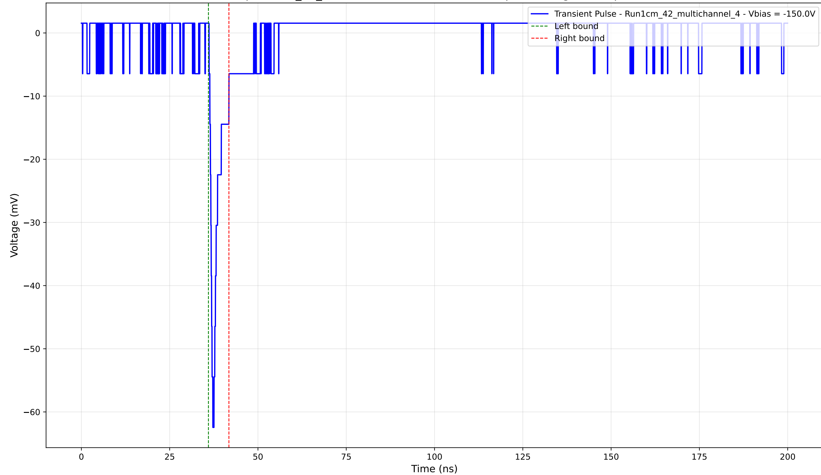
Transient Pulse - Sample: 1cm_42_multichannel - Position: 2135.0 \mu\text{m} - Charge: 2.96 pC - Rise Time: 1.06 ns
