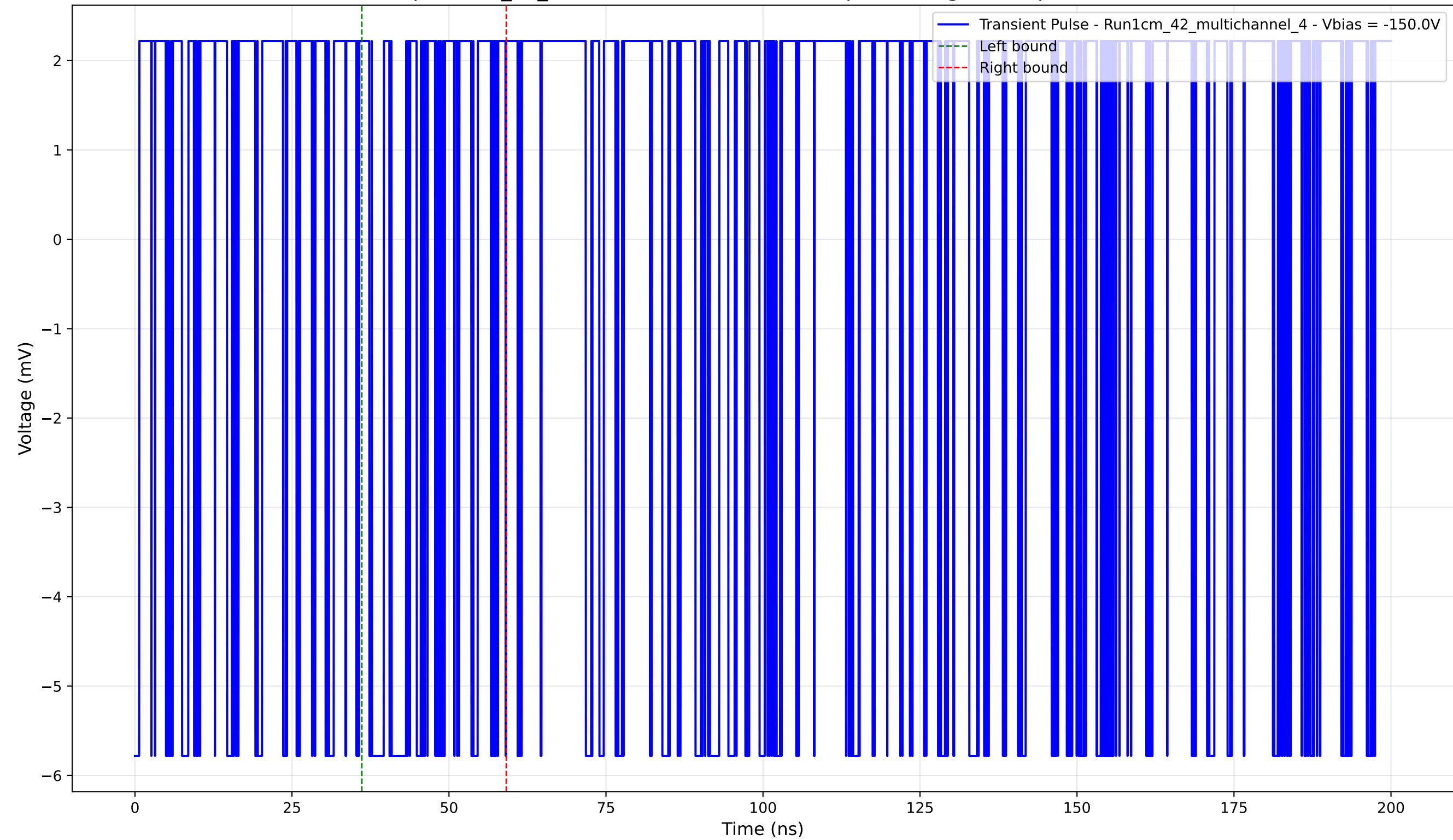
Transient Pulse - Sample: 1cm_42_multichannel - Position: 65.0 \mu\text{m} - Charge: 0.43 pC - Rise Time: 0.00 ns (N/A)
