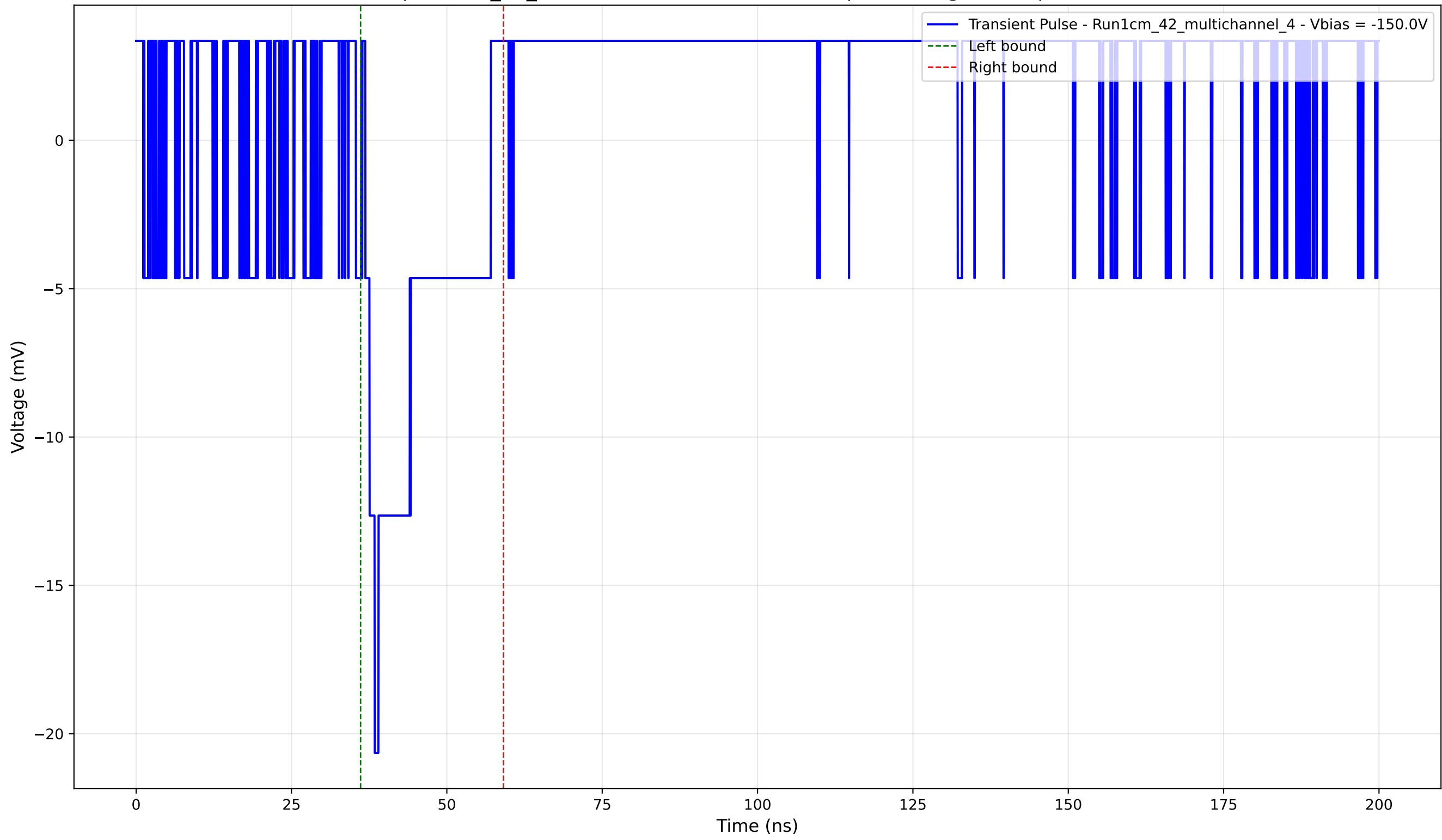
Transient Pulse - Sample: 1cm_42_multichannel - Position: 995.0 \mu\text{m} - Charge: 2.87 pC - Rise Time: 0.00 ns (N/A)
