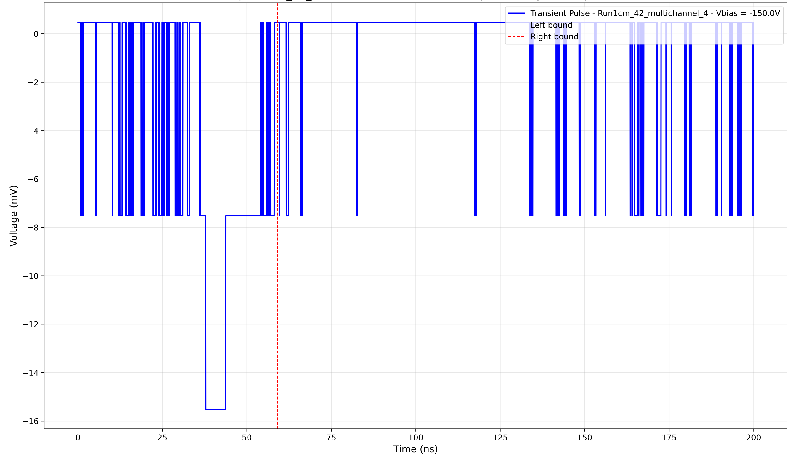
Transient Pulse - Sample: 1cm_42_multichannel - Position: 680.0 \mu\text{m} - Charge: 4.02 pC - Rise Time: 1.56 ns
