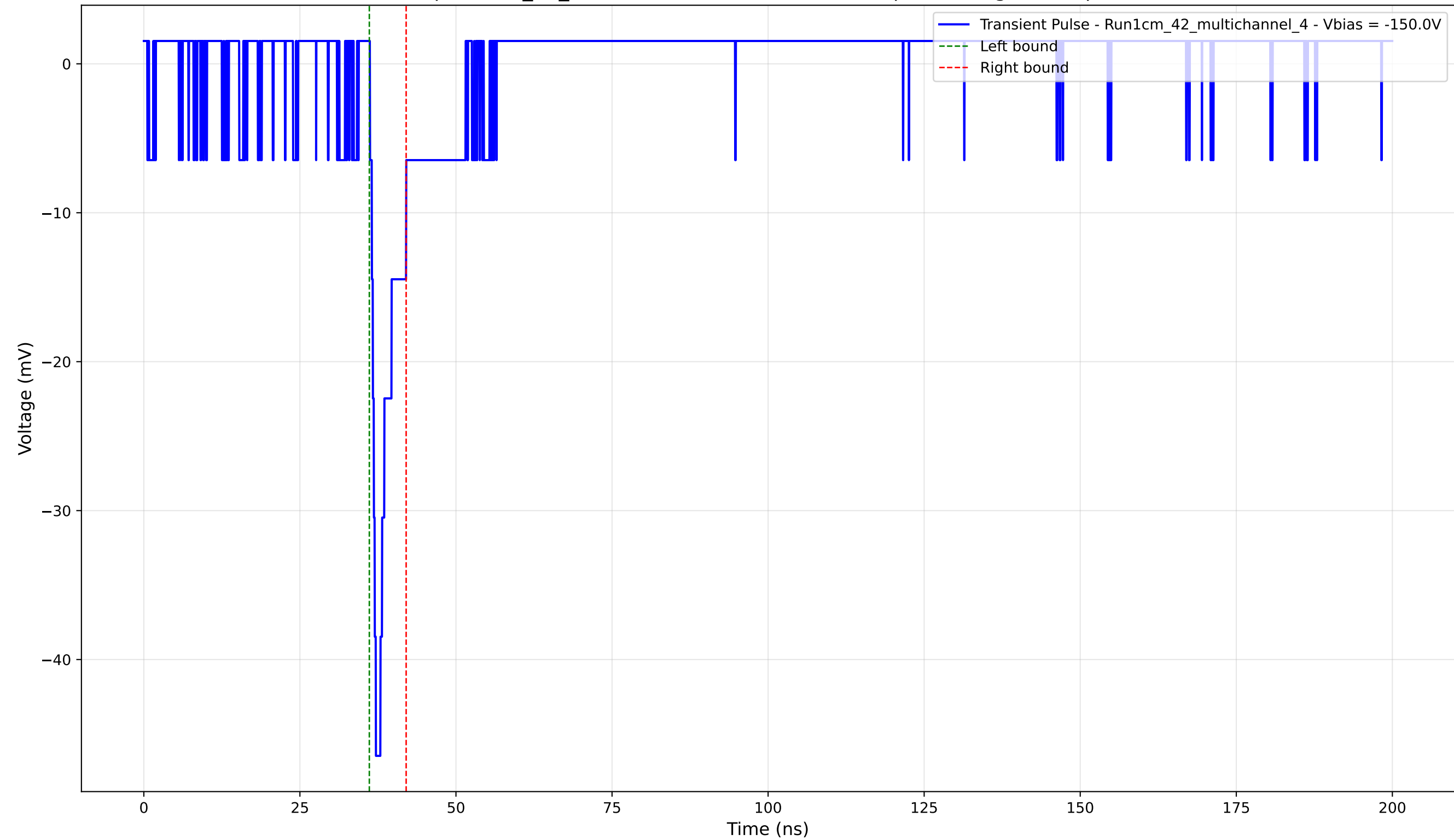
Transient Pulse - Sample: 1cm_42_multichannel - Position: 2800.0 \mu\text{m} - Charge: 2.68 pC - Rise Time: 0.95 ns
