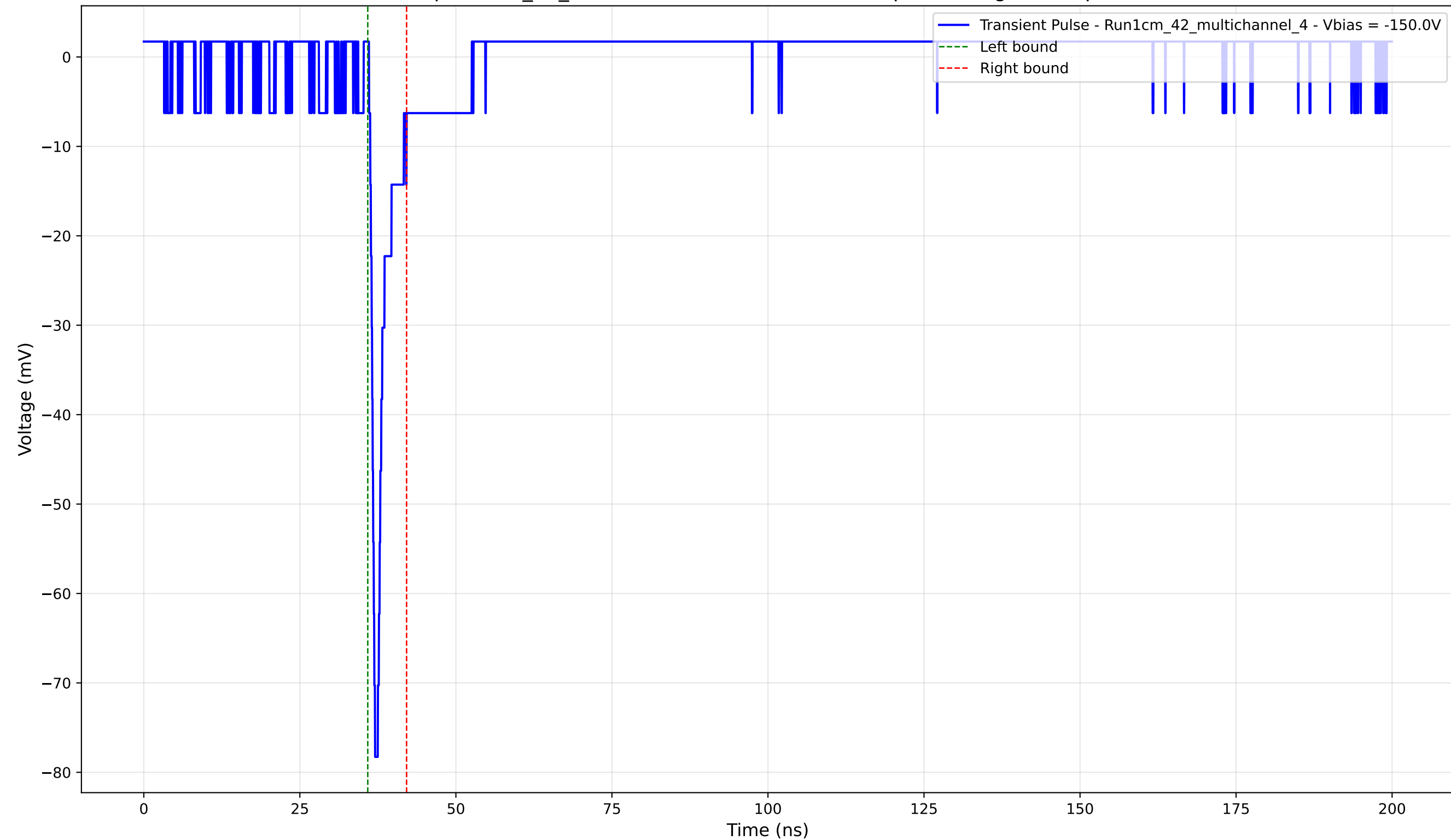
Transient Pulse - Sample: 1cm_42_multichannel - Position: 2260.0 \mu\text{m} - Charge: 3.49 pC - Rise Time: 0.78 ns
