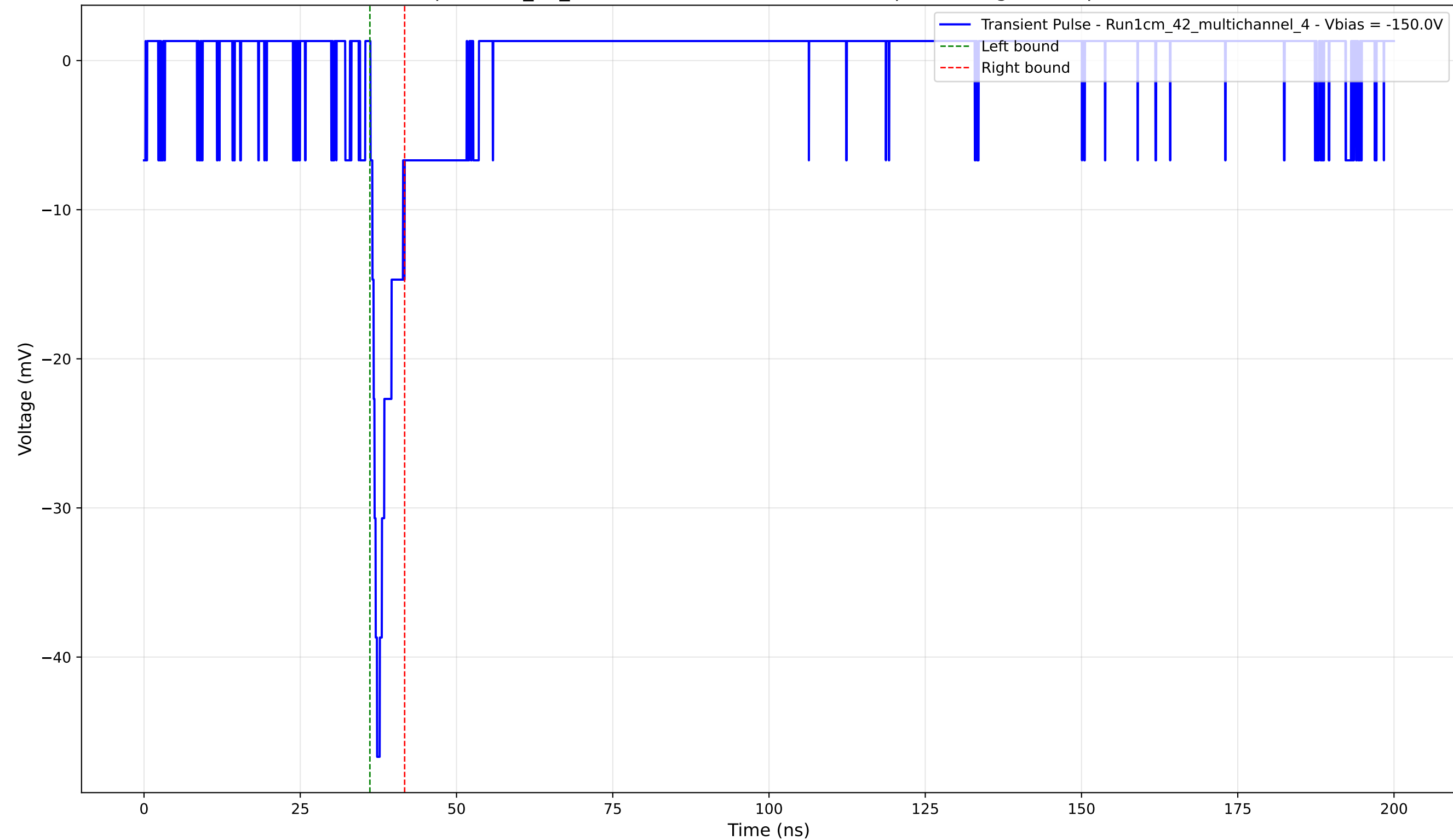
Transient Pulse - Sample: 1cm_42_multichannel - Position: 2815.0 \mu\text{m} - Charge: 2.47 pC - Rise Time: 1.05 ns
