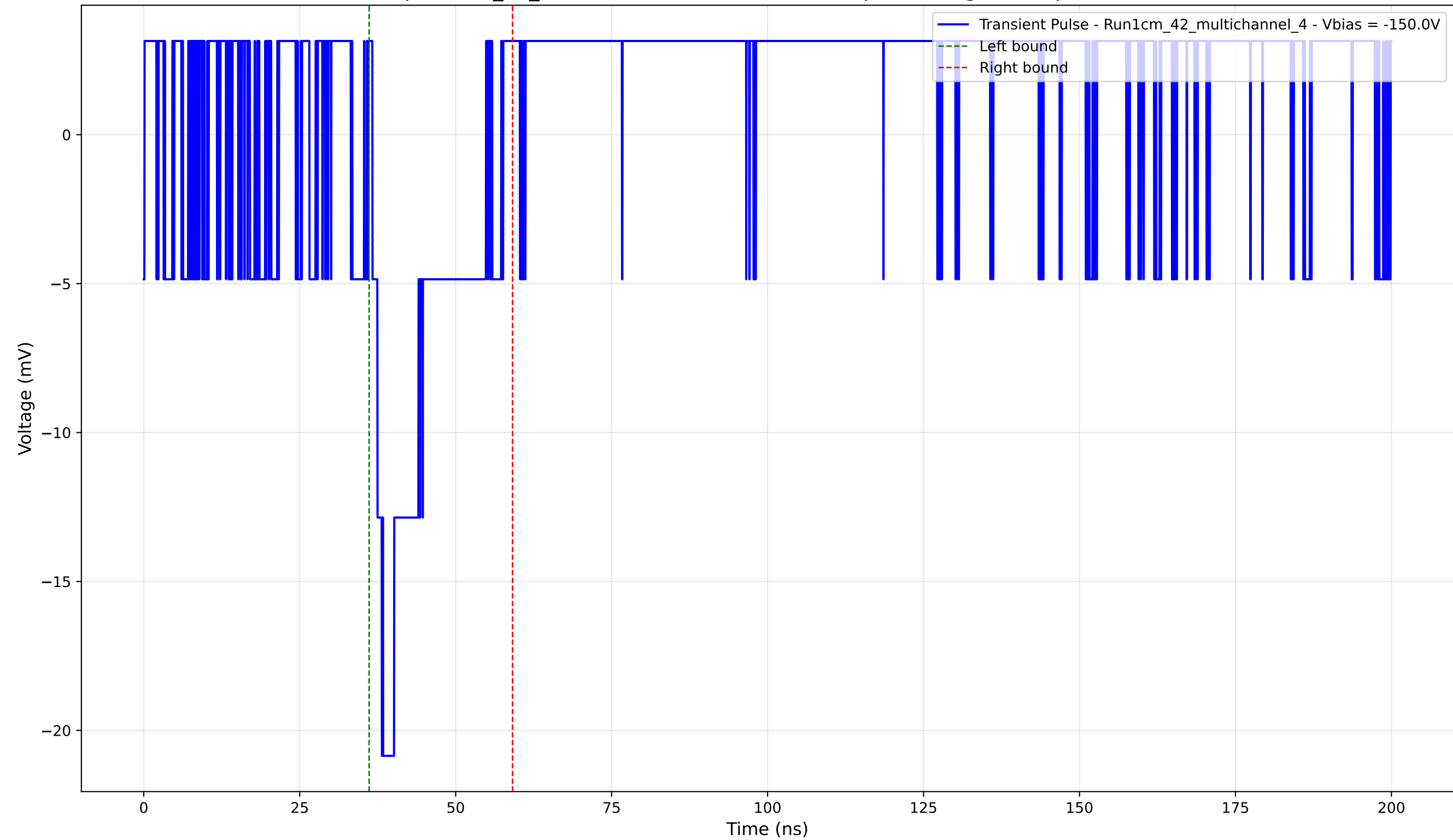
Transient Pulse - Sample: 1cm_42_multichannel - Position: 1055.0 \mu\text{m} - Charge: 3.17 pC - Rise Time: 0.00 ns (N/A)
