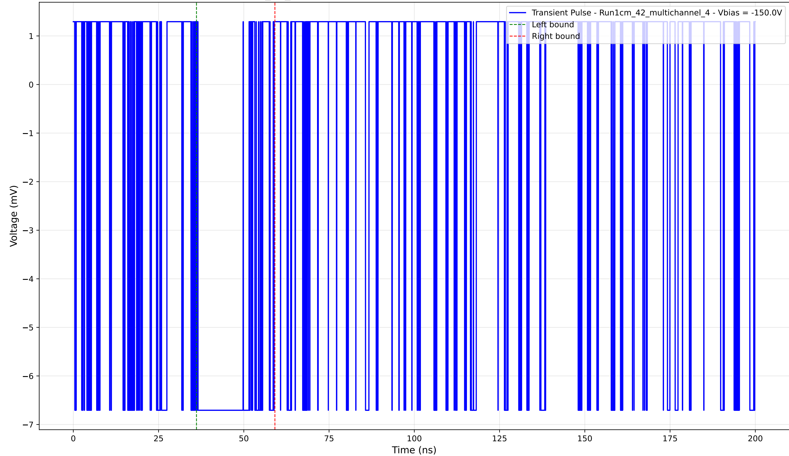
Transient Pulse - Sample: 1cm_42_multichannel - Position: 1415.0 \mu\text{m} - Charge: 2.37 pC - Rise Time: 0.00 ns (N/A)
