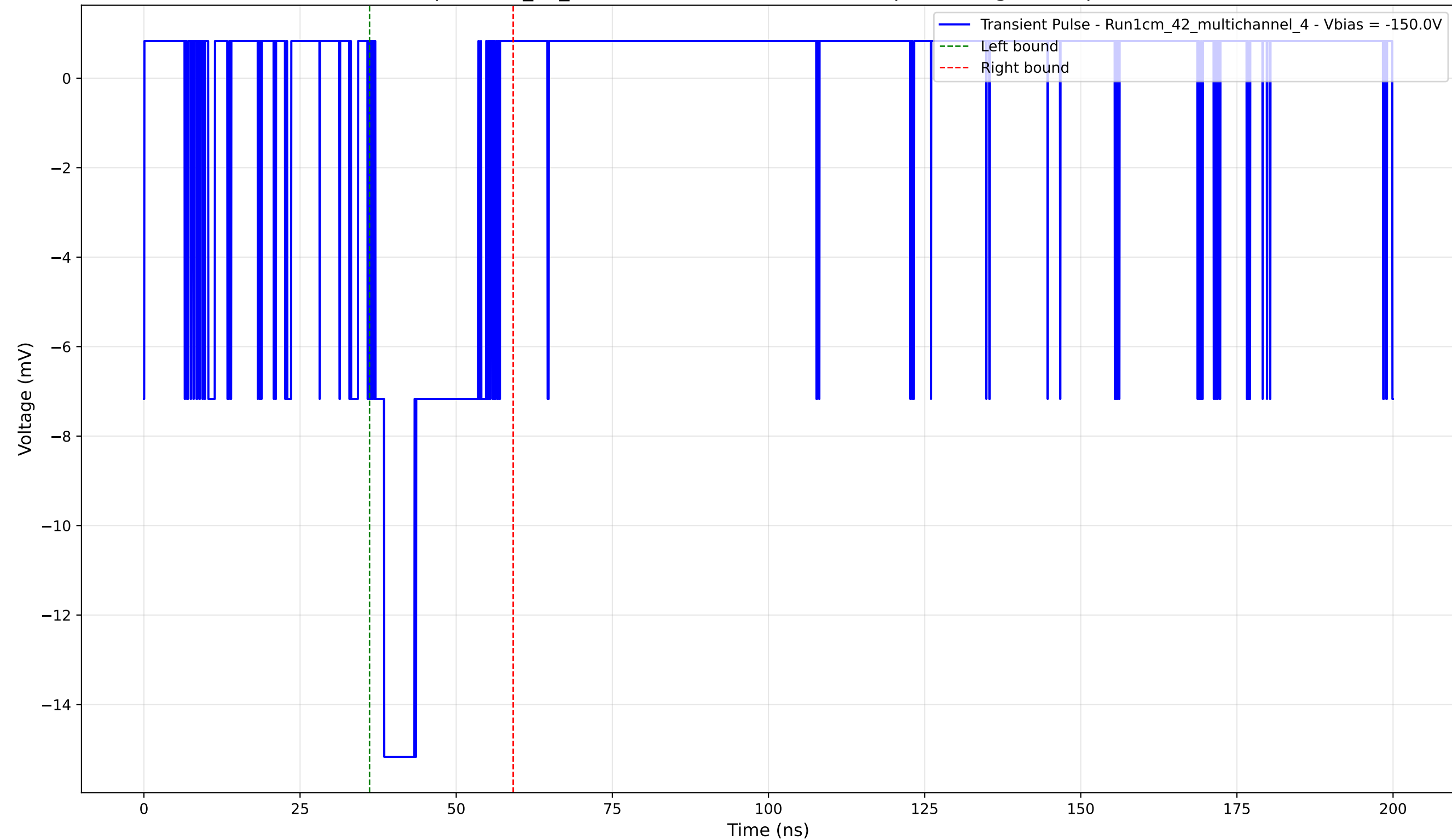
Transient Pulse - Sample: 1cm_42_multichannel - Position: 4500.0 \mu\text{m} - Charge: 3.42 pC - Rise Time: 1.42 ns
