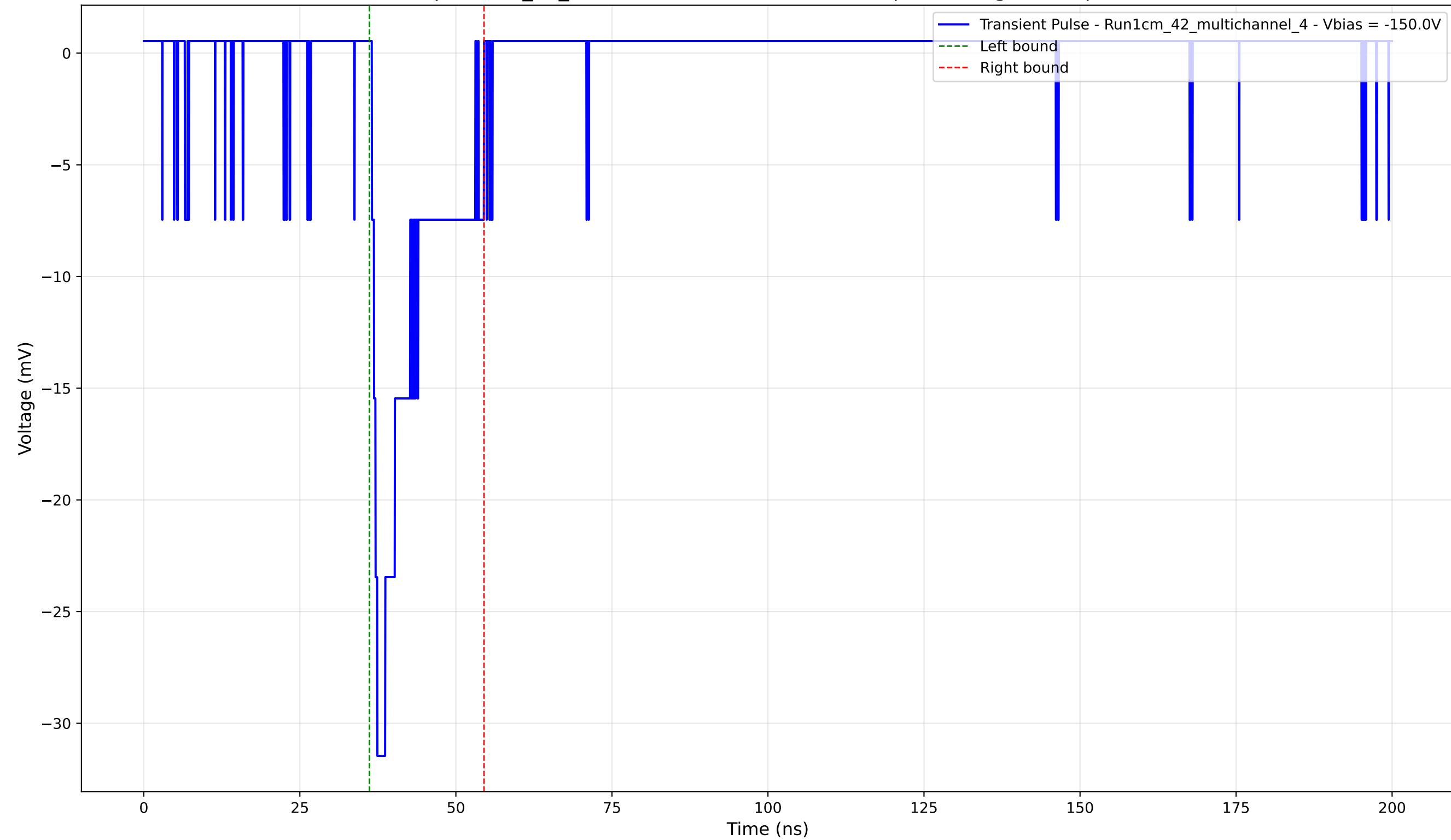
Transient Pulse - Sample: 1cm_42_multichannel - Position: 1550.0 \mu\text{m} - Charge: 4.36 pC - Rise Time: 0.87 ns
