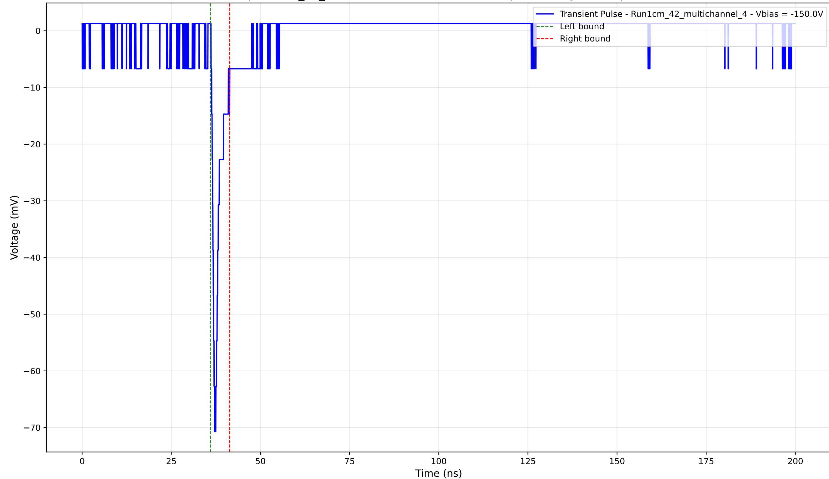
Transient Pulse - Sample: 1cm_42_multichannel - Position: 2580.0 \mu\text{m} - Charge: 3.02 pC - Rise Time: 0.86 ns
