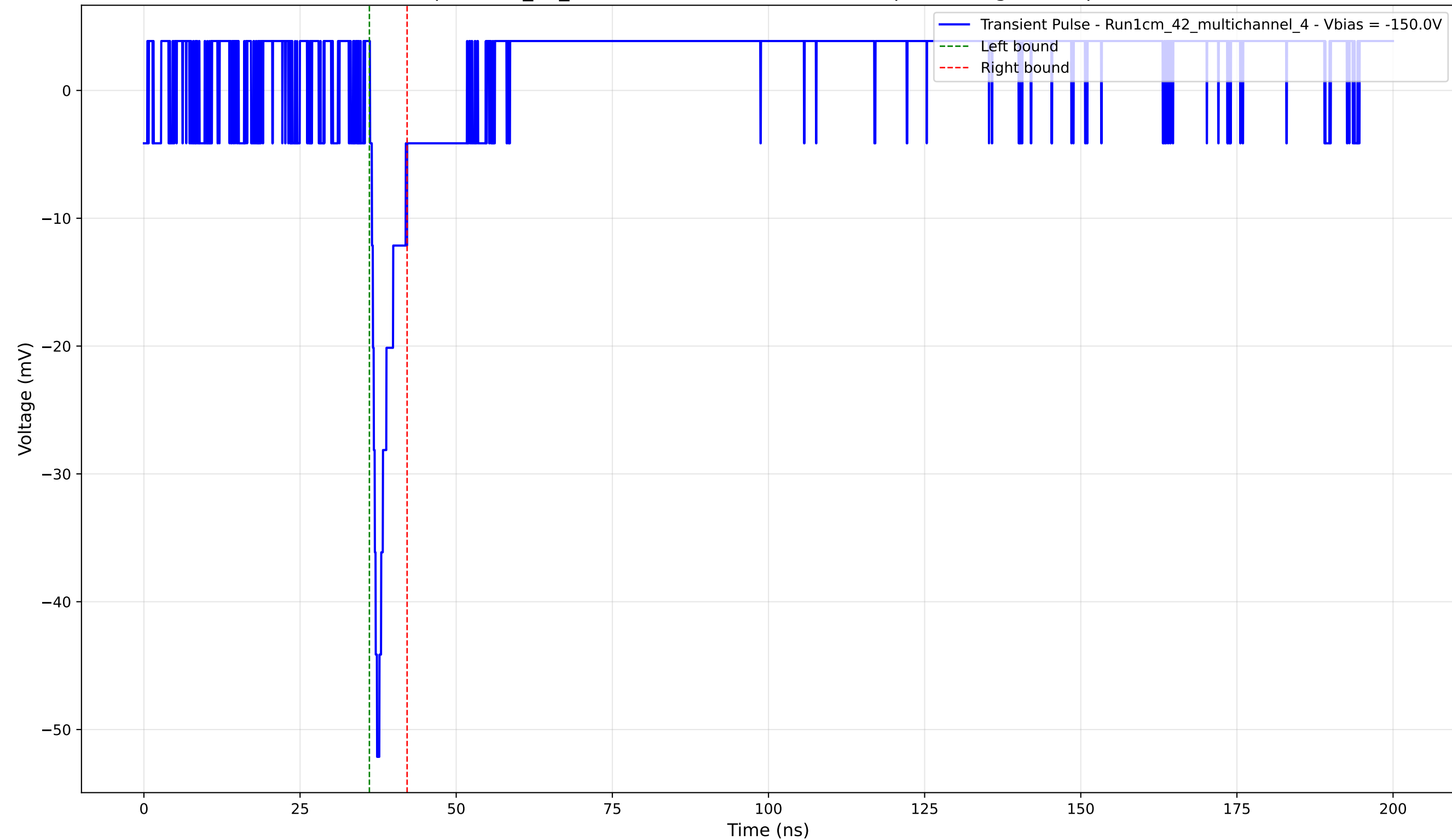
Transient Pulse - Sample: 1cm_42_multichannel - Position: 1965.0 \mu\text{m} - Charge: 2.62 pC - Rise Time: 0.84 ns
