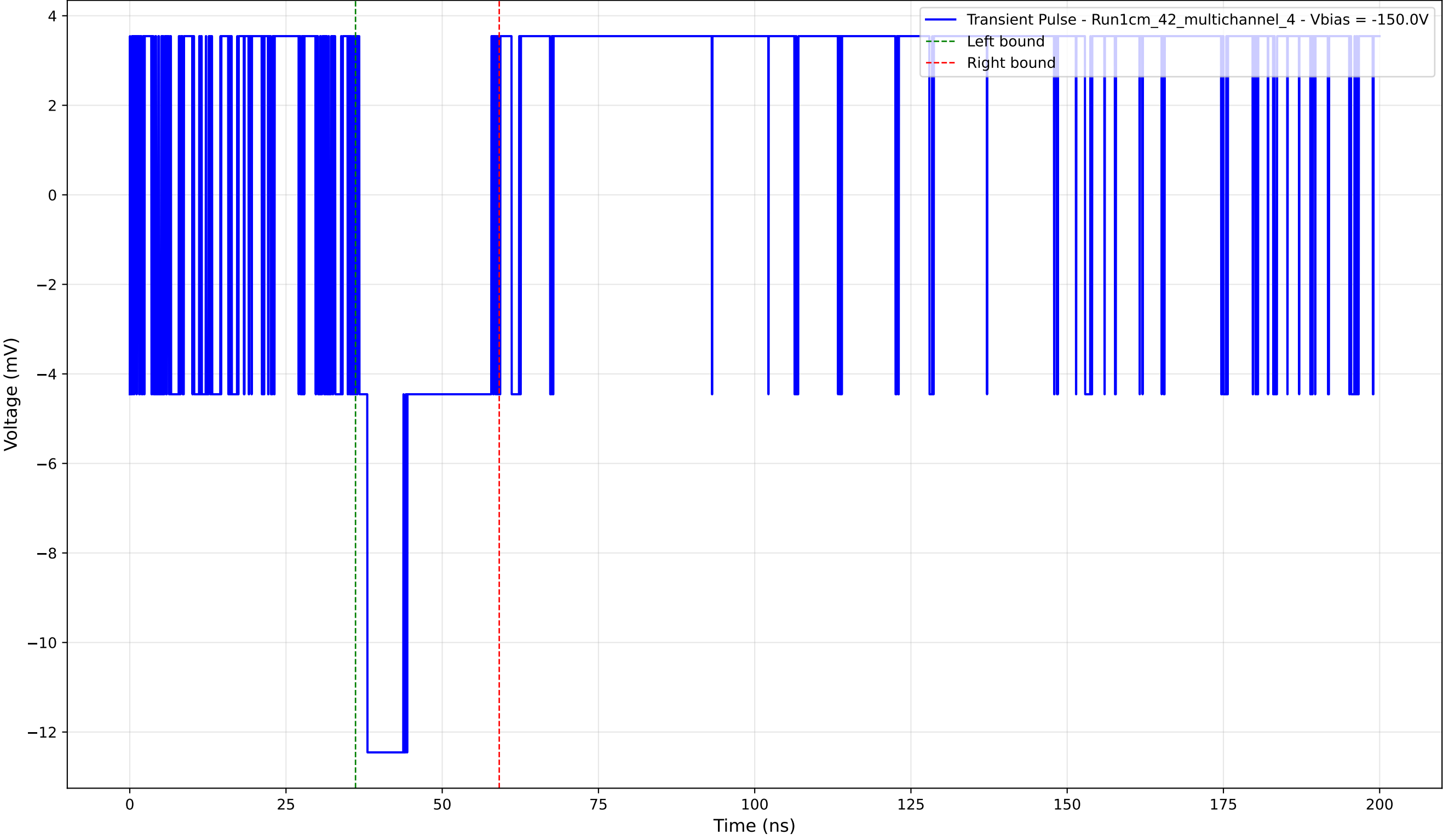
Transient Pulse - Sample: 1cm_42_multichannel - Position: 575.0 \mu\text{m} - Charge: 2.83 pC - Rise Time: 0.00 ns (N/A)
