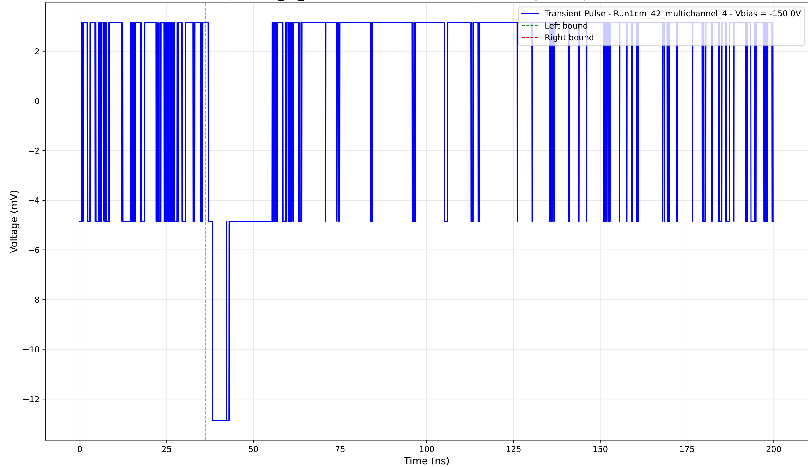
Transient Pulse - Sample: 1cm_42_multichannel - Position: 255.0 \mu\text{m} - Charge: 2.51 pC - Rise Time: 0.00 ns (N/A)
