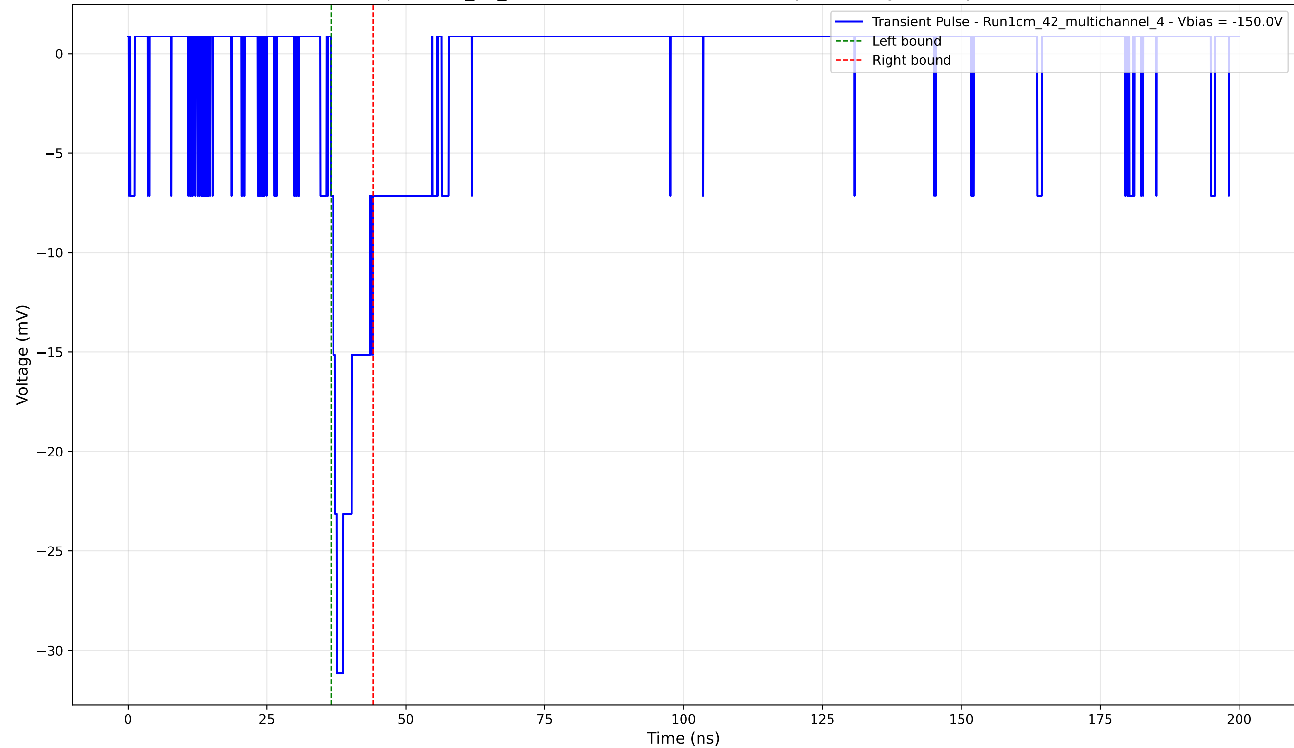
Transient Pulse - Sample: 1cm_42_multichannel - Position: 1480.0 \mu\text{m} - Charge: 2.83 pC - Rise Time: 1.13 ns
