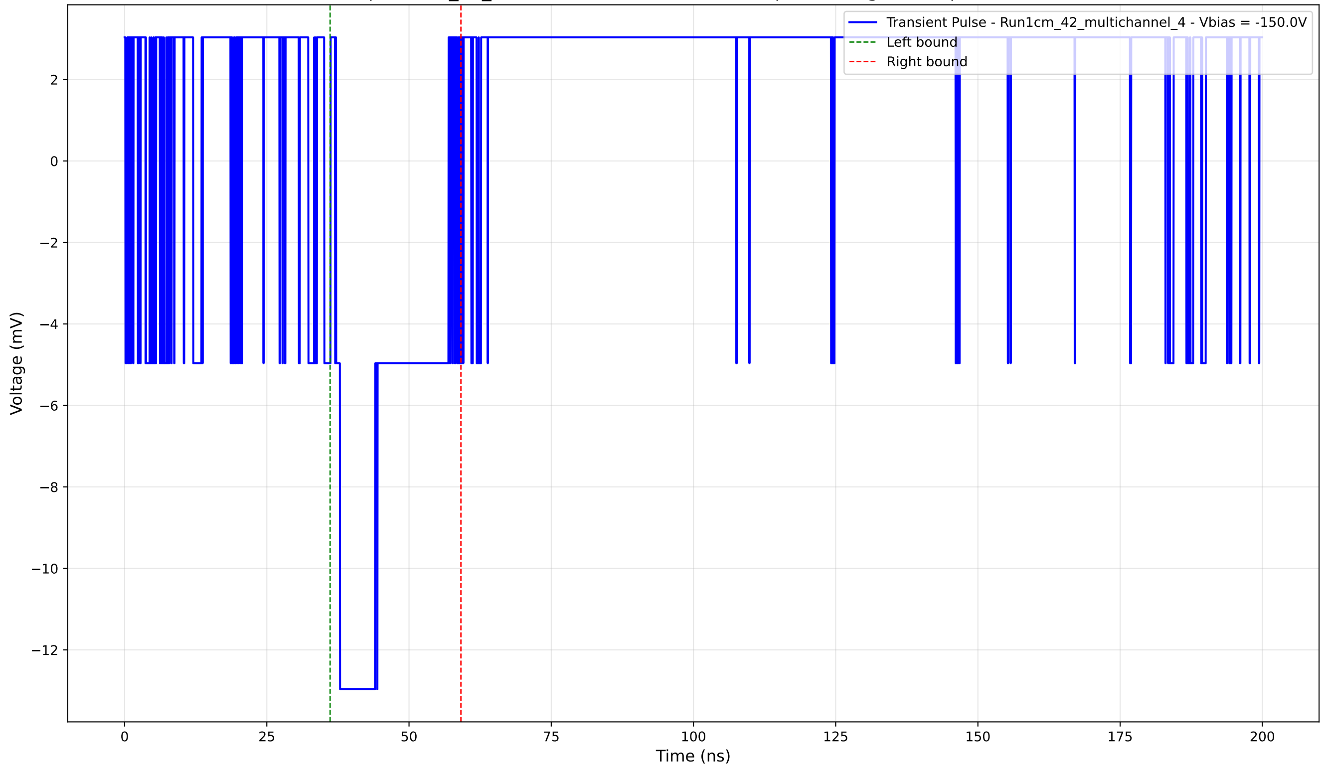
Transient Pulse - Sample: 1cm_42_multichannel - Position: 700.0 \mu\text{m} - Charge: 2.93 pC - Rise Time: 0.00 ns (N/A)
