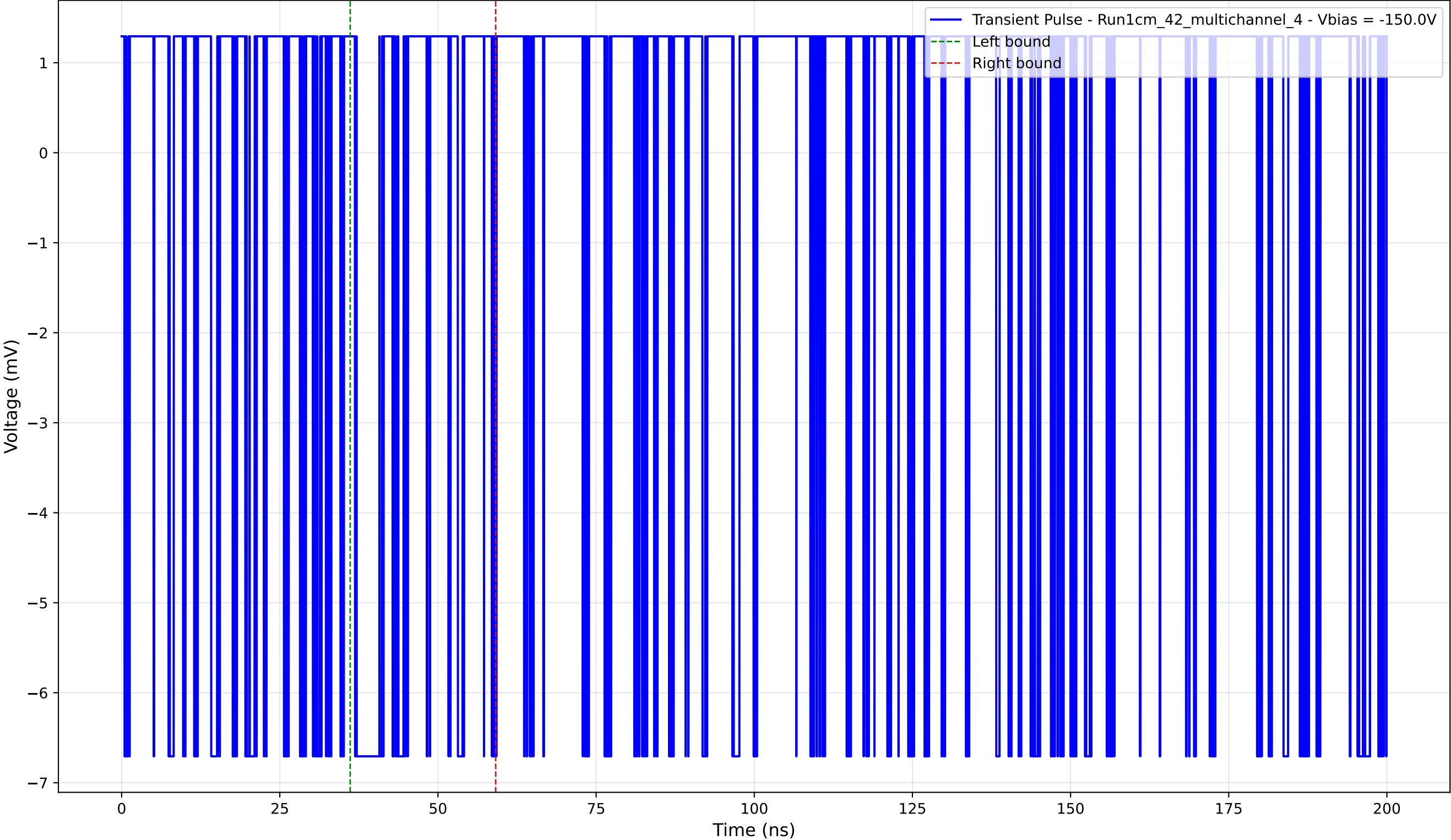
Transient Pulse - Sample: 1cm_42_multichannel - Position: 1865.0 \mu\text{m} - Charge: 0.57 pC - Rise Time: 0.00 ns (N/A)
