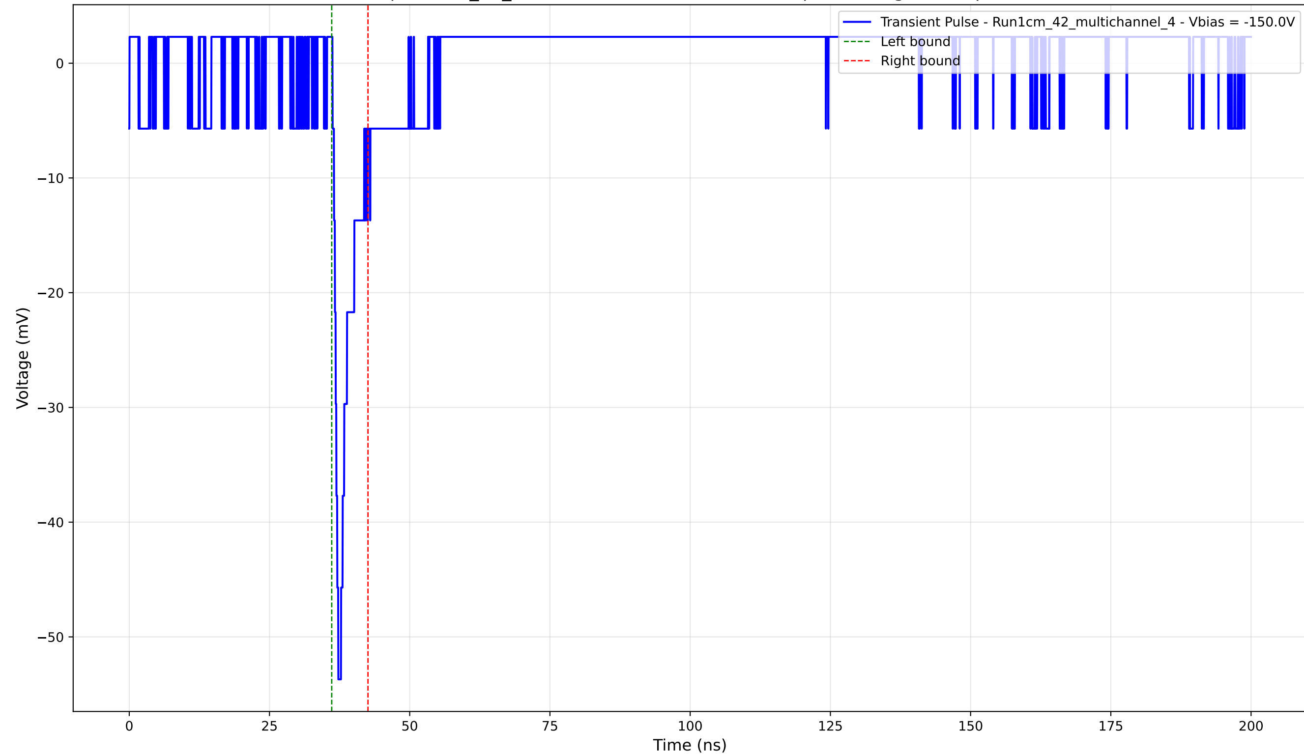
Transient Pulse - Sample: 1cm_42_multichannel - Position: 1975.0 \mu\text{m} - Charge: 2.95 pC - Rise Time: 1.02 ns
