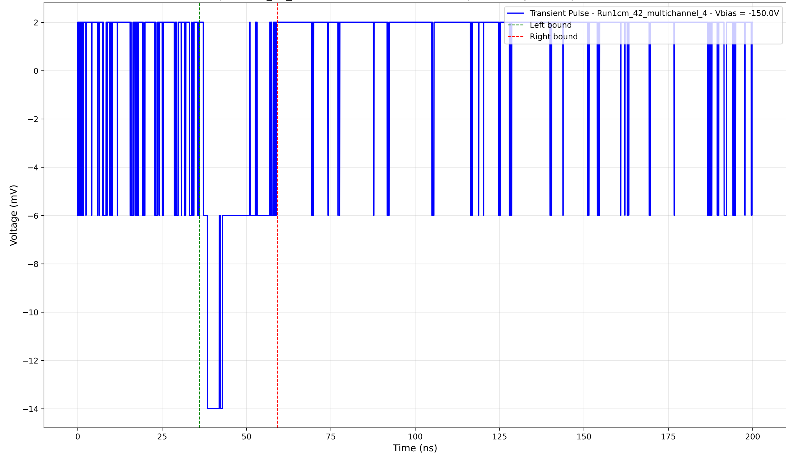
Transient Pulse - Sample: 1cm_42_multichannel - Position: 4335.0 \mu\text{m} - Charge: 3.06 pC - Rise Time: 0.00 ns (N/A)
