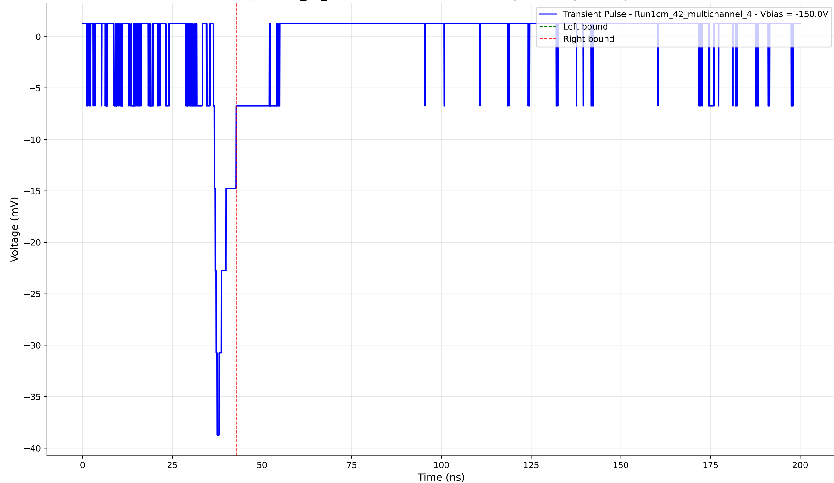
Transient Pulse - Sample: 1cm_42_multichannel - Position: 1695.0 \mu\text{m} - Charge: 2.65 pC - Rise Time: 1.07 ns
