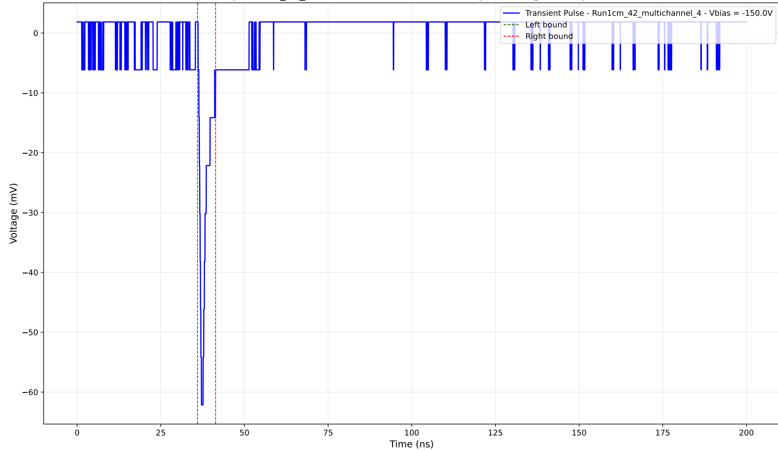
Transient Pulse - Sample: 1cm_42_multichannel - Position: 2140.0 \mu\text{m} - Charge: 2.89 pC - Rise Time: 0.78 ns
