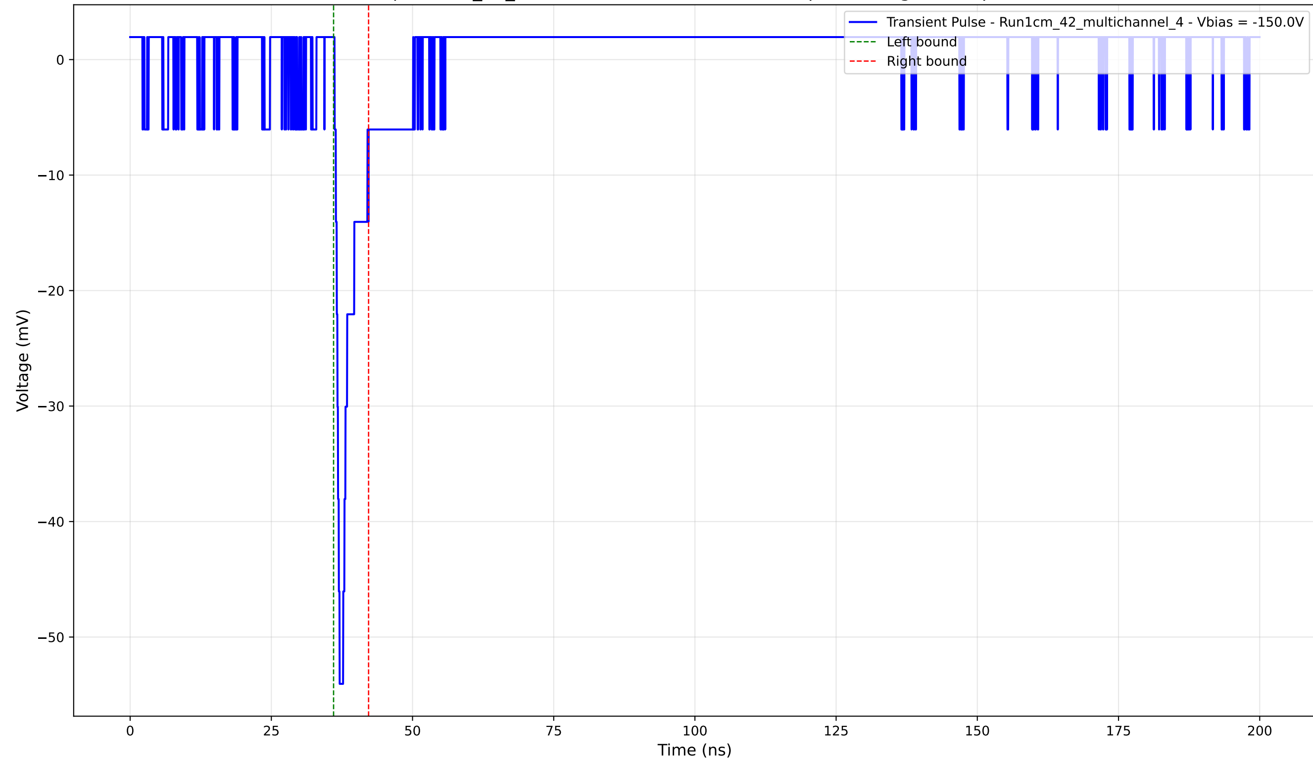
Transient Pulse - Sample: 1cm_42_multichannel - Position: 2665.0 \mu\text{m} - Charge: 2.87 pC - Rise Time: 0.88 ns
