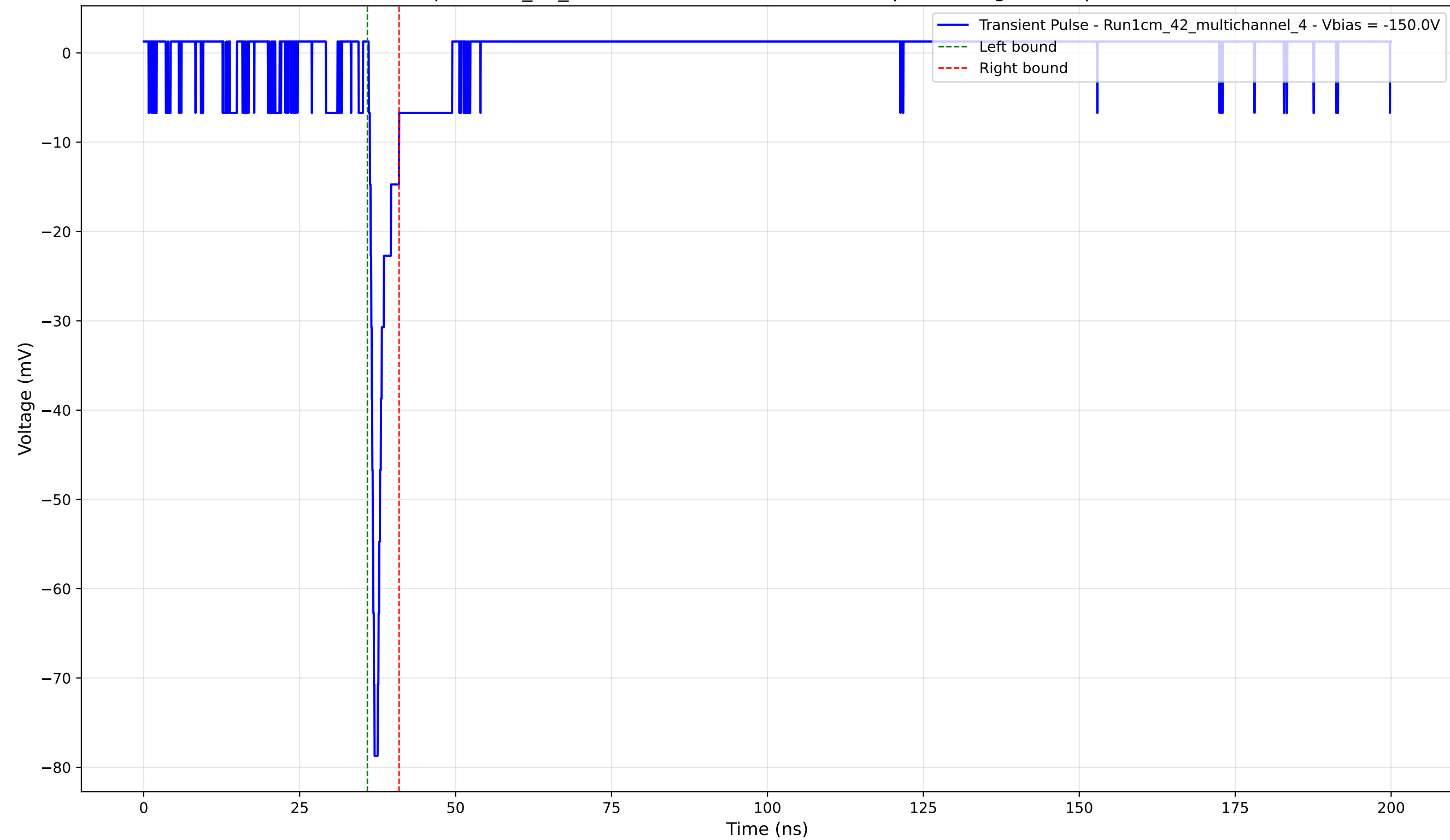
Transient Pulse - Sample: 1cm_42_multichannel - Position: 2295.0 \mu\text{m} - Charge: 3.26 pC - Rise Time: 0.76 ns
