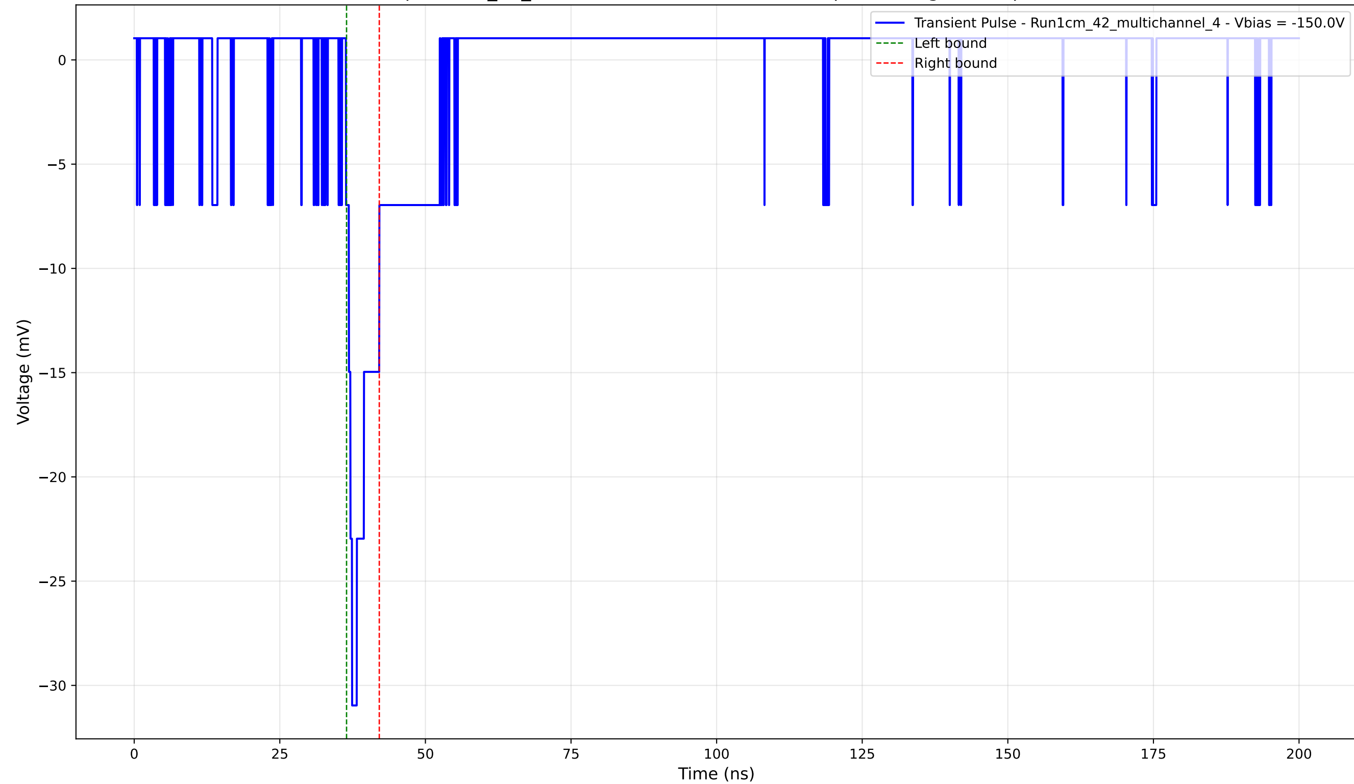
Transient Pulse - Sample: 1cm_42_multichannel - Position: 3115.0 \mu\text{m} - Charge: 2.12 pC - Rise Time: 1.05 ns
