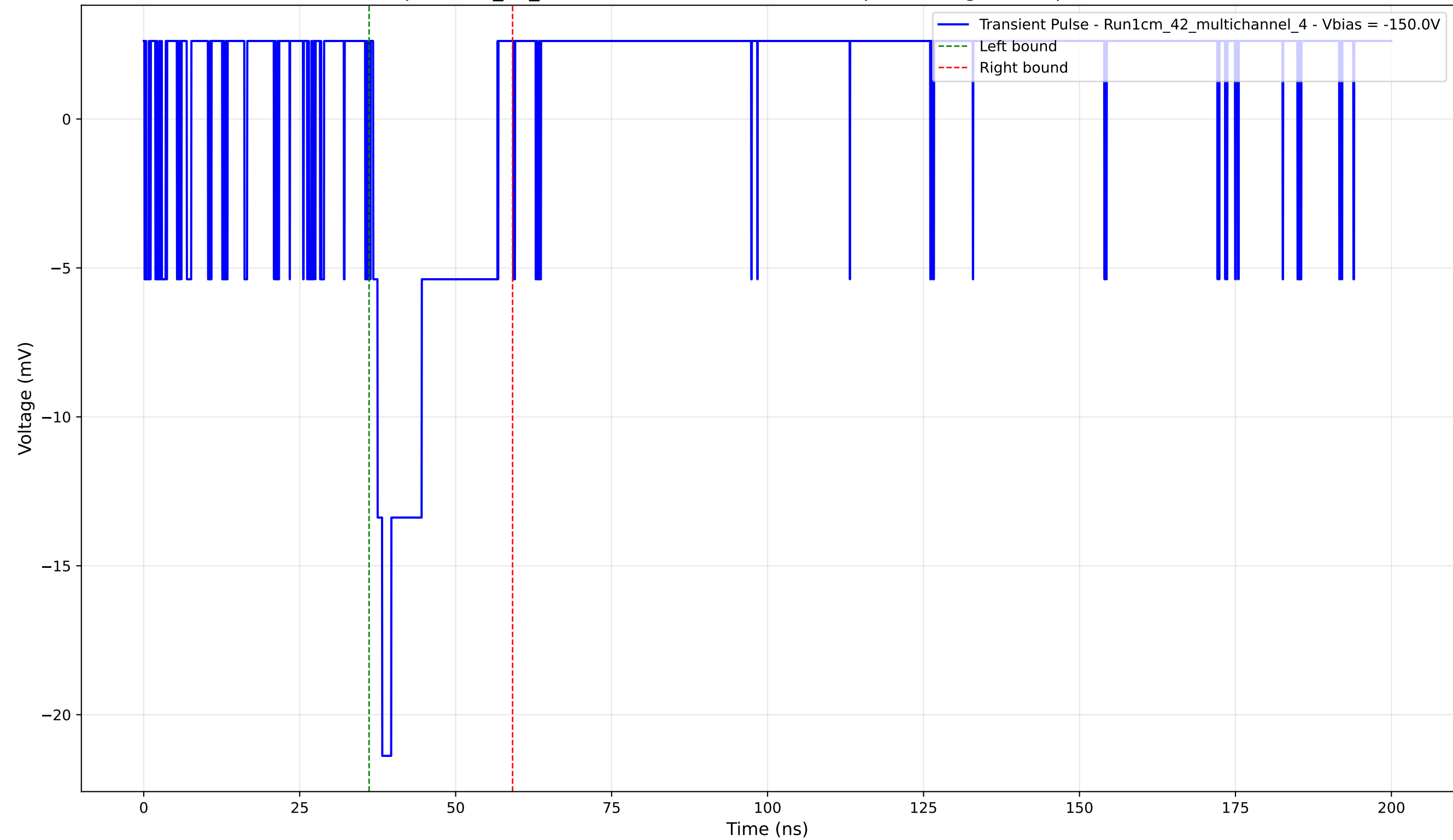
Transient Pulse - Sample: 1cm_42_multichannel - Position: 1015.0 \mu\text{m} - Charge: 3.38 pC - Rise Time: 0.00 ns (N/A)
