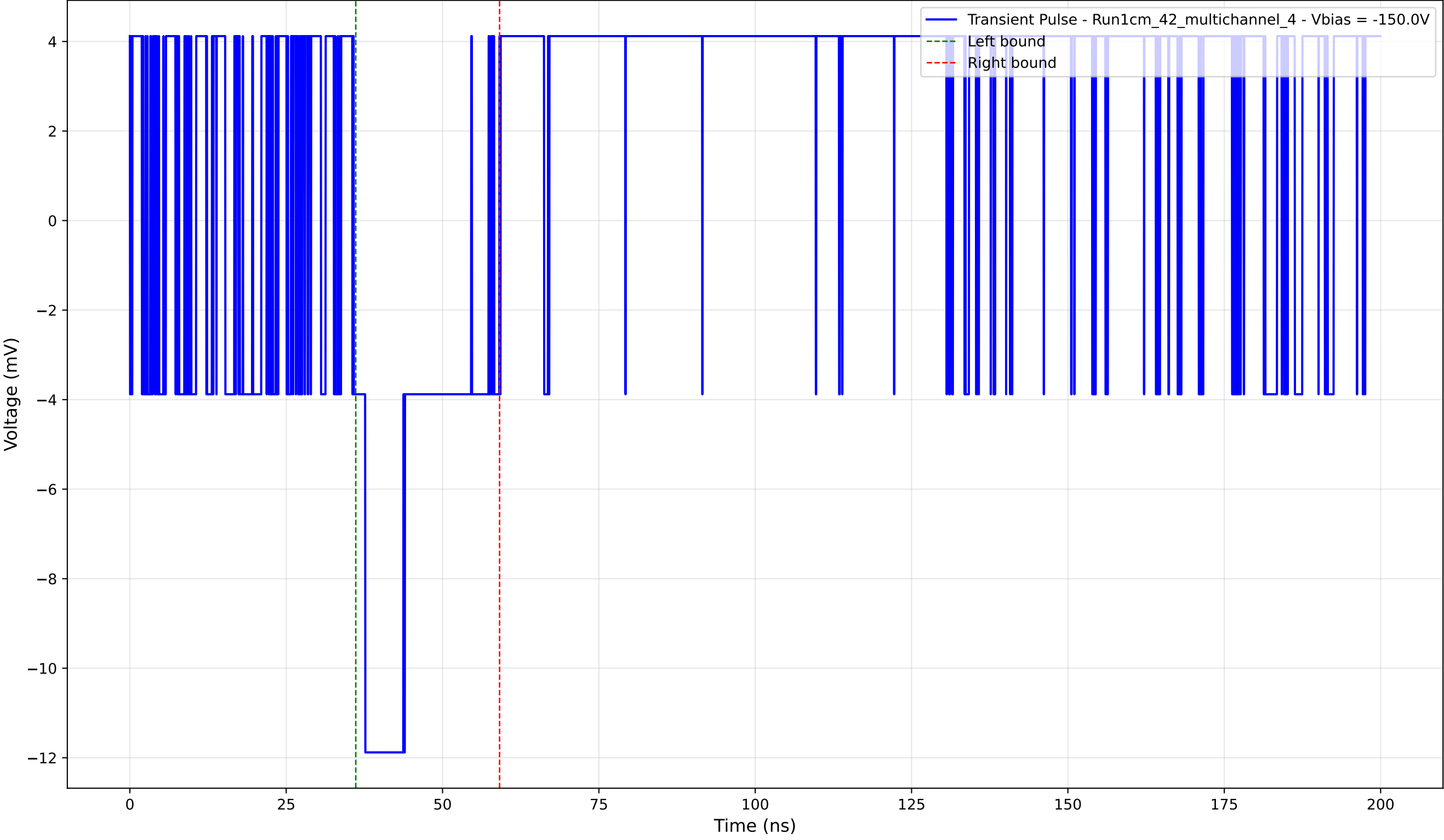
Transient Pulse - Sample: 1cm_42_multichannel - Position: 935.0 \mu\text{m} - Charge: 2.69 pC - Rise Time: 0.00 ns (N/A)
