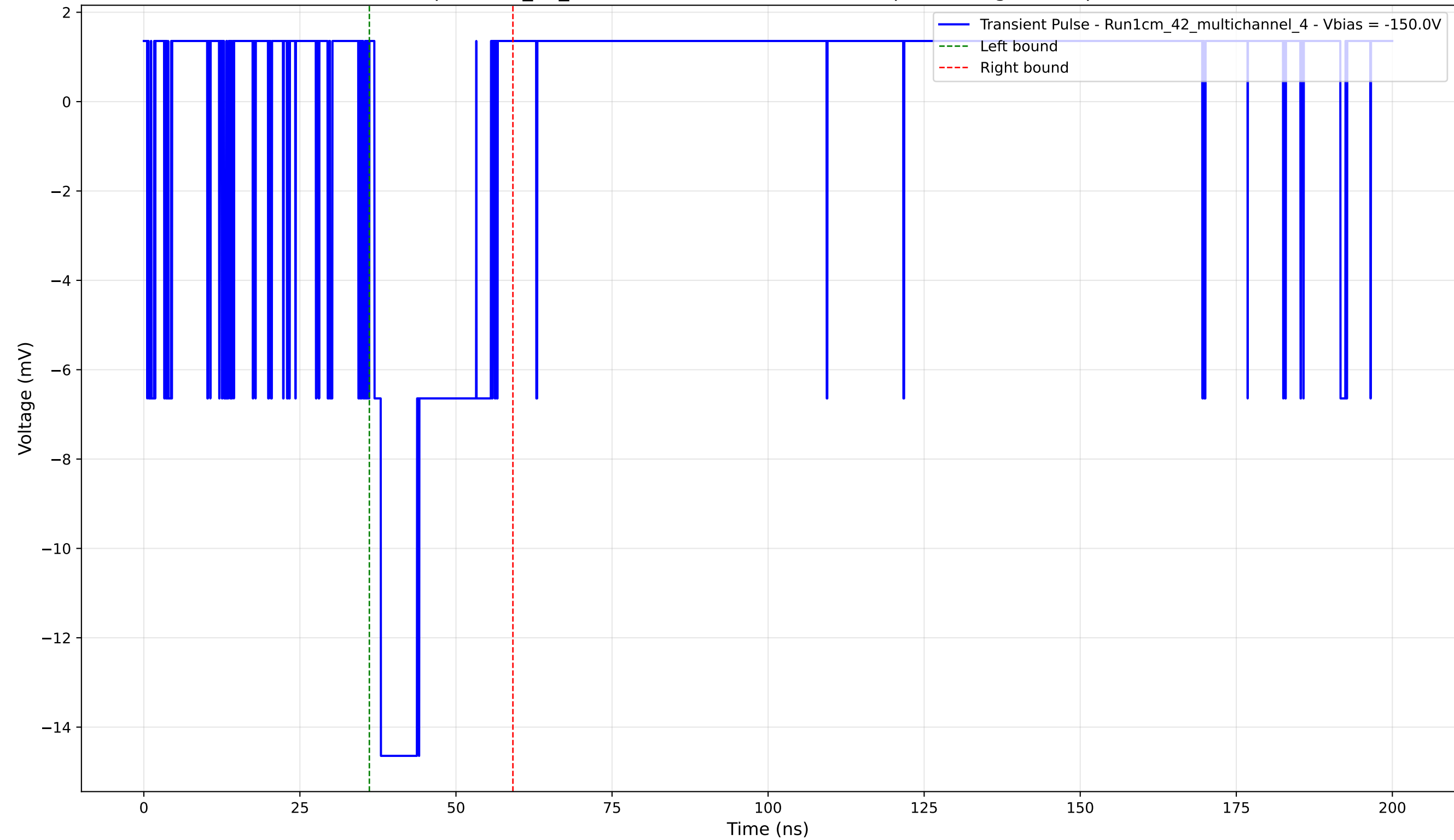
Transient Pulse - Sample: 1cm_42_multichannel - Position: 4055.0 \mu\text{m} - Charge: 3.35 pC - Rise Time: 1.04 ns
