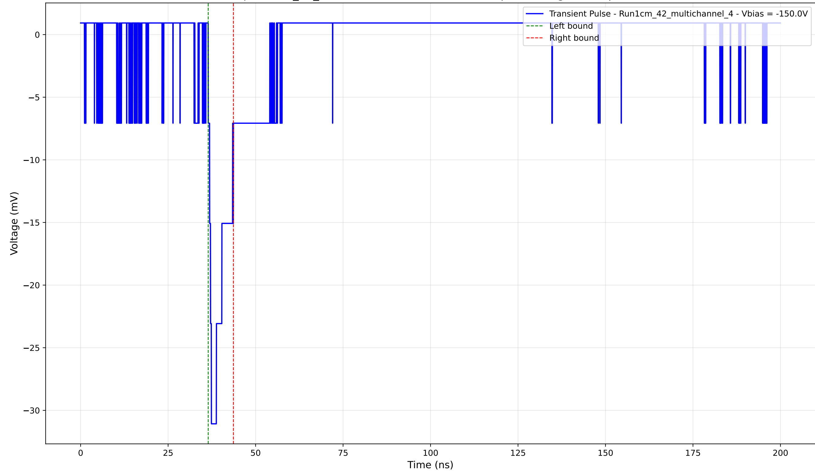
Transient Pulse - Sample: 1cm_42_multichannel - Position: 1540.0 \mu\text{m} - Charge: 2.85 pC - Rise Time: 0.91 ns
