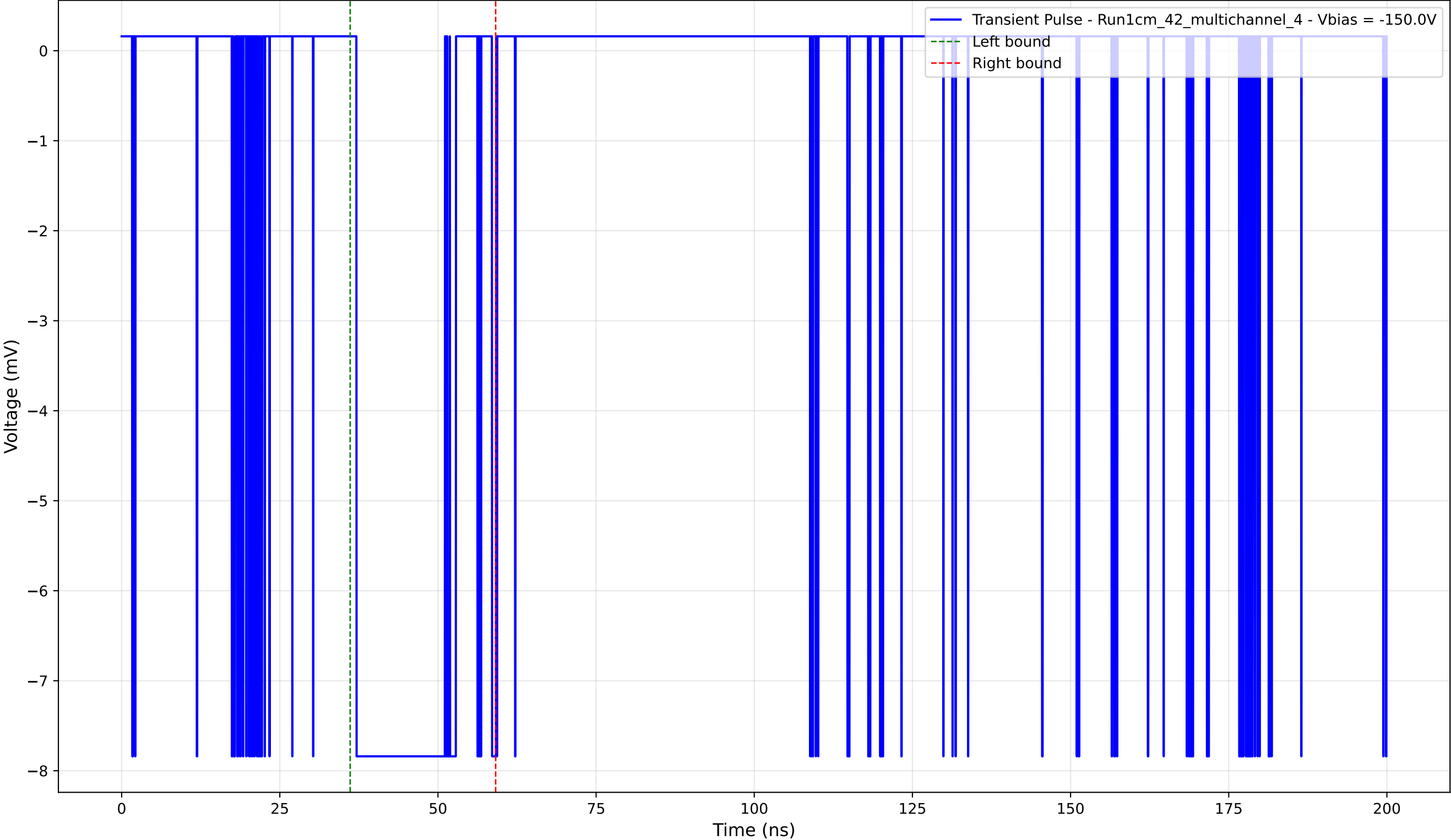
Transient Pulse - Sample: 1cm_42_multichannel - Position: 4855.0 \mu\text{m} - Charge: 2.54 pC - Rise Time: 0.02 ns
