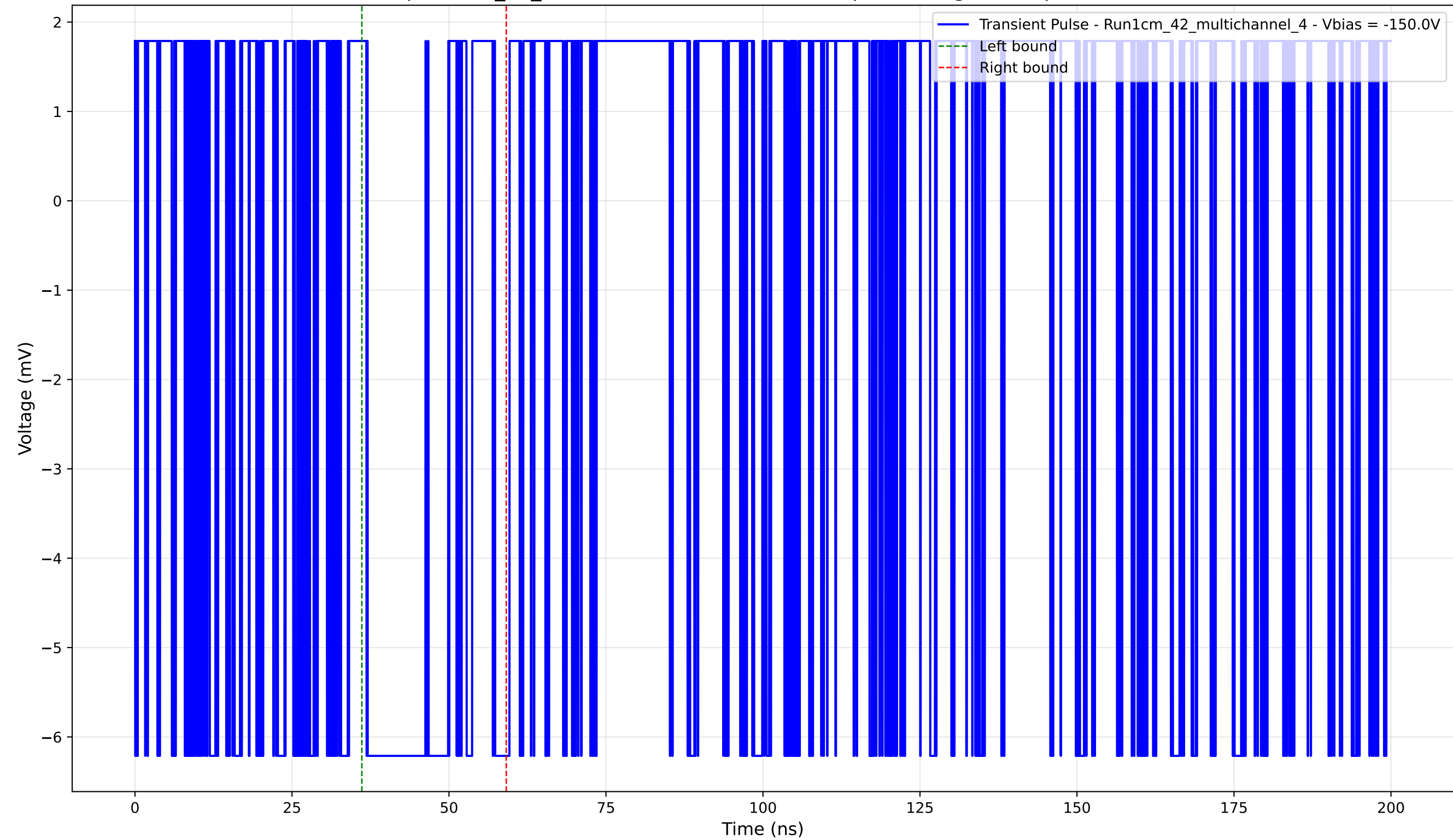
Transient Pulse - Sample: 1cm_42_multichannel - Position: 910.0 \mu\text{m} - Charge: 1.74 pC - Rise Time: 0.00 ns (N/A)
