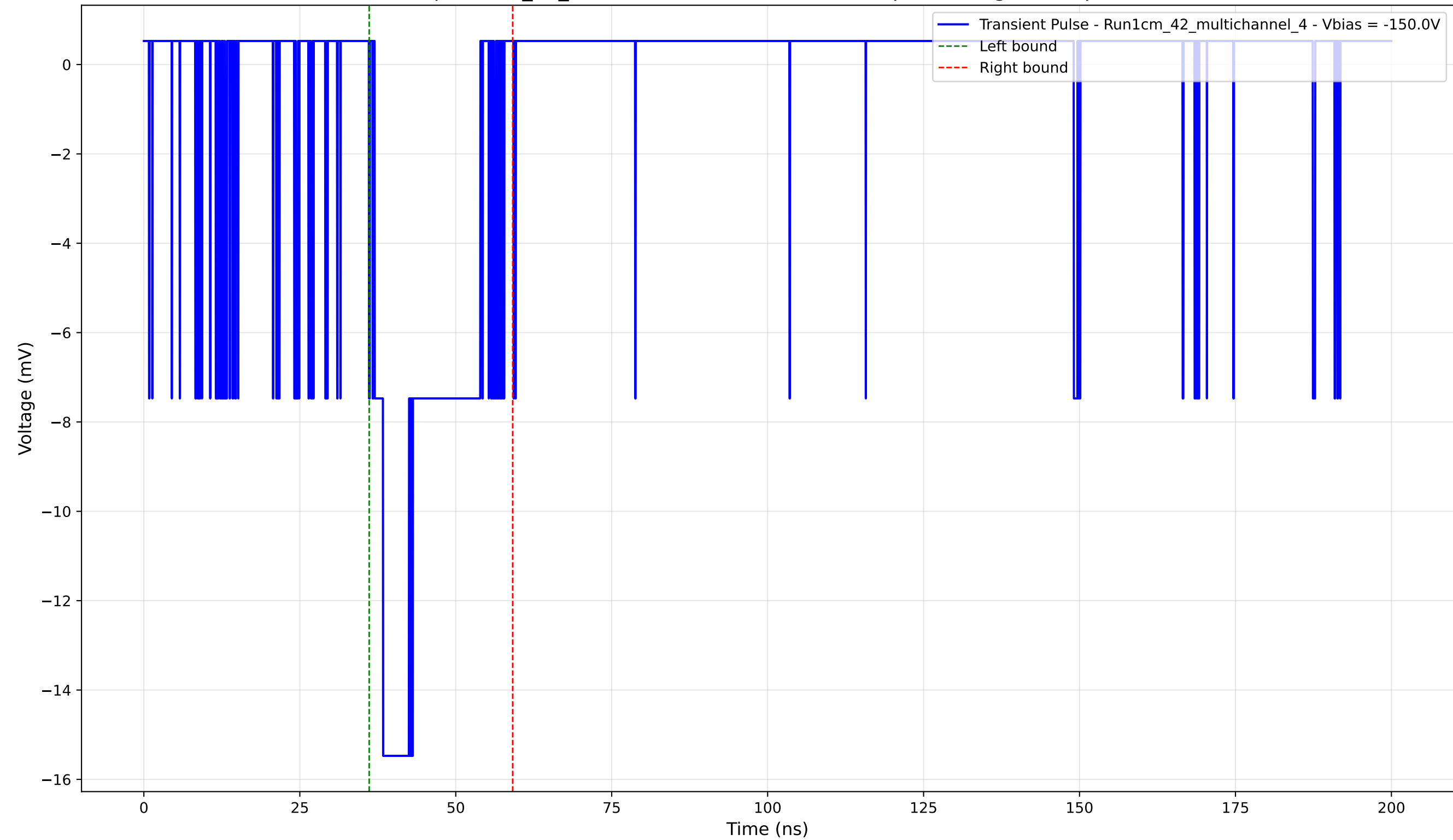
Transient Pulse - Sample: 1cm_42_multichannel - Position: 4200.0 \mu\text{m} - Charge: 3.39 pC - Rise Time: 1.36 ns
