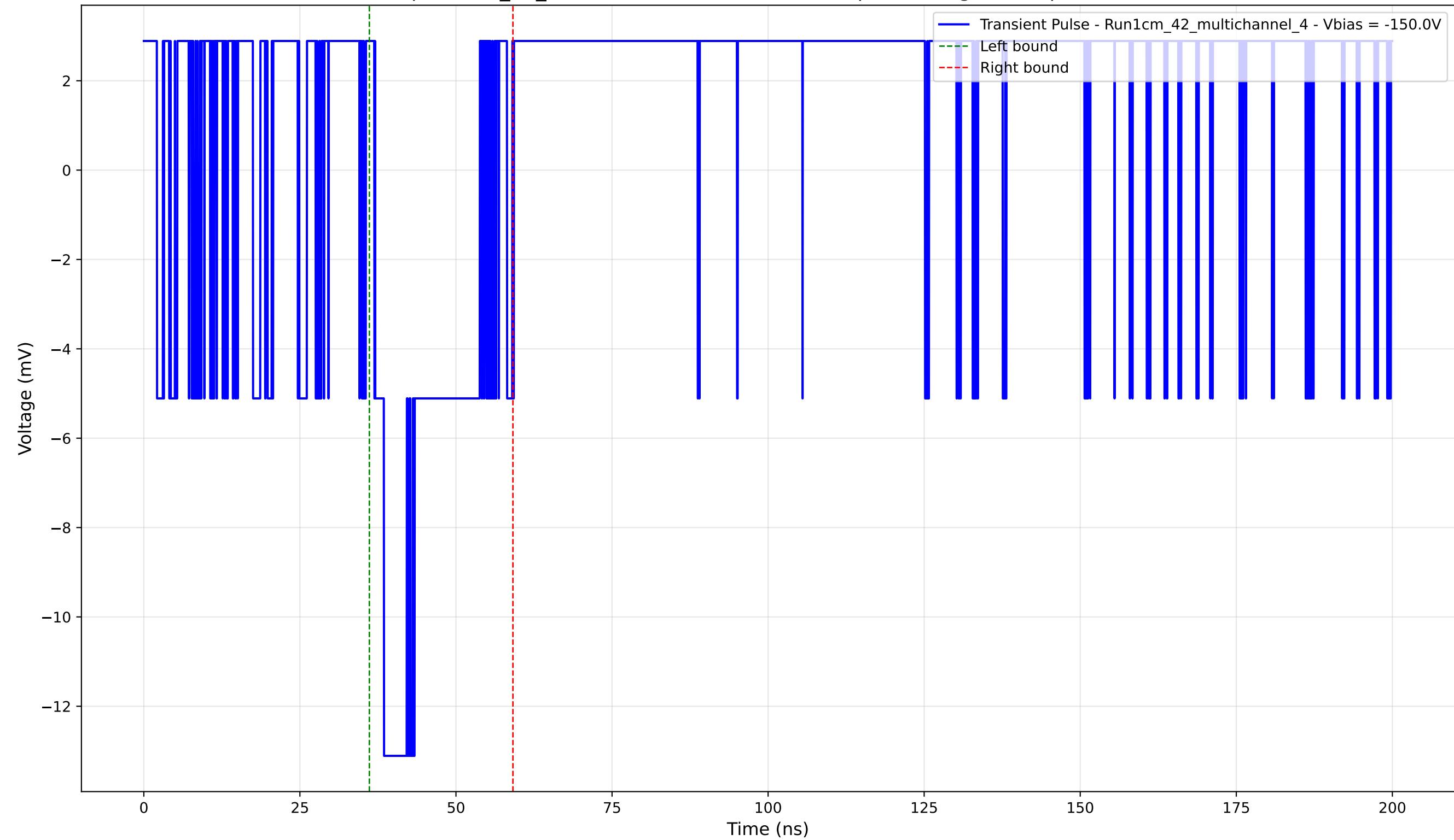
Transient Pulse - Sample: 1cm_42_multichannel - Position: 235.0 \mu\text{m} - Charge: 2.43 pC - Rise Time: 0.00 ns (N/A)
