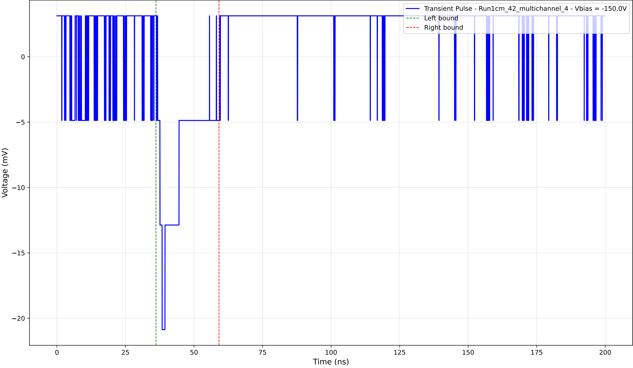
Transient Pulse - Sample: 1cm_42_multichannel - Position: 955.0 \mu\text{m} - Charge: 3.42 pC - Rise Time: 0.00 ns (N/A)
