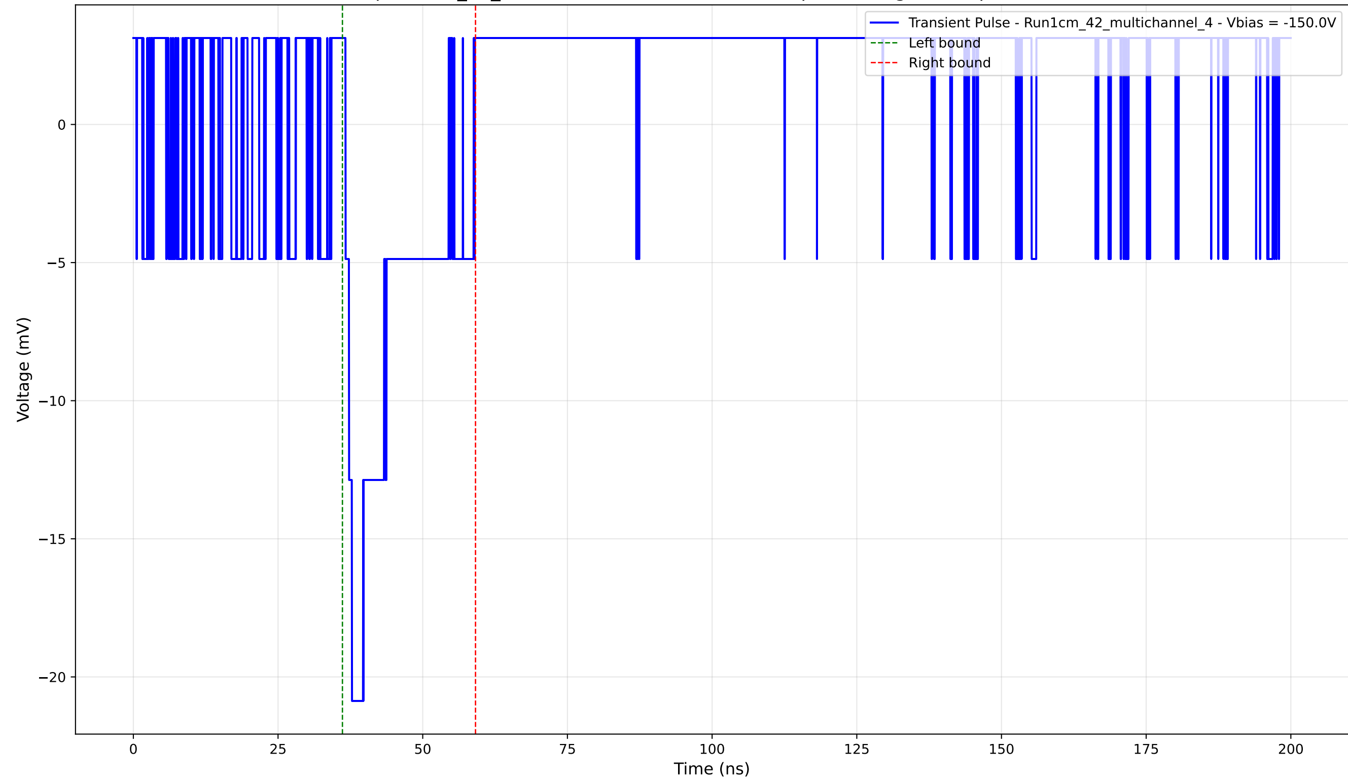
Transient Pulse - Sample: 1cm_42_multichannel - Position: 1180.0 \mu\text{m} - Charge: 3.35 pC - Rise Time: 0.00 ns (N/A)
