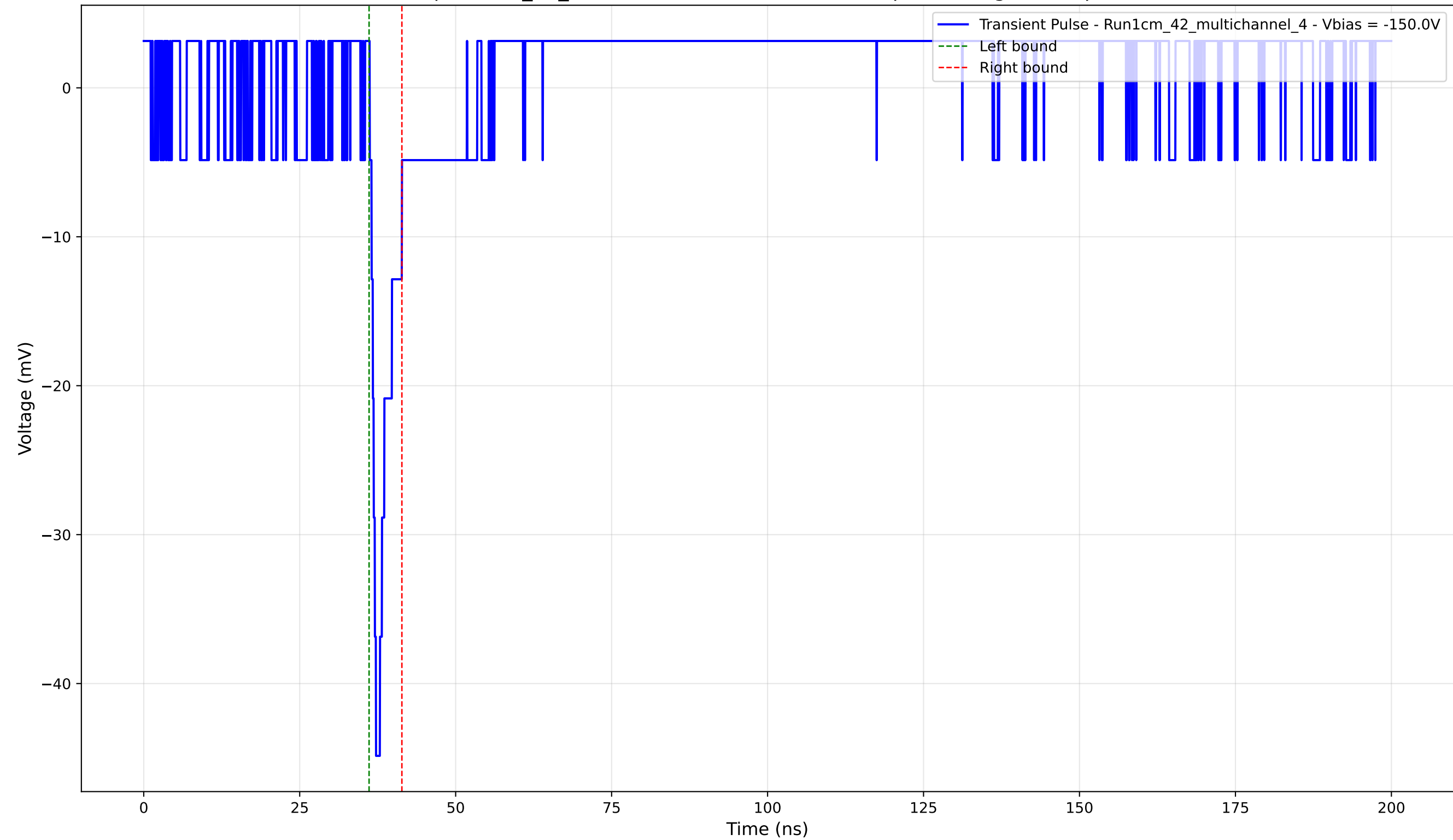
Transient Pulse - Sample: 1cm_42_multichannel - Position: 1950.0 \mu\text{m} - Charge: 2.32 pC - Rise Time: 1.00 ns
