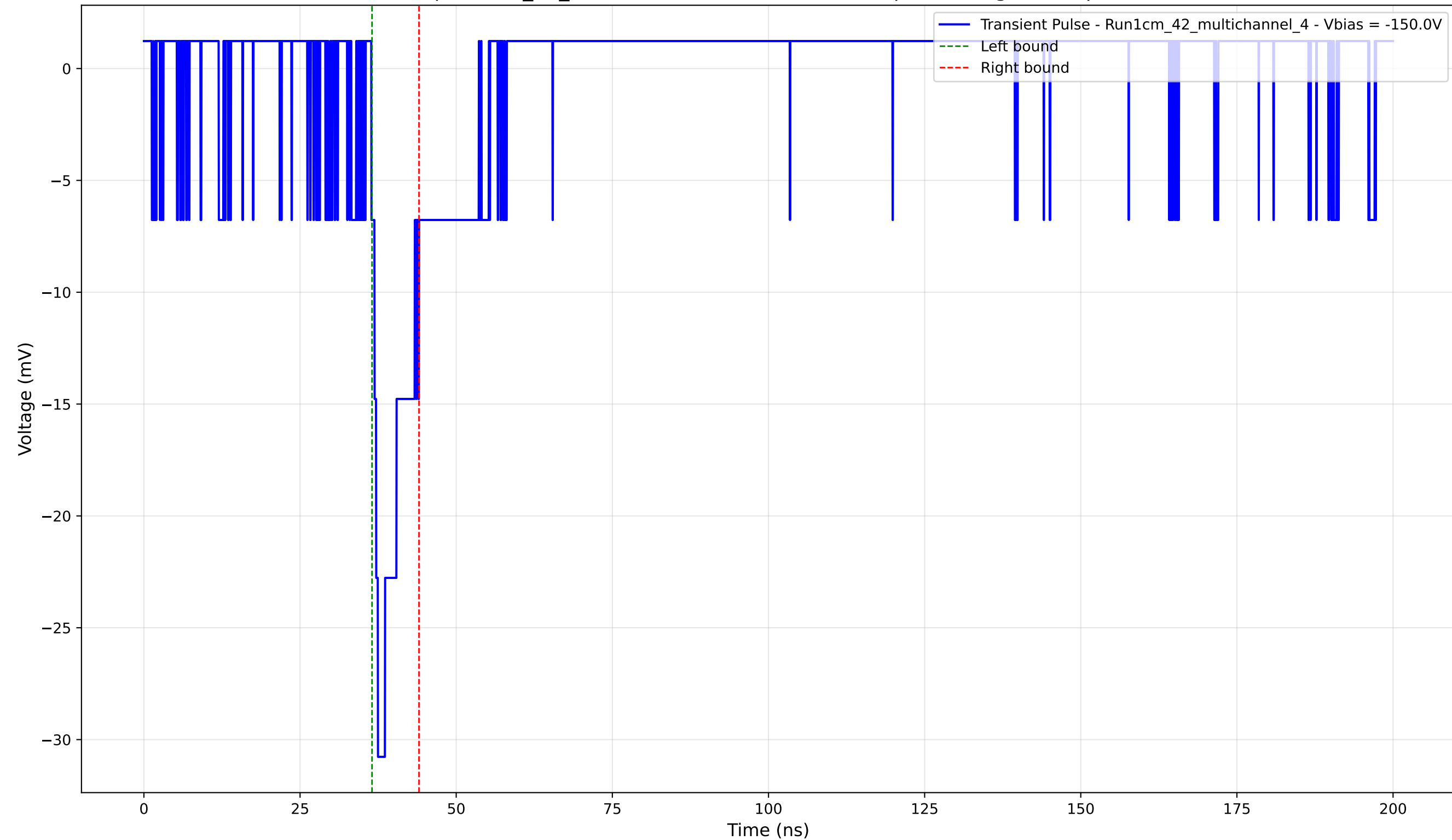
Transient Pulse - Sample: 1cm_42_multichannel - Position: 1520.0 \mu\text{m} - Charge: 2.78 pC - Rise Time: 1.05 ns
