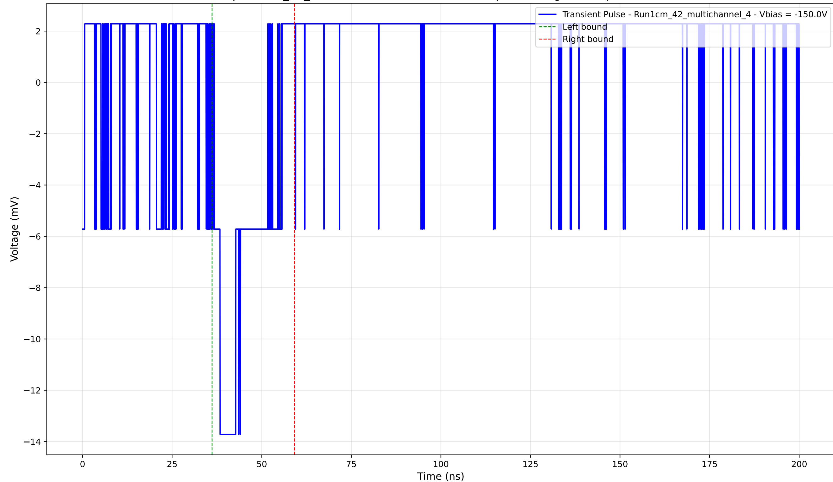
Transient Pulse - Sample: 1cm_42_multichannel - Position: 4305.0 \mu\text{m} - Charge: 2.60 pC - Rise Time: 0.00 ns (N/A)
