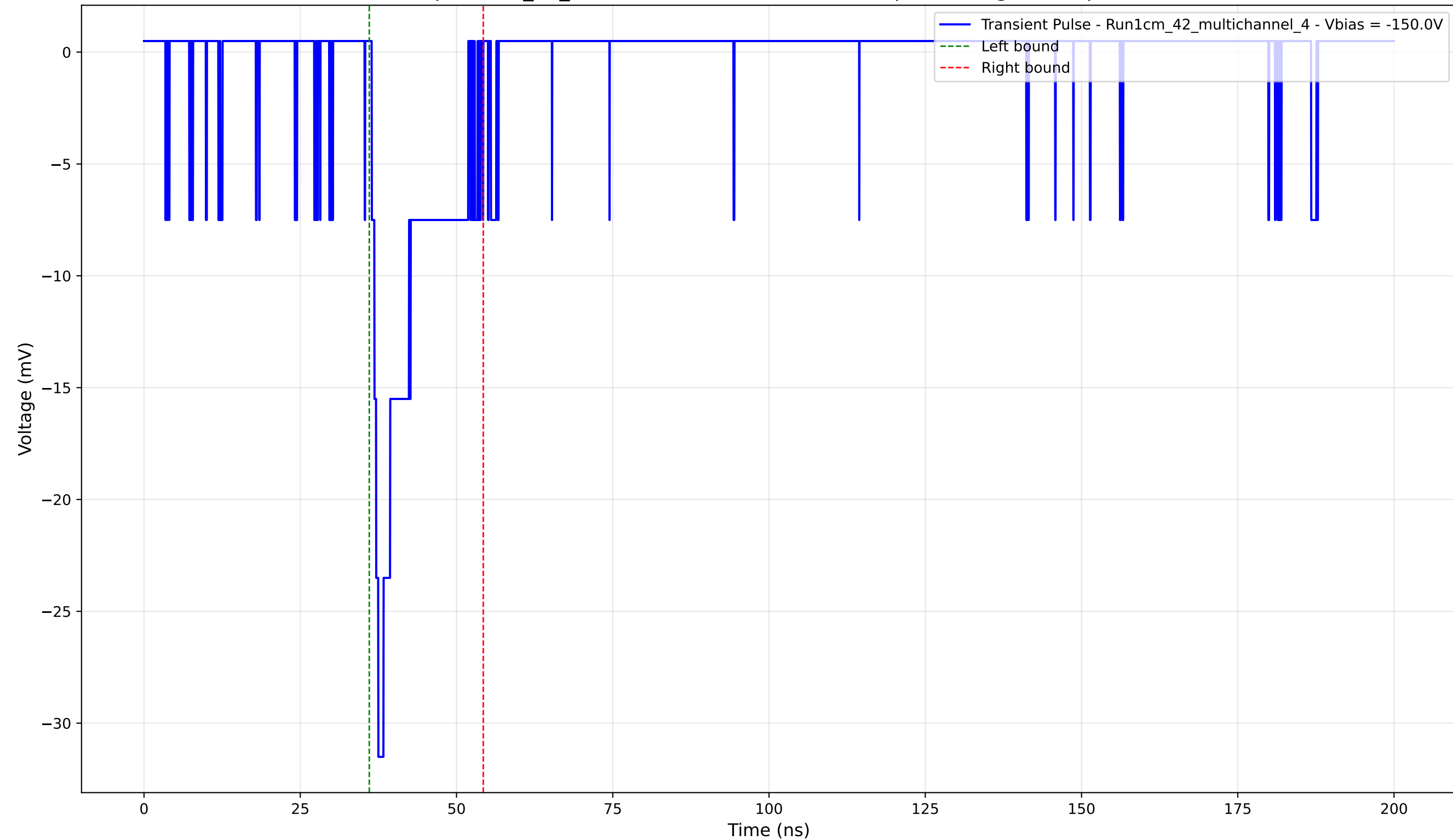
Transient Pulse - Sample: 1cm_42_multichannel - Position: 3155.0 \mu\text{m} - Charge: 3.87 pC - Rise Time: 1.05 ns
