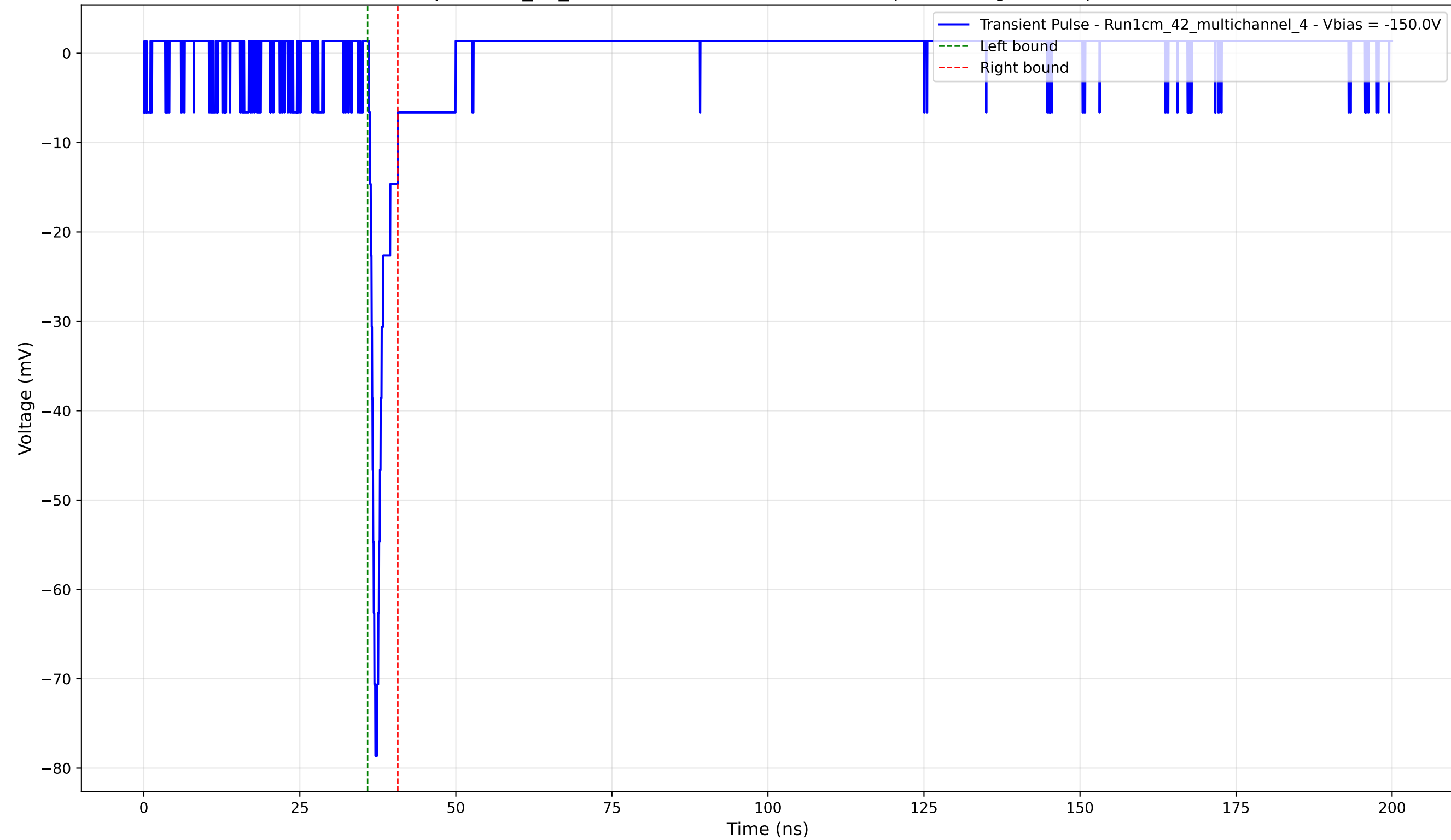
Transient Pulse - Sample: 1cm_42_multichannel - Position: 2310.0 \mu\text{m} - Charge: 3.01 pC - Rise Time: 0.86 ns
