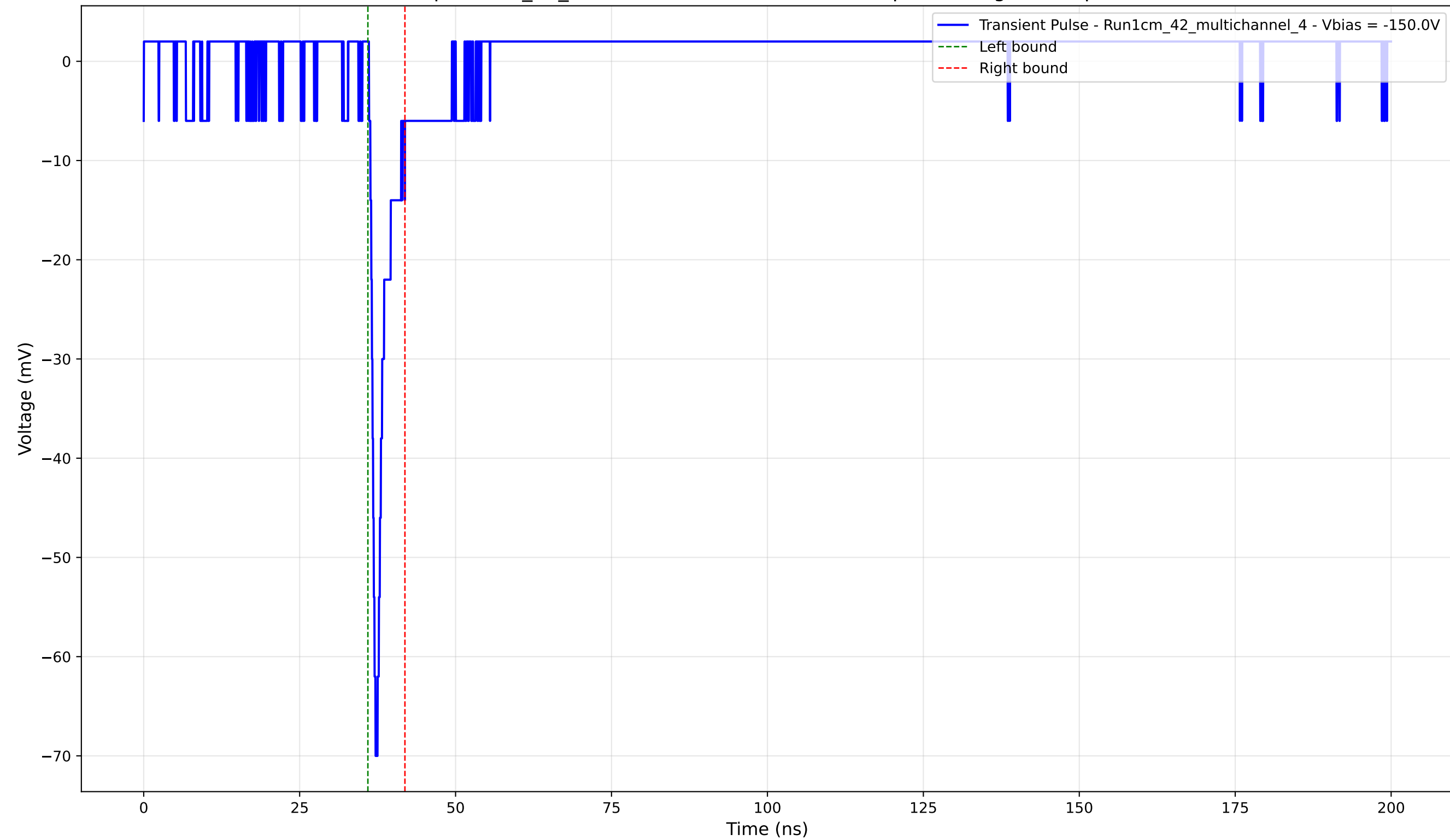
Transient Pulse - Sample: 1cm_42_multichannel - Position: 2185.0 \mu\text{m} - Charge: 3.09 pC - Rise Time: 0.84 ns
