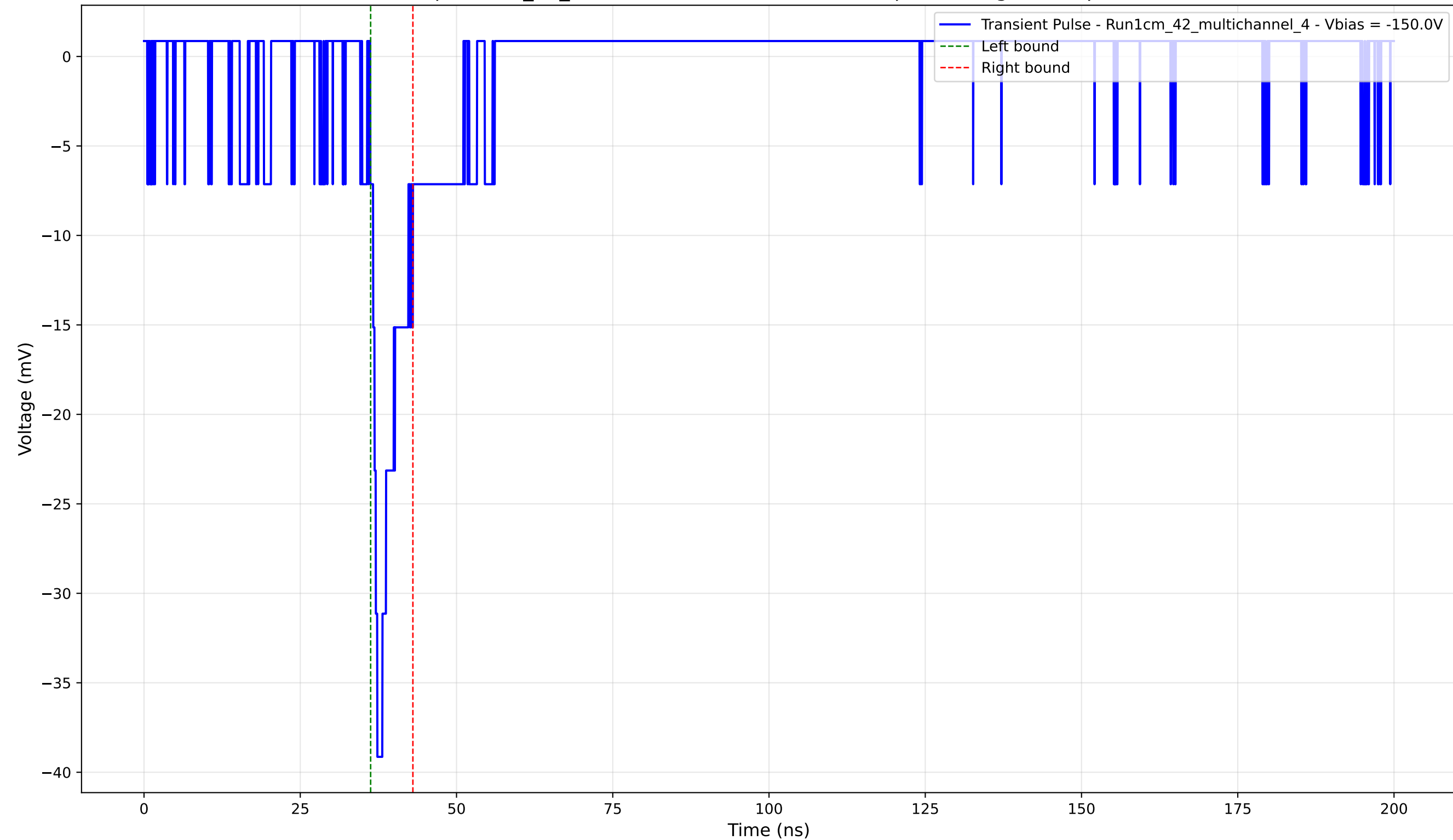
Transient Pulse - Sample: 1cm_42_multichannel - Position: 3000.0 \mu\text{m} - Charge: 2.81 pC - Rise Time: 1.13 ns
