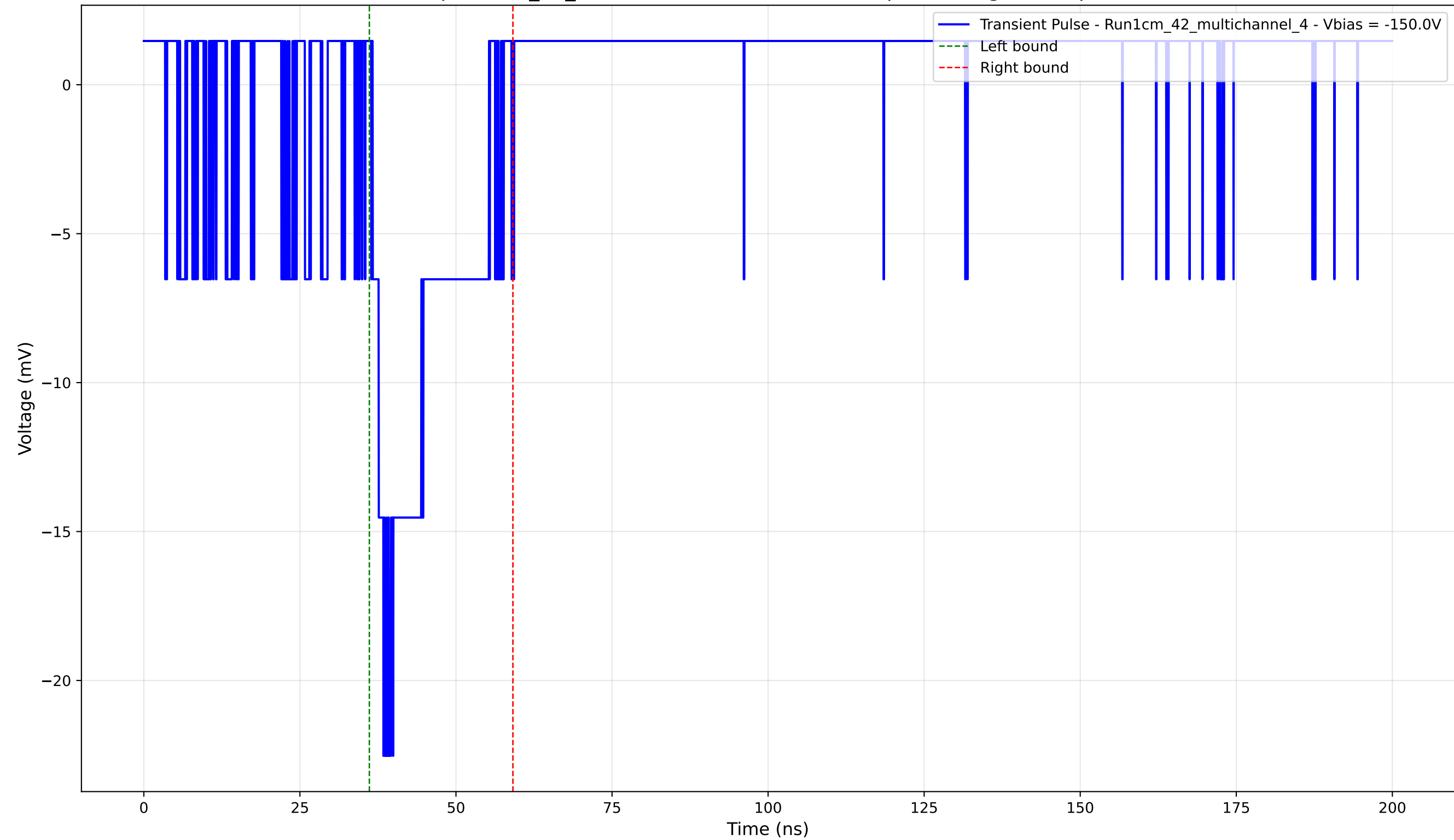
Transient Pulse - Sample: 1cm_42_multichannel - Position: 970.0 \mu\text{m} - Charge: 3.75 pC - Rise Time: 1.74 ns
