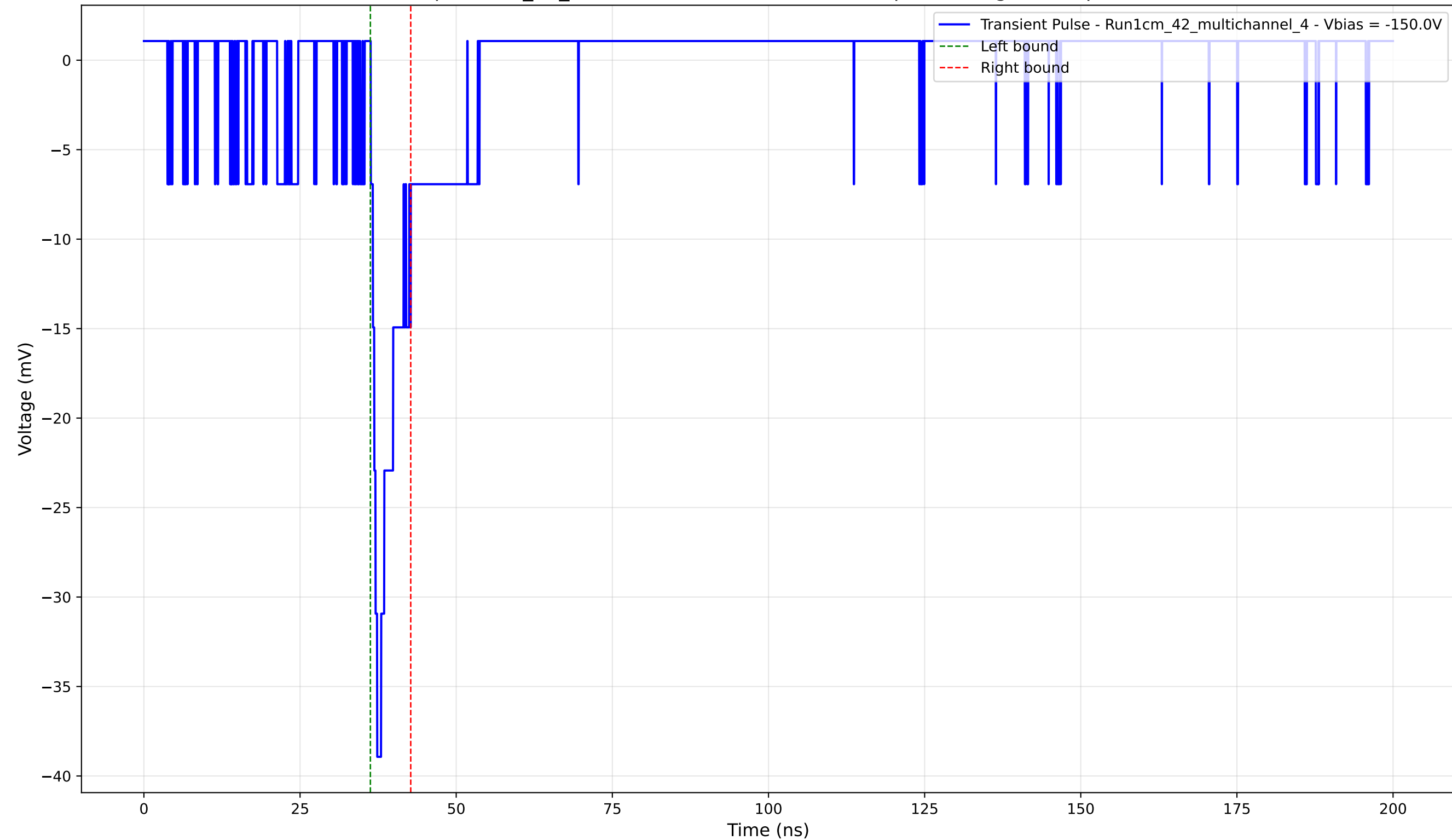
Transient Pulse - Sample: 1cm_42_multichannel - Position: 2975.0 \mu\text{m} - Charge: 2.61 pC - Rise Time: 1.03 ns
