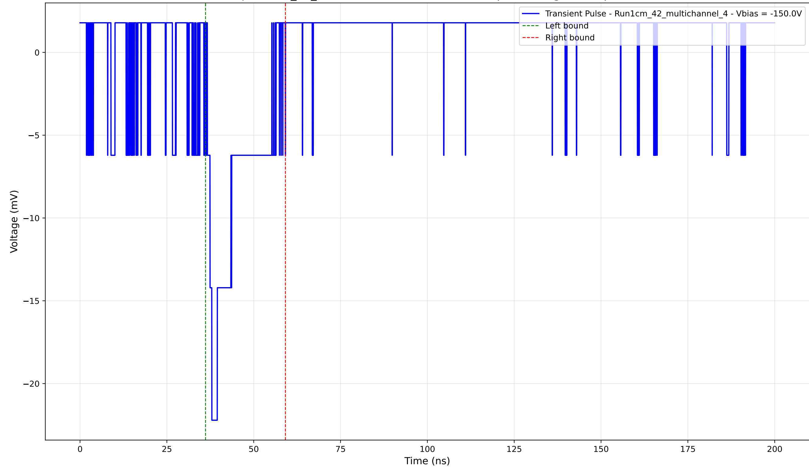
Transient Pulse - Sample: 1cm_42_multichannel - Position: 1145.0 \mu\text{m} - Charge: 3.62 pC - Rise Time: 1.30 ns
