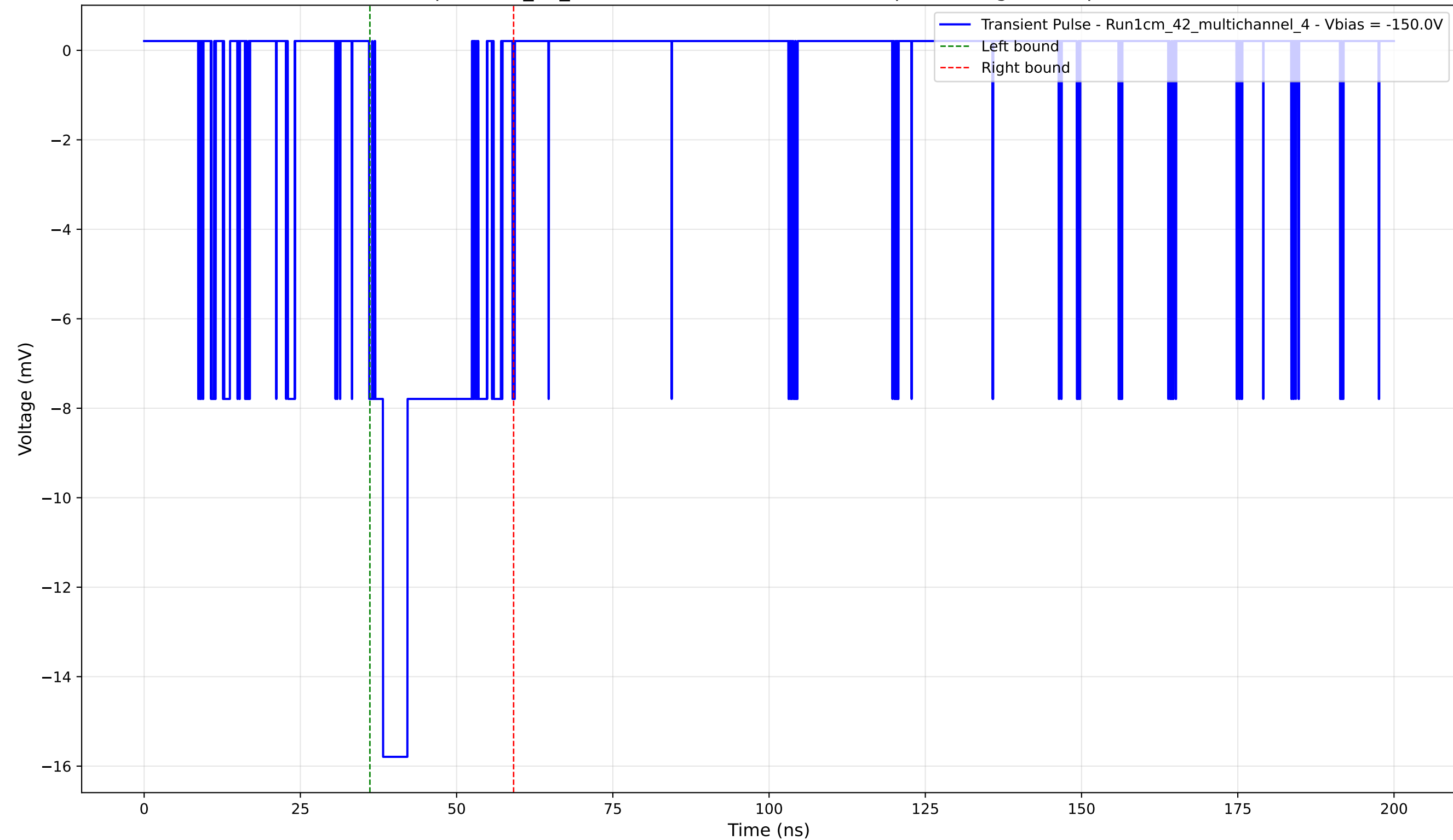
Transient Pulse - Sample: 1cm_42_multichannel - Position: 4745.0 \mu\text{m} - Charge: 3.65 pC - Rise Time: 1.26 ns
