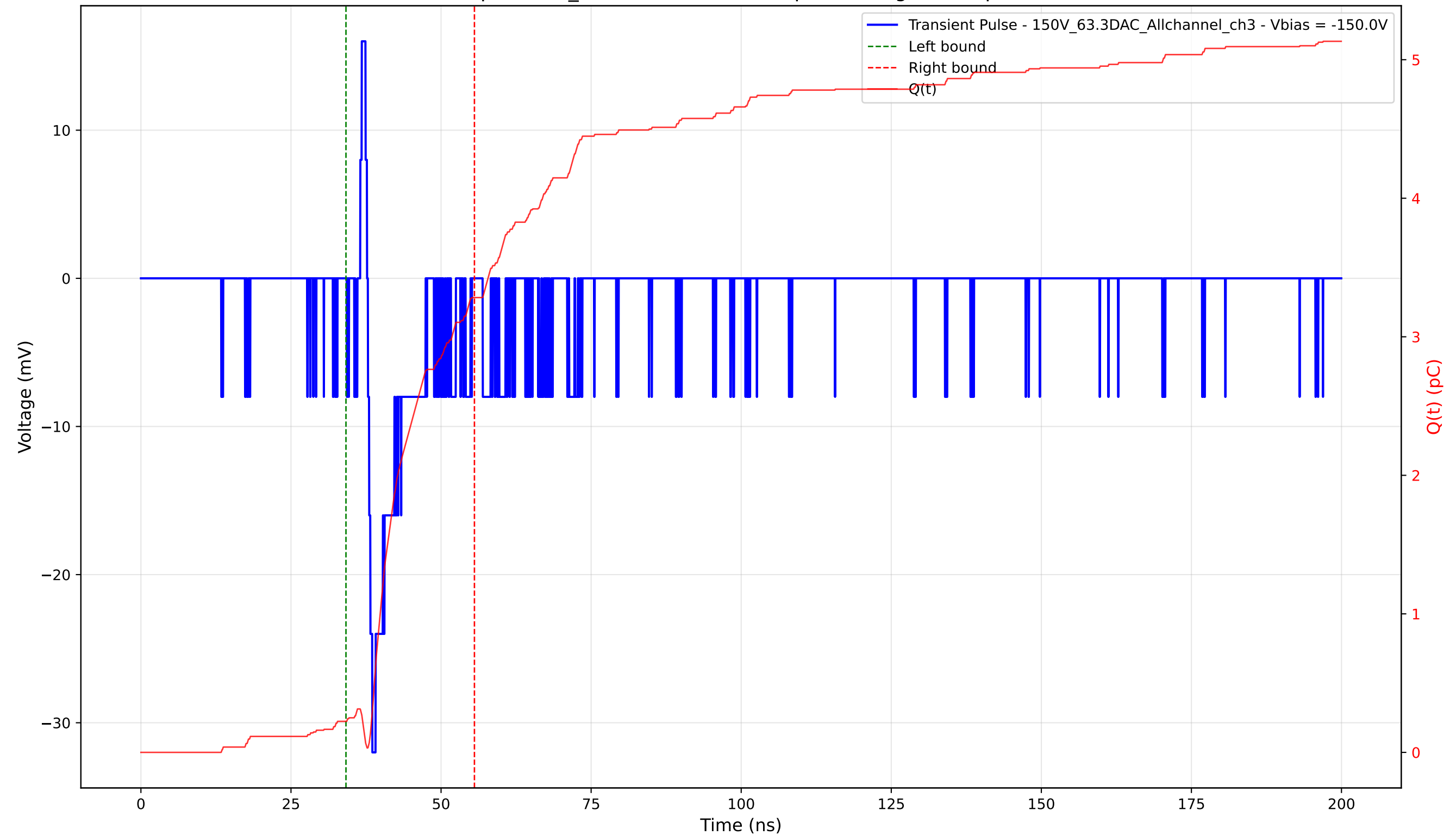
Transient Pulse - Sample: 1cm_42 - Position: 4555.0 \mu\text{m} - Charge: 3.06 pC - Rise Time: 0.74 ns
