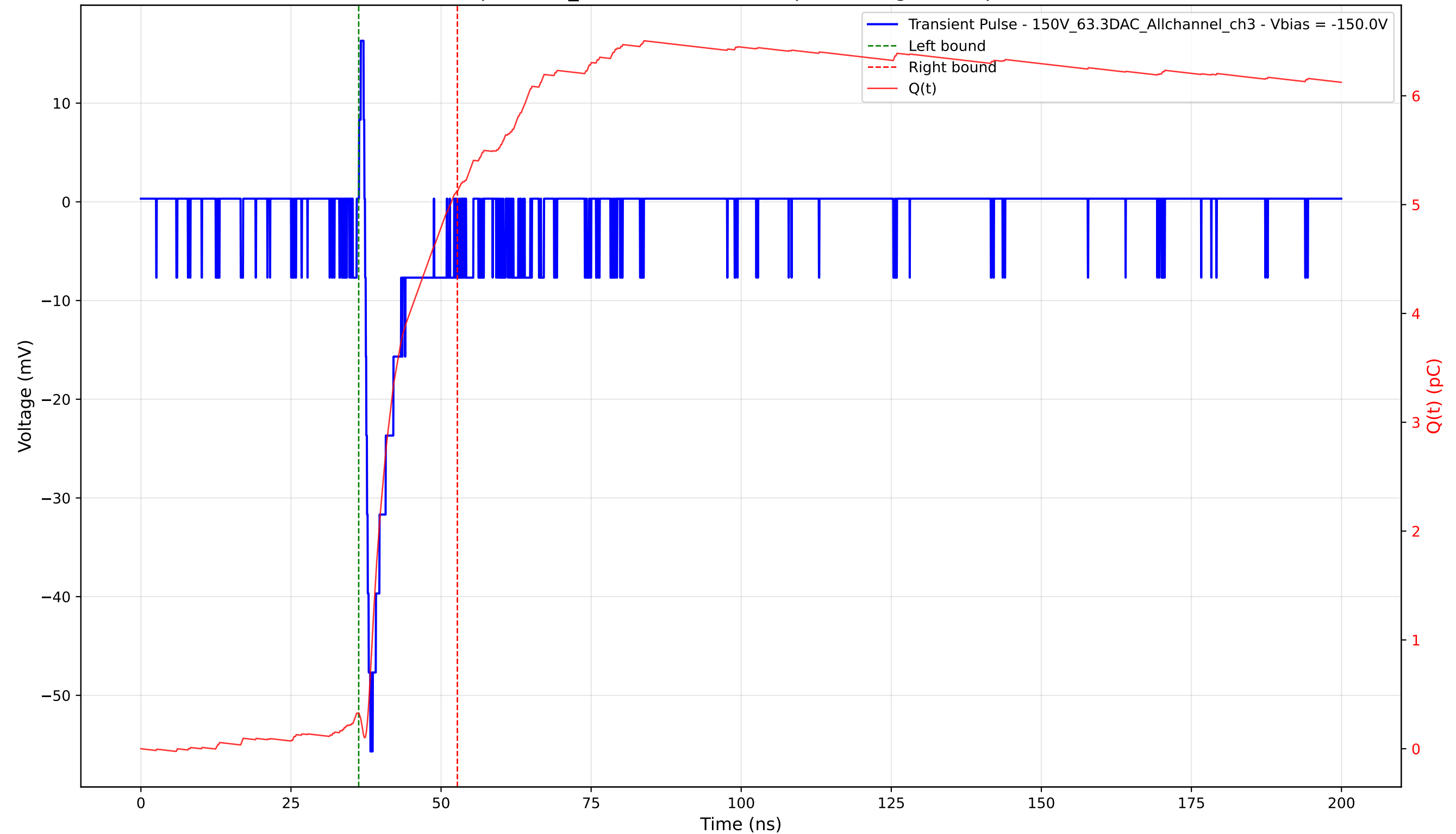
Transient Pulse - Sample: 1cm_42 - Position: 3860.0 \mu\text{m} - Charge: 4.80 pC - Rise Time: 0.89 ns
