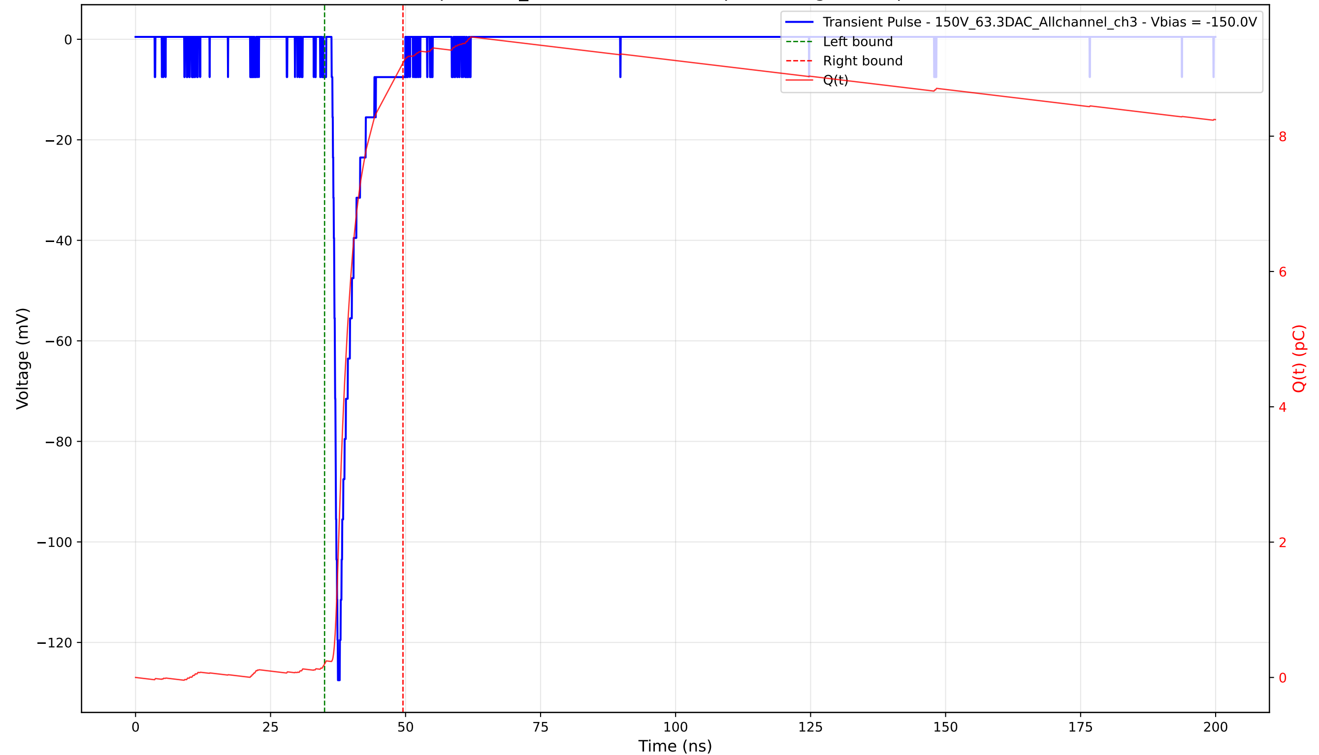
Transient Pulse - Sample: 1cm_42 - Position: 1675.0 \mu\text{m} - Charge: 8.89 pC - Rise Time: 0.93 ns
