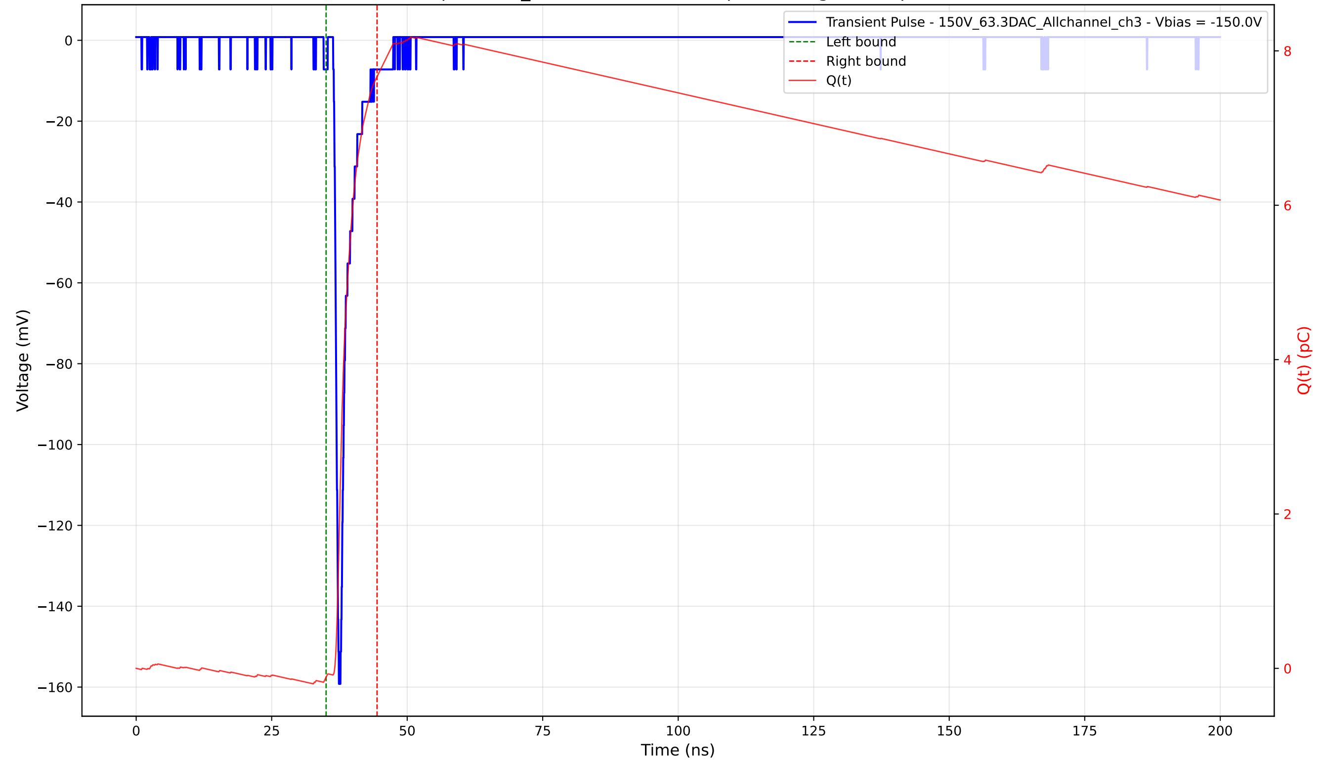
Transient Pulse - Sample: 1cm_42 - Position: 3150.0 \mu\text{m} - Charge: 7.78 pC - Rise Time: 0.80 ns
