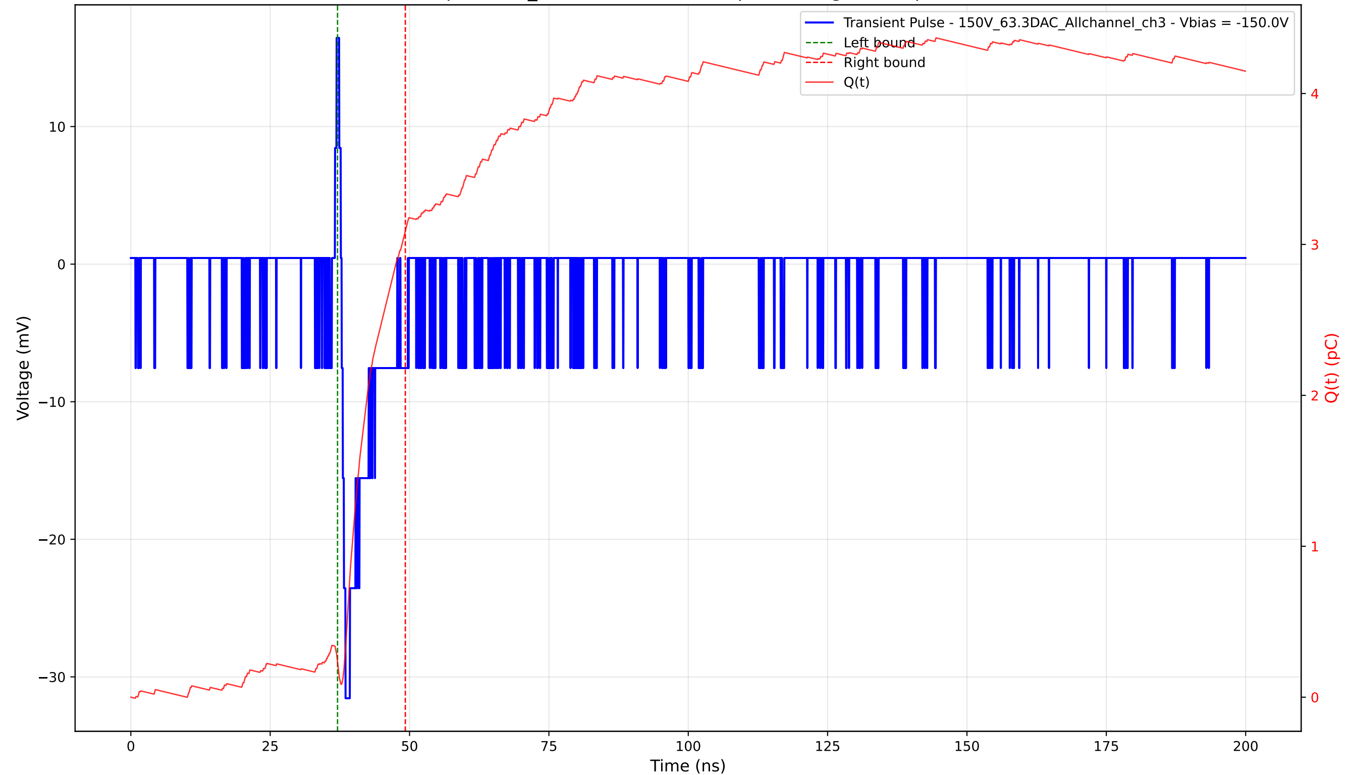
Transient Pulse - Sample: 1cm_42 - Position: 4695.0 \mu\text{m} - Charge: 2.86 pC - Rise Time: 0.70 ns
