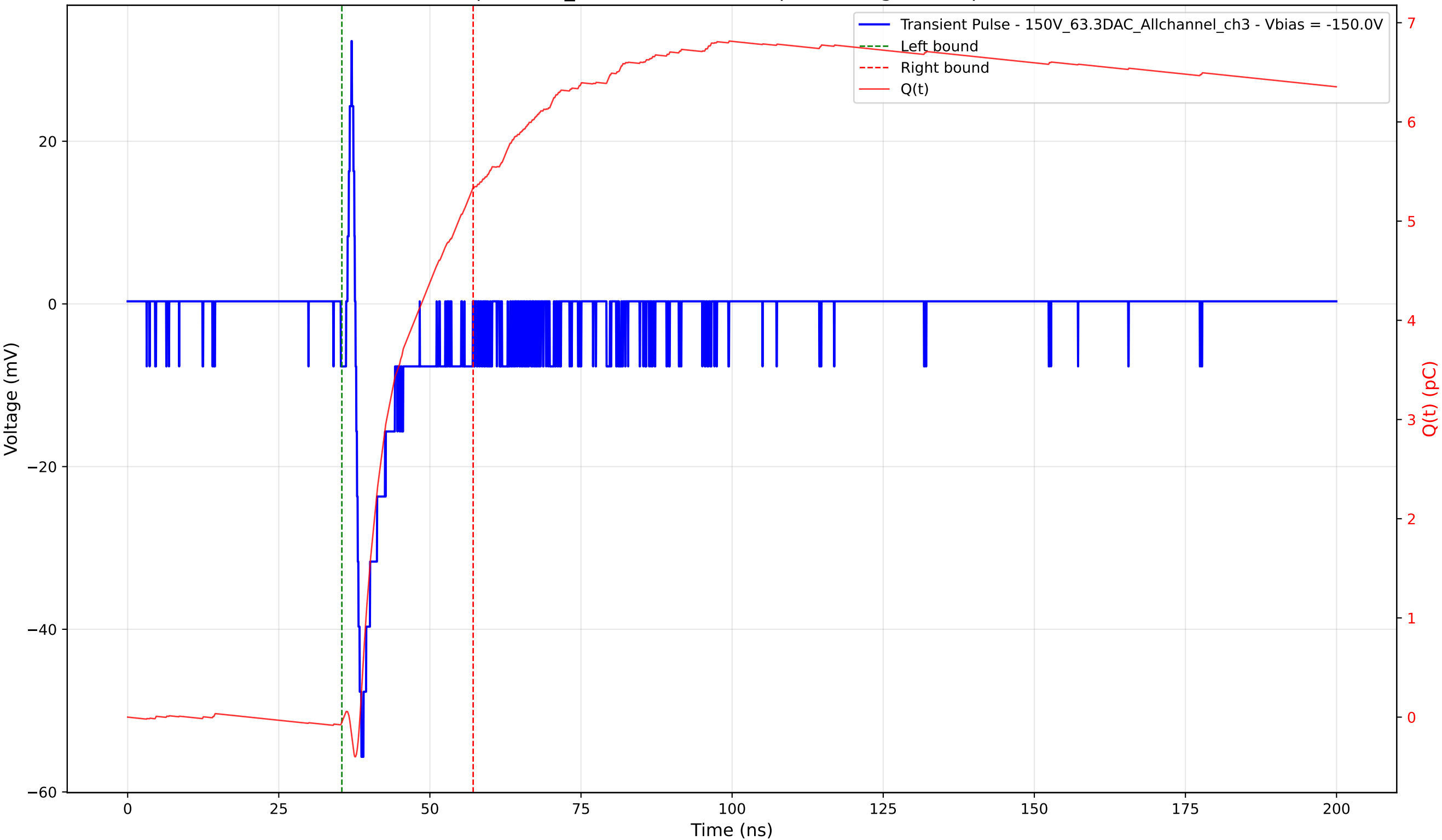
Transient Pulse - Sample: 1cm_42 - Position: 775.0 \mu\text{m} - Charge: 5.38 pC - Rise Time: 0.97 ns
