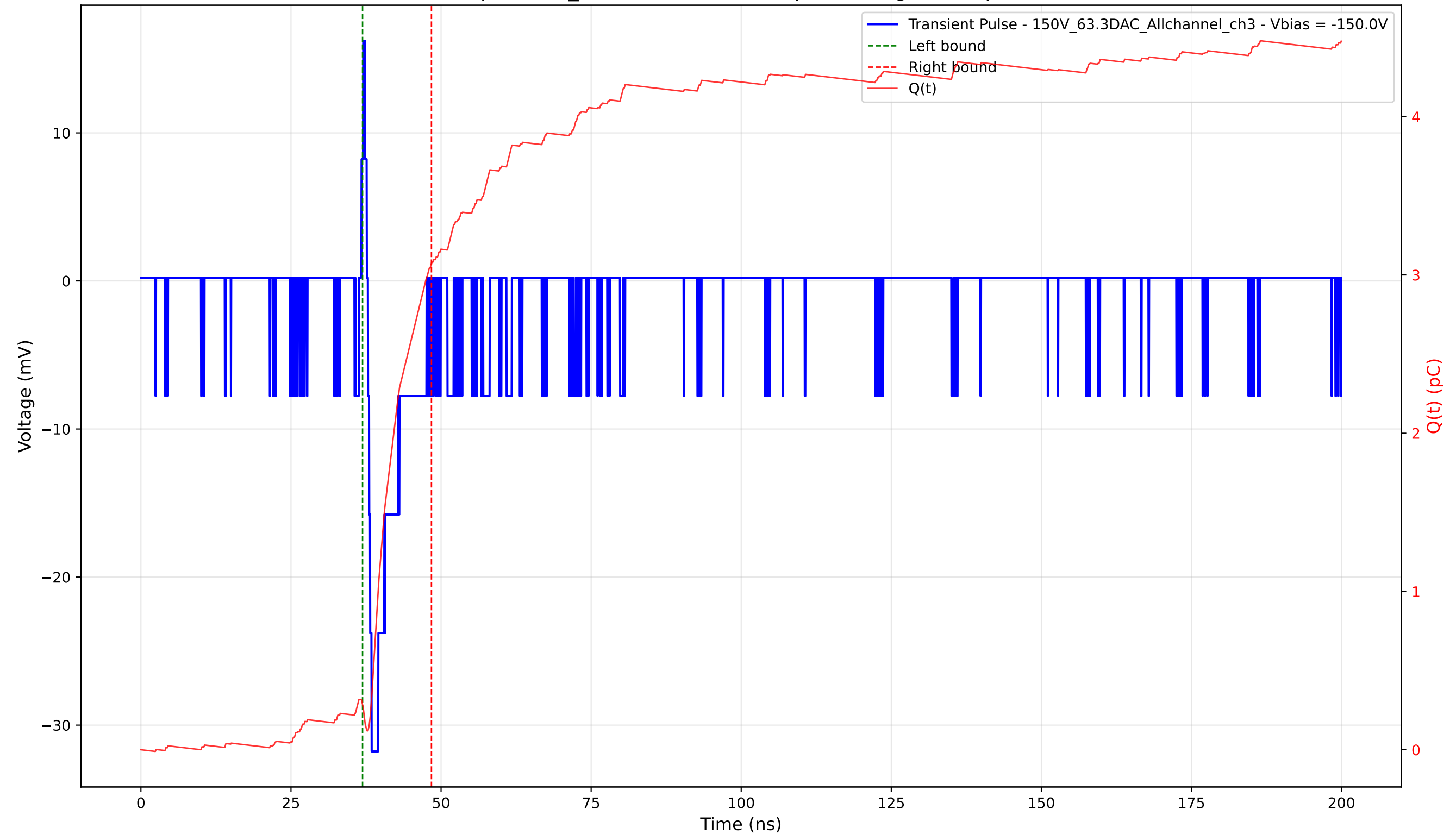
Transient Pulse - Sample: 1cm_42 - Position: 4825.0 \mu\text{m} - Charge: 2.79 pC - Rise Time: 0.62 ns
