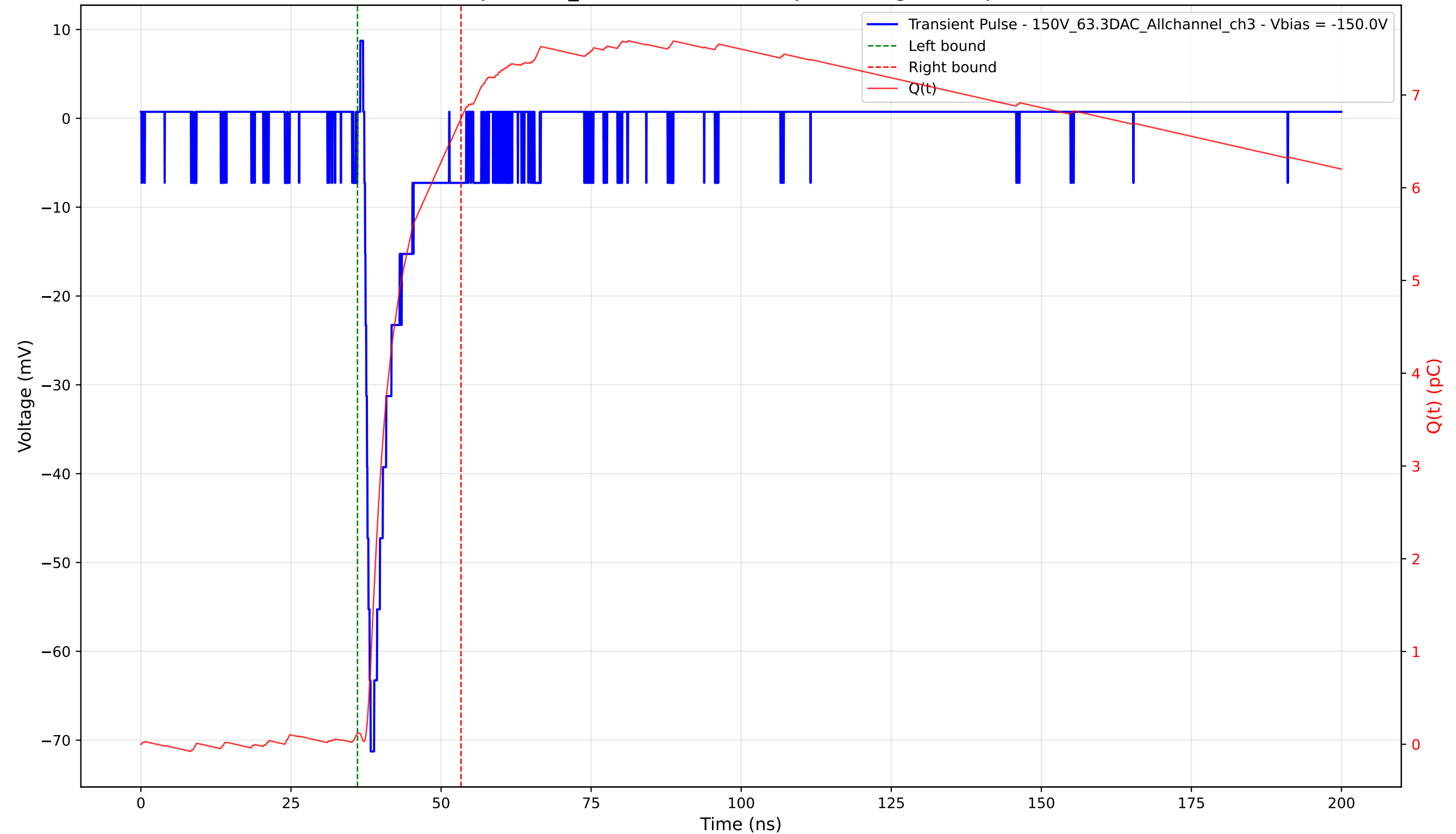
Transient Pulse - Sample: 1cm_42 - Position: 1265.0 \mu\text{m} - Charge: 6.62 pC - Rise Time: 1.04 ns
