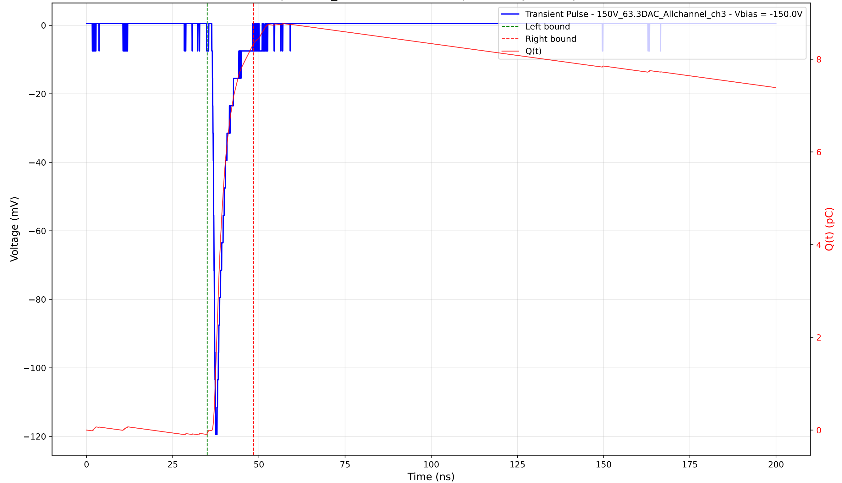
Transient Pulse - Sample: 1cm_42 - Position: 1660.0 \mu\text{m} - Charge: 8.40 pC - Rise Time: 0.86 ns
