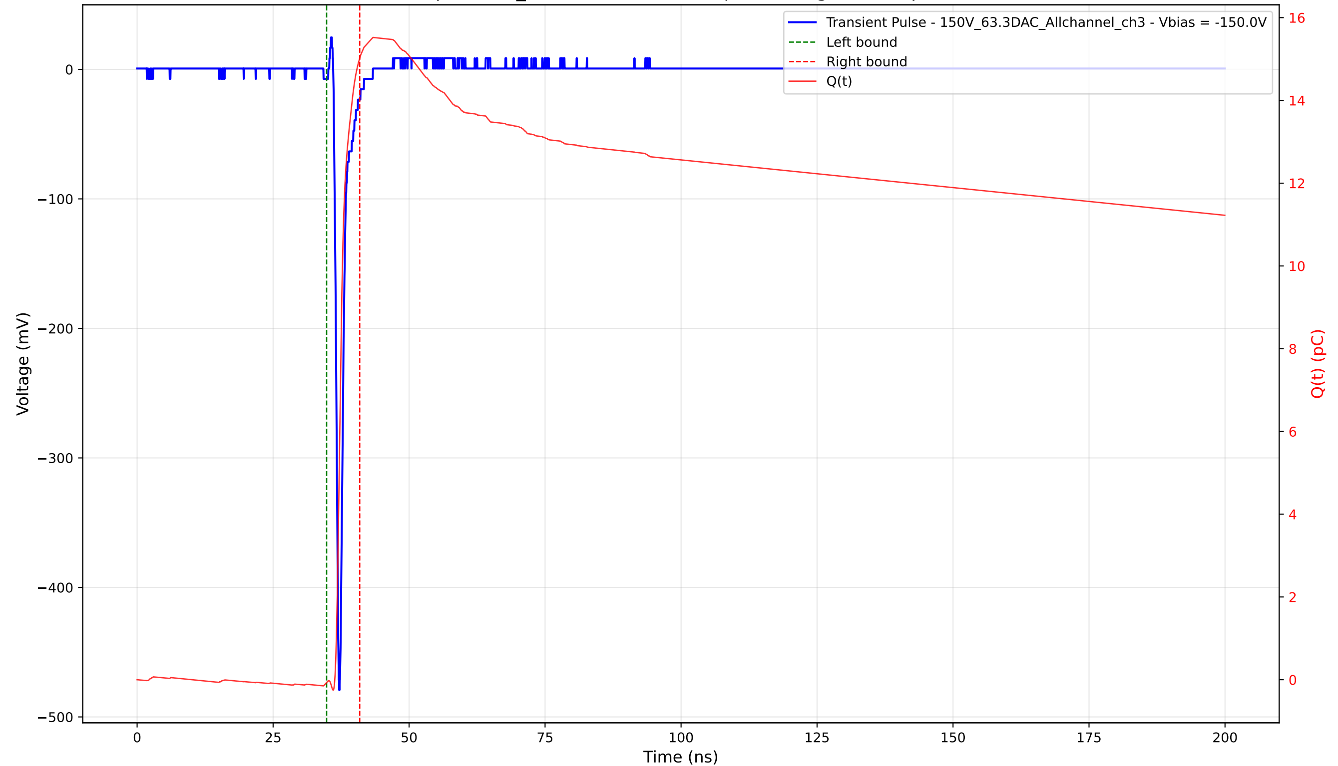
Transient Pulse - Sample: 1cm_42 - Position: 2345.0 \mu\text{m} - Charge: 15.09 pC - Rise Time: 0.70 ns
