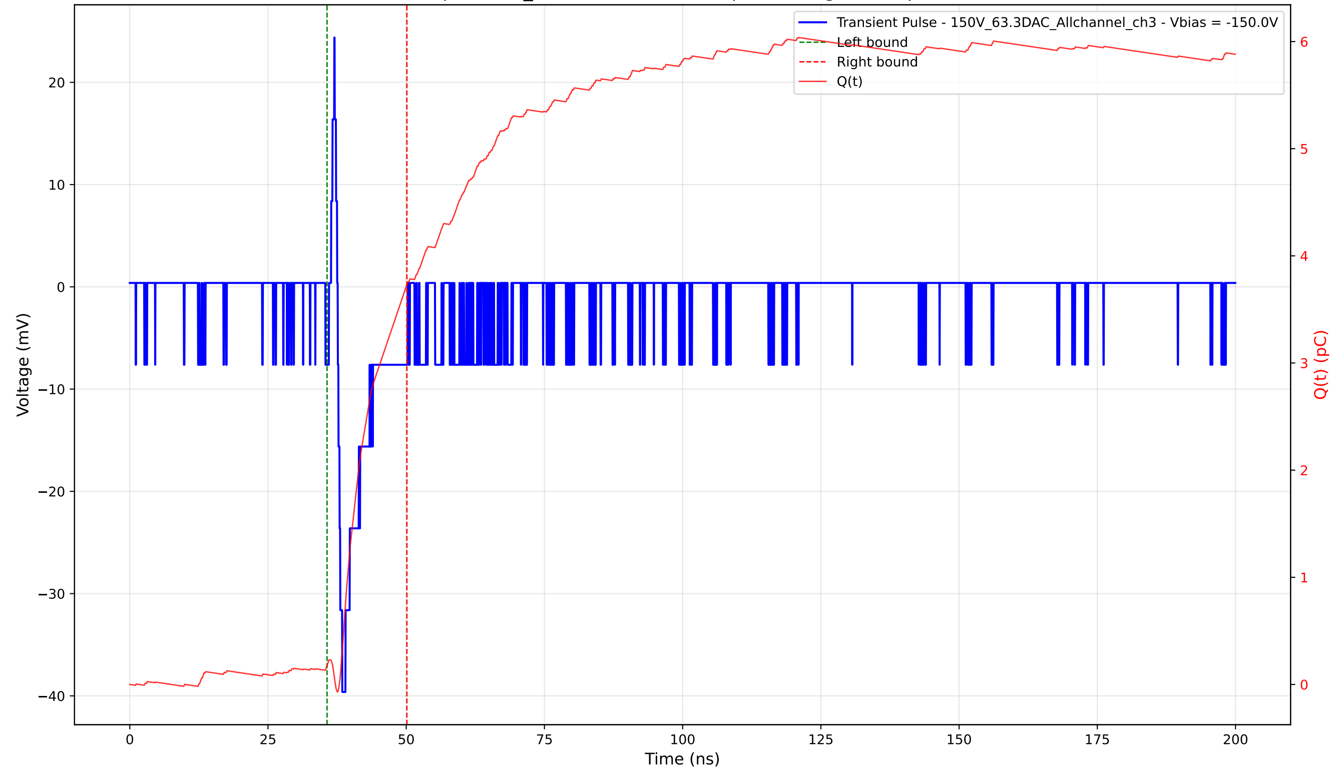
Transient Pulse - Sample: 1cm_42 - Position: 4100.0 \mu\text{m} - Charge: 3.56 pC - Rise Time: 0.82 ns
