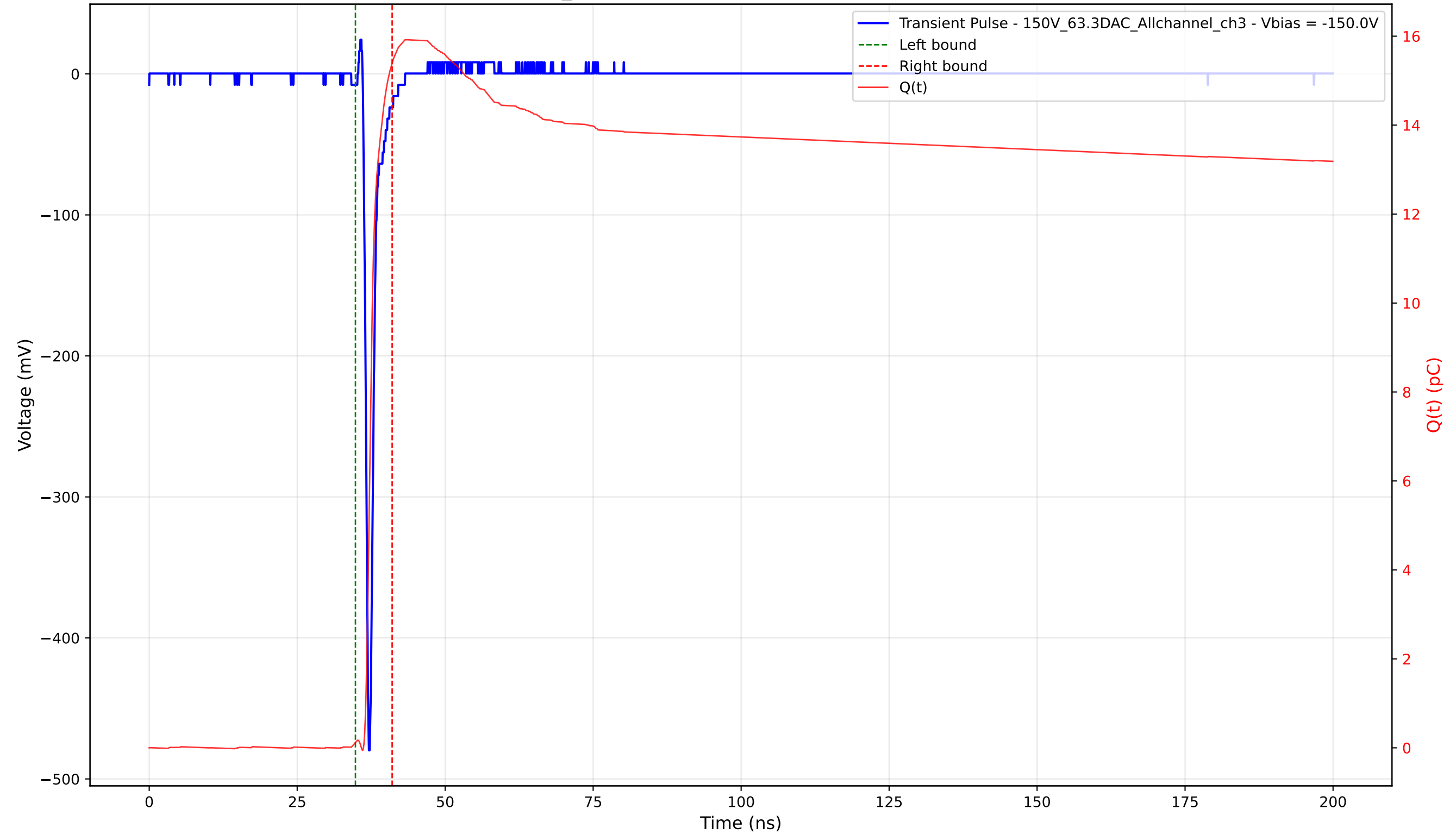
Transient Pulse - Sample: 1cm_42 - Position: 2700.0 \mu\text{m} - Charge: 15.27 pC - Rise Time: 0.70 ns
