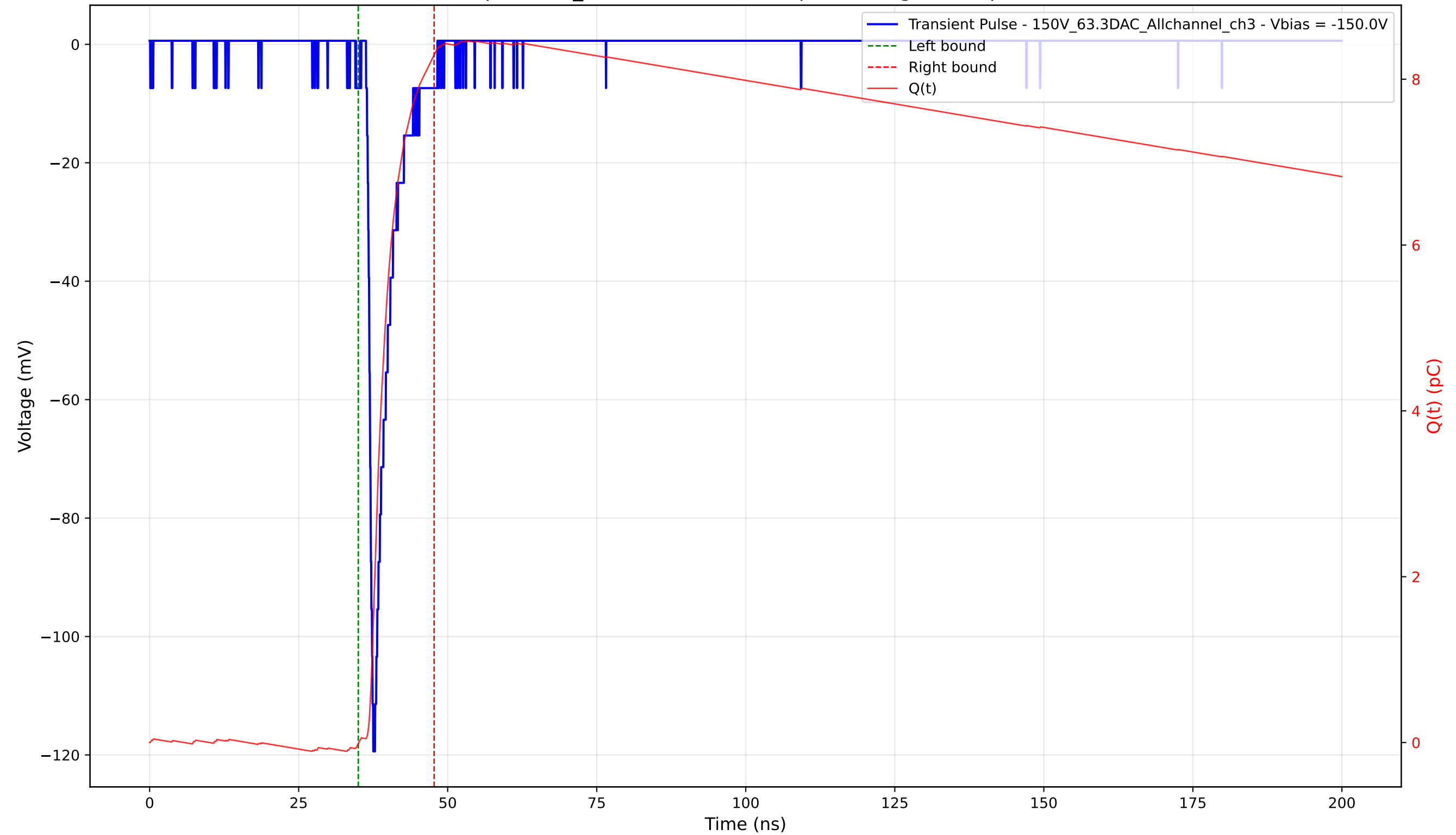
Transient Pulse - Sample: 1cm_42 - Position: 1655.0 \mu\text{m} - Charge: 8.31 pC - Rise Time: 0.94 ns
