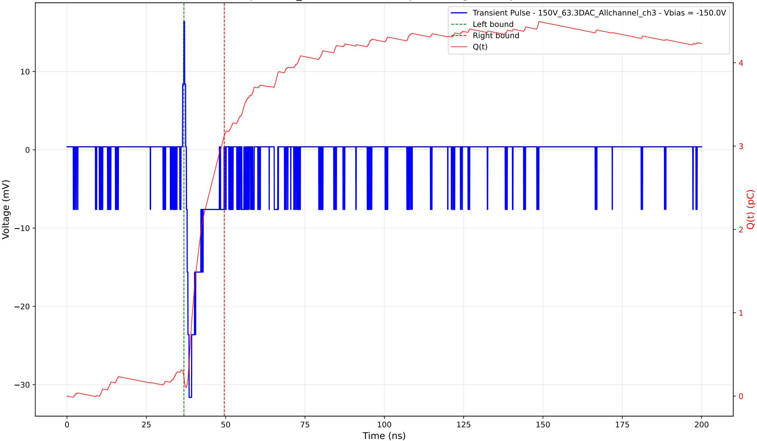
Transient Pulse - Sample: 1cm_42 - Position: 385.0 \mu\text{m} - Charge: 2.89 pC - Rise Time: 0.86 ns
