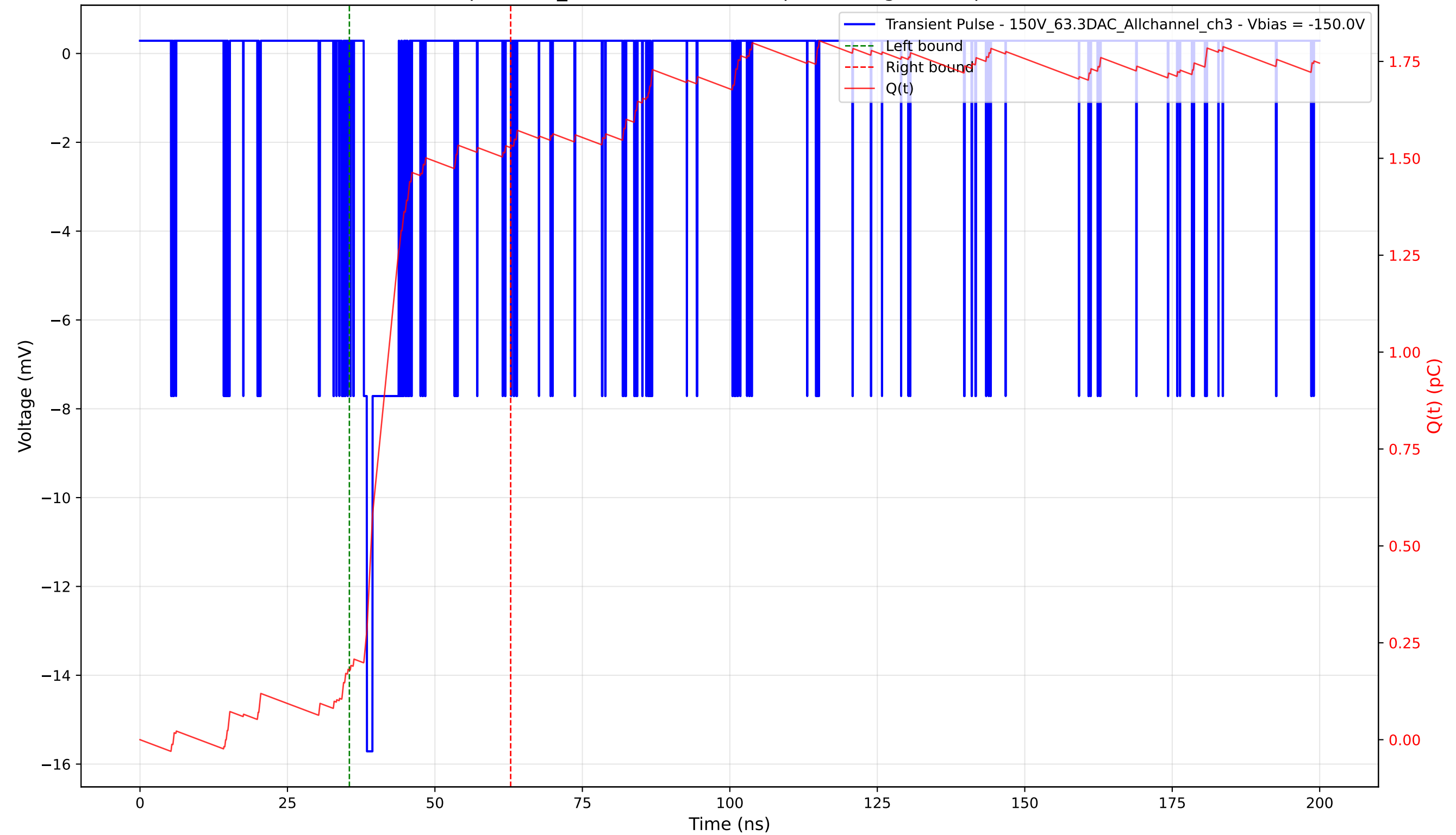
Transient Pulse - Sample: 1cm_42 - Position: 5065.0 \mu\text{m} - Charge: 1.35 pC - Rise Time: 0.55 ns
