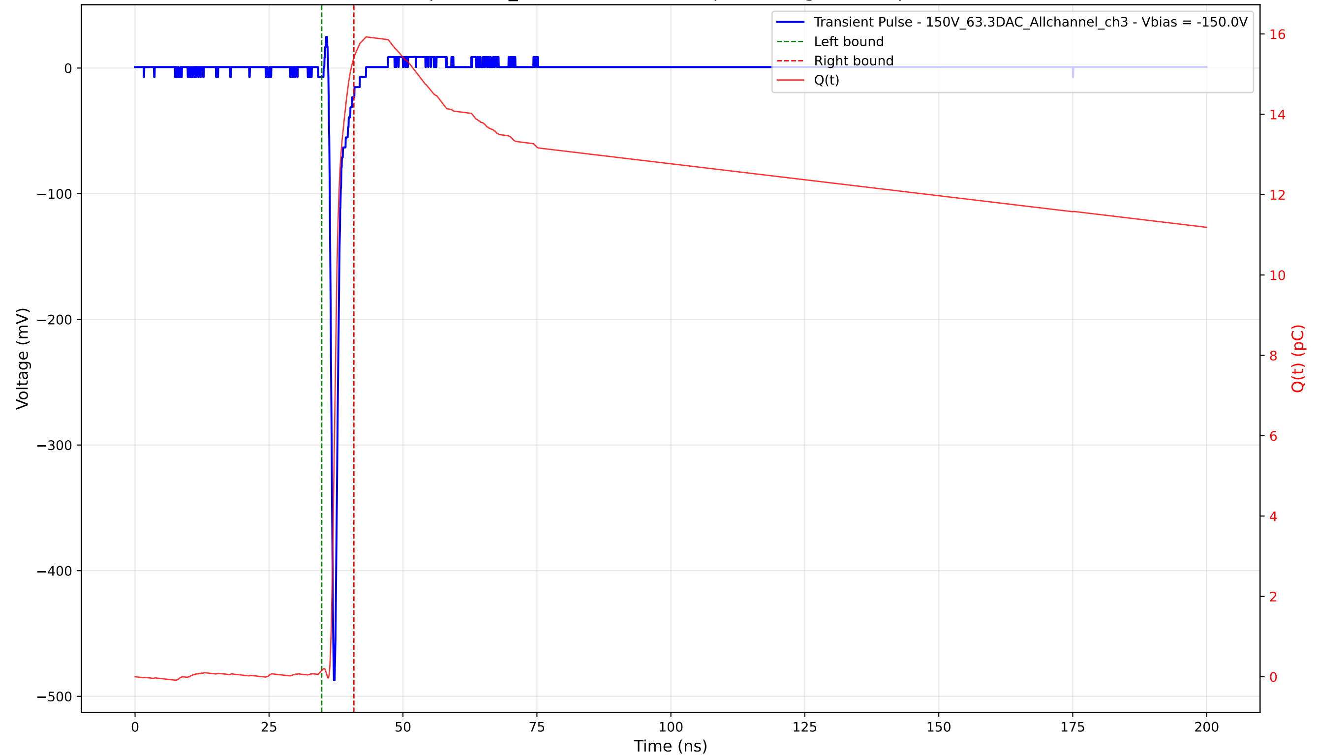
Transient Pulse - Sample: 1cm_42 - Position: 2660.0 \mu\text{m} - Charge: 15.25 pC - Rise Time: 0.73 ns
