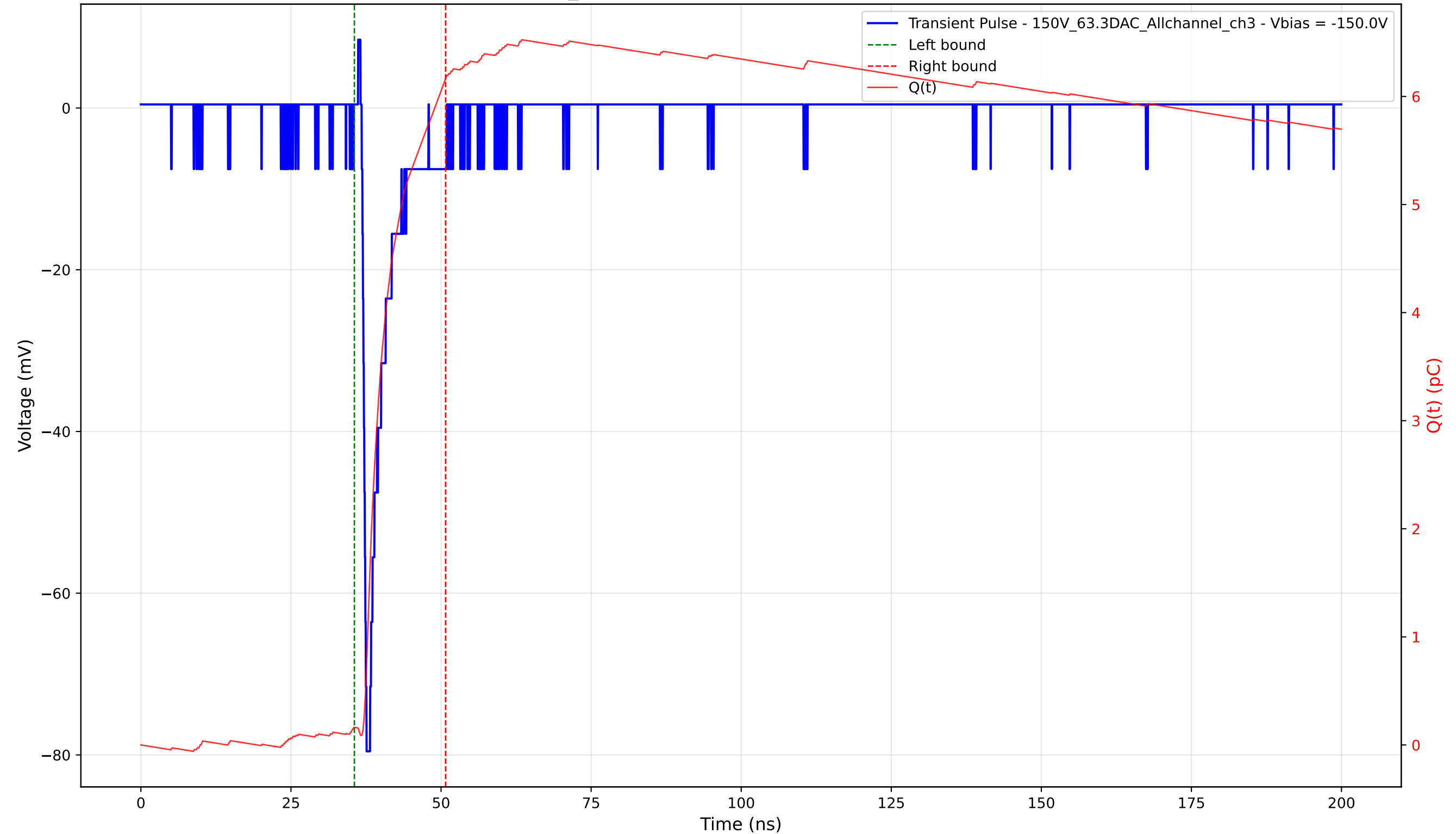
Transient Pulse - Sample: 1cm_42 - Position: 3475.0 \mu\text{m} - Charge: 6.01 pC - Rise Time: 0.72 ns
