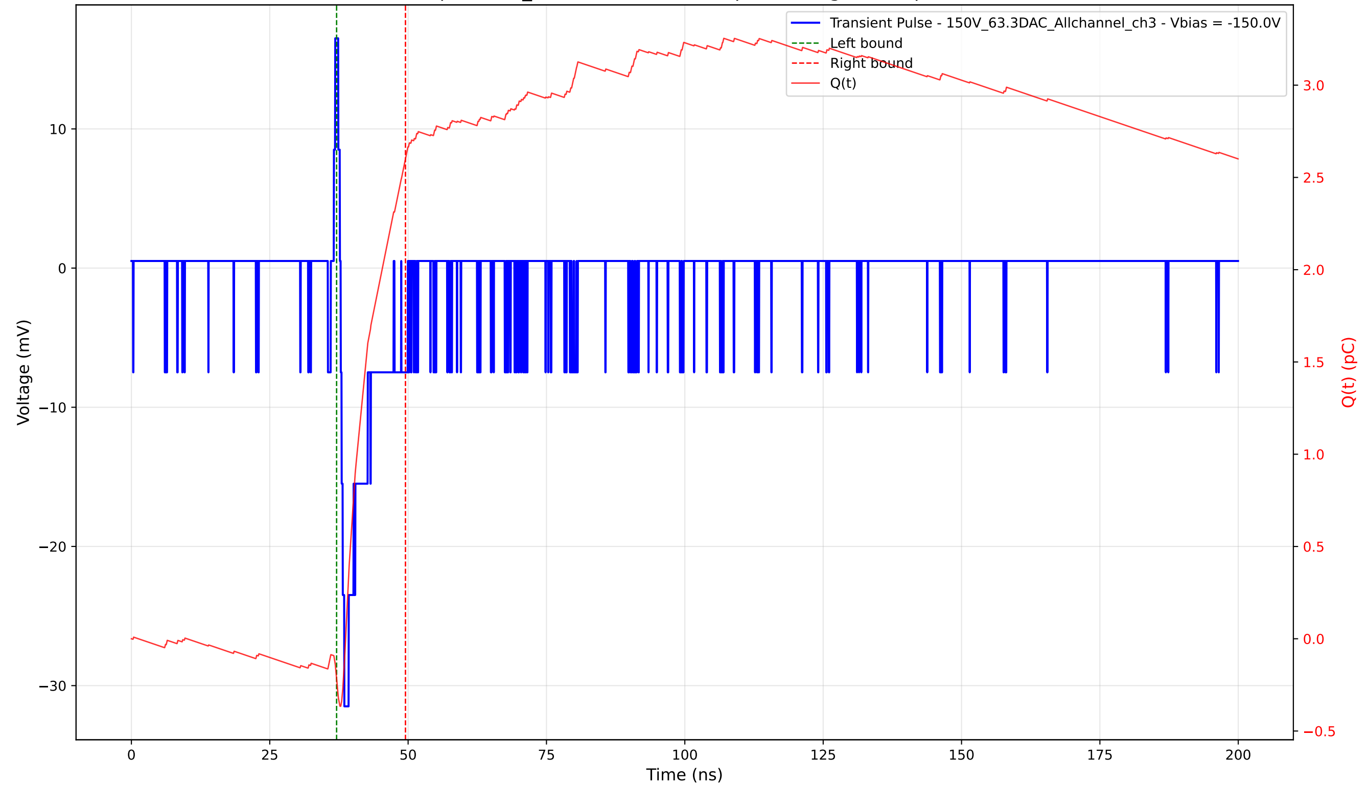
Transient Pulse - Sample: 1cm_42 - Position: 4690.0 \mu\text{m} - Charge: 2.82 pC - Rise Time: 0.66 ns
