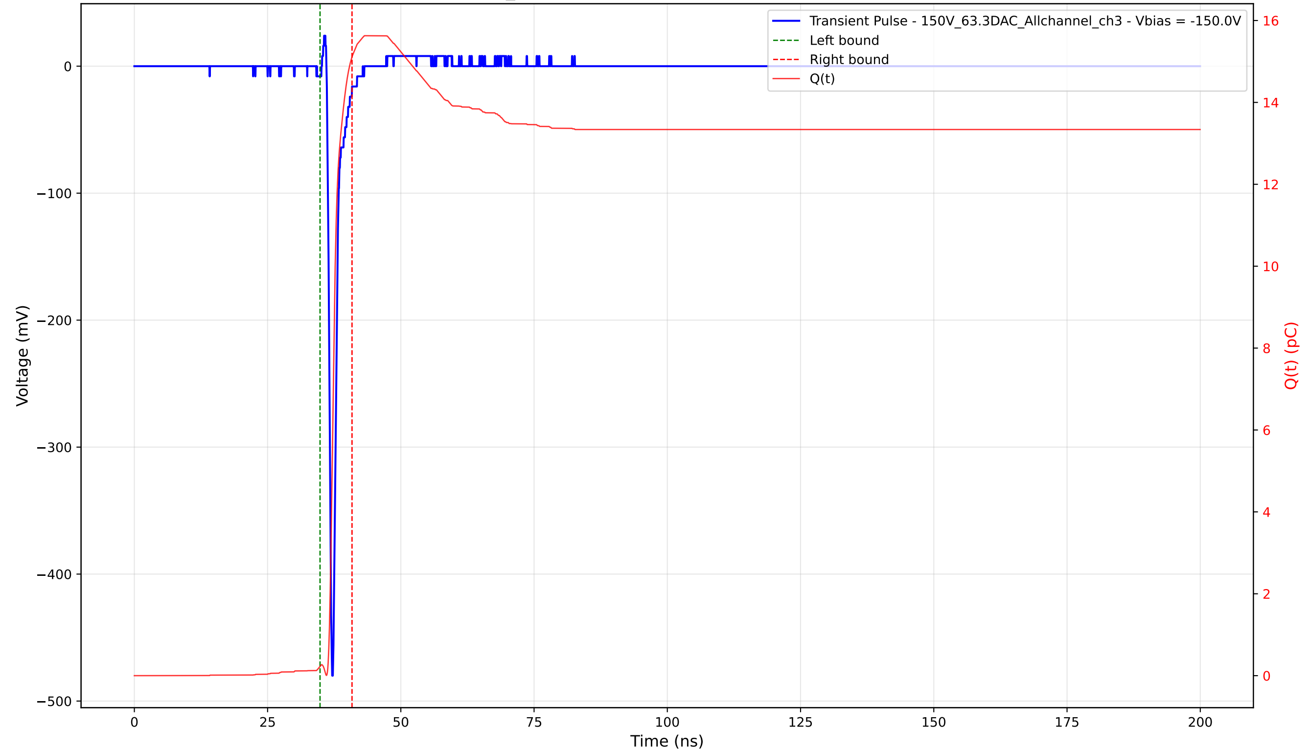
Transient Pulse - Sample: 1cm_42 - Position: 2395.0 \mu\text{m} - Charge: 14.89 pC - Rise Time: 0.70 ns
