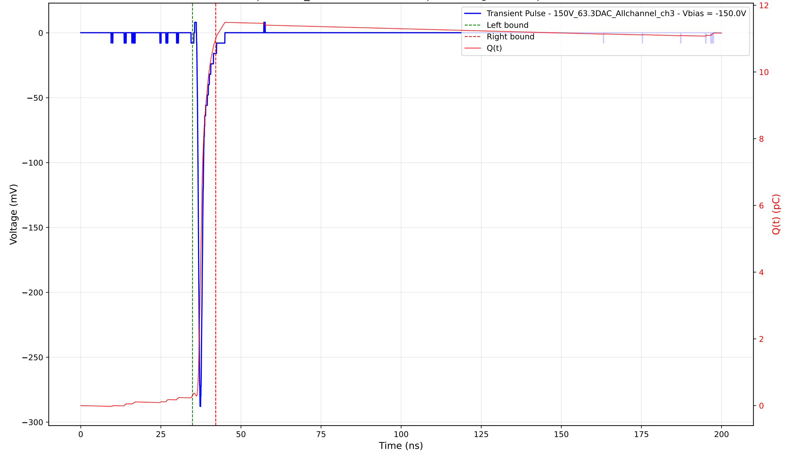
Transient Pulse - Sample: 1cm_42 - Position: 2950.0 \mu\text{m} - Charge: 10.69 pC - Rise Time: 0.75 ns
