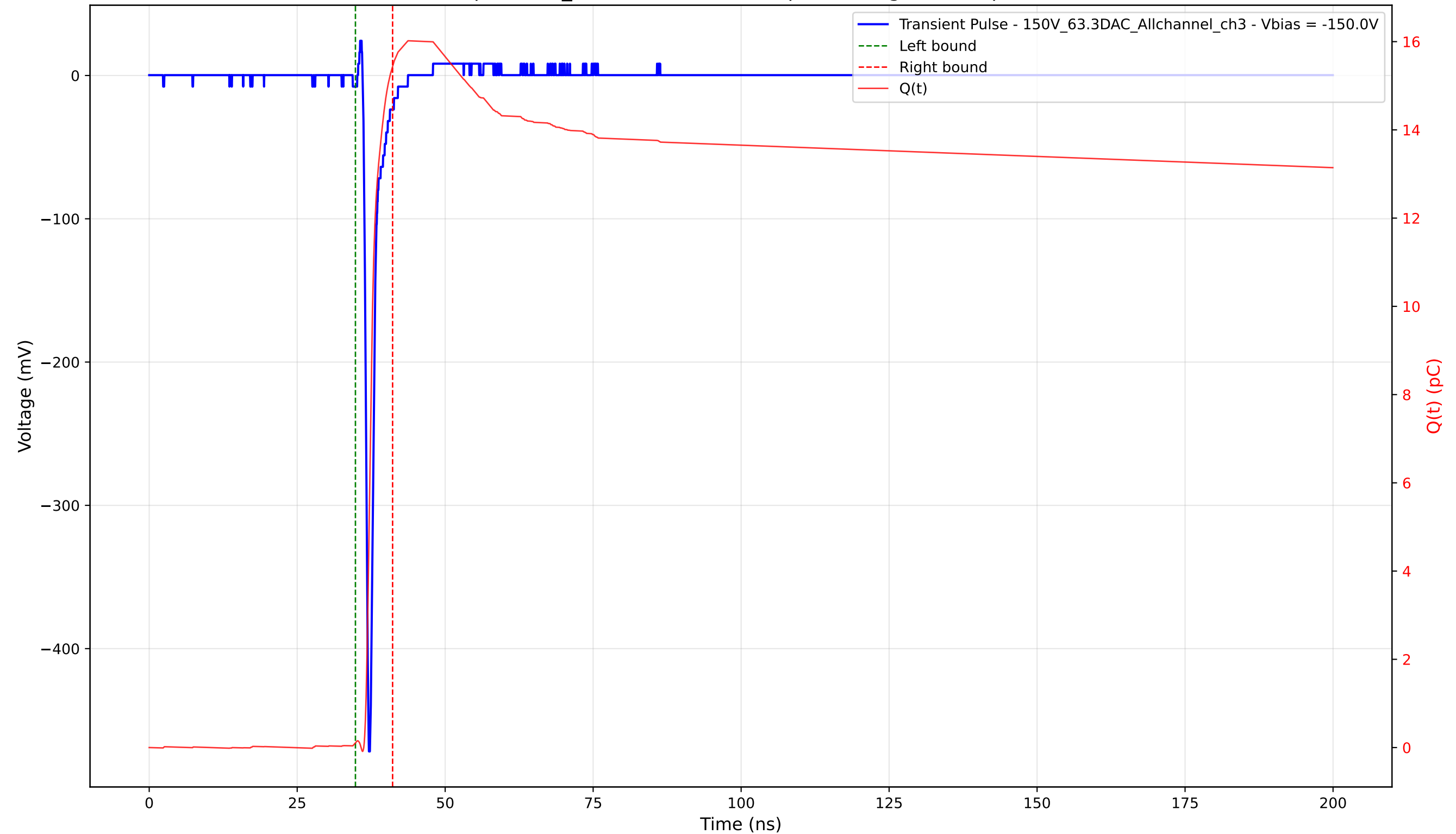
Transient Pulse - Sample: 1cm_42 - Position: 2290.0 \mu\text{m} - Charge: 15.33 pC - Rise Time: 0.72 ns
