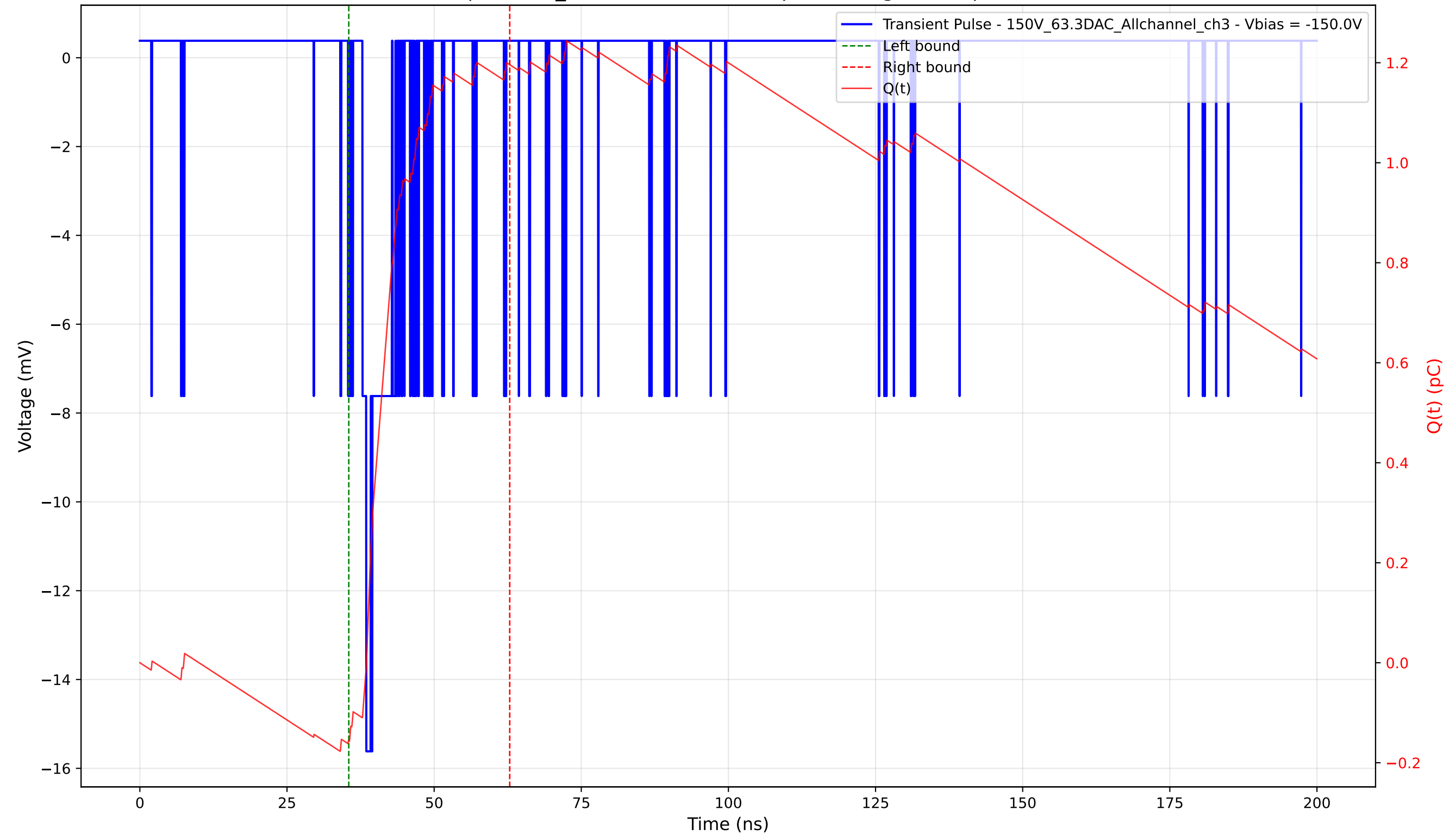
Transient Pulse - Sample: 1cm_42 - Position: 5075.0 \mu\text{m} - Charge: 1.35 pC - Rise Time: 0.67 ns
