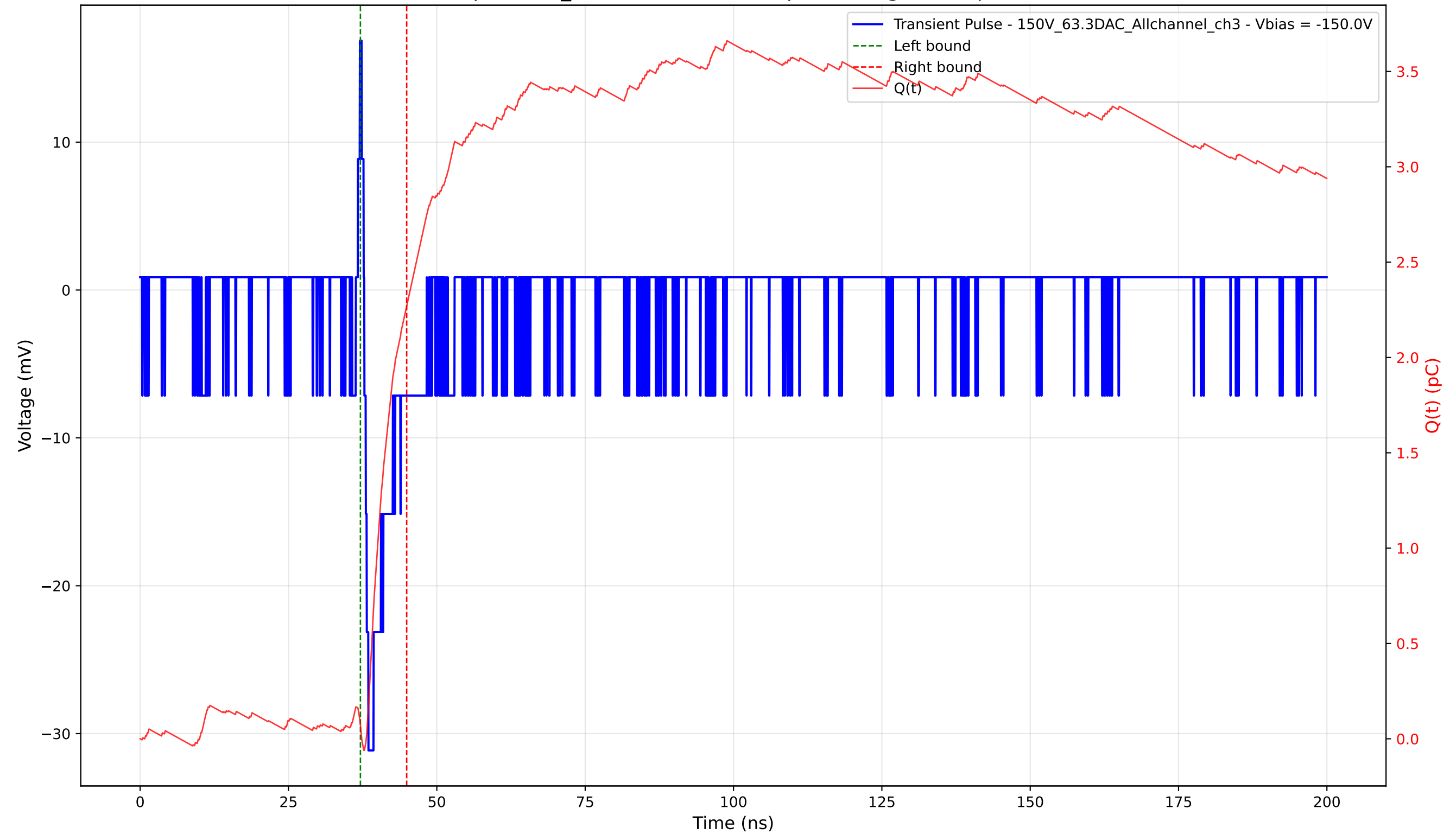
Transient Pulse - Sample: 1cm_42 - Position: 4820.0 \mu\text{m} - Charge: 2.20 pC - Rise Time: 0.71 ns
