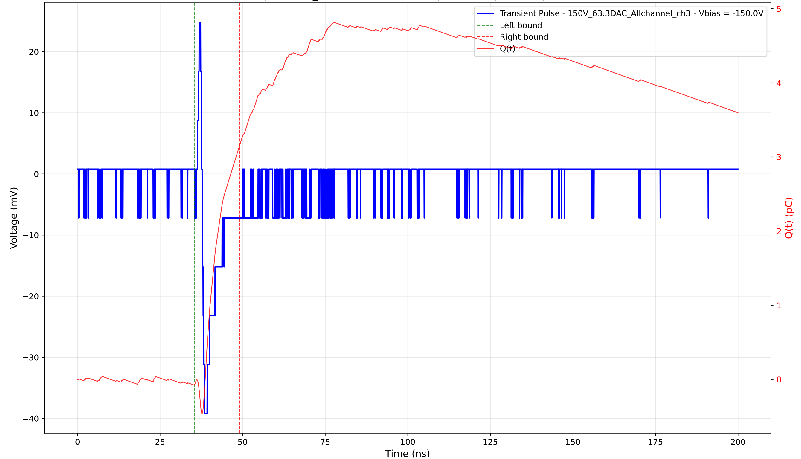
Transient Pulse - Sample: 1cm_42 - Position: 4290.0 \mu\text{m} - Charge: 3.21 pC - Rise Time: 0.70 ns
