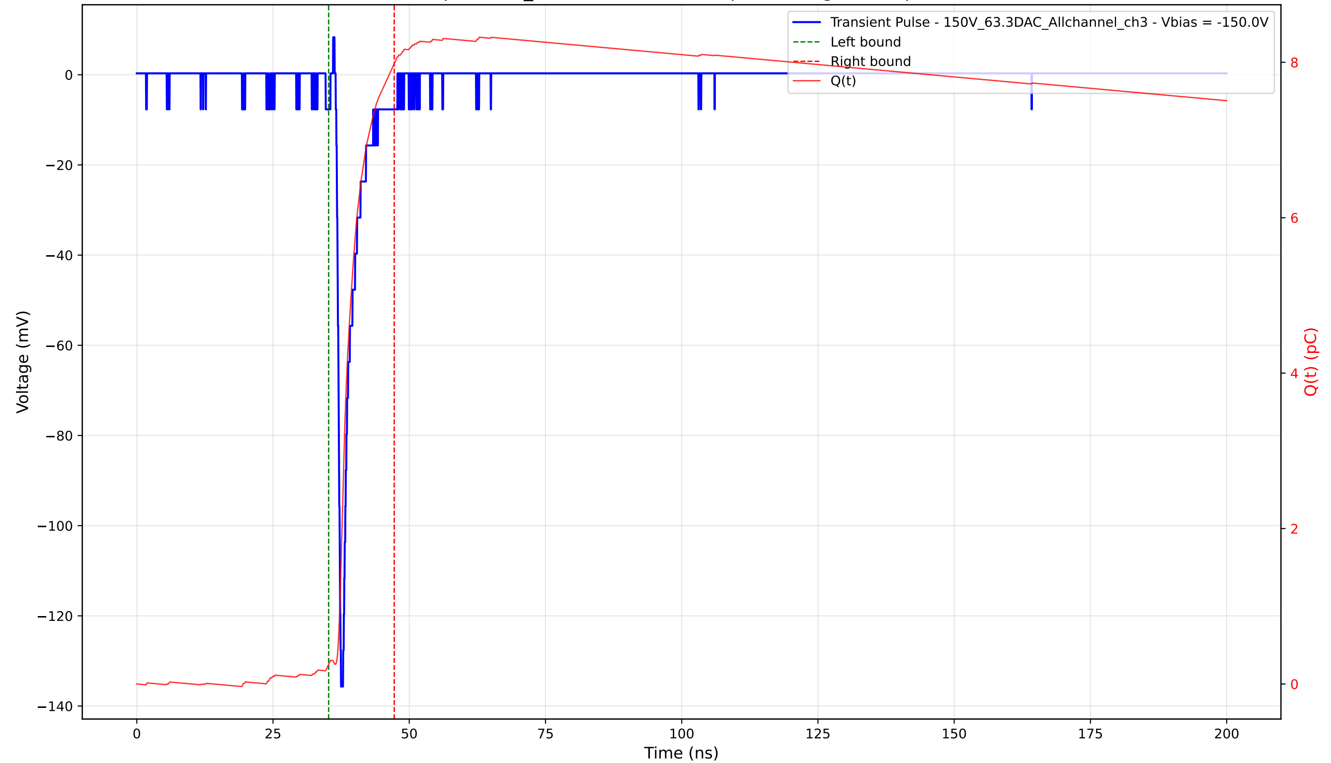
Transient Pulse - Sample: 1cm_42 - Position: 3275.0 \mu\text{m} - Charge: 7.73 pC - Rise Time: 0.77 ns
