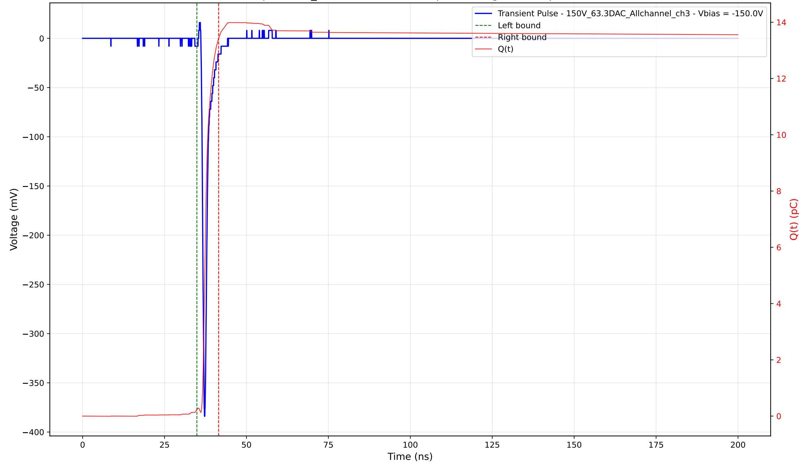
Transient Pulse - Sample: 1cm_42 - Position: 2180.0 \mu\text{m} - Charge: 13.20 pC - Rise Time: 0.77 ns
