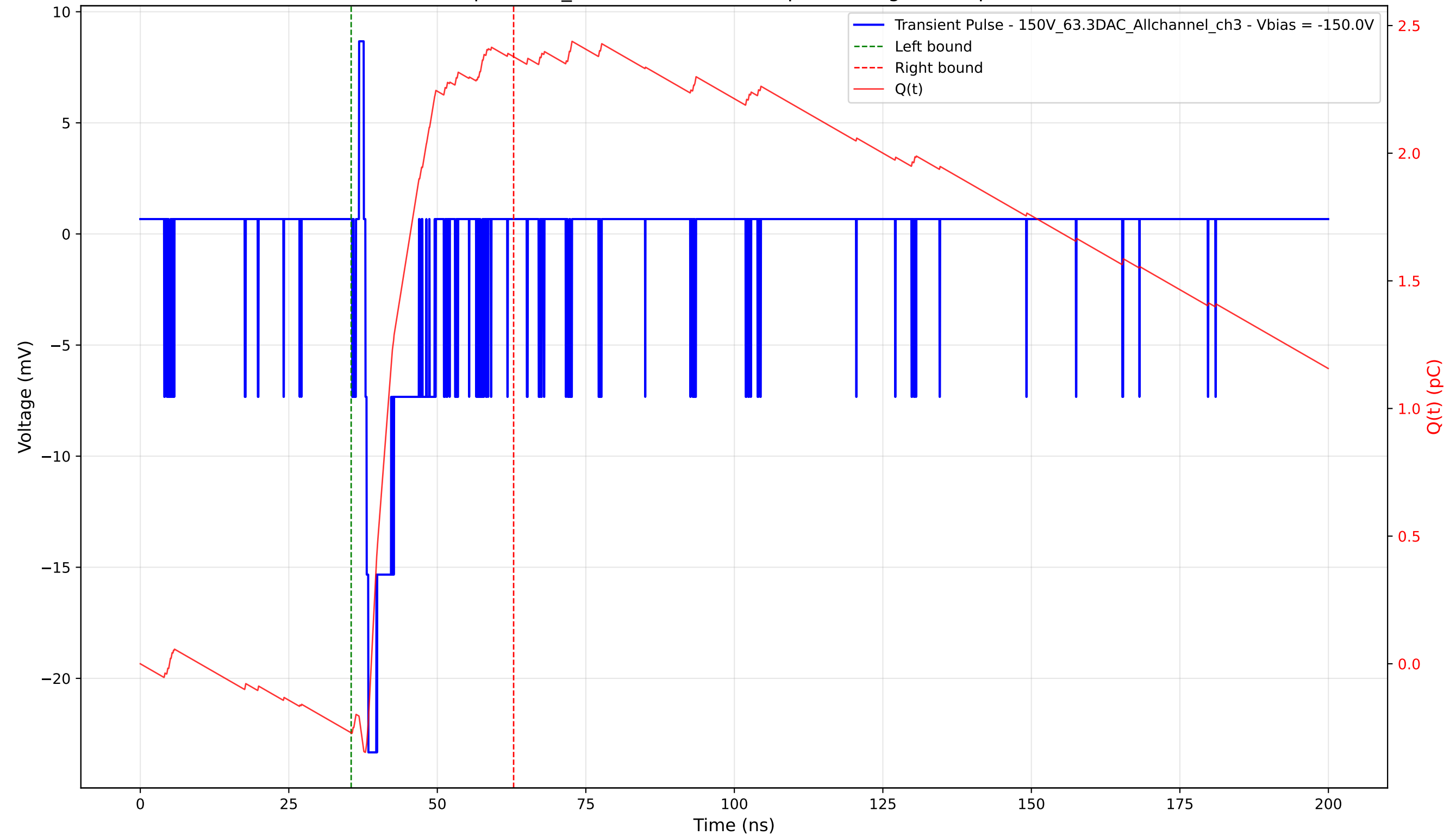
Transient Pulse - Sample: 1cm_42 - Position: 4915.0 \mu\text{m} - Charge: 2.65 pC - Rise Time: 0.51 ns
