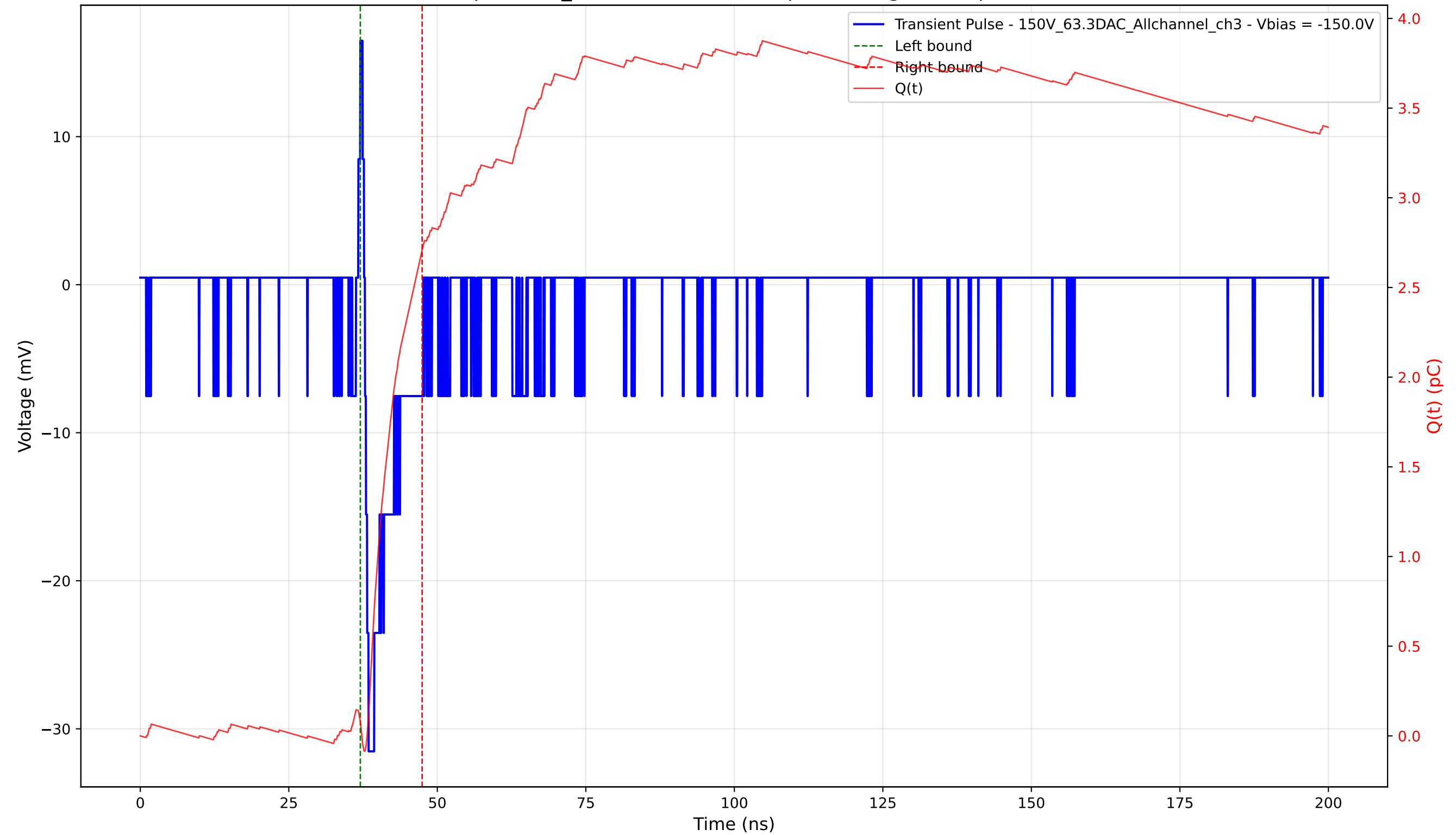
Transient Pulse - Sample: 1cm_42 - Position: 4745.0 \mu\text{m} - Charge: 2.63 pC - Rise Time: 0.62 ns
