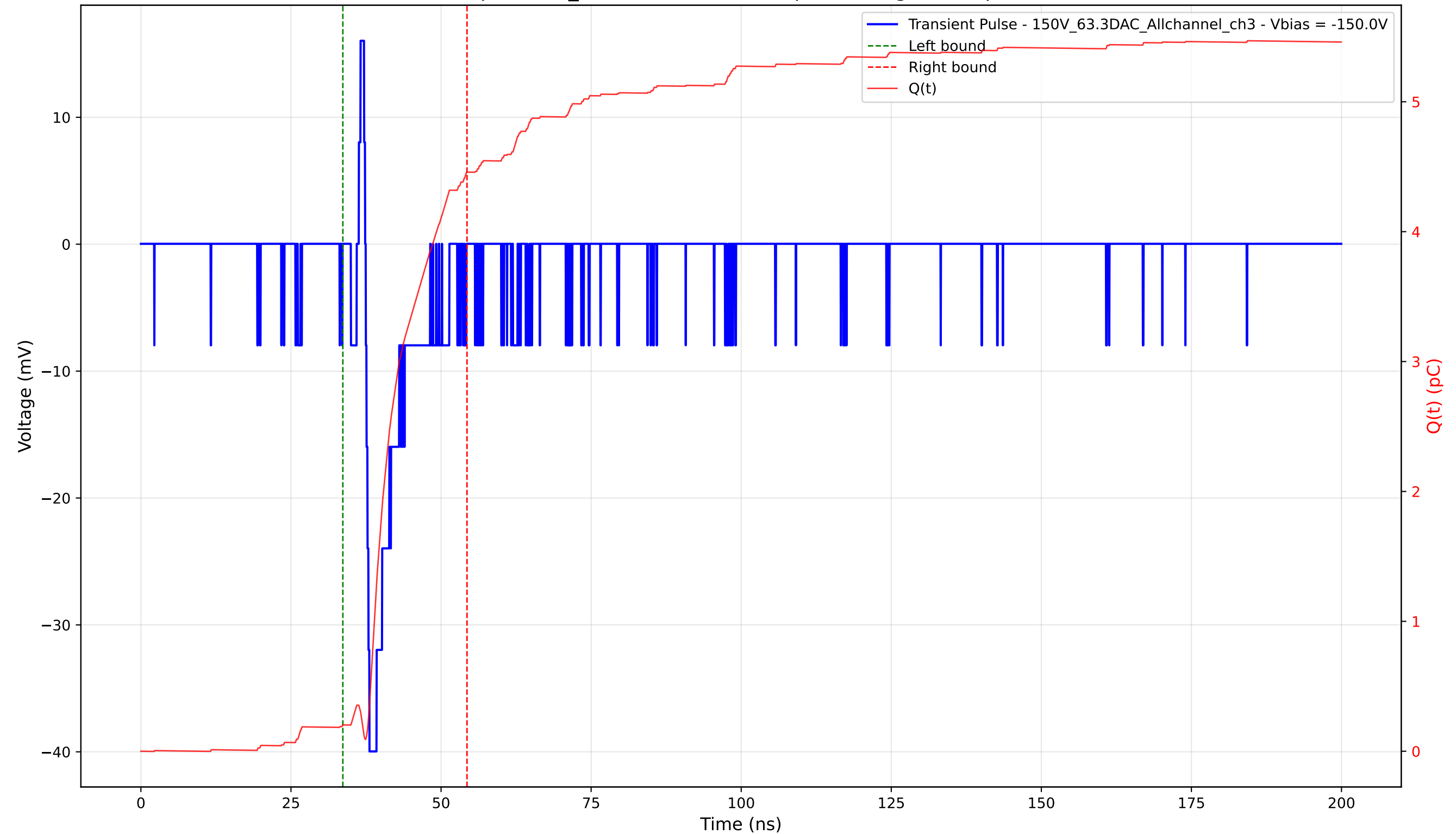
Transient Pulse - Sample: 1cm_42 - Position: 3970.0 \mu\text{m} - Charge: 4.26 pC - Rise Time: 0.62 ns
