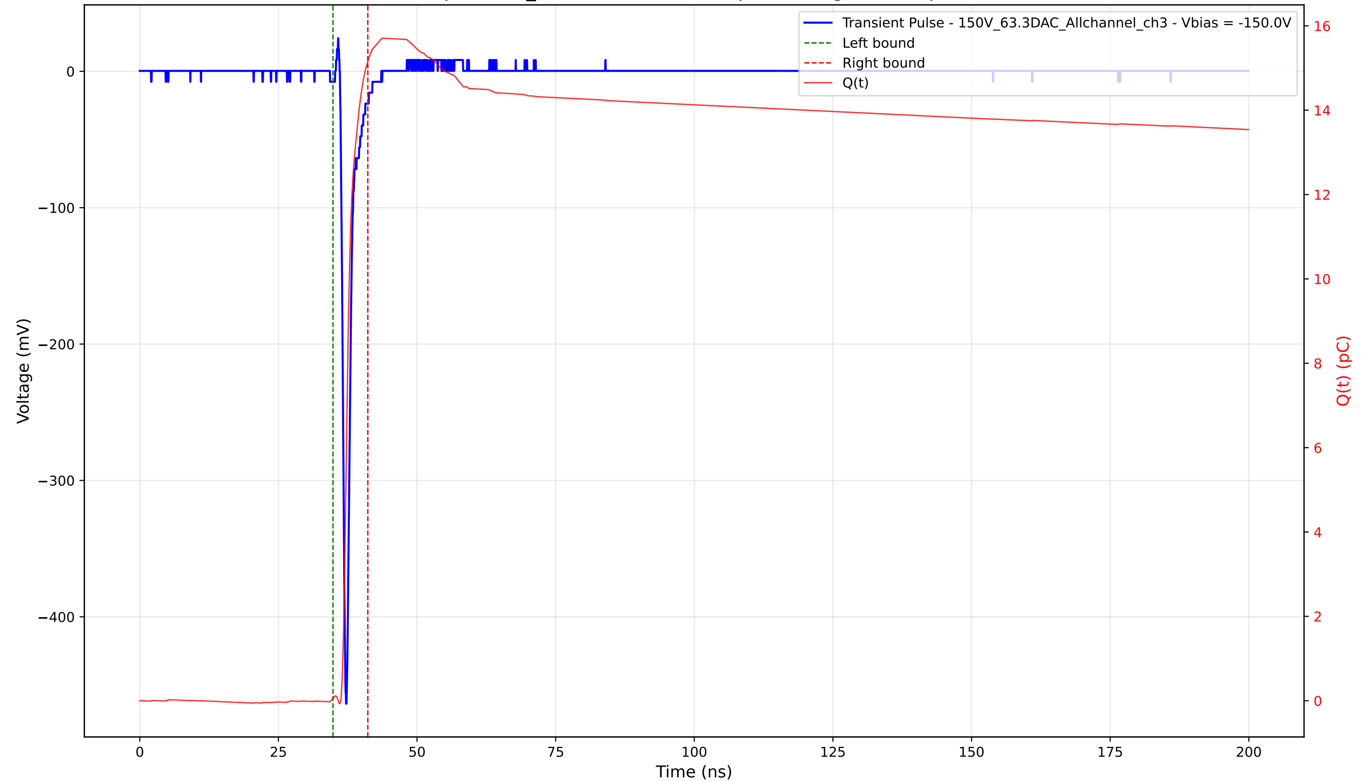
Transient Pulse - Sample: 1cm_42 - Position: 2770.0 \mu\text{m} - Charge: 15.10 pC - Rise Time: 0.75 ns
