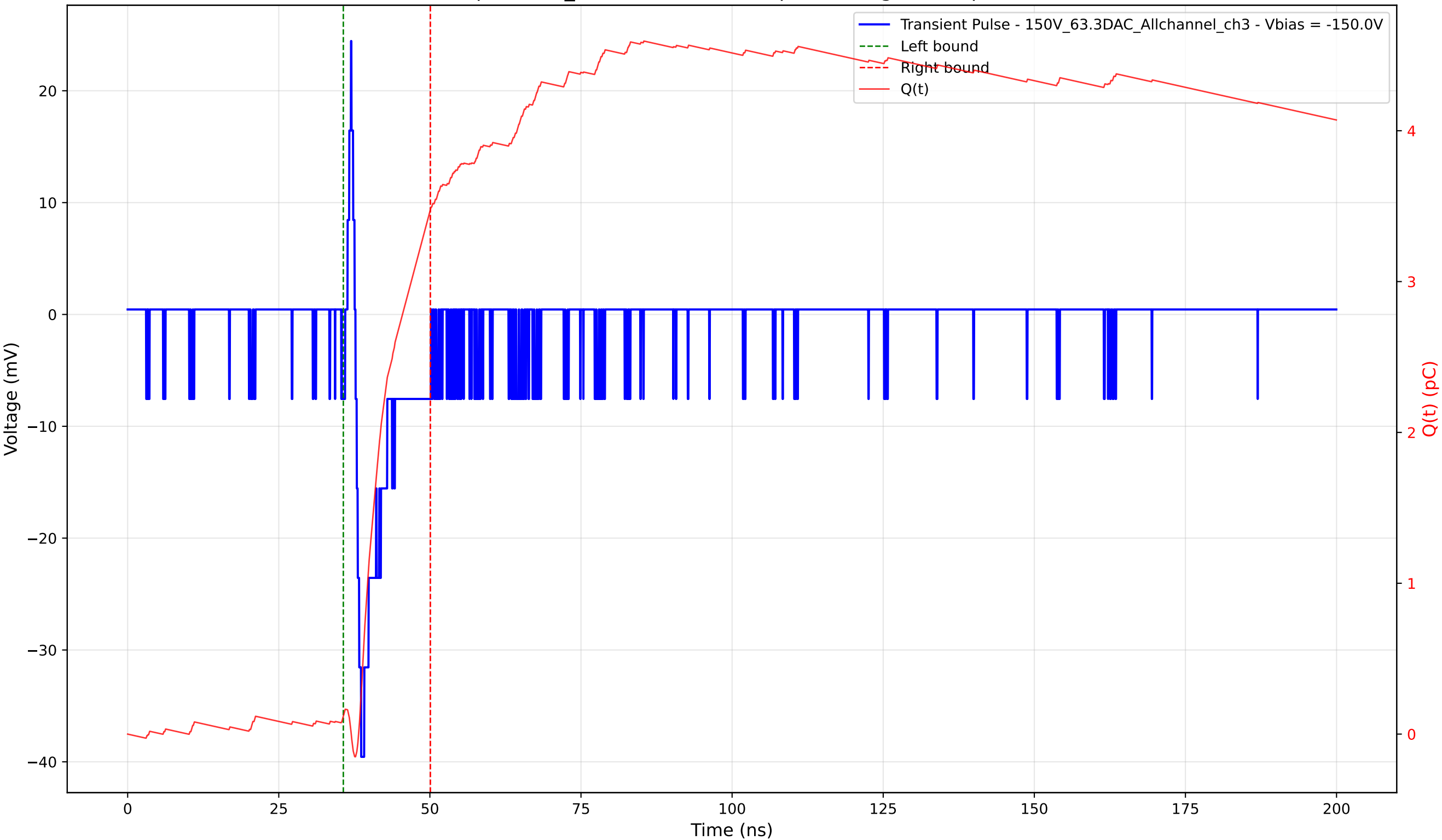
Transient Pulse - Sample: 1cm_42 - Position: 515.0 \mu\text{m} - Charge: 3.36 pC - Rise Time: 0.94 ns
