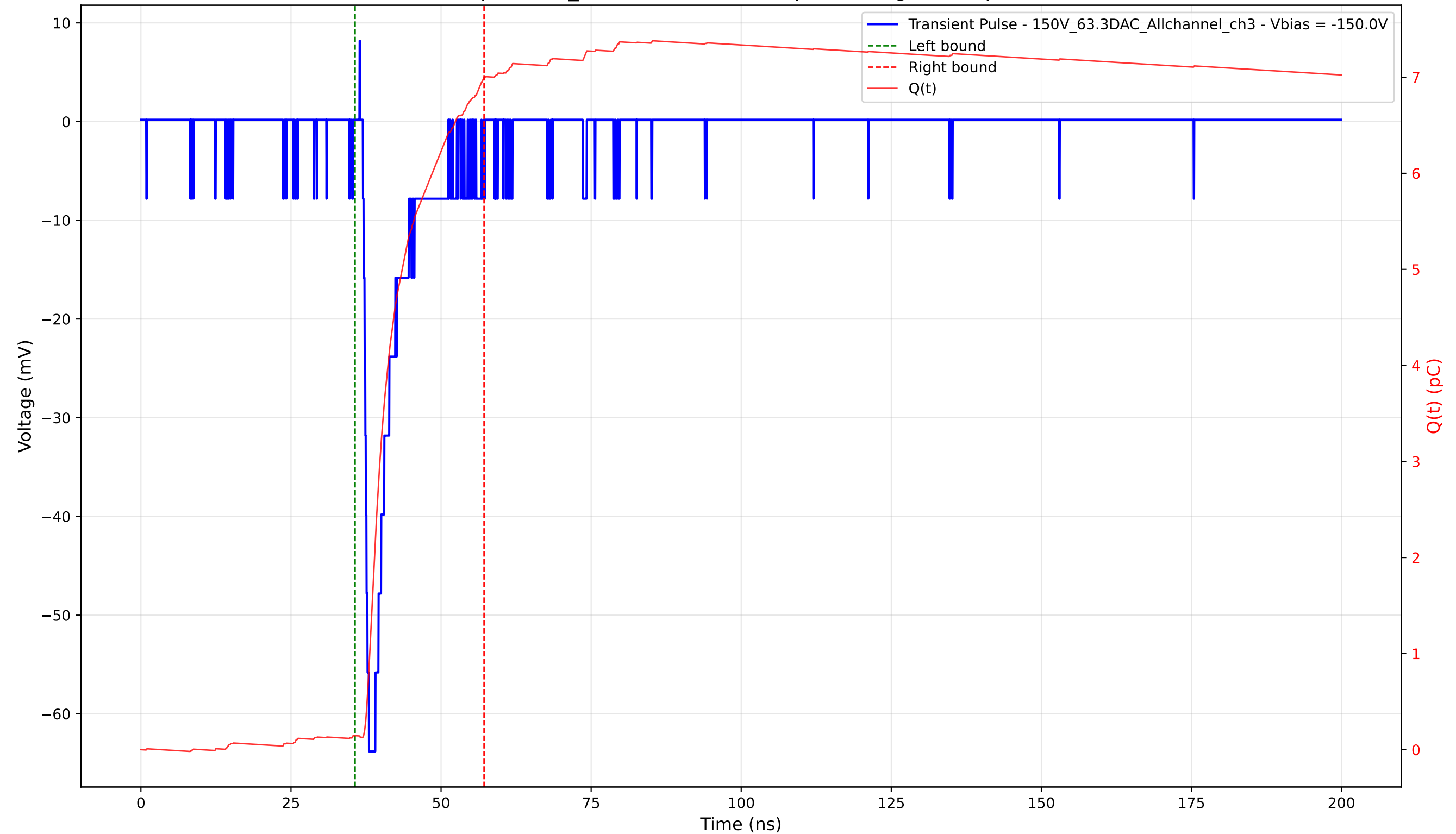
Transient Pulse - Sample: 1cm_42 - Position: 1400.0 \mu\text{m} - Charge: 6.85 pC - Rise Time: 1.01 ns
