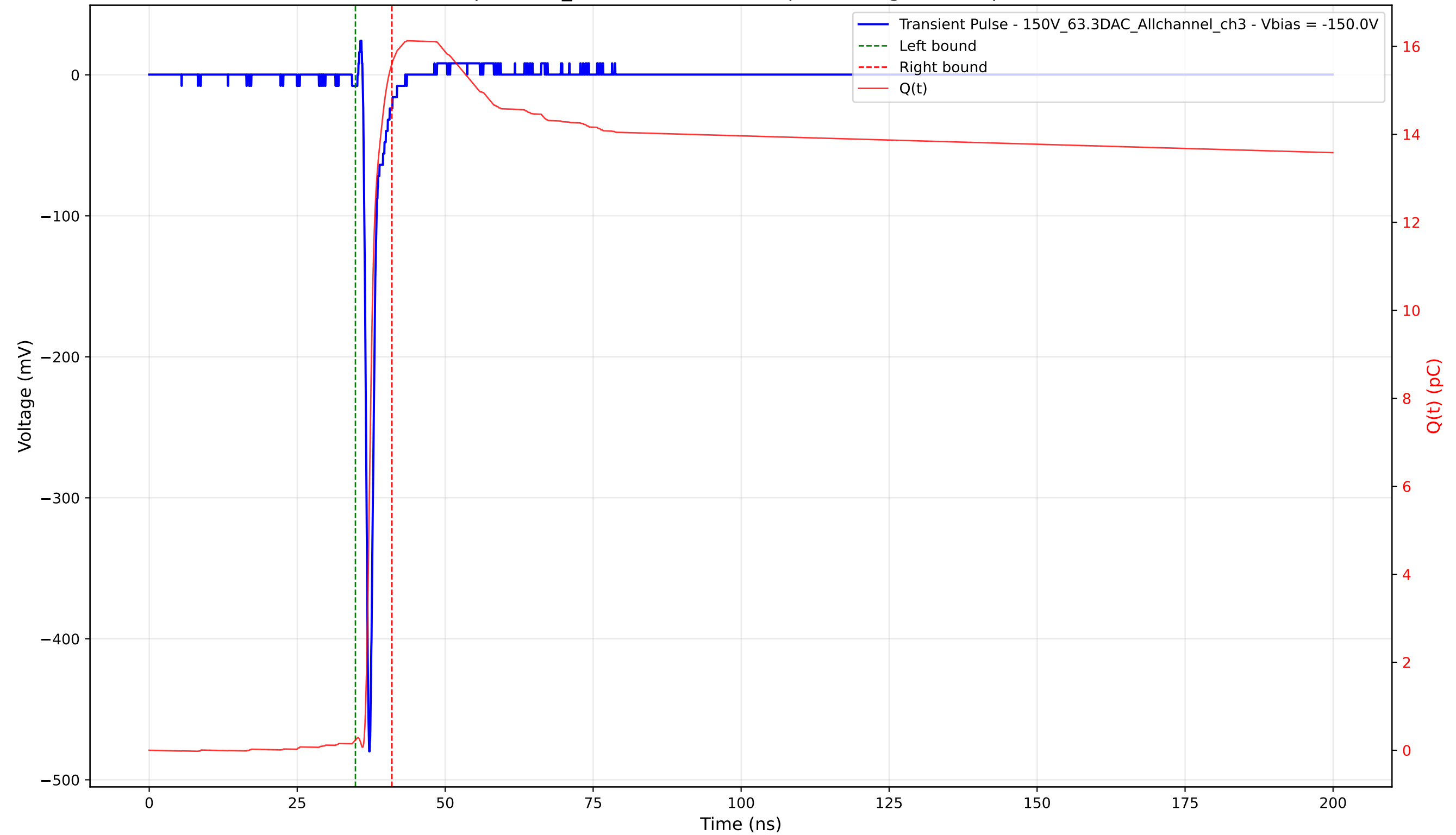
Transient Pulse - Sample: 1cm_42 - Position: 2715.0 \mu\text{m} - Charge: 15.37 pC - Rise Time: 0.70 ns
