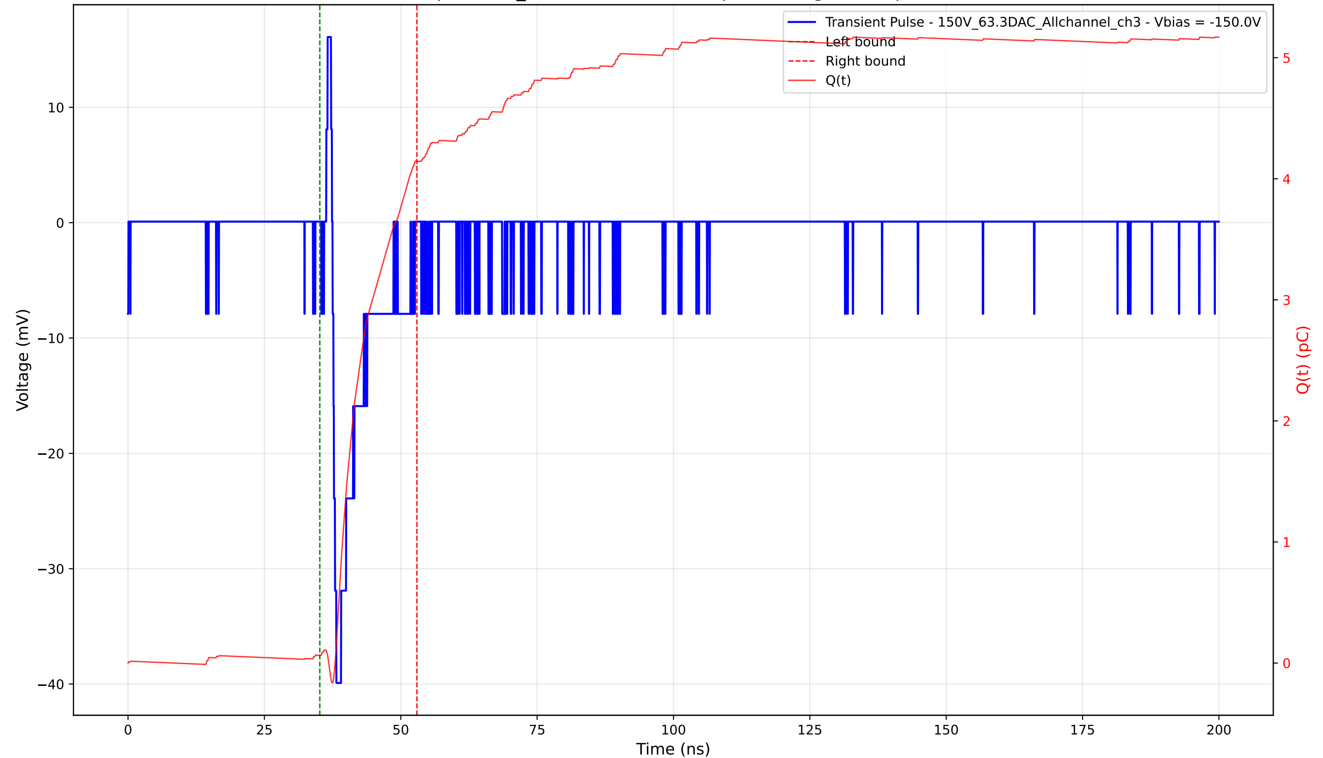
Transient Pulse - Sample: 1cm_42 - Position: 4000.0 \mu\text{m} - Charge: 4.08 pC - Rise Time: 0.70 ns
