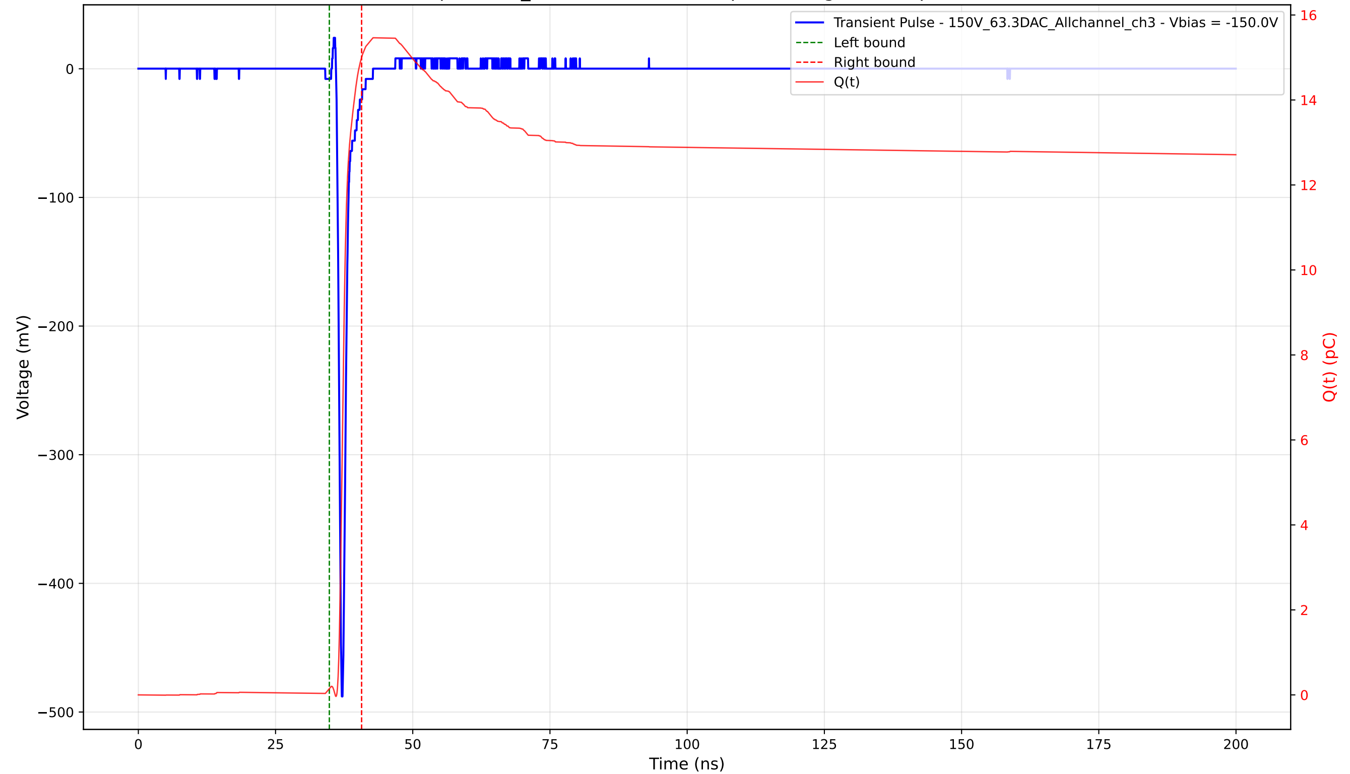
Transient Pulse - Sample: 1cm_42 - Position: 2460.0 \mu\text{m} - Charge: 14.86 pC - Rise Time: 0.67 ns
