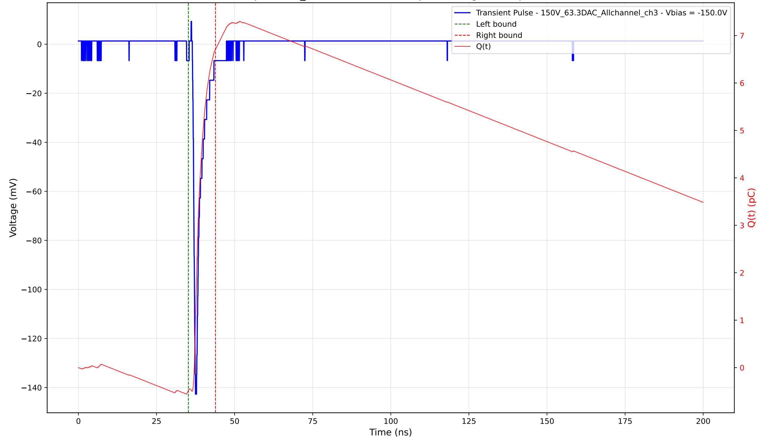
Transient Pulse - Sample: 1cm_42 - Position: 3225.0 \mu\text{m} - Charge: 7.19 pC - Rise Time: 0.80 ns
