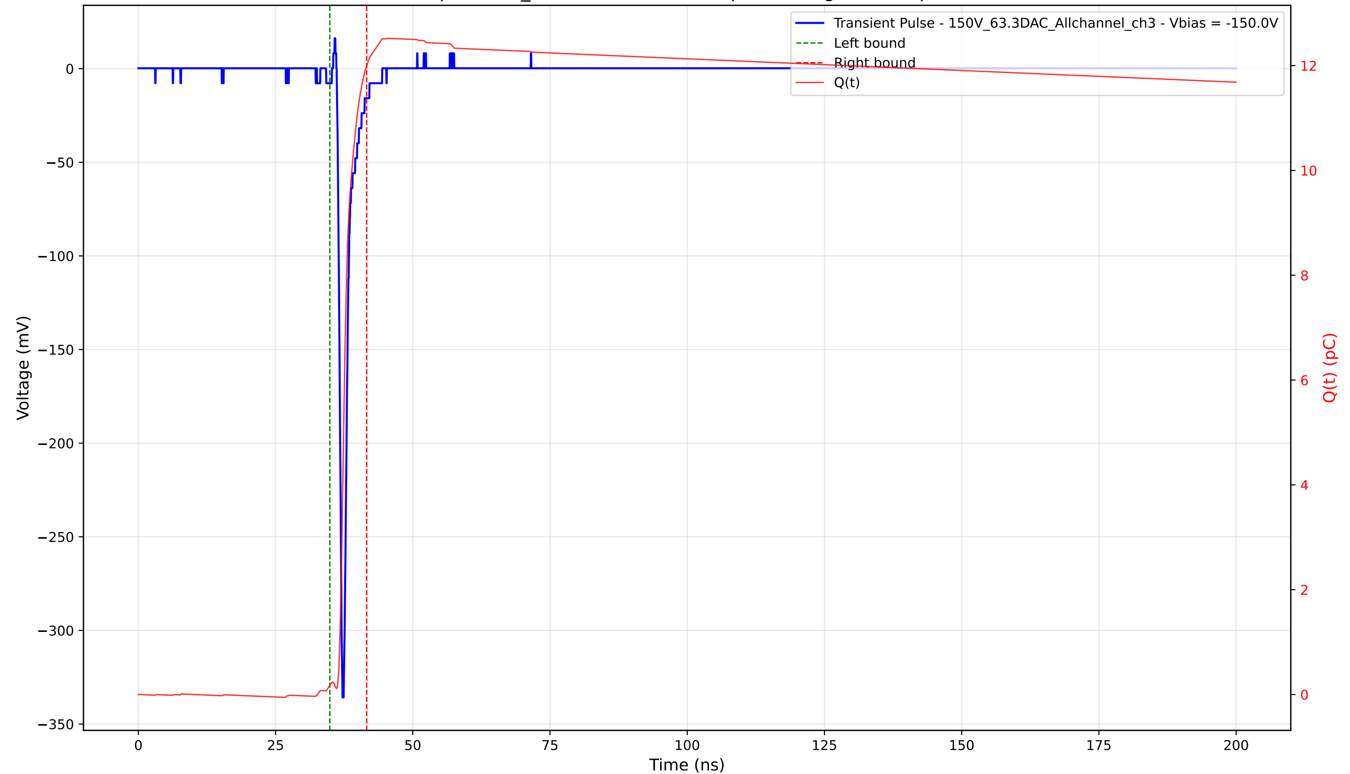
Transient Pulse - Sample: 1cm_42 - Position: 2900.0 \mu\text{m} - Charge: 11.82 pC - Rise Time: 0.74 ns
