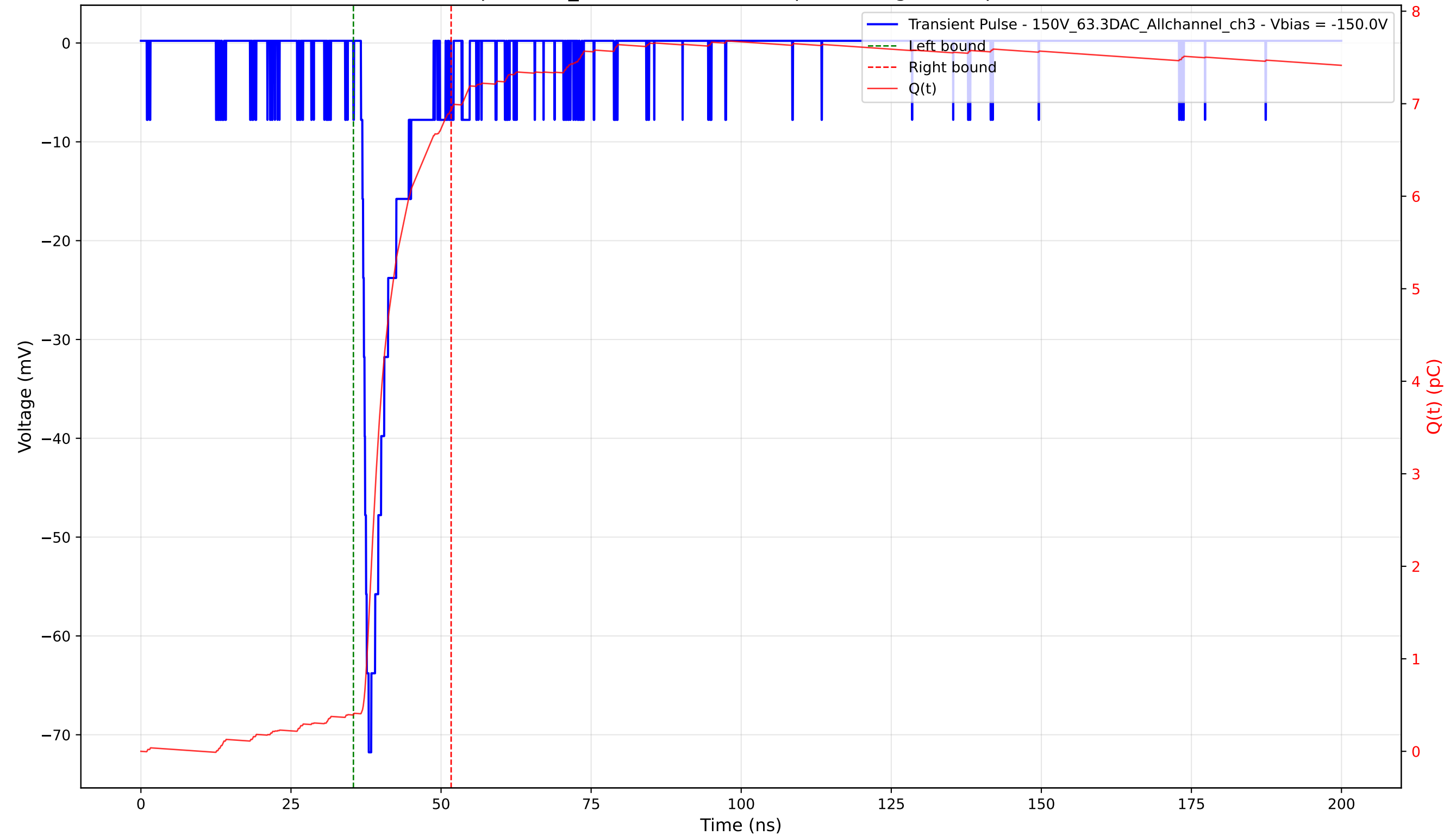
Transient Pulse - Sample: 1cm_42 - Position: 1480.0 \mu\text{m} - Charge: 6.54 pC - Rise Time: 1.28 ns
