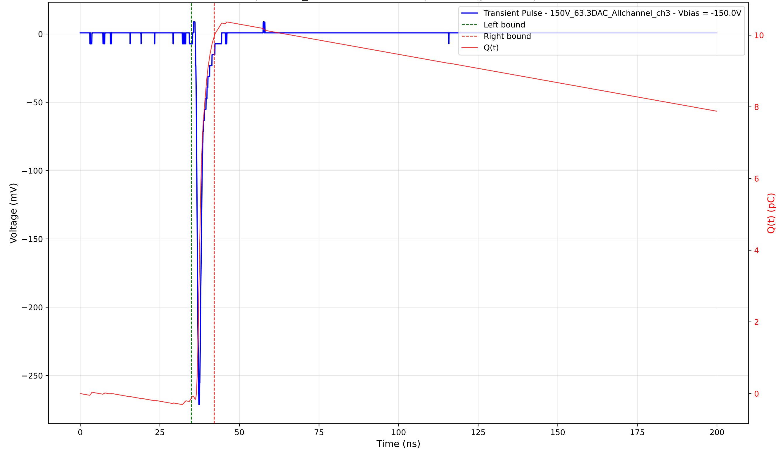
Transient Pulse - Sample: 1cm_42 - Position: 2965.0 \mu\text{m} - Charge: 10.09 pC - Rise Time: 0.76 ns
