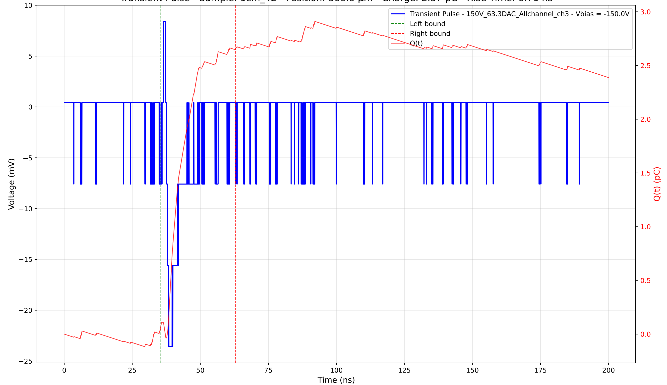
Transient Pulse - Sample: 1cm_42 - Position: 300.0 \mu\text{m} - Charge: 2.57 pC - Rise Time: 0.71 ns
