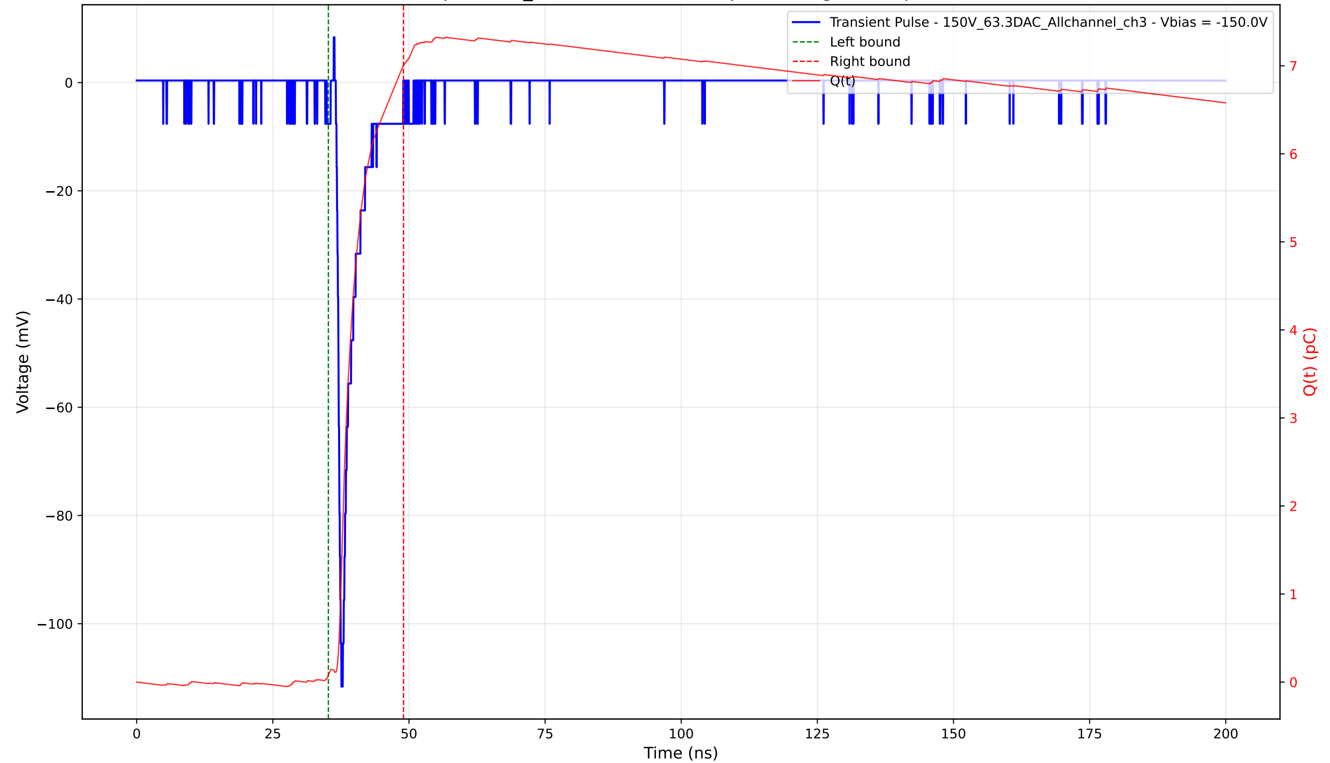
Transient Pulse - Sample: 1cm_42 - Position: 3385.0 \mu\text{m} - Charge: 6.92 pC - Rise Time: 0.78 ns
