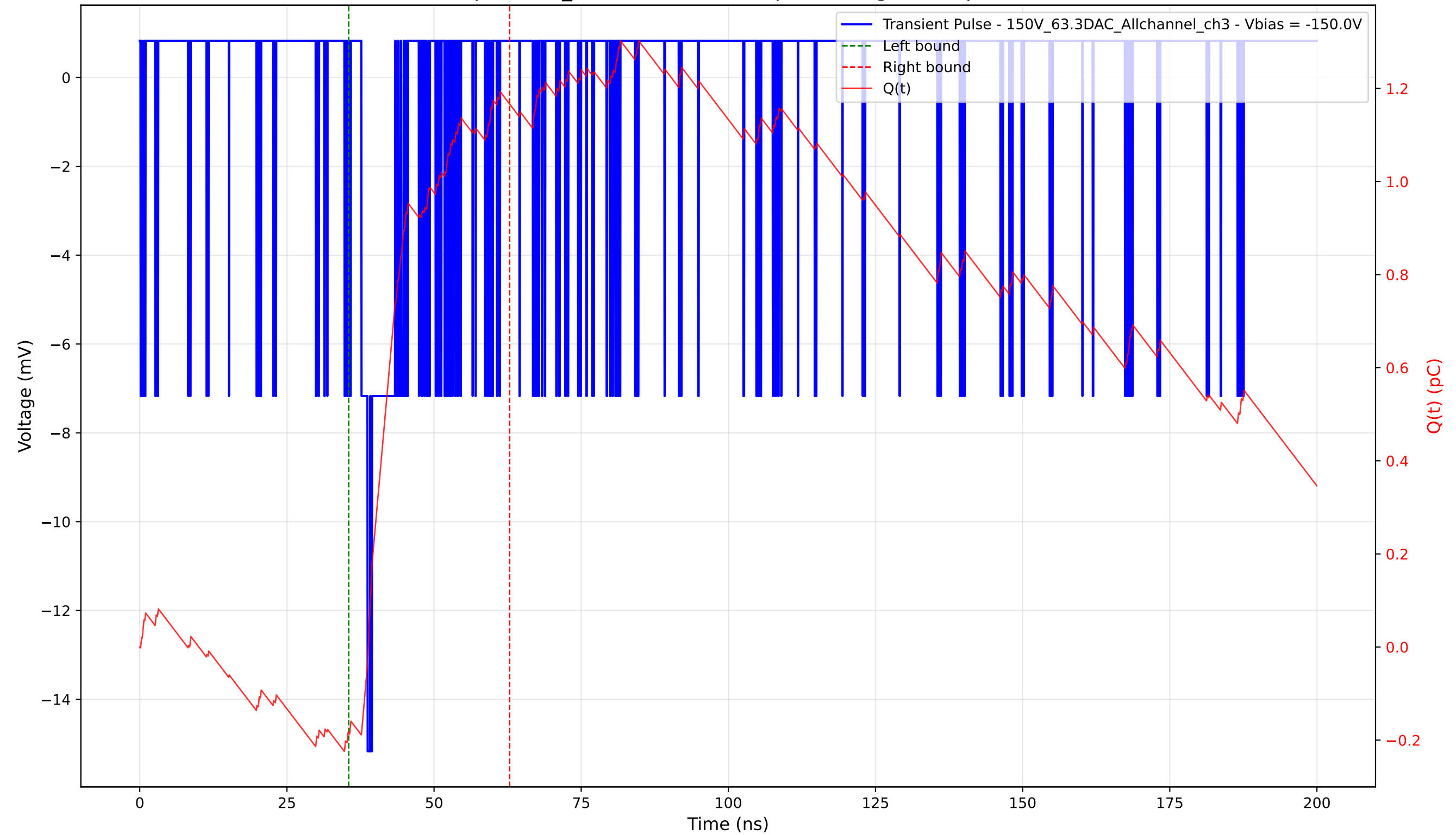
Transient Pulse - Sample: 1cm_42 - Position: 135.0 \mu\text{m} - Charge: 1.35 pC - Rise Time: 1.08 ns
