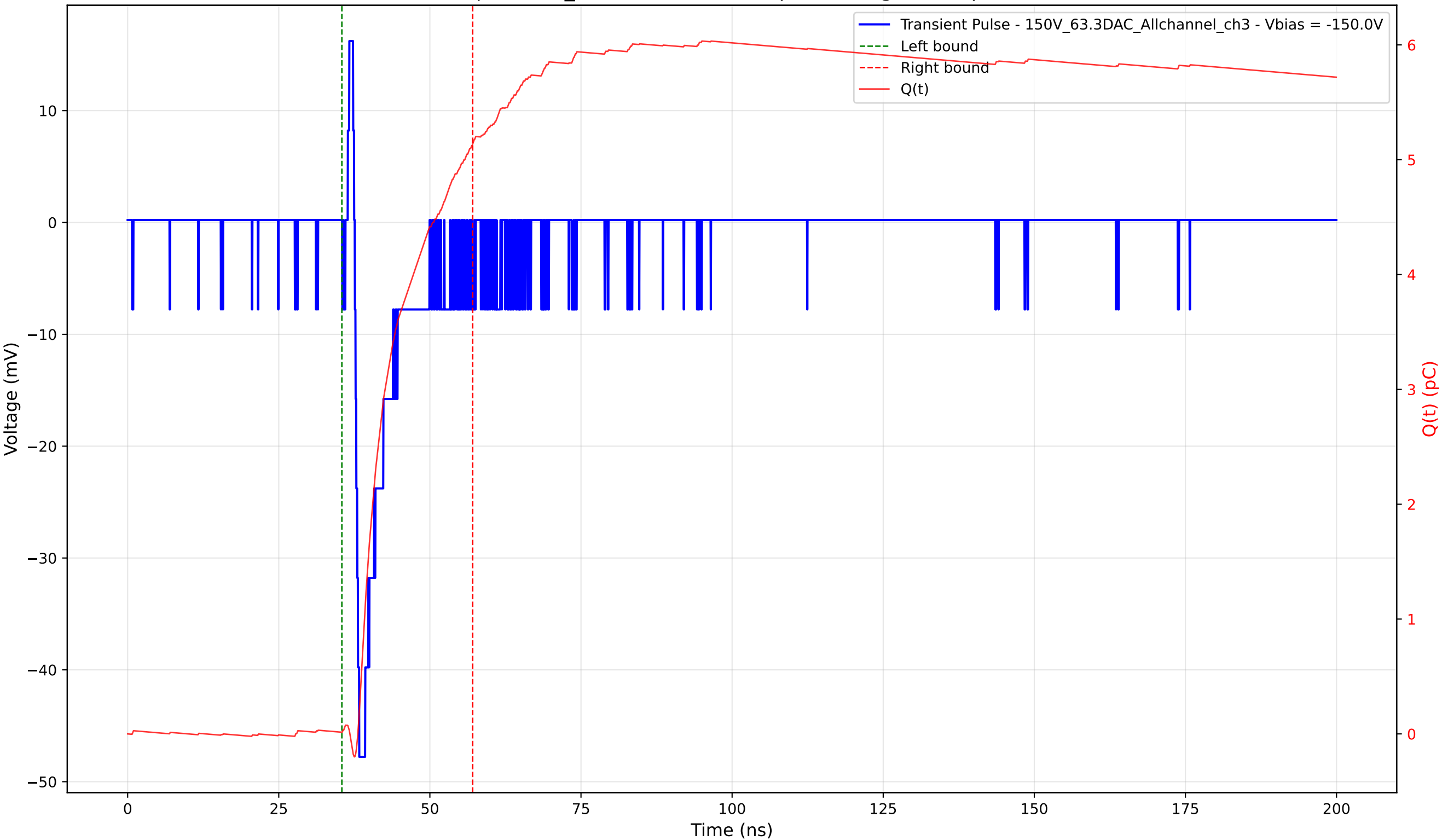
Transient Pulse - Sample: 1cm_42 - Position: 985.0 \mu\text{m} - Charge: 5.12 pC - Rise Time: 0.74 ns
