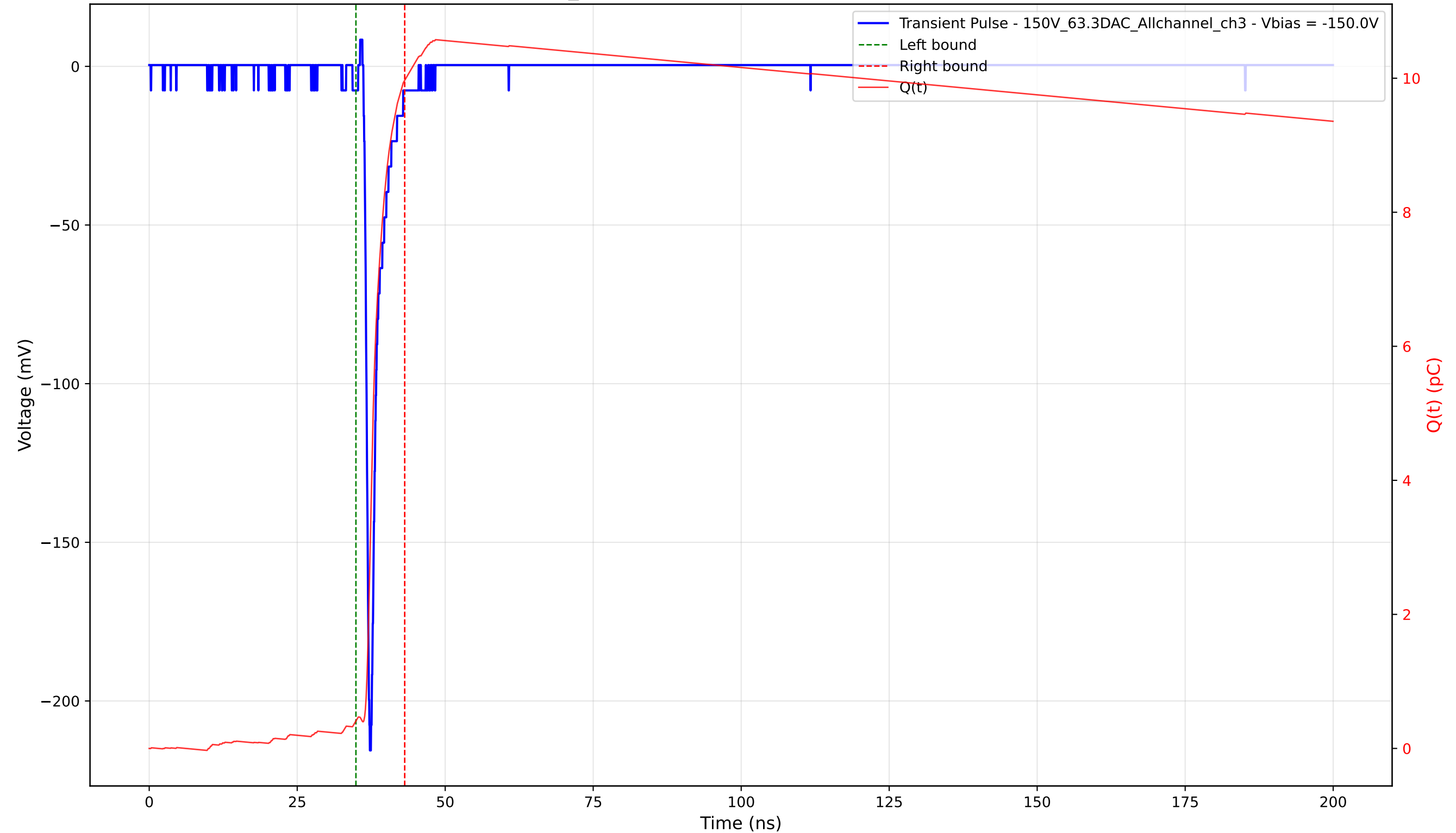
Transient Pulse - Sample: 1cm_42 - Position: 1990.0 \mu\text{m} - Charge: 9.56 pC - Rise Time: 0.81 ns
