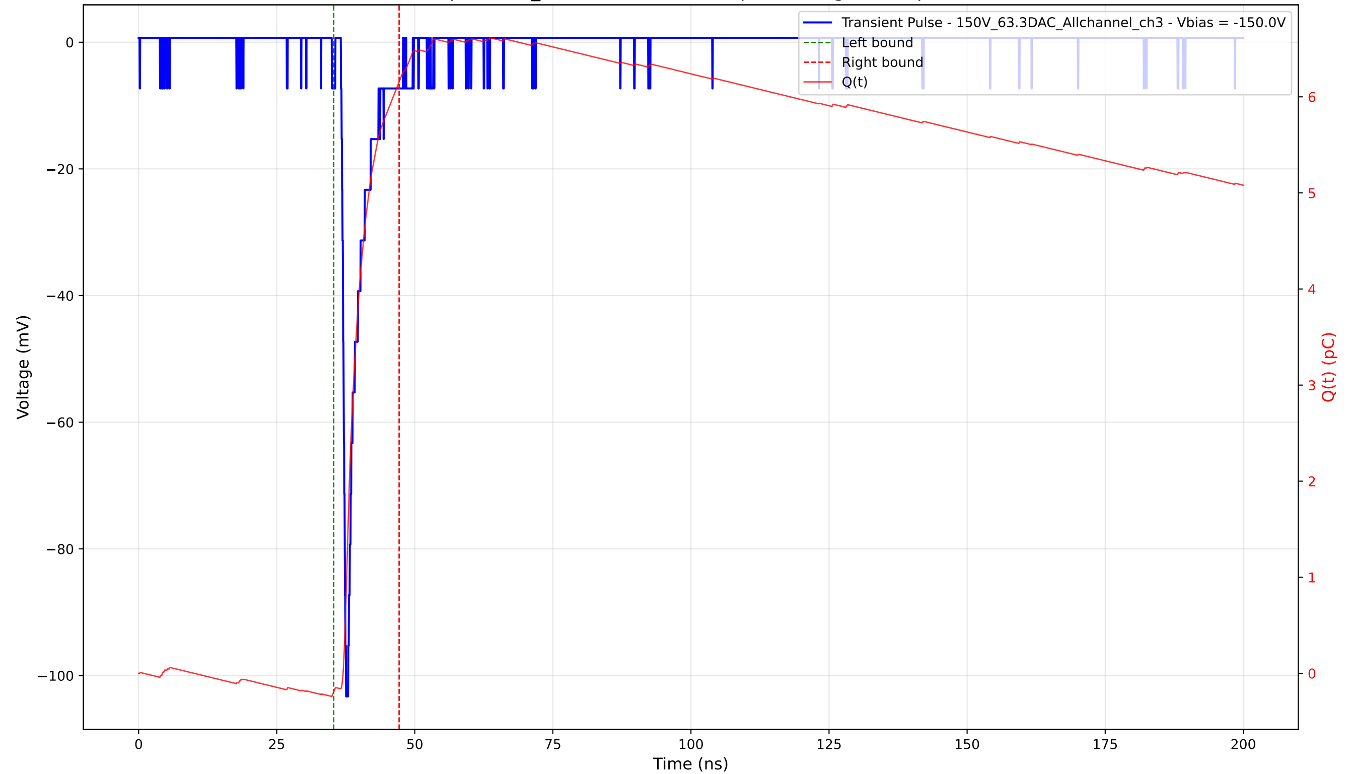
Transient Pulse - Sample: 1cm_42 - Position: 3405.0 \mu\text{m} - Charge: 6.35 pC - Rise Time: 0.70 ns
