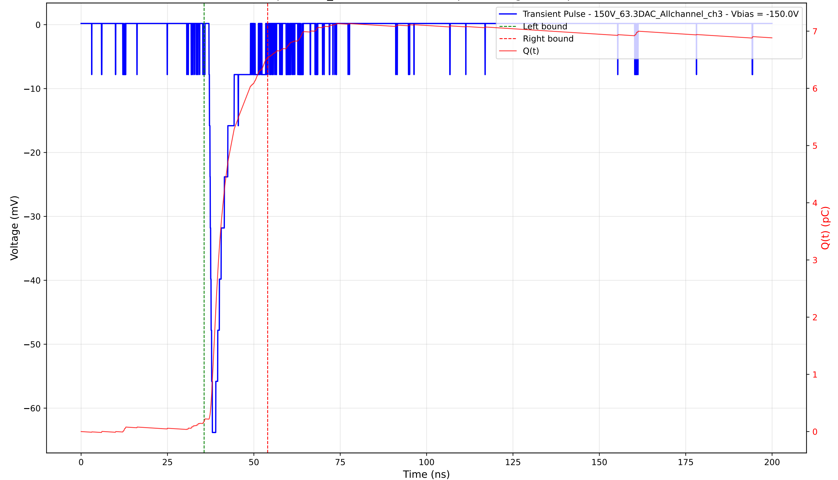
Transient Pulse - Sample: 1cm_42 - Position: 1390.0 \mu\text{m} - Charge: 6.35 pC - Rise Time: 0.97 ns
