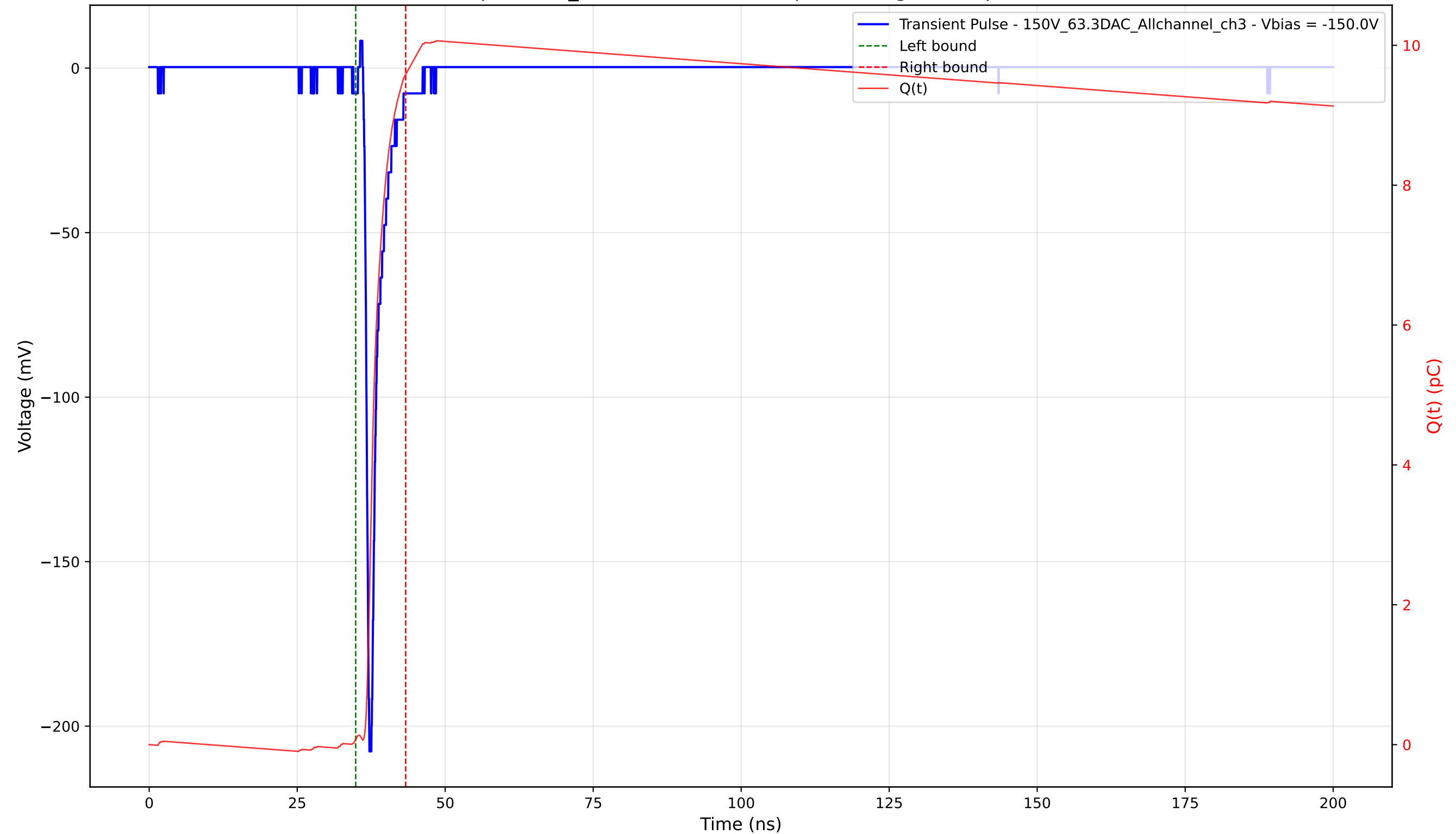
Transient Pulse - Sample: 1cm_42 - Position: 1985.0 \mu\text{m} - Charge: 9.51 pC - Rise Time: 0.77 ns
