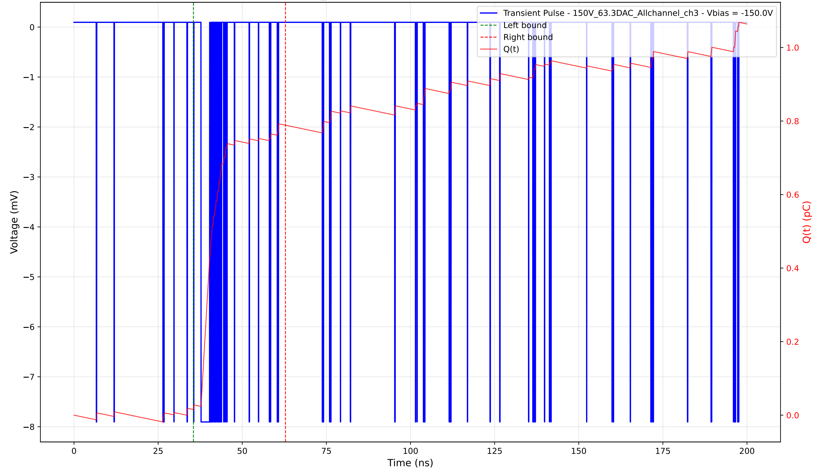
Transient Pulse - Sample: 1cm_42 - Position: 65.0 \mu\text{m} - Charge: 0.77 pC - Rise Time: 0.04 ns
