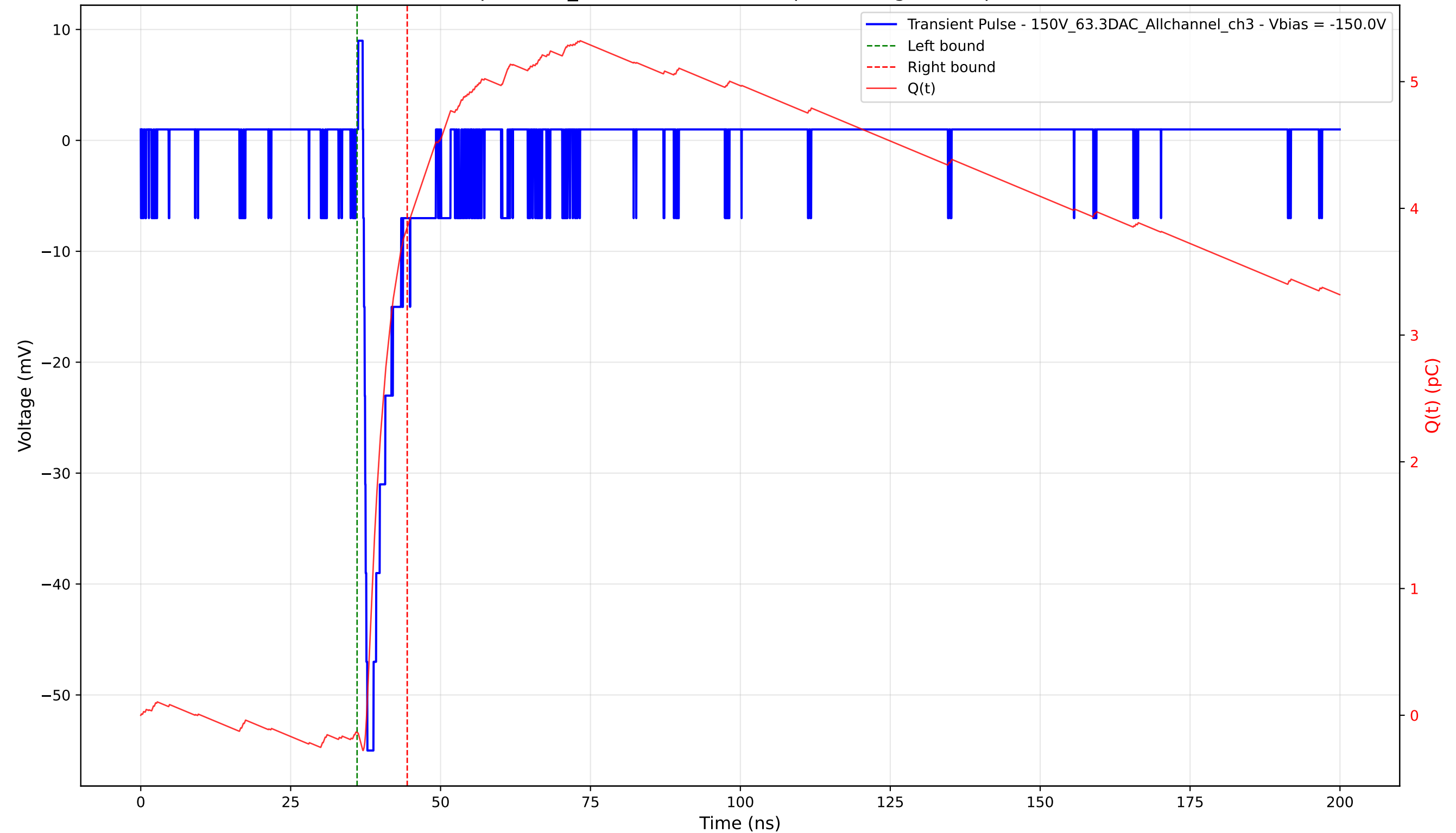
Transient Pulse - Sample: 1cm_42 - Position: 3645.0 \mu\text{m} - Charge: 3.99 pC - Rise Time: 0.69 ns
