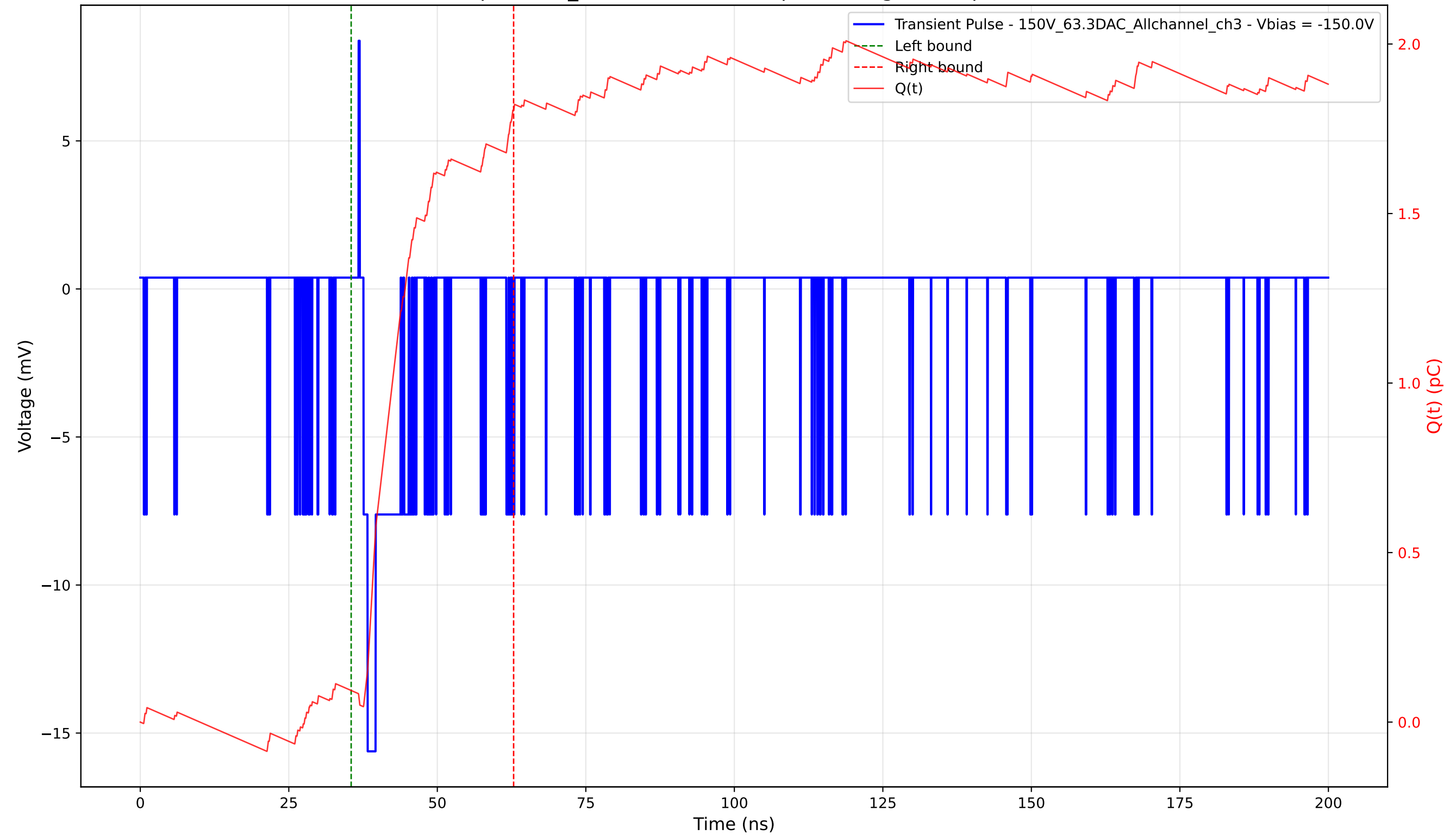
Transient Pulse - Sample: 1cm_42 - Position: 150.0 \mu\text{m} - Charge: 1.71 pC - Rise Time: 0.71 ns
