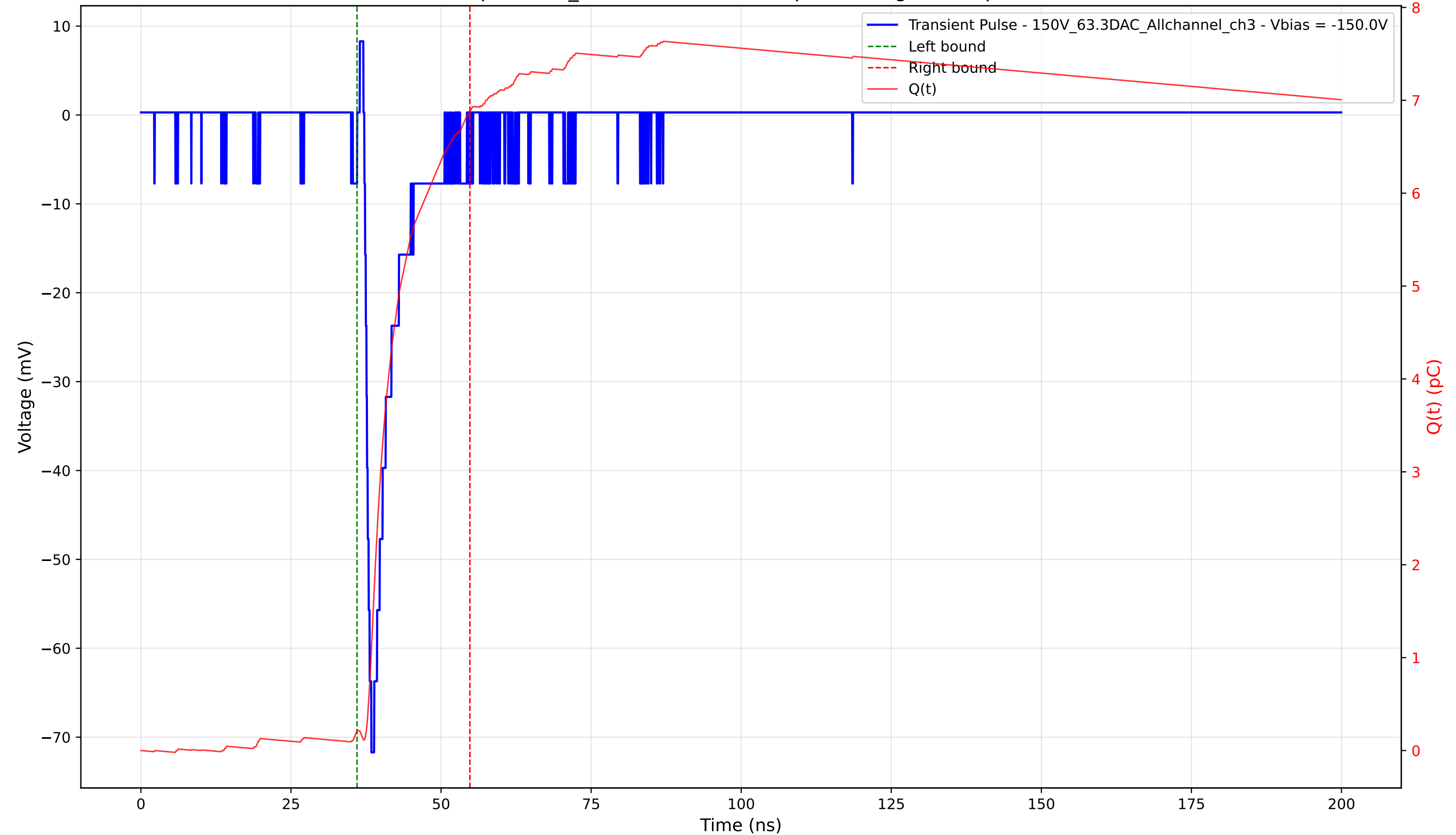
Transient Pulse - Sample: 1cm_42 - Position: 1240.0 \mu\text{m} - Charge: 6.66 pC - Rise Time: 1.16 ns
