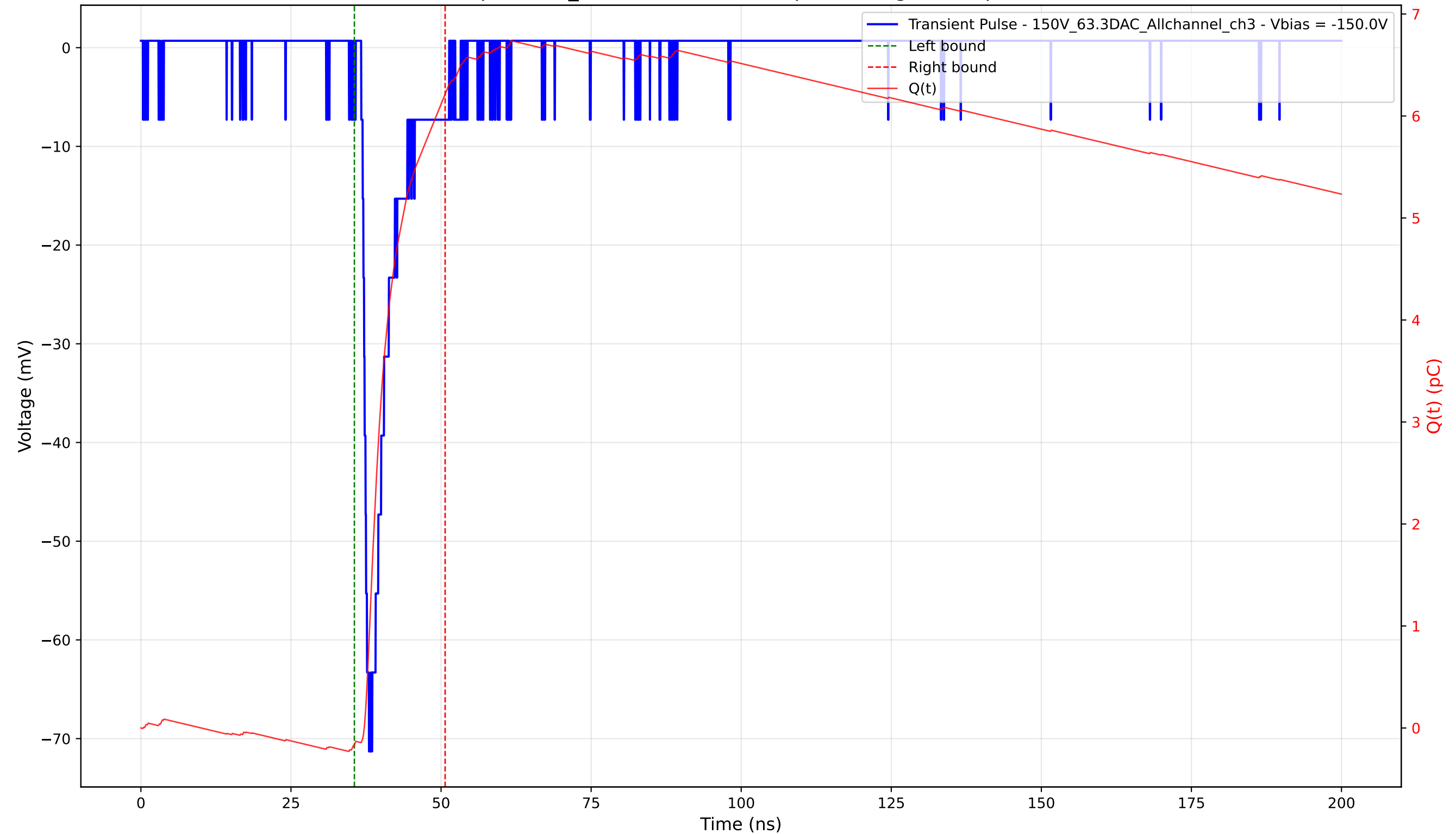
Transient Pulse - Sample: 1cm_42 - Position: 1470.0 \mu\text{m} - Charge: 6.38 pC - Rise Time: 1.28 ns
