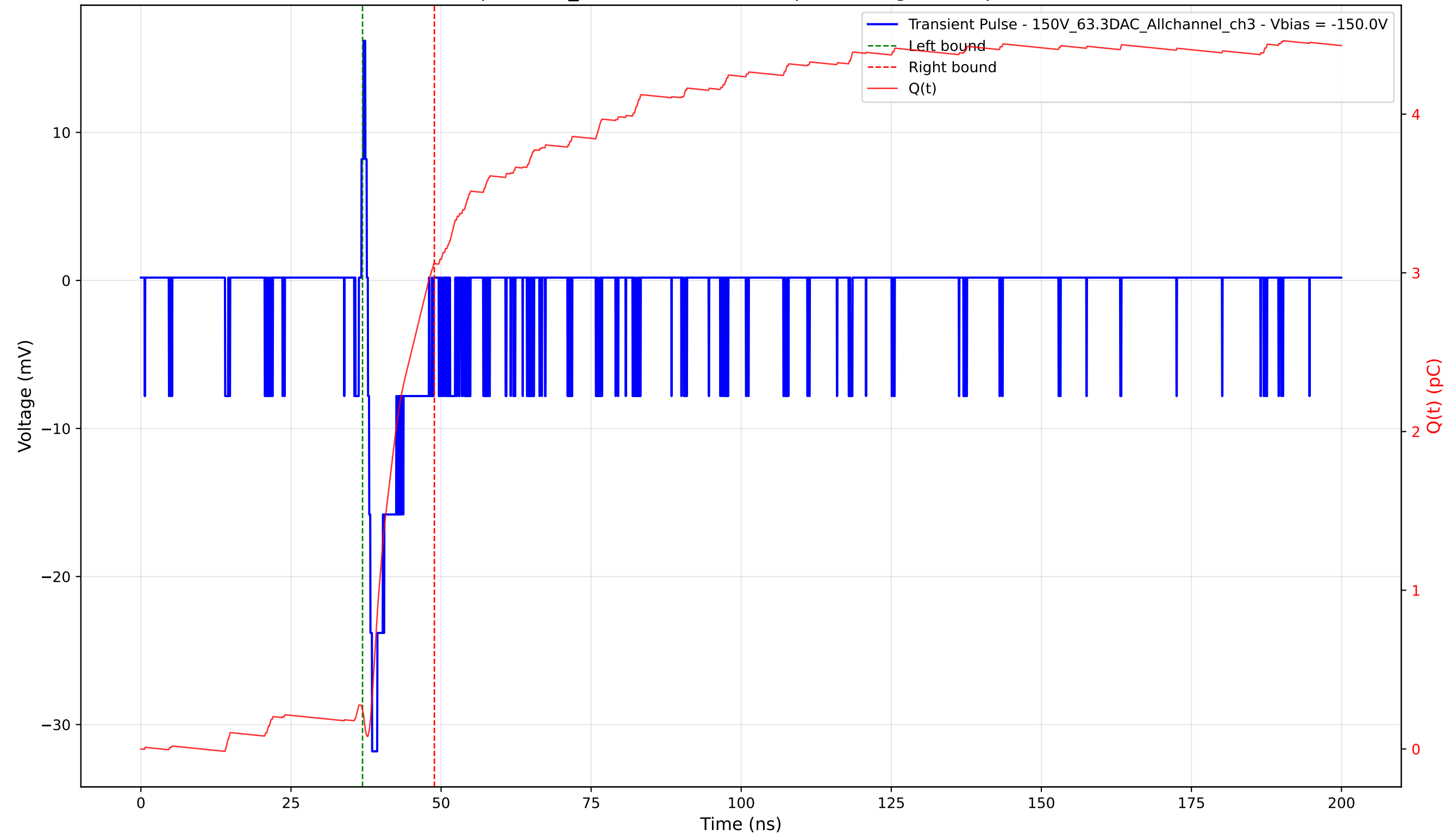
Transient Pulse - Sample: 1cm_42 - Position: 4845.0 \mu\text{m} - Charge: 2.81 pC - Rise Time: 0.70 ns
