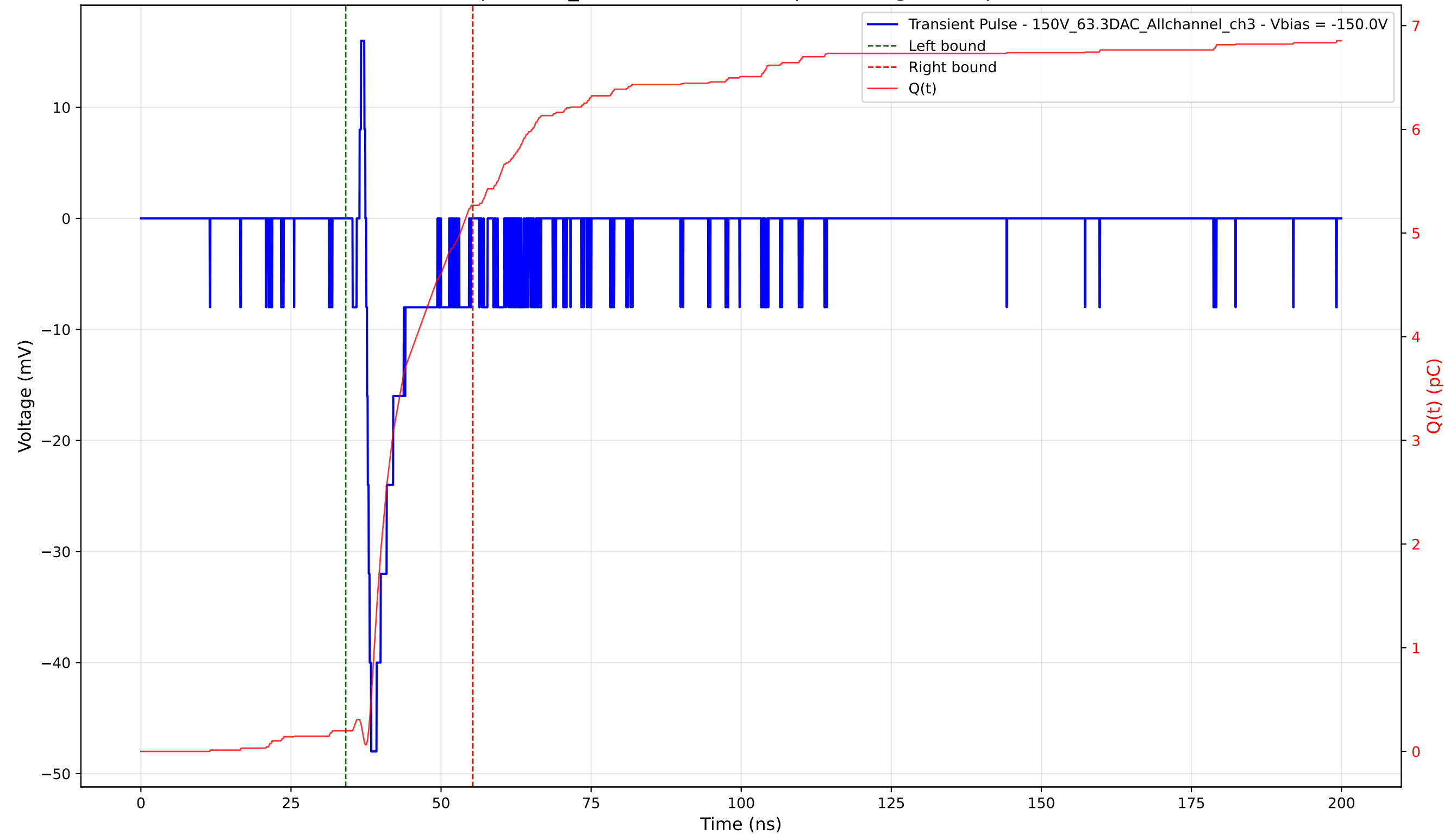
Transient Pulse - Sample: 1cm_42 - Position: 1015.0 \mu\text{m} - Charge: 5.07 pC - Rise Time: 0.82 ns
