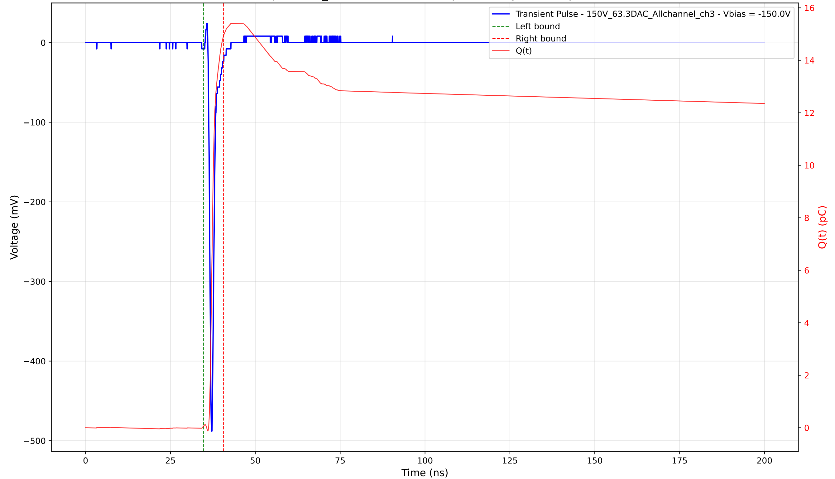
Transient Pulse - Sample: 1cm_42 - Position: 2560.0 \mu\text{m} - Charge: 14.88 pC - Rise Time: 0.67 ns
