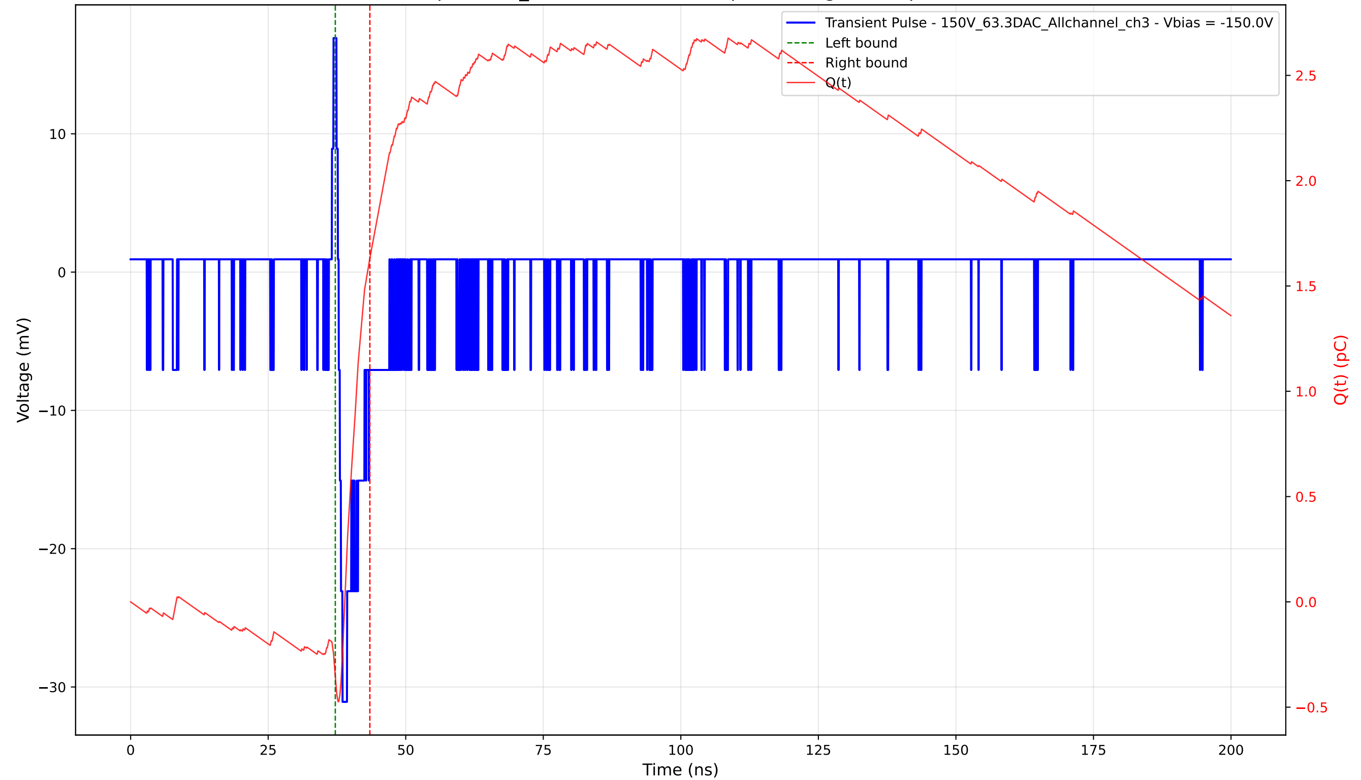
Transient Pulse - Sample: 1cm_42 - Position: 4670.0 \mu\text{m} - Charge: 1.99 pC - Rise Time: 0.71 ns
