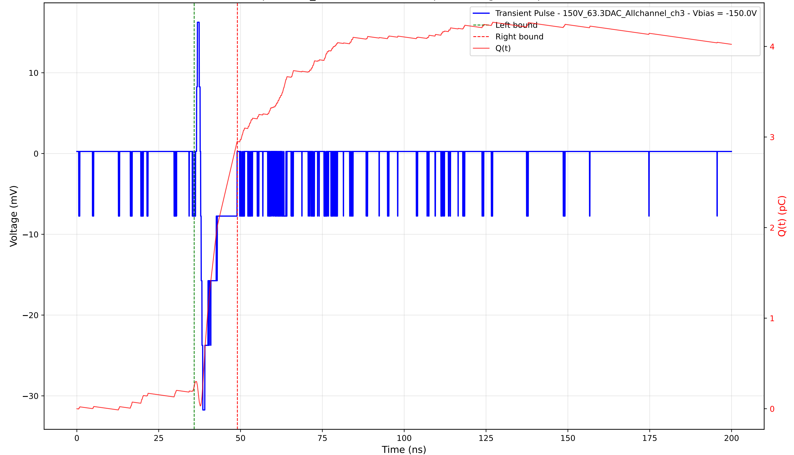
Transient Pulse - Sample: 1cm_42 - Position: 4610.0 \mu\text{m} - Charge: 2.70 pC - Rise Time: 0.66 ns
