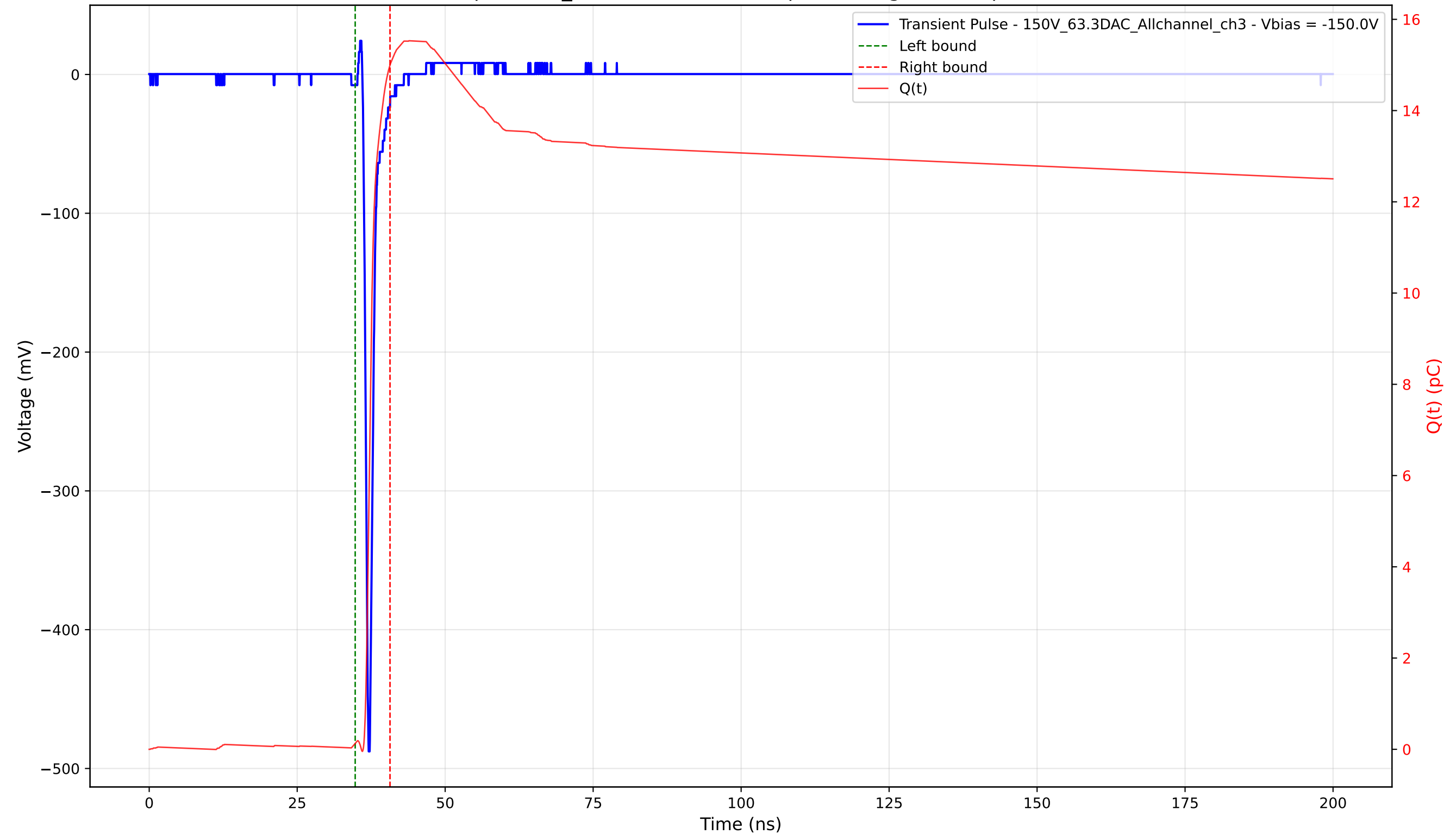
Transient Pulse - Sample: 1cm_42 - Position: 2485.0 \mu\text{m} - Charge: 14.87 pC - Rise Time: 0.67 ns
