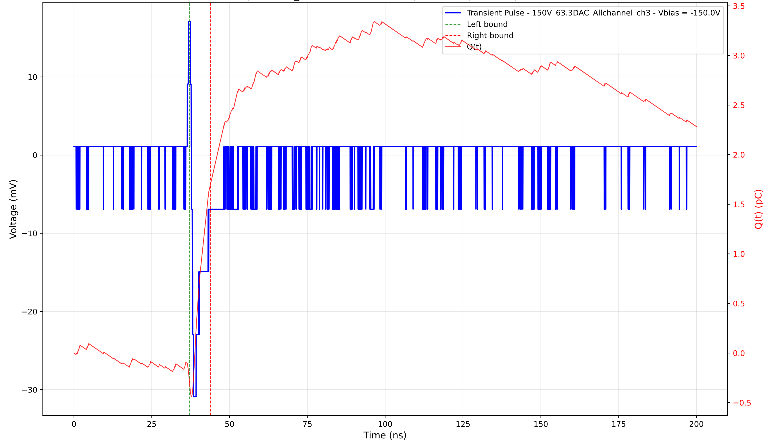
Transient Pulse - Sample: 1cm_42 - Position: 4530.0 \mu\text{m} - Charge: 2.05 pC - Rise Time: 0.67 ns
