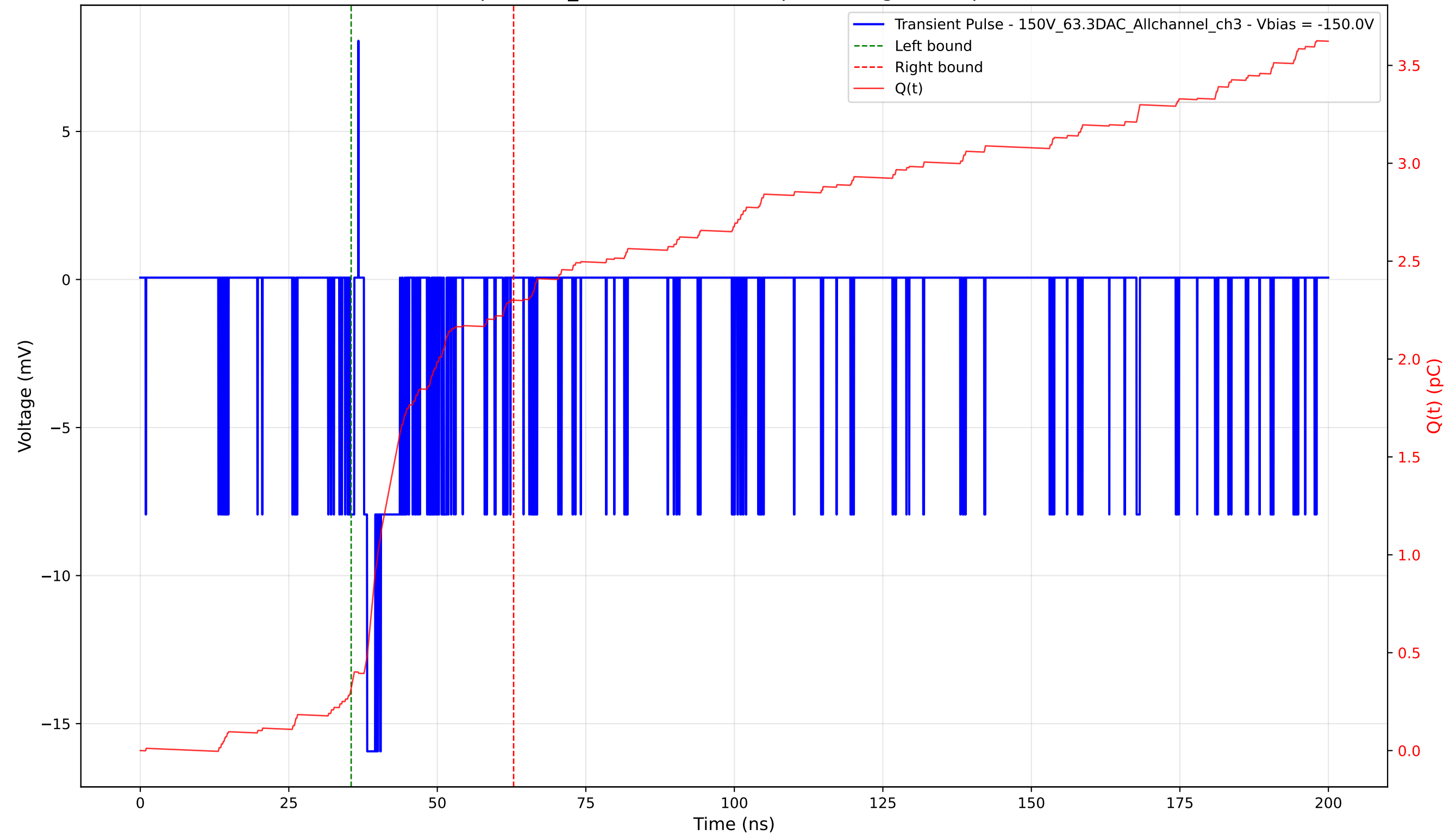
Transient Pulse - Sample: 1cm_42 - Position: 160.0 \mu\text{m} - Charge: 1.98 pC - Rise Time: 0.55 ns
