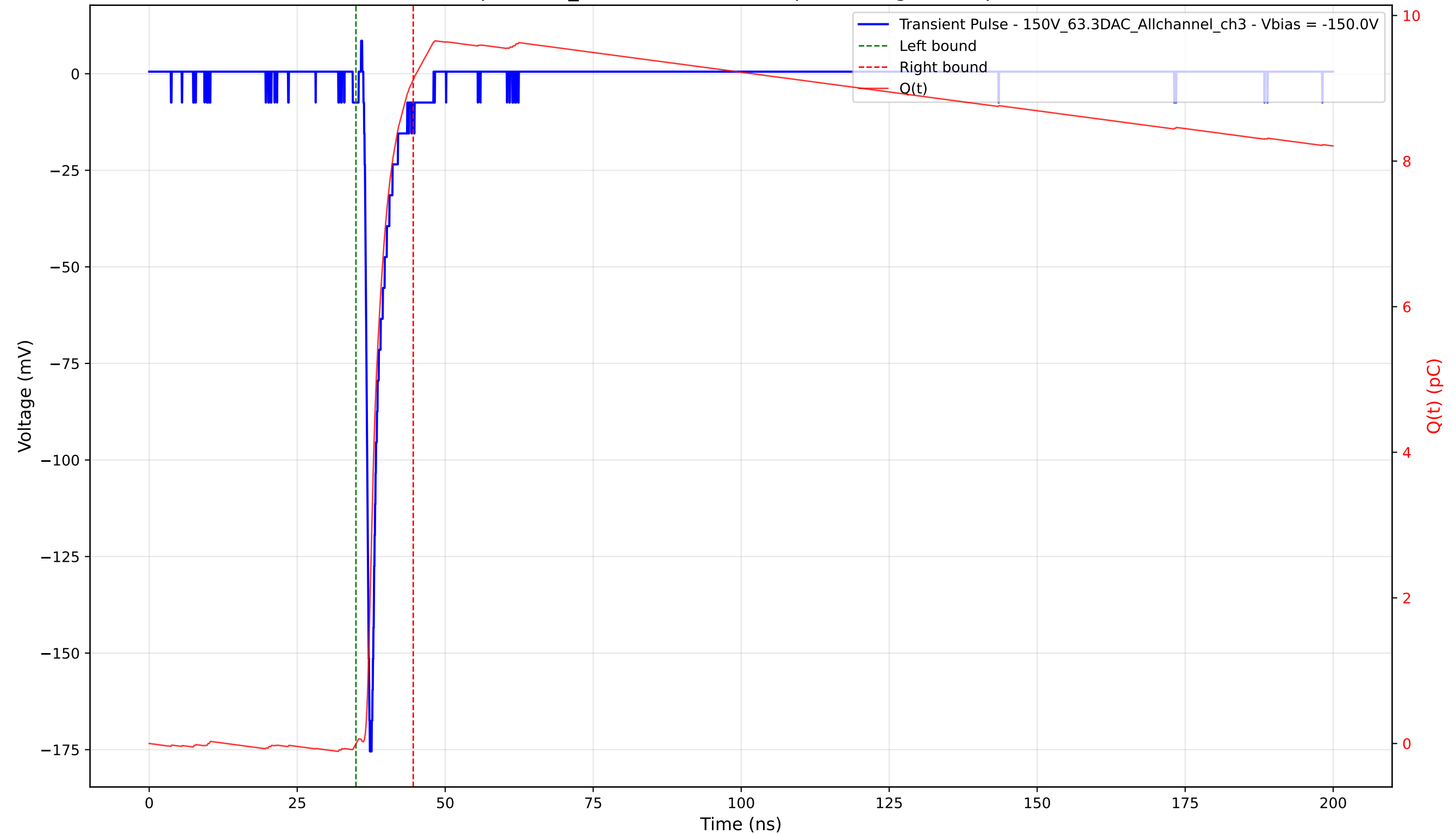
Transient Pulse - Sample: 1cm_42 - Position: 1915.0 \mu\text{m} - Charge: 9.12 pC - Rise Time: 0.78 ns
