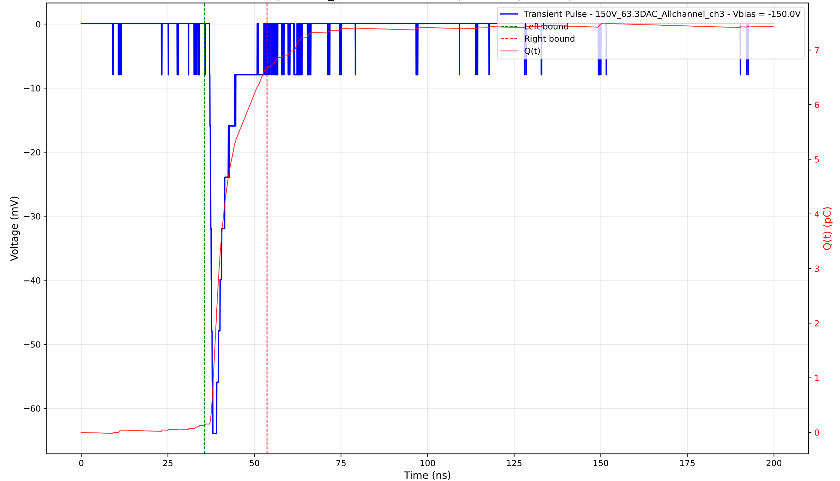
Transient Pulse - Sample: 1cm_42 - Position: 1385.0 \mu\text{m} - Charge: 6.55 pC - Rise Time: 0.97 ns
