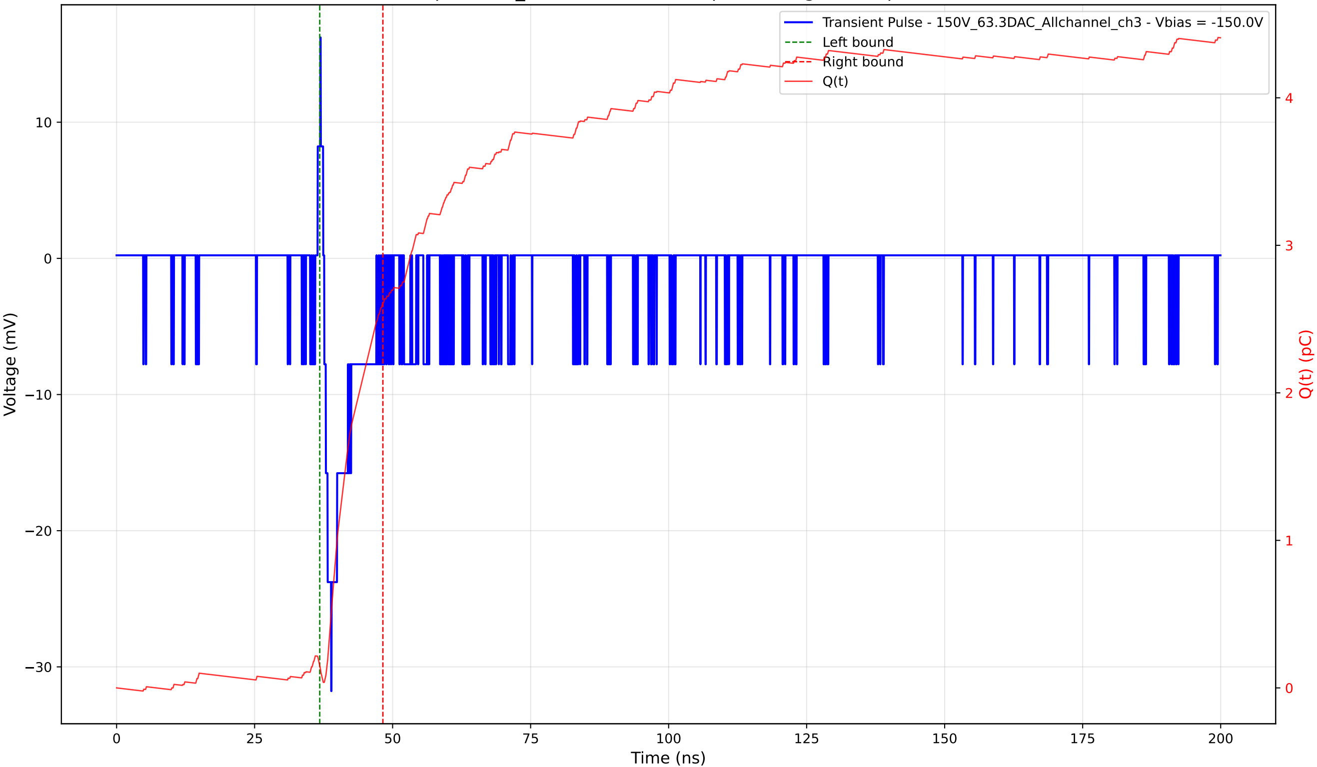
Transient Pulse - Sample: 1cm_42 - Position: 345.0 \mu\text{m} - Charge: 2.46 pC - Rise Time: 1.26 ns
