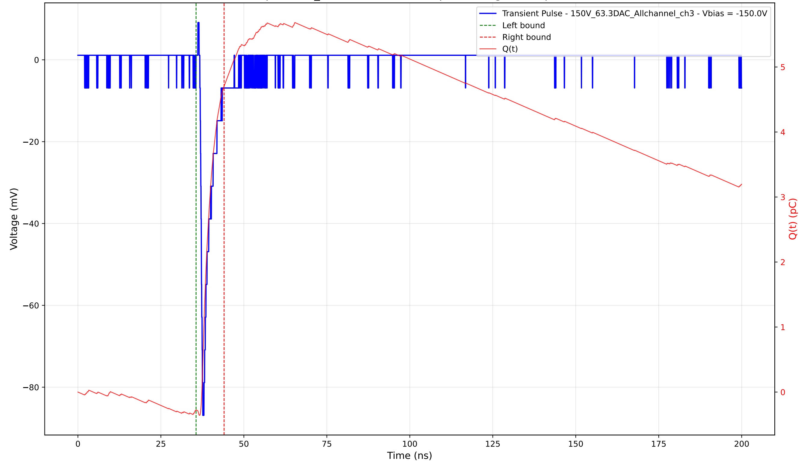
Transient Pulse - Sample: 1cm_42 - Position: 3460.0 \mu\text{m} - Charge: 4.98 pC - Rise Time: 0.67 ns
