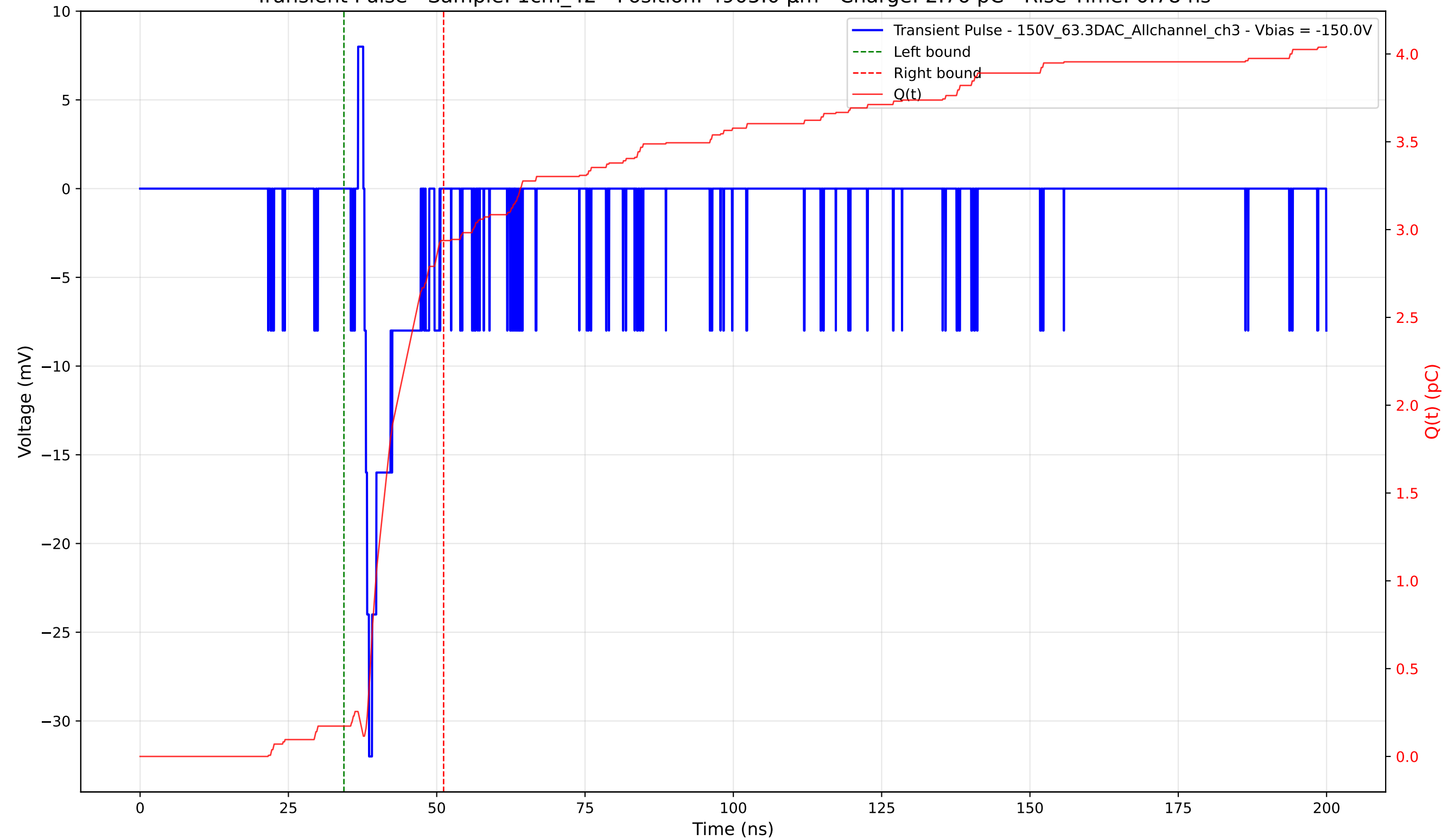
Transient Pulse - Sample: 1cm_42 - Position: 4905.0 \mu\text{m} - Charge: 2.76 pC - Rise Time: 0.78 ns
