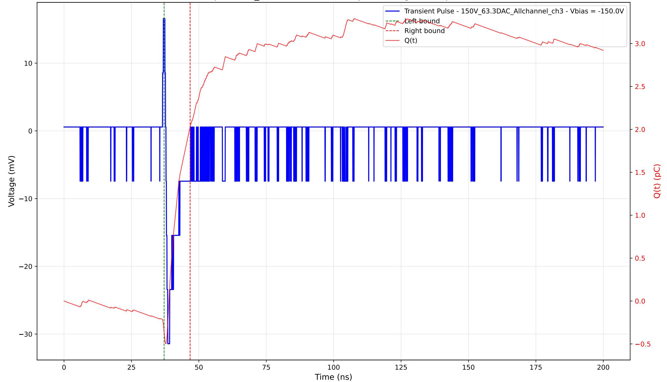
Transient Pulse - Sample: 1cm_42 - Position: 4590.0 \mu\text{m} - Charge: 2.39 pC - Rise Time: 0.67 ns
