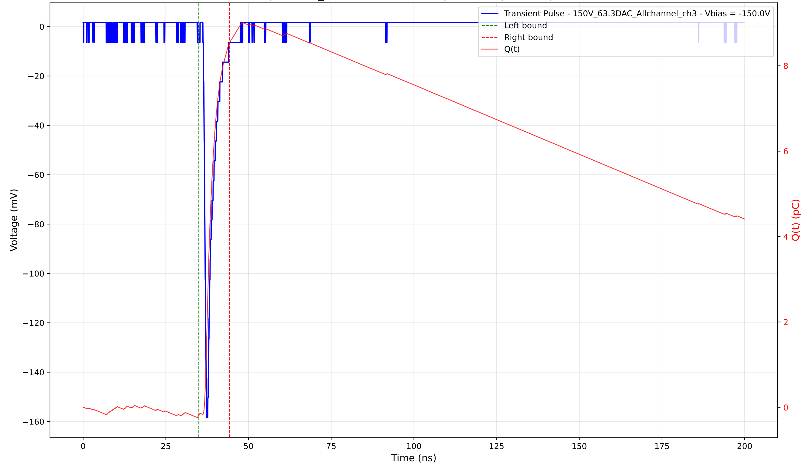
Transient Pulse - Sample: 1cm_42 - Position: 1865.0 \mu\text{m} - Charge: 8.72 pC - Rise Time: 0.87 ns
