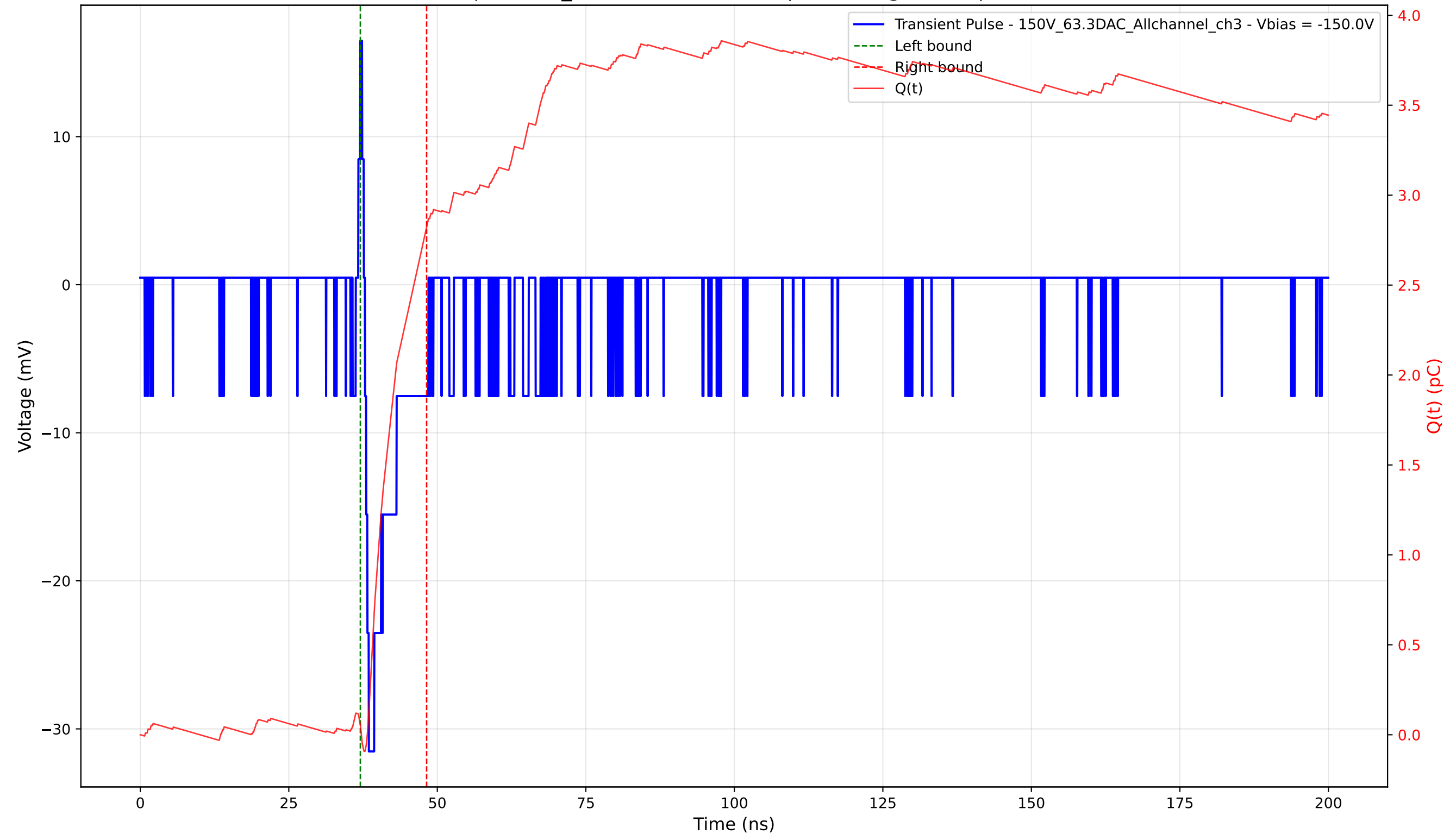
Transient Pulse - Sample: 1cm_42 - Position: 4830.0 \mu\text{m} - Charge: 2.77 pC - Rise Time: 0.66 ns
