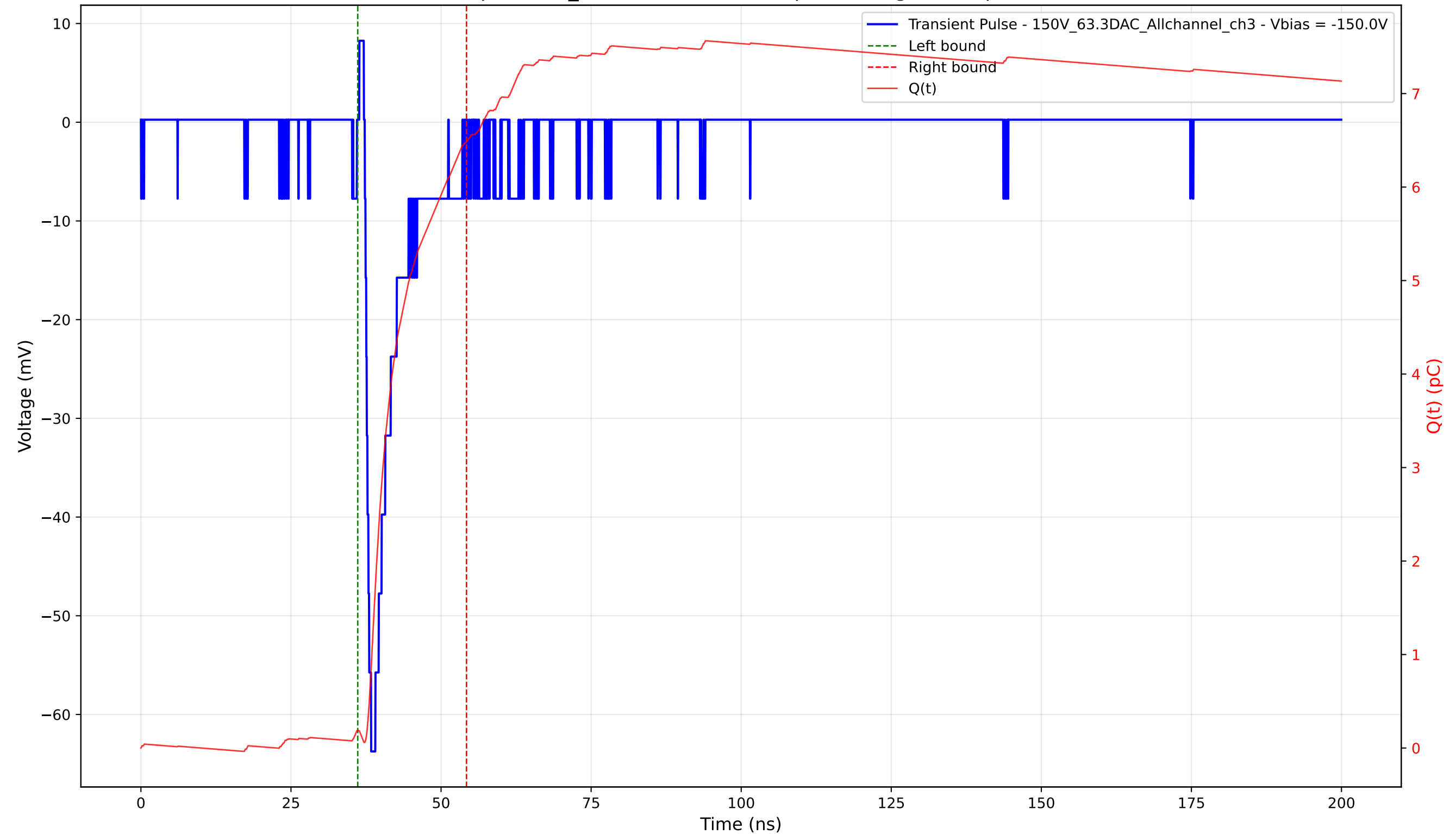
Transient Pulse - Sample: 1cm_42 - Position: 1185.0 \mu\text{m} - Charge: 6.30 pC - Rise Time: 1.05 ns
