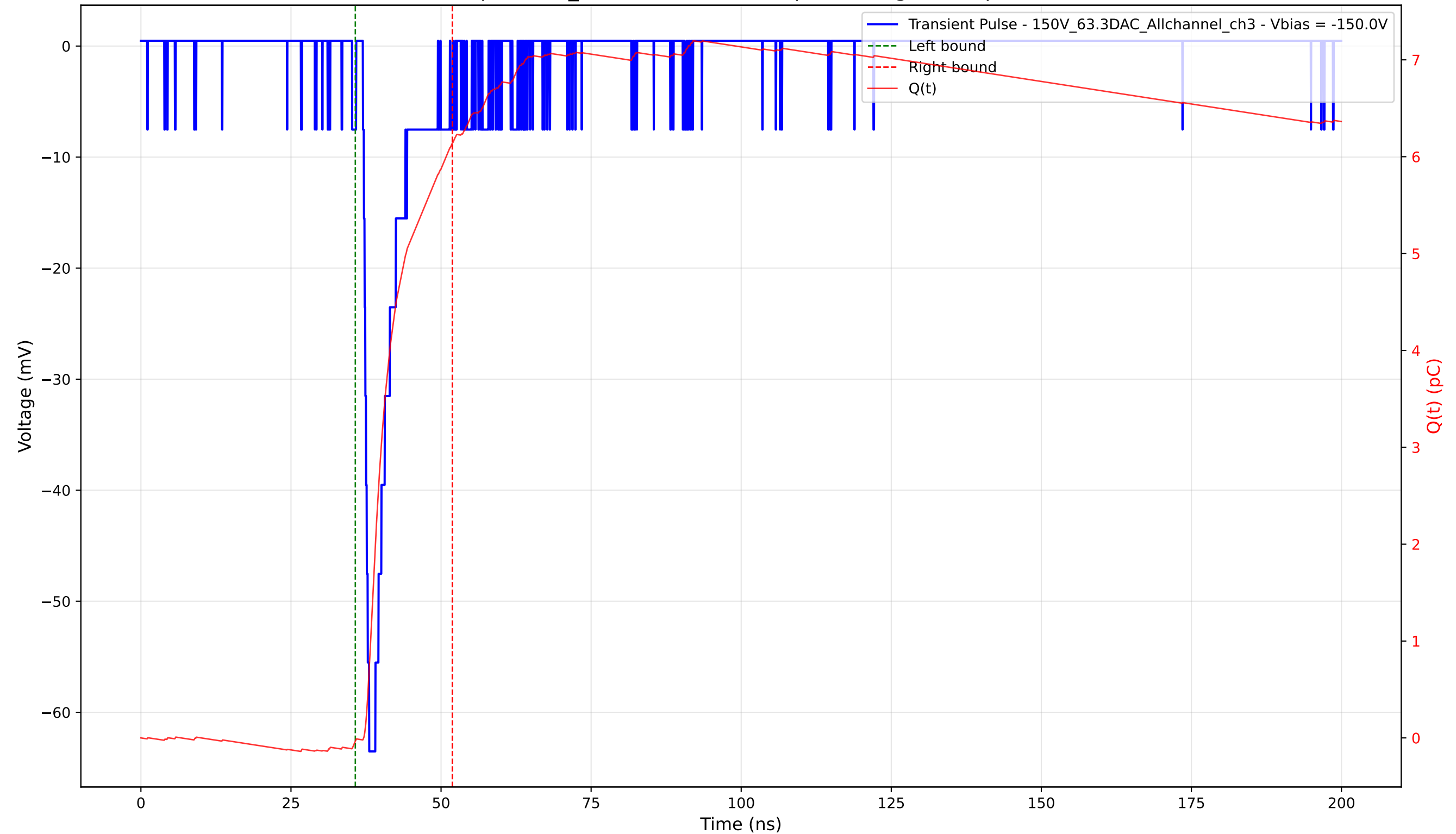
Transient Pulse - Sample: 1cm_42 - Position: 1395.0 \mu\text{m} - Charge: 6.18 pC - Rise Time: 1.05 ns
