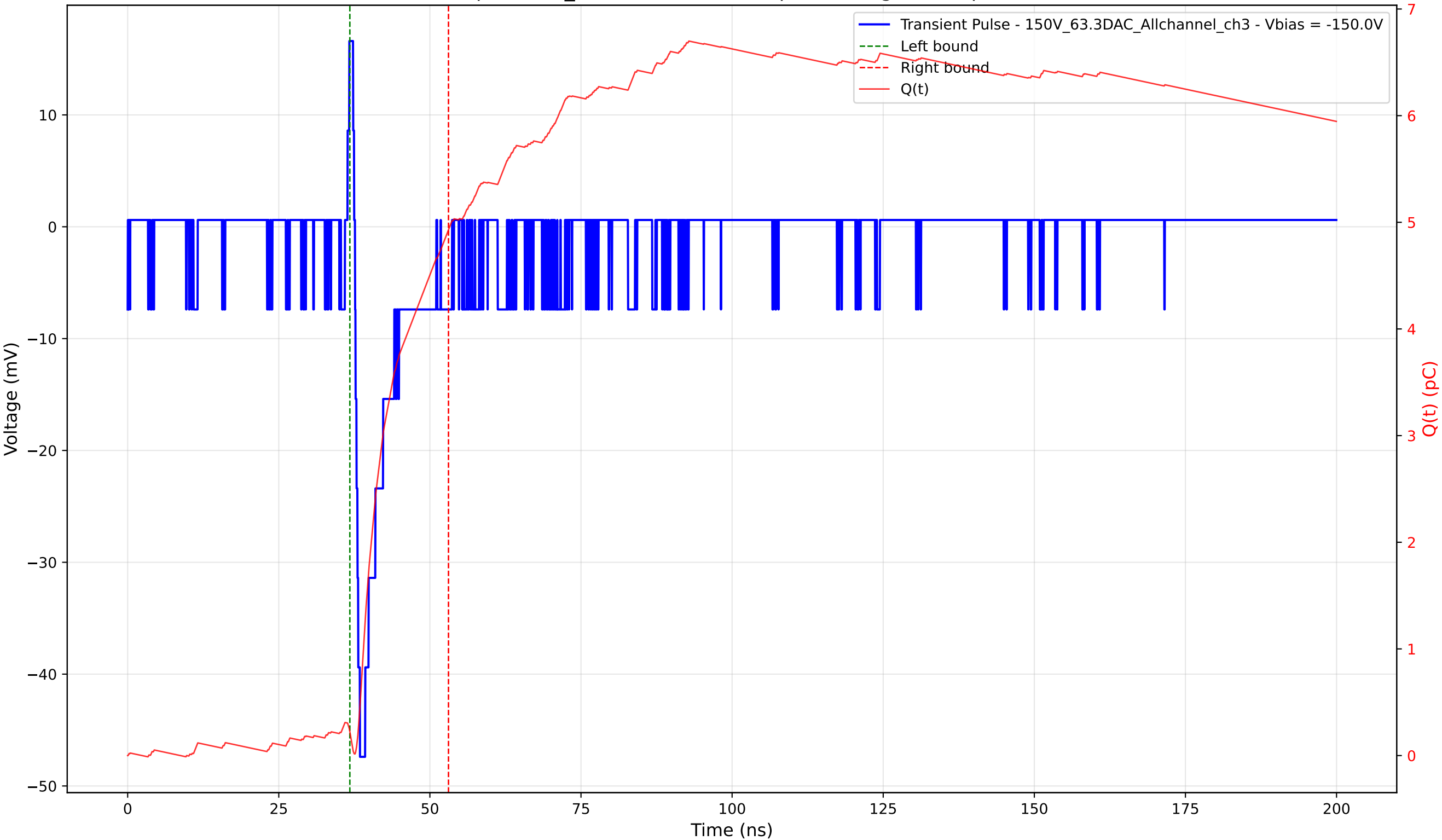
Transient Pulse - Sample: 1cm_42 - Position: 970.0 \mu\text{m} - Charge: 4.71 pC - Rise Time: 0.82 ns
