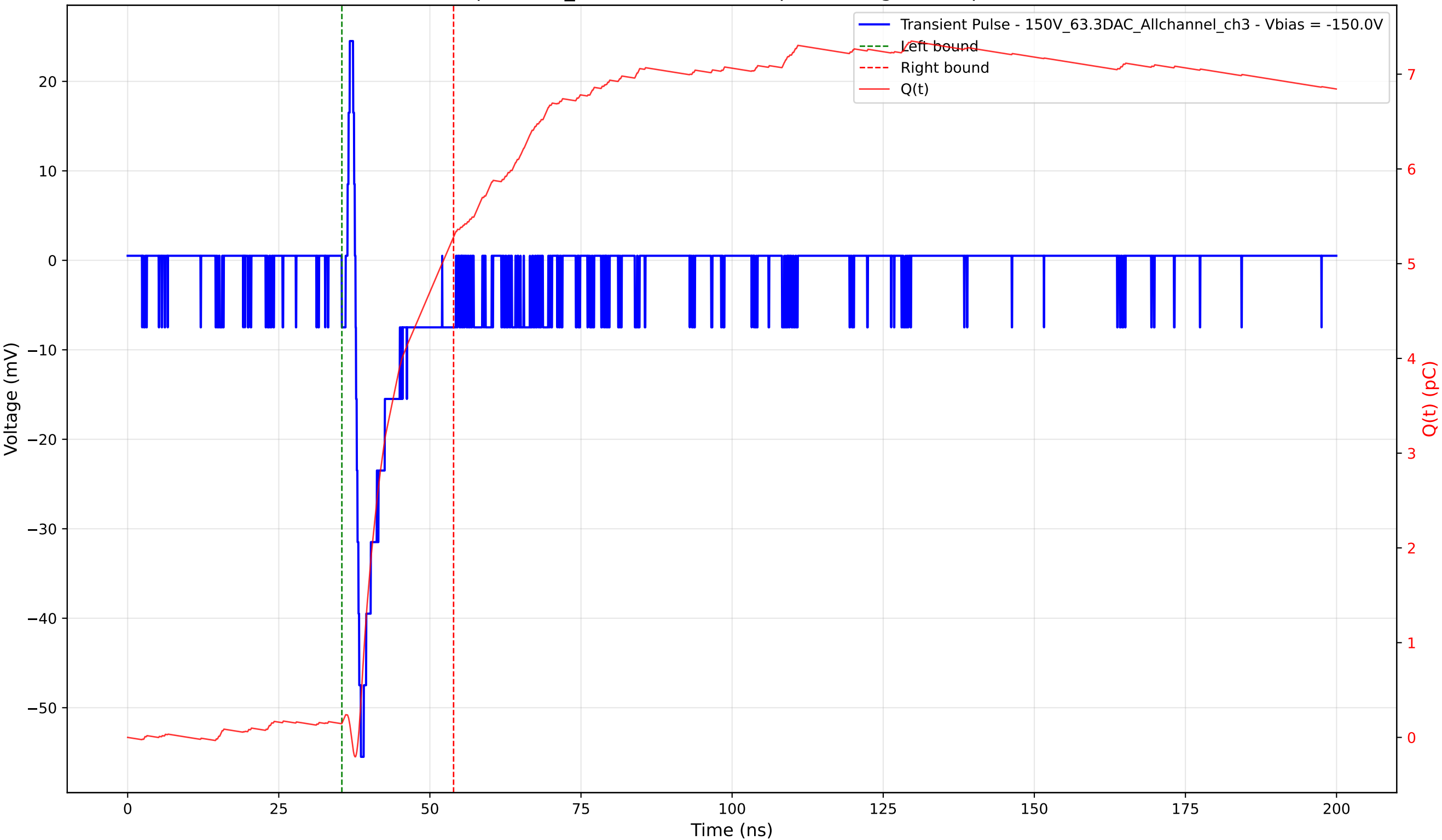
Transient Pulse - Sample: 1cm_42 - Position: 765.0 \mu\text{m} - Charge: 5.14 pC - Rise Time: 0.89 ns
