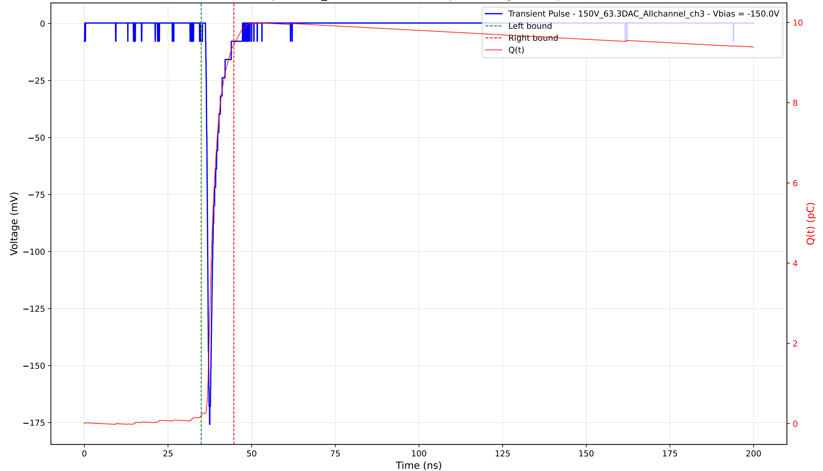
Transient Pulse - Sample: 1cm_42 - Position: 1895.0 \mu\text{m} - Charge: 9.25 pC - Rise Time: 0.83 ns
