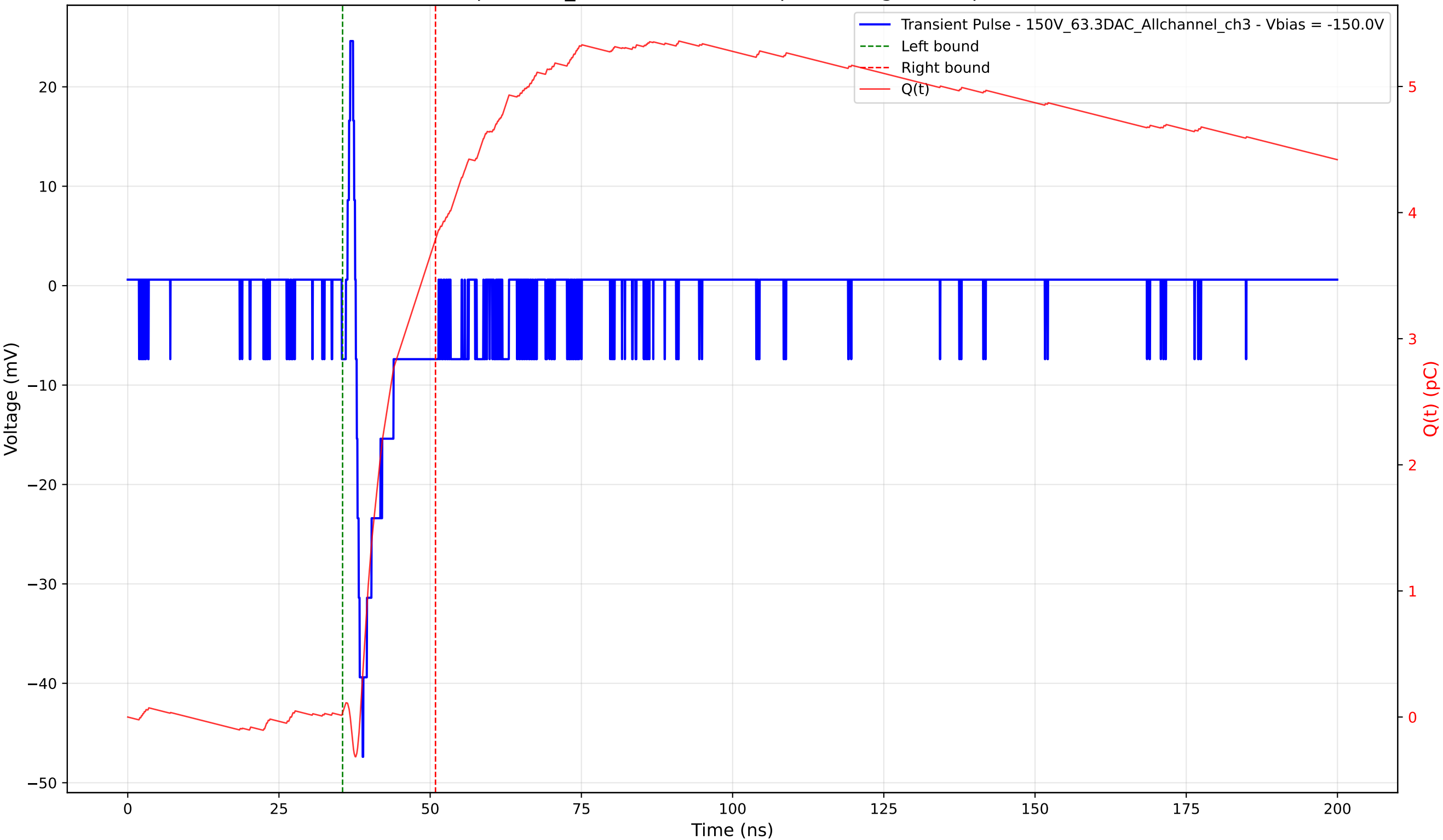
Transient Pulse - Sample: 1cm_42 - Position: 605.0 \mu\text{m} - Charge: 3.76 pC - Rise Time: 1.14 ns
