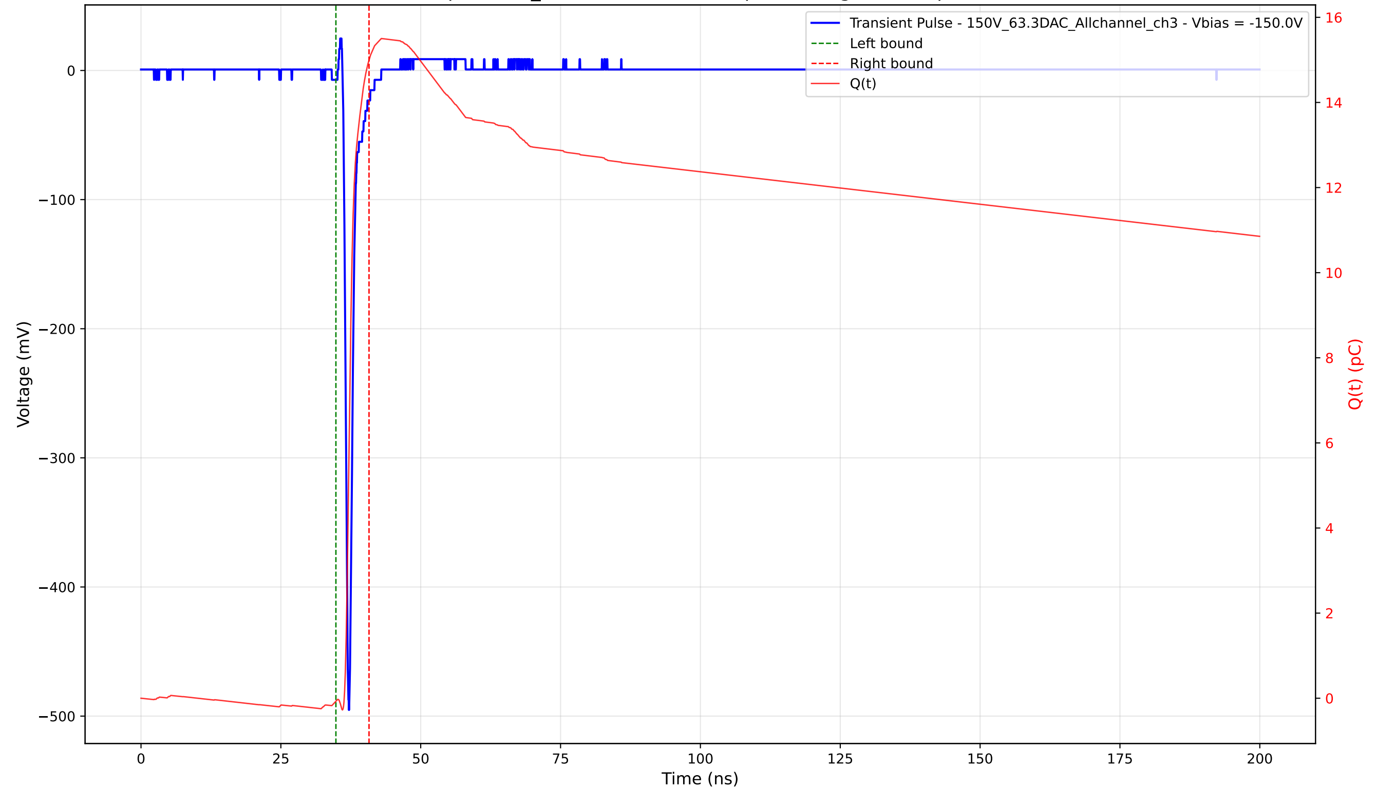
Transient Pulse - Sample: 1cm_42 - Position: 2595.0 \mu\text{m} - Charge: 15.06 pC - Rise Time: 0.71 ns
