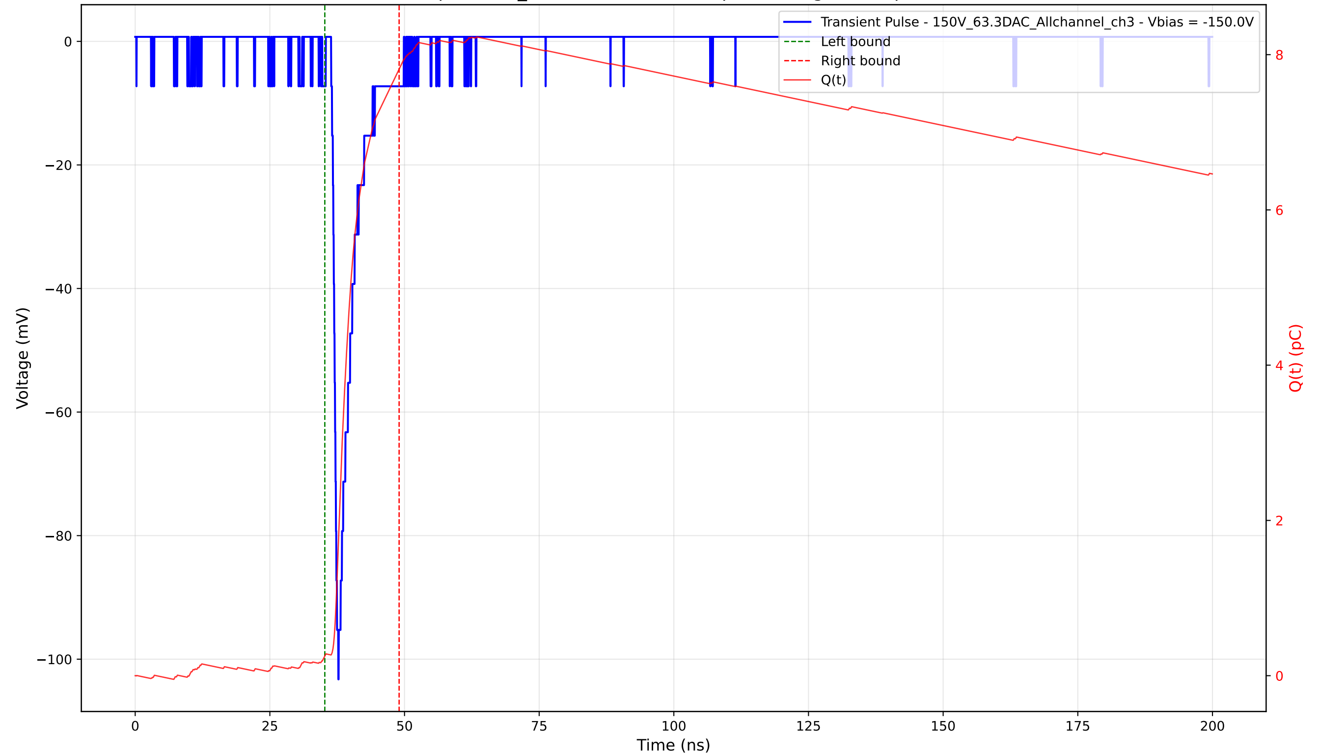
Transient Pulse - Sample: 1cm_42 - Position: 1605.0 \mu\text{m} - Charge: 7.56 pC - Rise Time: 0.94 ns
