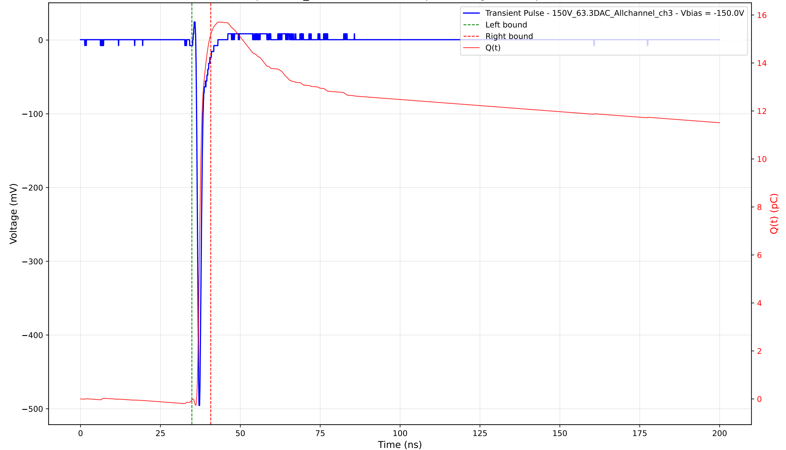
Transient Pulse - Sample: 1cm_42 - Position: 2620.0 \mu\text{m} - Charge: 15.24 pC - Rise Time: 0.71 ns
