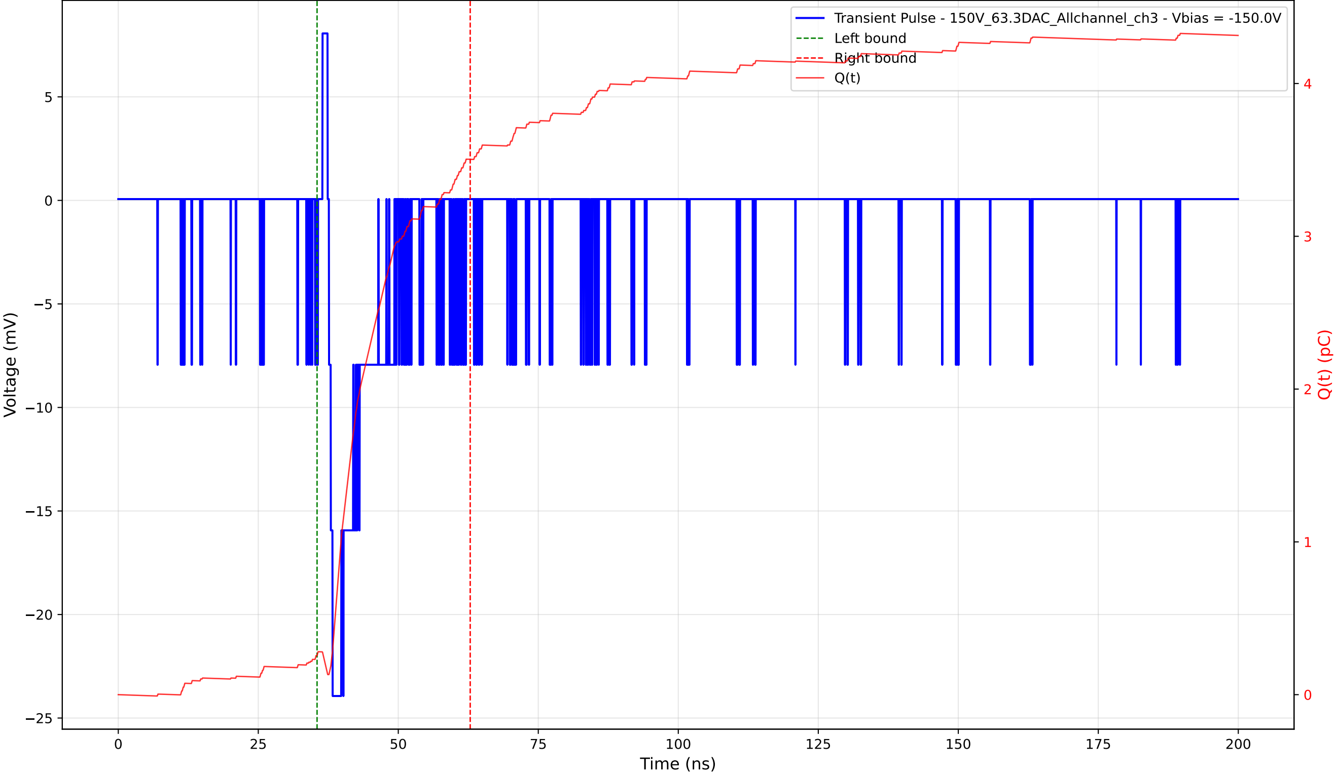
Transient Pulse - Sample: 1cm_42 - Position: 335.0 \mu\text{m} - Charge: 3.25 pC - Rise Time: 0.67 ns
