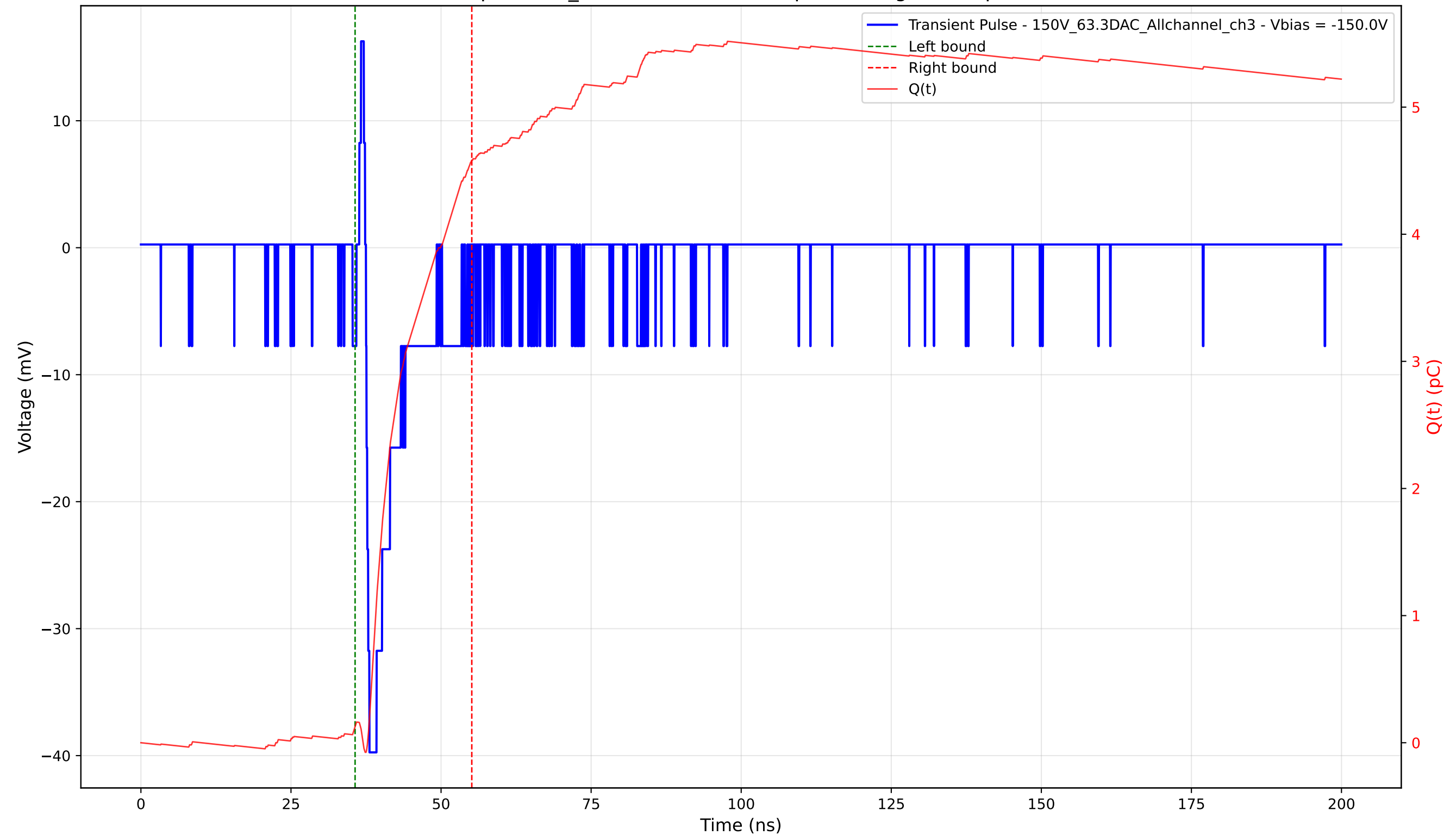
Transient Pulse - Sample: 1cm_42 - Position: 3965.0 \mu\text{m} - Charge: 4.45 pC - Rise Time: 0.58 ns
