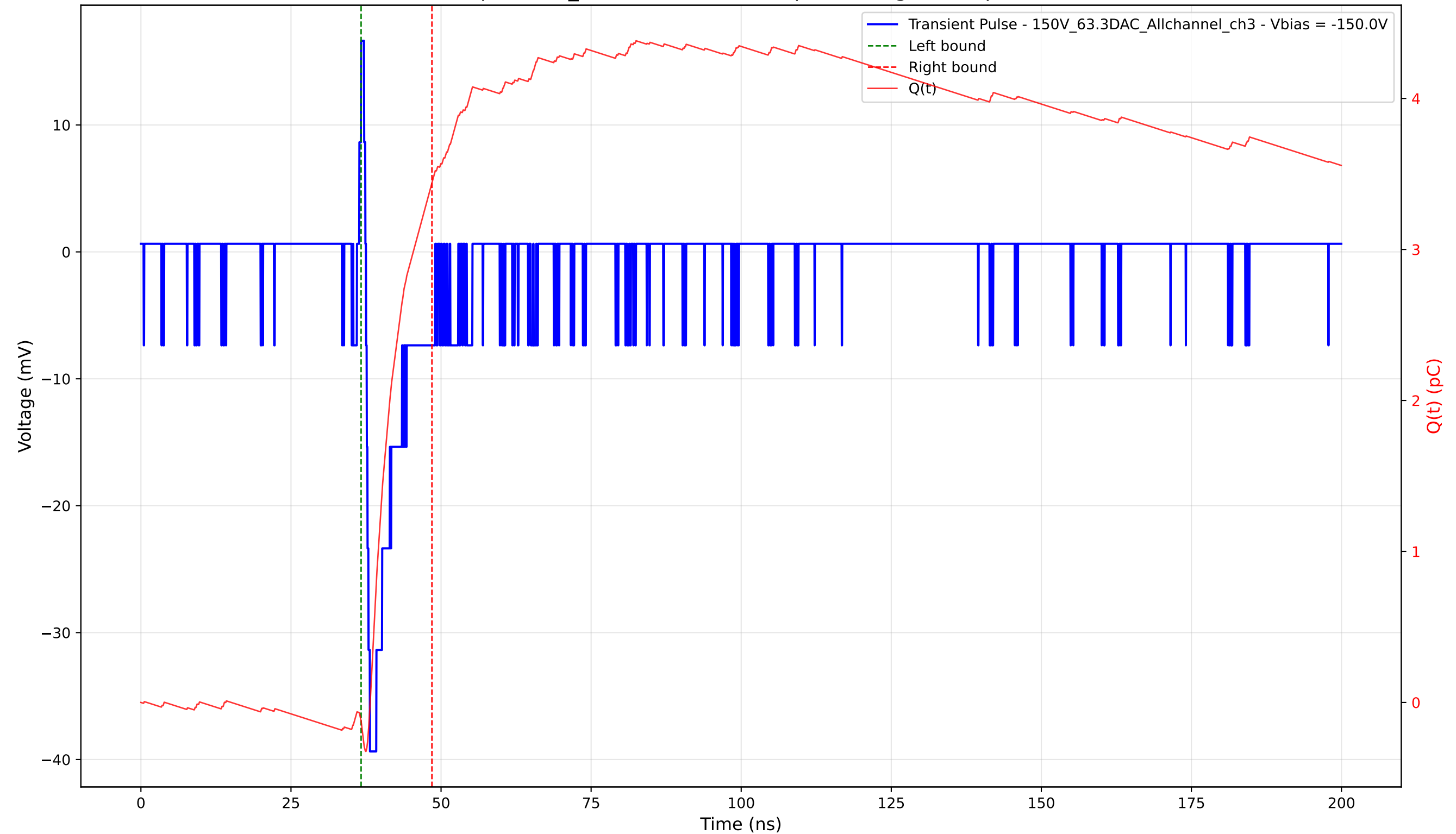
Transient Pulse - Sample: 1cm_42 - Position: 3990.0 \mu\text{m} - Charge: 3.56 pC - Rise Time: 0.66 ns
