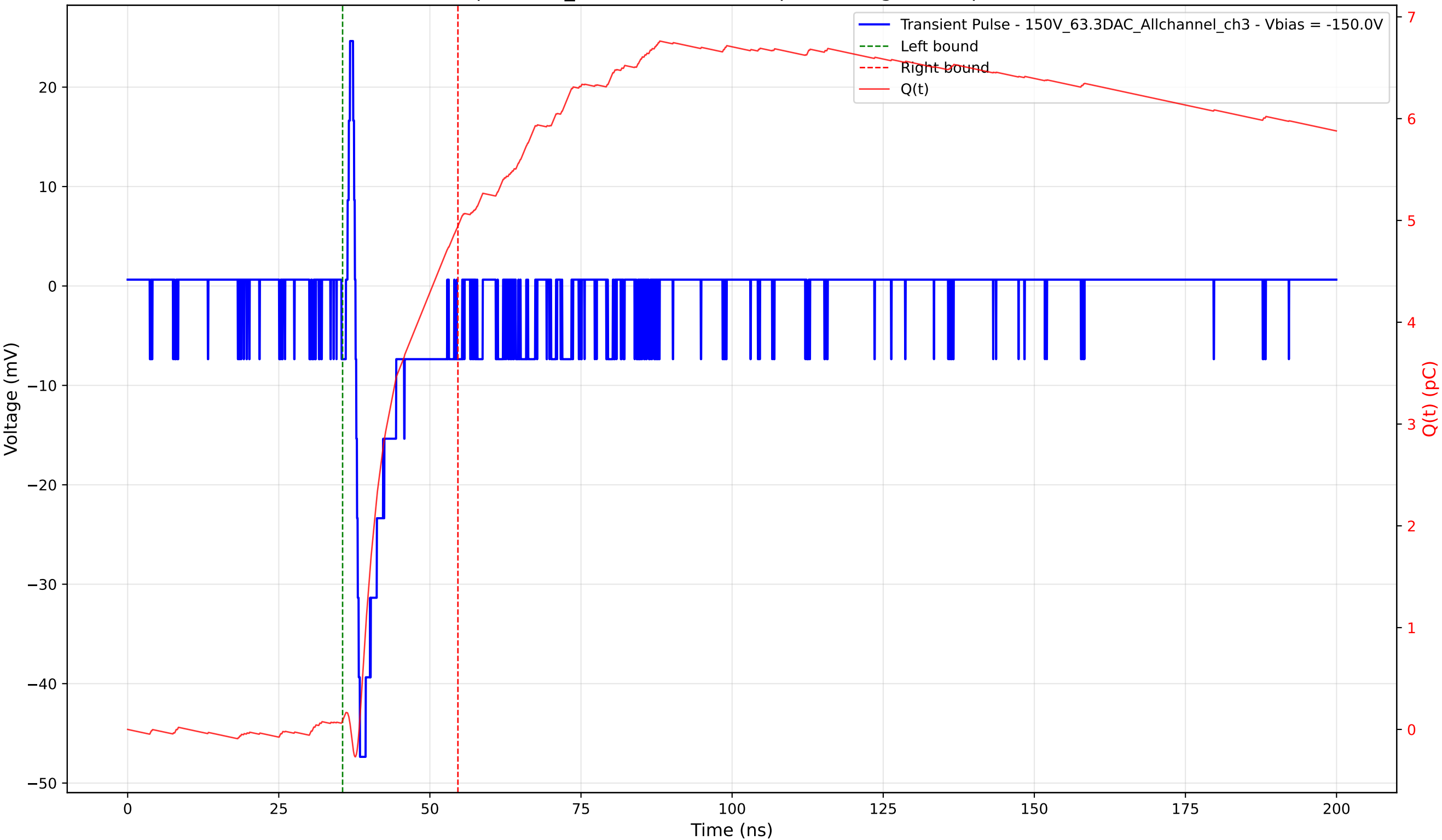
Transient Pulse - Sample: 1cm_42 - Position: 835.0 \mu\text{m} - Charge: 4.86 pC - Rise Time: 0.74 ns
