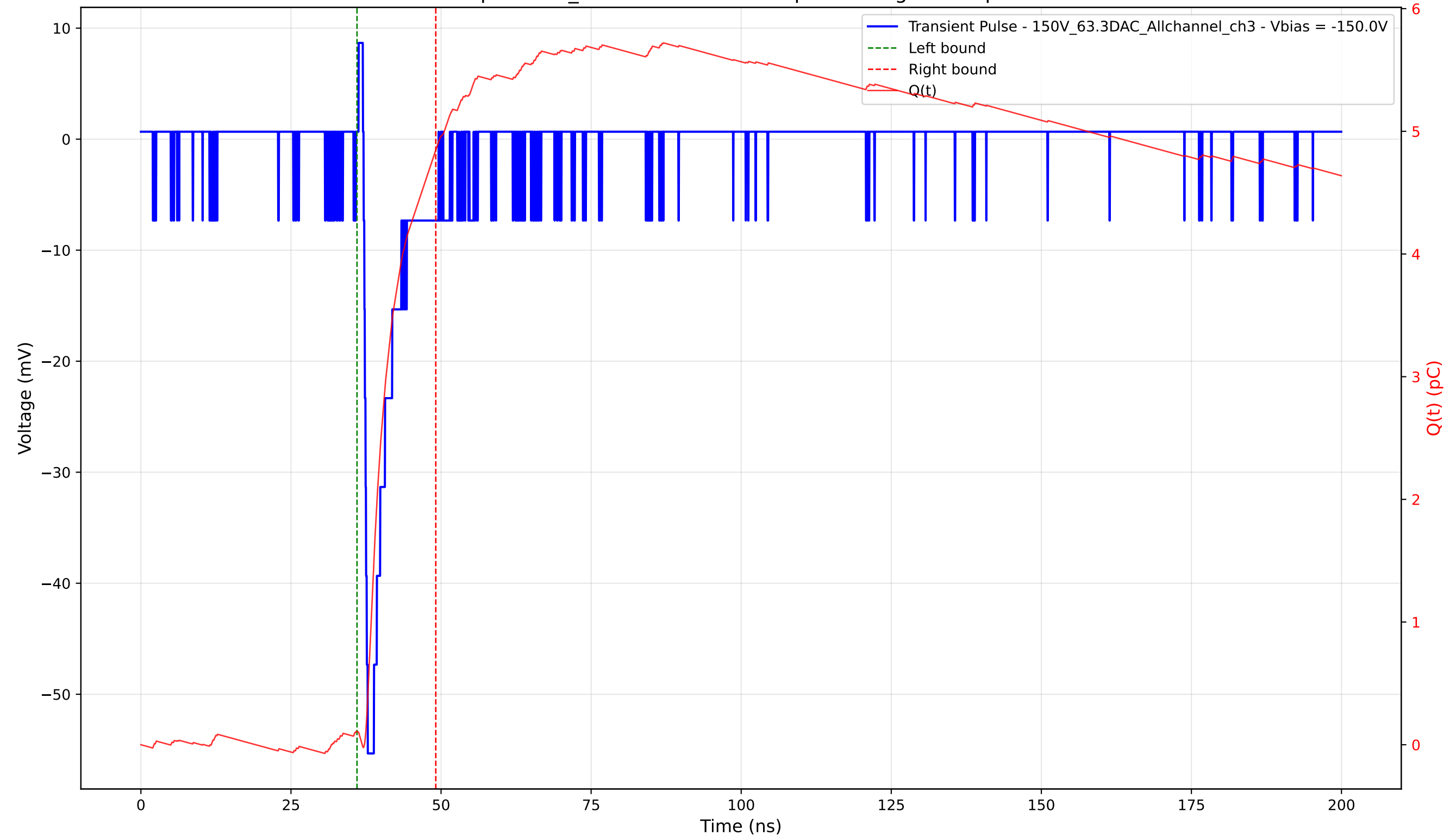
Transient Pulse - Sample: 1cm_42 - Position: 3640.0 \mu\text{m} - Charge: 4.74 pC - Rise Time: 0.69 ns
