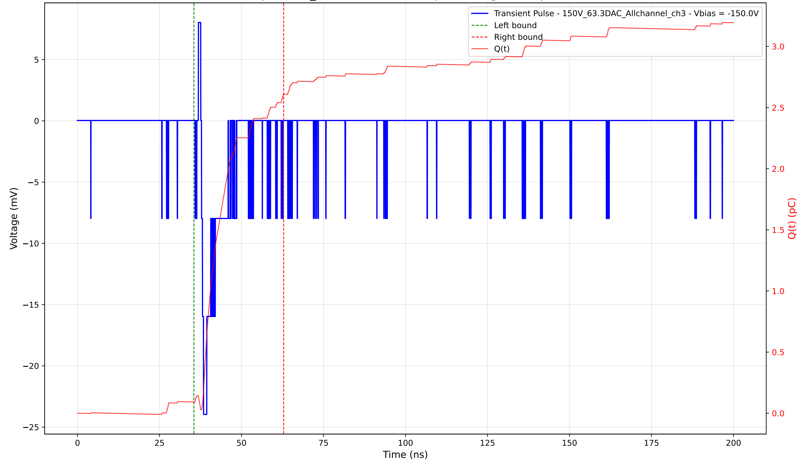
Transient Pulse - Sample: 1cm_42 - Position: 4965.0 \mu\text{m} - Charge: 2.52 pC - Rise Time: 0.63 ns
