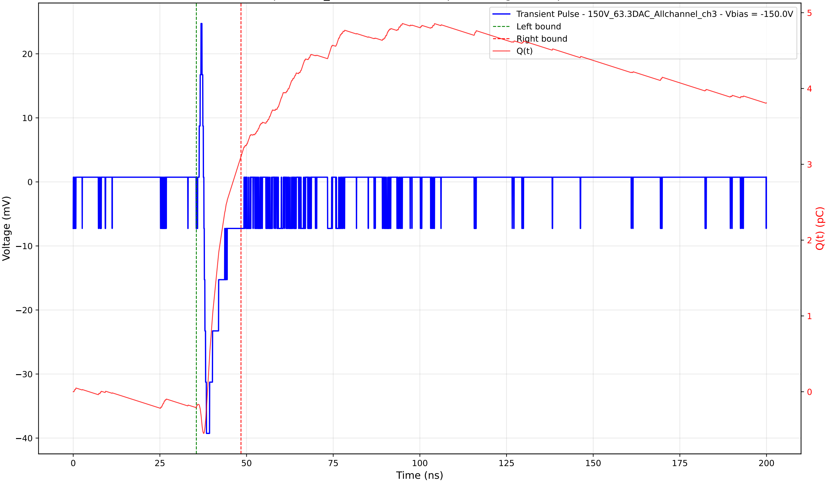
Transient Pulse - Sample: 1cm_42 - Position: 565.0 \mu\text{m} - Charge: 3.31 pC - Rise Time: 0.74 ns
