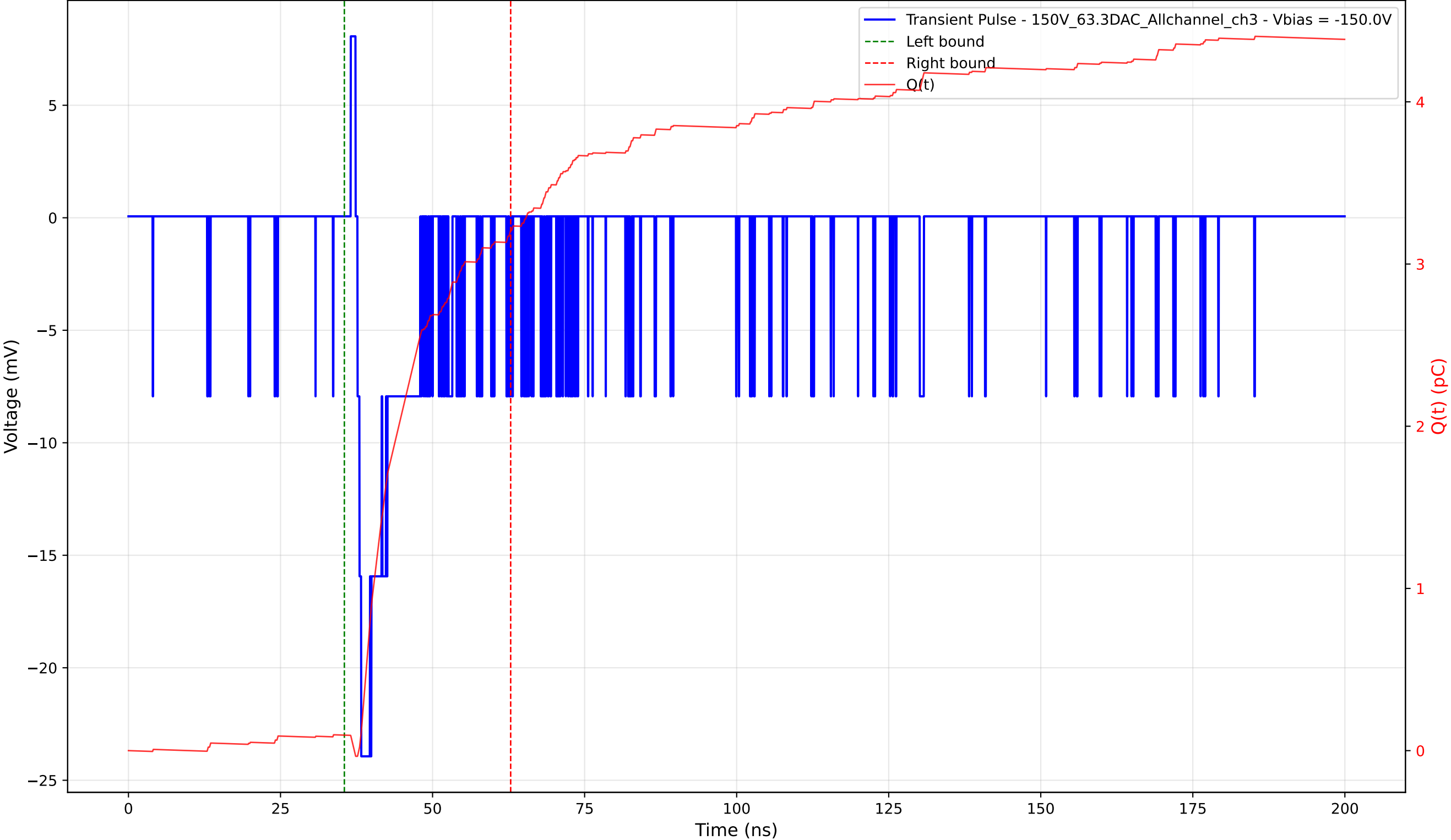
Transient Pulse - Sample: 1cm_42 - Position: 295.0 \mu\text{m} - Charge: 3.11 pC - Rise Time: 0.63 ns
