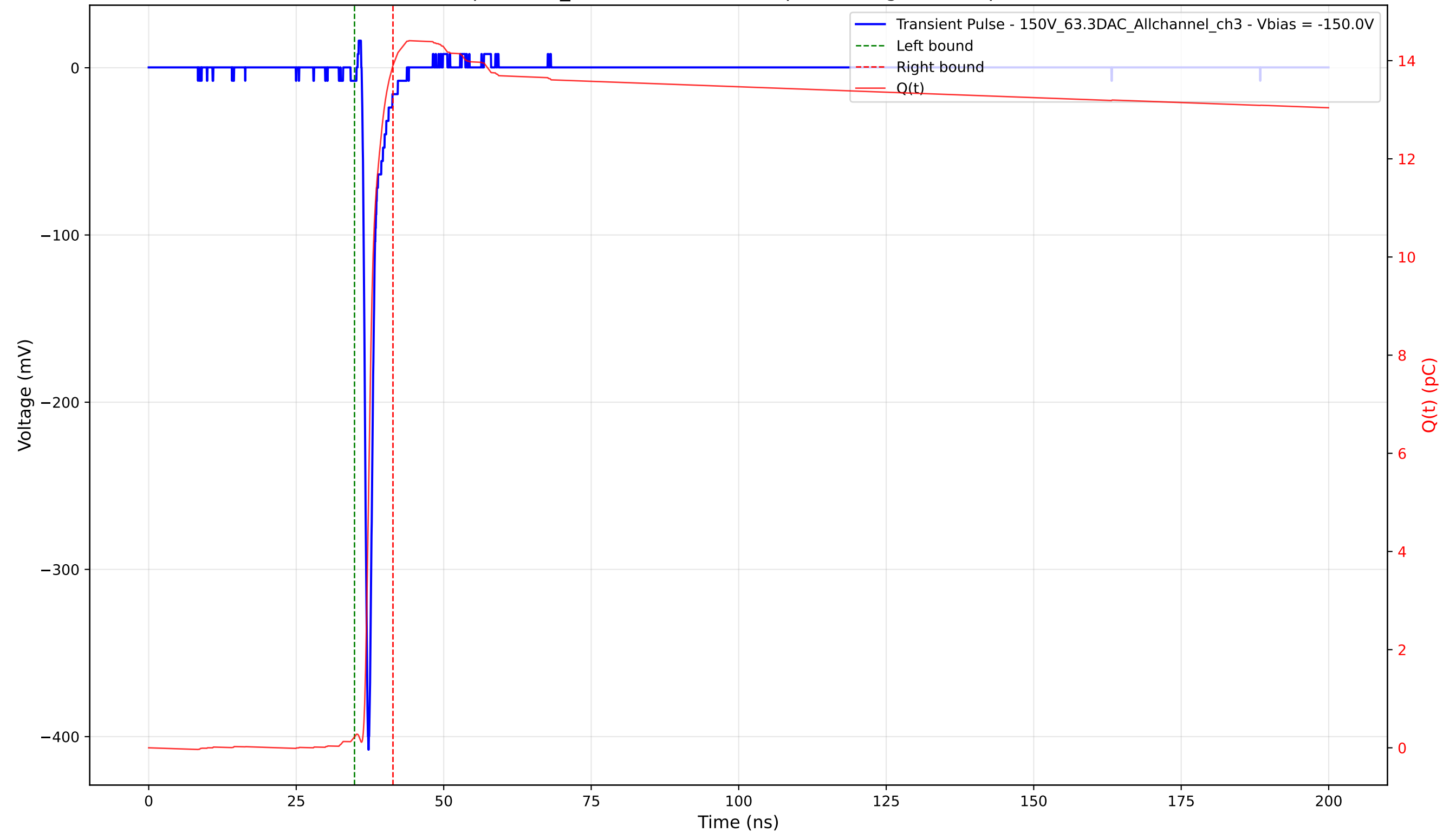
Transient Pulse - Sample: 1cm_42 - Position: 2845.0 \mu\text{m} - Charge: 13.68 pC - Rise Time: 0.75 ns
