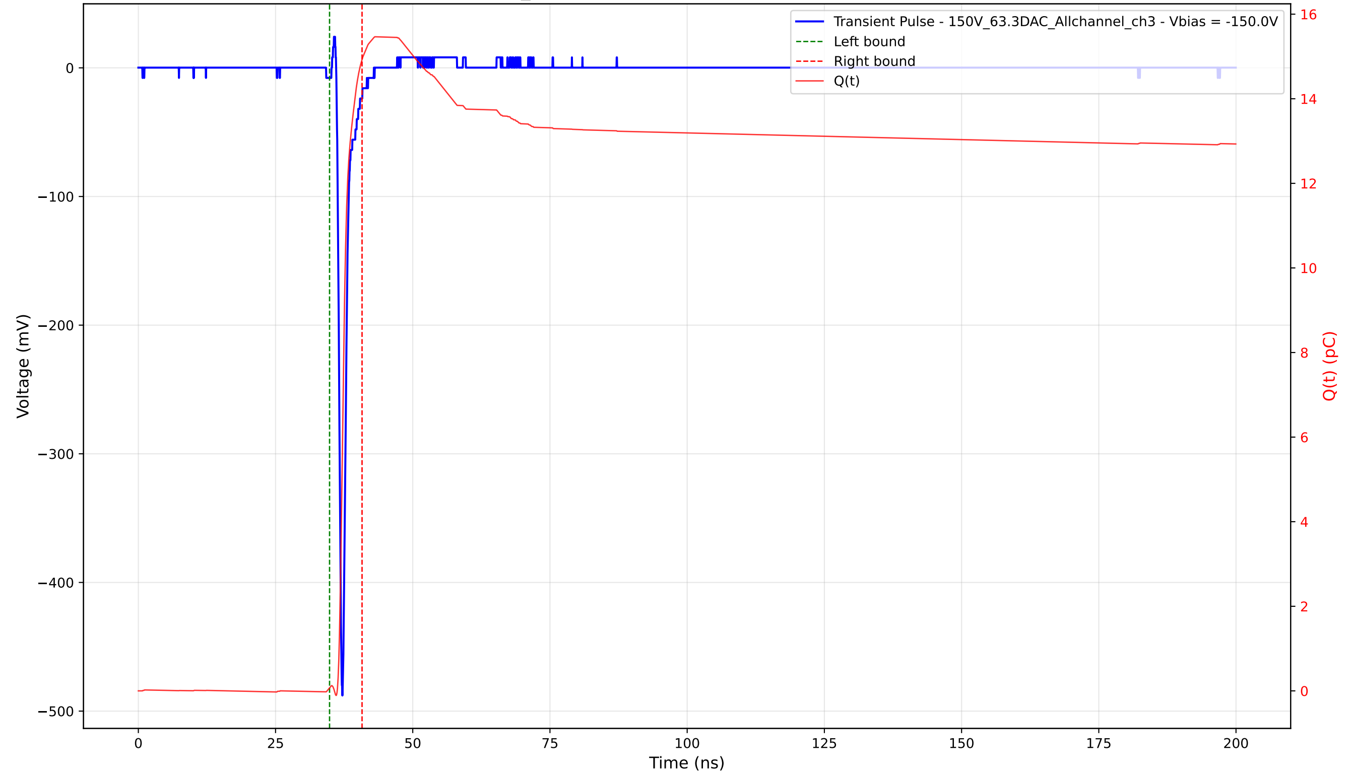
Transient Pulse - Sample: 1cm_42 - Position: 2425.0 \mu\text{m} - Charge: 14.86 pC - Rise Time: 0.73 ns
