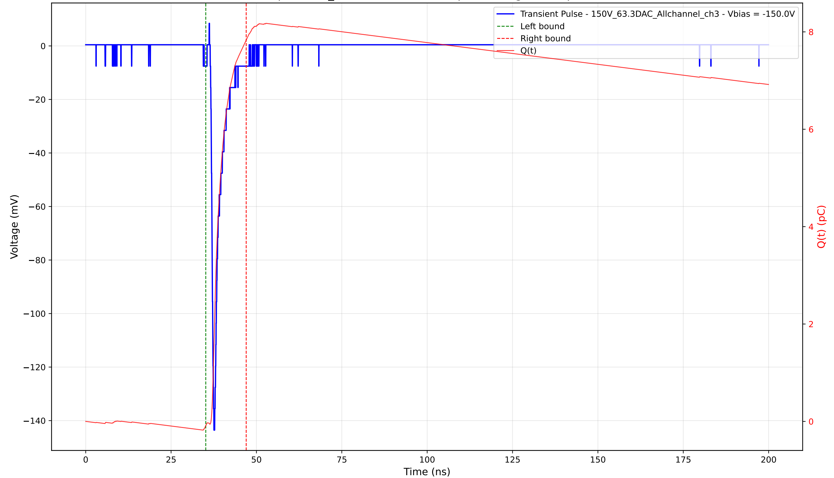
Transient Pulse - Sample: 1cm_42 - Position: 3255.0 \mu\text{m} - Charge: 7.92 pC - Rise Time: 0.85 ns
