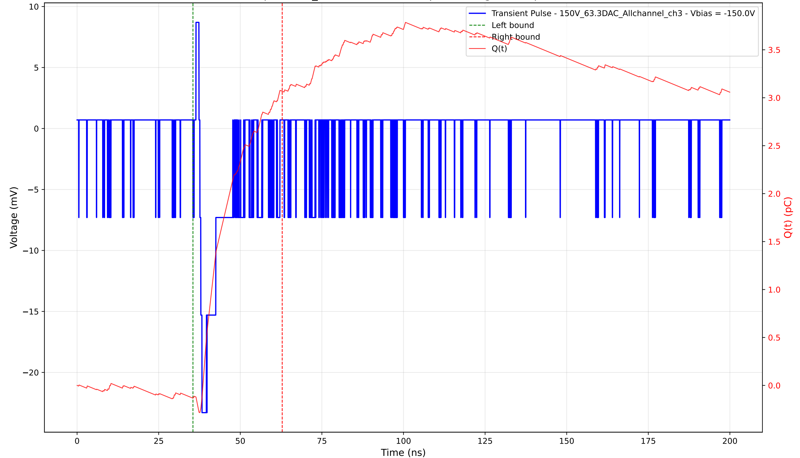
Transient Pulse - Sample: 1cm_42 - Position: 315.0 \mu\text{m} - Charge: 3.20 pC - Rise Time: 0.67 ns
