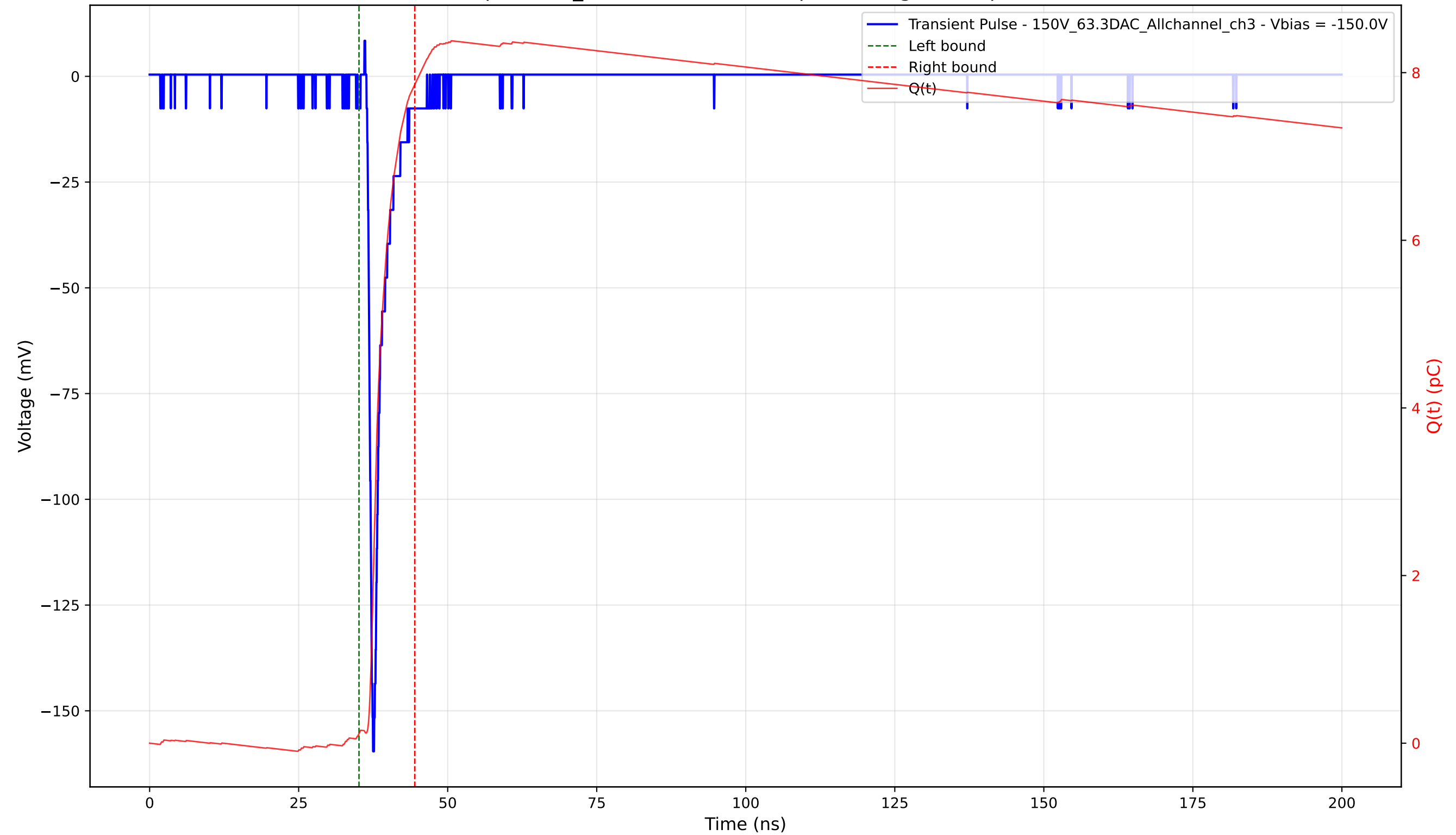
Transient Pulse - Sample: 1cm_42 - Position: 3175.0 \mu\text{m} - Charge: 7.74 pC - Rise Time: 0.84 ns
