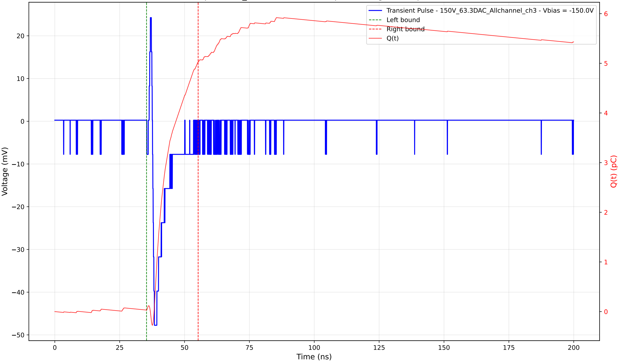
Transient Pulse - Sample: 1cm_42 - Position: 870.0 \mu\text{m} - Charge: 5.00 pC - Rise Time: 0.74 ns
