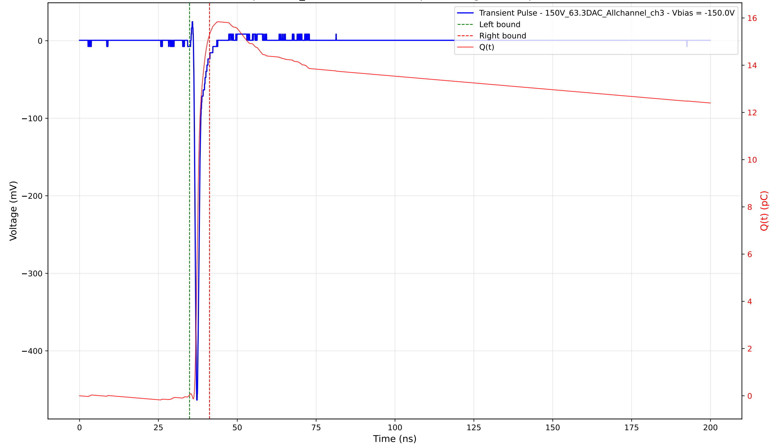
Transient Pulse - Sample: 1cm_42 - Position: 2775.0 \mu\text{m} - Charge: 15.26 pC - Rise Time: 0.73 ns
