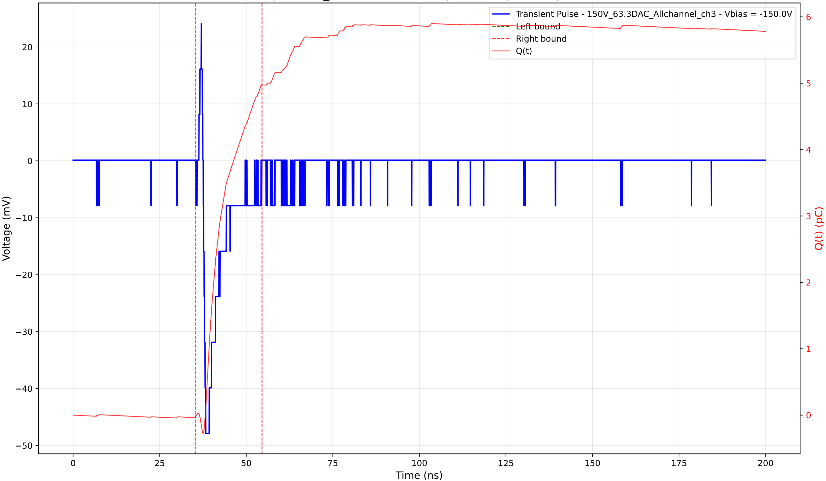
Transient Pulse - Sample: 1cm_42 - Position: 990.0 \mu\text{m} - Charge: 5.01 pC - Rise Time: 0.74 ns
