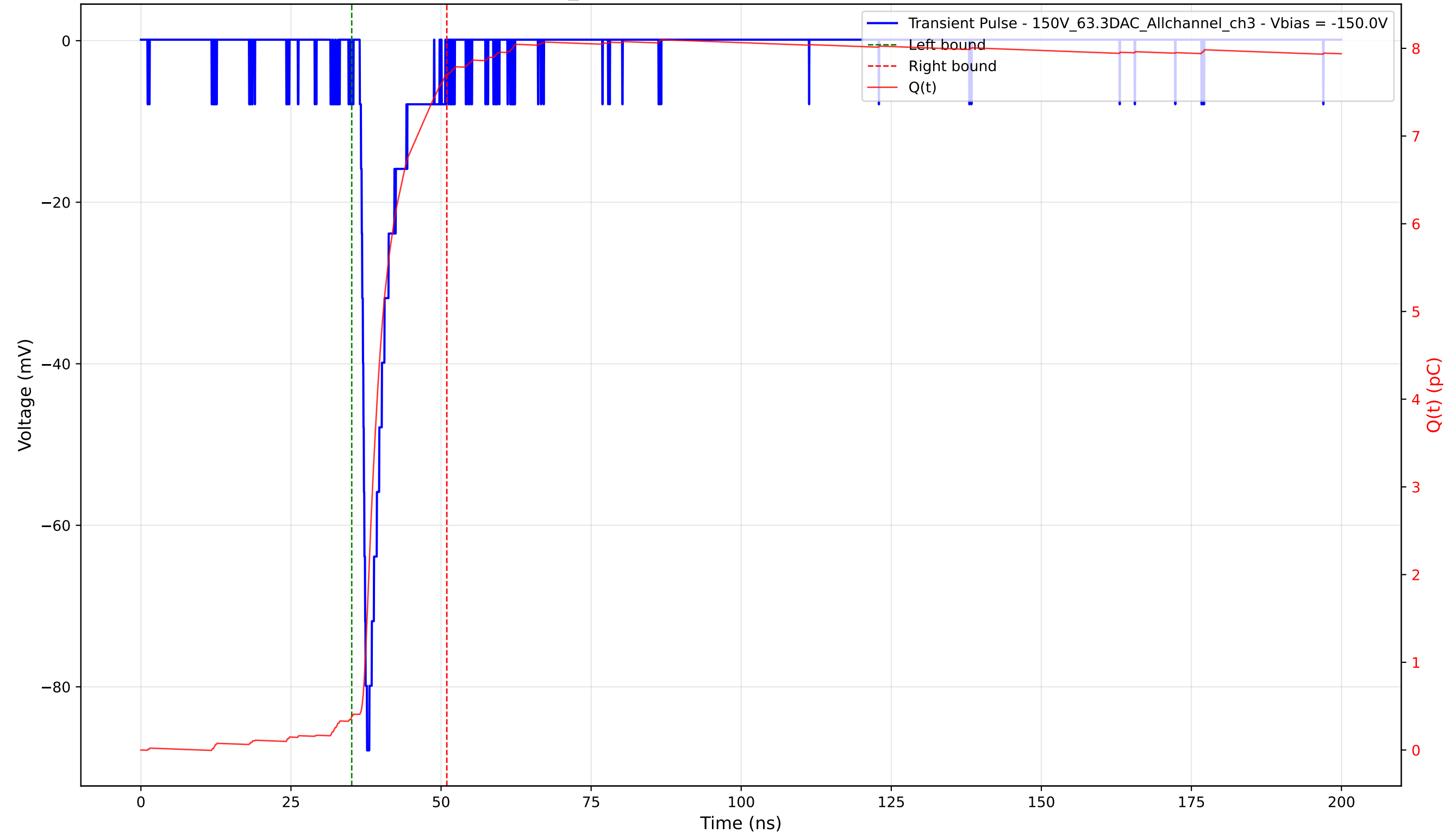
Transient Pulse - Sample: 1cm_42 - Position: 1560.0 \mu\text{m} - Charge: 7.32 pC - Rise Time: 0.80 ns
