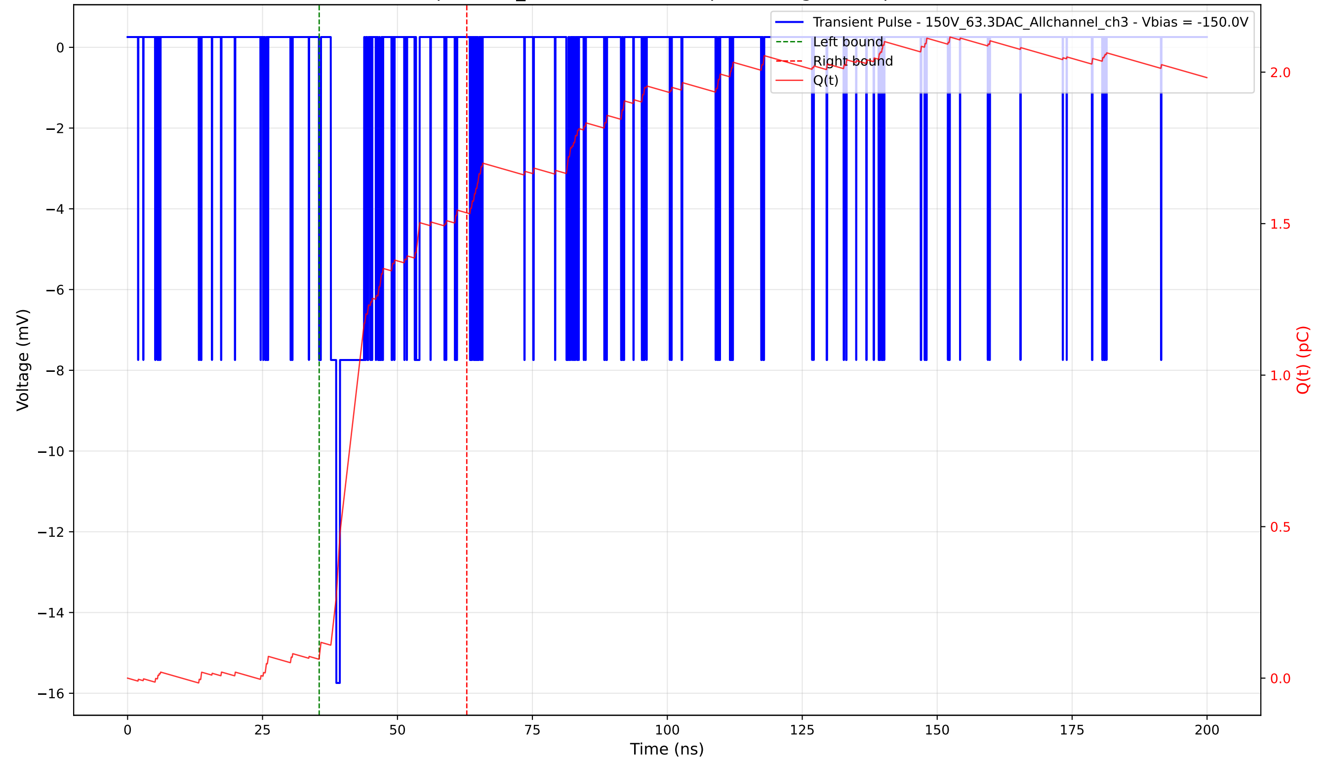
Transient Pulse - Sample: 1cm_42 - Position: 120.0 \mu\text{m} - Charge: 1.46 pC - Rise Time: 1.03 ns
