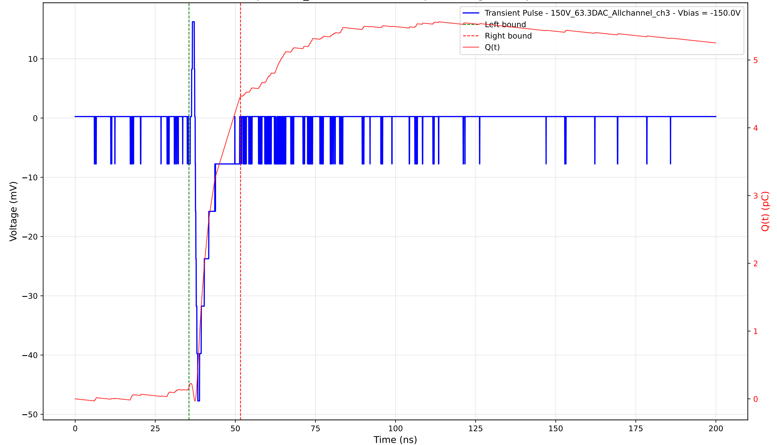
Transient Pulse - Sample: 1cm_42 - Position: 3935.0 \mu\text{m} - Charge: 4.30 pC - Rise Time: 0.82 ns
