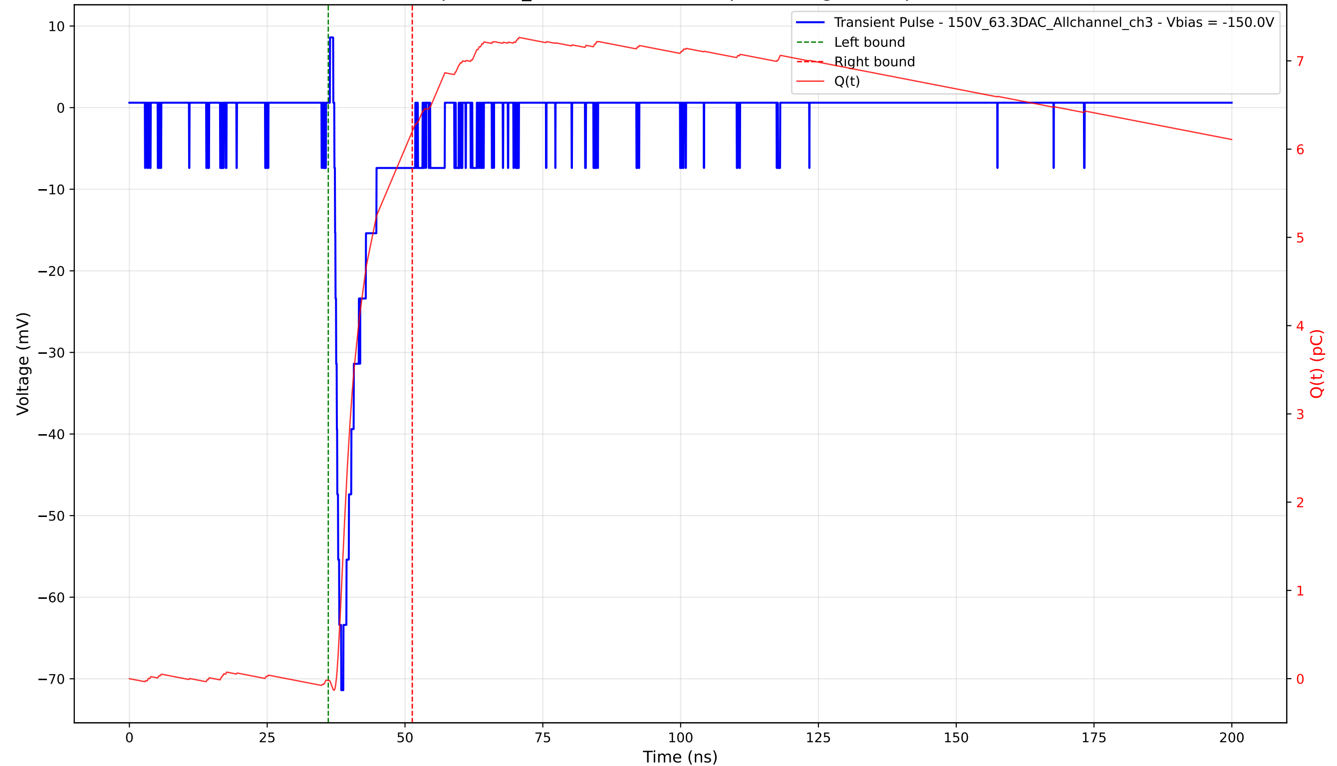
Transient Pulse - Sample: 1cm_42 - Position: 1310.0 \mu\text{m} - Charge: 6.23 pC - Rise Time: 1.24 ns
