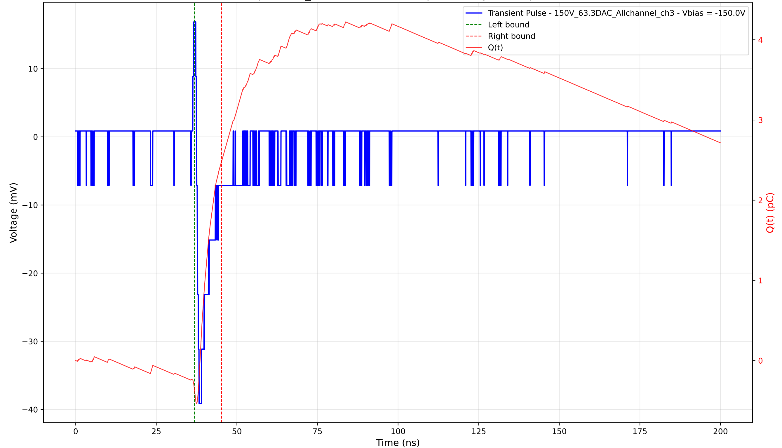
Transient Pulse - Sample: 1cm_42 - Position: 4035.0 \mu\text{m} - Charge: 2.84 pC - Rise Time: 0.74 ns
