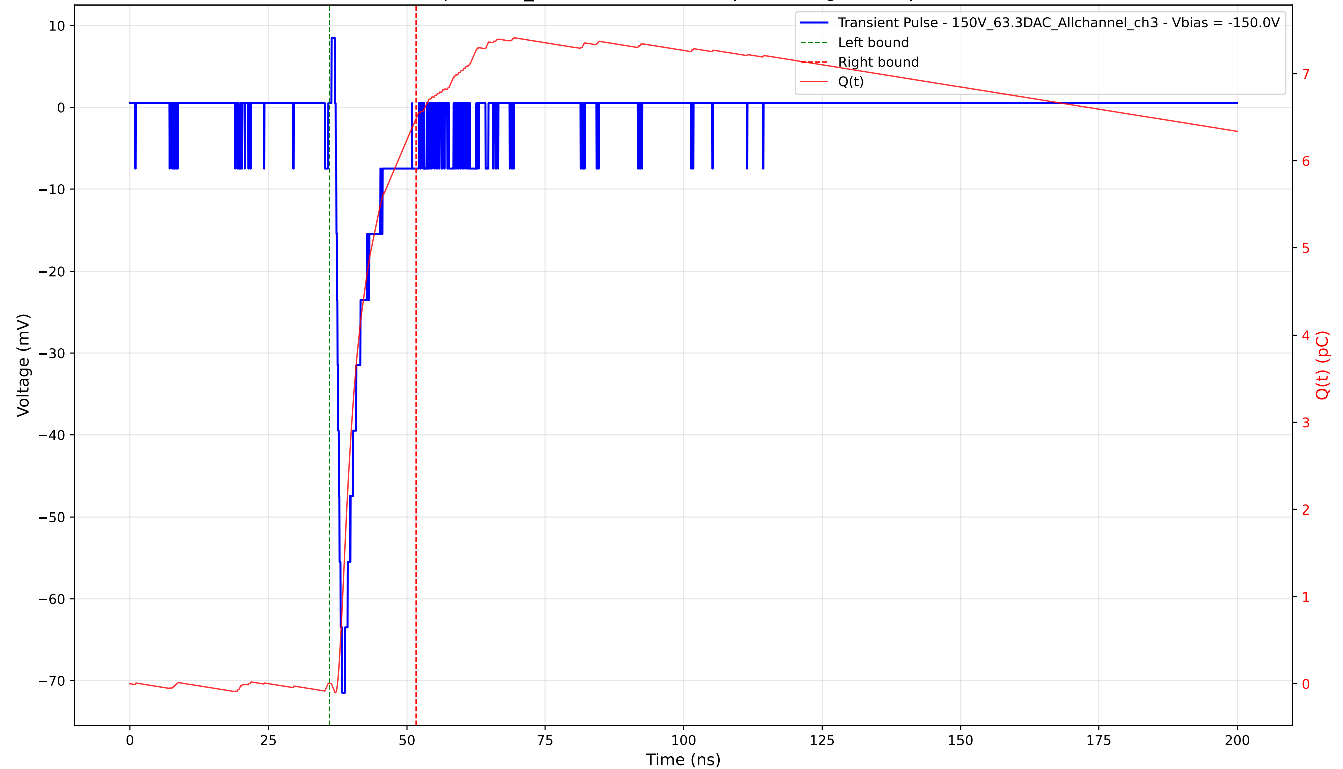
Transient Pulse - Sample: 1cm_42 - Position: 1300.0 \mu\text{m} - Charge: 6.48 pC - Rise Time: 1.16 ns
