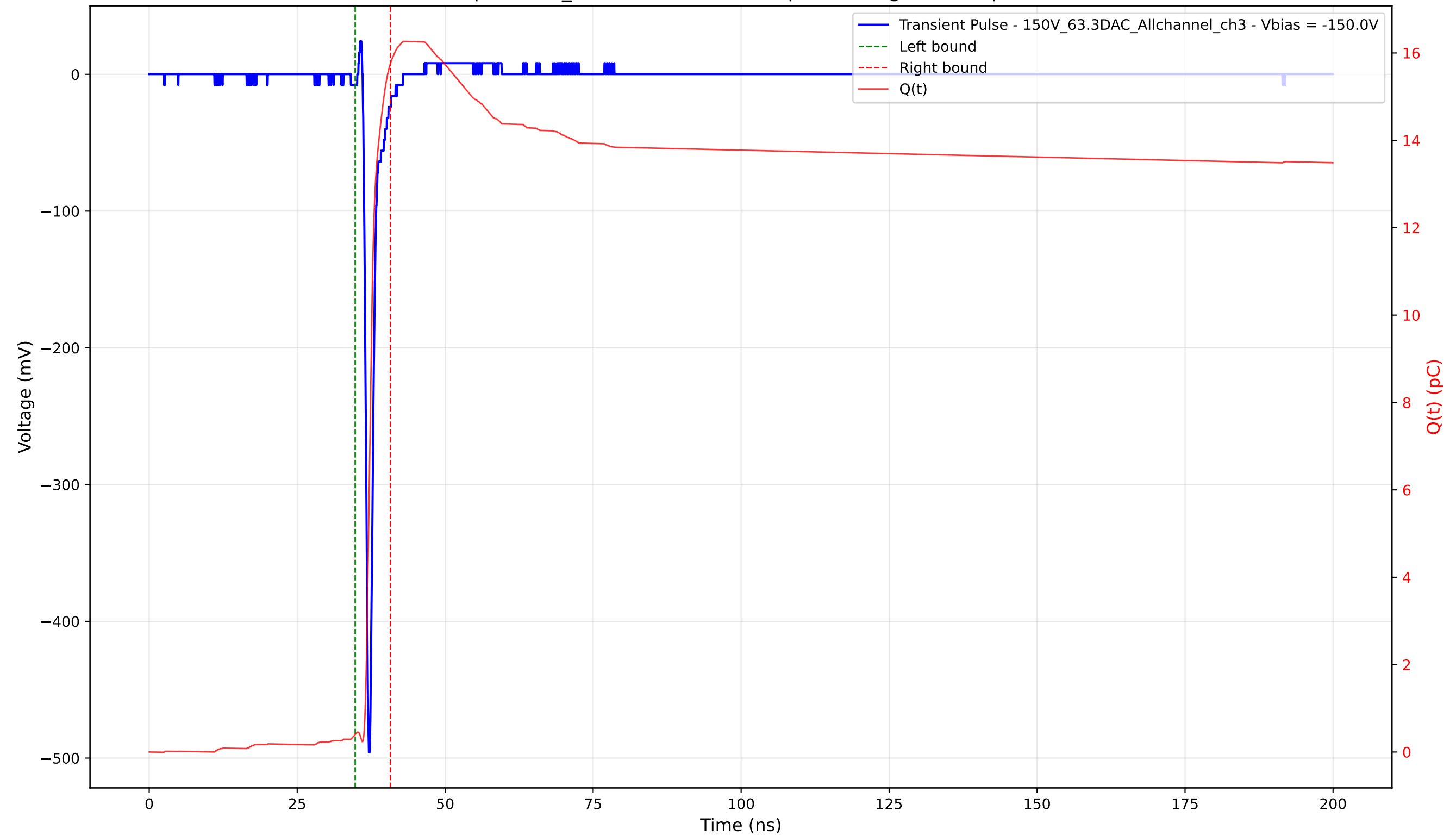
Transient Pulse - Sample: 1cm_42 - Position: 2625.0 \mu\text{m} - Charge: 15.36 pC - Rise Time: 0.71 ns
