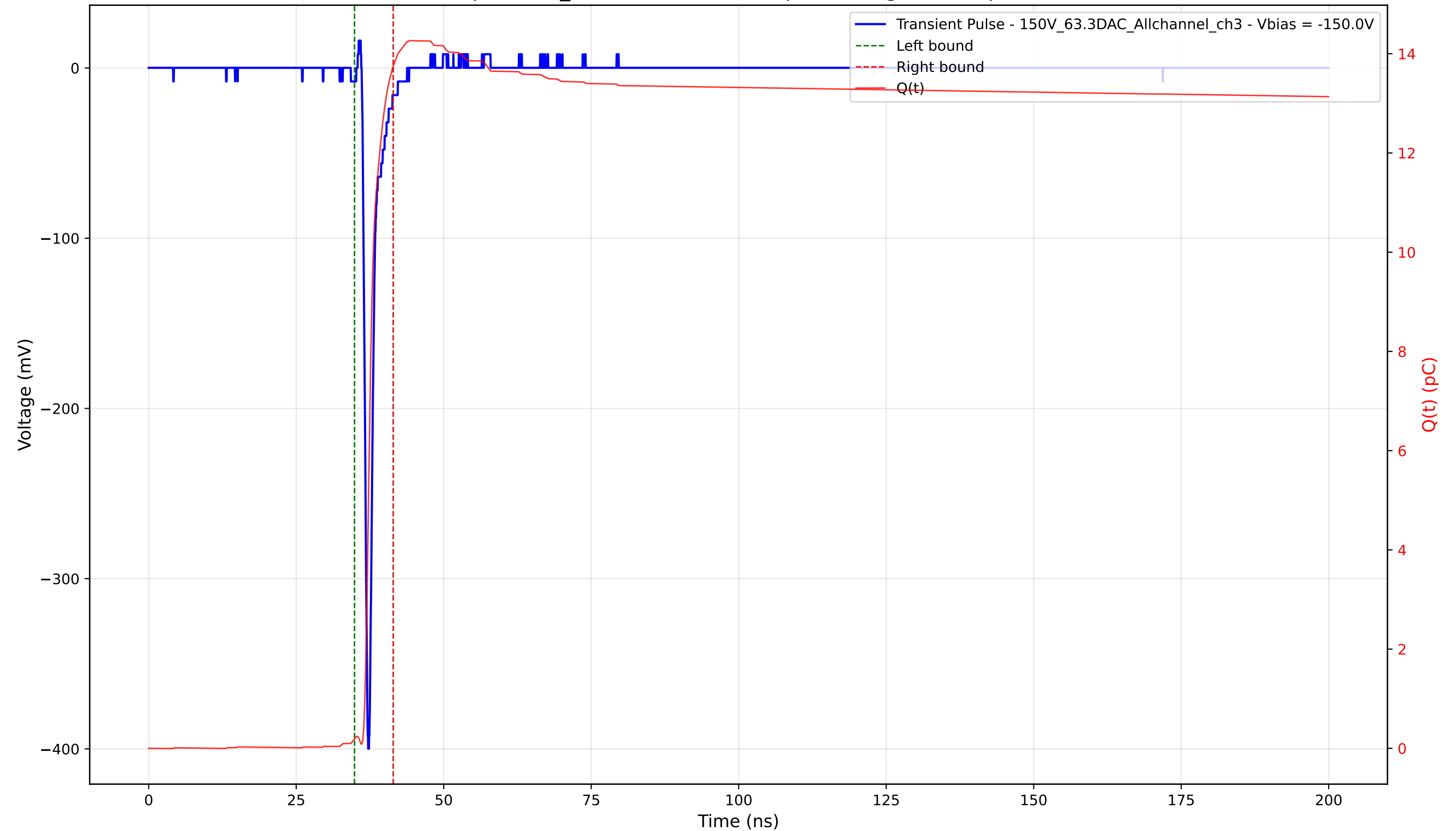
Transient Pulse - Sample: 1cm_42 - Position: 2850.0 \mu\text{m} - Charge: 13.56 pC - Rise Time: 0.70 ns
