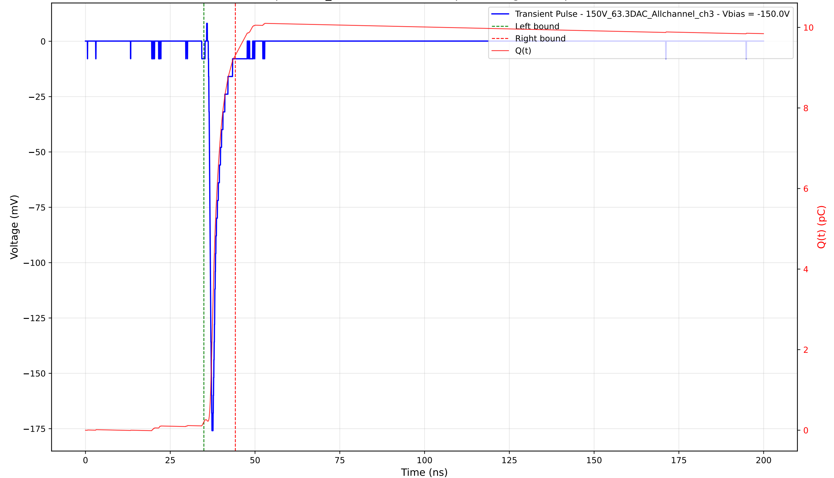
Transient Pulse - Sample: 1cm_42 - Position: 1910.0 \mu\text{m} - Charge: 9.10 pC - Rise Time: 0.79 ns
