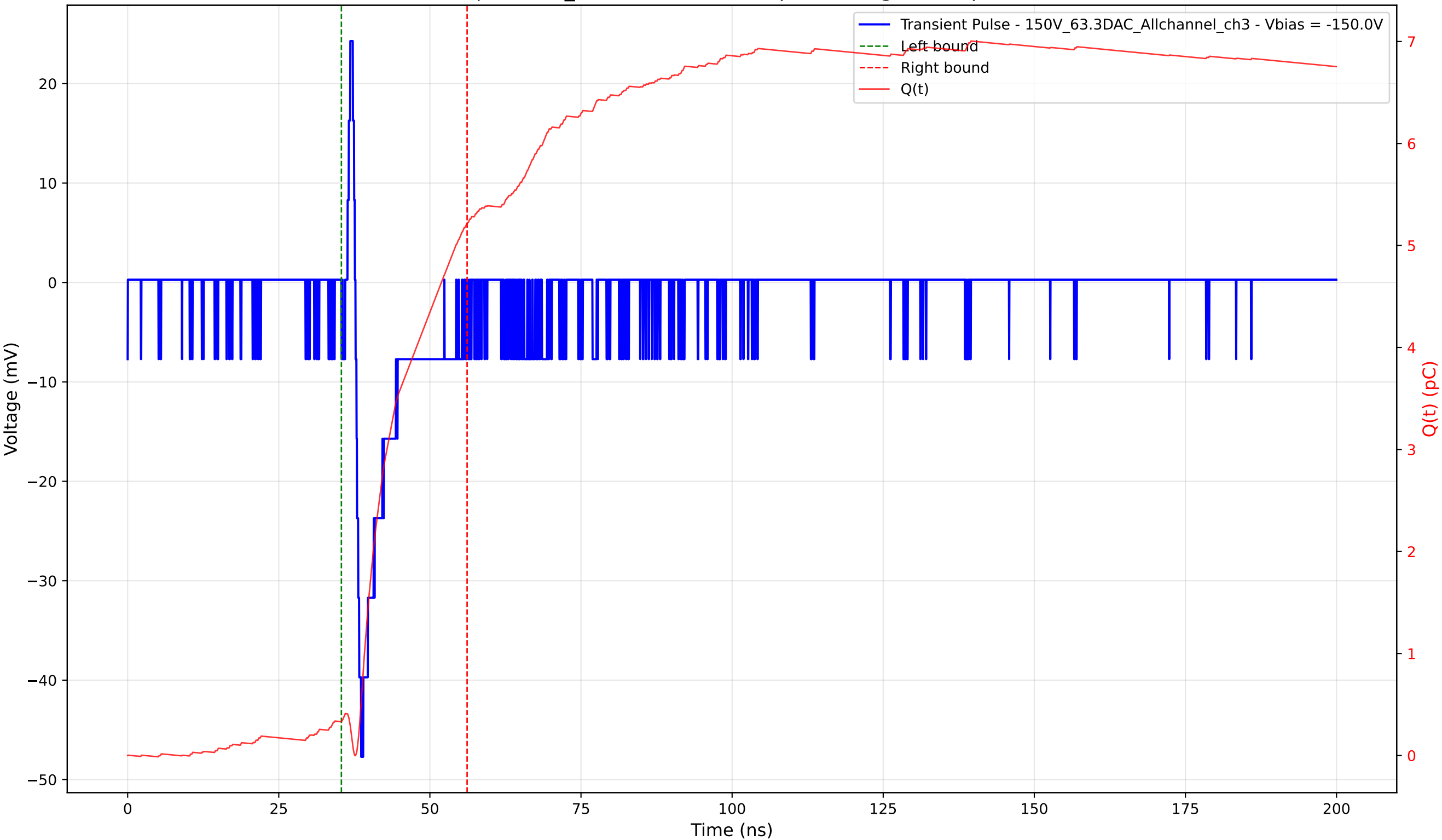
Transient Pulse - Sample: 1cm_42 - Position: 625.0 \mu\text{m} - Charge: 4.89 pC - Rise Time: 0.94 ns
