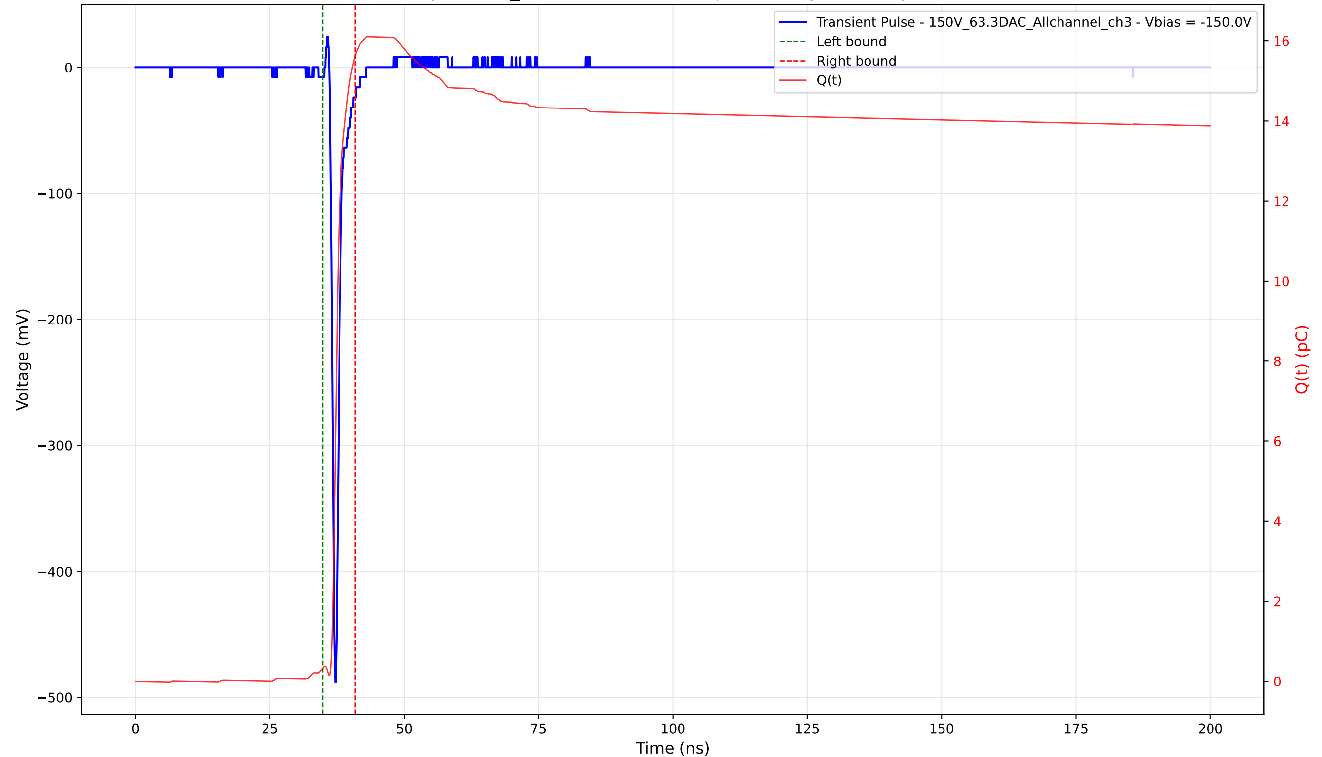
Transient Pulse - Sample: 1cm_42 - Position: 2670.0 \mu\text{m} - Charge: 15.30 pC - Rise Time: 0.69 ns
