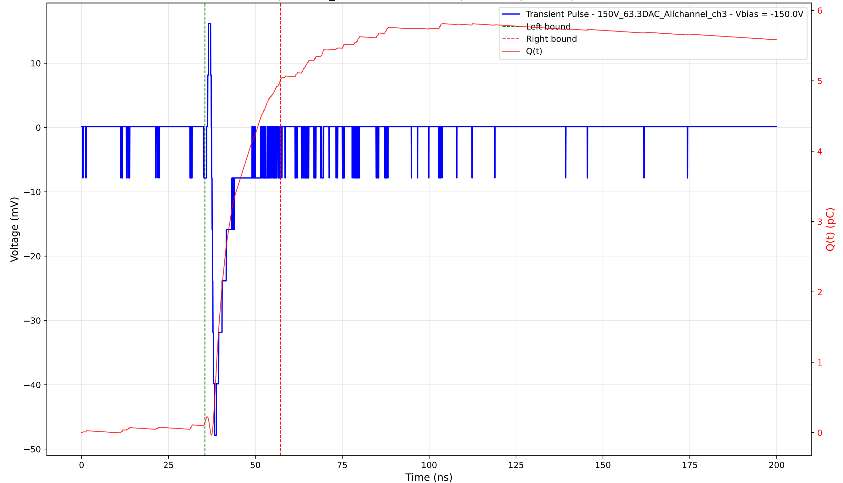
Transient Pulse - Sample: 1cm_42 - Position: 3925.0 \mu\text{m} - Charge: 4.86 pC - Rise Time: 0.82 ns
