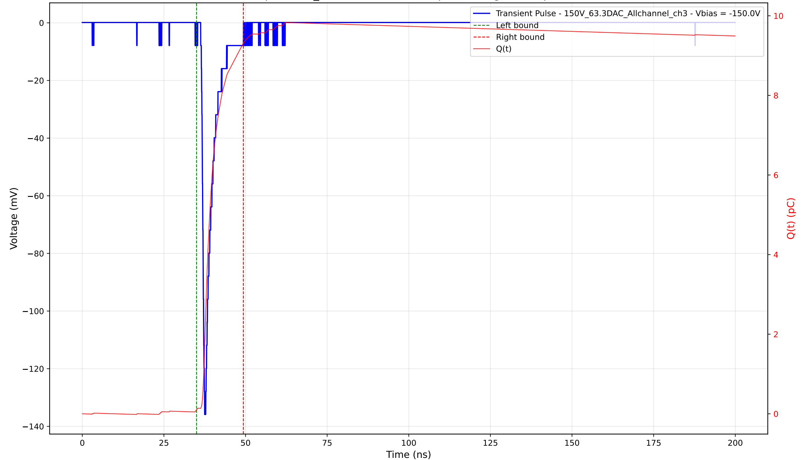
Transient Pulse - Sample: 1cm_42 - Position: 1695.0 \mu\text{m} - Charge: 9.21 pC - Rise Time: 0.93 ns
