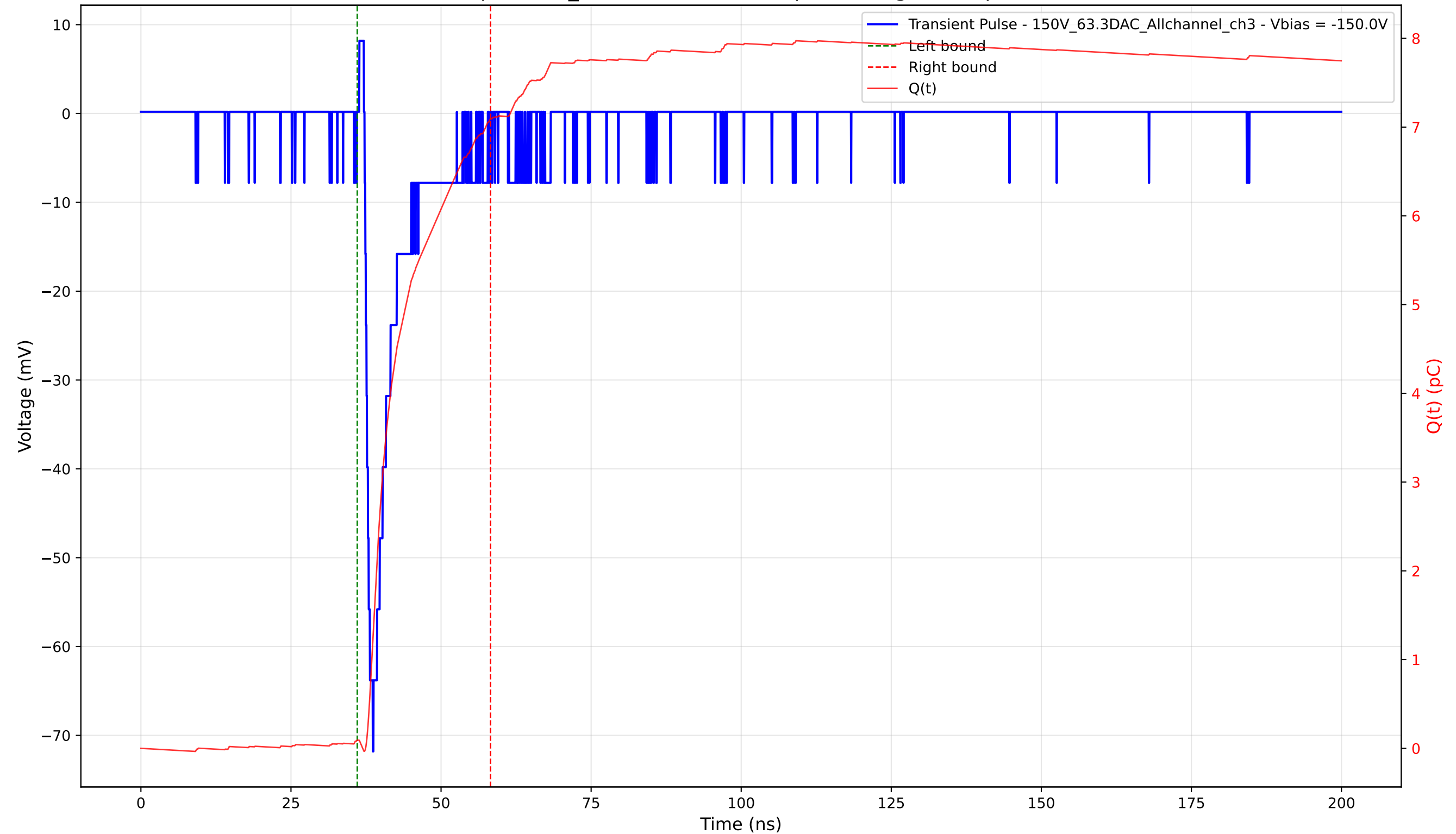
Transient Pulse - Sample: 1cm_42 - Position: 1225.0 \mu\text{m} - Charge: 7.00 pC - Rise Time: 1.36 ns
