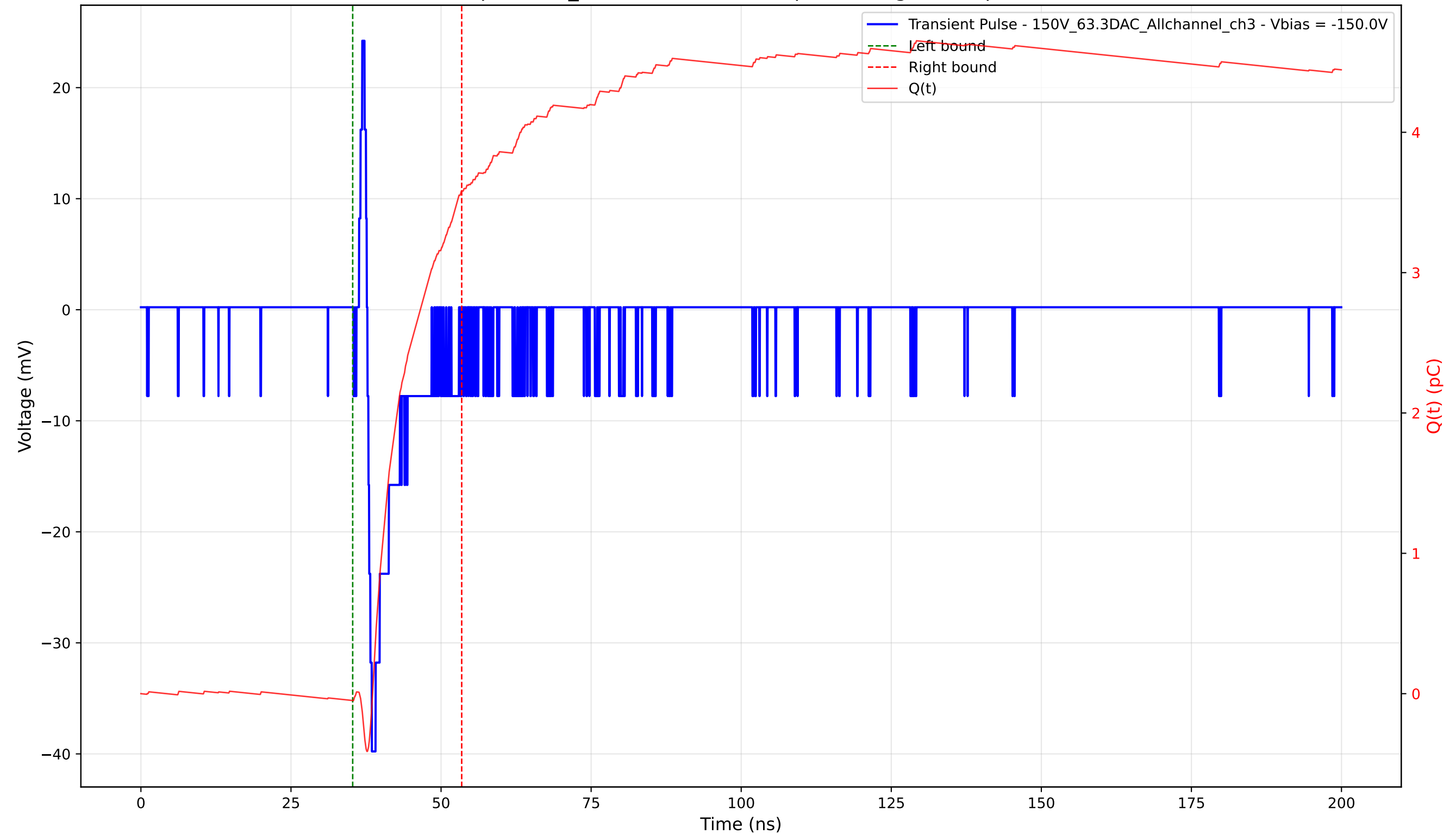
Transient Pulse - Sample: 1cm_42 - Position: 4340.0 \mu\text{m} - Charge: 3.63 pC - Rise Time: 0.74 ns
