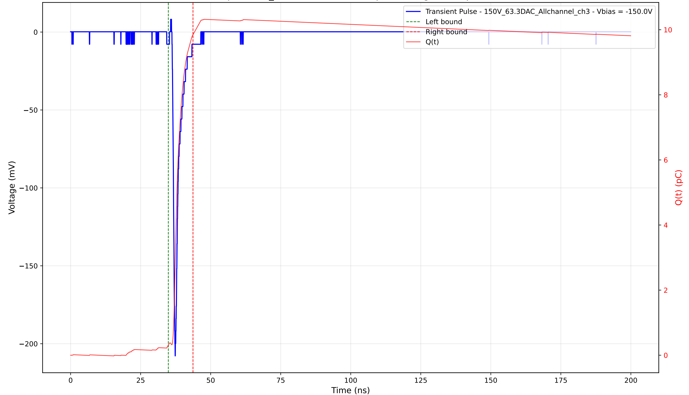
Transient Pulse - Sample: 1cm_42 - Position: 1970.0 \mu\text{m} - Charge: 9.53 pC - Rise Time: 0.86 ns
