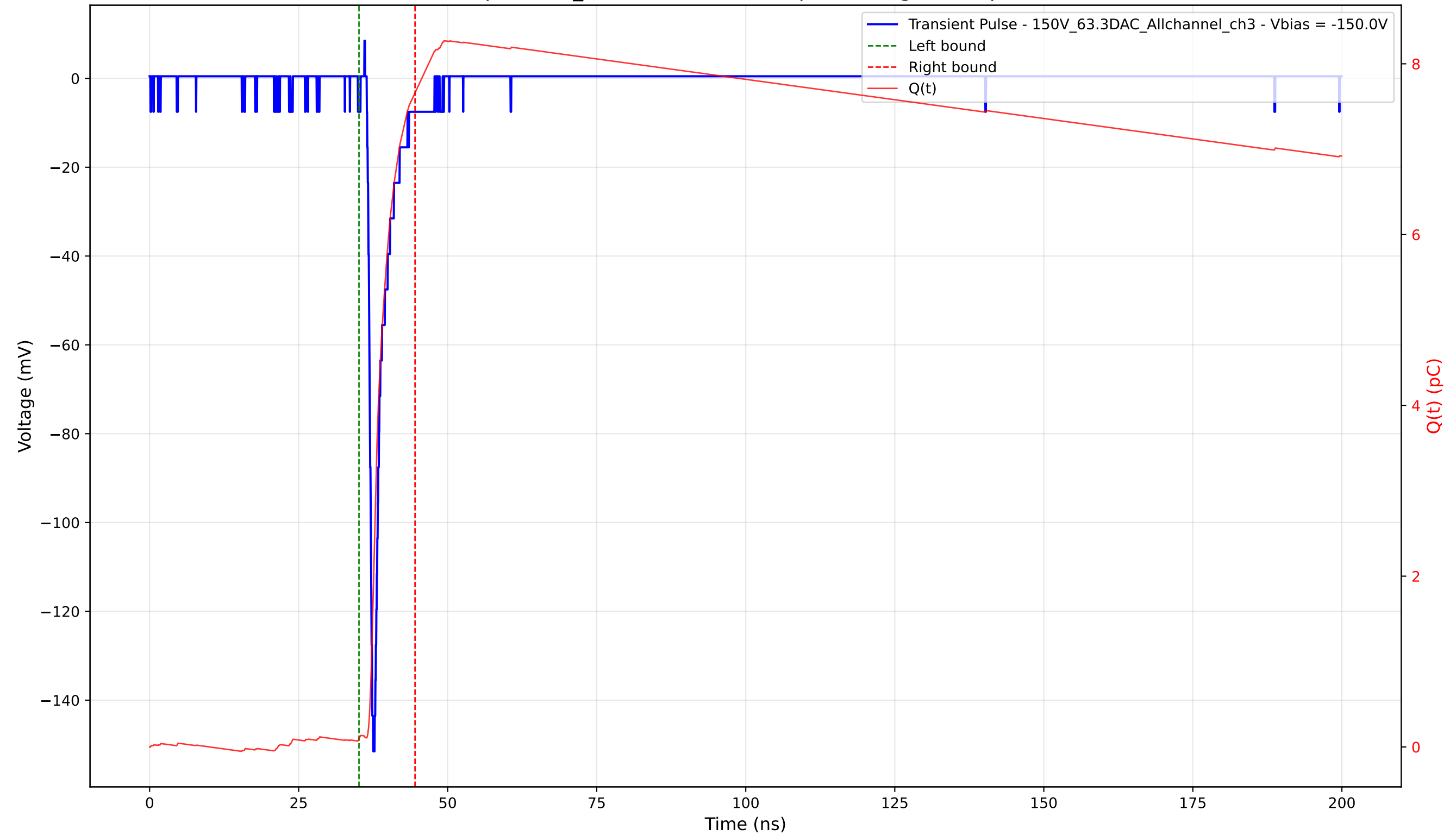
Transient Pulse - Sample: 1cm_42 - Position: 3195.0 \mu\text{m} - Charge: 7.56 pC - Rise Time: 0.84 ns
