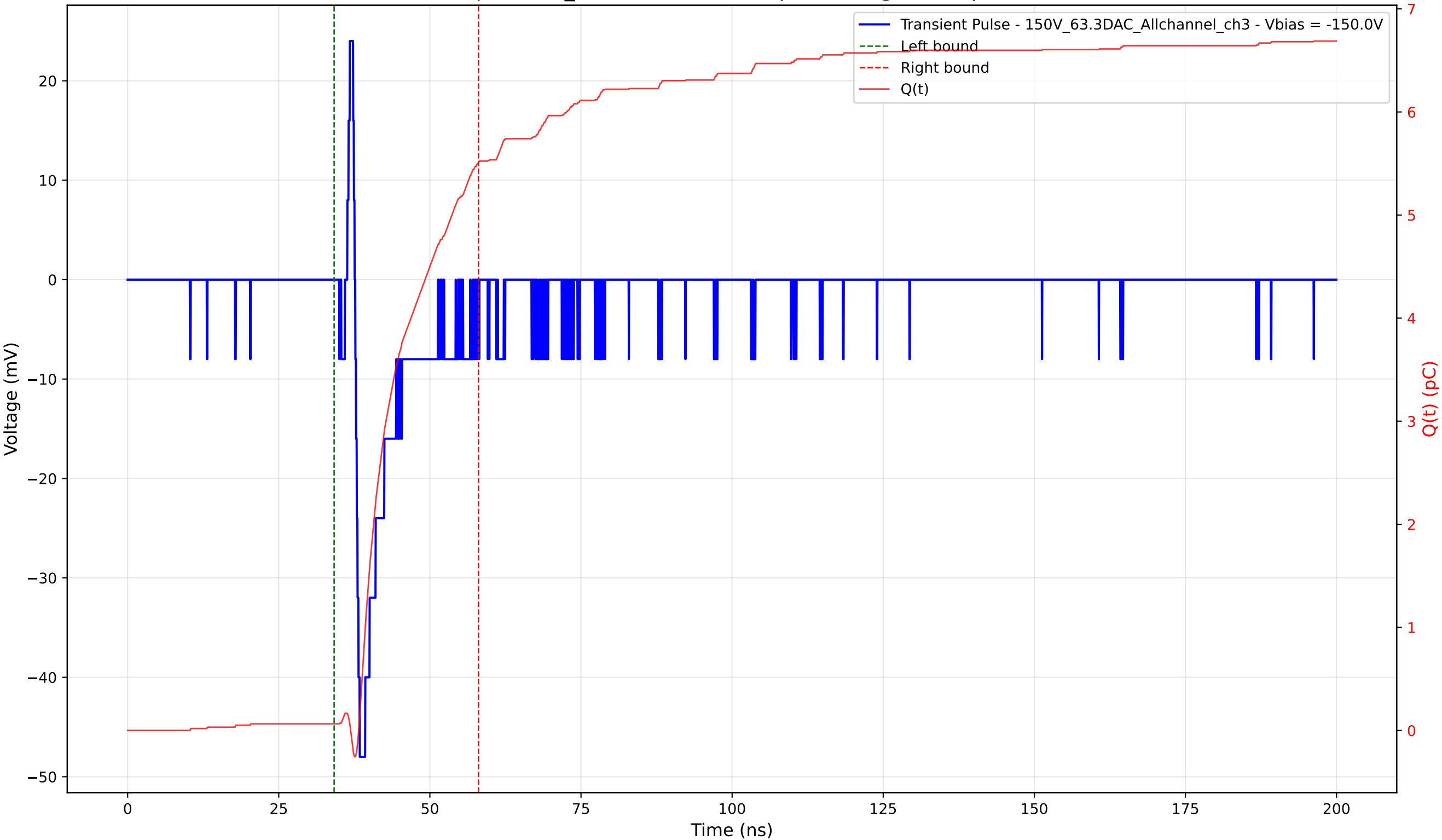
Transient Pulse - Sample: 1cm_42 - Position: 865.0 \mu\text{m} - Charge: 5.45 pC - Rise Time: 0.74 ns
