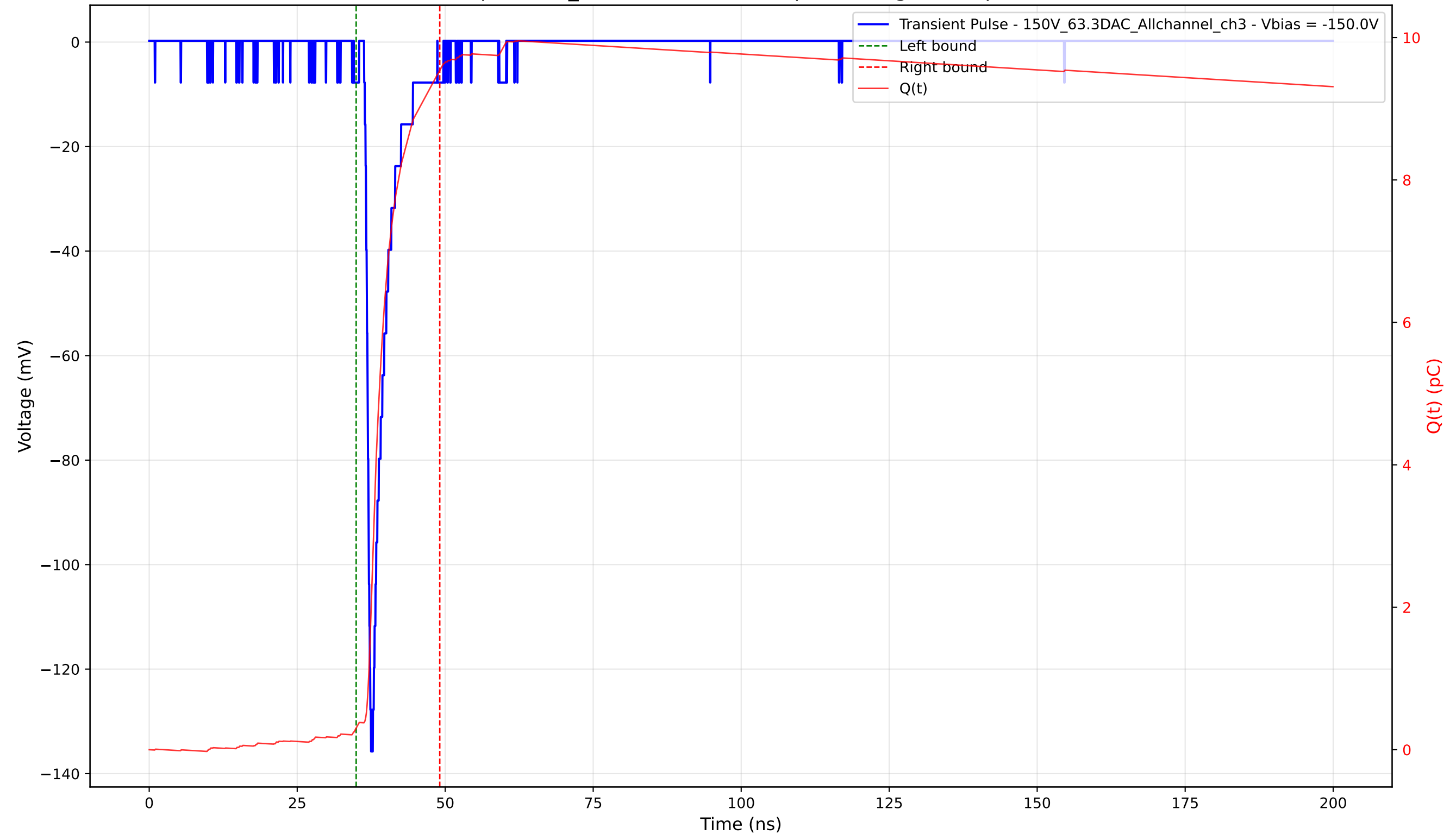
Transient Pulse - Sample: 1cm_42 - Position: 1700.0 \mu\text{m} - Charge: 9.23 pC - Rise Time: 0.93 ns
