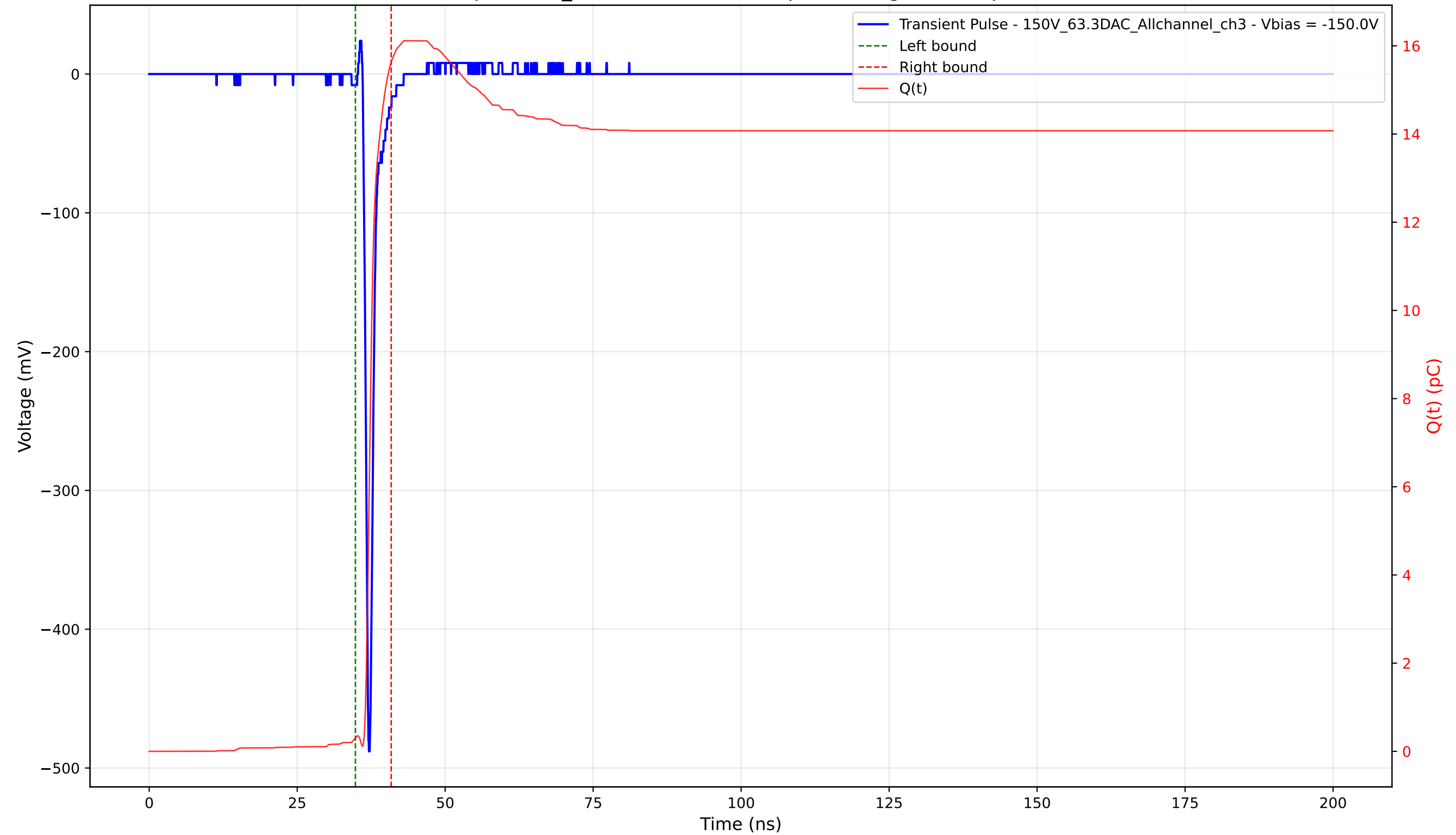
Transient Pulse - Sample: 1cm_42 - Position: 2655.0 \mu\text{m} - Charge: 15.33 pC - Rise Time: 0.72 ns
