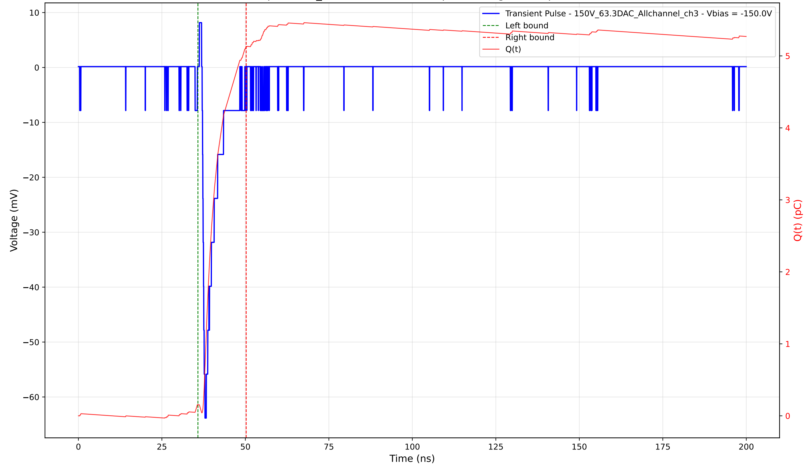
Transient Pulse - Sample: 1cm_42 - Position: 3600.0 \mu\text{m} - Charge: 4.97 pC - Rise Time: 0.85 ns
