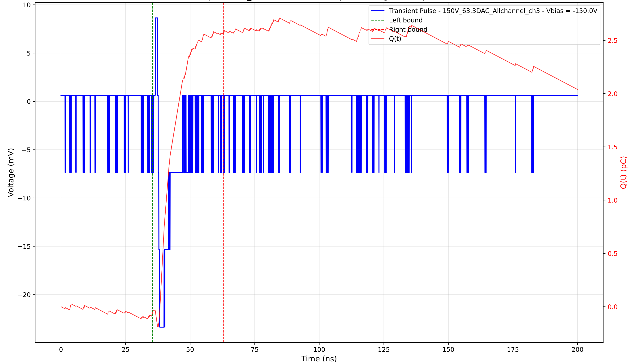
Transient Pulse - Sample: 1cm_42 - Position: 325.0 \mu\text{m} - Charge: 2.61 pC - Rise Time: 0.63 ns
