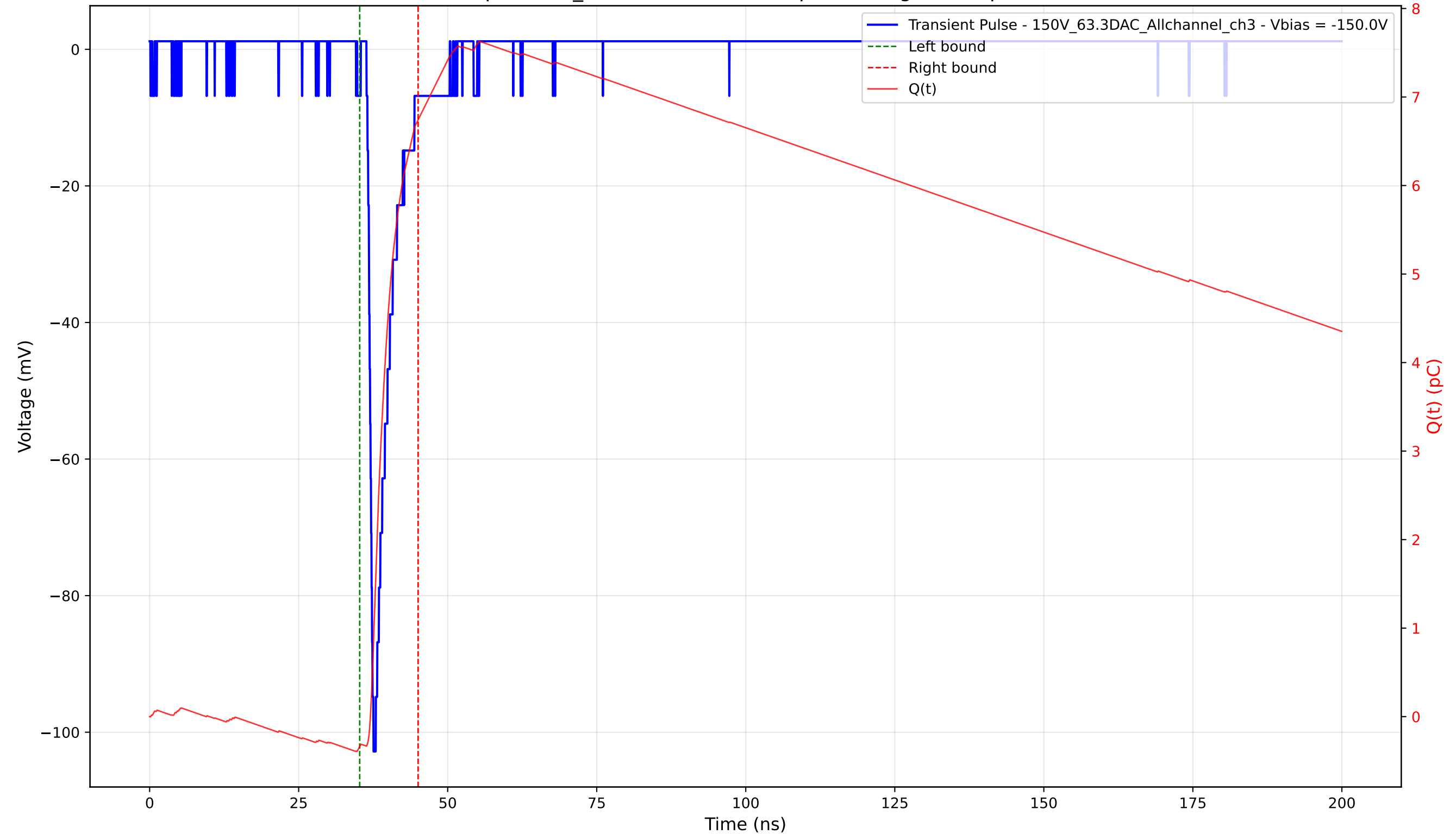
Transient Pulse - Sample: 1cm_42 - Position: 1610.0 \mu\text{m} - Charge: 7.08 pC - Rise Time: 0.86 ns
