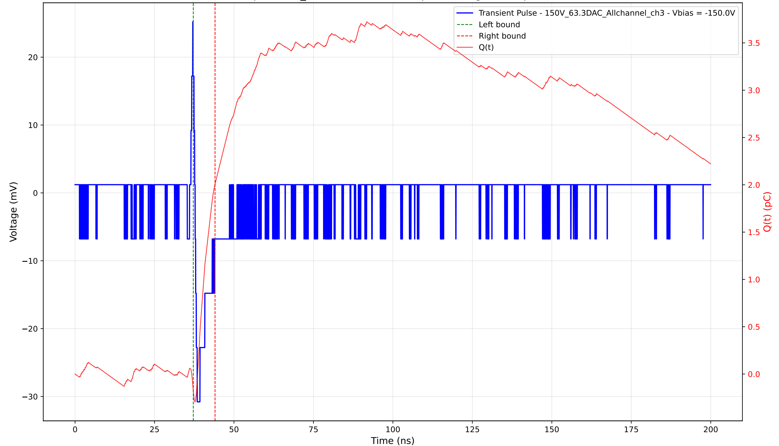
Transient Pulse - Sample: 1cm_42 - Position: 4450.0 \mu\text{m} - Charge: 2.19 pC - Rise Time: 0.67 ns
