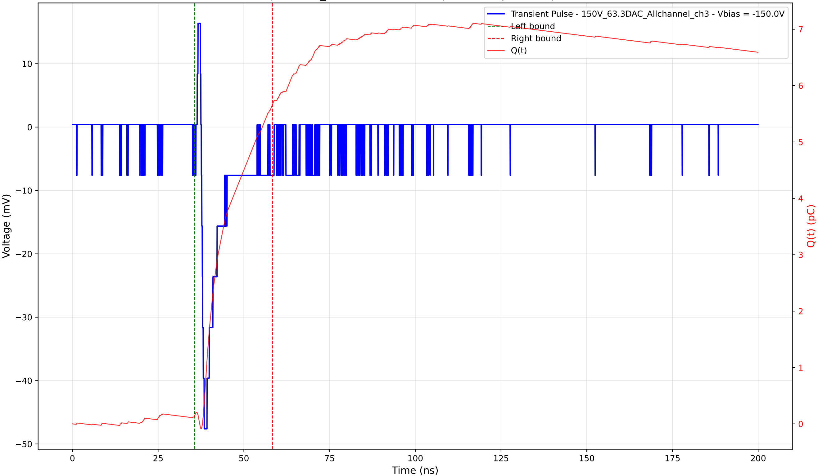
Transient Pulse - Sample: 1cm_42 - Position: 955.0 \mu\text{m} - Charge: 5.51 pC - Rise Time: 0.86 ns
