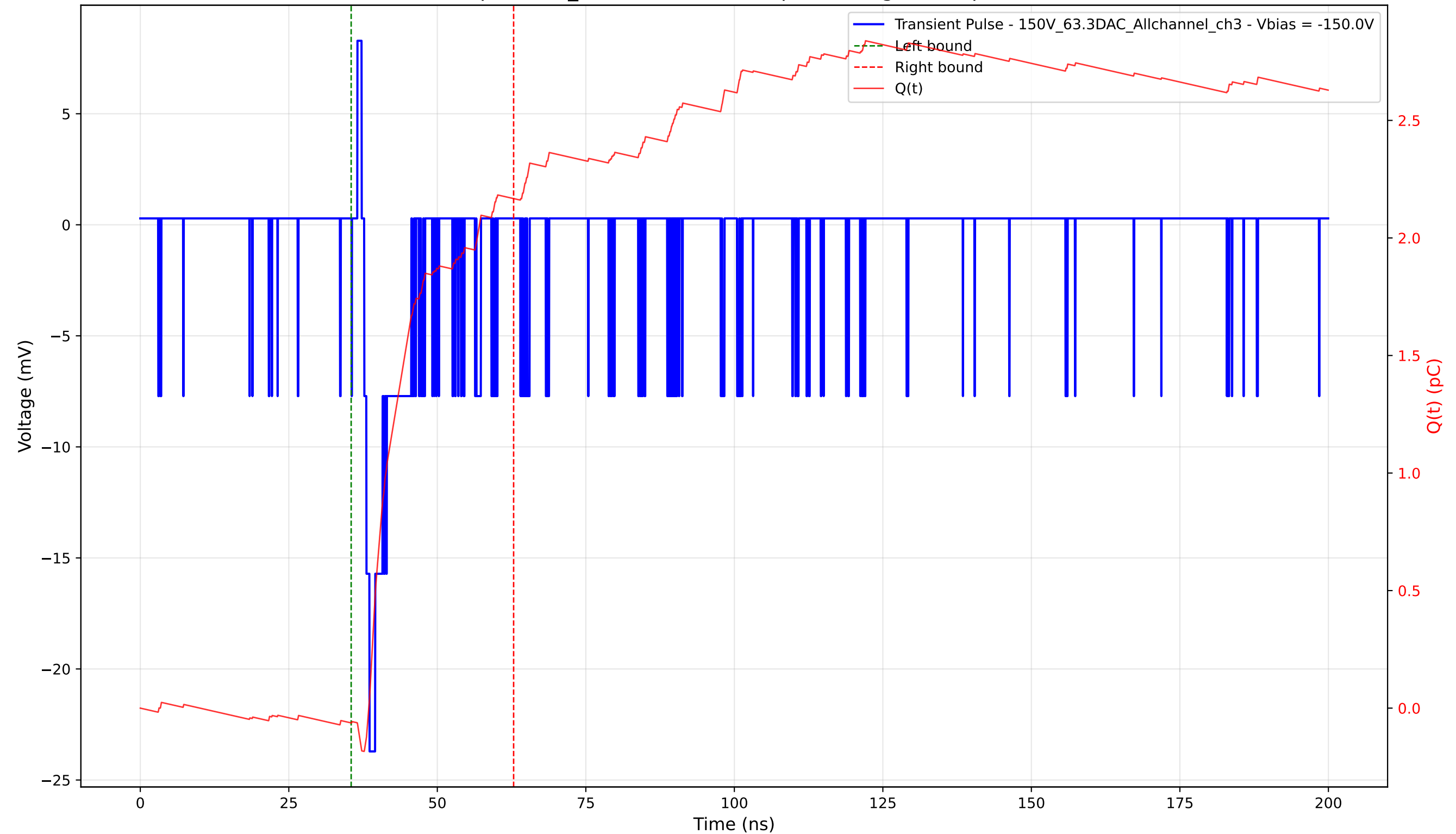
Transient Pulse - Sample: 1cm_42 - Position: 235.0 \mu\text{m} - Charge: 2.23 pC - Rise Time: 0.91 ns
