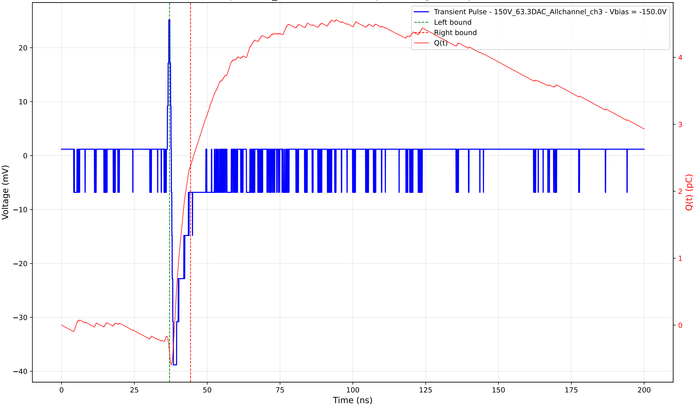
Transient Pulse - Sample: 1cm_42 - Position: 590.0 \mu\text{m} - Charge: 2.81 pC - Rise Time: 0.70 ns
