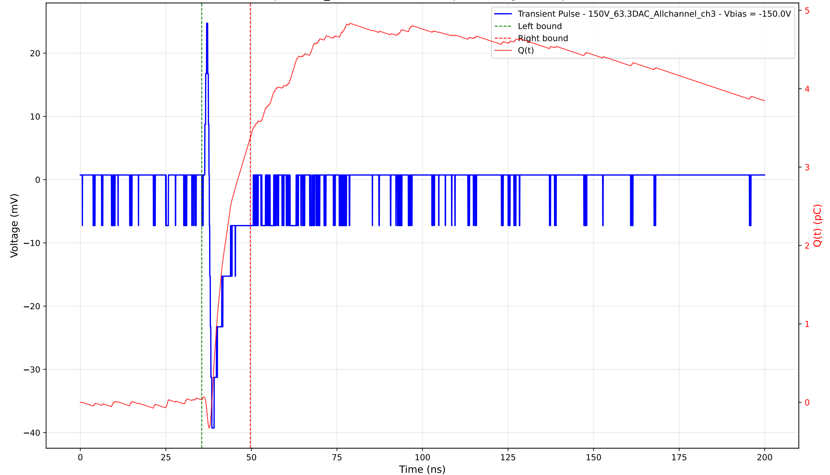
Transient Pulse - Sample: 1cm_42 - Position: 4190.0 \mu\text{m} - Charge: 3.35 pC - Rise Time: 0.74 ns
