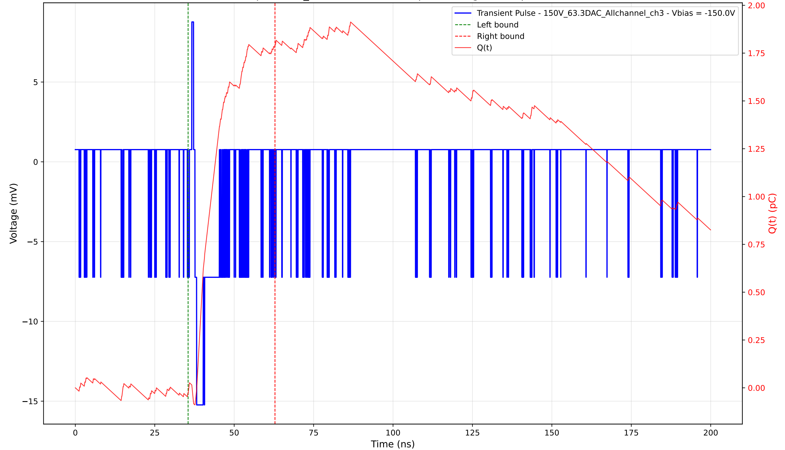
Transient Pulse - Sample: 1cm_42 - Position: 185.0 \mu\text{m} - Charge: 1.82 pC - Rise Time: 0.56 ns
