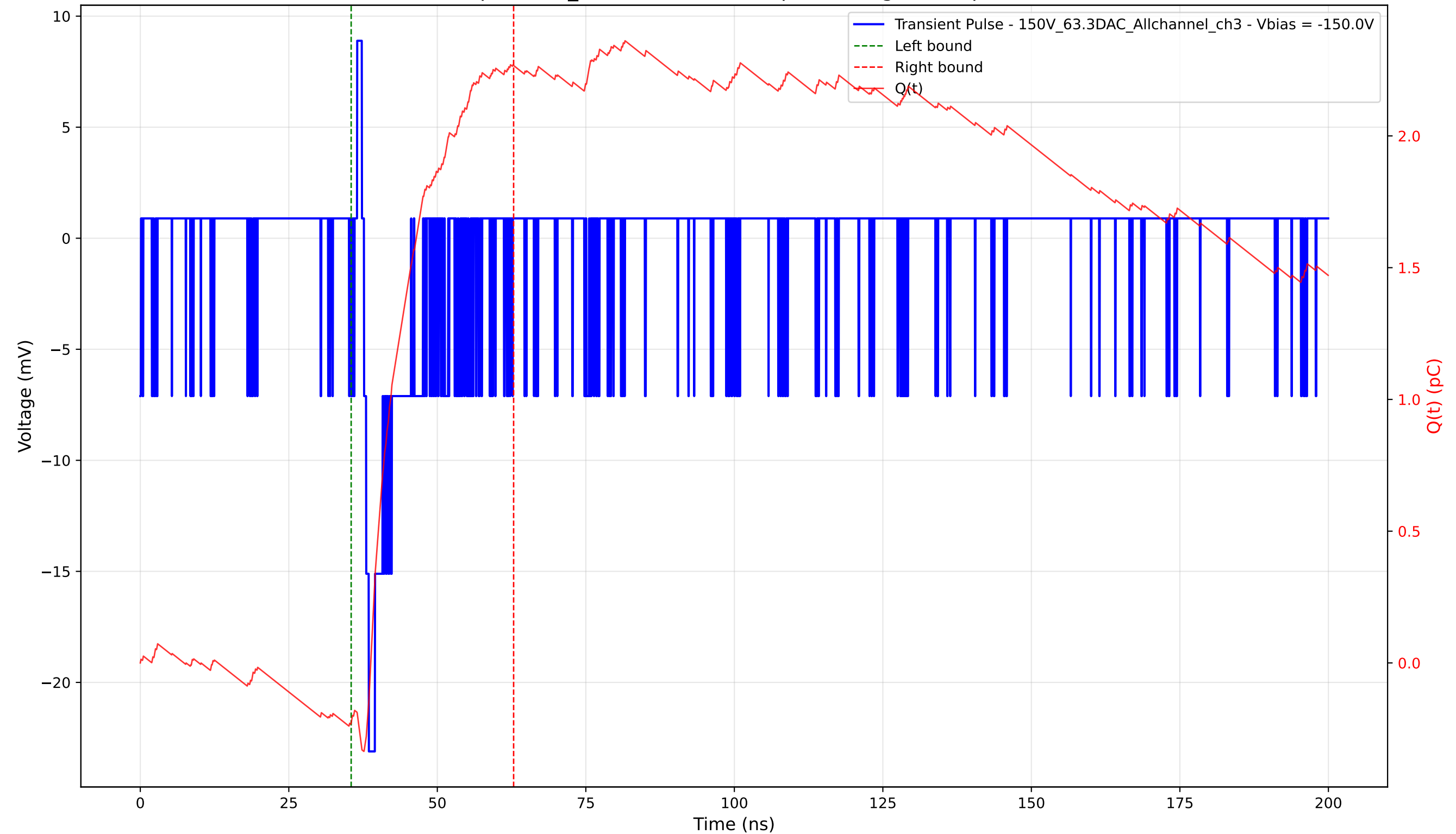
Transient Pulse - Sample: 1cm_42 - Position: 245.0 \mu\text{m} - Charge: 2.49 pC - Rise Time: 0.83 ns
