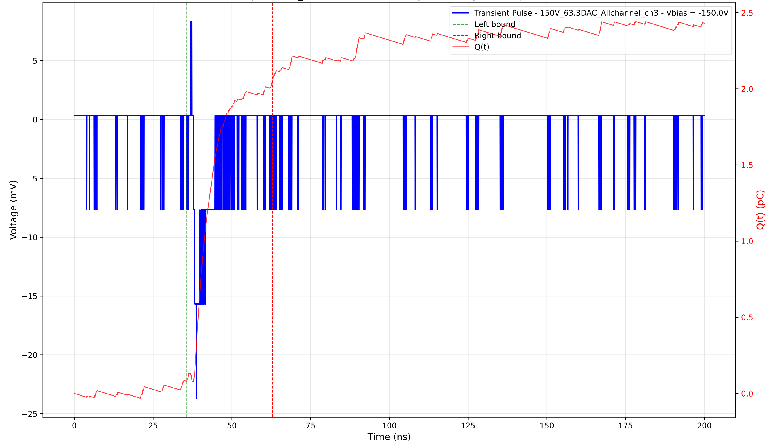
Transient Pulse - Sample: 1cm_42 - Position: 5005.0 \mu\text{m} - Charge: 1.97 pC - Rise Time: 0.91 ns
