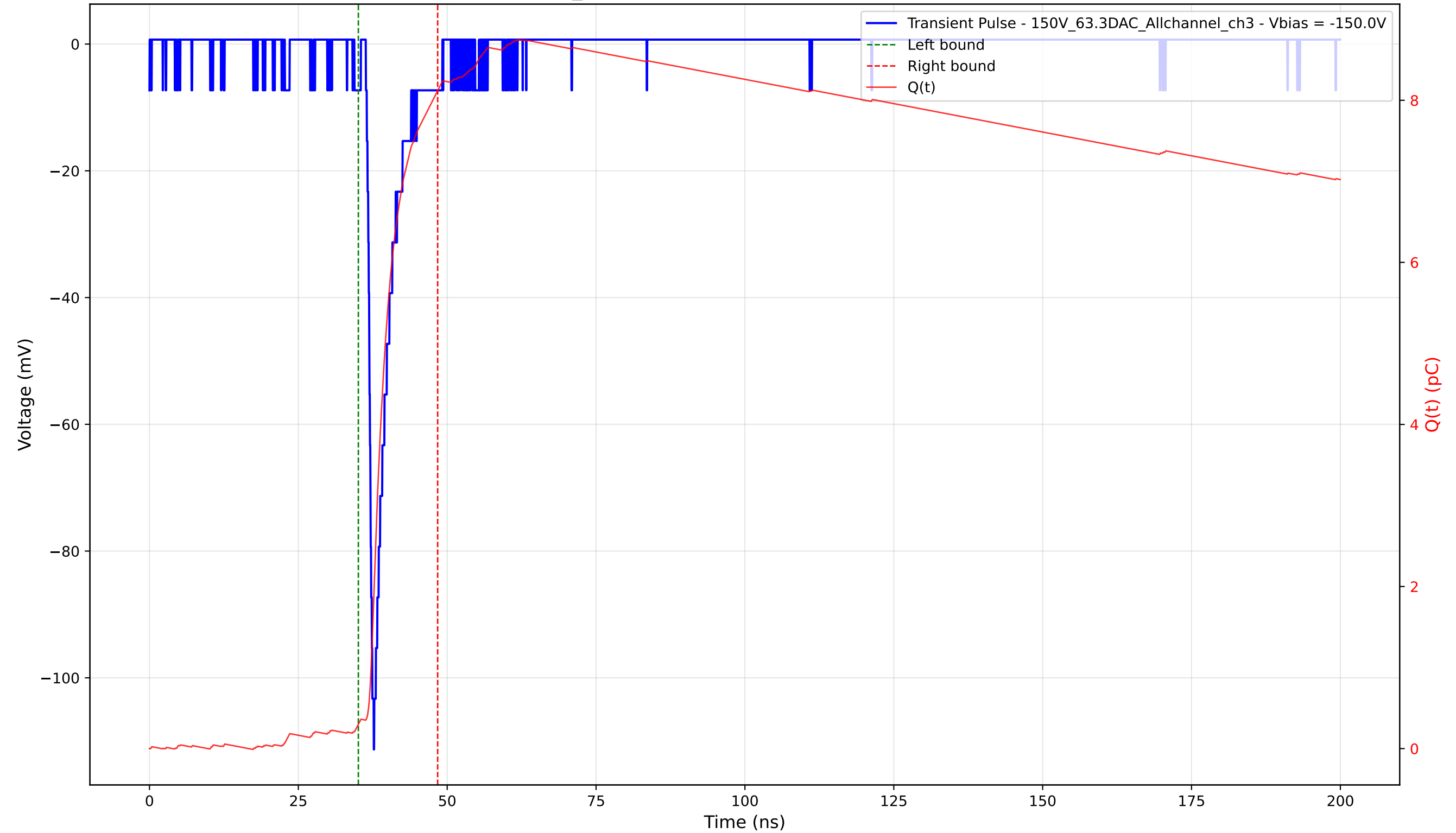
Transient Pulse - Sample: 1cm_42 - Position: 1625.0 \mu\text{m} - Charge: 7.82 pC - Rise Time: 0.94 ns
