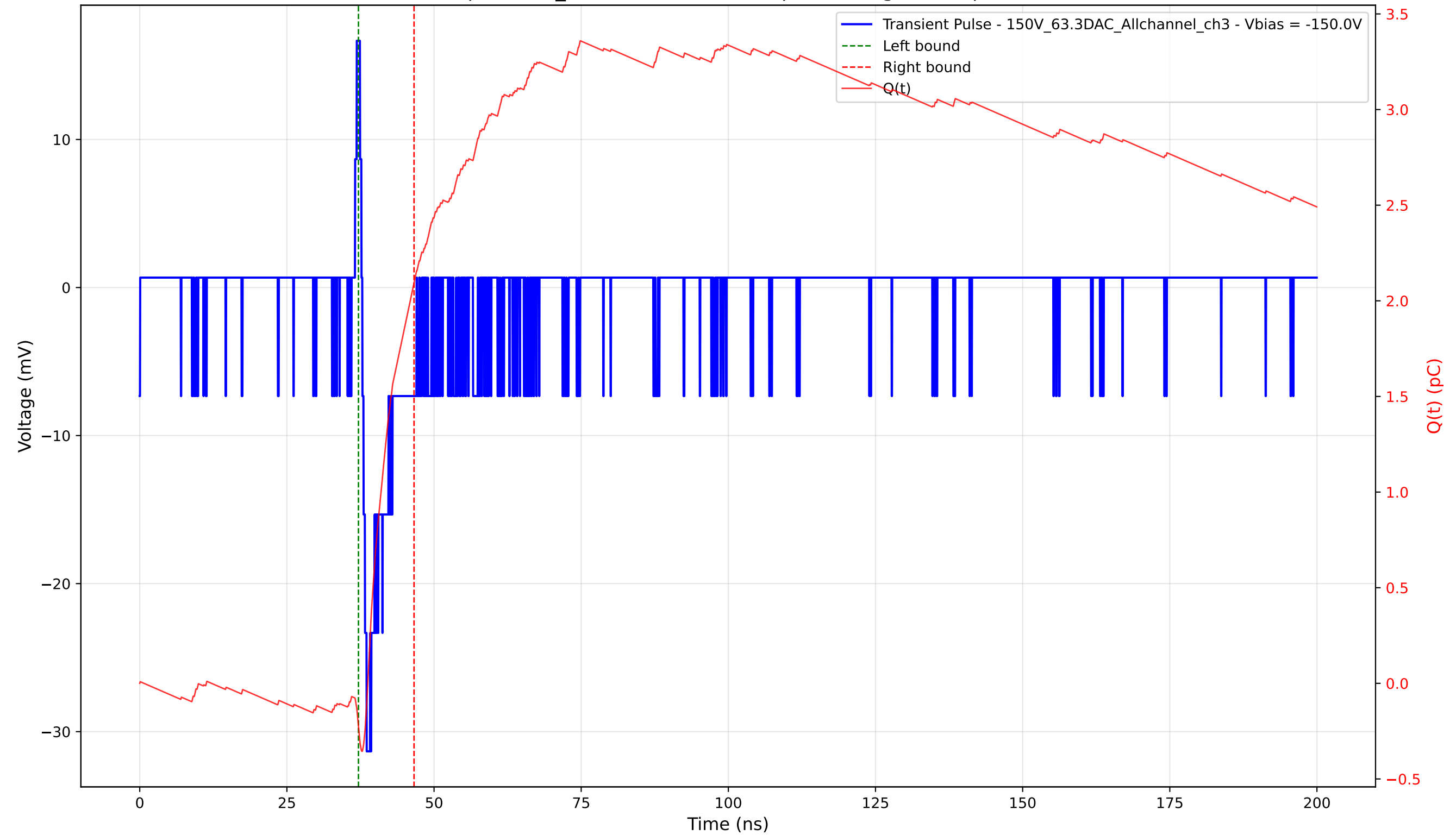
Transient Pulse - Sample: 1cm_42 - Position: 4600.0 \mu\text{m} - Charge: 2.32 pC - Rise Time: 0.75 ns
