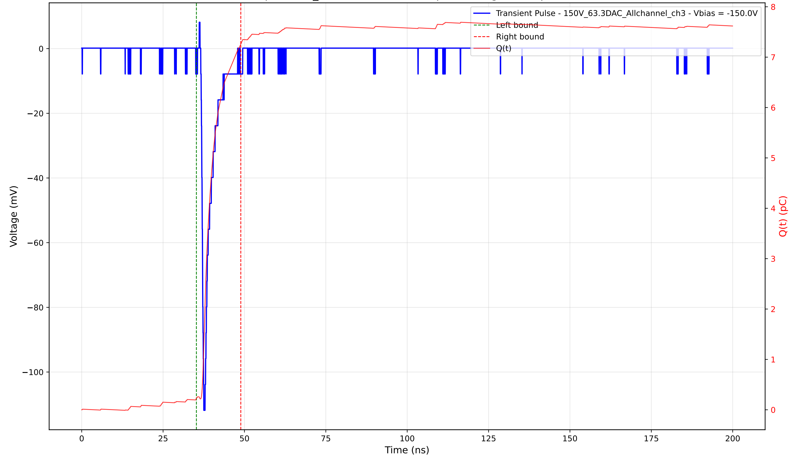
Transient Pulse - Sample: 1cm_42 - Position: 3380.0 \mu\text{m} - Charge: 7.03 pC - Rise Time: 0.74 ns
