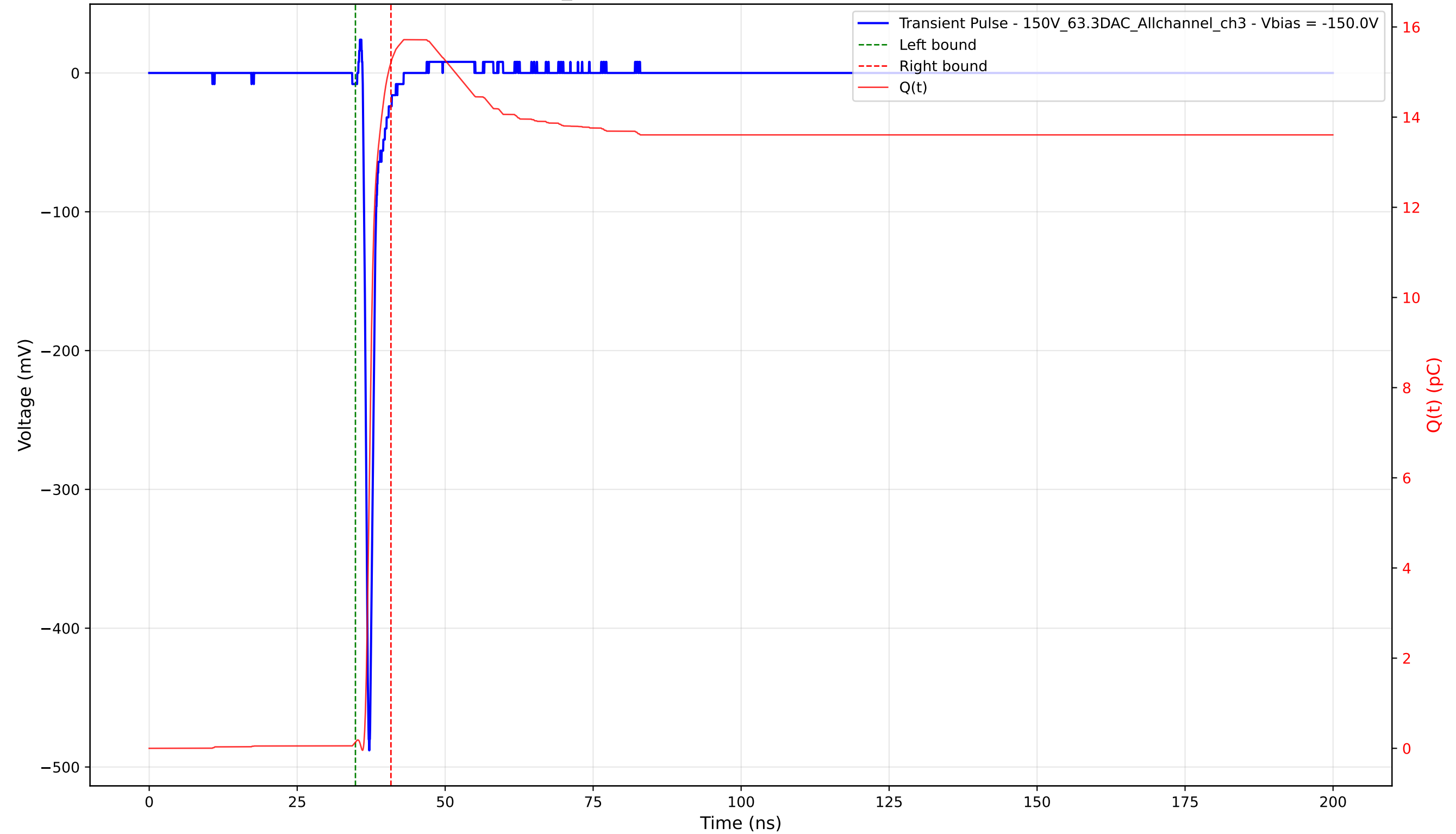
Transient Pulse - Sample: 1cm_42 - Position: 2400.0 \mu\text{m} - Charge: 15.08 pC - Rise Time: 0.74 ns
