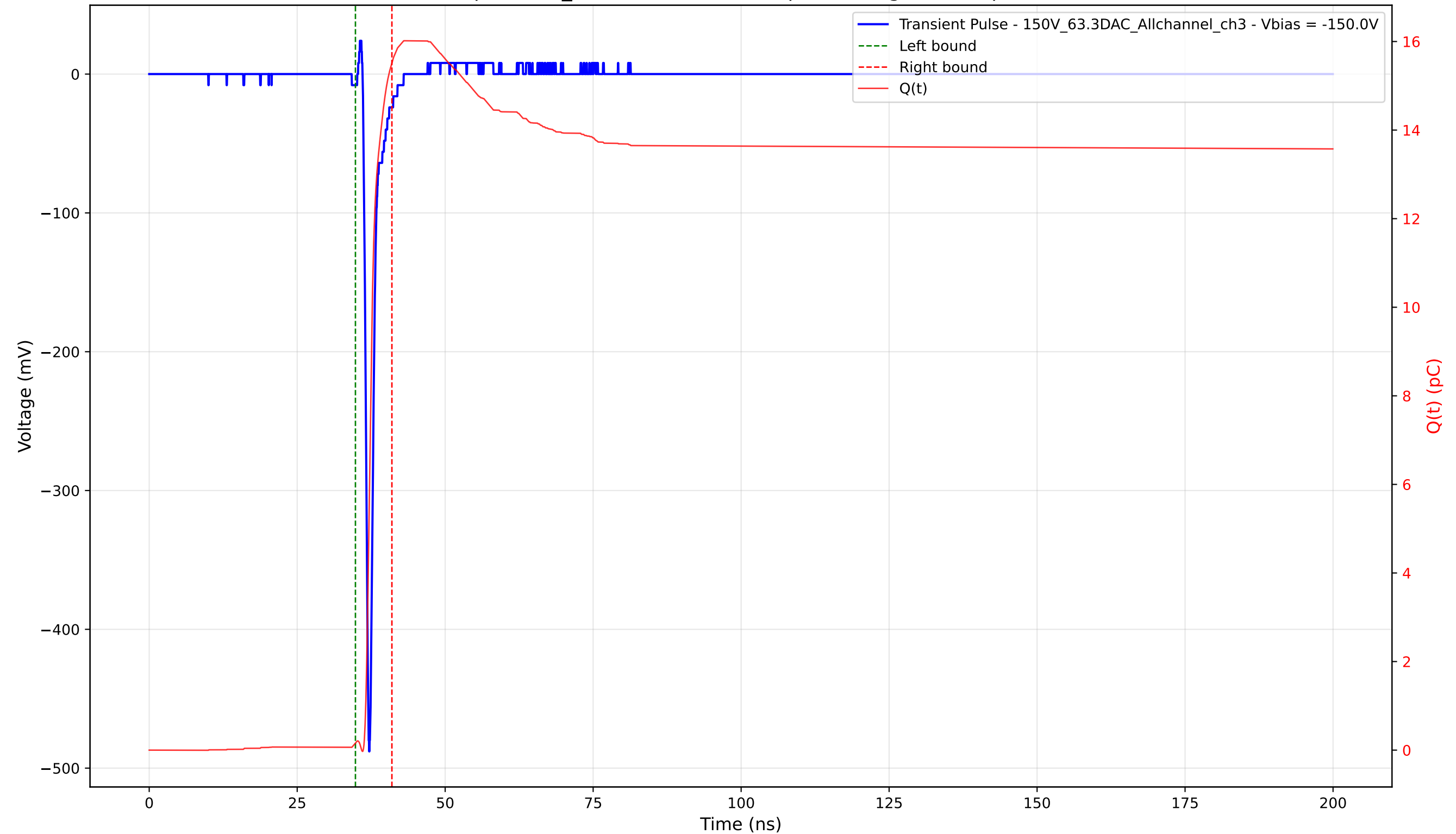
Transient Pulse - Sample: 1cm_42 - Position: 2685.0 \mu\text{m} - Charge: 15.36 pC - Rise Time: 0.74 ns
