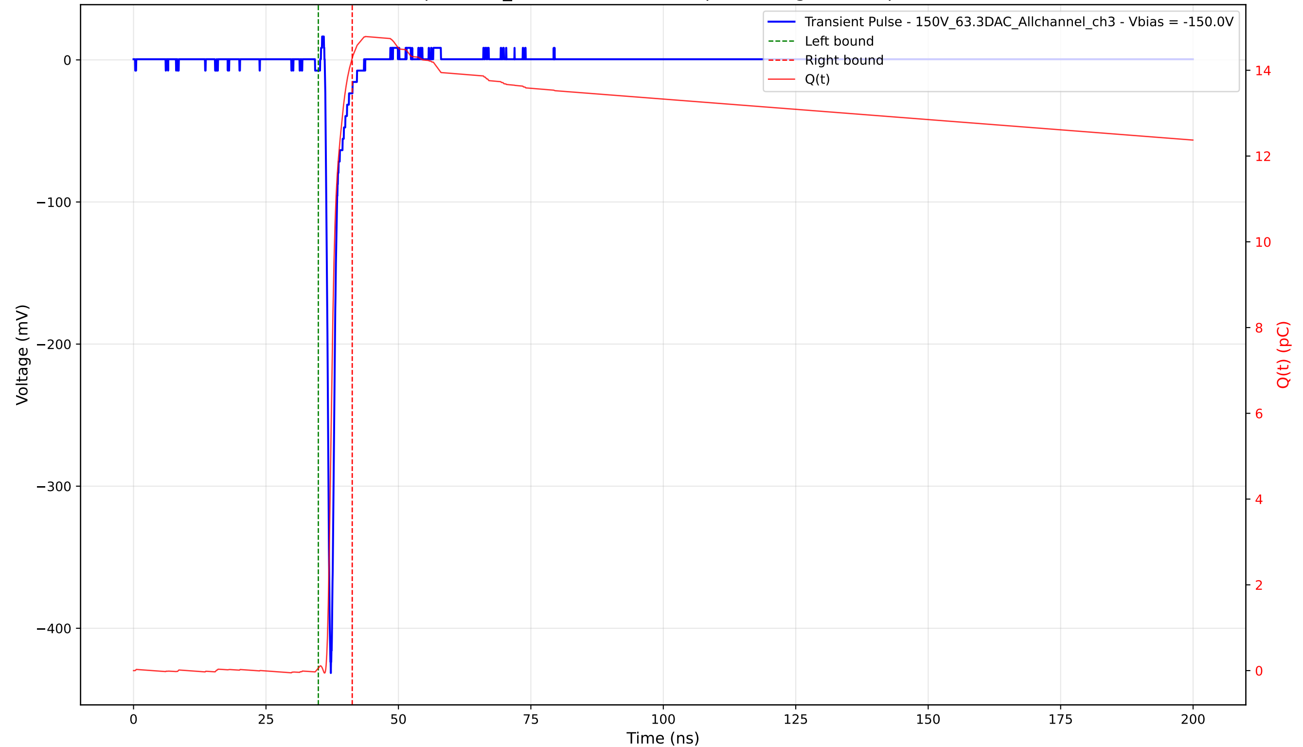
Transient Pulse - Sample: 1cm_42 - Position: 2825.0 \mu\text{m} - Charge: 14.23 pC - Rise Time: 0.73 ns
