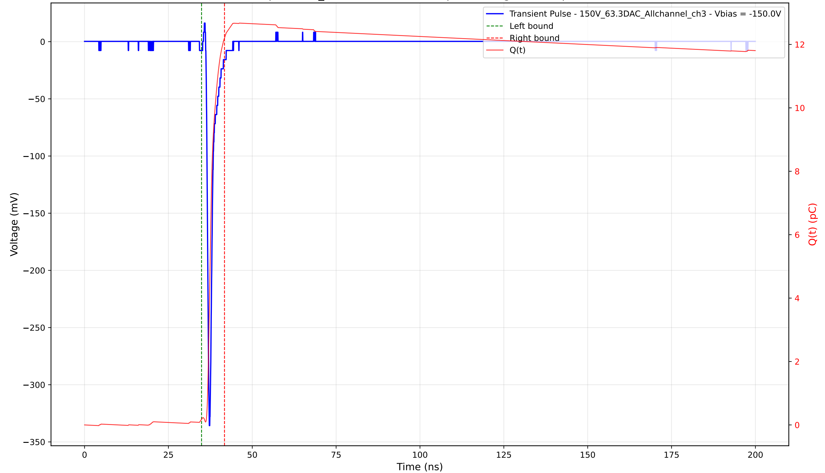
Transient Pulse - Sample: 1cm_42 - Position: 2130.0 \mu\text{m} - Charge: 12.03 pC - Rise Time: 0.75 ns
