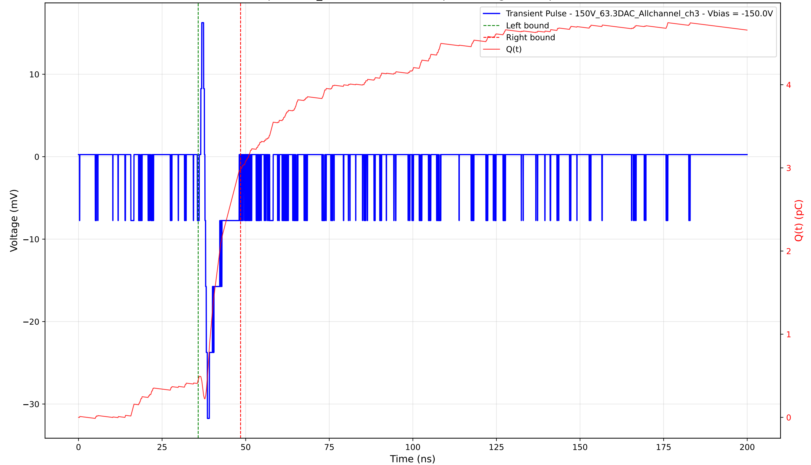
Transient Pulse - Sample: 1cm_42 - Position: 4605.0 \mu\text{m} - Charge: 2.53 pC - Rise Time: 0.74 ns
