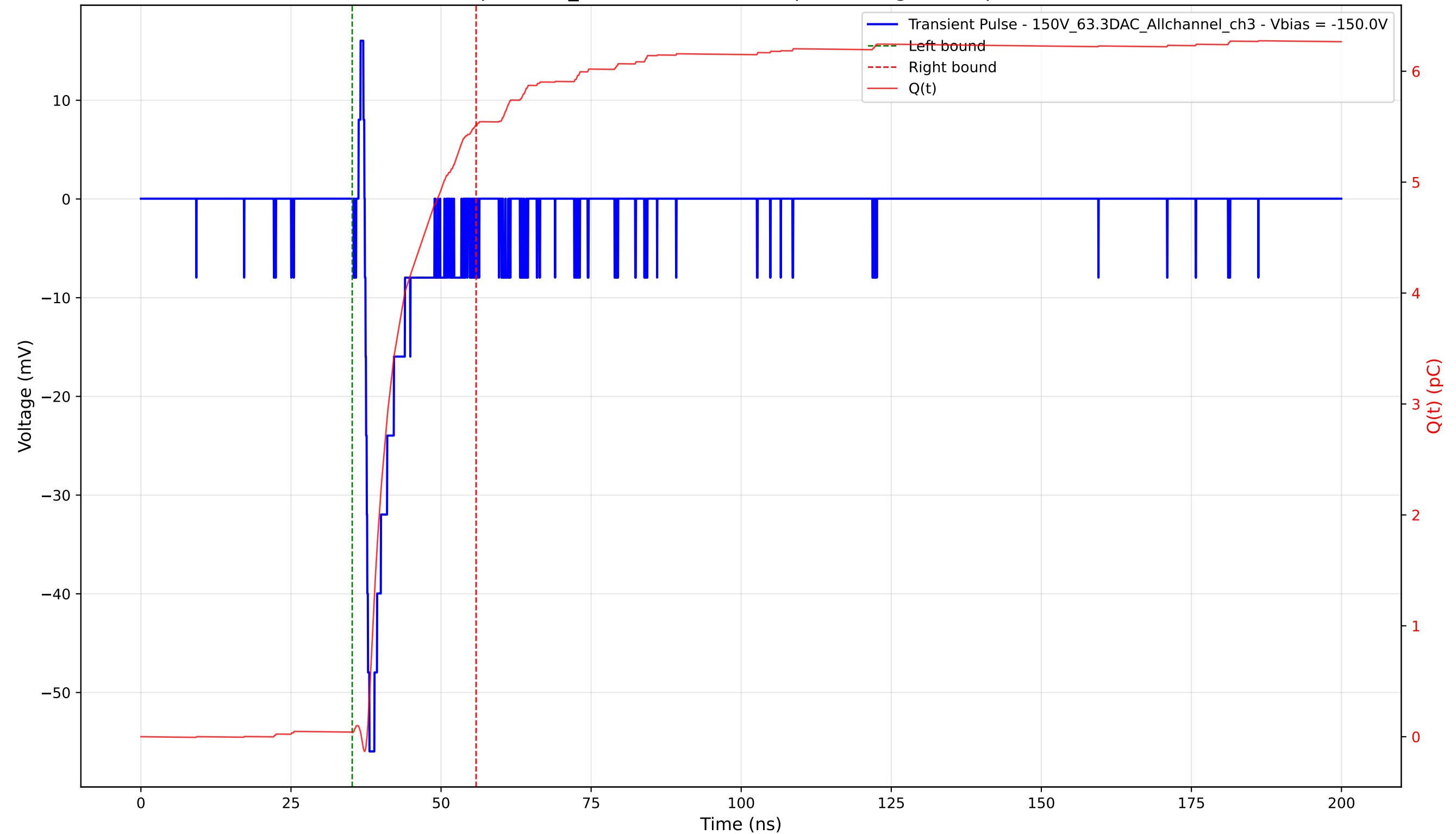
Transient Pulse - Sample: 1cm_42 - Position: 3785.0 \mu\text{m} - Charge: 5.47 pC - Rise Time: 0.77 ns
