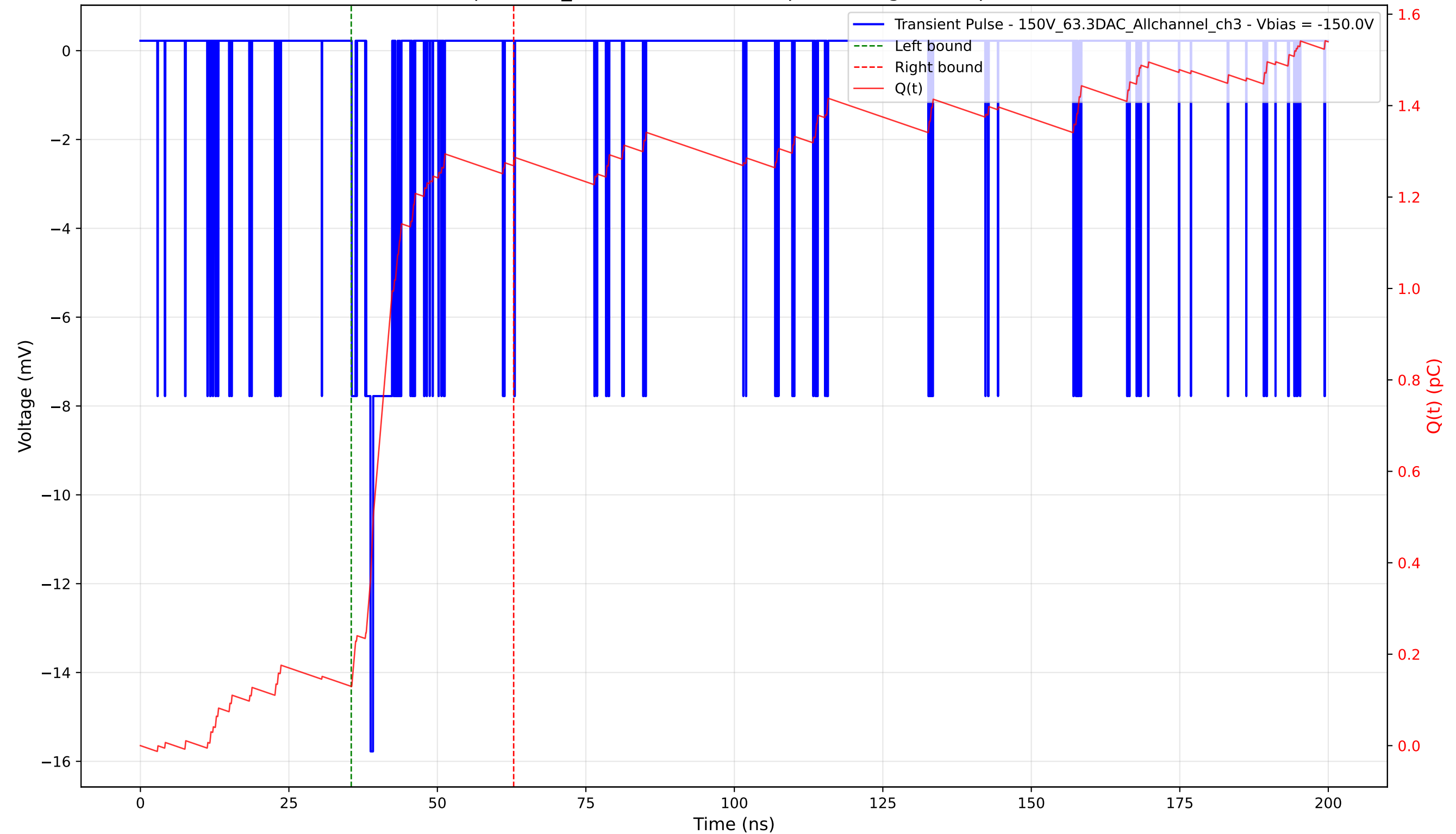
Transient Pulse - Sample: 1cm_42 - Position: 5095.0 \mu\text{m} - Charge: 1.14 pC - Rise Time: 0.75 ns
