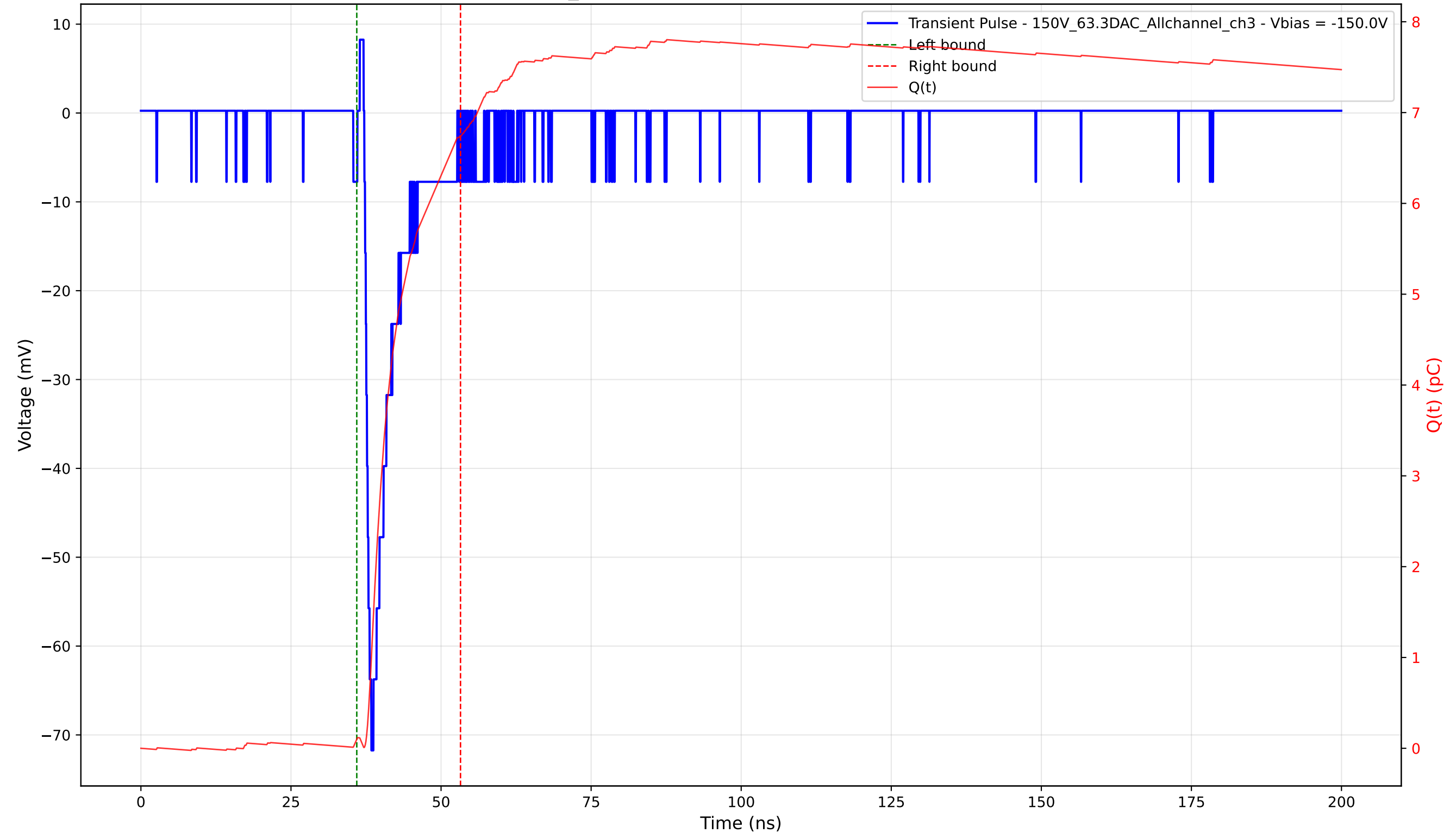
Transient Pulse - Sample: 1cm_42 - Position: 1250.0 \mu\text{m} - Charge: 6.64 pC - Rise Time: 1.16 ns
