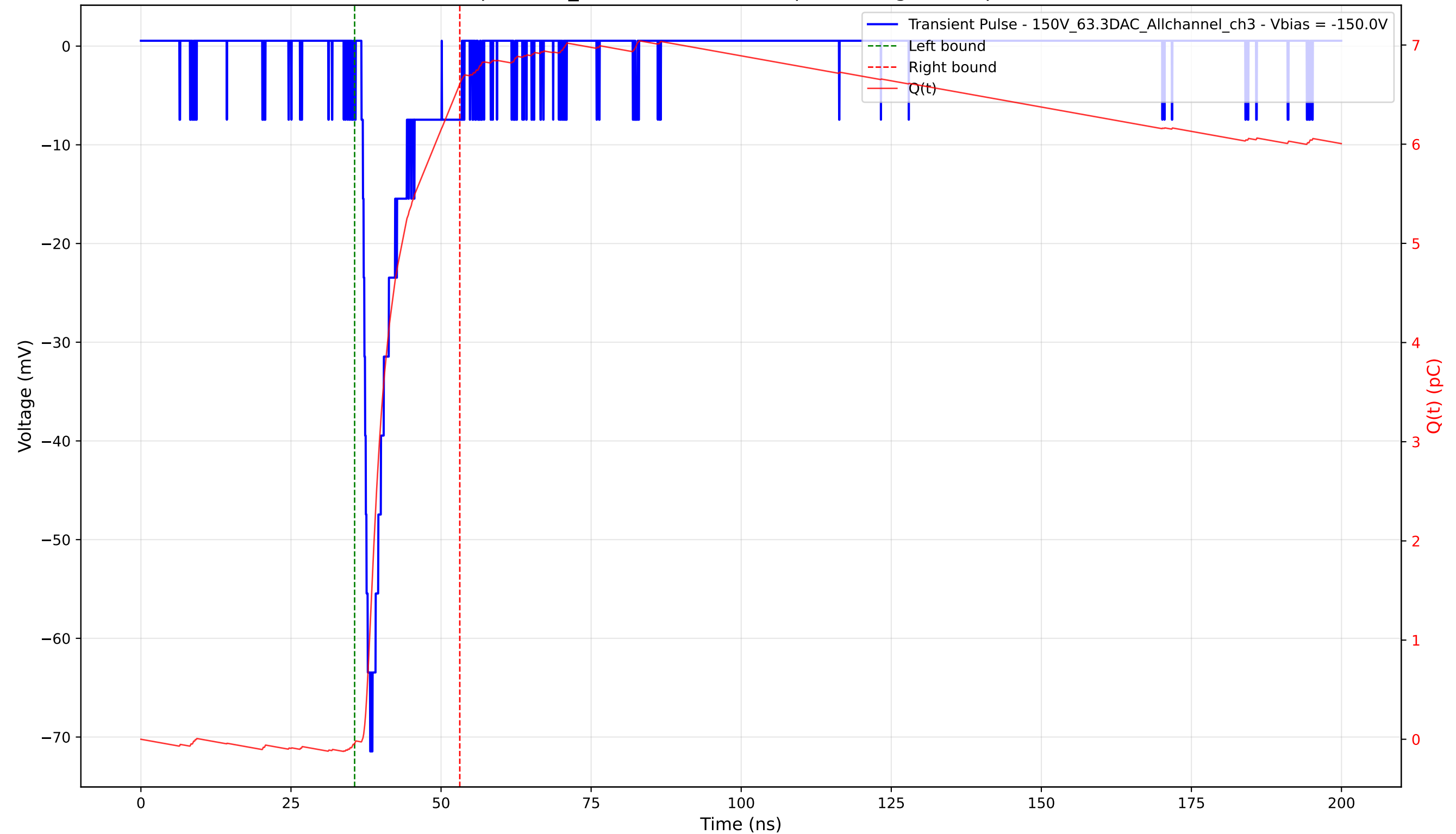
Transient Pulse - Sample: 1cm_42 - Position: 1450.0 \mu\text{m} - Charge: 6.65 pC - Rise Time: 1.44 ns
