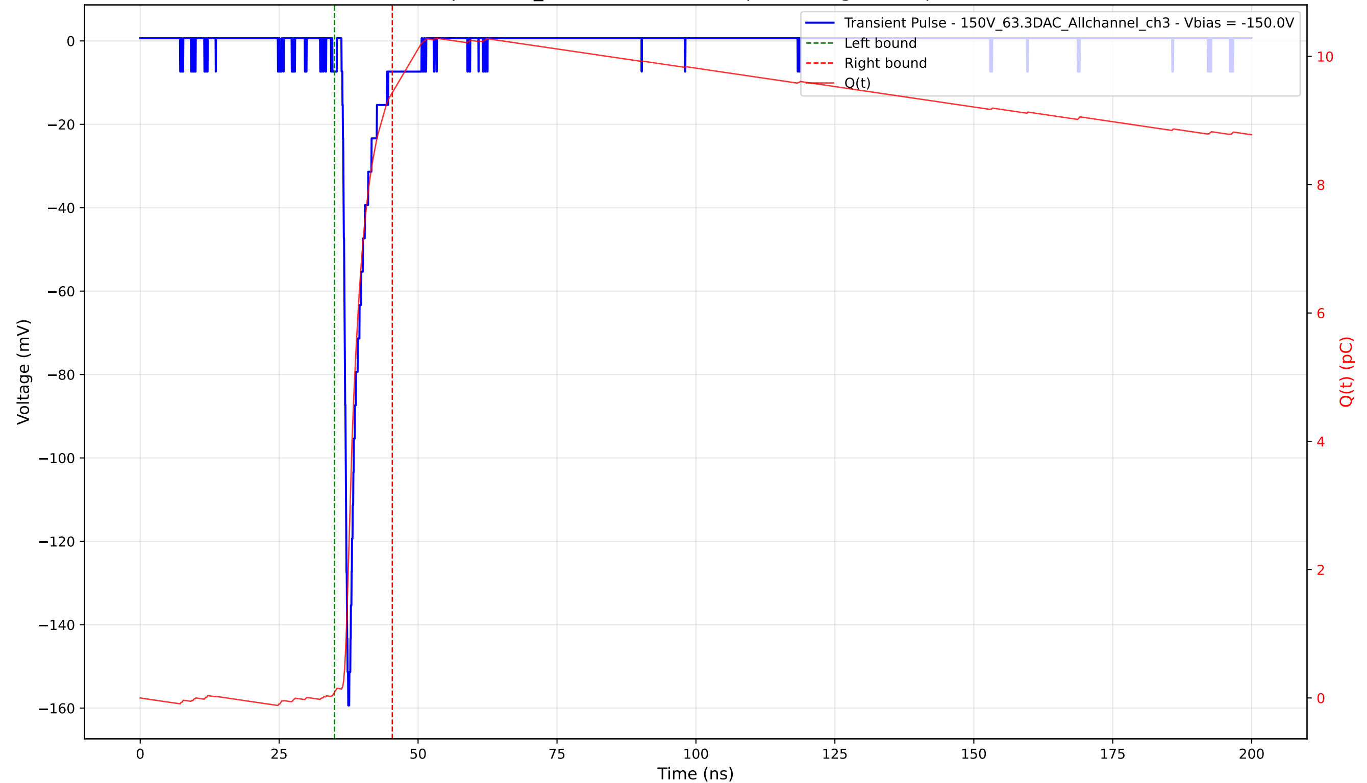
Transient Pulse - Sample: 1cm_42 - Position: 1805.0 \mu\text{m} - Charge: 9.35 pC - Rise Time: 0.88 ns
