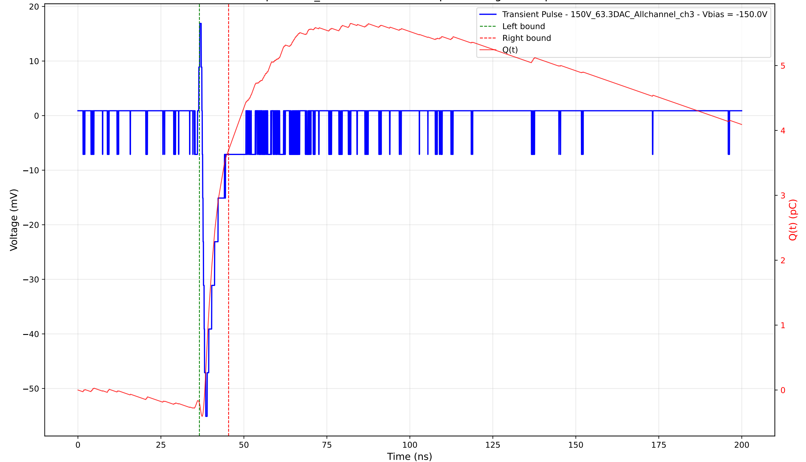
Transient Pulse - Sample: 1cm_42 - Position: 1070.0 \mu\text{m} - Charge: 3.90 pC - Rise Time: 1.05 ns
