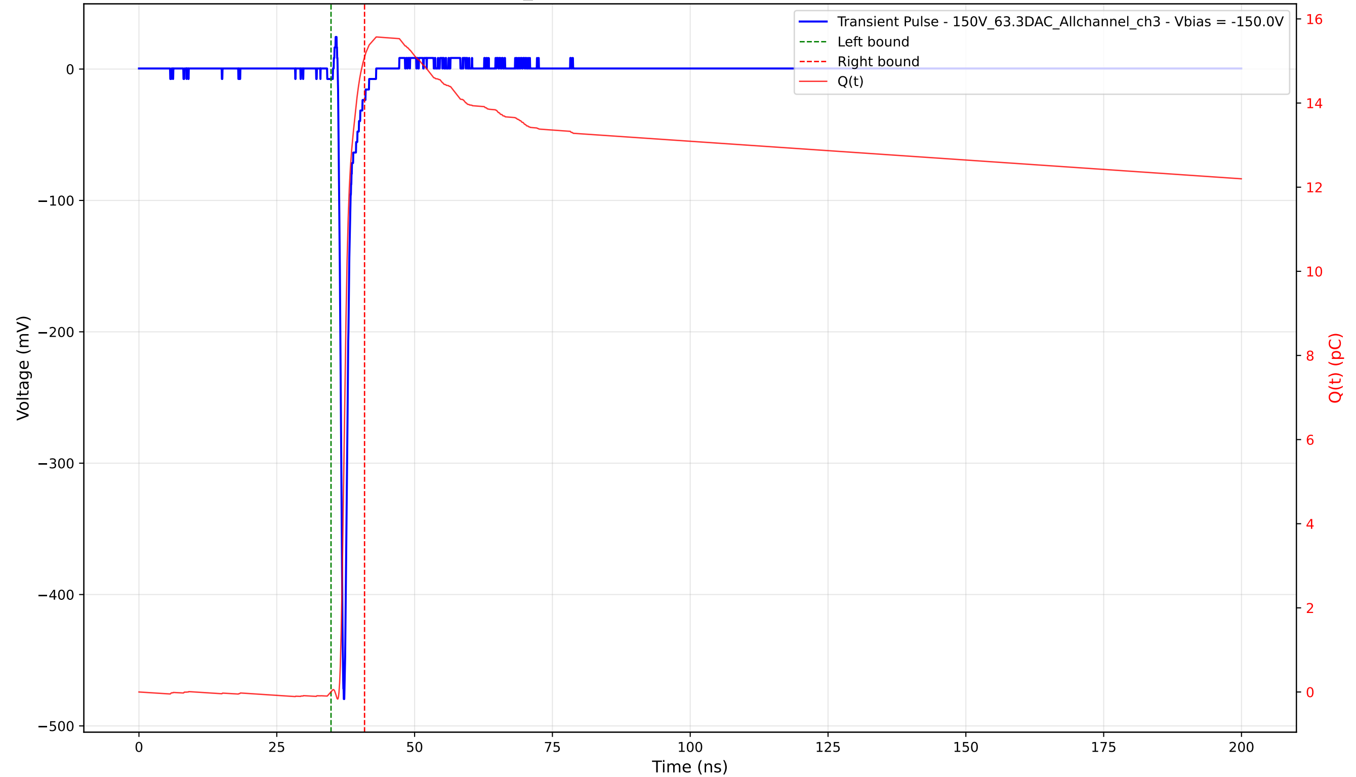
Transient Pulse - Sample: 1cm_42 - Position: 2360.0 \mu\text{m} - Charge: 15.09 pC - Rise Time: 0.70 ns
