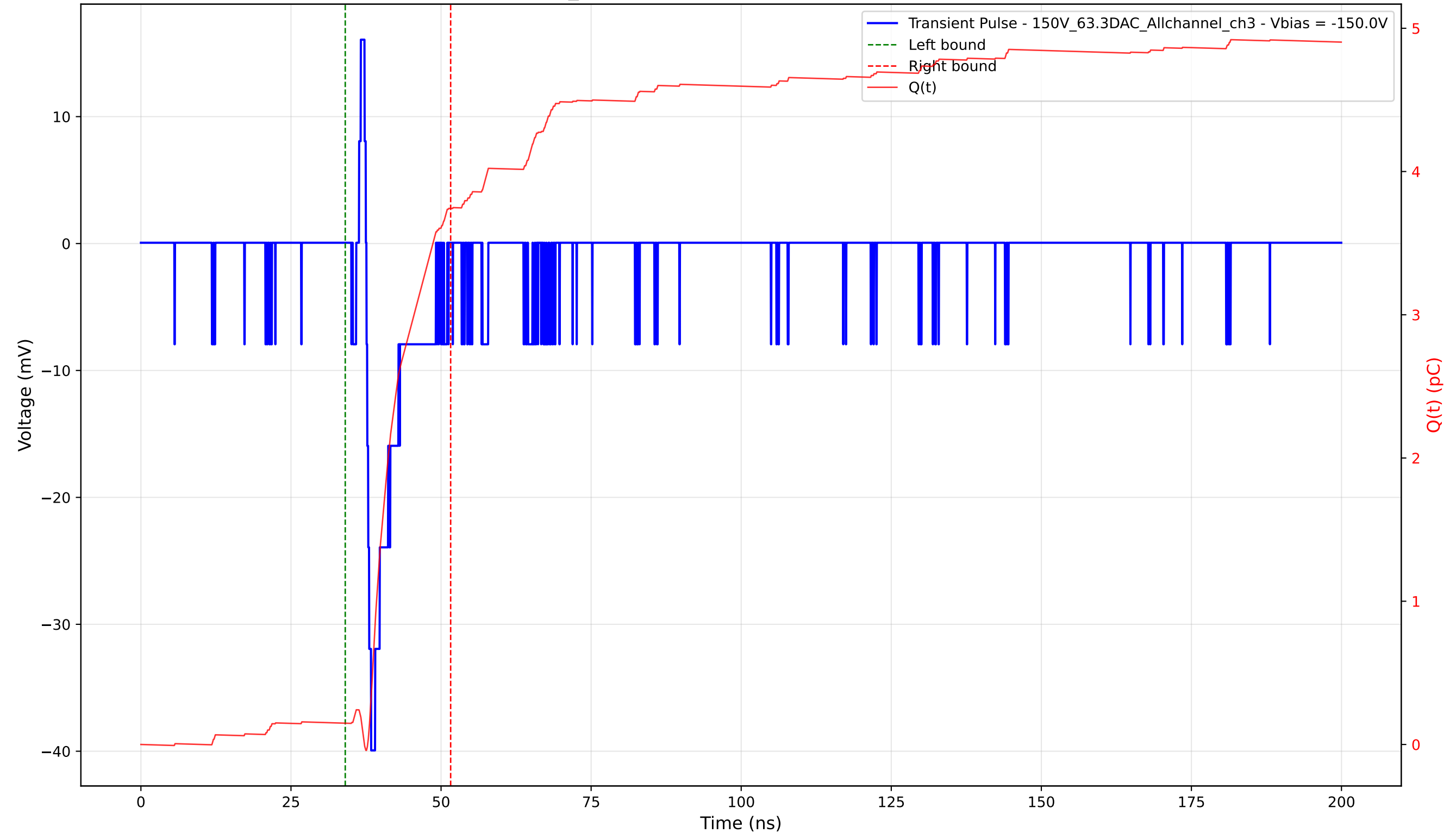
Transient Pulse - Sample: 1cm_42 - Position: 4055.0 \mu\text{m} - Charge: 3.59 pC - Rise Time: 0.78 ns
