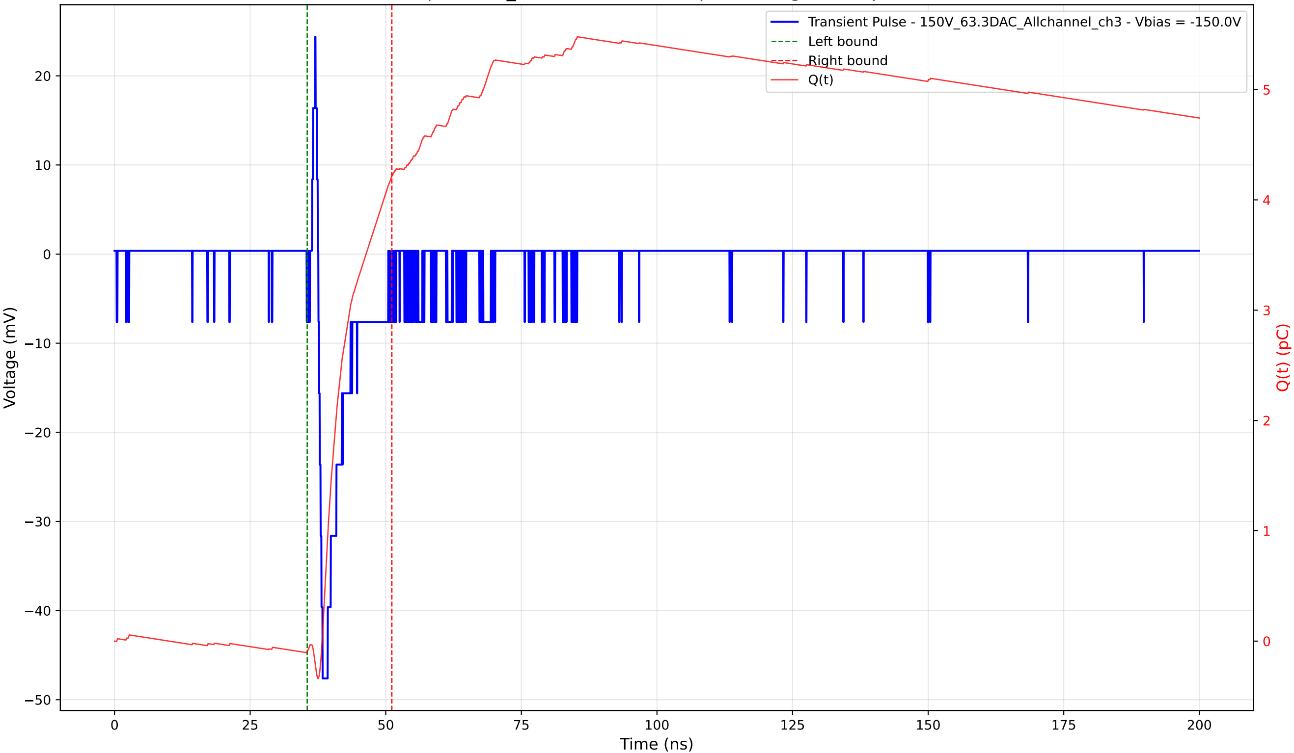
Transient Pulse - Sample: 1cm_42 - Position: 995.0 \mu\text{m} - Charge: 4.31 pC - Rise Time: 0.78 ns
