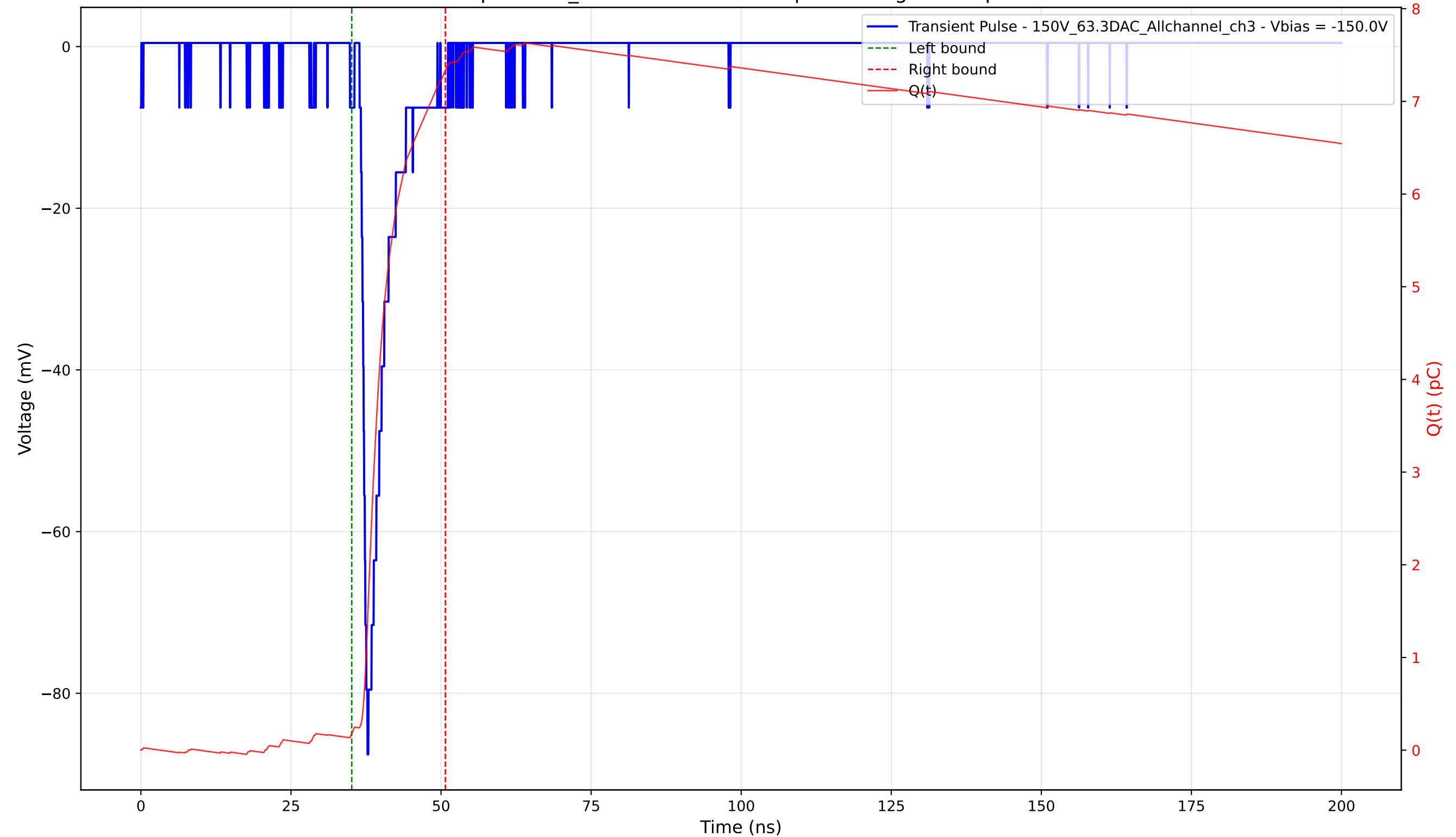
Transient Pulse - Sample: 1cm_42 - Position: 1550.0 \mu\text{m} - Charge: 7.16 pC - Rise Time: 0.91 ns
