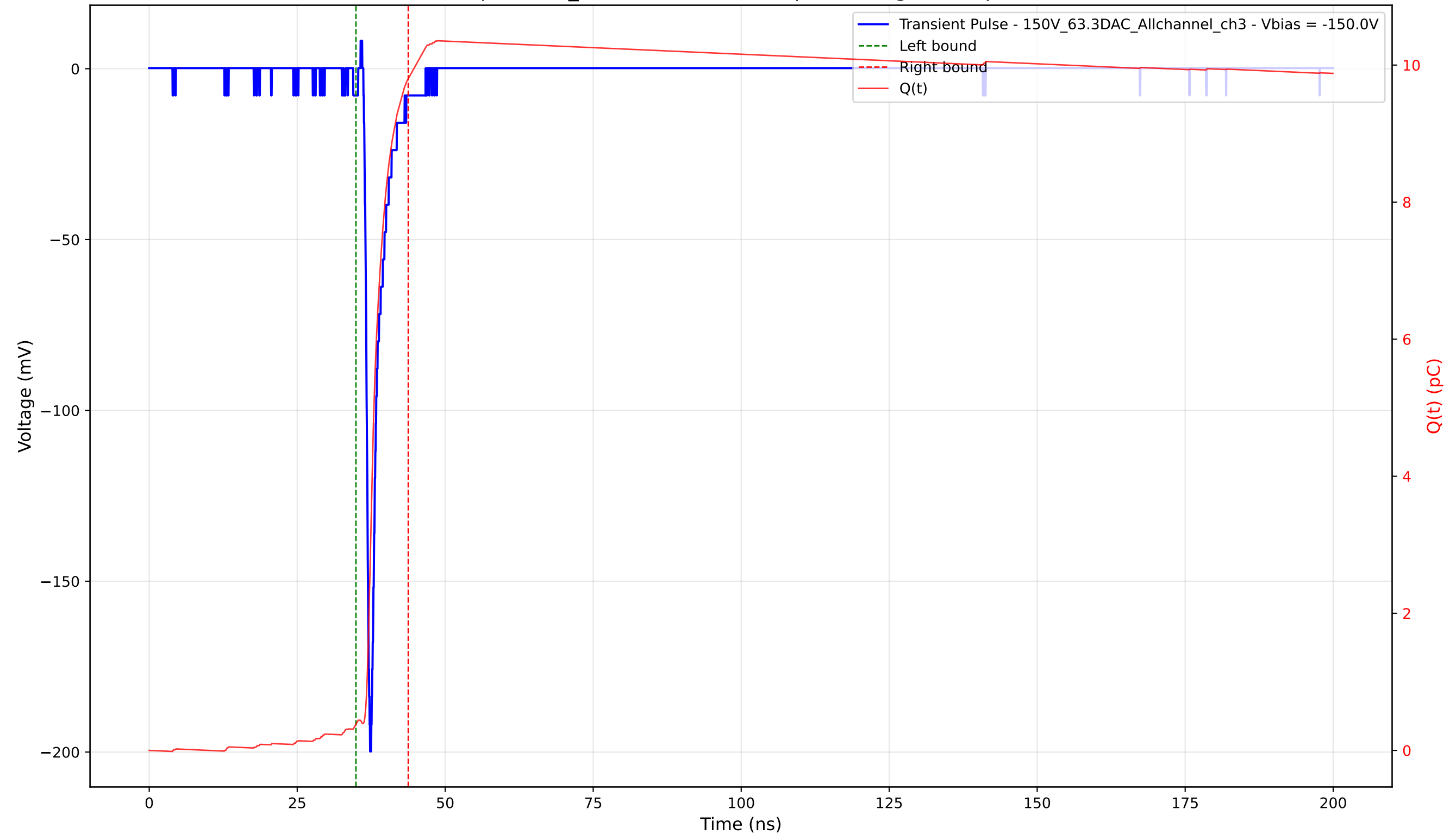
Transient Pulse - Sample: 1cm_42 - Position: 1960.0 \mu\text{m} - Charge: 9.42 pC - Rise Time: 0.82 ns
