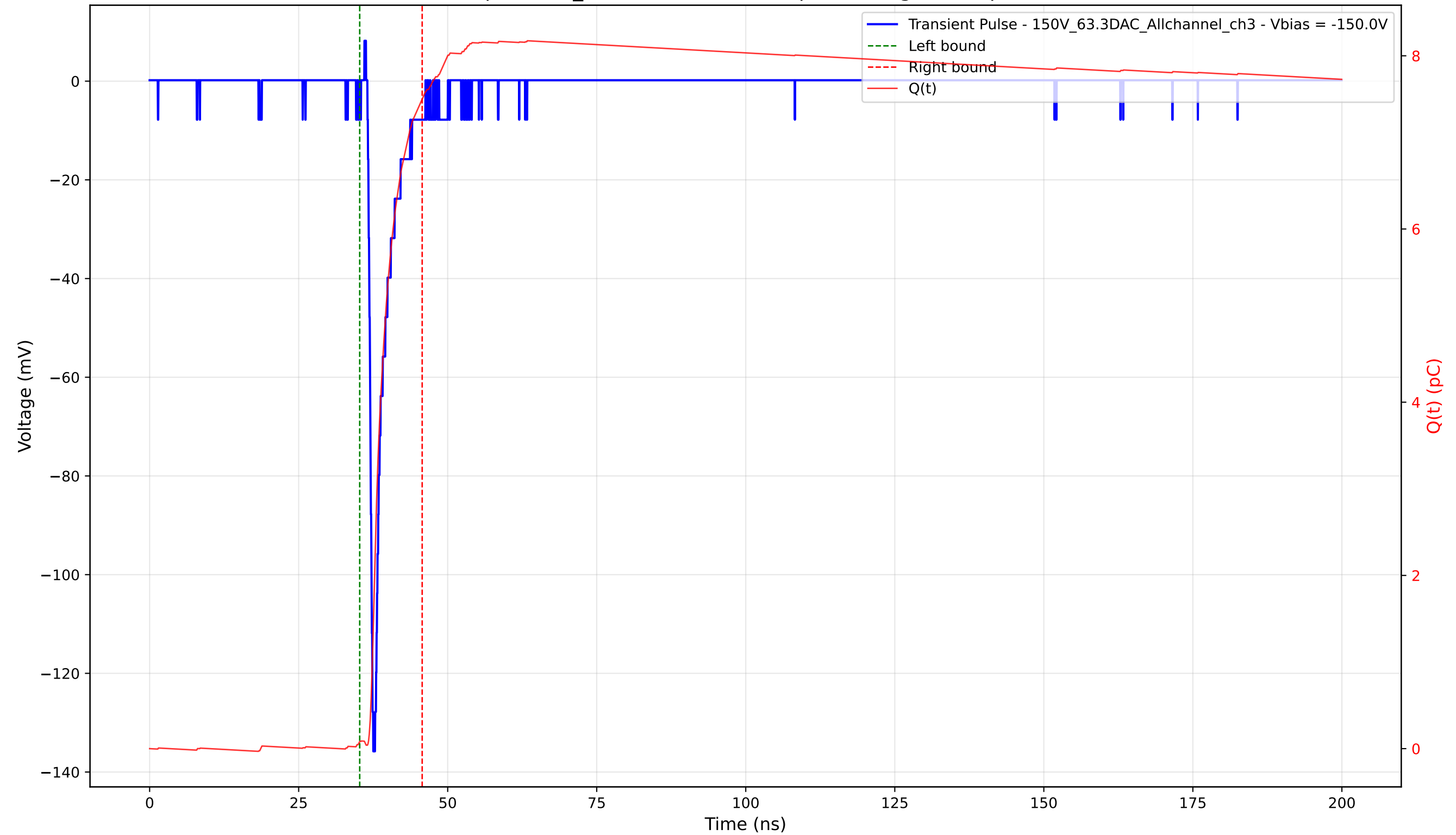
Transient Pulse - Sample: 1cm_42 - Position: 3290.0 \mu\text{m} - Charge: 7.42 pC - Rise Time: 0.77 ns
