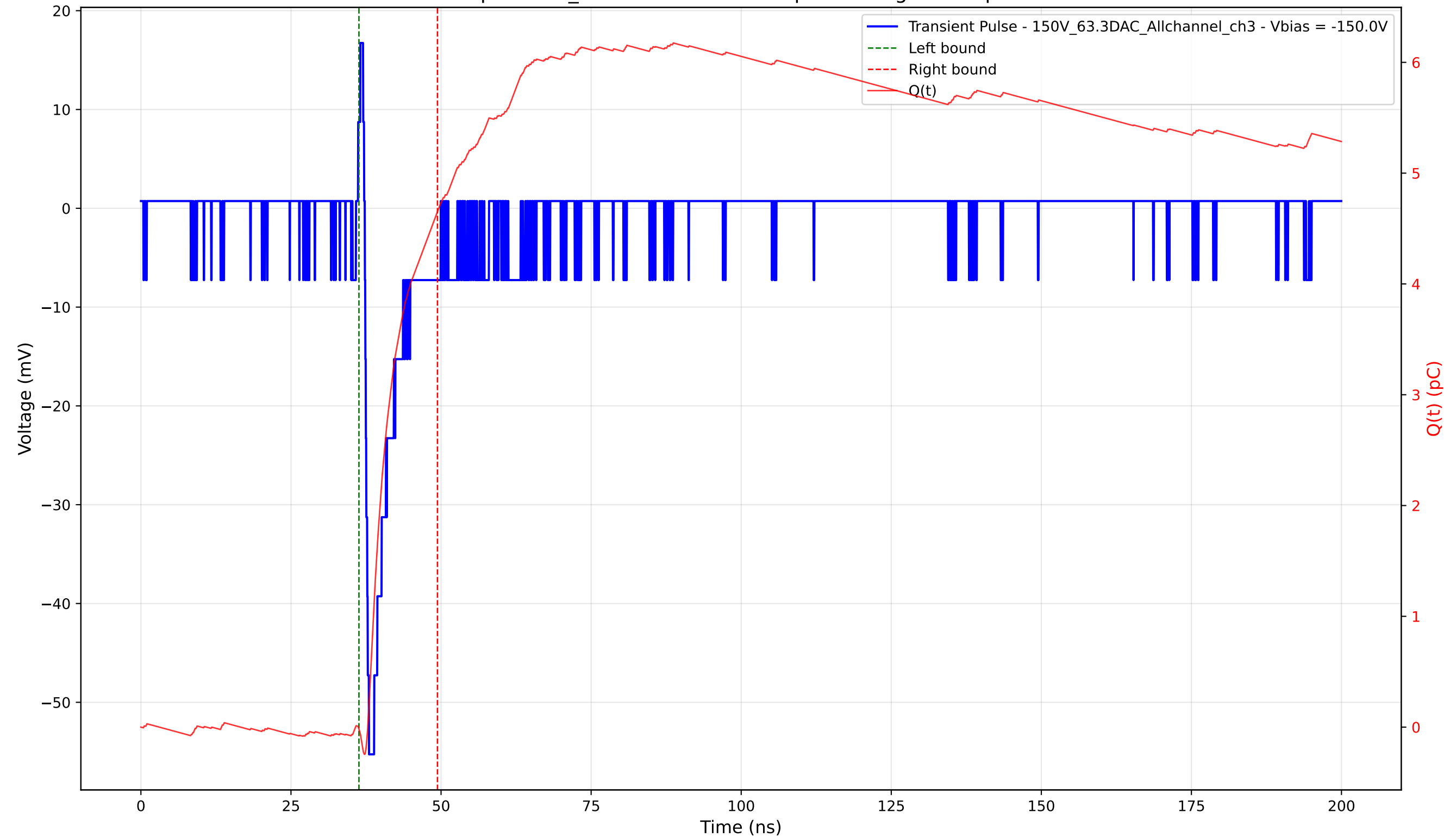
Transient Pulse - Sample: 1cm_42 - Position: 3765.0 \mu\text{m} - Charge: 4.67 pC - Rise Time: 0.69 ns
