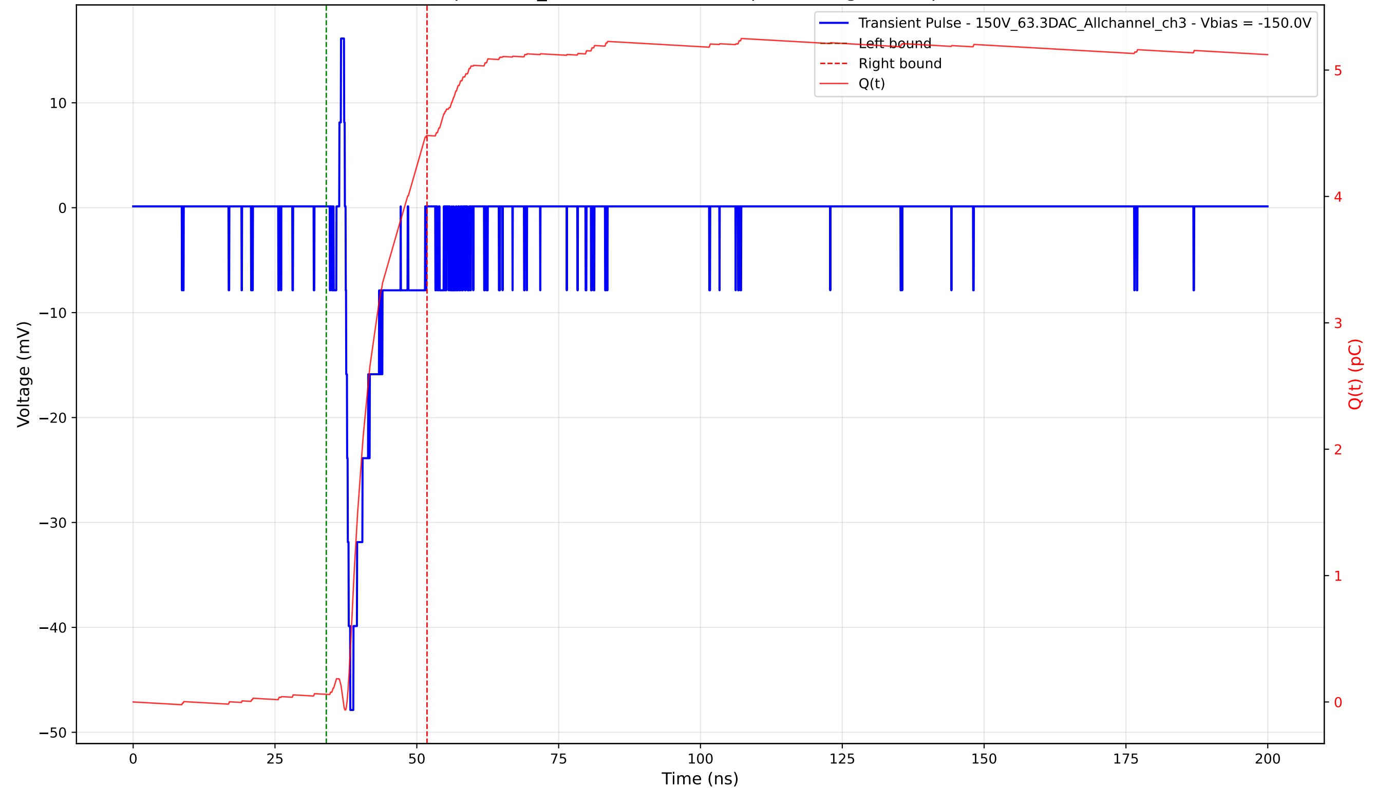
Transient Pulse - Sample: 1cm_42 - Position: 3940.0 \mu\text{m} - Charge: 4.42 pC - Rise Time: 0.82 ns
