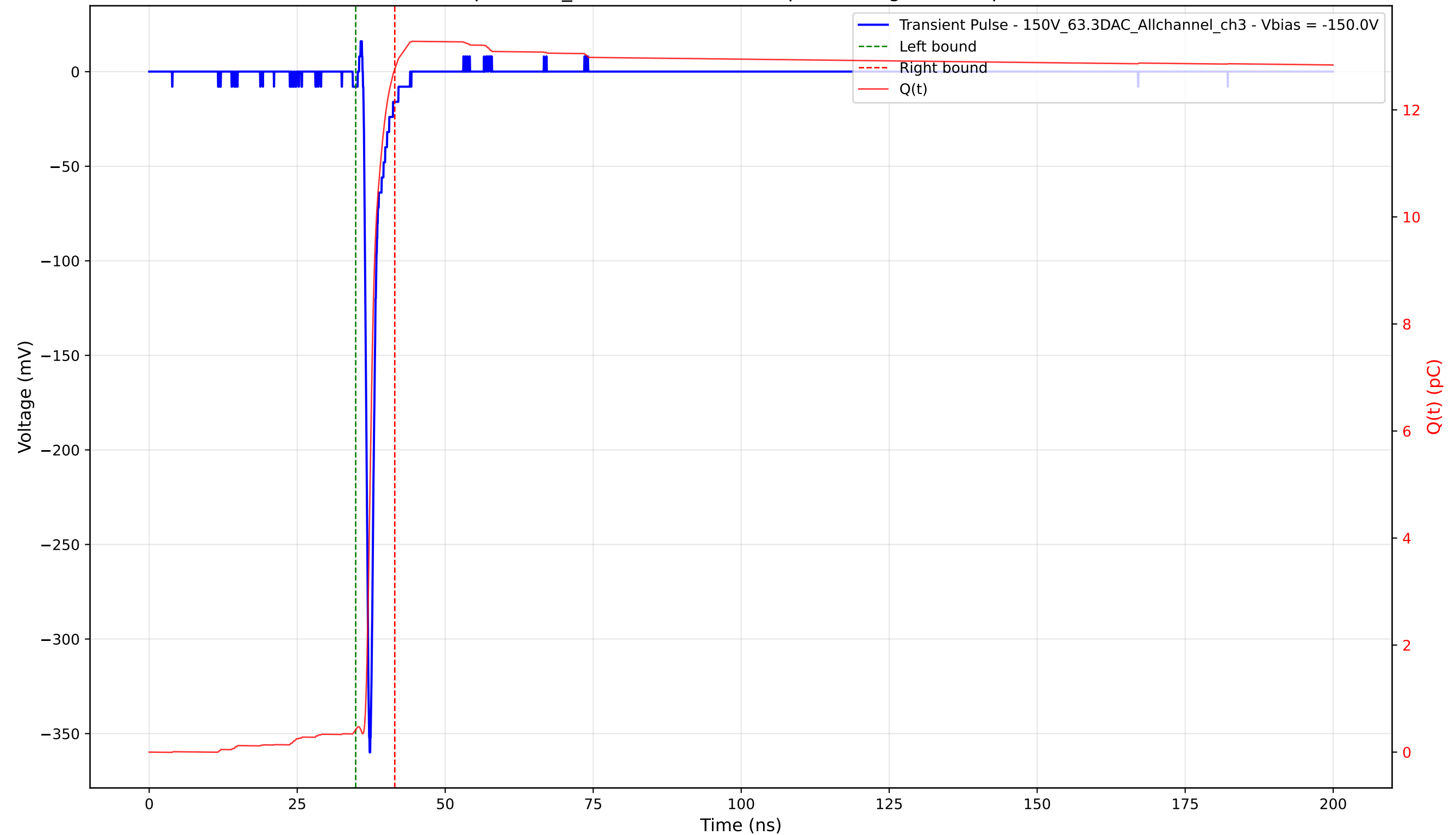
Transient Pulse - Sample: 1cm_42 - Position: 2885.0 \mu\text{m} - Charge: 12.34 pC - Rise Time: 0.73 ns
