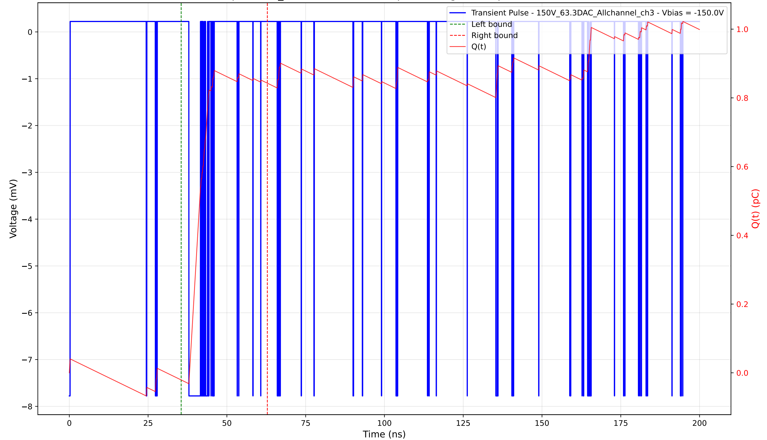
Transient Pulse - Sample: 1cm_42 - Position: 5120.0 \mu\text{m} - Charge: 0.86 pC - Rise Time: 0.00 ns (N/A)
