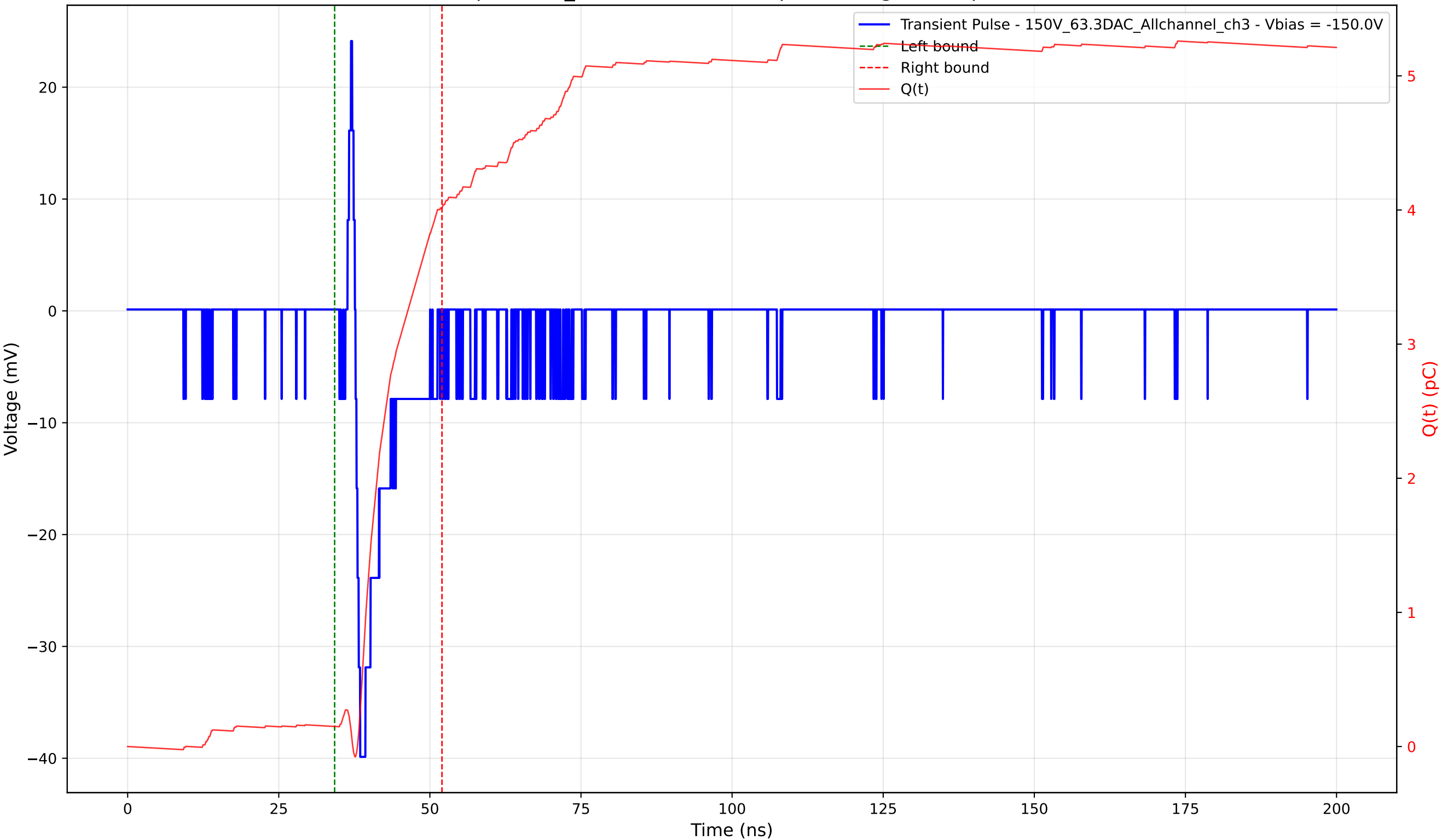
Transient Pulse - Sample: 1cm_42 - Position: 545.0 \mu\text{m} - Charge: 3.87 pC - Rise Time: 0.78 ns
