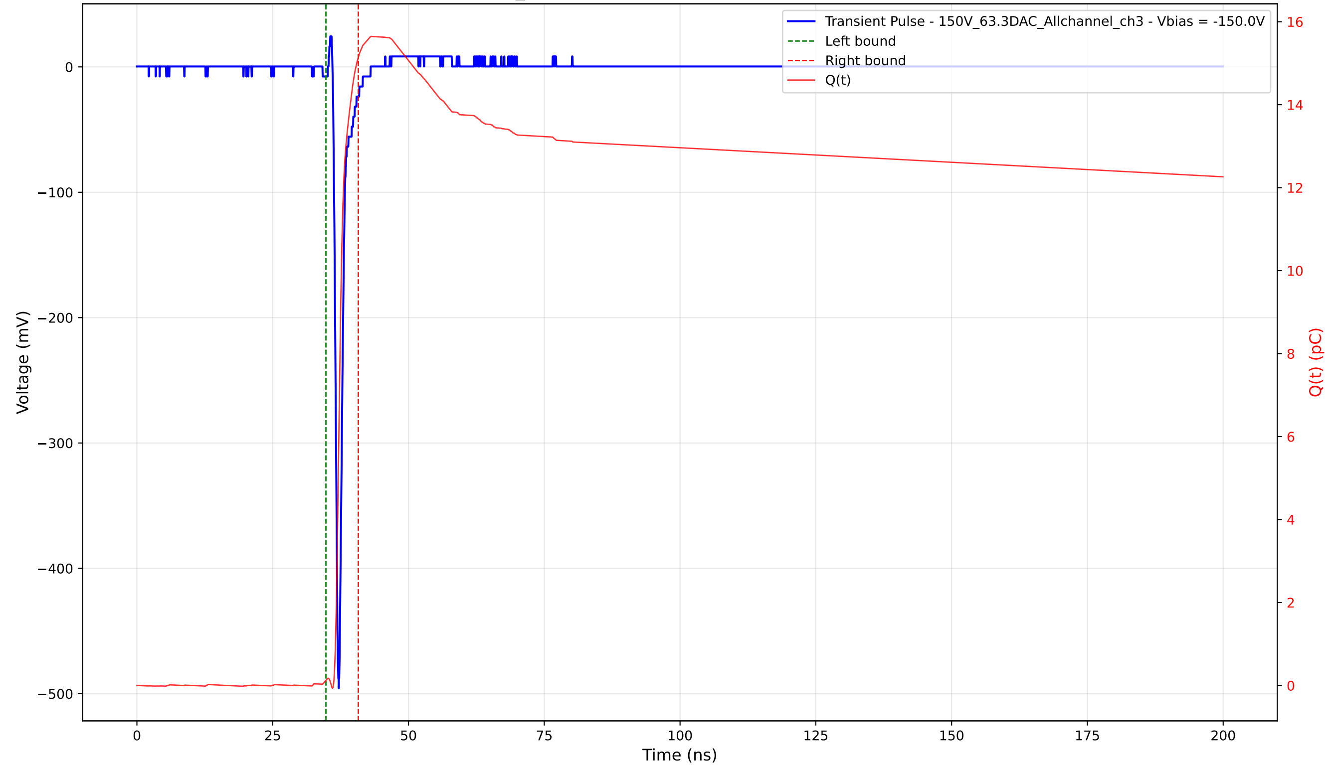
Transient Pulse - Sample: 1cm_42 - Position: 2575.0 \mu\text{m} - Charge: 15.02 pC - Rise Time: 0.73 ns
