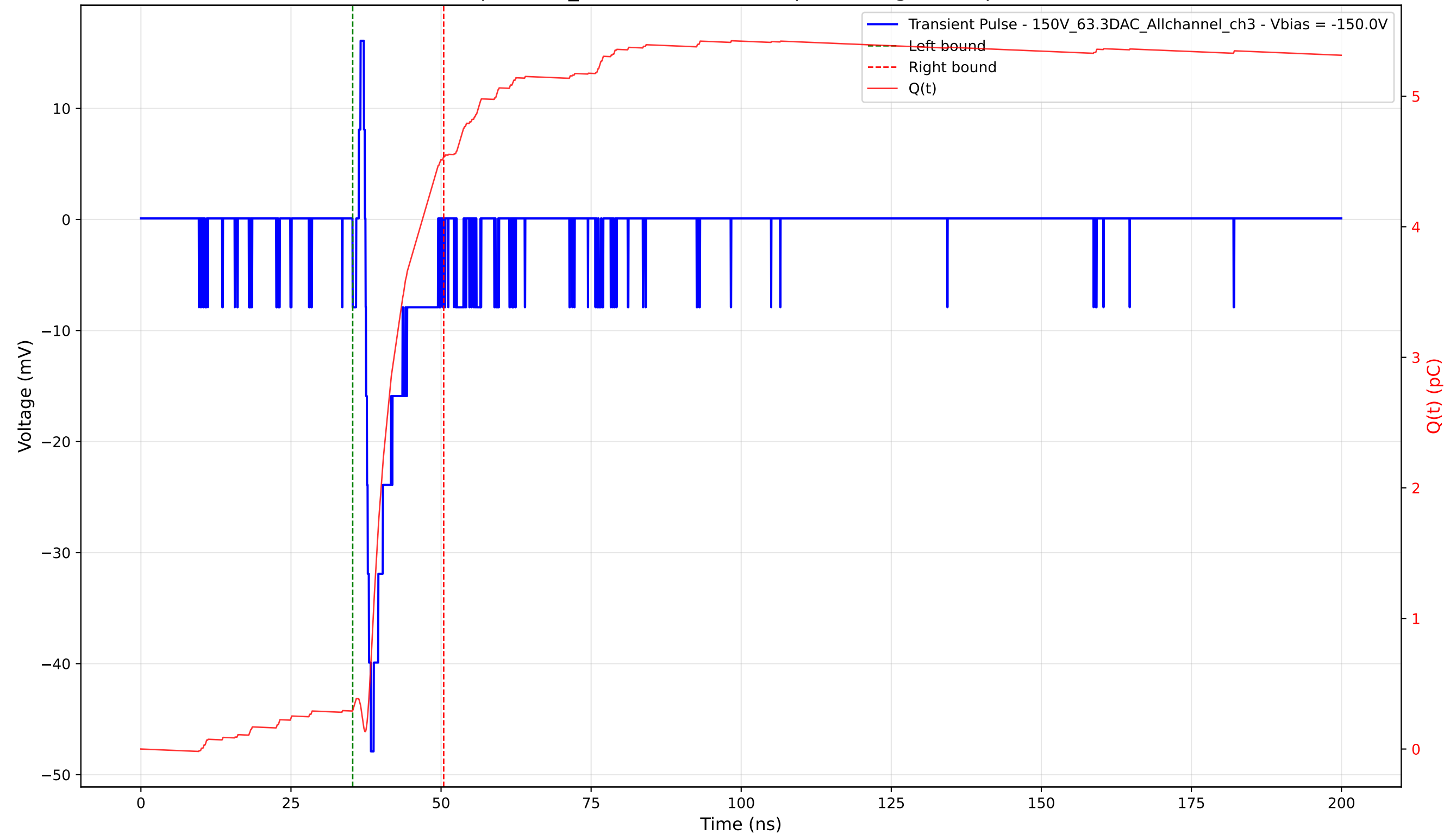
Transient Pulse - Sample: 1cm_42 - Position: 3915.0 \mu\text{m} - Charge: 4.24 pC - Rise Time: 0.90 ns
