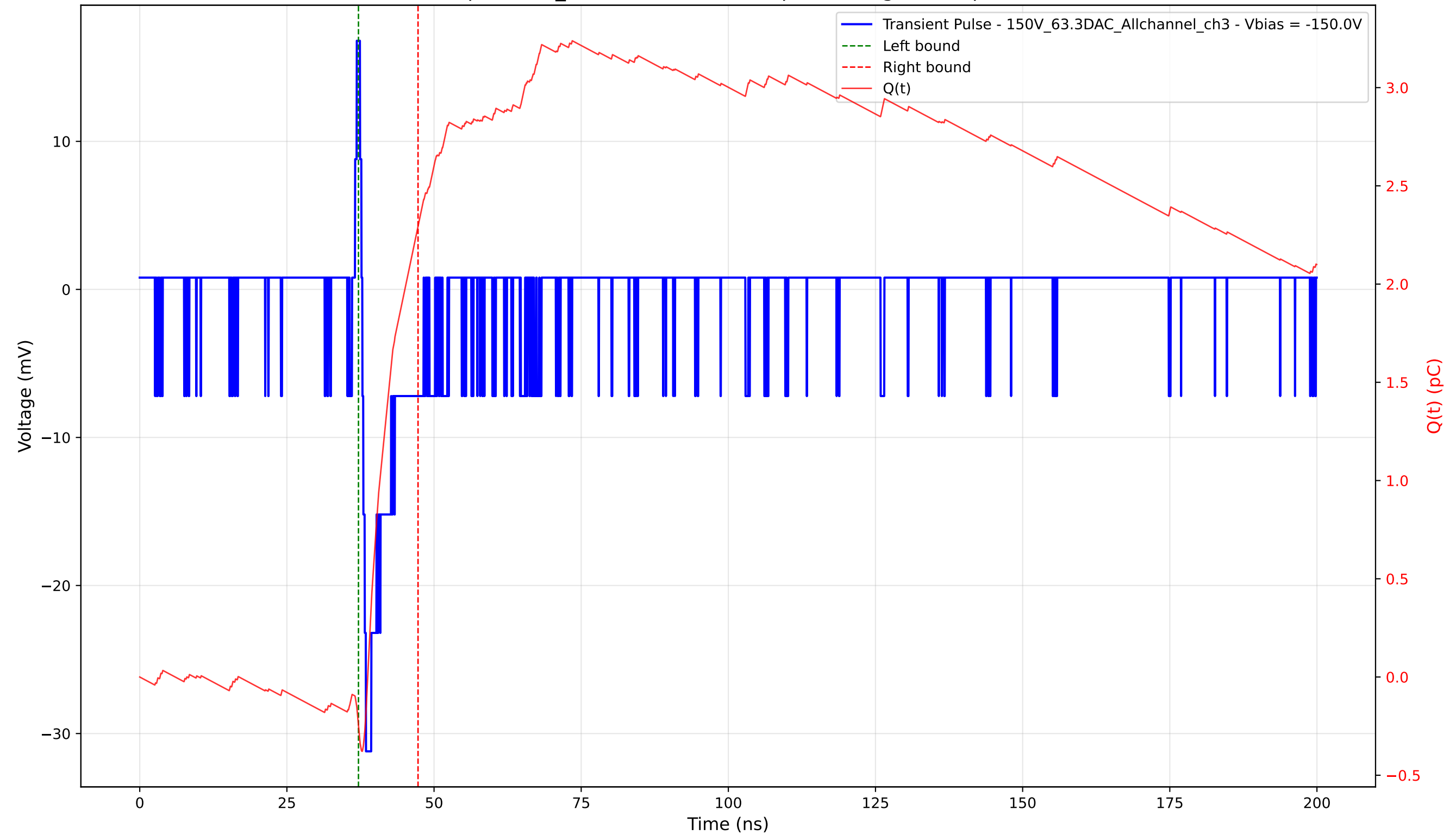
Transient Pulse - Sample: 1cm_42 - Position: 4655.0 \mu\text{m} - Charge: 2.54 pC - Rise Time: 0.63 ns
