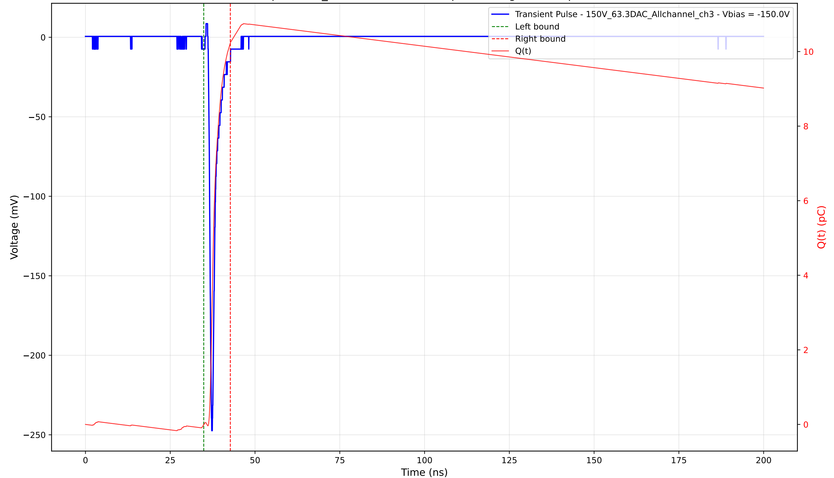
Transient Pulse - Sample: 1cm_42 - Position: 2035.0 \mu\text{m} - Charge: 10.24 pC - Rise Time: 0.79 ns
