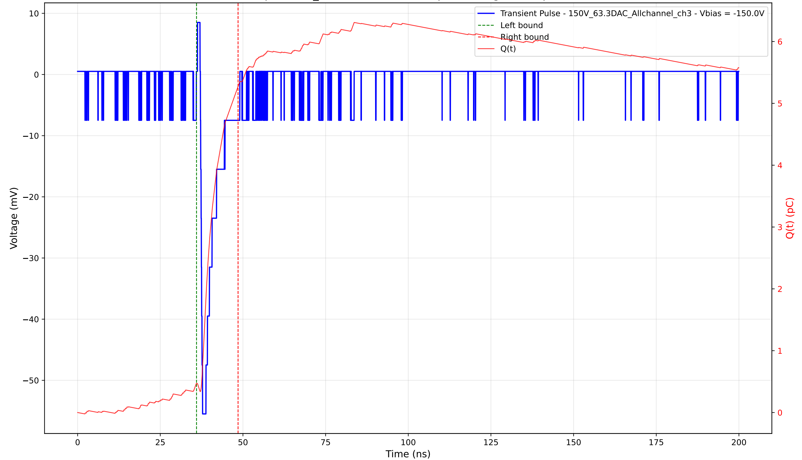
Transient Pulse - Sample: 1cm_42 - Position: 3650.0 \mu\text{m} - Charge: 4.80 pC - Rise Time: 0.65 ns
