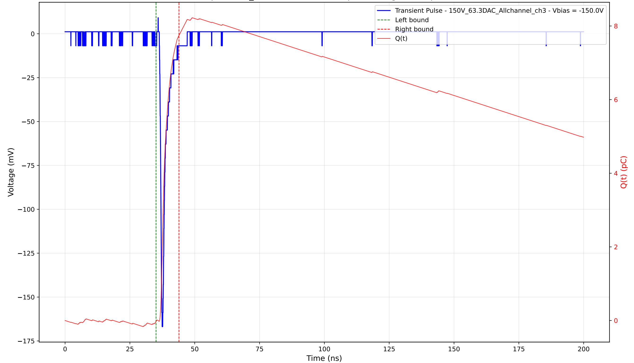
Transient Pulse - Sample: 1cm_42 - Position: 3135.0 \mu\text{m} - Charge: 7.77 pC - Rise Time: 0.75 ns
