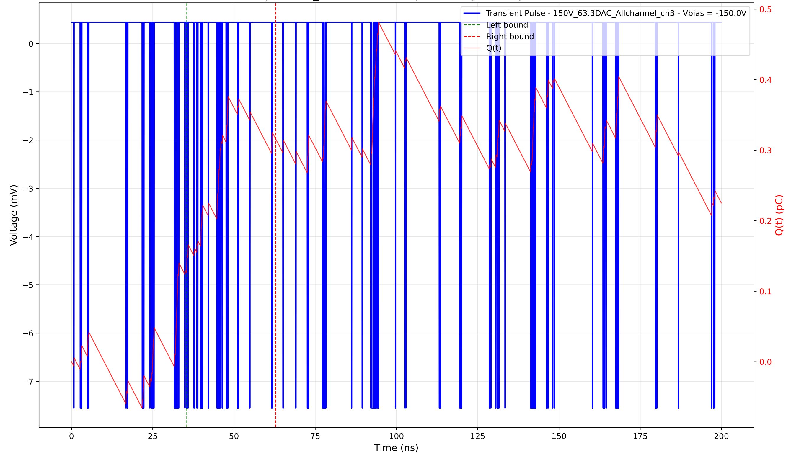
Transient Pulse - Sample: 1cm_42 - Position: 0.0 \mu\text{m} - Charge: 0.17 pC - Rise Time: 0.04 ns
