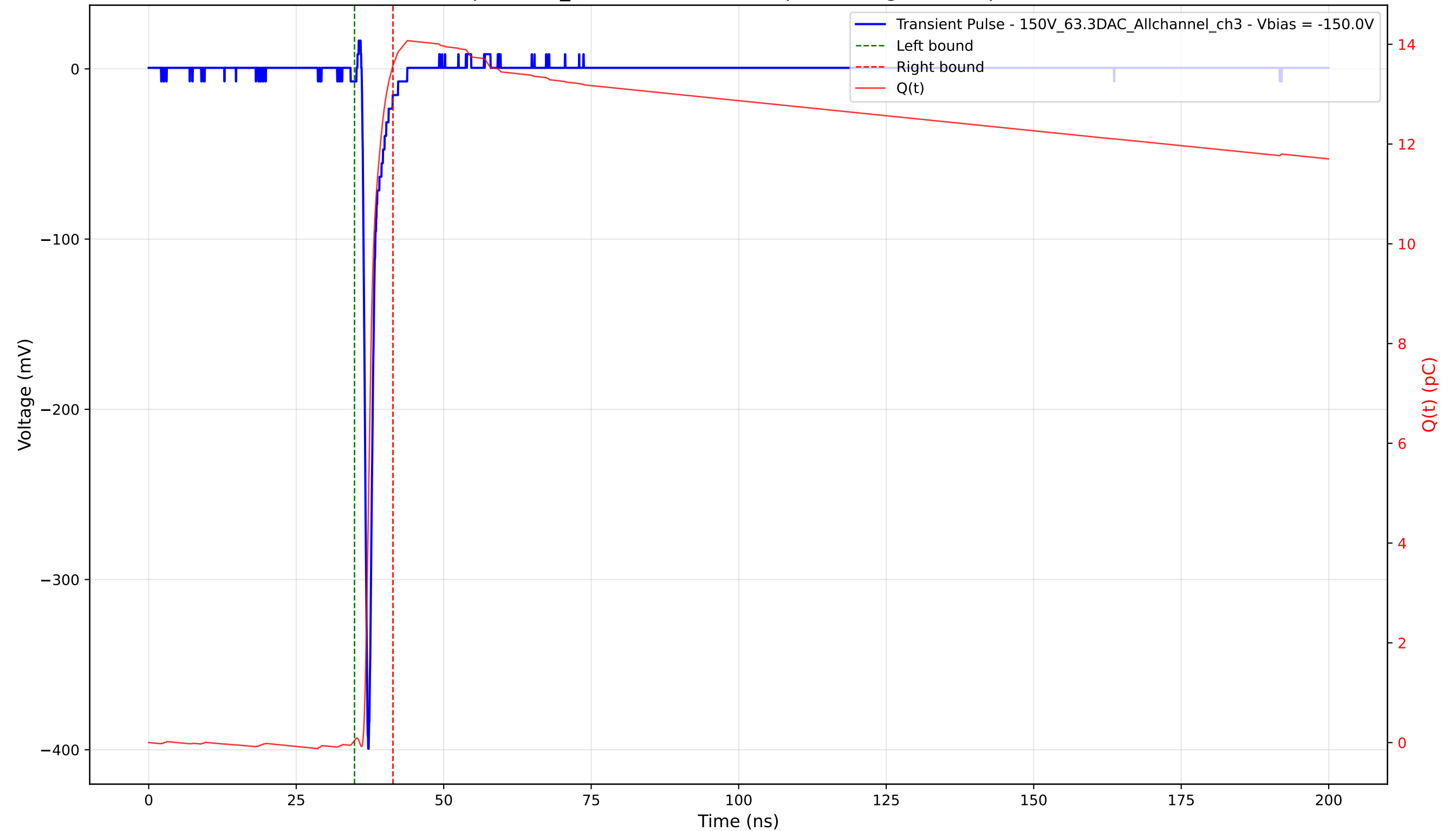
Transient Pulse - Sample: 1cm_42 - Position: 2195.0 \mu\text{m} - Charge: 13.54 pC - Rise Time: 0.72 ns
