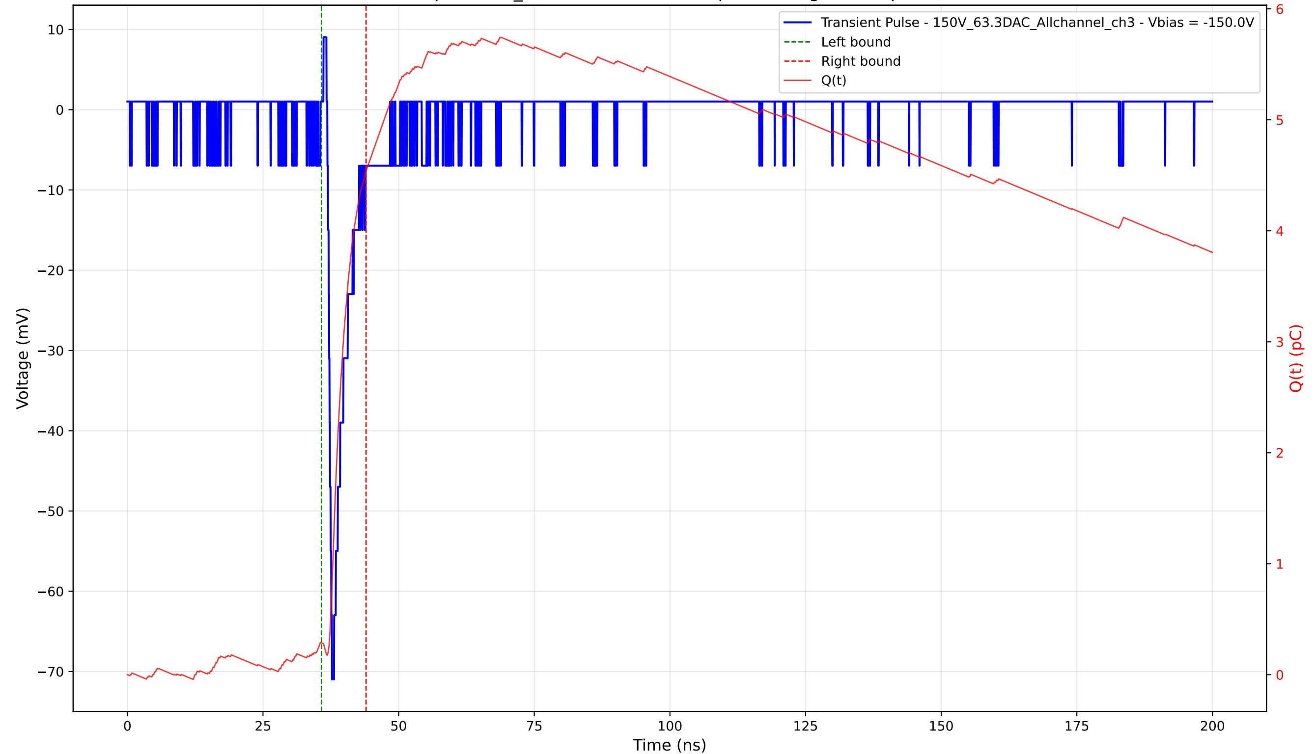
Transient Pulse - Sample: 1cm_42 - Position: 3530.0 \mu\text{m} - Charge: 4.25 pC - Rise Time: 0.76 ns
