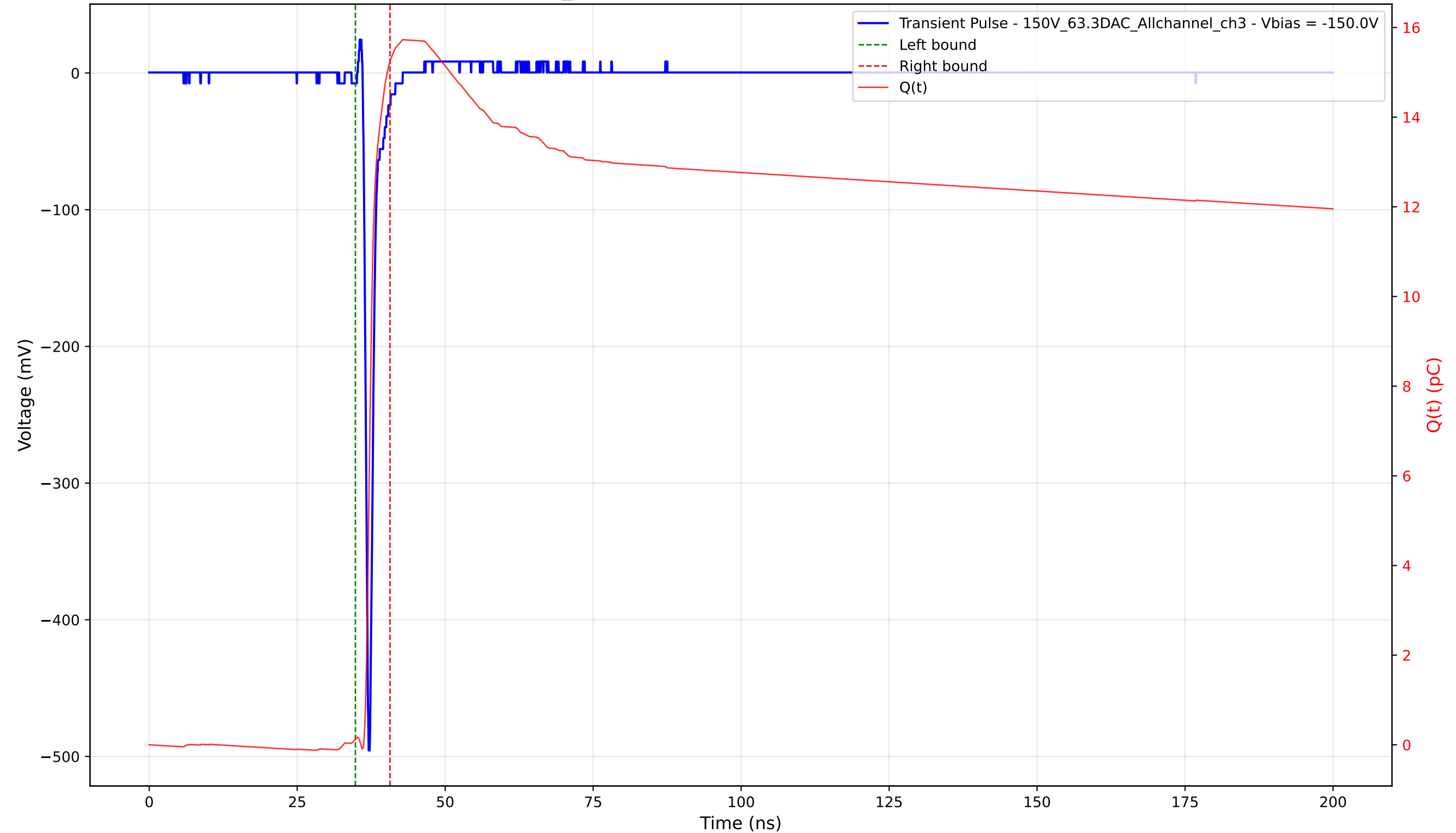
Transient Pulse - Sample: 1cm_42 - Position: 2590.0 \mu\text{m} - Charge: 15.11 pC - Rise Time: 0.71 ns
