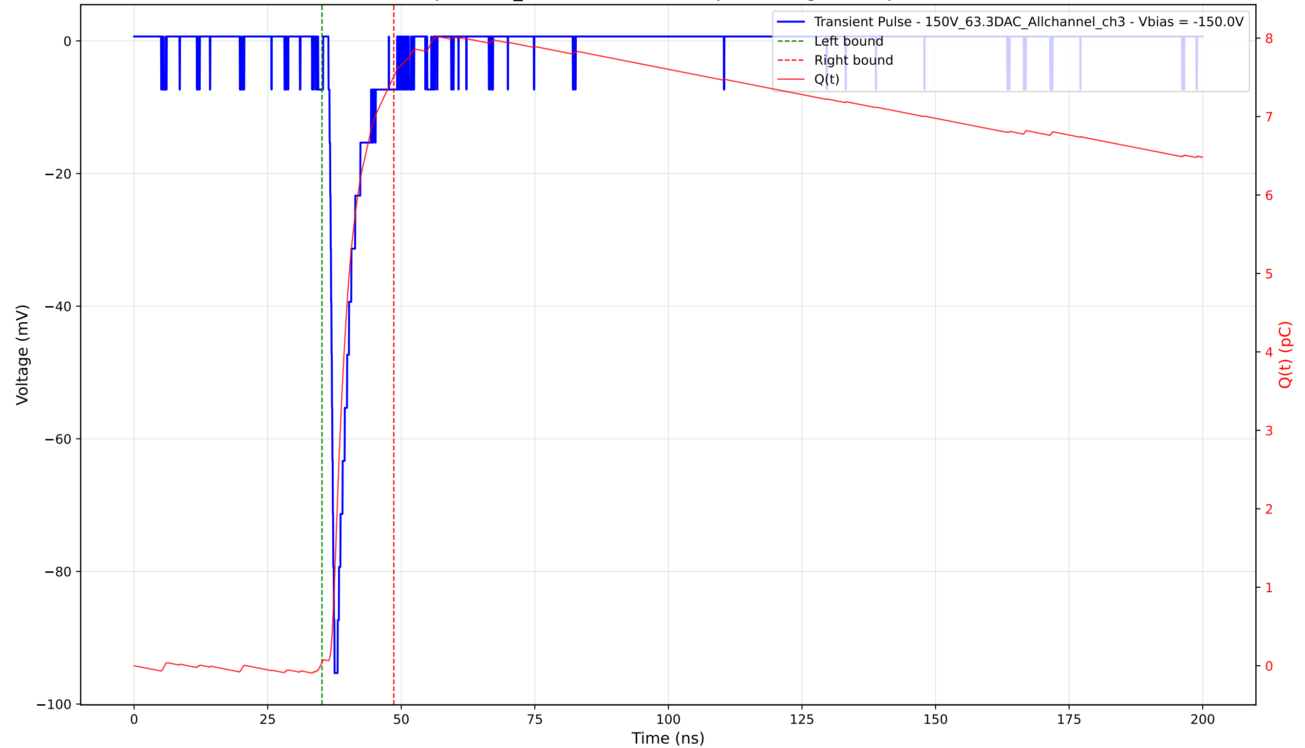
Transient Pulse - Sample: 1cm_42 - Position: 1600.0 \mu\text{m} - Charge: 7.47 pC - Rise Time: 0.83 ns
