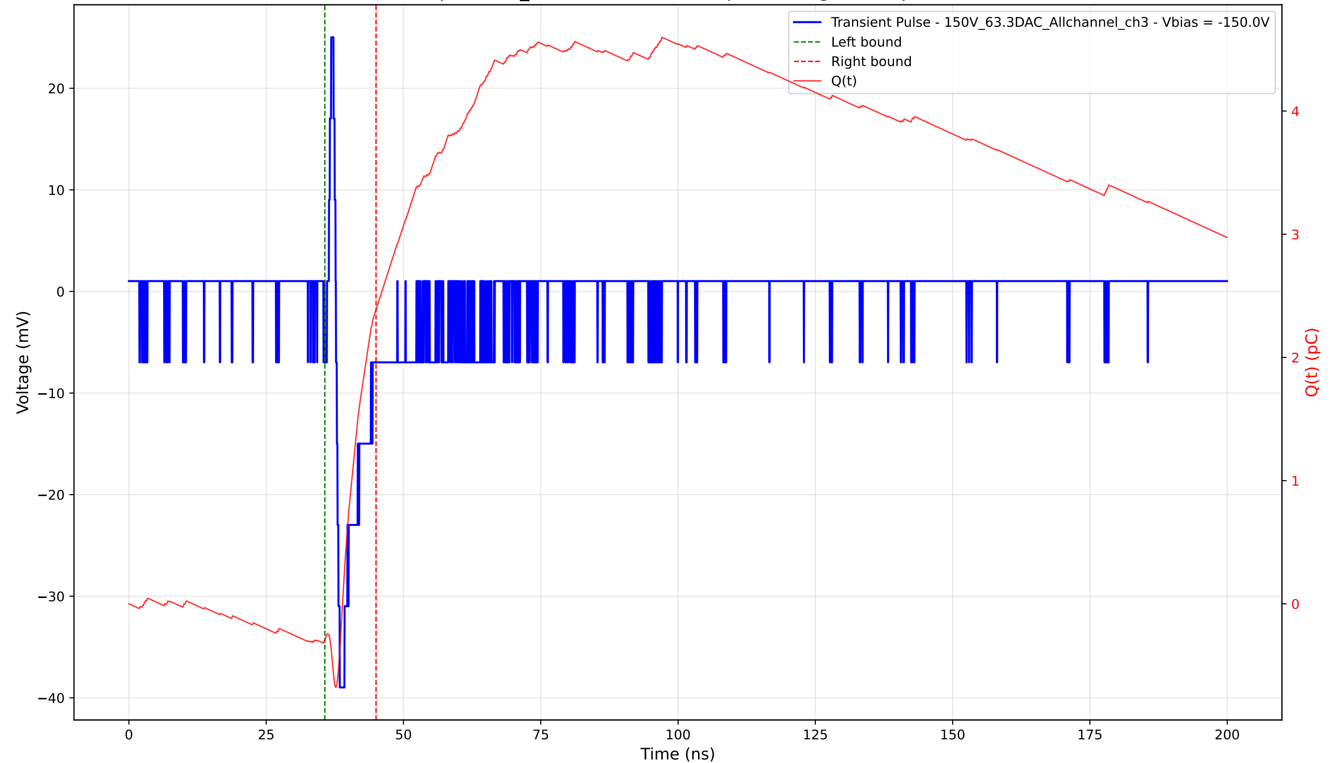
Transient Pulse - Sample: 1cm_42 - Position: 4250.0 \mu\text{m} - Charge: 2.68 pC - Rise Time: 0.70 ns
