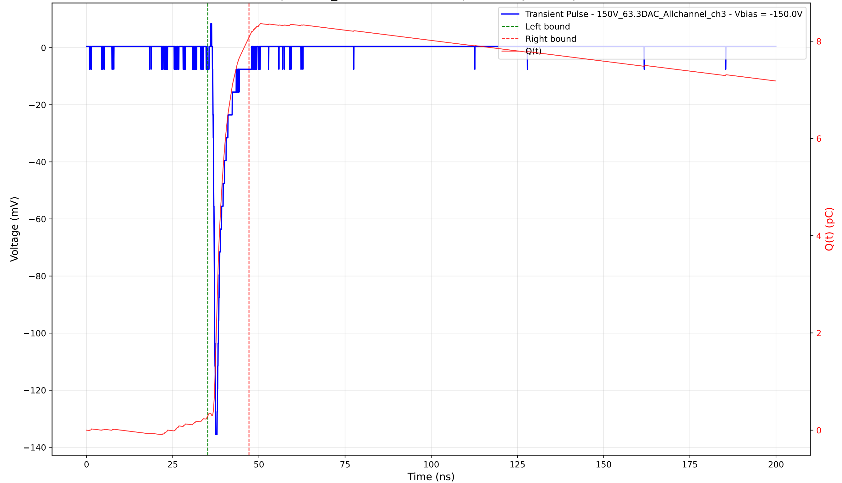
Transient Pulse - Sample: 1cm_42 - Position: 3280.0 \mu\text{m} - Charge: 7.79 pC - Rise Time: 0.77 ns
