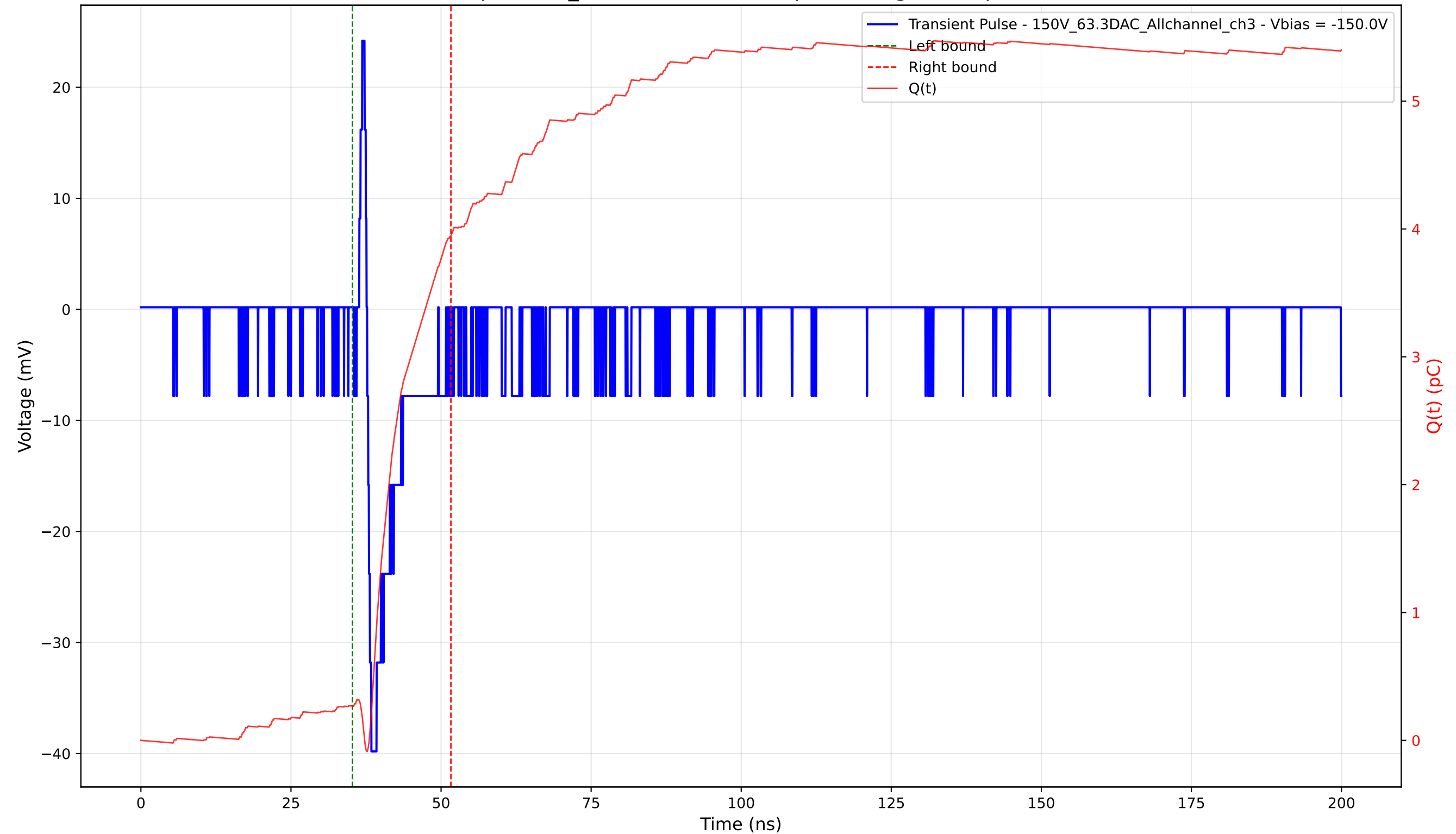
Transient Pulse - Sample: 1cm_42 - Position: 4235.0 \mu\text{m} - Charge: 3.68 pC - Rise Time: 0.70 ns
