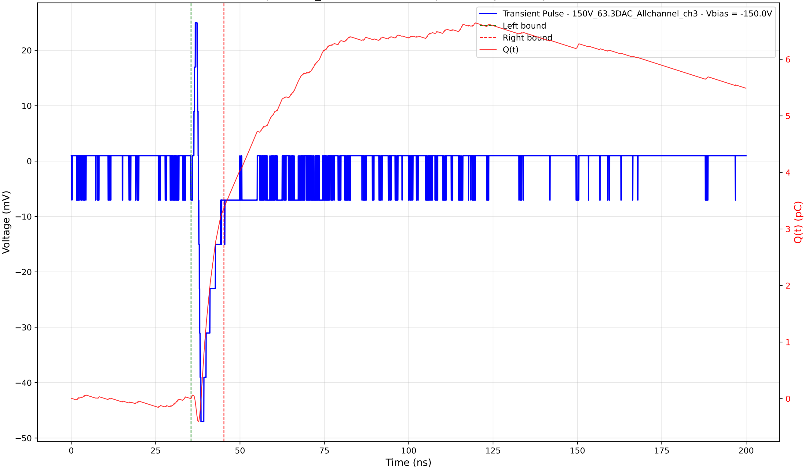
Transient Pulse - Sample: 1cm_42 - Position: 680.0 \mu\text{m} - Charge: 3.36 pC - Rise Time: 0.74 ns
