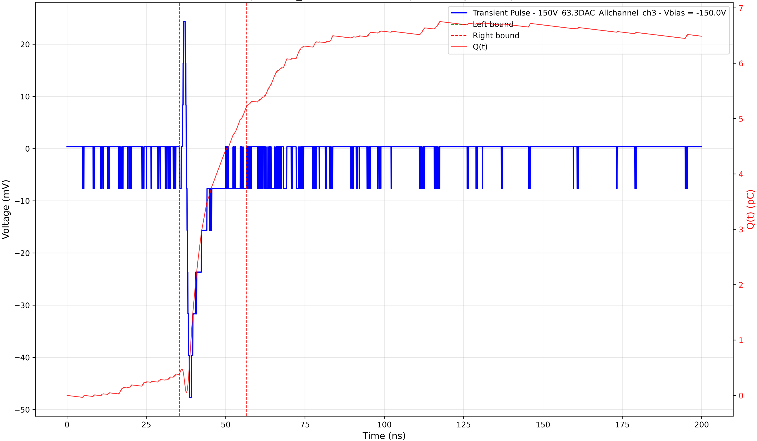
Transient Pulse - Sample: 1cm_42 - Position: 640.0 \mu\text{m} - Charge: 4.85 pC - Rise Time: 0.86 ns
