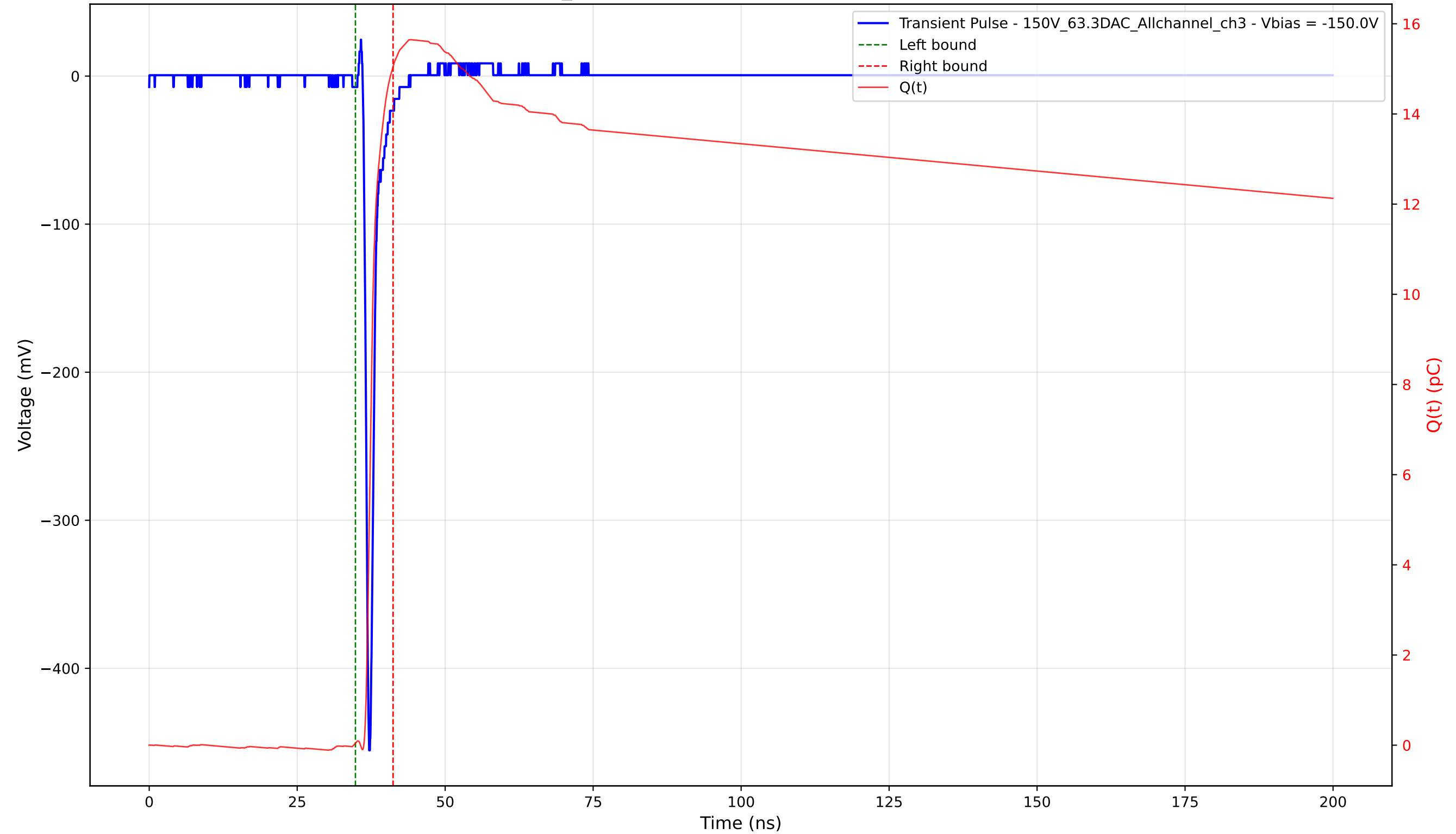
Transient Pulse - Sample: 1cm_42 - Position: 2785.0 \mu\text{m} - Charge: 15.01 pC - Rise Time: 0.75 ns
