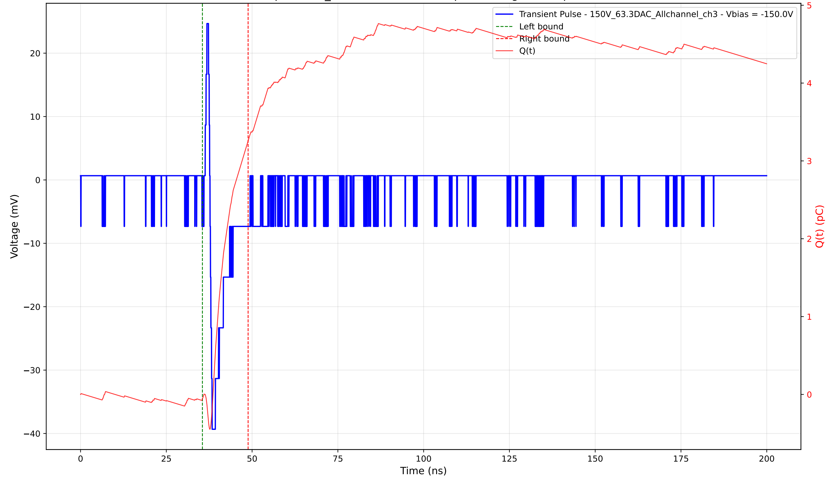
Transient Pulse - Sample: 1cm_42 - Position: 4275.0 \mu\text{m} - Charge: 3.32 pC - Rise Time: 0.62 ns
