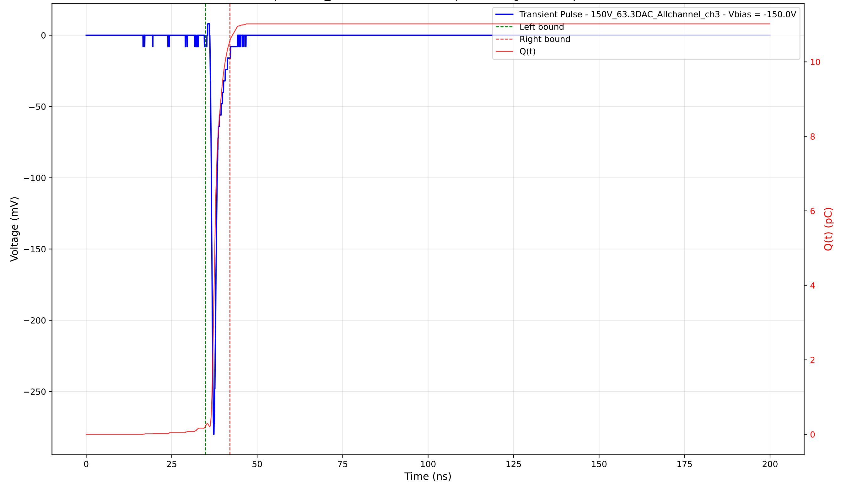
Transient Pulse - Sample: 1cm_42 - Position: 2960.0 \mu\text{m} - Charge: 10.35 pC - Rise Time: 0.80 ns
