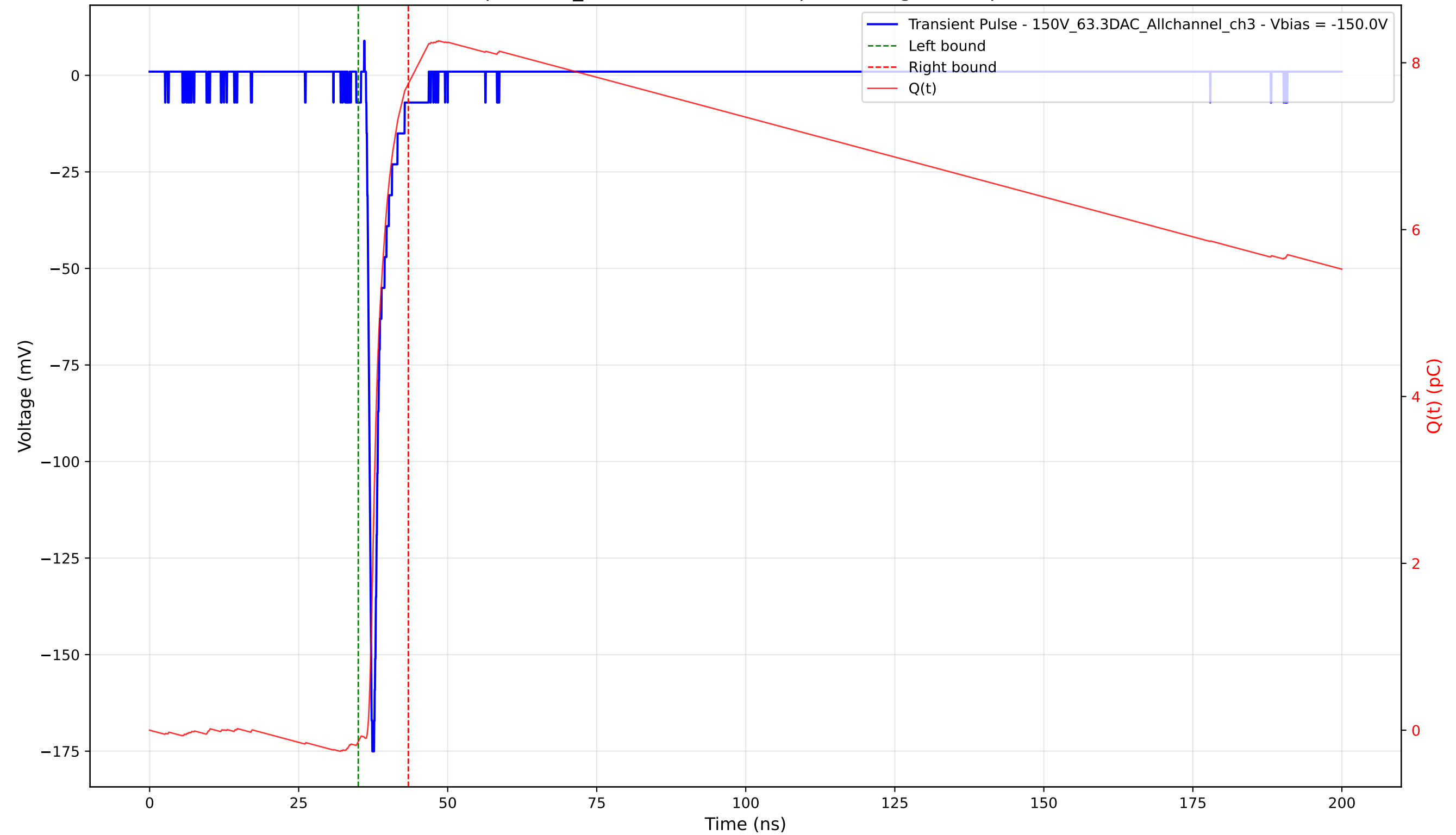
Transient Pulse - Sample: 1cm_42 - Position: 3100.0 \mu\text{m} - Charge: 7.88 pC - Rise Time: 0.74 ns
