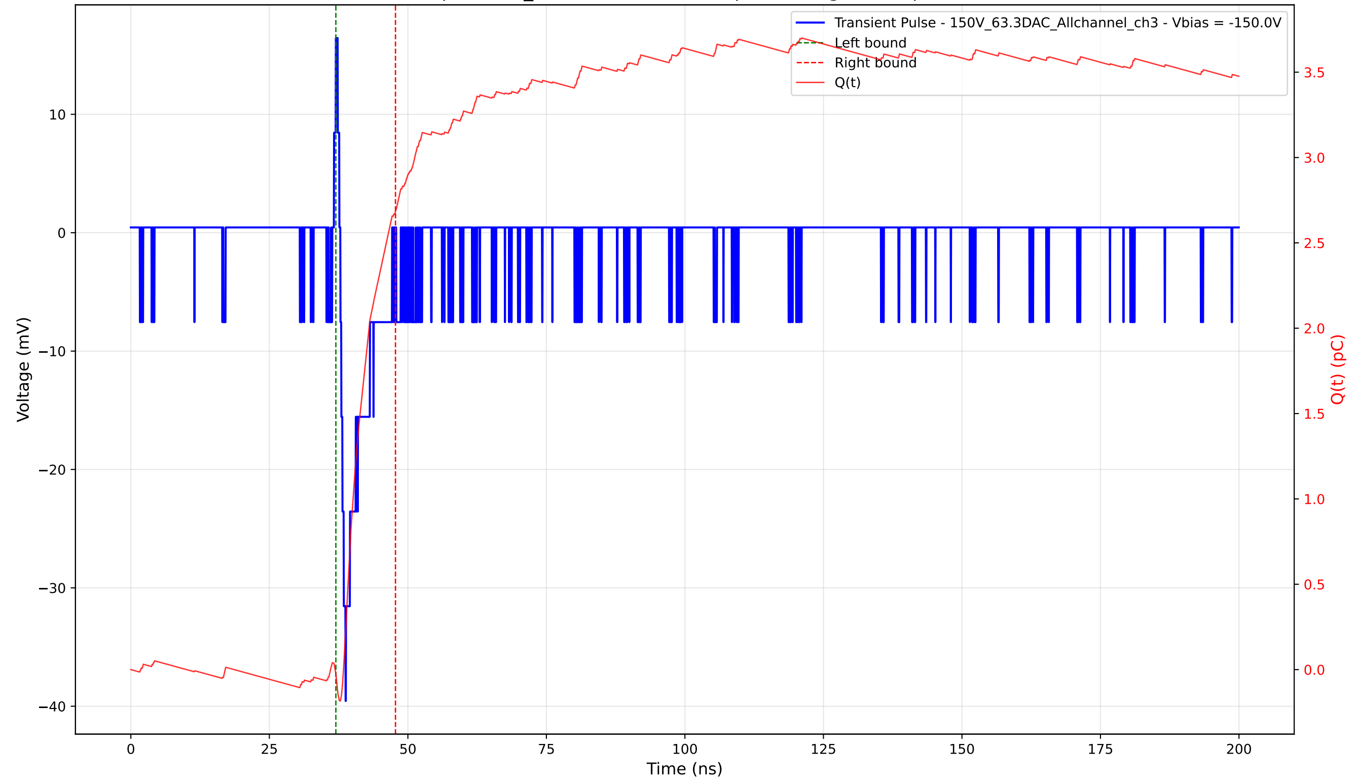
Transient Pulse - Sample: 1cm_42 - Position: 4750.0 \mu\text{m} - Charge: 2.71 pC - Rise Time: 0.94 ns
