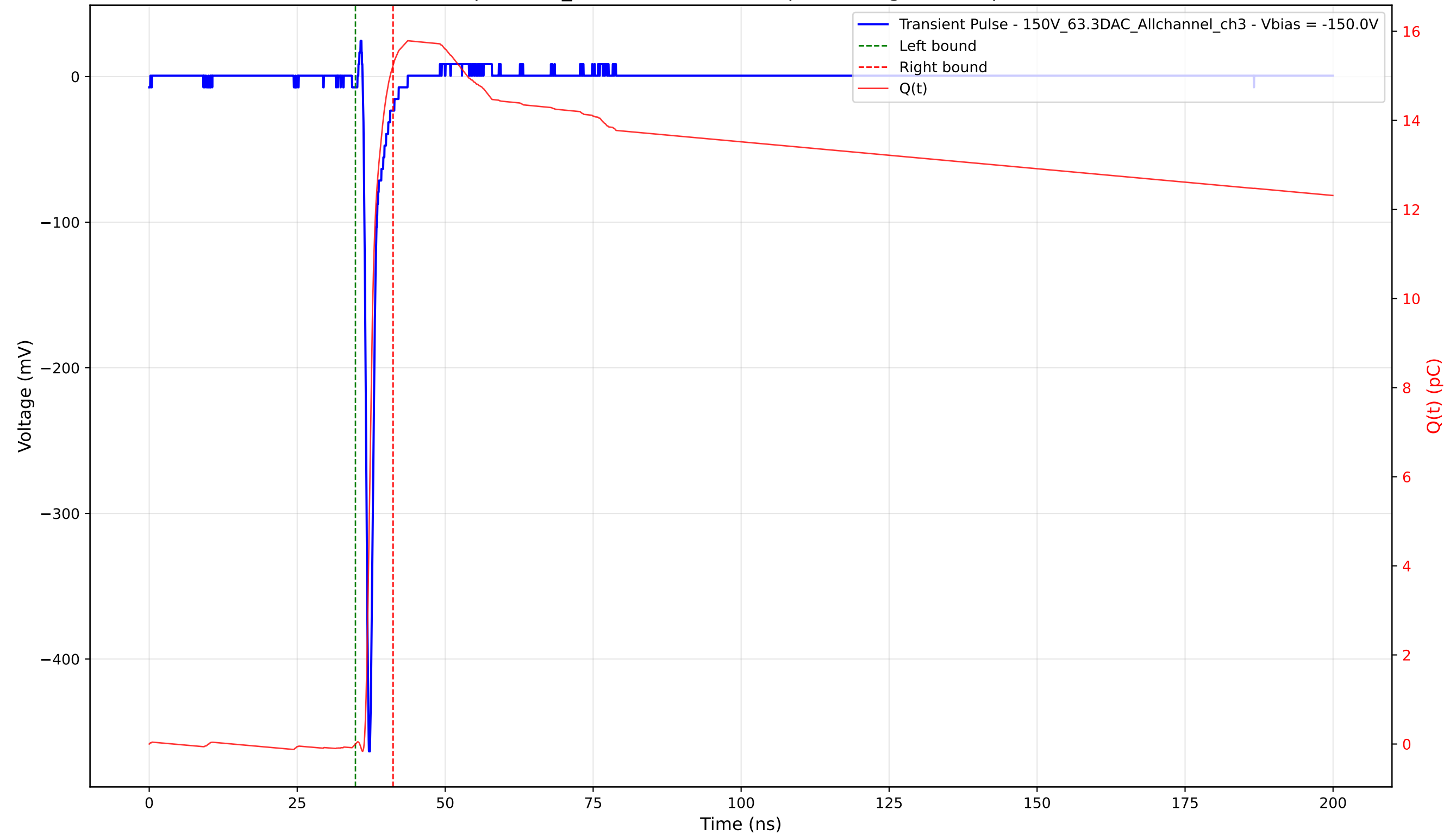
Transient Pulse - Sample: 1cm_42 - Position: 2265.0 \mu\text{m} - Charge: 15.24 pC - Rise Time: 0.73 ns
