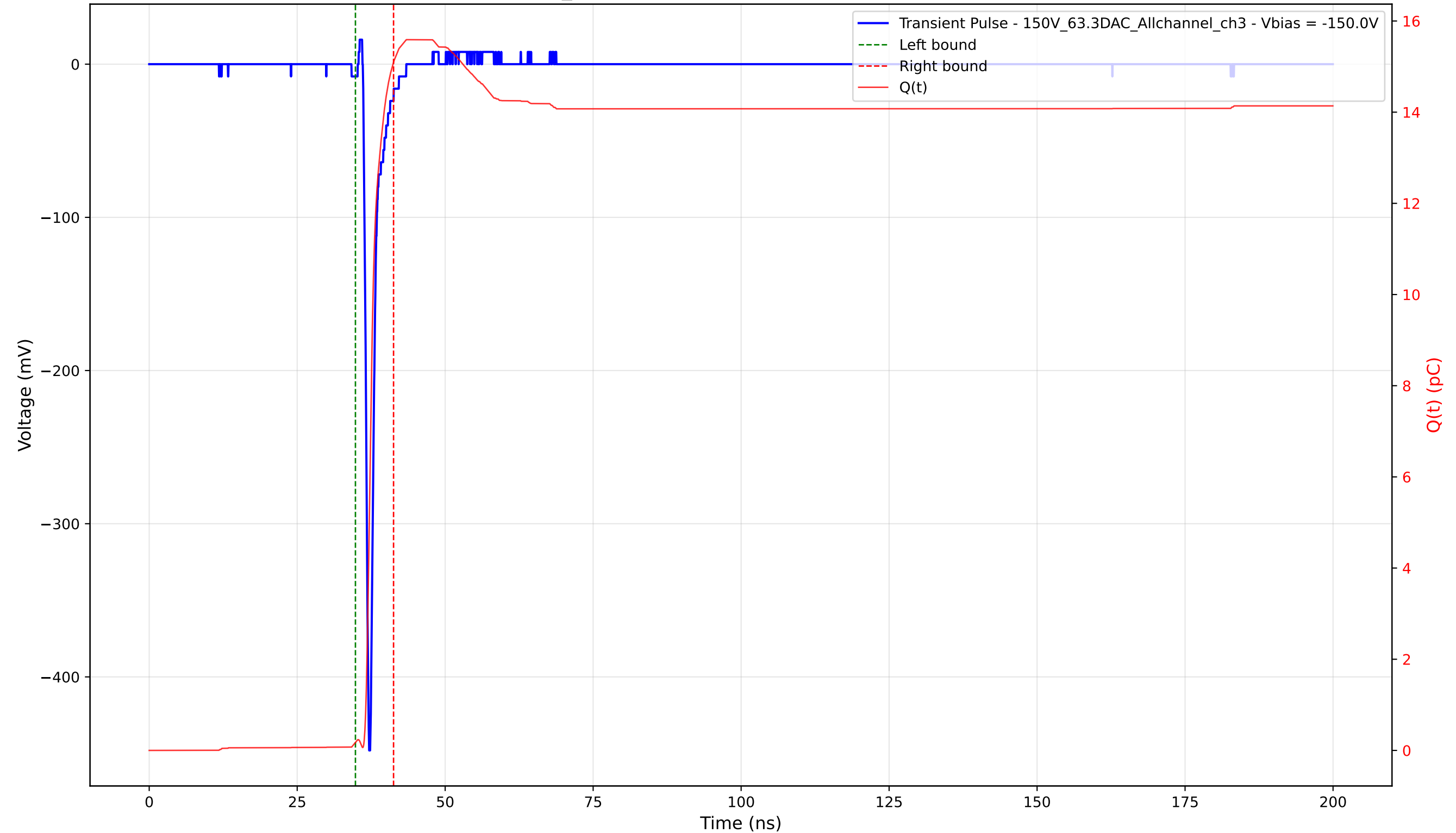
Transient Pulse - Sample: 1cm_42 - Position: 2790.0 \mu\text{m} - Charge: 14.92 pC - Rise Time: 0.74 ns
