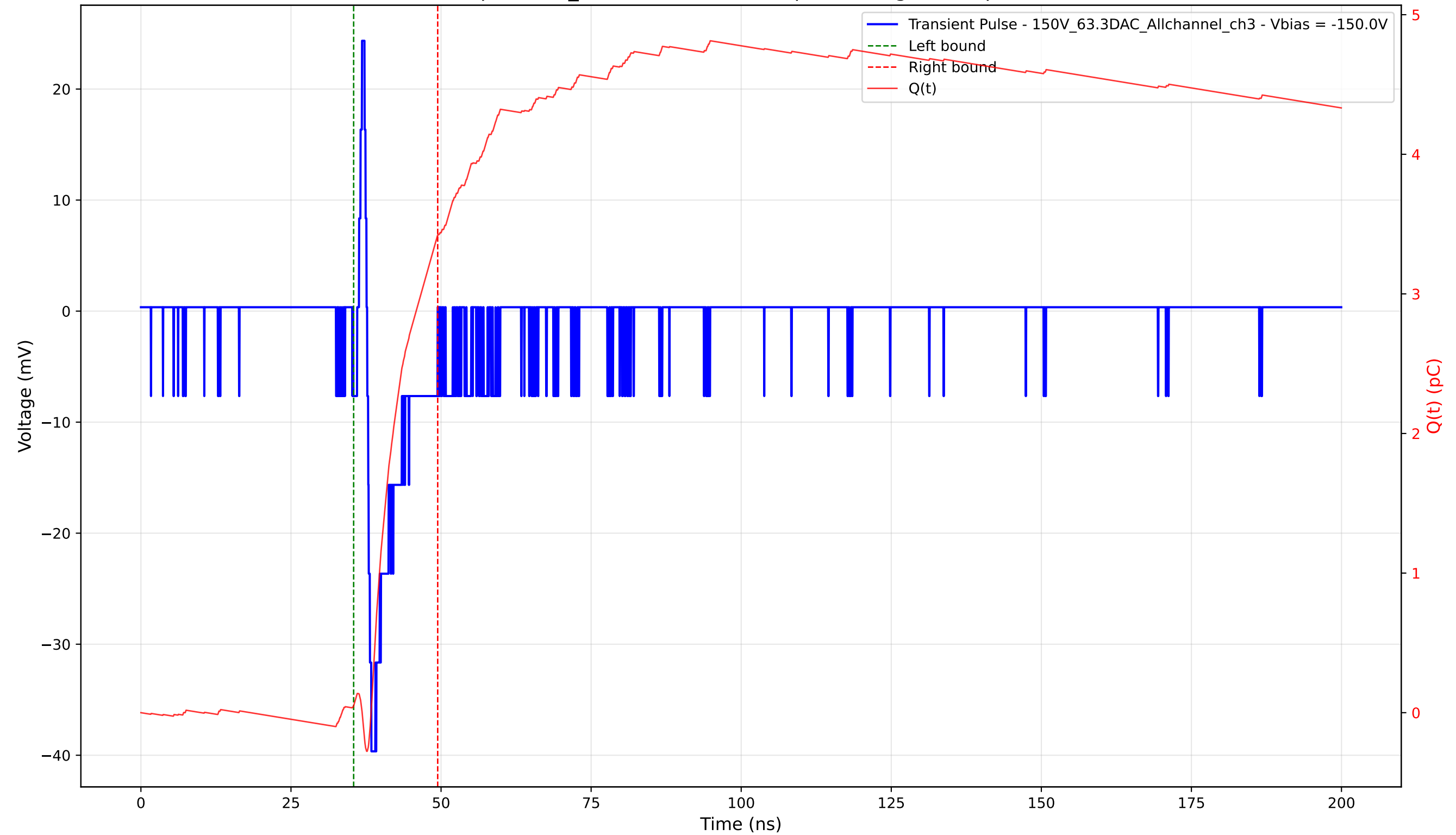
Transient Pulse - Sample: 1cm_42 - Position: 4210.0 \mu\text{m} - Charge: 3.37 pC - Rise Time: 0.70 ns
