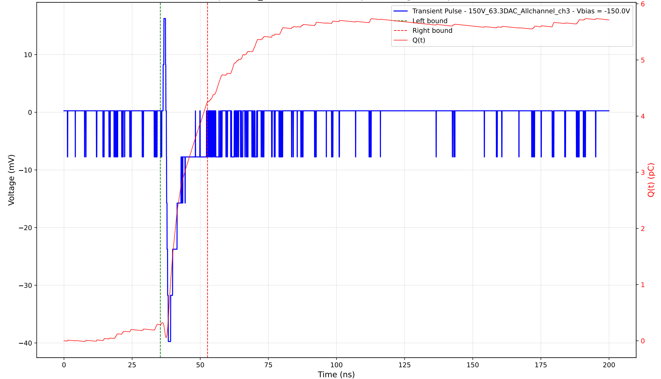
Transient Pulse - Sample: 1cm_42 - Position: 4040.0 \mu\text{m} - Charge: 3.96 pC - Rise Time: 0.70 ns
