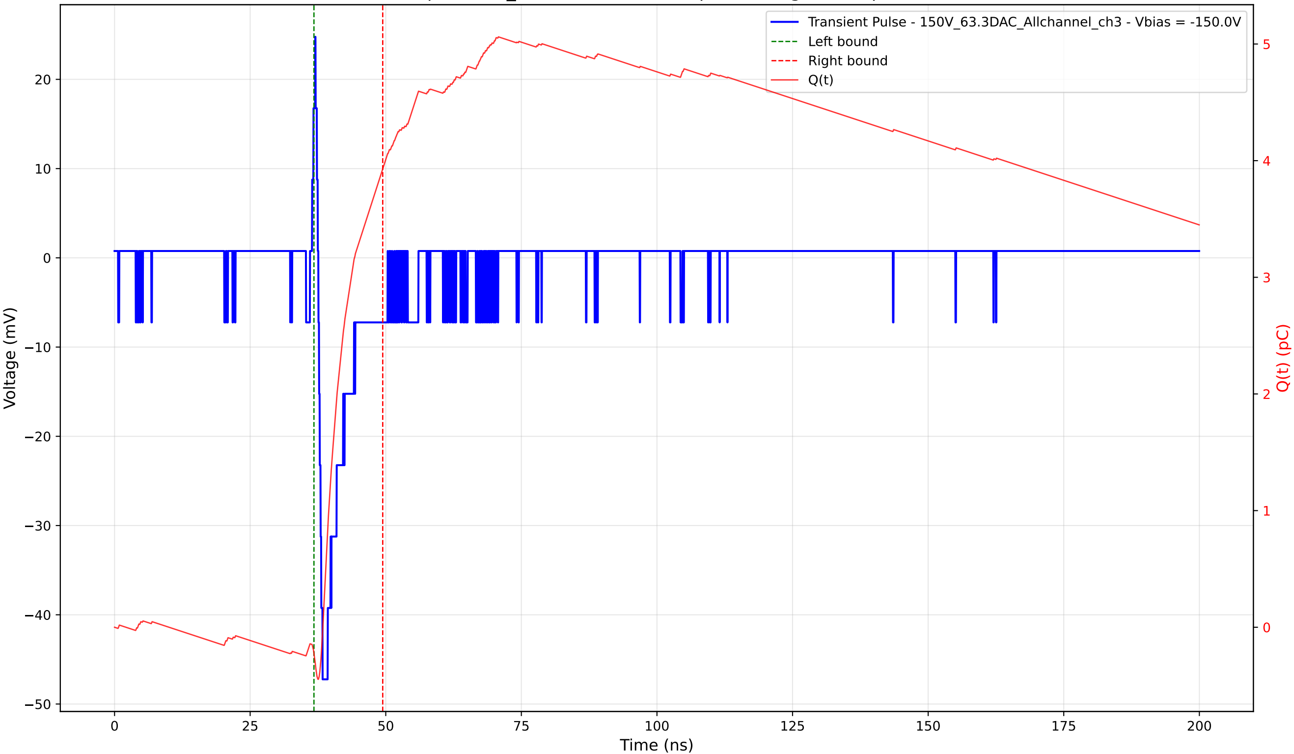
Transient Pulse - Sample: 1cm_42 - Position: 975.0 \mu\text{m} - Charge: 4.15 pC - Rise Time: 0.78 ns
