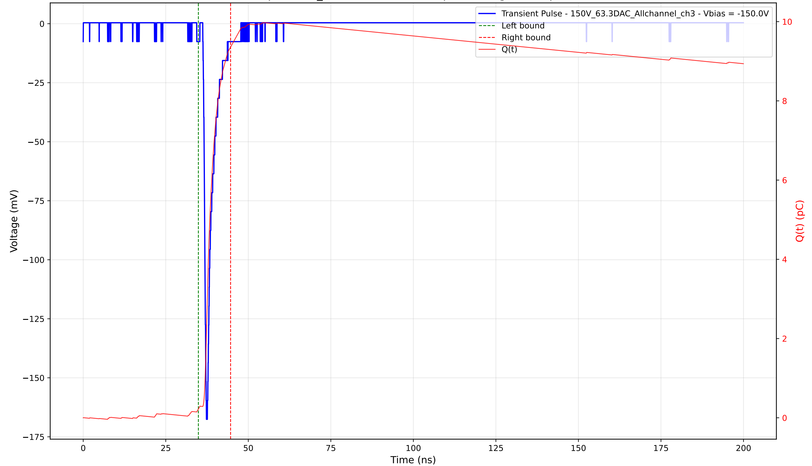
Transient Pulse - Sample: 1cm_42 - Position: 1885.0 \mu\text{m} - Charge: 9.14 pC - Rise Time: 0.79 ns
