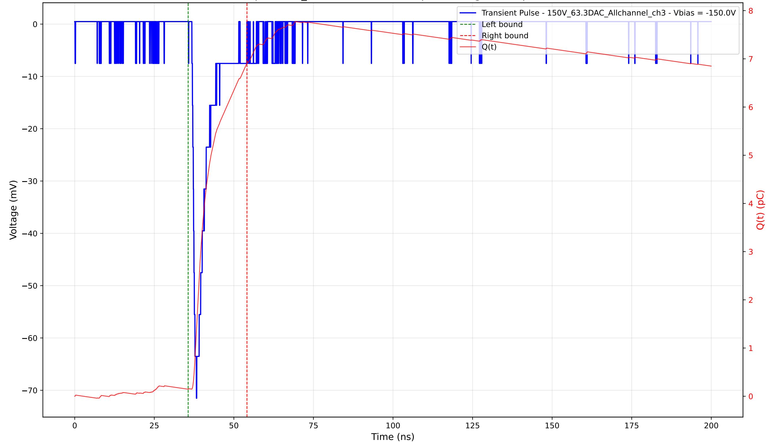
Transient Pulse - Sample: 1cm_42 - Position: 1440.0 \mu\text{m} - Charge: 6.76 pC - Rise Time: 1.40 ns
