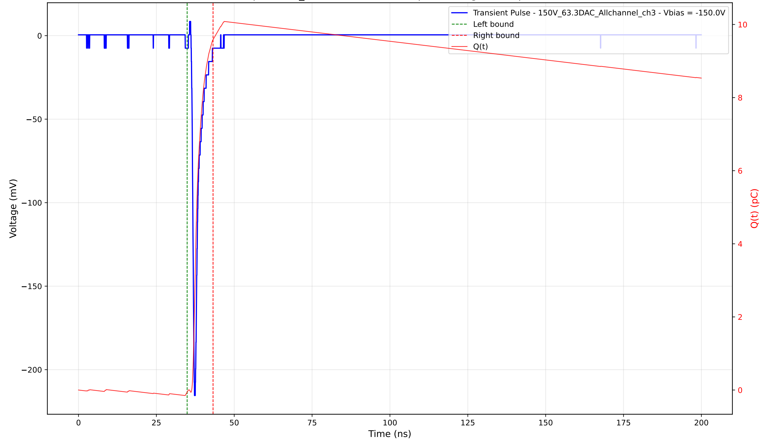
Transient Pulse - Sample: 1cm_42 - Position: 1995.0 \mu\text{m} - Charge: 9.64 pC - Rise Time: 0.78 ns
