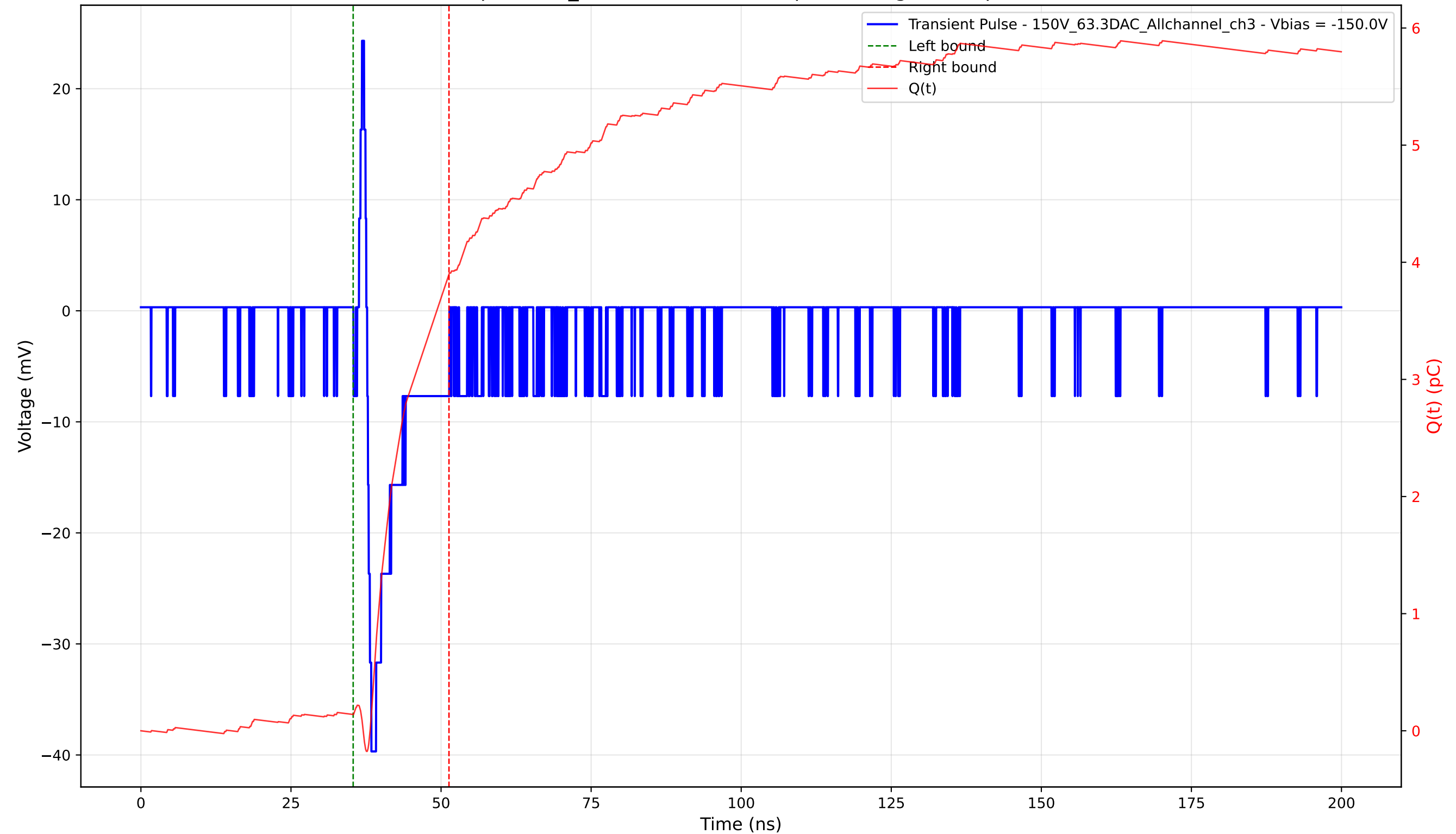
Transient Pulse - Sample: 1cm_42 - Position: 4175.0 \mu\text{m} - Charge: 3.76 pC - Rise Time: 0.70 ns
