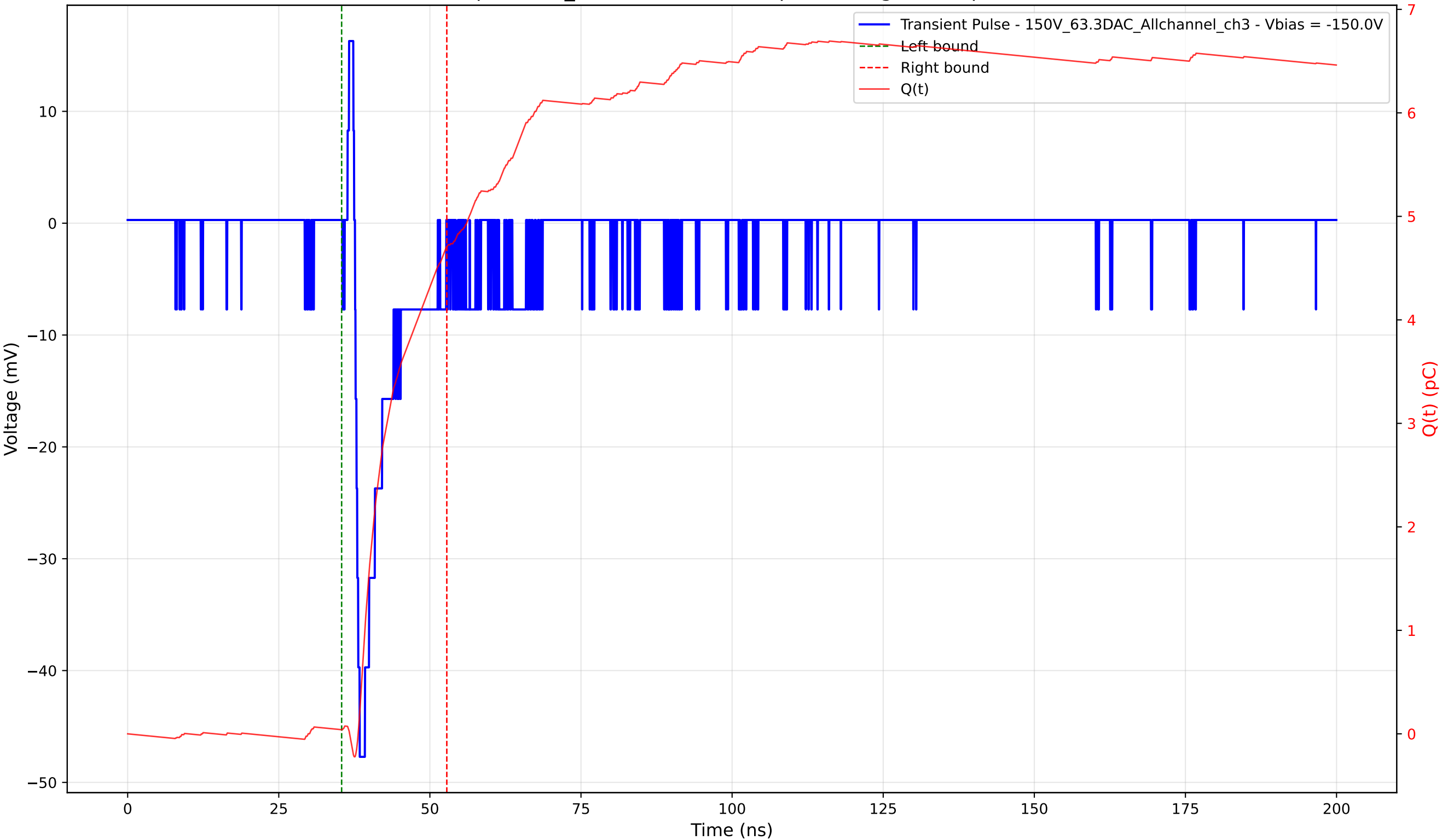
Transient Pulse - Sample: 1cm_42 - Position: 960.0 \mu\text{m} - Charge: 4.66 pC - Rise Time: 0.78 ns
