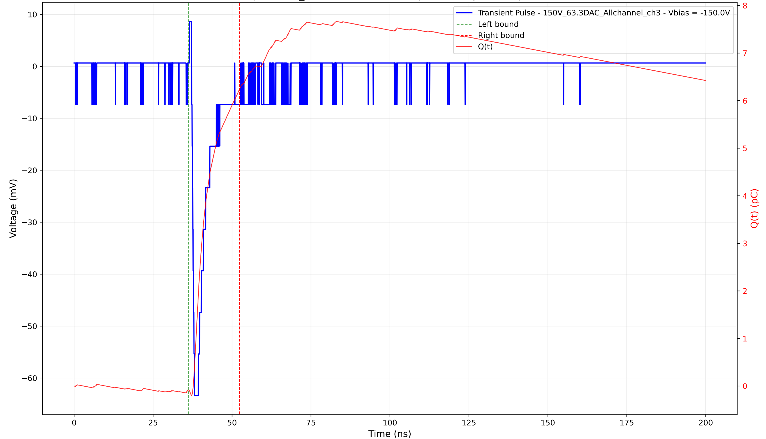
Transient Pulse - Sample: 1cm_42 - Position: 1220.0 \mu\text{m} - Charge: 6.32 pC - Rise Time: 0.93 ns
