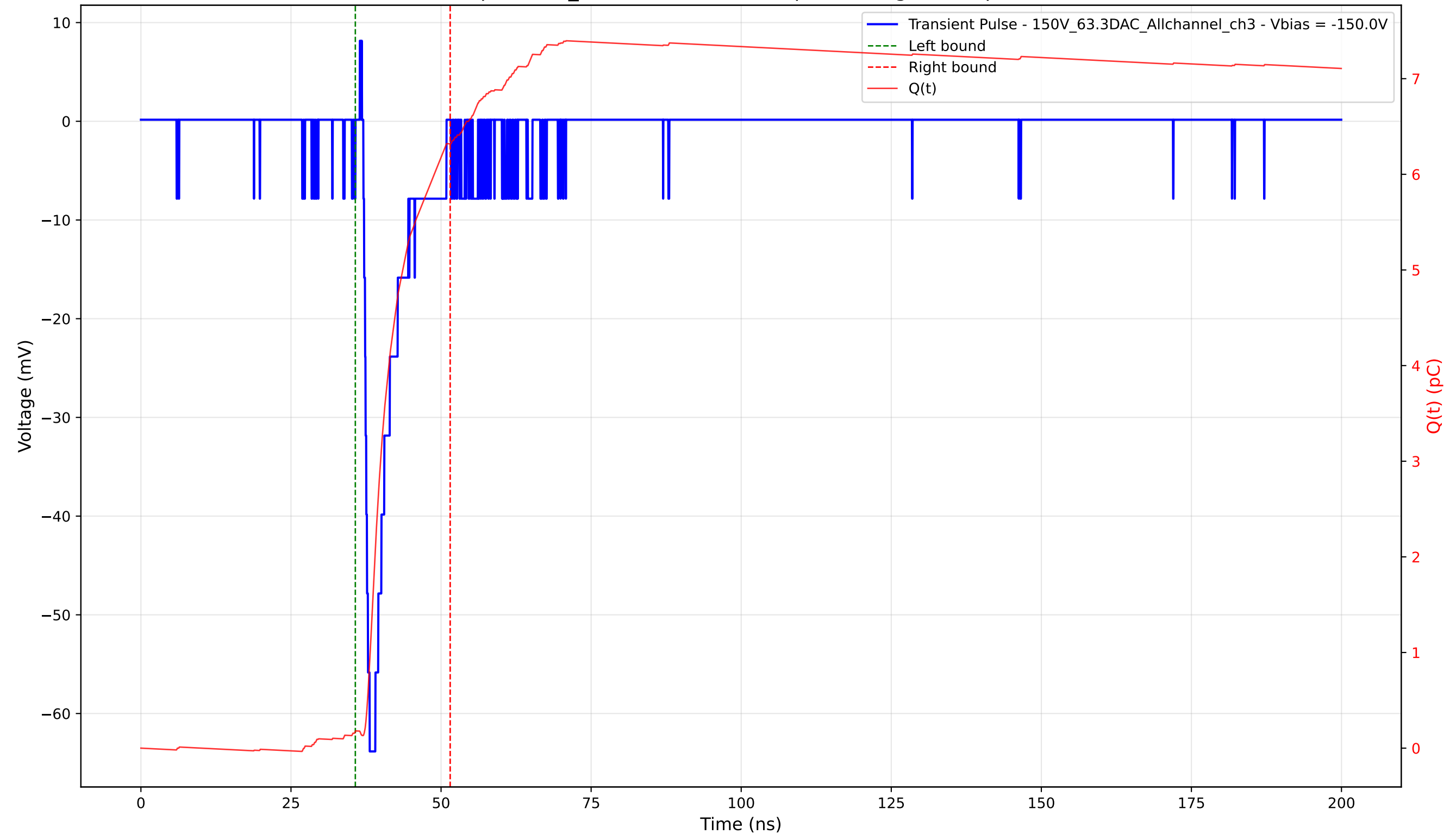
Transient Pulse - Sample: 1cm_42 - Position: 1370.0 \mu\text{m} - Charge: 6.14 pC - Rise Time: 1.05 ns
