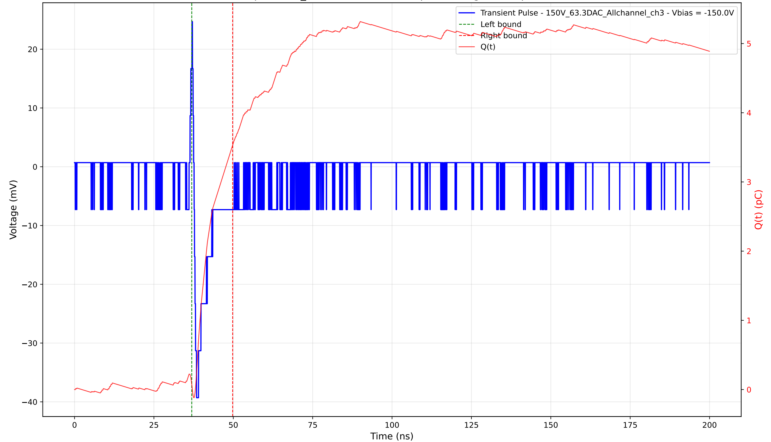
Transient Pulse - Sample: 1cm_42 - Position: 4130.0 \mu\text{m} - Charge: 3.46 pC - Rise Time: 0.78 ns
