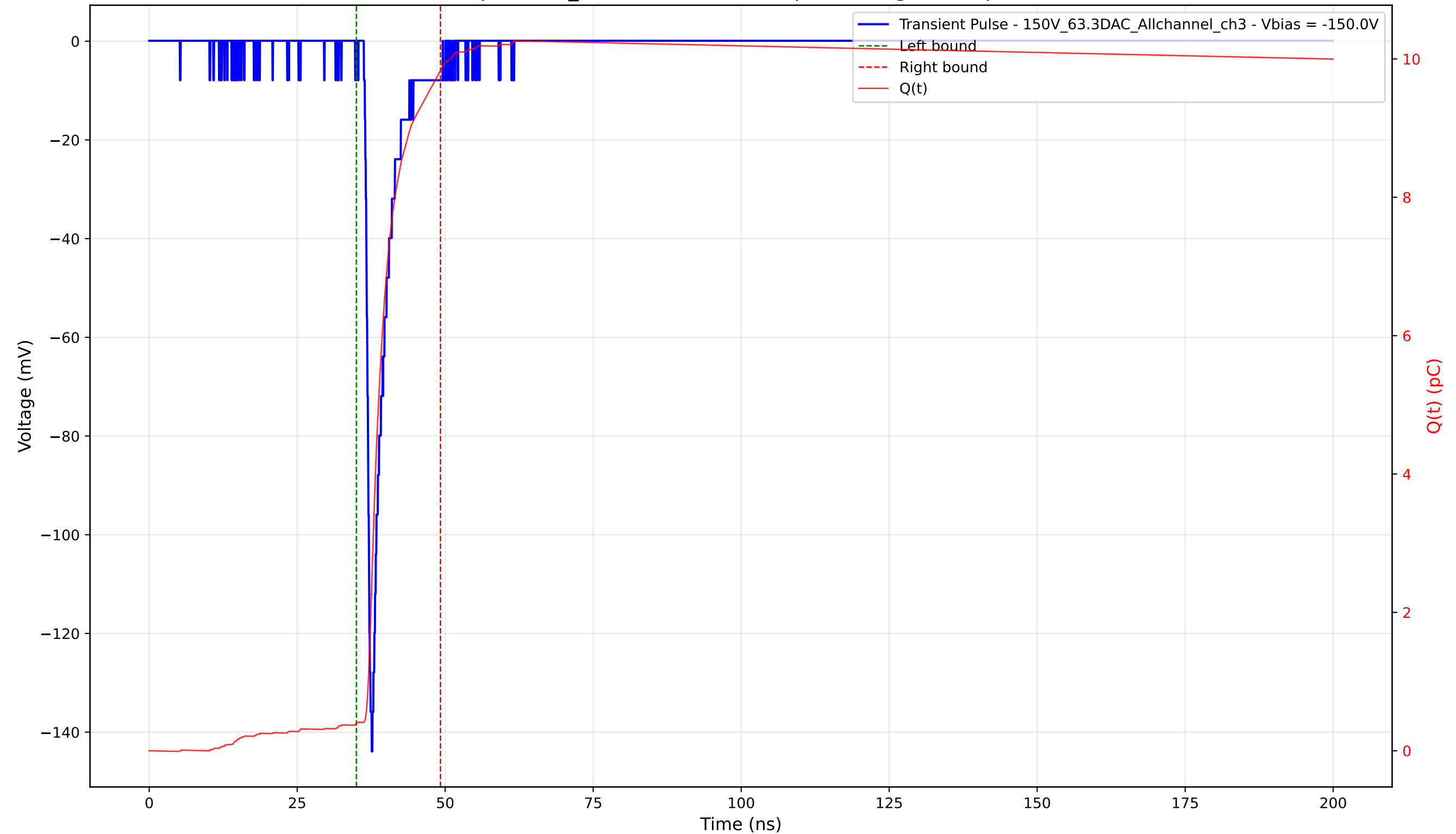
Transient Pulse - Sample: 1cm_42 - Position: 1705.0 \mu\text{m} - Charge: 9.44 pC - Rise Time: 0.97 ns
