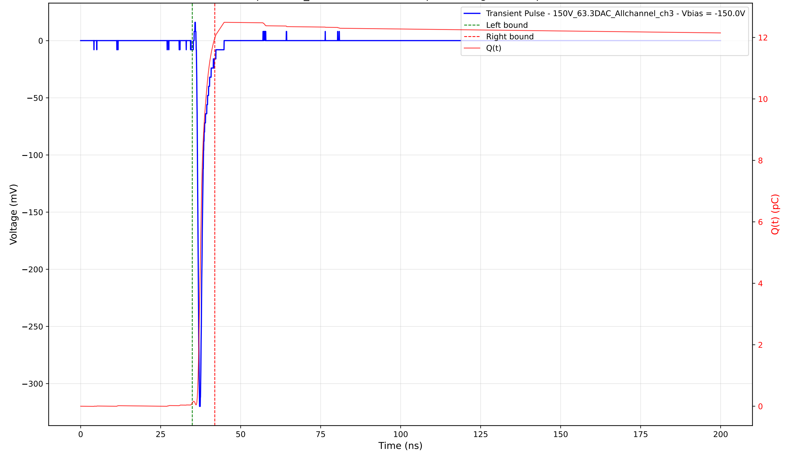
Transient Pulse - Sample: 1cm_42 - Position: 2115.0 \mu\text{m} - Charge: 11.87 pC - Rise Time: 0.72 ns
