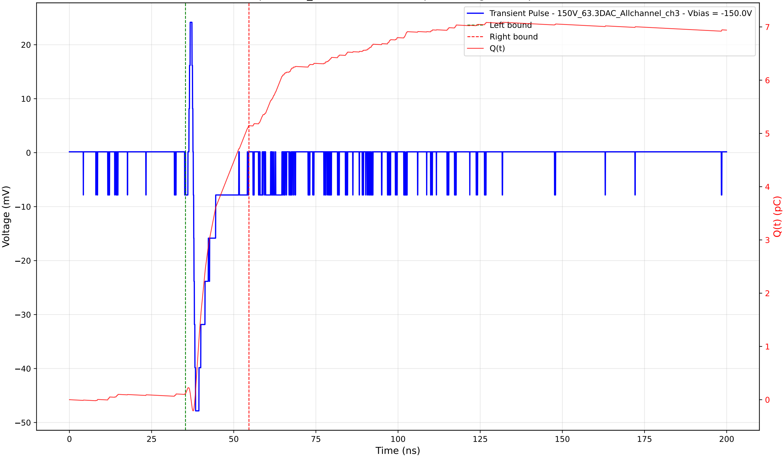
Transient Pulse - Sample: 1cm_42 - Position: 760.0 \mu\text{m} - Charge: 5.03 pC - Rise Time: 0.70 ns
