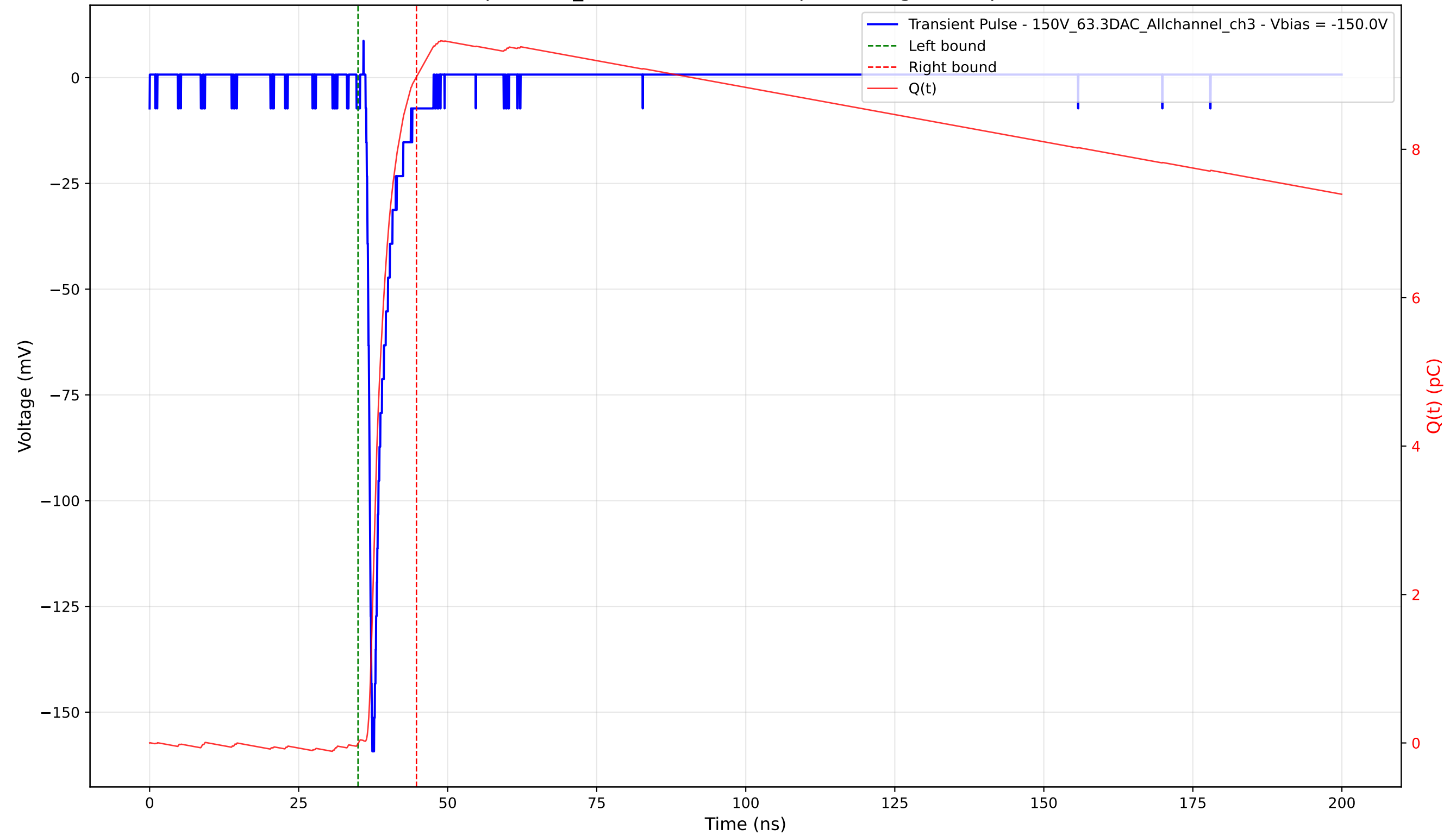
Transient Pulse - Sample: 1cm_42 - Position: 1855.0 \mu\text{m} - Charge: 8.98 pC - Rise Time: 0.88 ns
