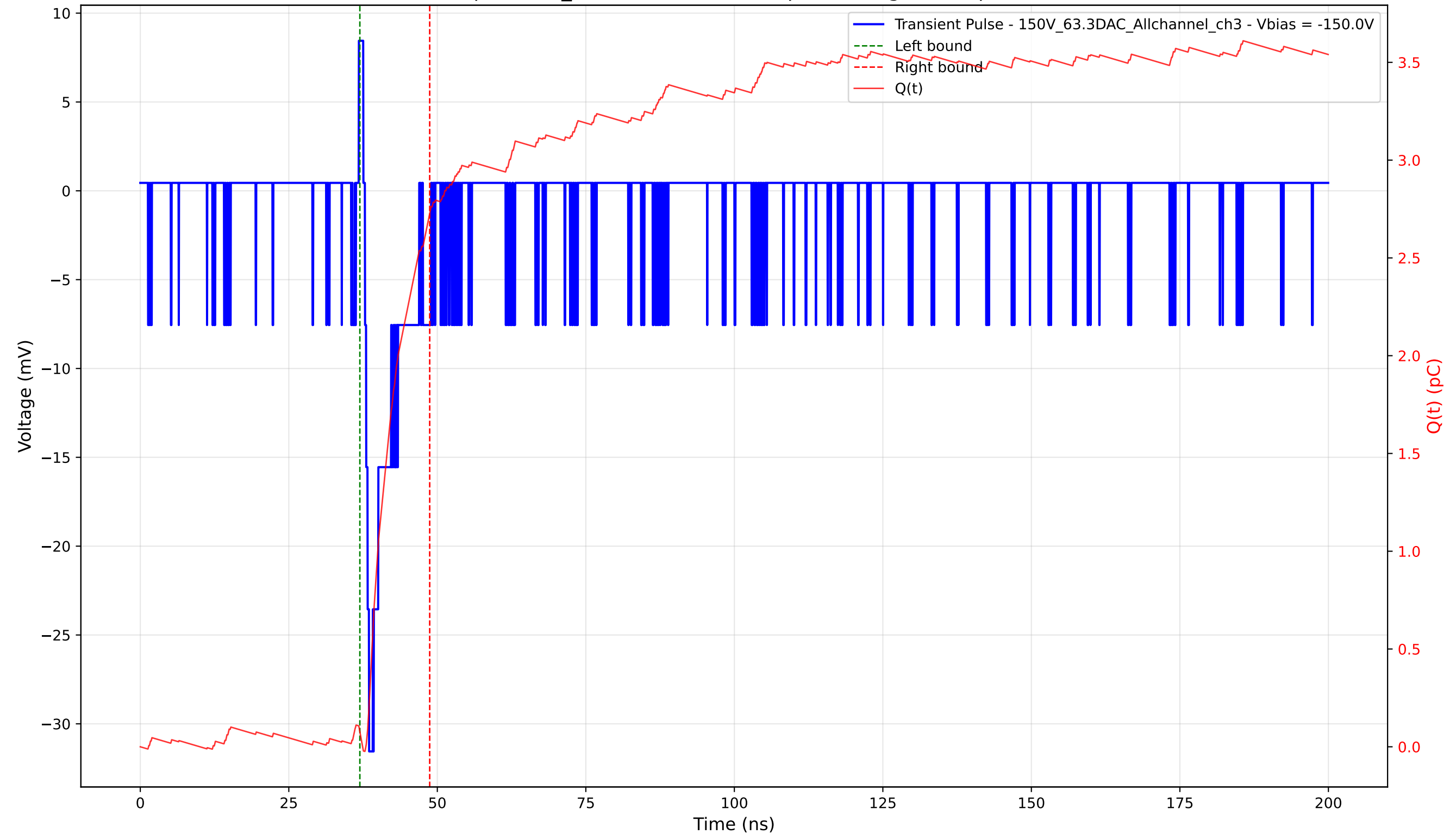
Transient Pulse - Sample: 1cm_42 - Position: 4895.0 \mu\text{m} - Charge: 2.65 pC - Rise Time: 0.70 ns
