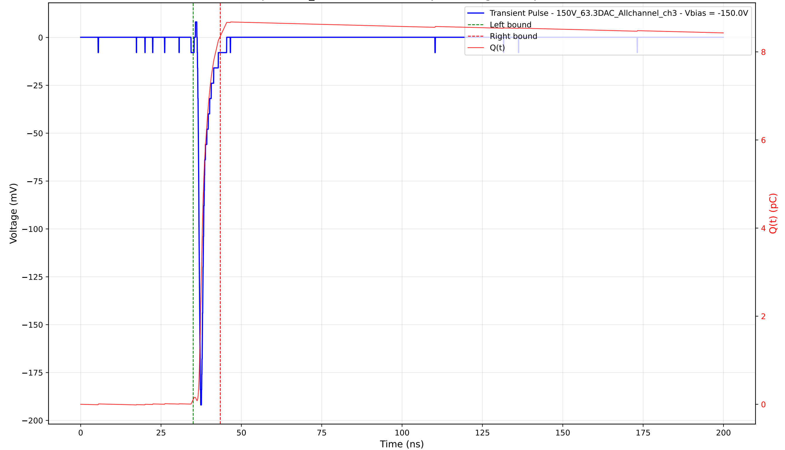
Transient Pulse - Sample: 1cm_42 - Position: 3065.0 \mu\text{m} - Charge: 8.25 pC - Rise Time: 0.77 ns
