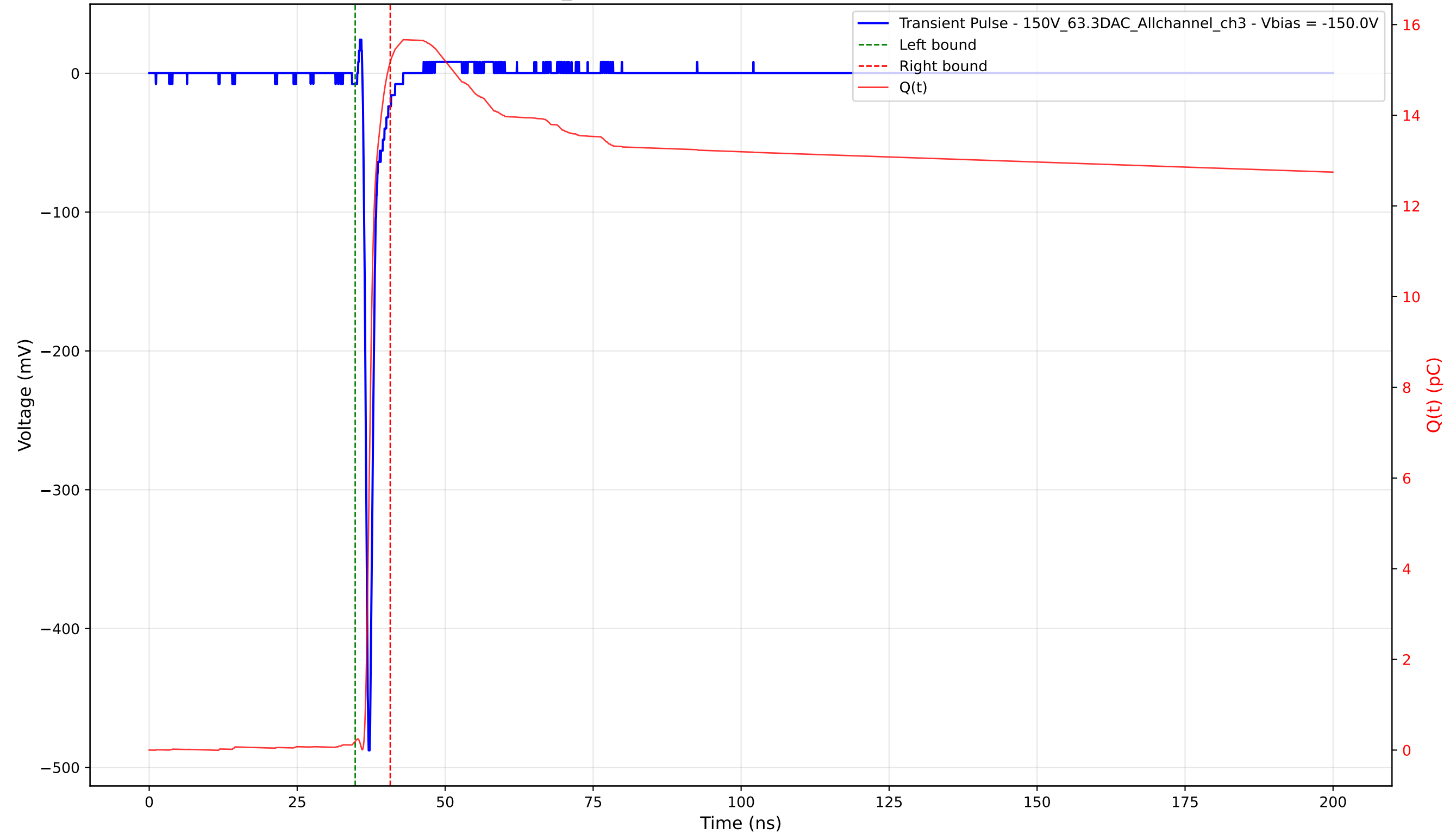
Transient Pulse - Sample: 1cm_42 - Position: 2455.0 \mu\text{m} - Charge: 14.98 pC - Rise Time: 0.67 ns
