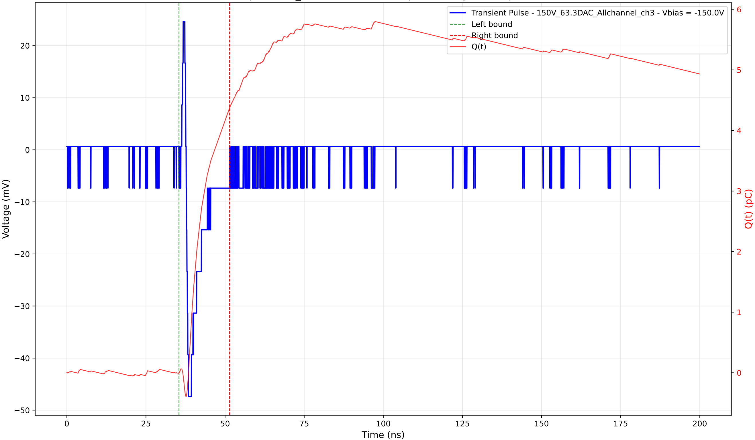
Transient Pulse - Sample: 1cm_42 - Position: 695.0 \mu\text{m} - Charge: 4.38 pC - Rise Time: 0.74 ns
