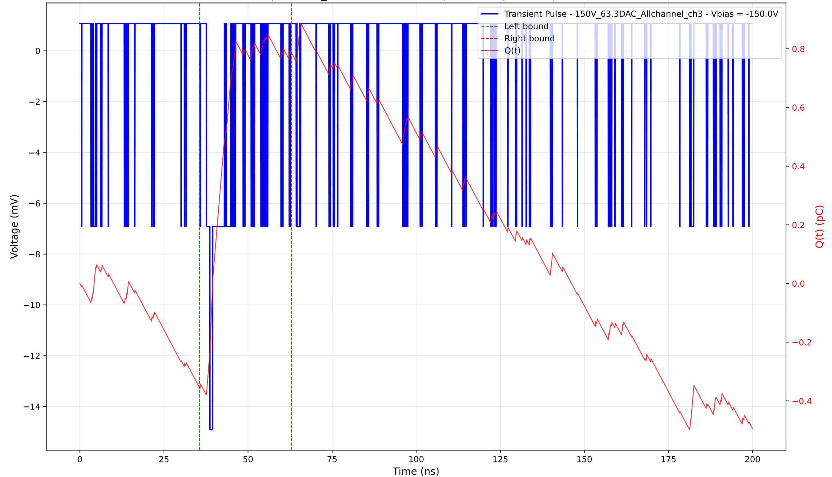
Transient Pulse - Sample: 1cm_42 - Position: 125.0 \mu\text{m} - Charge: 1.14 pC - Rise Time: 1.08 ns
