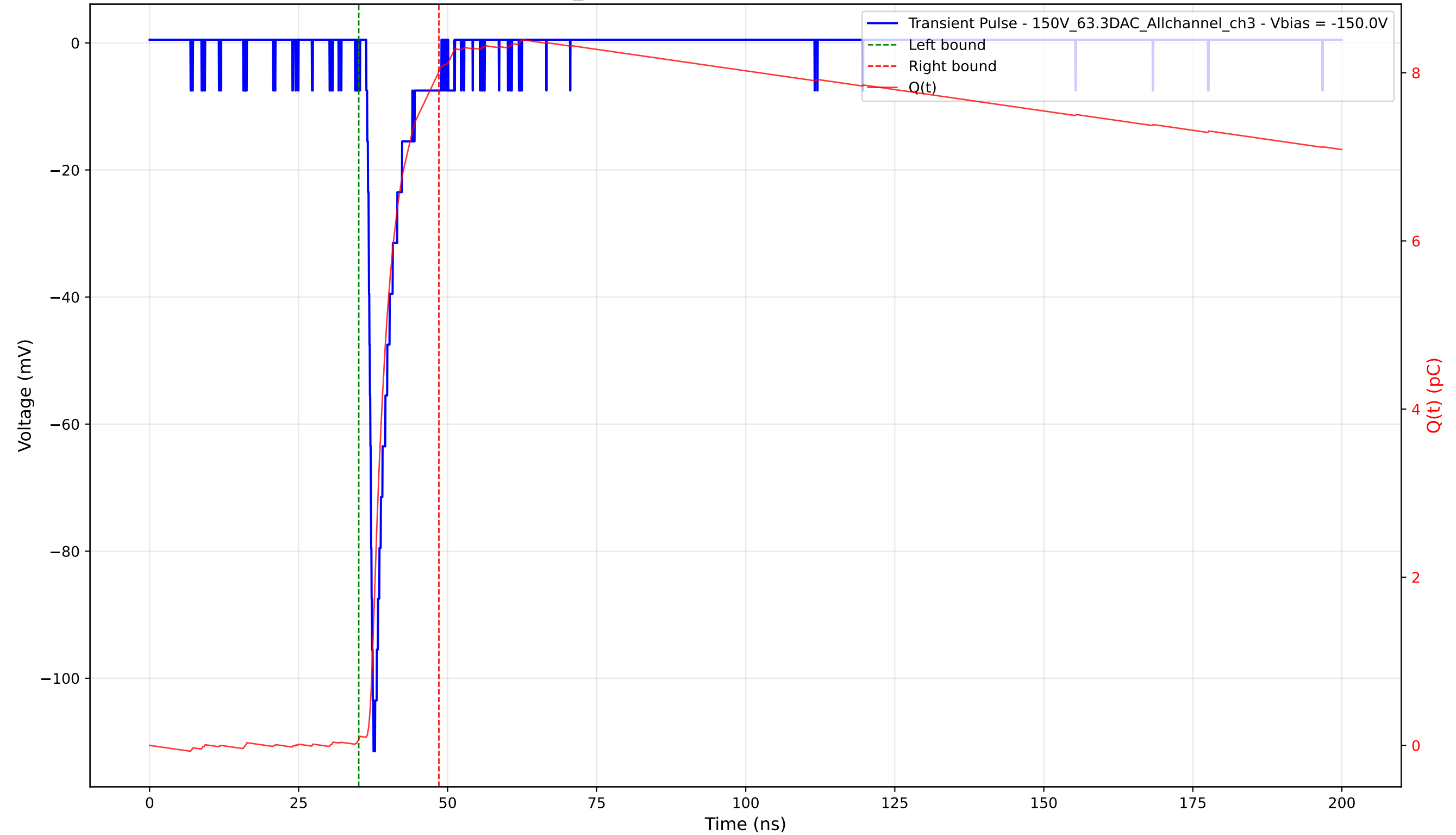
Transient Pulse - Sample: 1cm_42 - Position: 1630.0 \mu\text{m} - Charge: 7.94 pC - Rise Time: 0.94 ns
