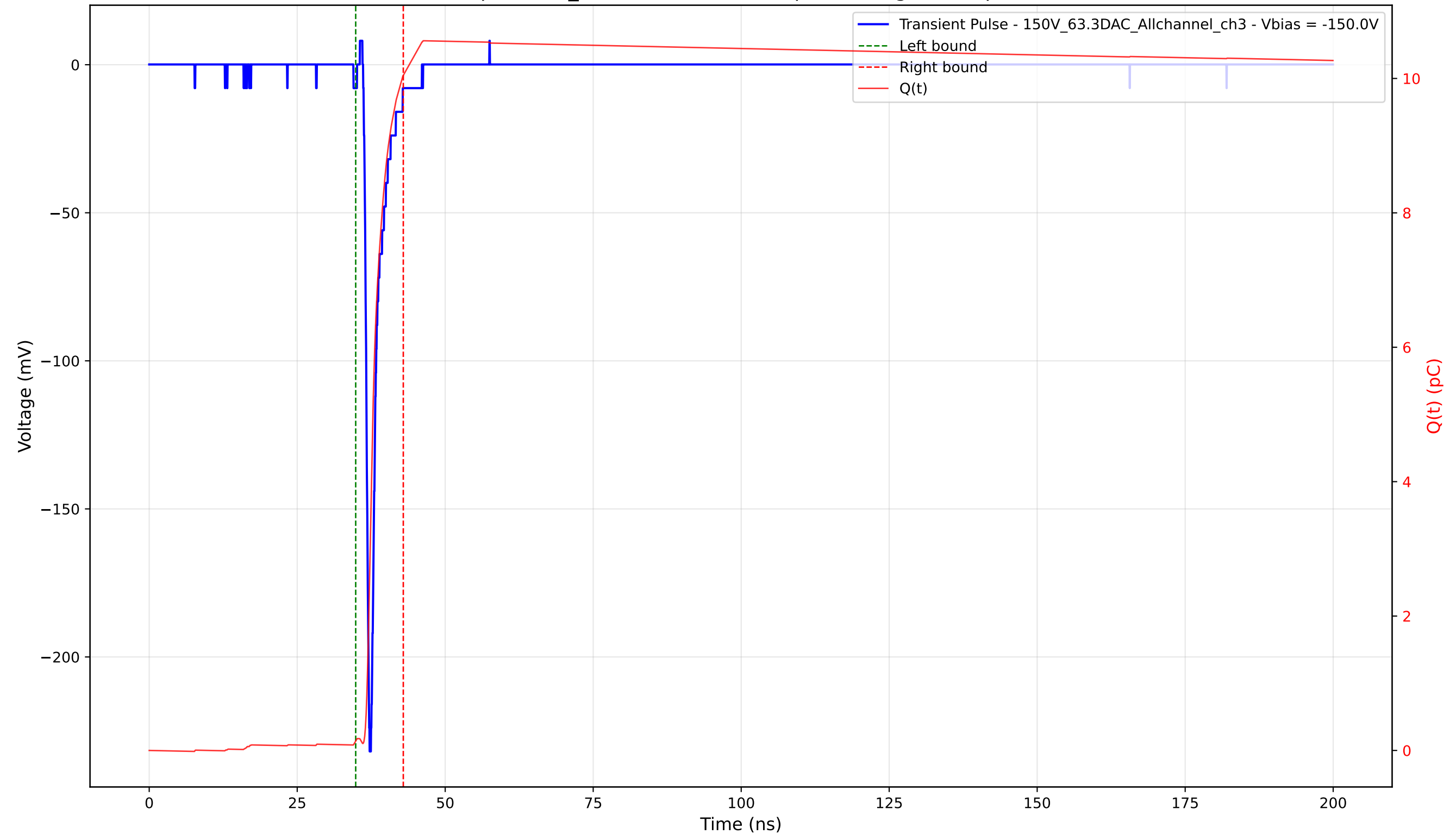
Transient Pulse - Sample: 1cm_42 - Position: 2015.0 \mu\text{m} - Charge: 9.90 pC - Rise Time: 0.81 ns
