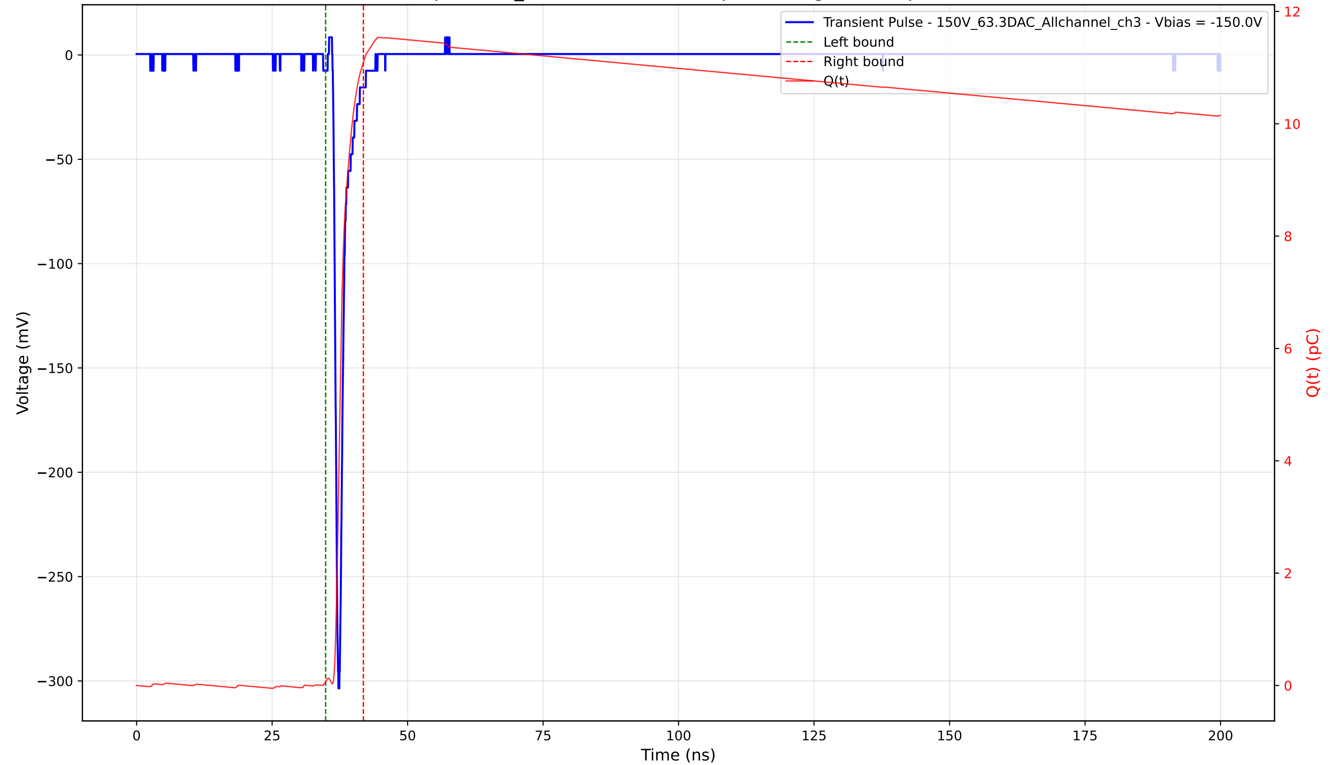
Transient Pulse - Sample: 1cm_42 - Position: 2930.0 \mu\text{m} - Charge: 11.02 pC - Rise Time: 0.73 ns
