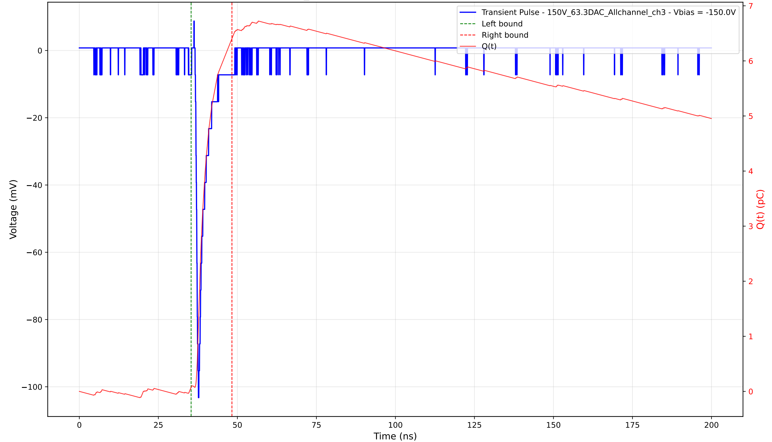
Transient Pulse - Sample: 1cm_42 - Position: 3415.0 \mu\text{m} - Charge: 6.33 pC - Rise Time: 0.82 ns
