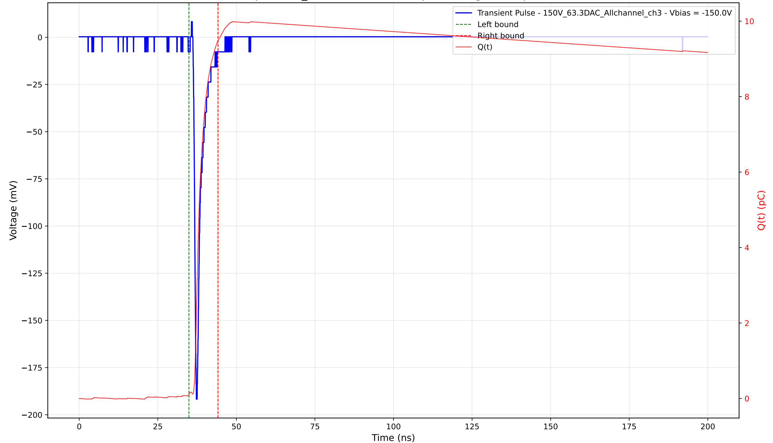
Transient Pulse - Sample: 1cm_42 - Position: 1950.0 \mu\text{m} - Charge: 9.37 pC - Rise Time: 0.78 ns
