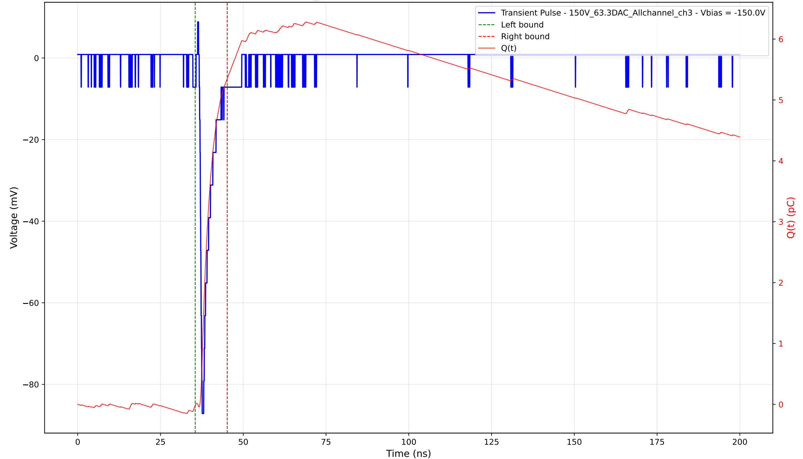
Transient Pulse - Sample: 1cm_42 - Position: 3455.0 \mu\text{m} - Charge: 5.37 pC - Rise Time: 0.67 ns
