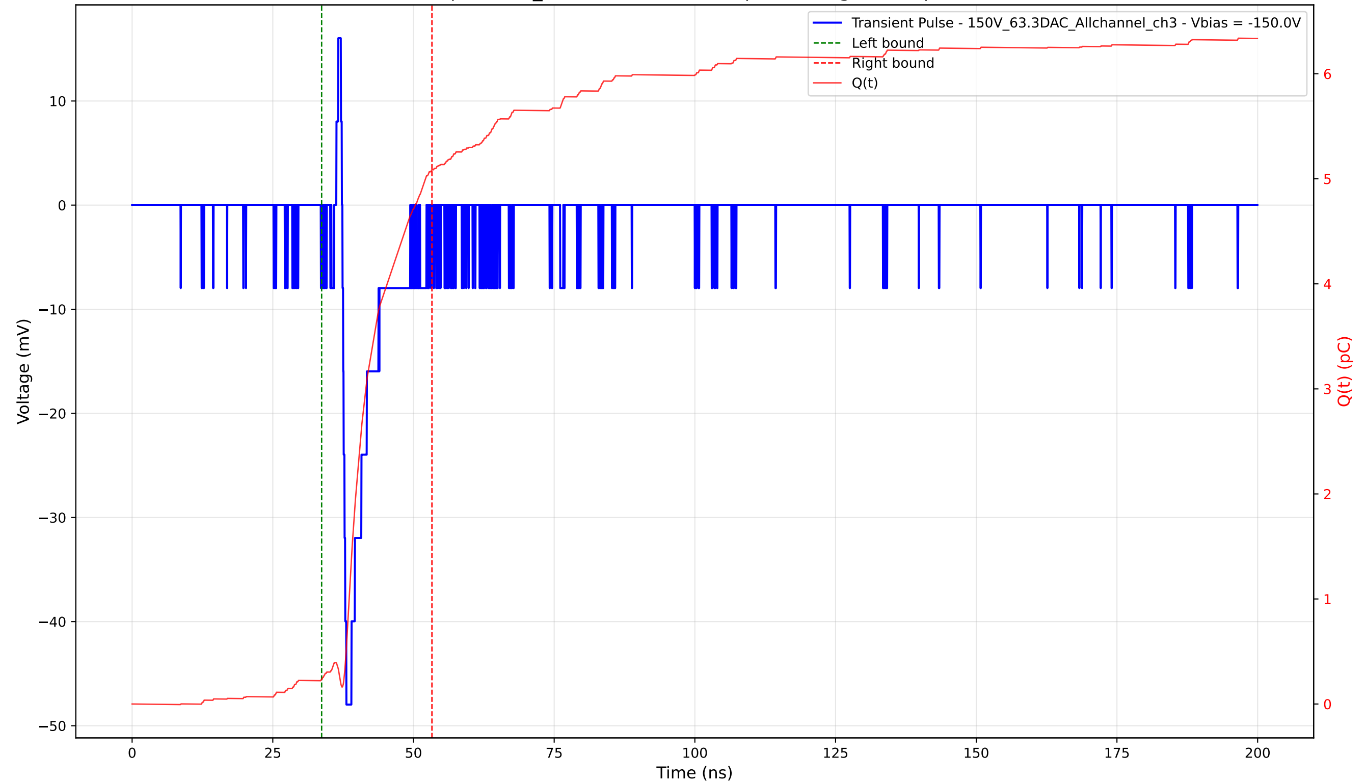
Transient Pulse - Sample: 1cm_42 - Position: 3885.0 \mu\text{m} - Charge: 4.85 pC - Rise Time: 0.70 ns
