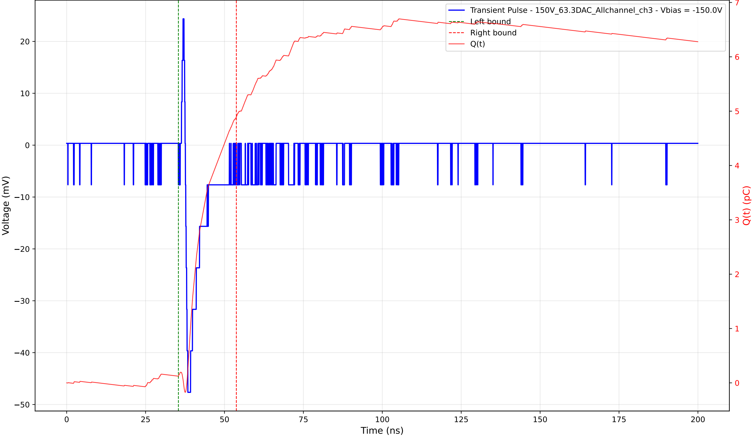
Transient Pulse - Sample: 1cm_42 - Position: 940.0 \mu\text{m} - Charge: 4.77 pC - Rise Time: 0.78 ns
