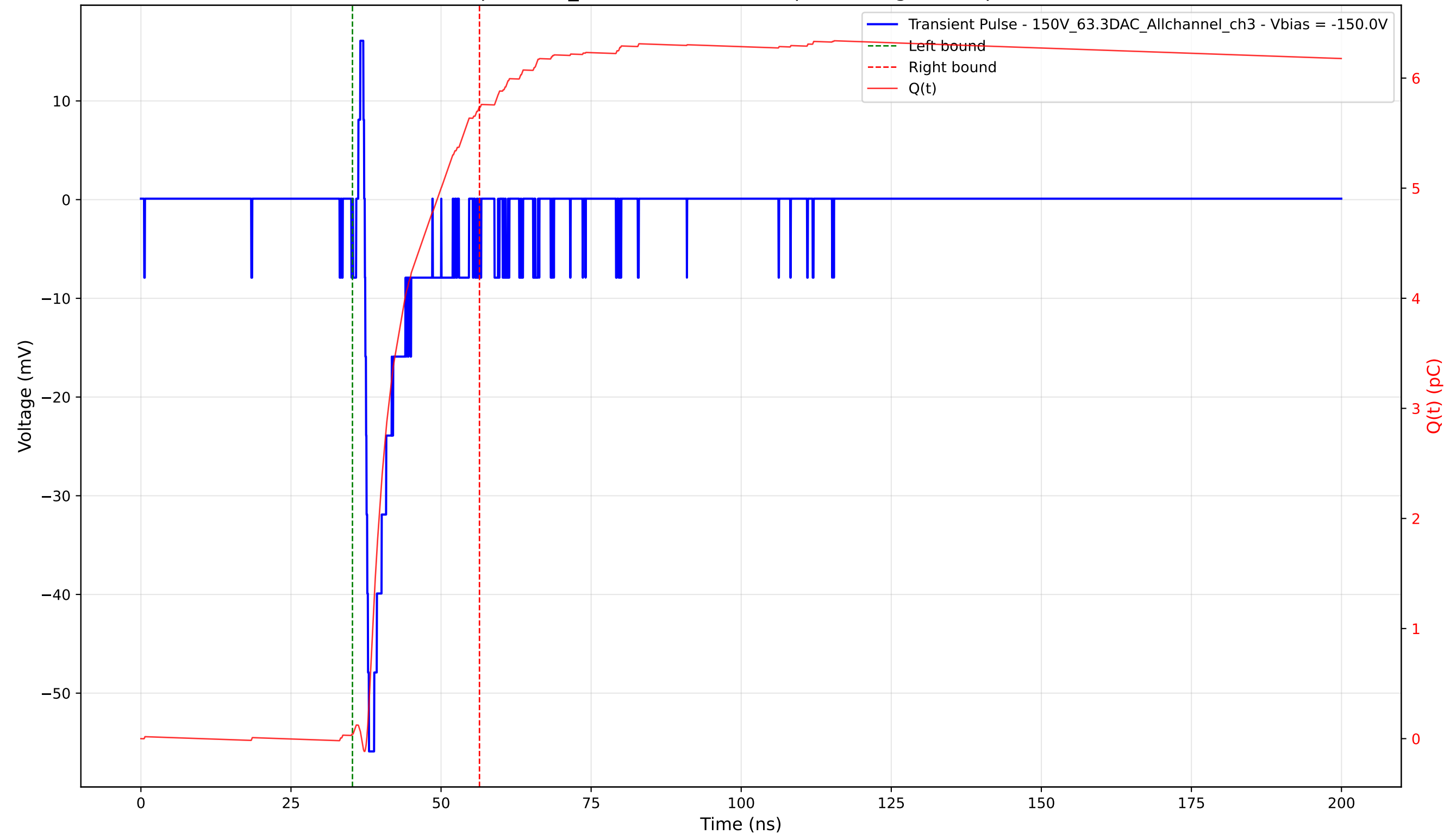
Transient Pulse - Sample: 1cm_42 - Position: 3780.0 \mu\text{m} - Charge: 5.69 pC - Rise Time: 0.69 ns
