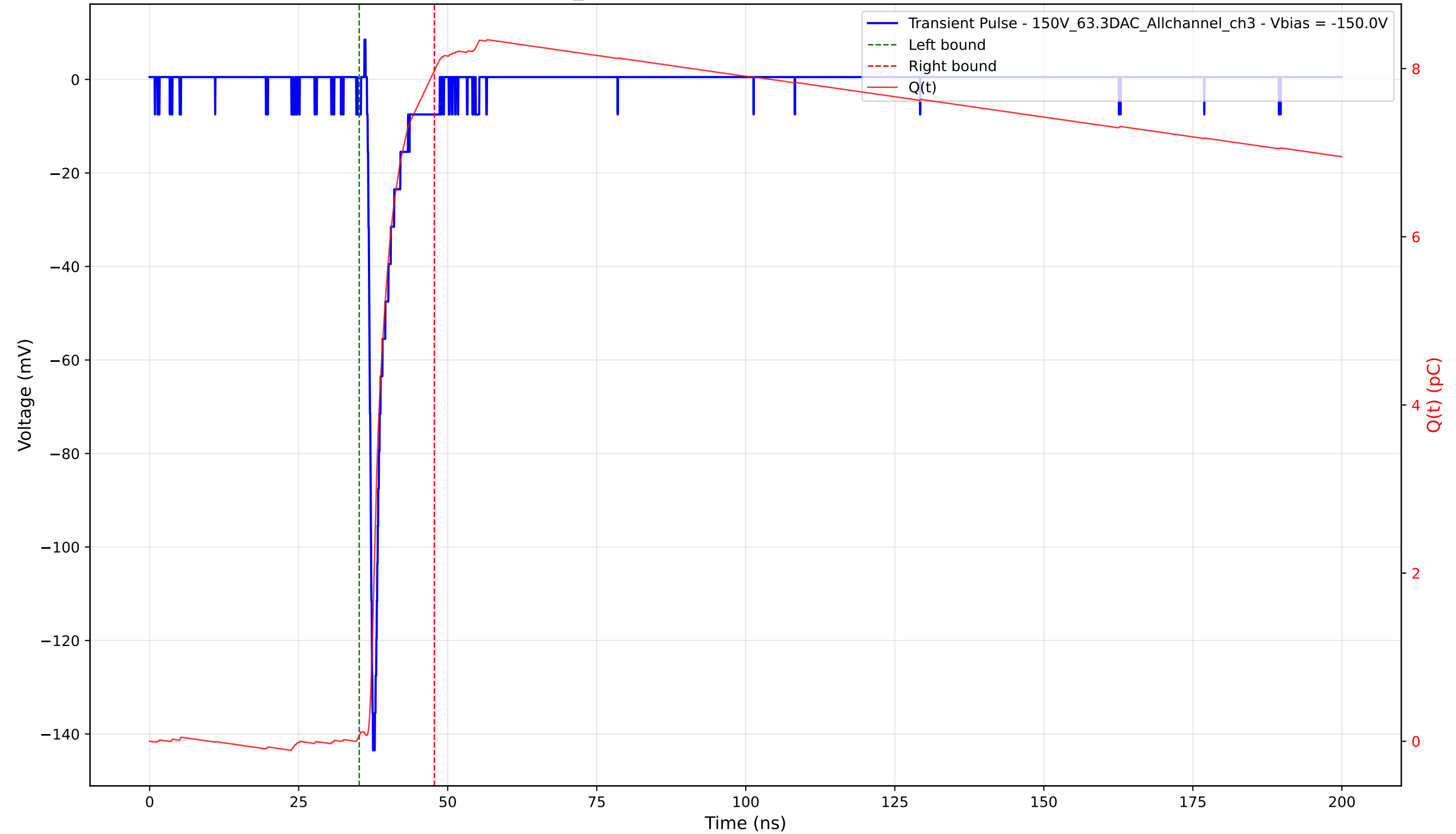
Transient Pulse - Sample: 1cm_42 - Position: 3235.0 \mu\text{m} - Charge: 7.91 pC - Rise Time: 0.81 ns
