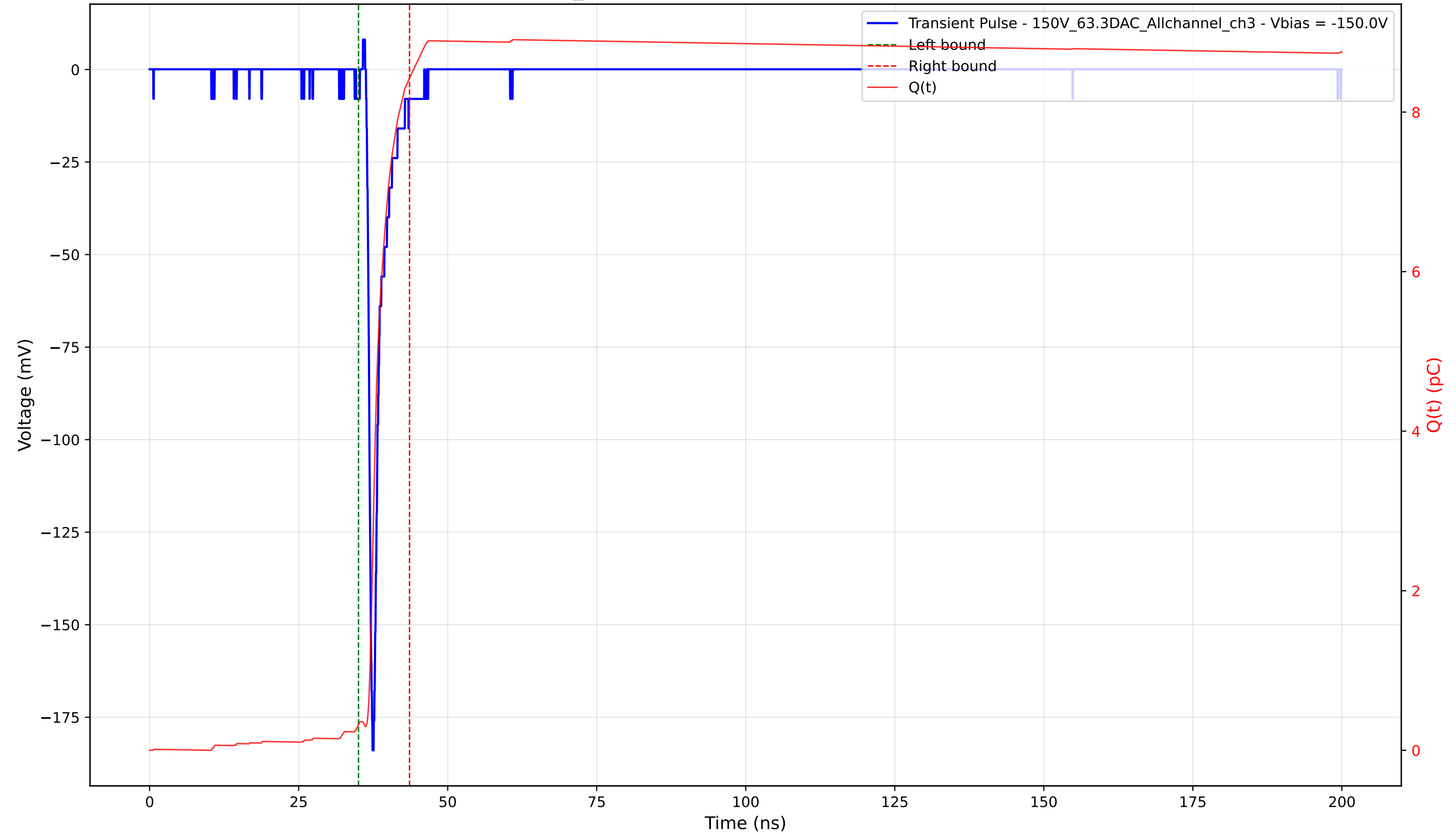
Transient Pulse - Sample: 1cm_42 - Position: 3090.0 \mu\text{m} - Charge: 8.10 pC - Rise Time: 0.79 ns
