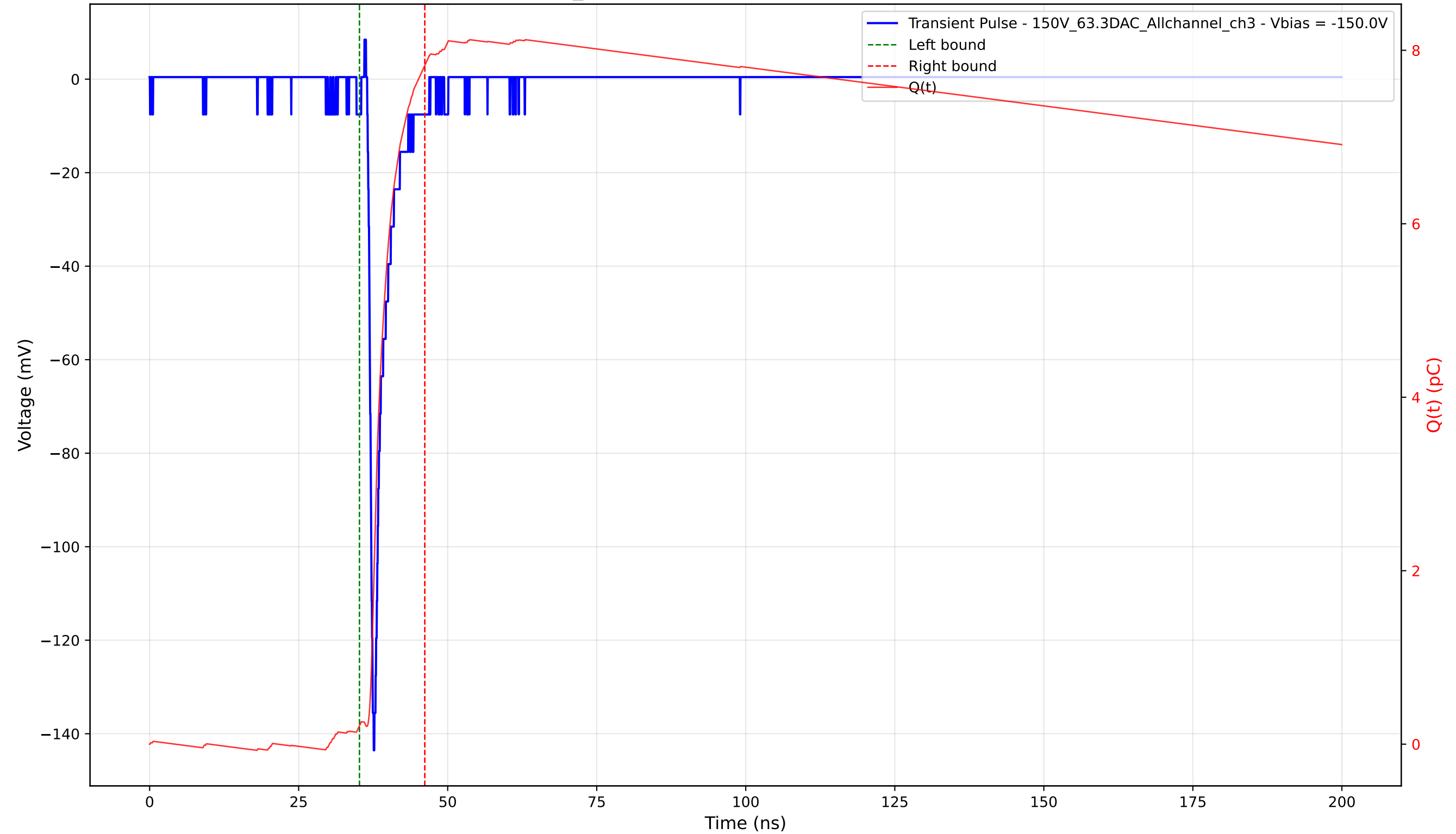
Transient Pulse - Sample: 1cm_42 - Position: 3265.0 \mu\text{m} - Charge: 7.61 pC - Rise Time: 0.85 ns
