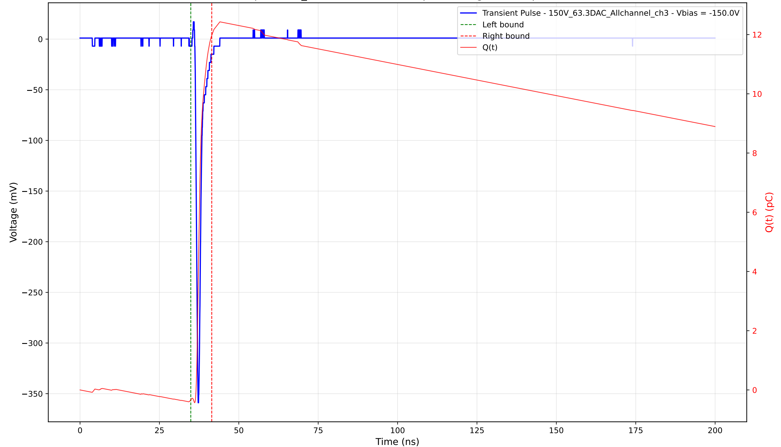
Transient Pulse - Sample: 1cm_42 - Position: 2880.0 \mu\text{m} - Charge: 12.31 pC - Rise Time: 0.73 ns
