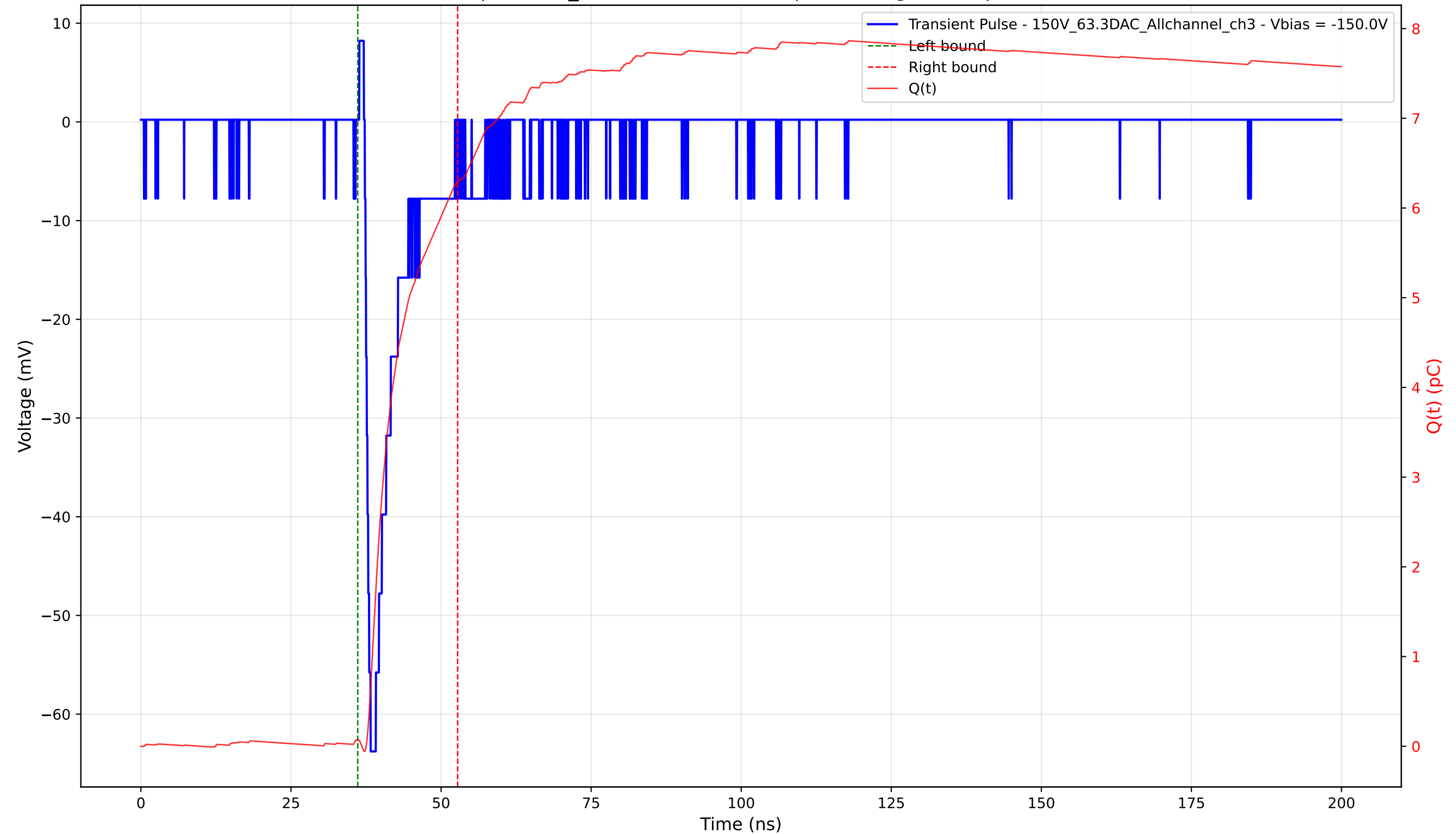
Transient Pulse - Sample: 1cm_42 - Position: 1190.0 \mu\text{m} - Charge: 6.22 pC - Rise Time: 0.97 ns
