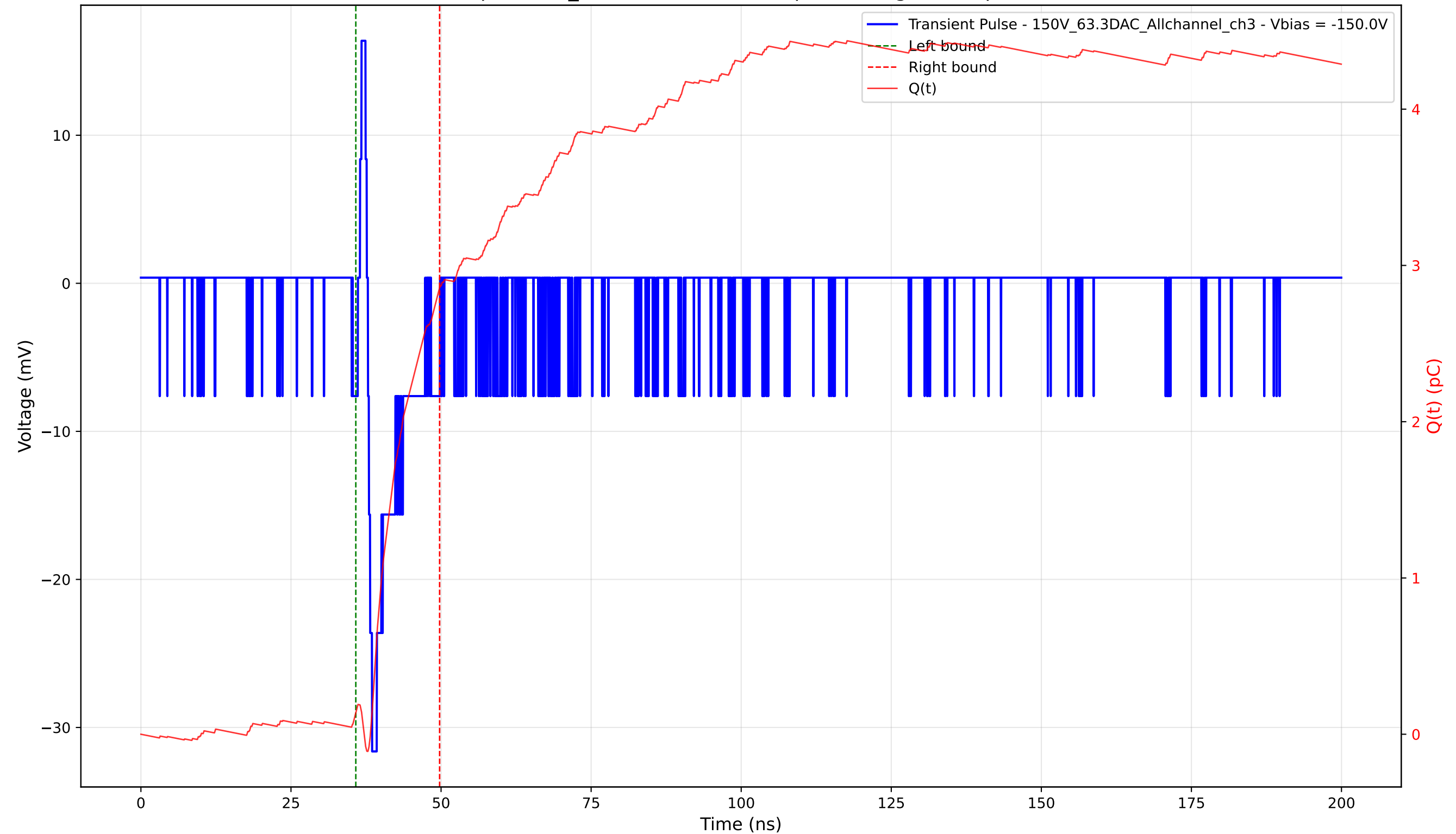
Transient Pulse - Sample: 1cm_42 - Position: 4520.0 \mu\text{m} - Charge: 2.72 pC - Rise Time: 0.70 ns
