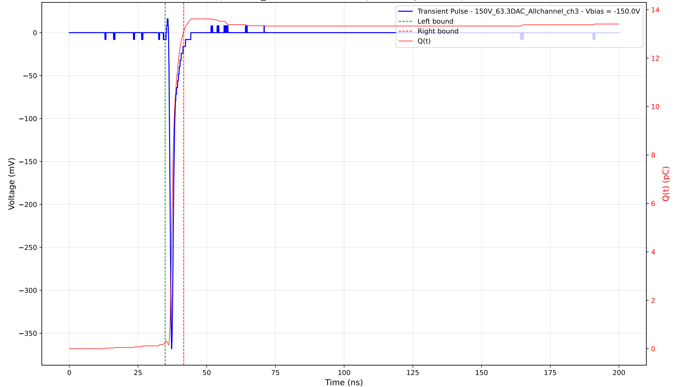
Transient Pulse - Sample: 1cm_42 - Position: 2165.0 \mu\text{m} - Charge: 12.84 pC - Rise Time: 0.75 ns
