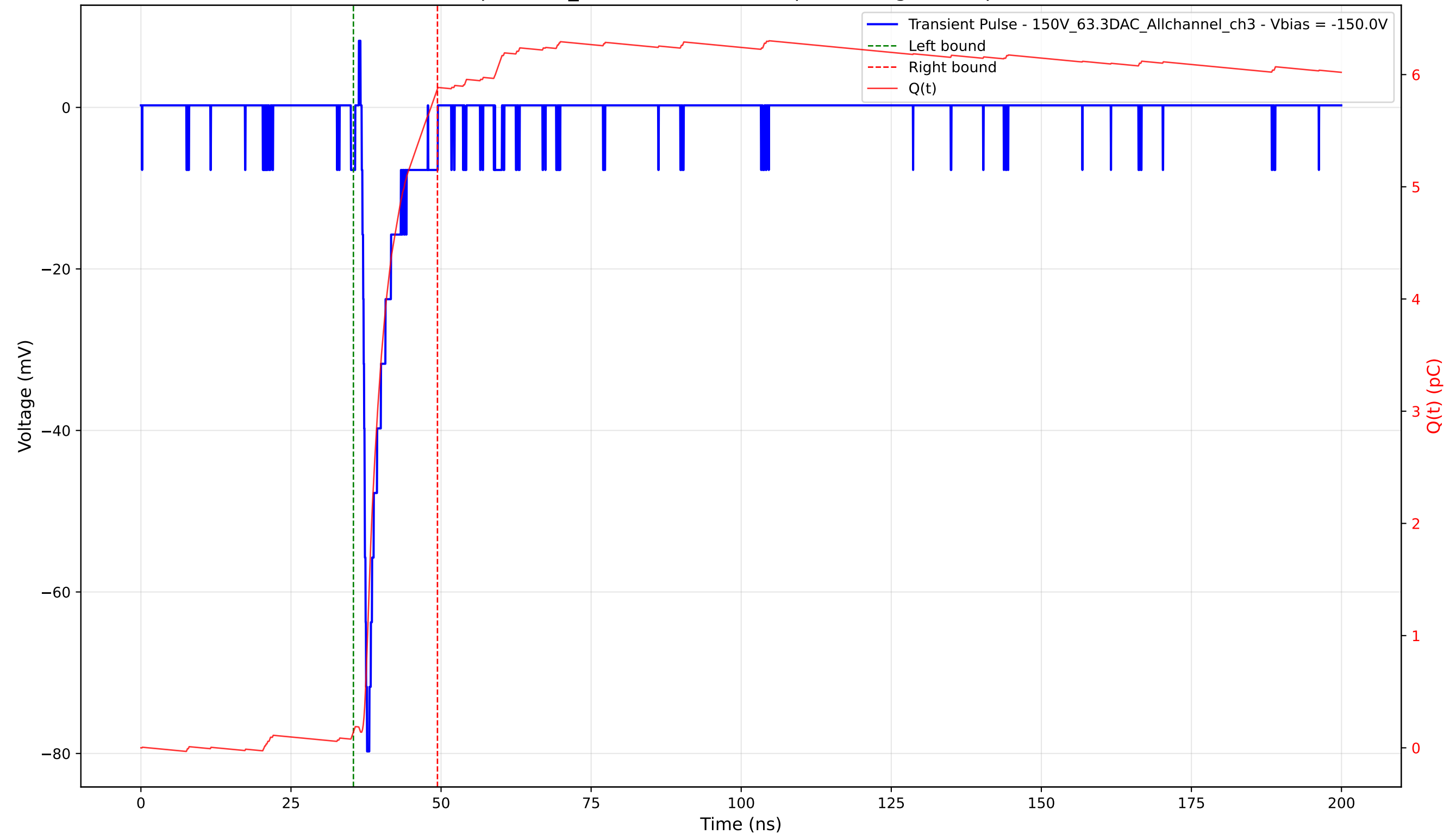
Transient Pulse - Sample: 1cm_42 - Position: 3490.0 \mu\text{m} - Charge: 5.73 pC - Rise Time: 0.80 ns
