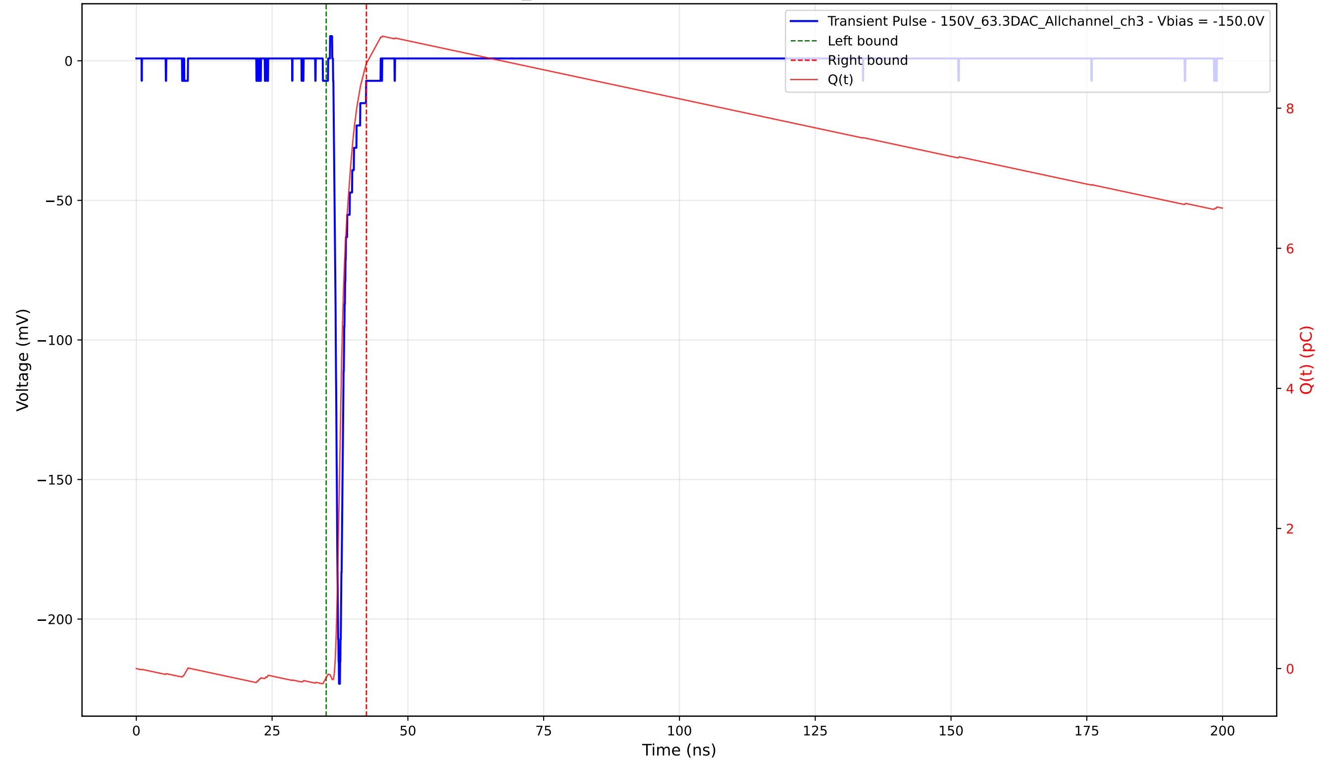
Transient Pulse - Sample: 1cm_42 - Position: 3015.0 \mu\text{m} - Charge: 8.77 pC - Rise Time: 0.80 ns
