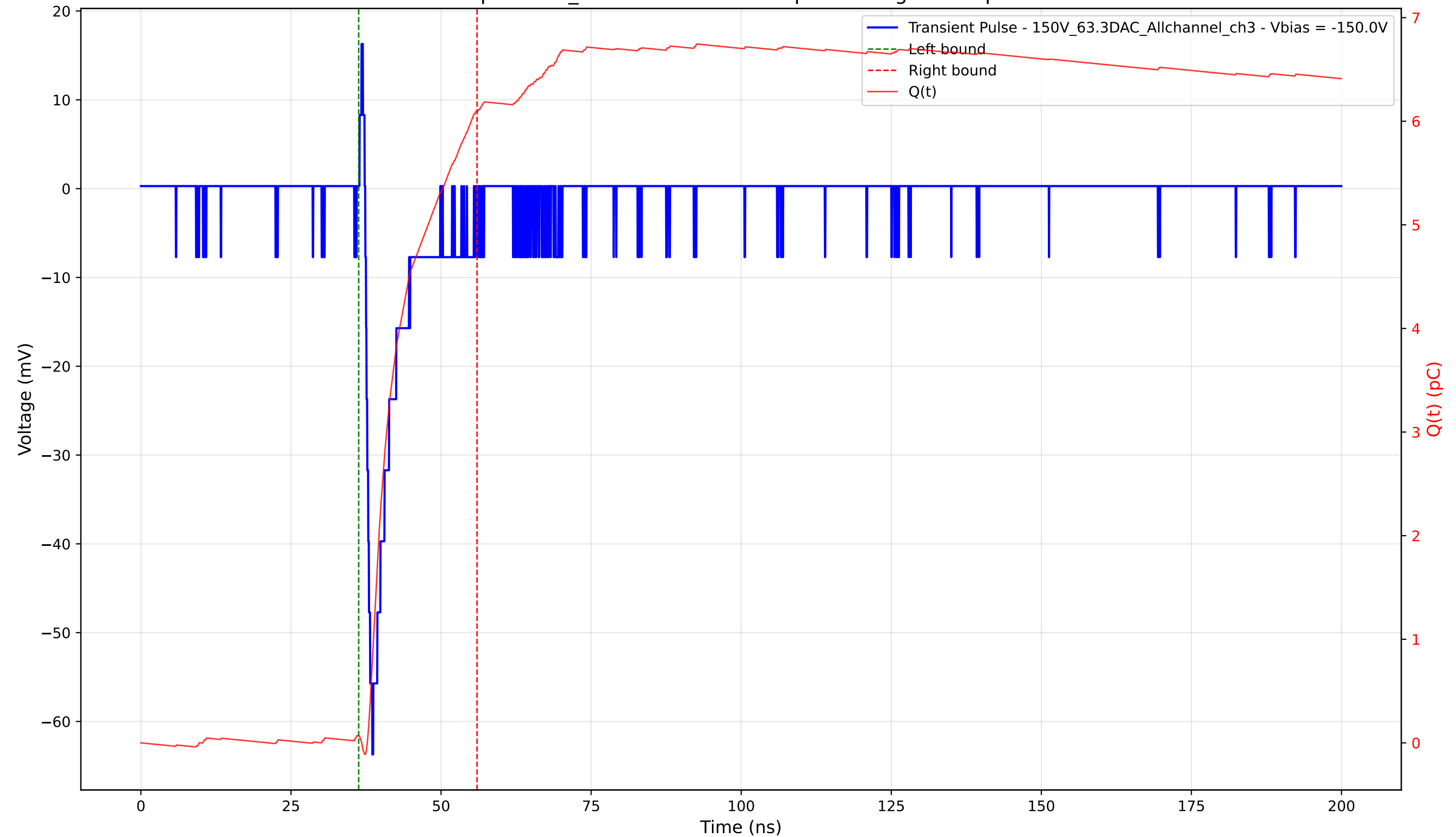
Transient Pulse - Sample: 1cm_42 - Position: 1140.0 \mu\text{m} - Charge: 6.02 pC - Rise Time: 1.17 ns
