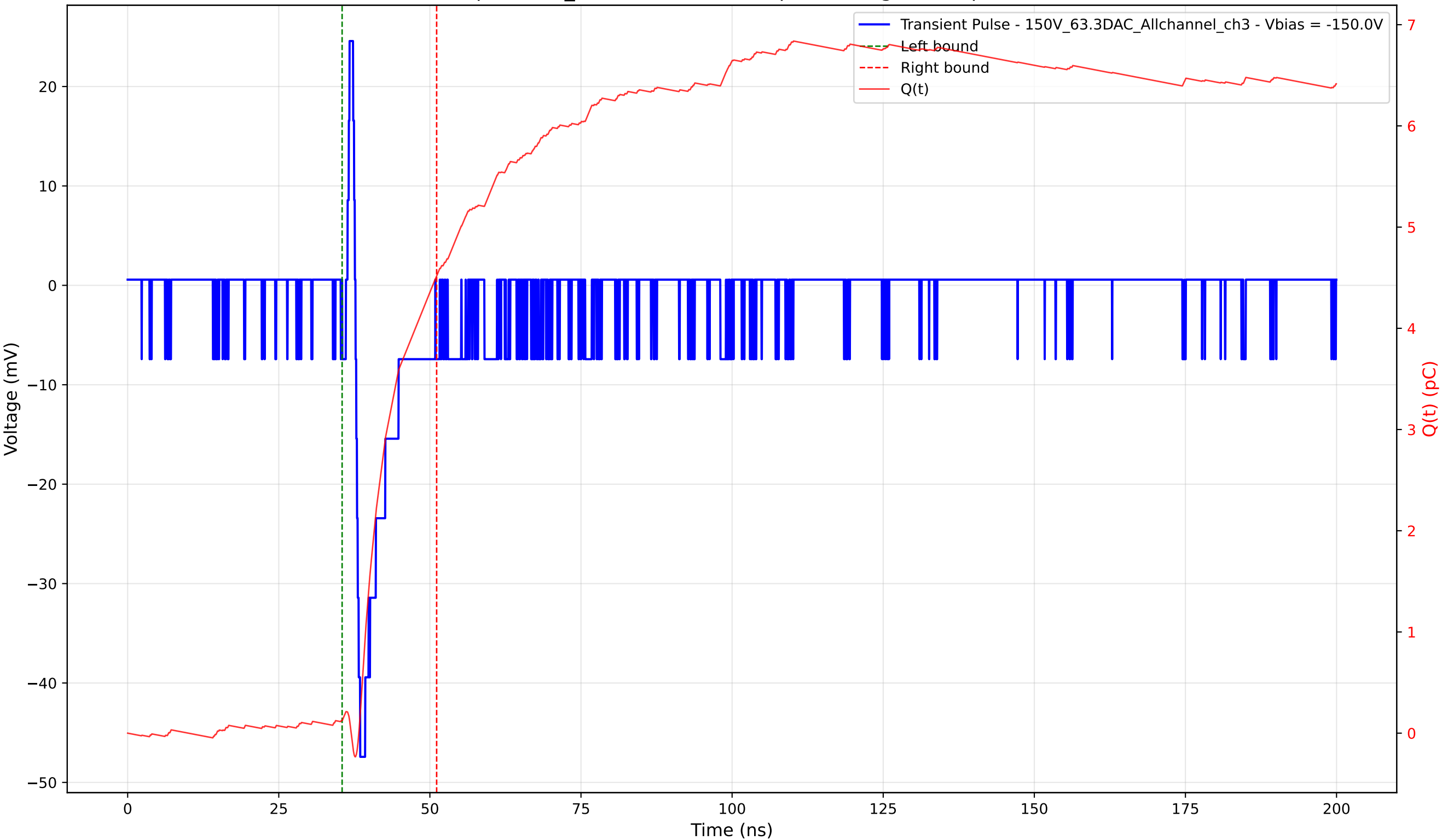
Transient Pulse - Sample: 1cm_42 - Position: 690.0 \mu\text{m} - Charge: 4.39 pC - Rise Time: 0.78 ns
