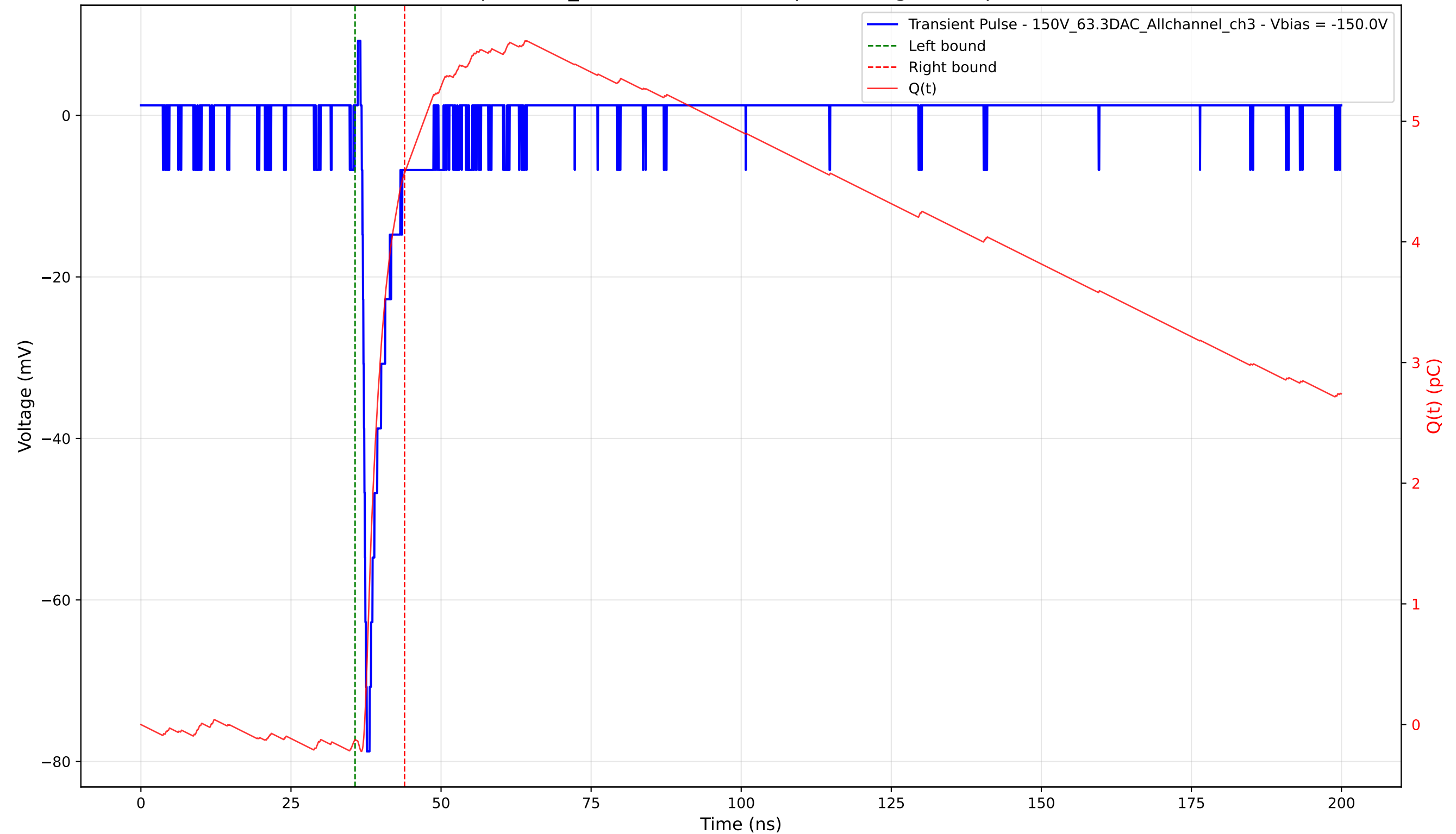
Transient Pulse - Sample: 1cm_42 - Position: 3480.0 \mu\text{m} - Charge: 4.69 pC - Rise Time: 0.75 ns
