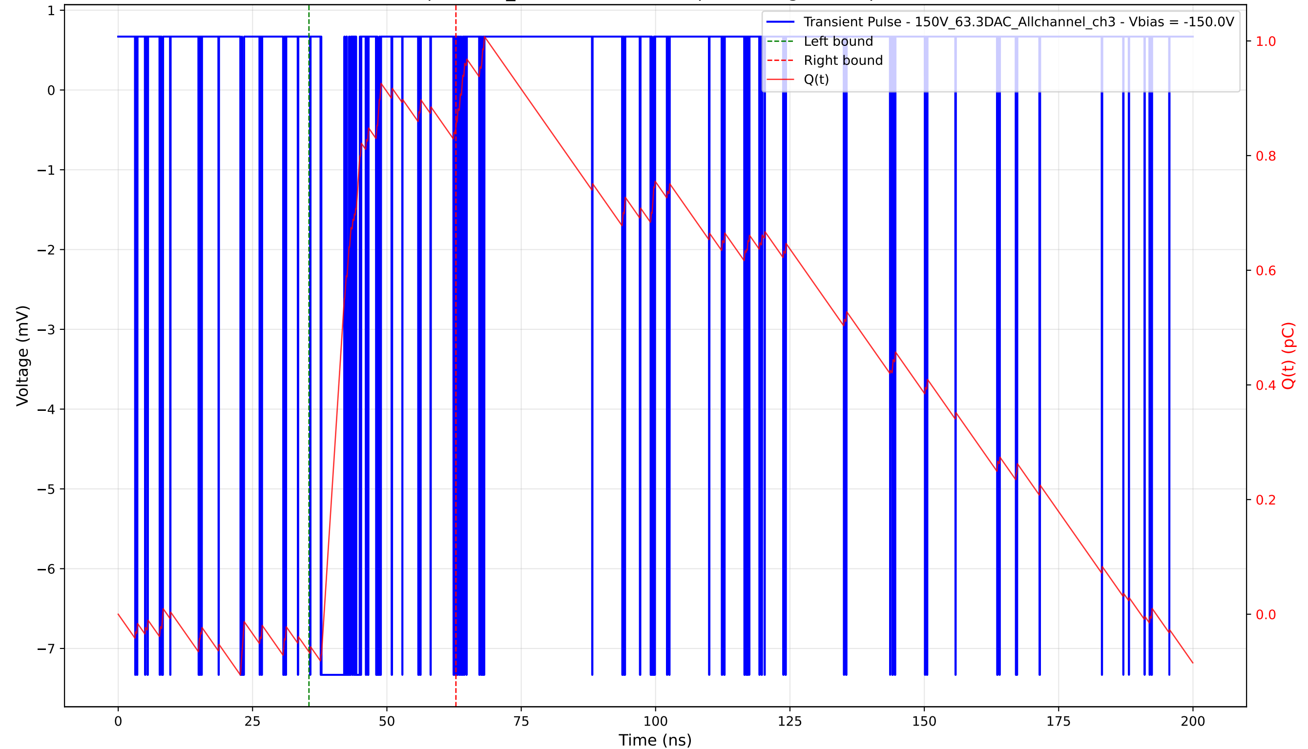
Transient Pulse - Sample: 1cm_42 - Position: 100.0 \mu\text{m} - Charge: 0.92 pC - Rise Time: 0.04 ns
