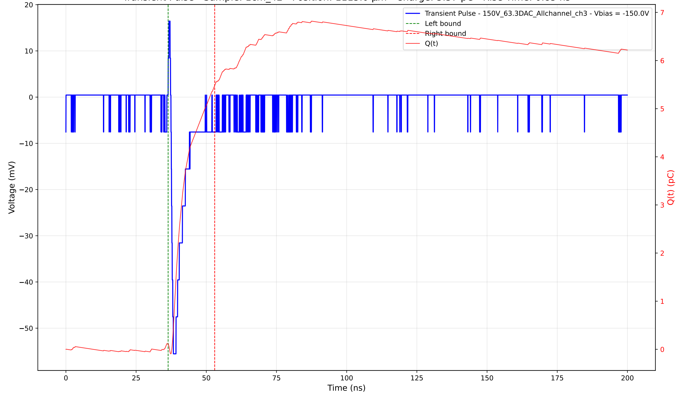
Transient Pulse - Sample: 1cm_42 - Position: 1115.0 \mu\text{m} - Charge: 5.37 pC - Rise Time: 0.85 ns
