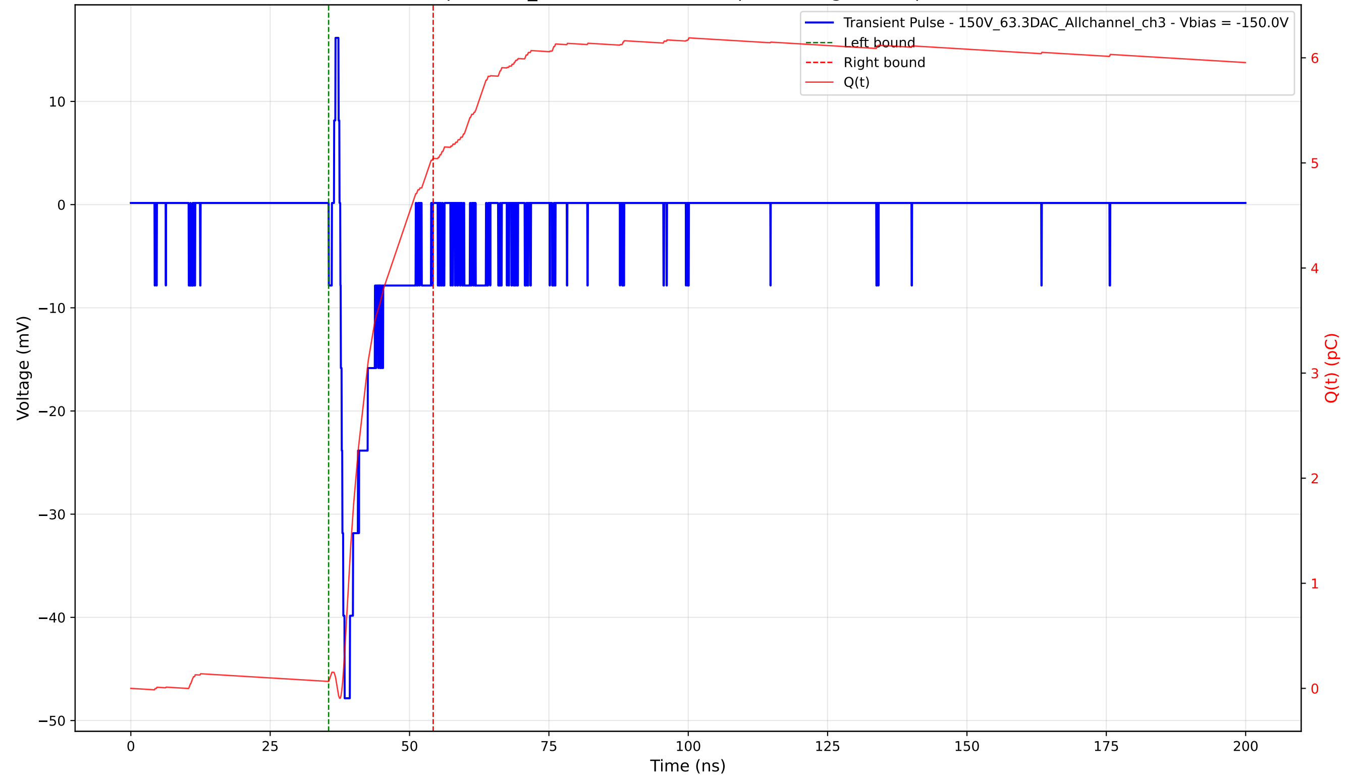
Transient Pulse - Sample: 1cm_42 - Position: 1005.0 \mu\text{m} - Charge: 4.98 pC - Rise Time: 0.78 ns
