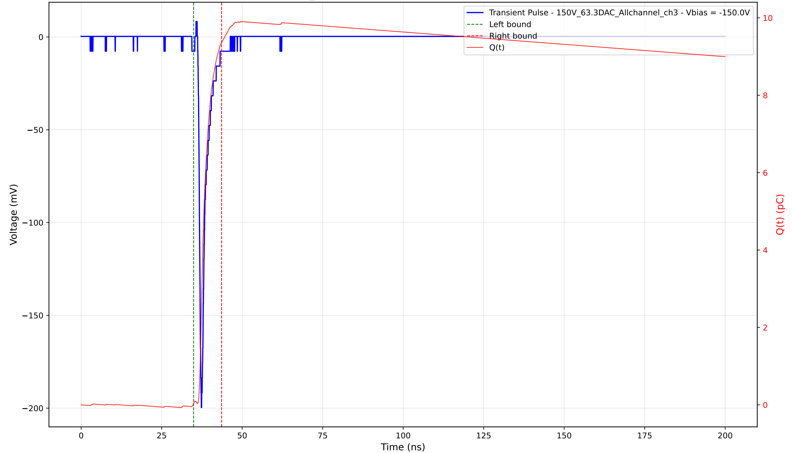
Transient Pulse - Sample: 1cm_42 - Position: 1955.0 \mu\text{m} - Charge: 9.32 pC - Rise Time: 0.82 ns
