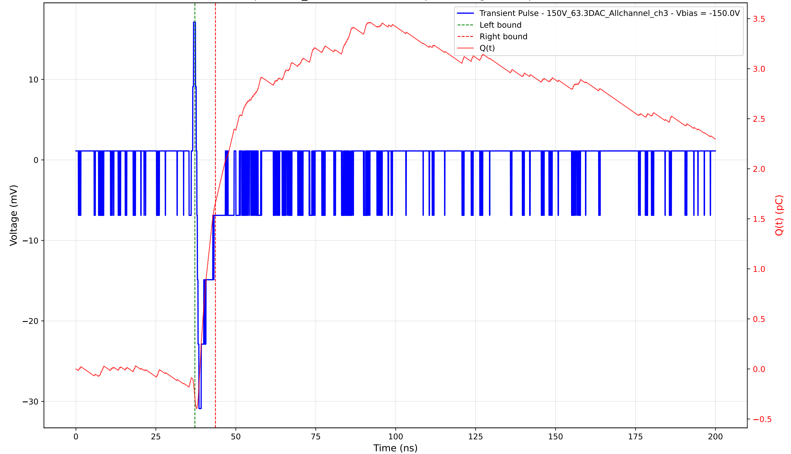
Transient Pulse - Sample: 1cm_42 - Position: 4575.0 \mu\text{m} - Charge: 1.95 pC - Rise Time: 0.67 ns
