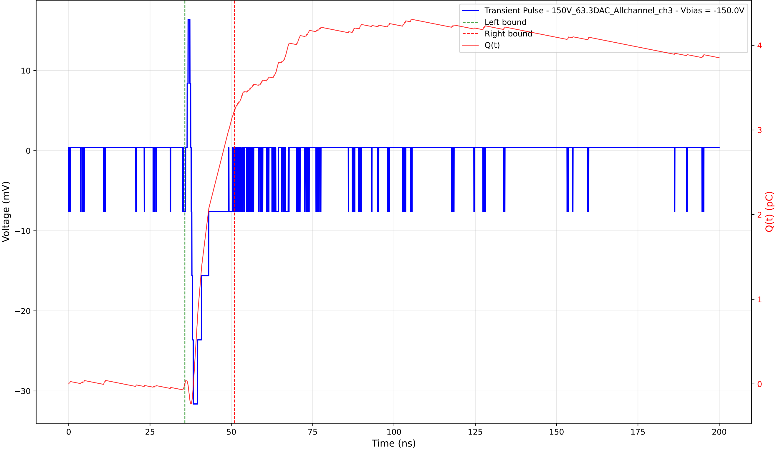
Transient Pulse - Sample: 1cm_42 - Position: 455.0 \mu\text{m} - Charge: 3.22 pC - Rise Time: 0.66 ns
