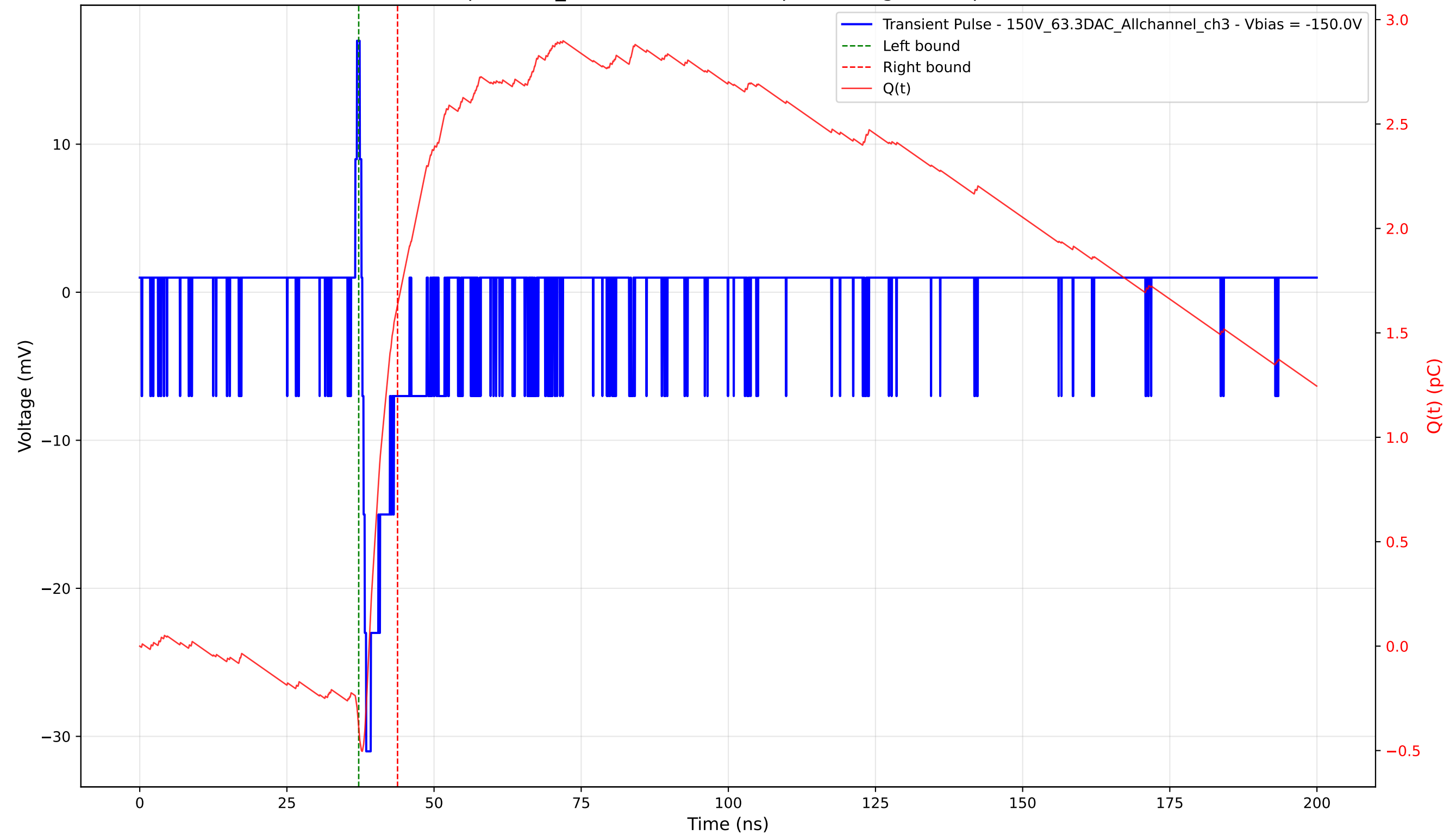
Transient Pulse - Sample: 1cm_42 - Position: 4680.0 \mu\text{m} - Charge: 2.02 pC - Rise Time: 0.67 ns
