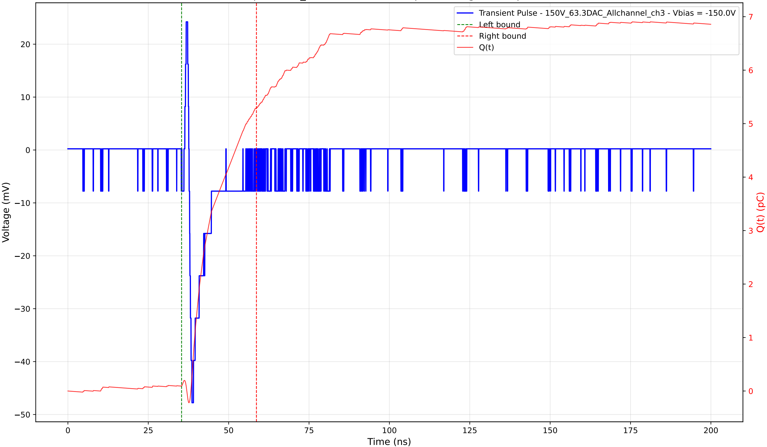
Transient Pulse - Sample: 1cm_42 - Position: 635.0 \mu\text{m} - Charge: 5.20 pC - Rise Time: 0.90 ns
