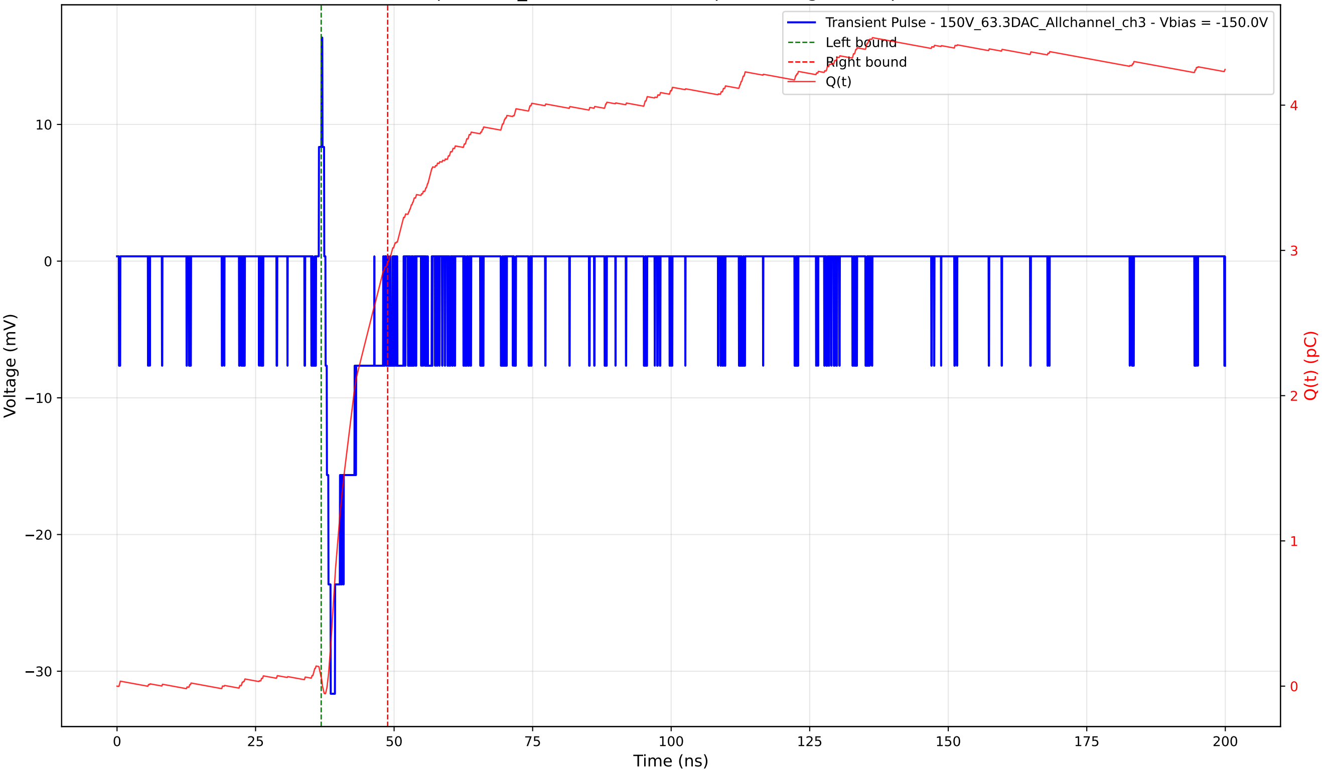
Transient Pulse - Sample: 1cm_42 - Position: 390.0 \mu\text{m} - Charge: 2.86 pC - Rise Time: 0.94 ns
