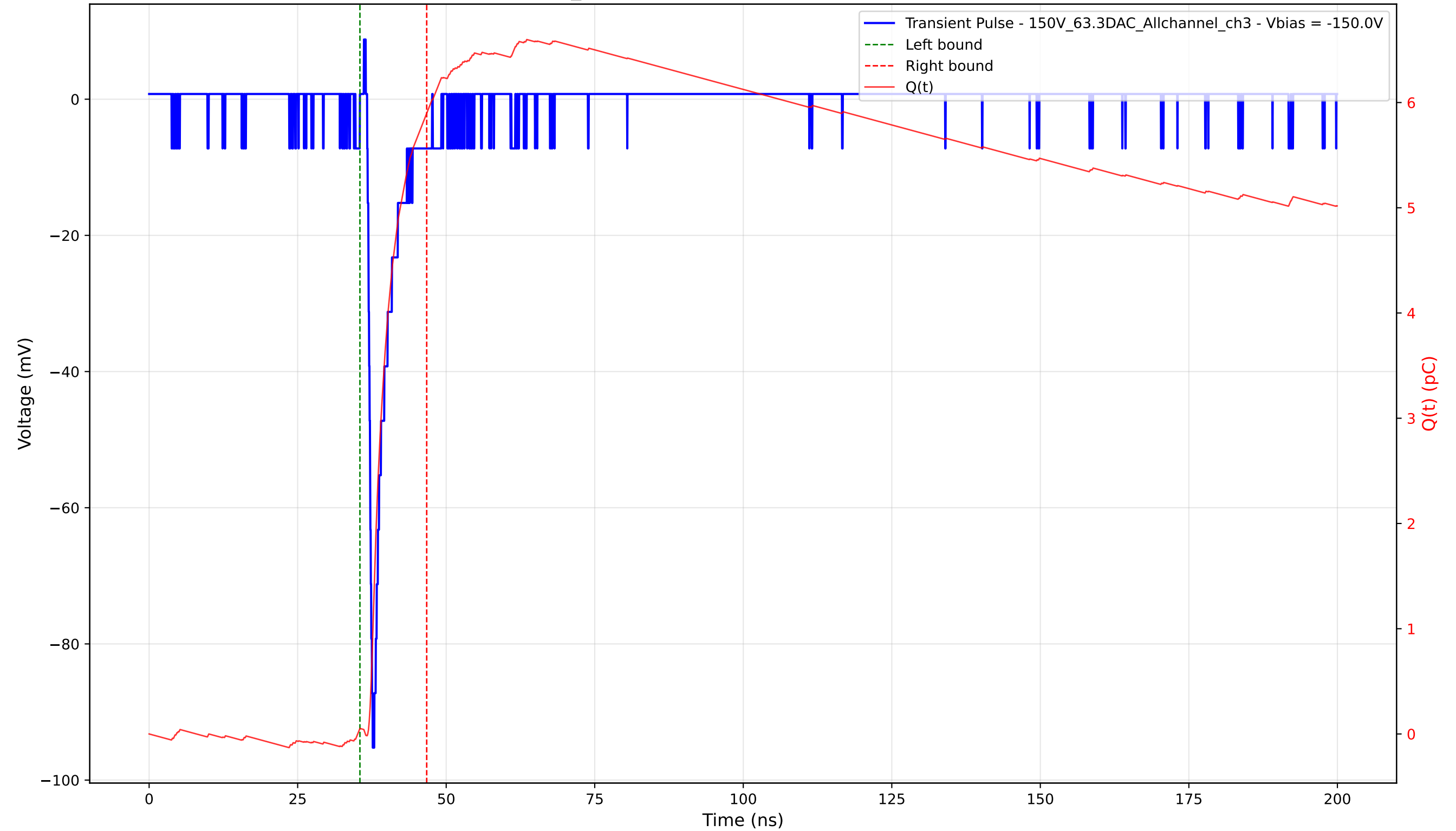
Transient Pulse - Sample: 1cm_42 - Position: 3435.0 \mu\text{m} - Charge: 5.85 pC - Rise Time: 0.75 ns
