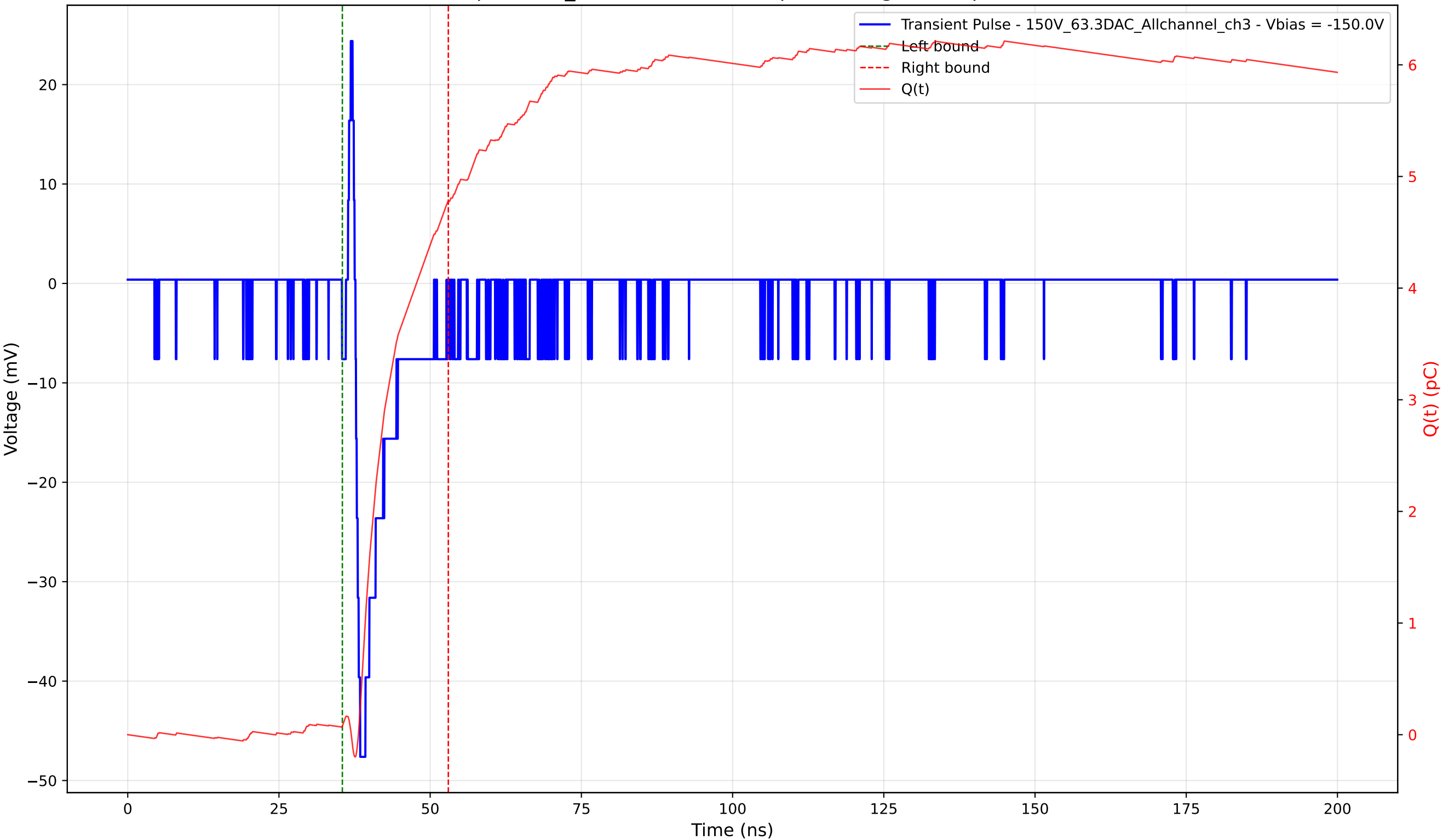
Transient Pulse - Sample: 1cm_42 - Position: 920.0 \mu\text{m} - Charge: 4.70 pC - Rise Time: 0.78 ns
