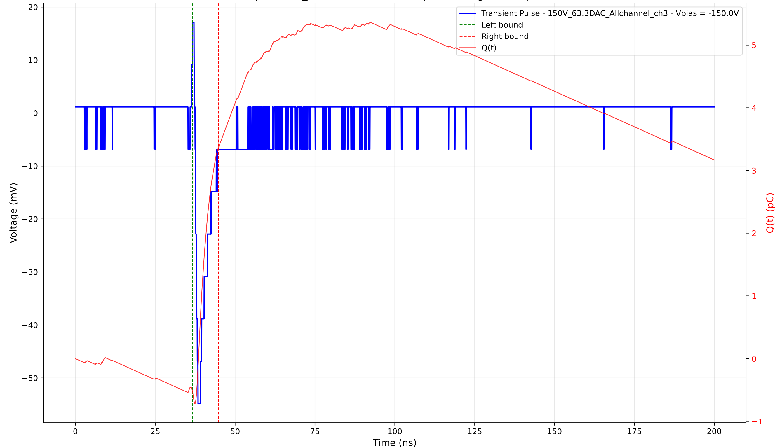
Transient Pulse - Sample: 1cm_42 - Position: 1075.0 \mu\text{m} - Charge: 3.88 pC - Rise Time: 0.93 ns
