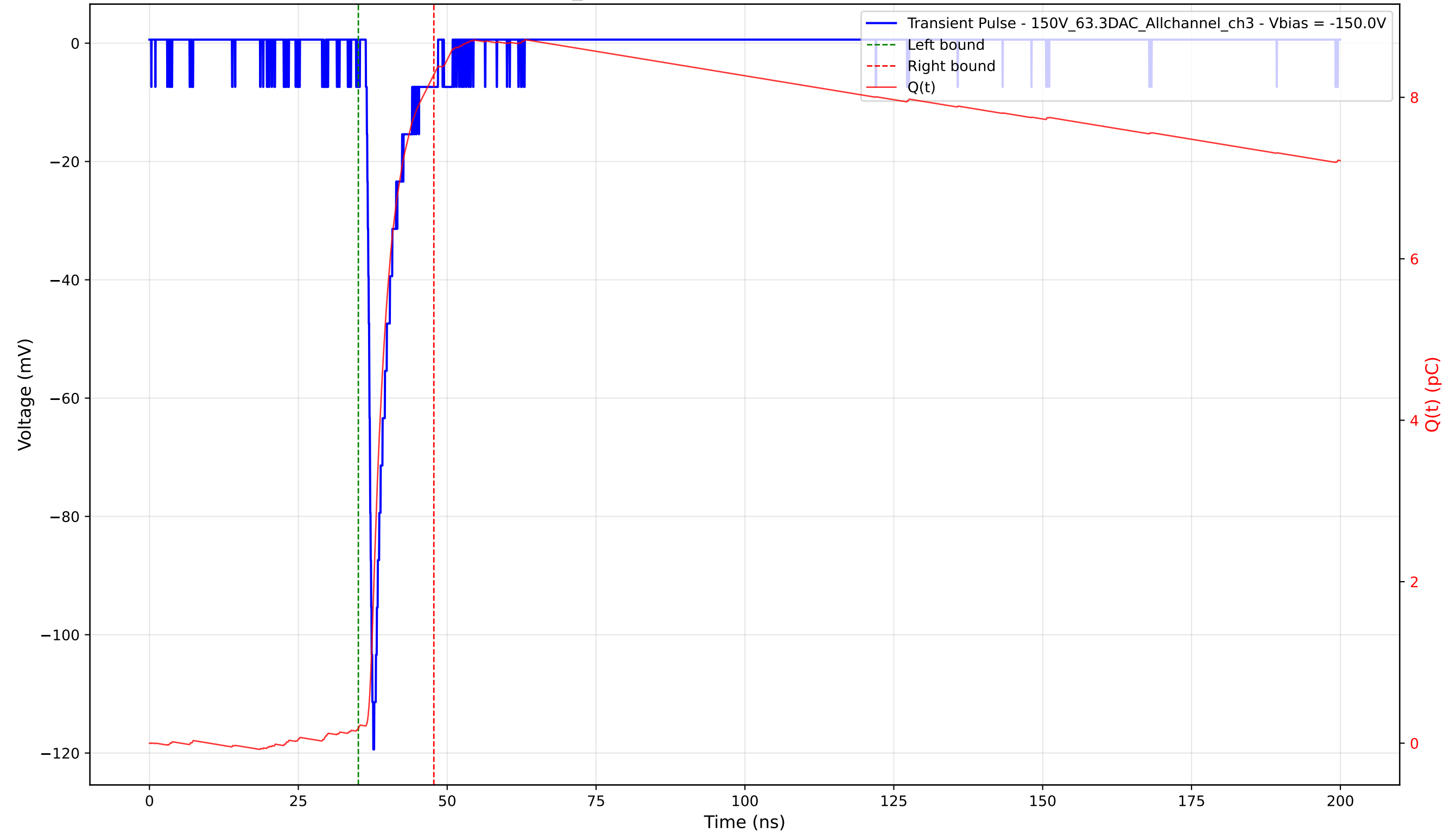
Transient Pulse - Sample: 1cm_42 - Position: 1650.0 \mu\text{m} - Charge: 8.10 pC - Rise Time: 0.94 ns
