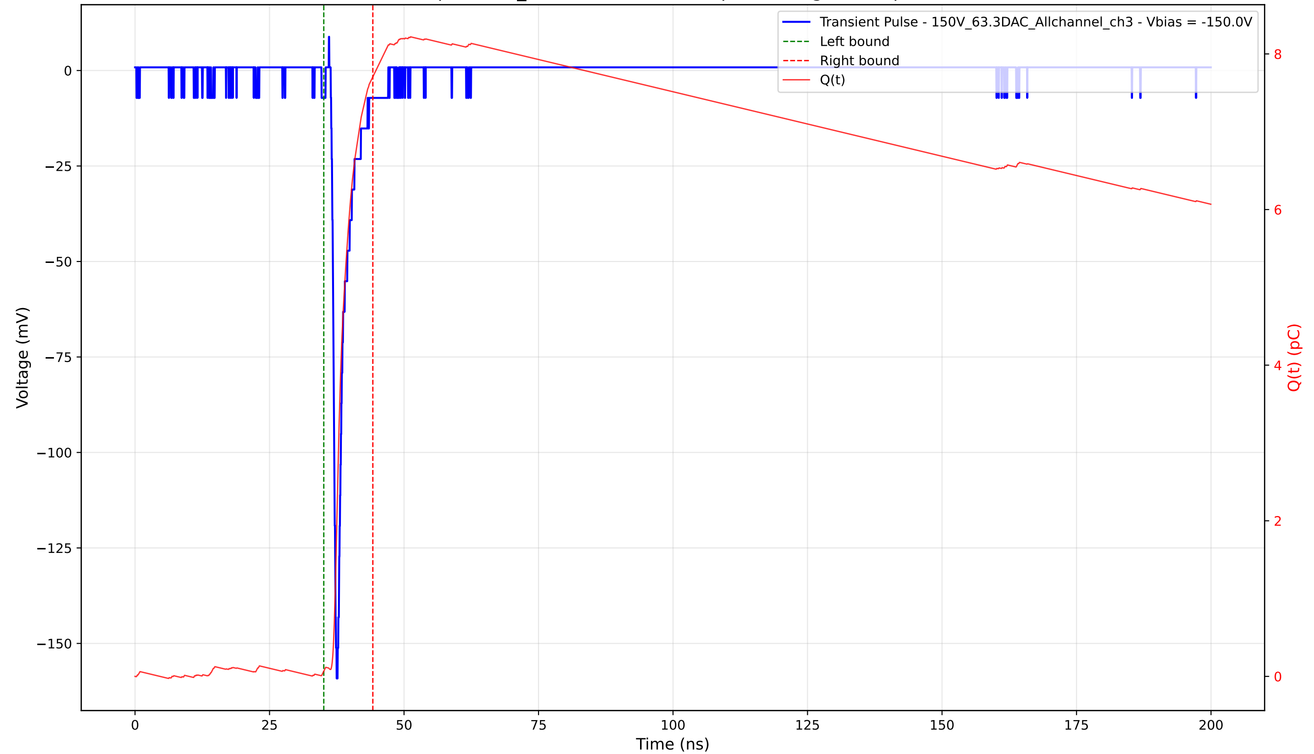
Transient Pulse - Sample: 1cm_42 - Position: 3165.0 \mu\text{m} - Charge: 7.64 pC - Rise Time: 0.84 ns
