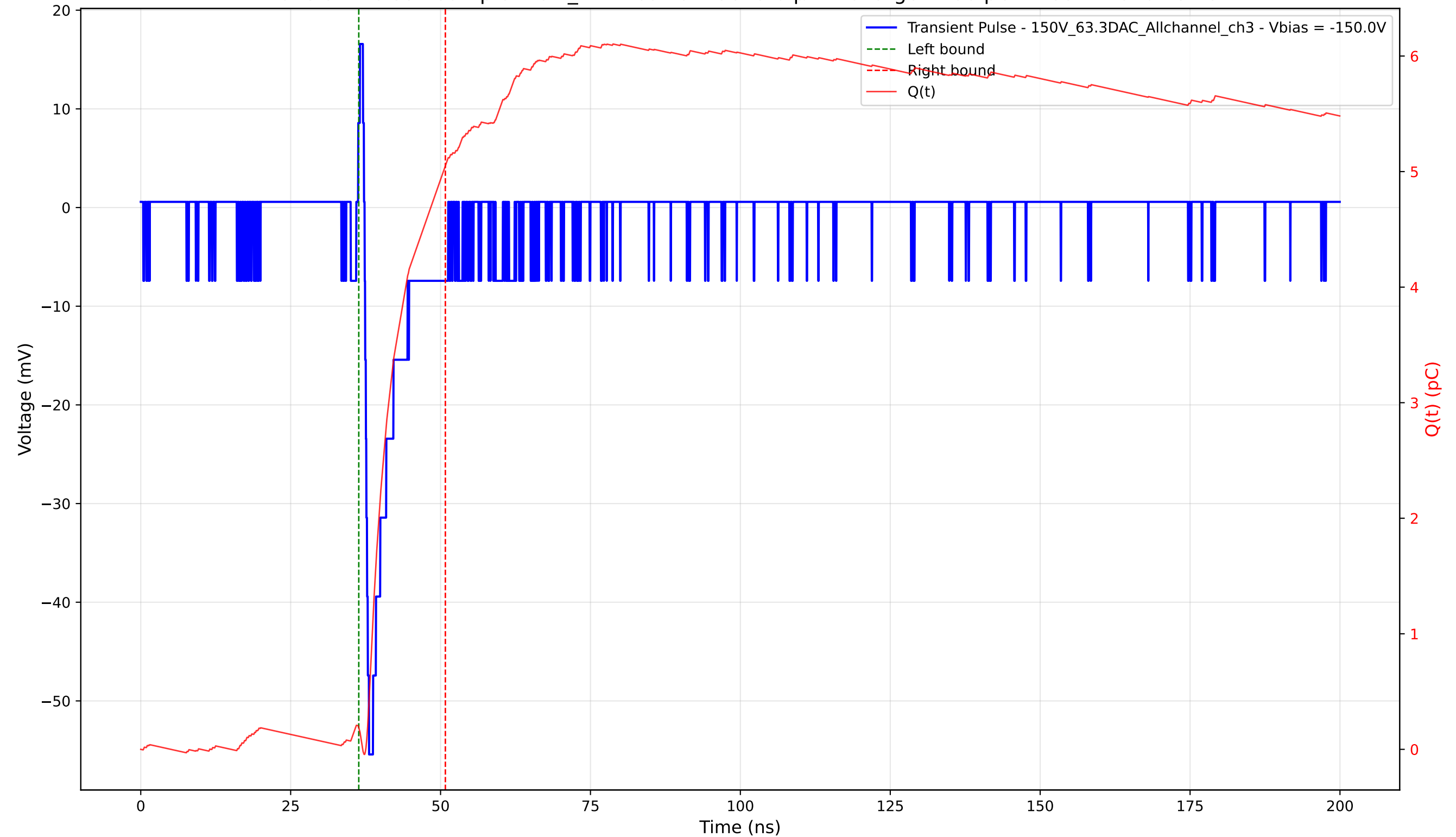
Transient Pulse - Sample: 1cm_42 - Position: 3825.0 \mu\text{m} - Charge: 4.86 pC - Rise Time: 0.73 ns
