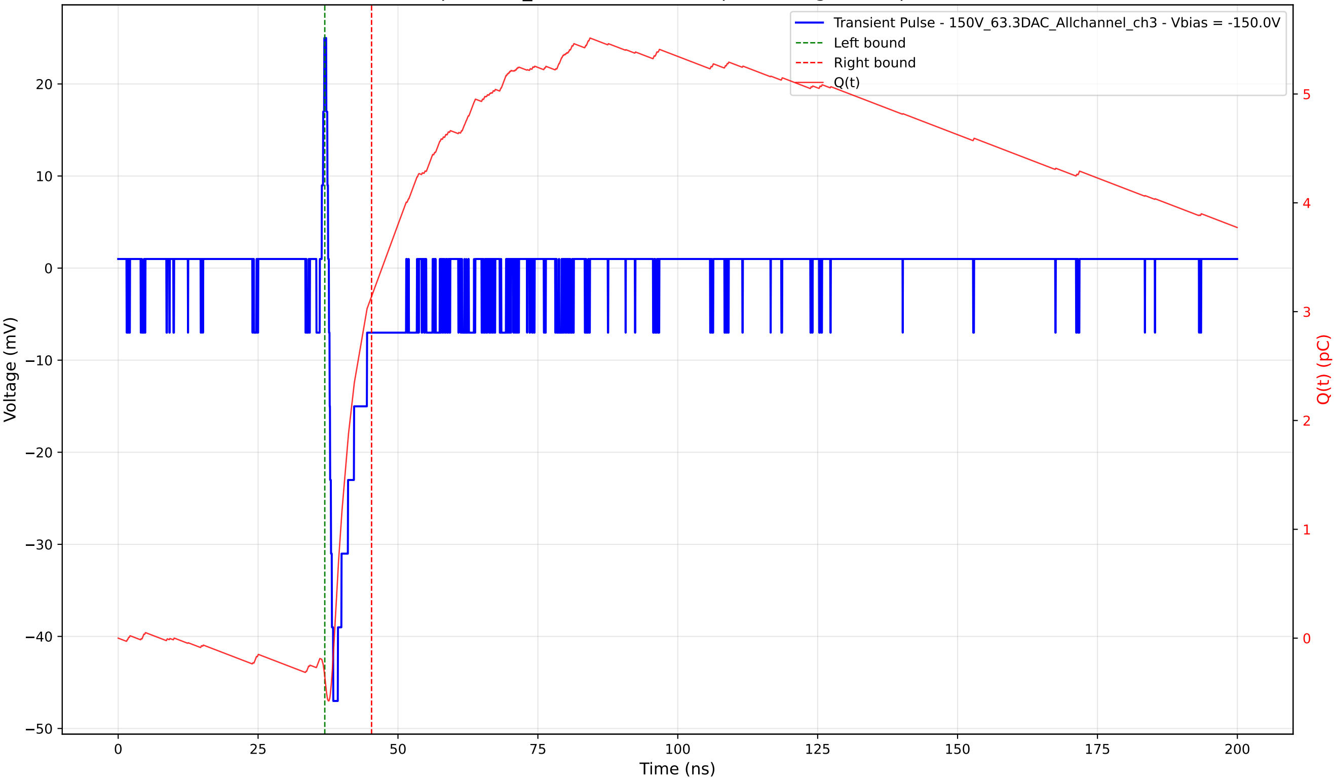
Transient Pulse - Sample: 1cm_42 - Position: 900.0 \mu\text{m} - Charge: 3.50 pC - Rise Time: 0.78 ns
