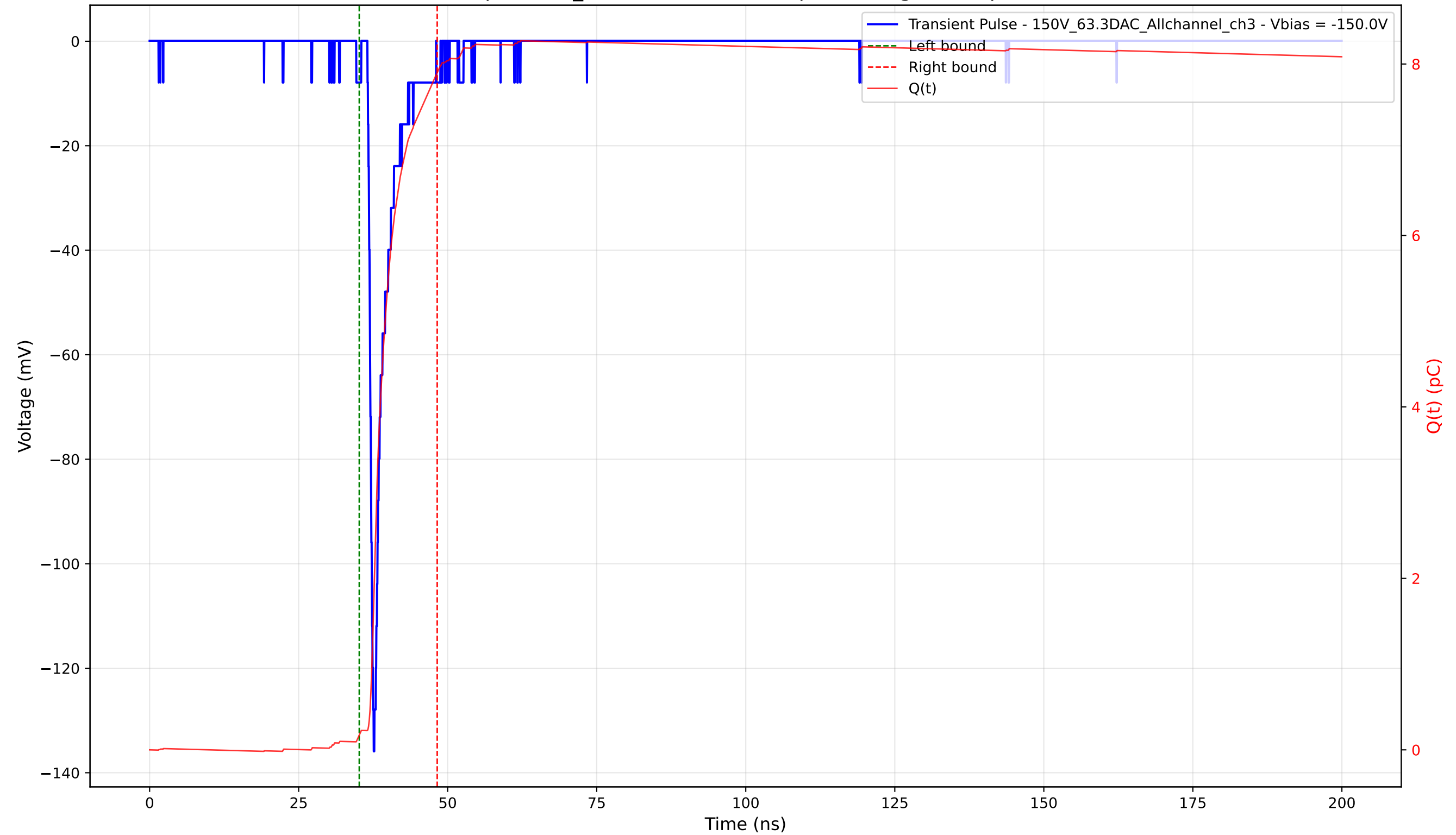
Transient Pulse - Sample: 1cm_42 - Position: 3310.0 \mu\text{m} - Charge: 7.73 pC - Rise Time: 0.85 ns
