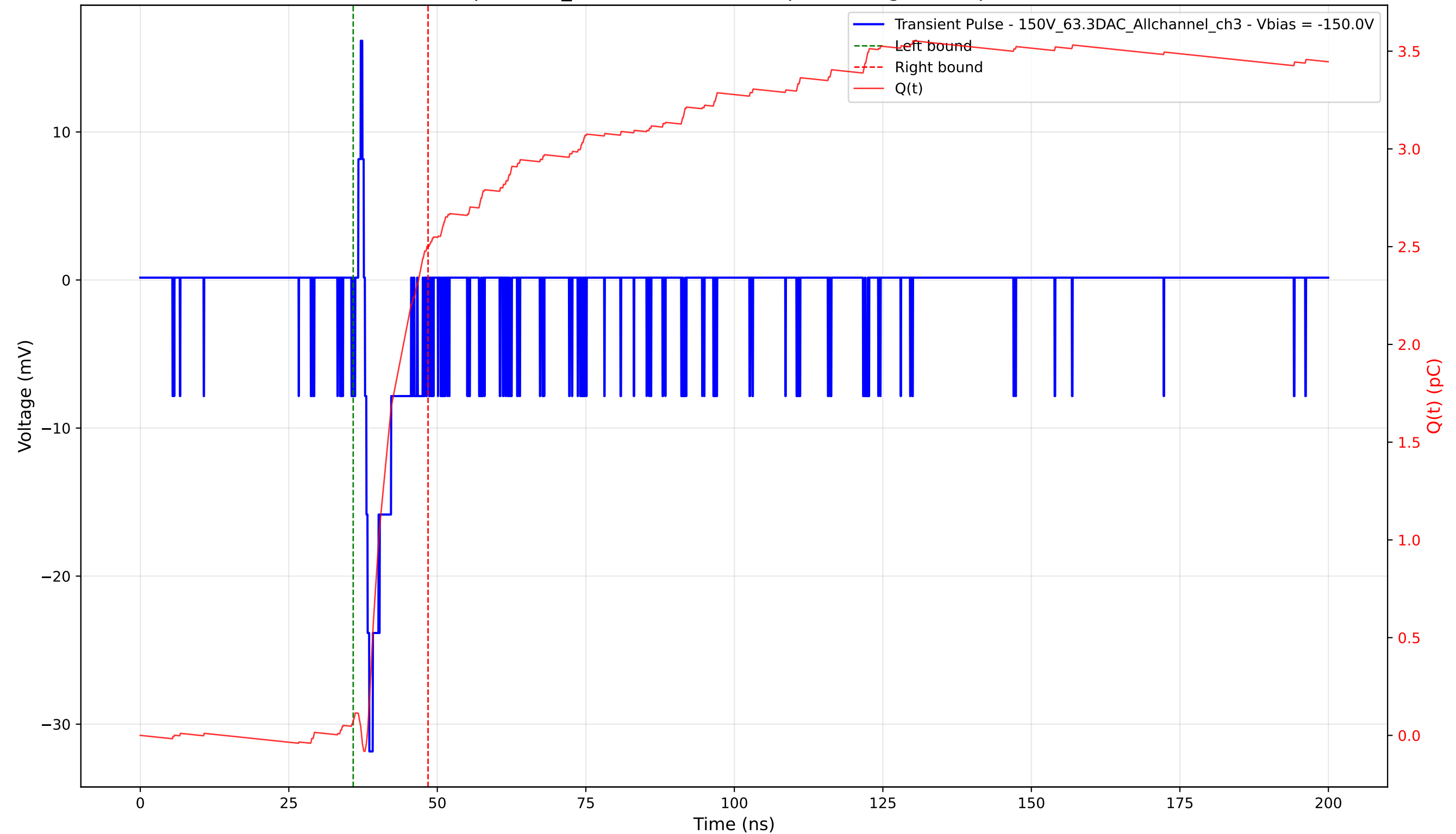
Transient Pulse - Sample: 1cm_42 - Position: 4880.0 \mu\text{m} - Charge: 2.43 pC - Rise Time: 0.74 ns
