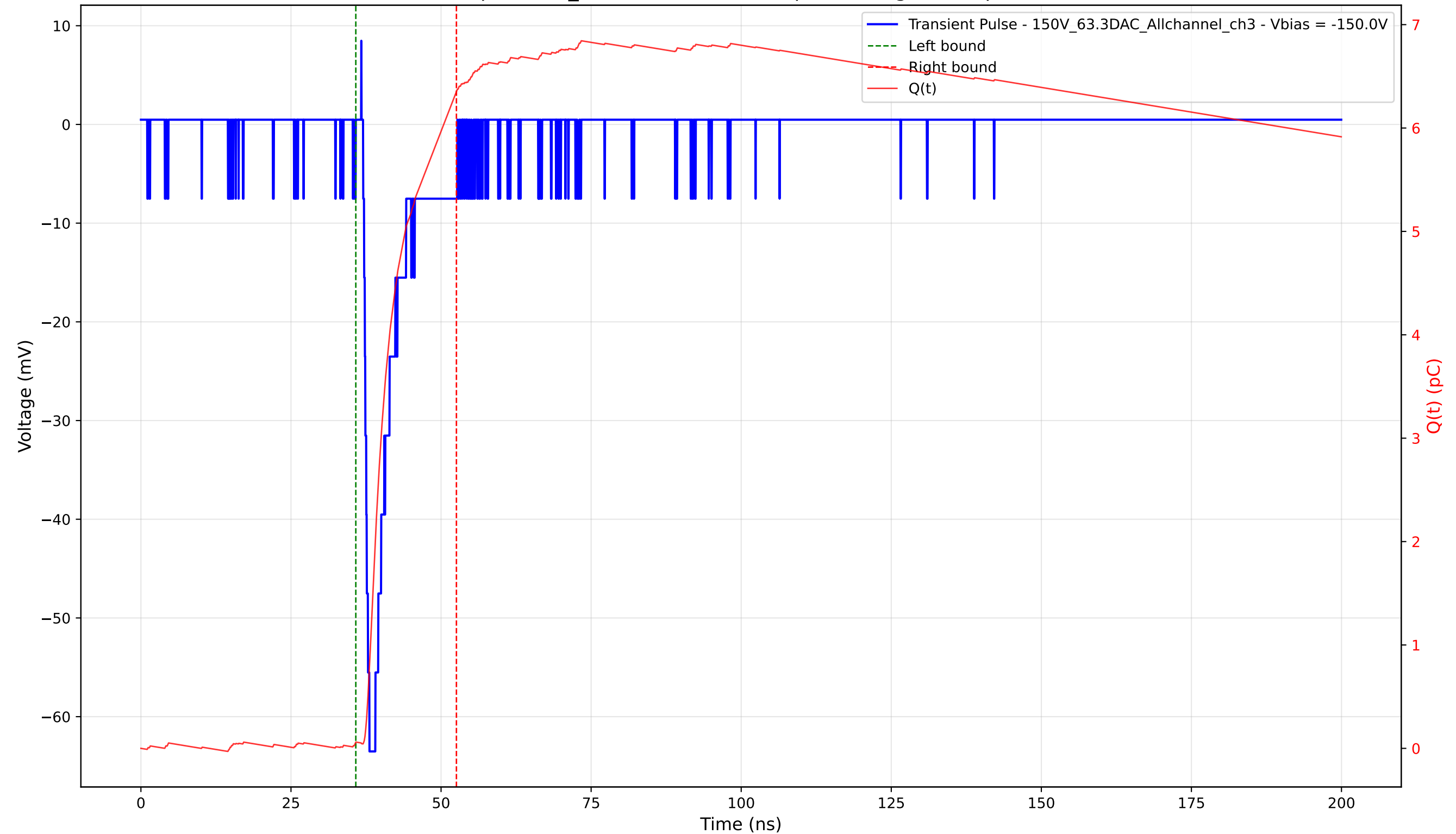
Transient Pulse - Sample: 1cm_42 - Position: 1380.0 \mu\text{m} - Charge: 6.29 pC - Rise Time: 1.05 ns
