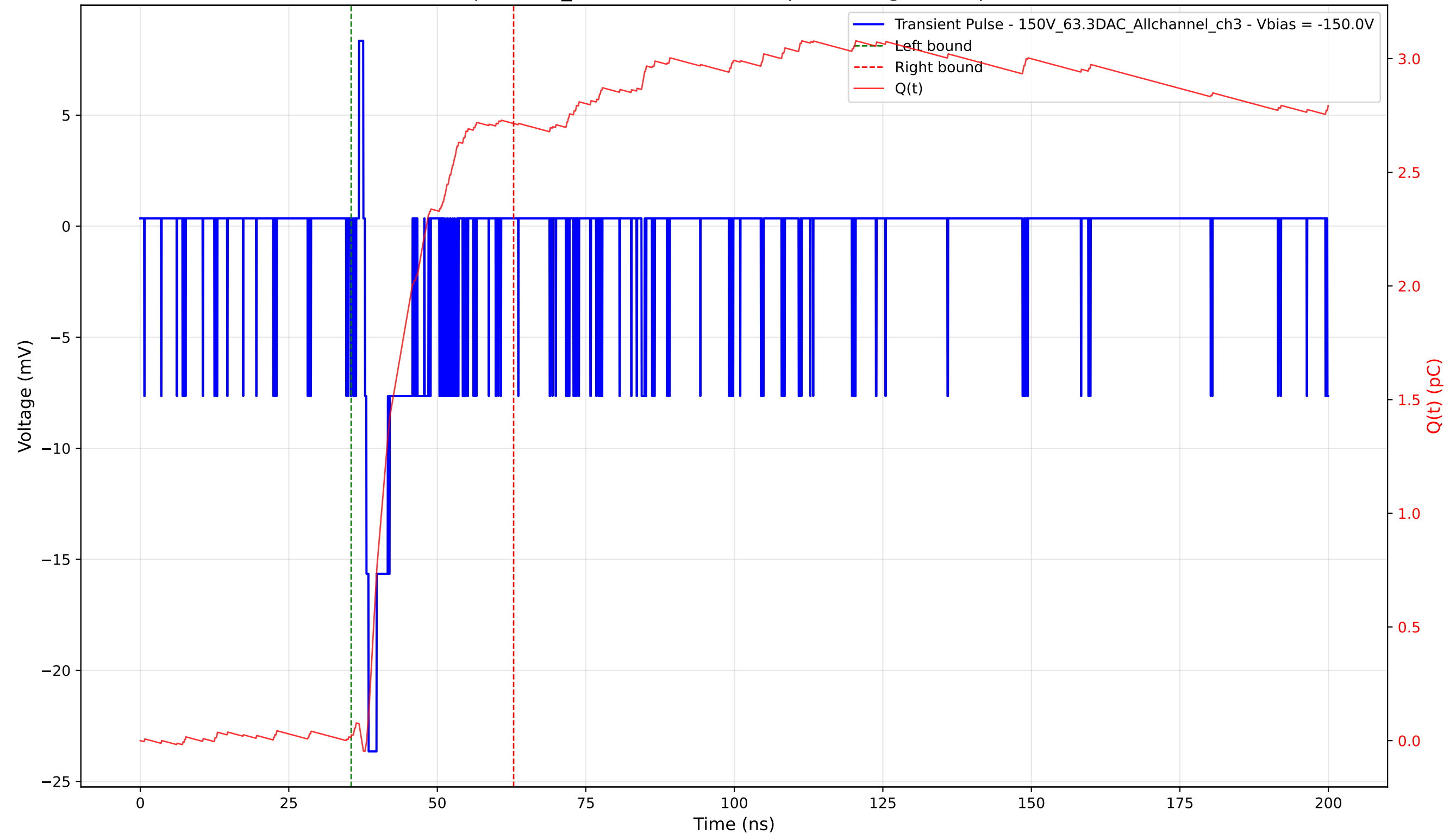
Transient Pulse - Sample: 1cm_42 - Position: 4940.0 \mu\text{m} - Charge: 2.69 pC - Rise Time: 0.63 ns
