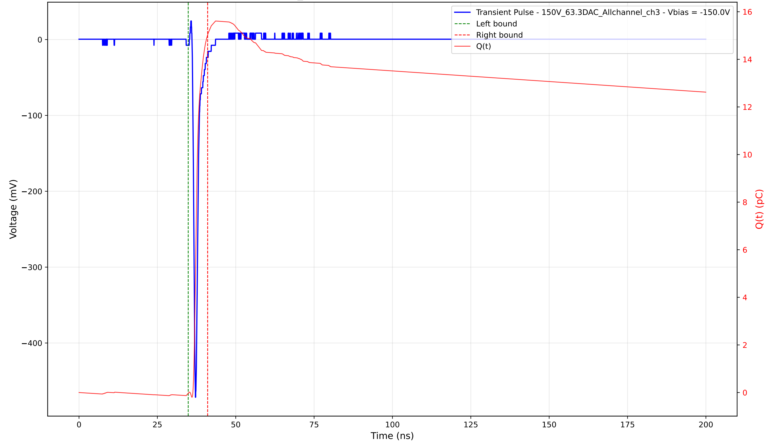
Transient Pulse - Sample: 1cm_42 - Position: 2300.0 \mu\text{m} - Charge: 15.07 pC - Rise Time: 0.69 ns
