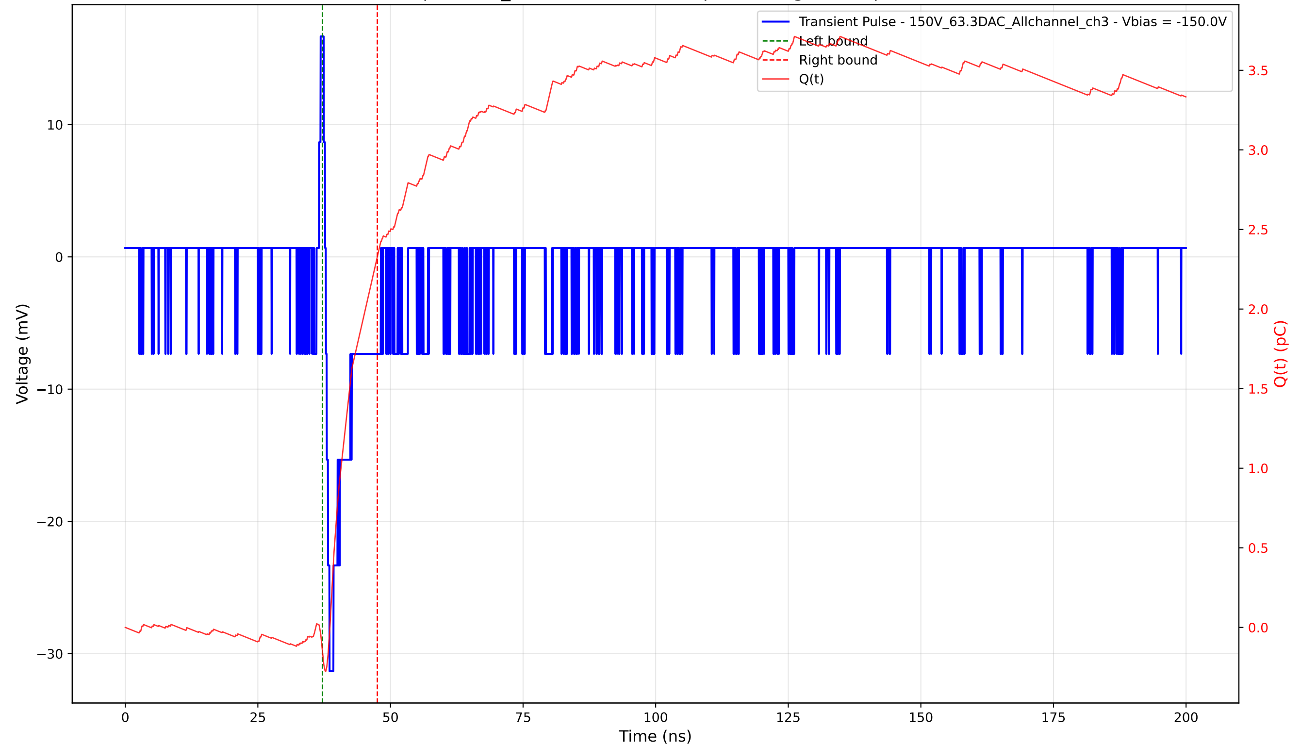
Transient Pulse - Sample: 1cm_42 - Position: 4580.0 \mu\text{m} - Charge: 2.48 pC - Rise Time: 0.71 ns
