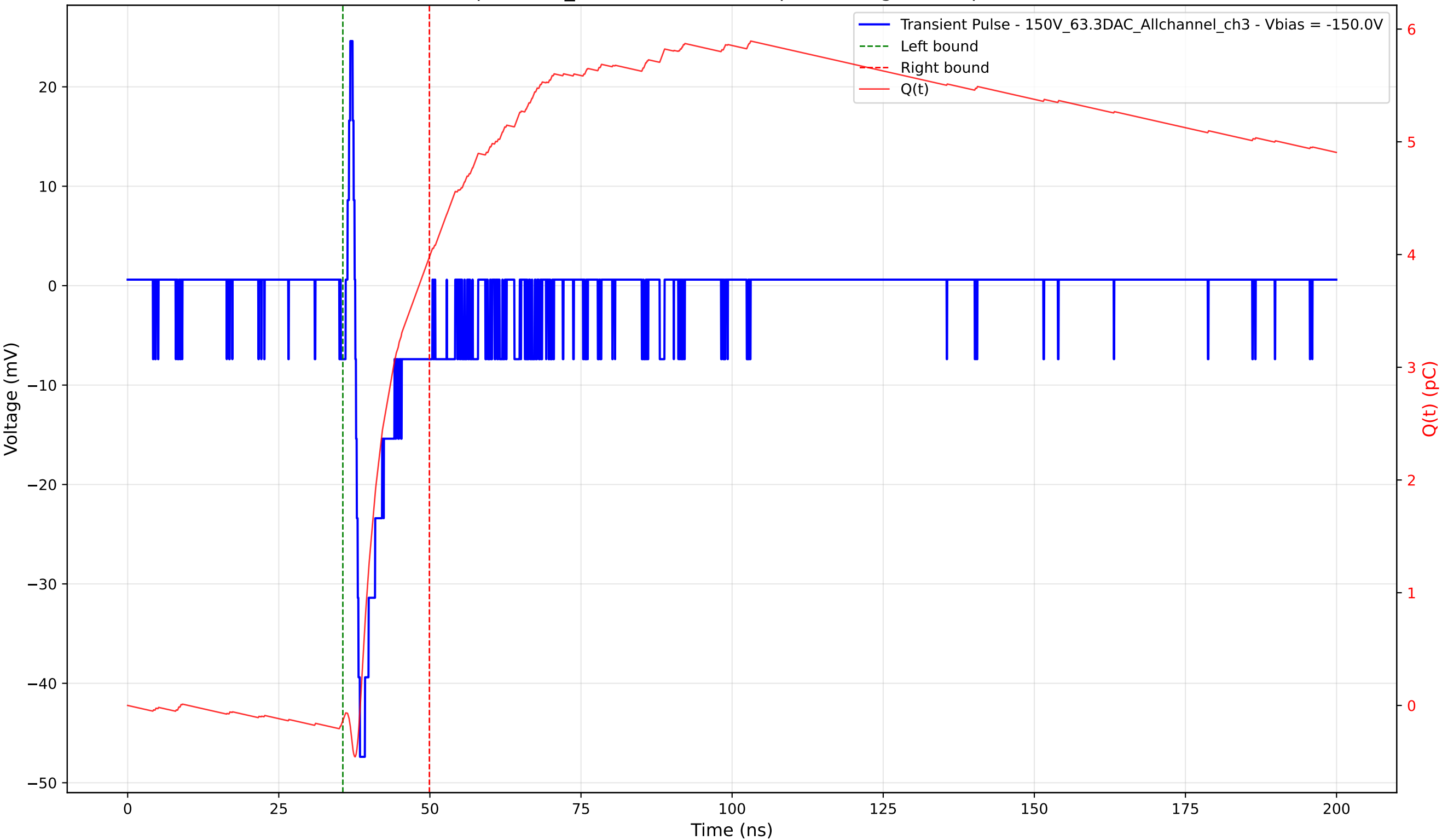
Transient Pulse - Sample: 1cm_42 - Position: 905.0 \mu\text{m} - Charge: 4.11 pC - Rise Time: 0.78 ns
