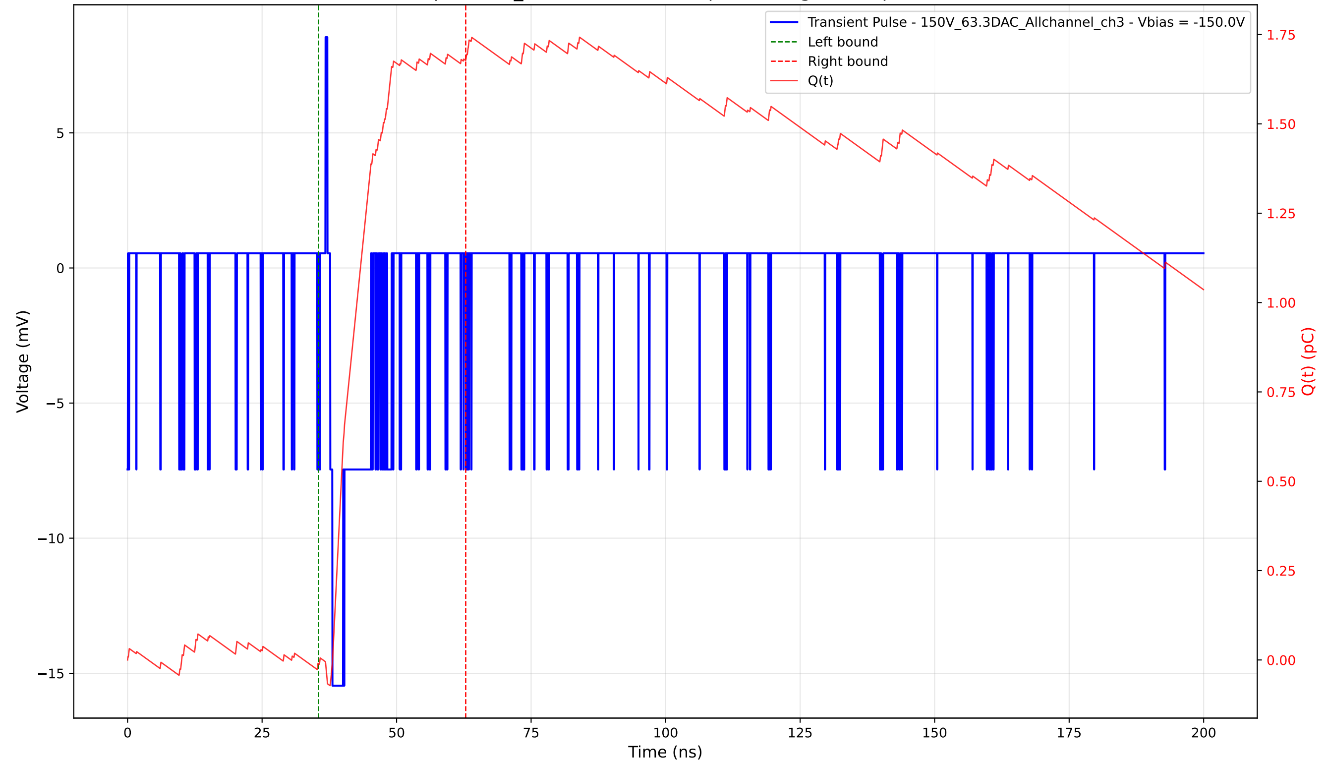
Transient Pulse - Sample: 1cm_42 - Position: 190.0 \mu\text{m} - Charge: 1.69 pC - Rise Time: 0.43 ns
