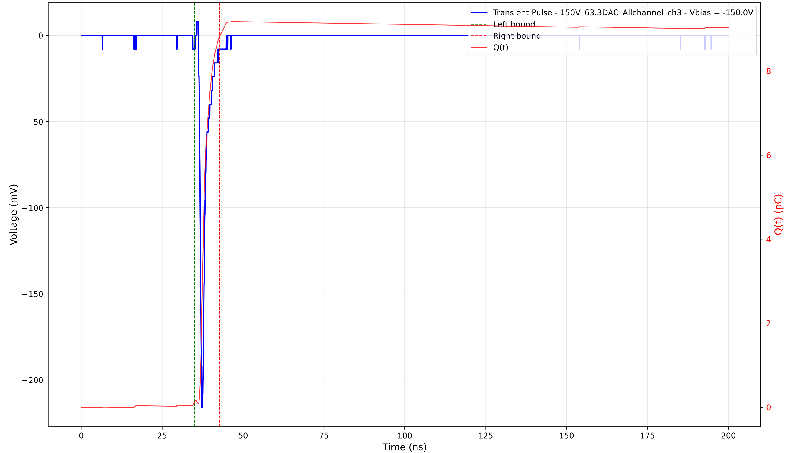
Transient Pulse - Sample: 1cm_42 - Position: 3030.0 \mu\text{m} - Charge: 8.69 pC - Rise Time: 0.81 ns
