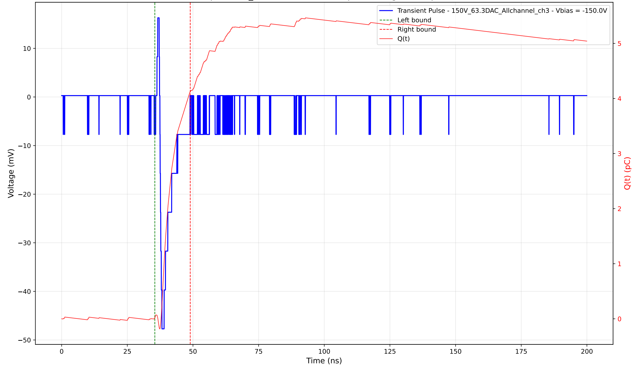
Transient Pulse - Sample: 1cm_42 - Position: 3905.0 \mu\text{m} - Charge: 4.11 pC - Rise Time: 0.78 ns
