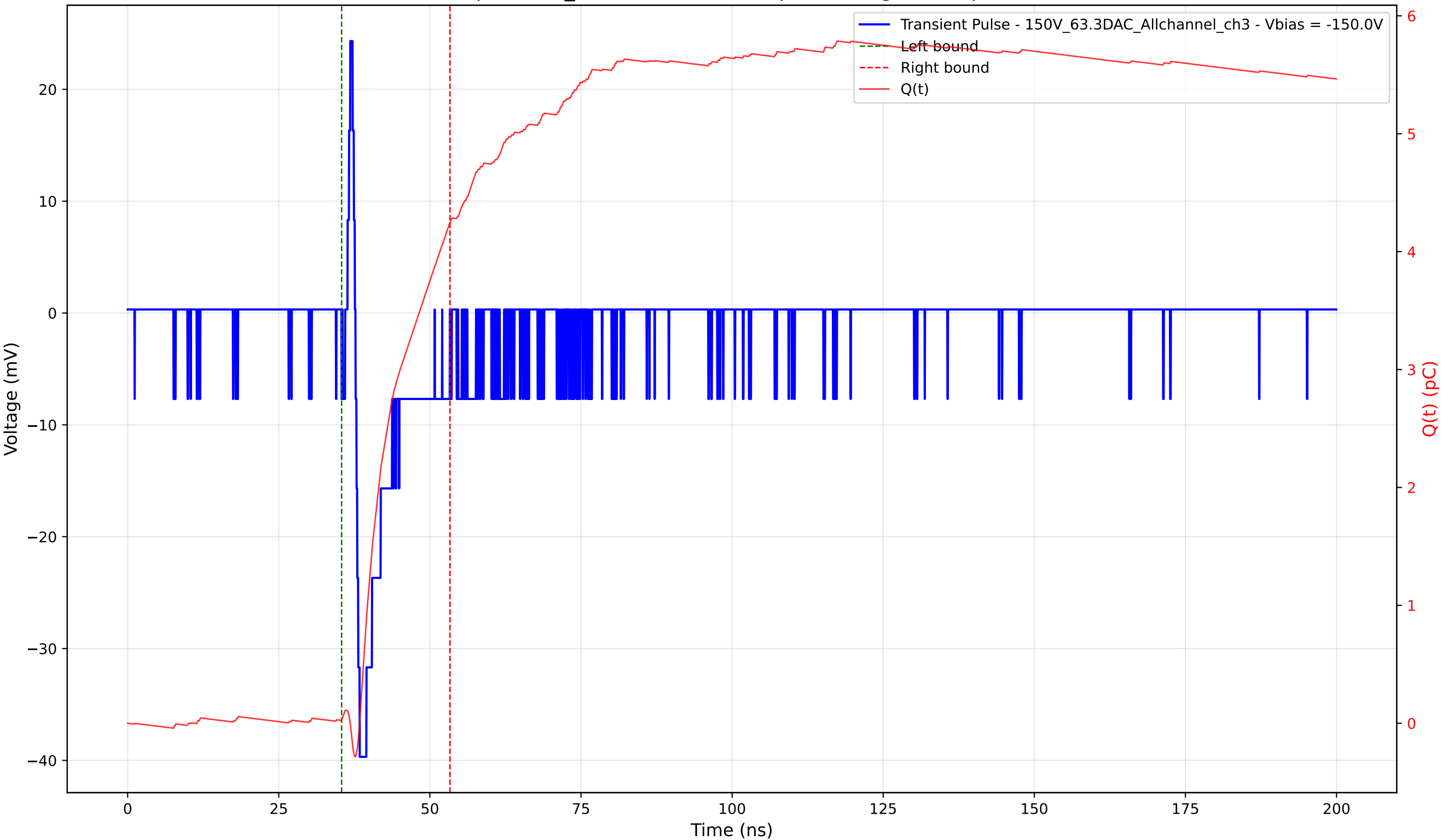
Transient Pulse - Sample: 1cm_42 - Position: 595.0 \mu\text{m} - Charge: 4.22 pC - Rise Time: 0.70 ns
