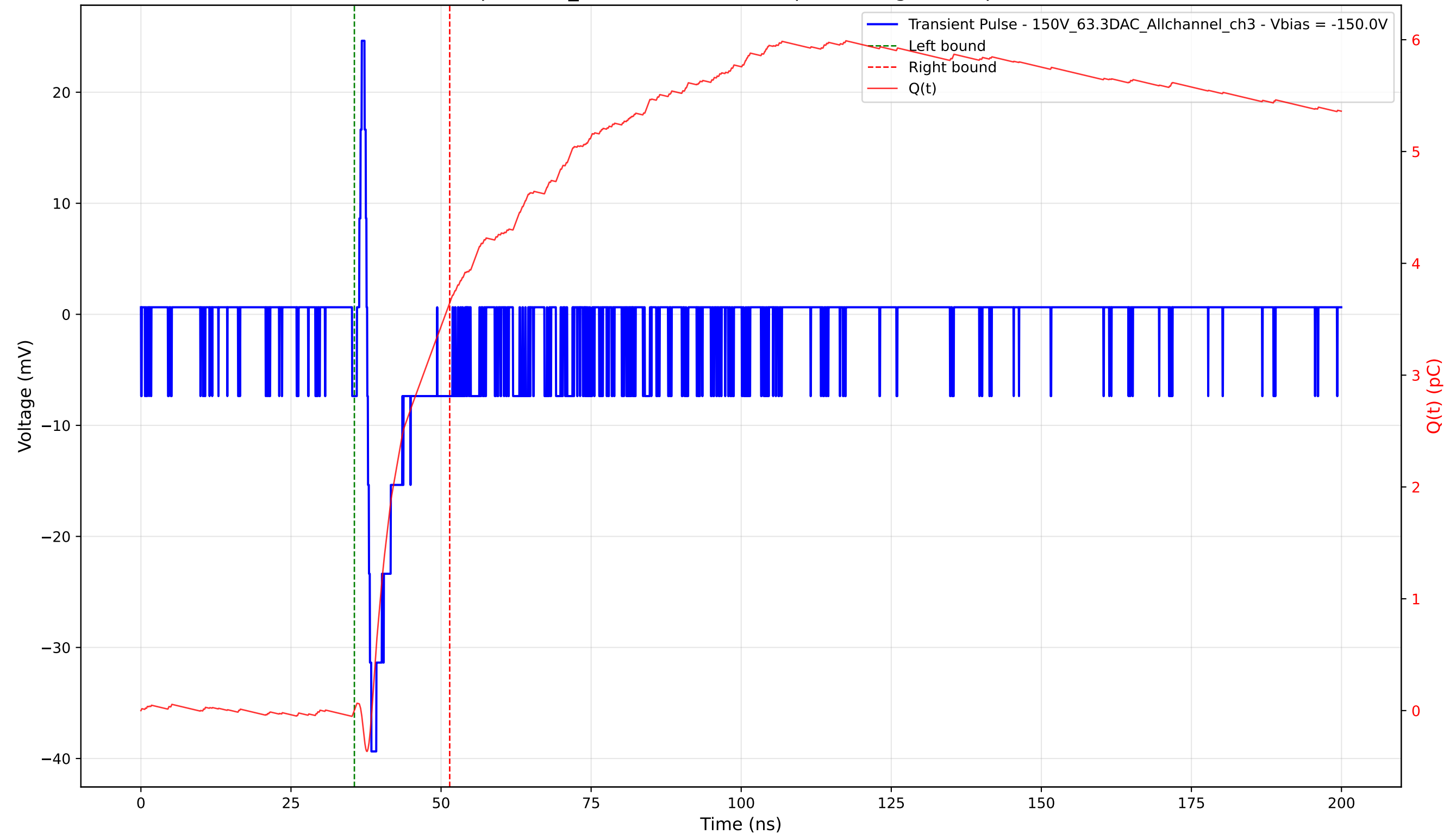
Transient Pulse - Sample: 1cm_42 - Position: 4240.0 \mu\text{m} - Charge: 3.64 pC - Rise Time: 0.70 ns
