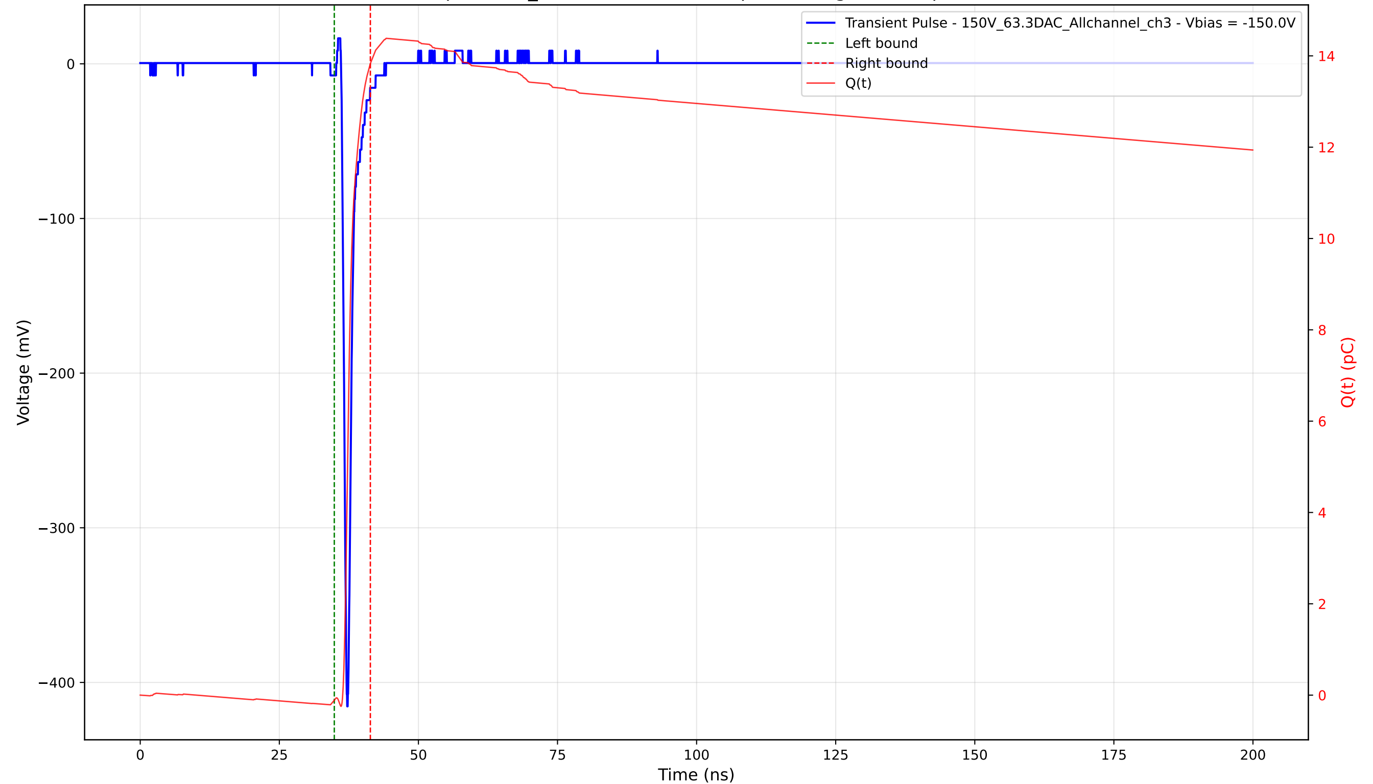
Transient Pulse - Sample: 1cm_42 - Position: 2205.0 \mu\text{m} - Charge: 13.94 pC - Rise Time: 0.74 ns
