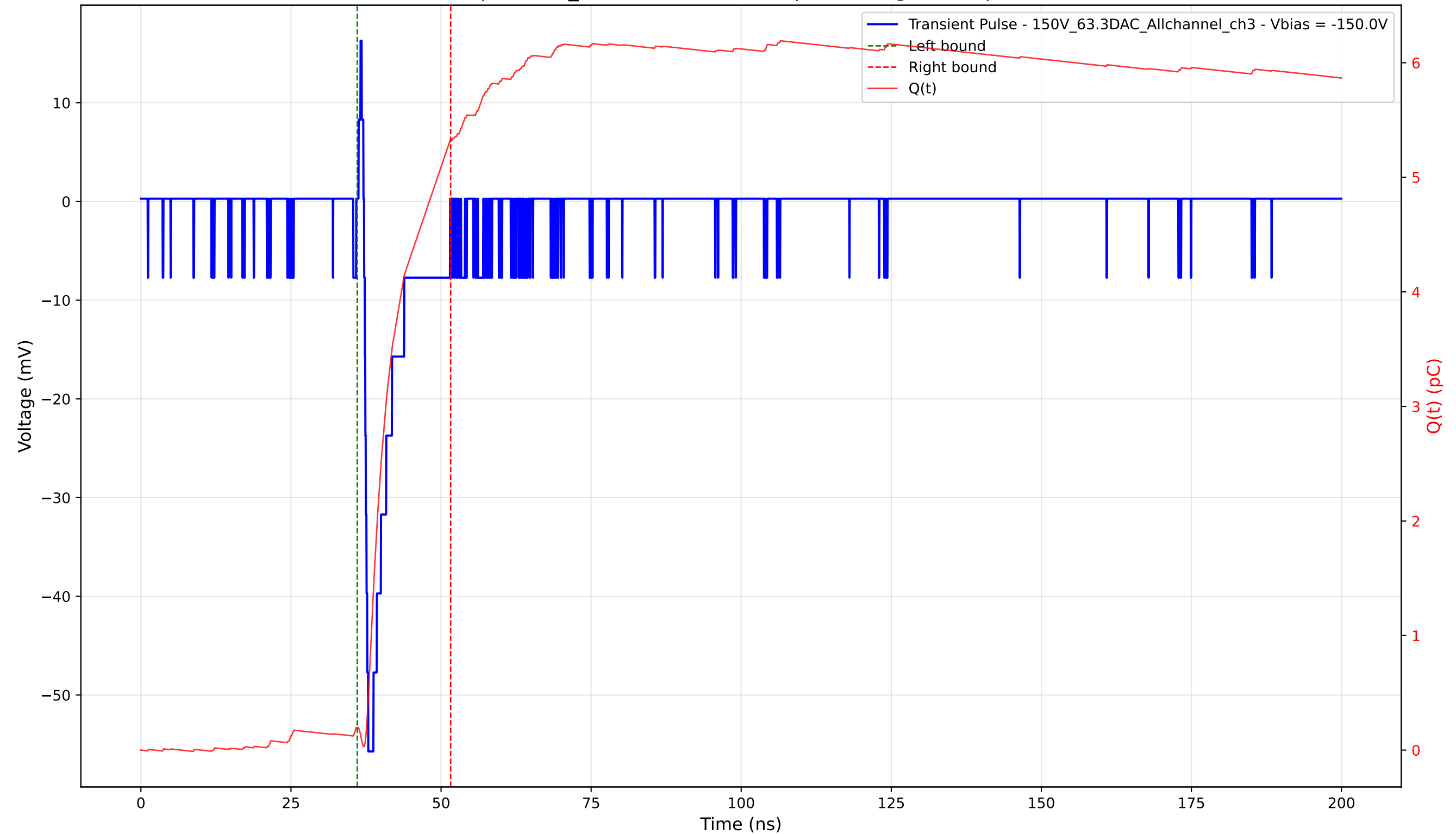
Transient Pulse - Sample: 1cm_42 - Position: 3680.0 \mu\text{m} - Charge: 5.13 pC - Rise Time: 0.69 ns
