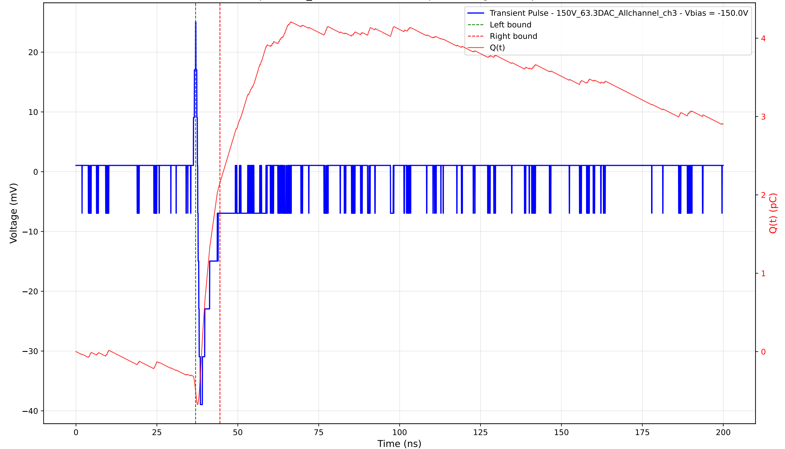
Transient Pulse - Sample: 1cm_42 - Position: 4105.0 \mu\text{m} - Charge: 2.65 pC - Rise Time: 0.82 ns
