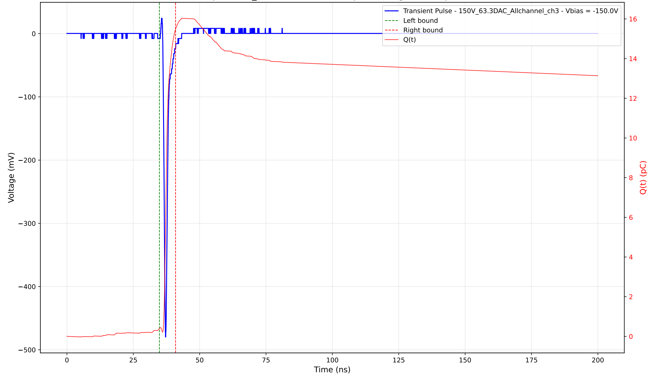
Transient Pulse - Sample: 1cm_42 - Position: 2350.0 \mu\text{m} - Charge: 15.10 pC - Rise Time: 0.74 ns
