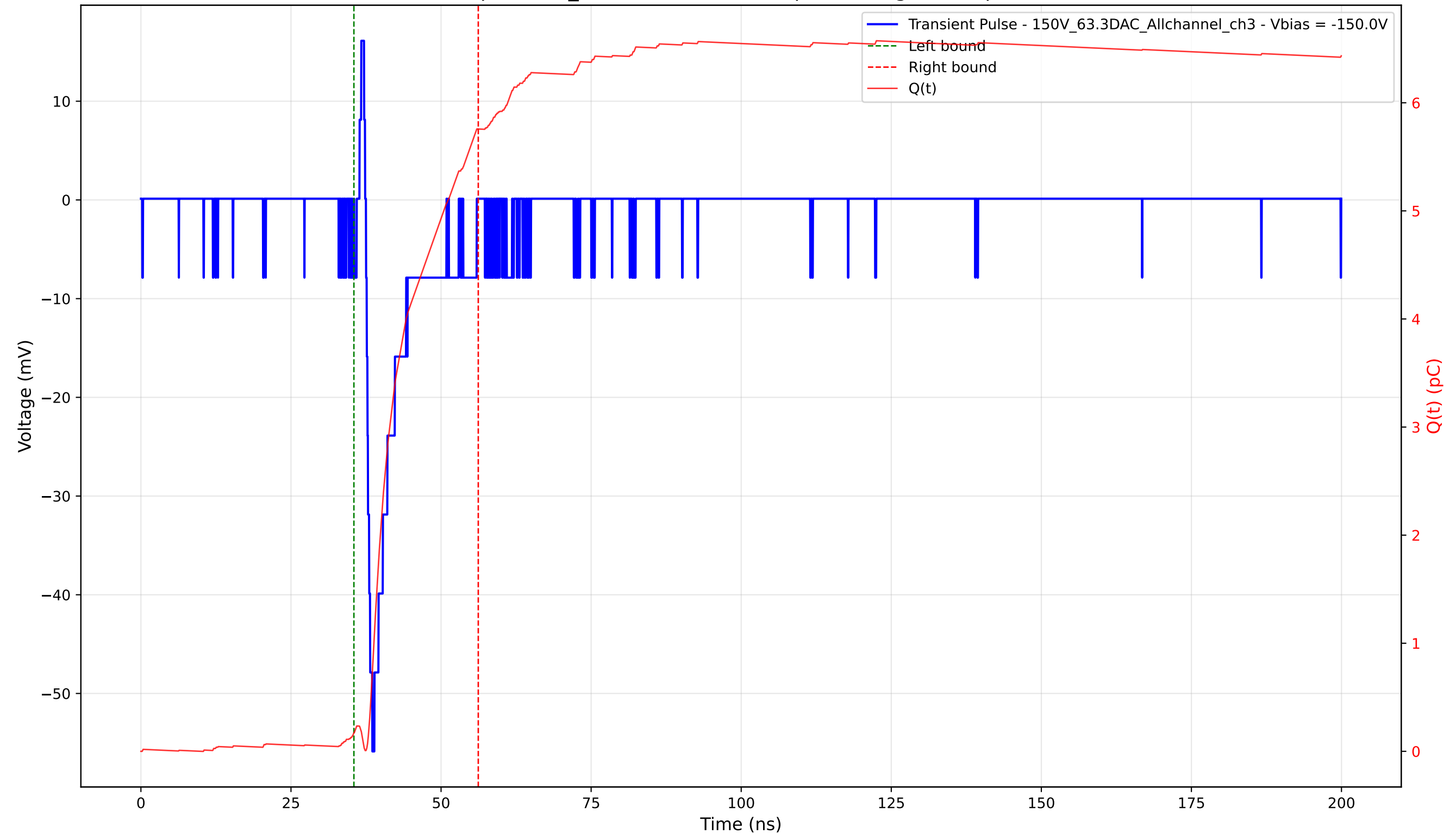
Transient Pulse - Sample: 1cm_42 - Position: 1060.0 \mu\text{m} - Charge: 5.59 pC - Rise Time: 1.05 ns
