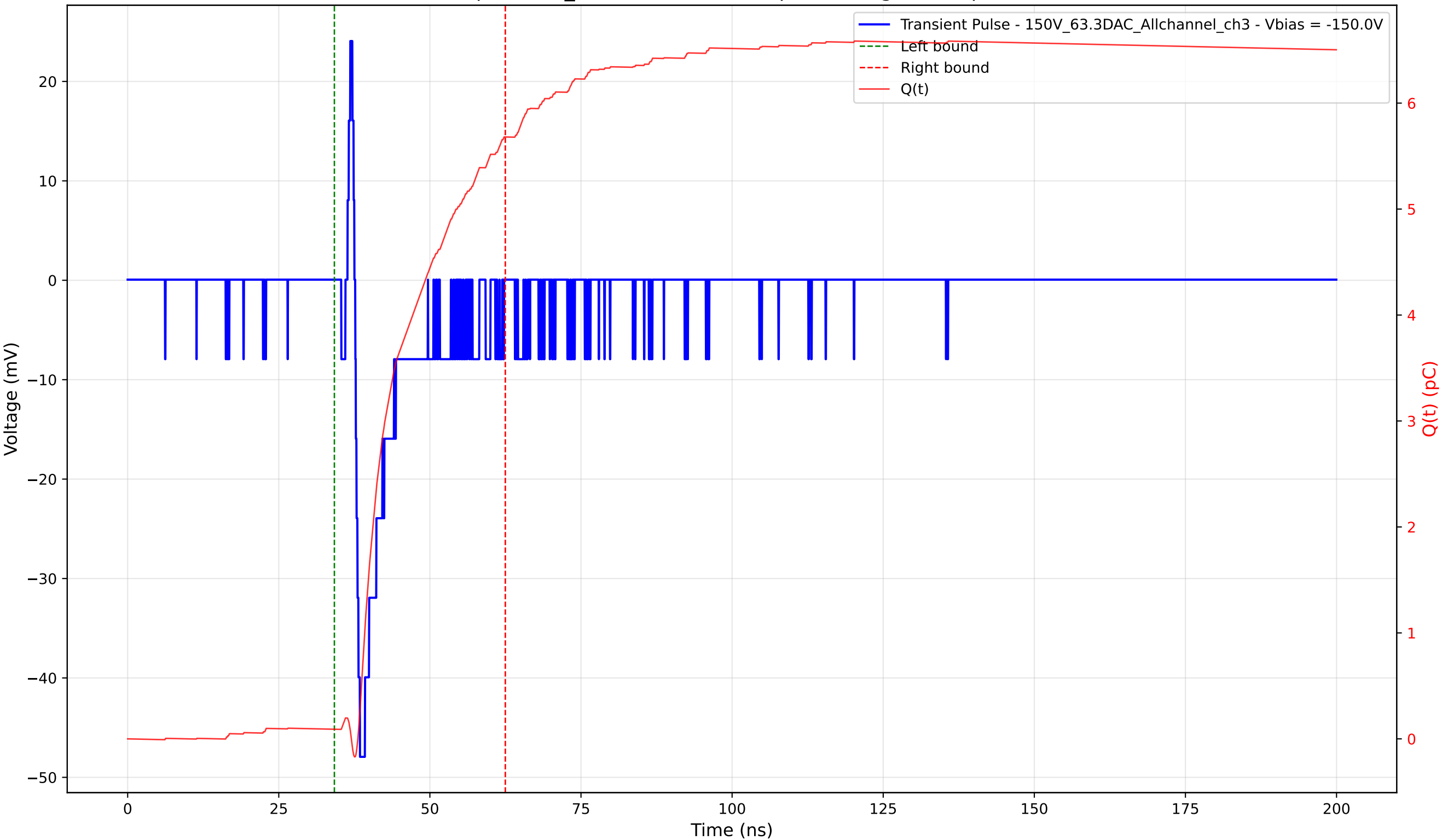
Transient Pulse - Sample: 1cm_42 - Position: 915.0 \mu\text{m} - Charge: 5.59 pC - Rise Time: 0.78 ns
