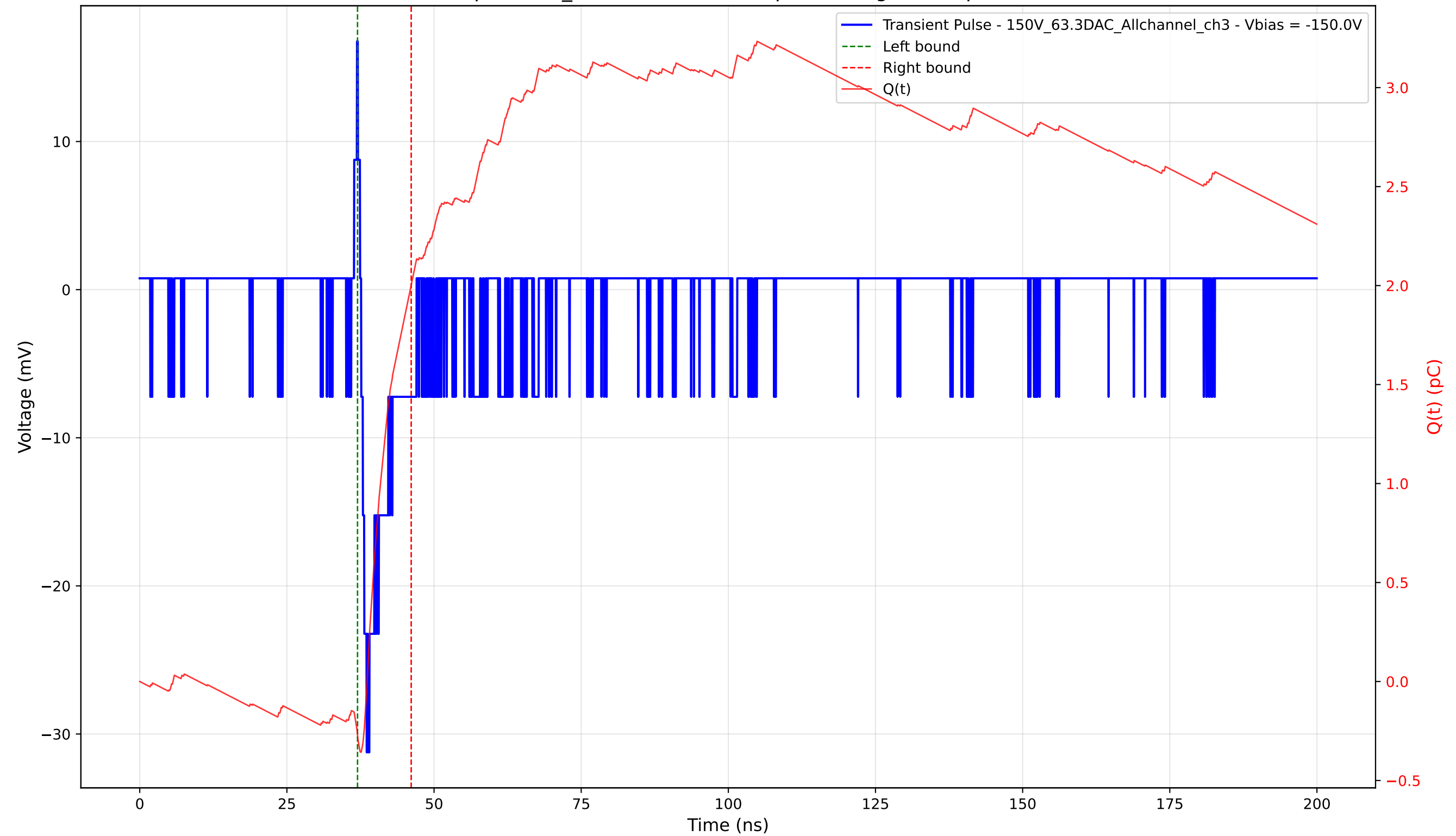
Transient Pulse - Sample: 1cm_42 - Position: 370.0 \mu\text{m} - Charge: 2.28 pC - Rise Time: 0.95 ns
