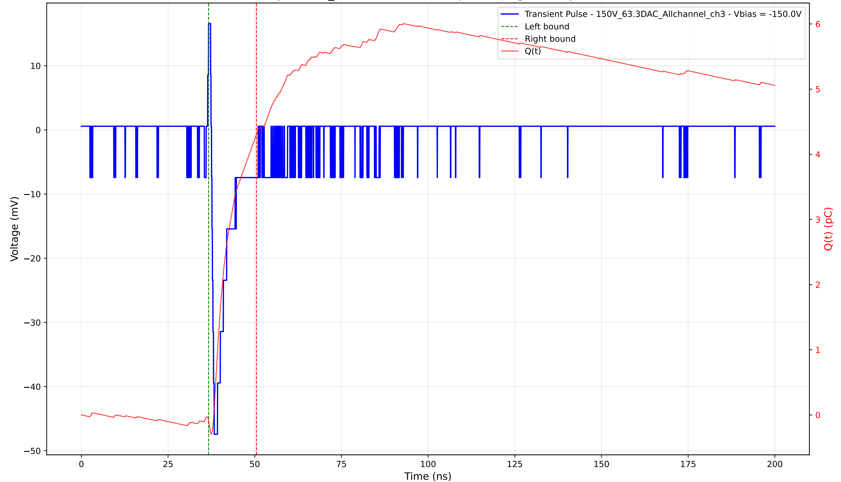
Transient Pulse - Sample: 1cm_42 - Position: 1010.0 \mu\text{m} - Charge: 4.39 pC - Rise Time: 0.78 ns
