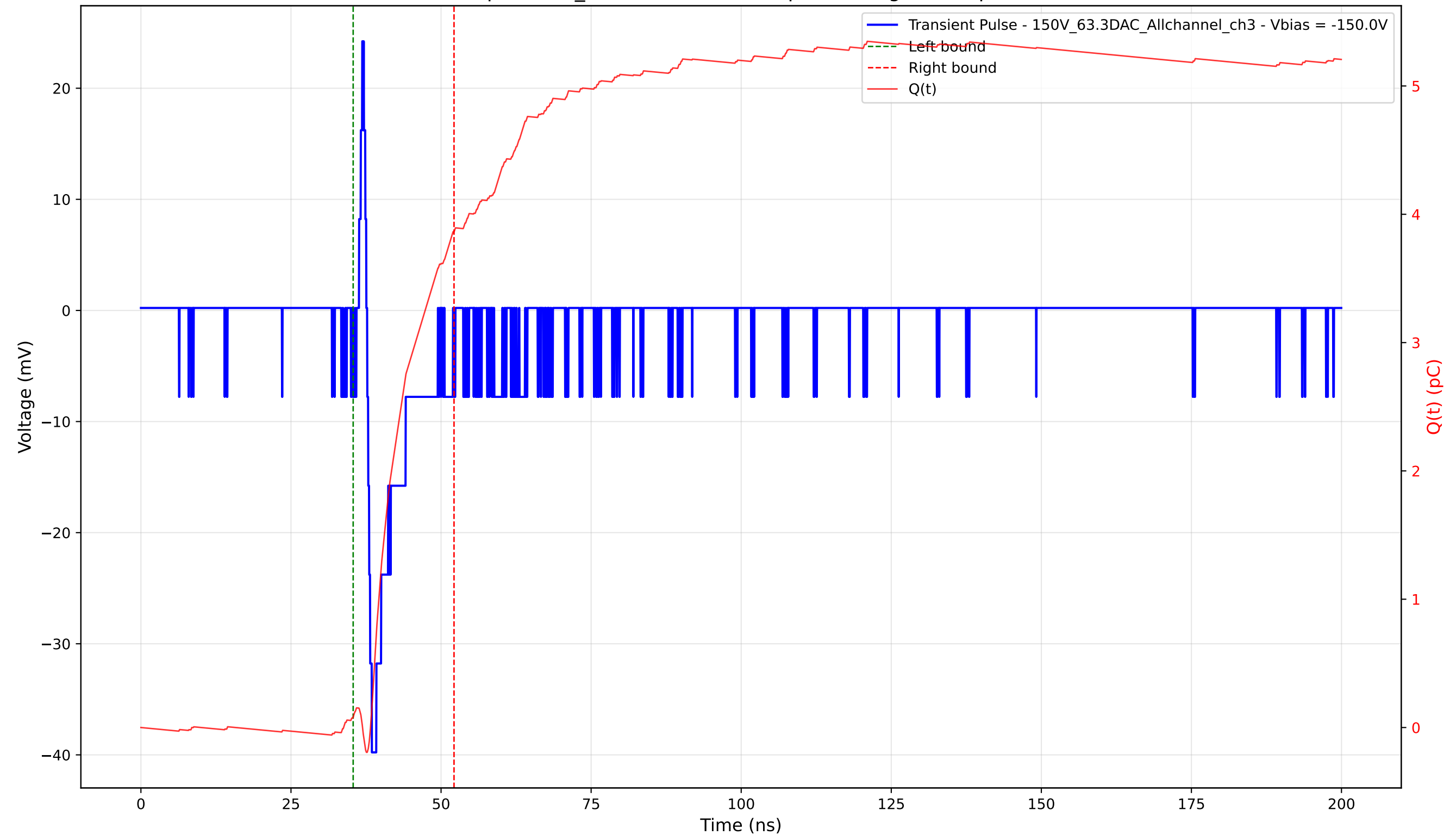
Transient Pulse - Sample: 1cm_42 - Position: 530.0 \mu\text{m} - Charge: 3.78 pC - Rise Time: 0.78 ns
