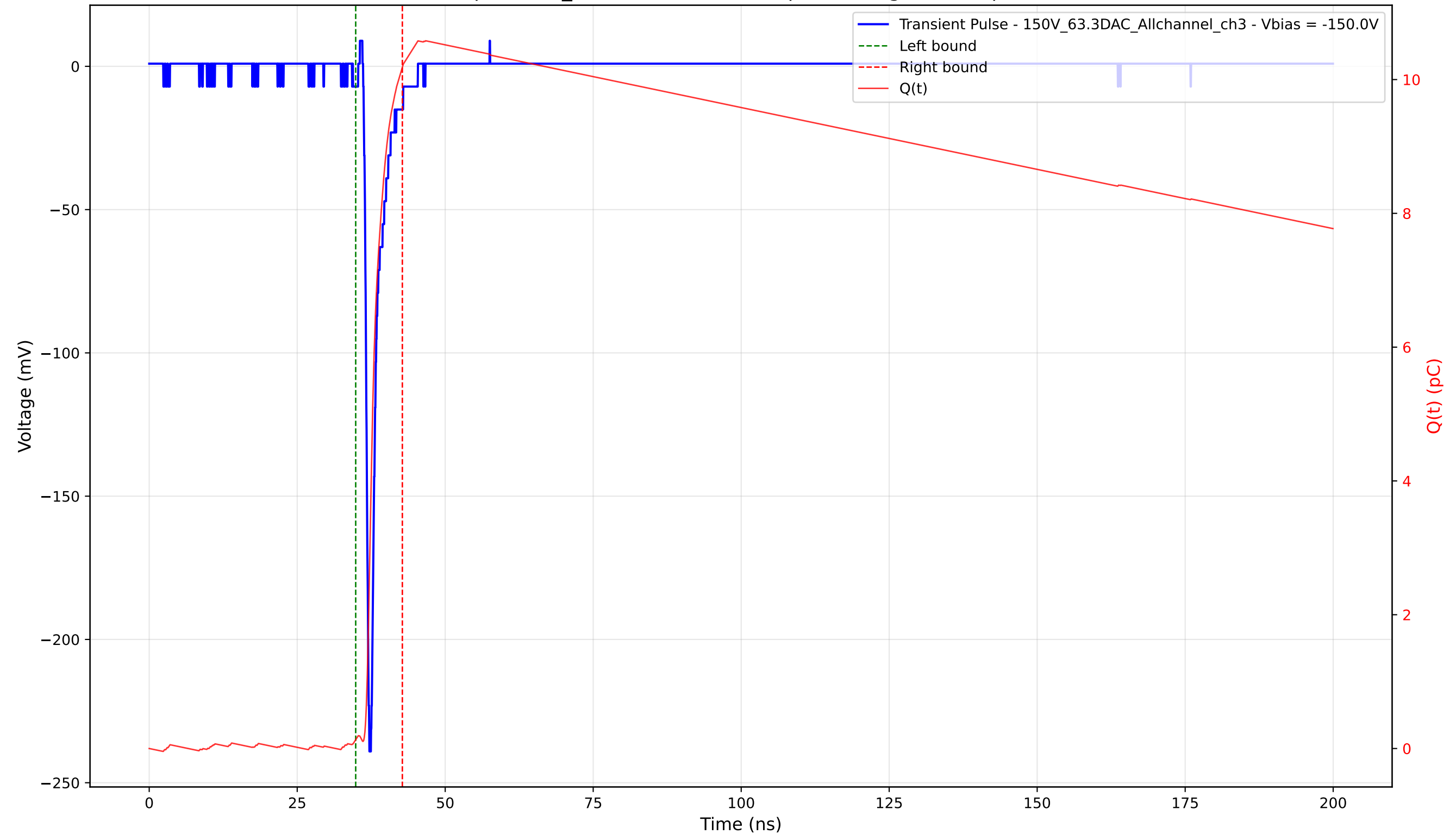
Transient Pulse - Sample: 1cm_42 - Position: 2030.0 \mu\text{m} - Charge: 10.05 pC - Rise Time: 0.80 ns
