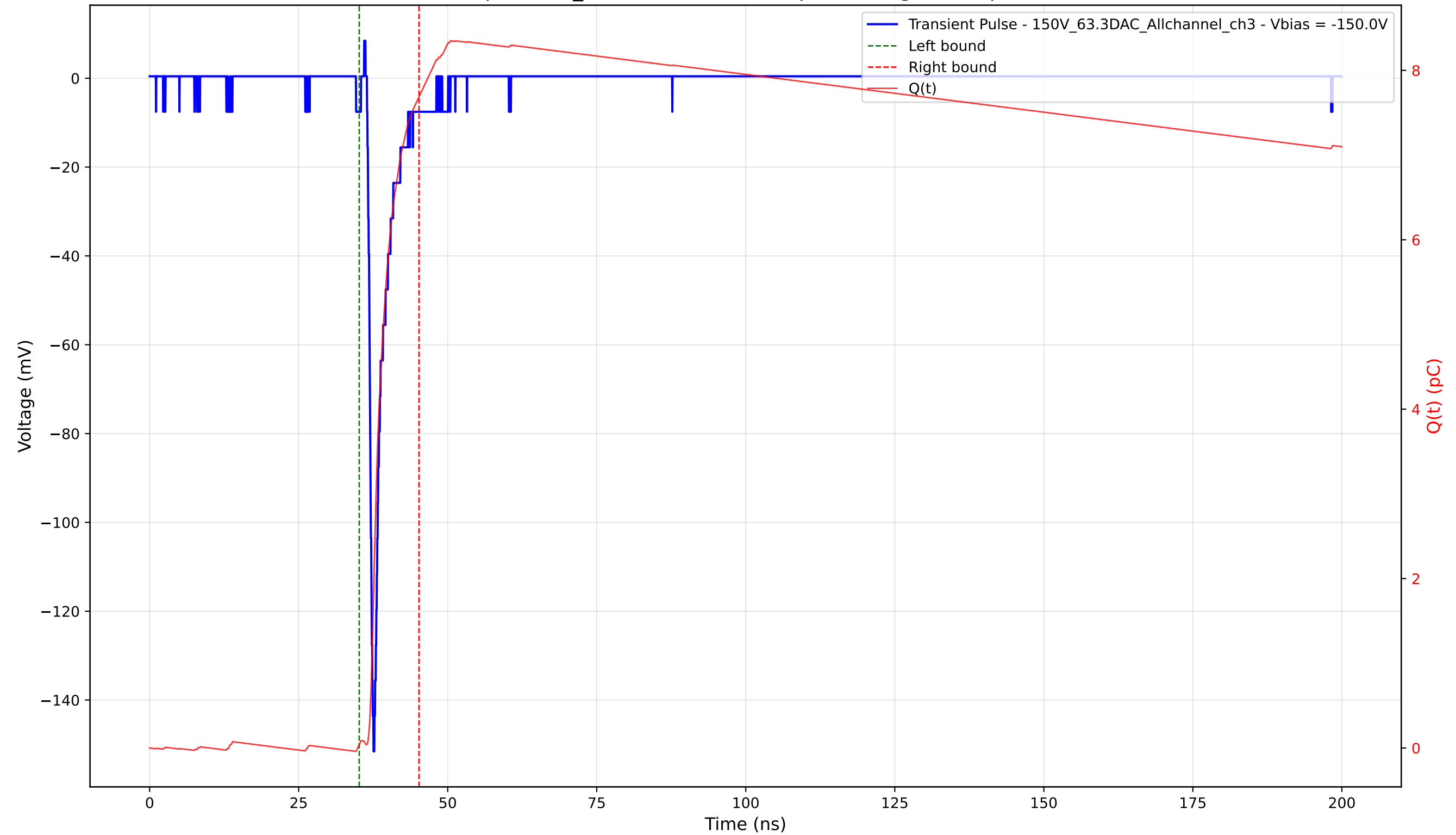
Transient Pulse - Sample: 1cm_42 - Position: 3215.0 \mu\text{m} - Charge: 7.65 pC - Rise Time: 0.88 ns
