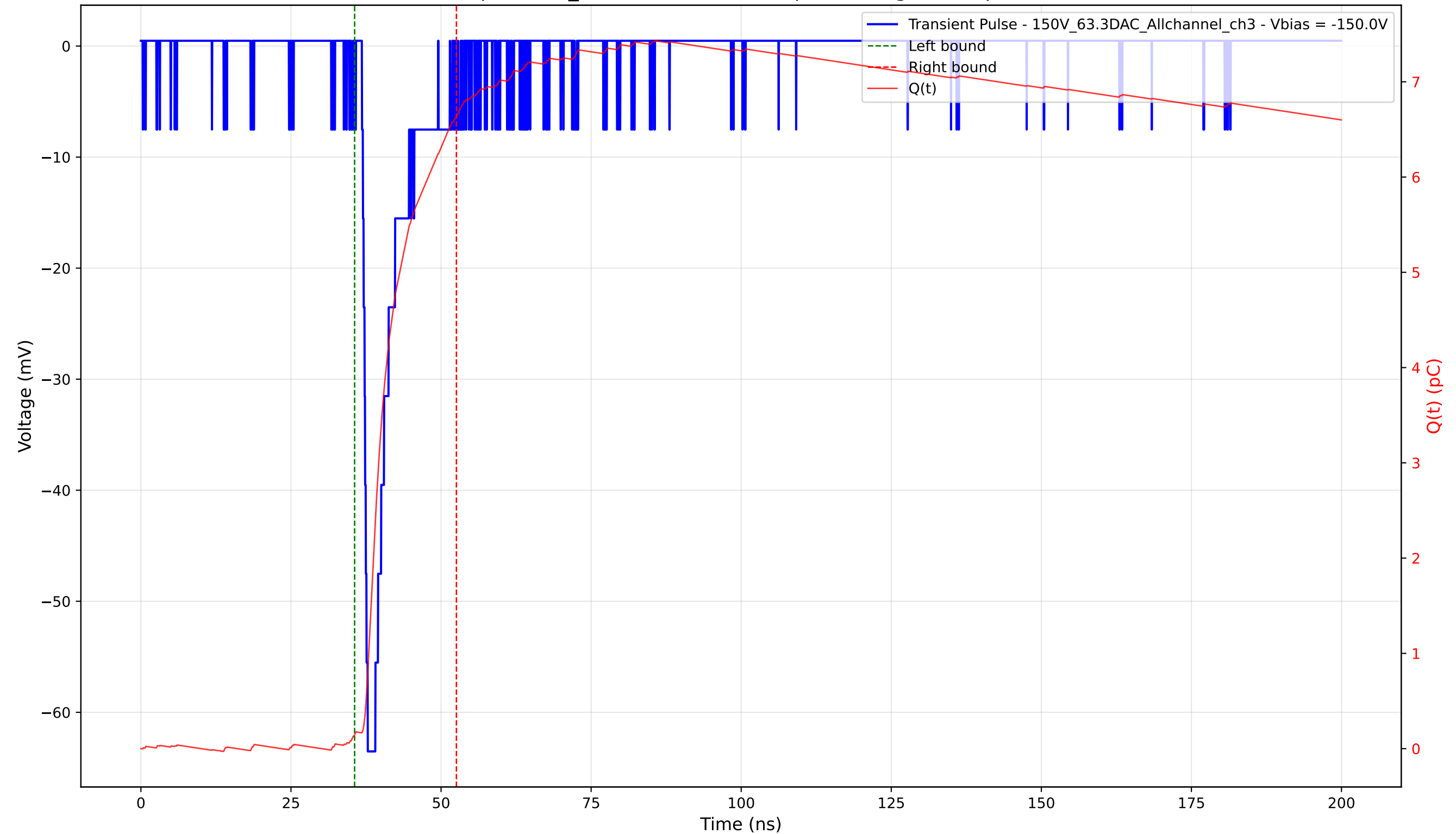
Transient Pulse - Sample: 1cm_42 - Position: 1445.0 \mu\text{m} - Charge: 6.48 pC - Rise Time: 0.97 ns
