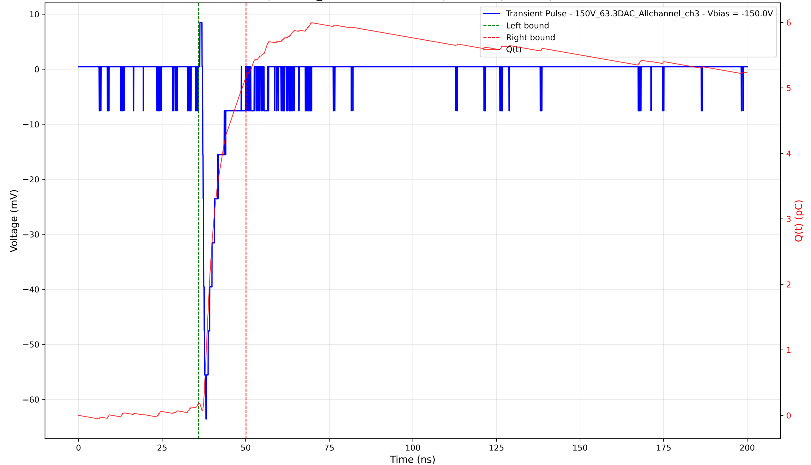
Transient Pulse - Sample: 1cm_42 - Position: 3620.0 \mu\text{m} - Charge: 4.98 pC - Rise Time: 1.01 ns
