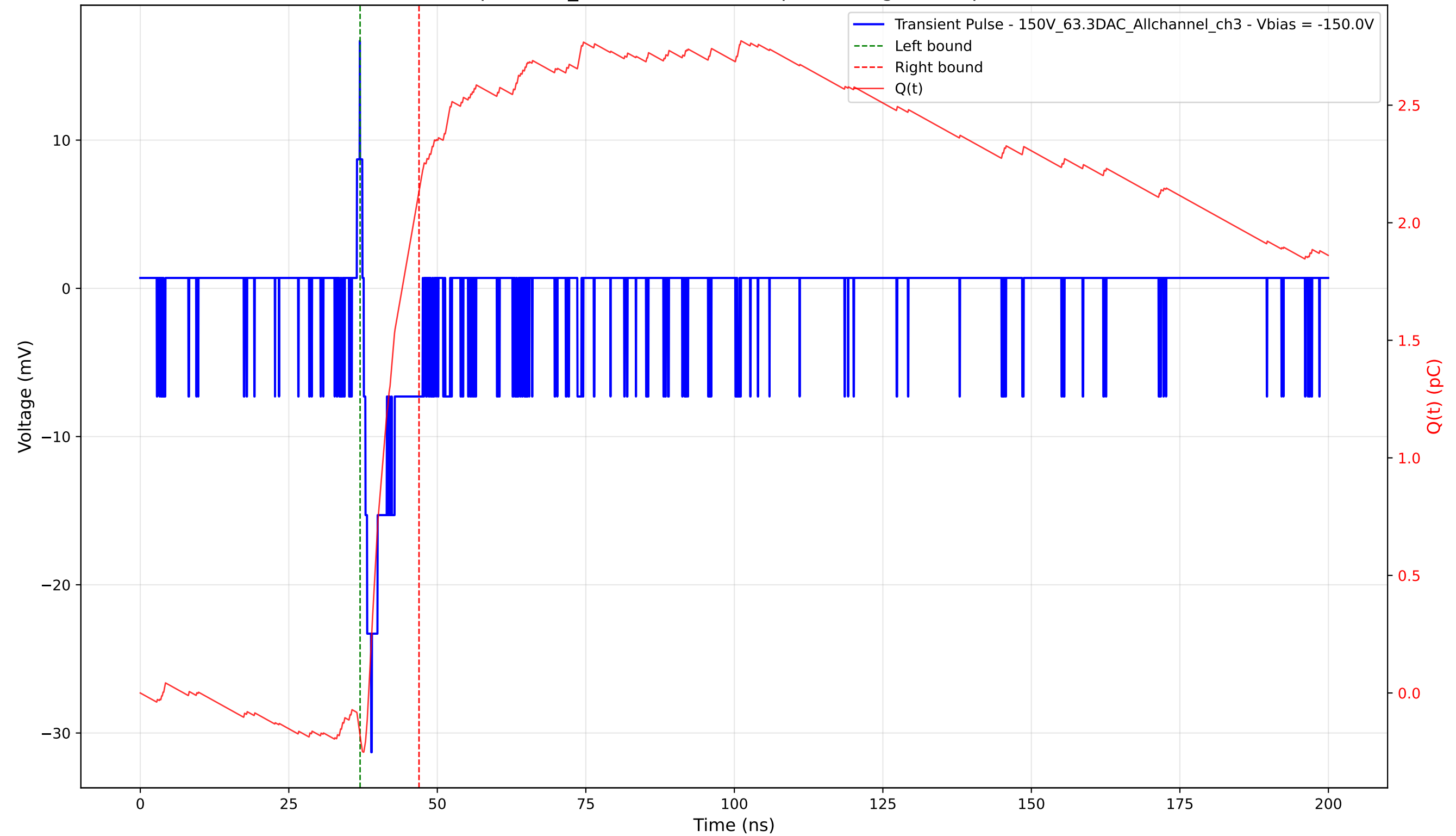
Transient Pulse - Sample: 1cm_42 - Position: 355.0 \mu\text{m} - Charge: 2.32 pC - Rise Time: 1.27 ns
