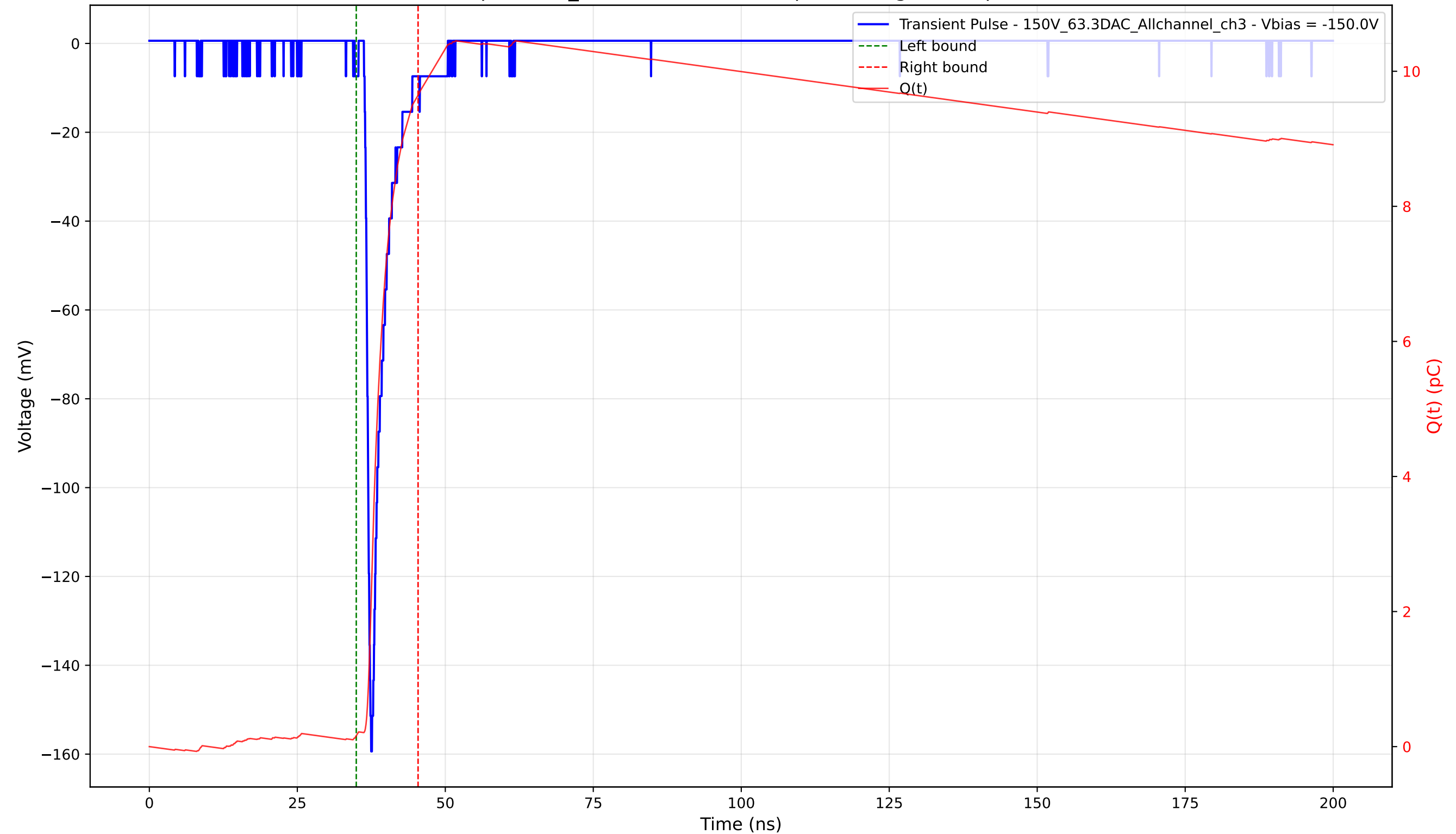
Transient Pulse - Sample: 1cm_42 - Position: 1785.0 \mu\text{m} - Charge: 9.48 pC - Rise Time: 0.92 ns
