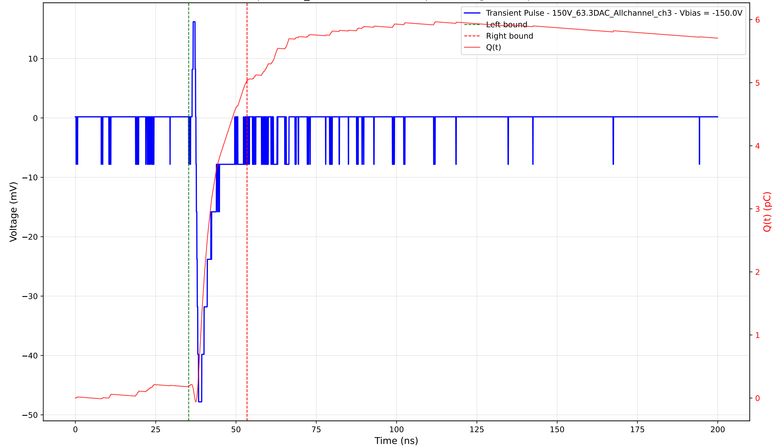
Transient Pulse - Sample: 1cm_42 - Position: 1000.0 \mu\text{m} - Charge: 4.85 pC - Rise Time: 0.82 ns
