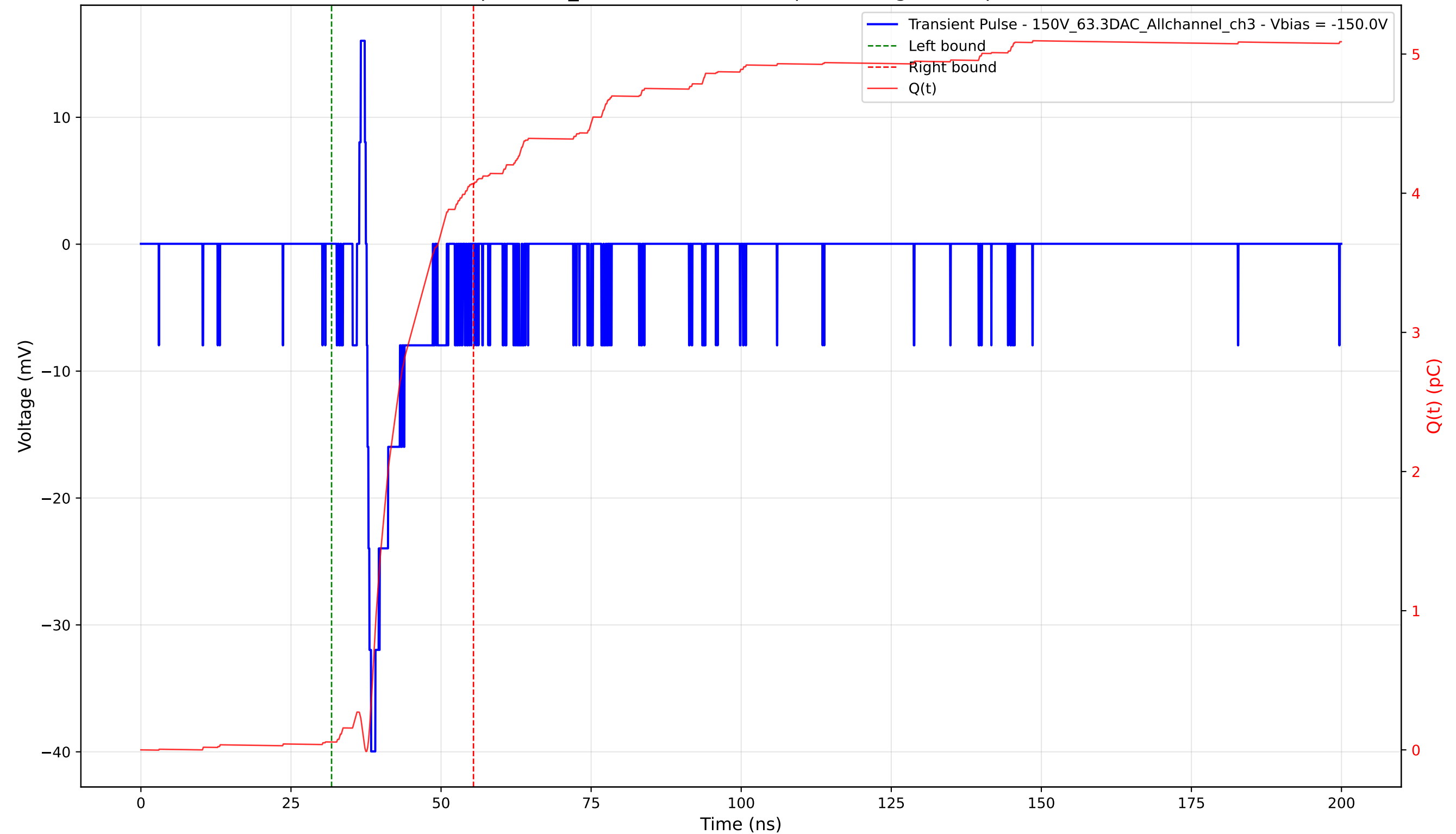
Transient Pulse - Sample: 1cm_42 - Position: 4070.0 \mu\text{m} - Charge: 4.01 pC - Rise Time: 0.74 ns
