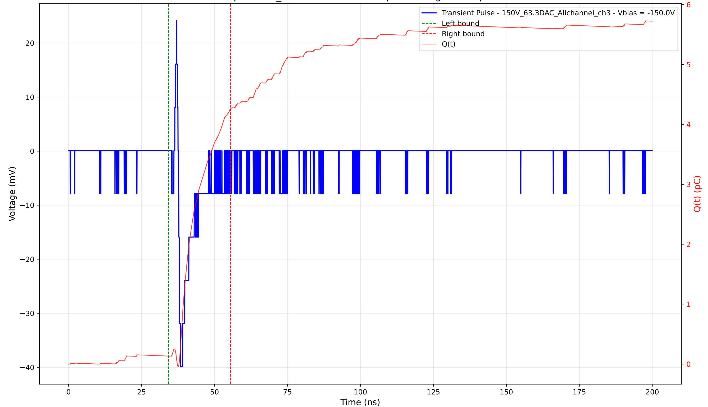
Transient Pulse - Sample: 1cm_42 - Position: 4115.0 \mu\text{m} - Charge: 4.12 pC - Rise Time: 0.78 ns
