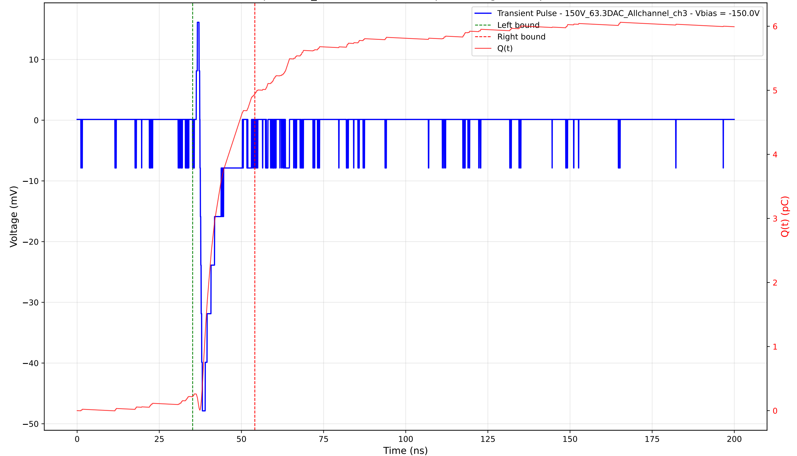
Transient Pulse - Sample: 1cm_42 - Position: 3895.0 \mu\text{m} - Charge: 4.72 pC - Rise Time: 0.74 ns
