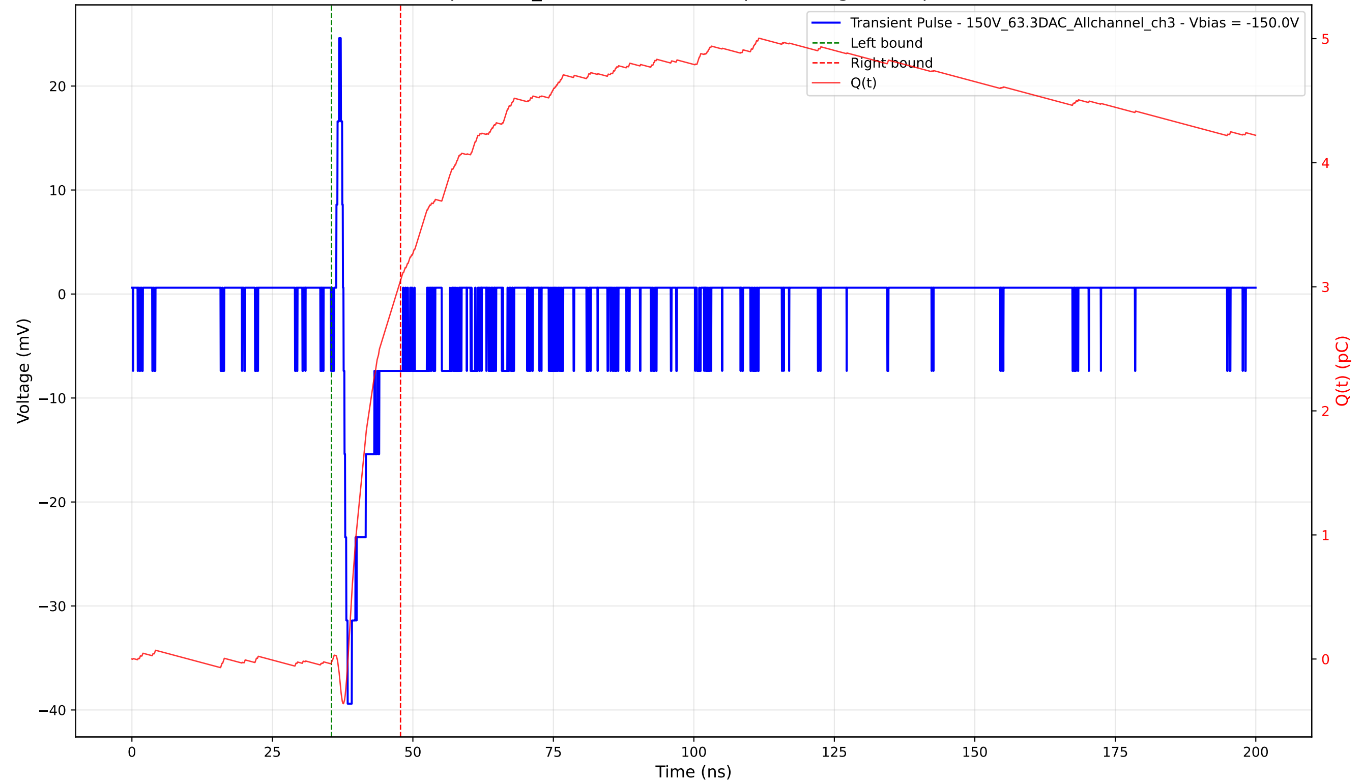
Transient Pulse - Sample: 1cm_42 - Position: 4165.0 \mu\text{m} - Charge: 3.08 pC - Rise Time: 0.74 ns
