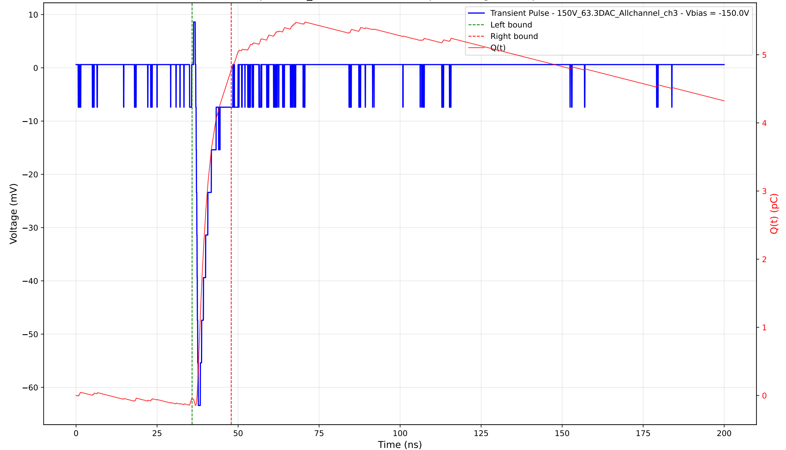
Transient Pulse - Sample: 1cm_42 - Position: 3555.0 \mu\text{m} - Charge: 4.83 pC - Rise Time: 0.77 ns
