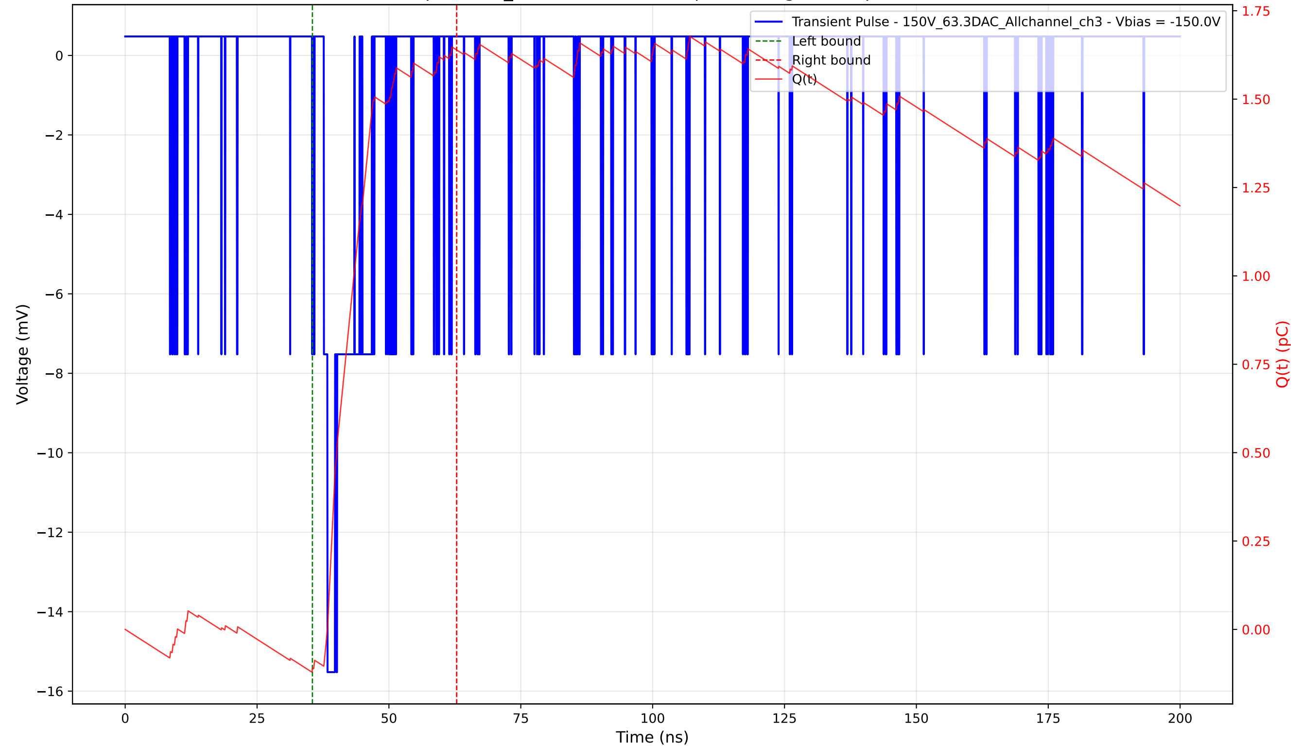
Transient Pulse - Sample: 1cm_42 - Position: 155.0 \mu\text{m} - Charge: 1.75 pC - Rise Time: 0.71 ns
