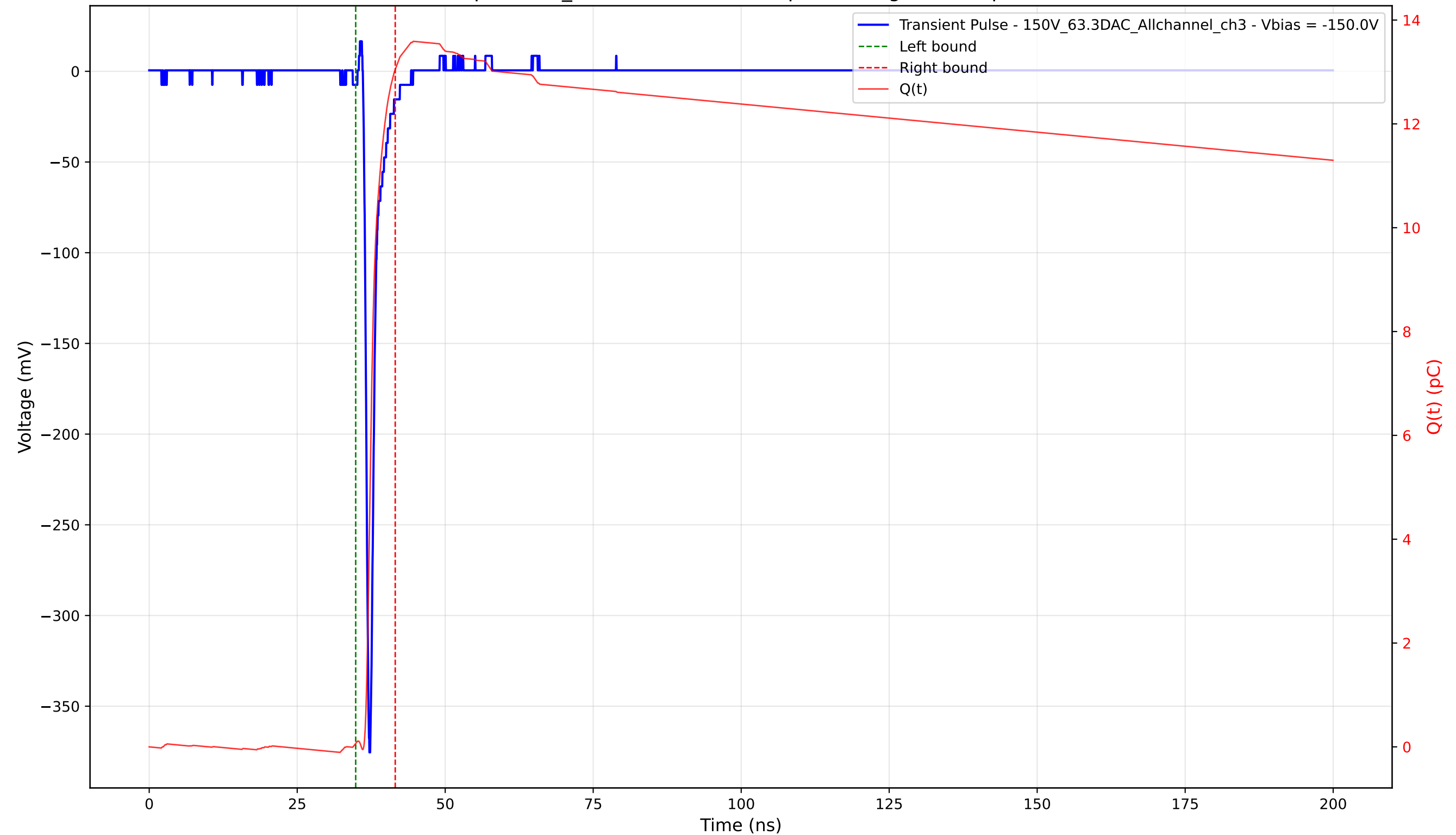
Transient Pulse - Sample: 1cm_42 - Position: 2175.0 \mu\text{m} - Charge: 12.98 pC - Rise Time: 0.72 ns
