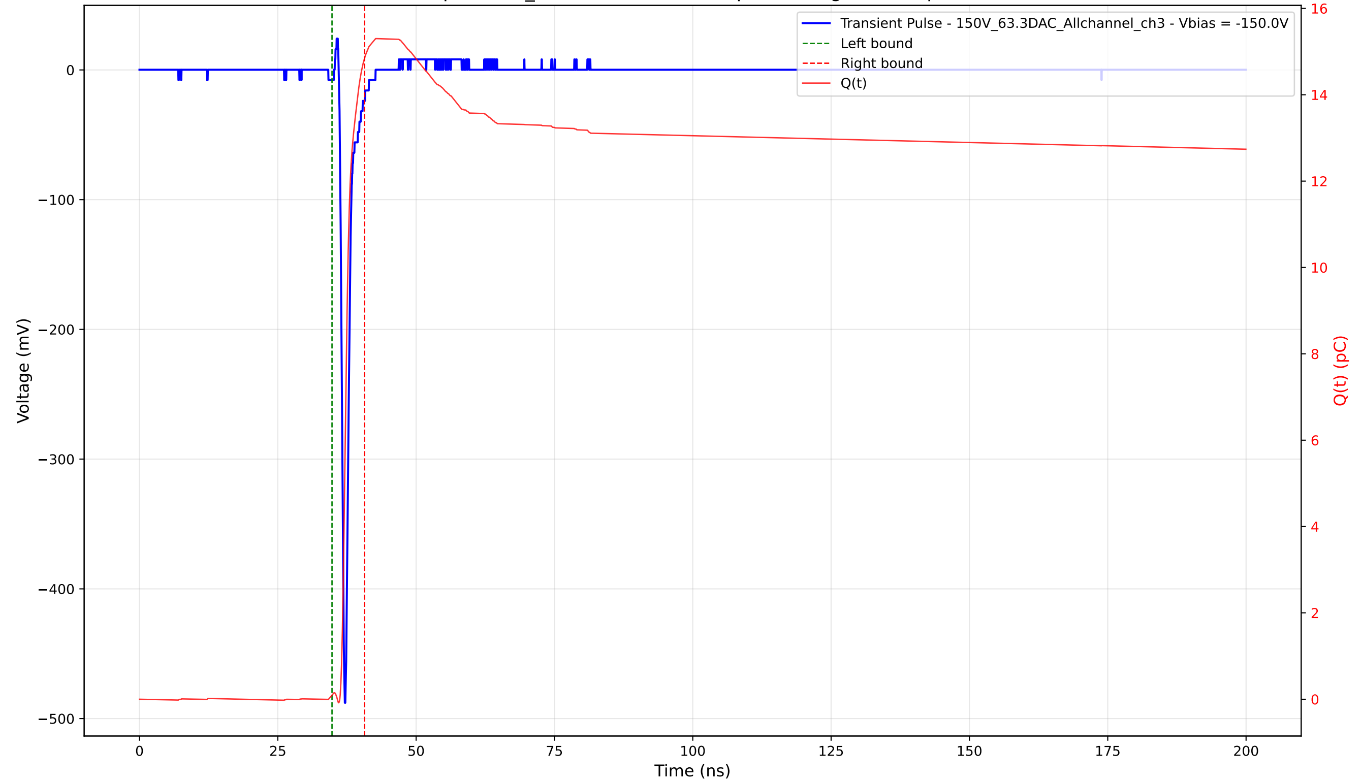
Transient Pulse - Sample: 1cm_42 - Position: 2540.0 \mu\text{m} - Charge: 14.75 pC - Rise Time: 0.72 ns
