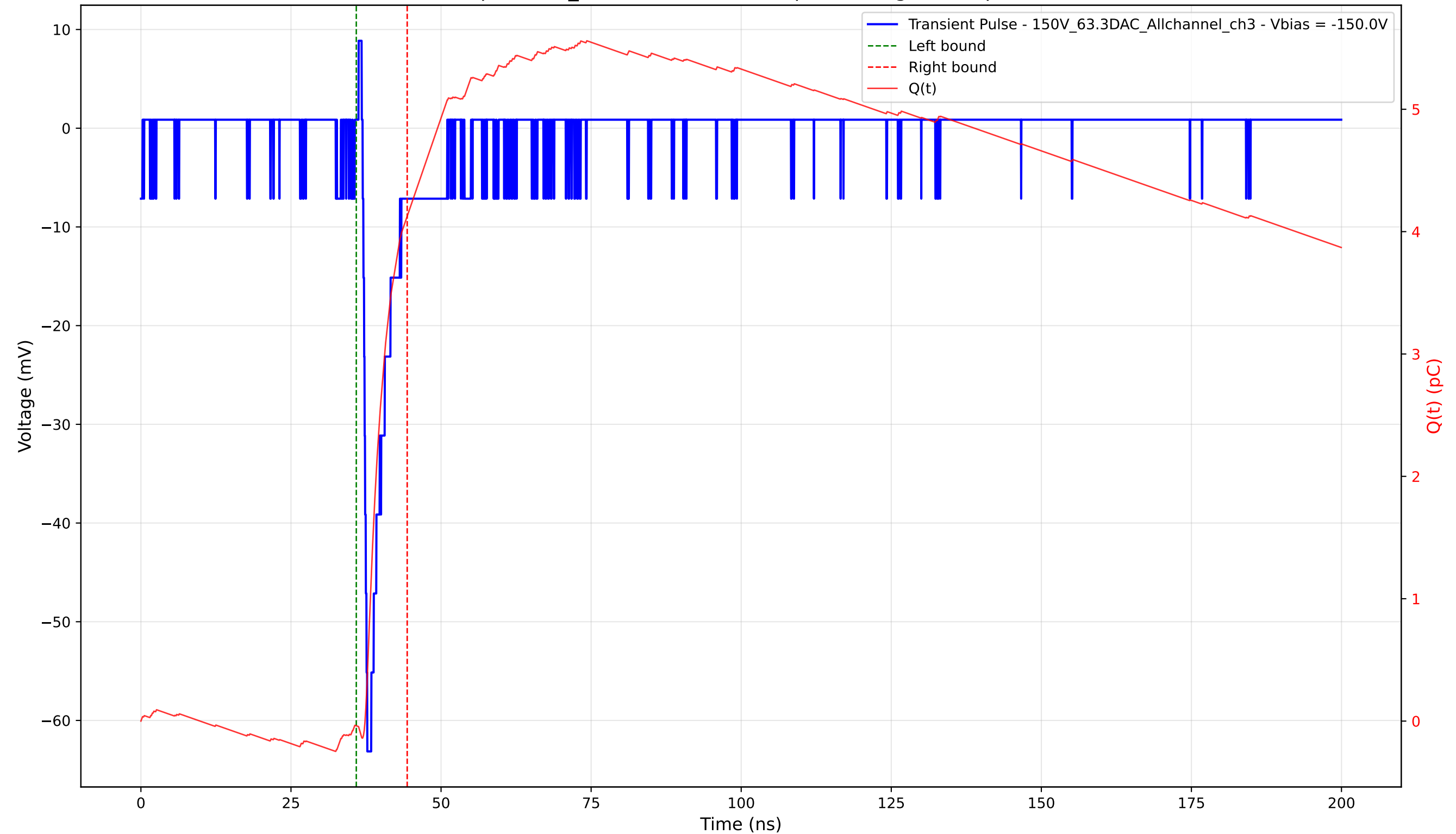
Transient Pulse - Sample: 1cm_42 - Position: 3565.0 \mu\text{m} - Charge: 4.16 pC - Rise Time: 0.77 ns
