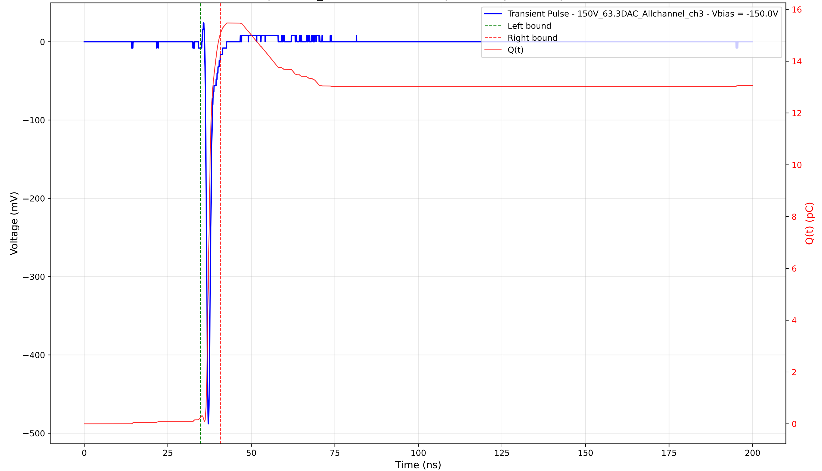
Transient Pulse - Sample: 1cm_42 - Position: 2535.0 \mu\text{m} - Charge: 14.79 pC - Rise Time: 0.72 ns
