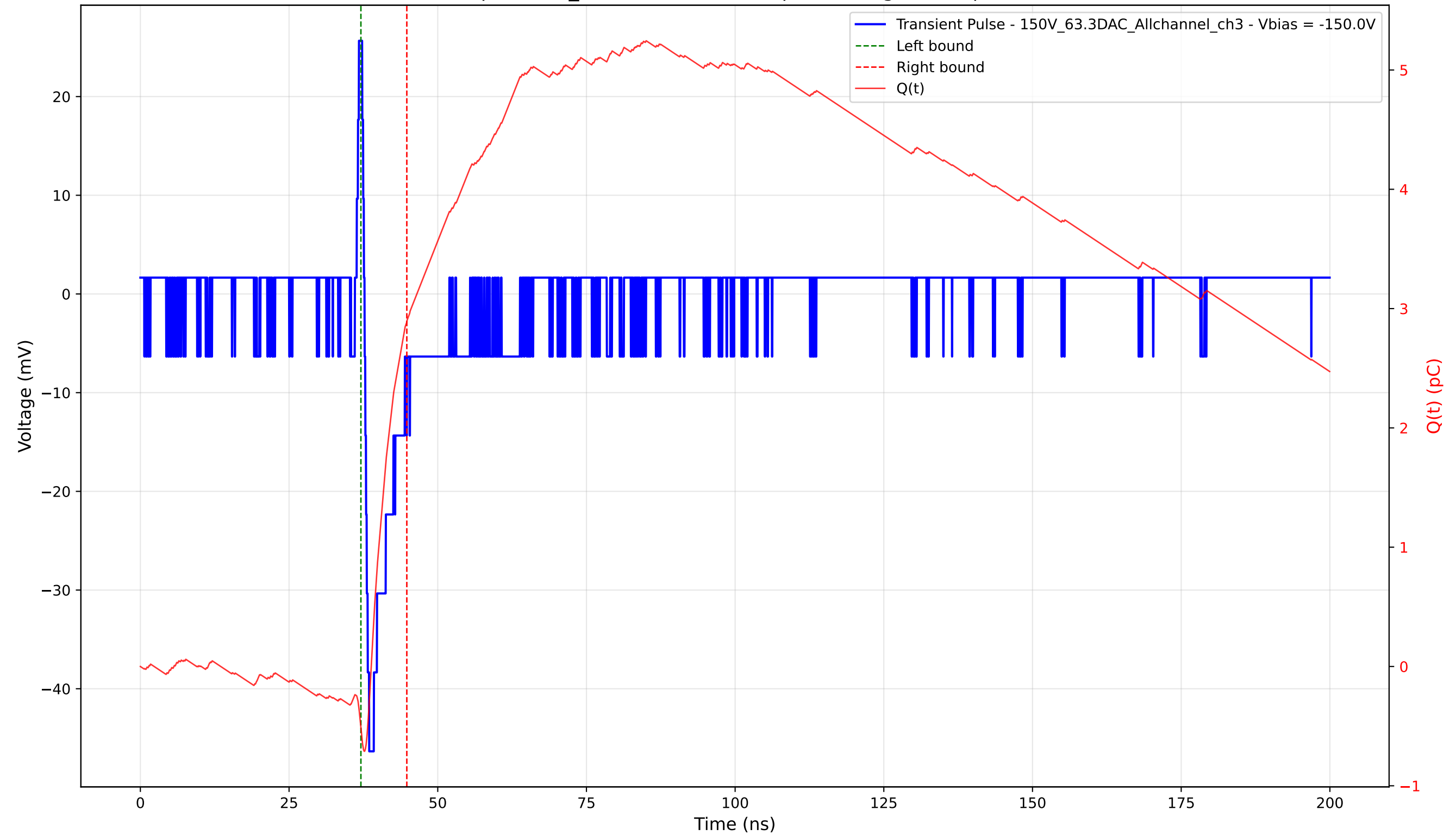
Transient Pulse - Sample: 1cm_42 - Position: 675.0 \mu\text{m} - Charge: 3.41 pC - Rise Time: 0.77 ns
