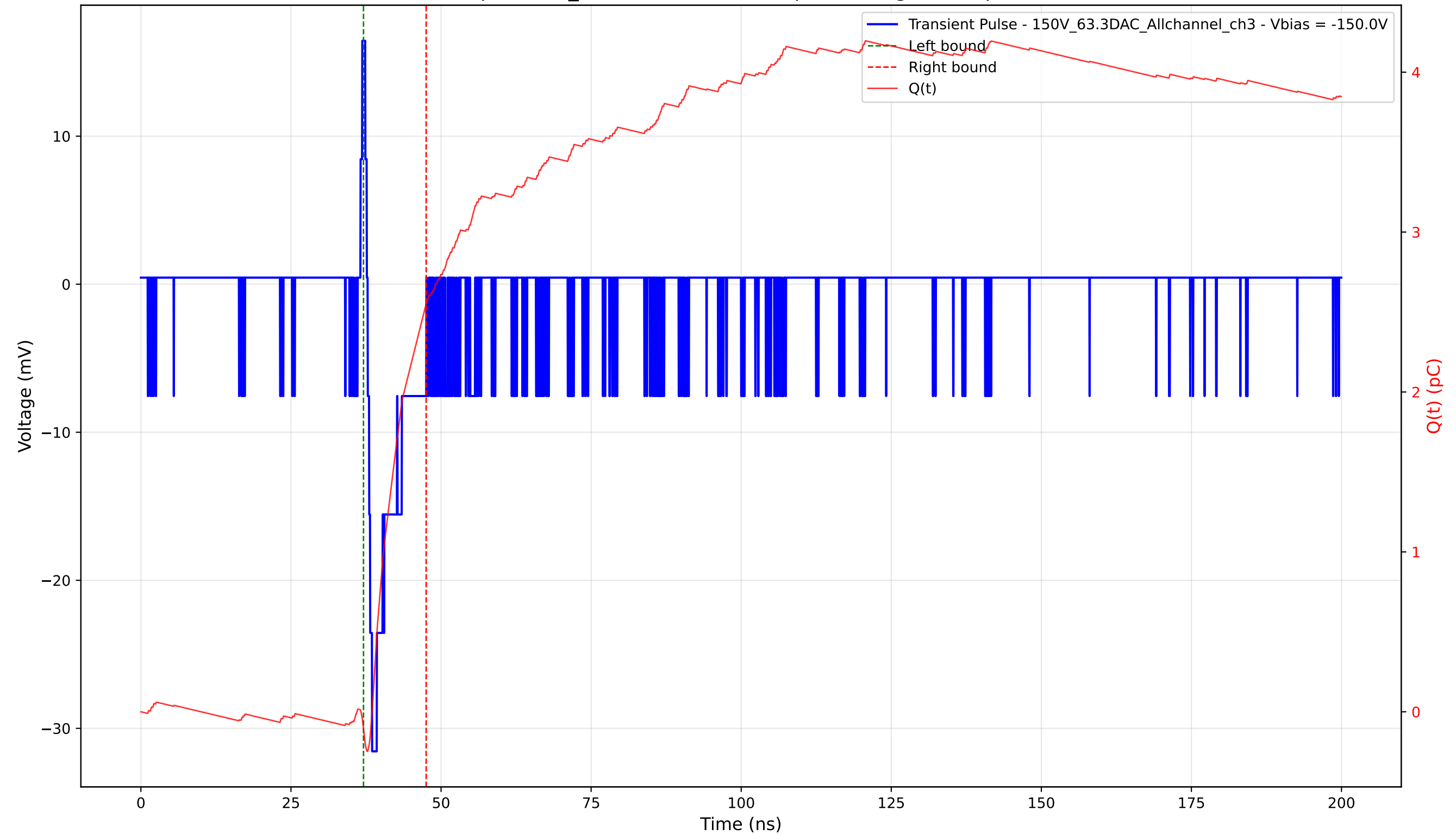
Transient Pulse - Sample: 1cm_42 - Position: 4630.0 \mu\text{m} - Charge: 2.66 pC - Rise Time: 0.74 ns
