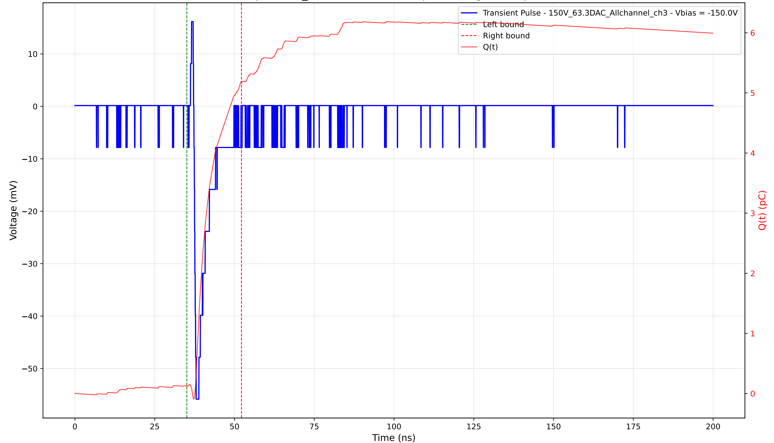
Transient Pulse - Sample: 1cm_42 - Position: 3775.0 \mu\text{m} - Charge: 5.06 pC - Rise Time: 0.69 ns
