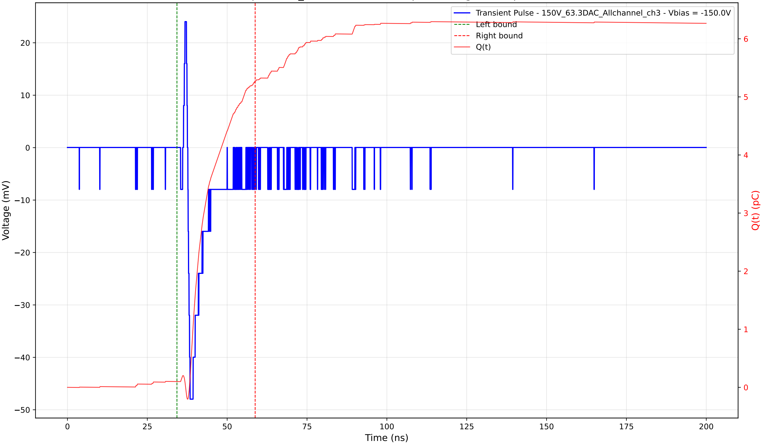
Transient Pulse - Sample: 1cm_42 - Position: 860.0 \mu\text{m} - Charge: 5.17 pC - Rise Time: 0.70 ns
