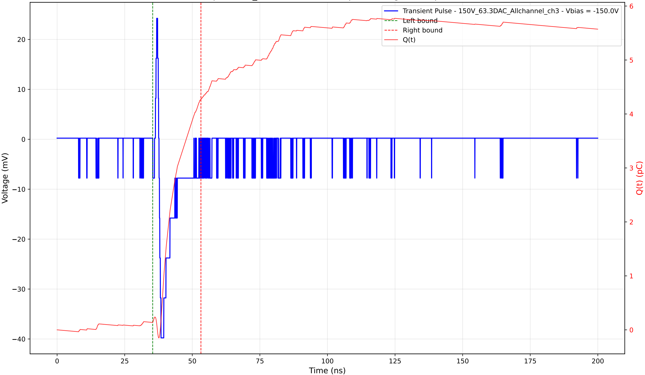
Transient Pulse - Sample: 1cm_42 - Position: 570.0 \mu\text{m} - Charge: 4.14 pC - Rise Time: 0.74 ns
