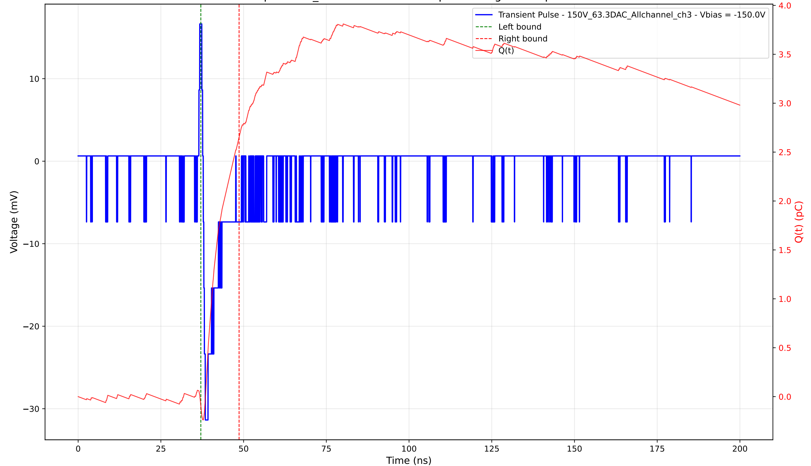
Transient Pulse - Sample: 1cm_42 - Position: 4495.0 \mu\text{m} - Charge: 2.75 pC - Rise Time: 0.63 ns
