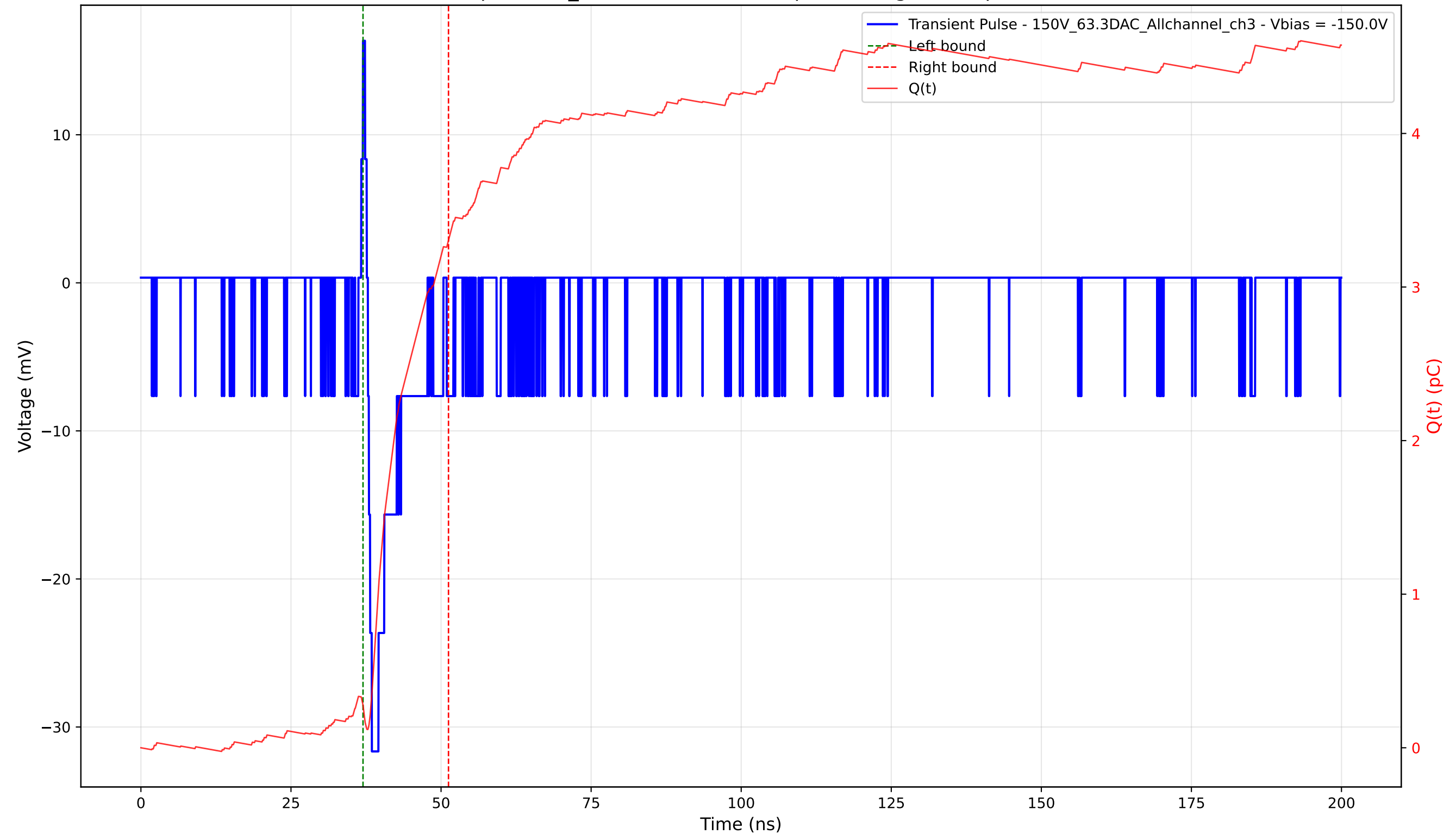
Transient Pulse - Sample: 1cm_42 - Position: 4780.0 \mu\text{m} - Charge: 3.03 pC - Rise Time: 0.66 ns
