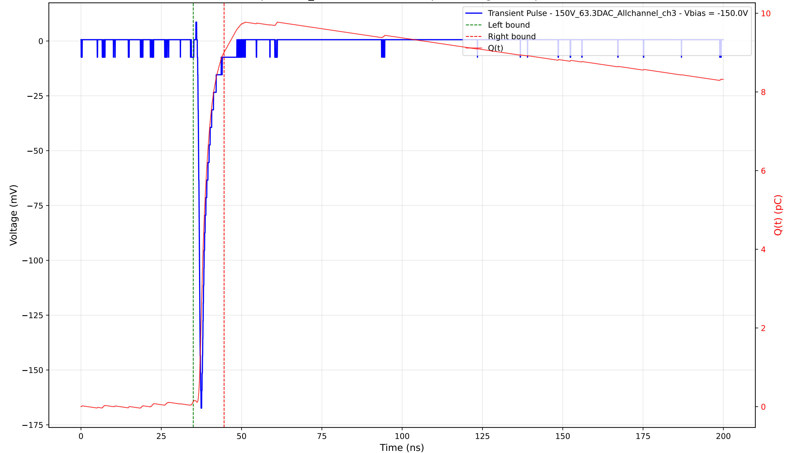
Transient Pulse - Sample: 1cm_42 - Position: 1880.0 \mu\text{m} - Charge: 8.88 pC - Rise Time: 0.79 ns
