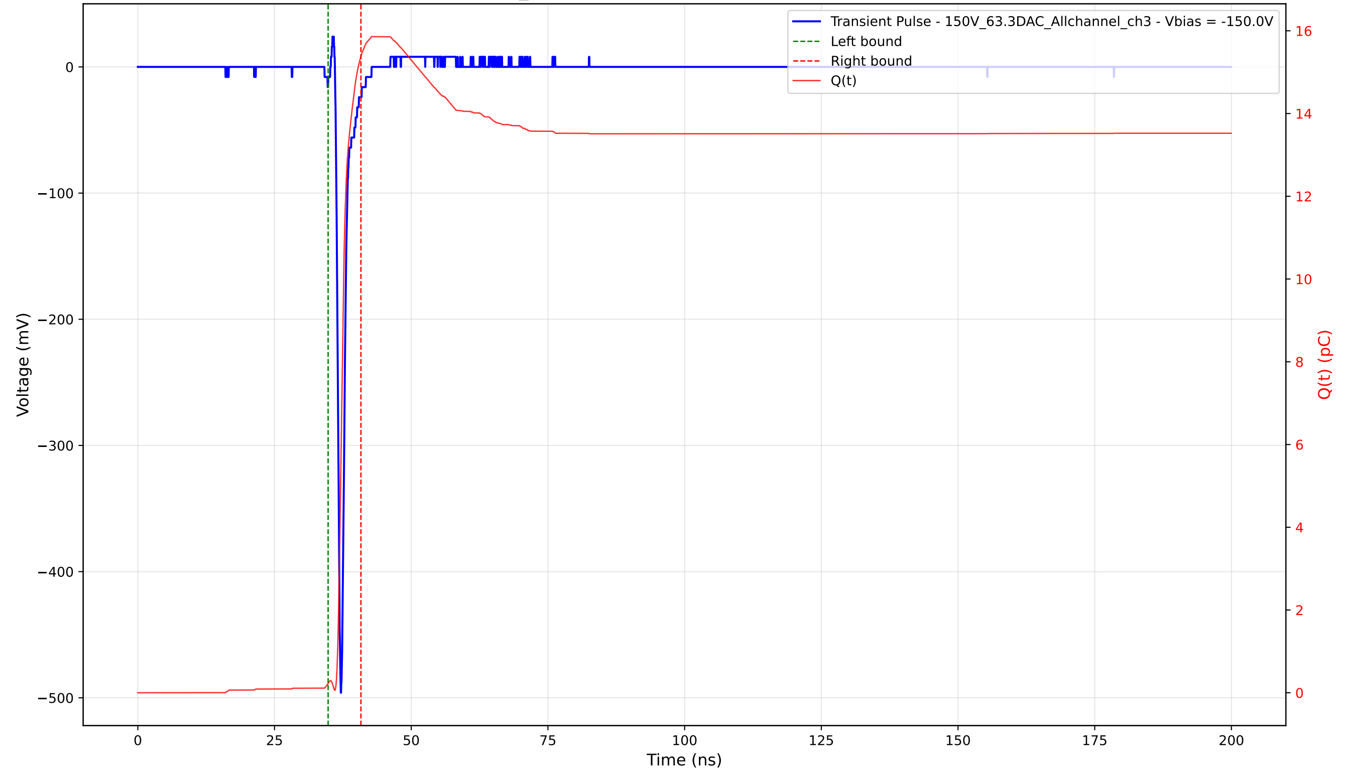
Transient Pulse - Sample: 1cm_42 - Position: 2580.0 \mu\text{m} - Charge: 15.15 pC - Rise Time: 0.71 ns
