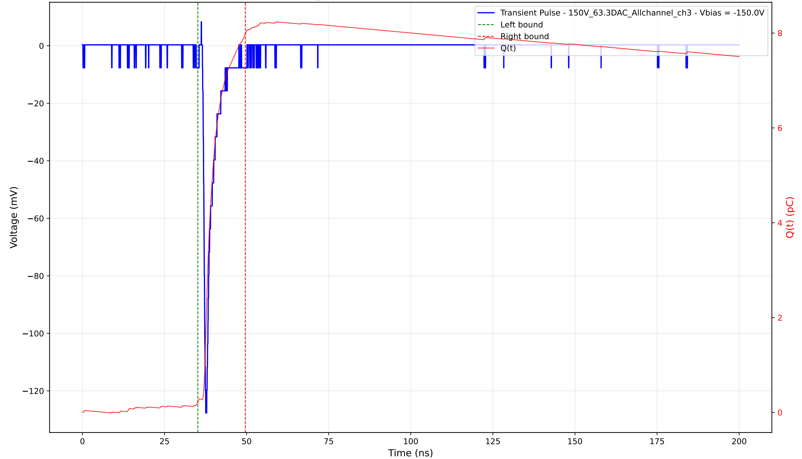
Transient Pulse - Sample: 1cm_42 - Position: 3330.0 \mu\text{m} - Charge: 7.75 pC - Rise Time: 0.81 ns
