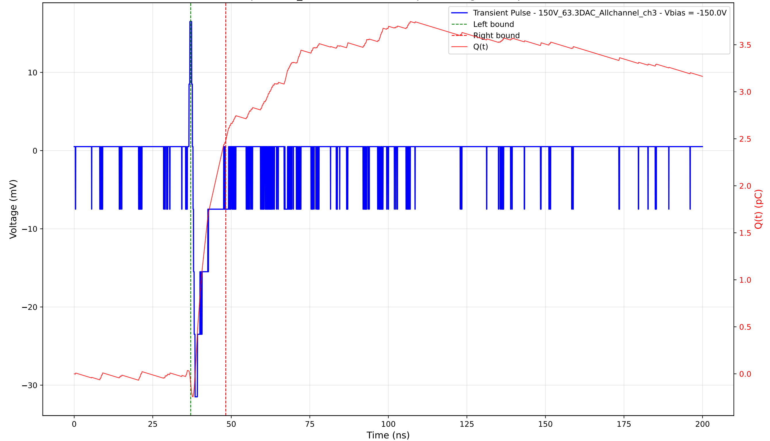
Transient Pulse - Sample: 1cm_42 - Position: 4560.0 \mu\text{m} - Charge: 2.58 pC - Rise Time: 0.66 ns
