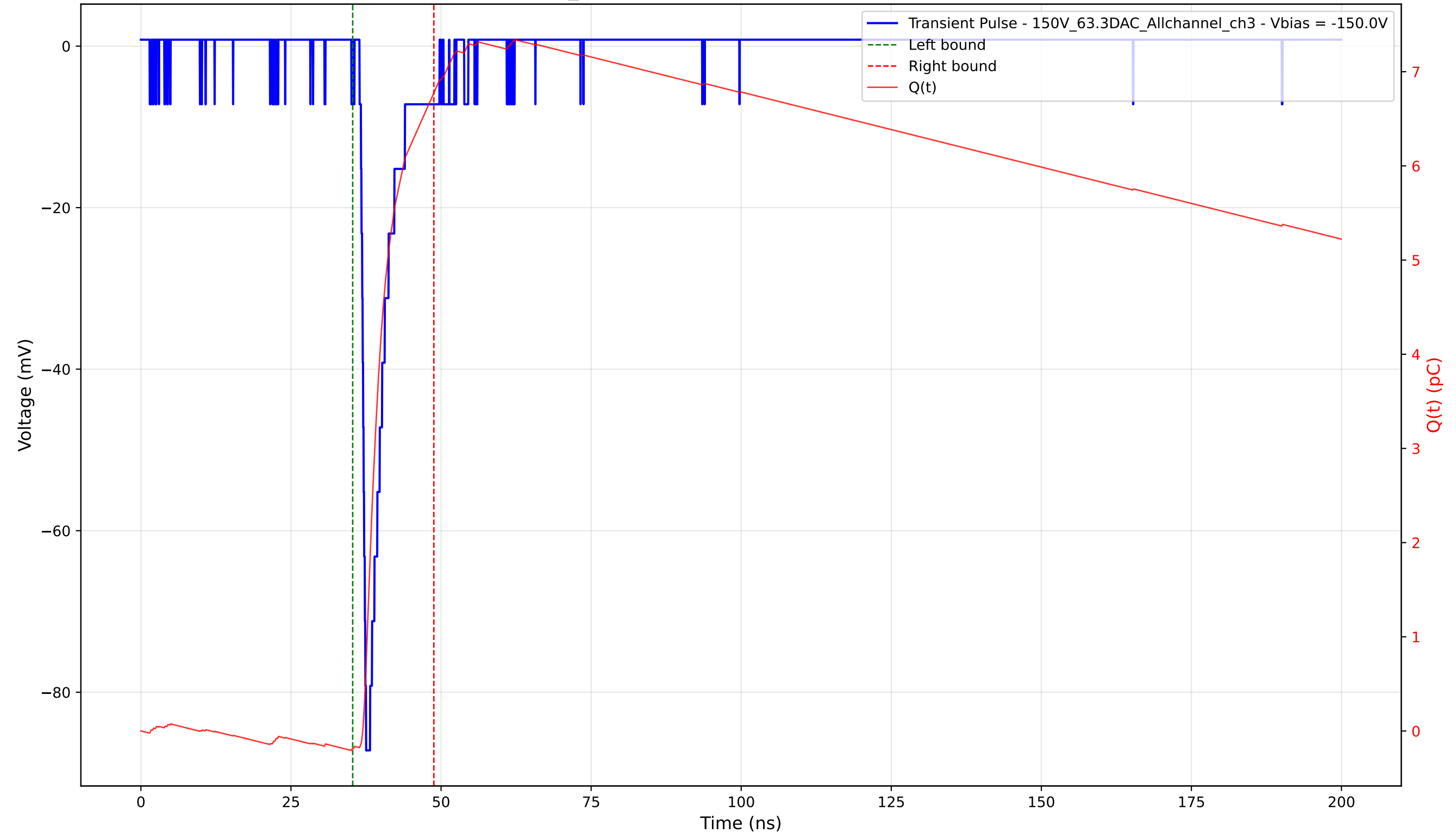
Transient Pulse - Sample: 1cm_42 - Position: 1575.0 \mu\text{m} - Charge: 6.96 pC - Rise Time: 0.75 ns
