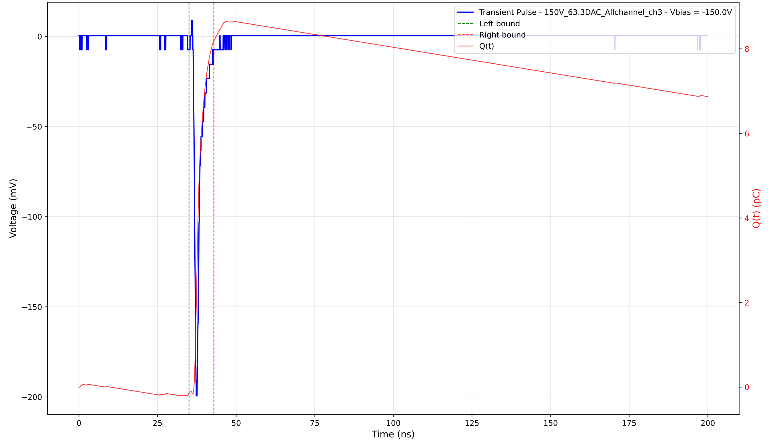
Transient Pulse - Sample: 1cm_42 - Position: 3055.0 \mu\text{m} - Charge: 8.33 pC - Rise Time: 0.78 ns
