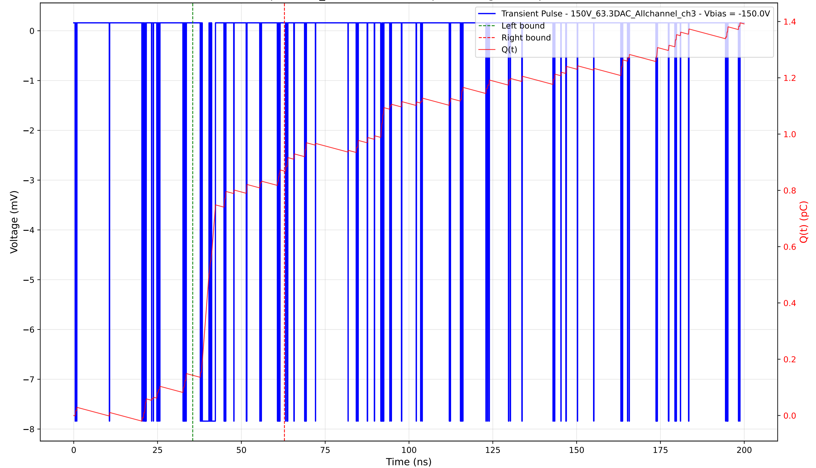
Transient Pulse - Sample: 1cm_42 - Position: 45.0 \mu\text{m} - Charge: 0.73 pC - Rise Time: 0.04 ns
