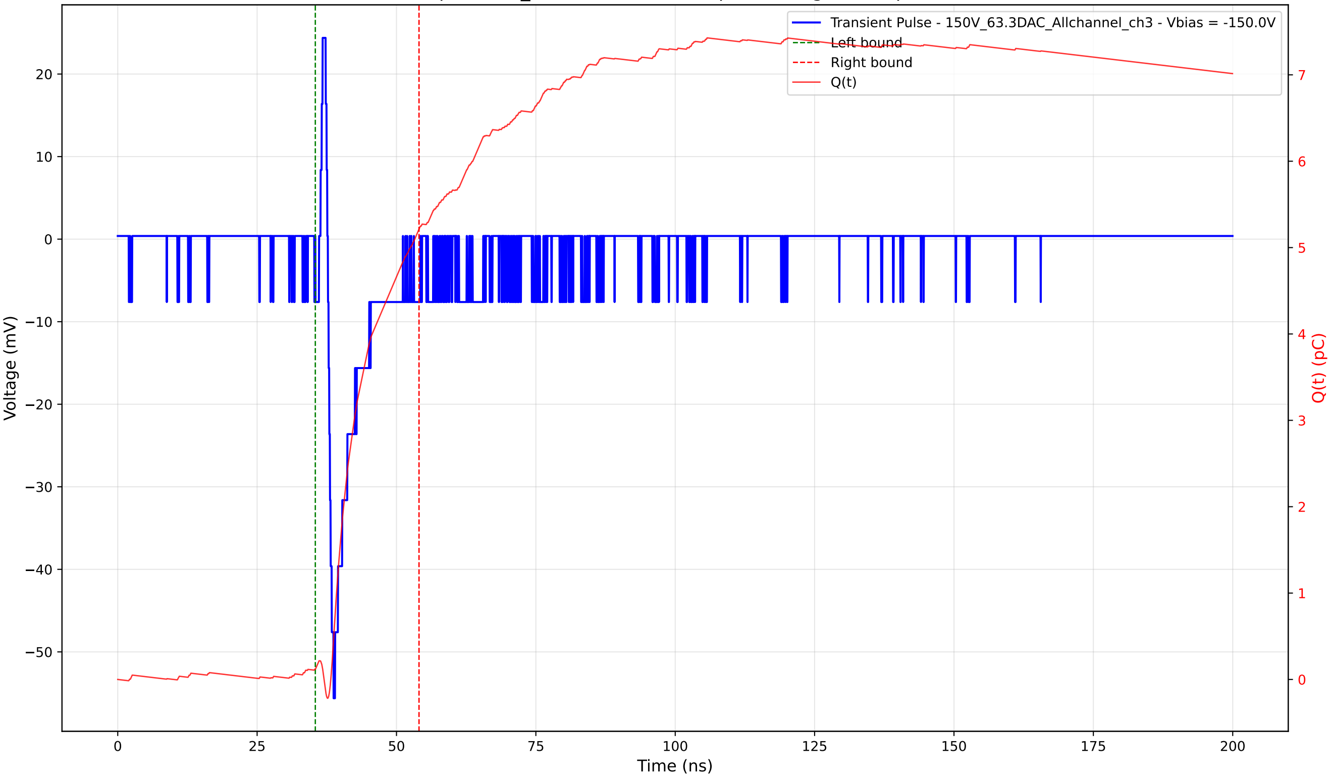
Transient Pulse - Sample: 1cm_42 - Position: 730.0 \mu\text{m} - Charge: 5.10 pC - Rise Time: 1.01 ns
