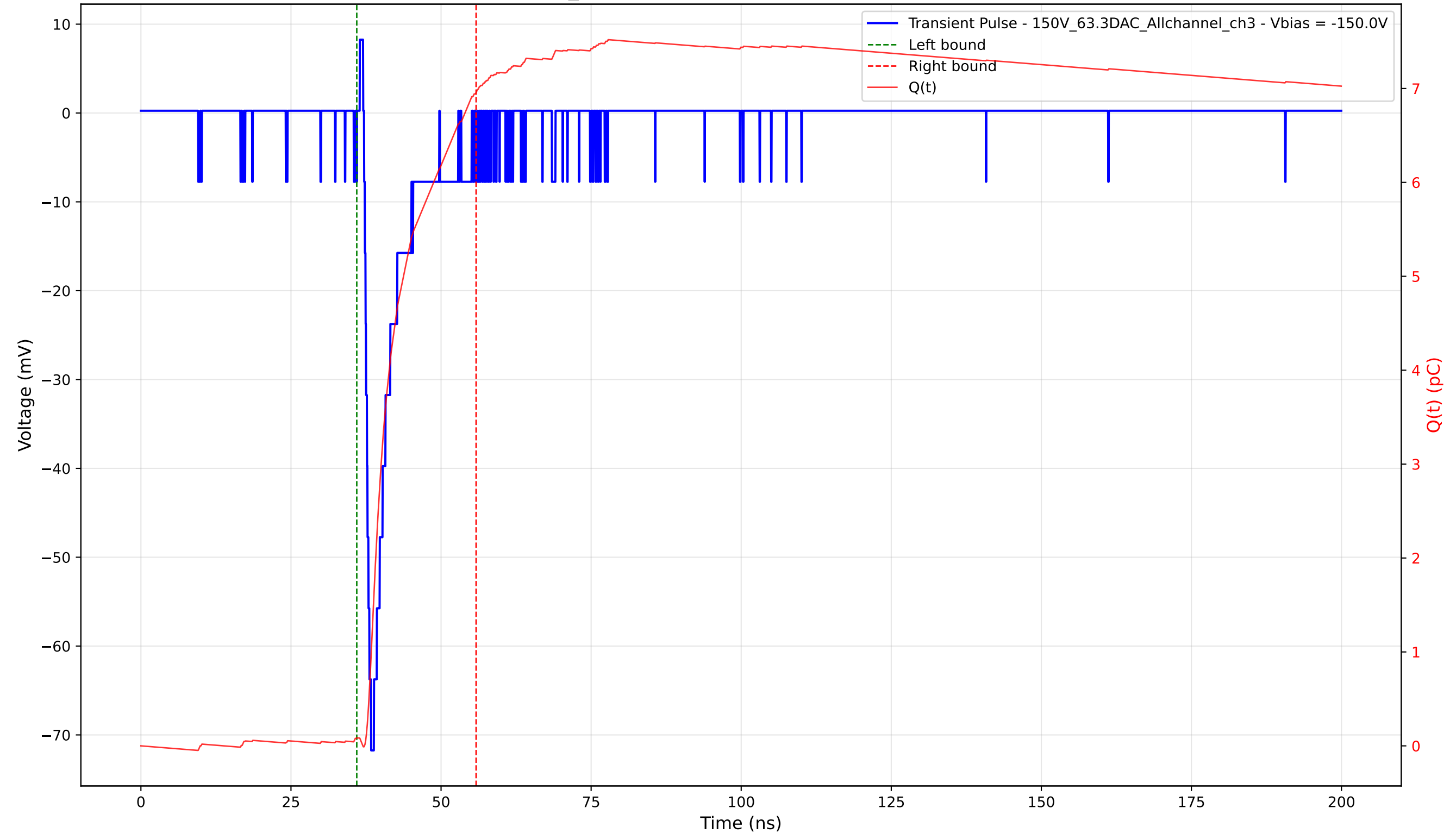
Transient Pulse - Sample: 1cm_42 - Position: 1295.0 \mu\text{m} - Charge: 6.87 pC - Rise Time: 1.16 ns
