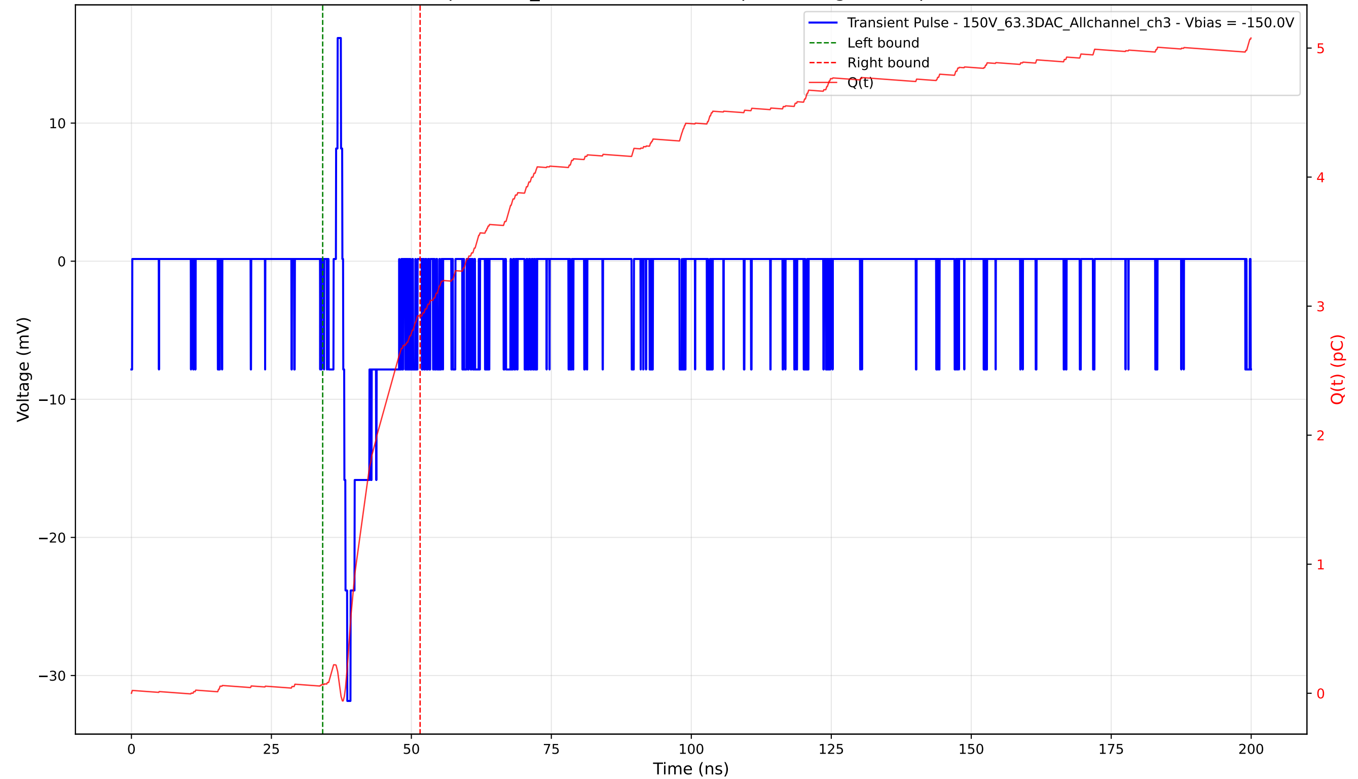
Transient Pulse - Sample: 1cm_42 - Position: 4570.0 \mu\text{m} - Charge: 2.86 pC - Rise Time: 0.74 ns
