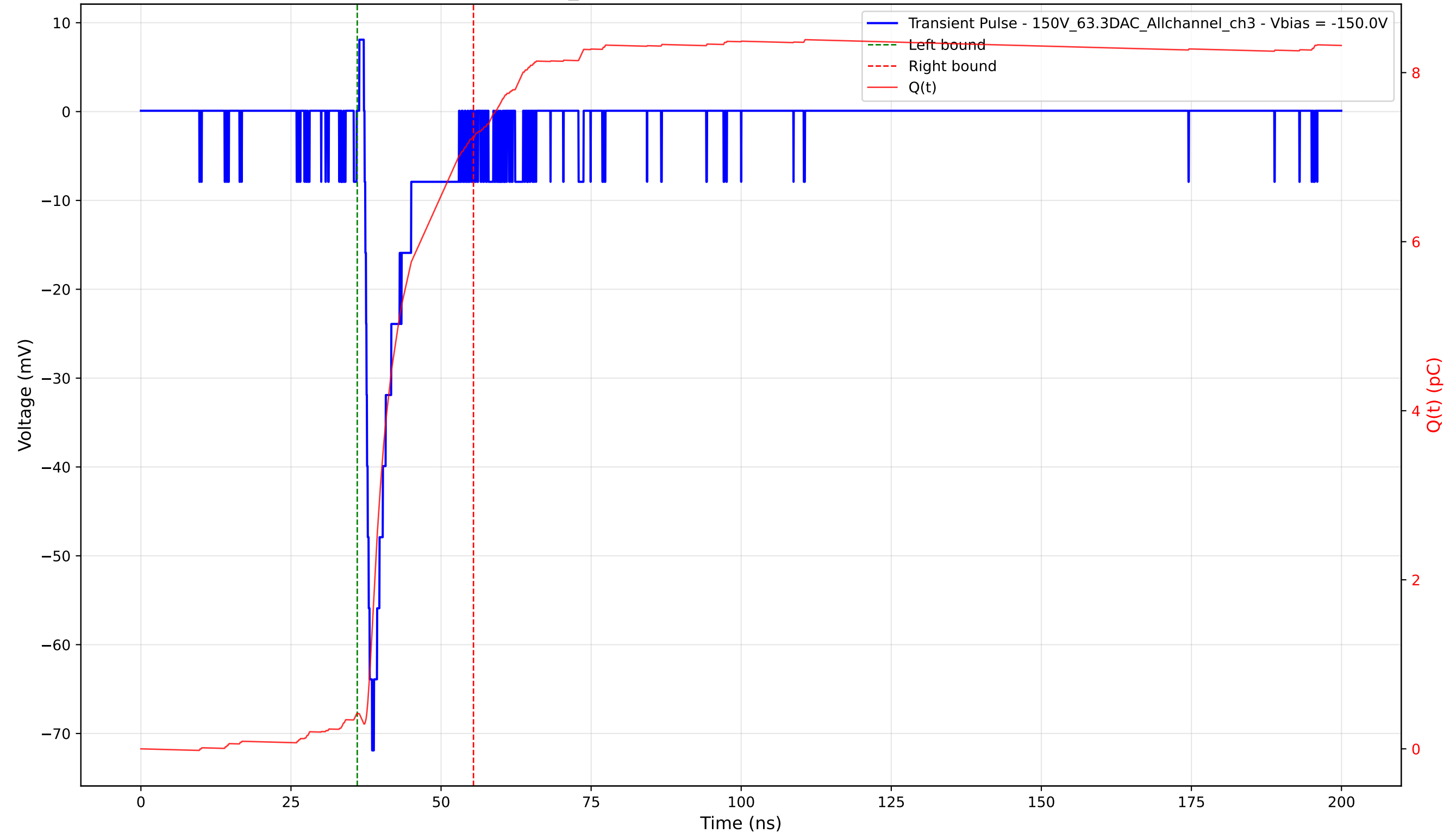
Transient Pulse - Sample: 1cm_42 - Position: 1230.0 \mu\text{m} - Charge: 6.82 pC - Rise Time: 1.24 ns
