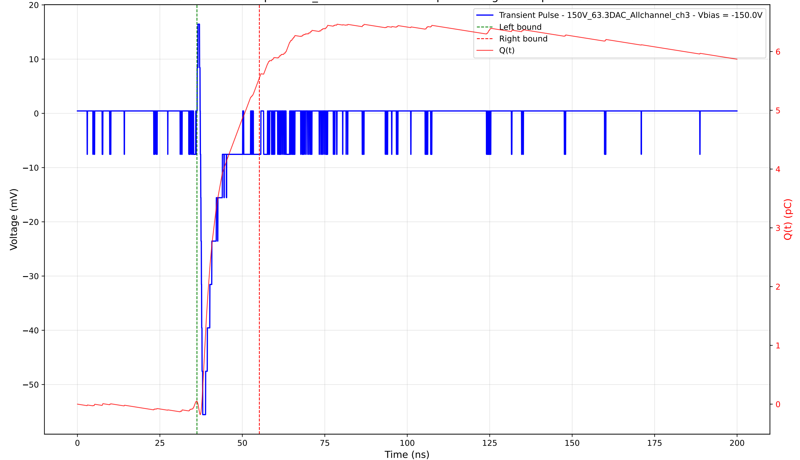
Transient Pulse - Sample: 1cm_42 - Position: 3745.0 \mu\text{m} - Charge: 5.50 pC - Rise Time: 0.73 ns
