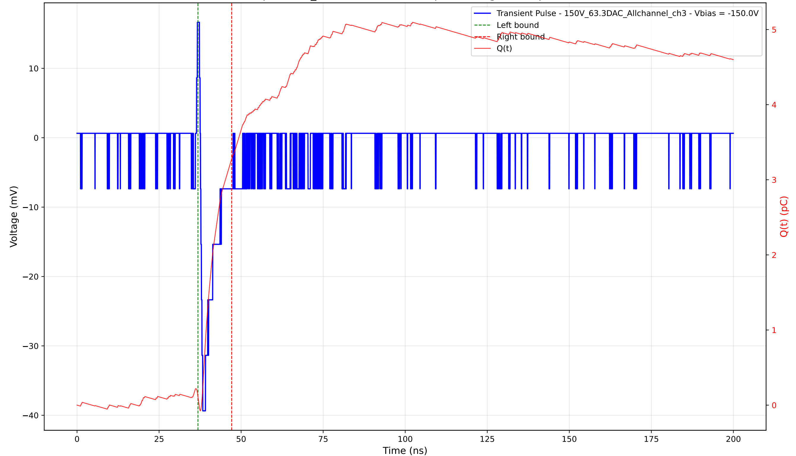
Transient Pulse - Sample: 1cm_42 - Position: 4095.0 \mu\text{m} - Charge: 3.17 pC - Rise Time: 0.70 ns
