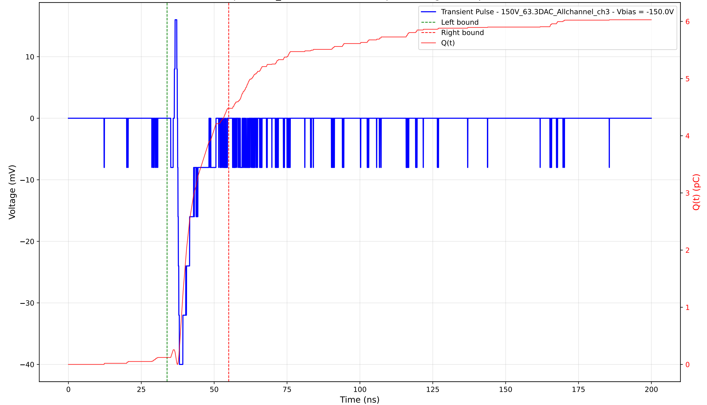
Transient Pulse - Sample: 1cm_42 - Position: 3955.0 \mu\text{m} - Charge: 4.36 pC - Rise Time: 0.62 ns
