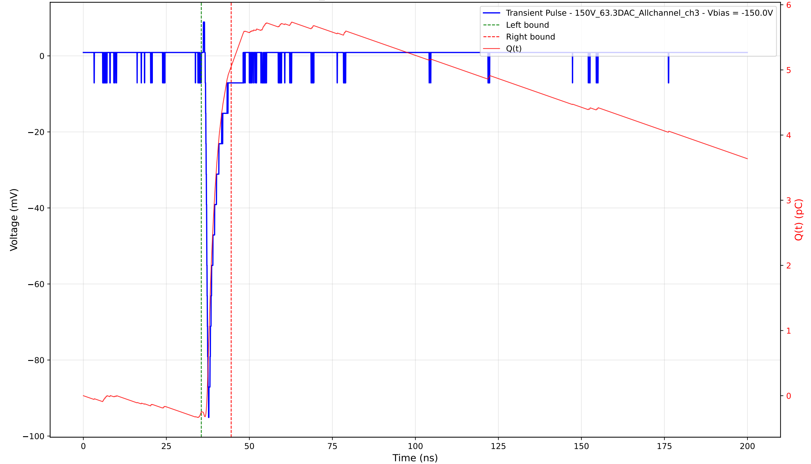
Transient Pulse - Sample: 1cm_42 - Position: 3445.0 \mu\text{m} - Charge: 5.30 pC - Rise Time: 0.75 ns
