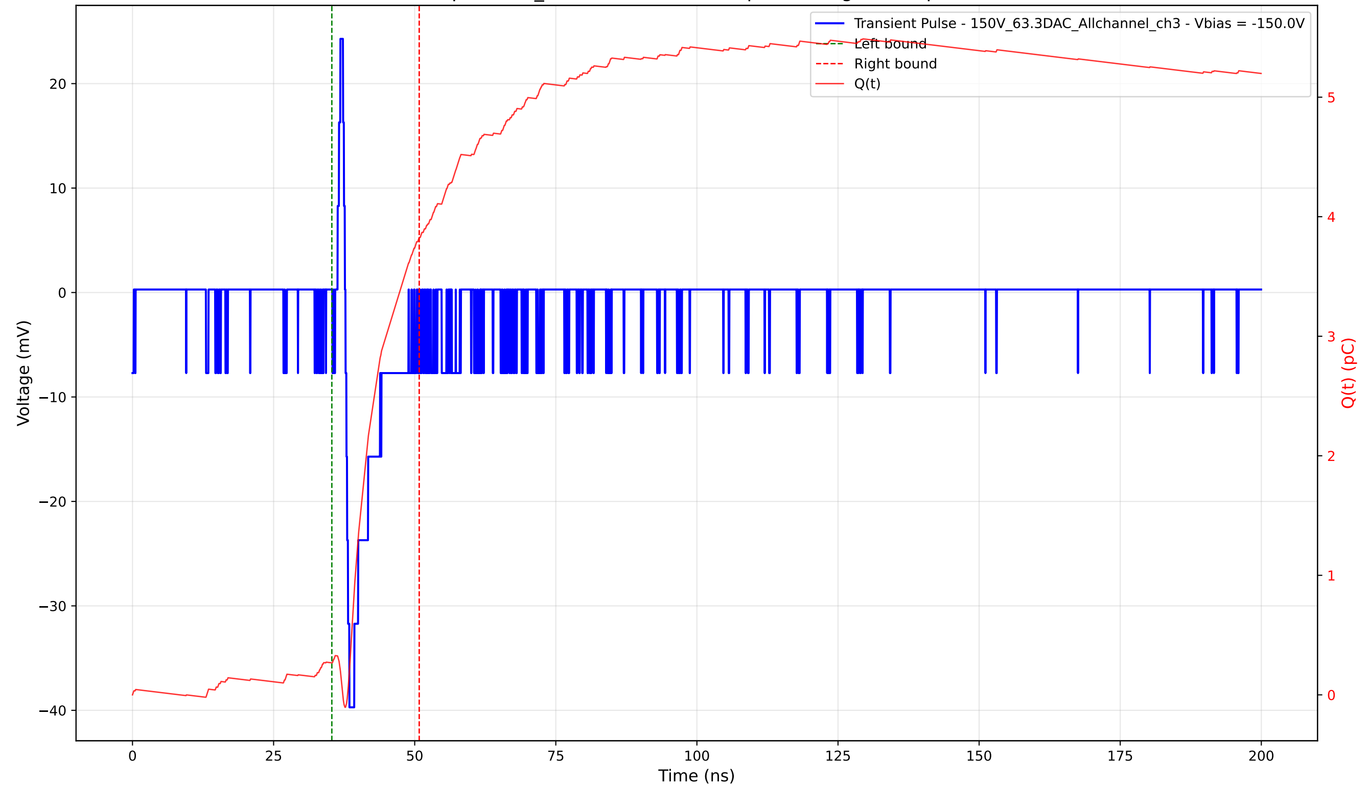
Transient Pulse - Sample: 1cm_42 - Position: 4315.0 \mu\text{m} - Charge: 3.56 pC - Rise Time: 0.70 ns
