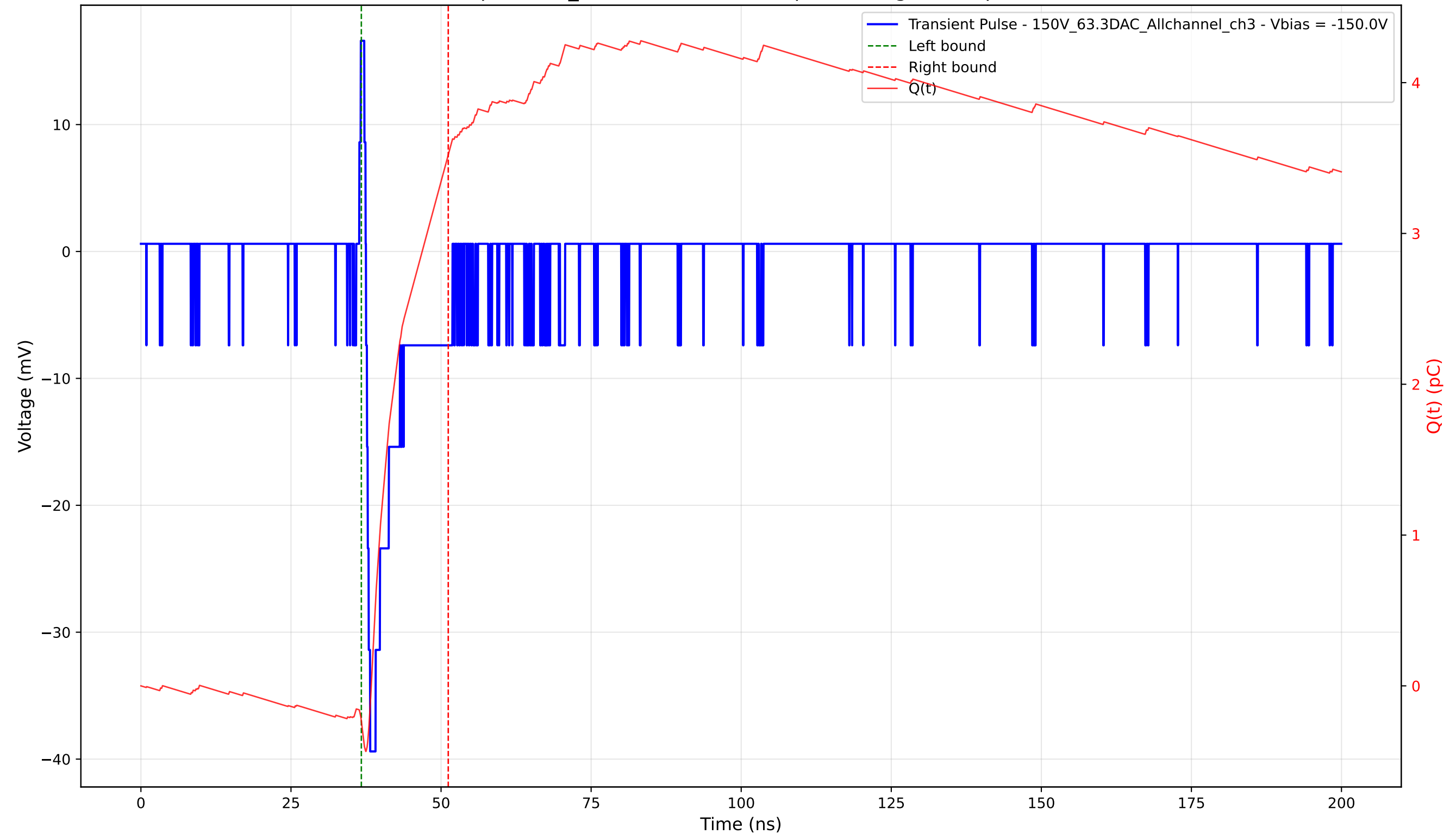
Transient Pulse - Sample: 1cm_42 - Position: 4005.0 \mu\text{m} - Charge: 3.76 pC - Rise Time: 0.70 ns
