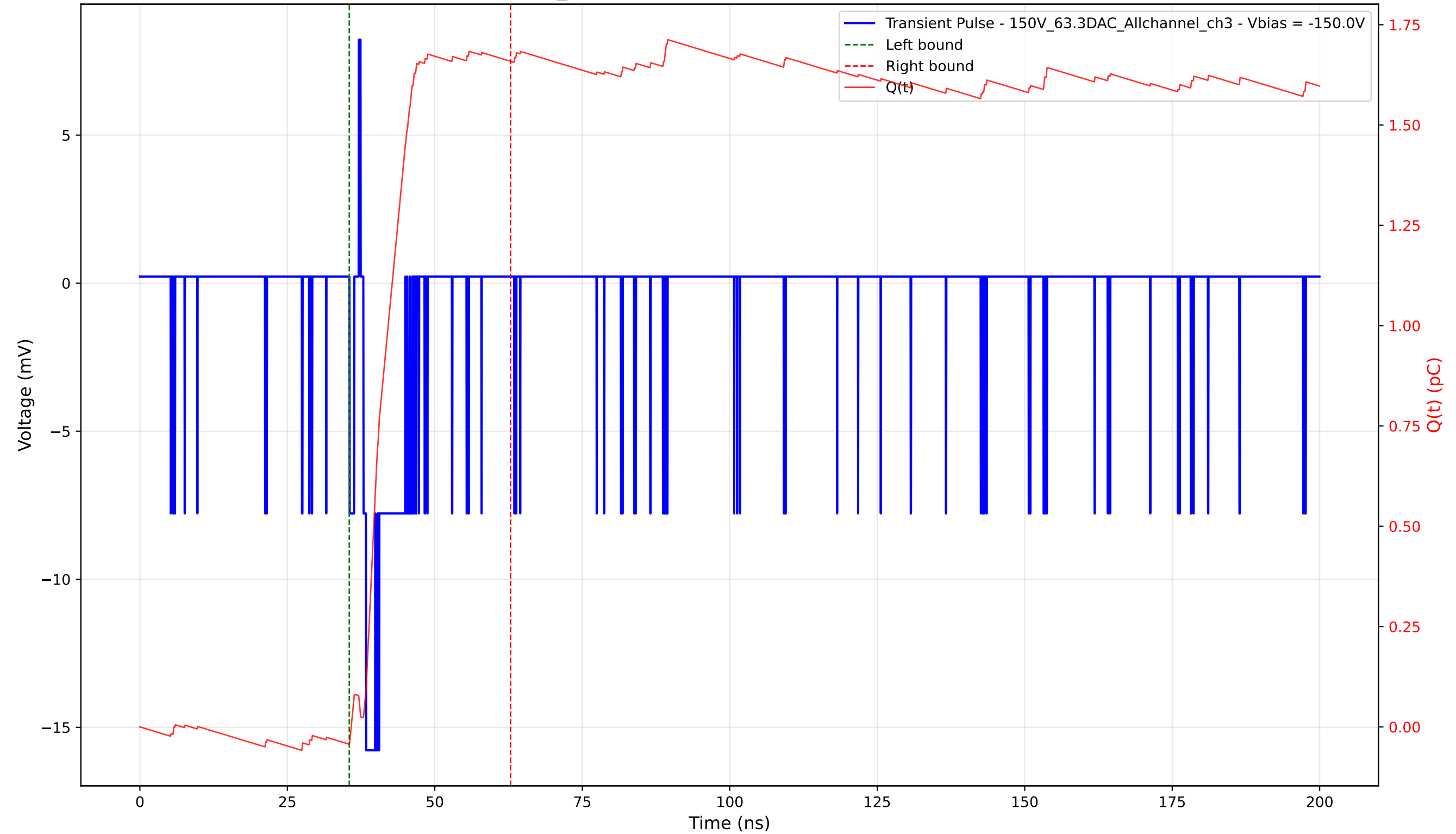
Transient Pulse - Sample: 1cm_42 - Position: 5015.0 \mu\text{m} - Charge: 1.70 pC - Rise Time: 0.47 ns
