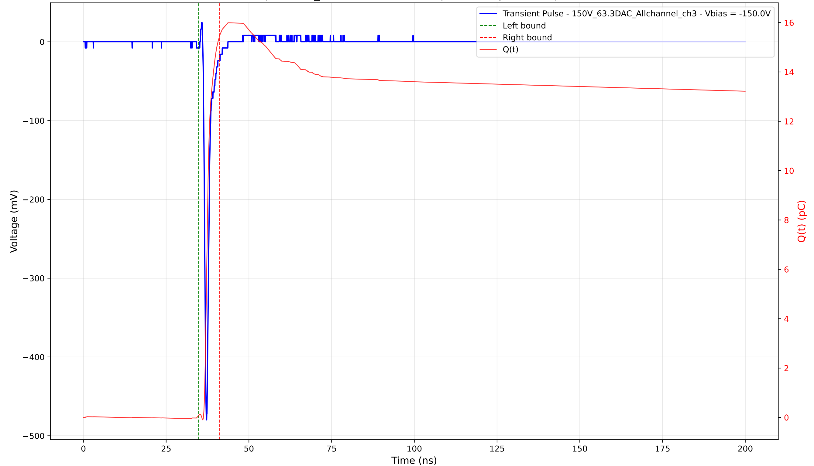
Transient Pulse - Sample: 1cm_42 - Position: 2315.0 \mu\text{m} - Charge: 15.32 pC - Rise Time: 0.68 ns
