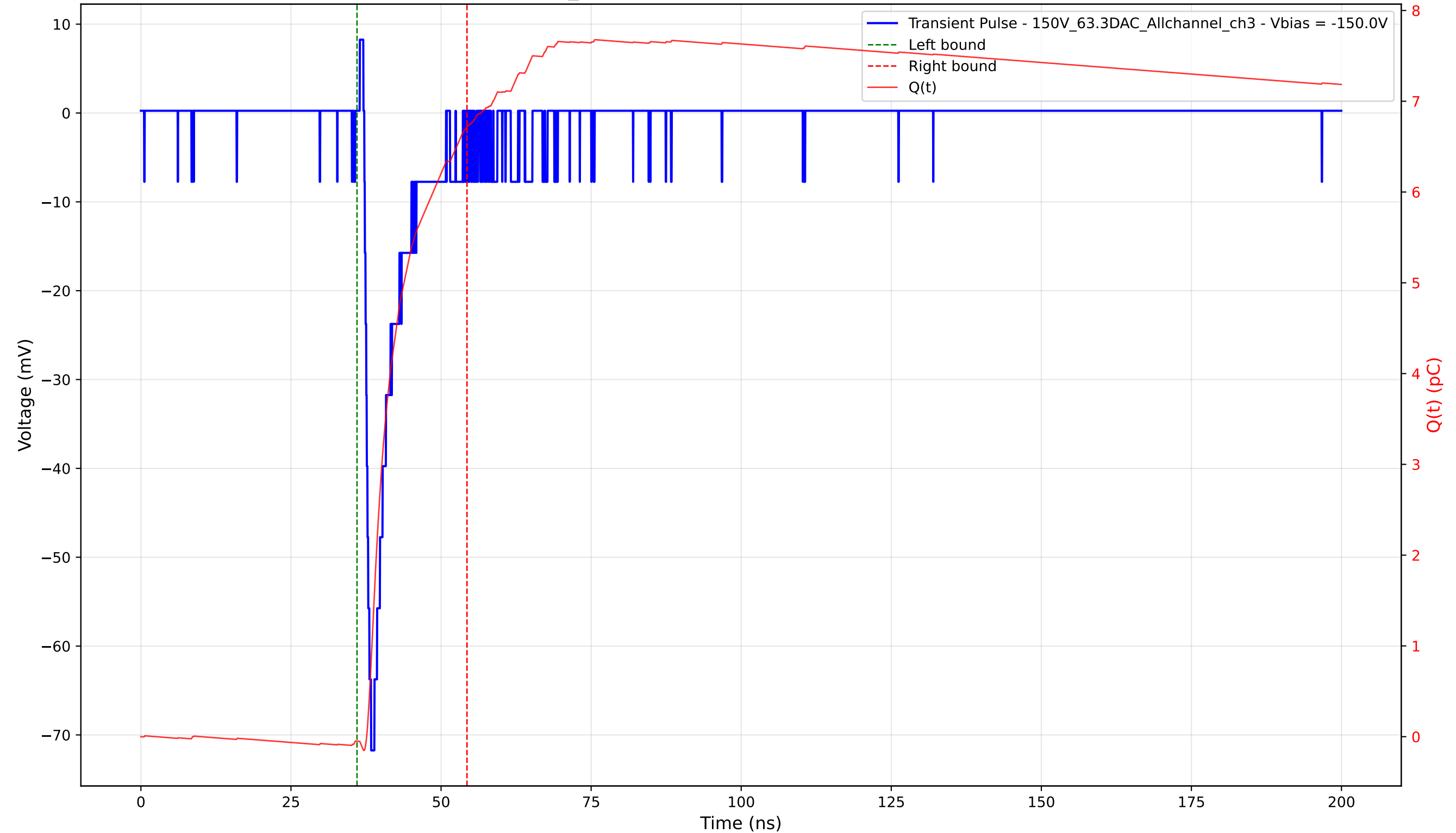
Transient Pulse - Sample: 1cm_42 - Position: 1290.0 \mu\text{m} - Charge: 6.77 pC - Rise Time: 1.12 ns
