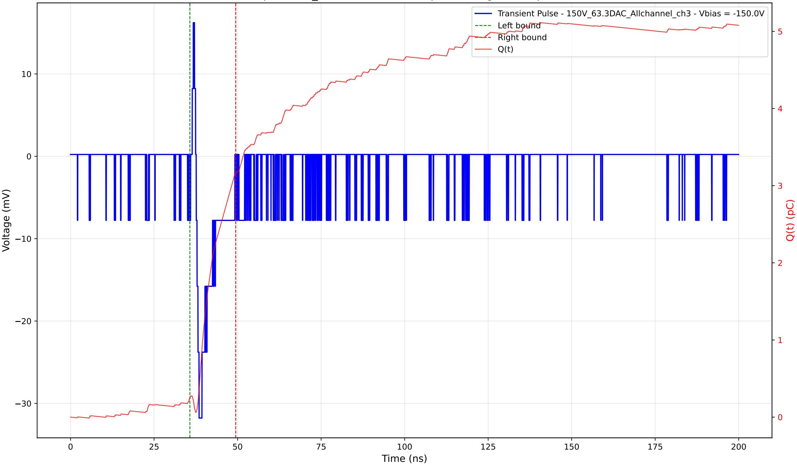
Transient Pulse - Sample: 1cm_42 - Position: 395.0 \mu\text{m} - Charge: 2.91 pC - Rise Time: 0.86 ns
