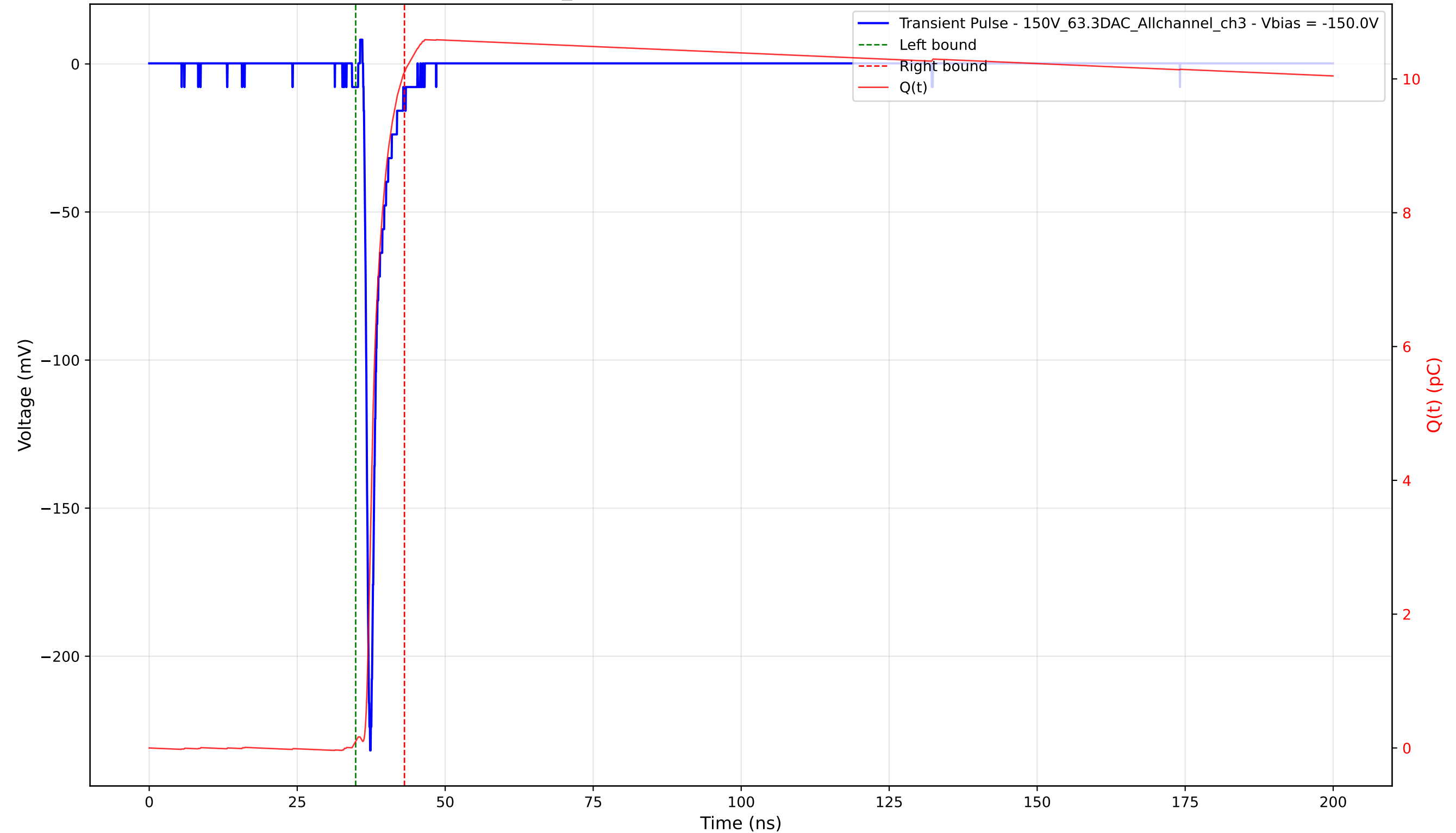
Transient Pulse - Sample: 1cm_42 - Position: 2010.0 \mu\text{m} - Charge: 10.00 pC - Rise Time: 0.80 ns
