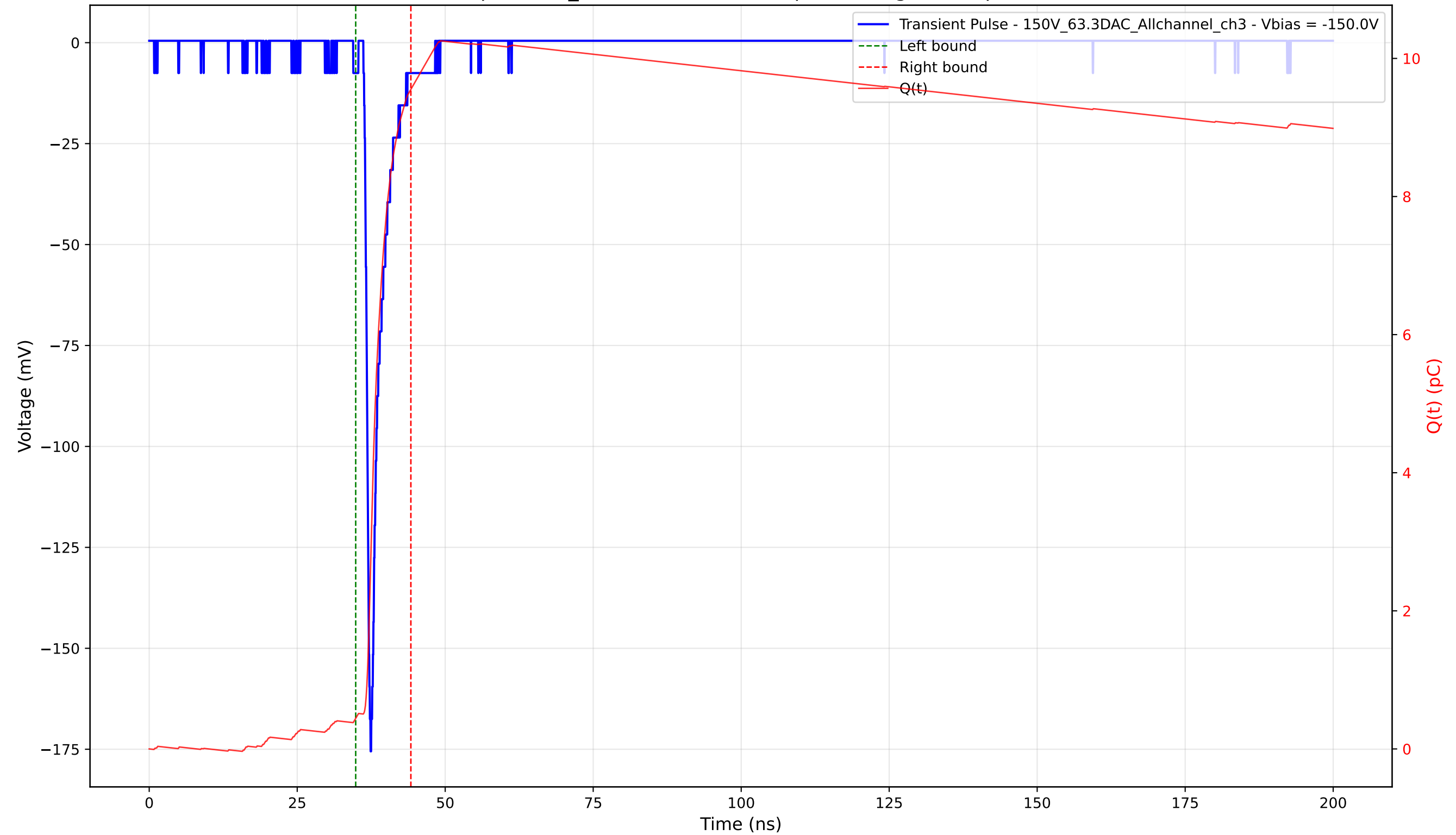
Transient Pulse - Sample: 1cm_42 - Position: 1900.0 \mu\text{m} - Charge: 9.11 pC - Rise Time: 0.83 ns
