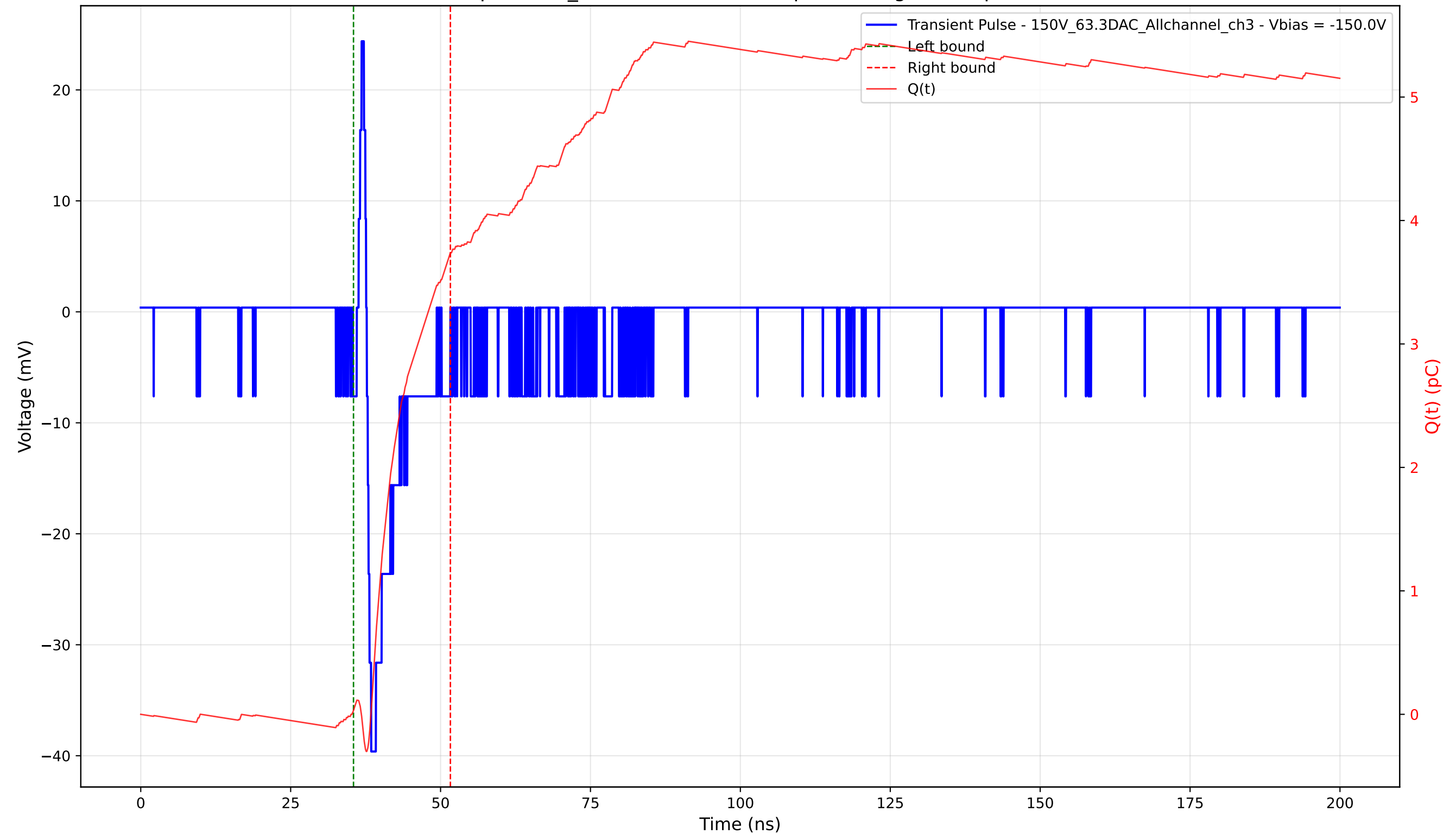
Transient Pulse - Sample: 1cm_42 - Position: 4195.0 \mu\text{m} - Charge: 3.71 pC - Rise Time: 0.74 ns
