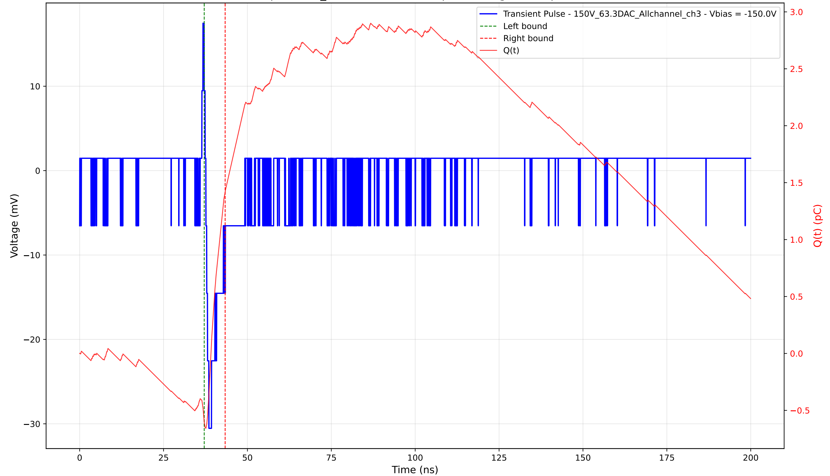
Transient Pulse - Sample: 1cm_42 - Position: 405.0 \mu\text{m} - Charge: 2.02 pC - Rise Time: 0.91 ns
