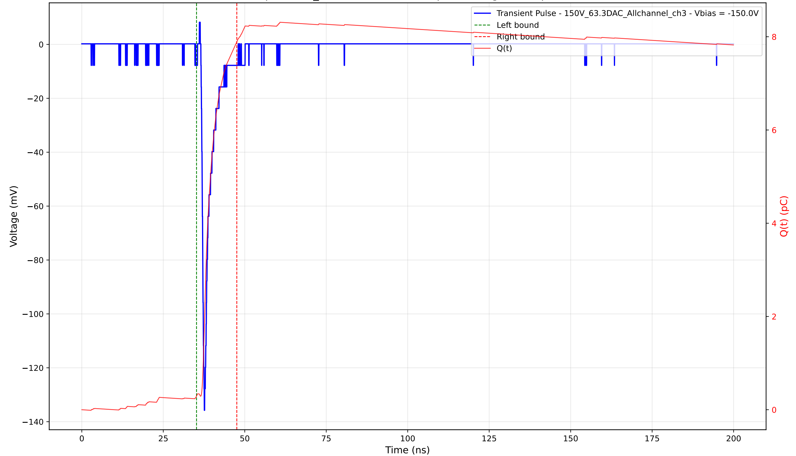
Transient Pulse - Sample: 1cm_42 - Position: 3320.0 \mu\text{m} - Charge: 7.60 pC - Rise Time: 0.89 ns
