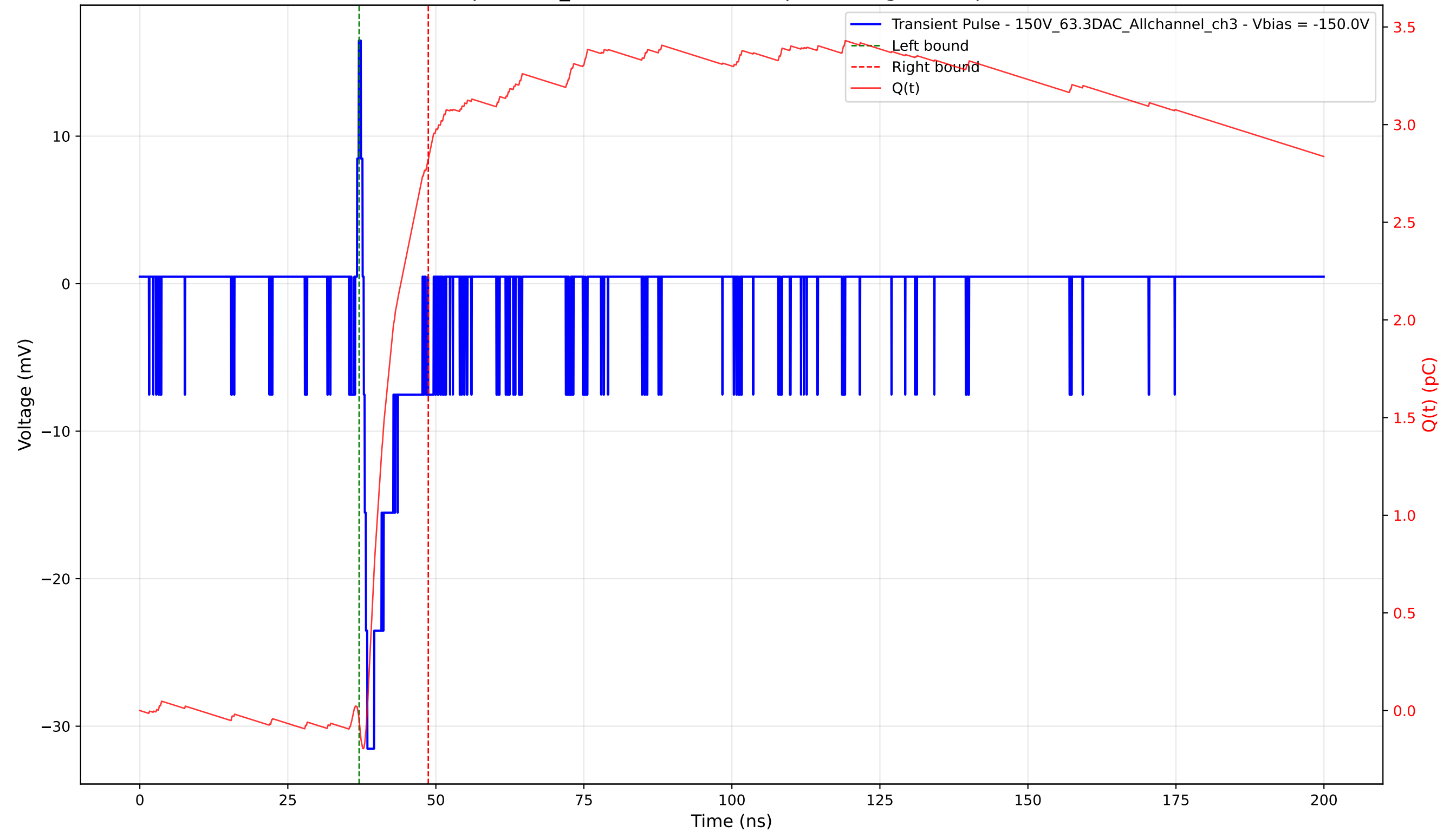
Transient Pulse - Sample: 1cm_42 - Position: 4785.0 \mu\text{m} - Charge: 2.87 pC - Rise Time: 0.62 ns
