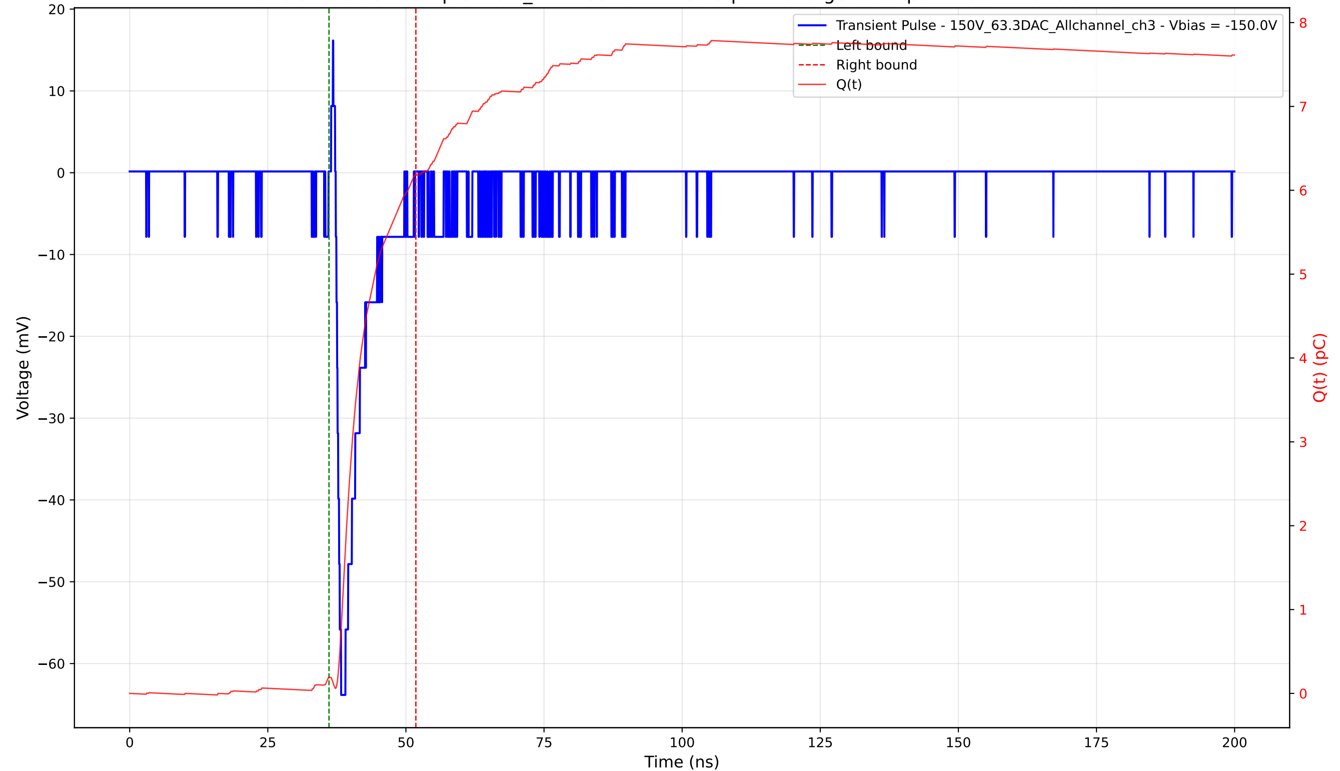
Transient Pulse - Sample: 1cm_42 - Position: 1180.0 \mu\text{m} - Charge: 5.99 pC - Rise Time: 0.97 ns
