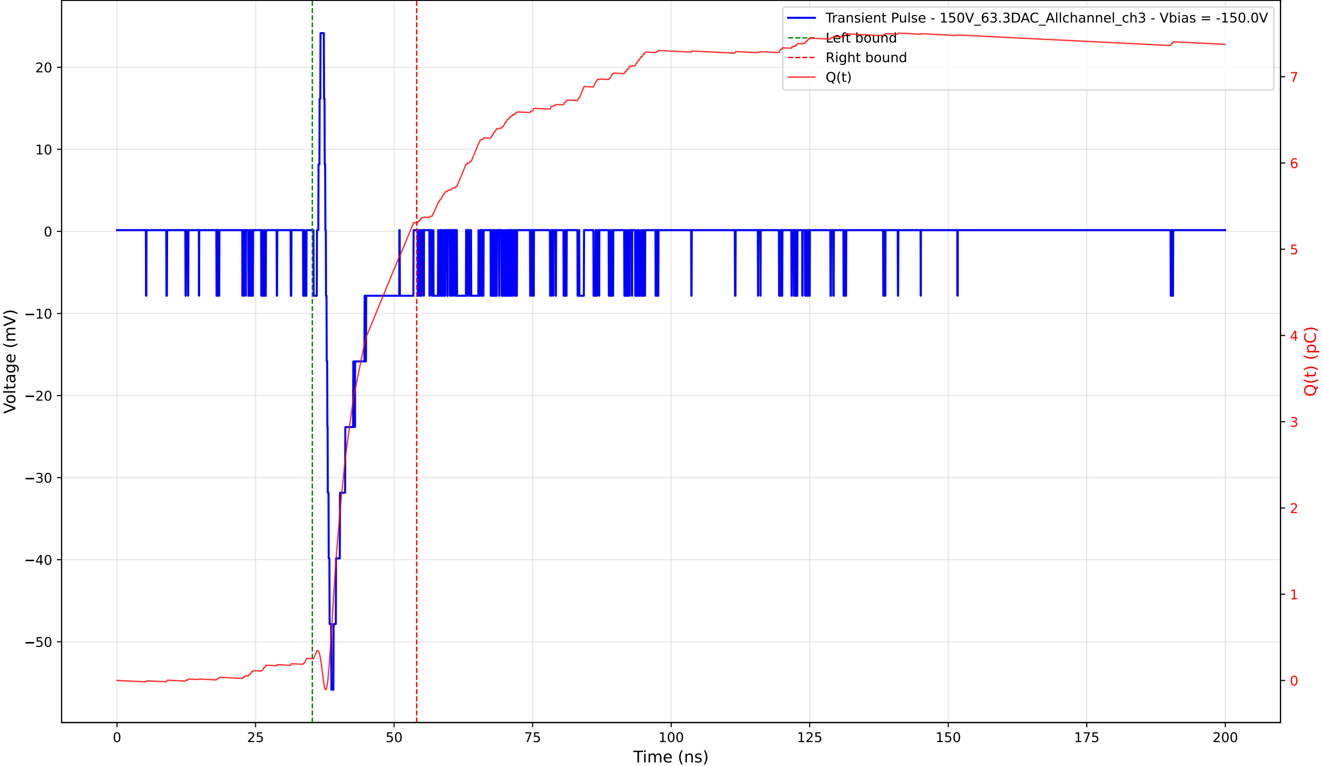
Transient Pulse - Sample: 1cm_42 - Position: 735.0 \mu\text{m} - Charge: 5.05 pC - Rise Time: 0.97 ns
