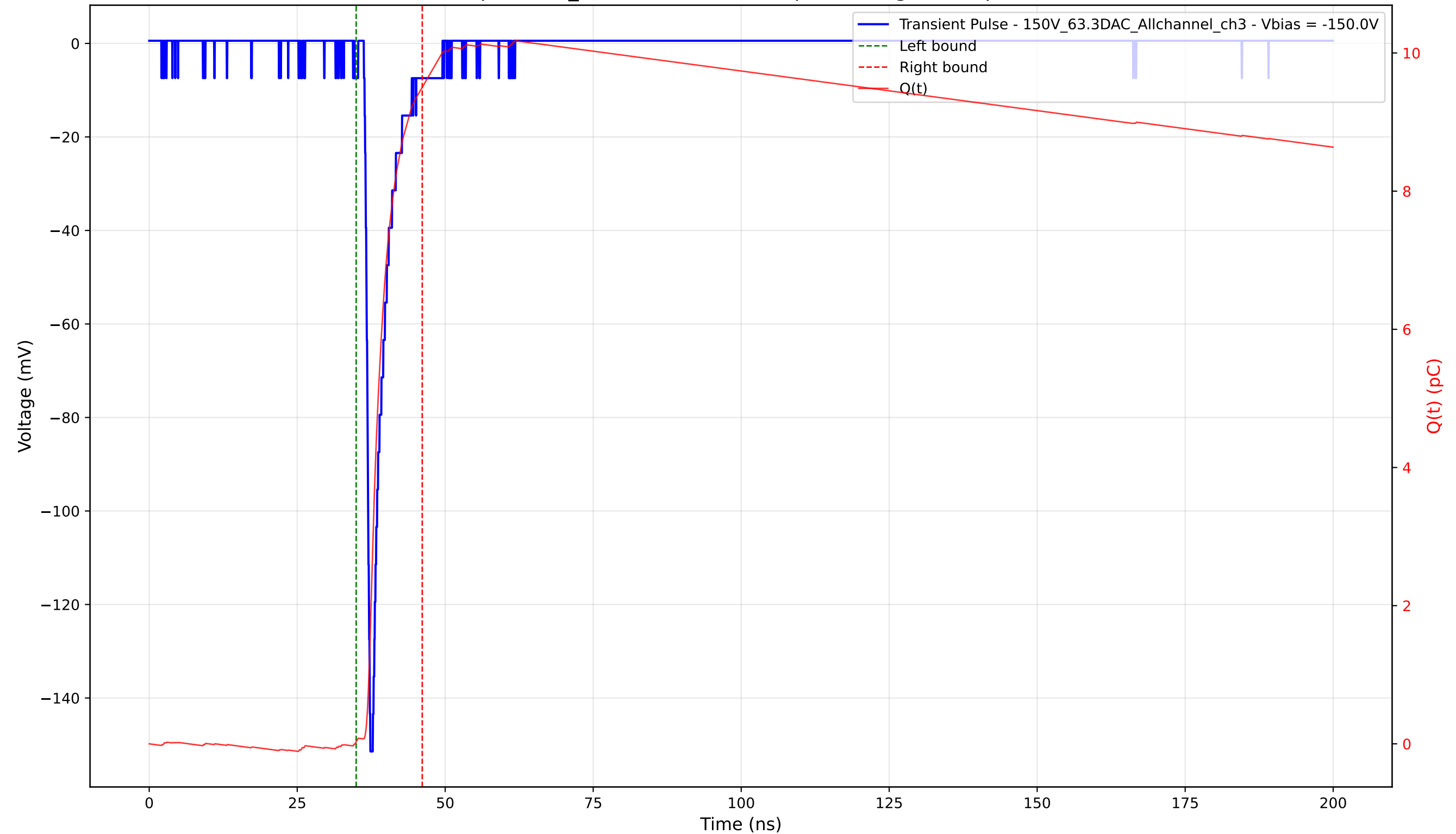
Transient Pulse - Sample: 1cm_42 - Position: 1780.0 \mu\text{m} - Charge: 9.47 pC - Rise Time: 0.88 ns
