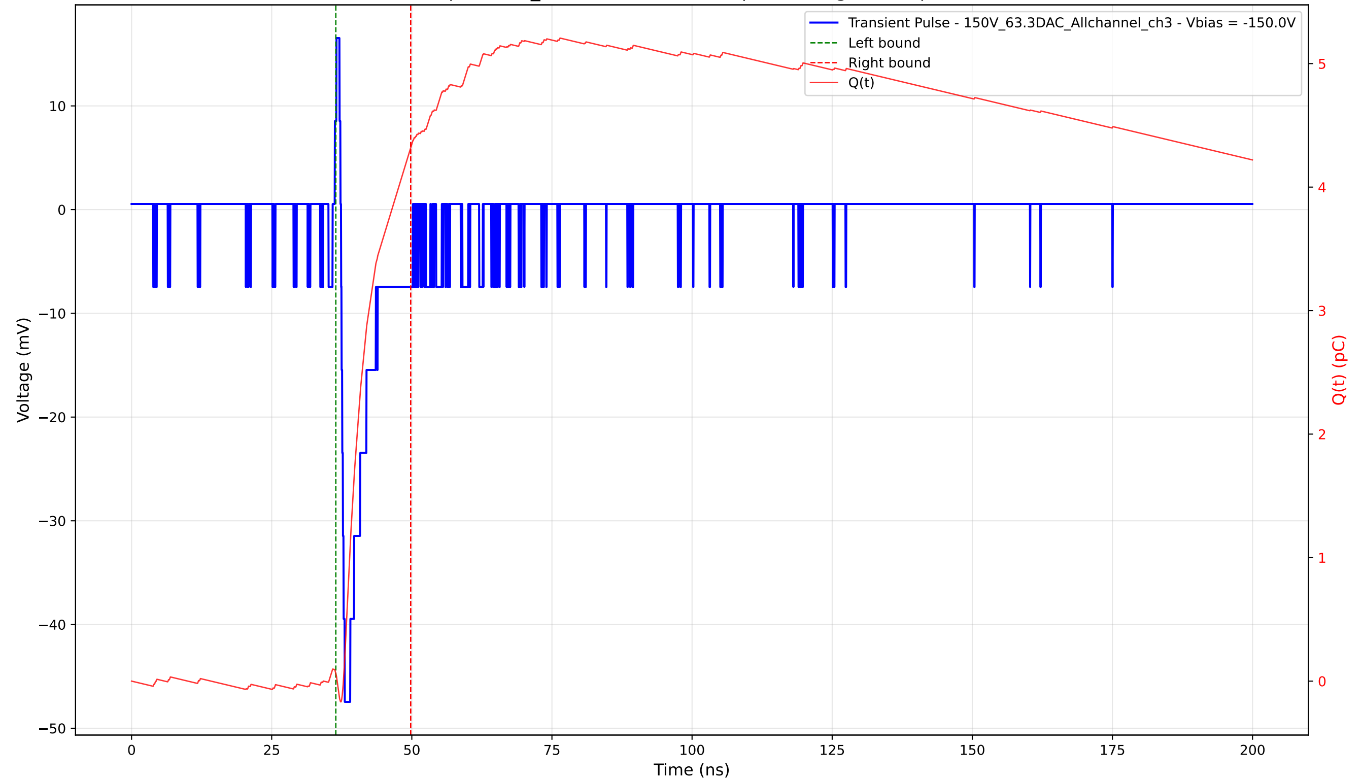
Transient Pulse - Sample: 1cm_42 - Position: 3875.0 \mu\text{m} - Charge: 4.26 pC - Rise Time: 0.66 ns
