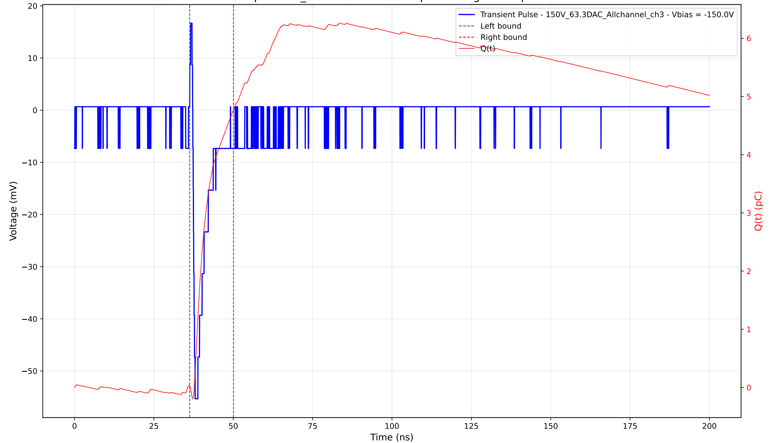
Transient Pulse - Sample: 1cm_42 - Position: 3760.0 \mu\text{m} - Charge: 4.75 pC - Rise Time: 0.73 ns
