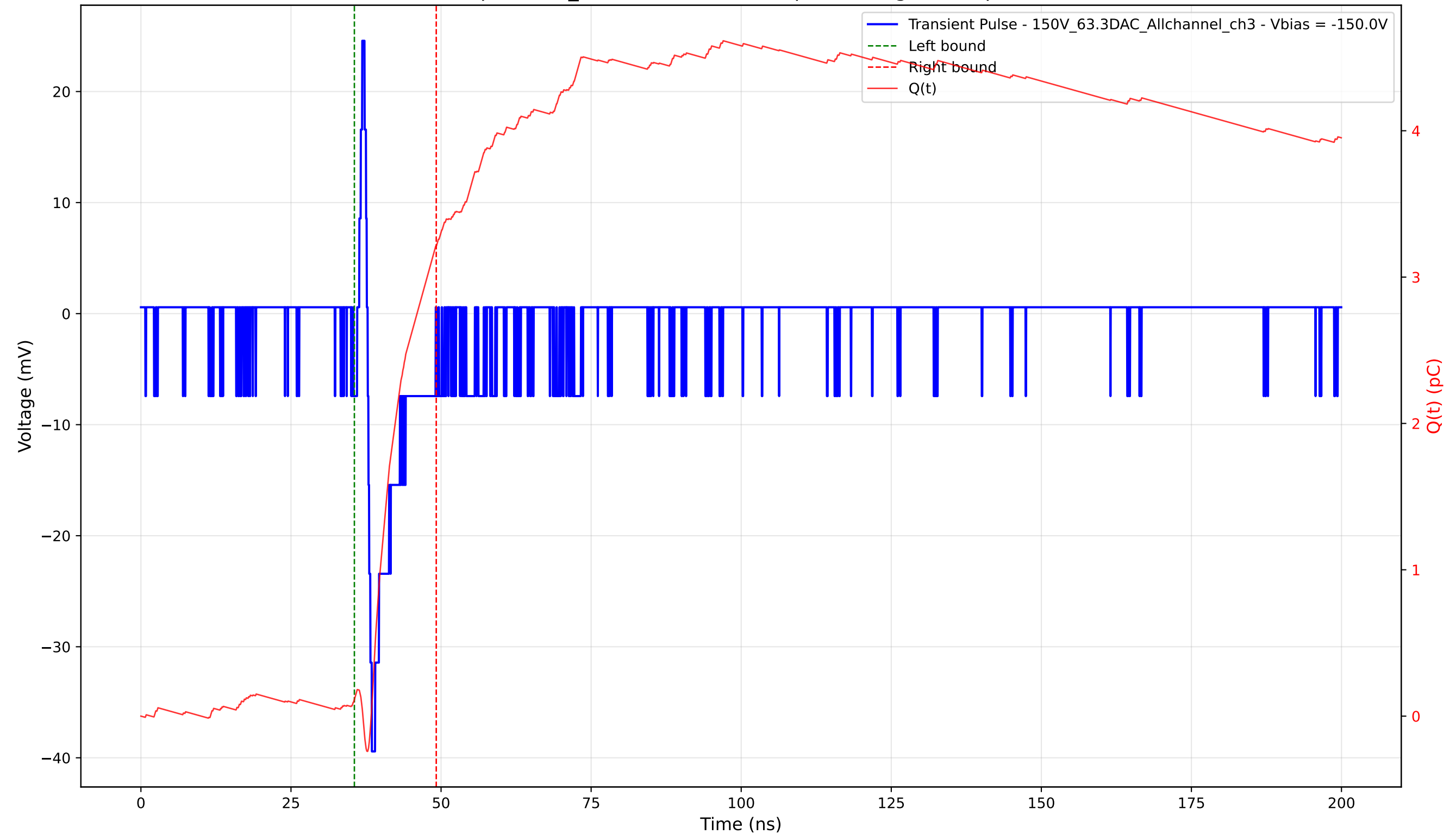
Transient Pulse - Sample: 1cm_42 - Position: 4370.0 \mu\text{m} - Charge: 3.10 pC - Rise Time: 0.70 ns
