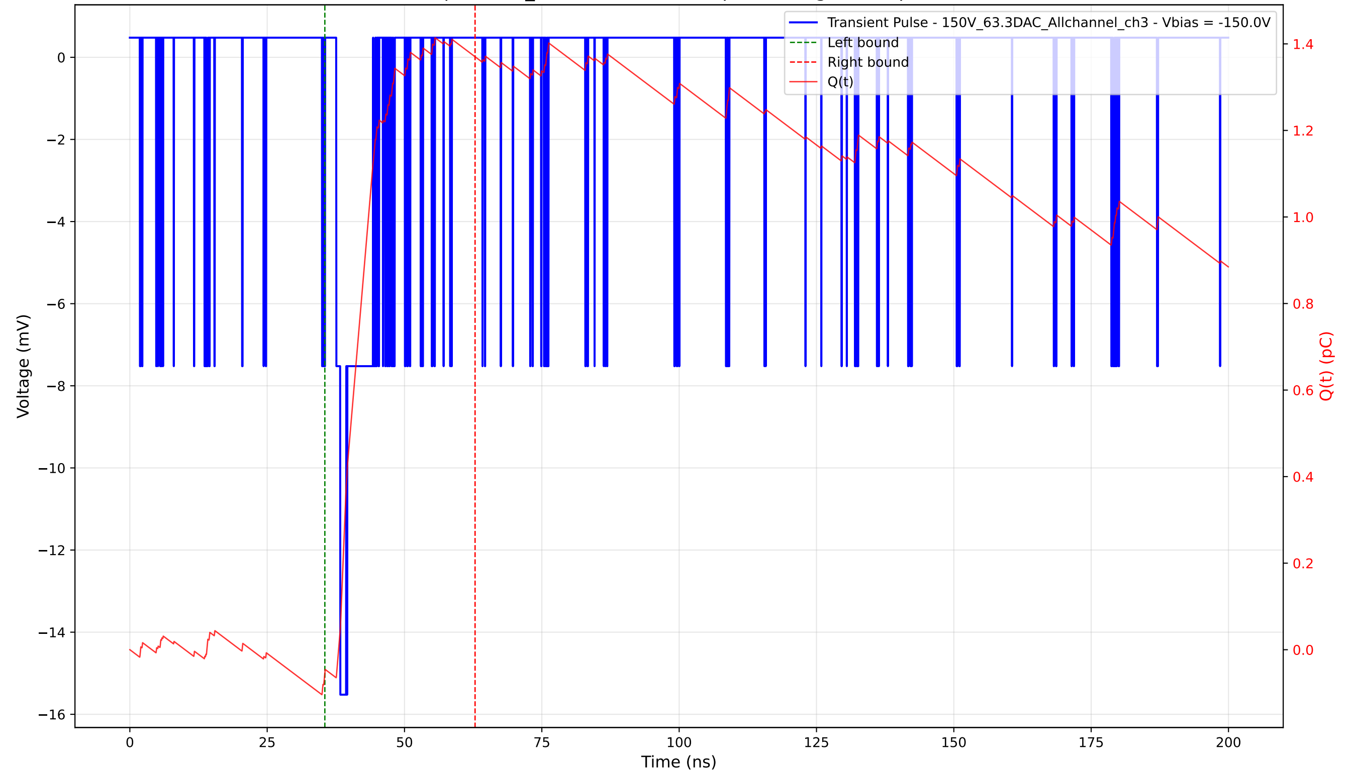
Transient Pulse - Sample: 1cm_42 - Position: 145.0 \mu\text{m} - Charge: 1.42 pC - Rise Time: 0.75 ns
