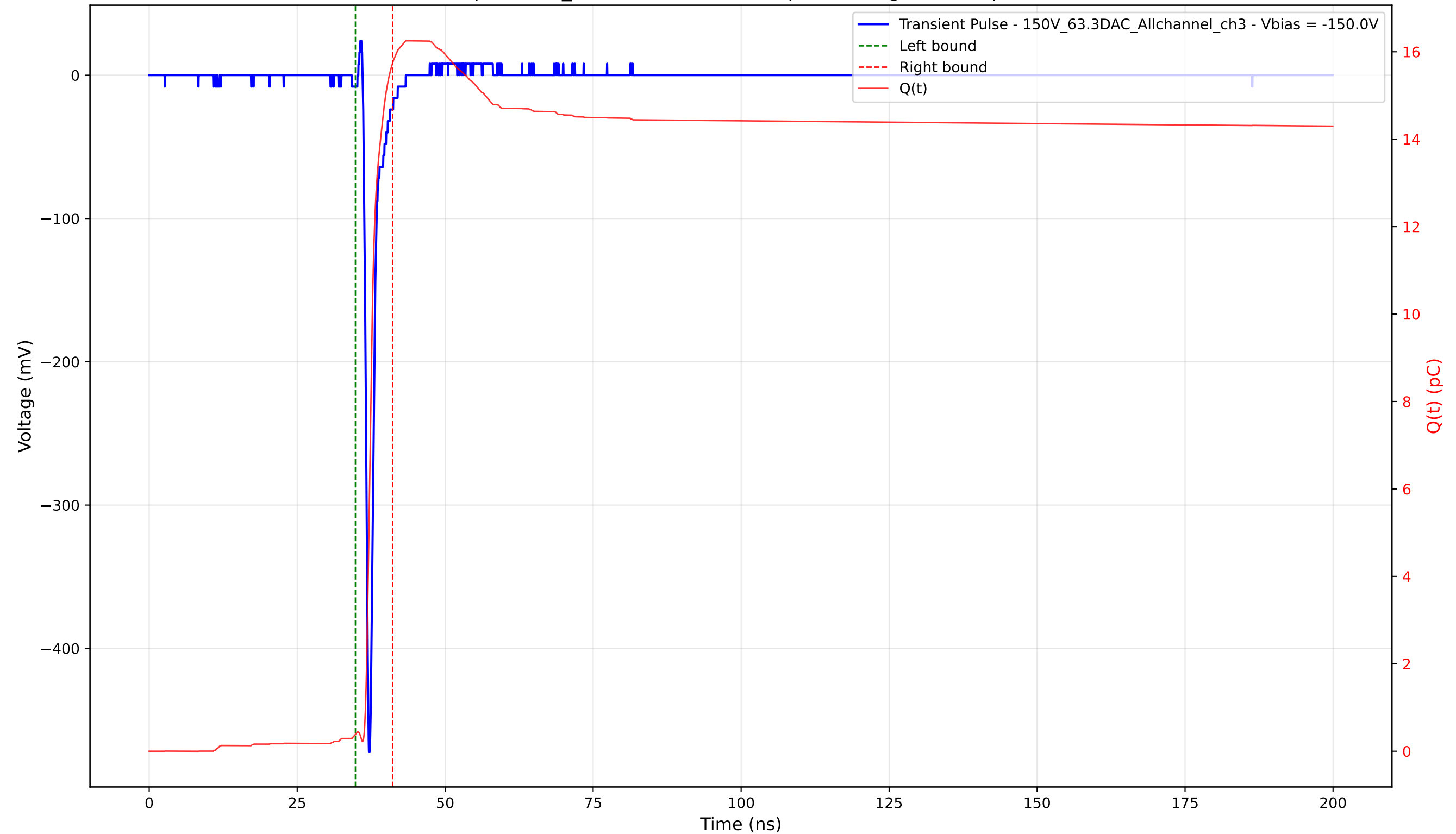
Transient Pulse - Sample: 1cm_42 - Position: 2725.0 \mu\text{m} - Charge: 15.36 pC - Rise Time: 0.73 ns
