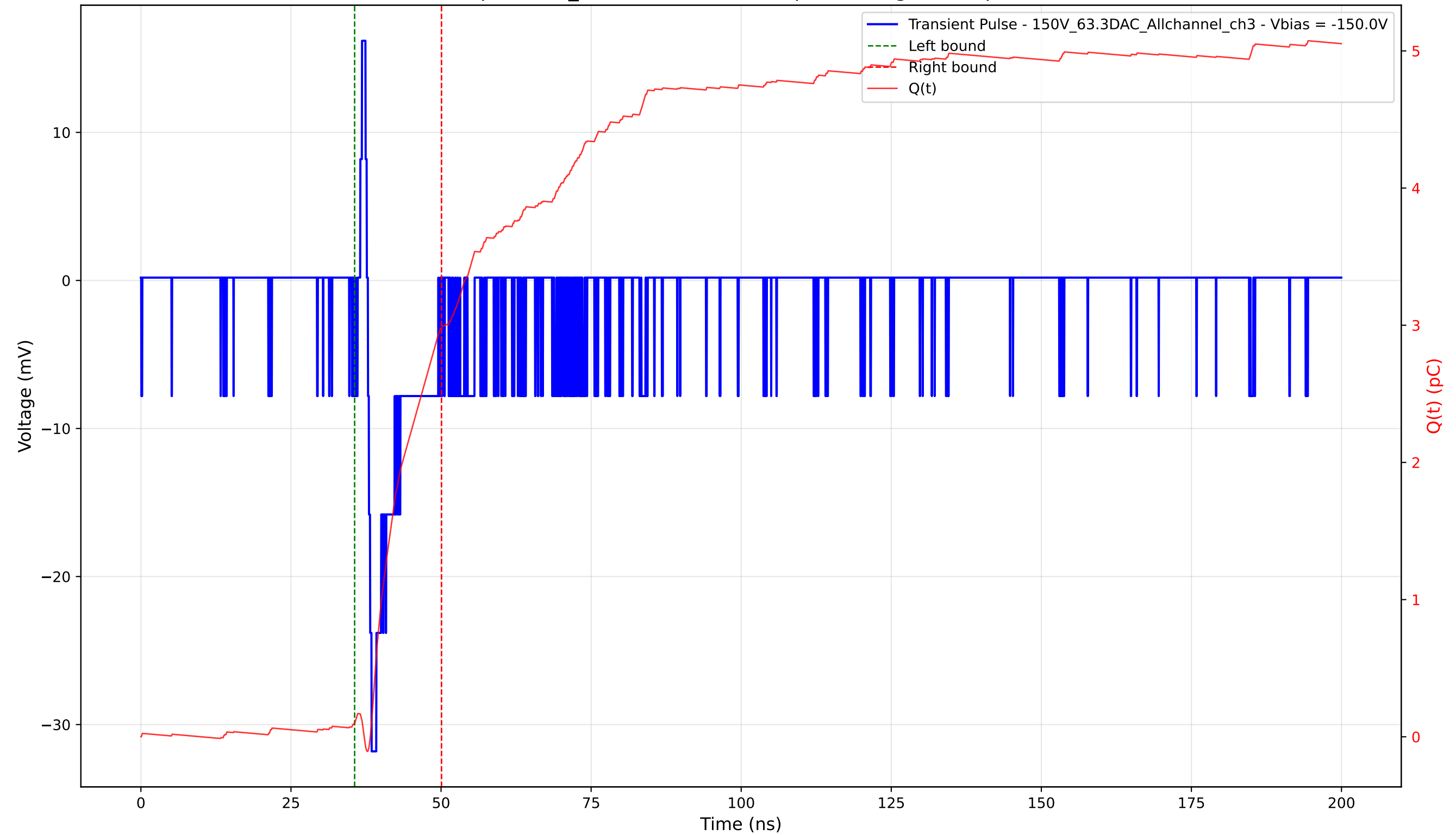
Transient Pulse - Sample: 1cm_42 - Position: 4540.0 \mu\text{m} - Charge: 2.88 pC - Rise Time: 0.62 ns
