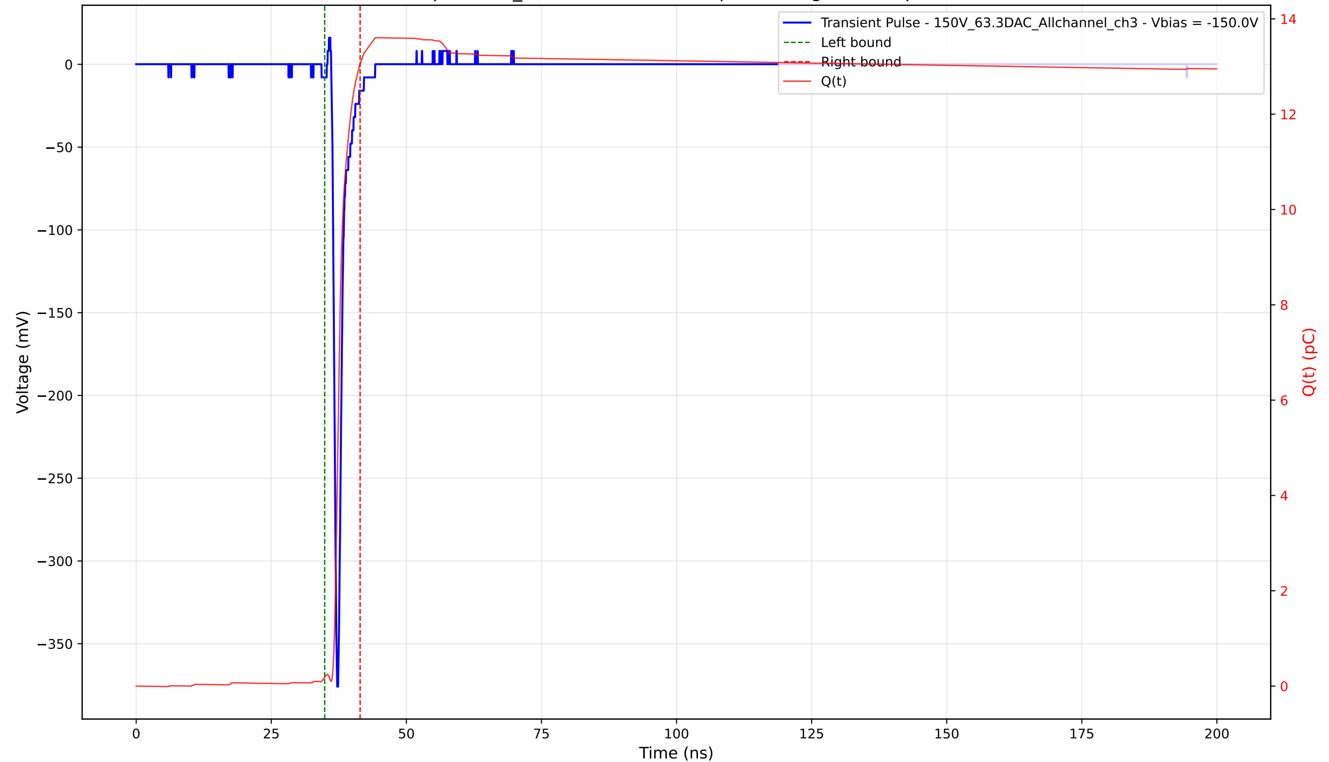
Transient Pulse - Sample: 1cm_42 - Position: 2870.0 \mu\text{m} - Charge: 12.87 pC - Rise Time: 0.74 ns
