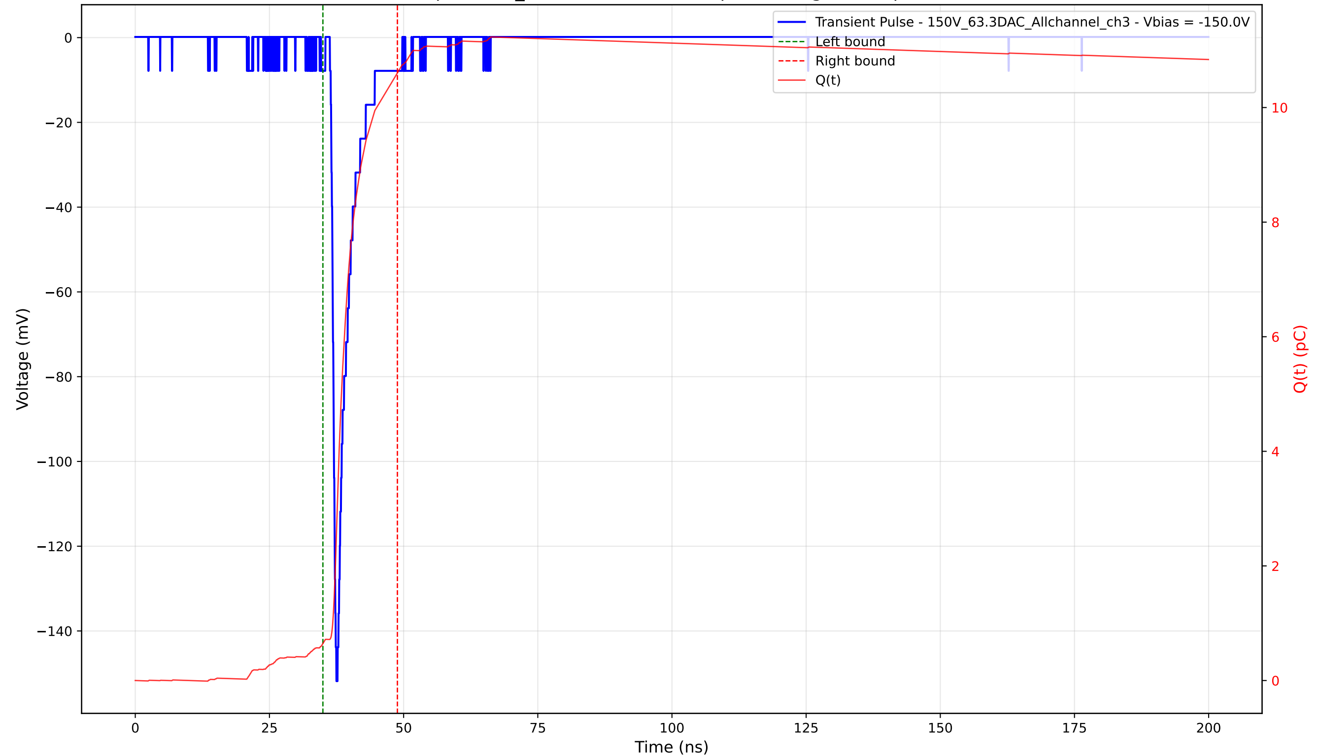
Transient Pulse - Sample: 1cm_42 - Position: 1740.0 \mu\text{m} - Charge: 9.96 pC - Rise Time: 0.92 ns
