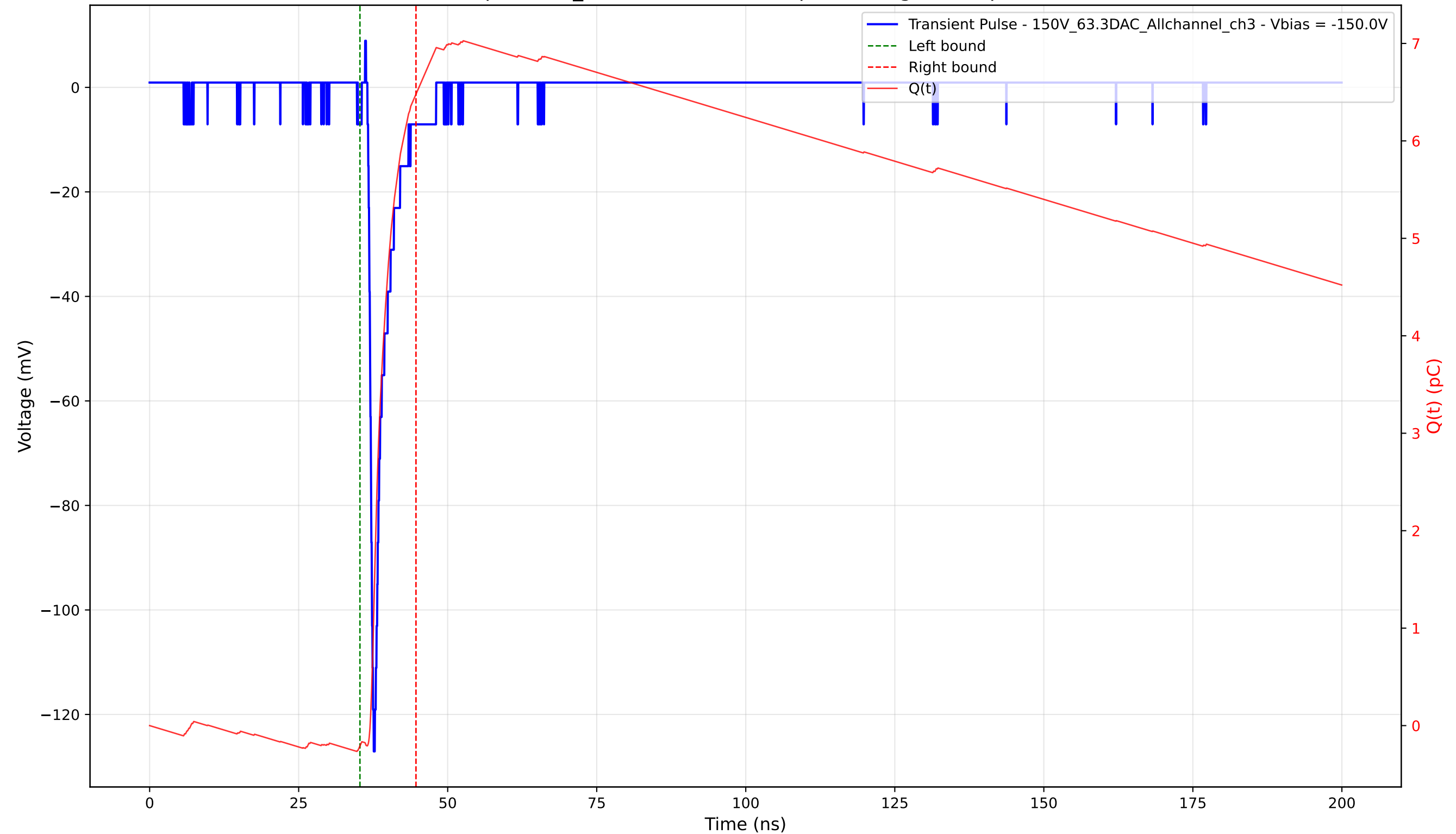
Transient Pulse - Sample: 1cm_42 - Position: 3345.0 \mu\text{m} - Charge: 6.69 pC - Rise Time: 0.81 ns
