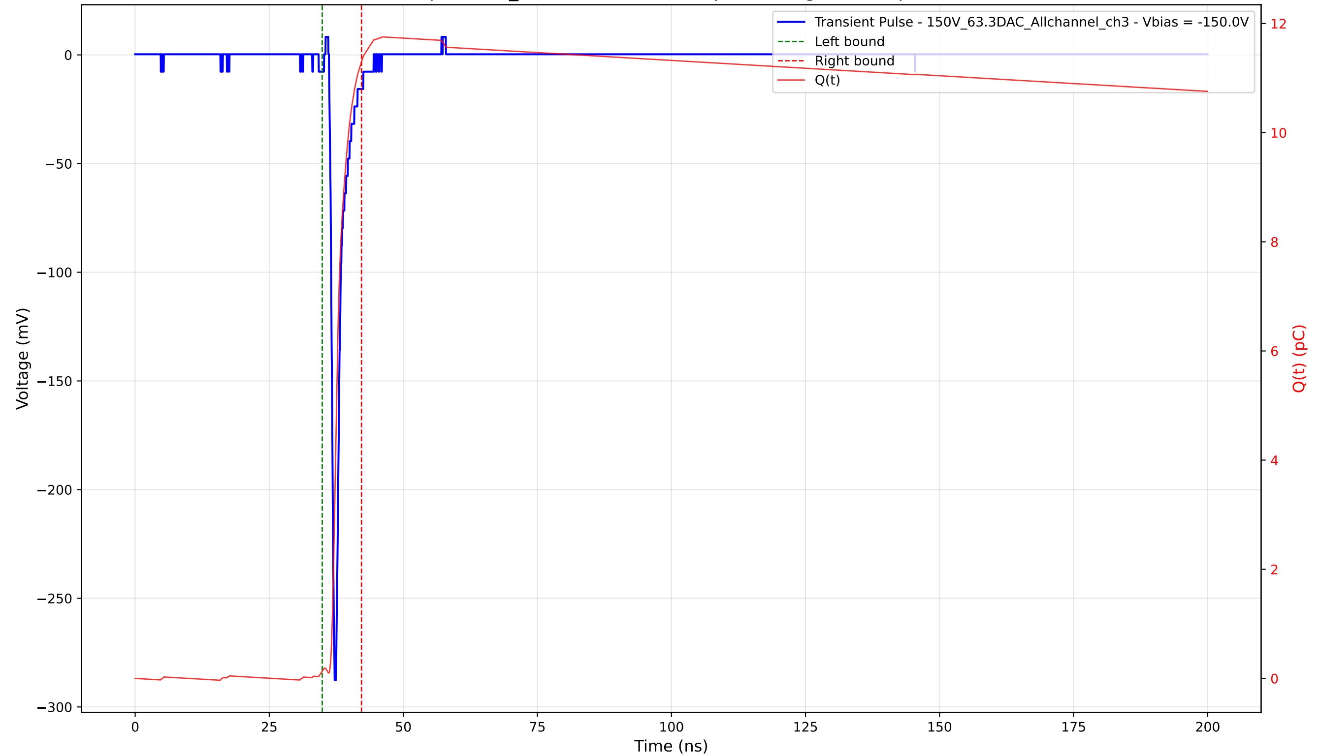
Transient Pulse - Sample: 1cm_42 - Position: 2080.0 \mu\text{m} - Charge: 11.16 pC - Rise Time: 0.75 ns
