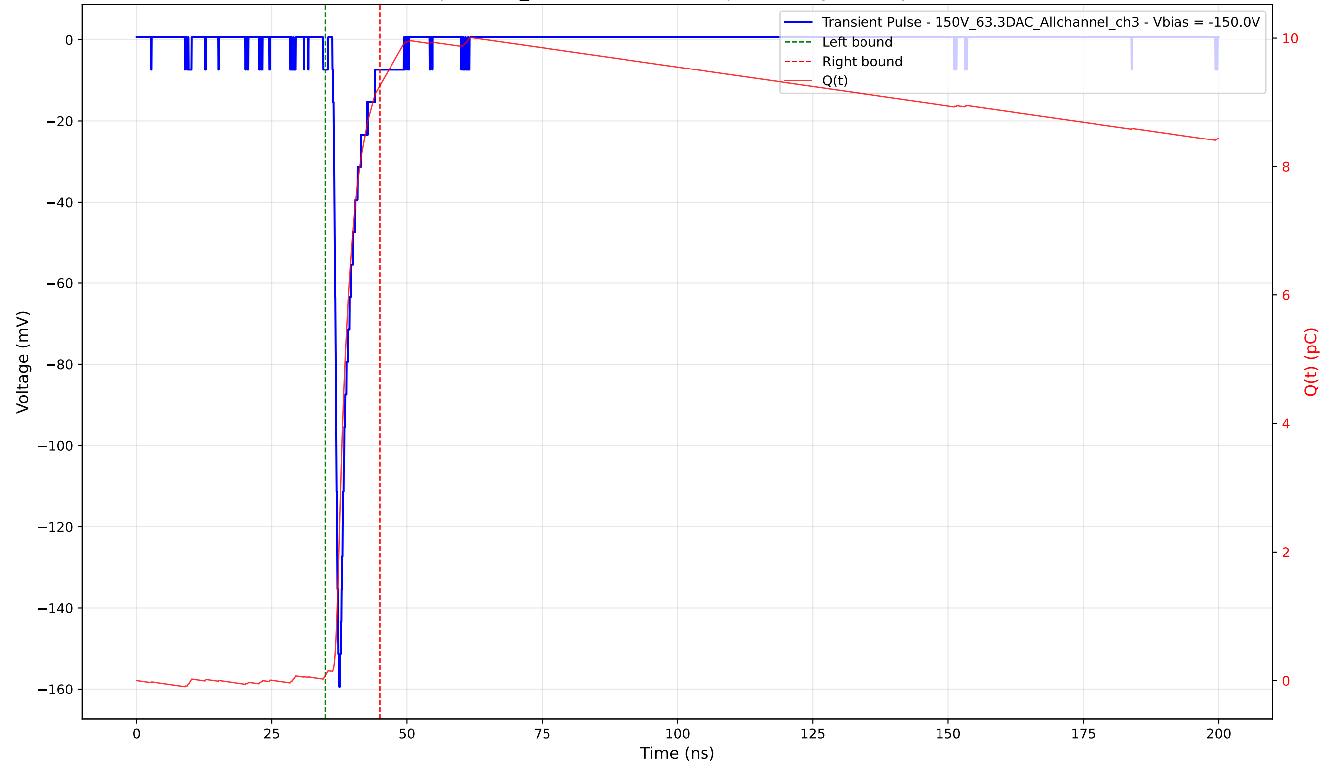
Transient Pulse - Sample: 1cm_42 - Position: 1830.0 \mu\text{m} - Charge: 9.18 pC - Rise Time: 0.88 ns
