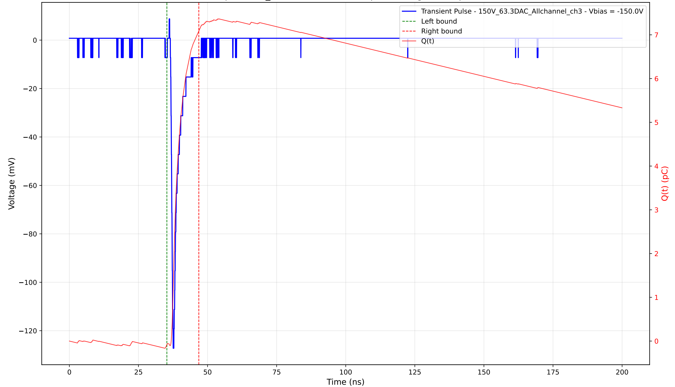
Transient Pulse - Sample: 1cm_42 - Position: 3340.0 \mu\text{m} - Charge: 7.17 pC - Rise Time: 0.81 ns
