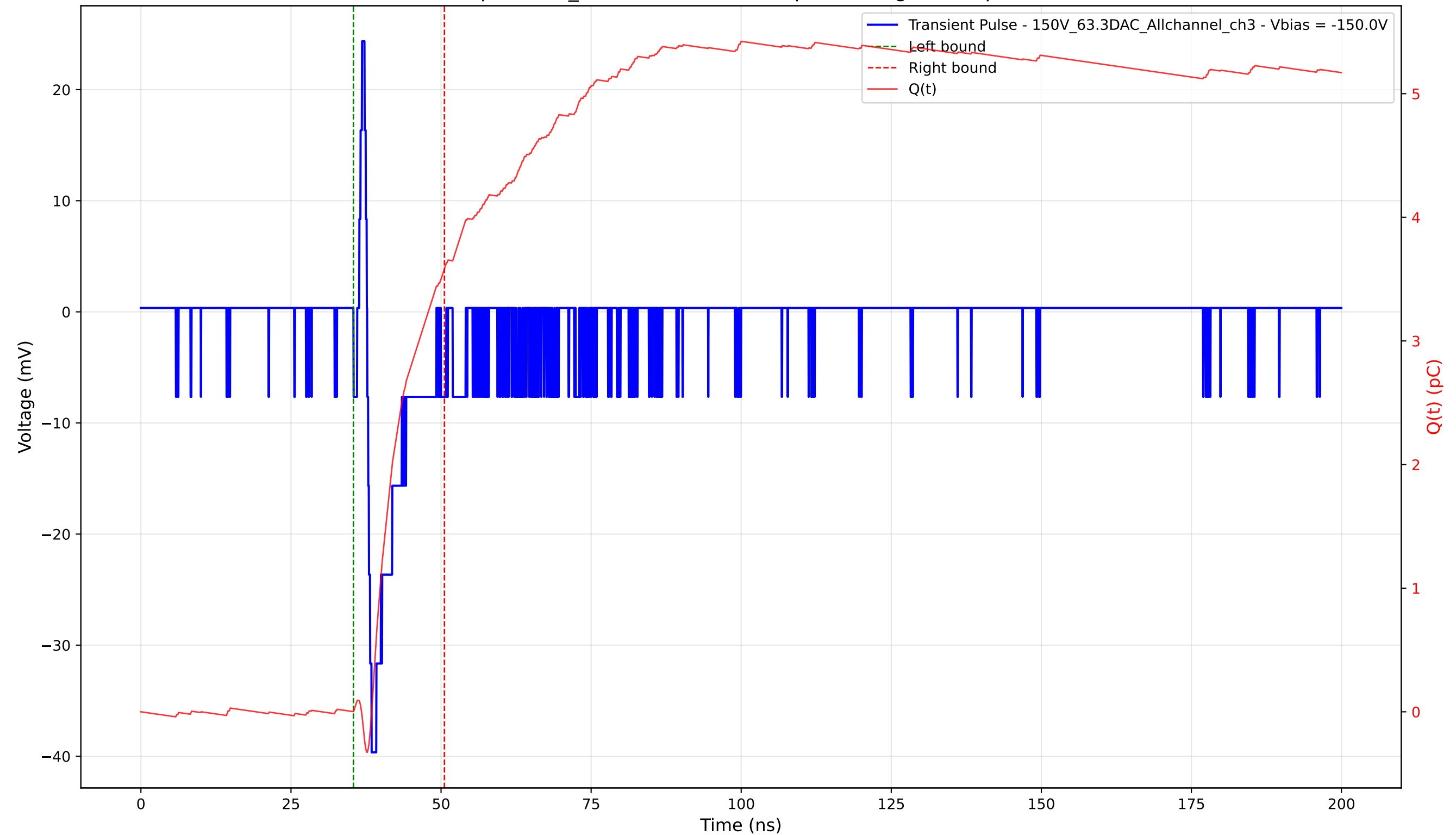
Transient Pulse - Sample: 1cm_42 - Position: 4265.0 \mu\text{m} - Charge: 3.58 pC - Rise Time: 0.74 ns
