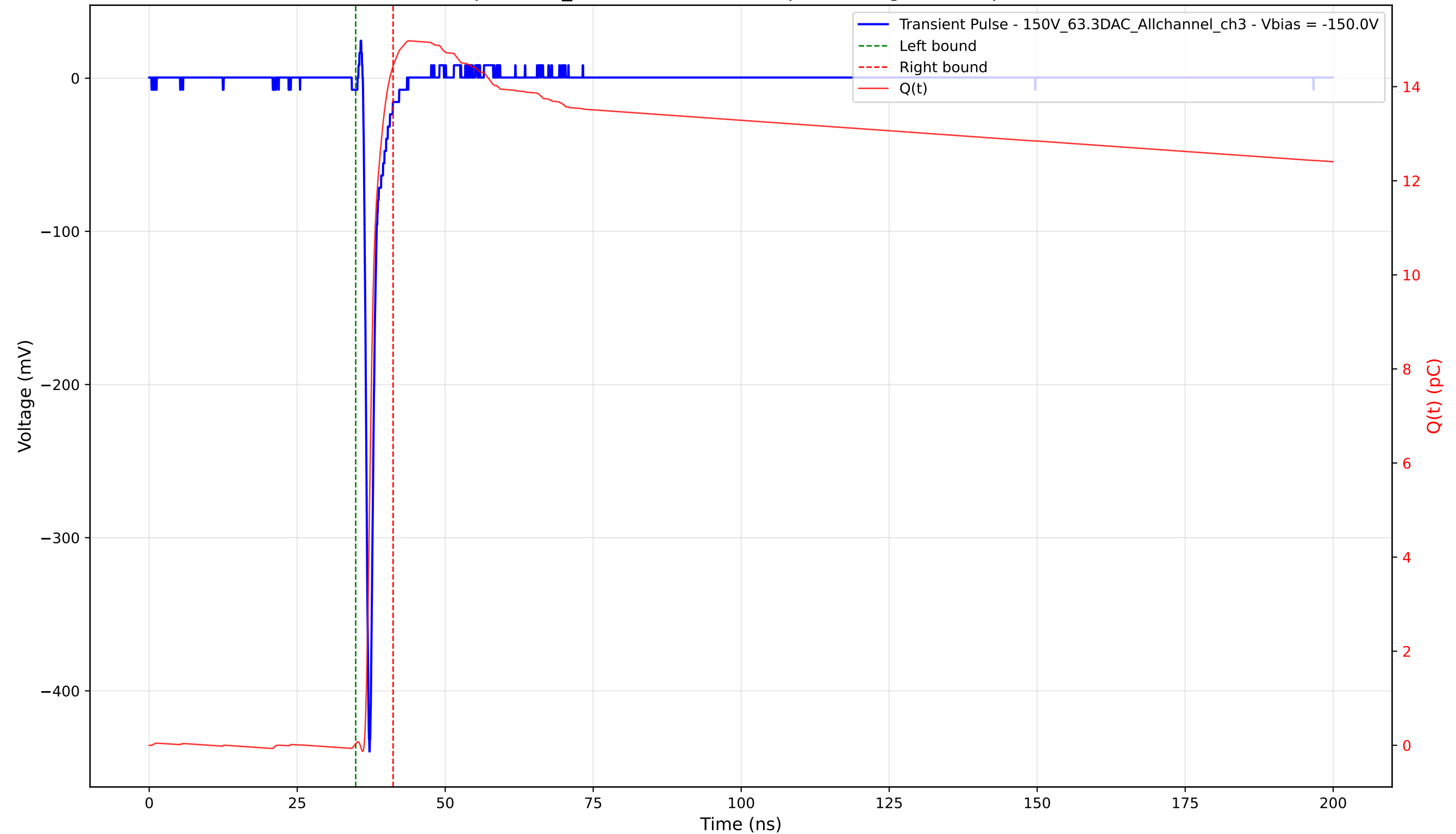
Transient Pulse - Sample: 1cm_42 - Position: 2225.0 \mu\text{m} - Charge: 14.42 pC - Rise Time: 0.74 ns
