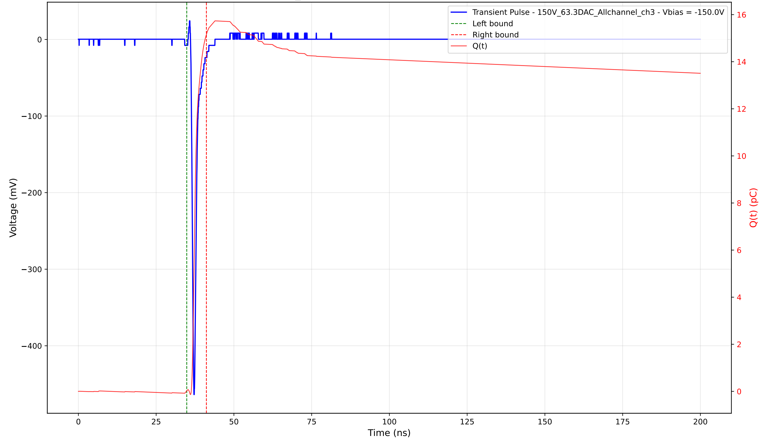
Transient Pulse - Sample: 1cm_42 - Position: 2270.0 \mu\text{m} - Charge: 15.14 pC - Rise Time: 0.69 ns
