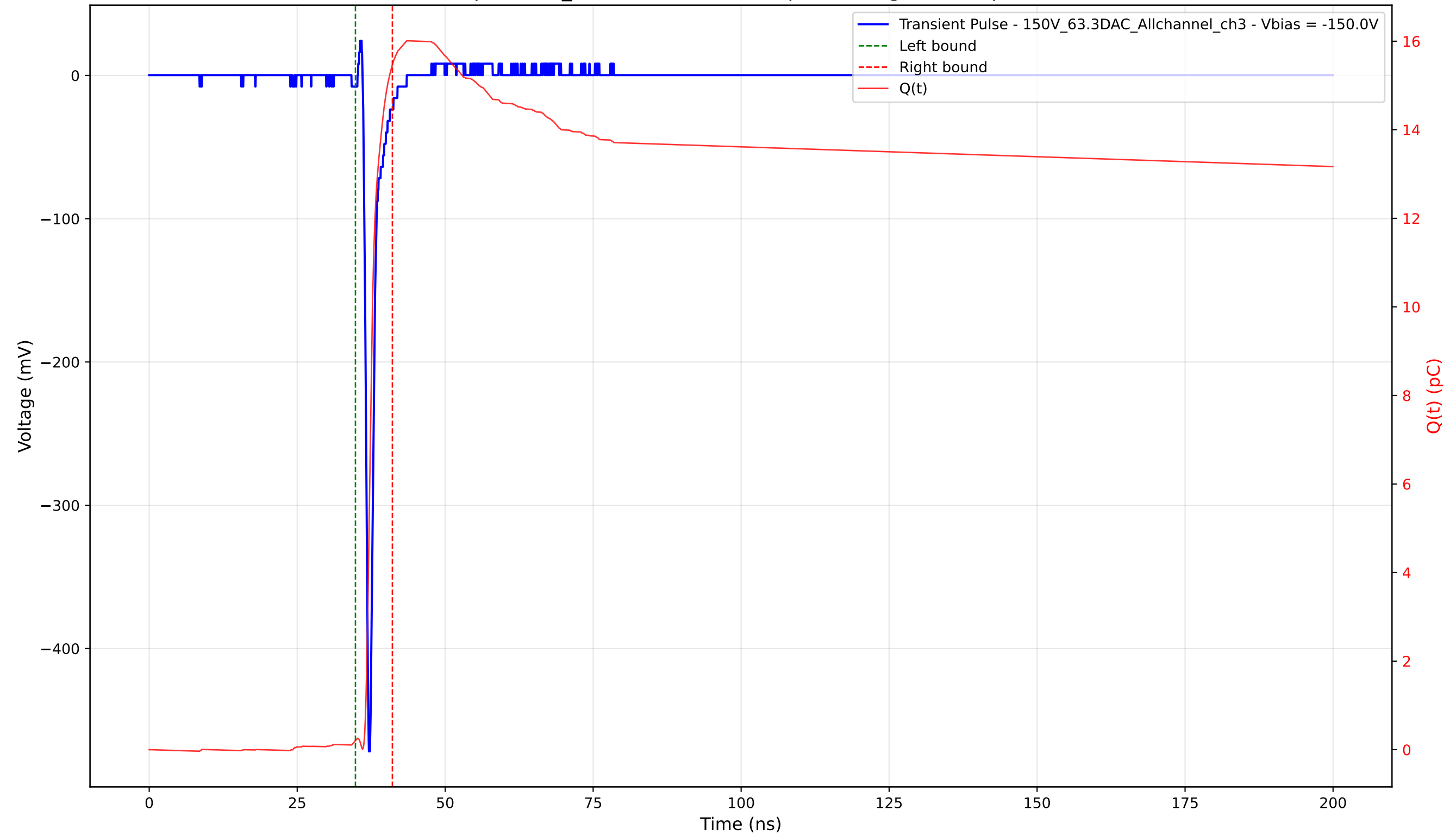
Transient Pulse - Sample: 1cm_42 - Position: 2310.0 \mu\text{m} - Charge: 15.26 pC - Rise Time: 0.73 ns
