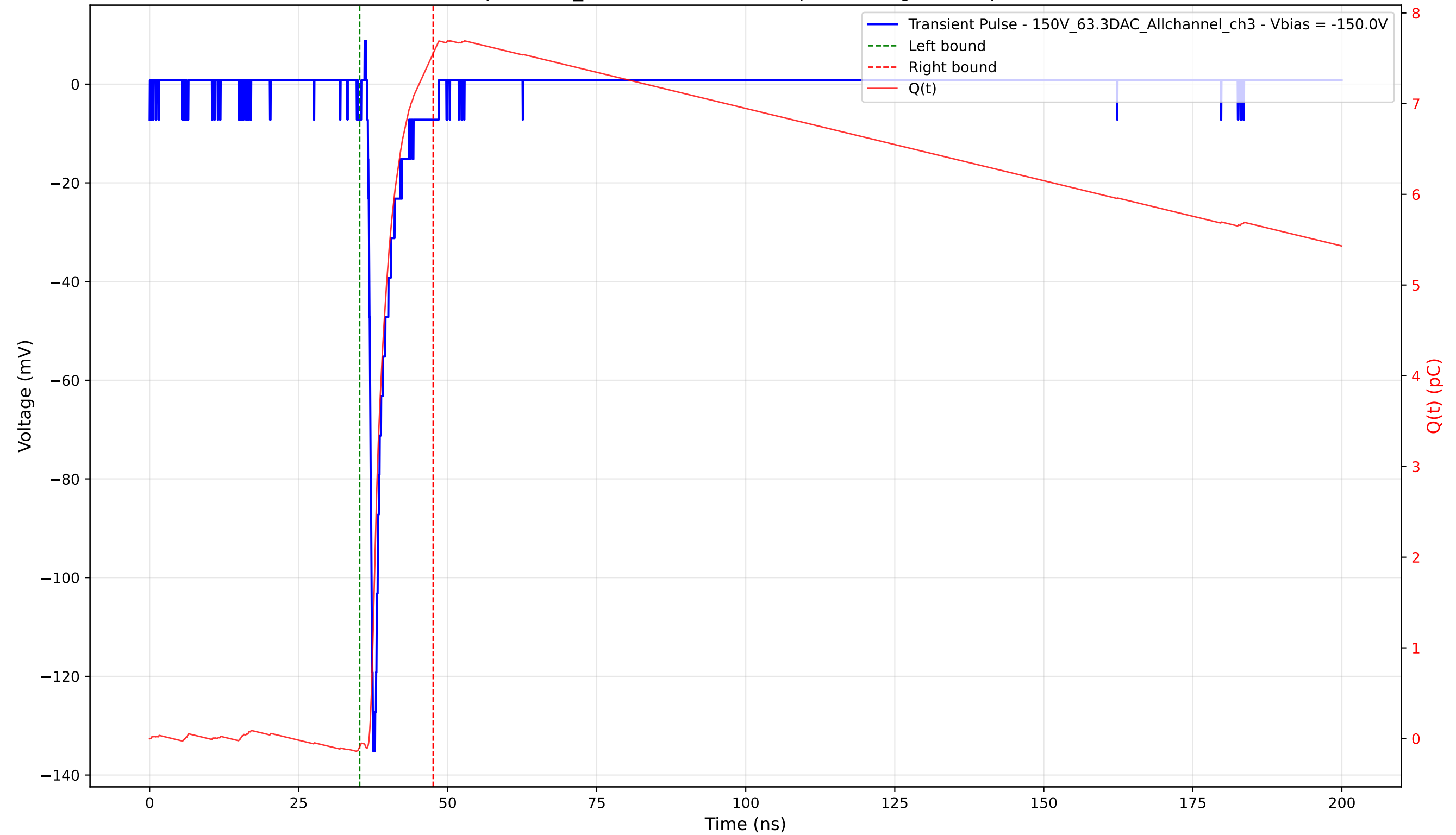
Transient Pulse - Sample: 1cm_42 - Position: 3300.0 \mu\text{m} - Charge: 7.64 pC - Rise Time: 0.81 ns
