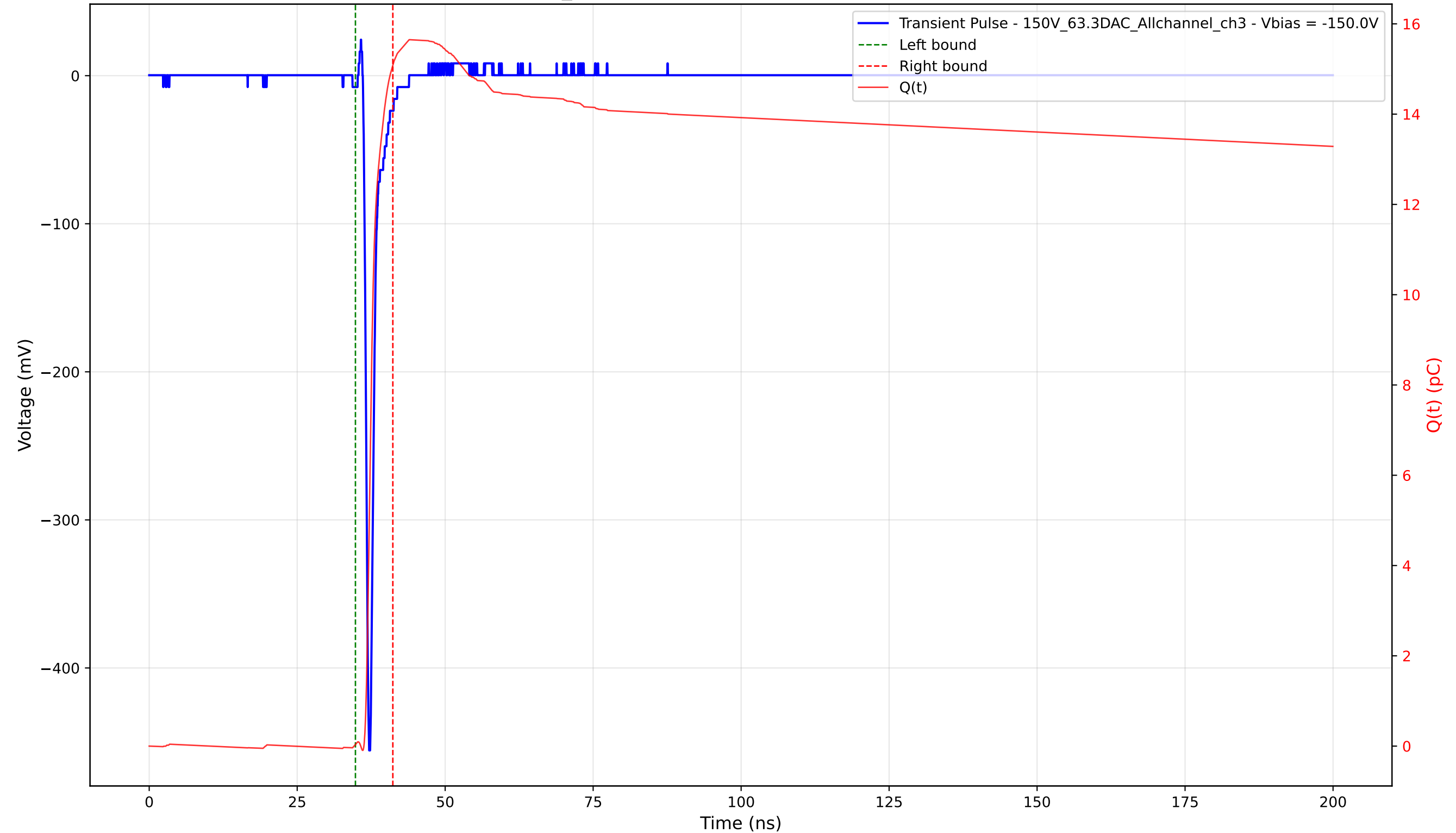
Transient Pulse - Sample: 1cm_42 - Position: 2780.0 \mu\text{m} - Charge: 15.05 pC - Rise Time: 0.73 ns
