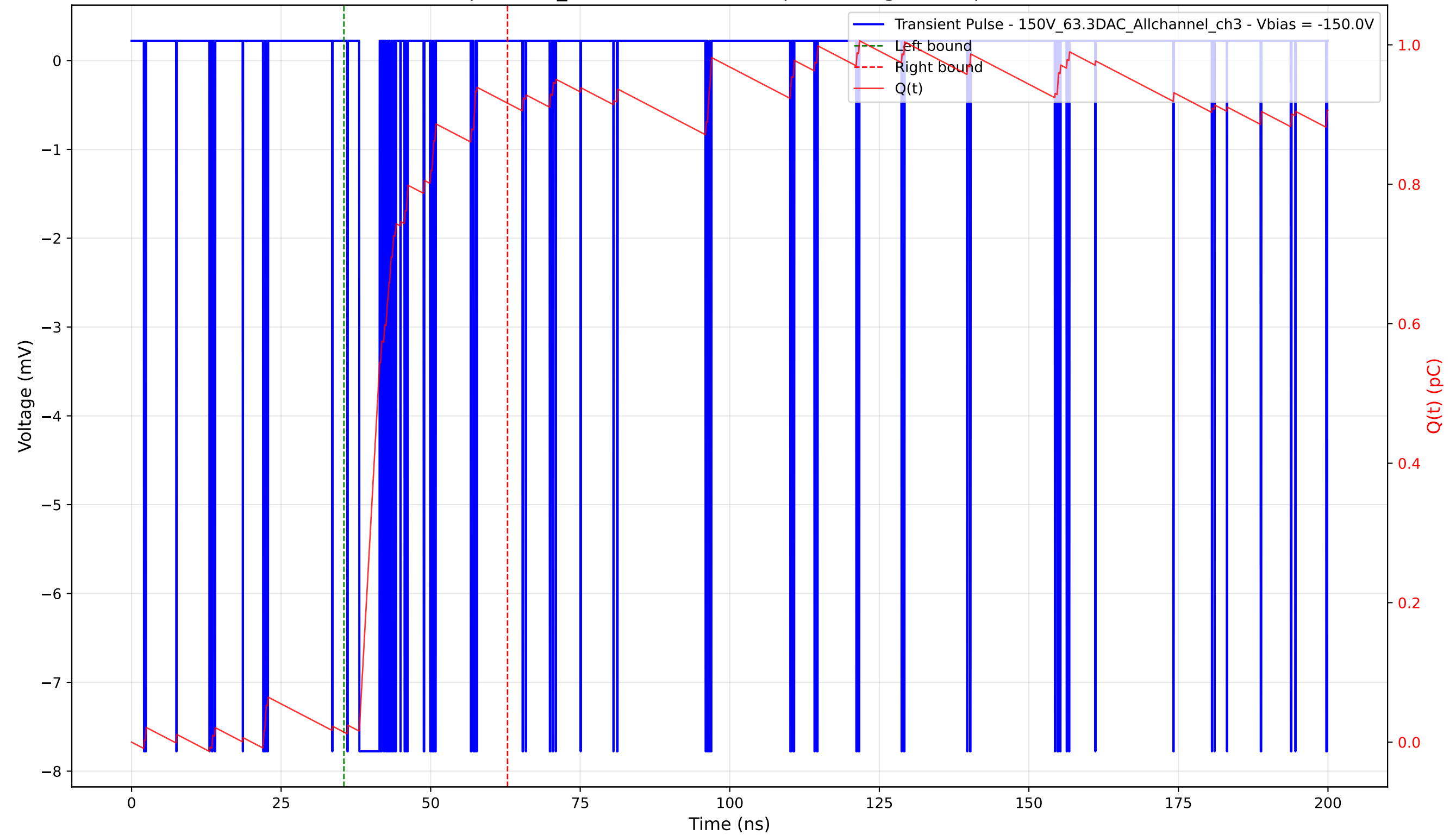
Transient Pulse - Sample: 1cm_42 - Position: 5140.0 \mu\text{m} - Charge: 0.90 pC - Rise Time: 0.04 ns
