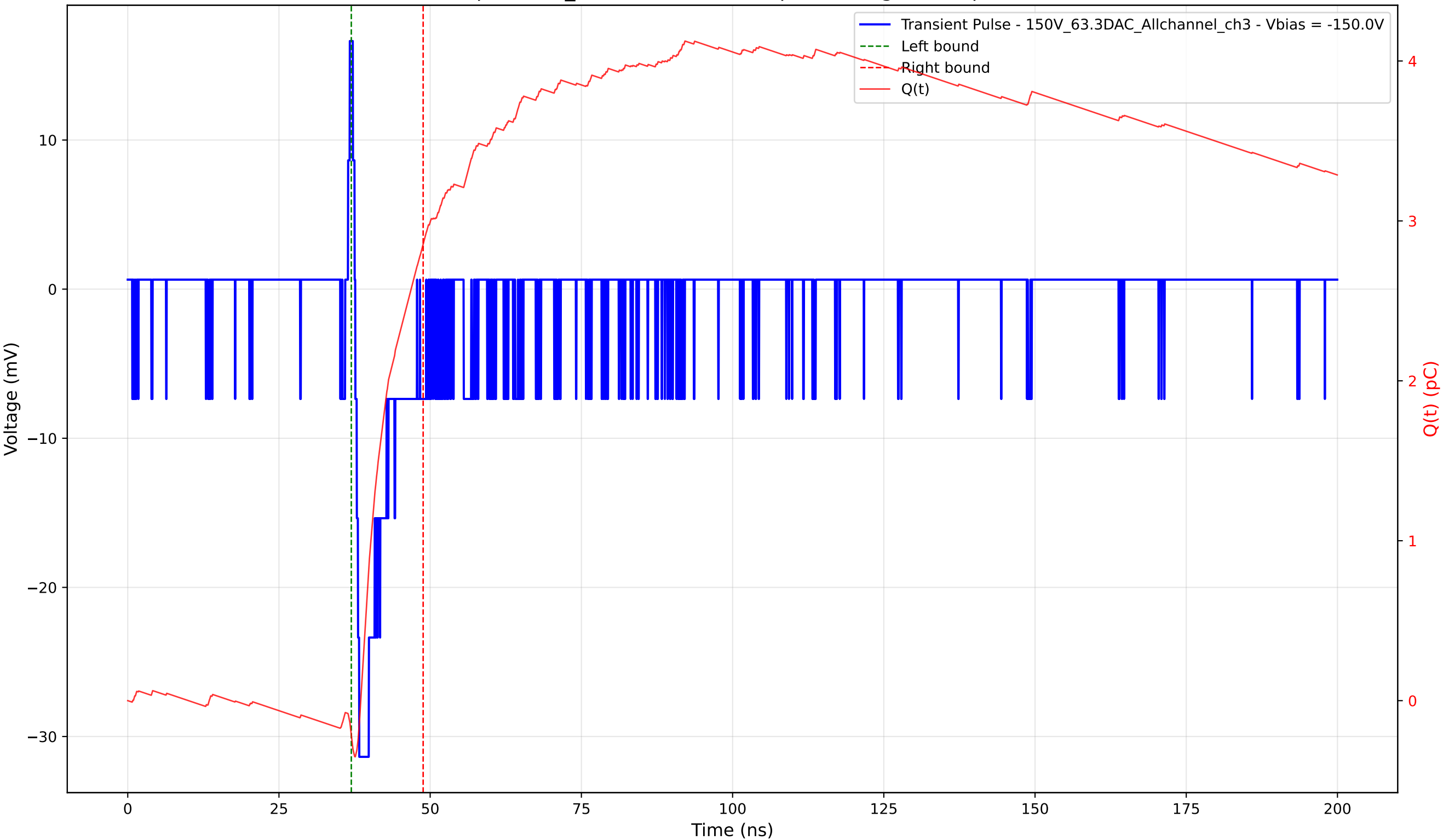
Transient Pulse - Sample: 1cm_42 - Position: 465.0 \mu\text{m} - Charge: 3.07 pC - Rise Time: 0.67 ns
