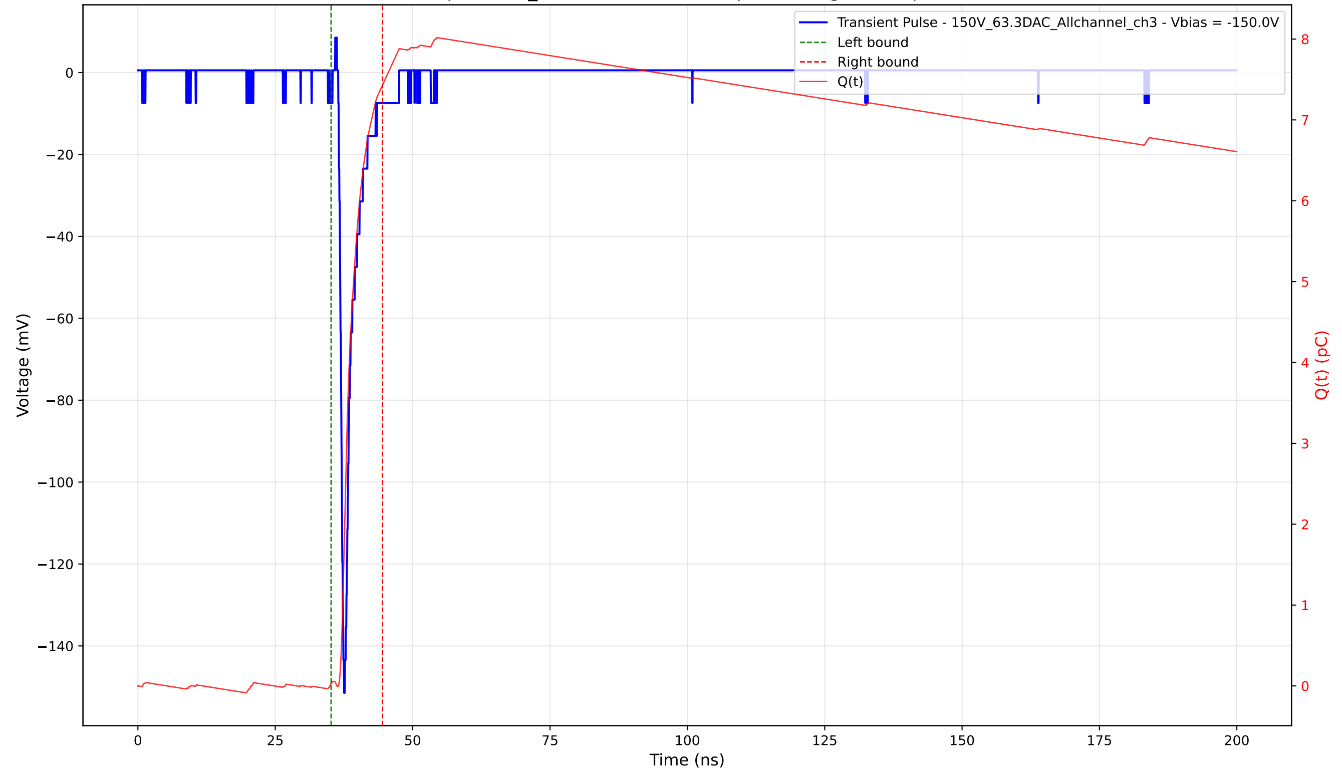
Transient Pulse - Sample: 1cm_42 - Position: 3205.0 \mu\text{m} - Charge: 7.40 pC - Rise Time: 0.84 ns
