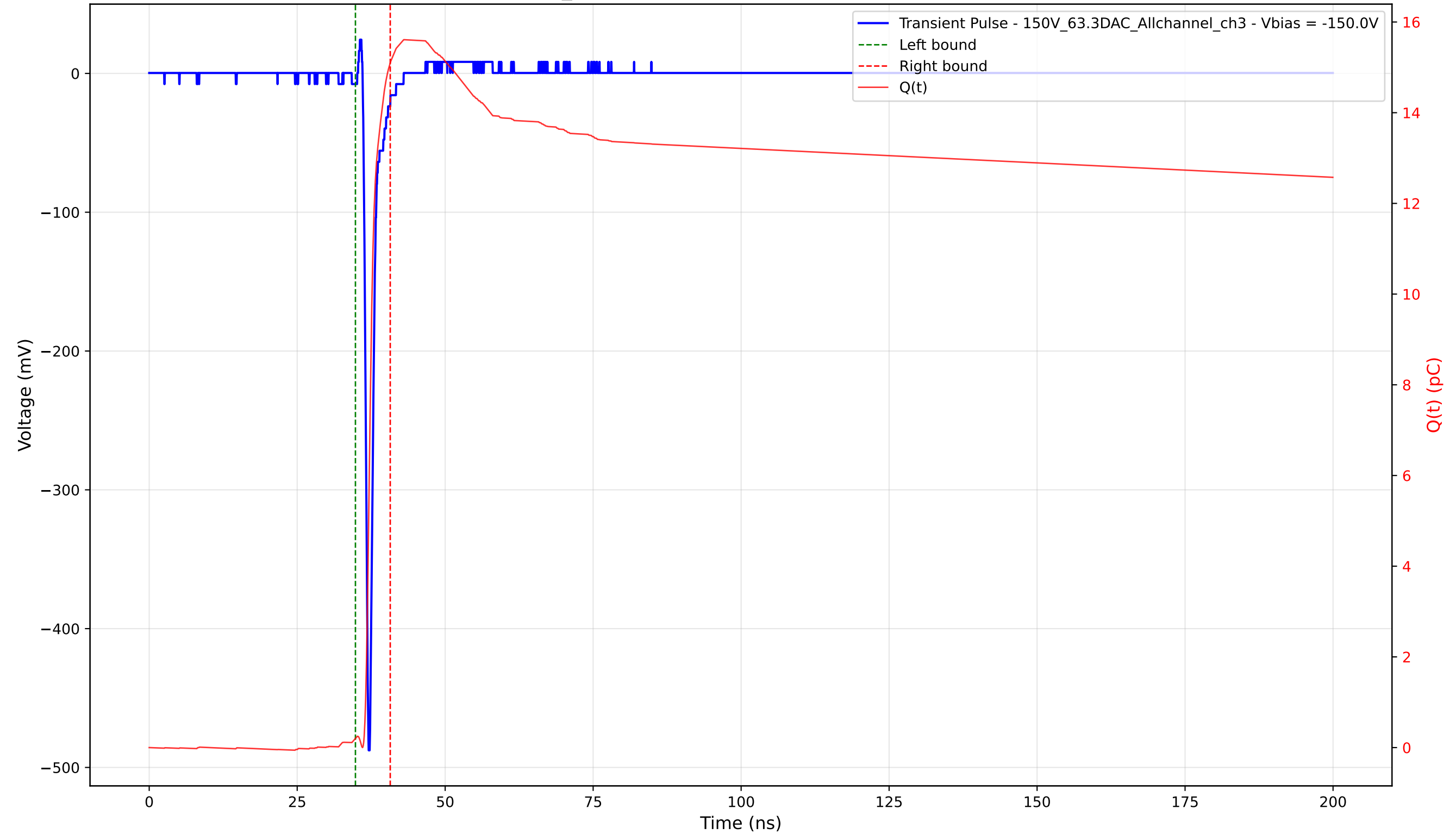
Transient Pulse - Sample: 1cm_42 - Position: 2465.0 \mu\text{m} - Charge: 14.90 pC - Rise Time: 0.72 ns
