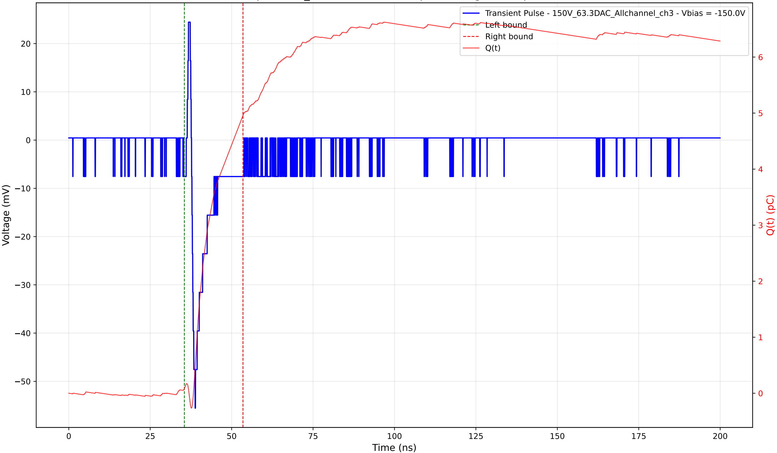
Transient Pulse - Sample: 1cm_42 - Position: 820.0 \mu\text{m} - Charge: 4.88 pC - Rise Time: 1.09 ns
