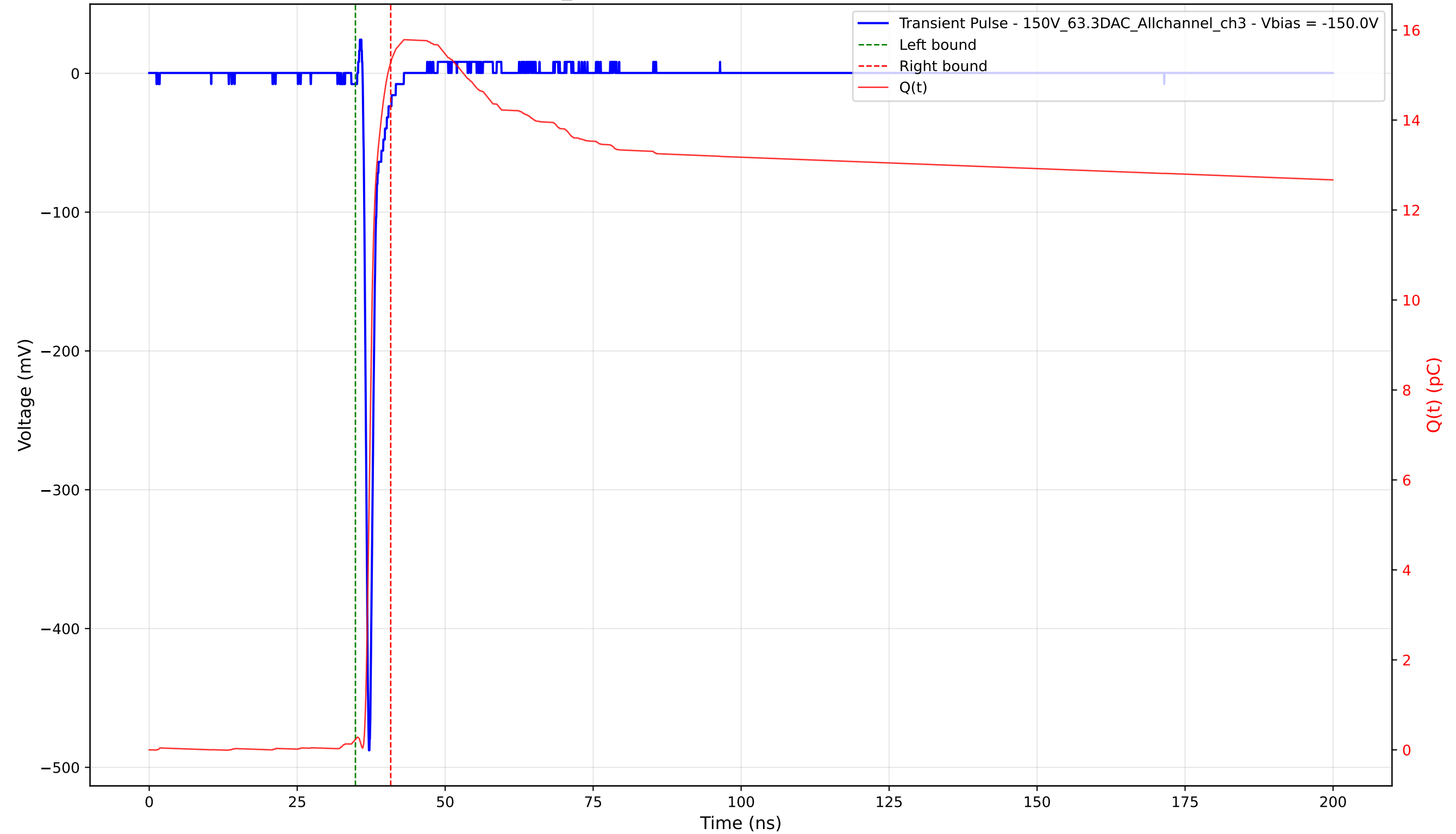
Transient Pulse - Sample: 1cm_42 - Position: 2405.0 \mu\text{m} - Charge: 15.05 pC - Rise Time: 0.73 ns
