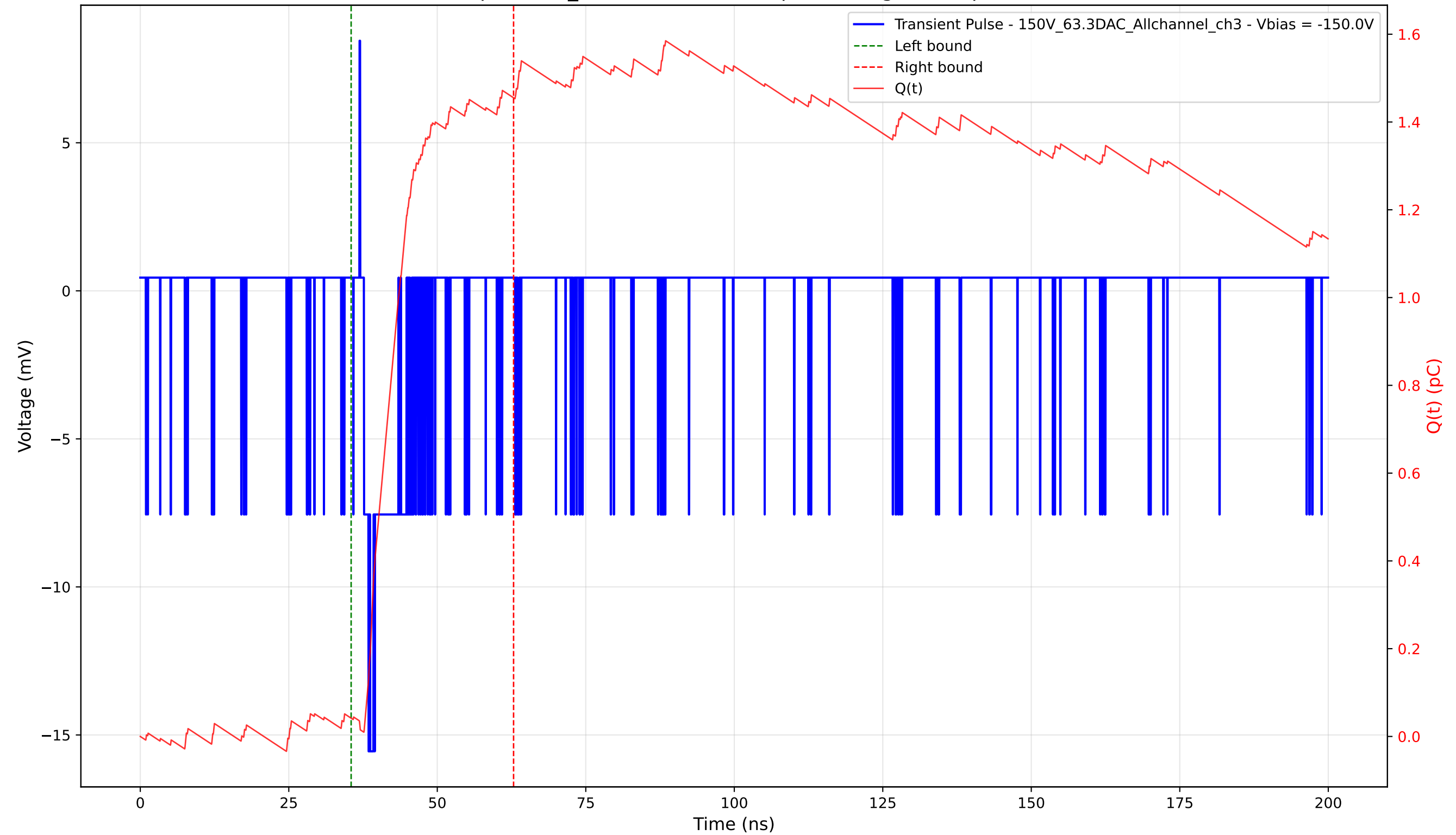
Transient Pulse - Sample: 1cm_42 - Position: 130.0 \mu\text{m} - Charge: 1.41 pC - Rise Time: 0.79 ns
