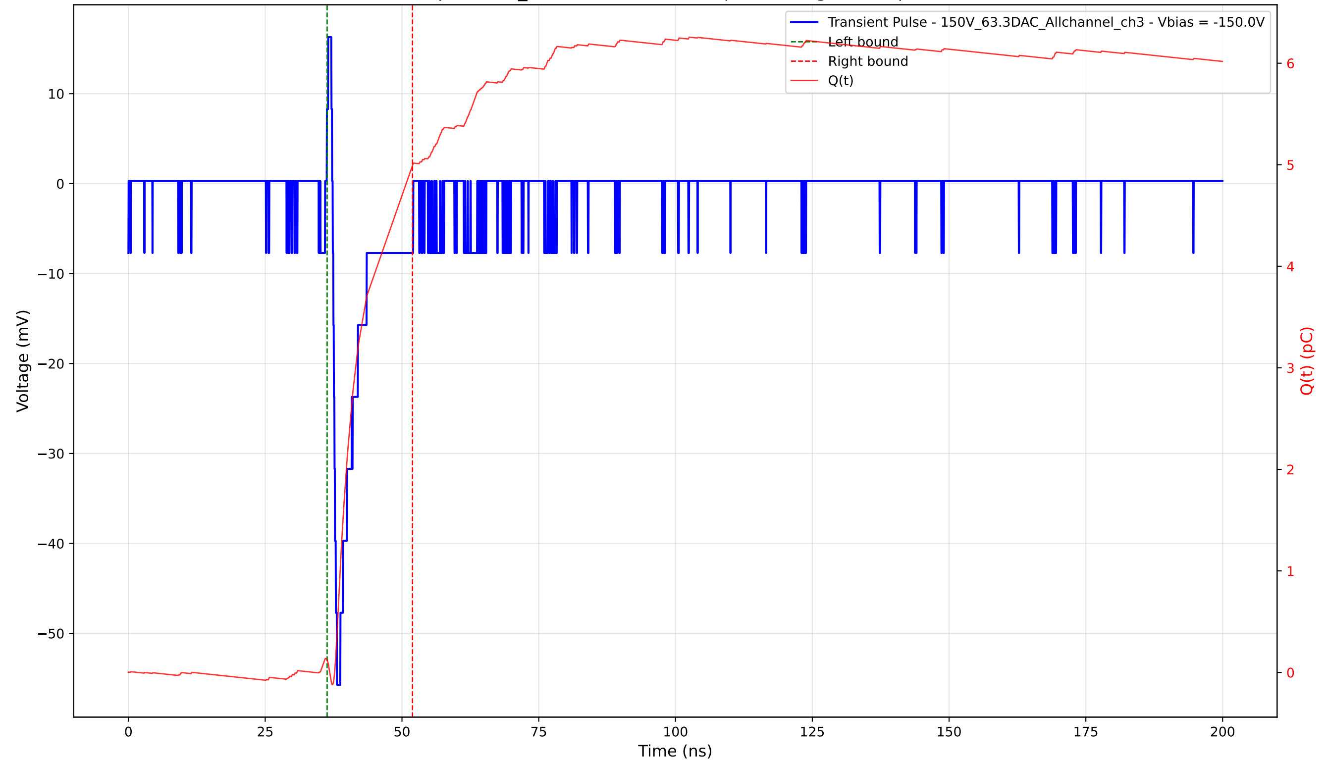
Transient Pulse - Sample: 1cm_42 - Position: 3835.0 \mu\text{m} - Charge: 4.87 pC - Rise Time: 0.77 ns
