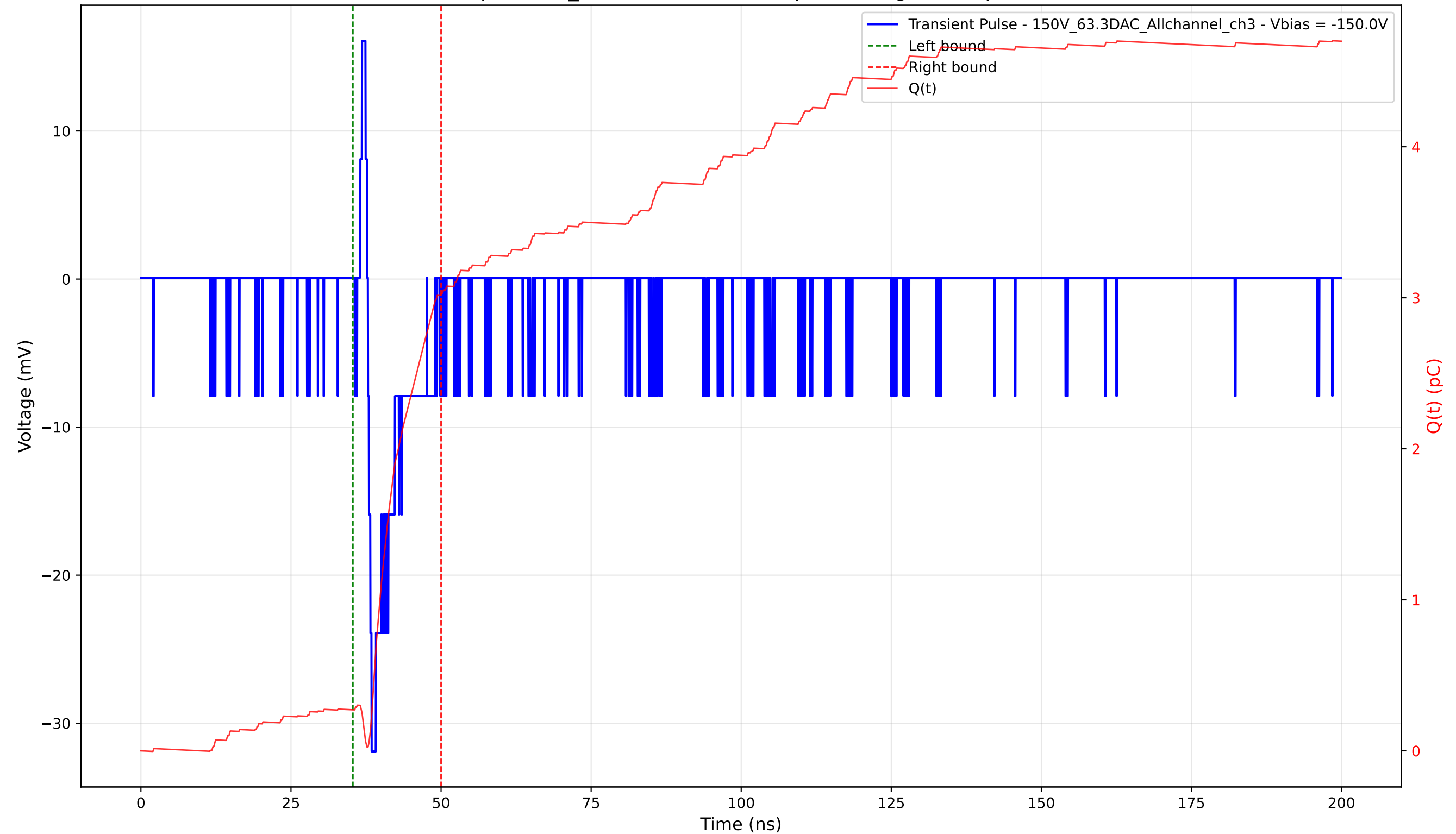
Transient Pulse - Sample: 1cm_42 - Position: 4615.0 \mu\text{m} - Charge: 2.76 pC - Rise Time: 0.62 ns
