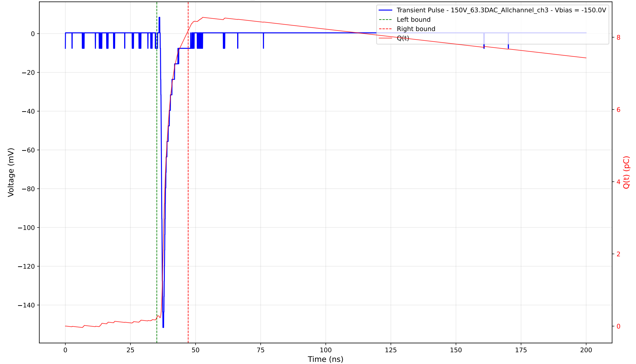
Transient Pulse - Sample: 1cm_42 - Position: 3200.0 \mu\text{m} - Charge: 7.95 pC - Rise Time: 0.80 ns
