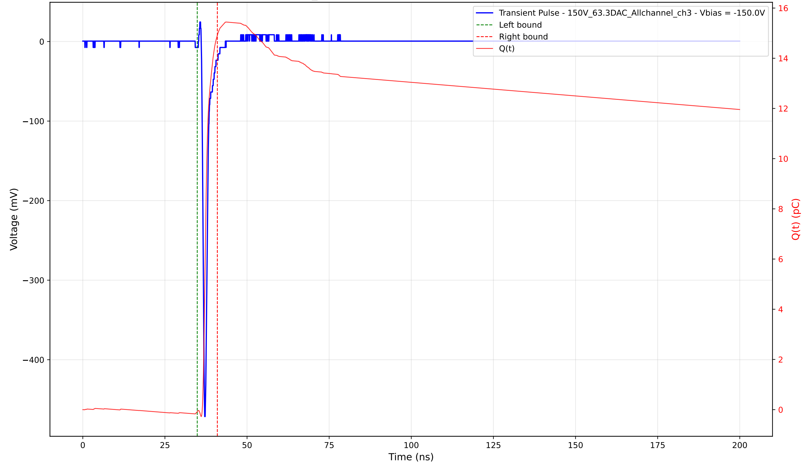
Transient Pulse - Sample: 1cm_42 - Position: 2335.0 \mu\text{m} - Charge: 15.00 pC - Rise Time: 0.71 ns
