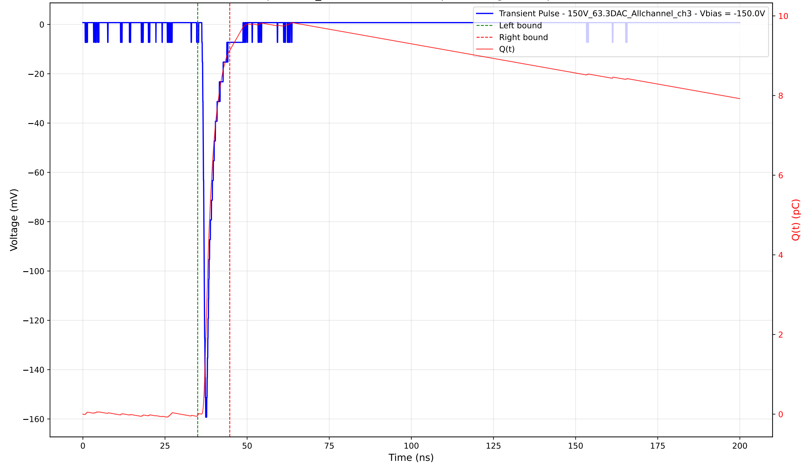
Transient Pulse - Sample: 1cm_42 - Position: 1835.0 \mu\text{m} - Charge: 9.16 pC - Rise Time: 0.84 ns
