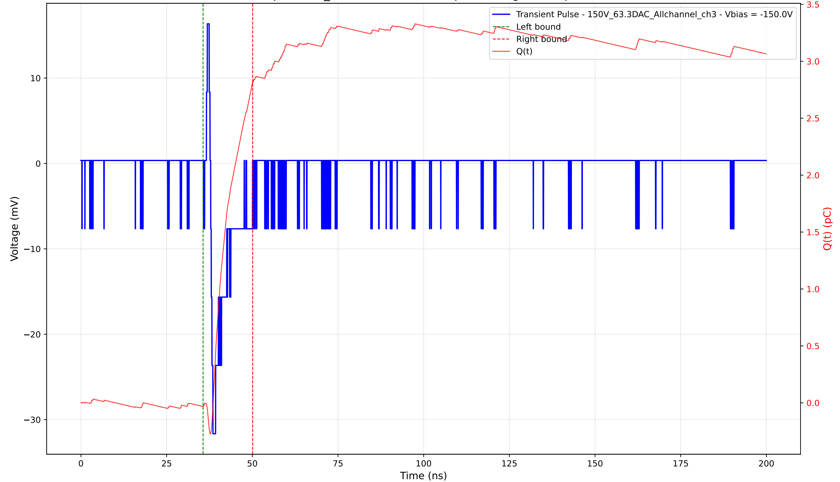
Transient Pulse - Sample: 1cm_42 - Position: 4685.0 \mu\text{m} - Charge: 2.85 pC - Rise Time: 0.66 ns
