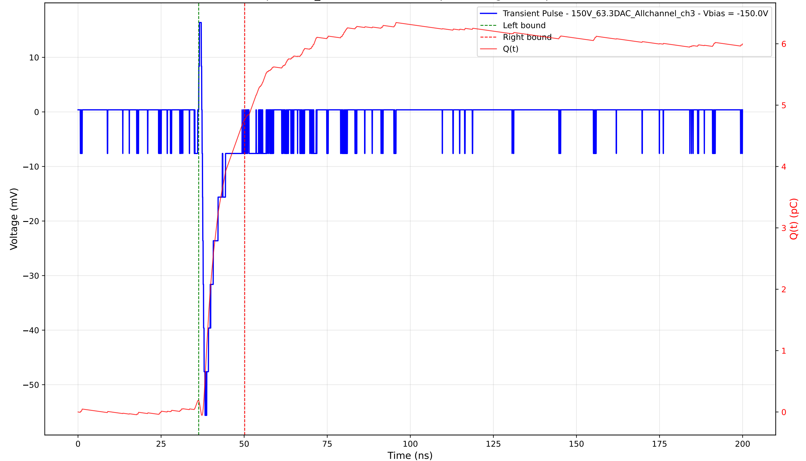
Transient Pulse - Sample: 1cm_42 - Position: 3850.0 \mu\text{m} - Charge: 4.58 pC - Rise Time: 0.89 ns
