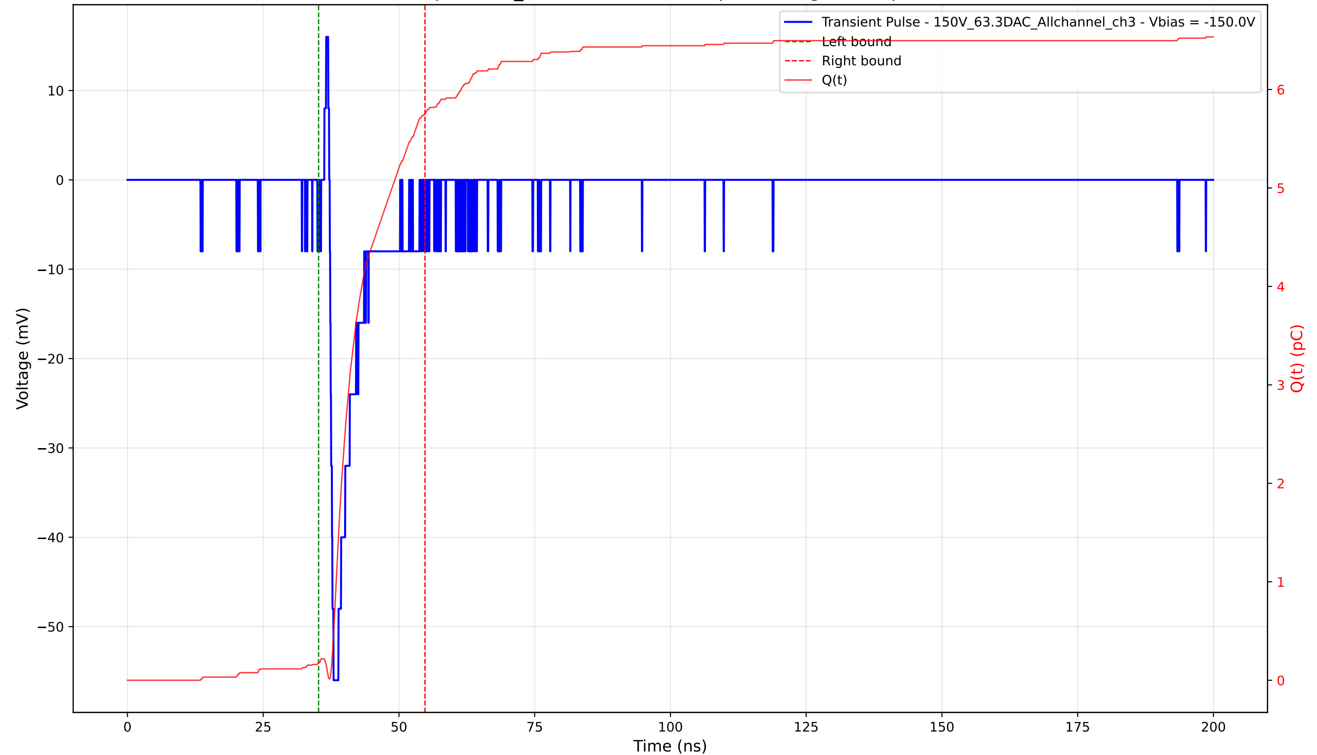
Transient Pulse - Sample: 1cm_42 - Position: 3730.0 \mu\text{m} - Charge: 5.57 pC - Rise Time: 0.69 ns
