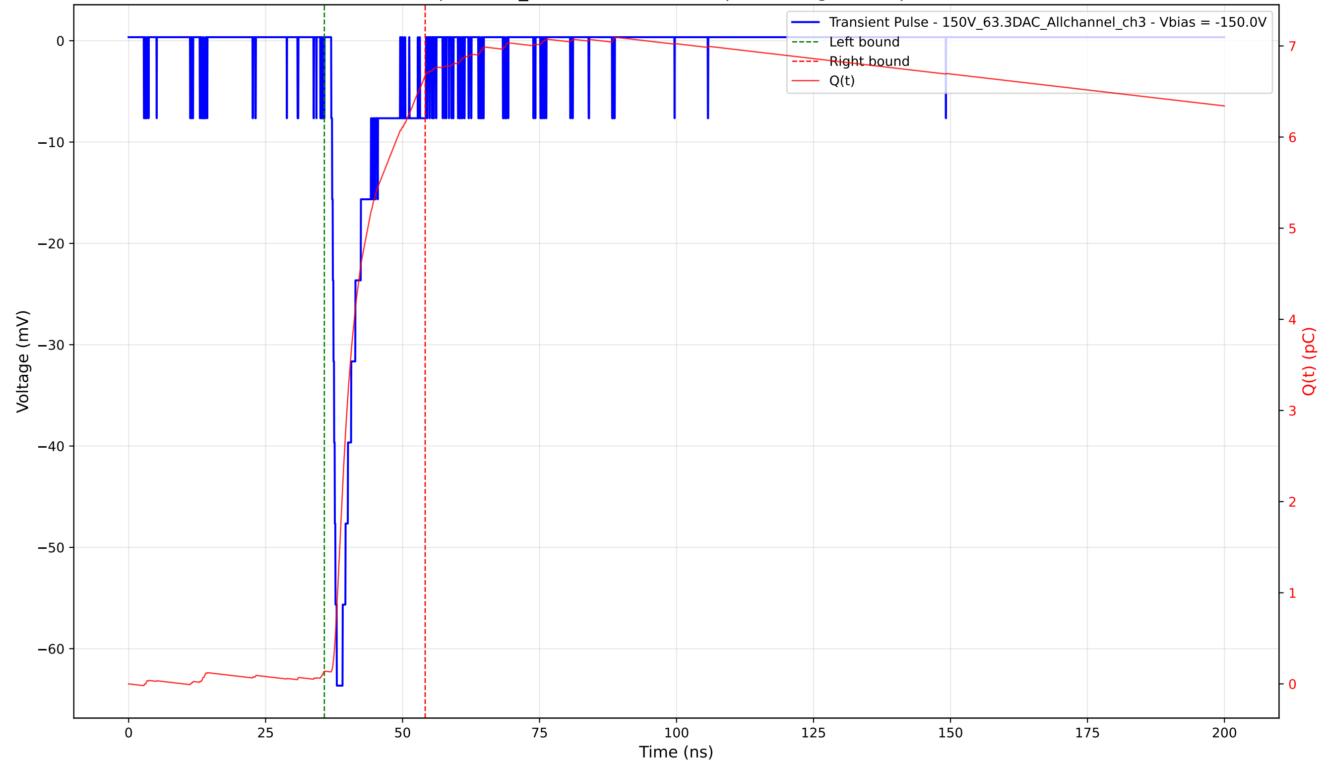
Transient Pulse - Sample: 1cm_42 - Position: 1405.0 \mu\text{m} - Charge: 6.54 pC - Rise Time: 1.01 ns
