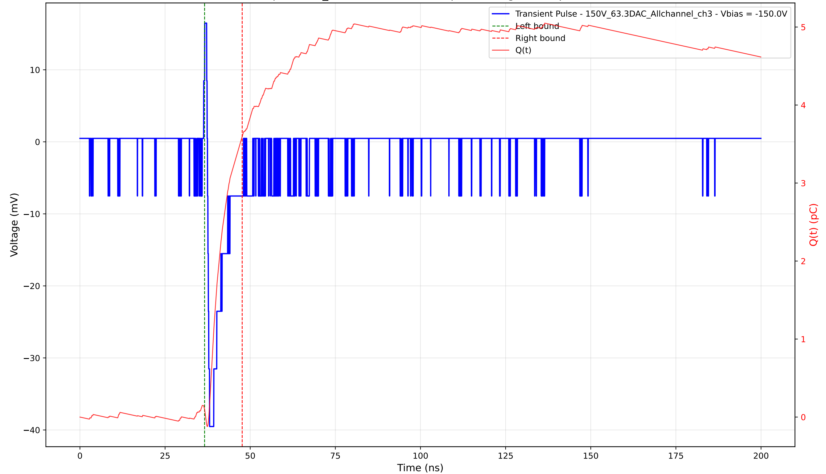
Transient Pulse - Sample: 1cm_42 - Position: 3960.0 \mu\text{m} - Charge: 3.50 pC - Rise Time: 0.62 ns
