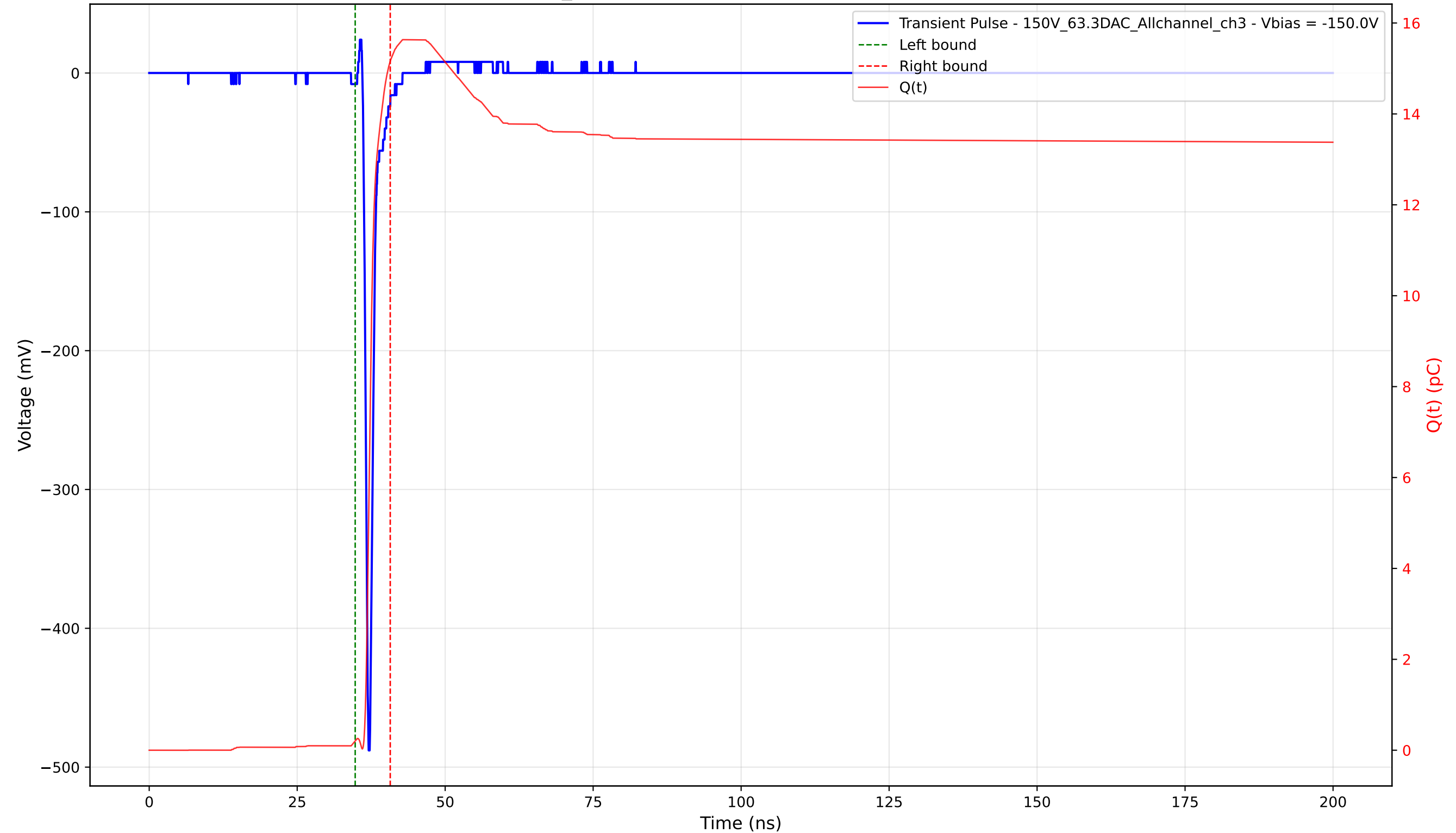
Transient Pulse - Sample: 1cm_42 - Position: 2550.0 \mu\text{m} - Charge: 14.96 pC - Rise Time: 0.67 ns
