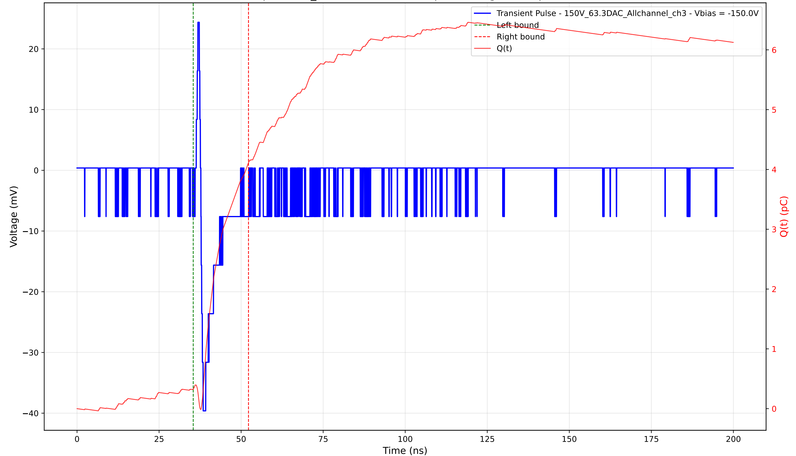
Transient Pulse - Sample: 1cm_42 - Position: 4220.0 \mu\text{m} - Charge: 3.79 pC - Rise Time: 0.70 ns
