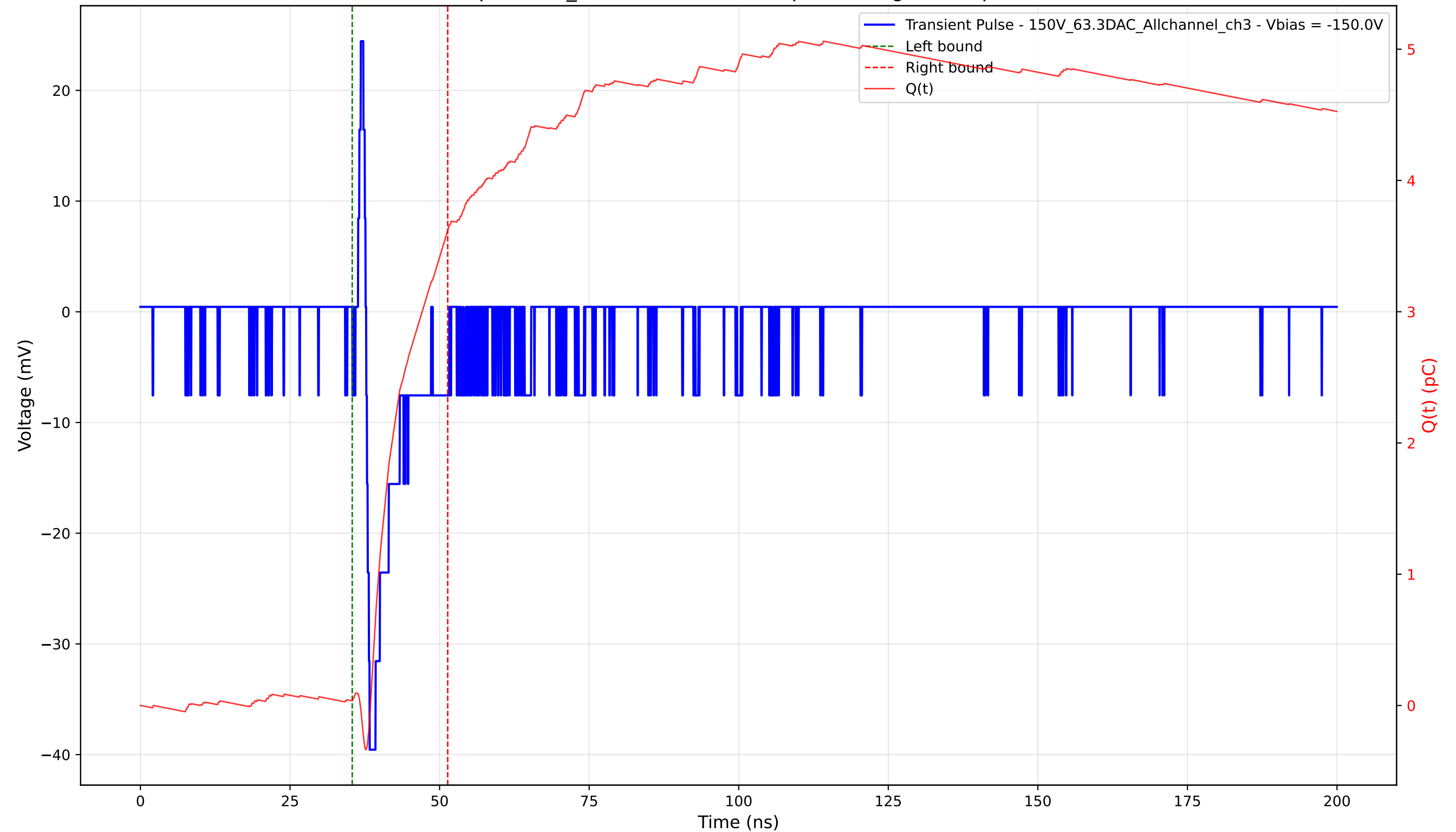
Transient Pulse - Sample: 1cm_42 - Position: 4255.0 \mu\text{m} - Charge: 3.59 pC - Rise Time: 0.58 ns
