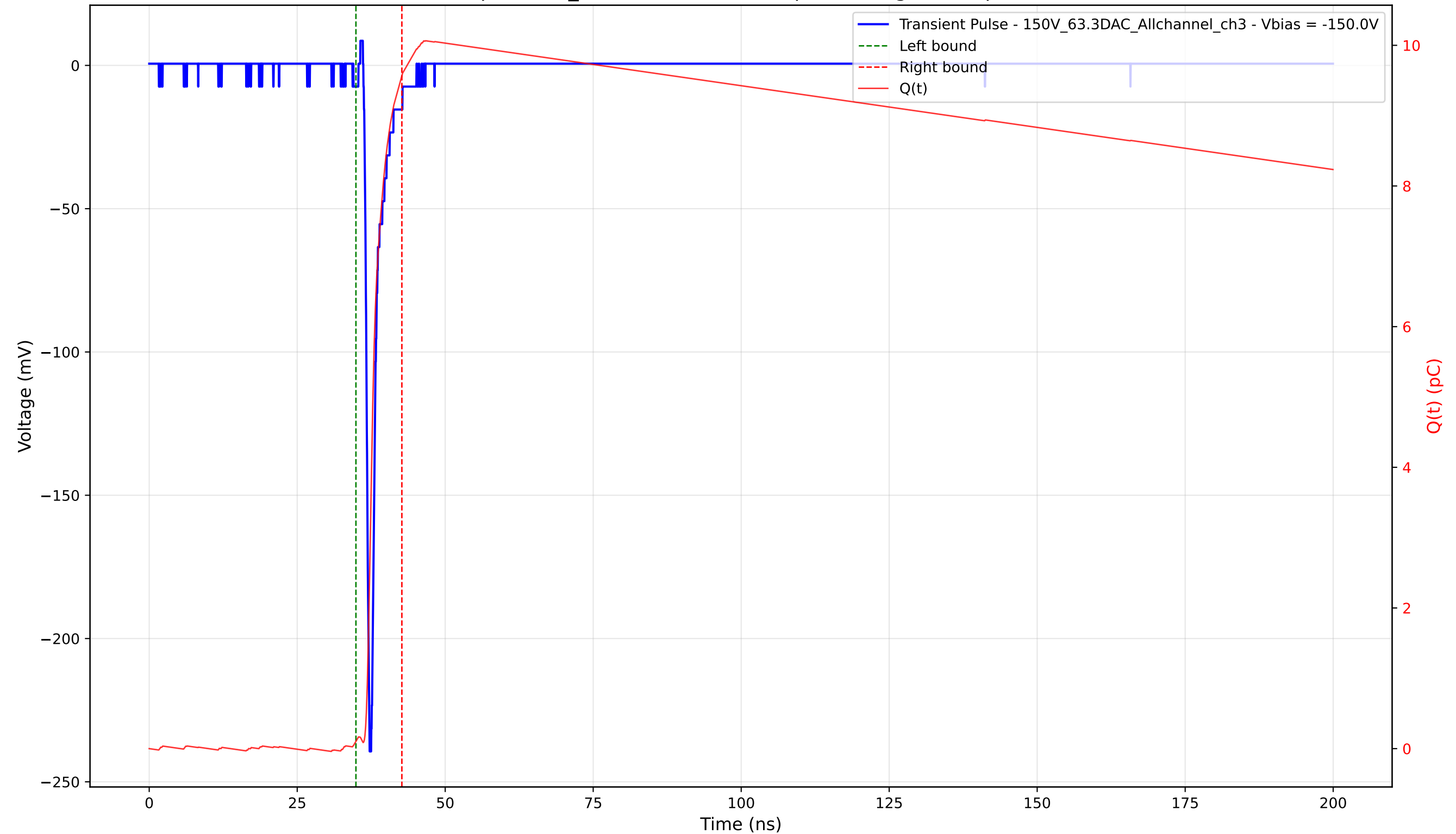
Transient Pulse - Sample: 1cm_42 - Position: 2995.0 \mu\text{m} - Charge: 9.46 pC - Rise Time: 0.76 ns
