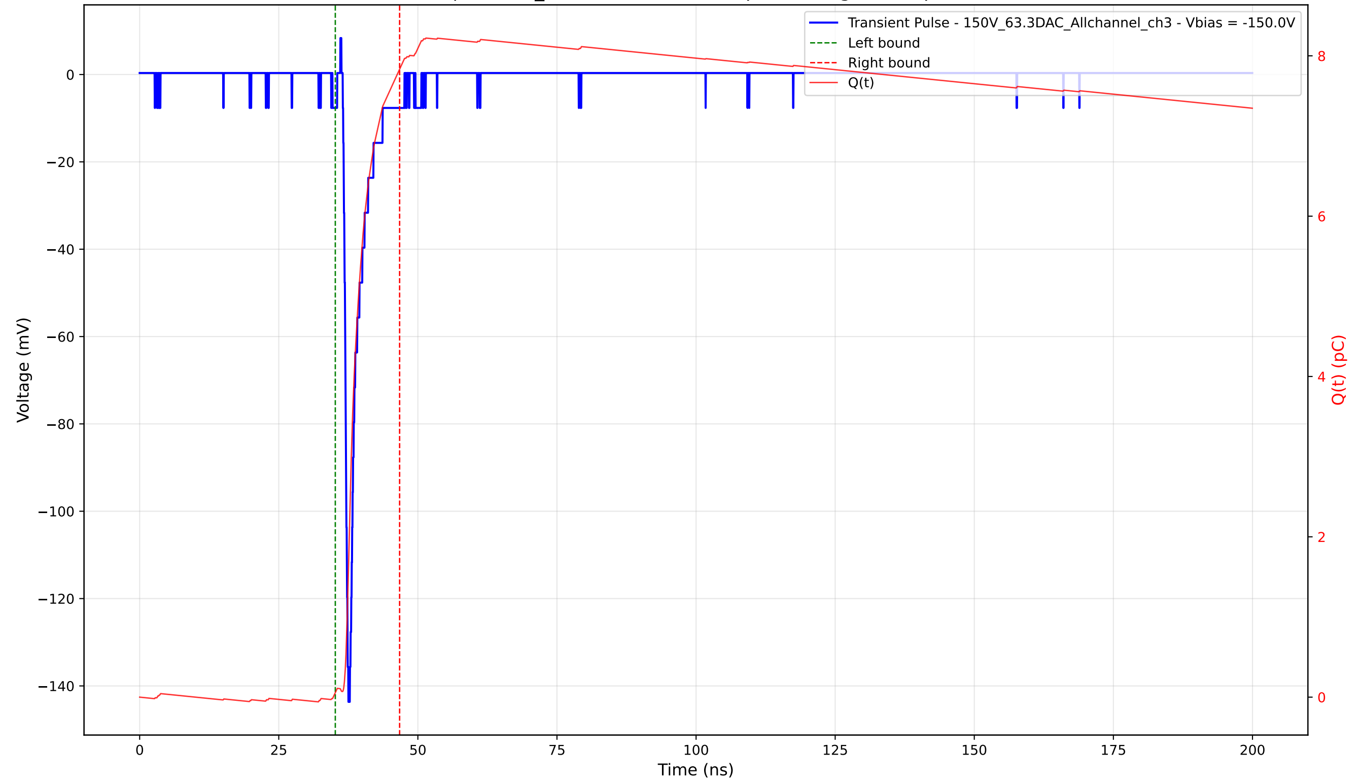
Transient Pulse - Sample: 1cm_42 - Position: 3250.0 \mu\text{m} - Charge: 7.78 pC - Rise Time: 0.81 ns
