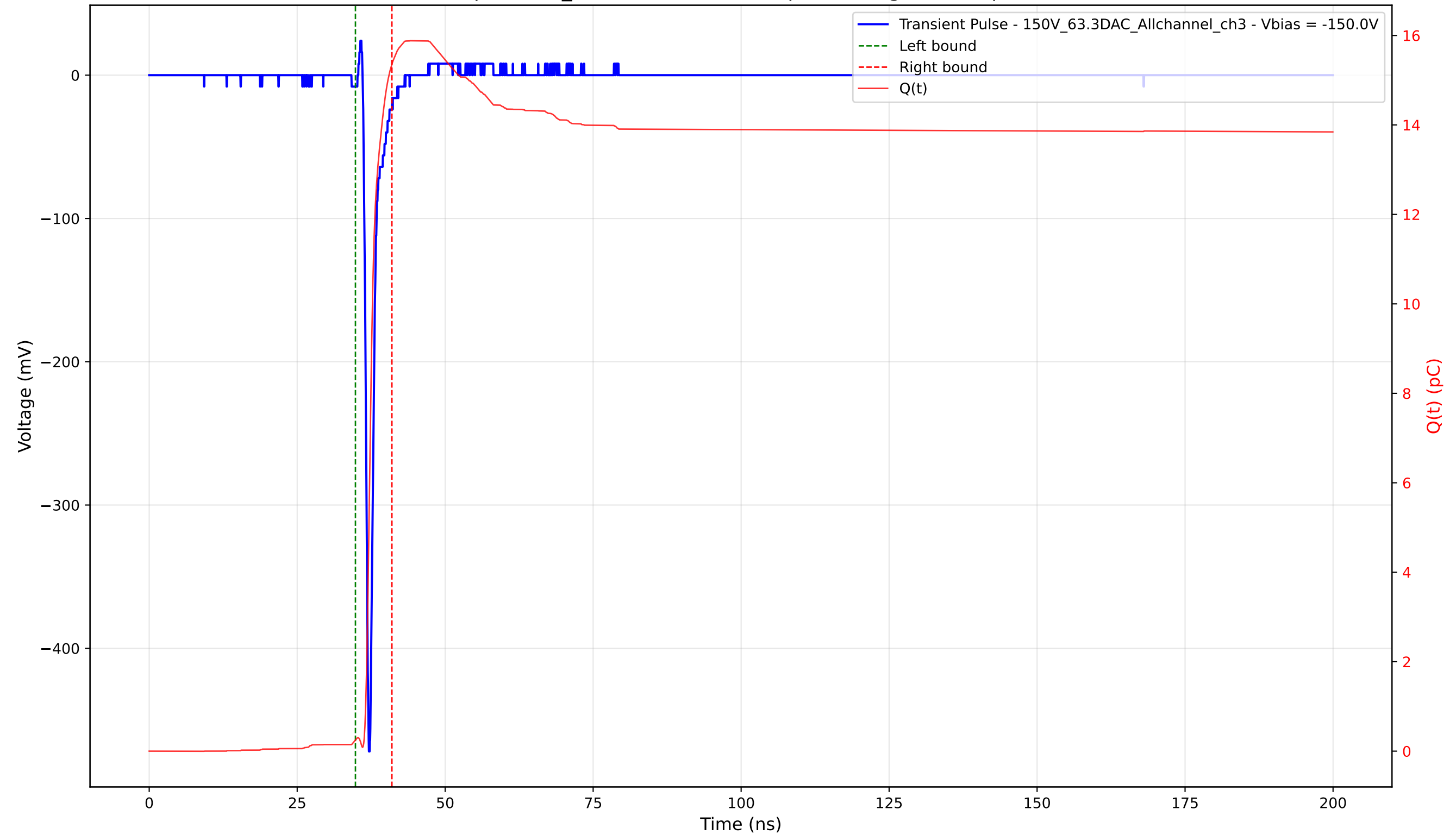
Transient Pulse - Sample: 1cm_42 - Position: 2325.0 \mu\text{m} - Charge: 15.11 pC - Rise Time: 0.73 ns
