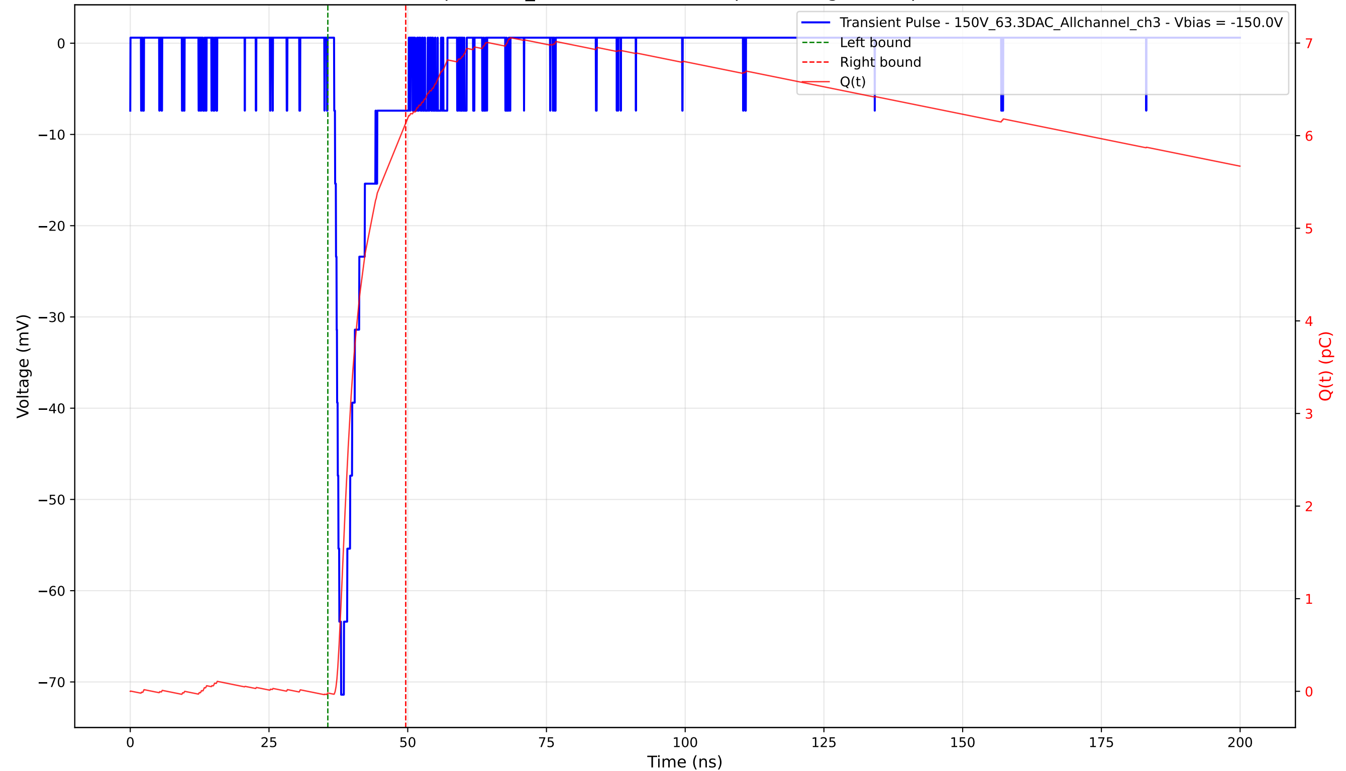
Transient Pulse - Sample: 1cm_42 - Position: 1465.0 \mu\text{m} - Charge: 6.16 pC - Rise Time: 1.24 ns
