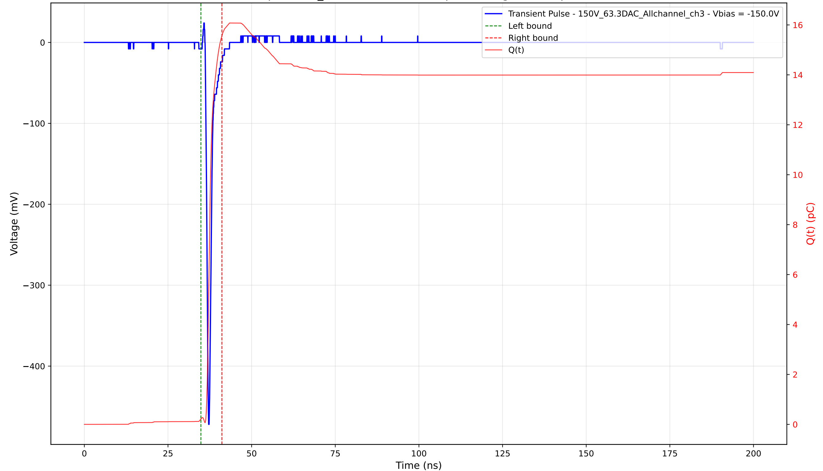
Transient Pulse - Sample: 1cm_42 - Position: 2730.0 \mu\text{m} - Charge: 15.35 pC - Rise Time: 0.74 ns
