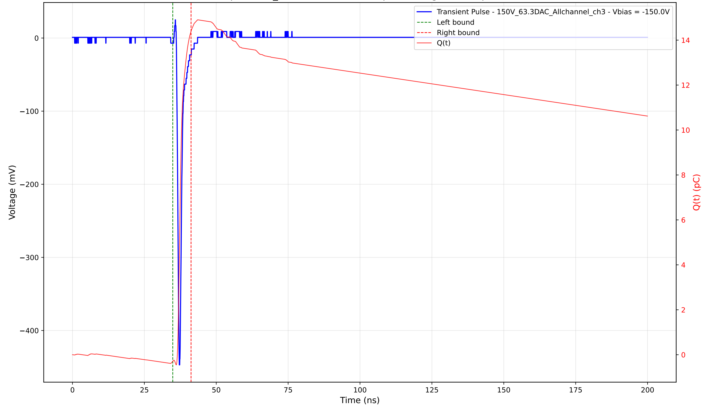
Transient Pulse - Sample: 1cm_42 - Position: 2805.0 \mu\text{m} - Charge: 14.69 pC - Rise Time: 0.72 ns
