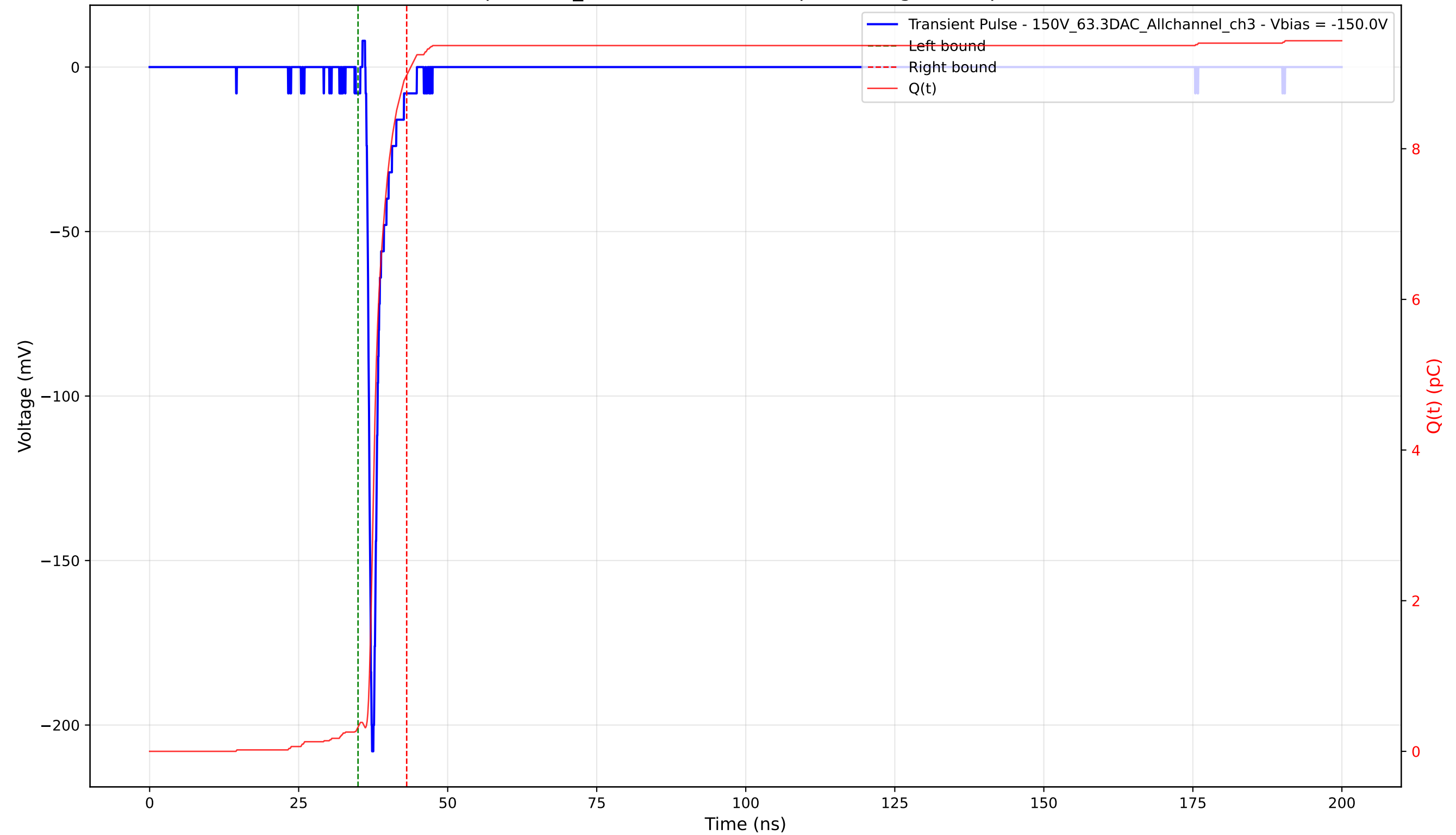
Transient Pulse - Sample: 1cm_42 - Position: 3040.0 \mu\text{m} - Charge: 8.65 pC - Rise Time: 0.79 ns
