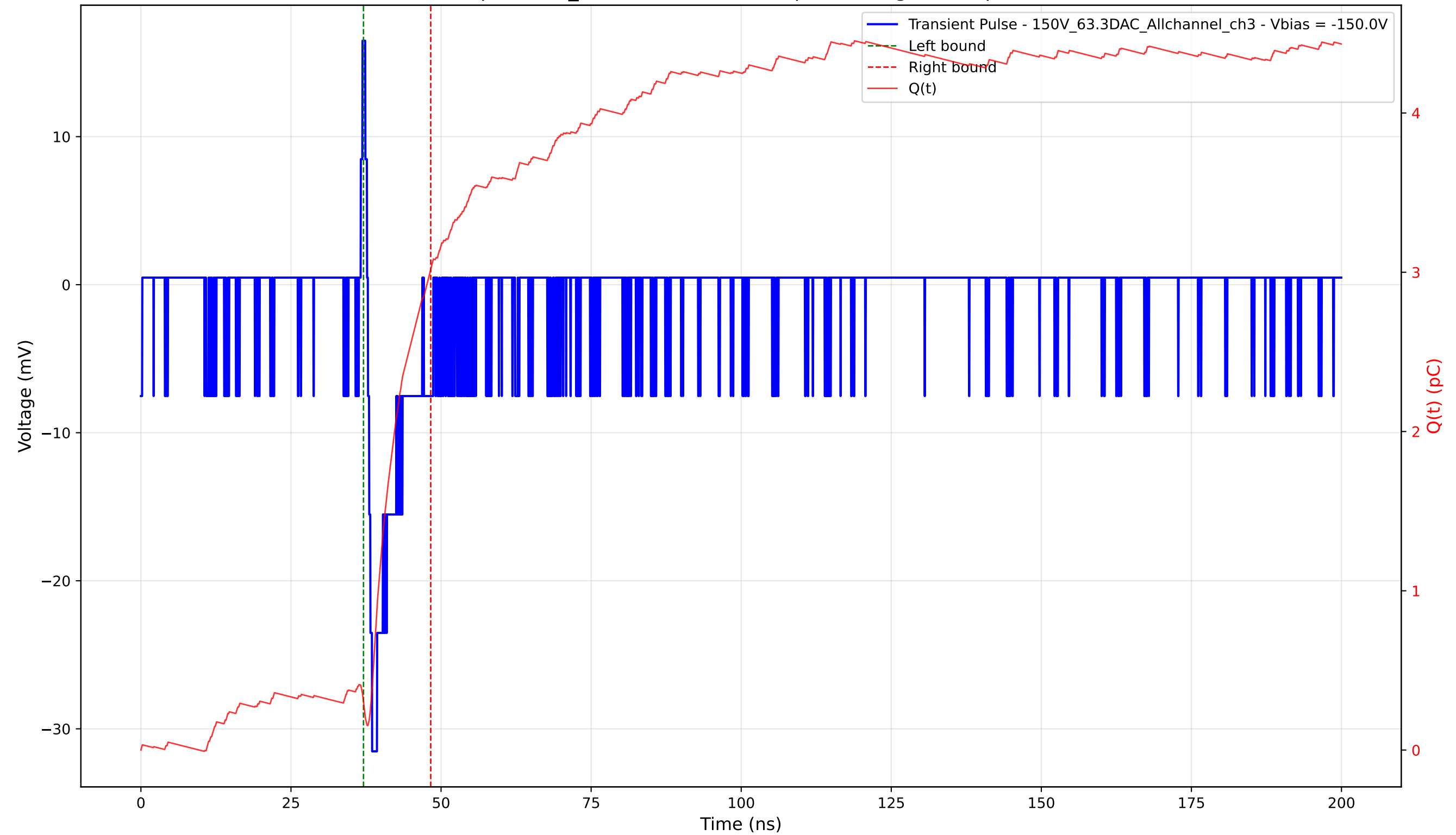
Transient Pulse - Sample: 1cm_42 - Position: 4675.0 \mu\text{m} - Charge: 2.72 pC - Rise Time: 0.70 ns
