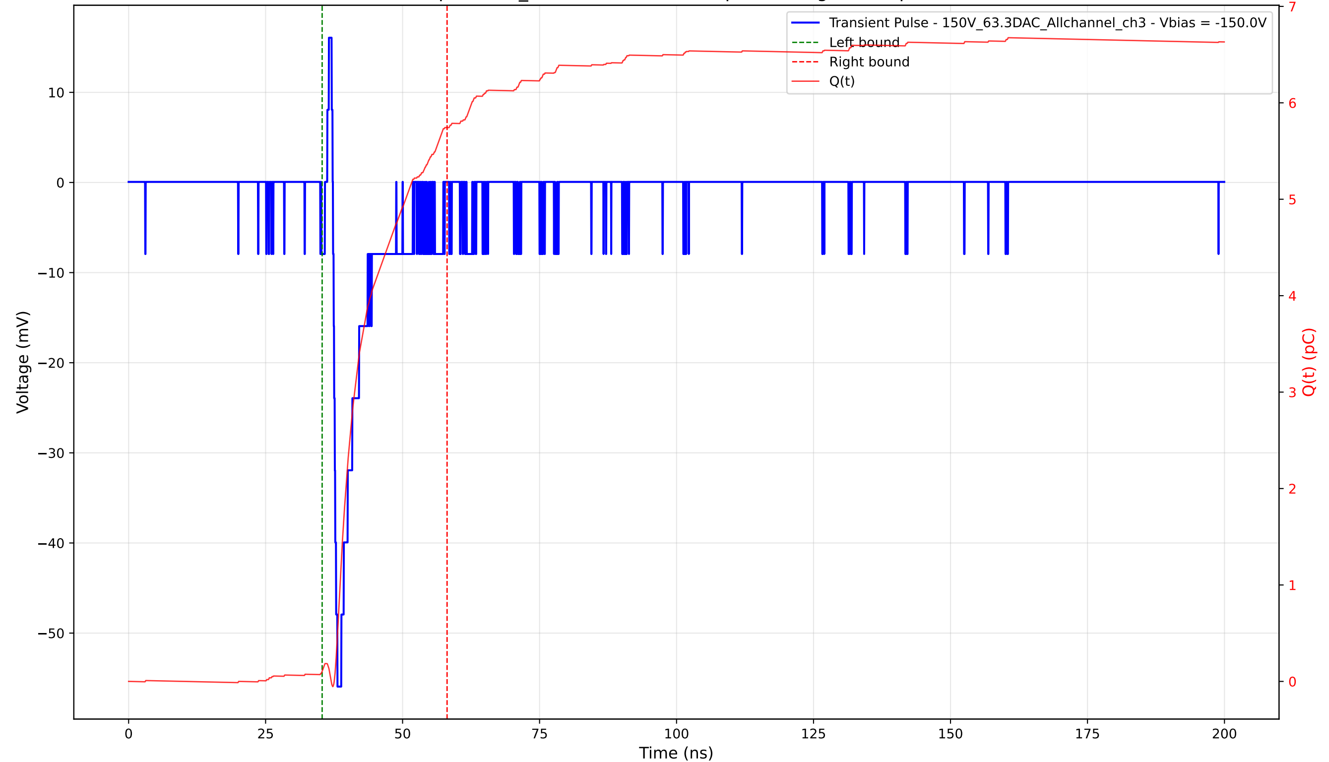
Transient Pulse - Sample: 1cm_42 - Position: 3815.0 \mu\text{m} - Charge: 5.64 pC - Rise Time: 0.81 ns
