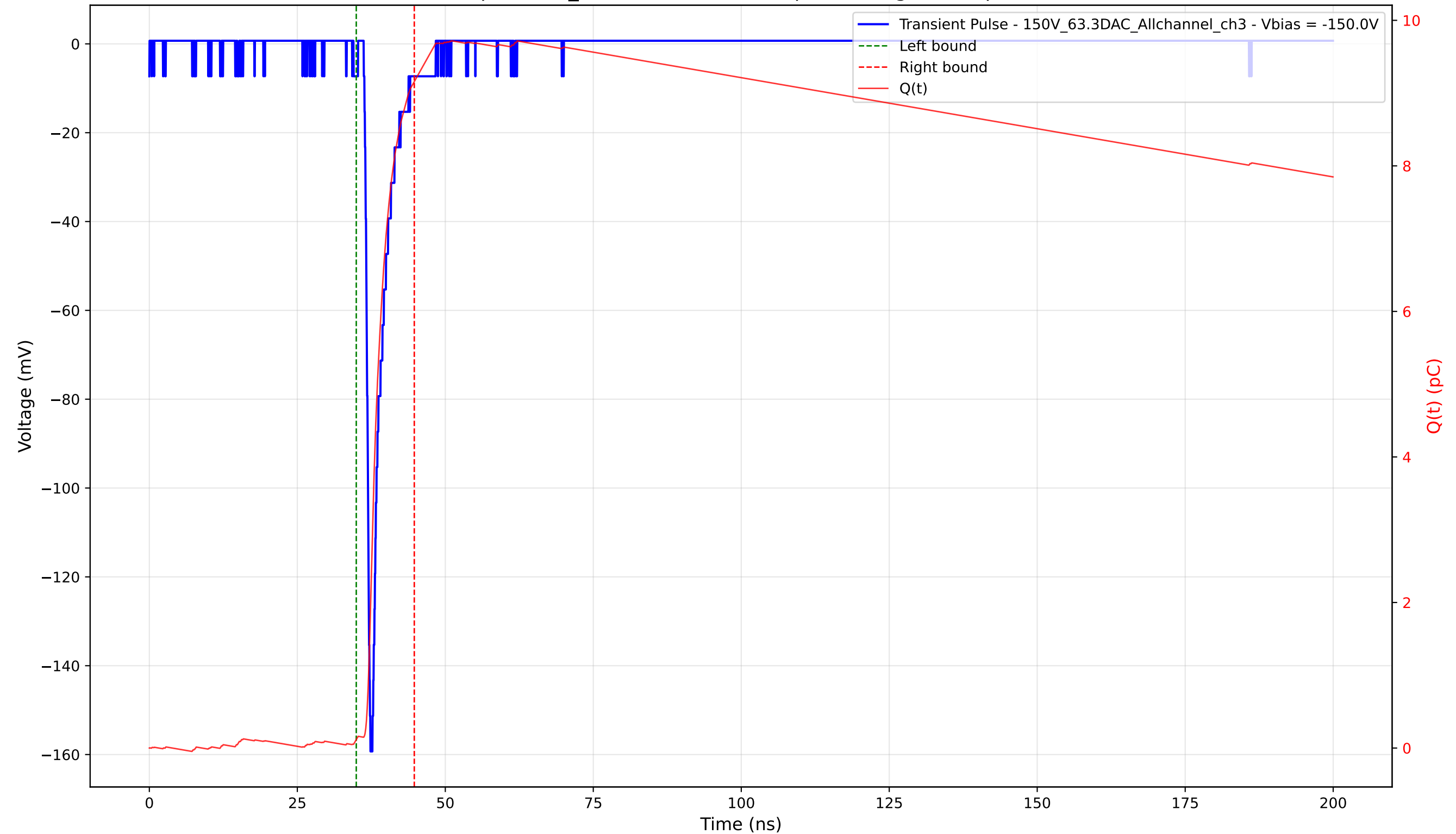
Transient Pulse - Sample: 1cm_42 - Position: 1860.0 \mu\text{m} - Charge: 9.04 pC - Rise Time: 0.88 ns
