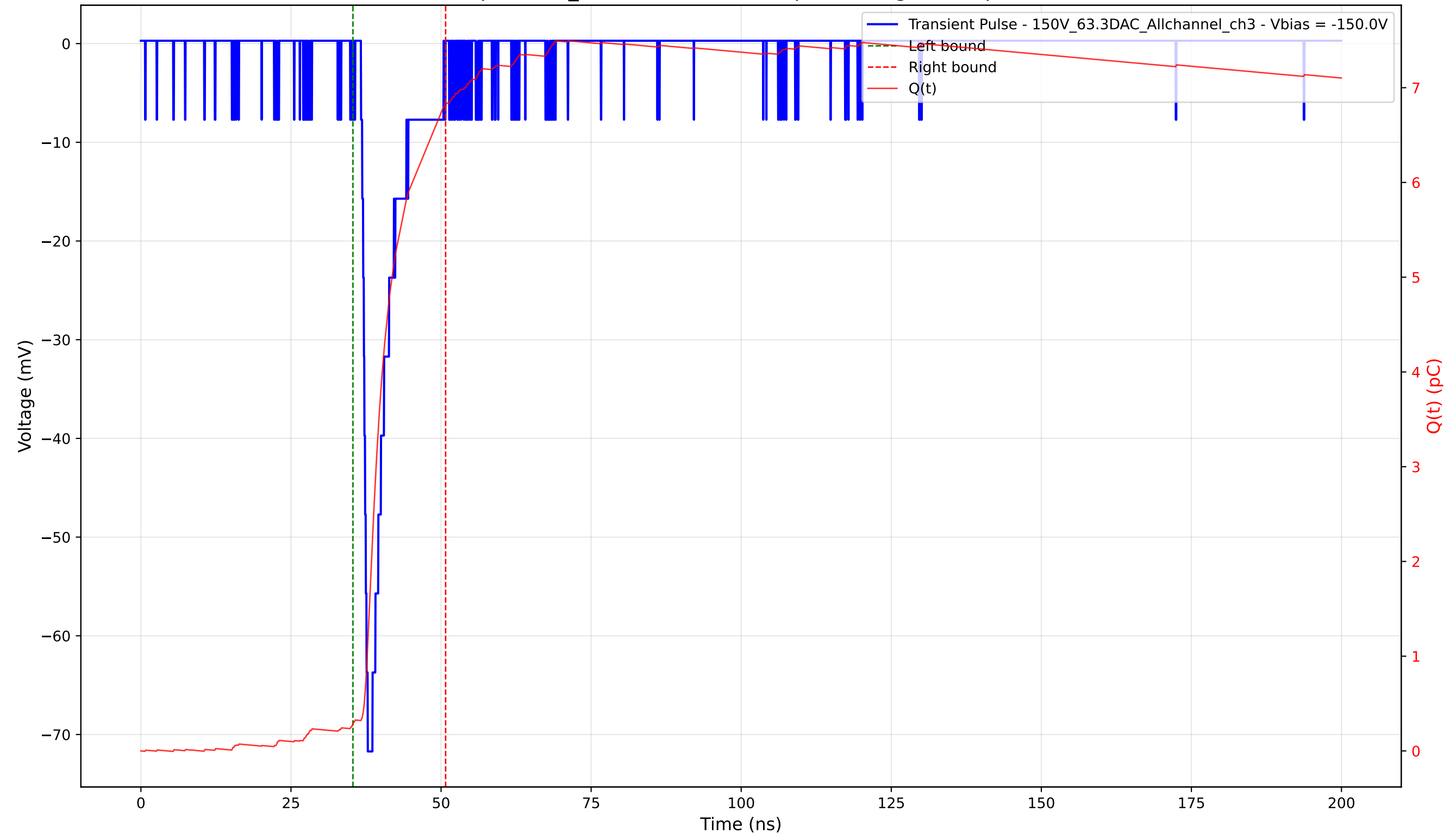
Transient Pulse - Sample: 1cm_42 - Position: 1485.0 \mu\text{m} - Charge: 6.55 pC - Rise Time: 1.12 ns
