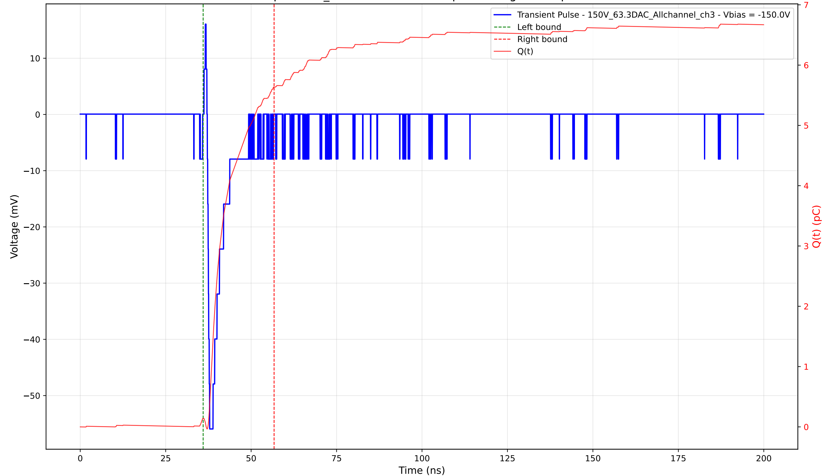
Transient Pulse - Sample: 1cm_42 - Position: 3685.0 \mu\text{m} - Charge: 5.50 pC - Rise Time: 0.69 ns
