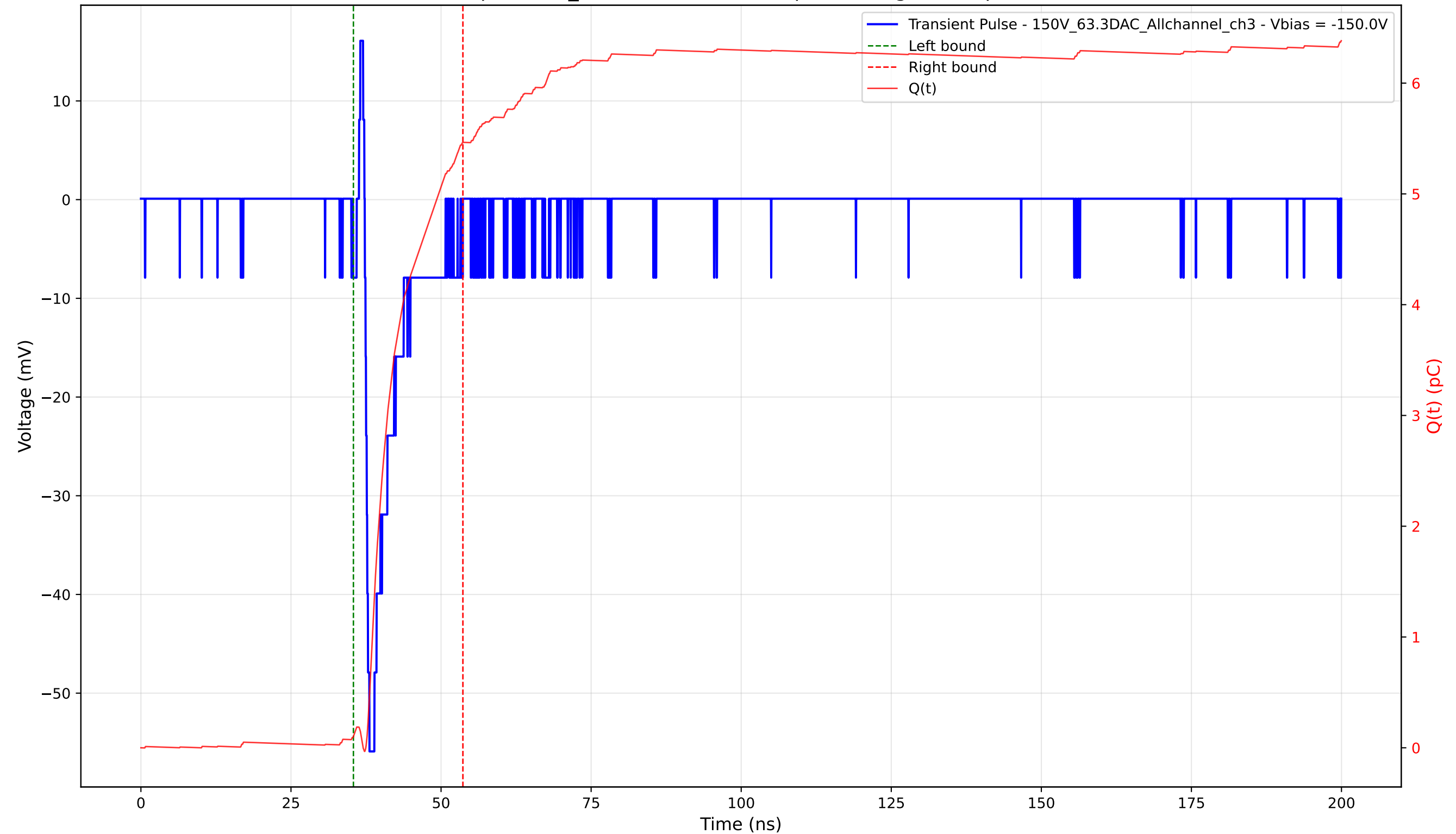
Transient Pulse - Sample: 1cm_42 - Position: 3790.0 \mu\text{m} - Charge: 5.36 pC - Rise Time: 0.77 ns
