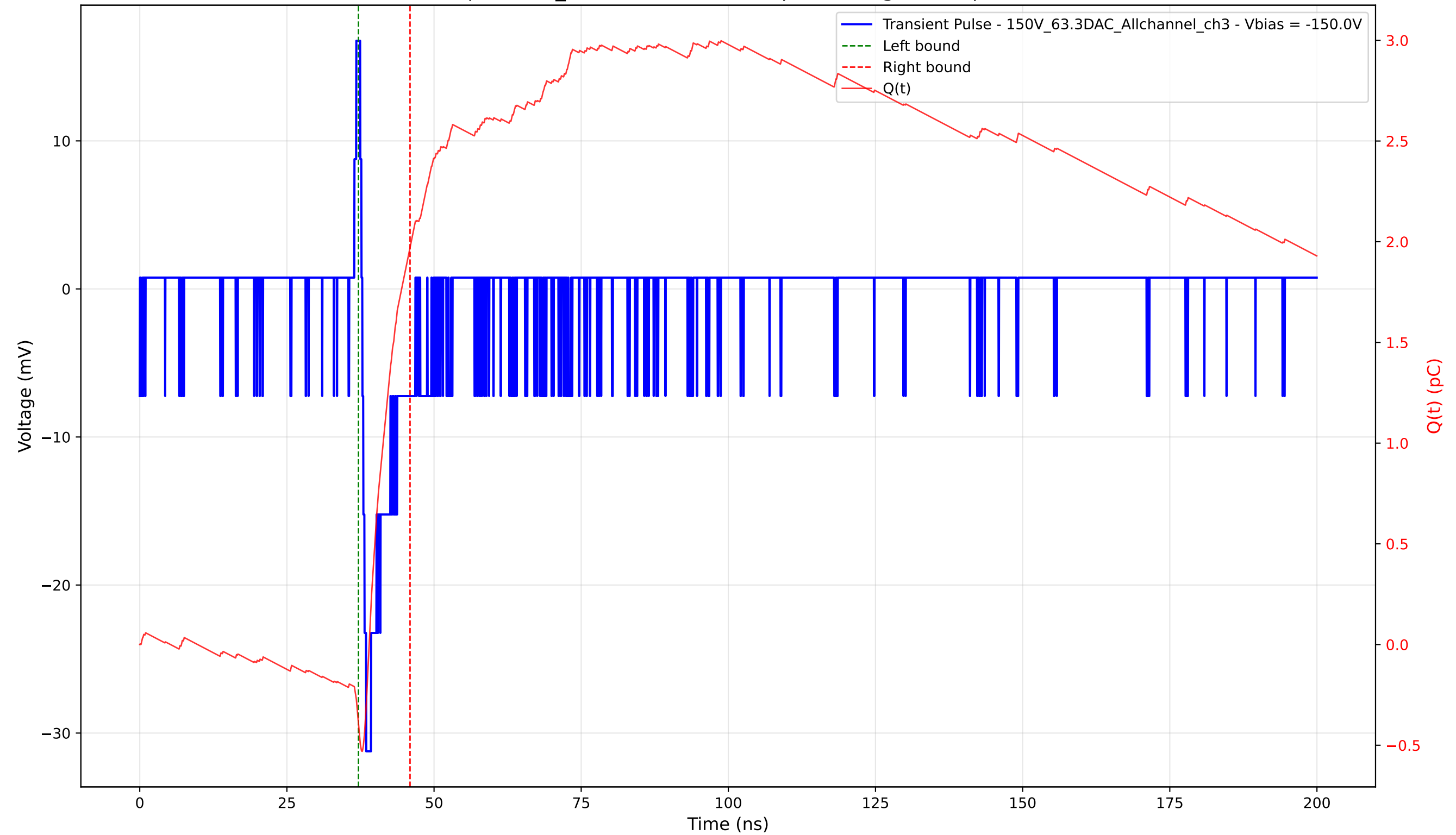
Transient Pulse - Sample: 1cm_42 - Position: 4510.0 \mu\text{m} - Charge: 2.37 pC - Rise Time: 0.67 ns
