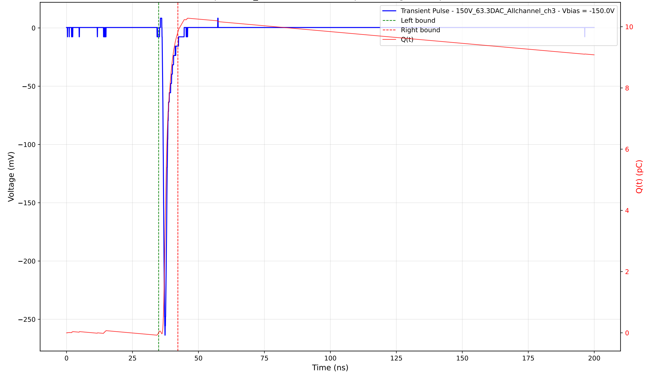
Transient Pulse - Sample: 1cm_42 - Position: 2975.0 \mu\text{m} - Charge: 9.82 pC - Rise Time: 0.77 ns
