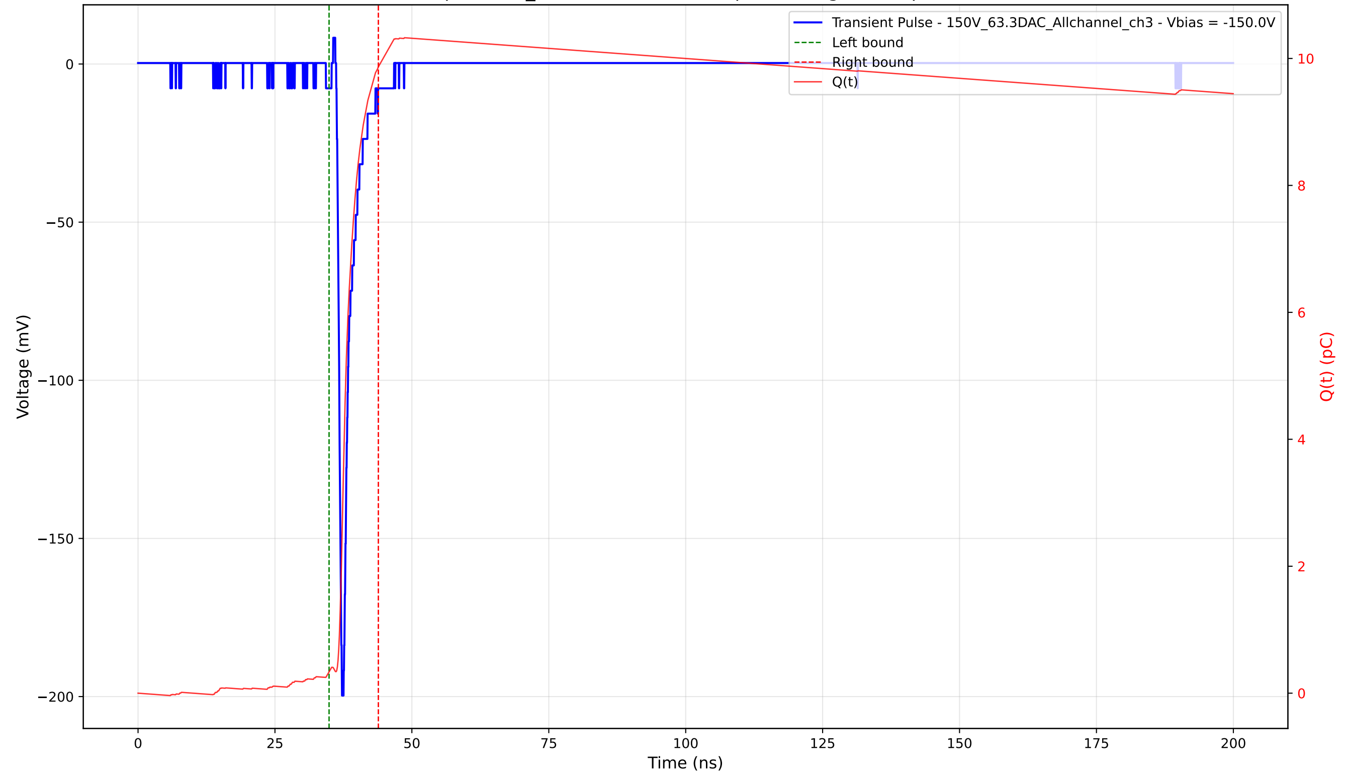
Transient Pulse - Sample: 1cm_42 - Position: 1965.0 \mu\text{m} - Charge: 9.53 pC - Rise Time: 0.82 ns
