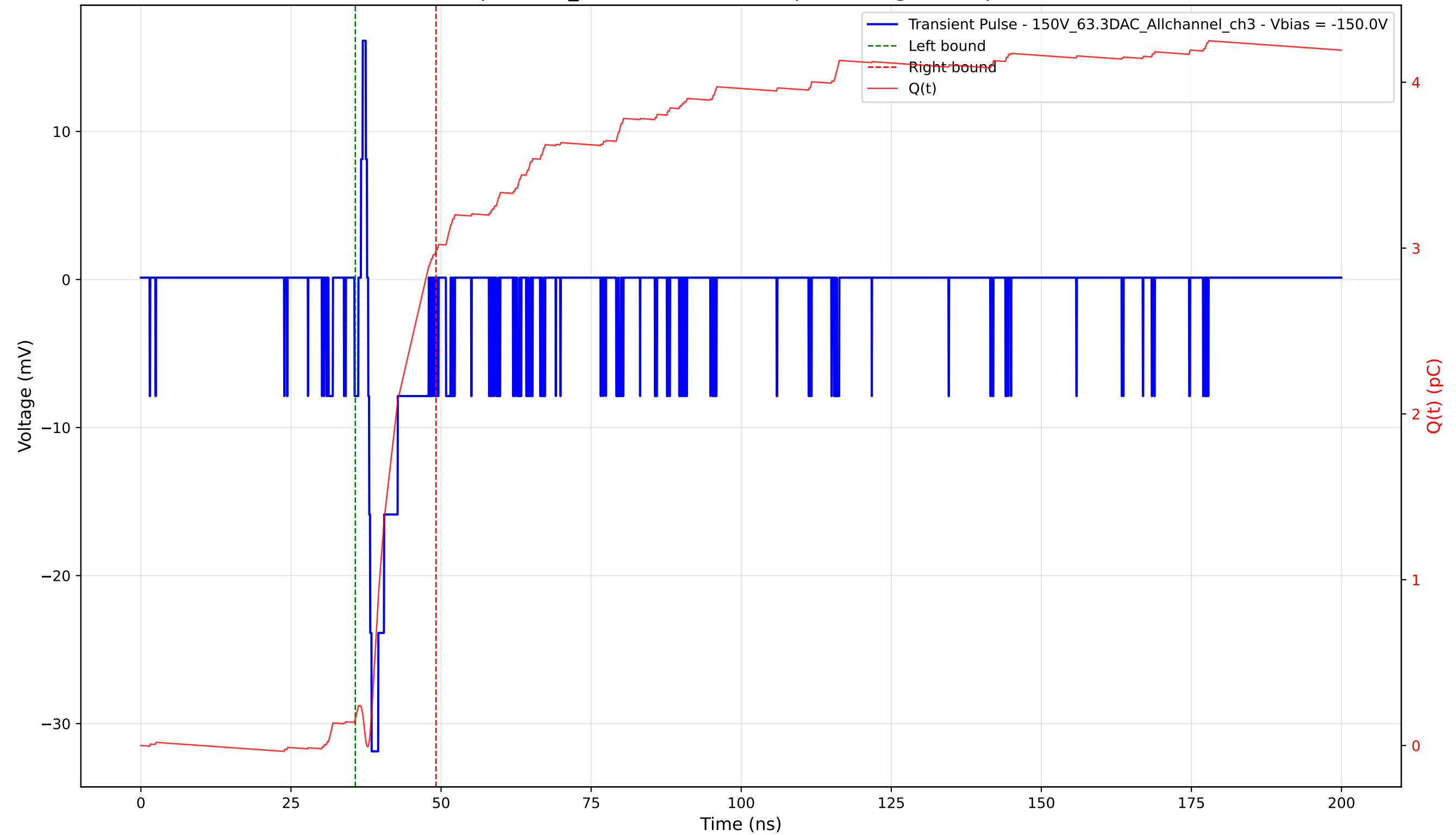
Transient Pulse - Sample: 1cm_42 - Position: 4765.0 \mu\text{m} - Charge: 2.83 pC - Rise Time: 0.58 ns
