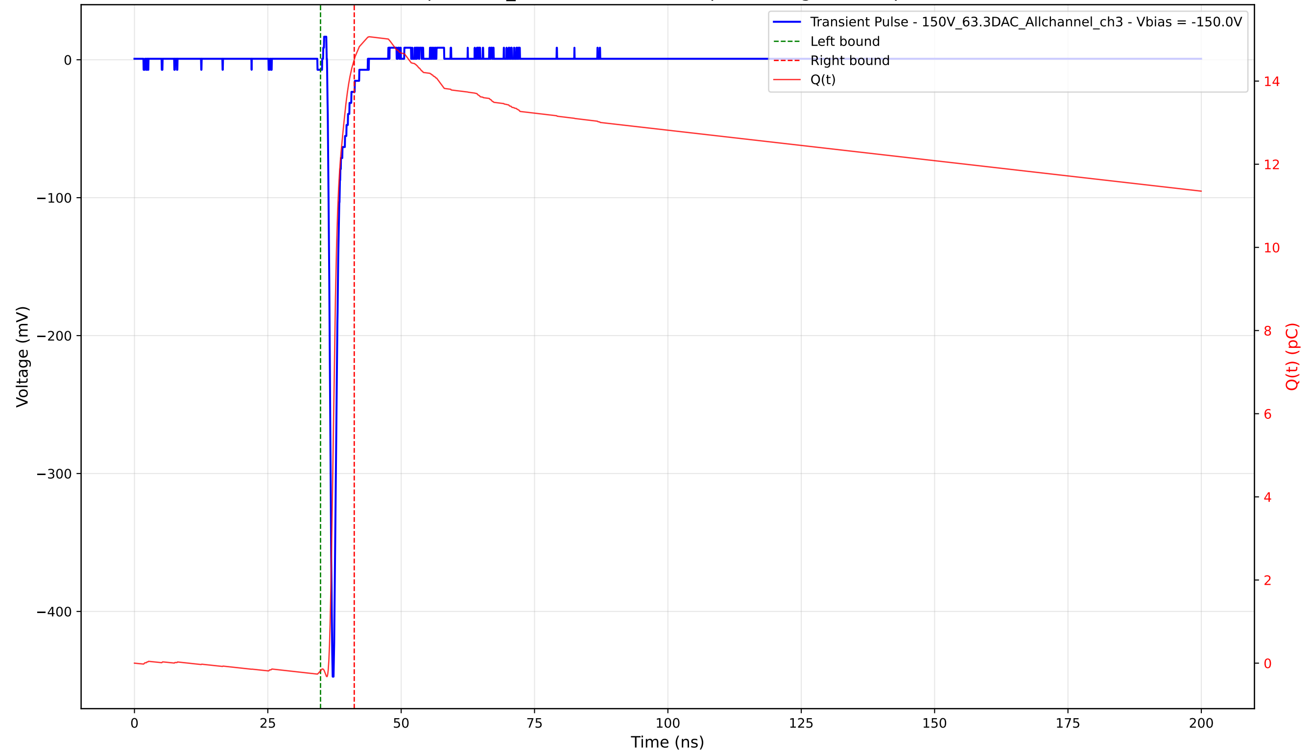
Transient Pulse - Sample: 1cm_42 - Position: 2795.0 \mu\text{m} - Charge: 14.70 pC - Rise Time: 0.73 ns
