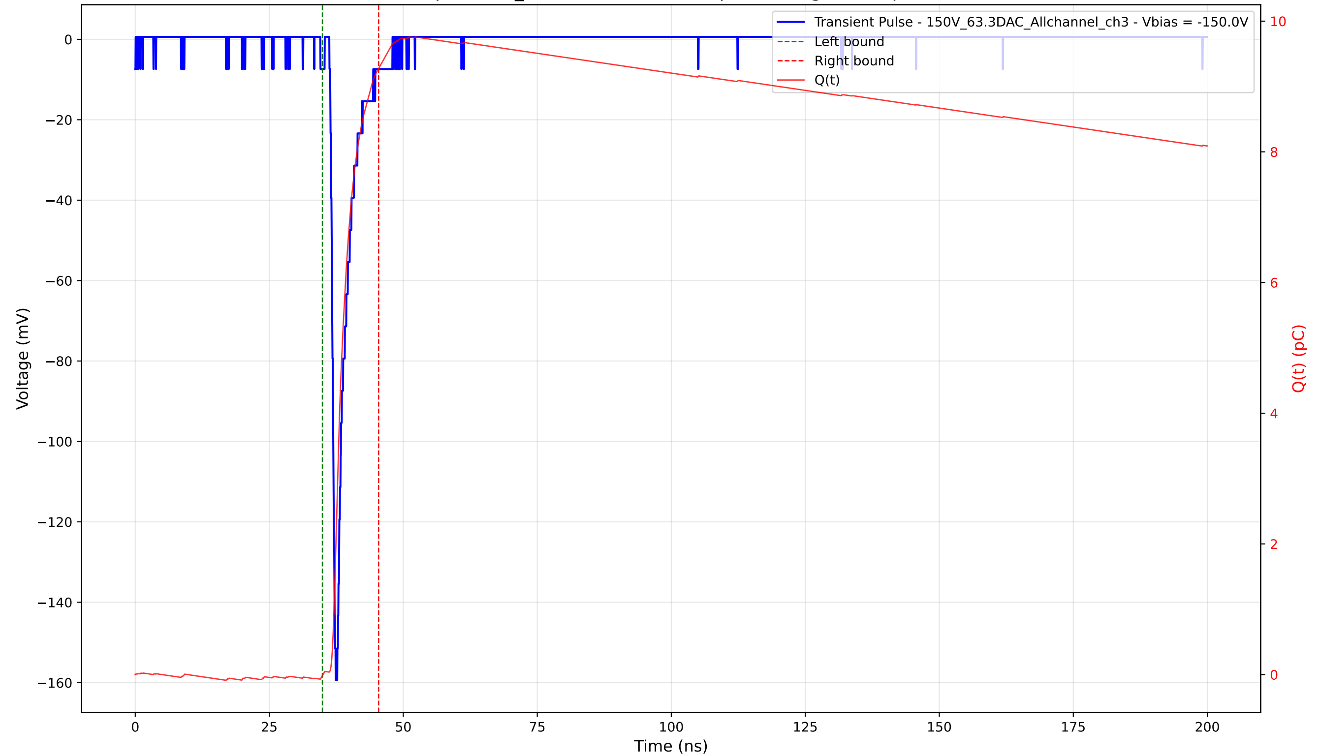
Transient Pulse - Sample: 1cm_42 - Position: 1845.0 \mu\text{m} - Charge: 9.29 pC - Rise Time: 0.88 ns
