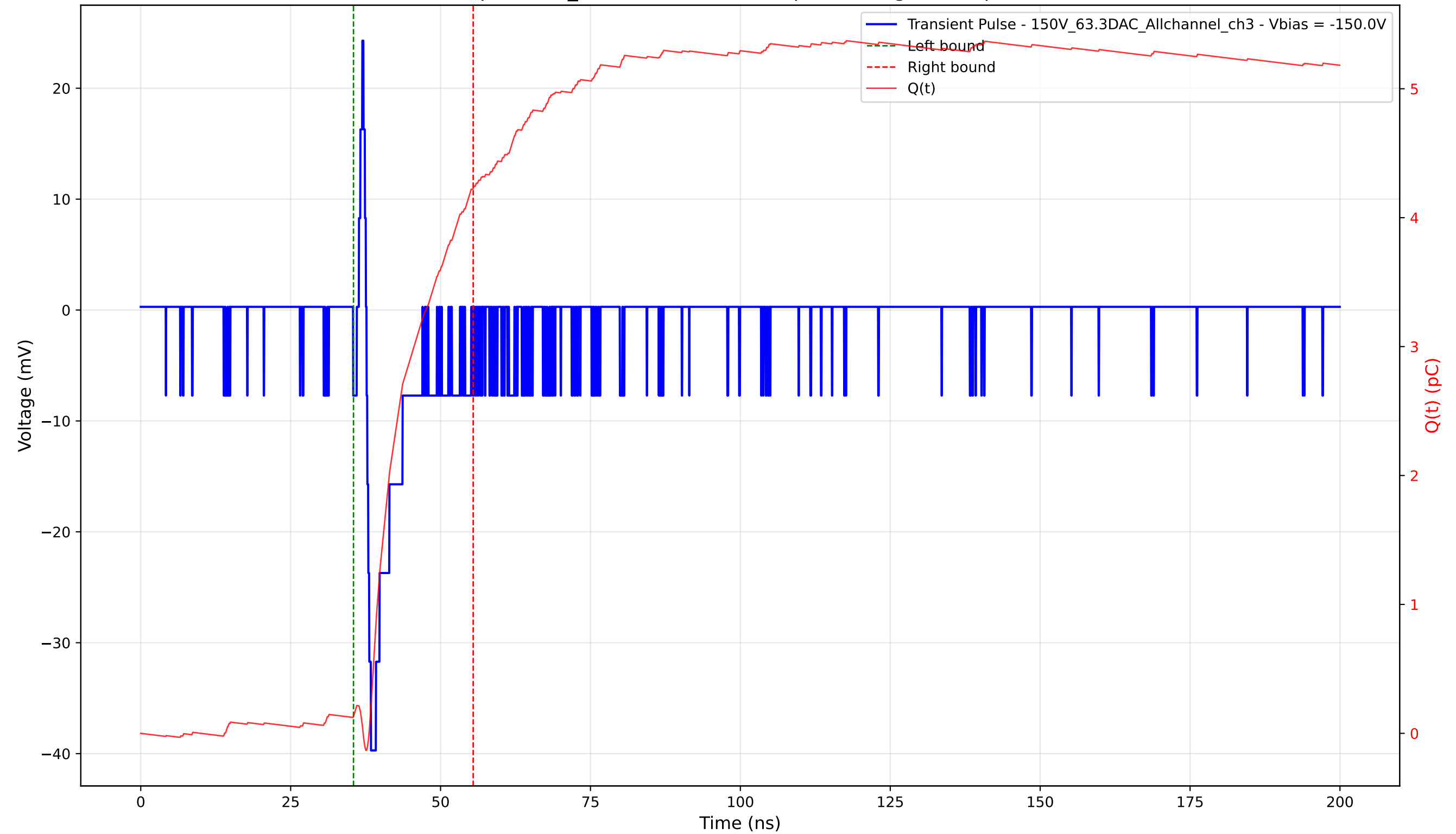
Transient Pulse - Sample: 1cm_42 - Position: 4150.0 \mu\text{m} - Charge: 4.10 pC - Rise Time: 0.74 ns
