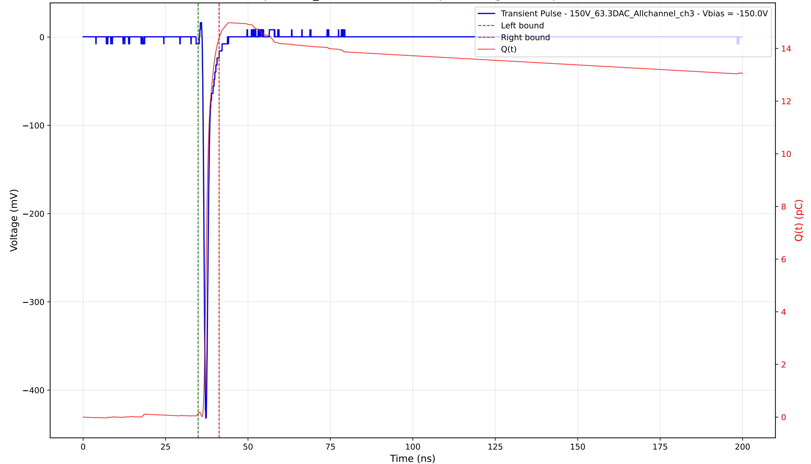
Transient Pulse - Sample: 1cm_42 - Position: 2820.0 \mu\text{m} - Charge: 14.28 pC - Rise Time: 0.73 ns
