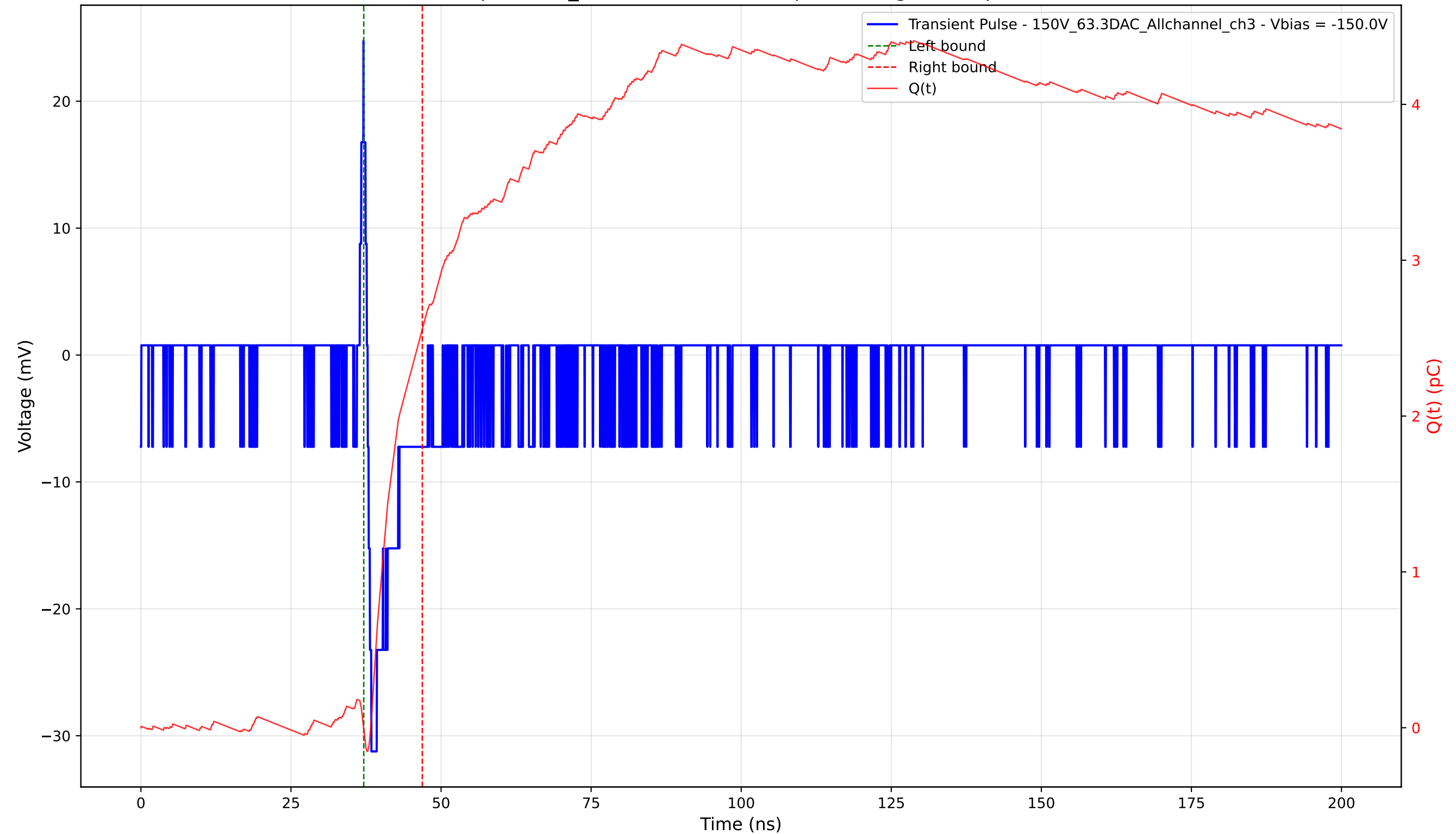
Transient Pulse - Sample: 1cm_42 - Position: 4460.0 \mu\text{m} - Charge: 2.57 pC - Rise Time: 0.63 ns
