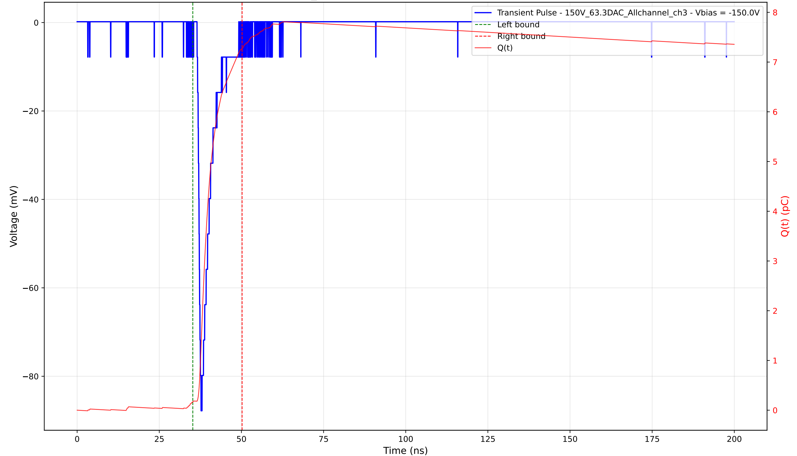
Transient Pulse - Sample: 1cm_42 - Position: 1555.0 \mu\text{m} - Charge: 7.11 pC - Rise Time: 0.88 ns
