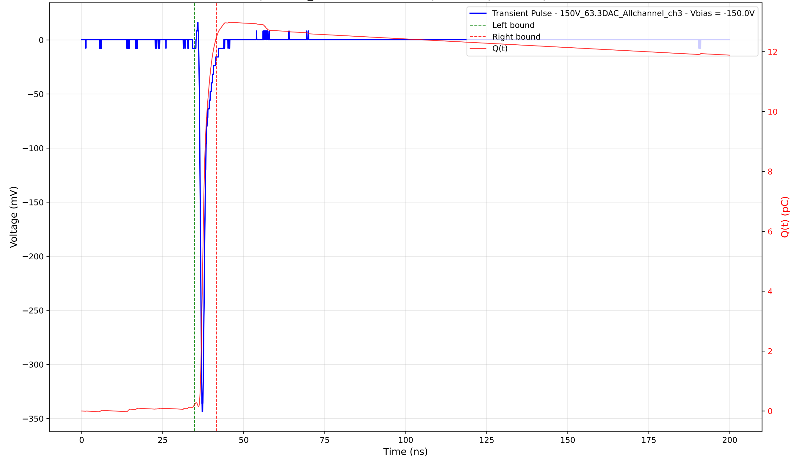
Transient Pulse - Sample: 1cm_42 - Position: 2145.0 \mu\text{m} - Charge: 12.29 pC - Rise Time: 0.73 ns
