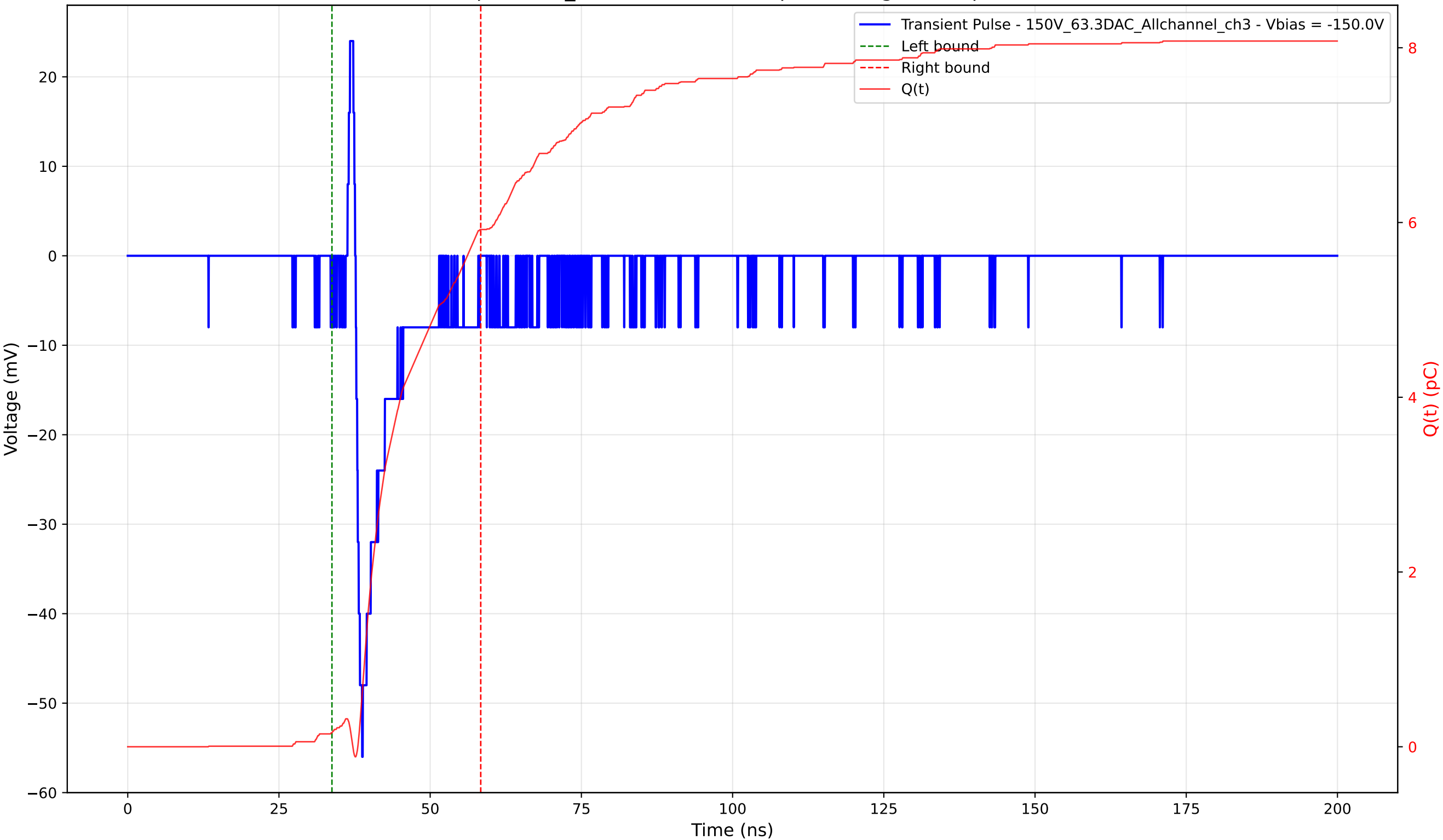
Transient Pulse - Sample: 1cm_42 - Position: 725.0 \mu\text{m} - Charge: 5.76 pC - Rise Time: 1.05 ns
