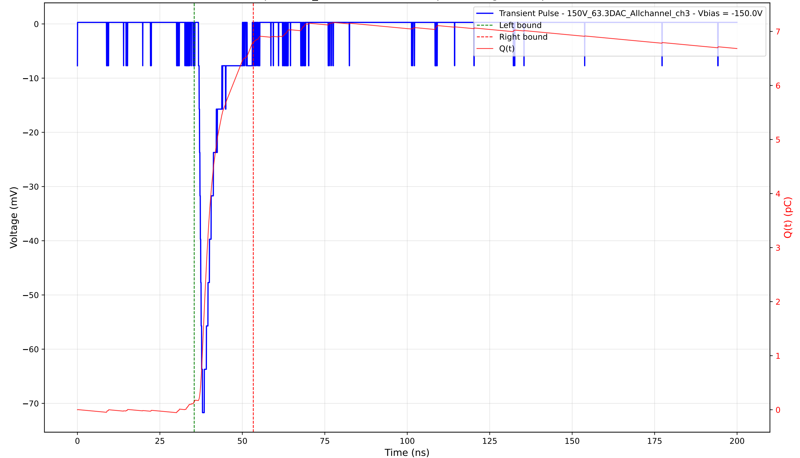
Transient Pulse - Sample: 1cm_42 - Position: 1475.0 \mu\text{m} - Charge: 6.66 pC - Rise Time: 1.20 ns
