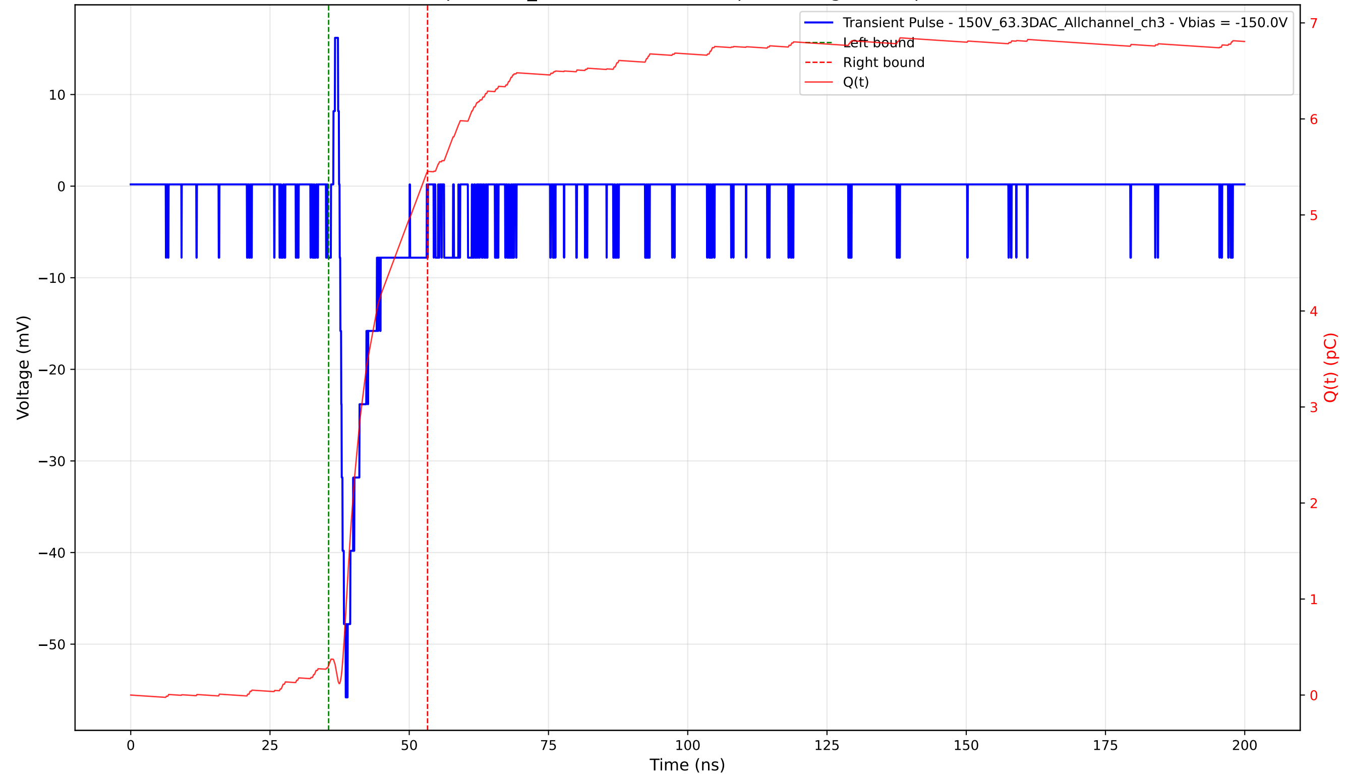
Transient Pulse - Sample: 1cm_42 - Position: 1040.0 \mu\text{m} - Charge: 5.14 pC - Rise Time: 1.09 ns
