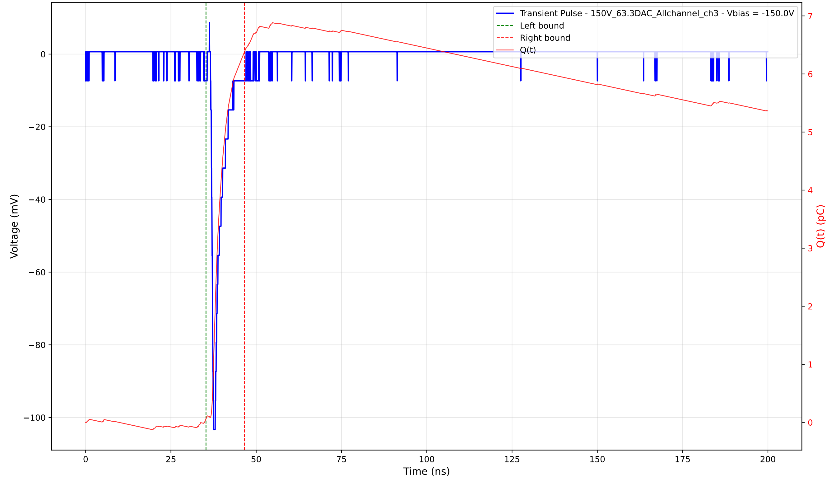
Transient Pulse - Sample: 1cm_42 - Position: 3390.0 \mu\text{m} - Charge: 6.31 pC - Rise Time: 0.71 ns
