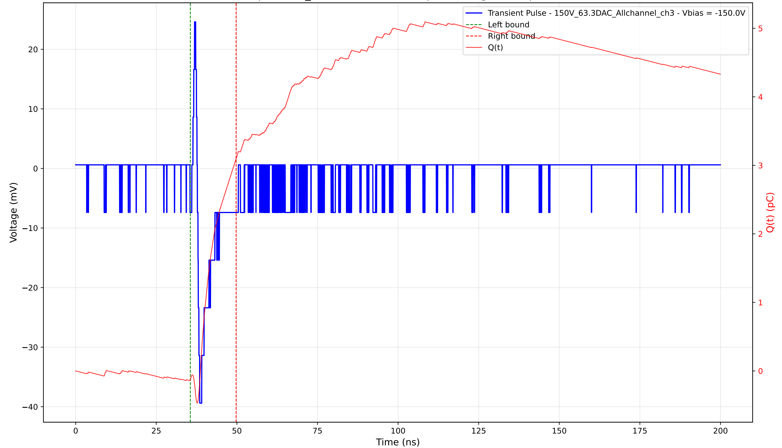
Transient Pulse - Sample: 1cm_42 - Position: 4365.0 \mu\text{m} - Charge: 3.23 pC - Rise Time: 0.74 ns
