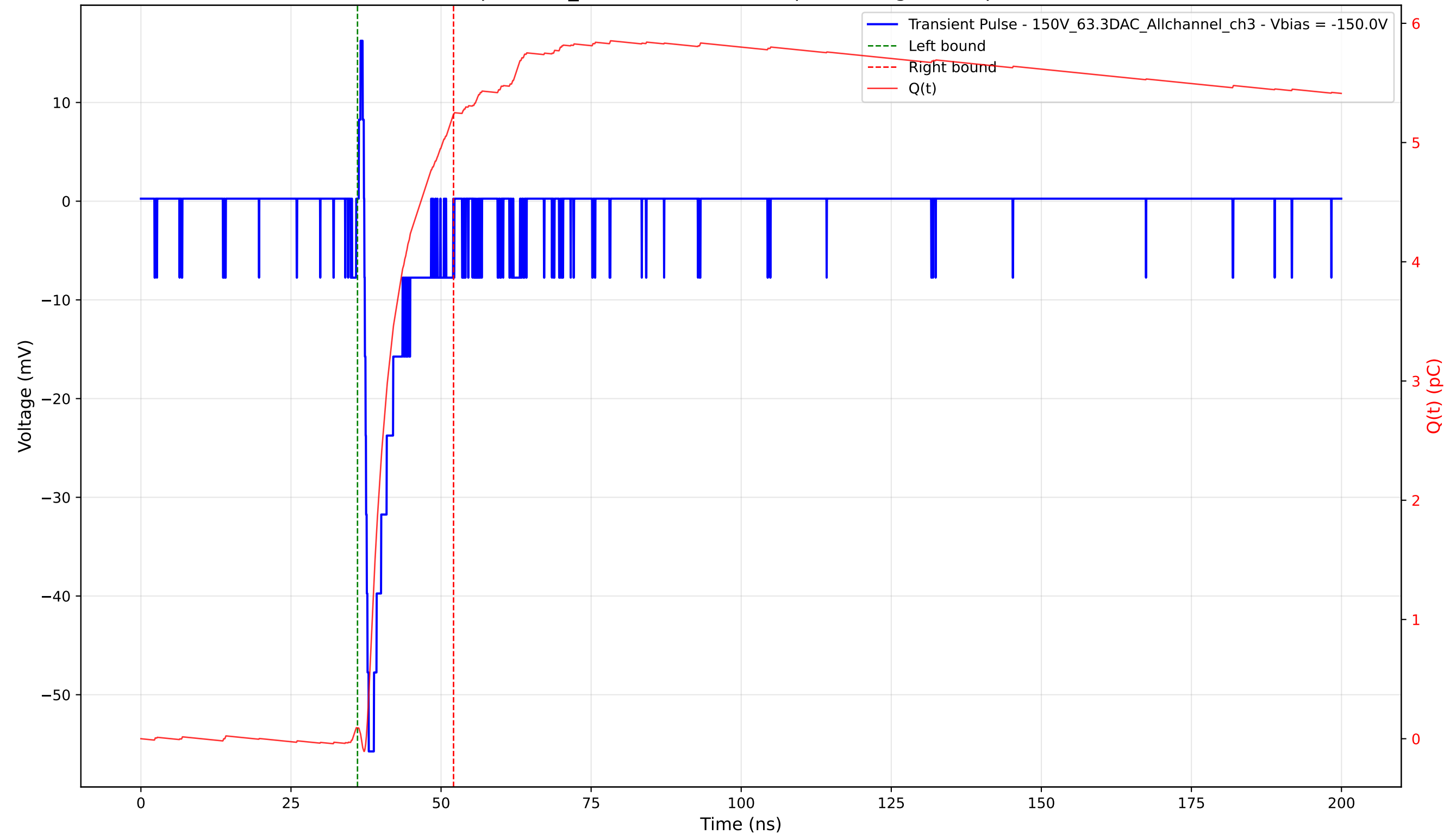
Transient Pulse - Sample: 1cm_42 - Position: 3715.0 \mu\text{m} - Charge: 5.14 pC - Rise Time: 0.73 ns
