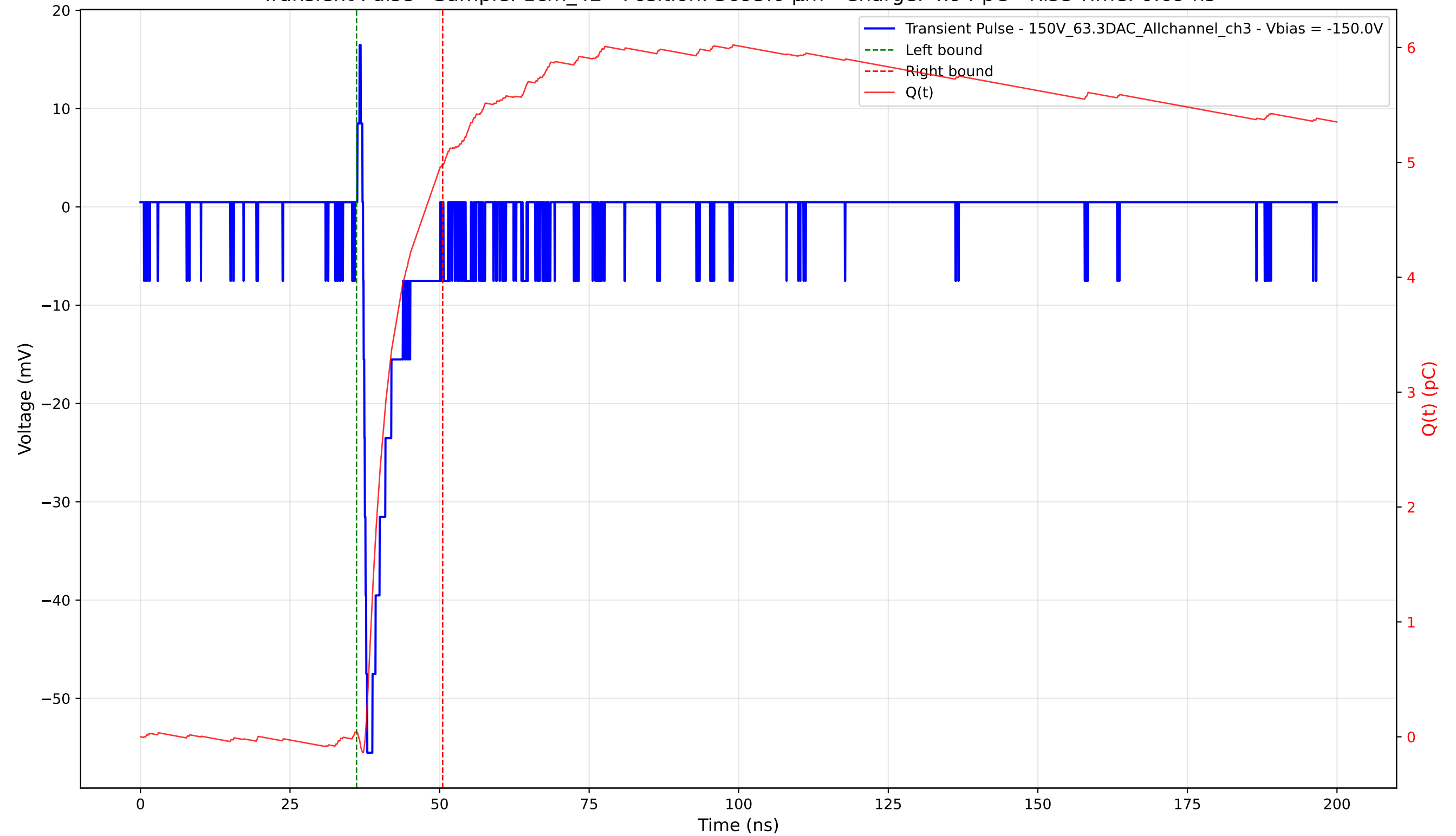
Transient Pulse - Sample: 1cm_42 - Position: 3695.0 \mu\text{m} - Charge: 4.94 pC - Rise Time: 0.69 ns
