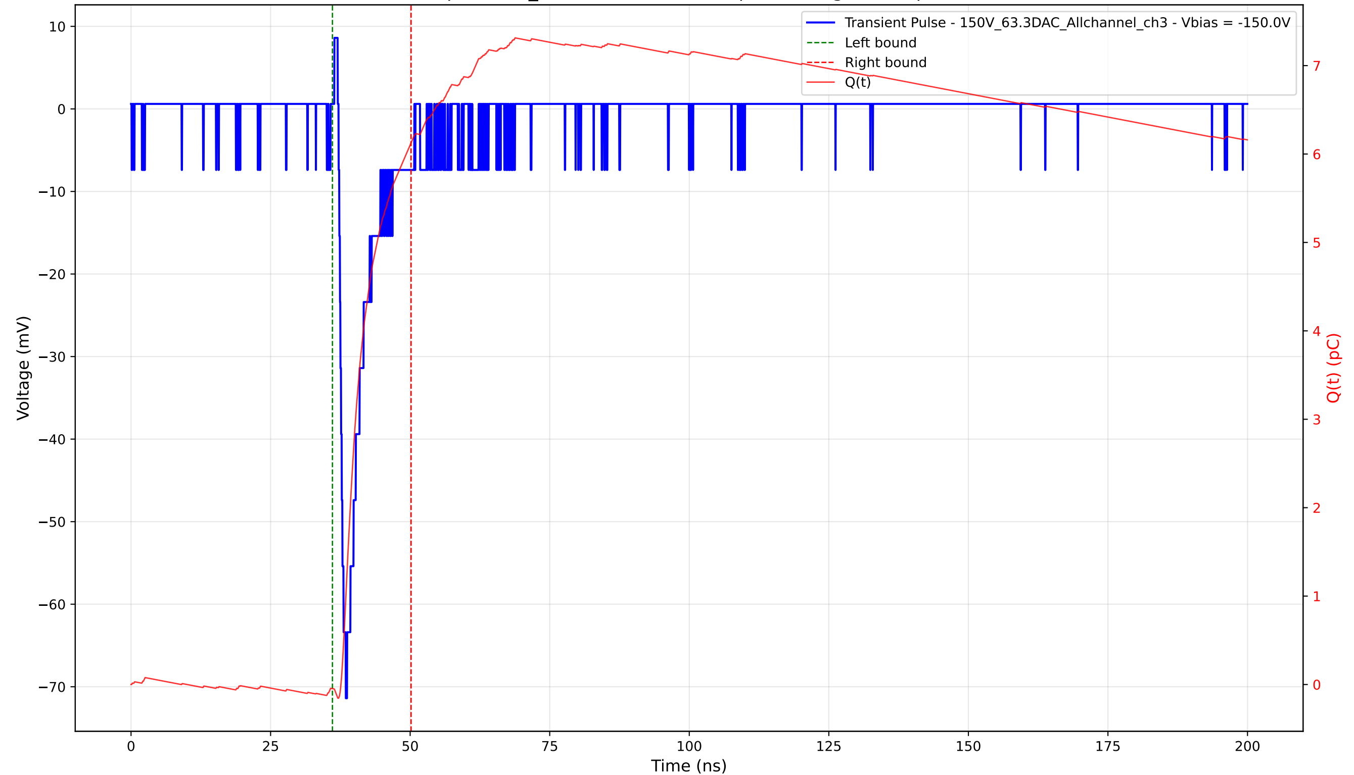
Transient Pulse - Sample: 1cm_42 - Position: 1305.0 \mu\text{m} - Charge: 6.18 pC - Rise Time: 1.28 ns
