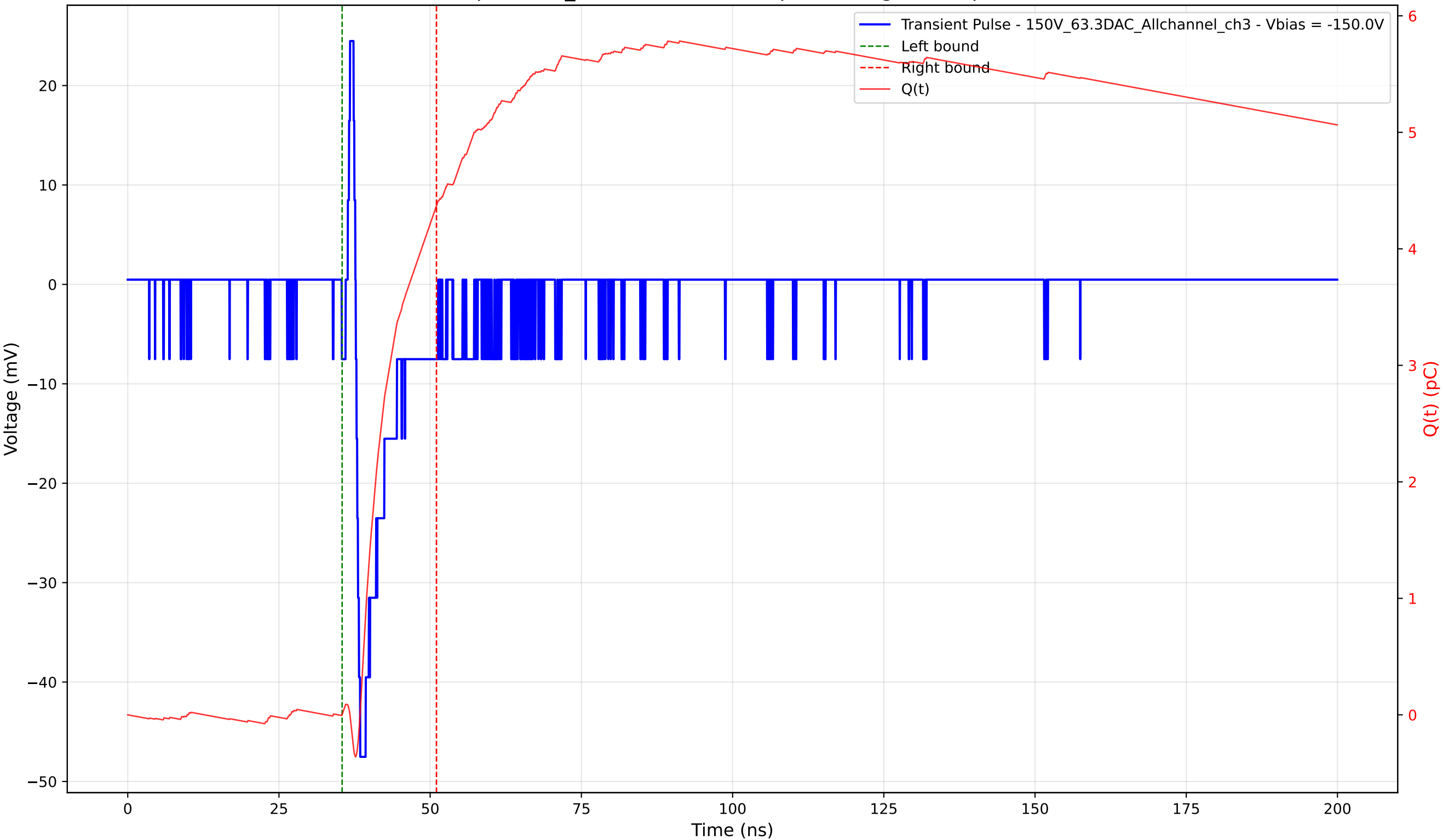
Transient Pulse - Sample: 1cm_42 - Position: 700.0 \mu\text{m} - Charge: 4.37 pC - Rise Time: 0.74 ns
