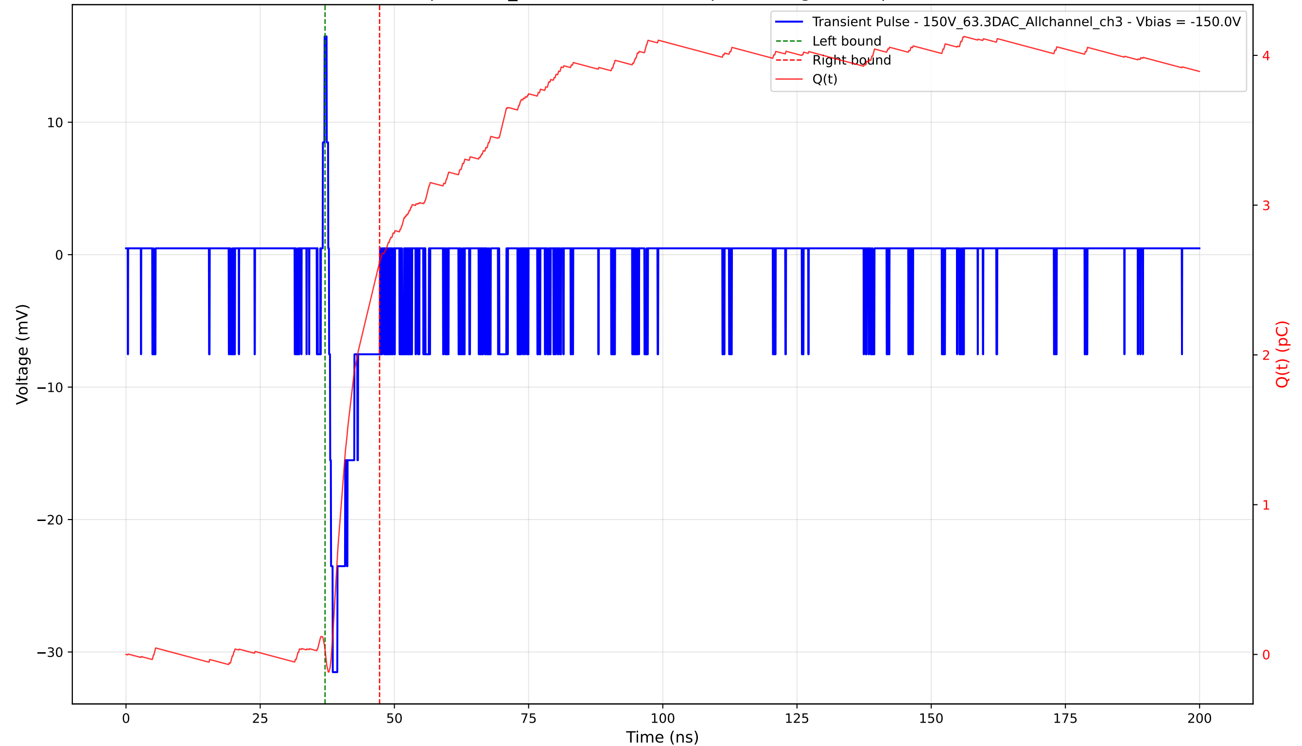
Transient Pulse - Sample: 1cm_42 - Position: 4710.0 \mu\text{m} - Charge: 2.59 pC - Rise Time: 0.70 ns
