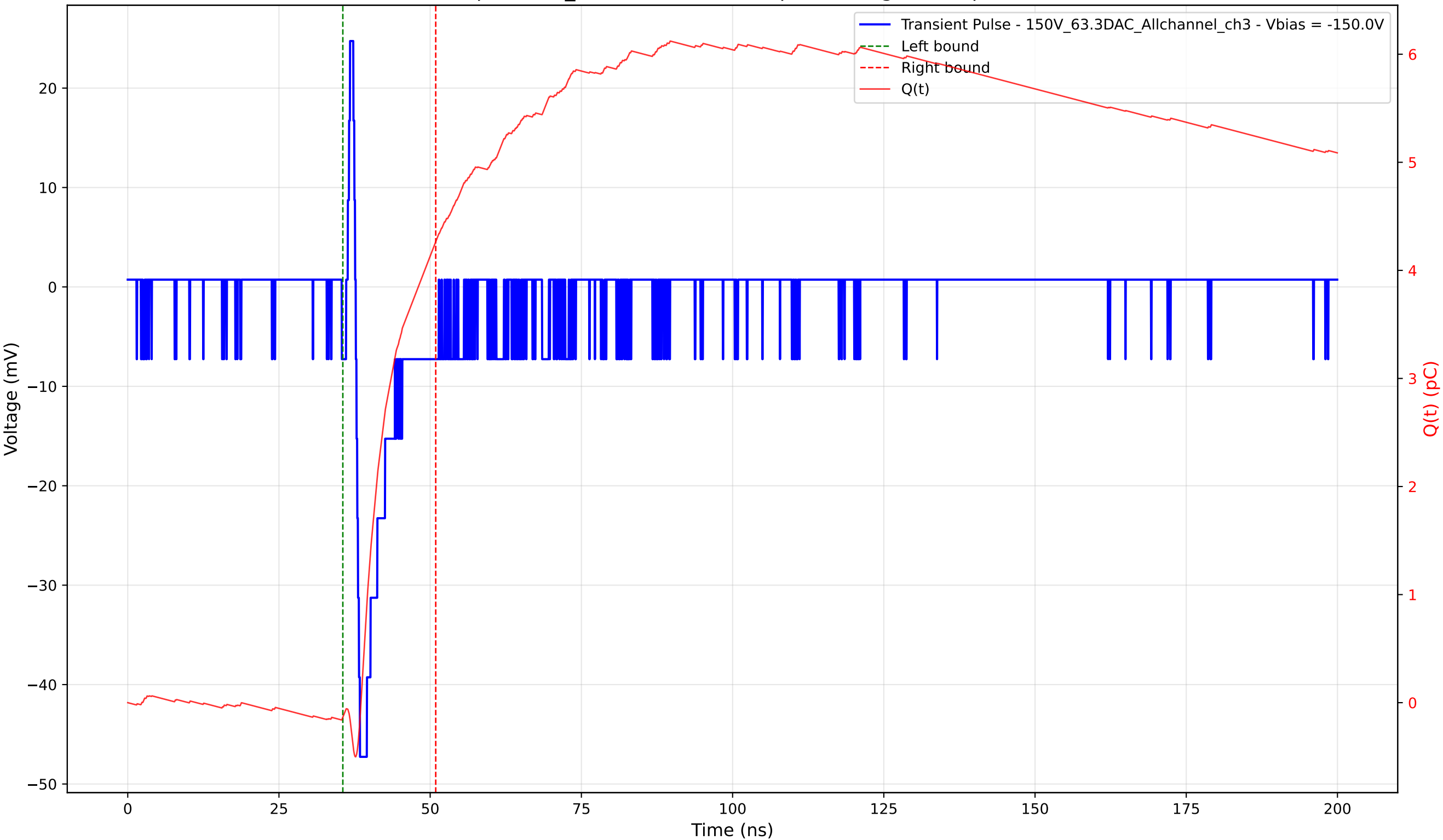
Transient Pulse - Sample: 1cm_42 - Position: 810.0 \mu\text{m} - Charge: 4.40 pC - Rise Time: 0.70 ns
