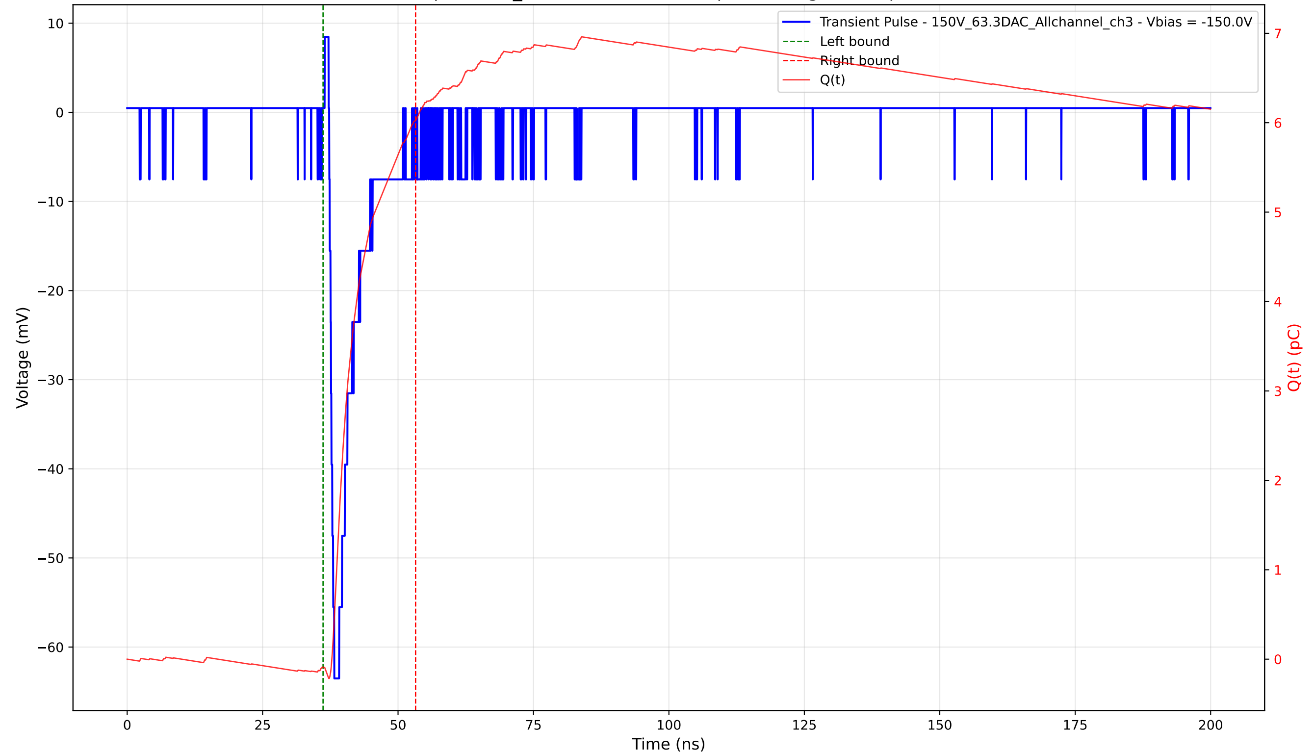
Transient Pulse - Sample: 1cm_42 - Position: 1195.0 \mu\text{m} - Charge: 6.12 pC - Rise Time: 0.93 ns
