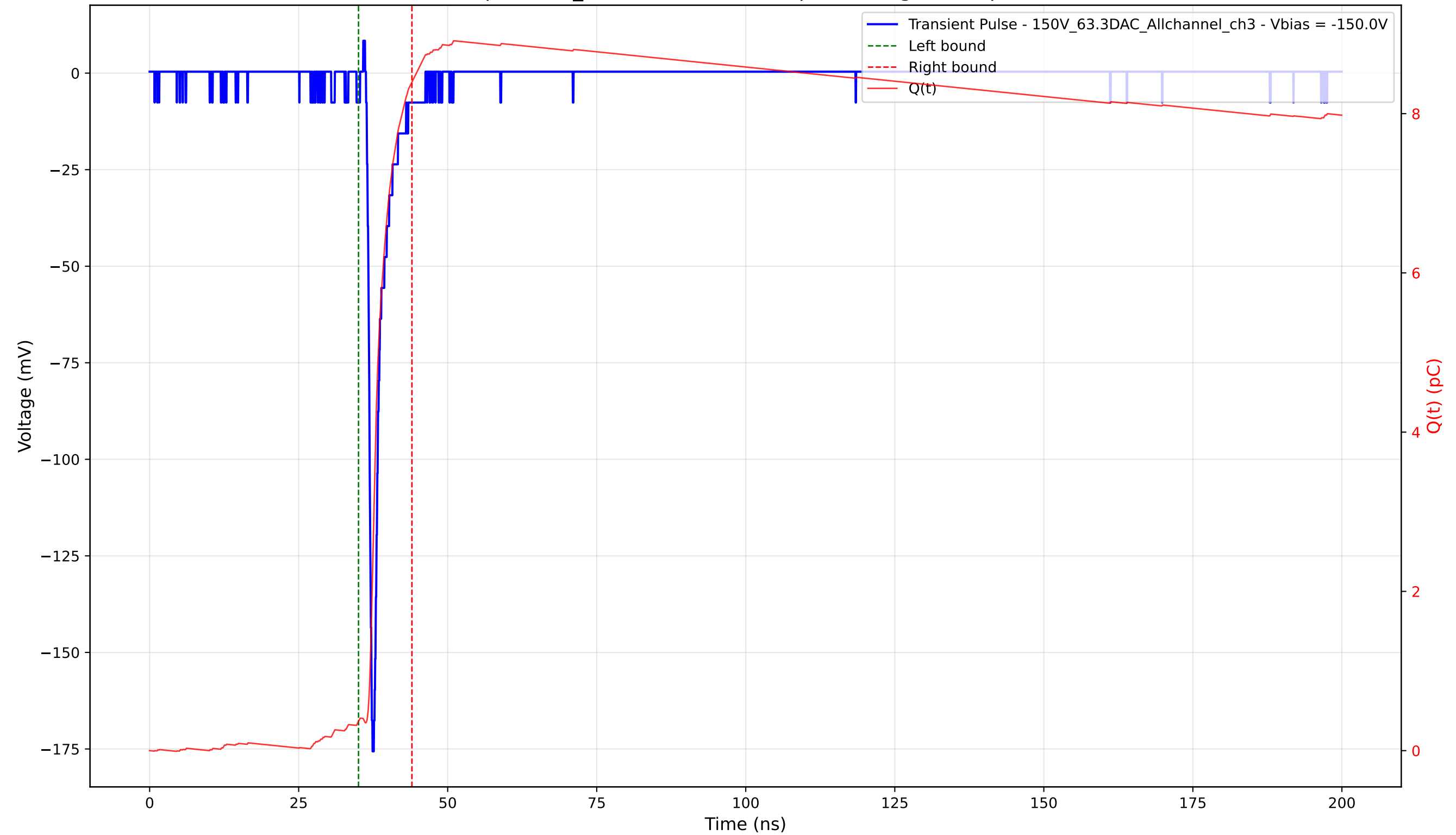
Transient Pulse - Sample: 1cm_42 - Position: 3110.0 \mu\text{m} - Charge: 8.03 pC - Rise Time: 0.78 ns
