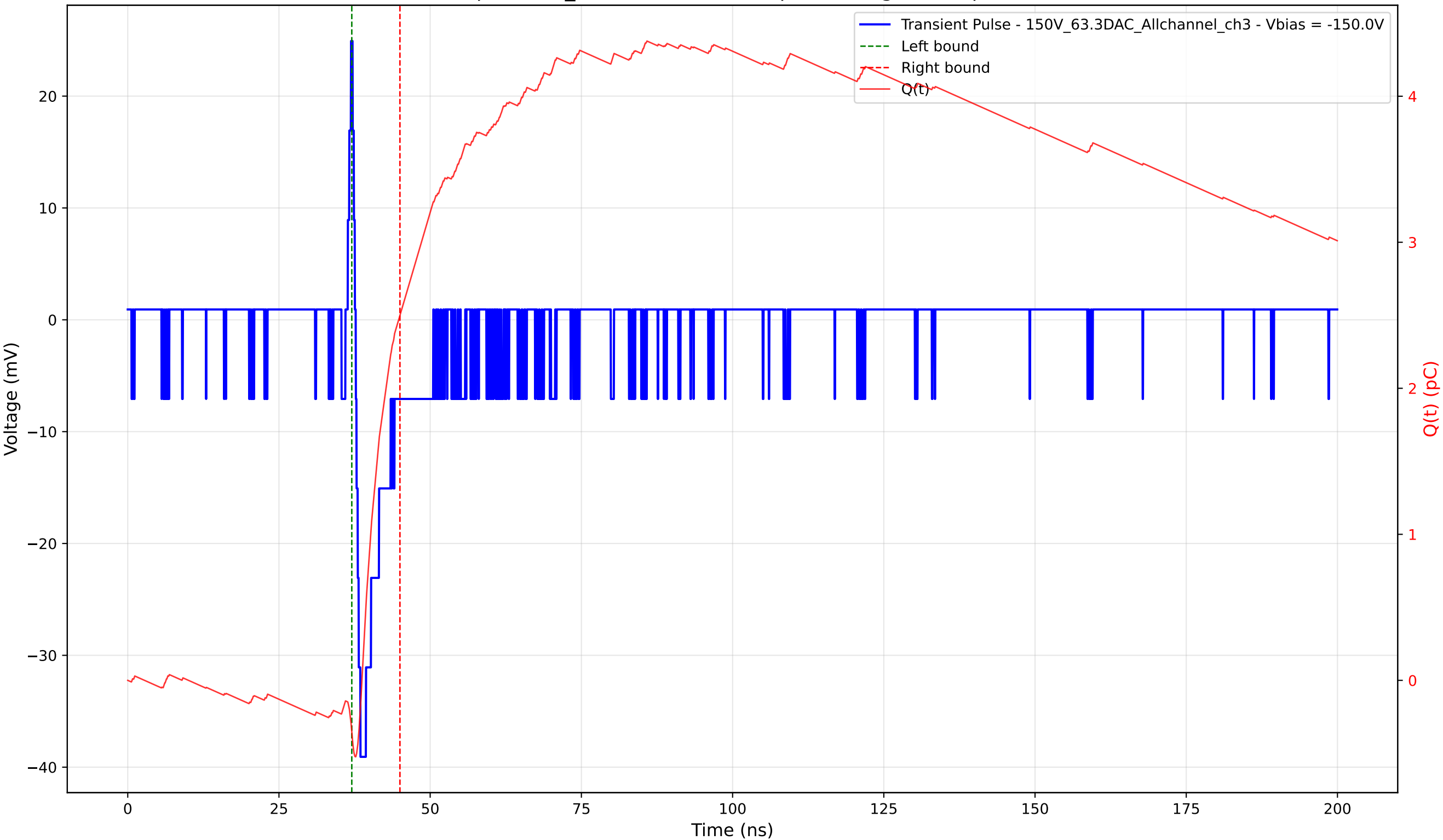
Transient Pulse - Sample: 1cm_42 - Position: 560.0 \mu\text{m} - Charge: 2.85 pC - Rise Time: 0.78 ns
