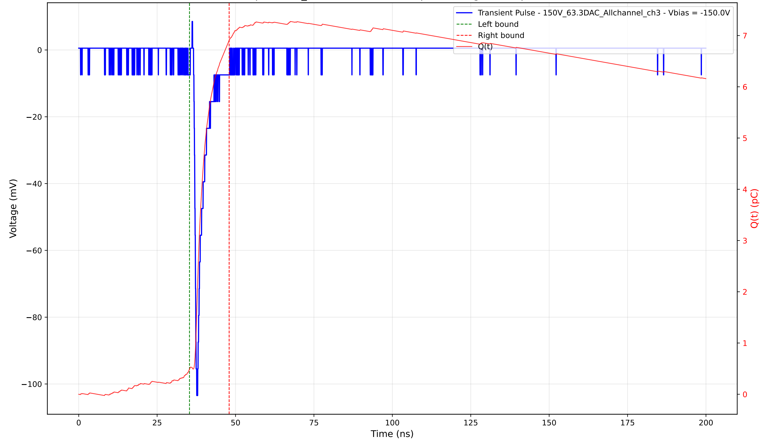
Transient Pulse - Sample: 1cm_42 - Position: 3410.0 \mu\text{m} - Charge: 6.42 pC - Rise Time: 0.71 ns
