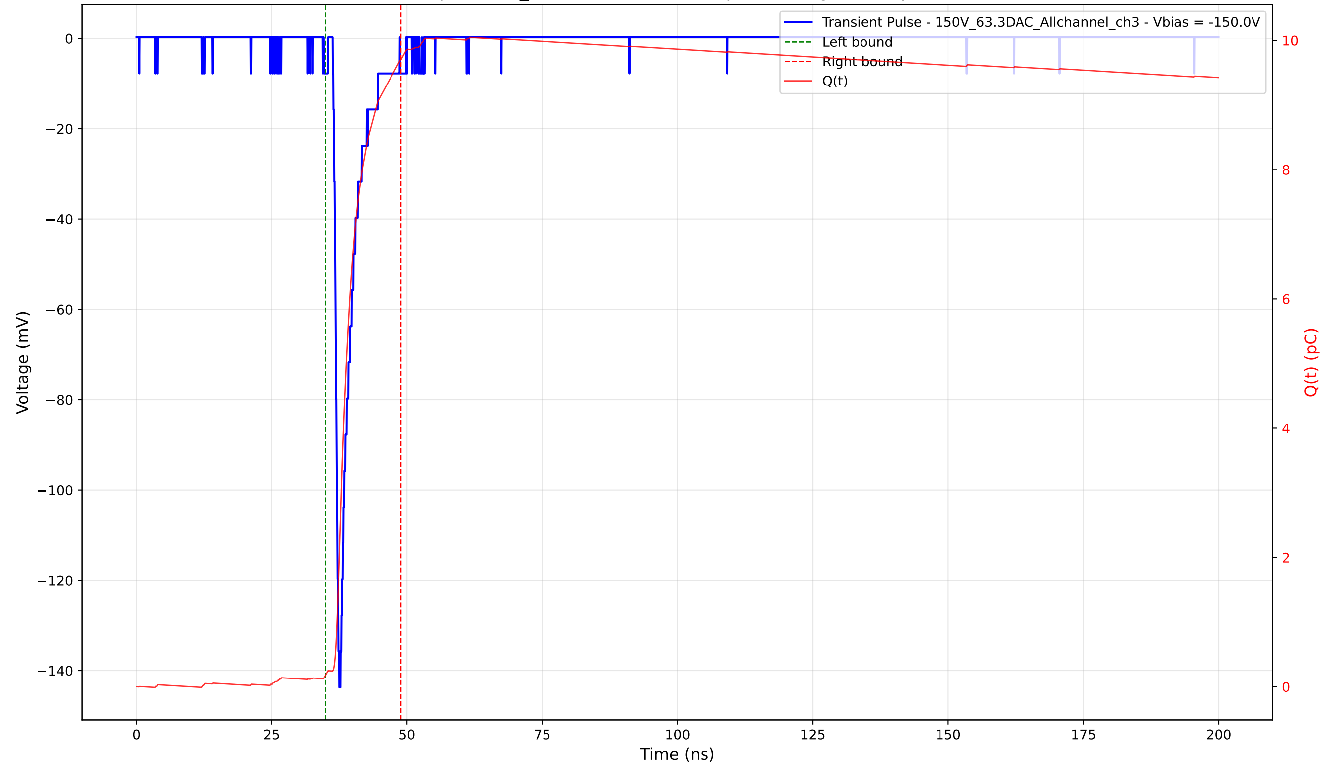
Transient Pulse - Sample: 1cm_42 - Position: 1715.0 \mu\text{m} - Charge: 9.52 pC - Rise Time: 0.93 ns
