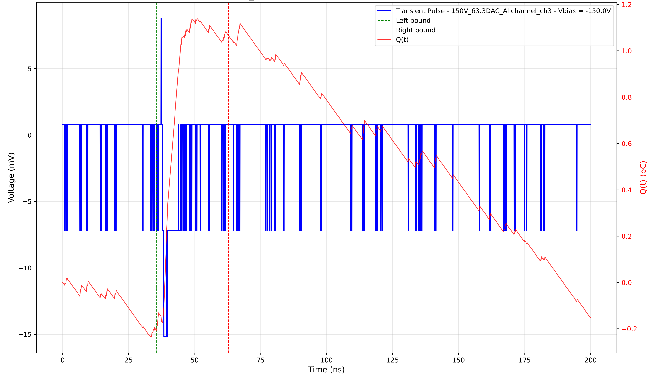
Transient Pulse - Sample: 1cm_42 - Position: 5050.0 \mu\text{m} - Charge: 1.27 pC - Rise Time: 0.48 ns
