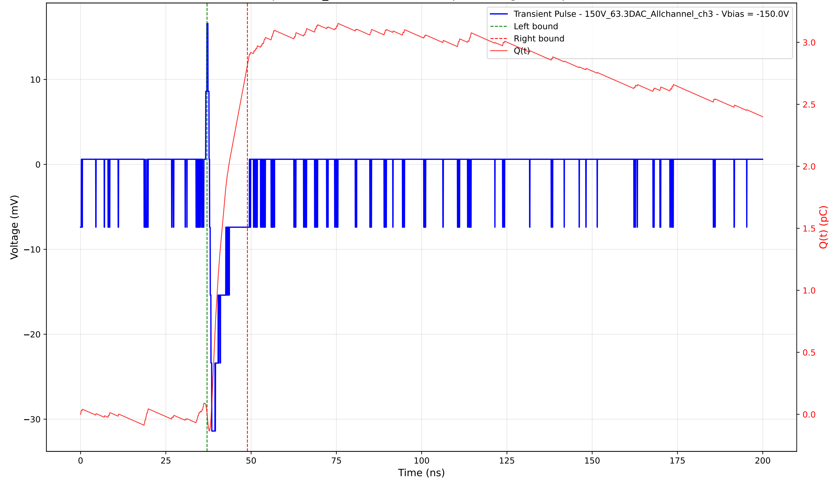
Transient Pulse - Sample: 1cm_42 - Position: 4835.0 \mu\text{m} - Charge: 2.81 pC - Rise Time: 0.67 ns
