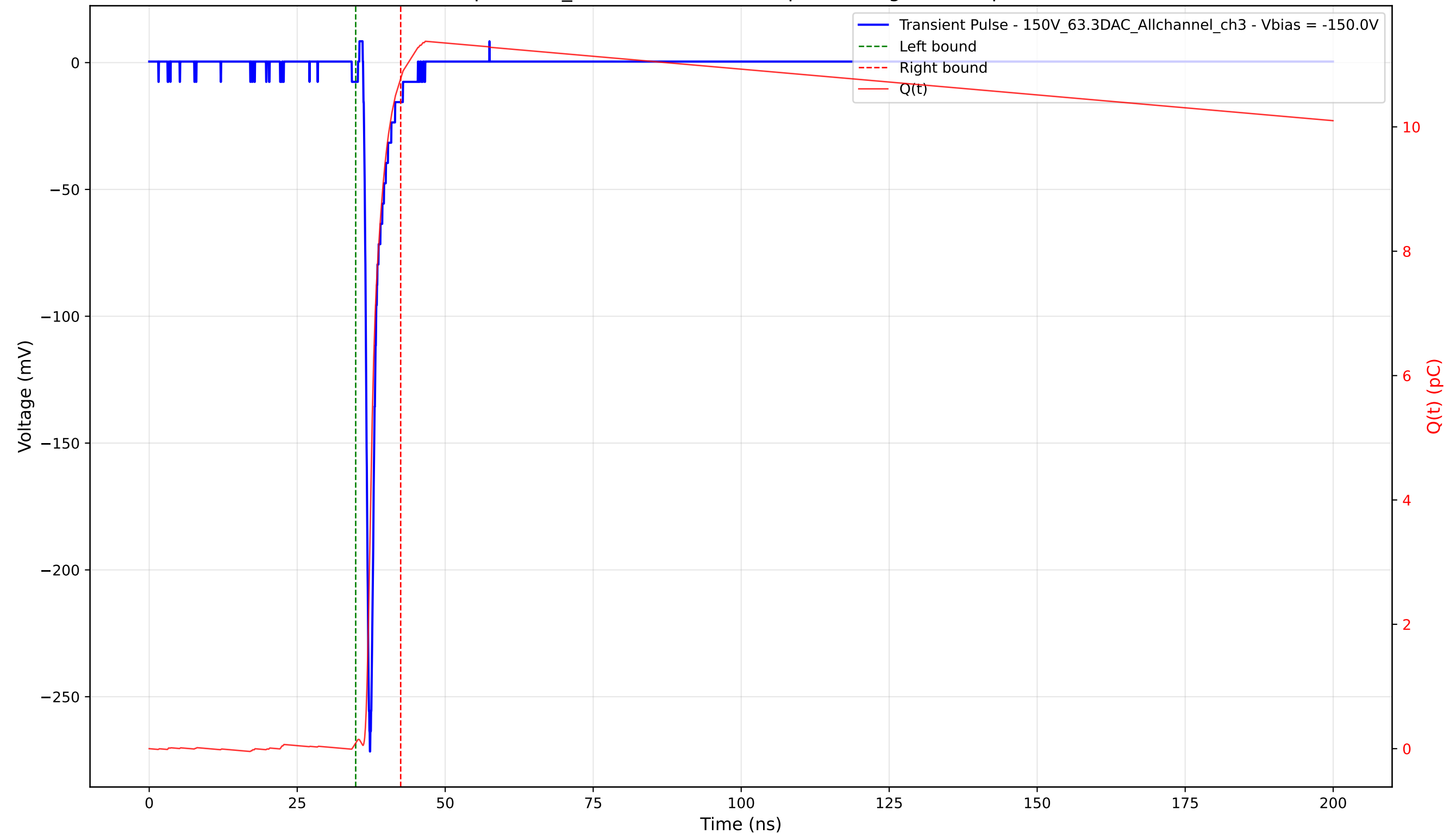
Transient Pulse - Sample: 1cm_42 - Position: 2060.0 \mu\text{m} - Charge: 10.69 pC - Rise Time: 0.77 ns
