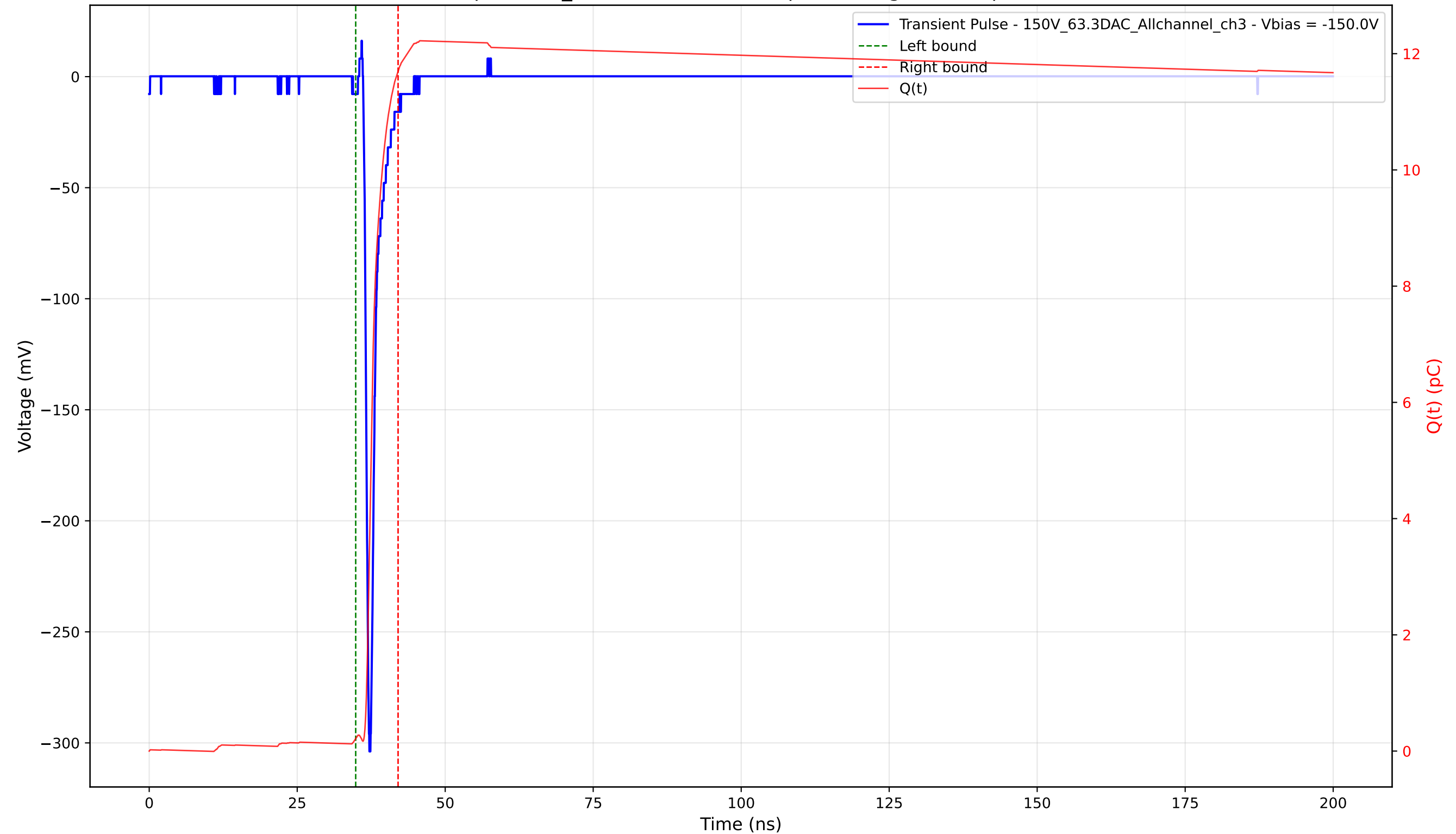
Transient Pulse - Sample: 1cm_42 - Position: 2100.0 \mu\text{m} - Charge: 11.48 pC - Rise Time: 0.74 ns
