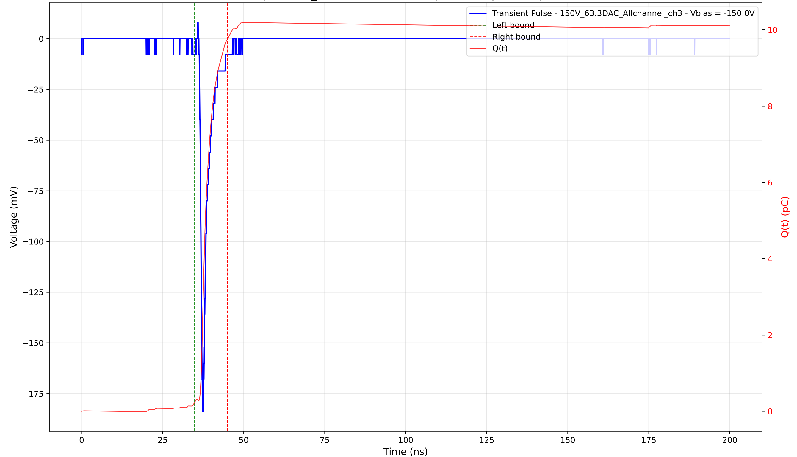
Transient Pulse - Sample: 1cm_42 - Position: 1925.0 \mu\text{m} - Charge: 9.53 pC - Rise Time: 0.83 ns
