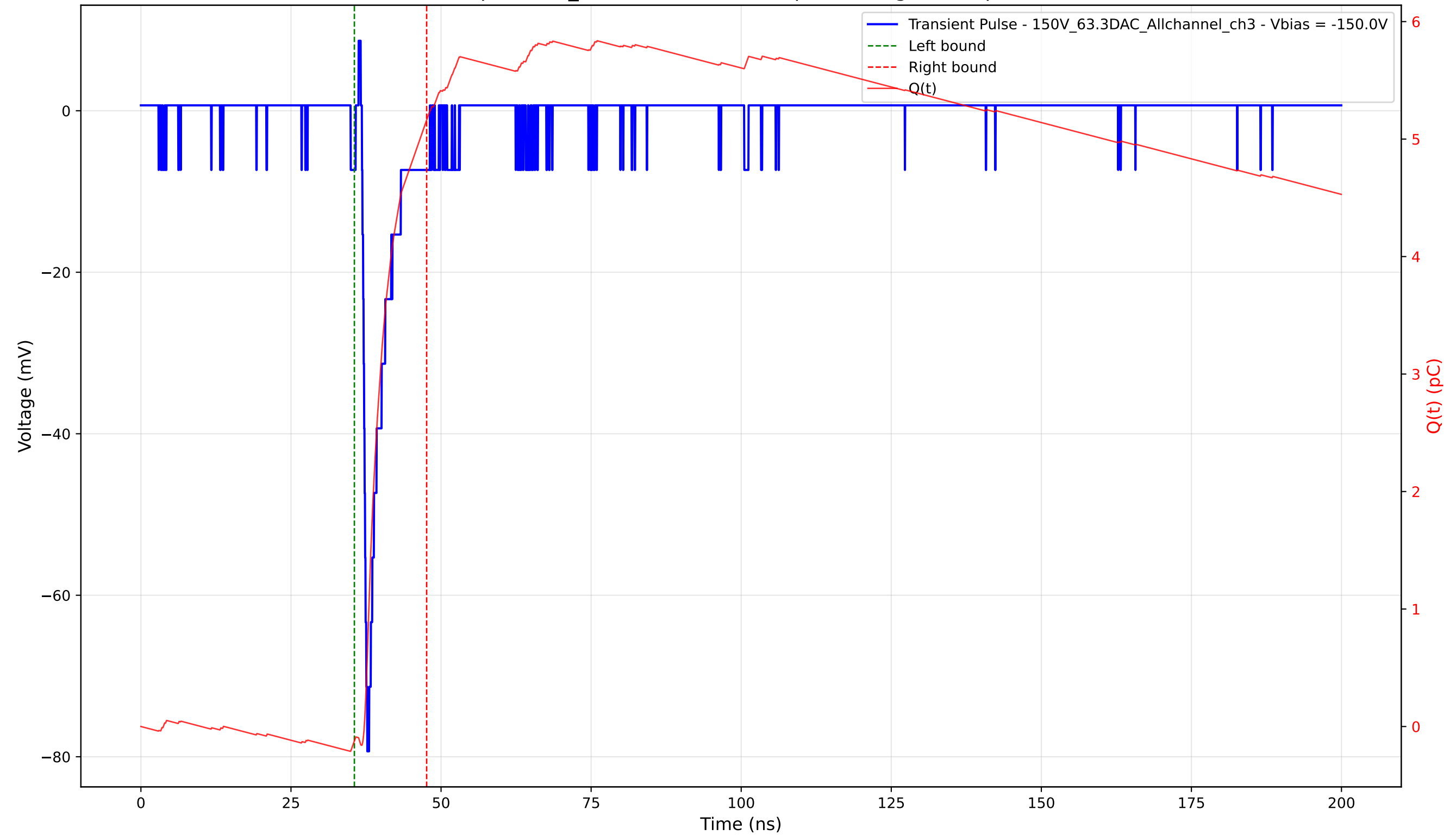
Transient Pulse - Sample: 1cm_42 - Position: 3495.0 \mu\text{m} - Charge: 5.29 pC - Rise Time: 0.84 ns
