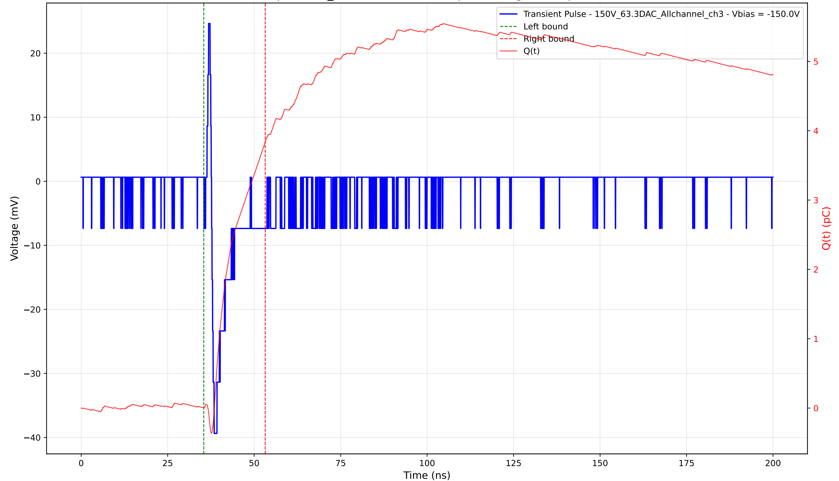
Transient Pulse - Sample: 1cm_42 - Position: 4225.0 \mu\text{m} - Charge: 3.83 pC - Rise Time: 0.74 ns
