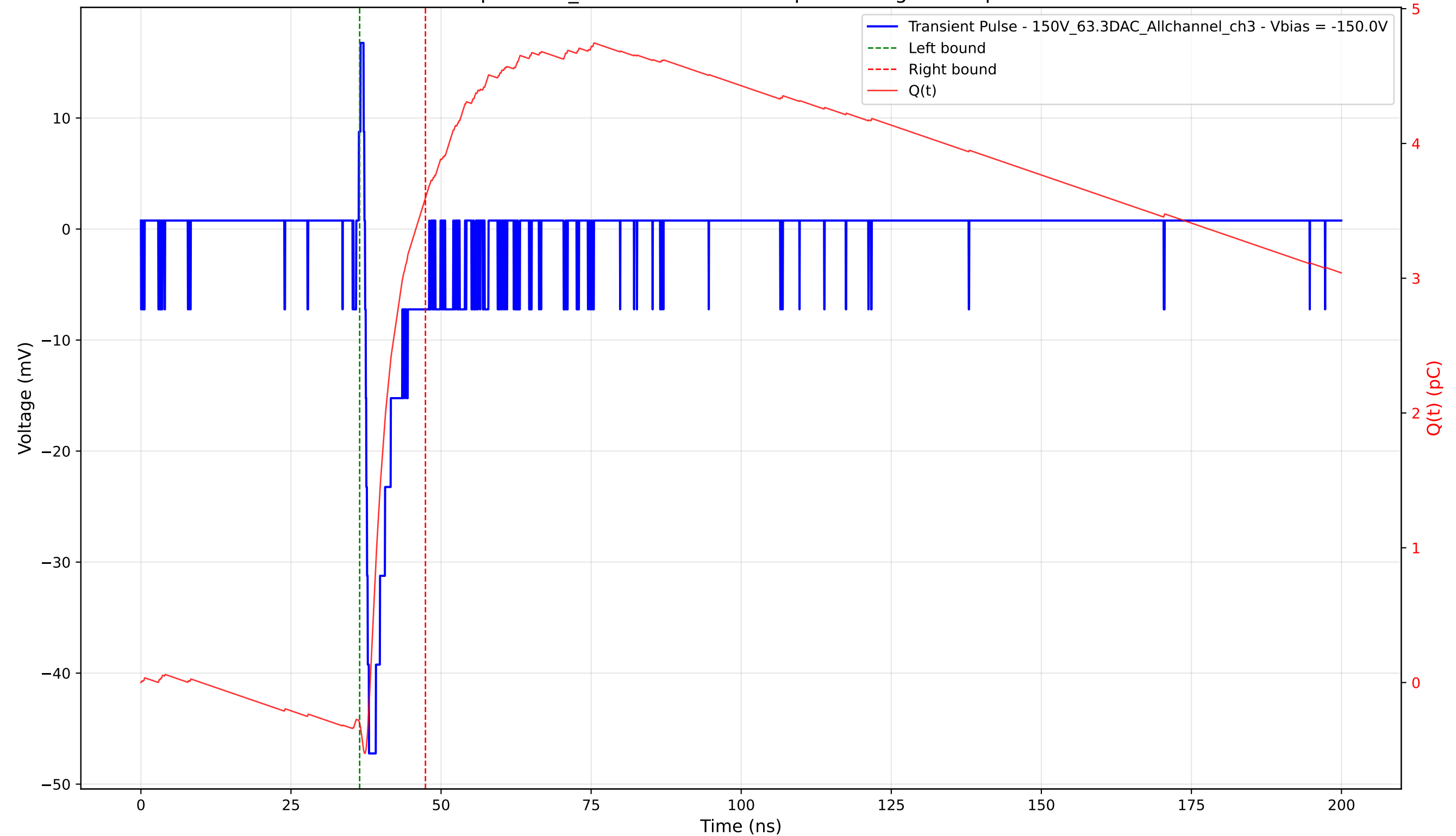
Transient Pulse - Sample: 1cm_42 - Position: 3855.0 \mu\text{m} - Charge: 3.90 pC - Rise Time: 0.66 ns
