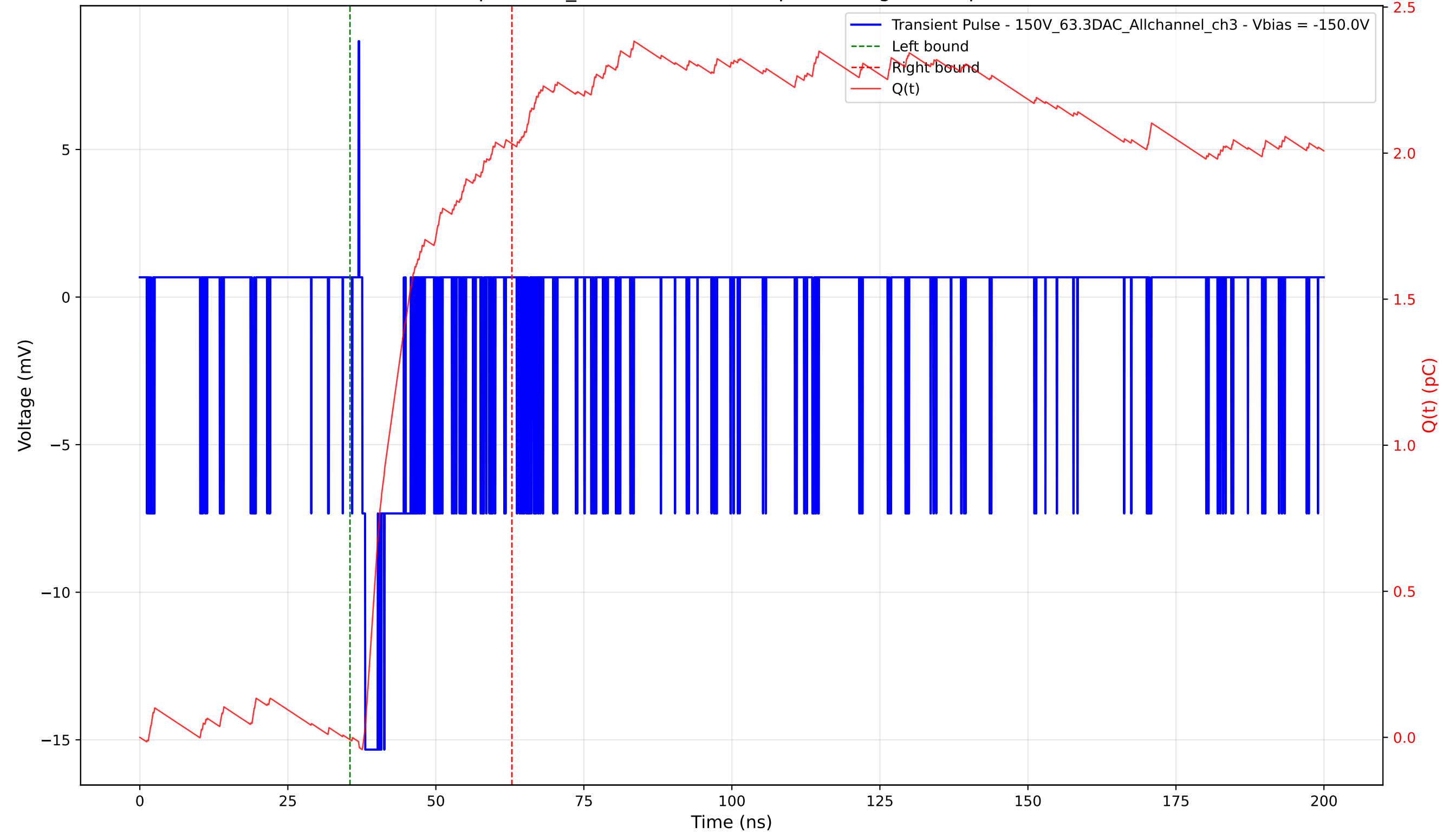
Transient Pulse - Sample: 1cm_42 - Position: 175.0 \mu\text{m} - Charge: 2.04 pC - Rise Time: 0.51 ns
