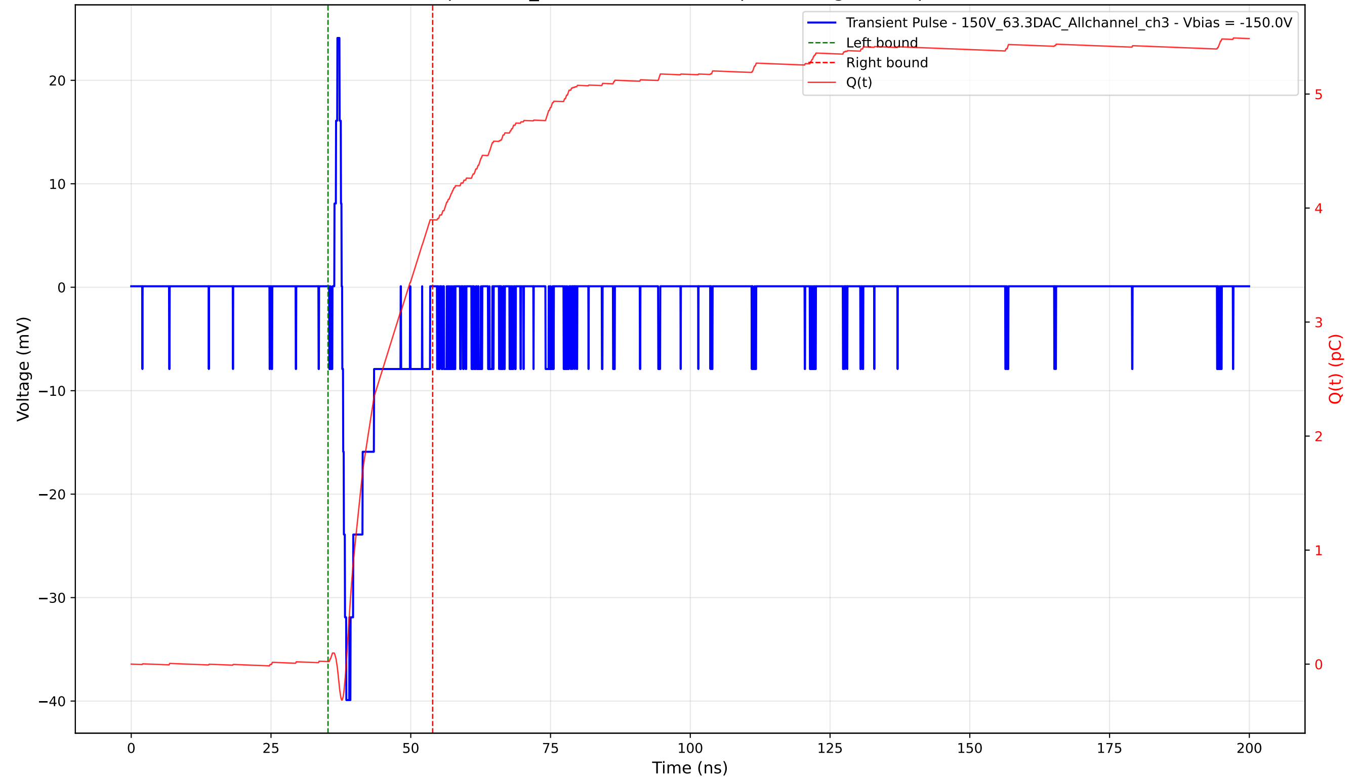
Transient Pulse - Sample: 1cm_42 - Position: 4350.0 \mu\text{m} - Charge: 3.87 pC - Rise Time: 0.74 ns
