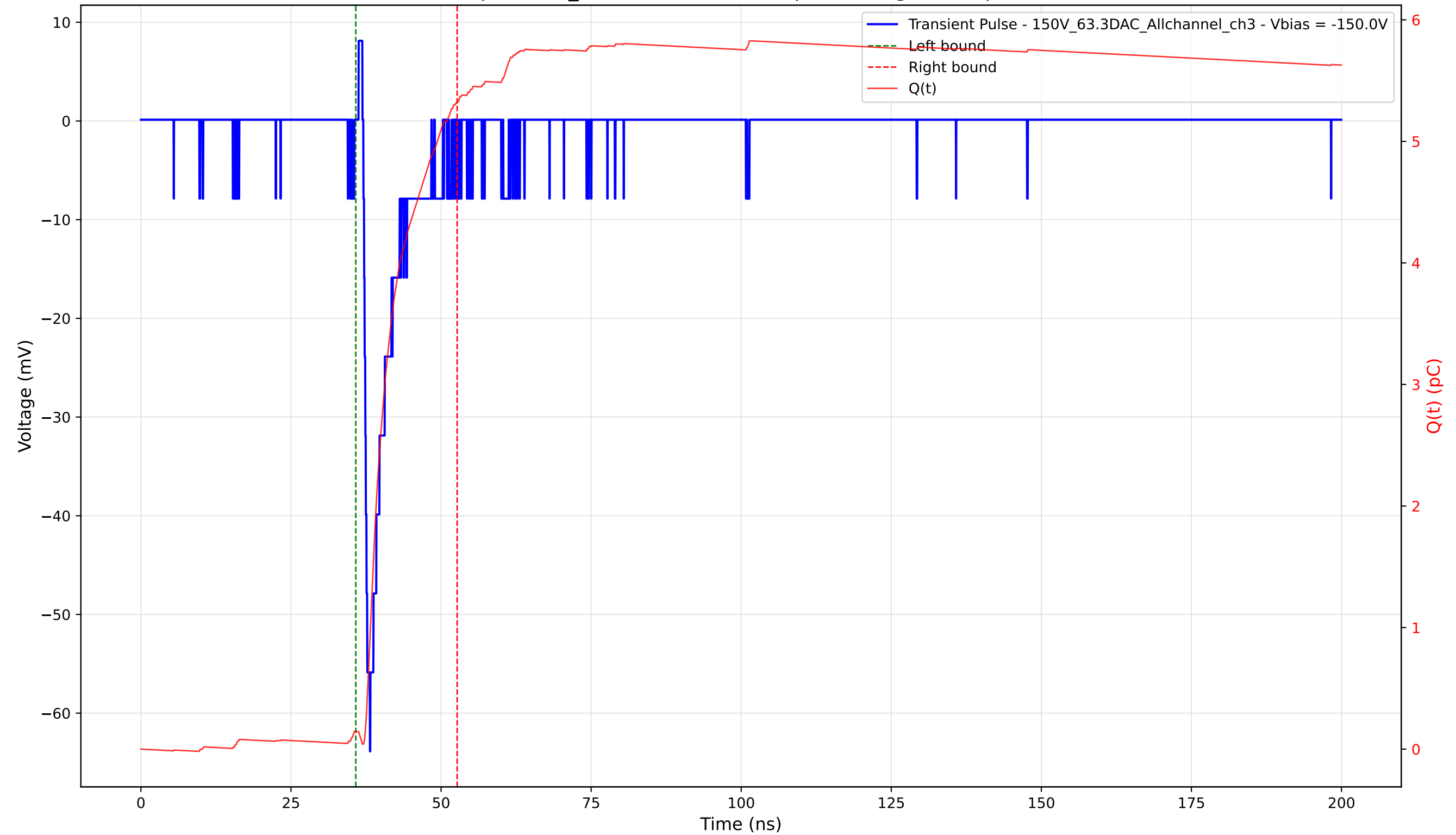
Transient Pulse - Sample: 1cm_42 - Position: 3615.0 \mu\text{m} - Charge: 5.18 pC - Rise Time: 1.09 ns
