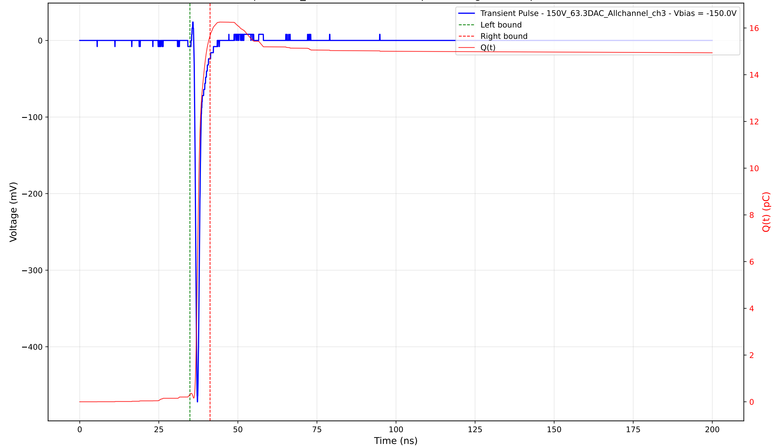
Transient Pulse - Sample: 1cm_42 - Position: 2760.0 \mu\text{m} - Charge: 15.36 pC - Rise Time: 0.73 ns
