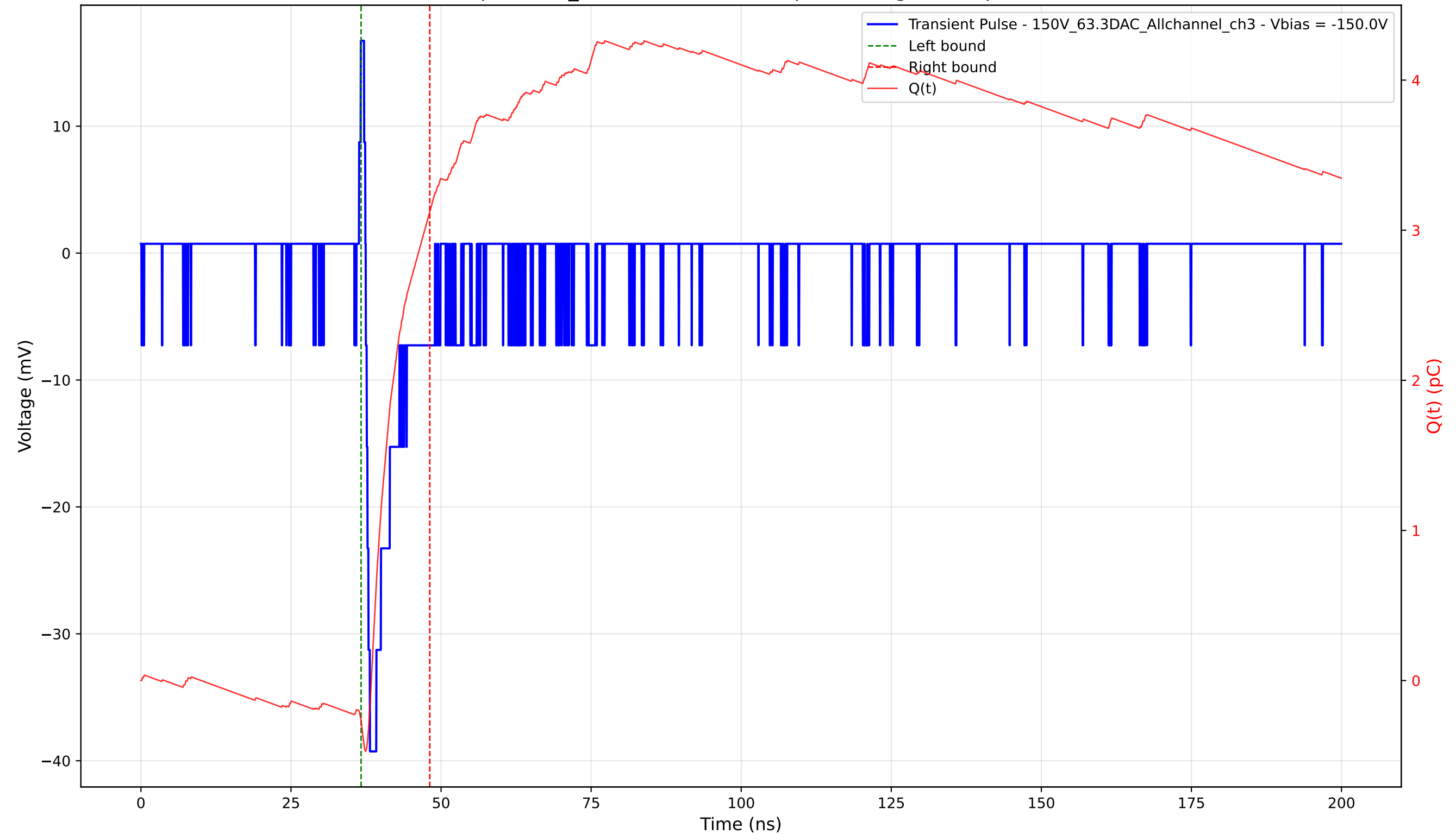
Transient Pulse - Sample: 1cm_42 - Position: 3985.0 \mu\text{m} - Charge: 3.39 pC - Rise Time: 0.70 ns
