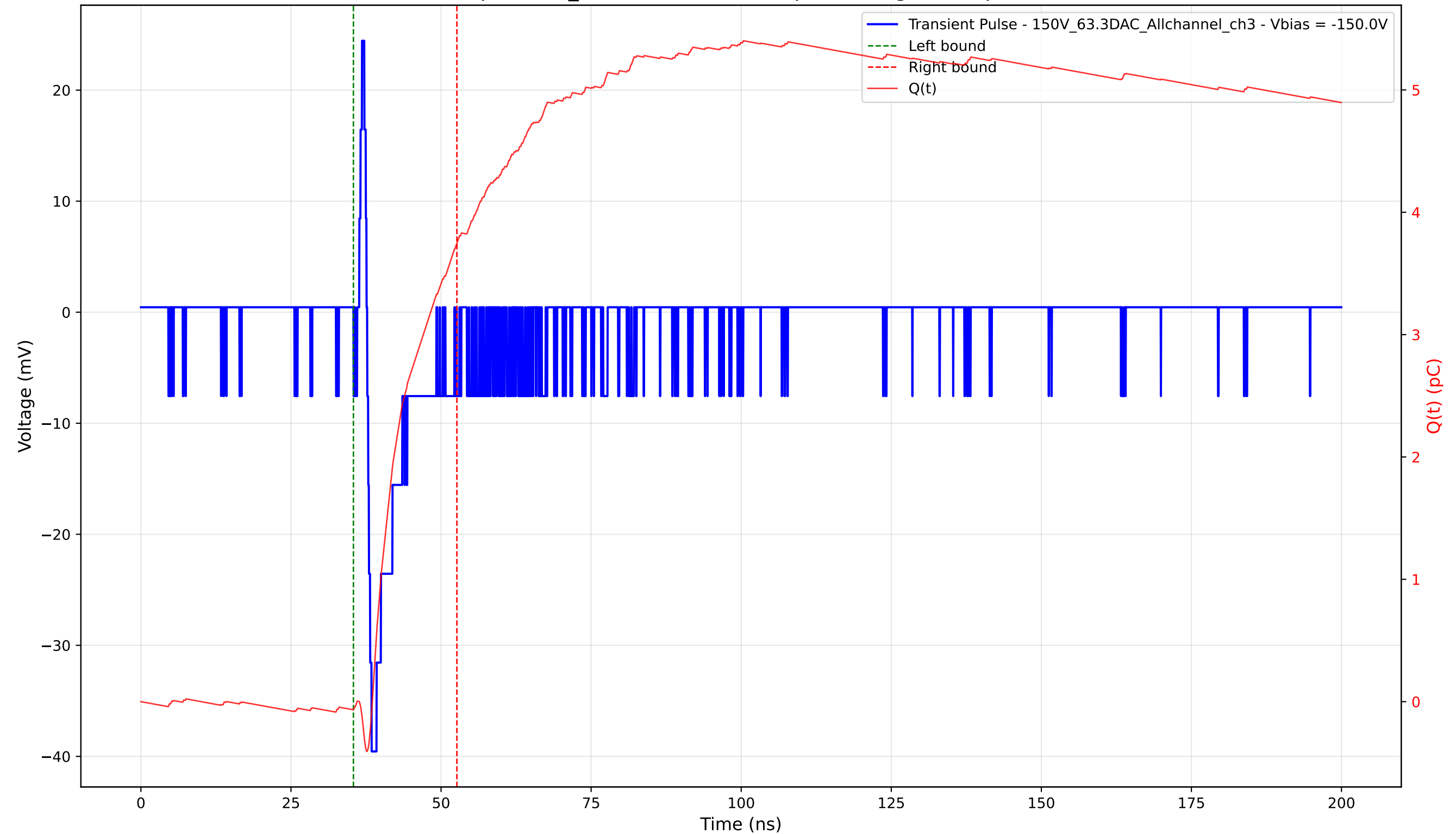
Transient Pulse - Sample: 1cm_42 - Position: 4205.0 \mu\text{m} - Charge: 3.81 pC - Rise Time: 0.74 ns
