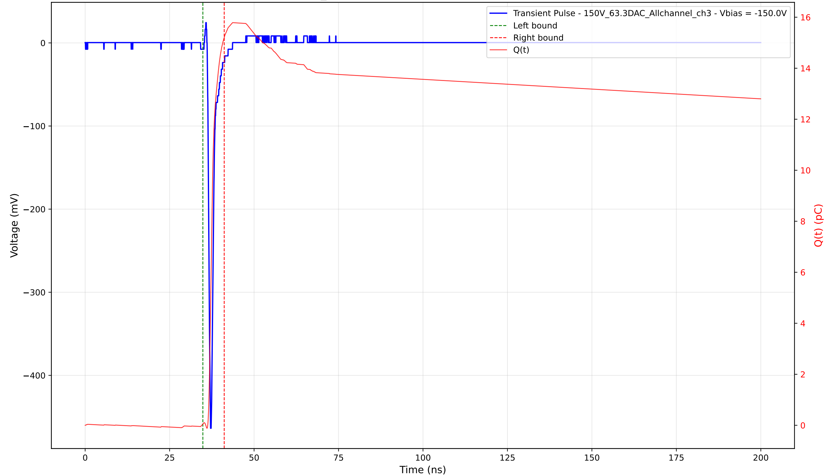
Transient Pulse - Sample: 1cm_42 - Position: 2285.0 \mu\text{m} - Charge: 15.16 pC - Rise Time: 0.69 ns
