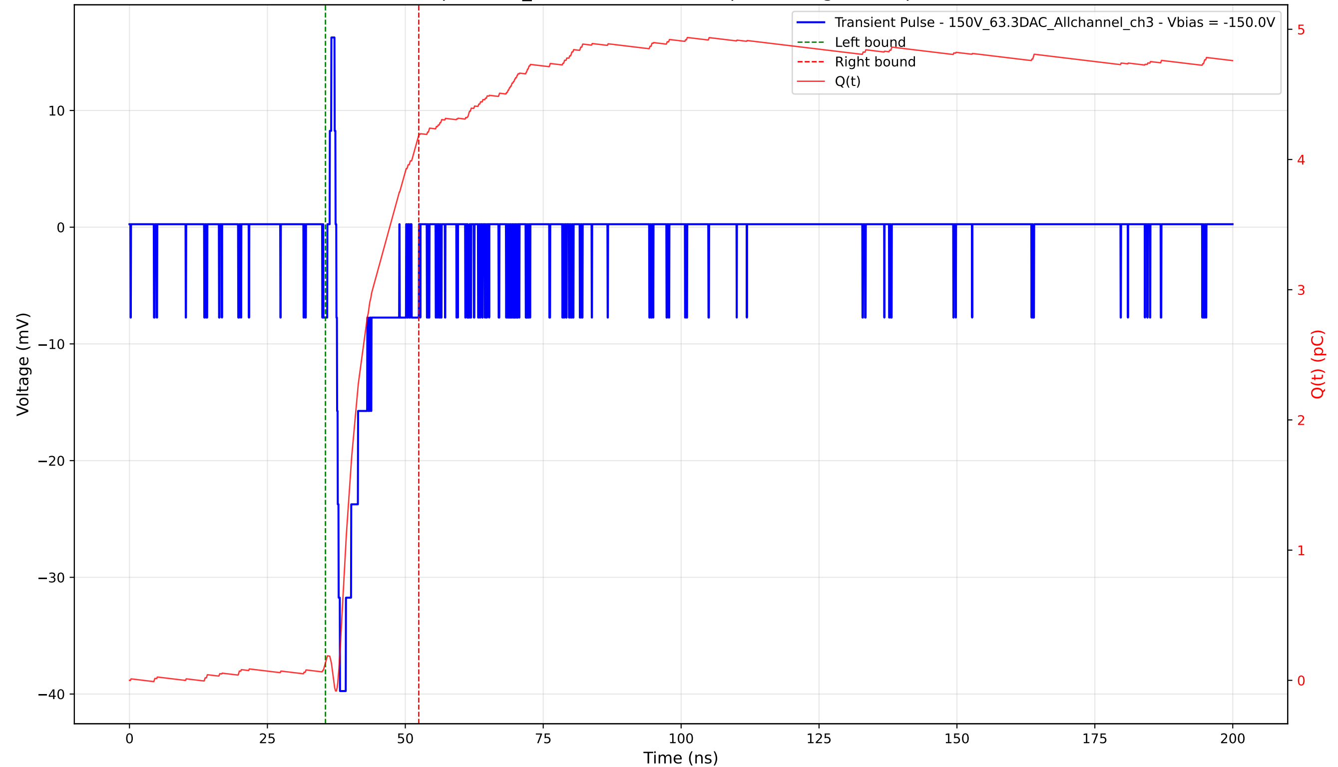
Transient Pulse - Sample: 1cm_42 - Position: 3980.0 \mu\text{m} - Charge: 4.05 pC - Rise Time: 0.66 ns
