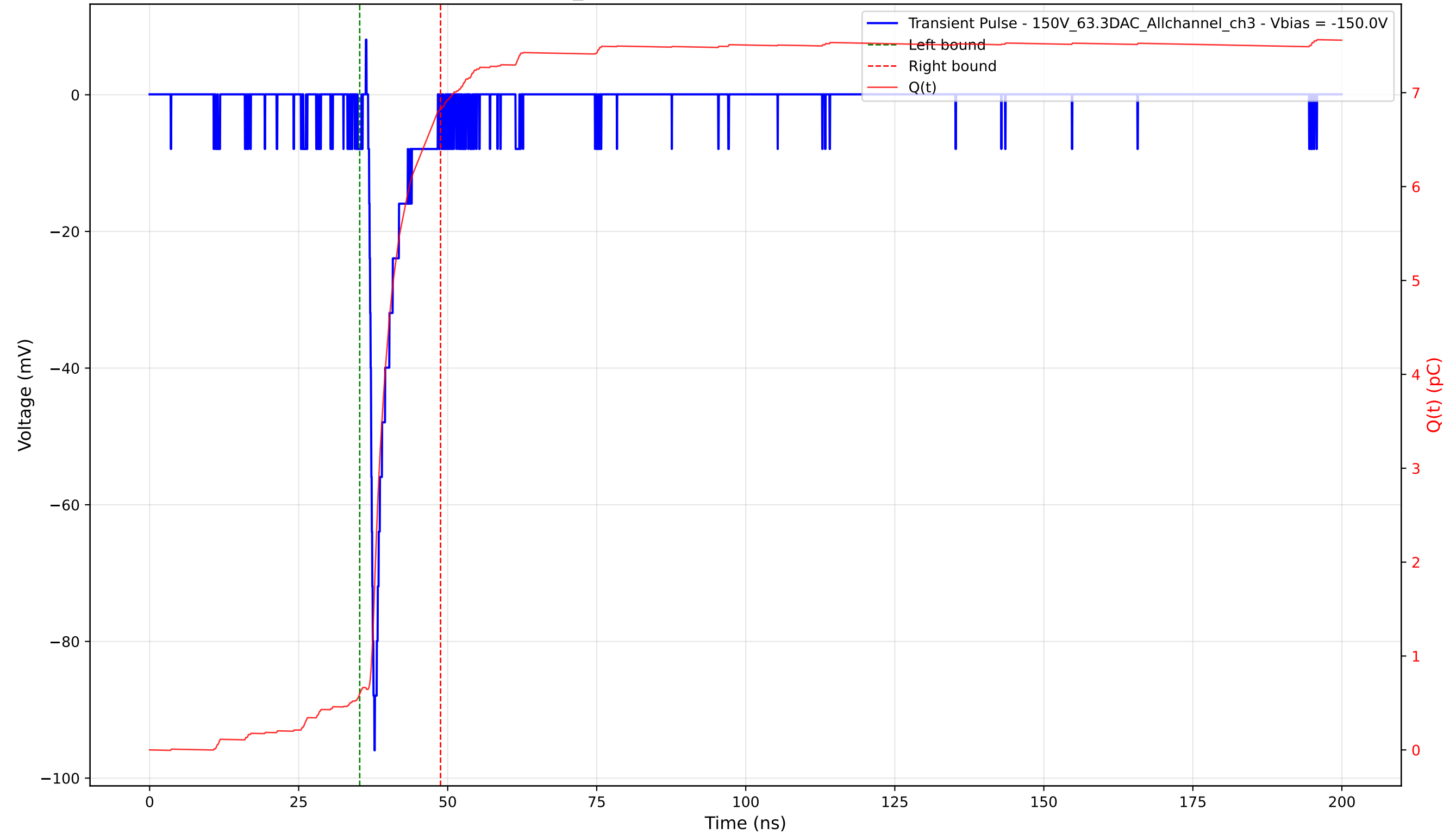
Transient Pulse - Sample: 1cm_42 - Position: 3440.0 \mu\text{m} - Charge: 6.23 pC - Rise Time: 0.75 ns
