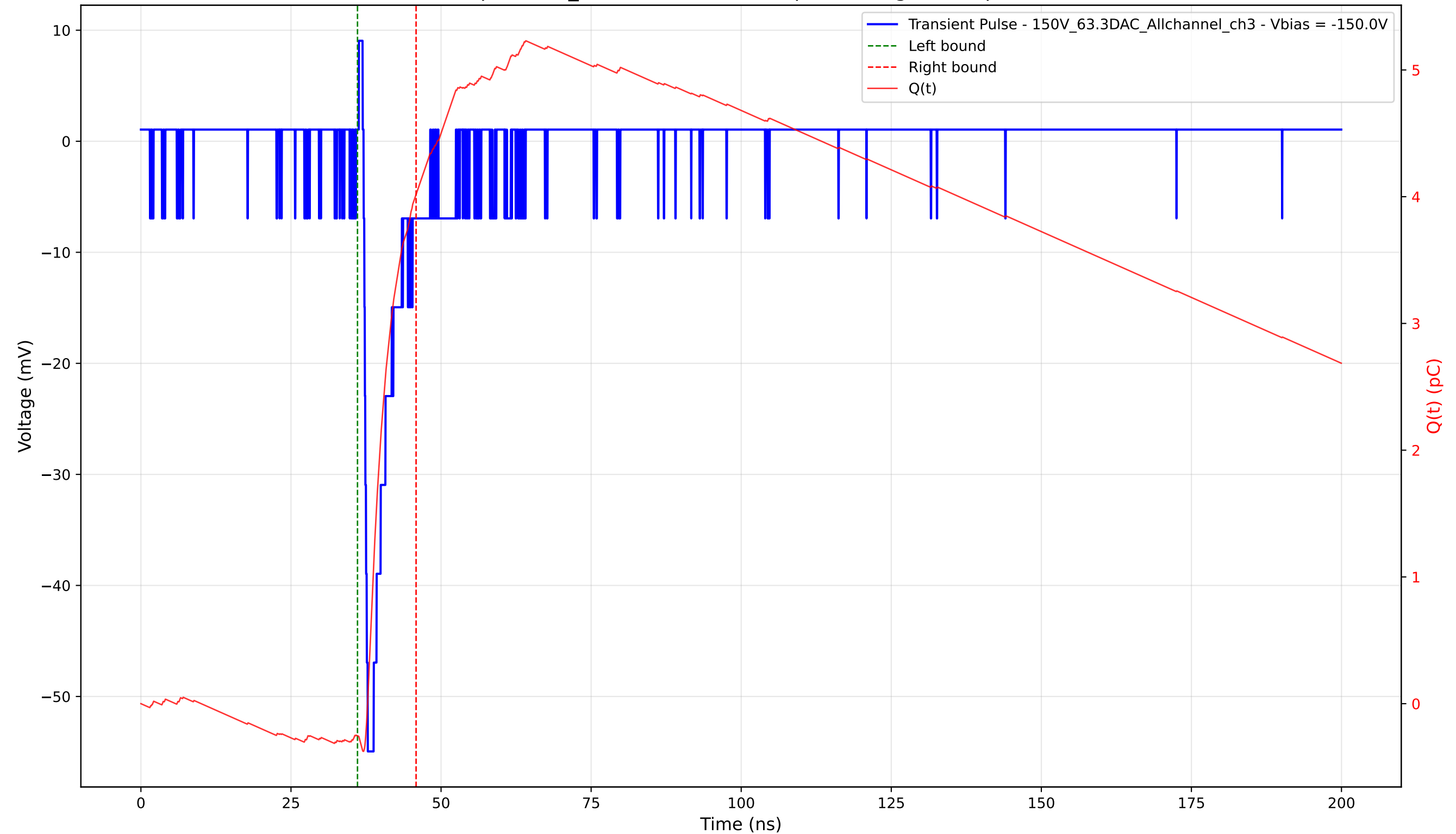
Transient Pulse - Sample: 1cm_42 - Position: 3635.0 \mu\text{m} - Charge: 4.27 pC - Rise Time: 0.69 ns
