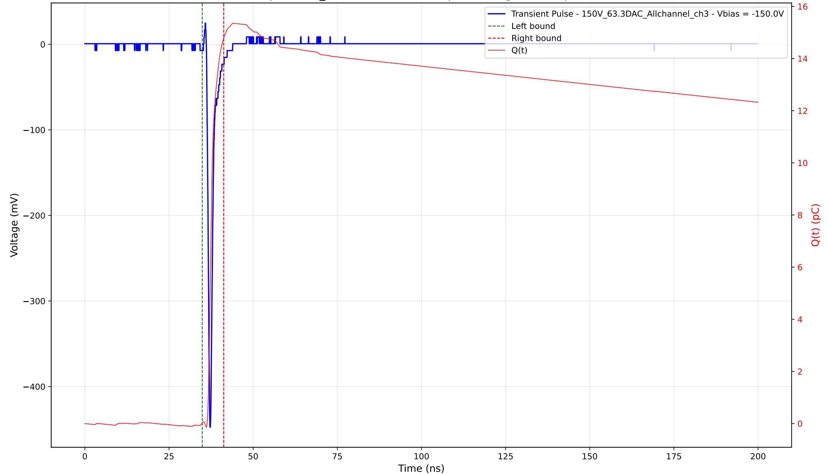
Transient Pulse - Sample: 1cm_42 - Position: 2800.0 \mu\text{m} - Charge: 14.77 pC - Rise Time: 0.72 ns
