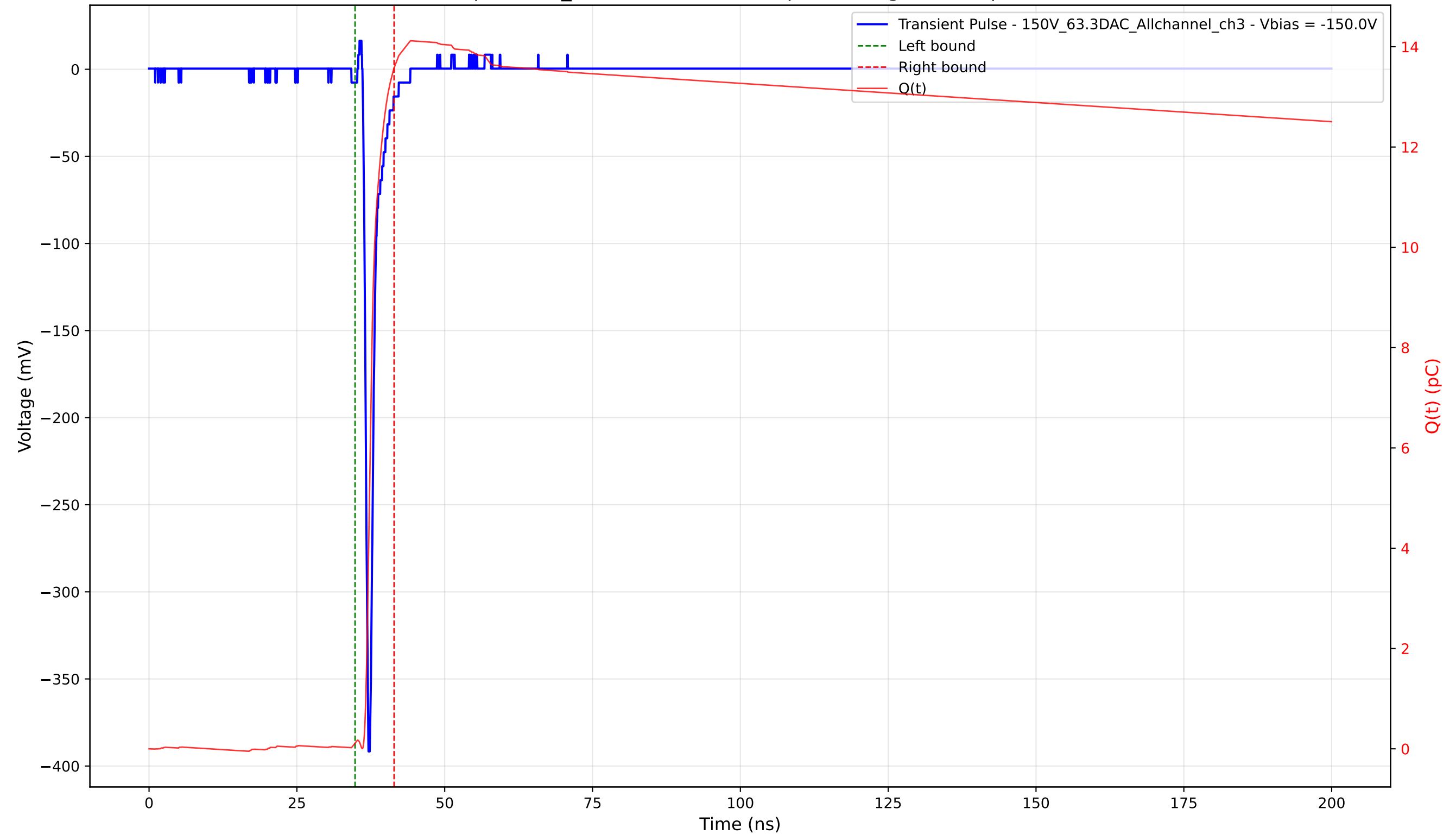
Transient Pulse - Sample: 1cm_42 - Position: 2190.0 \mu\text{m} - Charge: 13.46 pC - Rise Time: 0.74 ns
