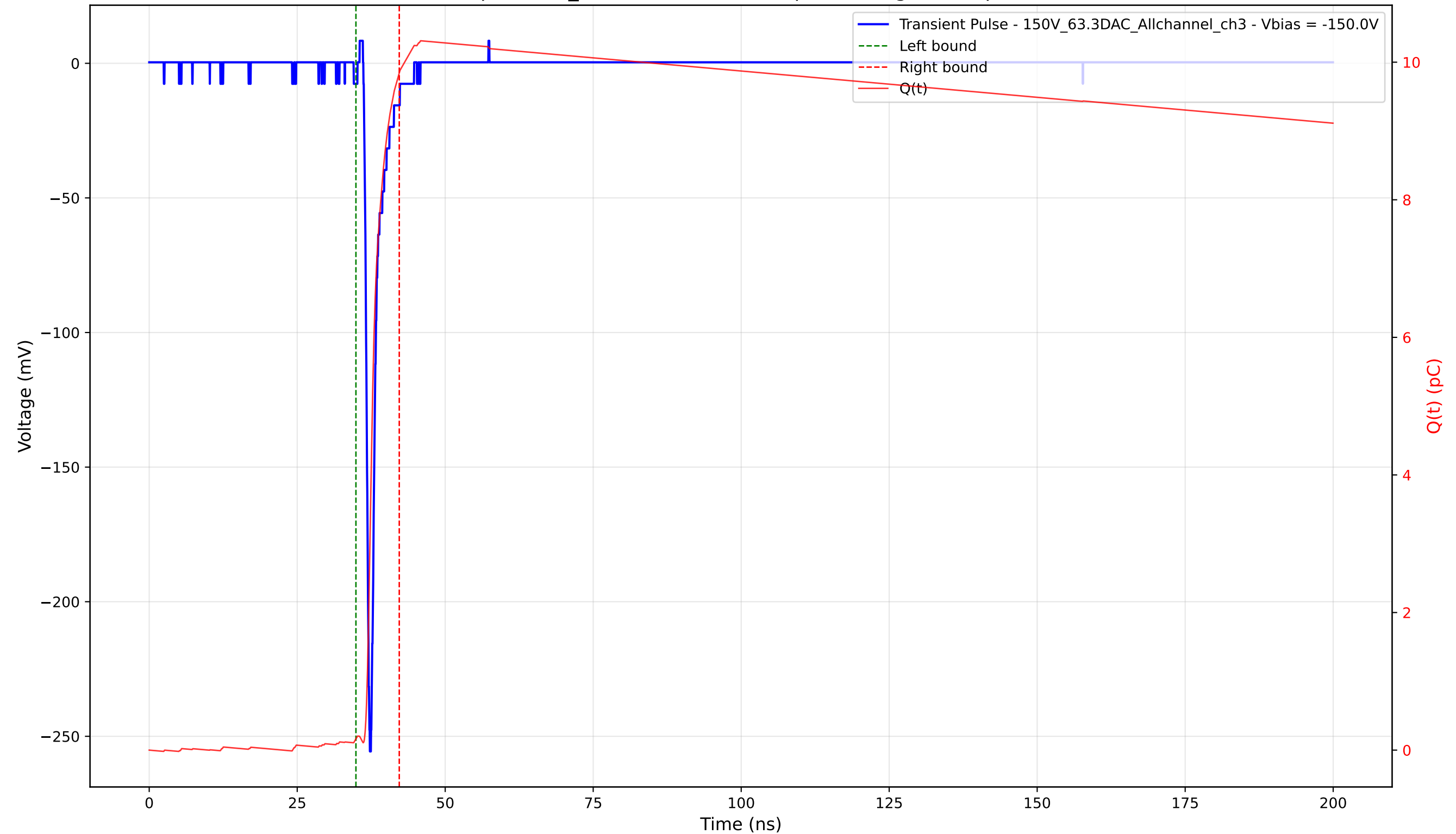
Transient Pulse - Sample: 1cm_42 - Position: 2980.0 \mu\text{m} - Charge: 9.68 pC - Rise Time: 0.75 ns
