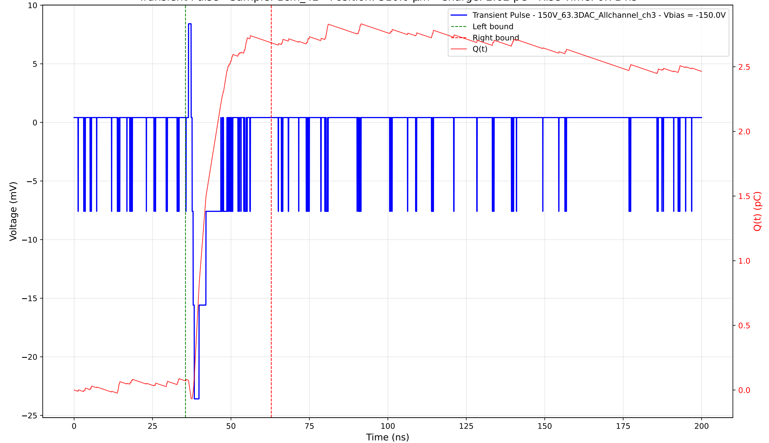
Transient Pulse - Sample: 1cm_42 - Position: 310.0 \mu\text{m} - Charge: 2.62 pC - Rise Time: 0.71 ns
