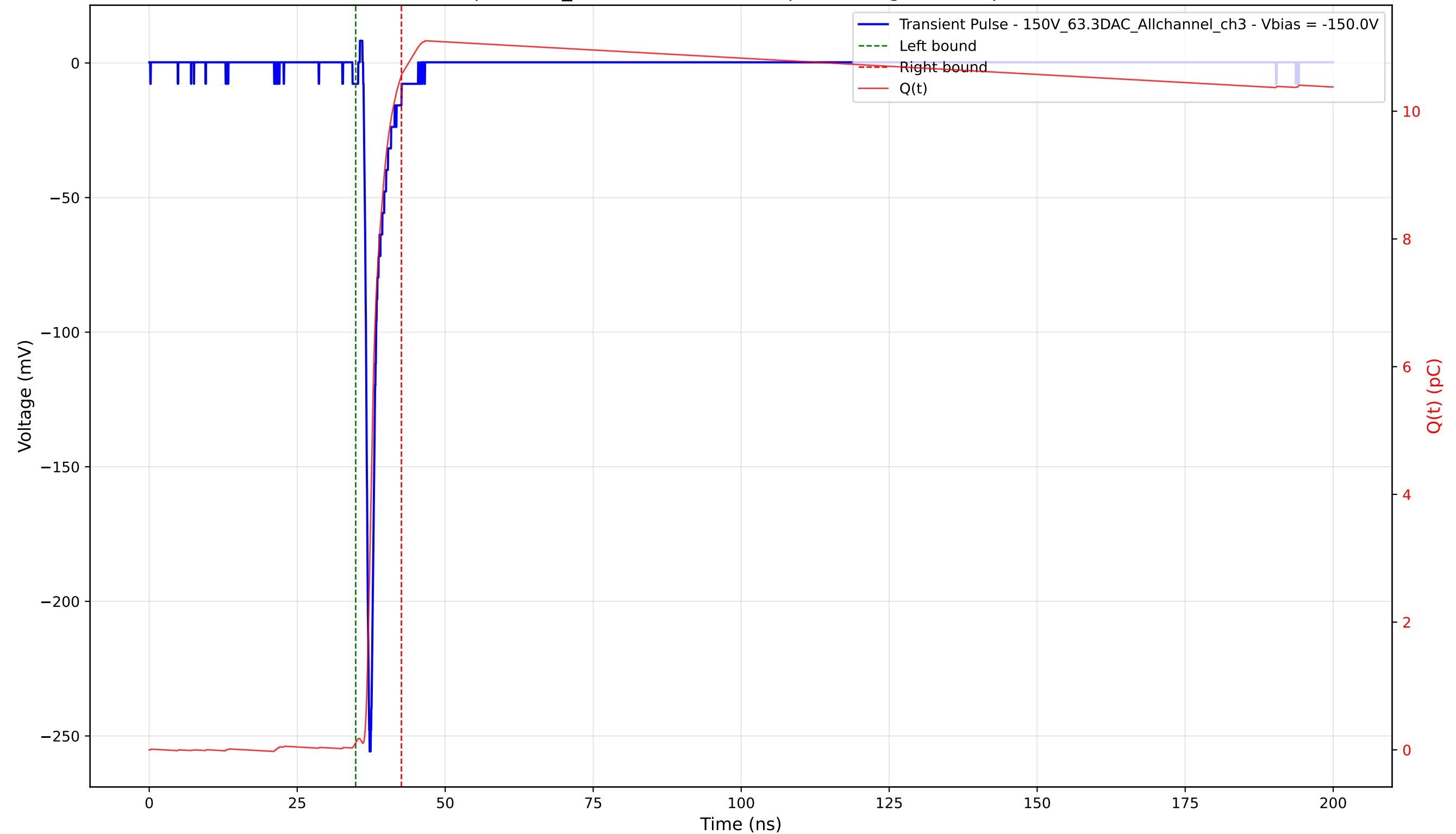
Transient Pulse - Sample: 1cm_42 - Position: 2045.0 \mu\text{m} - Charge: 10.45 pC - Rise Time: 0.78 ns
