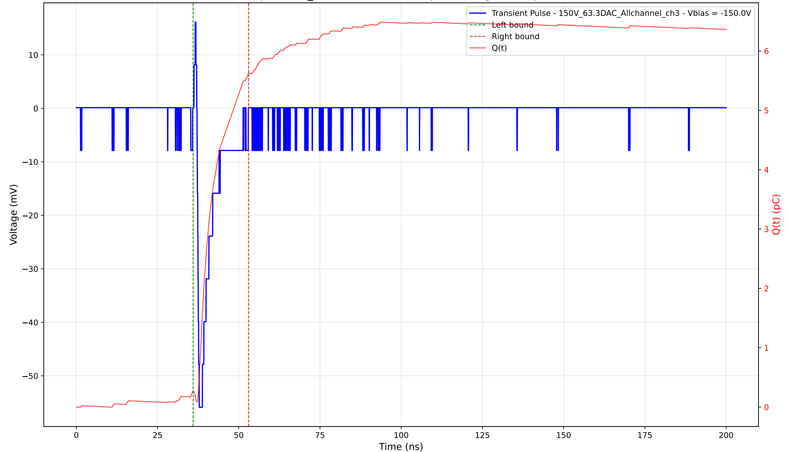
Transient Pulse - Sample: 1cm_42 - Position: 3670.0 \mu\text{m} - Charge: 5.36 pC - Rise Time: 0.65 ns
