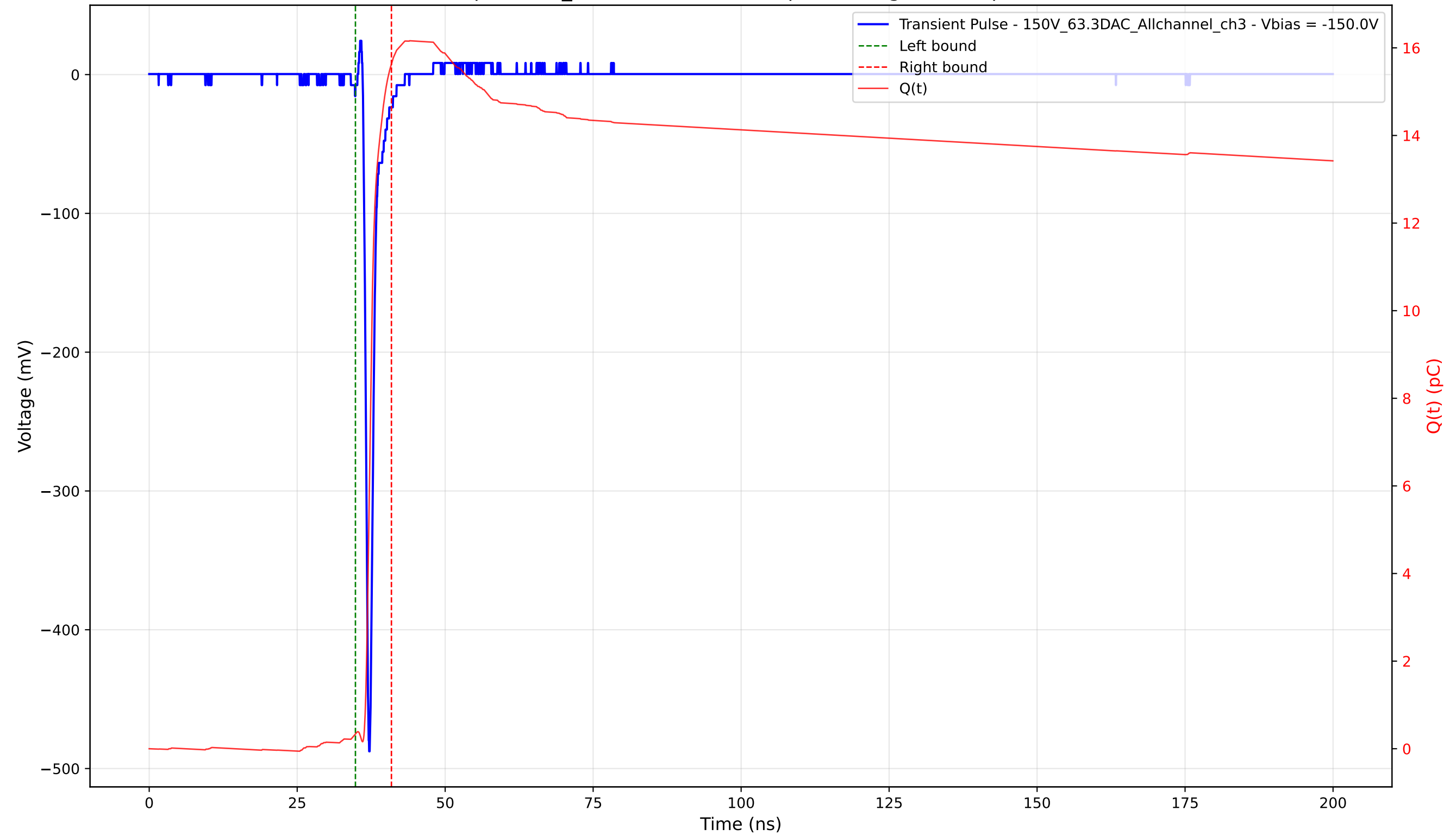
Transient Pulse - Sample: 1cm_42 - Position: 2680.0 \mu\text{m} - Charge: 15.29 pC - Rise Time: 0.69 ns
