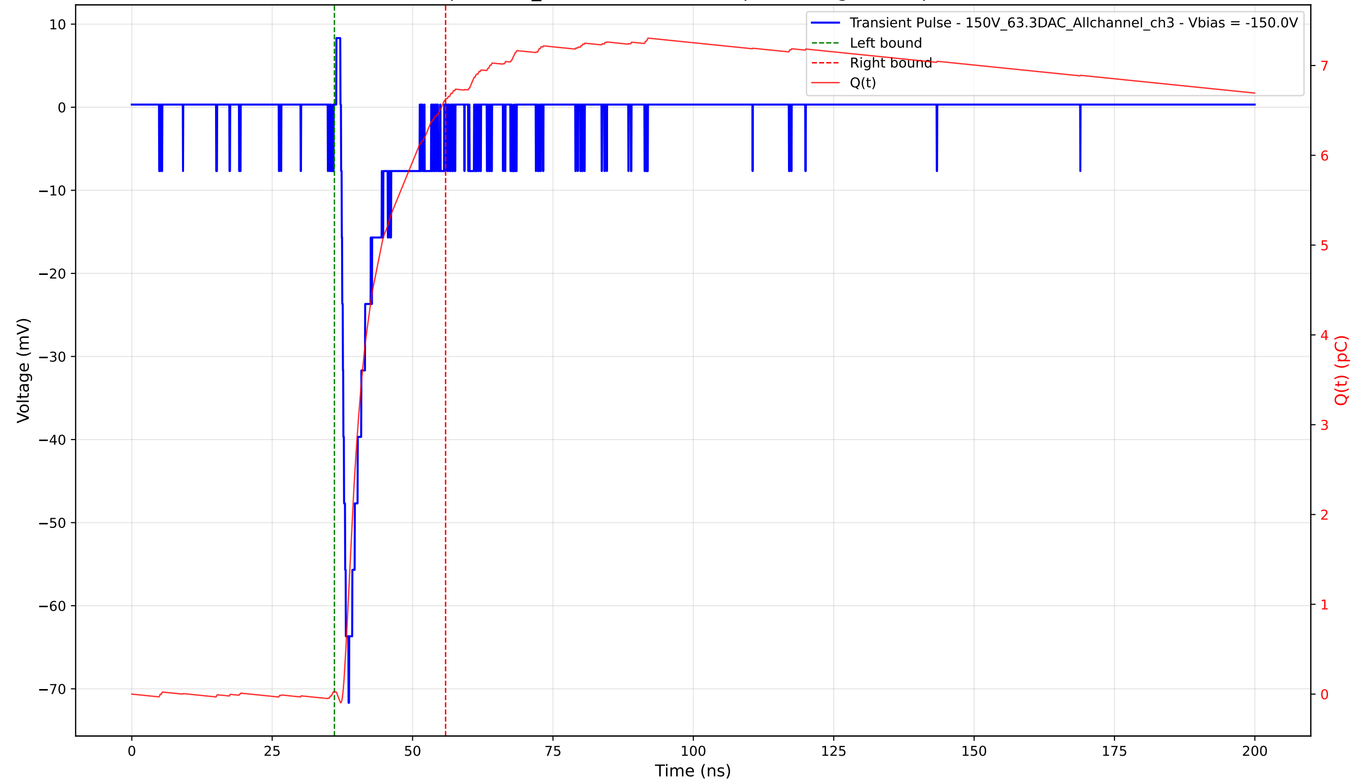
Transient Pulse - Sample: 1cm_42 - Position: 1215.0 \mu\text{m} - Charge: 6.60 pC - Rise Time: 1.32 ns
