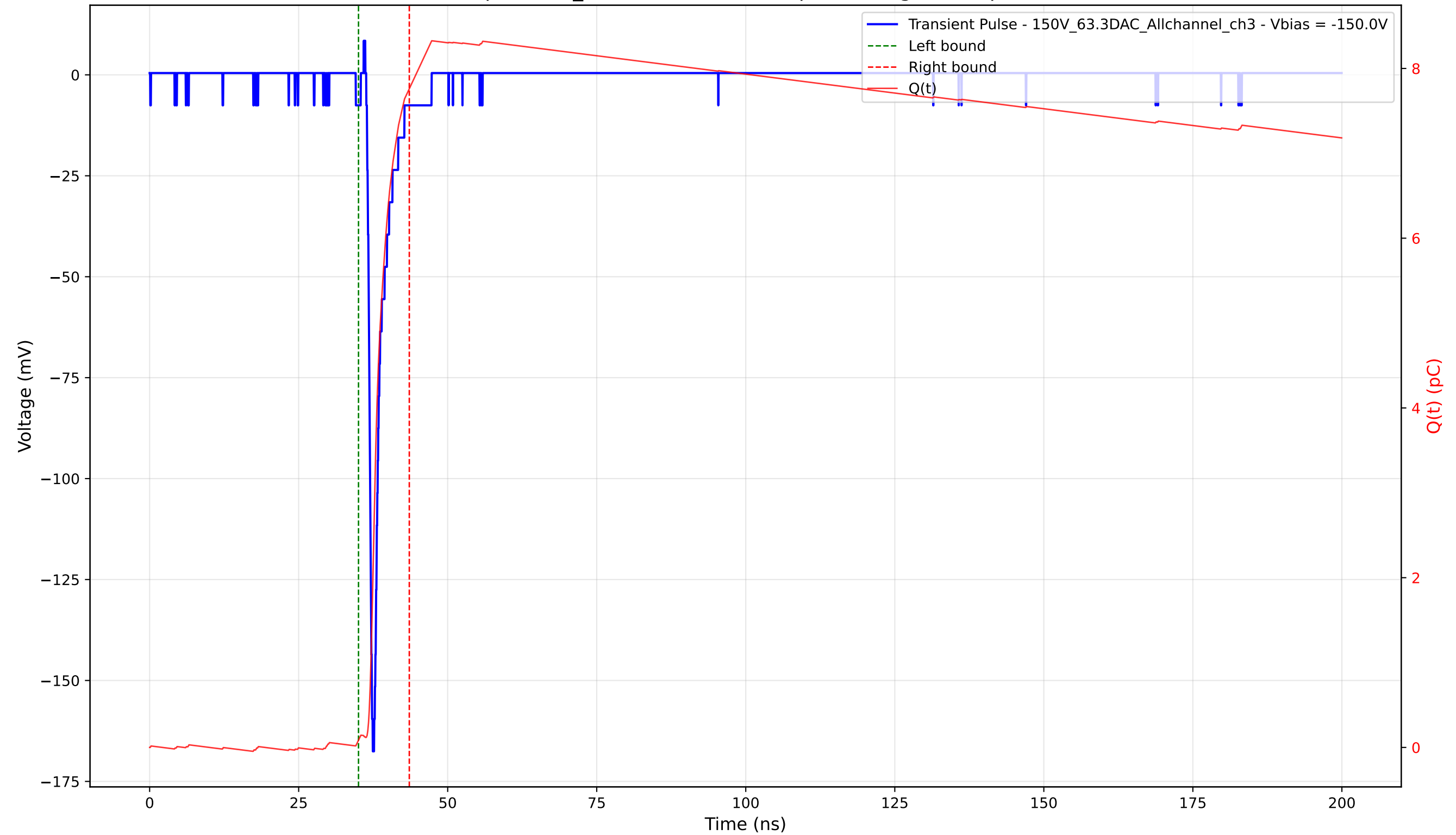
Transient Pulse - Sample: 1cm_42 - Position: 3140.0 \mu\text{m} - Charge: 7.67 pC - Rise Time: 0.79 ns
