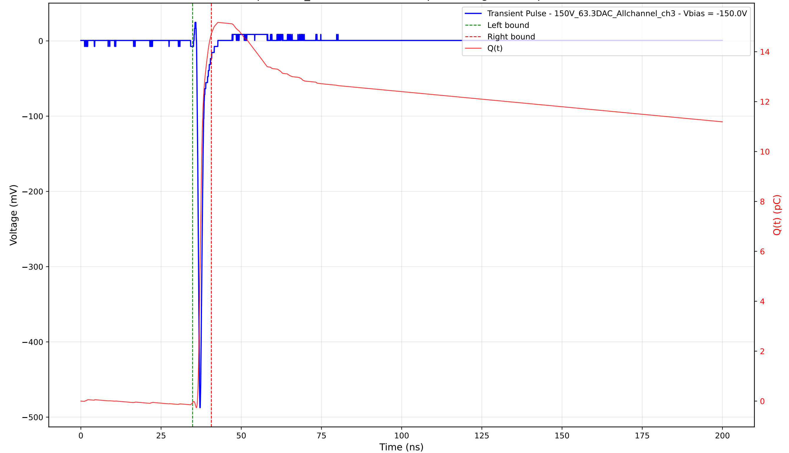
Transient Pulse - Sample: 1cm_42 - Position: 2435.0 \mu\text{m} - Charge: 14.78 pC - Rise Time: 0.71 ns
