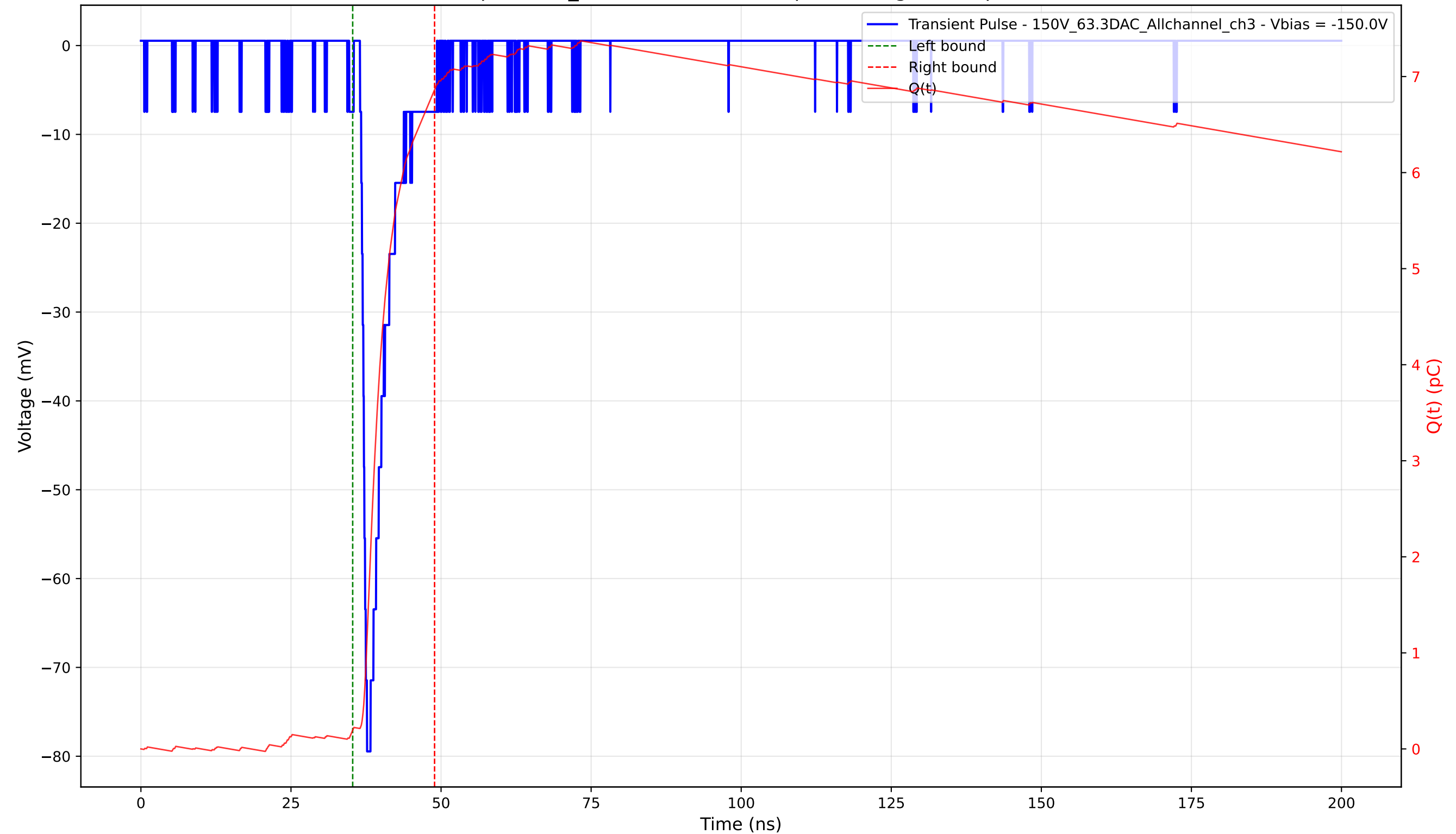
Transient Pulse - Sample: 1cm_42 - Position: 1535.0 \mu\text{m} - Charge: 6.67 pC - Rise Time: 1.00 ns
