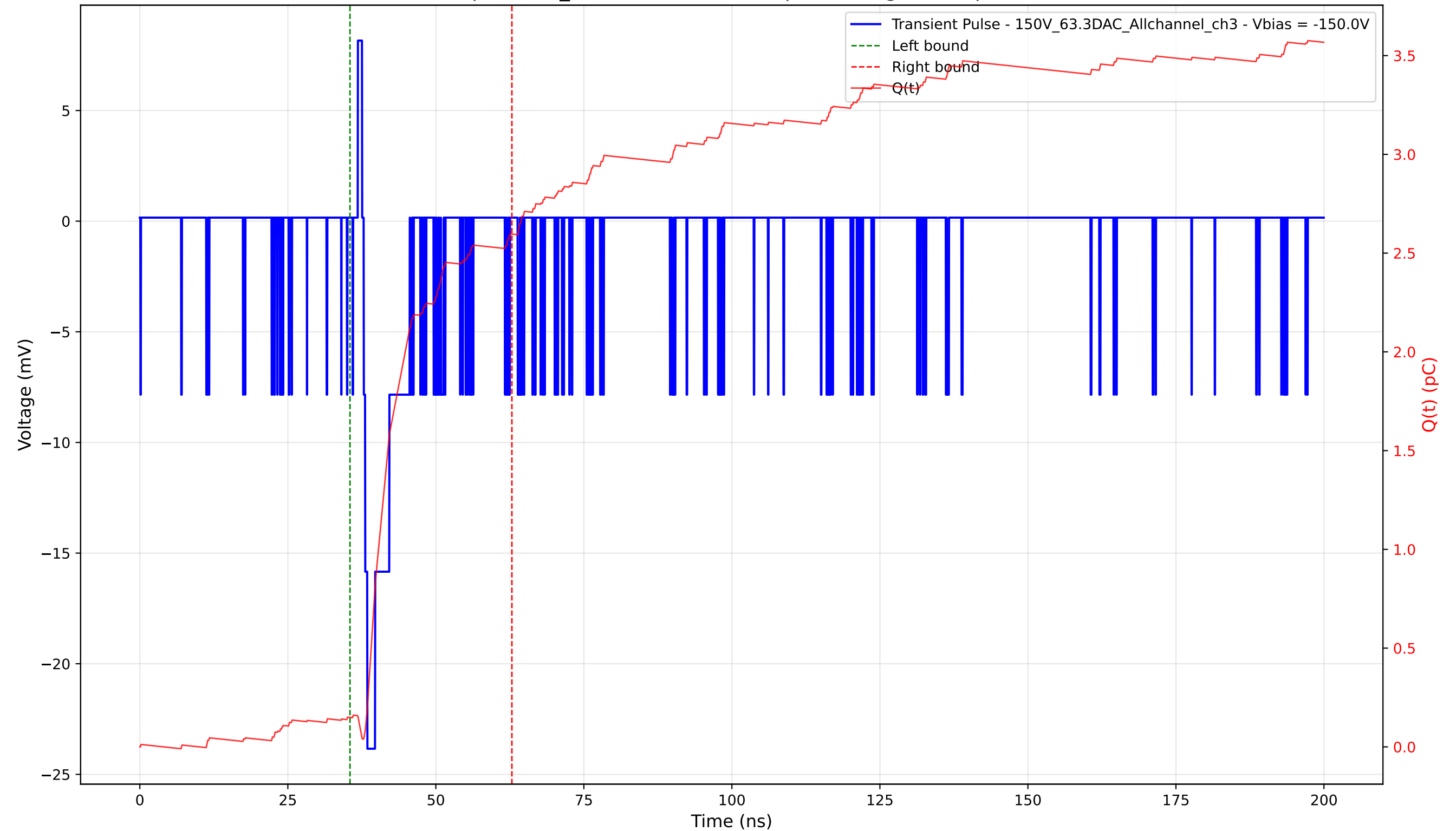
Transient Pulse - Sample: 1cm_42 - Position: 4945.0 \mu\text{m} - Charge: 2.45 pC - Rise Time: 0.63 ns
