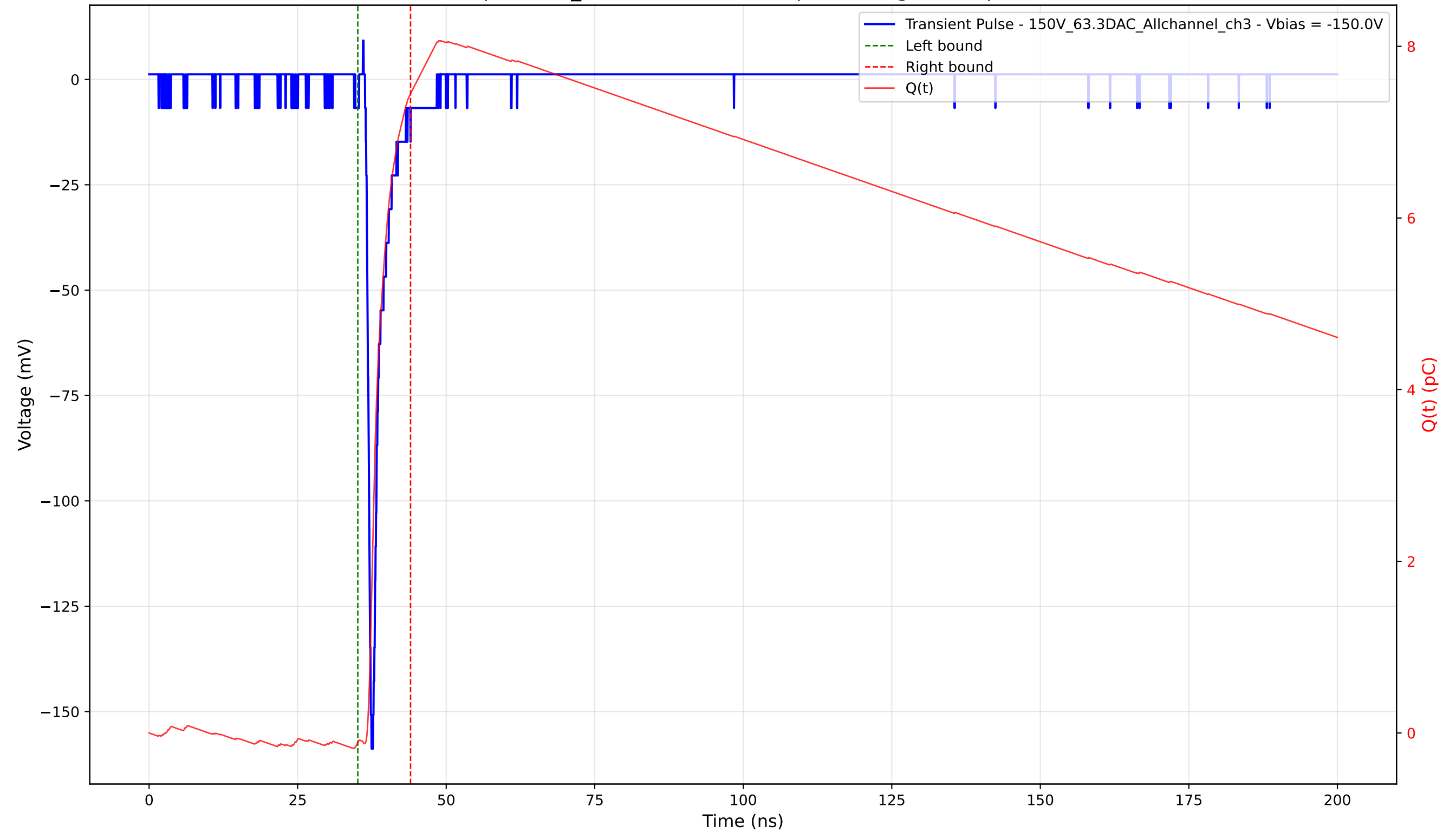
Transient Pulse - Sample: 1cm_42 - Position: 3155.0 \mu\text{m} - Charge: 7.56 pC - Rise Time: 0.79 ns
