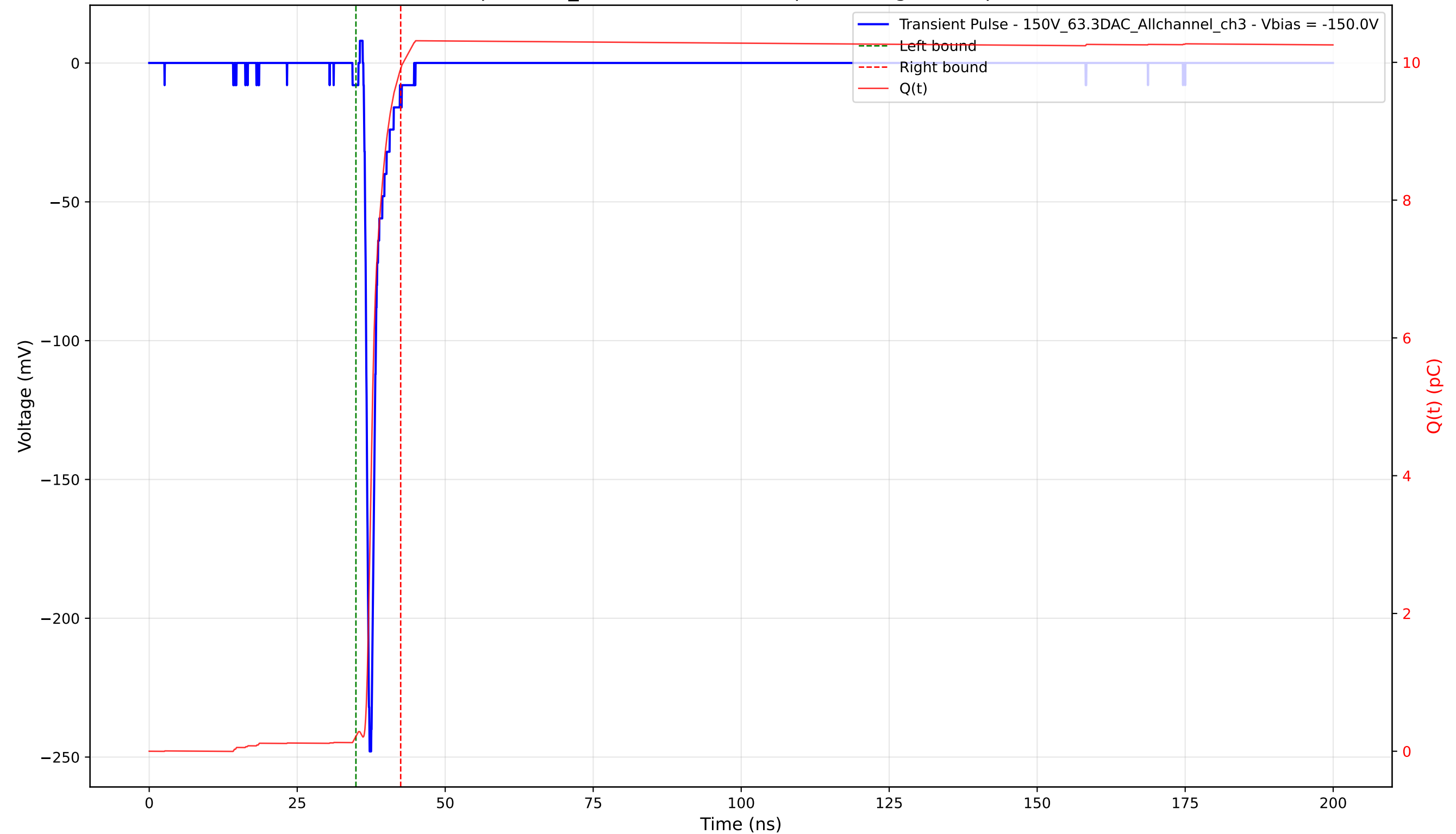
Transient Pulse - Sample: 1cm_42 - Position: 2985.0 \mu\text{m} - Charge: 9.68 pC - Rise Time: 0.75 ns
