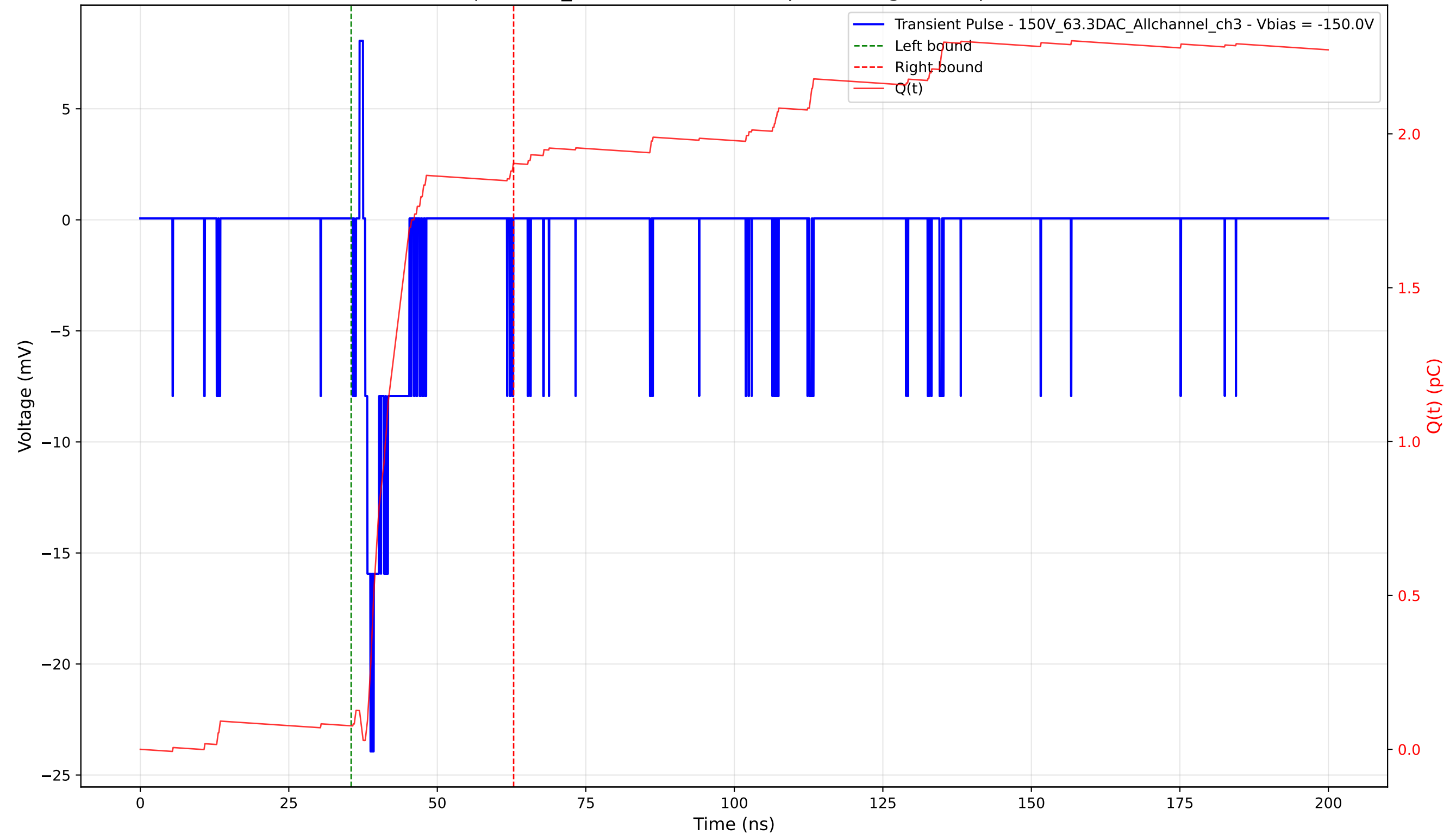
Transient Pulse - Sample: 1cm_42 - Position: 4990.0 \mu\text{m} - Charge: 1.83 pC - Rise Time: 0.91 ns
