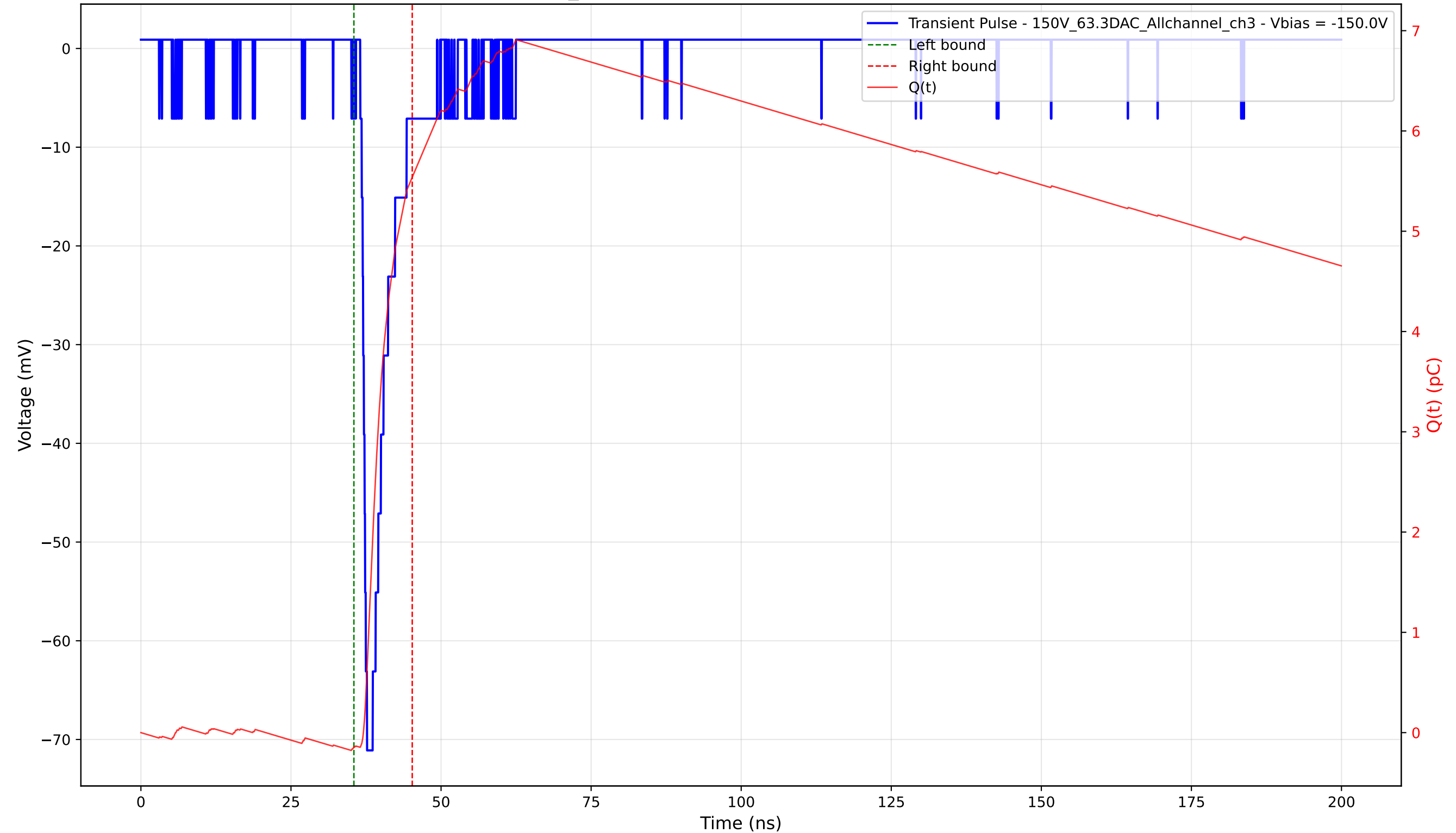
Transient Pulse - Sample: 1cm_42 - Position: 1505.0 \mu\text{m} - Charge: 5.69 pC - Rise Time: 0.92 ns
