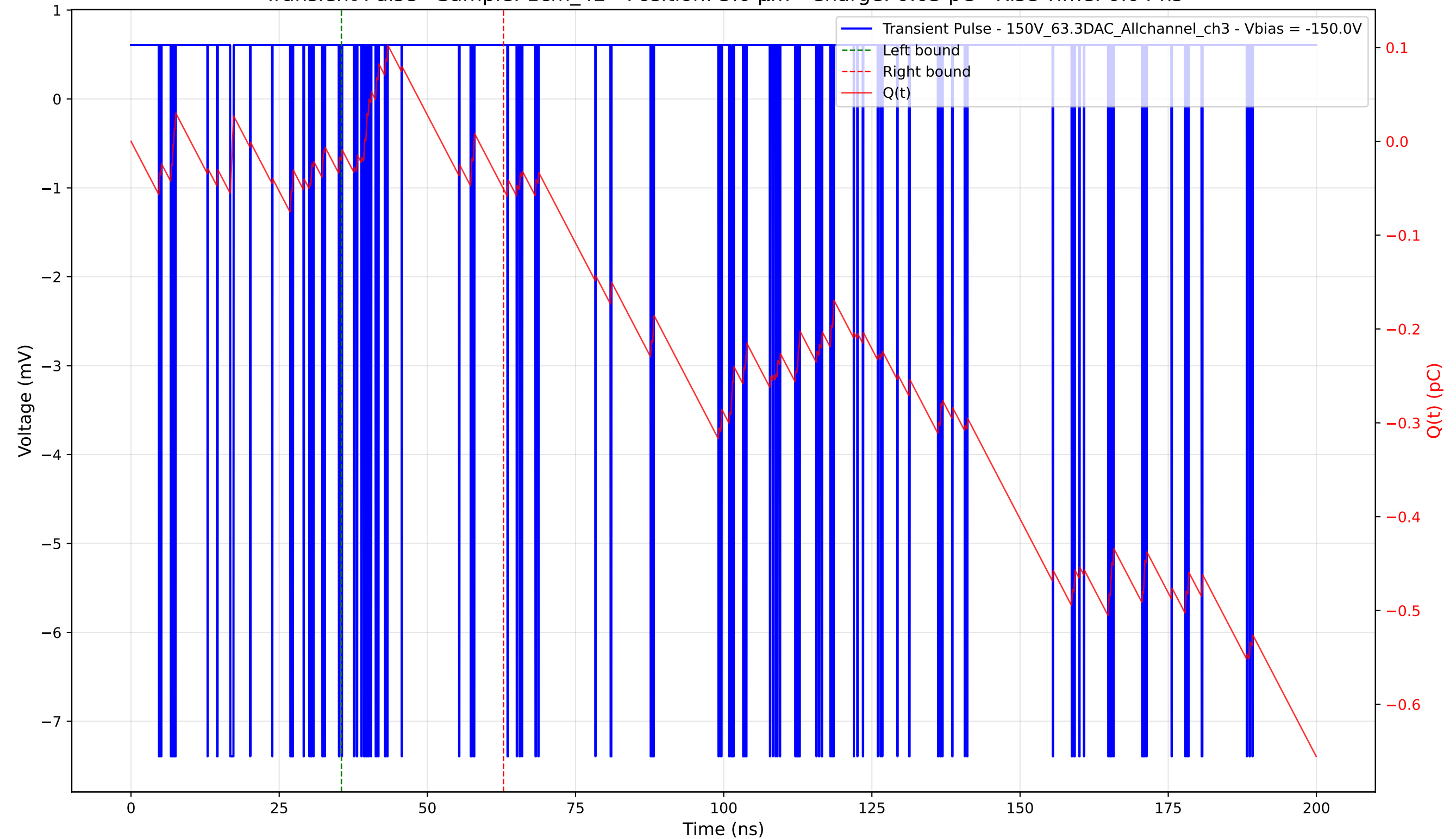
Transient Pulse - Sample: 1cm_42 - Position: 5.0 \mu\text{m} - Charge: 0.03 pC - Rise Time: 0.04 ns
