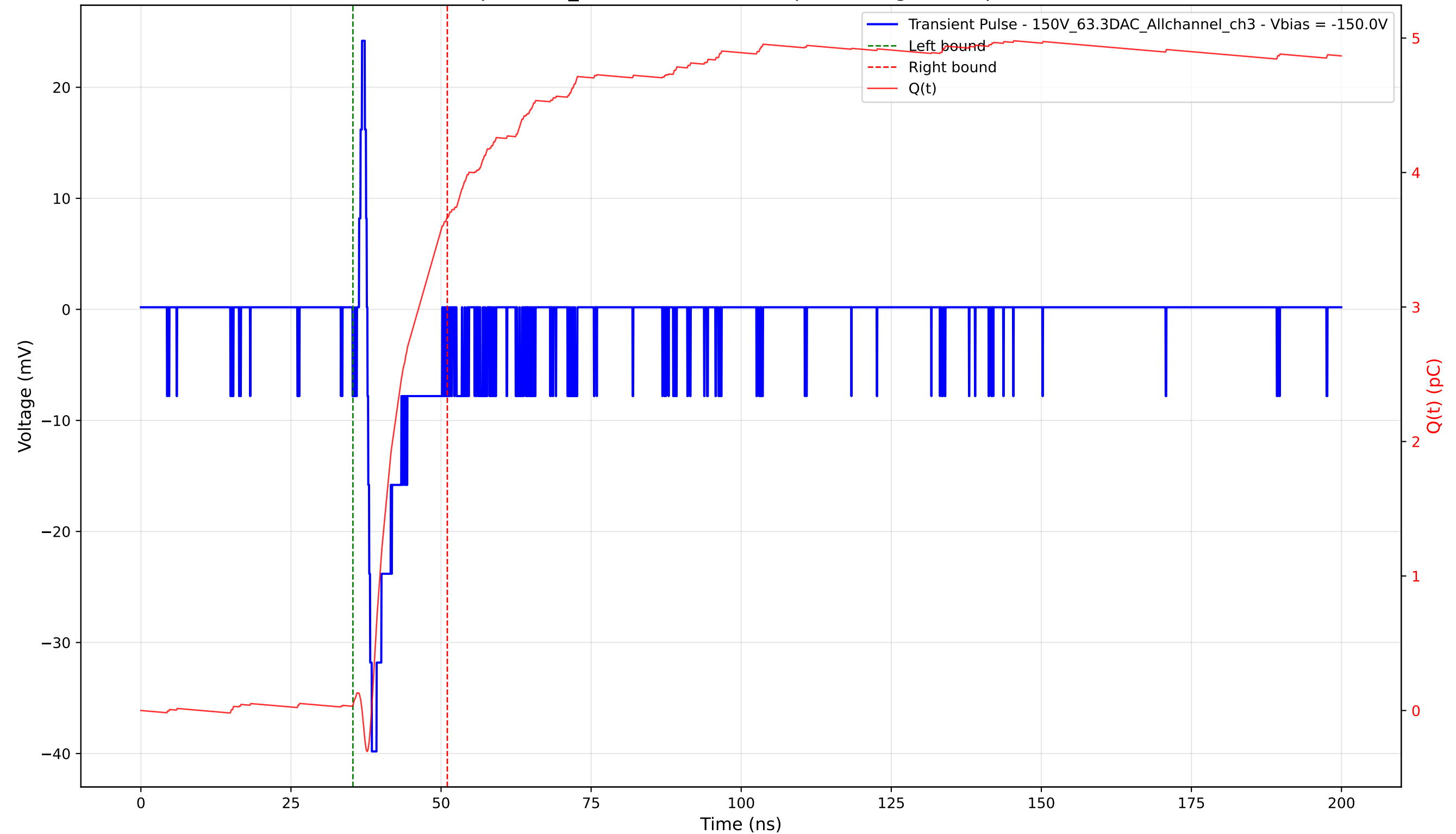
Transient Pulse - Sample: 1cm_42 - Position: 4295.0 \mu\text{m} - Charge: 3.63 pC - Rise Time: 0.74 ns
