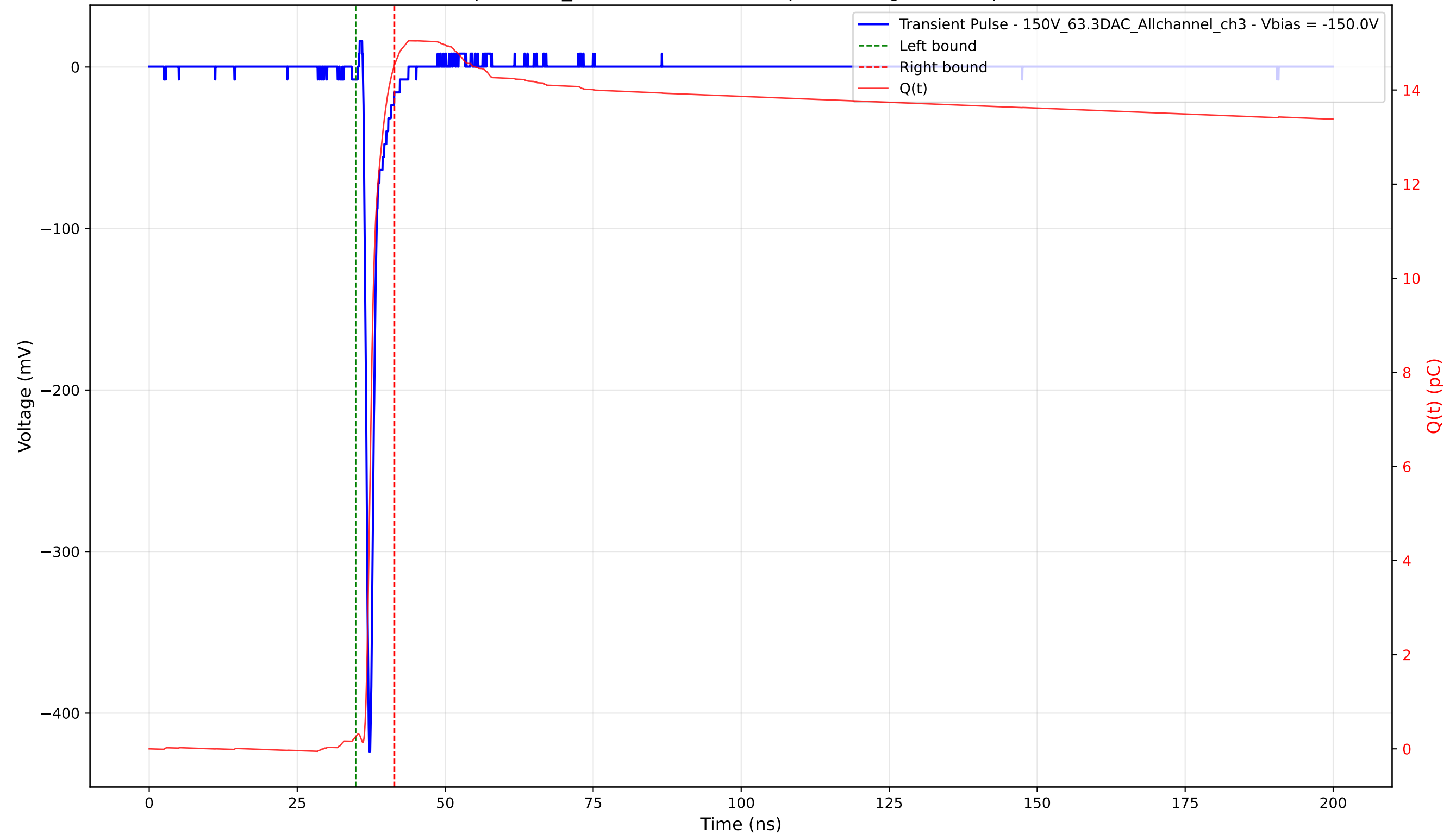
Transient Pulse - Sample: 1cm_42 - Position: 2830.0 \mu\text{m} - Charge: 14.28 pC - Rise Time: 0.73 ns
