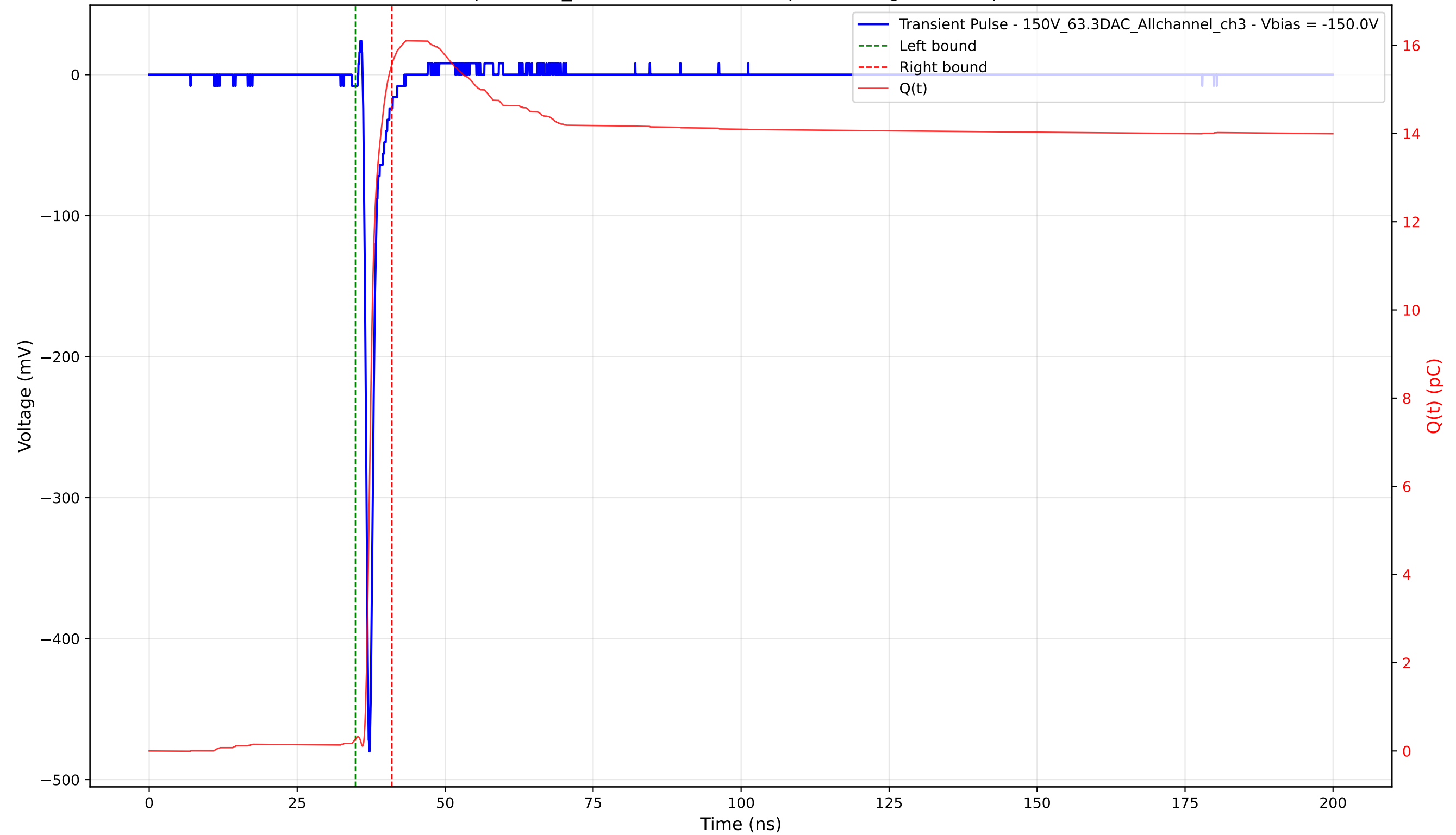
Transient Pulse - Sample: 1cm_42 - Position: 2340.0 \mu\text{m} - Charge: 15.31 pC - Rise Time: 0.70 ns
