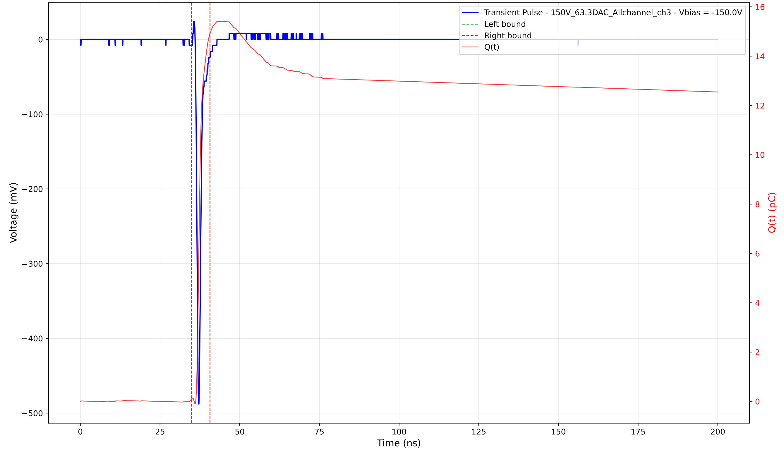
Transient Pulse - Sample: 1cm_42 - Position: 2495.0 \mu\text{m} - Charge: 14.84 pC - Rise Time: 0.72 ns
