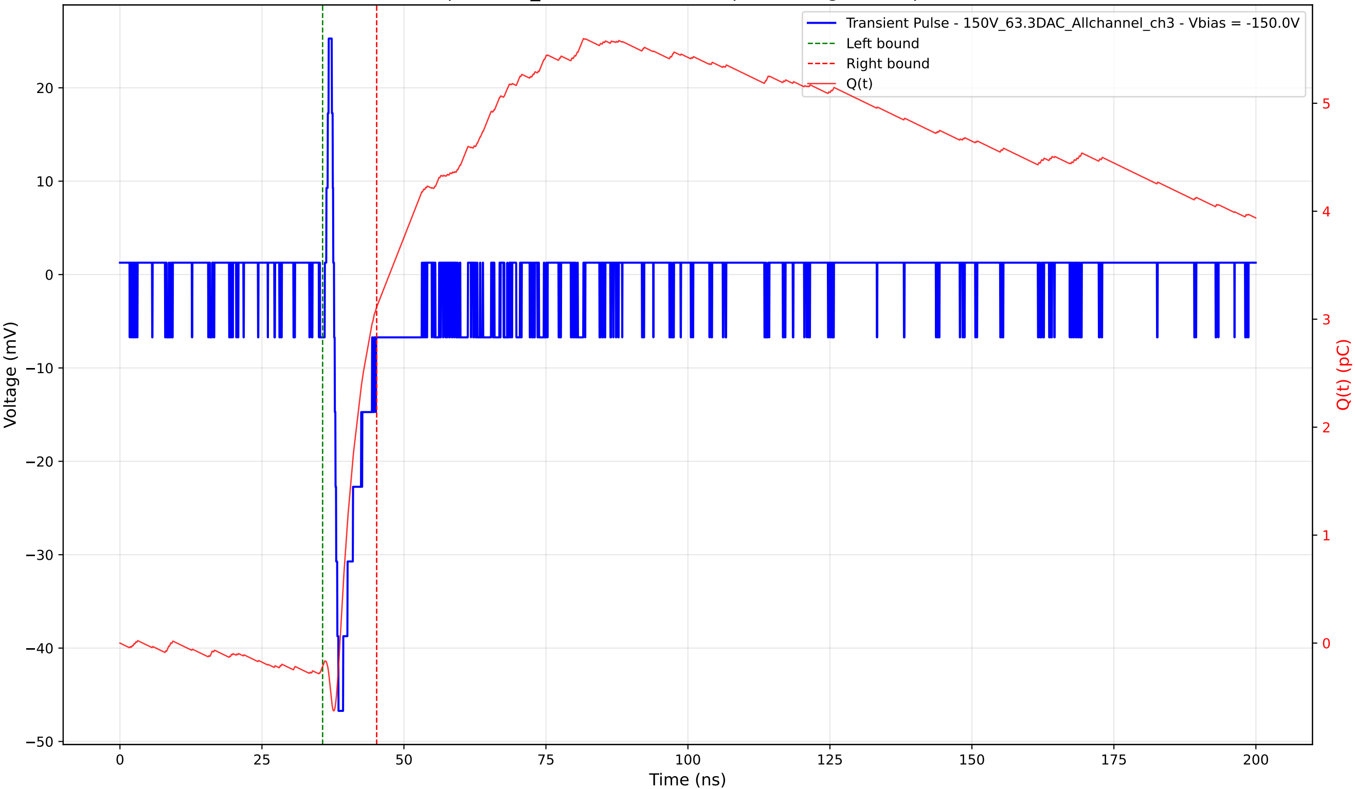
Transient Pulse - Sample: 1cm_42 - Position: 665.0 \mu\text{m} - Charge: 3.33 pC - Rise Time: 0.78 ns
