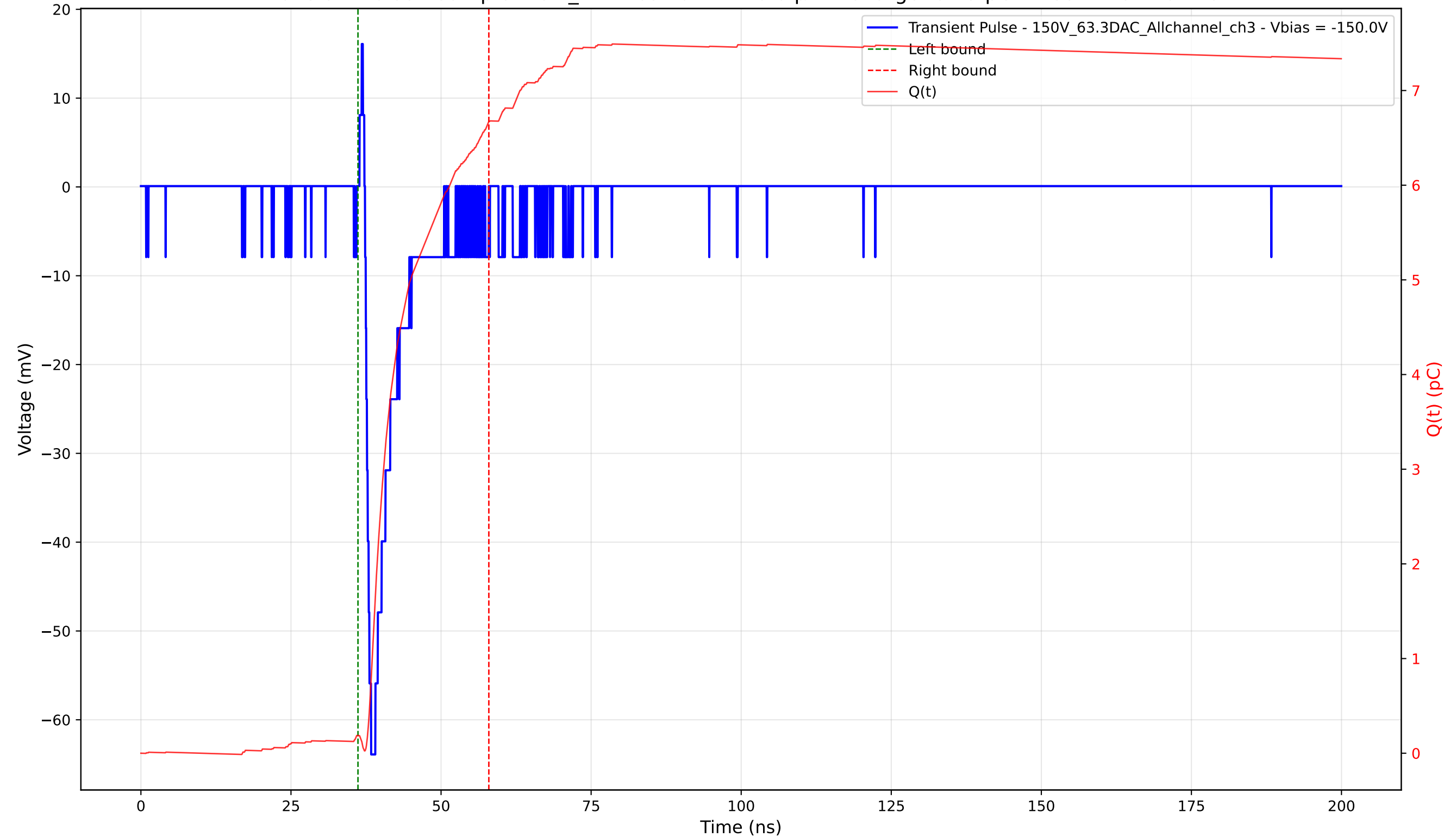
Transient Pulse - Sample: 1cm_42 - Position: 1170.0 \mu\text{m} - Charge: 6.49 pC - Rise Time: 1.01 ns
