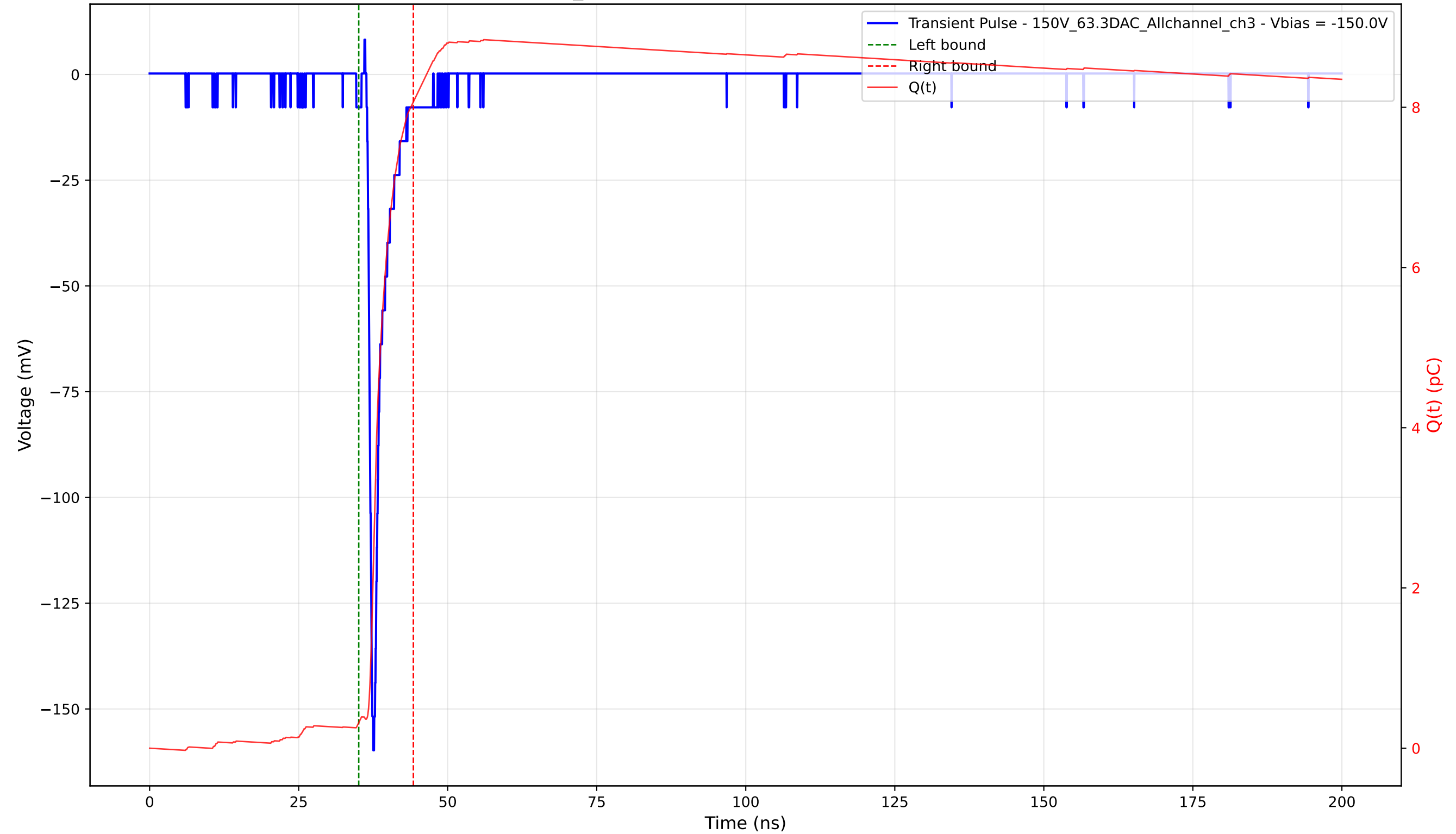
Transient Pulse - Sample: 1cm_42 - Position: 3170.0 \mu\text{m} - Charge: 7.75 pC - Rise Time: 0.80 ns
