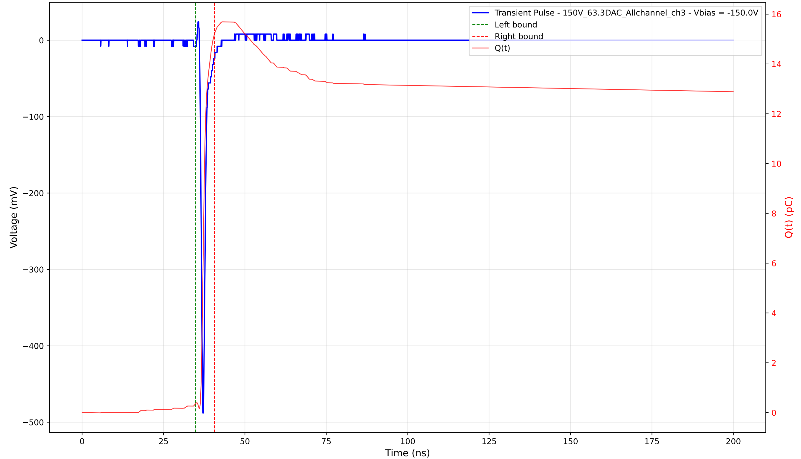
Transient Pulse - Sample: 1cm_42 - Position: 2515.0 \mu\text{m} - Charge: 14.87 pC - Rise Time: 0.67 ns
