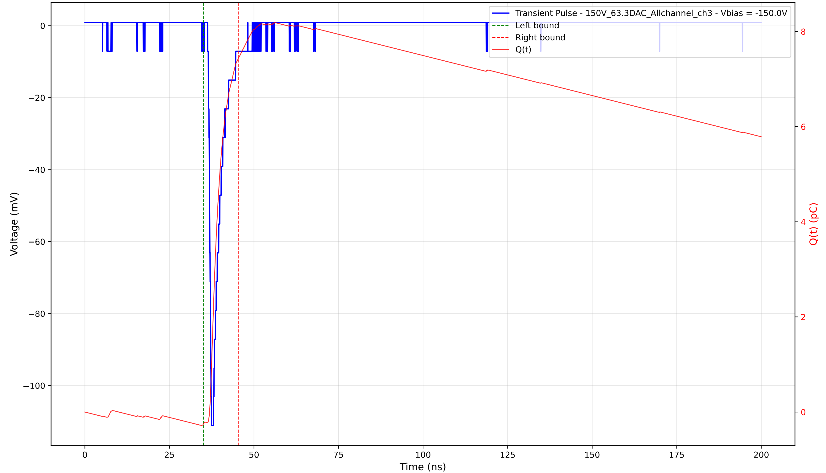
Transient Pulse - Sample: 1cm_42 - Position: 1645.0 \mu\text{m} - Charge: 7.69 pC - Rise Time: 0.82 ns
