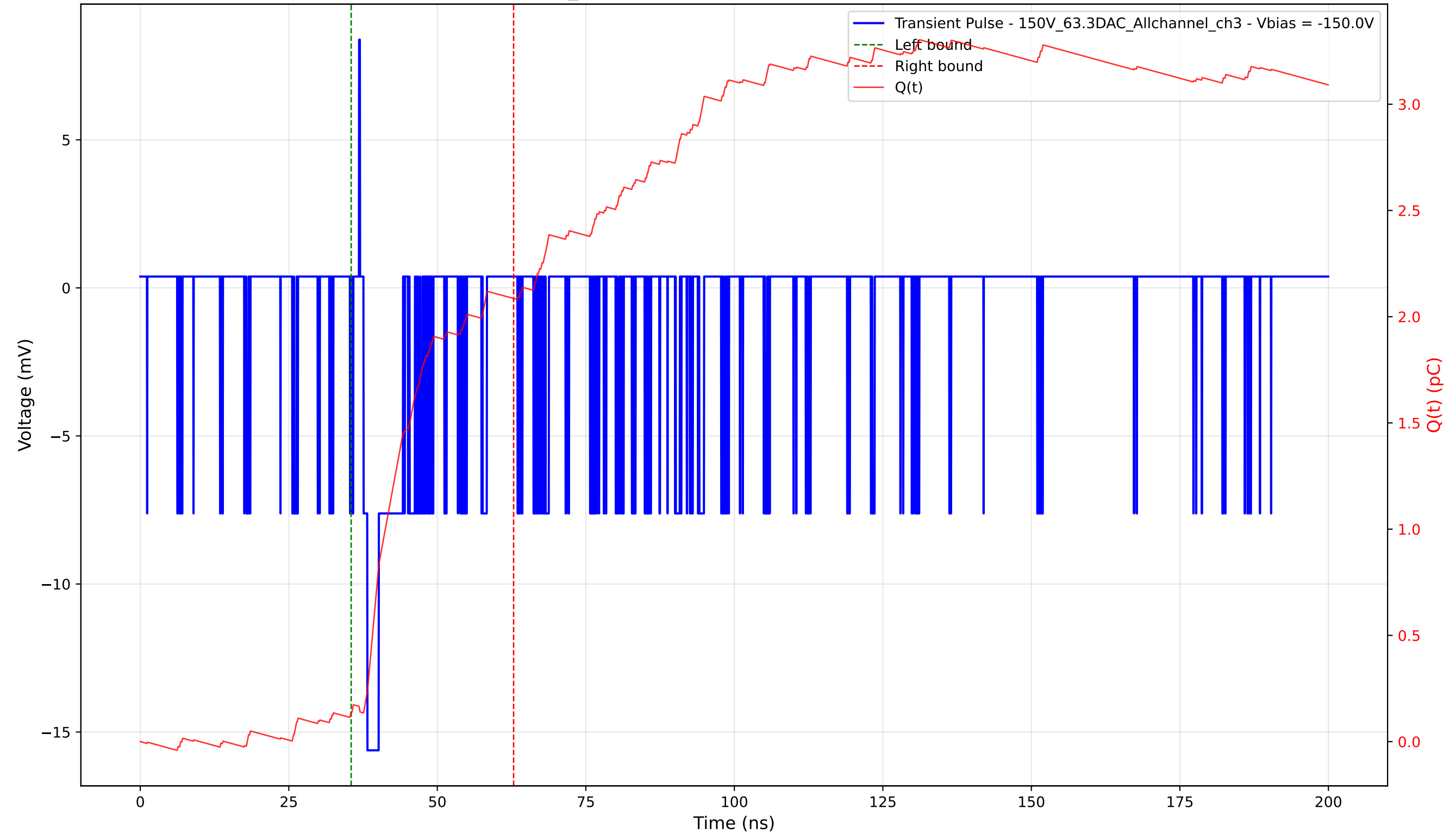
Transient Pulse - Sample: 1cm_42 - Position: 180.0 \mu\text{m} - Charge: 1.95 pC - Rise Time: 0.67 ns
