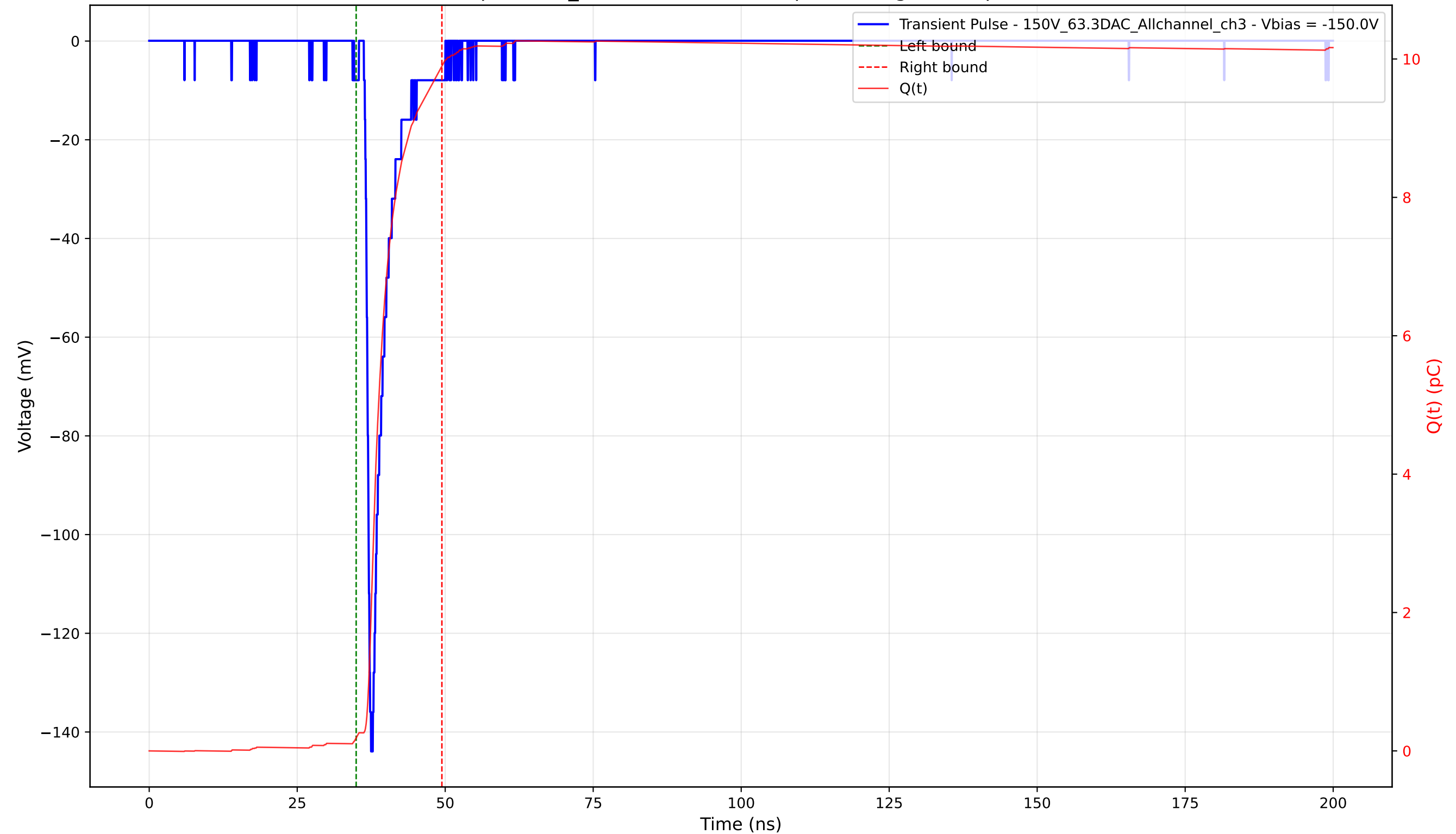
Transient Pulse - Sample: 1cm_42 - Position: 1720.0 \mu\text{m} - Charge: 9.71 pC - Rise Time: 0.89 ns
