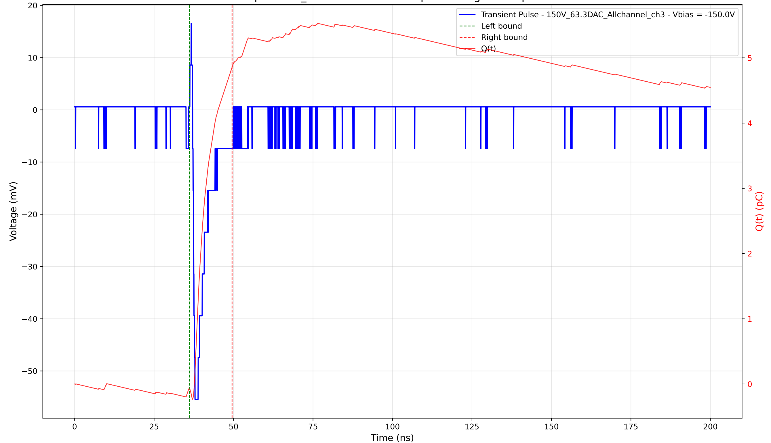
Transient Pulse - Sample: 1cm_42 - Position: 3675.0 \mu\text{m} - Charge: 4.93 pC - Rise Time: 0.73 ns
