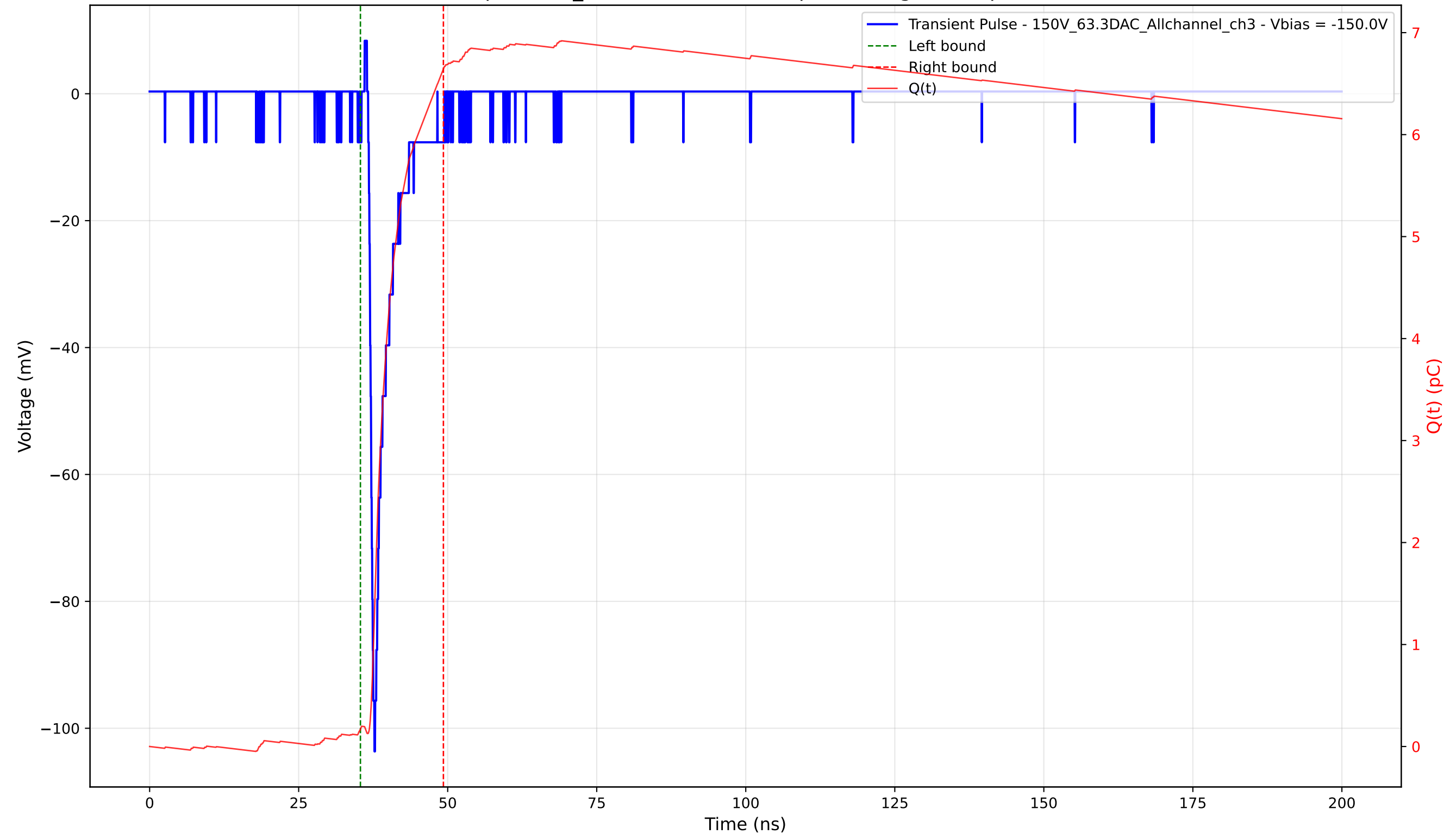
Transient Pulse - Sample: 1cm_42 - Position: 3420.0 \mu\text{m} - Charge: 6.48 pC - Rise Time: 0.75 ns
