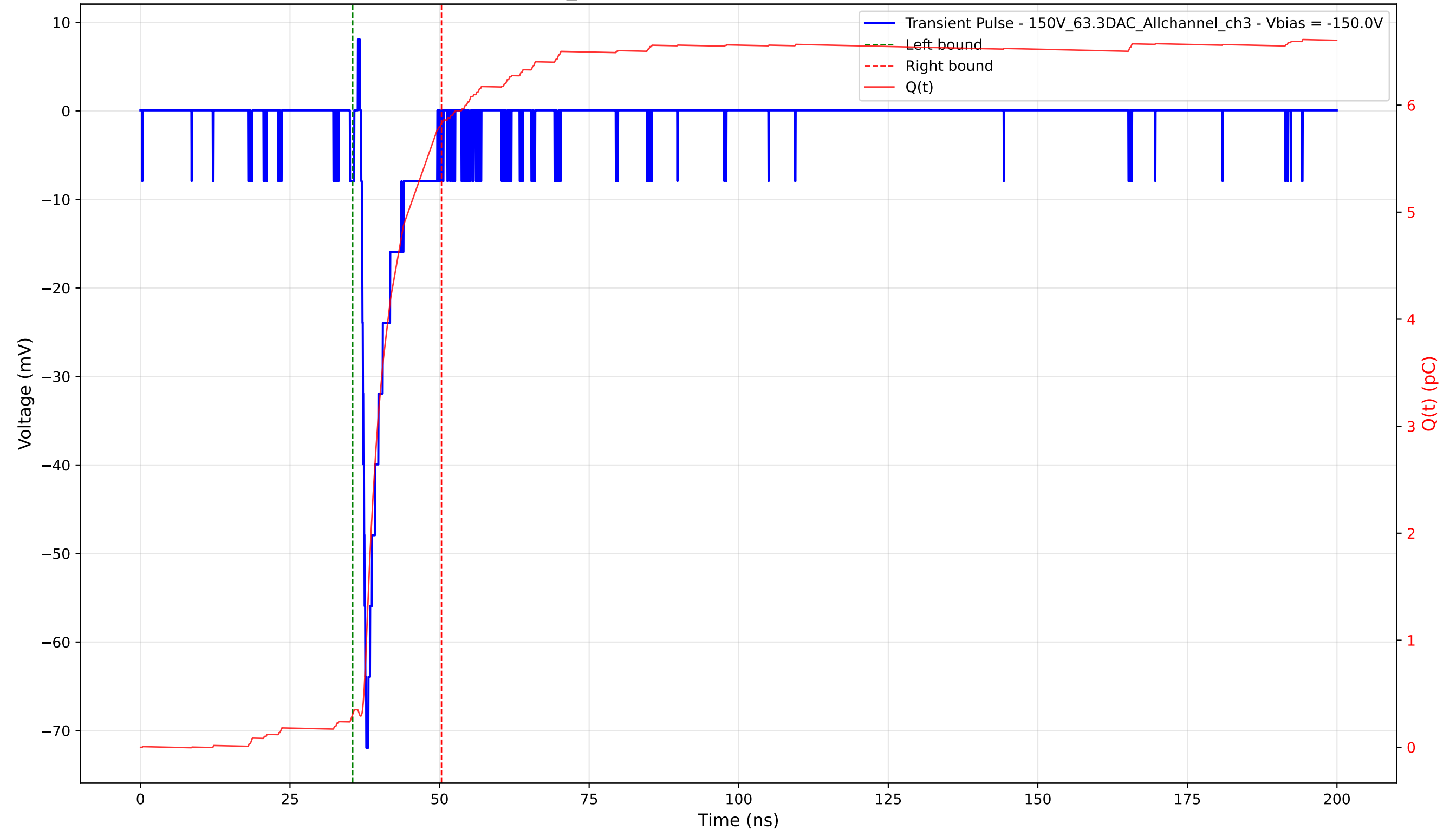
Transient Pulse - Sample: 1cm_42 - Position: 3535.0 \mu\text{m} - Charge: 5.52 pC - Rise Time: 0.84 ns
