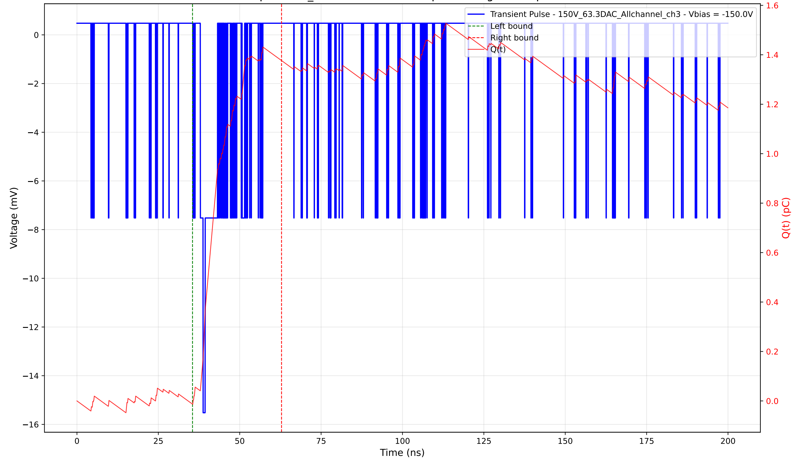
Transient Pulse - Sample: 1cm_42 - Position: 5090.0 \mu\text{m} - Charge: 1.39 pC - Rise Time: 0.87 ns
