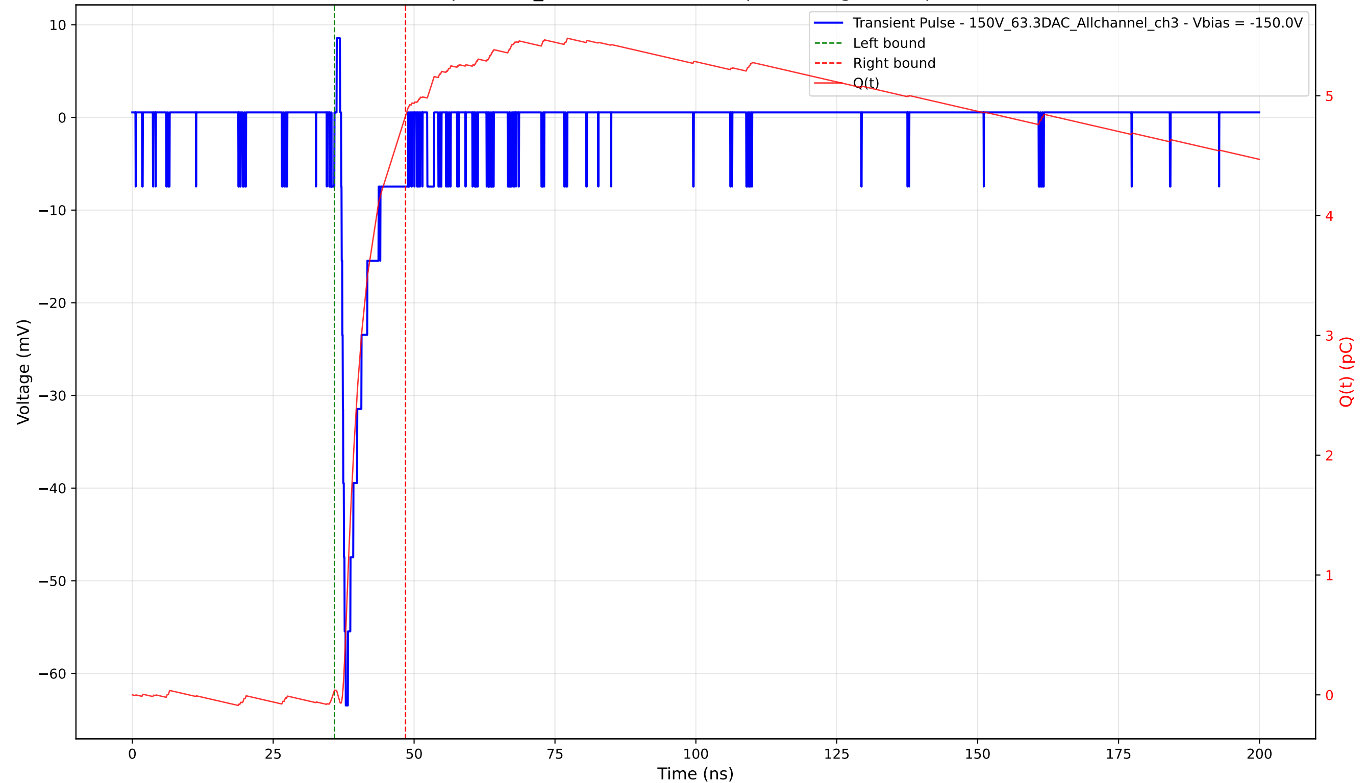
Transient Pulse - Sample: 1cm_42 - Position: 3605.0 \mu\text{m} - Charge: 4.79 pC - Rise Time: 0.81 ns
