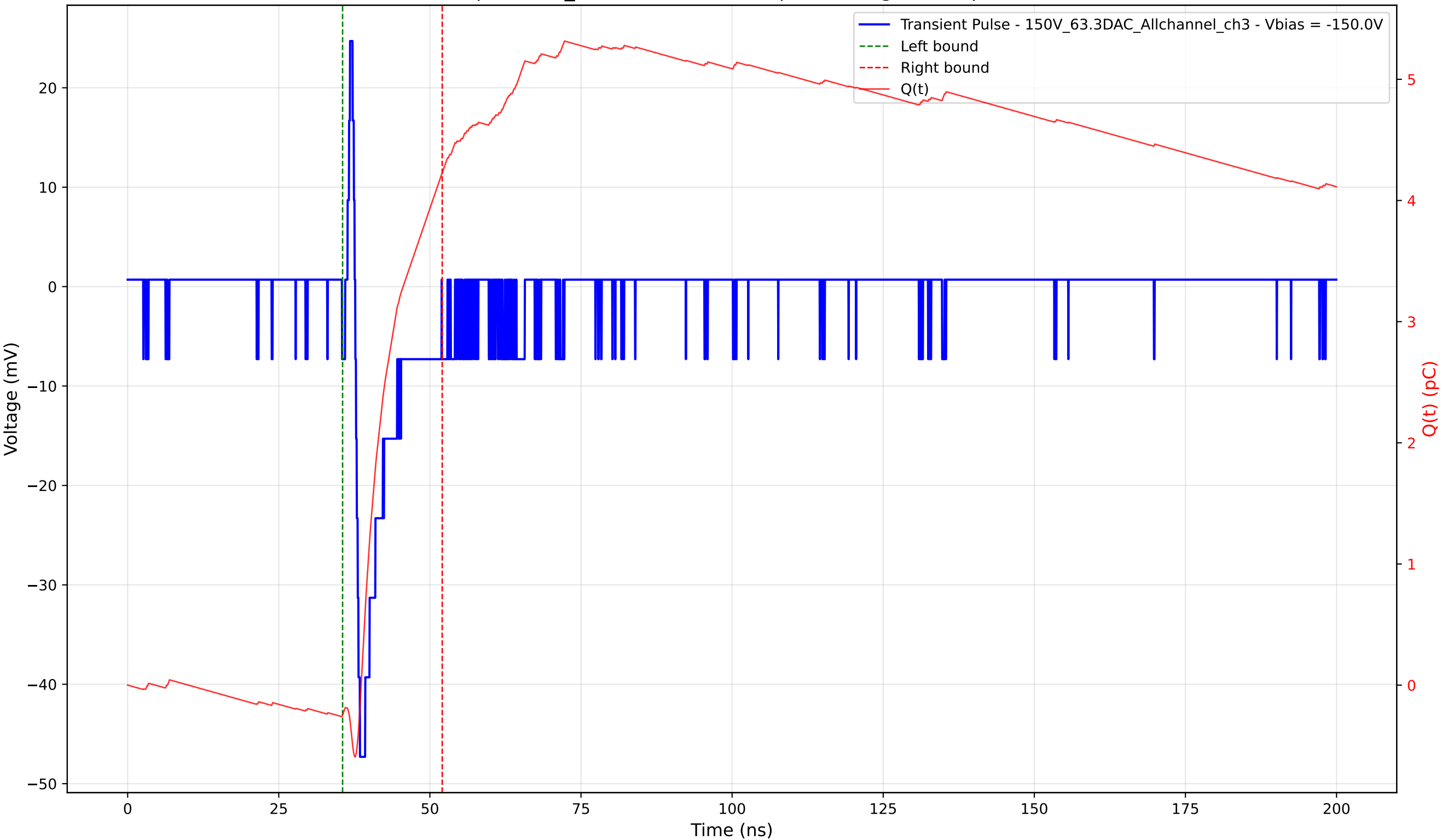
Transient Pulse - Sample: 1cm_42 - Position: 880.0 \mu\text{m} - Charge: 4.47 pC - Rise Time: 0.78 ns
