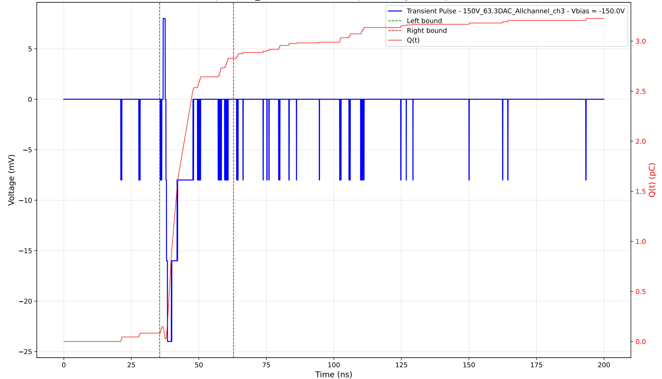
Transient Pulse - Sample: 1cm_42 - Position: 4920.0 \mu\text{m} - Charge: 2.75 pC - Rise Time: 0.59 ns
