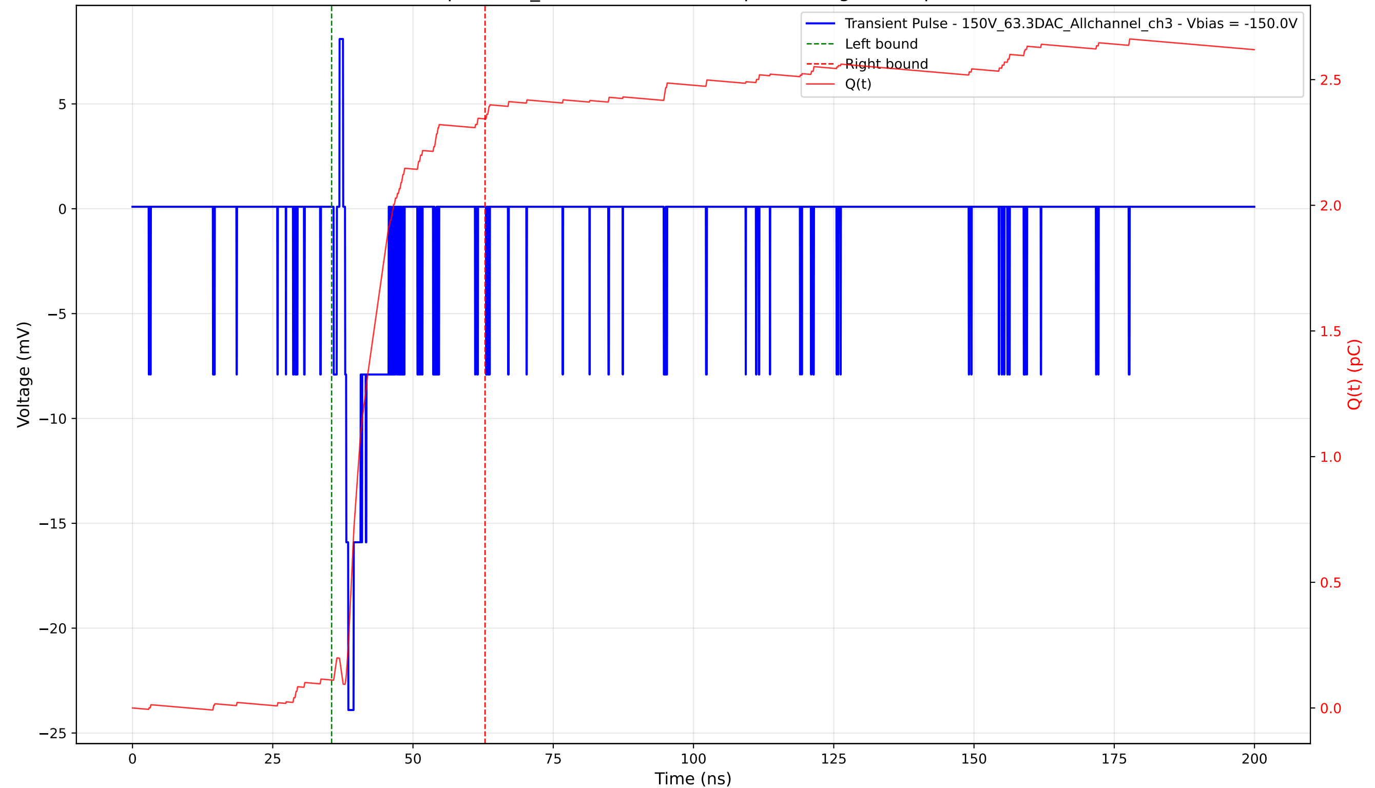
Transient Pulse - Sample: 1cm_42 - Position: 4970.0 \mu\text{m} - Charge: 2.23 pC - Rise Time: 0.59 ns
