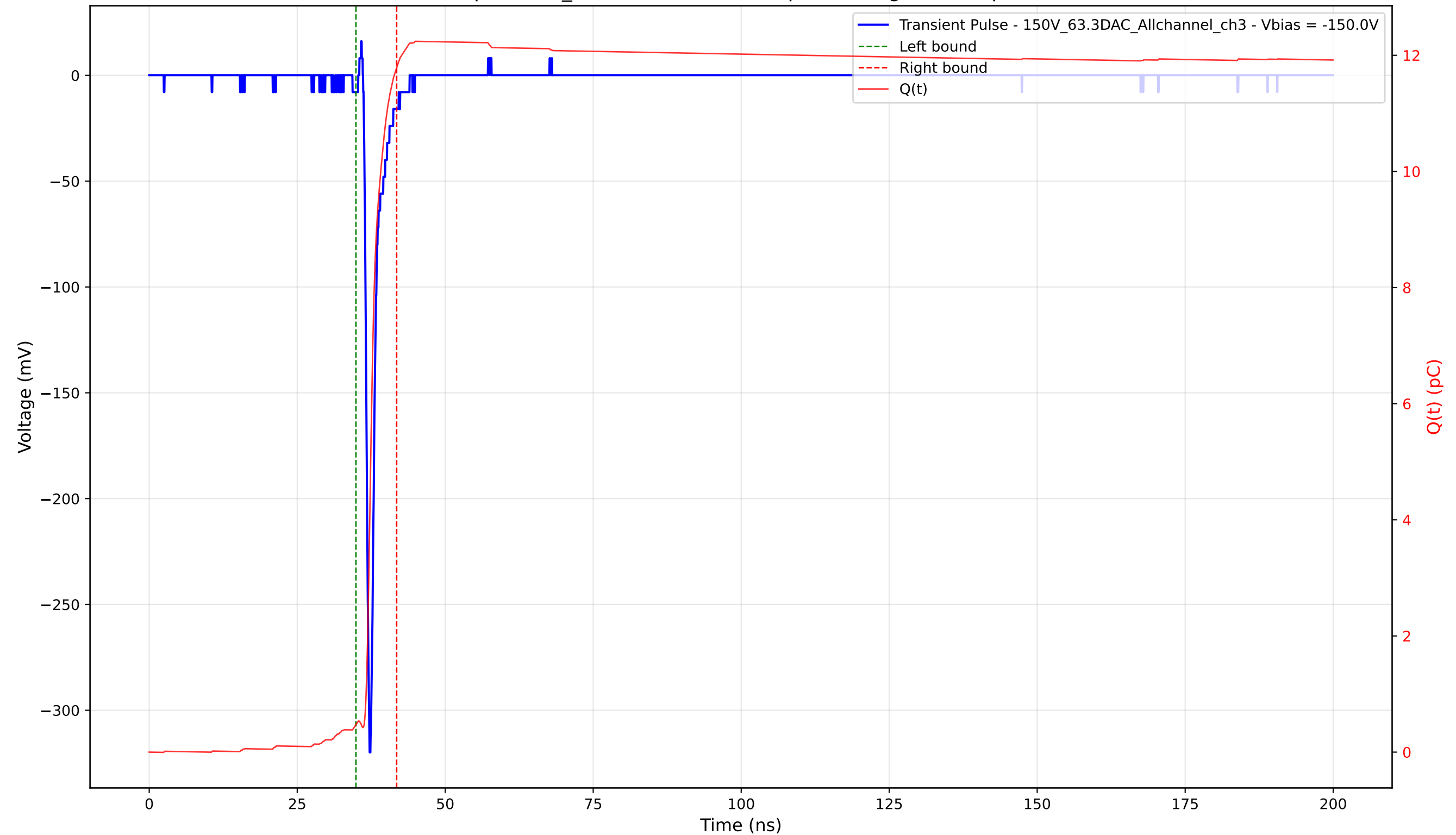
Transient Pulse - Sample: 1cm_42 - Position: 2920.0 \mu\text{m} - Charge: 11.31 pC - Rise Time: 0.76 ns
