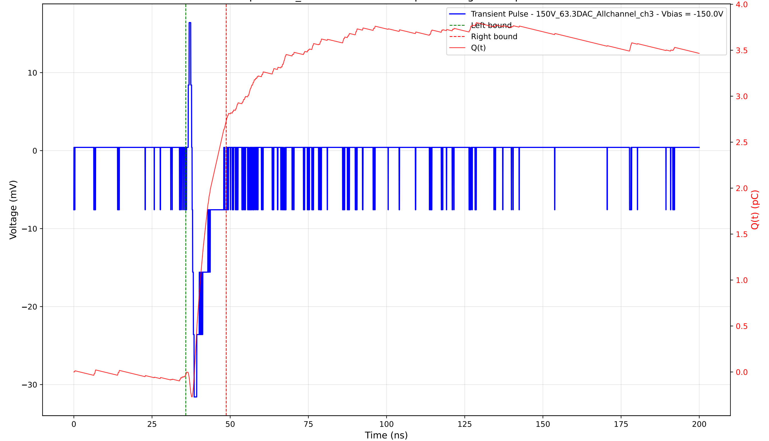
Transient Pulse - Sample: 1cm_42 - Position: 4660.0 \mu\text{m} - Charge: 2.76 pC - Rise Time: 0.66 ns
