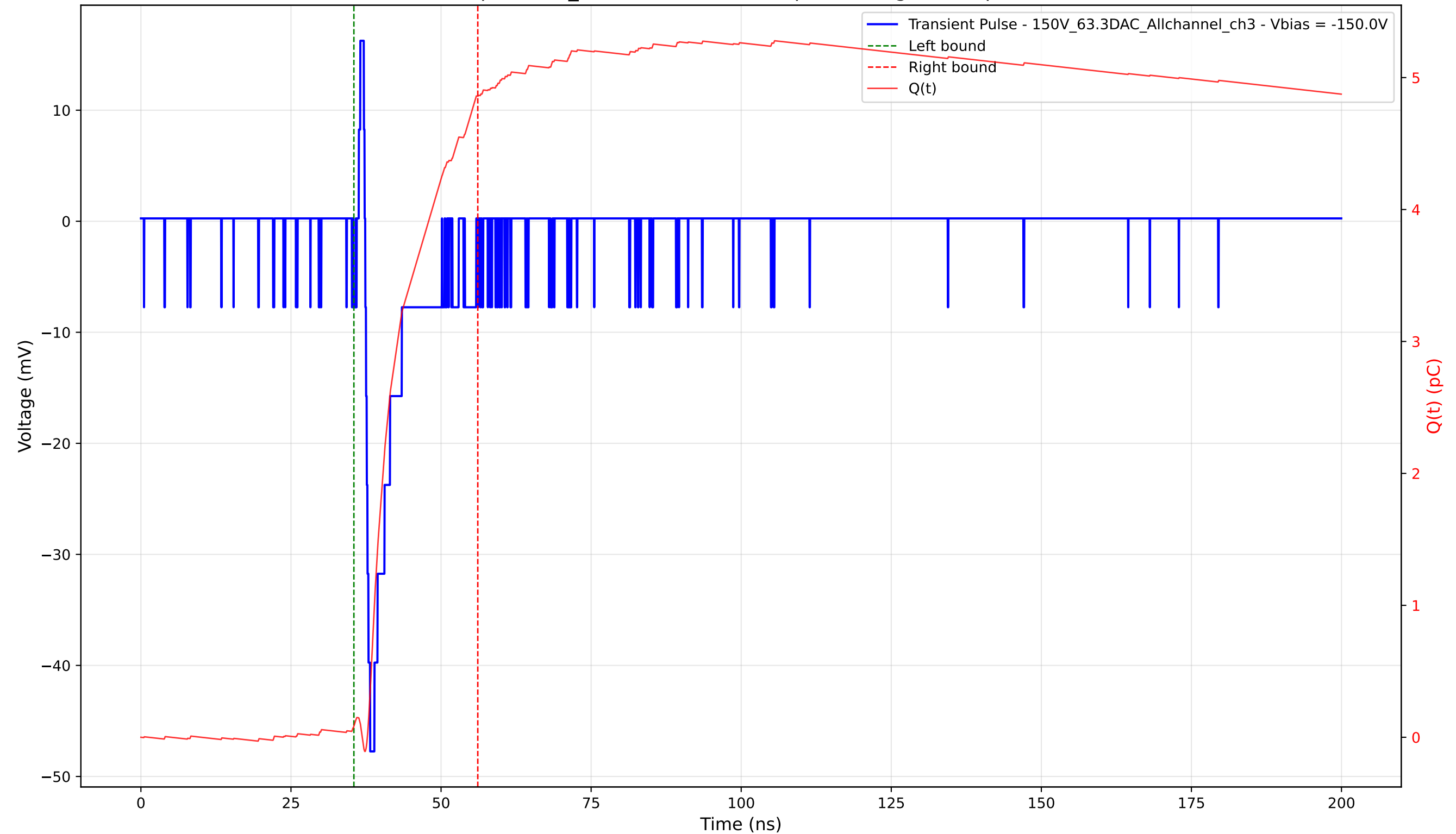
Transient Pulse - Sample: 1cm_42 - Position: 3910.0 \mu\text{m} - Charge: 4.77 pC - Rise Time: 0.82 ns
