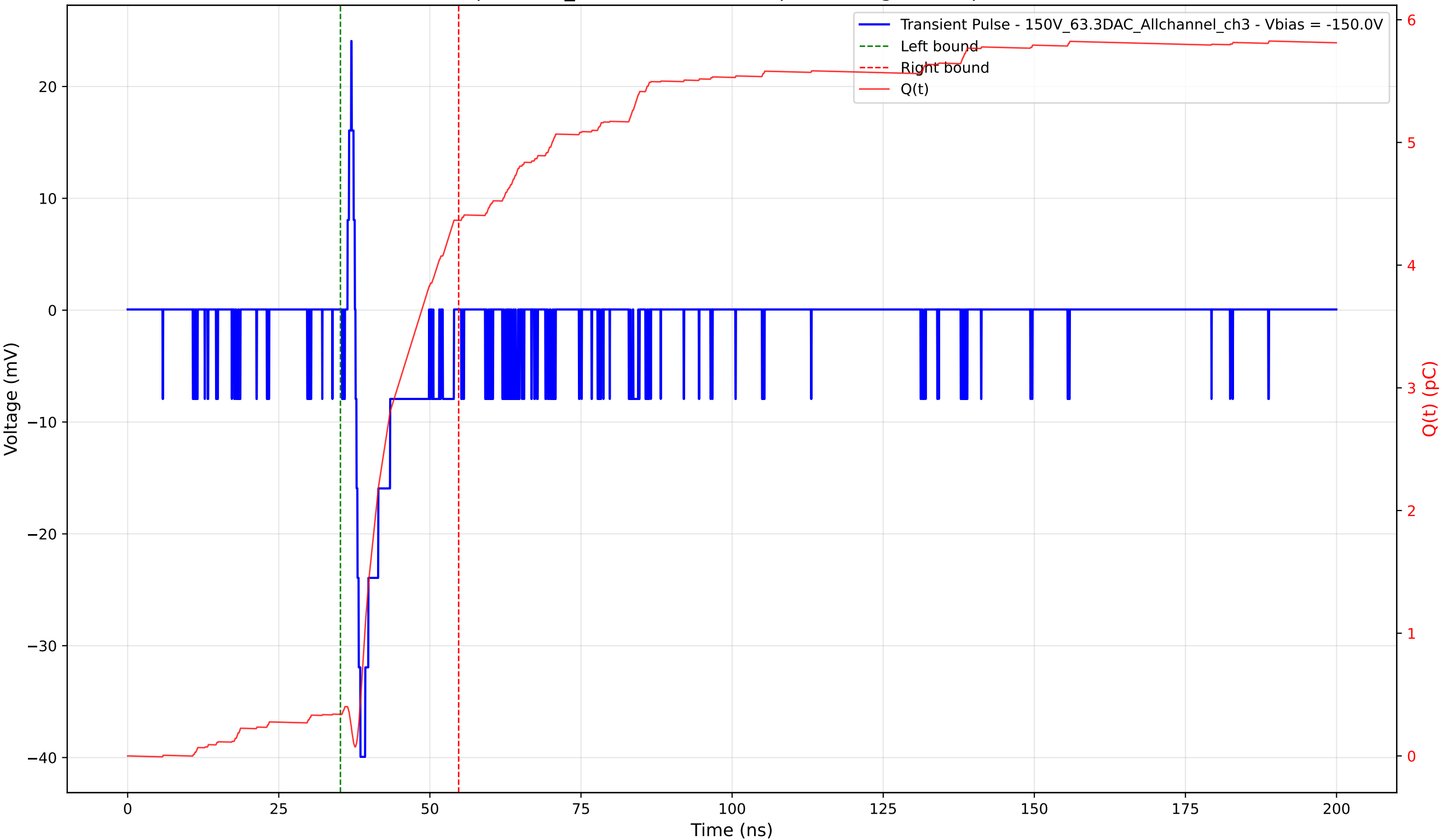
Transient Pulse - Sample: 1cm_42 - Position: 535.0 \mu\text{m} - Charge: 4.03 pC - Rise Time: 0.82 ns
