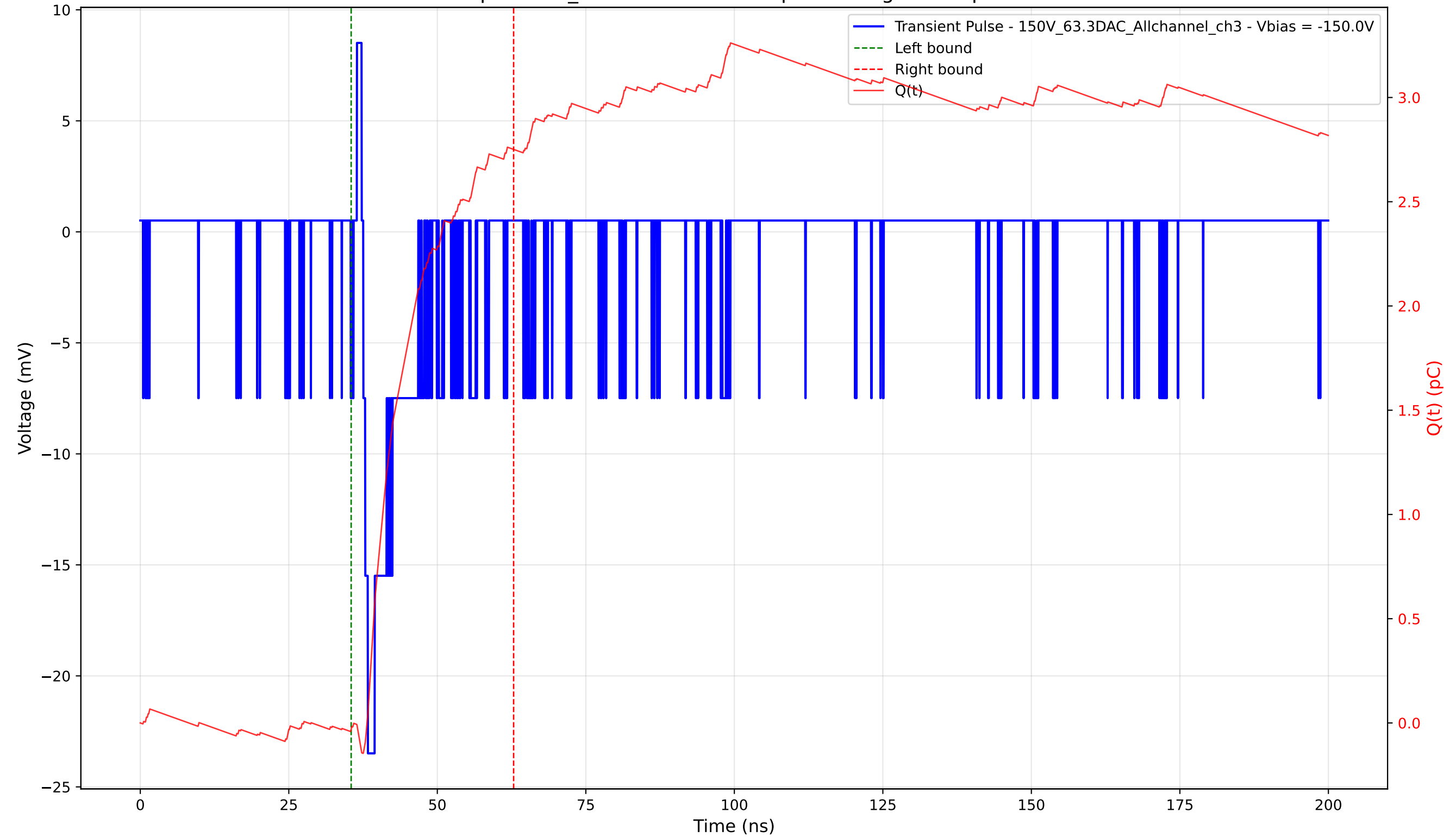
Transient Pulse - Sample: 1cm_42 - Position: 290.0 \mu\text{m} - Charge: 2.78 pC - Rise Time: 0.79 ns
