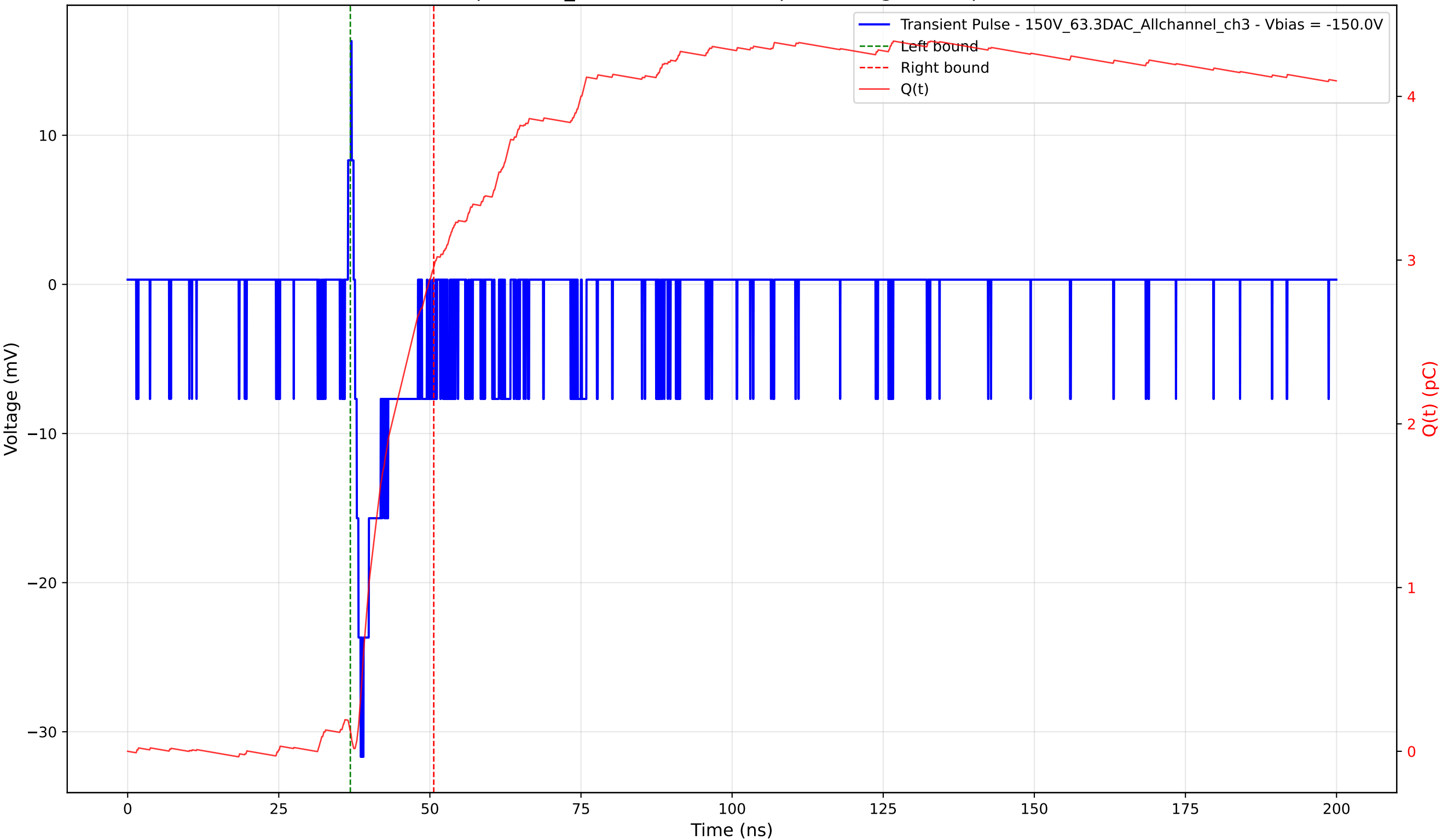
Transient Pulse - Sample: 1cm_42 - Position: 365.0 \mu\text{m} - Charge: 2.83 pC - Rise Time: 0.94 ns
