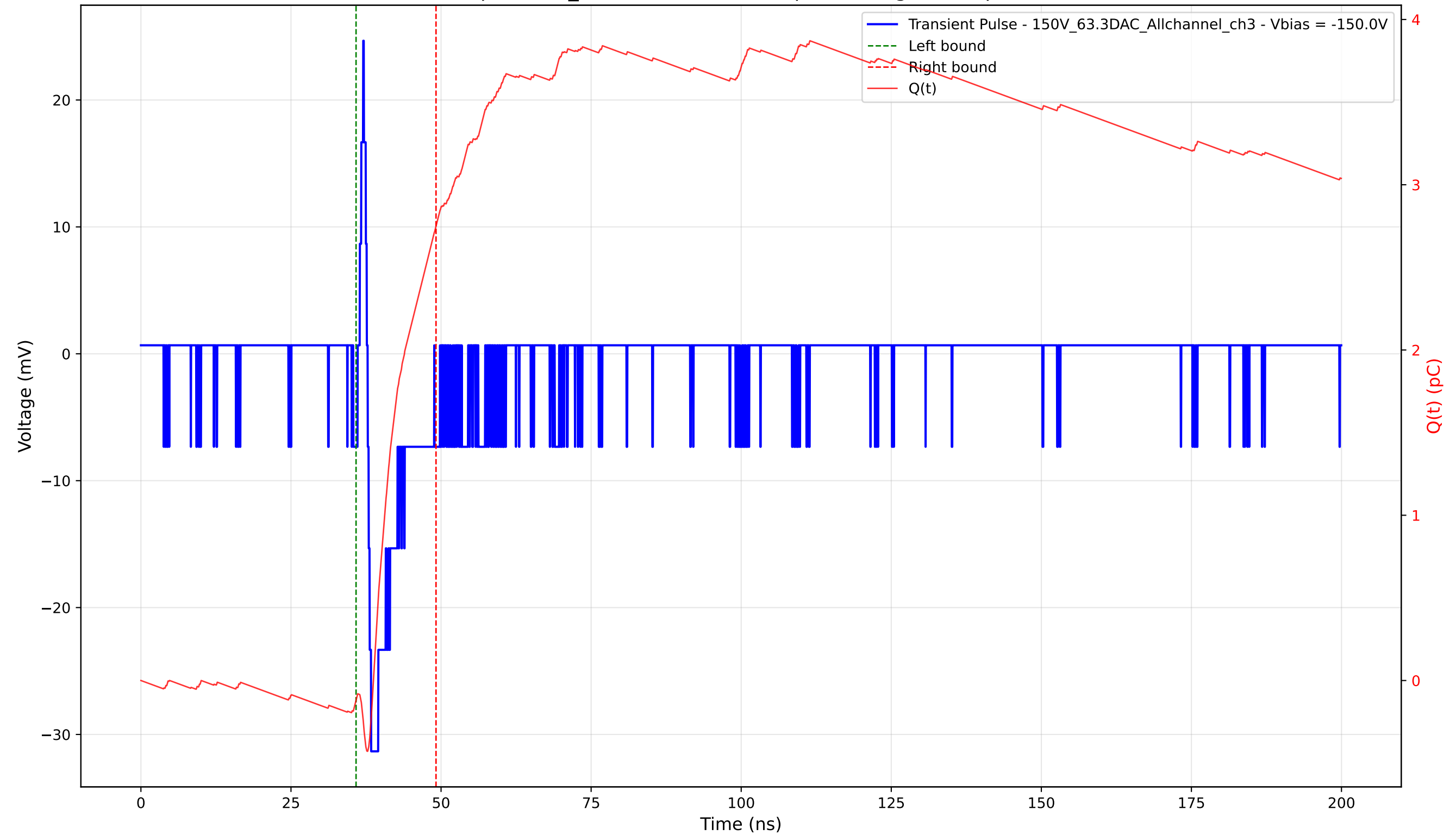
Transient Pulse - Sample: 1cm_42 - Position: 4415.0 \mu\text{m} - Charge: 2.87 pC - Rise Time: 0.59 ns
