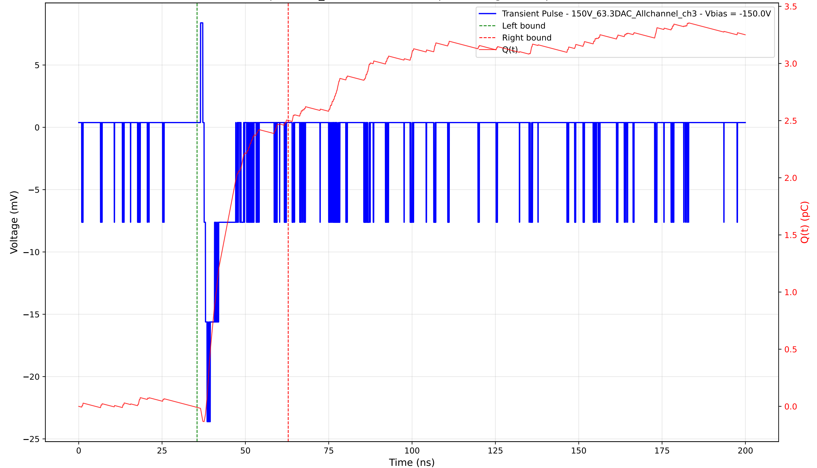
Transient Pulse - Sample: 1cm_42 - Position: 220.0 \mu\text{m} - Charge: 2.51 pC - Rise Time: 0.91 ns
