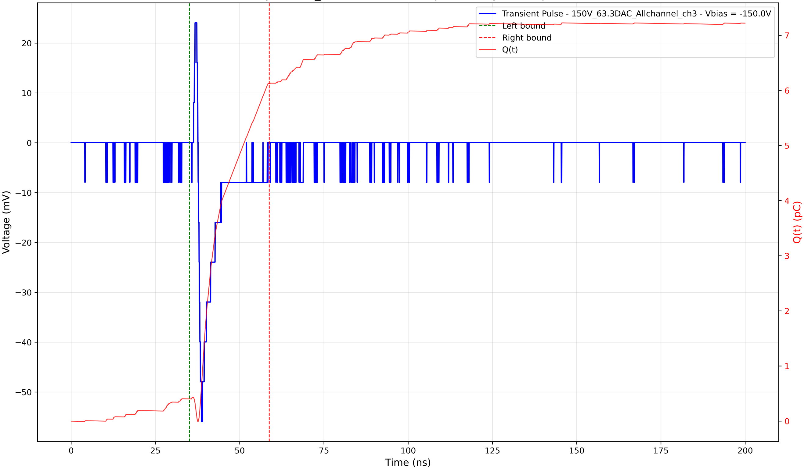
Transient Pulse - Sample: 1cm_42 - Position: 800.0 \mu\text{m} - Charge: 5.72 pC - Rise Time: 1.01 ns
