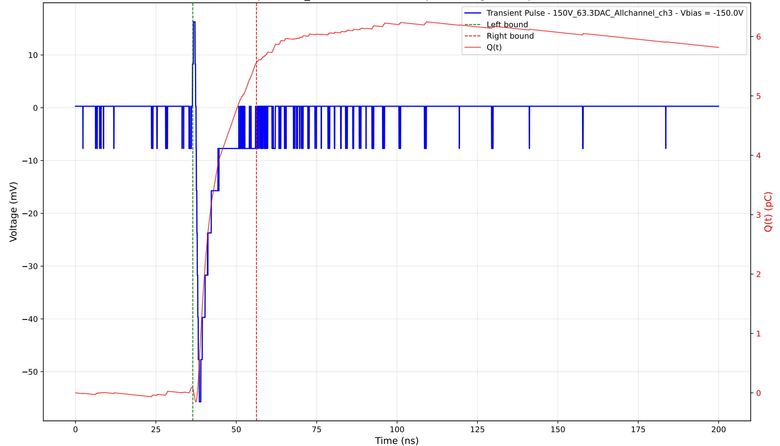
Transient Pulse - Sample: 1cm_42 - Position: 1065.0 \mu\text{m} - Charge: 5.49 pC - Rise Time: 1.01 ns
