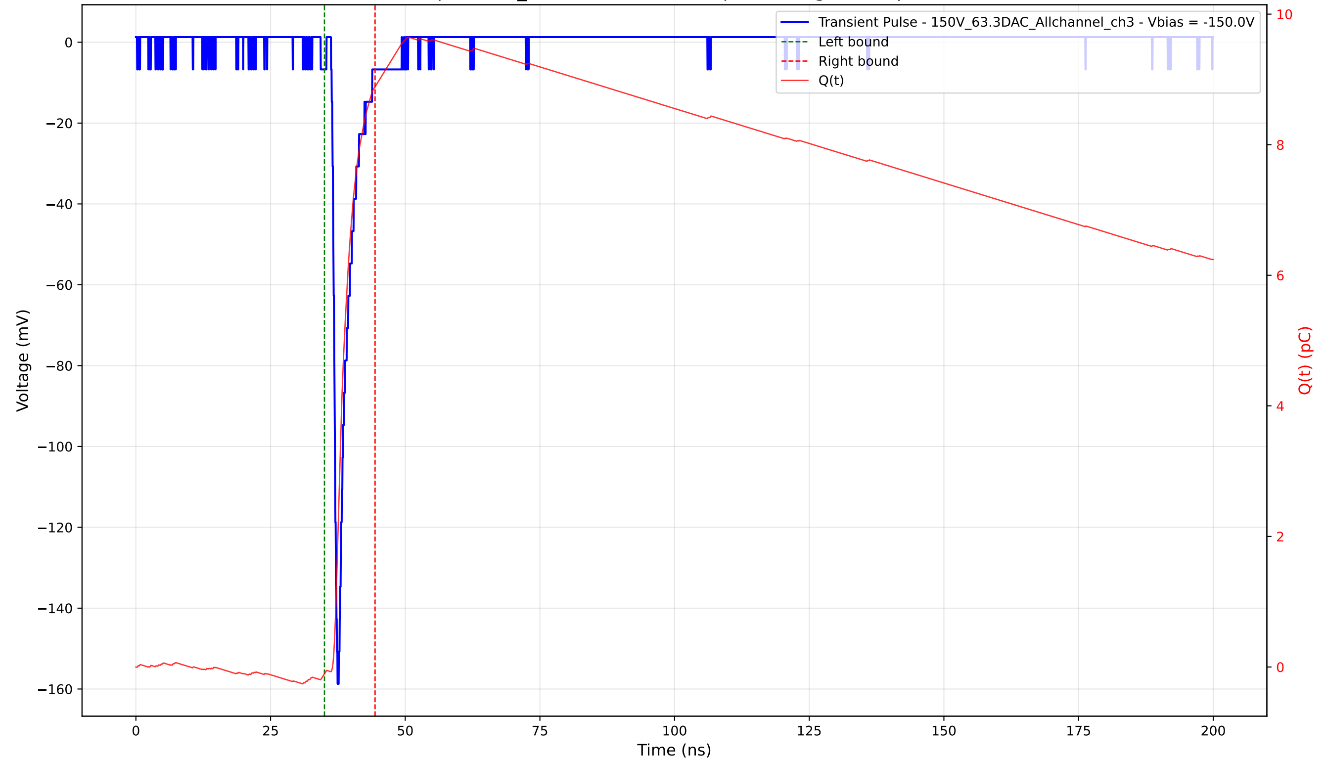
Transient Pulse - Sample: 1cm_42 - Position: 1825.0 \mu\text{m} - Charge: 8.99 pC - Rise Time: 0.87 ns
