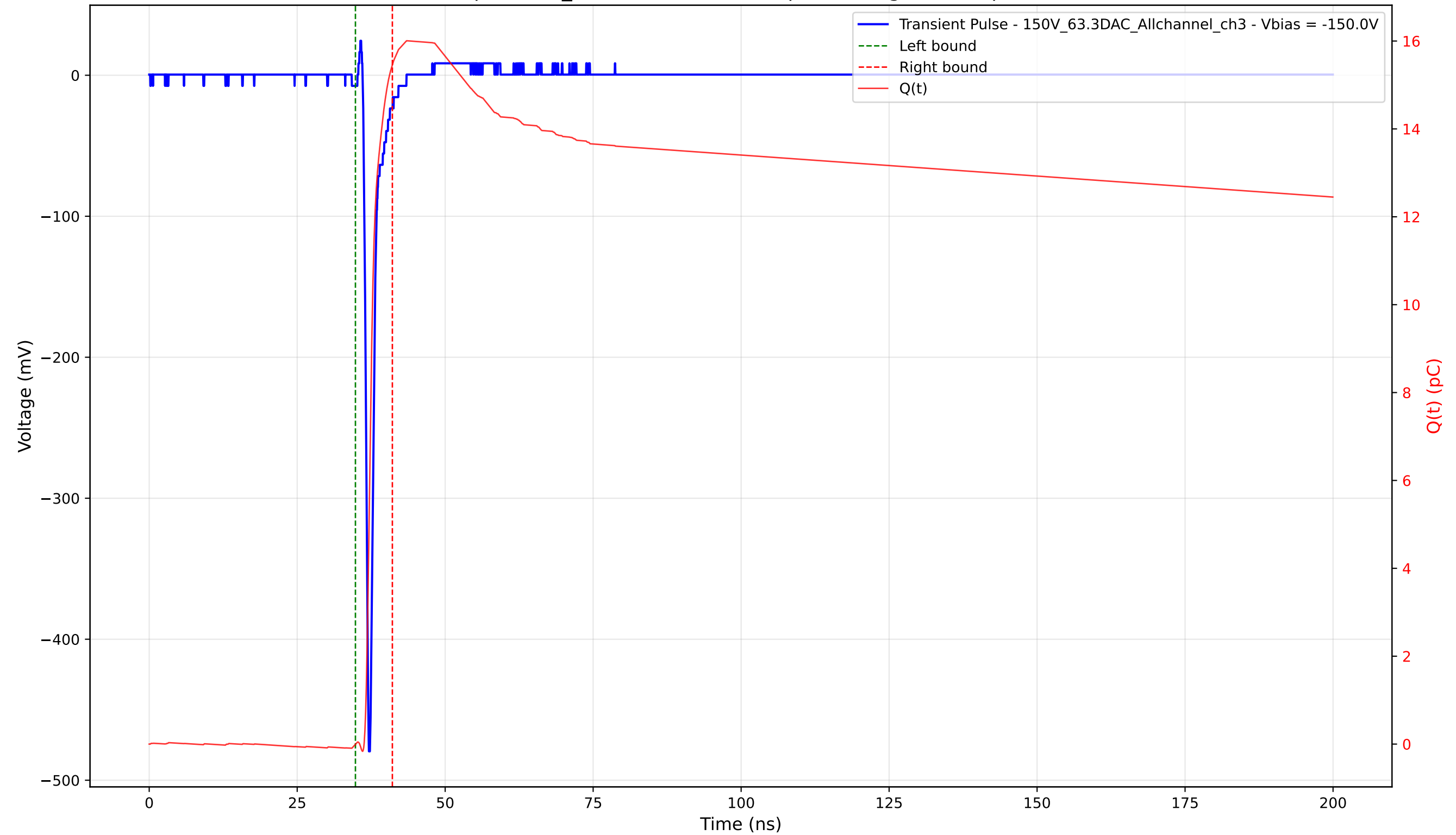
Transient Pulse - Sample: 1cm_42 - Position: 2720.0 \mu\text{m} - Charge: 15.47 pC - Rise Time: 0.68 ns
