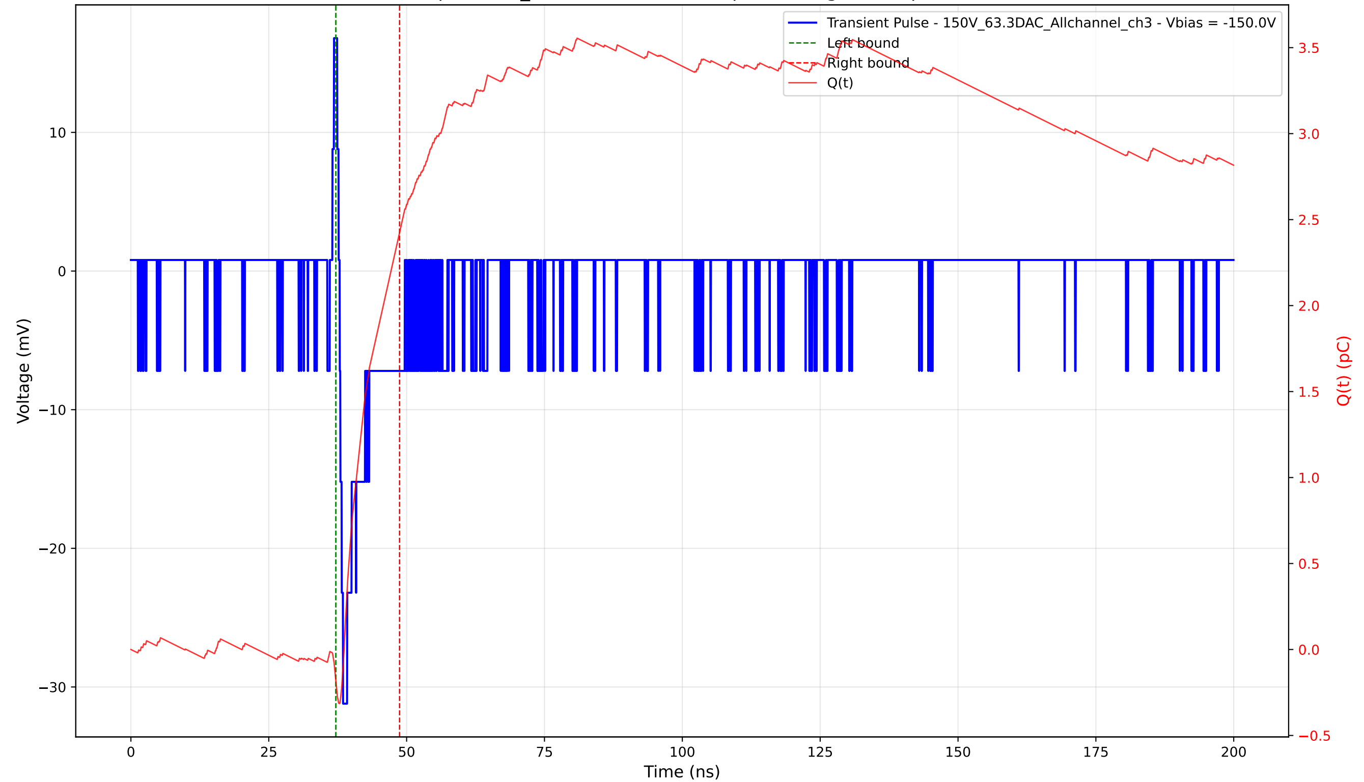
Transient Pulse - Sample: 1cm_42 - Position: 4525.0 \mu\text{m} - Charge: 2.61 pC - Rise Time: 0.63 ns
