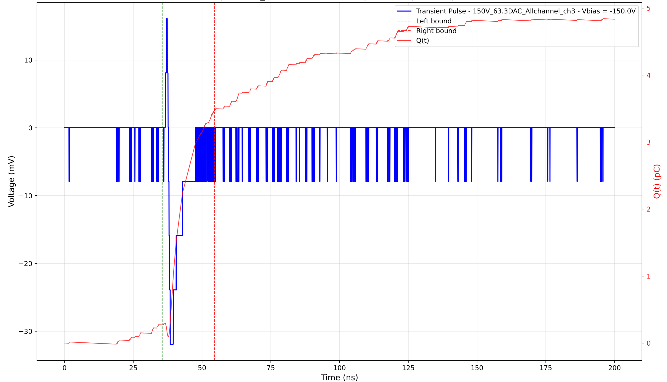
Transient Pulse - Sample: 1cm_42 - Position: 4760.0 \mu\text{m} - Charge: 3.19 pC - Rise Time: 0.62 ns
