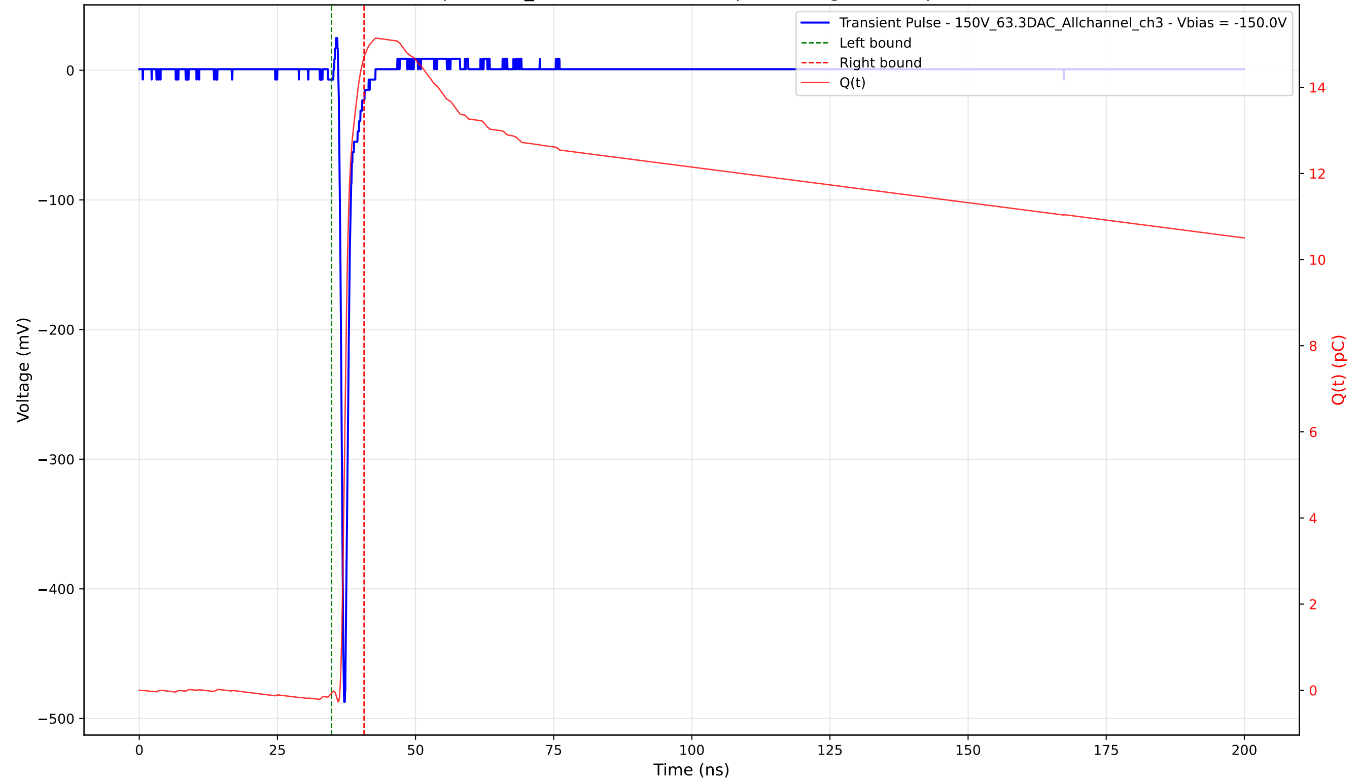
Transient Pulse - Sample: 1cm_42 - Position: 2530.0 \mu\text{m} - Charge: 14.76 pC - Rise Time: 0.67 ns
