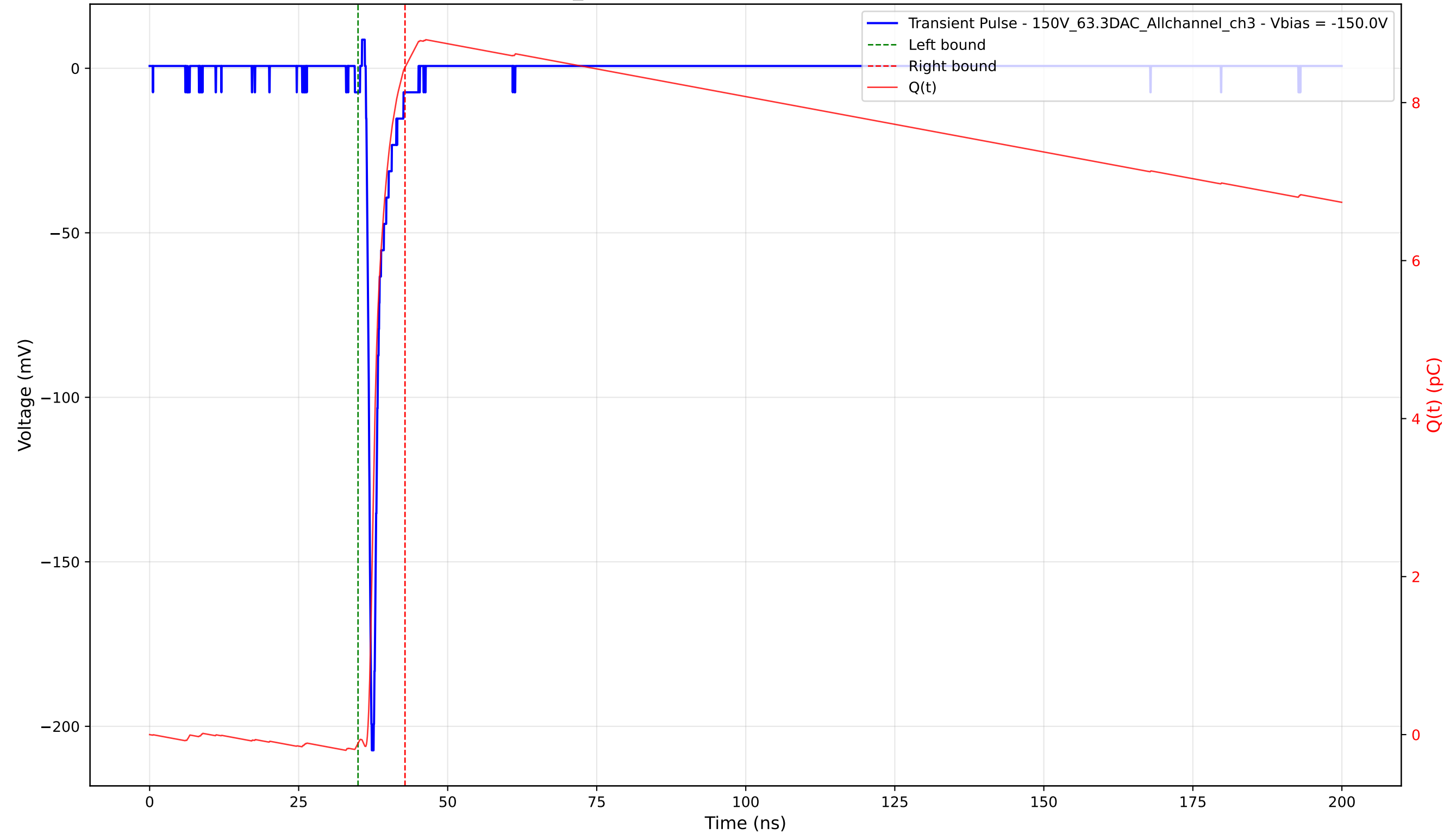
Transient Pulse - Sample: 1cm_42 - Position: 3035.0 \mu\text{m} - Charge: 8.56 pC - Rise Time: 0.75 ns
