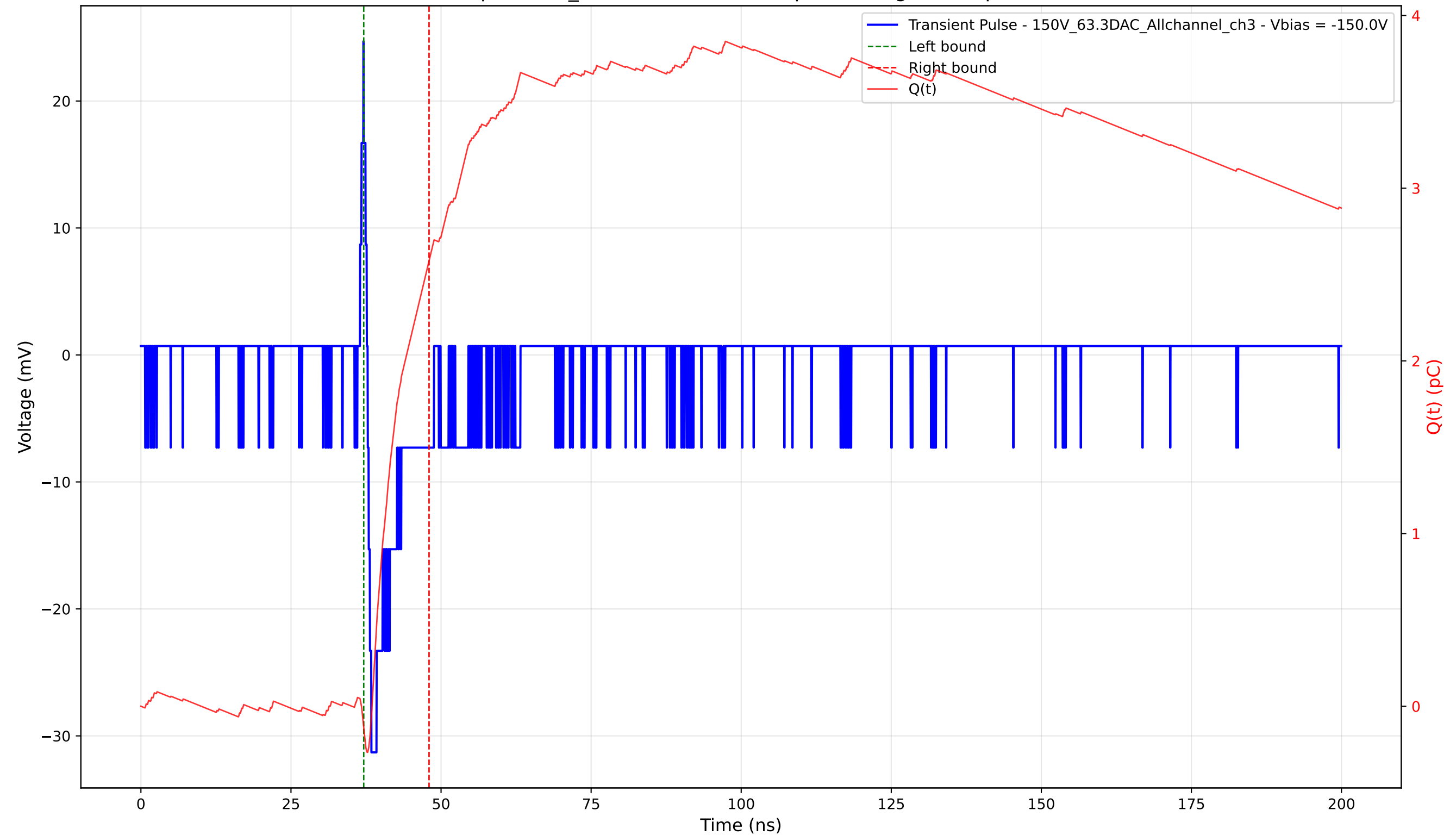
Transient Pulse - Sample: 1cm_42 - Position: 4475.0 \mu\text{m} - Charge: 2.71 pC - Rise Time: 0.63 ns
