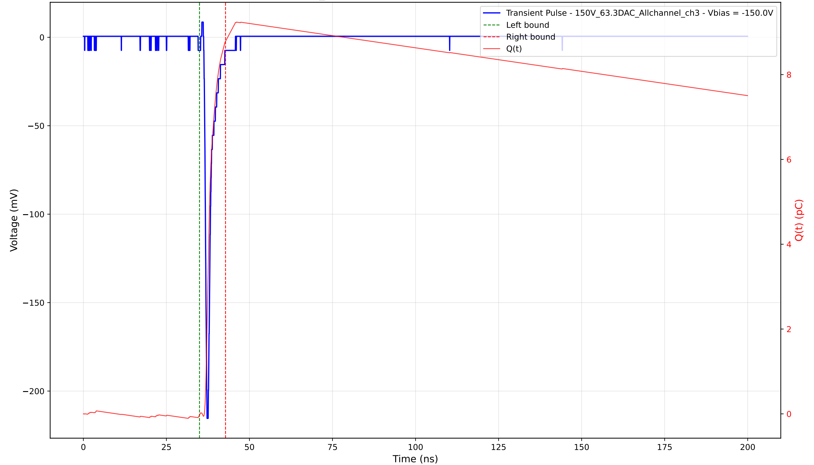
Transient Pulse - Sample: 1cm_42 - Position: 3020.0 \mu\text{m} - Charge: 8.81 pC - Rise Time: 0.77 ns
