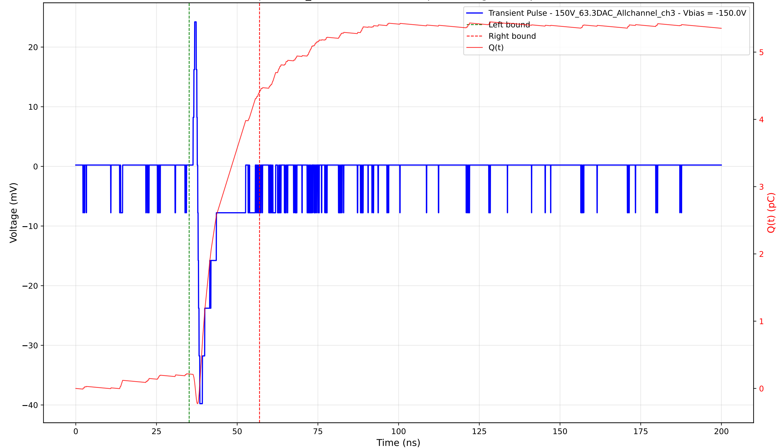
Transient Pulse - Sample: 1cm_42 - Position: 4325.0 \mu\text{m} - Charge: 4.20 pC - Rise Time: 0.66 ns
