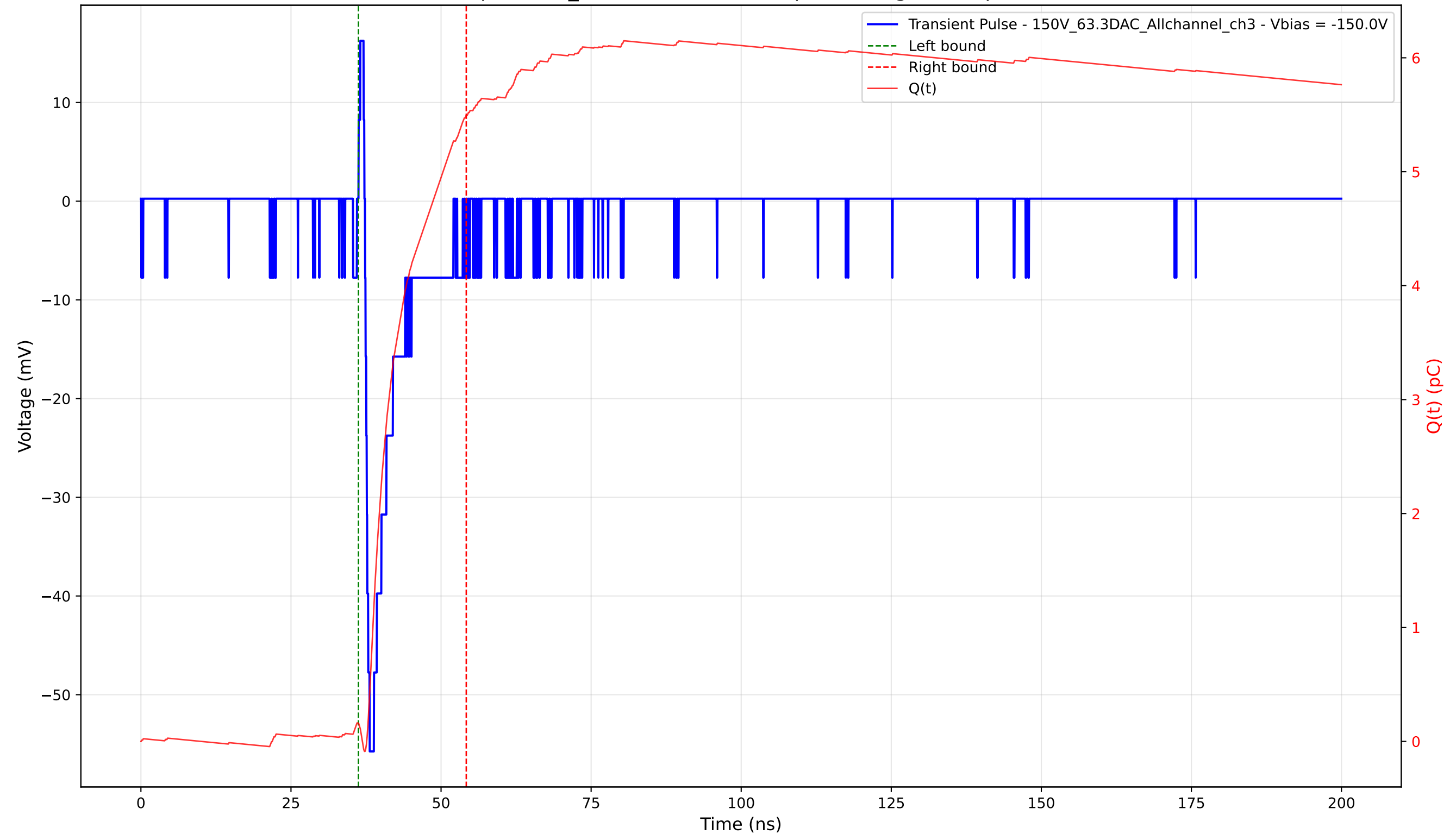
Transient Pulse - Sample: 1cm_42 - Position: 3810.0 \mu\text{m} - Charge: 5.34 pC - Rise Time: 0.77 ns
