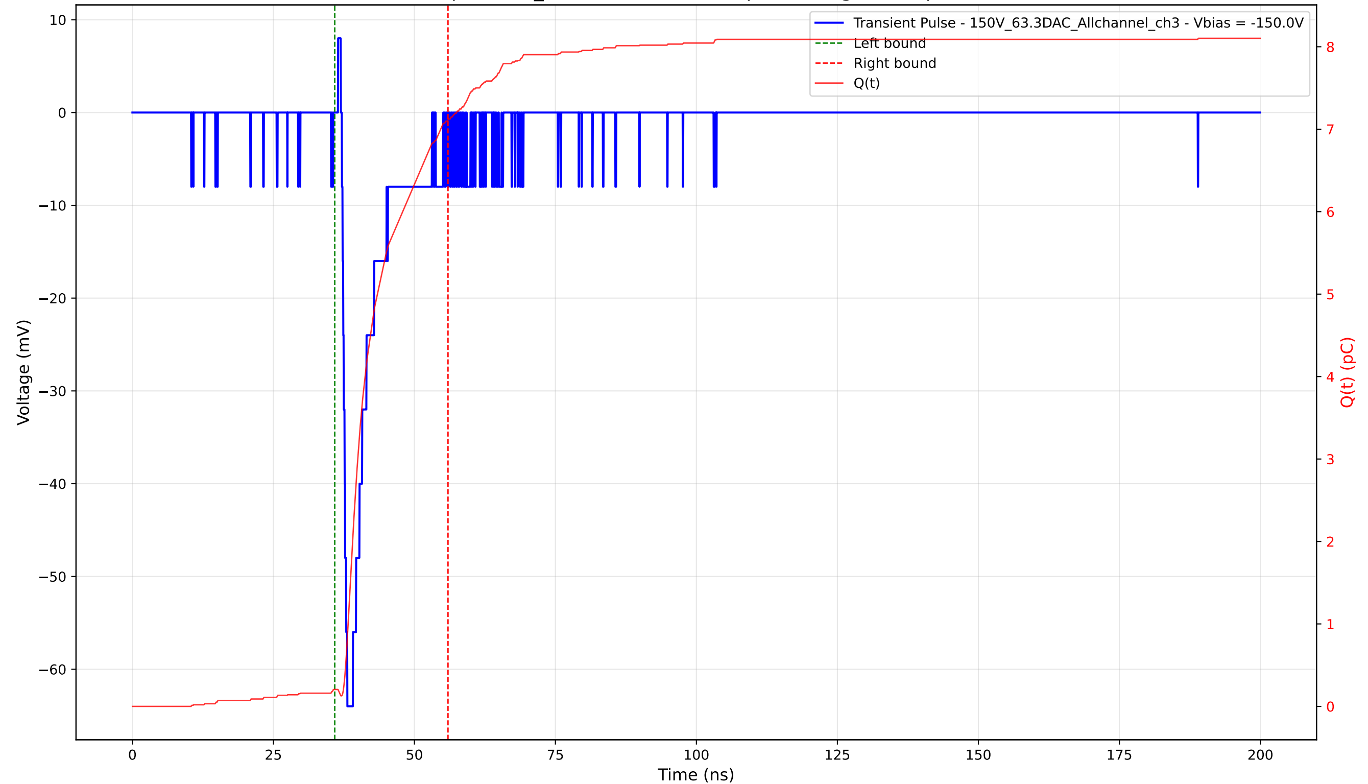
Transient Pulse - Sample: 1cm_42 - Position: 1335.0 \mu\text{m} - Charge: 6.91 pC - Rise Time: 0.97 ns
