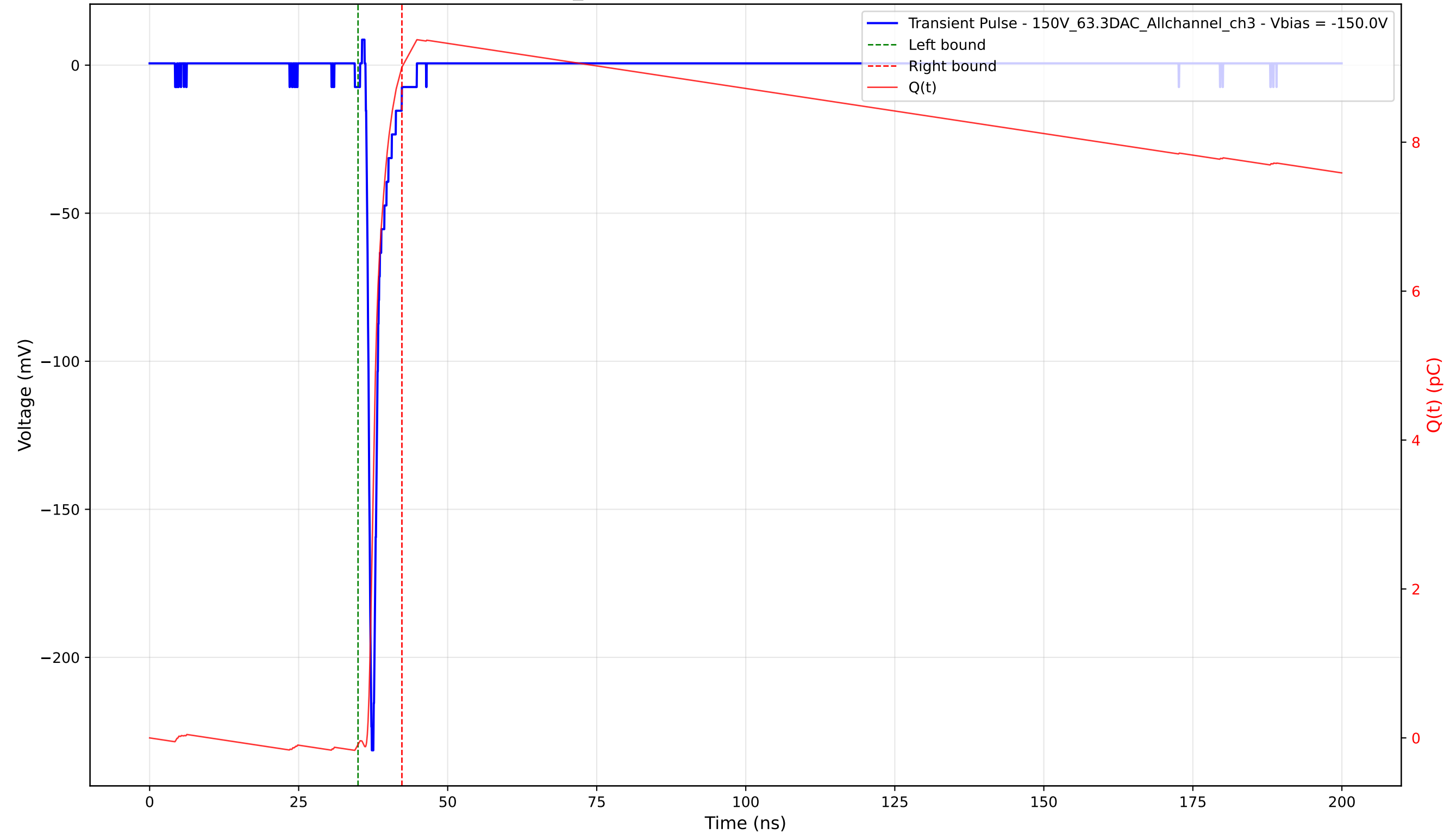
Transient Pulse - Sample: 1cm_42 - Position: 3005.0 \mu\text{m} - Charge: 9.09 pC - Rise Time: 0.77 ns
