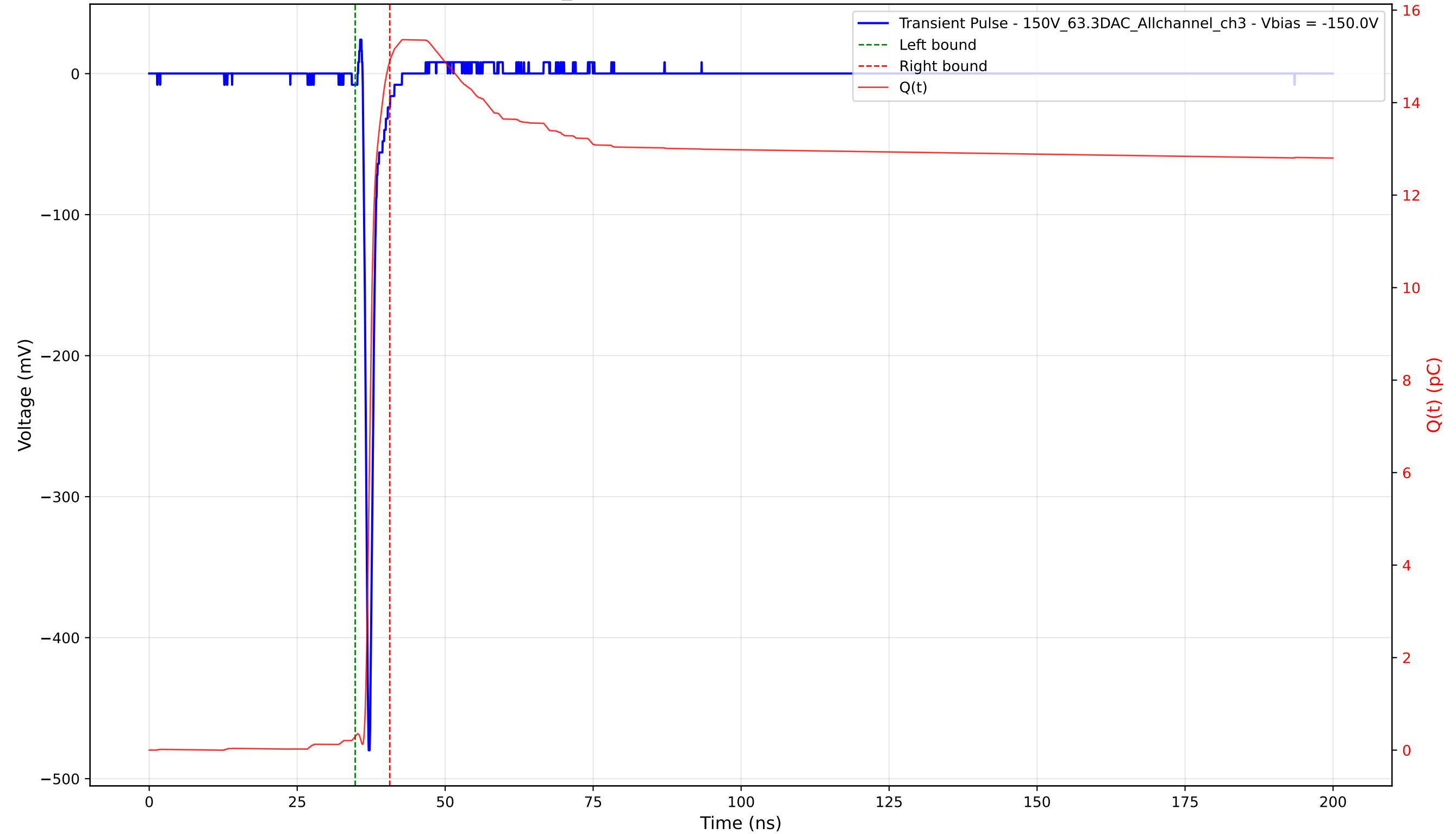
Transient Pulse - Sample: 1cm_42 - Position: 2545.0 \mu\text{m} - Charge: 14.61 pC - Rise Time: 0.72 ns
