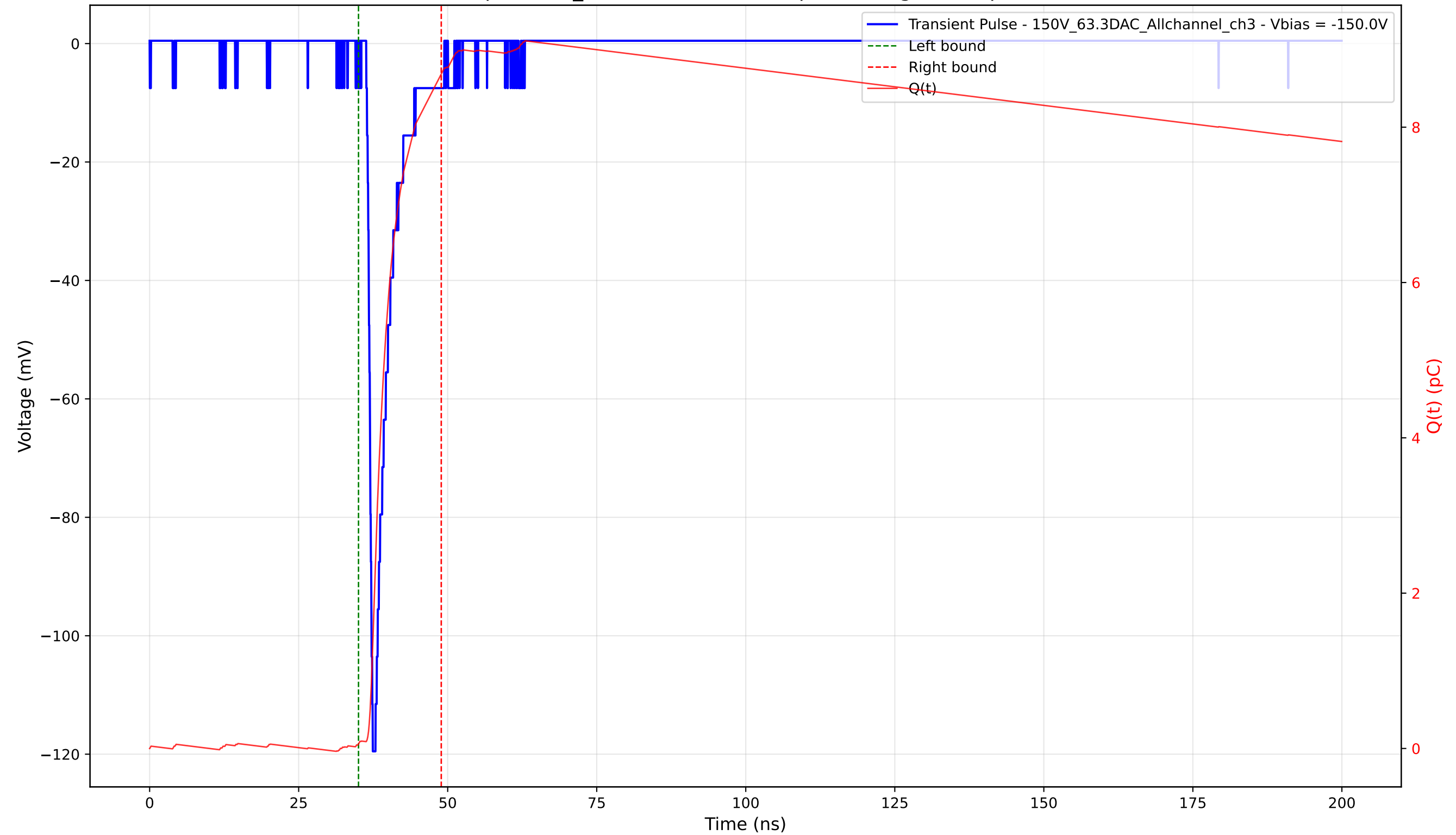
Transient Pulse - Sample: 1cm_42 - Position: 1665.0 \mu\text{m} - Charge: 8.63 pC - Rise Time: 0.90 ns
