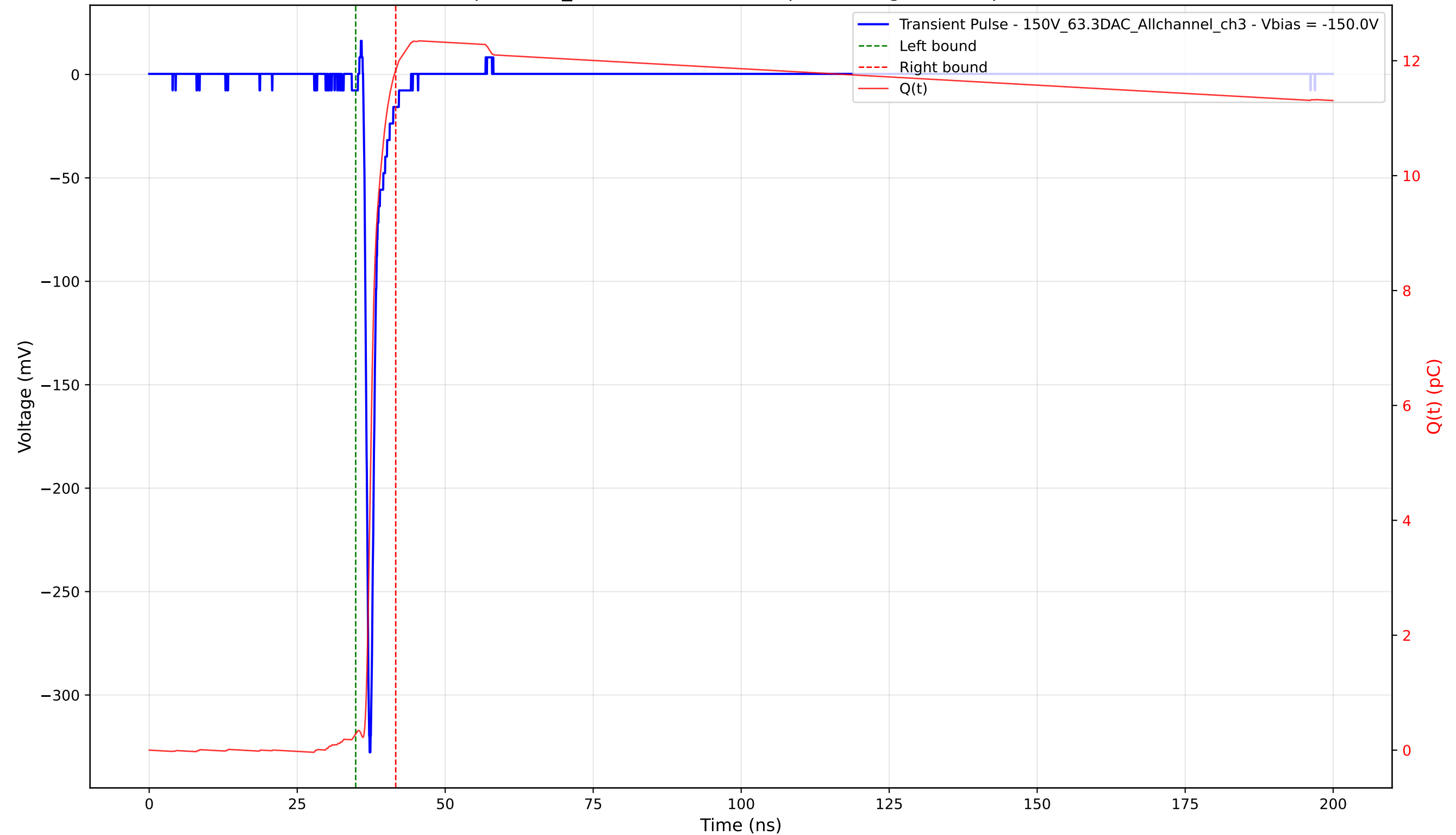
Transient Pulse - Sample: 1cm_42 - Position: 2910.0 \mu\text{m} - Charge: 11.55 pC - Rise Time: 0.75 ns
