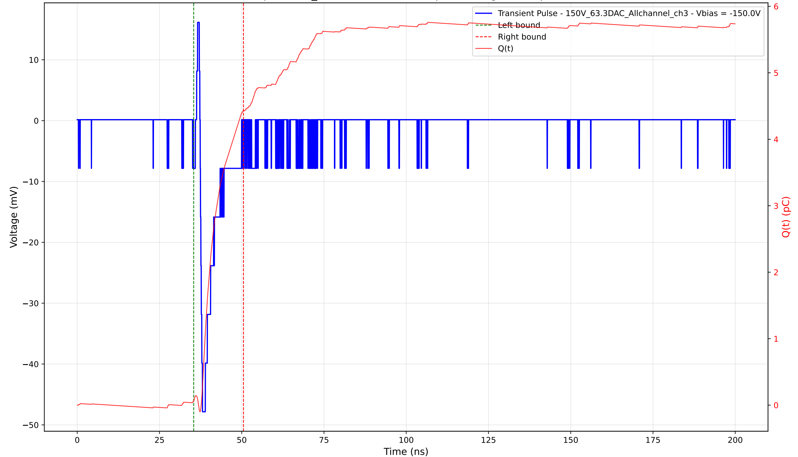
Transient Pulse - Sample: 1cm_42 - Position: 3890.0 \mu\text{m} - Charge: 4.36 pC - Rise Time: 0.70 ns
