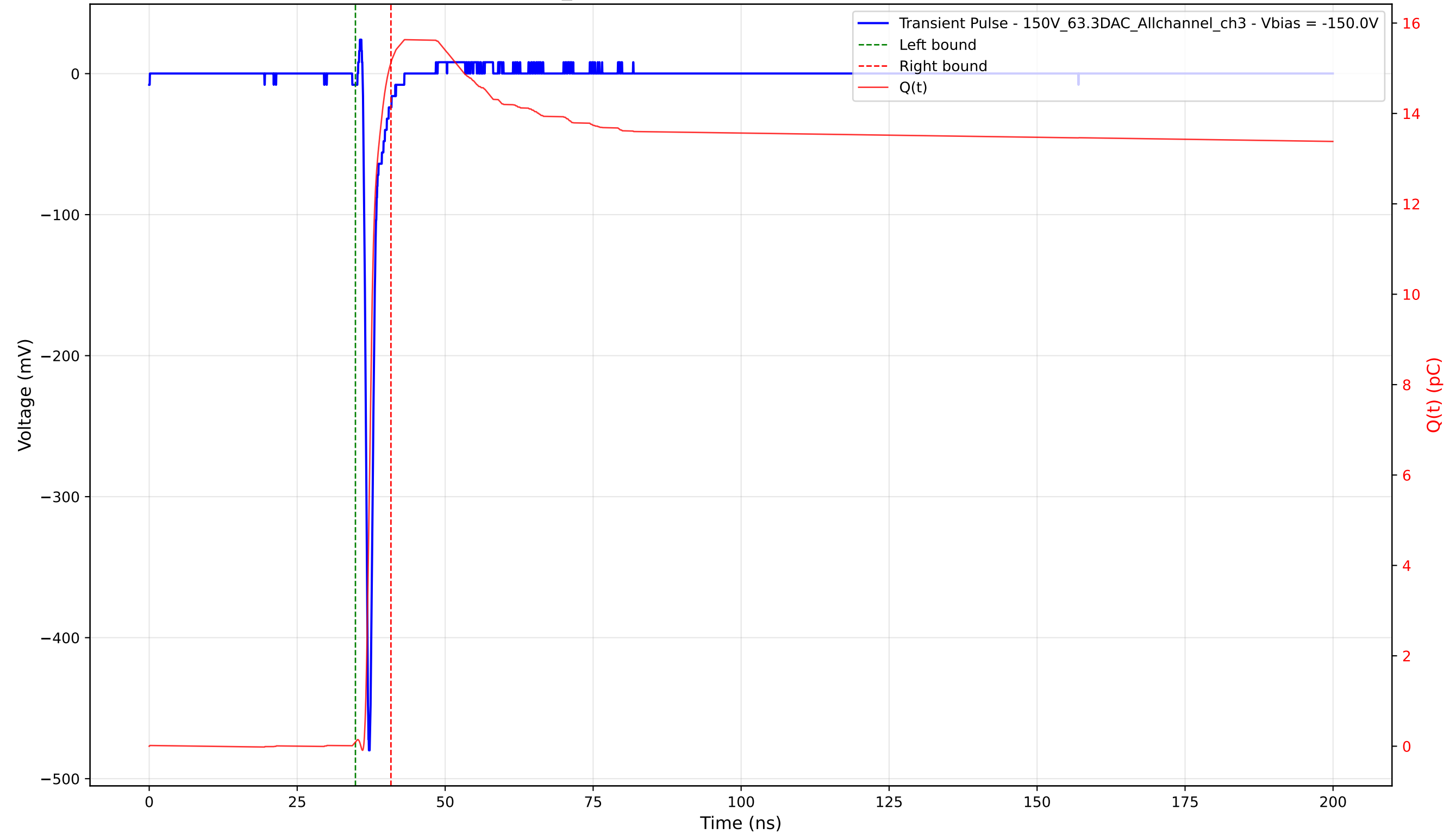
Transient Pulse - Sample: 1cm_42 - Position: 2390.0 \mu\text{m} - Charge: 15.03 pC - Rise Time: 0.68 ns
