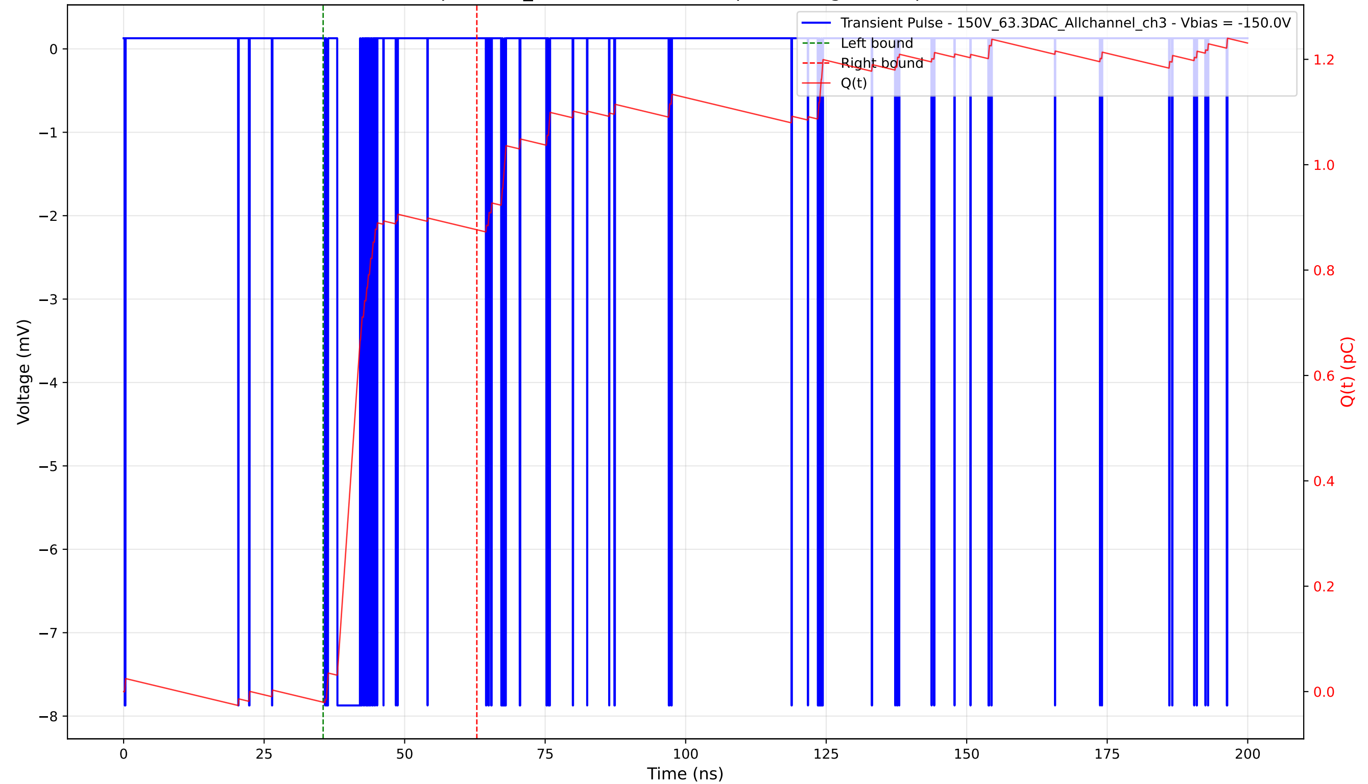
Transient Pulse - Sample: 1cm_42 - Position: 5125.0 \mu\text{m} - Charge: 0.90 pC - Rise Time: 0.04 ns
