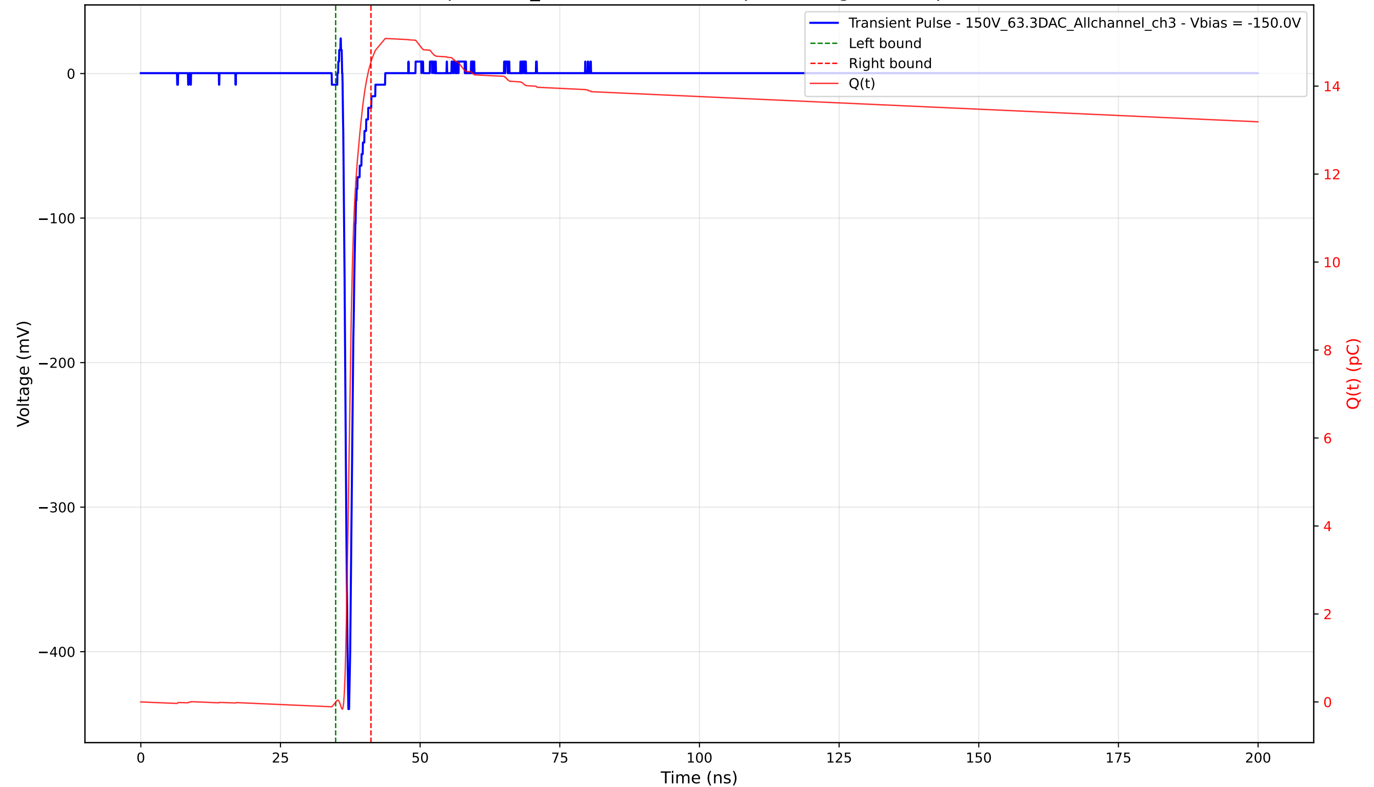
Transient Pulse - Sample: 1cm_42 - Position: 2230.0 \mu\text{m} - Charge: 14.56 pC - Rise Time: 0.69 ns
