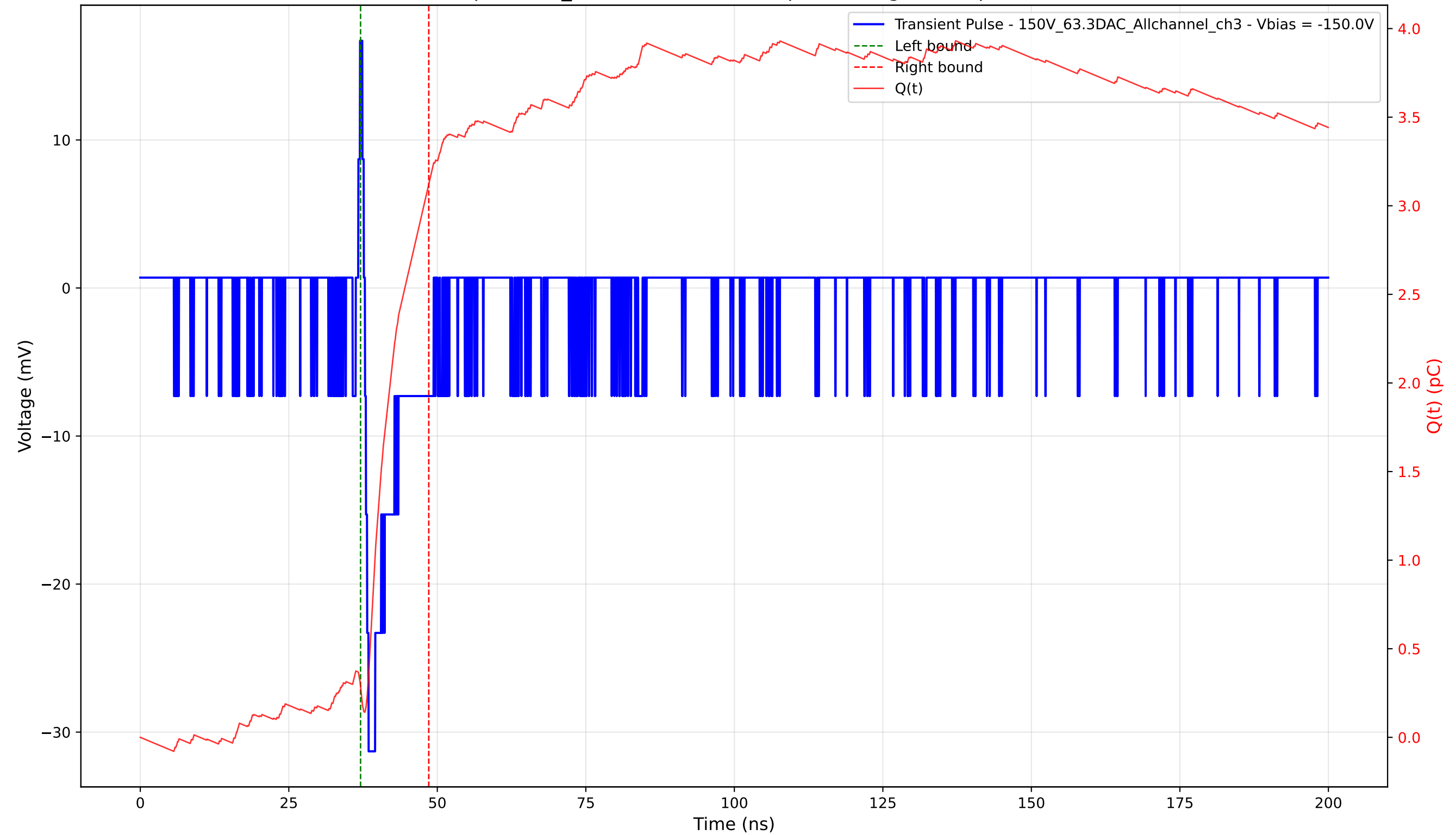
Transient Pulse - Sample: 1cm_42 - Position: 4805.0 \mu\text{m} - Charge: 2.84 pC - Rise Time: 0.63 ns
