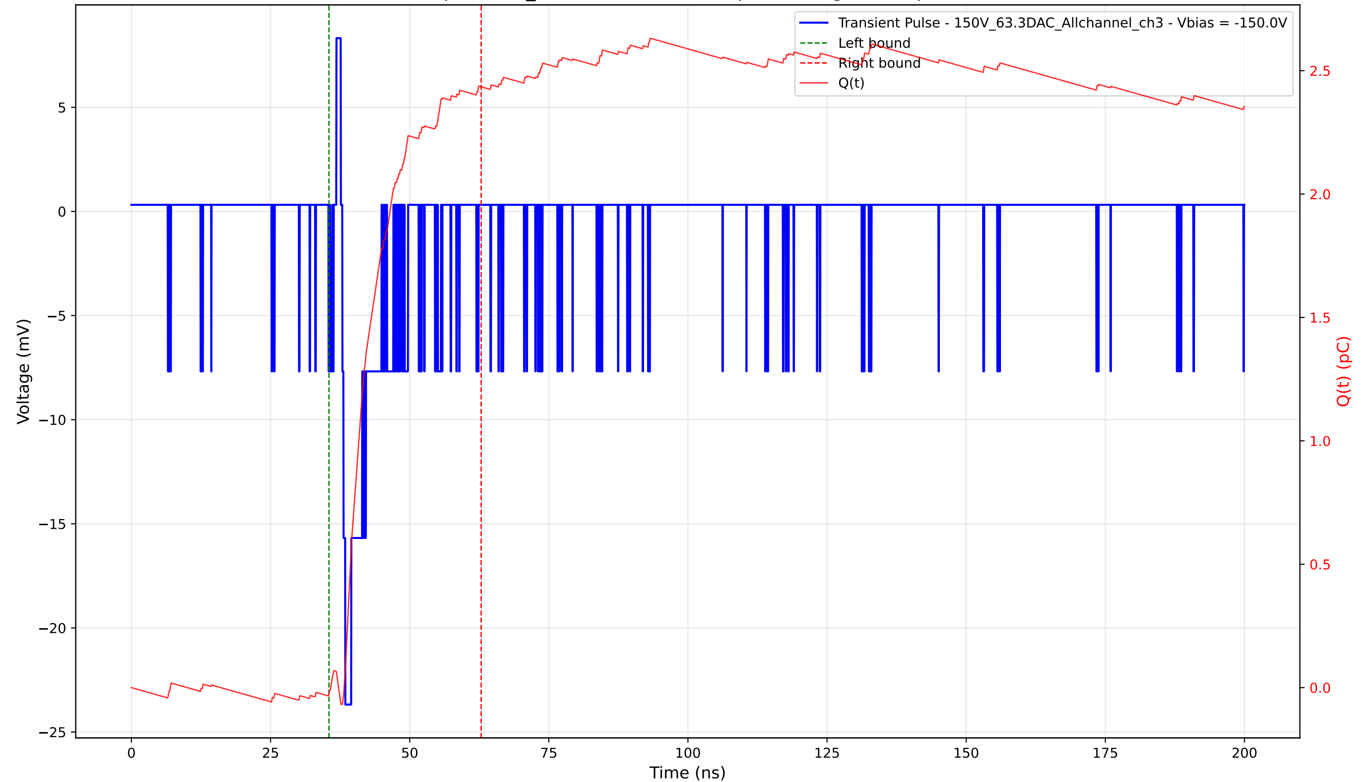
Transient Pulse - Sample: 1cm_42 - Position: 4950.0 \mu\text{m} - Charge: 2.45 pC - Rise Time: 0.55 ns
