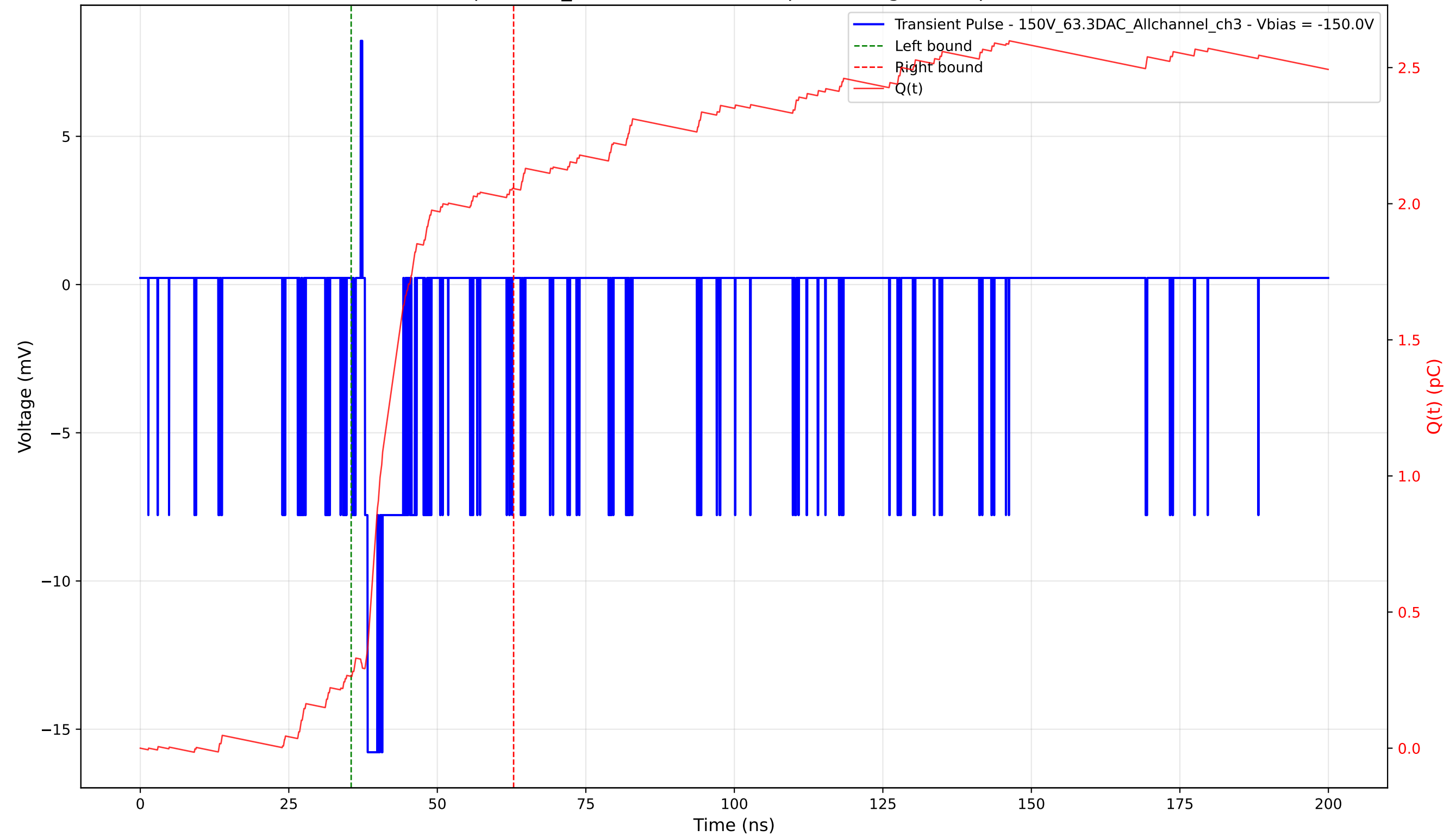
Transient Pulse - Sample: 1cm_42 - Position: 5035.0 \mu\text{m} - Charge: 1.79 pC - Rise Time: 0.47 ns
