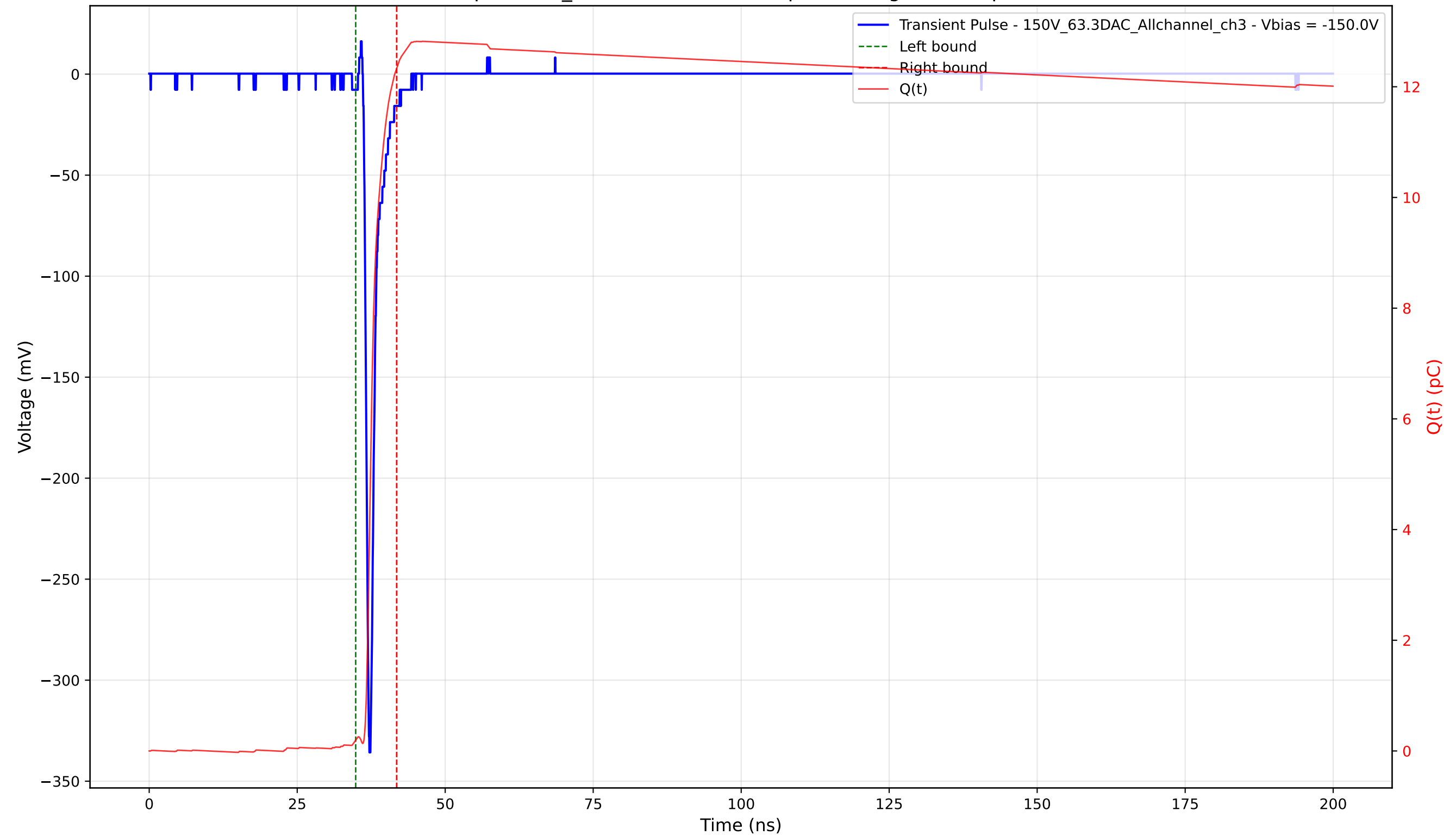
Transient Pulse - Sample: 1cm_42 - Position: 2135.0 \mu\text{m} - Charge: 12.13 pC - Rise Time: 0.73 ns
