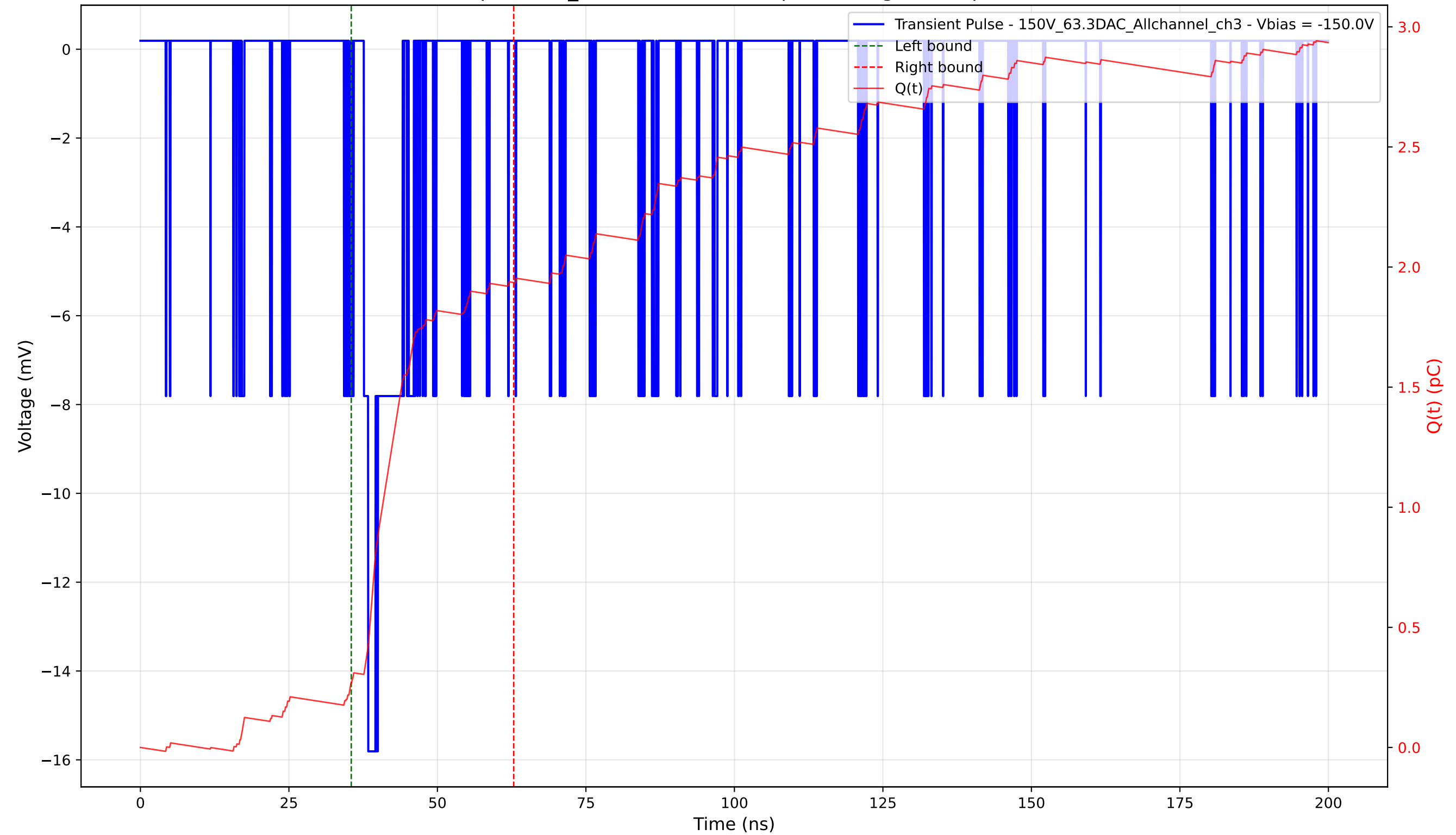
Transient Pulse - Sample: 1cm_42 - Position: 140.0 \mu\text{m} - Charge: 1.67 pC - Rise Time: 0.75 ns
