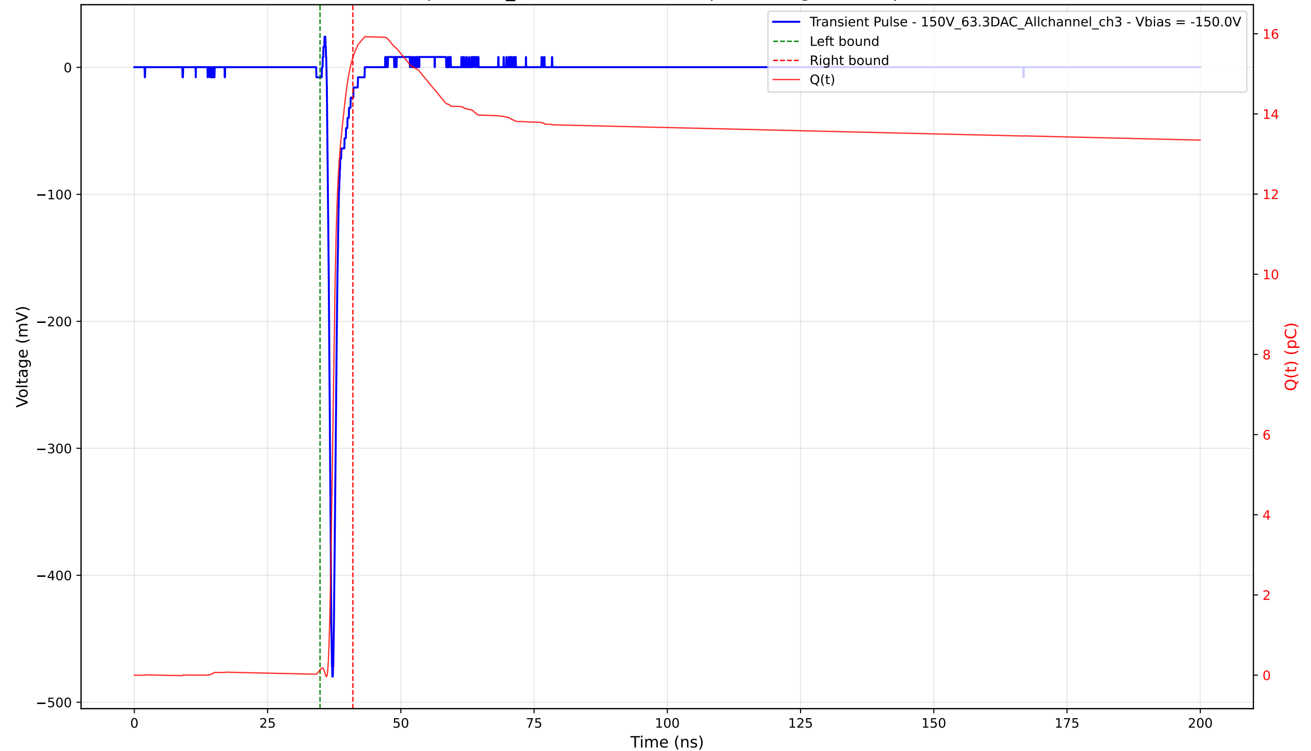
Transient Pulse - Sample: 1cm_42 - Position: 2695.0 \mu\text{m} - Charge: 15.28 pC - Rise Time: 0.70 ns
