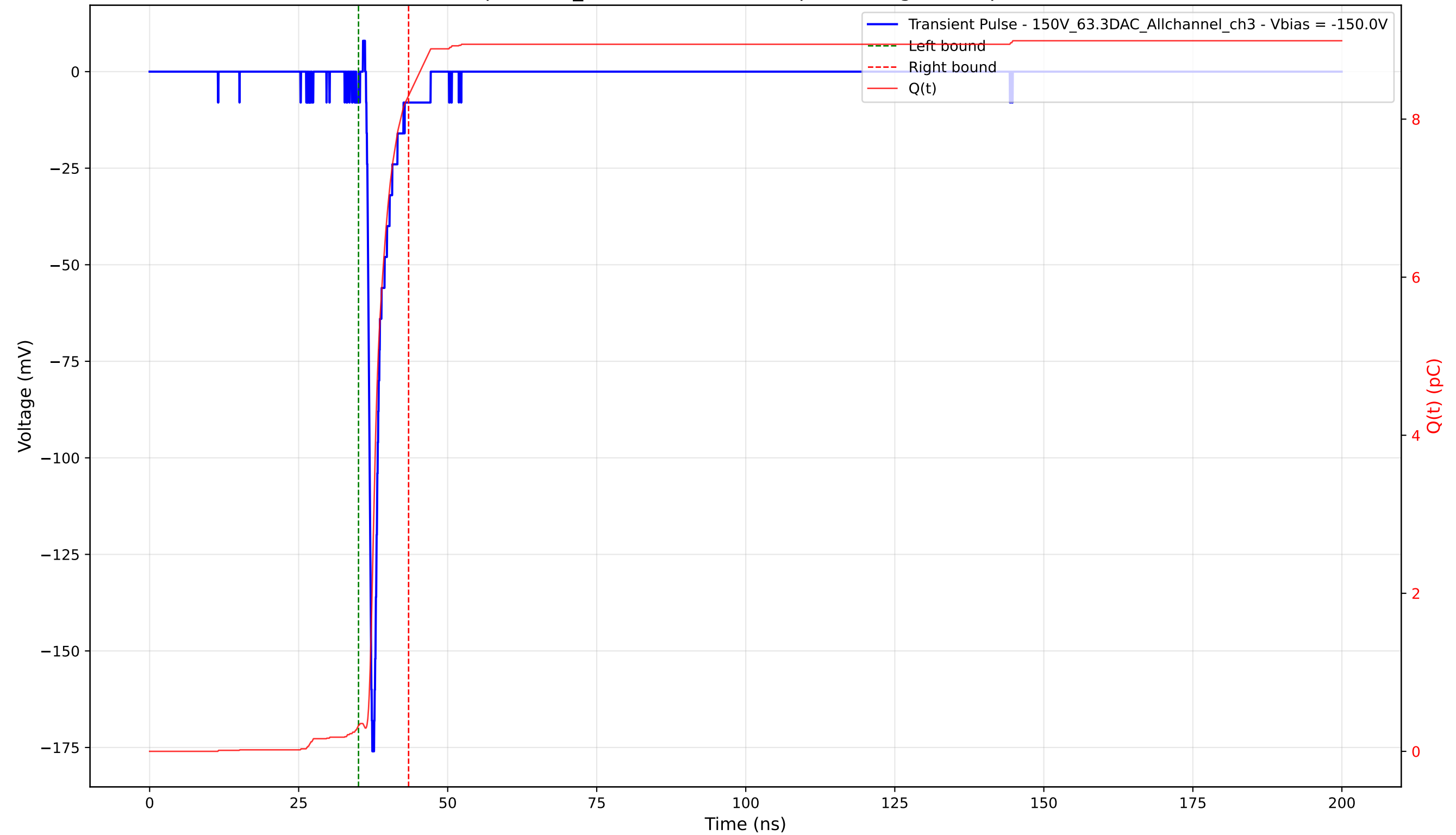
Transient Pulse - Sample: 1cm_42 - Position: 3105.0 \mu\text{m} - Charge: 7.97 pC - Rise Time: 0.75 ns
