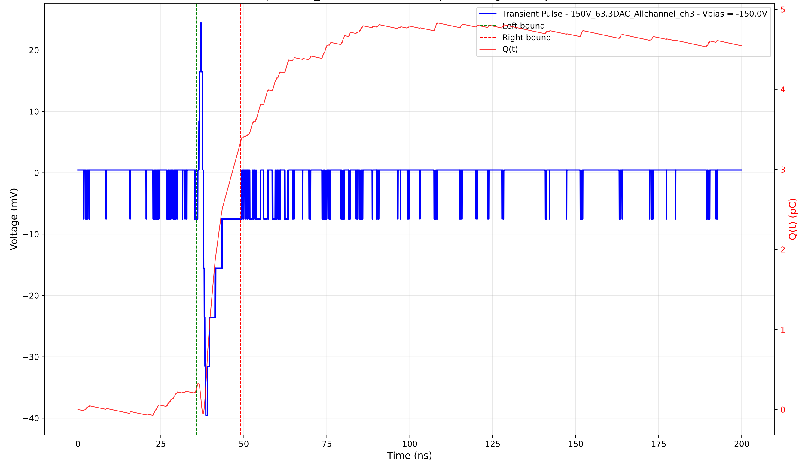
Transient Pulse - Sample: 1cm_42 - Position: 4385.0 \mu\text{m} - Charge: 3.09 pC - Rise Time: 0.78 ns
