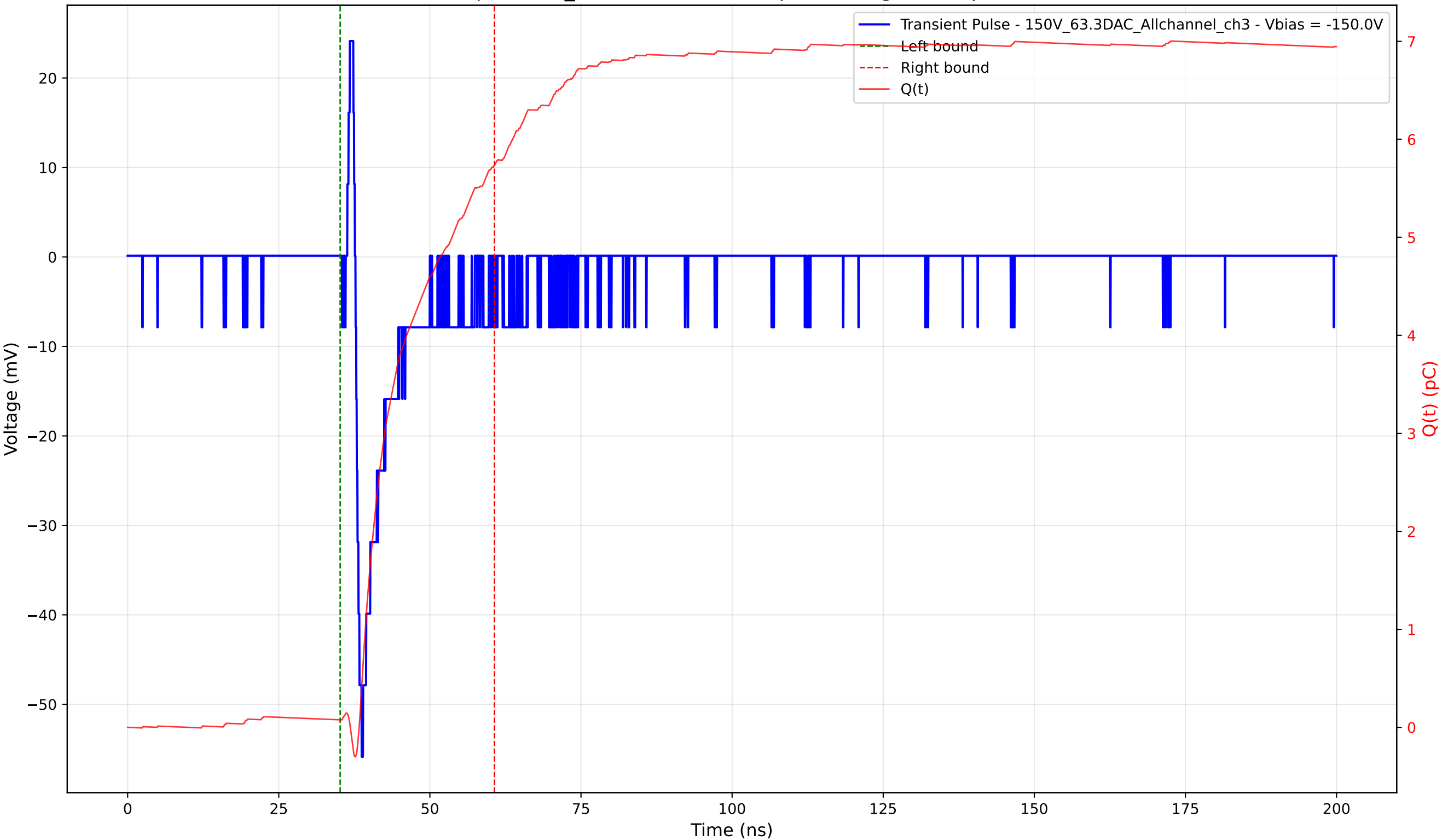
Transient Pulse - Sample: 1cm_42 - Position: 750.0 \mu\text{m} - Charge: 5.67 pC - Rise Time: 1.01 ns
