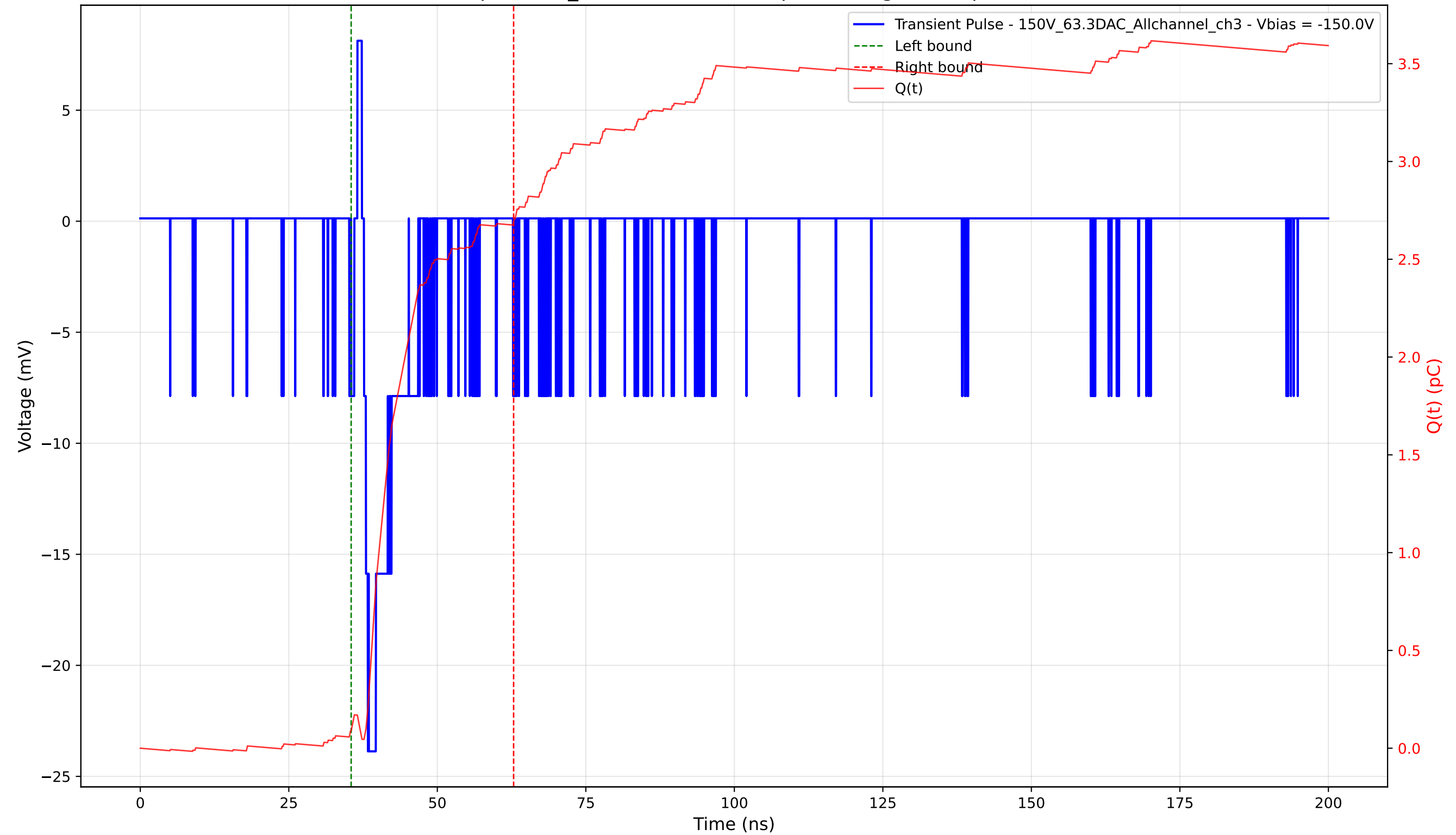
Transient Pulse - Sample: 1cm_42 - Position: 285.0 \mu\text{m} - Charge: 2.60 pC - Rise Time: 0.67 ns
