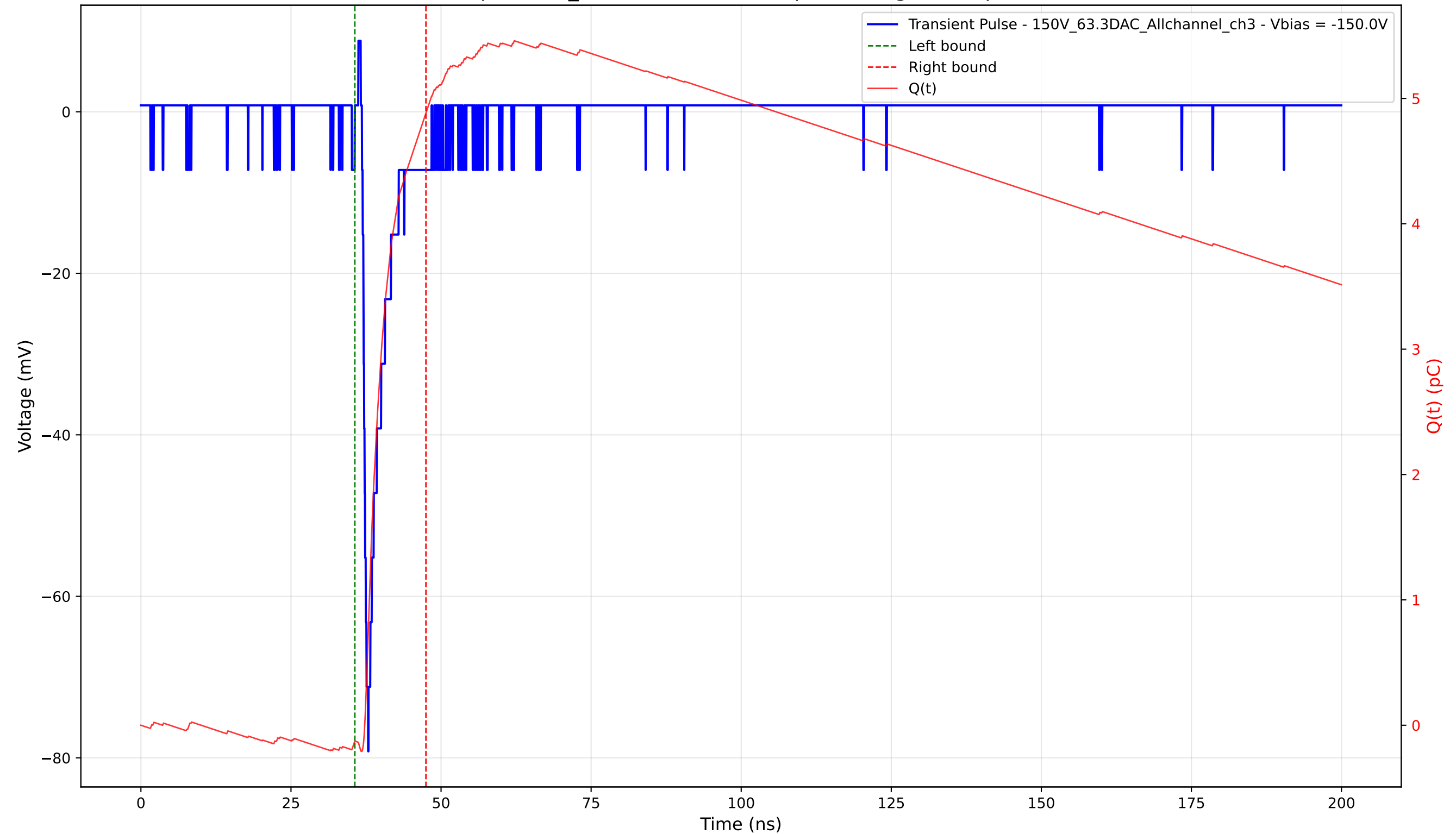
Transient Pulse - Sample: 1cm_42 - Position: 3500.0 \mu\text{m} - Charge: 5.01 pC - Rise Time: 0.96 ns
