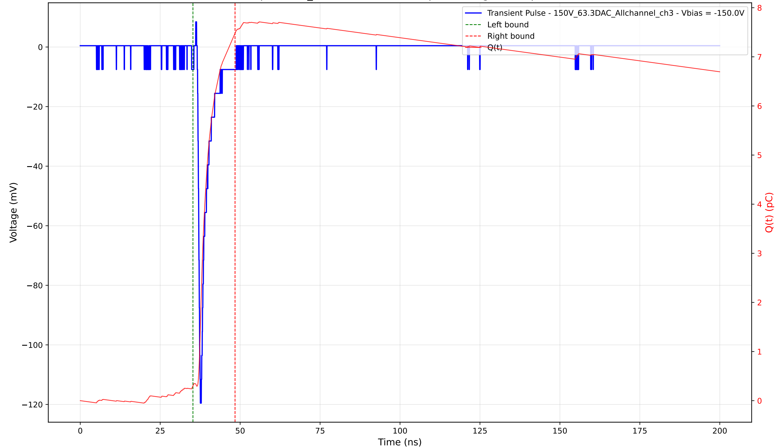
Transient Pulse - Sample: 1cm_42 - Position: 3360.0 \mu\text{m} - Charge: 7.18 pC - Rise Time: 0.78 ns
