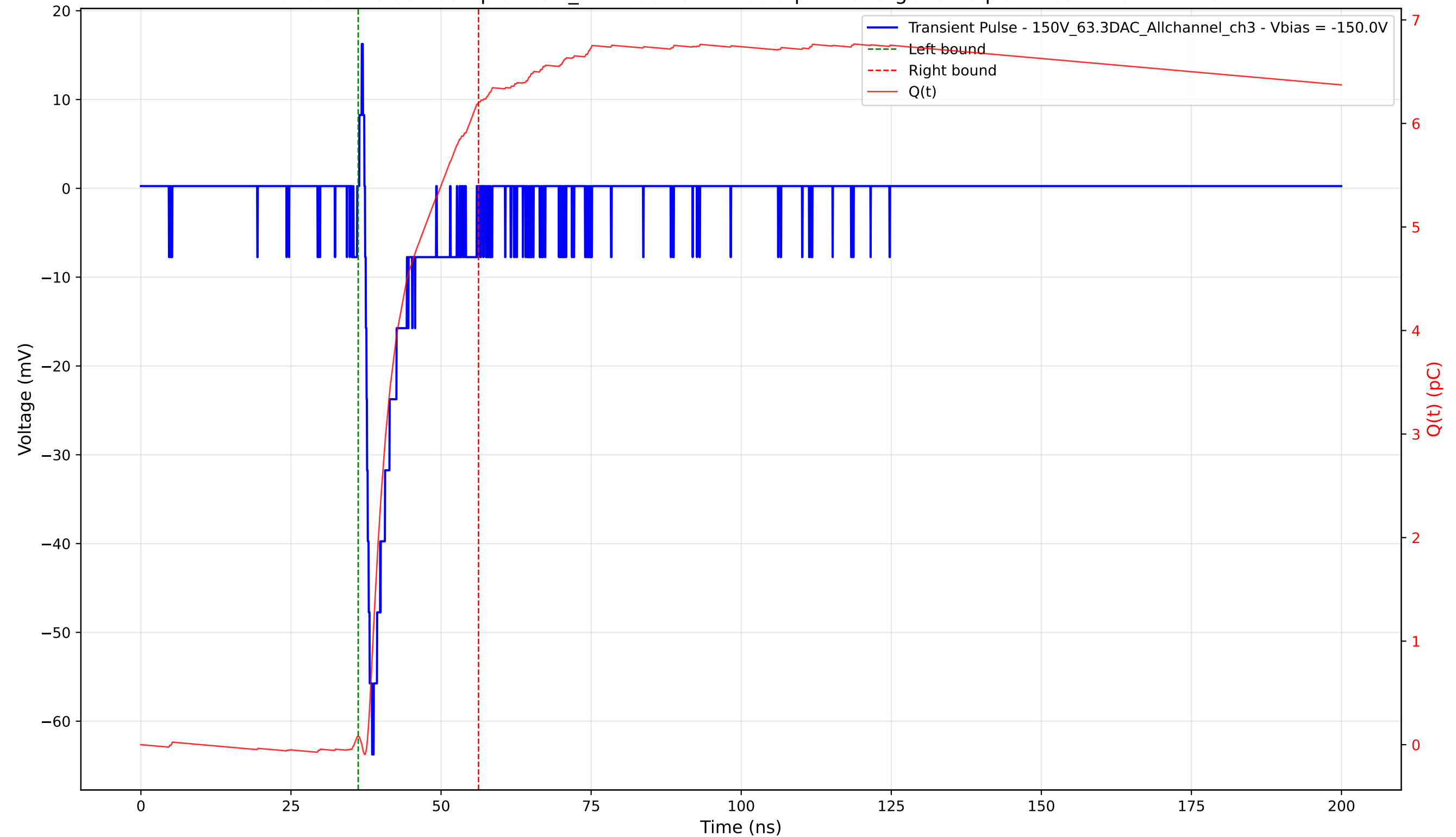
Transient Pulse - Sample: 1cm_42 - Position: 1160.0 \mu\text{m} - Charge: 6.13 pC - Rise Time: 1.17 ns
