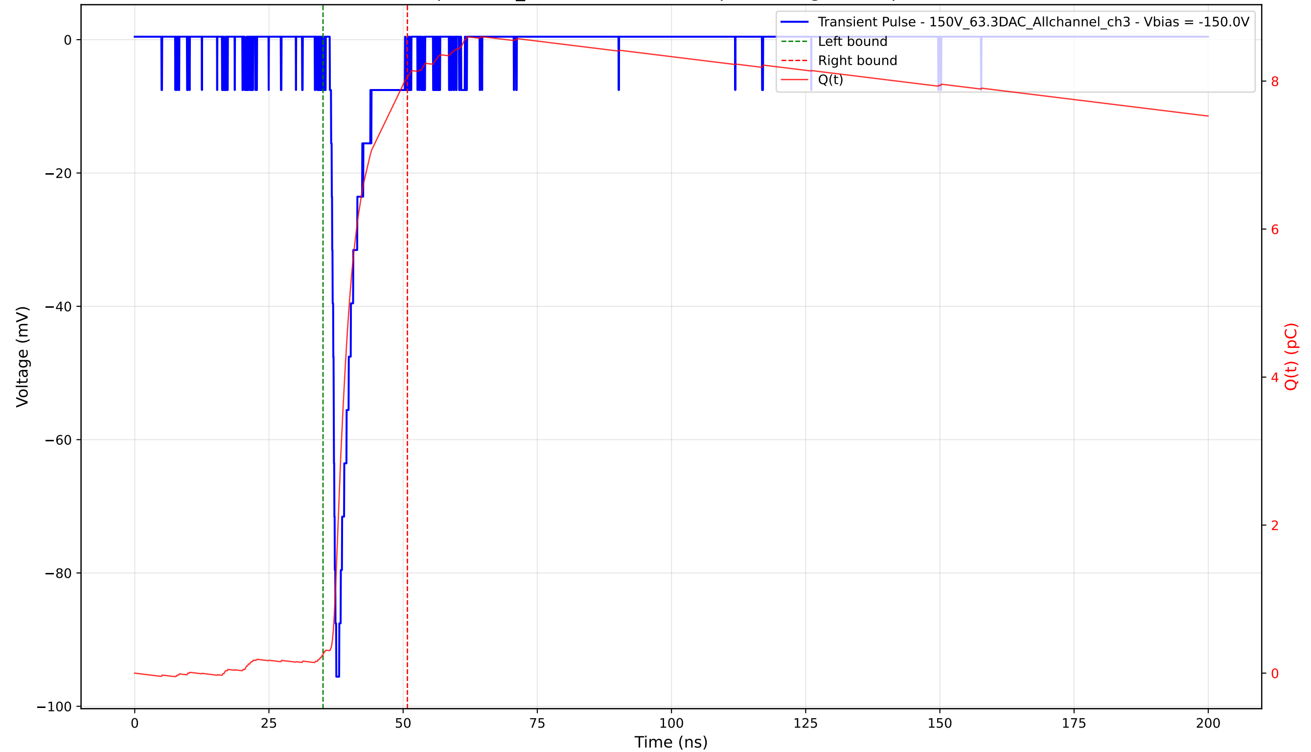
Transient Pulse - Sample: 1cm_42 - Position: 1595.0 \mu\text{m} - Charge: 7.81 pC - Rise Time: 0.83 ns
