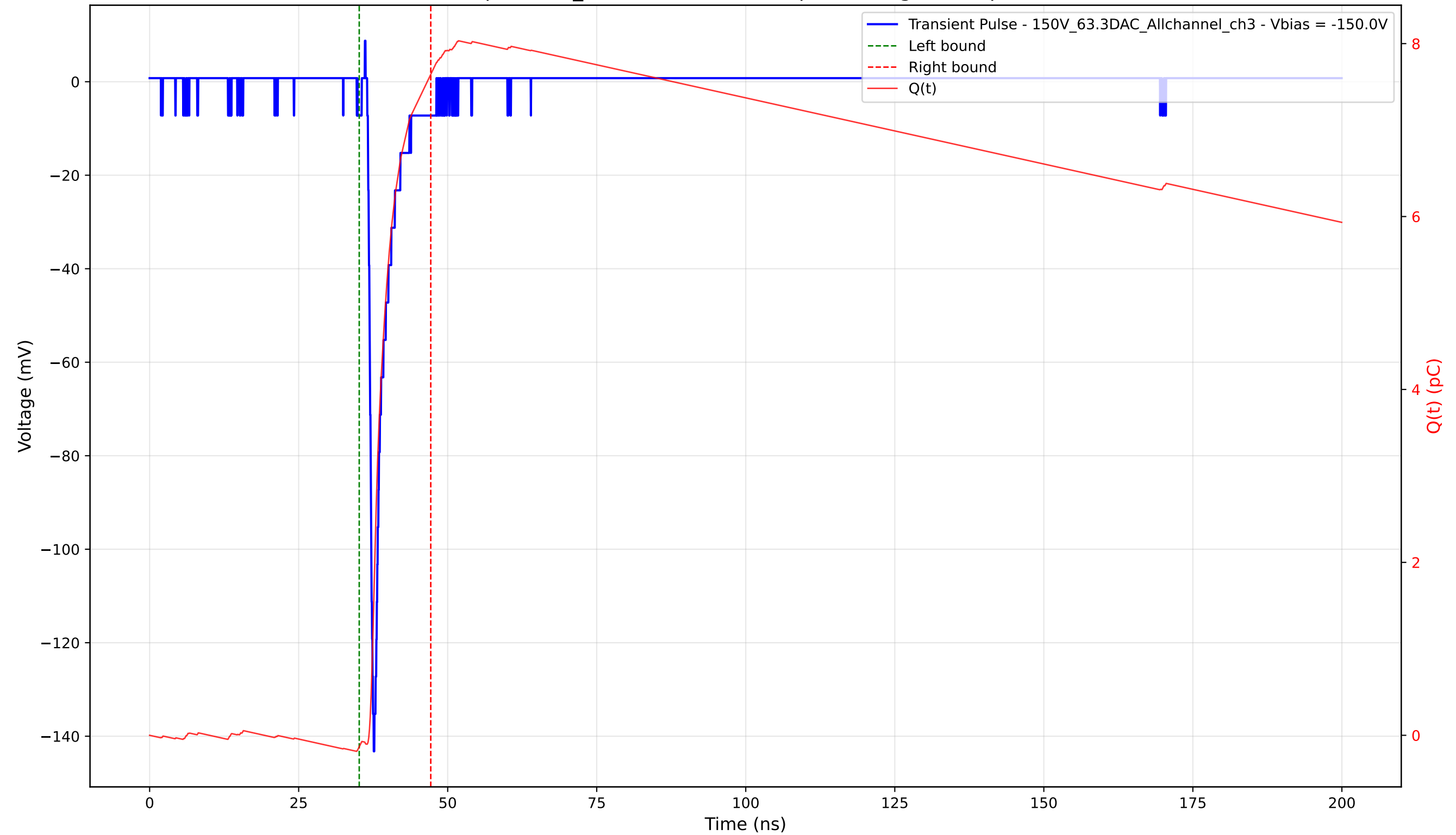
Transient Pulse - Sample: 1cm_42 - Position: 3270.0 \mu\text{m} - Charge: 7.78 pC - Rise Time: 0.84 ns
