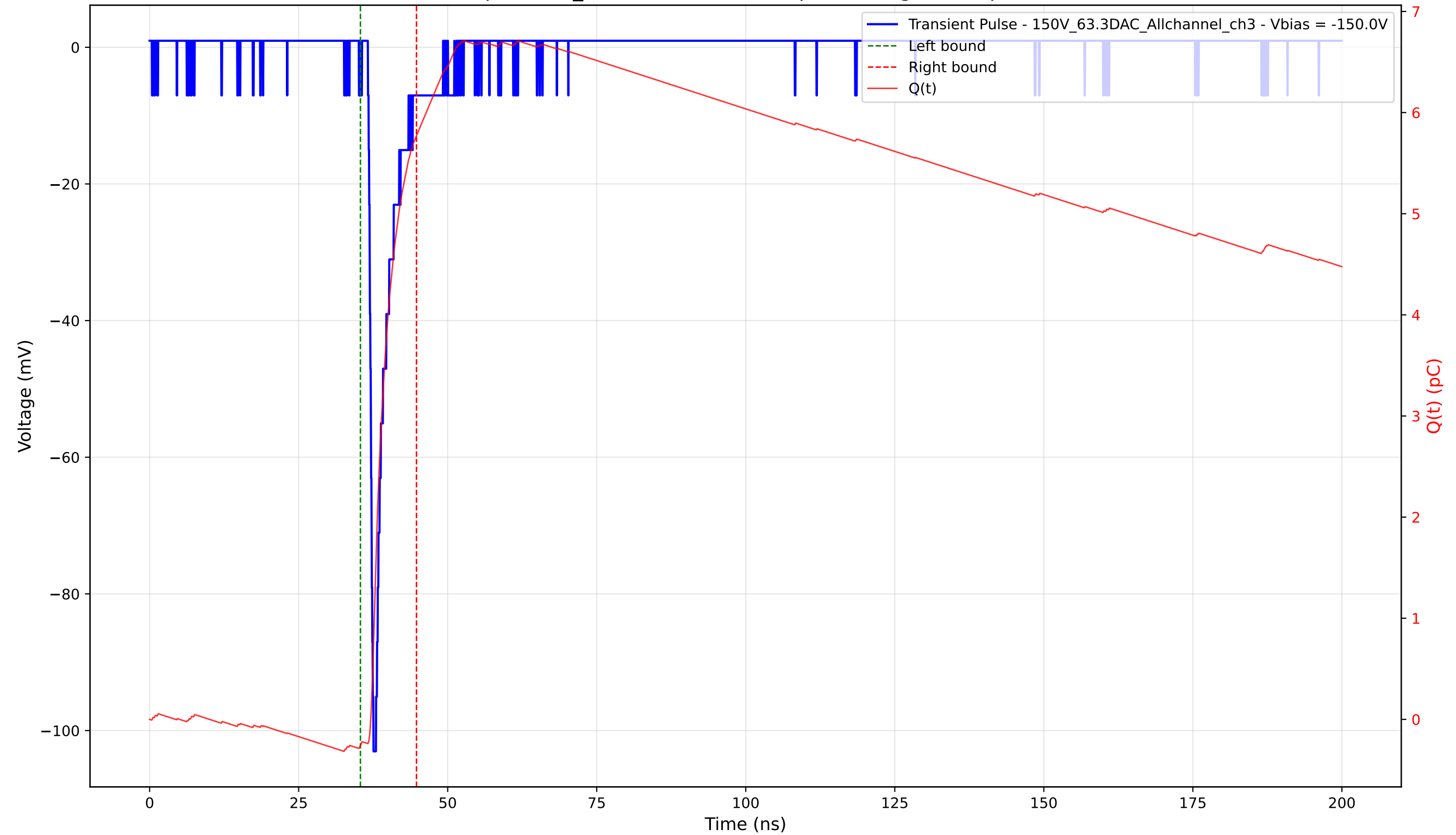
Transient Pulse - Sample: 1cm_42 - Position: 3400.0 \mu\text{m} - Charge: 6.03 pC - Rise Time: 0.70 ns
