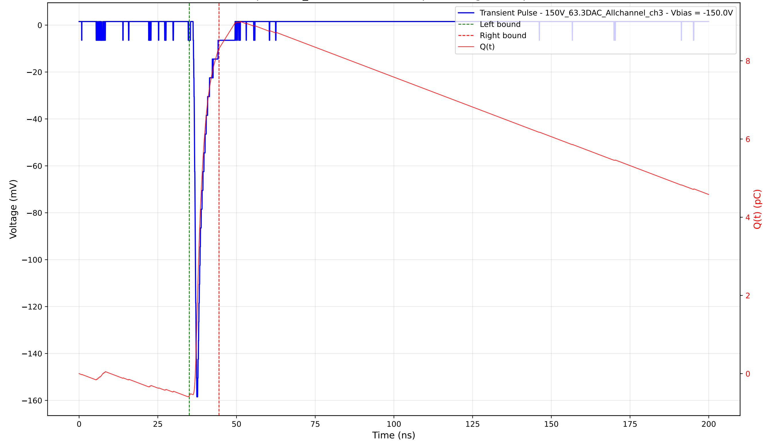
Transient Pulse - Sample: 1cm_42 - Position: 1840.0 \mu\text{m} - Charge: 8.88 pC - Rise Time: 0.91 ns
