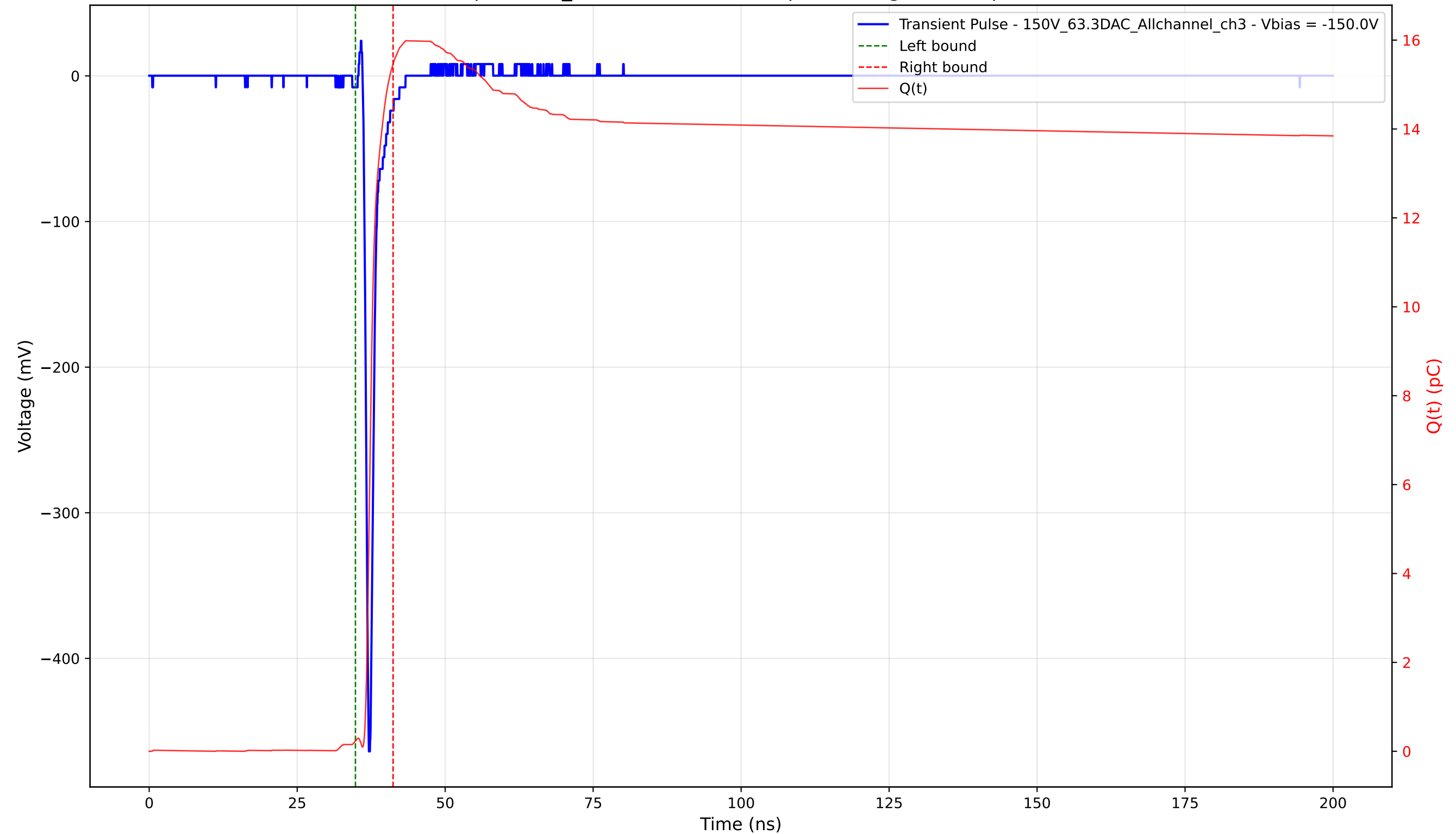
Transient Pulse - Sample: 1cm_42 - Position: 2755.0 \mu\text{m} - Charge: 15.23 pC - Rise Time: 0.69 ns
