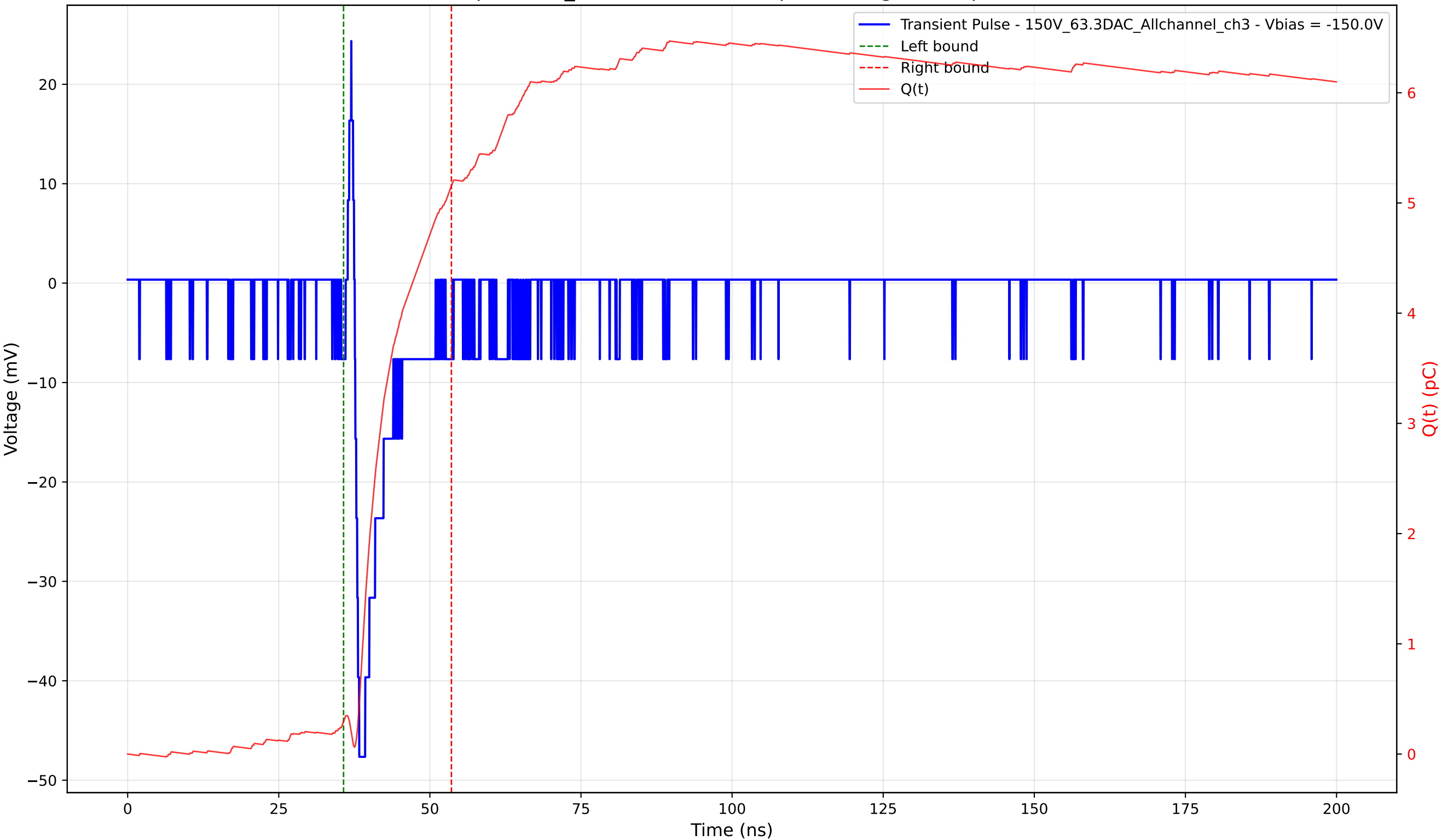
Transient Pulse - Sample: 1cm_42 - Position: 980.0 \mu\text{m} - Charge: 4.86 pC - Rise Time: 0.74 ns
