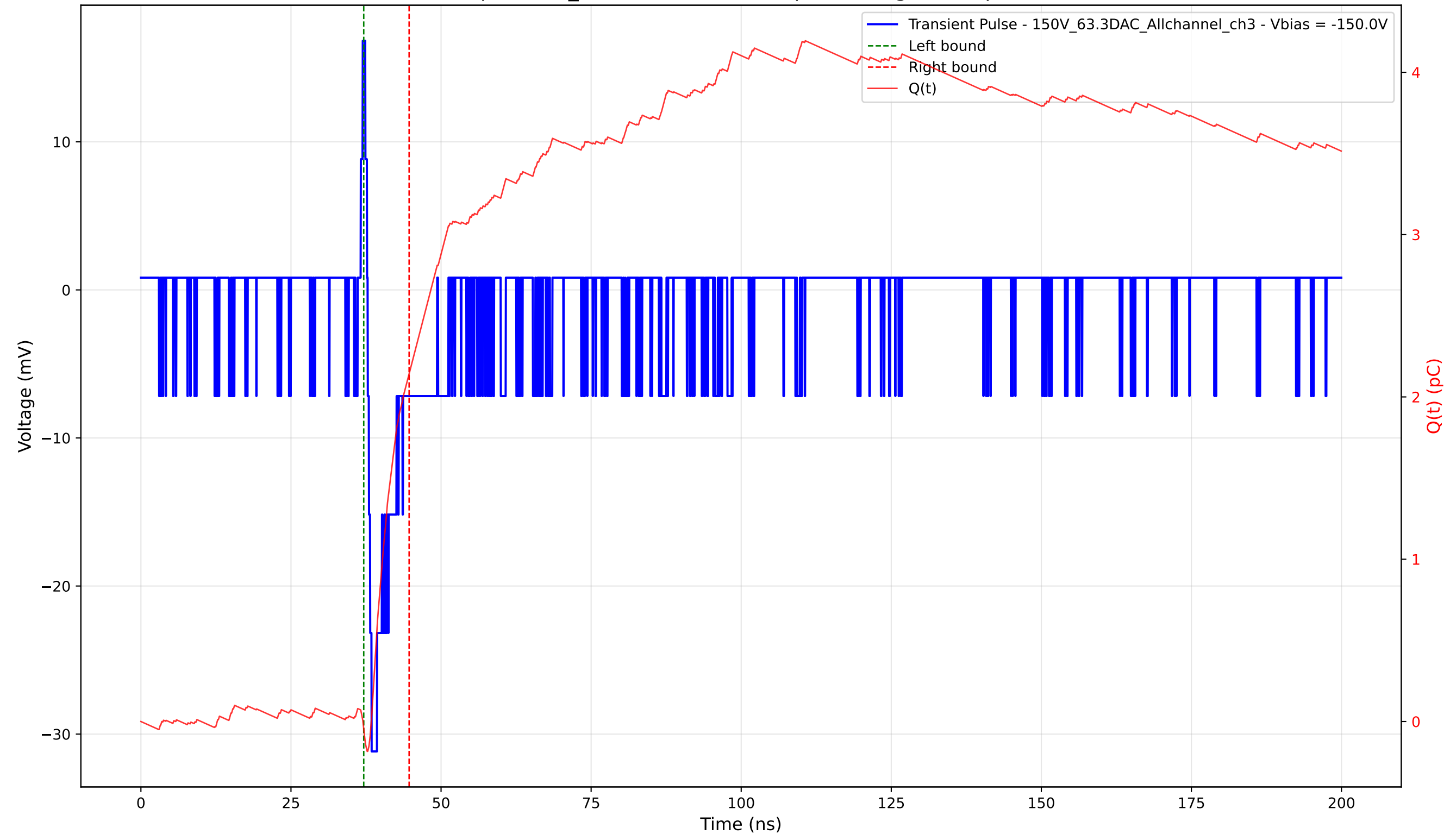
Transient Pulse - Sample: 1cm_42 - Position: 4725.0 \mu\text{m} - Charge: 2.19 pC - Rise Time: 0.67 ns
