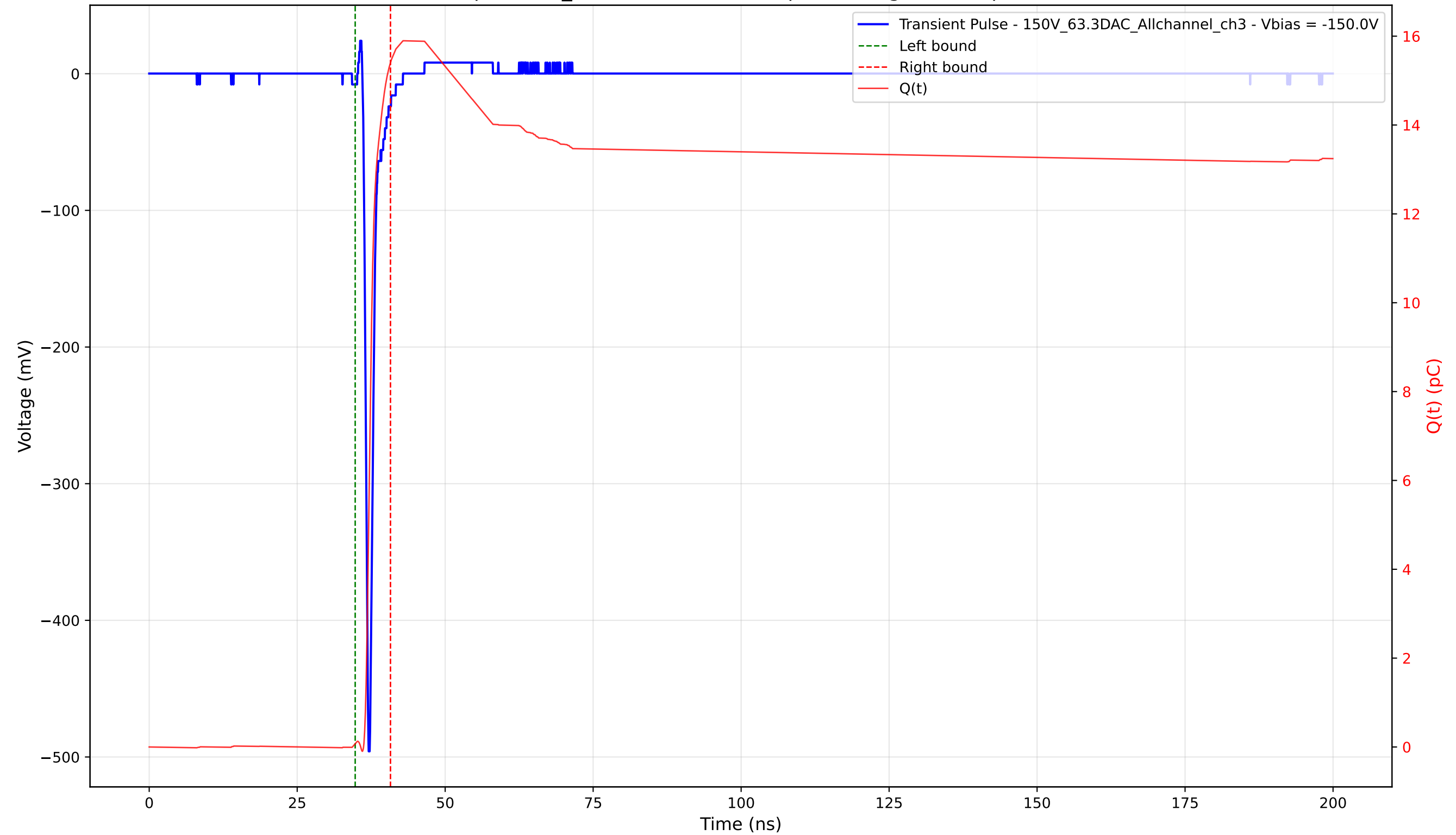
Transient Pulse - Sample: 1cm_42 - Position: 2605.0 \mu\text{m} - Charge: 15.33 pC - Rise Time: 0.71 ns
