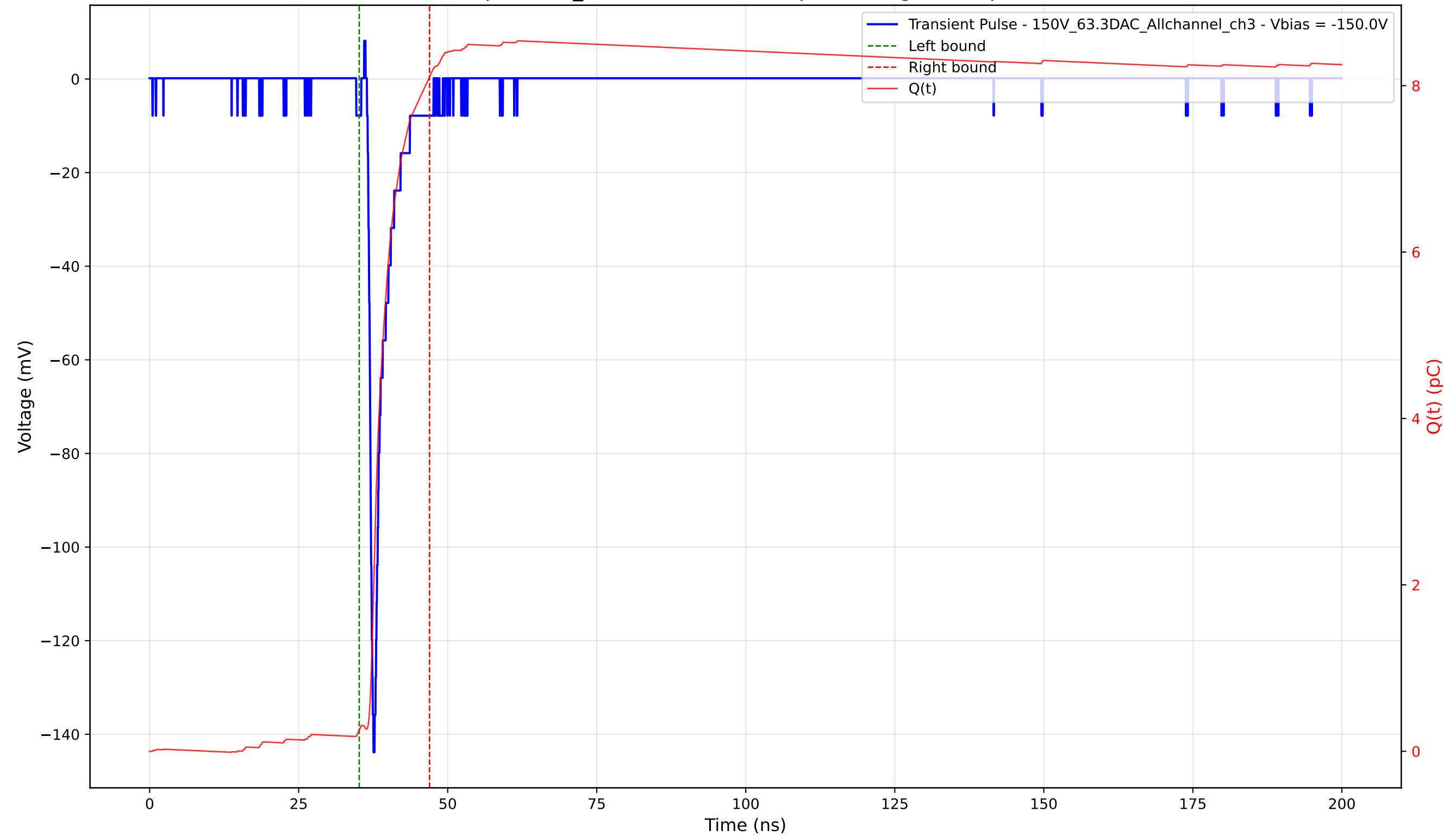
Transient Pulse - Sample: 1cm_42 - Position: 3240.0 \mu\text{m} - Charge: 7.85 pC - Rise Time: 0.85 ns
