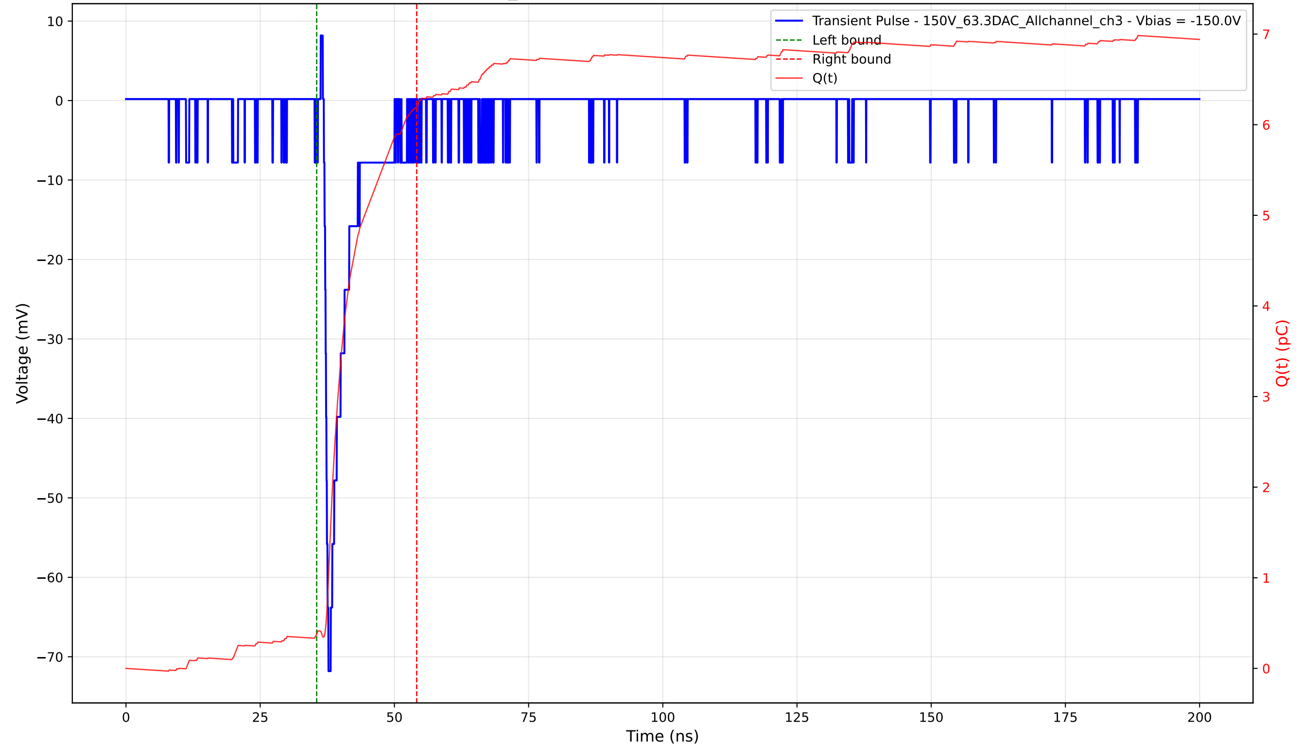
Transient Pulse - Sample: 1cm_42 - Position: 3520.0 \mu\text{m} - Charge: 5.83 pC - Rise Time: 0.84 ns
