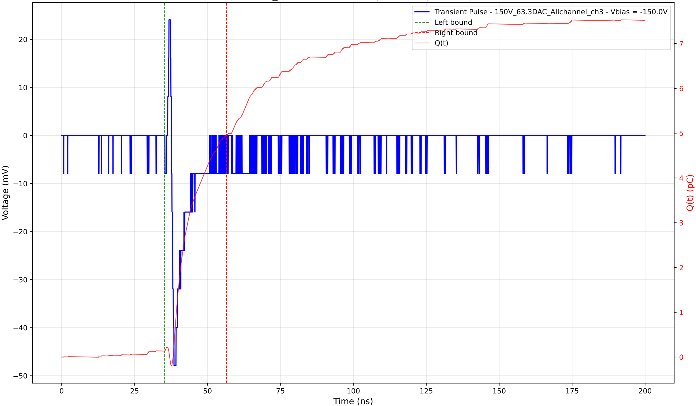
Transient Pulse - Sample: 1cm_42 - Position: 650.0 \mu\text{m} - Charge: 4.82 pC - Rise Time: 0.82 ns
