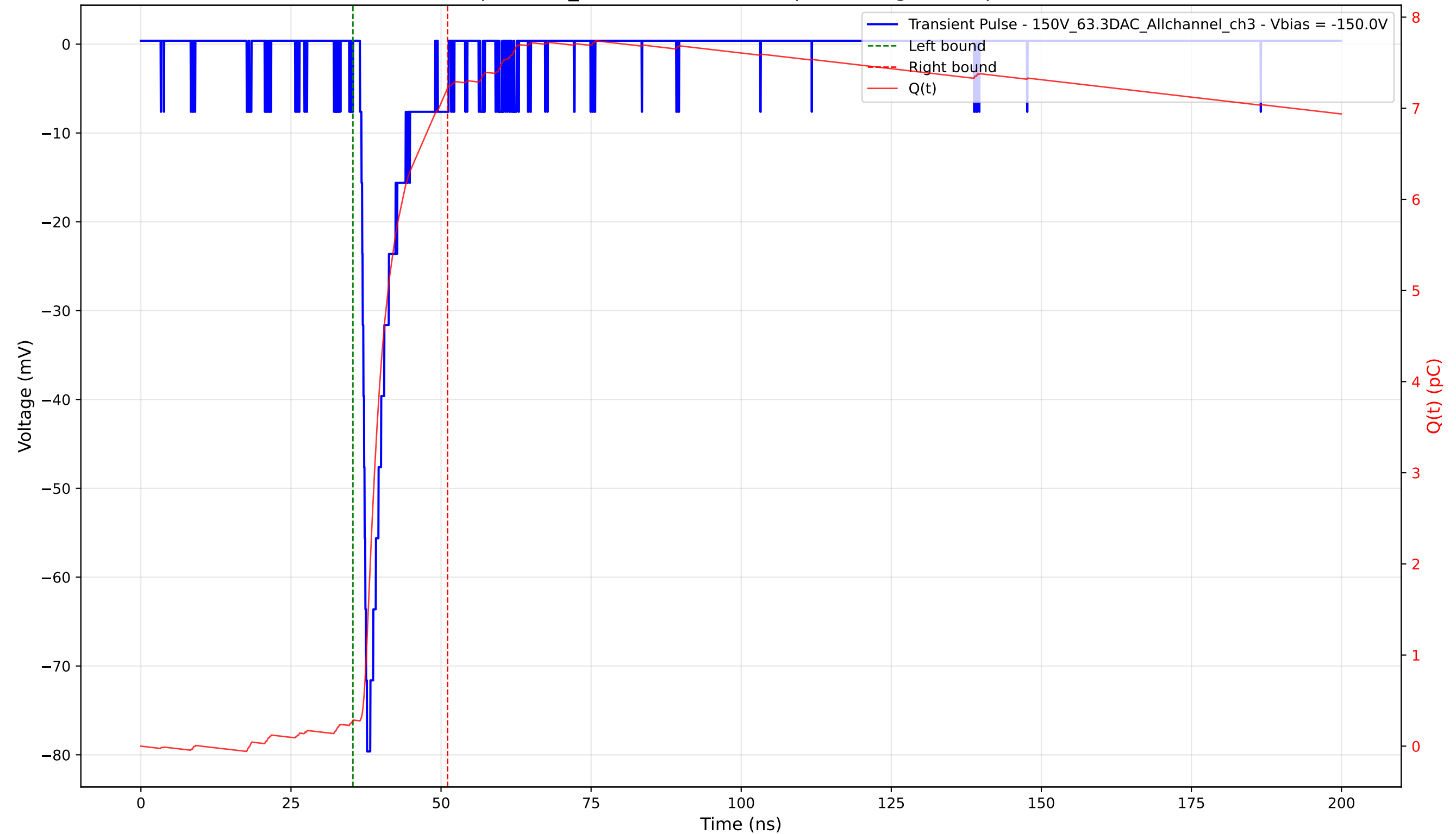
Transient Pulse - Sample: 1cm_42 - Position: 1530.0 \mu\text{m} - Charge: 6.94 pC - Rise Time: 0.96 ns
