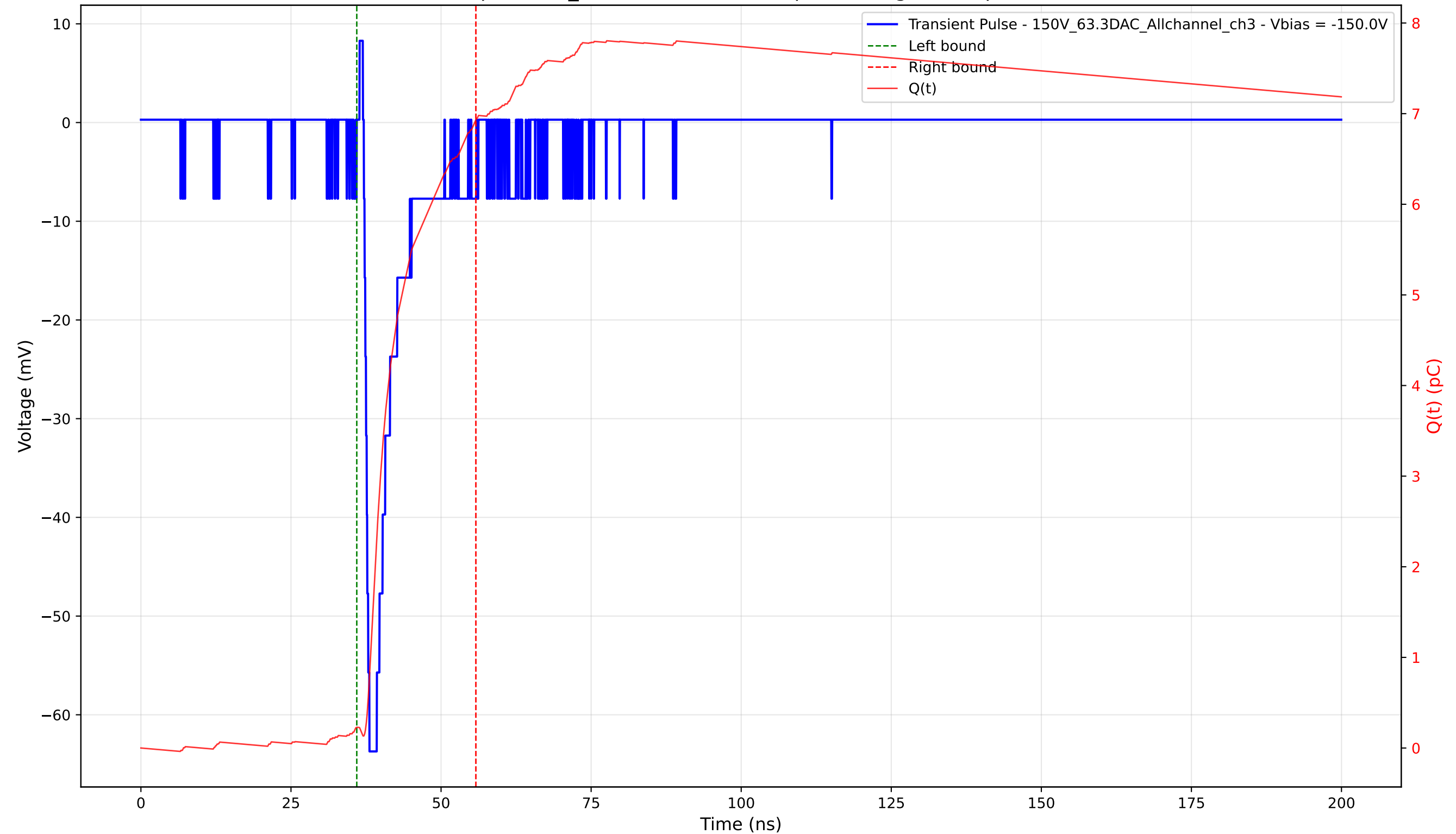
Transient Pulse - Sample: 1cm_42 - Position: 1330.0 \mu\text{m} - Charge: 6.71 pC - Rise Time: 0.93 ns
