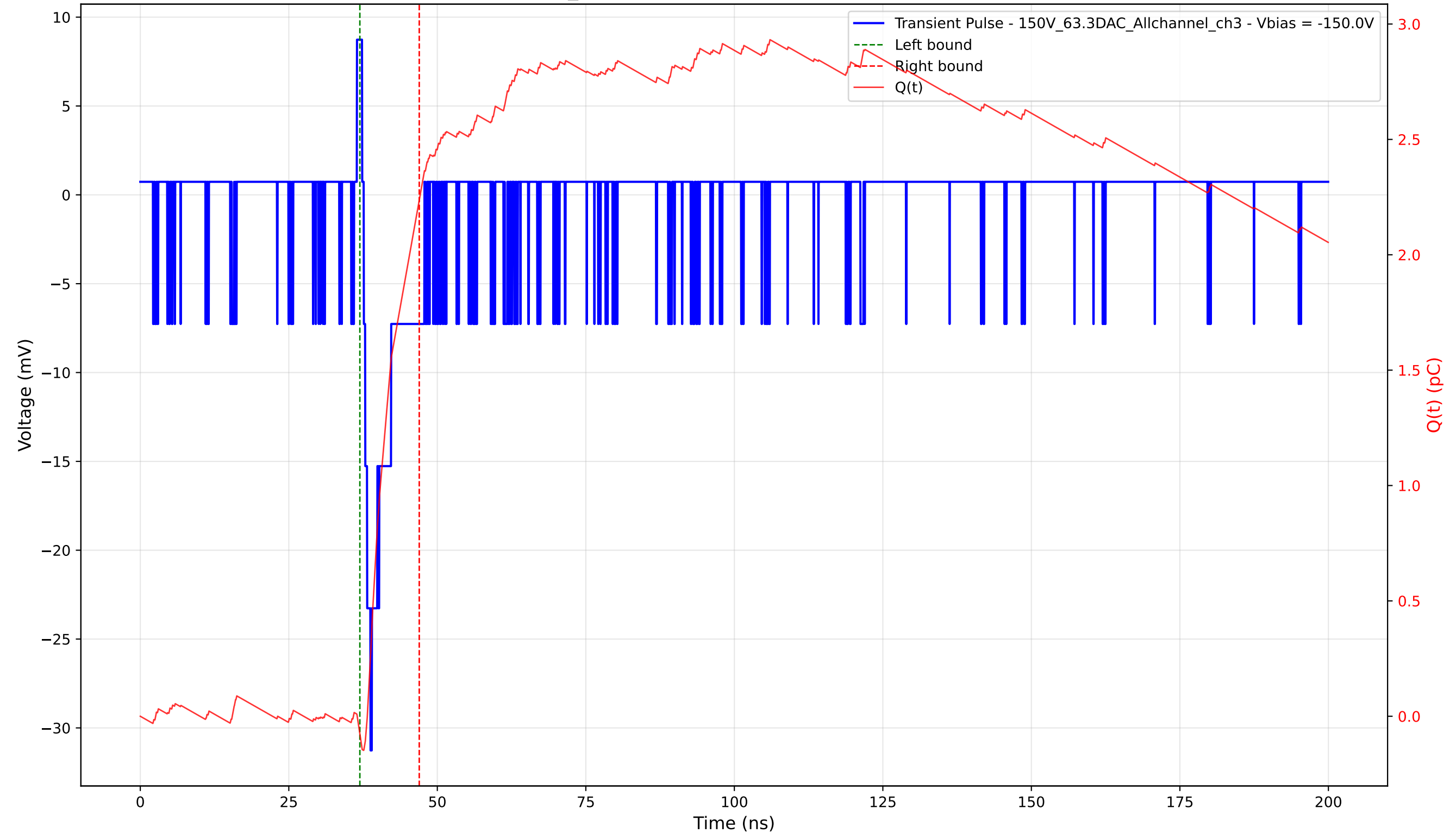
Transient Pulse - Sample: 1cm_42 - Position: 360.0 \mu\text{m} - Charge: 2.32 pC - Rise Time: 1.15 ns
