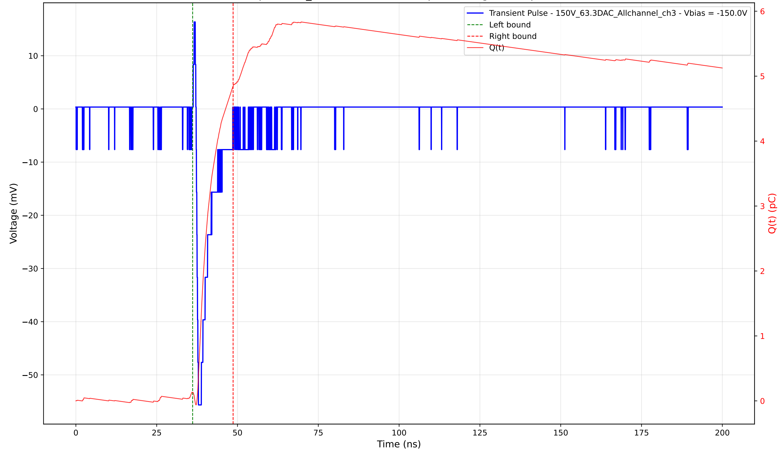
Transient Pulse - Sample: 1cm_42 - Position: 3705.0 \mu\text{m} - Charge: 4.72 pC - Rise Time: 0.69 ns
