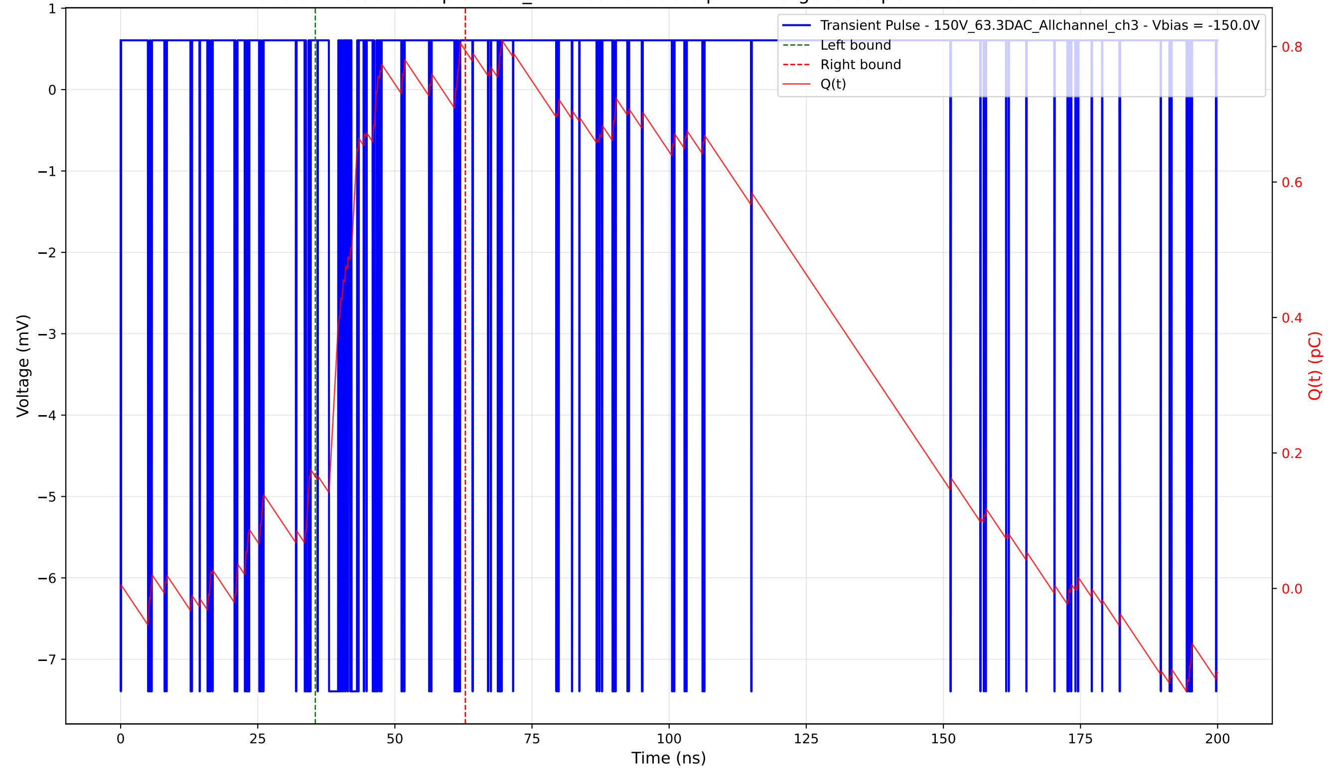
Transient Pulse - Sample: 1cm_42 - Position: 50.0 \mu\text{m} - Charge: 0.63 pC - Rise Time: 0.04 ns
