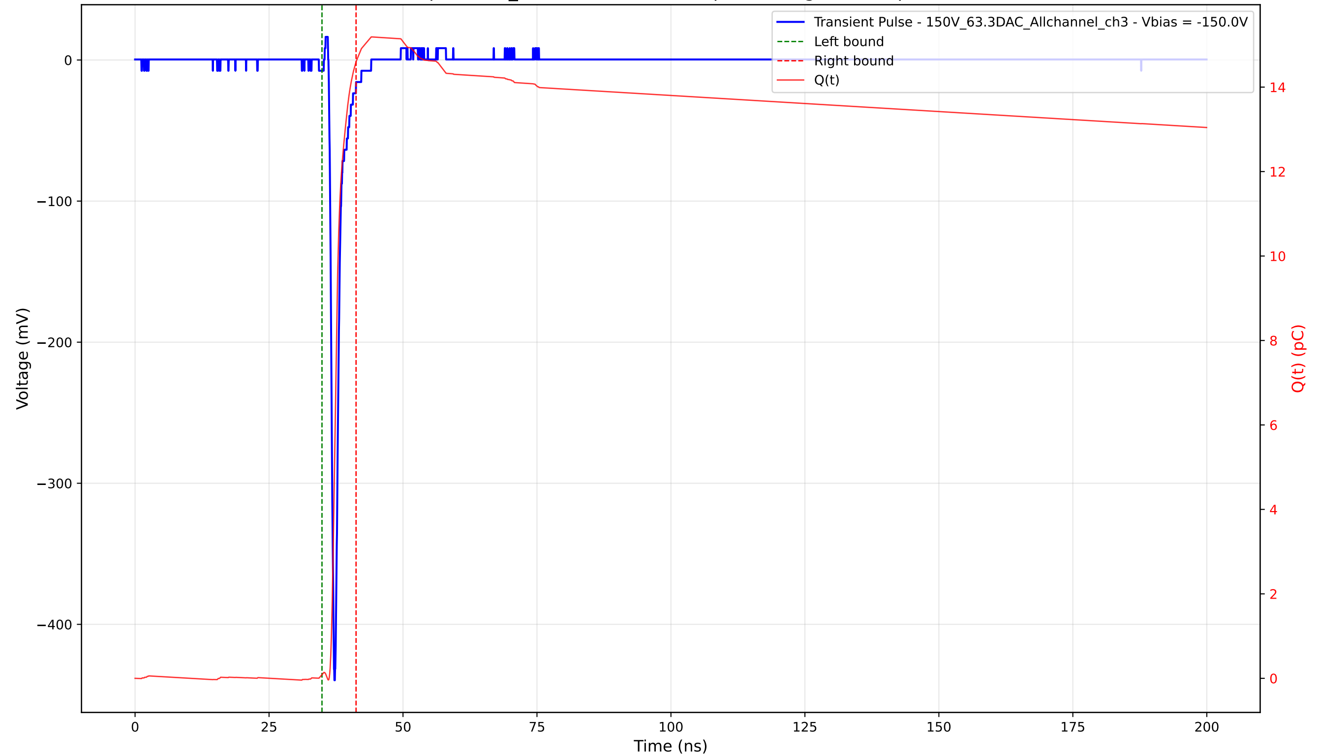
Transient Pulse - Sample: 1cm_42 - Position: 2815.0 \mu\text{m} - Charge: 14.51 pC - Rise Time: 0.73 ns
