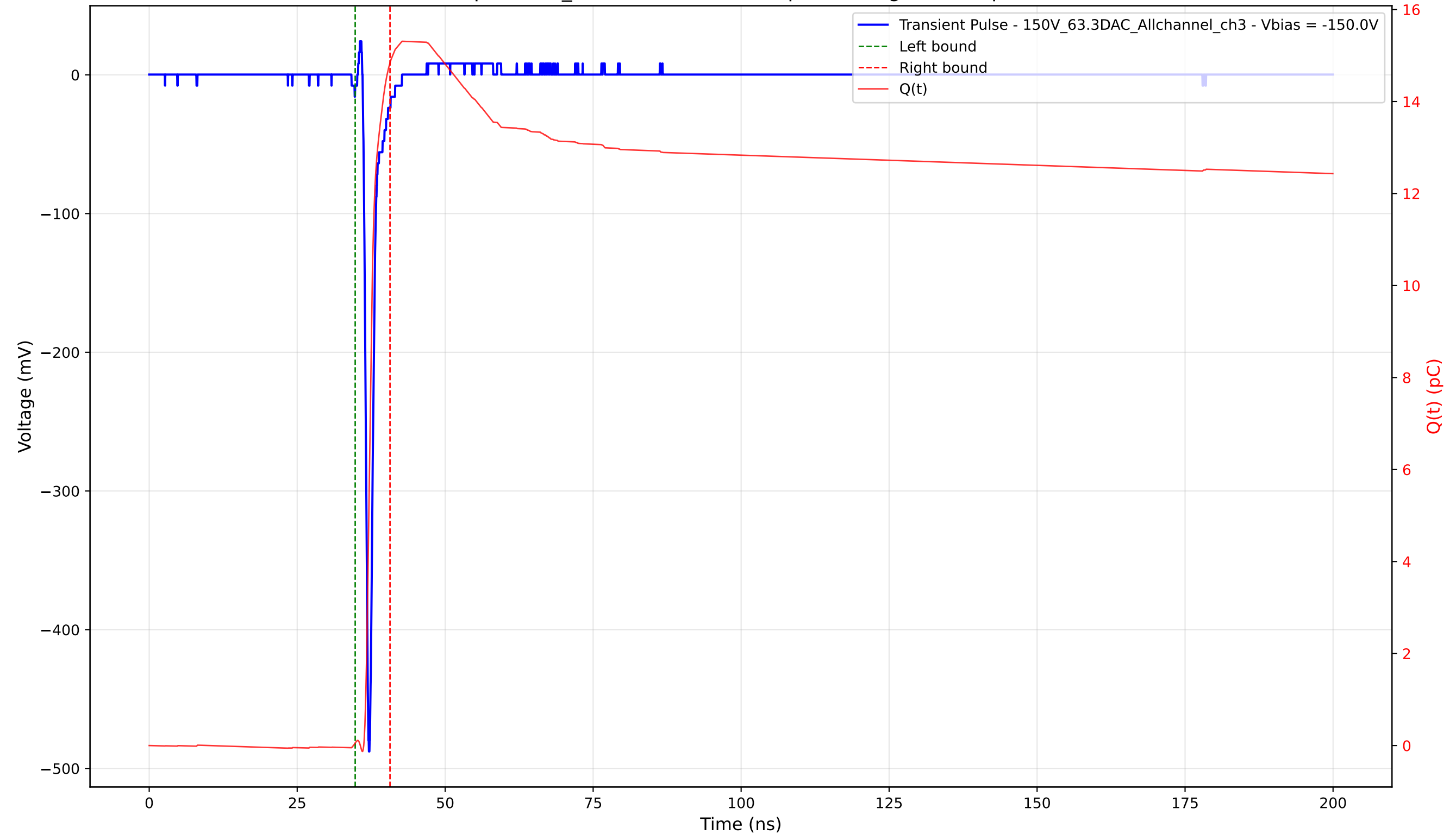
Transient Pulse - Sample: 1cm_42 - Position: 2500.0 \mu\text{m} - Charge: 14.78 pC - Rise Time: 0.72 ns
