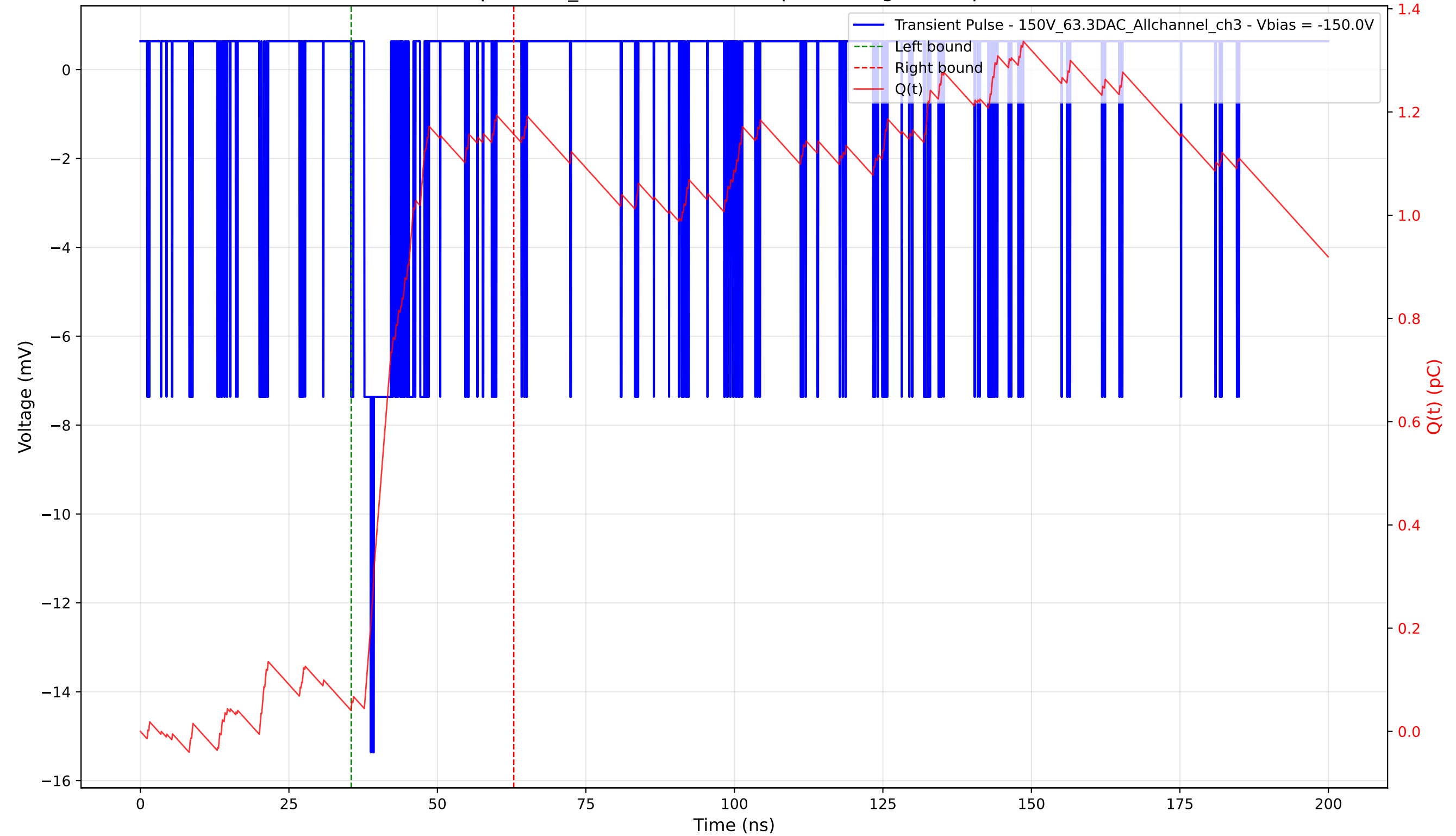
Transient Pulse - Sample: 1cm_42 - Position: 110.0 \mu\text{m} - Charge: 1.11 pC - Rise Time: 1.11 ns
