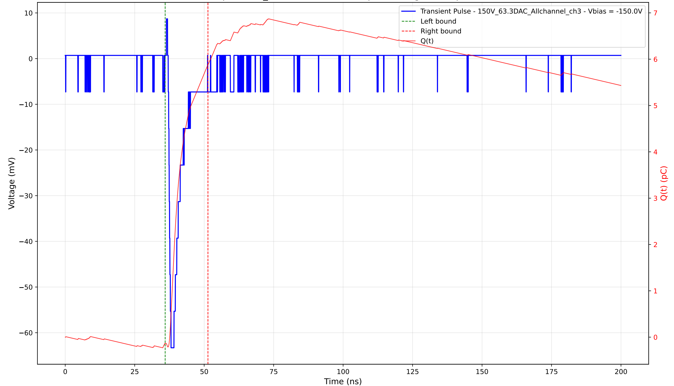
Transient Pulse - Sample: 1cm_42 - Position: 1365.0 \mu\text{m} - Charge: 6.01 pC - Rise Time: 1.01 ns
