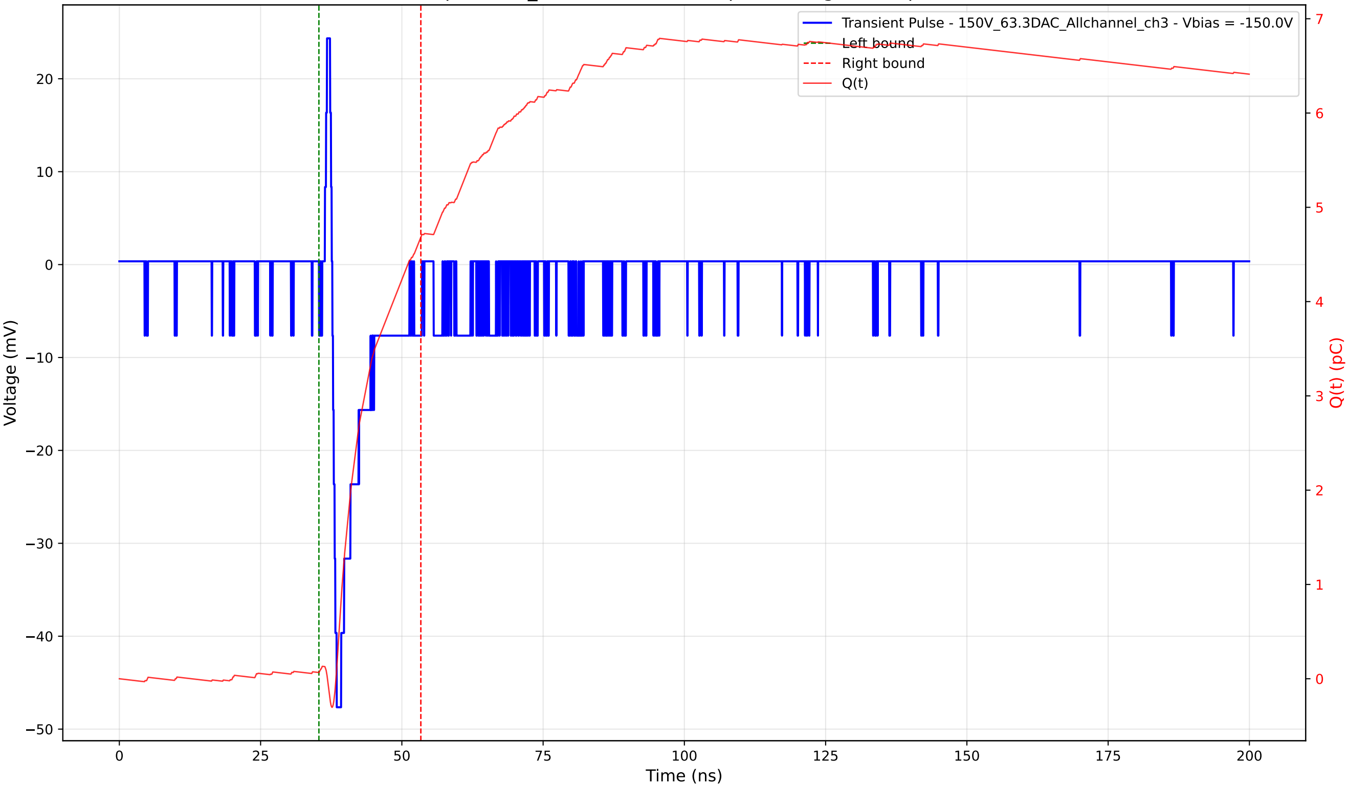
Transient Pulse - Sample: 1cm_42 - Position: 660.0 \mu\text{m} - Charge: 4.62 pC - Rise Time: 0.78 ns
