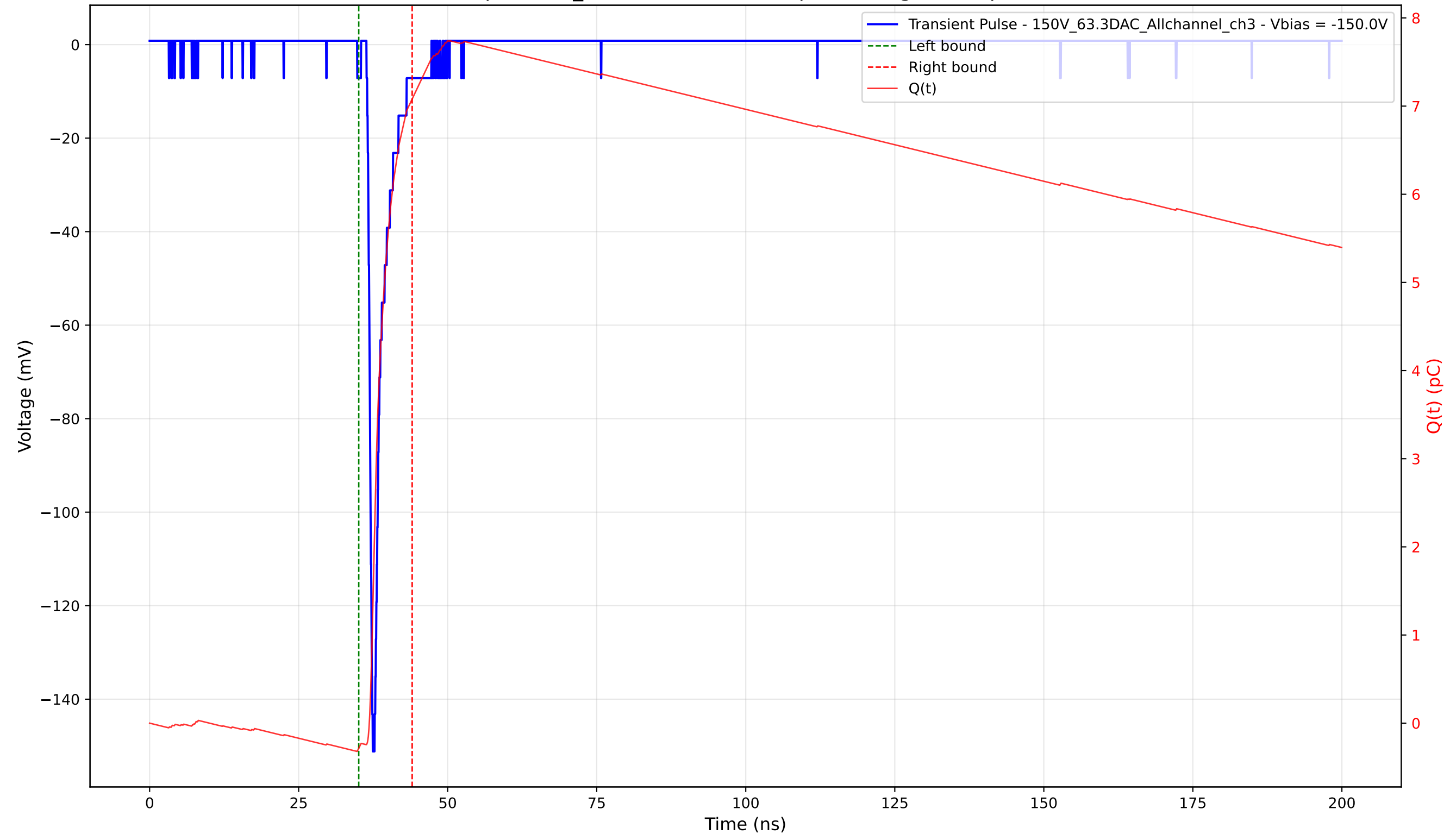
Transient Pulse - Sample: 1cm_42 - Position: 3180.0 \mu\text{m} - Charge: 7.37 pC - Rise Time: 0.84 ns
