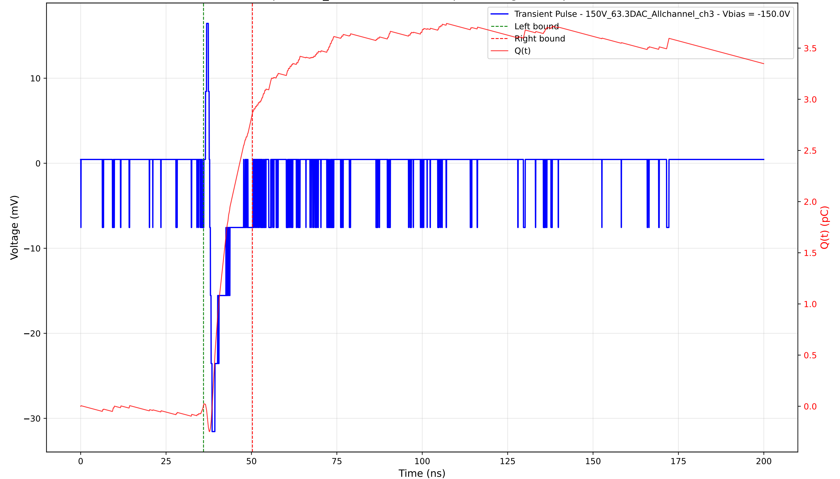
Transient Pulse - Sample: 1cm_42 - Position: 4640.0 \mu\text{m} - Charge: 2.85 pC - Rise Time: 0.70 ns
