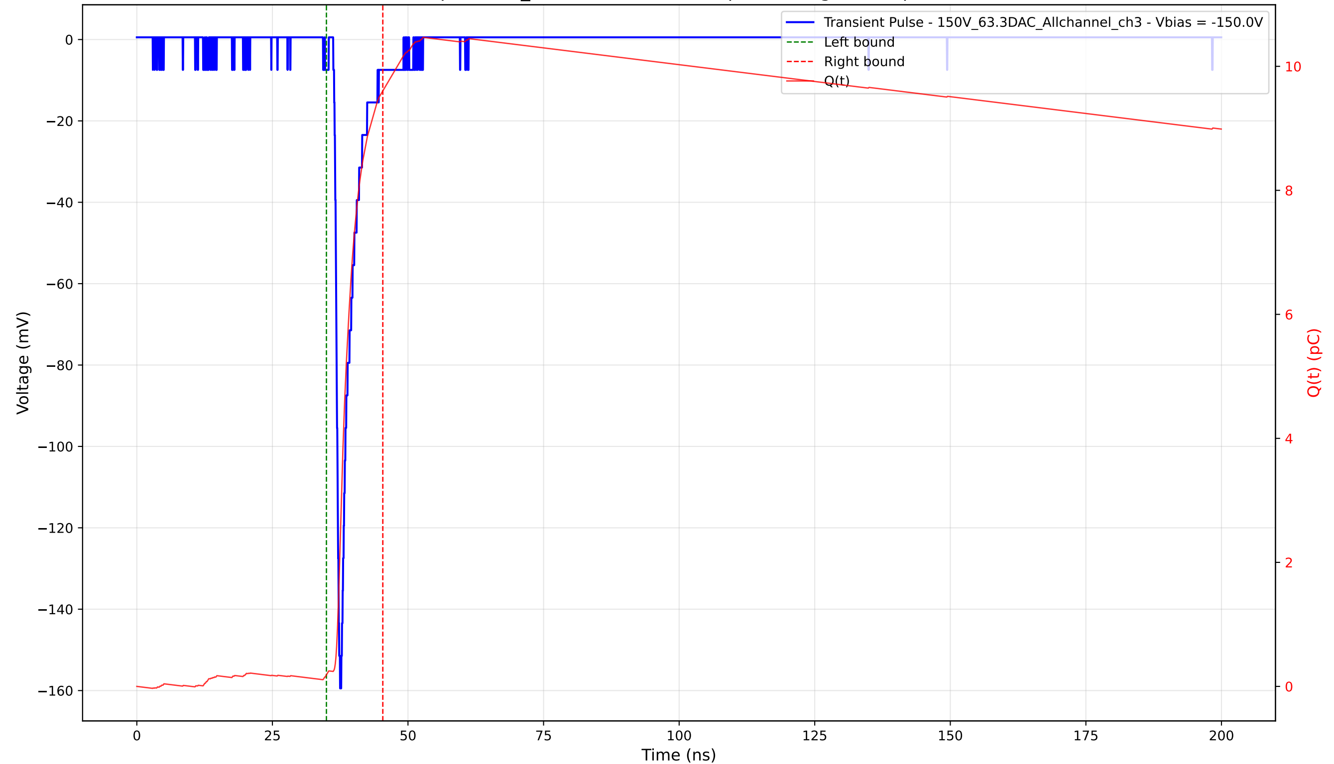
Transient Pulse - Sample: 1cm_42 - Position: 1795.0 \mu\text{m} - Charge: 9.42 pC - Rise Time: 0.88 ns
