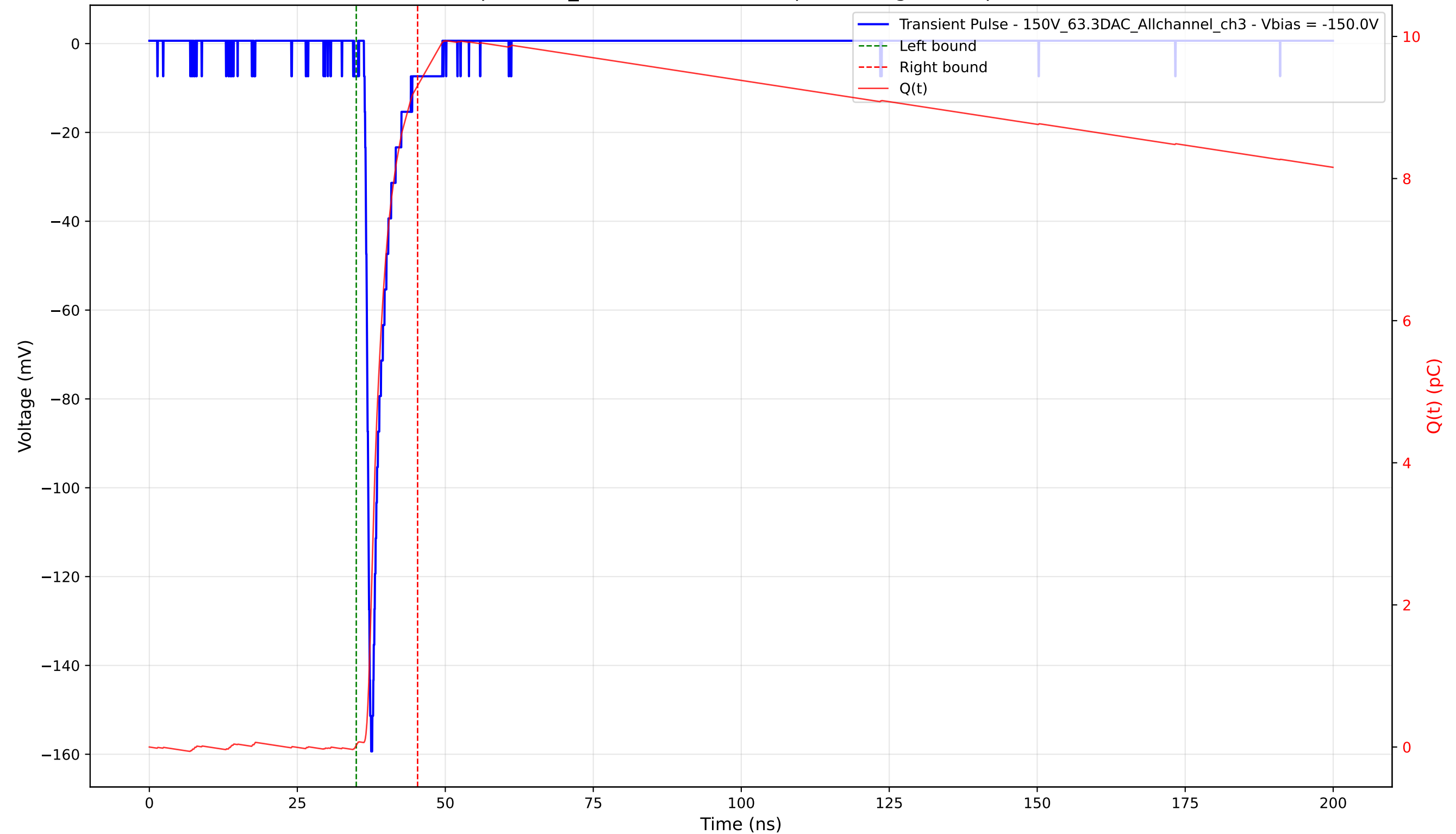
Transient Pulse - Sample: 1cm_42 - Position: 1820.0 \mu\text{m} - Charge: 9.28 pC - Rise Time: 0.88 ns
