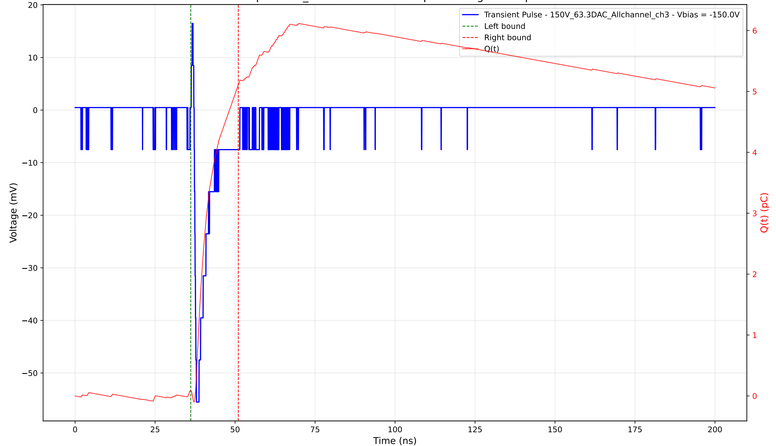
Transient Pulse - Sample: 1cm_42 - Position: 3700.0 \mu\text{m} - Charge: 5.03 pC - Rise Time: 0.69 ns
