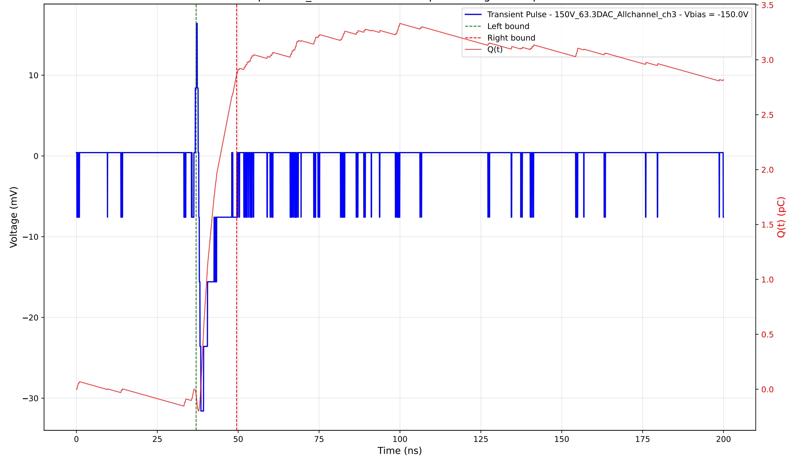
Transient Pulse - Sample: 1cm_42 - Position: 4850.0 \mu\text{m} - Charge: 2.92 pC - Rise Time: 0.66 ns
