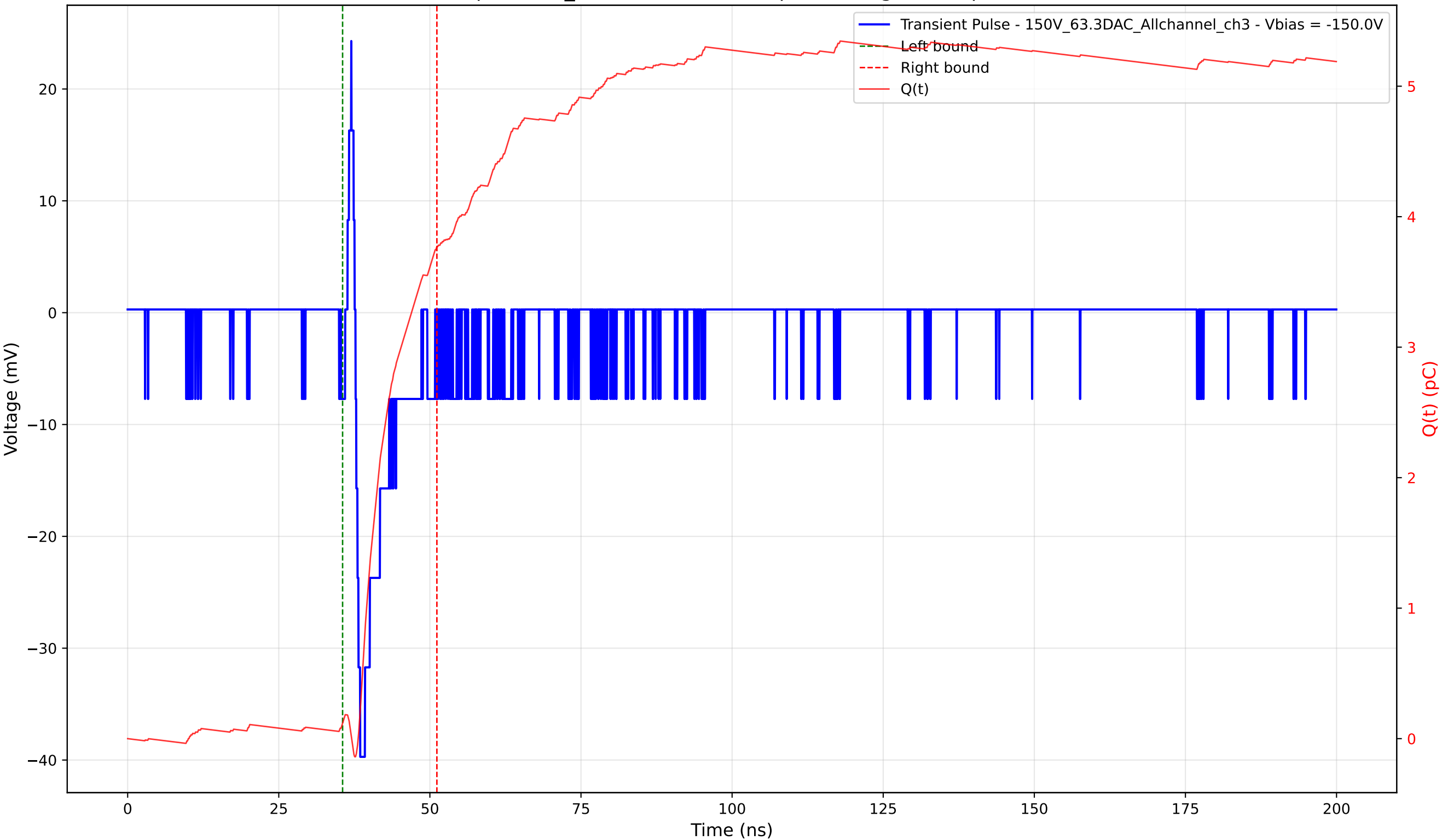
Transient Pulse - Sample: 1cm_42 - Position: 540.0 \mu\text{m} - Charge: 3.65 pC - Rise Time: 0.78 ns
