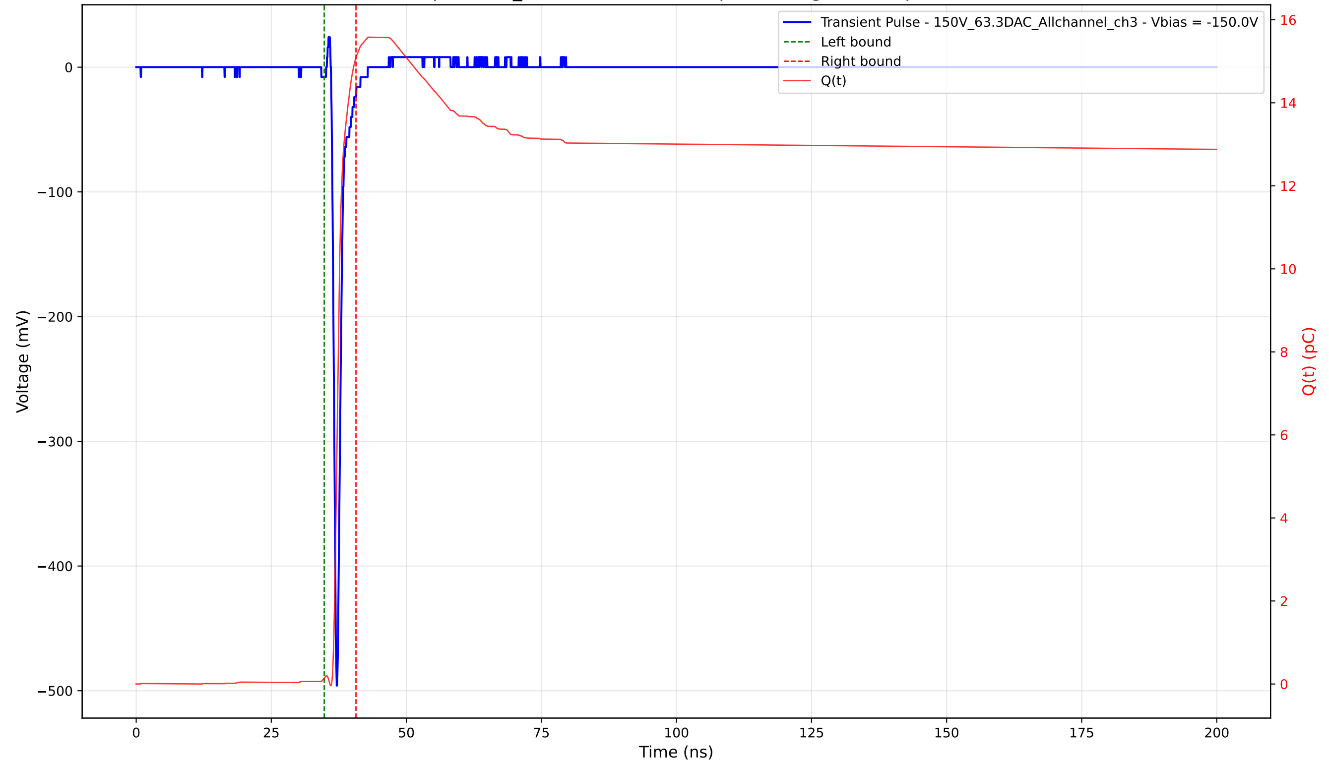
Transient Pulse - Sample: 1cm_42 - Position: 2480.0 \mu\text{m} - Charge: 14.95 pC - Rise Time: 0.71 ns
