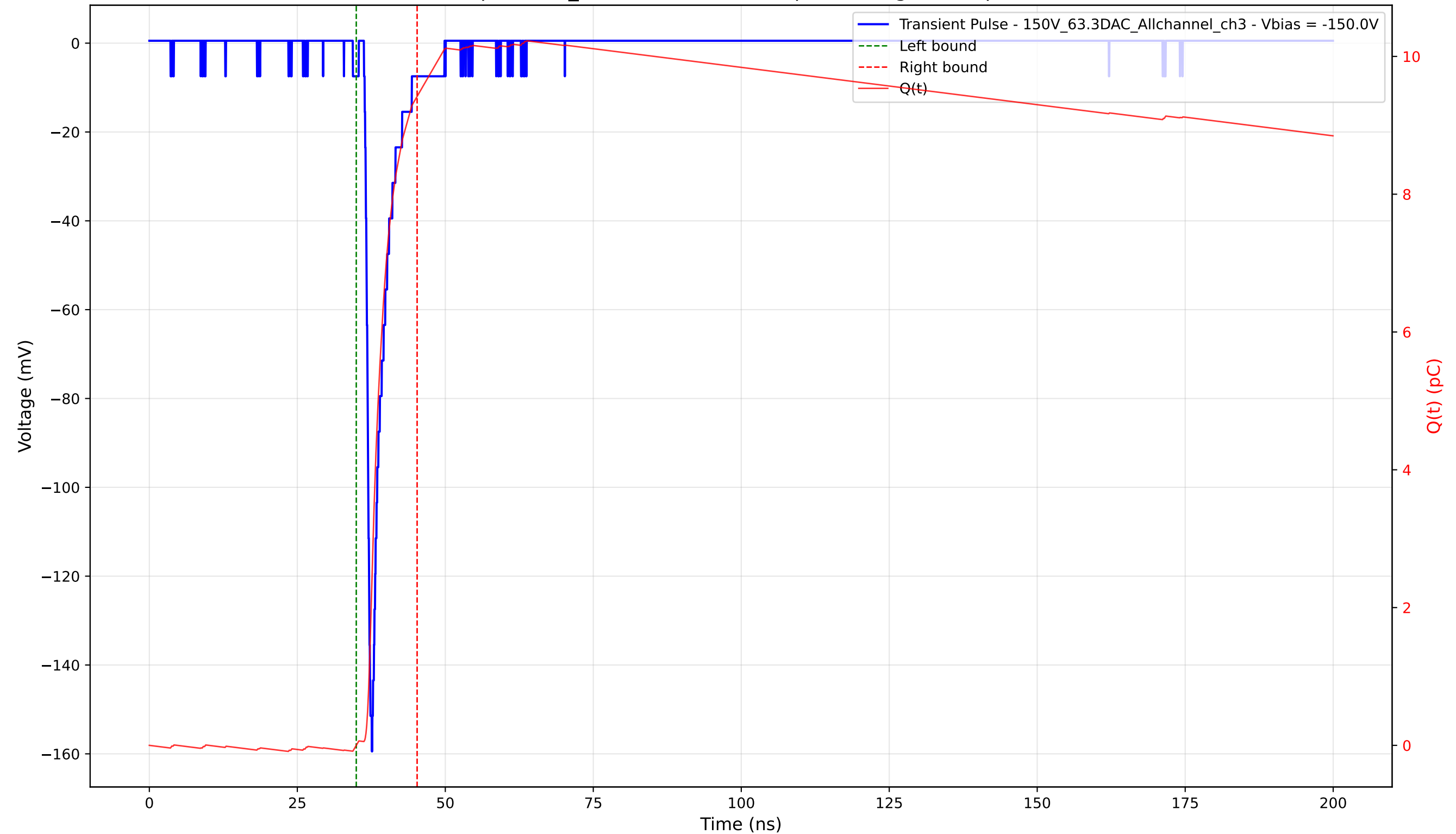
Transient Pulse - Sample: 1cm_42 - Position: 1765.0 \mu\text{m} - Charge: 9.42 pC - Rise Time: 0.92 ns
