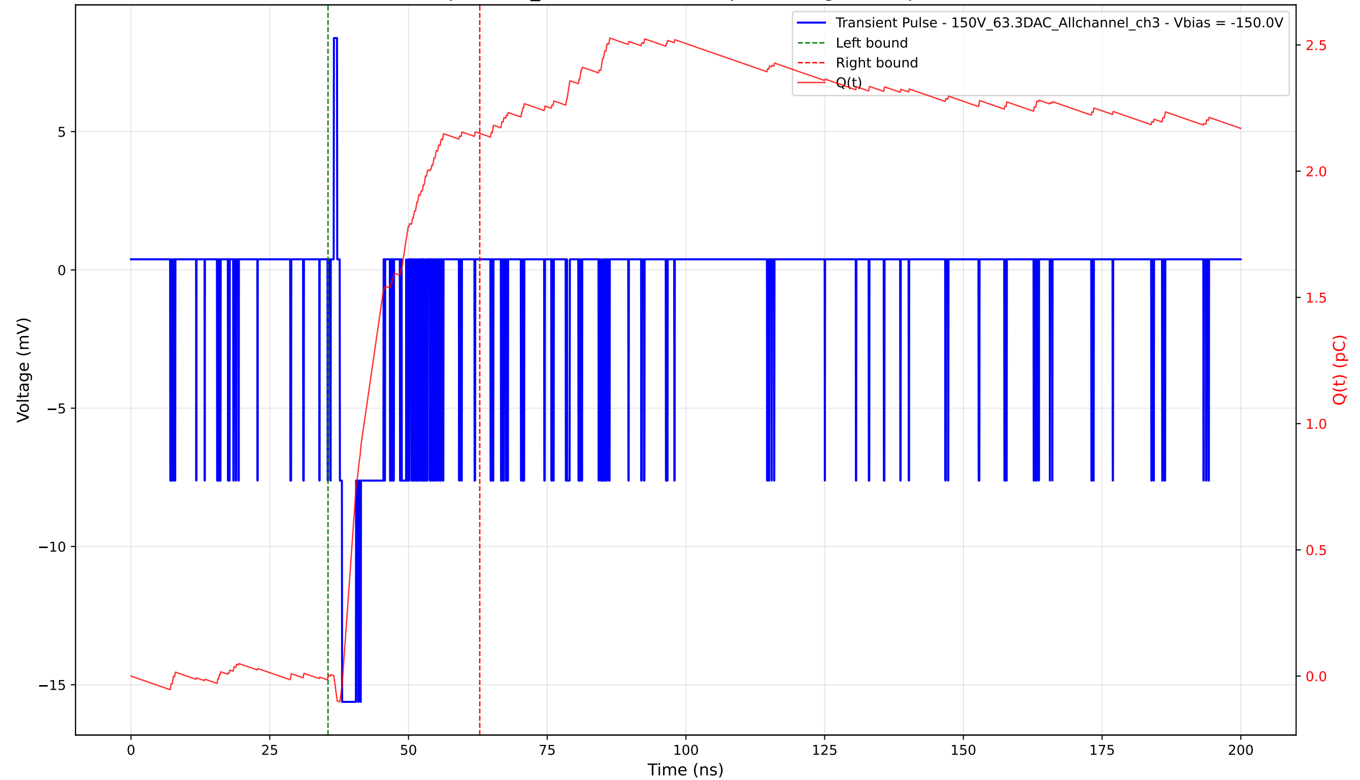
Transient Pulse - Sample: 1cm_42 - Position: 200.0 \mu\text{m} - Charge: 2.15 pC - Rise Time: 0.43 ns
