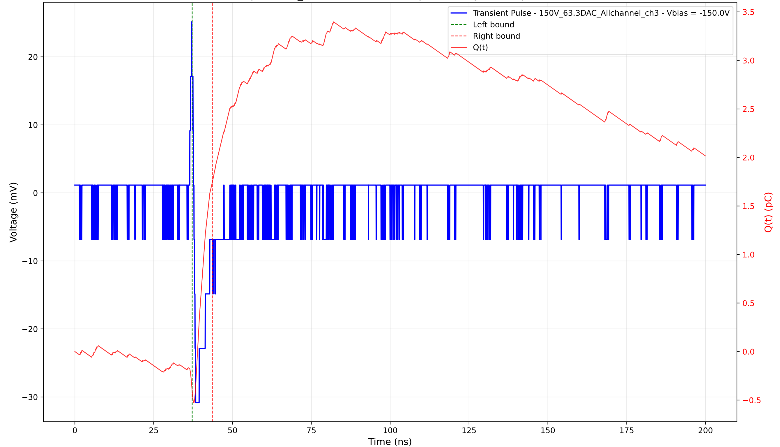
Transient Pulse - Sample: 1cm_42 - Position: 4425.0 \mu\text{m} - Charge: 2.14 pC - Rise Time: 0.55 ns
