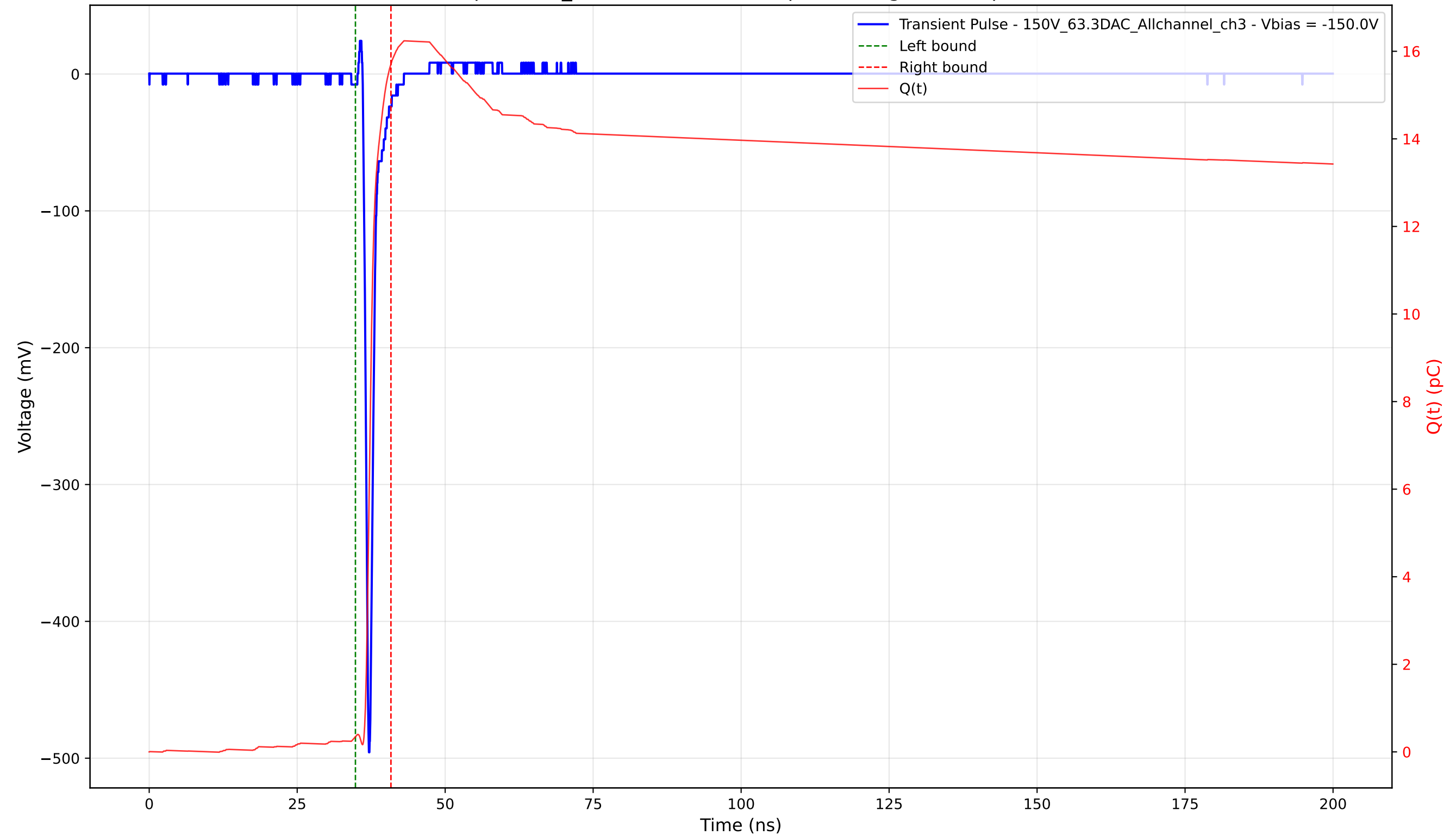
Transient Pulse - Sample: 1cm_42 - Position: 2645.0 \mu\text{m} - Charge: 15.36 pC - Rise Time: 0.73 ns
