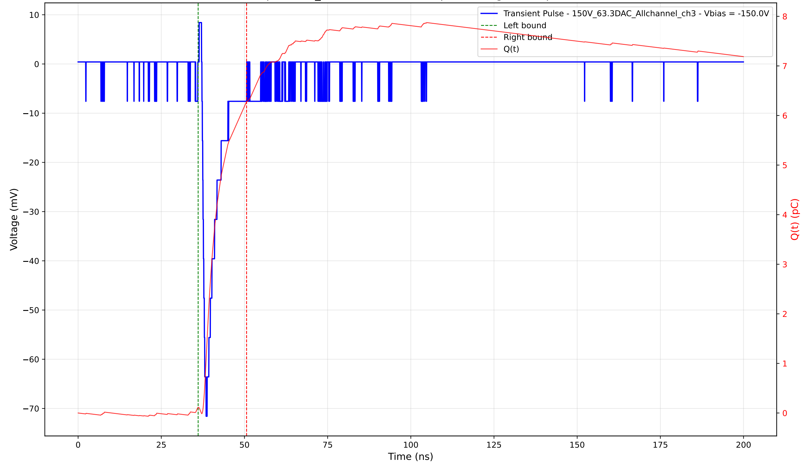
Transient Pulse - Sample: 1cm_42 - Position: 1235.0 \mu\text{m} - Charge: 6.17 pC - Rise Time: 1.24 ns
