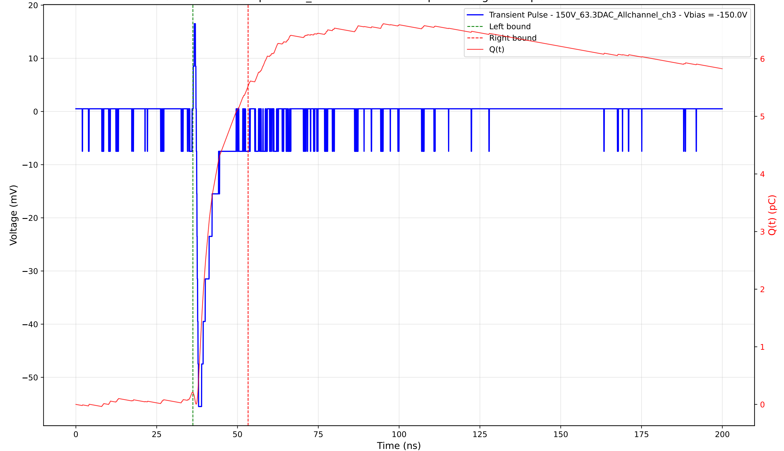
Transient Pulse - Sample: 1cm_42 - Position: 3735.0 \mu\text{m} - Charge: 5.32 pC - Rise Time: 0.69 ns
