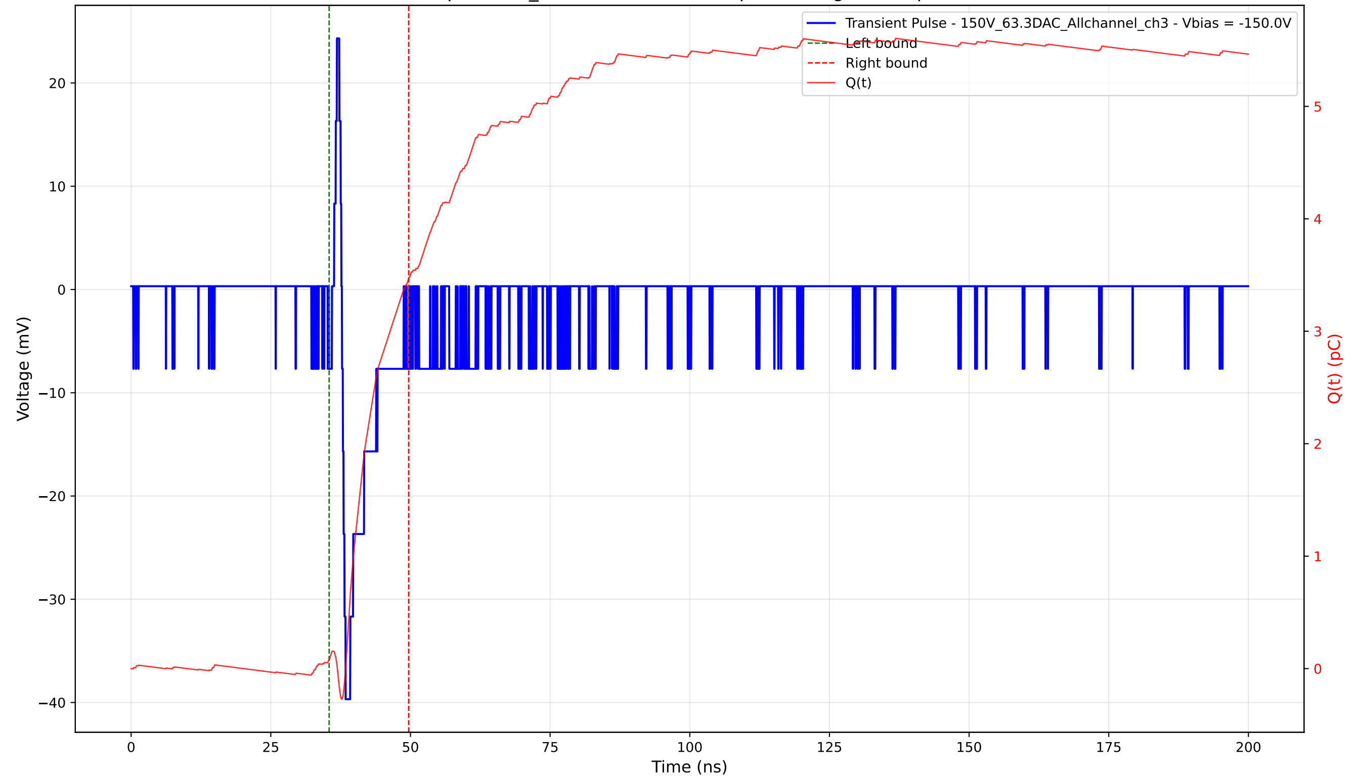
Transient Pulse - Sample: 1cm_42 - Position: 4305.0 \mu\text{m} - Charge: 3.39 pC - Rise Time: 0.66 ns
