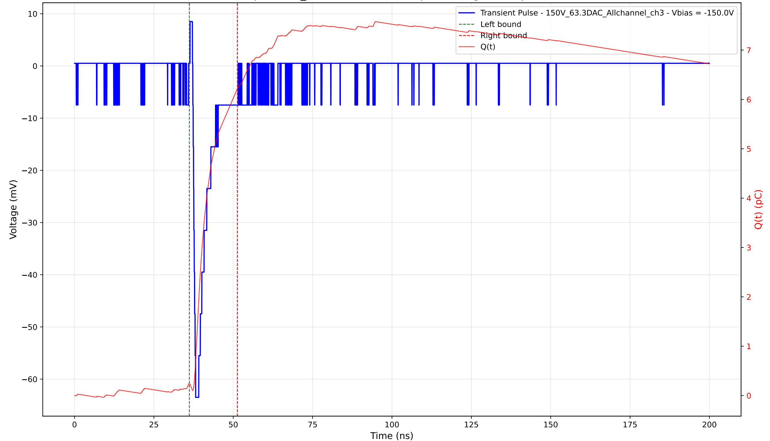
Transient Pulse - Sample: 1cm_42 - Position: 1205.0 \mu\text{m} - Charge: 5.99 pC - Rise Time: 0.89 ns
