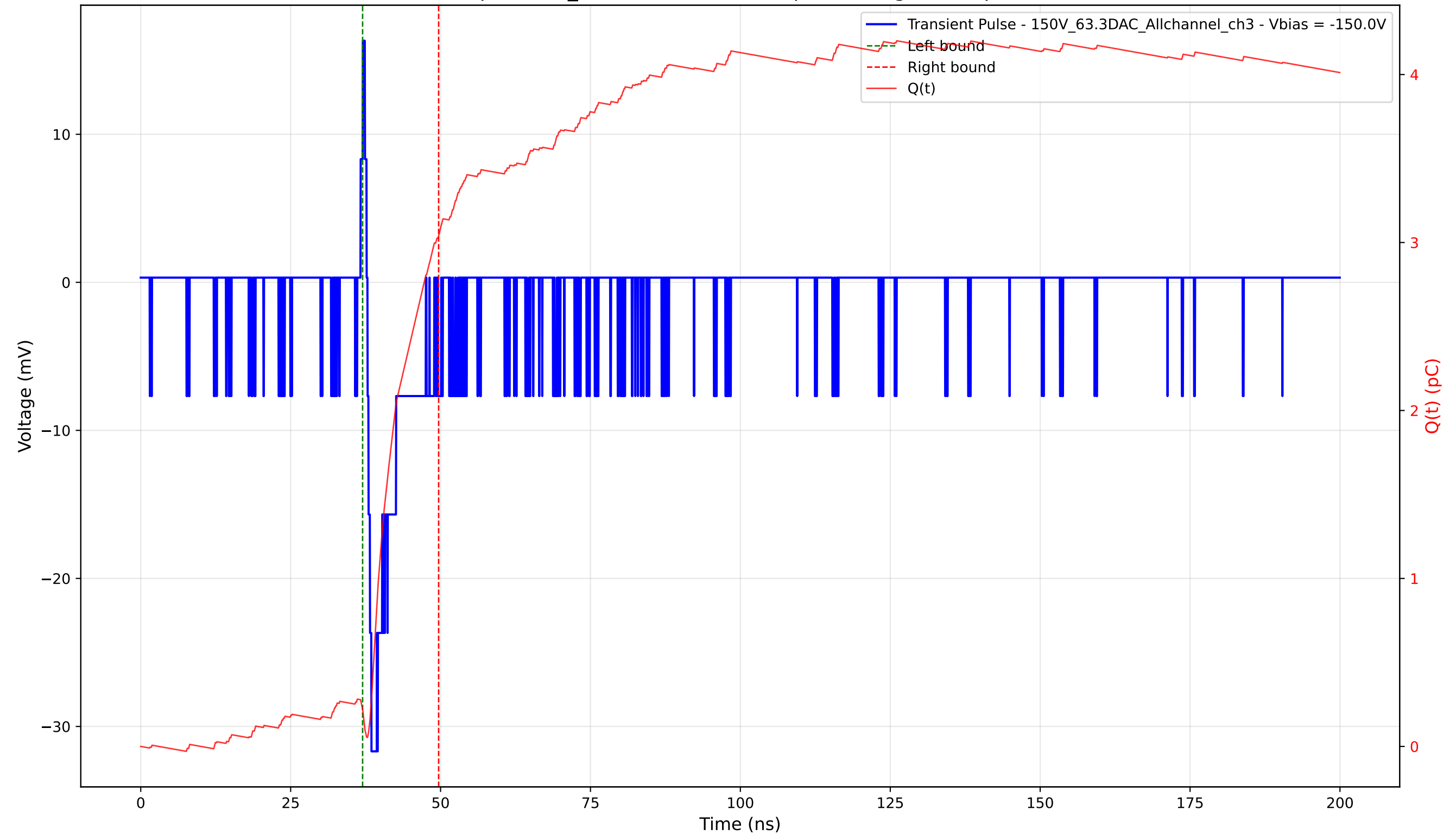
Transient Pulse - Sample: 1cm_42 - Position: 4810.0 \mu\text{m} - Charge: 2.82 pC - Rise Time: 0.66 ns
