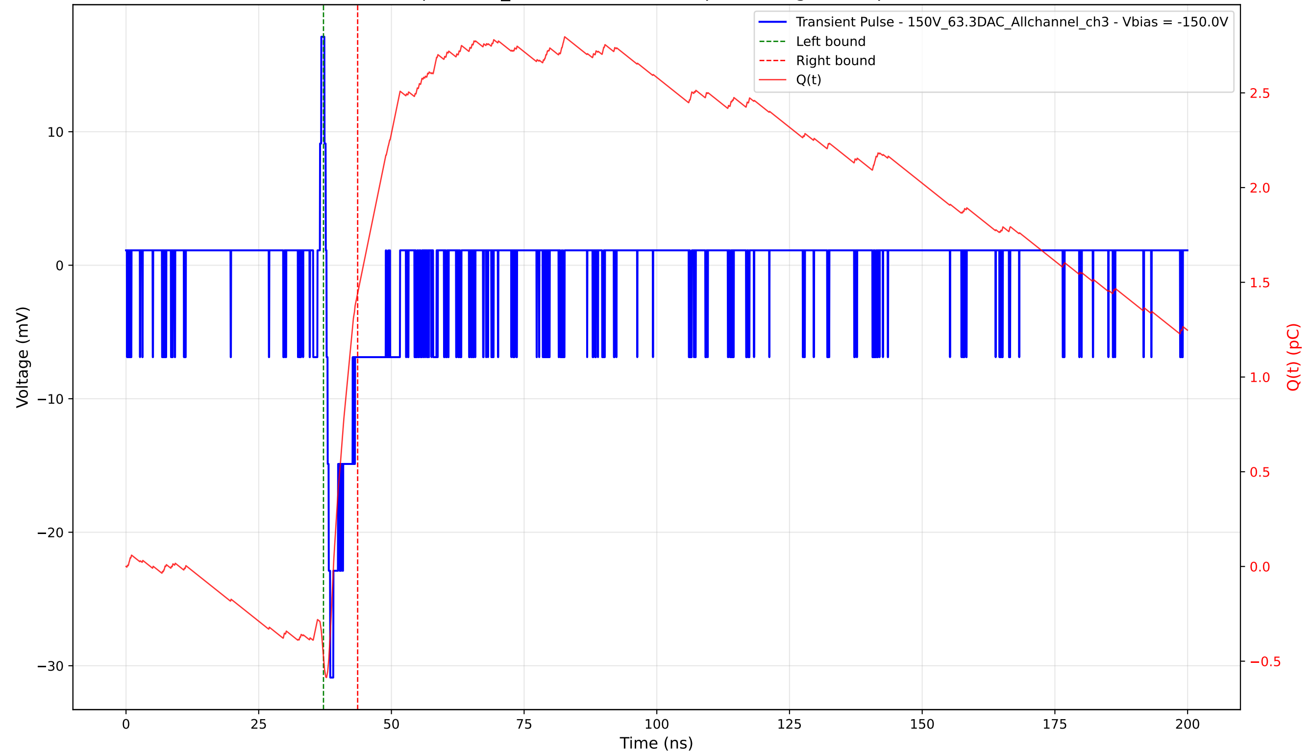
Transient Pulse - Sample: 1cm_42 - Position: 4535.0 \mu\text{m} - Charge: 1.92 pC - Rise Time: 0.71 ns
