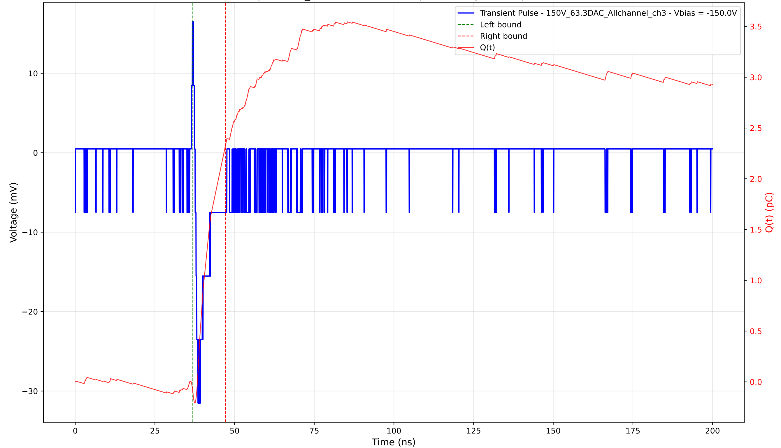
Transient Pulse - Sample: 1cm_42 - Position: 380.0 \mu\text{m} - Charge: 2.42 pC - Rise Time: 0.90 ns
