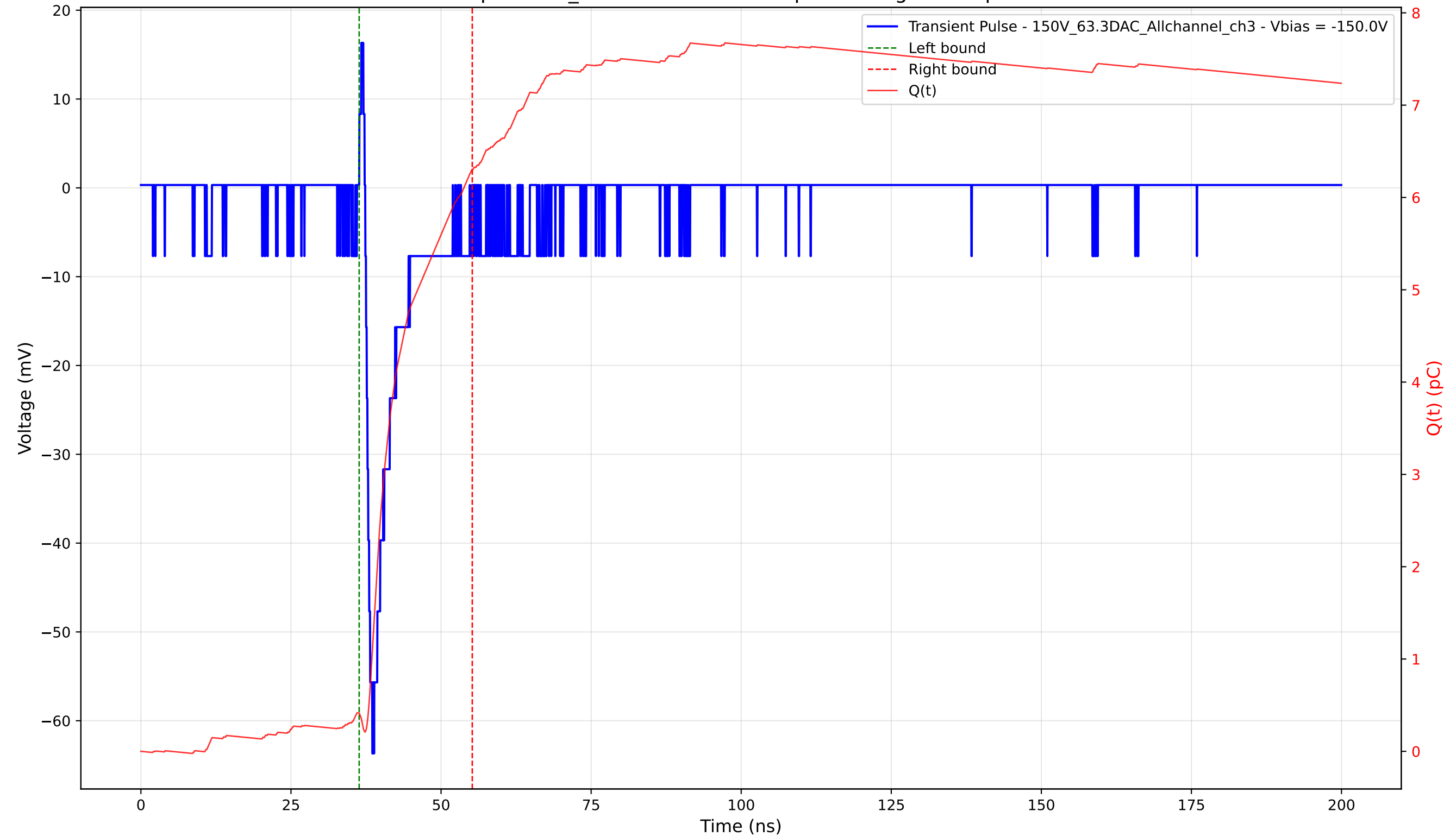
Transient Pulse - Sample: 1cm_42 - Position: 1130.0 \mu\text{m} - Charge: 5.89 pC - Rise Time: 1.17 ns
