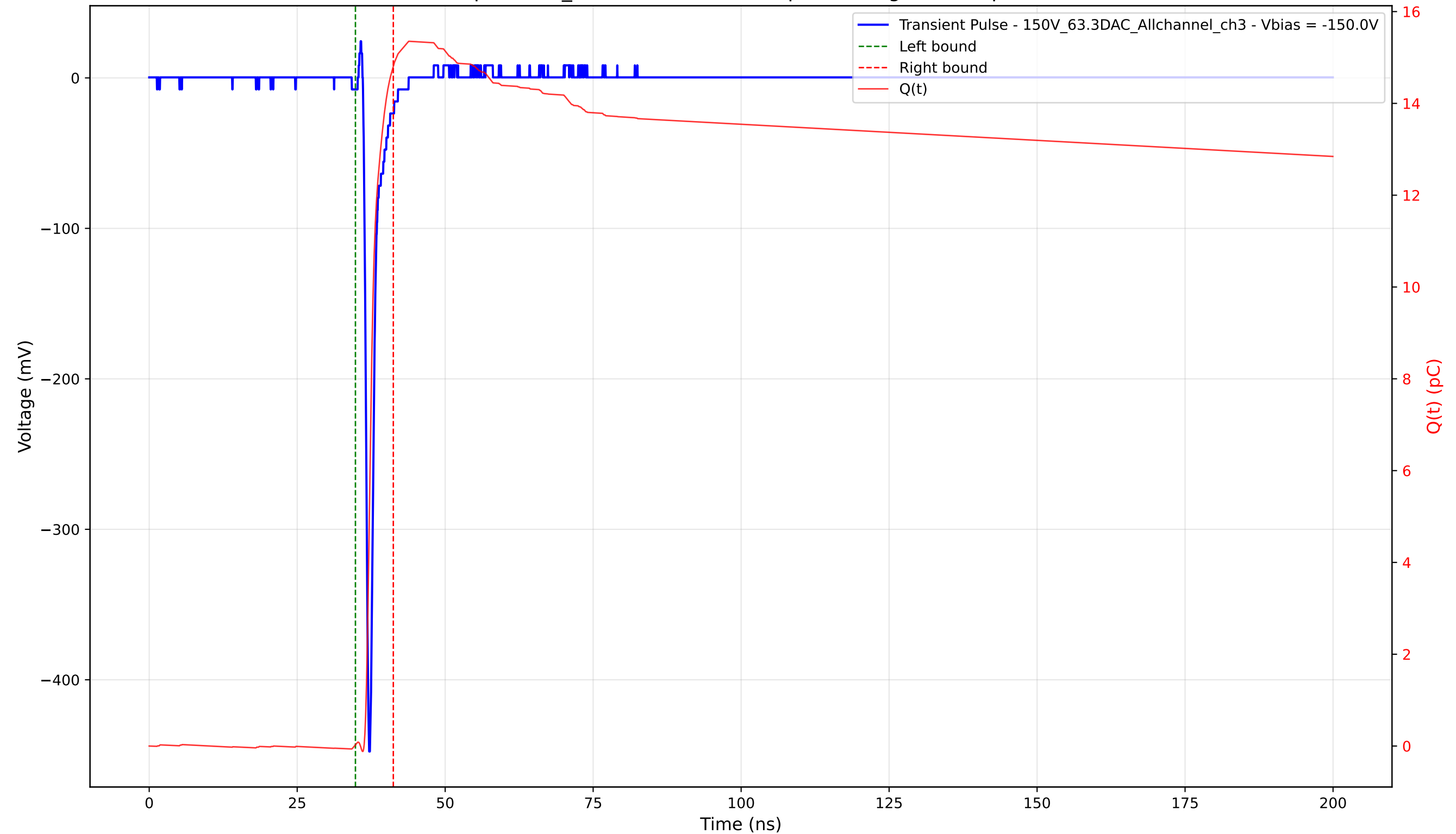
Transient Pulse - Sample: 1cm_42 - Position: 2245.0 \mu\text{m} - Charge: 14.78 pC - Rise Time: 0.68 ns
