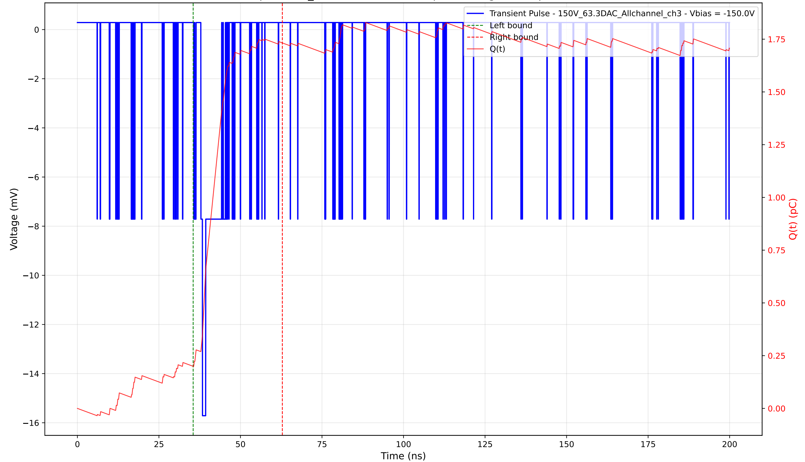
Transient Pulse - Sample: 1cm_42 - Position: 5060.0 \mu\text{m} - Charge: 1.53 pC - Rise Time: 0.51 ns
