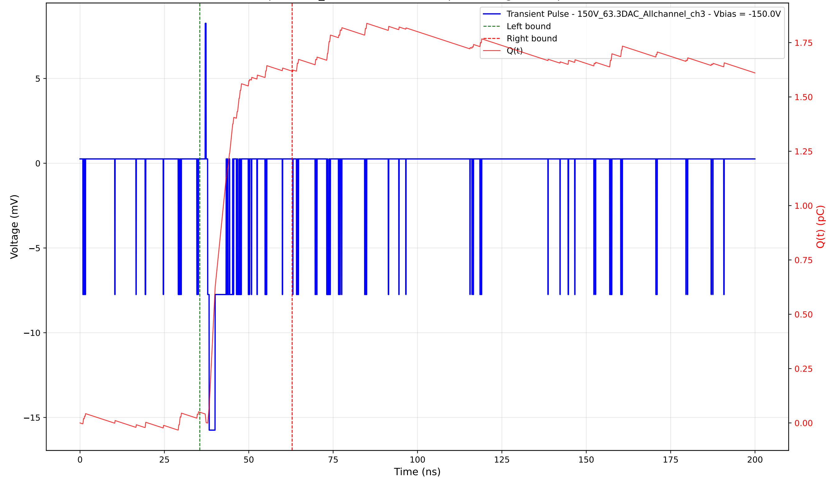
Transient Pulse - Sample: 1cm_42 - Position: 5020.0 \mu\text{m} - Charge: 1.57 pC - Rise Time: 0.47 ns
