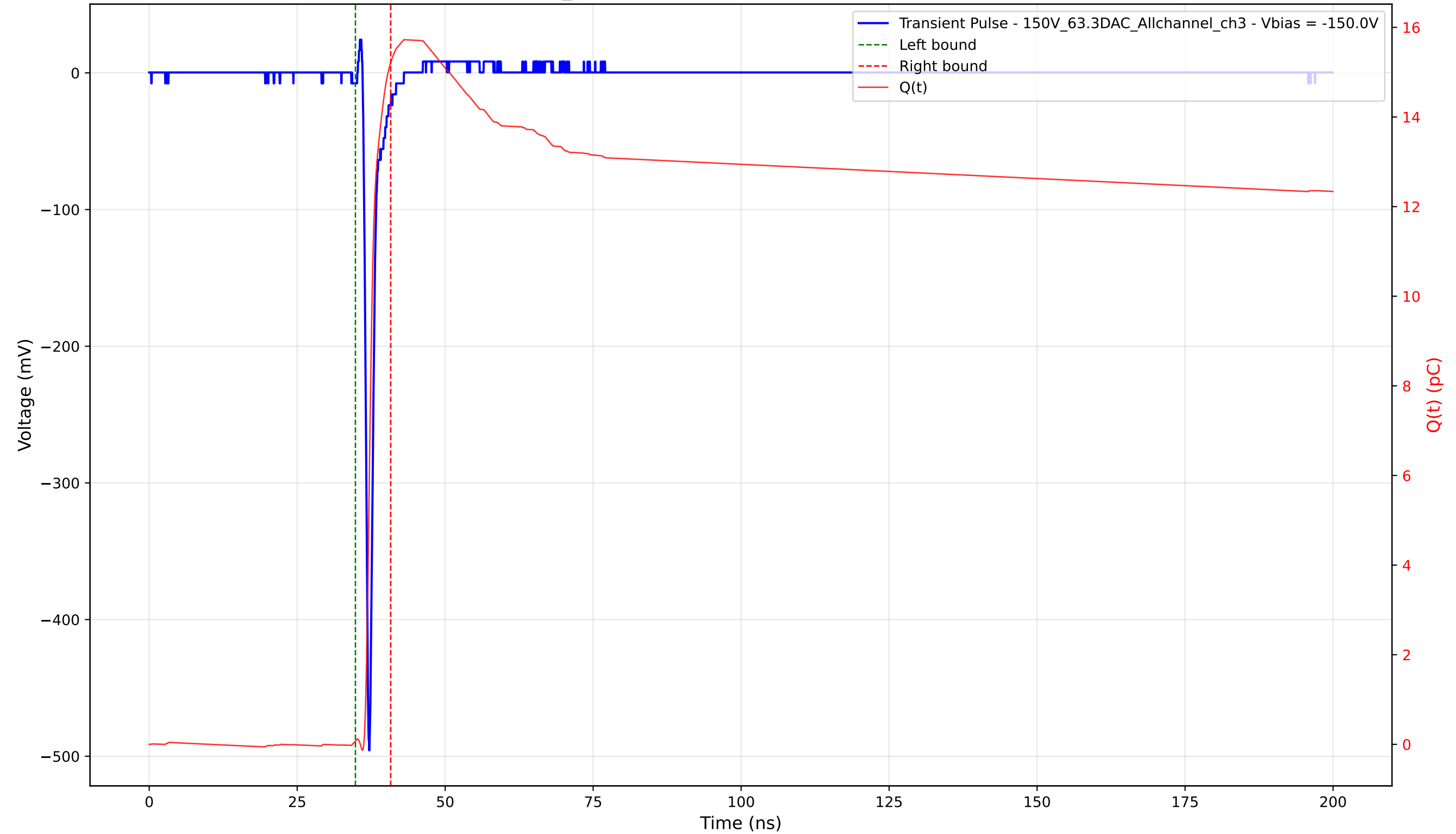
Transient Pulse - Sample: 1cm_42 - Position: 2615.0 \mu\text{m} - Charge: 15.14 pC - Rise Time: 0.73 ns
