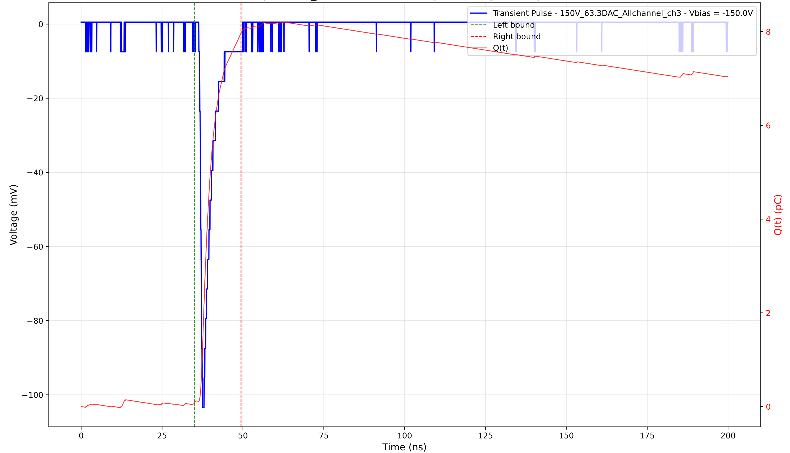
Transient Pulse - Sample: 1cm_42 - Position: 1615.0 \mu\text{m} - Charge: 7.87 pC - Rise Time: 0.87 ns
