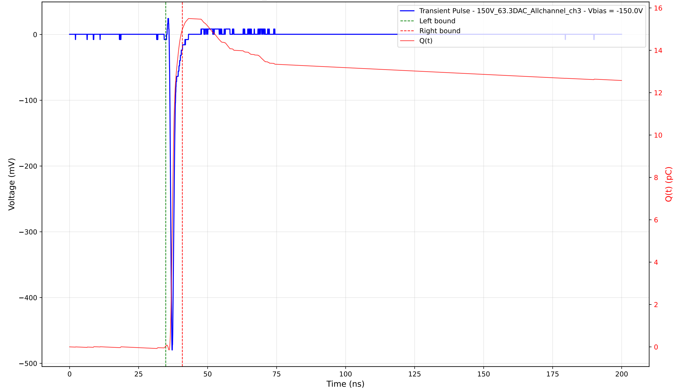
Transient Pulse - Sample: 1cm_42 - Position: 2380.0 \mu\text{m} - Charge: 14.95 pC - Rise Time: 0.74 ns
