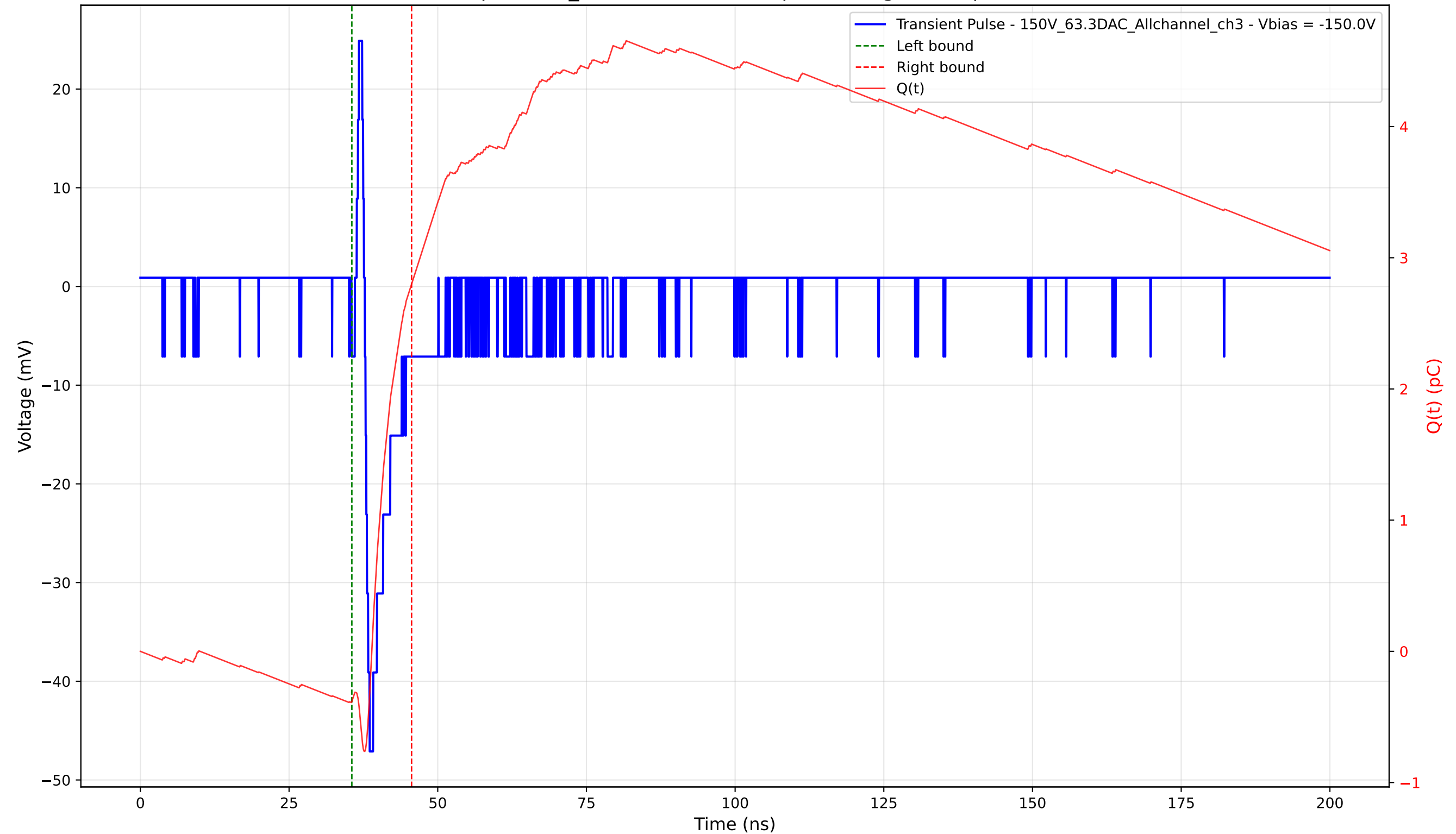
Transient Pulse - Sample: 1cm_42 - Position: 645.0 \mu\text{m} - Charge: 3.18 pC - Rise Time: 0.82 ns
