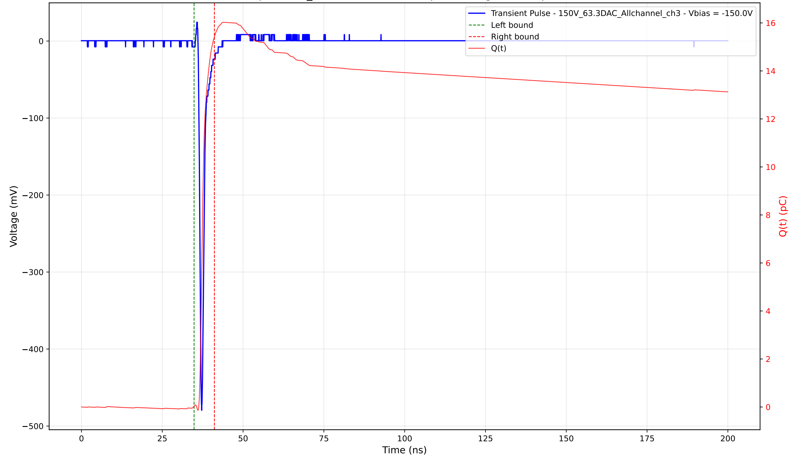
Transient Pulse - Sample: 1cm_42 - Position: 2295.0 \mu\text{m} - Charge: 15.38 pC - Rise Time: 0.68 ns
