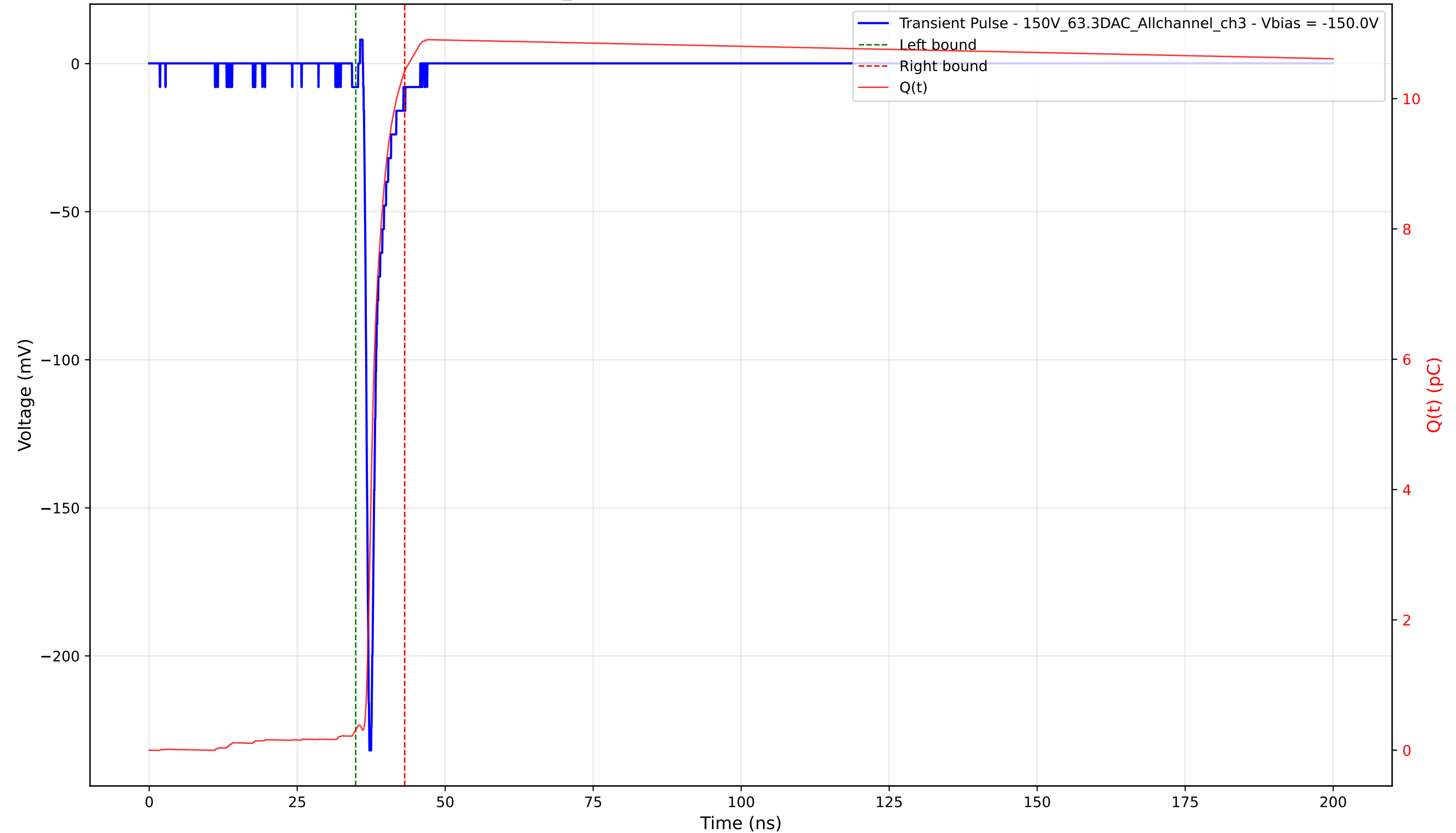
Transient Pulse - Sample: 1cm_42 - Position: 2020.0 \mu\text{m} - Charge: 10.10 pC - Rise Time: 0.76 ns
