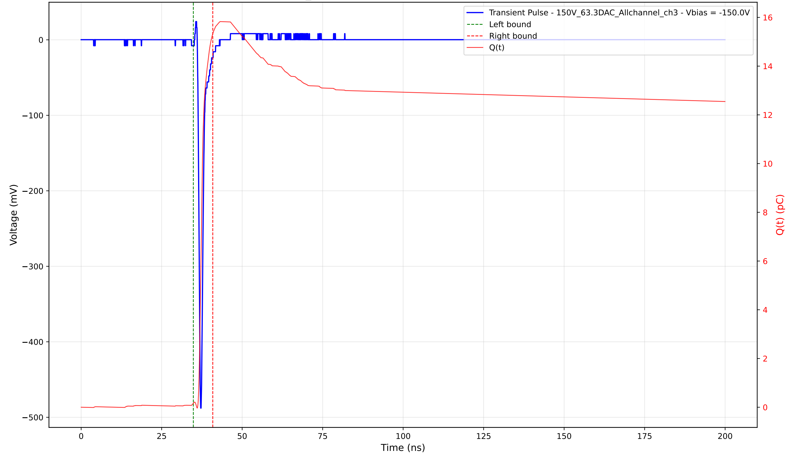
Transient Pulse - Sample: 1cm_42 - Position: 2640.0 \mu\text{m} - Charge: 15.17 pC - Rise Time: 0.71 ns
