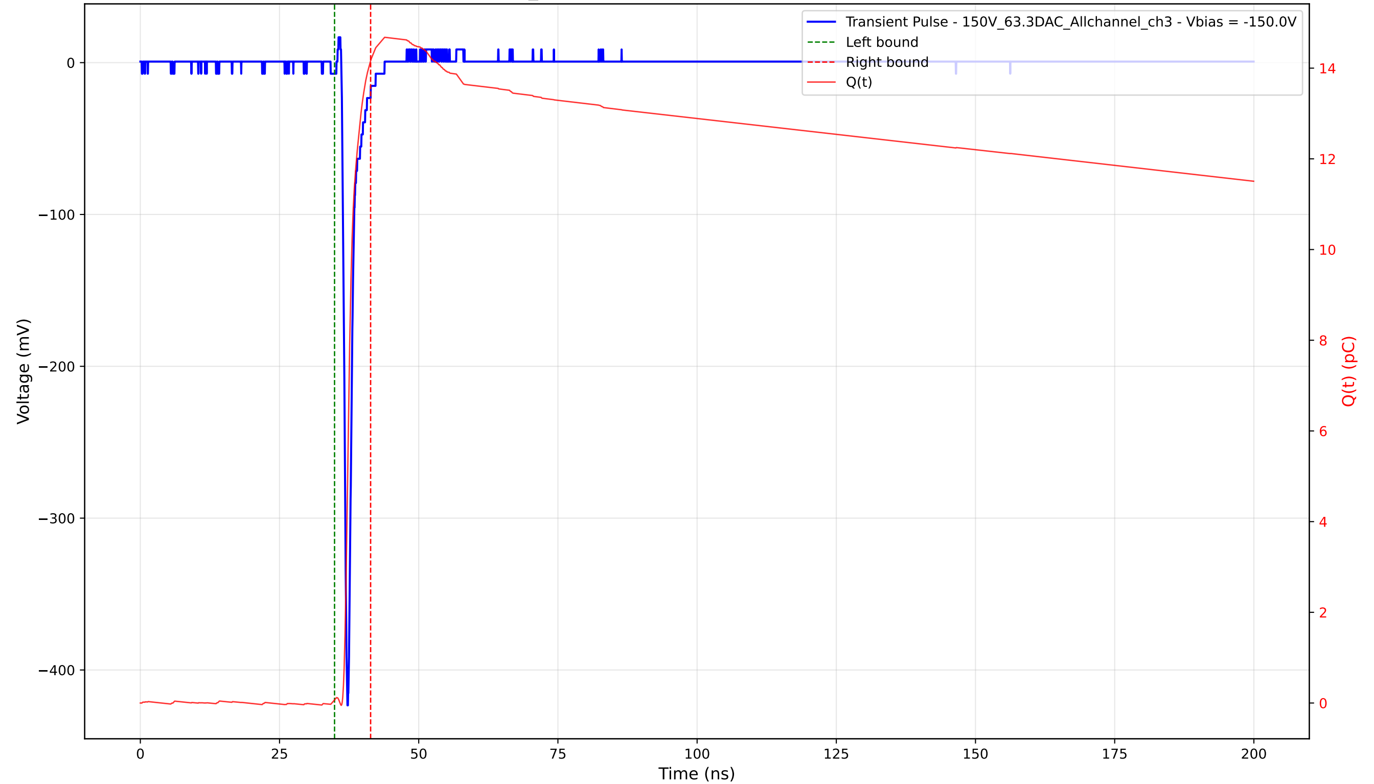
Transient Pulse - Sample: 1cm_42 - Position: 2835.0 \mu\text{m} - Charge: 14.10 pC - Rise Time: 0.73 ns
