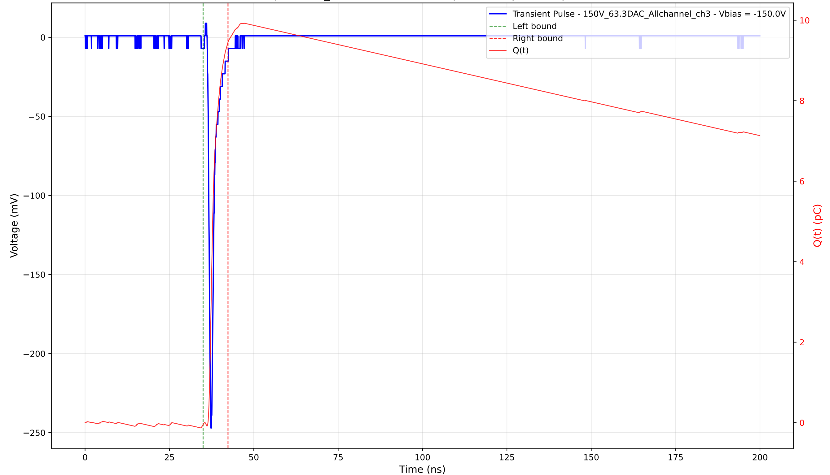
Transient Pulse - Sample: 1cm_42 - Position: 2990.0 \mu\text{m} - Charge: 9.51 pC - Rise Time: 0.75 ns
