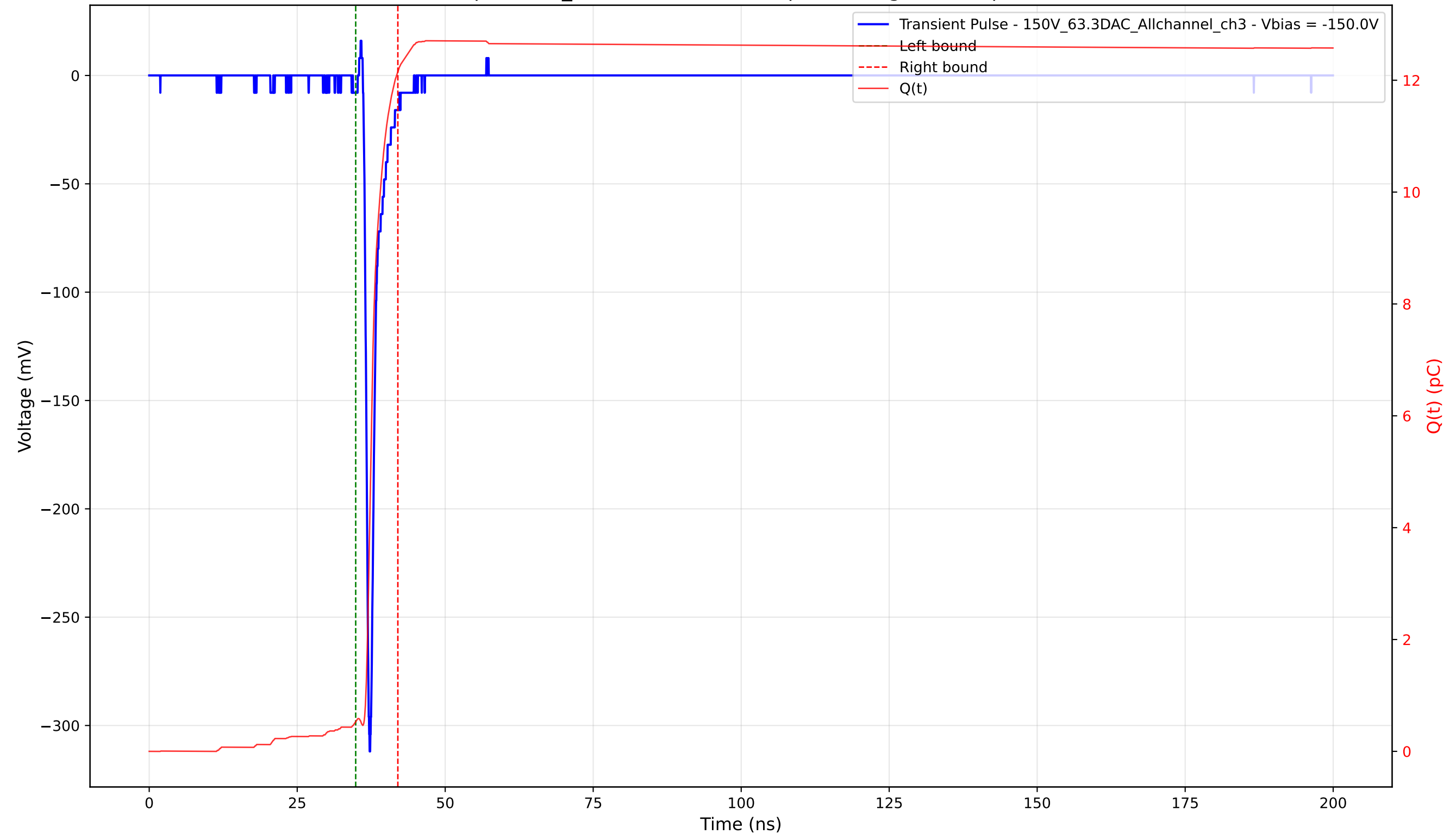
Transient Pulse - Sample: 1cm_42 - Position: 2105.0 \mu\text{m} - Charge: 11.62 pC - Rise Time: 0.73 ns
