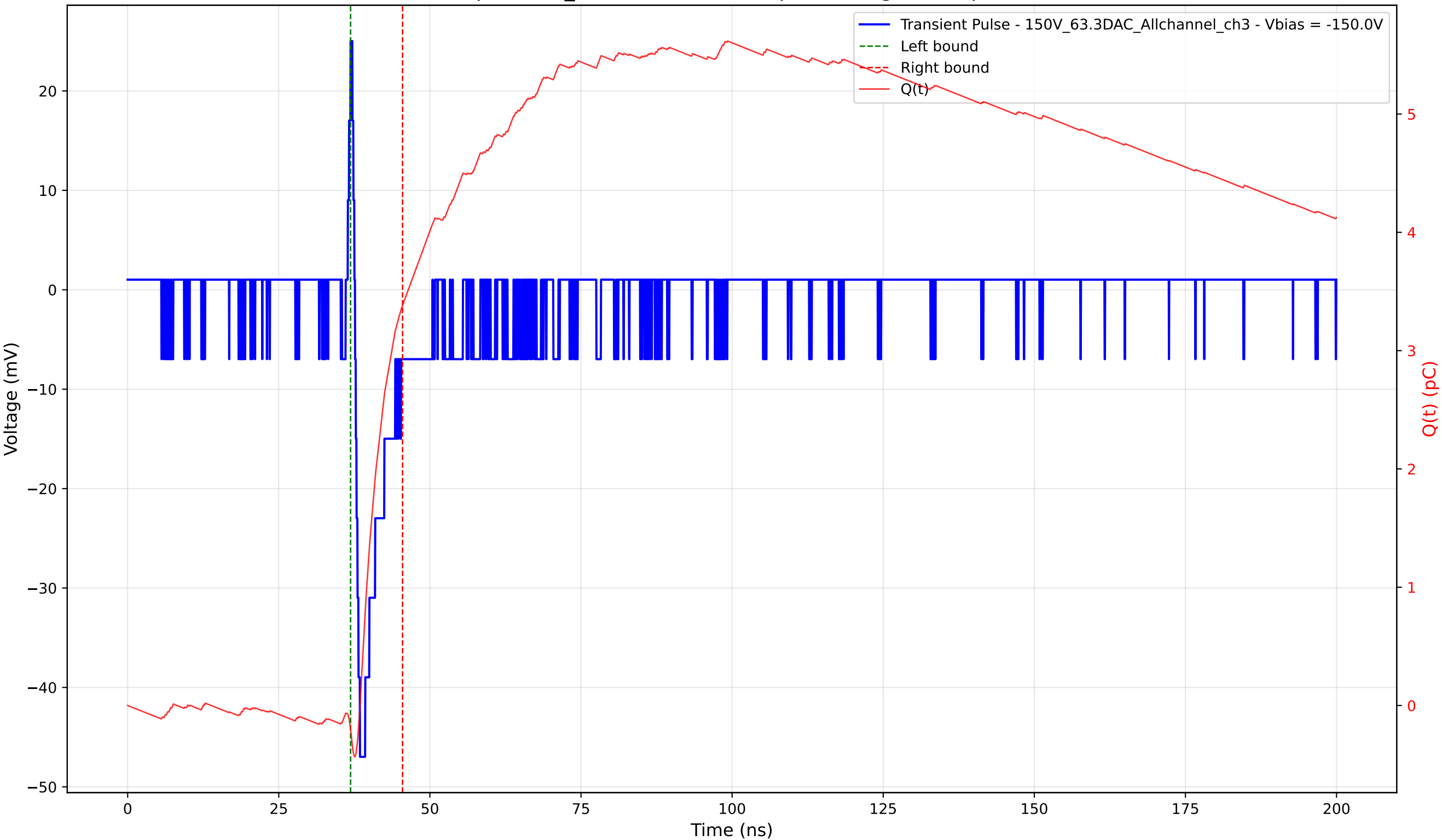
Transient Pulse - Sample: 1cm_42 - Position: 930.0 \mu\text{m} - Charge: 3.58 pC - Rise Time: 0.82 ns
