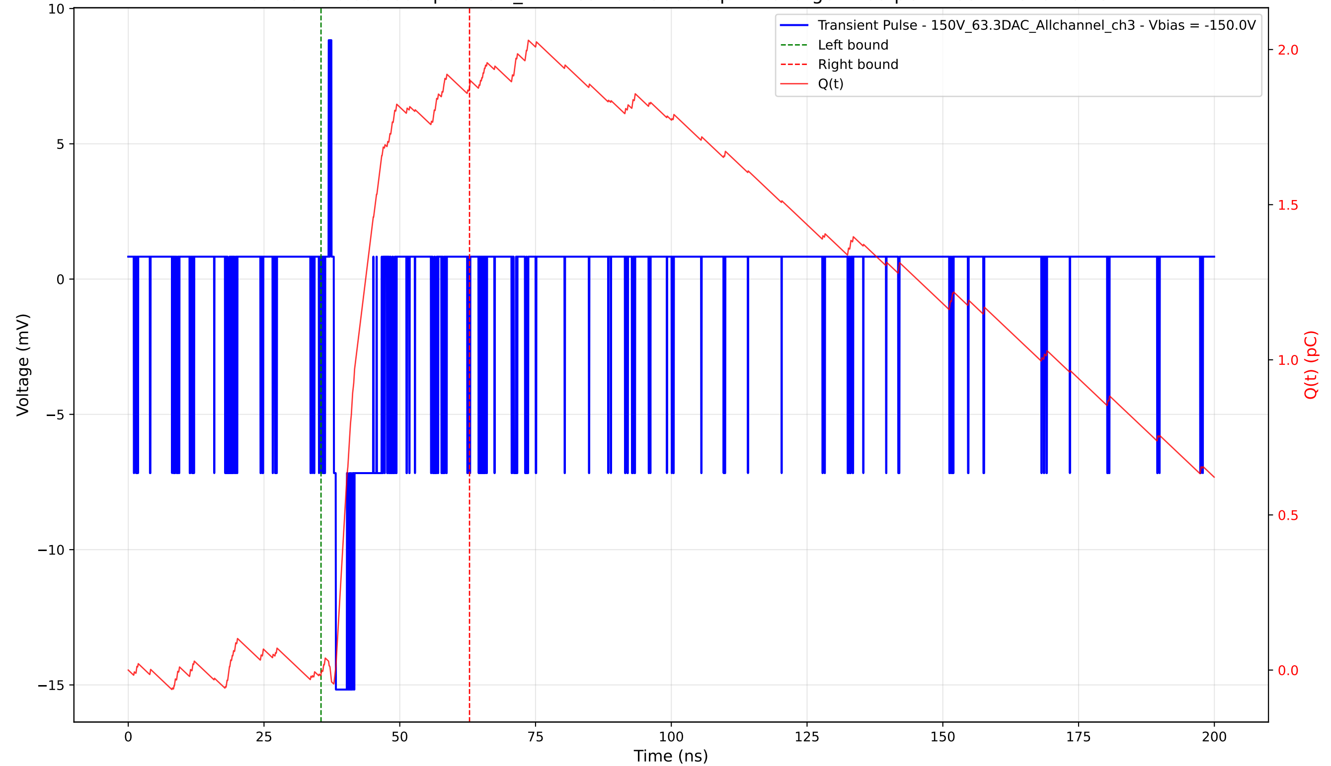
Transient Pulse - Sample: 1cm_42 - Position: 5000.0 \mu\text{m} - Charge: 1.89 pC - Rise Time: 0.40 ns
