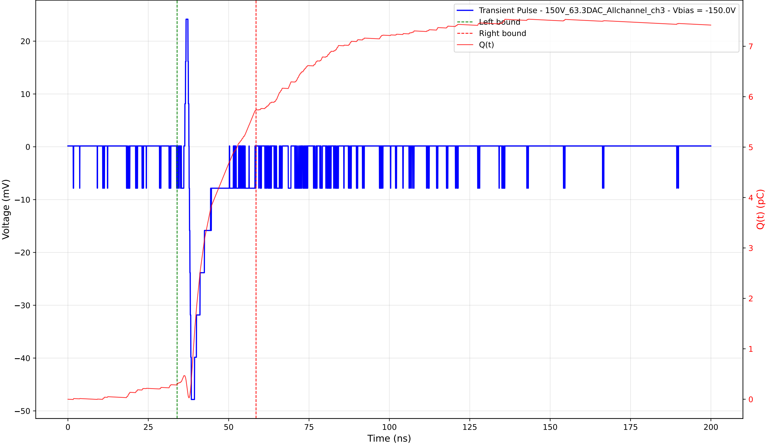
Transient Pulse - Sample: 1cm_42 - Position: 710.0 \mu\text{m} - Charge: 5.44 pC - Rise Time: 0.70 ns
