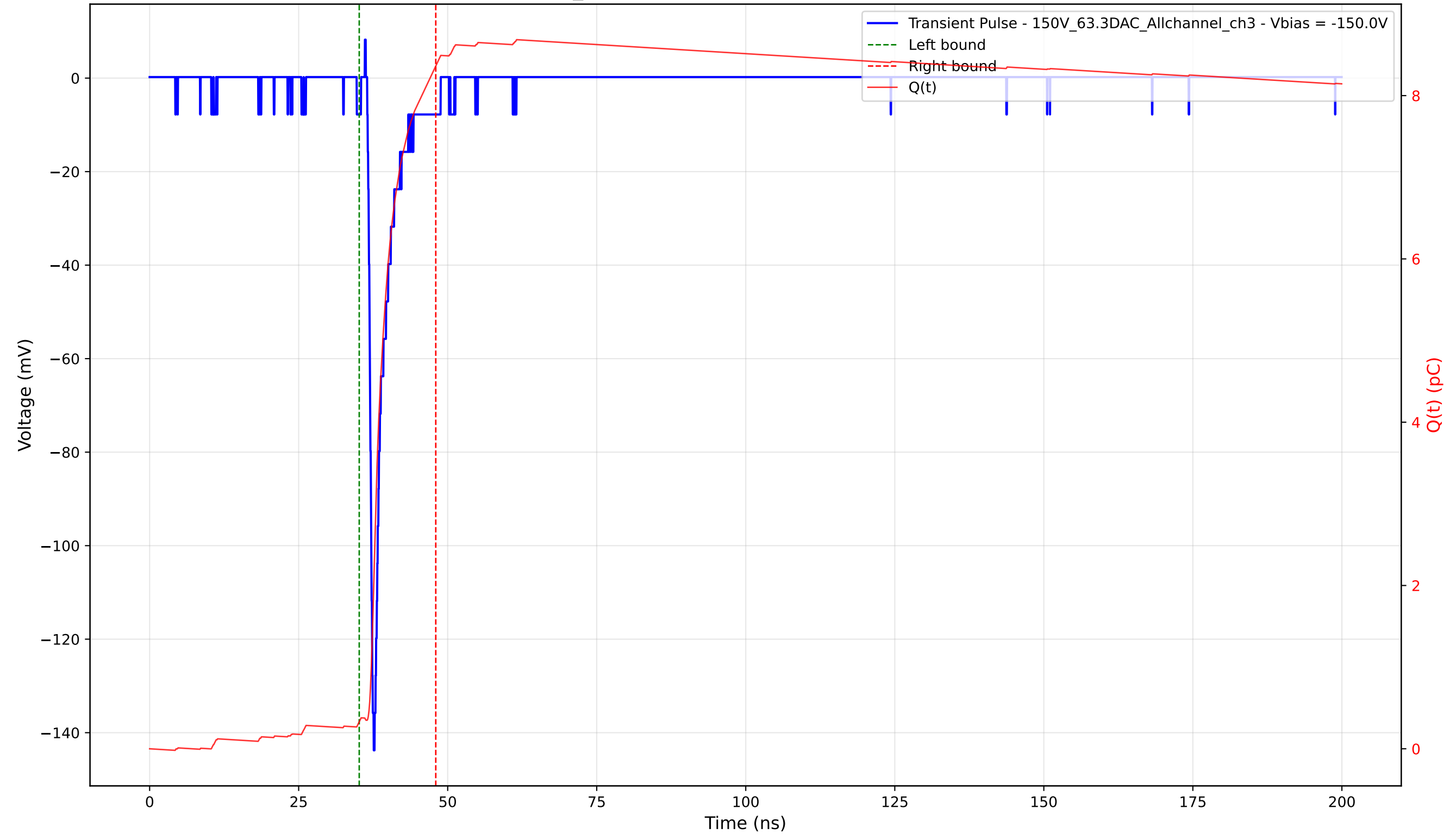
Transient Pulse - Sample: 1cm_42 - Position: 3260.0 \mu\text{m} - Charge: 8.03 pC - Rise Time: 0.85 ns
