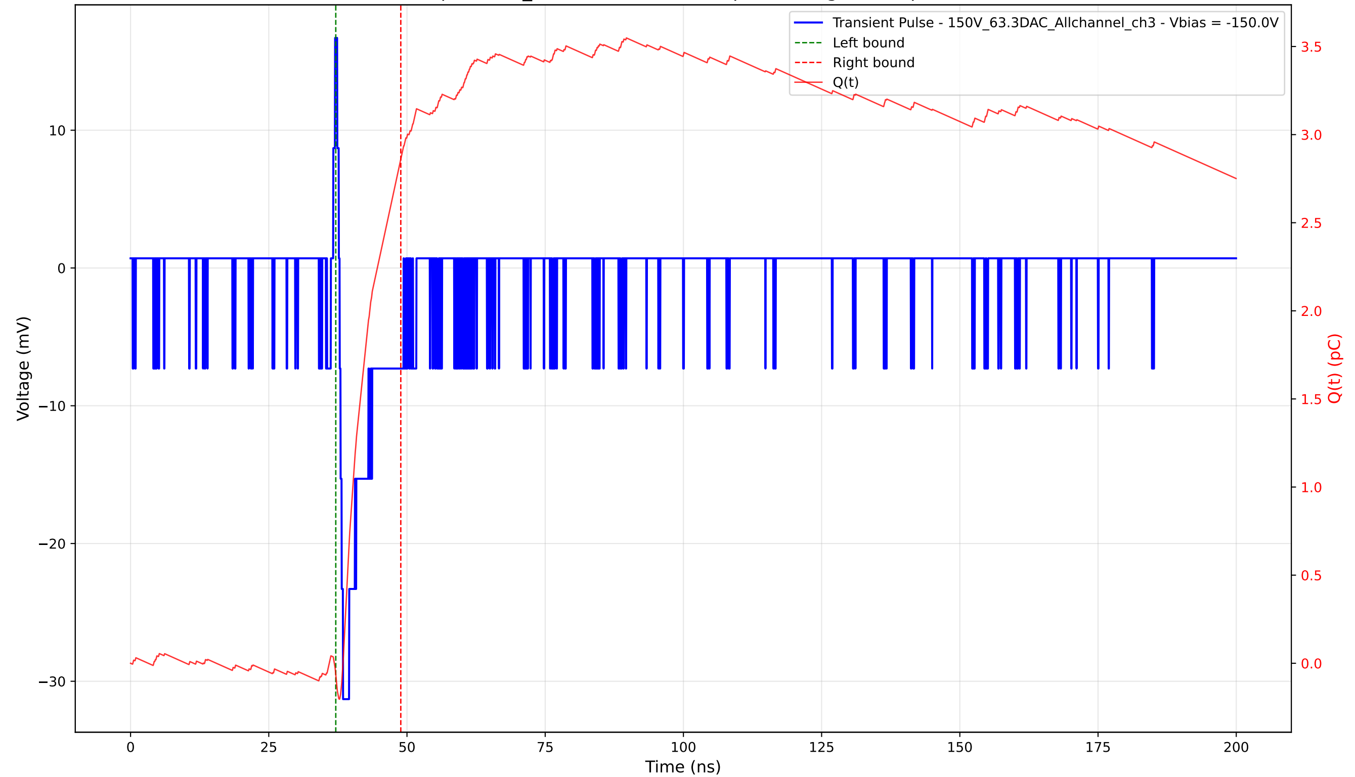
Transient Pulse - Sample: 1cm_42 - Position: 4790.0 \mu\text{m} - Charge: 2.93 pC - Rise Time: 0.63 ns
