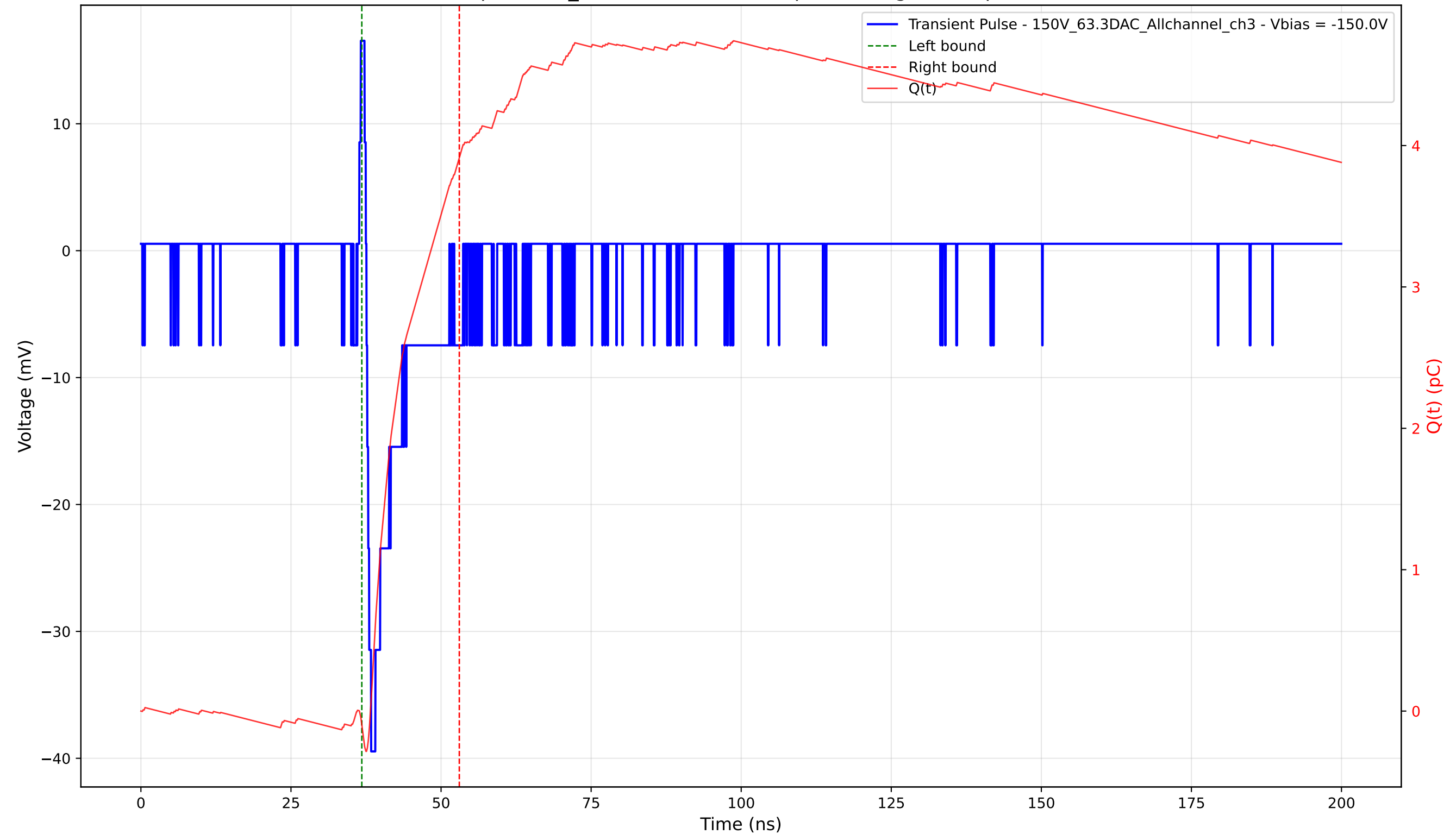
Transient Pulse - Sample: 1cm_42 - Position: 4050.0 \mu\text{m} - Charge: 4.01 pC - Rise Time: 0.78 ns
