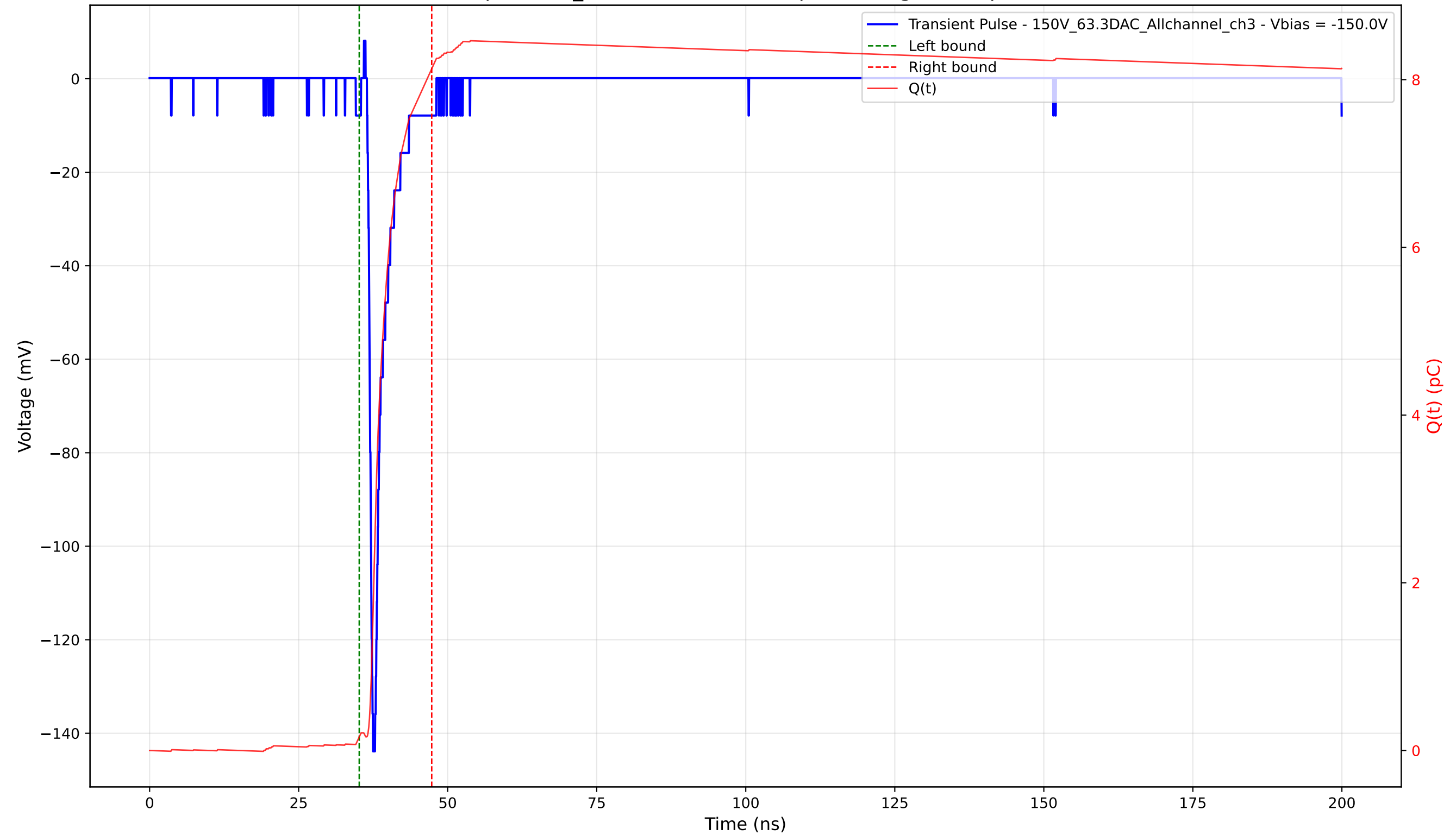
Transient Pulse - Sample: 1cm_42 - Position: 3220.0 \mu\text{m} - Charge: 7.97 pC - Rise Time: 0.85 ns
