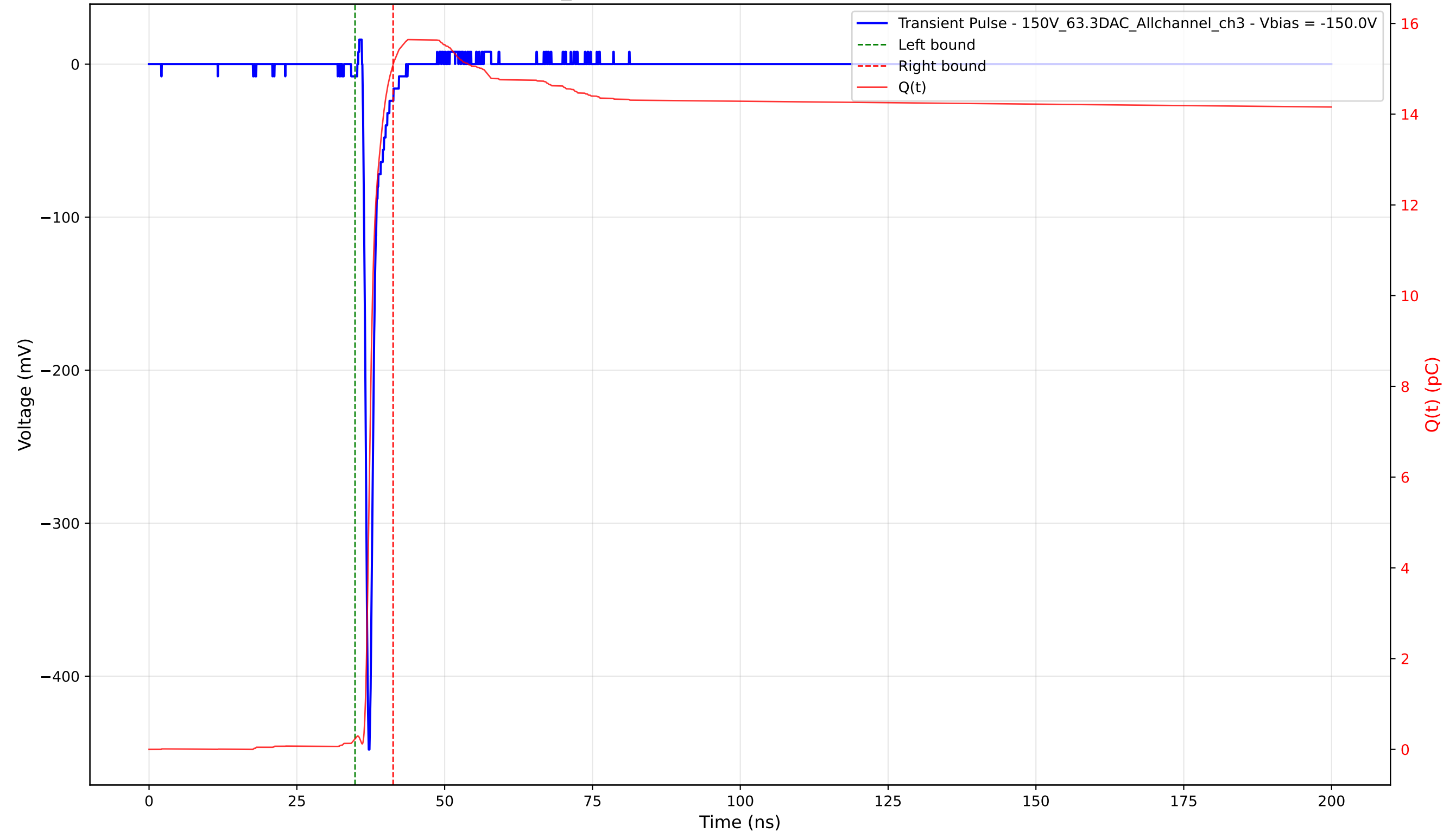
Transient Pulse - Sample: 1cm_42 - Position: 2240.0 \mu\text{m} - Charge: 14.87 pC - Rise Time: 0.76 ns
