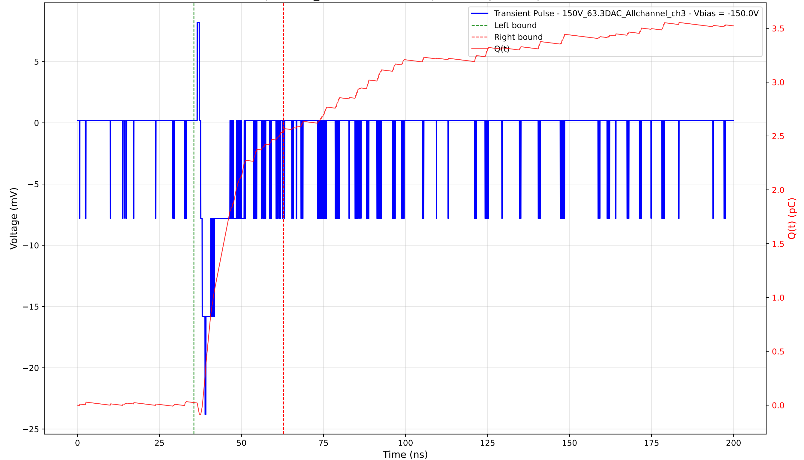
Transient Pulse - Sample: 1cm_42 - Position: 210.0 \mu\text{m} - Charge: 2.53 pC - Rise Time: 1.35 ns
