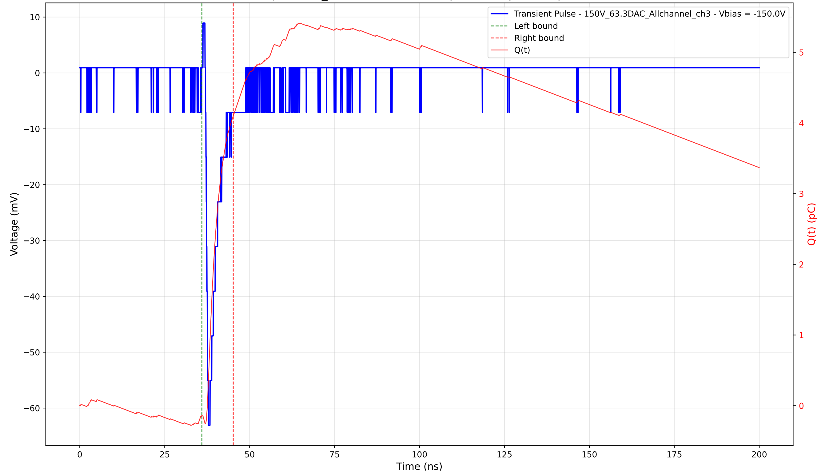
Transient Pulse - Sample: 1cm_42 - Position: 3590.0 \mu\text{m} - Charge: 4.24 pC - Rise Time: 0.80 ns
