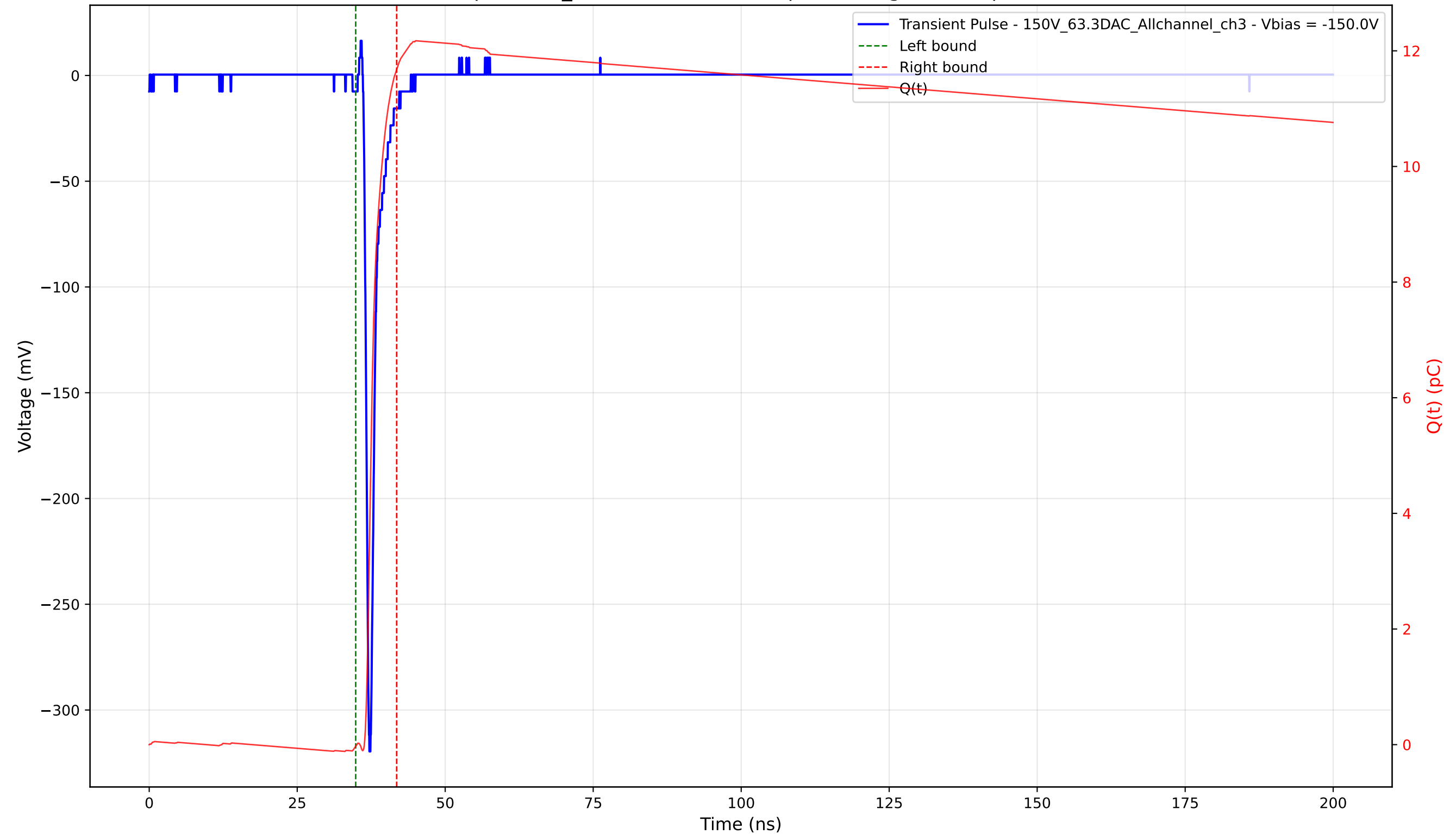
Transient Pulse - Sample: 1cm_42 - Position: 2120.0 \mu\text{m} - Charge: 11.70 pC - Rise Time: 0.72 ns
