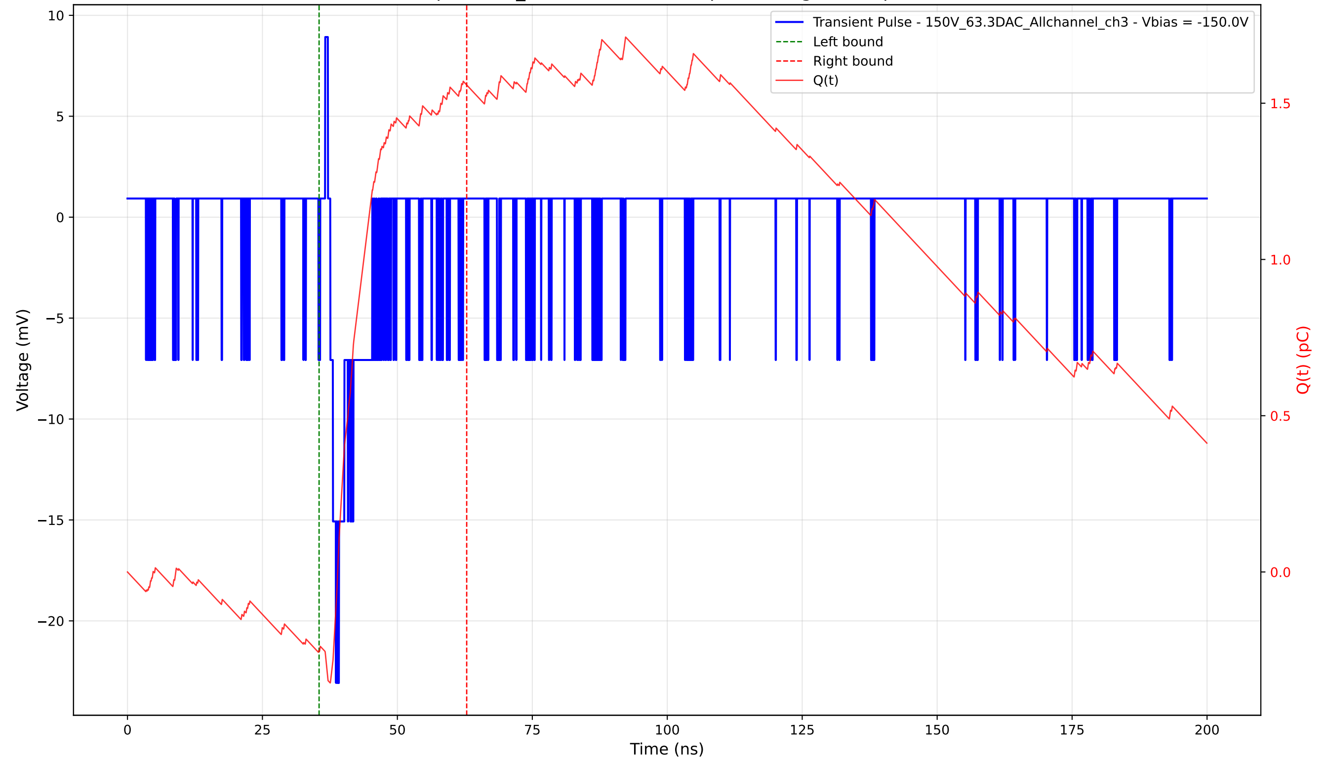
Transient Pulse - Sample: 1cm_42 - Position: 205.0 \mu\text{m} - Charge: 1.81 pC - Rise Time: 1.07 ns
