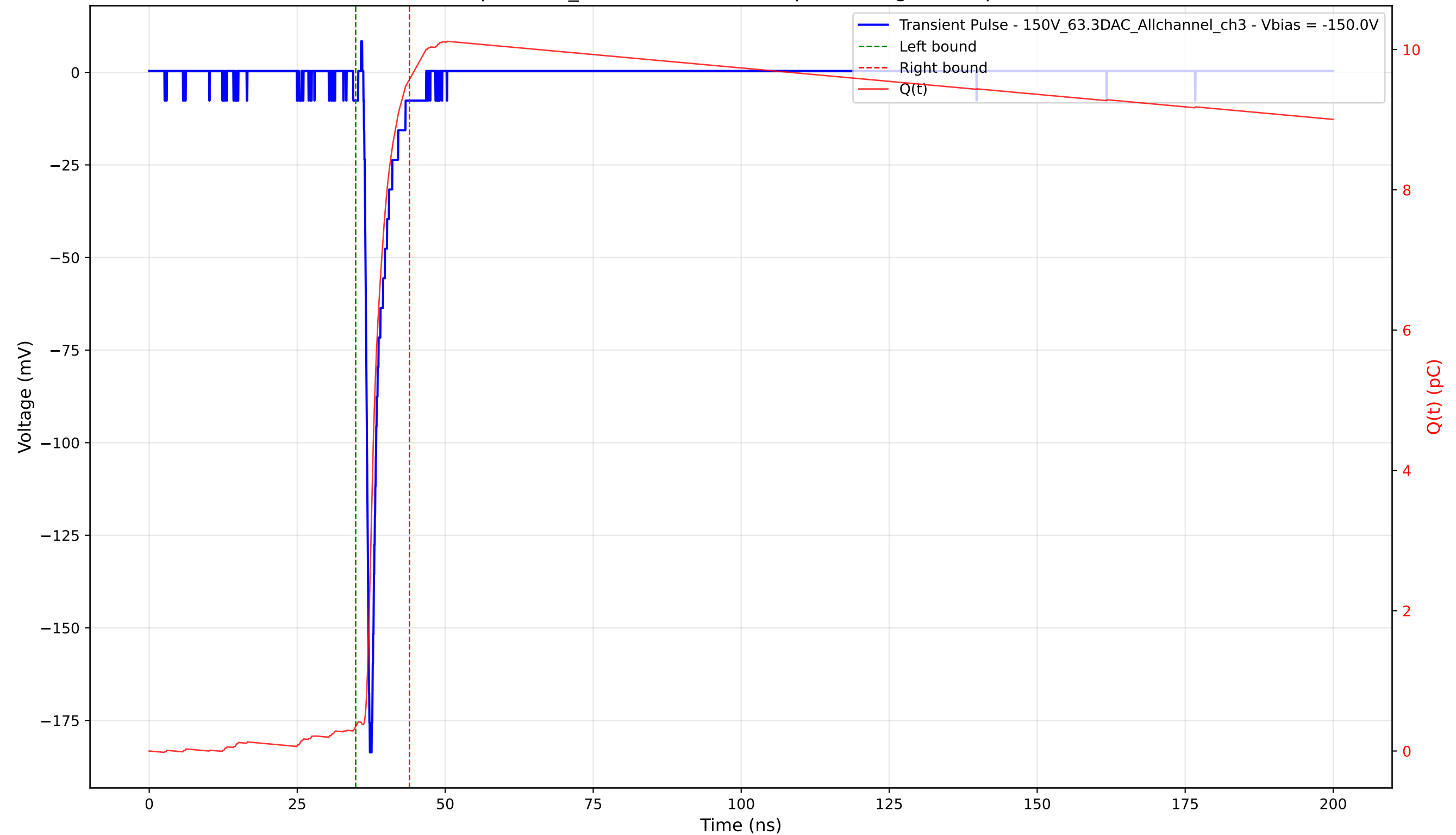
Transient Pulse - Sample: 1cm_42 - Position: 1935.0 \mu\text{m} - Charge: 9.22 pC - Rise Time: 0.79 ns
