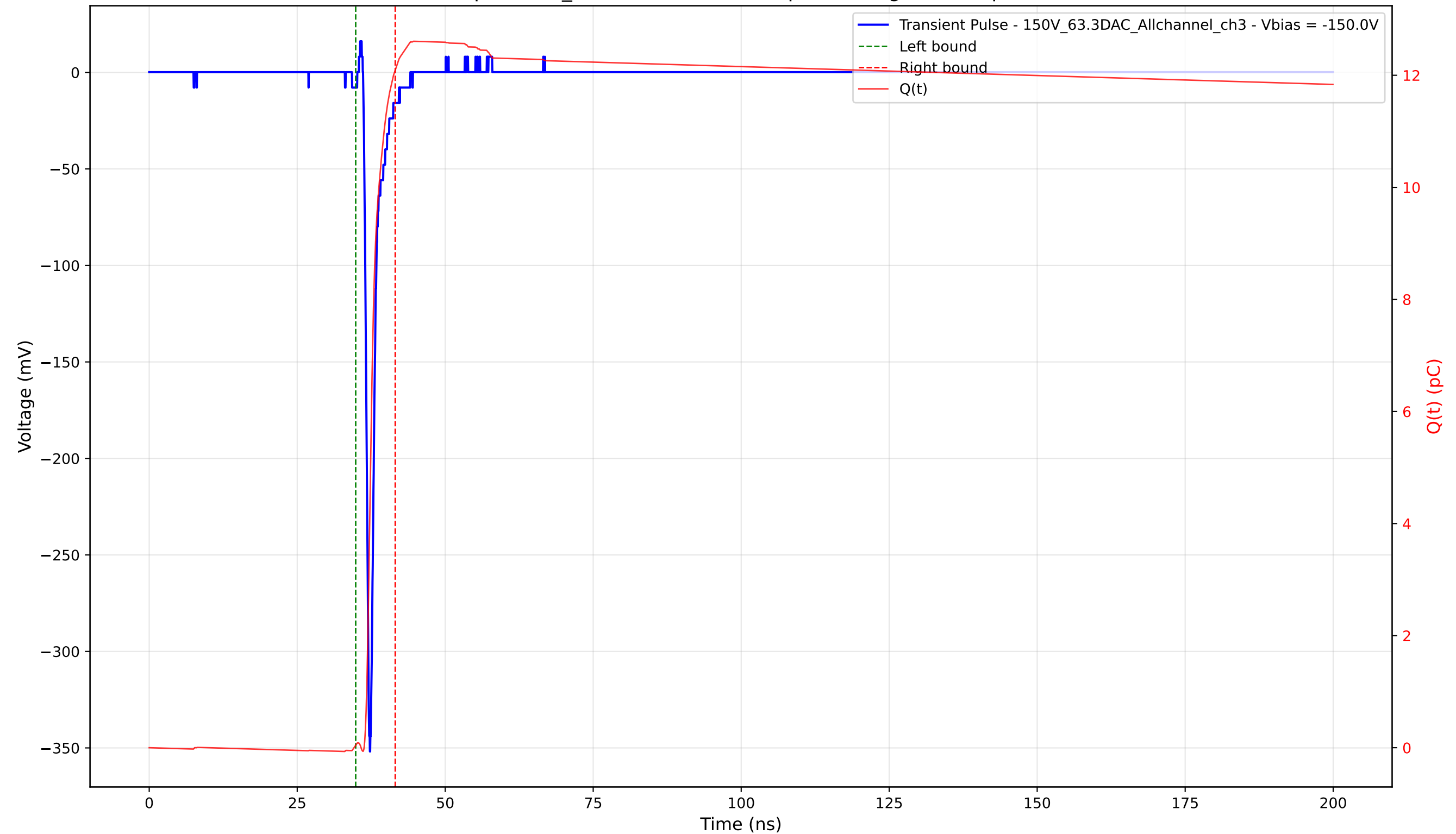
Transient Pulse - Sample: 1cm_42 - Position: 2890.0 \mu\text{m} - Charge: 12.05 pC - Rise Time: 0.74 ns
