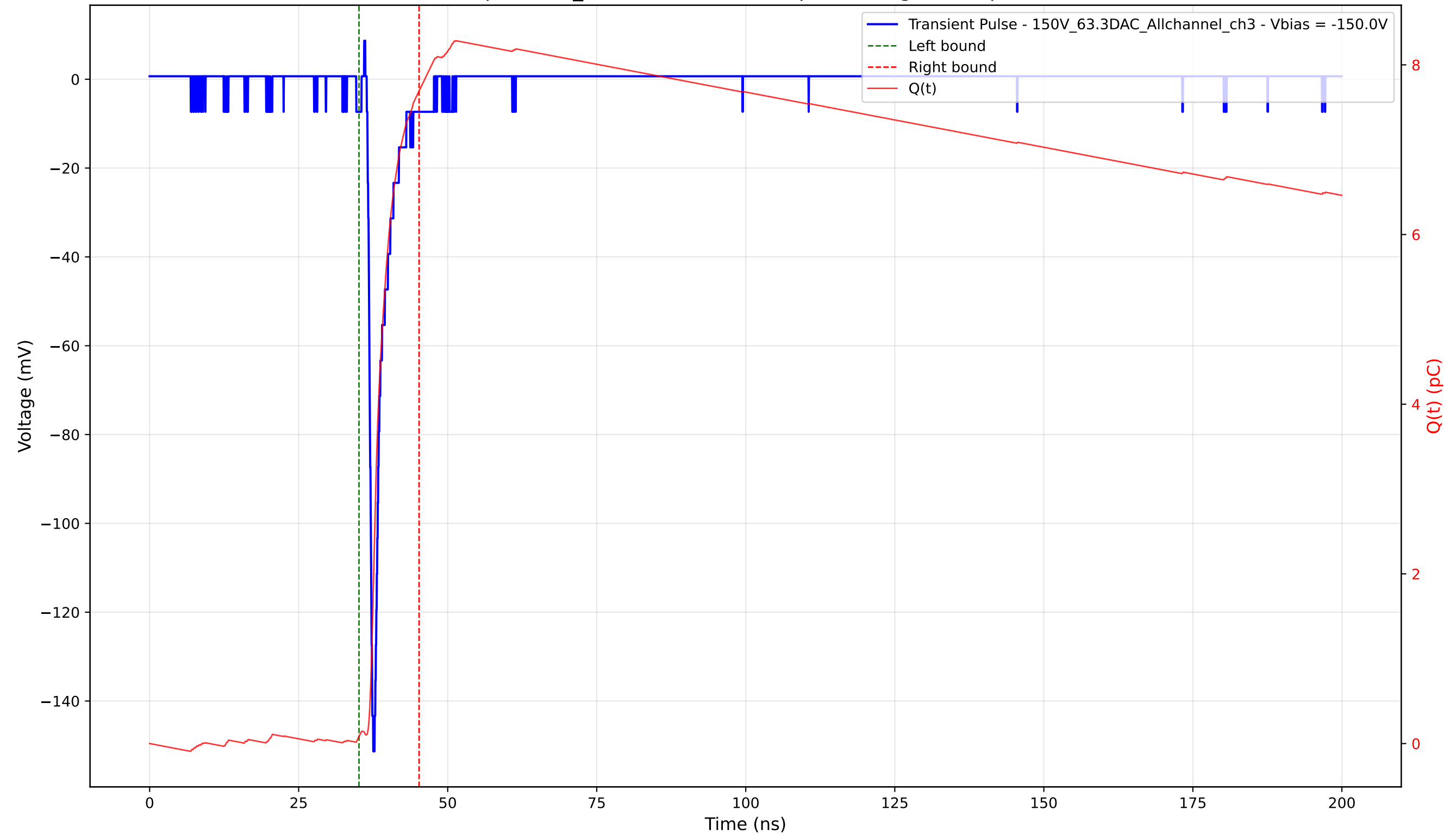
Transient Pulse - Sample: 1cm_42 - Position: 3190.0 \mu\text{m} - Charge: 7.61 pC - Rise Time: 0.80 ns
