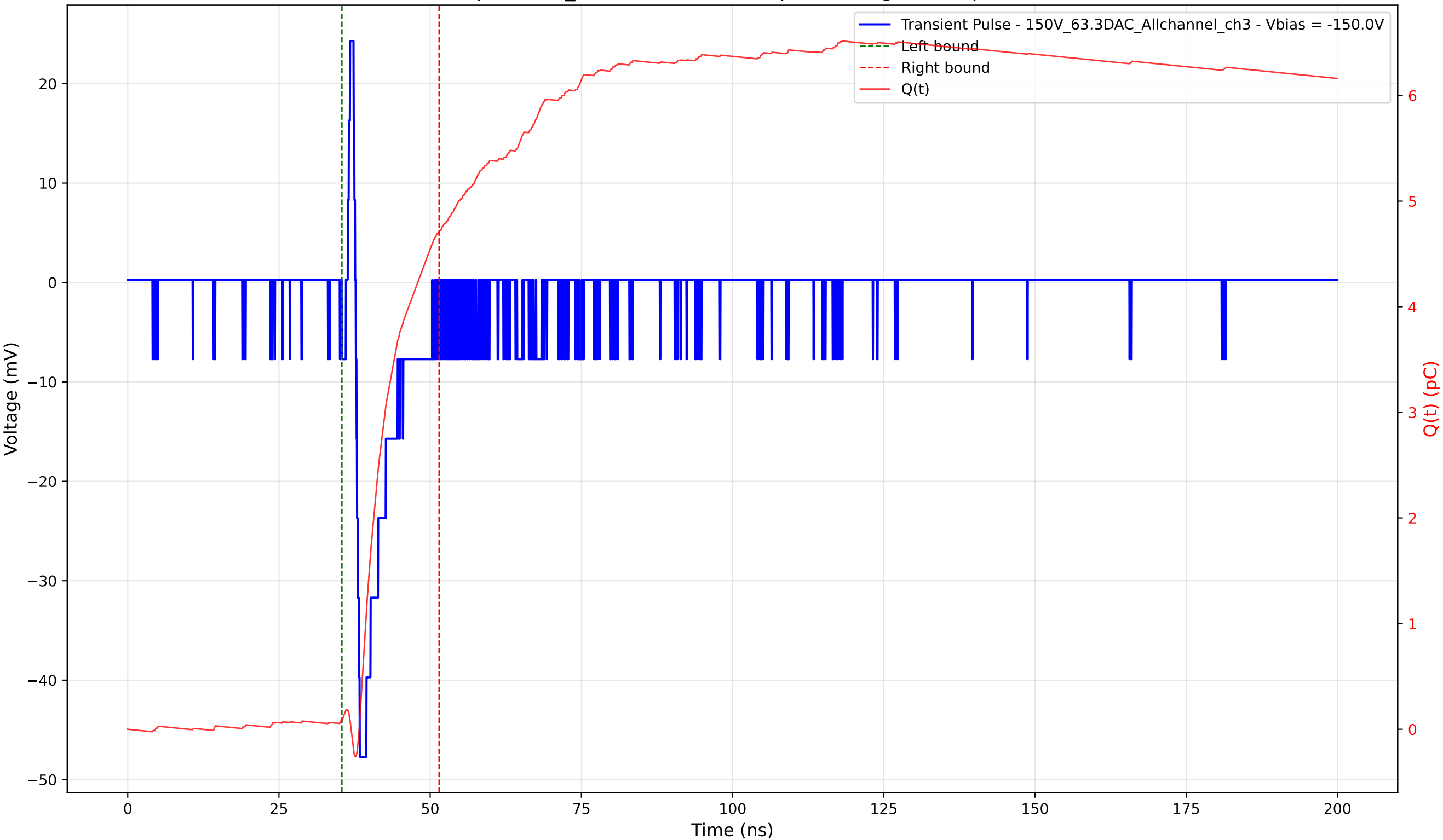
Transient Pulse - Sample: 1cm_42 - Position: 790.0 \mu\text{m} - Charge: 4.63 pC - Rise Time: 0.66 ns
