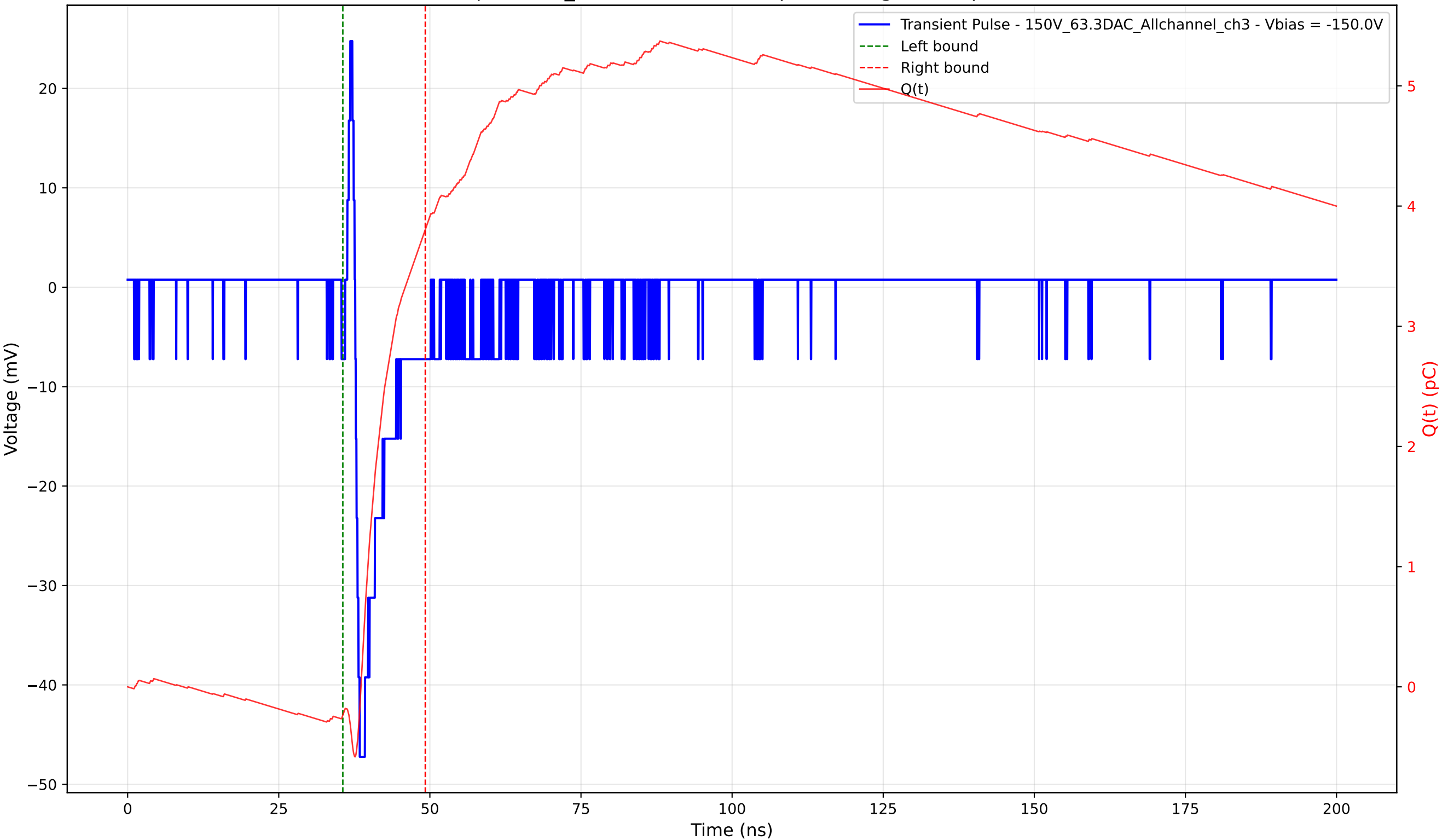
Transient Pulse - Sample: 1cm_42 - Position: 925.0 \mu\text{m} - Charge: 4.04 pC - Rise Time: 0.74 ns
