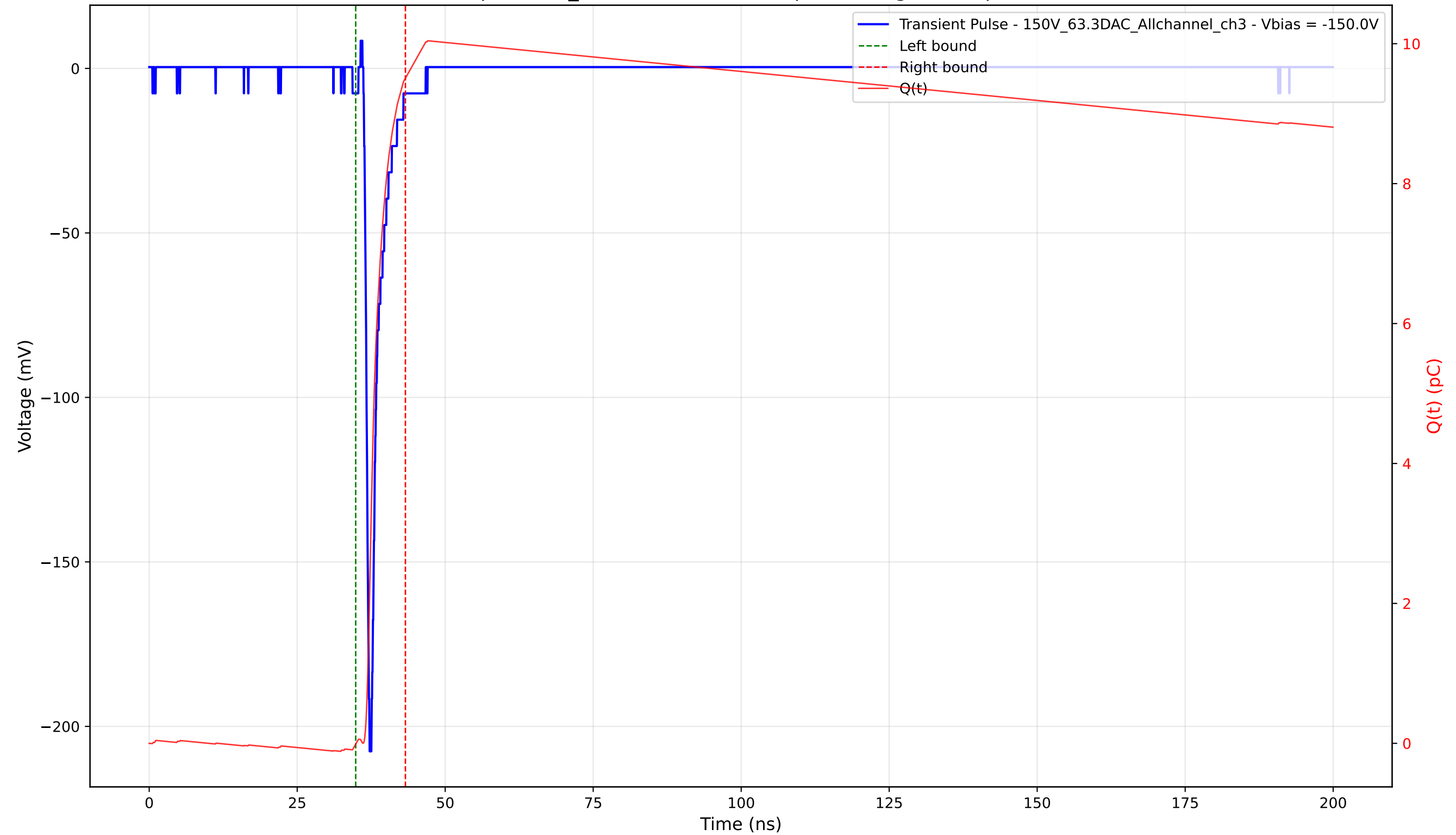
Transient Pulse - Sample: 1cm_42 - Position: 1980.0 \mu\text{m} - Charge: 9.52 pC - Rise Time: 0.81 ns
