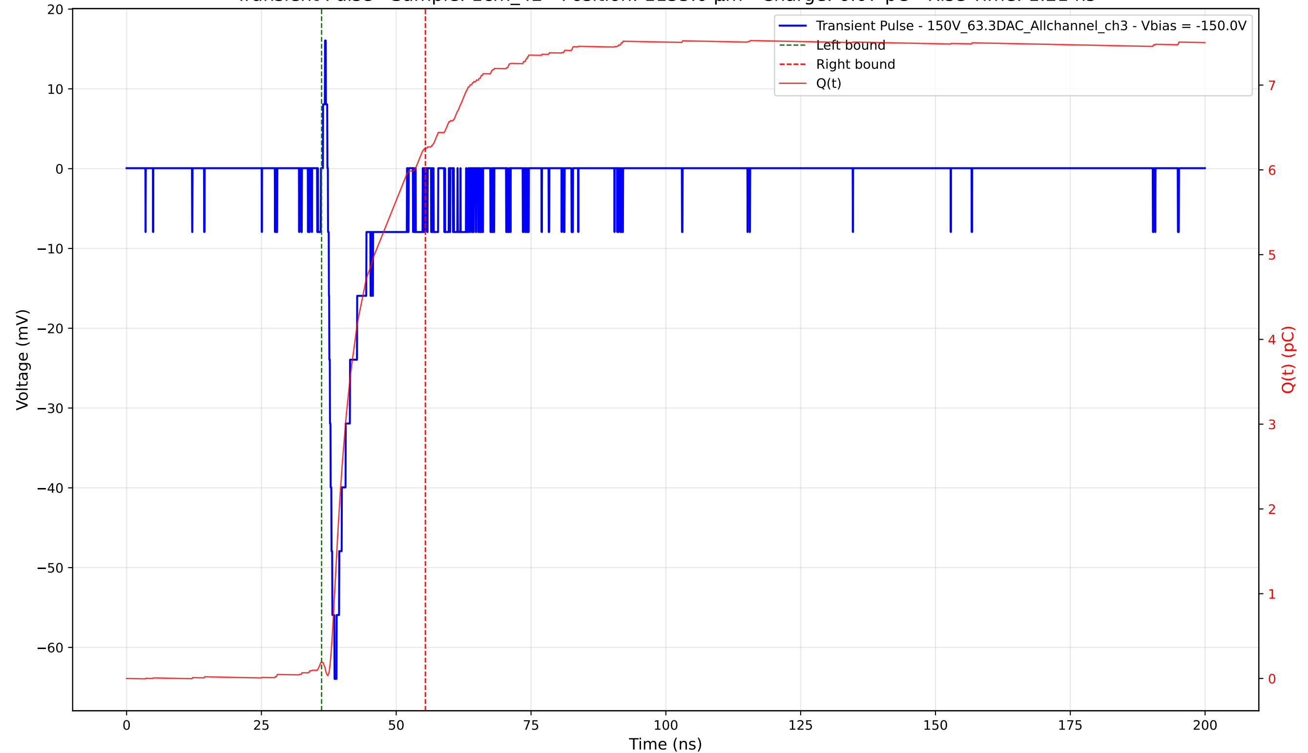
Transient Pulse - Sample: 1cm_42 - Position: 1155.0 \mu\text{m} - Charge: 6.07 pC - Rise Time: 1.21 ns
