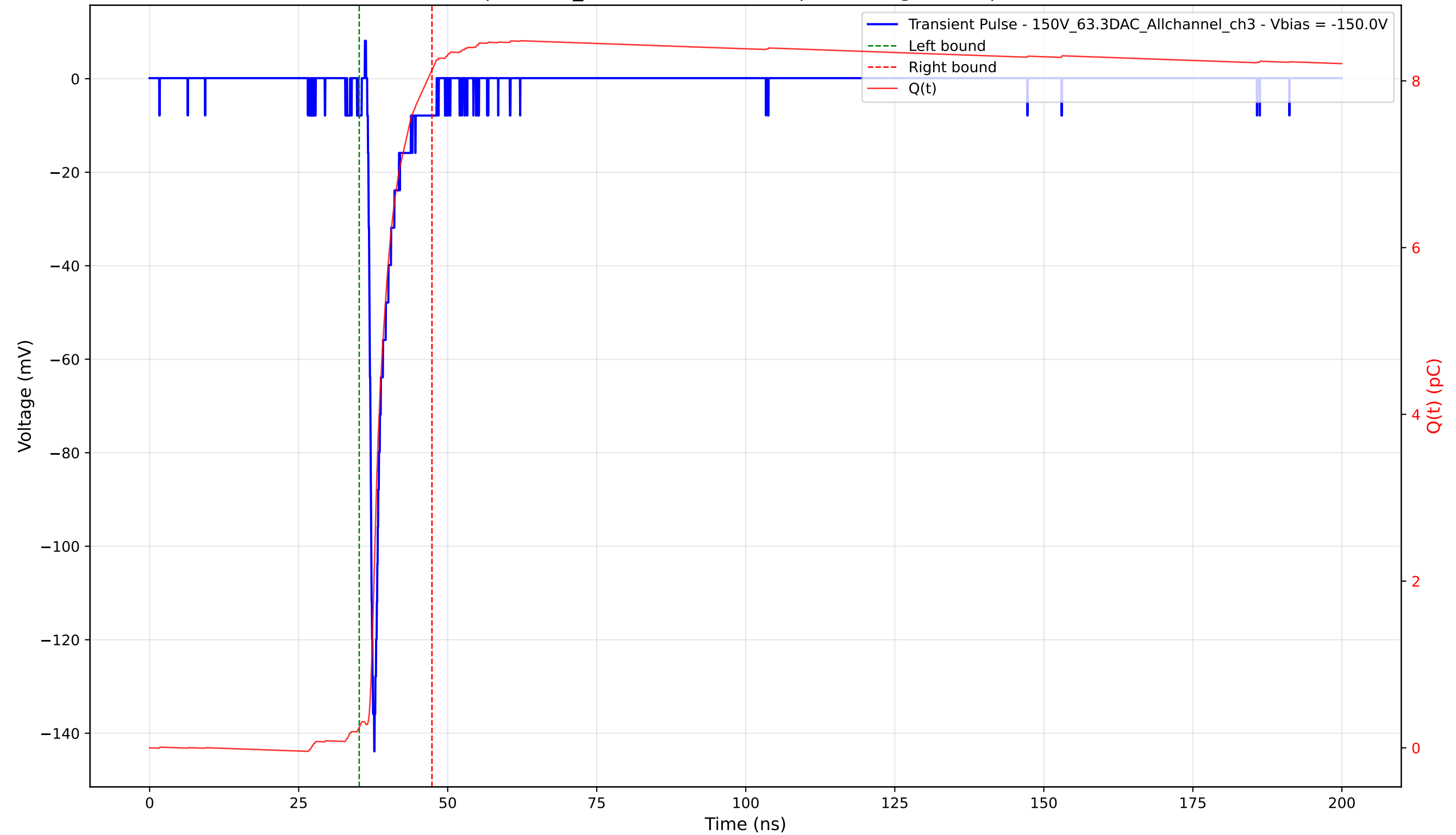
Transient Pulse - Sample: 1cm_42 - Position: 3285.0 \mu\text{m} - Charge: 7.89 pC - Rise Time: 0.85 ns
