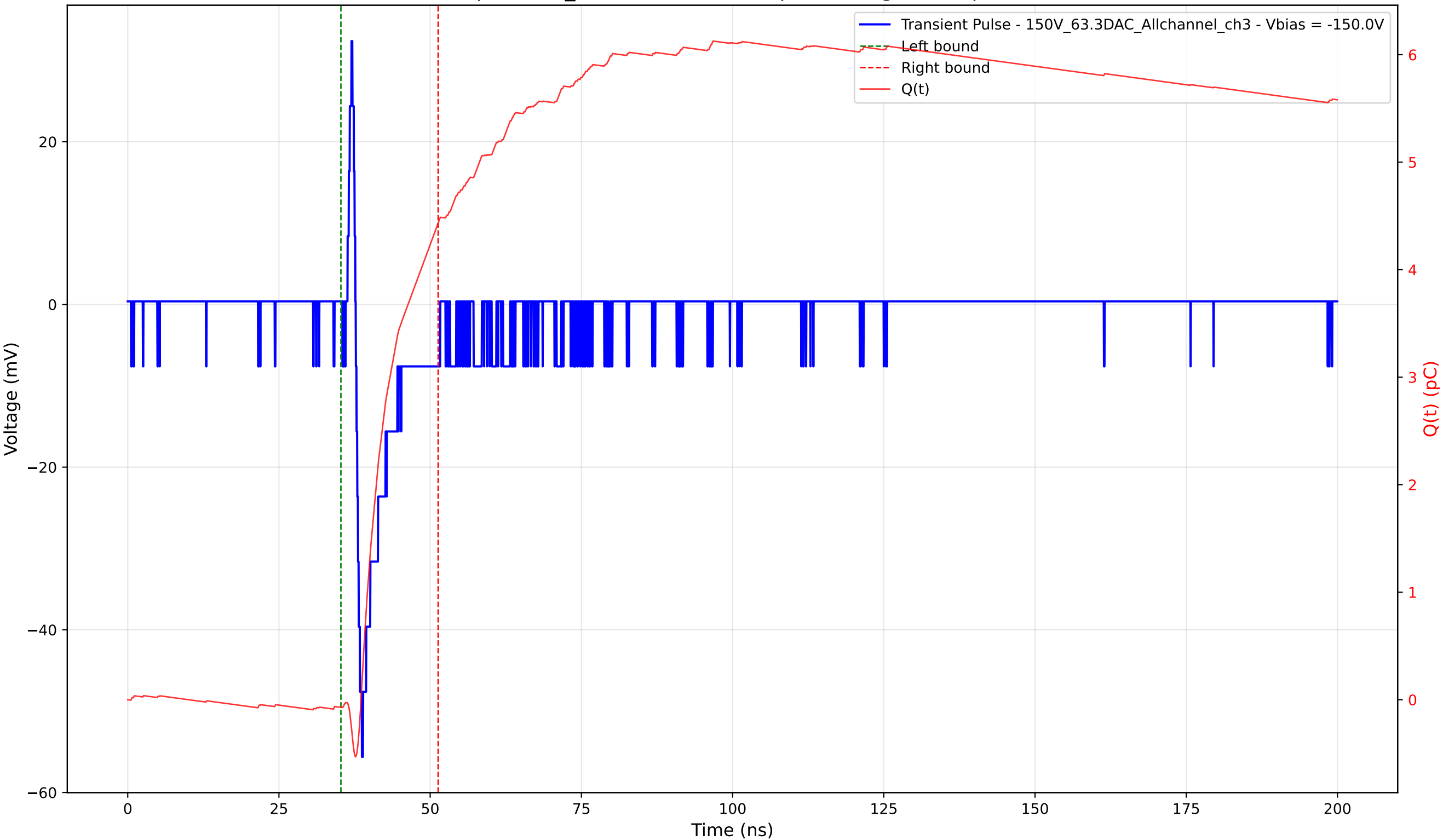
Transient Pulse - Sample: 1cm_42 - Position: 740.0 \mu\text{m} - Charge: 4.51 pC - Rise Time: 1.01 ns
