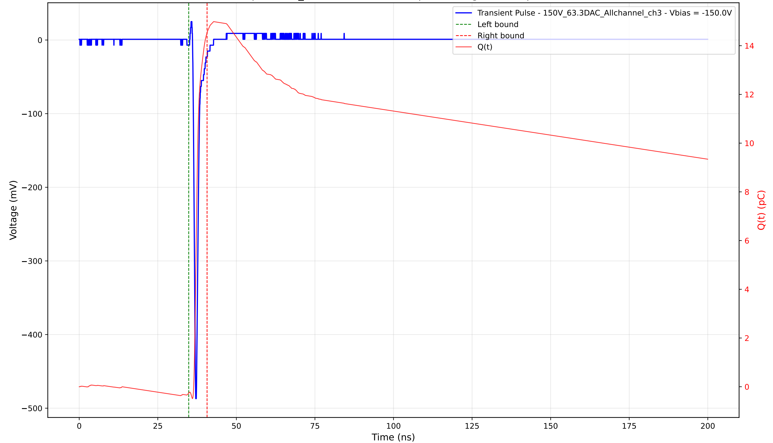
Transient Pulse - Sample: 1cm_42 - Position: 2555.0 \mu\text{m} - Charge: 14.80 pC - Rise Time: 0.71 ns
