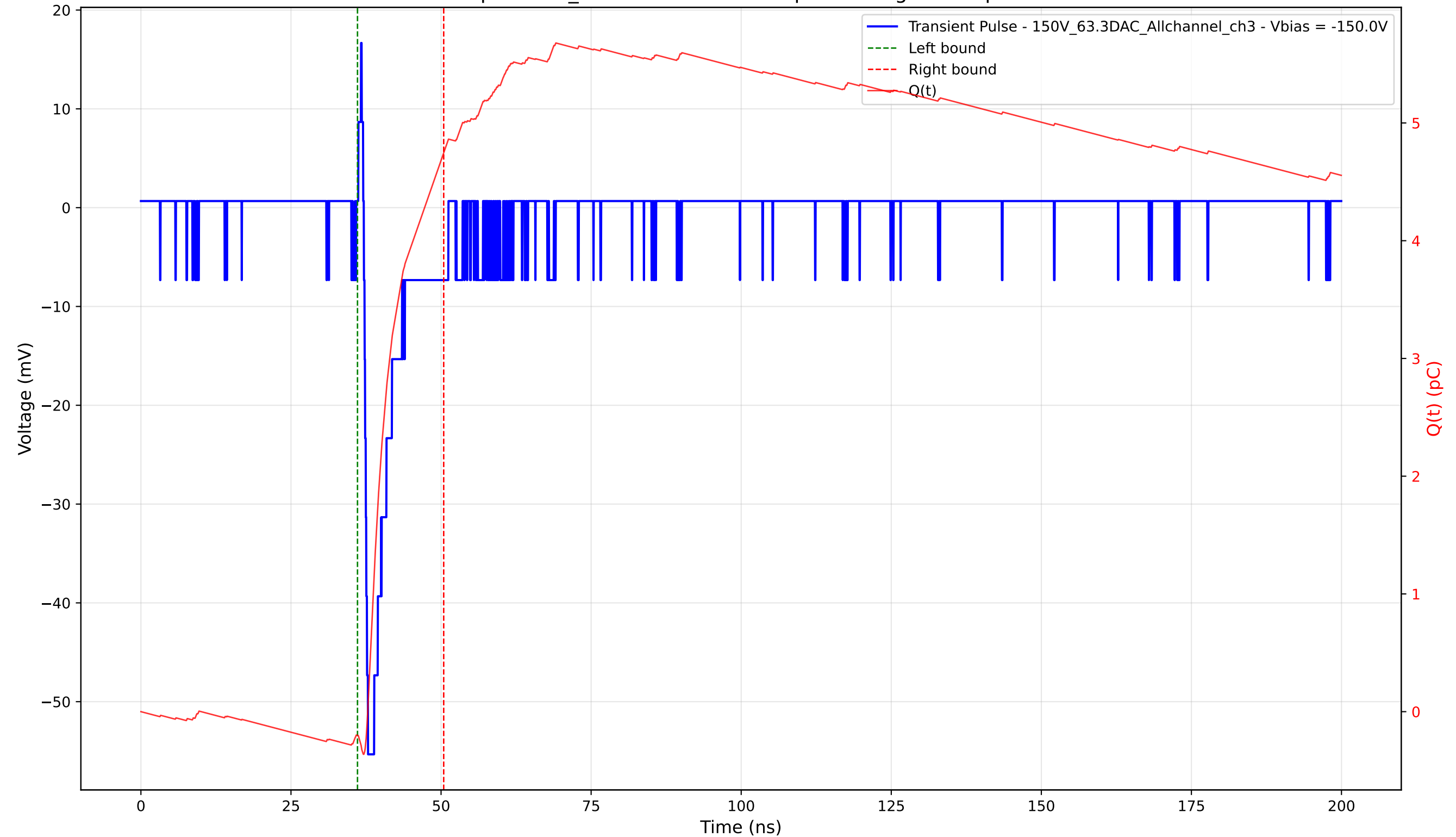
Transient Pulse - Sample: 1cm_42 - Position: 3660.0 \mu\text{m} - Charge: 4.95 pC - Rise Time: 0.69 ns
