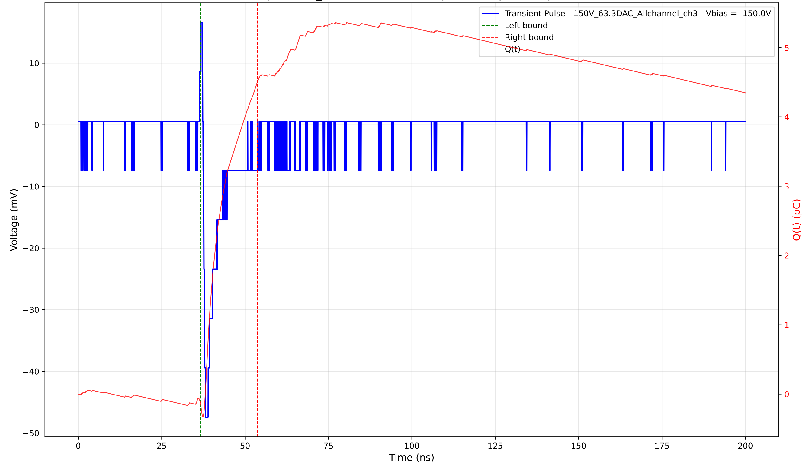
Transient Pulse - Sample: 1cm_42 - Position: 3920.0 \mu\text{m} - Charge: 4.61 pC - Rise Time: 0.74 ns
