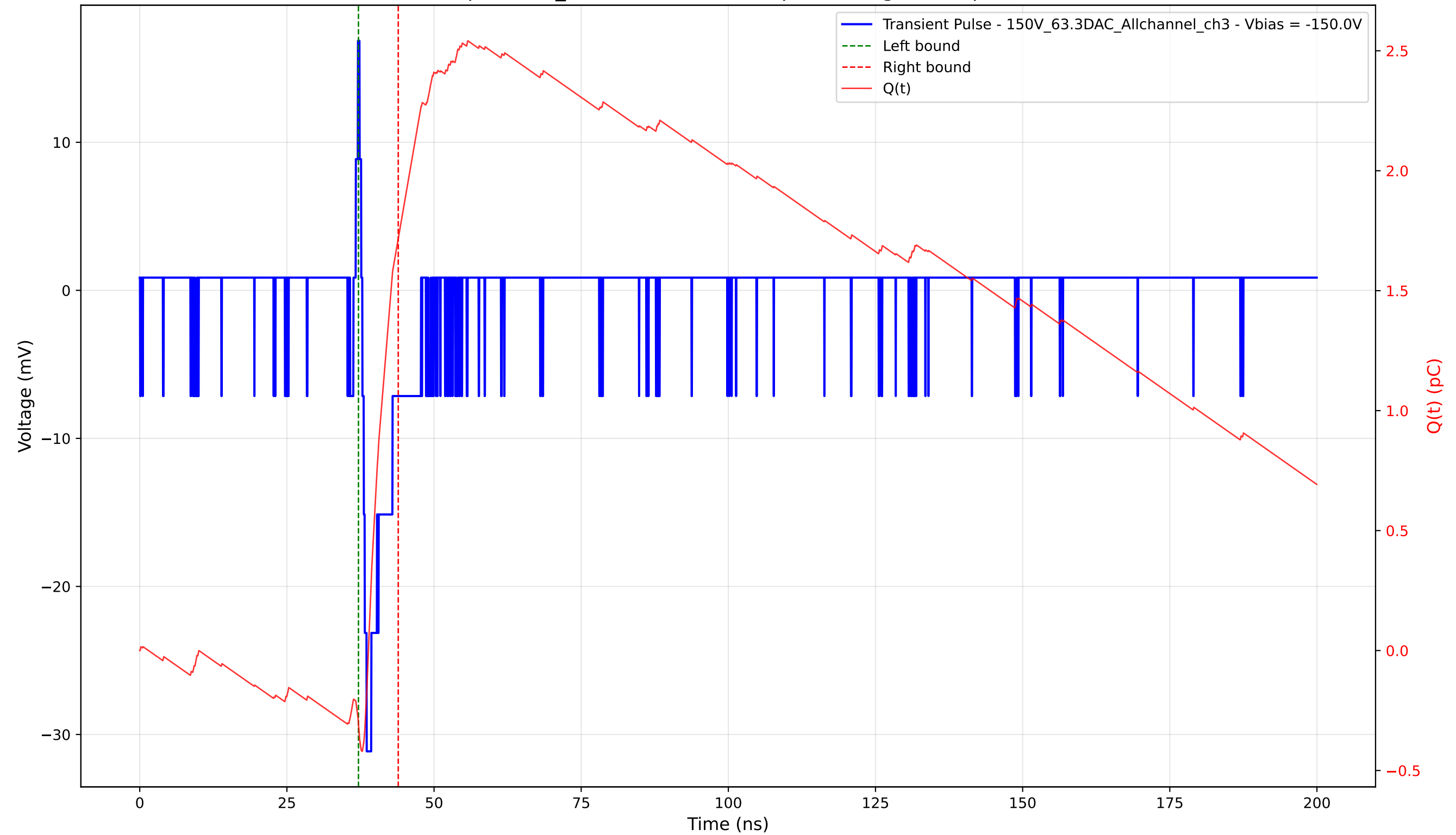
Transient Pulse - Sample: 1cm_42 - Position: 4870.0 \mu\text{m} - Charge: 2.02 pC - Rise Time: 0.75 ns
