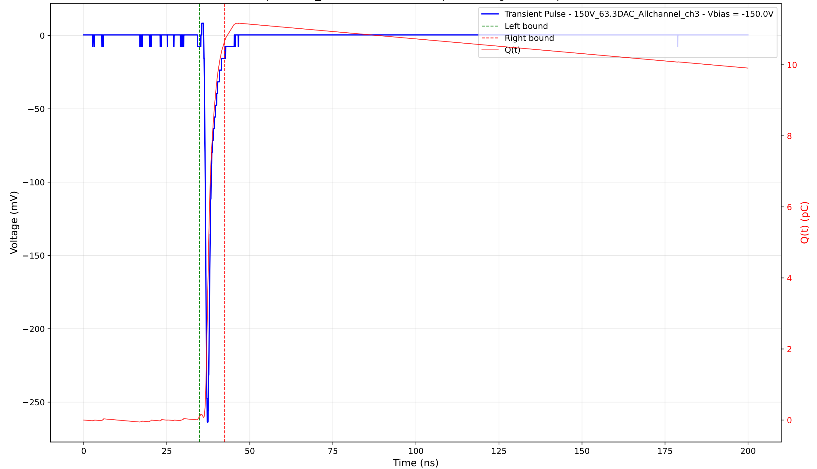
Transient Pulse - Sample: 1cm_42 - Position: 2055.0 \mu\text{m} - Charge: 10.57 pC - Rise Time: 0.73 ns
