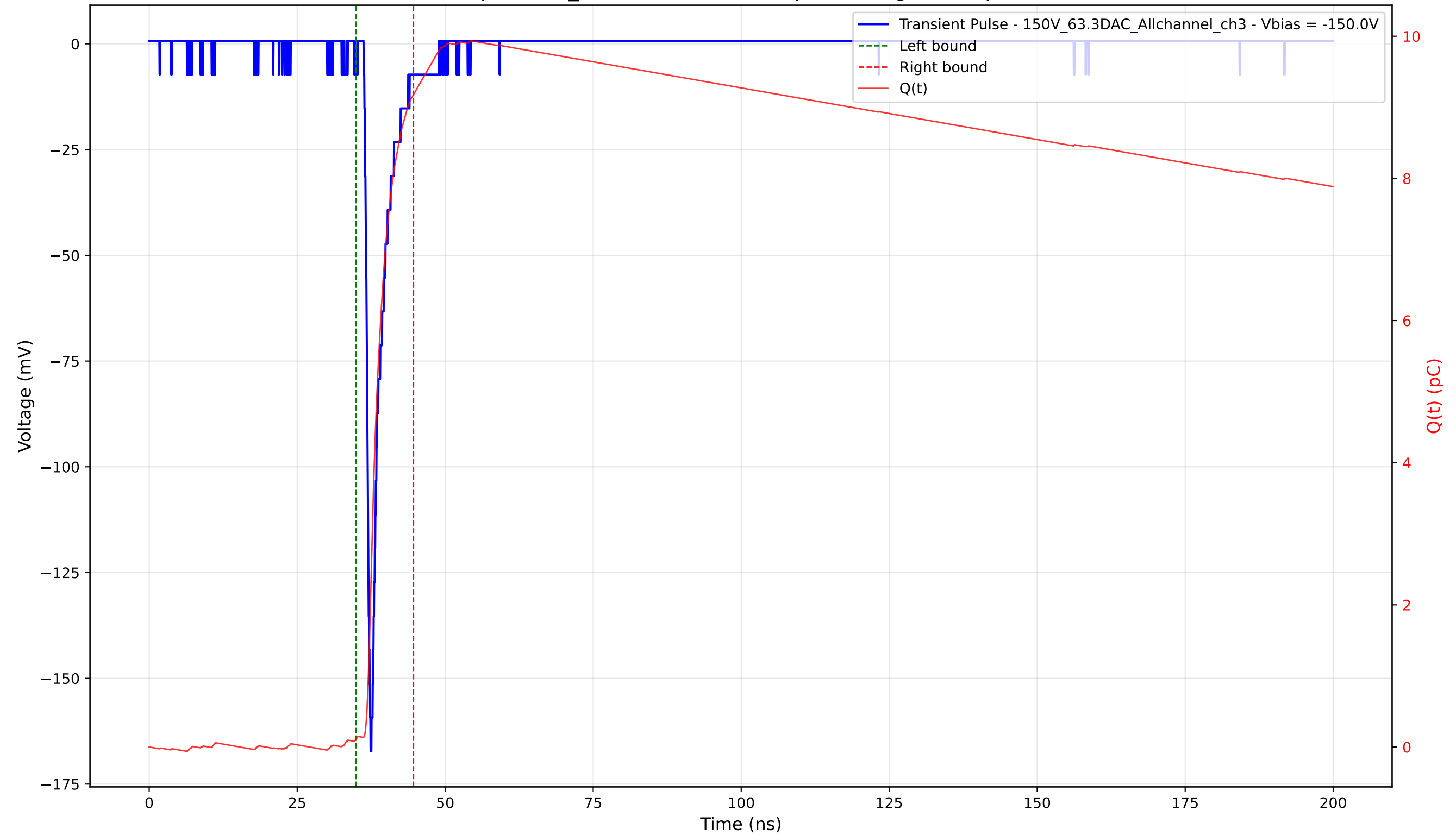
Transient Pulse - Sample: 1cm_42 - Position: 1875.0 \mu\text{m} - Charge: 9.07 pC - Rise Time: 0.83 ns
