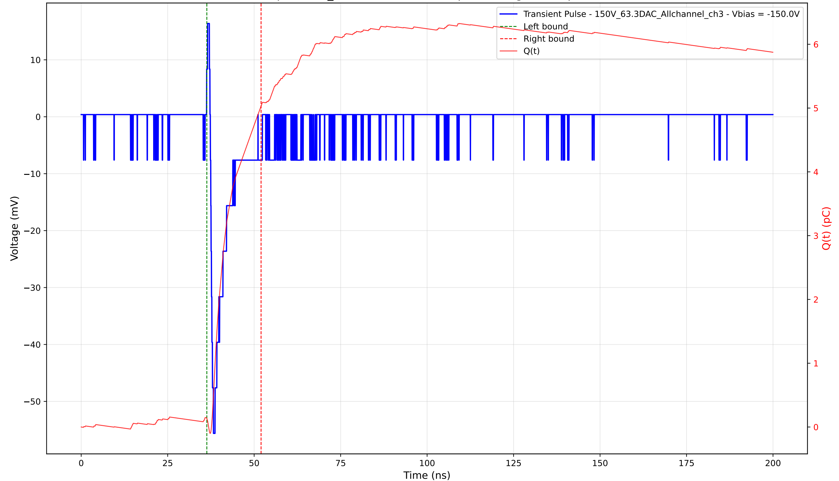
Transient Pulse - Sample: 1cm_42 - Position: 3845.0 \mu\text{m} - Charge: 4.90 pC - Rise Time: 0.89 ns
