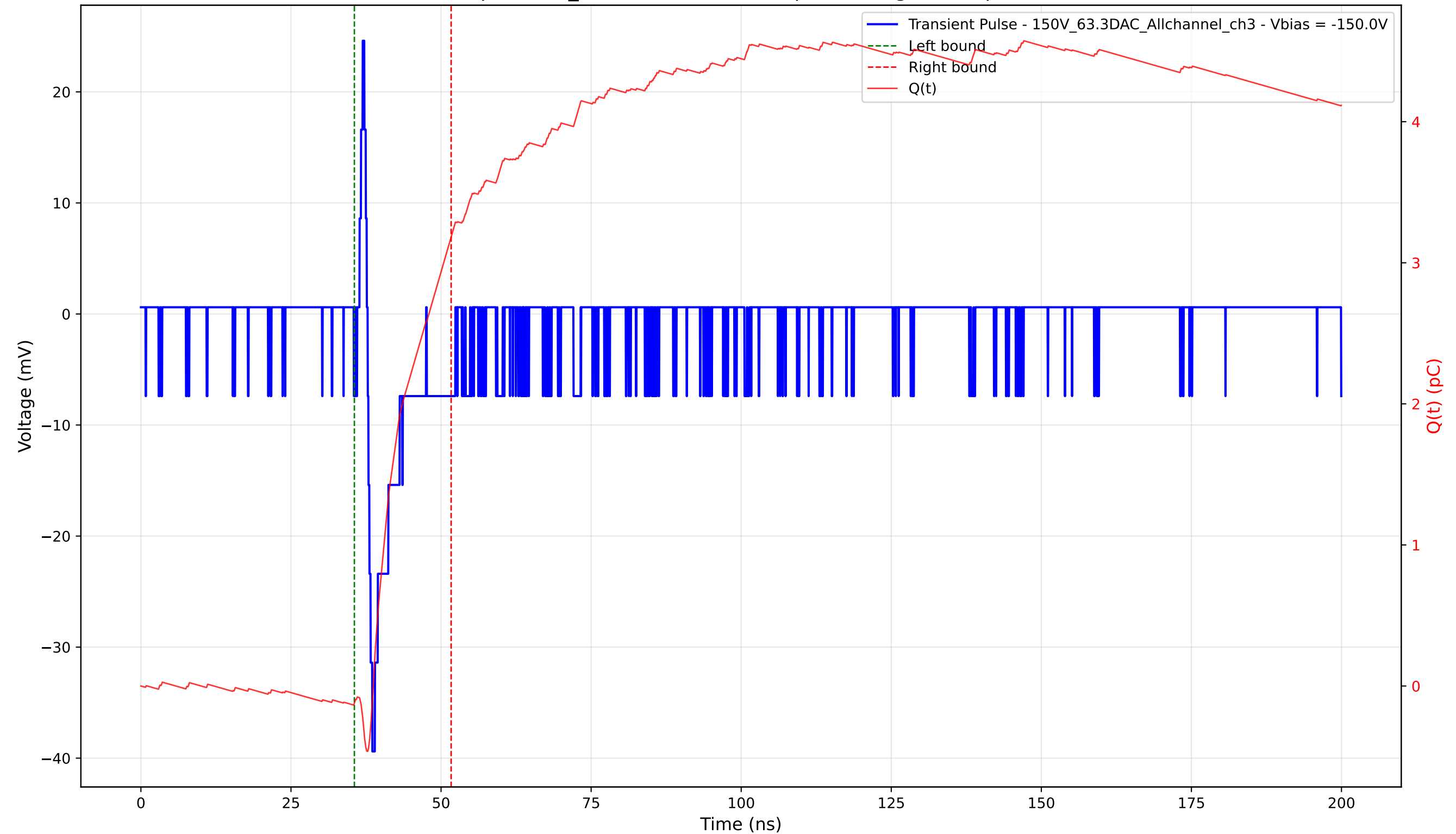
Transient Pulse - Sample: 1cm_42 - Position: 4400.0 \mu\text{m} - Charge: 3.31 pC - Rise Time: 0.78 ns
