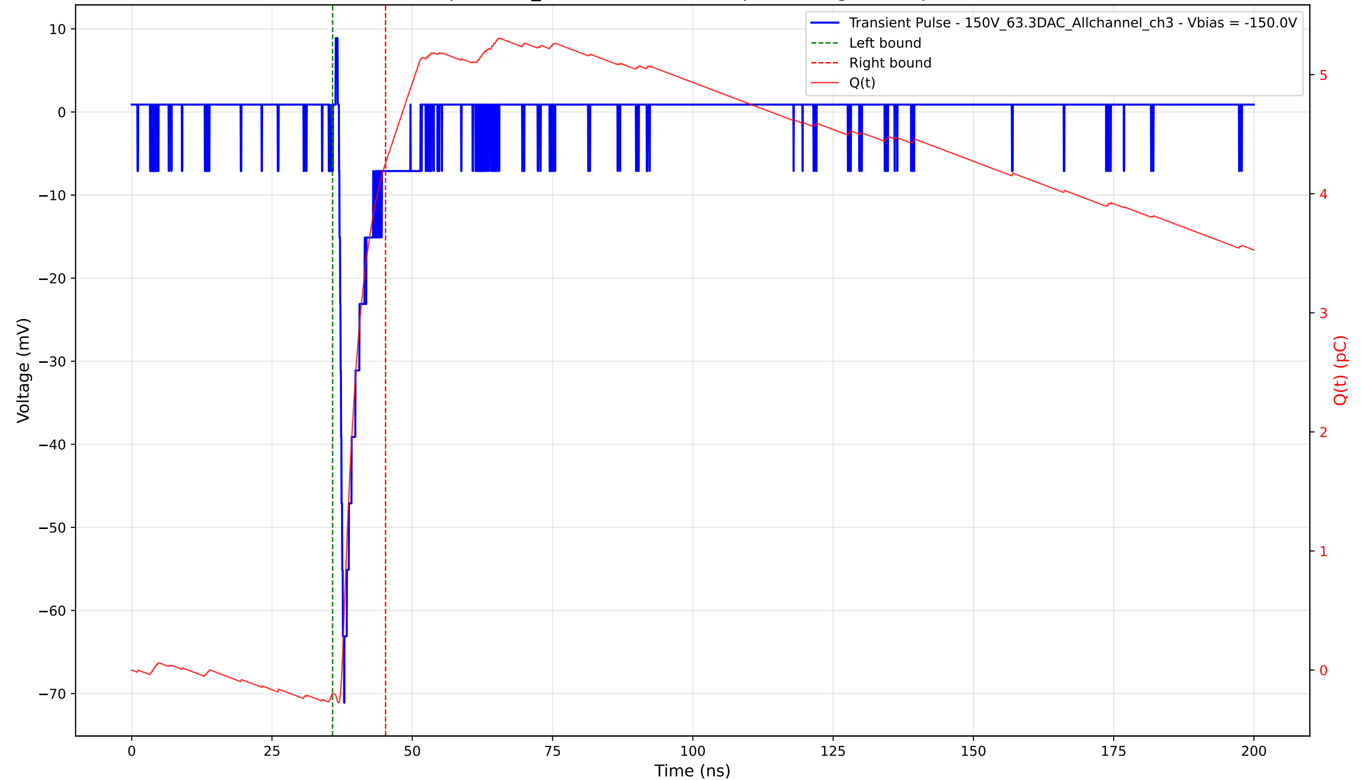
Transient Pulse - Sample: 1cm_42 - Position: 3545.0 \mu\text{m} - Charge: 4.46 pC - Rise Time: 0.88 ns
