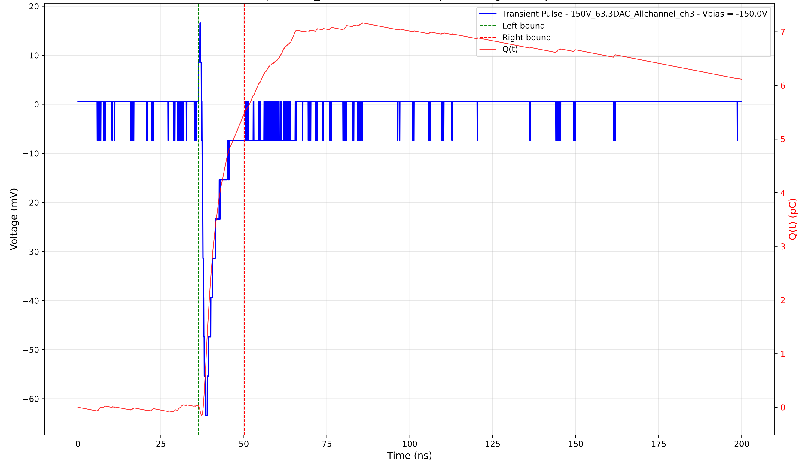
Transient Pulse - Sample: 1cm_42 - Position: 1165.0 \mu\text{m} - Charge: 5.45 pC - Rise Time: 1.09 ns
