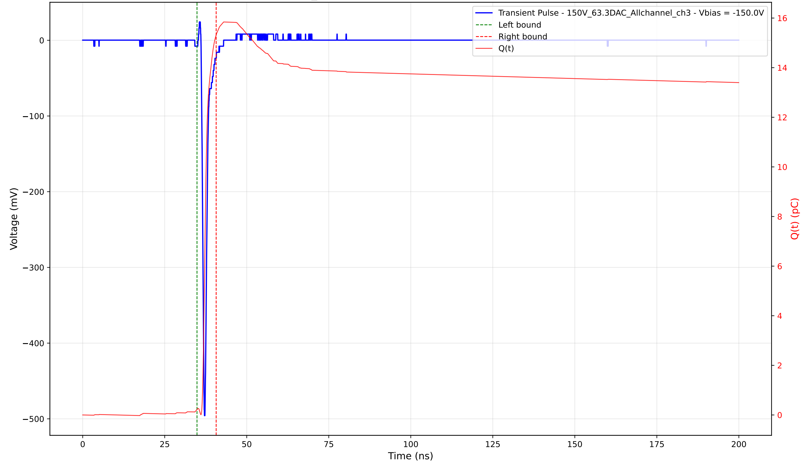
Transient Pulse - Sample: 1cm_42 - Position: 2445.0 \mu\text{m} - Charge: 15.10 pC - Rise Time: 0.71 ns
