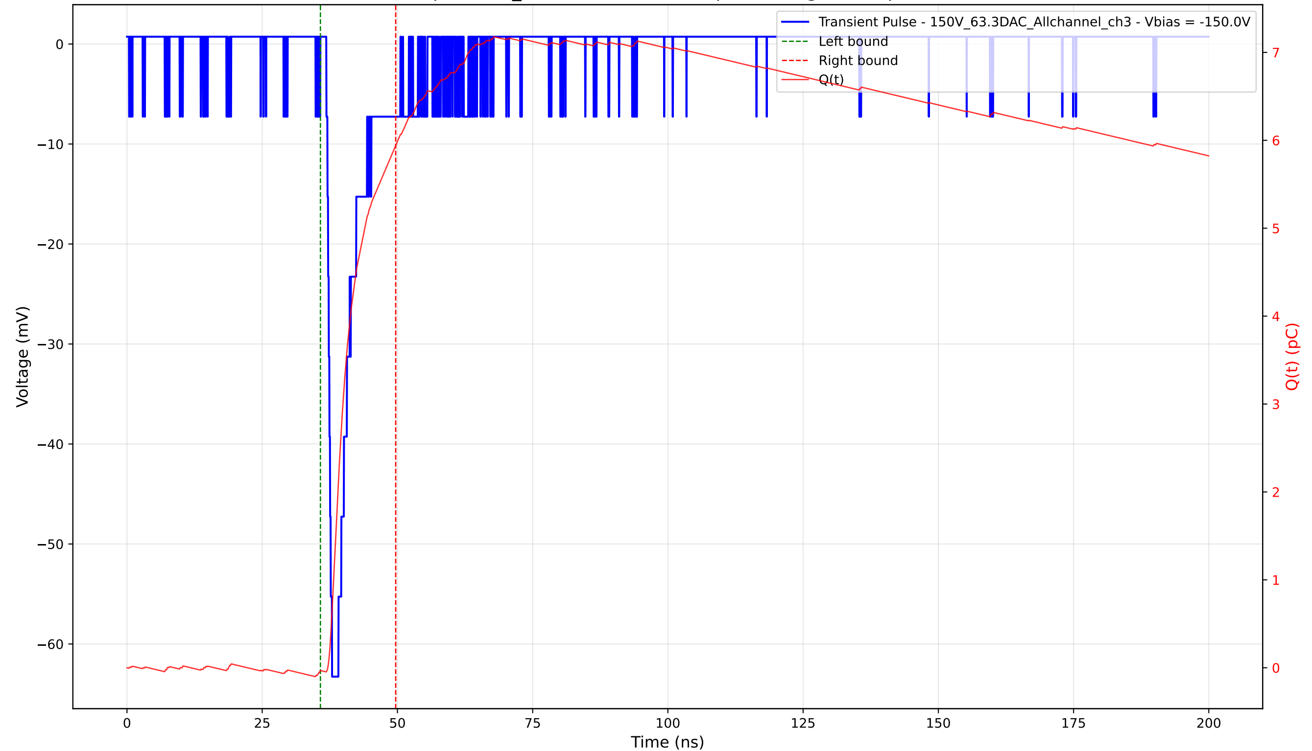
Transient Pulse - Sample: 1cm_42 - Position: 1415.0 \mu\text{m} - Charge: 5.98 pC - Rise Time: 1.05 ns
