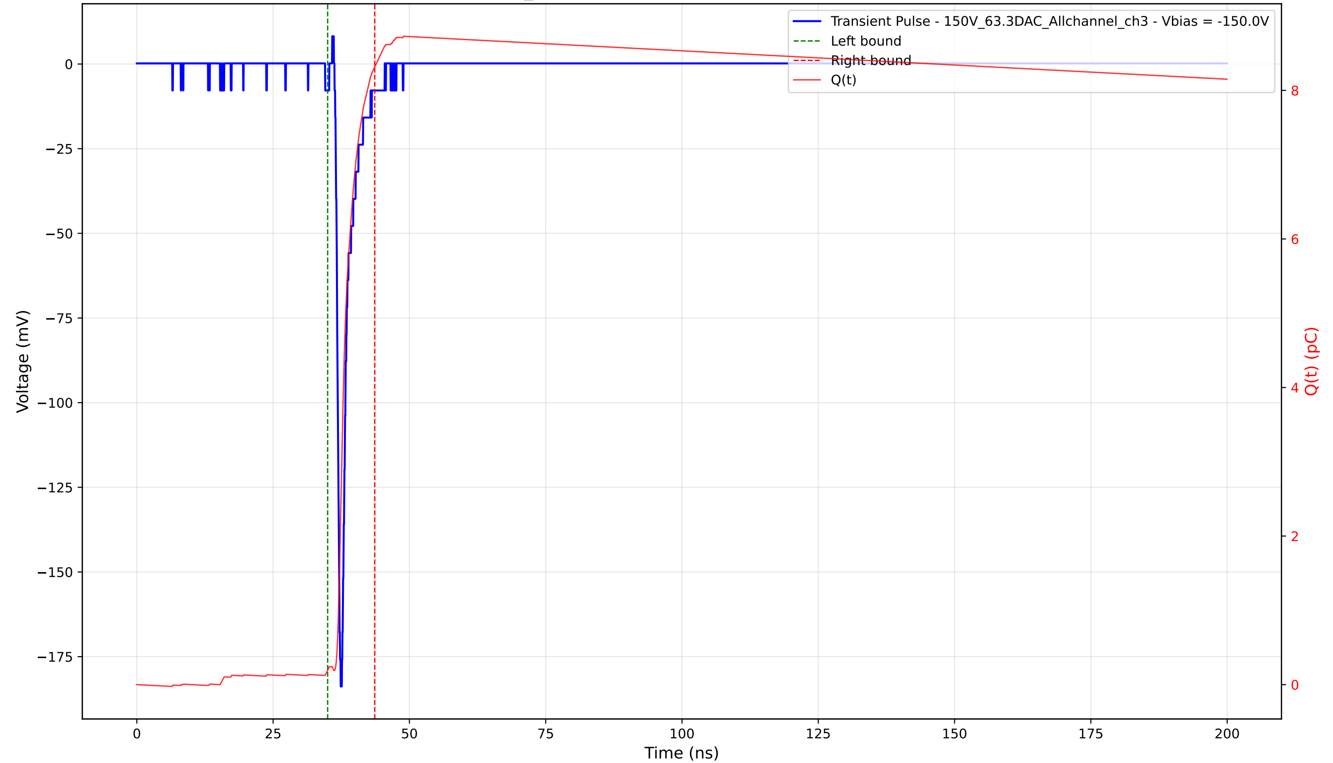
Transient Pulse - Sample: 1cm_42 - Position: 3085.0 \mu\text{m} - Charge: 8.12 pC - Rise Time: 0.75 ns
