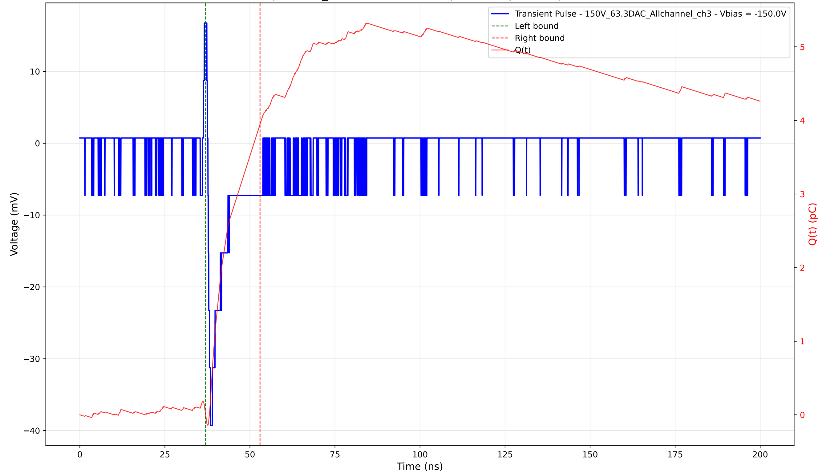
Transient Pulse - Sample: 1cm_42 - Position: 4110.0 \mu\text{m} - Charge: 3.91 pC - Rise Time: 0.74 ns
