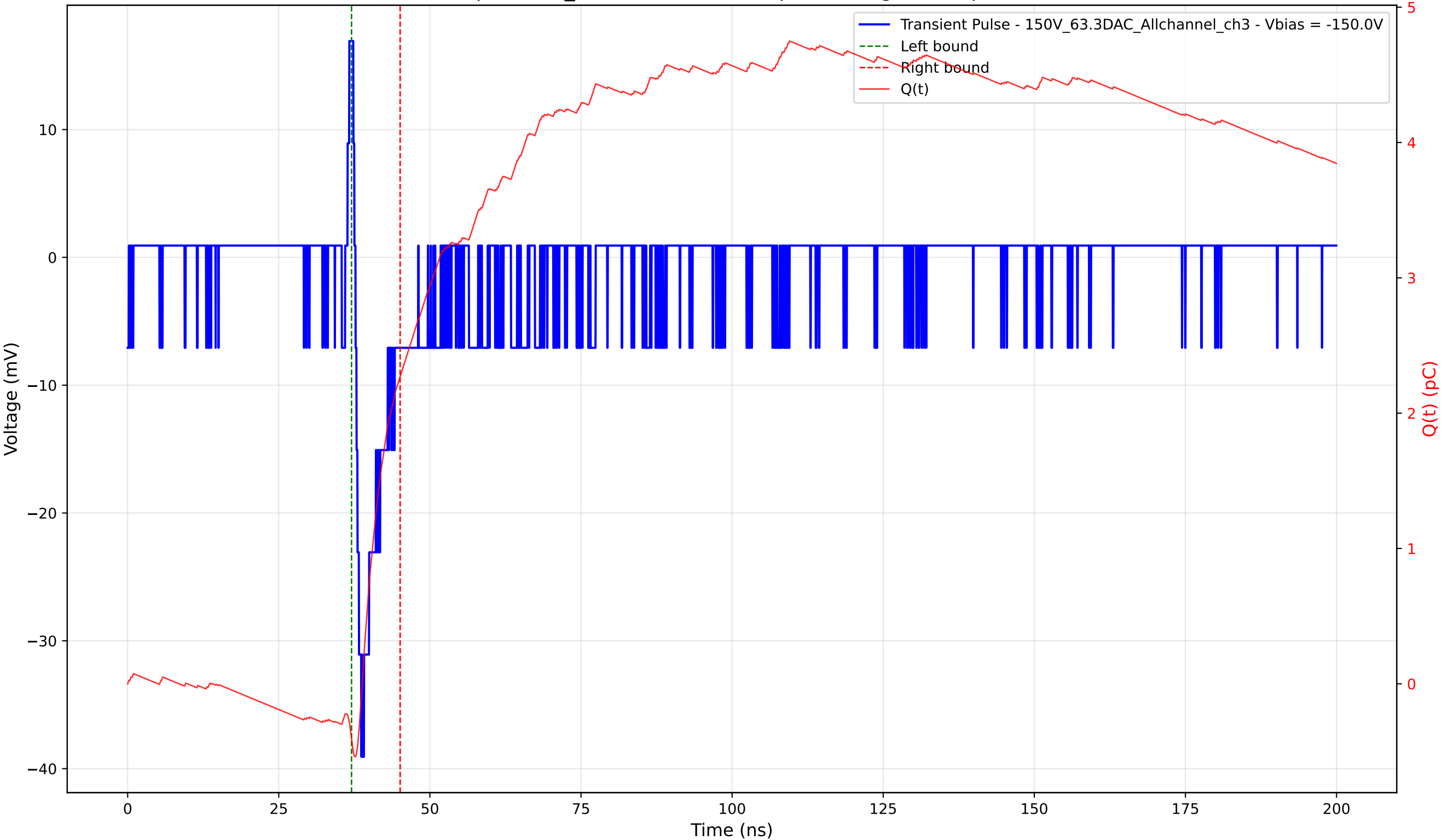
Transient Pulse - Sample: 1cm_42 - Position: 495.0 \mu\text{m} - Charge: 2.68 pC - Rise Time: 0.98 ns
