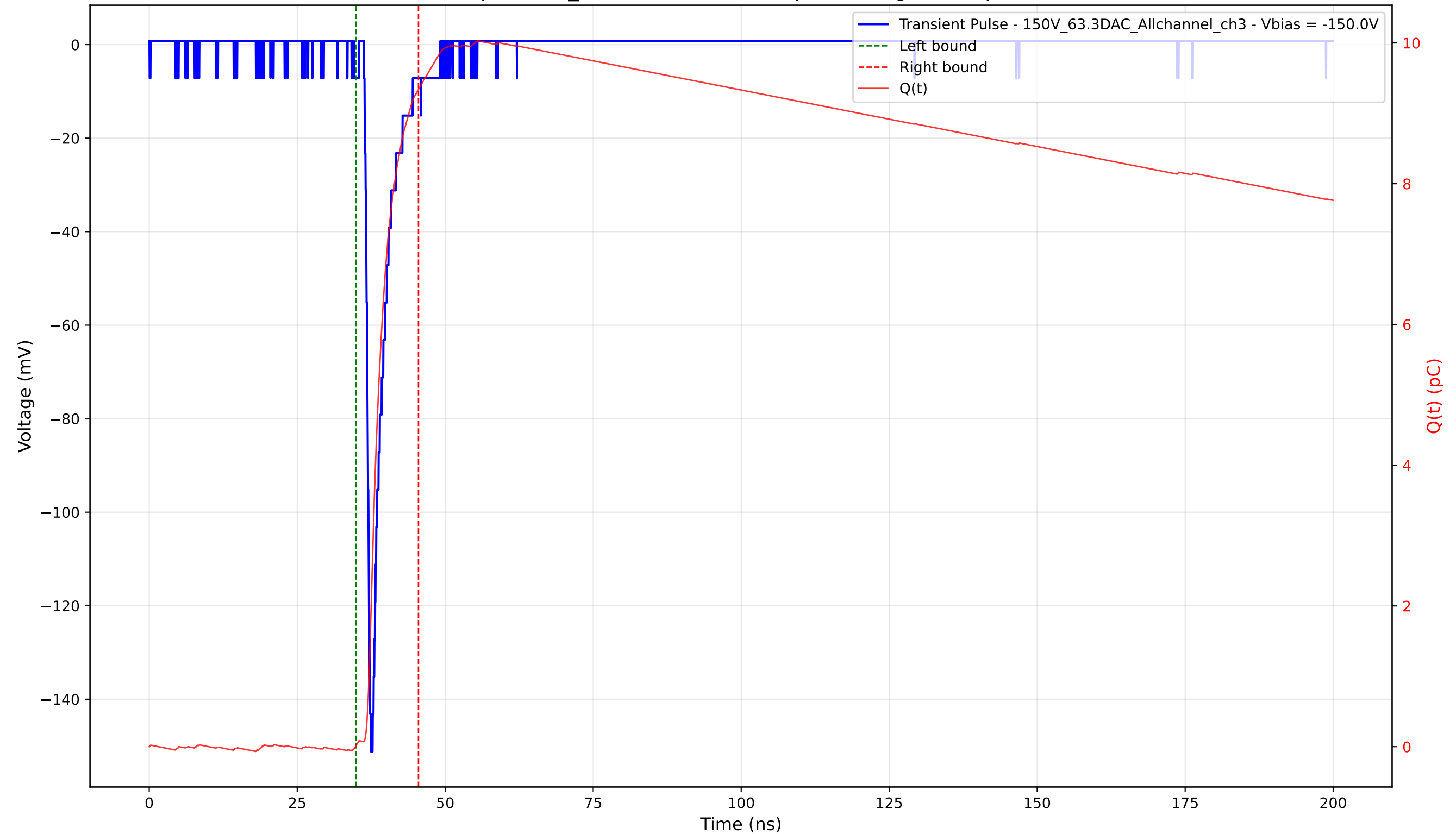
Transient Pulse - Sample: 1cm_42 - Position: 1755.0 \mu\text{m} - Charge: 9.32 pC - Rise Time: 0.92 ns
