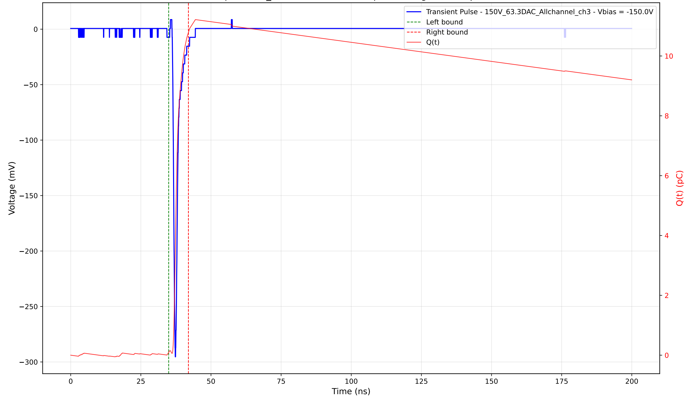
Transient Pulse - Sample: 1cm_42 - Position: 2945.0 \mu\text{m} - Charge: 10.69 pC - Rise Time: 0.78 ns
