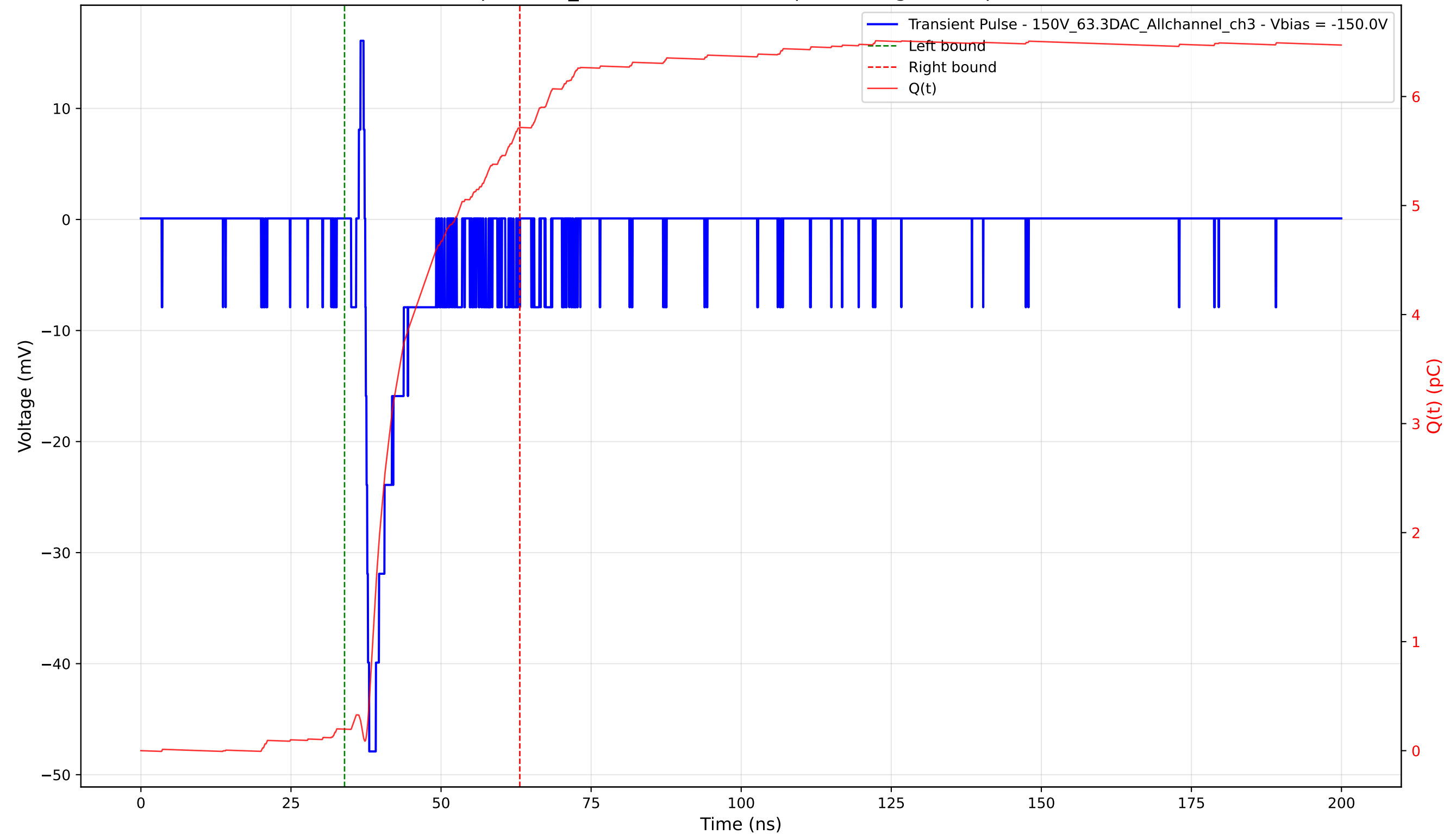
Transient Pulse - Sample: 1cm_42 - Position: 3880.0 \mu\text{m} - Charge: 5.52 pC - Rise Time: 0.66 ns
