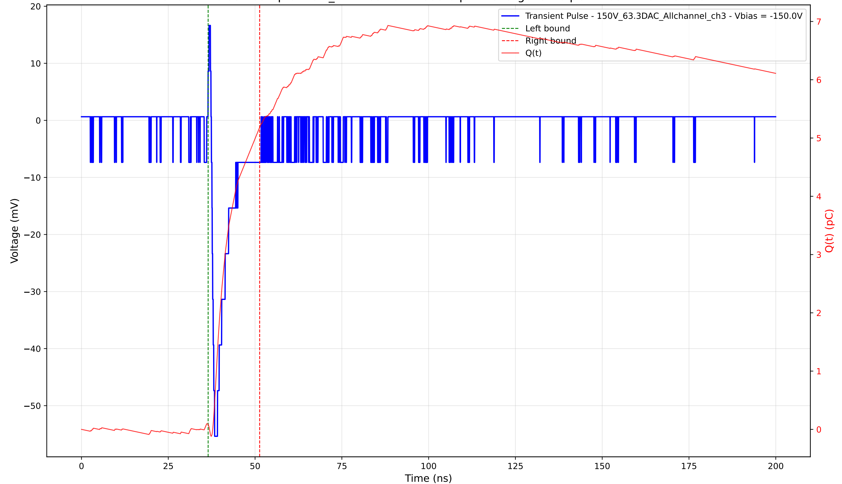
Transient Pulse - Sample: 1cm_42 - Position: 1095.0 \mu\text{m} - Charge: 5.10 pC - Rise Time: 0.93 ns
