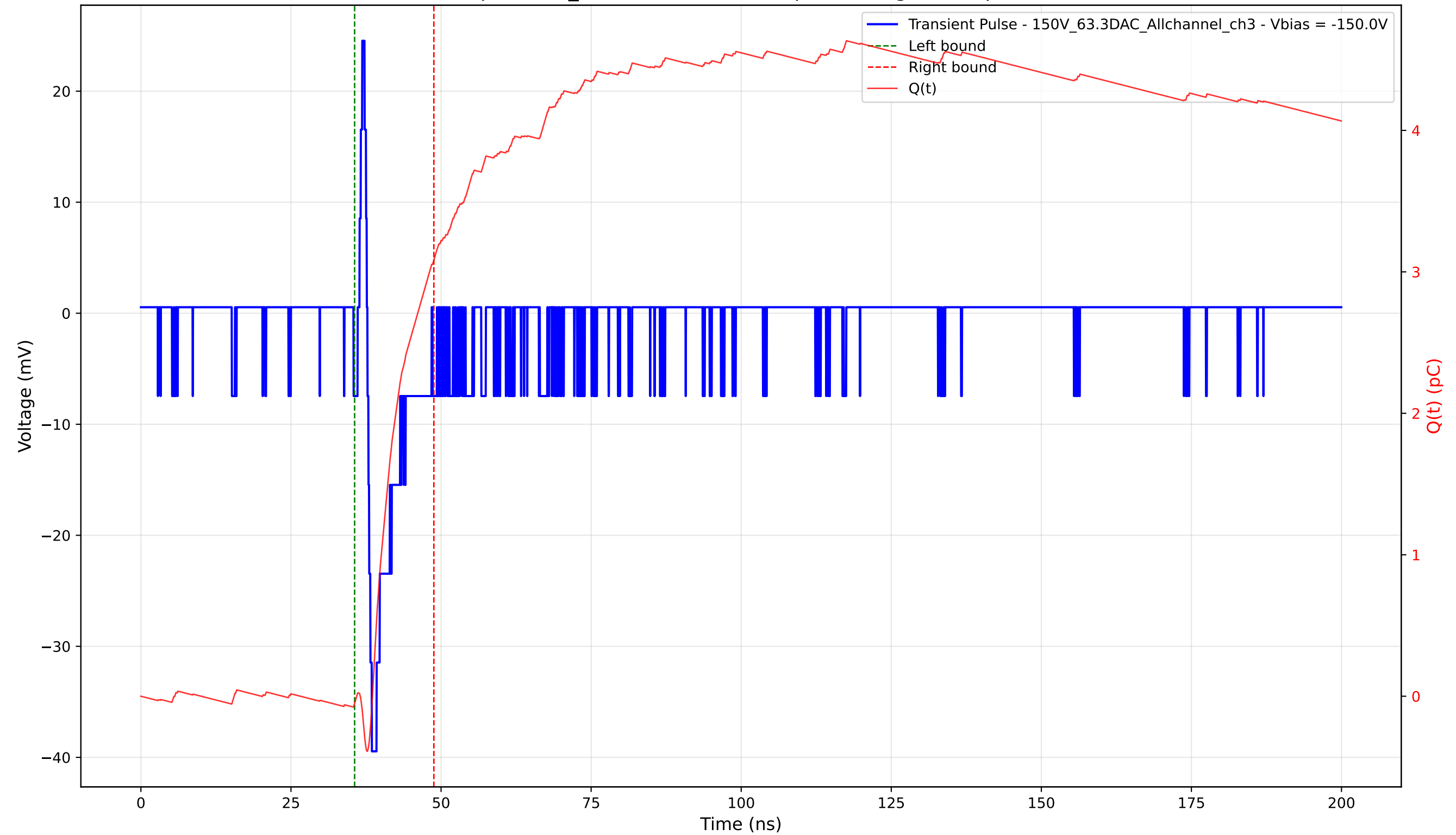
Transient Pulse - Sample: 1cm_42 - Position: 4355.0 \mu\text{m} - Charge: 3.13 pC - Rise Time: 0.74 ns
