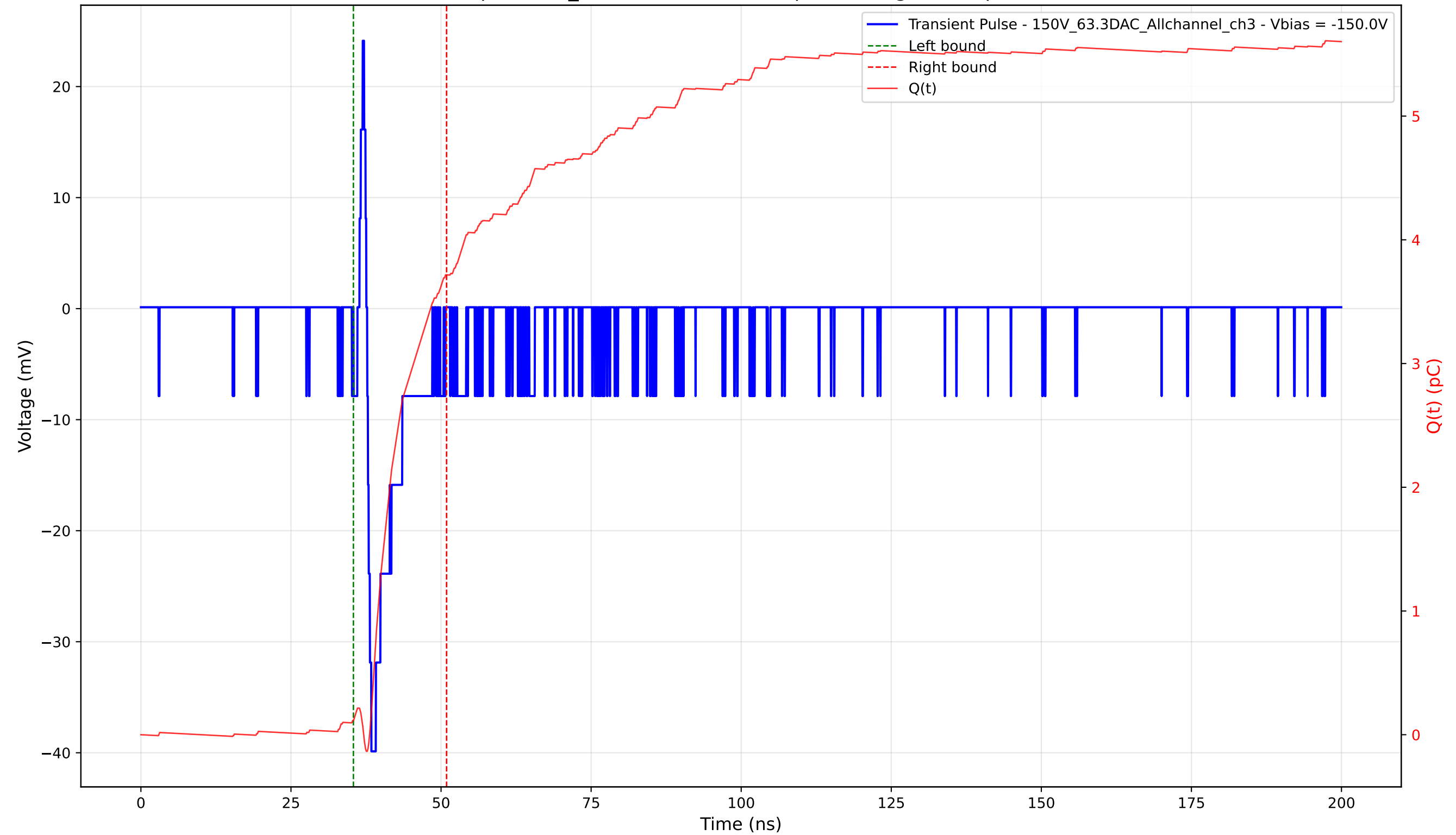
Transient Pulse - Sample: 1cm_42 - Position: 4180.0 \mu\text{m} - Charge: 3.60 pC - Rise Time: 0.70 ns
