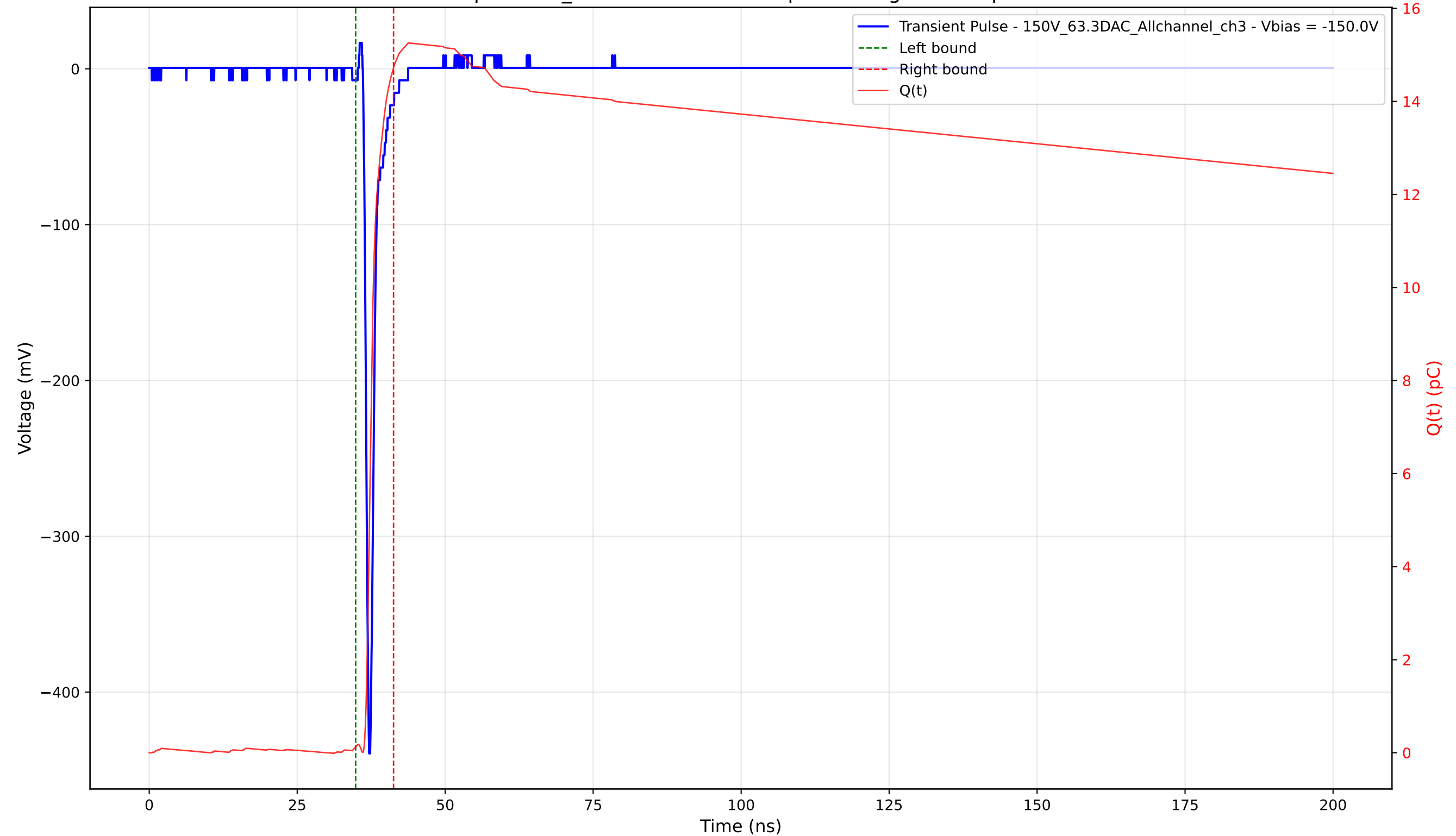
Transient Pulse - Sample: 1cm_42 - Position: 2810.0 \mu\text{m} - Charge: 14.60 pC - Rise Time: 0.74 ns
