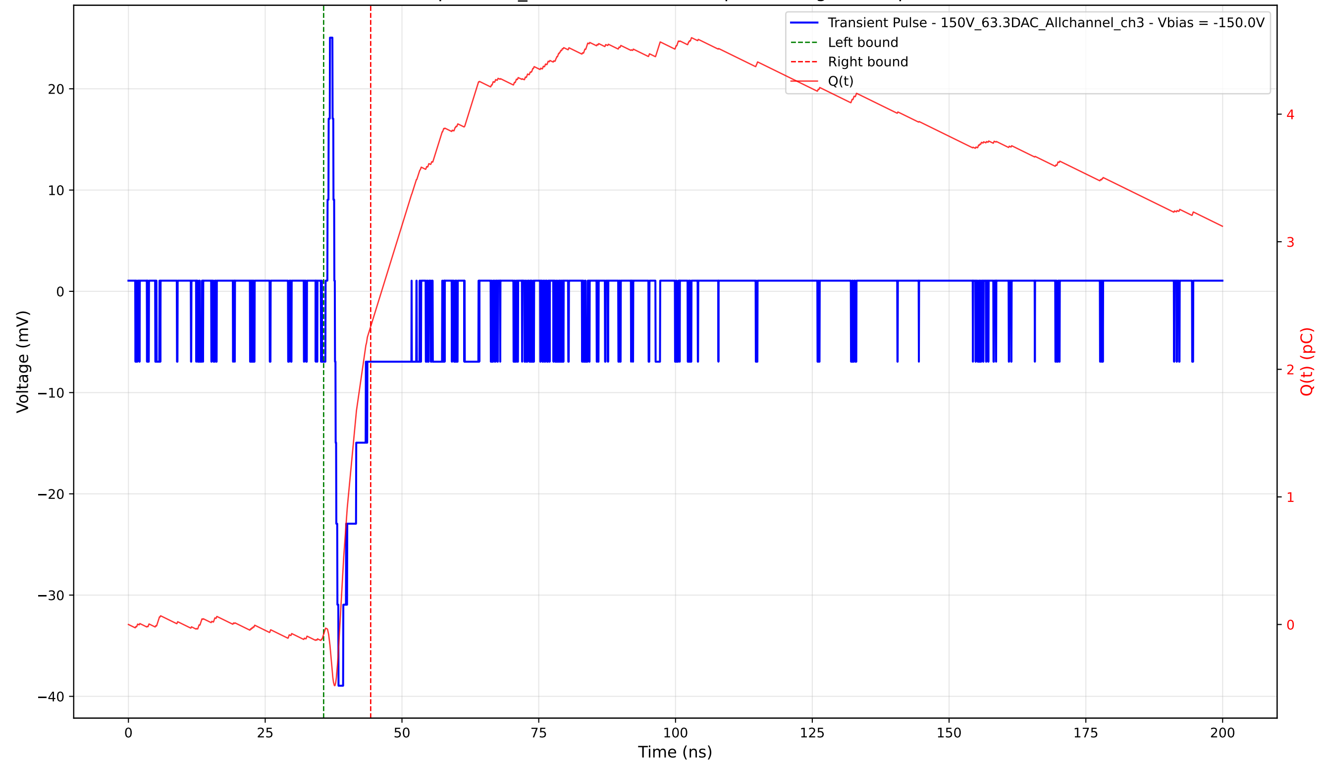
Transient Pulse - Sample: 1cm_42 - Position: 4270.0 \mu\text{m} - Charge: 2.41 pC - Rise Time: 0.66 ns
