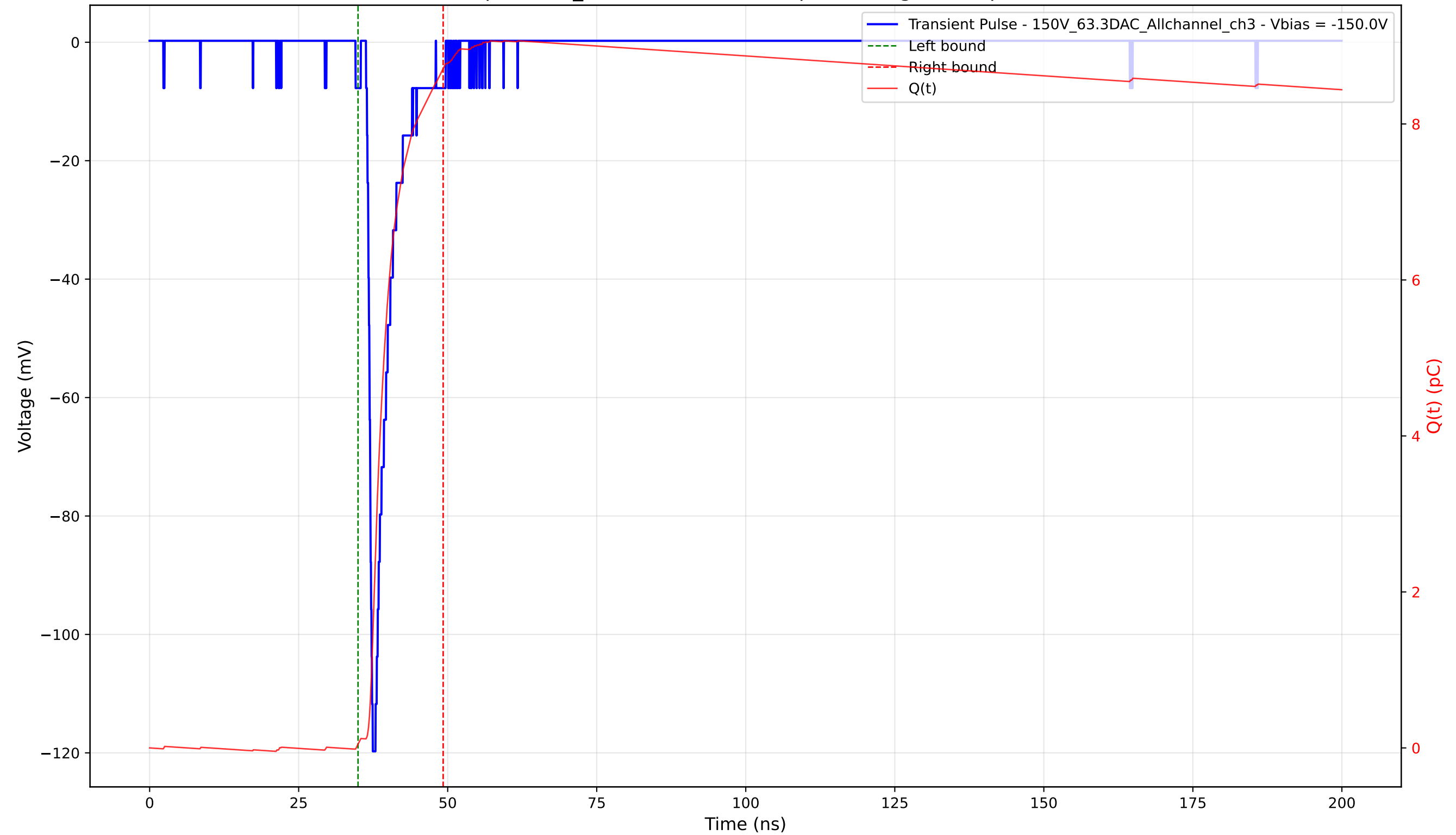
Transient Pulse - Sample: 1cm_42 - Position: 1670.0 \mu\text{m} - Charge: 8.66 pC - Rise Time: 0.86 ns
