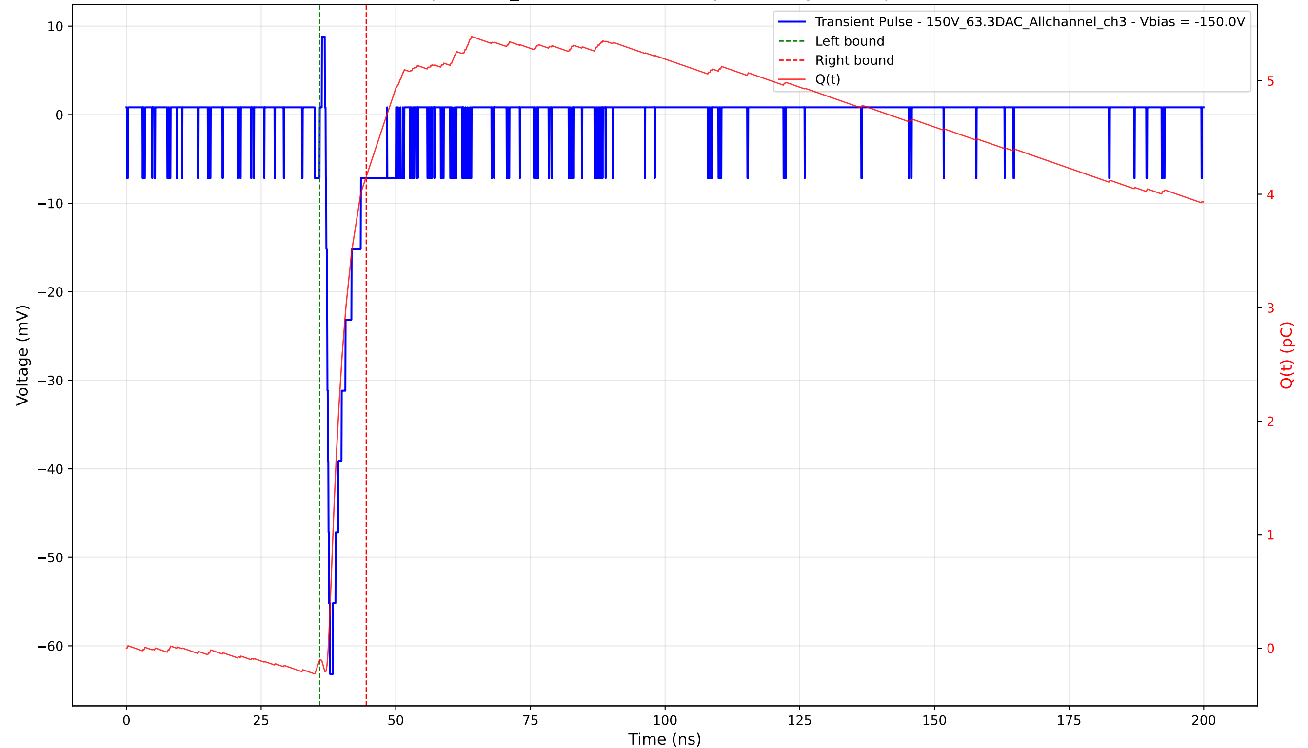
Transient Pulse - Sample: 1cm_42 - Position: 3575.0 \mu\text{m} - Charge: 4.26 pC - Rise Time: 0.81 ns
