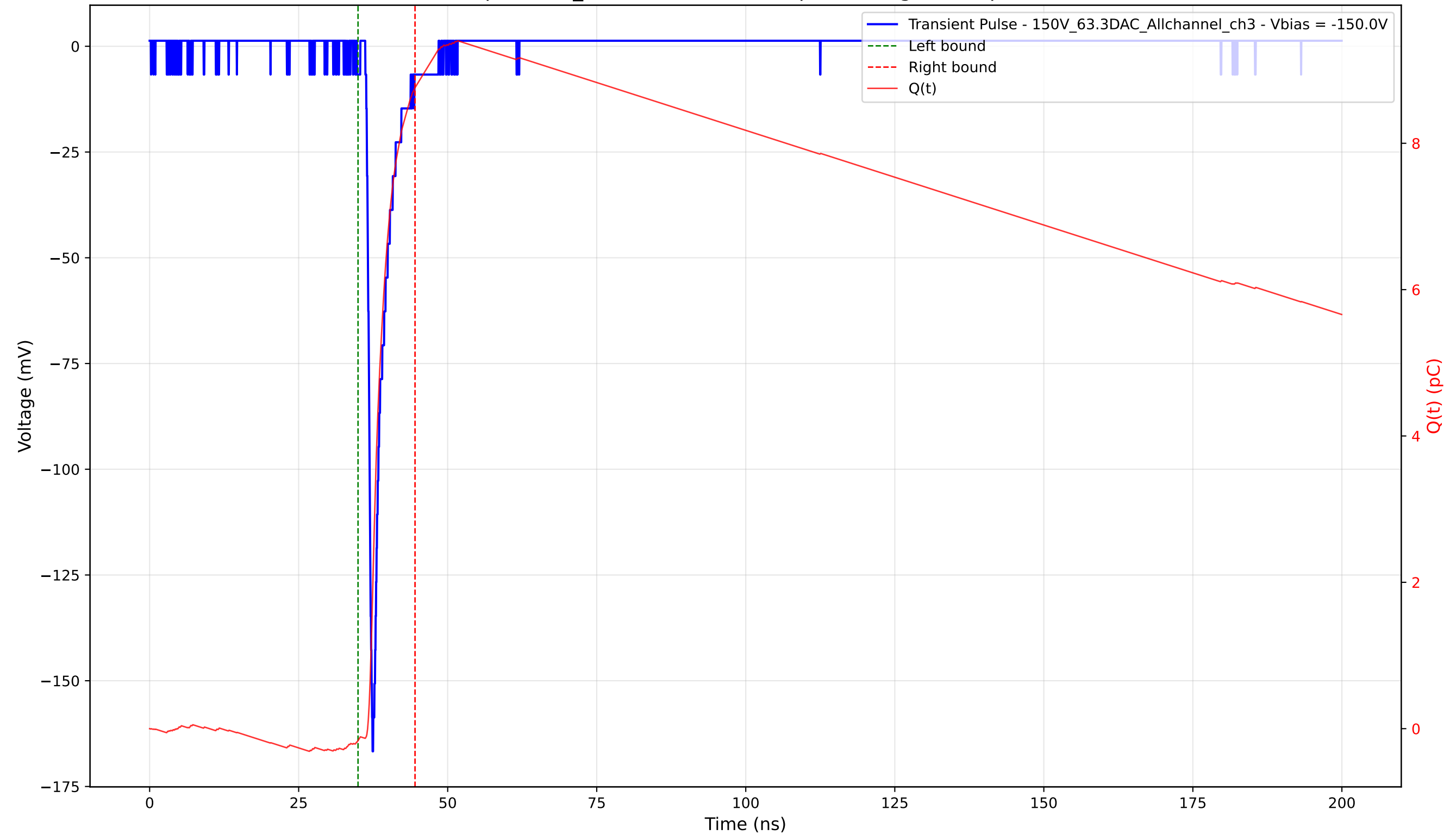
Transient Pulse - Sample: 1cm_42 - Position: 1870.0 \mu\text{m} - Charge: 8.92 pC - Rise Time: 0.83 ns
