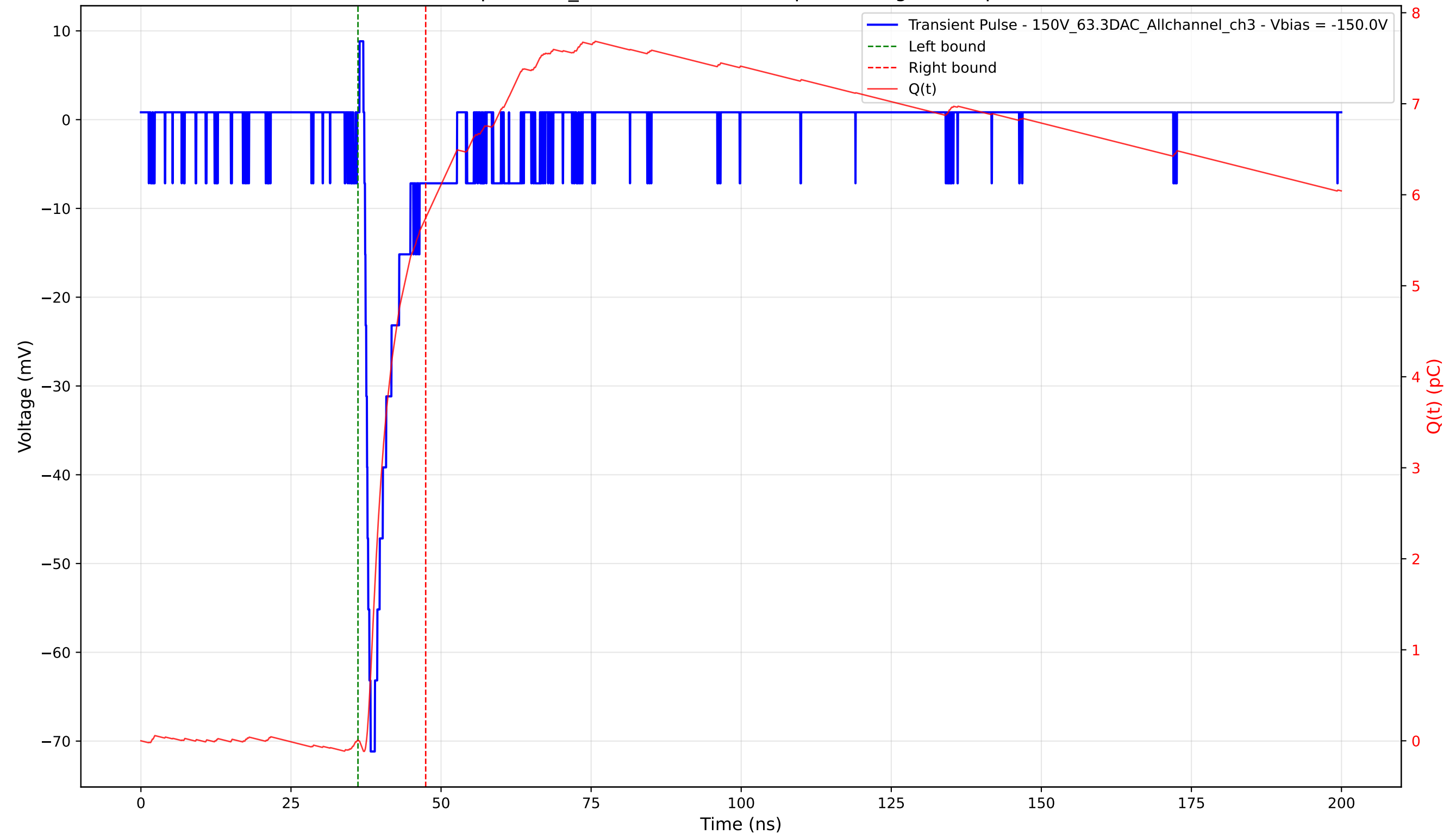
Transient Pulse - Sample: 1cm_42 - Position: 1260.0 \mu\text{m} - Charge: 5.74 pC - Rise Time: 1.04 ns
