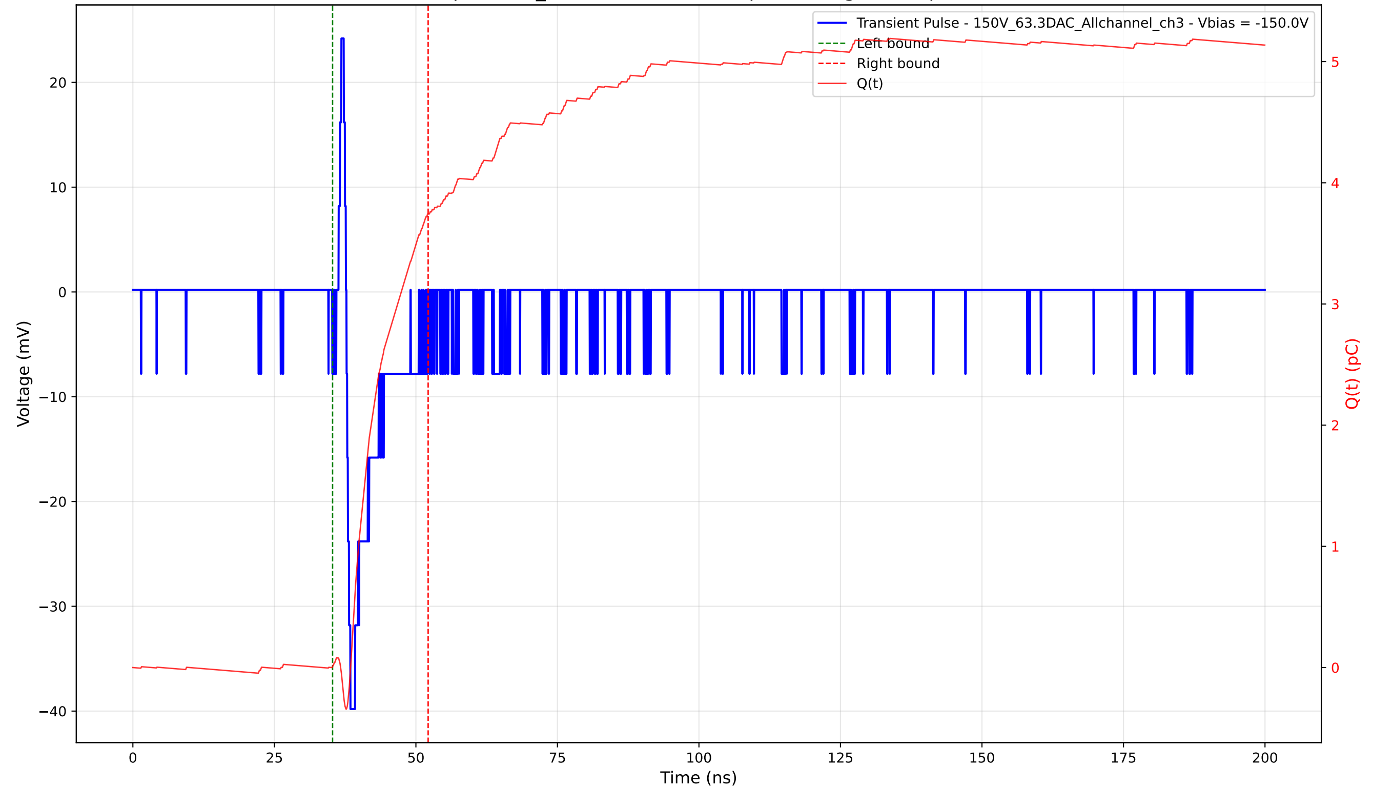
Transient Pulse - Sample: 1cm_42 - Position: 4280.0 \mu\text{m} - Charge: 3.73 pC - Rise Time: 0.70 ns
