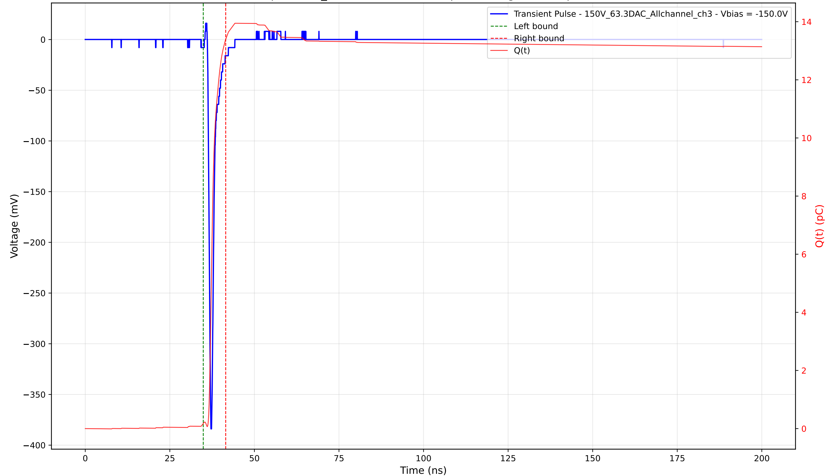
Transient Pulse - Sample: 1cm_42 - Position: 2185.0 \mu\text{m} - Charge: 13.22 pC - Rise Time: 0.71 ns
