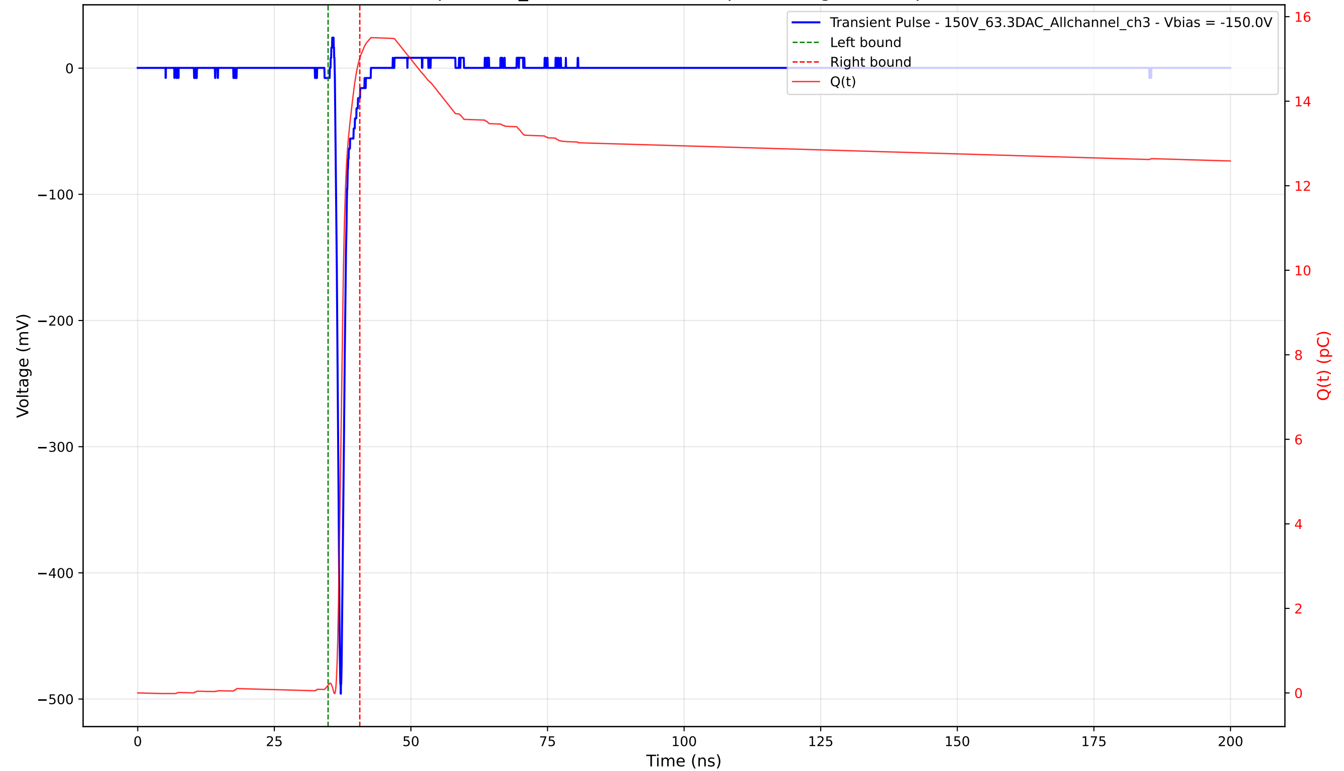
Transient Pulse - Sample: 1cm_42 - Position: 2570.0 \mu\text{m} - Charge: 14.84 pC - Rise Time: 0.73 ns
