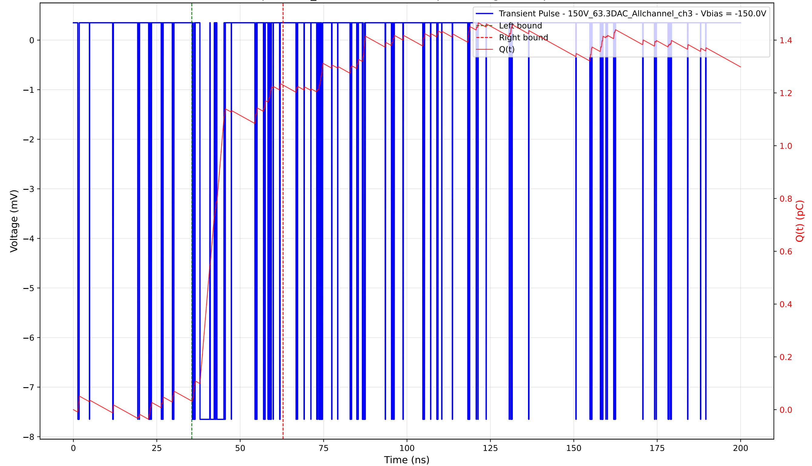
Transient Pulse - Sample: 1cm_42 - Position: 5105.0 \mu\text{m} - Charge: 1.20 pC - Rise Time: 0.04 ns
