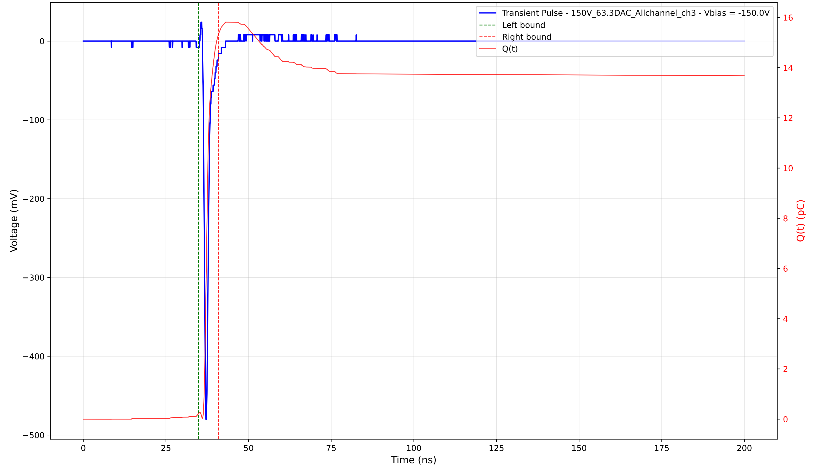
Transient Pulse - Sample: 1cm_42 - Position: 2385.0 \mu\text{m} - Charge: 15.09 pC - Rise Time: 0.68 ns
