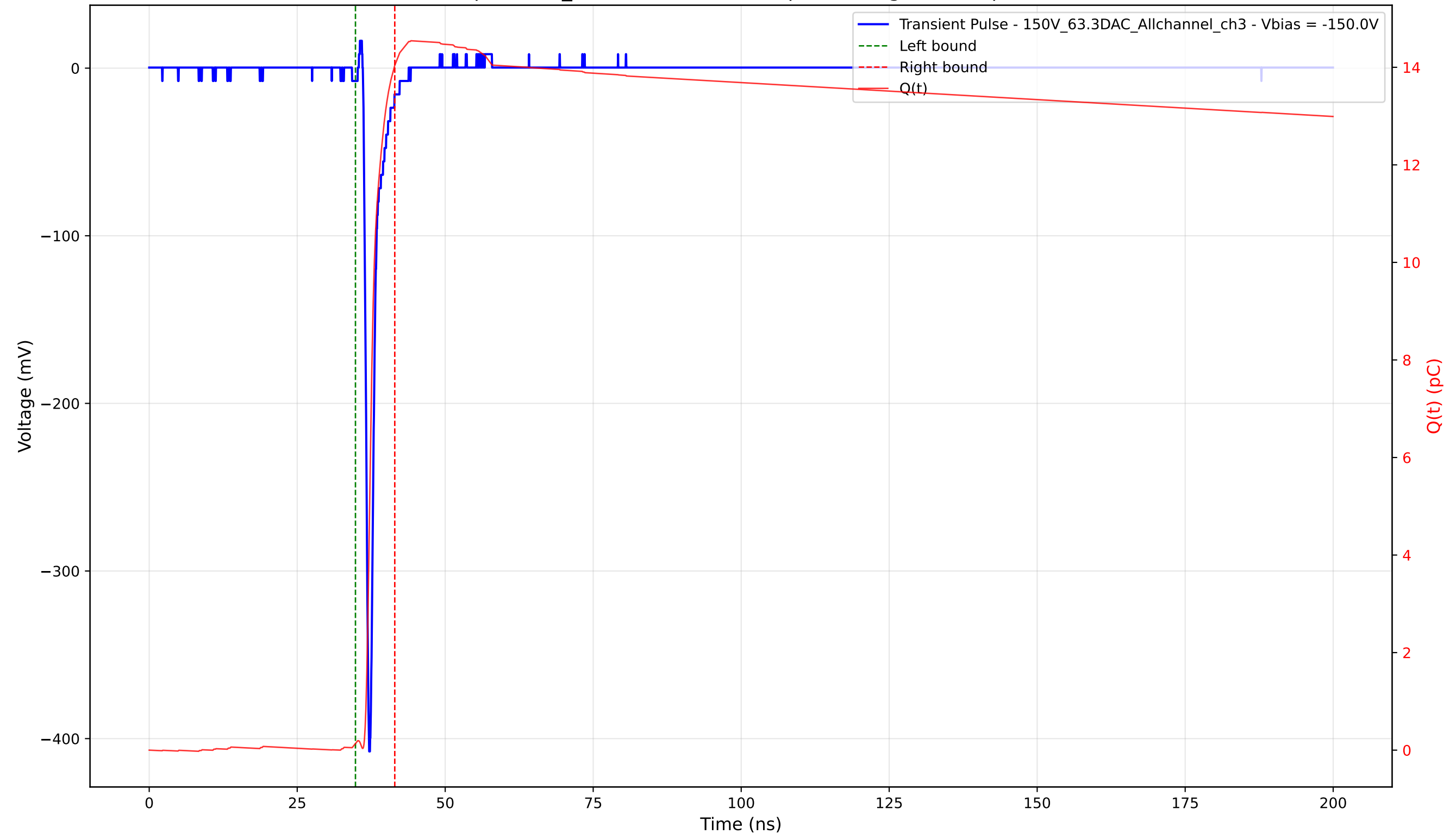
Transient Pulse - Sample: 1cm_42 - Position: 2200.0 \mu\text{m} - Charge: 13.90 pC - Rise Time: 0.71 ns
