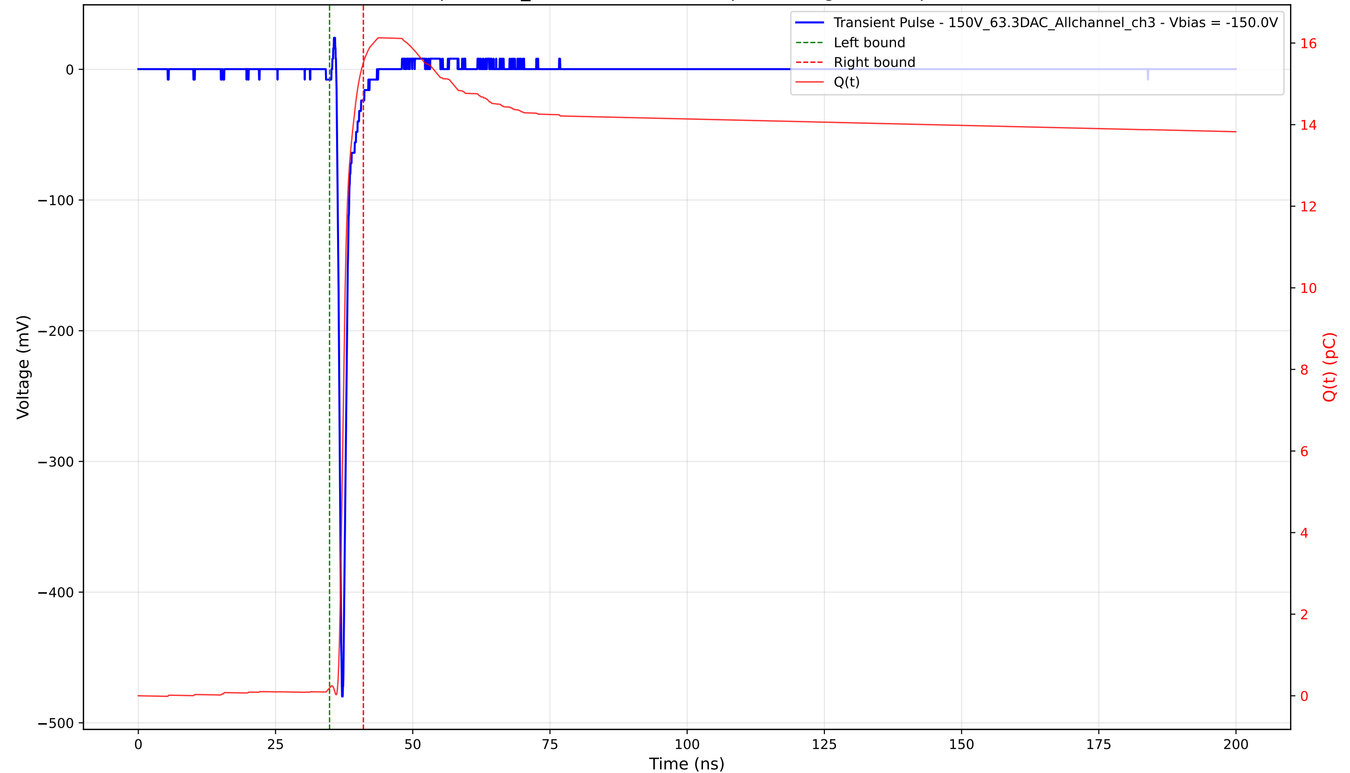
Transient Pulse - Sample: 1cm_42 - Position: 2705.0 \mu\text{m} - Charge: 15.33 pC - Rise Time: 0.70 ns
