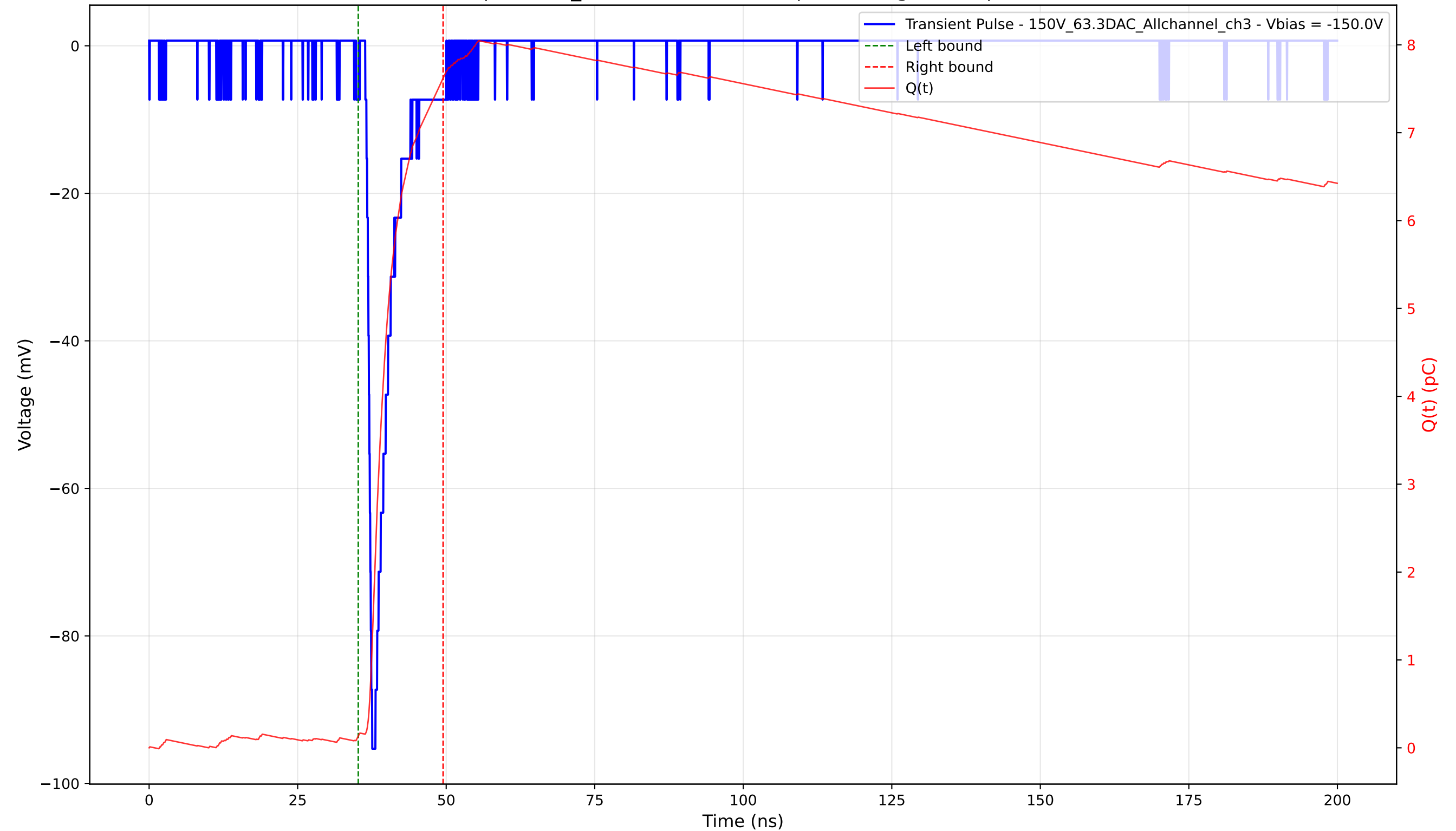
Transient Pulse - Sample: 1cm_42 - Position: 1590.0 \mu\text{m} - Charge: 7.49 pC - Rise Time: 0.83 ns
