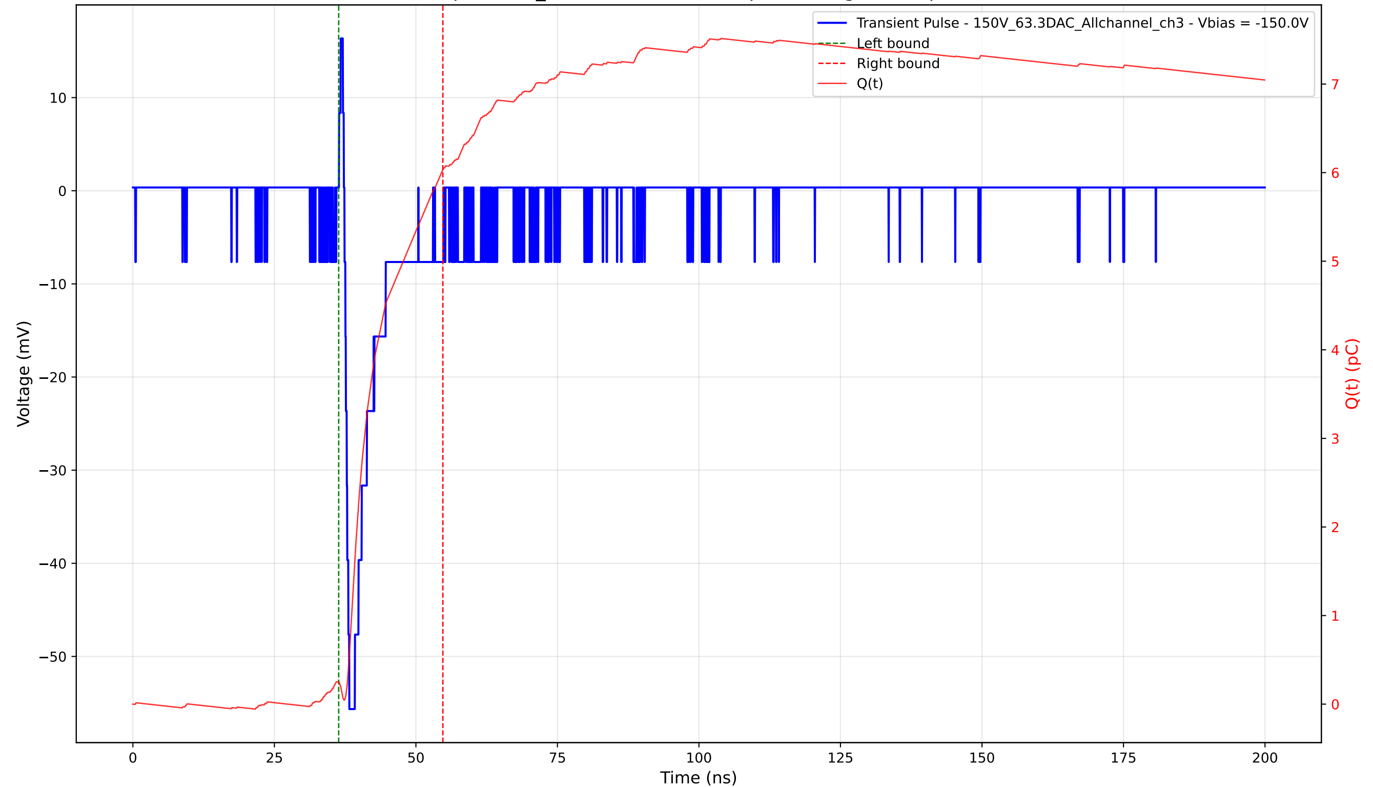
Transient Pulse - Sample: 1cm_42 - Position: 1110.0 \mu\text{m} - Charge: 5.79 pC - Rise Time: 0.85 ns
