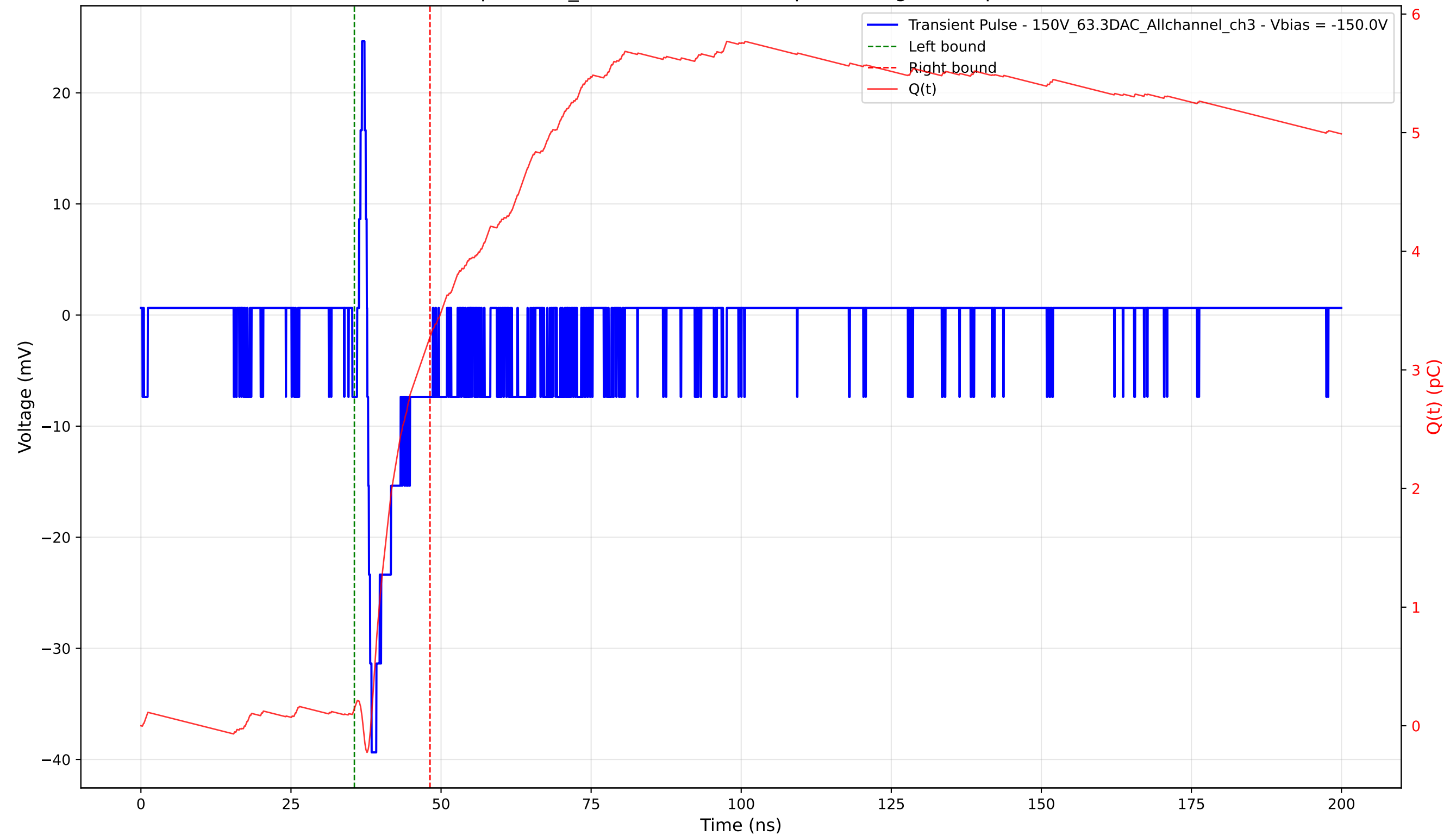
Transient Pulse - Sample: 1cm_42 - Position: 4215.0 \mu\text{m} - Charge: 3.14 pC - Rise Time: 0.74 ns
