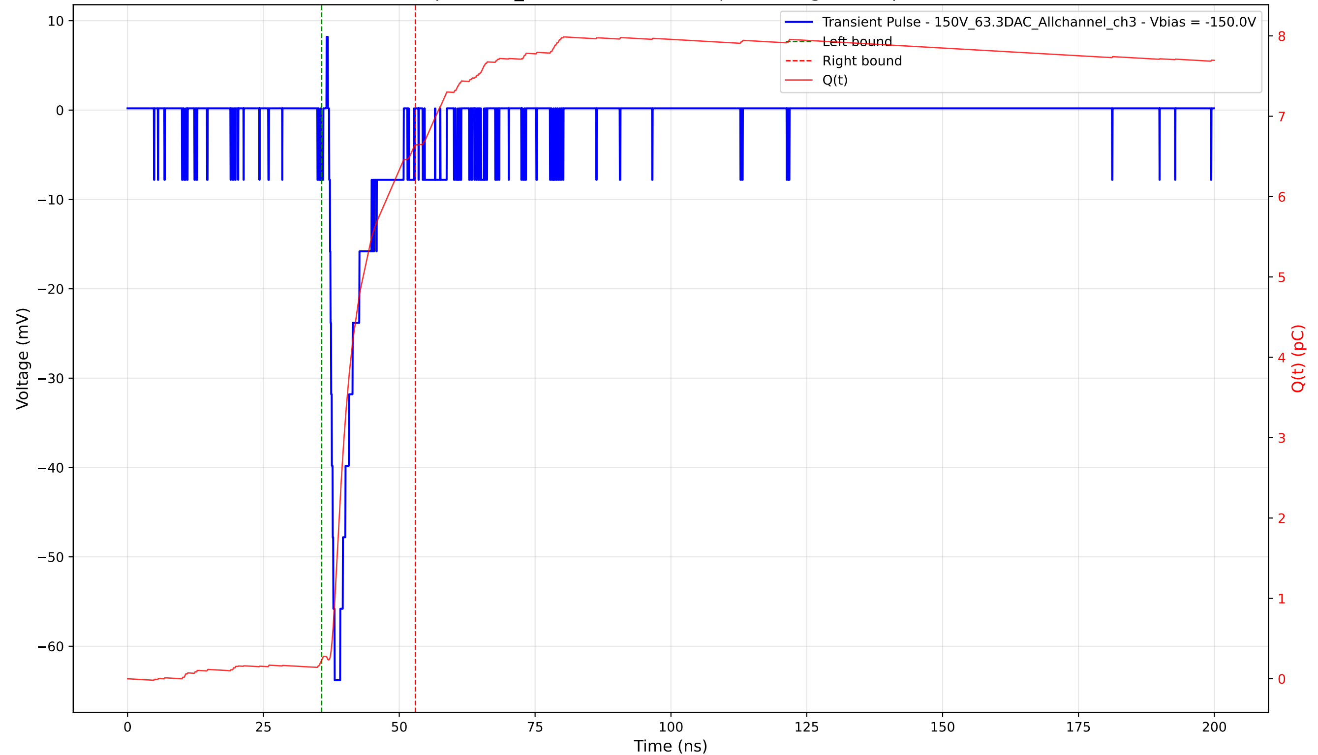
Transient Pulse - Sample: 1cm_42 - Position: 1355.0 \mu\text{m} - Charge: 6.41 pC - Rise Time: 1.01 ns
