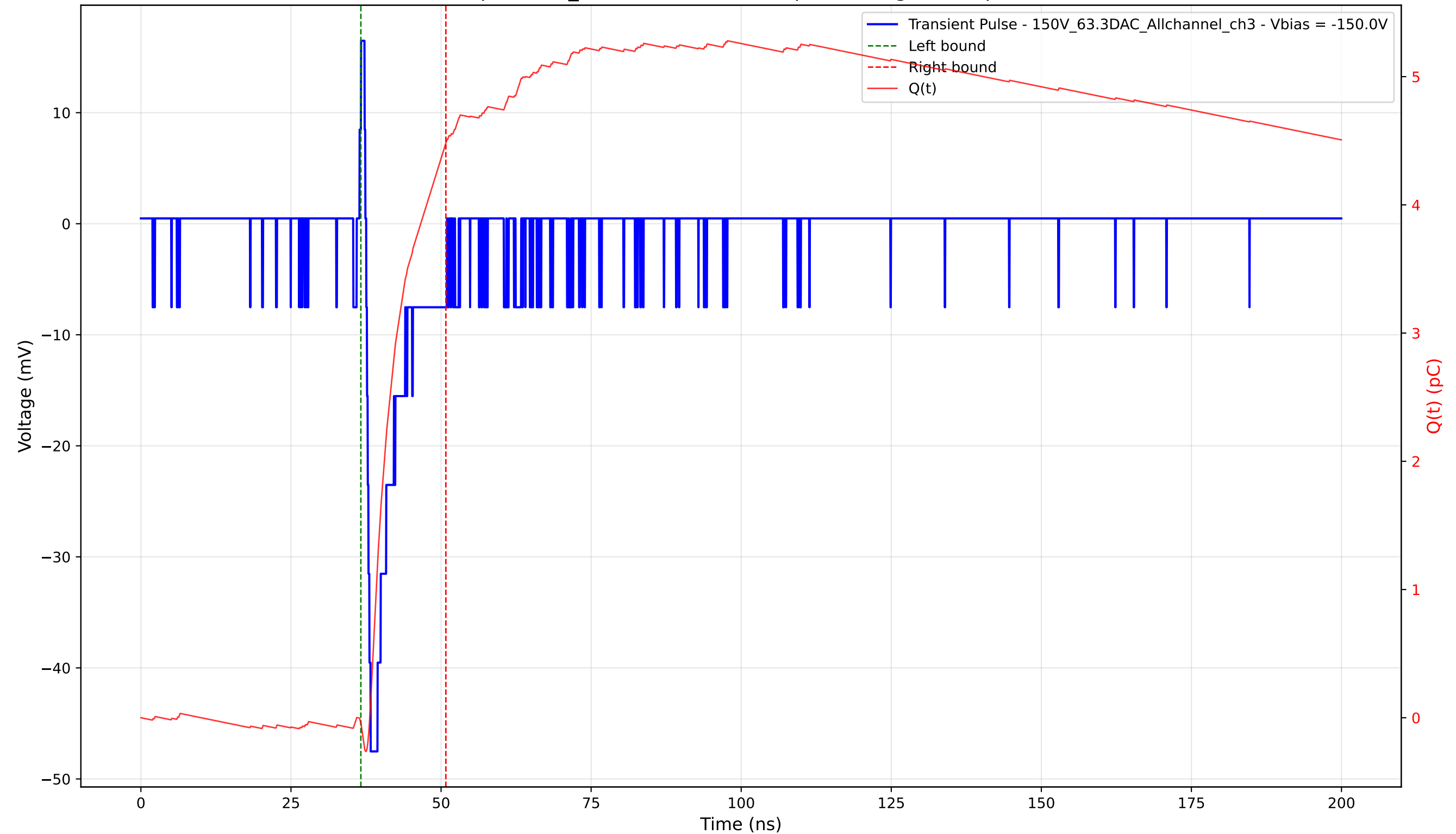
Transient Pulse - Sample: 1cm_42 - Position: 1025.0 \mu\text{m} - Charge: 4.52 pC - Rise Time: 0.74 ns
