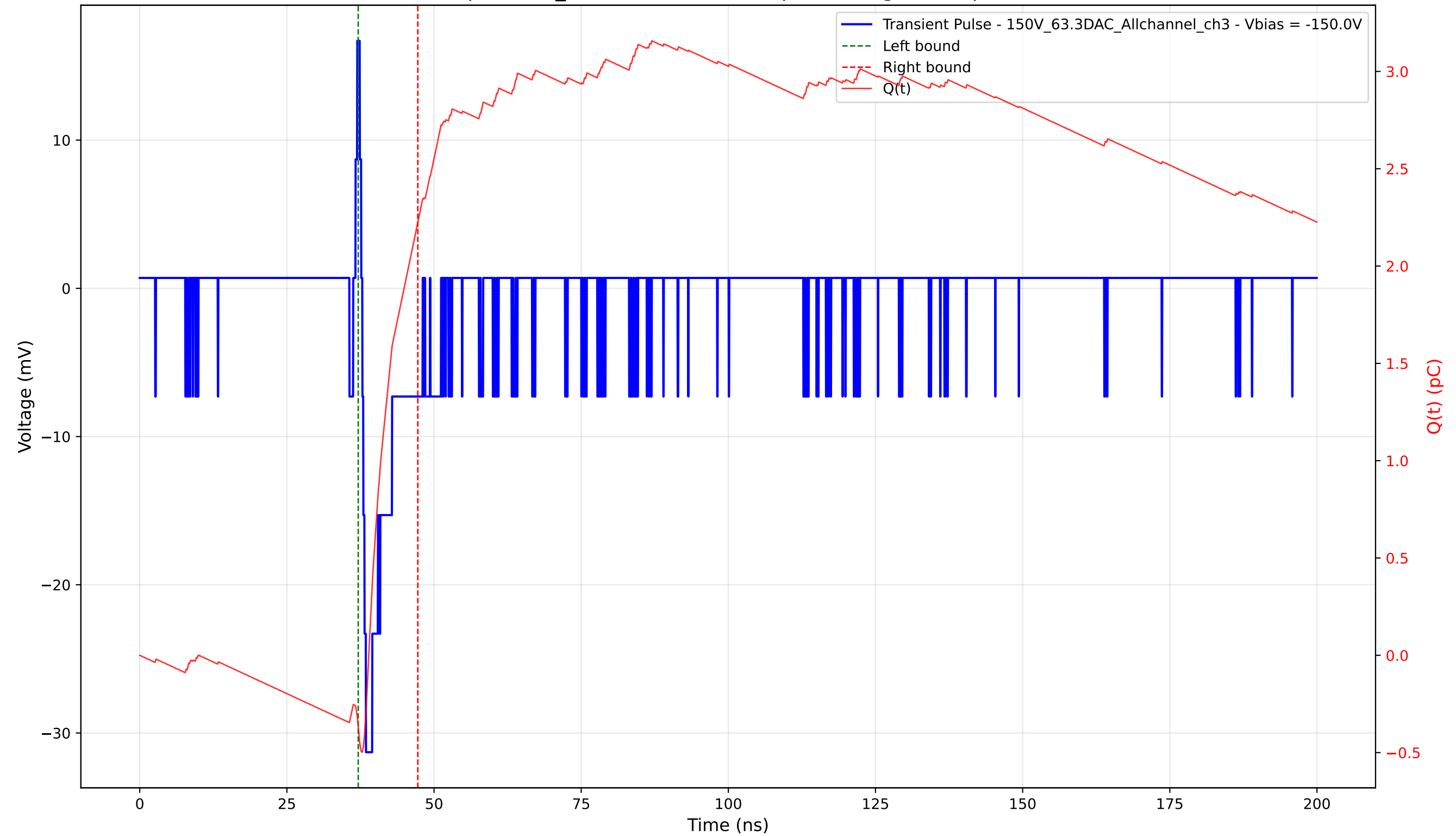
Transient Pulse - Sample: 1cm_42 - Position: 4770.0 \mu\text{m} - Charge: 2.59 pC - Rise Time: 0.63 ns
