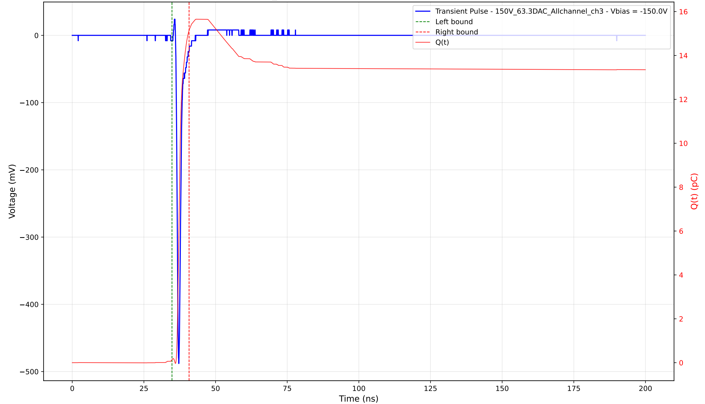
Transient Pulse - Sample: 1cm_42 - Position: 2410.0 \mu\text{m} - Charge: 15.01 pC - Rise Time: 0.71 ns
