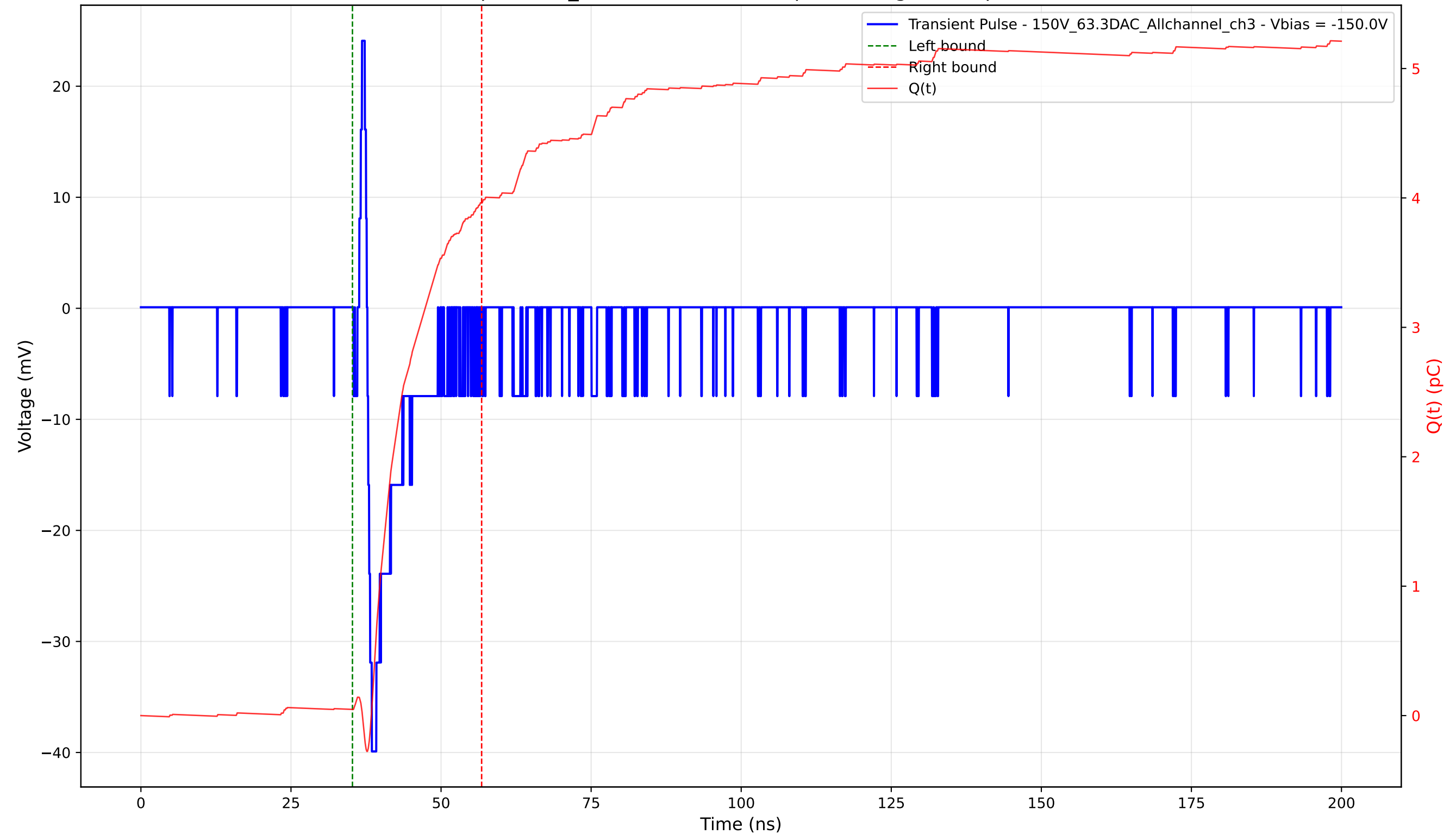
Transient Pulse - Sample: 1cm_42 - Position: 4335.0 \mu\text{m} - Charge: 3.91 pC - Rise Time: 0.74 ns
