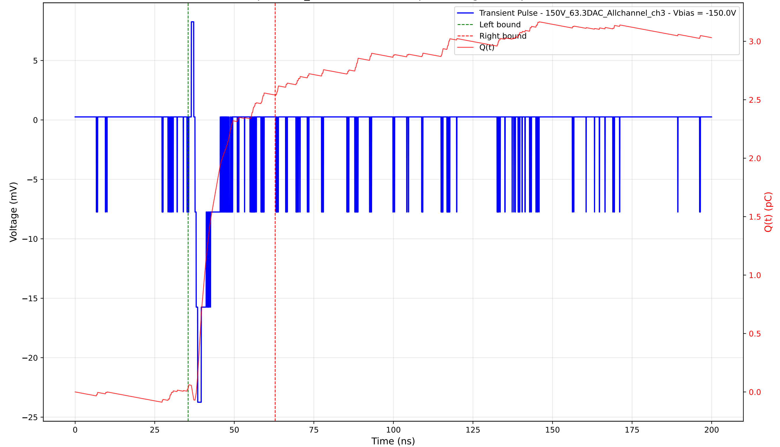
Transient Pulse - Sample: 1cm_42 - Position: 260.0 \mu\text{m} - Charge: 2.51 pC - Rise Time: 0.87 ns
