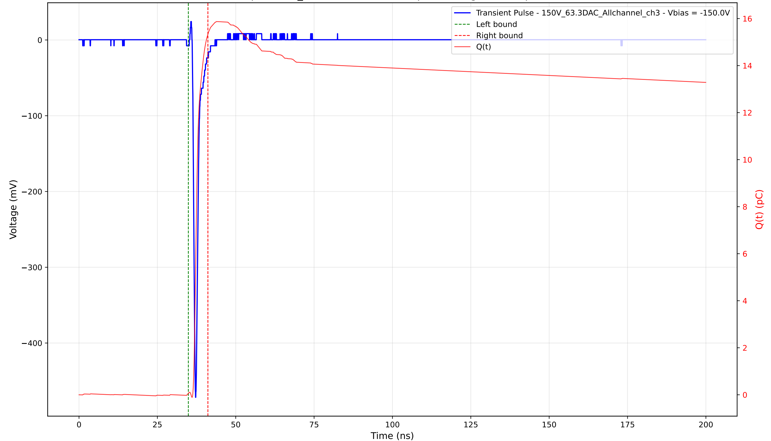
Transient Pulse - Sample: 1cm_42 - Position: 2745.0 \mu\text{m} - Charge: 15.28 pC - Rise Time: 0.74 ns
