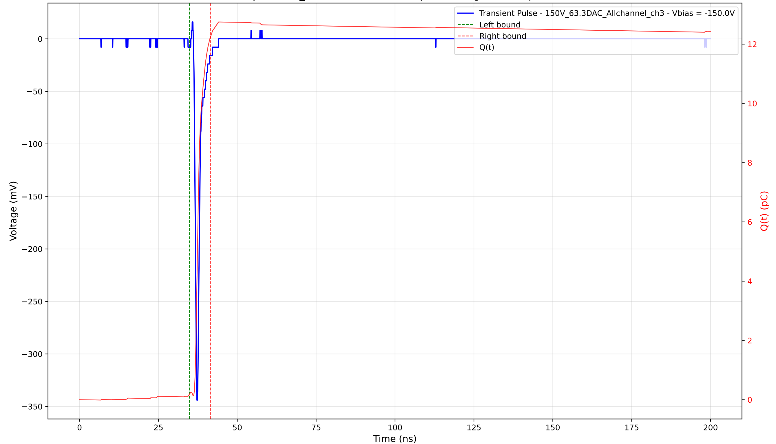
Transient Pulse - Sample: 1cm_42 - Position: 2895.0 \mu\text{m} - Charge: 12.08 pC - Rise Time: 0.75 ns
