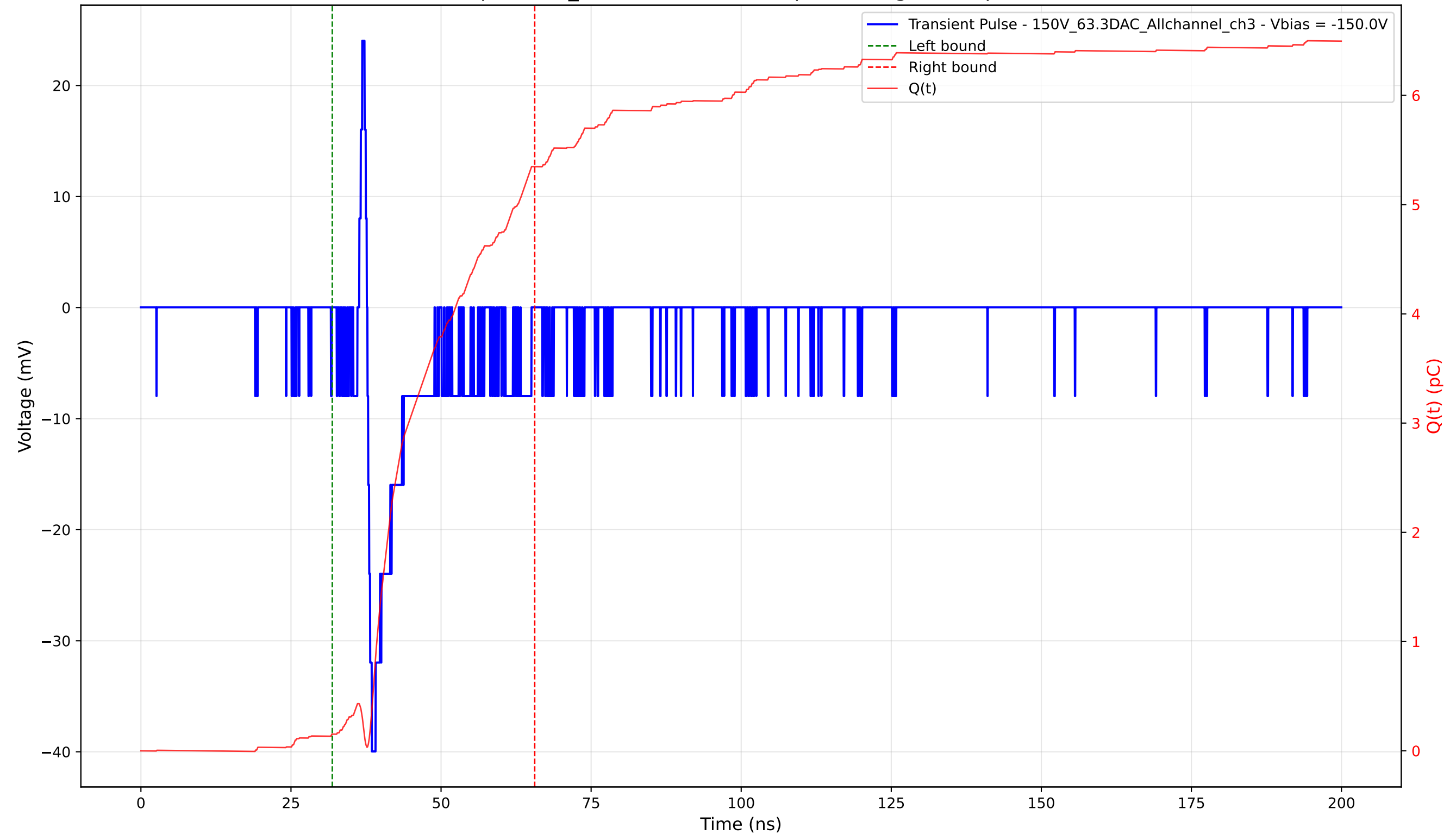
Transient Pulse - Sample: 1cm_42 - Position: 4345.0 \mu\text{m} - Charge: 5.19 pC - Rise Time: 0.74 ns
