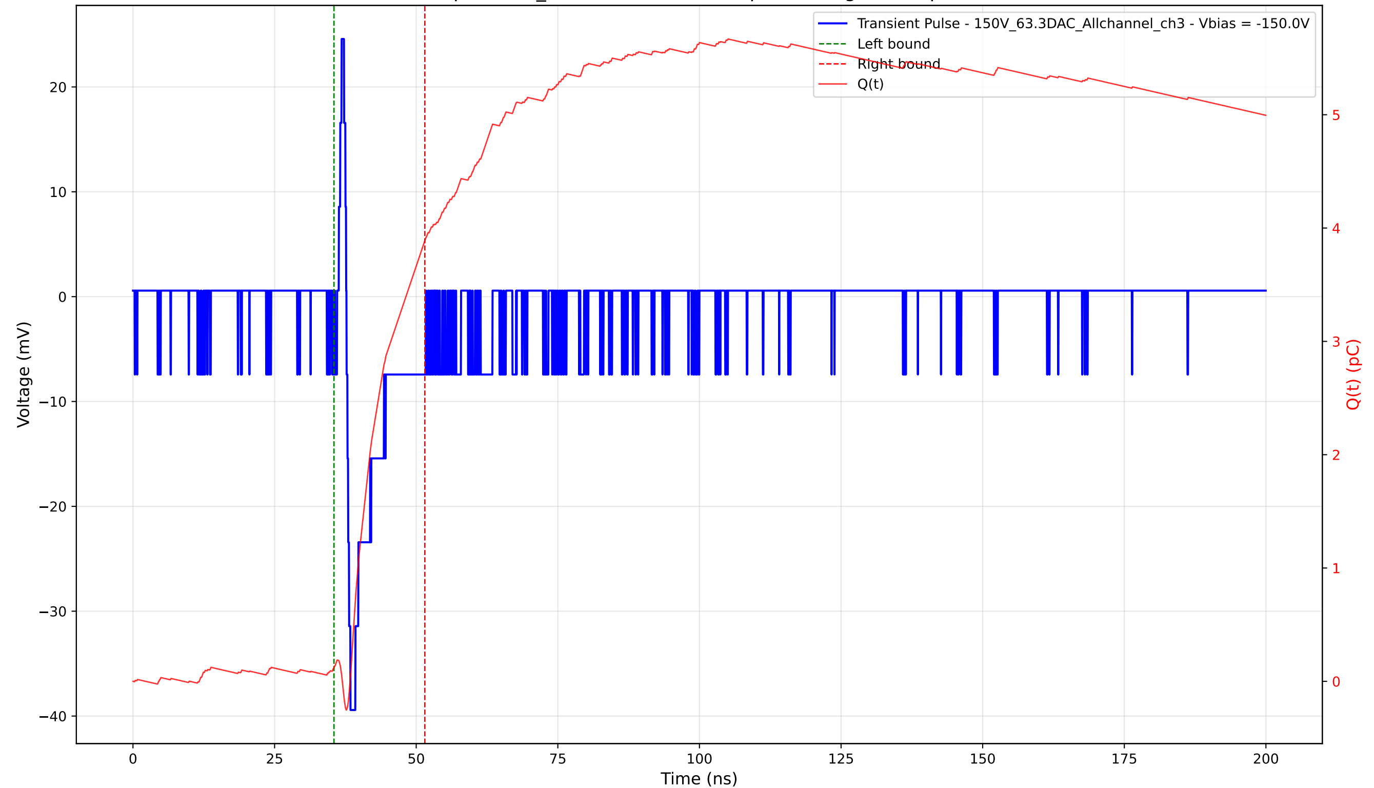
Transient Pulse - Sample: 1cm_42 - Position: 4285.0 \mu\text{m} - Charge: 3.77 pC - Rise Time: 0.70 ns
