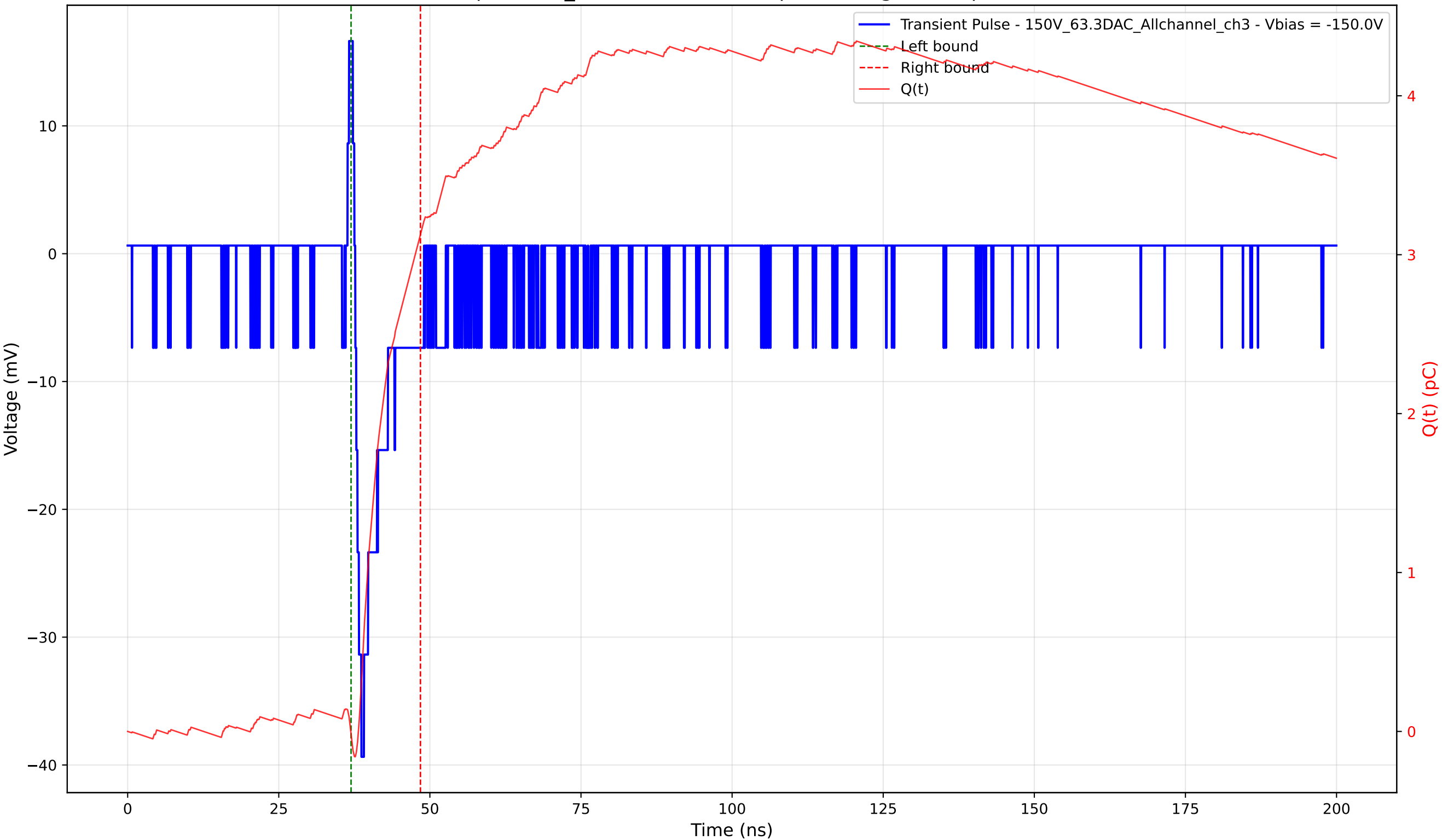
Transient Pulse - Sample: 1cm_42 - Position: 470.0 \mu\text{m} - Charge: 3.15 pC - Rise Time: 1.02 ns
