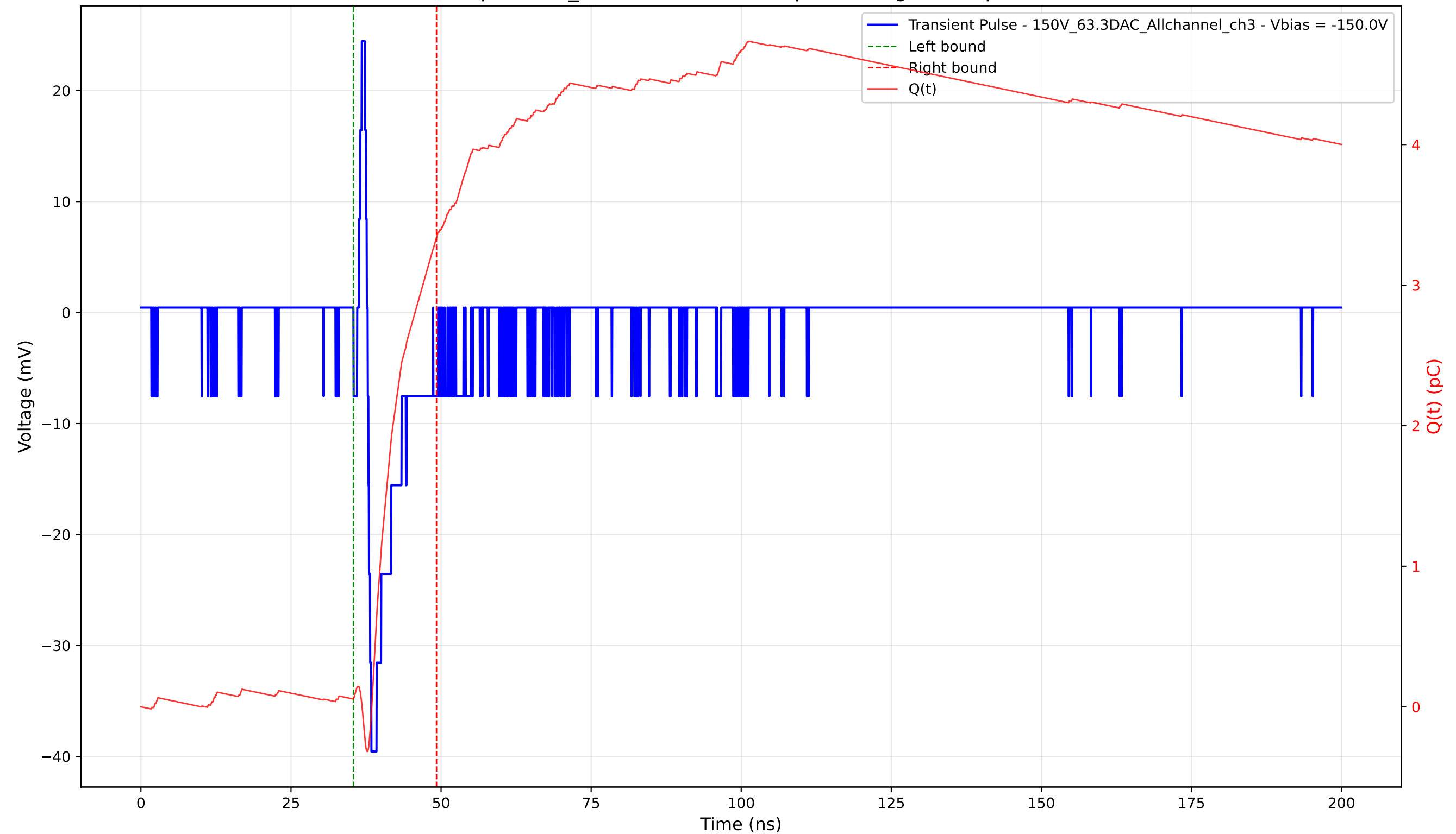
Transient Pulse - Sample: 1cm_42 - Position: 4310.0 \mu\text{m} - Charge: 3.28 pC - Rise Time: 0.62 ns
