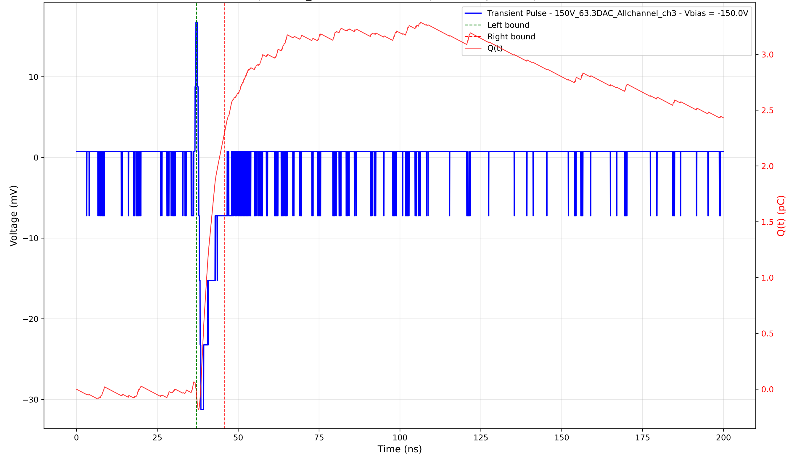
Transient Pulse - Sample: 1cm_42 - Position: 4730.0 \mu\text{m} - Charge: 2.34 pC - Rise Time: 0.67 ns
