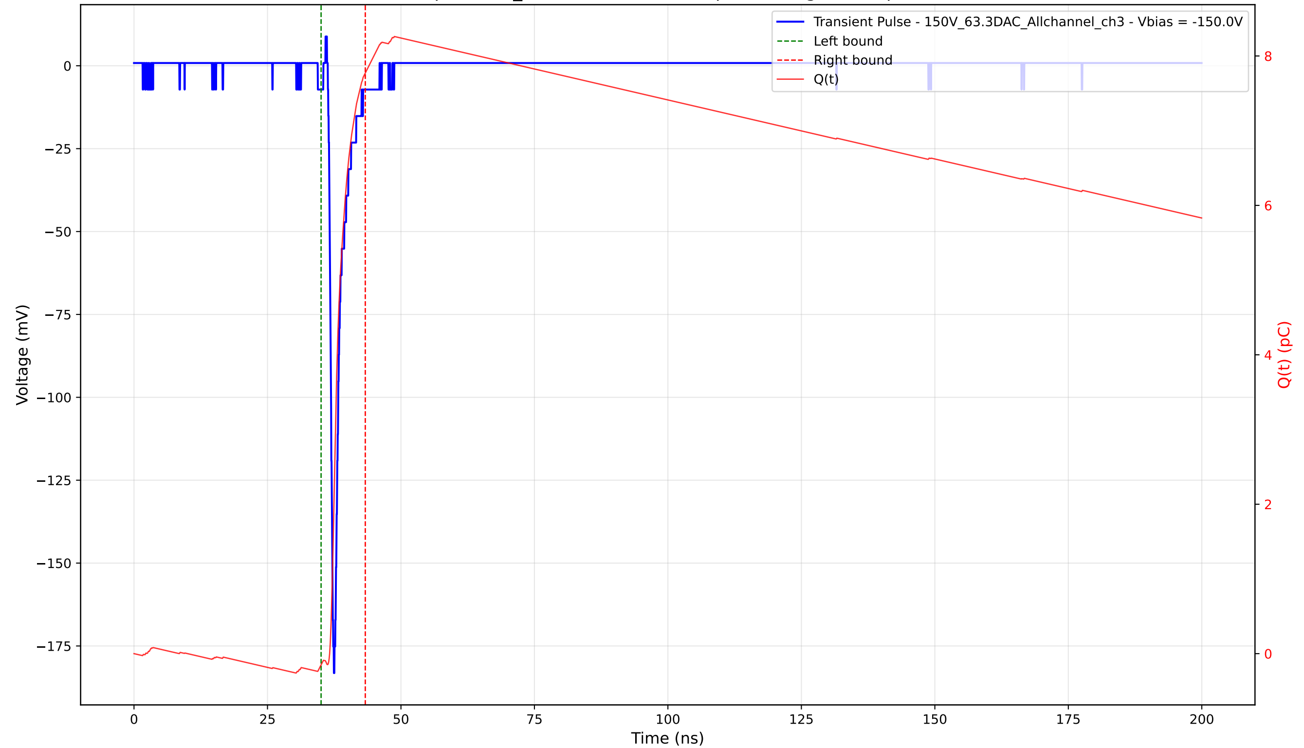
Transient Pulse - Sample: 1cm_42 - Position: 3095.0 \mu\text{m} - Charge: 7.92 pC - Rise Time: 0.78 ns
