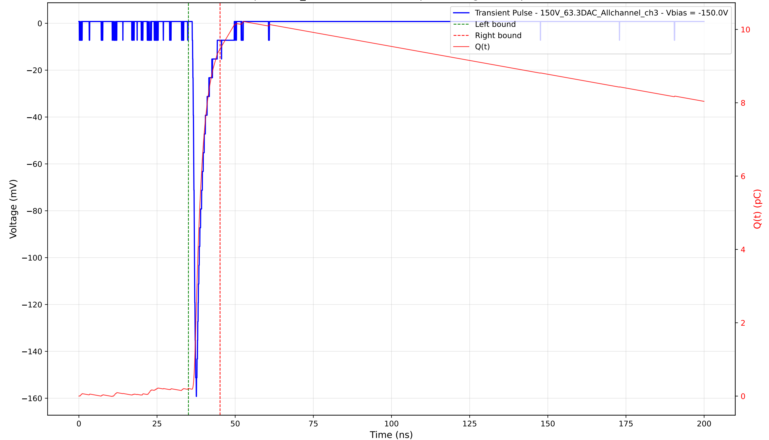
Transient Pulse - Sample: 1cm_42 - Position: 1770.0 \mu\text{m} - Charge: 9.26 pC - Rise Time: 0.92 ns
