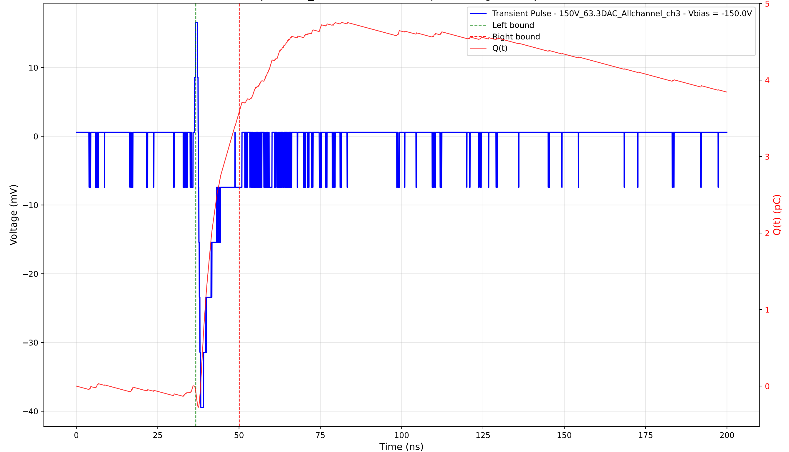
Transient Pulse - Sample: 1cm_42 - Position: 4015.0 \mu\text{m} - Charge: 3.69 pC - Rise Time: 0.70 ns
