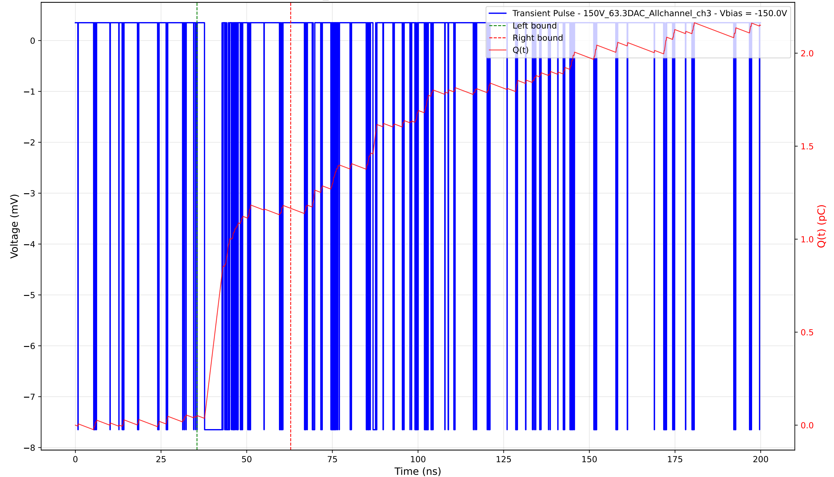
Transient Pulse - Sample: 1cm_42 - Position: 115.0 \mu\text{m} - Charge: 1.12 pC - Rise Time: 0.04 ns
