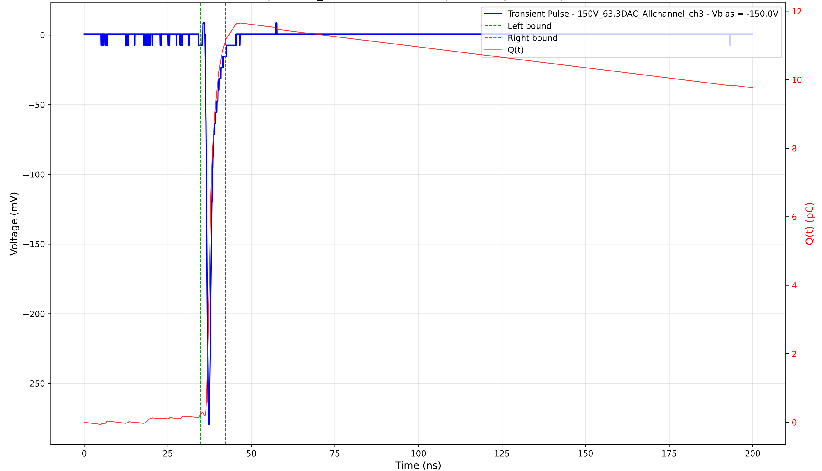
Transient Pulse - Sample: 1cm_42 - Position: 2070.0 \mu\text{m} - Charge: 10.87 pC - Rise Time: 0.76 ns
