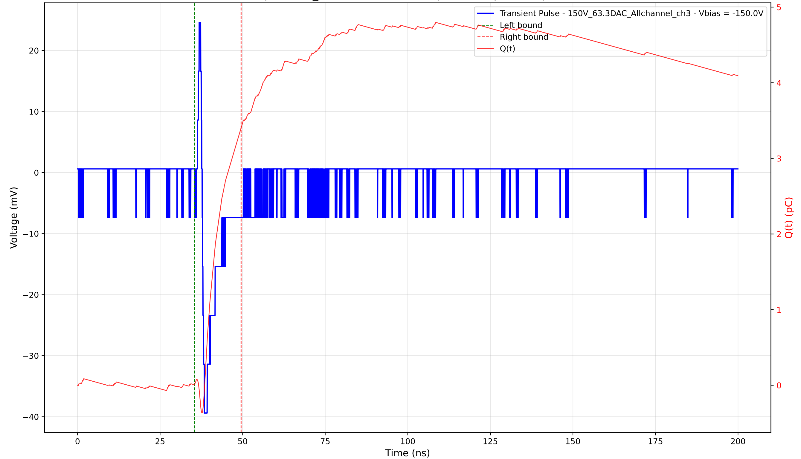
Transient Pulse - Sample: 1cm_42 - Position: 4320.0 \mu\text{m} - Charge: 3.39 pC - Rise Time: 0.66 ns
