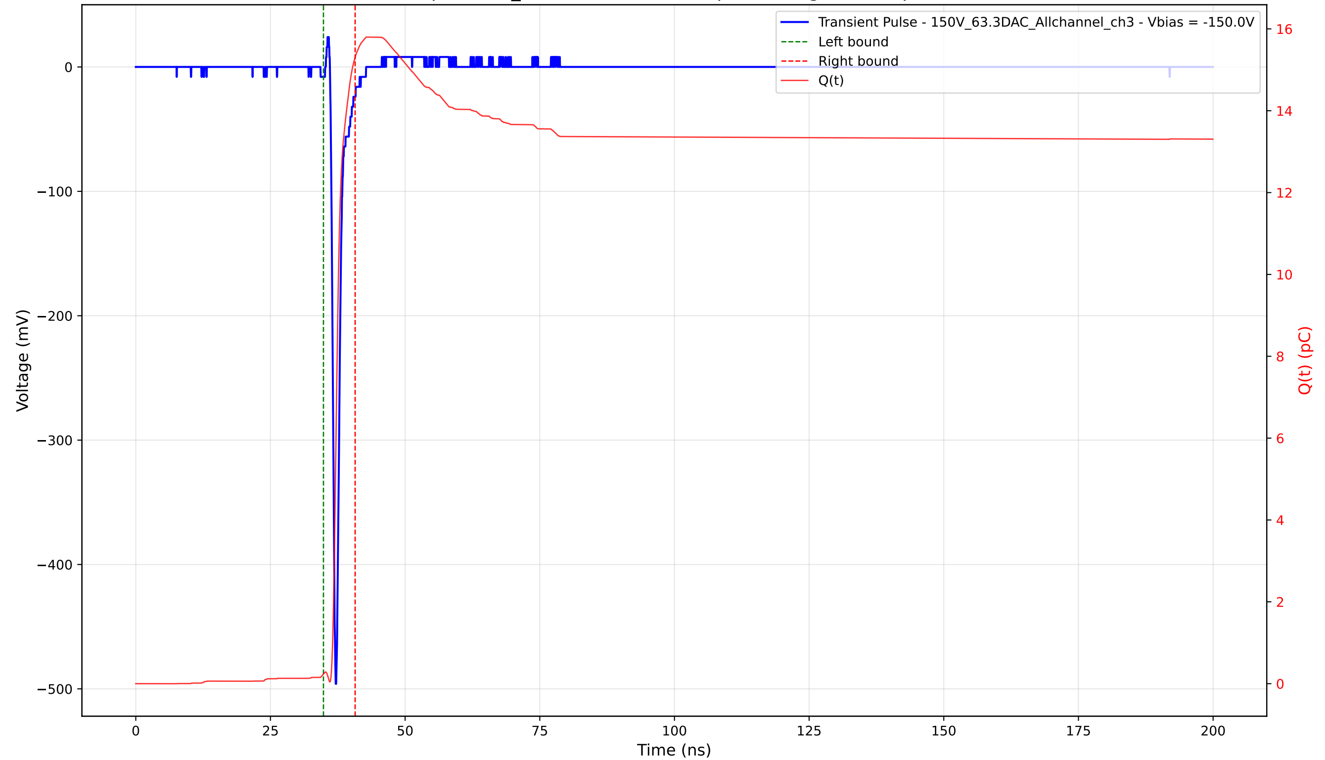
Transient Pulse - Sample: 1cm_42 - Position: 2585.0 \mu\text{m} - Charge: 15.07 pC - Rise Time: 0.71 ns
