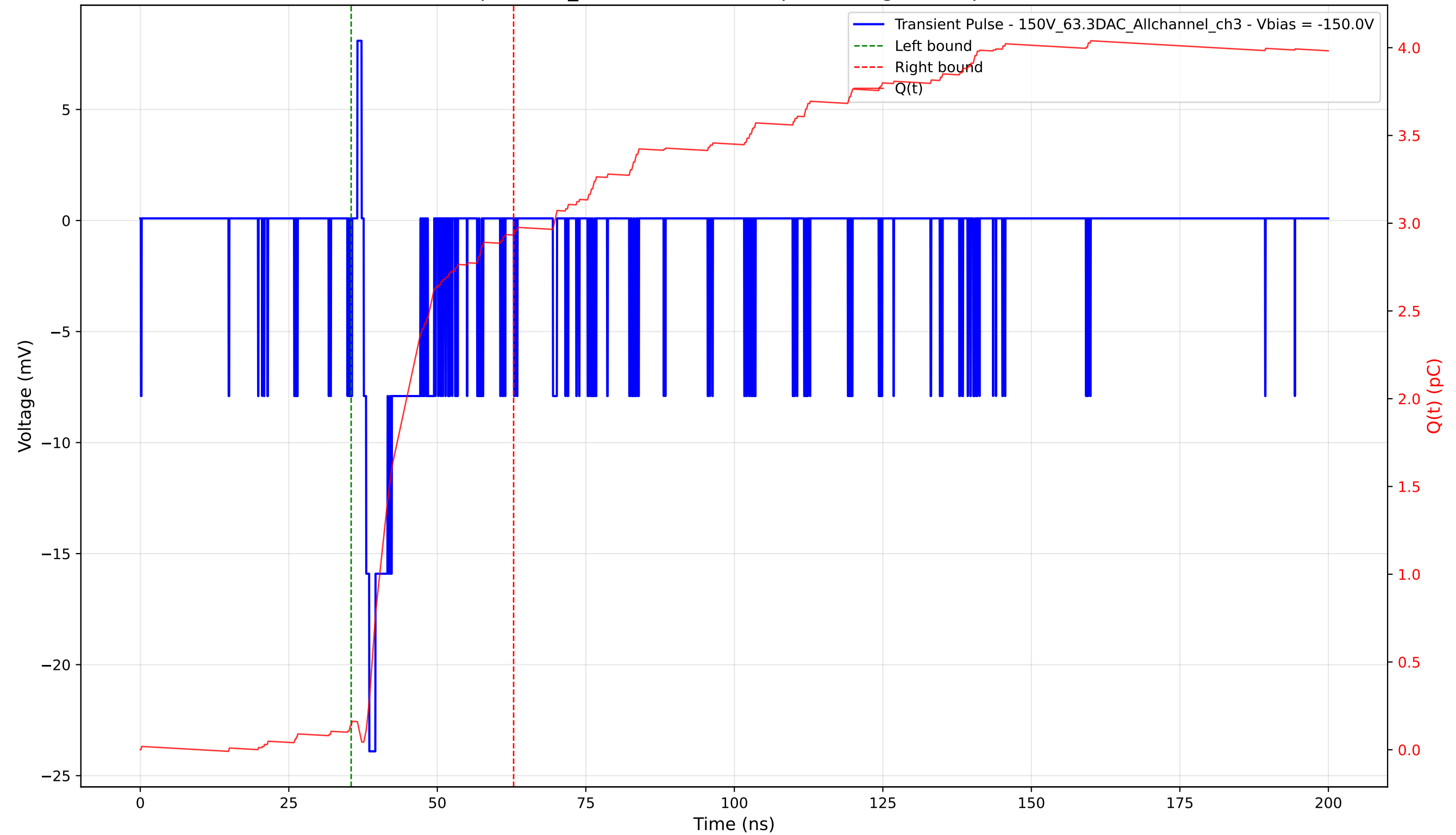
Transient Pulse - Sample: 1cm_42 - Position: 250.0 \mu\text{m} - Charge: 2.79 pC - Rise Time: 0.95 ns
