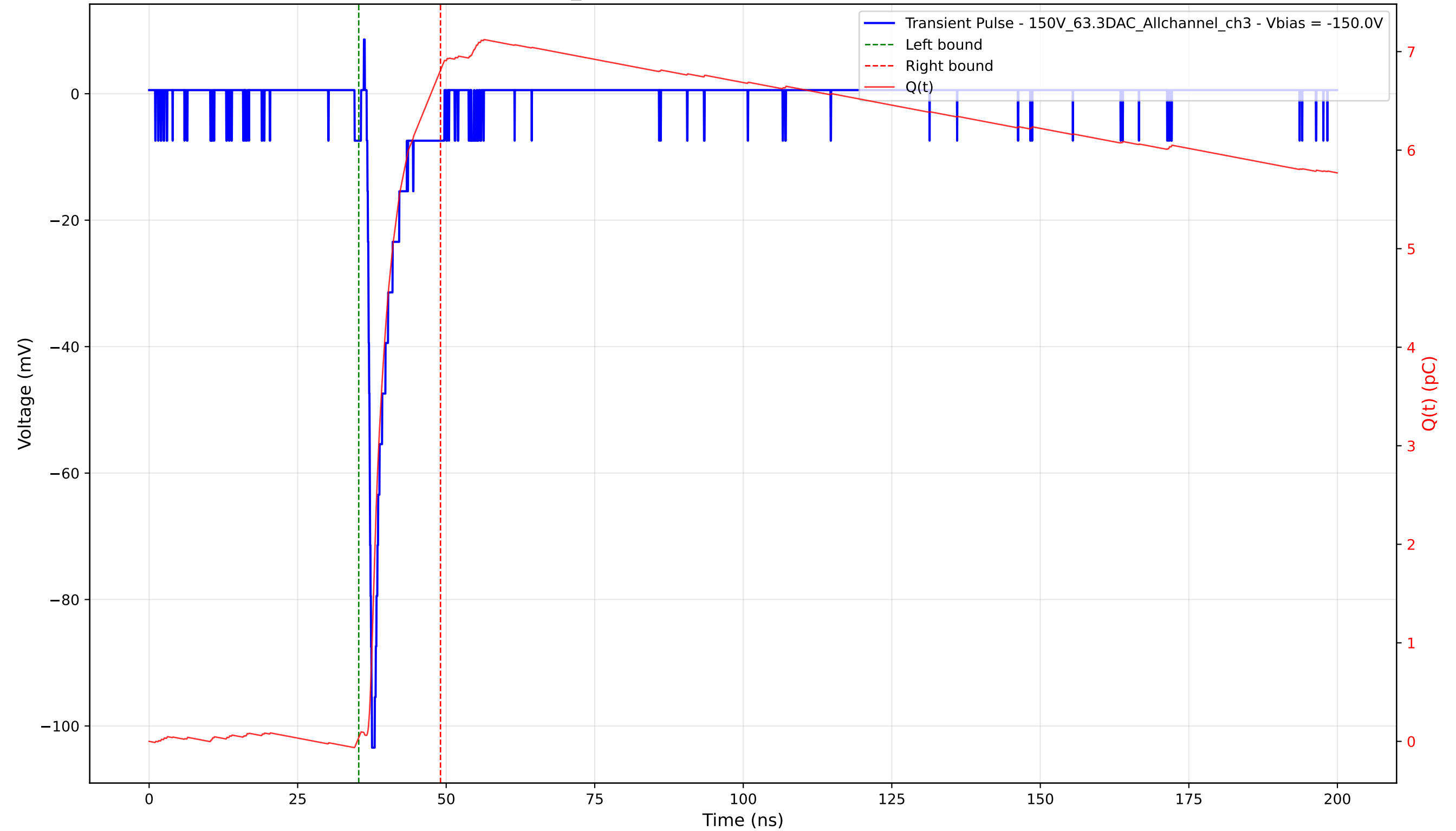
Transient Pulse - Sample: 1cm_42 - Position: 3395.0 \mu\text{m} - Charge: 6.77 pC - Rise Time: 0.71 ns
