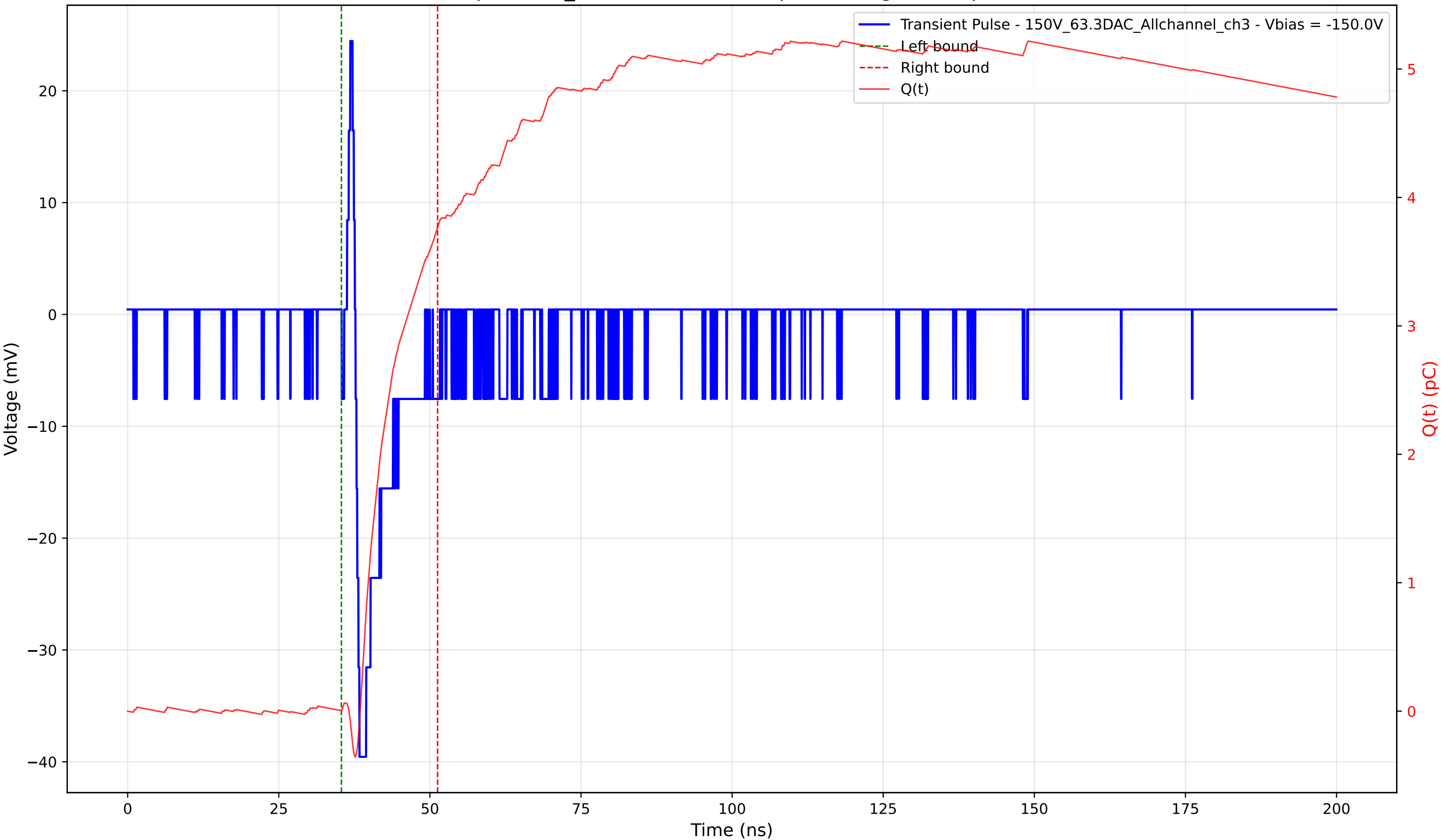
Transient Pulse - Sample: 1cm_42 - Position: 585.0 \mu\text{m} - Charge: 3.77 pC - Rise Time: 0.66 ns
