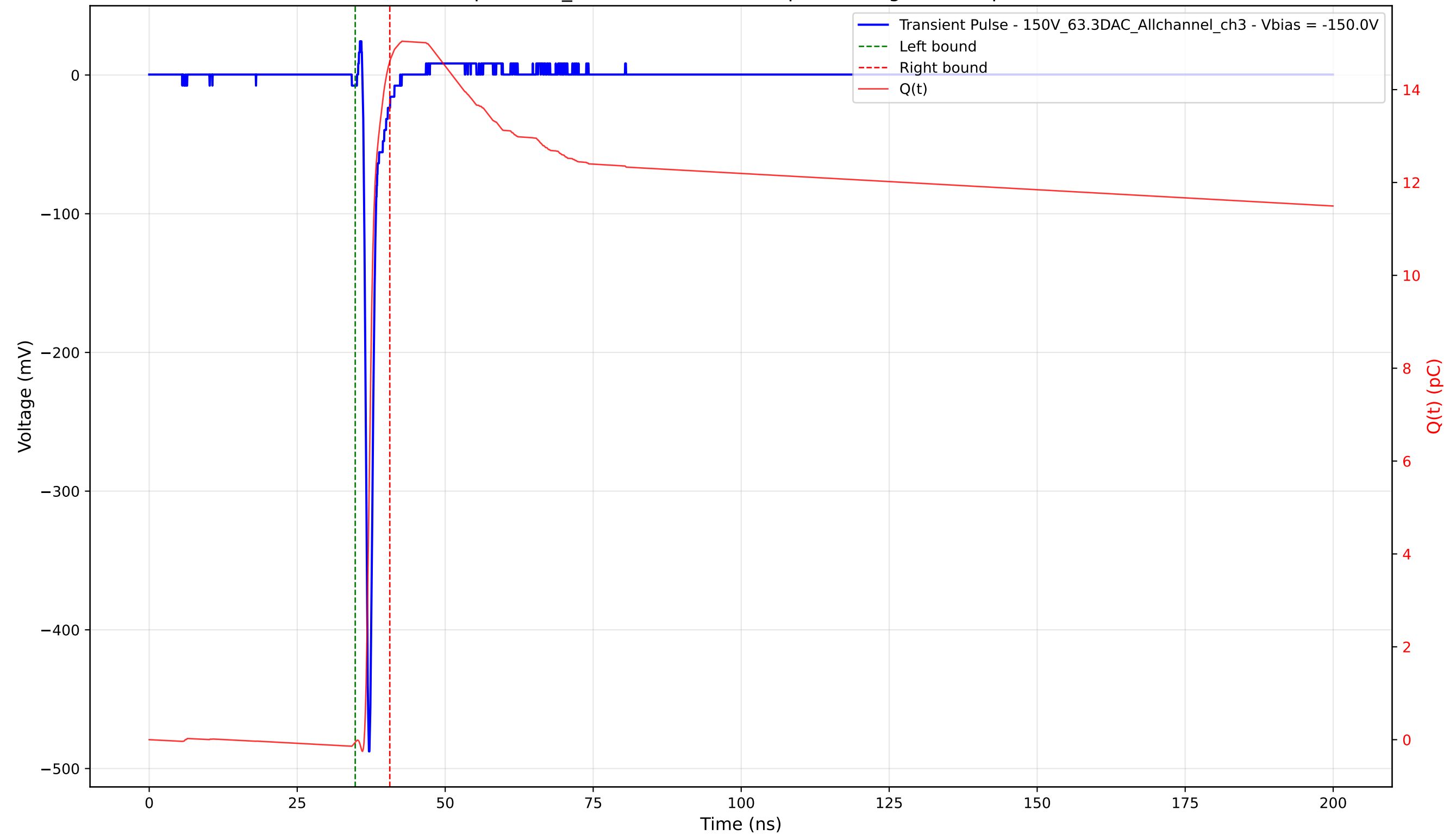
Transient Pulse - Sample: 1cm_42 - Position: 2520.0 \mu\text{m} - Charge: 14.67 pC - Rise Time: 0.72 ns
