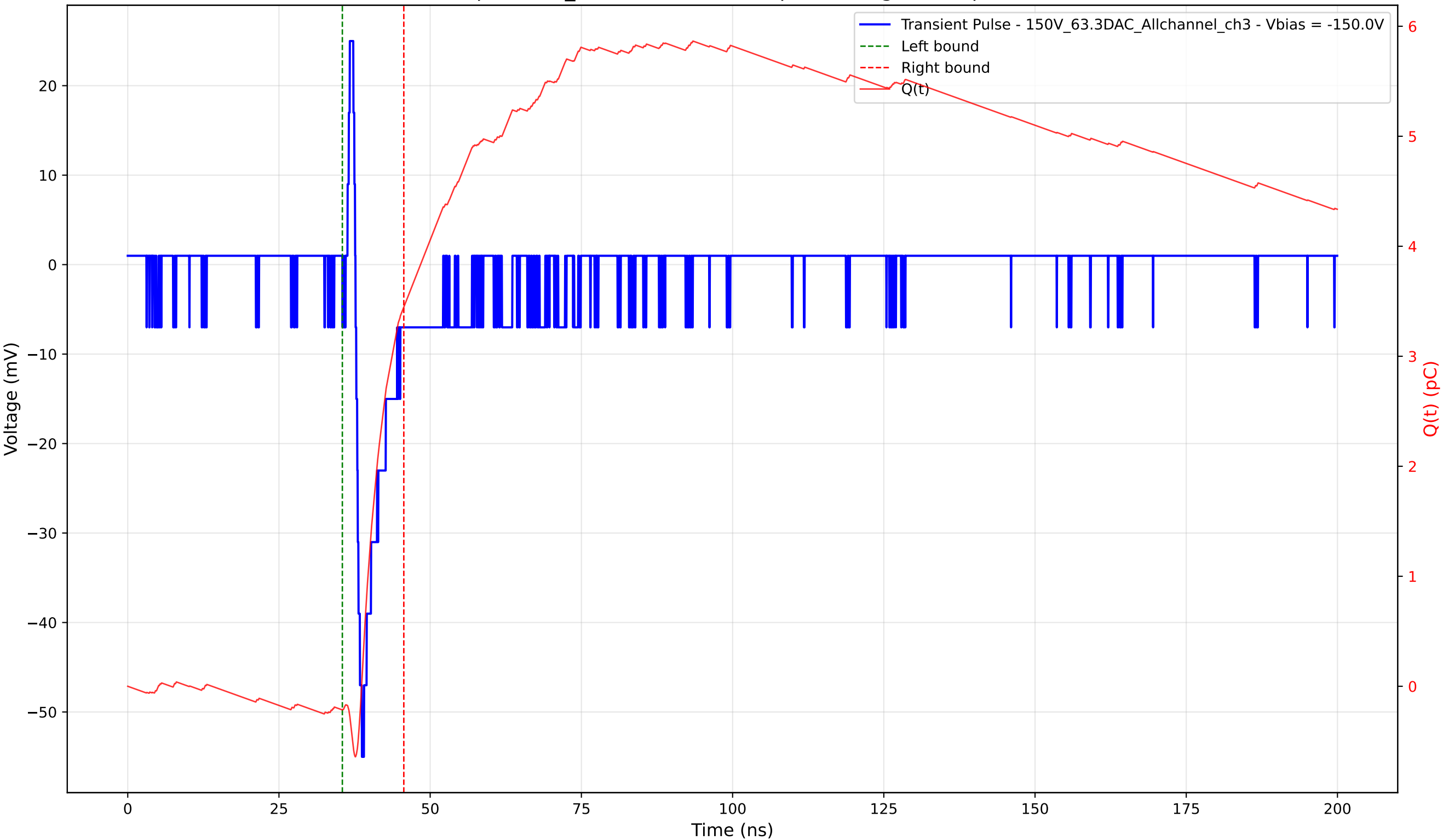
Transient Pulse - Sample: 1cm_42 - Position: 805.0 \mu\text{m} - Charge: 3.66 pC - Rise Time: 1.05 ns
