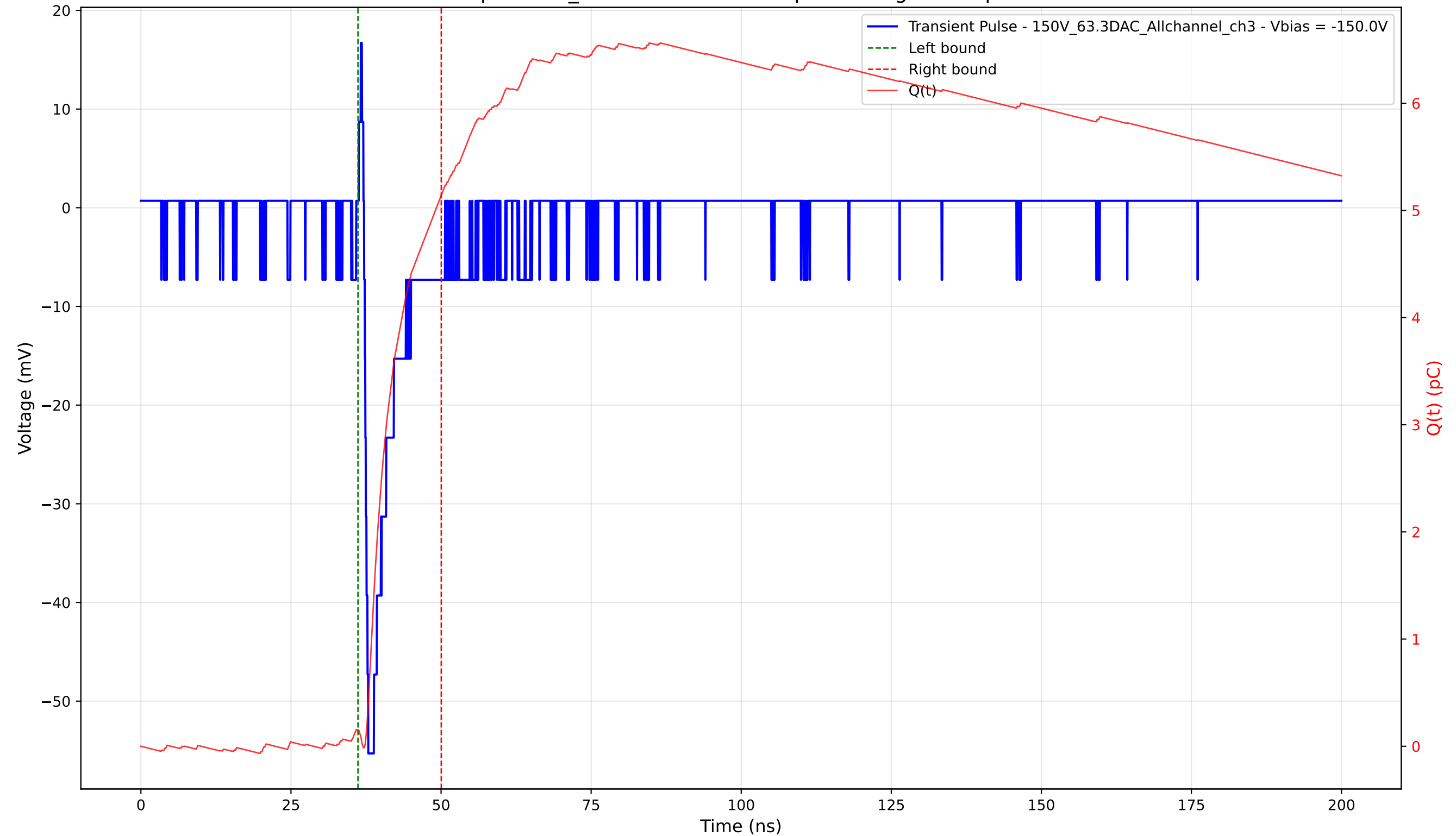
Transient Pulse - Sample: 1cm_42 - Position: 3690.0 \mu\text{m} - Charge: 4.99 pC - Rise Time: 0.69 ns
