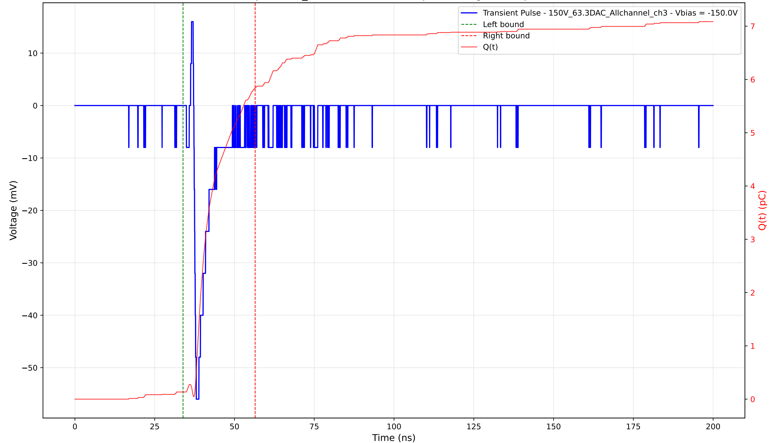
Transient Pulse - Sample: 1cm_42 - Position: 3770.0 \mu\text{m} - Charge: 5.71 pC - Rise Time: 0.73 ns
