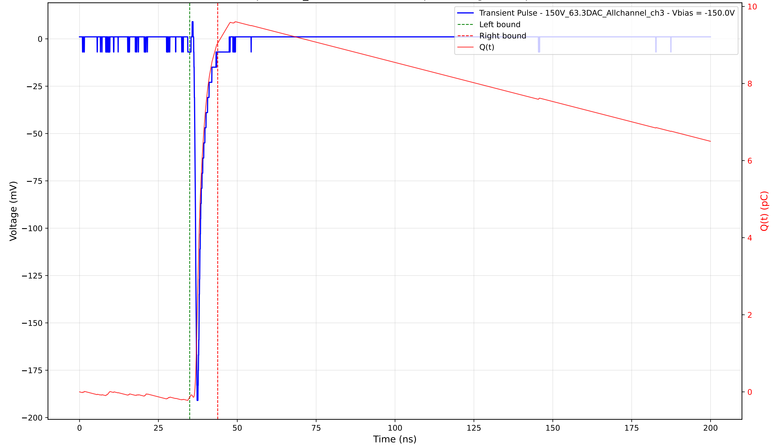
Transient Pulse - Sample: 1cm_42 - Position: 1945.0 \mu\text{m} - Charge: 9.18 pC - Rise Time: 0.80 ns
