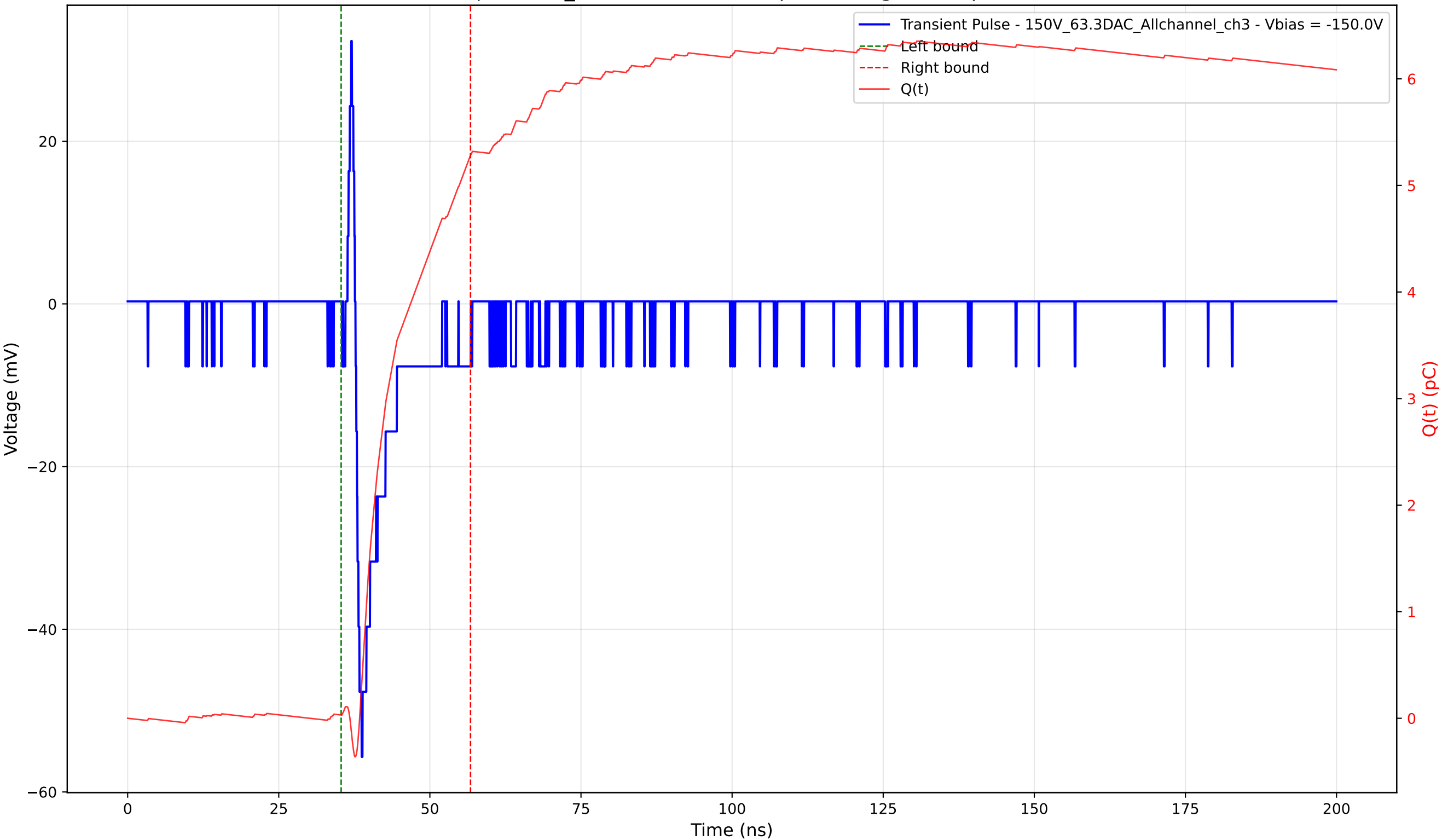
Transient Pulse - Sample: 1cm_42 - Position: 715.0 \mu\text{m} - Charge: 5.26 pC - Rise Time: 1.01 ns
