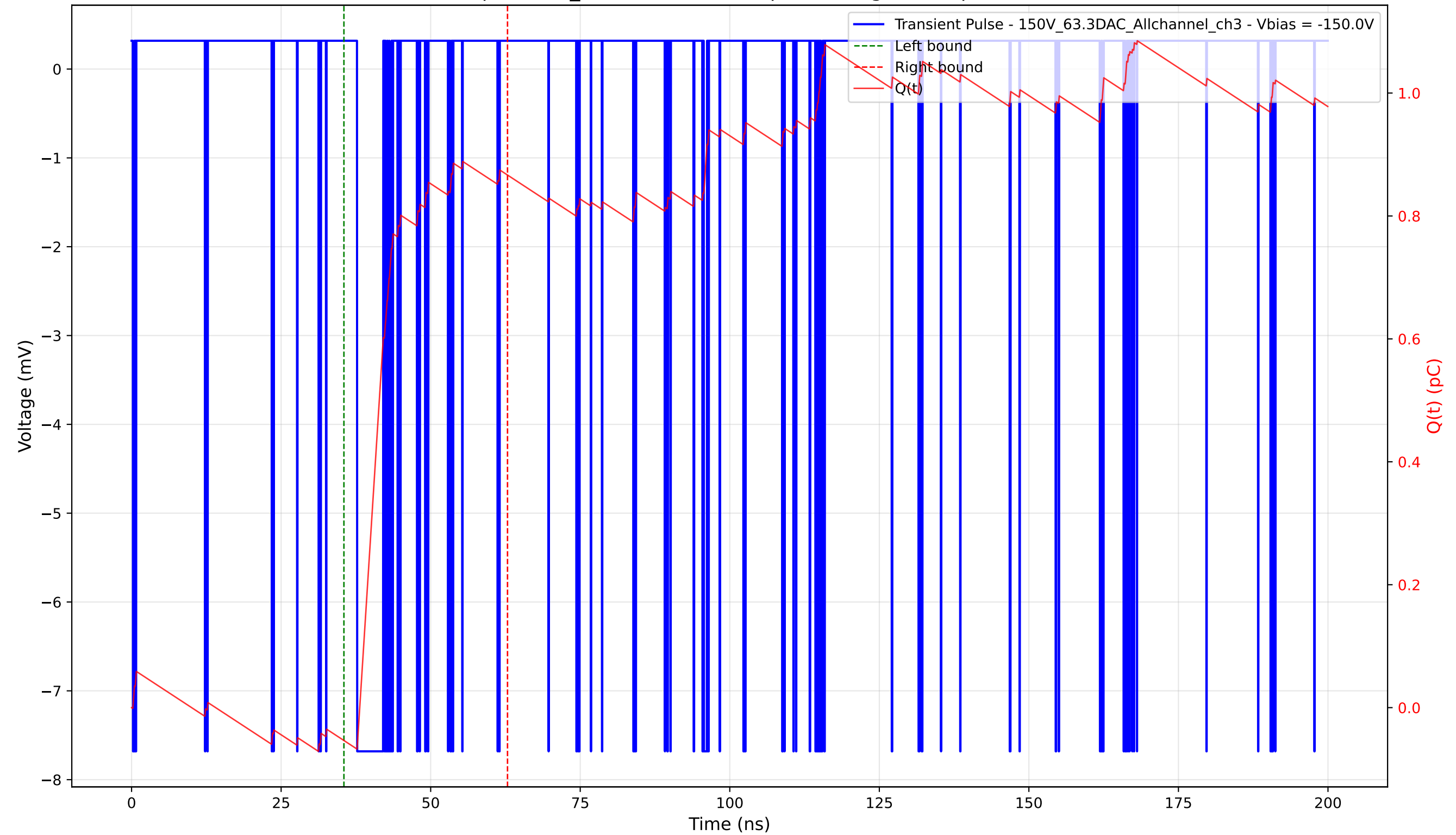
Transient Pulse - Sample: 1cm_42 - Position: 75.0 \mu\text{m} - Charge: 0.92 pC - Rise Time: 0.04 ns
