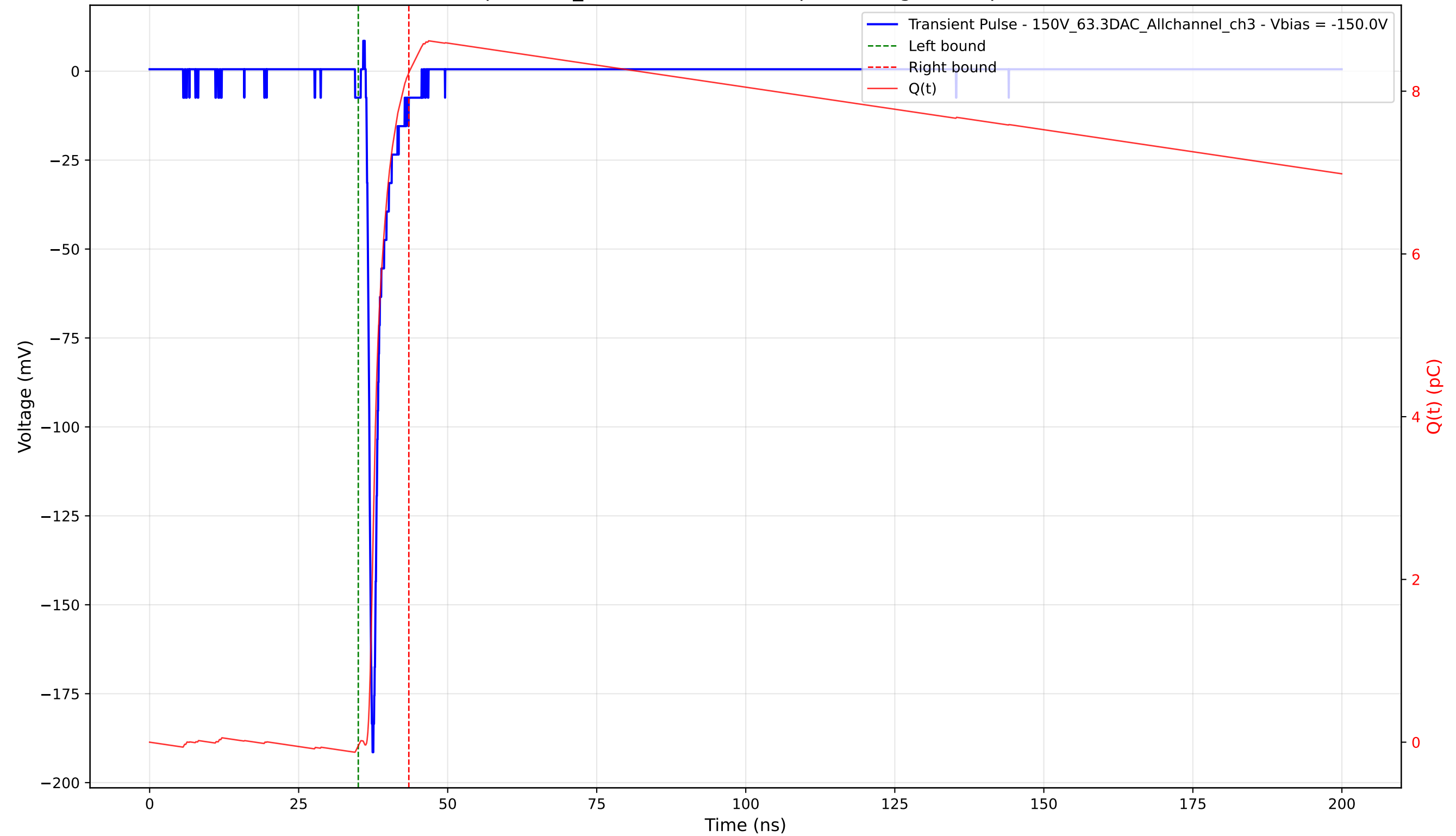
Transient Pulse - Sample: 1cm_42 - Position: 3075.0 \mu\text{m} - Charge: 8.27 pC - Rise Time: 0.81 ns
