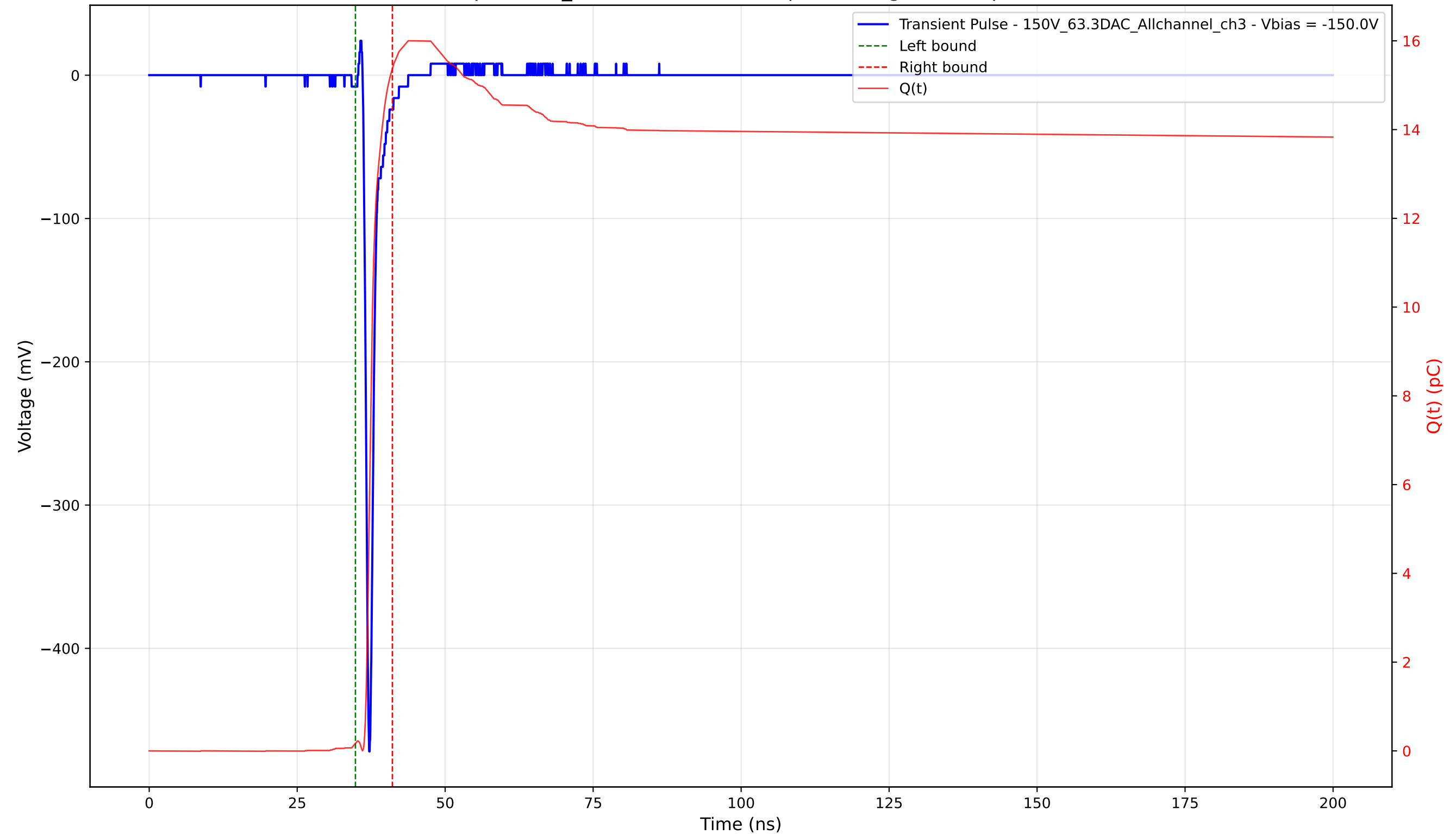
Transient Pulse - Sample: 1cm_42 - Position: 2305.0 \mu\text{m} - Charge: 15.20 pC - Rise Time: 0.69 ns
