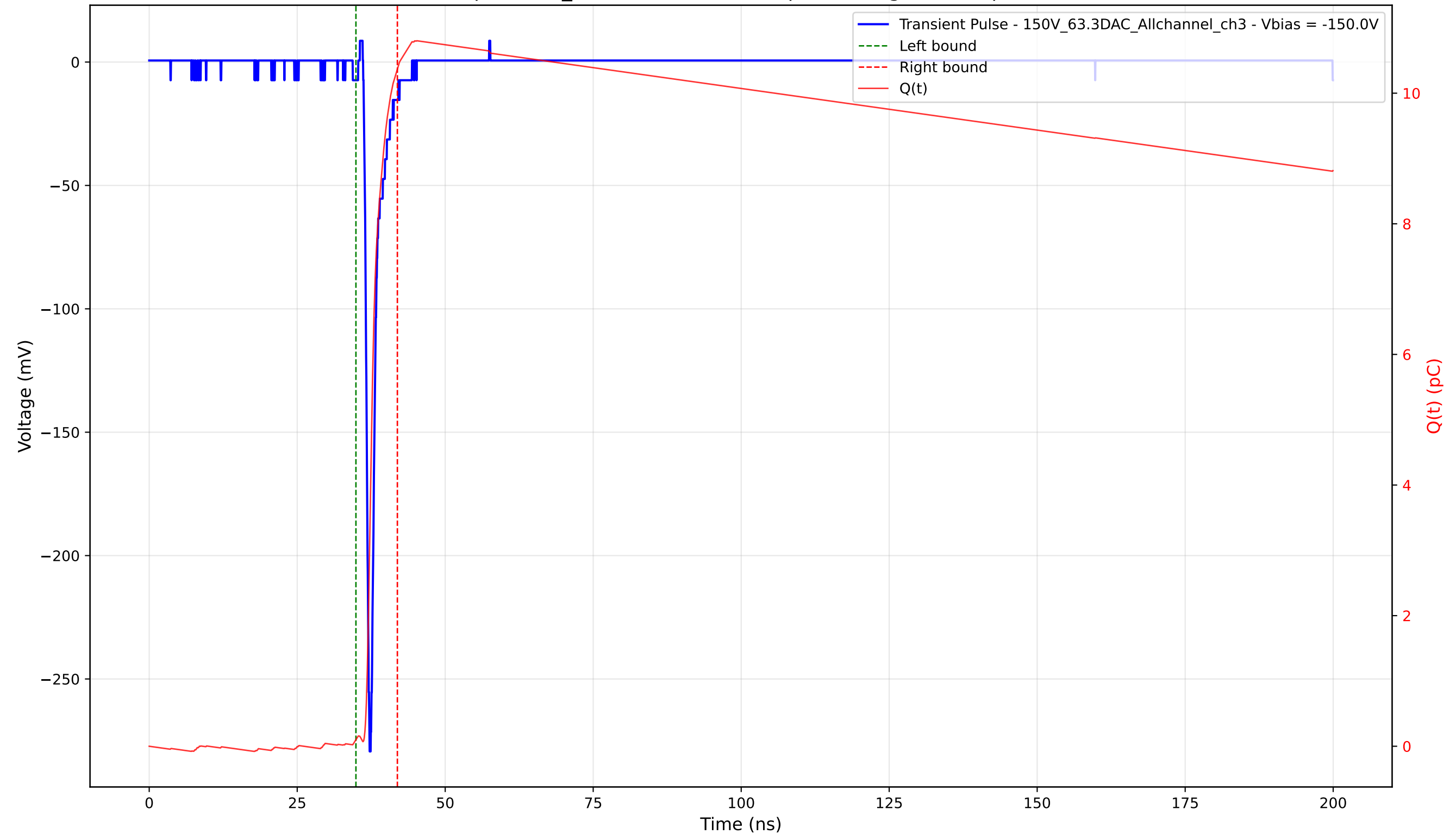
Transient Pulse - Sample: 1cm_42 - Position: 2955.0 \mu\text{m} - Charge: 10.28 pC - Rise Time: 0.78 ns
