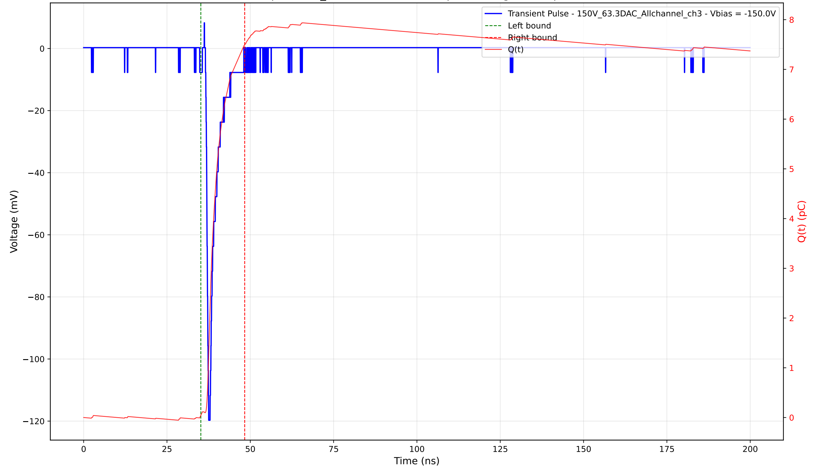
Transient Pulse - Sample: 1cm_42 - Position: 3350.0 \mu\text{m} - Charge: 7.44 pC - Rise Time: 0.78 ns
