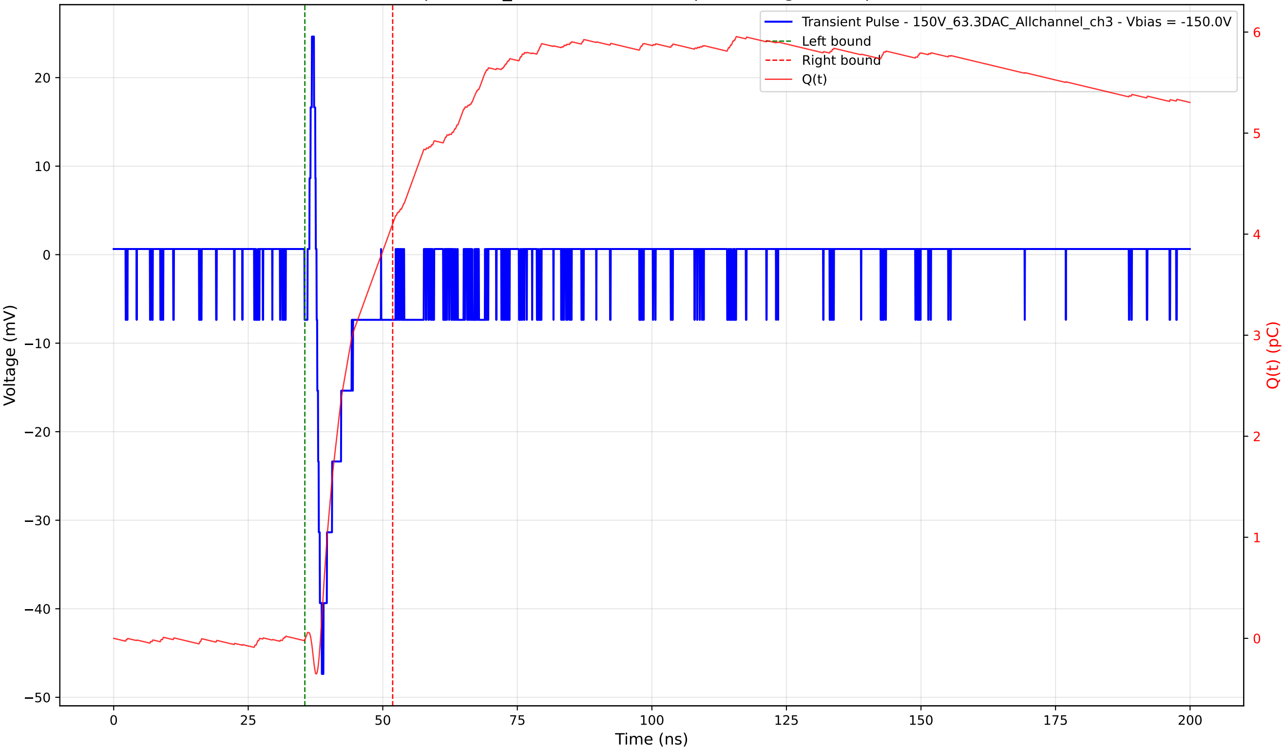
Transient Pulse - Sample: 1cm_42 - Position: 620.0 \mu\text{m} - Charge: 4.12 pC - Rise Time: 0.98 ns
