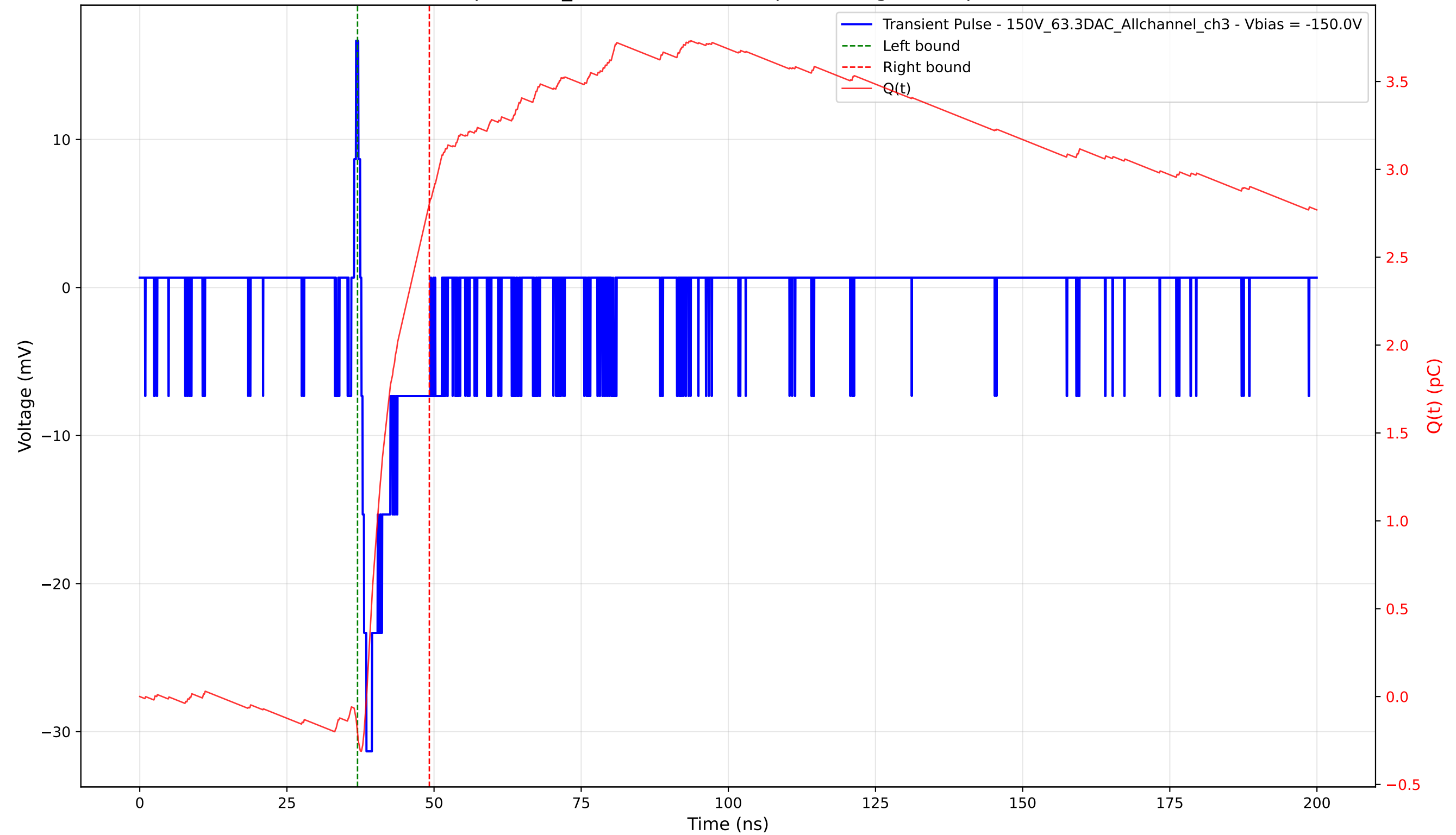
Transient Pulse - Sample: 1cm_42 - Position: 415.0 \mu\text{m} - Charge: 3.01 pC - Rise Time: 0.87 ns
