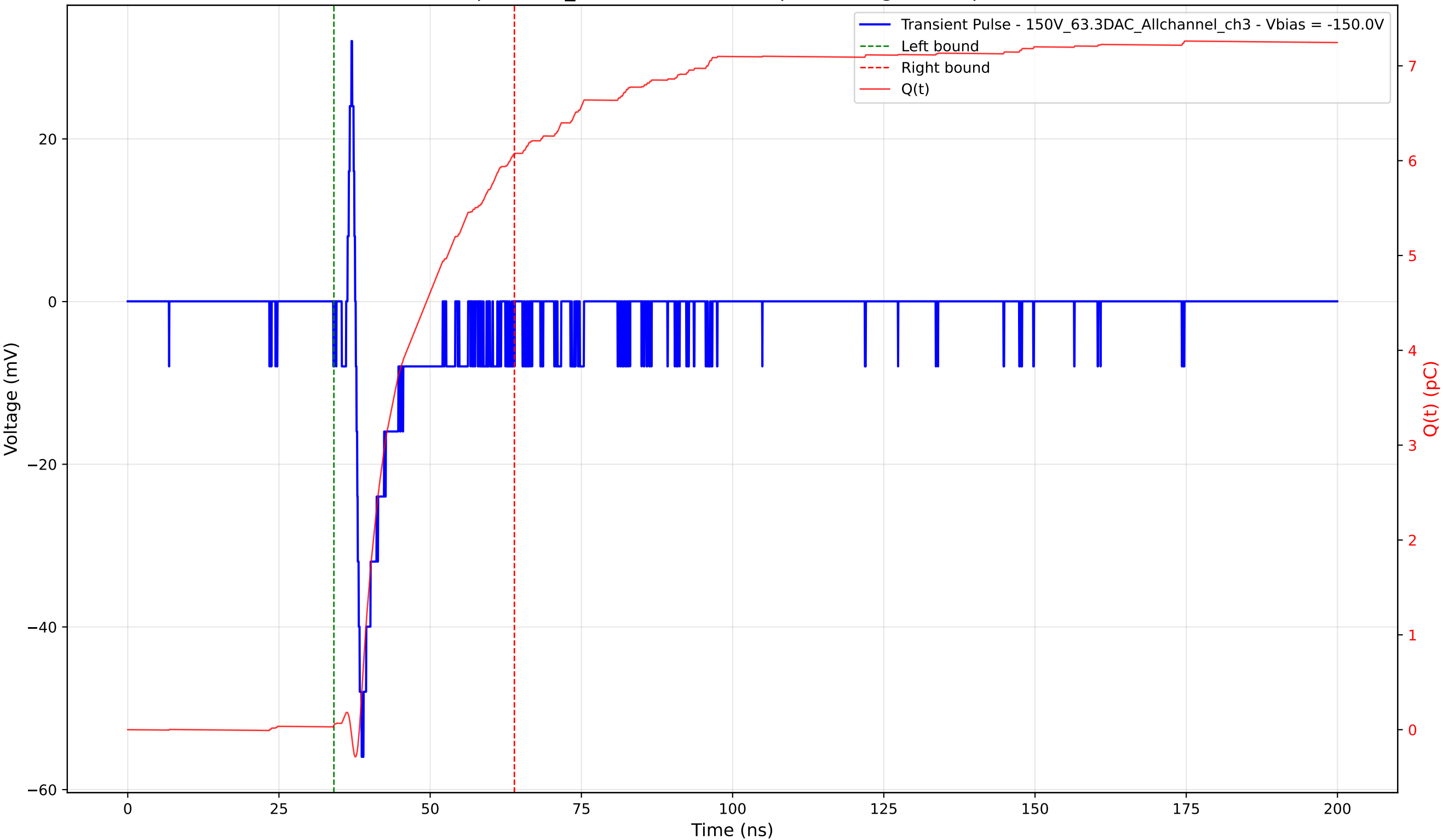
Transient Pulse - Sample: 1cm_42 - Position: 755.0 \mu\text{m} - Charge: 6.02 pC - Rise Time: 0.97 ns
