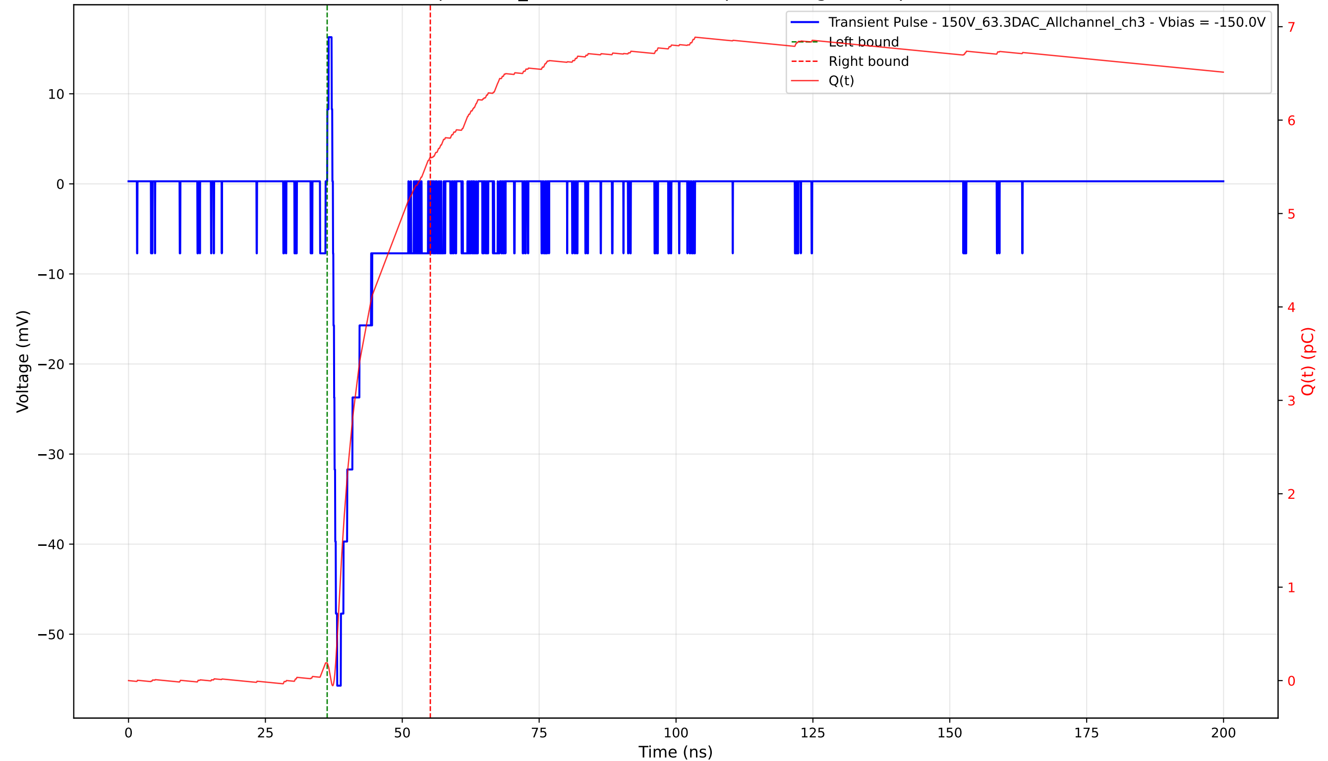
Transient Pulse - Sample: 1cm_42 - Position: 3820.0 \mu\text{m} - Charge: 5.41 pC - Rise Time: 0.77 ns
