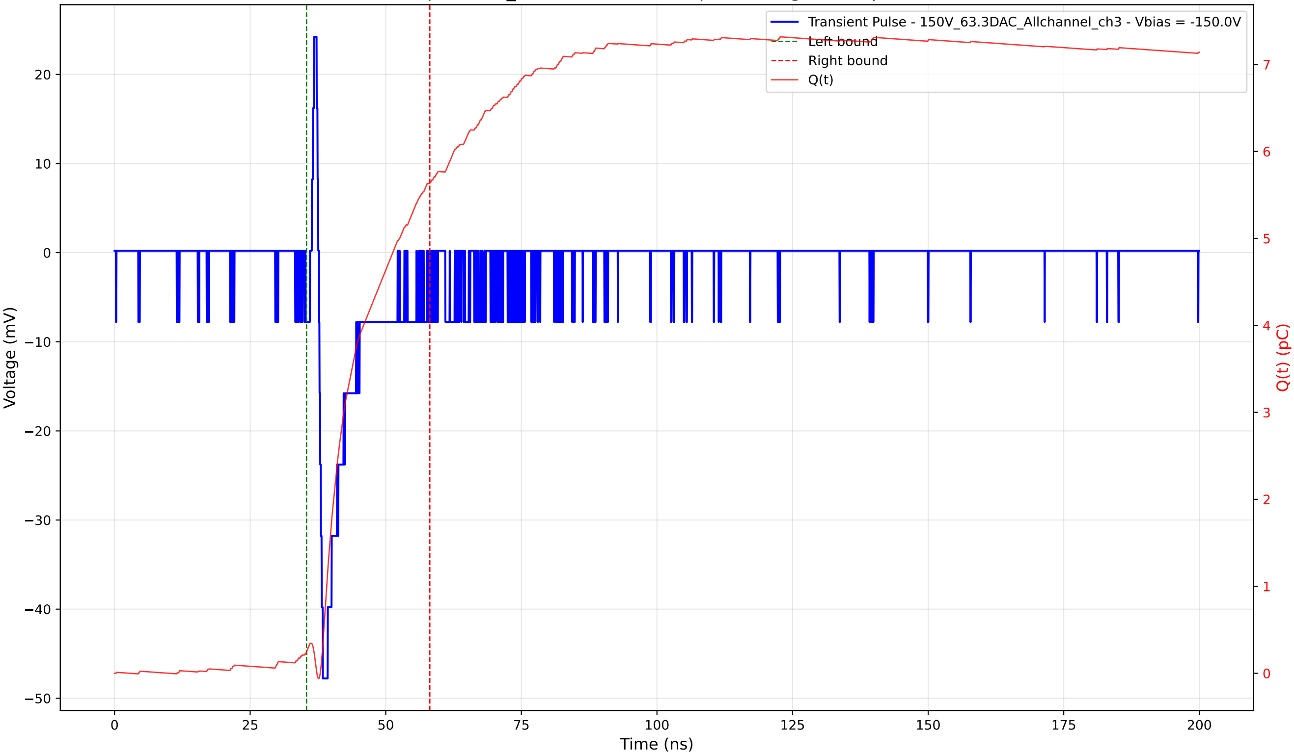
Transient Pulse - Sample: 1cm_42 - Position: 840.0 \mu\text{m} - Charge: 5.39 pC - Rise Time: 0.70 ns
