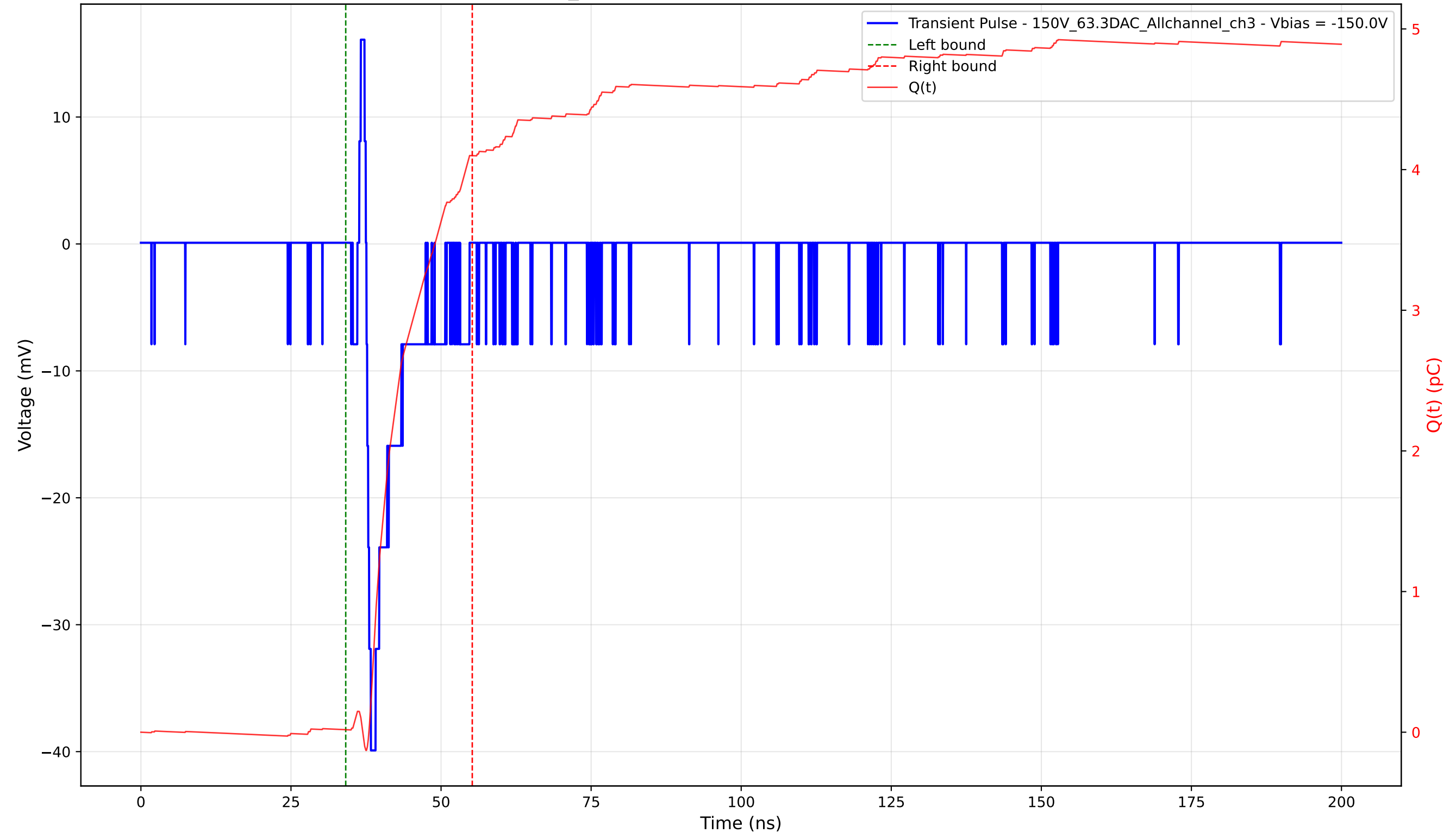
Transient Pulse - Sample: 1cm_42 - Position: 4045.0 \mu\text{m} - Charge: 4.08 pC - Rise Time: 0.74 ns
