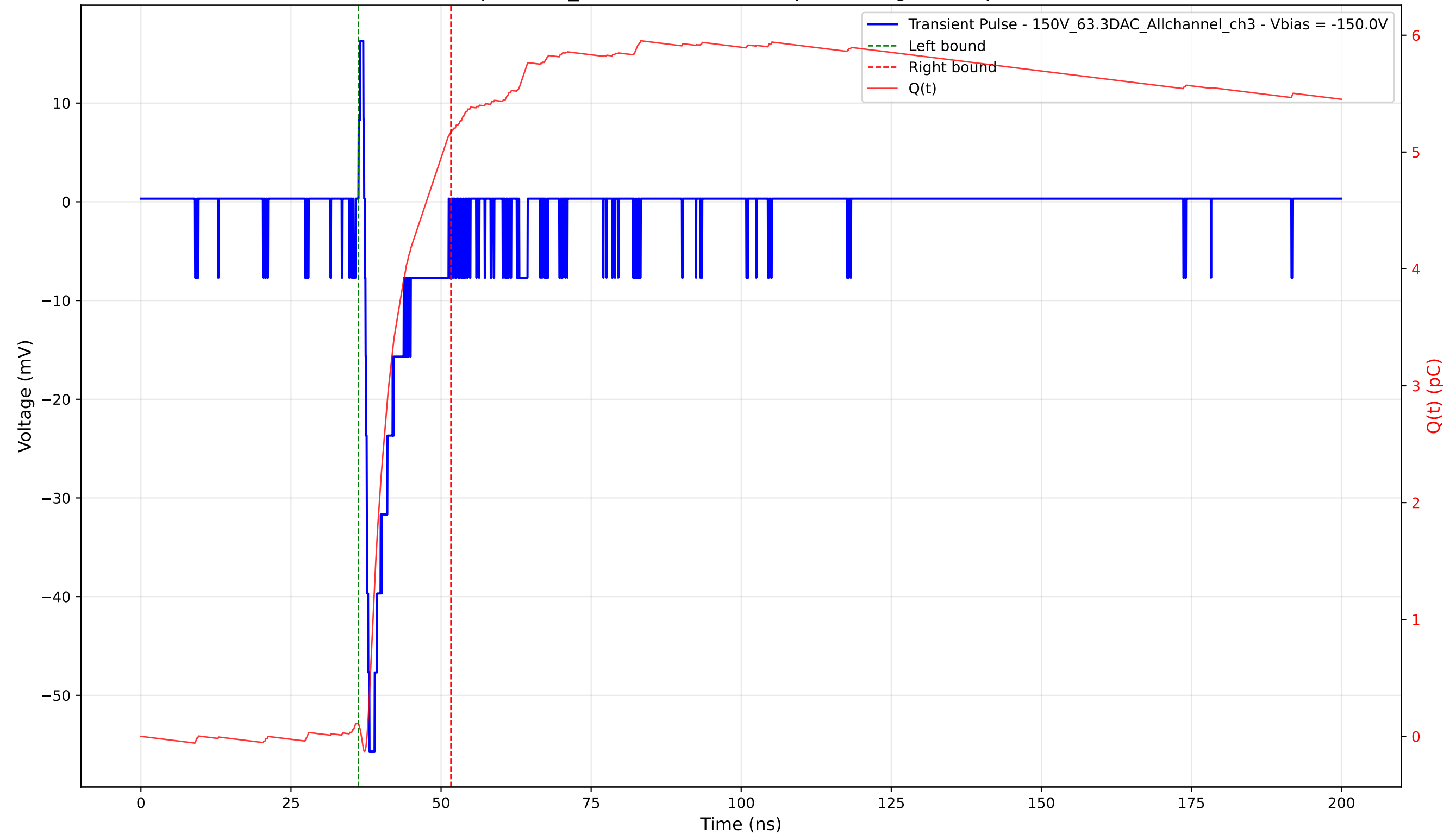
Transient Pulse - Sample: 1cm_42 - Position: 3805.0 \mu\text{m} - Charge: 5.07 pC - Rise Time: 0.77 ns
