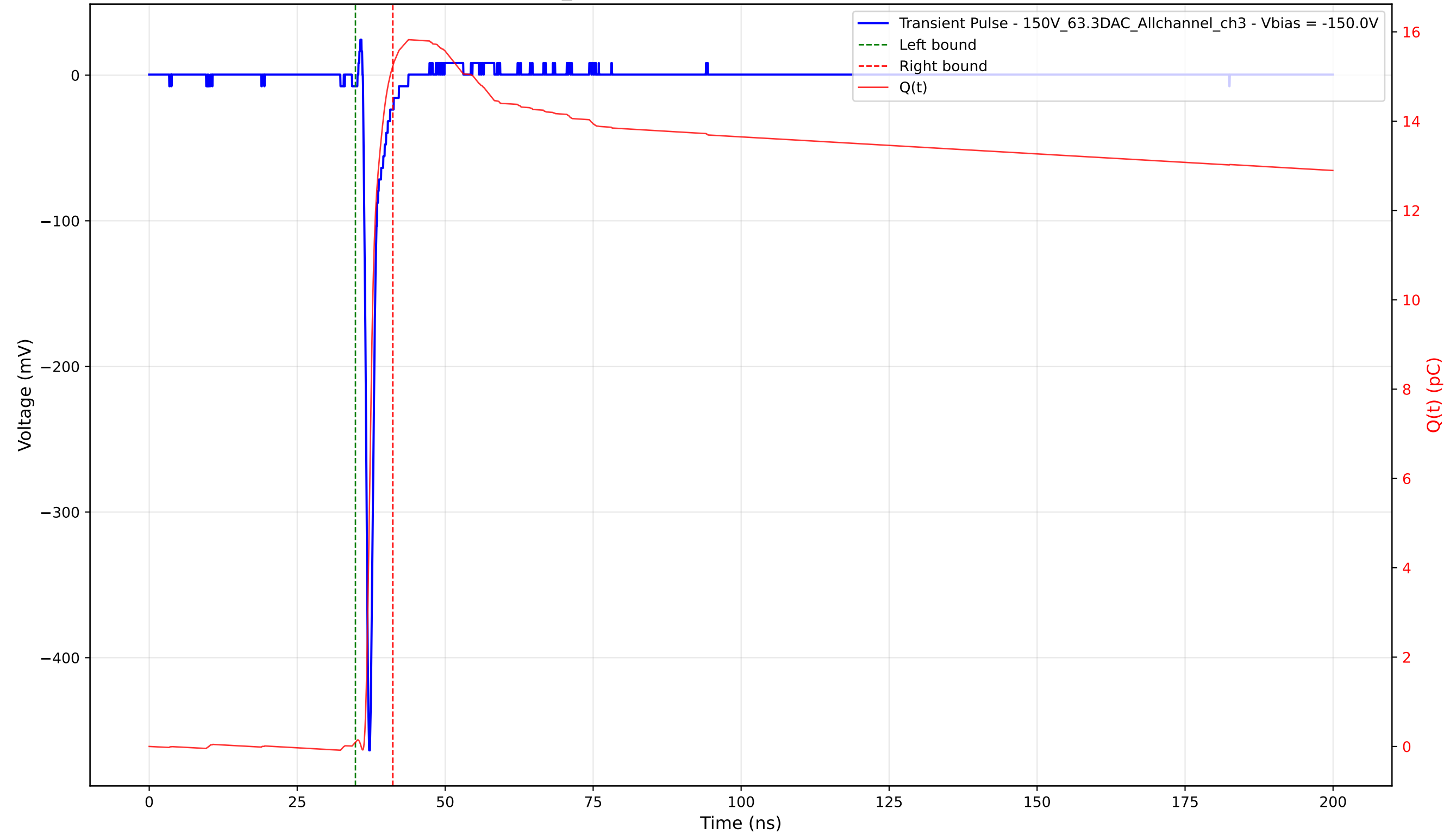
Transient Pulse - Sample: 1cm_42 - Position: 2260.0 \mu\text{m} - Charge: 15.15 pC - Rise Time: 0.69 ns
