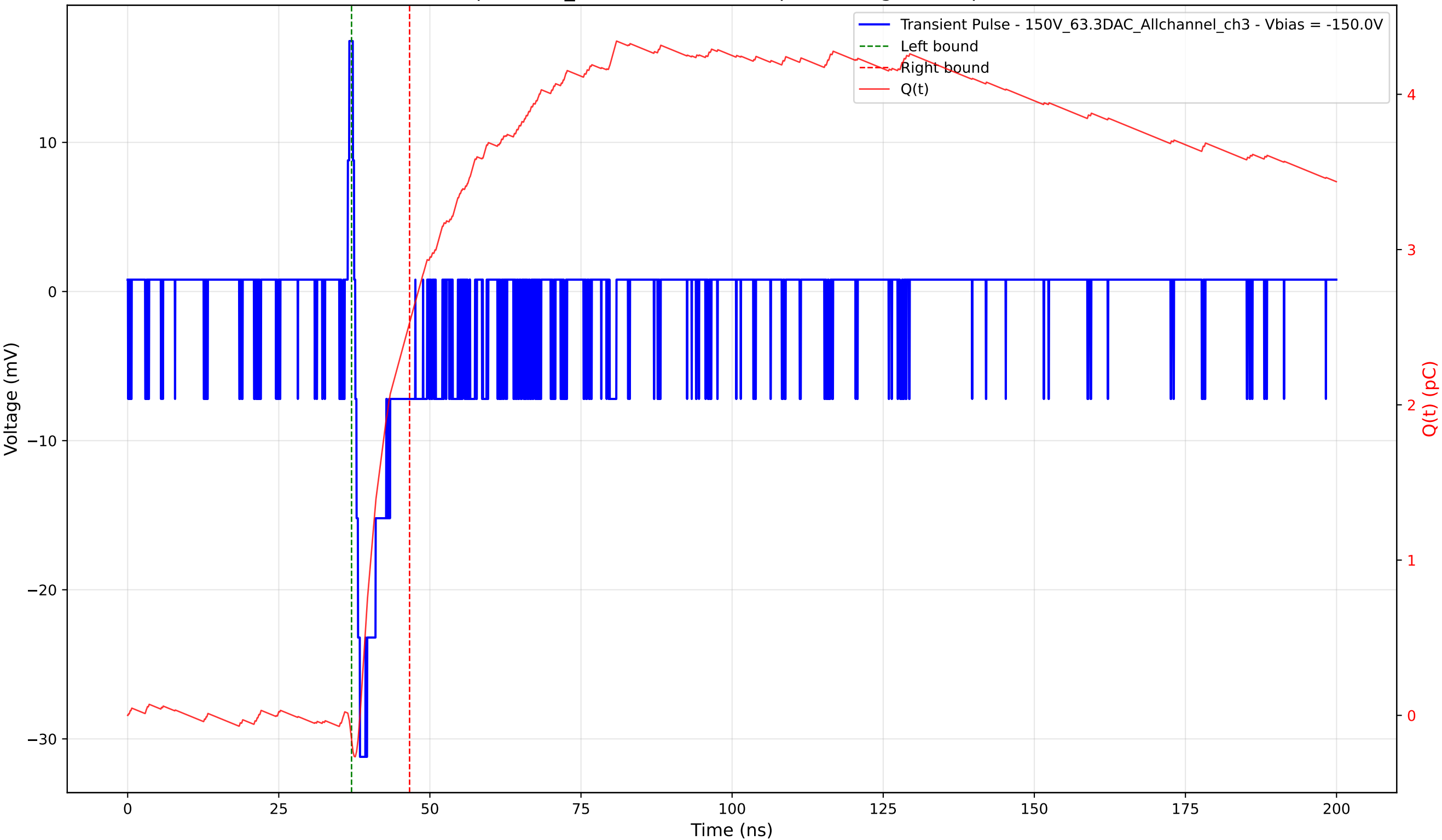
Transient Pulse - Sample: 1cm_42 - Position: 435.0 \mu\text{m} - Charge: 2.69 pC - Rise Time: 0.79 ns
