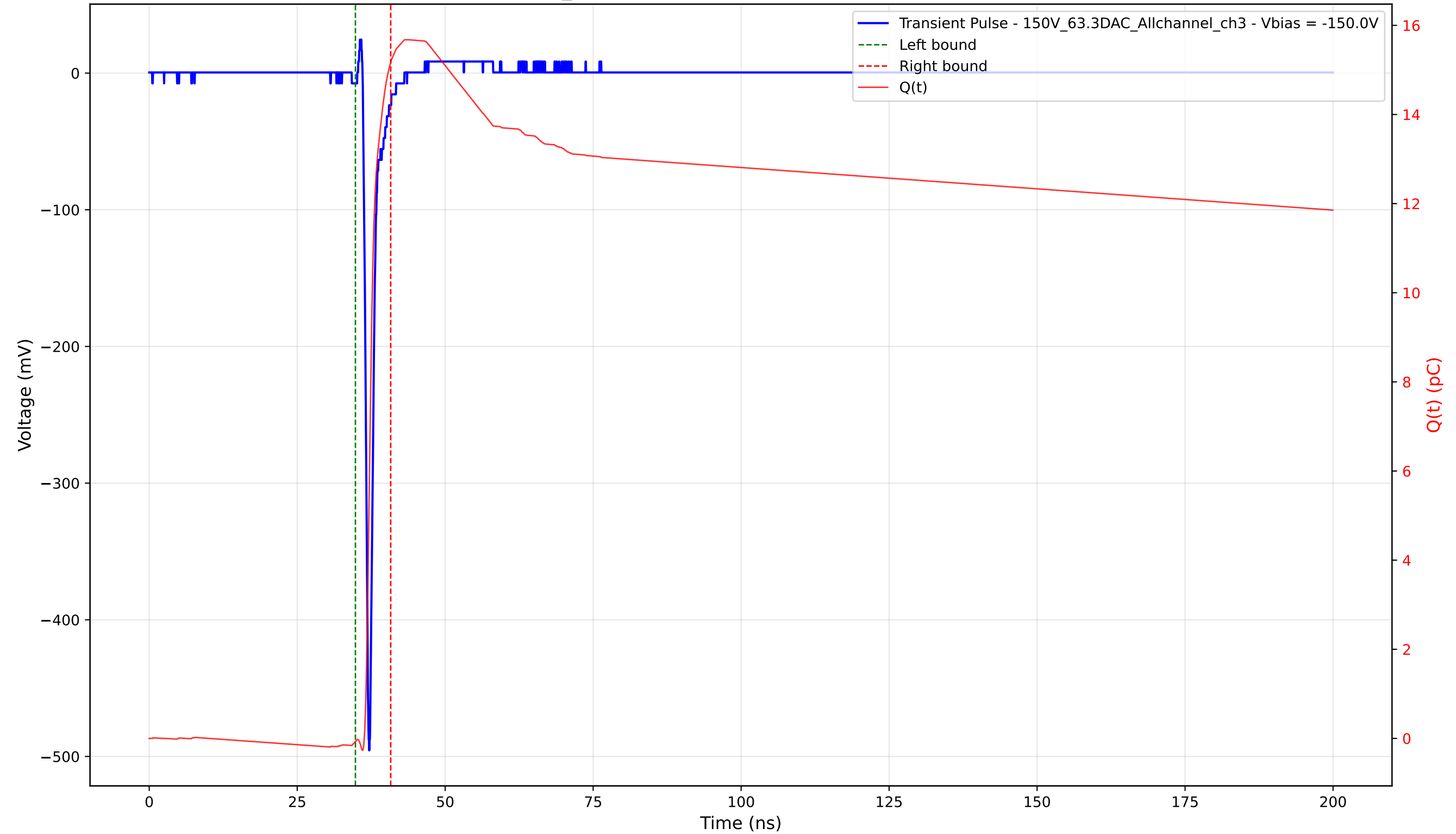
Transient Pulse - Sample: 1cm_42 - Position: 2630.0 \mu\text{m} - Charge: 15.24 pC - Rise Time: 0.73 ns
