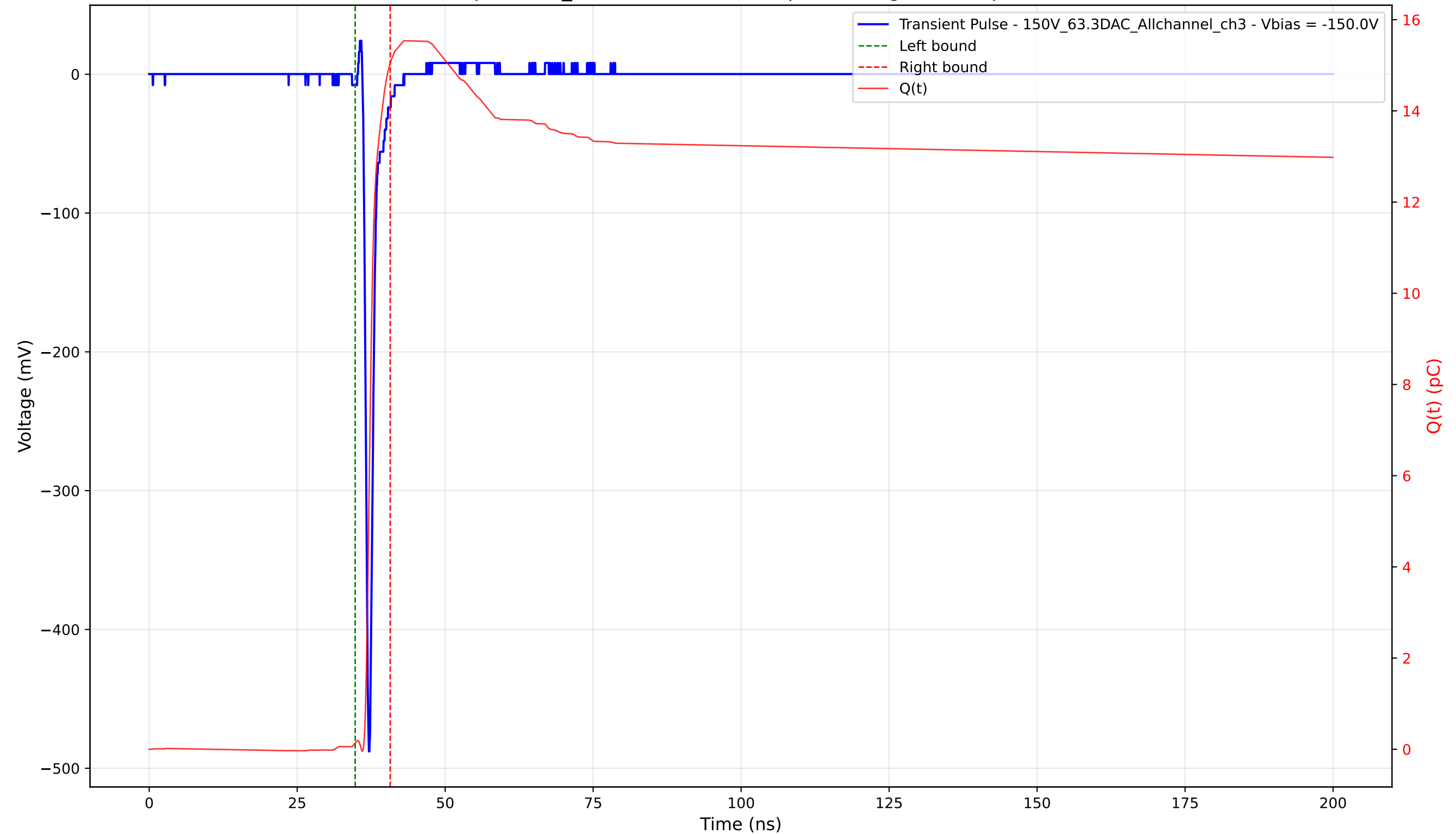
Transient Pulse - Sample: 1cm_42 - Position: 2440.0 \mu\text{m} - Charge: 14.91 pC - Rise Time: 0.72 ns
