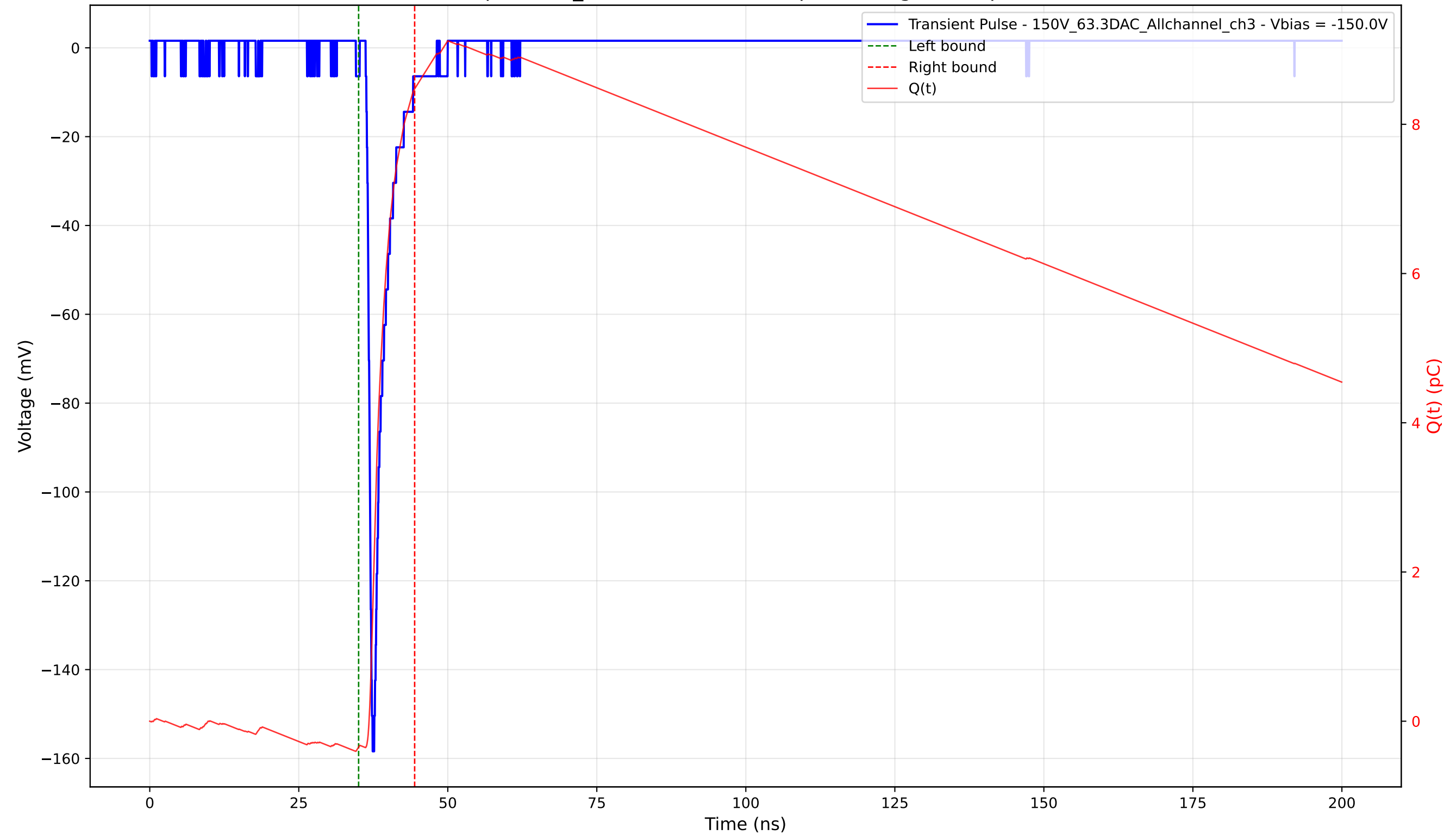
Transient Pulse - Sample: 1cm_42 - Position: 1850.0 \mu\text{m} - Charge: 8.82 pC - Rise Time: 0.87 ns
