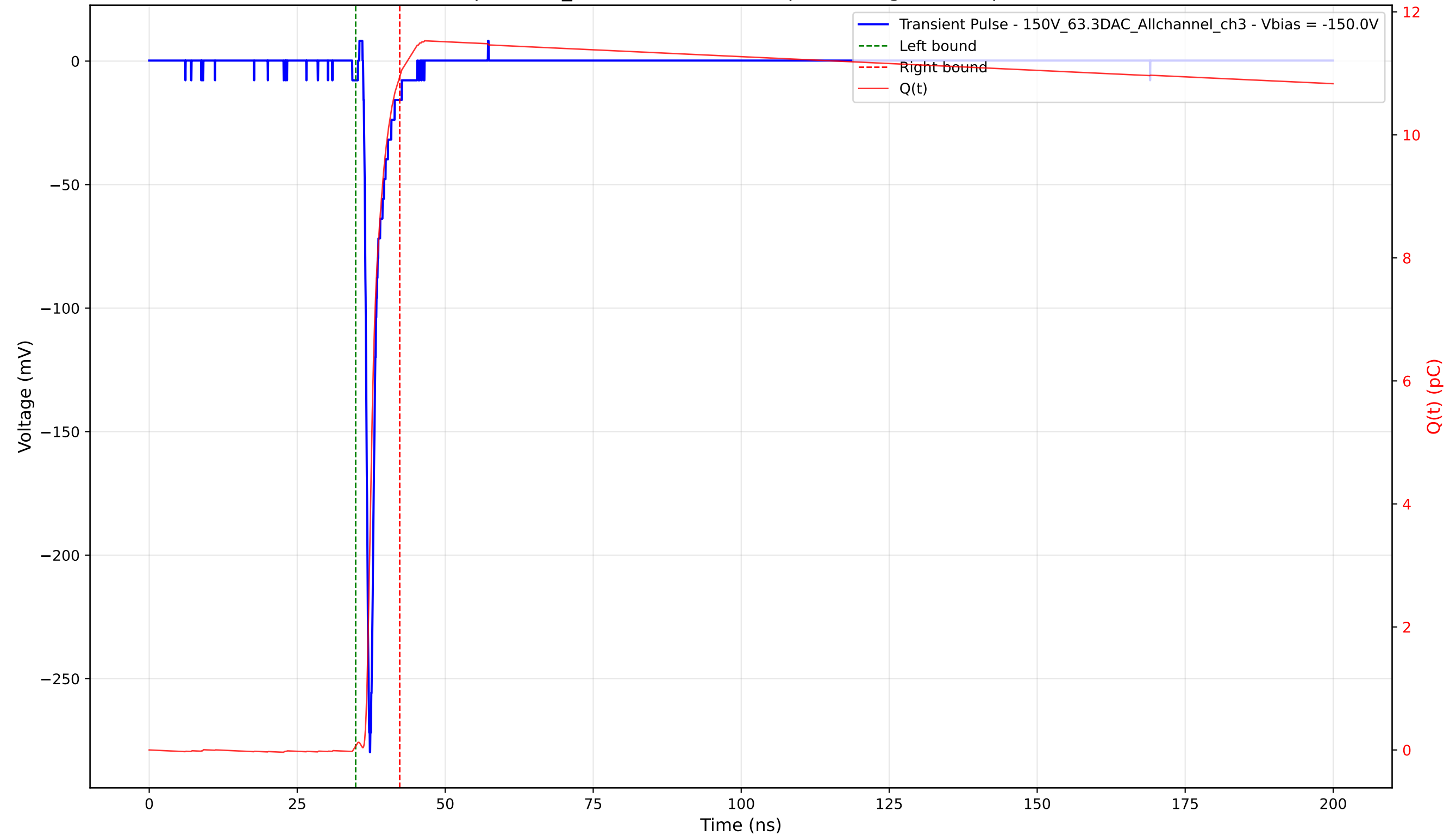
Transient Pulse - Sample: 1cm_42 - Position: 2065.0 \mu\text{m} - Charge: 10.88 pC - Rise Time: 0.76 ns
