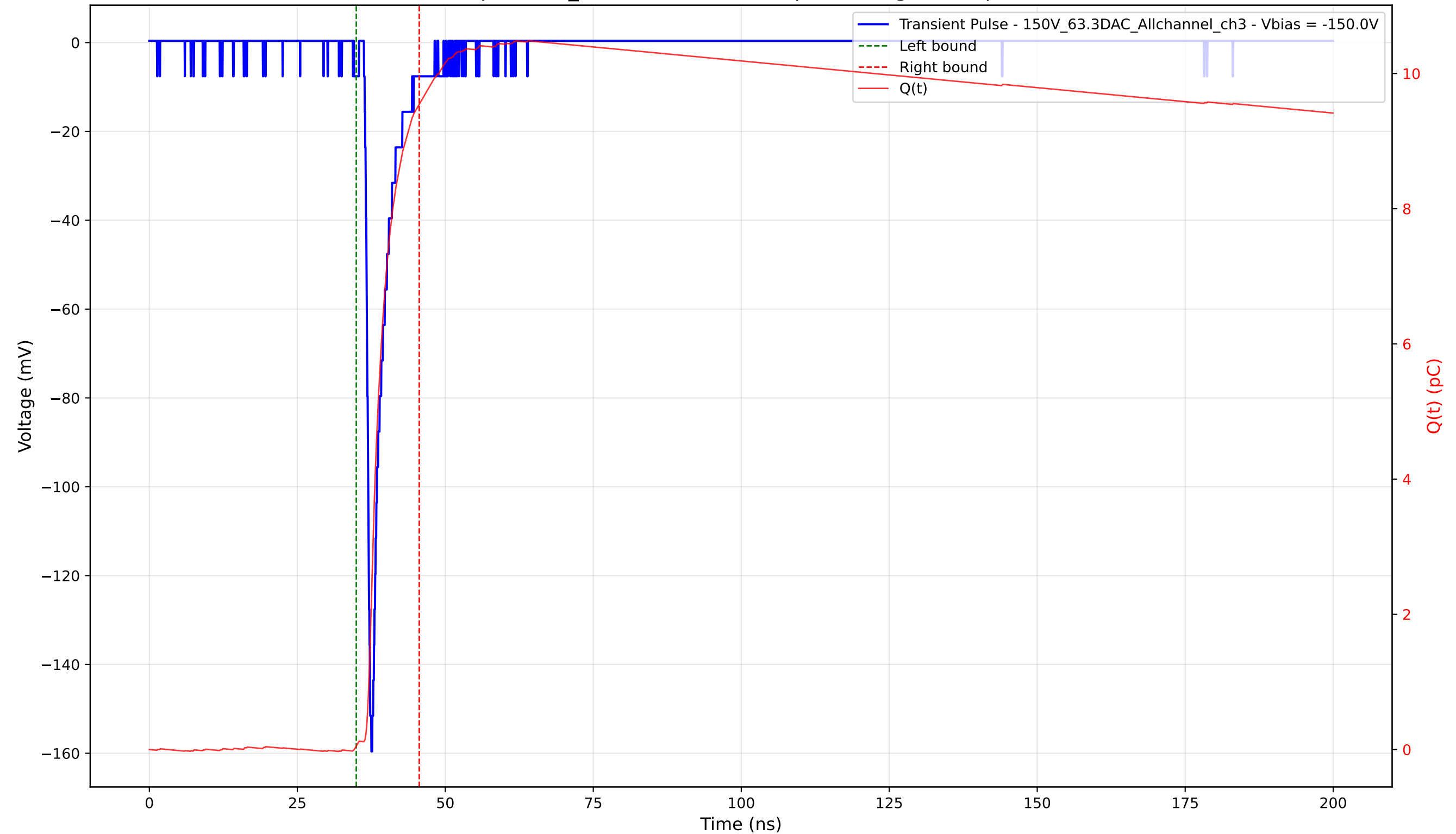
Transient Pulse - Sample: 1cm_42 - Position: 1790.0 \mu\text{m} - Charge: 9.49 pC - Rise Time: 0.88 ns
