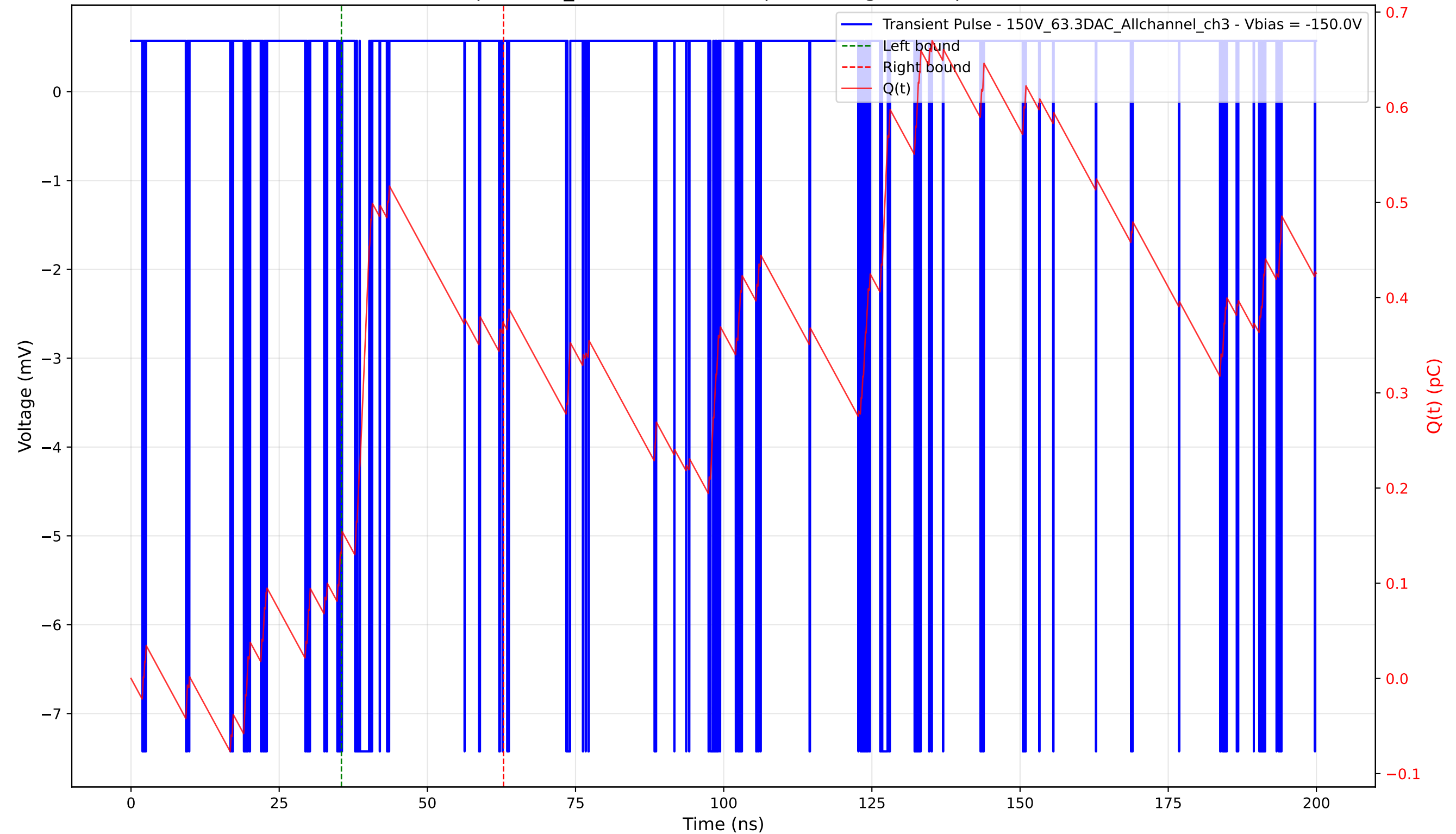
Transient Pulse - Sample: 1cm_42 - Position: 20.0 \mu\text{m} - Charge: 0.23 pC - Rise Time: 0.04 ns
