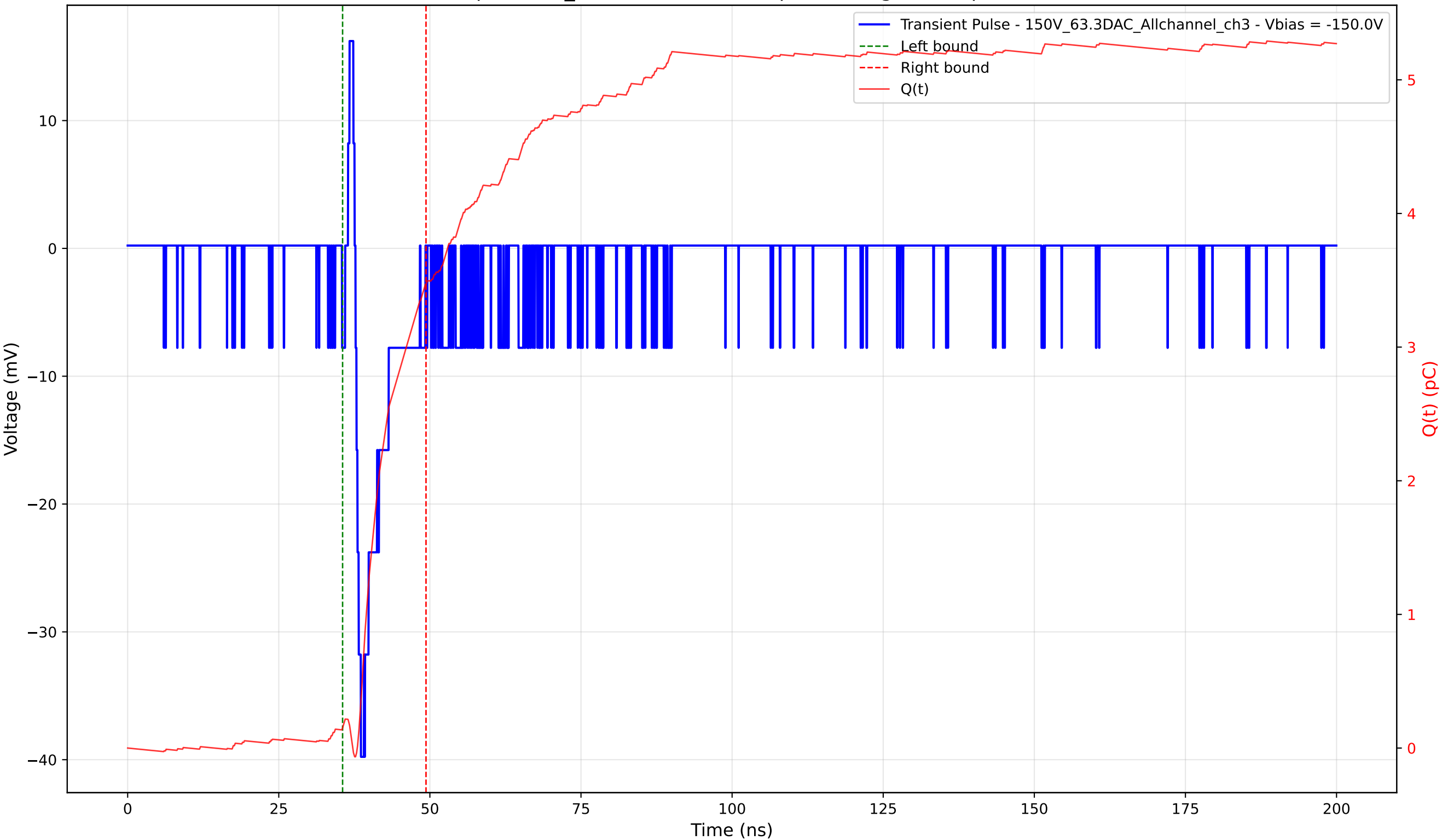
Transient Pulse - Sample: 1cm_42 - Position: 500.0 \mu\text{m} - Charge: 3.32 pC - Rise Time: 0.90 ns
