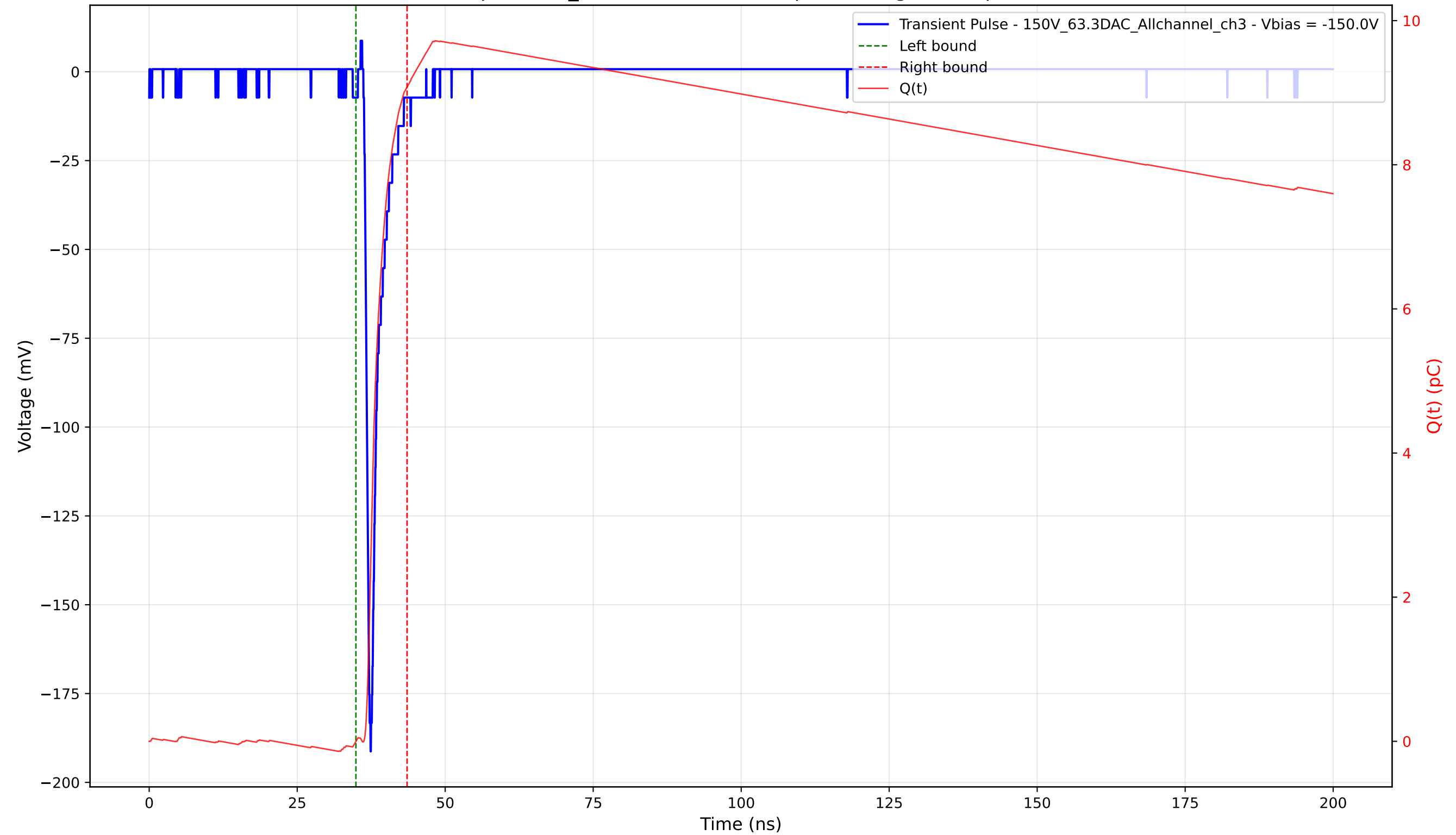
Transient Pulse - Sample: 1cm_42 - Position: 1940.0 \mu\text{m} - Charge: 9.08 pC - Rise Time: 0.82 ns
