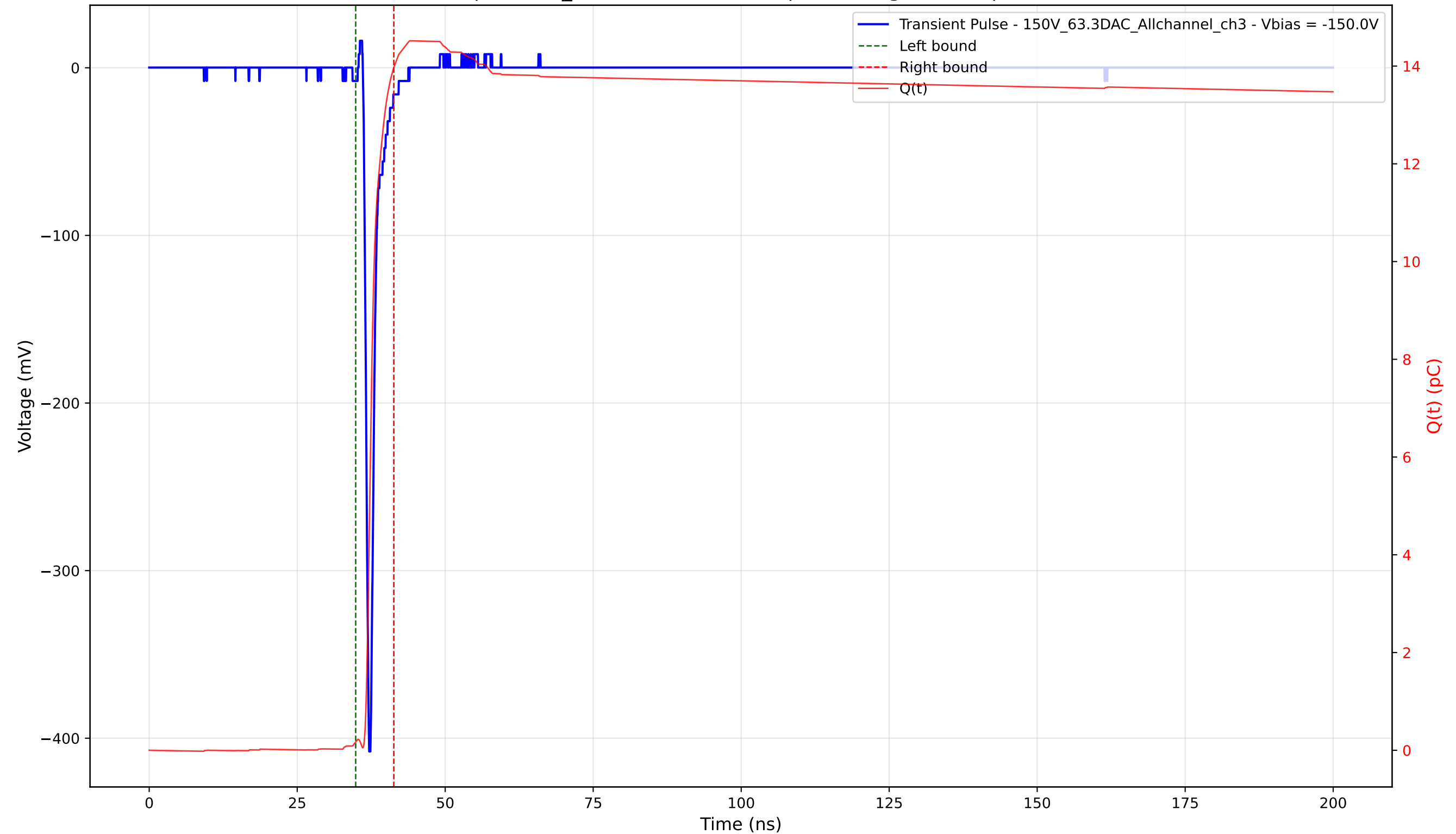
Transient Pulse - Sample: 1cm_42 - Position: 2840.0 \mu\text{m} - Charge: 13.80 pC - Rise Time: 0.74 ns
