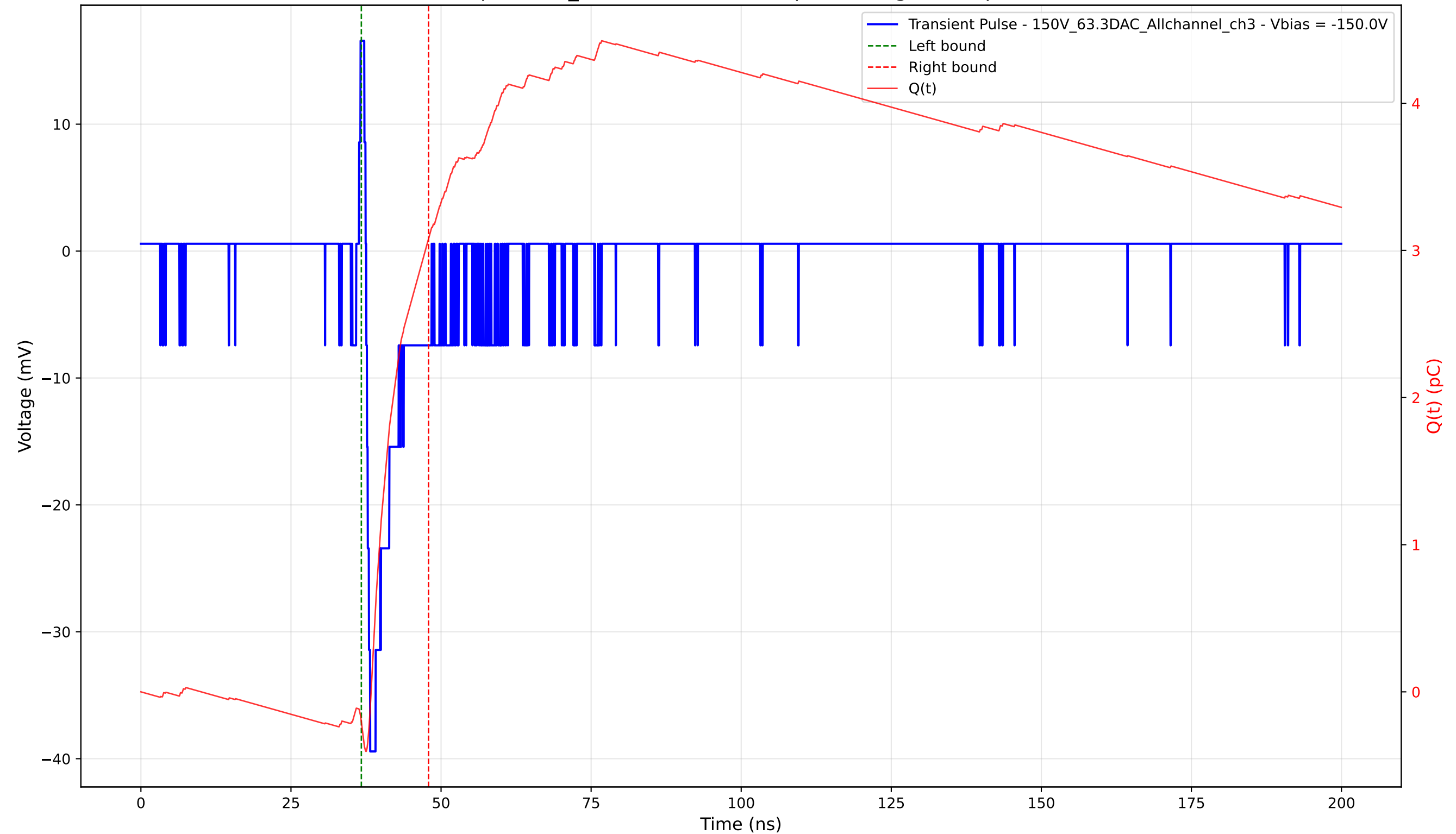
Transient Pulse - Sample: 1cm_42 - Position: 4010.0 \mu\text{m} - Charge: 3.29 pC - Rise Time: 0.66 ns
