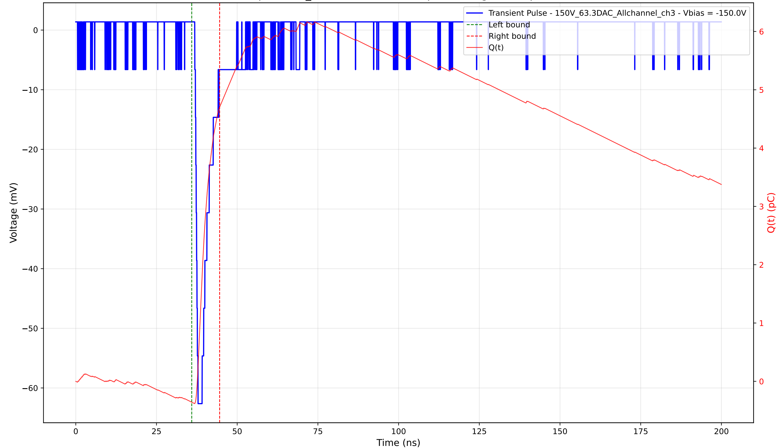
Transient Pulse - Sample: 1cm_42 - Position: 1425.0 \mu\text{m} - Charge: 5.06 pC - Rise Time: 1.00 ns
