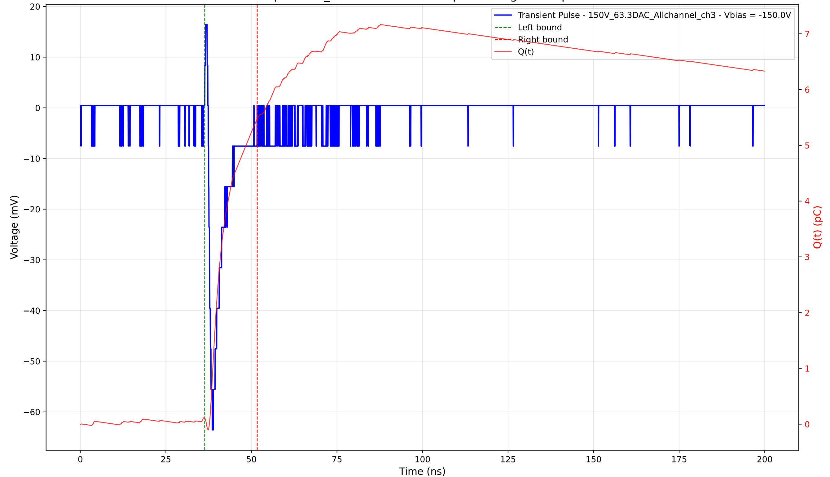
Transient Pulse - Sample: 1cm_42 - Position: 1135.0 \mu\text{m} - Charge: 5.37 pC - Rise Time: 1.17 ns
