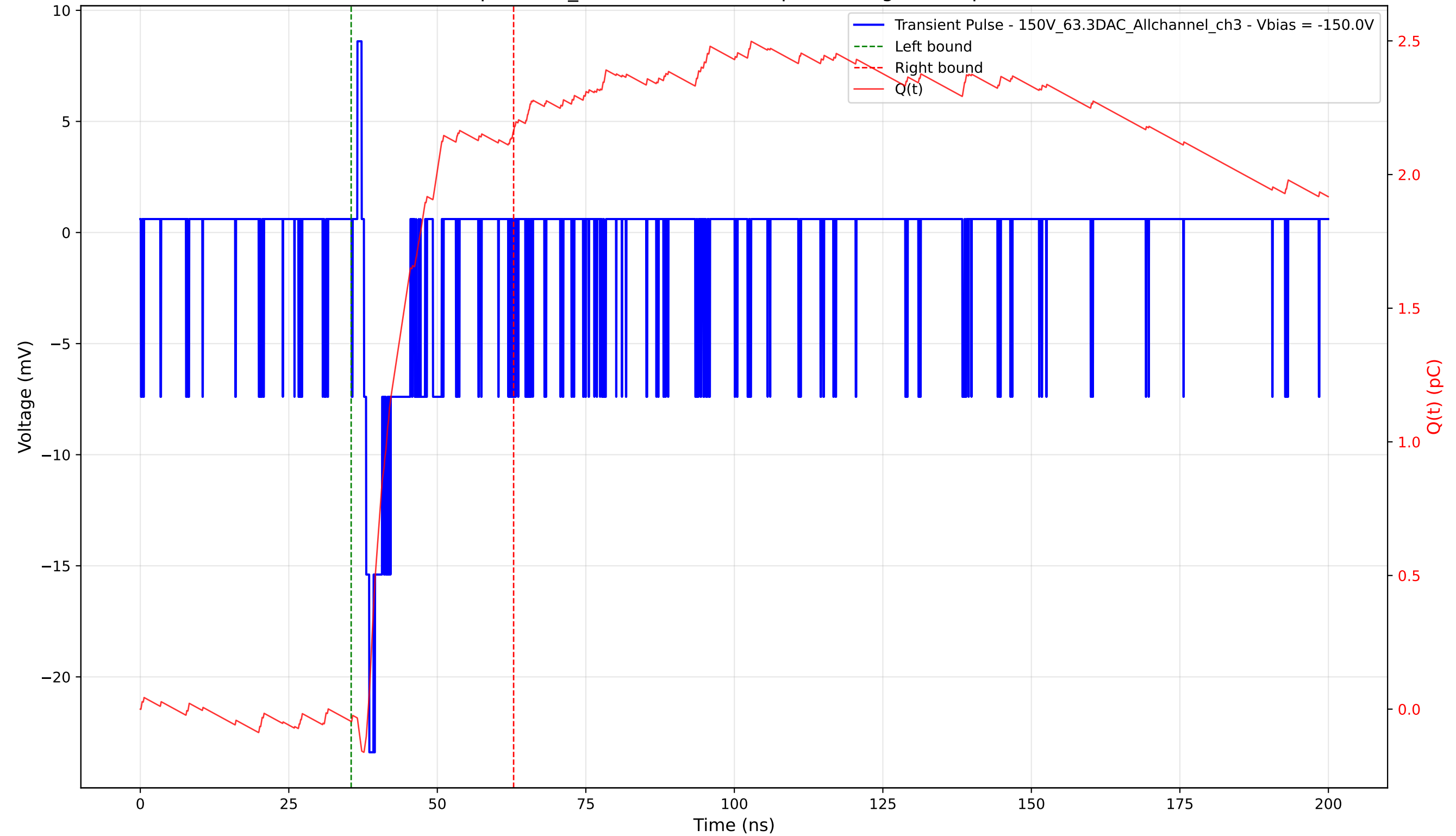
Transient Pulse - Sample: 1cm_42 - Position: 225.0 \mu\text{m} - Charge: 2.21 pC - Rise Time: 0.91 ns
