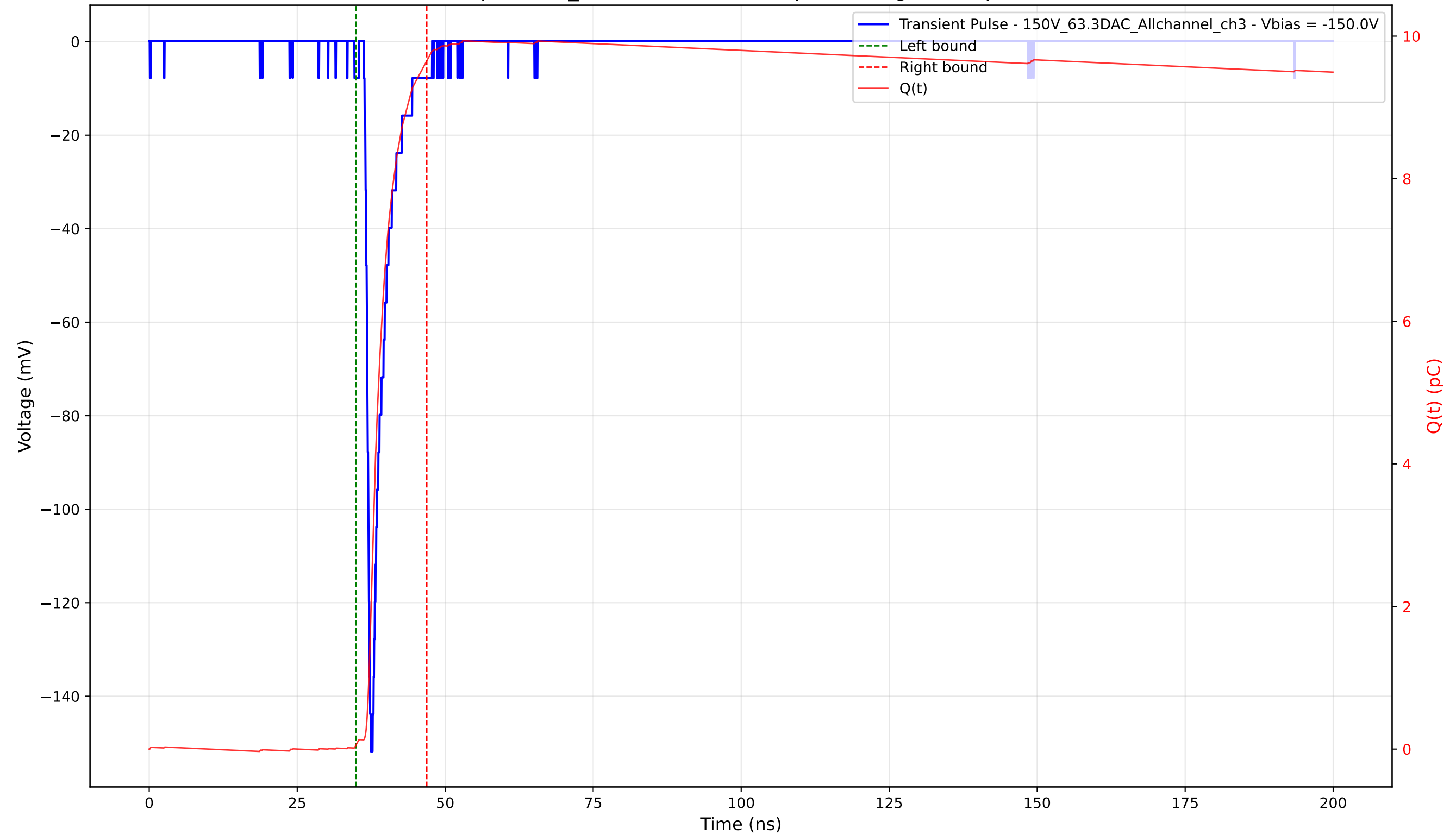
Transient Pulse - Sample: 1cm_42 - Position: 1750.0 \mu\text{m} - Charge: 9.60 pC - Rise Time: 0.92 ns
