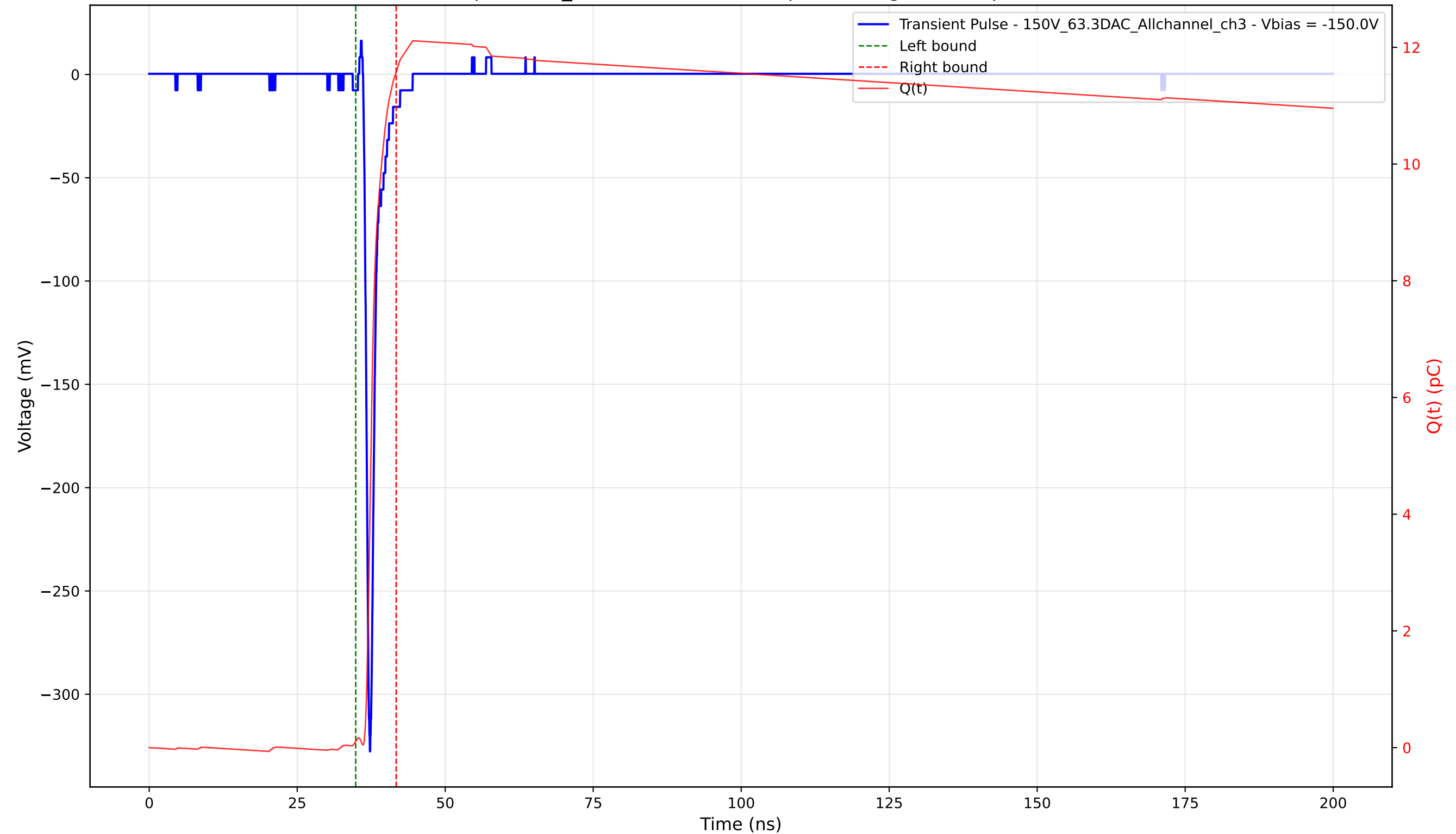
Transient Pulse - Sample: 1cm_42 - Position: 2915.0 \mu\text{m} - Charge: 11.47 pC - Rise Time: 0.75 ns
