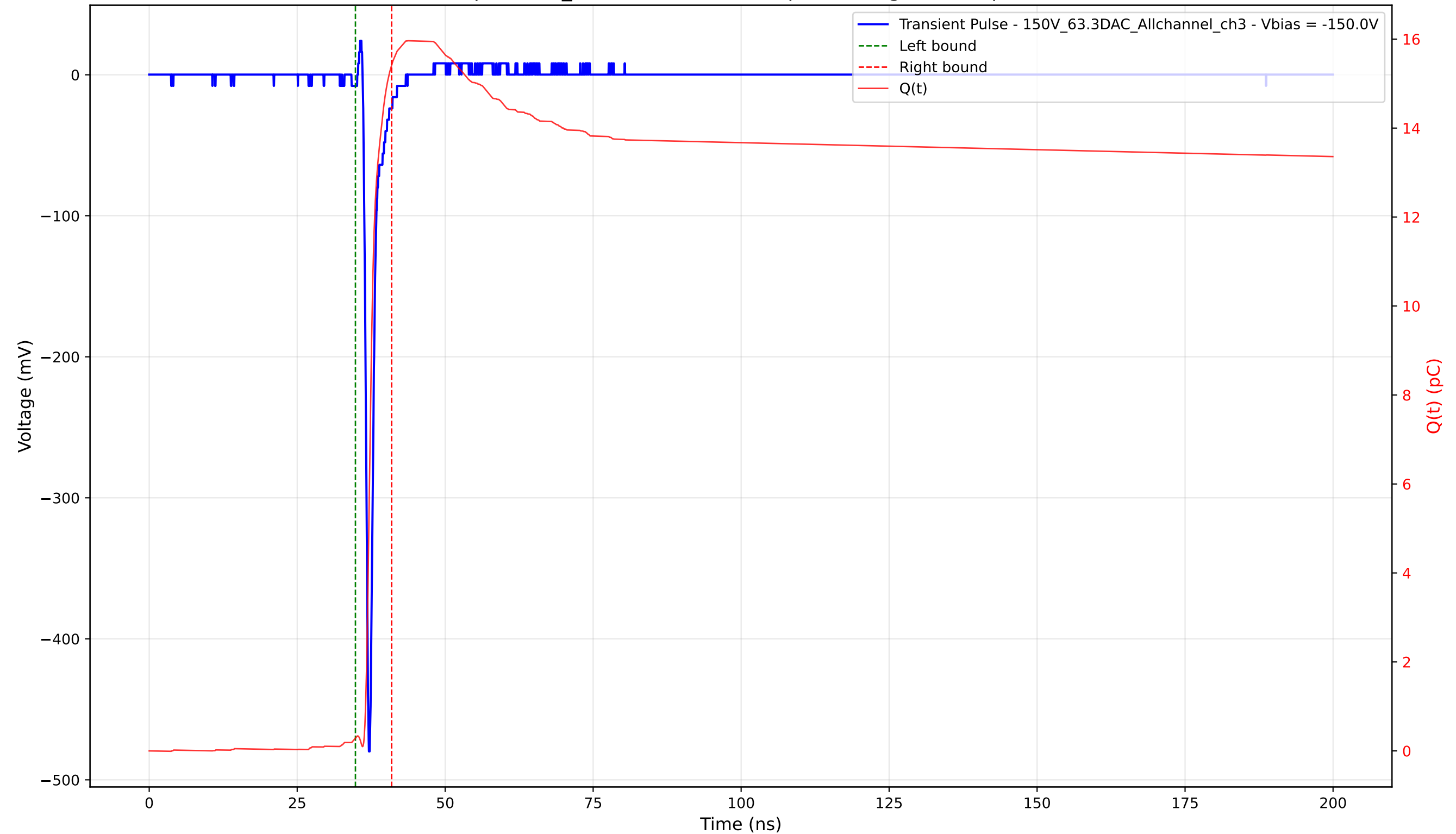
Transient Pulse - Sample: 1cm_42 - Position: 2355.0 \mu\text{m} - Charge: 15.13 pC - Rise Time: 0.70 ns
