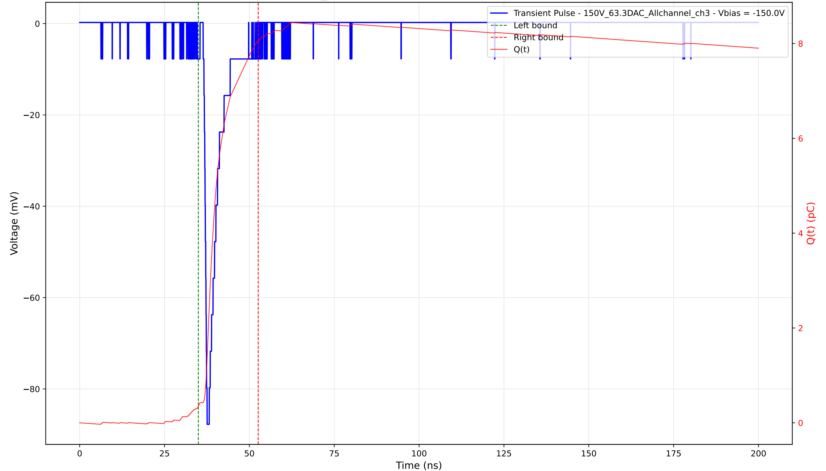
Transient Pulse - Sample: 1cm_42 - Position: 1570.0 \mu\text{m} - Charge: 7.70 pC - Rise Time: 0.79 ns
