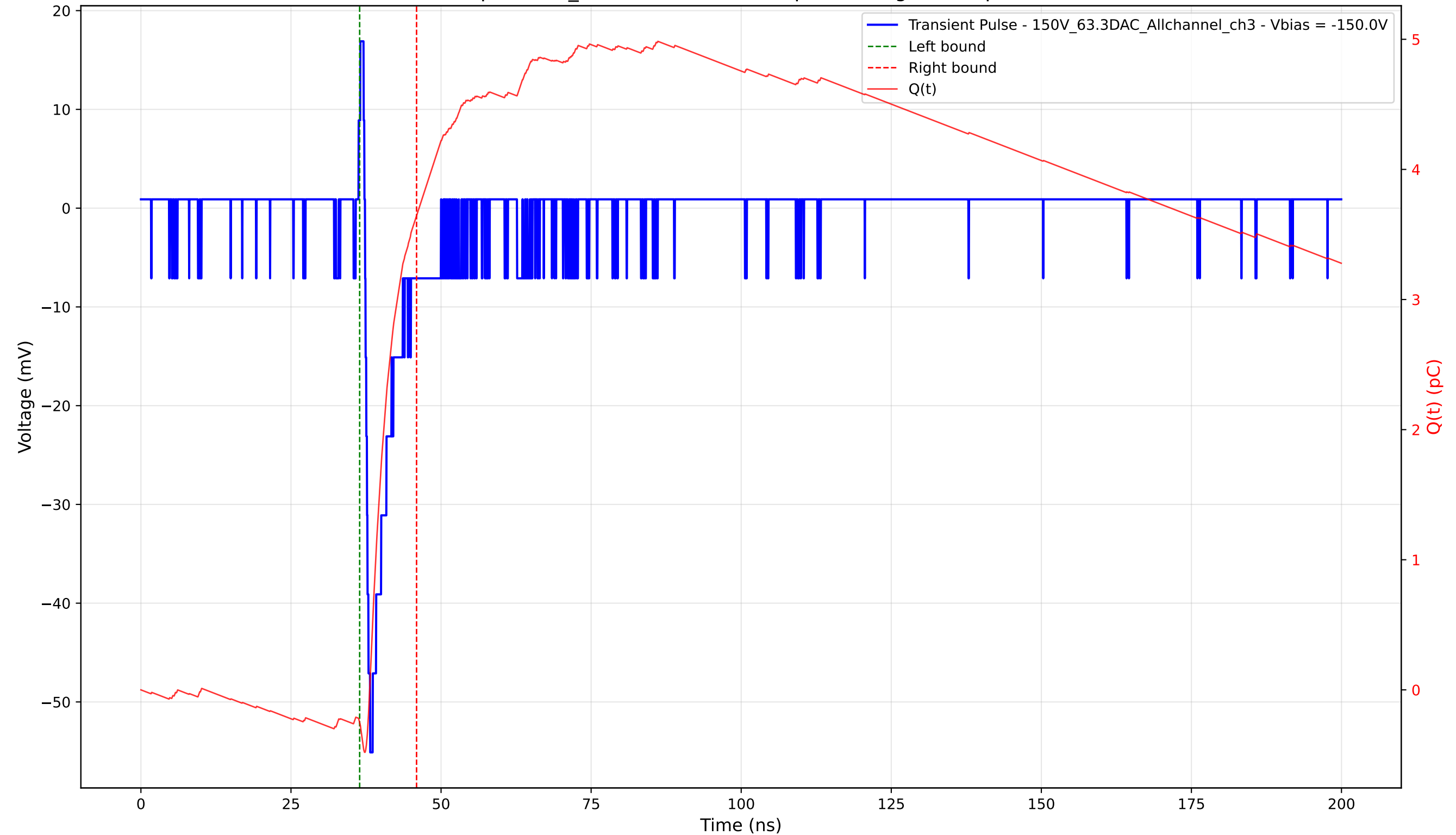
Transient Pulse - Sample: 1cm_42 - Position: 3840.0 \mu\text{m} - Charge: 3.89 pC - Rise Time: 0.85 ns
