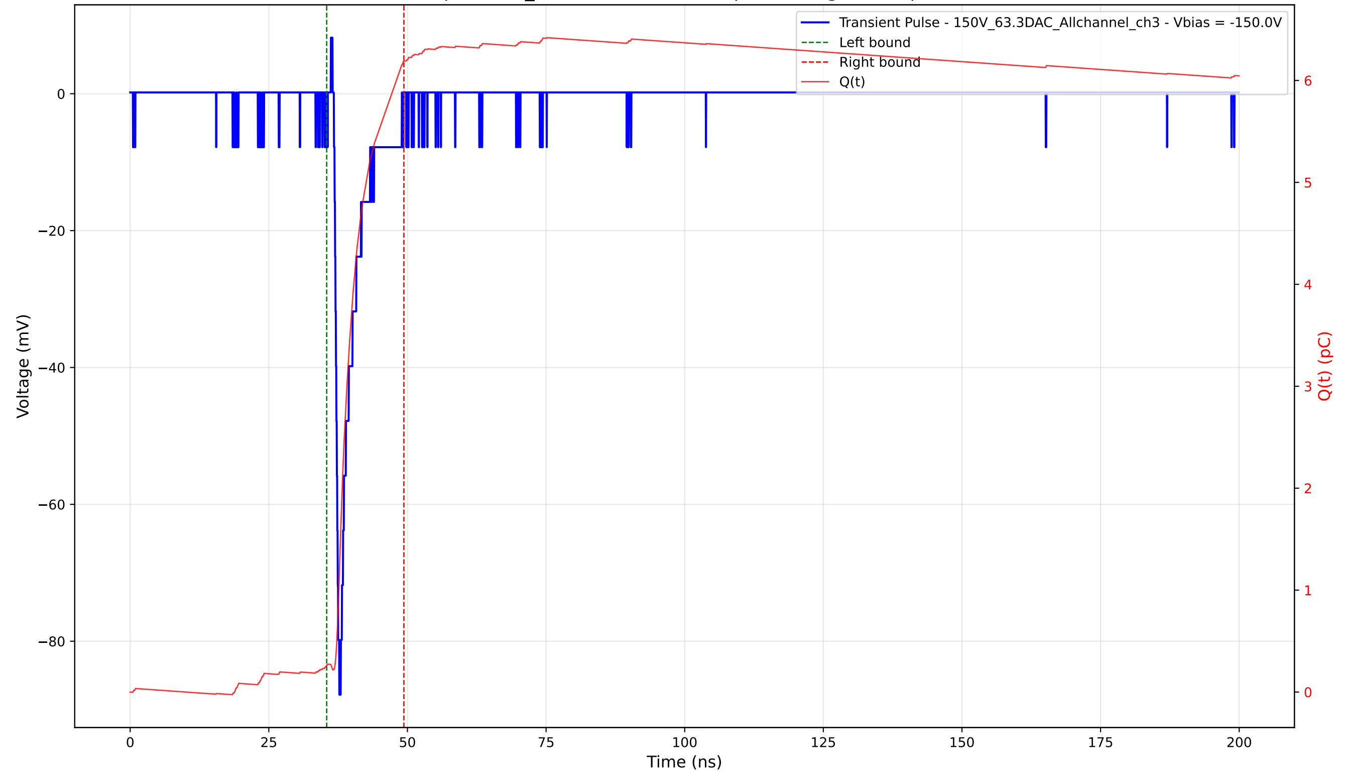
Transient Pulse - Sample: 1cm_42 - Position: 3465.0 \mu\text{m} - Charge: 5.93 pC - Rise Time: 0.68 ns
