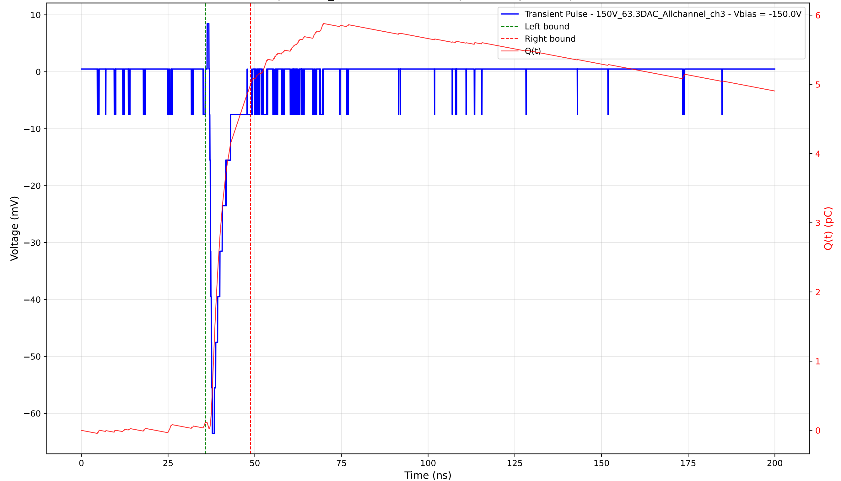
Transient Pulse - Sample: 1cm_42 - Position: 3570.0 \mu\text{m} - Charge: 4.88 pC - Rise Time: 0.81 ns
