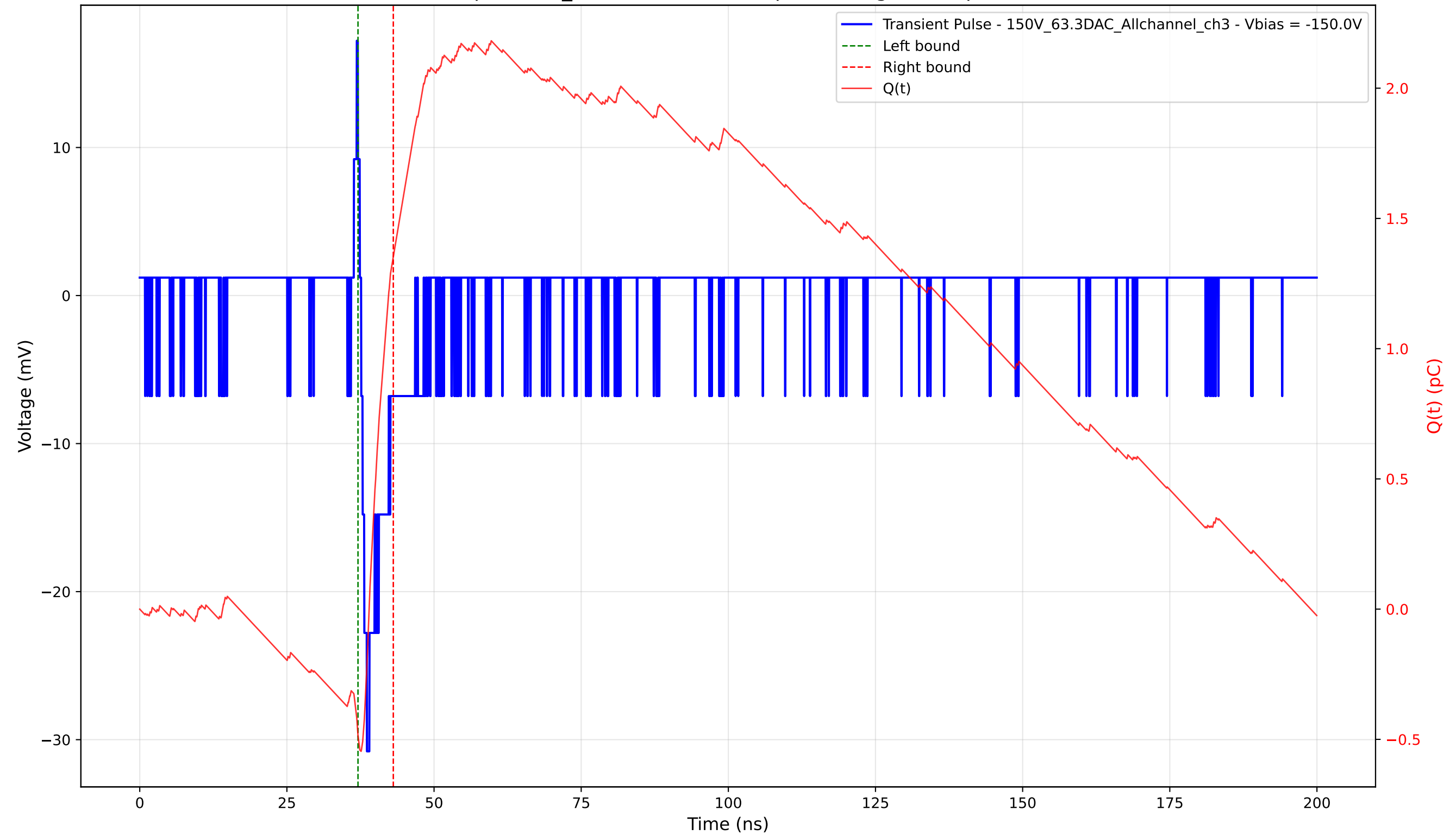
Transient Pulse - Sample: 1cm_42 - Position: 375.0 \mu\text{m} - Charge: 1.84 pC - Rise Time: 0.99 ns
