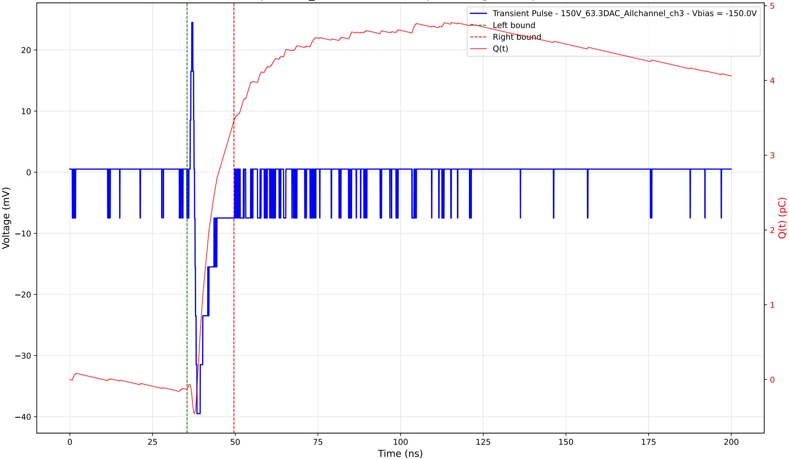
Transient Pulse - Sample: 1cm_42 - Position: 575.0 \mu\text{m} - Charge: 3.58 pC - Rise Time: 0.74 ns
