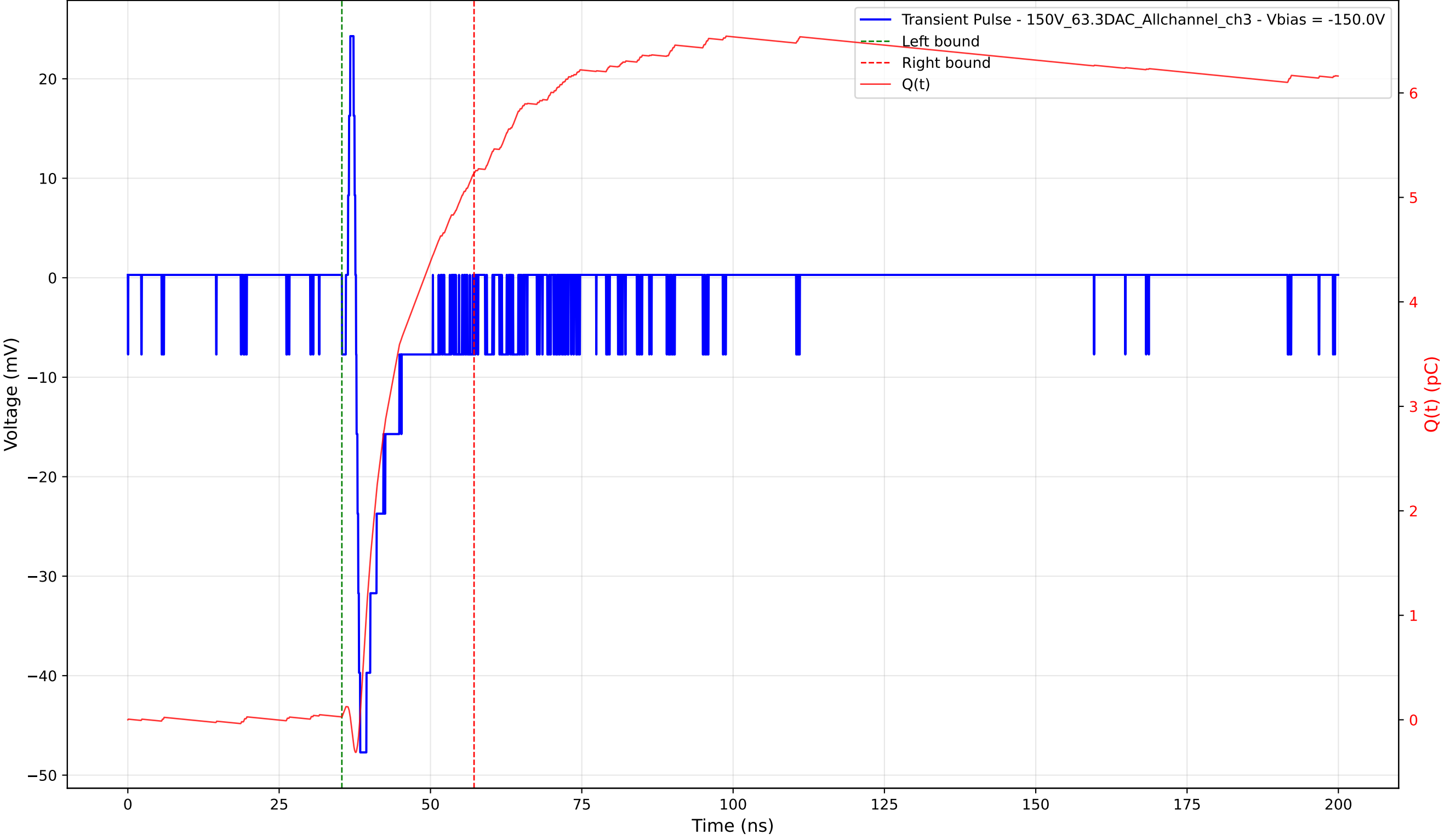
Transient Pulse - Sample: 1cm_42 - Position: 815.0 \mu\text{m} - Charge: 5.21 pC - Rise Time: 0.70 ns
