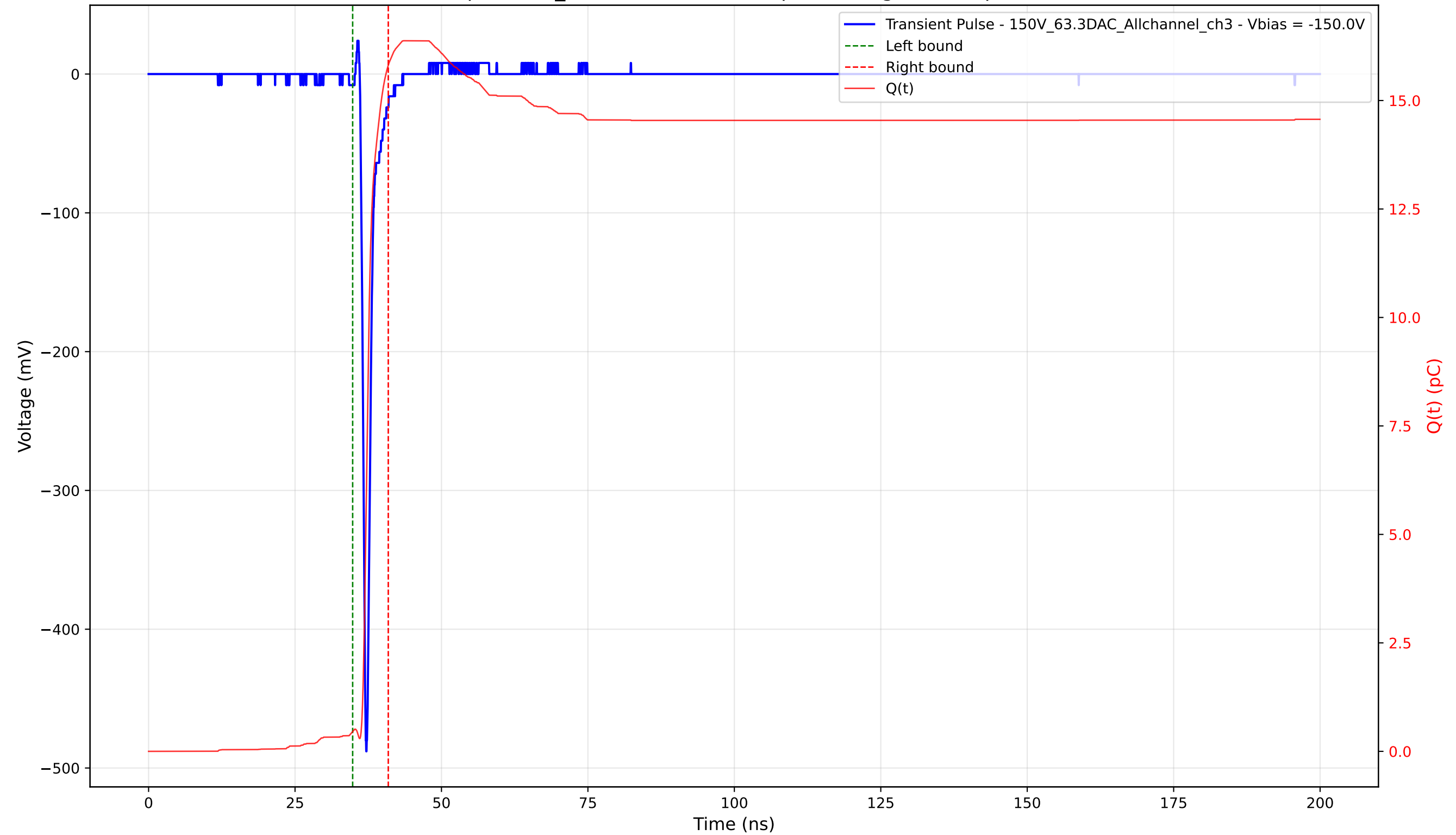
Transient Pulse - Sample: 1cm_42 - Position: 2690.0 \mu\text{m} - Charge: 15.36 pC - Rise Time: 0.74 ns
