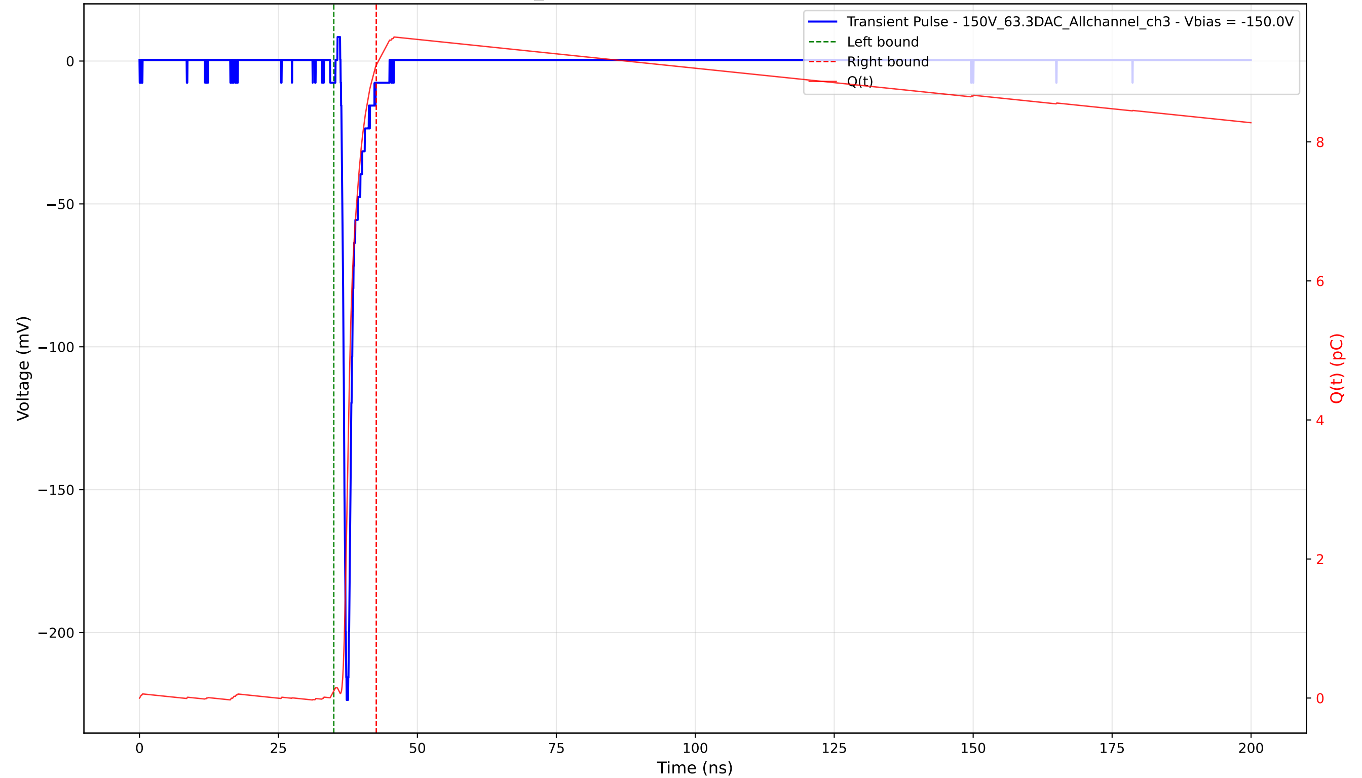
Transient Pulse - Sample: 1cm_42 - Position: 3010.0 \mu\text{m} - Charge: 9.00 pC - Rise Time: 0.77 ns
