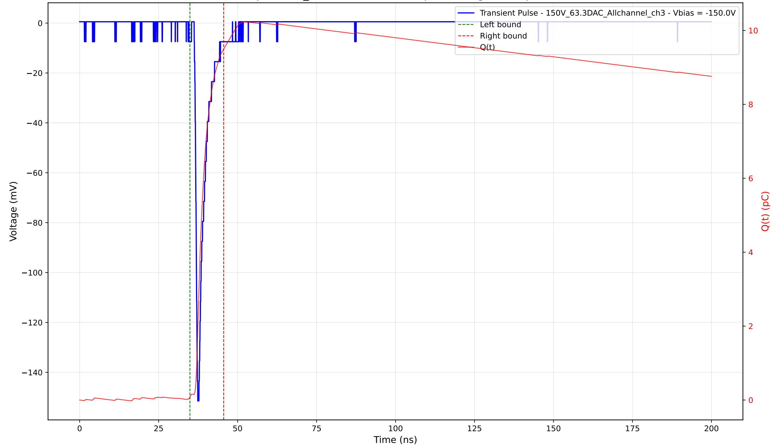
Transient Pulse - Sample: 1cm_42 - Position: 1775.0 \mu\text{m} - Charge: 9.41 pC - Rise Time: 0.92 ns
