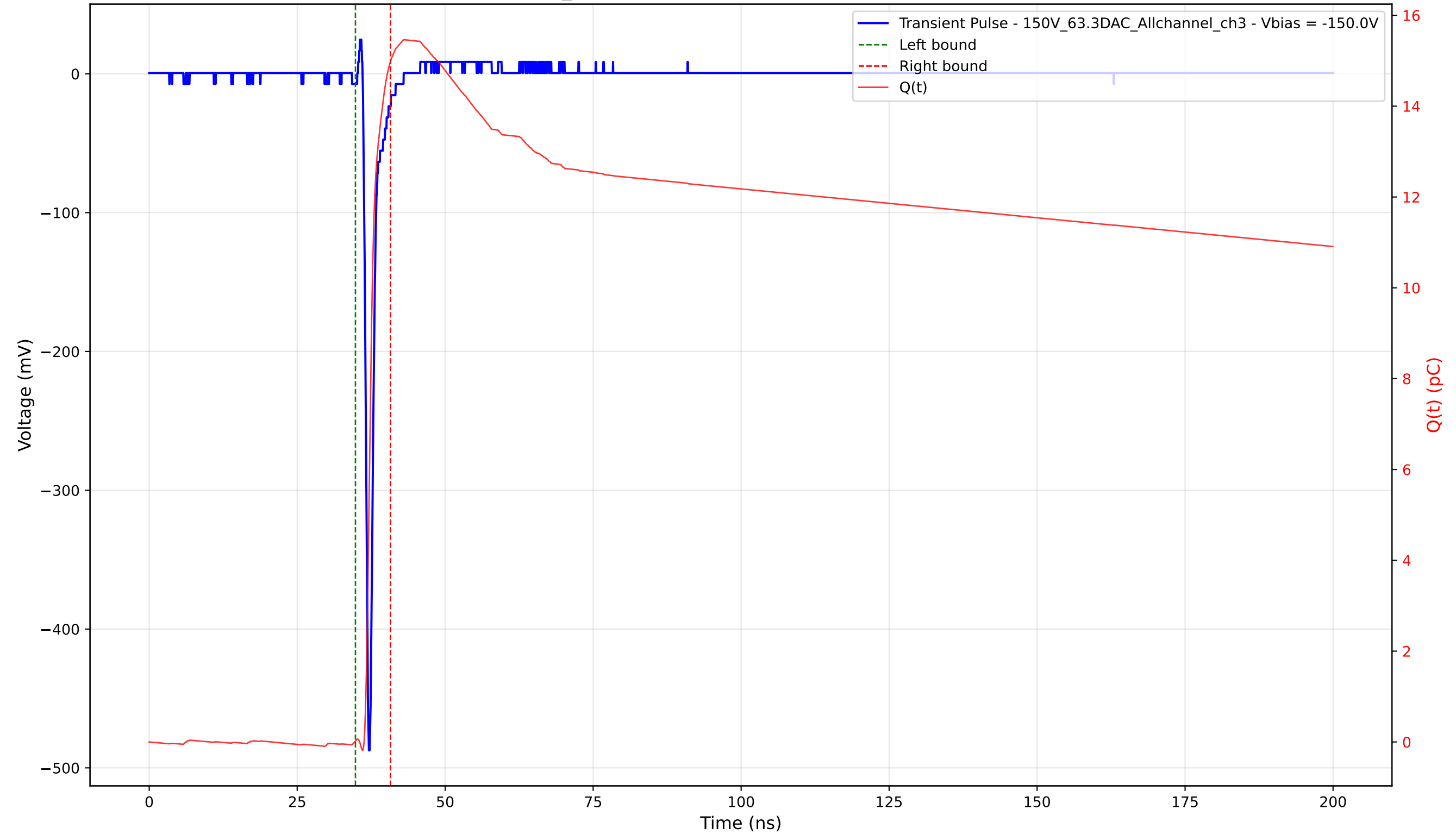
Transient Pulse - Sample: 1cm_42 - Position: 2610.0 \mu\text{m} - Charge: 14.97 pC - Rise Time: 0.69 ns
