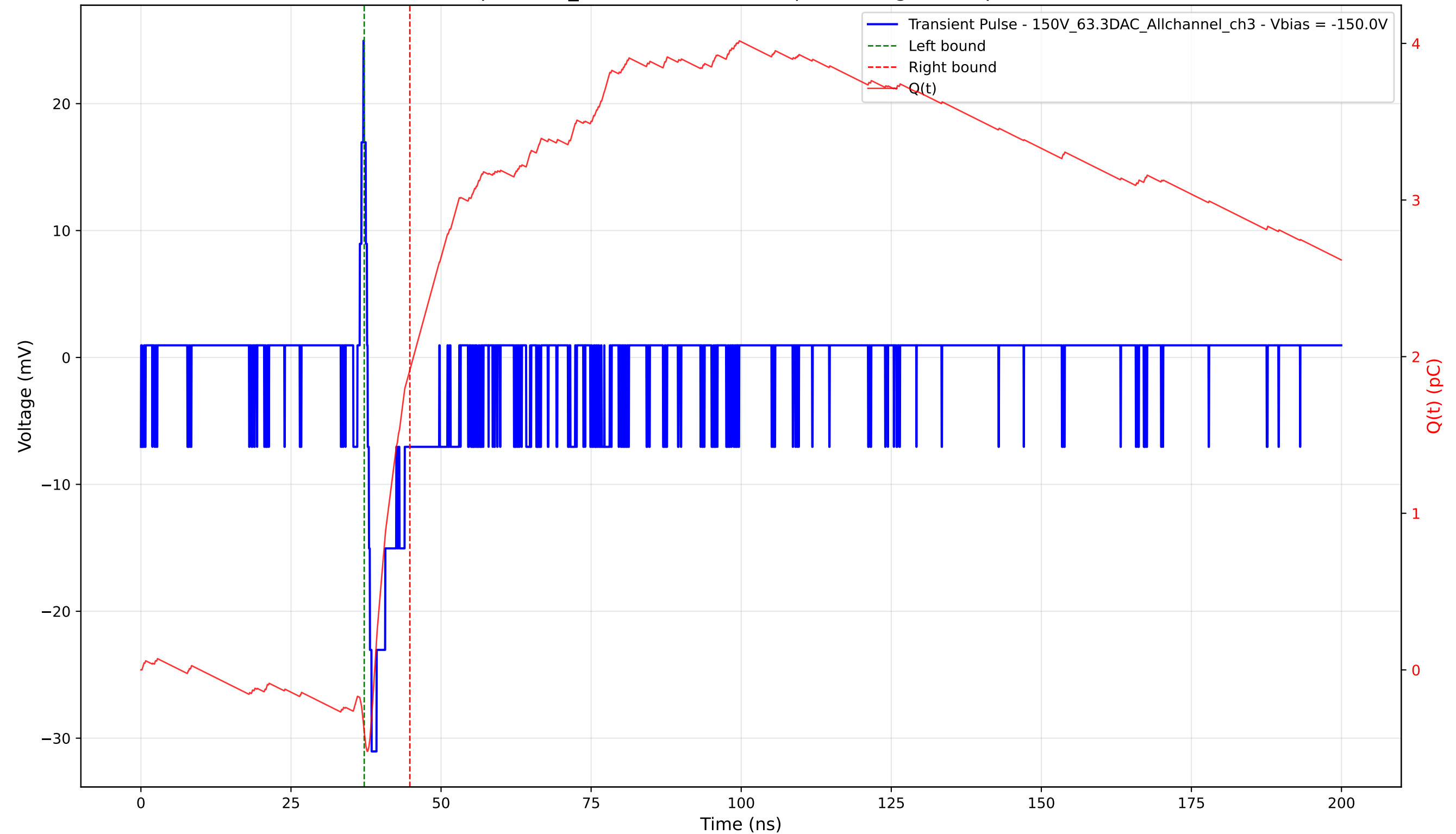
Transient Pulse - Sample: 1cm_42 - Position: 4470.0 \mu\text{m} - Charge: 2.31 pC - Rise Time: 0.67 ns
