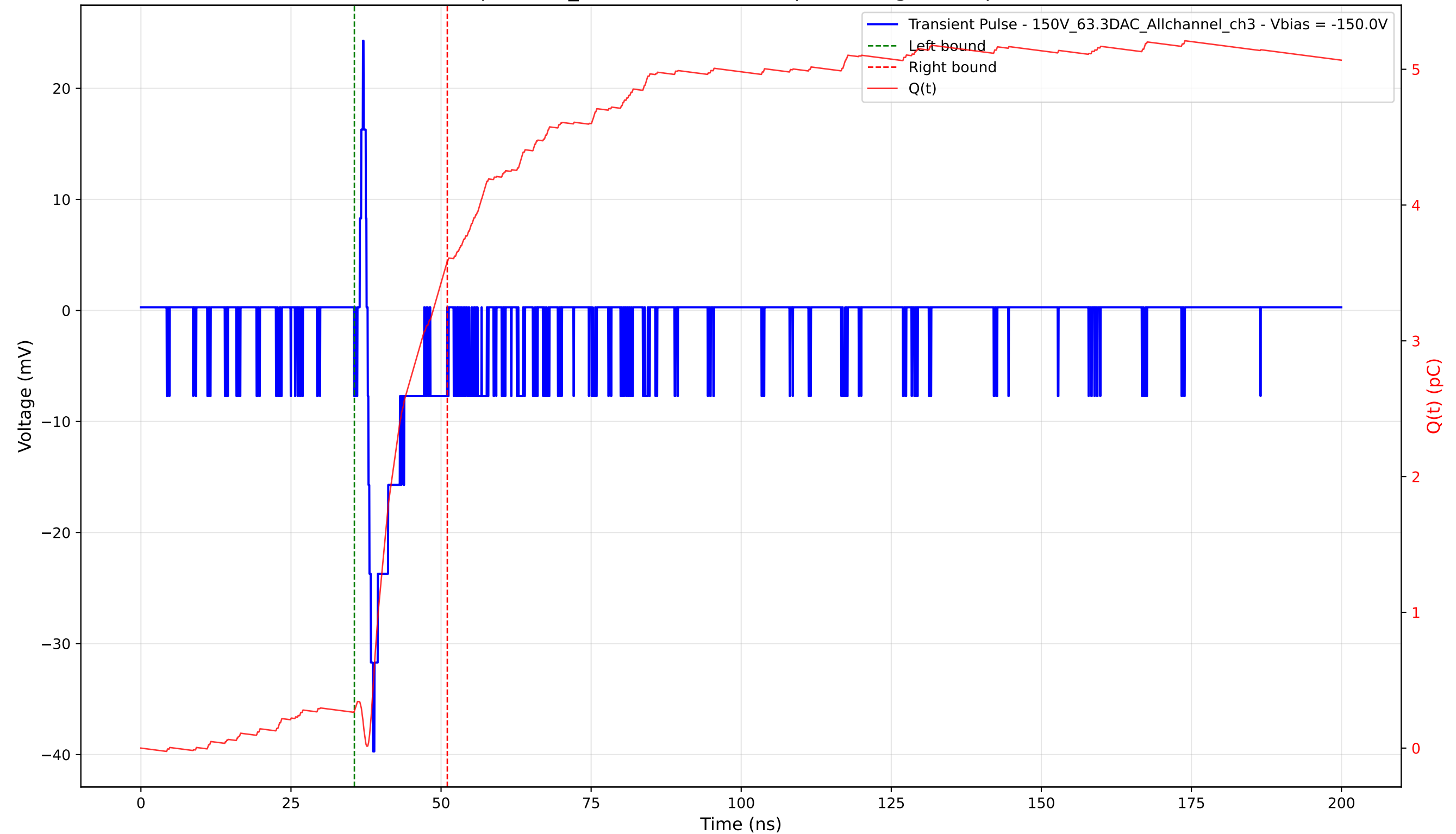
Transient Pulse - Sample: 1cm_42 - Position: 4410.0 \mu\text{m} - Charge: 3.31 pC - Rise Time: 0.90 ns
