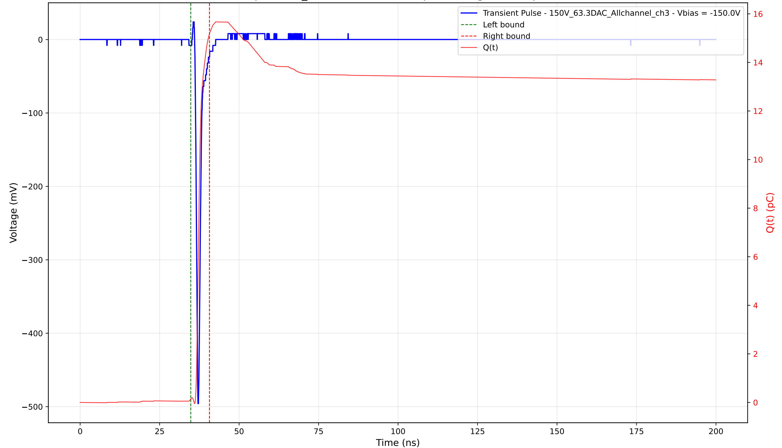
Transient Pulse - Sample: 1cm_42 - Position: 2505.0 \mu\text{m} - Charge: 15.04 pC - Rise Time: 0.73 ns
