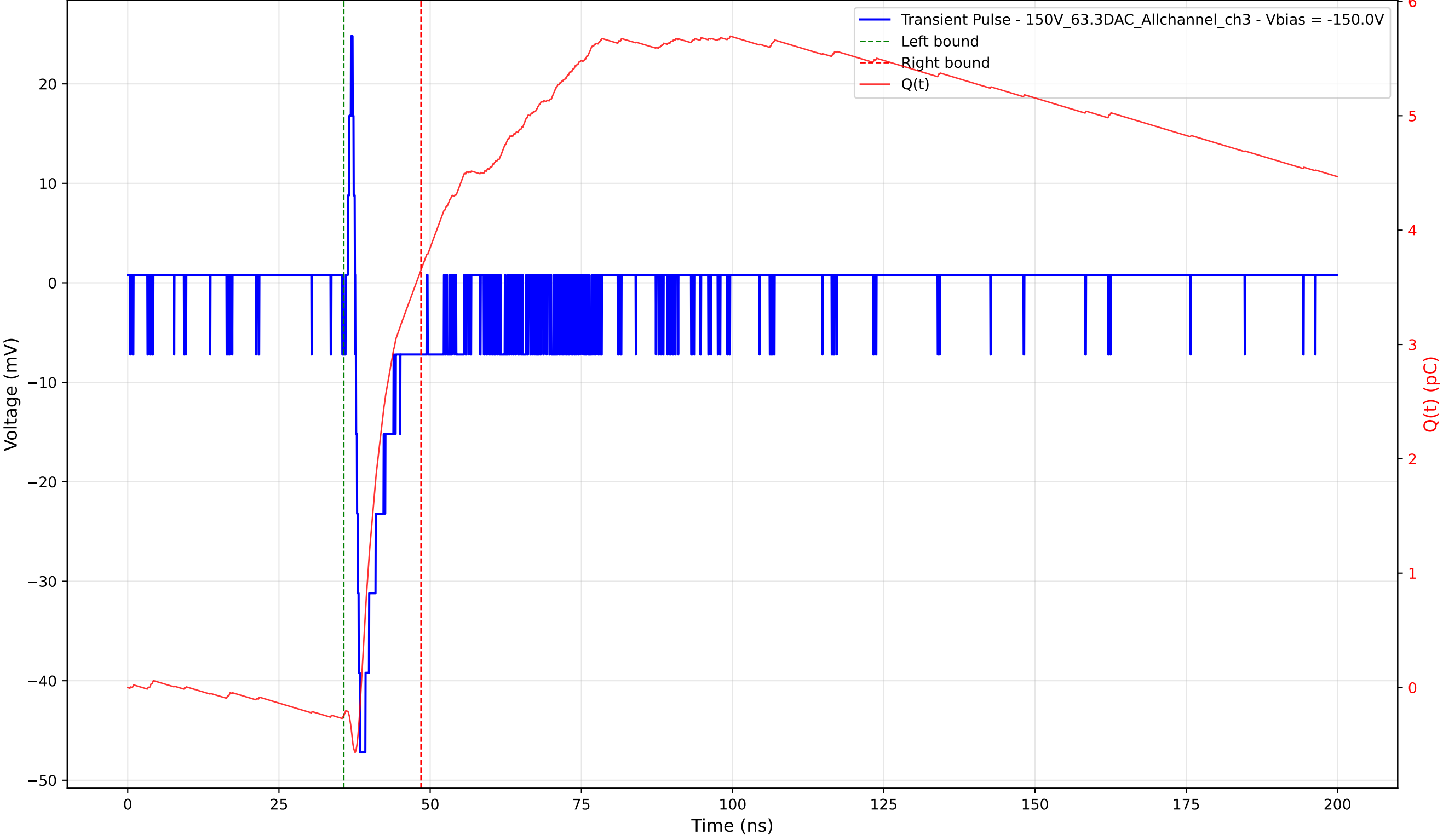
Transient Pulse - Sample: 1cm_42 - Position: 910.0 \mu\text{m} - Charge: 3.90 pC - Rise Time: 0.78 ns
