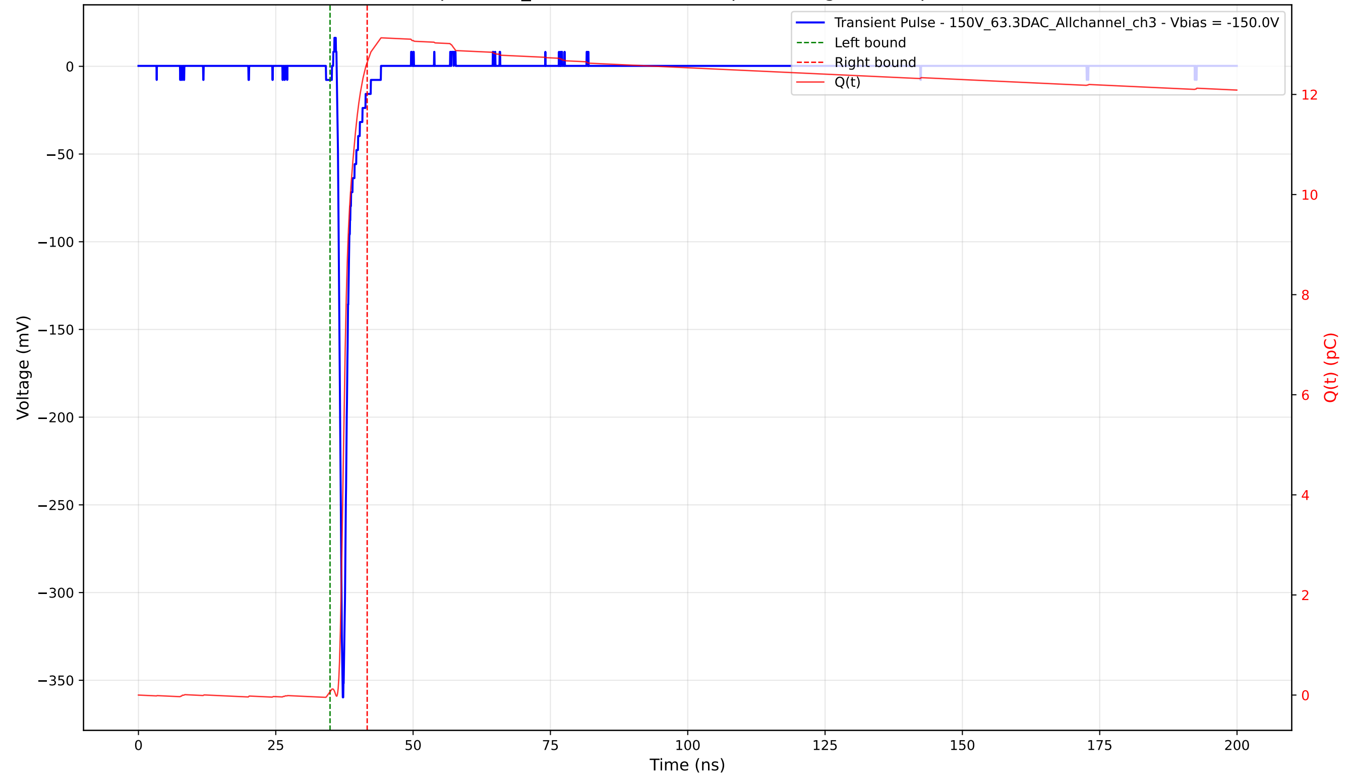
Transient Pulse - Sample: 1cm_42 - Position: 2155.0 \mu\text{m} - Charge: 12.57 pC - Rise Time: 0.76 ns
