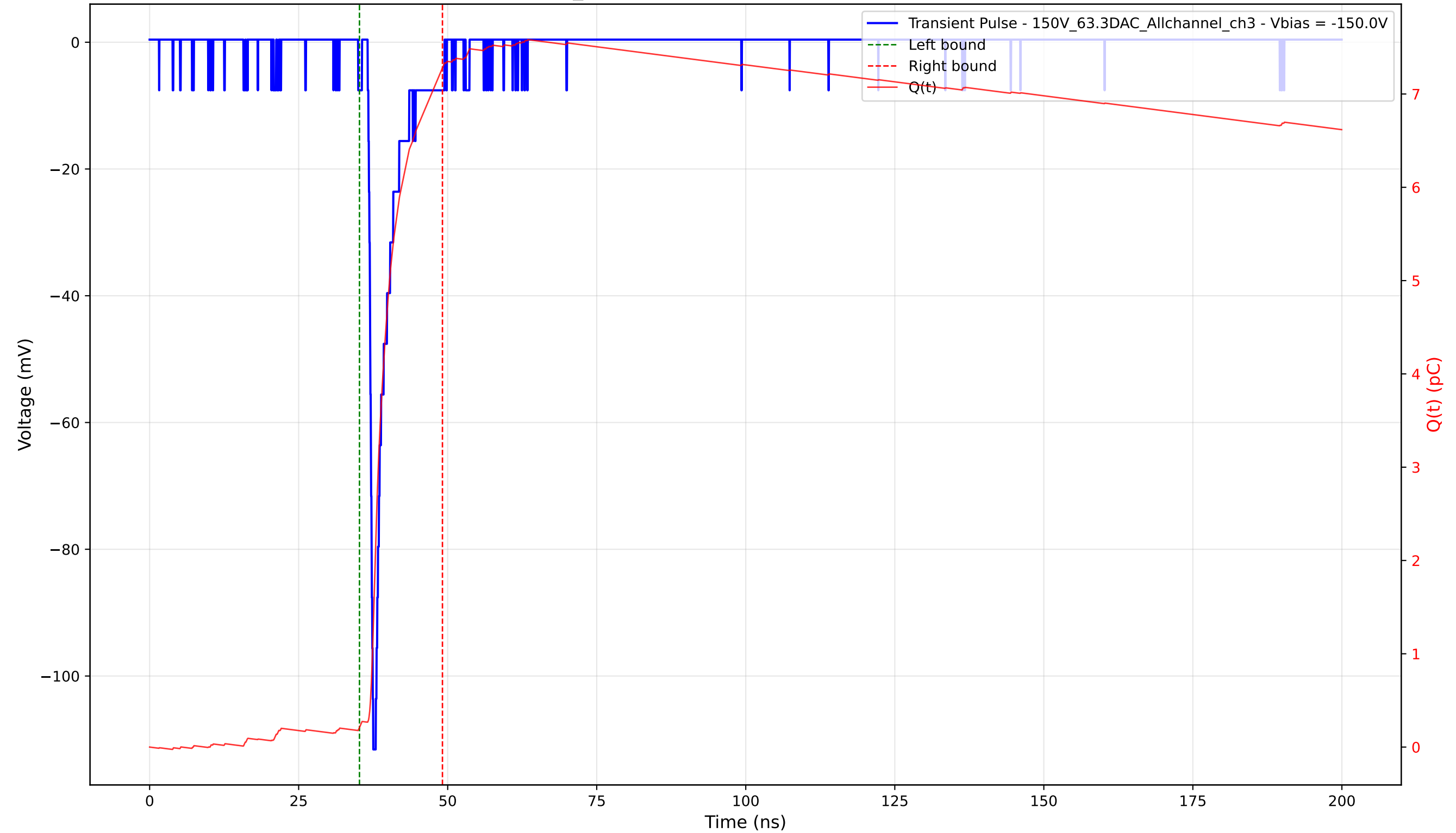
Transient Pulse - Sample: 1cm_42 - Position: 3375.0 \mu\text{m} - Charge: 7.07 pC - Rise Time: 0.74 ns
