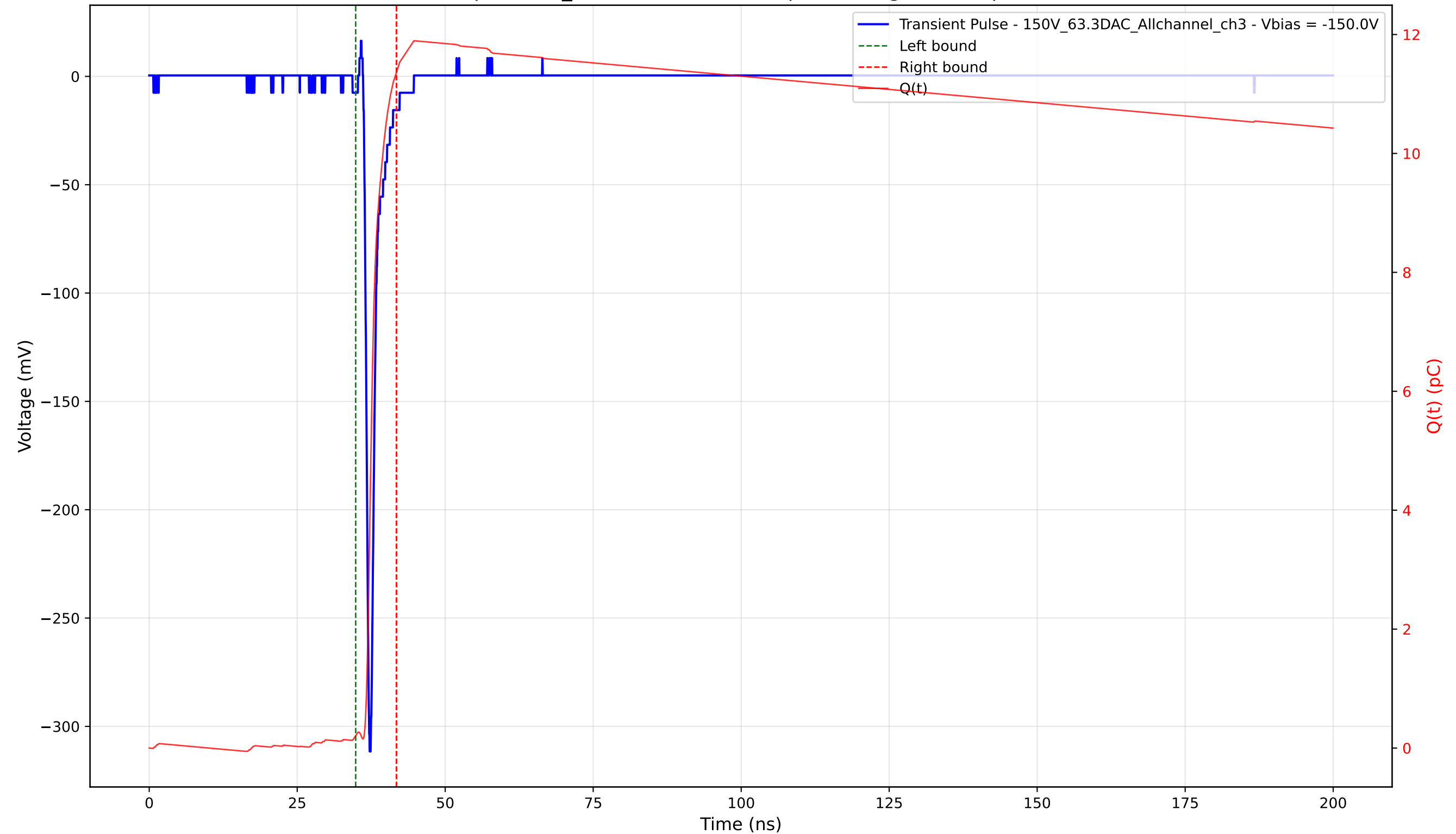
Transient Pulse - Sample: 1cm_42 - Position: 2925.0 \mu\text{m} - Charge: 11.15 pC - Rise Time: 0.75 ns
