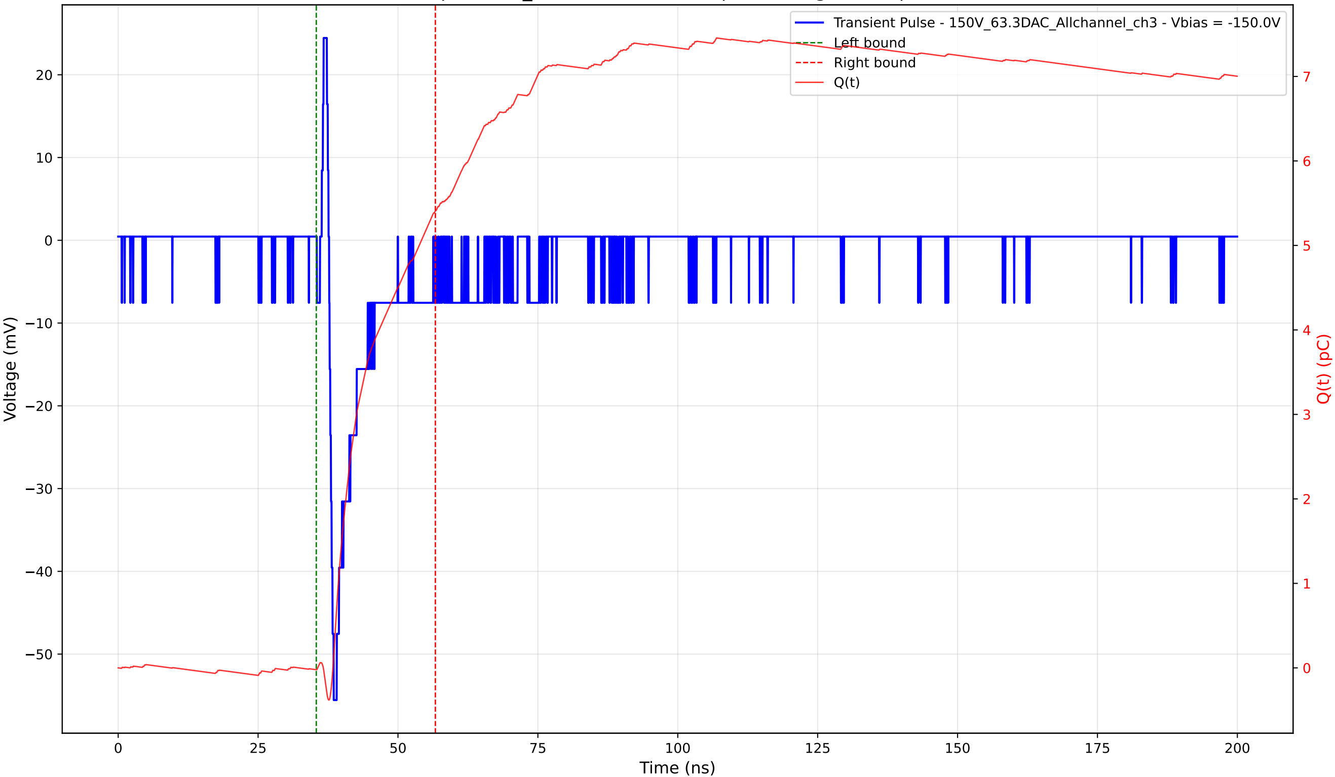
Transient Pulse - Sample: 1cm_42 - Position: 795.0 \mu\text{m} - Charge: 5.43 pC - Rise Time: 0.81 ns
