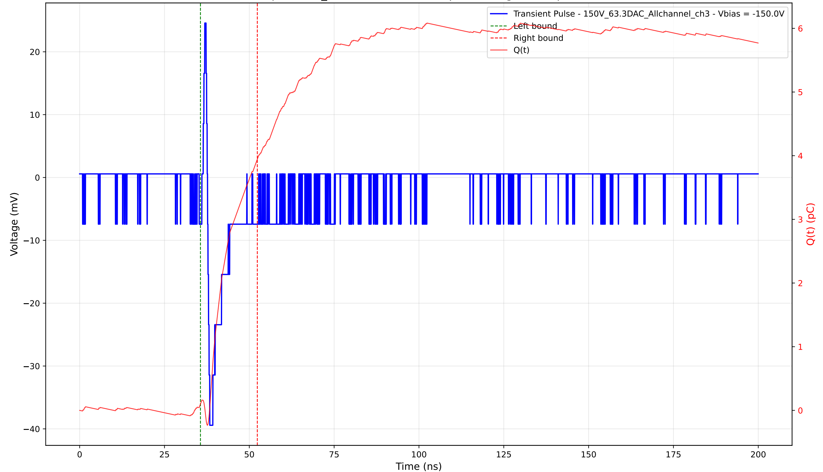
Transient Pulse - Sample: 1cm_42 - Position: 4200.0 \mu\text{m} - Charge: 3.85 pC - Rise Time: 0.66 ns
