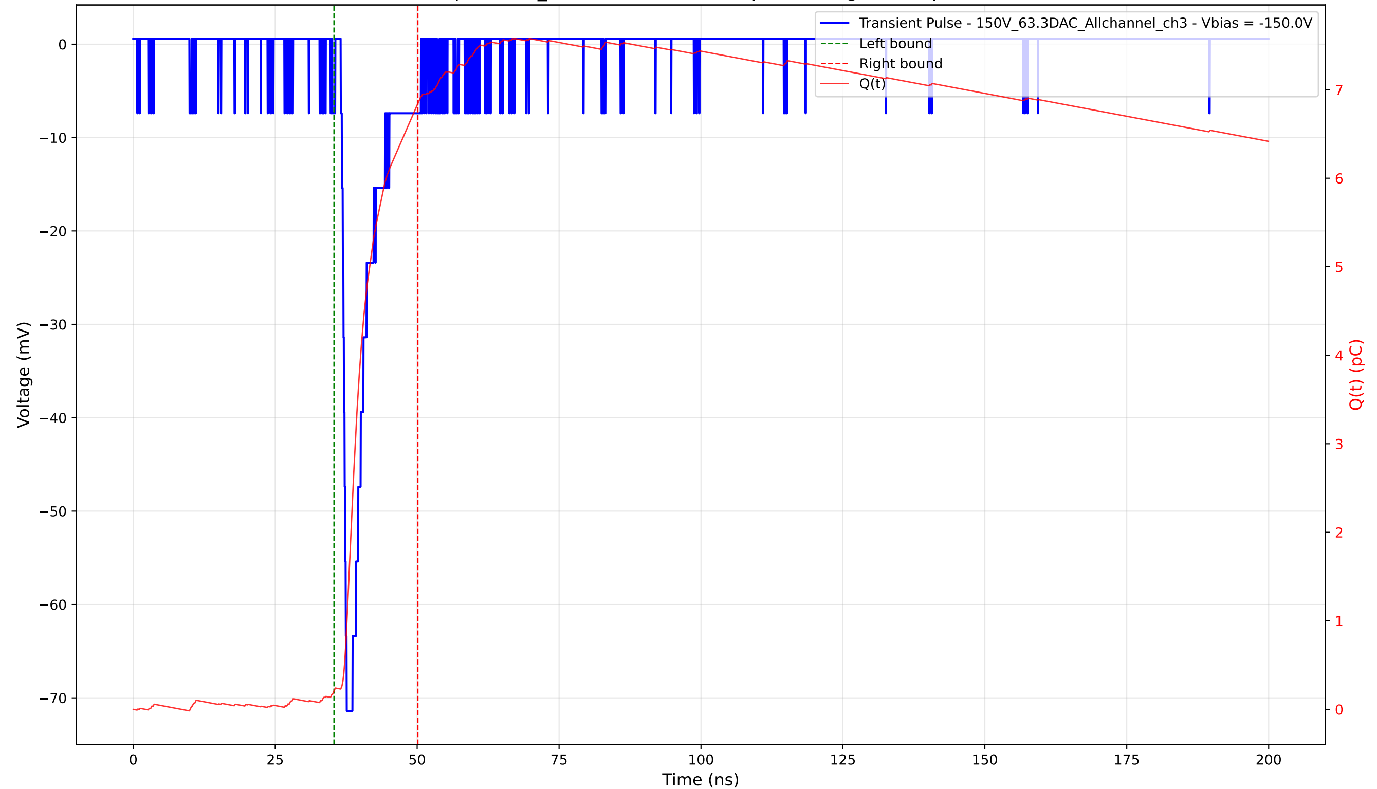
Transient Pulse - Sample: 1cm_42 - Position: 1515.0 \mu\text{m} - Charge: 6.64 pC - Rise Time: 1.04 ns
