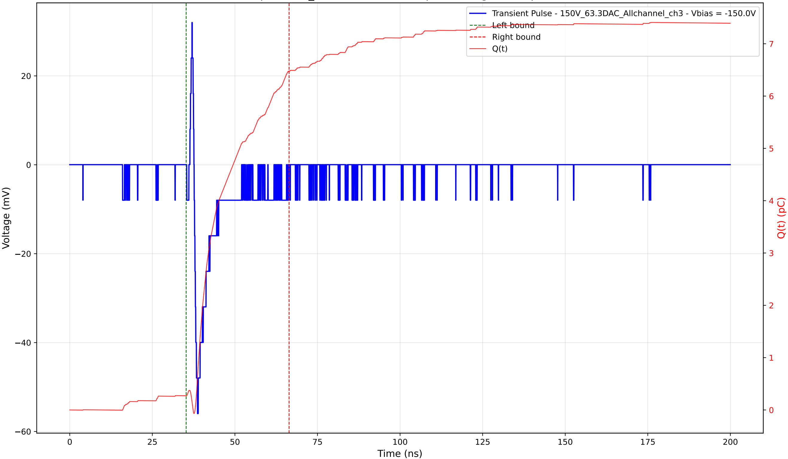
Transient Pulse - Sample: 1cm_42 - Position: 780.0 \mu\text{m} - Charge: 6.21 pC - Rise Time: 1.01 ns
