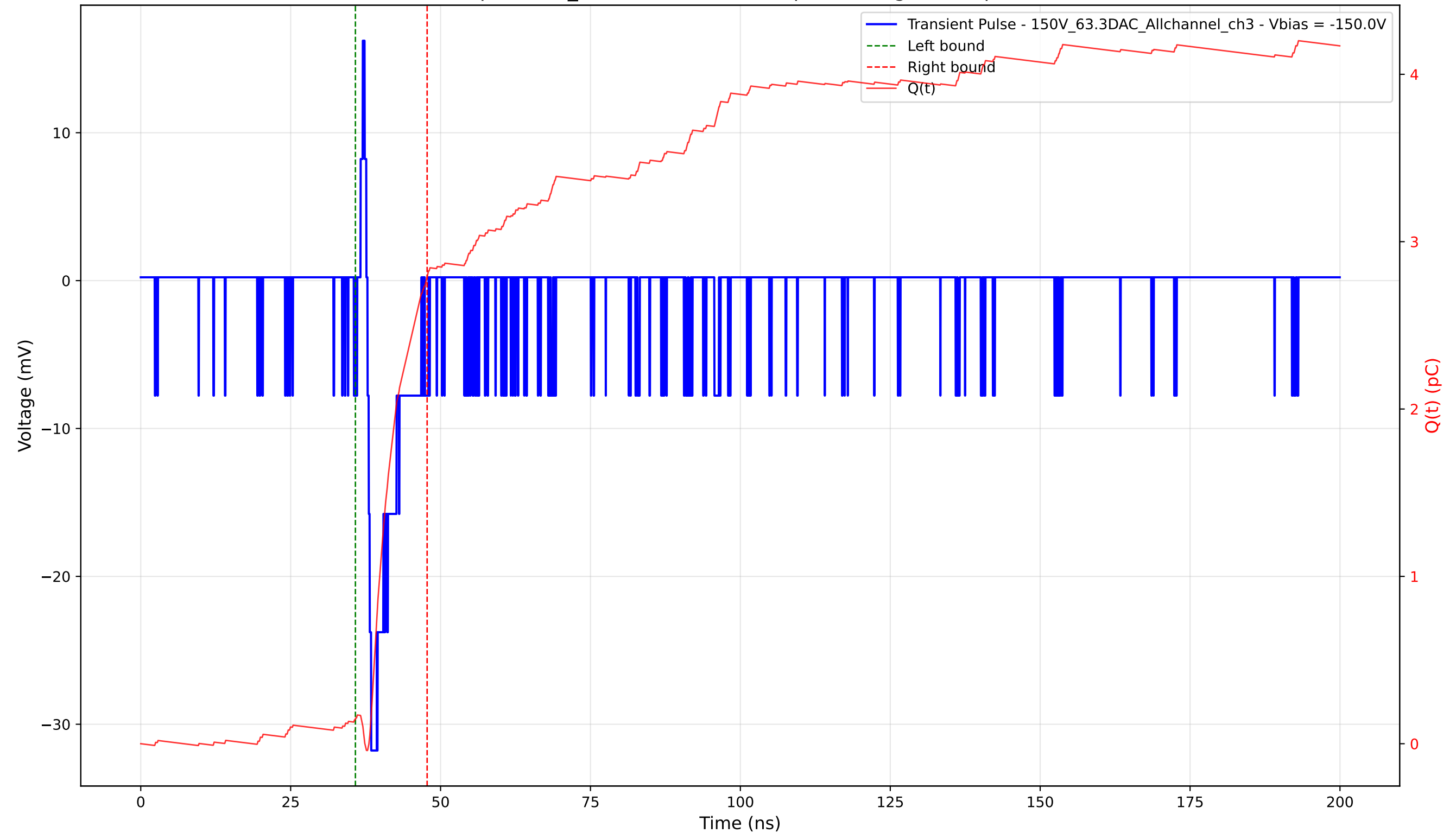
Transient Pulse - Sample: 1cm_42 - Position: 4840.0 \mu\text{m} - Charge: 2.64 pC - Rise Time: 0.62 ns
