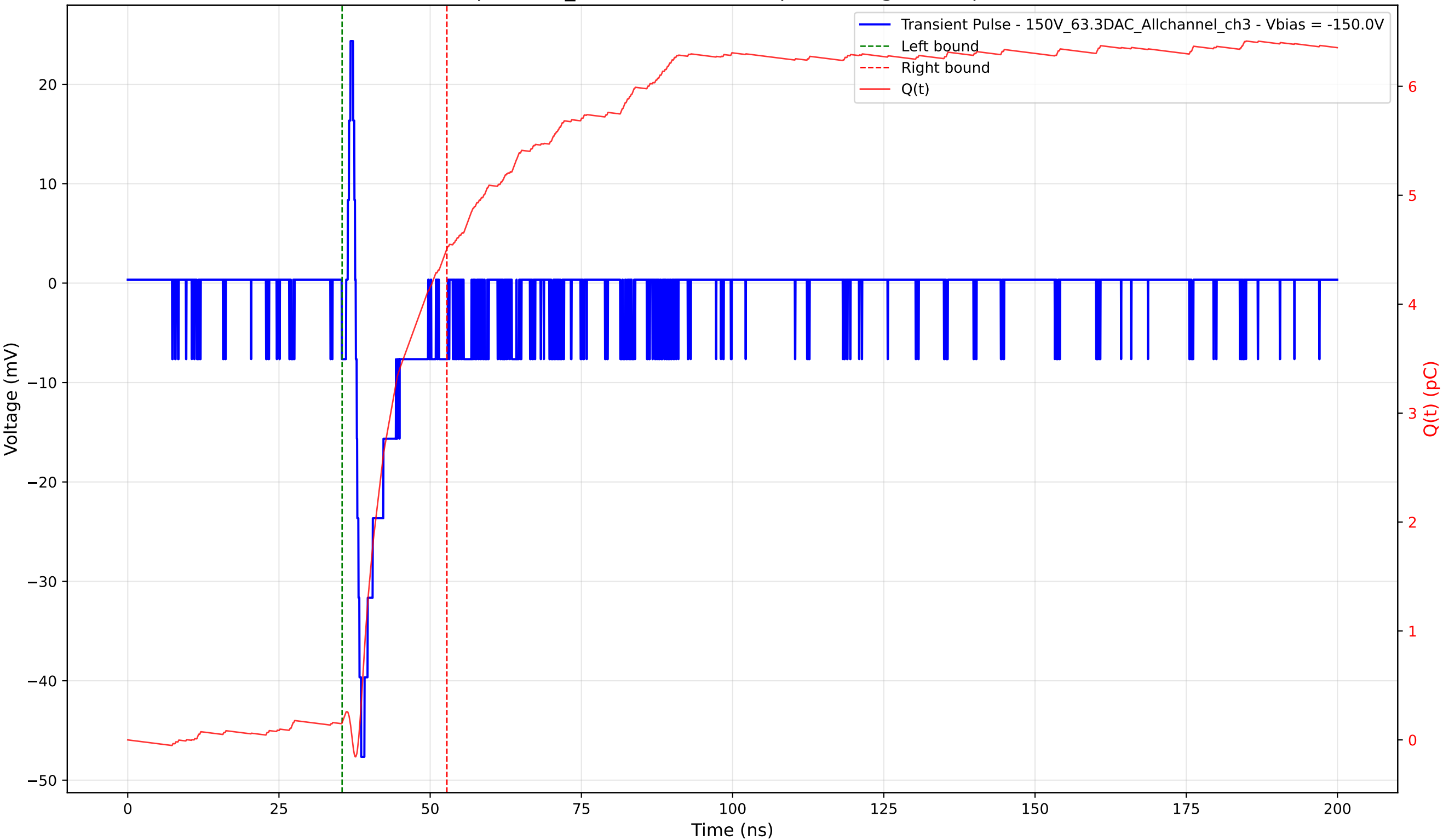
Transient Pulse - Sample: 1cm_42 - Position: 615.0 \mu\text{m} - Charge: 4.35 pC - Rise Time: 0.90 ns
