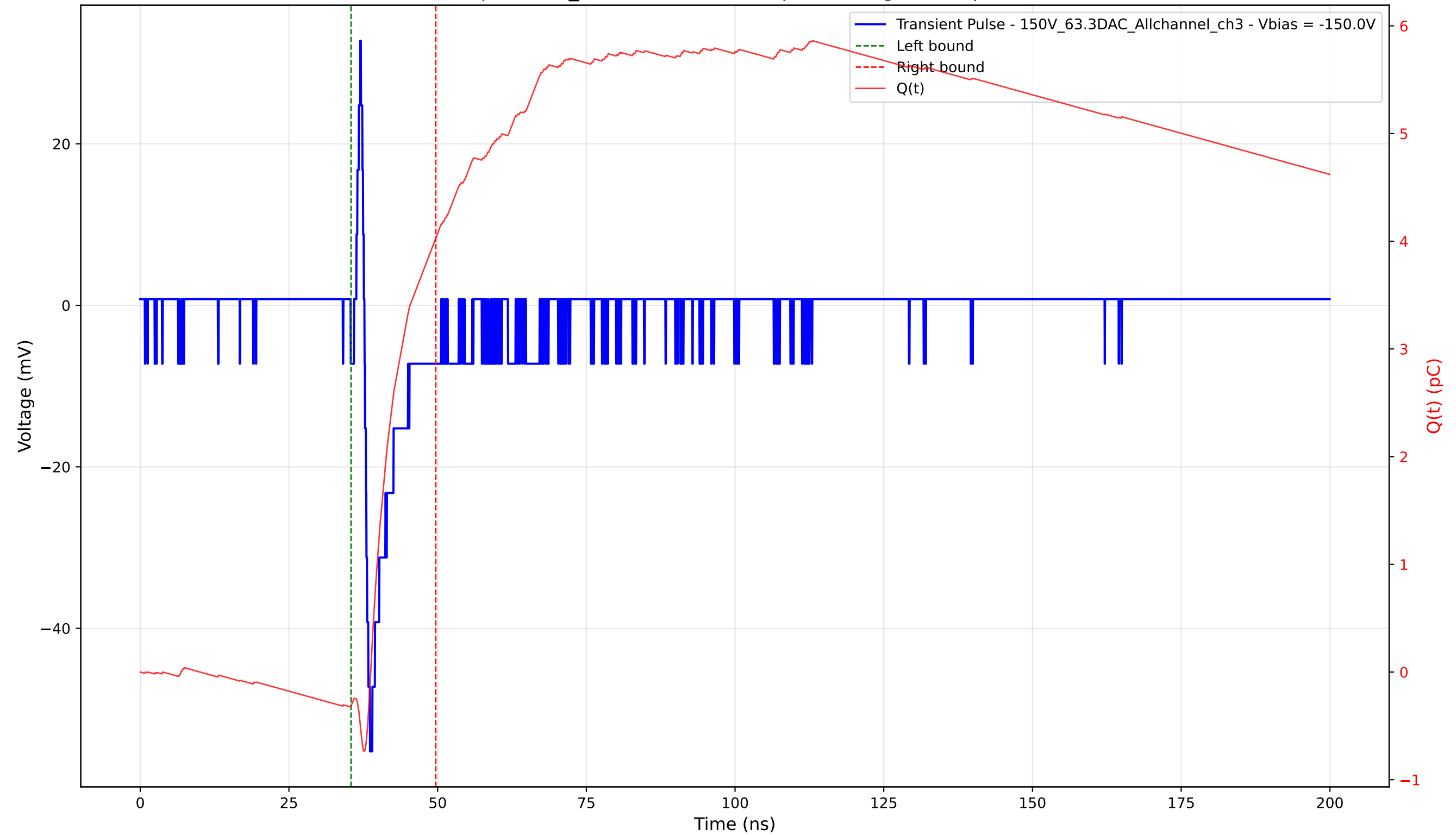
Transient Pulse - Sample: 1cm_42 - Position: 745.0 \mu\text{m} - Charge: 4.35 pC - Rise Time: 0.93 ns
