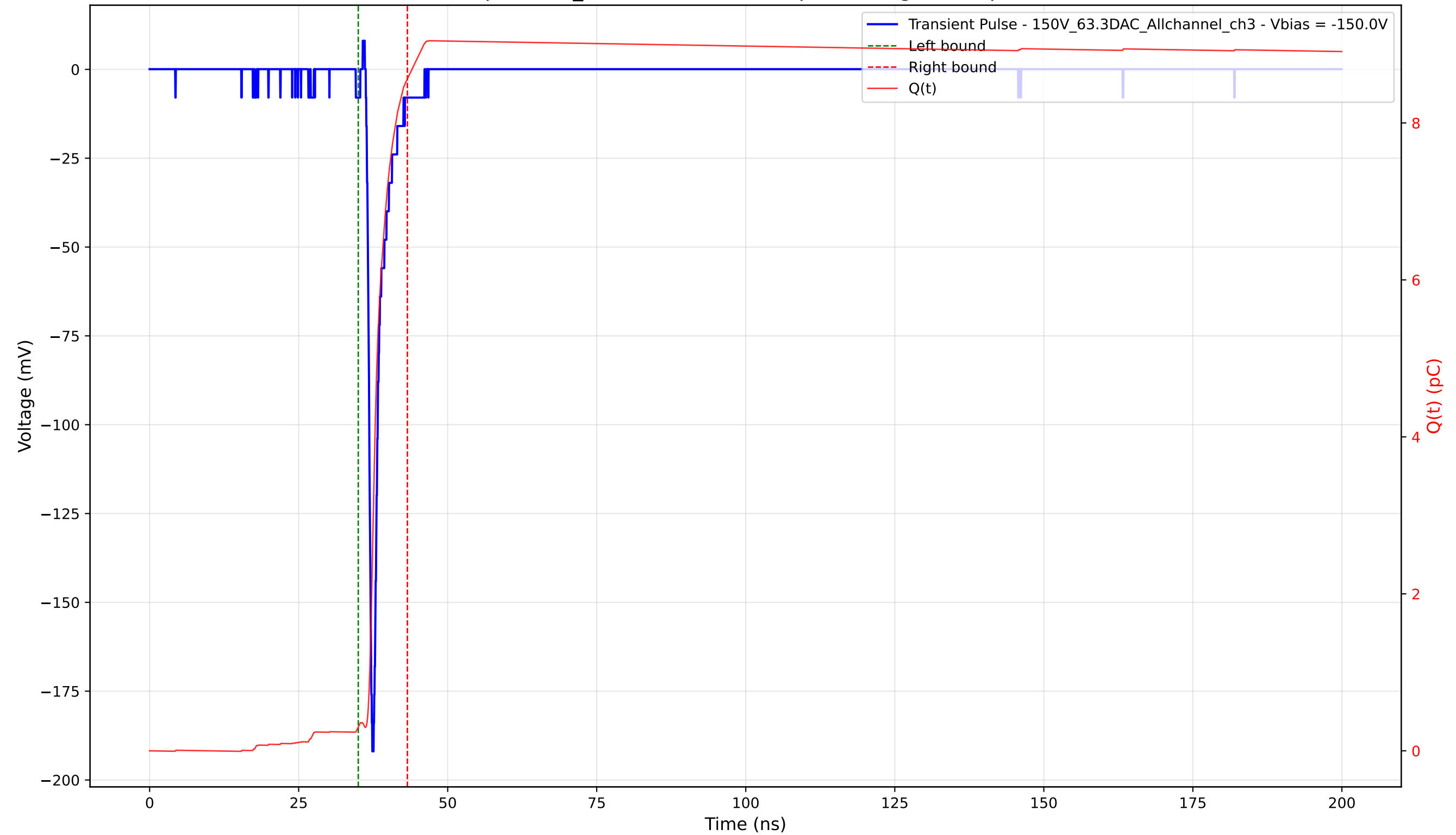
Transient Pulse - Sample: 1cm_42 - Position: 3070.0 \mu\text{m} - Charge: 8.26 pC - Rise Time: 0.78 ns
