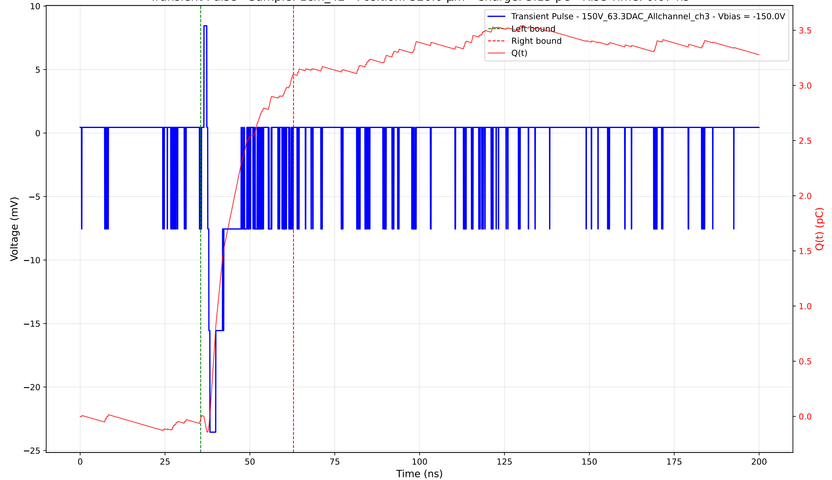
Transient Pulse - Sample: 1cm_42 - Position: 320.0 \mu\text{m} - Charge: 3.13 pC - Rise Time: 0.67 ns
