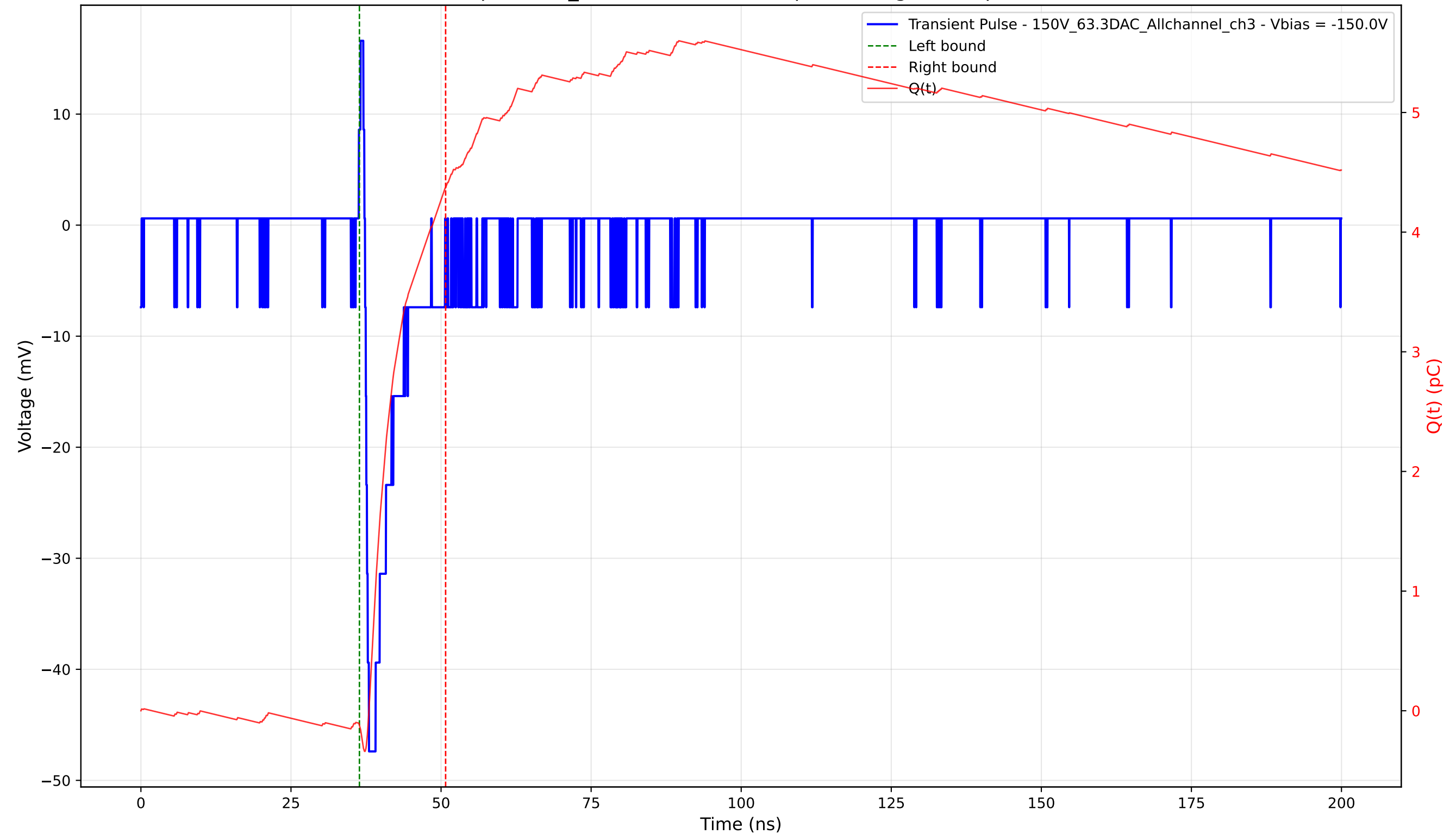
Transient Pulse - Sample: 1cm_42 - Position: 3865.0 \mu\text{m} - Charge: 4.49 pC - Rise Time: 0.66 ns
