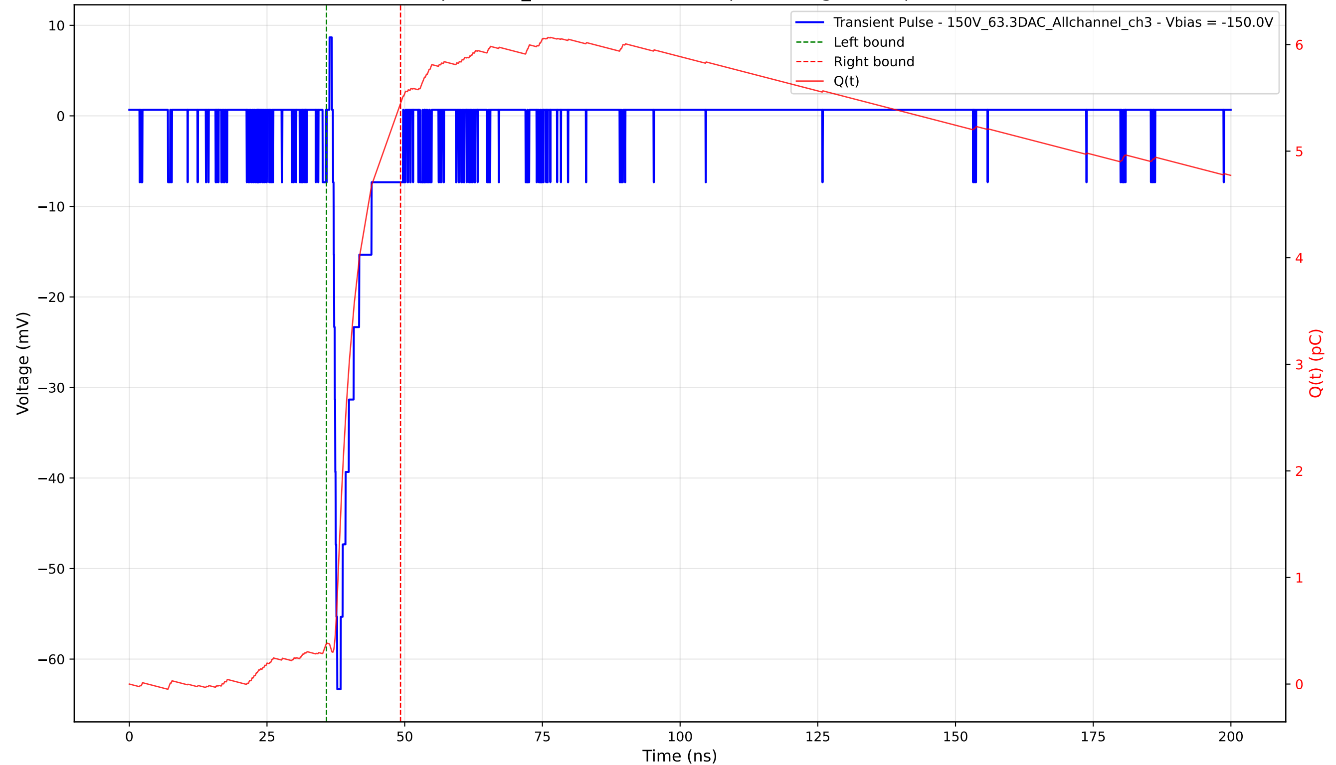
Transient Pulse - Sample: 1cm_42 - Position: 3580.0 \mu\text{m} - Charge: 5.07 pC - Rise Time: 0.77 ns
