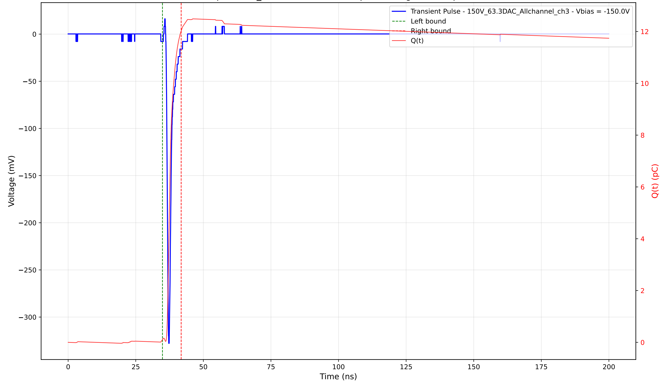
Transient Pulse - Sample: 1cm_42 - Position: 2125.0 \mu\text{m} - Charge: 11.91 pC - Rise Time: 0.71 ns
