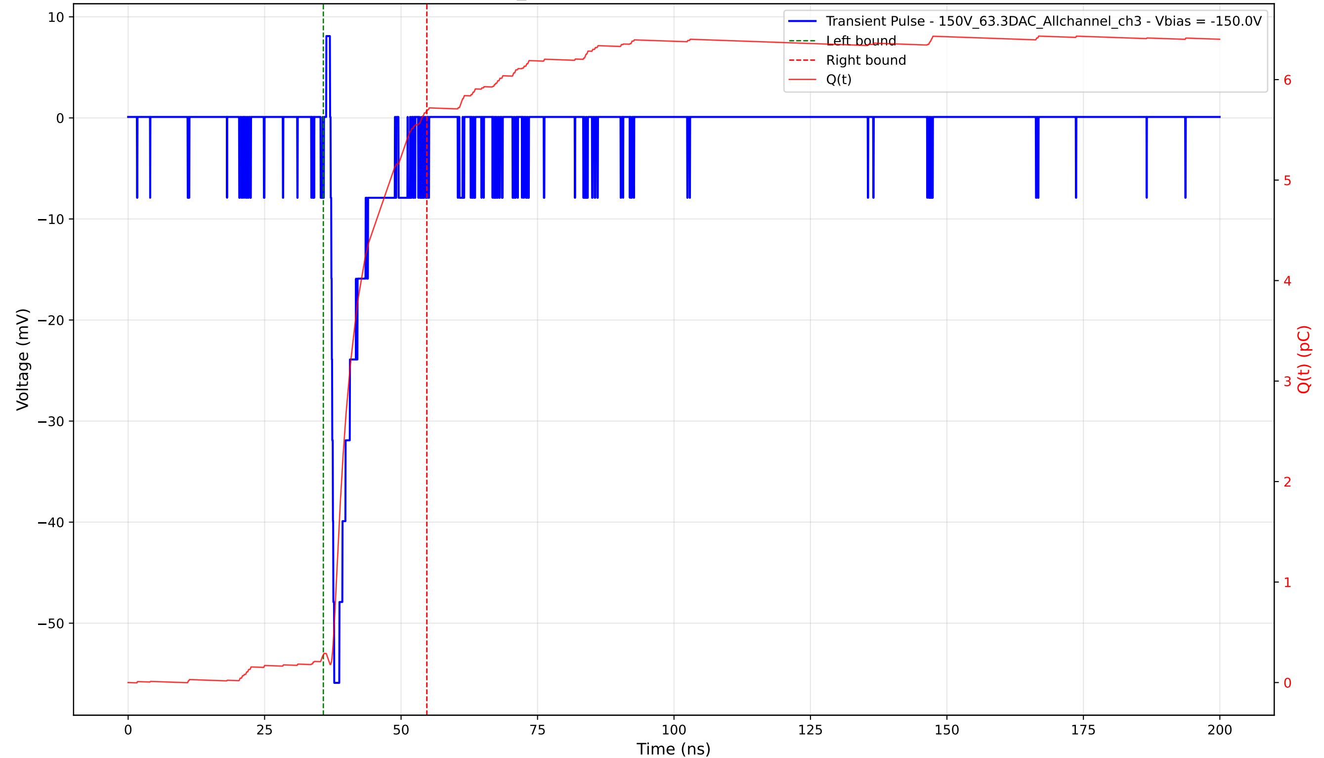
Transient Pulse - Sample: 1cm_42 - Position: 3630.0 \mu\text{m} - Charge: 5.42 pC - Rise Time: 0.65 ns
