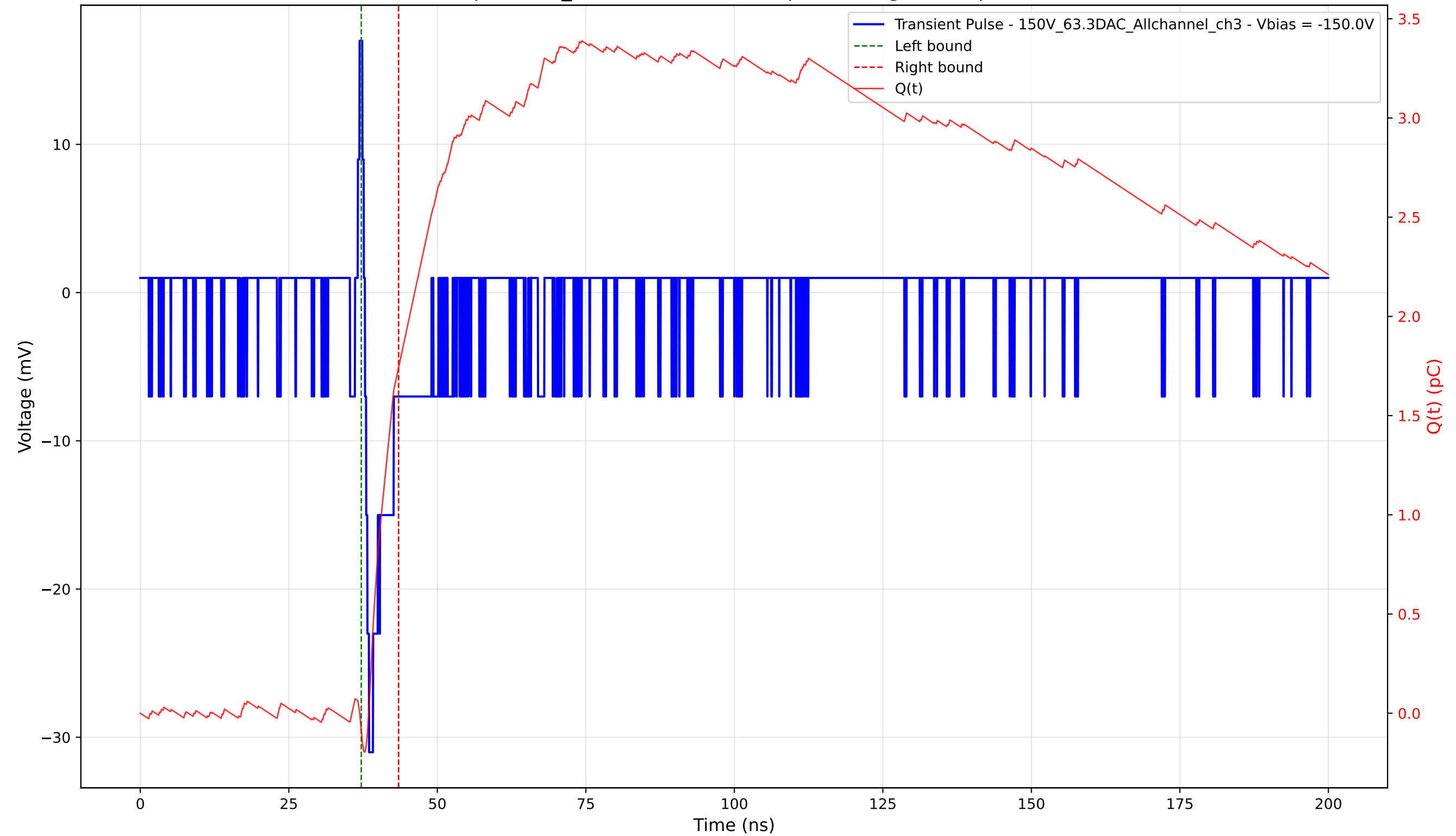
Transient Pulse - Sample: 1cm_42 - Position: 4625.0 \mu\text{m} - Charge: 1.83 pC - Rise Time: 0.71 ns
