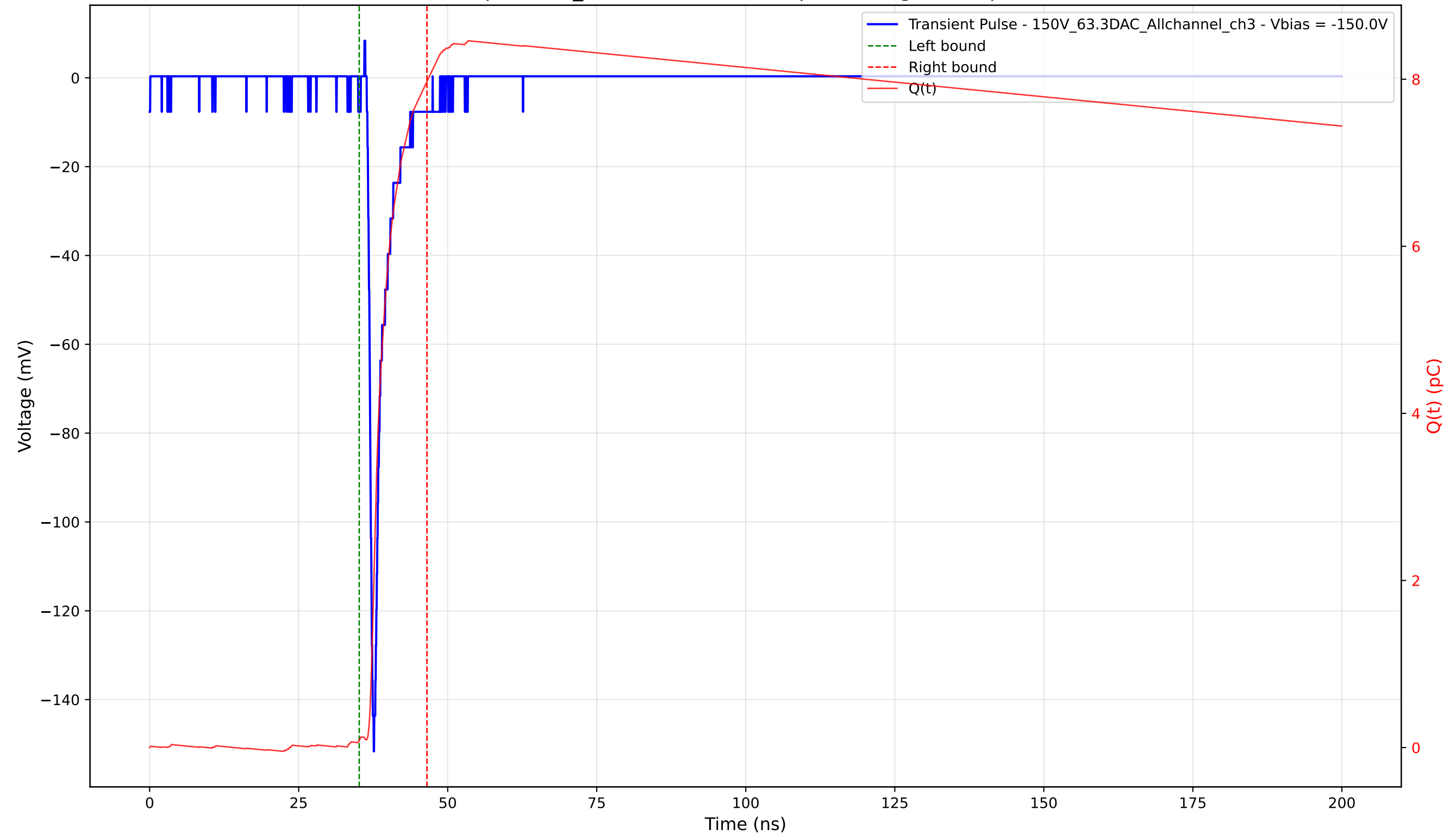
Transient Pulse - Sample: 1cm_42 - Position: 3210.0 \mu\text{m} - Charge: 7.89 pC - Rise Time: 0.88 ns
