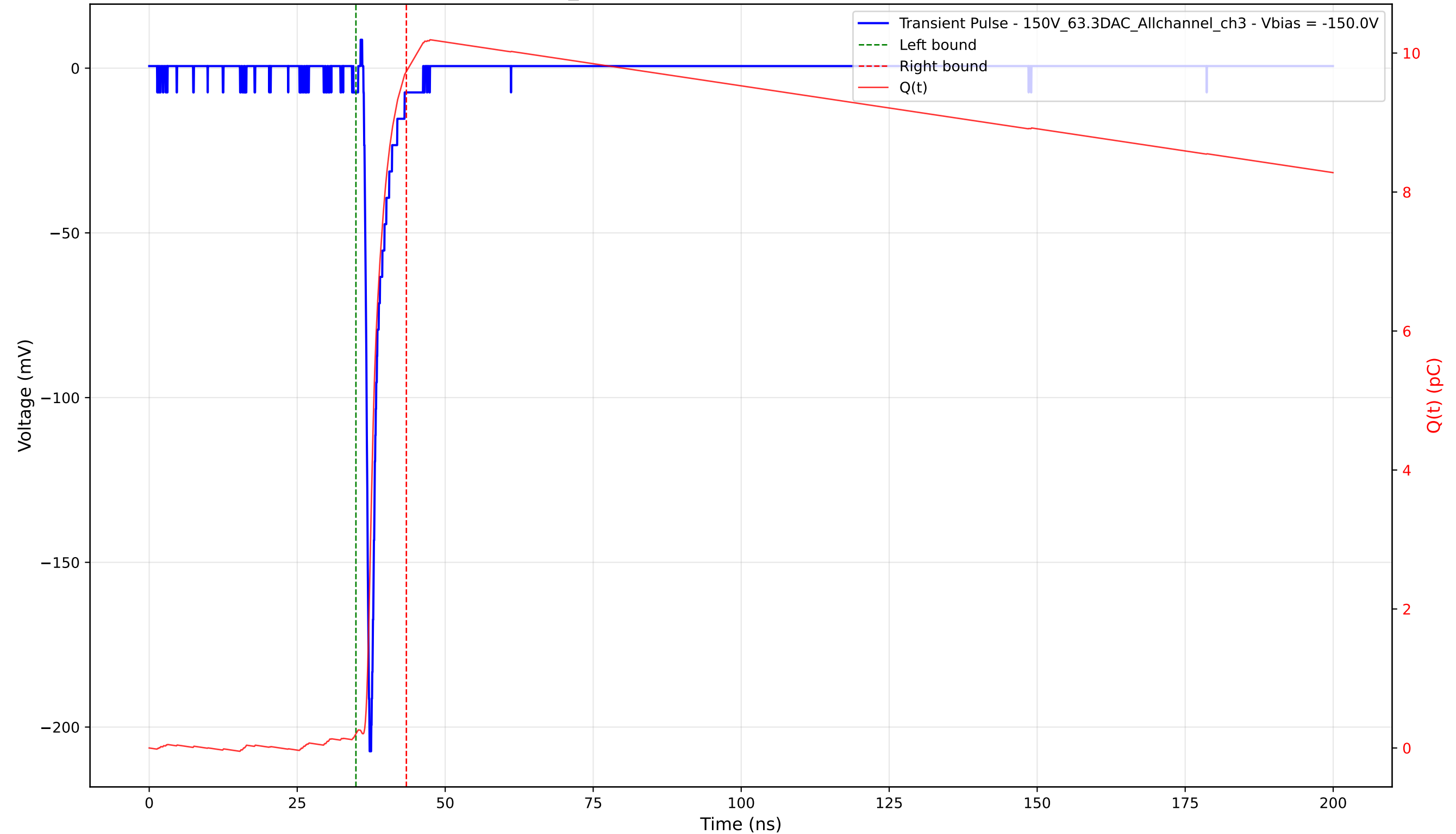
Transient Pulse - Sample: 1cm_42 - Position: 1975.0 \mu\text{m} - Charge: 9.53 pC - Rise Time: 0.81 ns
