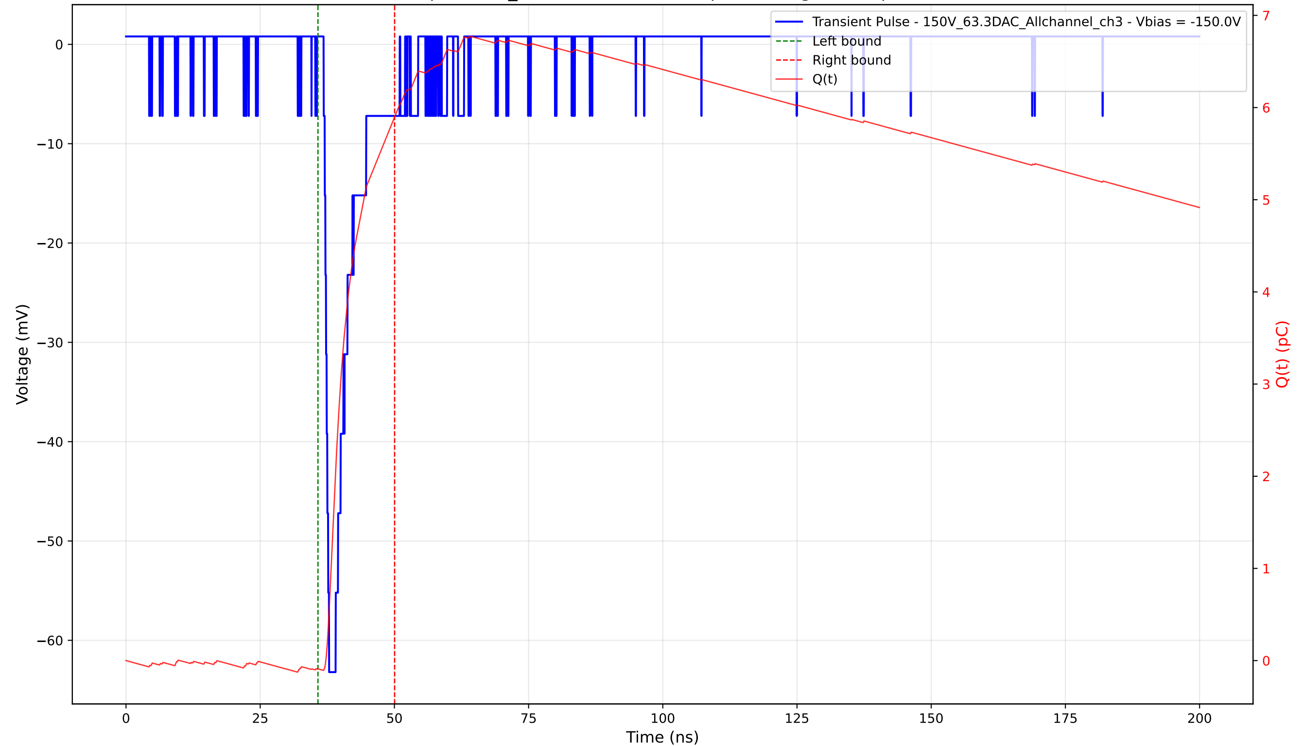
Transient Pulse - Sample: 1cm_42 - Position: 1435.0 \mu\text{m} - Charge: 5.99 pC - Rise Time: 1.01 ns
