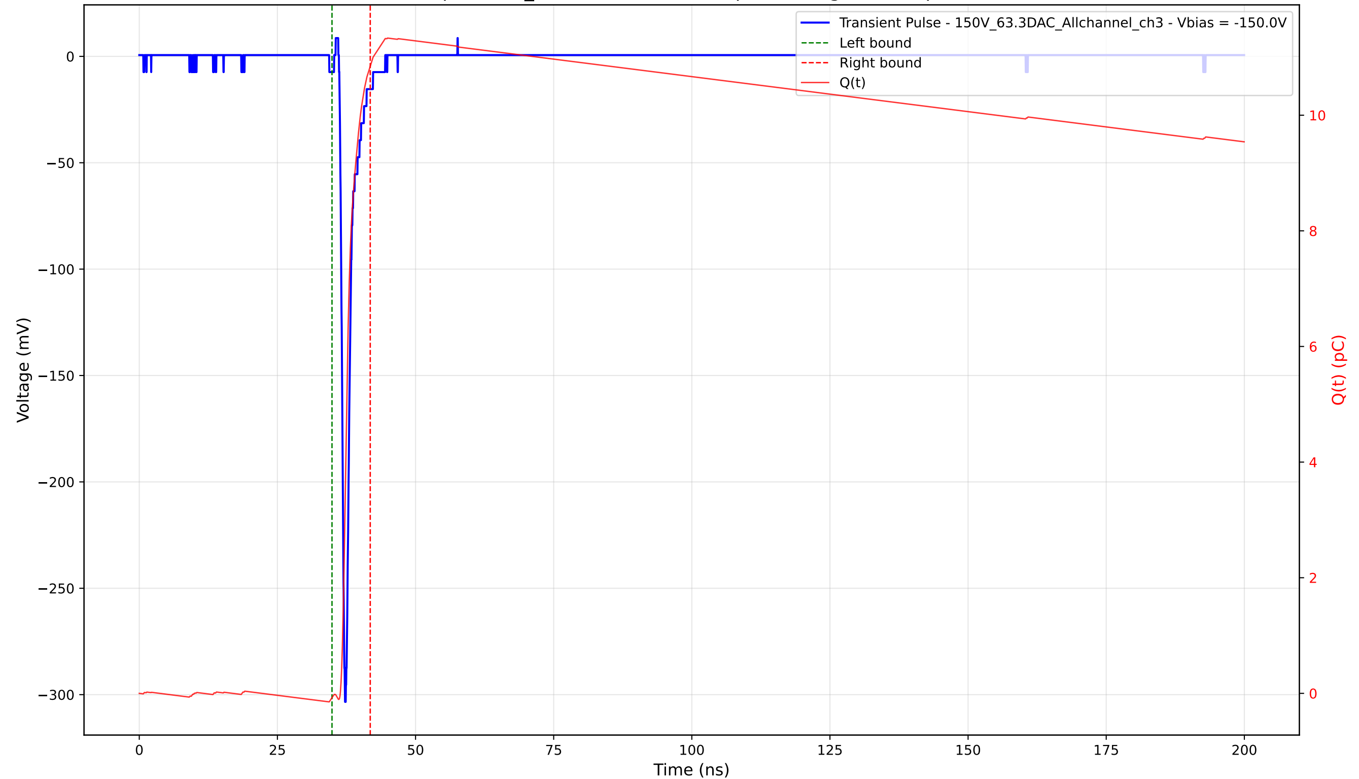
Transient Pulse - Sample: 1cm_42 - Position: 2935.0 \mu\text{m} - Charge: 10.92 pC - Rise Time: 0.73 ns
