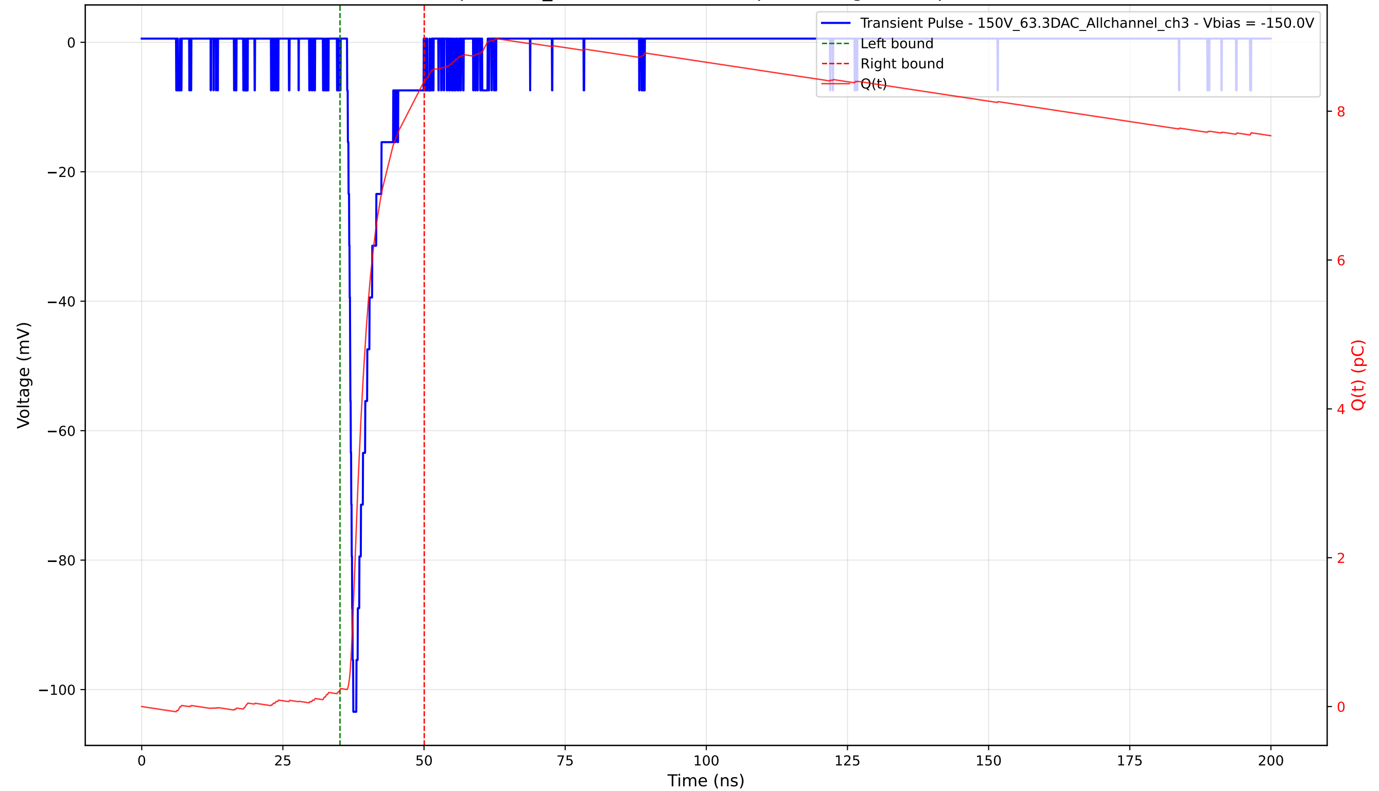
Transient Pulse - Sample: 1cm_42 - Position: 1620.0 \mu\text{m} - Charge: 8.16 pC - Rise Time: 0.87 ns
