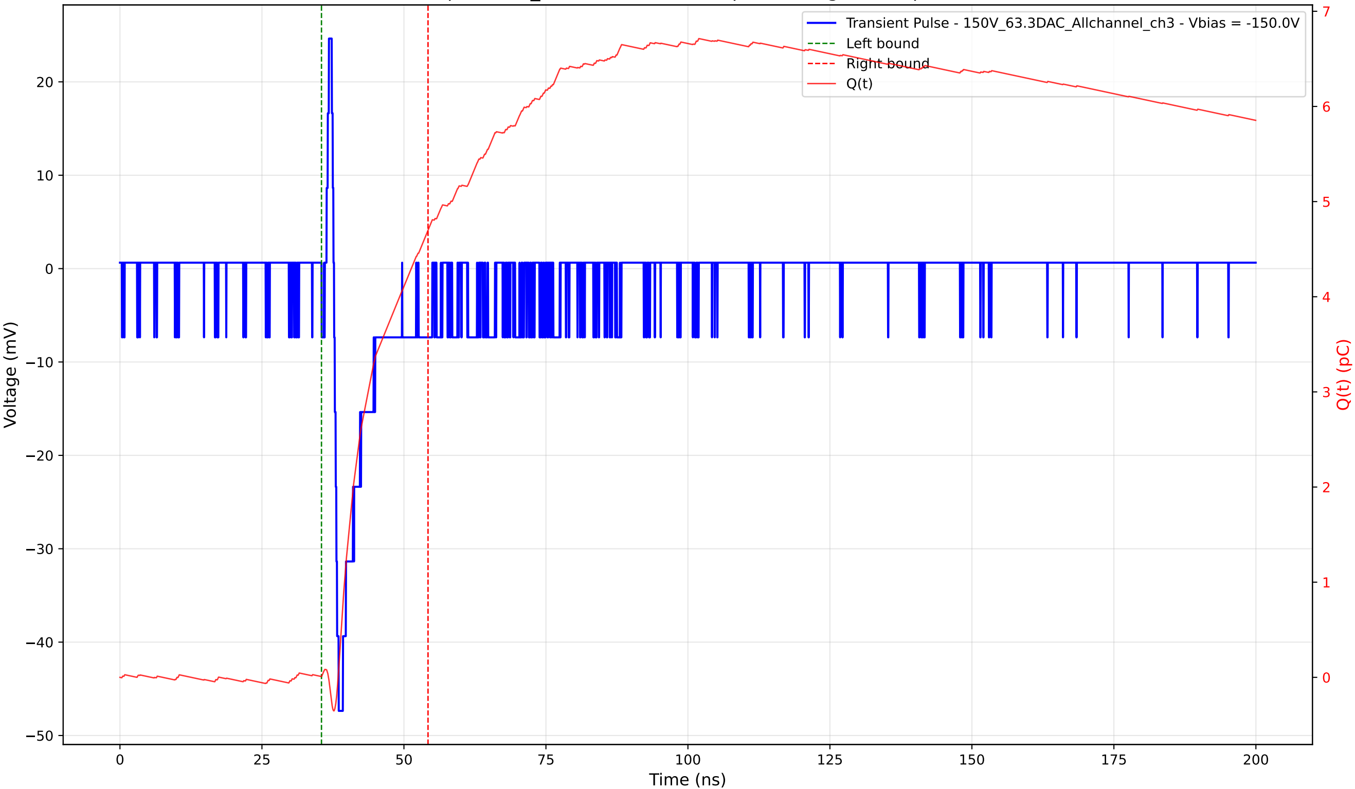
Transient Pulse - Sample: 1cm_42 - Position: 670.0 \mu\text{m} - Charge: 4.69 pC - Rise Time: 0.82 ns
