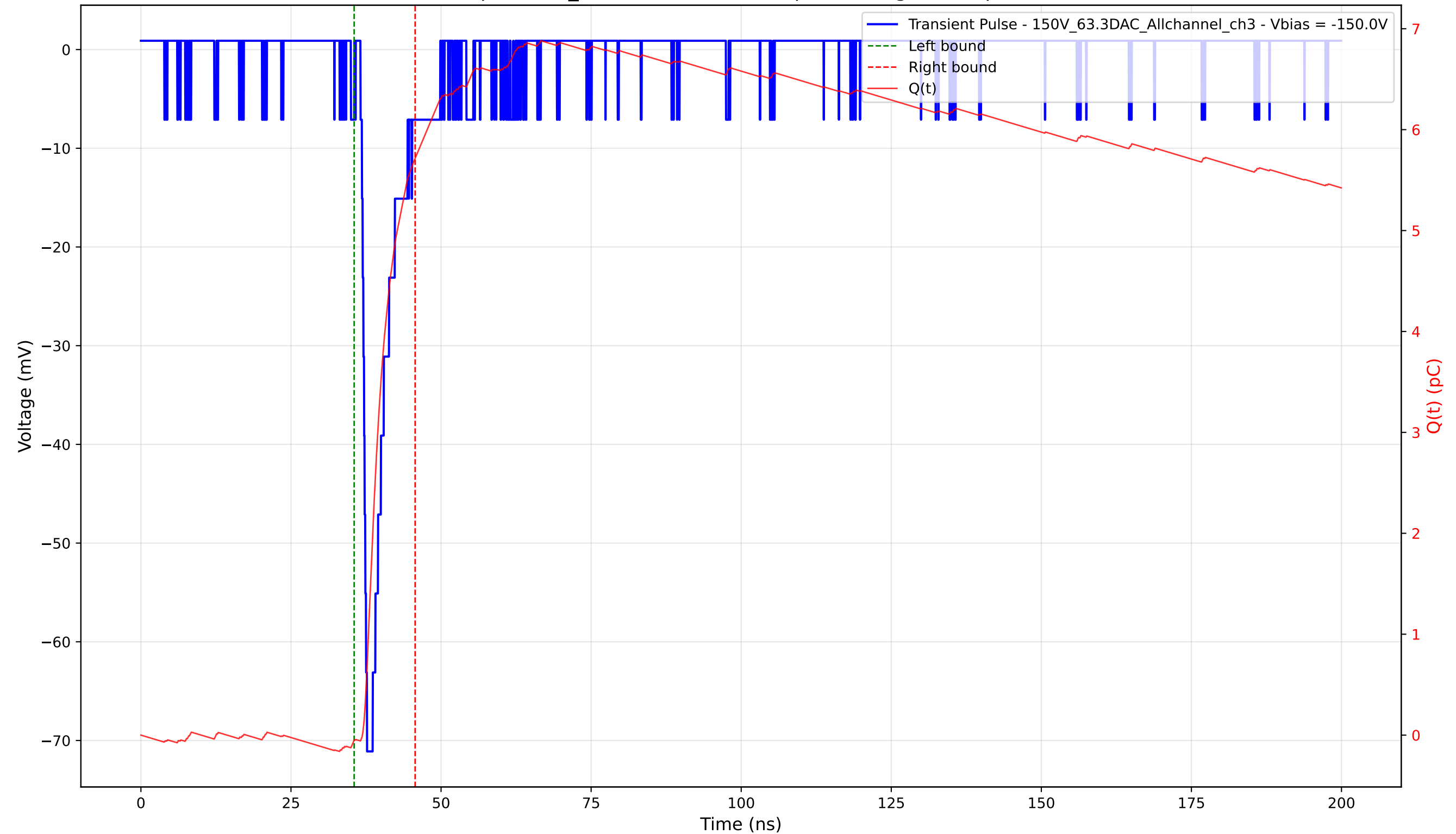
Transient Pulse - Sample: 1cm_42 - Position: 1500.0 \mu\text{m} - Charge: 5.76 pC - Rise Time: 0.88 ns
