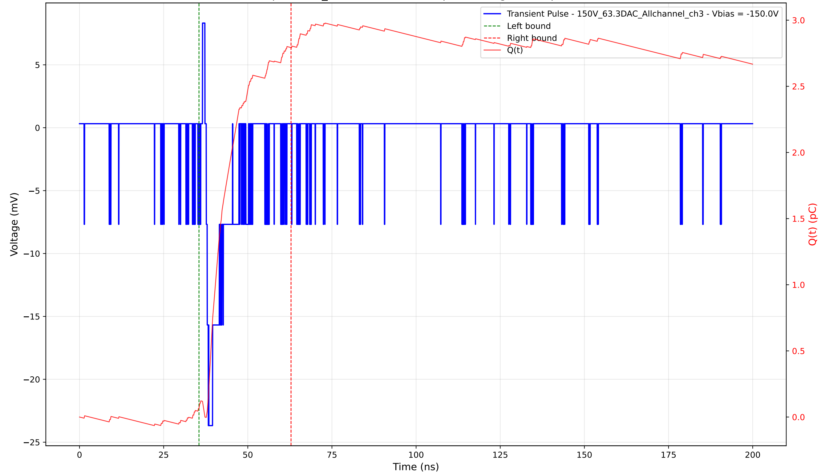
Transient Pulse - Sample: 1cm_42 - Position: 280.0 \mu\text{m} - Charge: 2.72 pC - Rise Time: 0.63 ns
