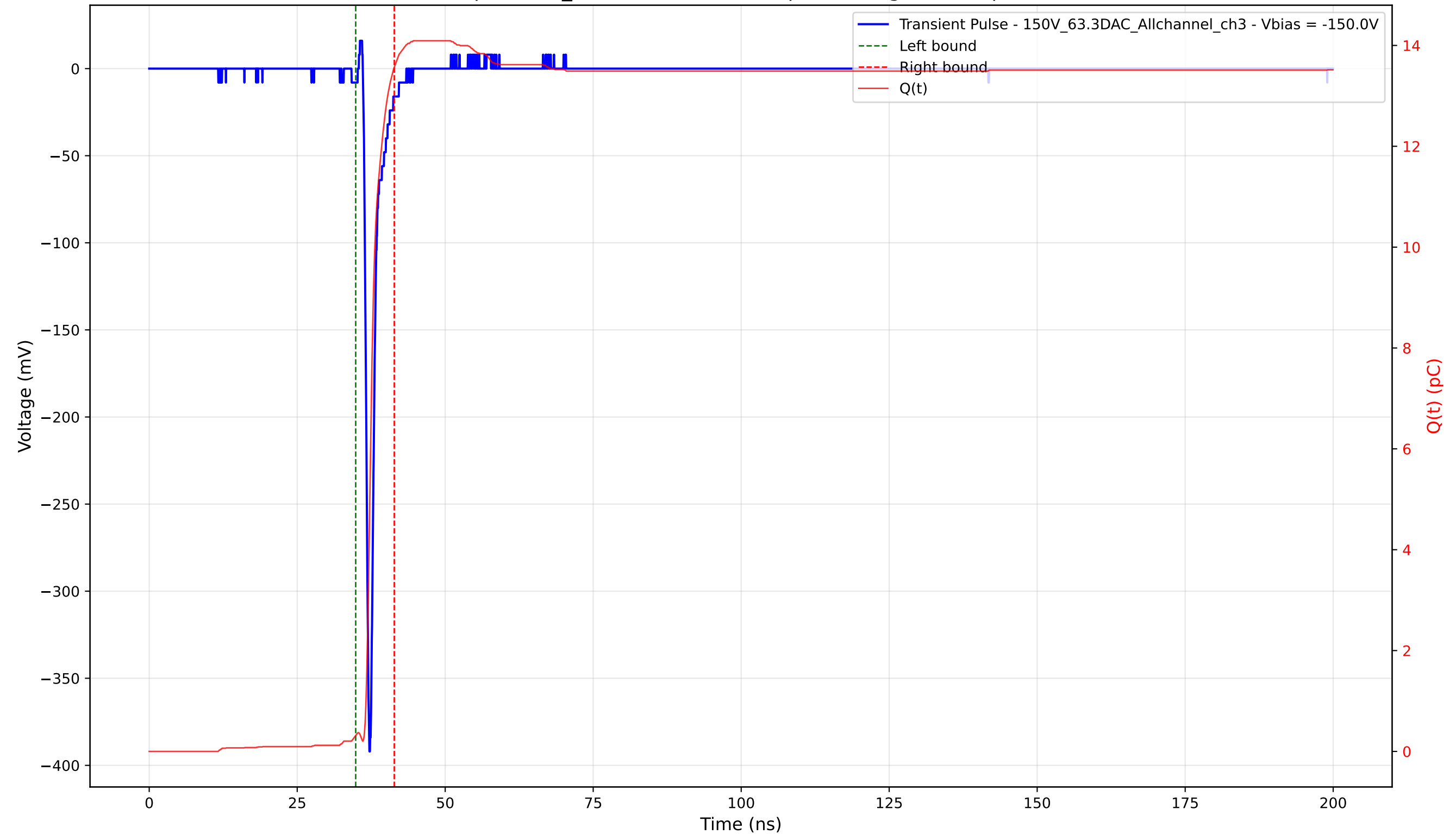
Transient Pulse - Sample: 1cm_42 - Position: 2860.0 \mu\text{m} - Charge: 13.25 pC - Rise Time: 0.73 ns
