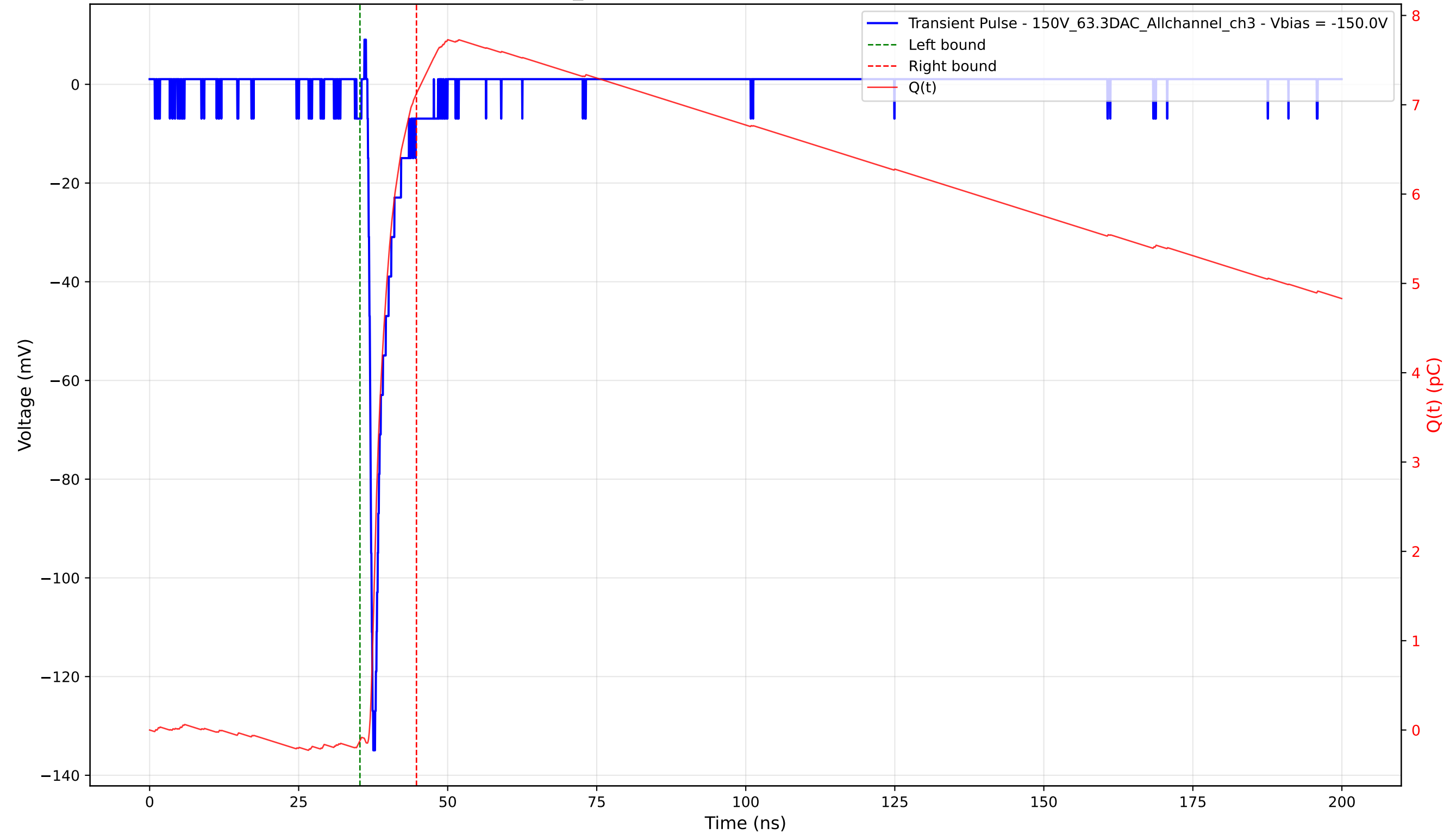
Transient Pulse - Sample: 1cm_42 - Position: 3295.0 \mu\text{m} - Charge: 7.24 pC - Rise Time: 0.77 ns
