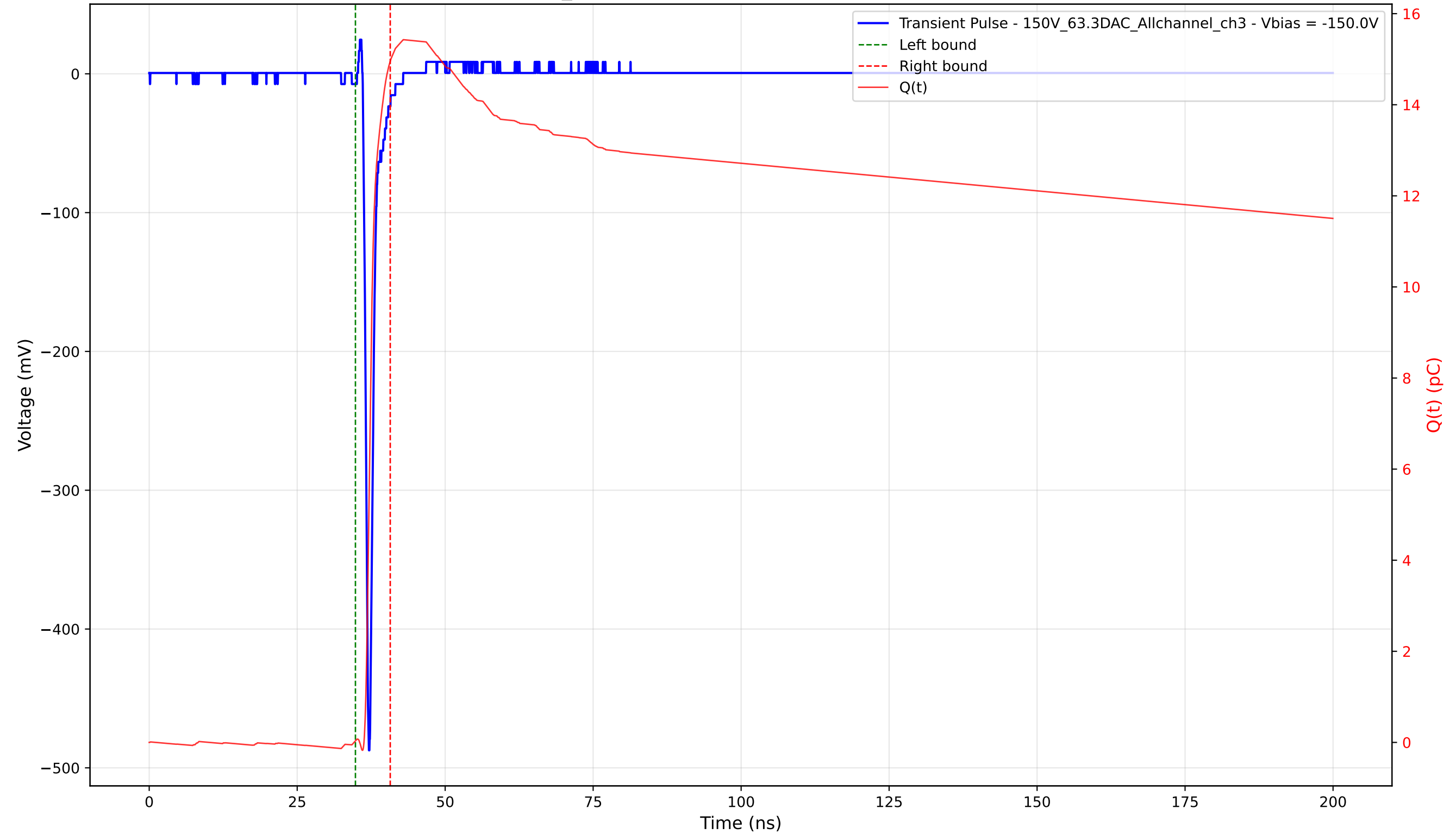
Transient Pulse - Sample: 1cm_42 - Position: 2415.0 \mu\text{m} - Charge: 14.92 pC - Rise Time: 0.71 ns
