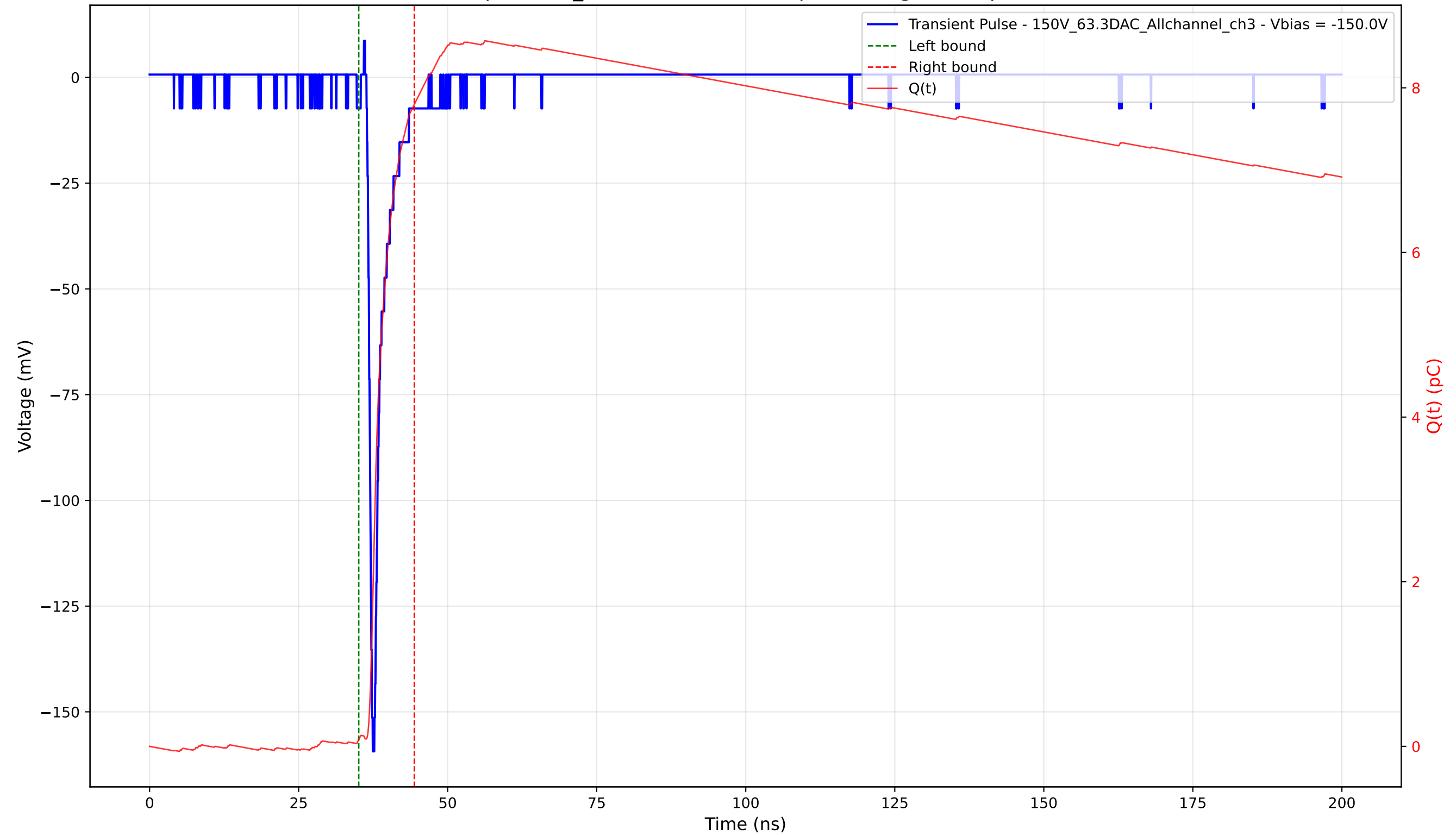
Transient Pulse - Sample: 1cm_42 - Position: 3160.0 \mu\text{m} - Charge: 7.72 pC - Rise Time: 0.80 ns
