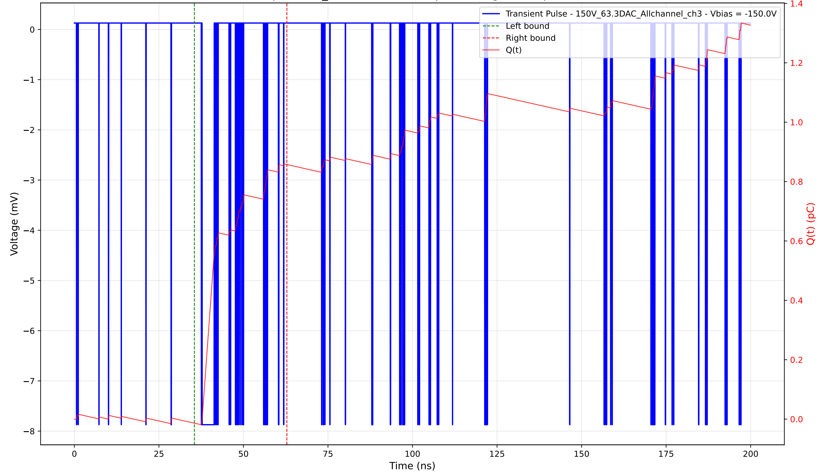
Transient Pulse - Sample: 1cm_42 - Position: 60.0 \mu\text{m} - Charge: 0.87 pC - Rise Time: 0.04 ns
