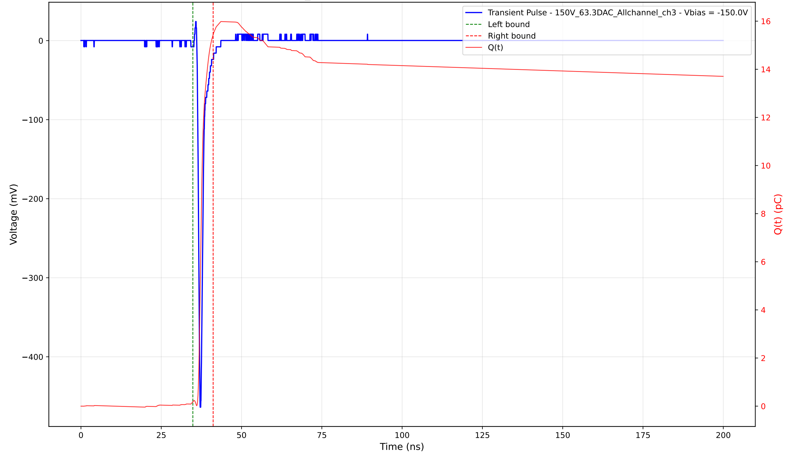
Transient Pulse - Sample: 1cm_42 - Position: 2275.0 \mu\text{m} - Charge: 15.26 pC - Rise Time: 0.73 ns
