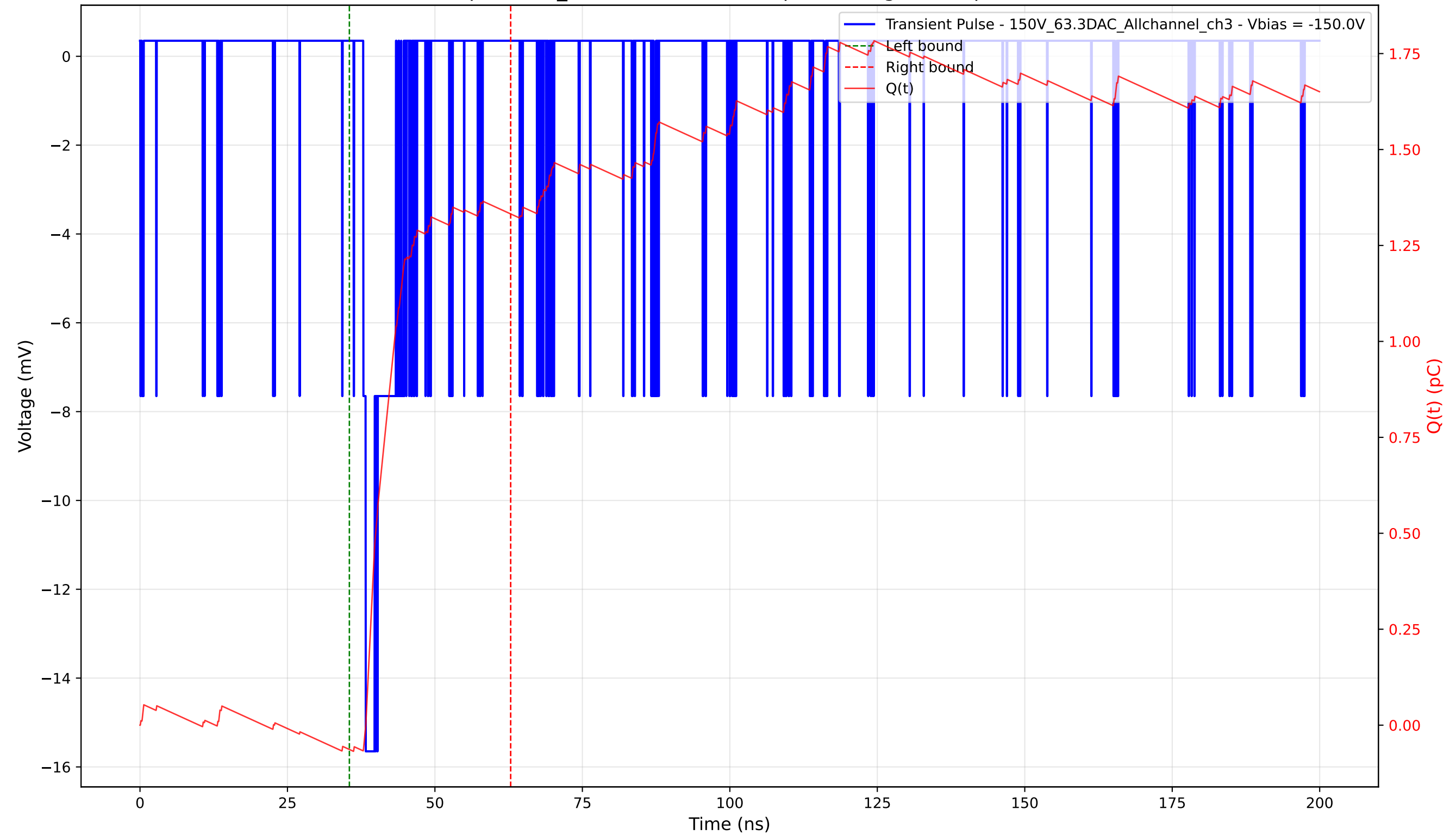
Transient Pulse - Sample: 1cm_42 - Position: 5045.0 \mu\text{m} - Charge: 1.40 pC - Rise Time: 0.43 ns
