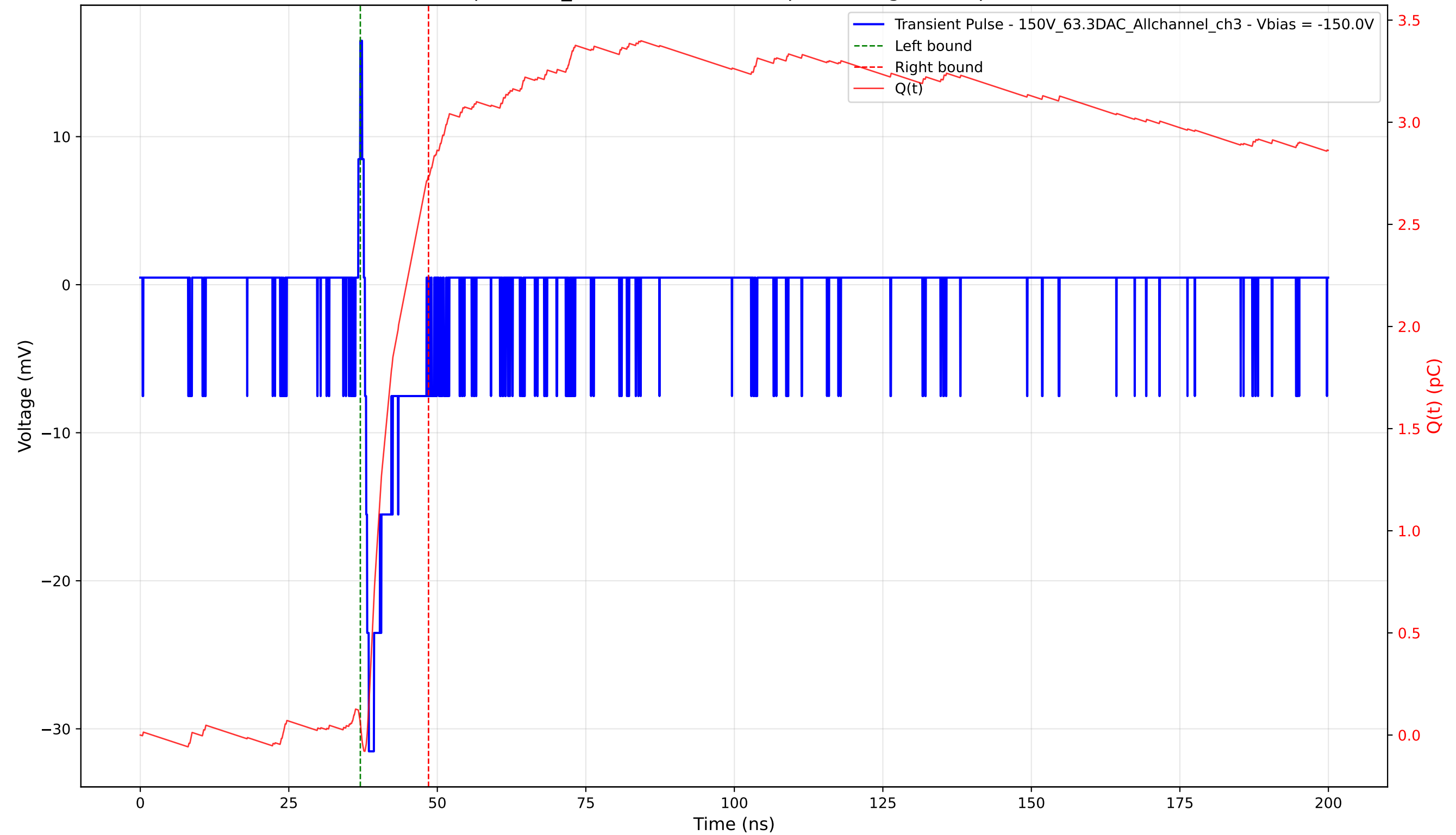
Transient Pulse - Sample: 1cm_42 - Position: 4865.0 \mu\text{m} - Charge: 2.67 pC - Rise Time: 0.66 ns
