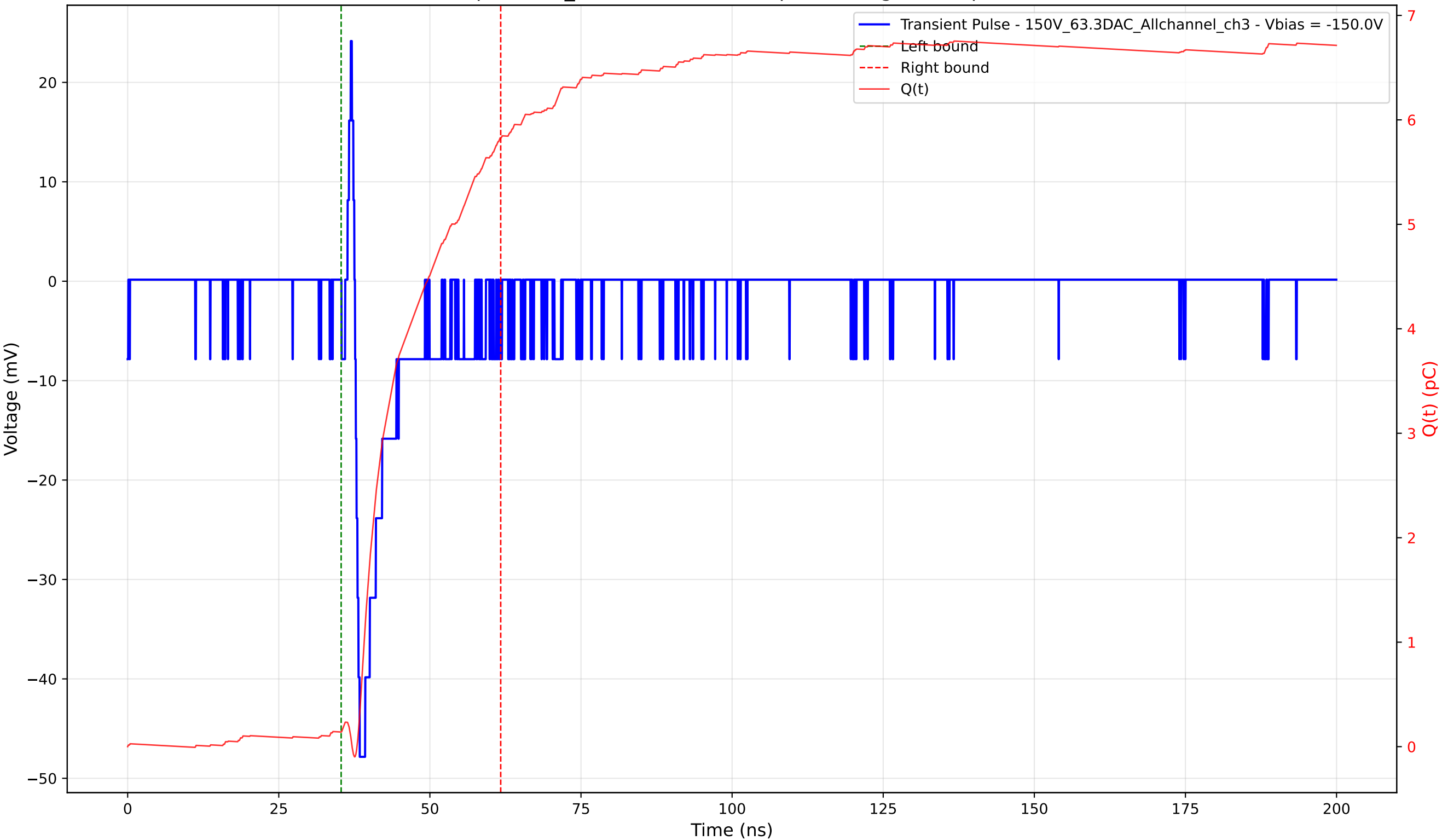
Transient Pulse - Sample: 1cm_42 - Position: 945.0 \mu\text{m} - Charge: 5.69 pC - Rise Time: 0.78 ns
