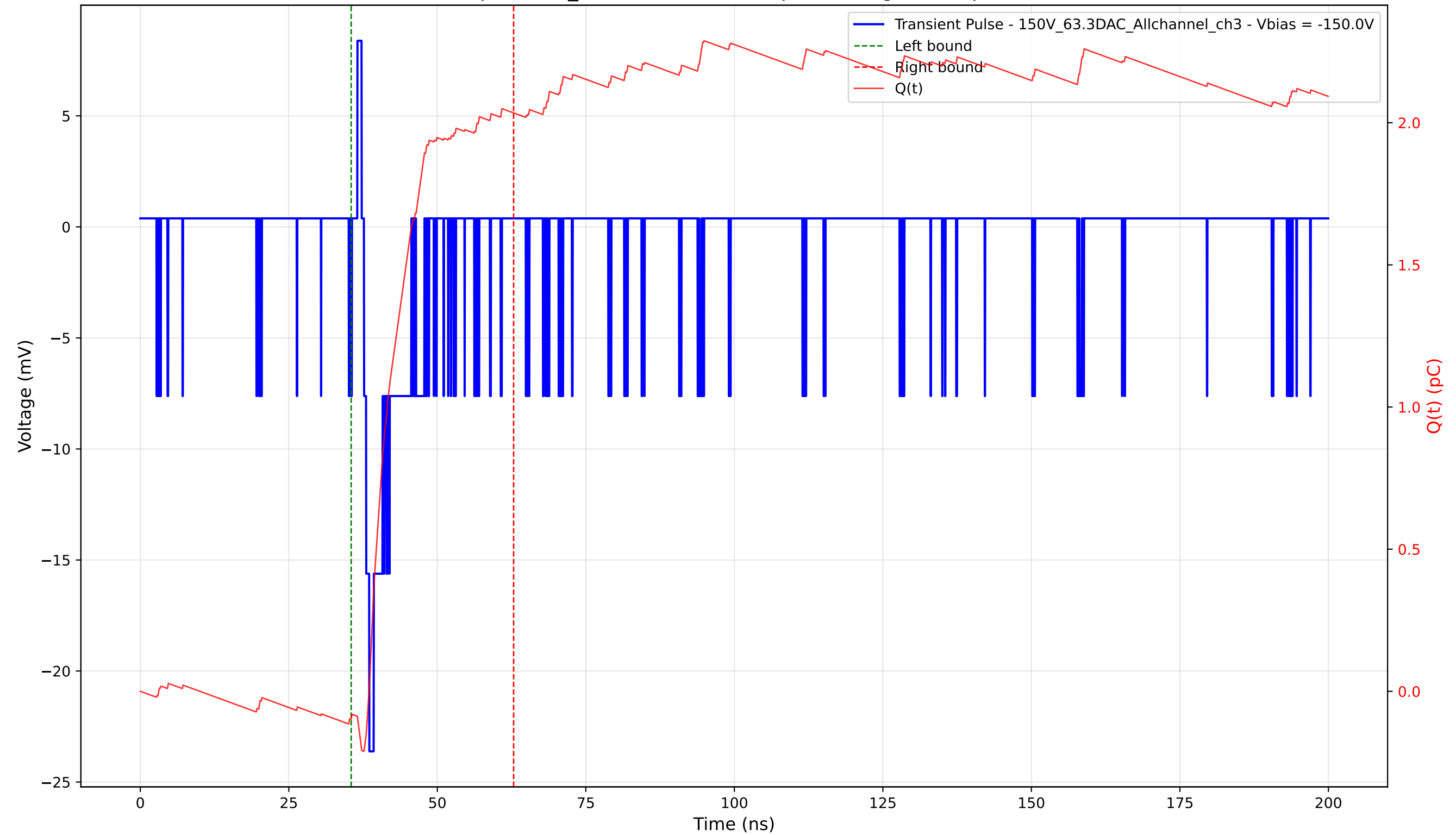
Transient Pulse - Sample: 1cm_42 - Position: 230.0 \mu\text{m} - Charge: 2.13 pC - Rise Time: 0.91 ns
