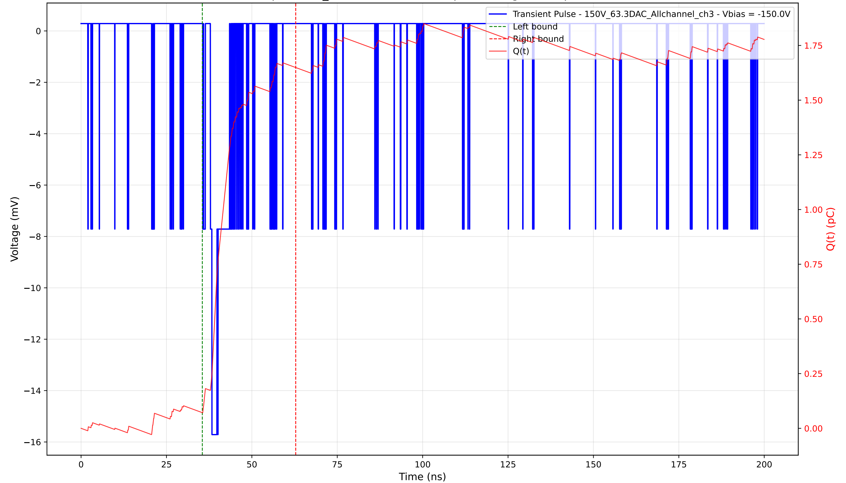
Transient Pulse - Sample: 1cm_42 - Position: 5040.0 \mu\text{m} - Charge: 1.58 pC - Rise Time: 0.47 ns
