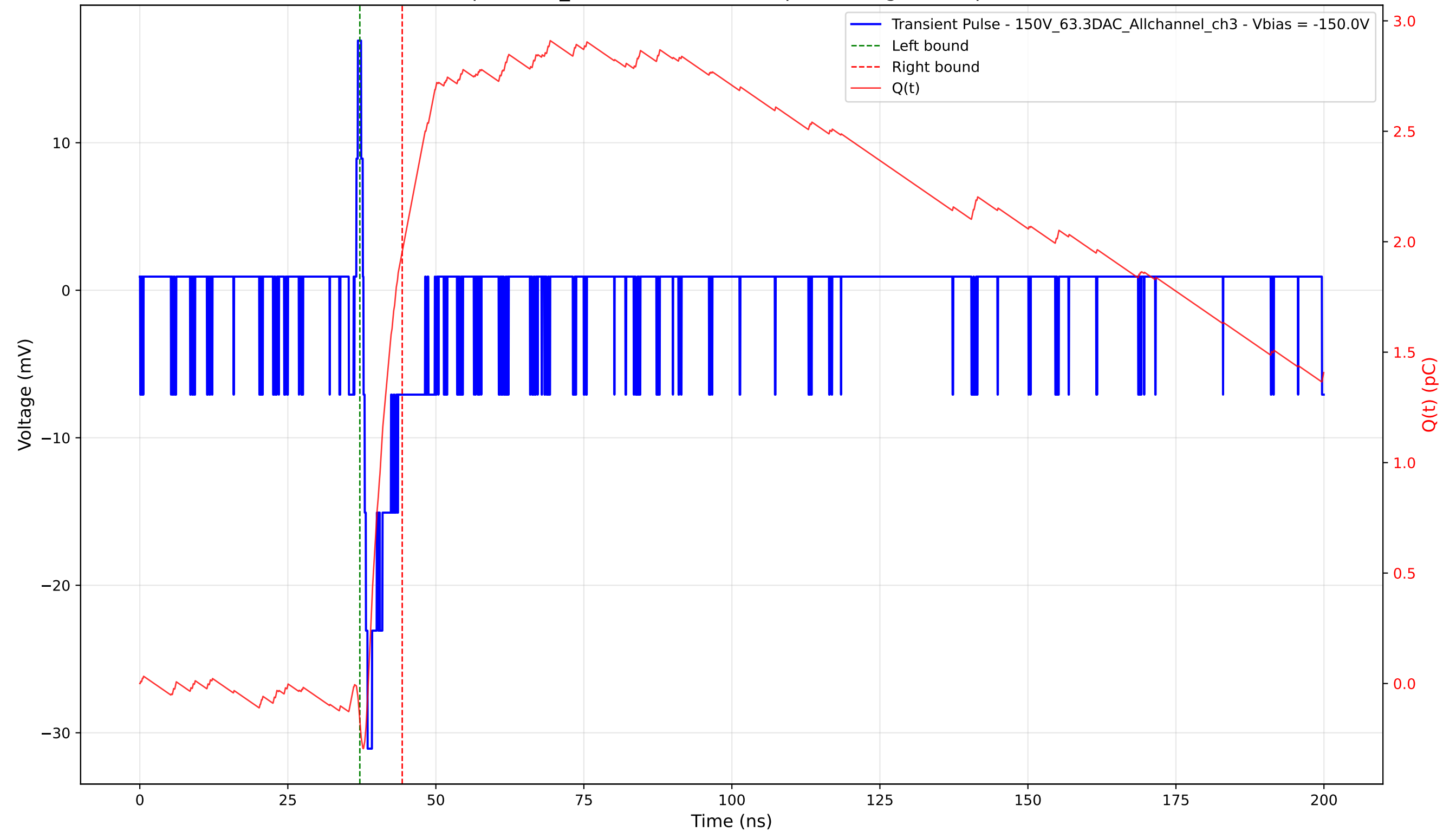
Transient Pulse - Sample: 1cm_42 - Position: 4620.0 \mu\text{m} - Charge: 2.12 pC - Rise Time: 0.71 ns
