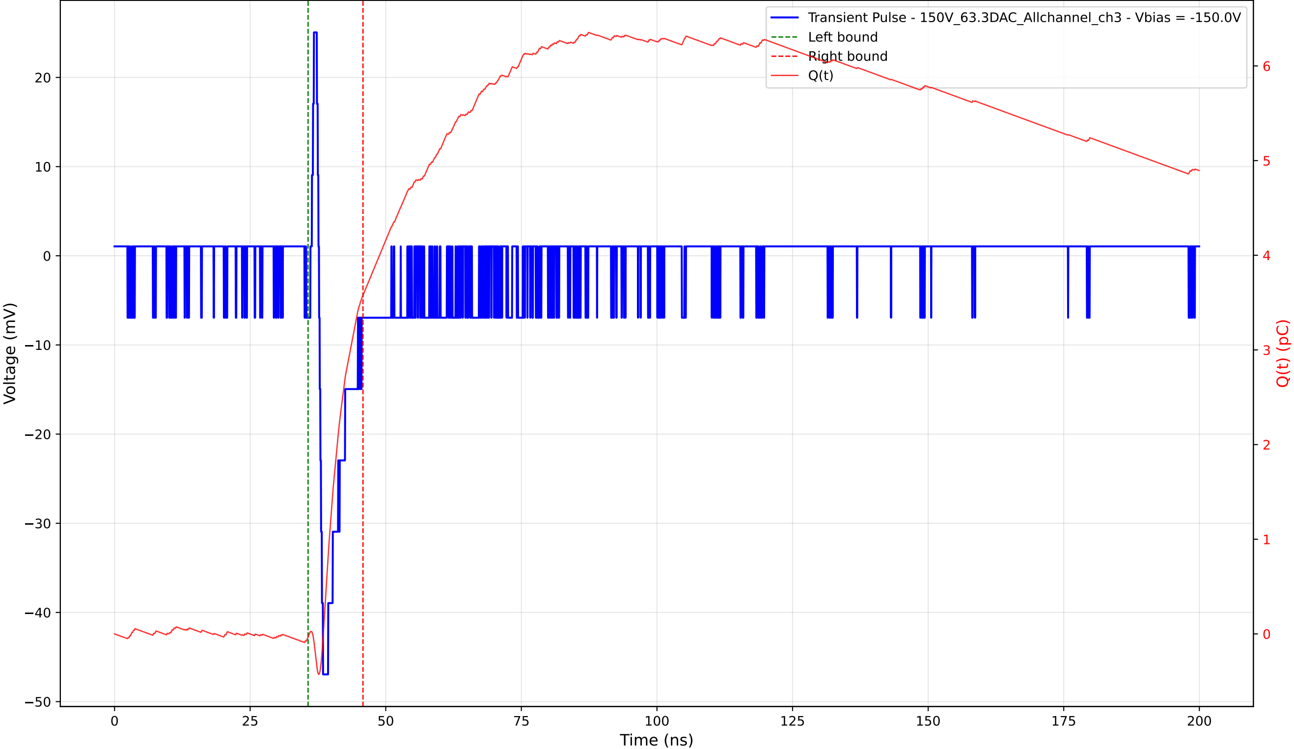
Transient Pulse - Sample: 1cm_42 - Position: 705.0 \mu\text{m} - Charge: 3.61 pC - Rise Time: 0.74 ns
