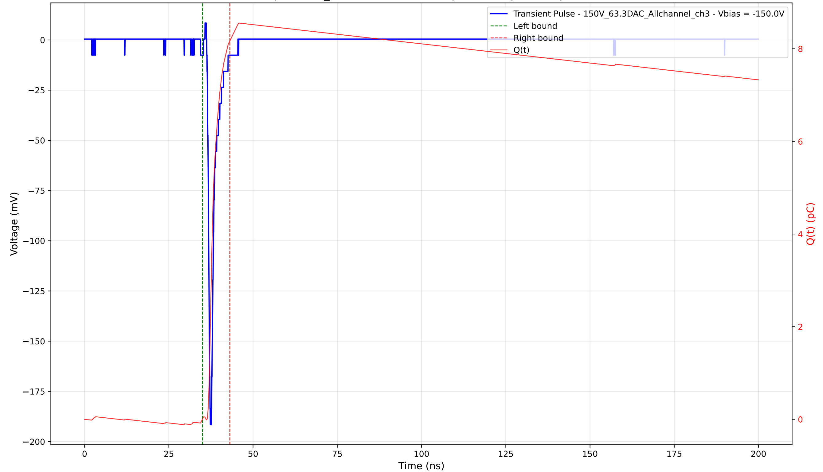
Transient Pulse - Sample: 1cm_42 - Position: 3060.0 \mu\text{m} - Charge: 8.16 pC - Rise Time: 0.77 ns
