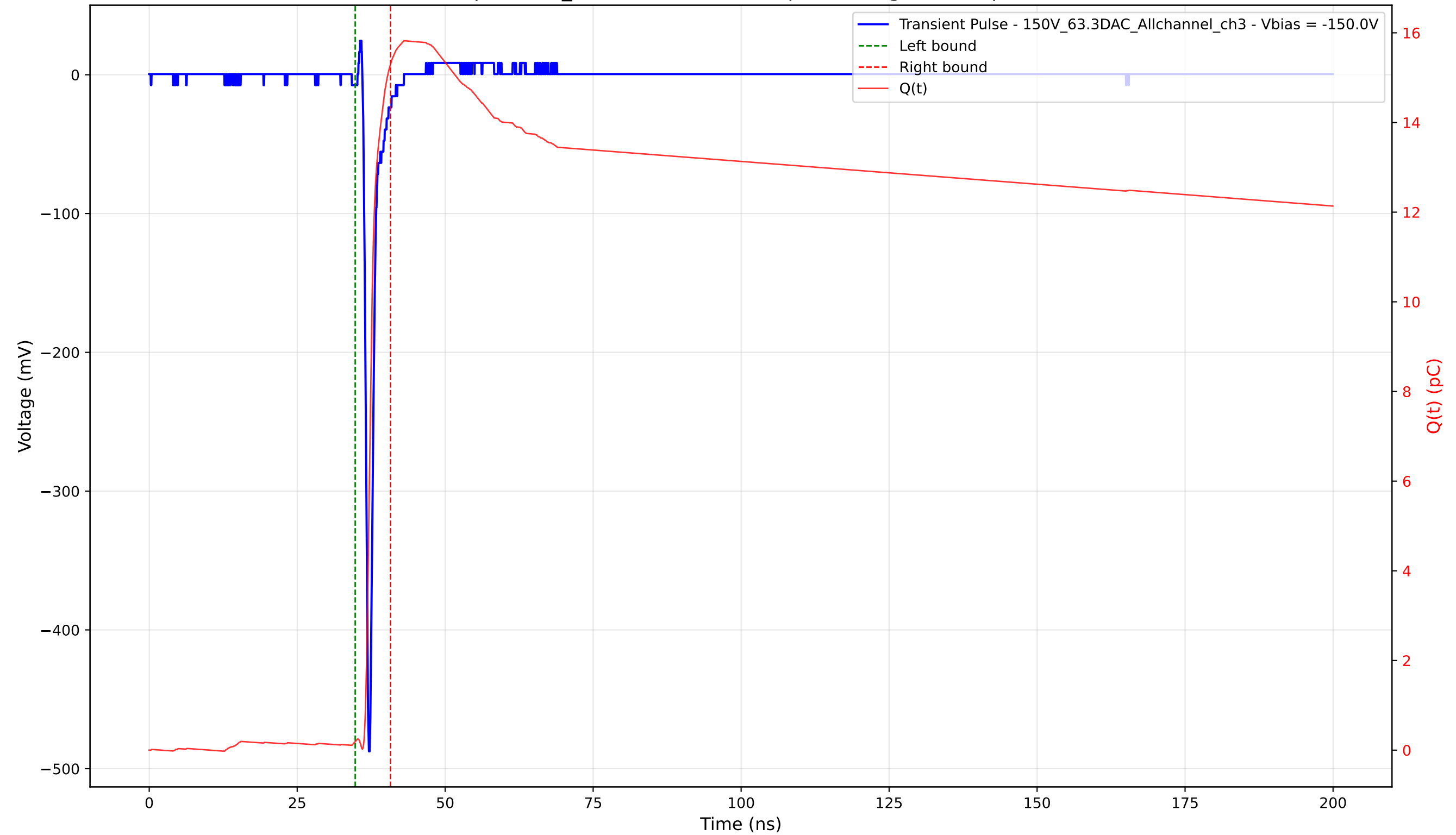
Transient Pulse - Sample: 1cm_42 - Position: 2635.0 \mu\text{m} - Charge: 15.11 pC - Rise Time: 0.71 ns
