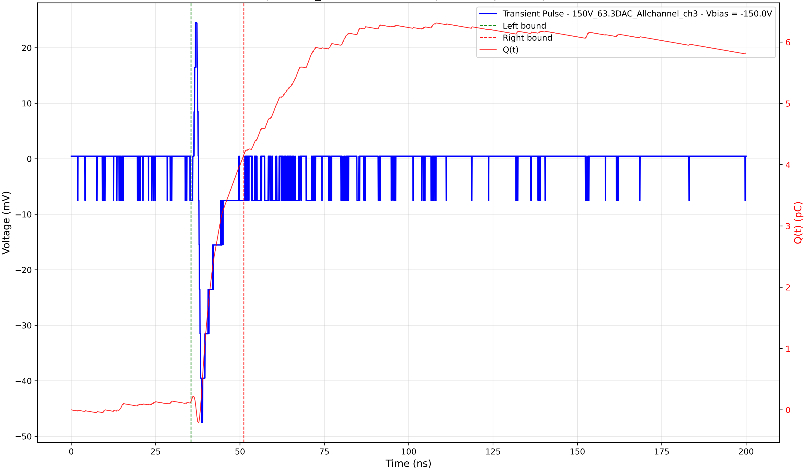
Transient Pulse - Sample: 1cm_42 - Position: 610.0 \mu\text{m} - Charge: 4.03 pC - Rise Time: 0.98 ns
