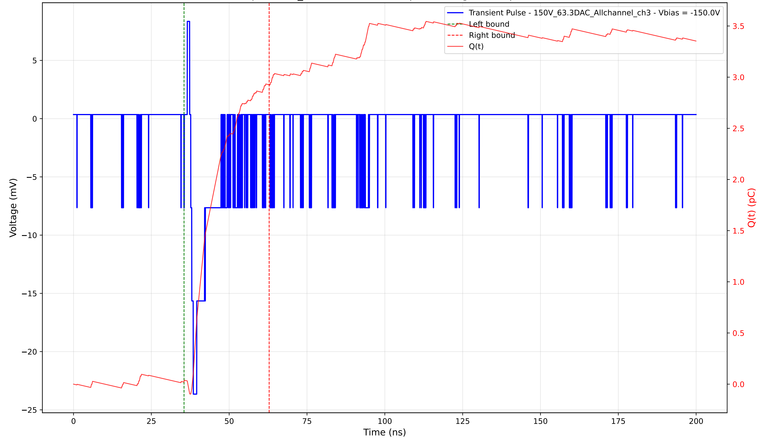
Transient Pulse - Sample: 1cm_42 - Position: 265.0 \mu\text{m} - Charge: 2.90 pC - Rise Time: 0.83 ns
