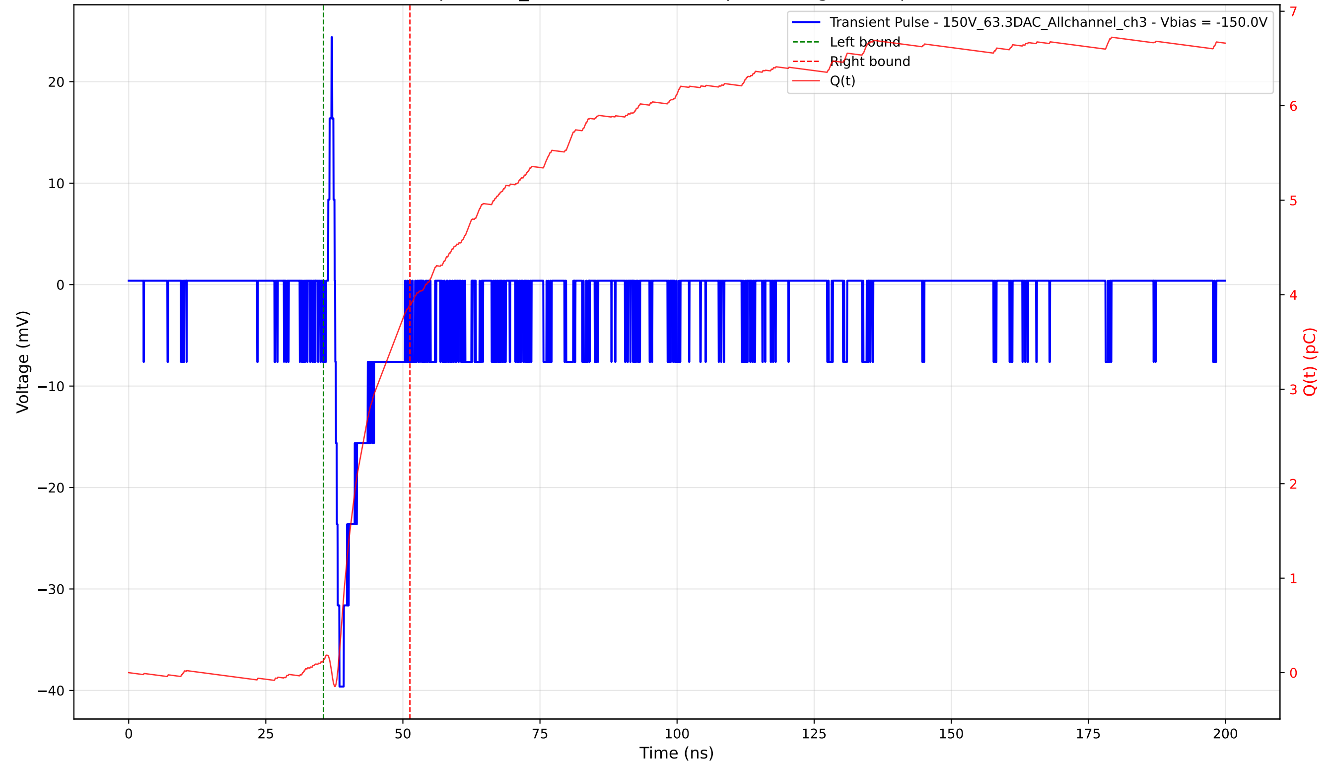
Transient Pulse - Sample: 1cm_42 - Position: 4145.0 \mu\text{m} - Charge: 3.75 pC - Rise Time: 0.78 ns
