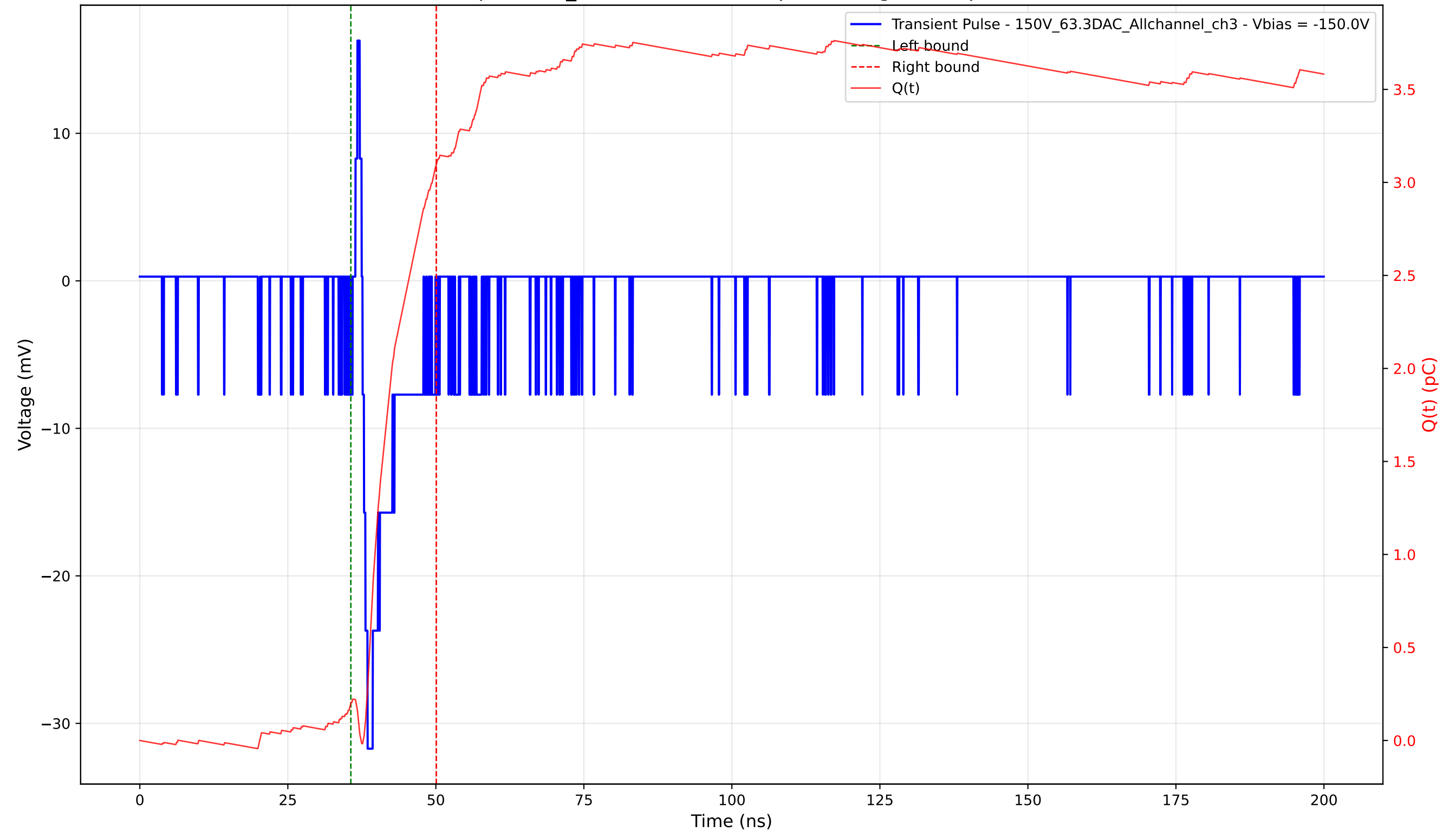
Transient Pulse - Sample: 1cm_42 - Position: 410.0 \mu\text{m} - Charge: 2.89 pC - Rise Time: 0.86 ns
