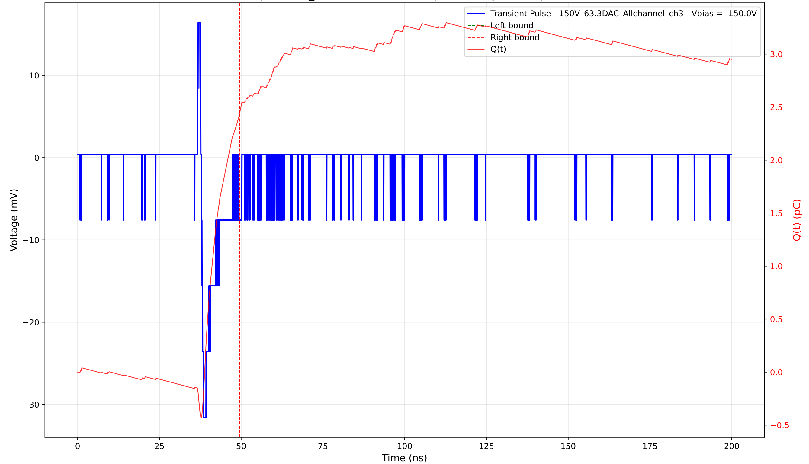
Transient Pulse - Sample: 1cm_42 - Position: 4645.0 \mu\text{m} - Charge: 2.61 pC - Rise Time: 0.70 ns
