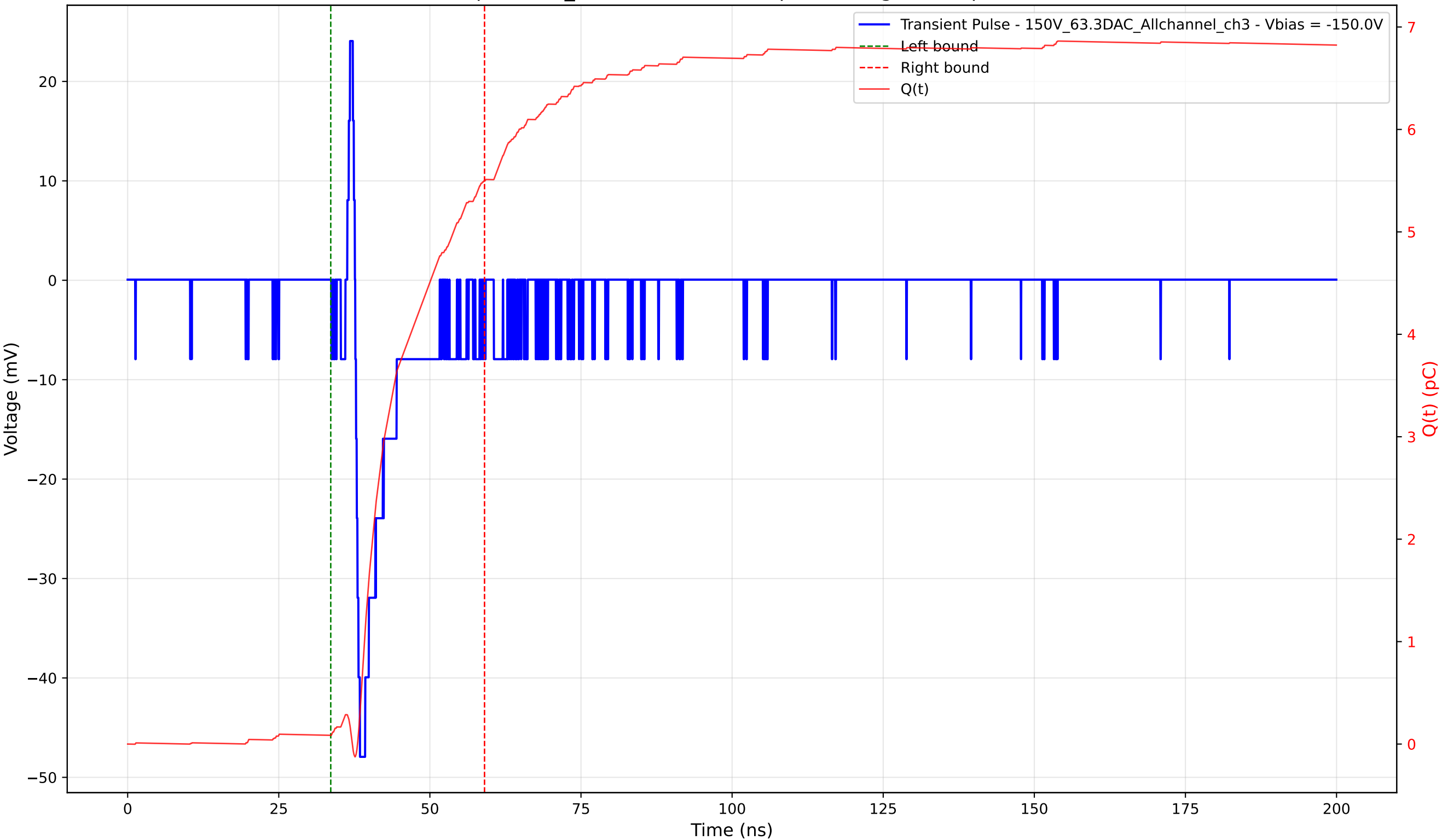
Transient Pulse - Sample: 1cm_42 - Position: 855.0 \mu\text{m} - Charge: 5.41 pC - Rise Time: 0.78 ns
