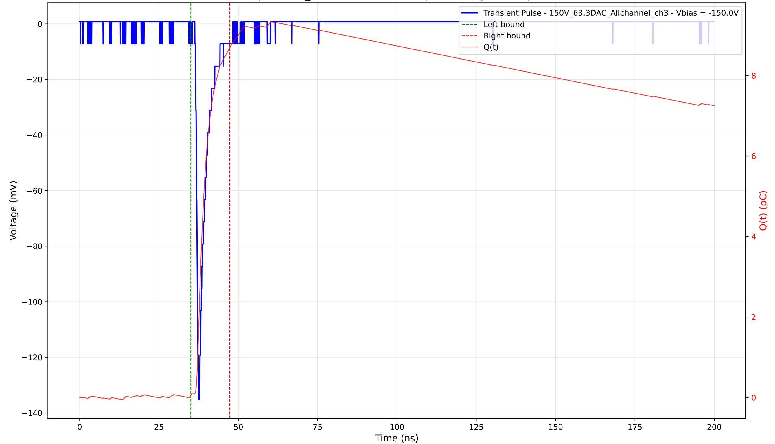
Transient Pulse - Sample: 1cm_42 - Position: 1690.0 \mu\text{m} - Charge: 8.64 pC - Rise Time: 0.93 ns
