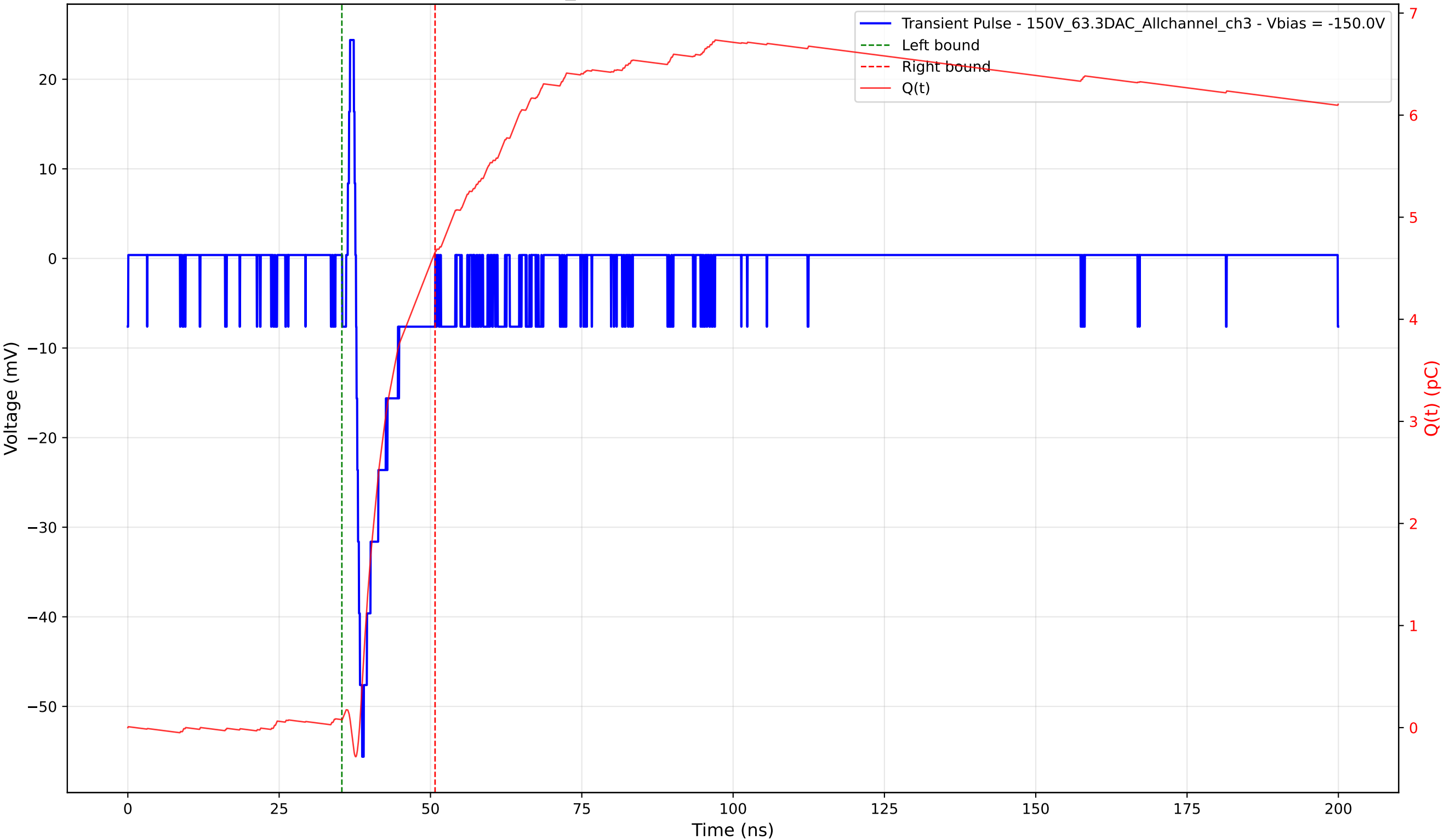
Transient Pulse - Sample: 1cm_42 - Position: 770.0 \mu\text{m} - Charge: 4.58 pC - Rise Time: 1.01 ns
