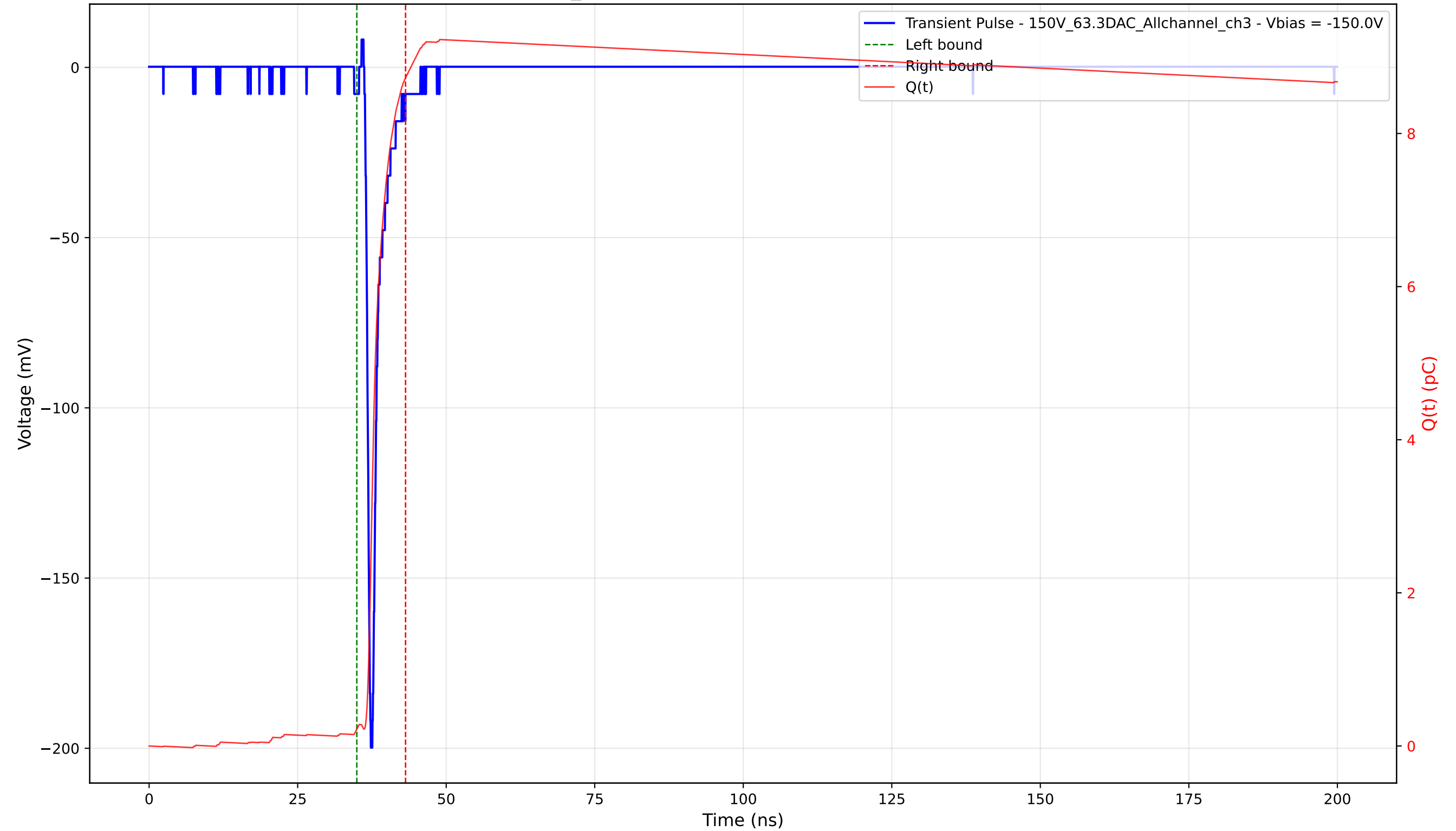
Transient Pulse - Sample: 1cm_42 - Position: 3050.0 \mu\text{m} - Charge: 8.51 pC - Rise Time: 0.78 ns
