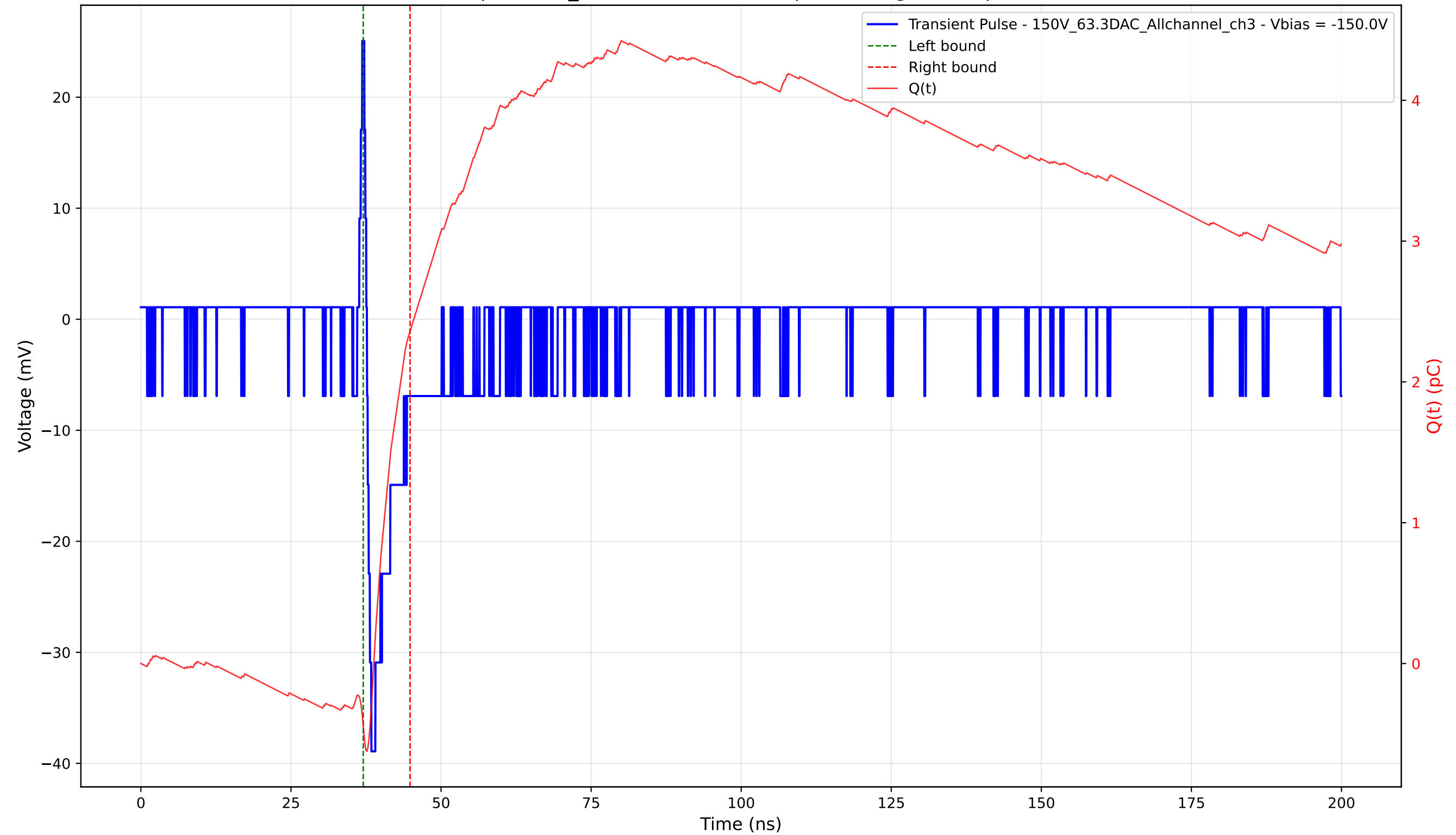
Transient Pulse - Sample: 1cm_42 - Position: 4155.0 \mu\text{m} - Charge: 2.81 pC - Rise Time: 0.74 ns
