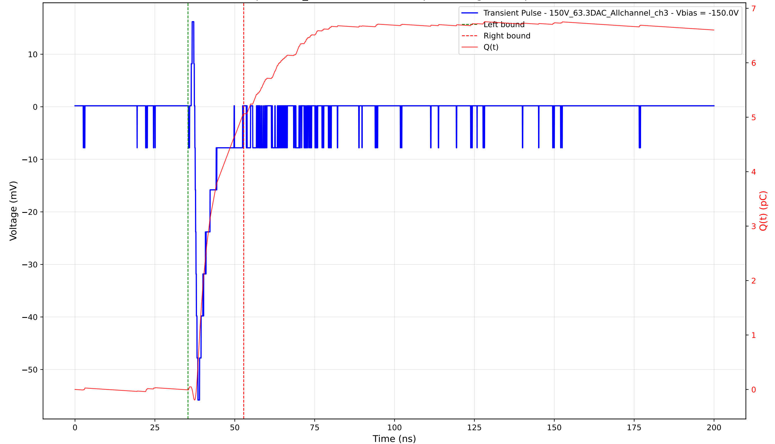
Transient Pulse - Sample: 1cm_42 - Position: 1055.0 \mu\text{m} - Charge: 5.07 pC - Rise Time: 0.97 ns
