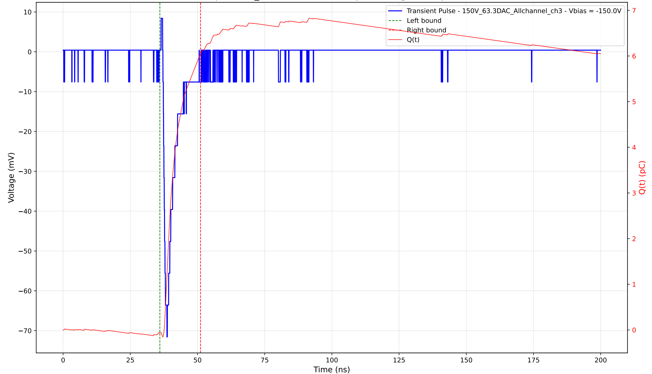
Transient Pulse - Sample: 1cm_42 - Position: 1325.0 \mu\text{m} - Charge: 6.11 pC - Rise Time: 1.48 ns
