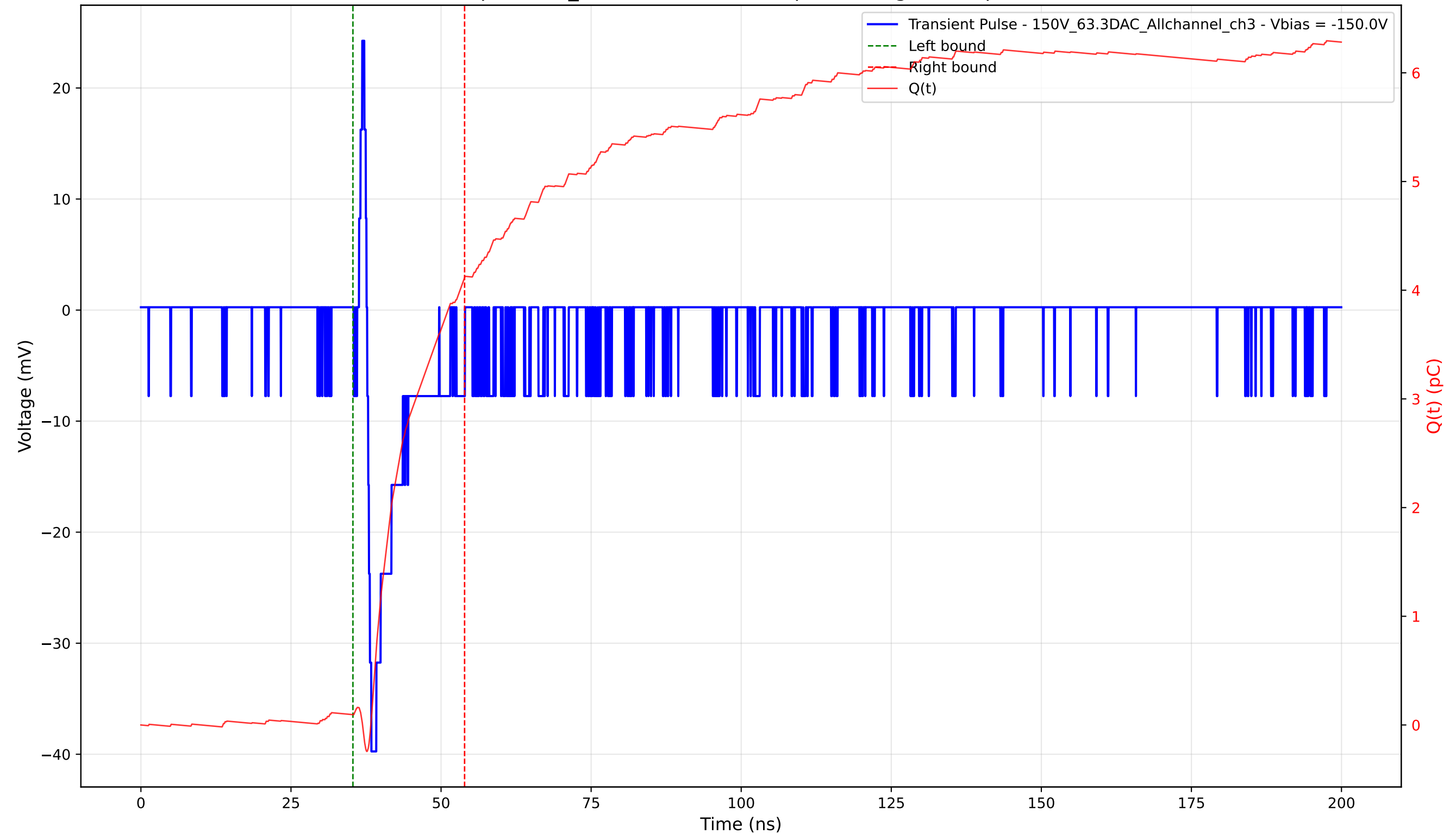
Transient Pulse - Sample: 1cm_42 - Position: 4230.0 \mu\text{m} - Charge: 4.02 pC - Rise Time: 0.70 ns
