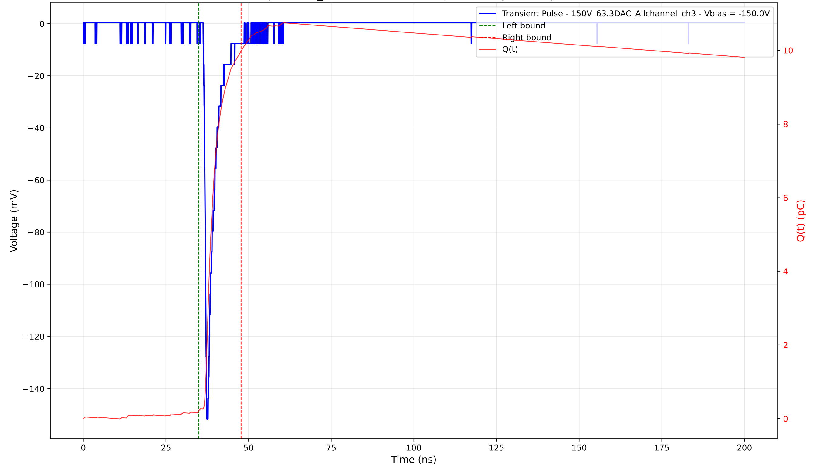
Transient Pulse - Sample: 1cm_42 - Position: 1760.0 \mu\text{m} - Charge: 9.77 pC - Rise Time: 0.92 ns
