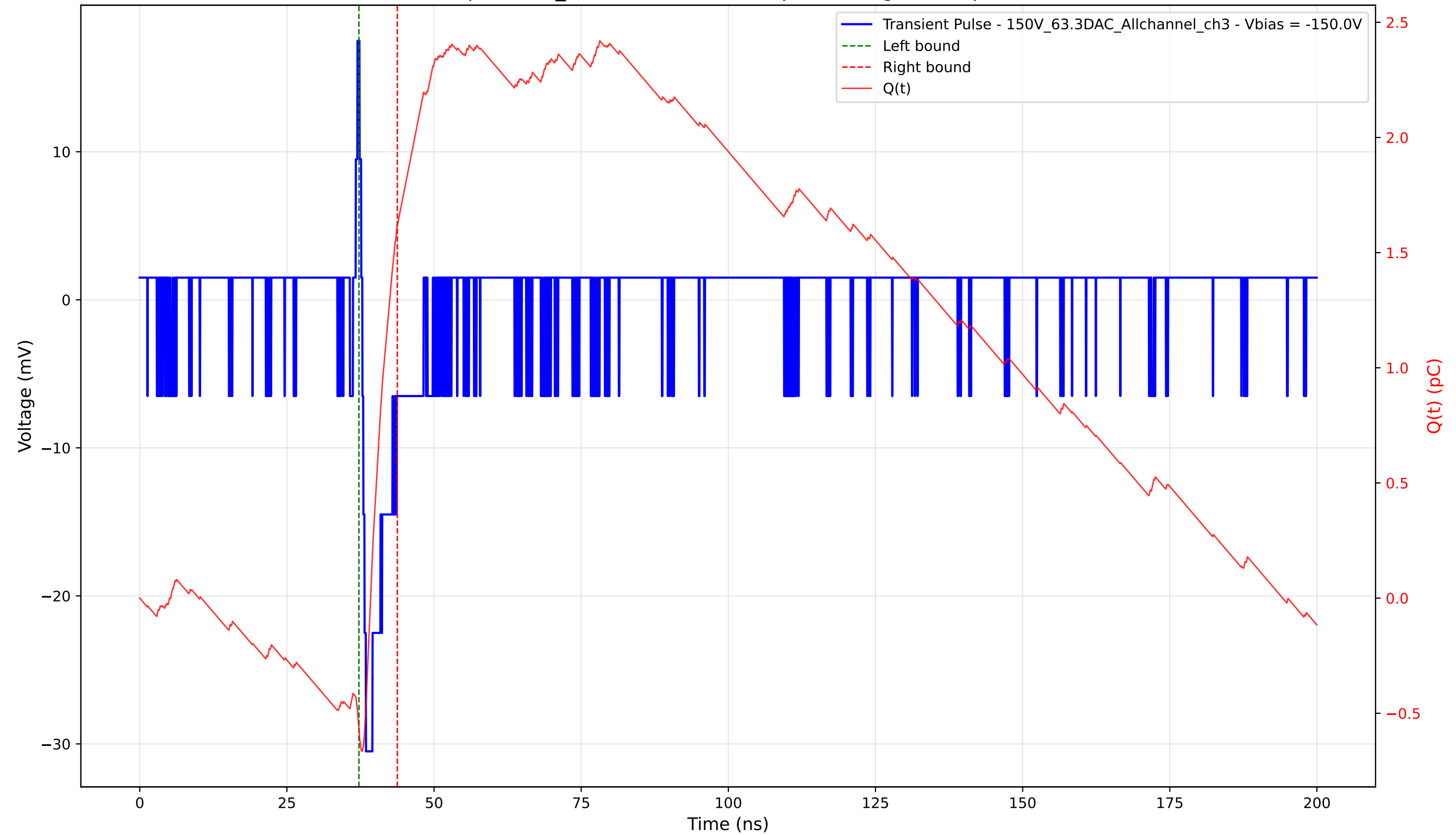
Transient Pulse - Sample: 1cm_42 - Position: 4815.0 \mu\text{m} - Charge: 2.19 pC - Rise Time: 0.63 ns
