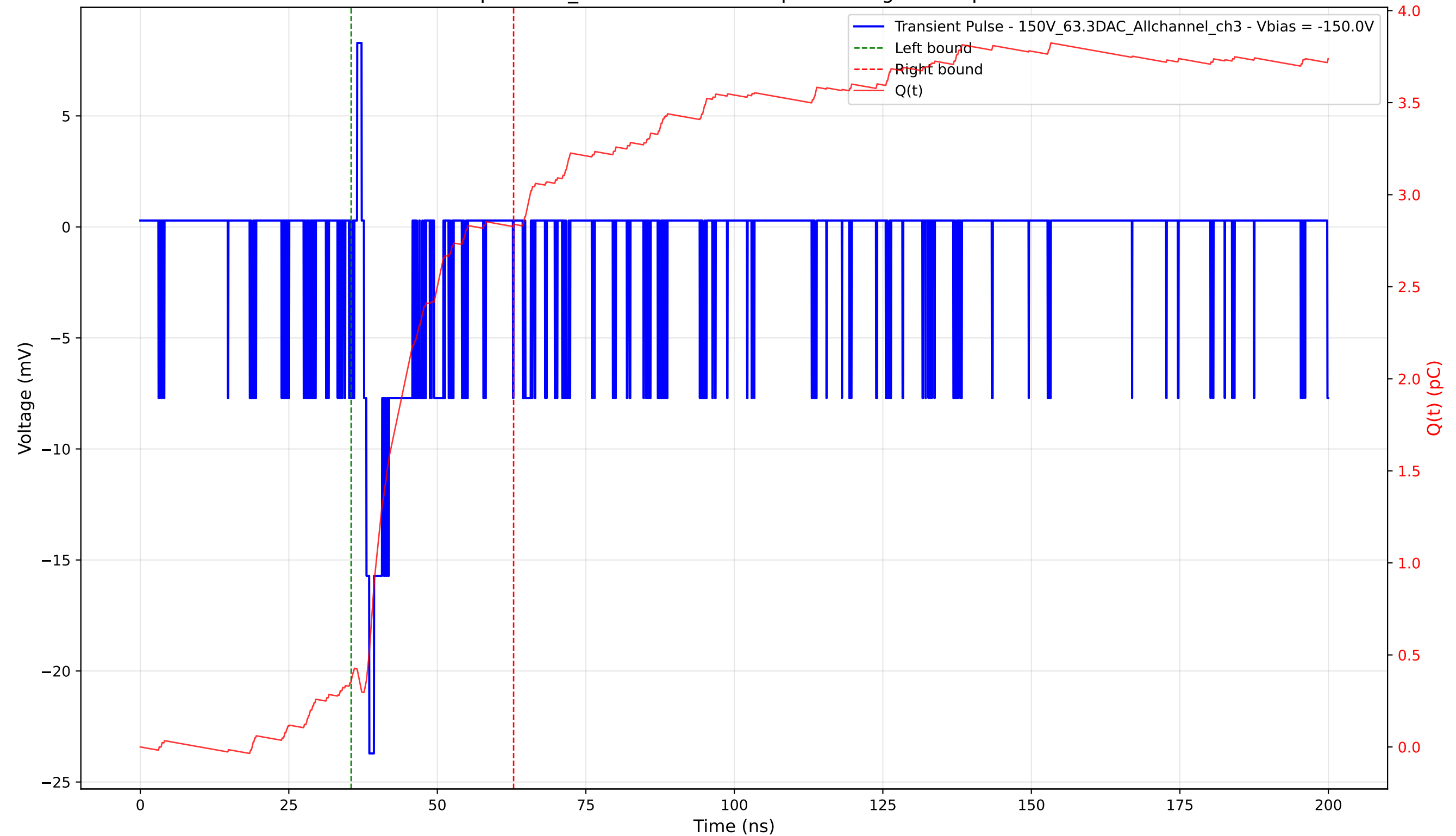
Transient Pulse - Sample: 1cm_42 - Position: 240.0 \mu\text{m} - Charge: 2.48 pC - Rise Time: 0.91 ns
