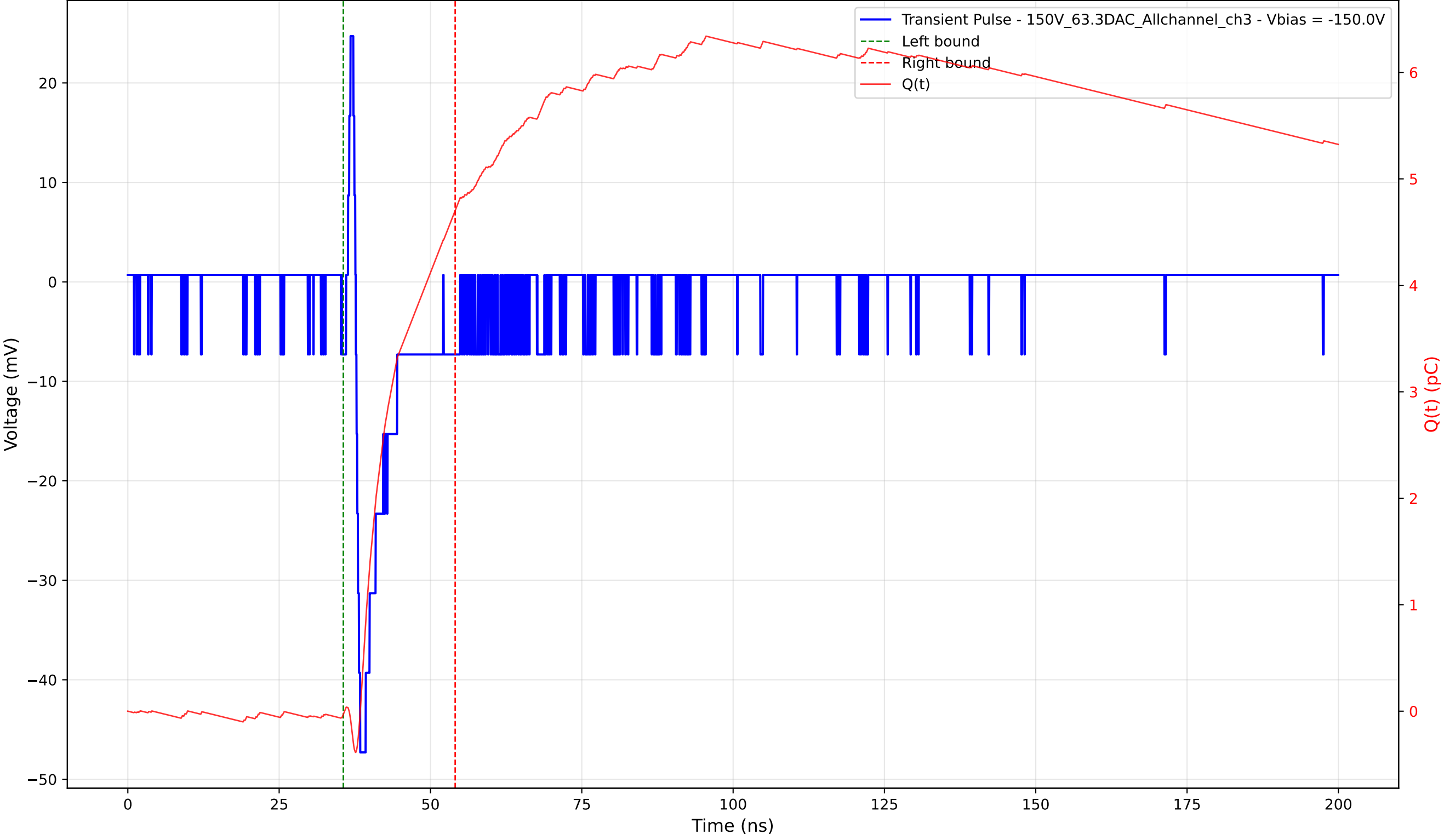
Transient Pulse - Sample: 1cm_42 - Position: 875.0 \mu\text{m} - Charge: 4.73 pC - Rise Time: 0.74 ns
