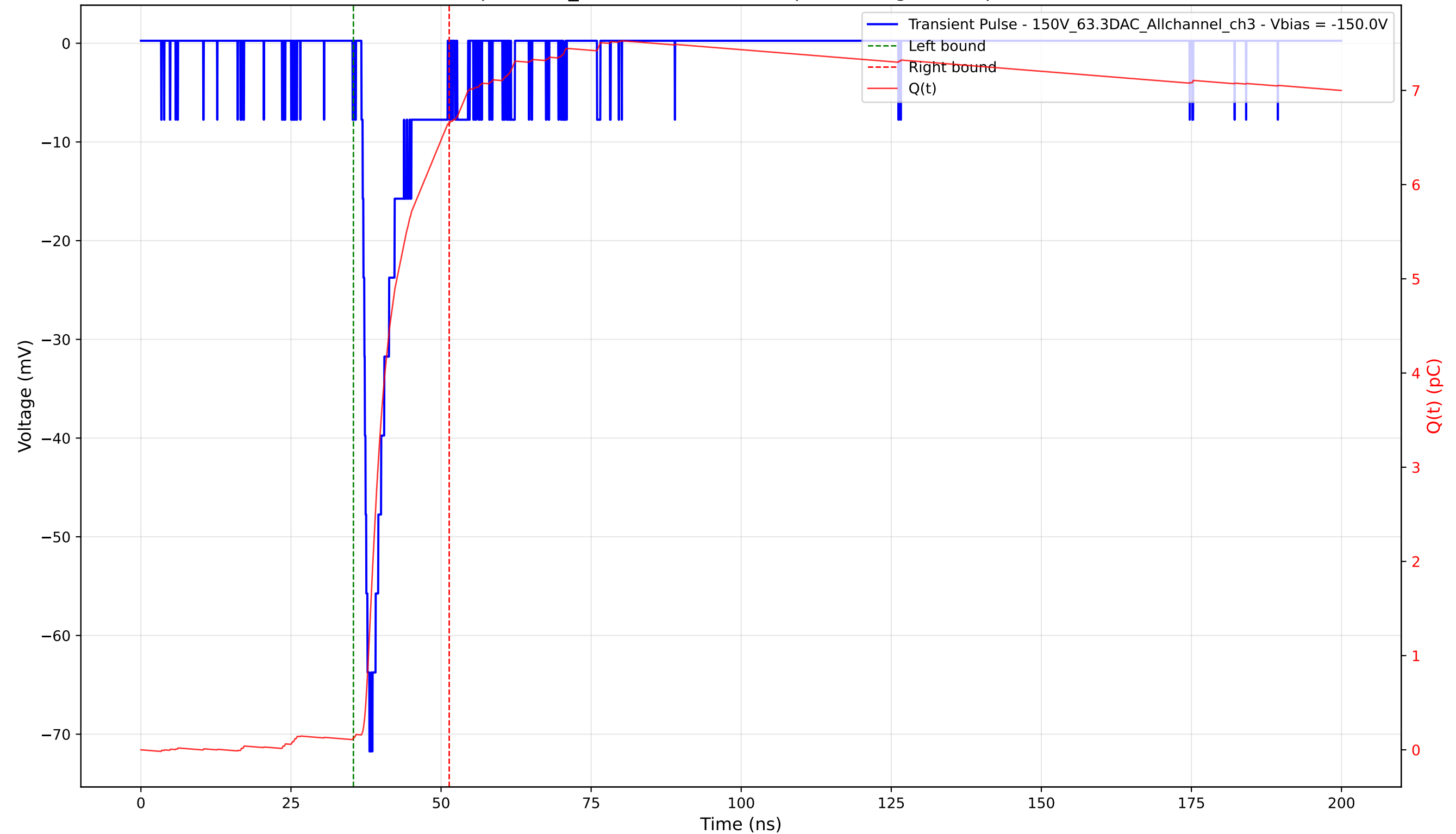
Transient Pulse - Sample: 1cm_42 - Position: 1460.0 \mu\text{m} - Charge: 6.51 pC - Rise Time: 1.32 ns
