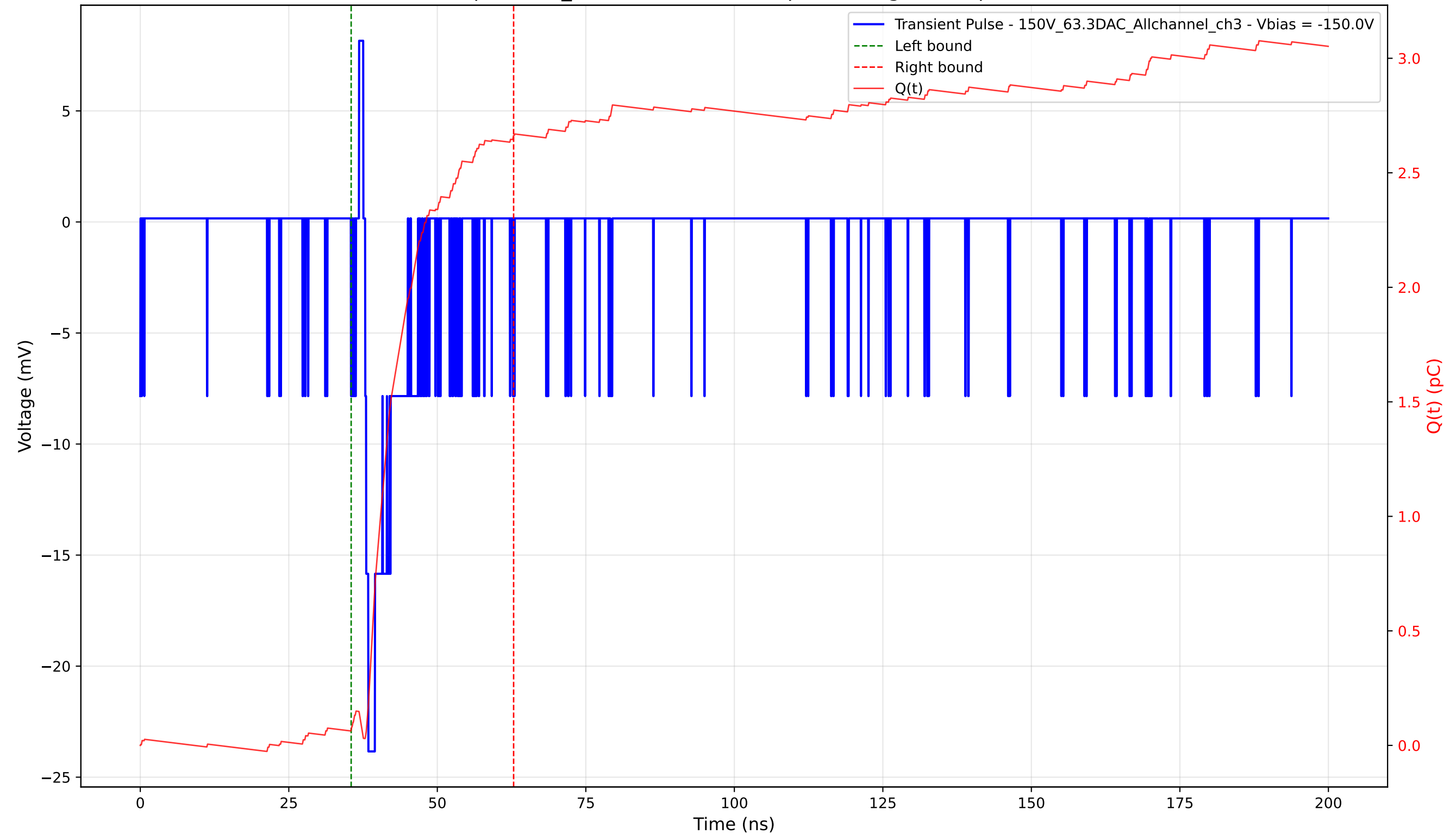
Transient Pulse - Sample: 1cm_42 - Position: 4955.0 \mu\text{m} - Charge: 2.59 pC - Rise Time: 0.55 ns
