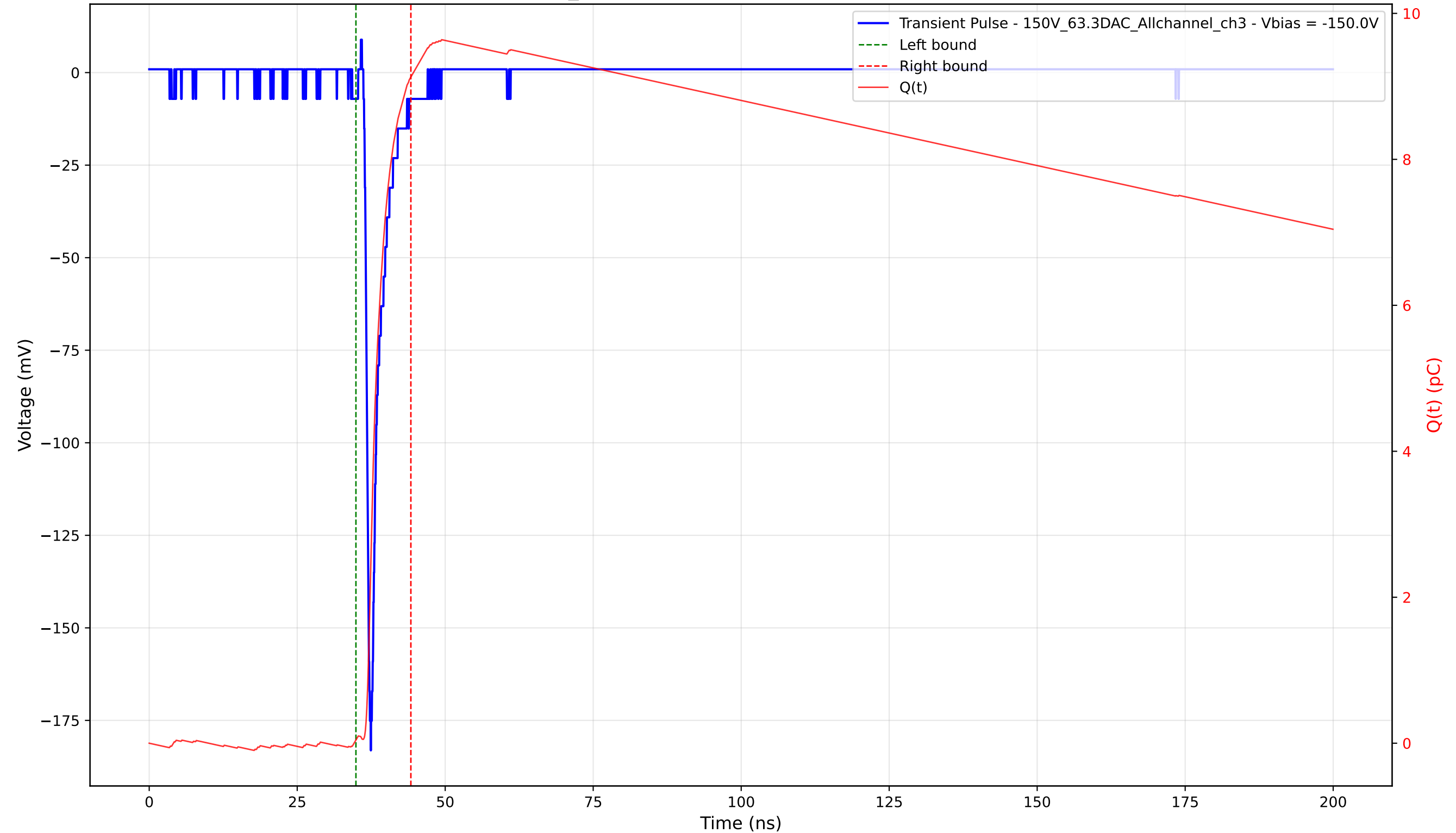
Transient Pulse - Sample: 1cm_42 - Position: 1920.0 \mu\text{m} - Charge: 9.08 pC - Rise Time: 0.82 ns
