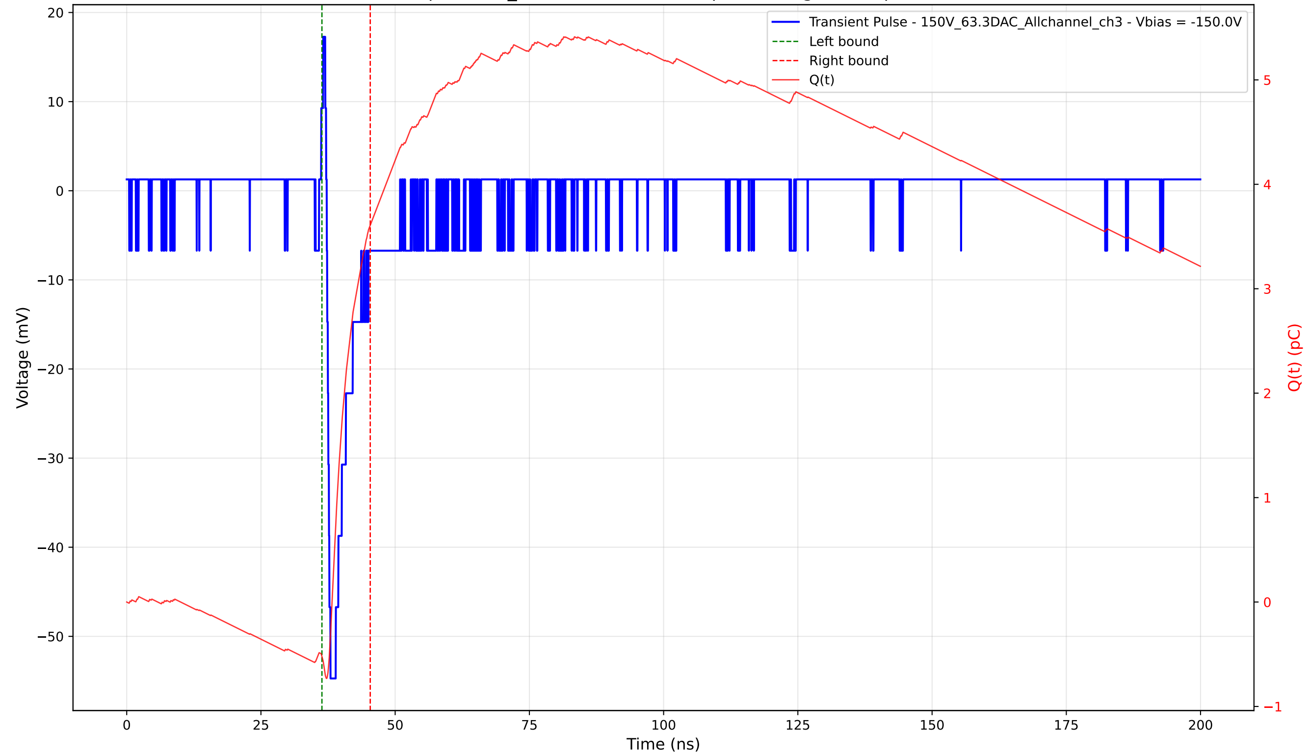
Transient Pulse - Sample: 1cm_42 - Position: 3725.0 \mu\text{m} - Charge: 4.13 pC - Rise Time: 0.69 ns
