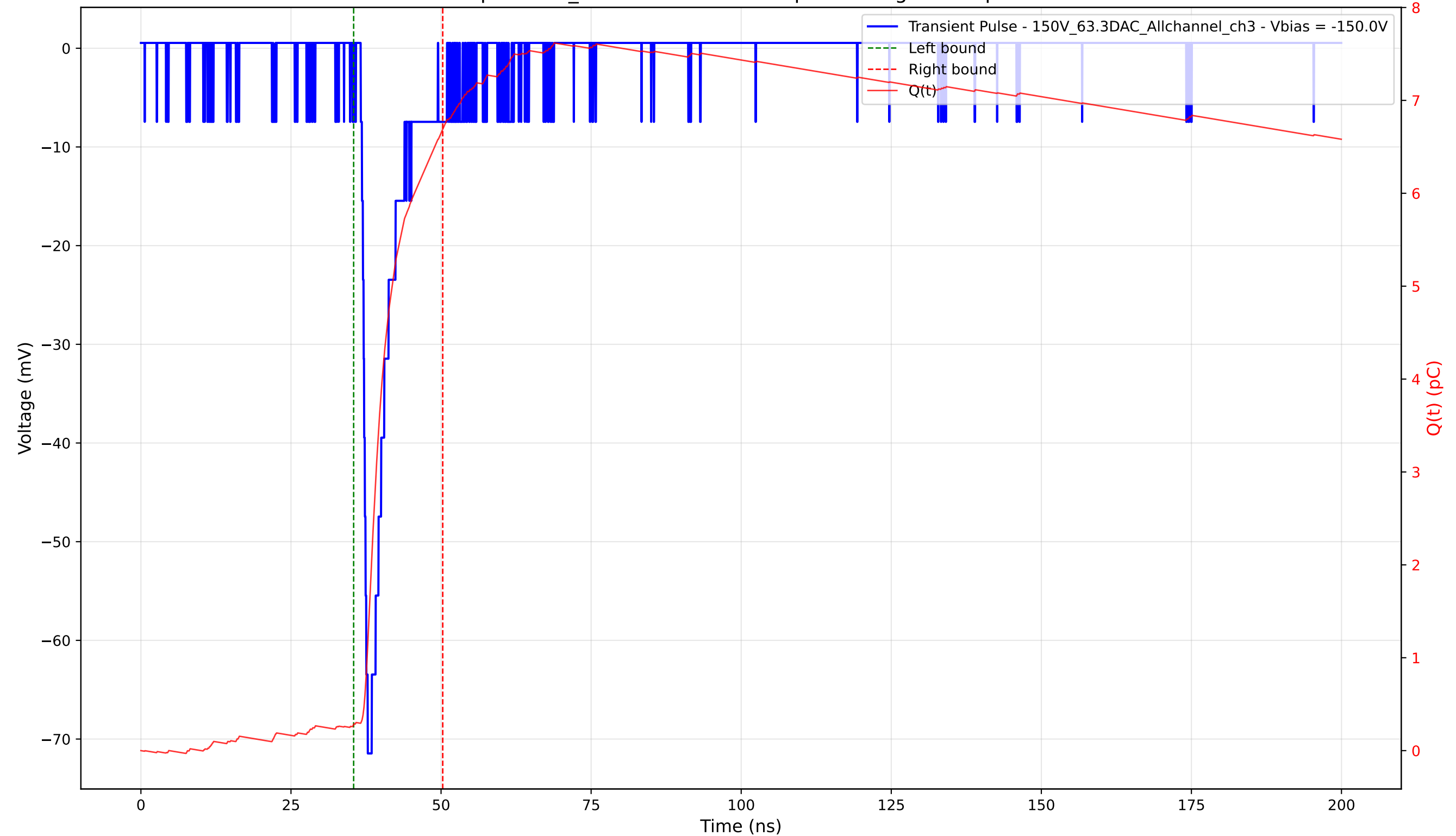
Transient Pulse - Sample: 1cm_42 - Position: 1495.0 \mu\text{m} - Charge: 6.41 pC - Rise Time: 1.16 ns
