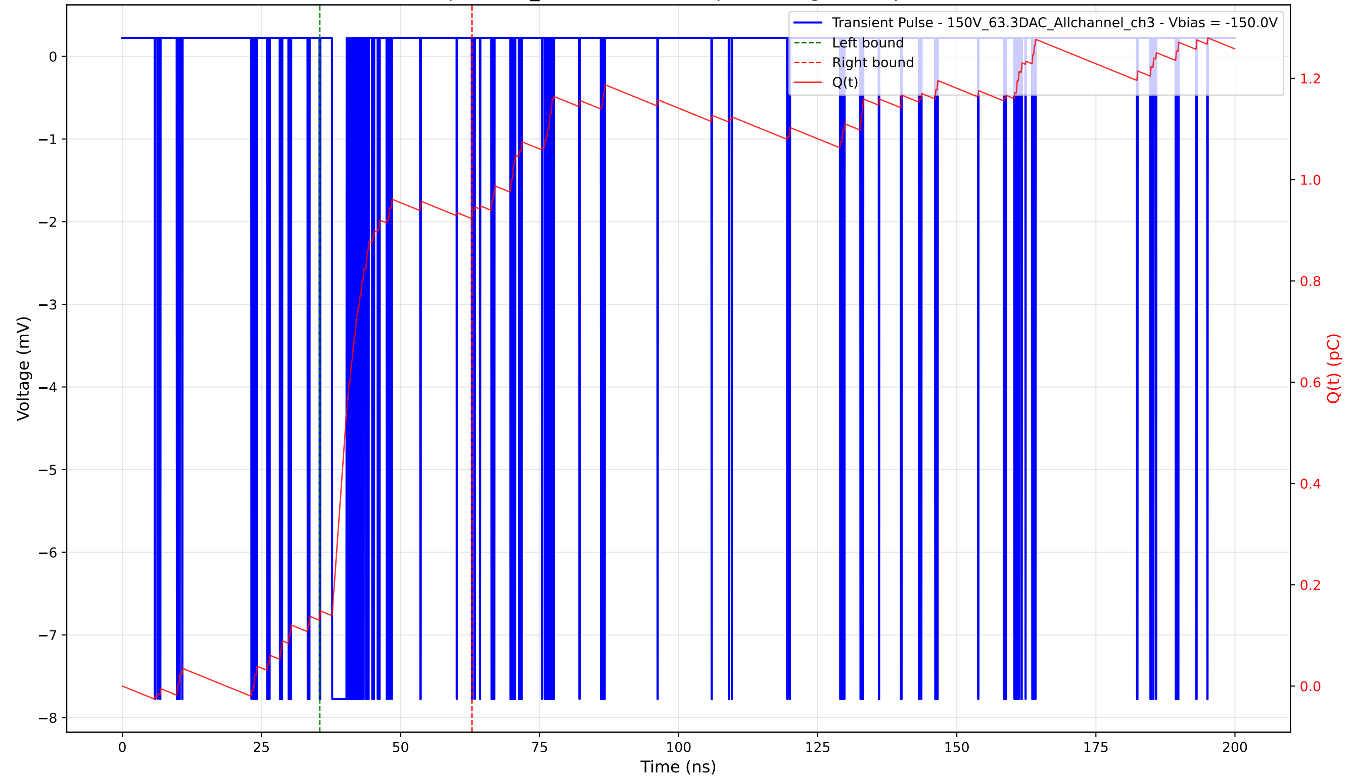
Transient Pulse - Sample: 1cm_42 - Position: 70.0 \mu\text{m} - Charge: 0.79 pC - Rise Time: 0.04 ns
