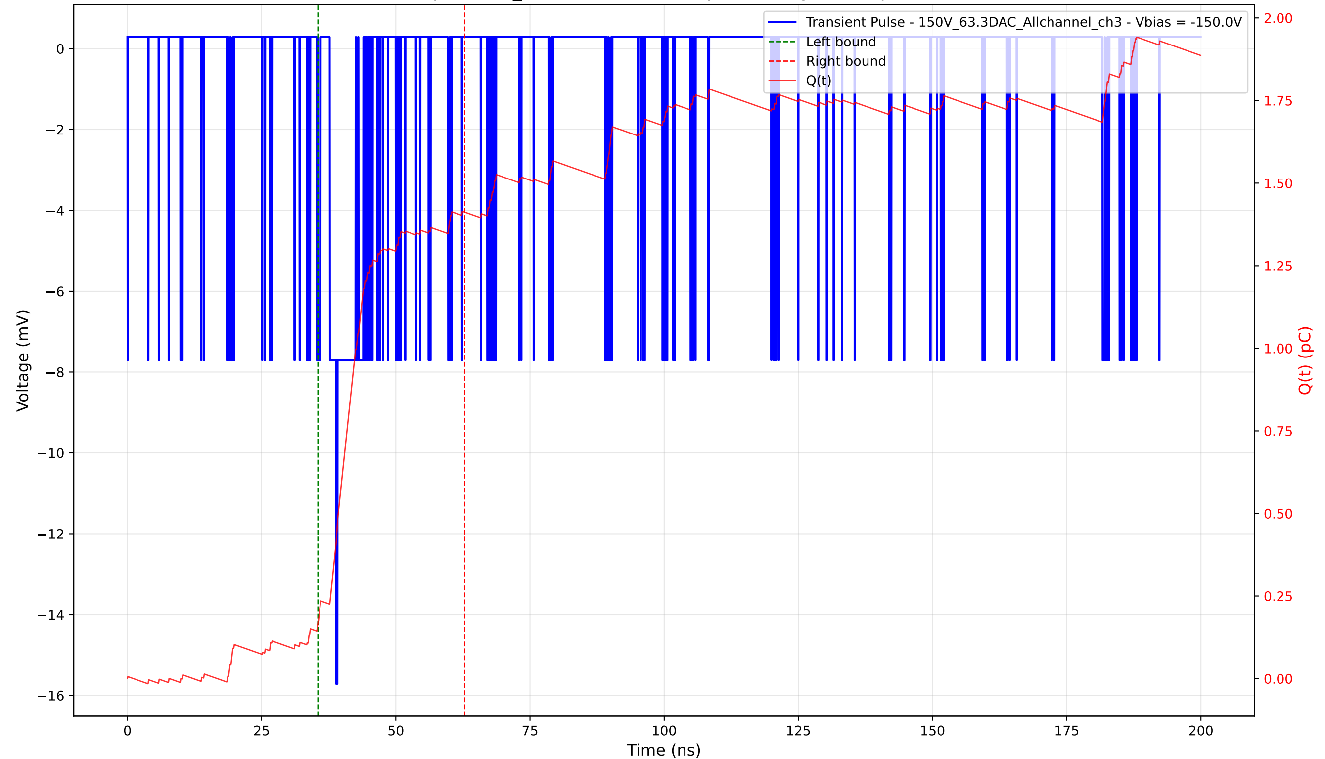
Transient Pulse - Sample: 1cm_42 - Position: 105.0 \mu\text{m} - Charge: 1.24 pC - Rise Time: 1.19 ns
