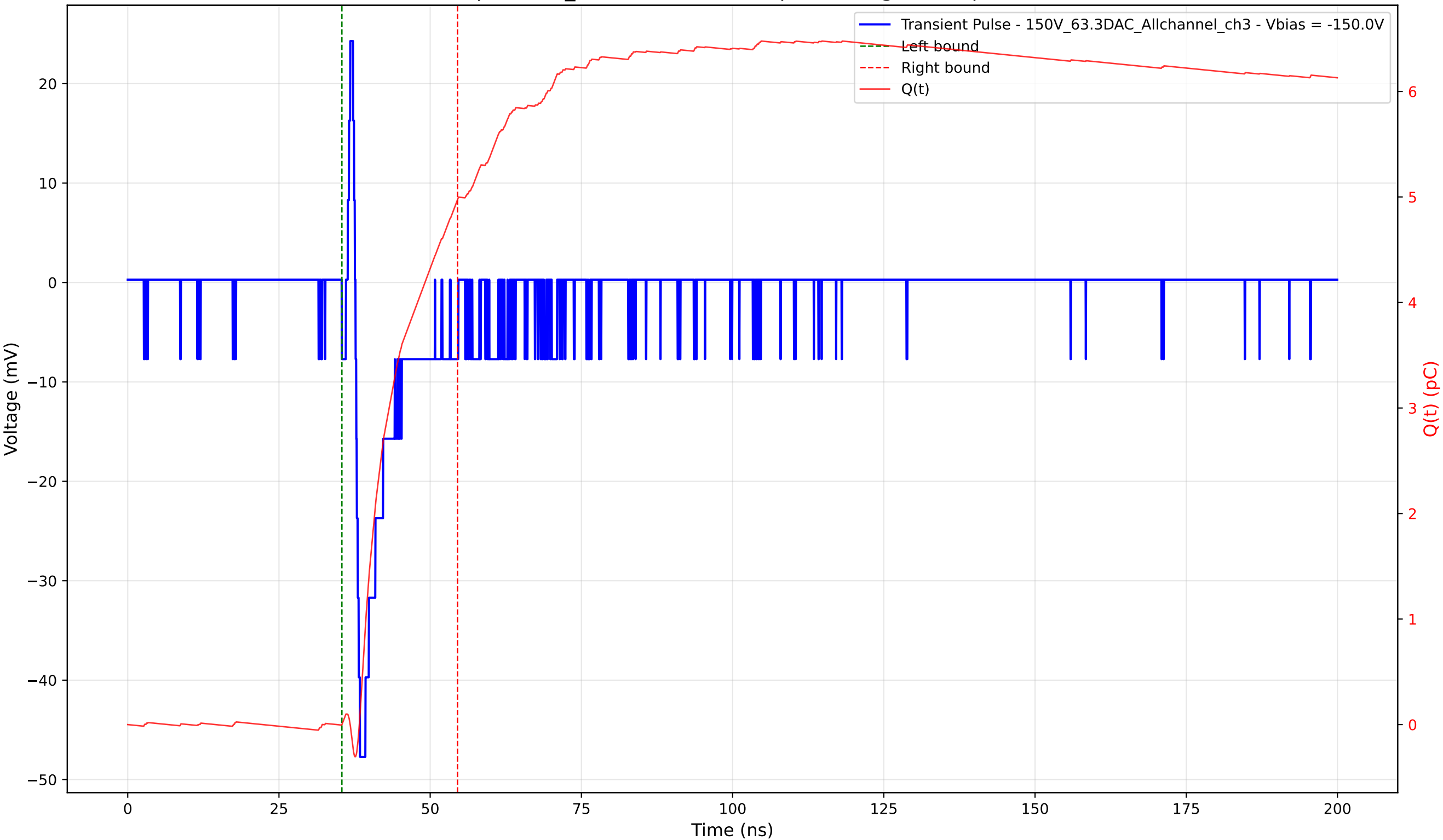
Transient Pulse - Sample: 1cm_42 - Position: 890.0 \mu\text{m} - Charge: 4.98 pC - Rise Time: 0.74 ns
