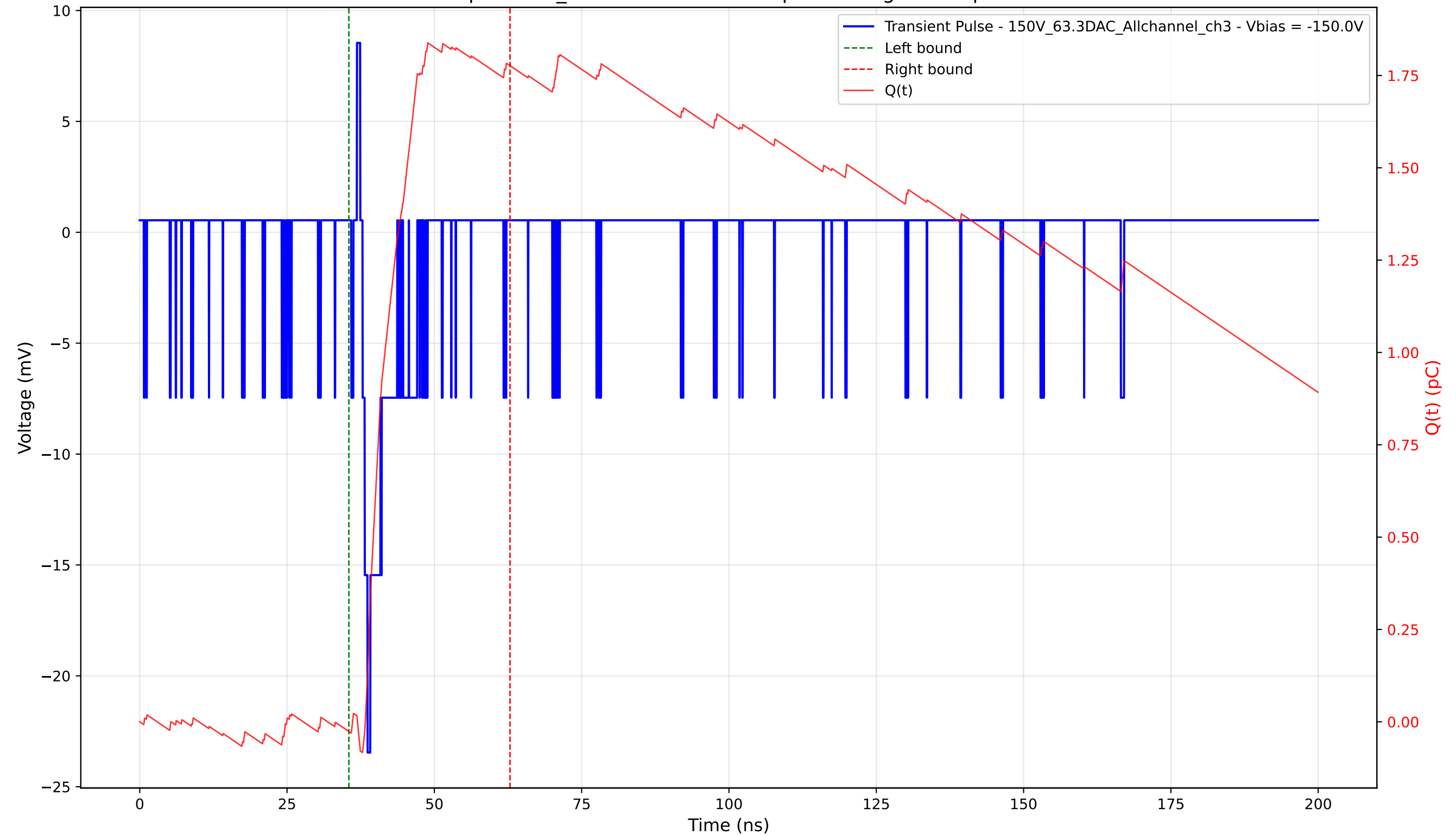
Transient Pulse - Sample: 1cm_42 - Position: 4985.0 \mu\text{m} - Charge: 1.80 pC - Rise Time: 0.87 ns
