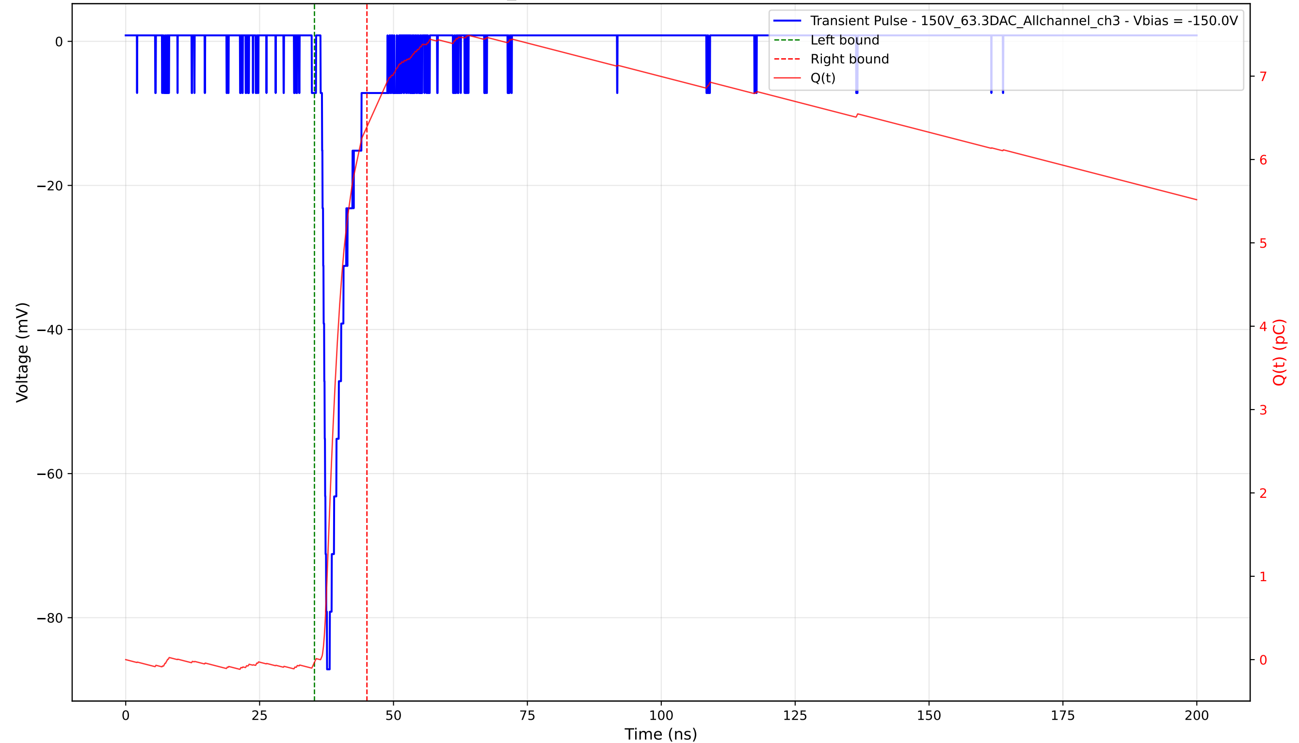
Transient Pulse - Sample: 1cm_42 - Position: 1565.0 \mu\text{m} - Charge: 6.42 pC - Rise Time: 0.79 ns
