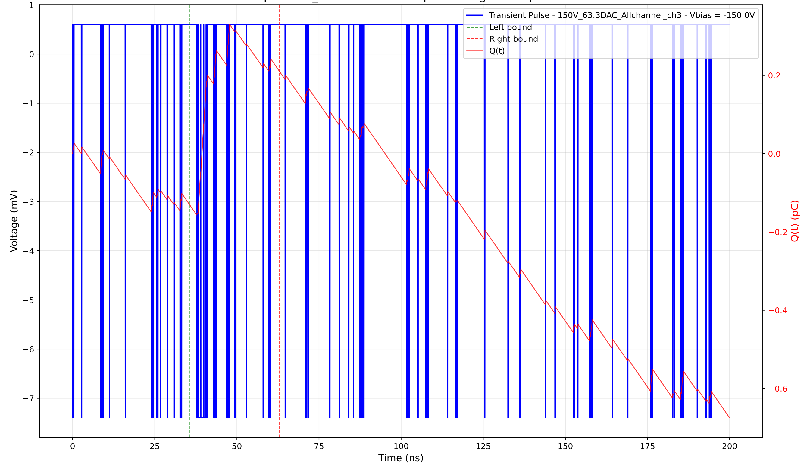
Transient Pulse - Sample: 1cm_42 - Position: 15.0 \mu\text{m} - Charge: 0.34 pC - Rise Time: 0.04 ns
