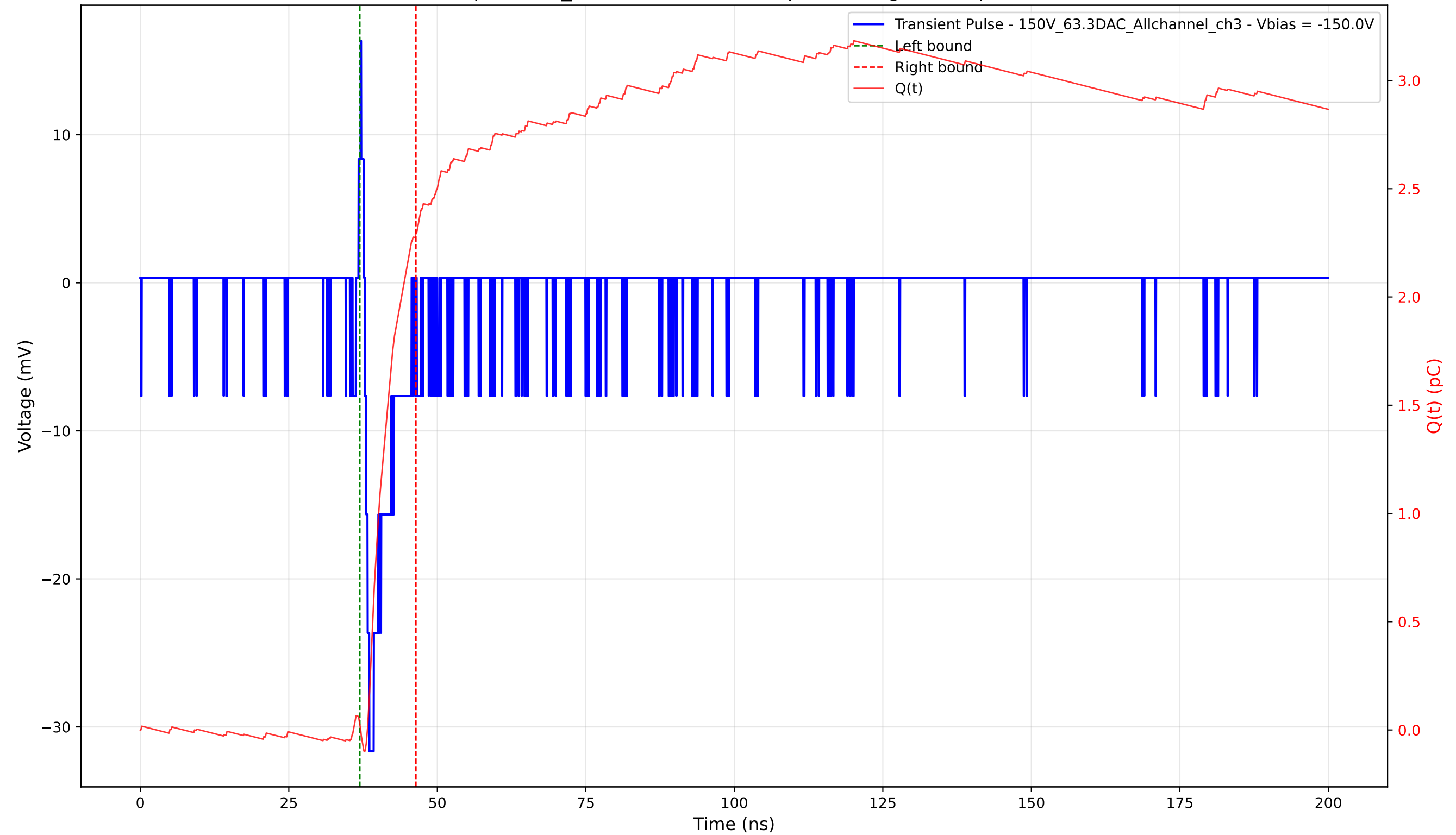
Transient Pulse - Sample: 1cm_42 - Position: 4890.0 \mu\text{m} - Charge: 2.27 pC - Rise Time: 0.74 ns
