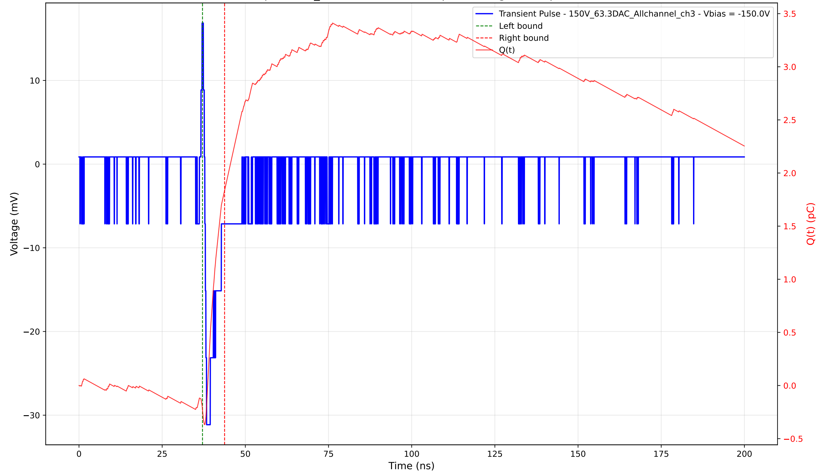
Transient Pulse - Sample: 1cm_42 - Position: 4755.0 \mu\text{m} - Charge: 2.06 pC - Rise Time: 0.55 ns
