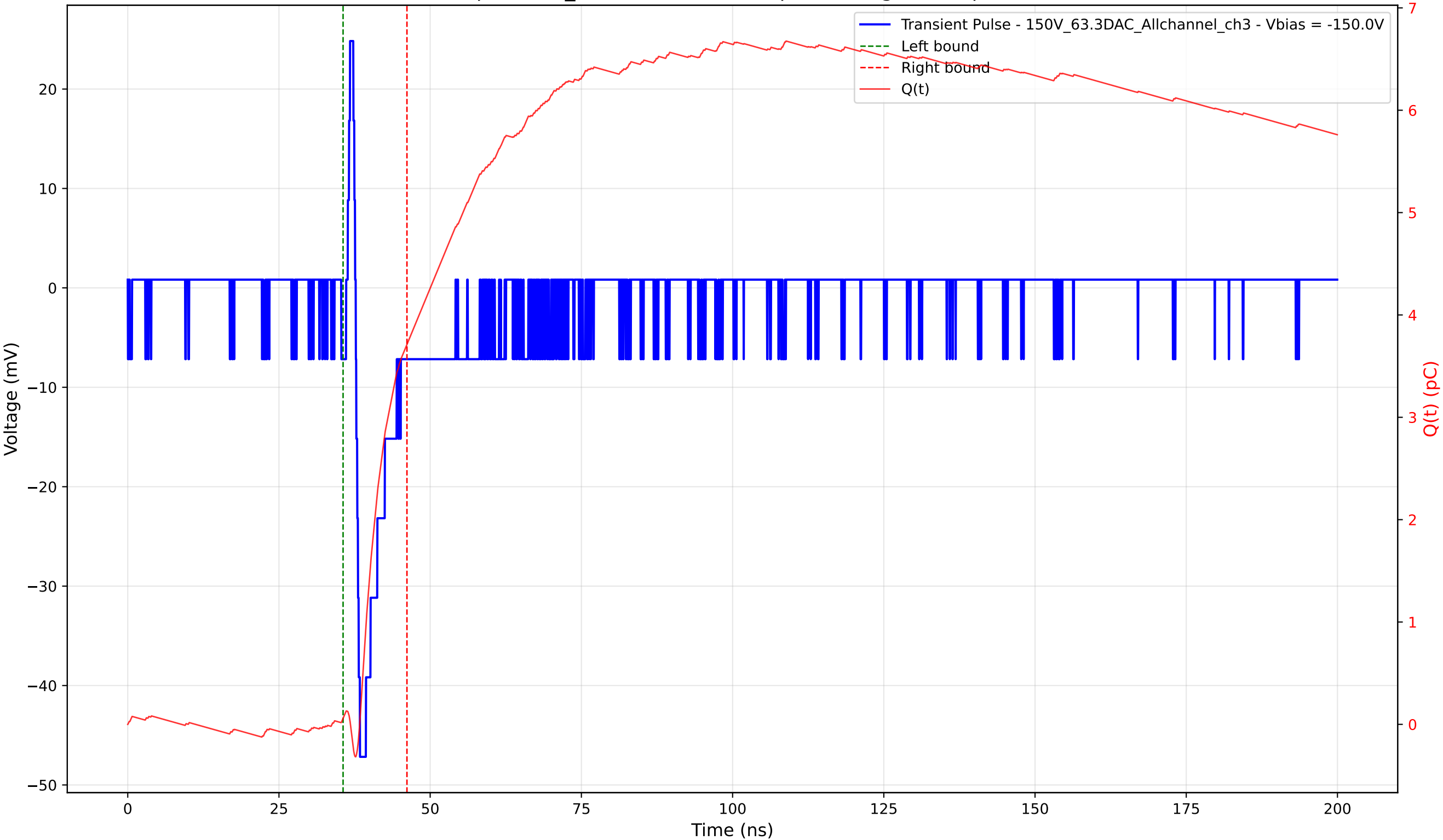
Transient Pulse - Sample: 1cm_42 - Position: 825.0 \mu\text{m} - Charge: 3.65 pC - Rise Time: 0.70 ns
