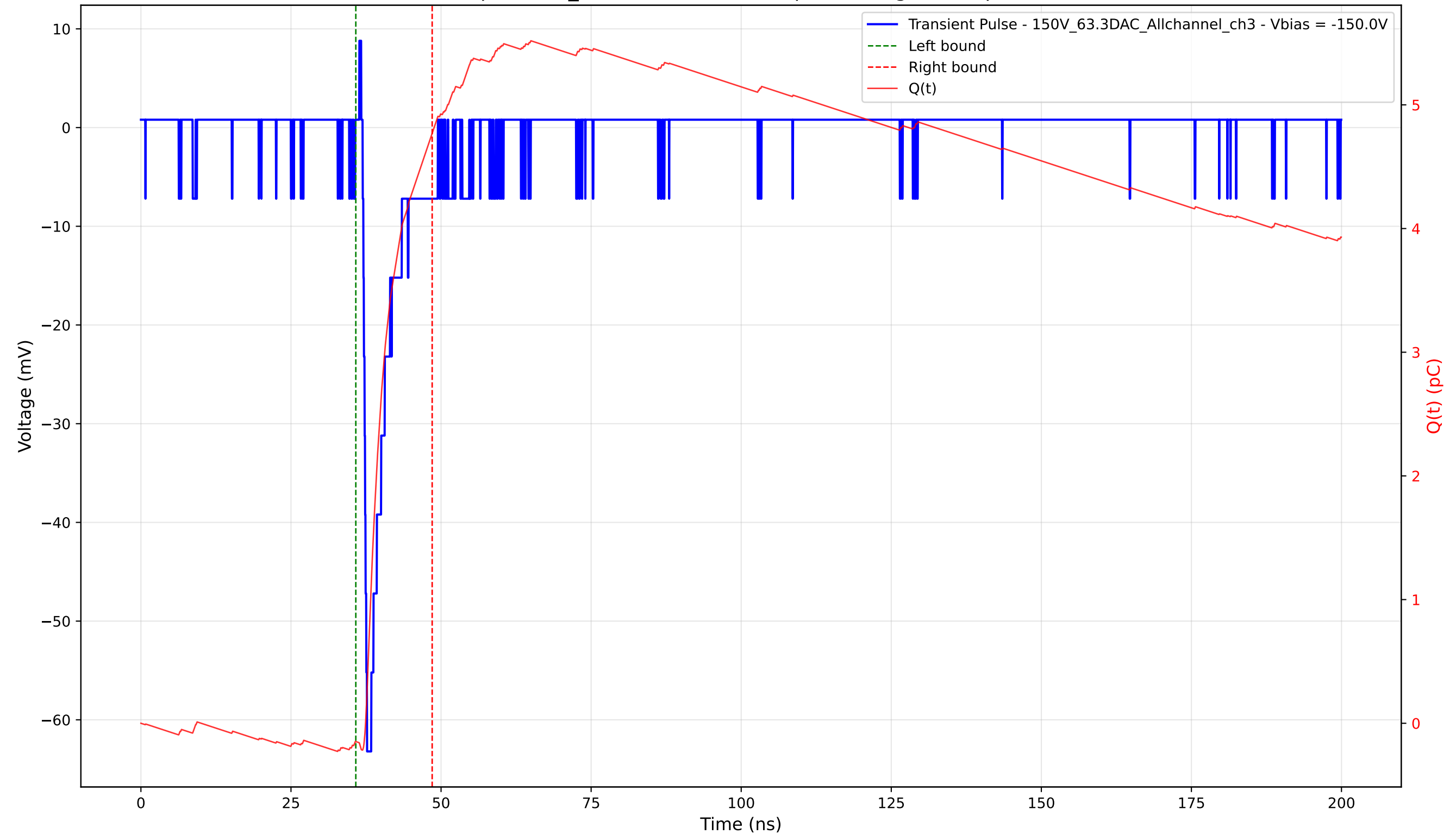
Transient Pulse - Sample: 1cm_42 - Position: 3550.0 \mu\text{m} - Charge: 4.92 pC - Rise Time: 0.73 ns
