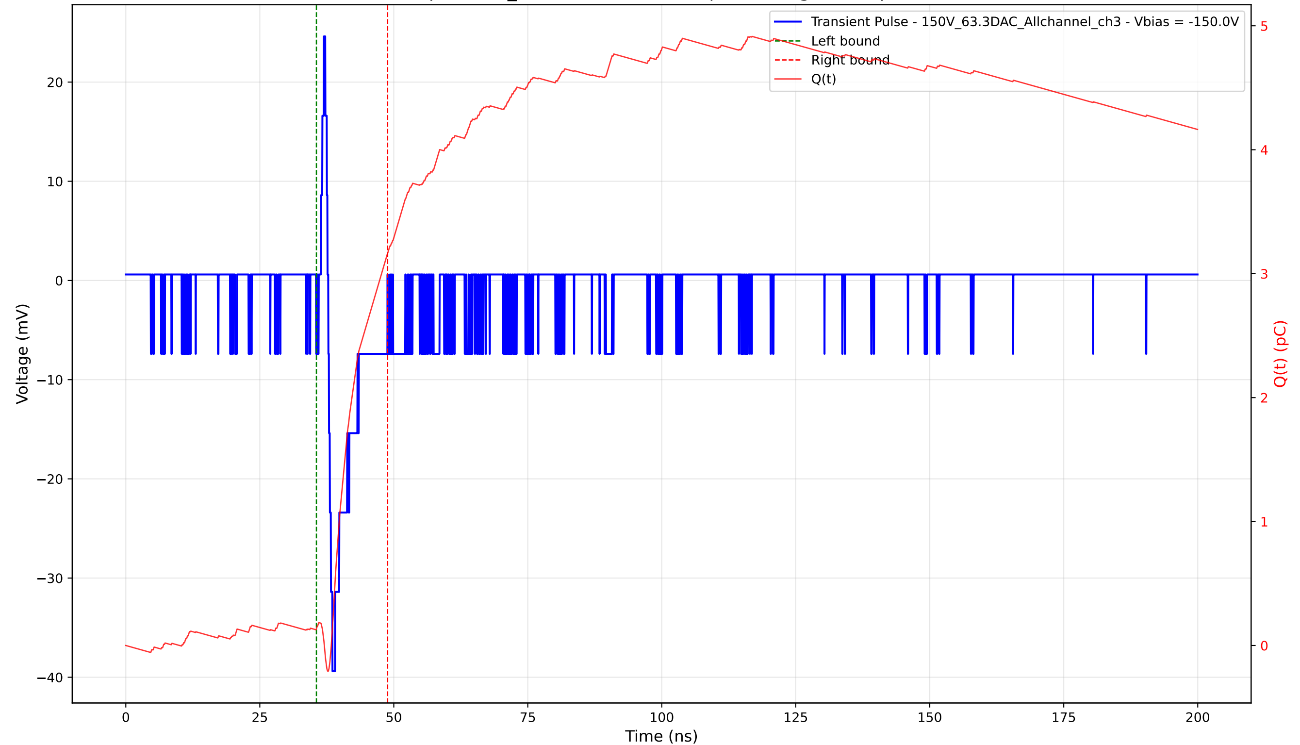
Transient Pulse - Sample: 1cm_42 - Position: 4390.0 \mu\text{m} - Charge: 3.03 pC - Rise Time: 0.78 ns
