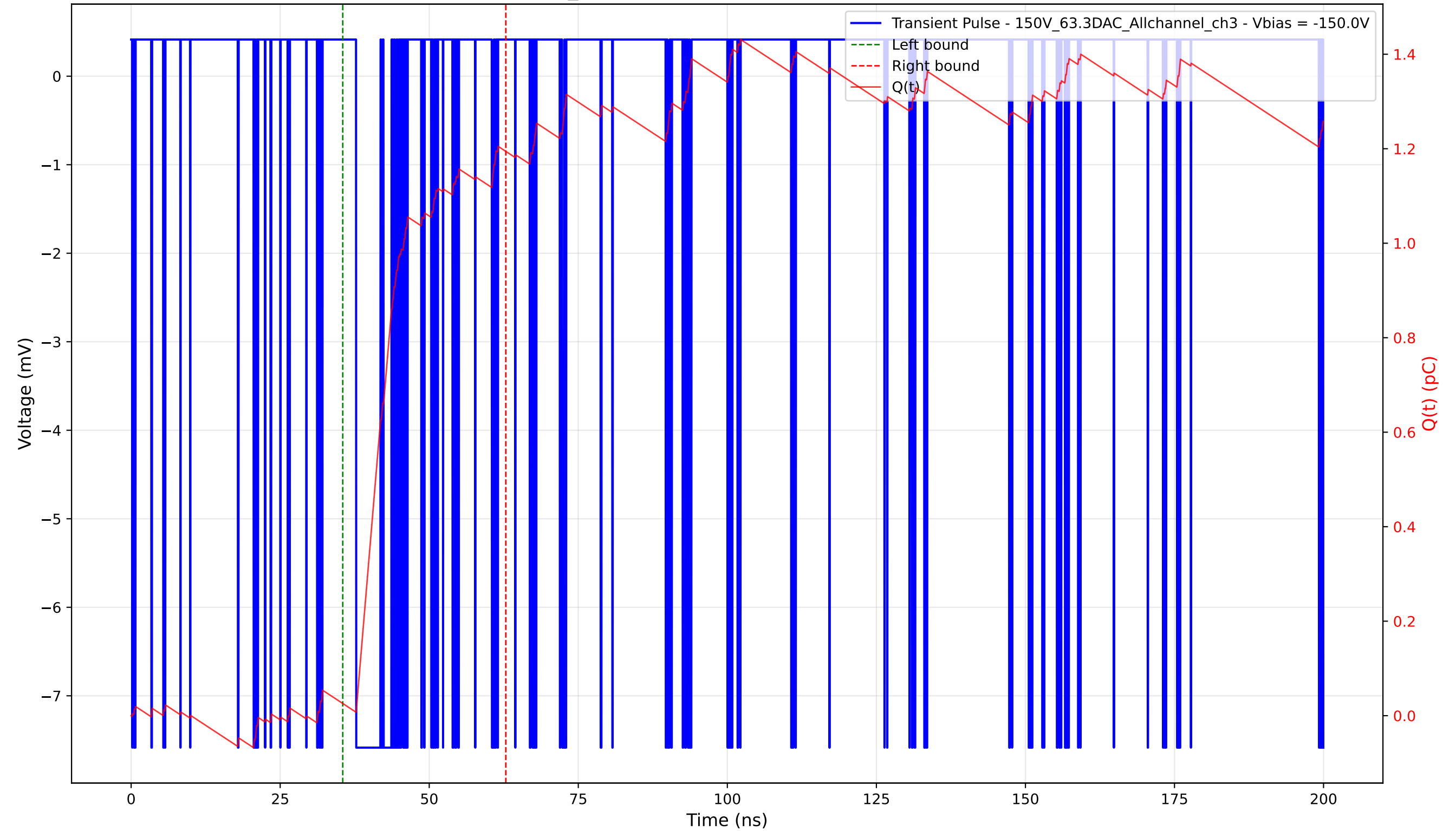
Transient Pulse - Sample: 1cm_42 - Position: 90.0 \mu\text{m} - Charge: 1.17 pC - Rise Time: 0.04 ns
