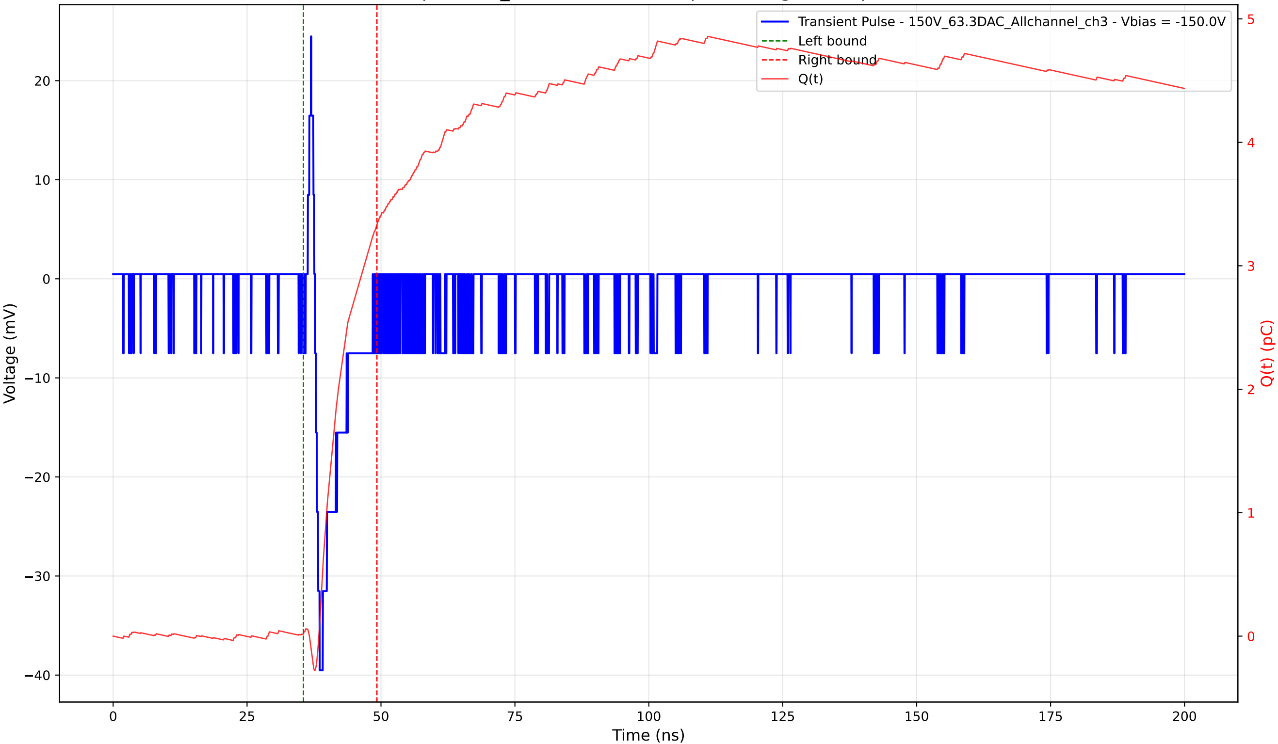
Transient Pulse - Sample: 1cm_42 - Position: 510.0 \mu\text{m} - Charge: 3.31 pC - Rise Time: 0.86 ns
