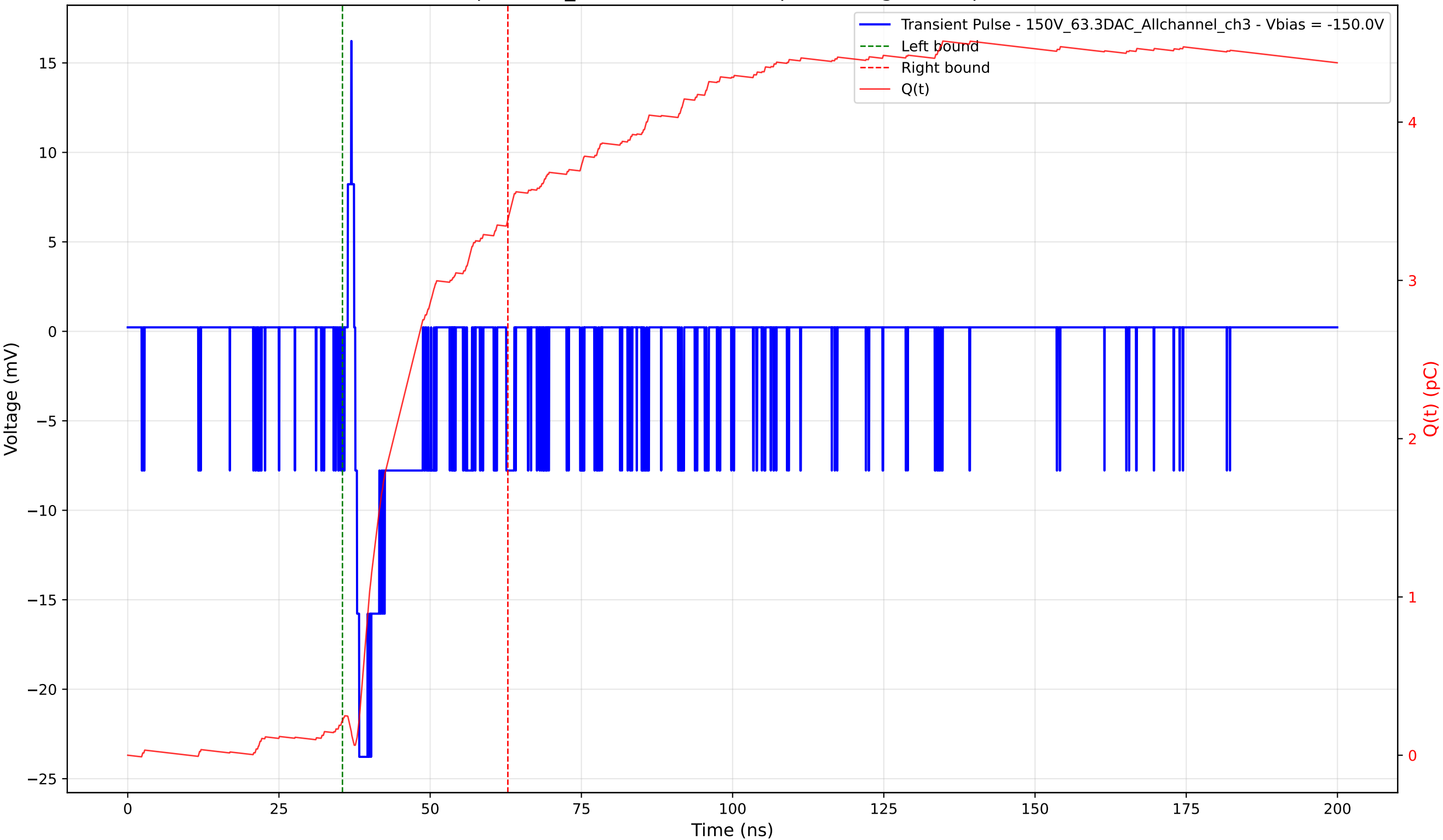
Transient Pulse - Sample: 1cm_42 - Position: 330.0 \mu\text{m} - Charge: 3.17 pC - Rise Time: 0.67 ns
