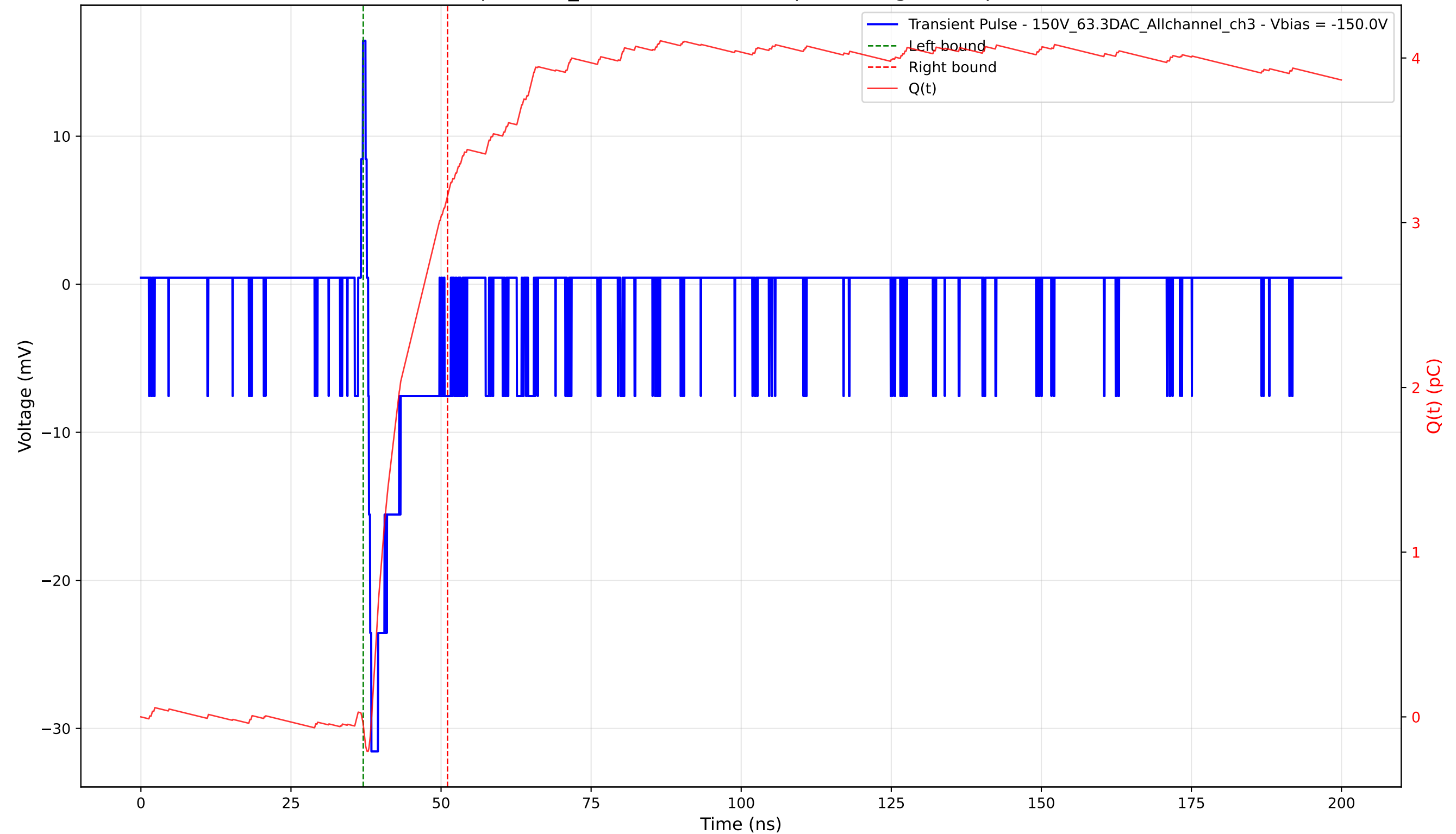
Transient Pulse - Sample: 1cm_42 - Position: 4800.0 \mu\text{m} - Charge: 3.21 pC - Rise Time: 0.54 ns
