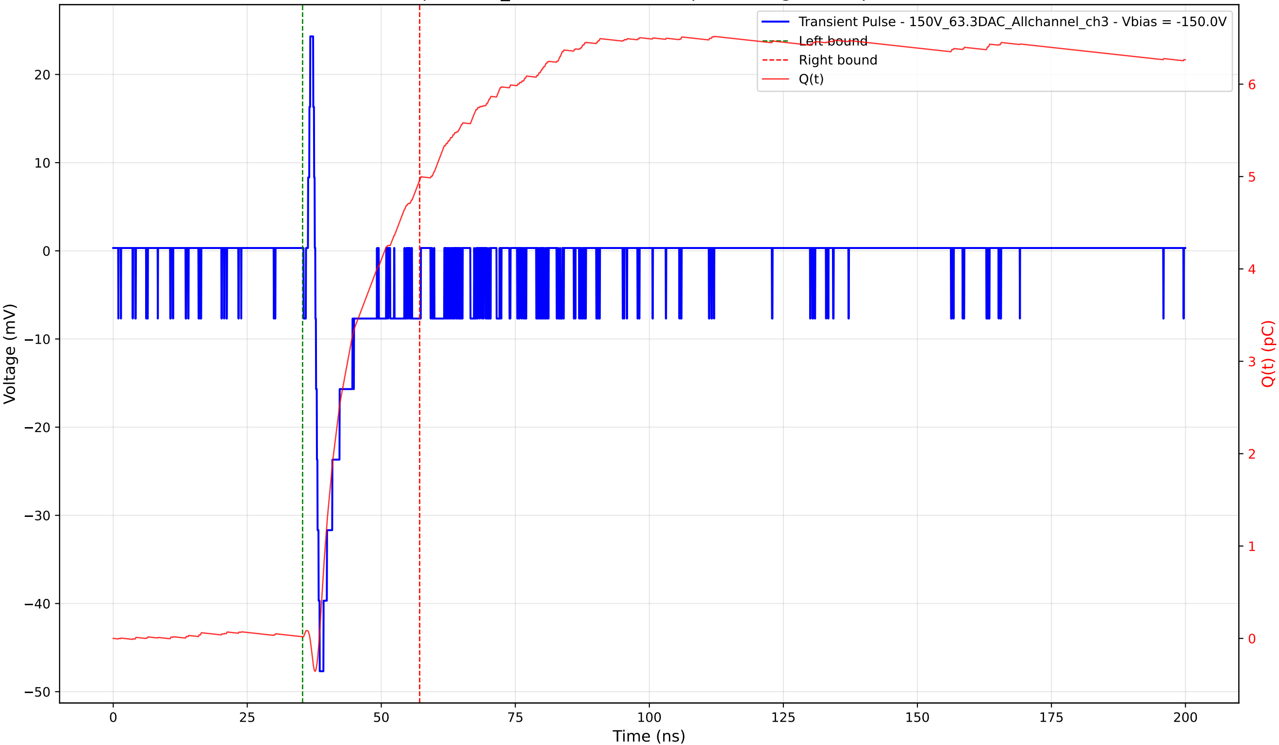
Transient Pulse - Sample: 1cm_42 - Position: 655.0 \mu\text{m} - Charge: 4.95 pC - Rise Time: 0.82 ns
