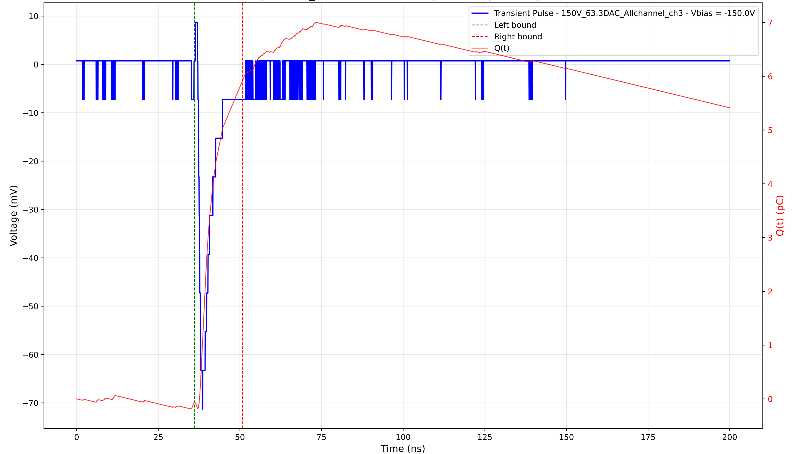
Transient Pulse - Sample: 1cm_42 - Position: 1320.0 \mu\text{m} - Charge: 6.00 pC - Rise Time: 1.32 ns
