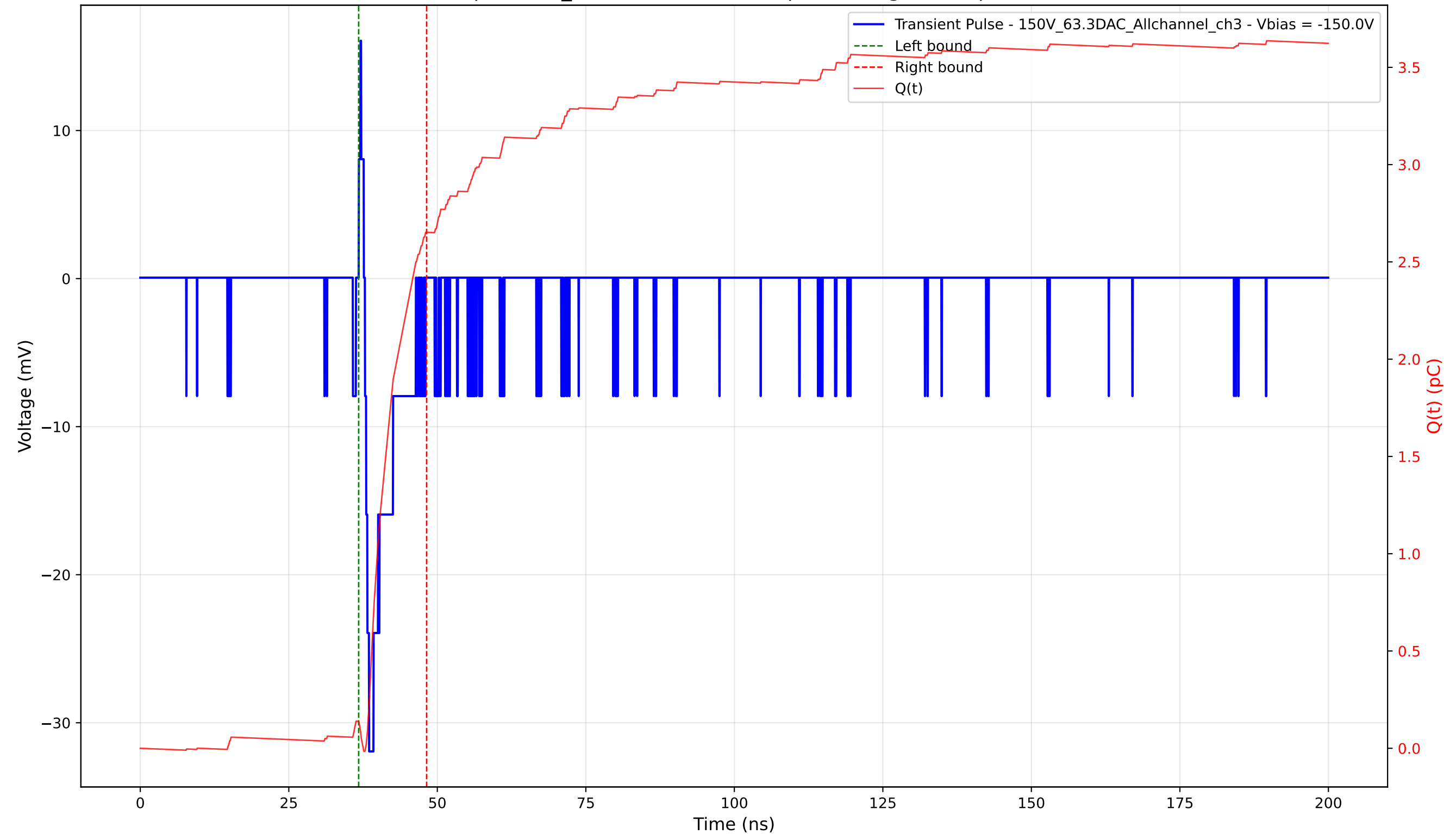
Transient Pulse - Sample: 1cm_42 - Position: 4875.0 \mu\text{m} - Charge: 2.51 pC - Rise Time: 0.70 ns
