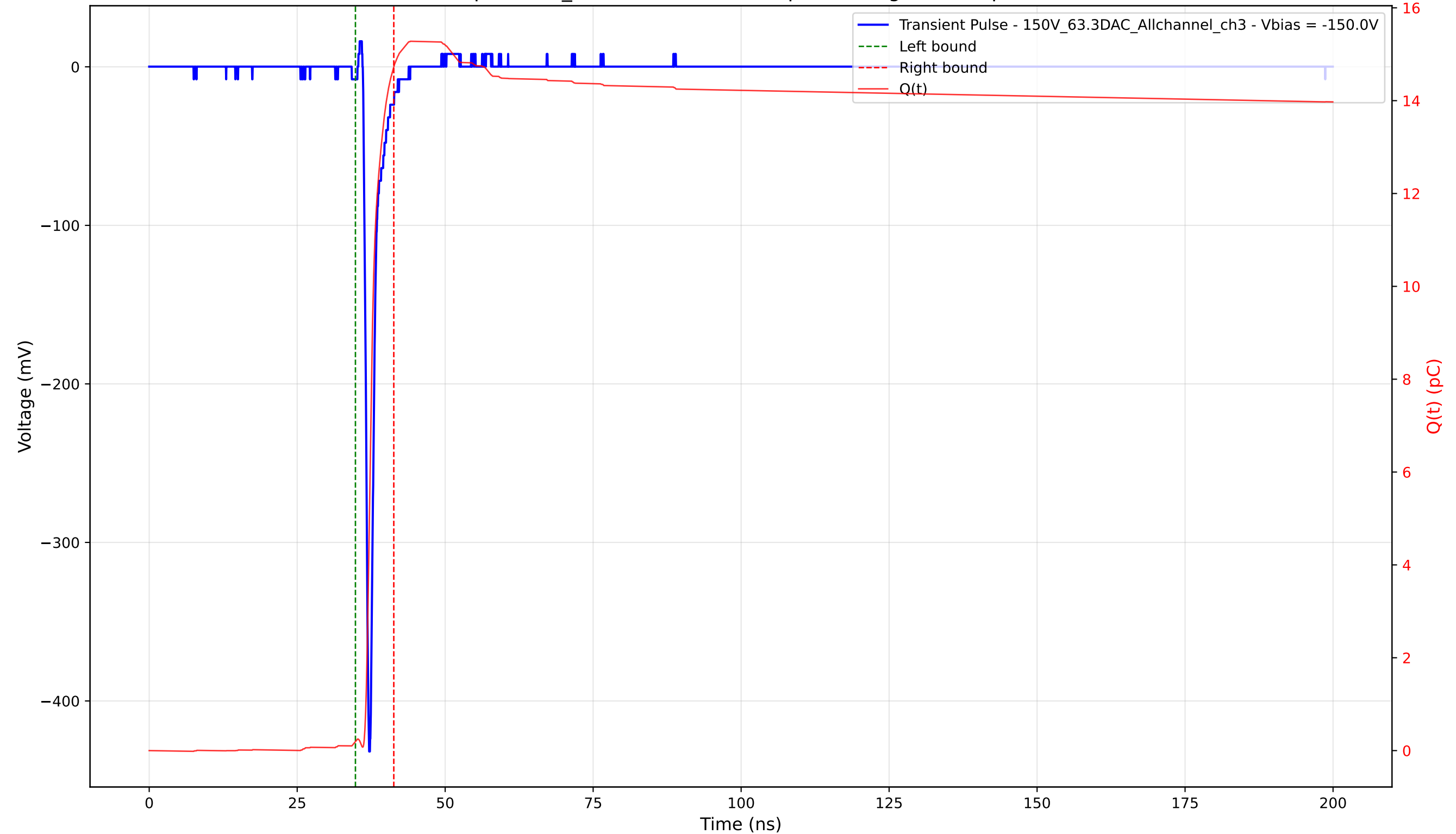
Transient Pulse - Sample: 1cm_42 - Position: 2220.0 \mu\text{m} - Charge: 14.54 pC - Rise Time: 0.70 ns
