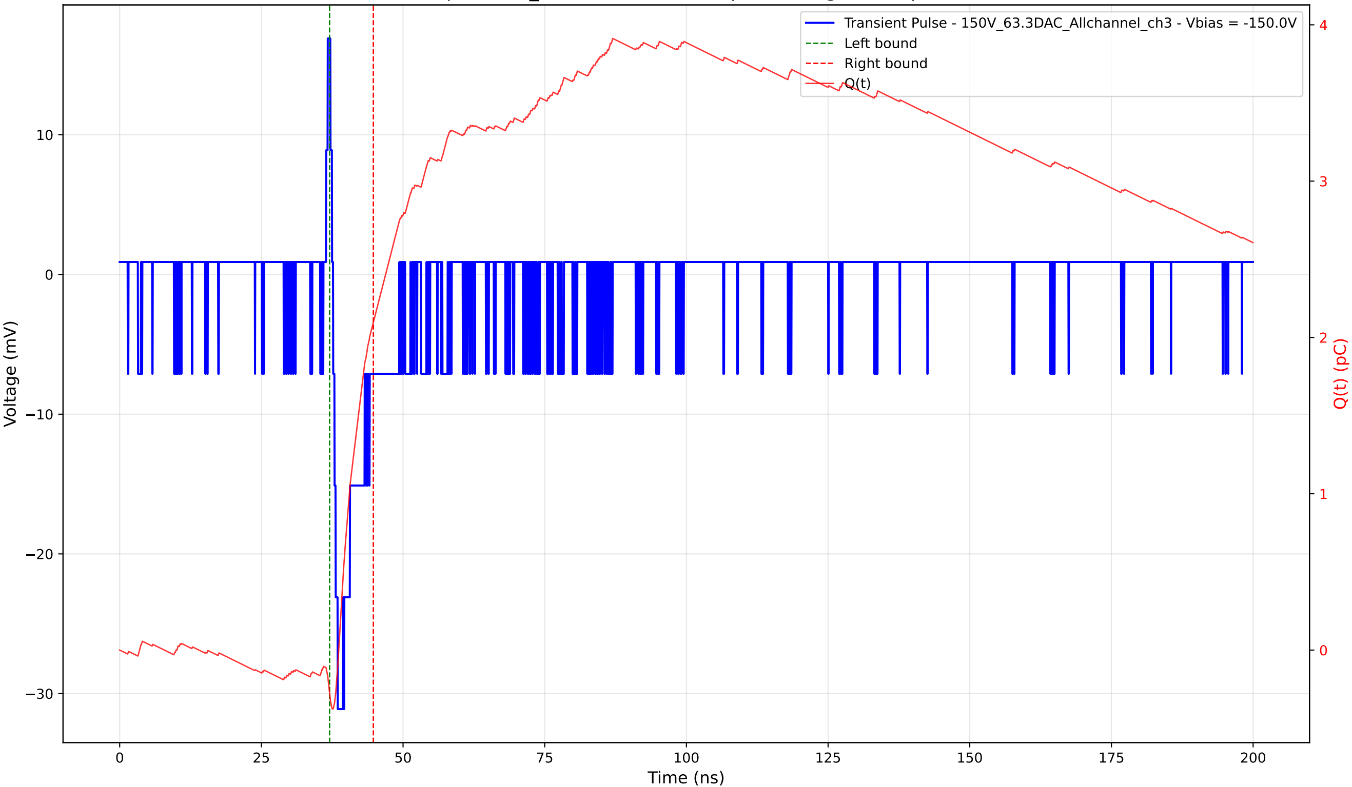
Transient Pulse - Sample: 1cm_42 - Position: 430.0 \mu\text{m} - Charge: 2.37 pC - Rise Time: 0.83 ns
