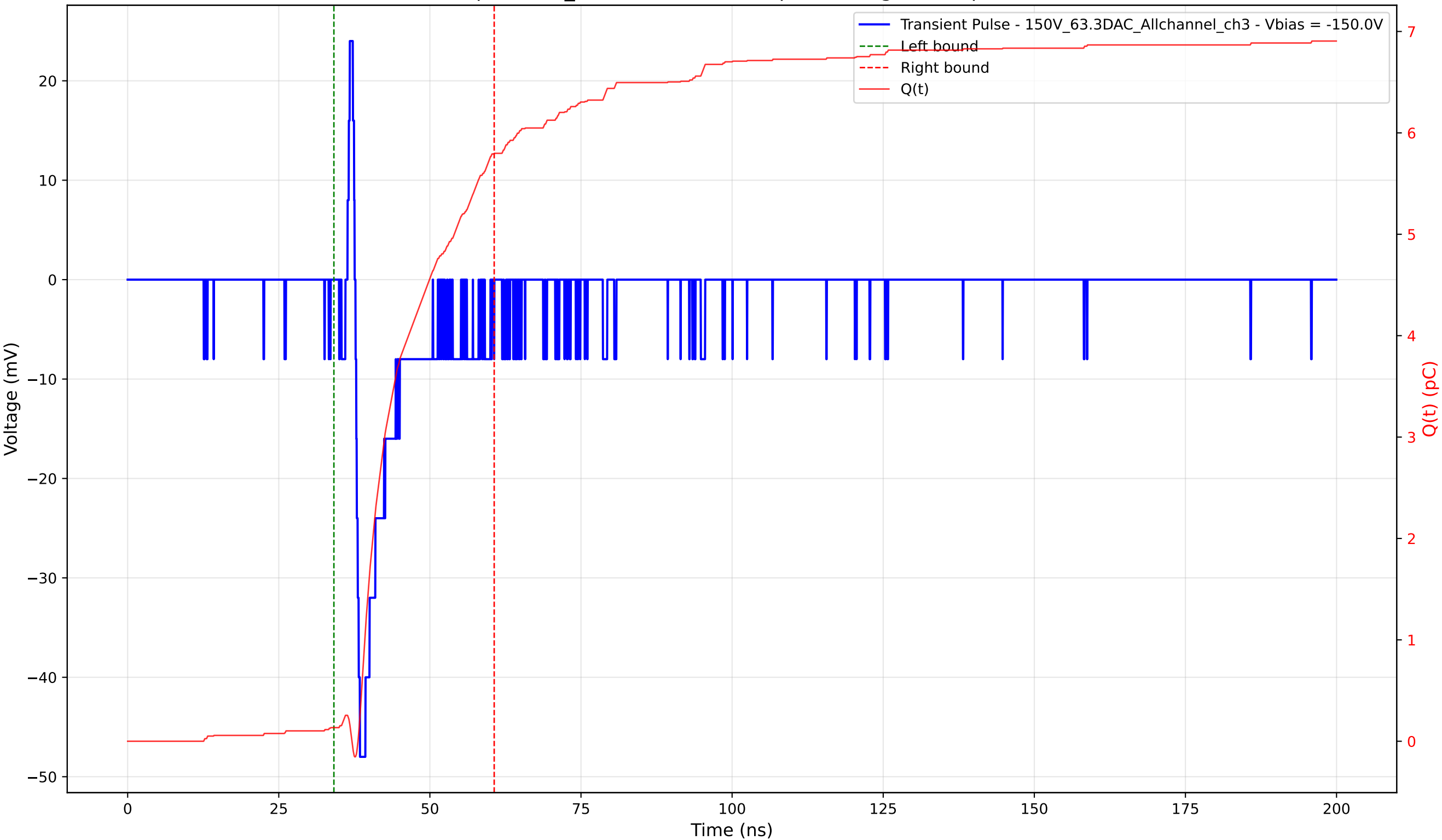
Transient Pulse - Sample: 1cm_42 - Position: 850.0 \mu\text{m} - Charge: 5.66 pC - Rise Time: 0.74 ns
