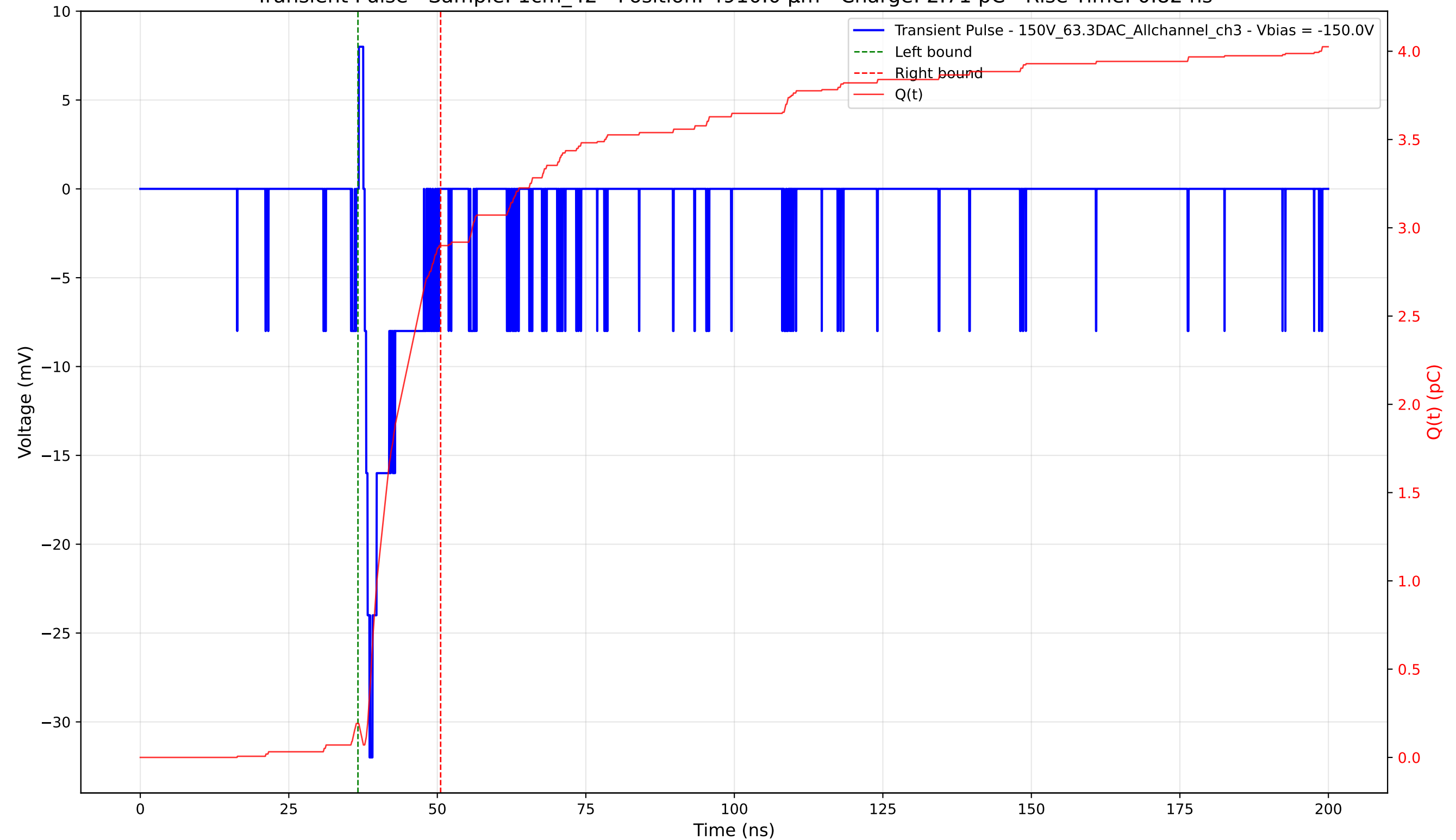
Transient Pulse - Sample: 1cm_42 - Position: 4910.0 \mu\text{m} - Charge: 2.71 pC - Rise Time: 0.82 ns
