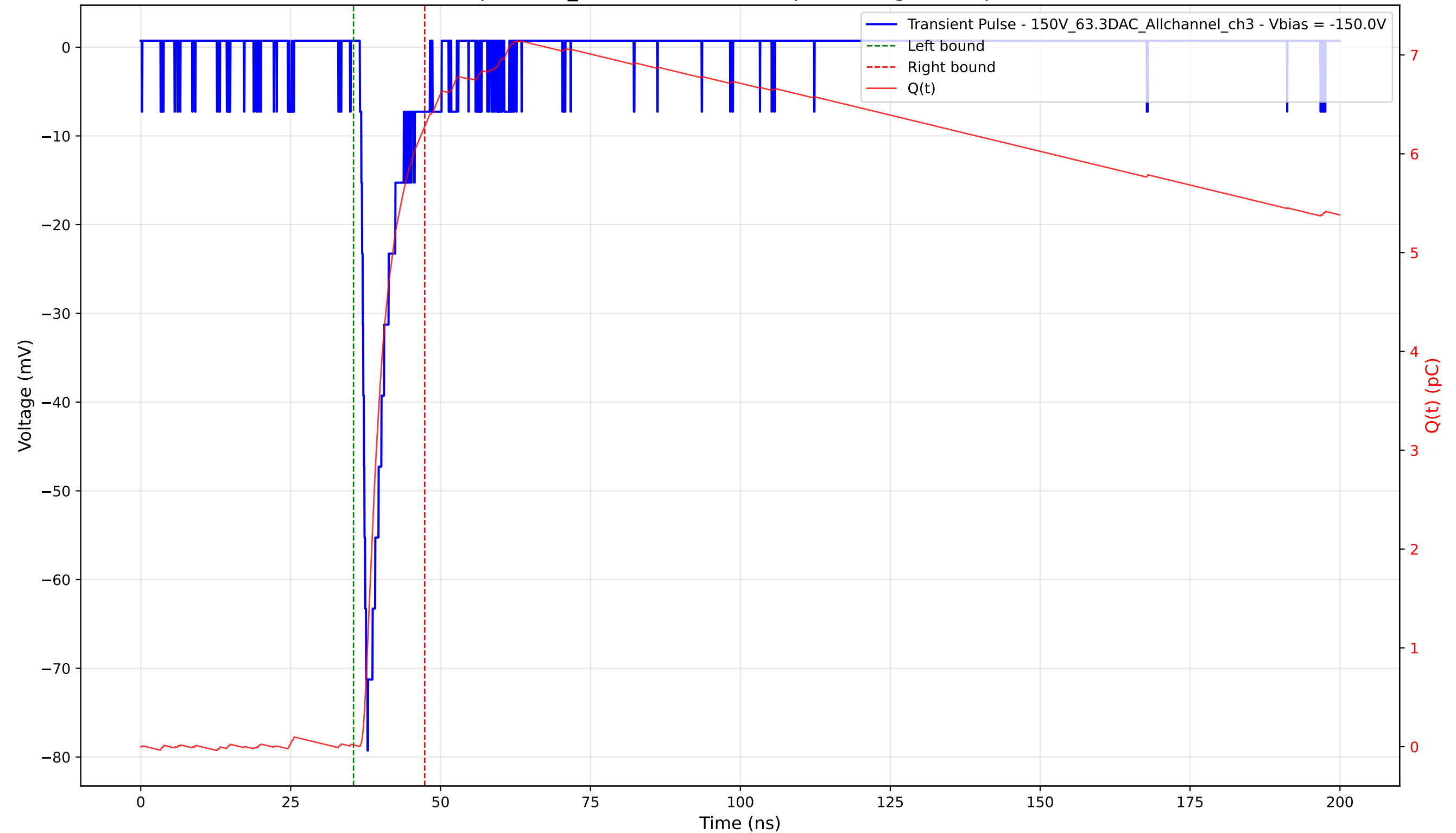
Transient Pulse - Sample: 1cm_42 - Position: 1520.0 \mu\text{m} - Charge: 6.26 pC - Rise Time: 1.08 ns
