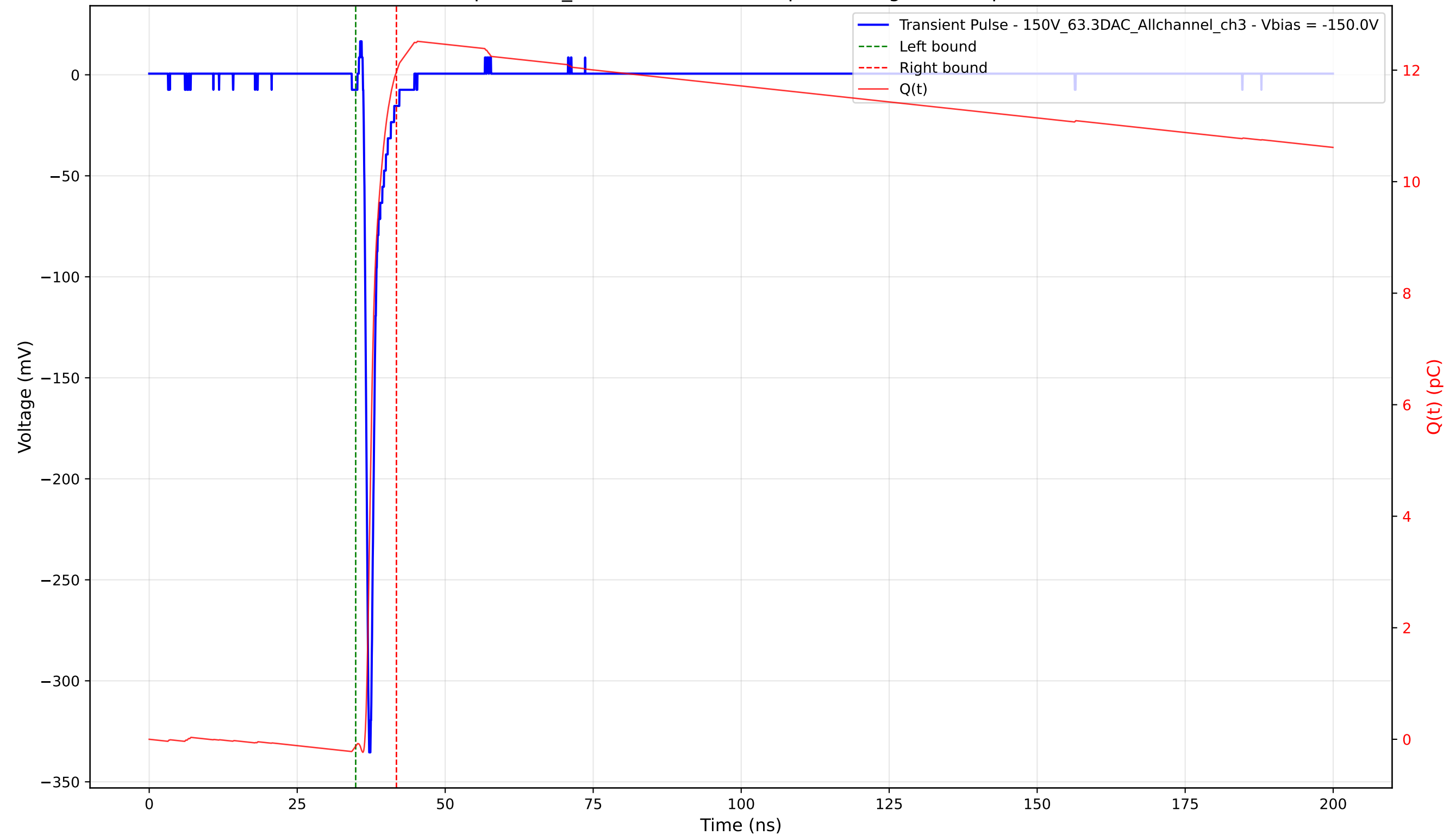
Transient Pulse - Sample: 1cm_42 - Position: 2140.0 \mu\text{m} - Charge: 12.09 pC - Rise Time: 0.73 ns
