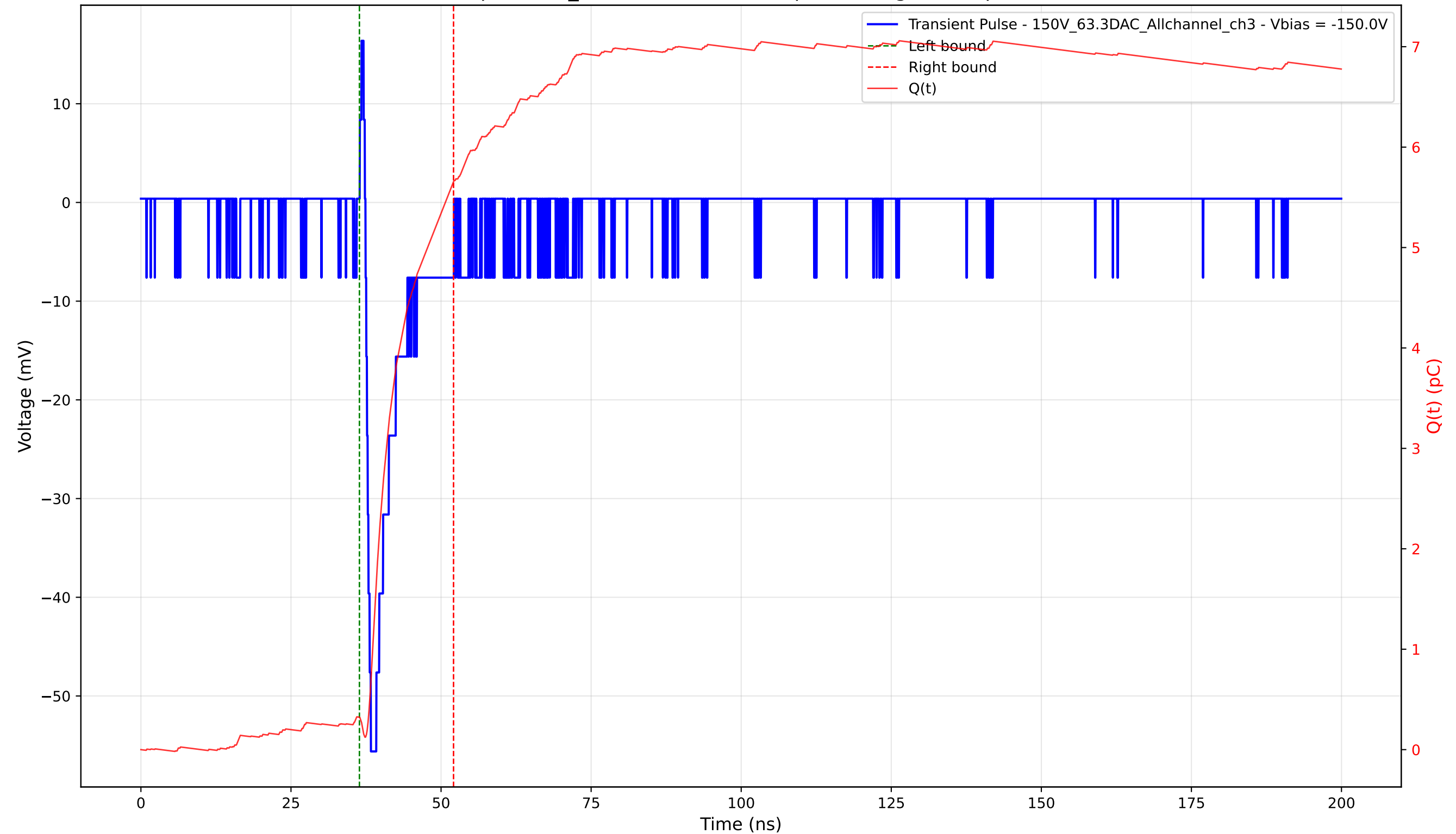
Transient Pulse - Sample: 1cm_42 - Position: 1100.0 \mu\text{m} - Charge: 5.34 pC - Rise Time: 0.89 ns
