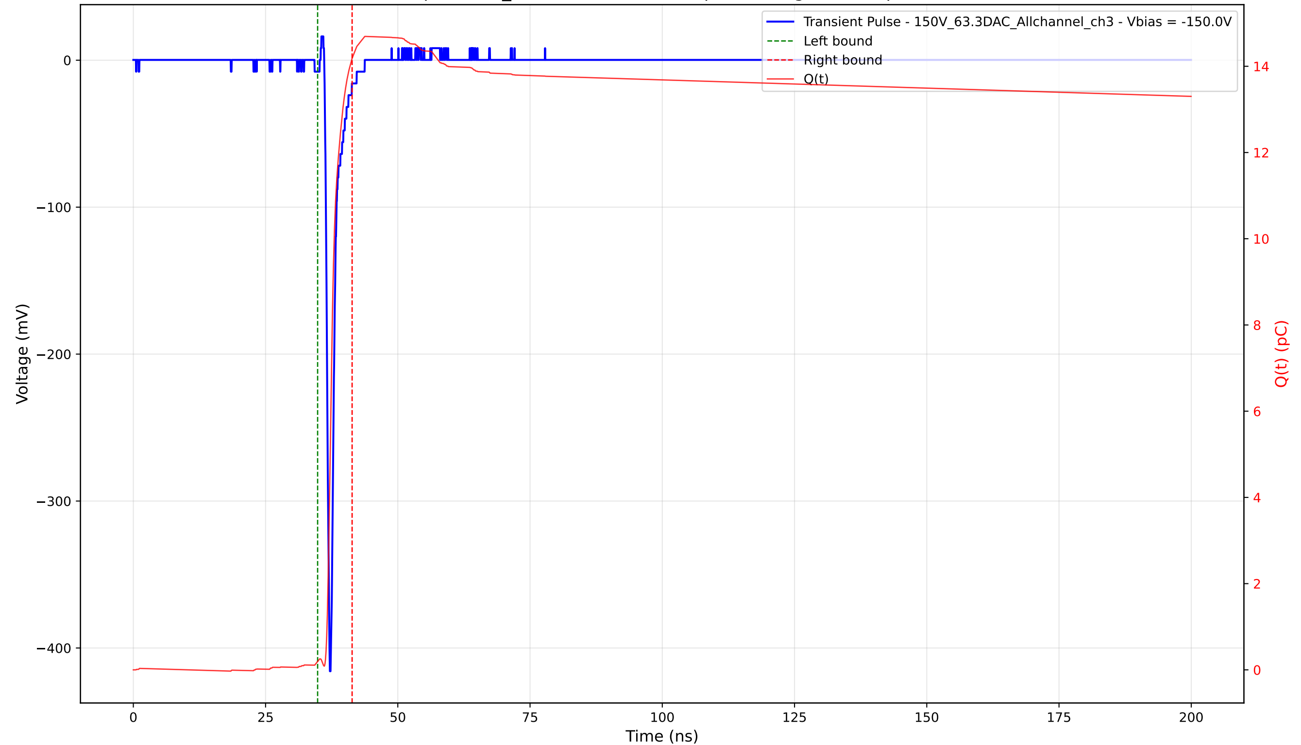
Transient Pulse - Sample: 1cm_42 - Position: 2210.0 \mu\text{m} - Charge: 13.99 pC - Rise Time: 0.75 ns
