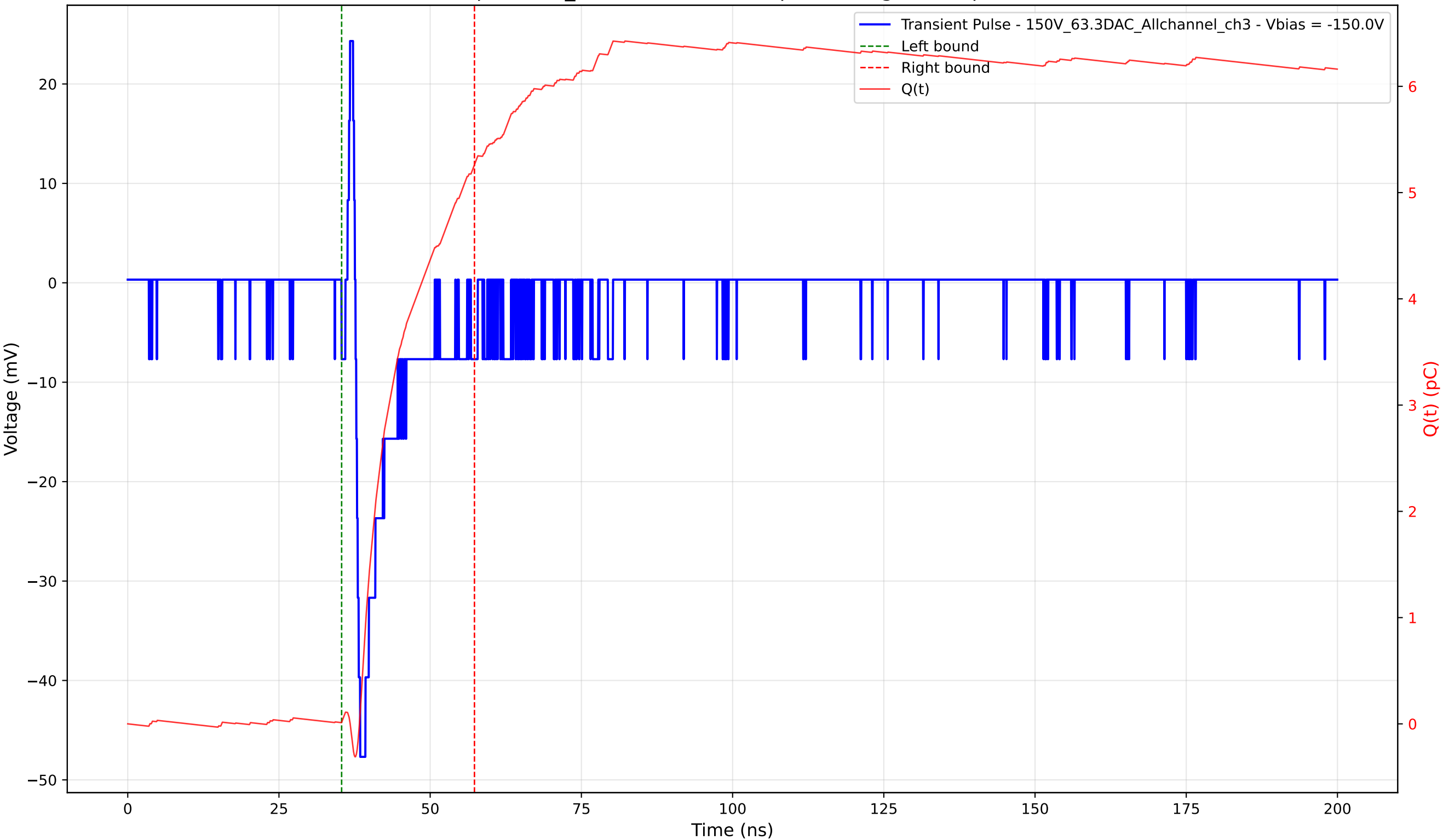
Transient Pulse - Sample: 1cm_42 - Position: 885.0 \mu\text{m} - Charge: 5.25 pC - Rise Time: 0.78 ns
