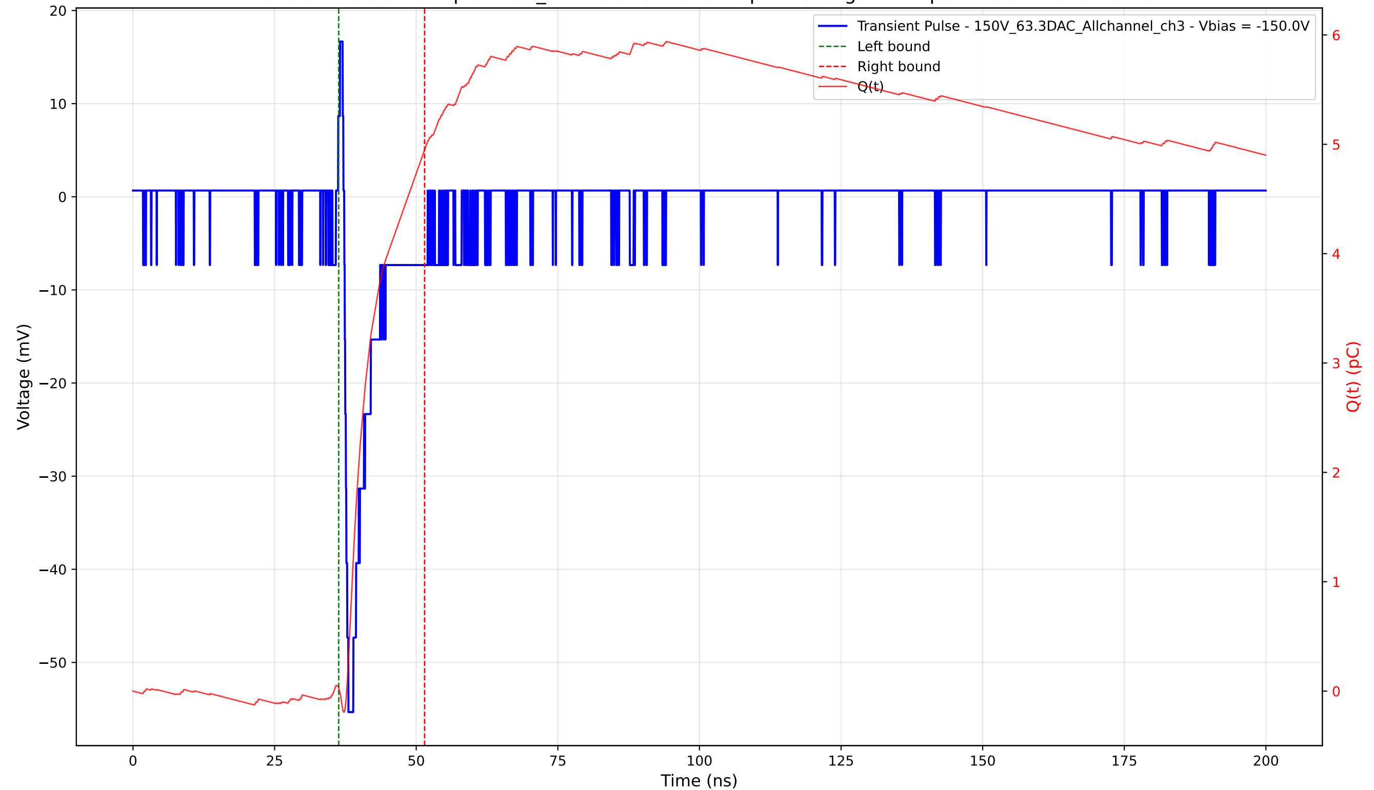
Transient Pulse - Sample: 1cm_42 - Position: 3750.0 \mu\text{m} - Charge: 4.92 pC - Rise Time: 0.73 ns
