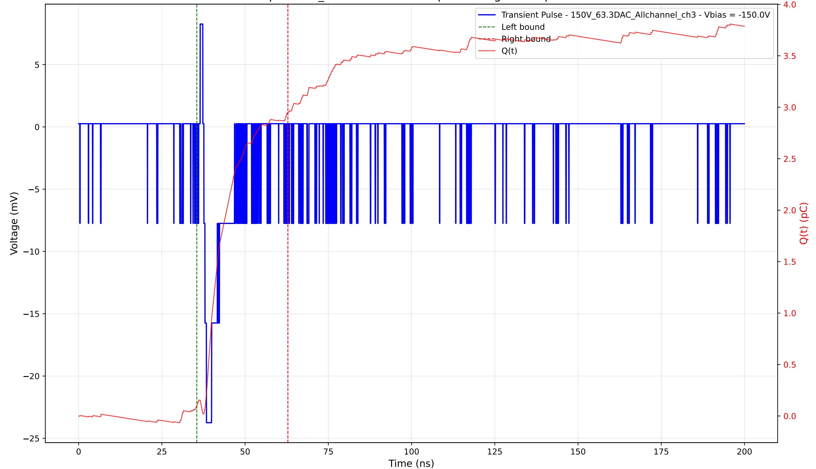
Transient Pulse - Sample: 1cm_42 - Position: 275.0 \mu\text{m} - Charge: 2.85 pC - Rise Time: 0.79 ns
