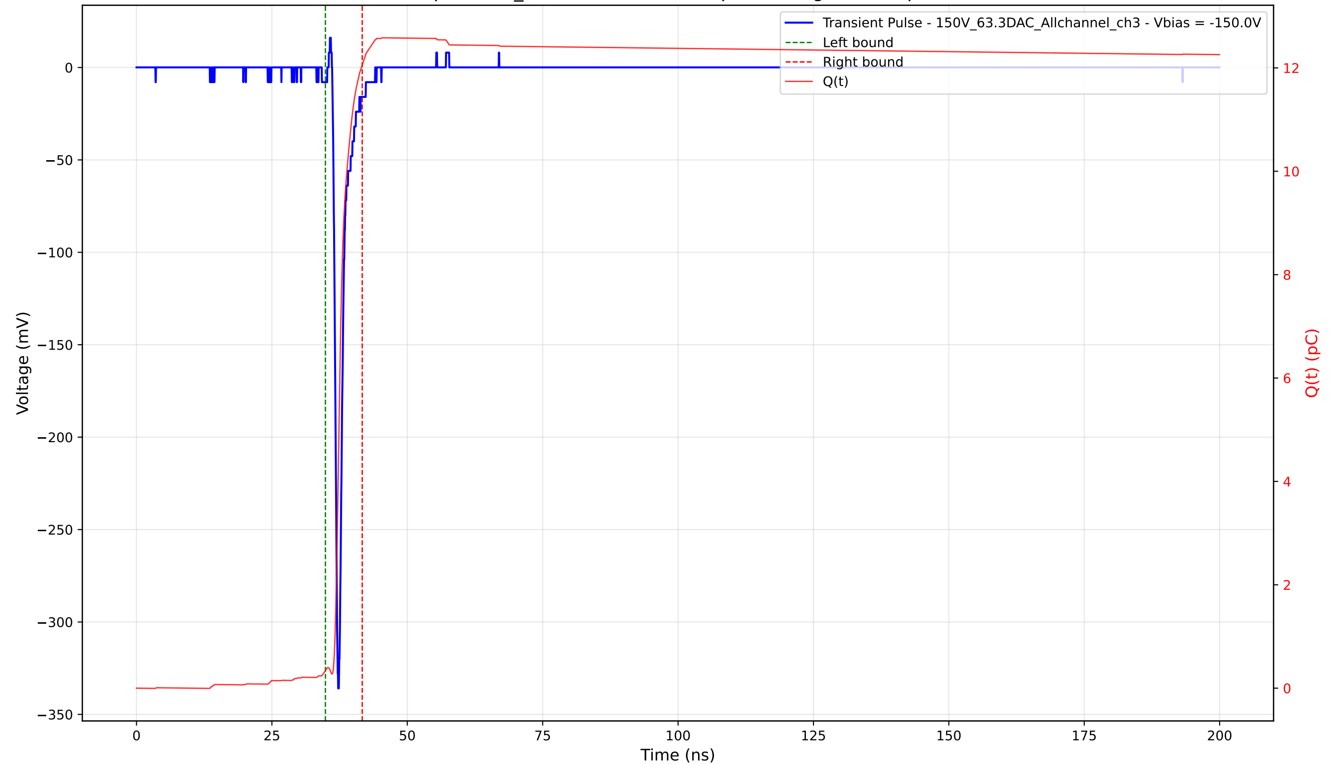
Transient Pulse - Sample: 1cm_42 - Position: 2905.0 \mu\text{m} - Charge: 11.72 pC - Rise Time: 0.74 ns
