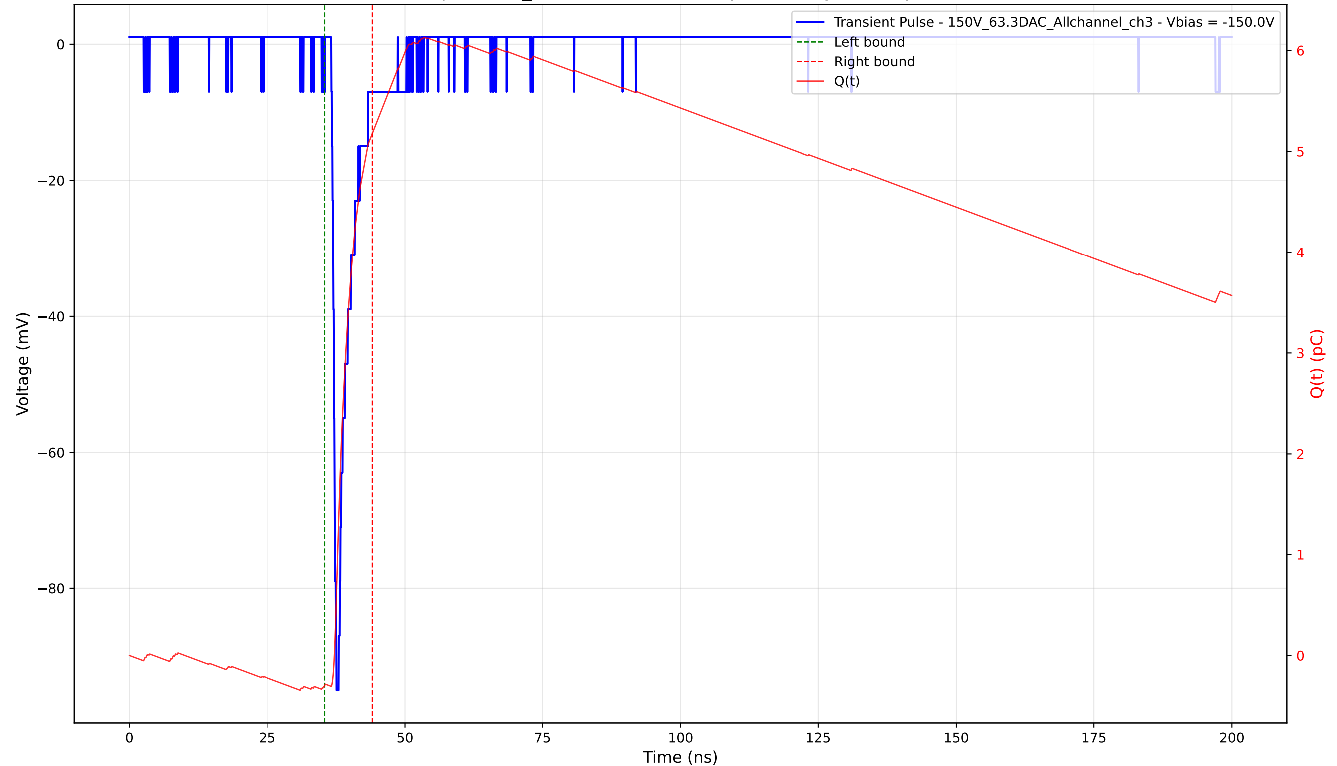
Transient Pulse - Sample: 1cm_42 - Position: 3425.0 \mu\text{m} - Charge: 5.47 pC - Rise Time: 0.75 ns
