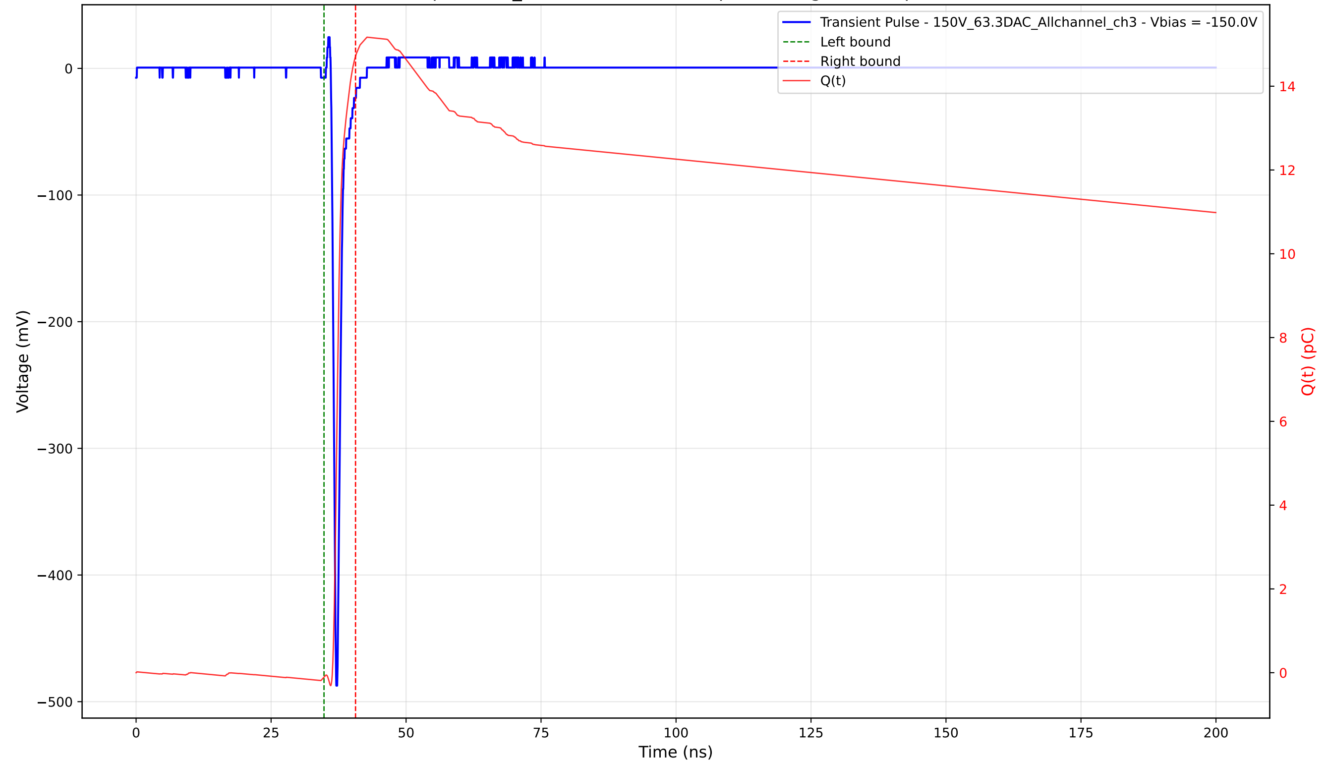
Transient Pulse - Sample: 1cm_42 - Position: 2470.0 \mu\text{m} - Charge: 14.82 pC - Rise Time: 0.71 ns
