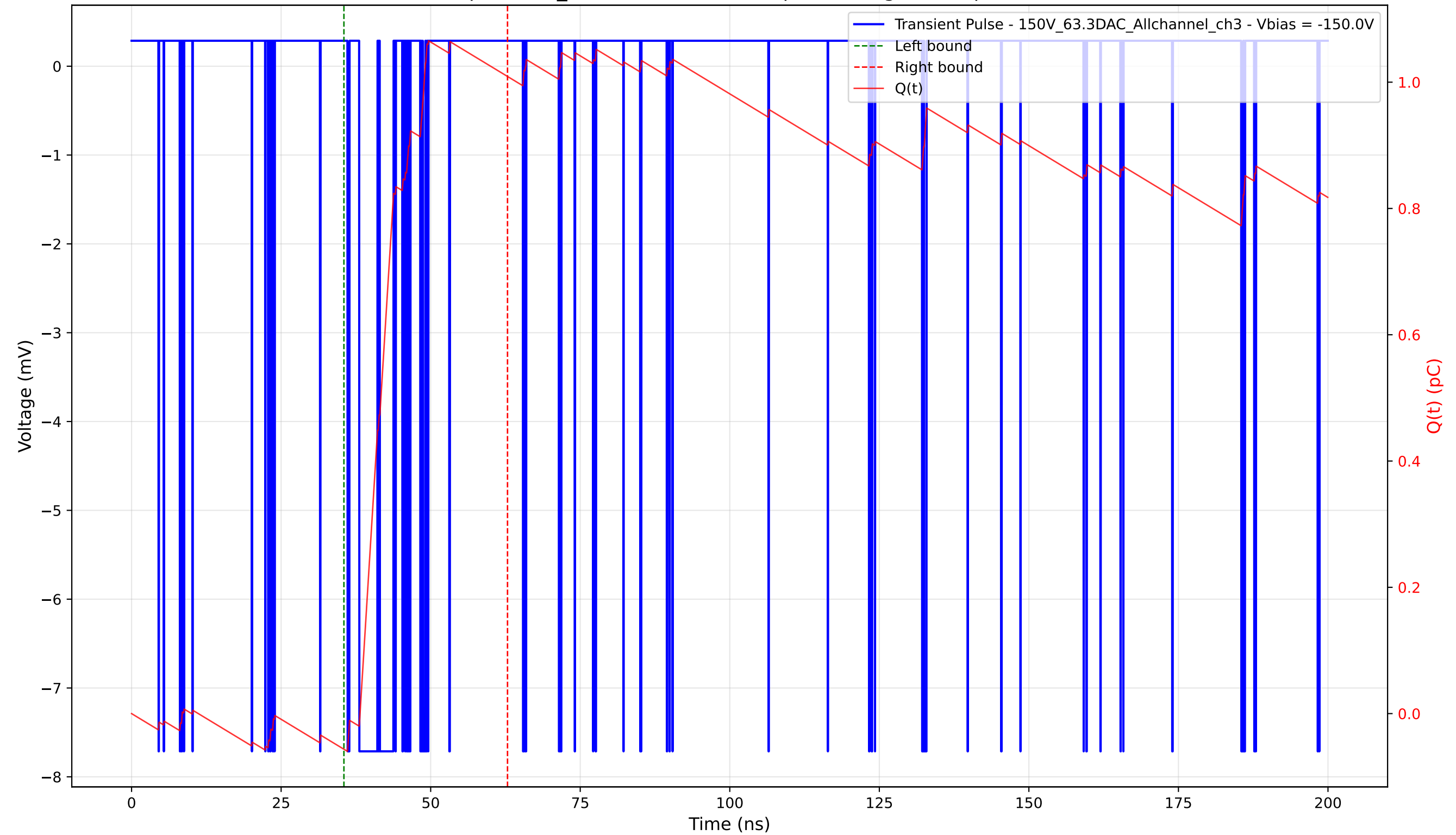
Transient Pulse - Sample: 1cm_42 - Position: 5130.0 \mu\text{m} - Charge: 1.07 pC - Rise Time: 0.04 ns
