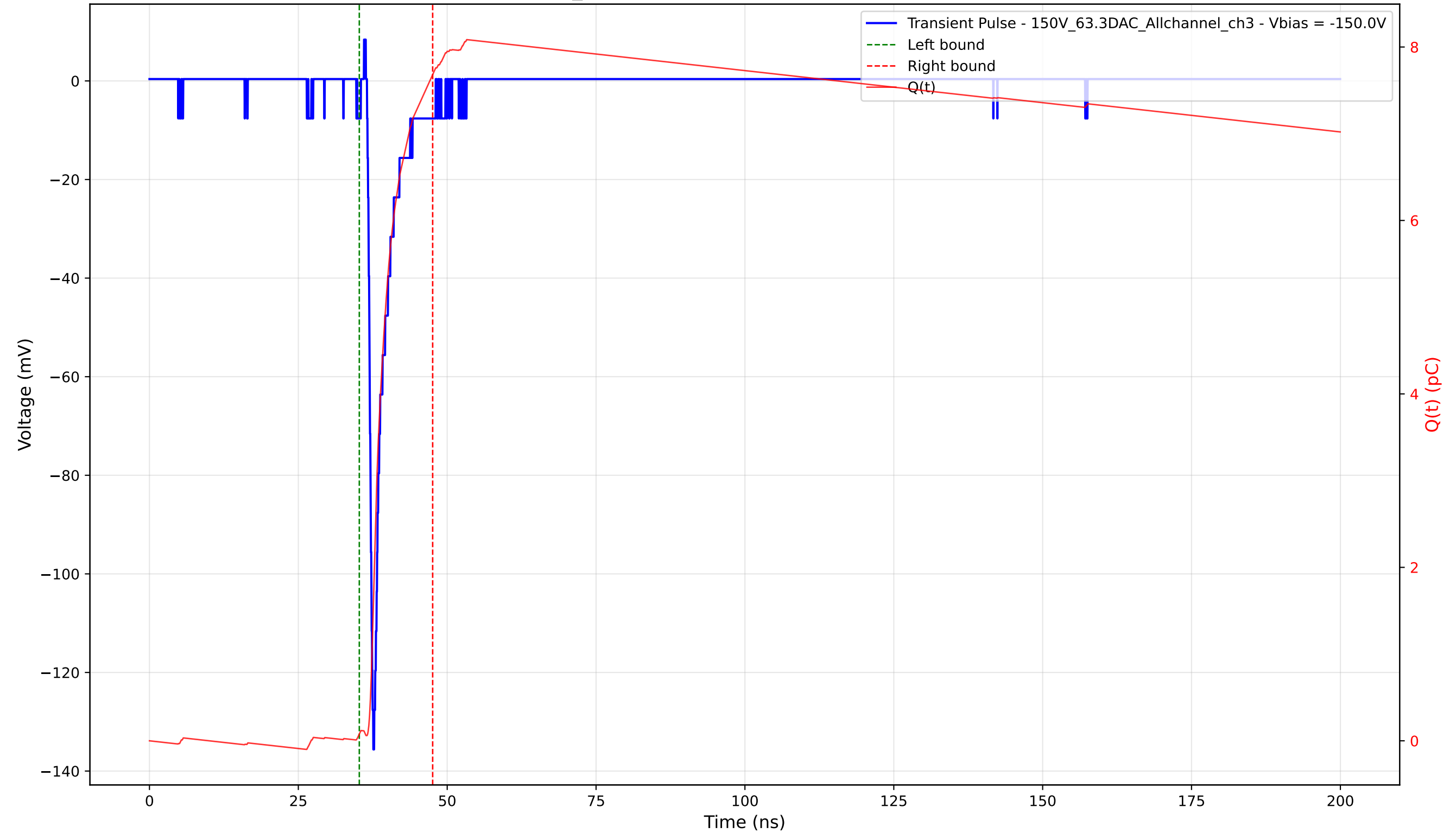
Transient Pulse - Sample: 1cm_42 - Position: 3315.0 \mu\text{m} - Charge: 7.60 pC - Rise Time: 0.85 ns
