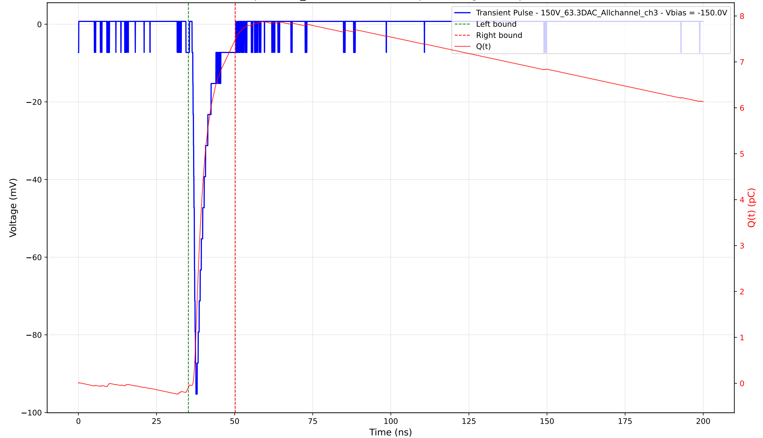
Transient Pulse - Sample: 1cm_42 - Position: 1585.0 \mu\text{m} - Charge: 7.58 pC - Rise Time: 0.87 ns
