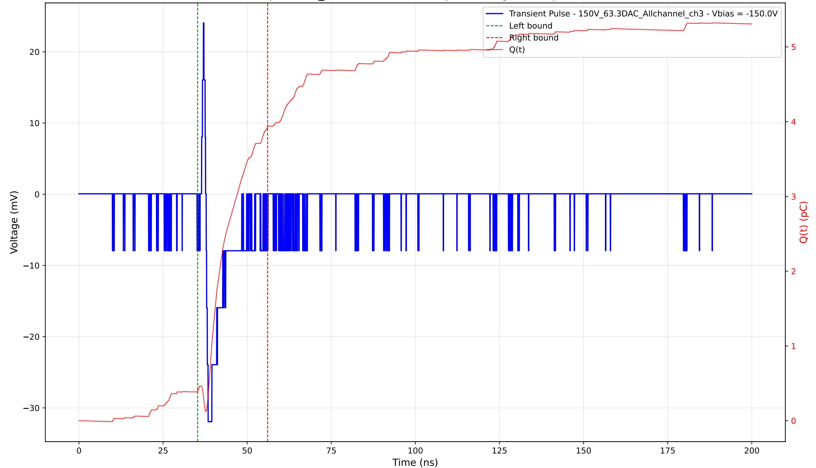
Transient Pulse - Sample: 1cm_42 - Position: 4440.0 \mu\text{m} - Charge: 3.52 pC - Rise Time: 0.58 ns
