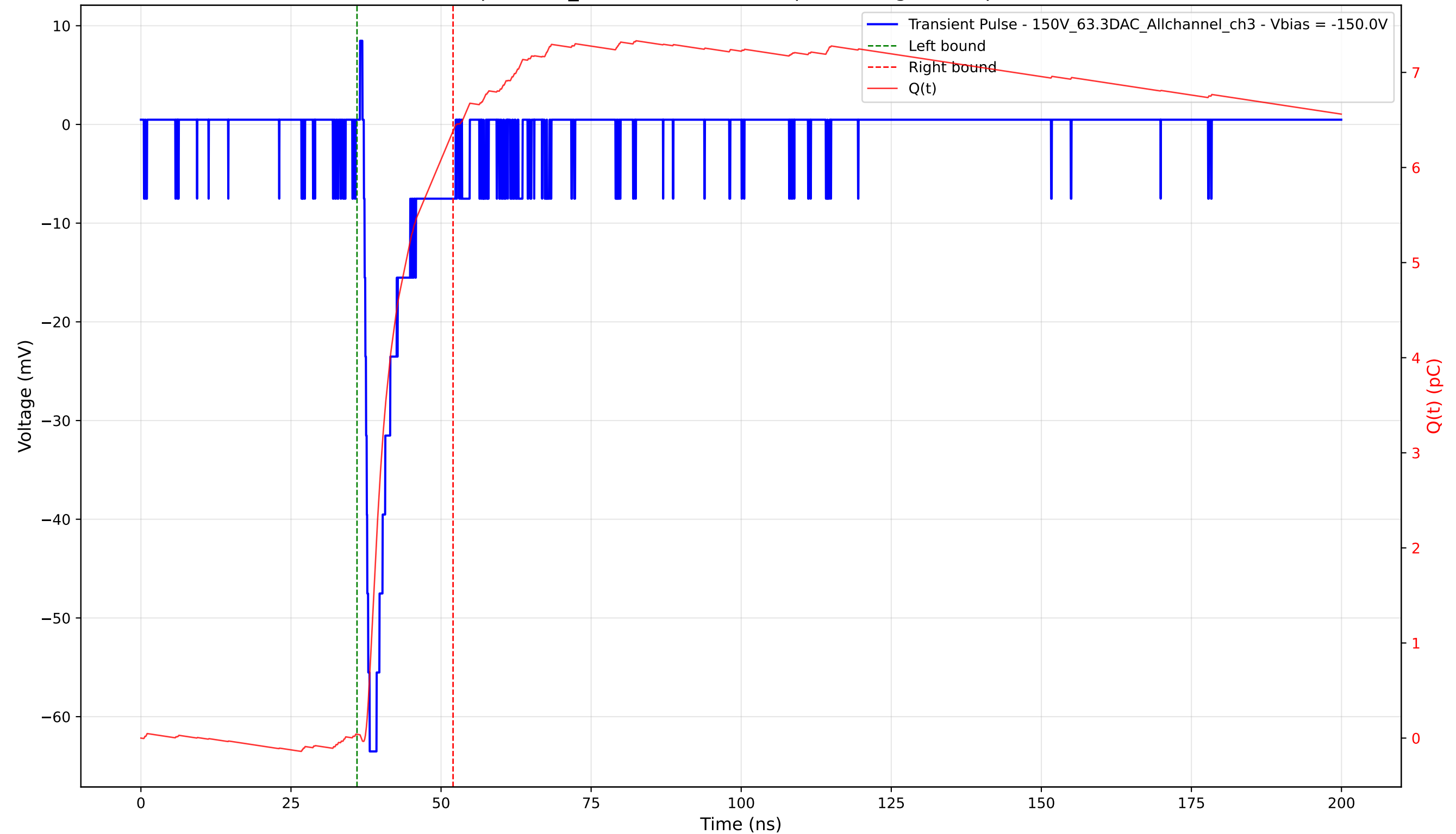
Transient Pulse - Sample: 1cm_42 - Position: 1340.0 \mu\text{m} - Charge: 6.35 pC - Rise Time: 0.97 ns
