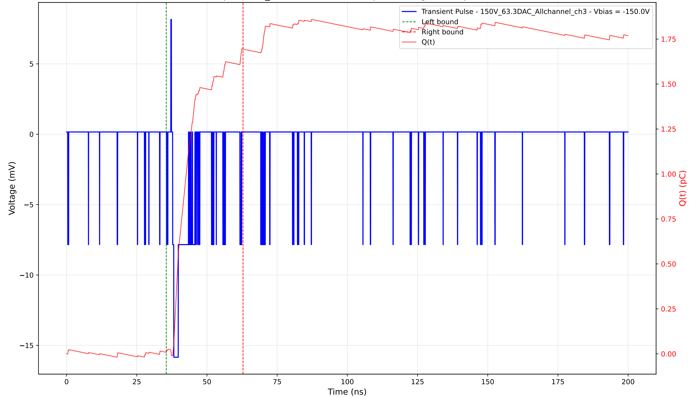
Transient Pulse - Sample: 1cm_42 - Position: 5030.0 \mu\text{m} - Charge: 1.69 pC - Rise Time: 0.43 ns
