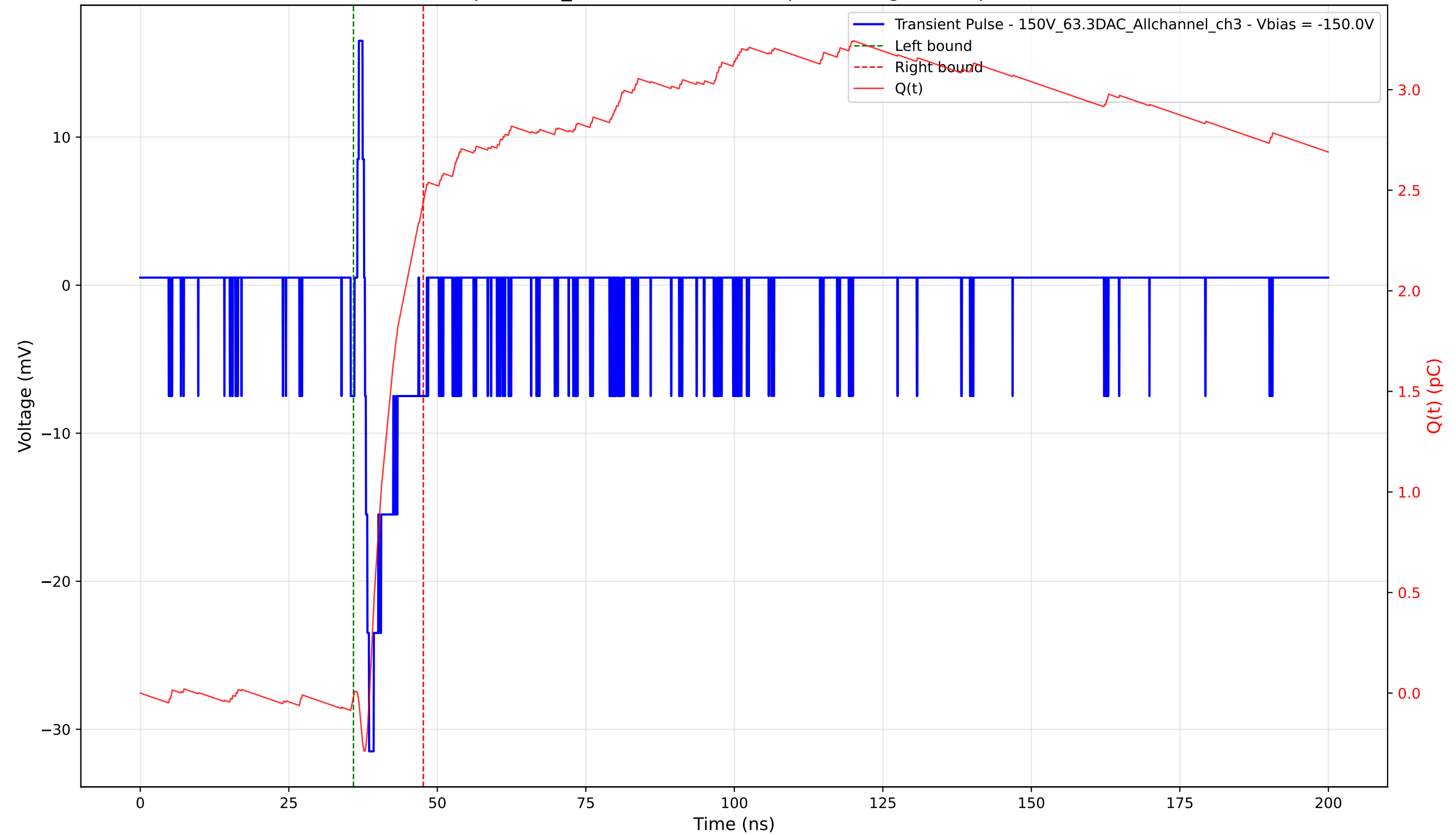
Transient Pulse - Sample: 1cm_42 - Position: 4500.0 \mu\text{m} - Charge: 2.46 pC - Rise Time: 0.70 ns
