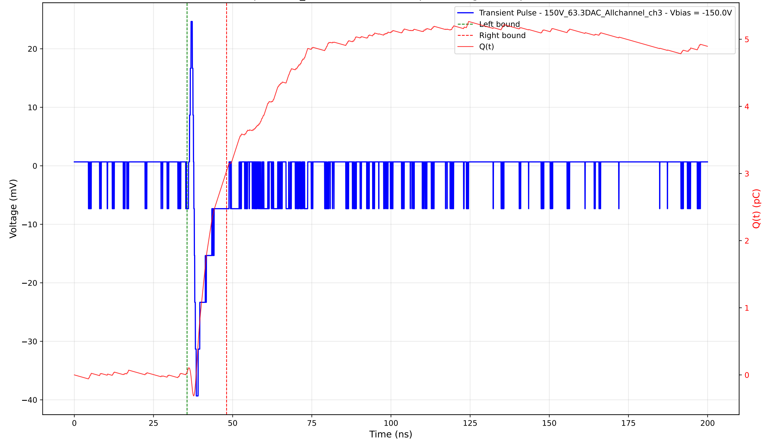
Transient Pulse - Sample: 1cm_42 - Position: 4375.0 \mu\text{m} - Charge: 3.00 pC - Rise Time: 0.78 ns
