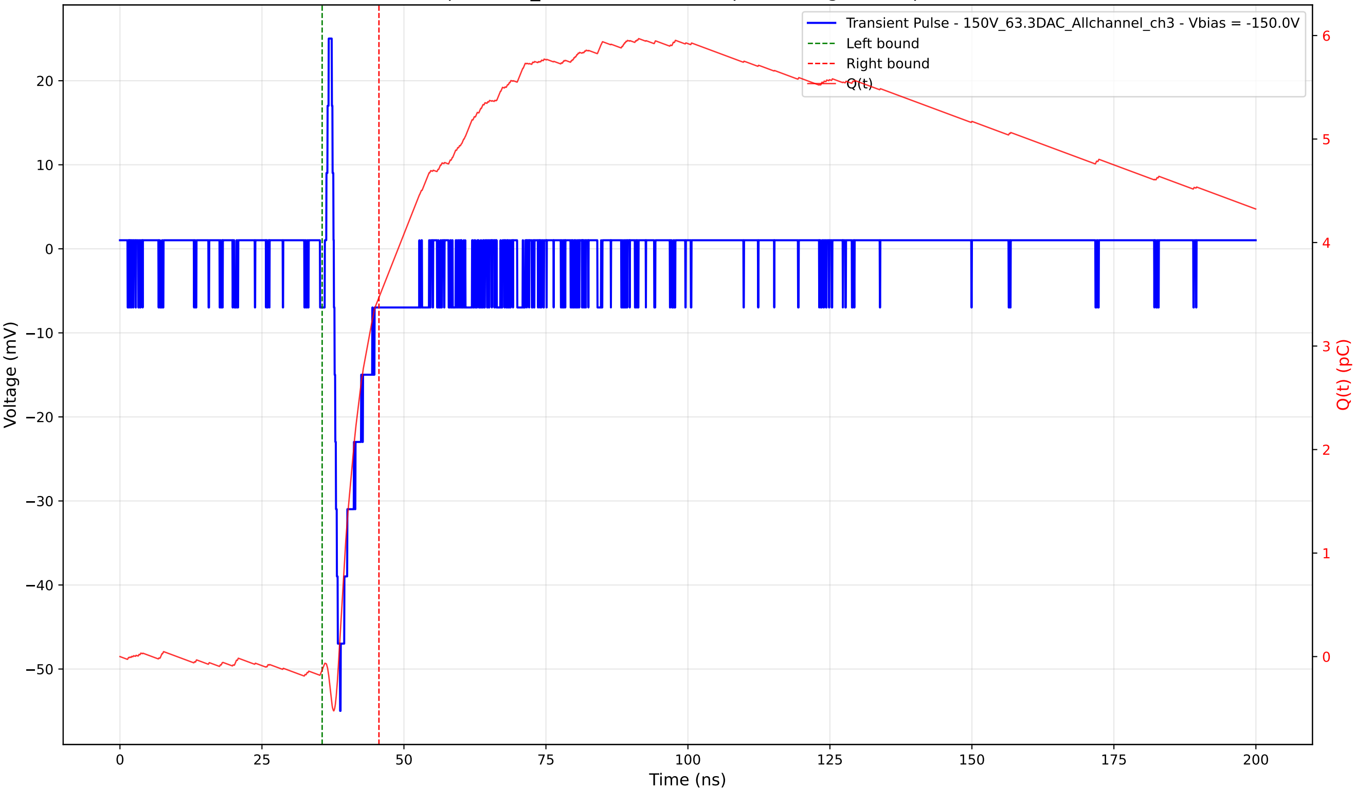
Transient Pulse - Sample: 1cm_42 - Position: 830.0 \mu\text{m} - Charge: 3.60 pC - Rise Time: 1.09 ns
