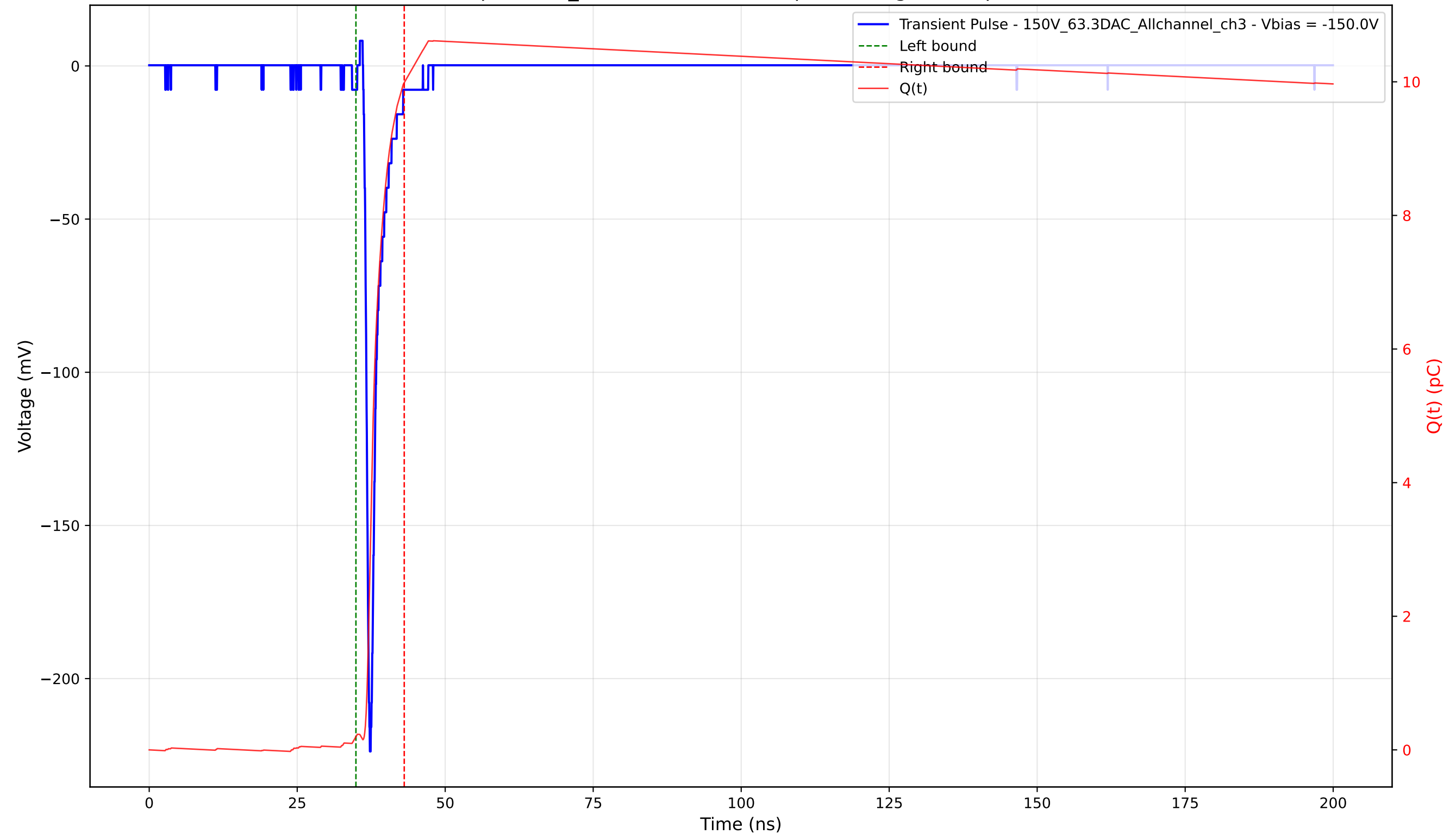
Transient Pulse - Sample: 1cm_42 - Position: 2000.0 \mu\text{m} - Charge: 9.79 pC - Rise Time: 0.81 ns
