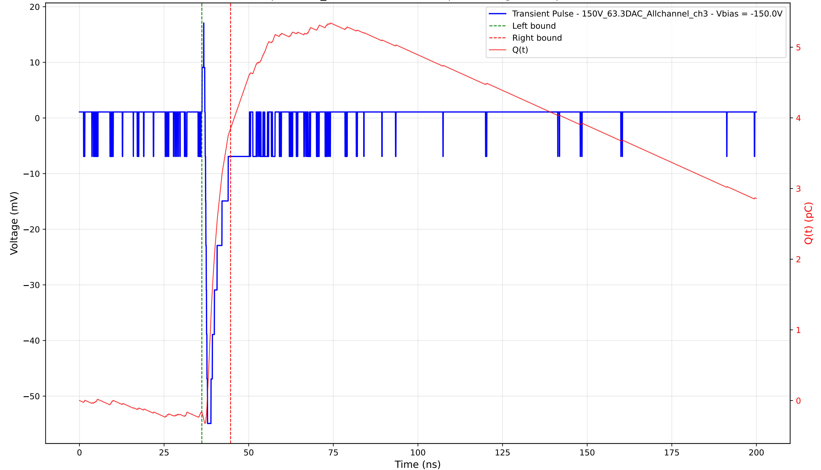
Transient Pulse - Sample: 1cm_42 - Position: 3665.0 \mu\text{m} - Charge: 4.02 pC - Rise Time: 0.69 ns
