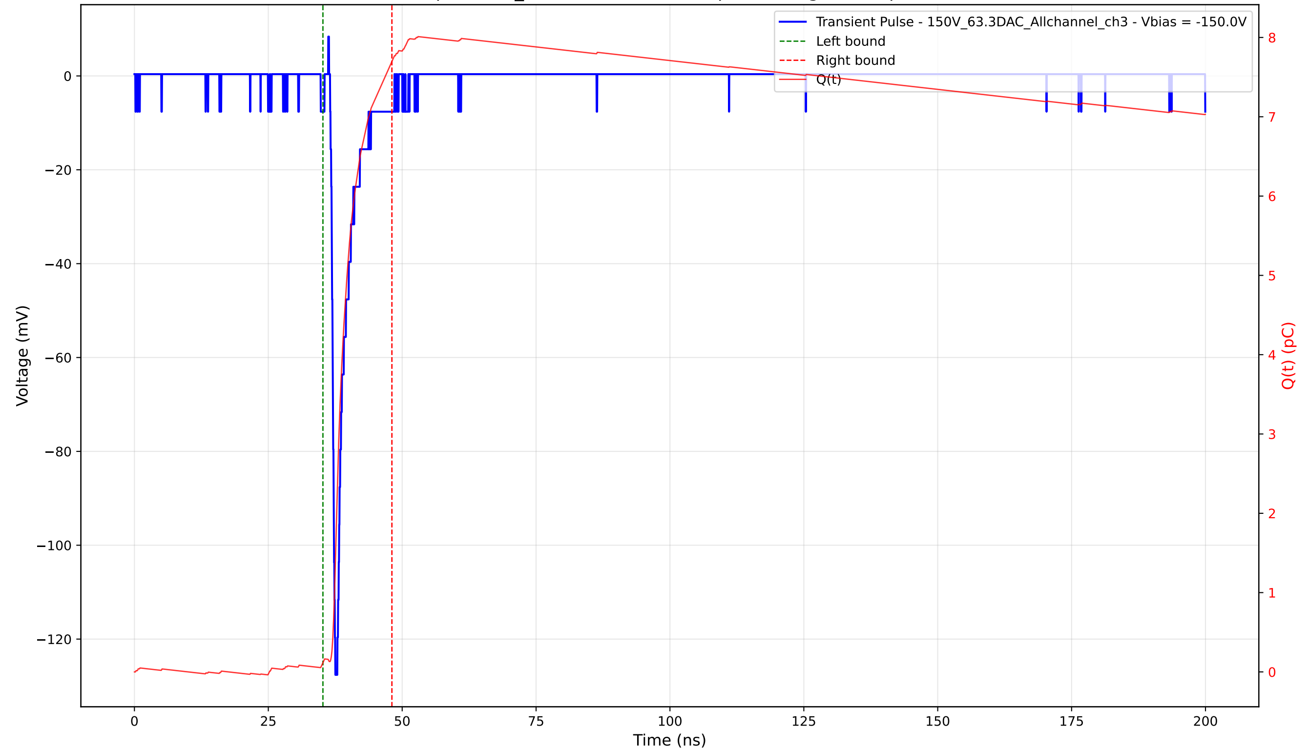
Transient Pulse - Sample: 1cm_42 - Position: 3325.0 \mu\text{m} - Charge: 7.58 pC - Rise Time: 0.81 ns
