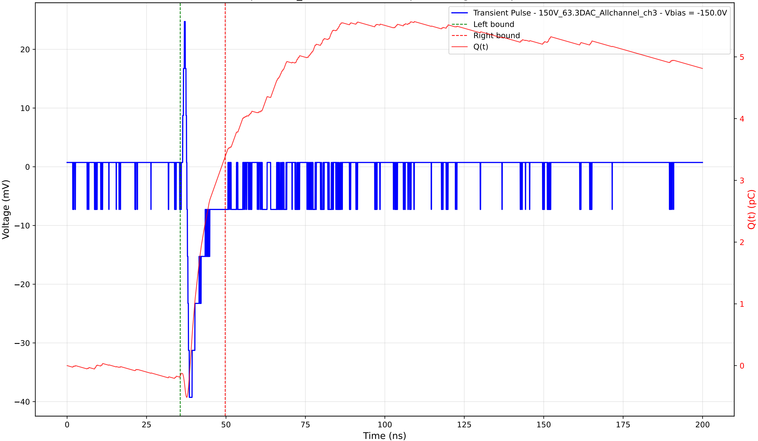
Transient Pulse - Sample: 1cm_42 - Position: 550.0 \mu\text{m} - Charge: 3.55 pC - Rise Time: 0.78 ns
