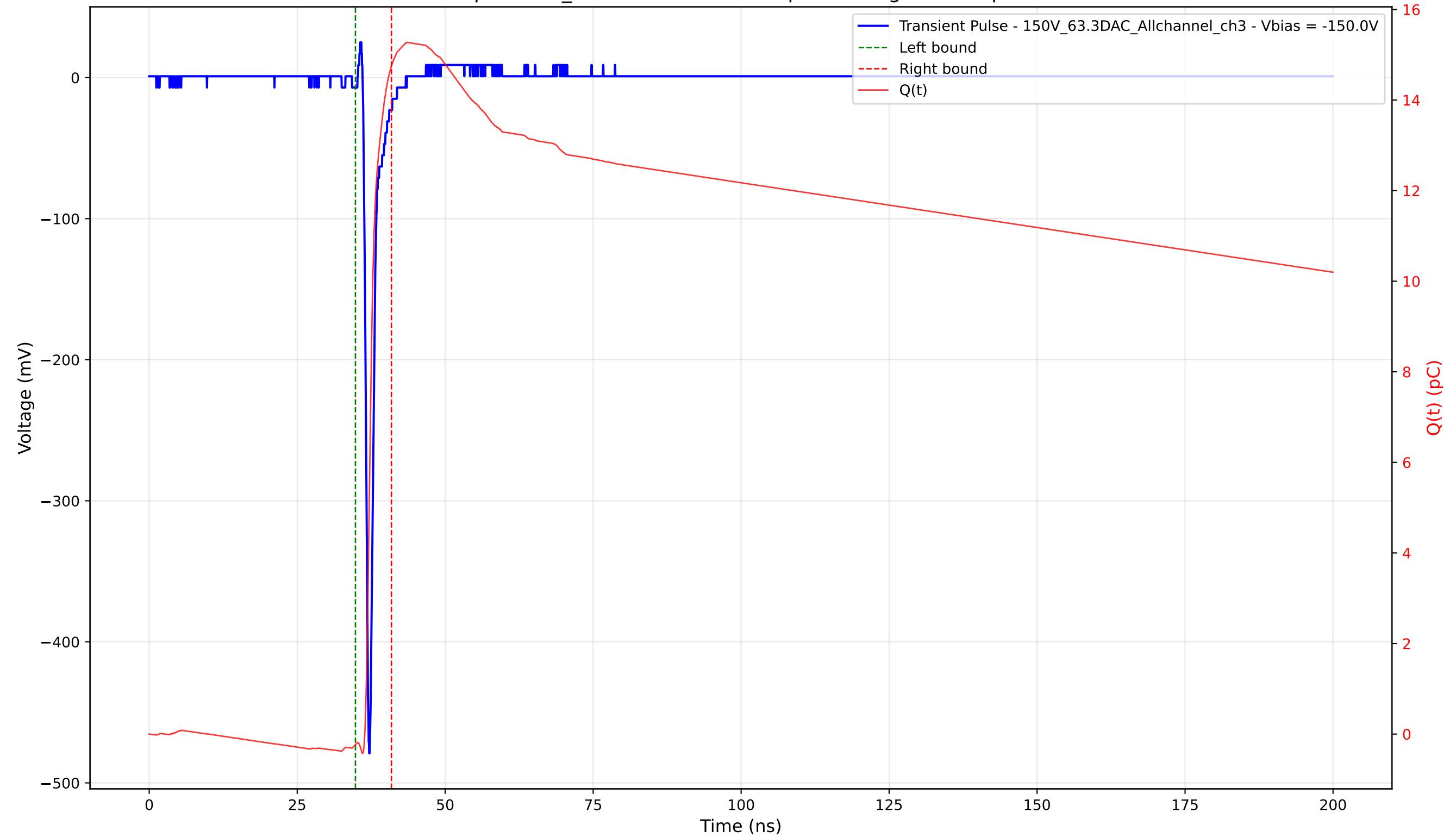
Transient Pulse - Sample: 1cm_42 - Position: 2365.0 \mu\text{m} - Charge: 14.98 pC - Rise Time: 0.70 ns
