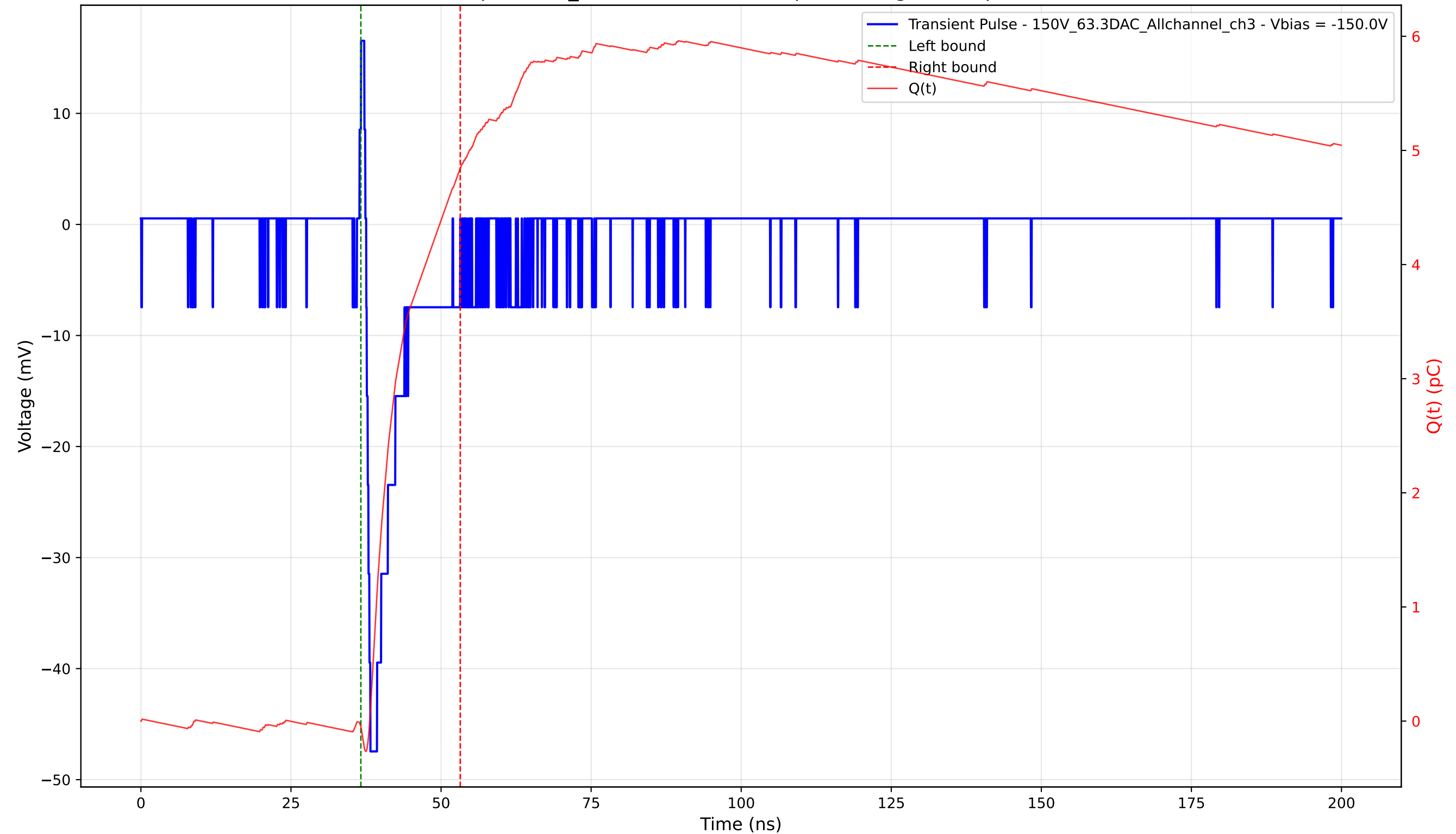
Transient Pulse - Sample: 1cm_42 - Position: 1030.0 \mu\text{m} - Charge: 4.89 pC - Rise Time: 0.70 ns
