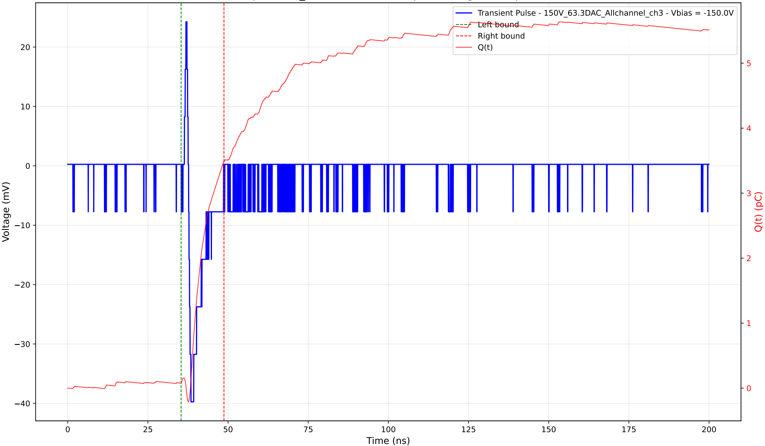
Transient Pulse - Sample: 1cm_42 - Position: 555.0 \mu\text{m} - Charge: 3.41 pC - Rise Time: 0.74 ns
