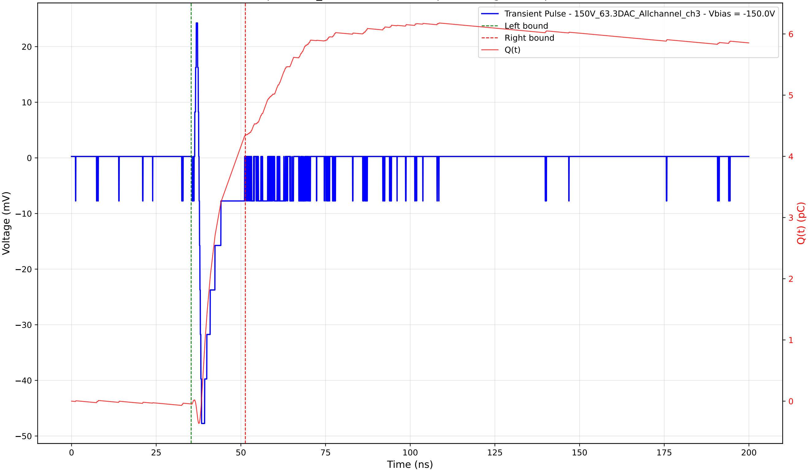
Transient Pulse - Sample: 1cm_42 - Position: 895.0 \mu\text{m} - Charge: 4.39 pC - Rise Time: 0.74 ns
