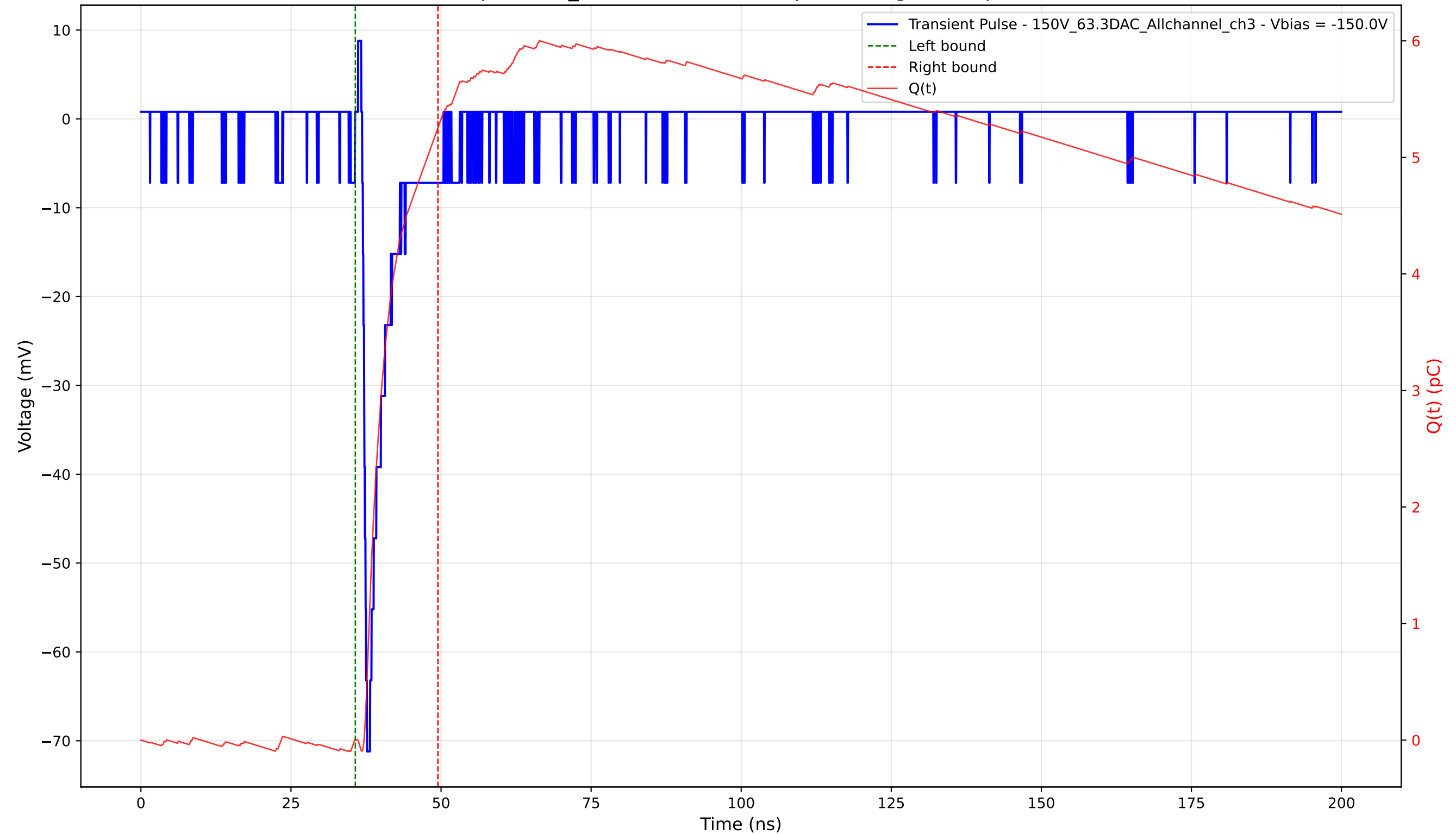
Transient Pulse - Sample: 1cm_42 - Position: 3515.0 \mu\text{m} - Charge: 5.25 pC - Rise Time: 0.80 ns
