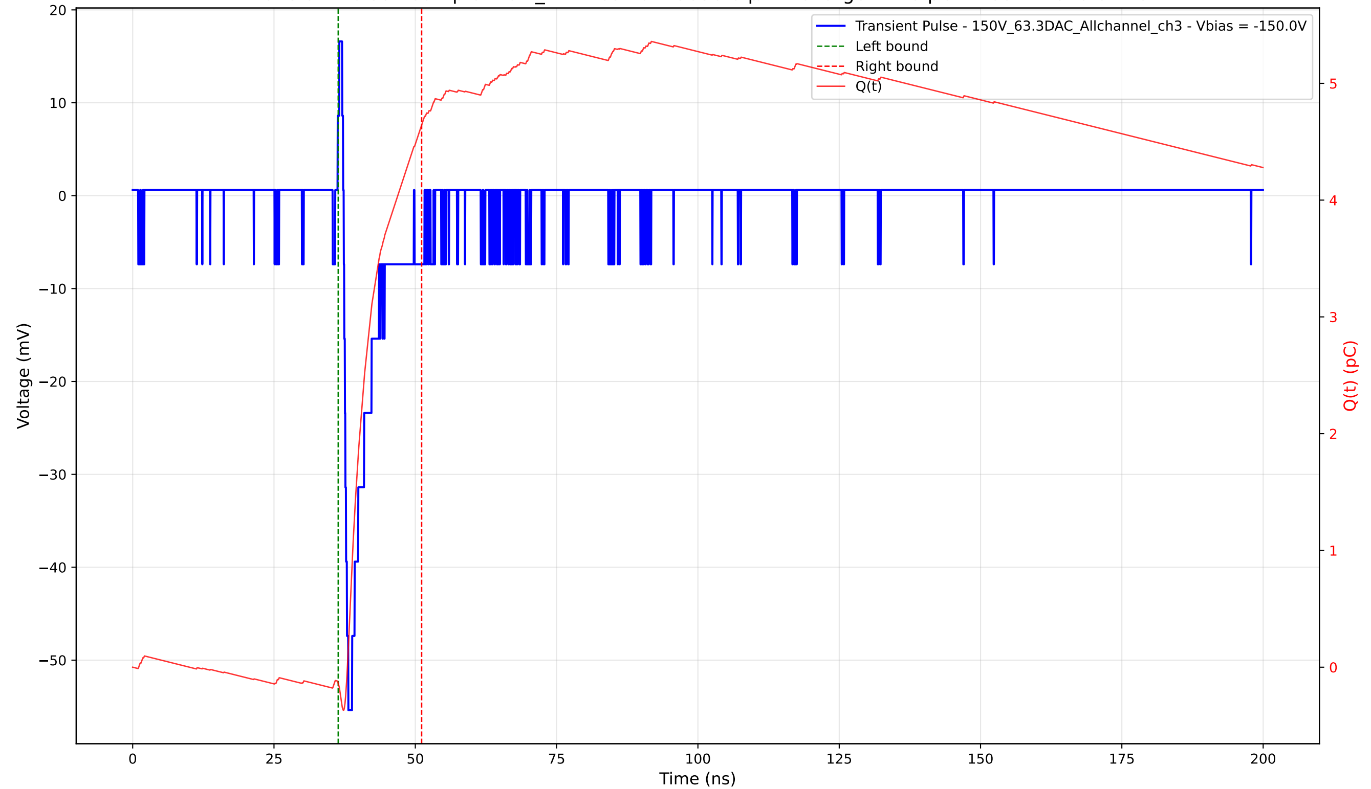
Transient Pulse - Sample: 1cm_42 - Position: 3830.0 \mu\text{m} - Charge: 4.78 pC - Rise Time: 0.81 ns
