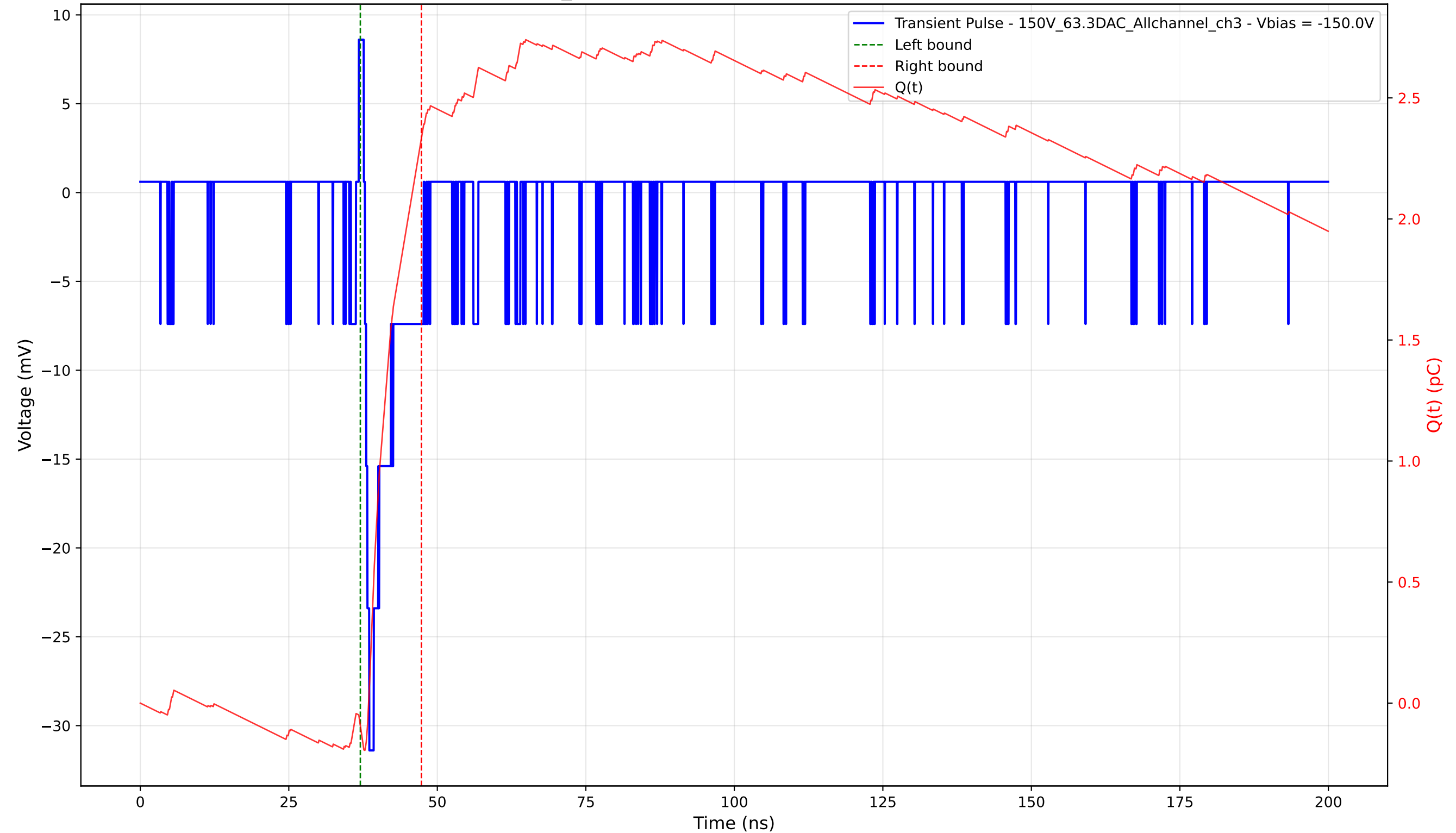
Transient Pulse - Sample: 1cm_42 - Position: 4885.0 \mu\text{m} - Charge: 2.43 pC - Rise Time: 0.75 ns
