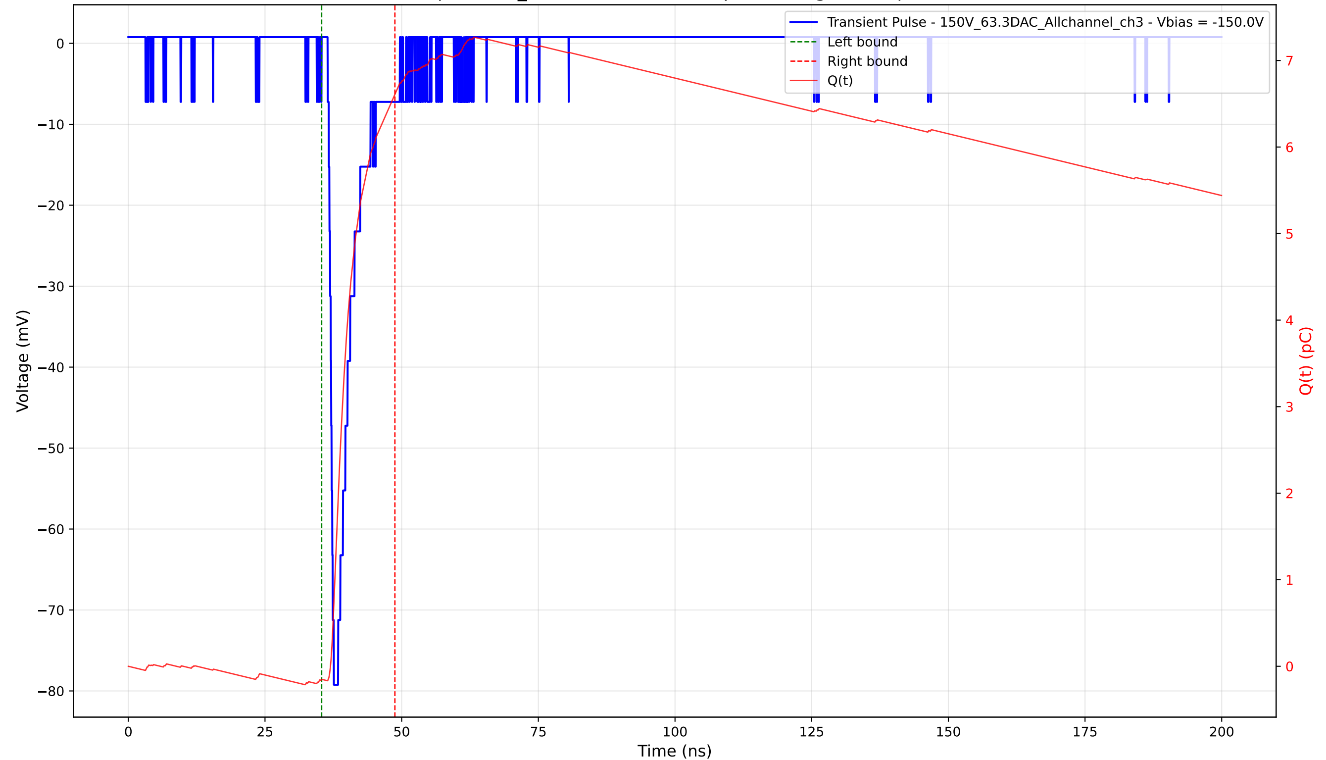
Transient Pulse - Sample: 1cm_42 - Position: 1545.0 \mu\text{m} - Charge: 6.76 pC - Rise Time: 0.96 ns
