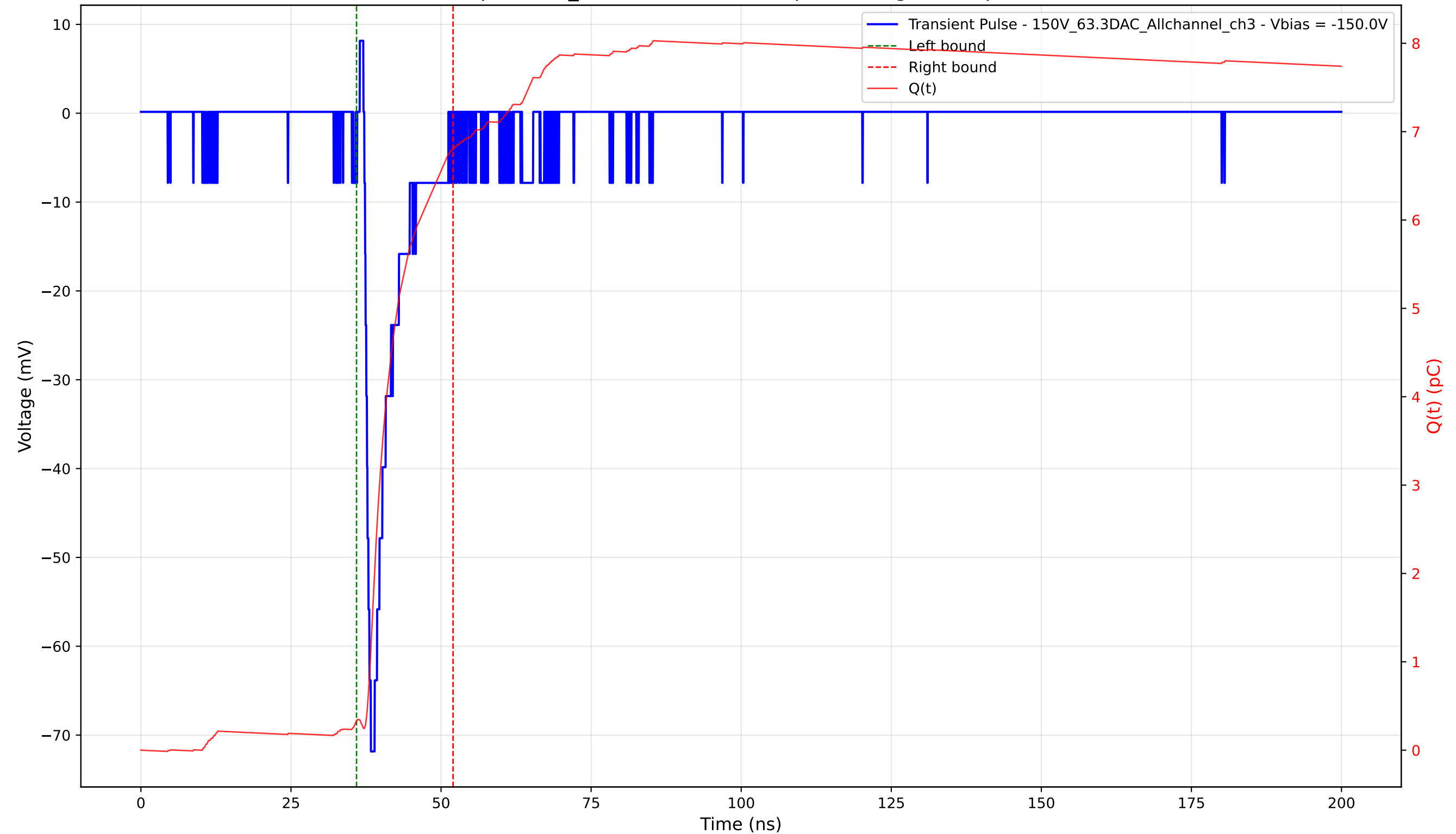
Transient Pulse - Sample: 1cm_42 - Position: 1275.0 \mu\text{m} - Charge: 6.47 pC - Rise Time: 1.08 ns
