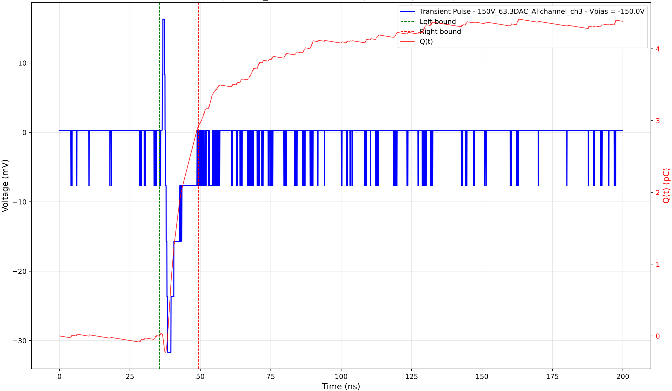
Transient Pulse - Sample: 1cm_42 - Position: 425.0 \mu\text{m} - Charge: 2.94 pC - Rise Time: 0.74 ns
