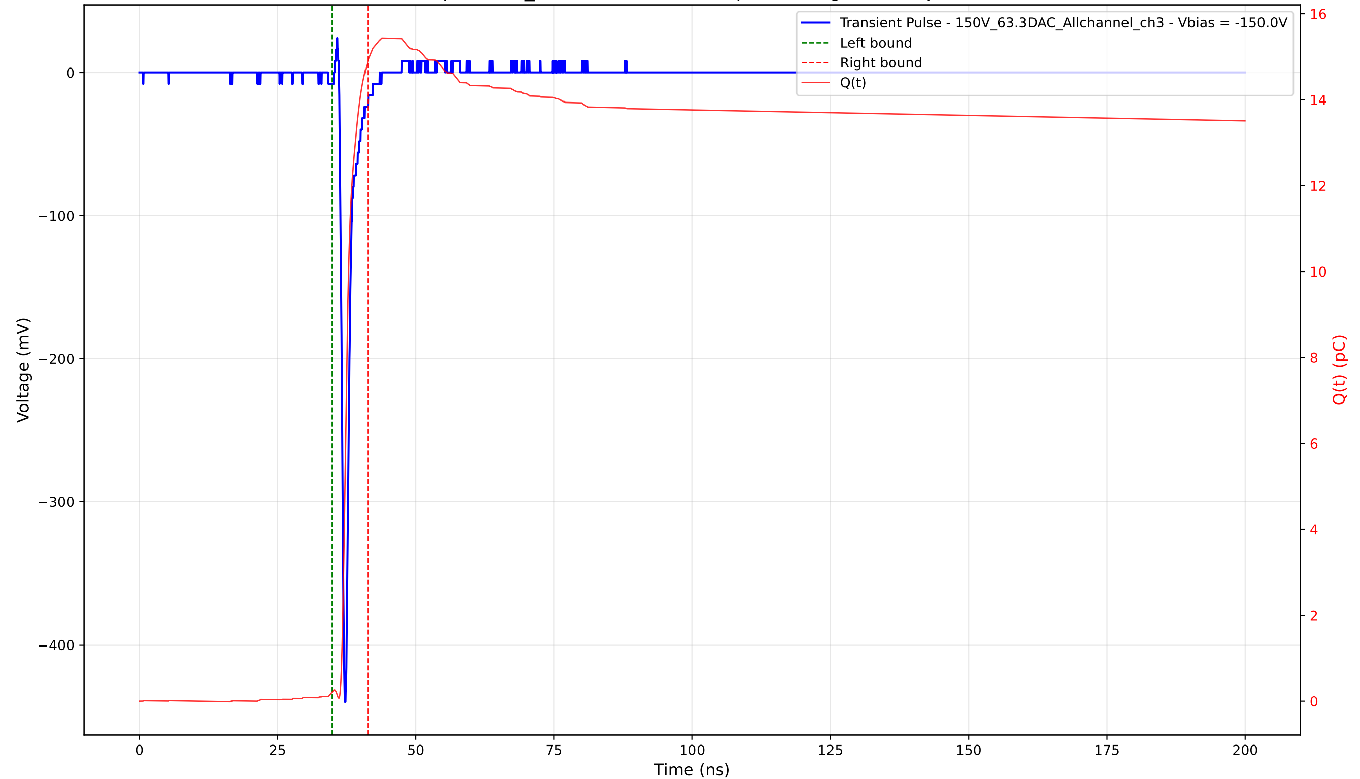
Transient Pulse - Sample: 1cm_42 - Position: 2235.0 \mu\text{m} - Charge: 14.68 pC - Rise Time: 0.69 ns
