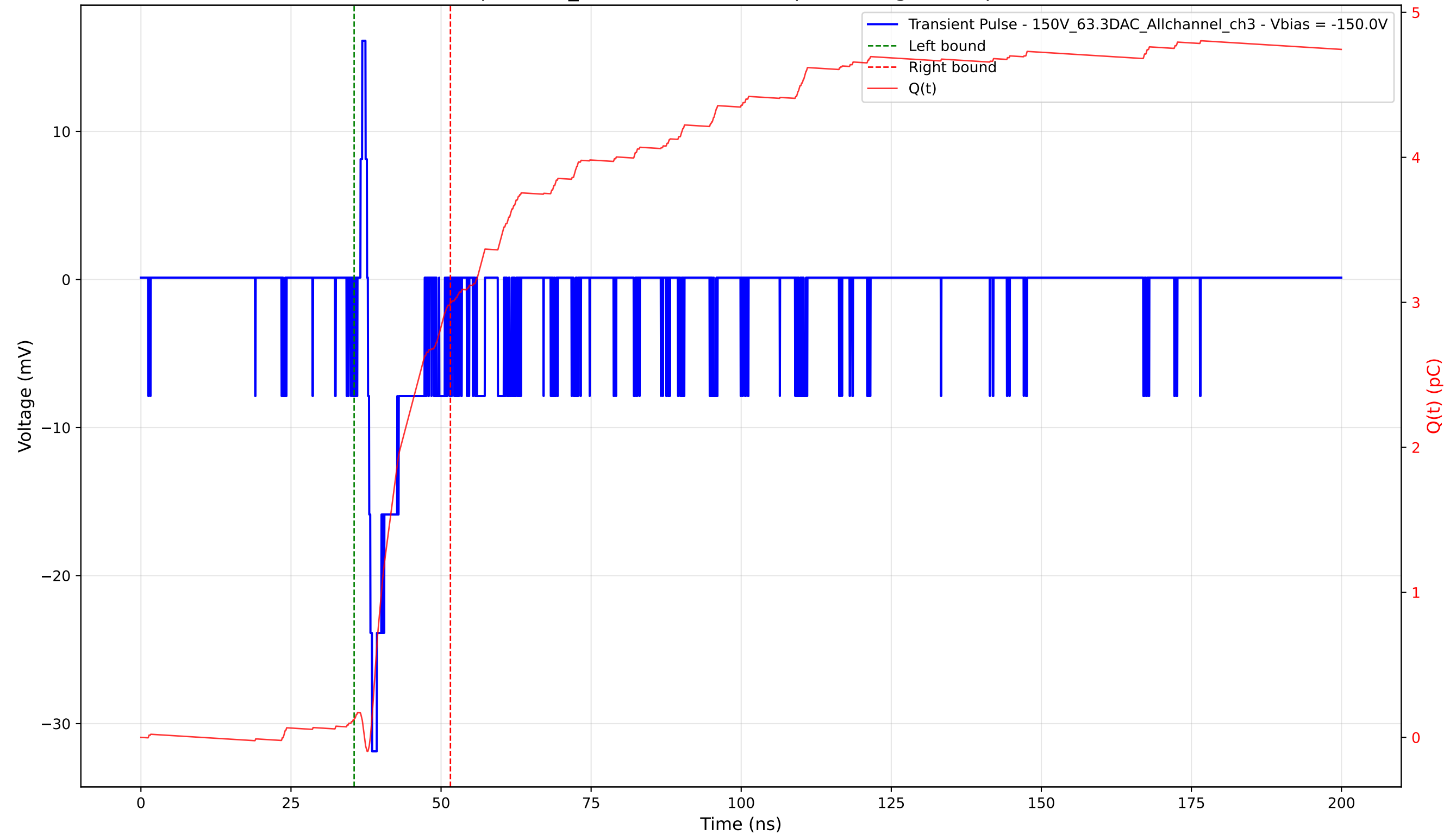
Transient Pulse - Sample: 1cm_42 - Position: 4635.0 \mu\text{m} - Charge: 2.87 pC - Rise Time: 0.70 ns
