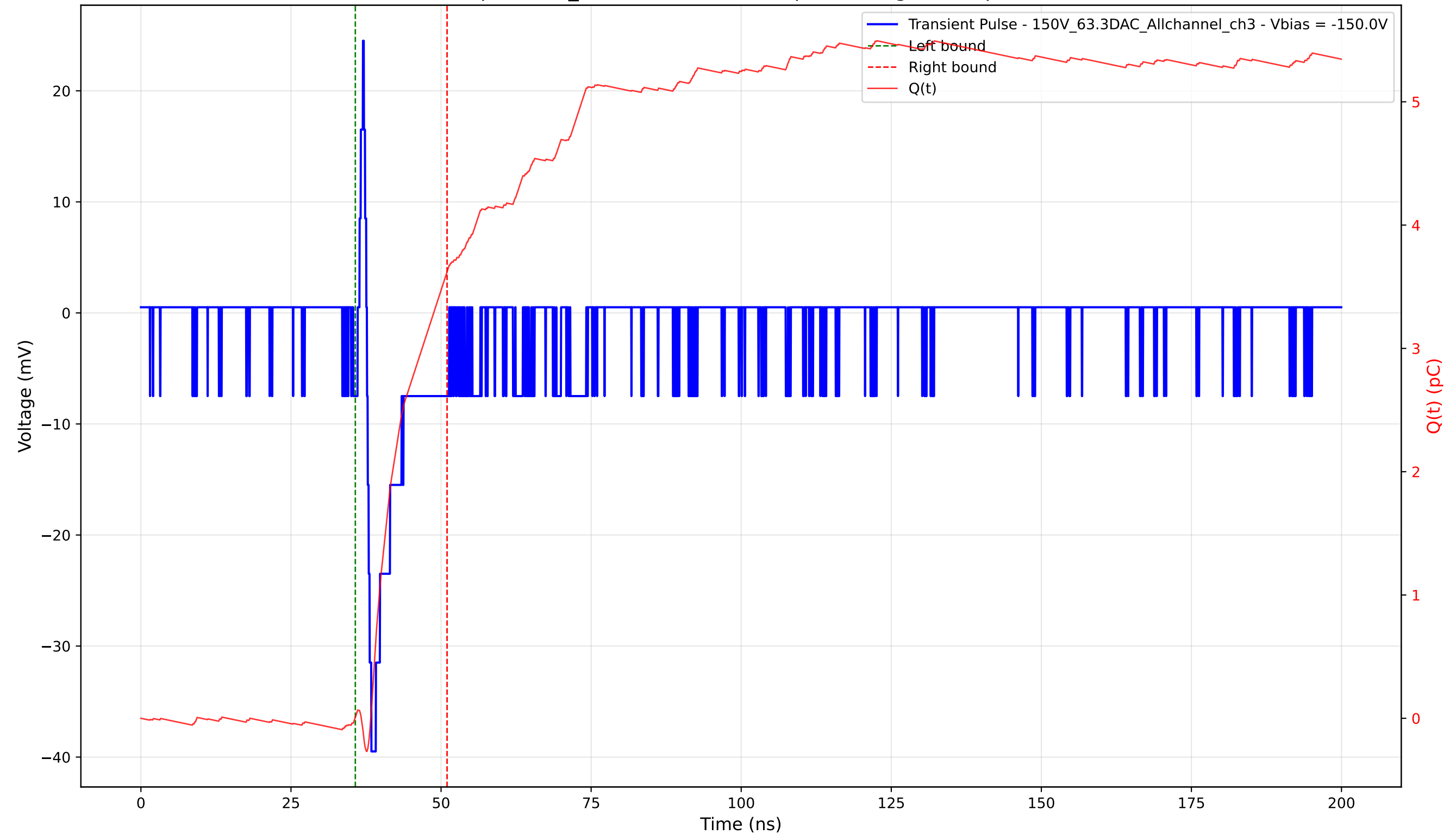
Transient Pulse - Sample: 1cm_42 - Position: 4135.0 \mu\text{m} - Charge: 3.61 pC - Rise Time: 0.74 ns
