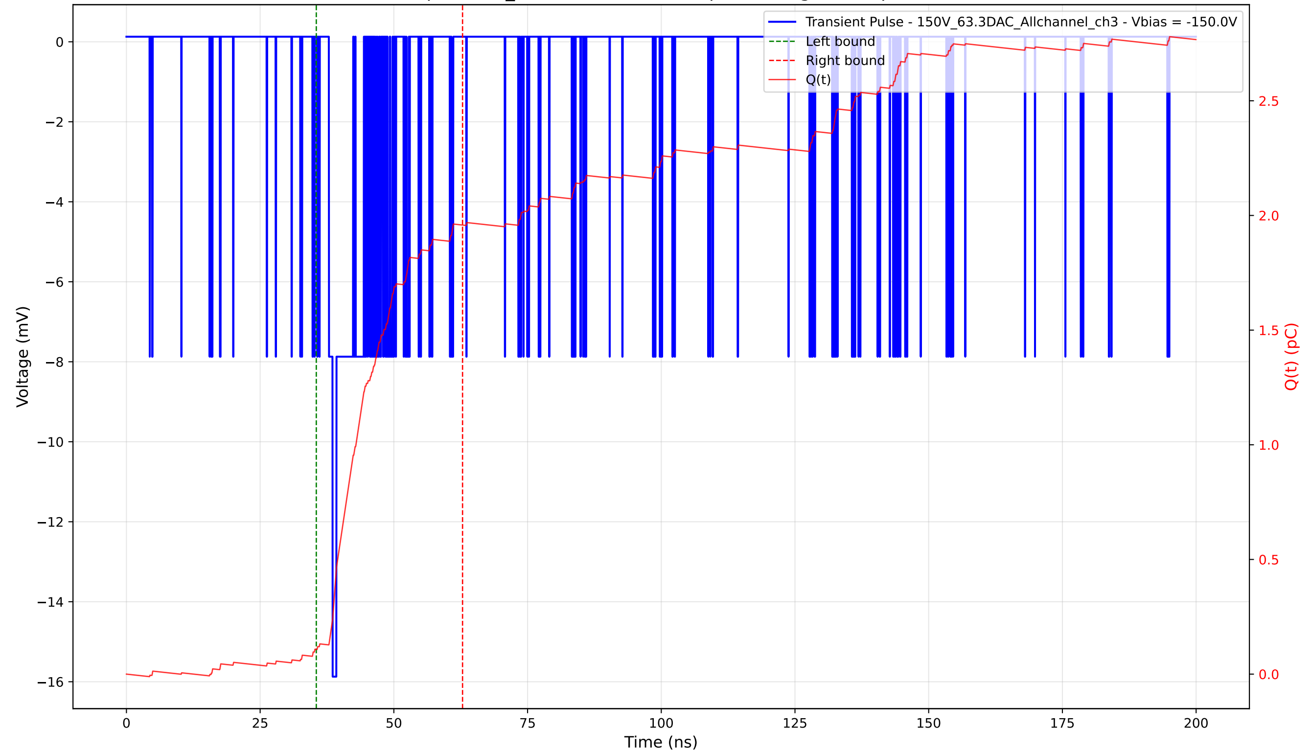
Transient Pulse - Sample: 1cm_42 - Position: 5070.0 \mu\text{m} - Charge: 1.85 pC - Rise Time: 0.71 ns
