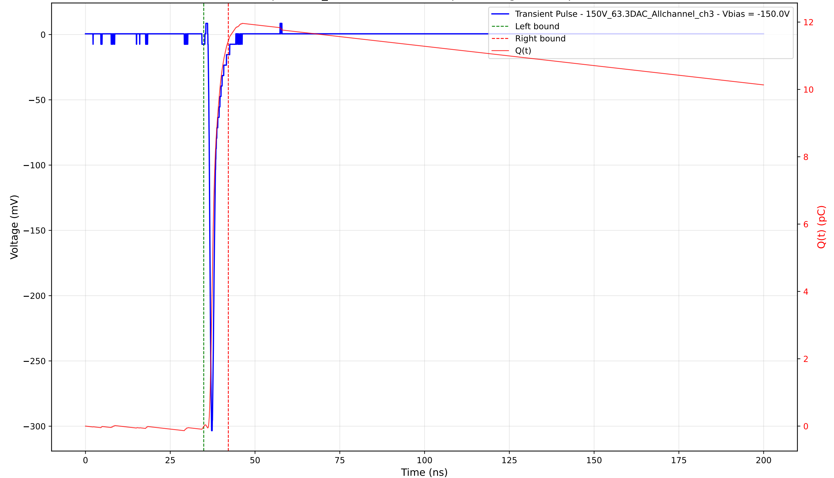
Transient Pulse - Sample: 1cm_42 - Position: 2095.0 \mu\text{m} - Charge: 11.45 pC - Rise Time: 0.77 ns
