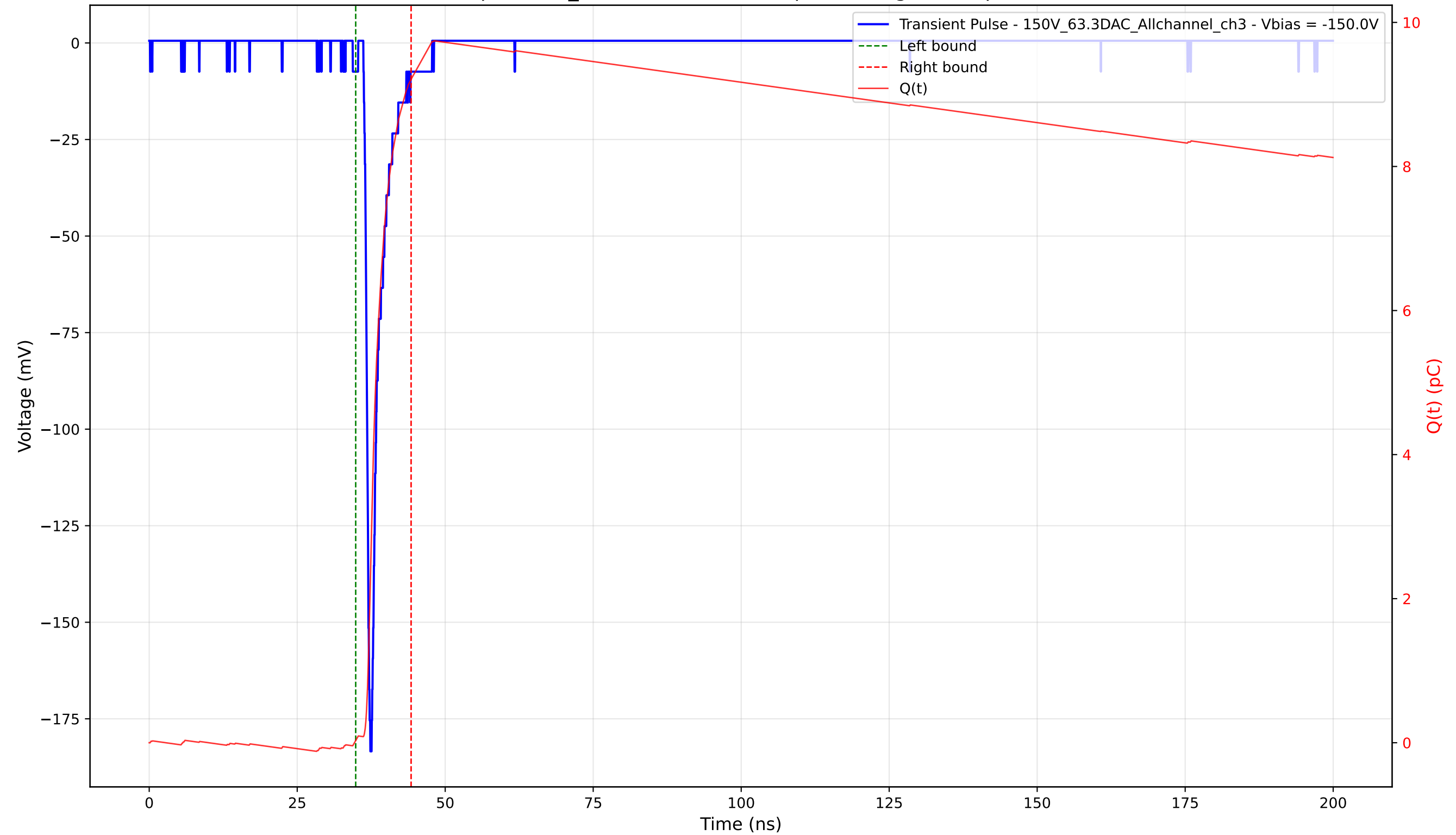
Transient Pulse - Sample: 1cm_42 - Position: 1930.0 \mu\text{m} - Charge: 9.18 pC - Rise Time: 0.83 ns
