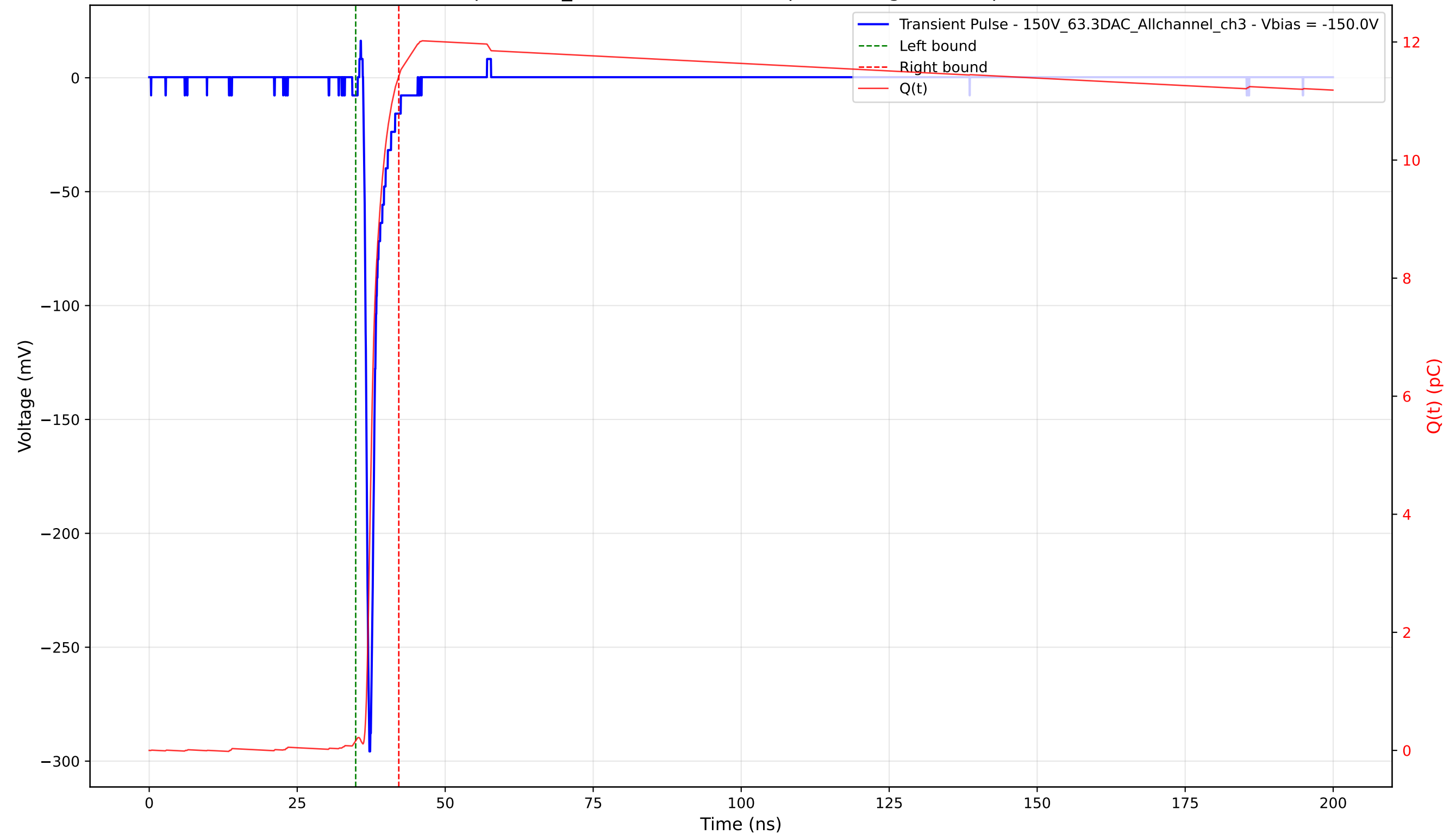
Transient Pulse - Sample: 1cm_42 - Position: 2085.0 \mu\text{m} - Charge: 11.26 pC - Rise Time: 0.78 ns
