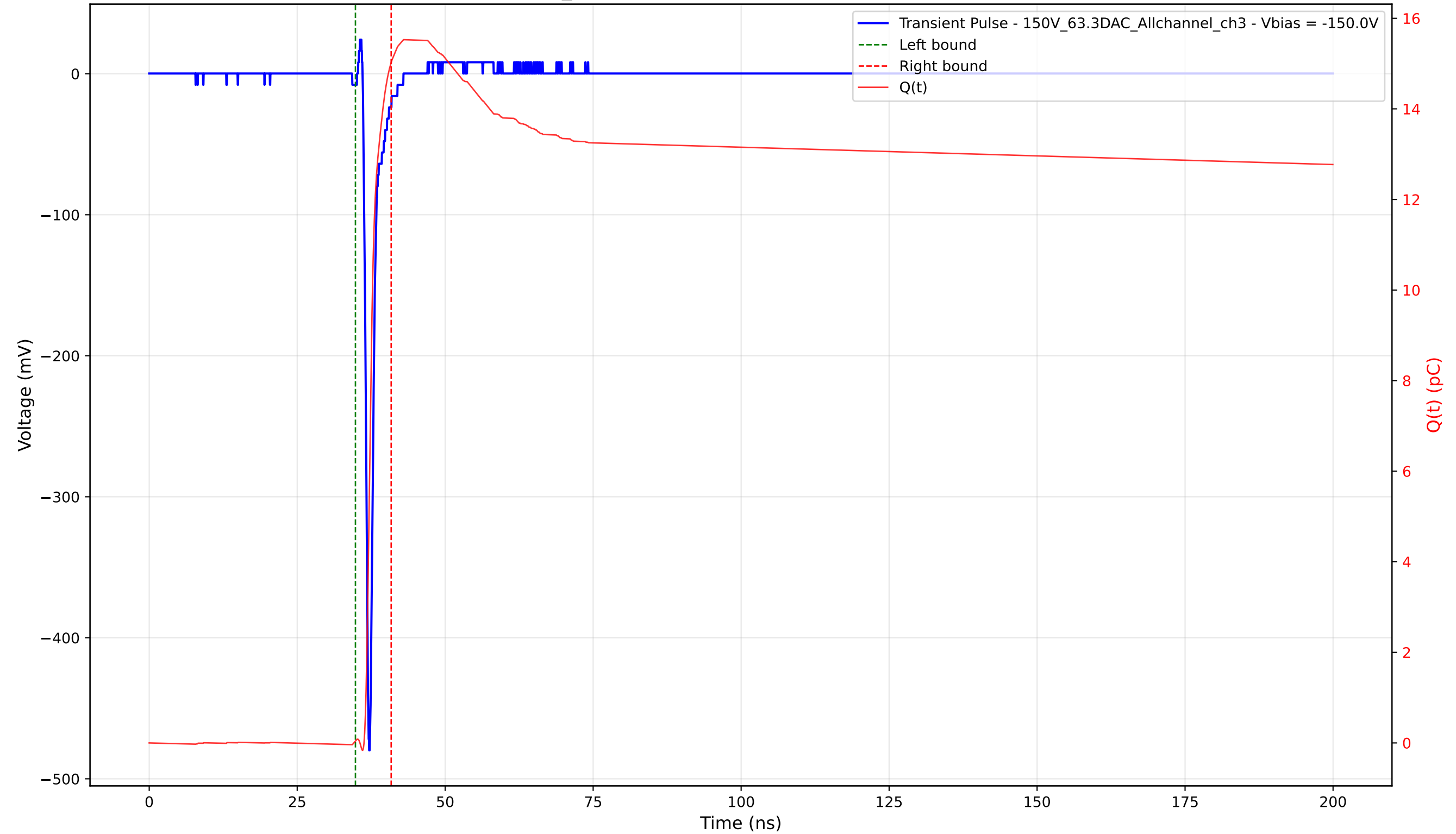
Transient Pulse - Sample: 1cm_42 - Position: 2370.0 \mu\text{m} - Charge: 14.98 pC - Rise Time: 0.70 ns
