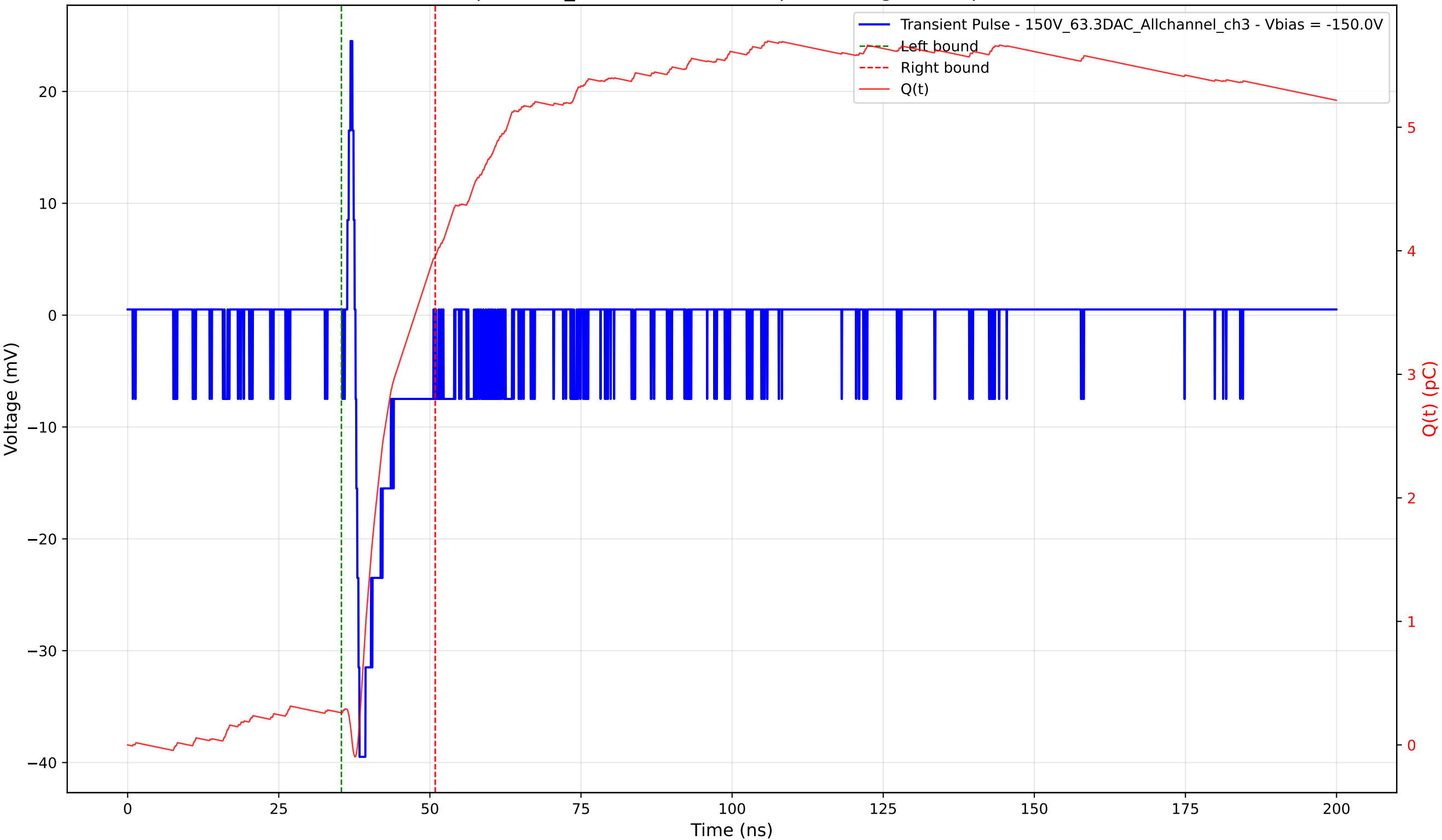
Transient Pulse - Sample: 1cm_42 - Position: 580.0 \mu\text{m} - Charge: 3.70 pC - Rise Time: 0.66 ns
