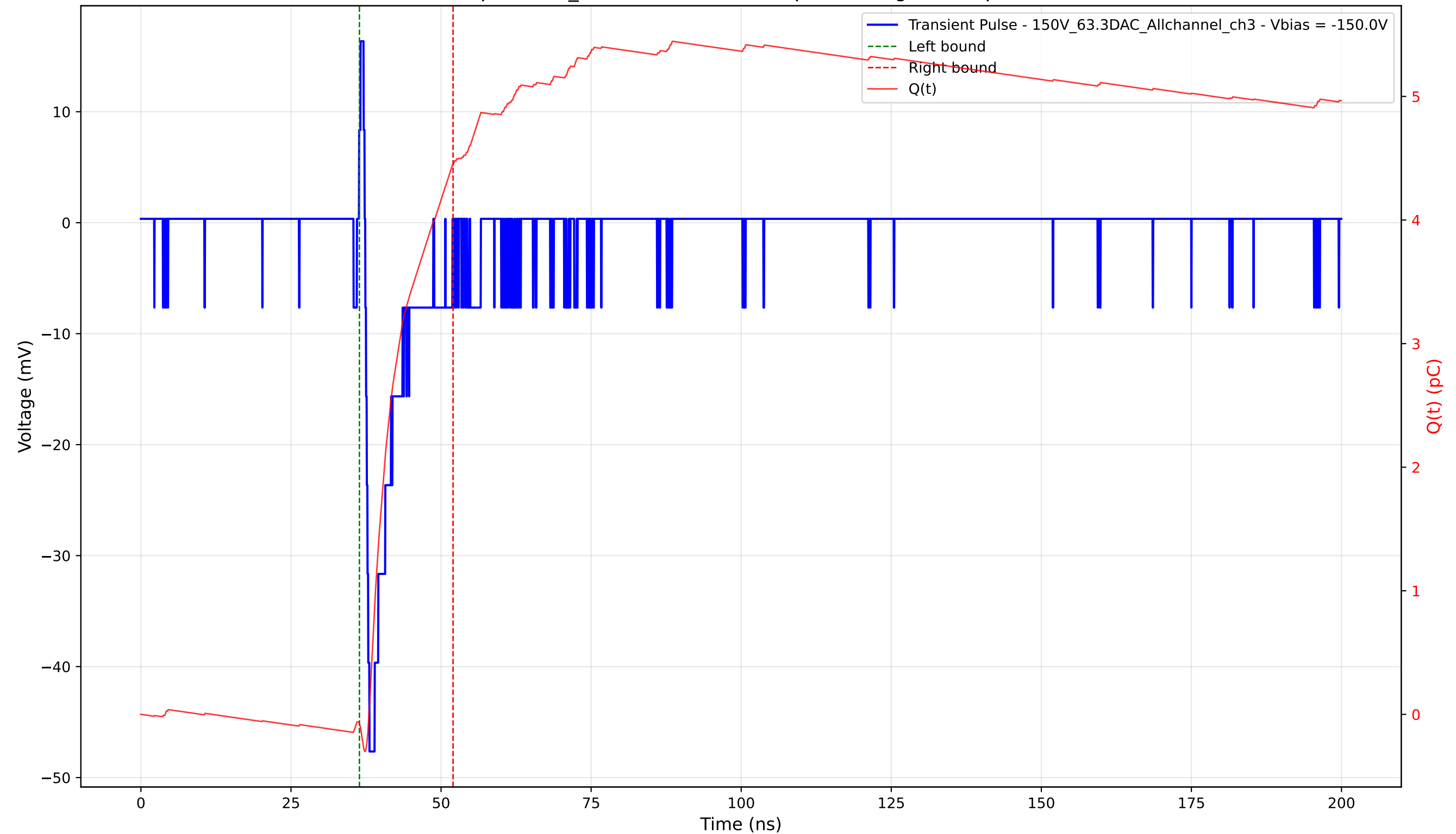
Transient Pulse - Sample: 1cm_42 - Position: 3900.0 \mu\text{m} - Charge: 4.52 pC - Rise Time: 0.70 ns
