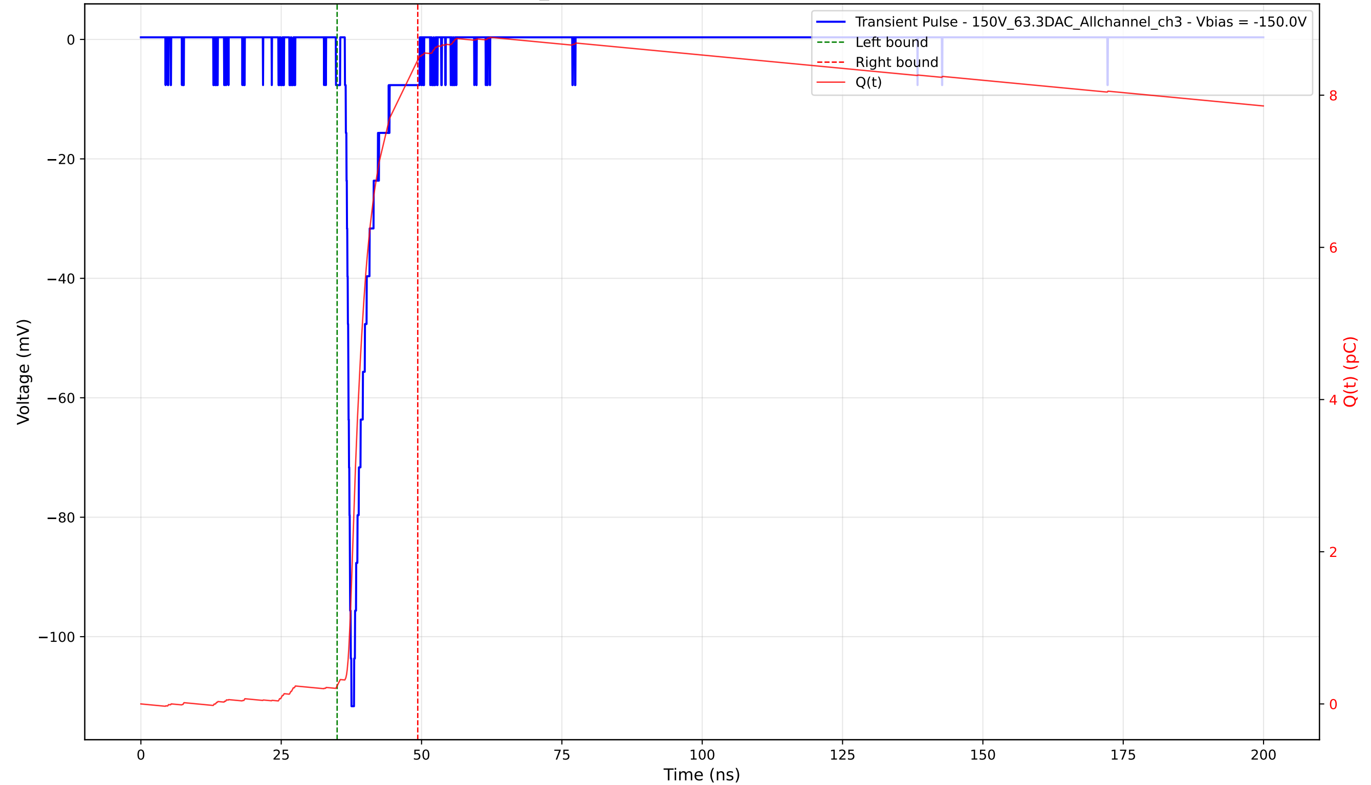
Transient Pulse - Sample: 1cm_42 - Position: 1635.0 \mu\text{m} - Charge: 8.23 pC - Rise Time: 0.90 ns
