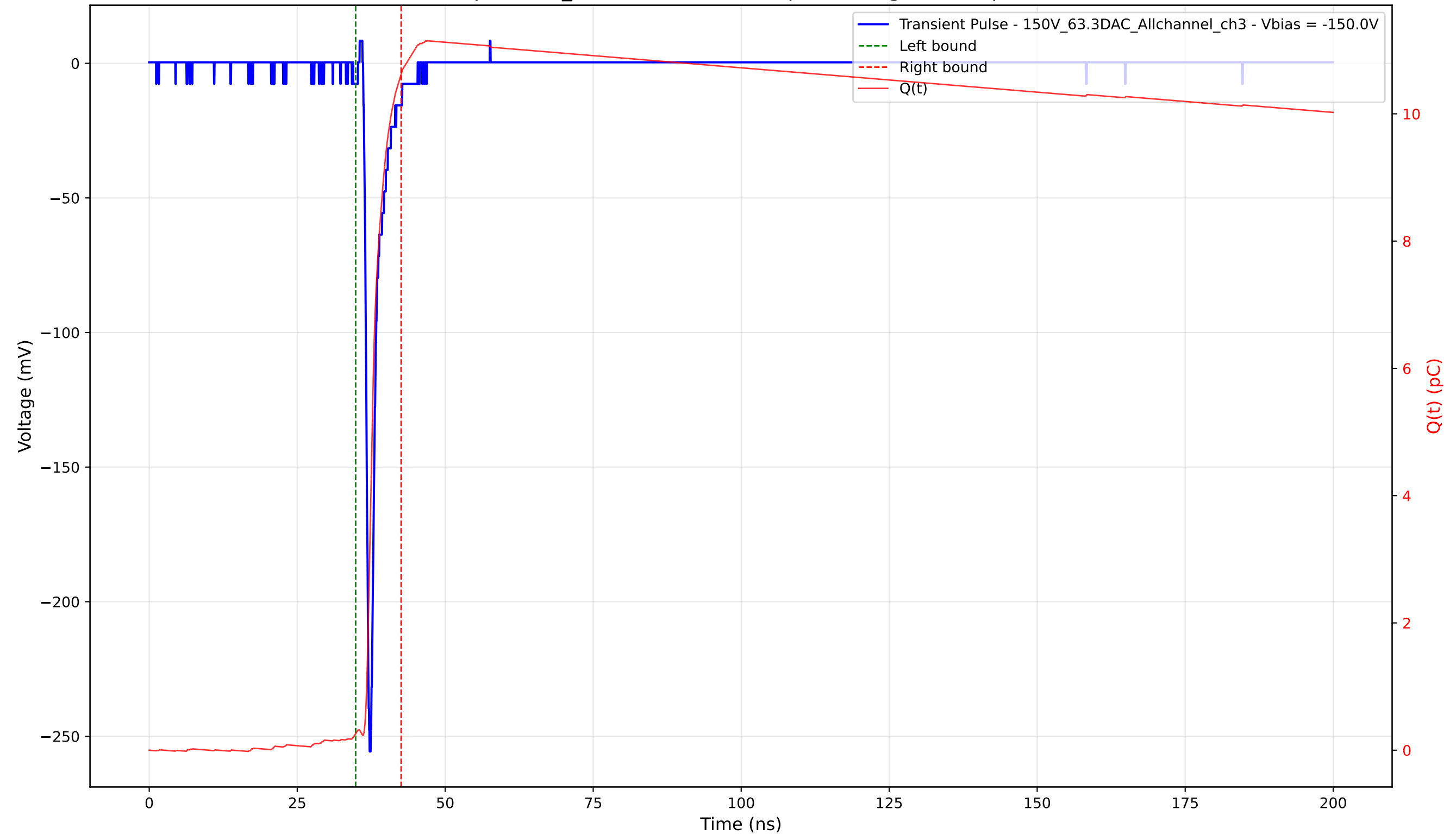
Transient Pulse - Sample: 1cm_42 - Position: 2050.0 \mu\text{m} - Charge: 10.37 pC - Rise Time: 0.74 ns
