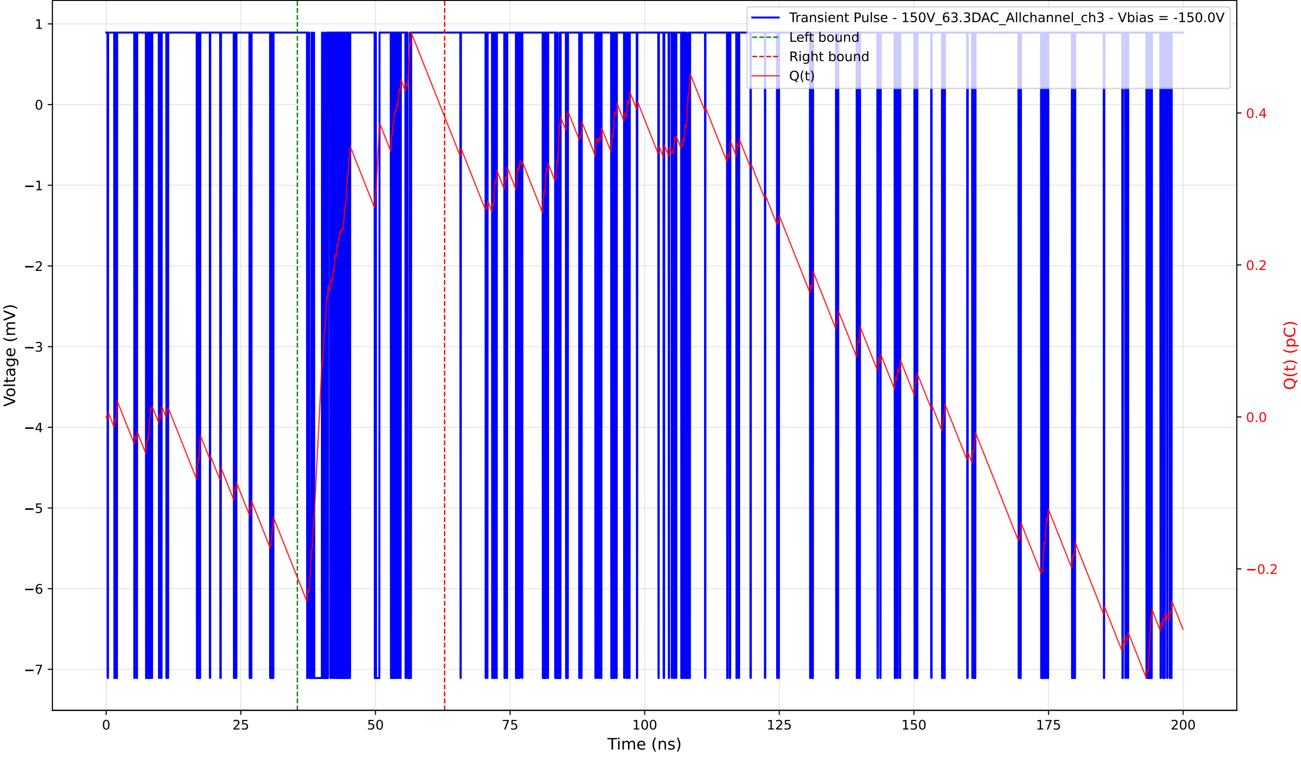
Transient Pulse - Sample: 1cm_42 - Position: 35.0 \mu\text{m} - Charge: 0.61 pC - Rise Time: 0.00 ns (N/A)
