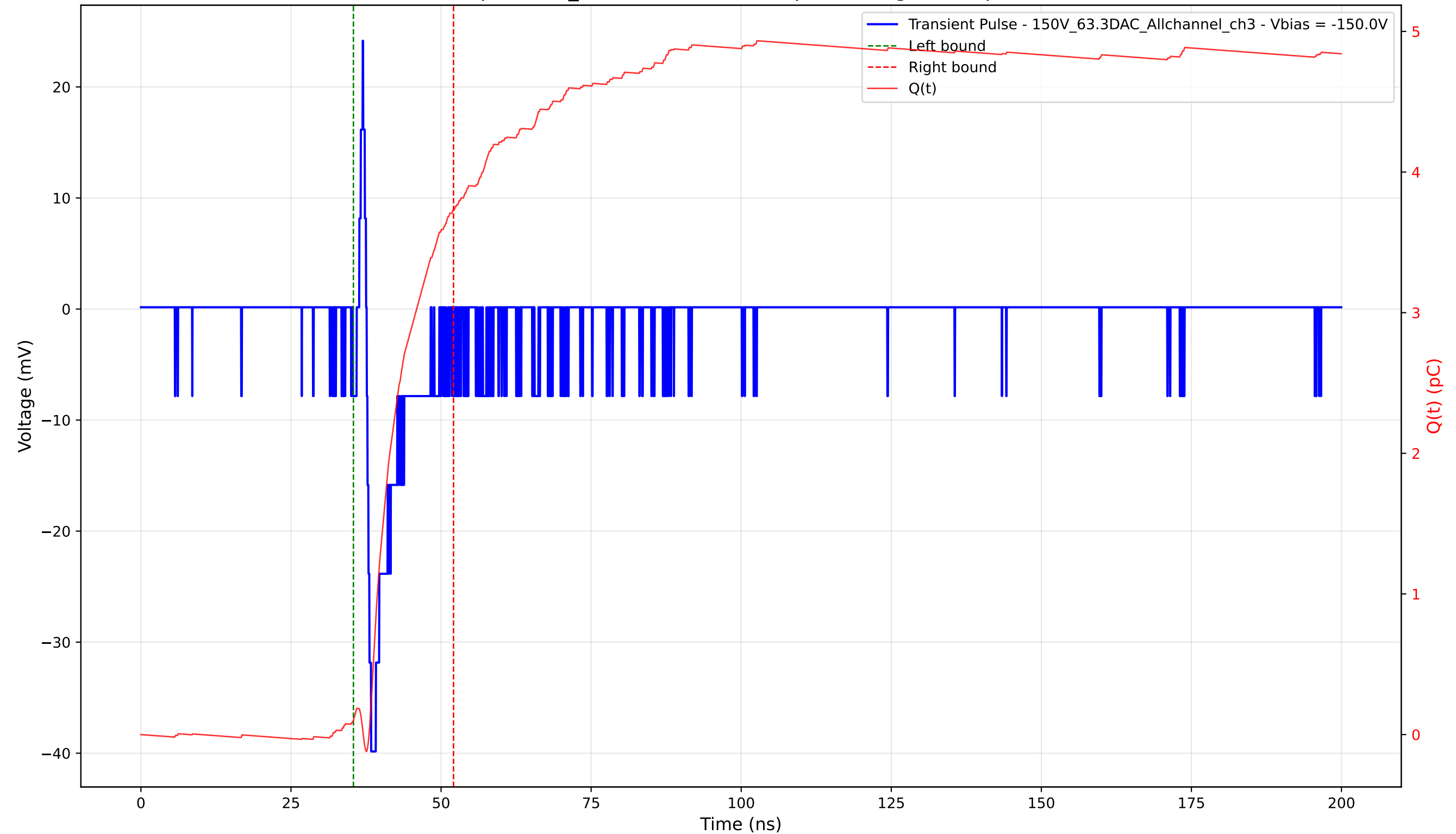
Transient Pulse - Sample: 1cm_42 - Position: 4075.0 \mu\text{m} - Charge: 3.63 pC - Rise Time: 0.74 ns
