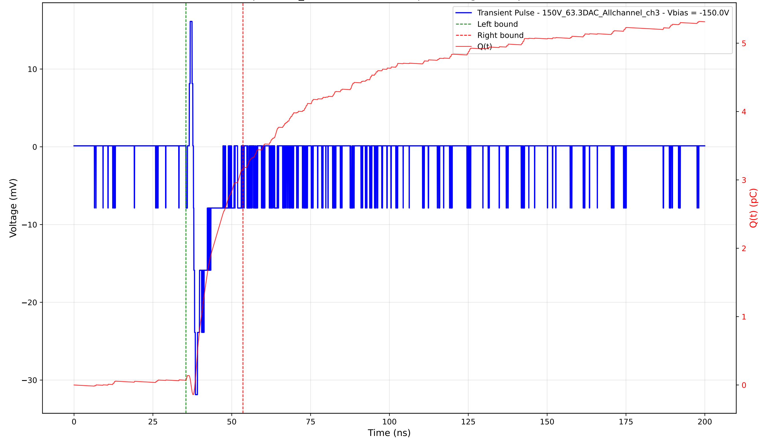
Transient Pulse - Sample: 1cm_42 - Position: 4565.0 \mu\text{m} - Charge: 3.10 pC - Rise Time: 0.62 ns
