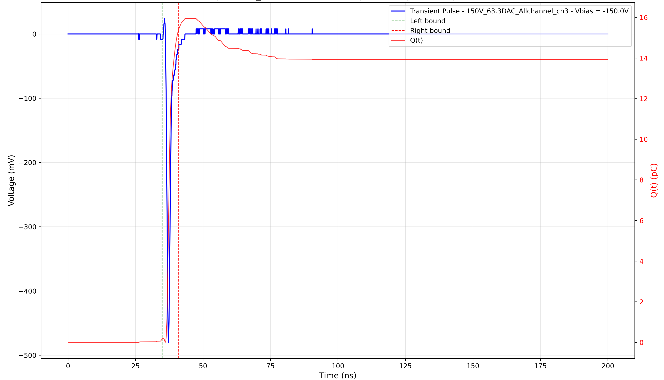
Transient Pulse - Sample: 1cm_42 - Position: 2320.0 \mu\text{m} - Charge: 15.26 pC - Rise Time: 0.74 ns
