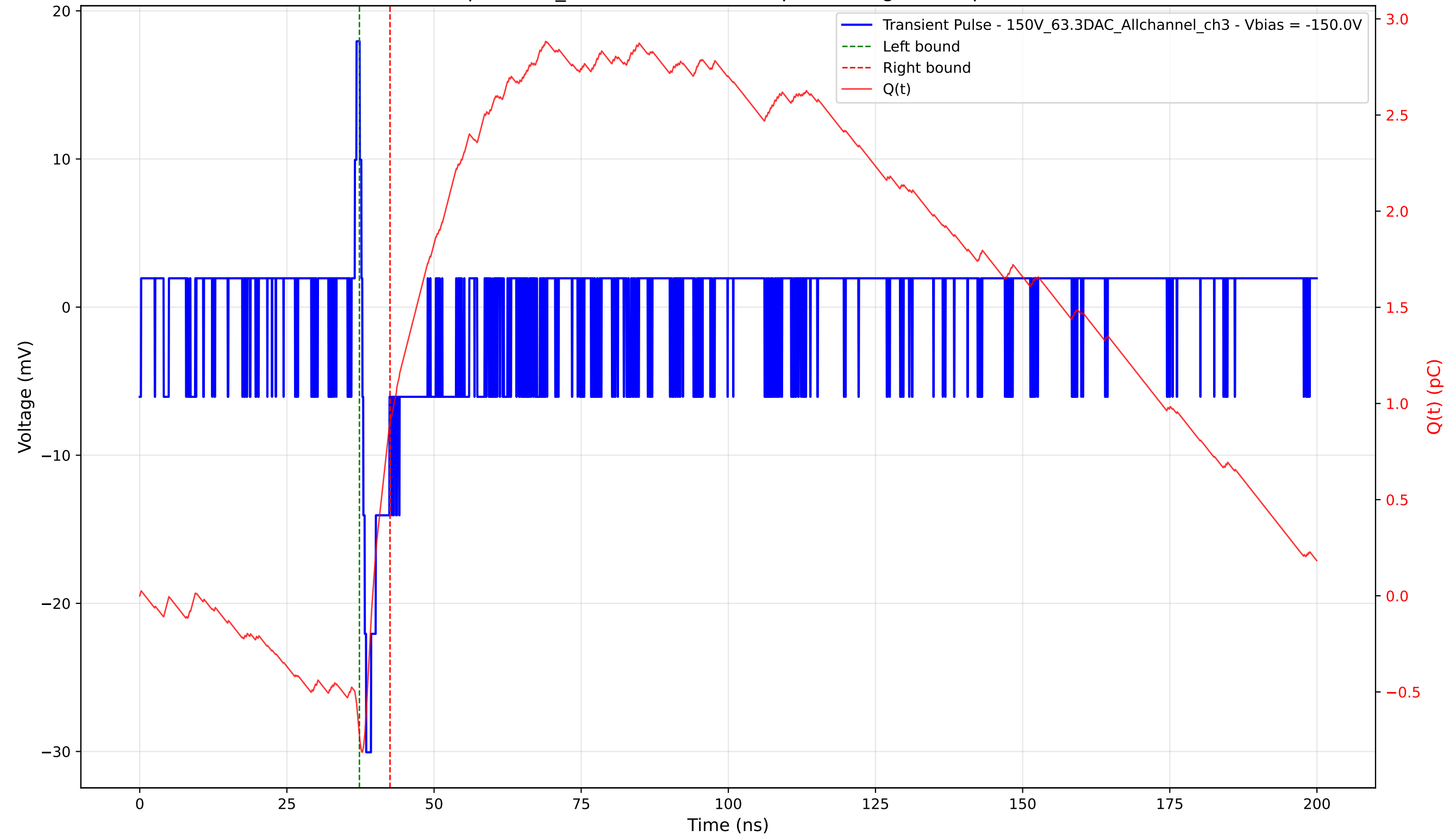
Transient Pulse - Sample: 1cm_42 - Position: 4545.0 \mu\text{m} - Charge: 1.63 pC - Rise Time: 0.67 ns
