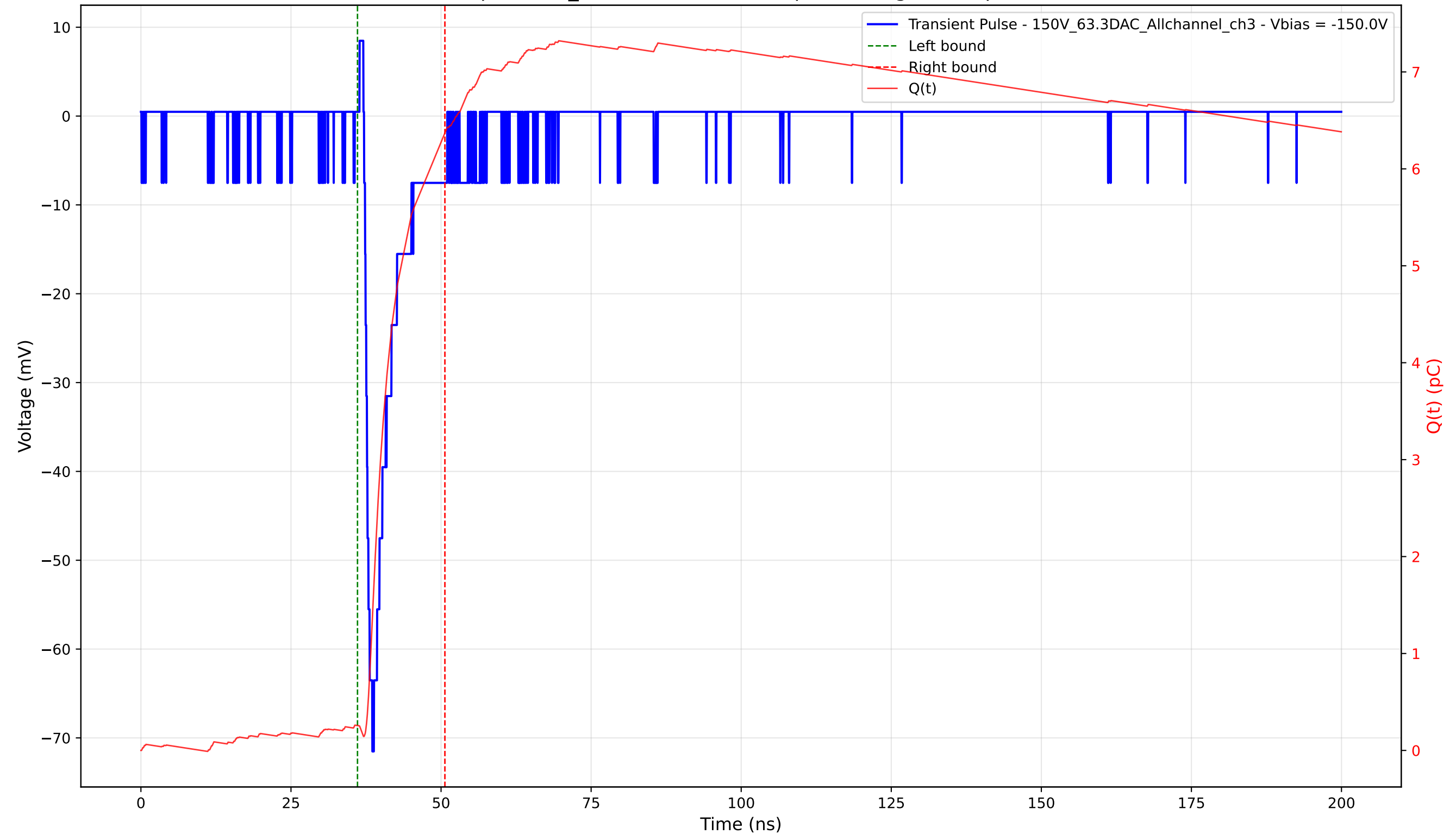
Transient Pulse - Sample: 1cm_42 - Position: 1270.0 \mu\text{m} - Charge: 6.12 pC - Rise Time: 1.36 ns
