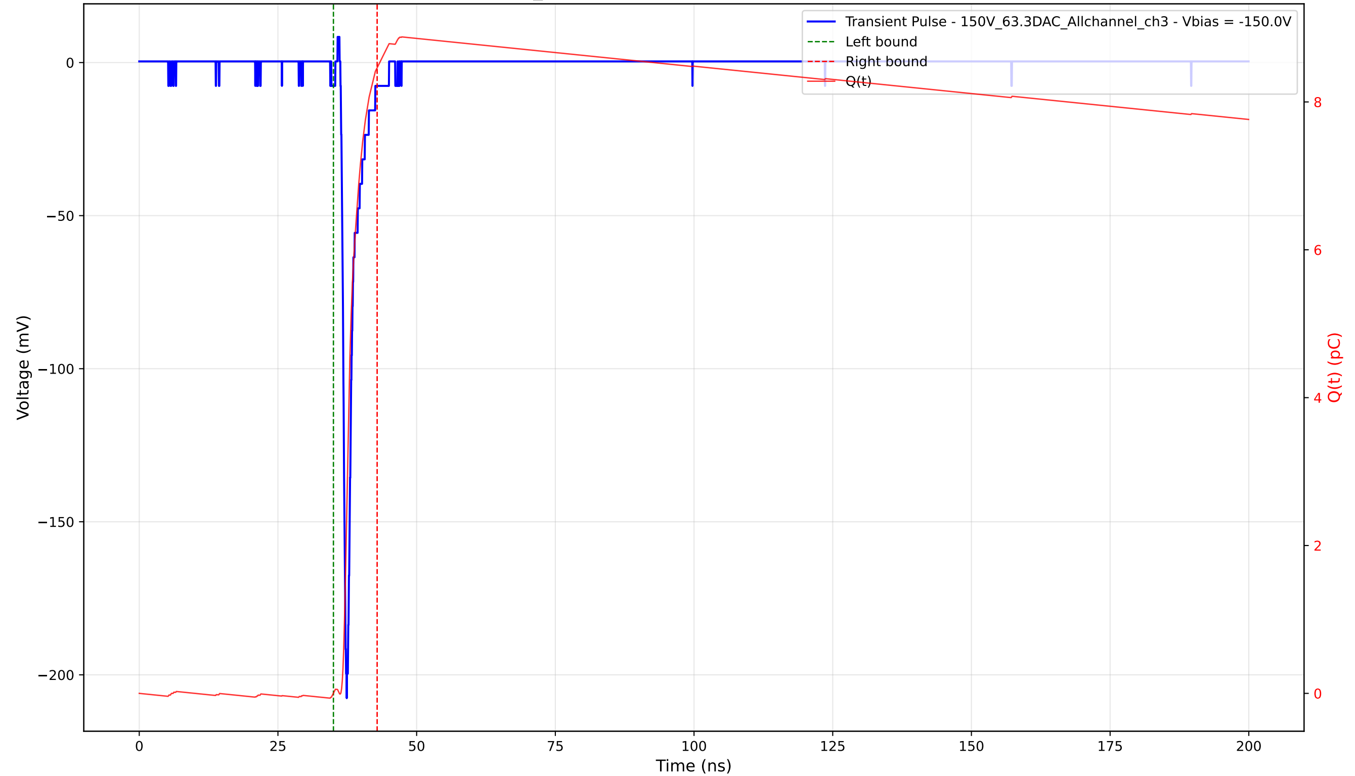
Transient Pulse - Sample: 1cm_42 - Position: 3045.0 \mu\text{m} - Charge: 8.46 pC - Rise Time: 0.81 ns
