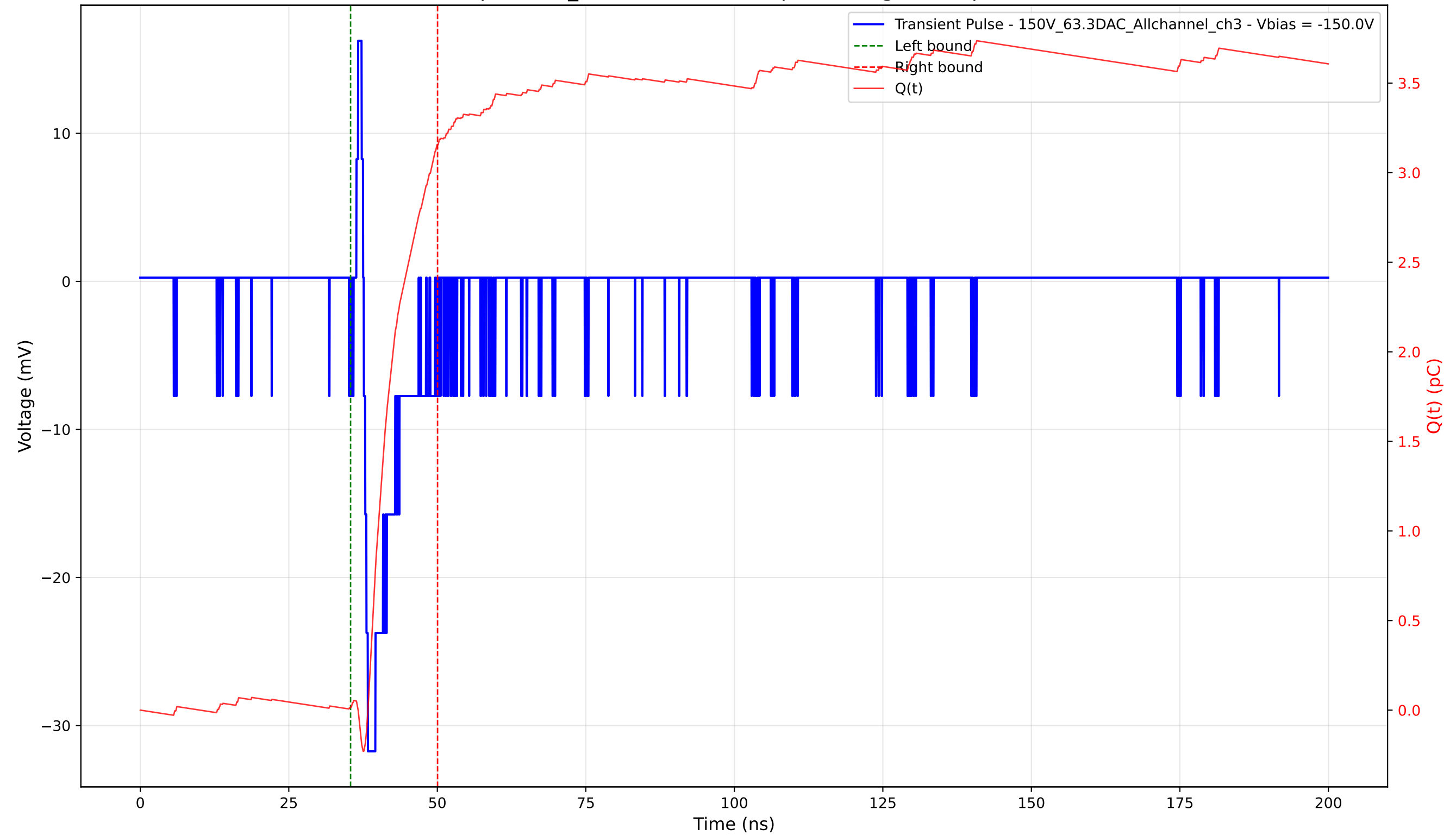
Transient Pulse - Sample: 1cm_42 - Position: 460.0 \mu\text{m} - Charge: 3.14 pC - Rise Time: 0.70 ns
