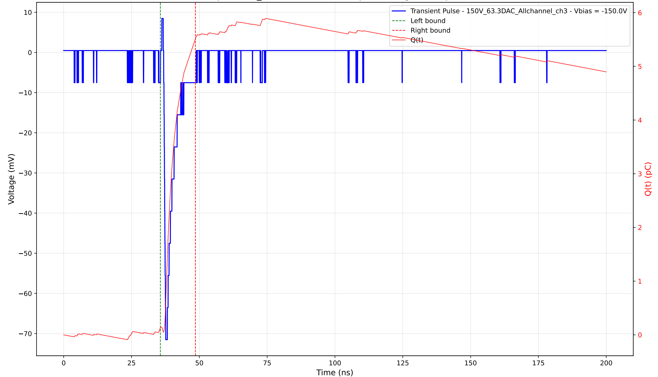
Transient Pulse - Sample: 1cm_42 - Position: 3510.0 \mu\text{m} - Charge: 5.38 pC - Rise Time: 0.76 ns
