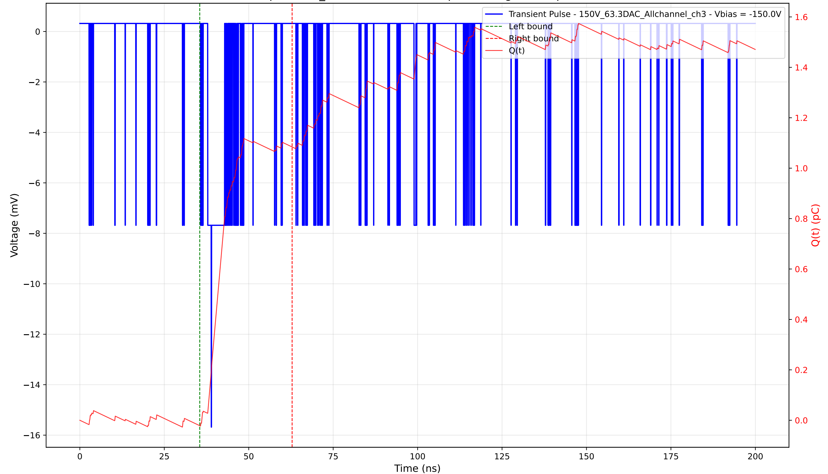
Transient Pulse - Sample: 1cm_42 - Position: 5100.0 \mu\text{m} - Charge: 1.11 pC - Rise Time: 1.07 ns
