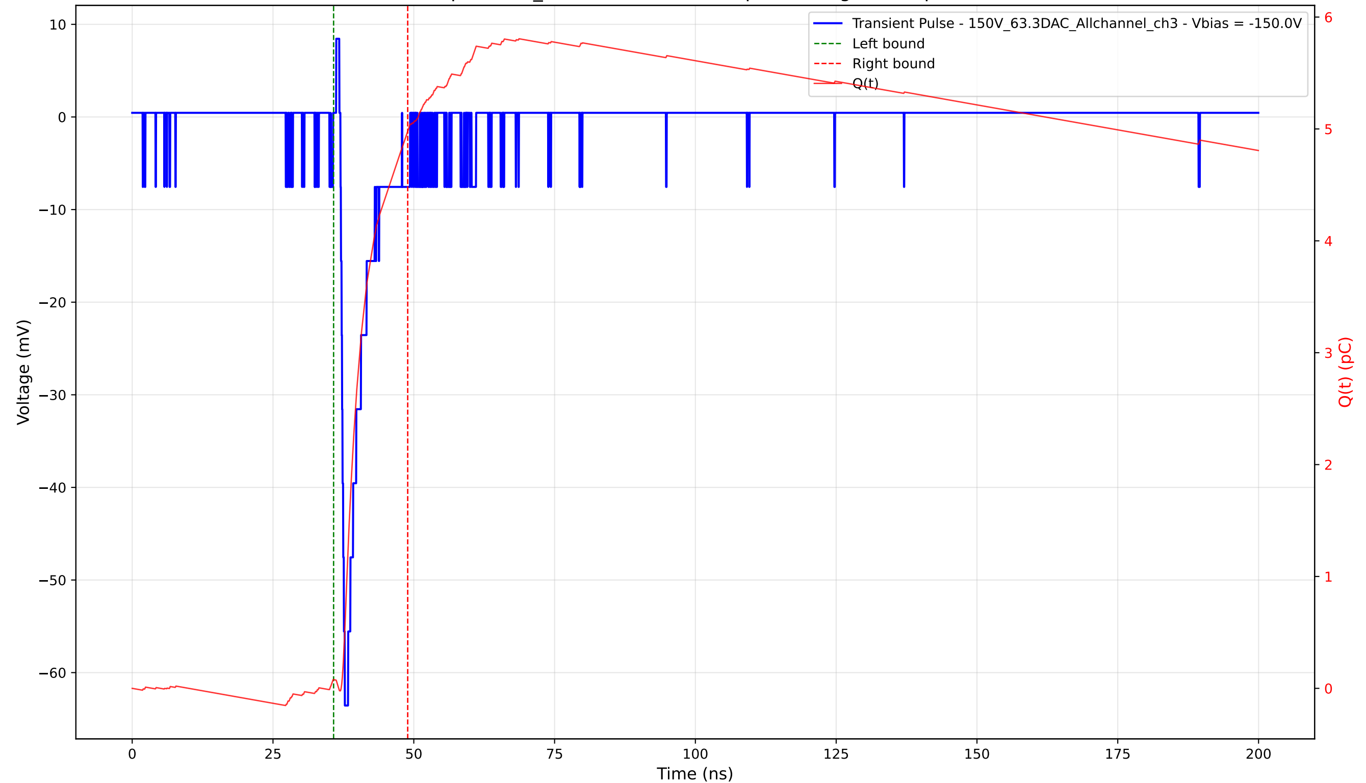
Transient Pulse - Sample: 1cm_42 - Position: 3560.0 \mu\text{m} - Charge: 4.90 pC - Rise Time: 0.77 ns
