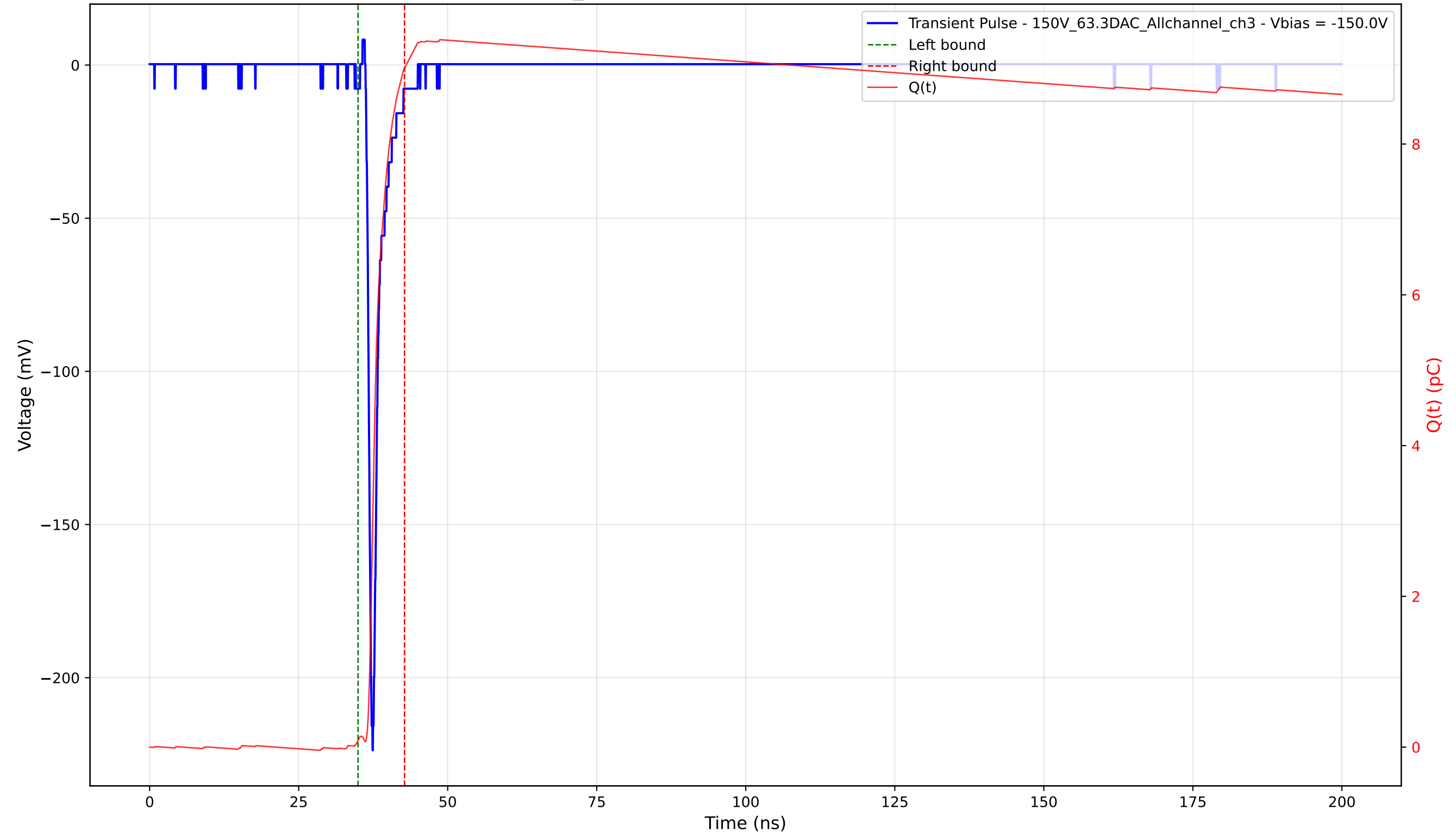
Transient Pulse - Sample: 1cm_42 - Position: 3025.0 \mu\text{m} - Charge: 8.92 pC - Rise Time: 0.81 ns
