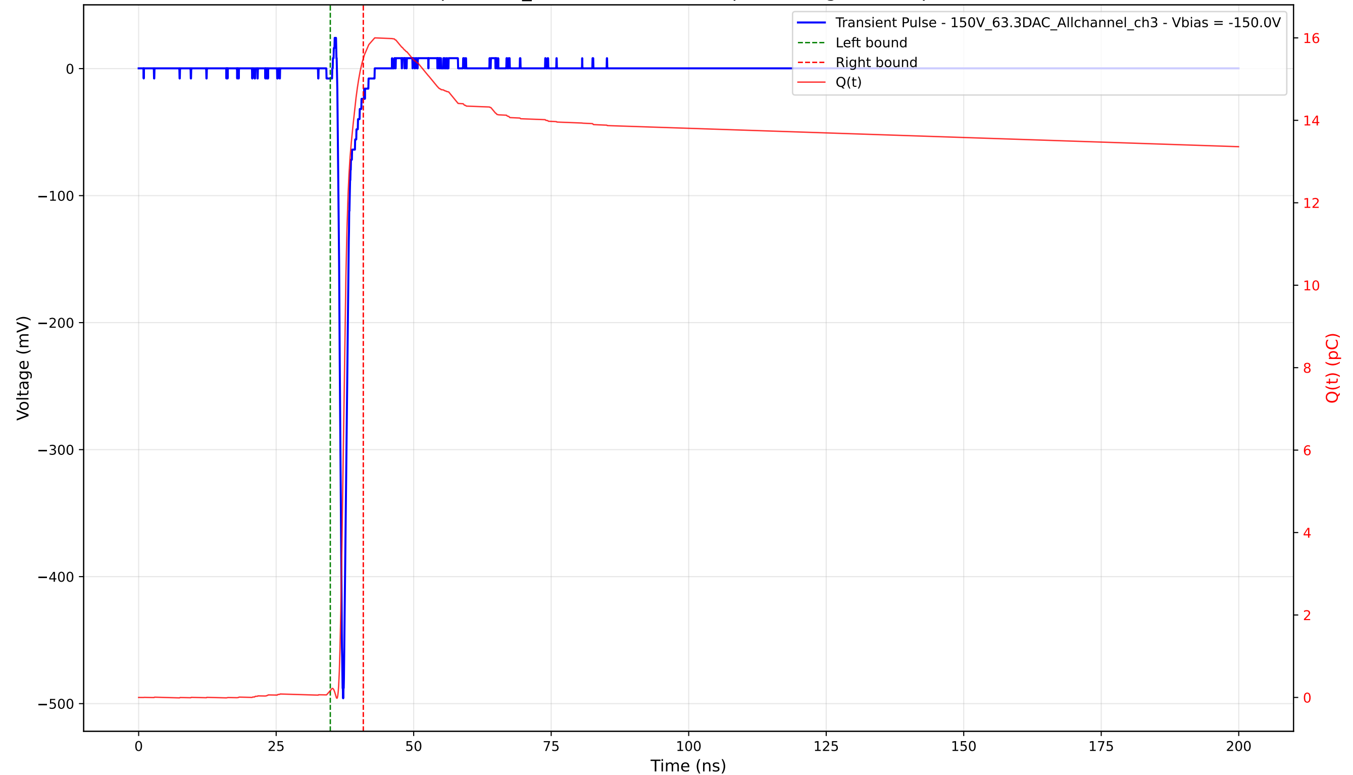
Transient Pulse - Sample: 1cm_42 - Position: 2650.0 \mu\text{m} - Charge: 15.33 pC - Rise Time: 0.70 ns
