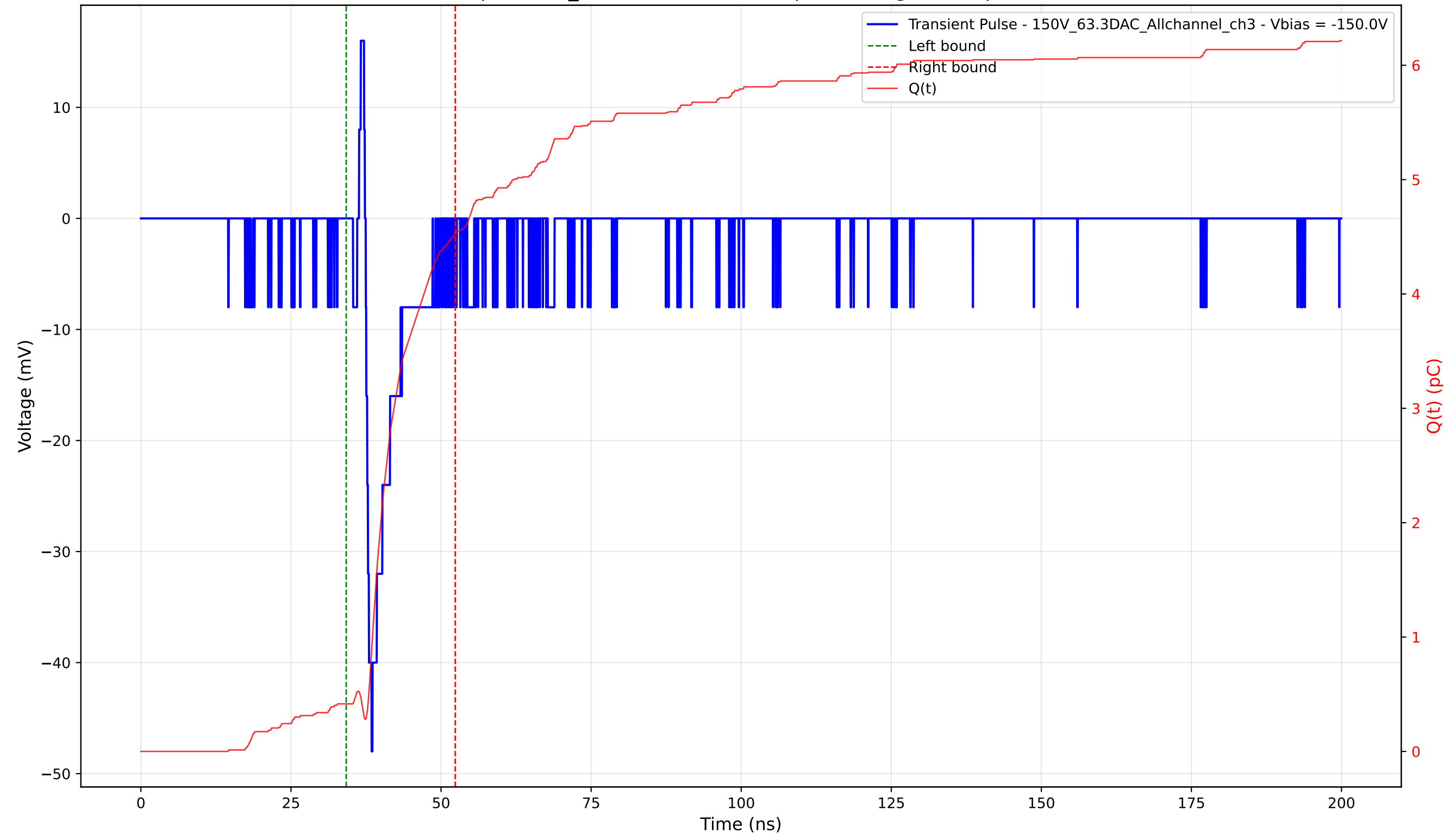
Transient Pulse - Sample: 1cm_42 - Position: 3950.0 \mu\text{m} - Charge: 4.11 pC - Rise Time: 0.98 ns
