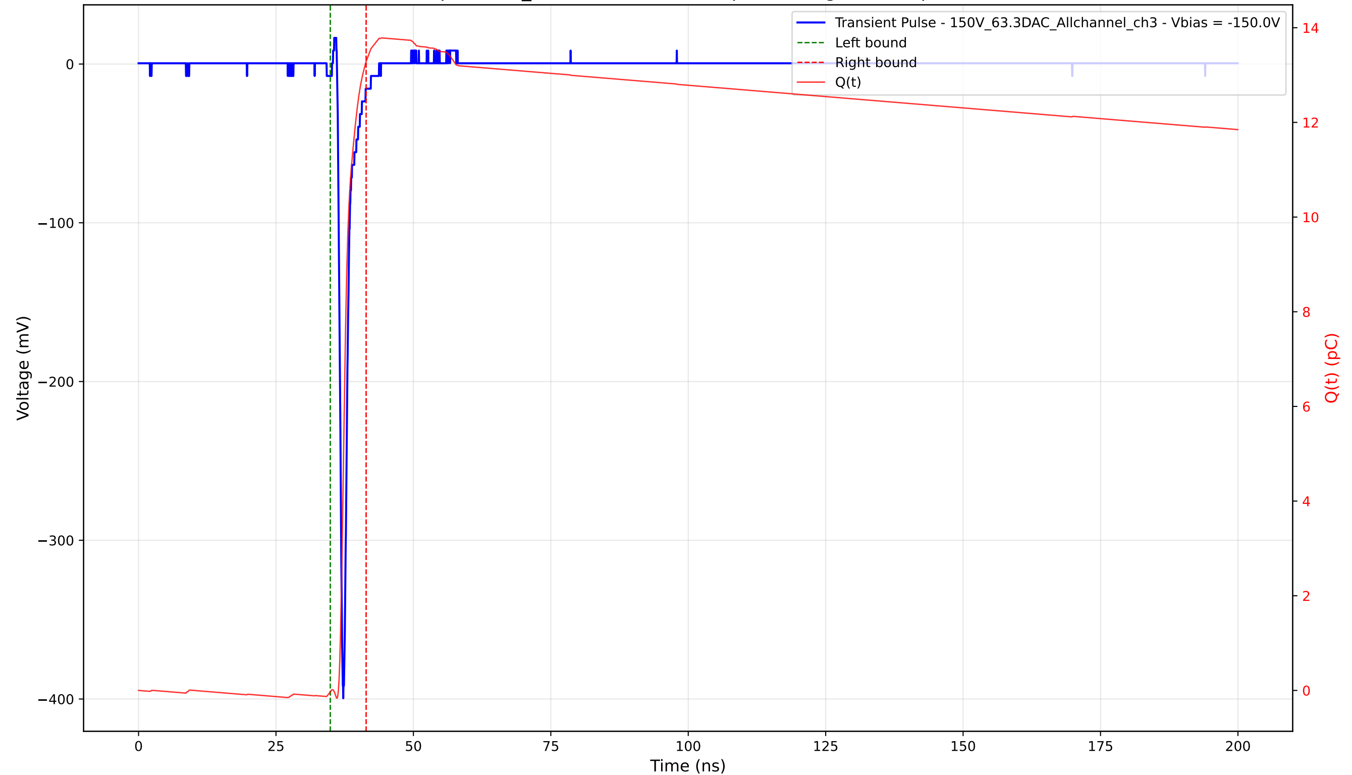
Transient Pulse - Sample: 1cm_42 - Position: 2855.0 \mu\text{m} - Charge: 13.32 pC - Rise Time: 0.74 ns
