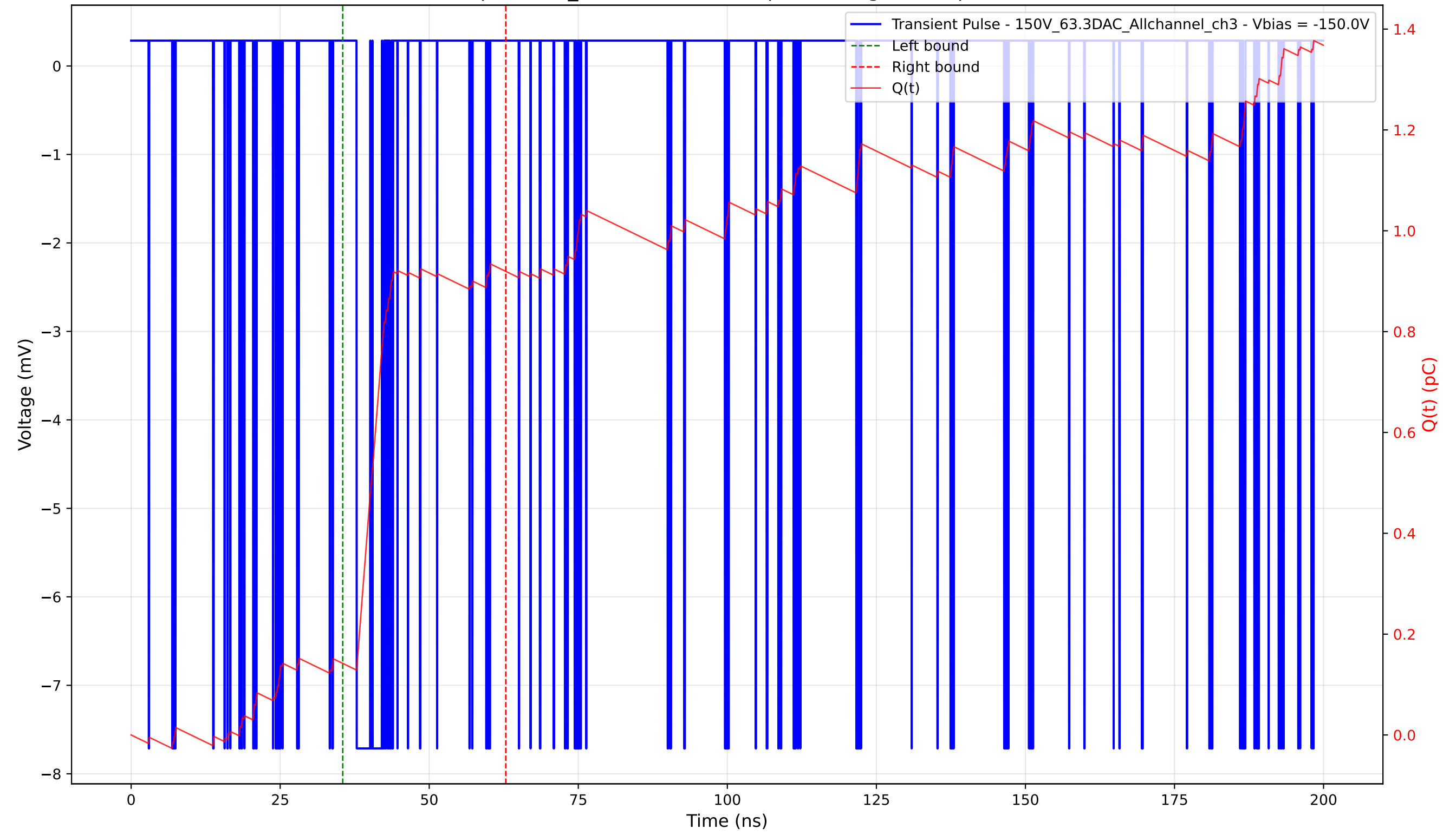
Transient Pulse - Sample: 1cm_42 - Position: 80.0 \mu\text{m} - Charge: 0.78 pC - Rise Time: 0.04 ns
