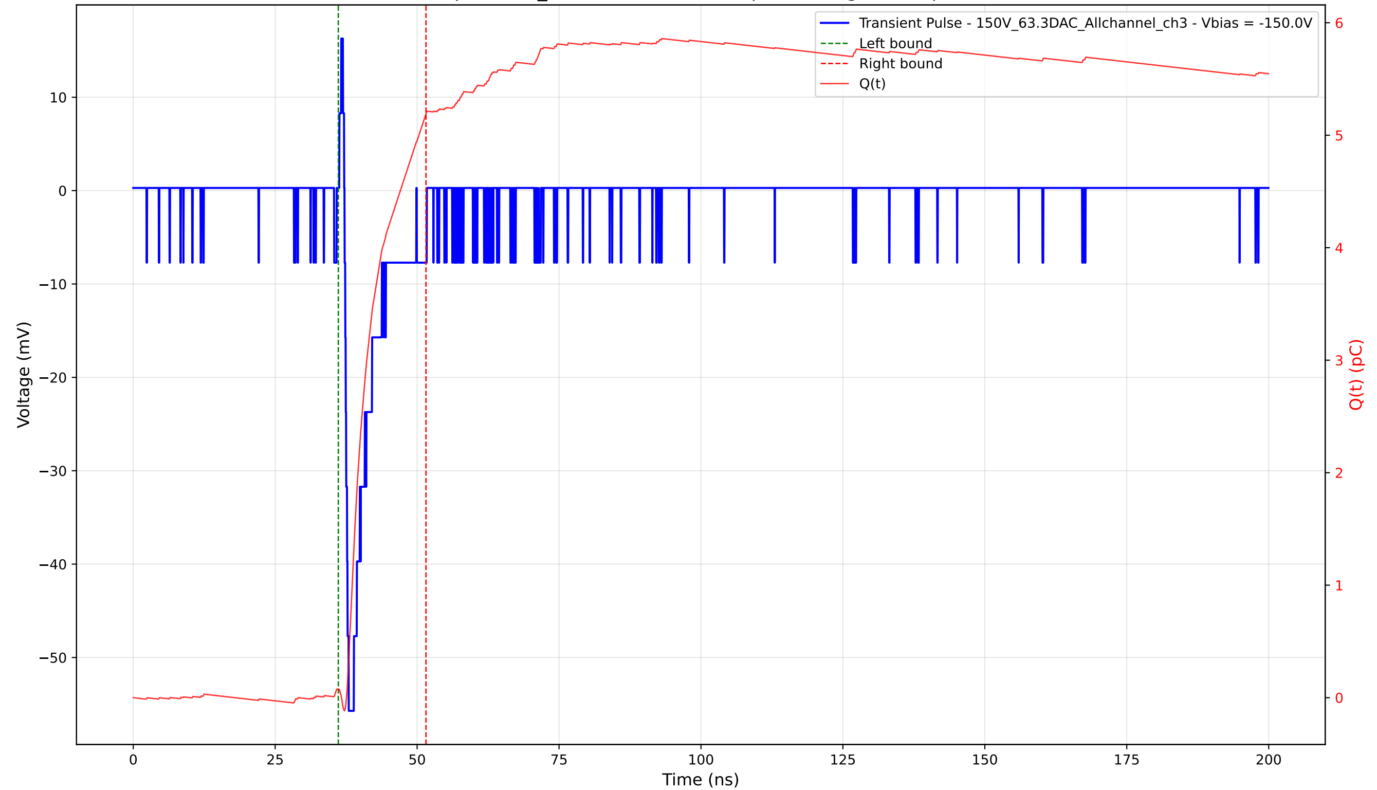
Transient Pulse - Sample: 1cm_42 - Position: 3710.0 \mu\text{m} - Charge: 5.12 pC - Rise Time: 0.73 ns
