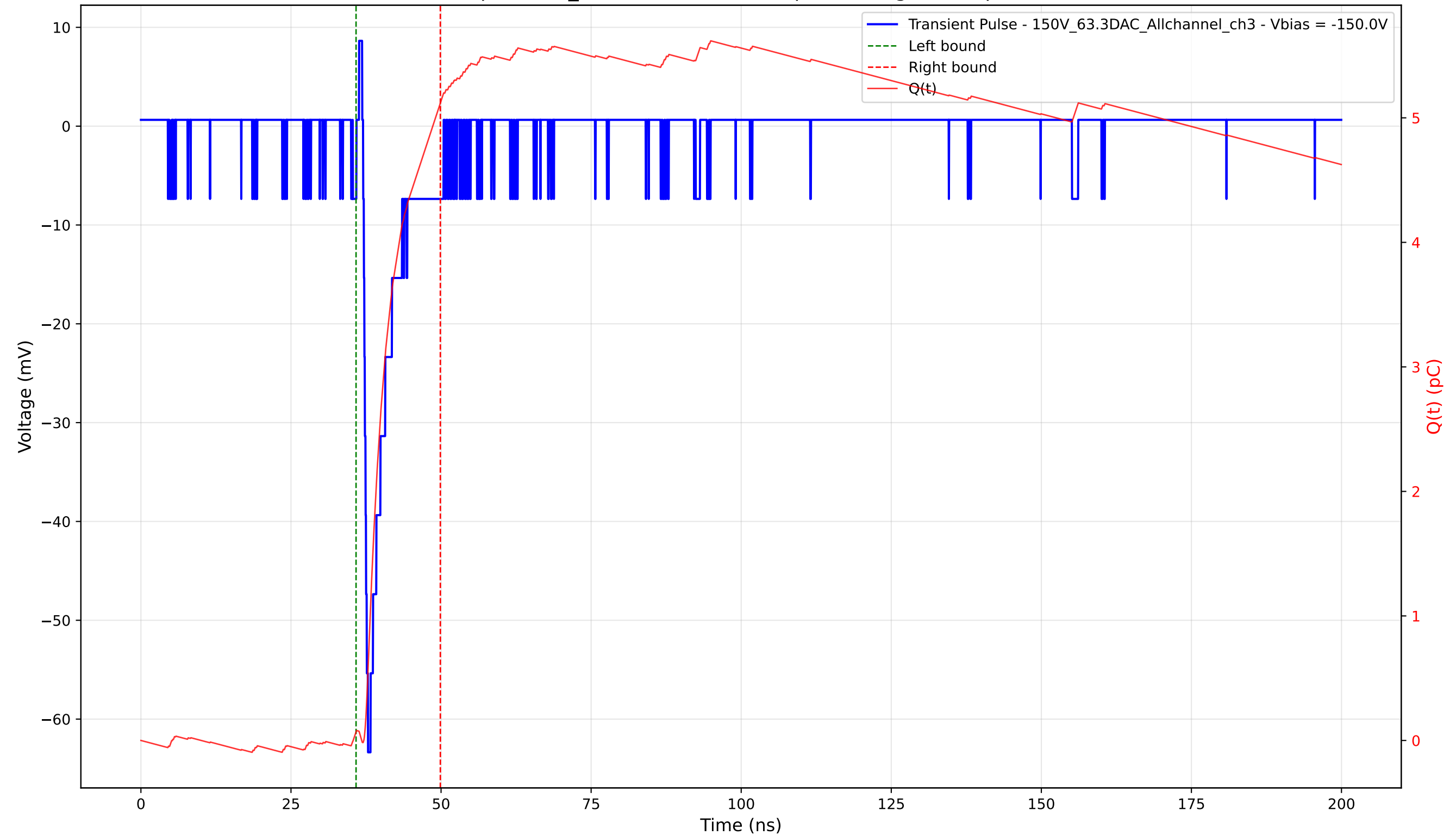
Transient Pulse - Sample: 1cm_42 - Position: 3585.0 \mu\text{m} - Charge: 5.05 pC - Rise Time: 0.81 ns
