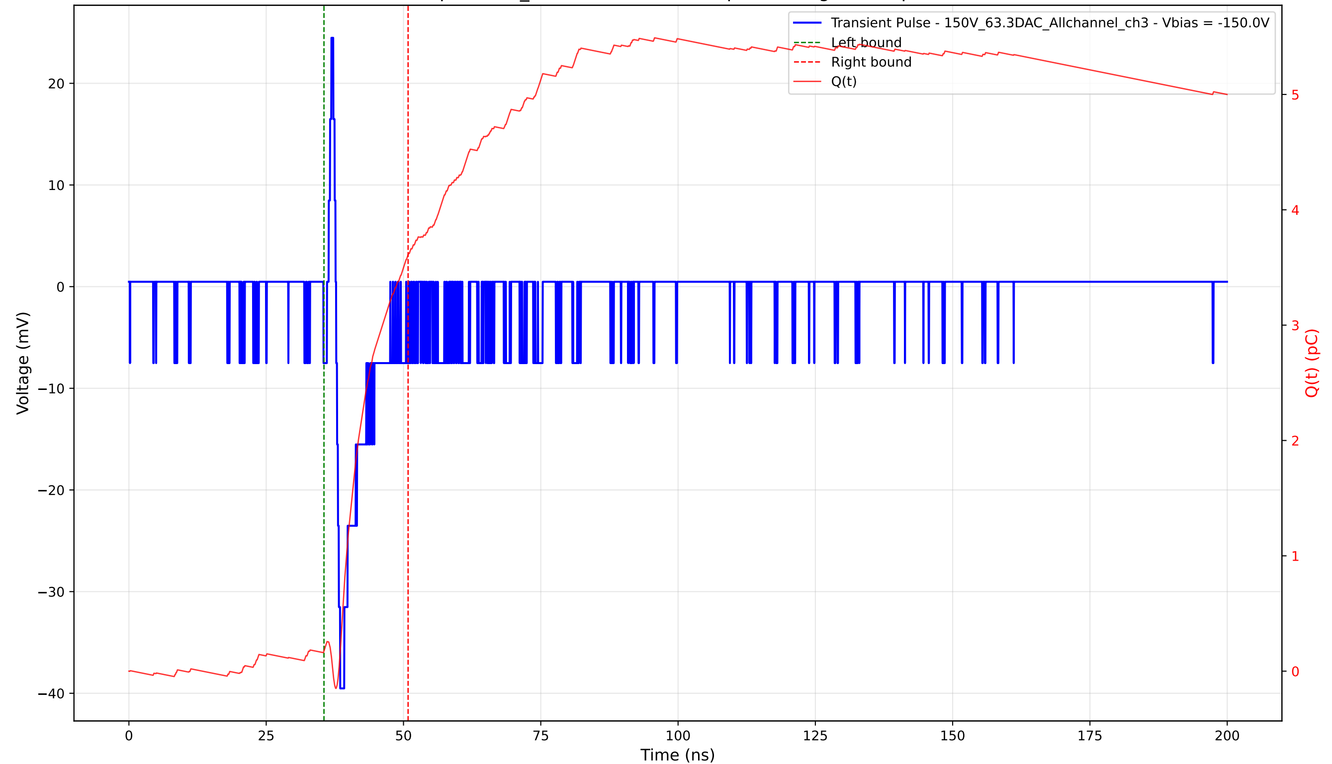
Transient Pulse - Sample: 1cm_42 - Position: 4360.0 \mu\text{m} - Charge: 3.44 pC - Rise Time: 0.74 ns
