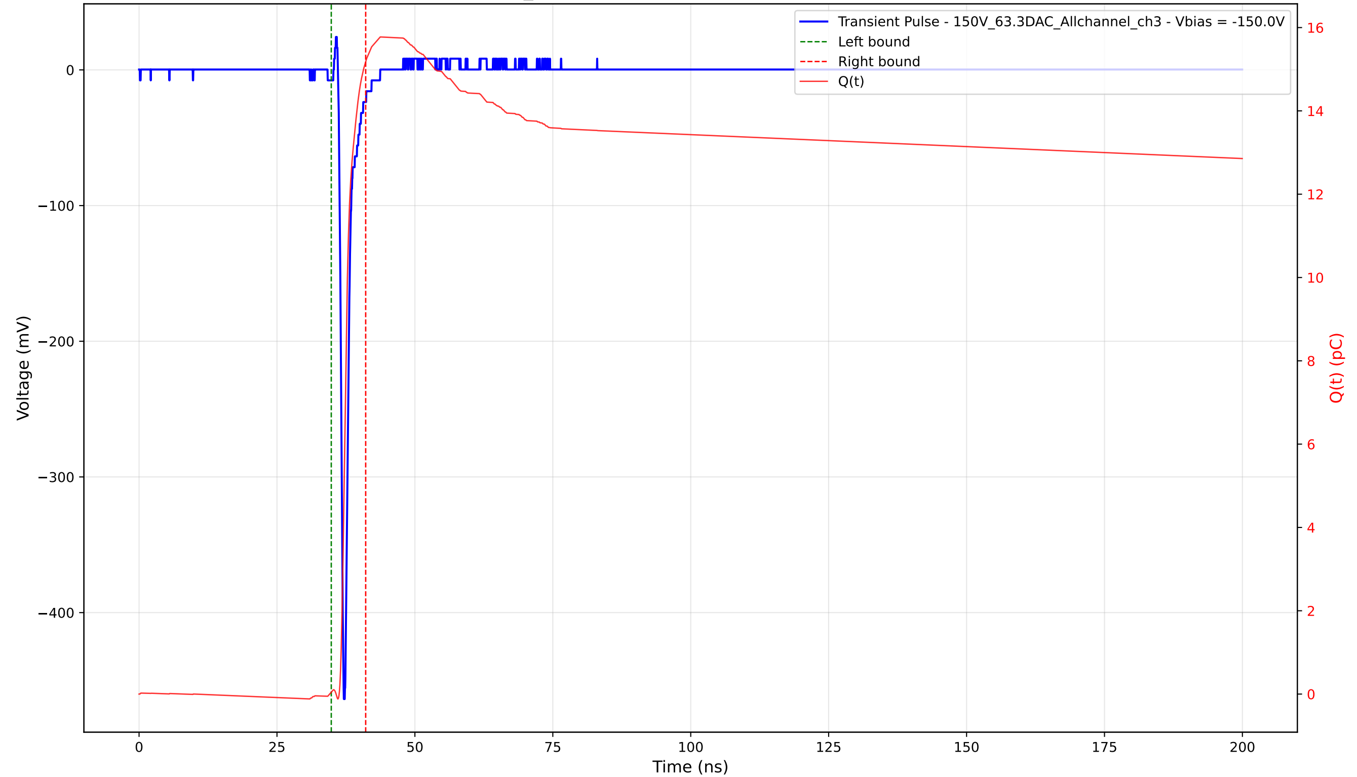
Transient Pulse - Sample: 1cm_42 - Position: 2750.0 \mu\text{m} - Charge: 15.14 pC - Rise Time: 0.69 ns
