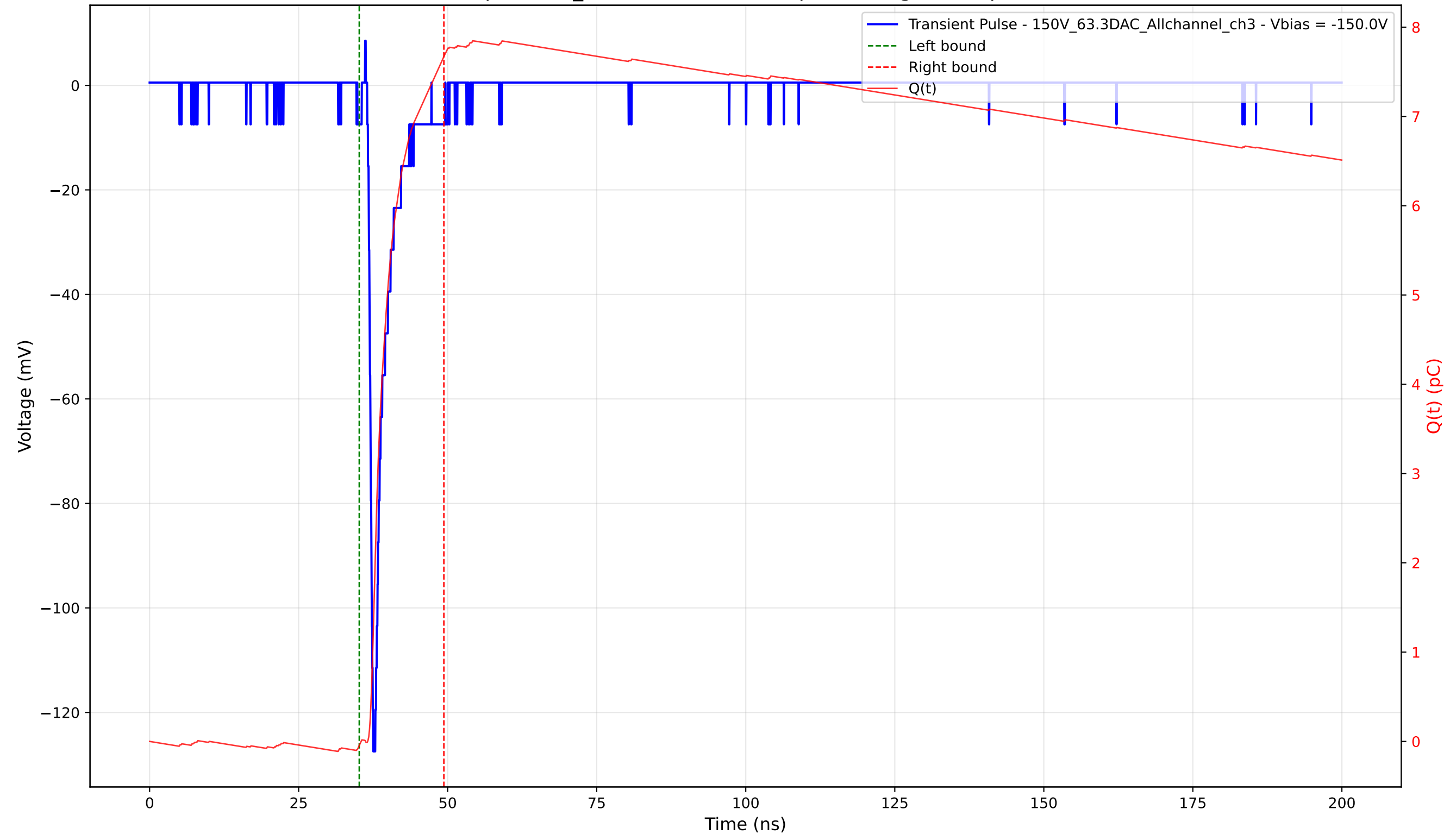
Transient Pulse - Sample: 1cm_42 - Position: 3335.0 \mu\text{m} - Charge: 7.72 pC - Rise Time: 0.81 ns
