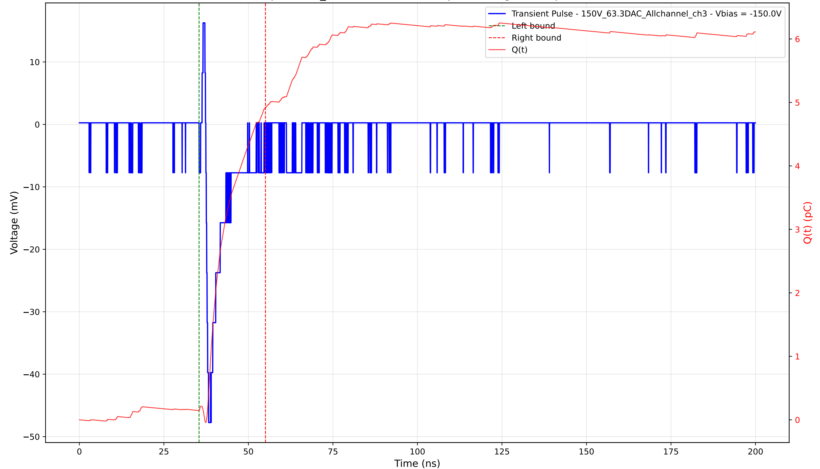
Transient Pulse - Sample: 1cm_42 - Position: 3930.0 \mu\text{m} - Charge: 4.78 pC - Rise Time: 0.82 ns
