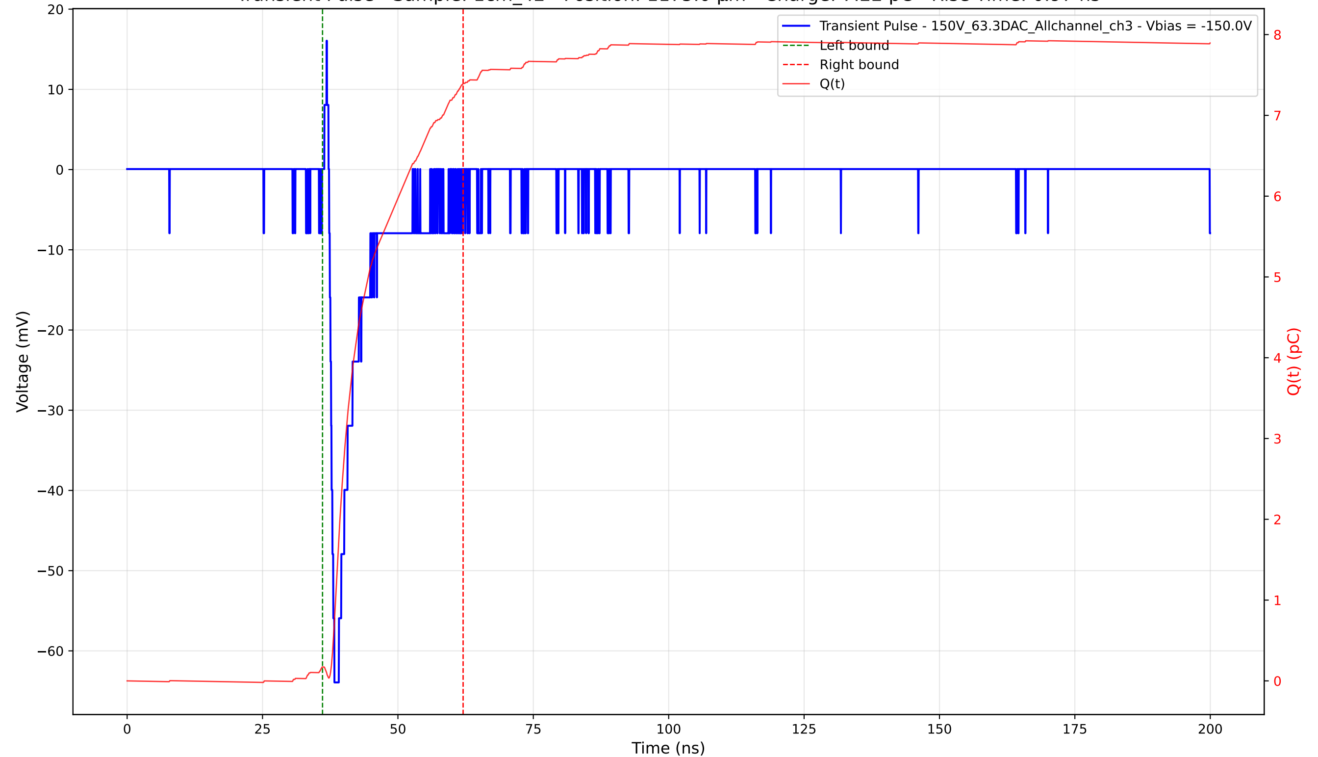
Transient Pulse - Sample: 1cm_42 - Position: 1175.0 \mu\text{m} - Charge: 7.22 pC - Rise Time: 0.97 ns
