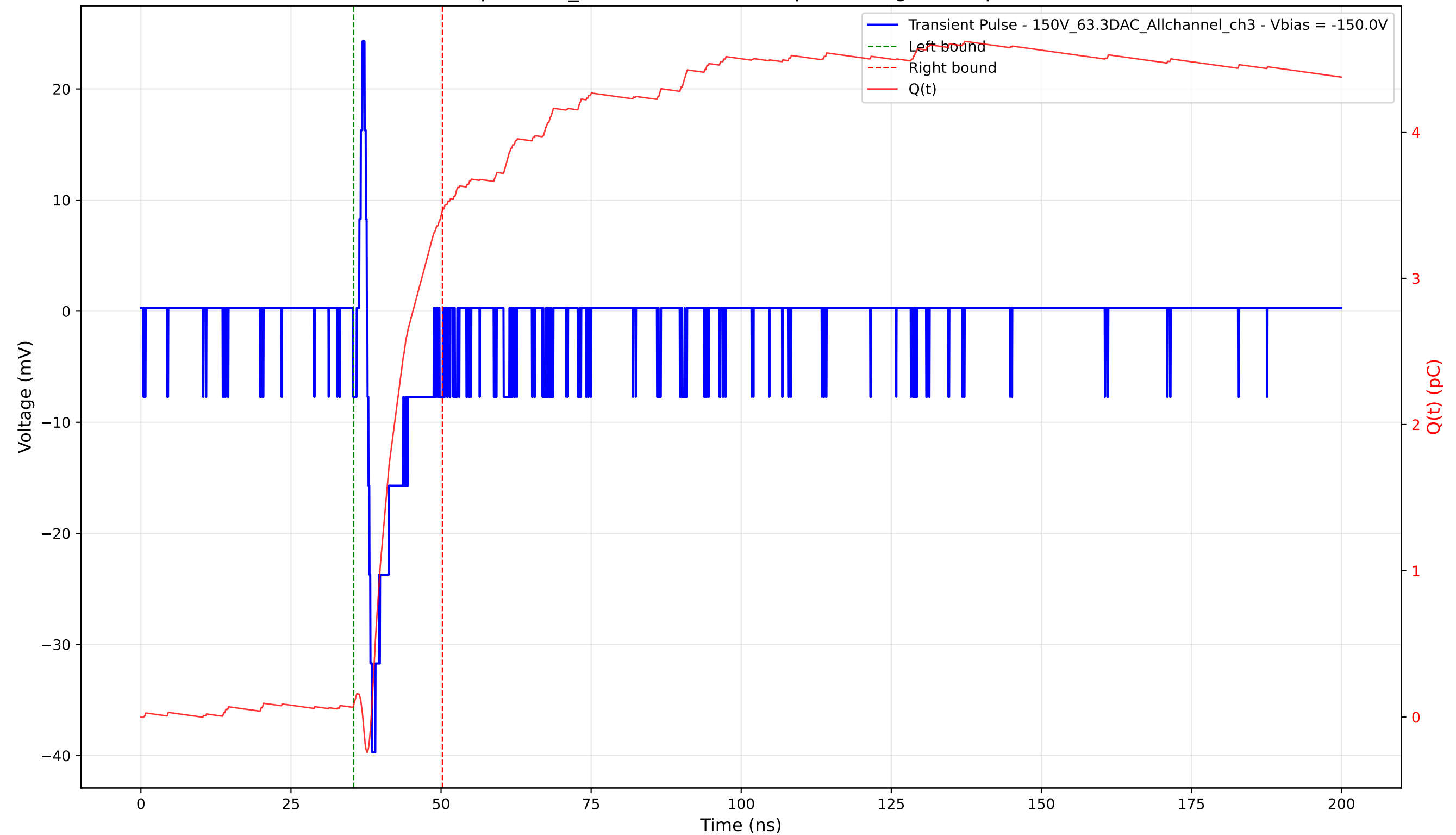
Transient Pulse - Sample: 1cm_42 - Position: 4380.0 \mu\text{m} - Charge: 3.38 pC - Rise Time: 0.78 ns
