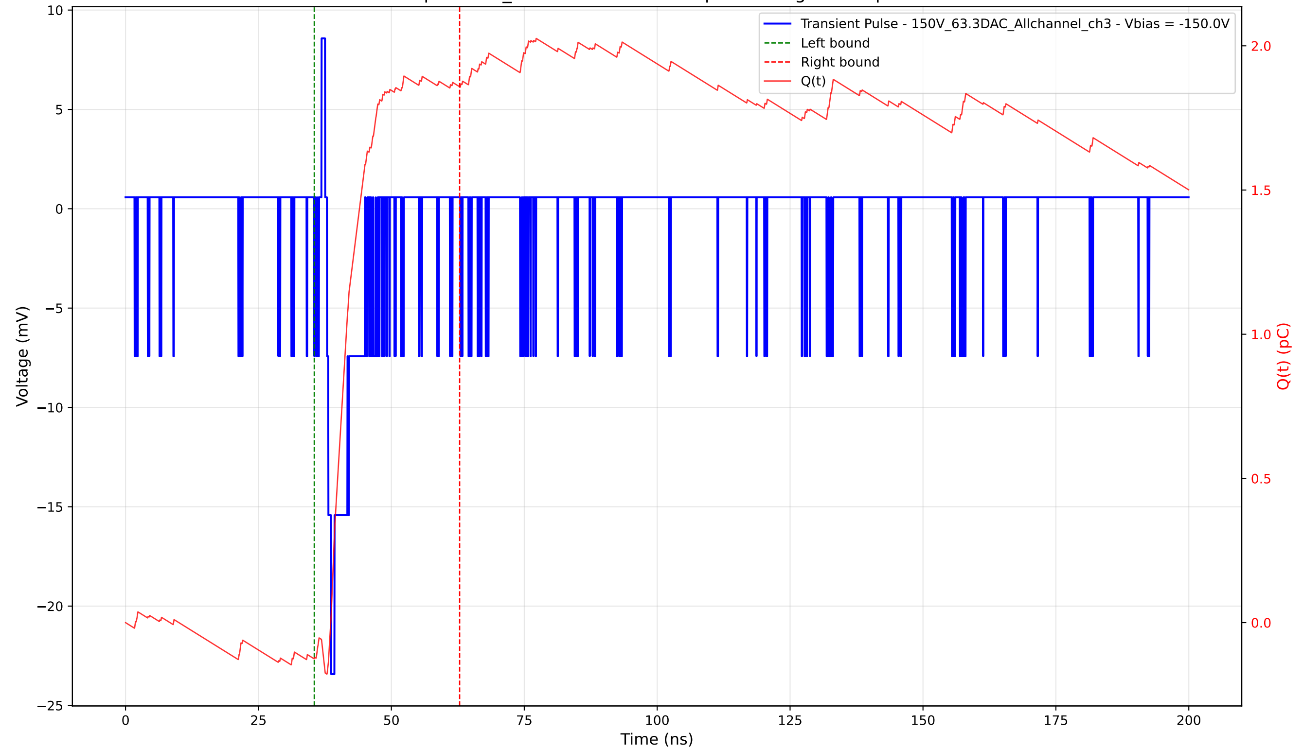
Transient Pulse - Sample: 1cm_42 - Position: 4975.0 \mu\text{m} - Charge: 1.98 pC - Rise Time: 0.79 ns
