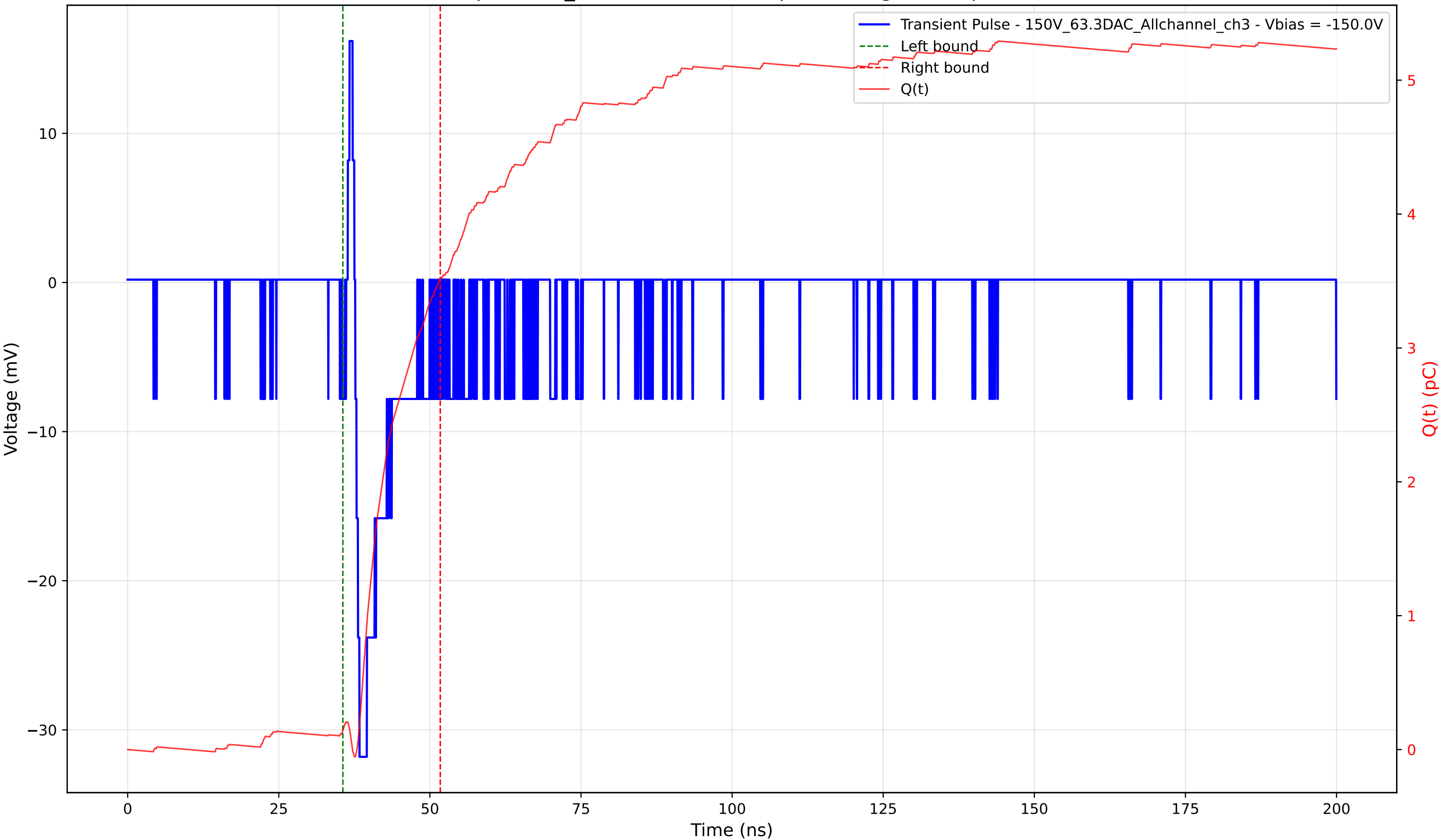
Transient Pulse - Sample: 1cm_42 - Position: 450.0 \mu\text{m} - Charge: 3.37 pC - Rise Time: 0.70 ns
