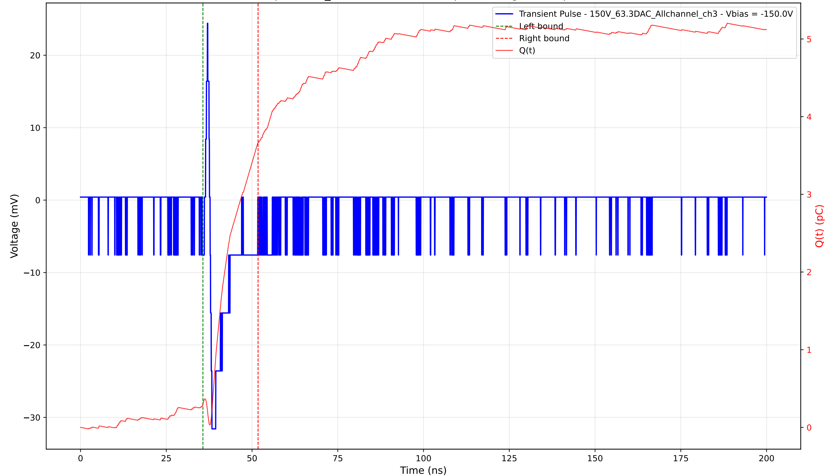
Transient Pulse - Sample: 1cm_42 - Position: 4435.0 \mu\text{m} - Charge: 3.36 pC - Rise Time: 0.54 ns
