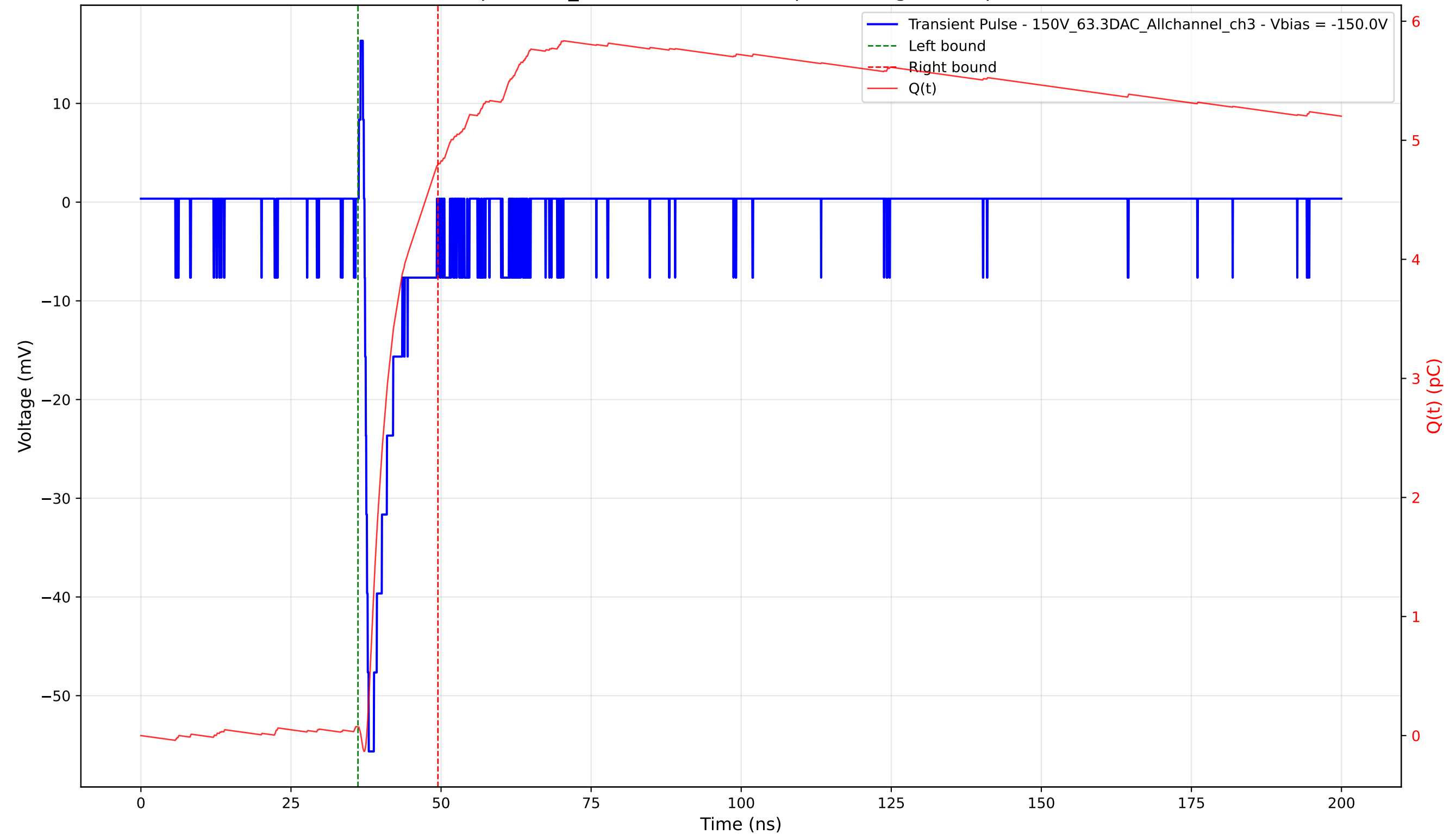
Transient Pulse - Sample: 1cm_42 - Position: 3720.0 \mu\text{m} - Charge: 4.72 pC - Rise Time: 0.69 ns
