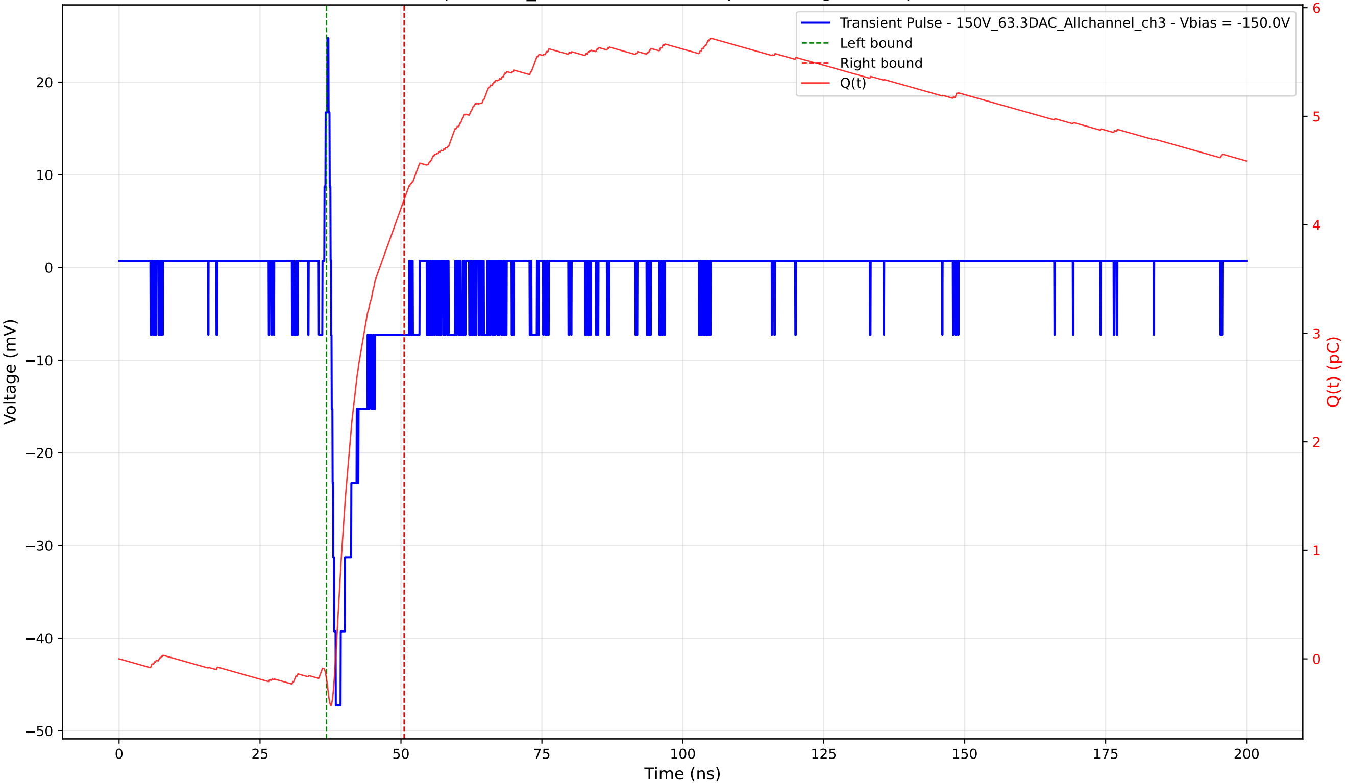
Transient Pulse - Sample: 1cm_42 - Position: 950.0 \mu\text{m} - Charge: 4.42 pC - Rise Time: 0.82 ns
