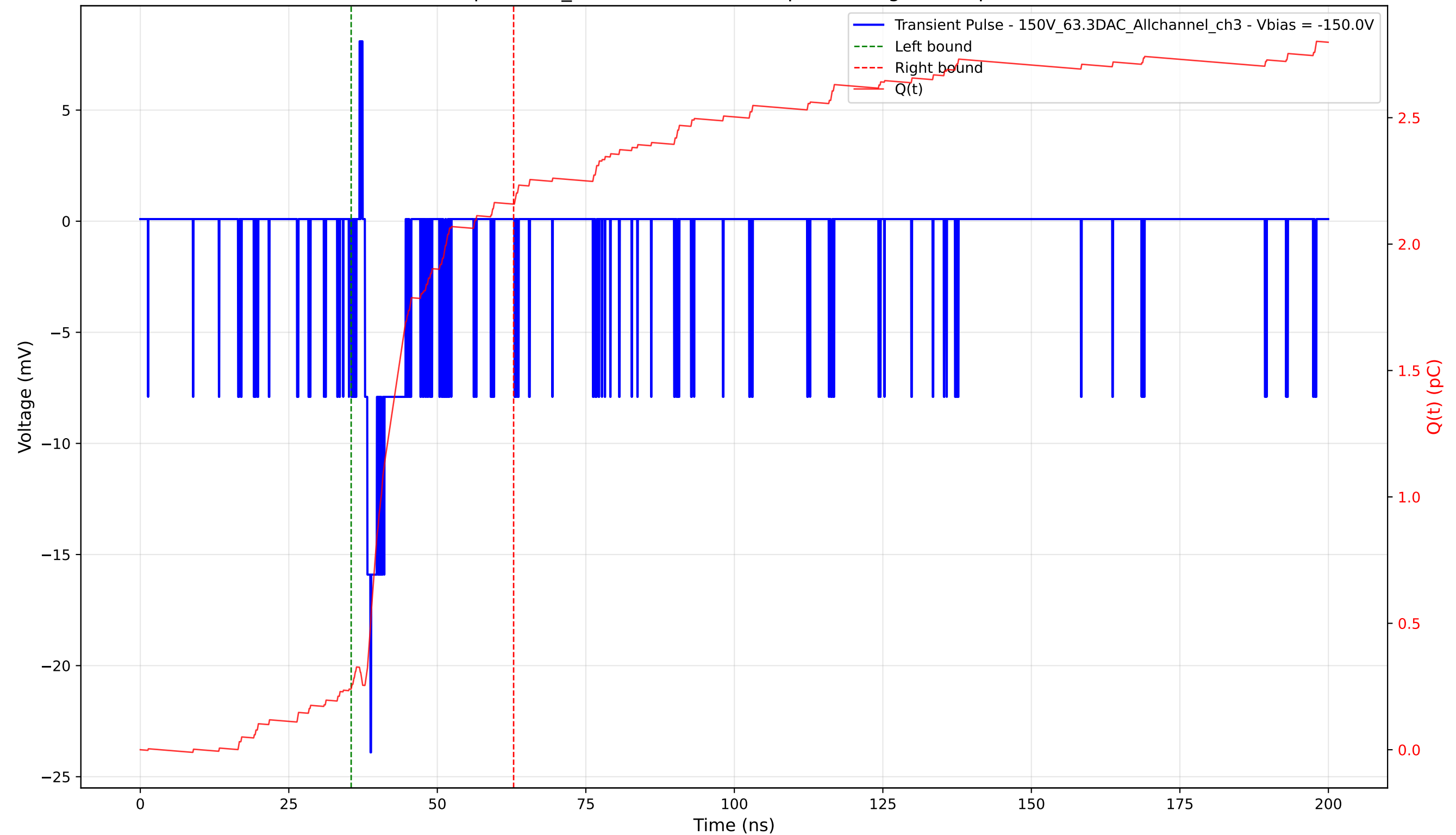
Transient Pulse - Sample: 1cm_42 - Position: 5010.0 \mu\text{m} - Charge: 1.92 pC - Rise Time: 0.95 ns
