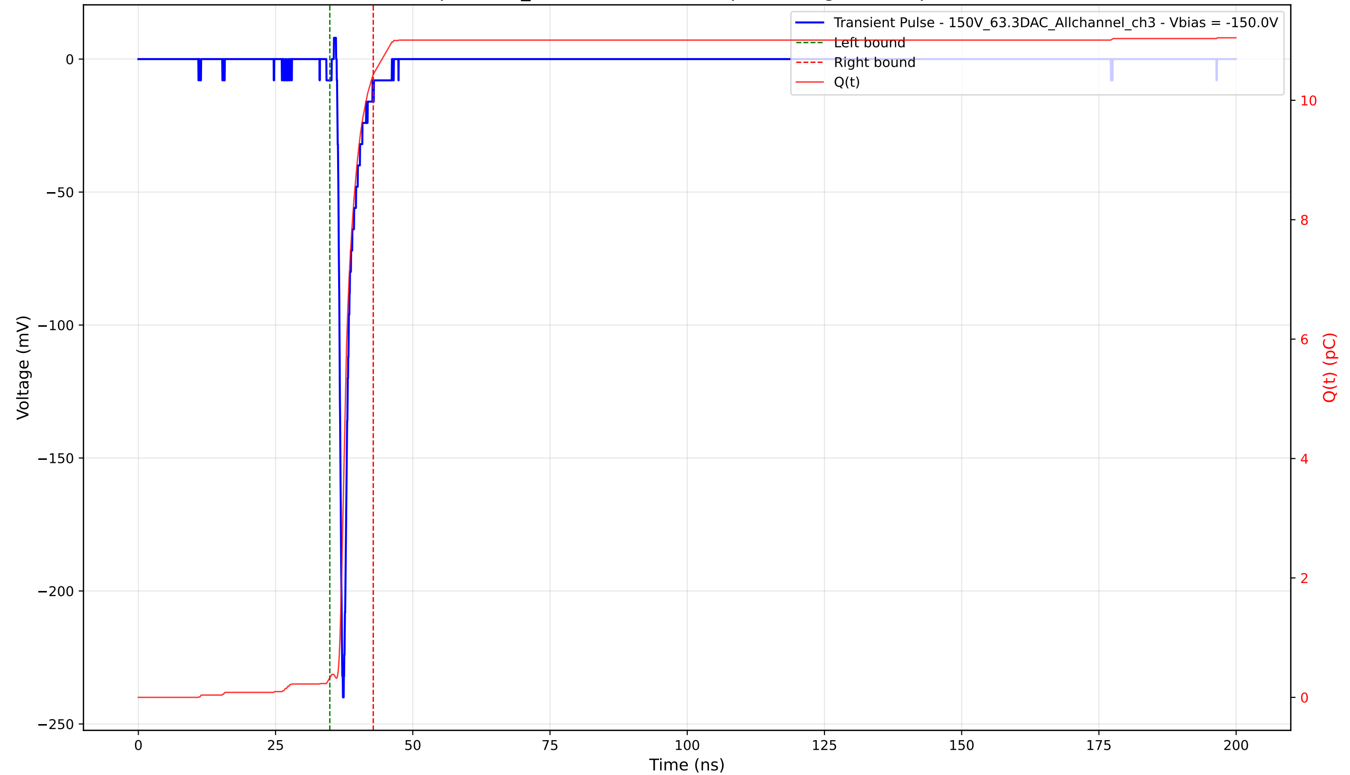
Transient Pulse - Sample: 1cm_42 - Position: 2025.0 \mu\text{m} - Charge: 10.09 pC - Rise Time: 0.80 ns
