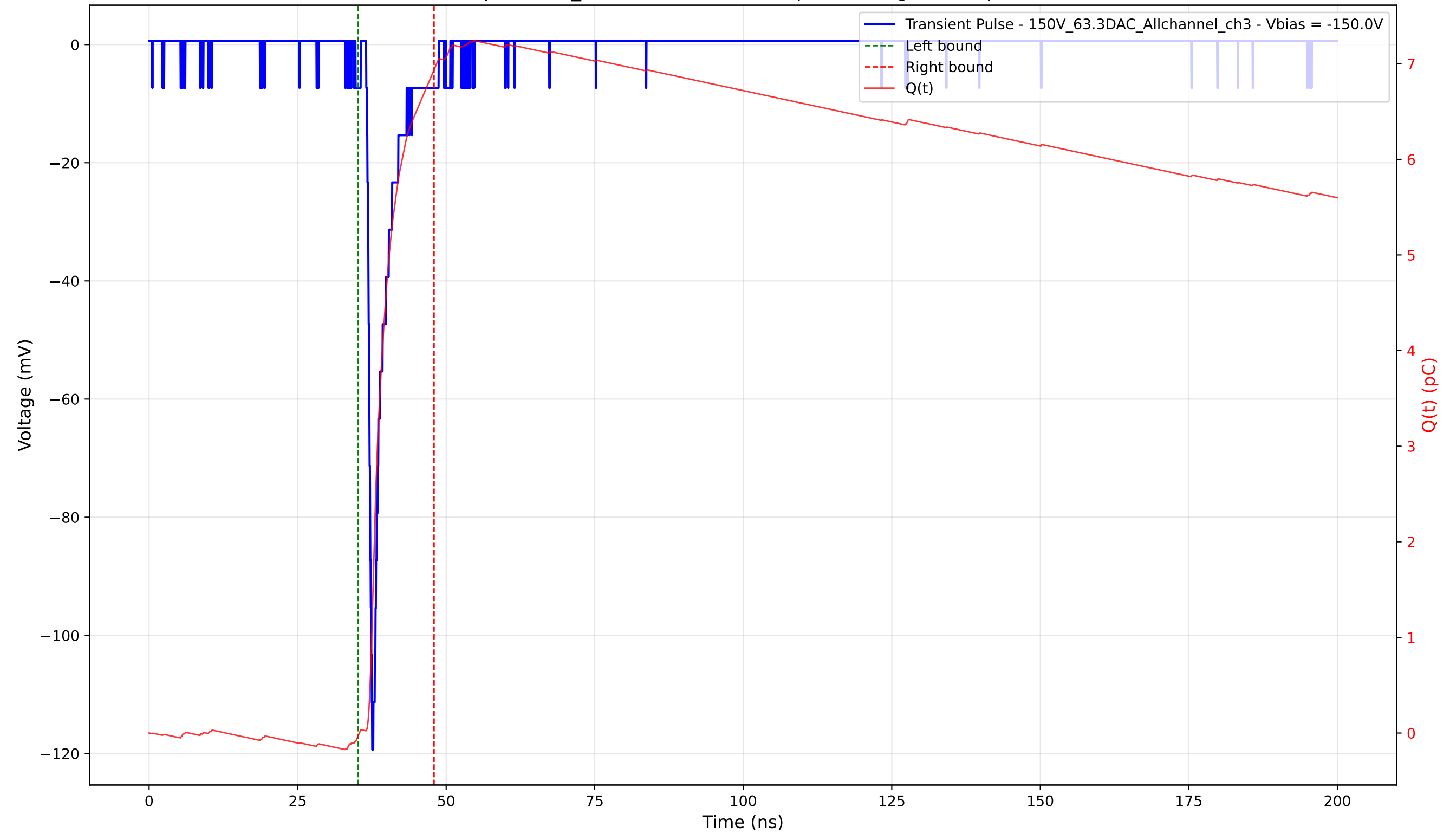
Transient Pulse - Sample: 1cm_42 - Position: 3365.0 \mu\text{m} - Charge: 6.97 pC - Rise Time: 0.82 ns
