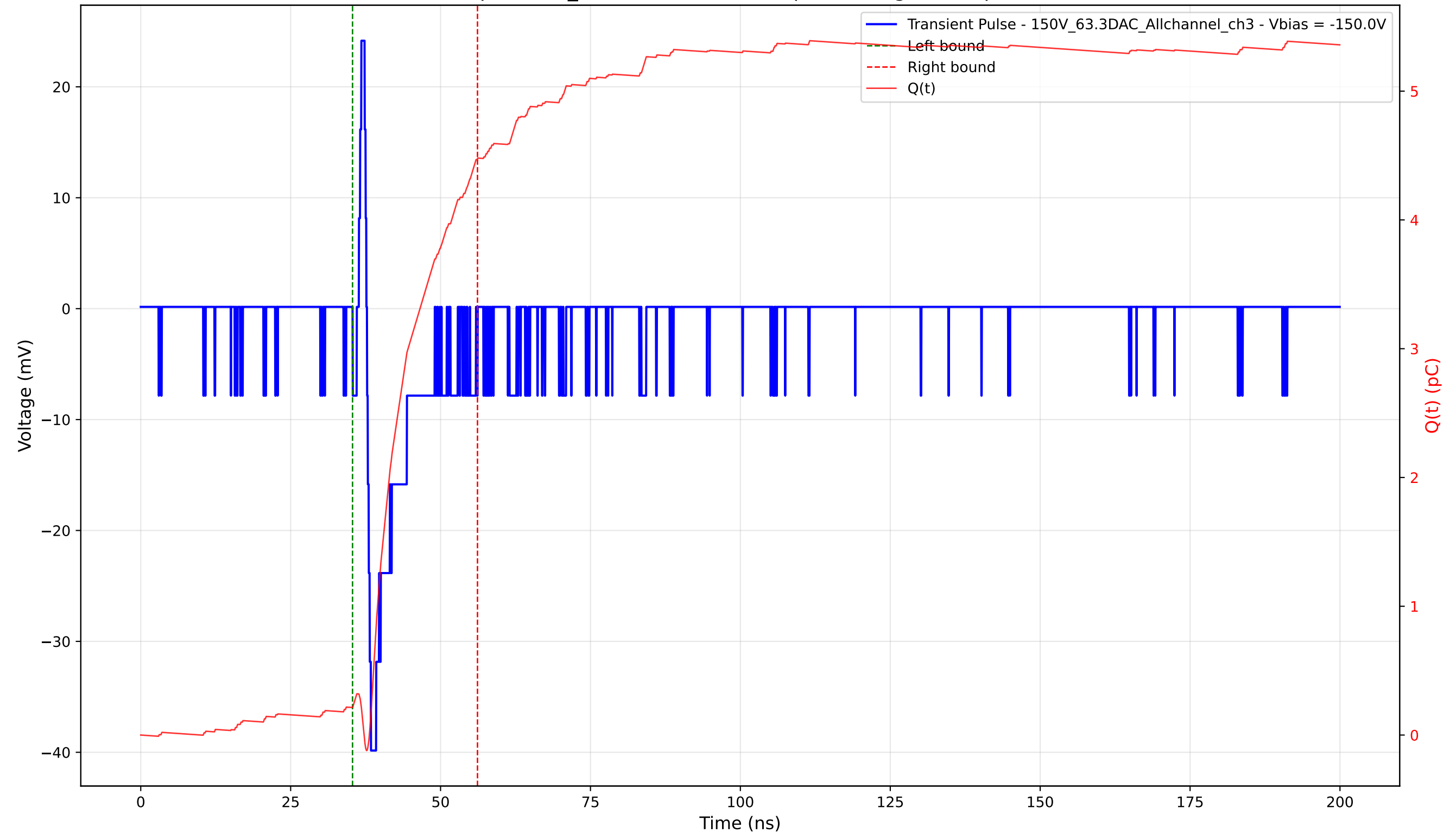
Transient Pulse - Sample: 1cm_42 - Position: 4300.0 \mu\text{m} - Charge: 4.26 pC - Rise Time: 0.66 ns
