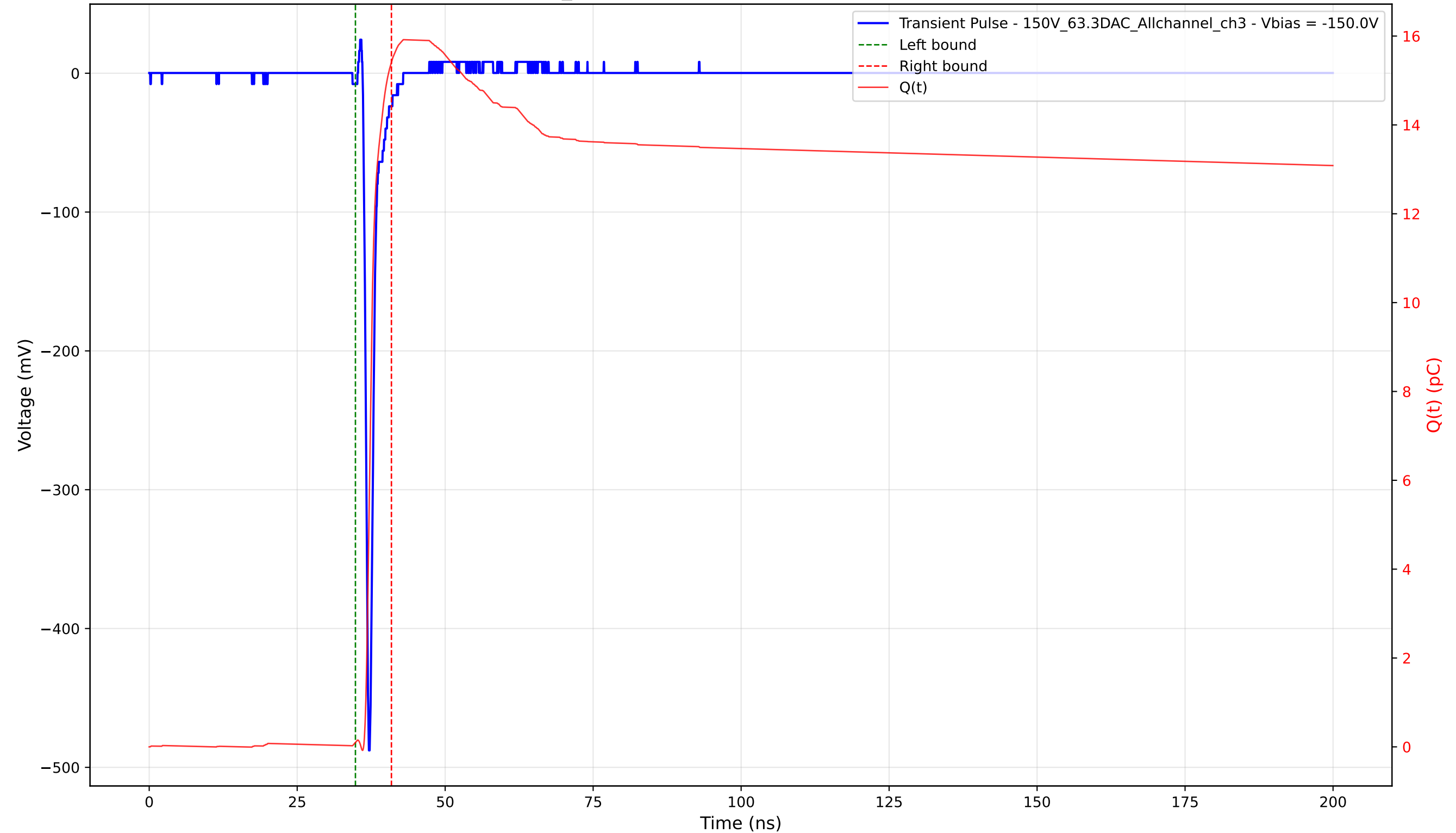
Transient Pulse - Sample: 1cm_42 - Position: 2665.0 \mu\text{m} - Charge: 15.31 pC - Rise Time: 0.69 ns
