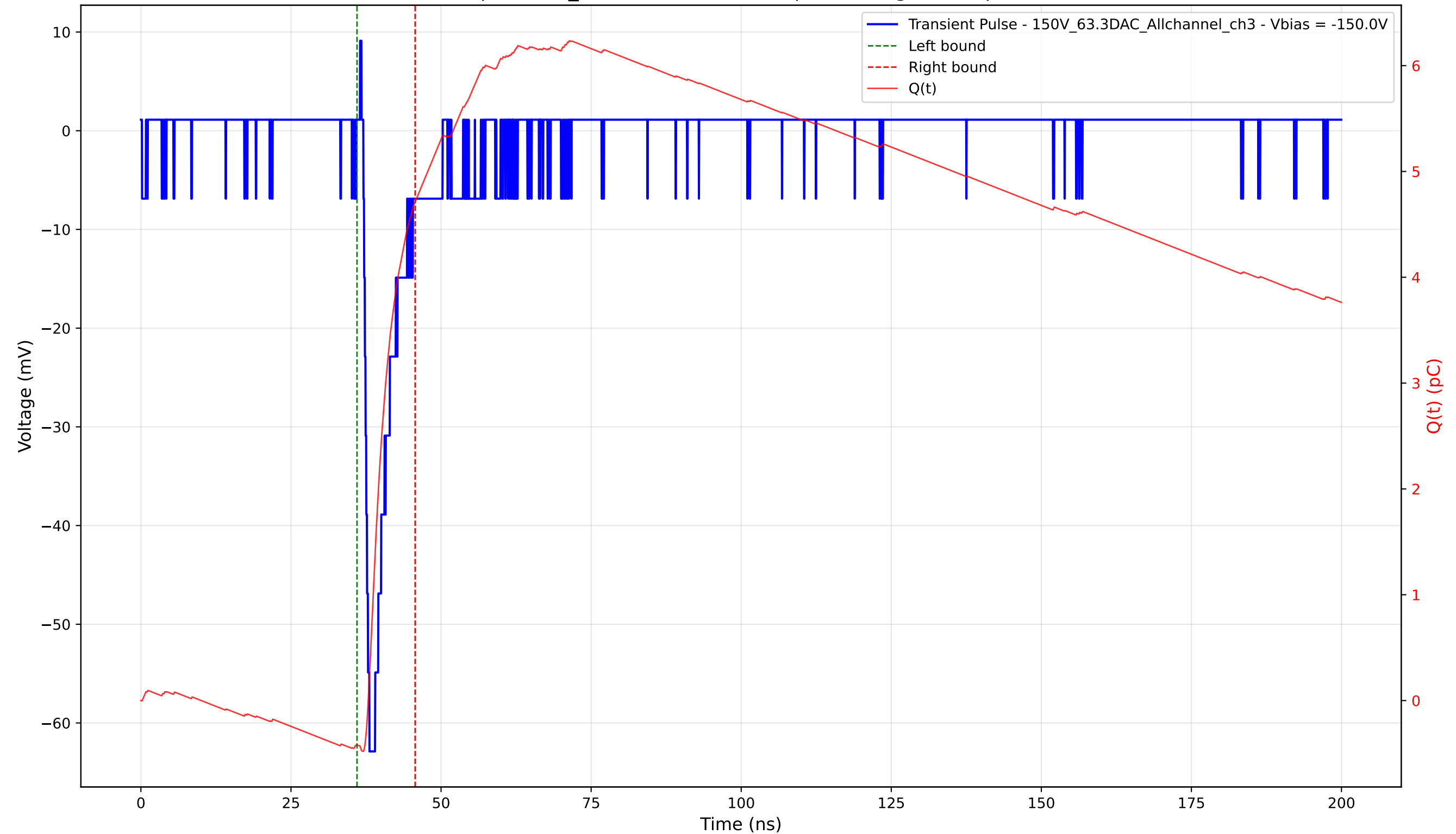
Transient Pulse - Sample: 1cm_42 - Position: 1375.0 \mu\text{m} - Charge: 5.13 pC - Rise Time: 1.00 ns
