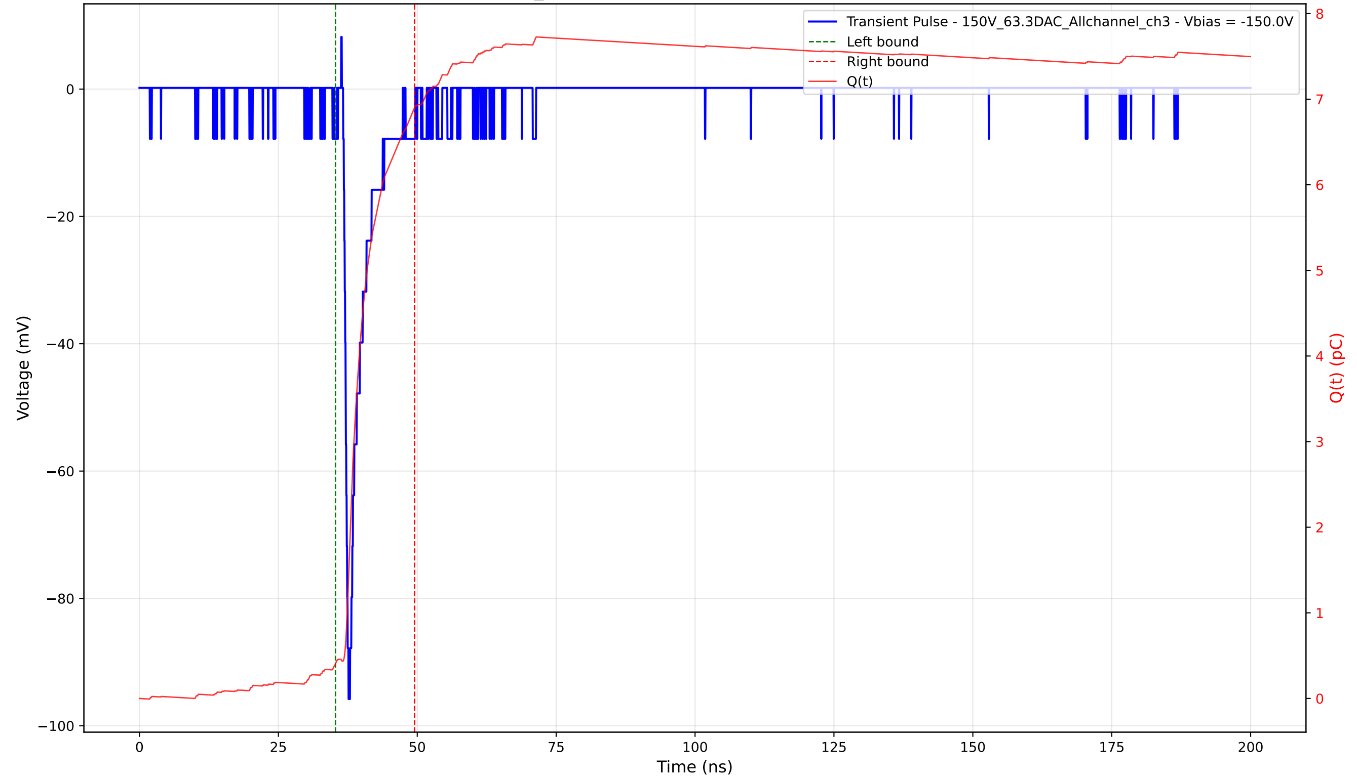
Transient Pulse - Sample: 1cm_42 - Position: 3430.0 \mu\text{m} - Charge: 6.50 pC - Rise Time: 0.71 ns
