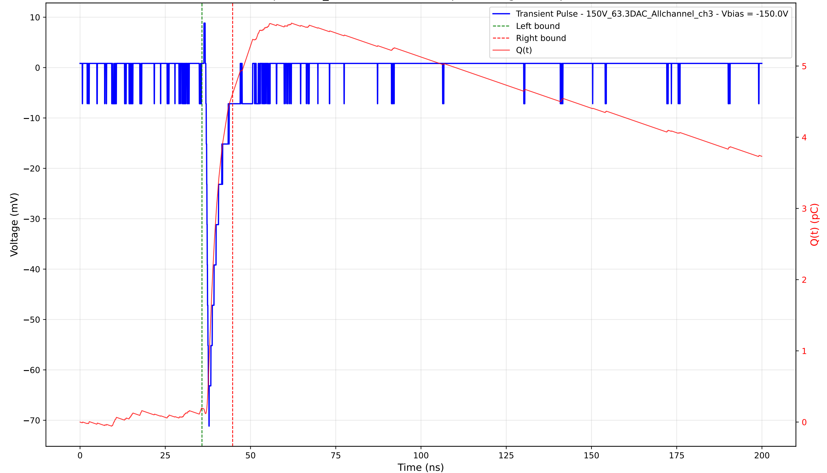
Transient Pulse - Sample: 1cm_42 - Position: 3540.0 \mu\text{m} - Charge: 4.42 pC - Rise Time: 0.92 ns
