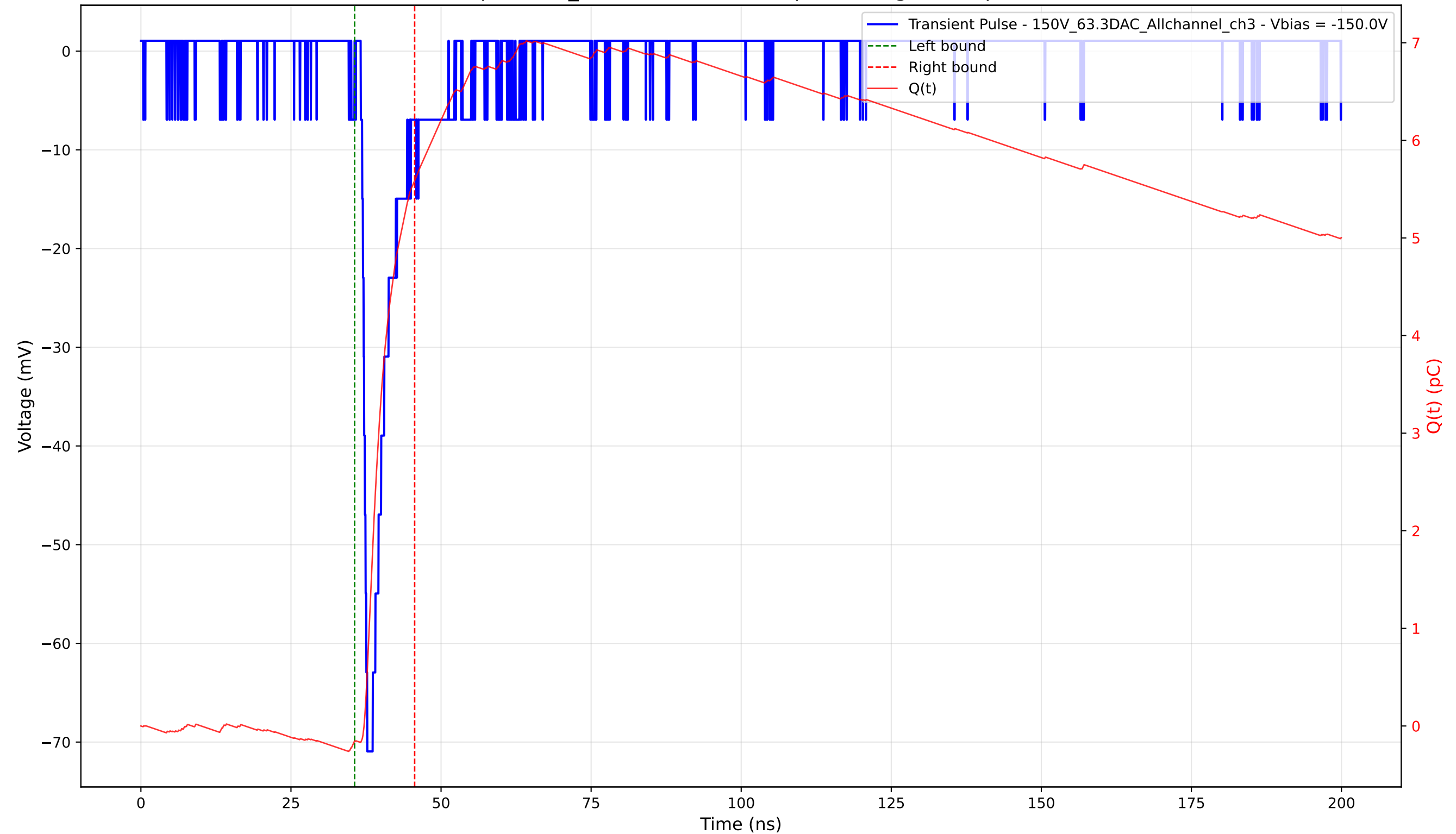
Transient Pulse - Sample: 1cm_42 - Position: 1490.0 \mu\text{m} - Charge: 5.74 pC - Rise Time: 0.88 ns
