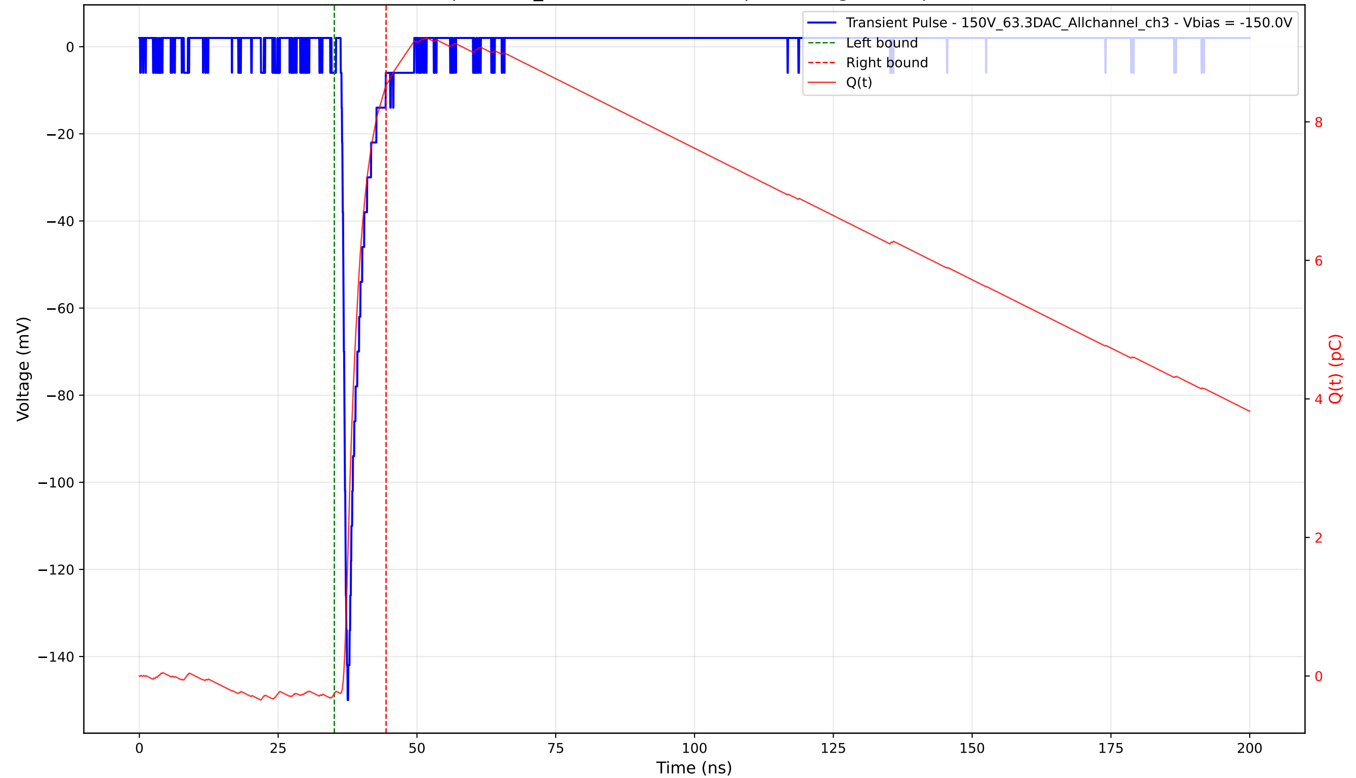
Transient Pulse - Sample: 1cm_42 - Position: 1730.0 \mu\text{m} - Charge: 8.78 pC - Rise Time: 0.91 ns
