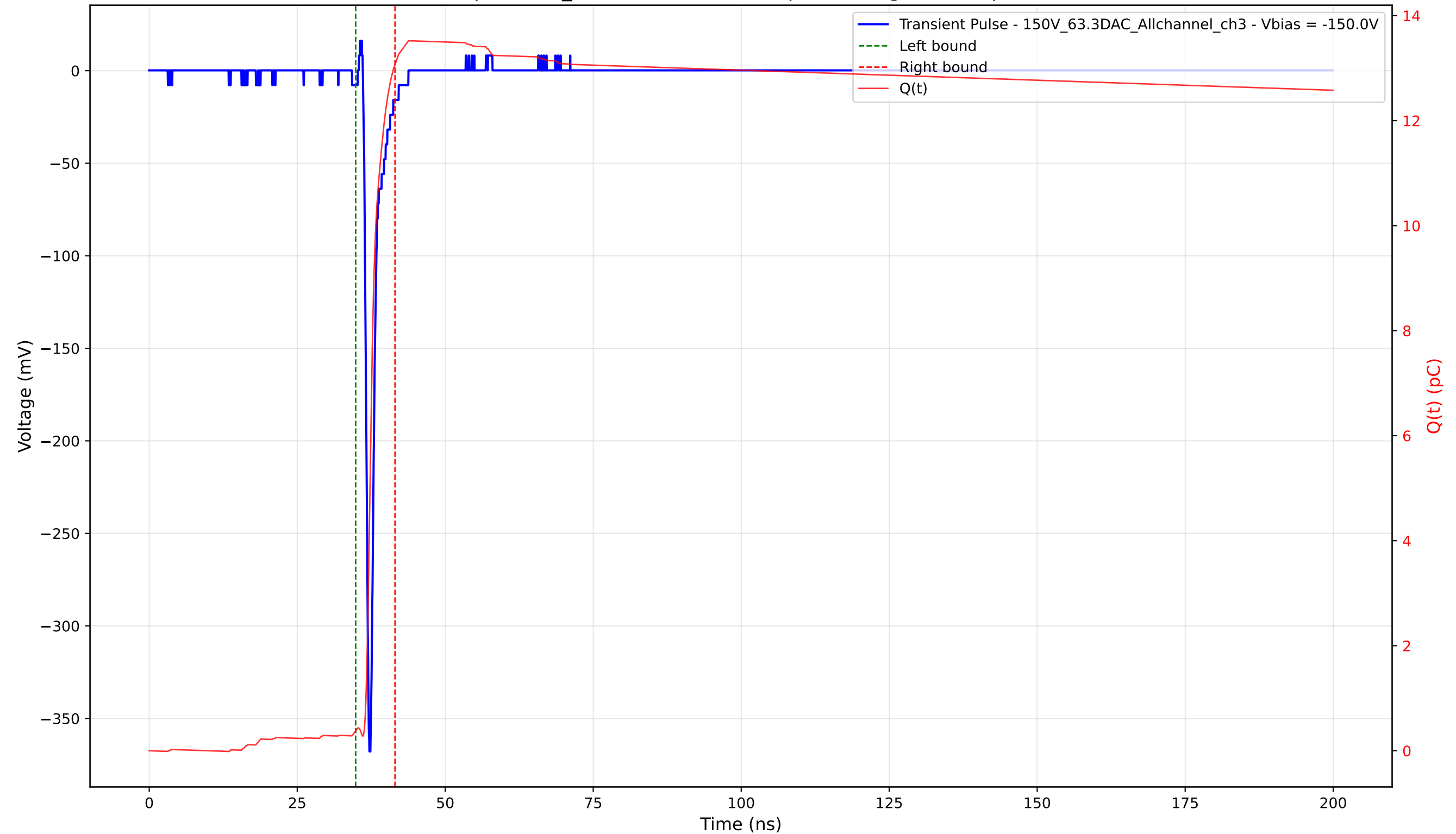
Transient Pulse - Sample: 1cm_42 - Position: 2875.0 \mu\text{m} - Charge: 12.69 pC - Rise Time: 0.76 ns
