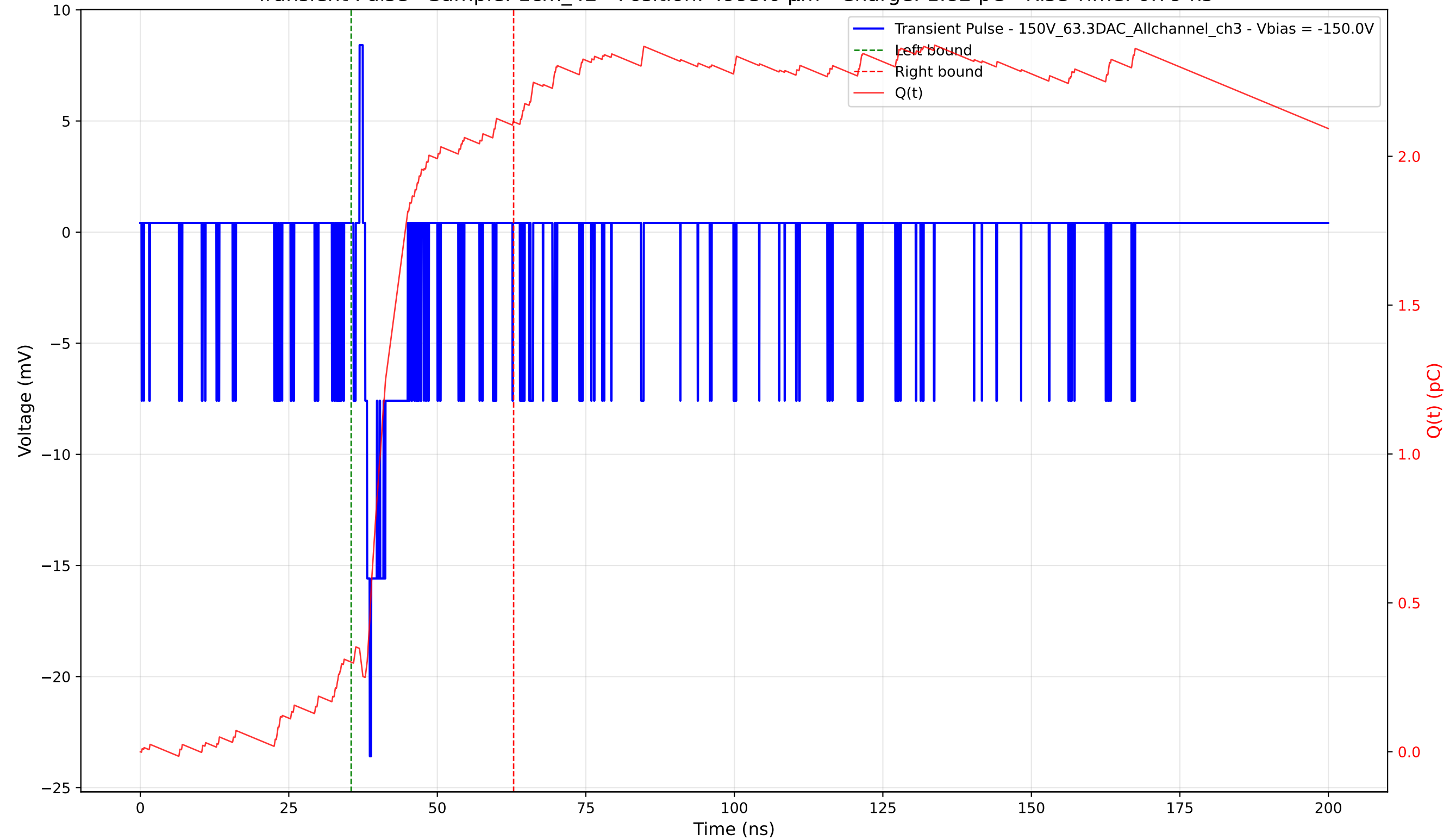
Transient Pulse - Sample: 1cm_42 - Position: 4995.0 \mu\text{m} - Charge: 1.82 pC - Rise Time: 0.79 ns
