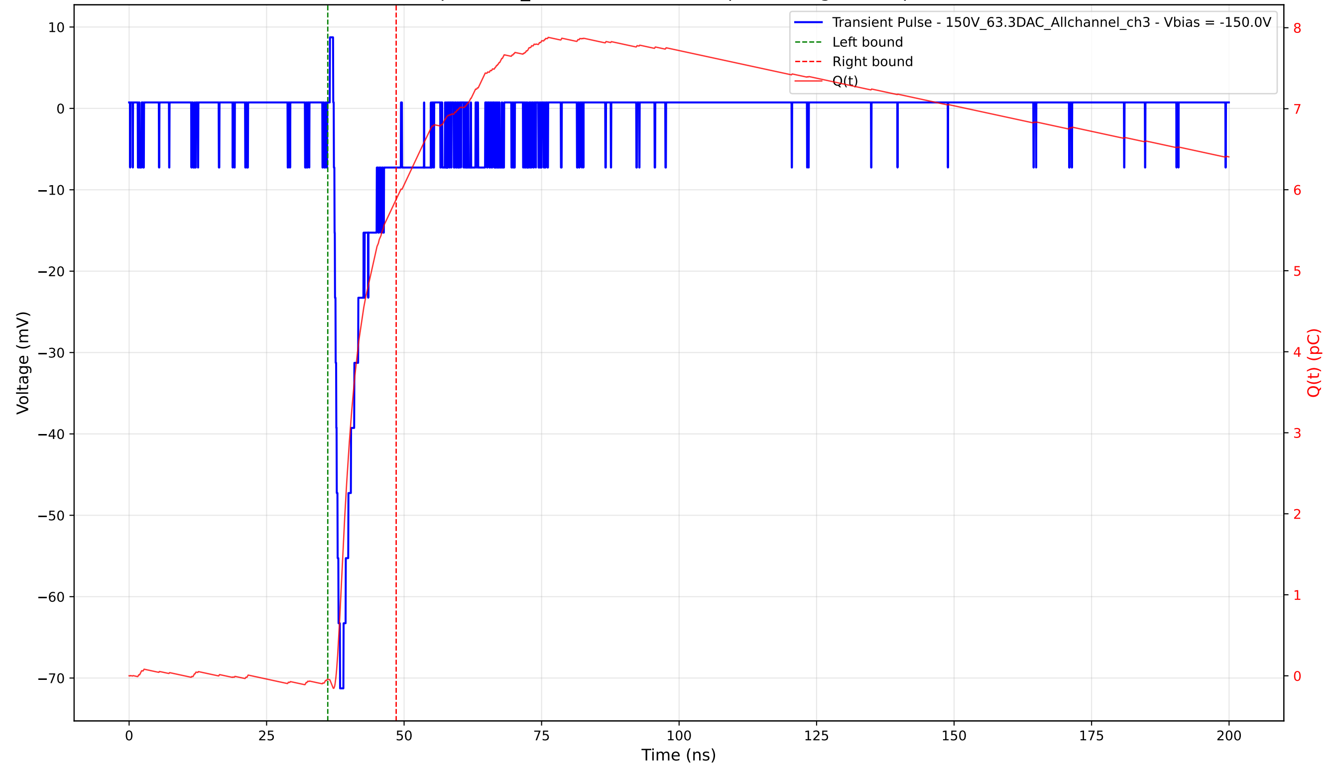
Transient Pulse - Sample: 1cm_42 - Position: 1255.0 \mu\text{m} - Charge: 5.93 pC - Rise Time: 1.12 ns
