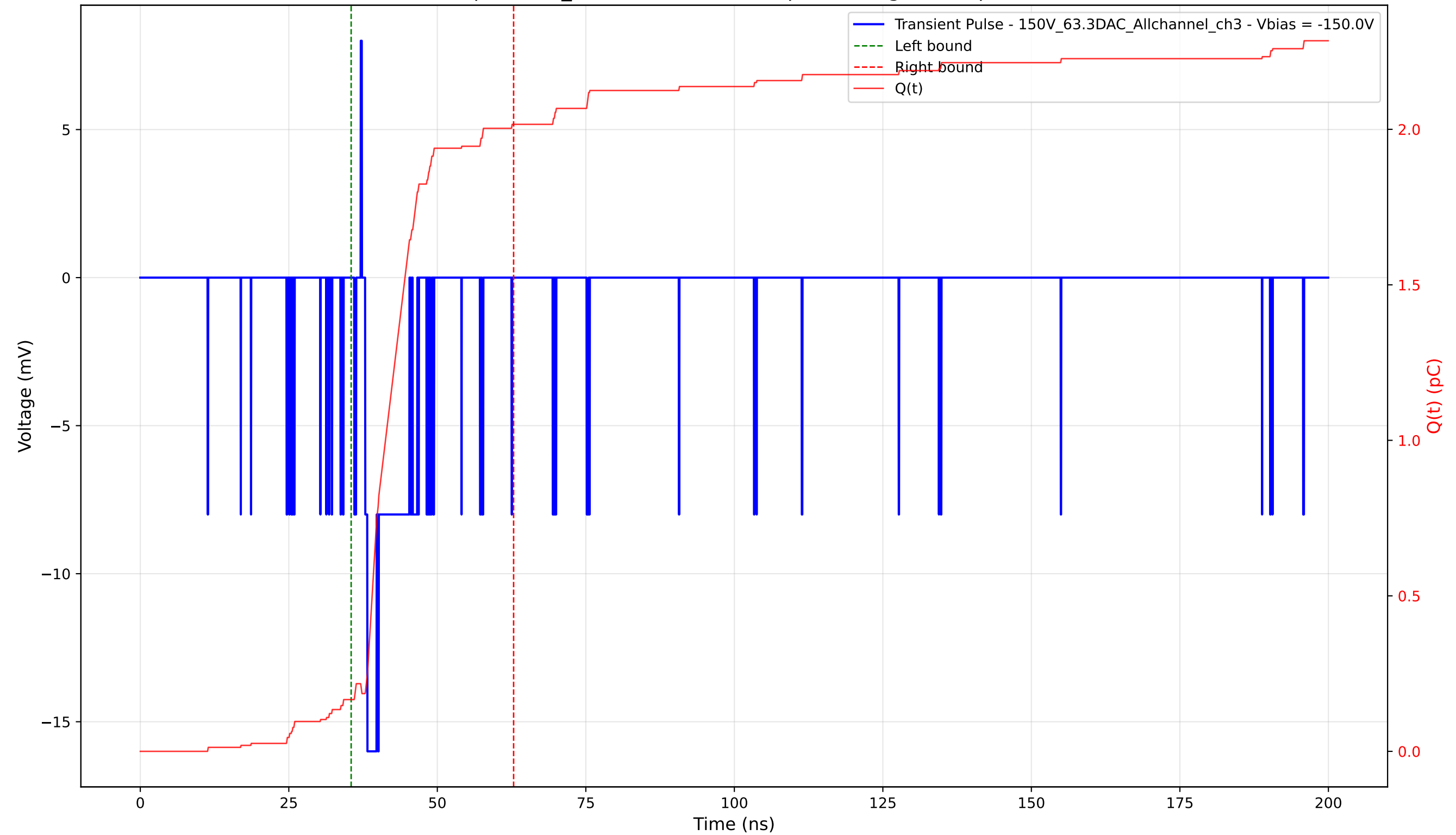
Transient Pulse - Sample: 1cm_42 - Position: 5025.0 \mu\text{m} - Charge: 1.85 pC - Rise Time: 0.39 ns
