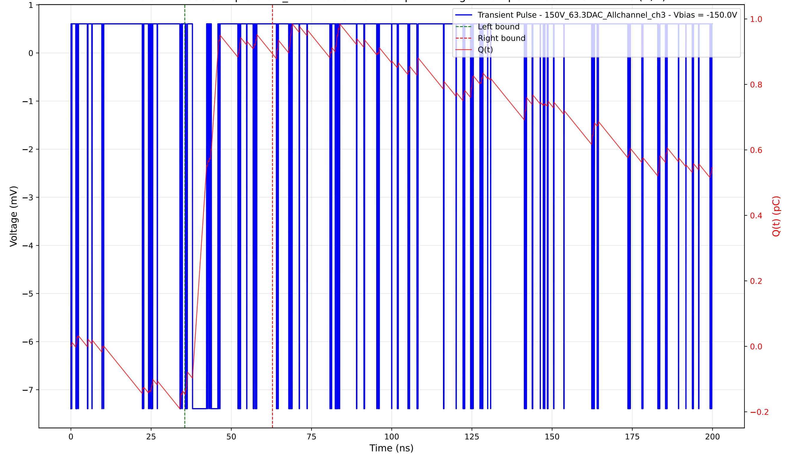
Transient Pulse - Sample: 1cm_42 - Position: 5110.0 \mu\text{m} - Charge: 1.04 pC - Rise Time: 0.00 ns (N/A)
