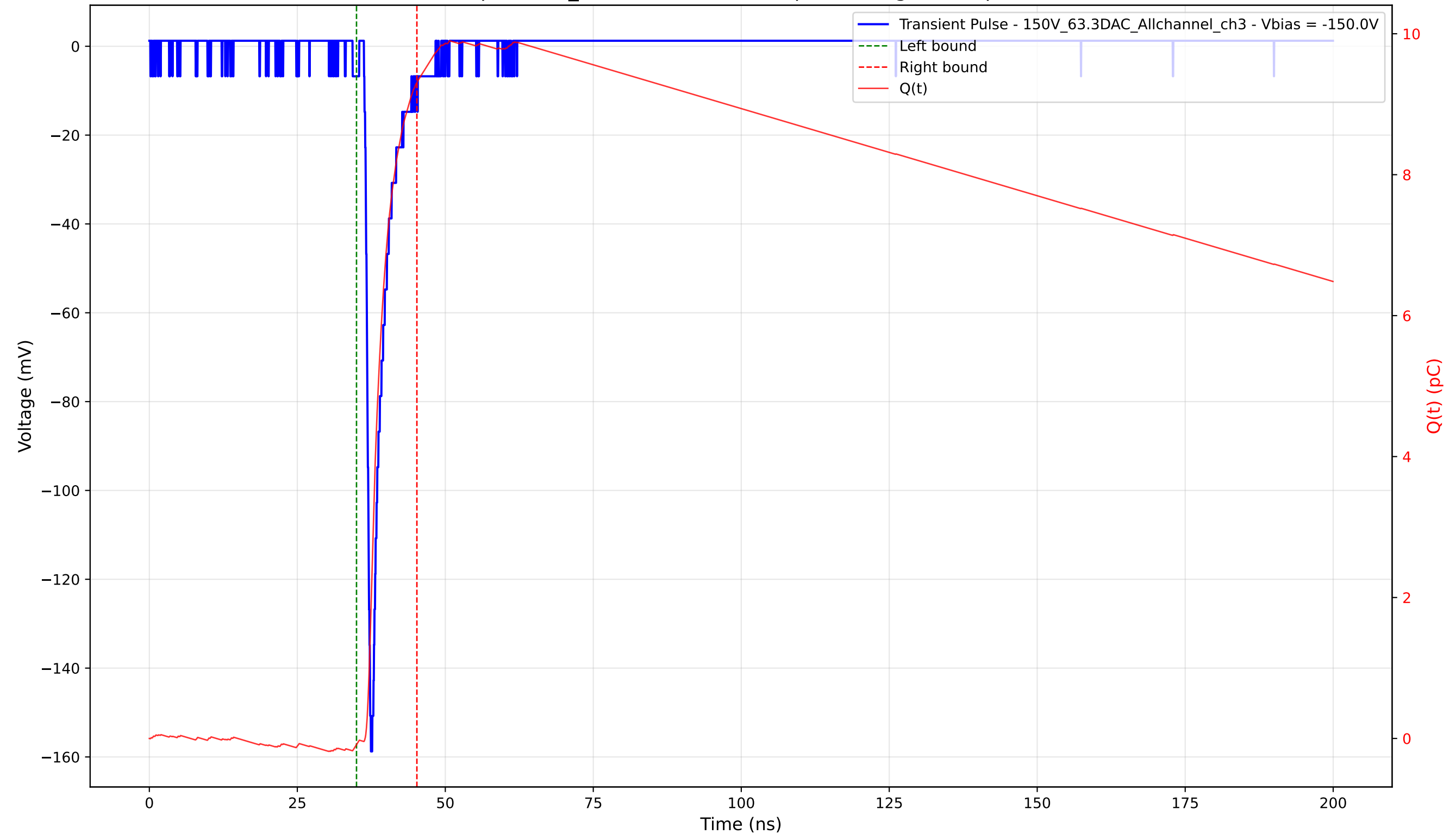
Transient Pulse - Sample: 1cm_42 - Position: 1800.0 \mu\text{m} - Charge: 9.39 pC - Rise Time: 0.87 ns
