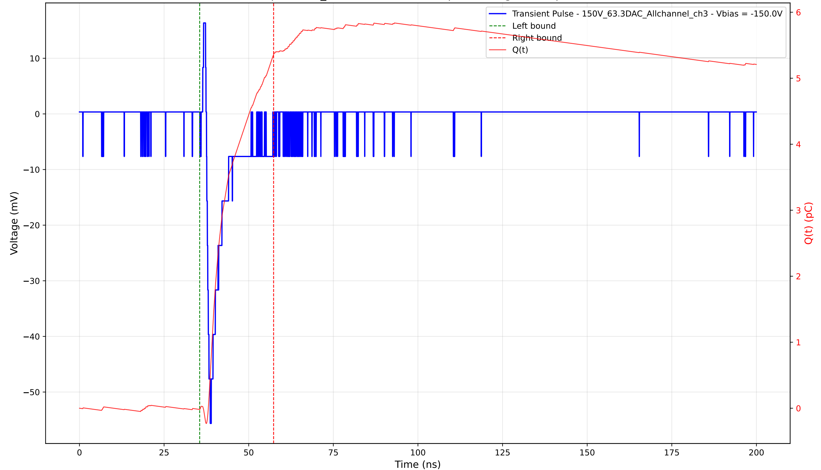
Transient Pulse - Sample: 1cm_42 - Position: 1035.0 \mu\text{m} - Charge: 5.38 pC - Rise Time: 1.13 ns
