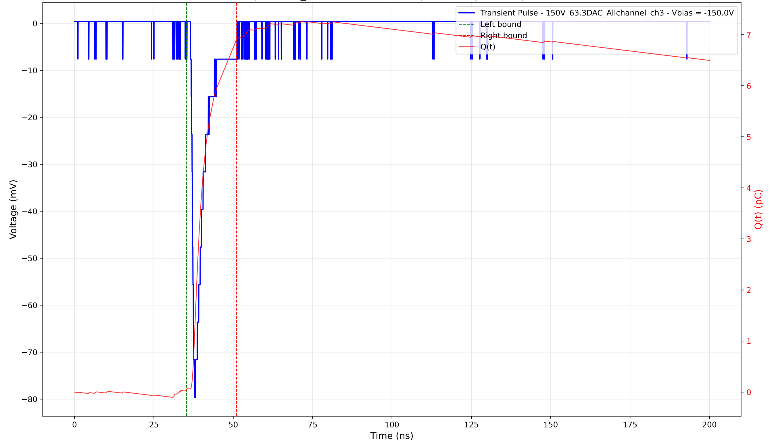
Transient Pulse - Sample: 1cm_42 - Position: 1525.0 \mu\text{m} - Charge: 6.85 pC - Rise Time: 1.08 ns
