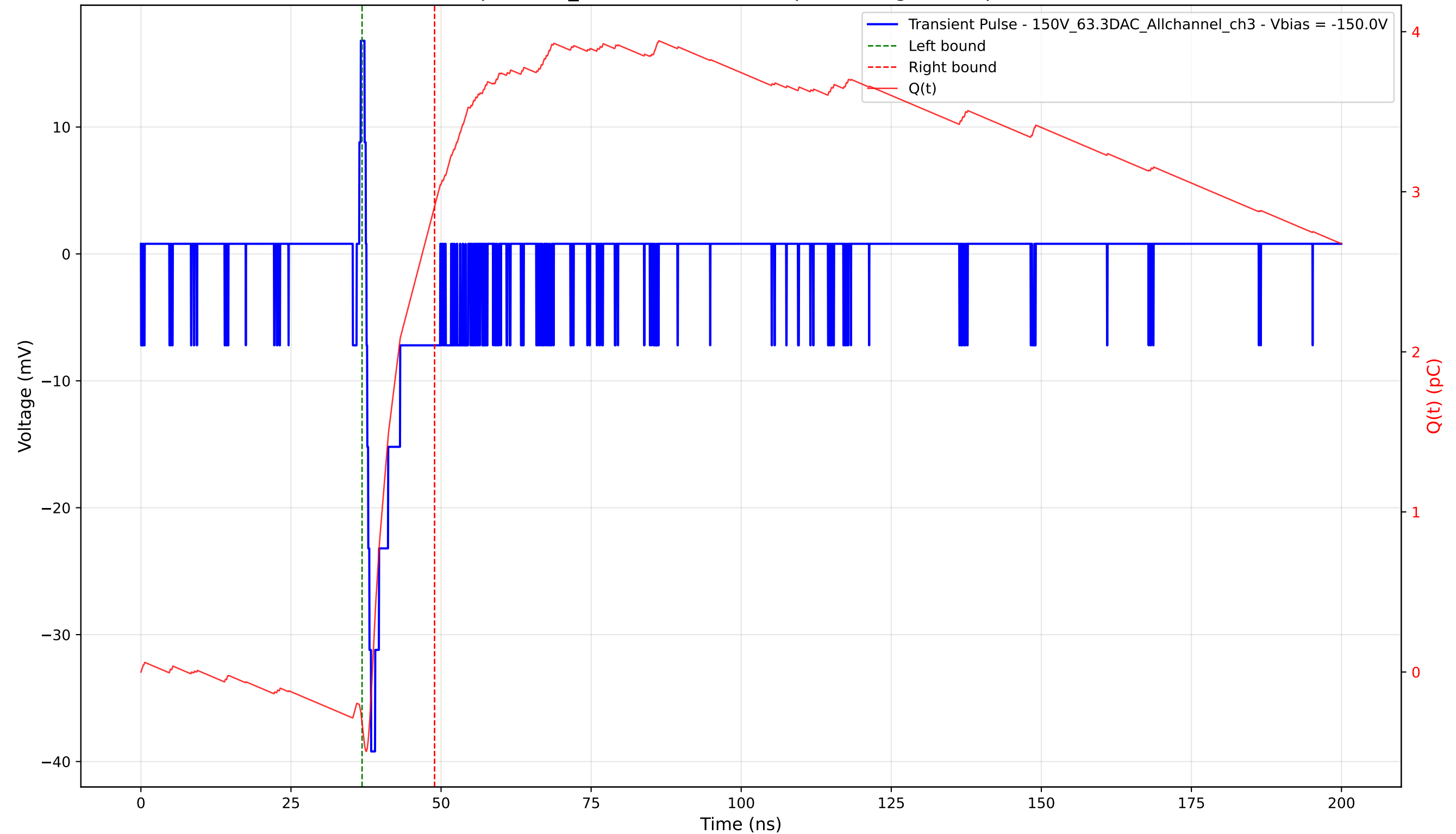
Transient Pulse - Sample: 1cm_42 - Position: 4060.0 \mu\text{m} - Charge: 3.23 pC - Rise Time: 0.78 ns
