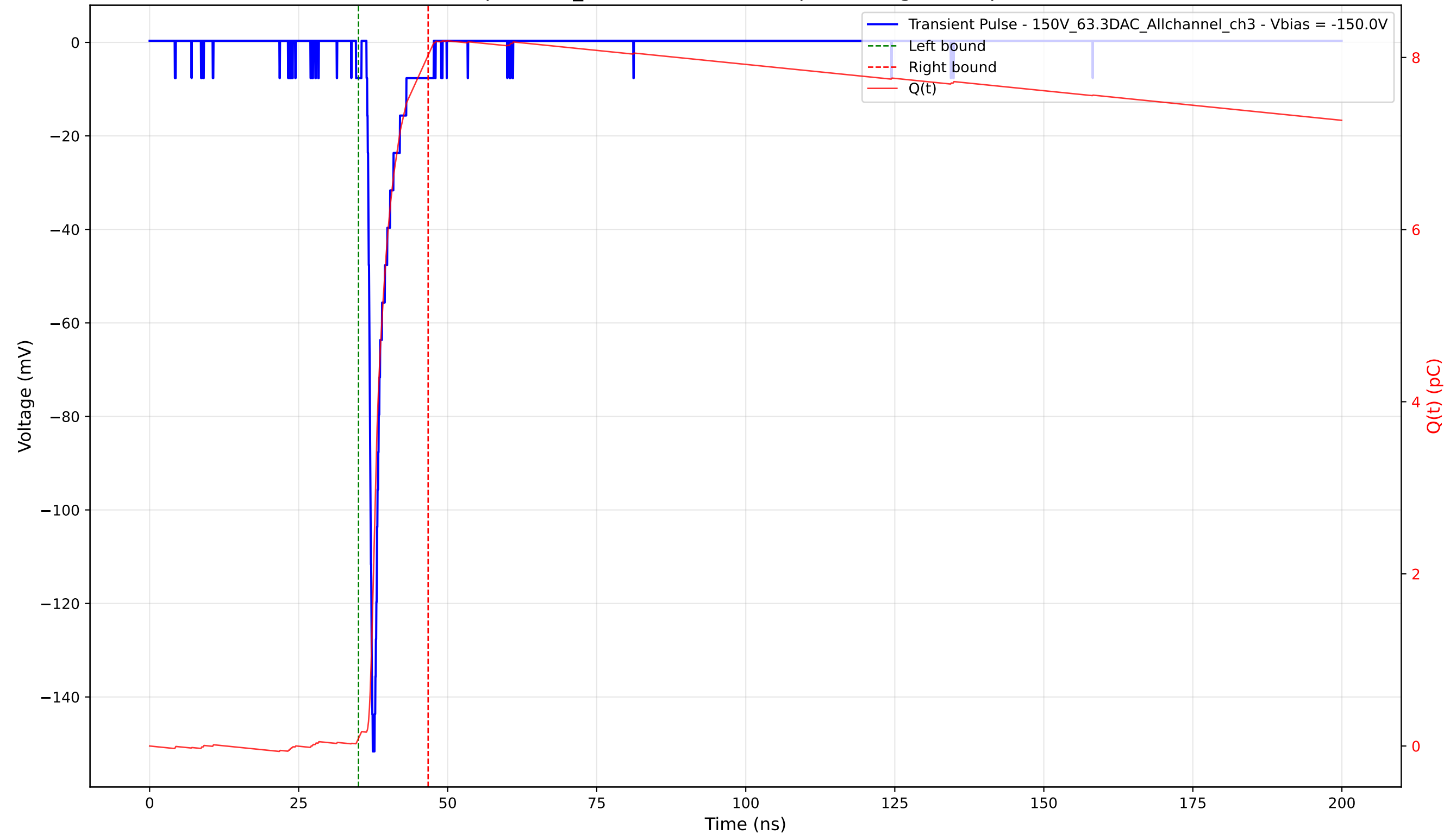
Transient Pulse - Sample: 1cm_42 - Position: 3185.0 \mu\text{m} - Charge: 7.94 pC - Rise Time: 0.84 ns
