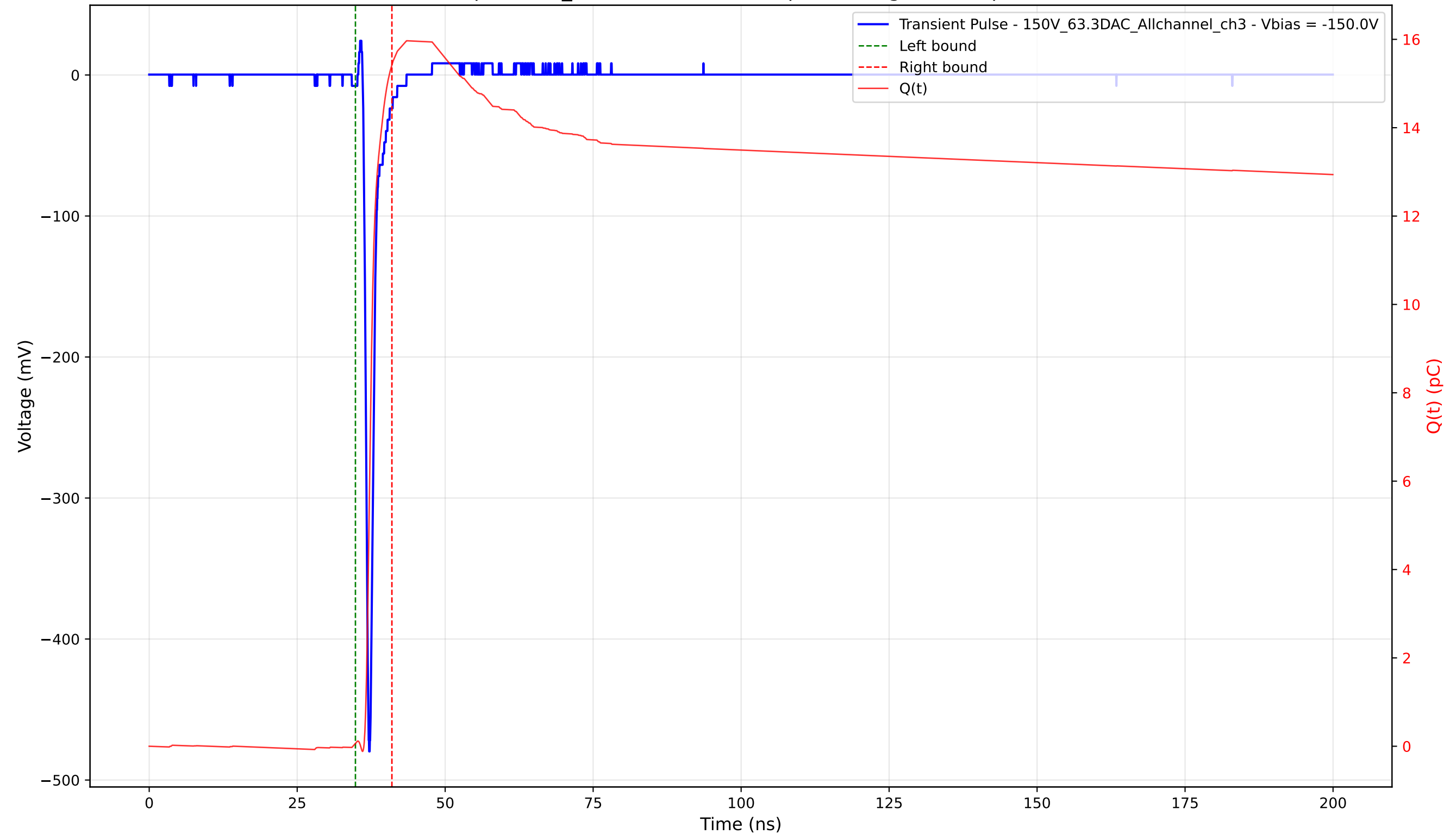
Transient Pulse - Sample: 1cm_42 - Position: 2710.0 \mu\text{m} - Charge: 15.36 pC - Rise Time: 0.68 ns
