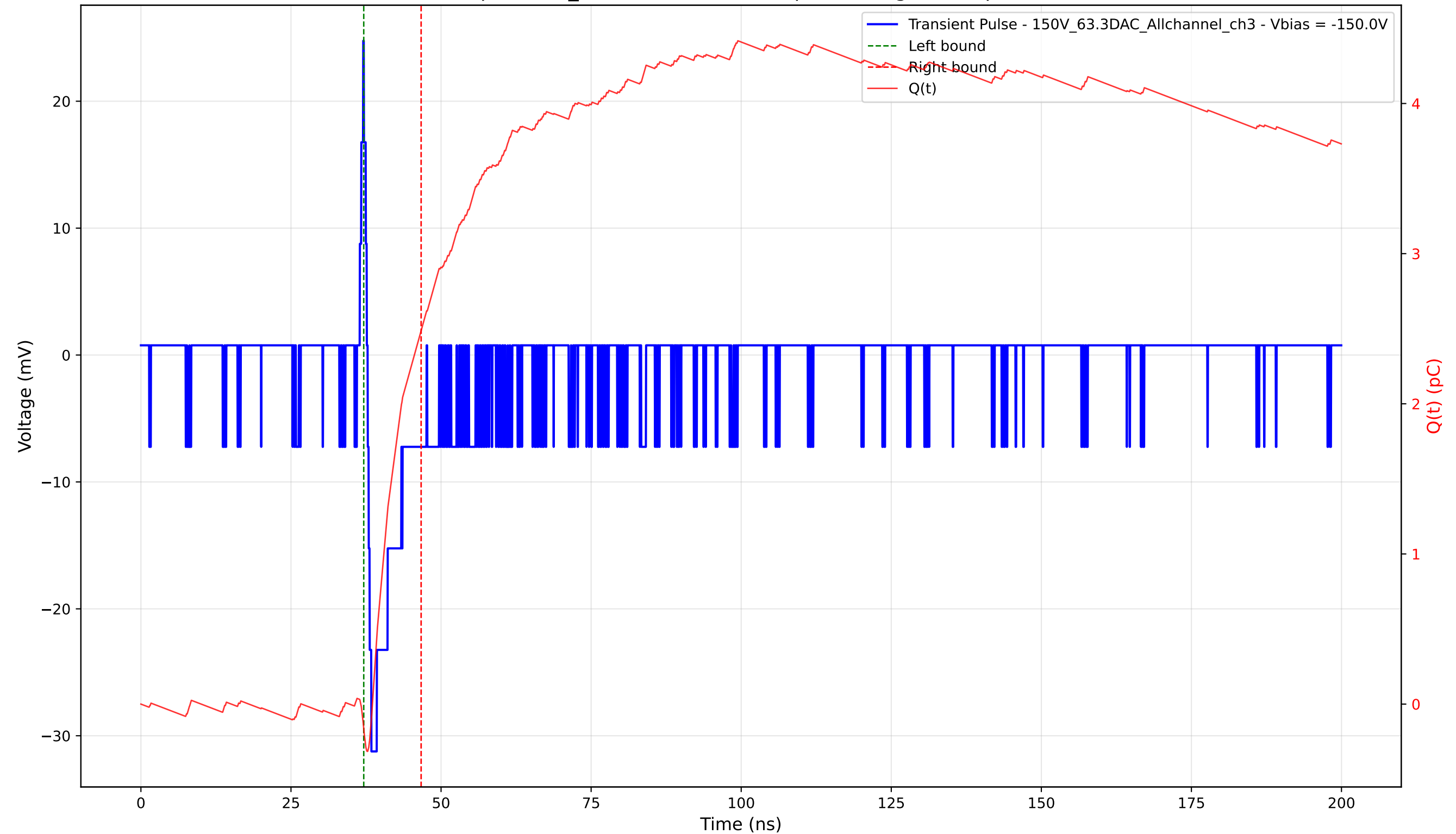
Transient Pulse - Sample: 1cm_42 - Position: 4445.0 \mu\text{m} - Charge: 2.66 pC - Rise Time: 0.63 ns
