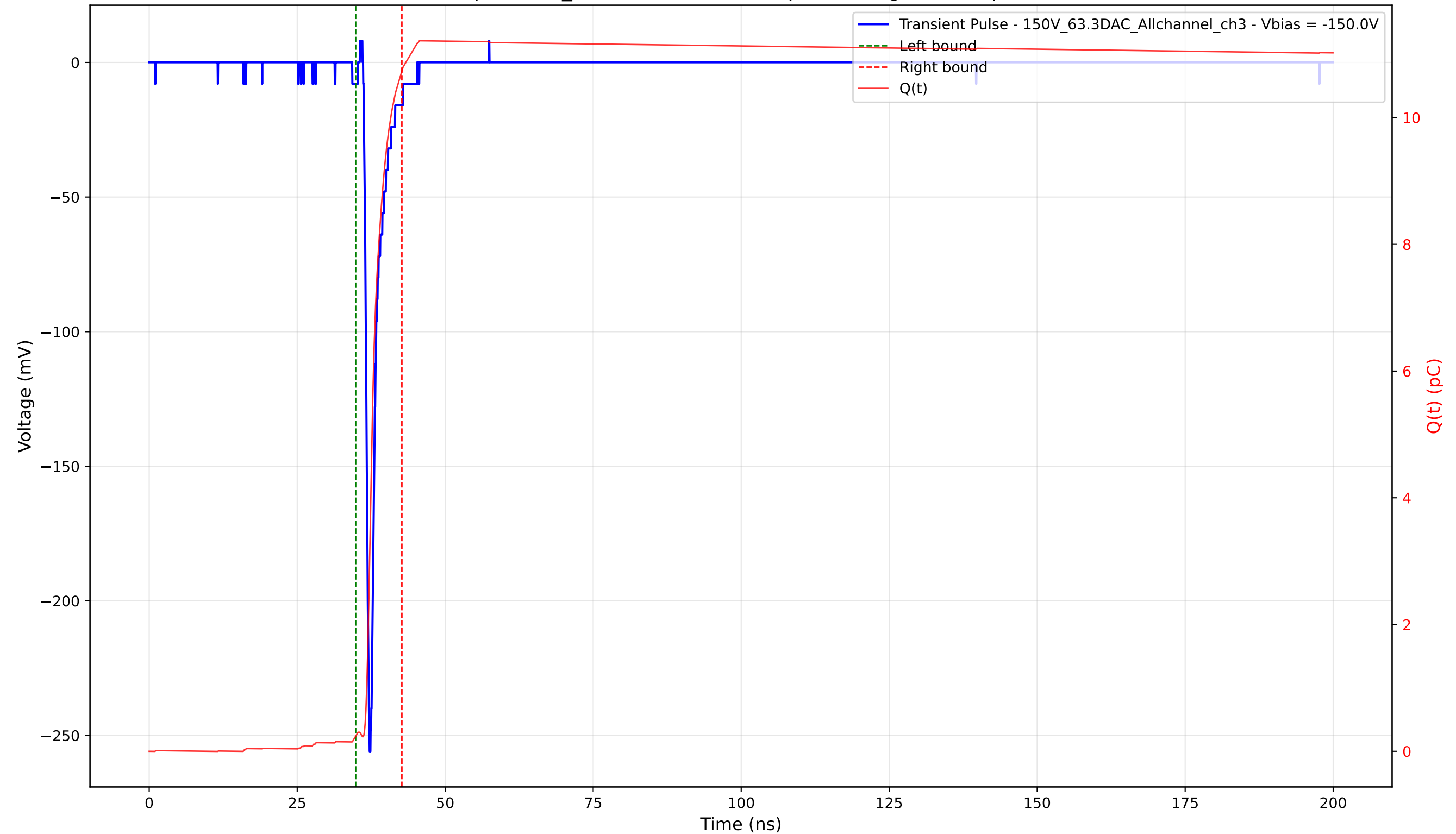
Transient Pulse - Sample: 1cm_42 - Position: 2040.0 \mu\text{m} - Charge: 10.50 pC - Rise Time: 0.78 ns
