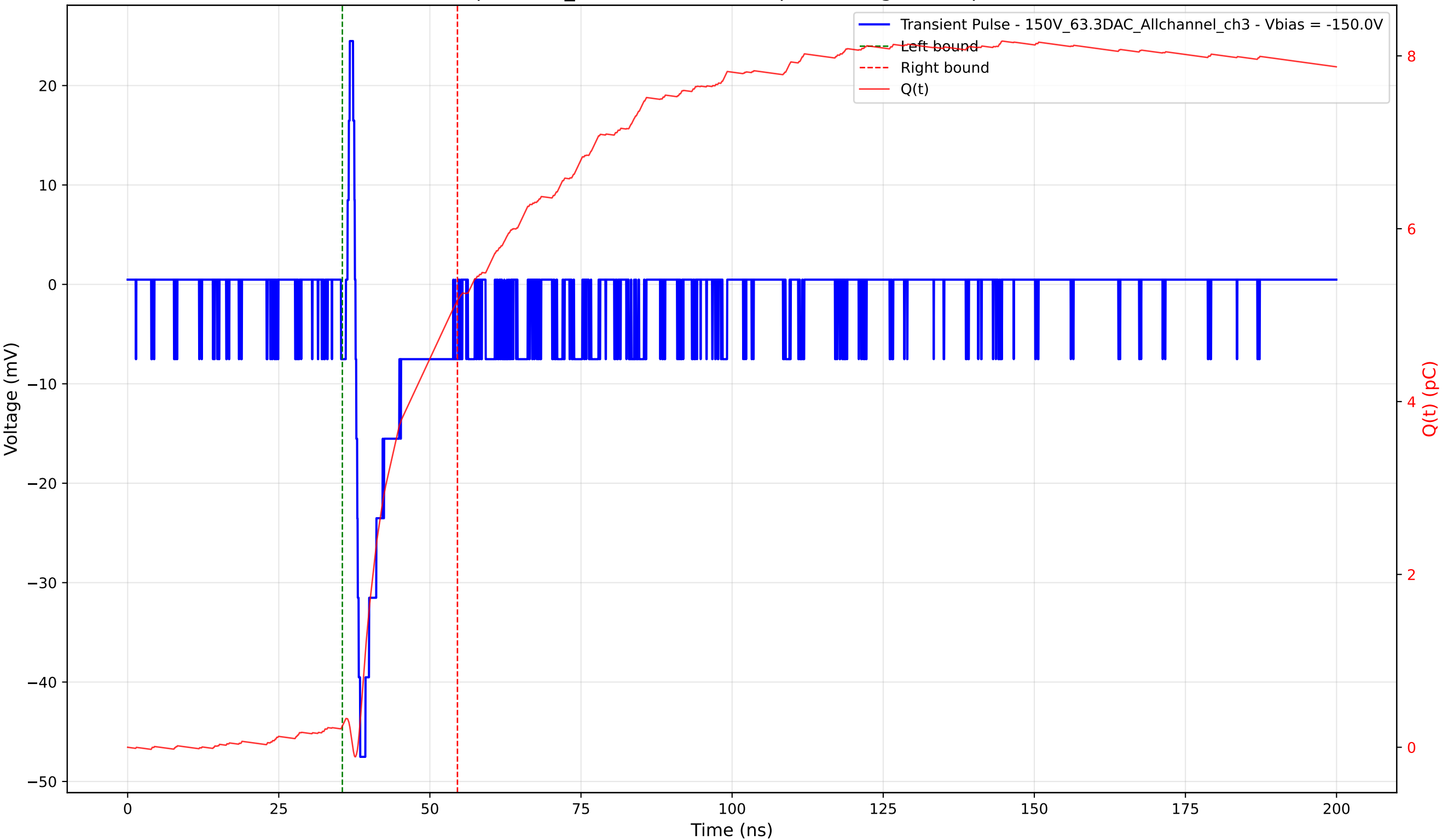
Transient Pulse - Sample: 1cm_42 - Position: 685.0 \mu\text{m} - Charge: 4.93 pC - Rise Time: 0.78 ns
