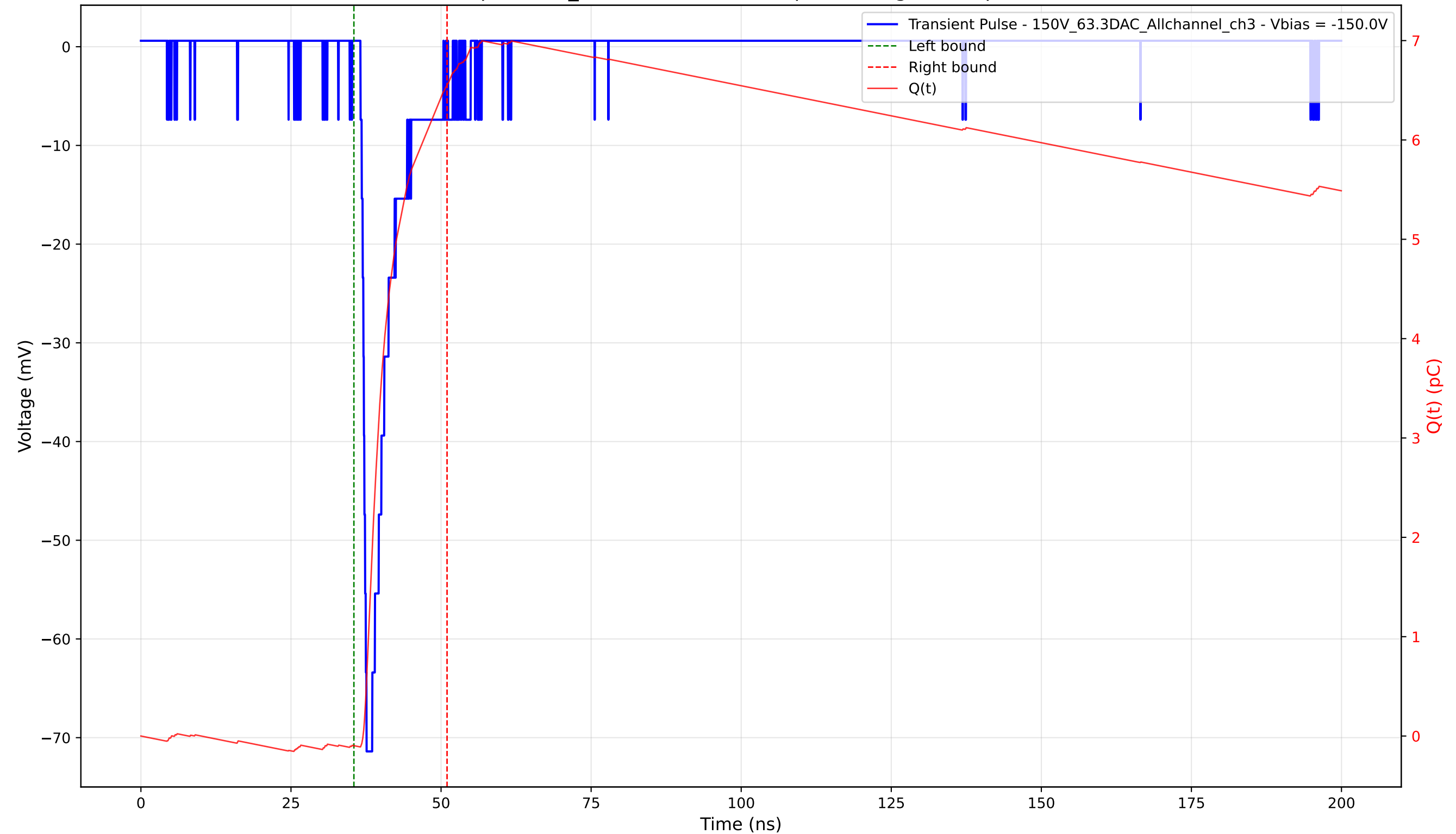
Transient Pulse - Sample: 1cm_42 - Position: 1510.0 \mu\text{m} - Charge: 6.65 pC - Rise Time: 1.00 ns
