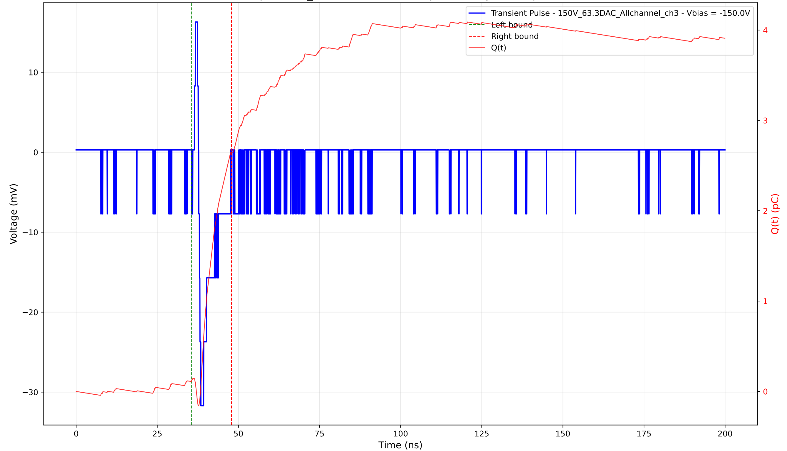
Transient Pulse - Sample: 1cm_42 - Position: 4505.0 \mu\text{m} - Charge: 2.54 pC - Rise Time: 0.66 ns
