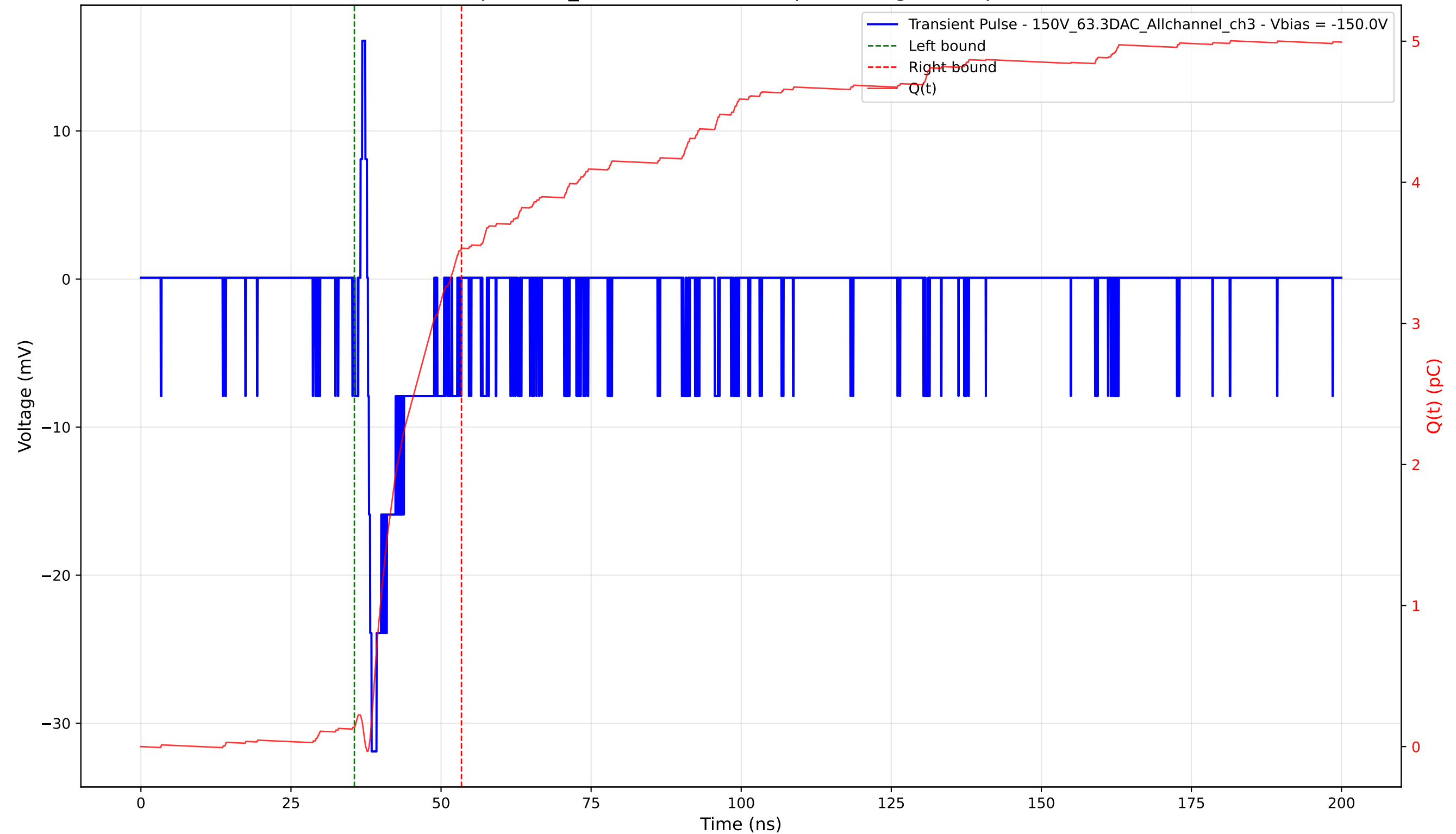
Transient Pulse - Sample: 1cm_42 - Position: 4650.0 \mu\text{m} - Charge: 3.40 pC - Rise Time: 0.62 ns
