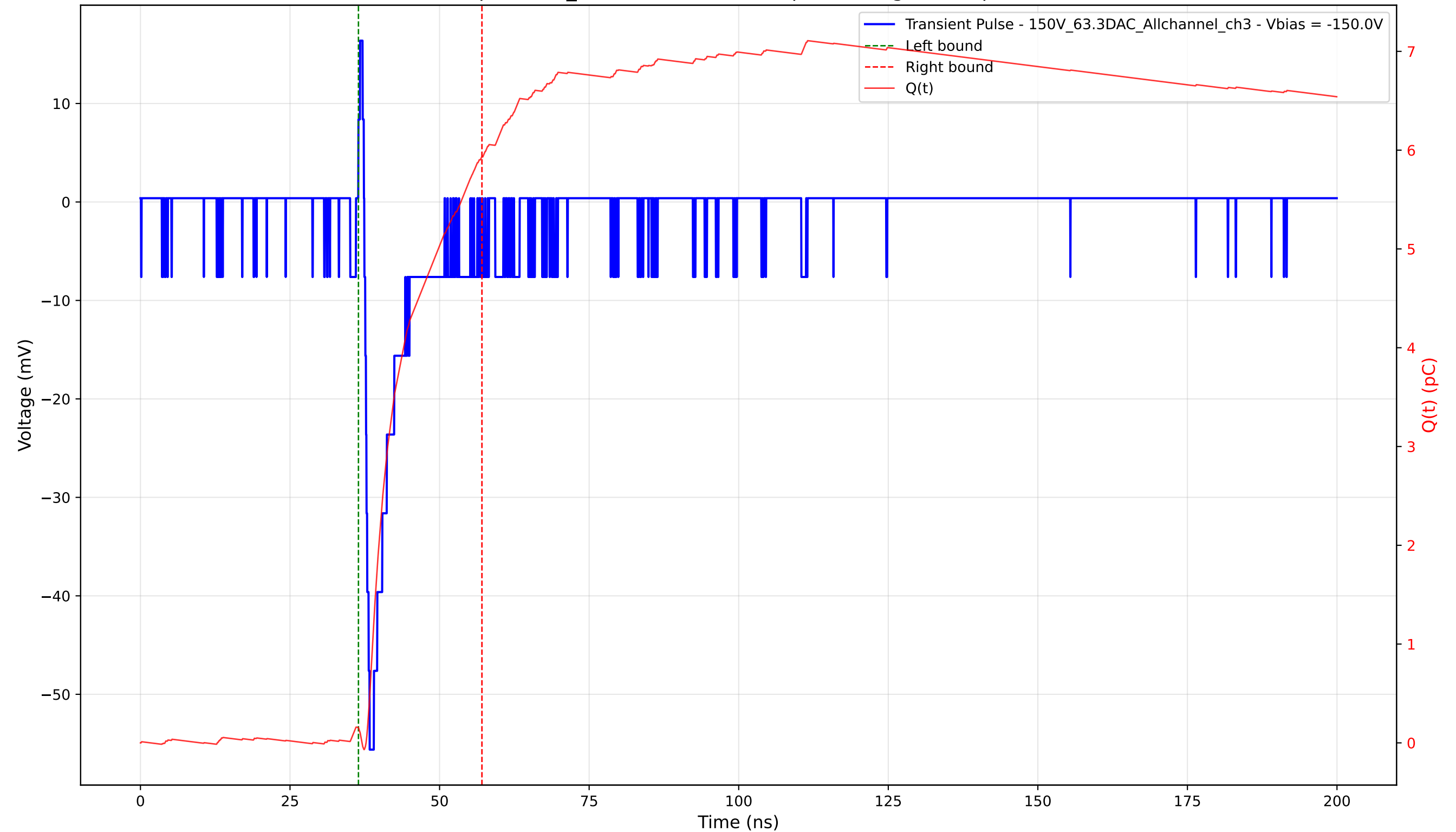
Transient Pulse - Sample: 1cm_42 - Position: 1090.0 \mu\text{m} - Charge: 5.78 pC - Rise Time: 0.89 ns
