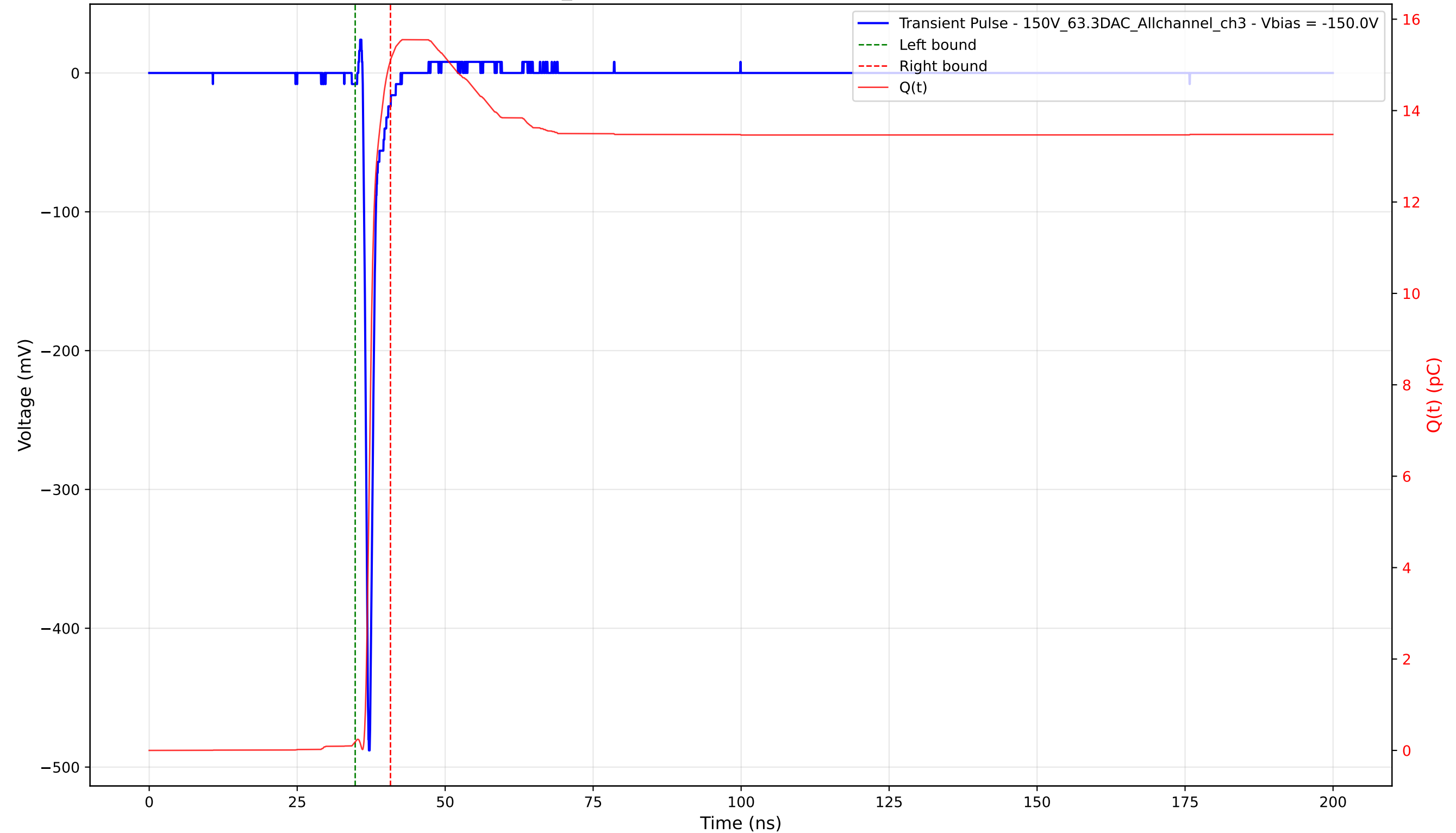
Transient Pulse - Sample: 1cm_42 - Position: 2490.0 \mu\text{m} - Charge: 14.91 pC - Rise Time: 0.72 ns
