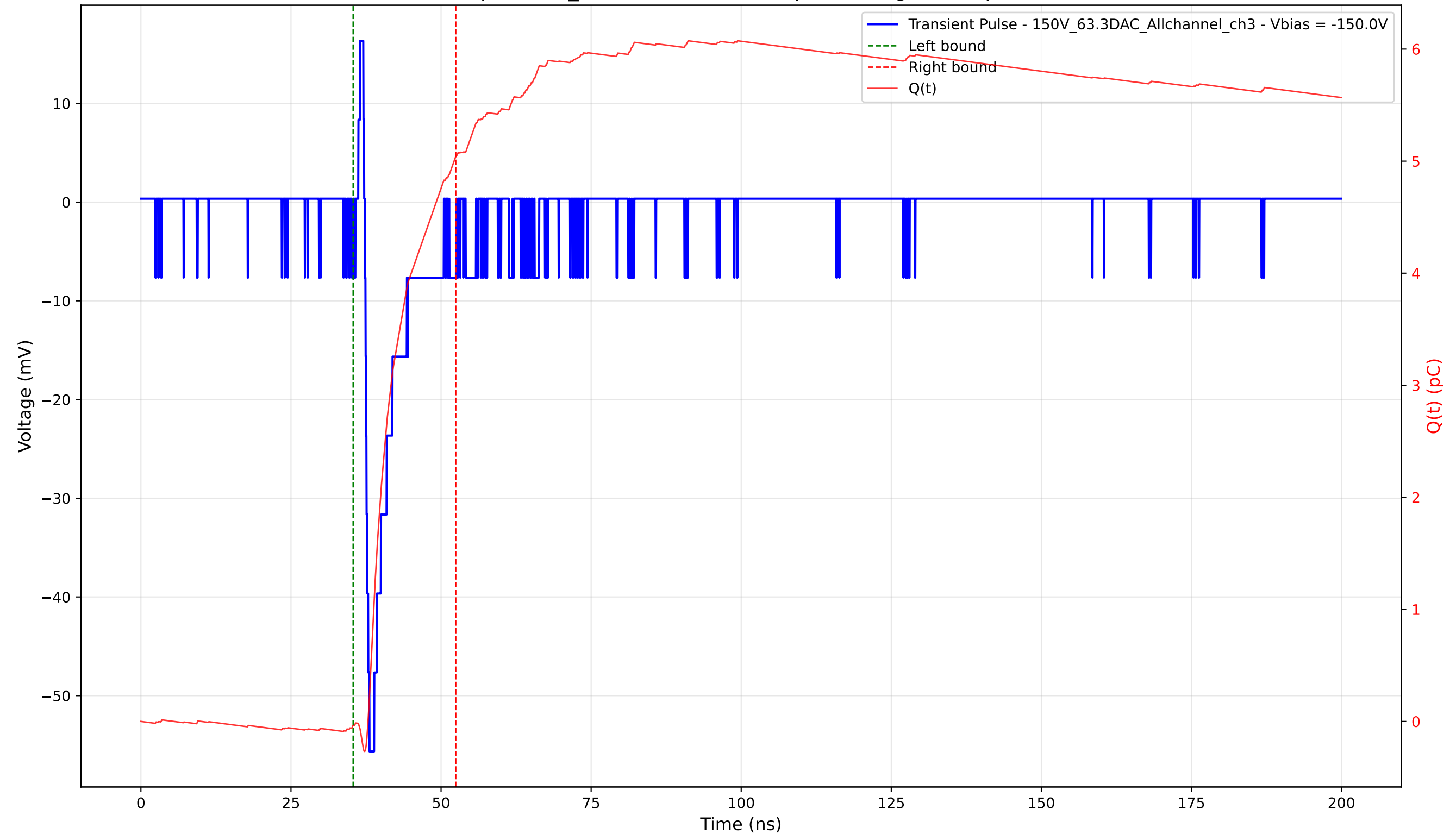
Transient Pulse - Sample: 1cm_42 - Position: 3795.0 \mu\text{m} - Charge: 5.08 pC - Rise Time: 0.77 ns
