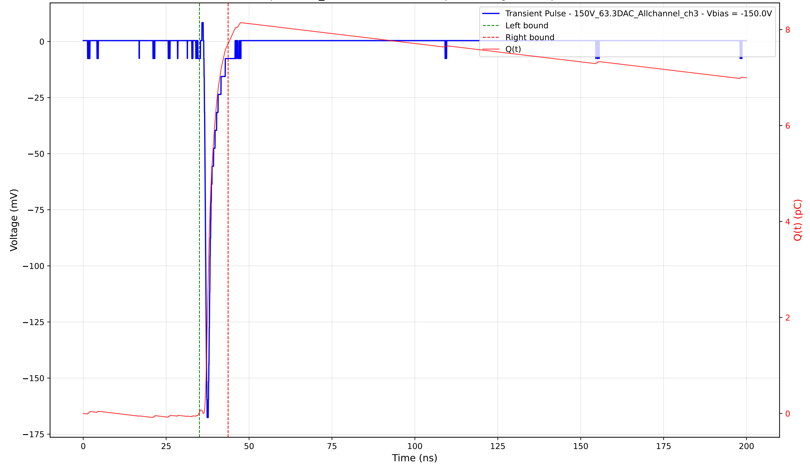
Transient Pulse - Sample: 1cm_42 - Position: 3115.0 \mu\text{m} - Charge: 7.68 pC - Rise Time: 0.71 ns
