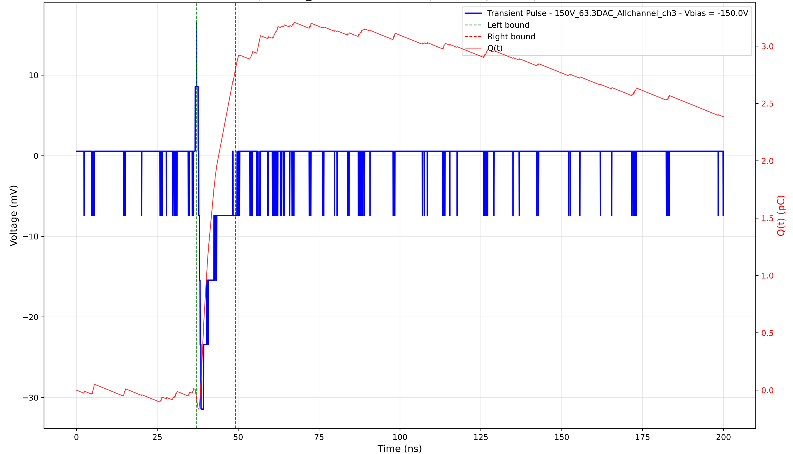
Transient Pulse - Sample: 1cm_42 - Position: 4860.0 \mu\text{m} - Charge: 2.86 pC - Rise Time: 0.71 ns
