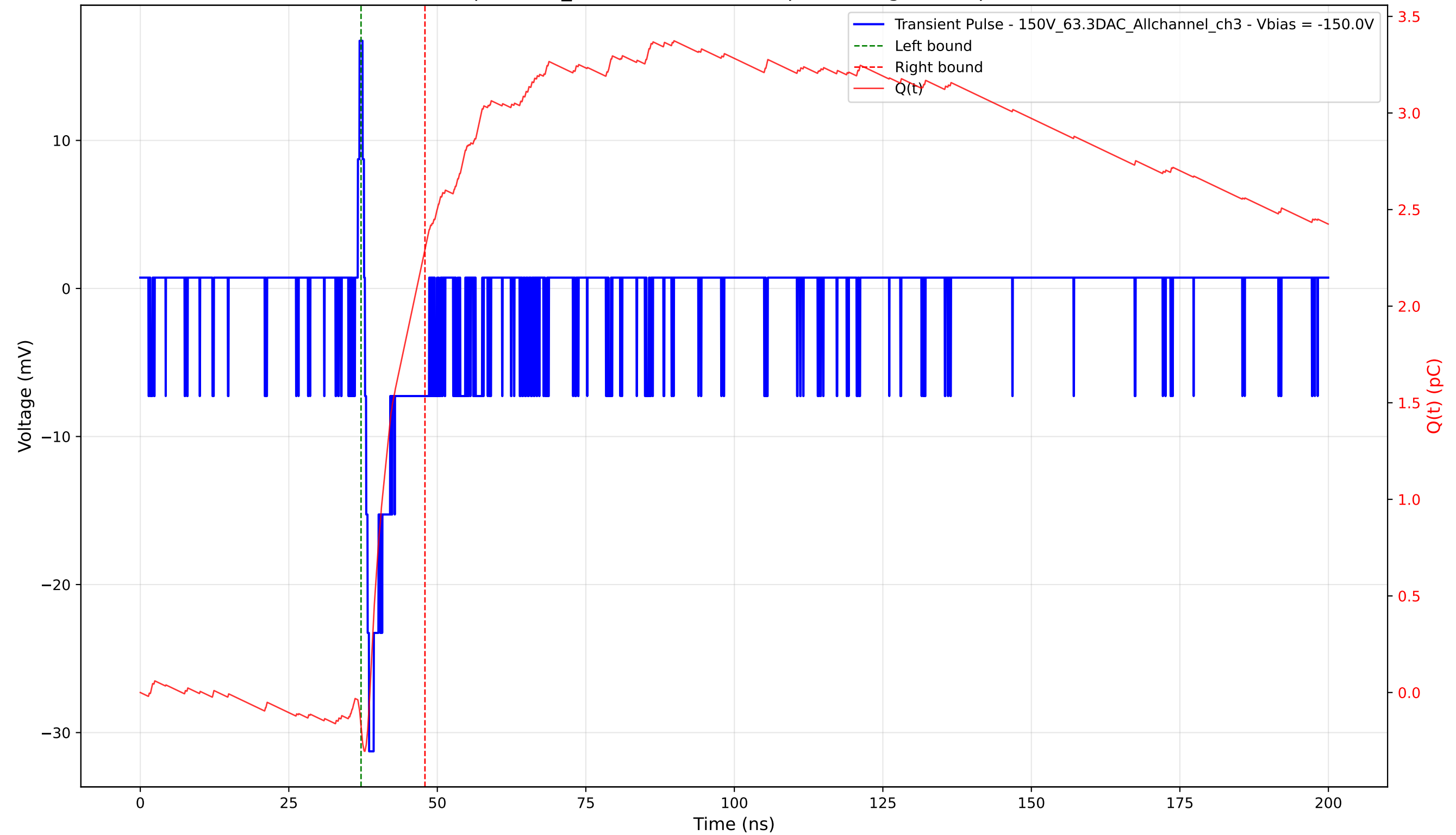
Transient Pulse - Sample: 1cm_42 - Position: 4665.0 \mu\text{m} - Charge: 2.47 pC - Rise Time: 0.71 ns
