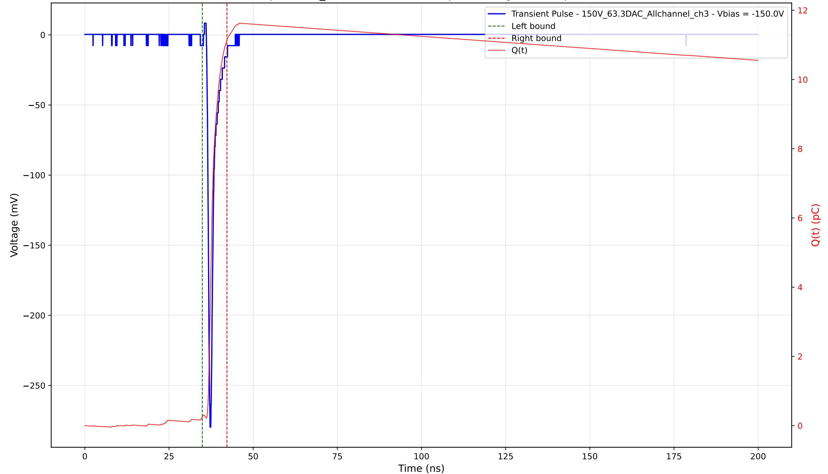
Transient Pulse - Sample: 1cm_42 - Position: 2075.0 \mu\text{m} - Charge: 10.89 pC - Rise Time: 0.76 ns
