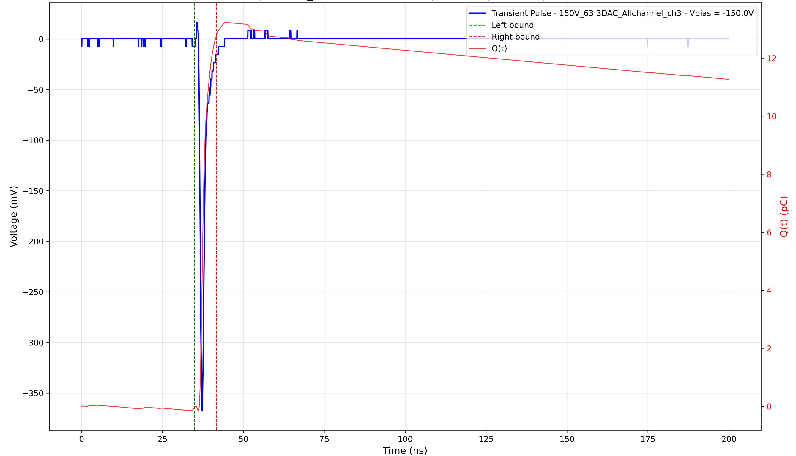
Transient Pulse - Sample: 1cm_42 - Position: 2170.0 \mu\text{m} - Charge: 12.79 pC - Rise Time: 0.72 ns
