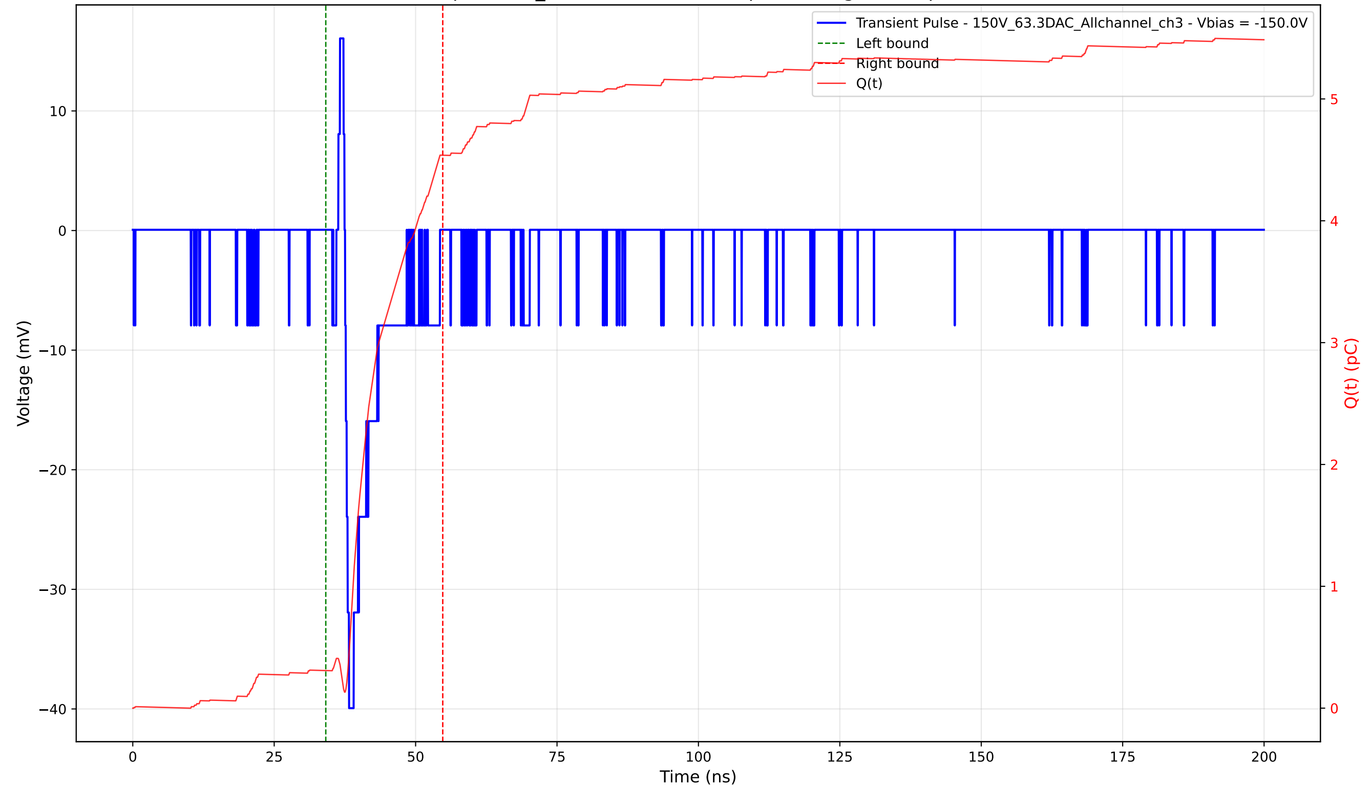
Transient Pulse - Sample: 1cm_42 - Position: 4025.0 \mu\text{m} - Charge: 4.23 pC - Rise Time: 0.70 ns
