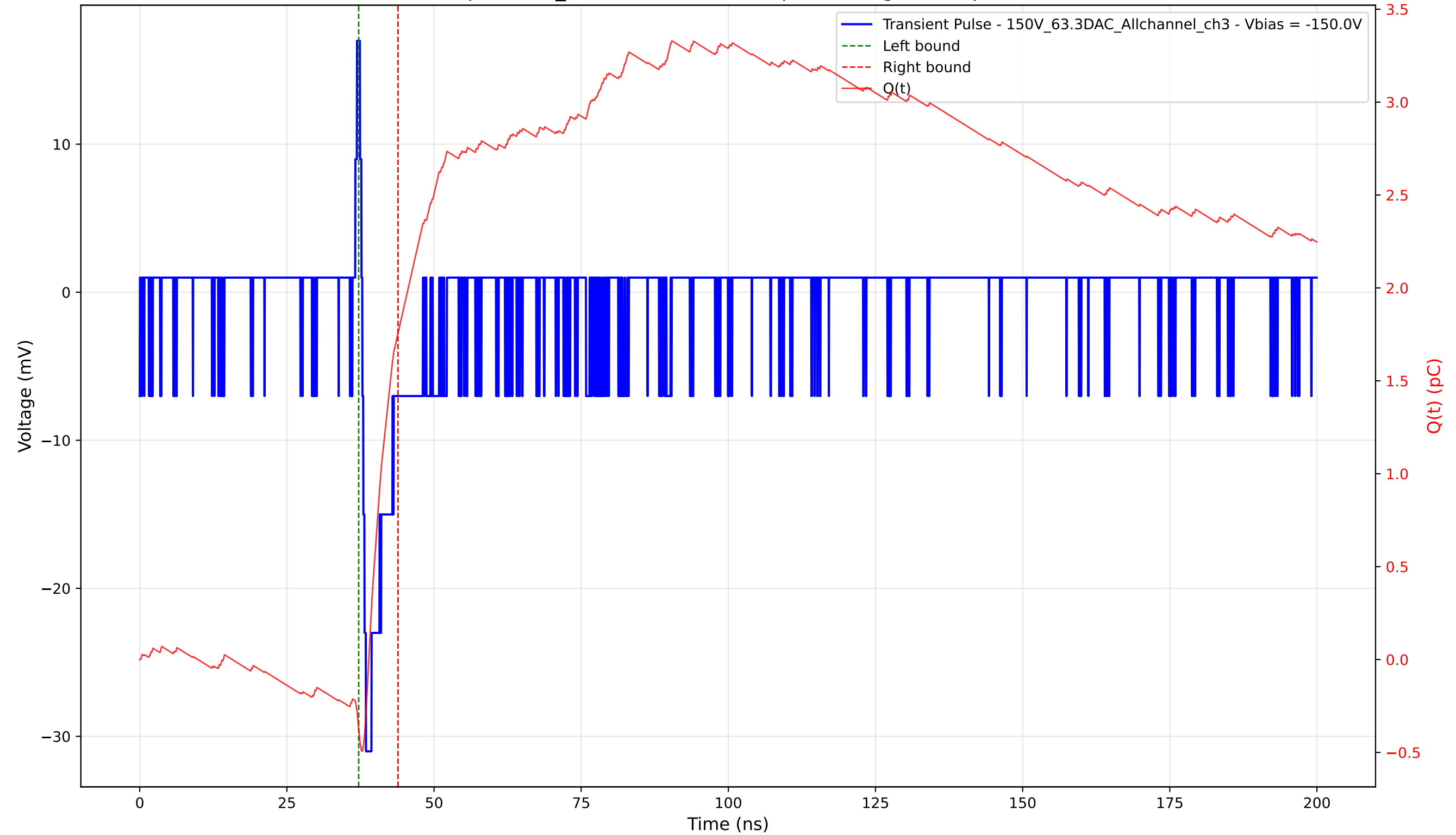
Transient Pulse - Sample: 1cm_42 - Position: 4700.0 \mu\text{m} - Charge: 2.13 pC - Rise Time: 0.63 ns
