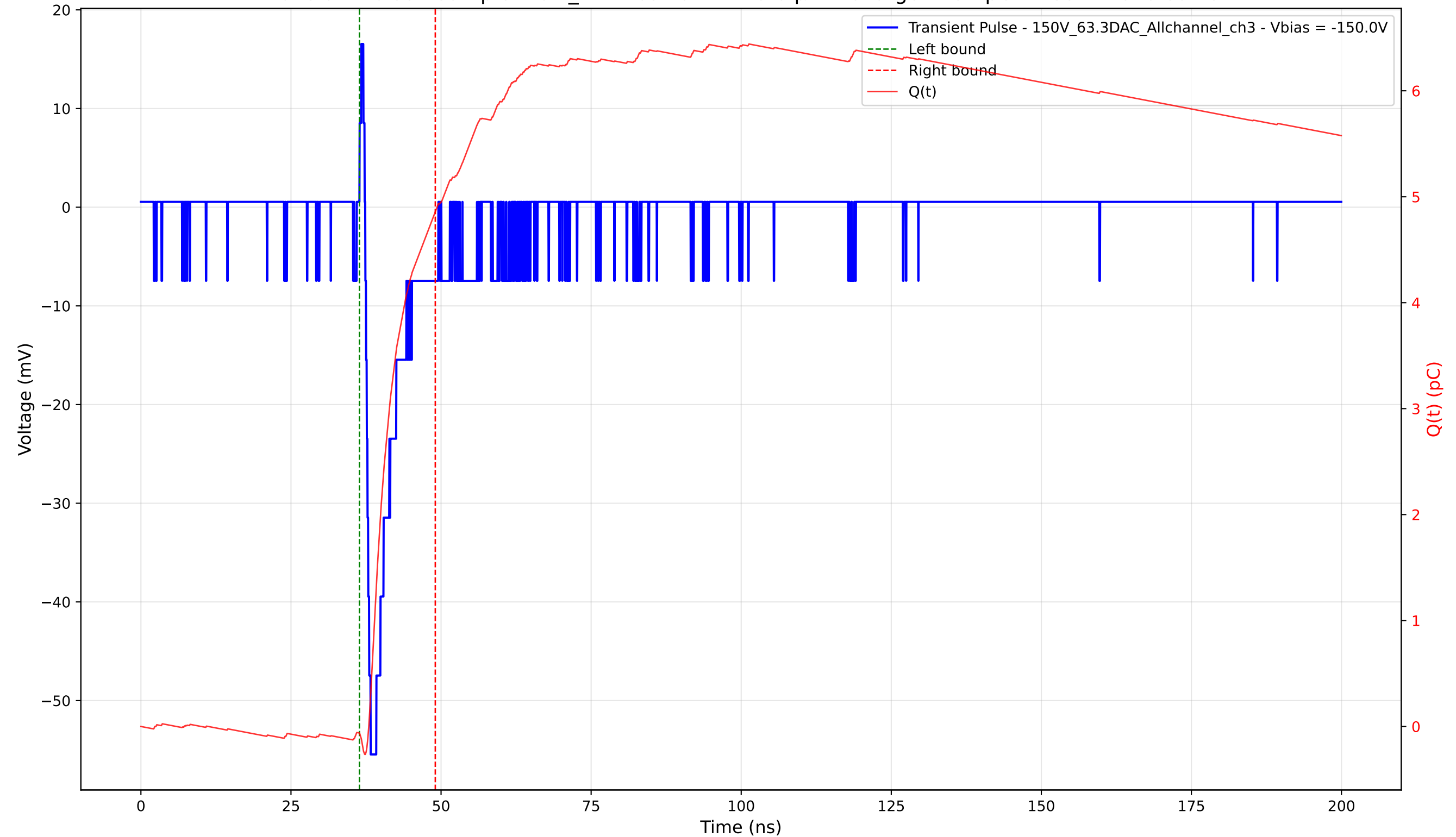
Transient Pulse - Sample: 1cm_42 - Position: 1125.0 \mu\text{m} - Charge: 4.92 pC - Rise Time: 0.89 ns
