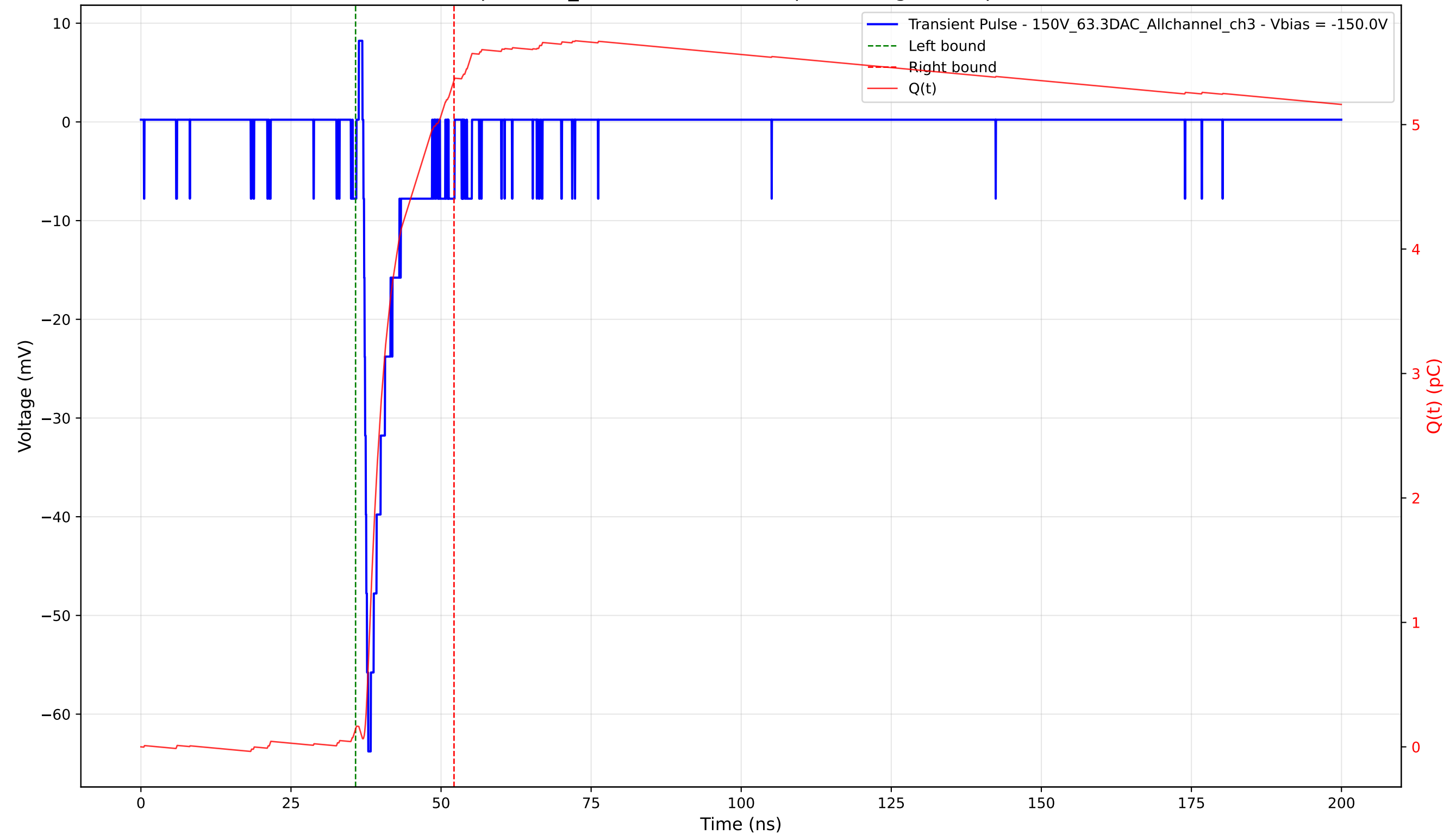
Transient Pulse - Sample: 1cm_42 - Position: 3610.0 \mu\text{m} - Charge: 5.21 pC - Rise Time: 0.81 ns
