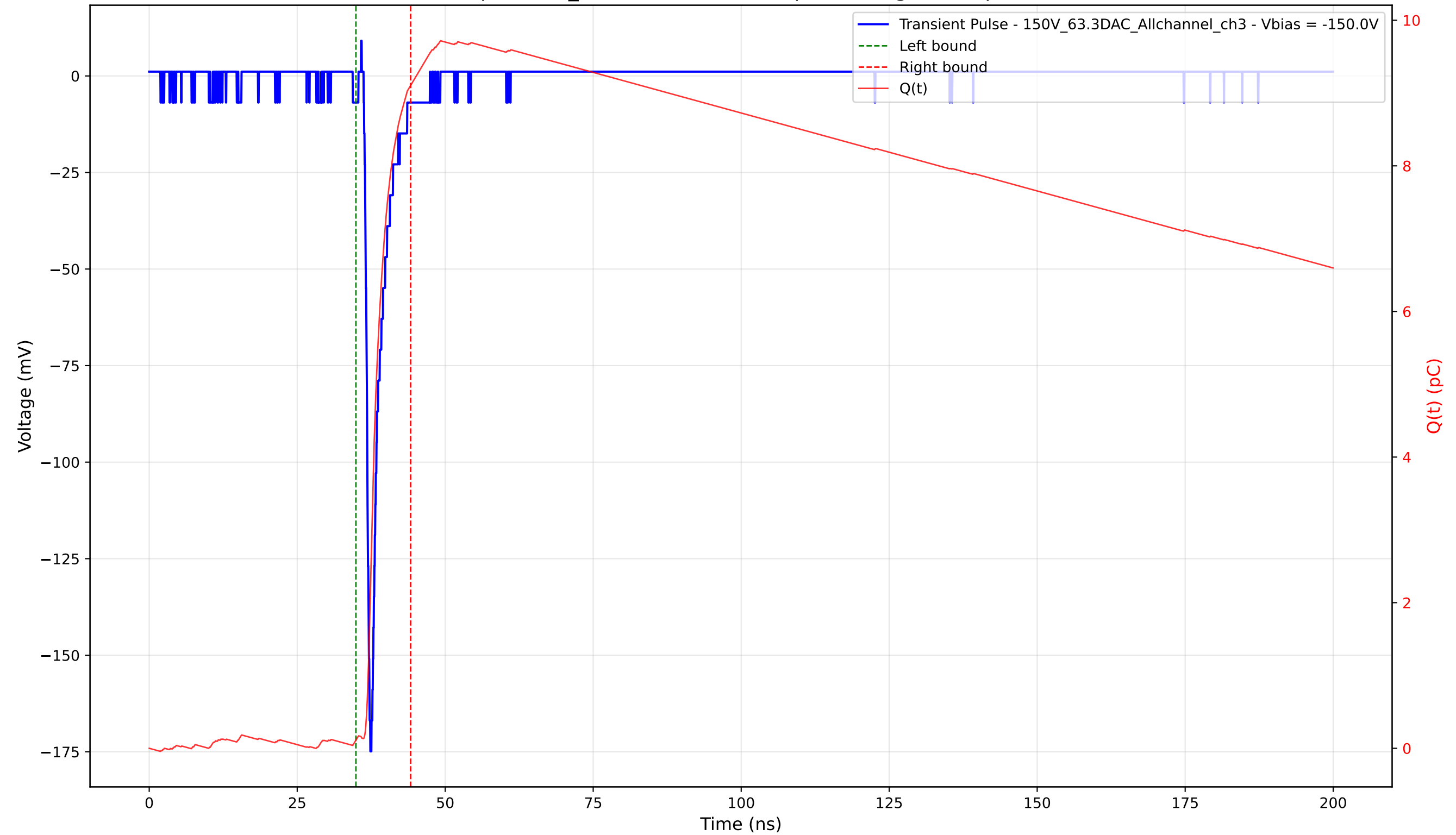
Transient Pulse - Sample: 1cm_42 - Position: 1905.0 \mu\text{m} - Charge: 8.99 pC - Rise Time: 0.82 ns
