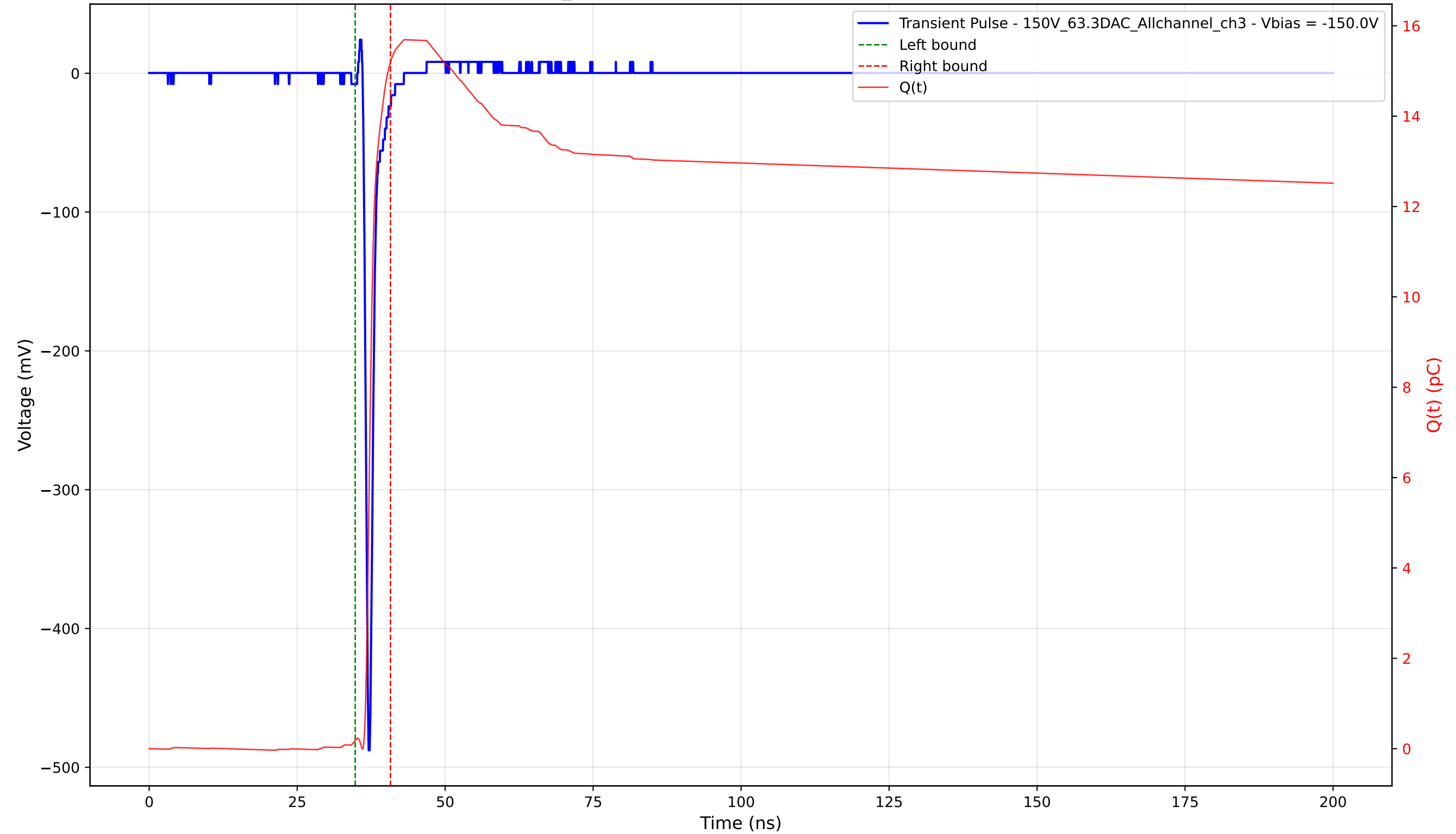
Transient Pulse - Sample: 1cm_42 - Position: 2430.0 \mu\text{m} - Charge: 15.02 pC - Rise Time: 0.72 ns
