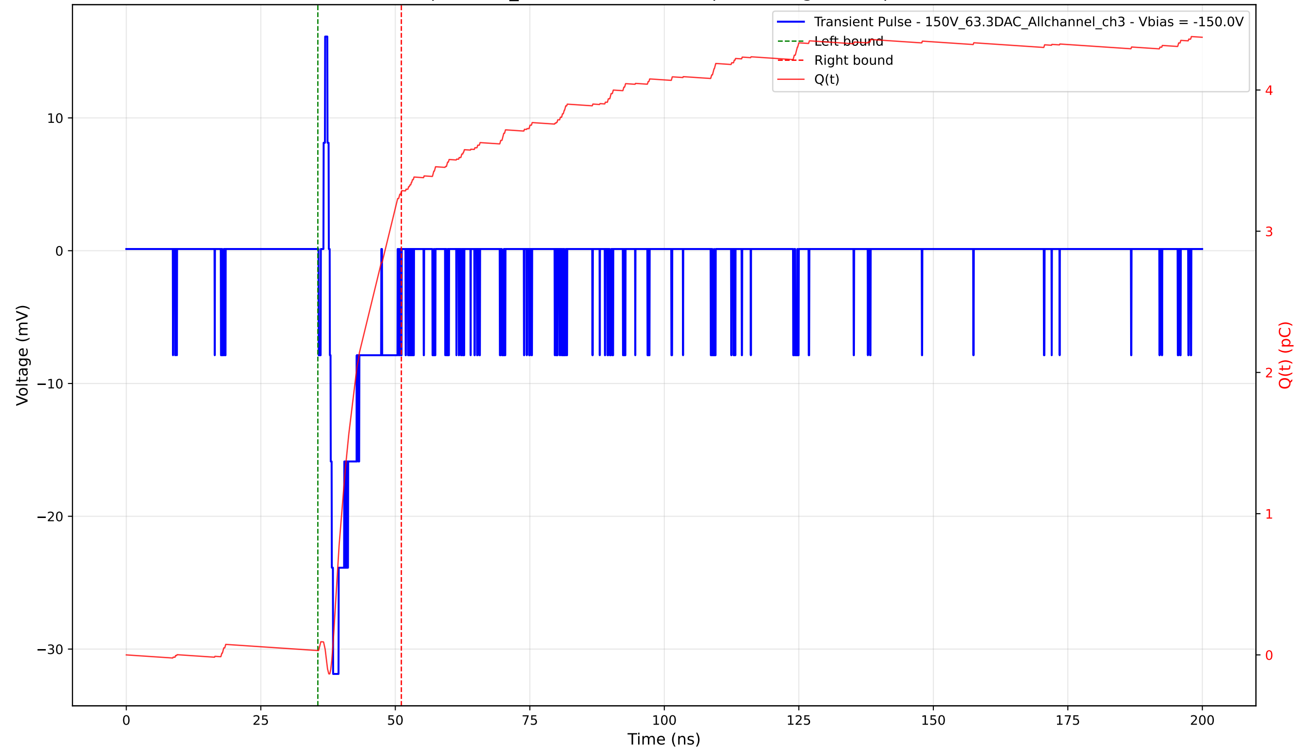
Transient Pulse - Sample: 1cm_42 - Position: 4735.0 \mu\text{m} - Charge: 3.25 pC - Rise Time: 0.62 ns
