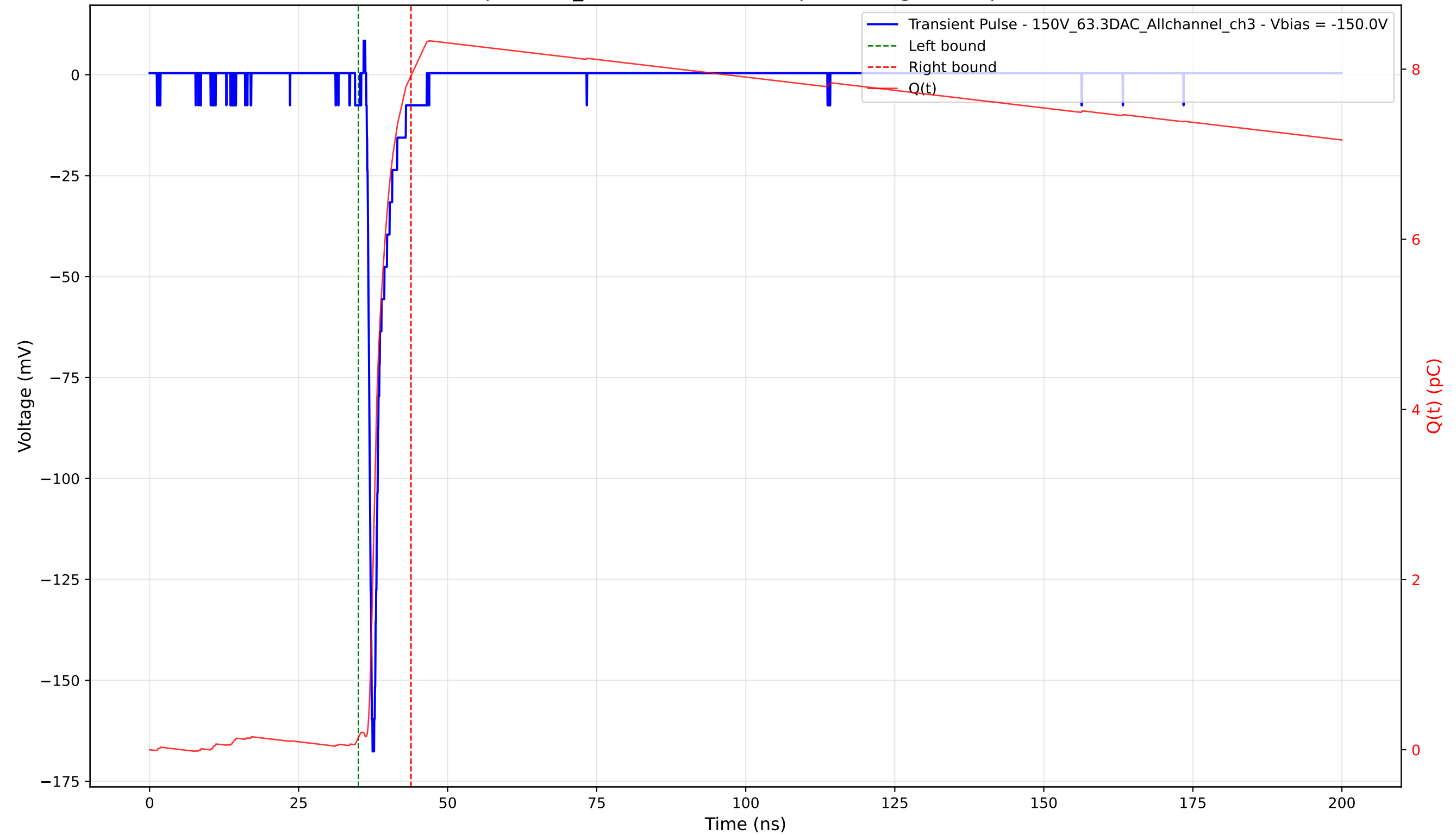
Transient Pulse - Sample: 1cm_42 - Position: 3125.0 \mu\text{m} - Charge: 7.77 pC - Rise Time: 0.75 ns
