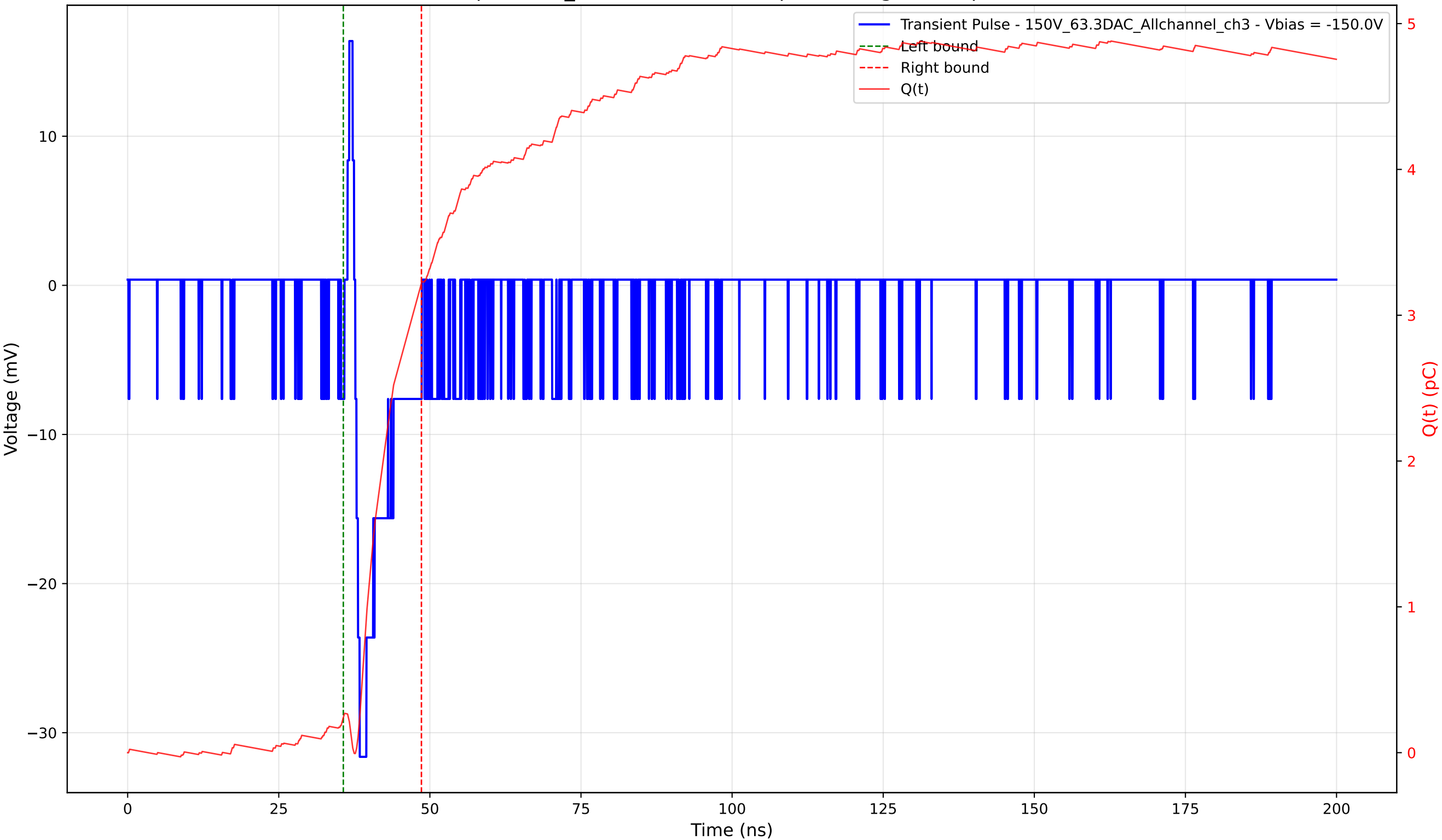
Transient Pulse - Sample: 1cm_42 - Position: 440.0 \mu\text{m} - Charge: 2.98 pC - Rise Time: 0.74 ns
