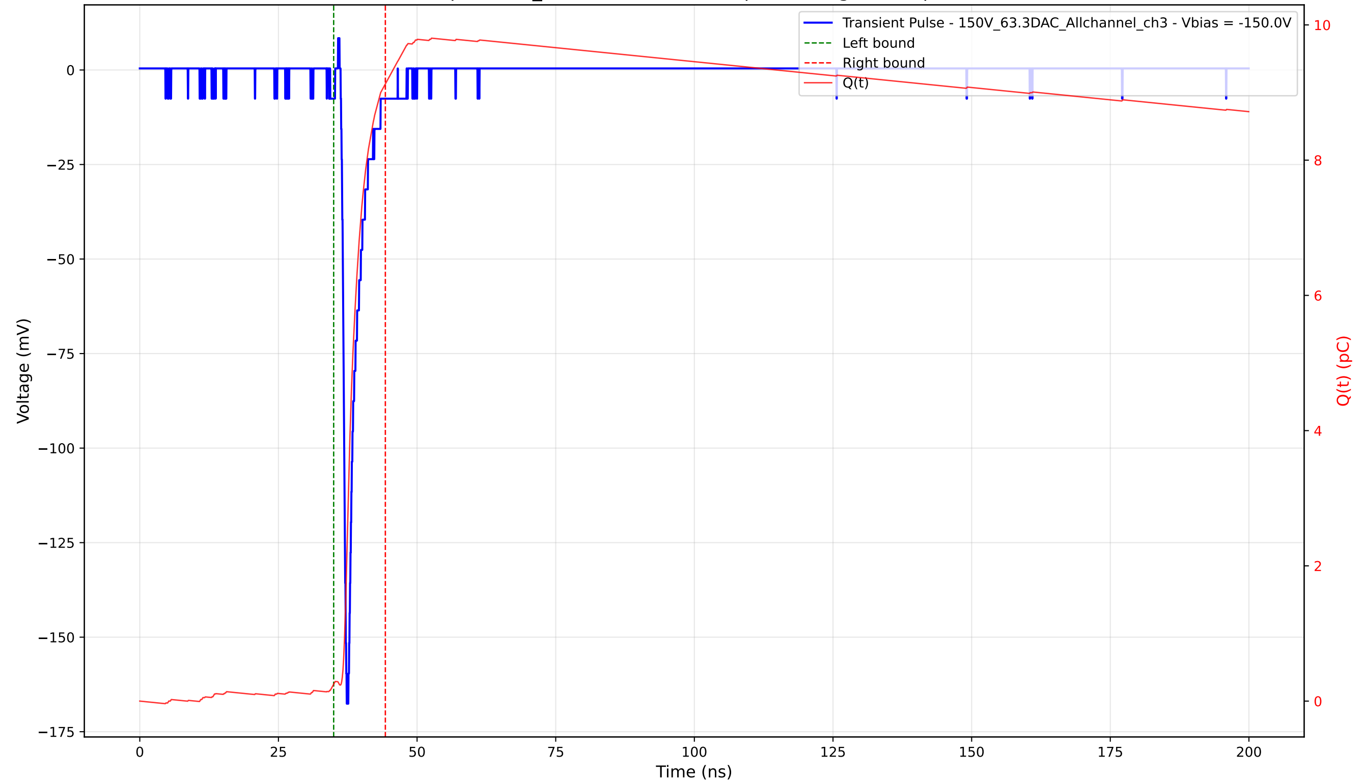
Transient Pulse - Sample: 1cm_42 - Position: 1890.0 \mu\text{m} - Charge: 8.88 pC - Rise Time: 0.79 ns
