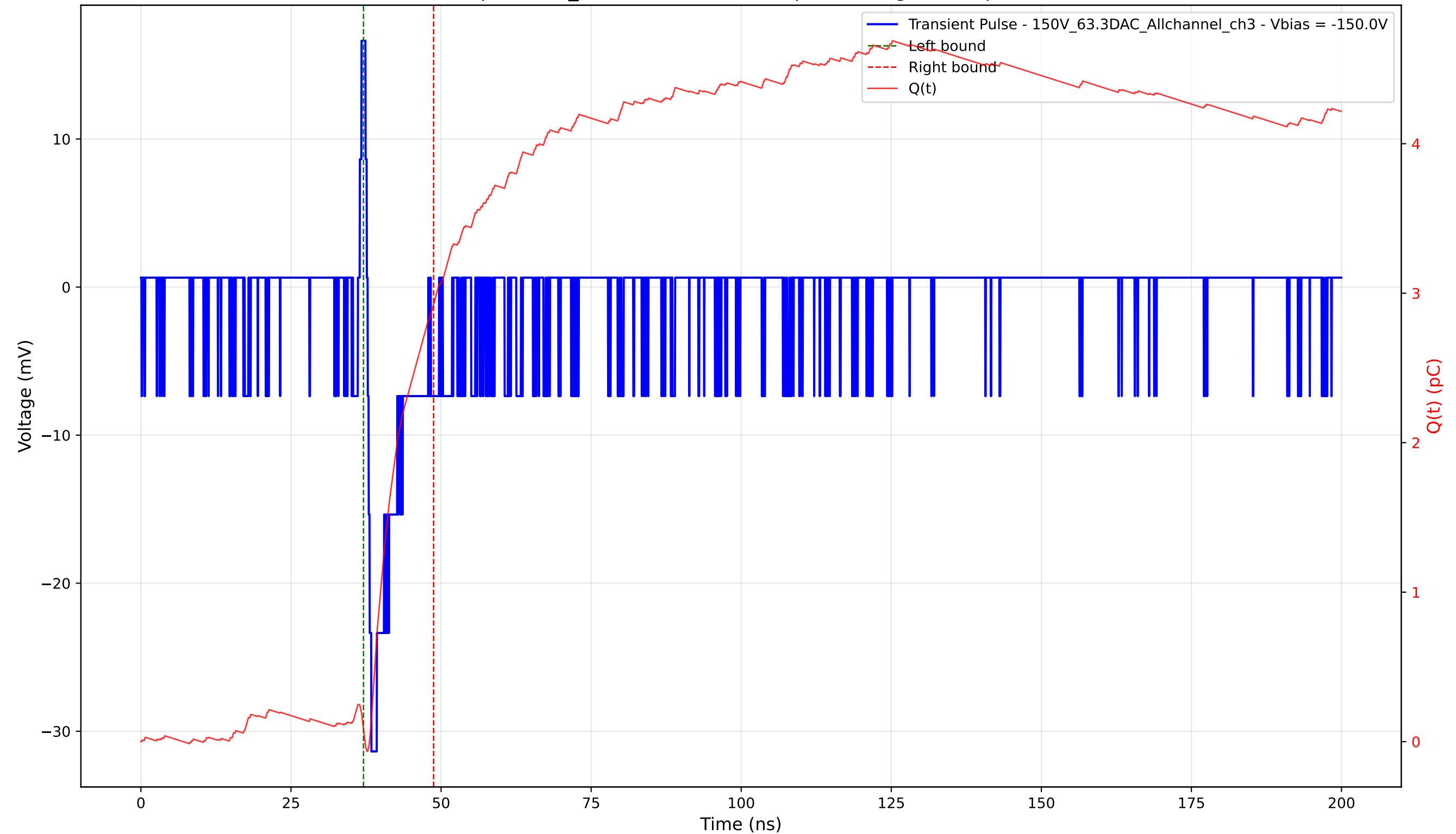
Transient Pulse - Sample: 1cm_42 - Position: 4465.0 \mu\text{m} - Charge: 2.84 pC - Rise Time: 0.63 ns
