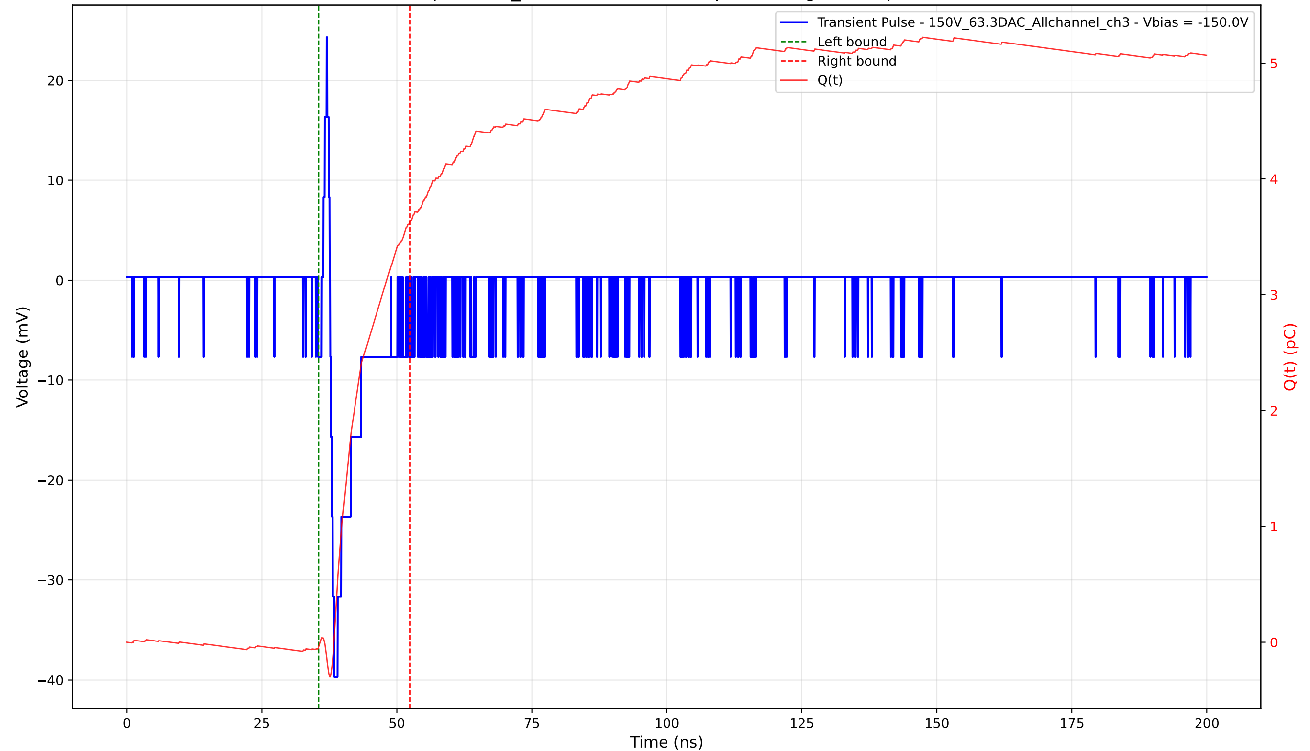
Transient Pulse - Sample: 1cm_42 - Position: 4120.0 \mu\text{m} - Charge: 3.67 pC - Rise Time: 0.78 ns
