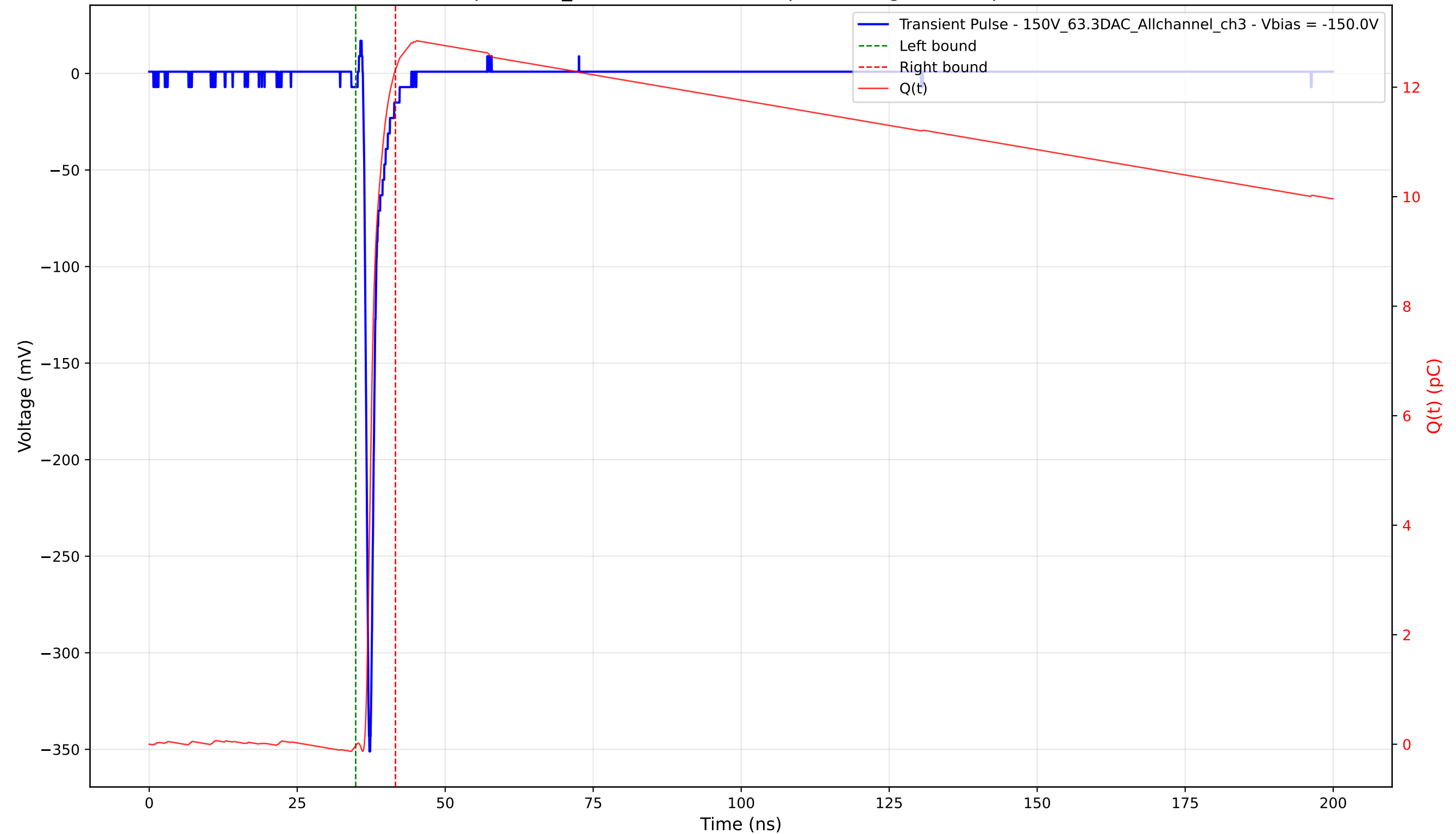
Transient Pulse - Sample: 1cm_42 - Position: 2150.0 \mu\text{m} - Charge: 12.35 pC - Rise Time: 0.72 ns
