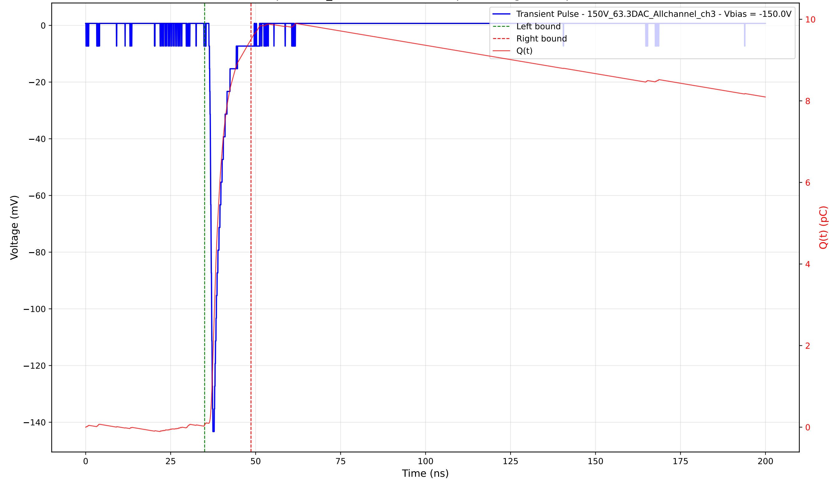
Transient Pulse - Sample: 1cm_42 - Position: 1725.0 \mu\text{m} - Charge: 9.45 pC - Rise Time: 0.88 ns
