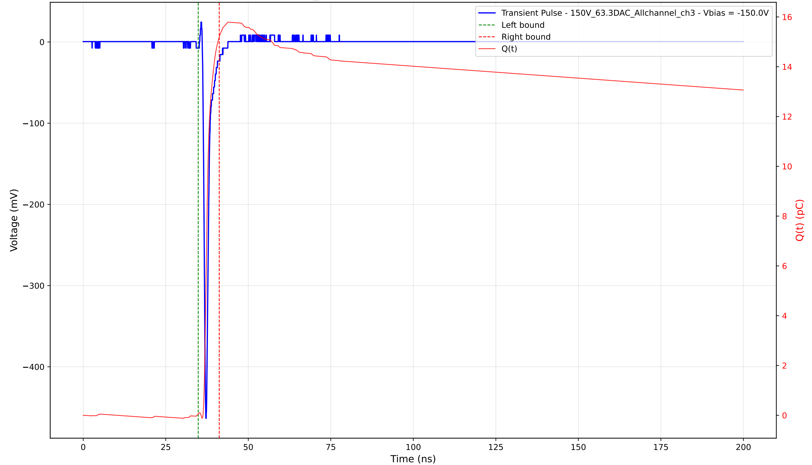
Transient Pulse - Sample: 1cm_42 - Position: 2250.0 \mu\text{m} - Charge: 15.13 pC - Rise Time: 0.75 ns
