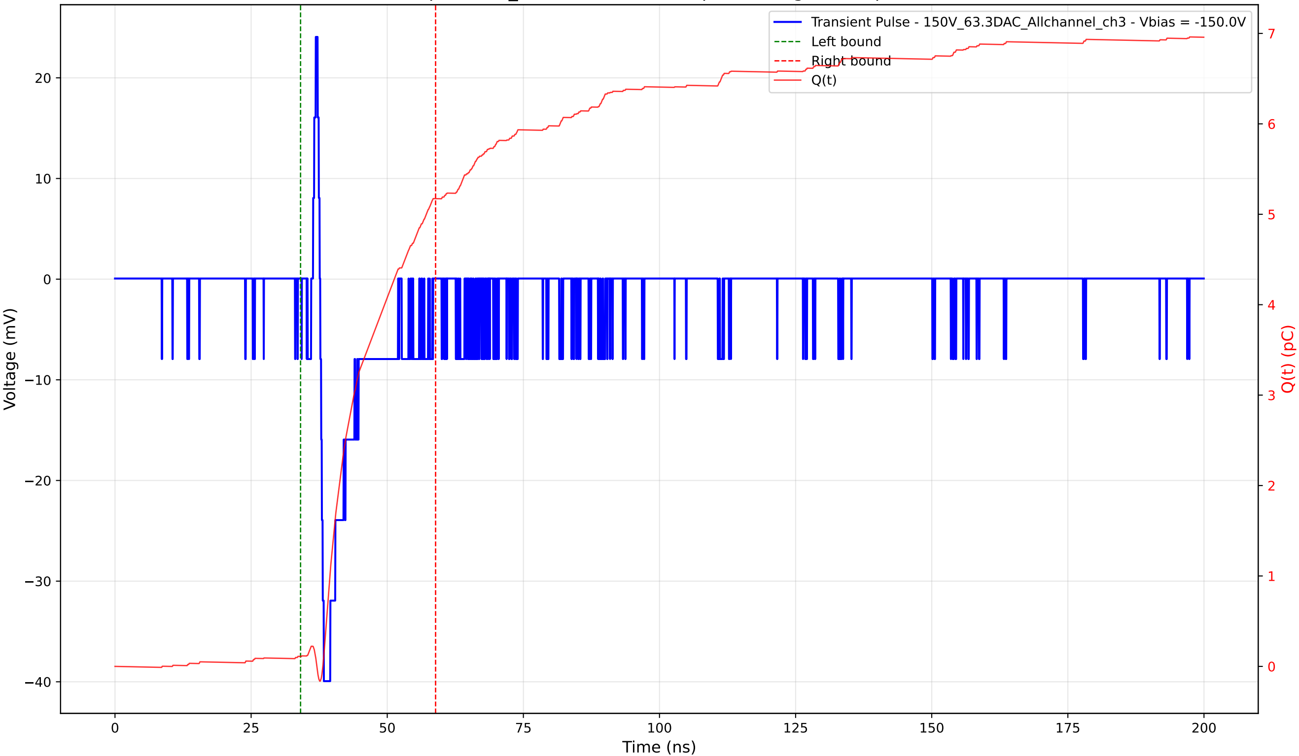
Transient Pulse - Sample: 1cm_42 - Position: 600.0 \mu\text{m} - Charge: 5.06 pC - Rise Time: 0.66 ns
