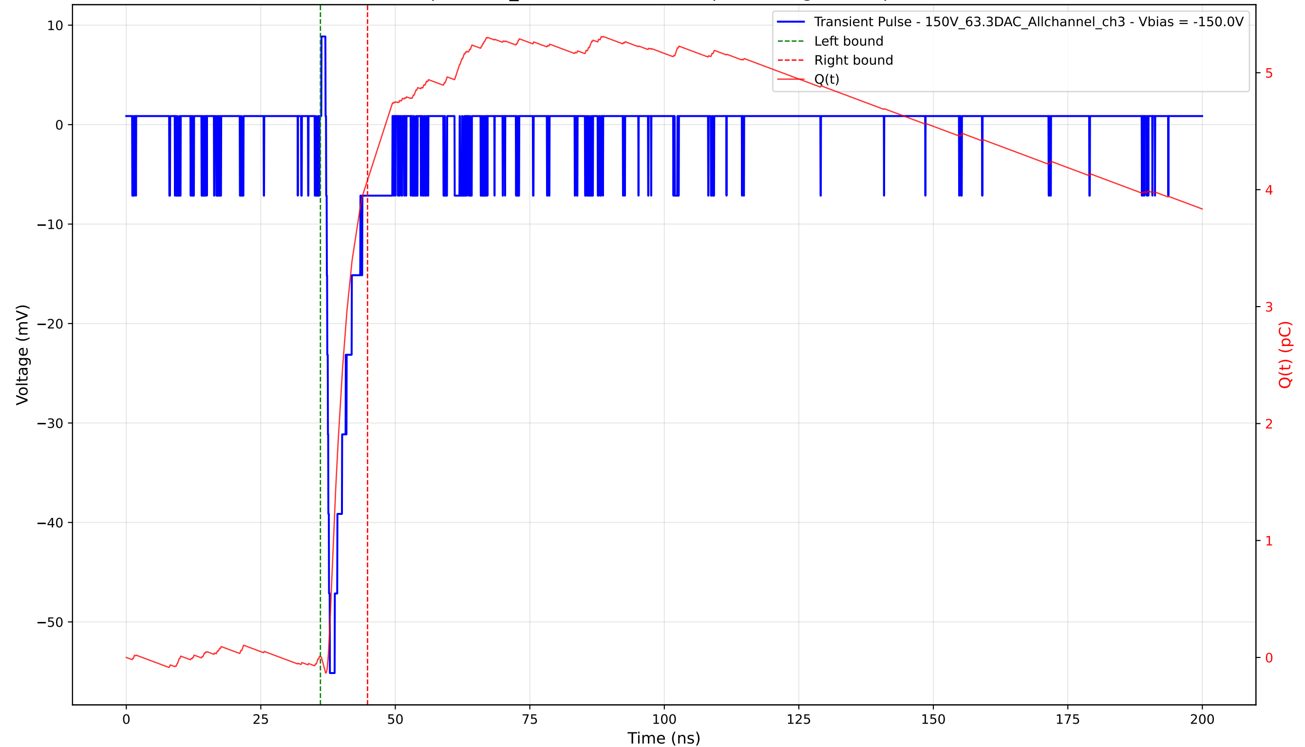
Transient Pulse - Sample: 1cm_42 - Position: 3655.0 \mu\text{m} - Charge: 4.08 pC - Rise Time: 0.69 ns
