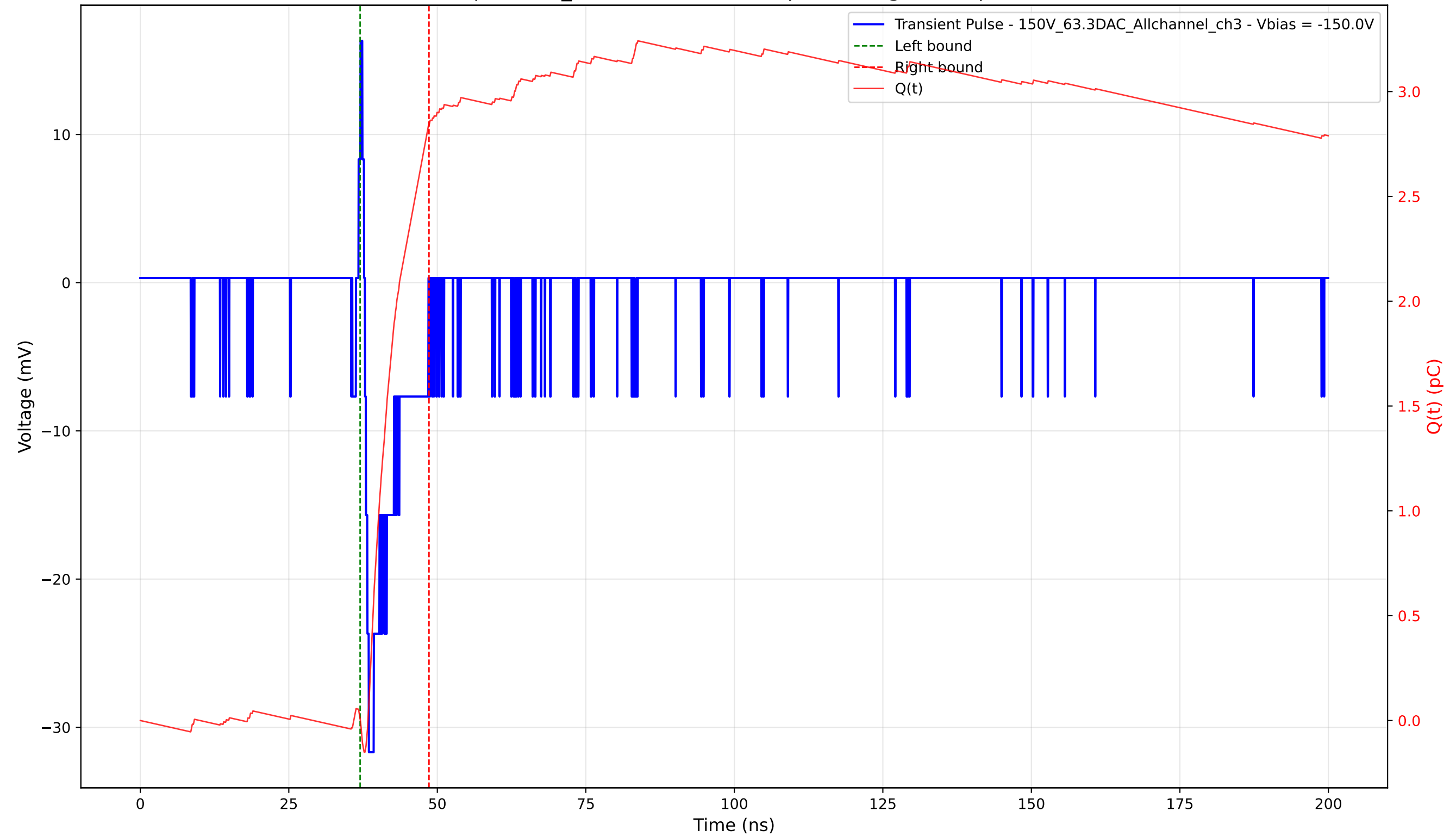
Transient Pulse - Sample: 1cm_42 - Position: 4855.0 \mu\text{m} - Charge: 2.83 pC - Rise Time: 0.66 ns
