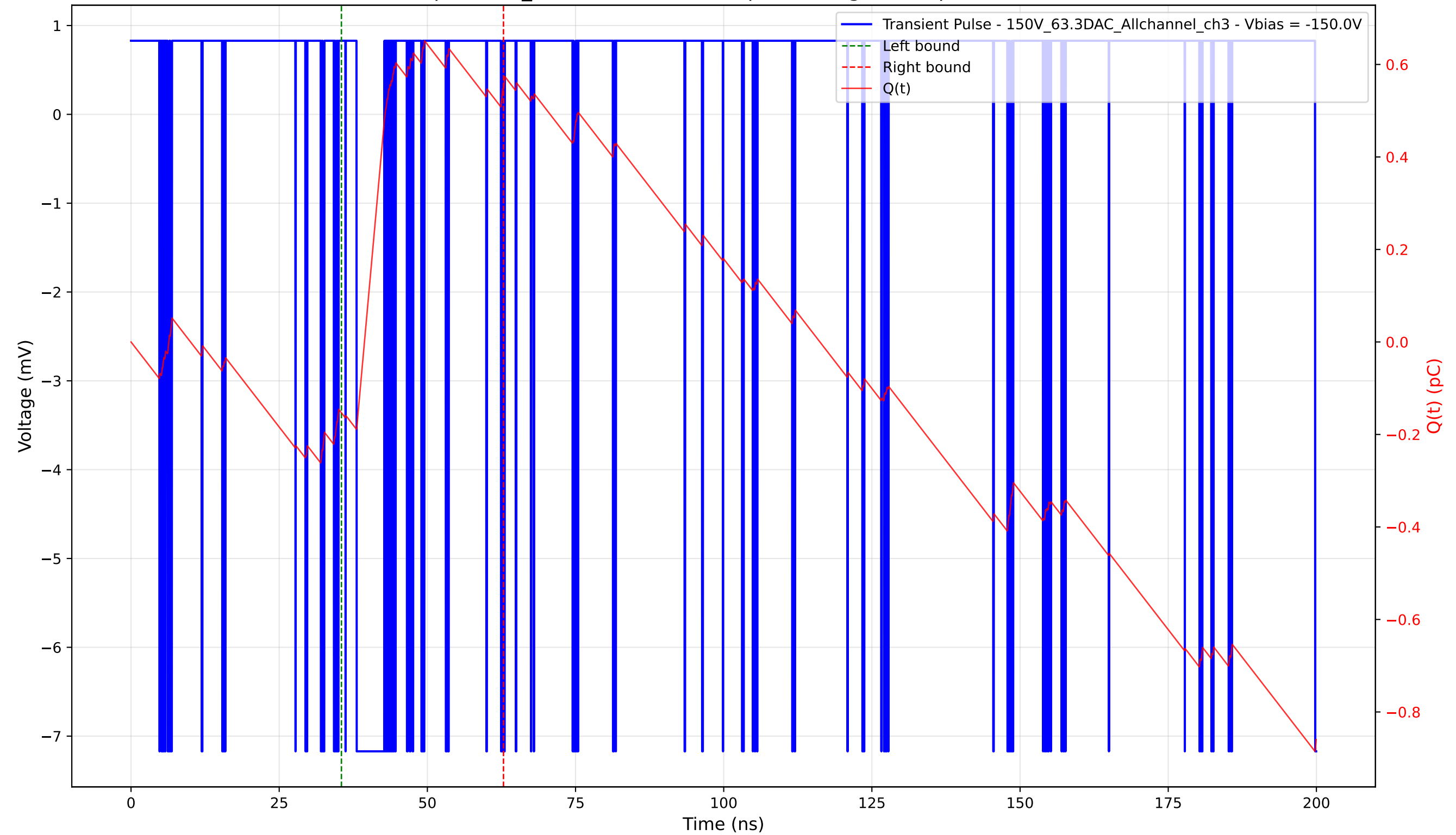
Transient Pulse - Sample: 1cm_42 - Position: 5115.0 \mu\text{m} - Charge: 0.70 pC - Rise Time: 0.00 ns (N/A)
