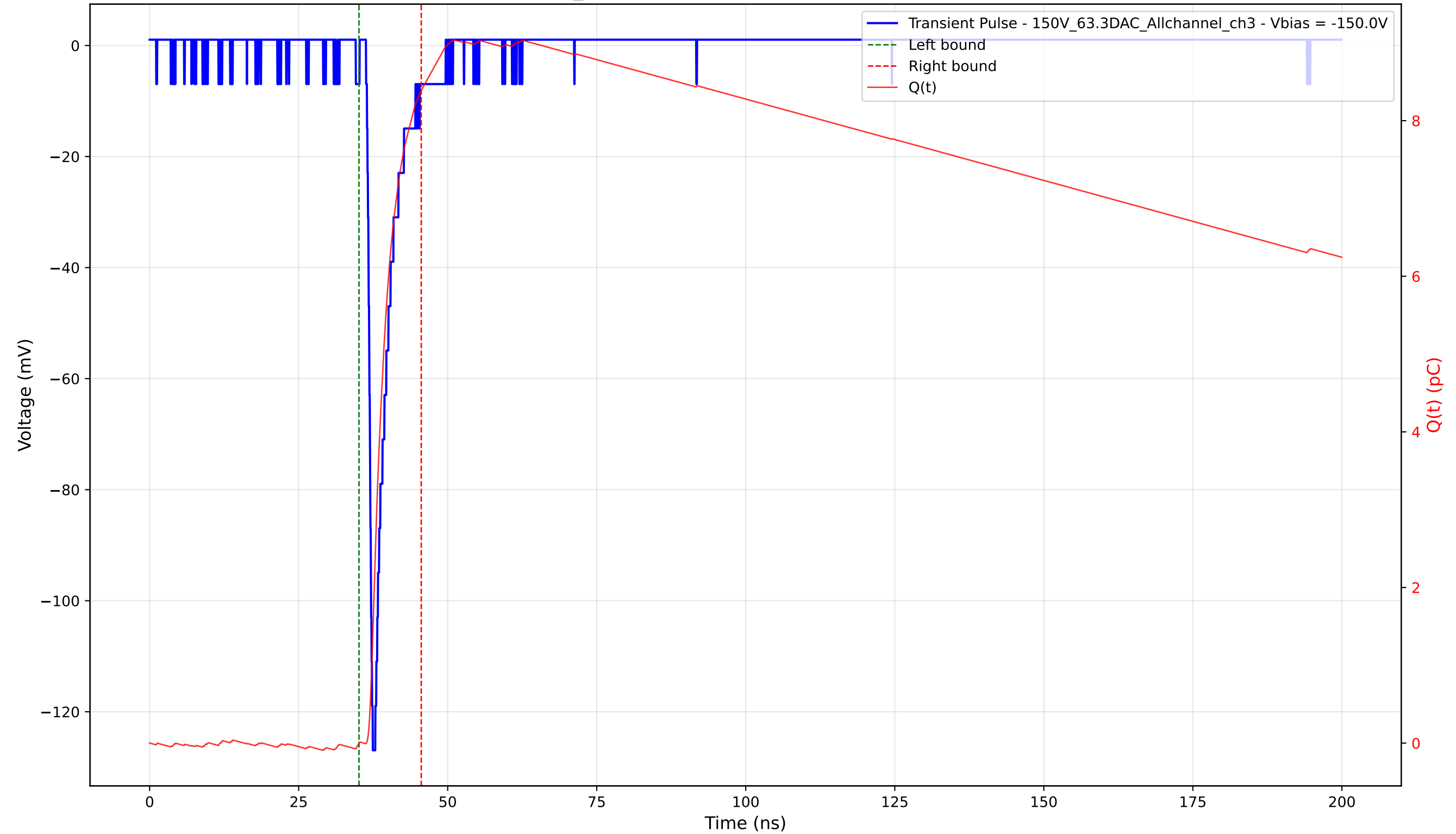
Transient Pulse - Sample: 1cm_42 - Position: 1685.0 \mu\text{m} - Charge: 8.39 pC - Rise Time: 0.85 ns
