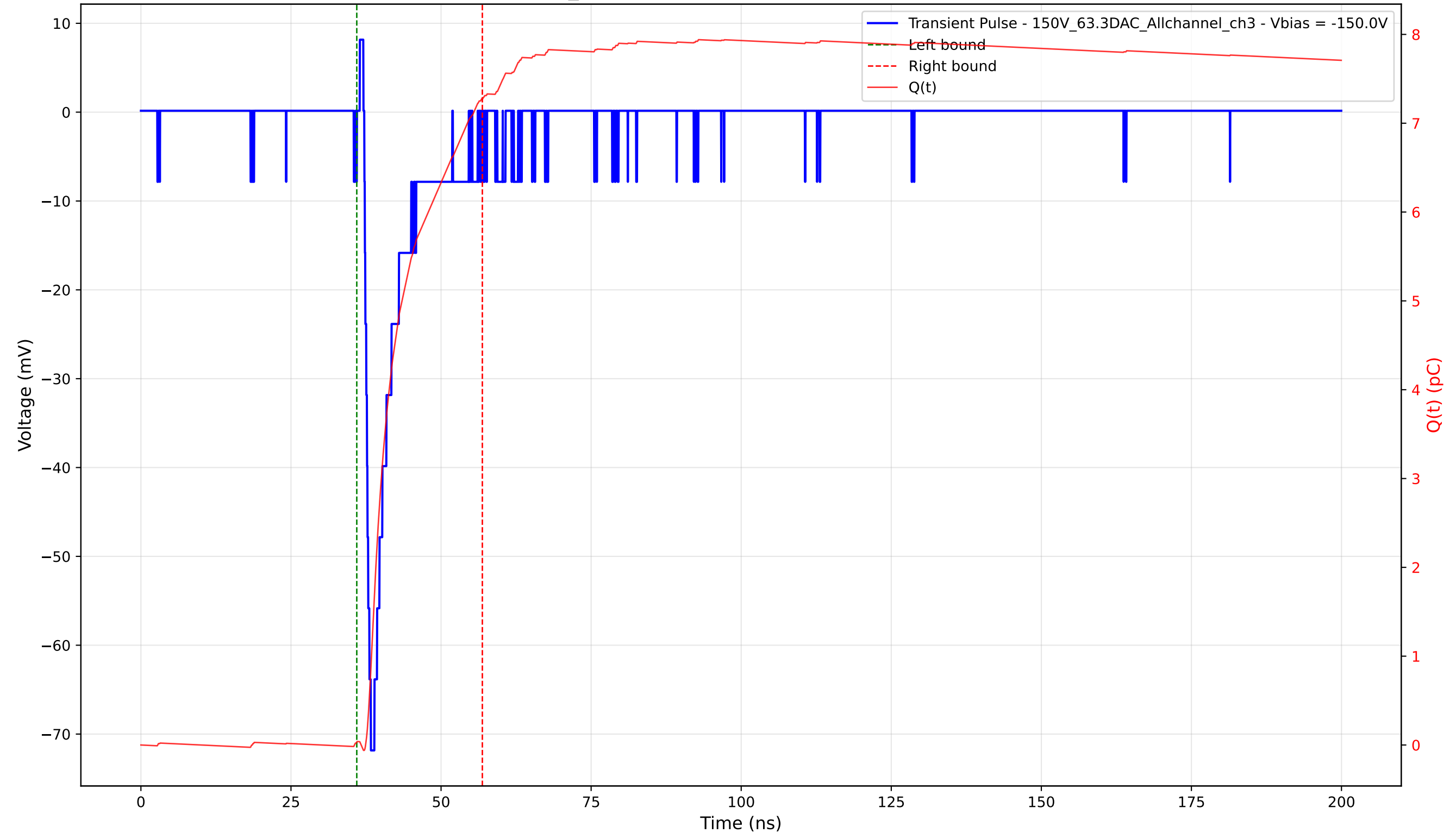
Transient Pulse - Sample: 1cm_42 - Position: 1285.0 \mu\text{m} - Charge: 7.24 pC - Rise Time: 1.08 ns
