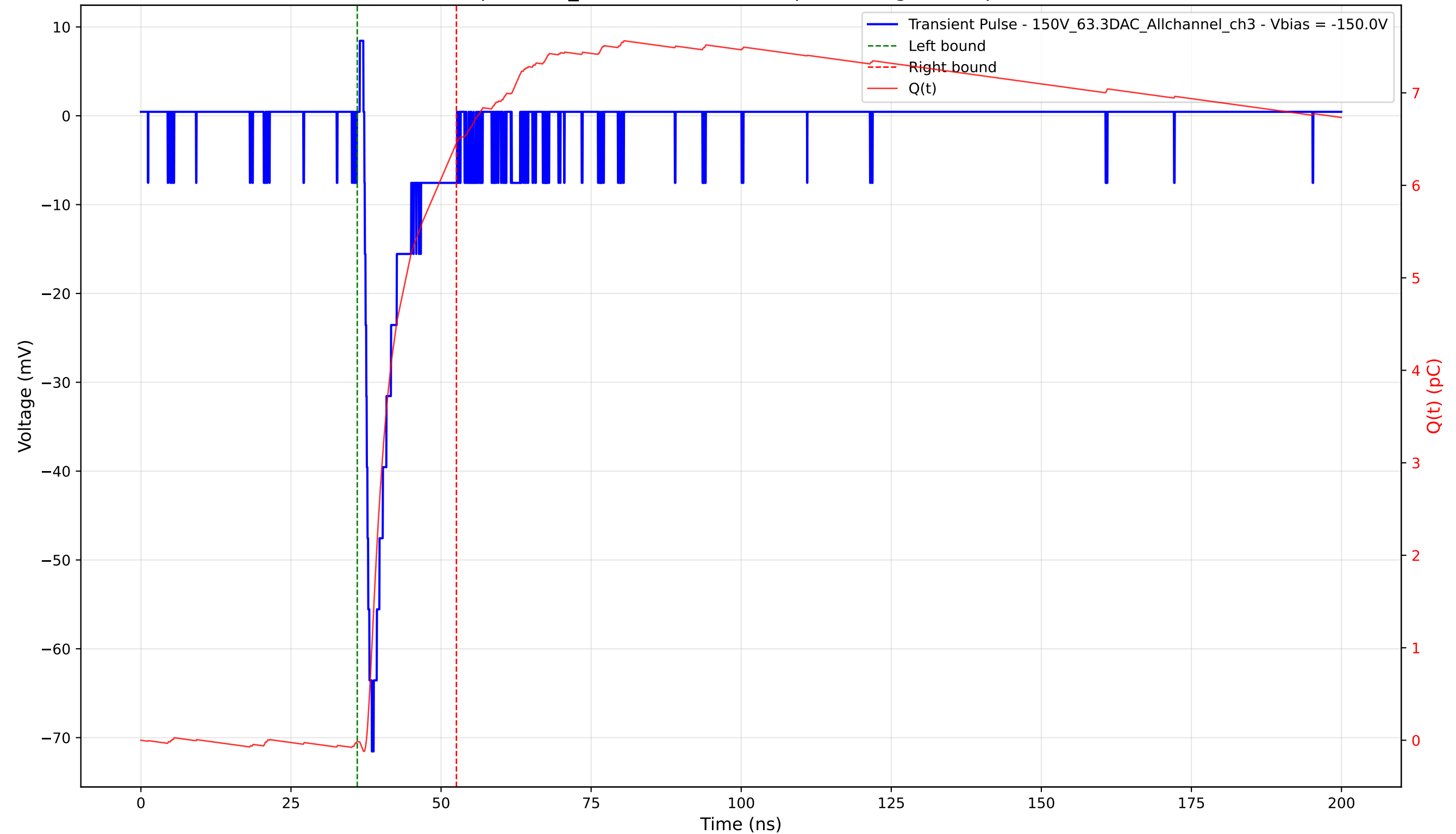
Transient Pulse - Sample: 1cm_42 - Position: 1280.0 \mu\text{m} - Charge: 6.47 pC - Rise Time: 1.24 ns
