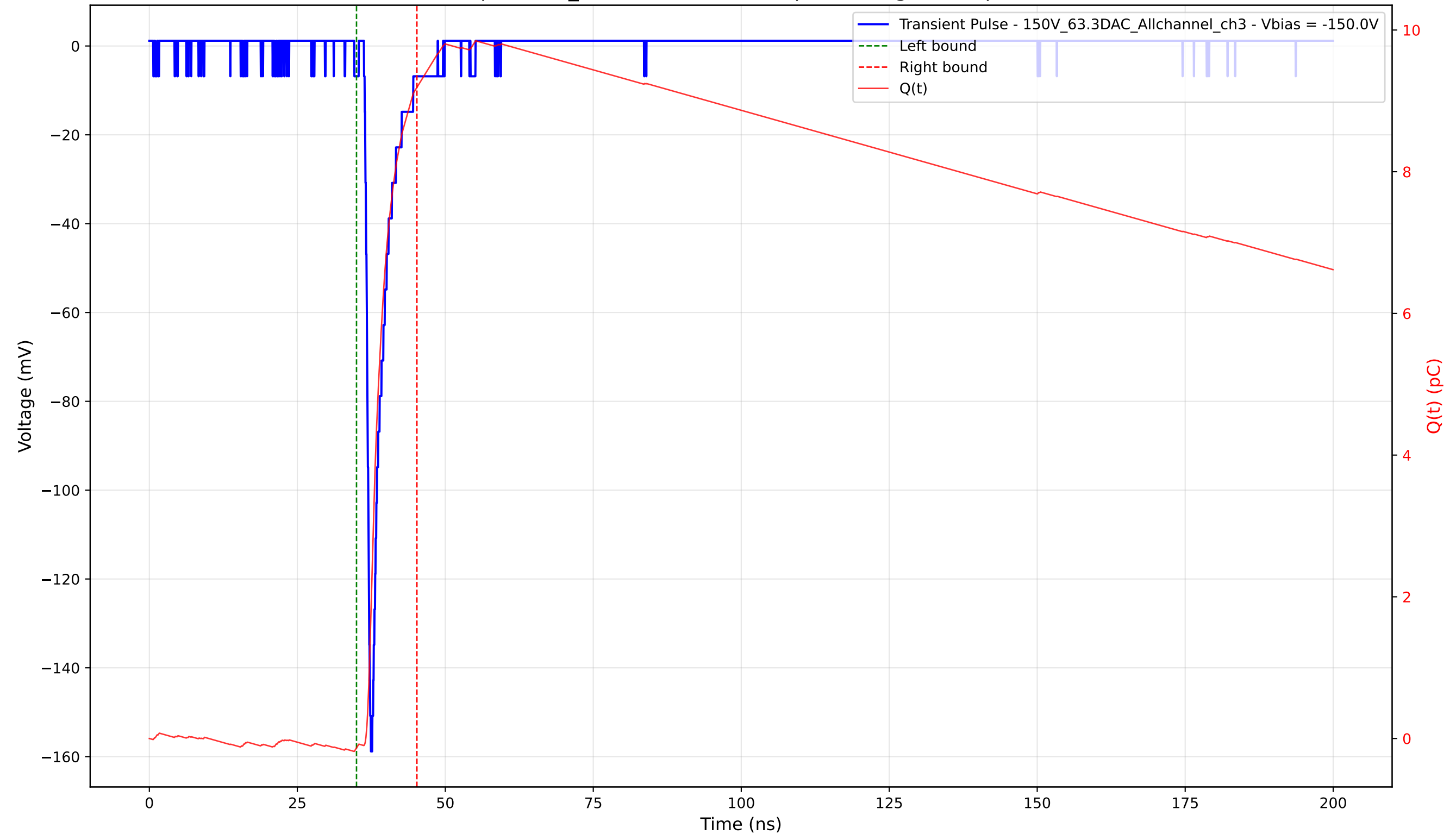
Transient Pulse - Sample: 1cm_42 - Position: 1810.0 \mu\text{m} - Charge: 9.32 pC - Rise Time: 0.87 ns
