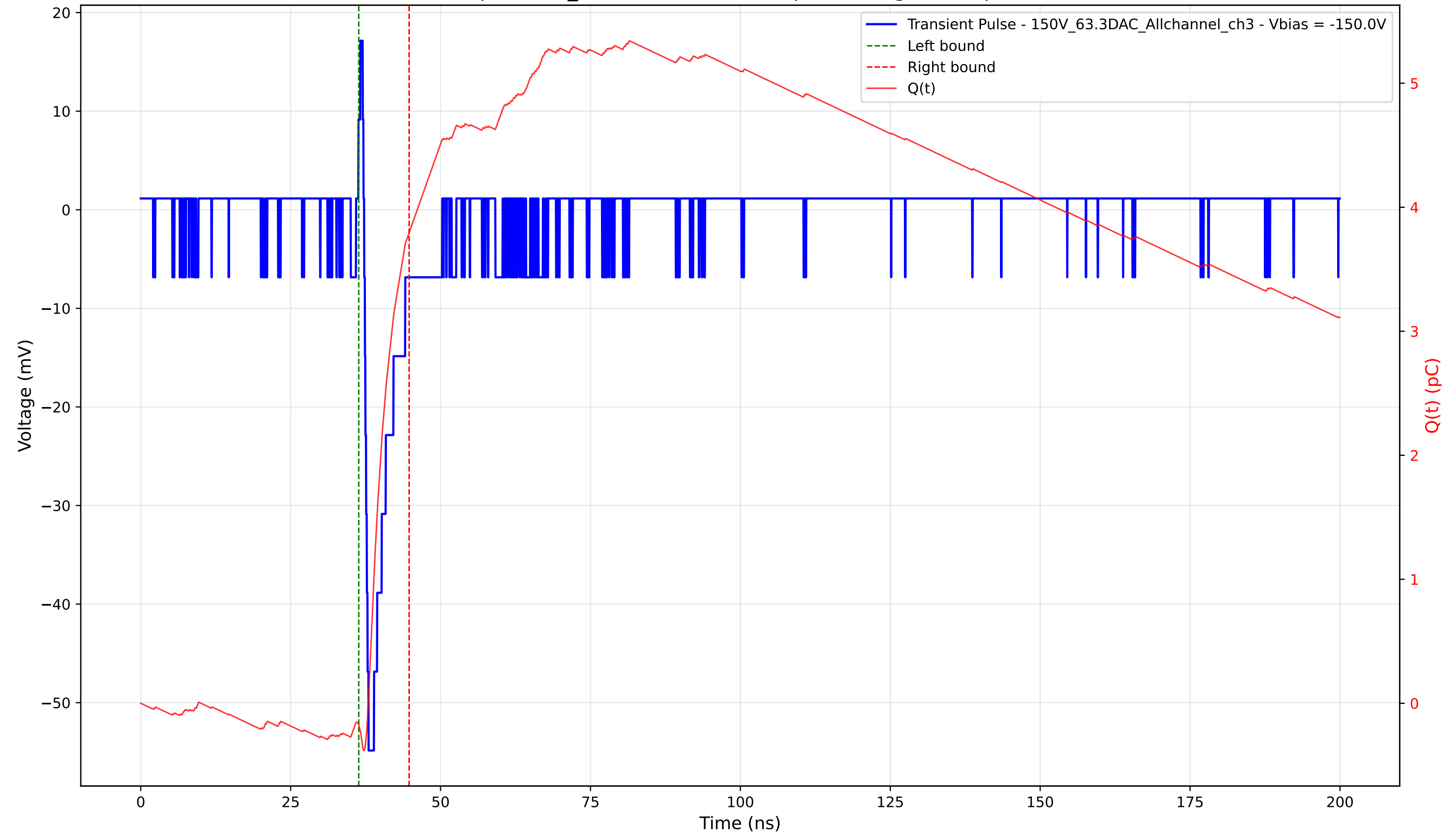
Transient Pulse - Sample: 1cm_42 - Position: 3740.0 \mu\text{m} - Charge: 3.97 pC - Rise Time: 0.73 ns
