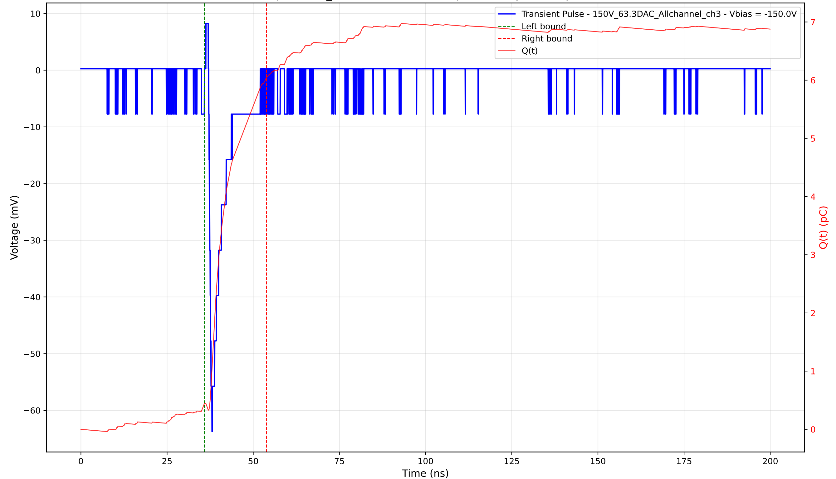
Transient Pulse - Sample: 1cm_42 - Position: 3625.0 \mu\text{m} - Charge: 5.60 pC - Rise Time: 0.93 ns
