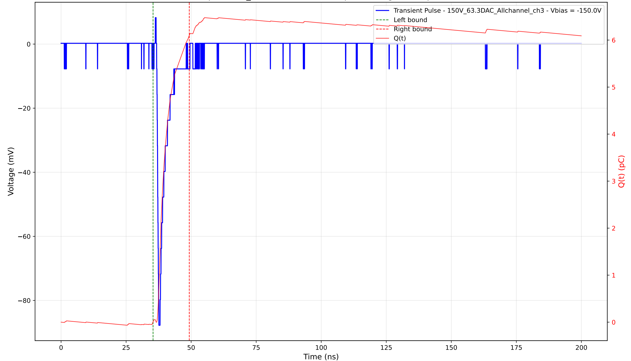
Transient Pulse - Sample: 1cm_42 - Position: 3450.0 \mu\text{m} - Charge: 6.09 pC - Rise Time: 0.63 ns
