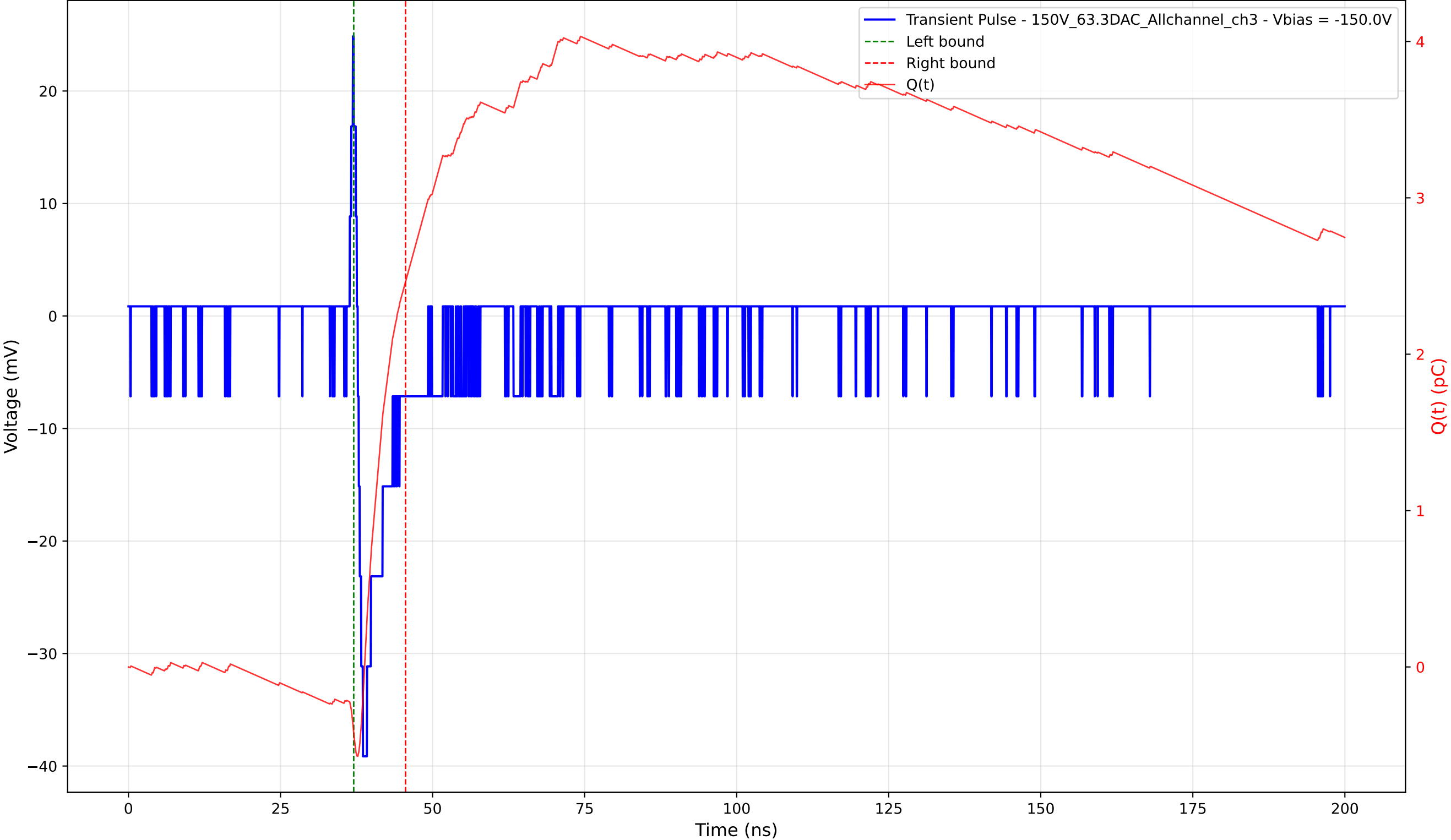
Transient Pulse - Sample: 1cm_42 - Position: 520.0 \mu\text{m} - Charge: 2.89 pC - Rise Time: 0.86 ns
