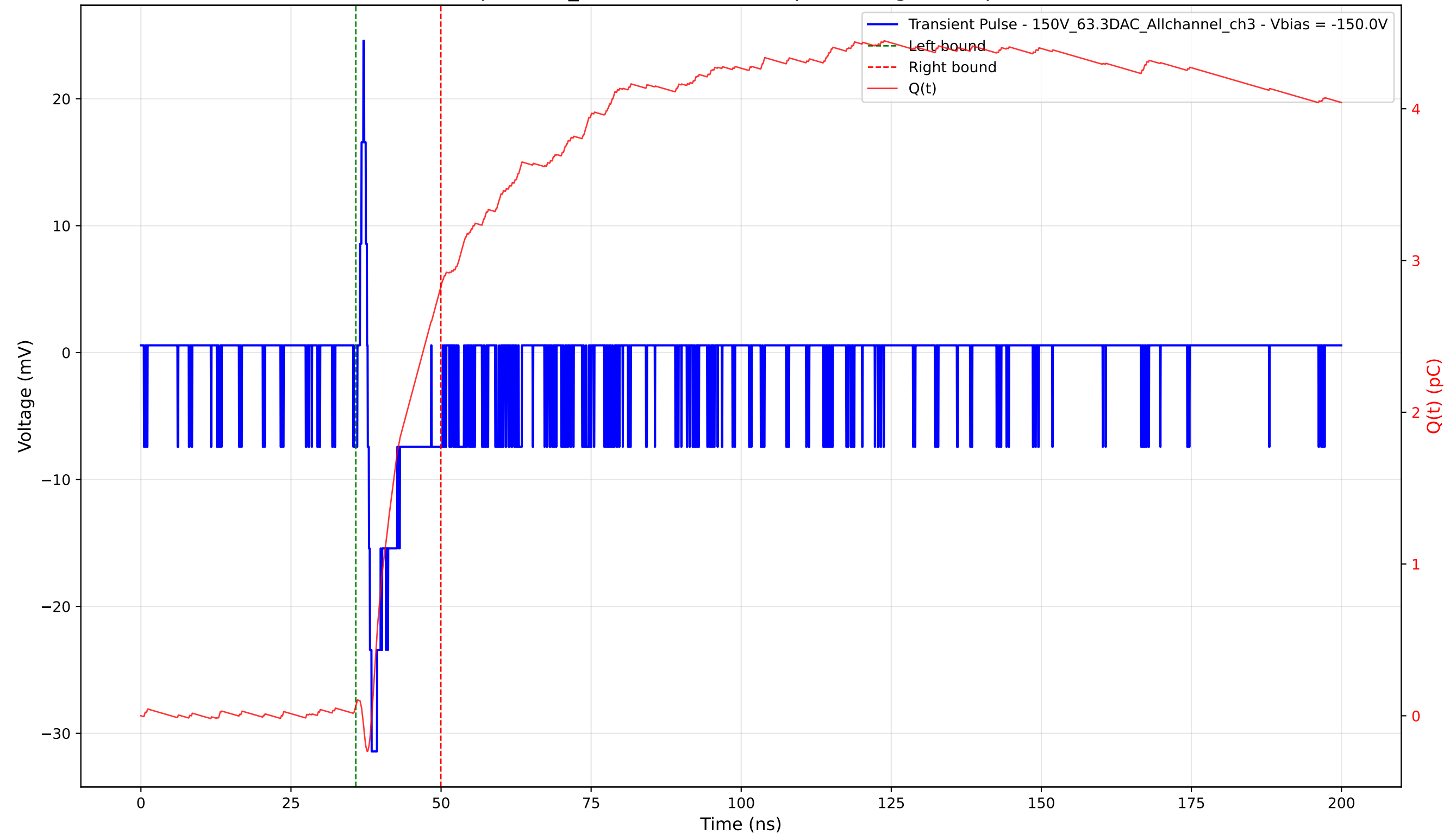
Transient Pulse - Sample: 1cm_42 - Position: 4490.0 \mu\text{m} - Charge: 2.76 pC - Rise Time: 0.67 ns
