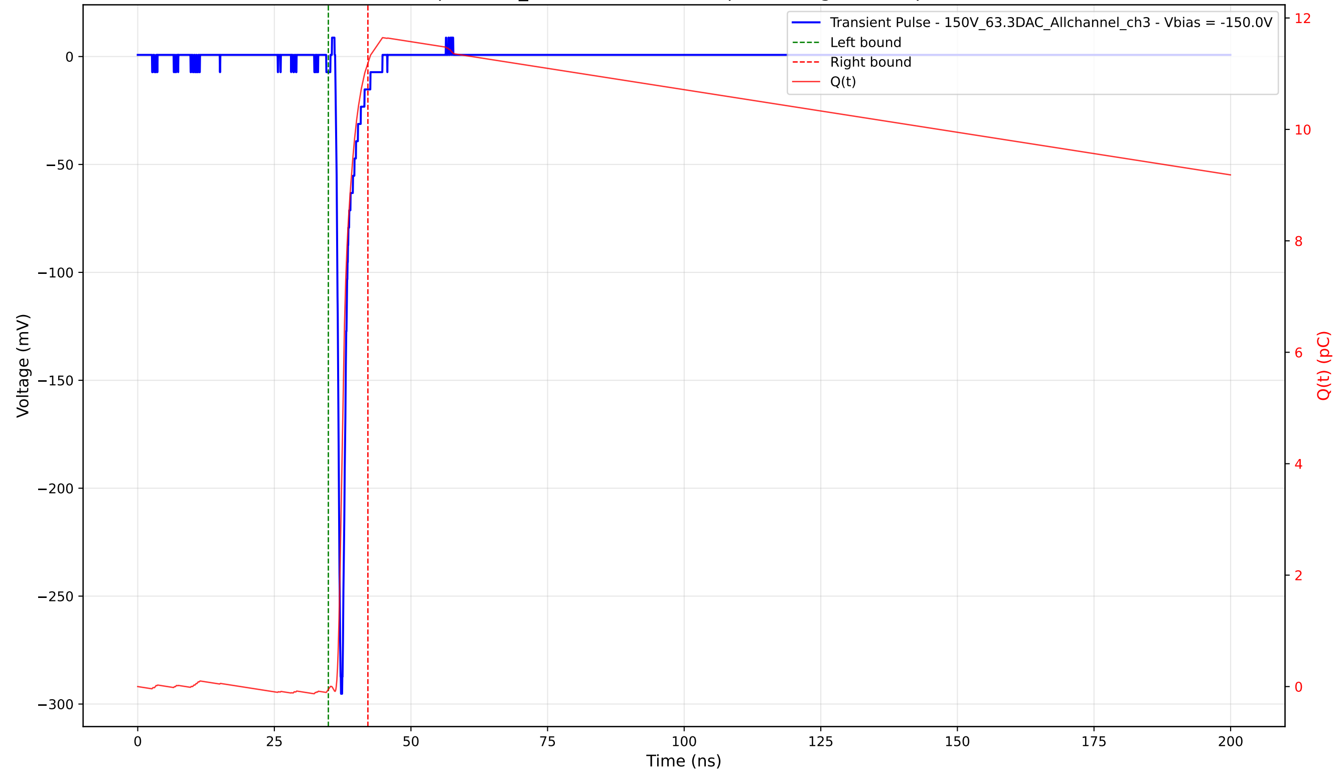
Transient Pulse - Sample: 1cm_42 - Position: 2090.0 \mu\text{m} - Charge: 11.24 pC - Rise Time: 0.74 ns
