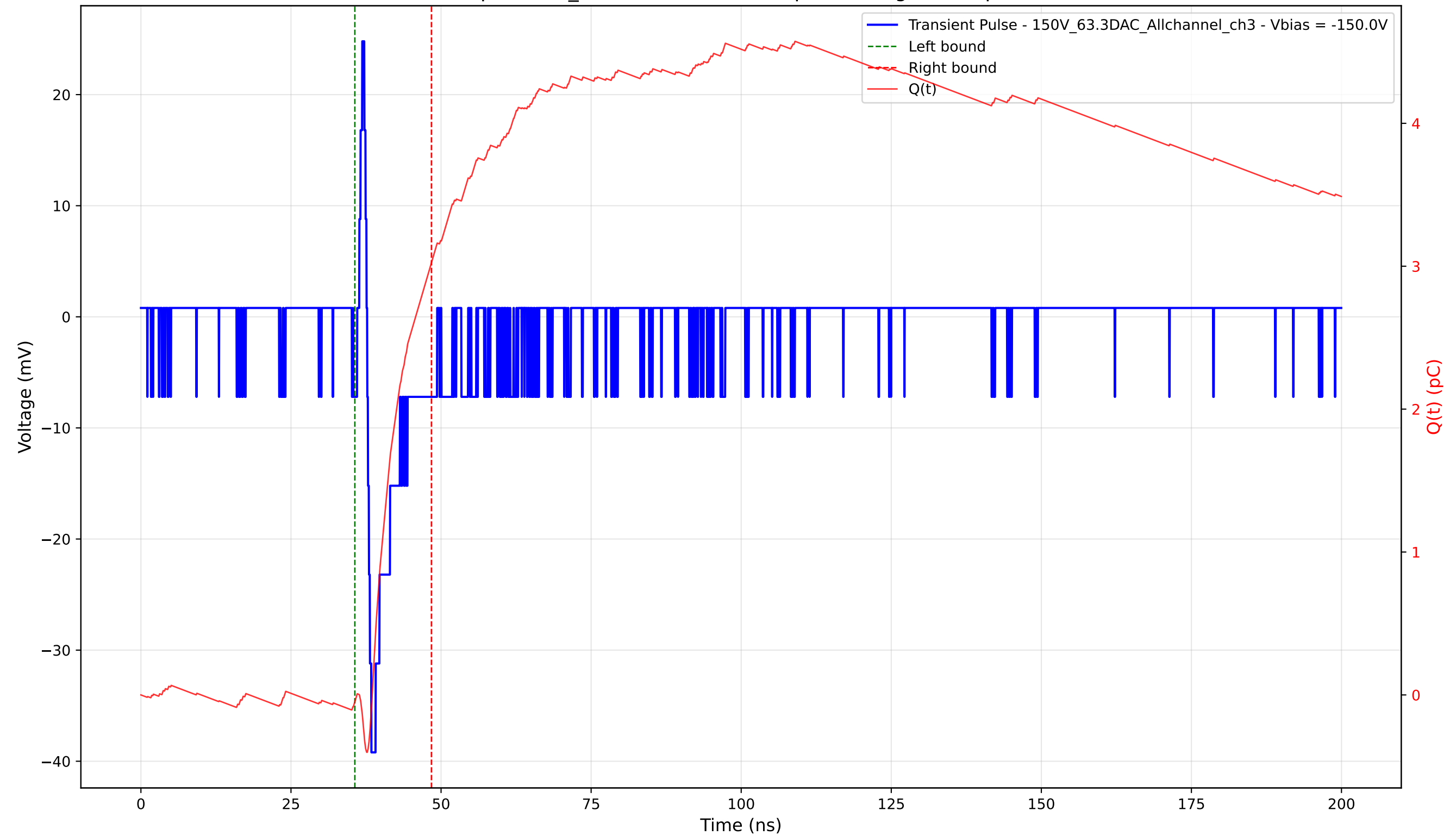
Transient Pulse - Sample: 1cm_42 - Position: 4170.0 \mu\text{m} - Charge: 3.07 pC - Rise Time: 0.70 ns
