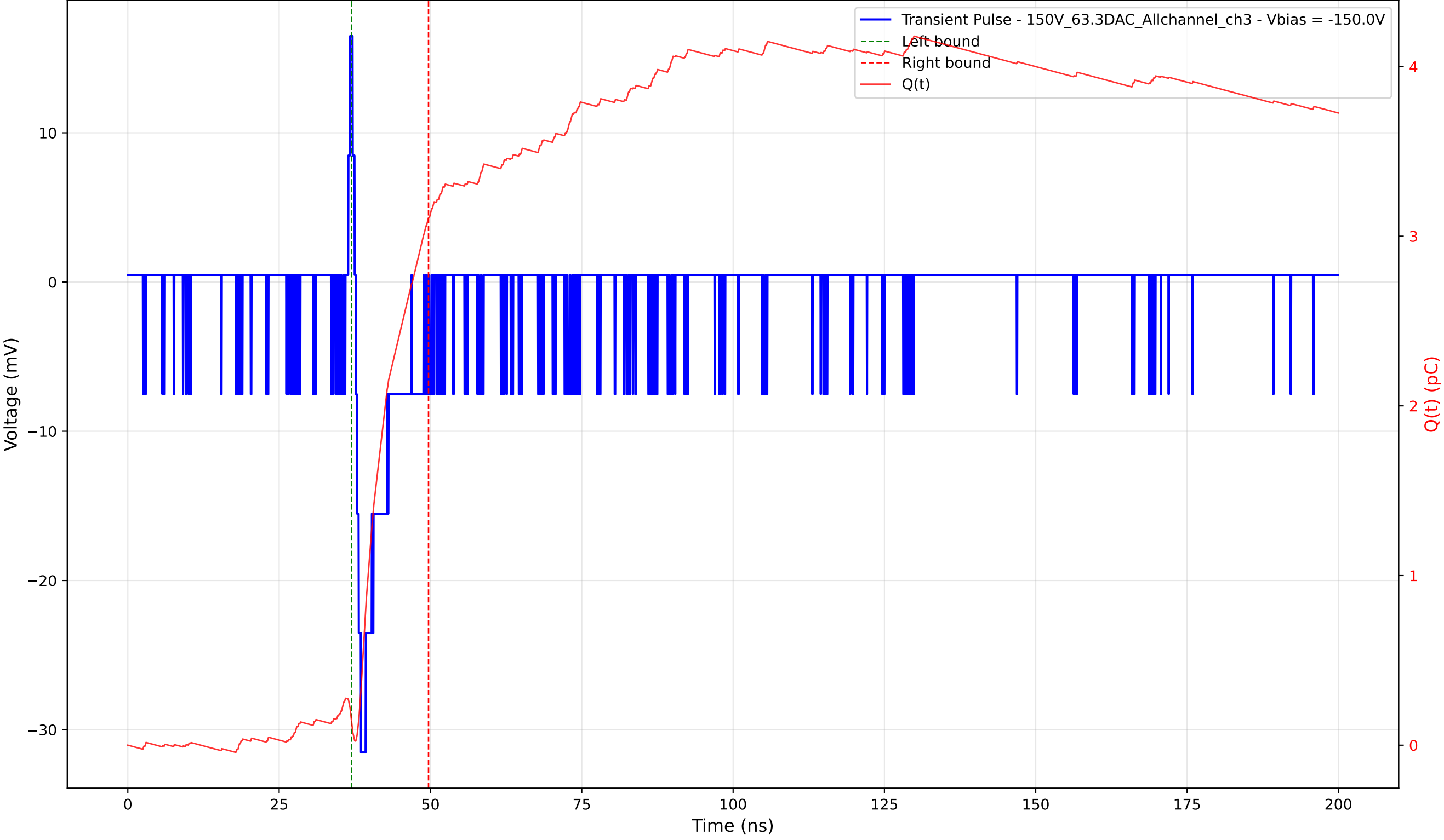
Transient Pulse - Sample: 1cm_42 - Position: 400.0 \mu\text{m} - Charge: 2.97 pC - Rise Time: 0.86 ns
