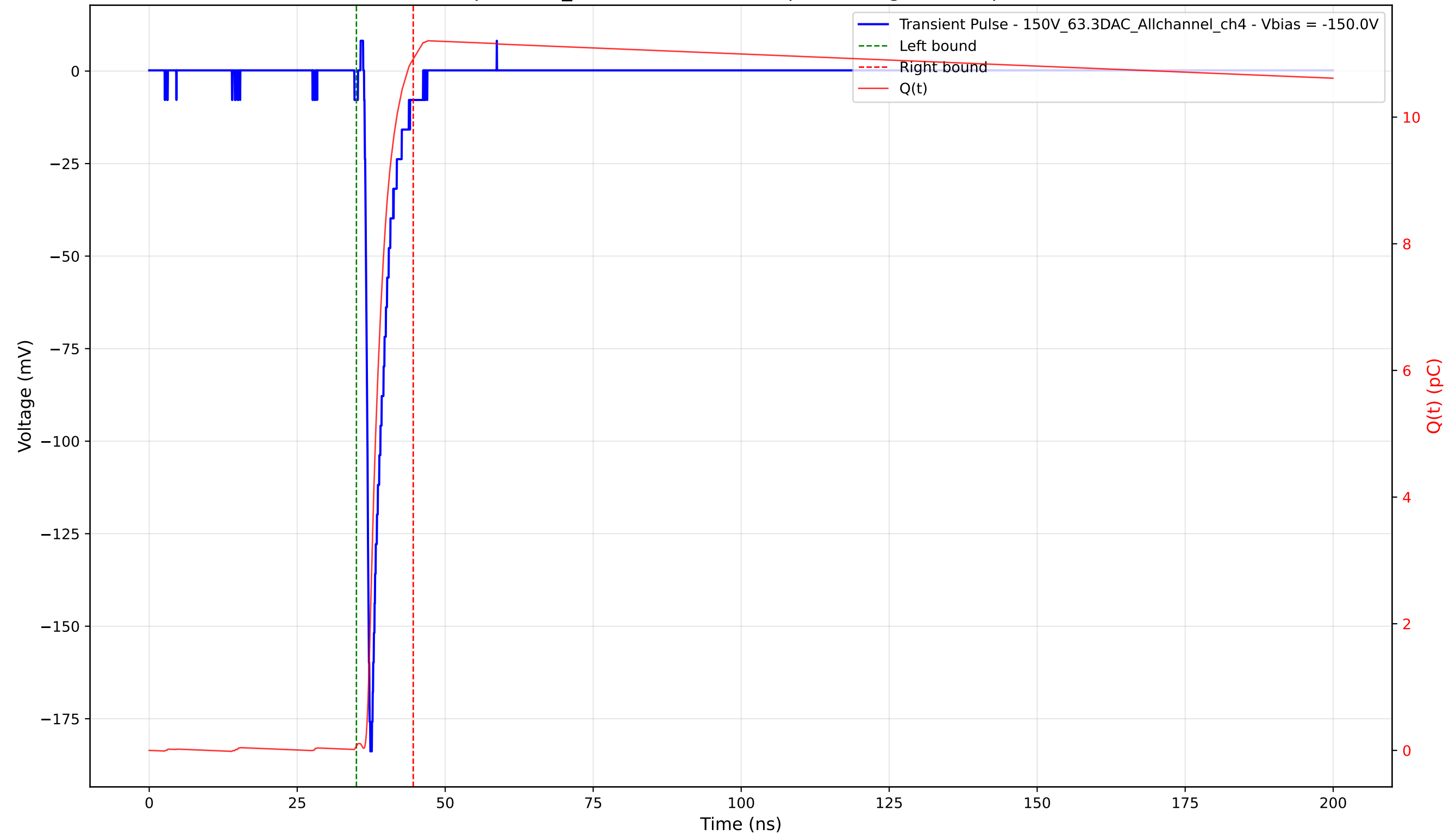
Transient Pulse - Sample: 1cm_42 - Position: 1250.0 \mu\text{m} - Charge: 10.85 pC - Rise Time: 0.78 ns
