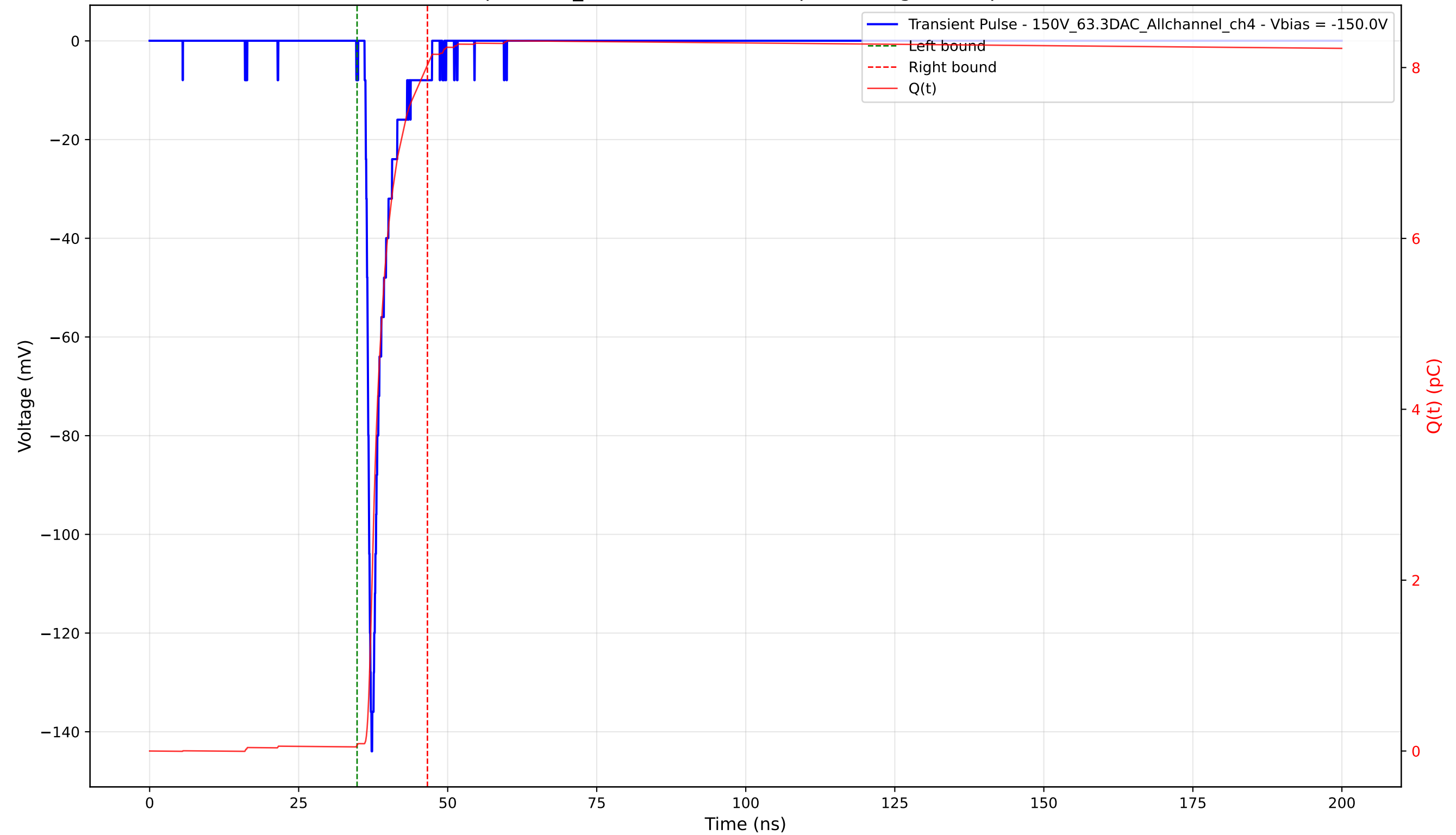
Transient Pulse - Sample: 1cm_42 - Position: 2745.0 \mu\text{m} - Charge: 7.96 pC - Rise Time: 0.89 ns
