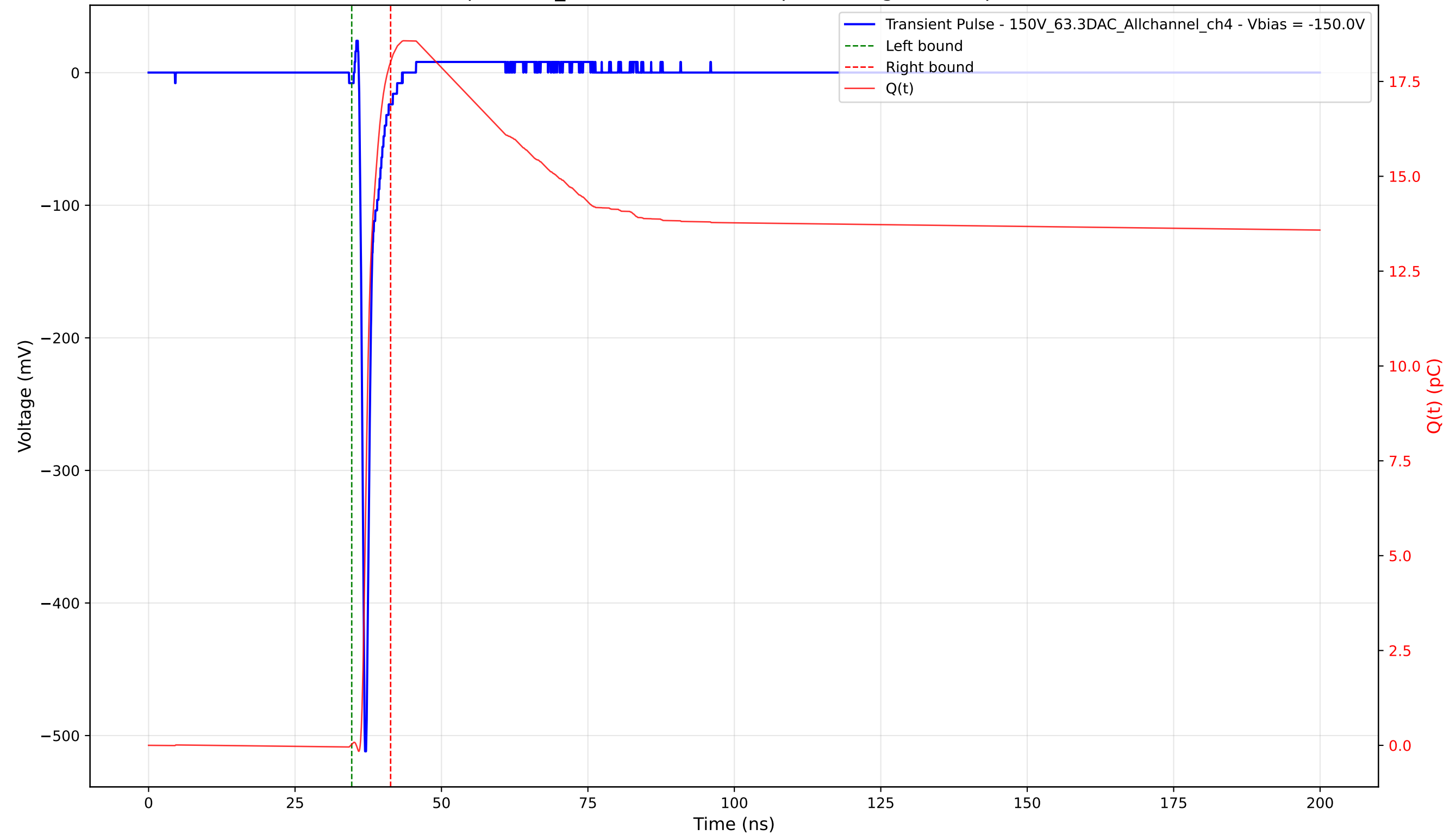
Transient Pulse - Sample: 1cm_42 - Position: 1700.0 \mu\text{m} - Charge: 17.99 pC - Rise Time: 0.72 ns
