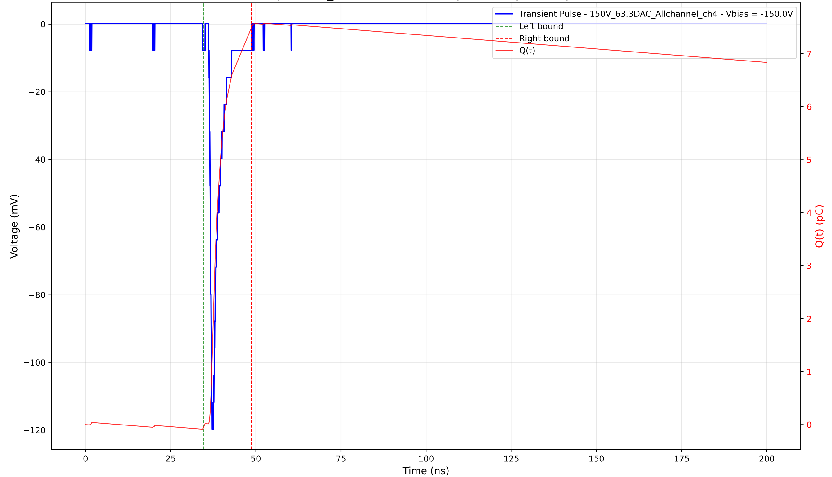
Transient Pulse - Sample: 1cm_42 - Position: 2840.0 \mu\text{m} - Charge: 7.52 pC - Rise Time: 0.82 ns
