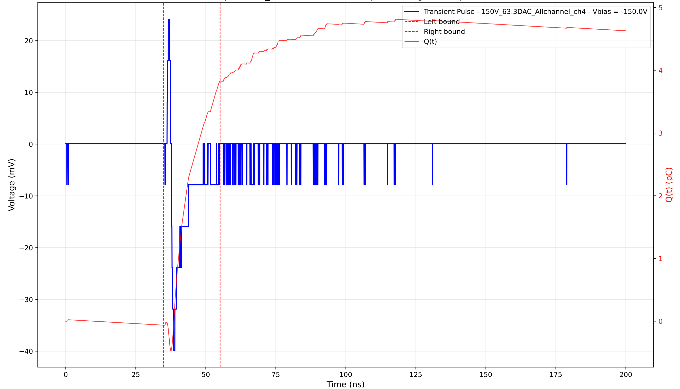
Transient Pulse - Sample: 1cm_42 - Position: 3710.0 \mu\text{m} - Charge: 3.89 pC - Rise Time: 0.90 ns
