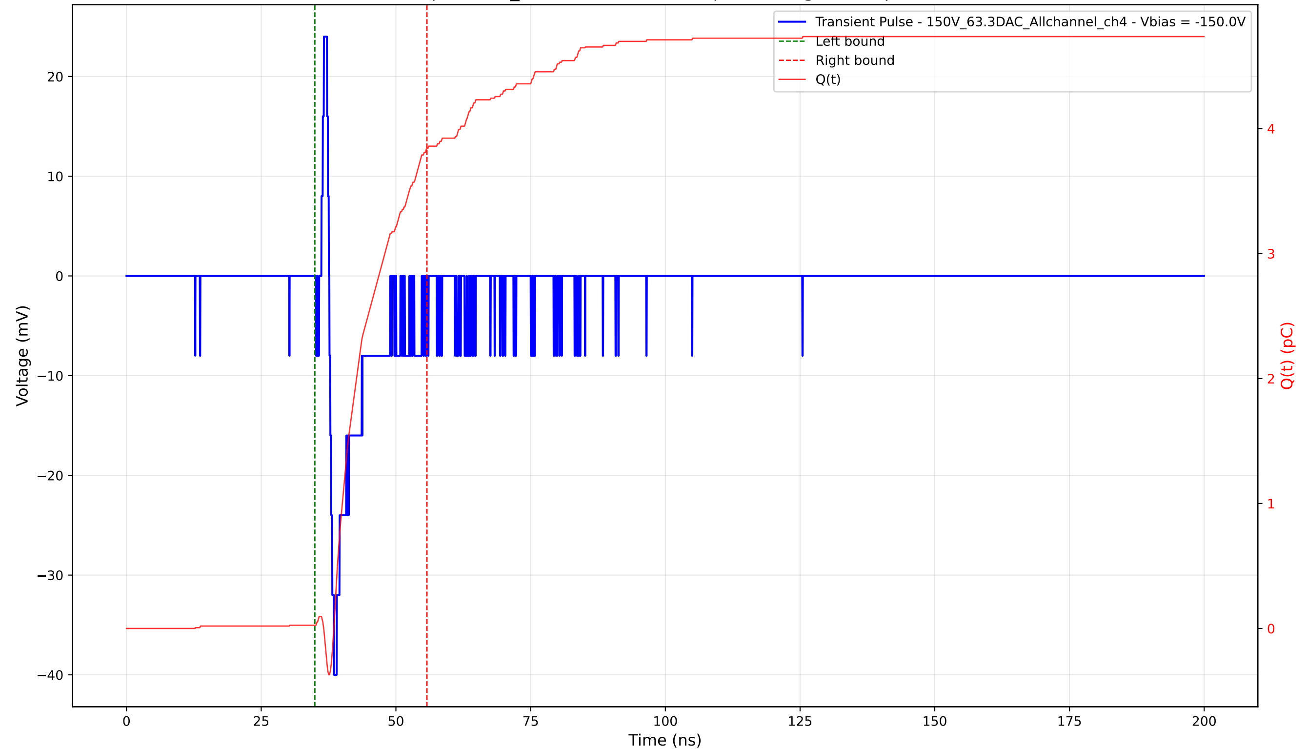
Transient Pulse - Sample: 1cm_42 - Position: 3760.0 \mu\text{m} - Charge: 3.81 pC - Rise Time: 0.86 ns
