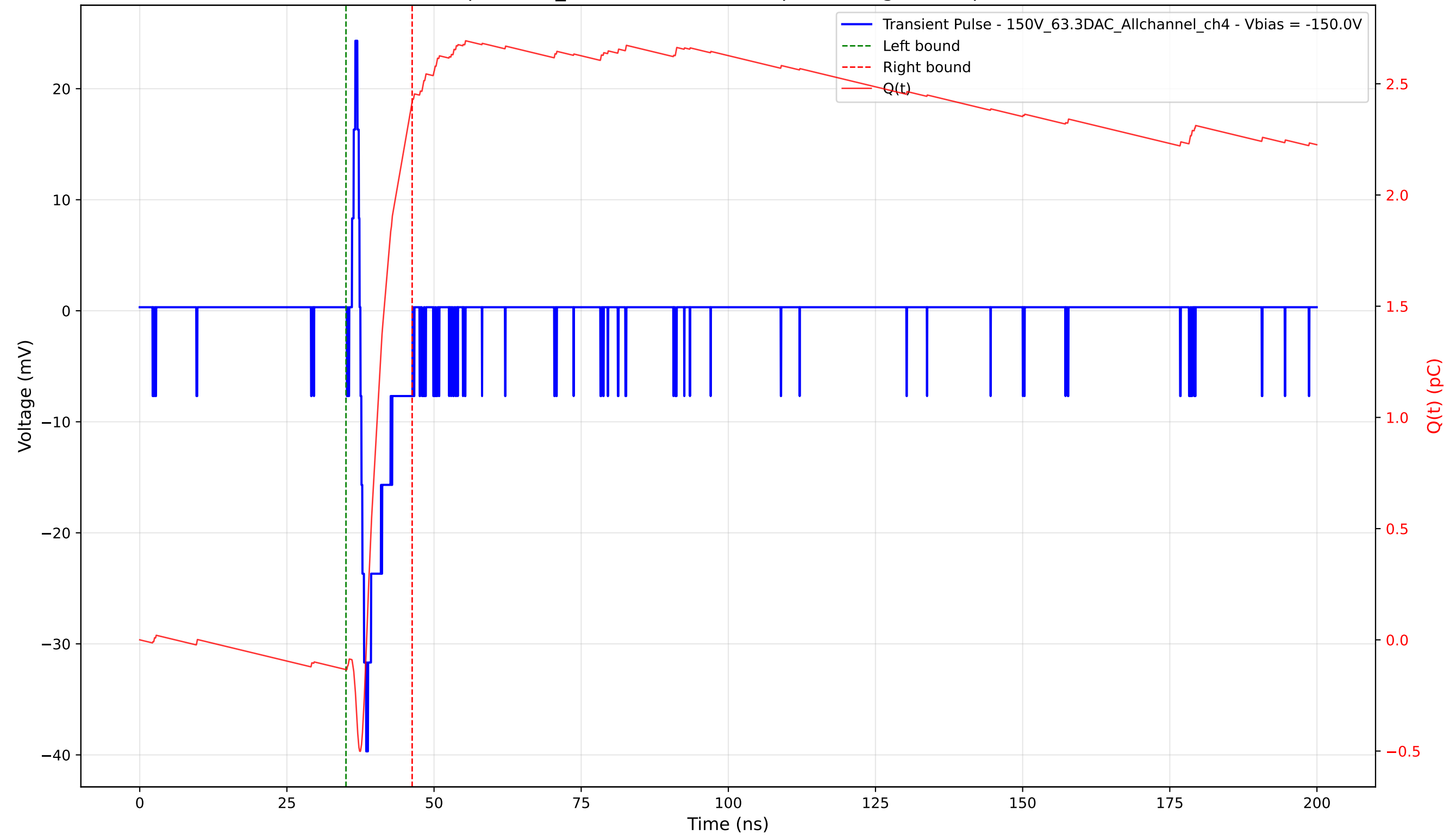
Transient Pulse - Sample: 1cm_42 - Position: 4755.0 \mu\text{m} - Charge: 2.56 pC - Rise Time: 0.98 ns
