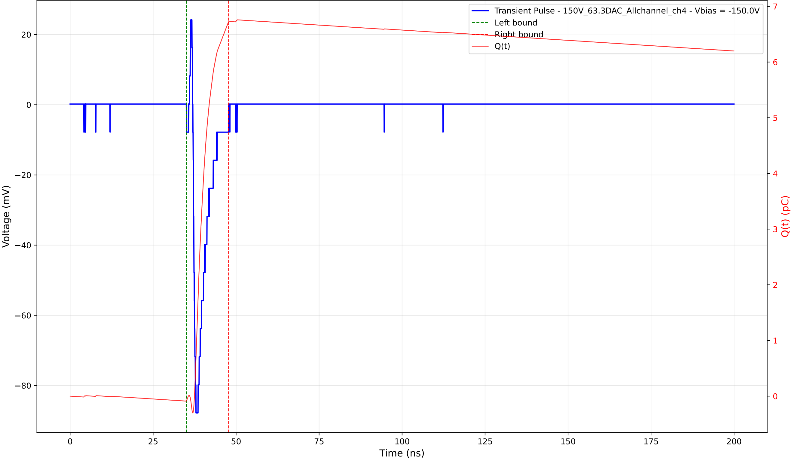
Transient Pulse - Sample: 1cm_42 - Position: 805.0 \mu\text{m} - Charge: 6.80 pC - Rise Time: 0.68 ns
