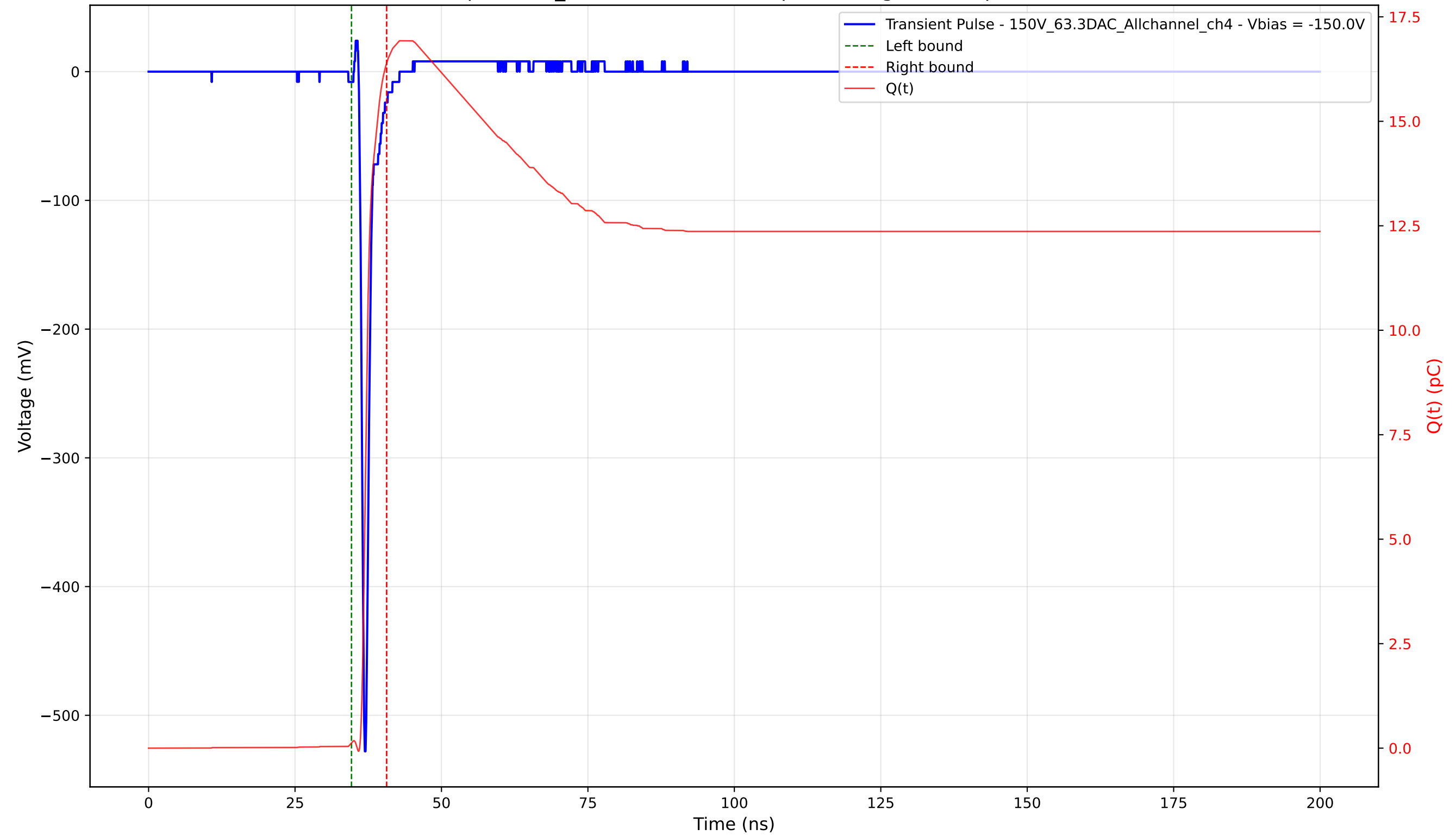
Transient Pulse - Sample: 1cm_42 - Position: 2175.0 \mu\text{m} - Charge: 16.27 pC - Rise Time: 0.70 ns
