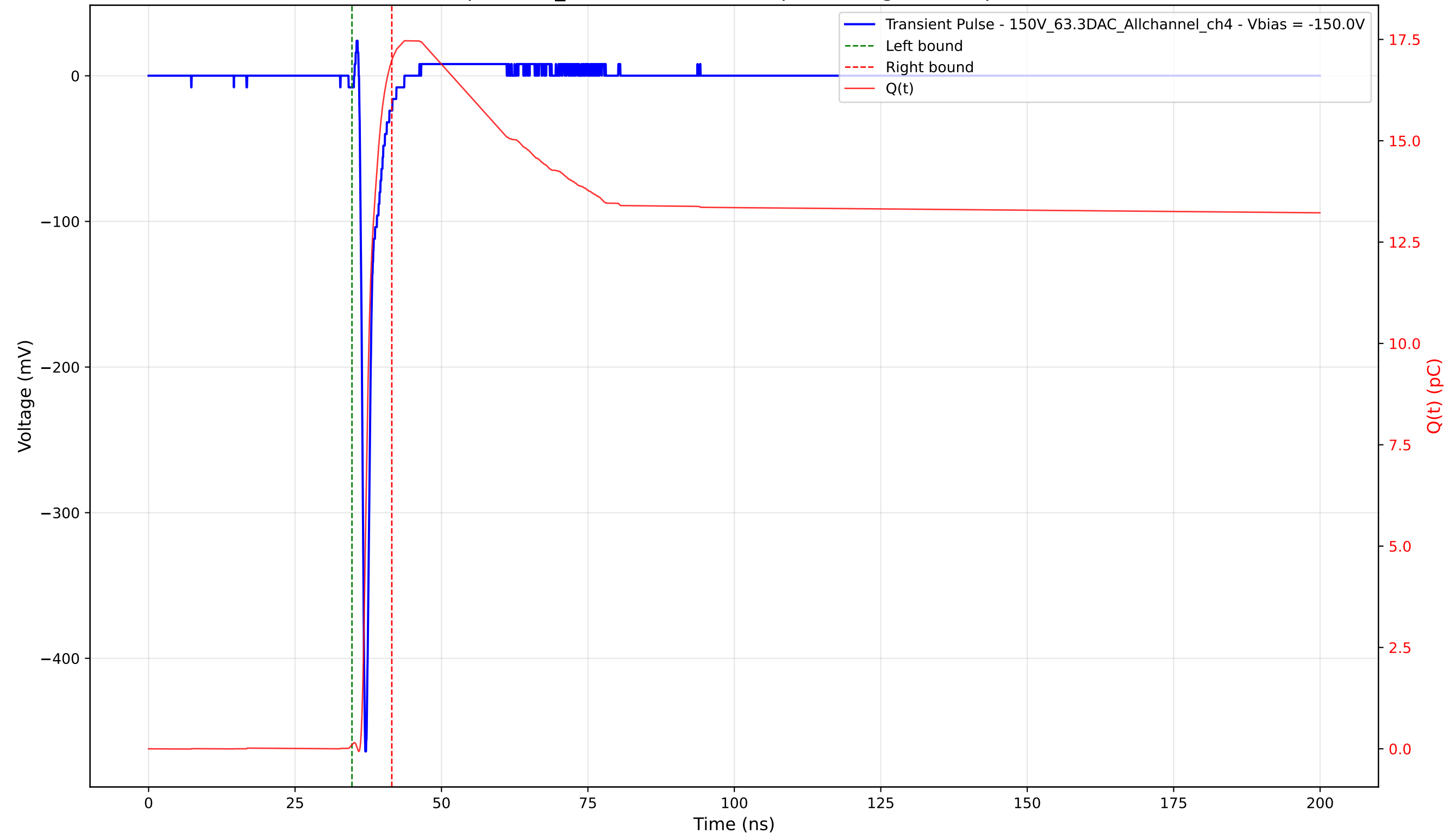
Transient Pulse - Sample: 1cm_42 - Position: 1665.0 \mu\text{m} - Charge: 16.89 pC - Rise Time: 0.75 ns
