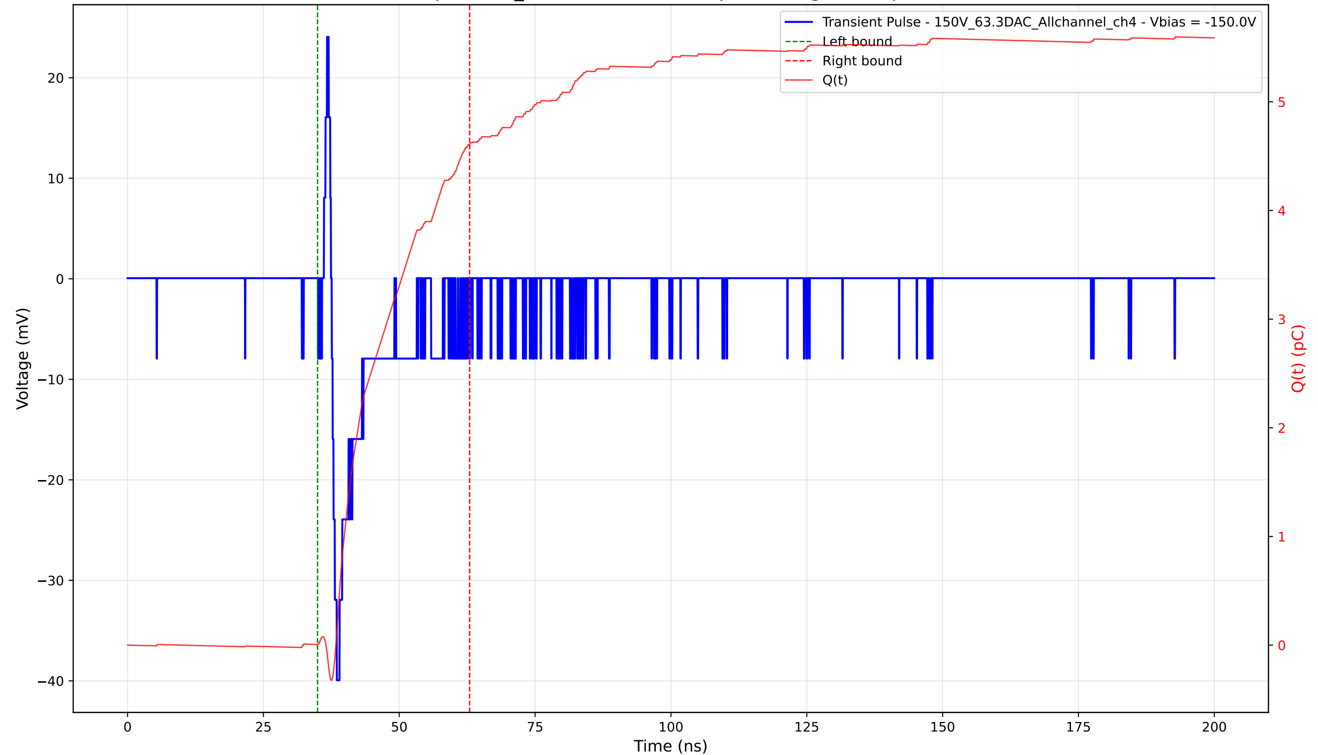
Transient Pulse - Sample: 1cm_42 - Position: 3655.0 \mu\text{m} - Charge: 4.60 pC - Rise Time: 0.94 ns
