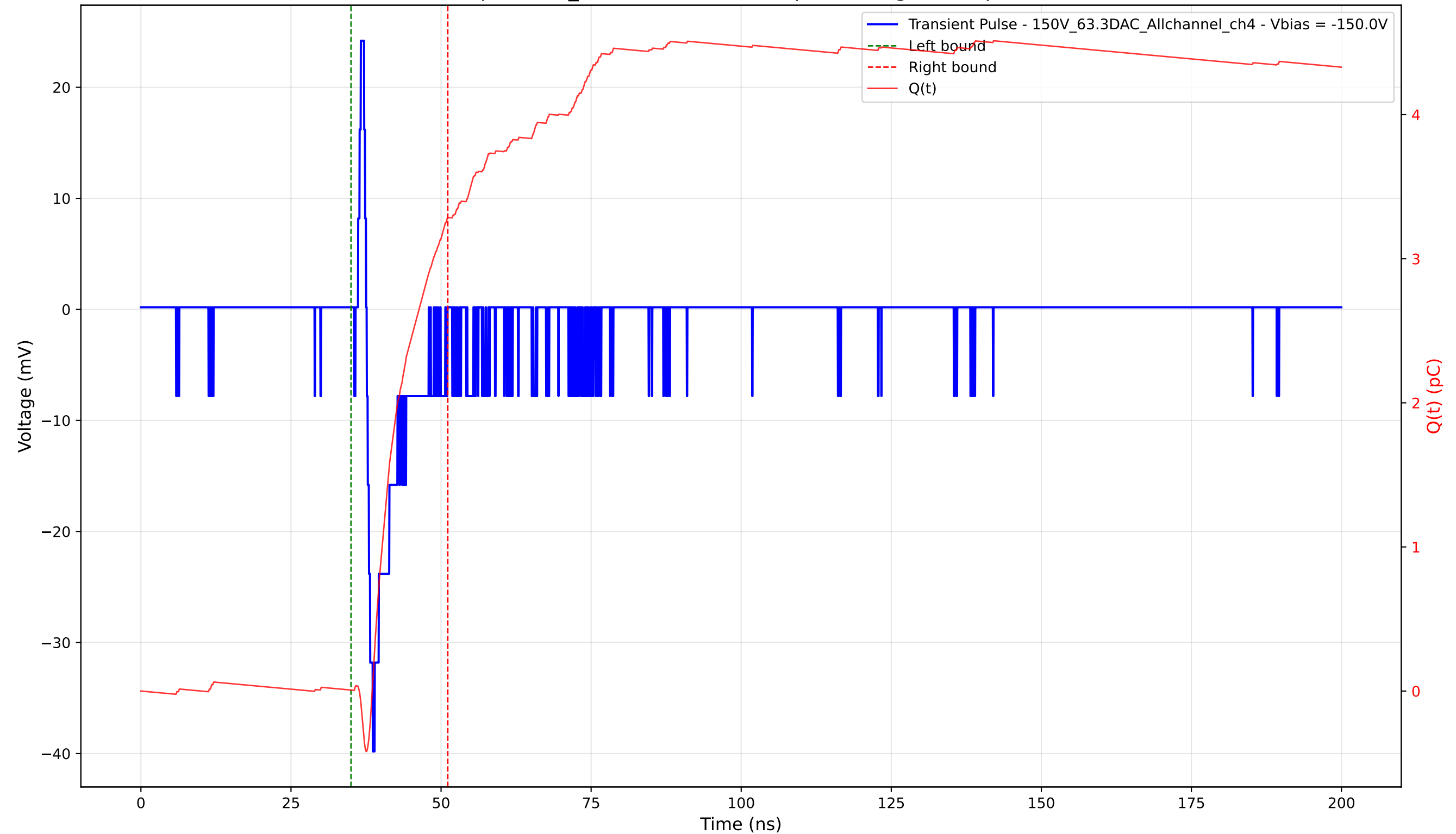
Transient Pulse - Sample: 1cm_42 - Position: 3730.0 \mu\text{m} - Charge: 3.28 pC - Rise Time: 1.02 ns
