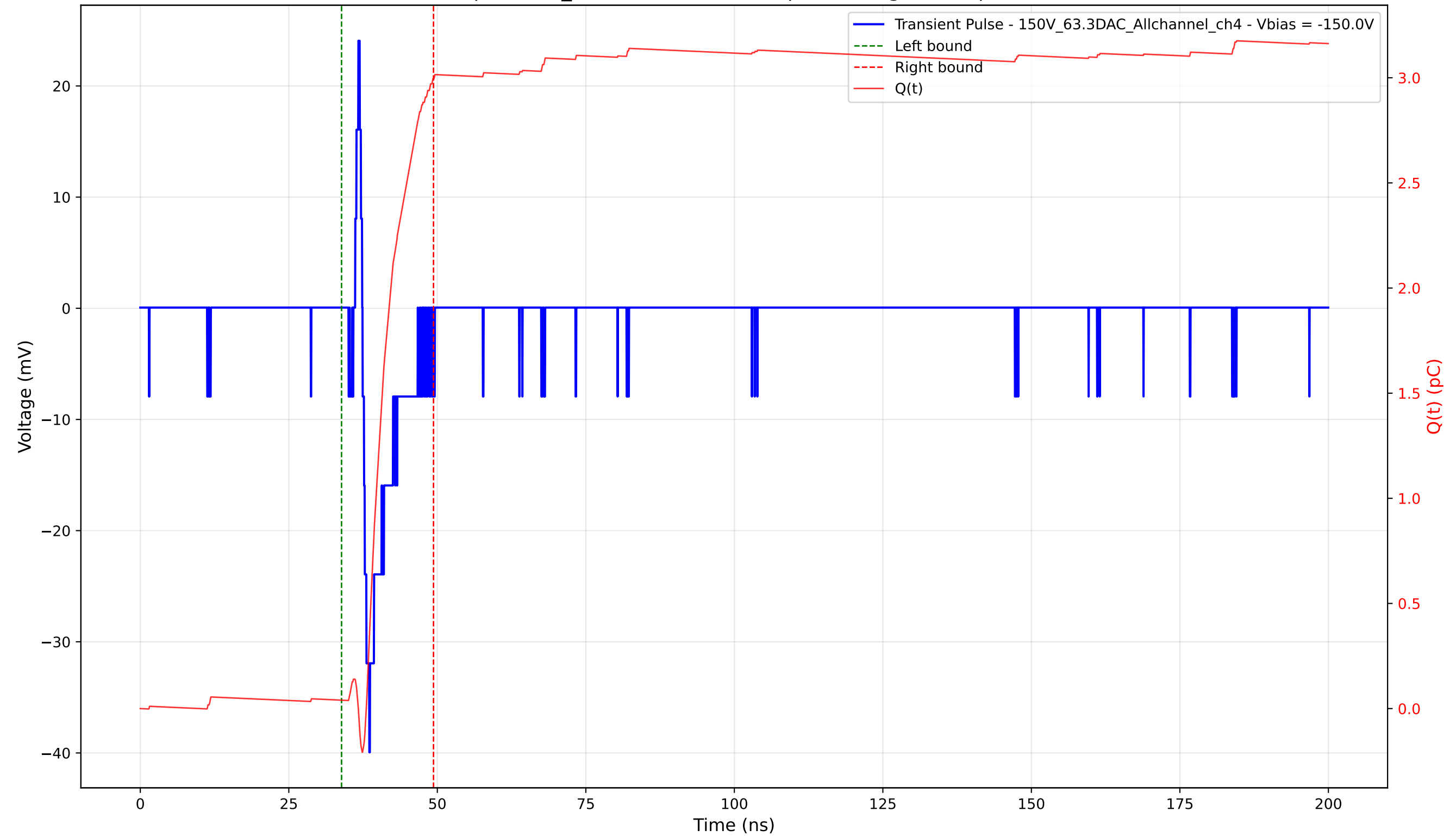
Transient Pulse - Sample: 1cm_42 - Position: 4835.0 \mu\text{m} - Charge: 2.96 pC - Rise Time: 1.14 ns
