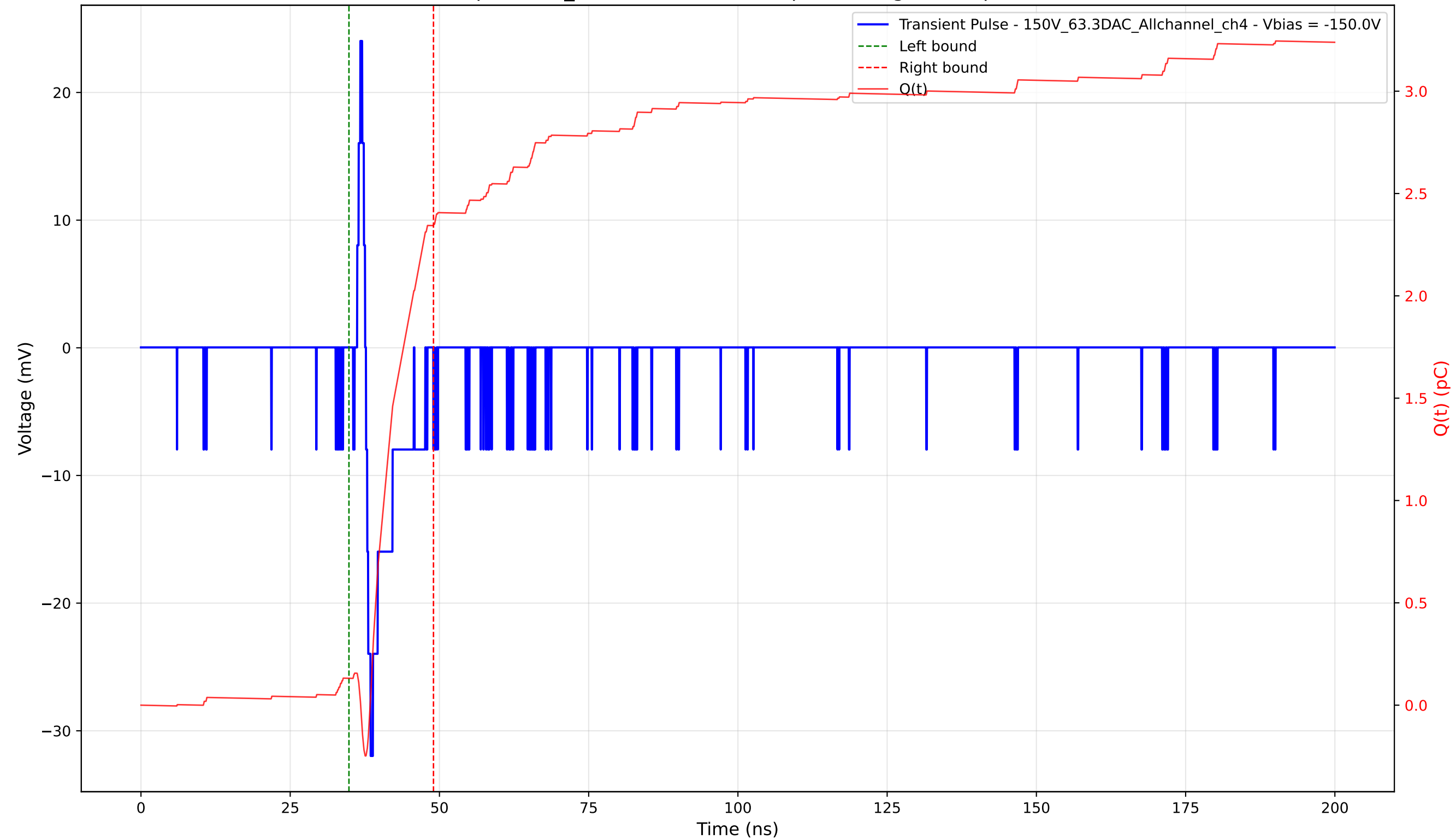
Transient Pulse - Sample: 1cm_42 - Position: 4550.0 \mu\text{m} - Charge: 2.21 pC - Rise Time: 0.78 ns
