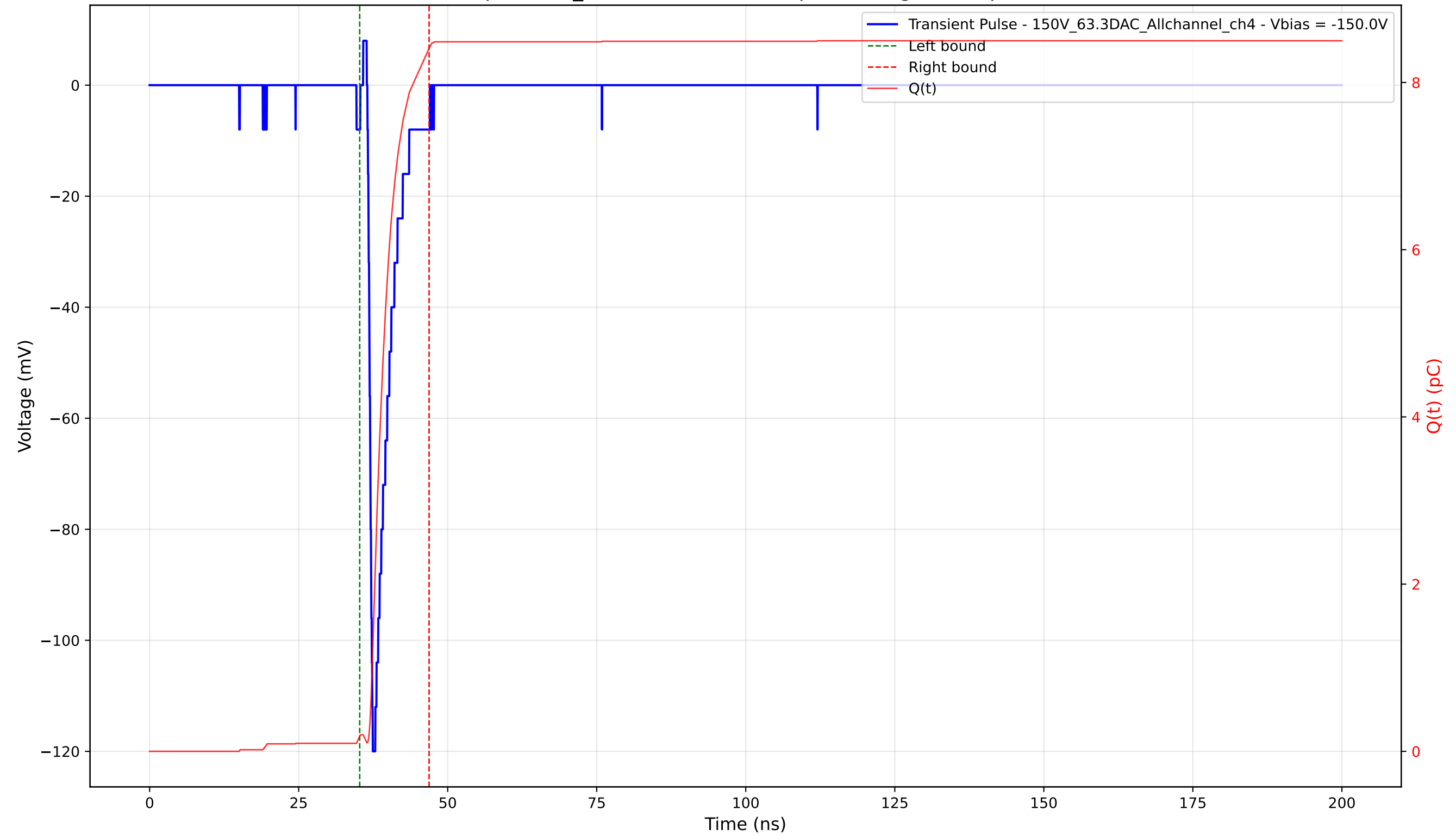
Transient Pulse - Sample: 1cm_42 - Position: 1085.0 \mu\text{m} - Charge: 8.23 pC - Rise Time: 0.74 ns
