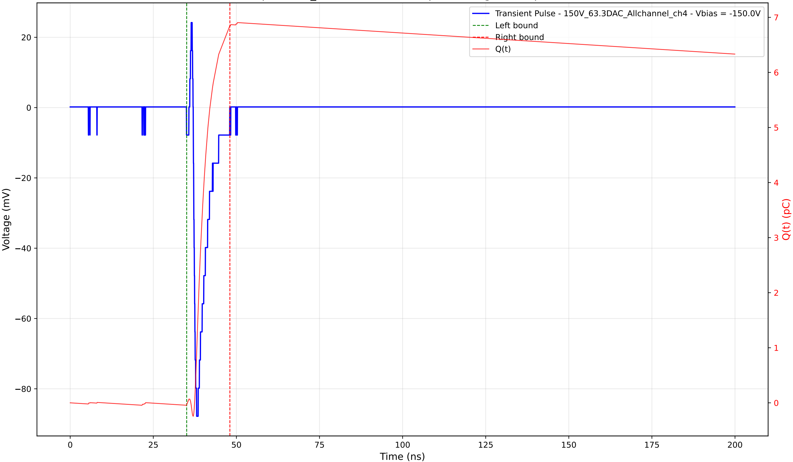
Transient Pulse - Sample: 1cm_42 - Position: 785.0 \mu\text{m} - Charge: 6.88 pC - Rise Time: 0.72 ns
