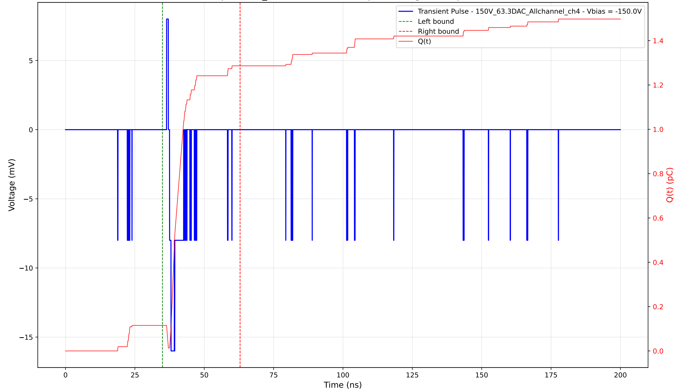
Transient Pulse - Sample: 1cm_42 - Position: 5065.0 \mu\text{m} - Charge: 1.17 pC - Rise Time: 0.55 ns
