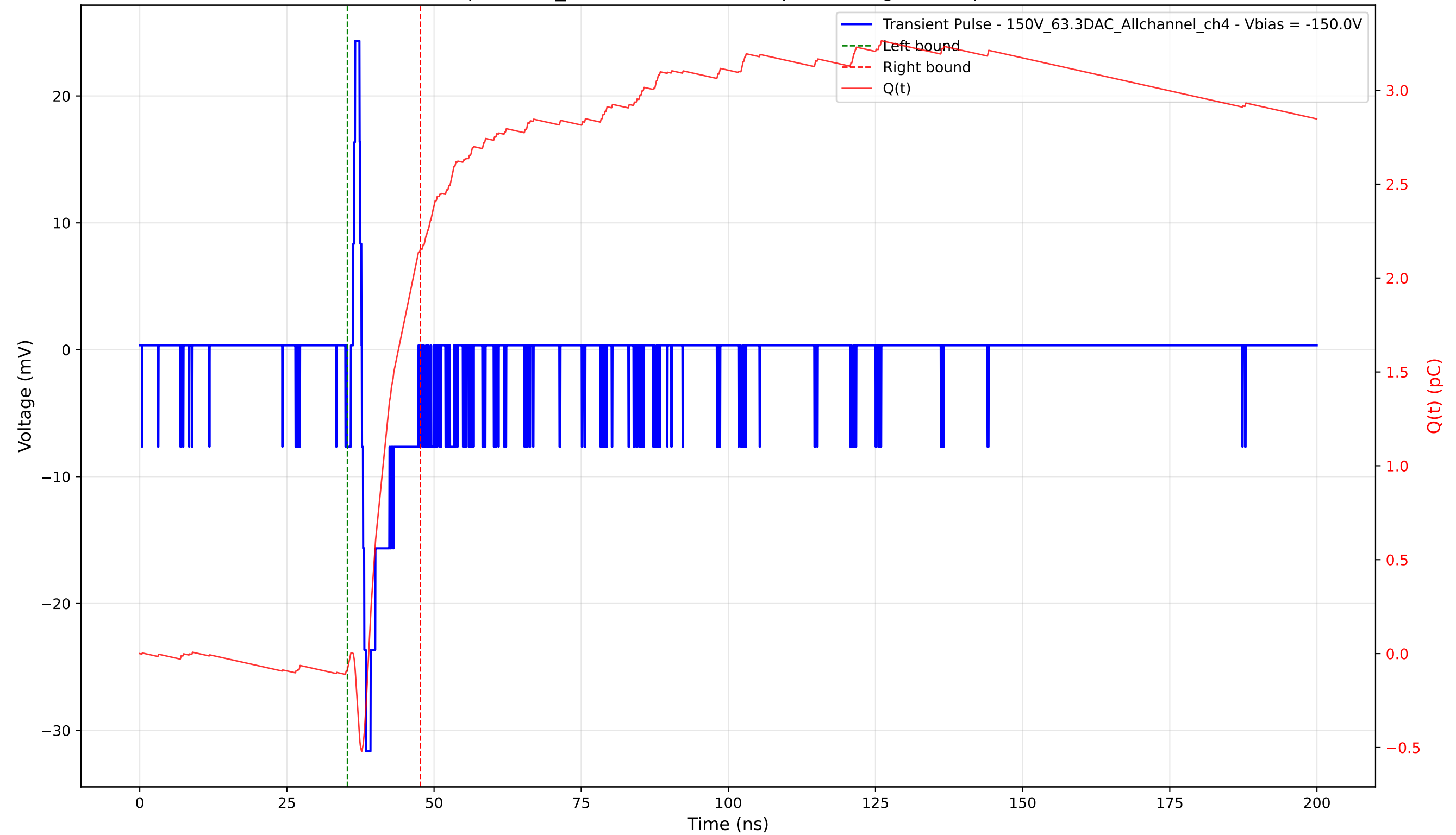
Transient Pulse - Sample: 1cm_42 - Position: 4165.0 \mu\text{m} - Charge: 2.24 pC - Rise Time: 0.70 ns
