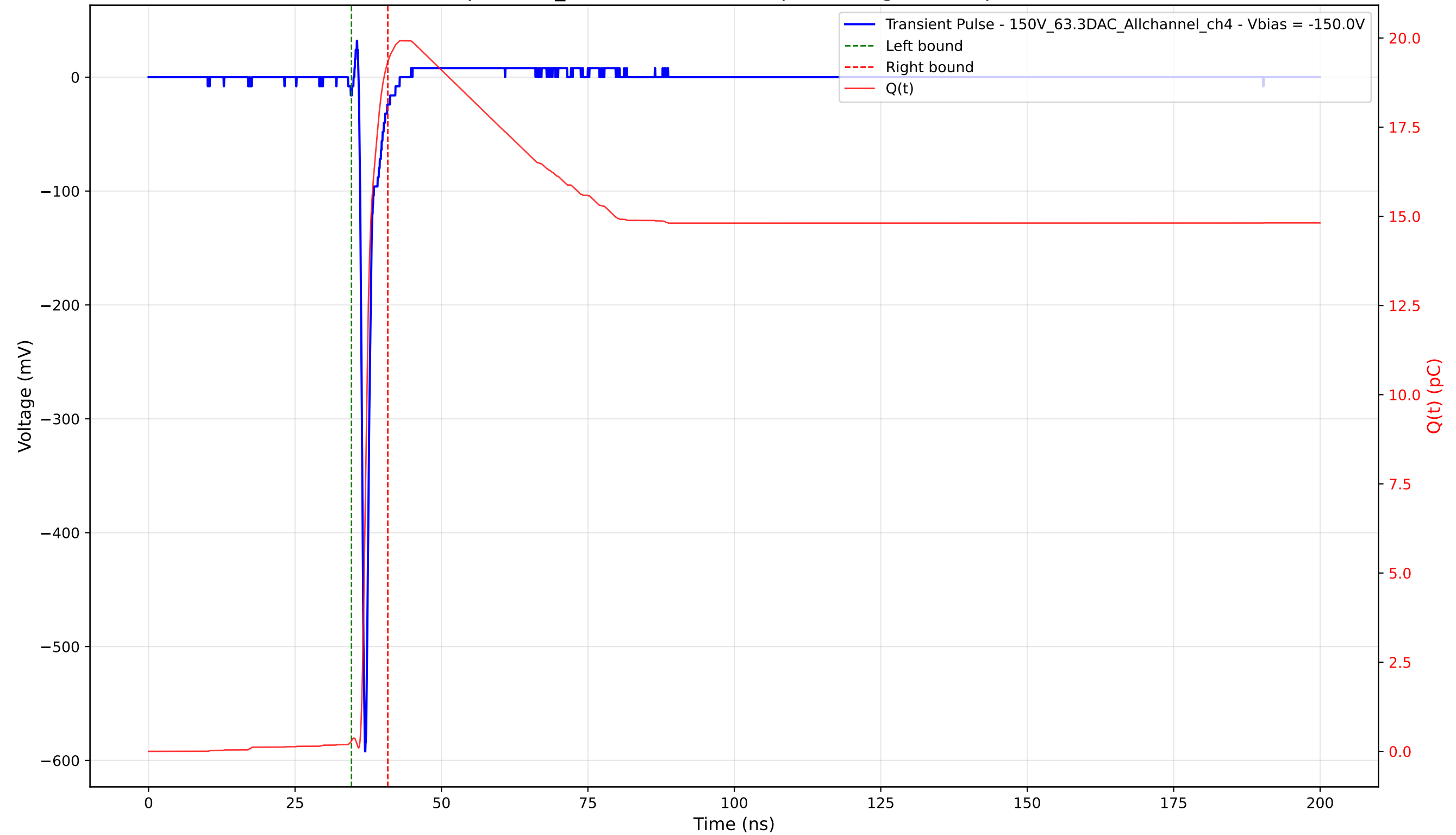
Transient Pulse - Sample: 1cm_42 - Position: 1855.0 \mu\text{m} - Charge: 19.03 pC - Rise Time: 0.72 ns
