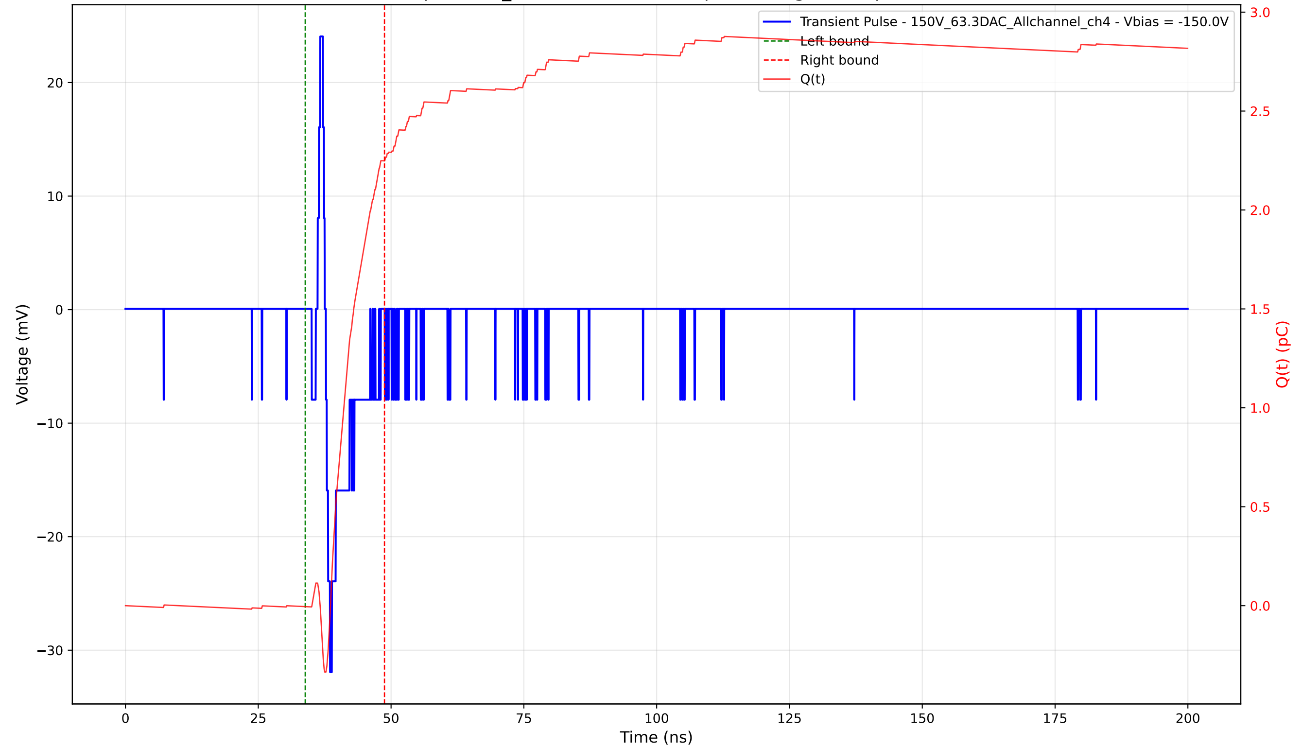
Transient Pulse - Sample: 1cm_42 - Position: 4495.0 \mu\text{m} - Charge: 2.25 pC - Rise Time: 0.78 ns
