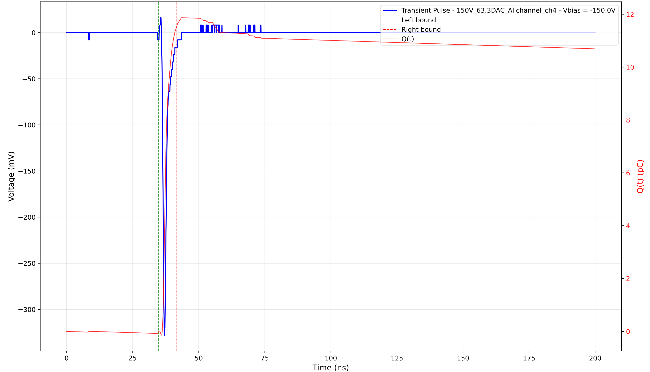
Transient Pulse - Sample: 1cm_42 - Position: 2430.0 \mu\text{m} - Charge: 11.50 pC - Rise Time: 0.71 ns
