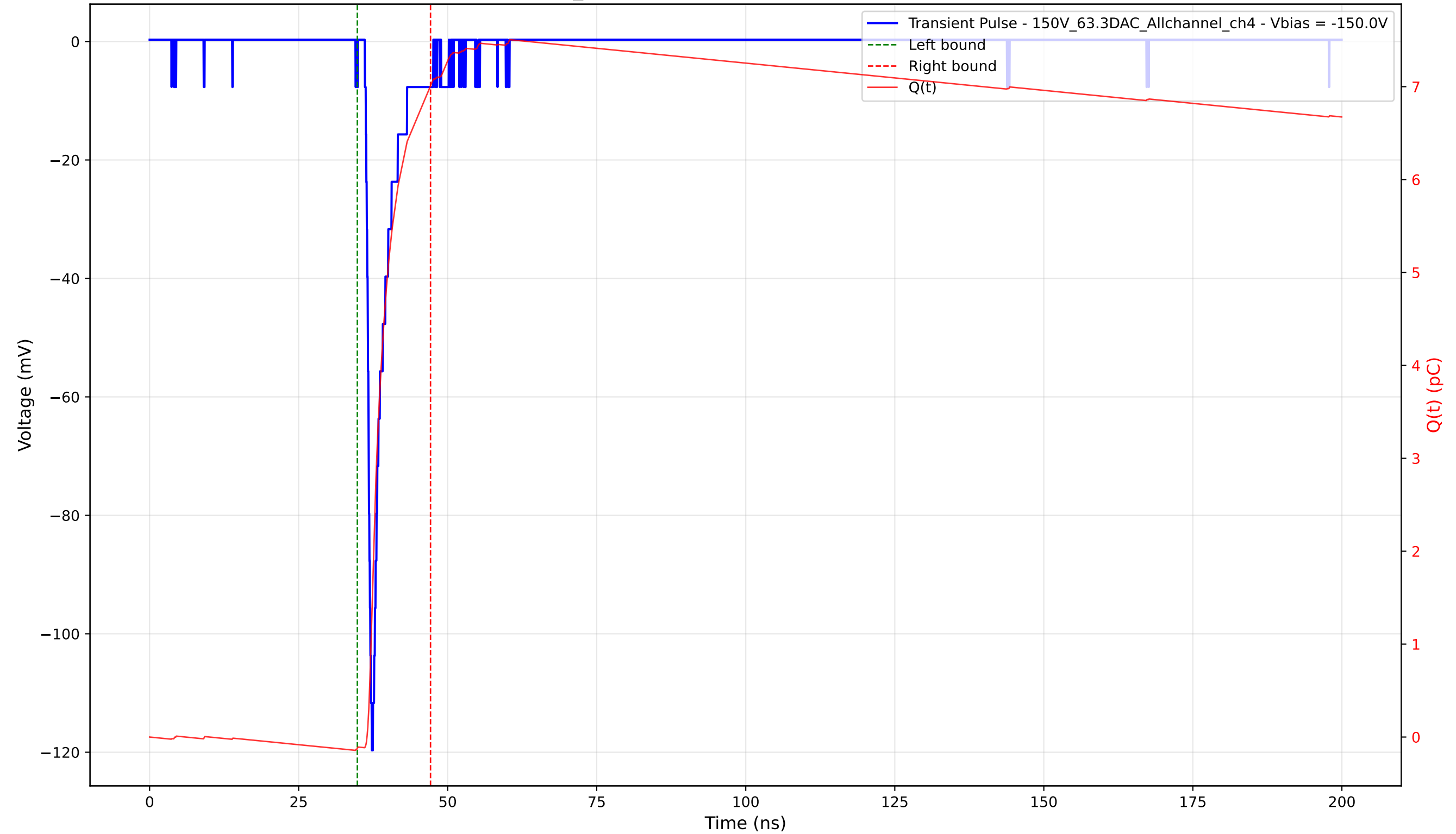
Transient Pulse - Sample: 1cm_42 - Position: 2850.0 \mu\text{m} - Charge: 7.13 pC - Rise Time: 0.86 ns
