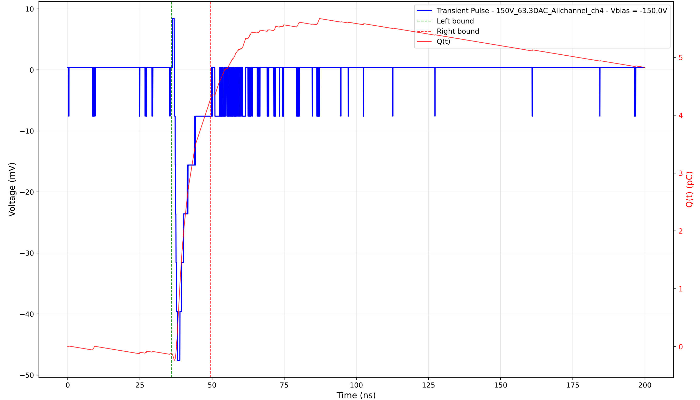
Transient Pulse - Sample: 1cm_42 - Position: 3320.0 \mu\text{m} - Charge: 4.42 pC - Rise Time: 0.94 ns
