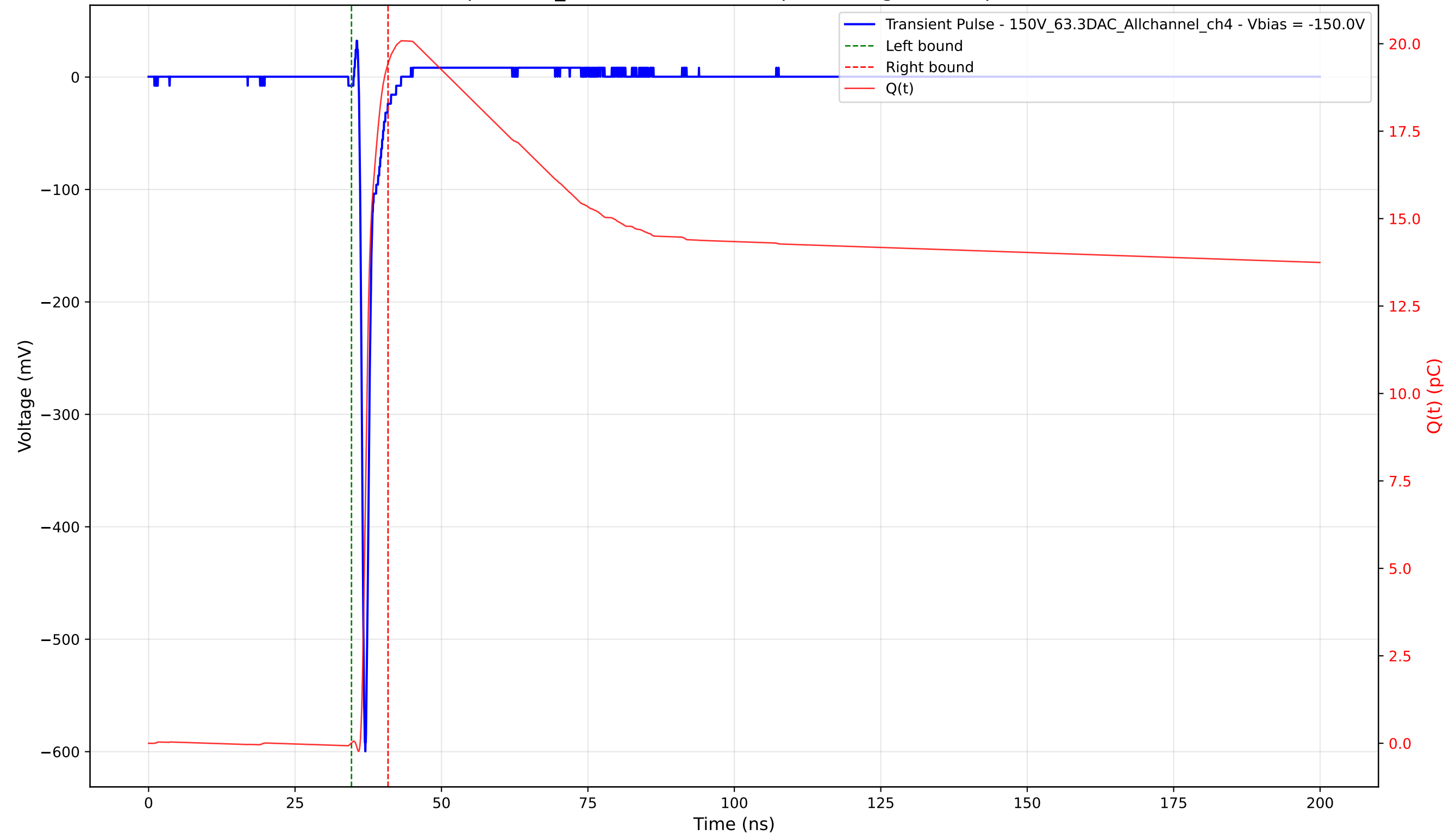
Transient Pulse - Sample: 1cm_42 - Position: 1835.0 \mu\text{m} - Charge: 19.43 pC - Rise Time: 0.72 ns
