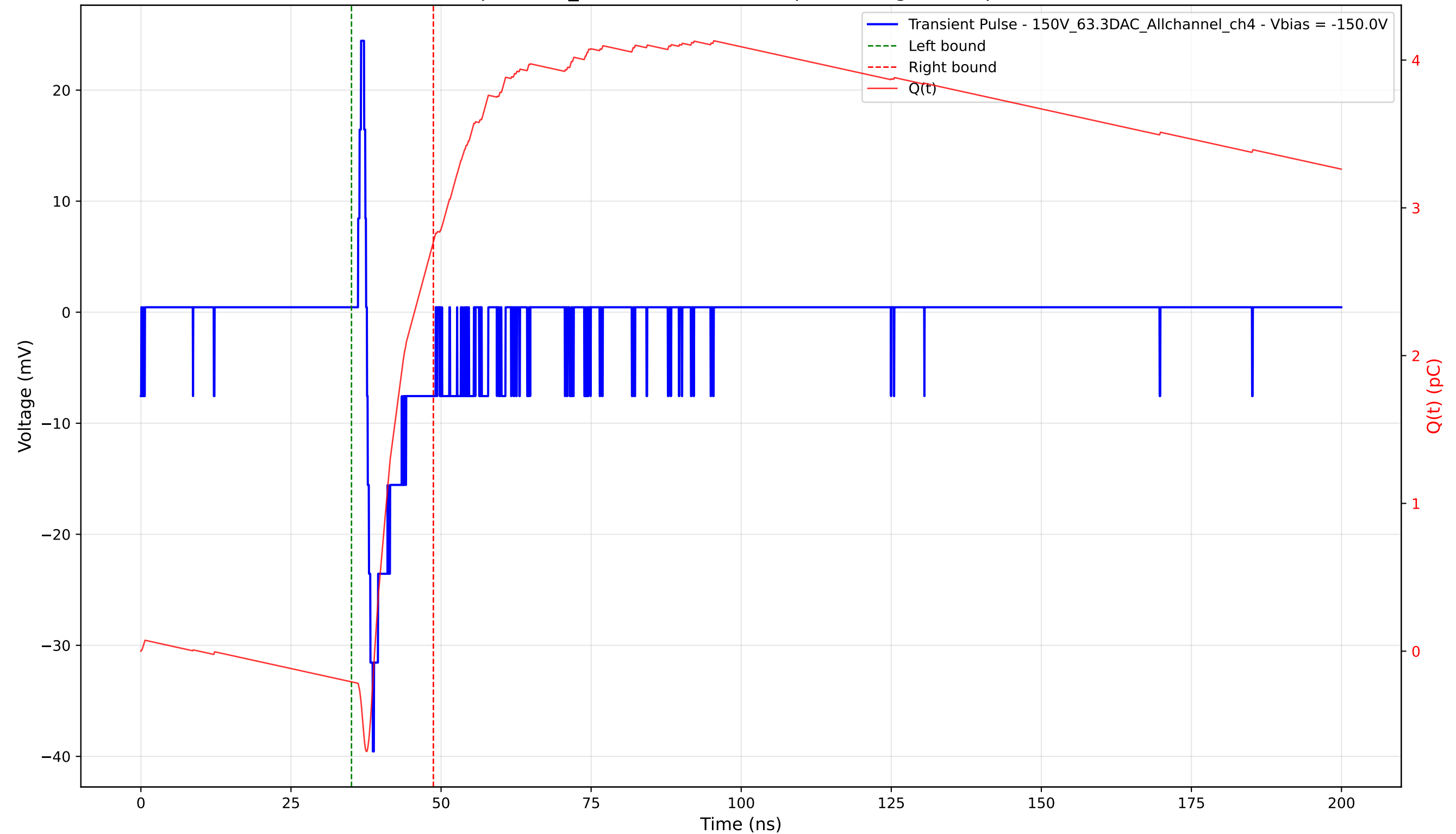
Transient Pulse - Sample: 1cm_42 - Position: 3720.0 \mu\text{m} - Charge: 2.98 pC - Rise Time: 0.98 ns
