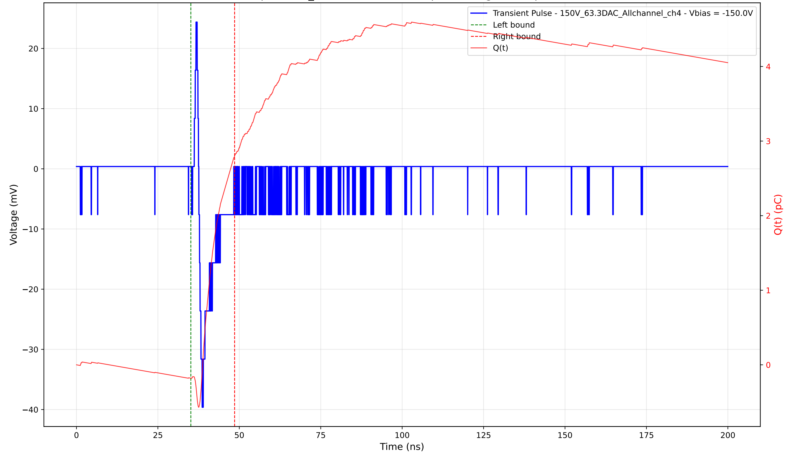
Transient Pulse - Sample: 1cm_42 - Position: 3680.0 \mu\text{m} - Charge: 2.98 pC - Rise Time: 1.02 ns
