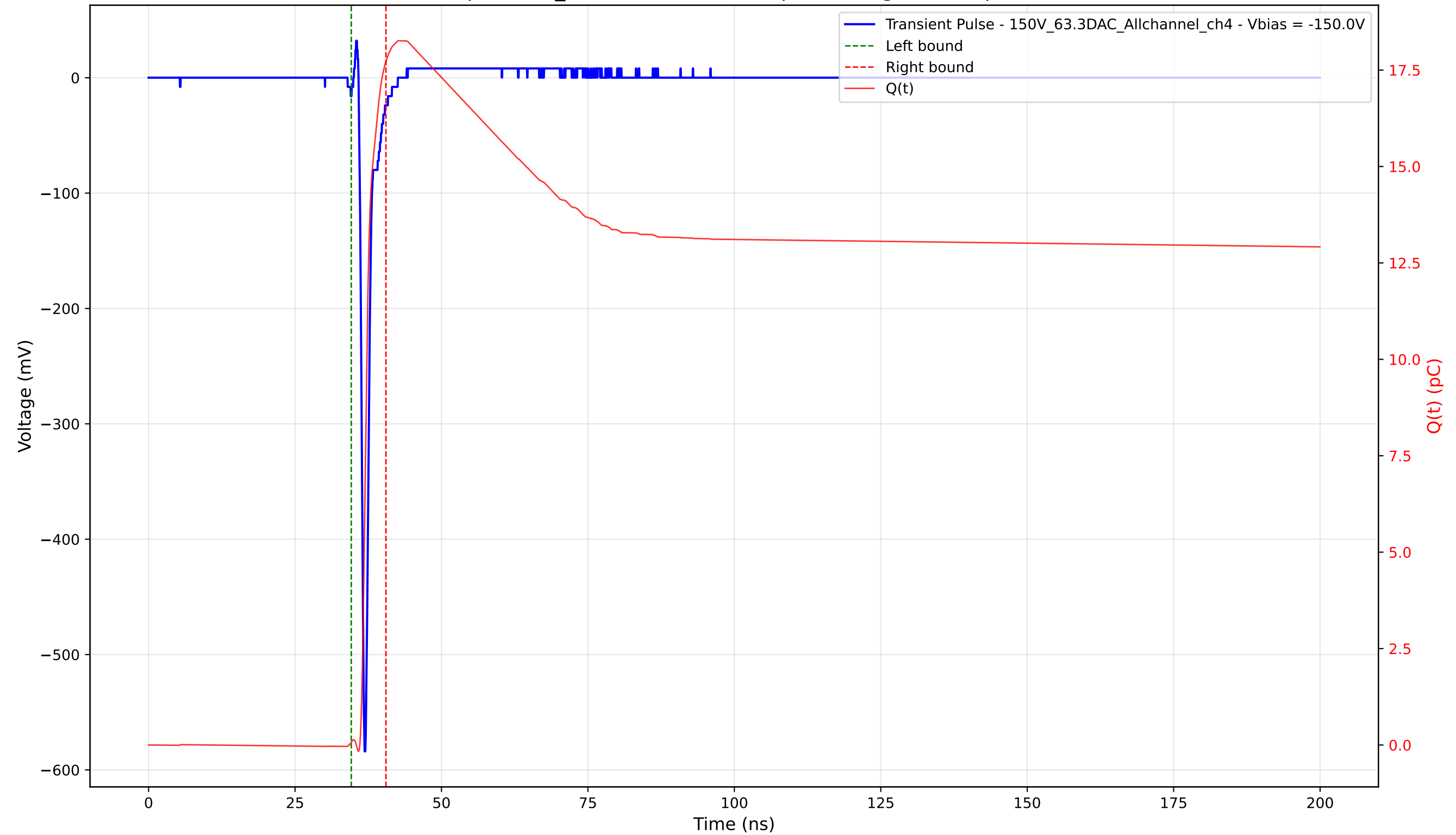
Transient Pulse - Sample: 1cm_42 - Position: 2025.0 \mu\text{m} - Charge: 17.65 pC - Rise Time: 0.69 ns
