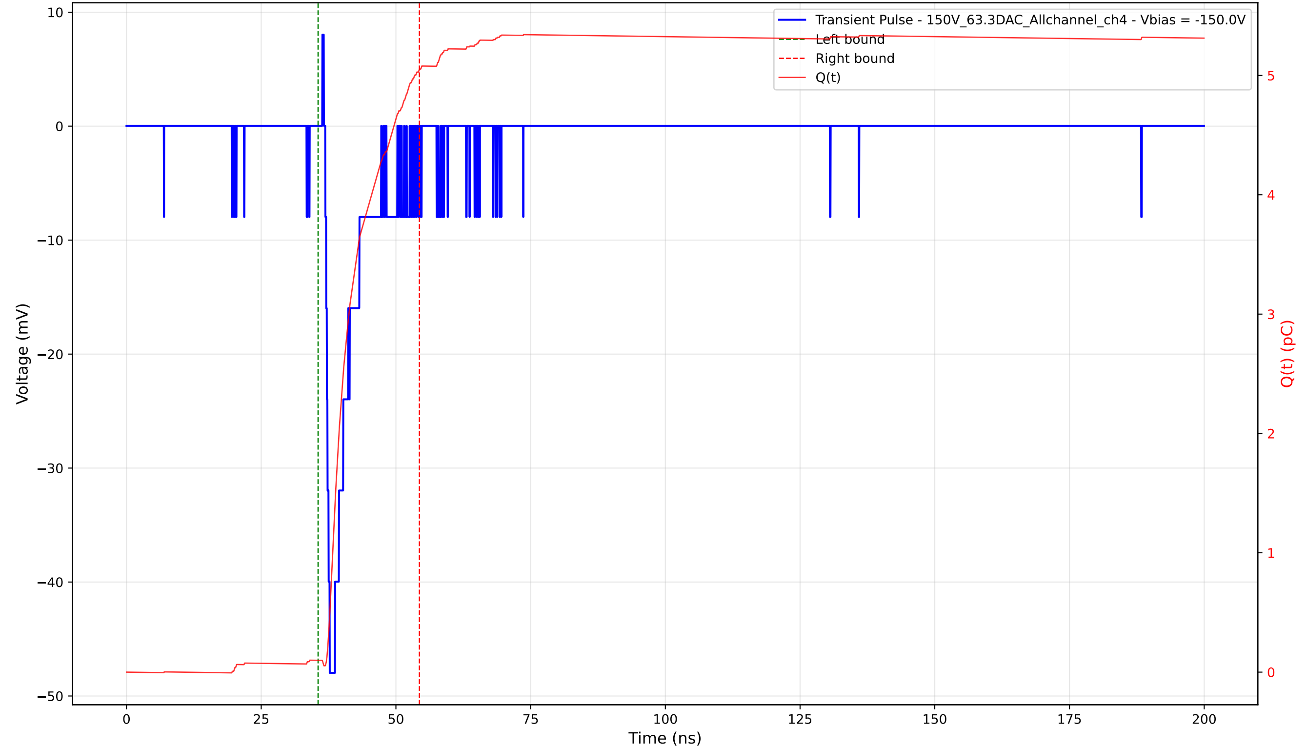
Transient Pulse - Sample: 1cm_42 - Position: 3190.0 \mu\text{m} - Charge: 4.95 pC - Rise Time: 0.82 ns
