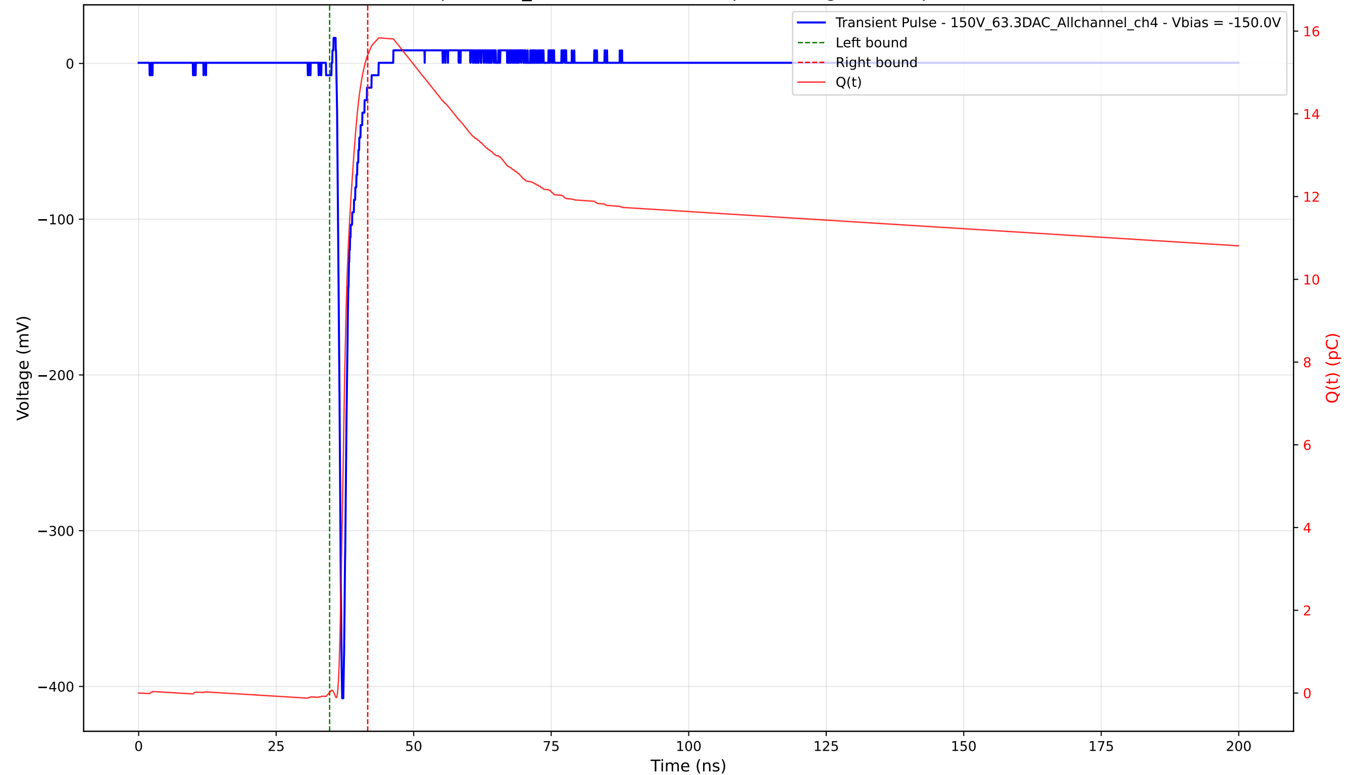
Transient Pulse - Sample: 1cm_42 - Position: 1630.0 \mu\text{m} - Charge: 15.41 pC - Rise Time: 0.73 ns
