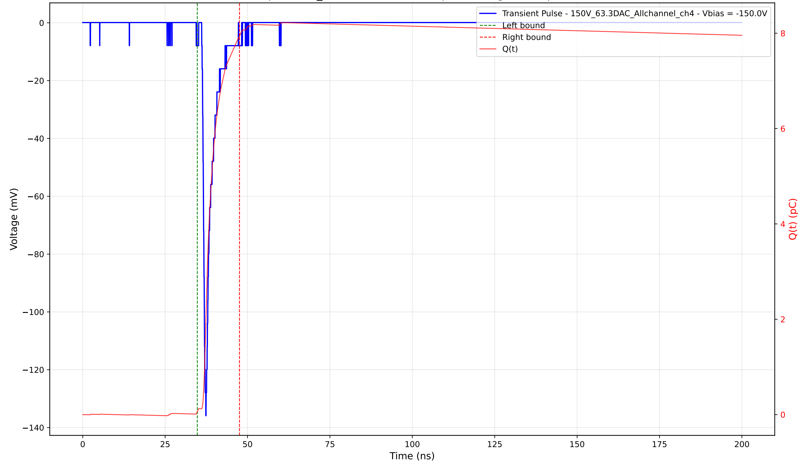
Transient Pulse - Sample: 1cm_42 - Position: 2805.0 \mu\text{m} - Charge: 7.88 pC - Rise Time: 0.93 ns
