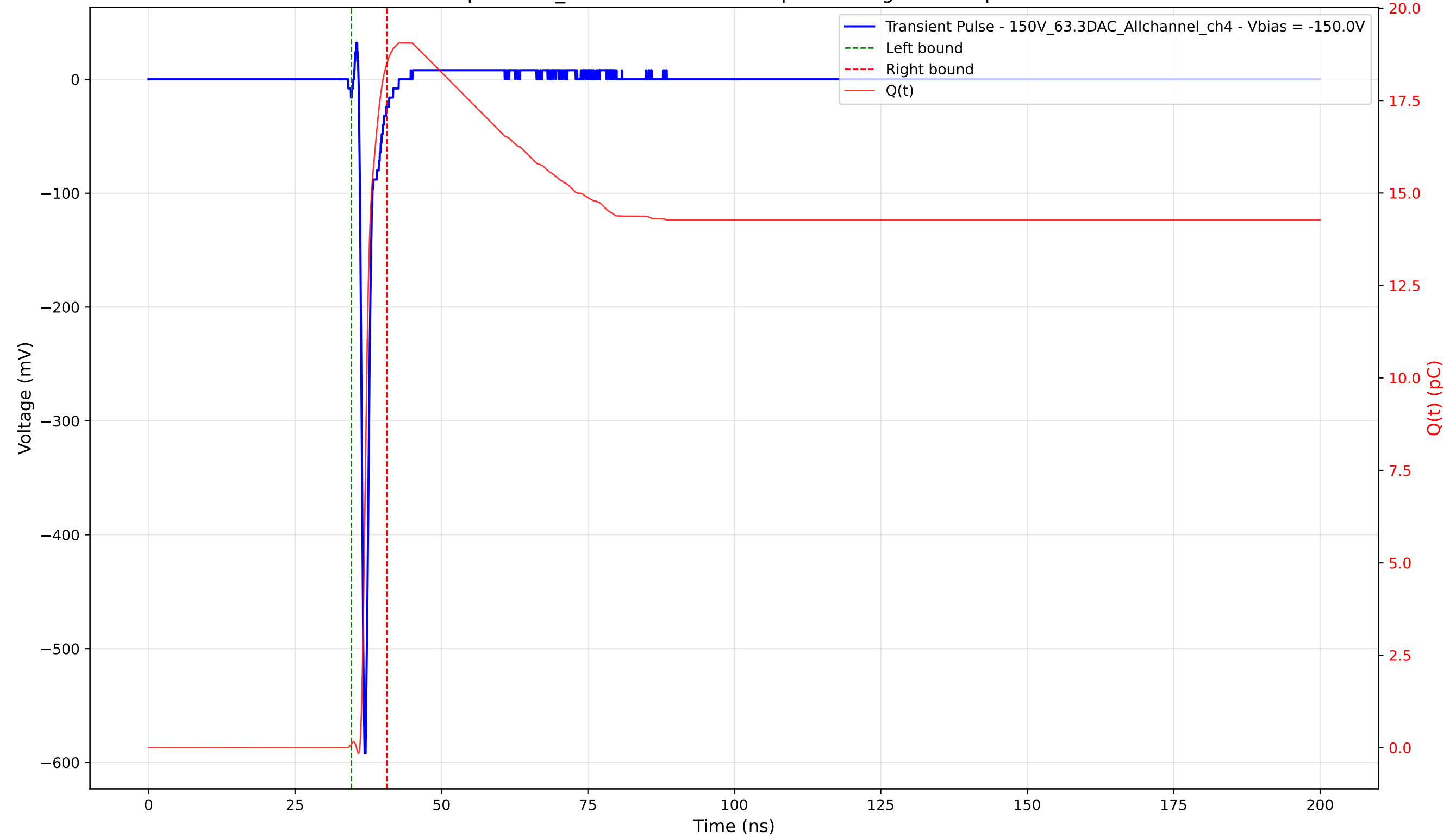
Transient Pulse - Sample: 1cm_42 - Position: 1935.0 \mu\text{m} - Charge: 18.40 pC - Rise Time: 0.70 ns
