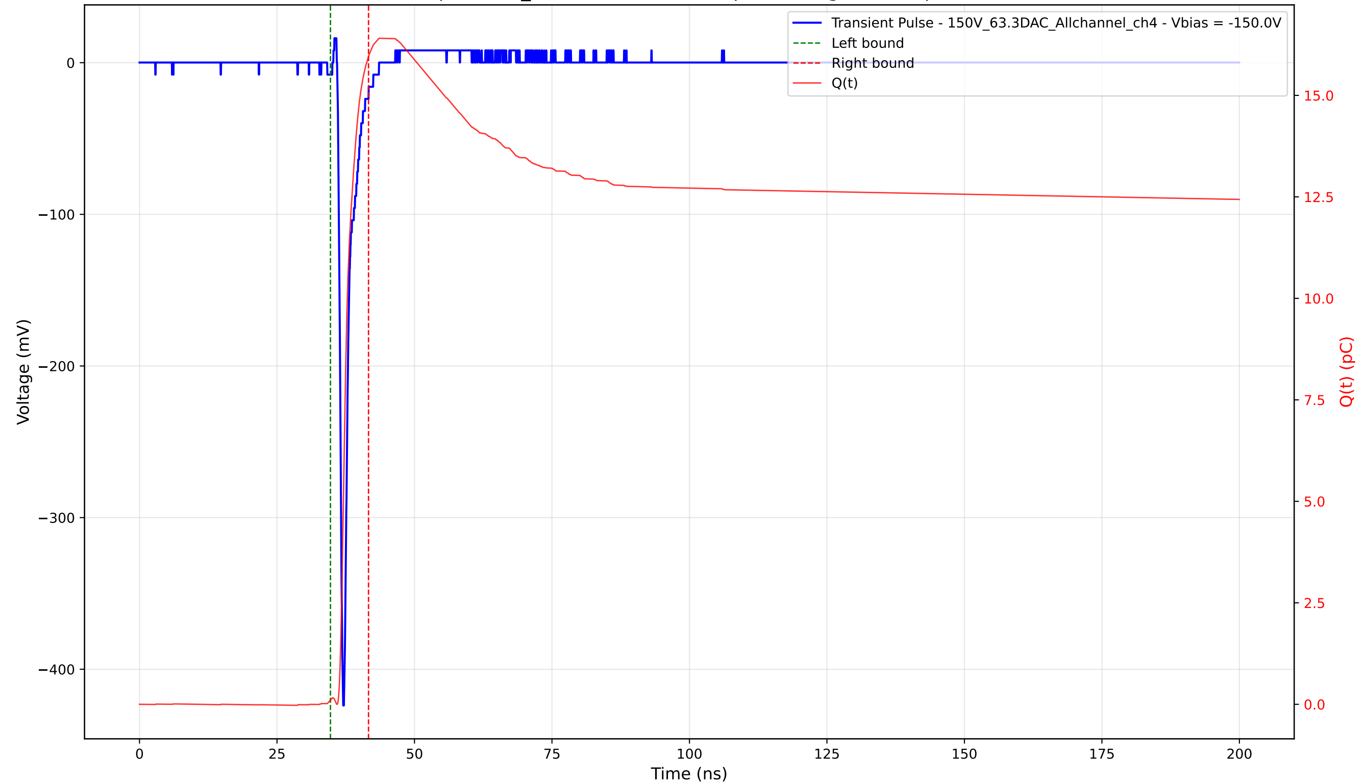
Transient Pulse - Sample: 1cm_42 - Position: 1635.0 \mu\text{m} - Charge: 15.86 pC - Rise Time: 0.72 ns
