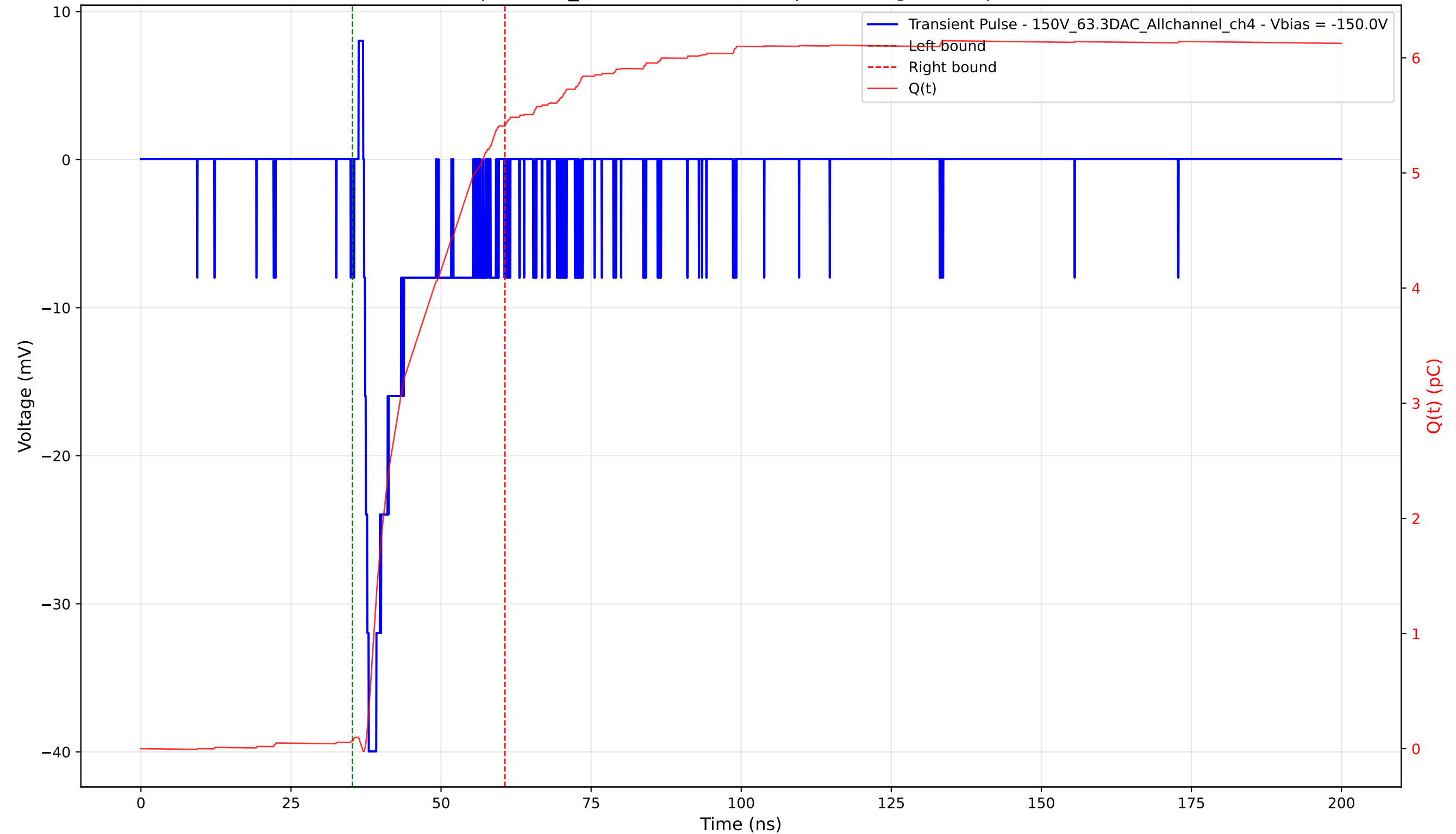
Transient Pulse - Sample: 1cm_42 - Position: 3400.0 \mu\text{m} - Charge: 5.36 pC - Rise Time: 0.78 ns
