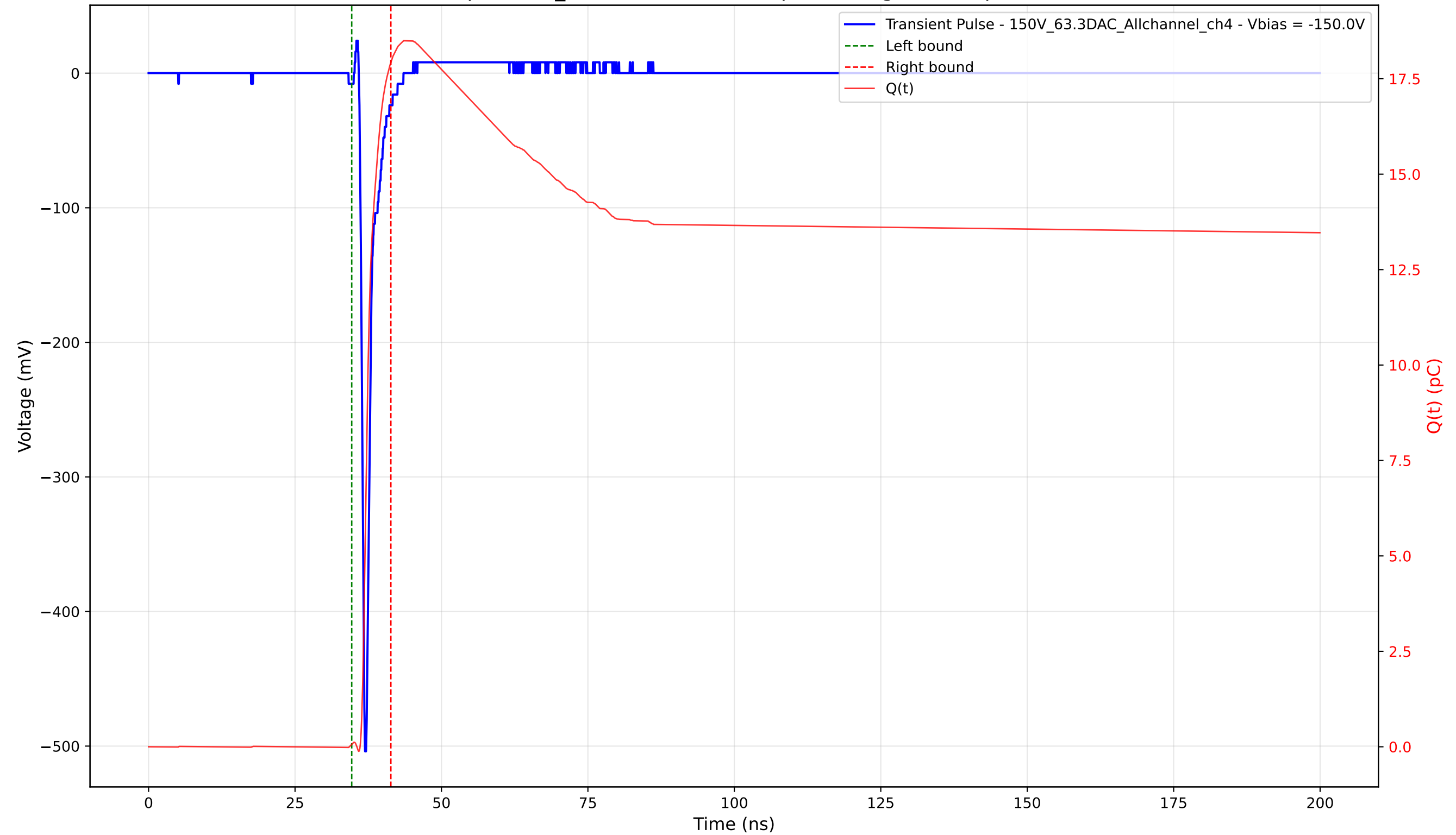
Transient Pulse - Sample: 1cm_42 - Position: 1695.0 \mu\text{m} - Charge: 17.86 pC - Rise Time: 0.73 ns
