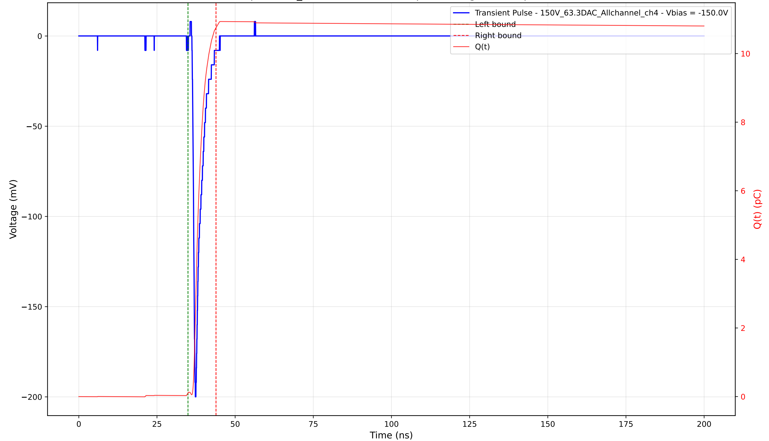
Transient Pulse - Sample: 1cm_42 - Position: 1385.0 \mu\text{m} - Charge: 10.65 pC - Rise Time: 0.80 ns
