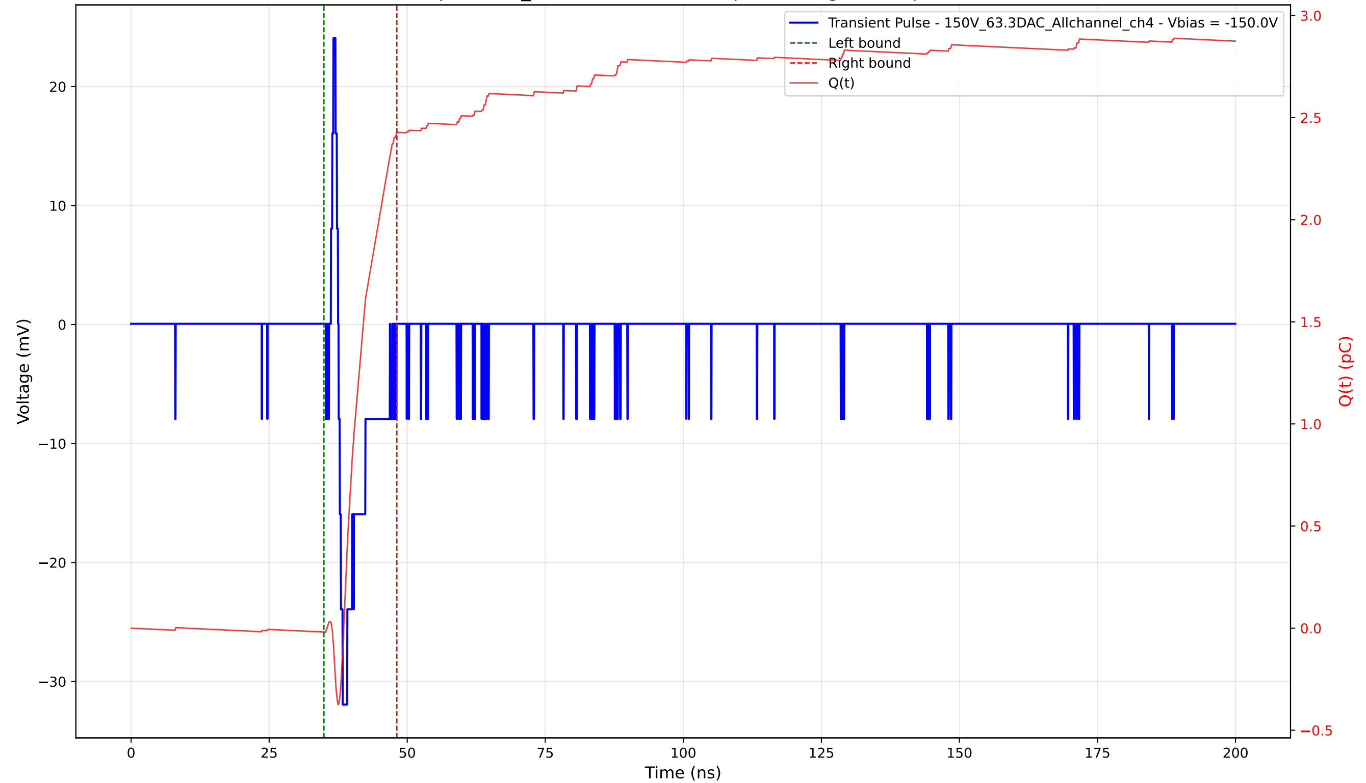
Transient Pulse - Sample: 1cm_42 - Position: 4645.0 \mu\text{m} - Charge: 2.45 pC - Rise Time: 0.74 ns
