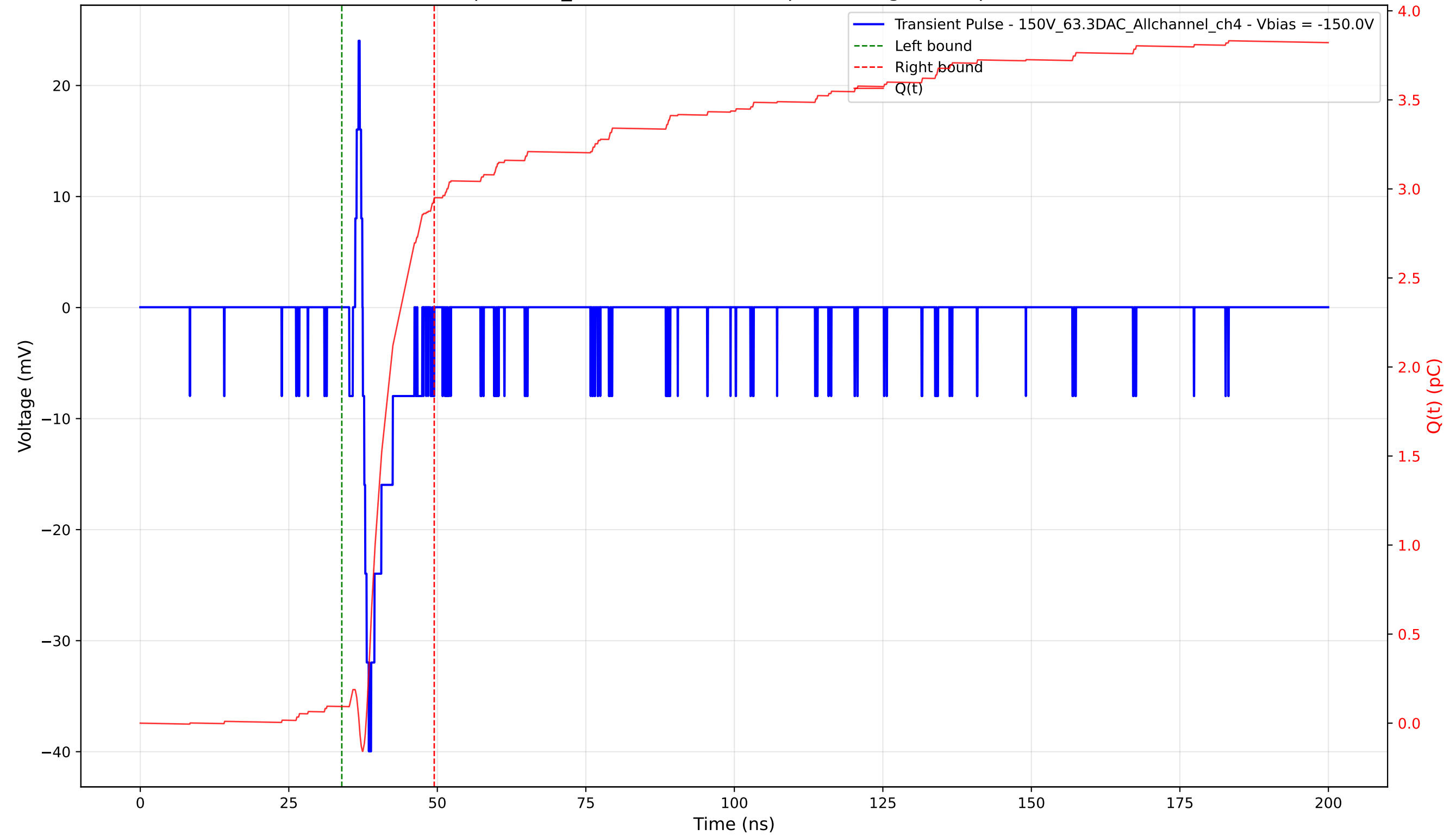
Transient Pulse - Sample: 1cm_42 - Position: 4815.0 \mu\text{m} - Charge: 2.85 pC - Rise Time: 1.02 ns
