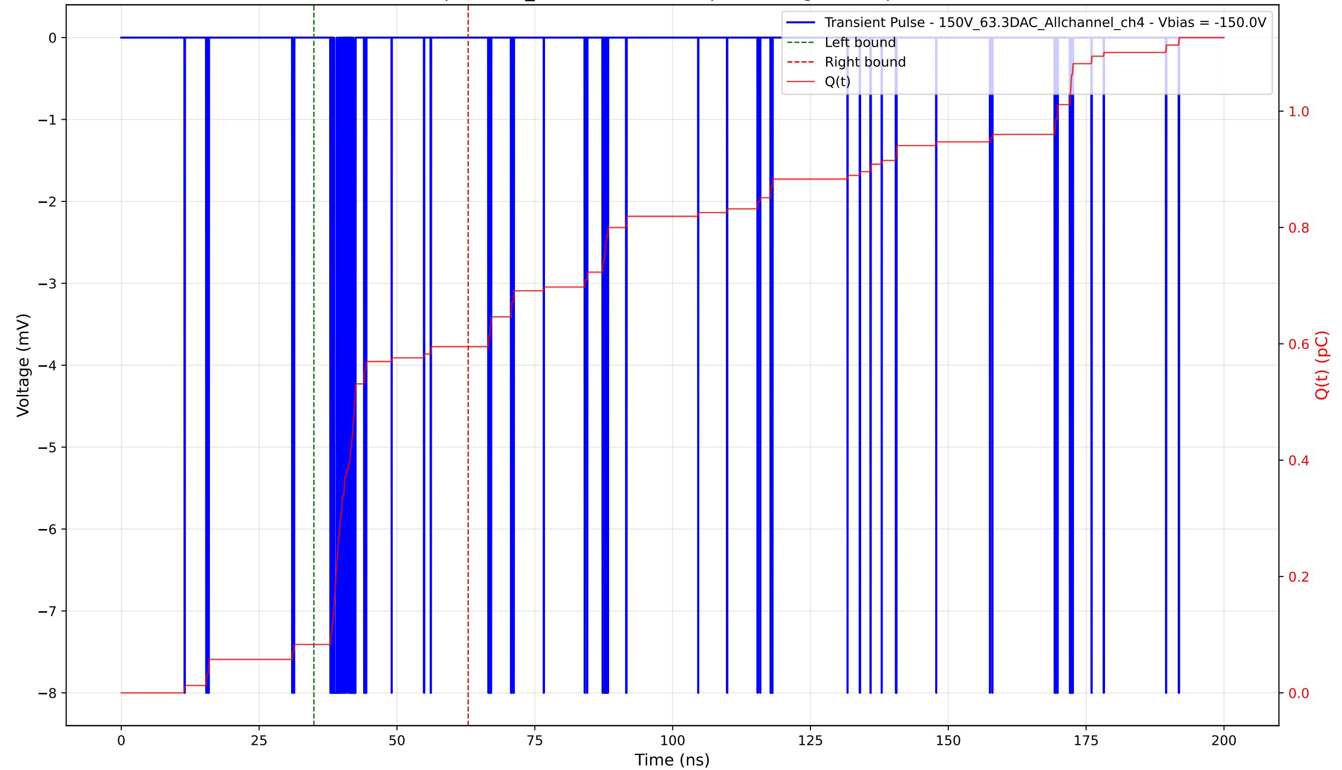
Transient Pulse - Sample: 1cm_42 - Position: 15.0 \mu\text{m} - Charge: 0.51 pC - Rise Time: 0.04 ns
