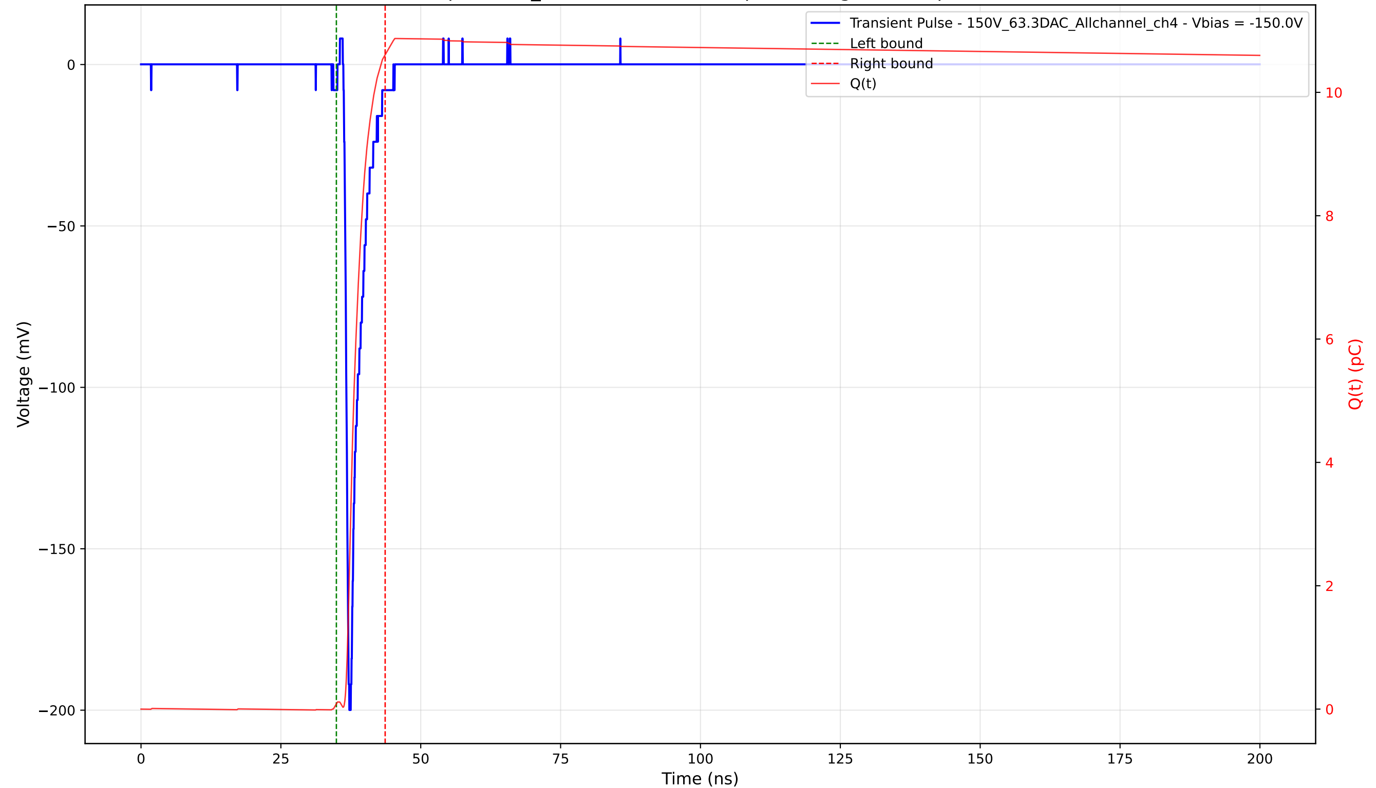
Transient Pulse - Sample: 1cm_42 - Position: 1395.0 \mu\text{m} - Charge: 10.52 pC - Rise Time: 0.76 ns
