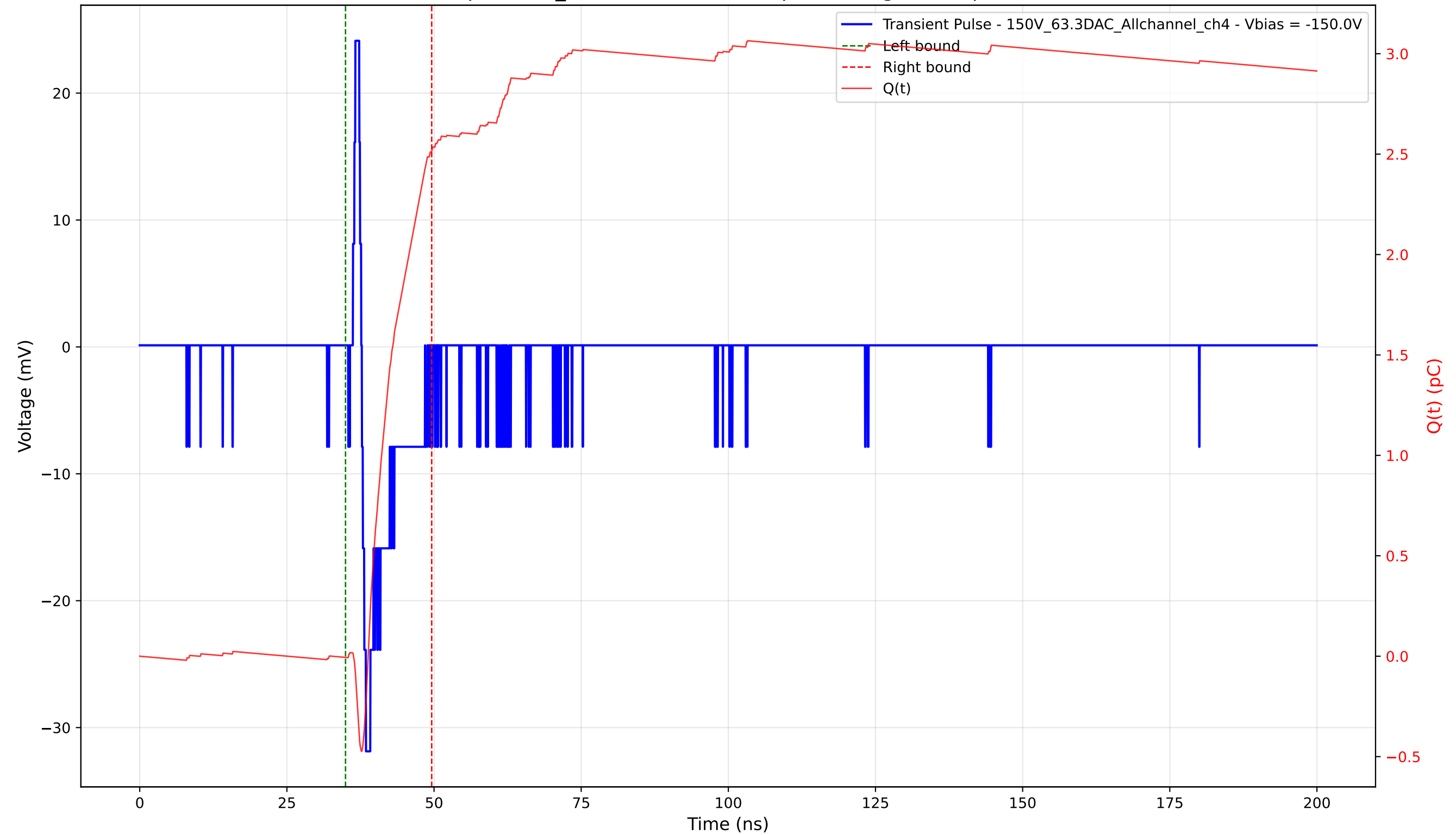
Transient Pulse - Sample: 1cm_42 - Position: 4410.0 \mu\text{m} - Charge: 2.52 pC - Rise Time: 0.70 ns
