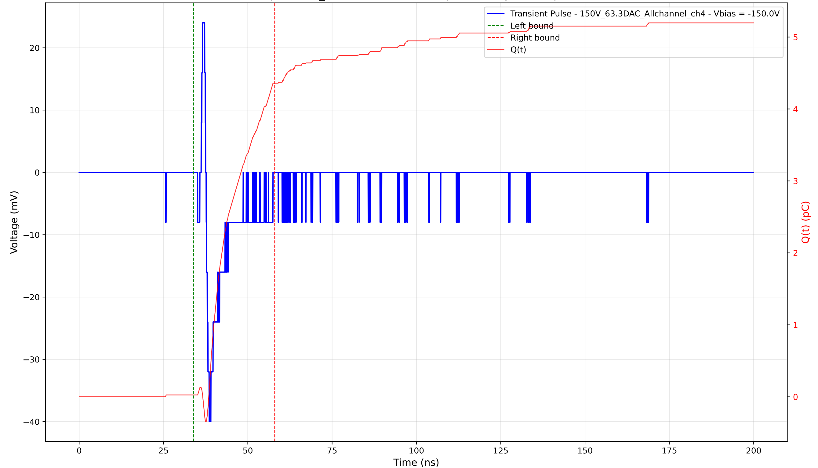
Transient Pulse - Sample: 1cm_42 - Position: 3735.0 \mu\text{m} - Charge: 4.33 pC - Rise Time: 0.90 ns
