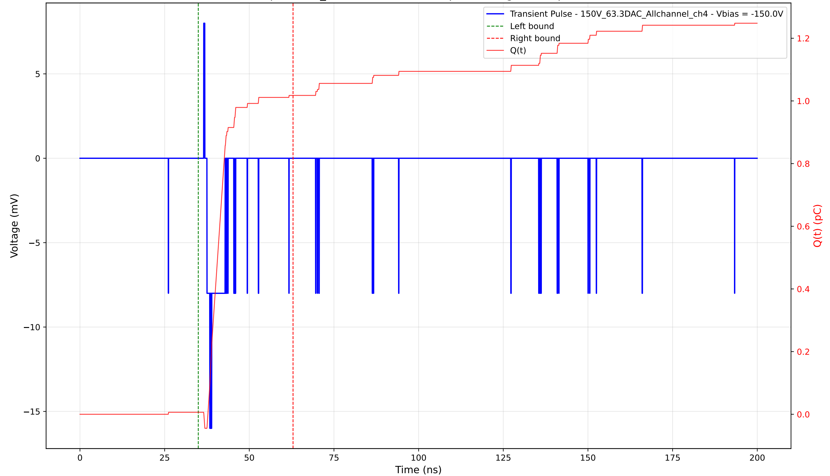
Transient Pulse - Sample: 1cm_42 - Position: 5100.0 \mu\text{m} - Charge: 1.01 pC - Rise Time: 0.87 ns
