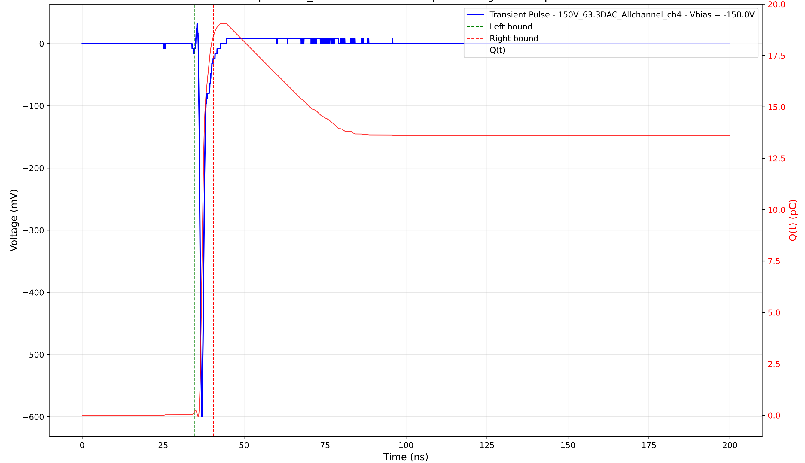
Transient Pulse - Sample: 1cm_42 - Position: 1955.0 \mu\text{m} - Charge: 18.32 pC - Rise Time: 0.70 ns
