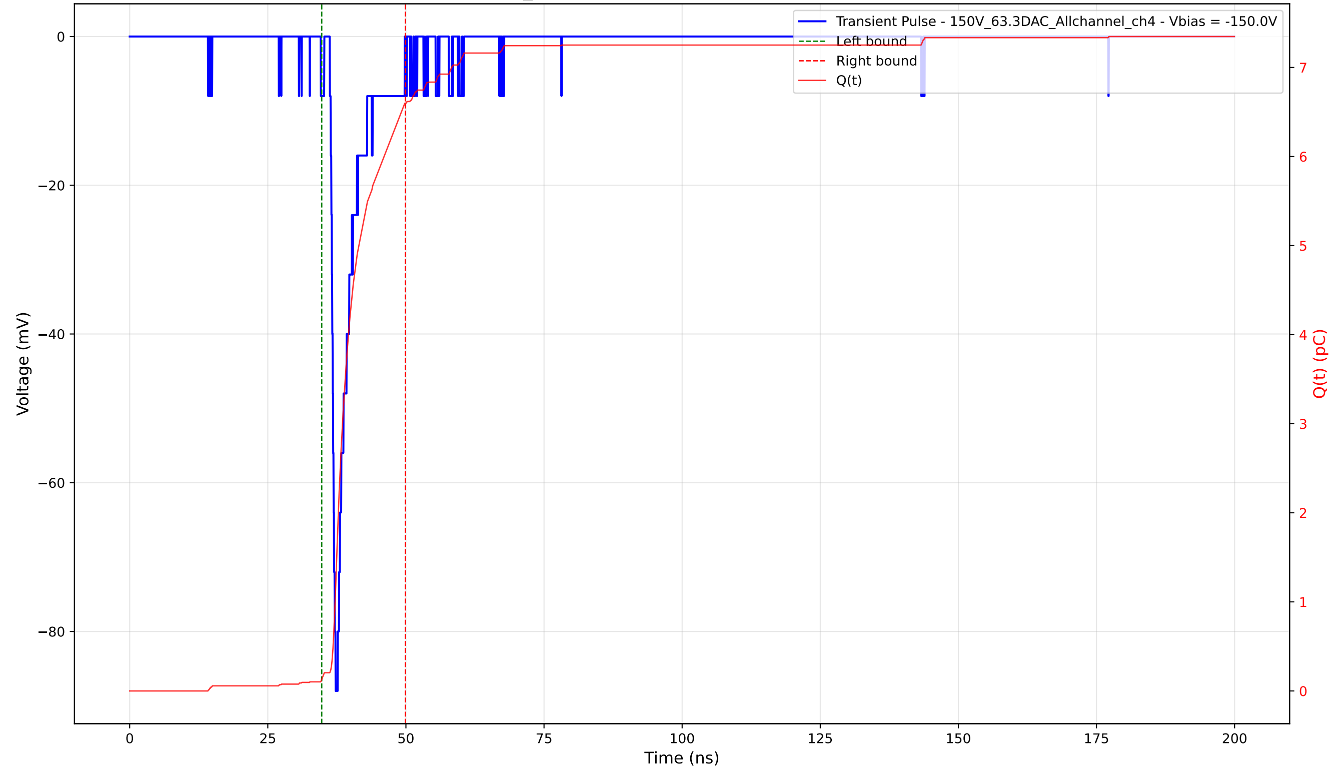
Transient Pulse - Sample: 1cm_42 - Position: 2930.0 \mu\text{m} - Charge: 6.47 pC - Rise Time: 0.76 ns
