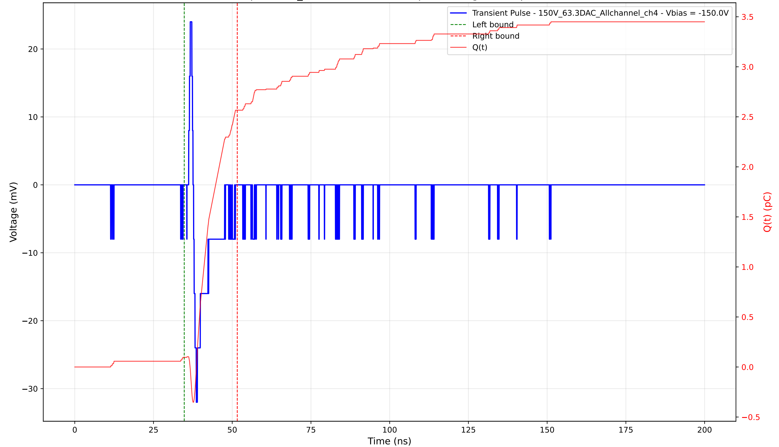
Transient Pulse - Sample: 1cm_42 - Position: 4465.0 \mu\text{m} - Charge: 2.47 pC - Rise Time: 0.86 ns
