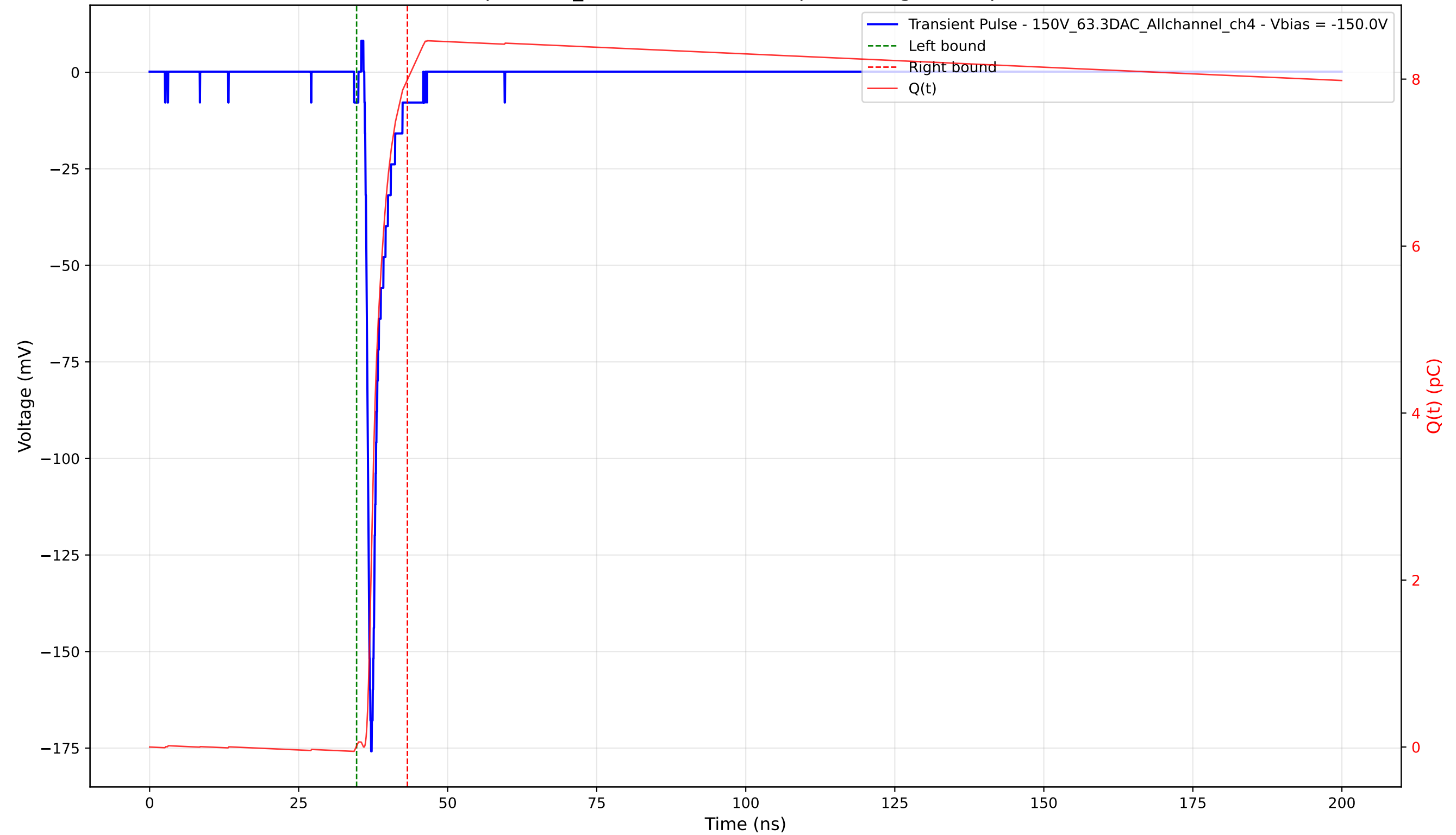
Transient Pulse - Sample: 1cm_42 - Position: 2625.0 \mu\text{m} - Charge: 7.98 pC - Rise Time: 0.79 ns
