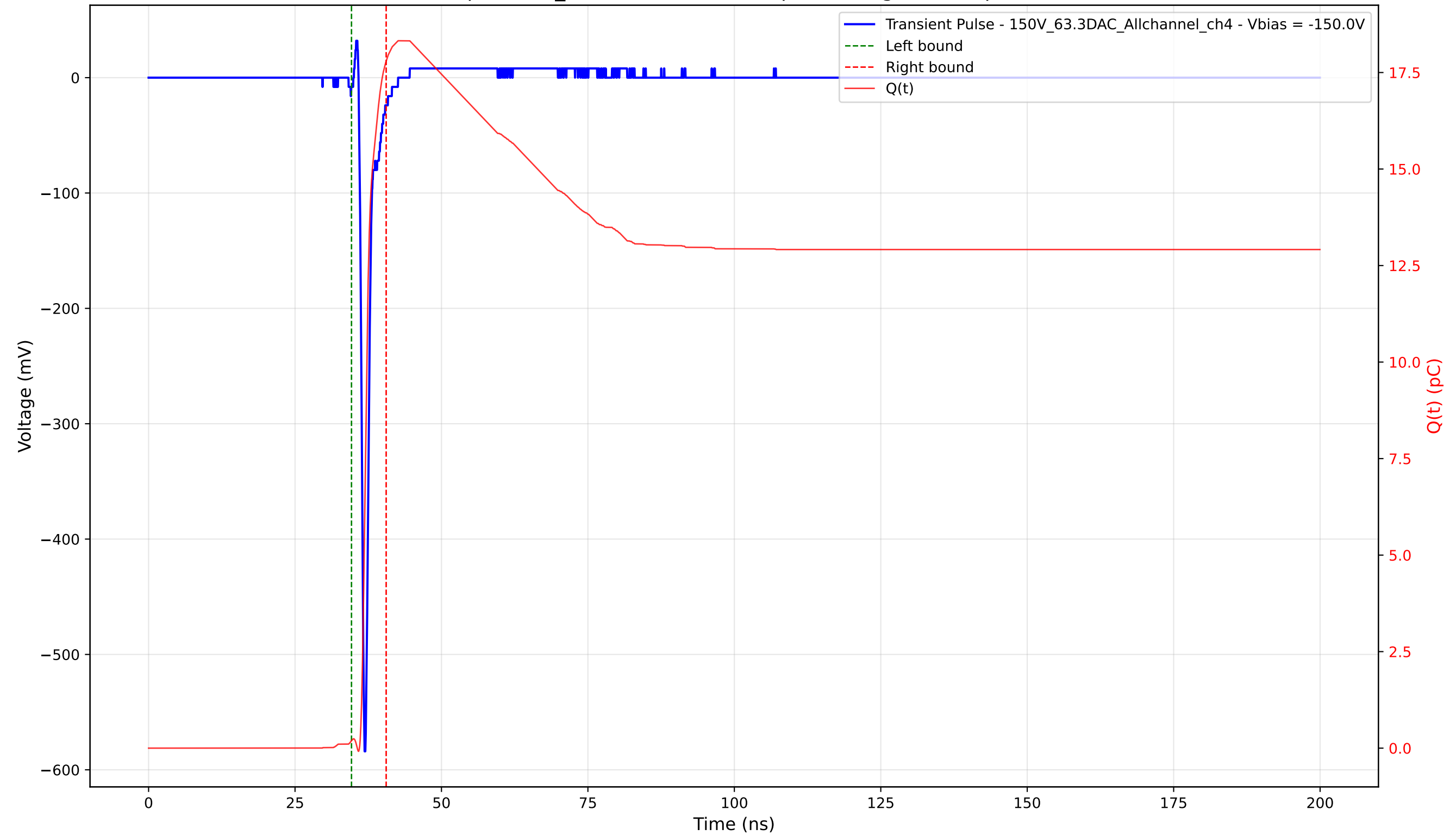
Transient Pulse - Sample: 1cm_42 - Position: 2020.0 \mu\text{m} - Charge: 17.60 pC - Rise Time: 0.71 ns
