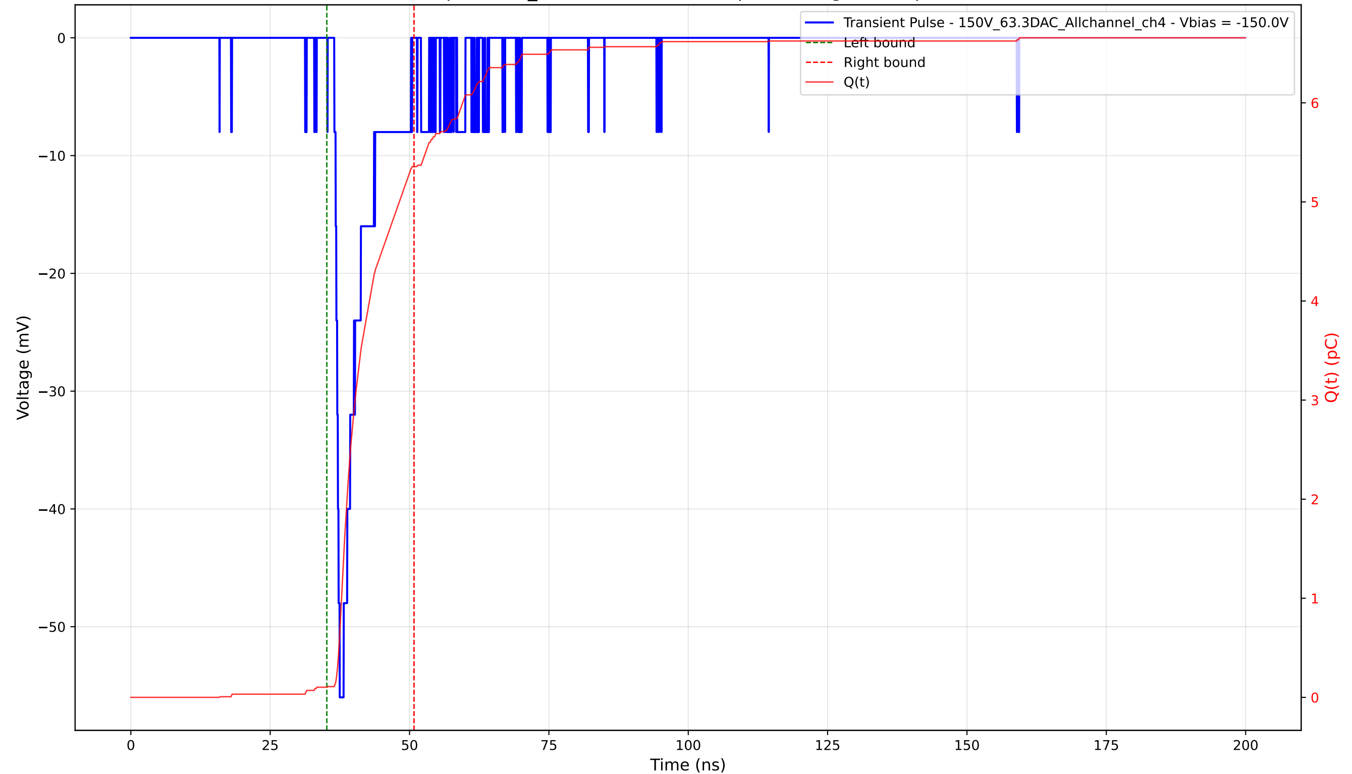
Transient Pulse - Sample: 1cm_42 - Position: 3080.0 \mu\text{m} - Charge: 5.25 pC - Rise Time: 0.97 ns
