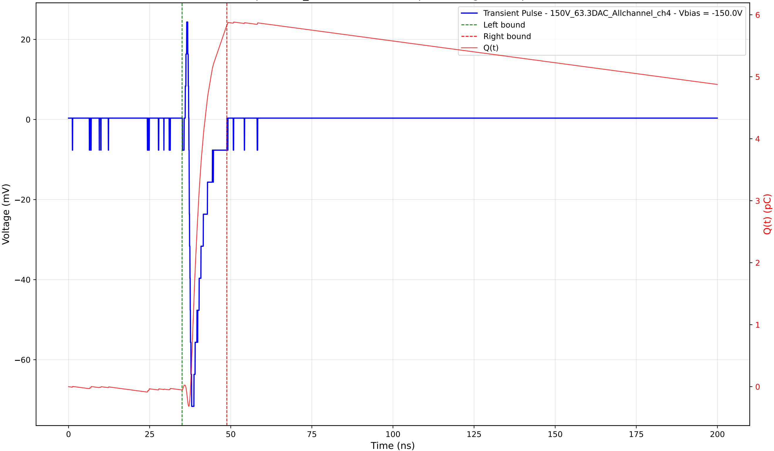
Transient Pulse - Sample: 1cm_42 - Position: 640.0 \mu\text{m} - Charge: 5.89 pC - Rise Time: 0.84 ns
