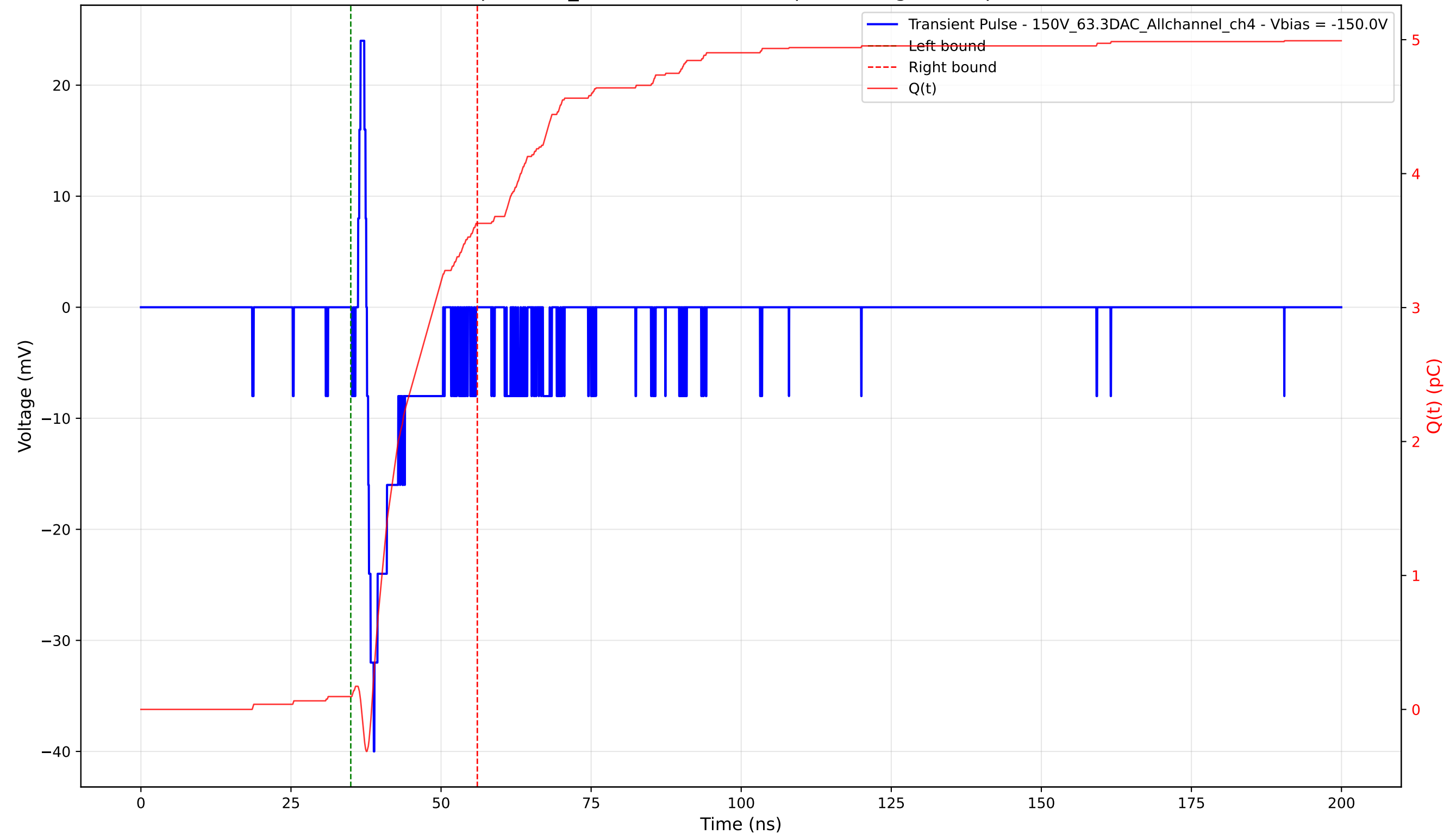
Transient Pulse - Sample: 1cm_42 - Position: 3845.0 \mu\text{m} - Charge: 3.53 pC - Rise Time: 1.14 ns
