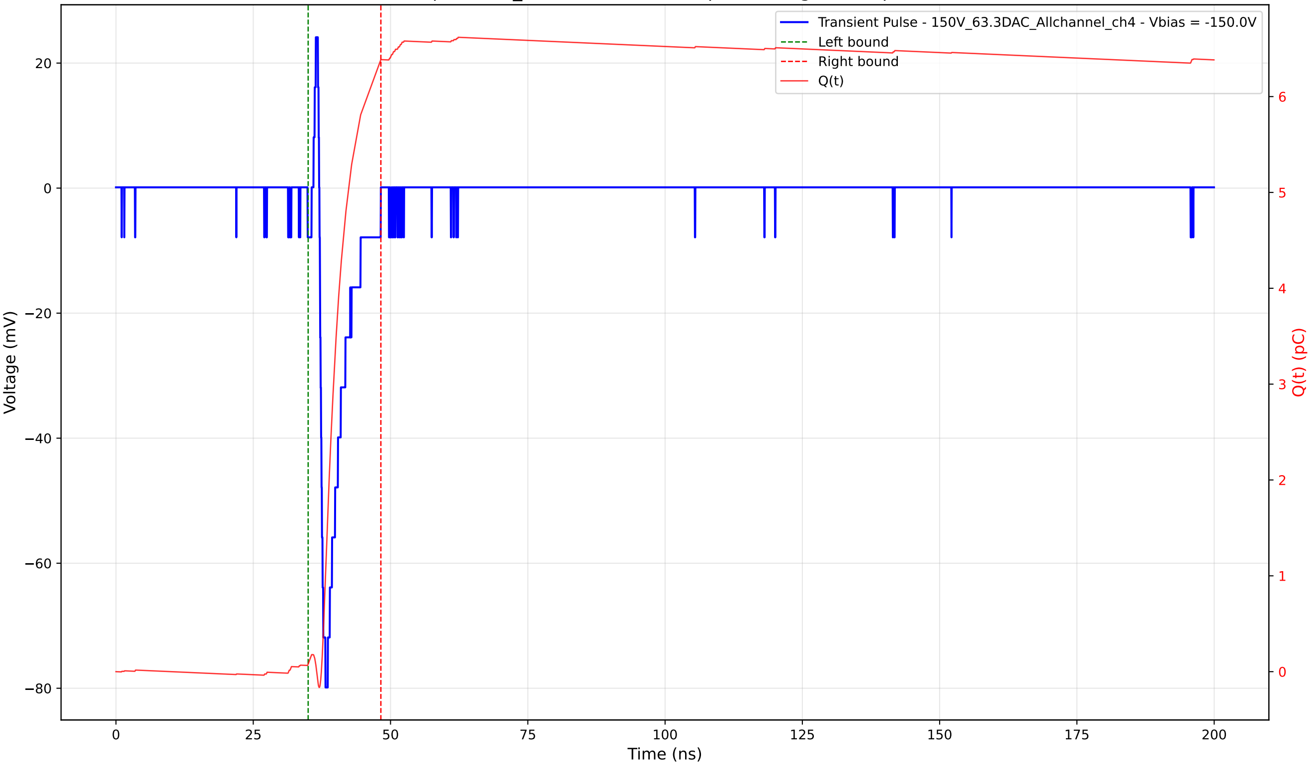
Transient Pulse - Sample: 1cm_42 - Position: 675.0 \mu\text{m} - Charge: 6.31 pC - Rise Time: 1.04 ns
