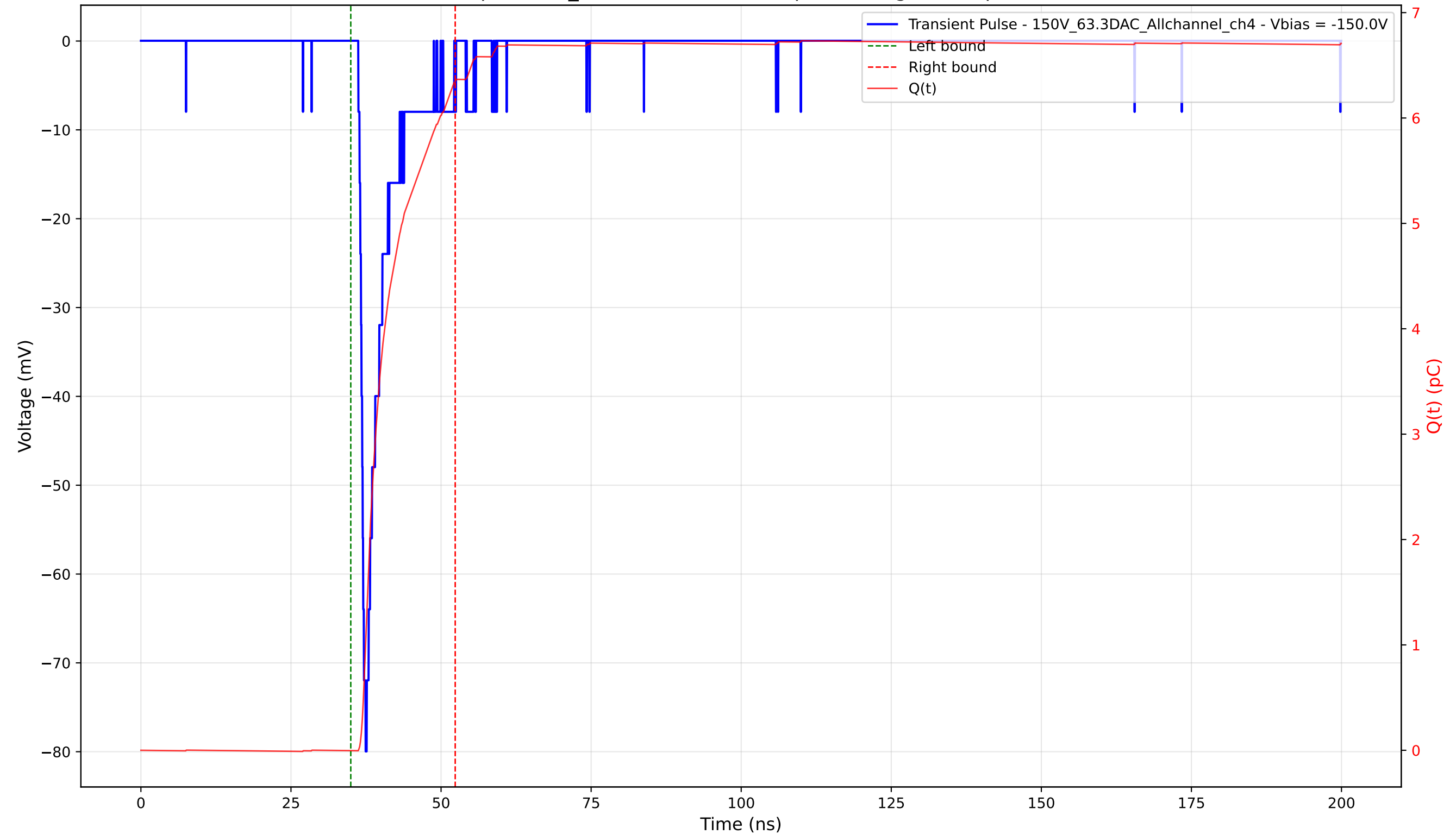
Transient Pulse - Sample: 1cm_42 - Position: 2965.0 \mu\text{m} - Charge: 6.35 pC - Rise Time: 1.04 ns
