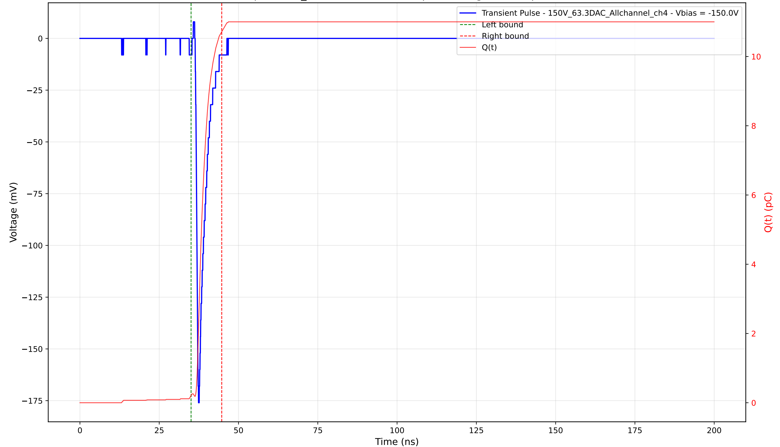
Transient Pulse - Sample: 1cm_42 - Position: 1220.0 \mu\text{m} - Charge: 10.51 pC - Rise Time: 0.75 ns
