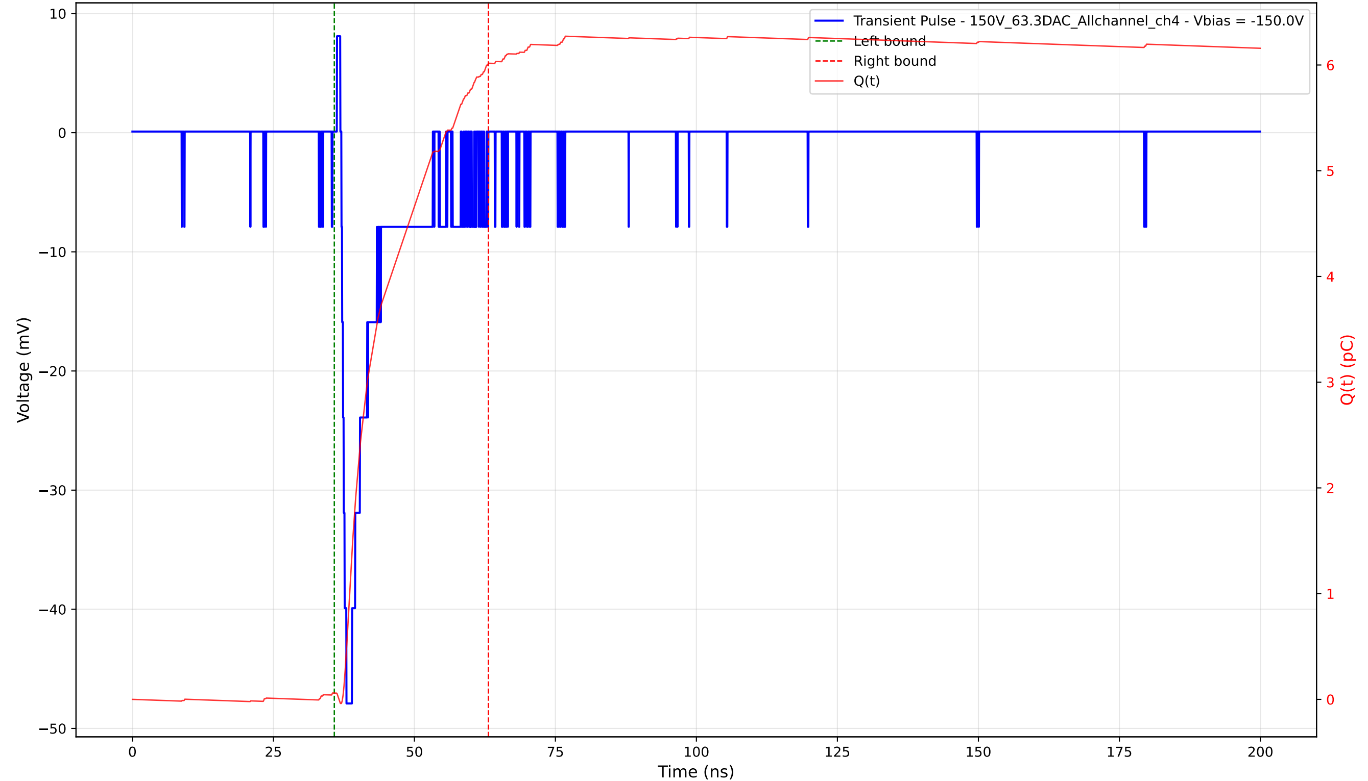
Transient Pulse - Sample: 1cm_42 - Position: 3300.0 \mu\text{m} - Charge: 5.96 pC - Rise Time: 0.90 ns
