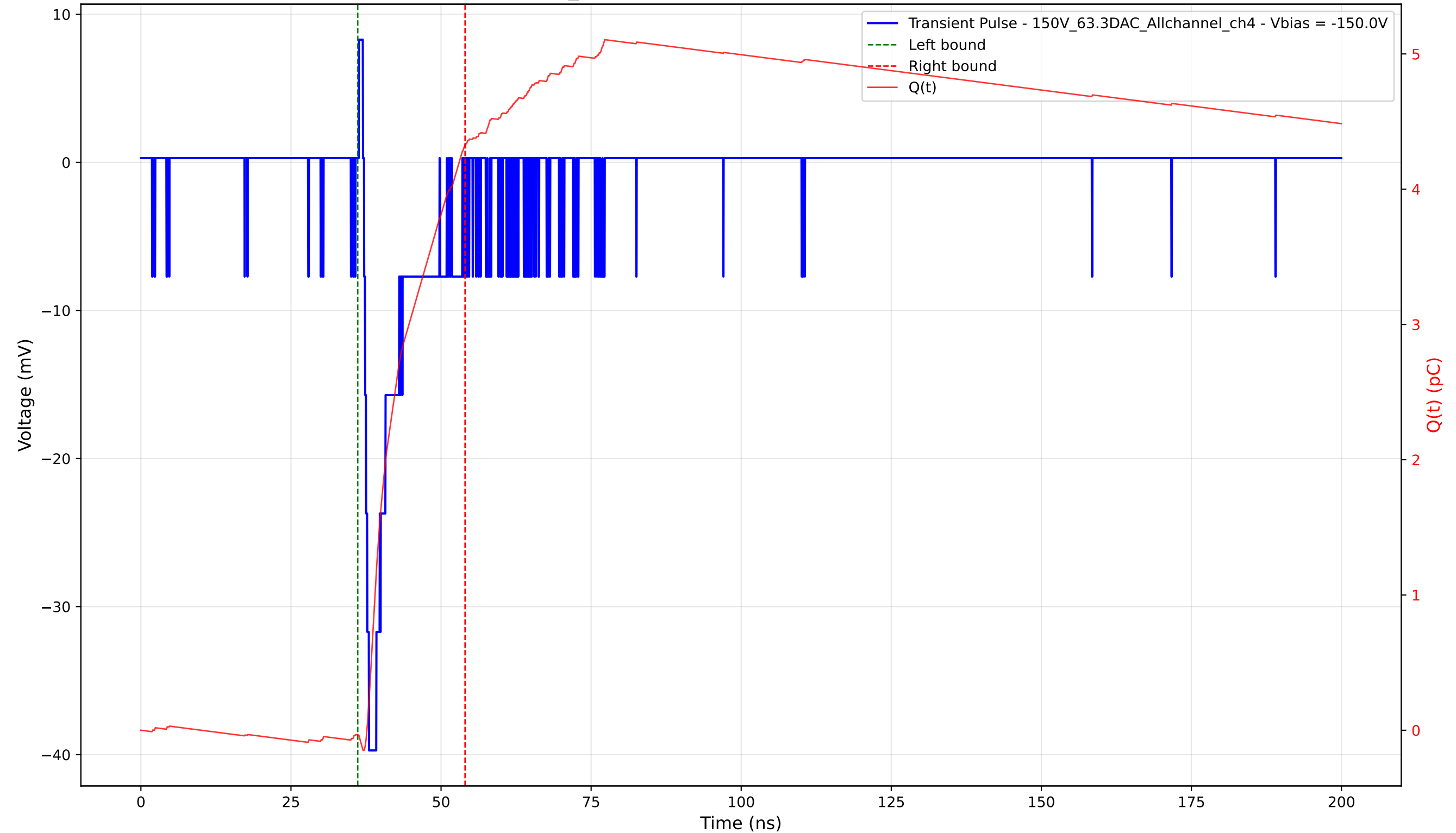
Transient Pulse - Sample: 1cm_42 - Position: 3410.0 \mu\text{m} - Charge: 4.37 pC - Rise Time: 0.82 ns
