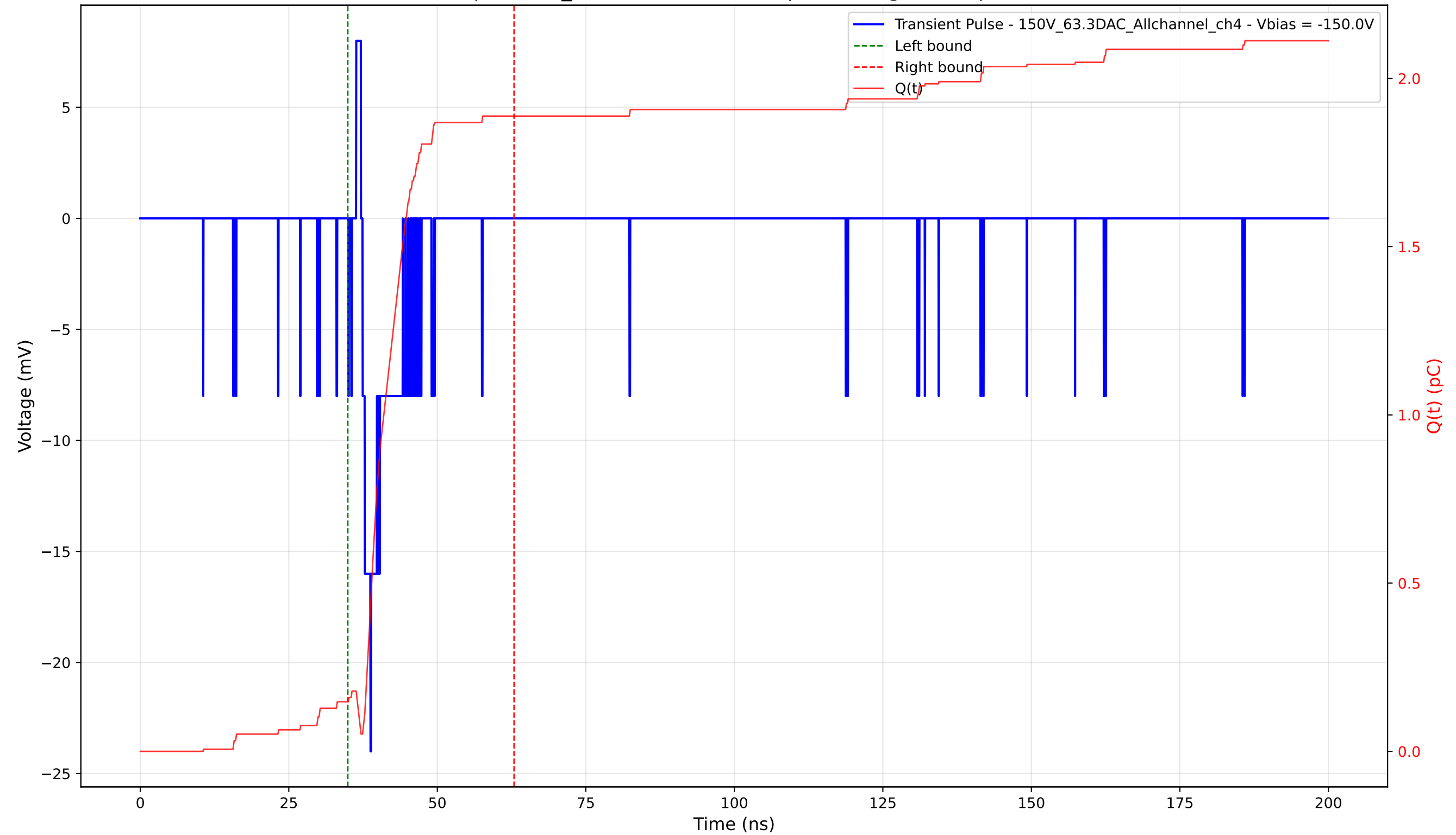
Transient Pulse - Sample: 1cm_42 - Position: 5020.0 \mu\text{m} - Charge: 1.74 pC - Rise Time: 1.35 ns
