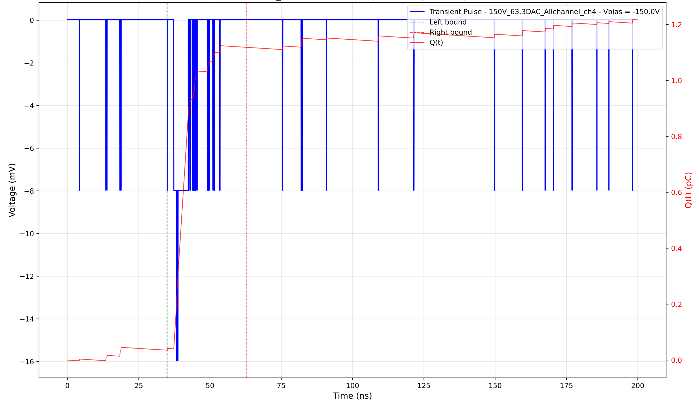
Transient Pulse - Sample: 1cm_42 - Position: 90.0 \mu\text{m} - Charge: 1.08 pC - Rise Time: 0.95 ns
