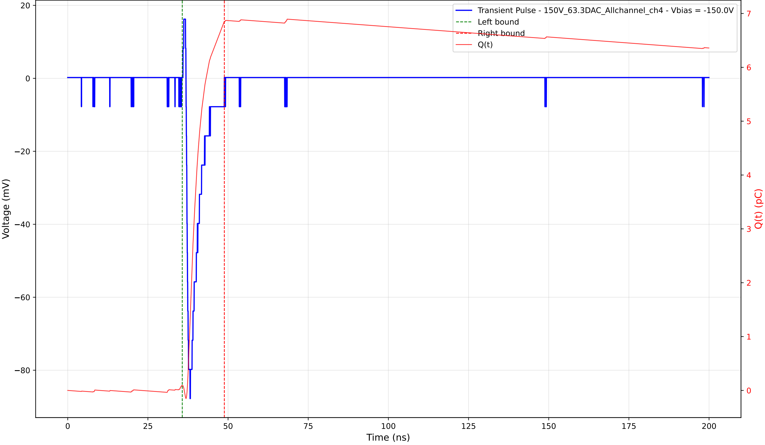
Transient Pulse - Sample: 1cm_42 - Position: 865.0 \mu\text{m} - Charge: 6.76 pC - Rise Time: 0.71 ns
