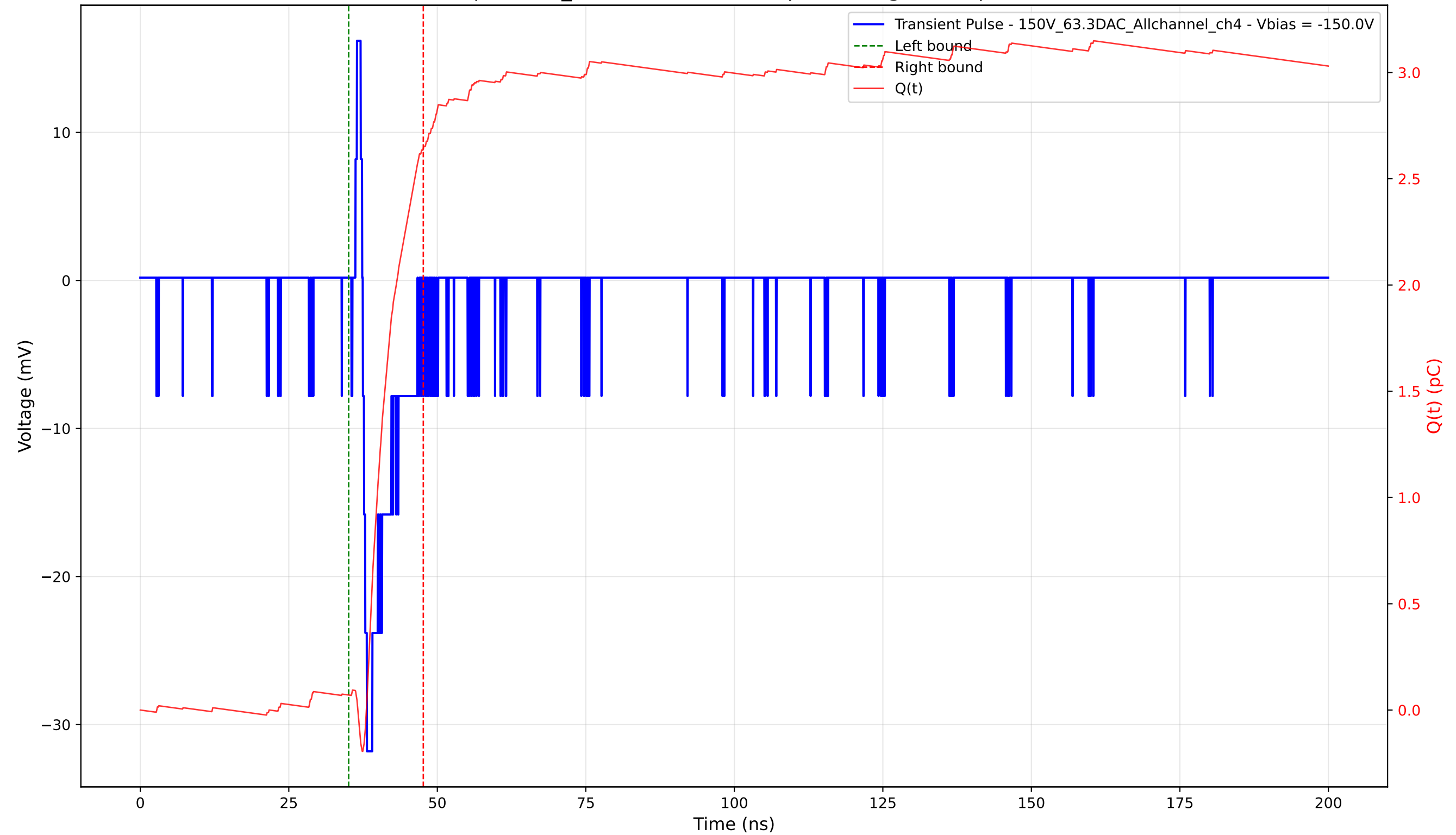
Transient Pulse - Sample: 1cm_42 - Position: 4890.0 \mu\text{m} - Charge: 2.57 pC - Rise Time: 0.70 ns
