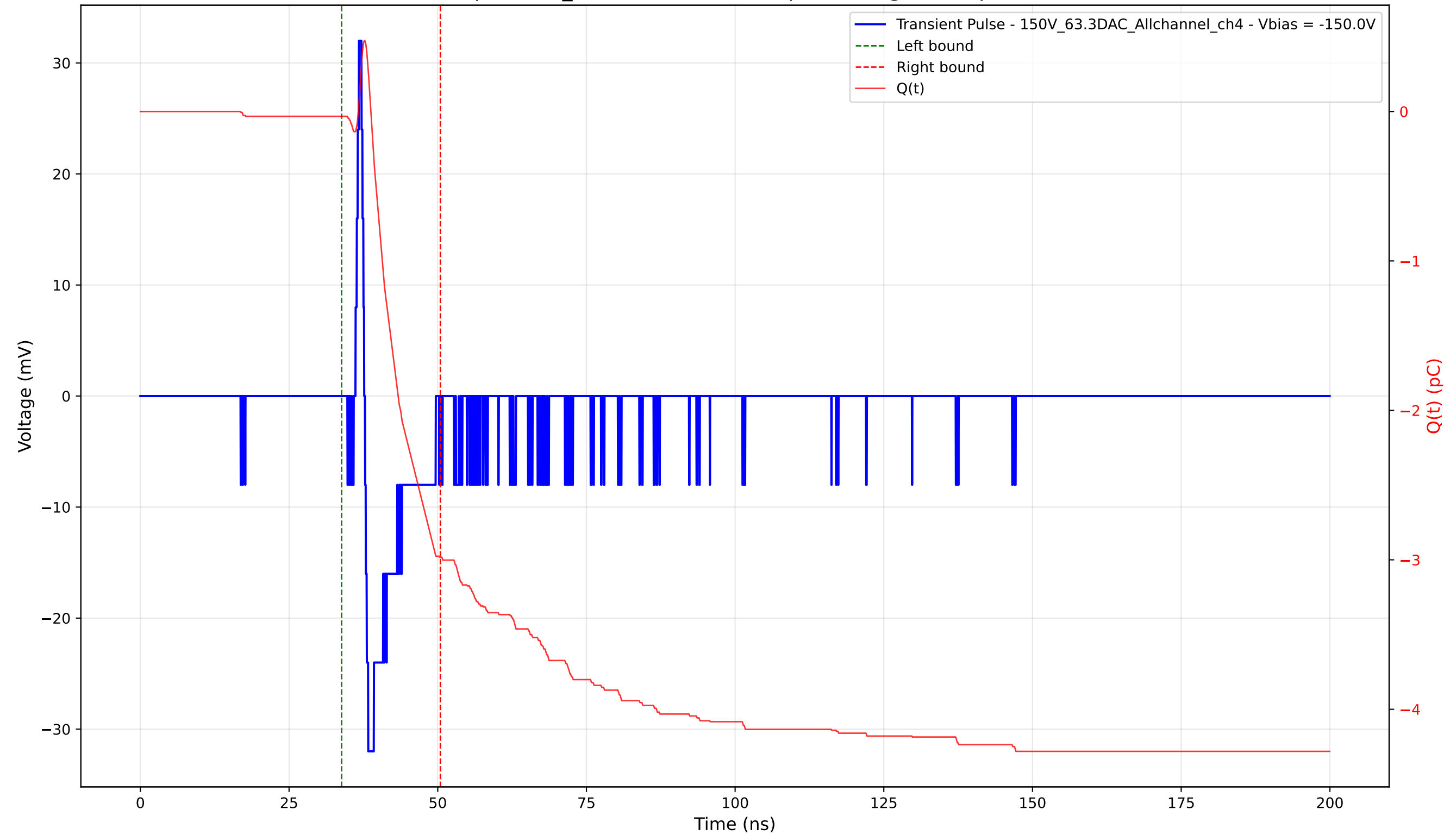
Transient Pulse - Sample: 1cm_42 - Position: 4275.0 \mu\text{m} - Charge: 2.95 pC - Rise Time: 0.58 ns
