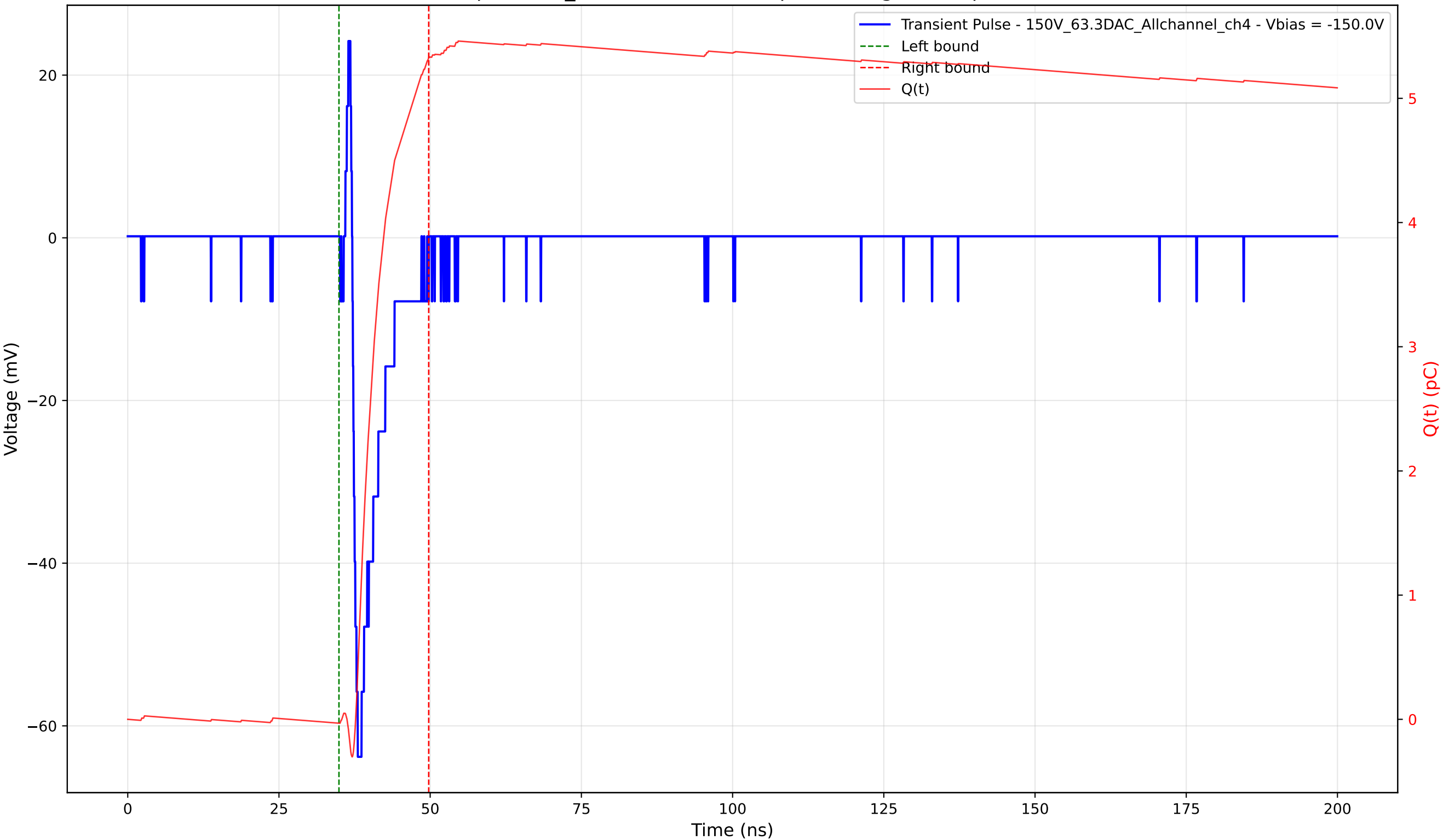
Transient Pulse - Sample: 1cm_42 - Position: 570.0 \mu\text{m} - Charge: 5.36 pC - Rise Time: 0.89 ns
