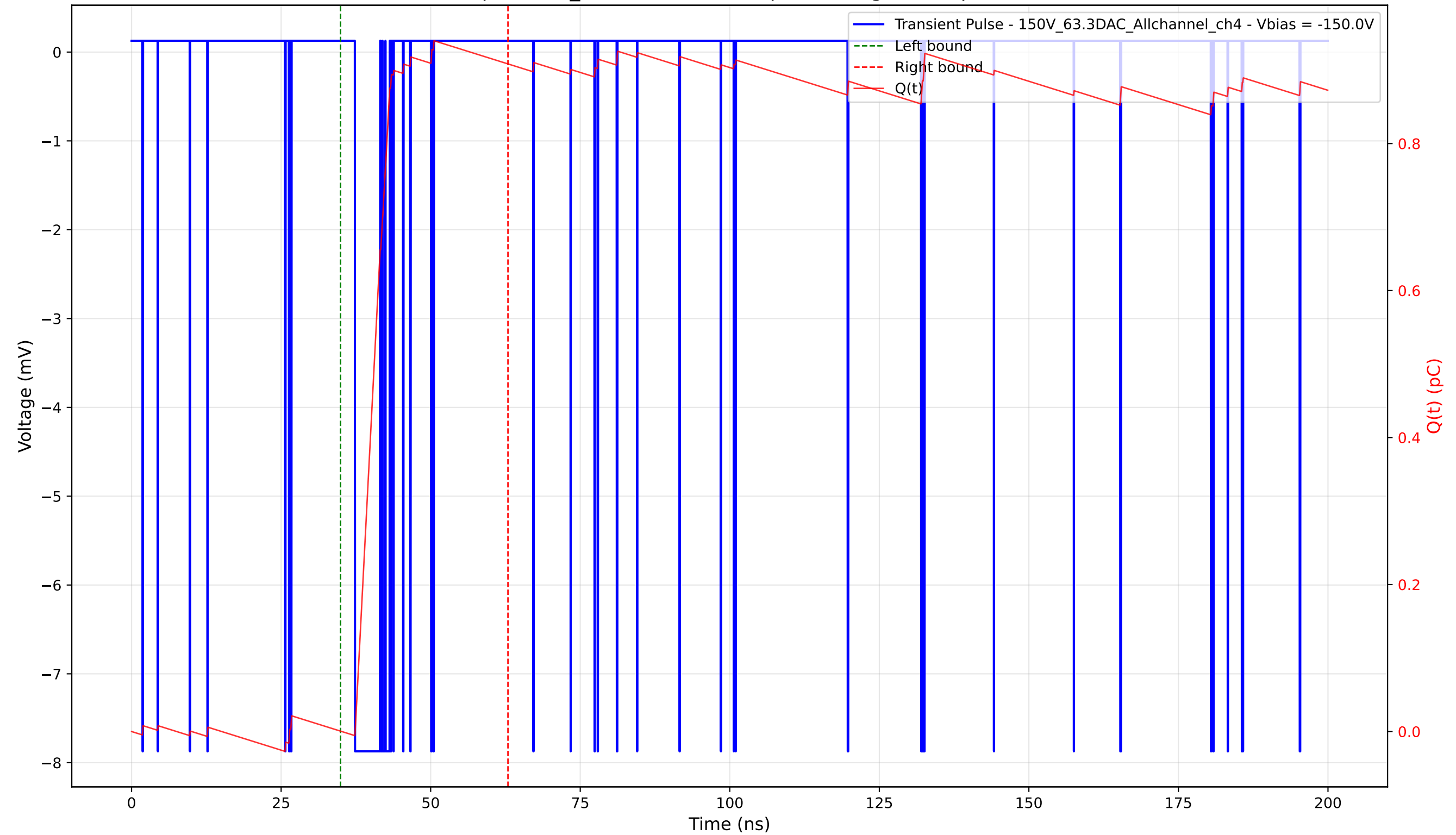
Transient Pulse - Sample: 1cm_42 - Position: 85.0 \mu\text{m} - Charge: 0.91 pC - Rise Time: 0.04 ns
