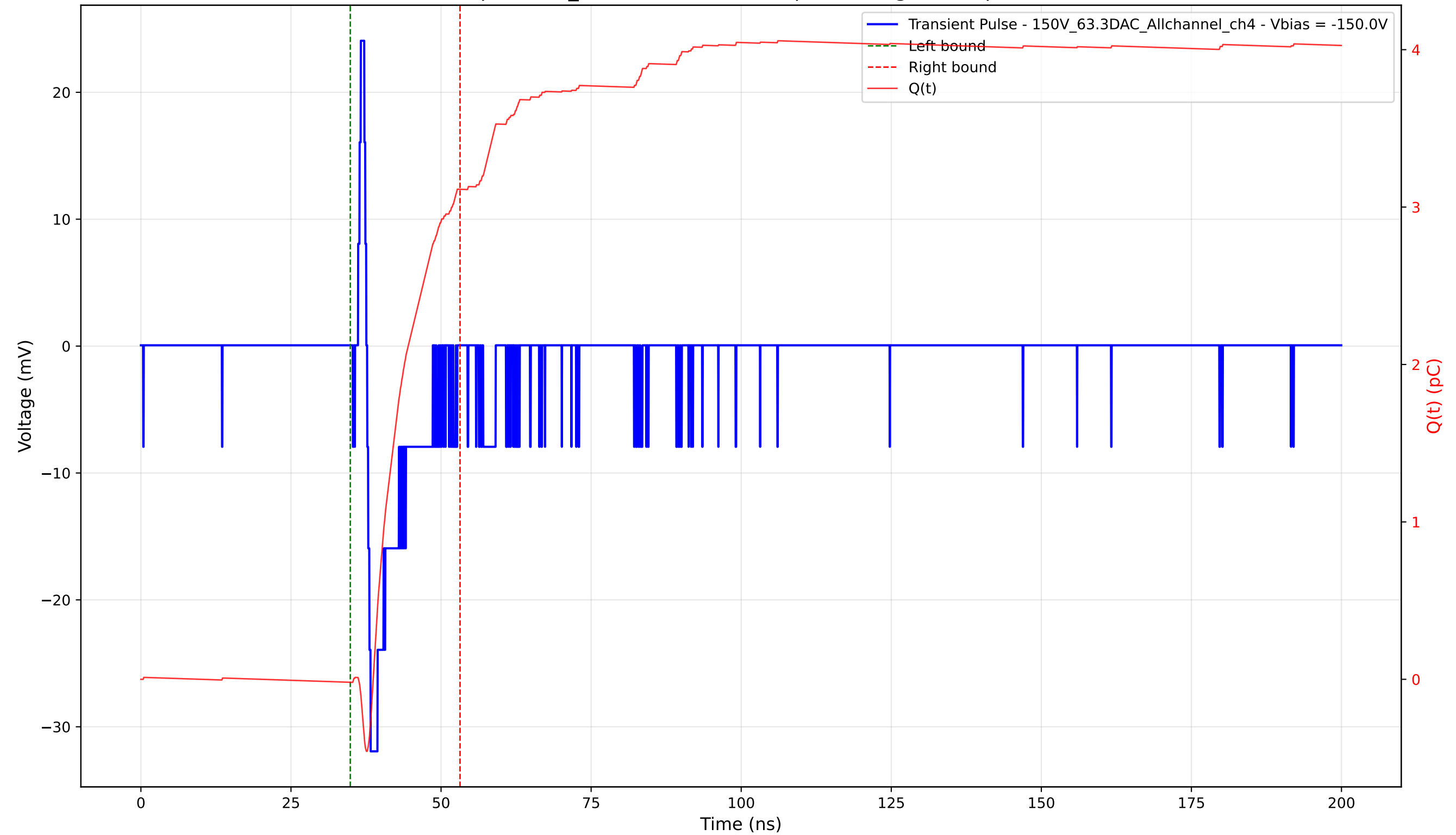
Transient Pulse - Sample: 1cm_42 - Position: 3875.0 \mu\text{m} - Charge: 3.13 pC - Rise Time: 0.58 ns
