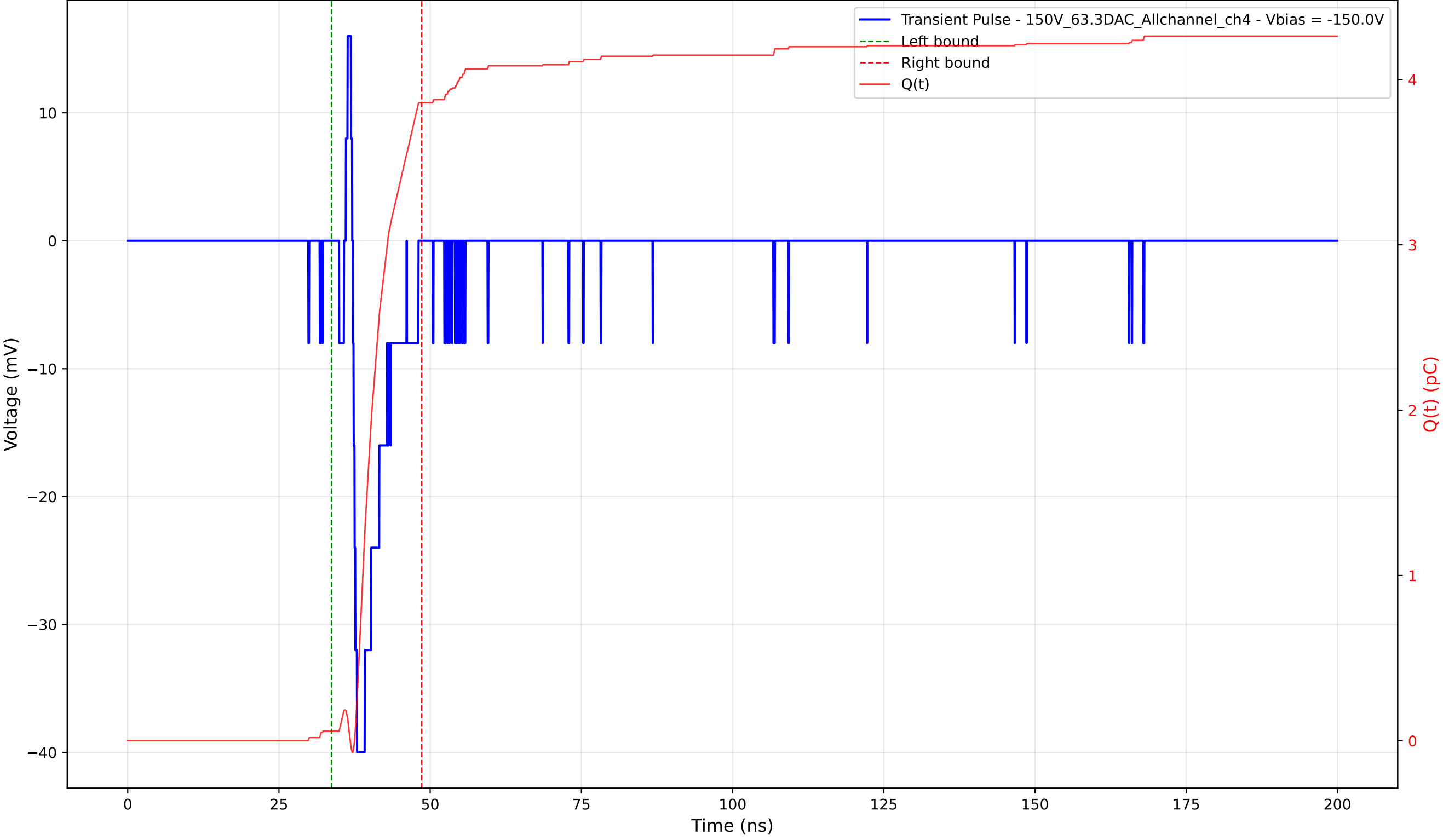
Transient Pulse - Sample: 1cm_42 - Position: 405.0 \mu\text{m} - Charge: 3.80 pC - Rise Time: 0.70 ns
