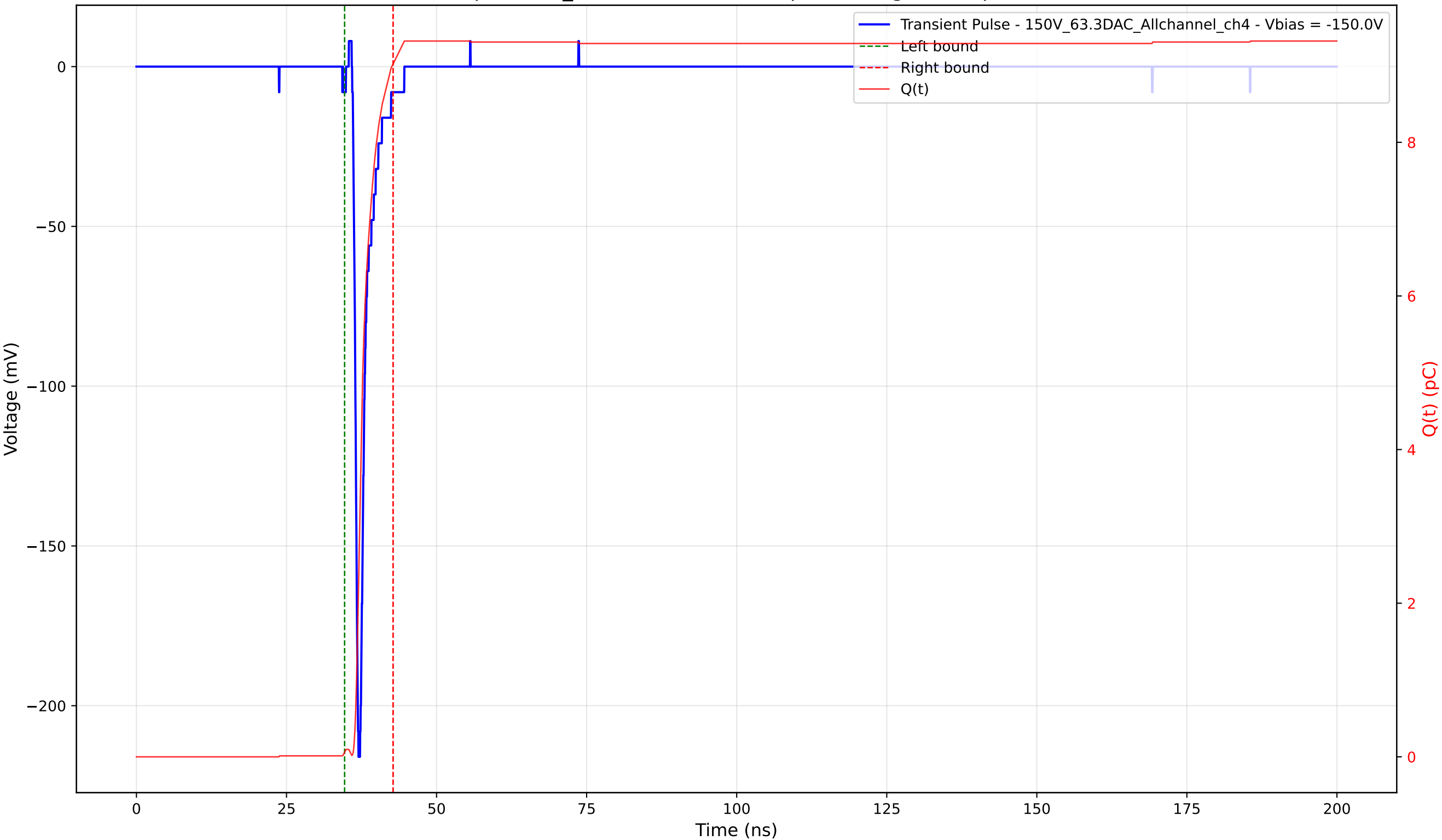
Transient Pulse - Sample: 1cm_42 - Position: 2535.0 \mu\text{m} - Charge: 8.96 pC - Rise Time: 0.74 ns
