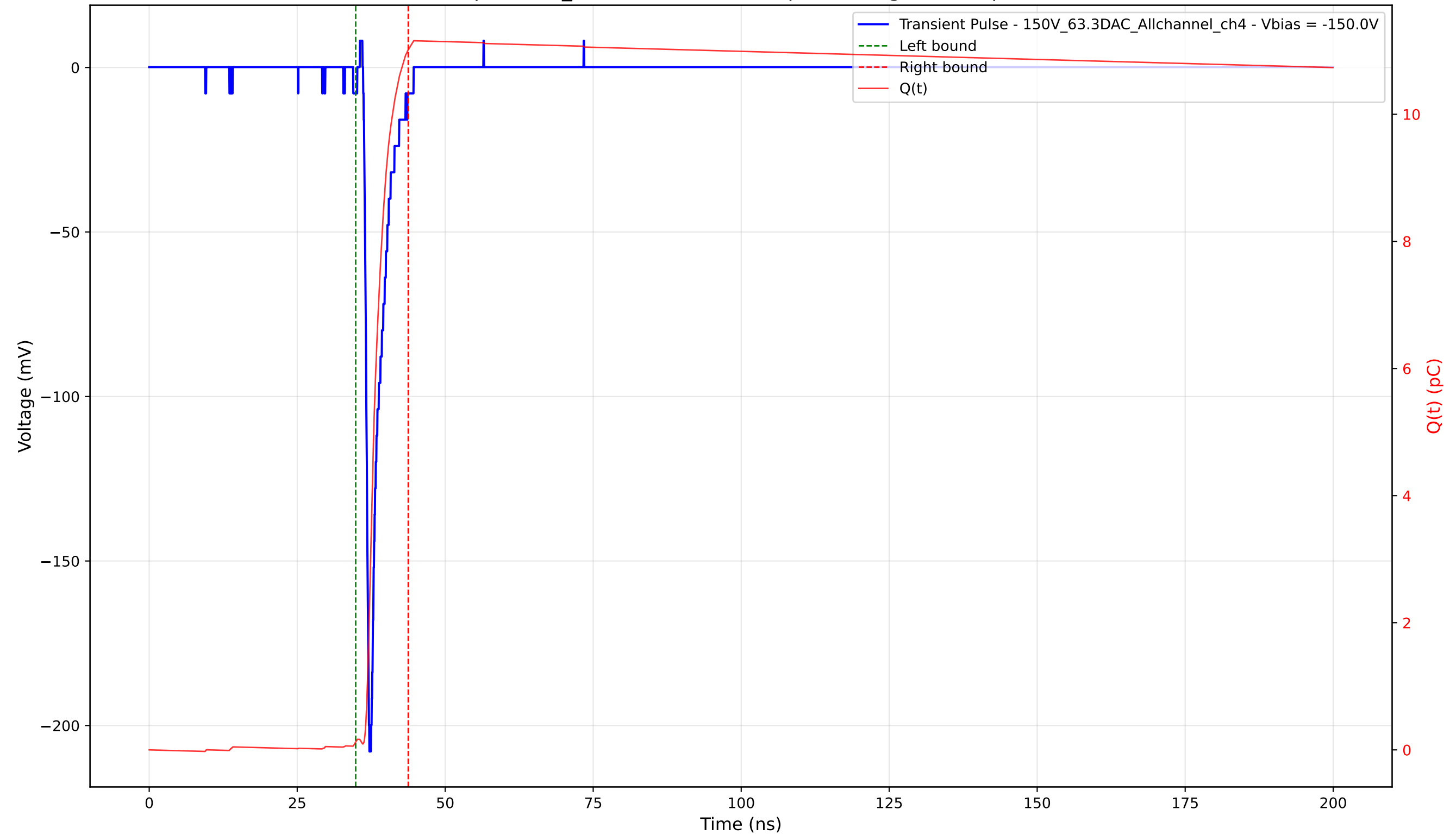
Transient Pulse - Sample: 1cm_42 - Position: 1410.0 \mu\text{m} - Charge: 10.89 pC - Rise Time: 0.75 ns
