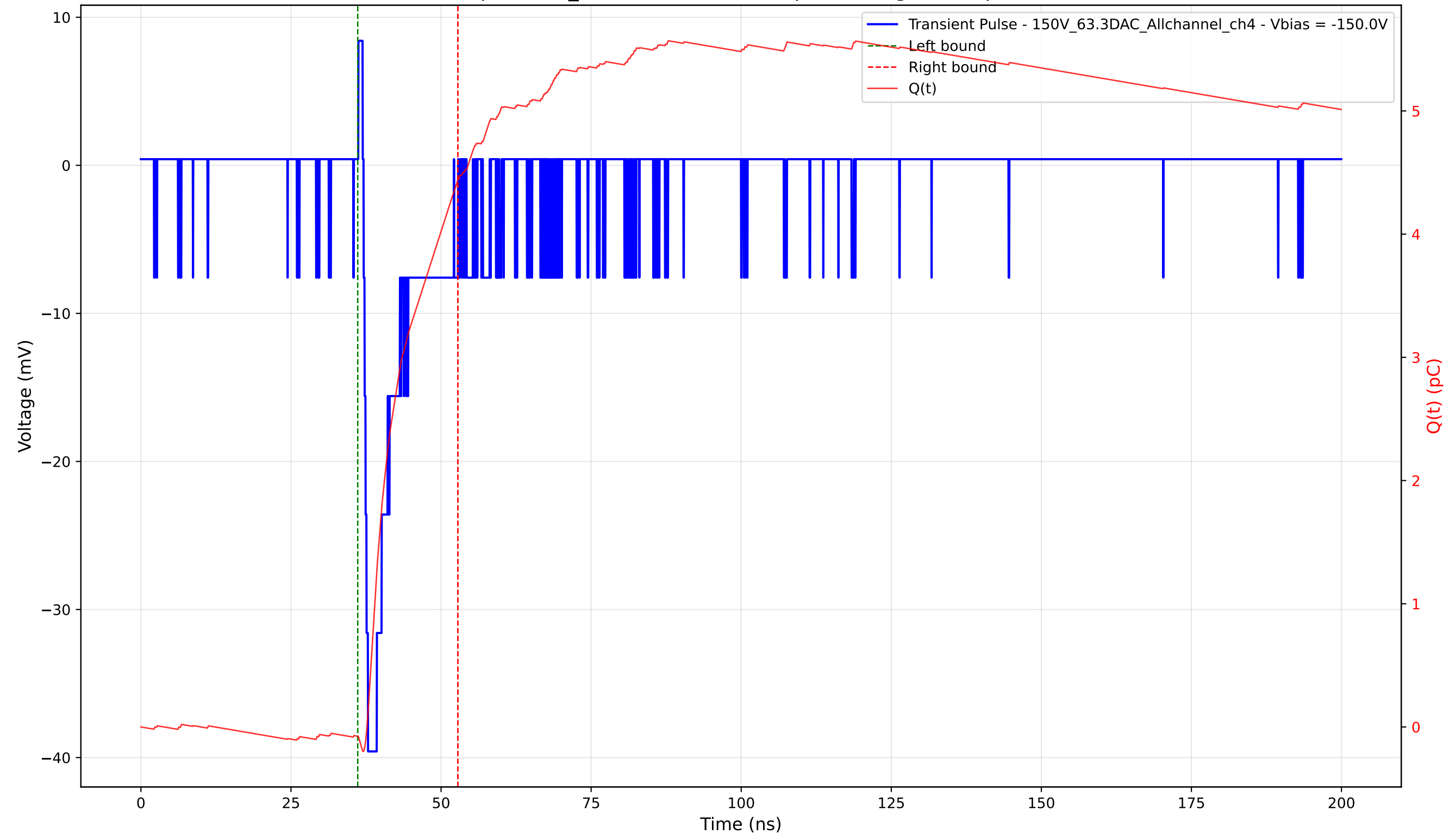
Transient Pulse - Sample: 1cm_42 - Position: 3365.0 \mu\text{m} - Charge: 4.52 pC - Rise Time: 0.74 ns
