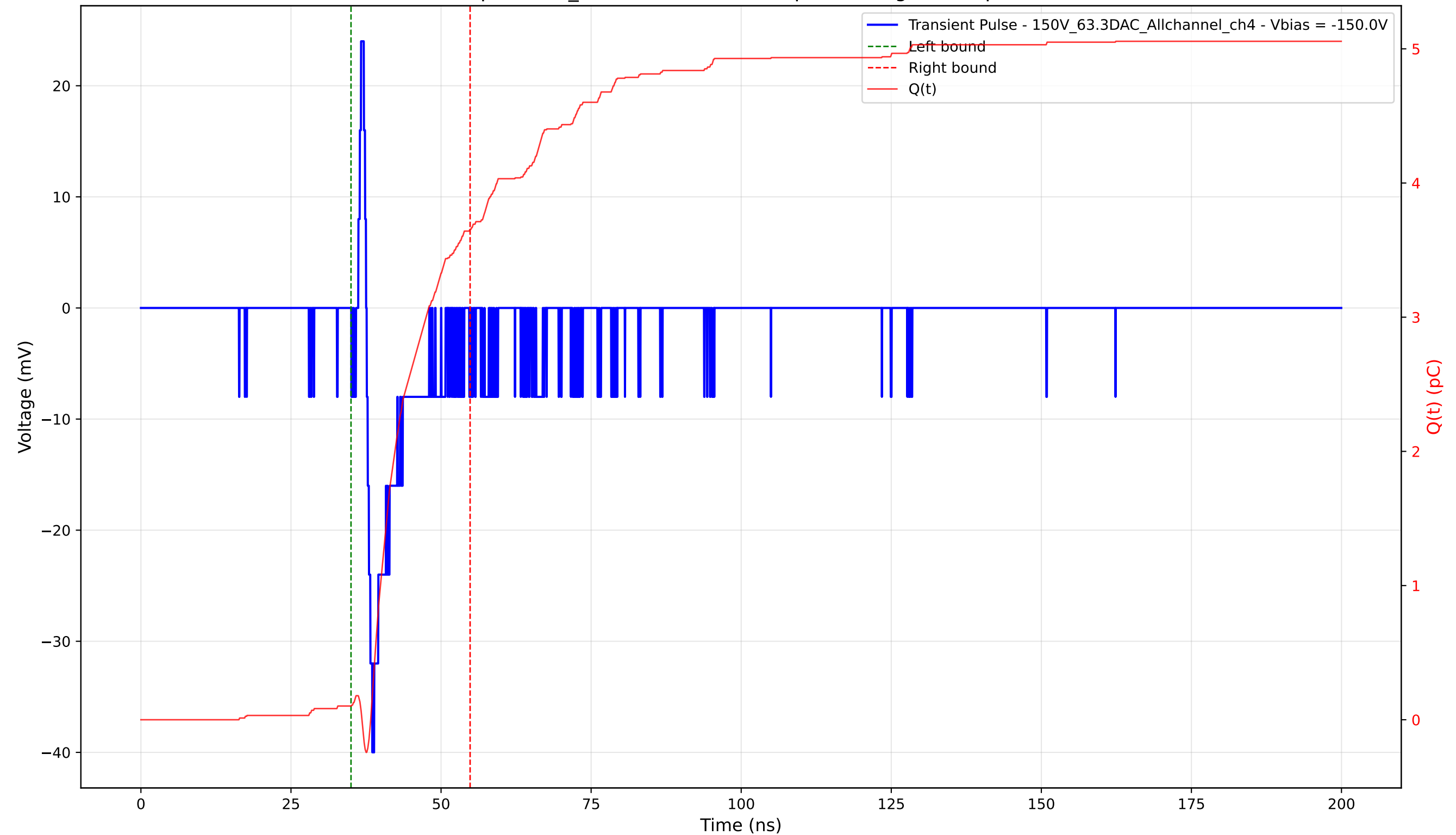
Transient Pulse - Sample: 1cm_42 - Position: 3685.0 \mu\text{m} - Charge: 3.55 pC - Rise Time: 0.94 ns
