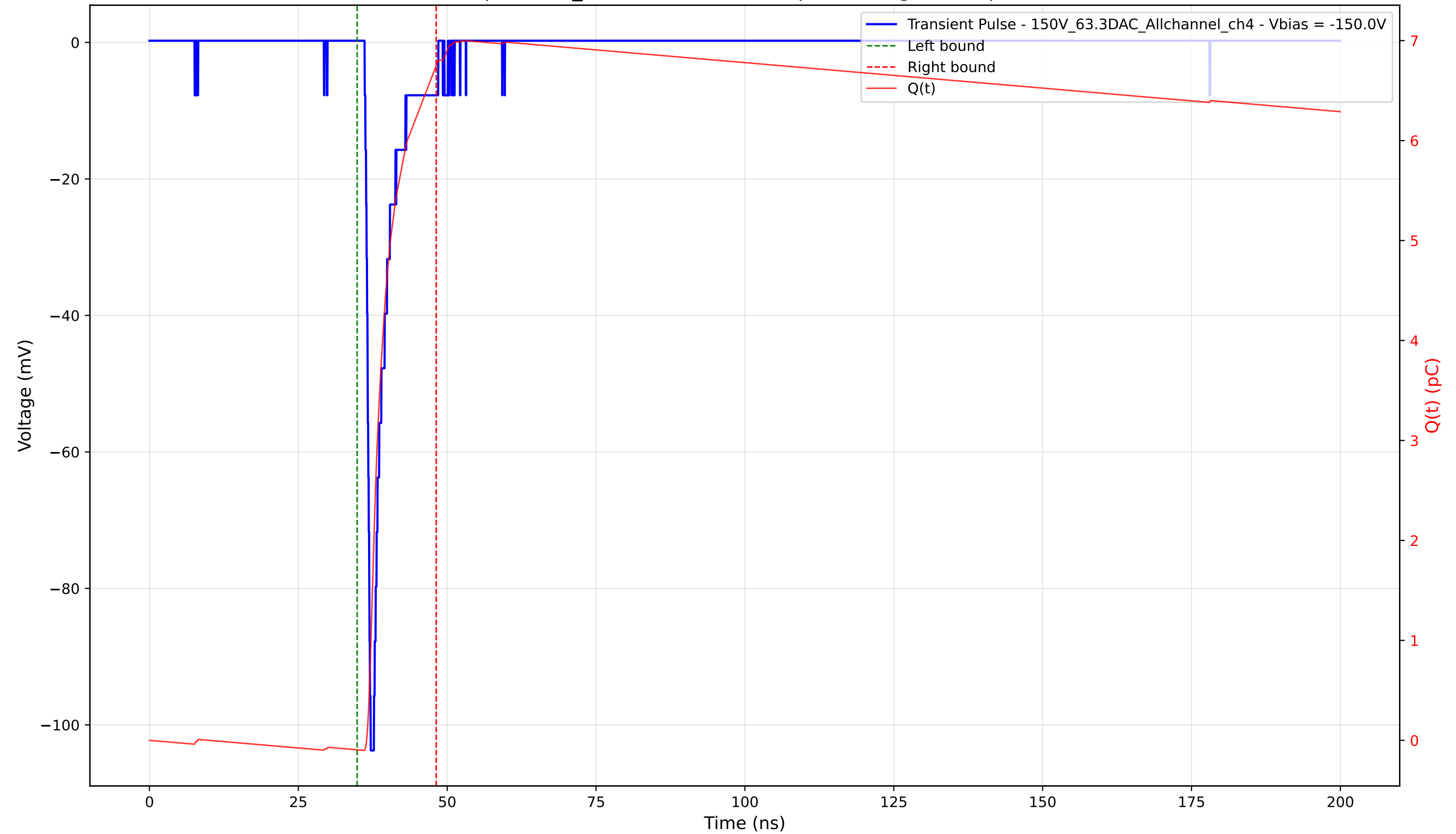
Transient Pulse - Sample: 1cm_42 - Position: 2875.0 \mu\text{m} - Charge: 6.85 pC - Rise Time: 0.79 ns
