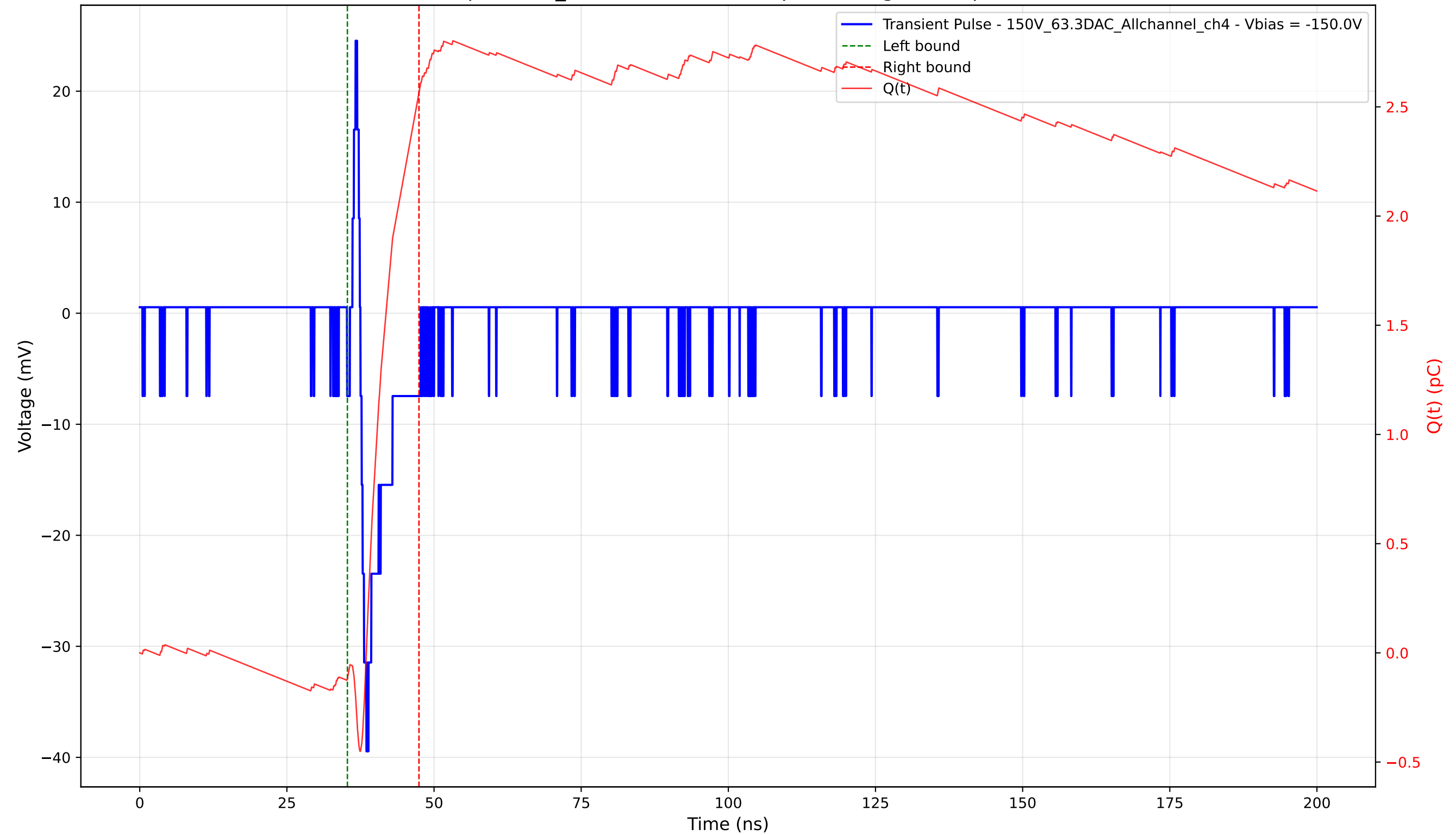
Transient Pulse - Sample: 1cm_42 - Position: 4745.0 \mu\text{m} - Charge: 2.68 pC - Rise Time: 1.02 ns
