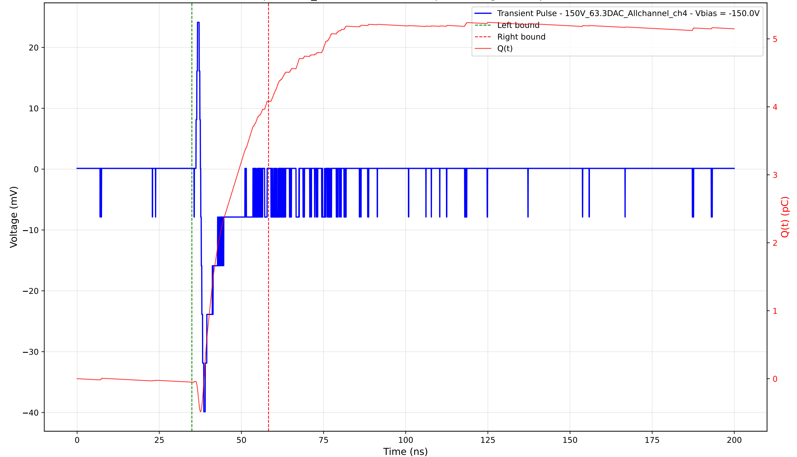
Transient Pulse - Sample: 1cm_42 - Position: 3715.0 \mu\text{m} - Charge: 4.13 pC - Rise Time: 0.94 ns
