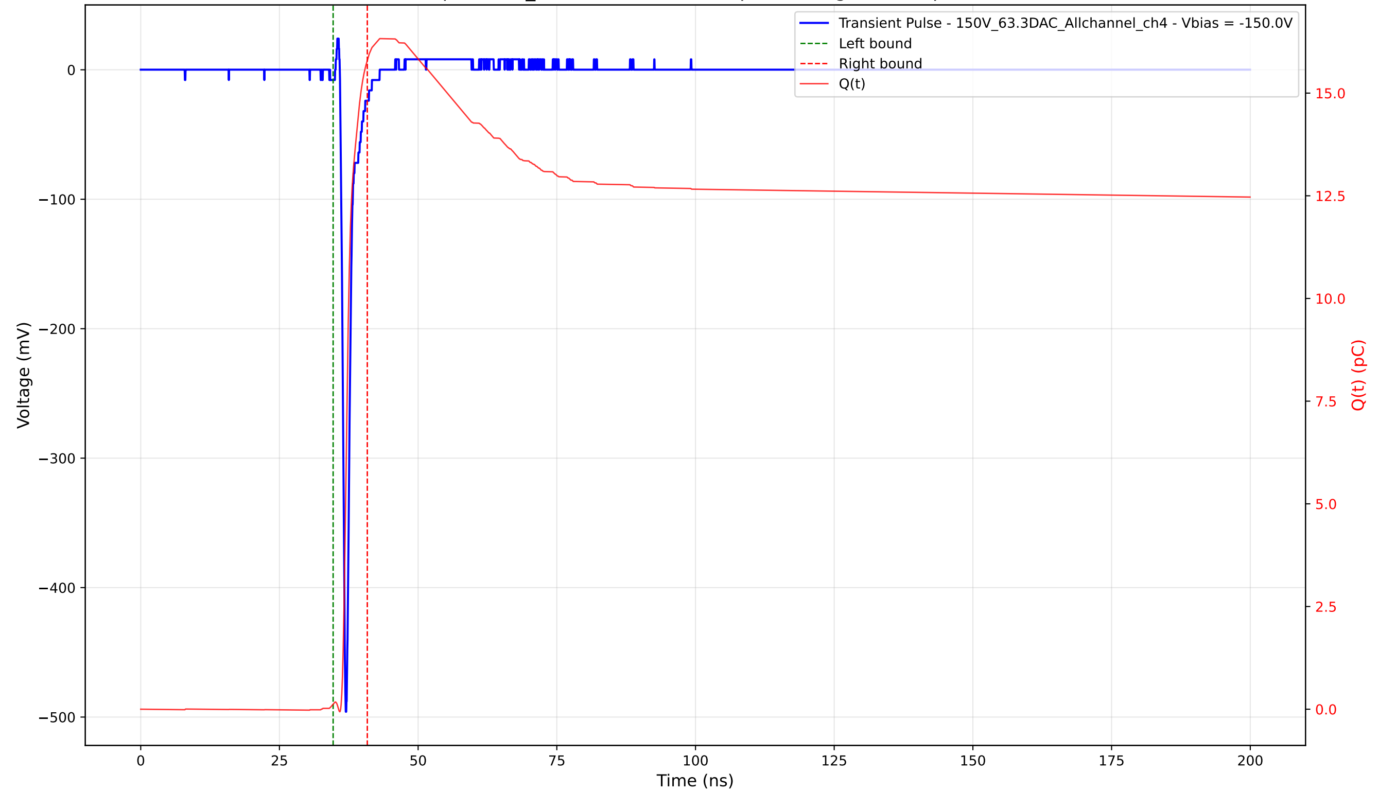
Transient Pulse - Sample: 1cm_42 - Position: 2270.0 \mu\text{m} - Charge: 15.67 pC - Rise Time: 0.73 ns
