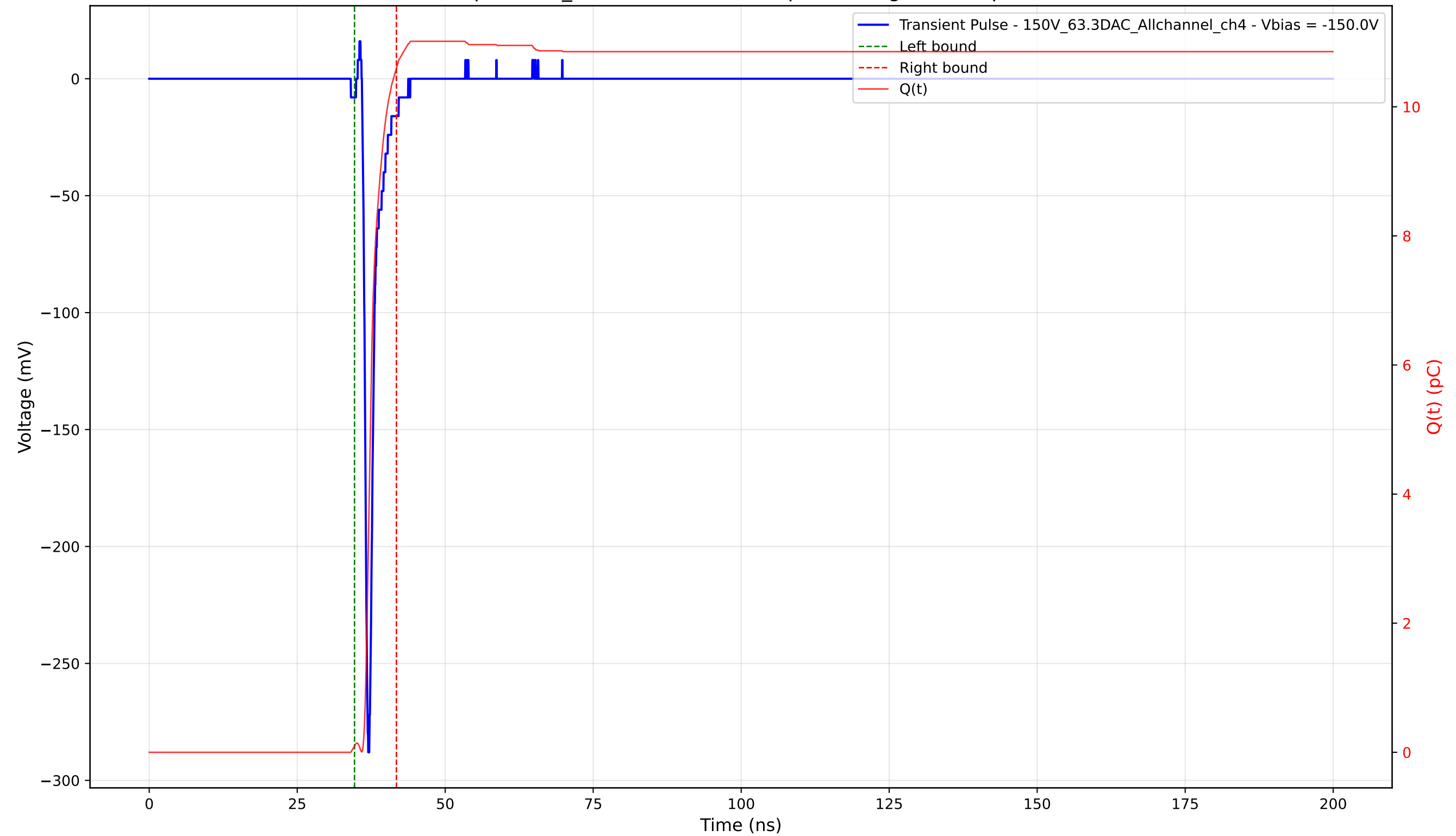
Transient Pulse - Sample: 1cm_42 - Position: 2460.0 \mu\text{m} - Charge: 10.50 pC - Rise Time: 0.75 ns
