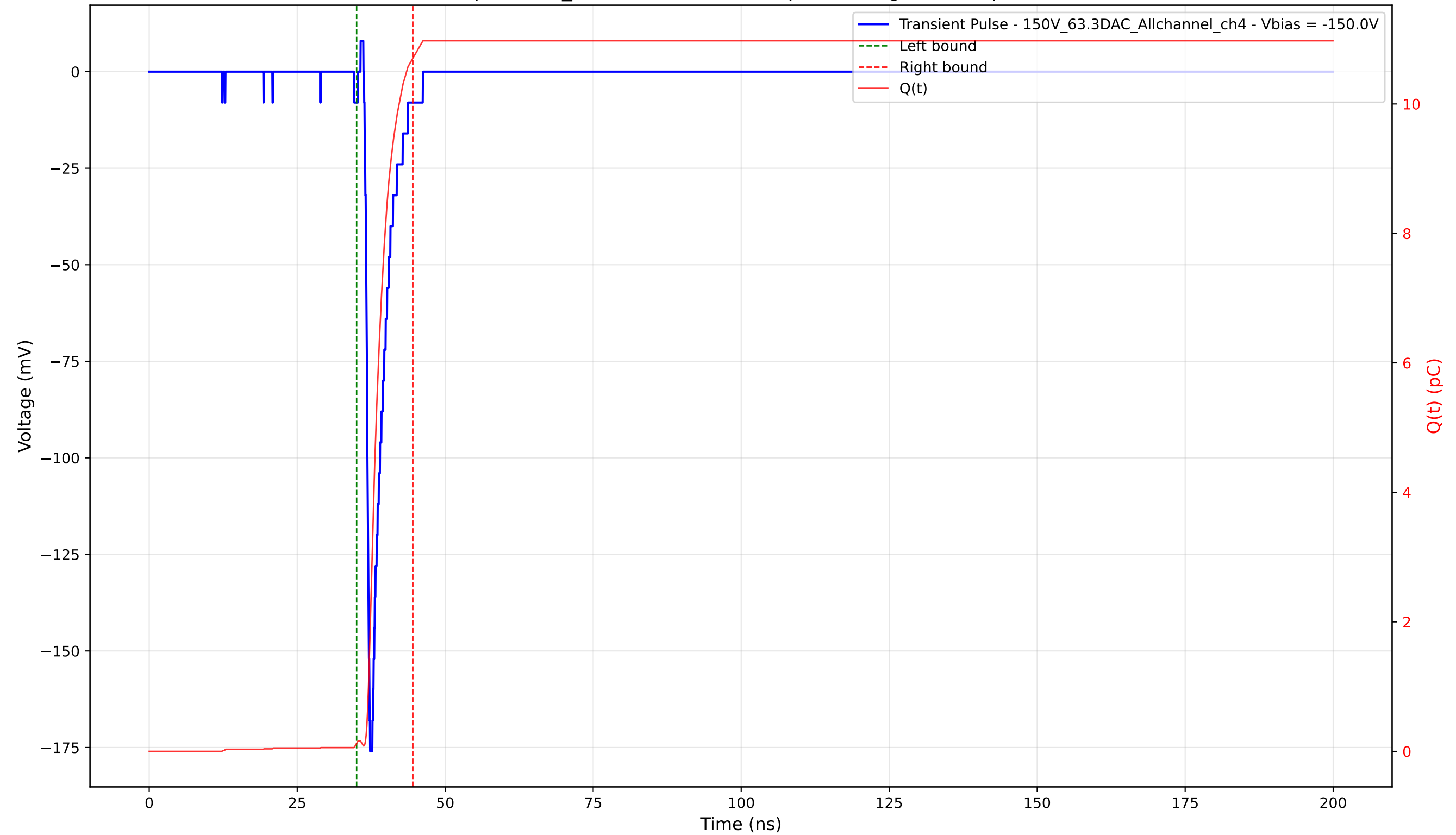
Transient Pulse - Sample: 1cm_42 - Position: 1235.0 \mu\text{m} - Charge: 10.58 pC - Rise Time: 0.74 ns
