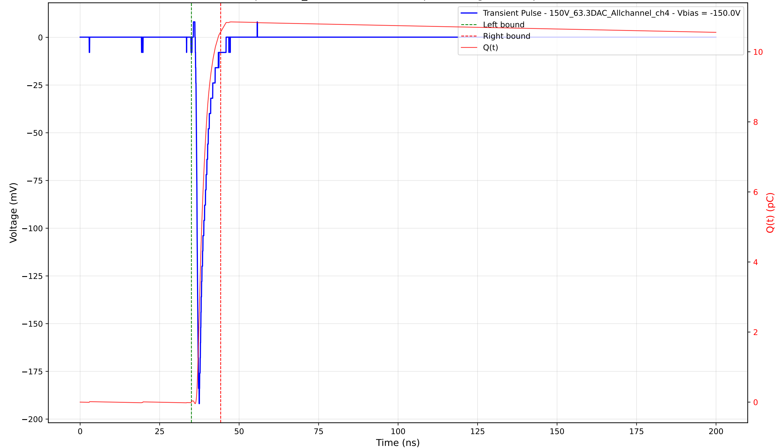
Transient Pulse - Sample: 1cm_42 - Position: 1330.0 \mu\text{m} - Charge: 10.56 pC - Rise Time: 0.81 ns
