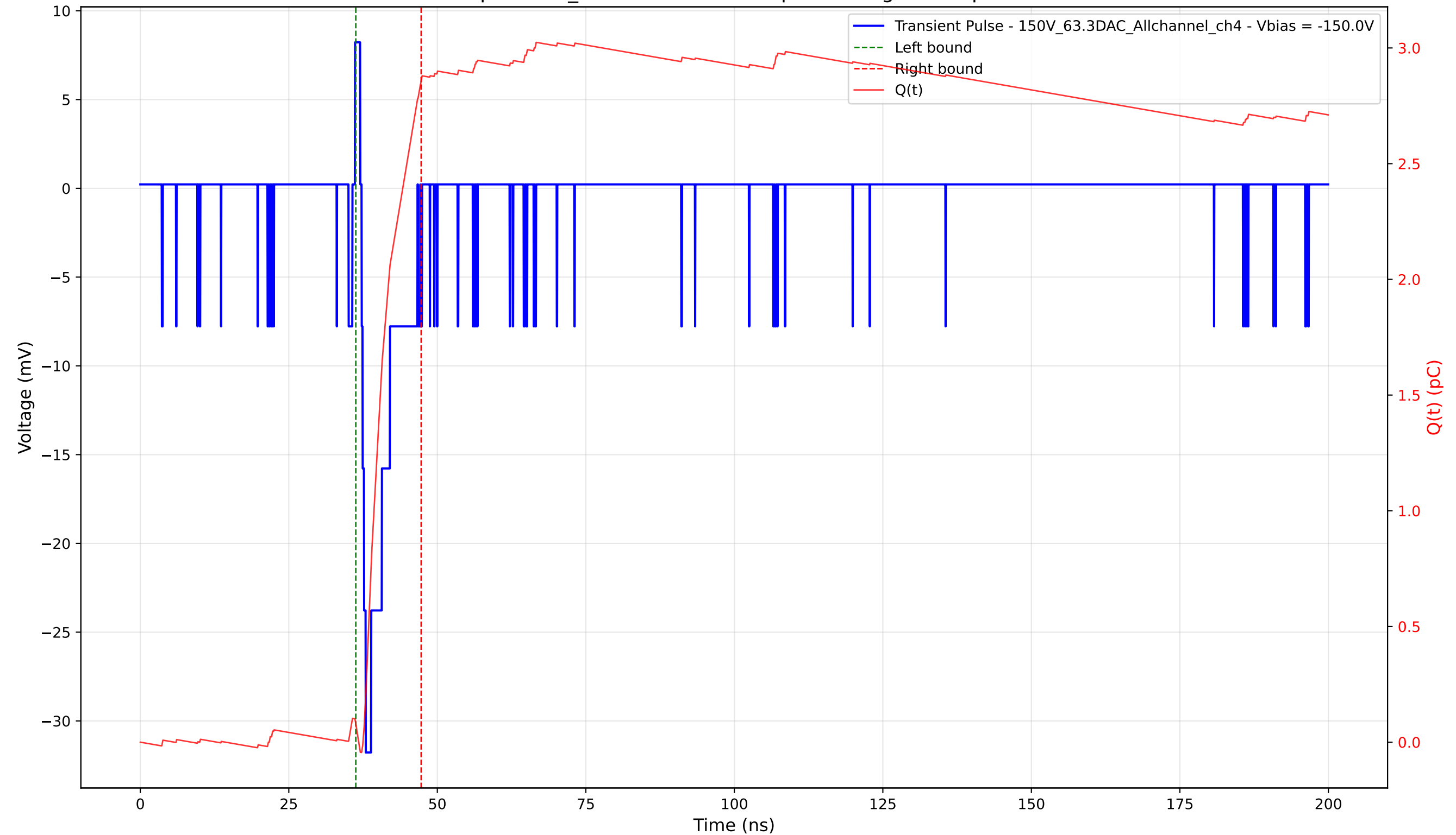
Transient Pulse - Sample: 1cm_42 - Position: 260.0 \mu\text{m} - Charge: 2.78 pC - Rise Time: 0.70 ns
