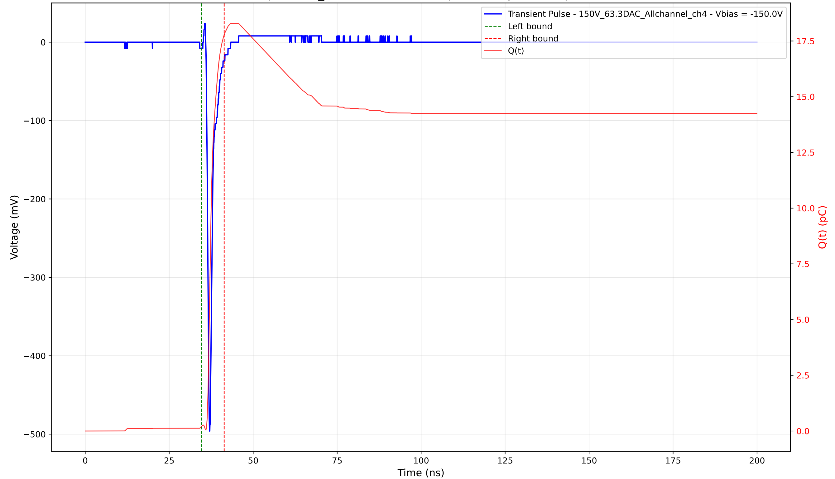
Transient Pulse - Sample: 1cm_42 - Position: 1685.0 \mu\text{m} - Charge: 17.56 pC - Rise Time: 0.75 ns
