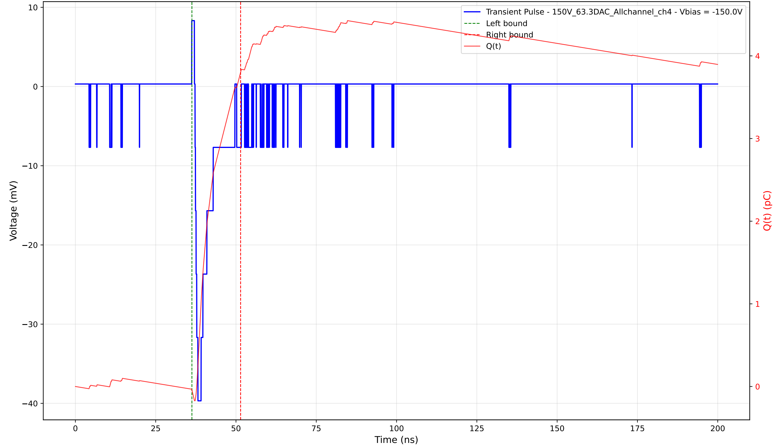
Transient Pulse - Sample: 1cm_42 - Position: 3425.0 \mu\text{m} - Charge: 3.85 pC - Rise Time: 0.90 ns
