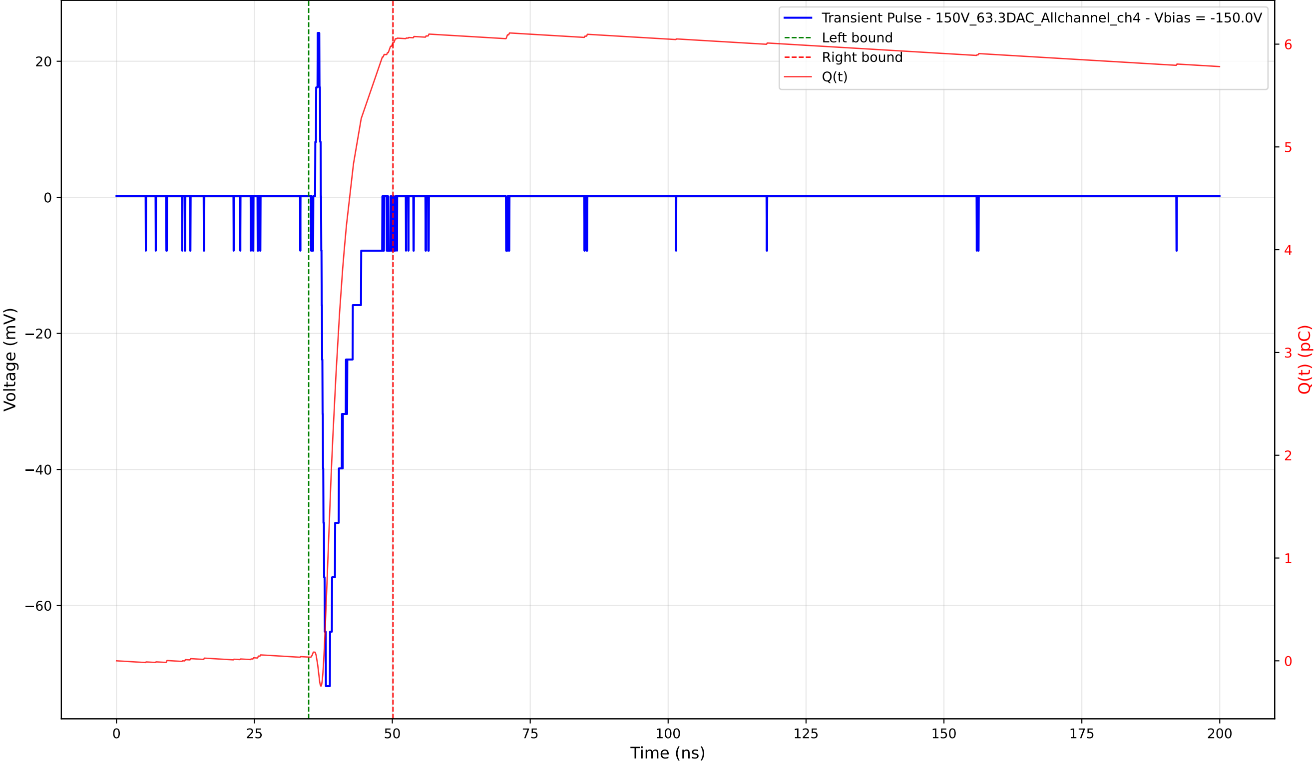
Transient Pulse - Sample: 1cm_42 - Position: 645.0 \mu\text{m} - Charge: 5.98 pC - Rise Time: 0.84 ns
