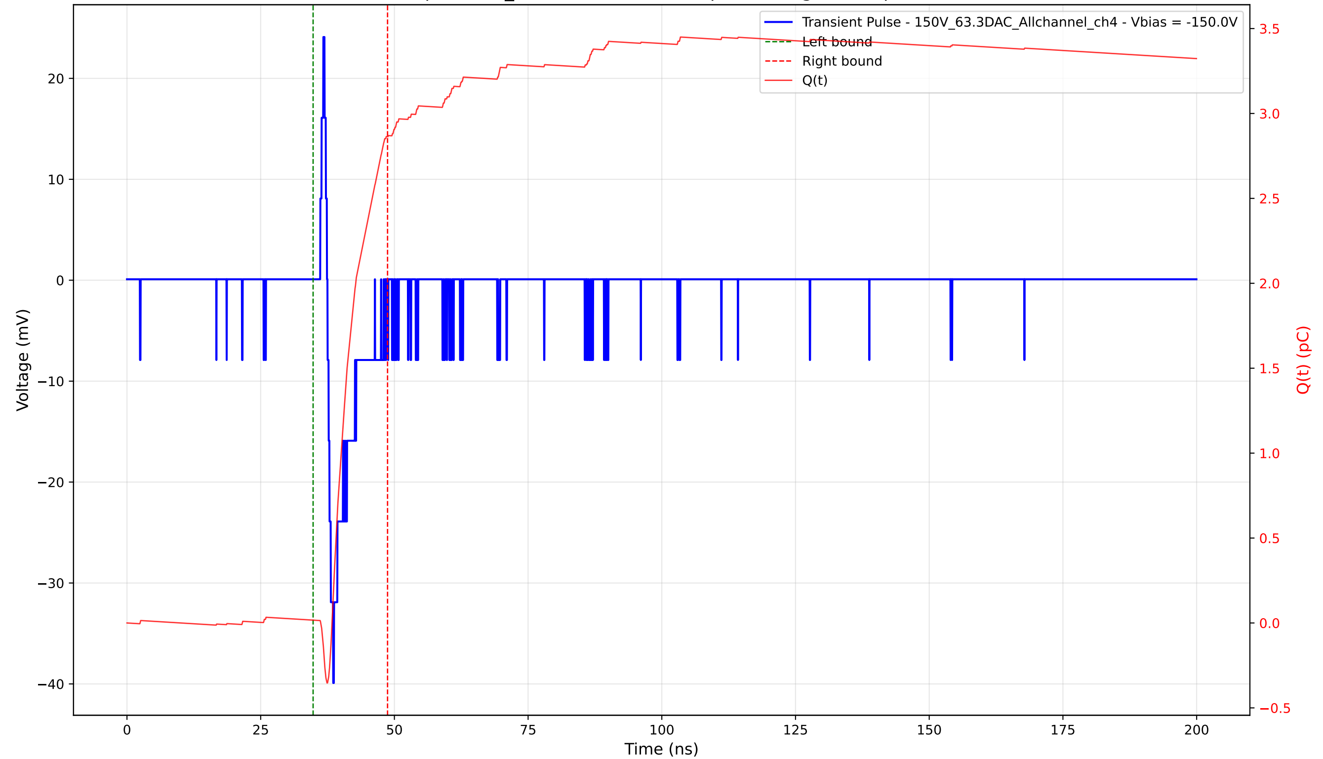
Transient Pulse - Sample: 1cm_42 - Position: 4760.0 \mu\text{m} - Charge: 2.85 pC - Rise Time: 1.06 ns
