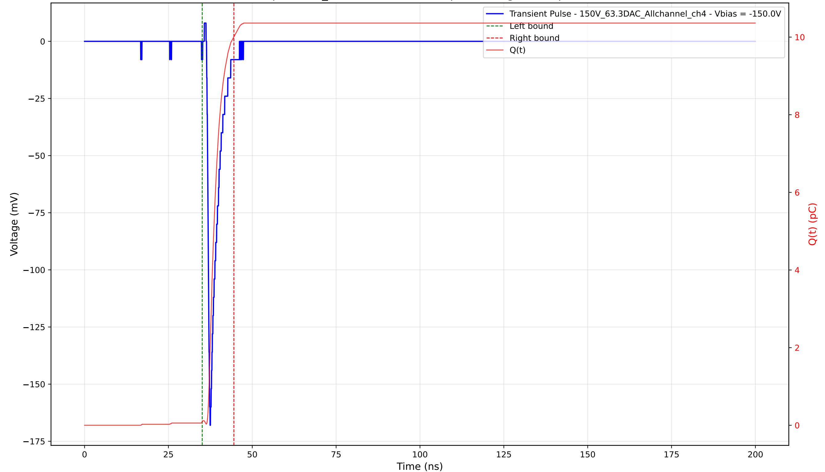
Transient Pulse - Sample: 1cm_42 - Position: 1195.0 \mu\text{m} - Charge: 9.91 pC - Rise Time: 0.76 ns
