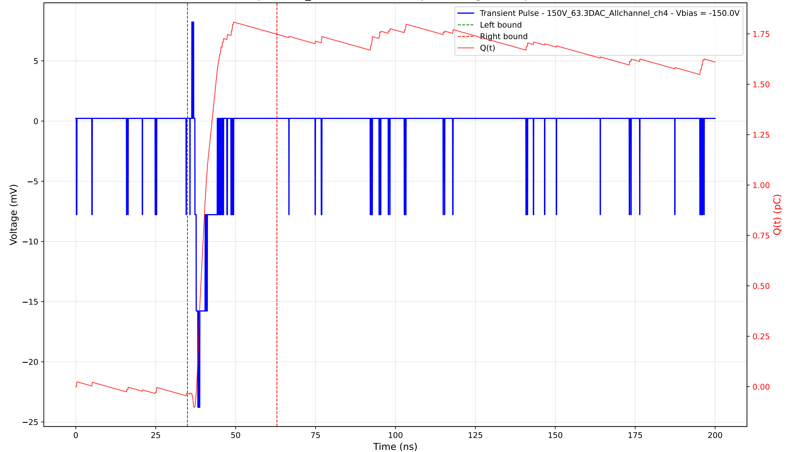
Transient Pulse - Sample: 1cm_42 - Position: 155.0 \mu\text{m} - Charge: 1.78 pC - Rise Time: 0.95 ns
