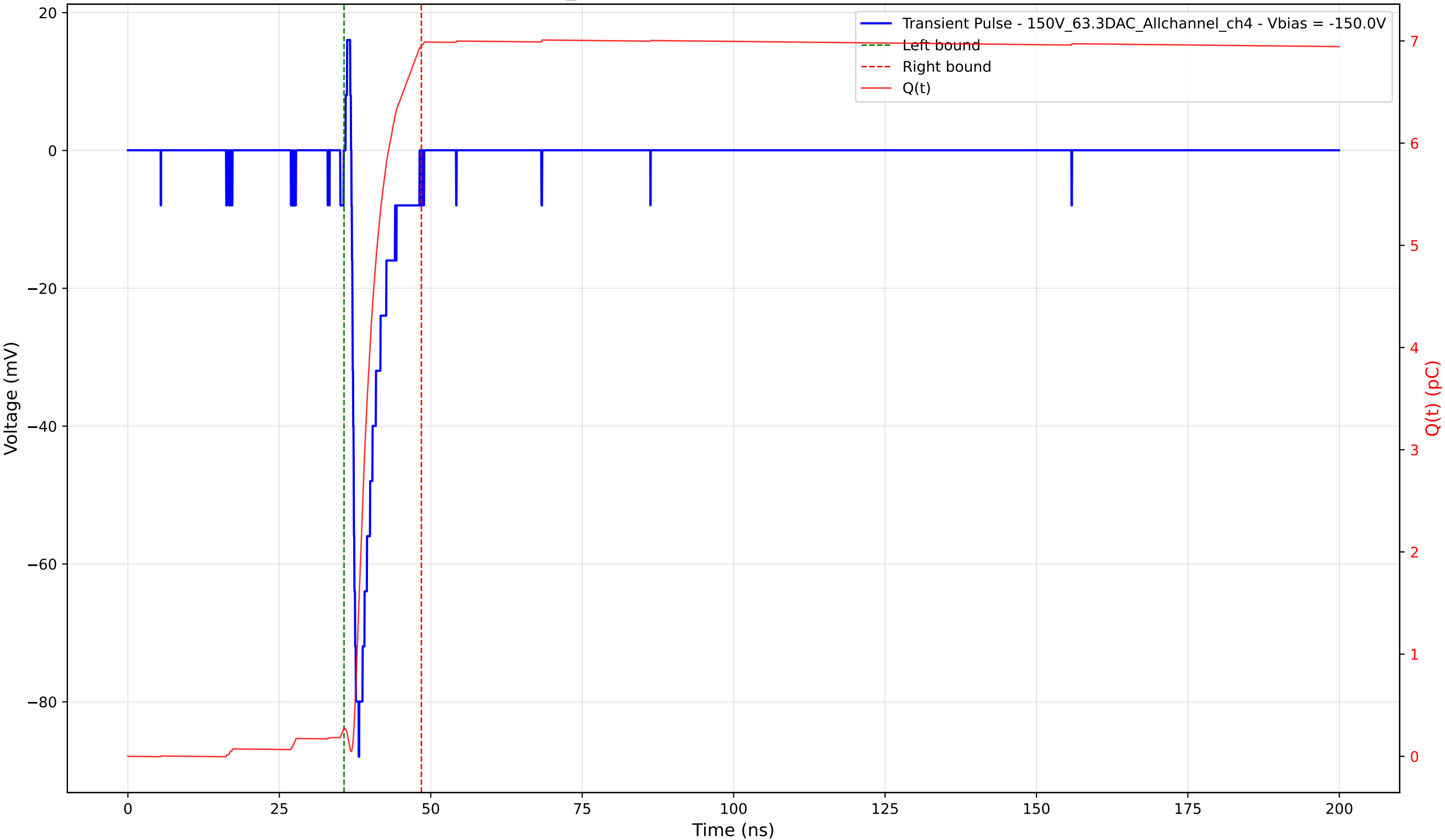
Transient Pulse - Sample: 1cm_42 - Position: 890.0 \mu\text{m} - Charge: 6.68 pC - Rise Time: 0.68 ns
