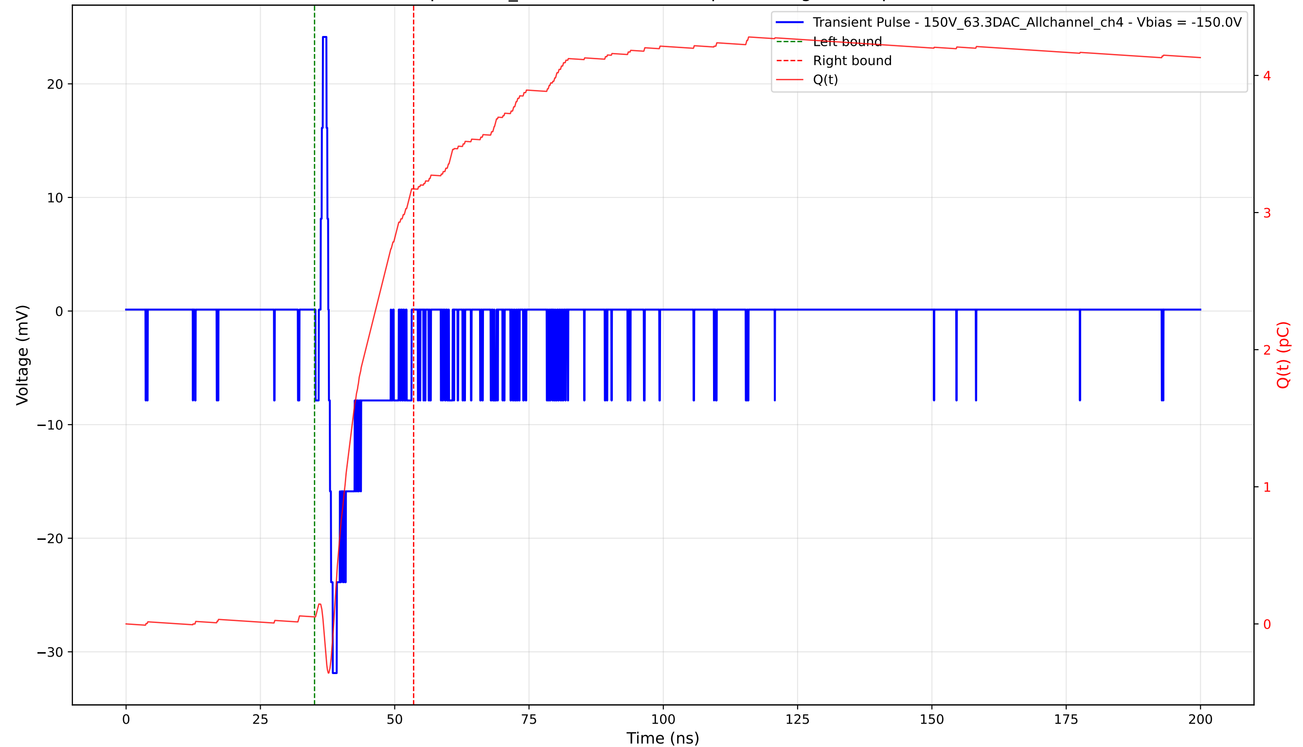
Transient Pulse - Sample: 1cm_42 - Position: 4125.0 \mu\text{m} - Charge: 3.12 pC - Rise Time: 0.74 ns
