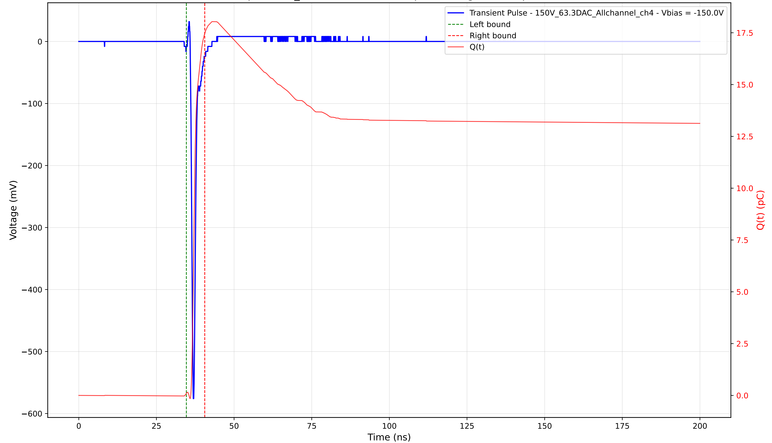
Transient Pulse - Sample: 1cm_42 - Position: 2060.0 \mu\text{m} - Charge: 17.36 pC - Rise Time: 0.69 ns
