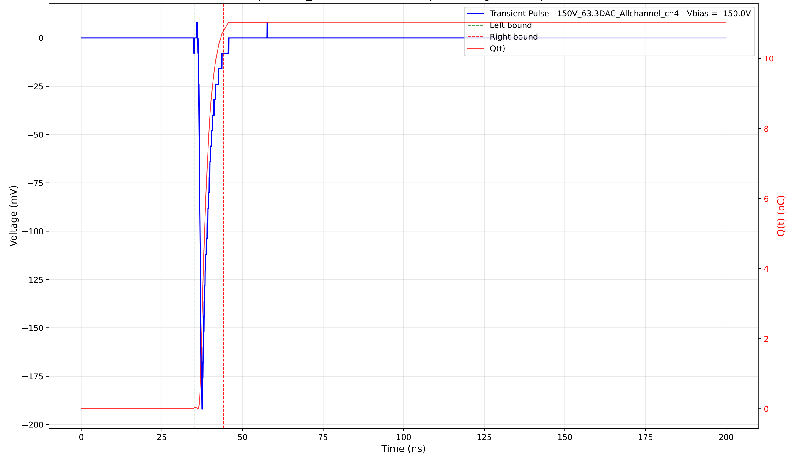
Transient Pulse - Sample: 1cm_42 - Position: 1320.0 \mu\text{m} - Charge: 10.79 pC - Rise Time: 0.82 ns
