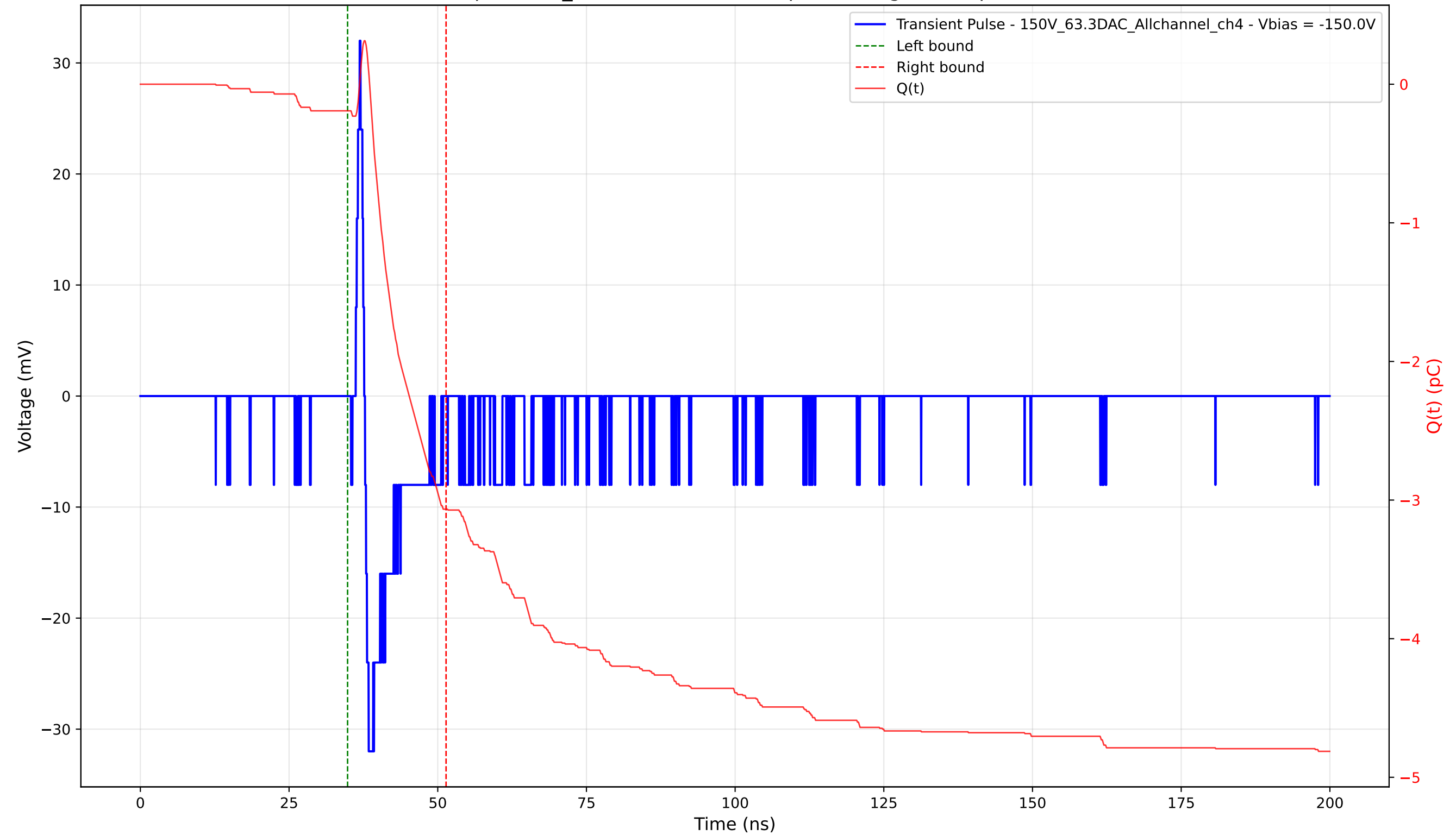
Transient Pulse - Sample: 1cm_42 - Position: 4185.0 \mu\text{m} - Charge: 2.87 pC - Rise Time: 0.66 ns
