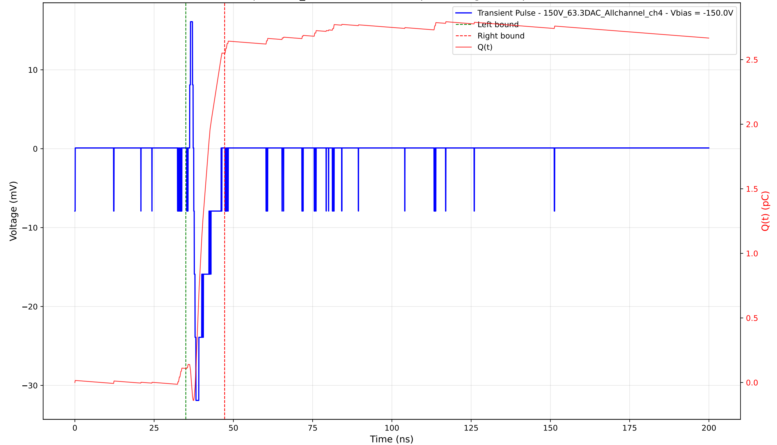
Transient Pulse - Sample: 1cm_42 - Position: 4895.0 \mu\text{m} - Charge: 2.44 pC - Rise Time: 0.70 ns
