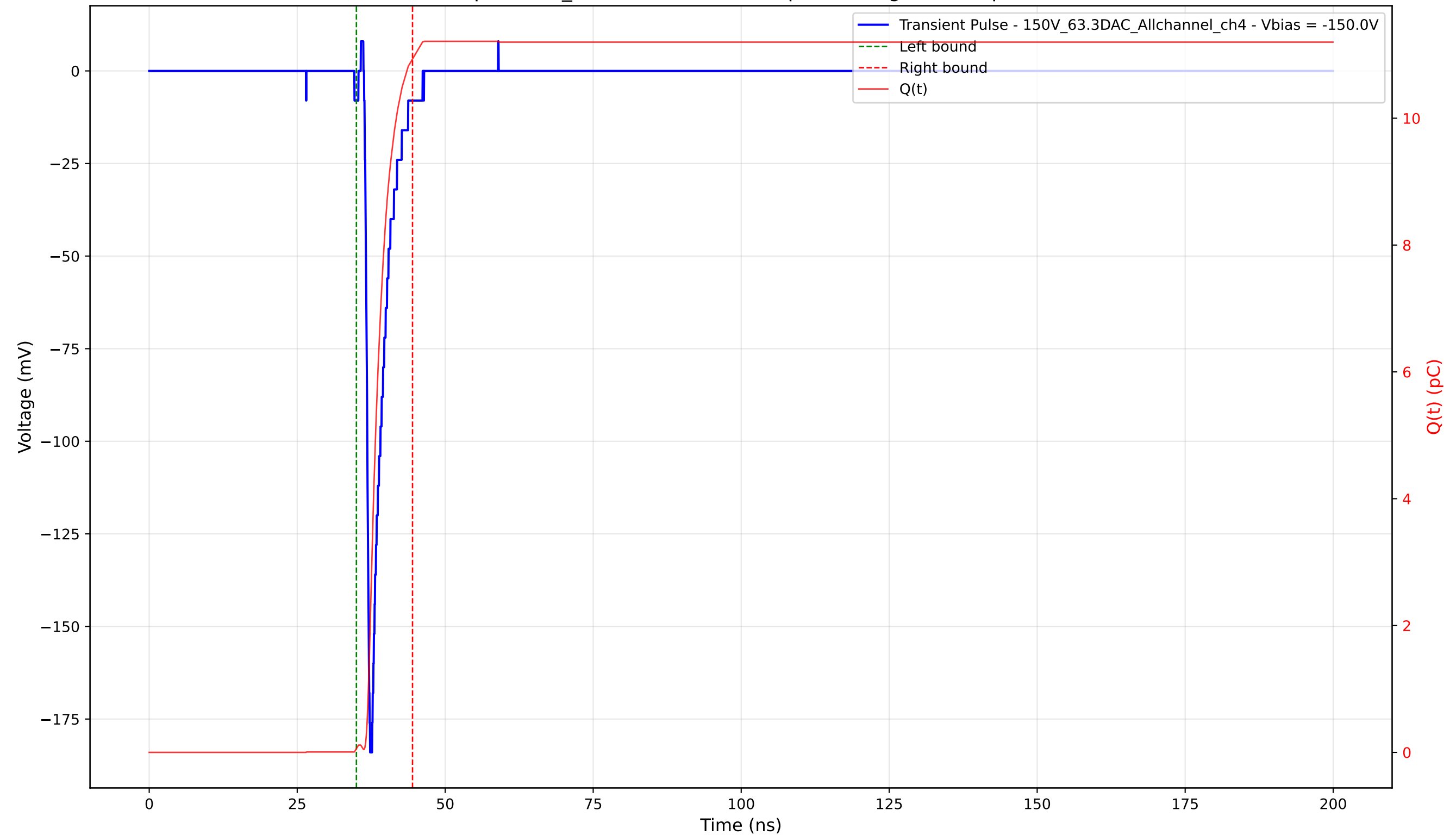
Transient Pulse - Sample: 1cm_42 - Position: 1270.0 \mu\text{m} - Charge: 10.87 pC - Rise Time: 0.75 ns
