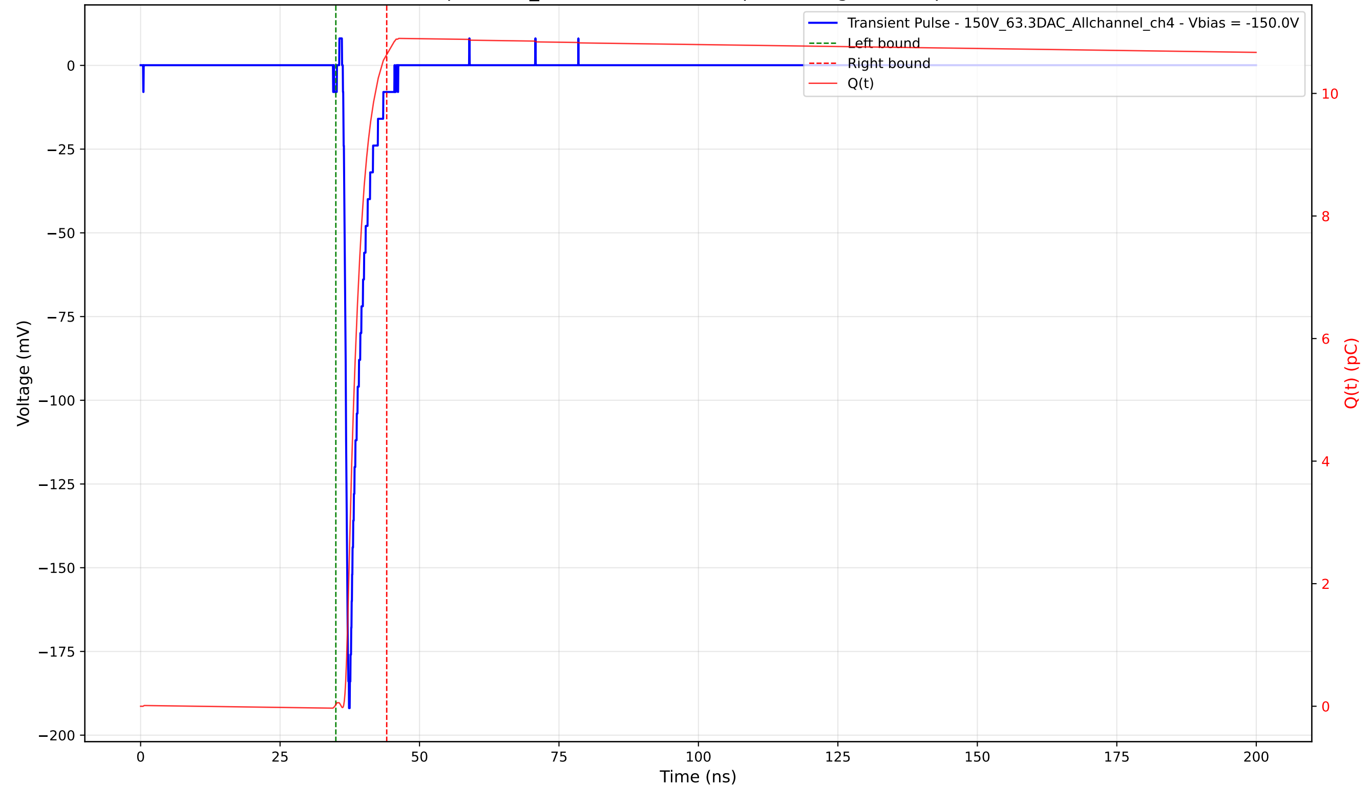
Transient Pulse - Sample: 1cm_42 - Position: 1335.0 \mu\text{m} - Charge: 10.61 pC - Rise Time: 0.78 ns
