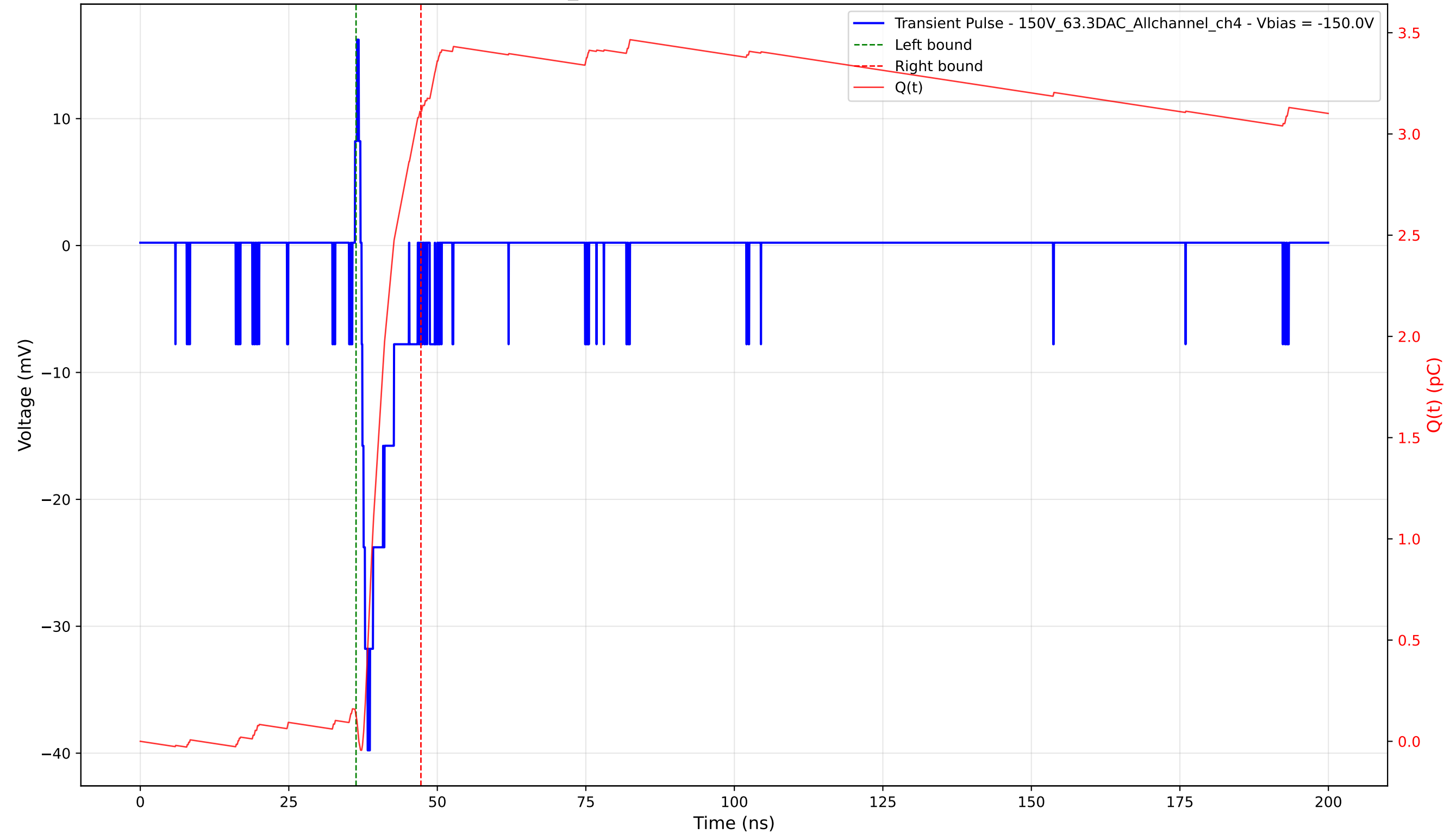
Transient Pulse - Sample: 1cm_42 - Position: 330.0 \mu\text{m} - Charge: 2.98 pC - Rise Time: 1.02 ns
