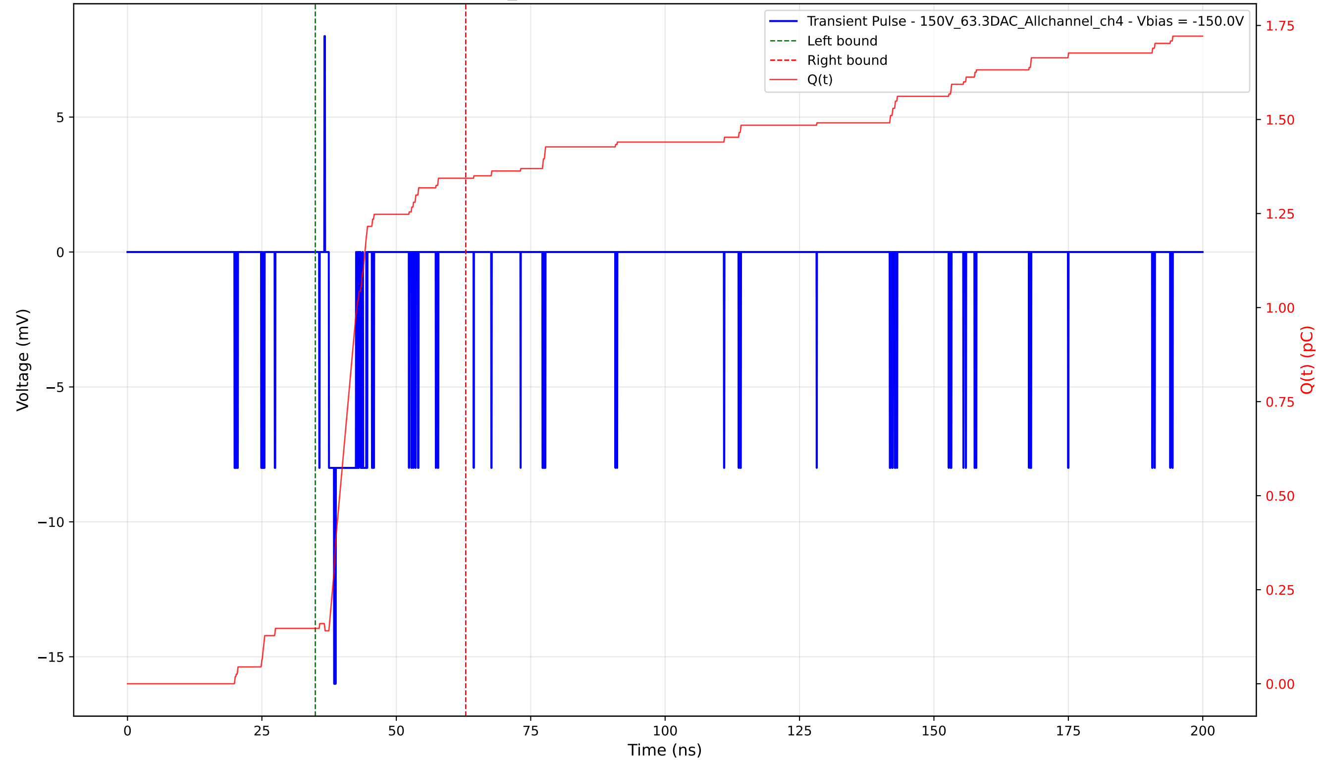
Transient Pulse - Sample: 1cm_42 - Position: 5105.0 \mu\text{m} - Charge: 1.20 pC - Rise Time: 0.99 ns
