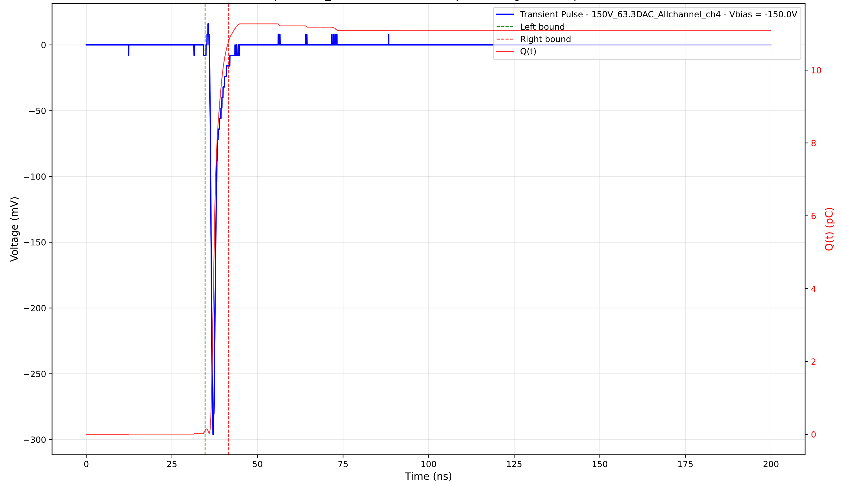
Transient Pulse - Sample: 1cm_42 - Position: 2455.0 \mu\text{m} - Charge: 10.70 pC - Rise Time: 0.74 ns
