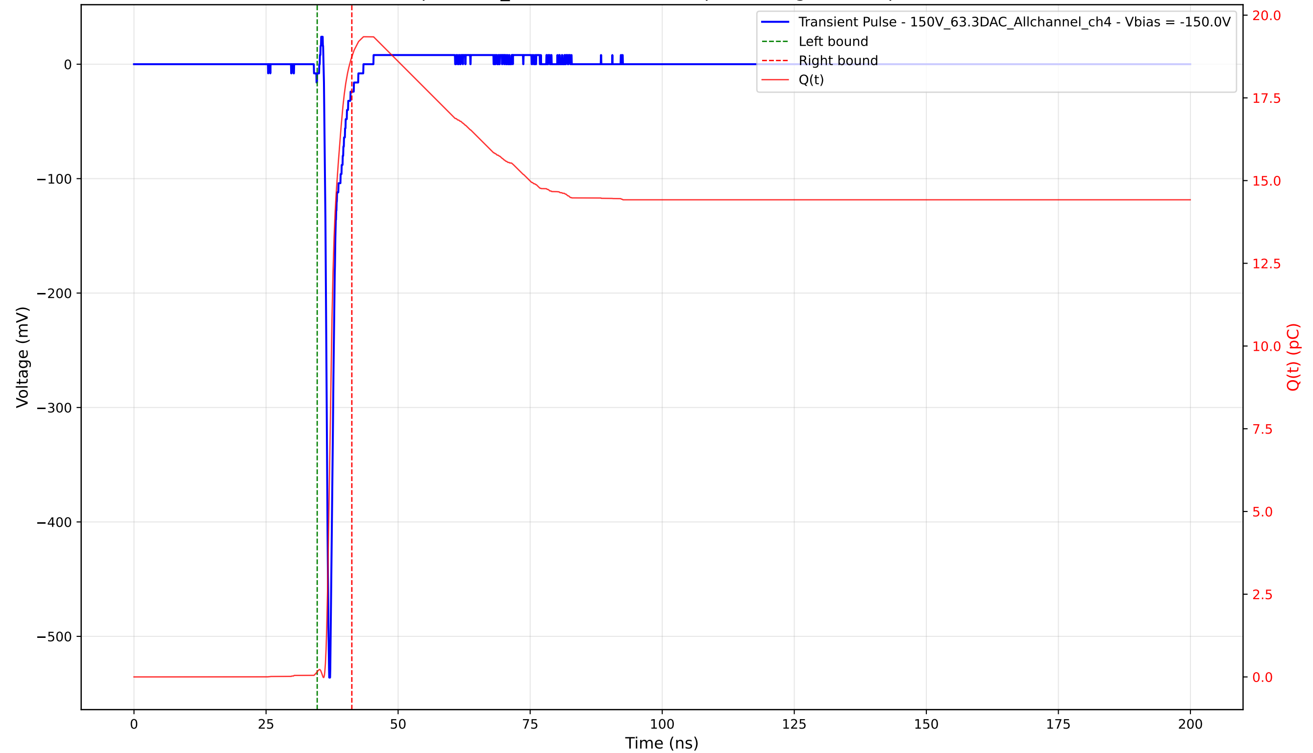
Transient Pulse - Sample: 1cm_42 - Position: 1715.0 \mu\text{m} - Charge: 18.58 pC - Rise Time: 0.73 ns
