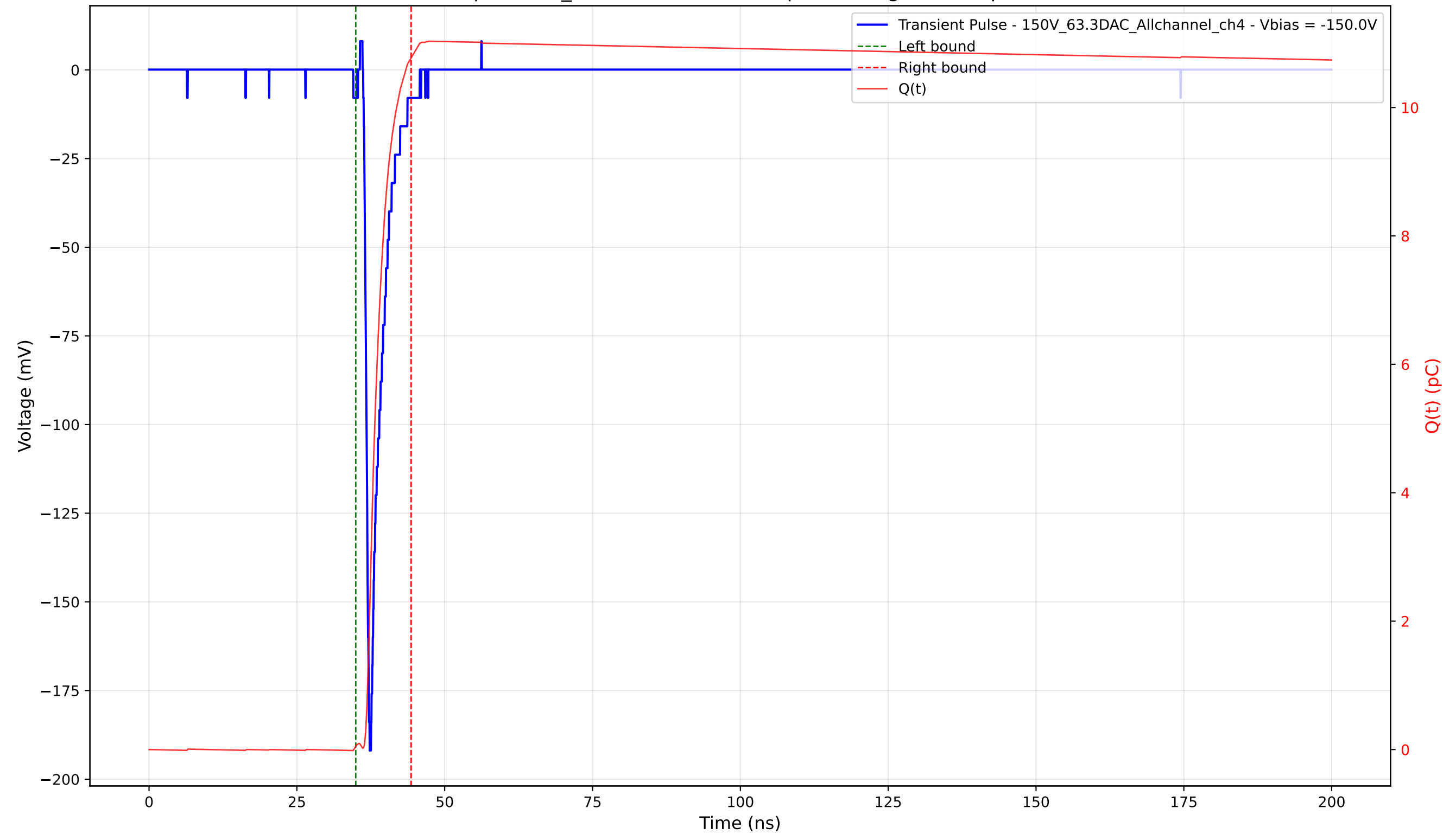
Transient Pulse - Sample: 1cm_42 - Position: 1345.0 \mu\text{m} - Charge: 10.72 pC - Rise Time: 0.77 ns
