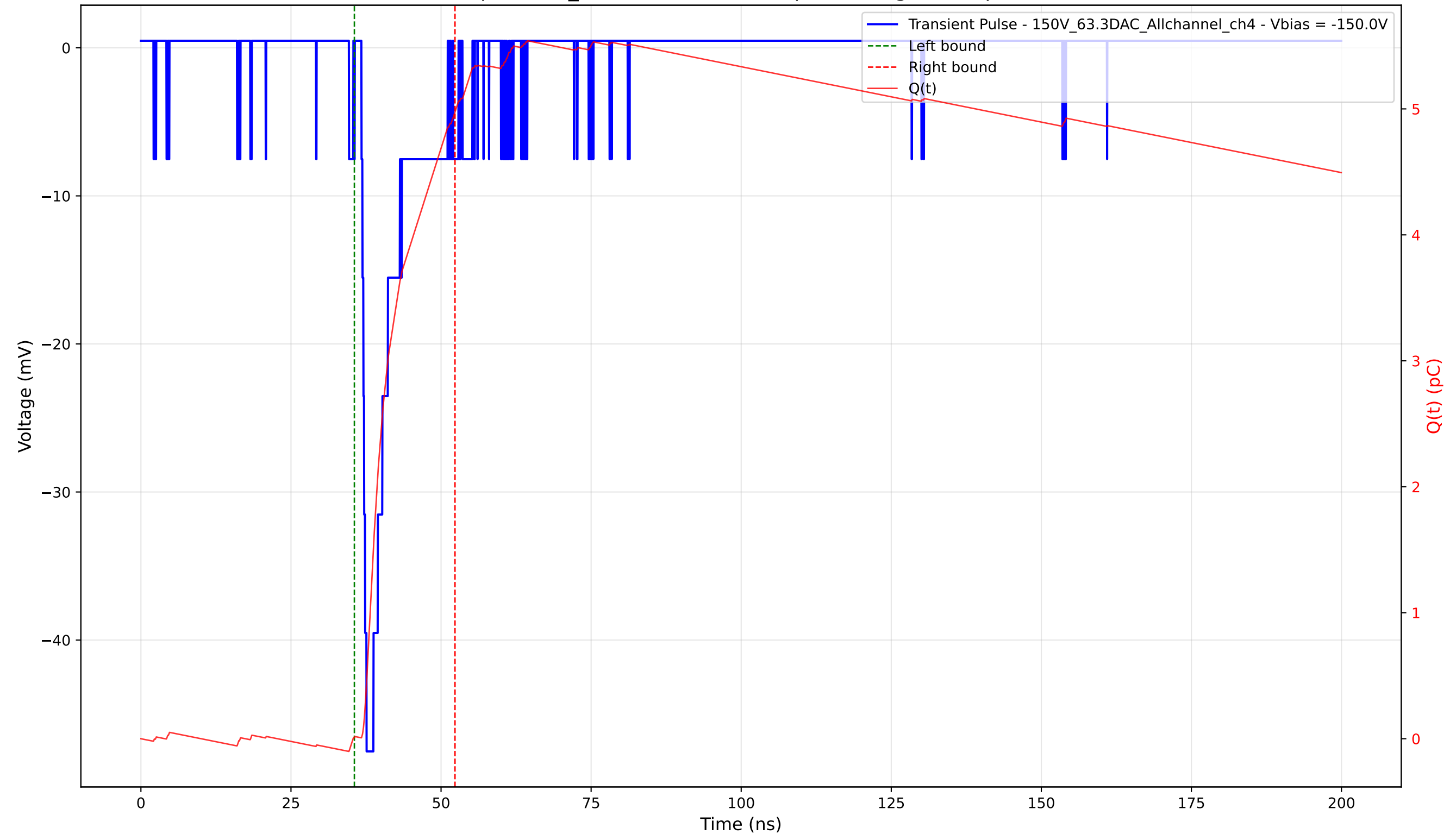
Transient Pulse - Sample: 1cm_42 - Position: 3145.0 \mu\text{m} - Charge: 4.97 pC - Rise Time: 0.86 ns
