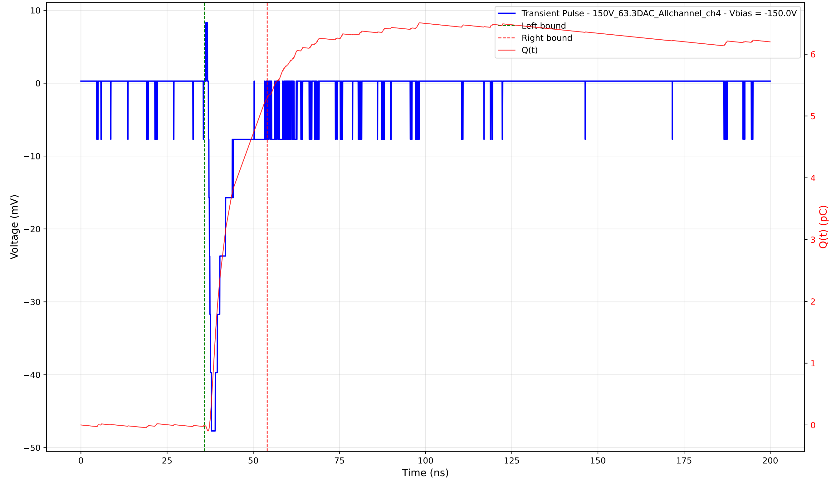
Transient Pulse - Sample: 1cm_42 - Position: 3225.0 \mu\text{m} - Charge: 5.31 pC - Rise Time: 0.90 ns
