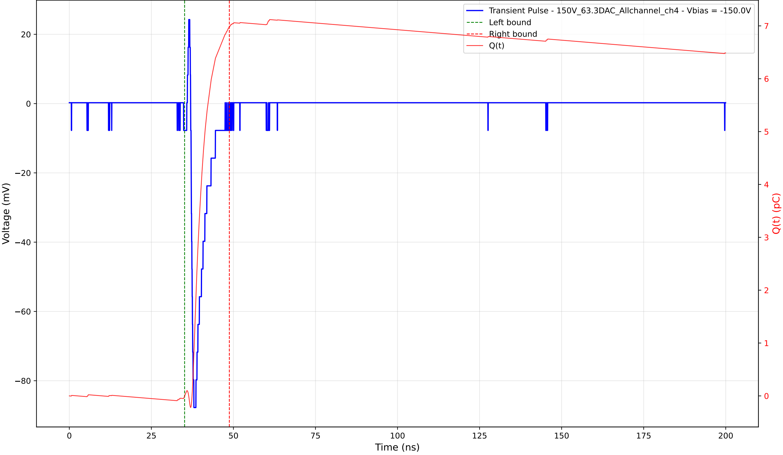
Transient Pulse - Sample: 1cm_42 - Position: 770.0 \mu\text{m} - Charge: 6.99 pC - Rise Time: 0.63 ns
