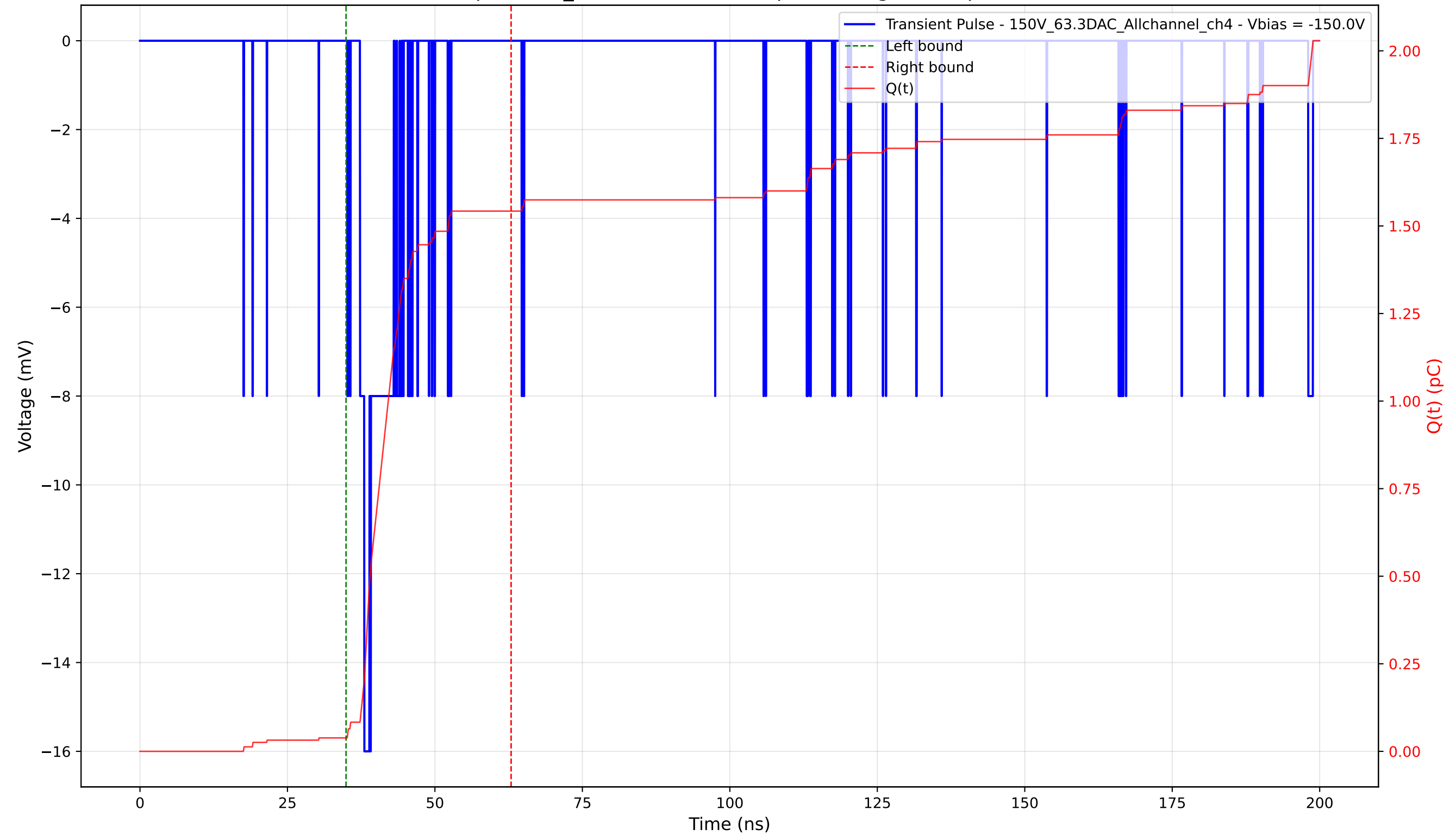
Transient Pulse - Sample: 1cm_42 - Position: 110.0 \mu\text{m} - Charge: 1.50 pC - Rise Time: 0.75 ns
