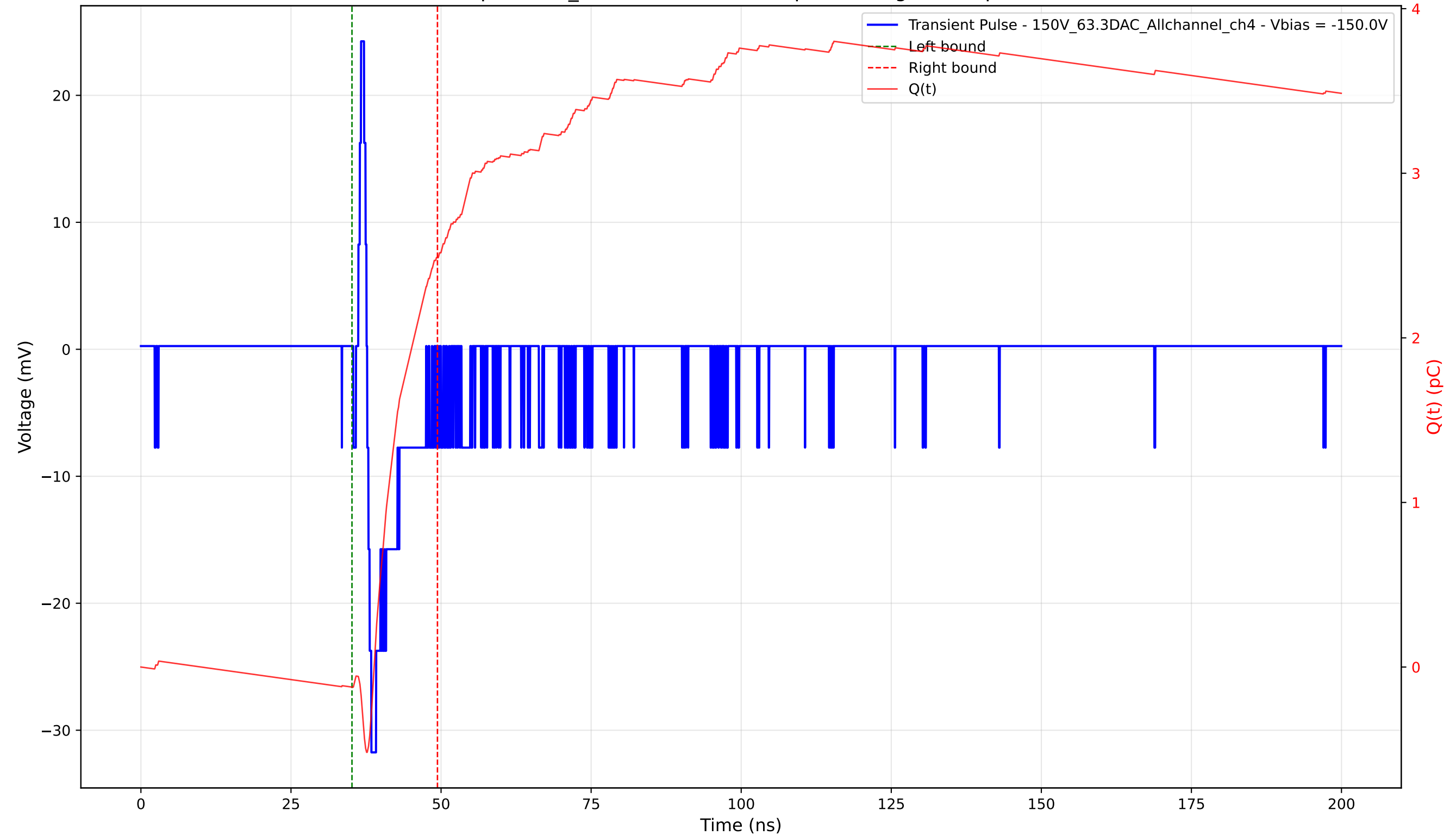
Transient Pulse - Sample: 1cm_42 - Position: 3960.0 \mu\text{m} - Charge: 2.61 pC - Rise Time: 0.70 ns
