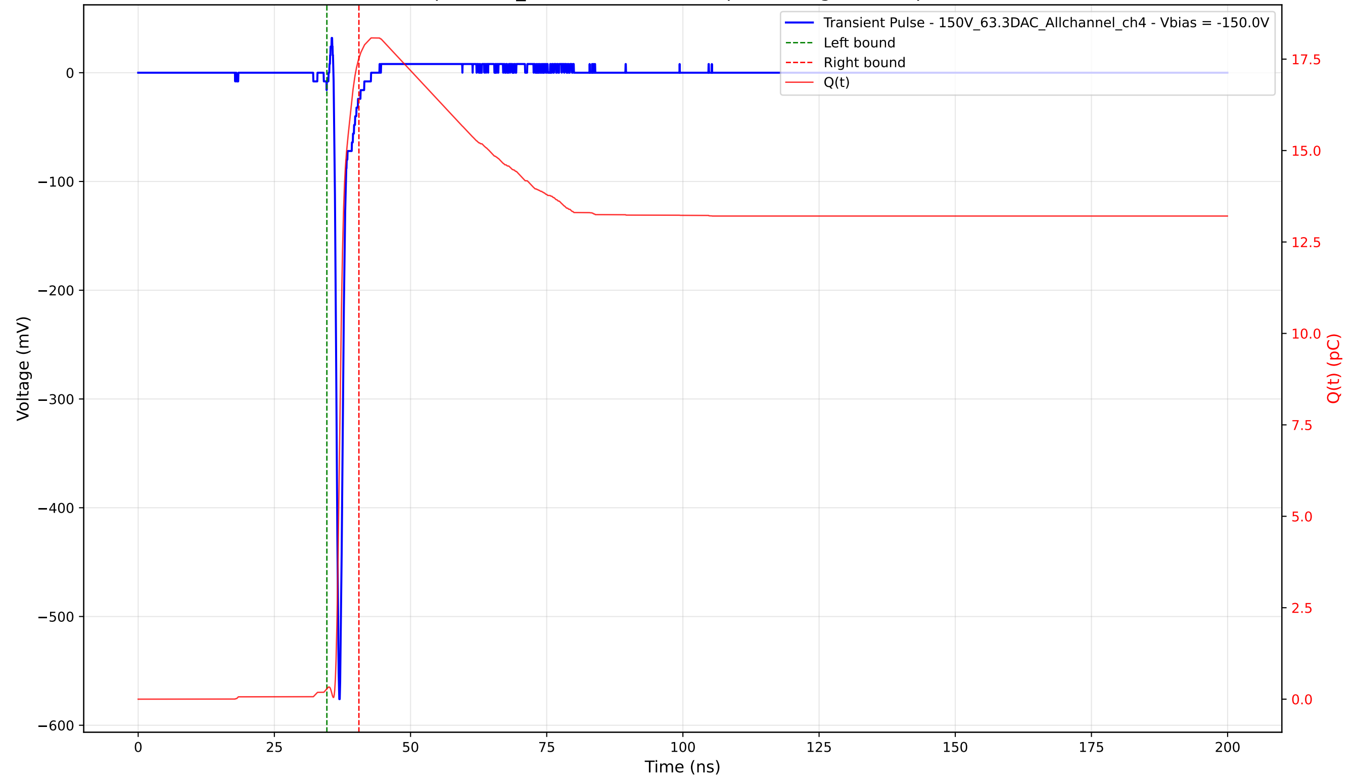
Transient Pulse - Sample: 1cm_42 - Position: 2090.0 \mu\text{m} - Charge: 17.24 pC - Rise Time: 0.71 ns
