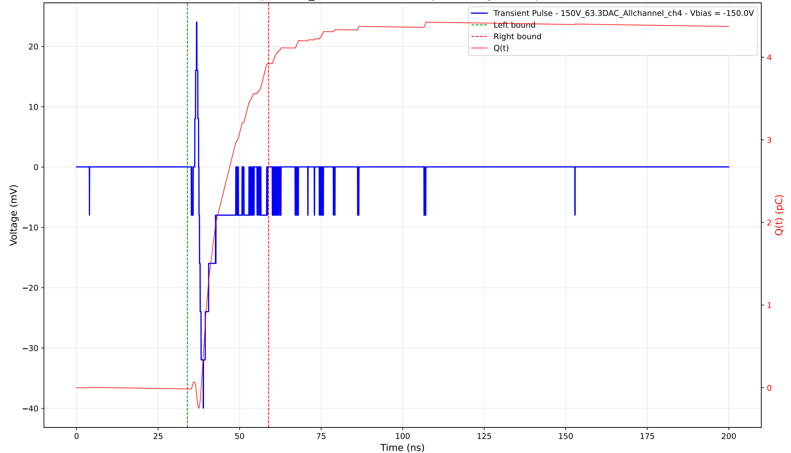
Transient Pulse - Sample: 1cm_42 - Position: 3620.0 \mu\text{m} - Charge: 3.94 pC - Rise Time: 1.34 ns
