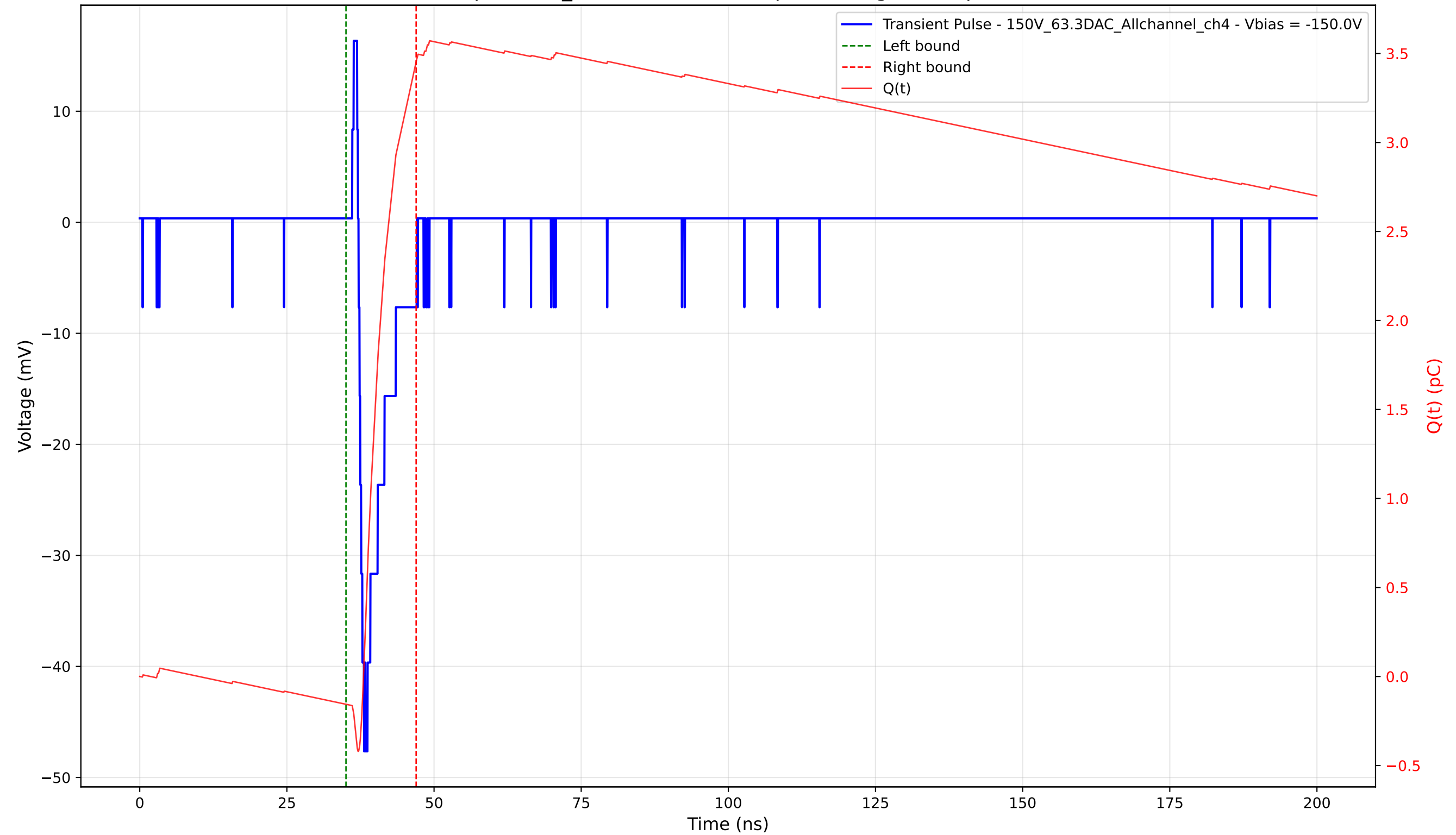
Transient Pulse - Sample: 1cm_42 - Position: 420.0 \mu\text{m} - Charge: 3.61 pC - Rise Time: 0.94 ns
