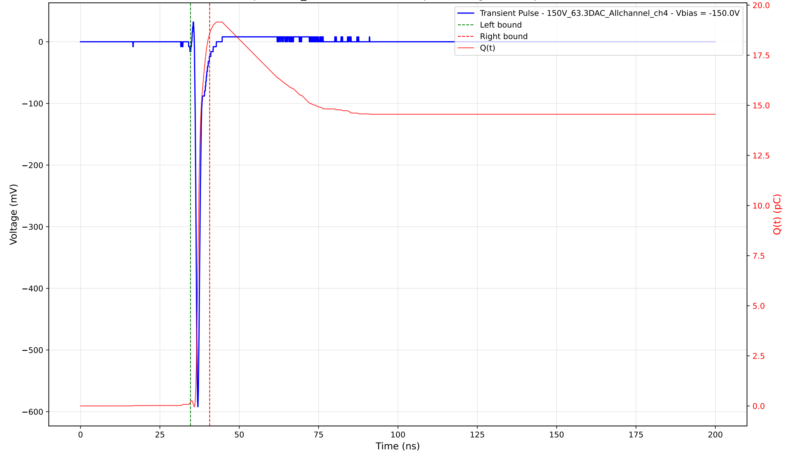
Transient Pulse - Sample: 1cm_42 - Position: 1915.0 \mu\text{m} - Charge: 18.38 pC - Rise Time: 0.72 ns
