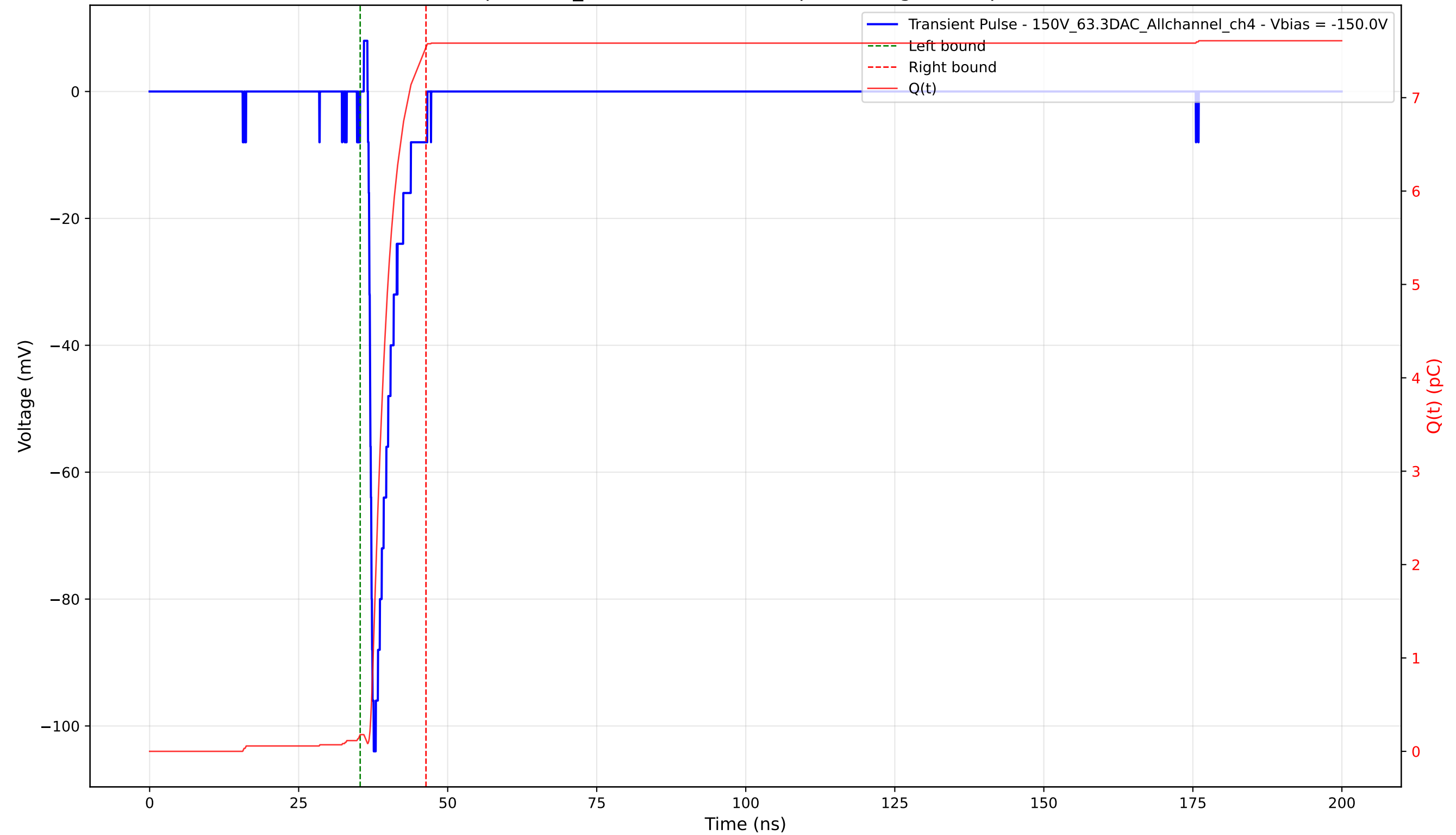
Transient Pulse - Sample: 1cm_42 - Position: 1025.0 \mu\text{m} - Charge: 7.36 pC - Rise Time: 0.67 ns
