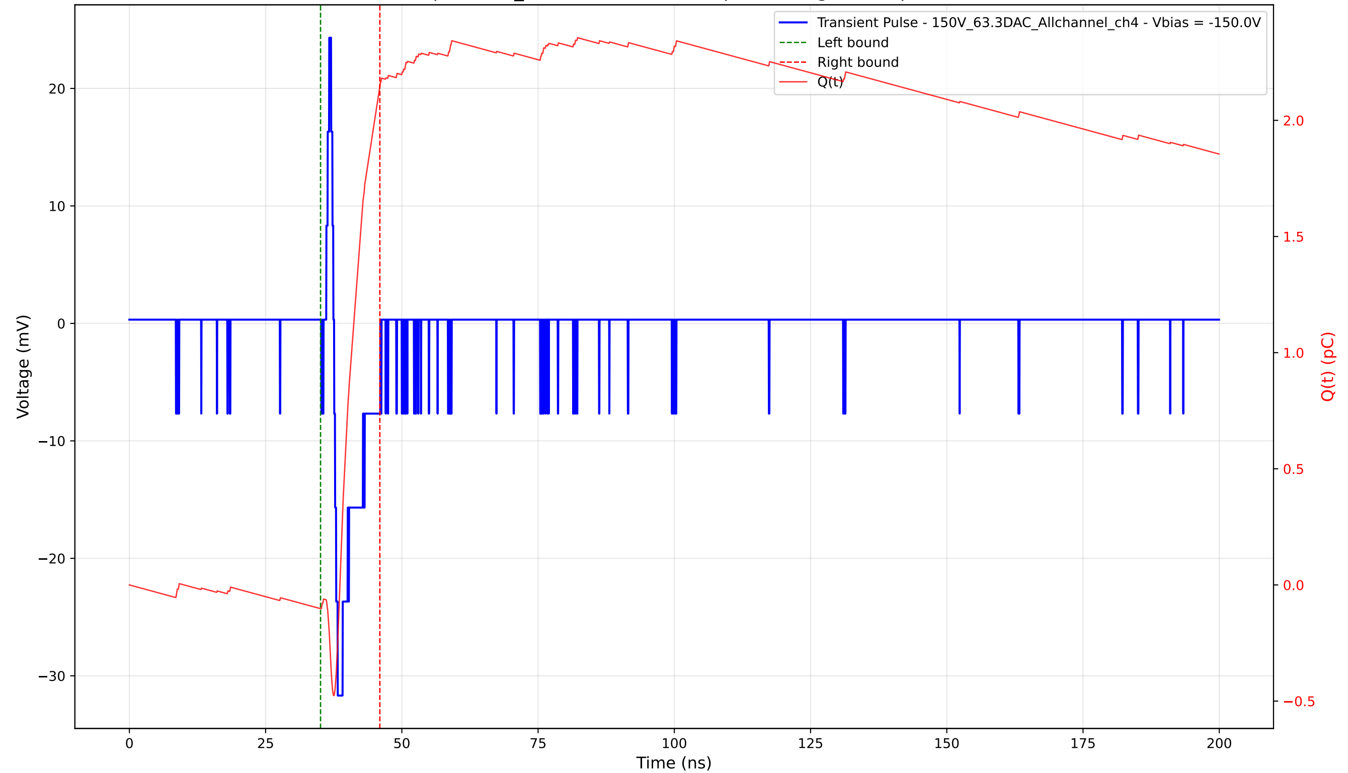
Transient Pulse - Sample: 1cm_42 - Position: 4690.0 \mu\text{m} - Charge: 2.25 pC - Rise Time: 0.66 ns
