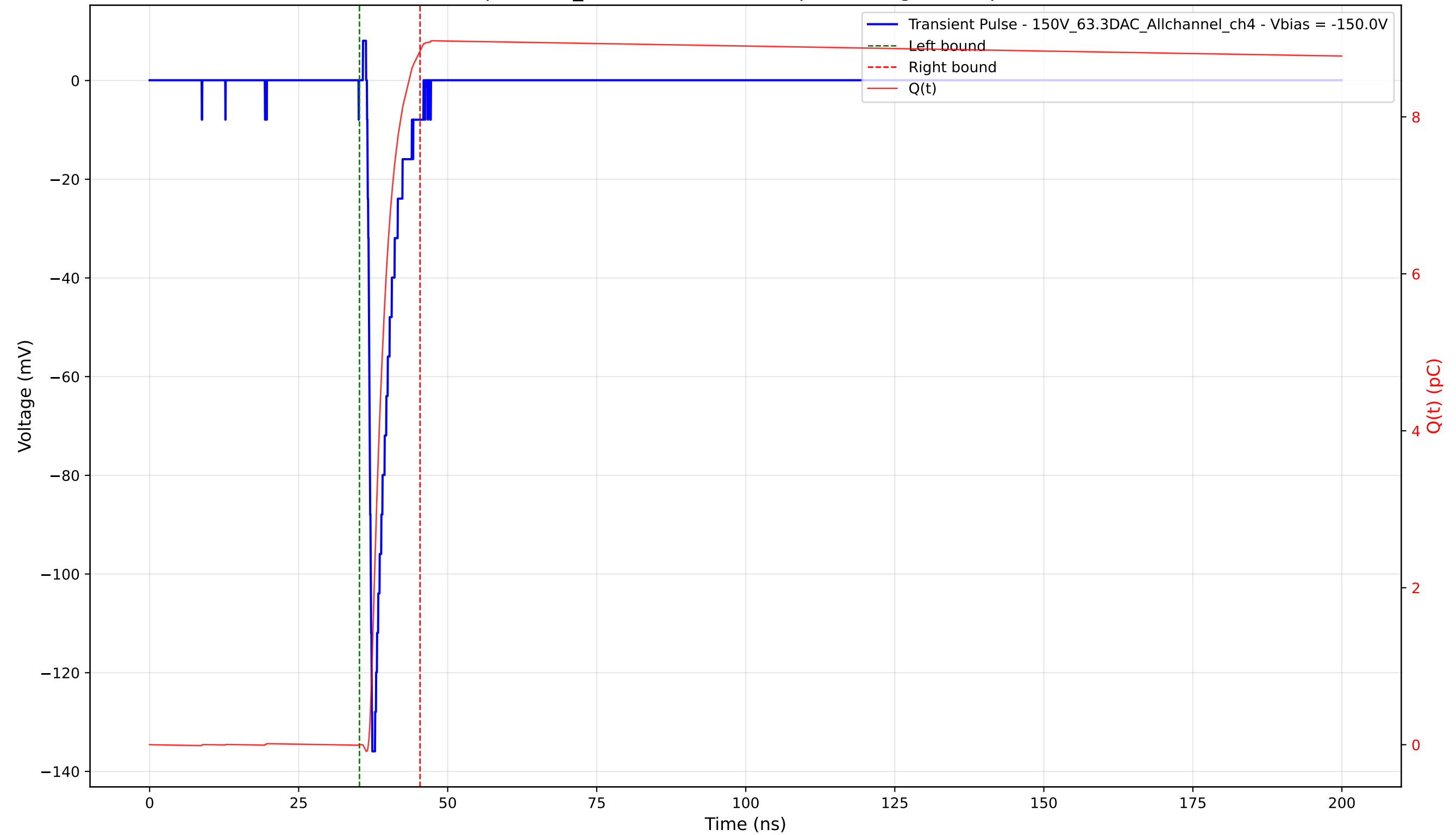
Transient Pulse - Sample: 1cm_42 - Position: 1130.0 \mu\text{m} - Charge: 8.84 pC - Rise Time: 0.73 ns
