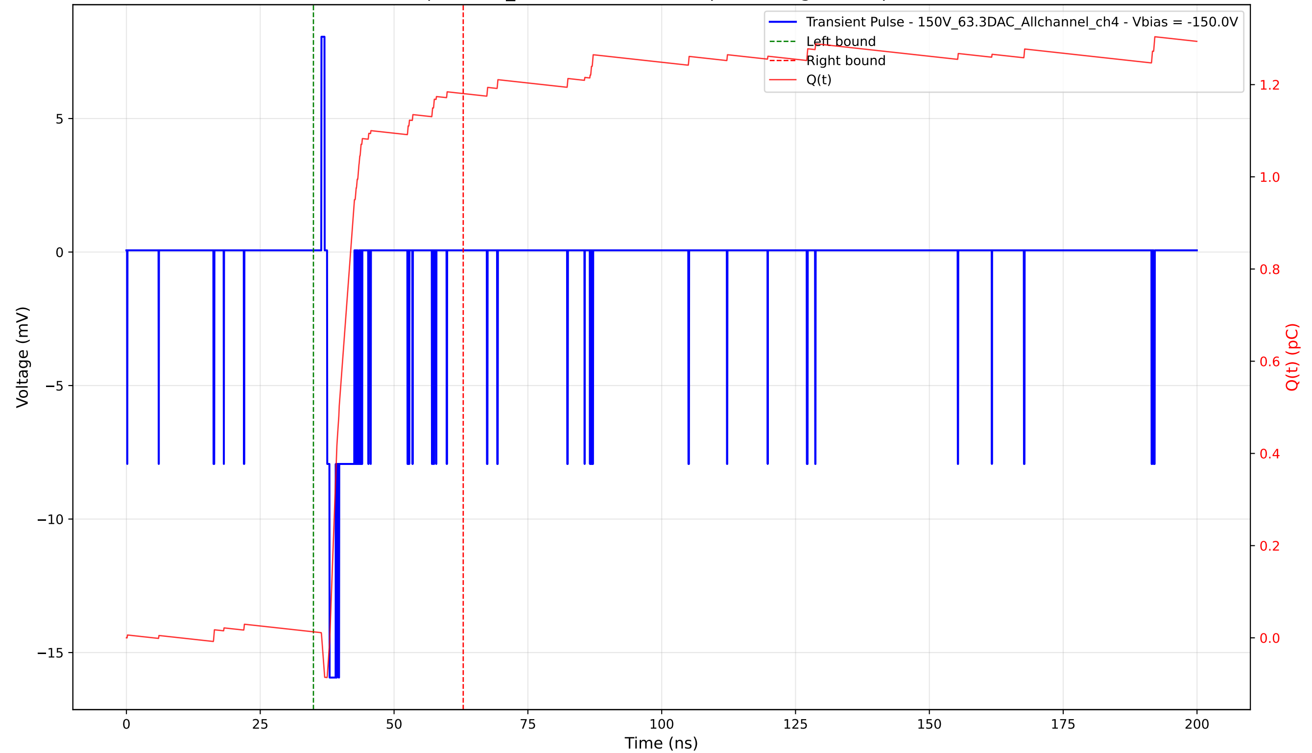
Transient Pulse - Sample: 1cm_42 - Position: 5055.0 \mu\text{m} - Charge: 1.17 pC - Rise Time: 0.47 ns
