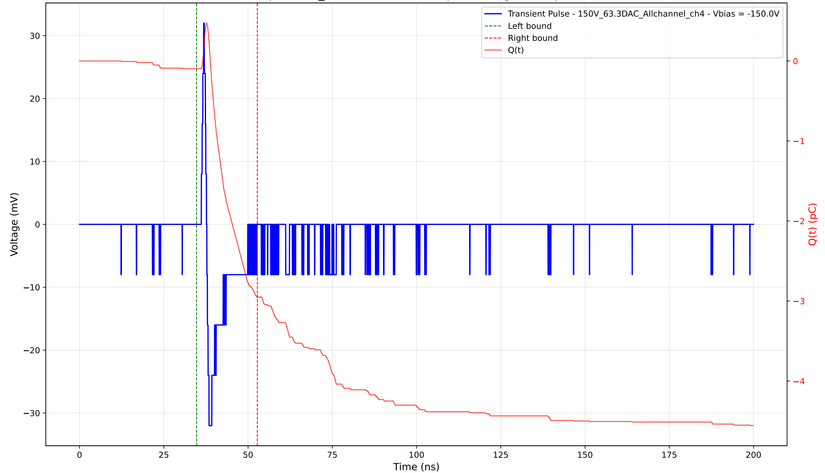
Transient Pulse - Sample: 1cm_42 - Position: 4175.0 \mu\text{m} - Charge: 2.85 pC - Rise Time: 0.70 ns
