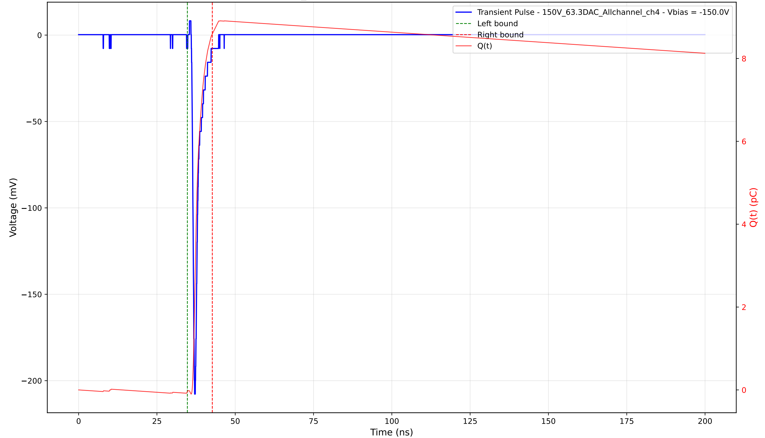
Transient Pulse - Sample: 1cm_42 - Position: 2555.0 \mu\text{m} - Charge: 8.63 pC - Rise Time: 0.75 ns
