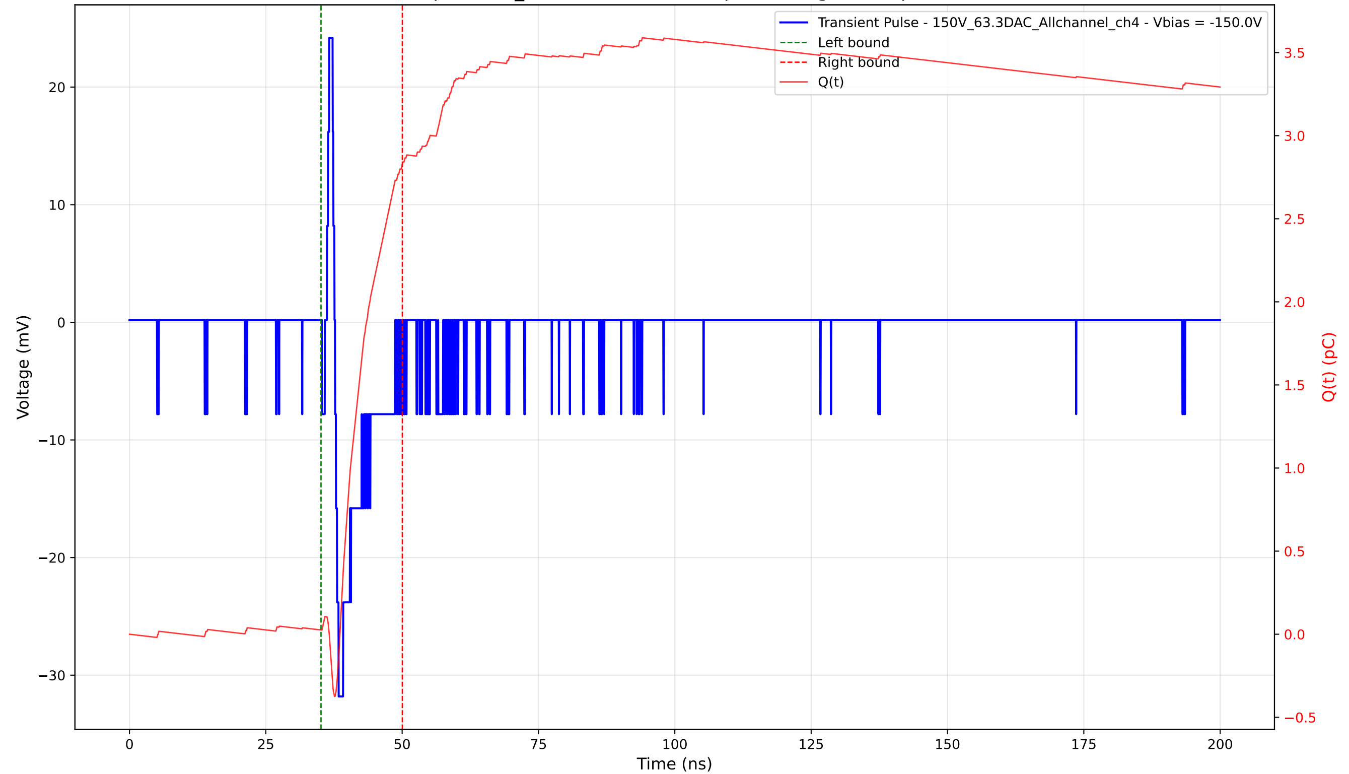
Transient Pulse - Sample: 1cm_42 - Position: 3910.0 \mu\text{m} - Charge: 2.81 pC - Rise Time: 0.66 ns
