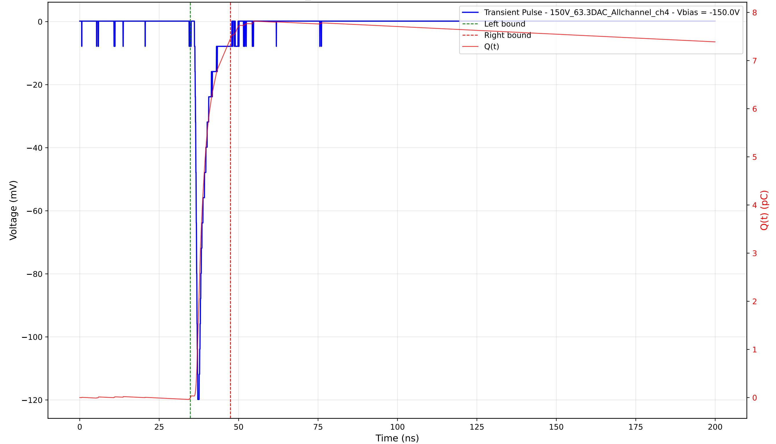
Transient Pulse - Sample: 1cm_42 - Position: 2835.0 \mu\text{m} - Charge: 7.47 pC - Rise Time: 0.82 ns
