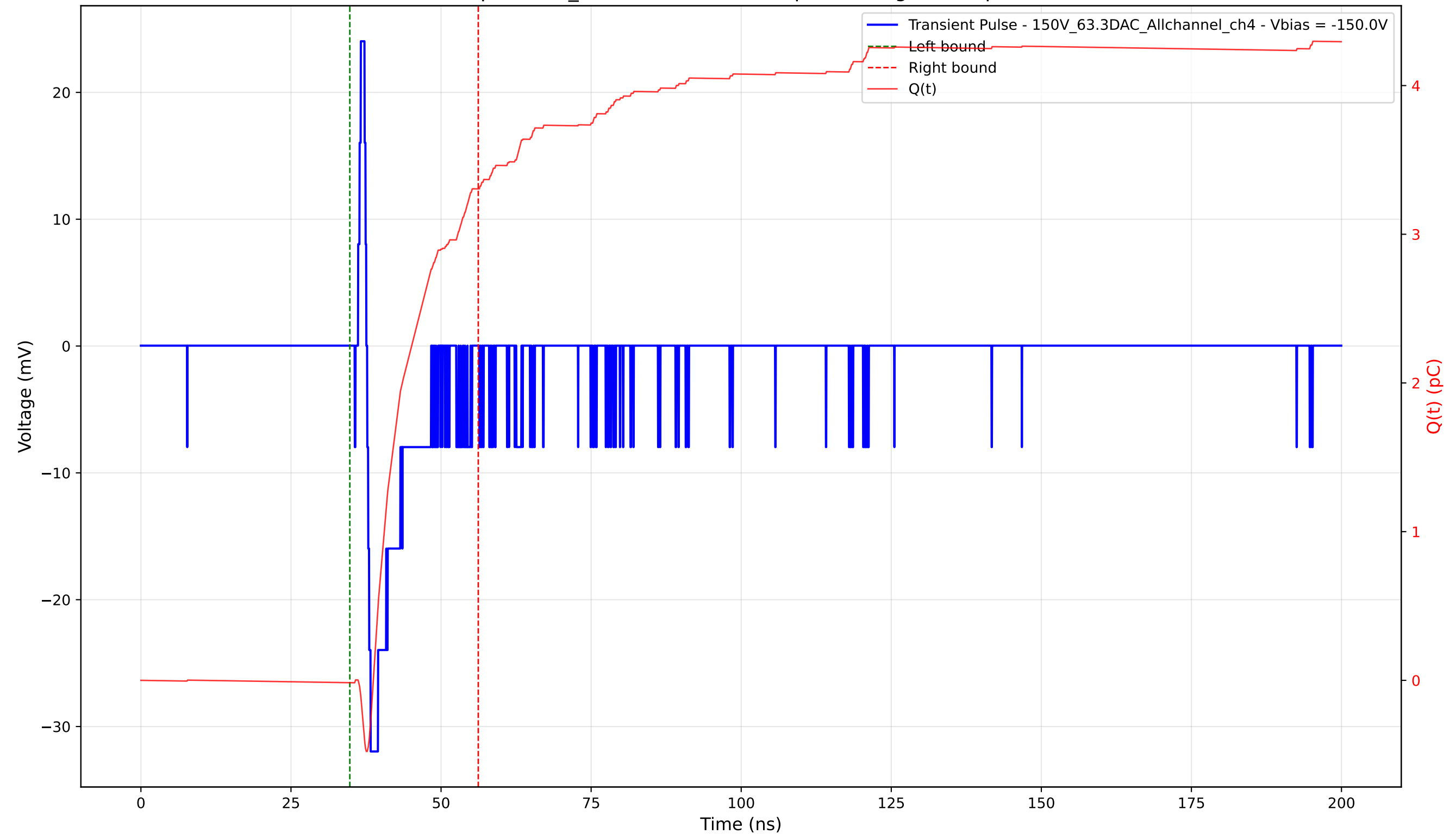
Transient Pulse - Sample: 1cm_42 - Position: 3850.0 \mu\text{m} - Charge: 3.32 pC - Rise Time: 0.58 ns
