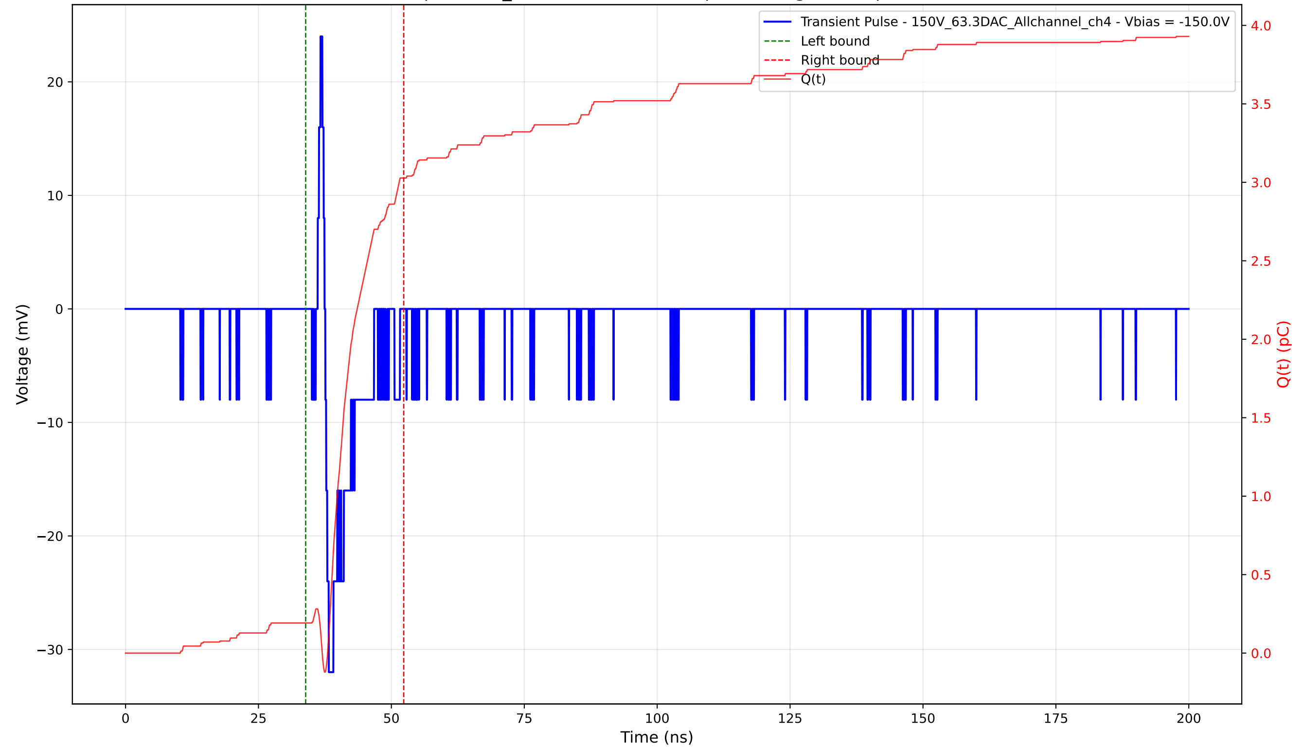
Transient Pulse - Sample: 1cm_42 - Position: 4660.0 \mu\text{m} - Charge: 2.84 pC - Rise Time: 0.66 ns
