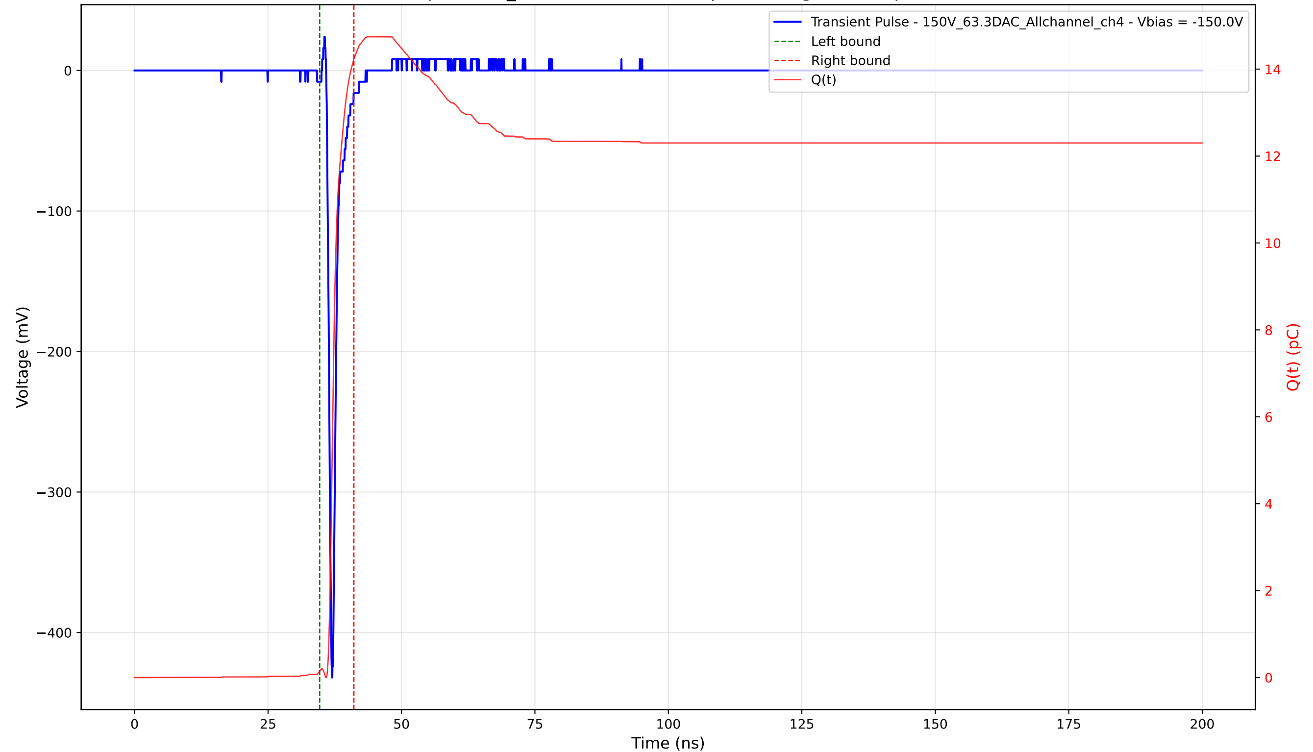
Transient Pulse - Sample: 1cm_42 - Position: 2350.0 \mu\text{m} - Charge: 14.08 pC - Rise Time: 0.74 ns
