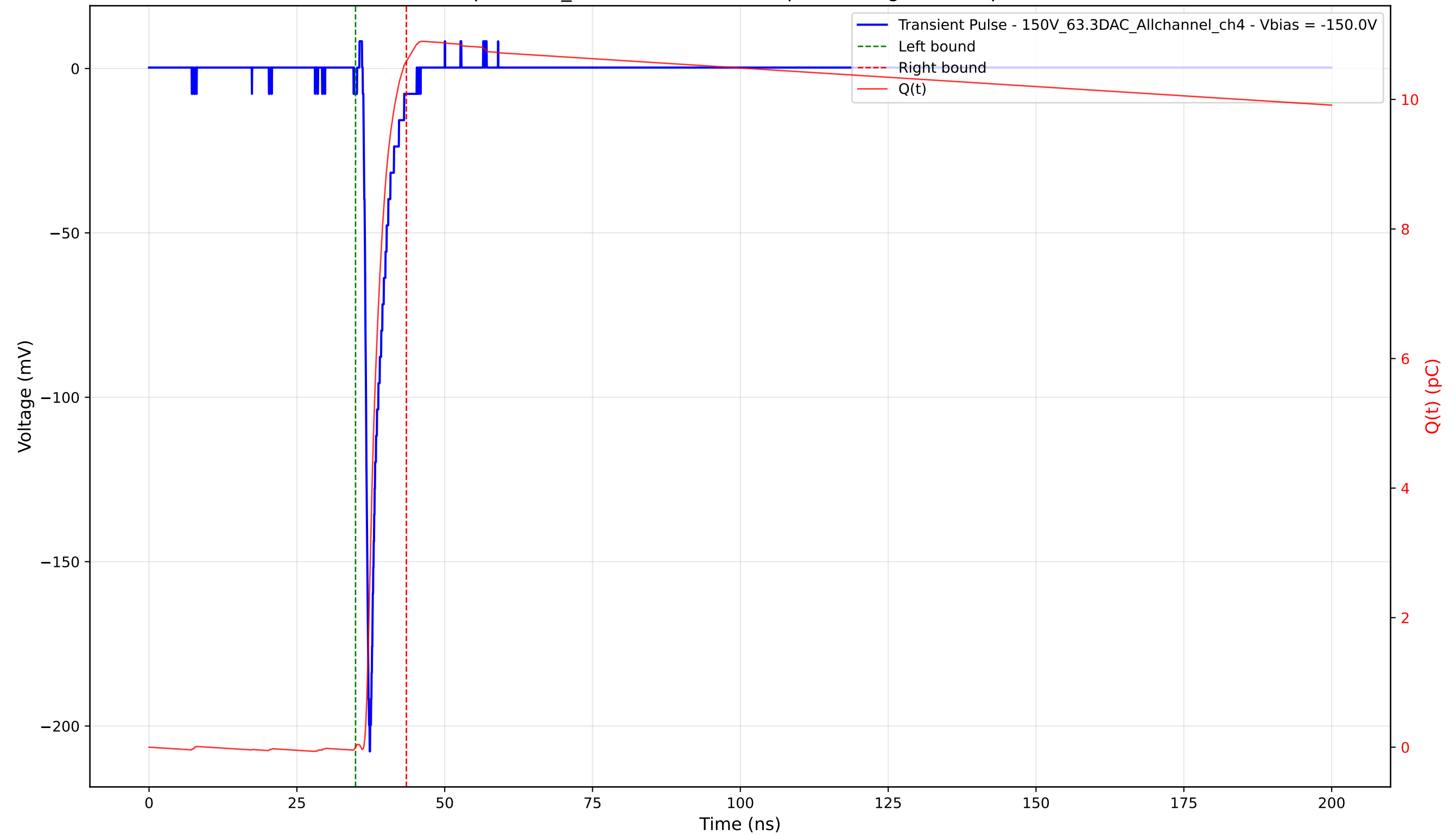
Transient Pulse - Sample: 1cm_42 - Position: 1405.0 \mu\text{m} - Charge: 10.59 pC - Rise Time: 0.81 ns
