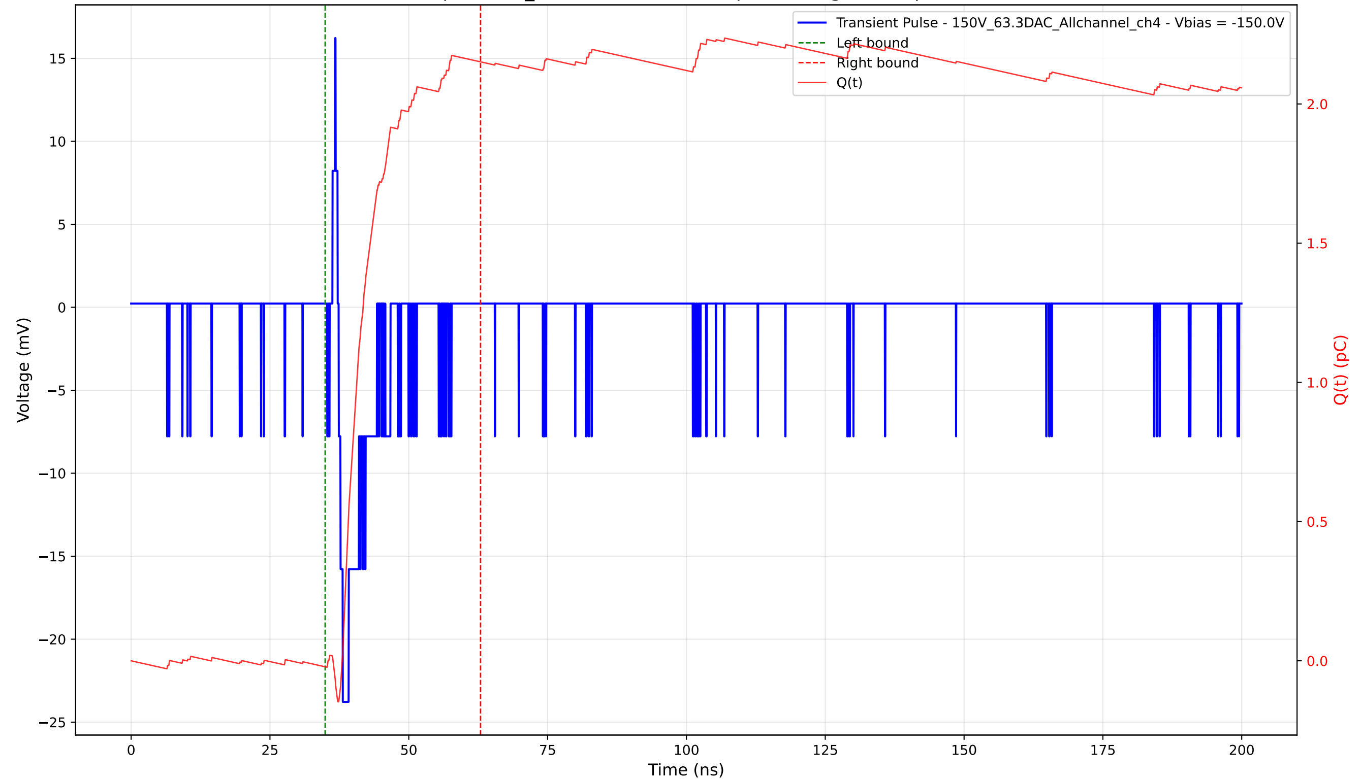
Transient Pulse - Sample: 1cm_42 - Position: 4990.0 \mu\text{m} - Charge: 2.17 pC - Rise Time: 0.75 ns
