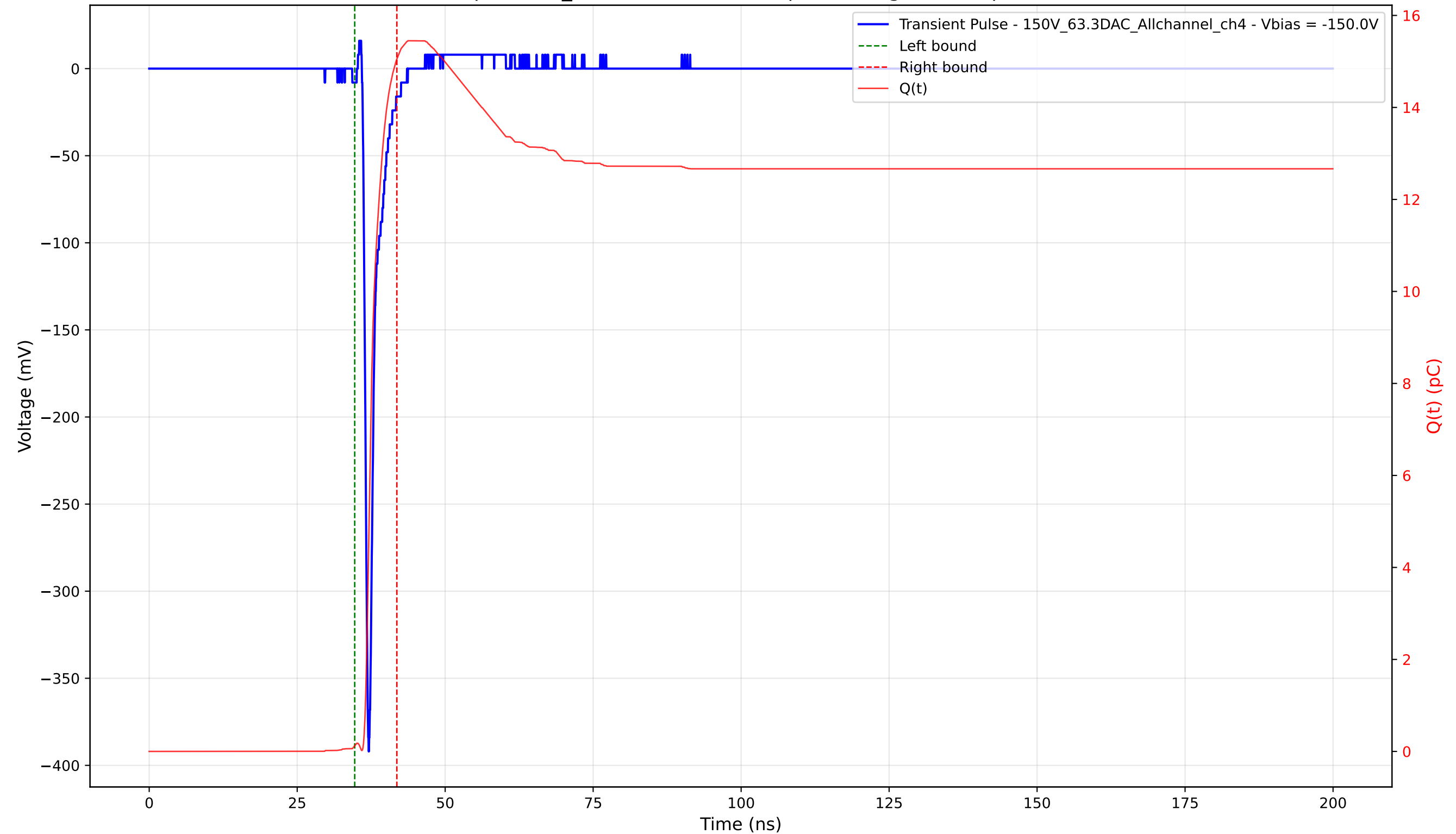
Transient Pulse - Sample: 1cm_42 - Position: 1610.0 \mu\text{m} - Charge: 14.93 pC - Rise Time: 0.73 ns
