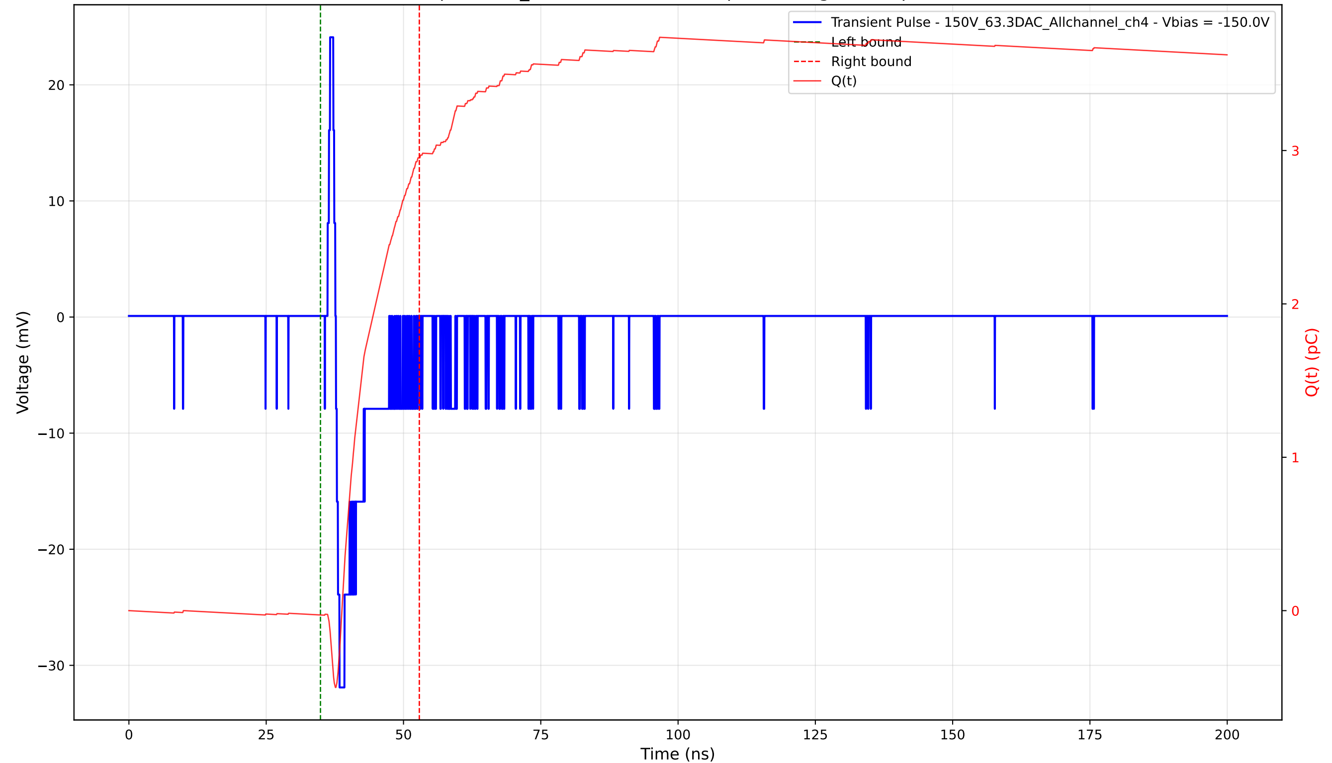
Transient Pulse - Sample: 1cm_42 - Position: 3900.0 \mu\text{m} - Charge: 2.98 pC - Rise Time: 0.66 ns
