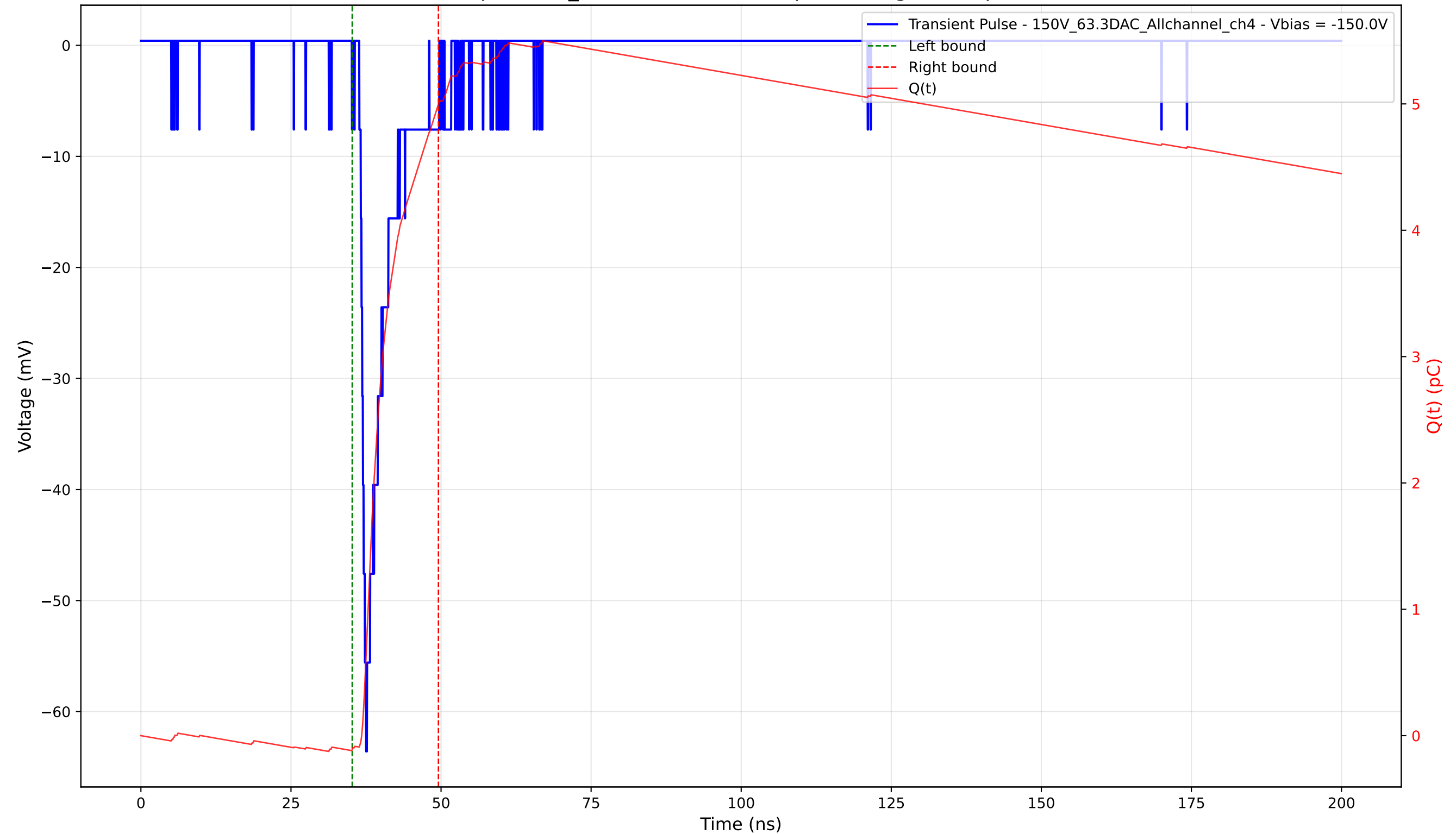
Transient Pulse - Sample: 1cm_42 - Position: 3035.0 \mu\text{m} - Charge: 5.11 pC - Rise Time: 1.13 ns
