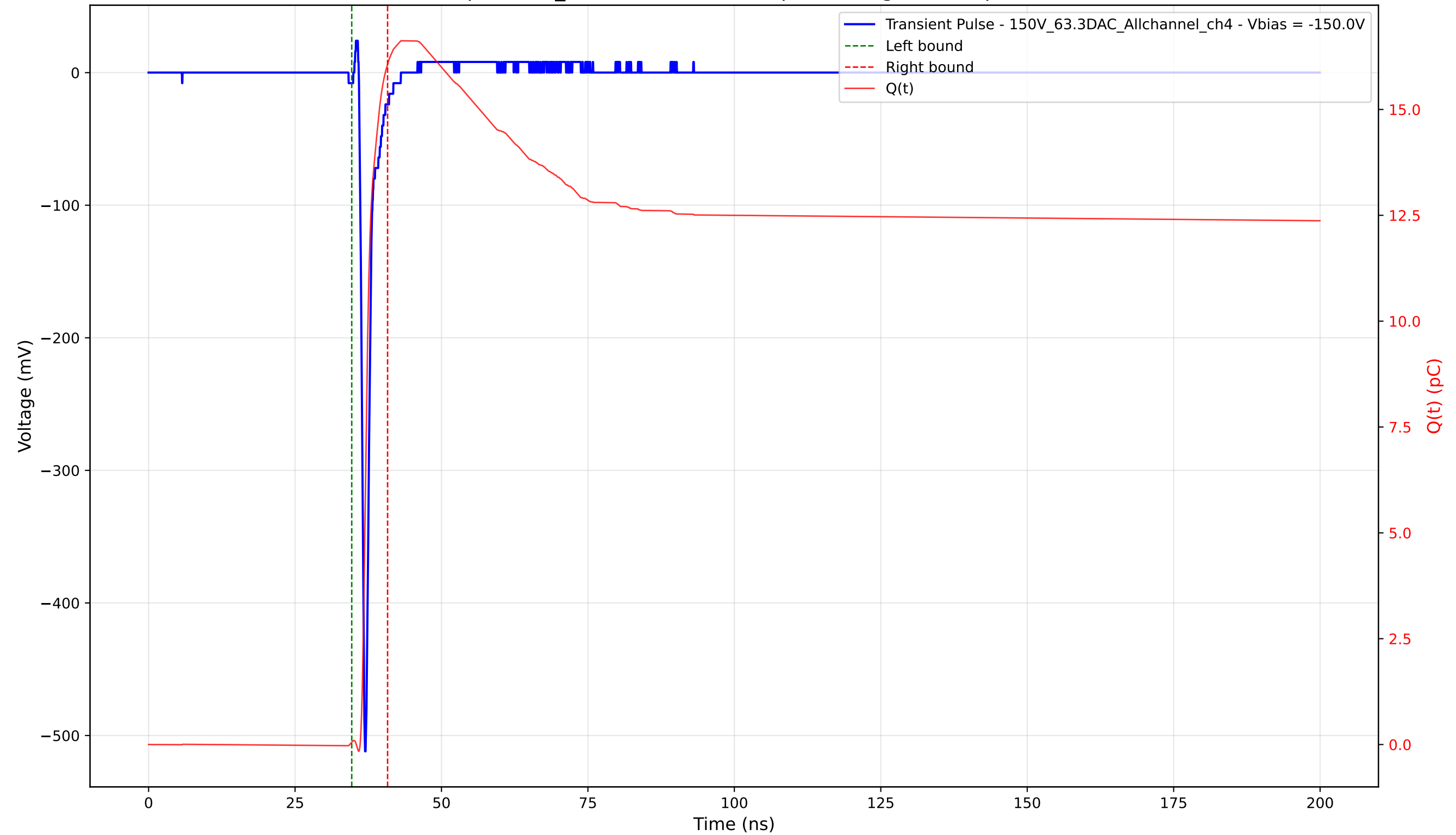
Transient Pulse - Sample: 1cm_42 - Position: 2235.0 \mu\text{m} - Charge: 16.01 pC - Rise Time: 0.70 ns
