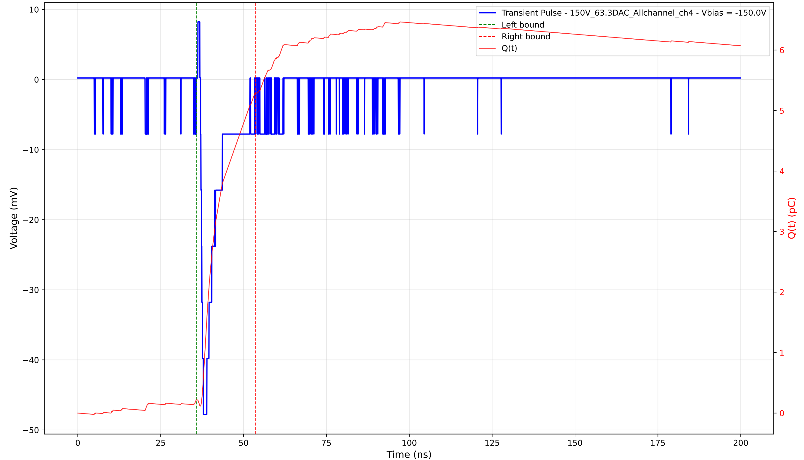
Transient Pulse - Sample: 1cm_42 - Position: 3270.0 \mu\text{m} - Charge: 5.06 pC - Rise Time: 0.82 ns
