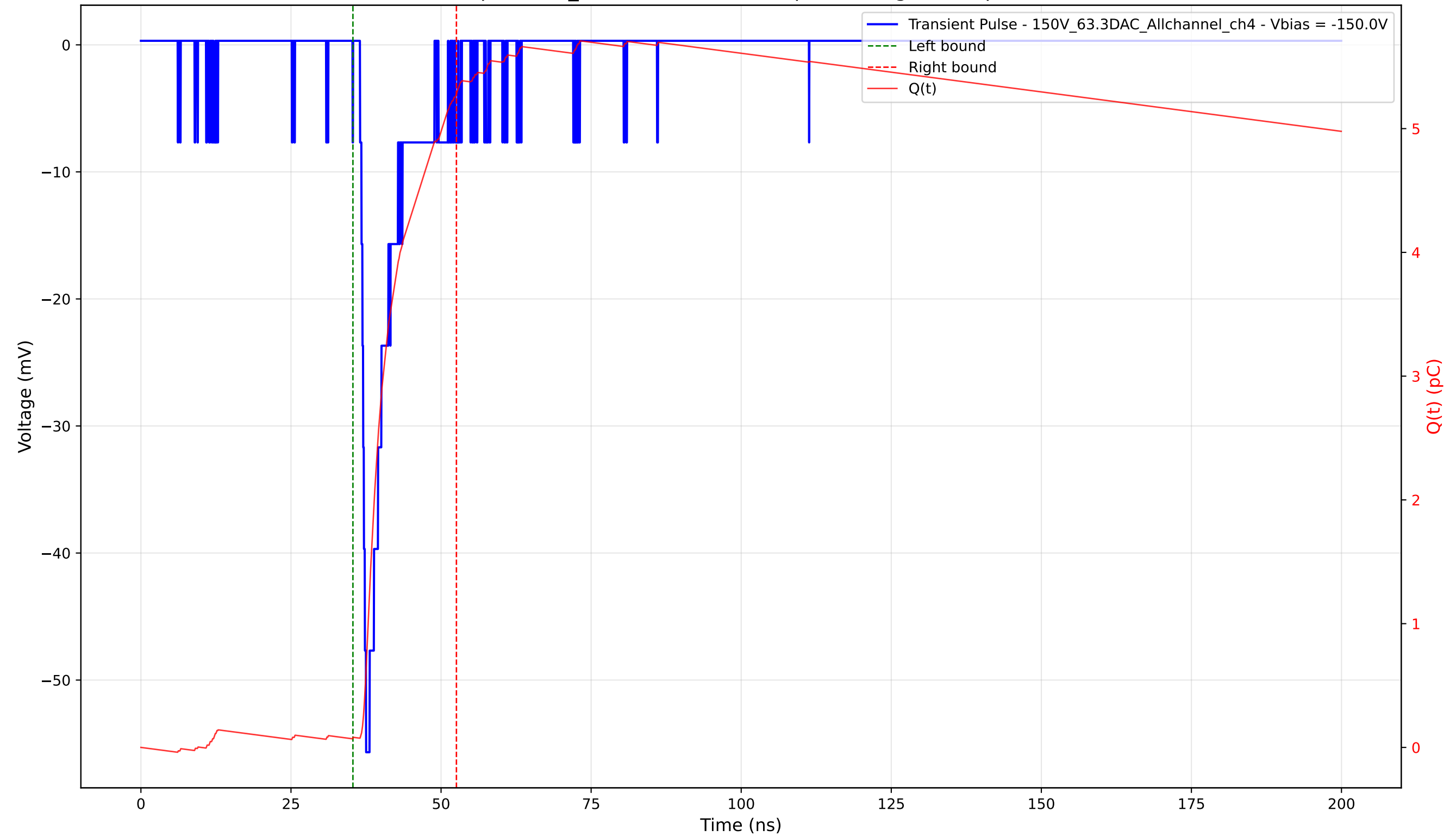
Transient Pulse - Sample: 1cm_42 - Position: 3085.0 \mu\text{m} - Charge: 5.20 pC - Rise Time: 1.01 ns
