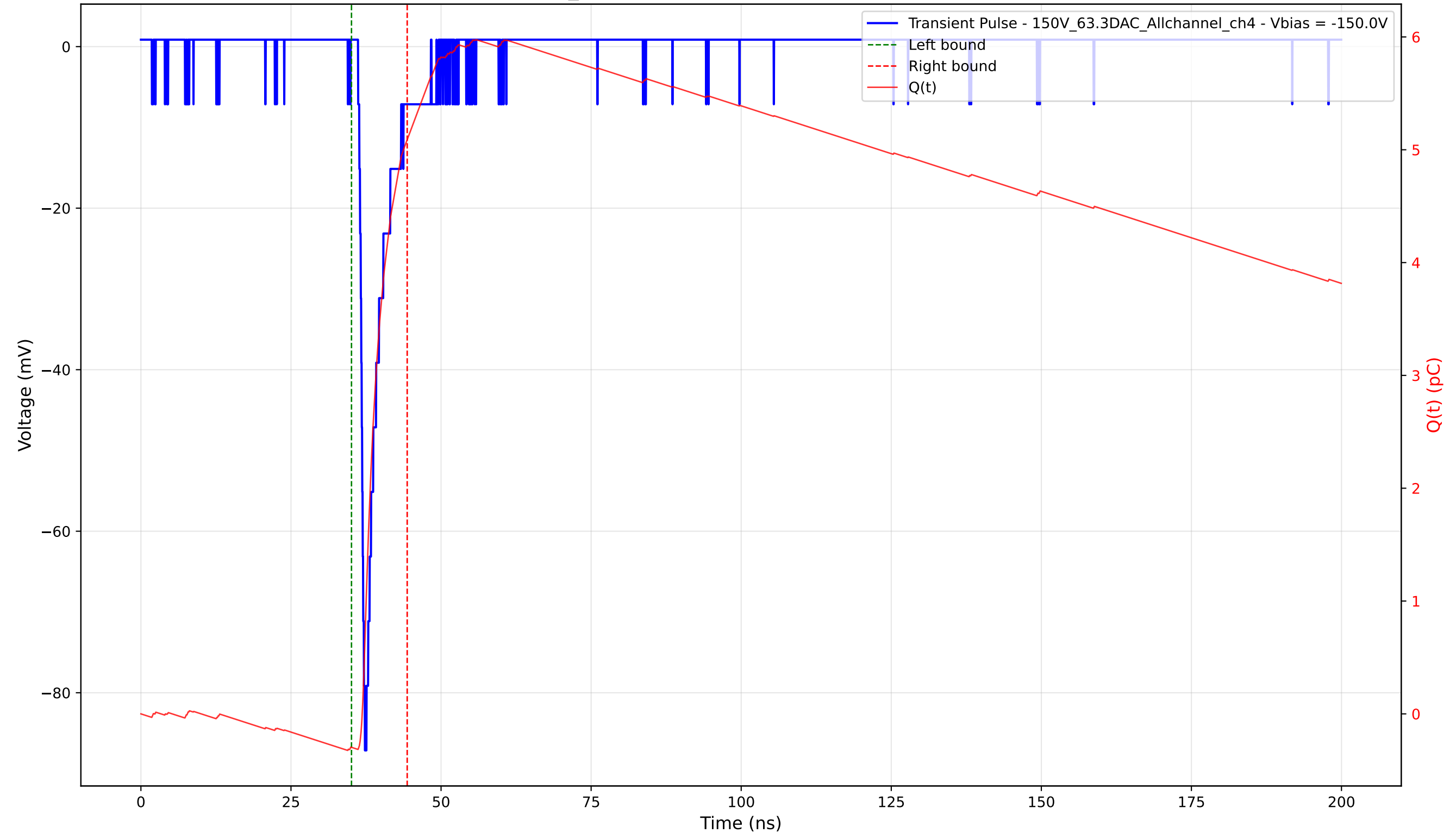
Transient Pulse - Sample: 1cm_42 - Position: 2940.0 \mu\text{m} - Charge: 5.39 pC - Rise Time: 0.79 ns
