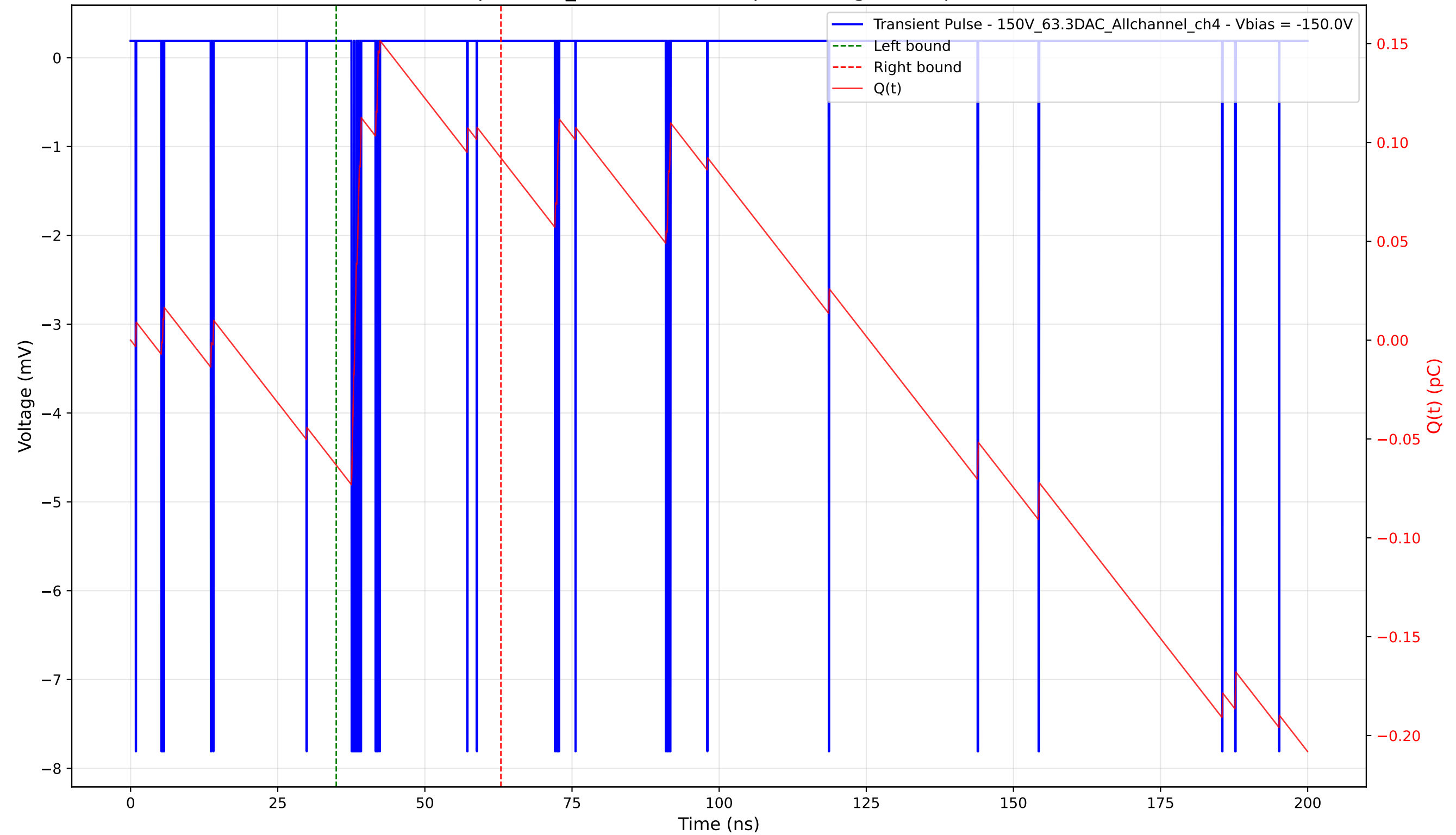
Transient Pulse - Sample: 1cm_42 - Position: 5.0 \mu\text{m} - Charge: 0.16 pC - Rise Time: 0.04 ns
