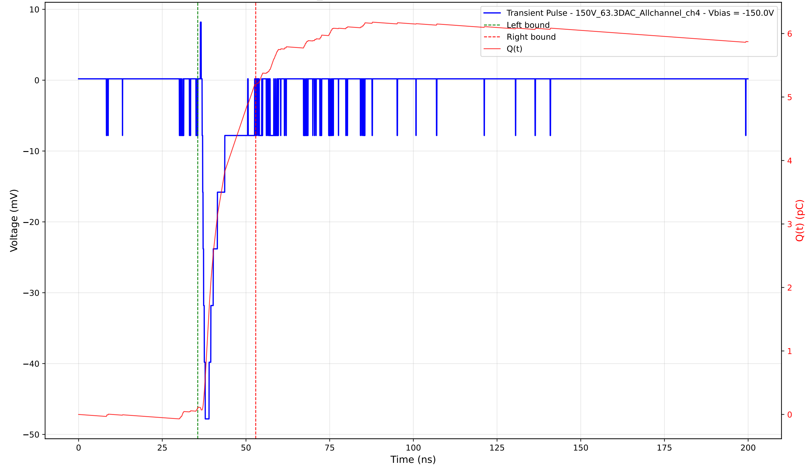
Transient Pulse - Sample: 1cm_42 - Position: 3210.0 \mu\text{m} - Charge: 5.09 pC - Rise Time: 0.94 ns
