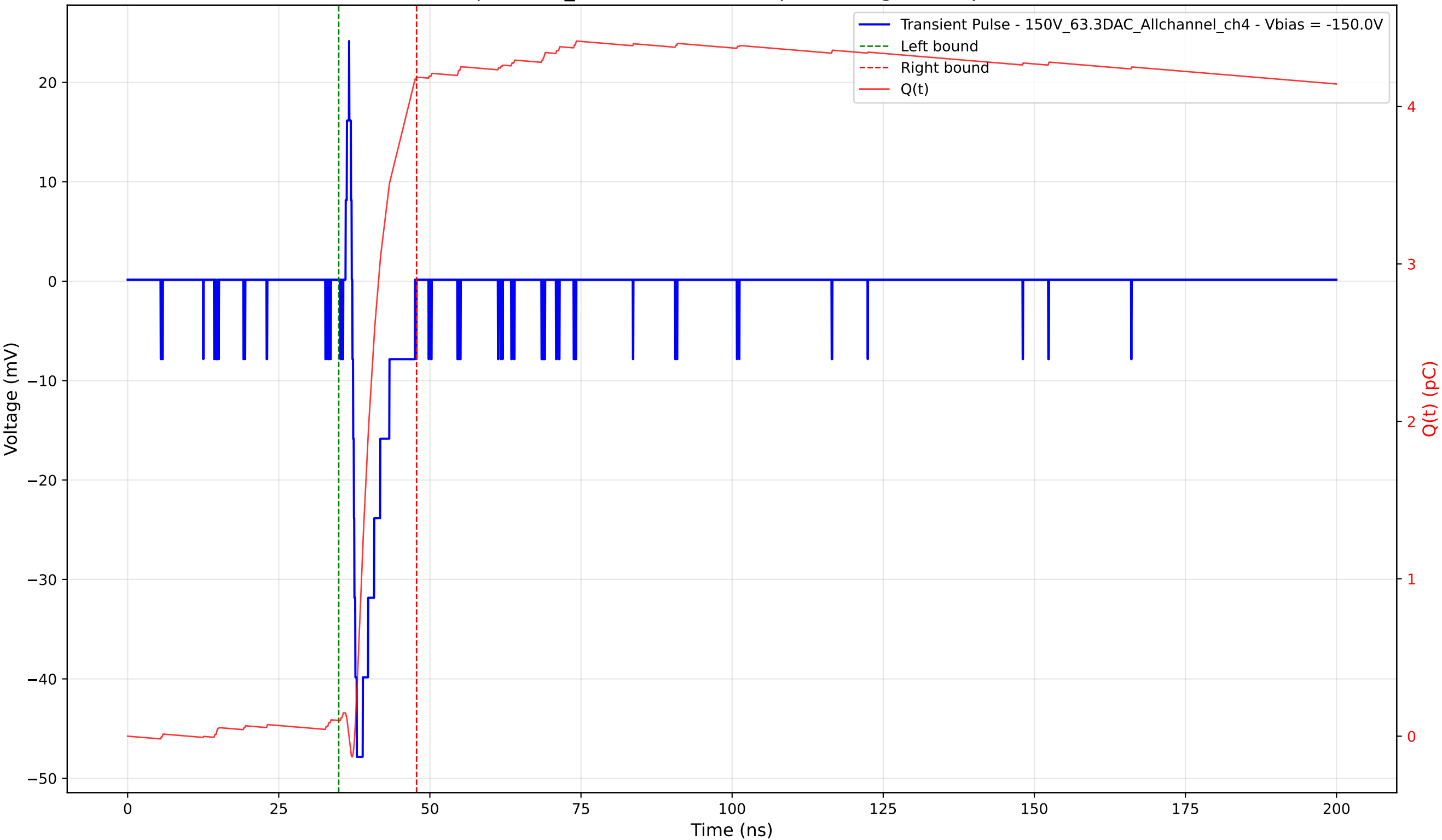
Transient Pulse - Sample: 1cm_42 - Position: 470.0 \mu\text{m} - Charge: 4.09 pC - Rise Time: 0.74 ns
