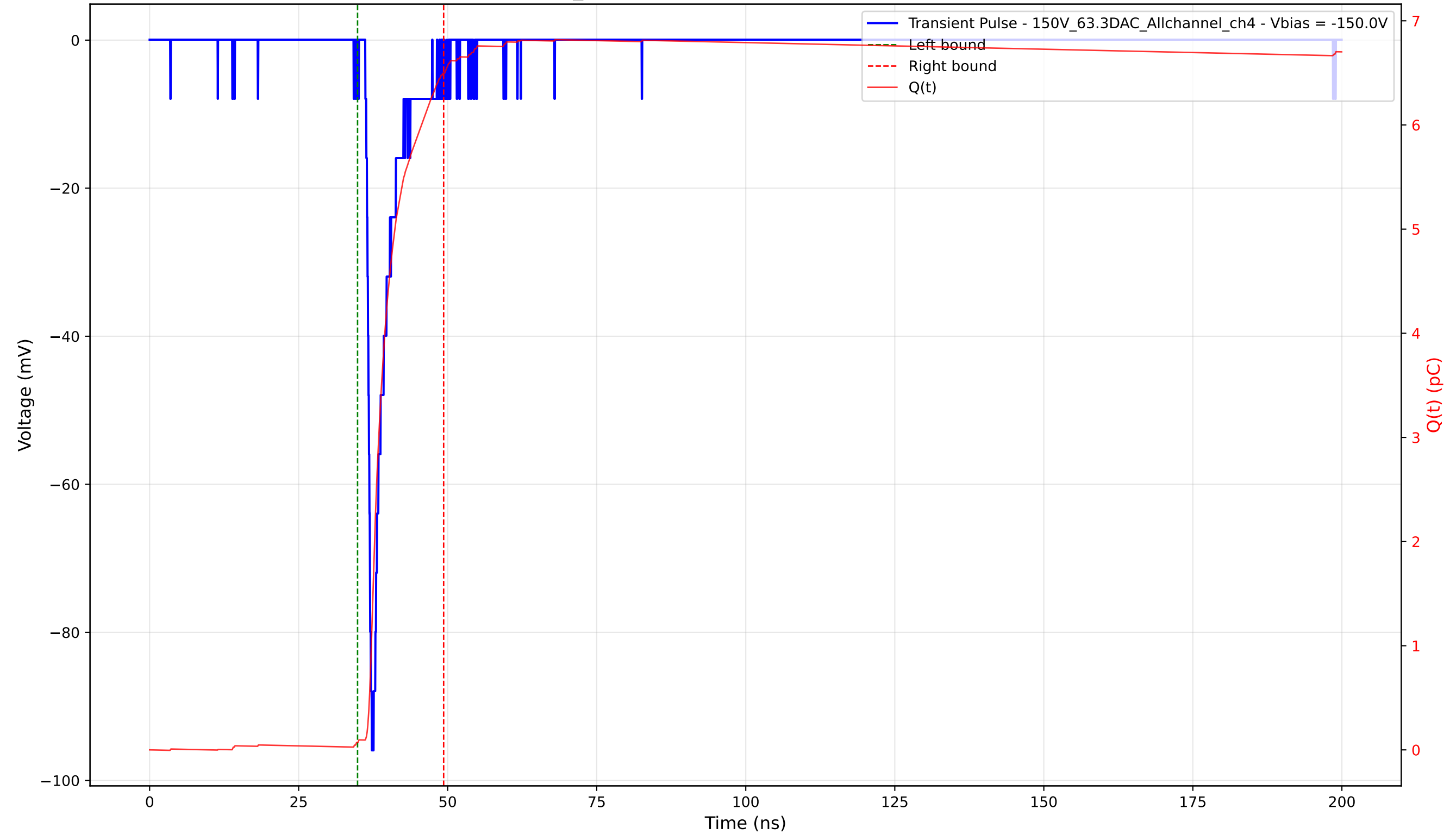
Transient Pulse - Sample: 1cm_42 - Position: 2910.0 \mu\text{m} - Charge: 6.43 pC - Rise Time: 0.79 ns
