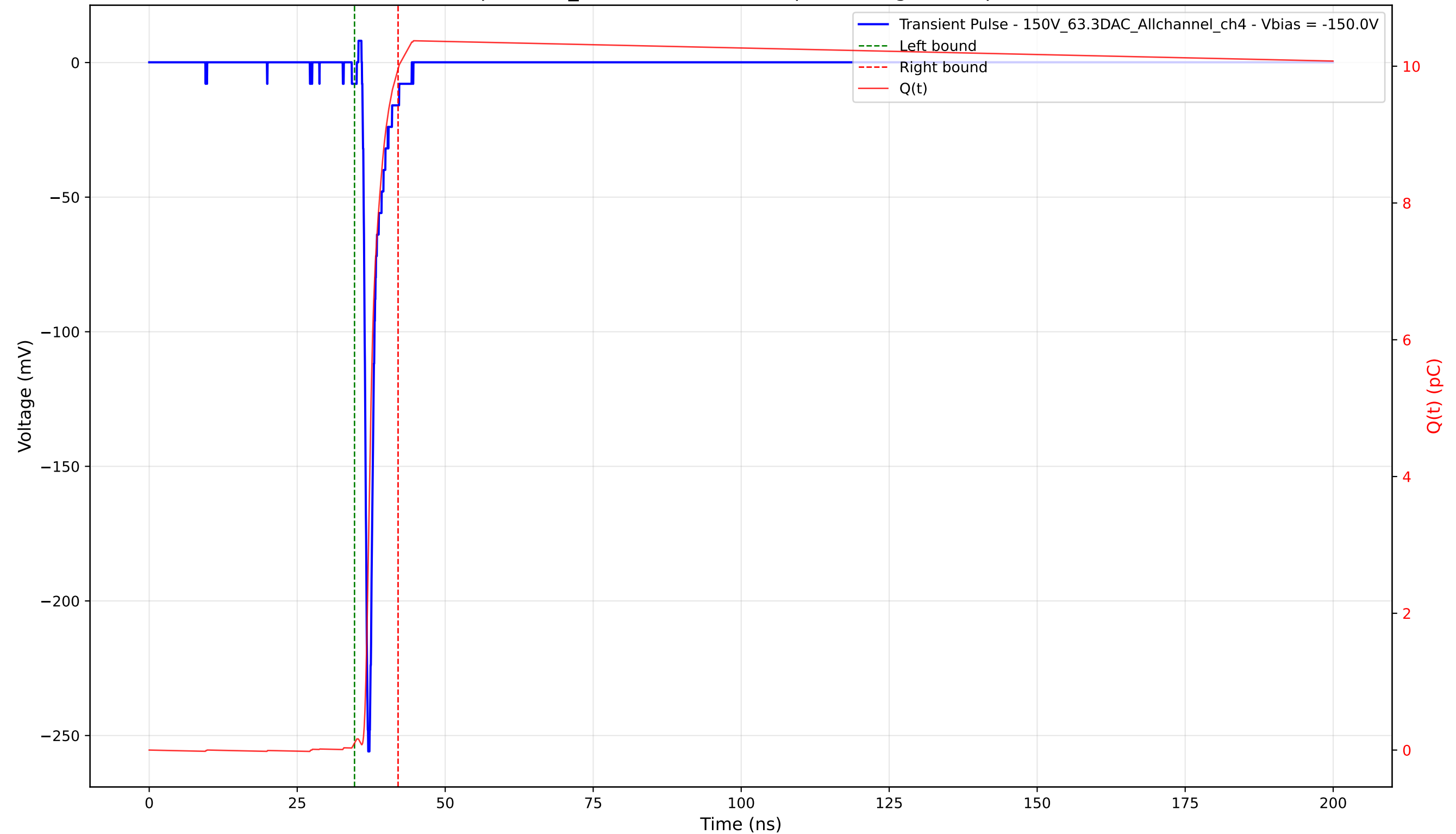
Transient Pulse - Sample: 1cm_42 - Position: 2490.0 \mu\text{m} - Charge: 9.86 pC - Rise Time: 0.74 ns
