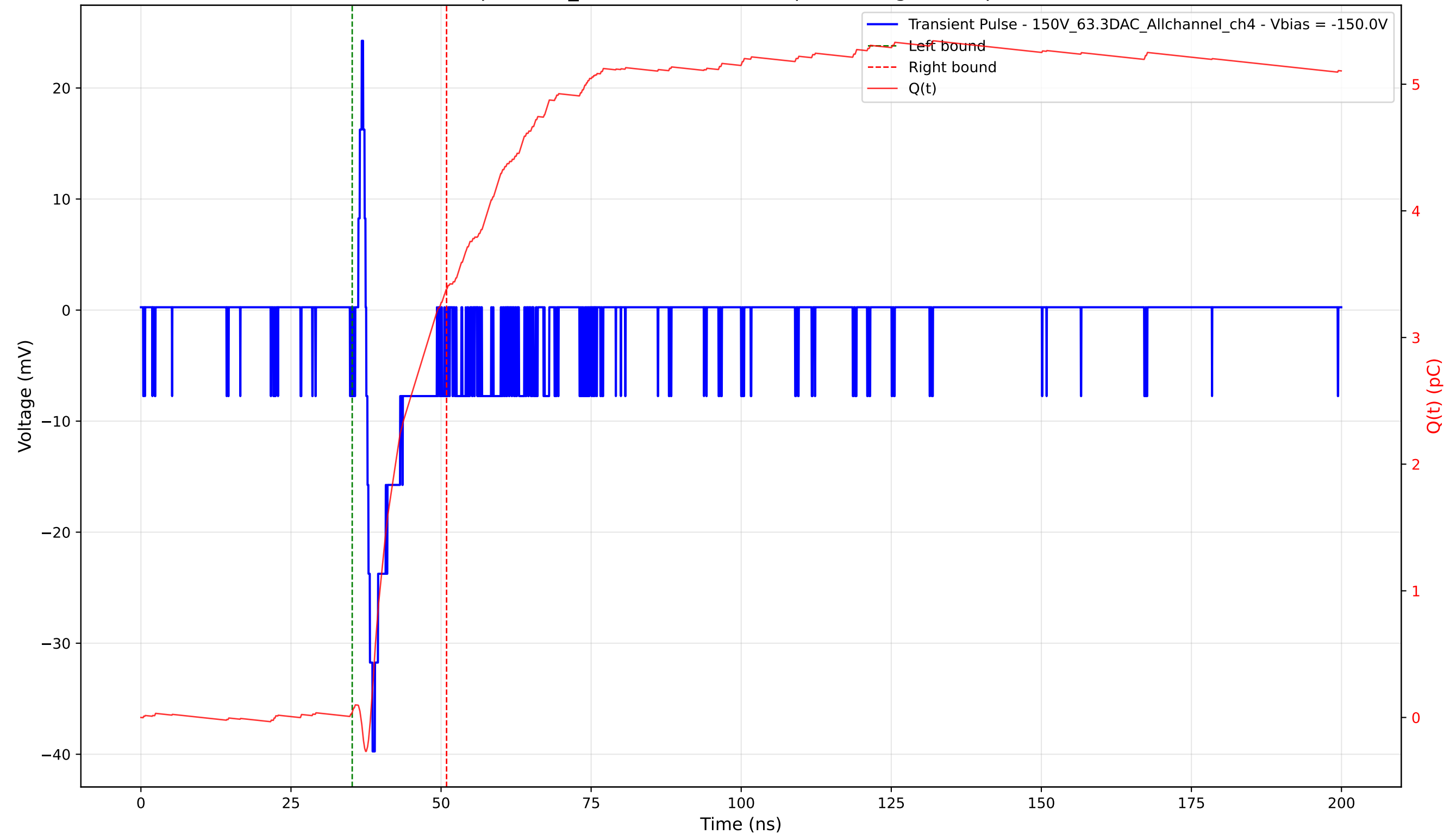
Transient Pulse - Sample: 1cm_42 - Position: 3635.0 \mu\text{m} - Charge: 3.34 pC - Rise Time: 1.06 ns
