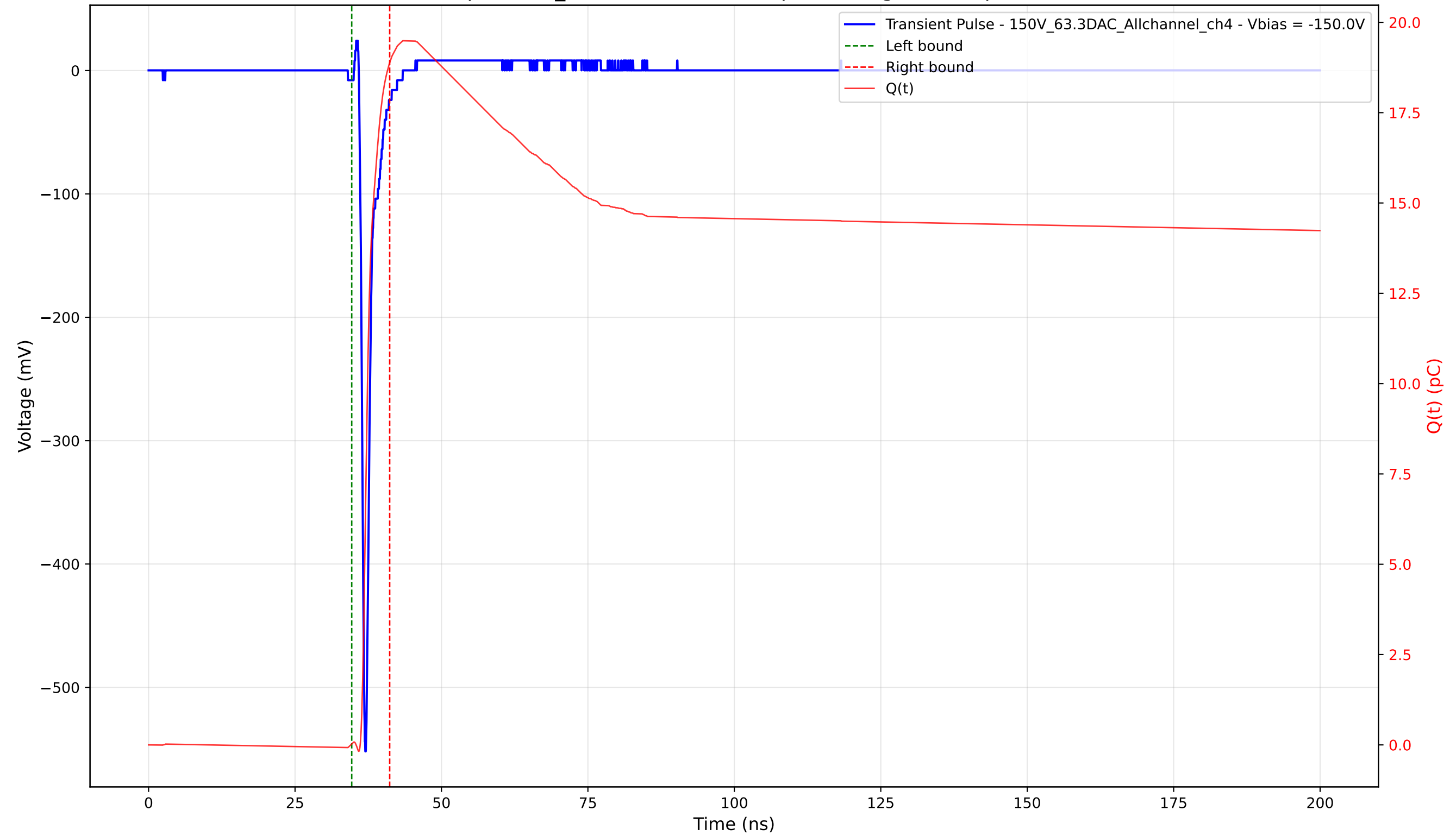
Transient Pulse - Sample: 1cm_42 - Position: 1725.0 \mu\text{m} - Charge: 18.86 pC - Rise Time: 0.72 ns
