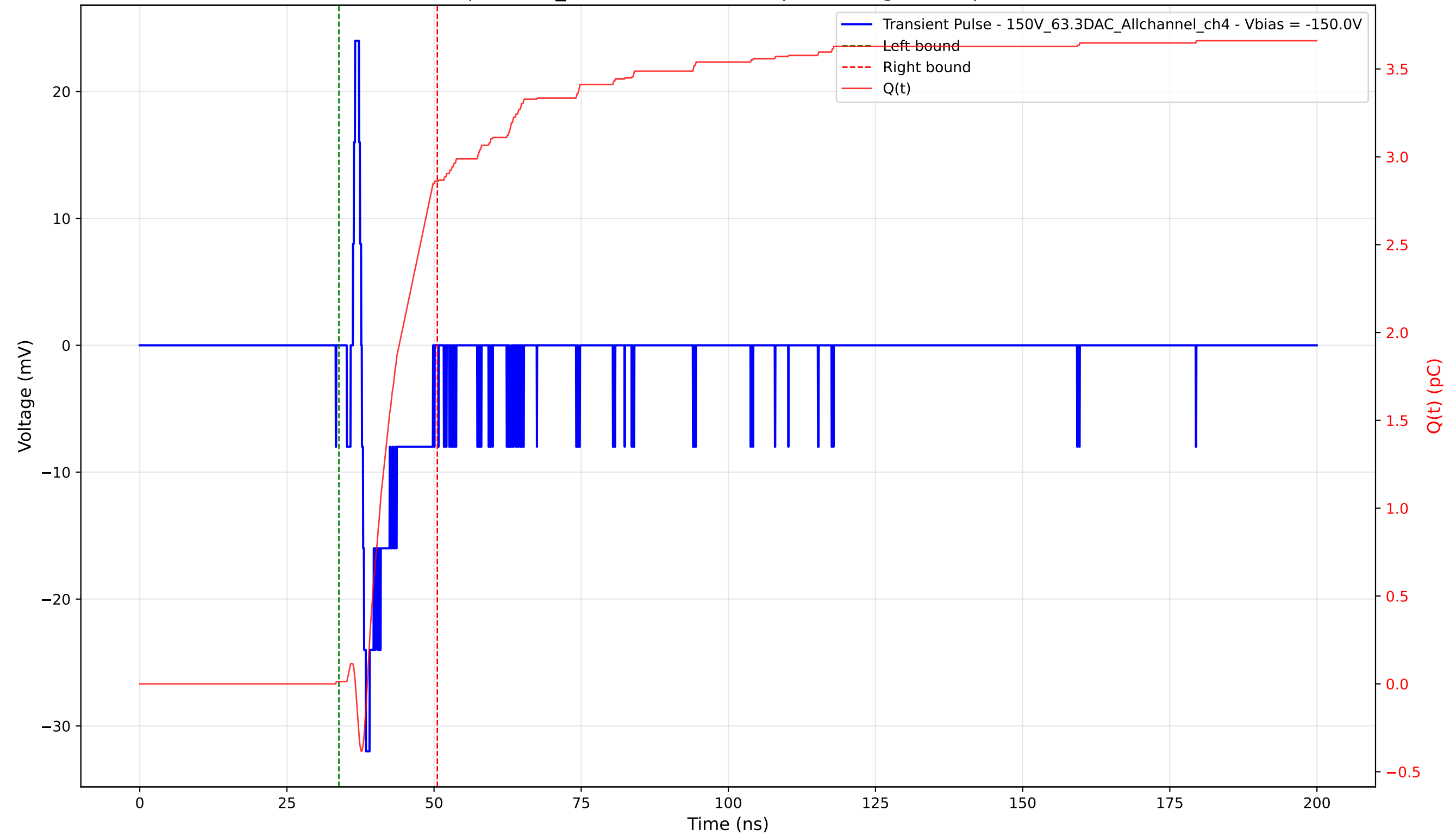
Transient Pulse - Sample: 1cm_42 - Position: 4395.0 \mu\text{m} - Charge: 2.85 pC - Rise Time: 0.70 ns
