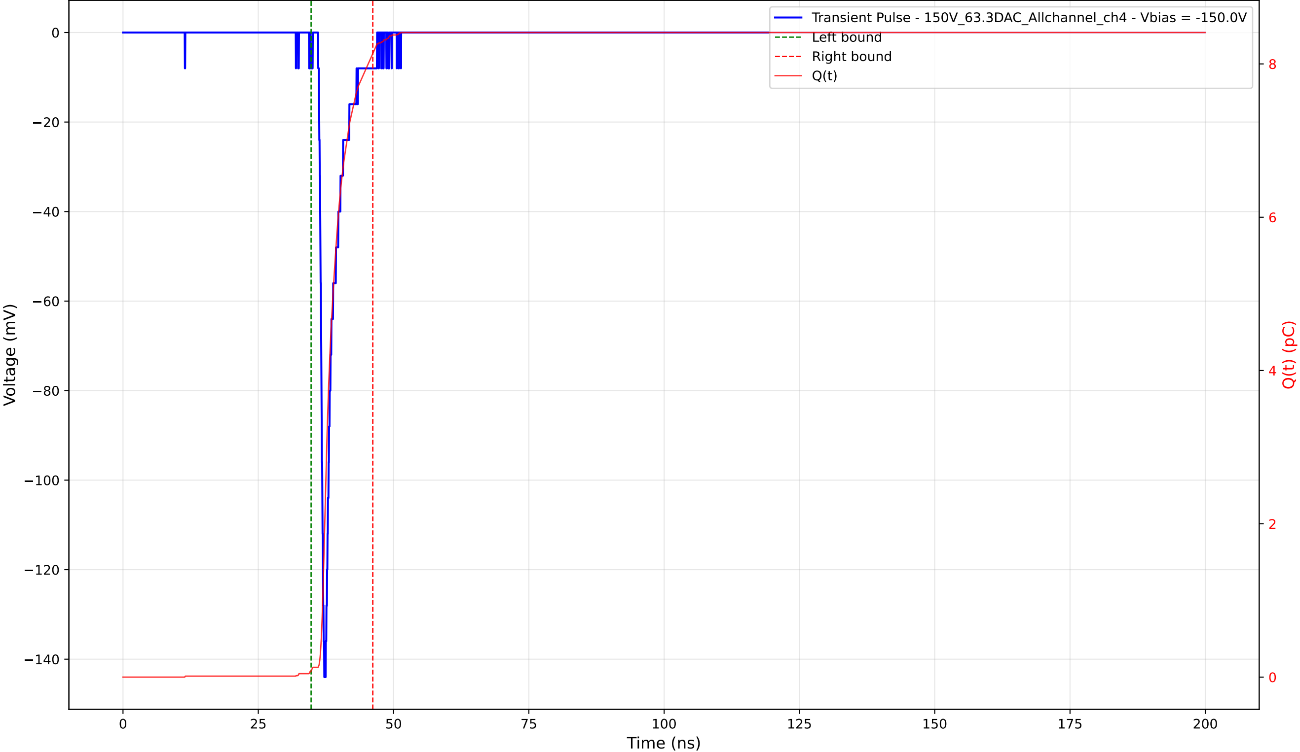
Transient Pulse - Sample: 1cm_42 - Position: 2730.0 \mu\text{m} - Charge: 8.06 pC - Rise Time: 0.85 ns
