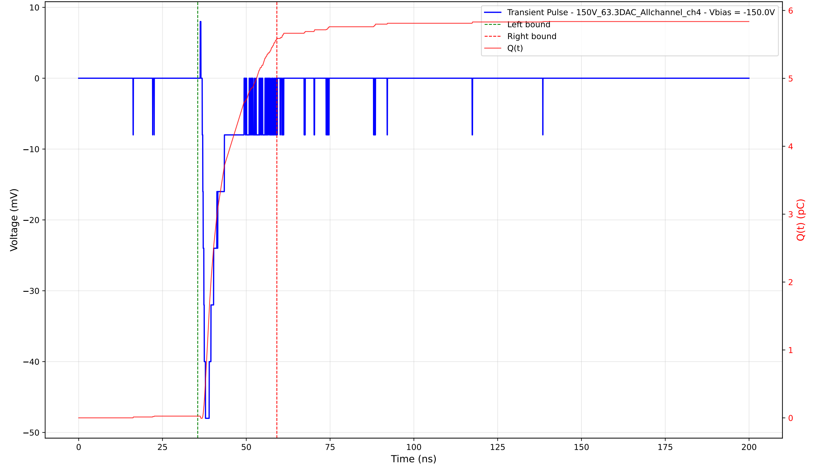
Transient Pulse - Sample: 1cm_42 - Position: 3185.0 \mu\text{m} - Charge: 5.56 pC - Rise Time: 0.98 ns
