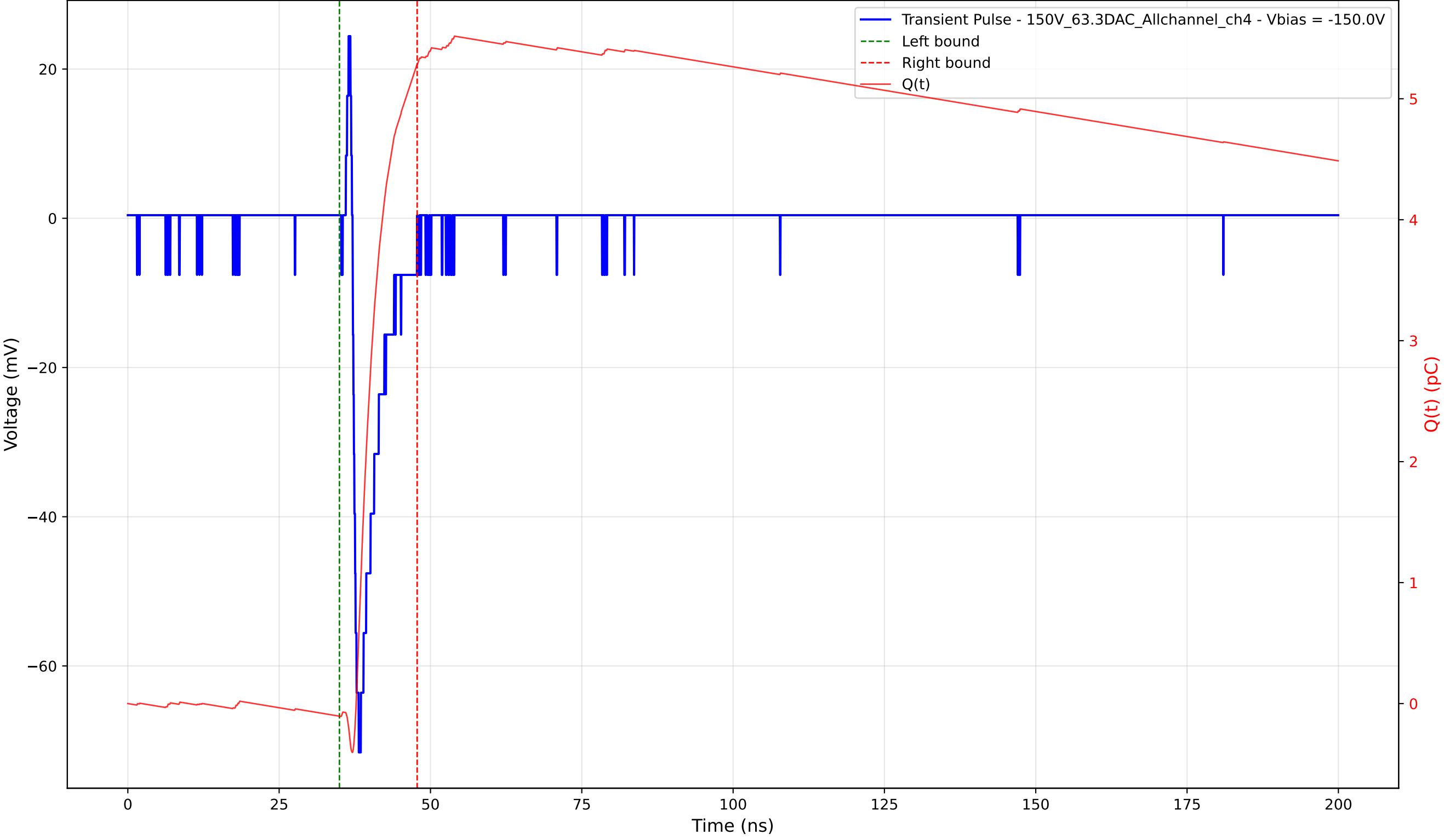
Transient Pulse - Sample: 1cm_42 - Position: 620.0 \mu\text{m} - Charge: 5.39 pC - Rise Time: 1.00 ns
