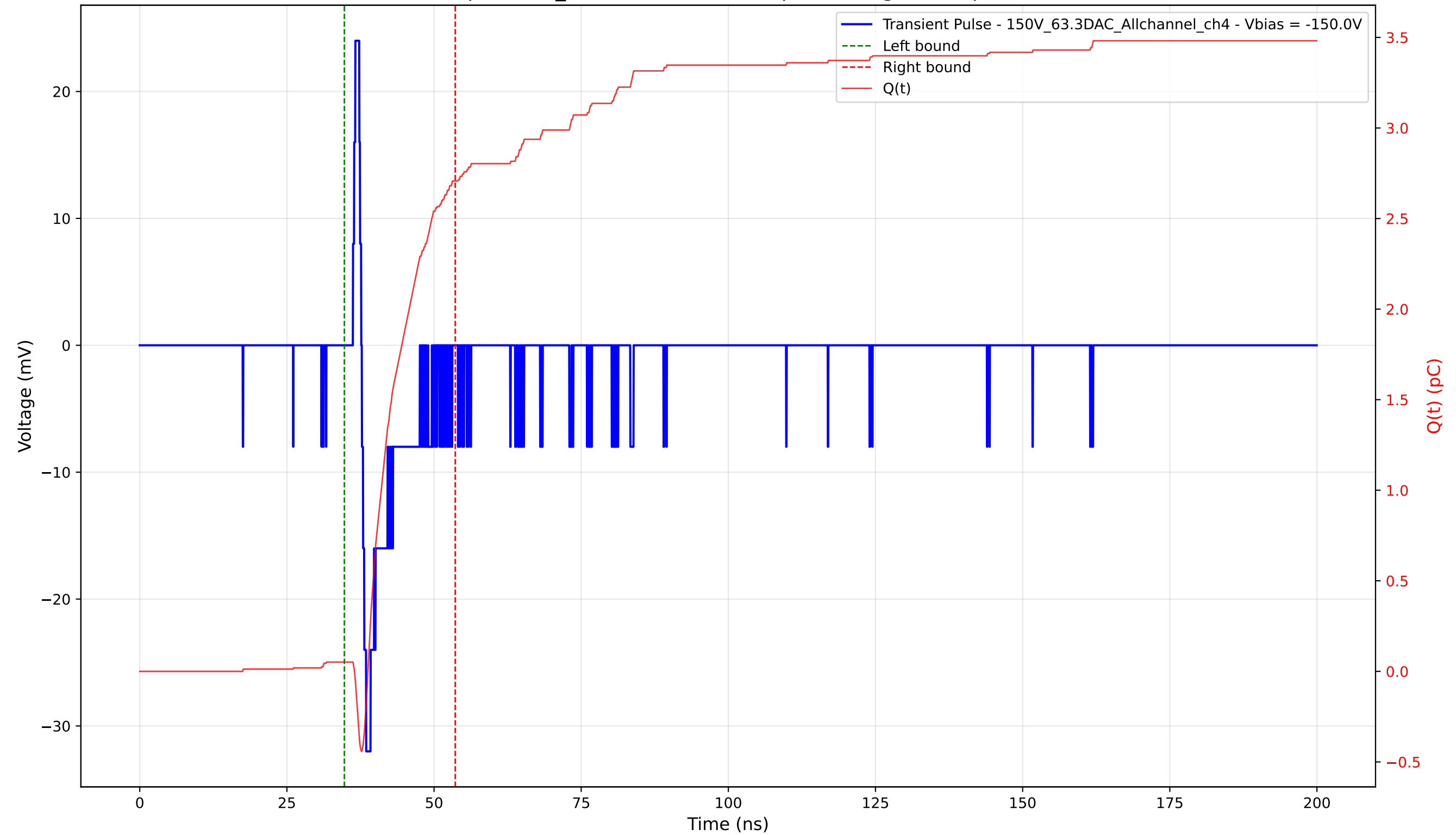
Transient Pulse - Sample: 1cm_42 - Position: 4090.0 \mu\text{m} - Charge: 2.66 pC - Rise Time: 0.74 ns
