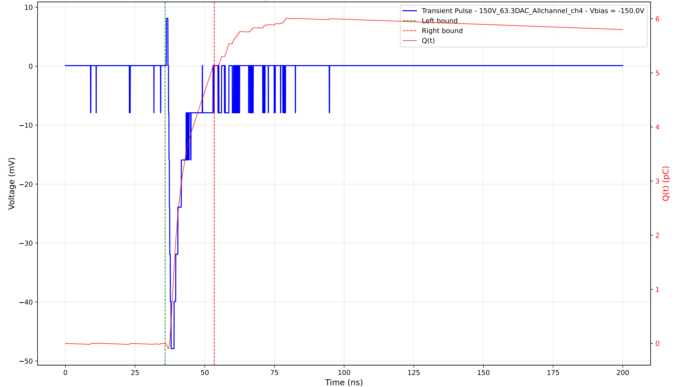
Transient Pulse - Sample: 1cm_42 - Position: 3260.0 \mu\text{m} - Charge: 5.14 pC - Rise Time: 0.94 ns
