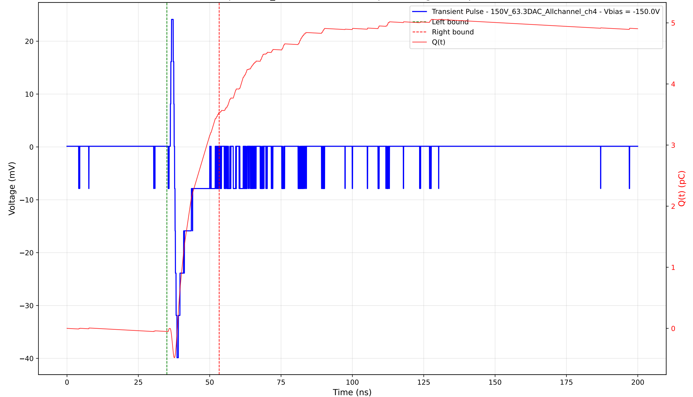
Transient Pulse - Sample: 1cm_42 - Position: 3835.0 \mu\text{m} - Charge: 3.58 pC - Rise Time: 0.86 ns
