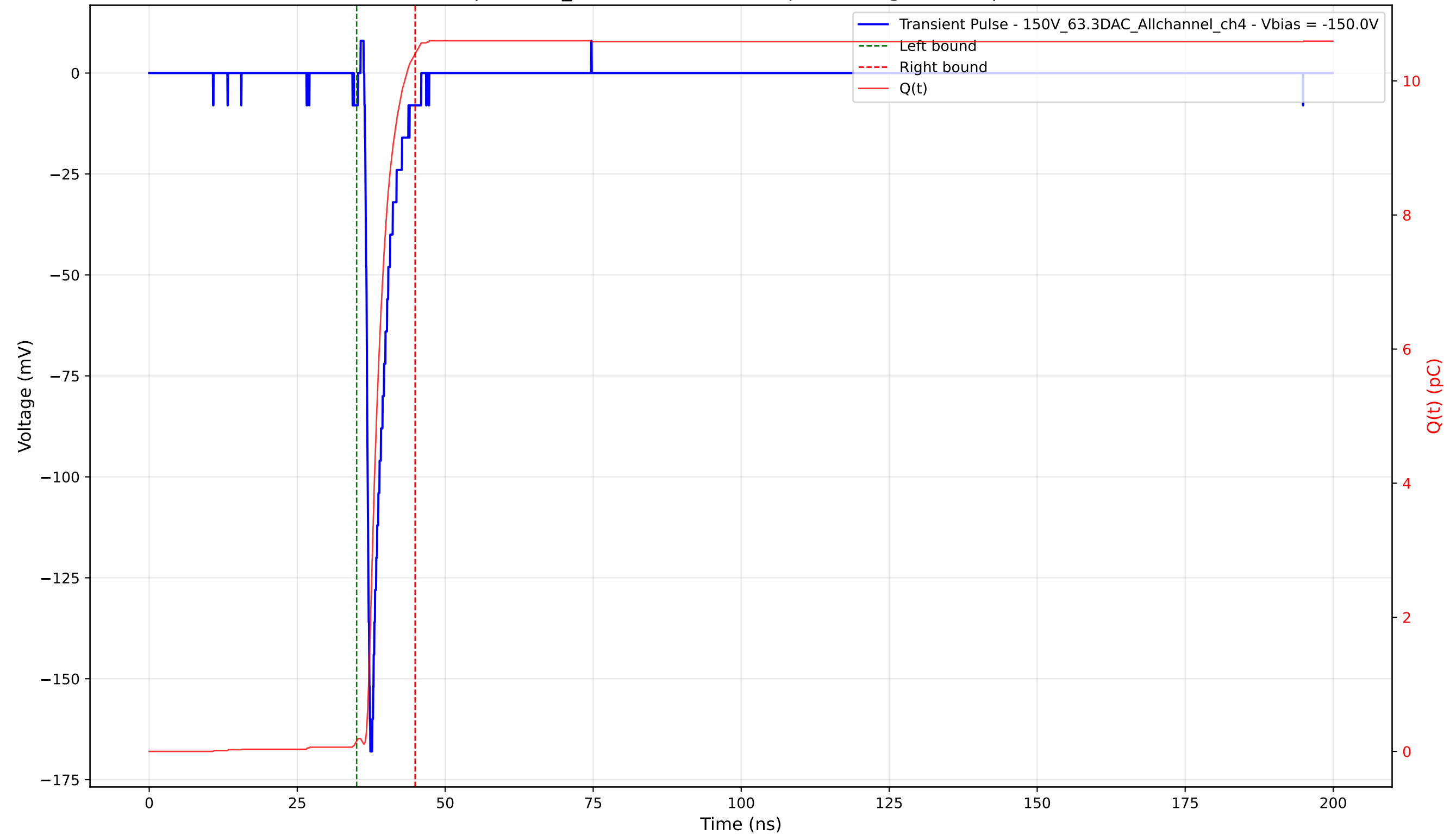
Transient Pulse - Sample: 1cm_42 - Position: 1205.0 \mu\text{m} - Charge: 10.25 pC - Rise Time: 0.72 ns
