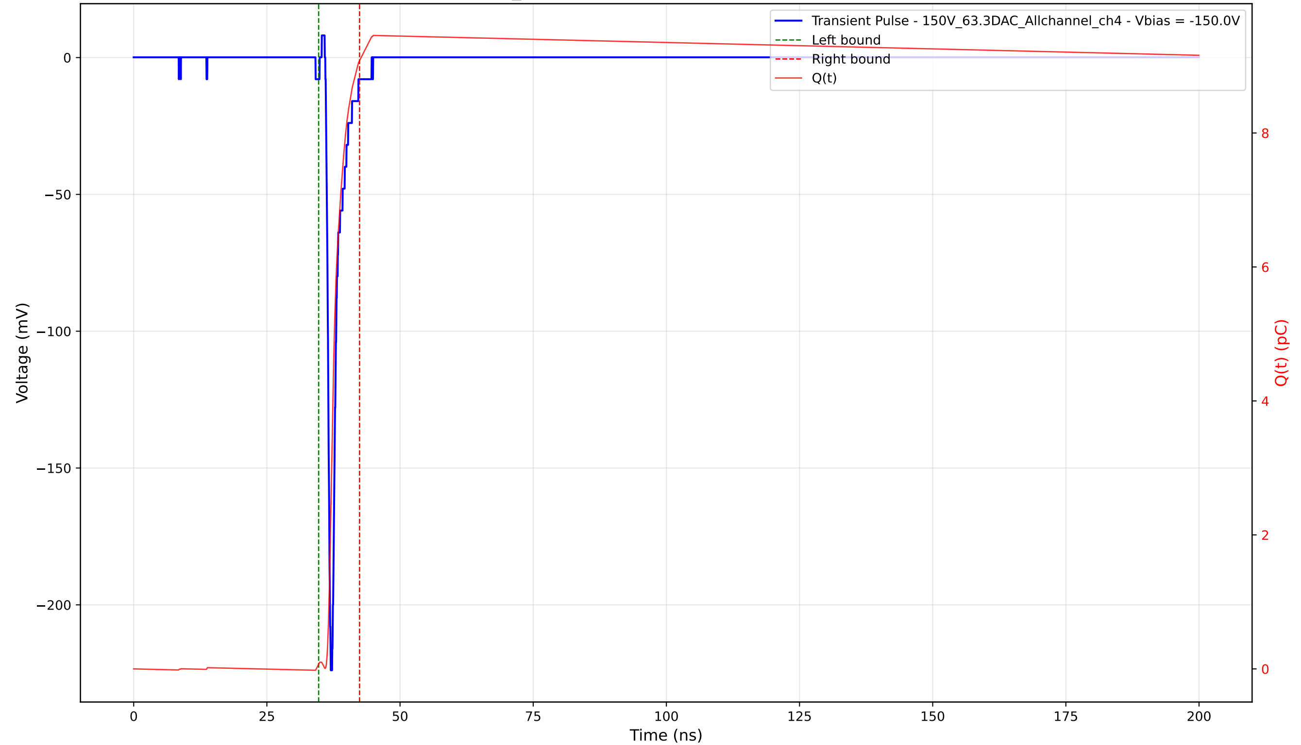
Transient Pulse - Sample: 1cm_42 - Position: 2530.0 \mu\text{m} - Charge: 9.01 pC - Rise Time: 0.77 ns
