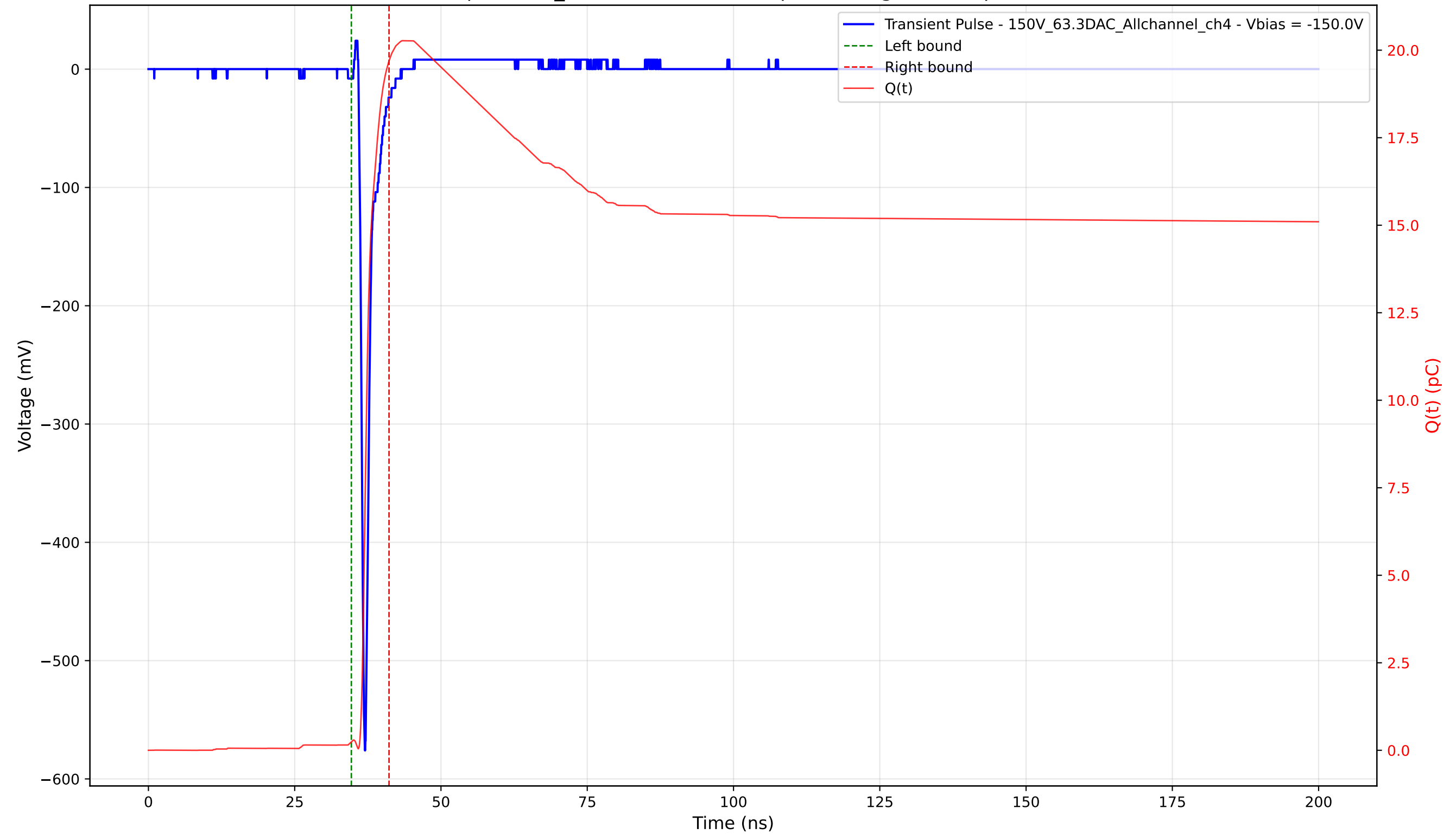
Transient Pulse - Sample: 1cm_42 - Position: 1745.0 \mu\text{m} - Charge: 19.45 pC - Rise Time: 0.73 ns
