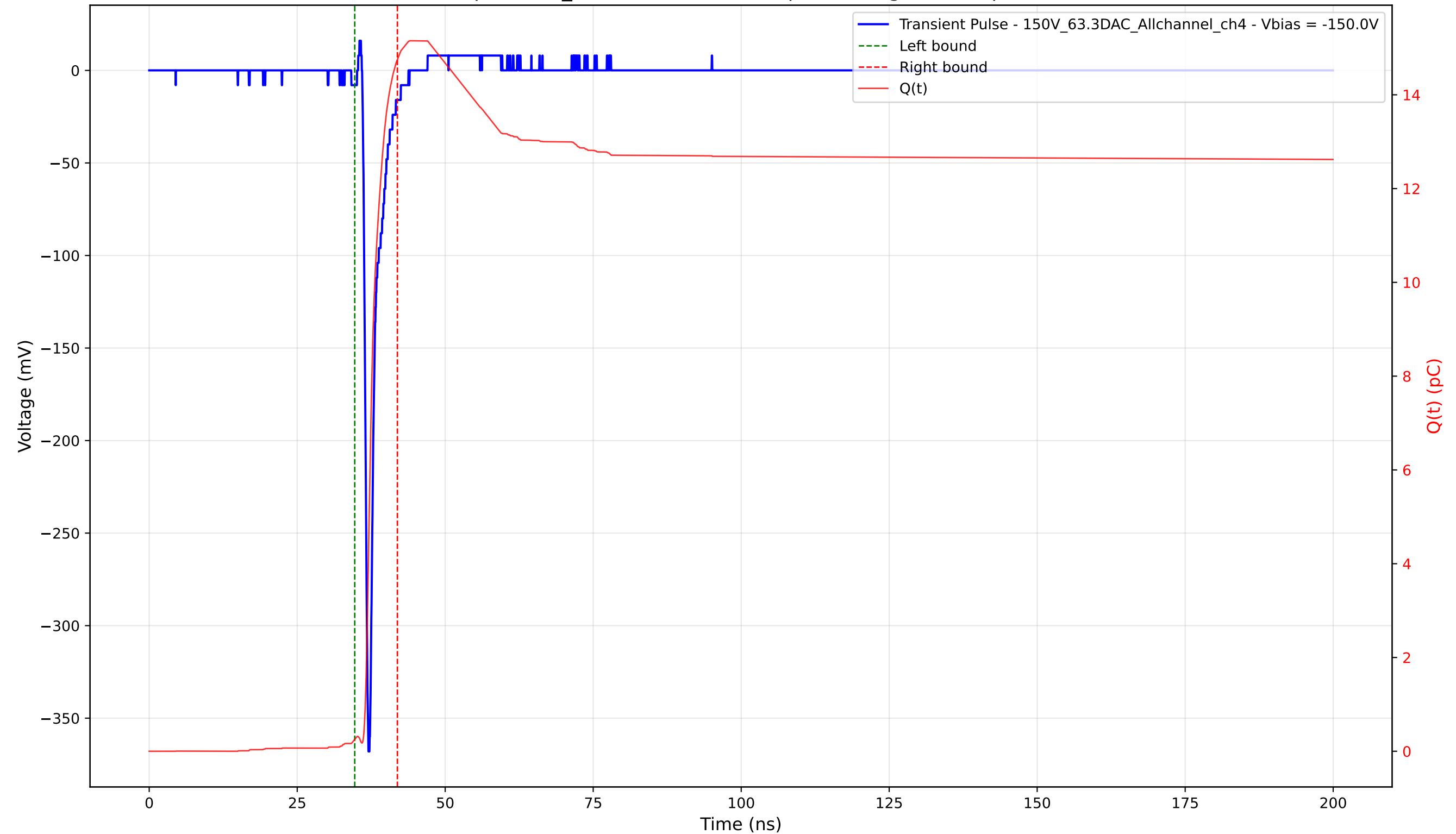
Transient Pulse - Sample: 1cm_42 - Position: 1600.0 \mu\text{m} - Charge: 14.49 pC - Rise Time: 0.74 ns
