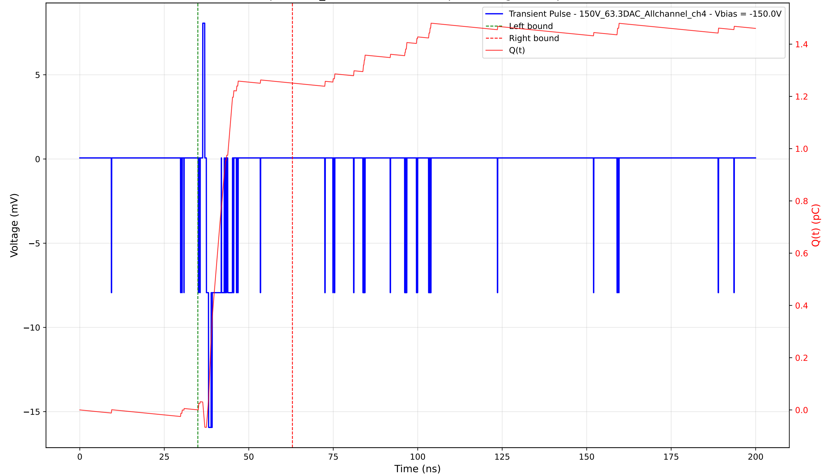
Transient Pulse - Sample: 1cm_42 - Position: 5080.0 \mu\text{m} - Charge: 1.25 pC - Rise Time: 0.67 ns
