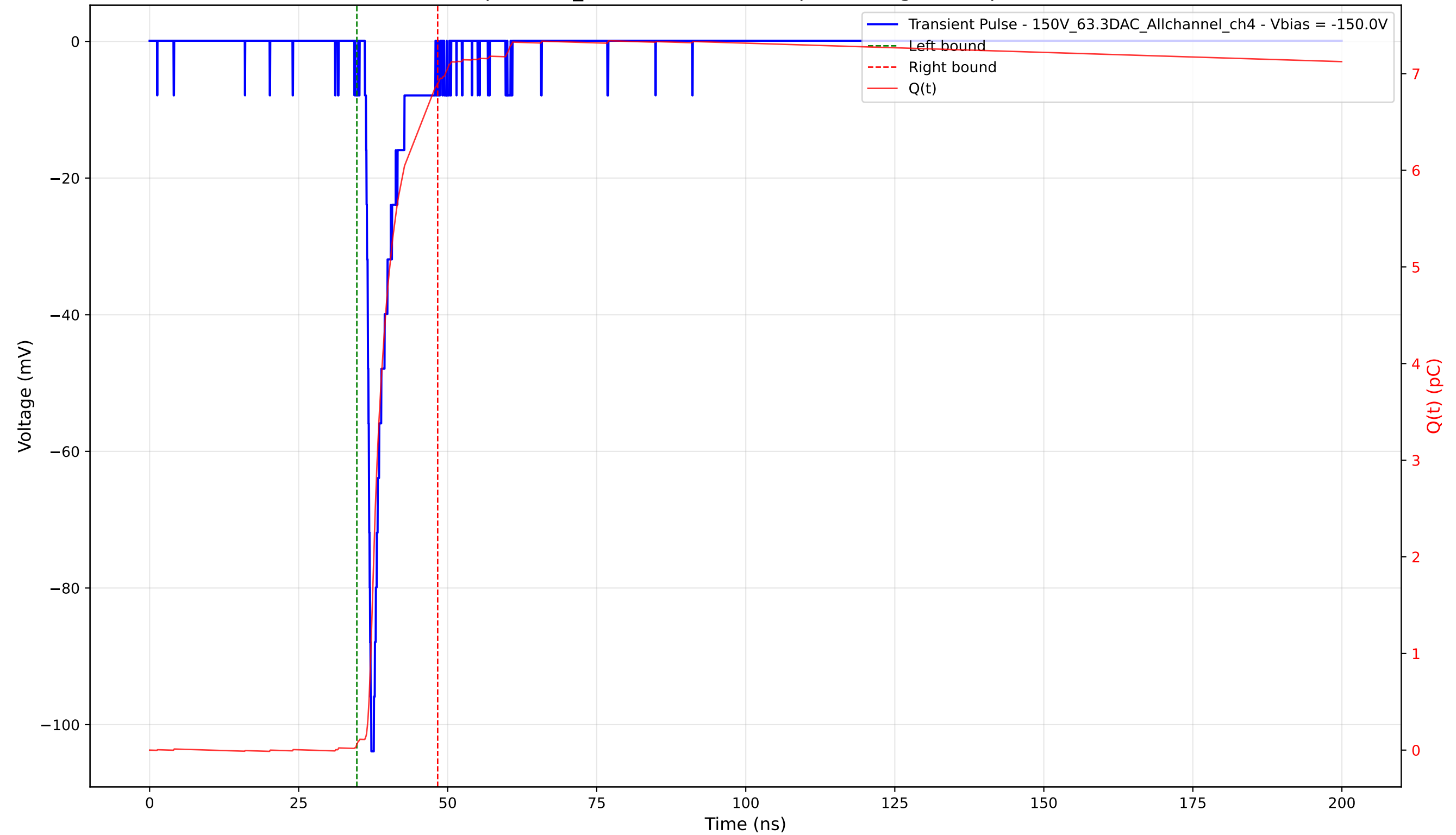
Transient Pulse - Sample: 1cm_42 - Position: 2880.0 \mu\text{m} - Charge: 6.84 pC - Rise Time: 0.79 ns
