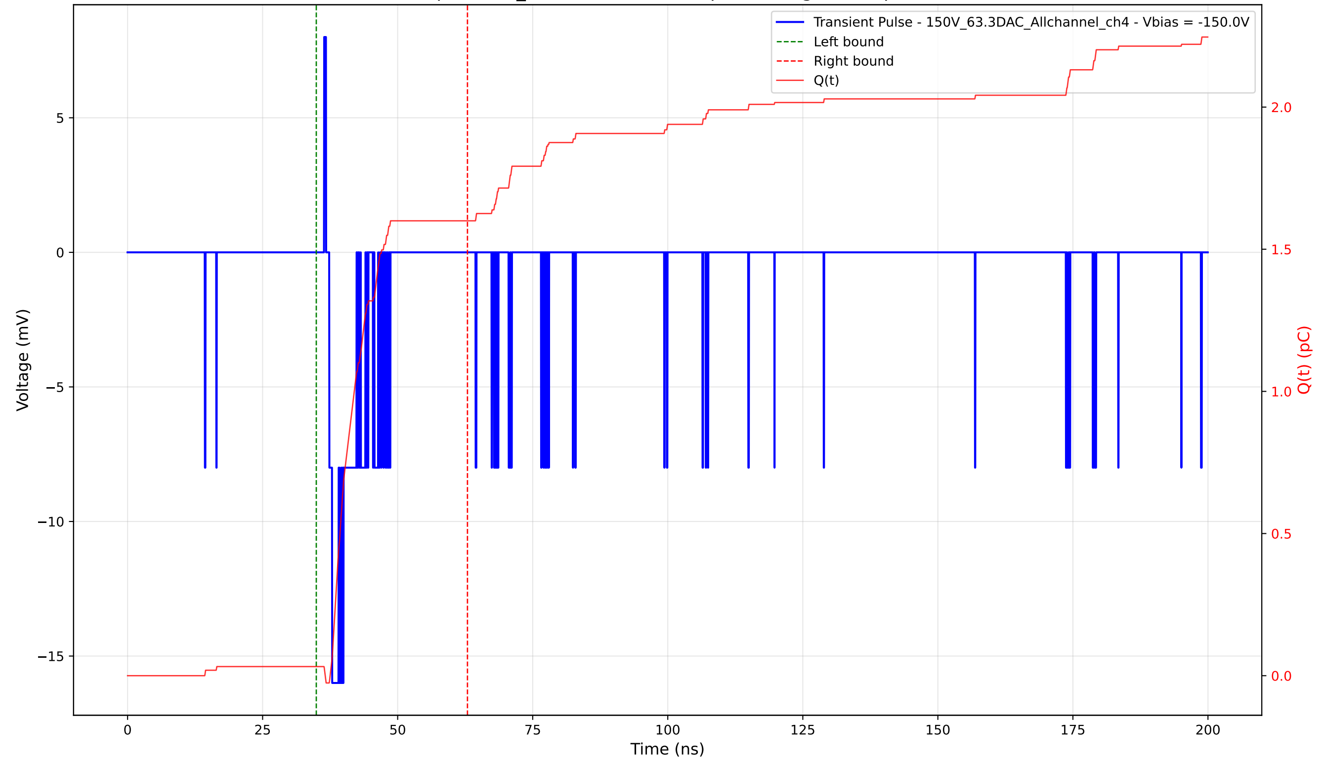
Transient Pulse - Sample: 1cm_42 - Position: 120.0 \mu\text{m} - Charge: 1.57 pC - Rise Time: 0.55 ns
