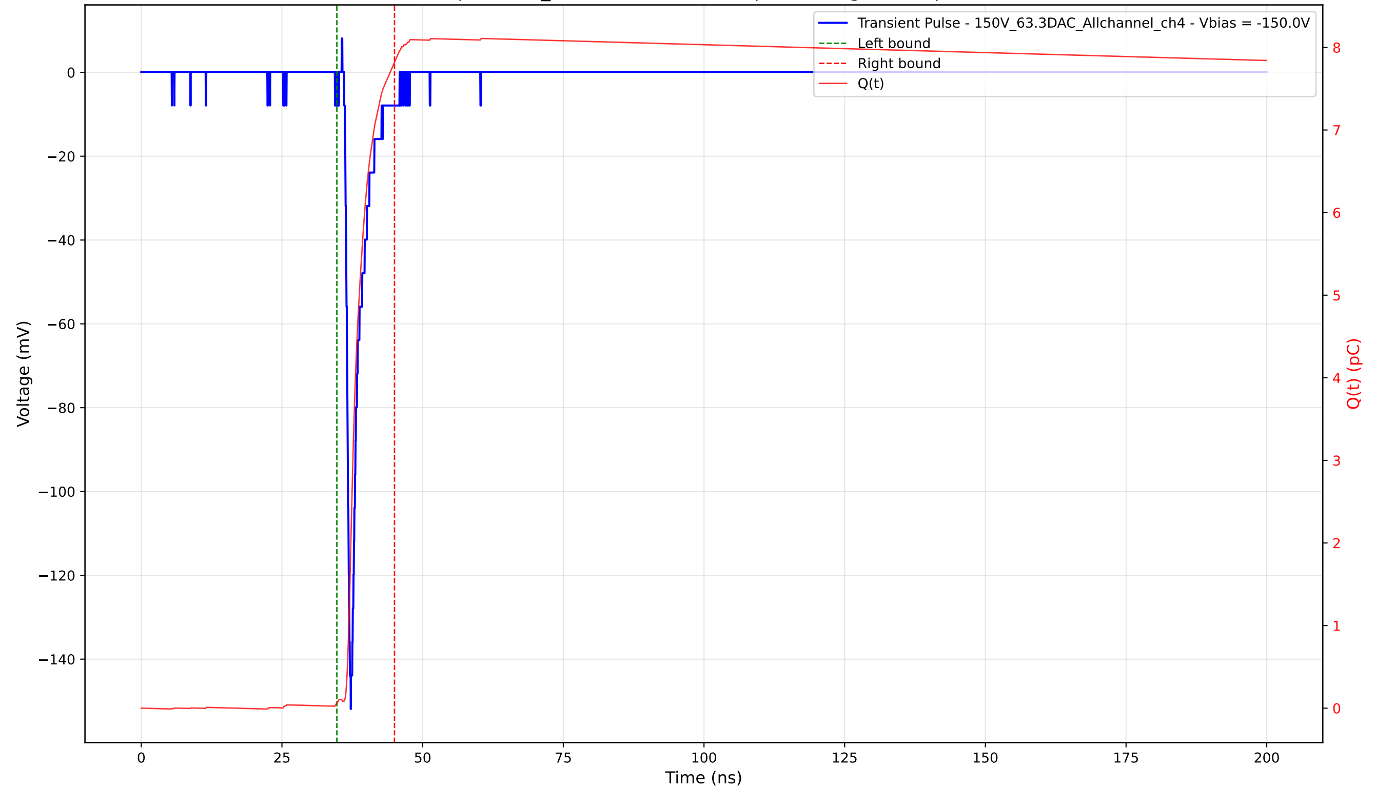
Transient Pulse - Sample: 1cm_42 - Position: 2695.0 \mu\text{m} - Charge: 7.76 pC - Rise Time: 0.88 ns
