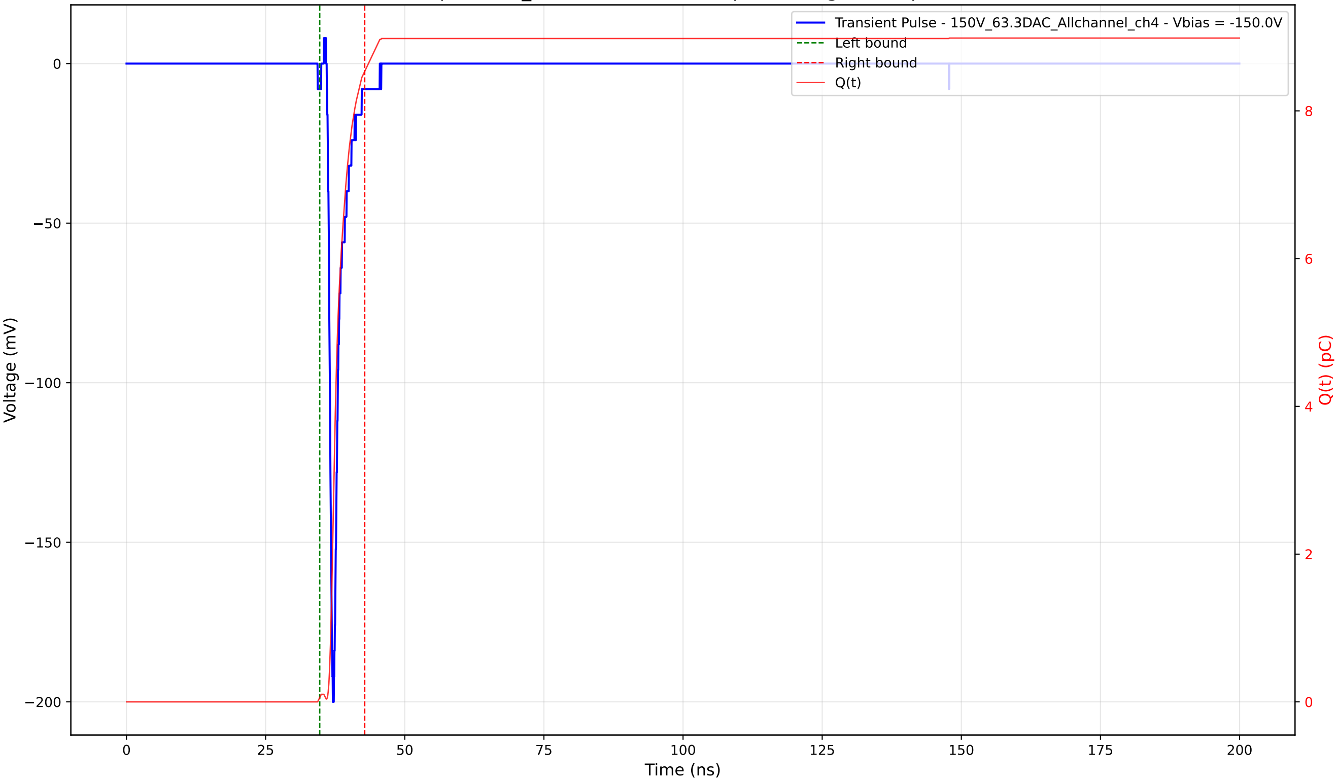
Transient Pulse - Sample: 1cm_42 - Position: 2570.0 \mu\text{m} - Charge: 8.47 pC - Rise Time: 0.78 ns
