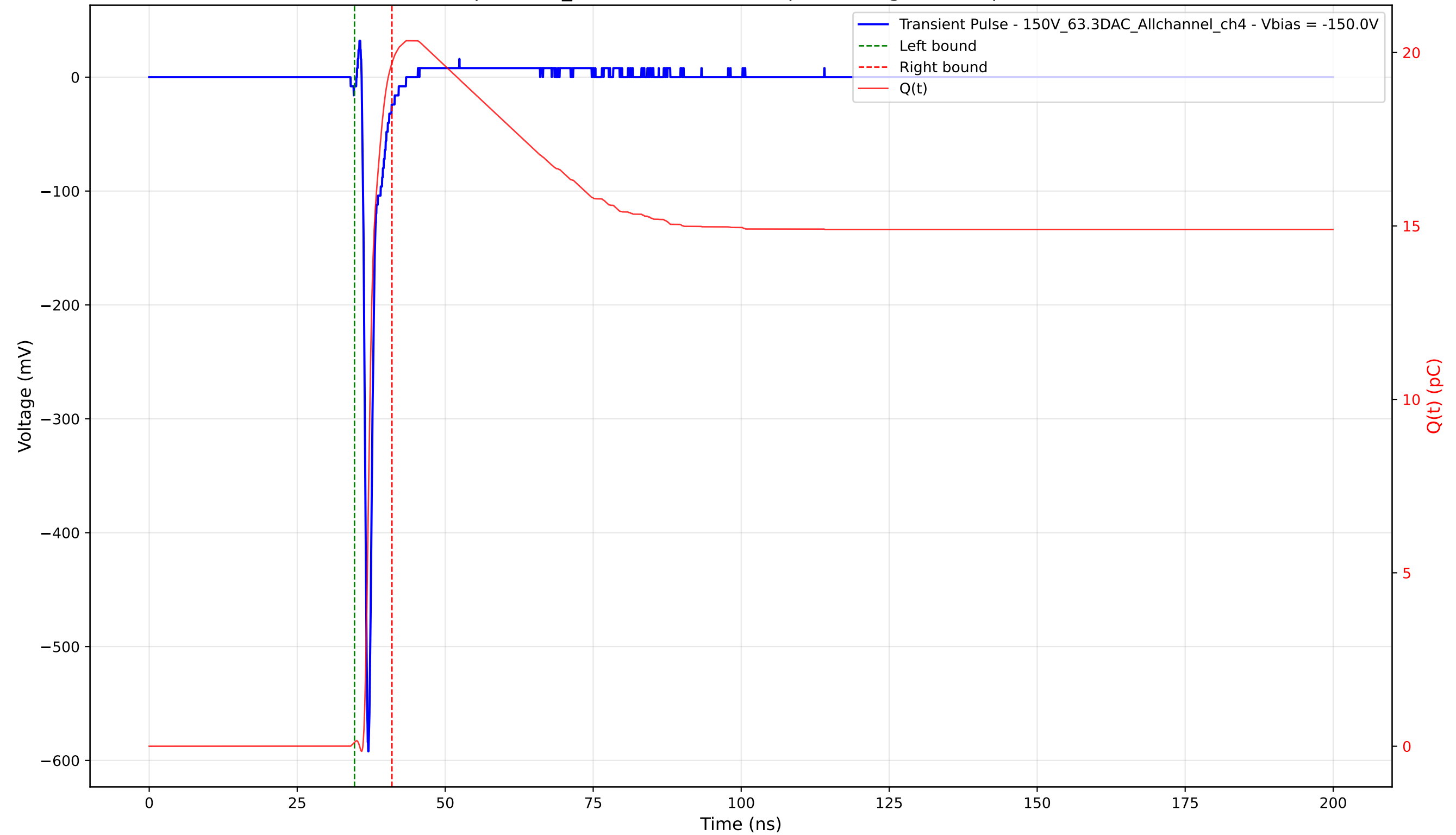
Transient Pulse - Sample: 1cm_42 - Position: 1780.0 \mu\text{m} - Charge: 19.59 pC - Rise Time: 0.72 ns
