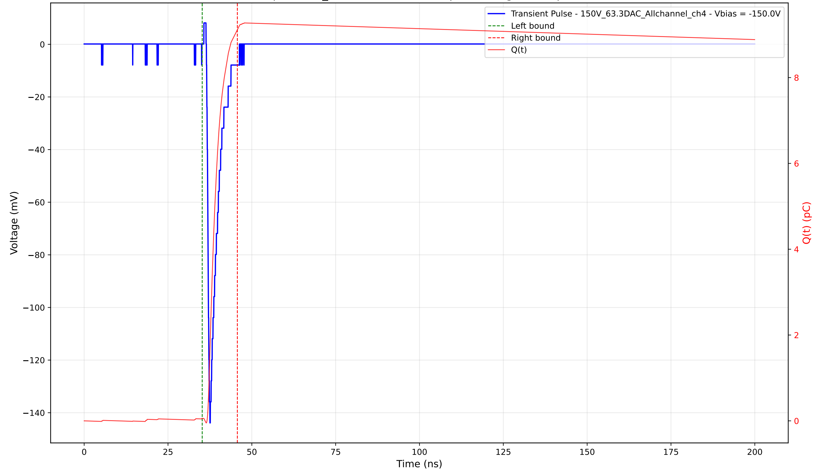
Transient Pulse - Sample: 1cm_42 - Position: 1135.0 \mu\text{m} - Charge: 9.06 pC - Rise Time: 0.81 ns
