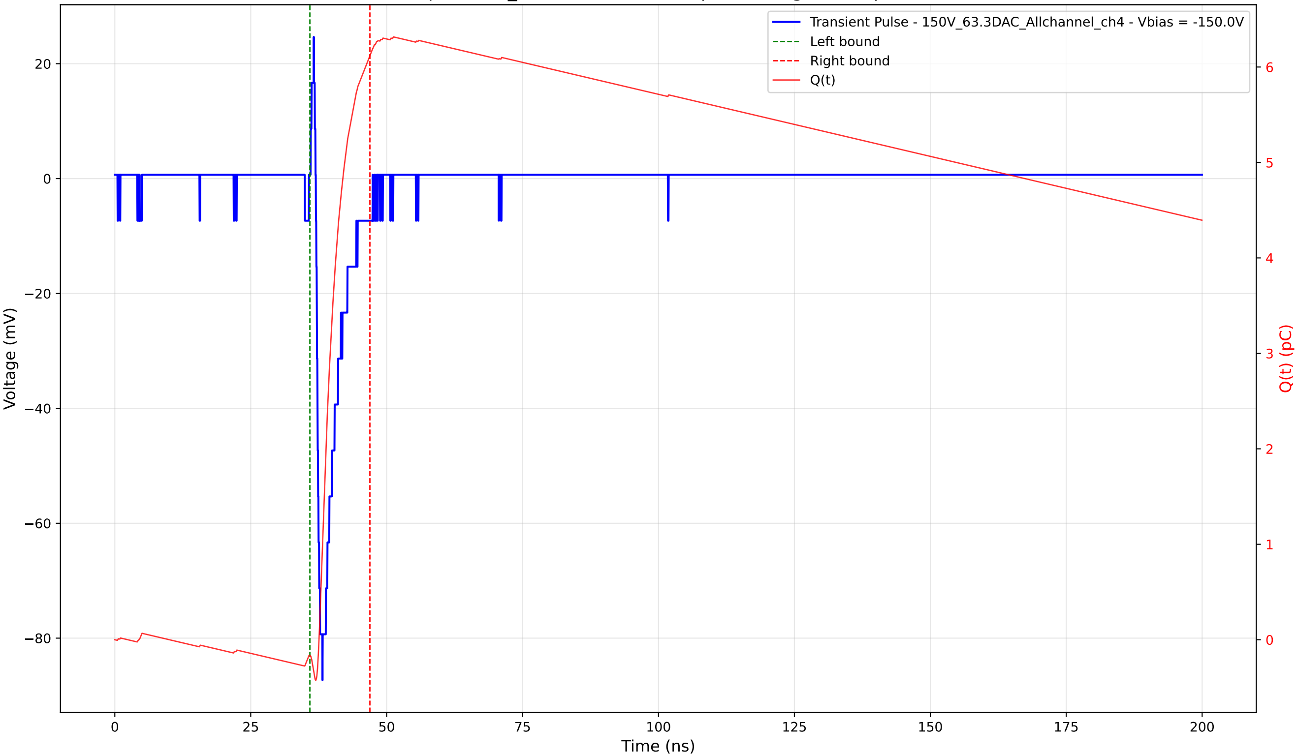
Transient Pulse - Sample: 1cm_42 - Position: 825.0 \mu\text{m} - Charge: 6.29 pC - Rise Time: 0.71 ns
