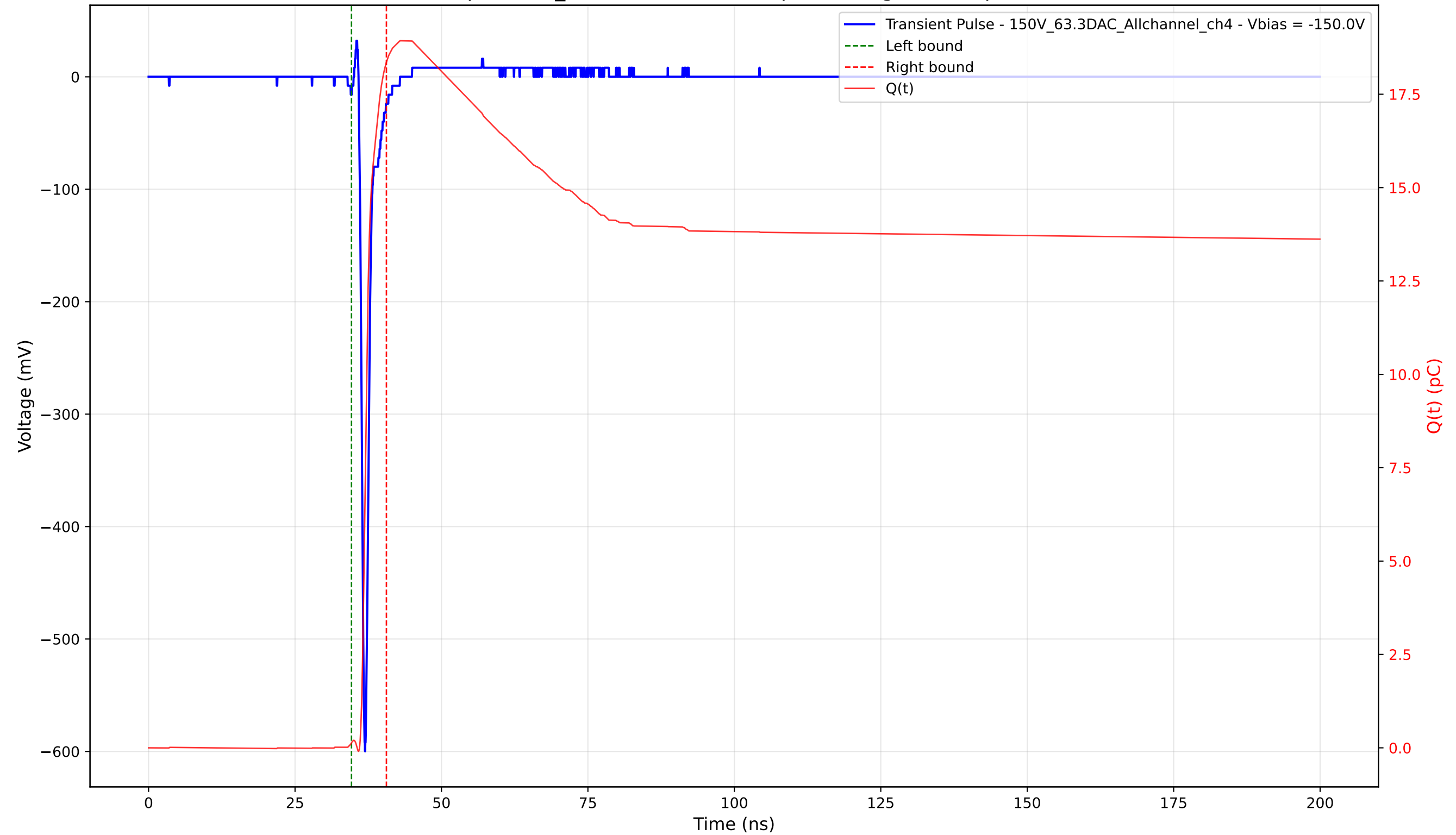
Transient Pulse - Sample: 1cm_42 - Position: 1950.0 \mu\text{m} - Charge: 18.22 pC - Rise Time: 0.65 ns
