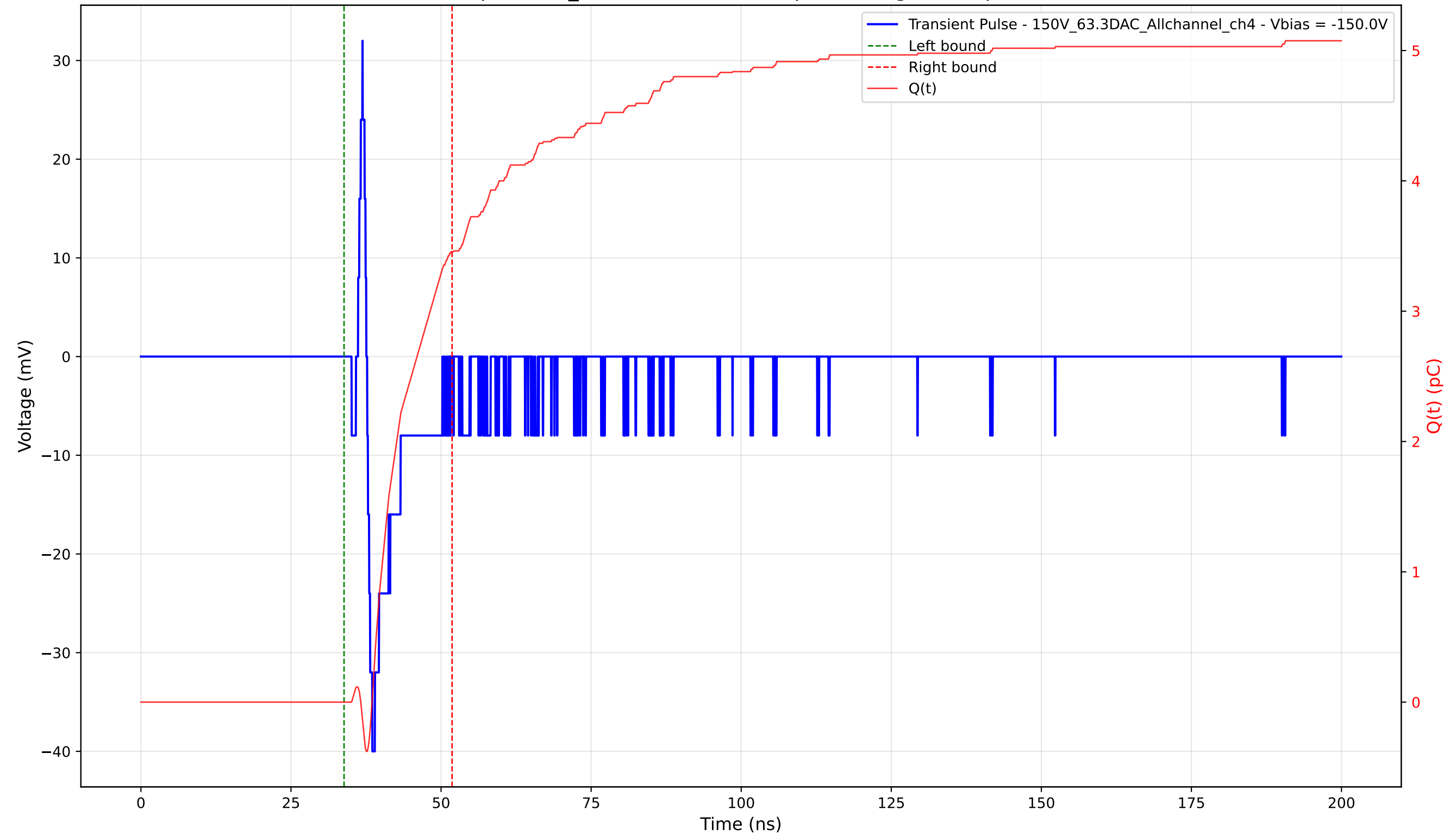
Transient Pulse - Sample: 1cm_42 - Position: 3805.0 \mu\text{m} - Charge: 3.46 pC - Rise Time: 0.86 ns
