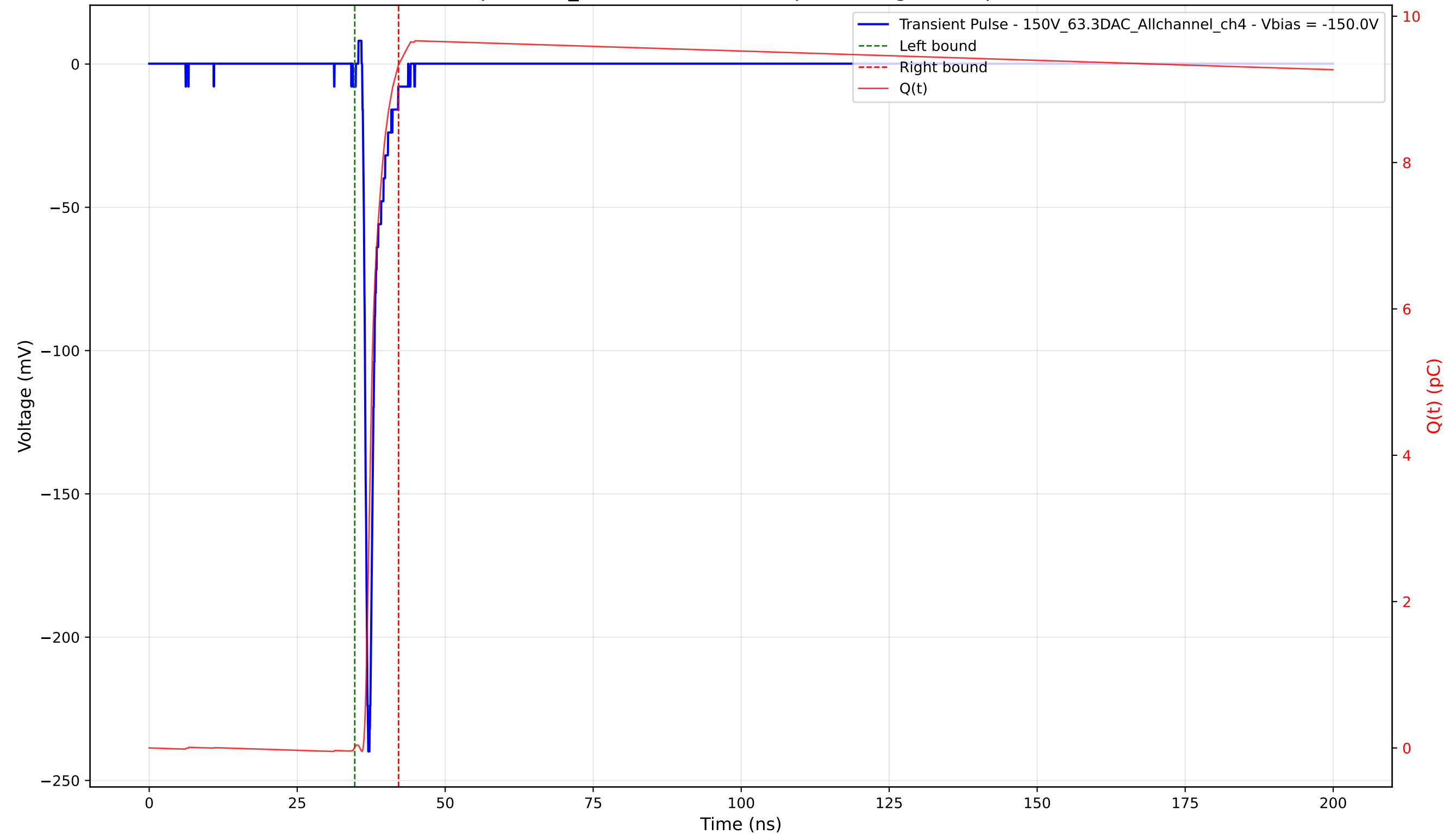
Transient Pulse - Sample: 1cm_42 - Position: 2510.0 \mu\text{m} - Charge: 9.33 pC - Rise Time: 0.76 ns
