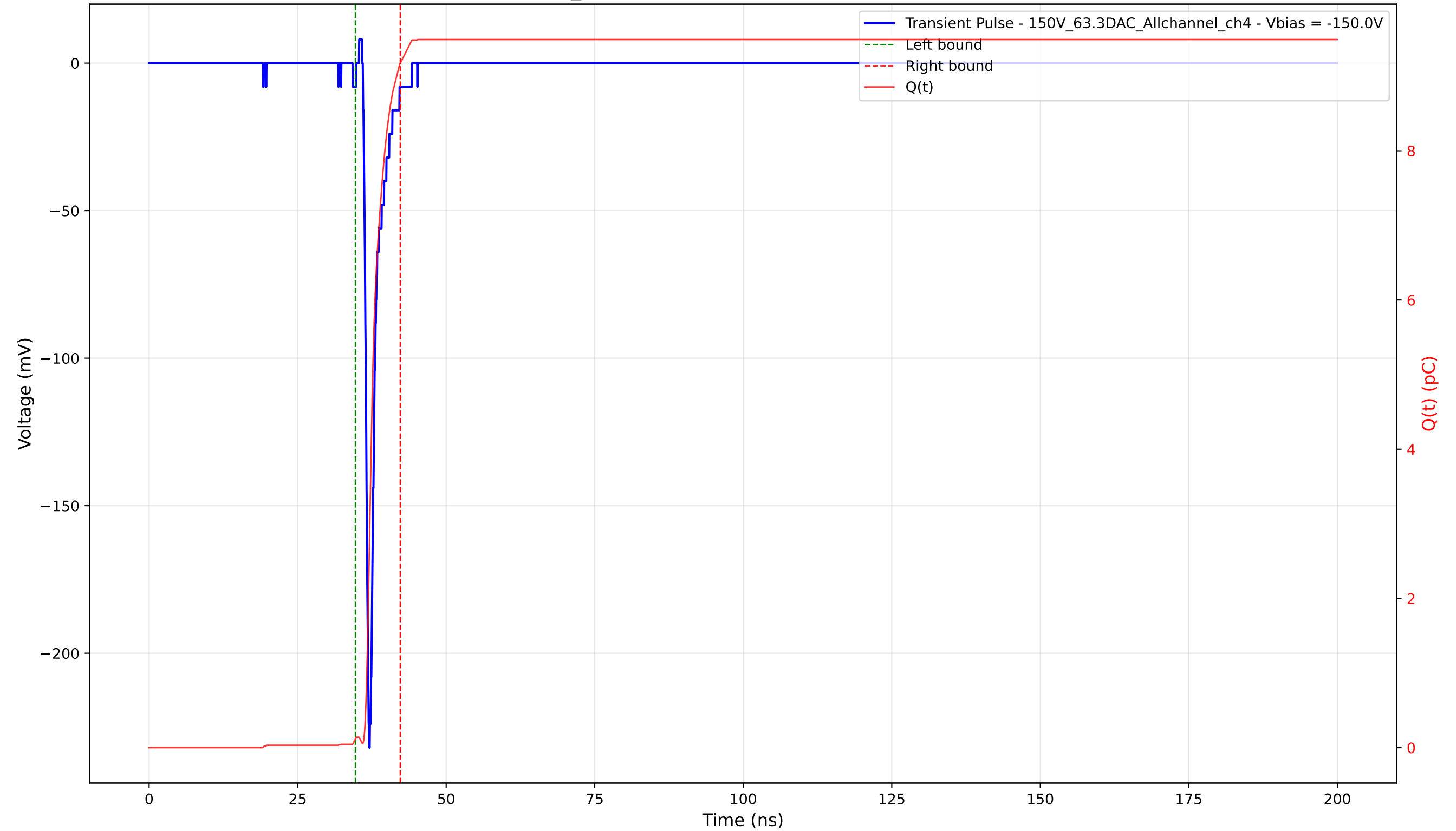
Transient Pulse - Sample: 1cm_42 - Position: 2525.0 \mu\text{m} - Charge: 9.06 pC - Rise Time: 0.77 ns
