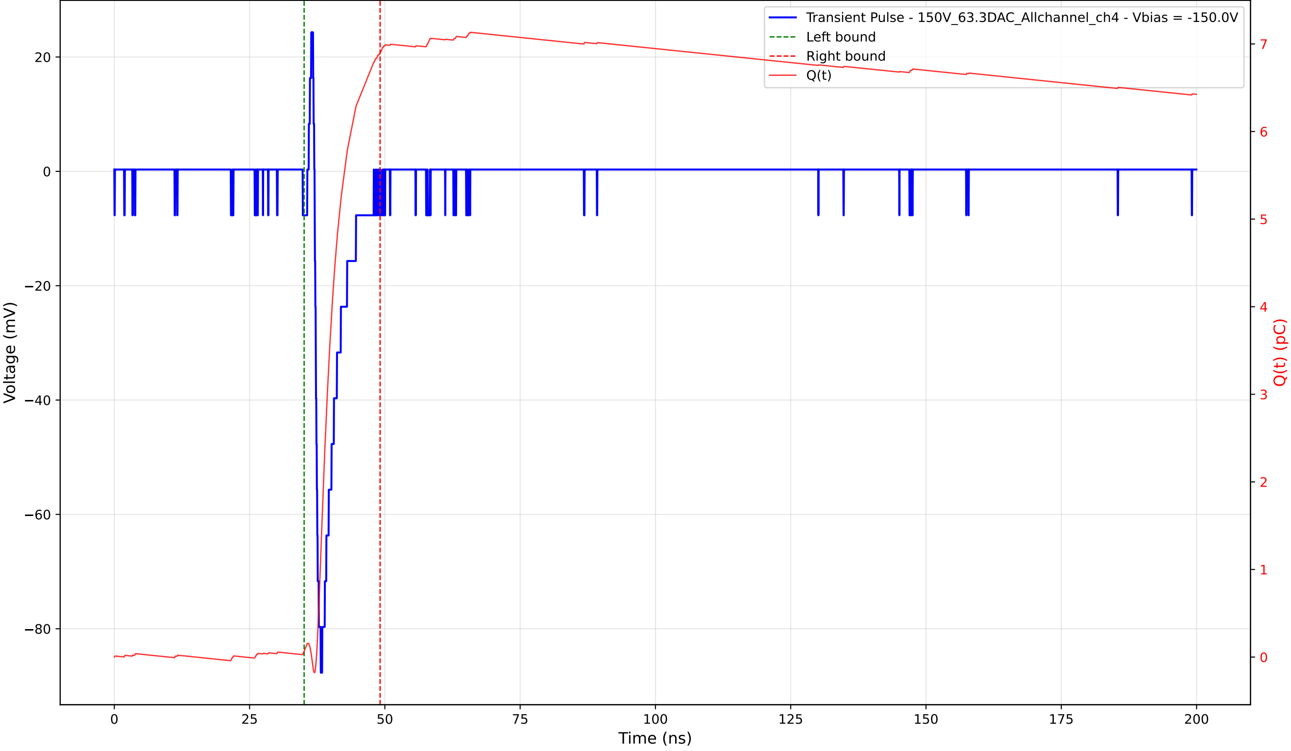
Transient Pulse - Sample: 1cm_42 - Position: 760.0 \mu\text{m} - Charge: 6.84 pC - Rise Time: 0.75 ns
