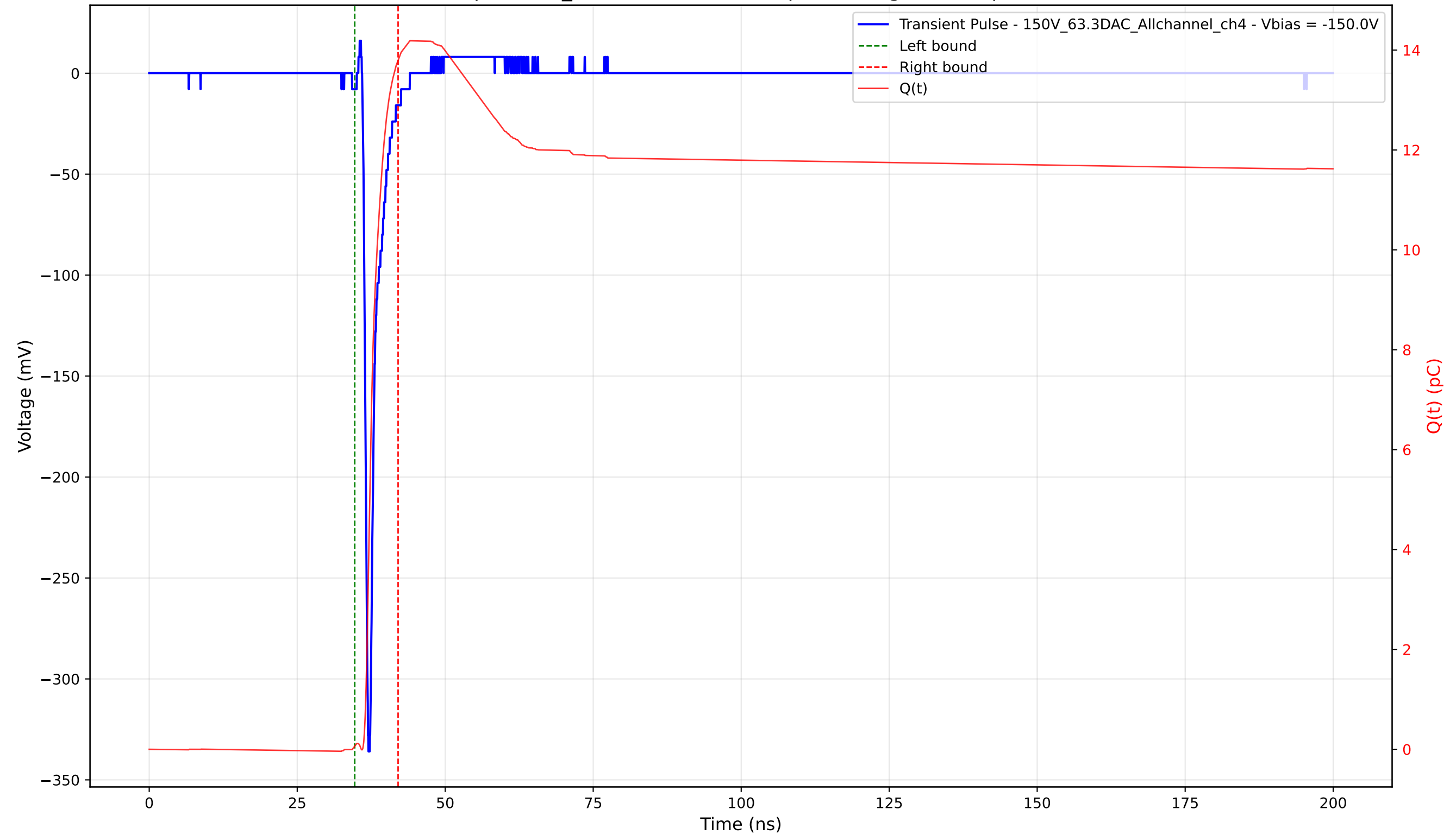
Transient Pulse - Sample: 1cm_42 - Position: 1575.0 \mu\text{m} - Charge: 13.73 pC - Rise Time: 0.74 ns
