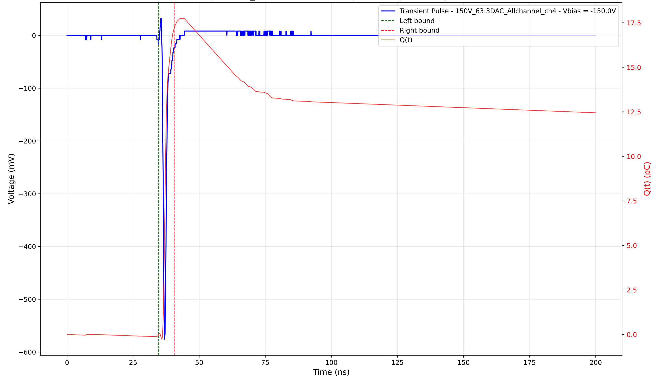
Transient Pulse - Sample: 1cm_42 - Position: 2050.0 \mu\text{m} - Charge: 17.19 pC - Rise Time: 0.71 ns
