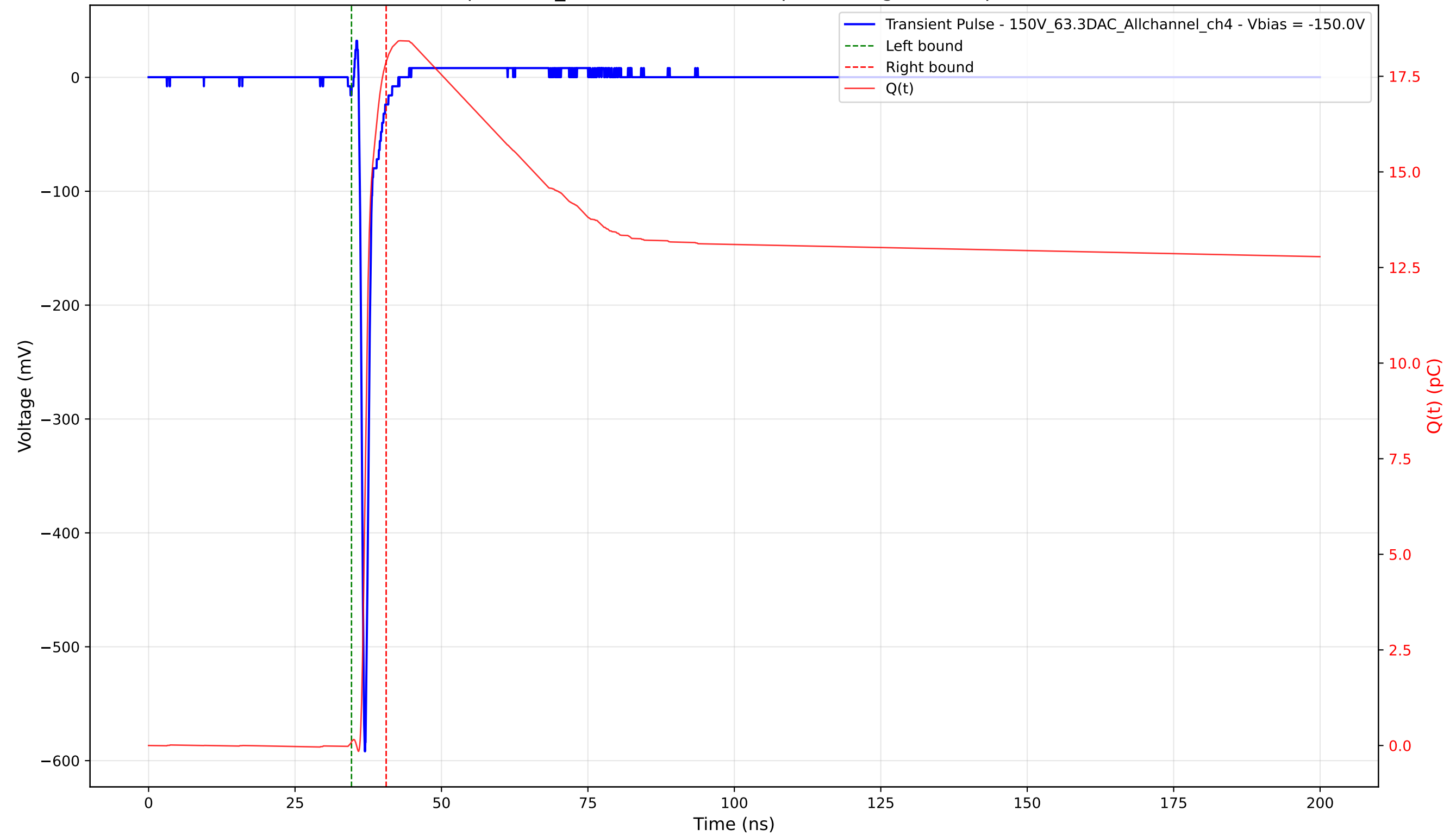
Transient Pulse - Sample: 1cm_42 - Position: 2000.0 \mu\text{m} - Charge: 17.78 pC - Rise Time: 0.70 ns
