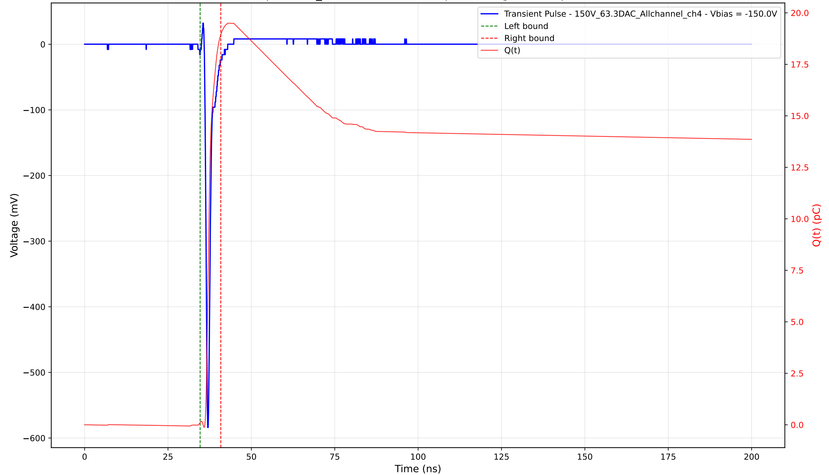
Transient Pulse - Sample: 1cm_42 - Position: 1850.0 \mu\text{m} - Charge: 18.83 pC - Rise Time: 0.71 ns
