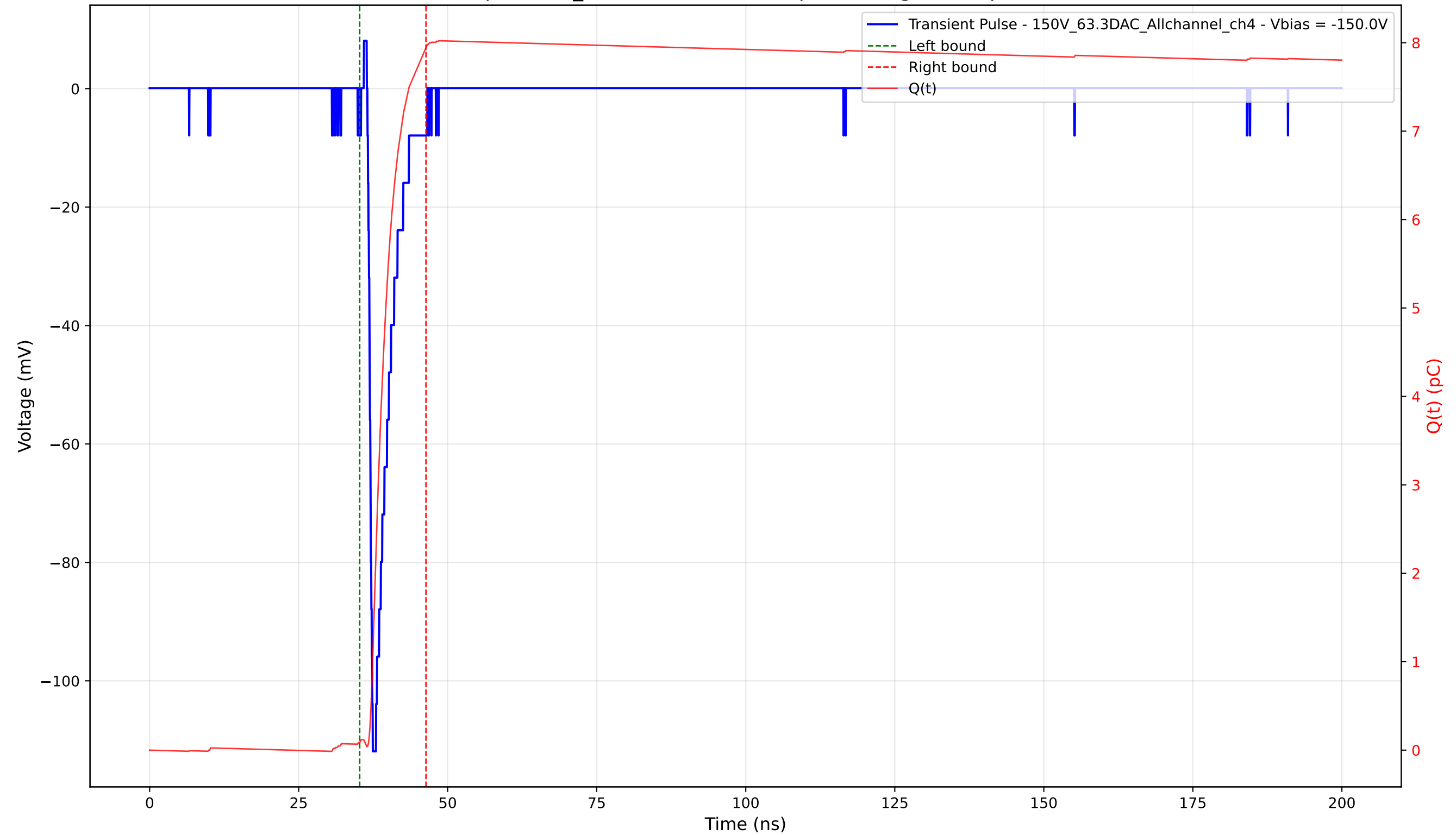
Transient Pulse - Sample: 1cm_42 - Position: 1070.0 \mu\text{m} - Charge: 7.86 pC - Rise Time: 0.74 ns
