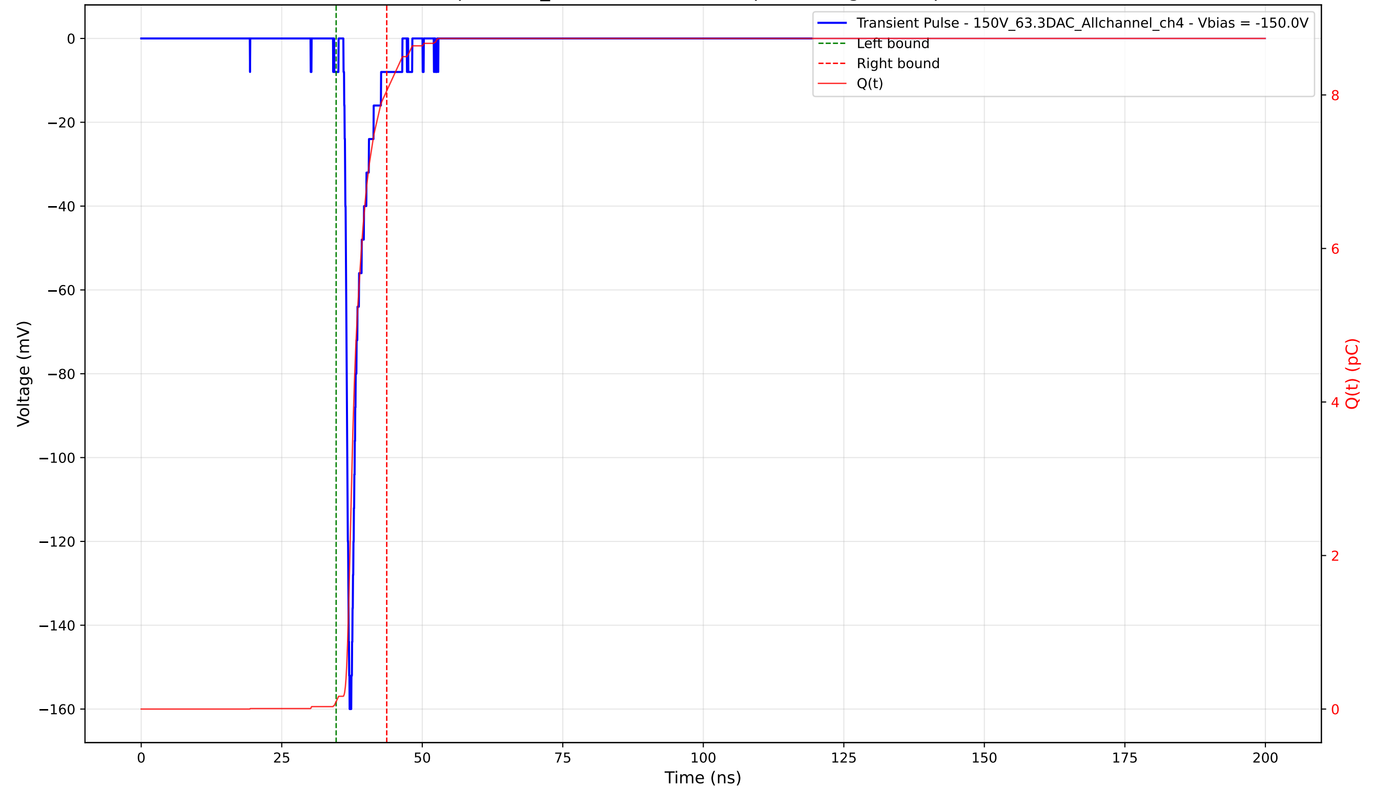
Transient Pulse - Sample: 1cm_42 - Position: 2655.0 \mu\text{m} - Charge: 7.96 pC - Rise Time: 0.76 ns
