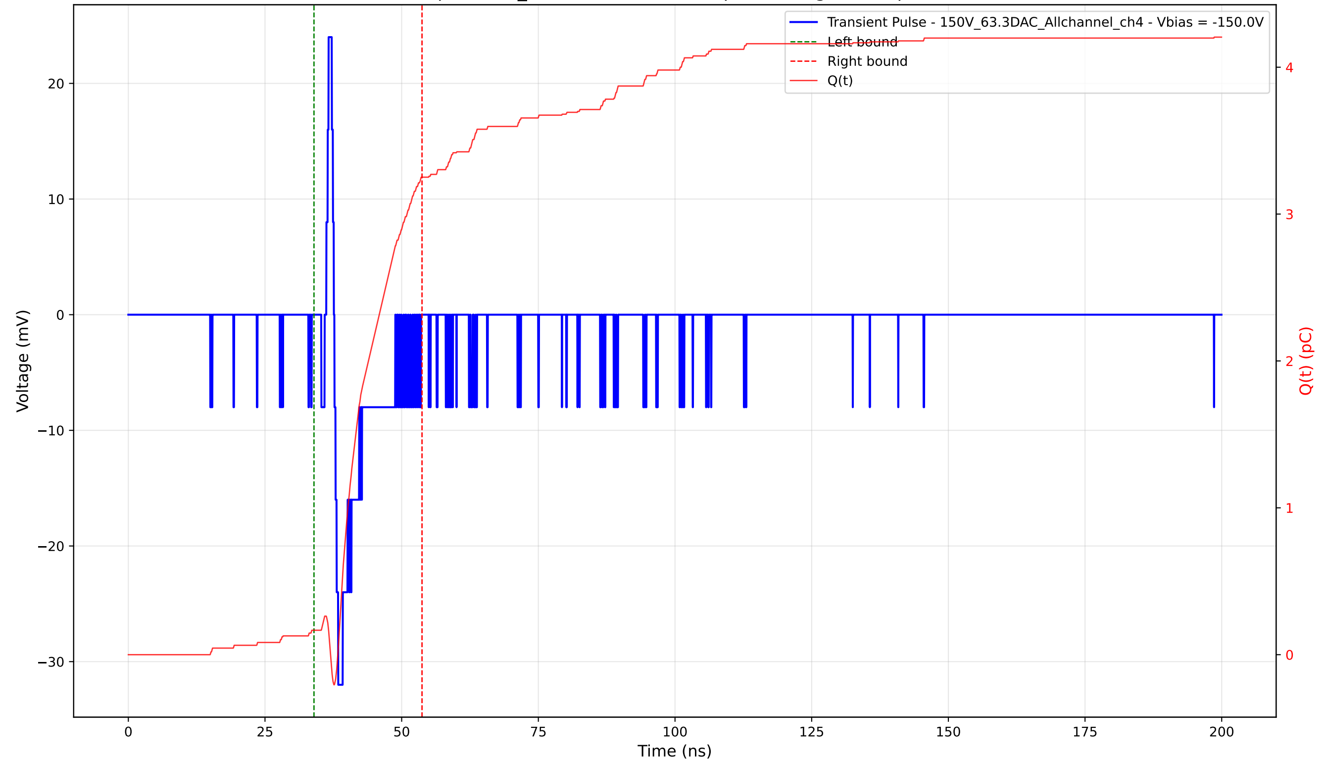
Transient Pulse - Sample: 1cm_42 - Position: 3950.0 \mu\text{m} - Charge: 3.08 pC - Rise Time: 0.70 ns
