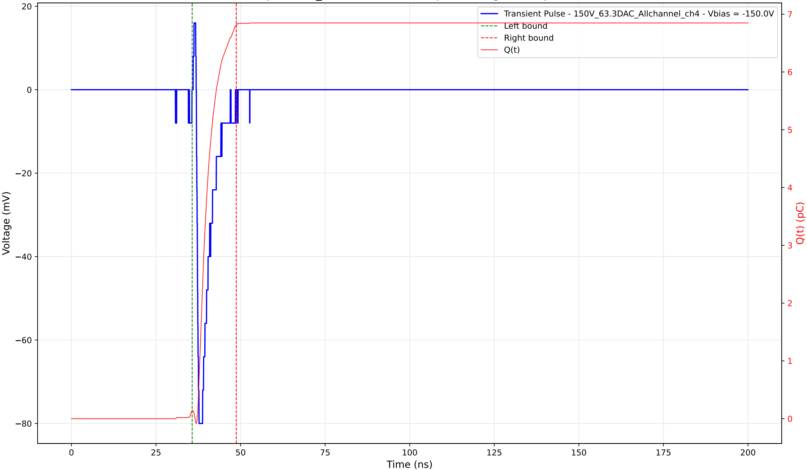
Transient Pulse - Sample: 1cm_42 - Position: 870.0 \mu\text{m} - Charge: 6.67 pC - Rise Time: 0.60 ns
