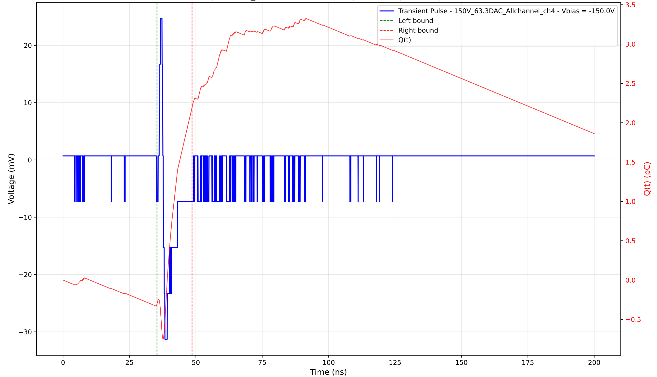
Transient Pulse - Sample: 1cm_42 - Position: 3895.0 \mu\text{m} - Charge: 2.50 pC - Rise Time: 0.67 ns
