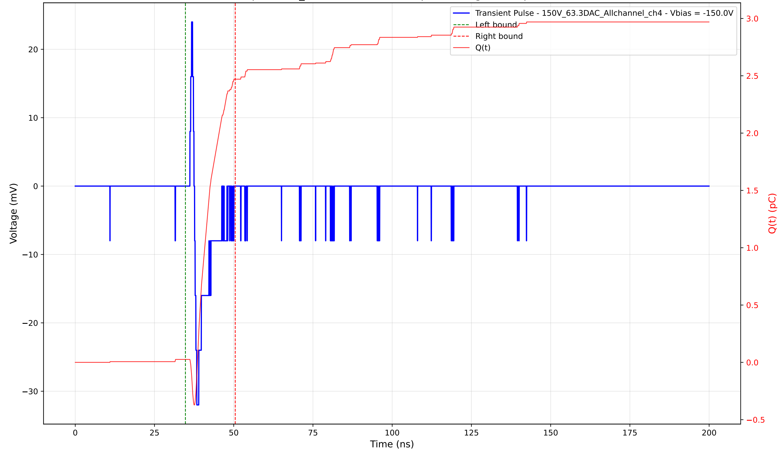
Transient Pulse - Sample: 1cm_42 - Position: 4605.0 \mu\text{m} - Charge: 2.44 pC - Rise Time: 0.70 ns
