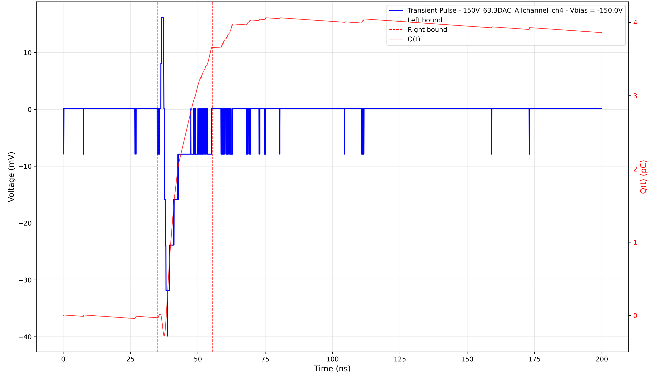
Transient Pulse - Sample: 1cm_42 - Position: 3580.0 \mu\text{m} - Charge: 3.69 pC - Rise Time: 1.18 ns
