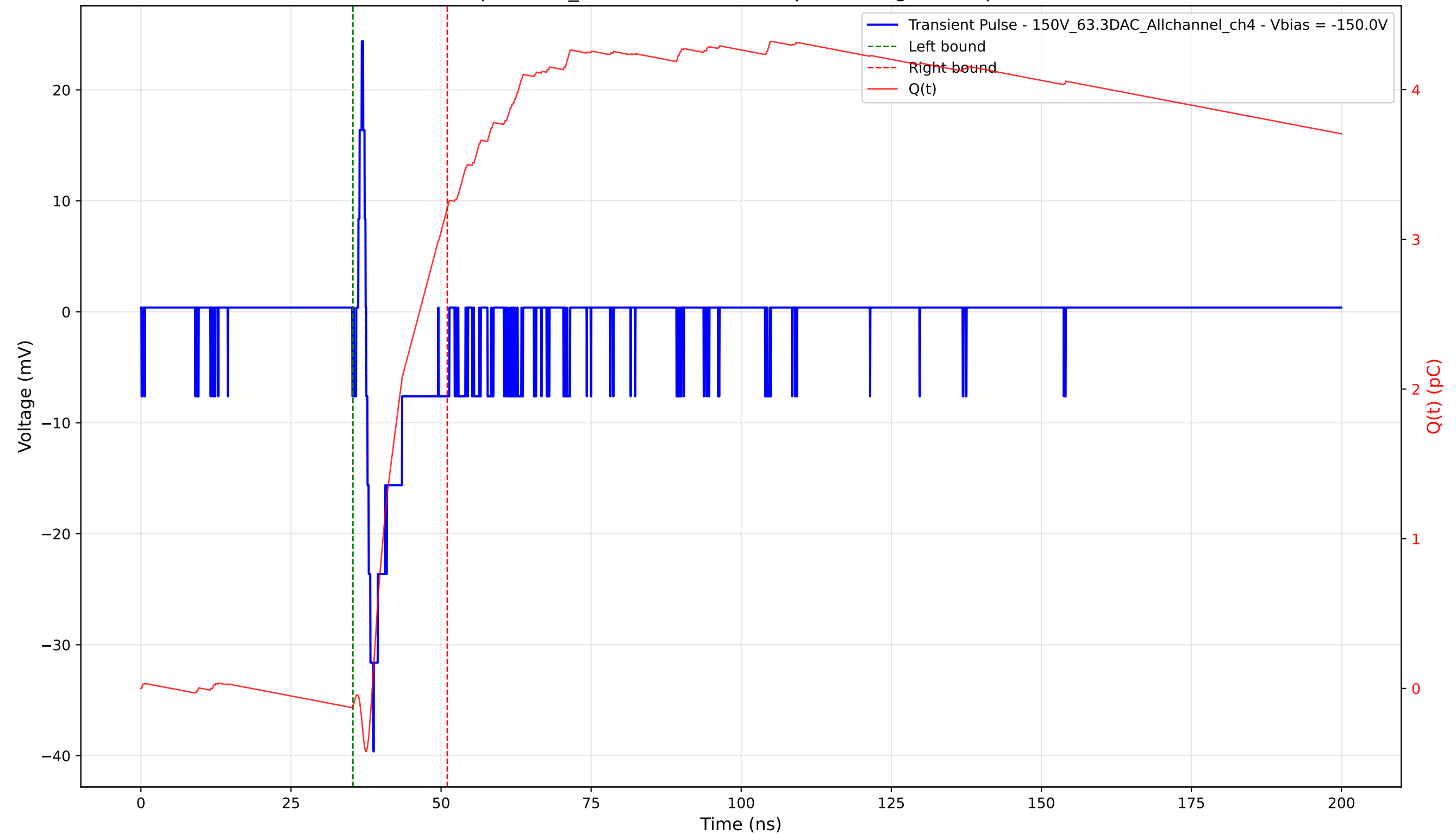
Transient Pulse - Sample: 1cm_42 - Position: 3645.0 \mu\text{m} - Charge: 3.32 pC - Rise Time: 1.22 ns
