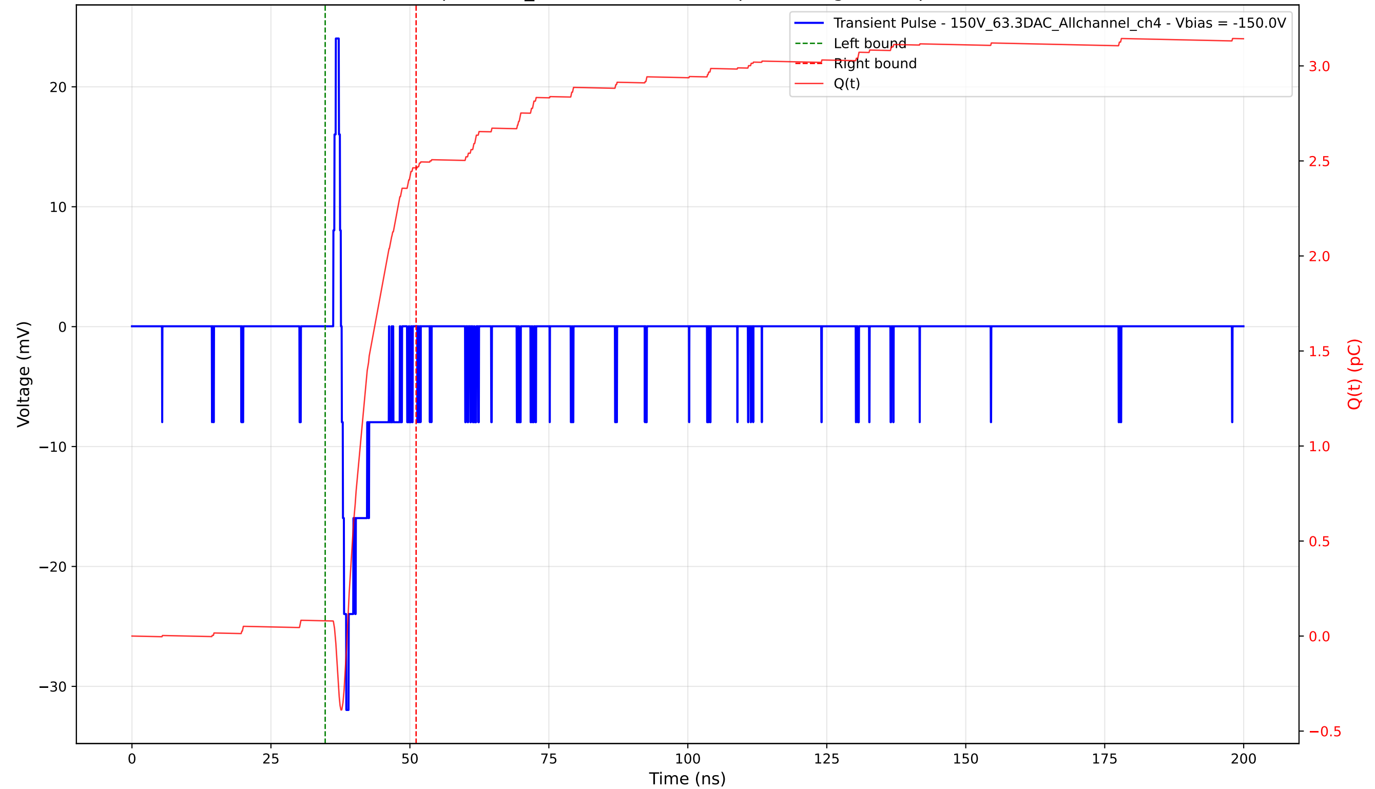
Transient Pulse - Sample: 1cm_42 - Position: 4460.0 \mu\text{m} - Charge: 2.38 pC - Rise Time: 0.82 ns
