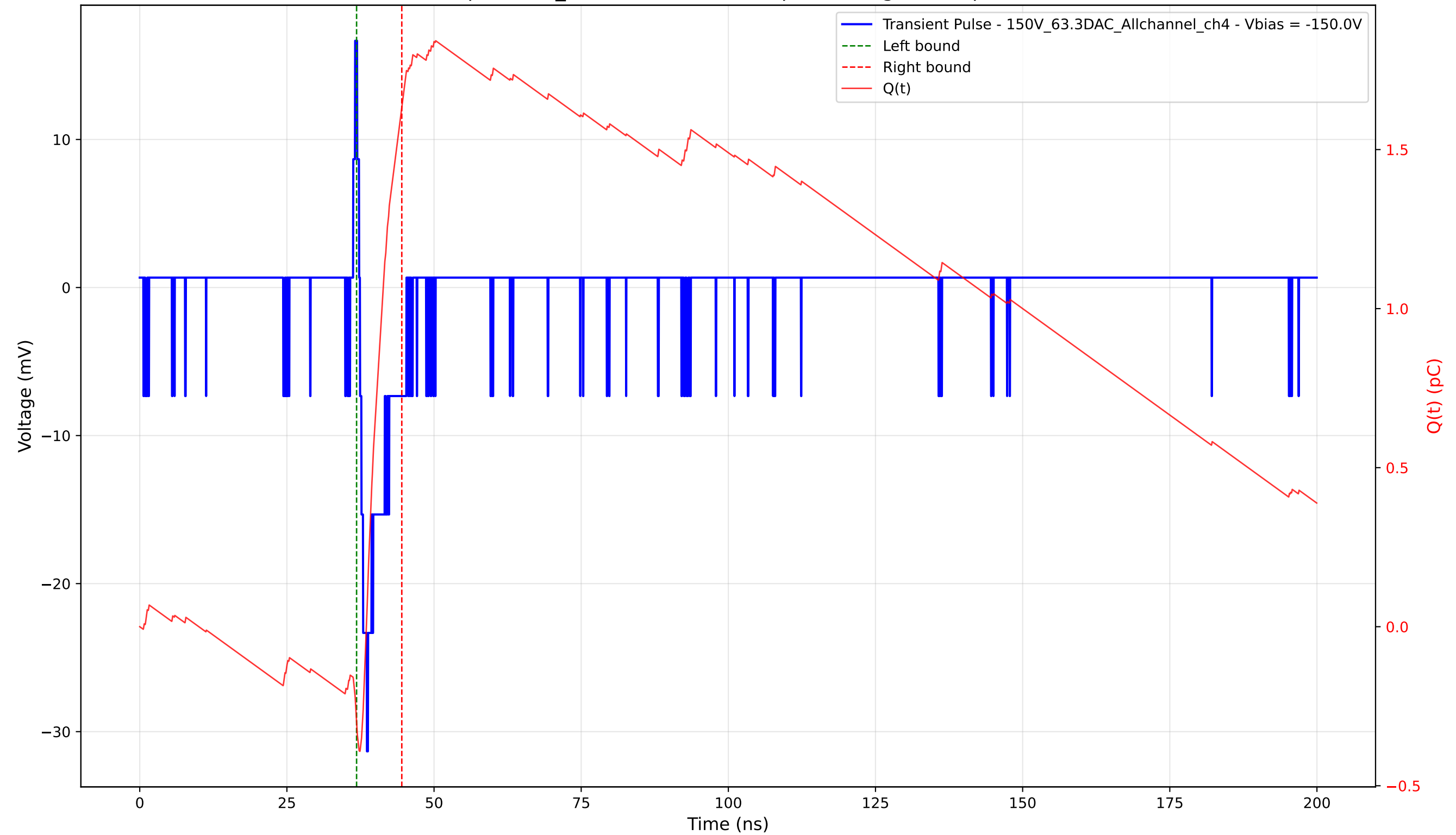
Transient Pulse - Sample: 1cm_42 - Position: 4945.0 \mu\text{m} - Charge: 1.94 pC - Rise Time: 1.19 ns
