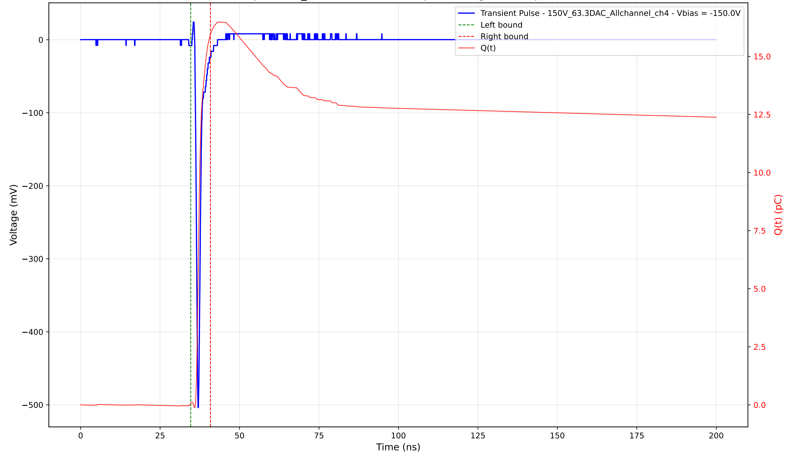
Transient Pulse - Sample: 1cm_42 - Position: 2265.0 \mu\text{m} - Charge: 15.89 pC - Rise Time: 0.73 ns
