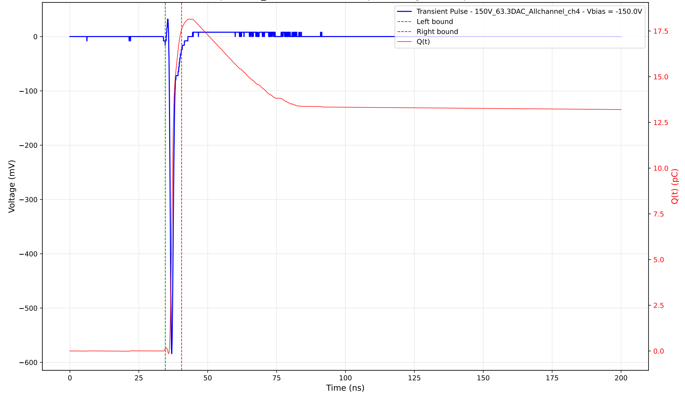
Transient Pulse - Sample: 1cm_42 - Position: 2035.0 \mu\text{m} - Charge: 17.47 pC - Rise Time: 0.71 ns
