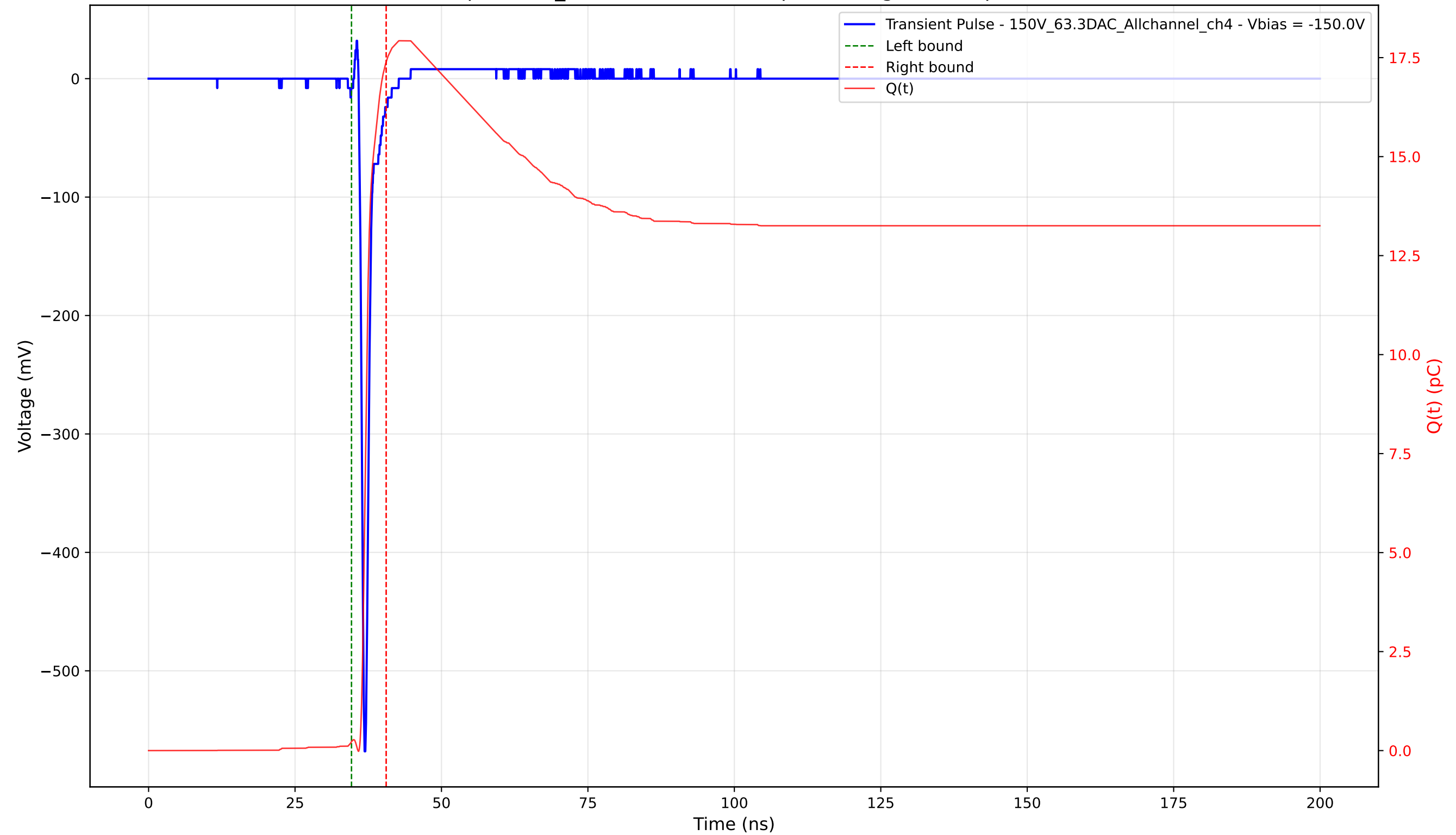
Transient Pulse - Sample: 1cm_42 - Position: 2115.0 \mu\text{m} - Charge: 17.16 pC - Rise Time: 0.72 ns
