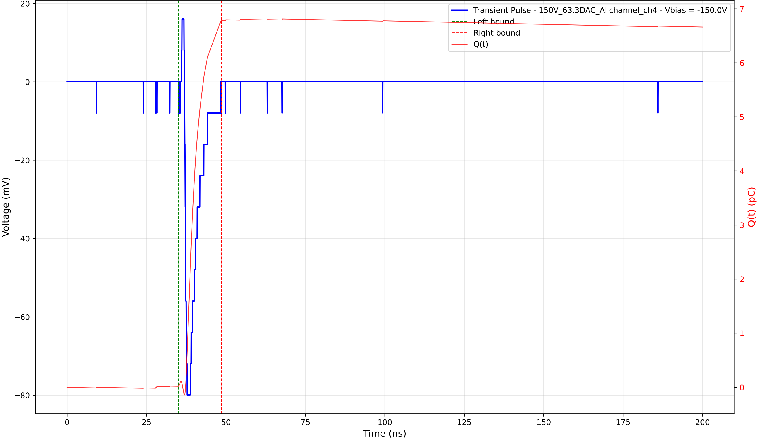
Transient Pulse - Sample: 1cm_42 - Position: 855.0 \mu\text{m} - Charge: 6.74 pC - Rise Time: 0.76 ns
