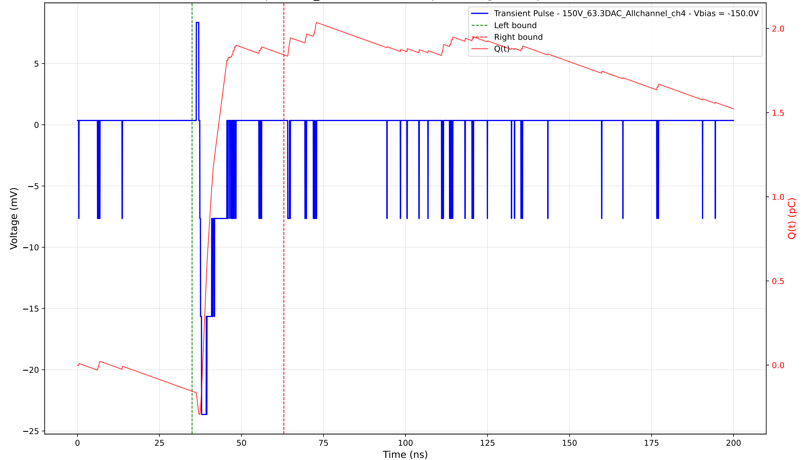
Transient Pulse - Sample: 1cm_42 - Position: 195.0 \mu\text{m} - Charge: 2.00 pC - Rise Time: 0.55 ns
