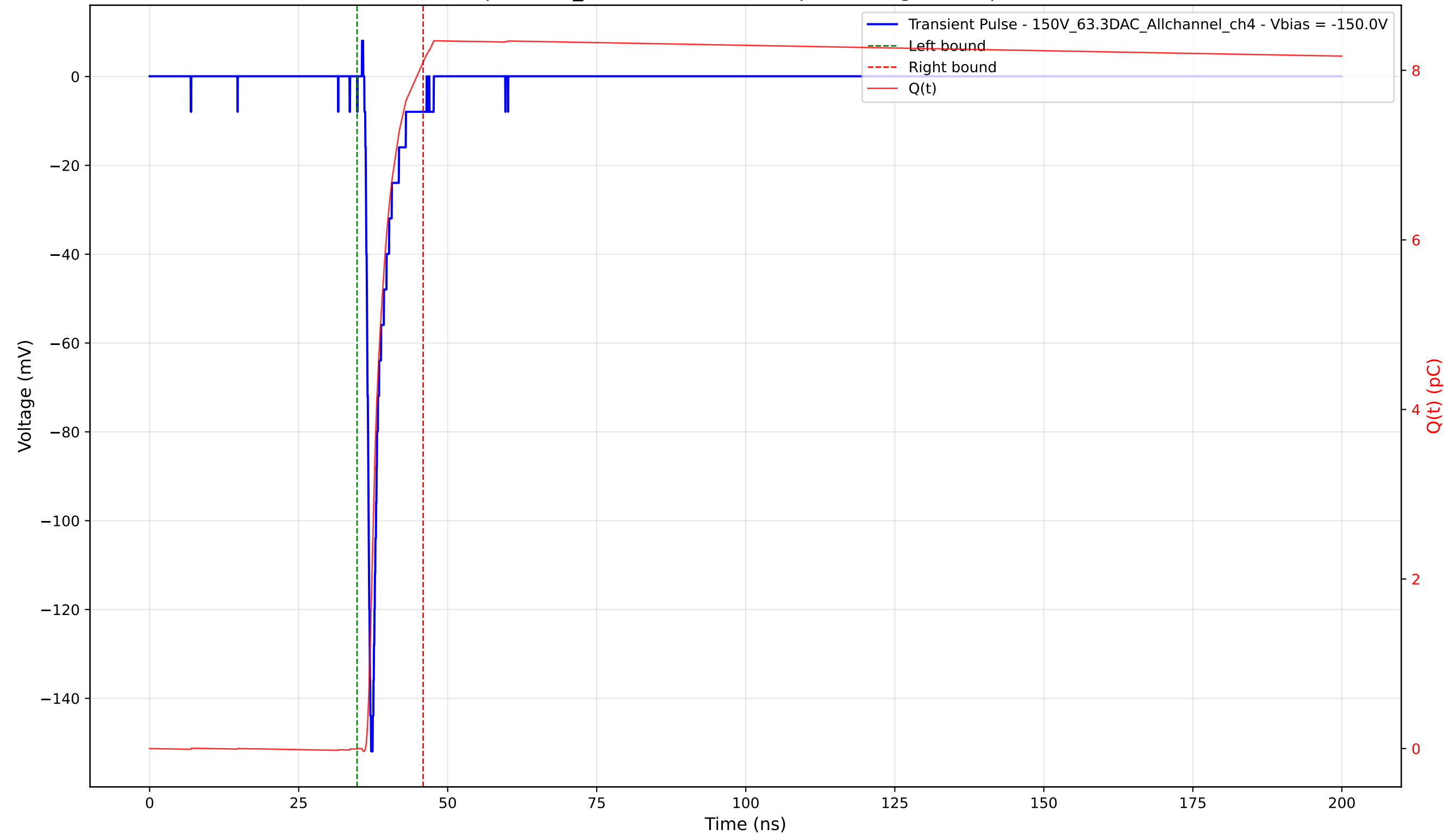
Transient Pulse - Sample: 1cm_42 - Position: 2690.0 \mu\text{m} - Charge: 8.10 pC - Rise Time: 0.84 ns
