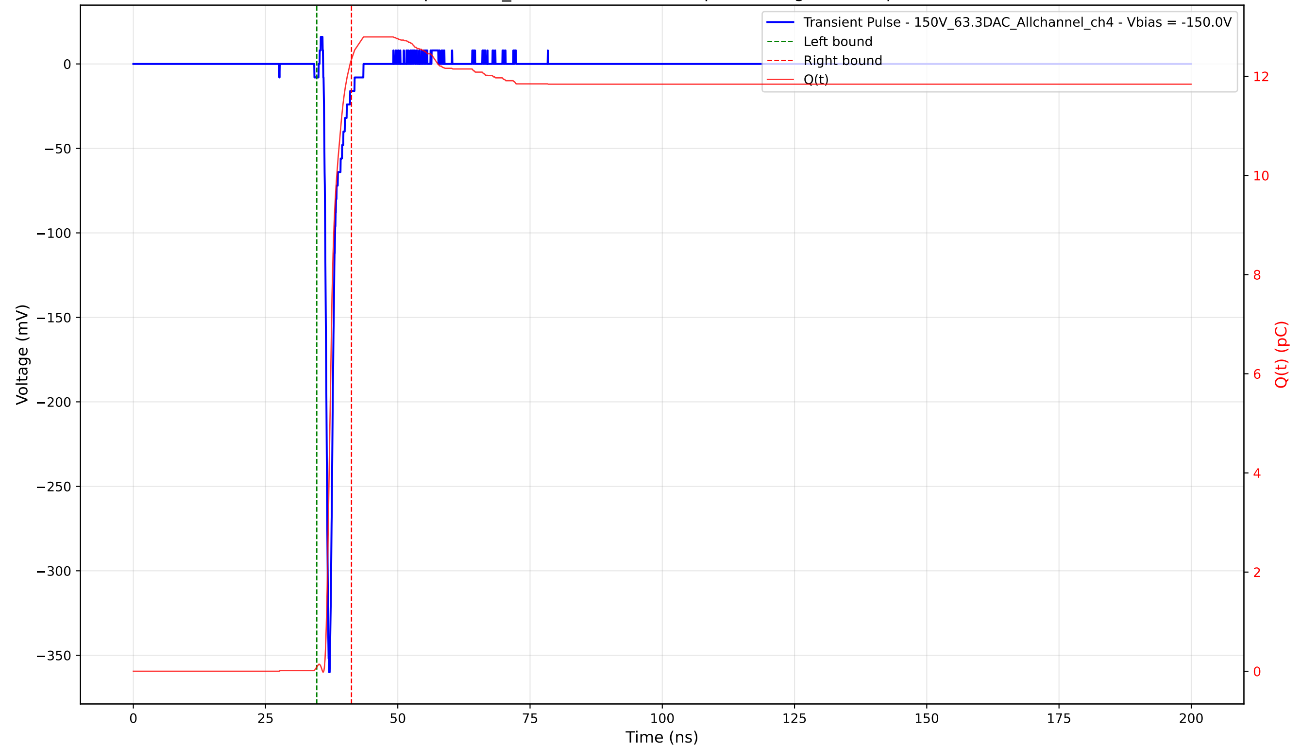
Transient Pulse - Sample: 1cm_42 - Position: 2405.0 \mu\text{m} - Charge: 12.25 pC - Rise Time: 0.71 ns
