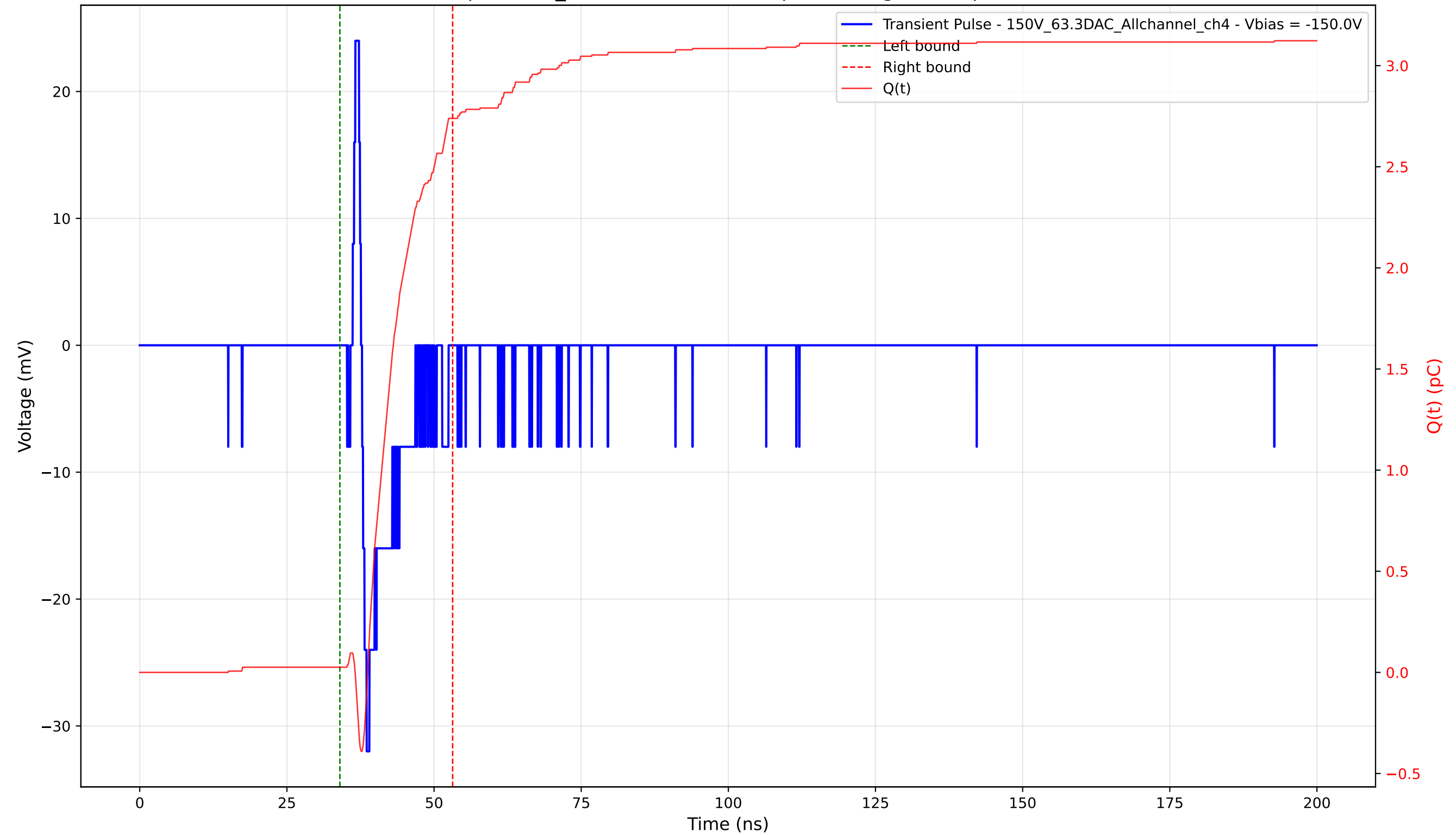
Transient Pulse - Sample: 1cm_42 - Position: 4060.0 \mu\text{m} - Charge: 2.71 pC - Rise Time: 0.78 ns
