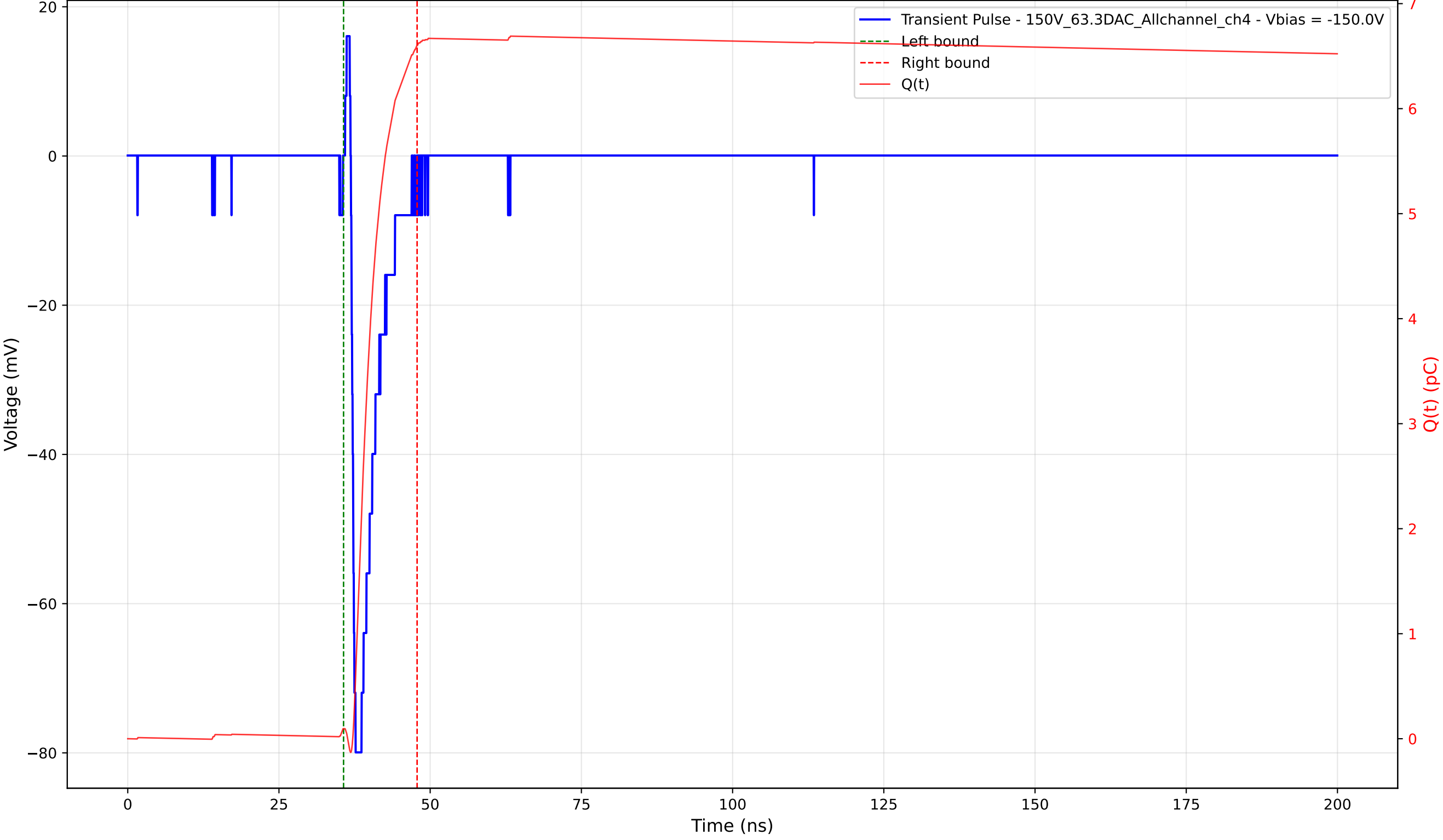
Transient Pulse - Sample: 1cm_42 - Position: 895.0 \mu\text{m} - Charge: 6.51 pC - Rise Time: 0.72 ns
