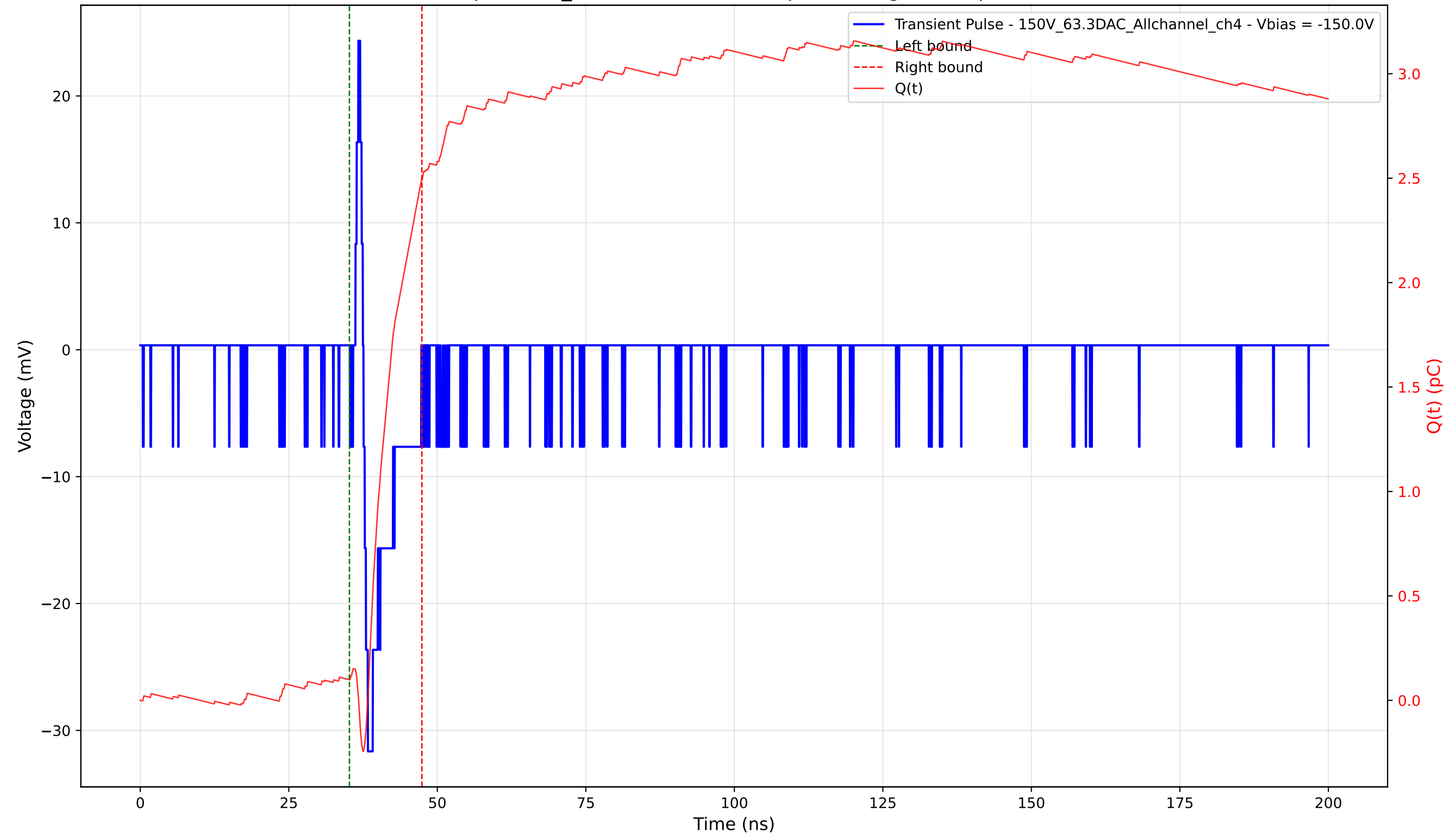
Transient Pulse - Sample: 1cm_42 - Position: 4630.0 \mu\text{m} - Charge: 2.39 pC - Rise Time: 0.74 ns
