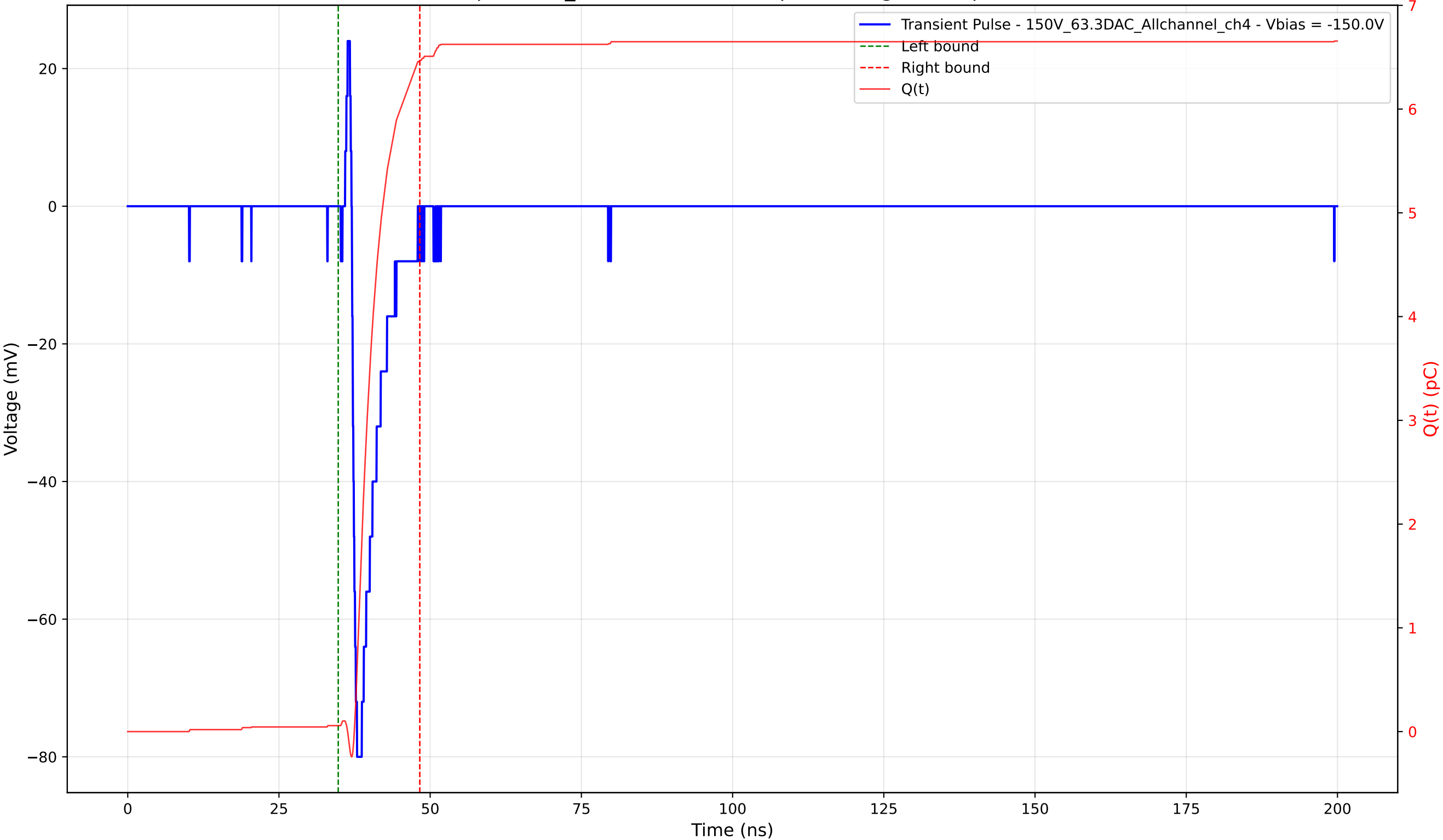
Transient Pulse - Sample: 1cm_42 - Position: 700.0 \mu\text{m} - Charge: 6.41 pC - Rise Time: 0.64 ns
