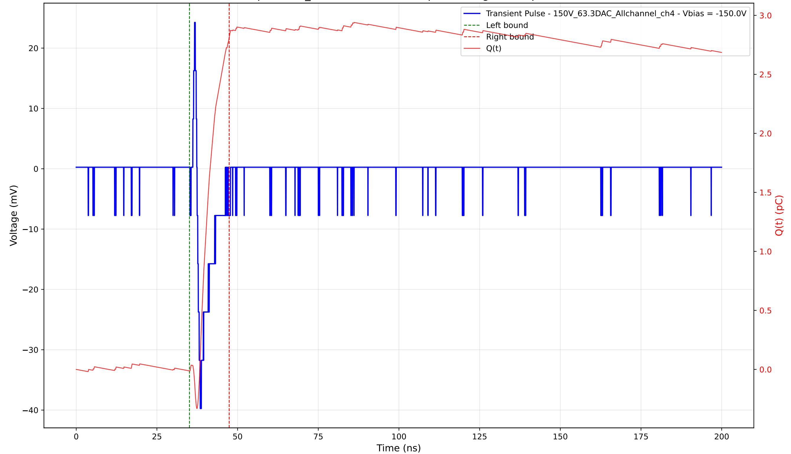
Transient Pulse - Sample: 1cm_42 - Position: 4795.0 \mu\text{m} - Charge: 2.83 pC - Rise Time: 0.98 ns
