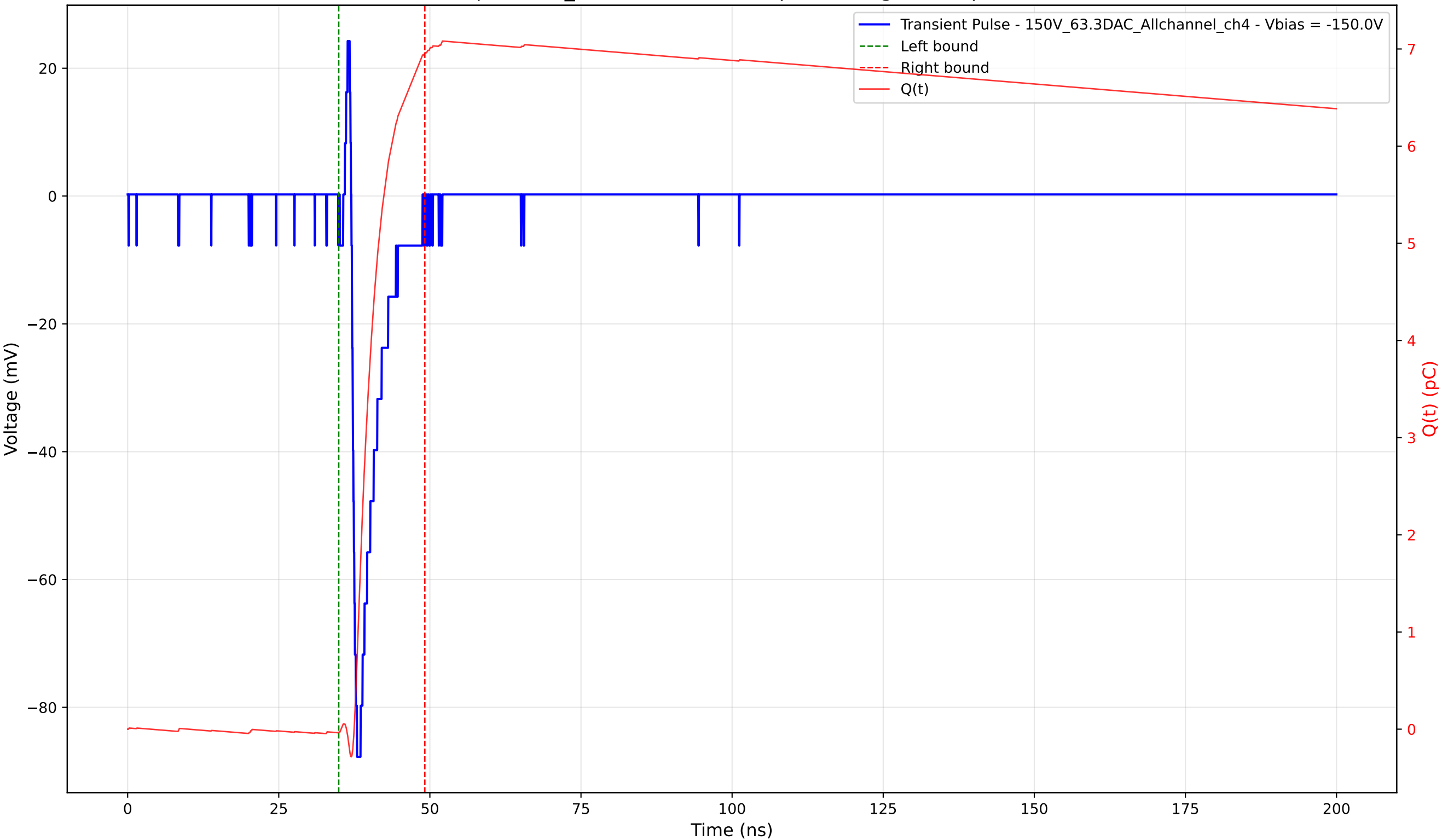
Transient Pulse - Sample: 1cm_42 - Position: 745.0 \mu\text{m} - Charge: 6.99 pC - Rise Time: 0.67 ns
