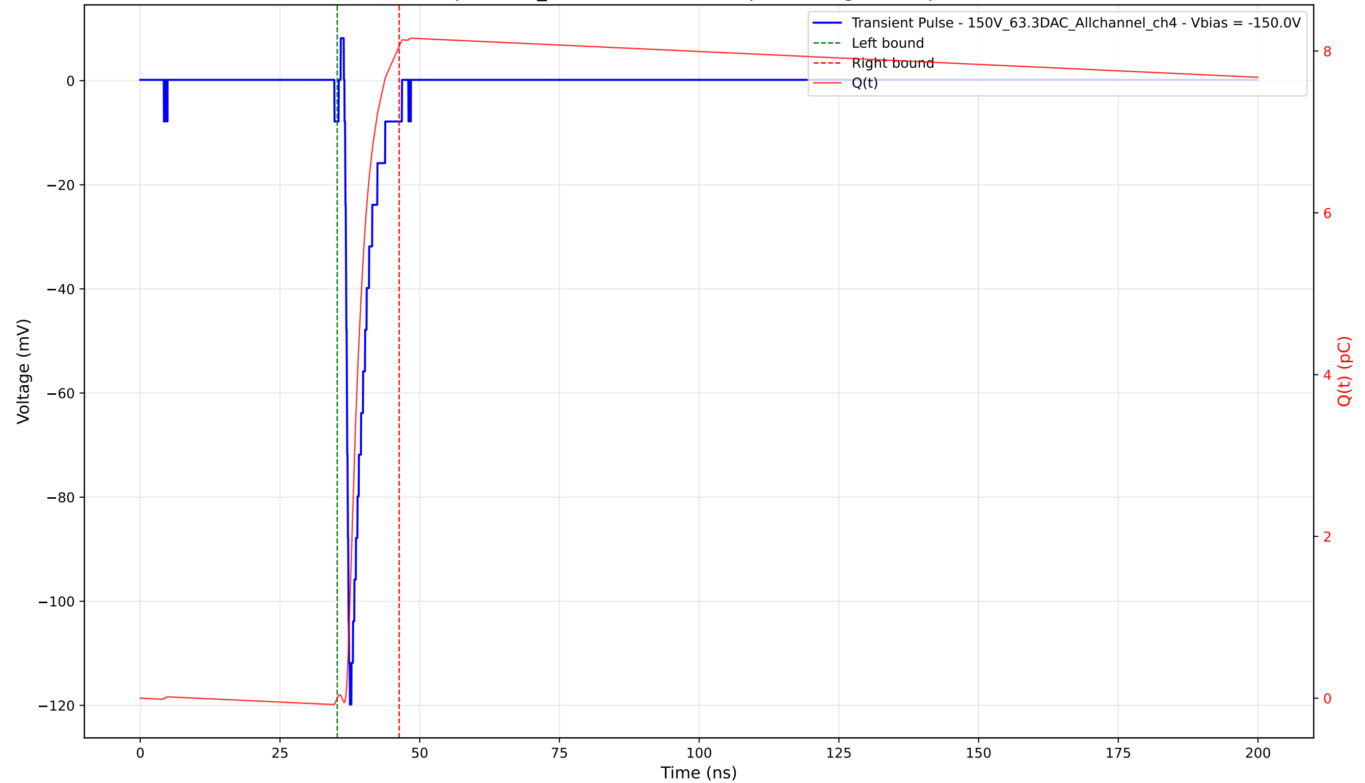
Transient Pulse - Sample: 1cm_42 - Position: 1080.0 \mu\text{m} - Charge: 8.06 pC - Rise Time: 0.70 ns
