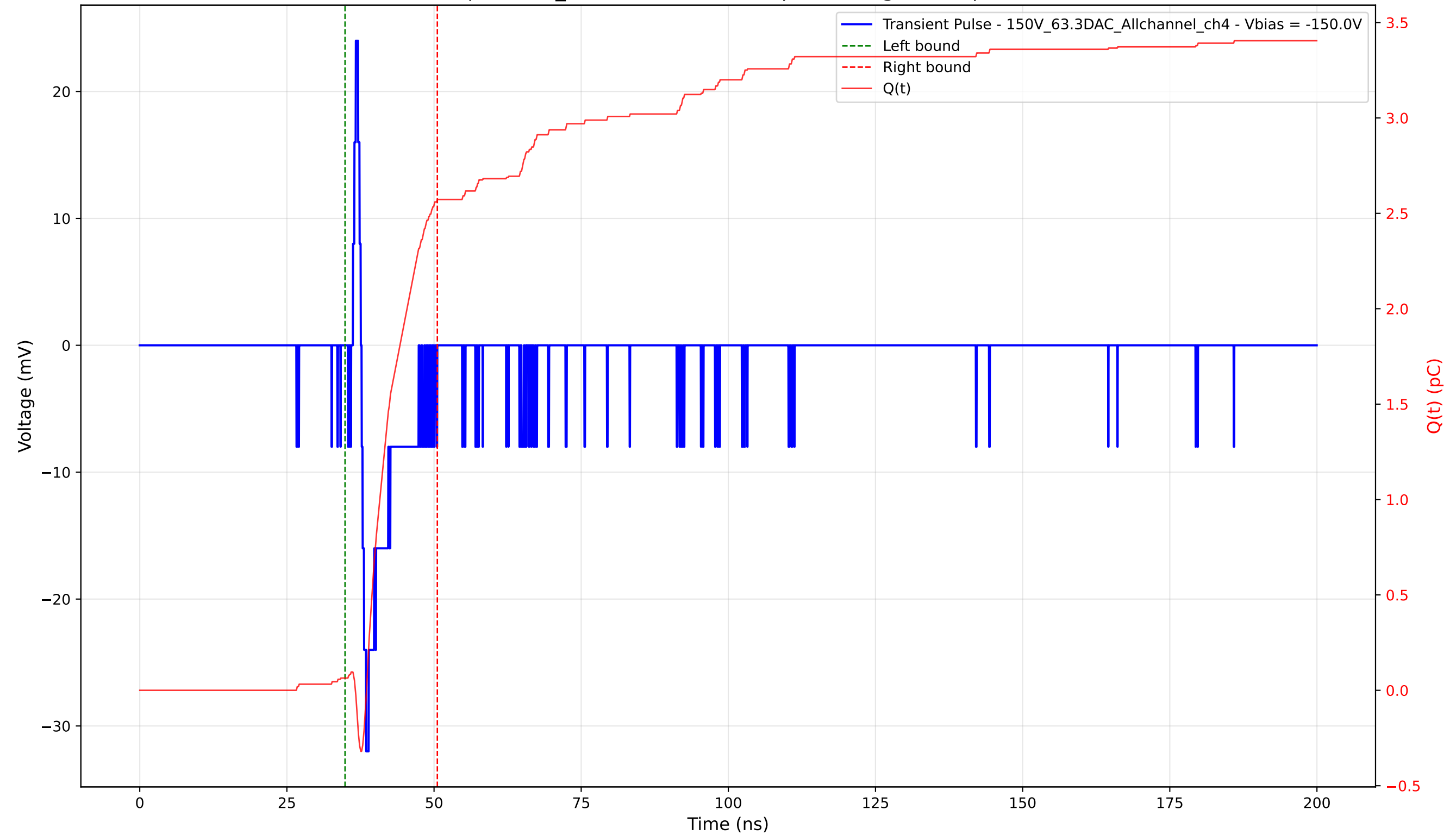
Transient Pulse - Sample: 1cm_42 - Position: 4515.0 \mu\text{m} - Charge: 2.51 pC - Rise Time: 0.78 ns
