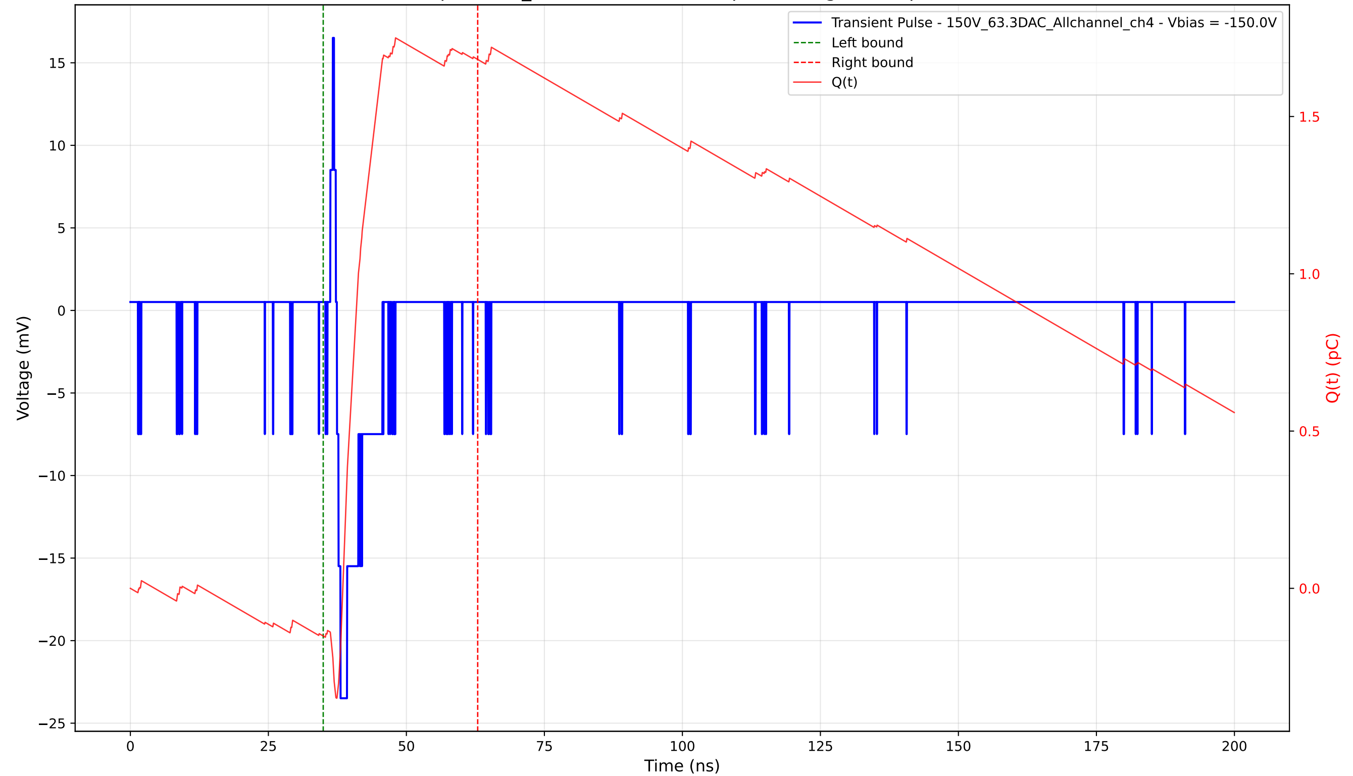
Transient Pulse - Sample: 1cm_42 - Position: 4965.0 \mu\text{m} - Charge: 1.83 pC - Rise Time: 0.67 ns
