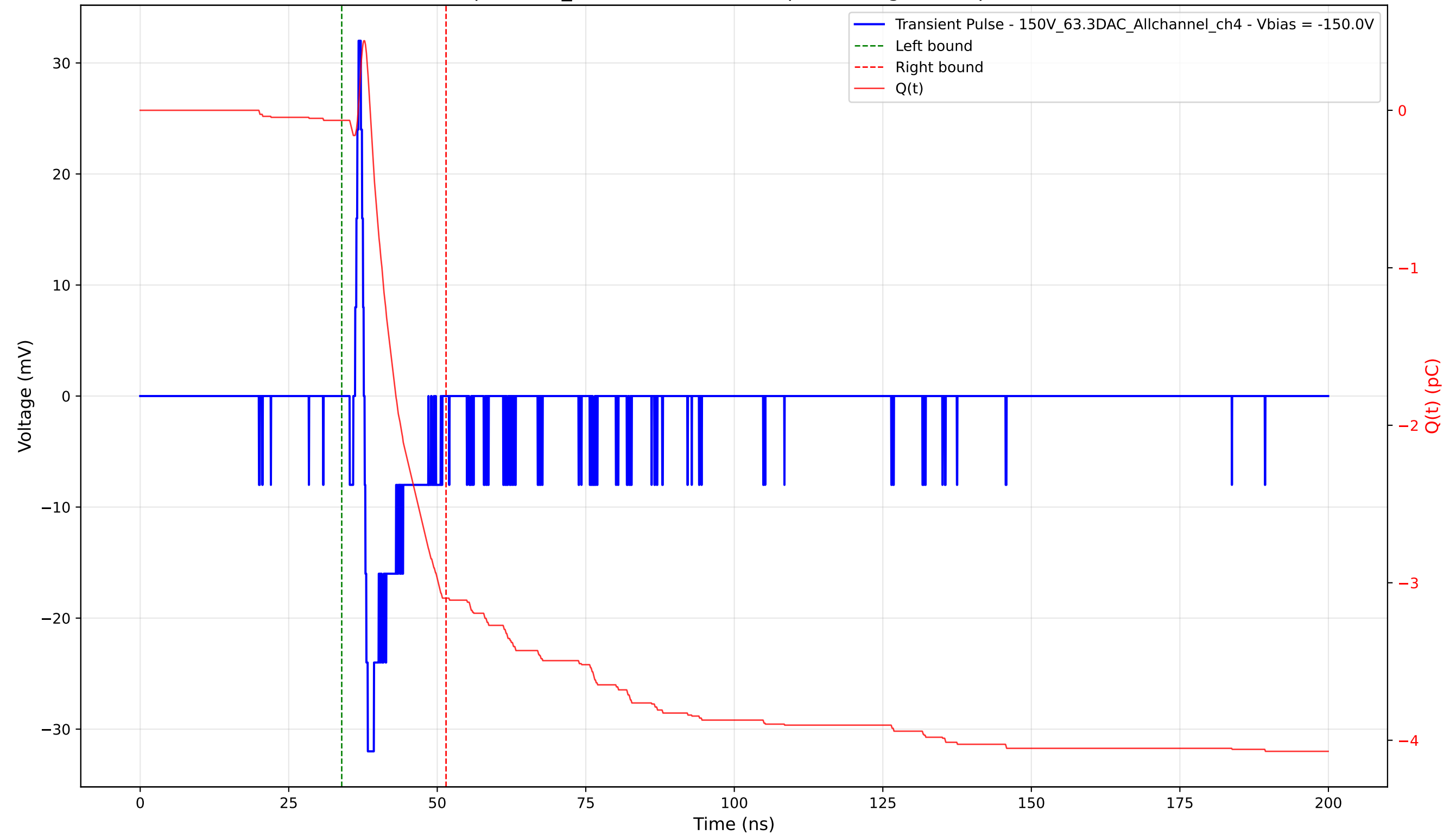
Transient Pulse - Sample: 1cm_42 - Position: 4300.0 \mu\text{m} - Charge: 3.03 pC - Rise Time: 0.58 ns
