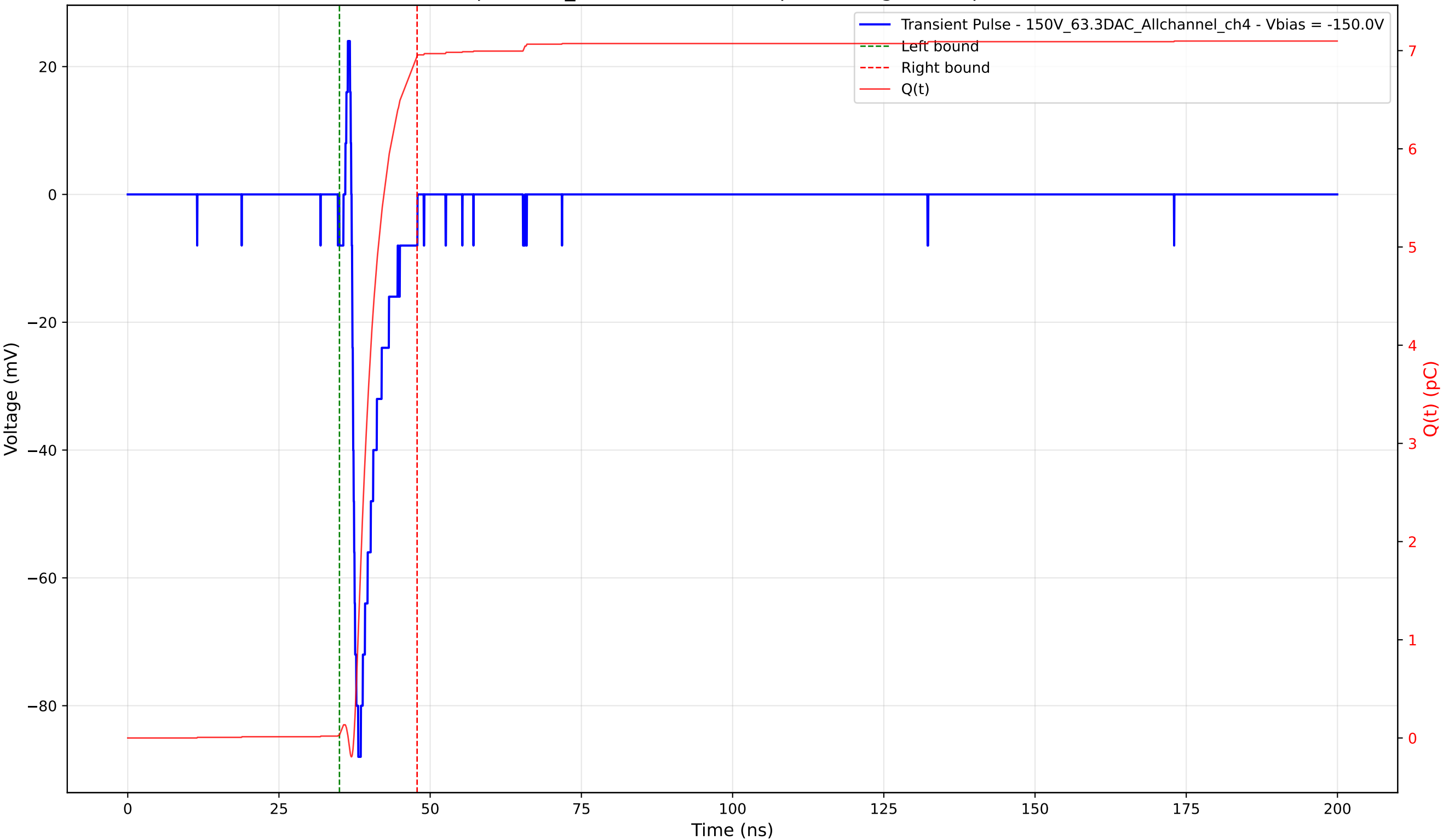
Transient Pulse - Sample: 1cm_42 - Position: 755.0 \mu\text{m} - Charge: 6.92 pC - Rise Time: 0.72 ns
