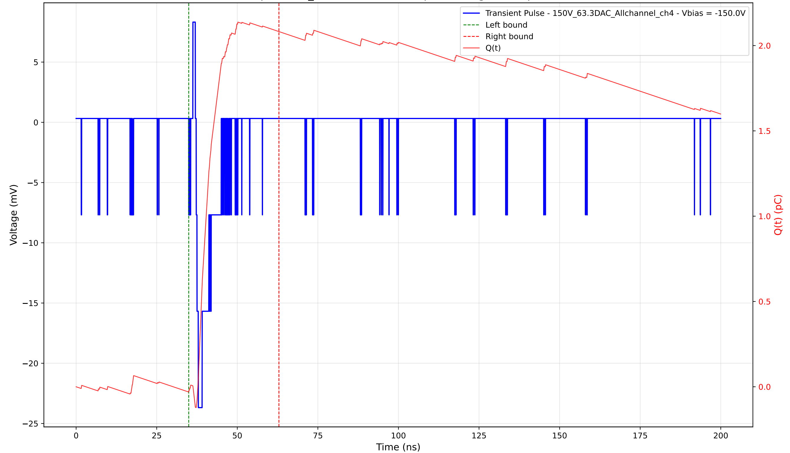
Transient Pulse - Sample: 1cm_42 - Position: 190.0 \mu\text{m} - Charge: 2.11 pC - Rise Time: 0.67 ns
