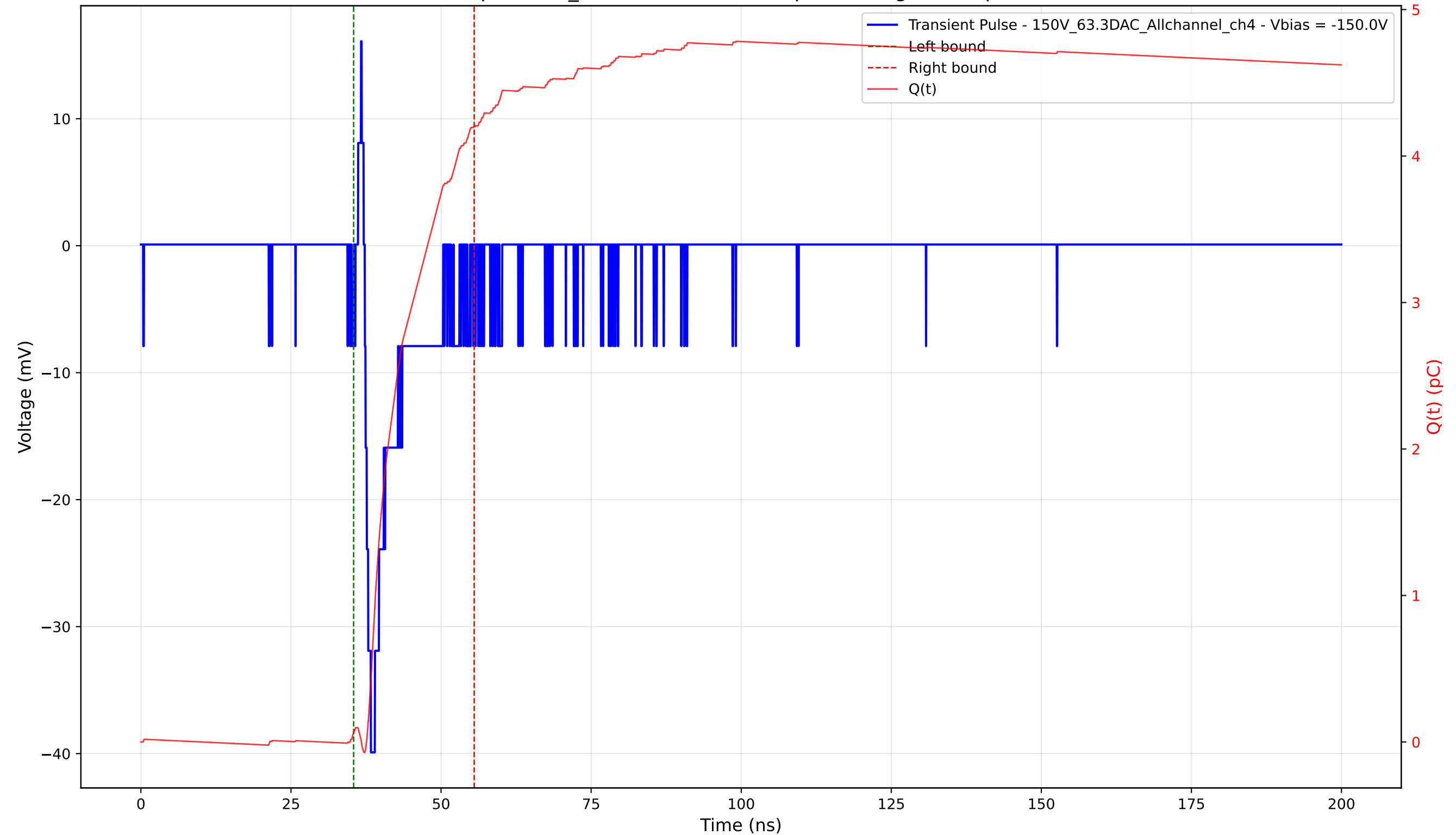
Transient Pulse - Sample: 1cm_42 - Position: 3465.0 \mu\text{m} - Charge: 4.13 pC - Rise Time: 1.02 ns
