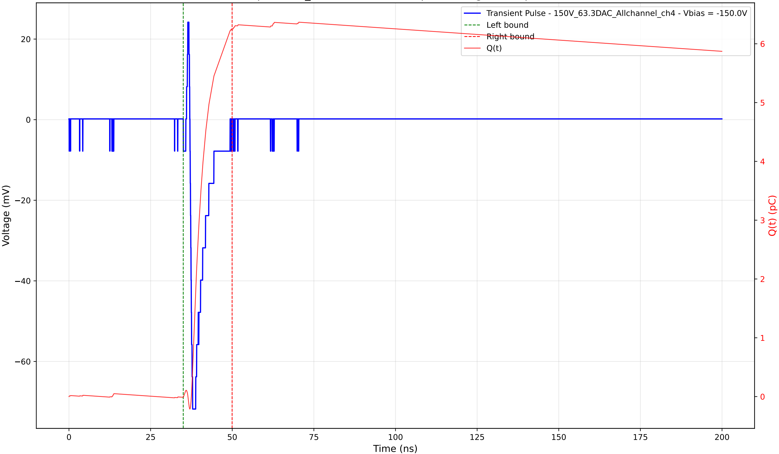
Transient Pulse - Sample: 1cm_42 - Position: 655.0 \mu\text{m} - Charge: 6.27 pC - Rise Time: 0.80 ns
