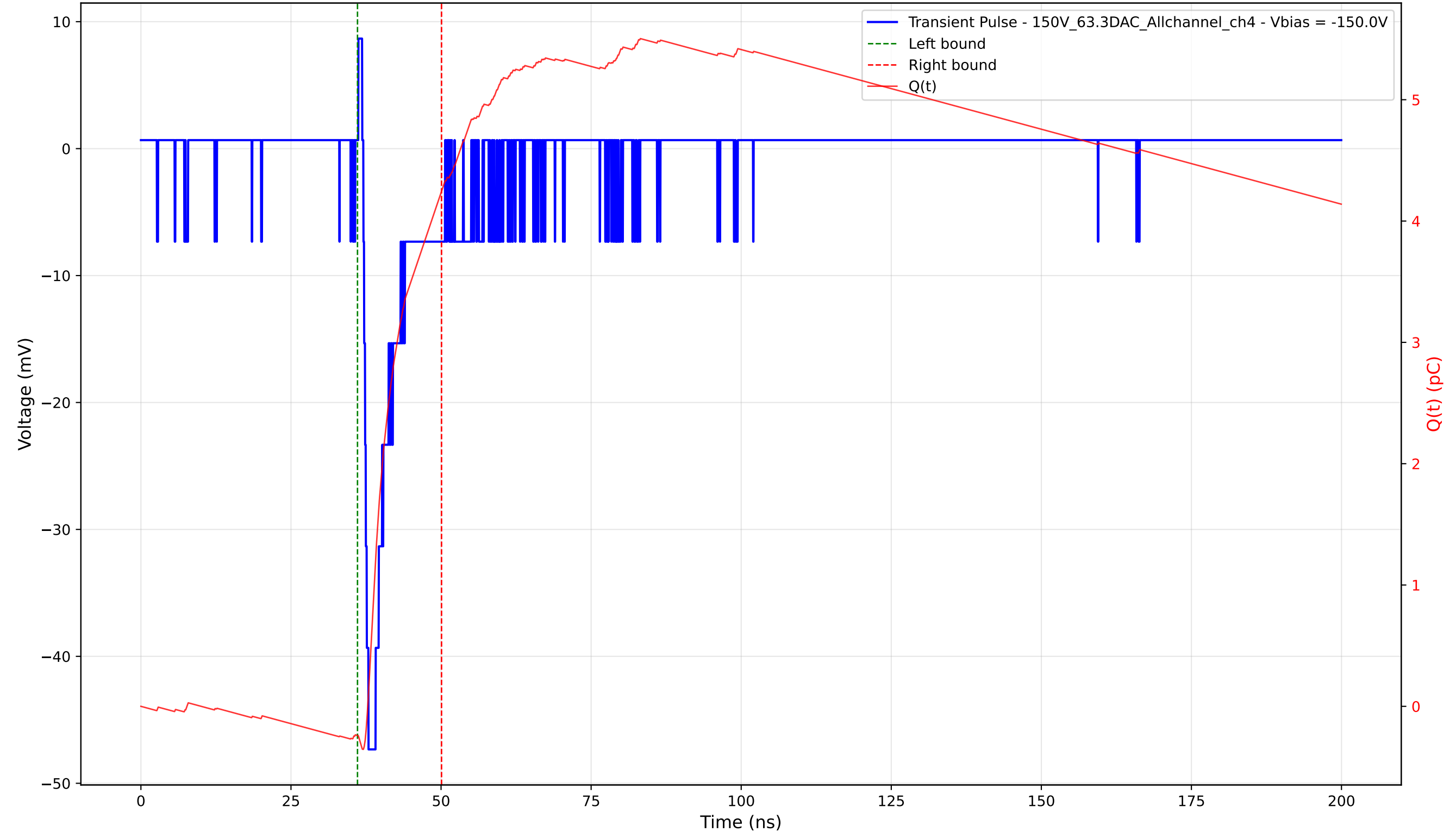
Transient Pulse - Sample: 1cm_42 - Position: 3280.0 \mu\text{m} - Charge: 4.49 pC - Rise Time: 0.86 ns
