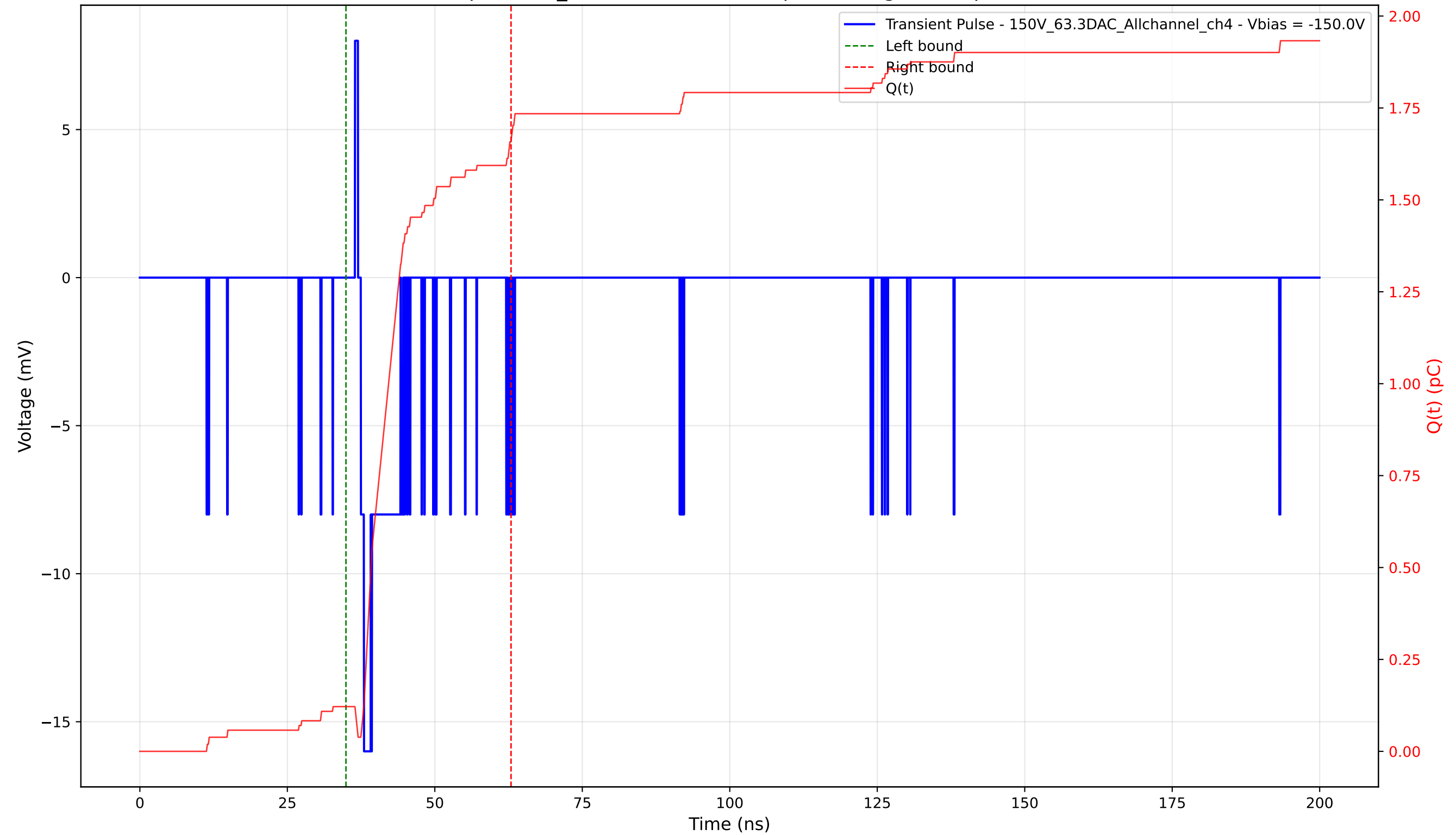
Transient Pulse - Sample: 1cm_42 - Position: 5070.0 \mu\text{m} - Charge: 1.54 pC - Rise Time: 0.55 ns
