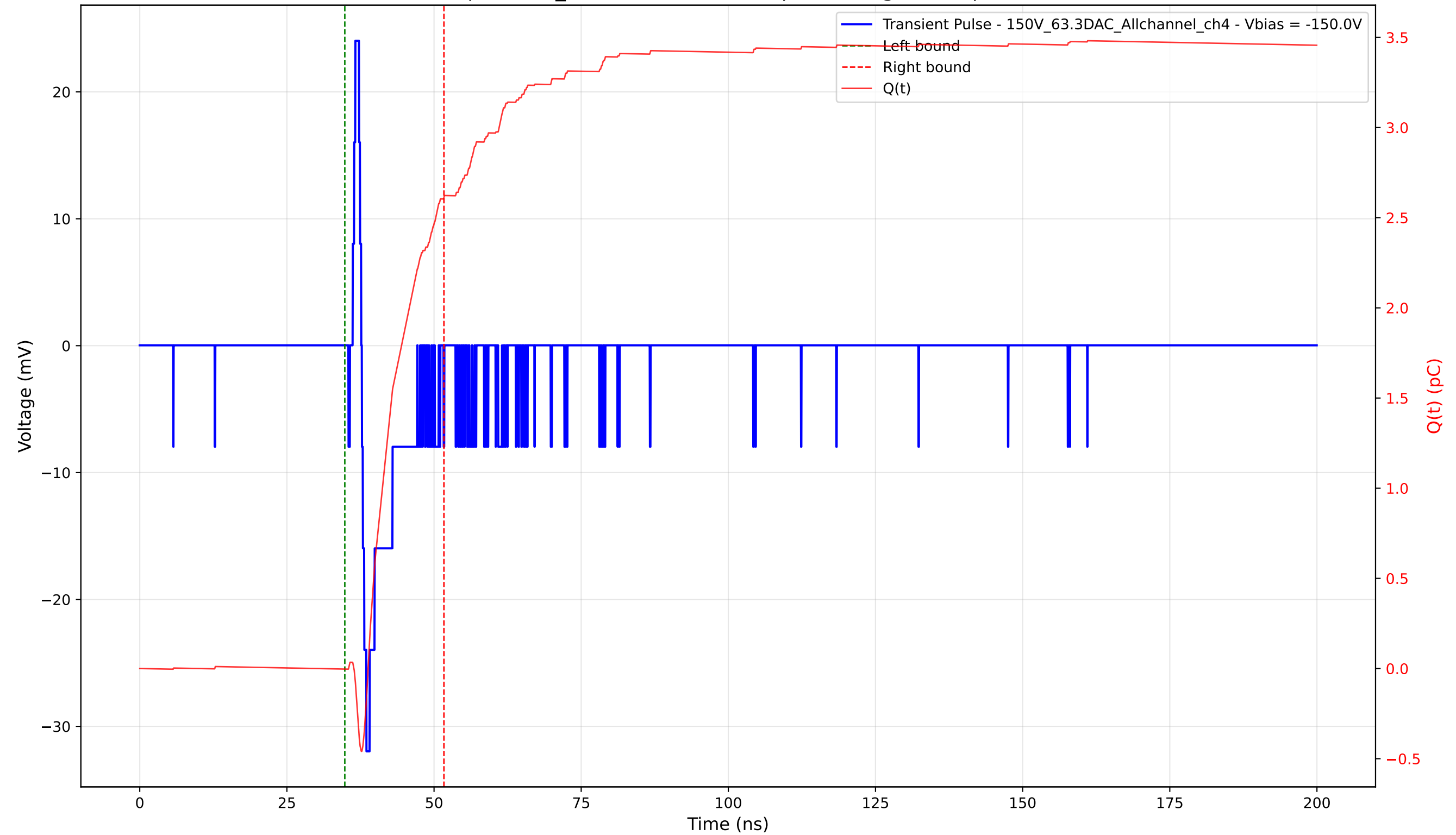
Transient Pulse - Sample: 1cm_42 - Position: 3995.0 \mu\text{m} - Charge: 2.62 pC - Rise Time: 0.78 ns
