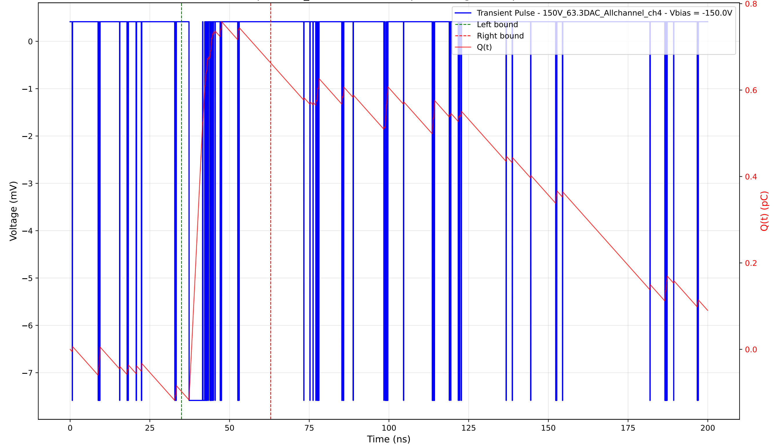
Transient Pulse - Sample: 1cm_42 - Position: 70.0 \mu\text{m} - Charge: 0.76 pC - Rise Time: 0.04 ns
