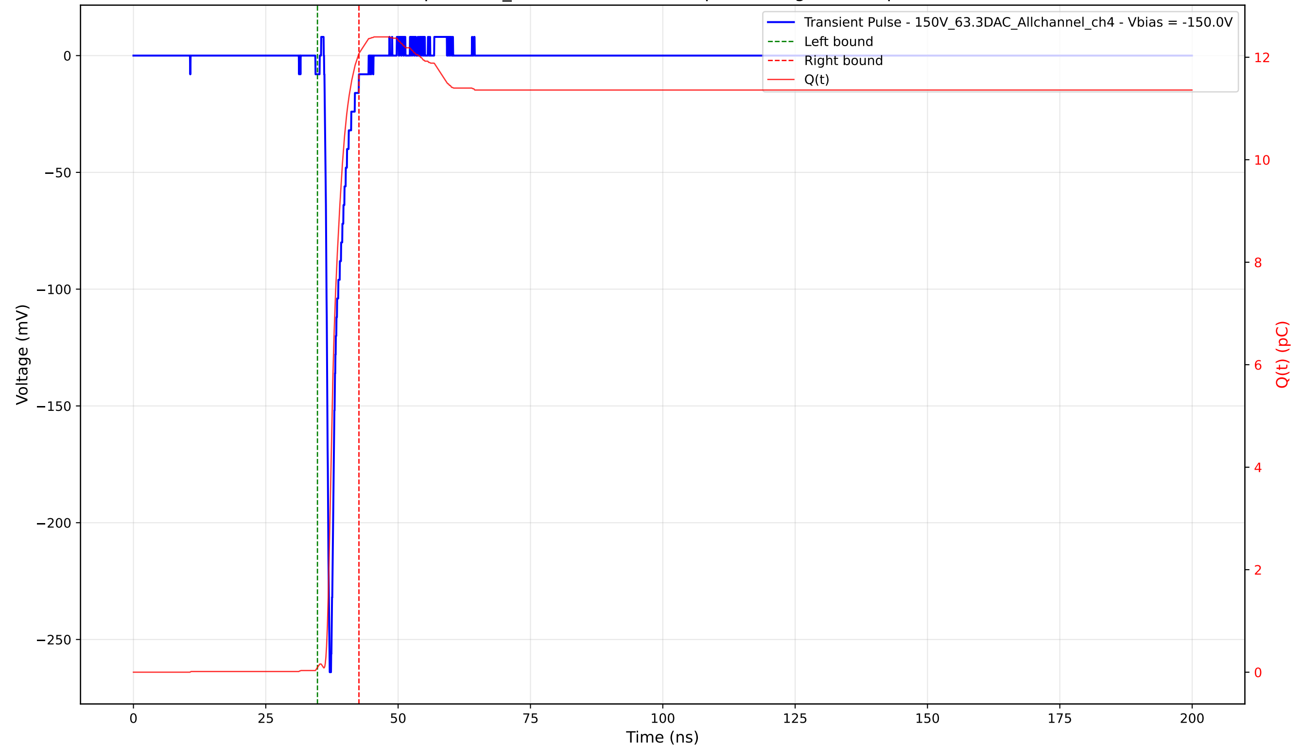
Transient Pulse - Sample: 1cm_42 - Position: 1505.0 \mu\text{m} - Charge: 11.98 pC - Rise Time: 0.78 ns
