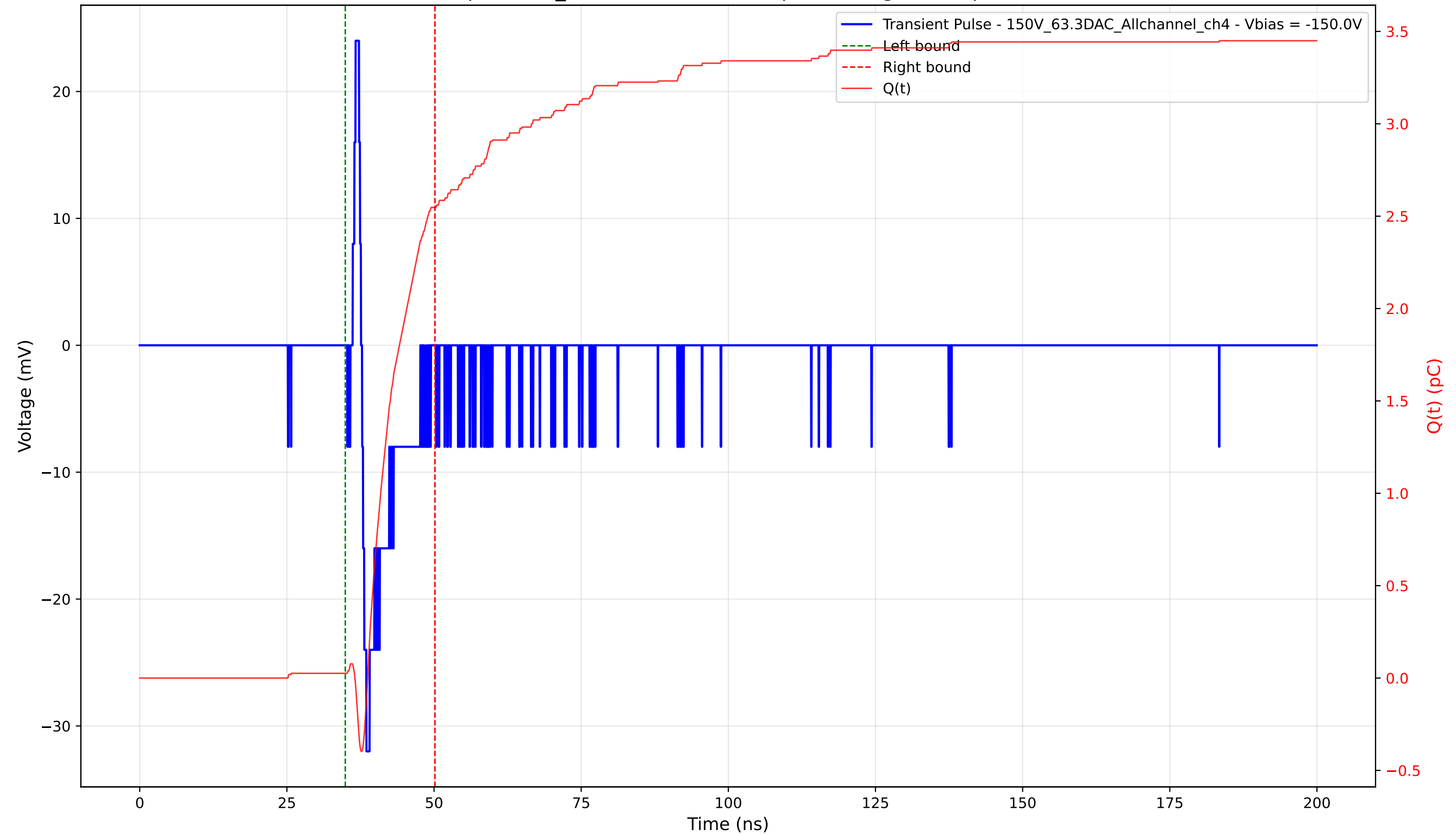
Transient Pulse - Sample: 1cm_42 - Position: 4055.0 \mu\text{m} - Charge: 2.52 pC - Rise Time: 0.74 ns
