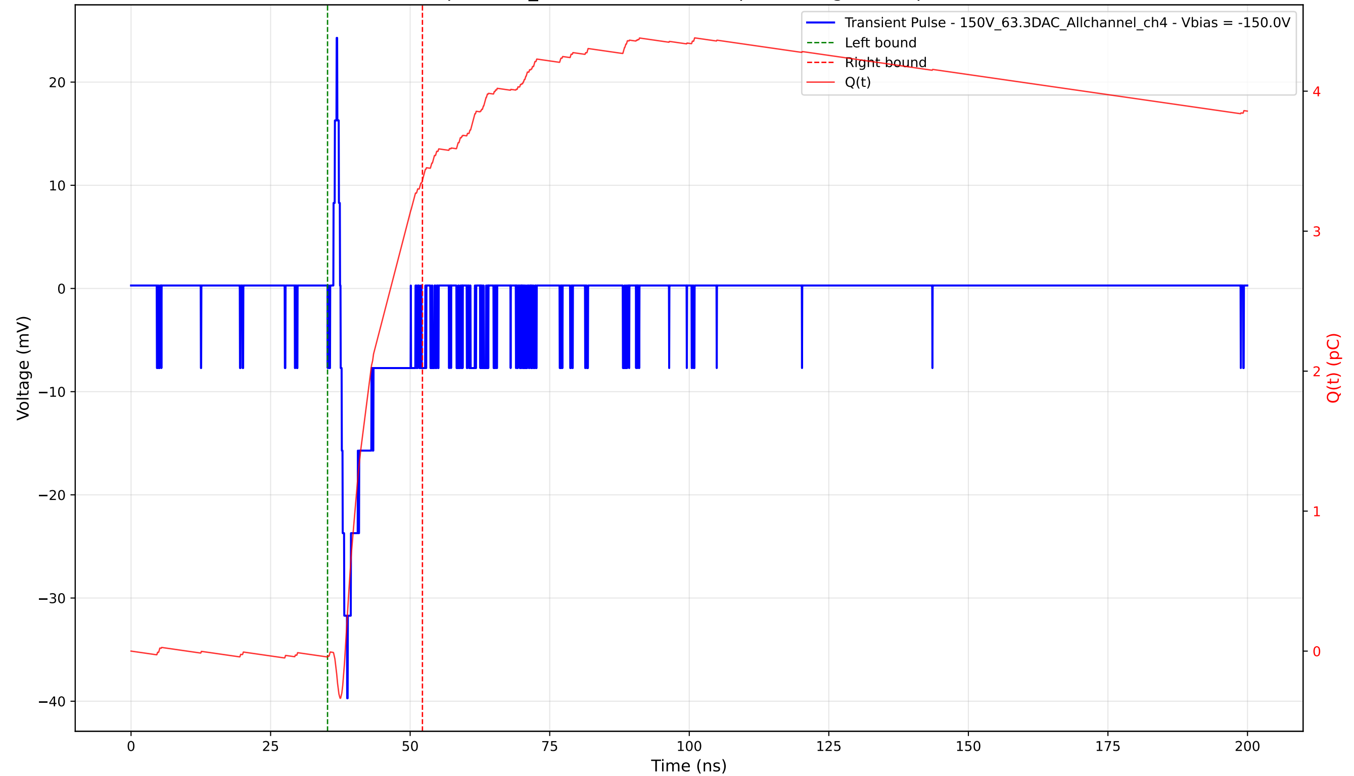
Transient Pulse - Sample: 1cm_42 - Position: 3630.0 \mu\text{m} - Charge: 3.41 pC - Rise Time: 1.18 ns
