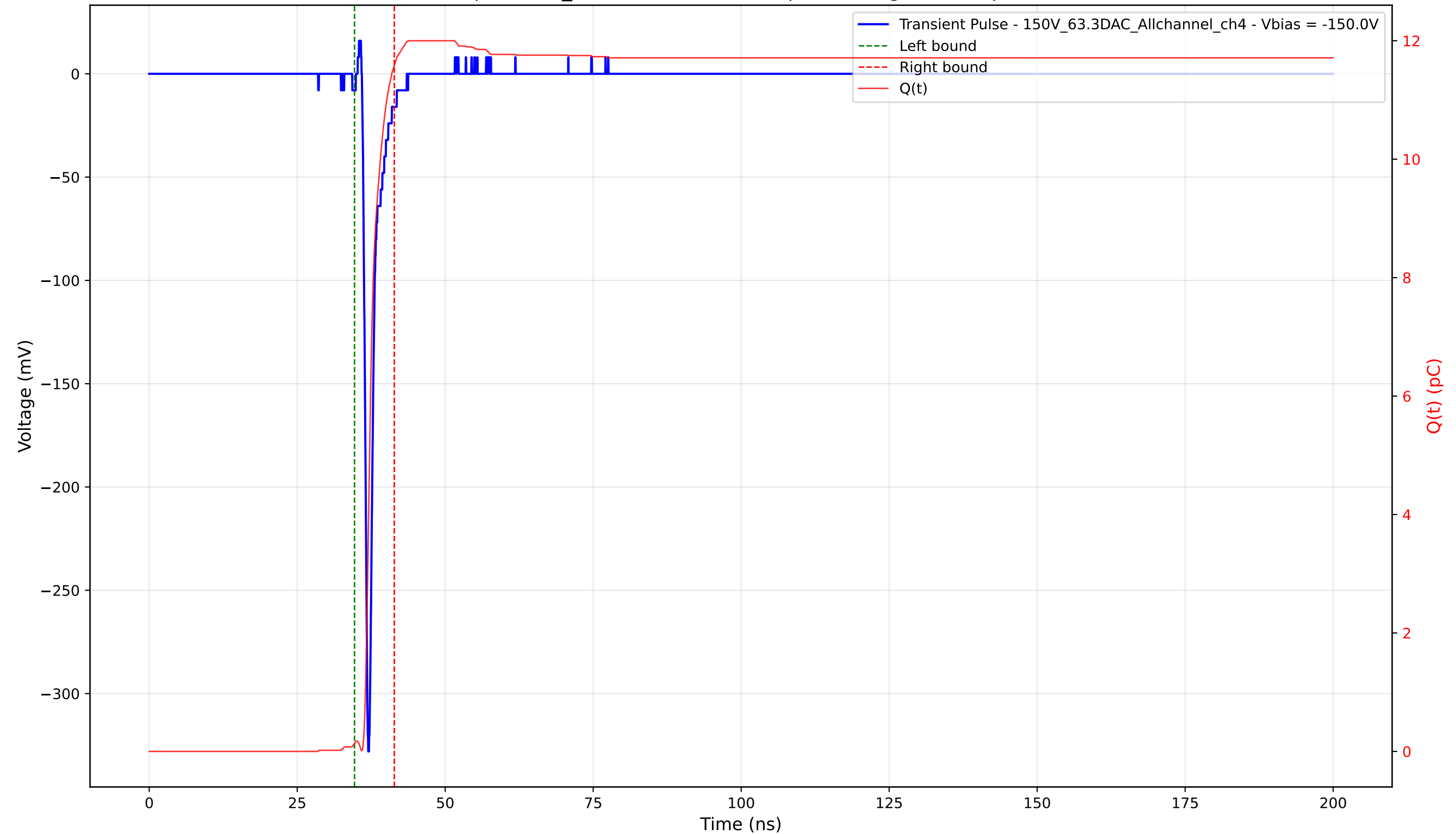
Transient Pulse - Sample: 1cm_42 - Position: 2425.0 \mu\text{m} - Charge: 11.45 pC - Rise Time: 0.71 ns
