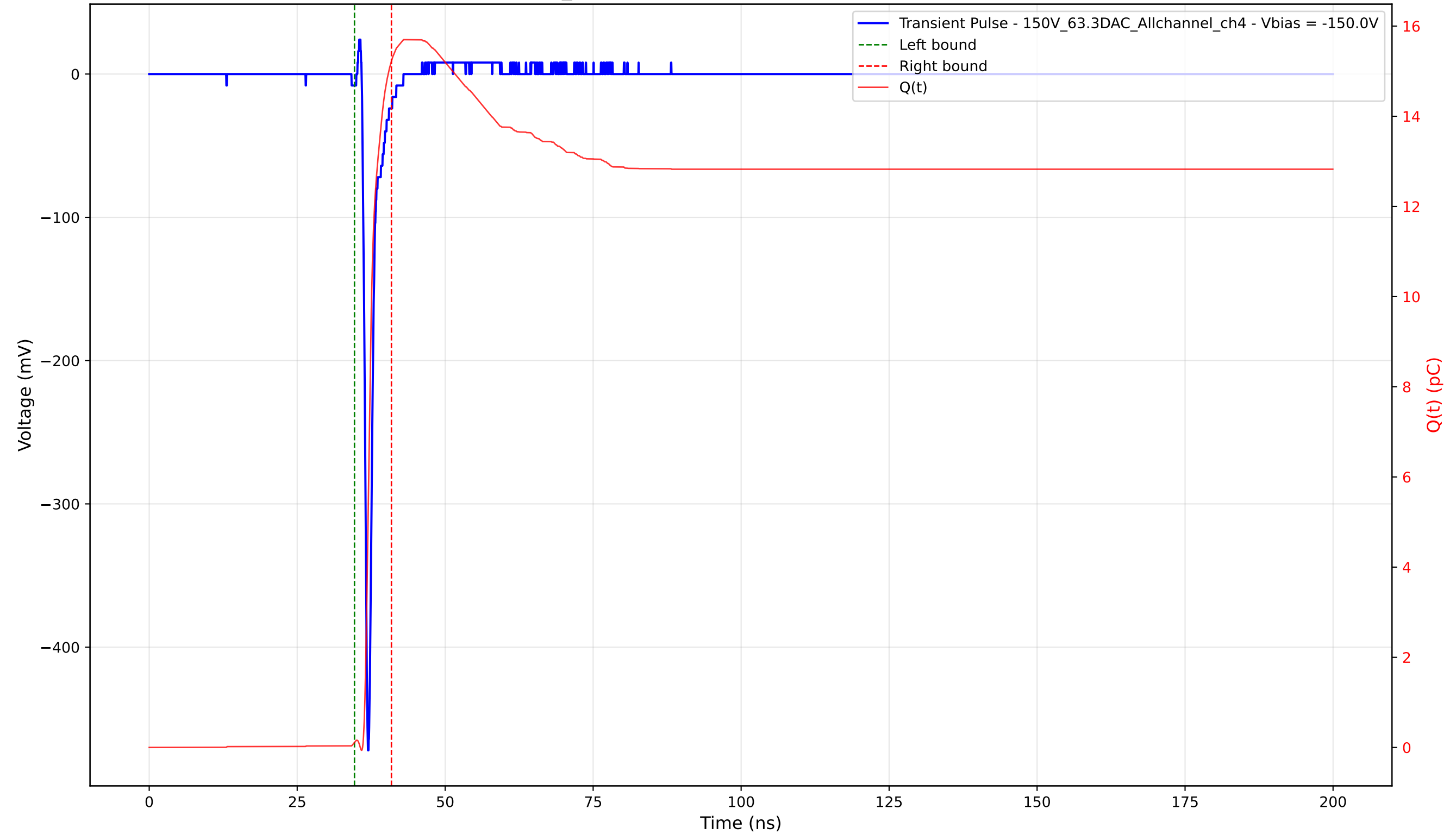
Transient Pulse - Sample: 1cm_42 - Position: 2305.0 \mu\text{m} - Charge: 15.11 pC - Rise Time: 0.72 ns
