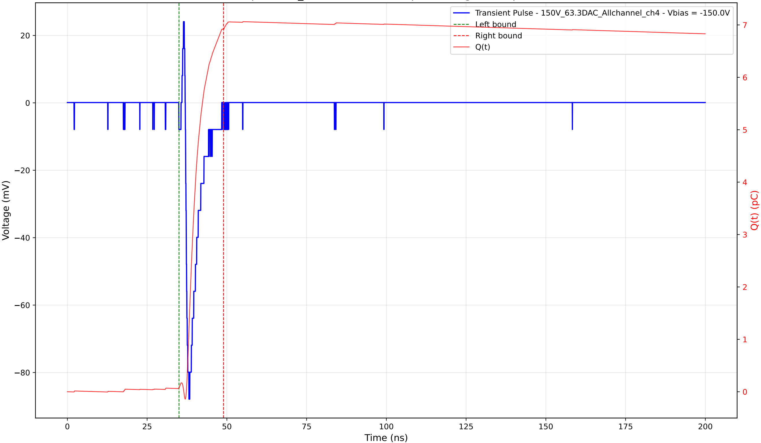
Transient Pulse - Sample: 1cm_42 - Position: 830.0 \mu\text{m} - Charge: 6.85 pC - Rise Time: 0.72 ns
