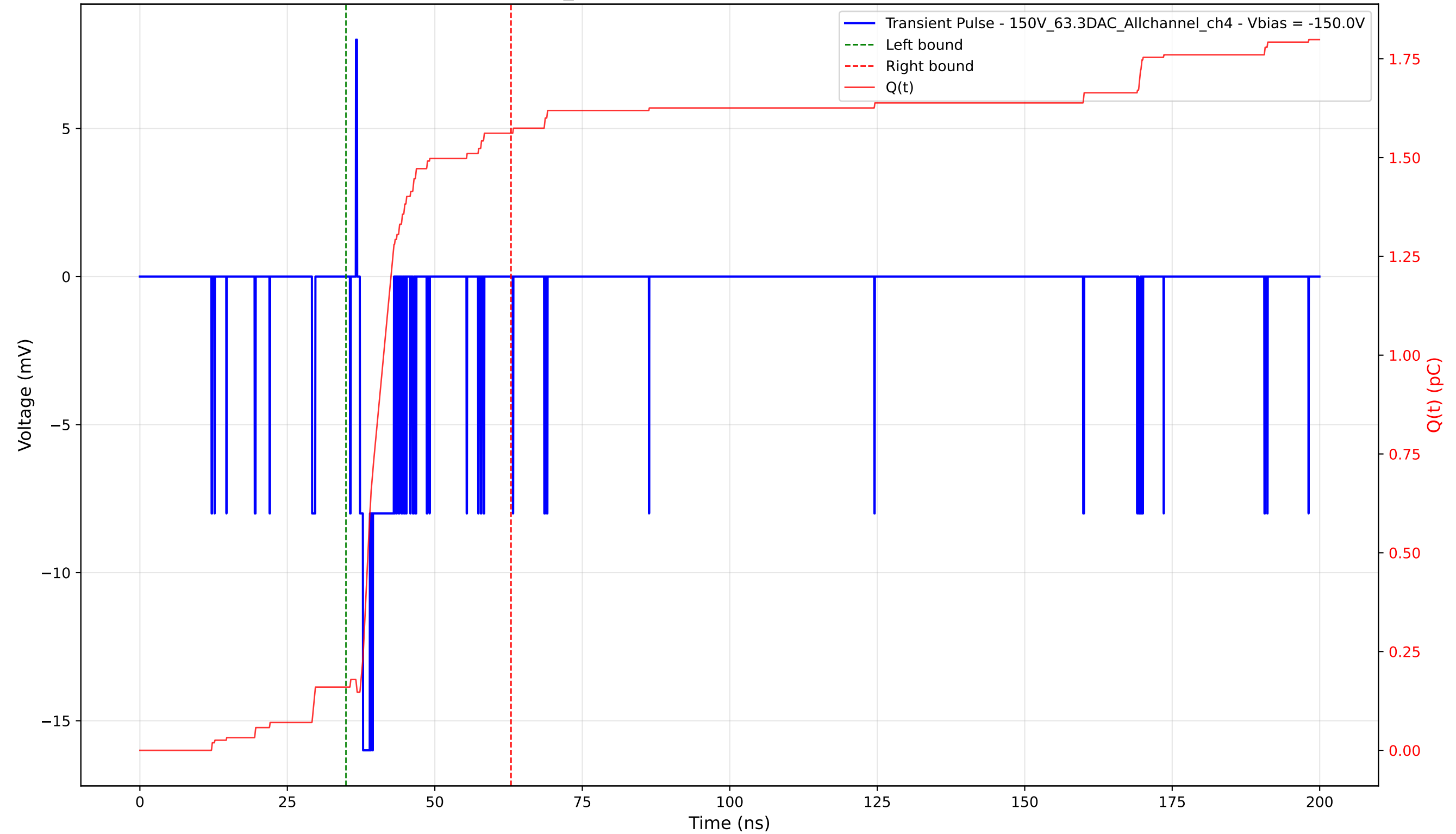
Transient Pulse - Sample: 1cm_42 - Position: 125.0 \mu\text{m} - Charge: 1.40 pC - Rise Time: 0.55 ns
