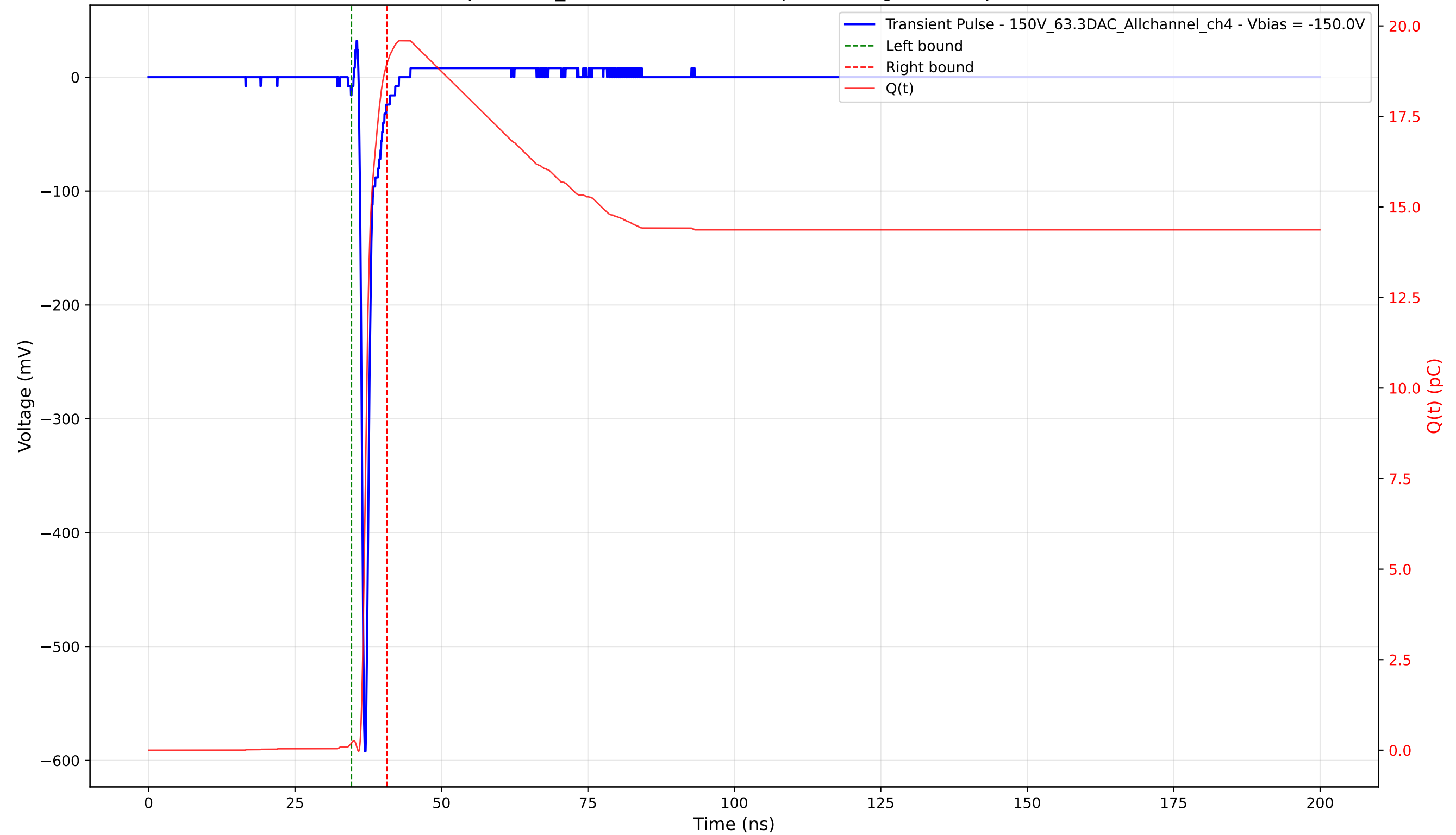
Transient Pulse - Sample: 1cm_42 - Position: 1885.0 \mu\text{m} - Charge: 18.77 pC - Rise Time: 0.70 ns
