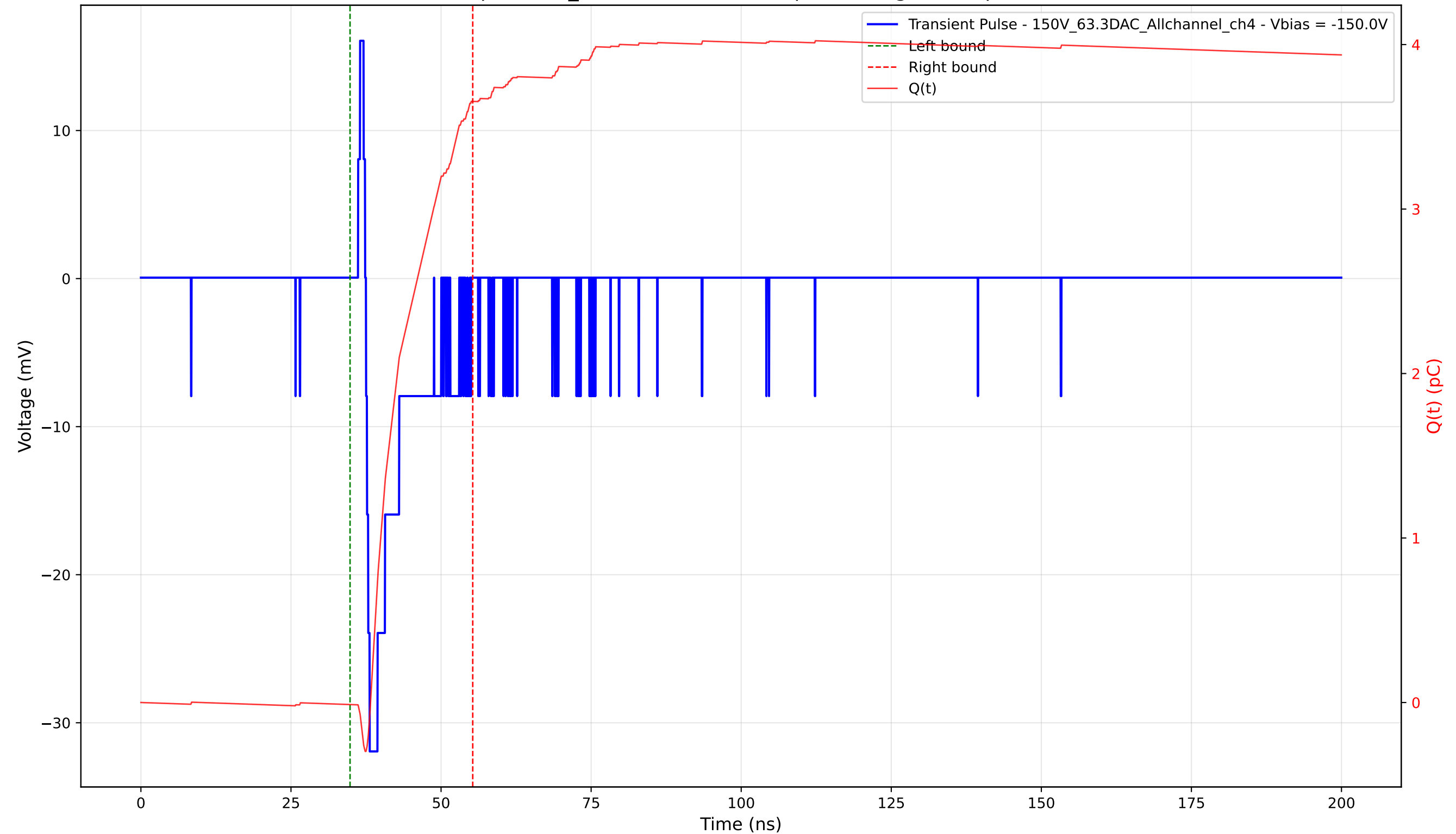
Transient Pulse - Sample: 1cm_42 - Position: 3565.0 \mu\text{m} - Charge: 3.67 pC - Rise Time: 0.62 ns
