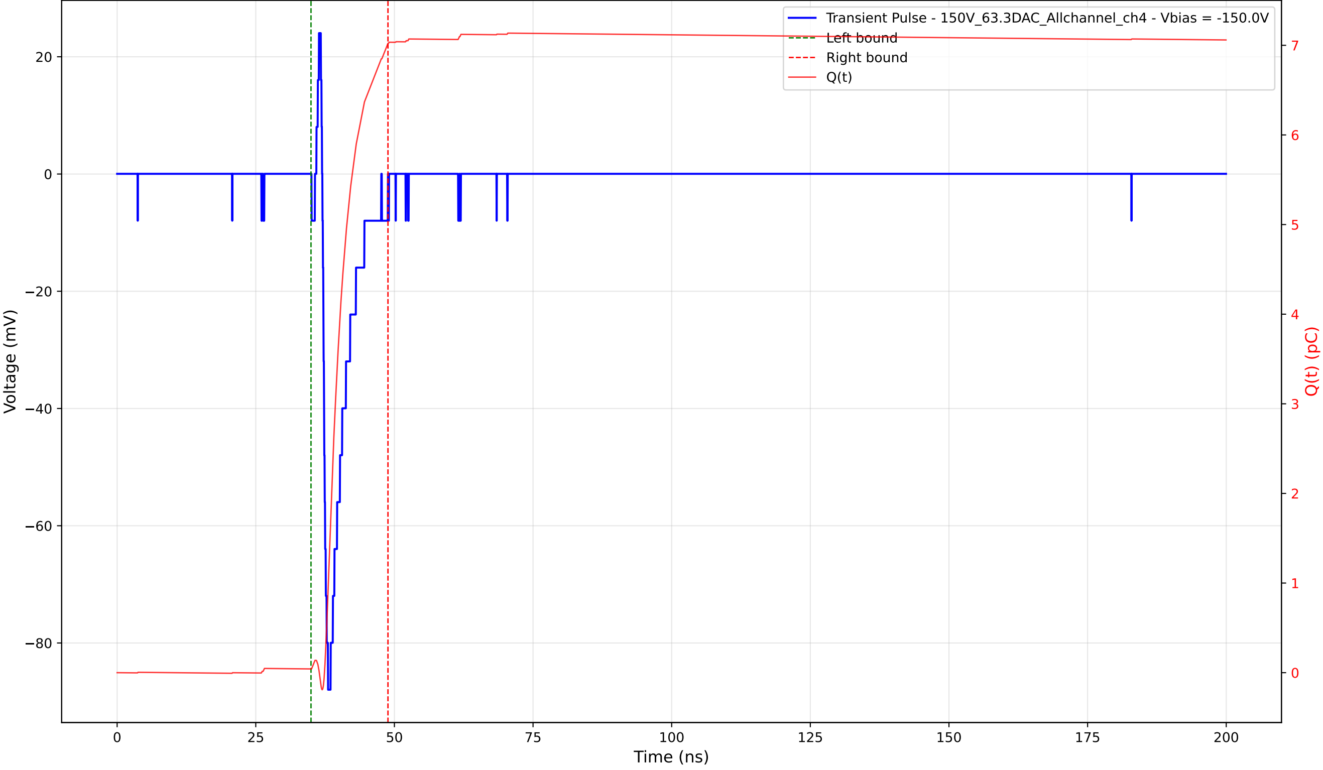
Transient Pulse - Sample: 1cm_42 - Position: 735.0 \mu\text{m} - Charge: 6.98 pC - Rise Time: 0.72 ns
