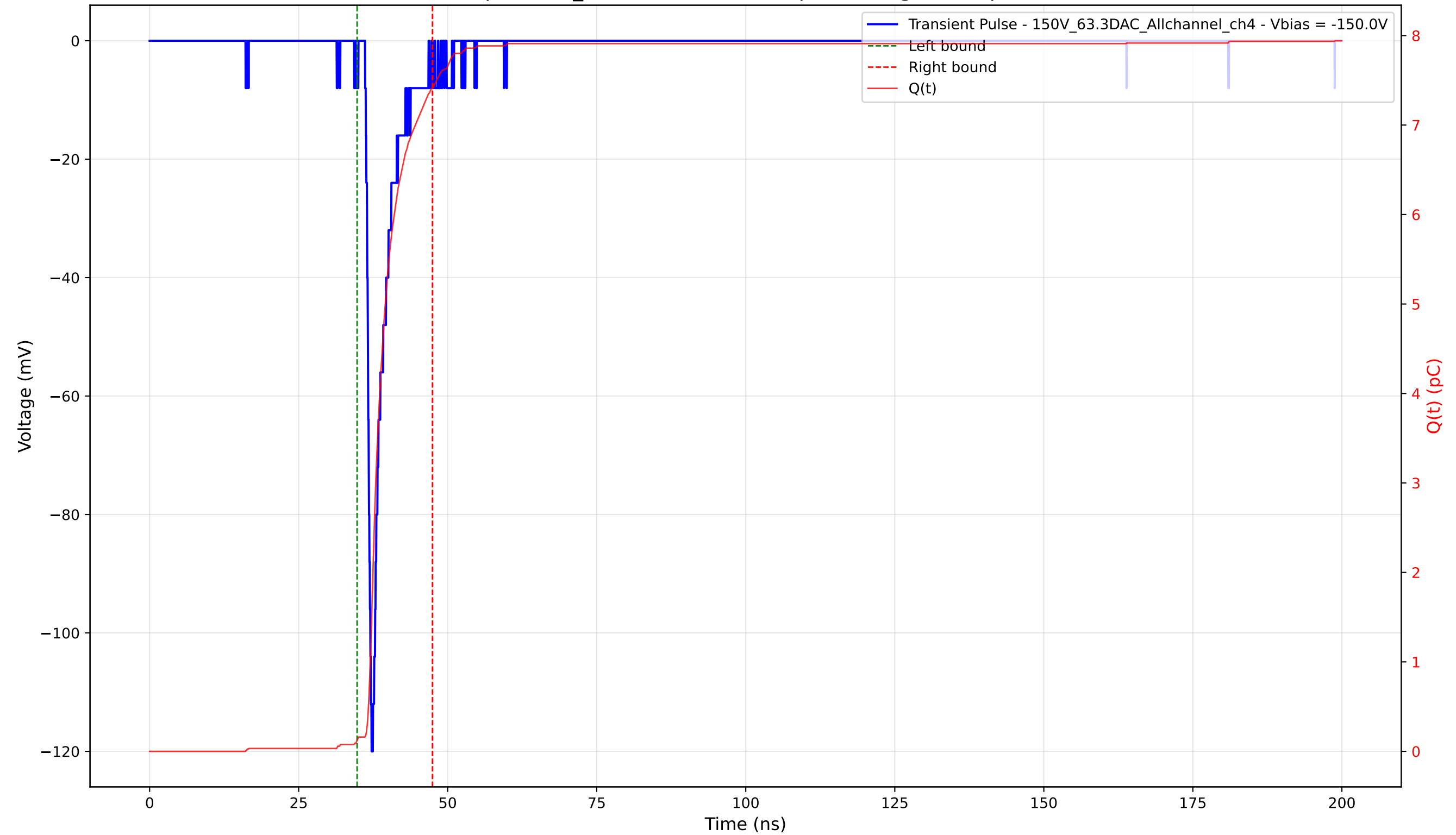
Transient Pulse - Sample: 1cm_42 - Position: 2845.0 \mu\text{m} - Charge: 7.29 pC - Rise Time: 0.86 ns
