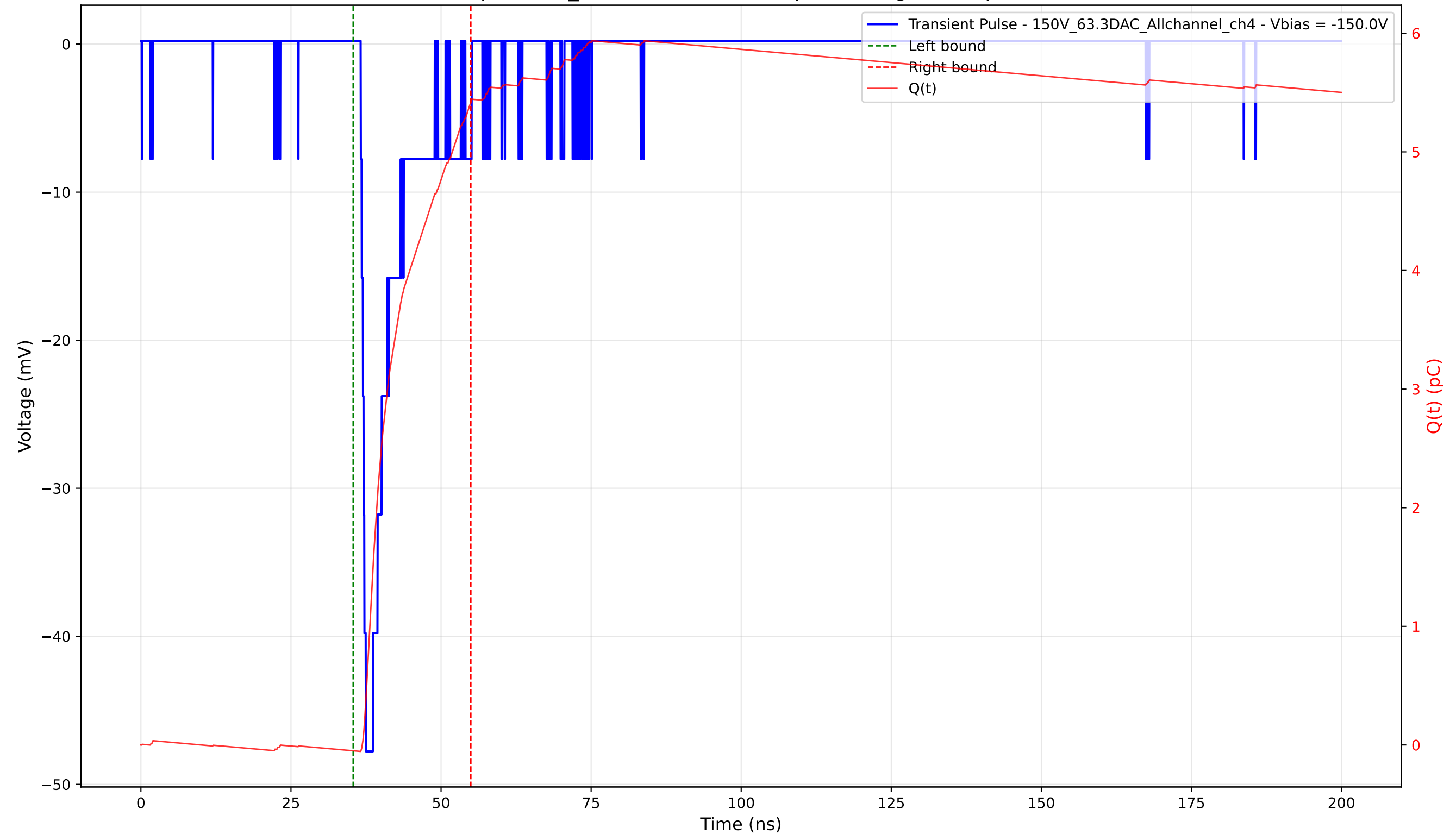
Transient Pulse - Sample: 1cm_42 - Position: 3115.0 \mu\text{m} - Charge: 5.47 pC - Rise Time: 0.86 ns
