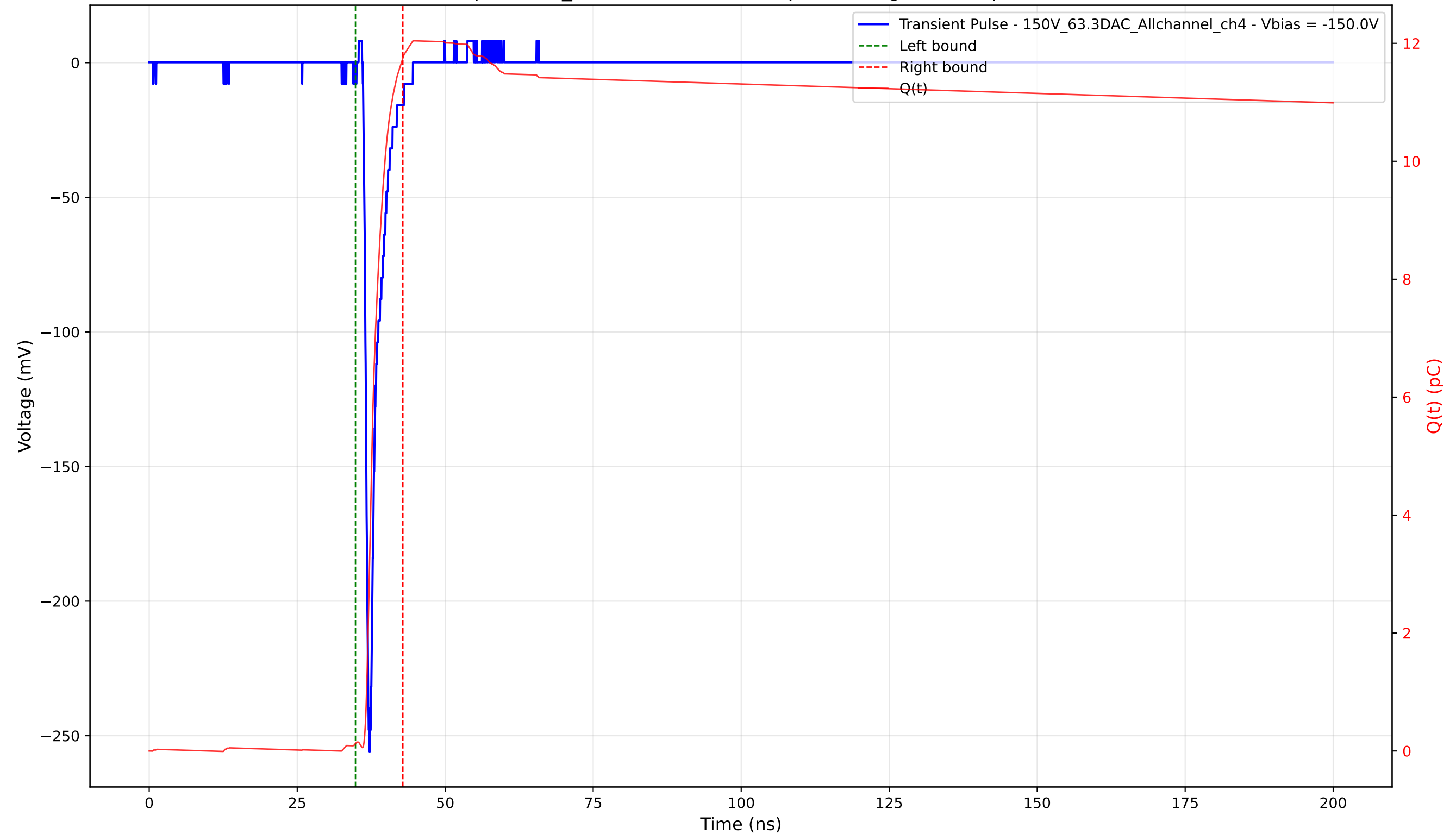
Transient Pulse - Sample: 1cm_42 - Position: 1490.0 \mu\text{m} - Charge: 11.62 pC - Rise Time: 0.74 ns
