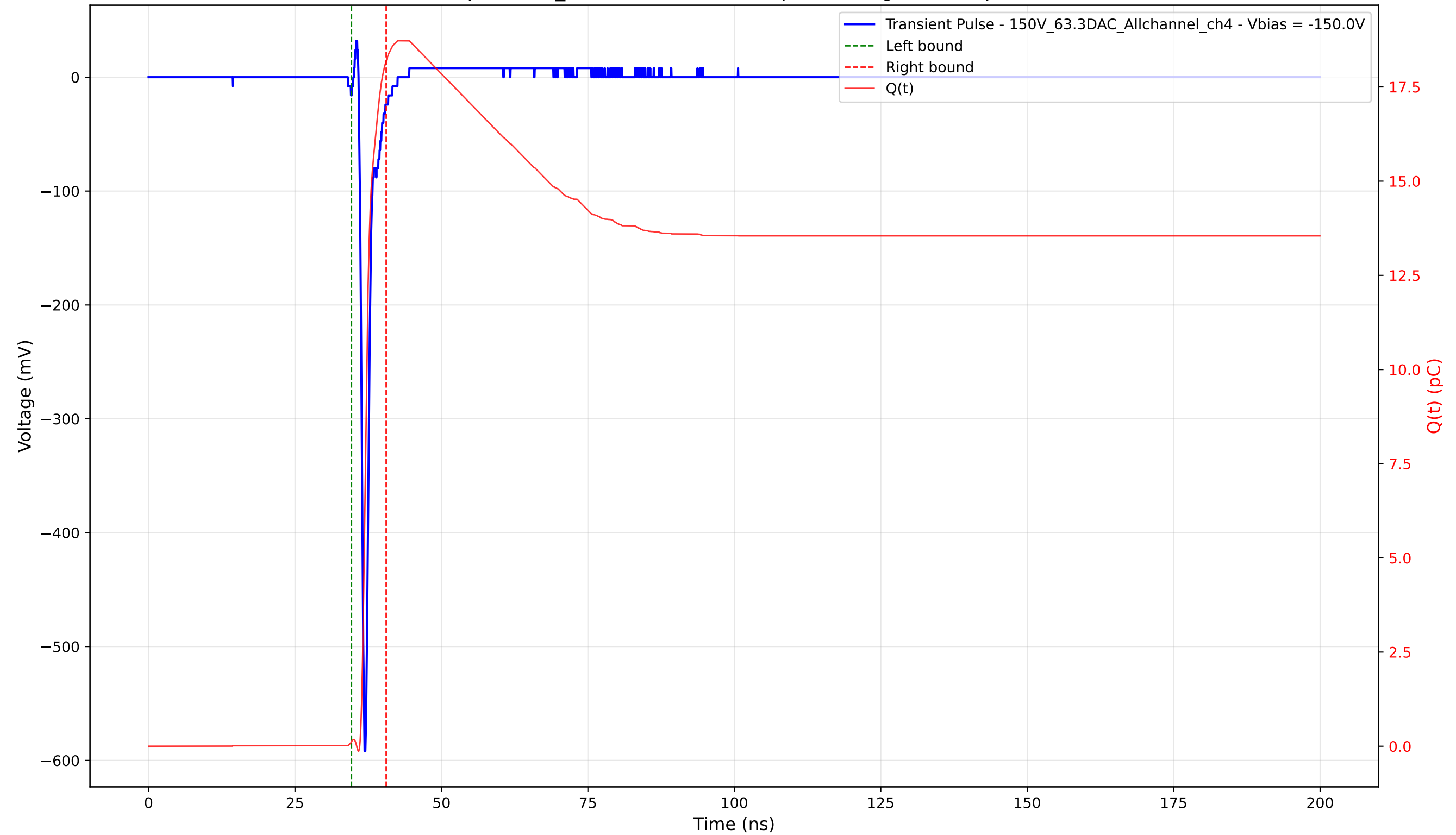
Transient Pulse - Sample: 1cm_42 - Position: 1960.0 \mu\text{m} - Charge: 18.07 pC - Rise Time: 0.70 ns
