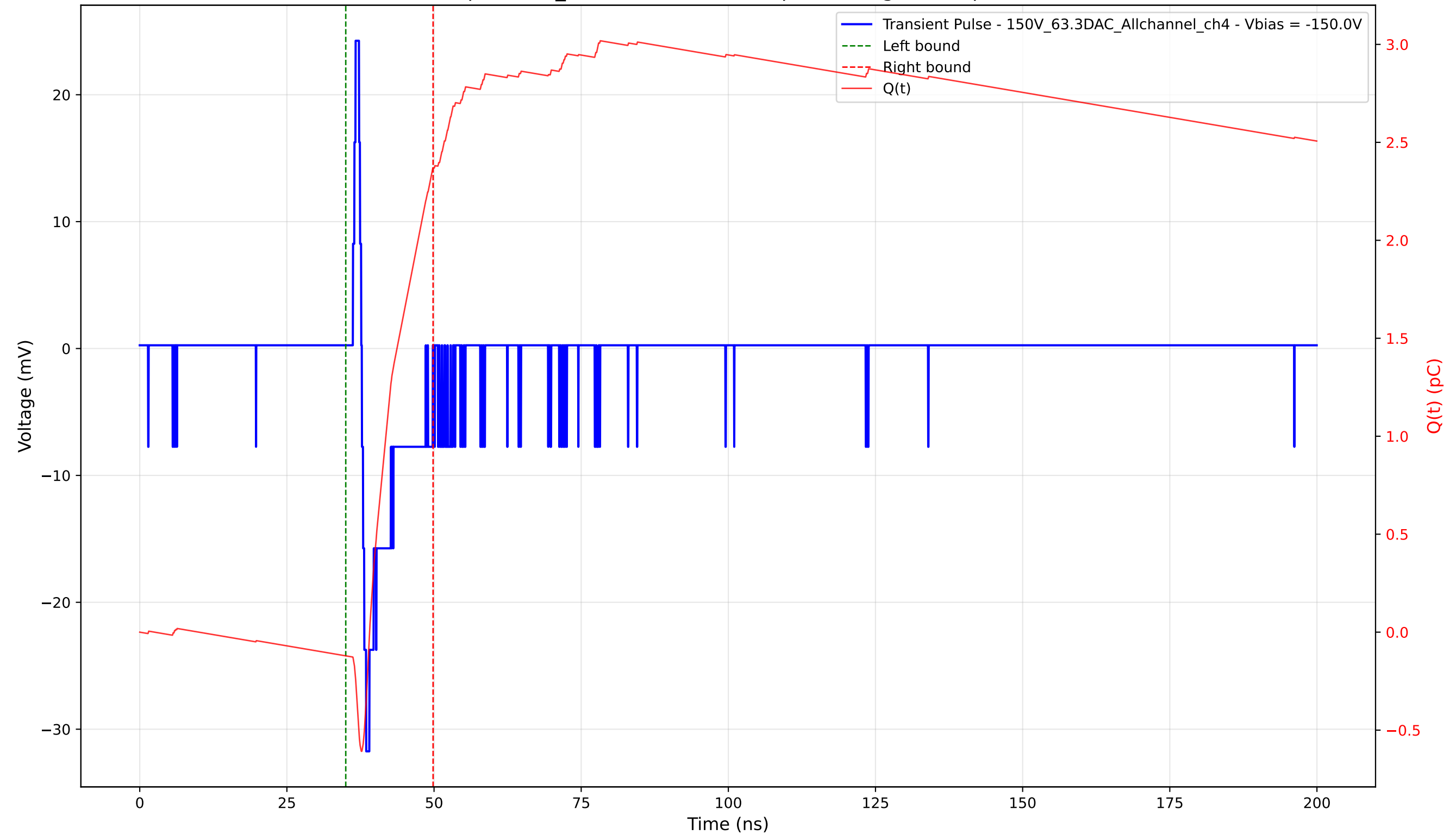
Transient Pulse - Sample: 1cm_42 - Position: 4000.0 \mu\text{m} - Charge: 2.49 pC - Rise Time: 0.74 ns
