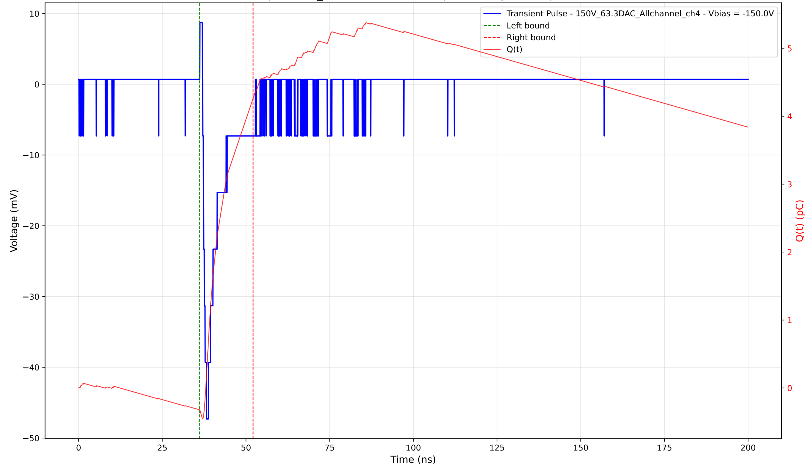
Transient Pulse - Sample: 1cm_42 - Position: 3345.0 \mu\text{m} - Charge: 4.59 pC - Rise Time: 1.14 ns
