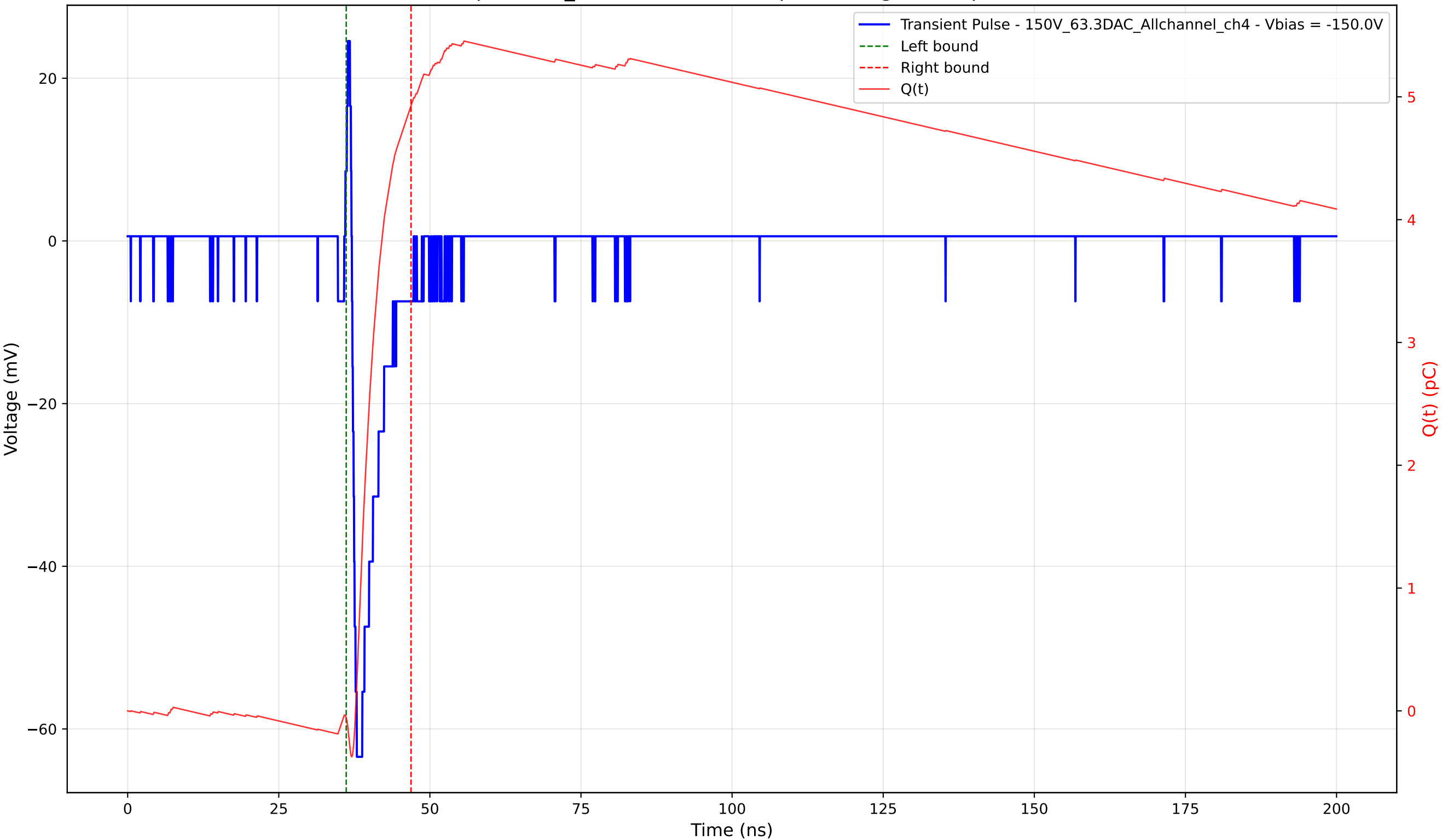
Transient Pulse - Sample: 1cm_42 - Position: 595.0 \mu\text{m} - Charge: 4.99 pC - Rise Time: 0.81 ns
