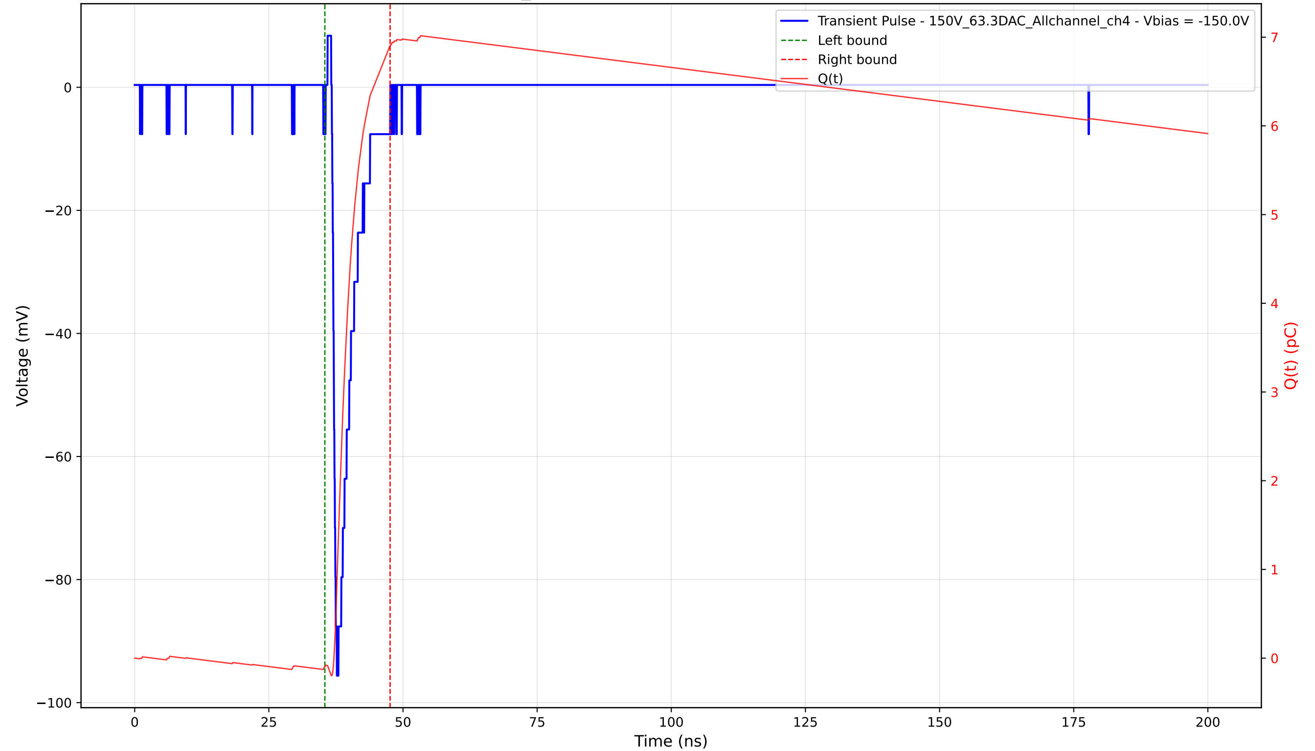
Transient Pulse - Sample: 1cm_42 - Position: 980.0 \mu\text{m} - Charge: 7.01 pC - Rise Time: 0.67 ns
