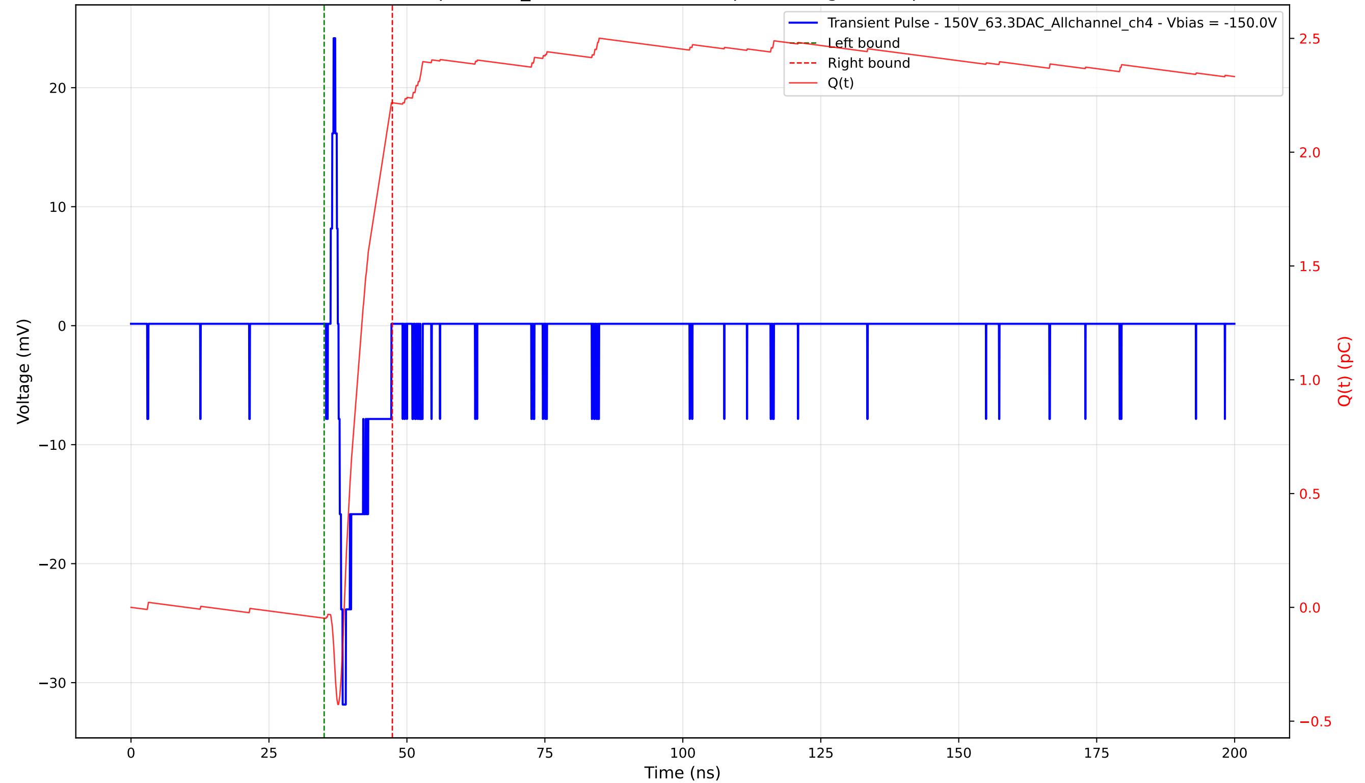
Transient Pulse - Sample: 1cm_42 - Position: 4590.0 \mu\text{m} - Charge: 2.26 pC - Rise Time: 0.74 ns
