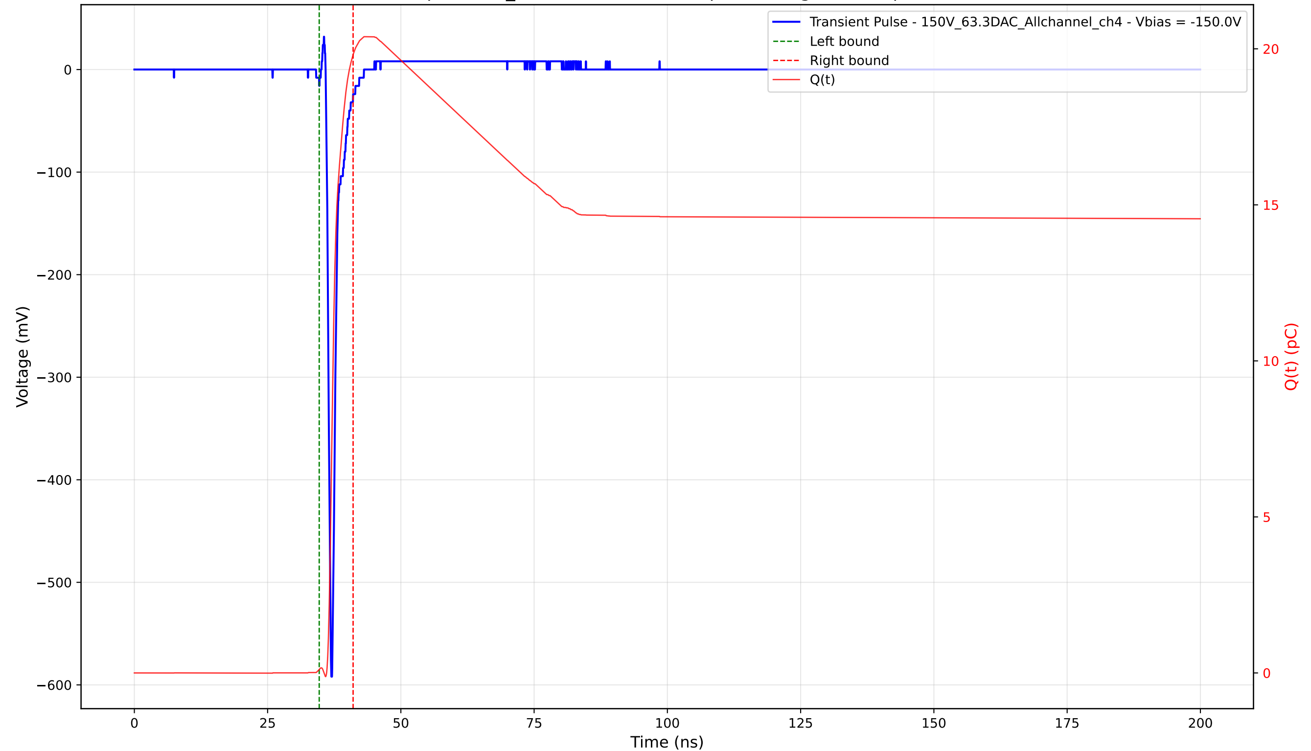
Transient Pulse - Sample: 1cm_42 - Position: 1785.0 \mu\text{m} - Charge: 19.71 pC - Rise Time: 0.72 ns
