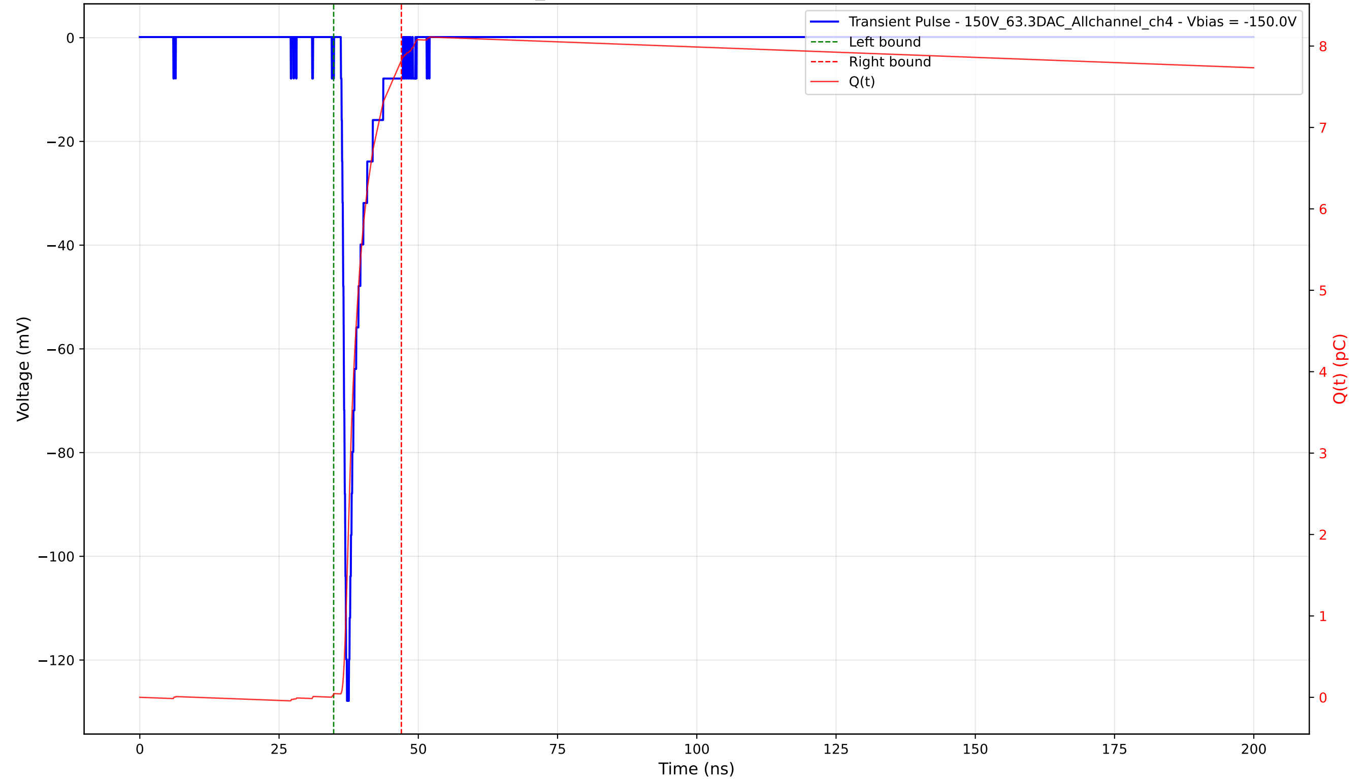
Transient Pulse - Sample: 1cm_42 - Position: 2810.0 \mu\text{m} - Charge: 7.79 pC - Rise Time: 0.82 ns
