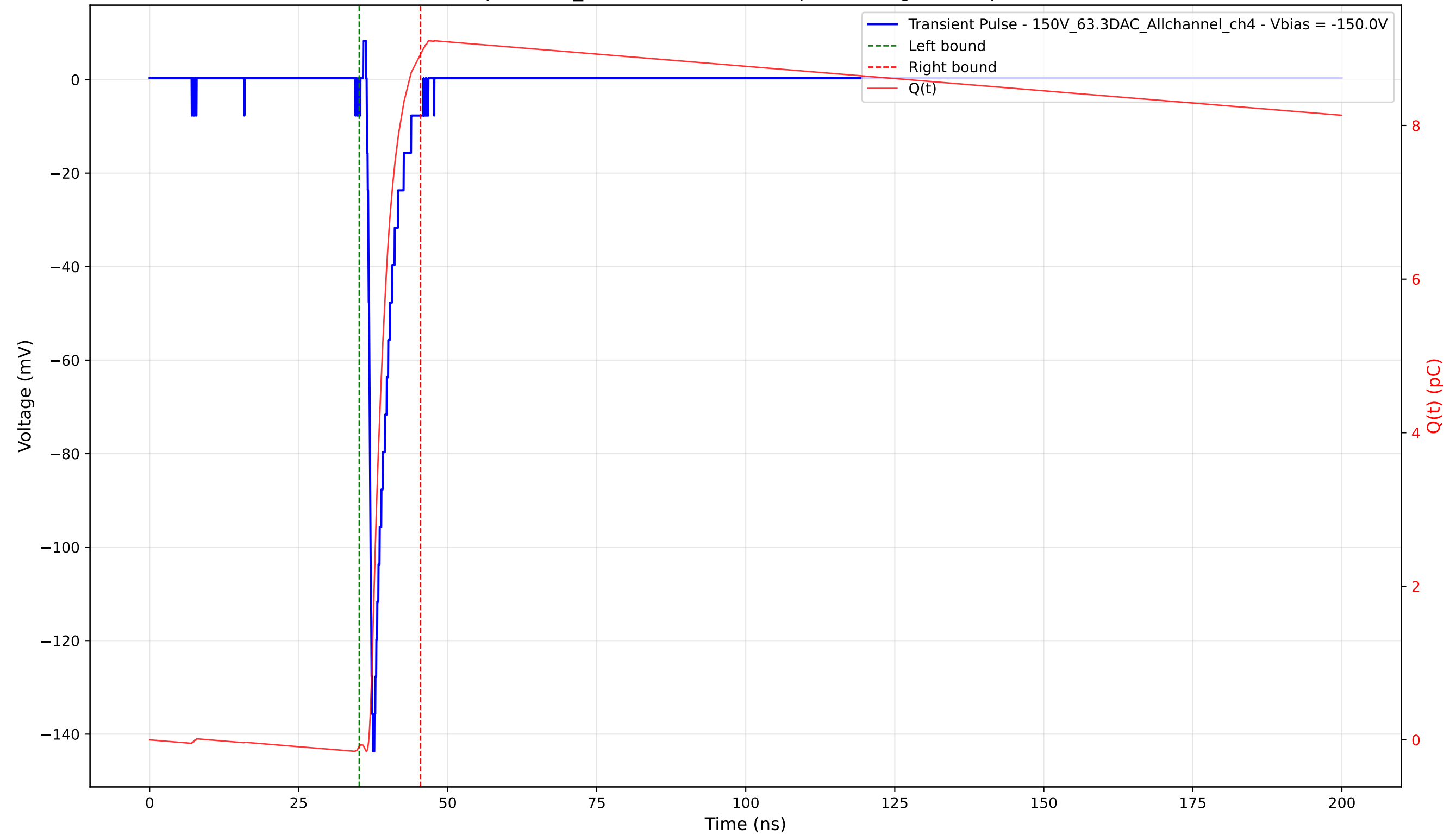
Transient Pulse - Sample: 1cm_42 - Position: 1140.0 \mu\text{m} - Charge: 9.02 pC - Rise Time: 0.81 ns
