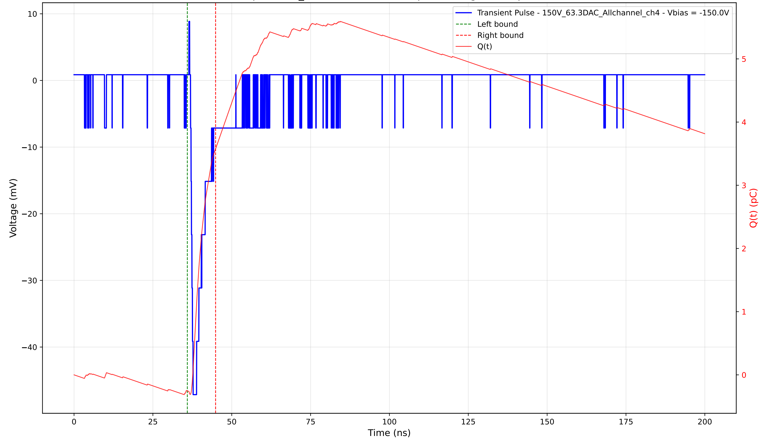
Transient Pulse - Sample: 1cm_42 - Position: 3215.0 \mu\text{m} - Charge: 3.83 pC - Rise Time: 0.82 ns
