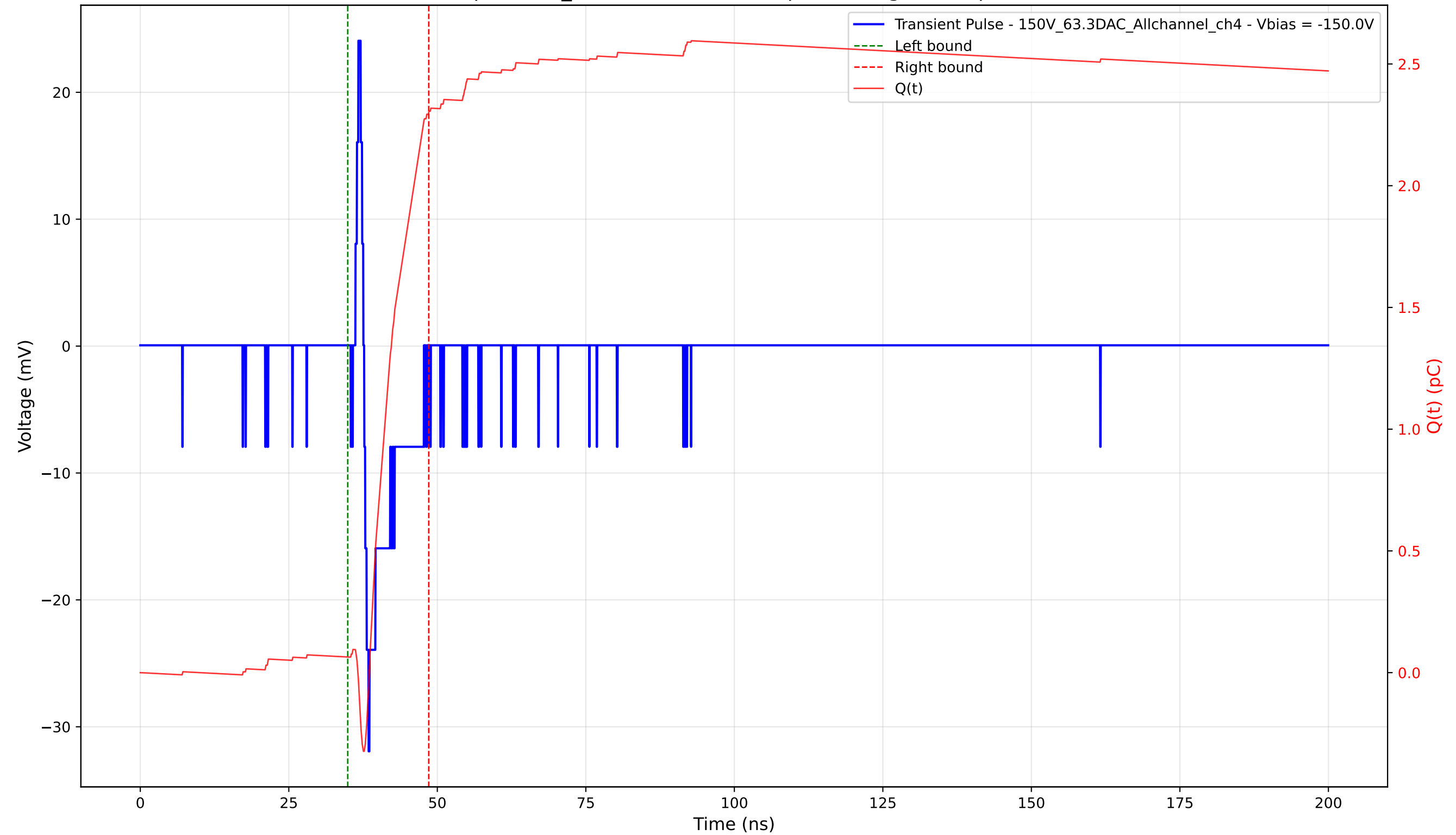
Transient Pulse - Sample: 1cm_42 - Position: 4525.0 \mu\text{m} - Charge: 2.24 pC - Rise Time: 0.74 ns
