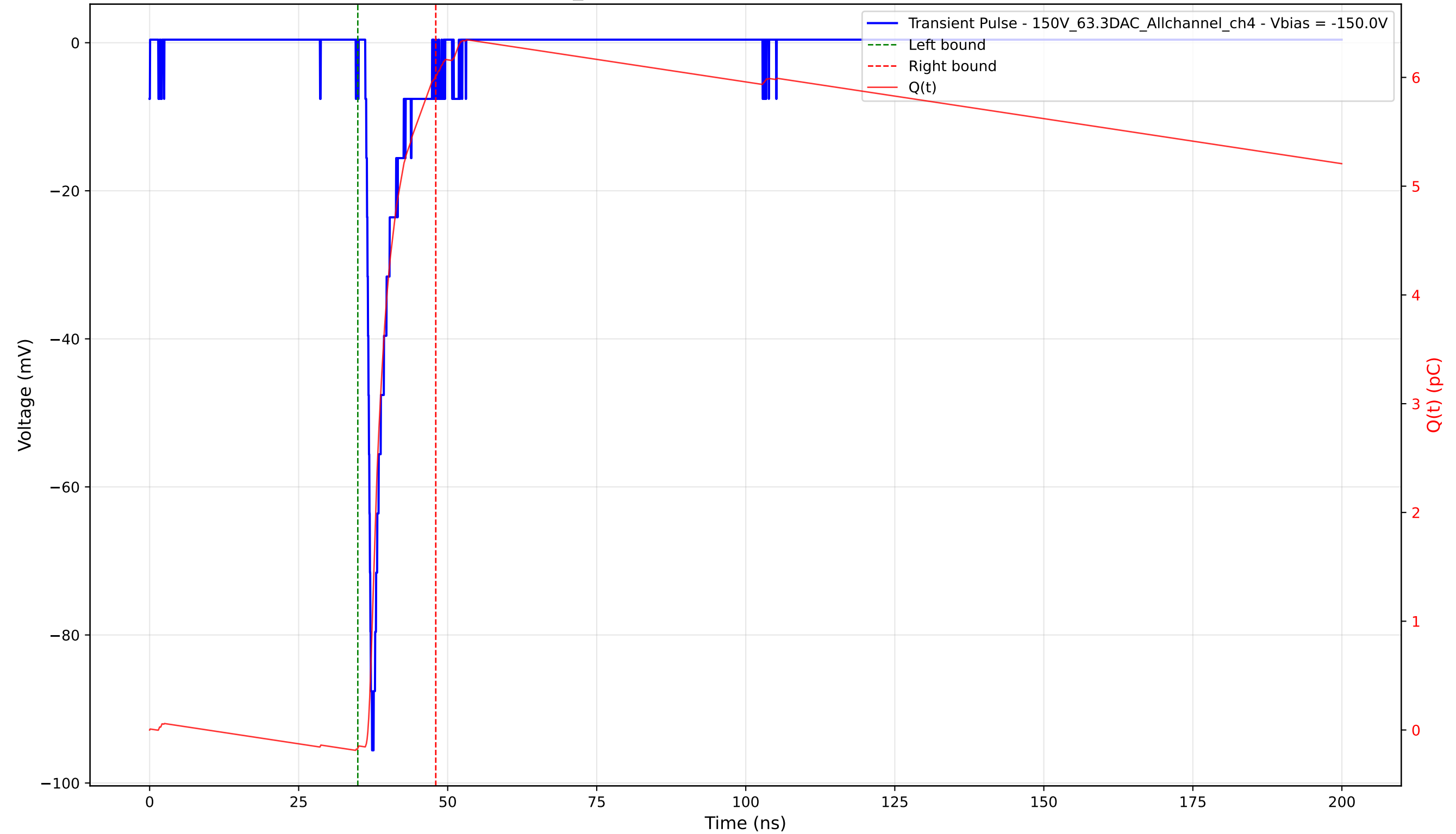
Transient Pulse - Sample: 1cm_42 - Position: 2915.0 \mu\text{m} - Charge: 6.19 pC - Rise Time: 0.79 ns
