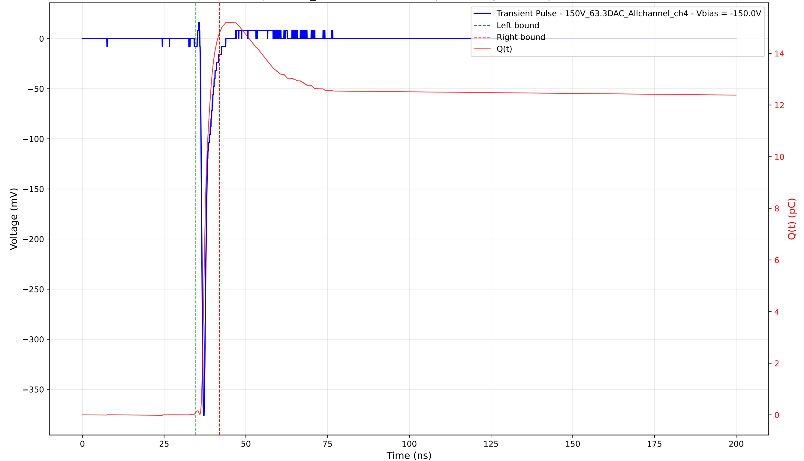
Transient Pulse - Sample: 1cm_42 - Position: 1605.0 \mu\text{m} - Charge: 14.67 pC - Rise Time: 0.74 ns
