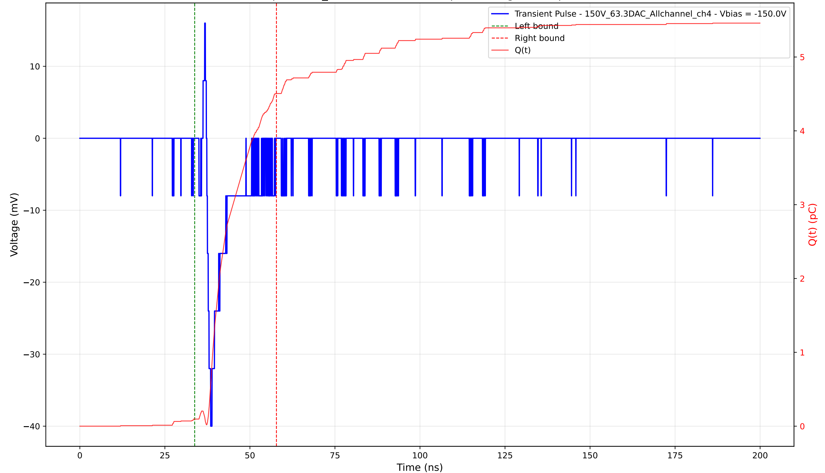
Transient Pulse - Sample: 1cm_42 - Position: 3485.0 \mu\text{m} - Charge: 4.41 pC - Rise Time: 1.14 ns
