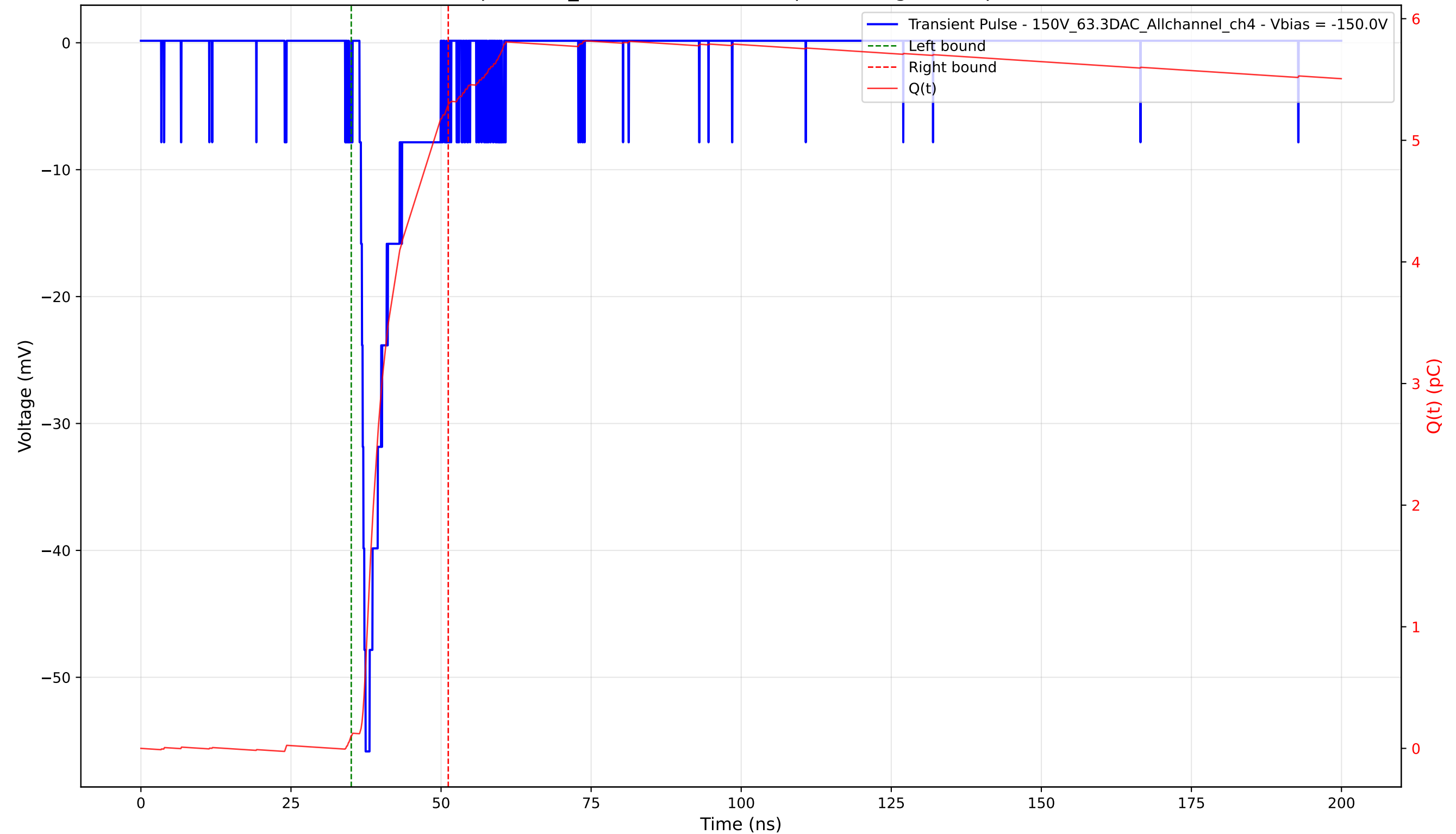
Transient Pulse - Sample: 1cm_42 - Position: 3060.0 \mu\text{m} - Charge: 5.19 pC - Rise Time: 1.01 ns
