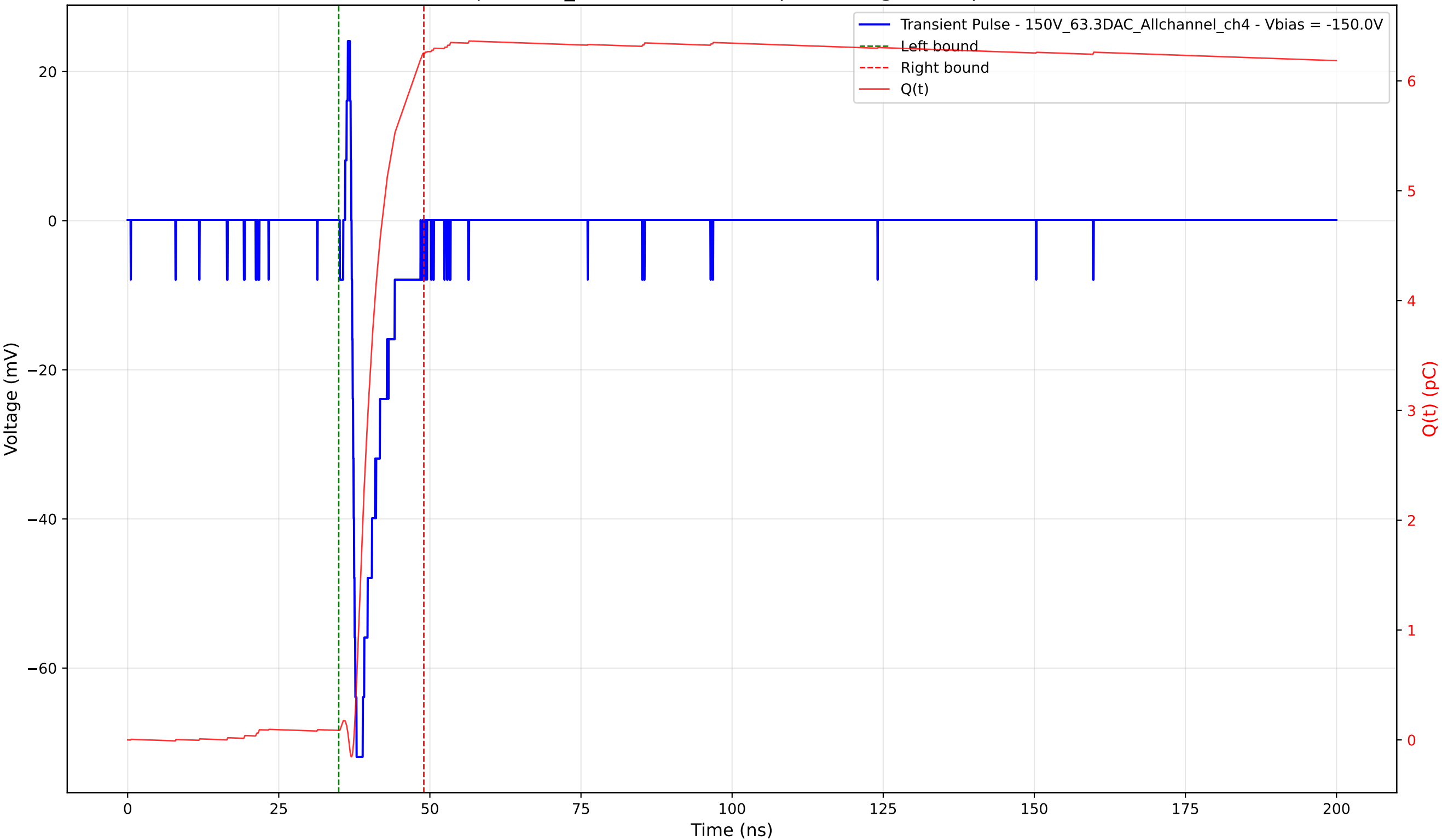
Transient Pulse - Sample: 1cm_42 - Position: 665.0 \mu\text{m} - Charge: 6.16 pC - Rise Time: 0.80 ns
