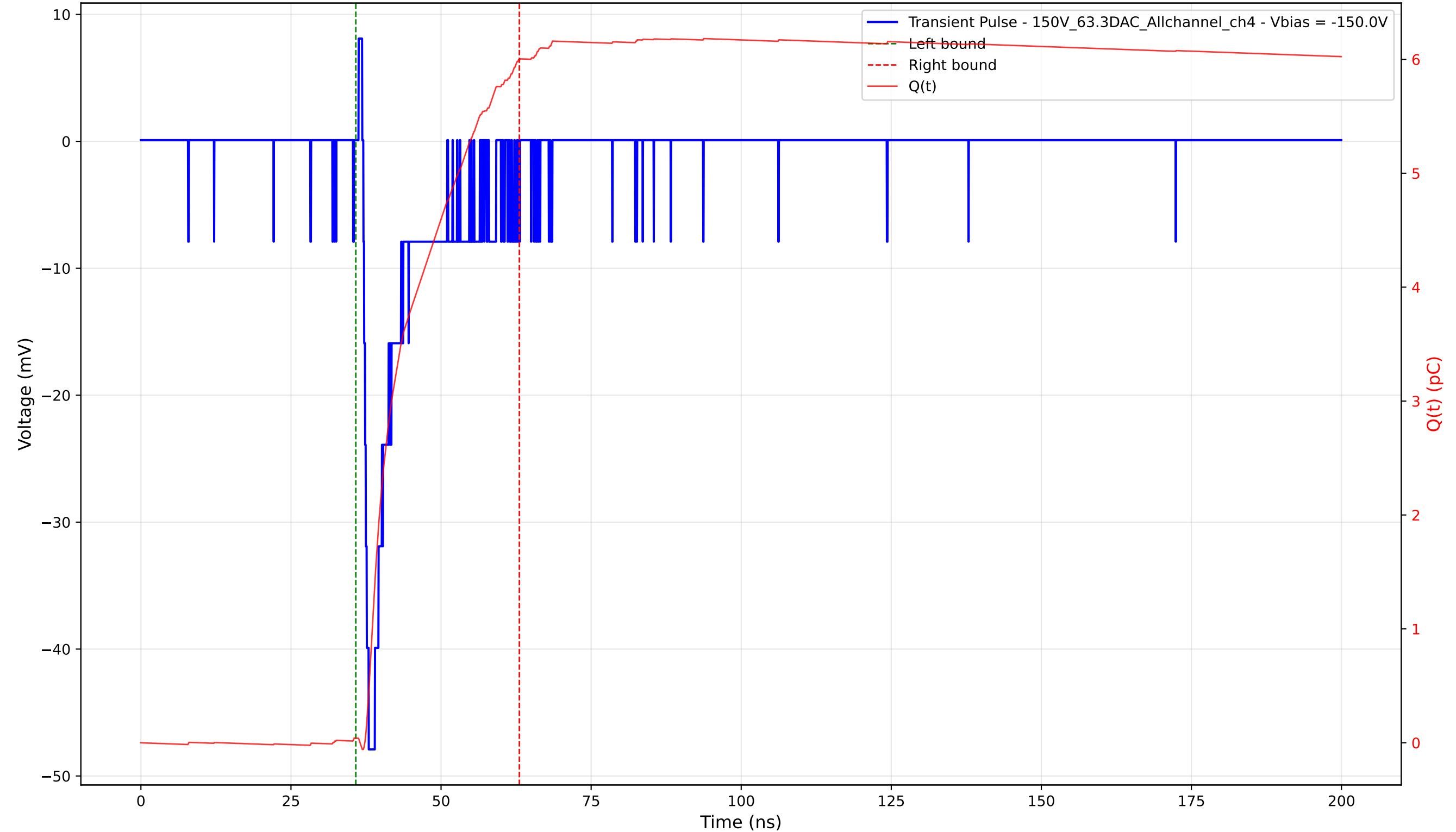
Transient Pulse - Sample: 1cm_42 - Position: 3275.0 \mu\text{m} - Charge: 5.96 pC - Rise Time: 0.90 ns
