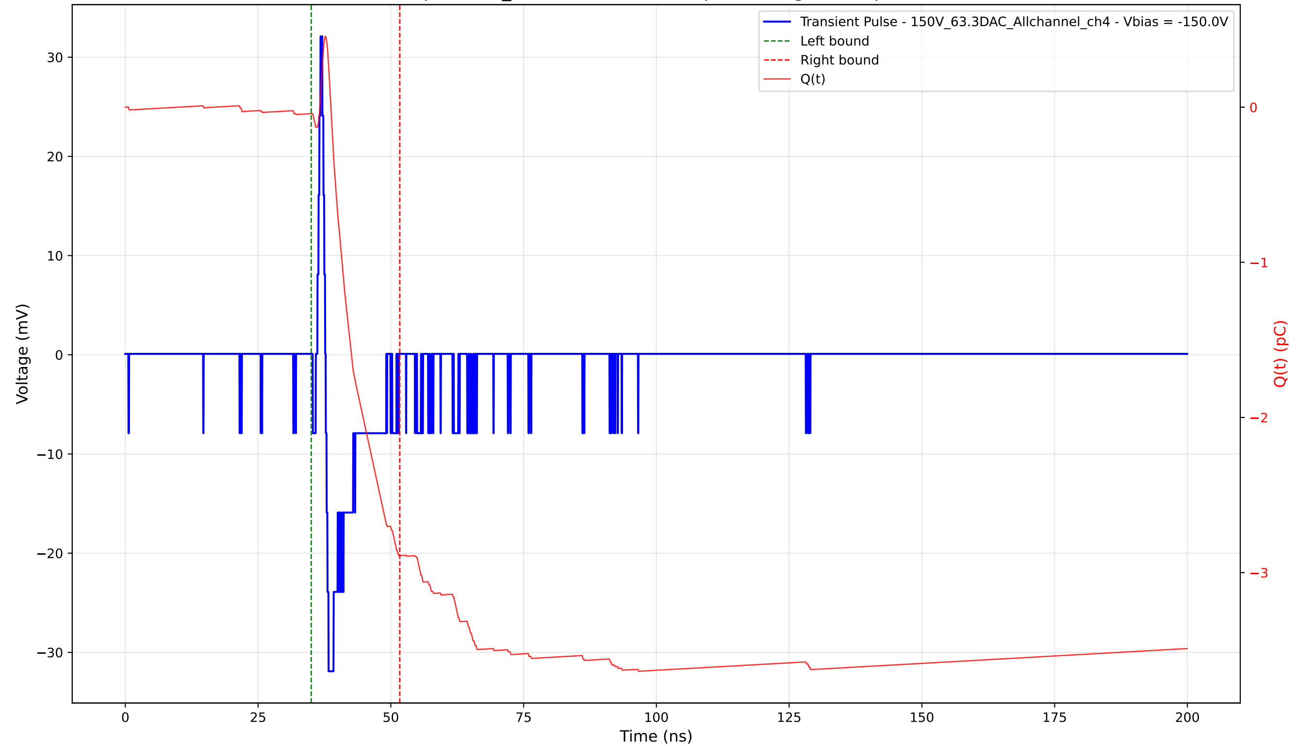
Transient Pulse - Sample: 1cm_42 - Position: 4350.0 \mu\text{m} - Charge: 2.85 pC - Rise Time: 0.58 ns
