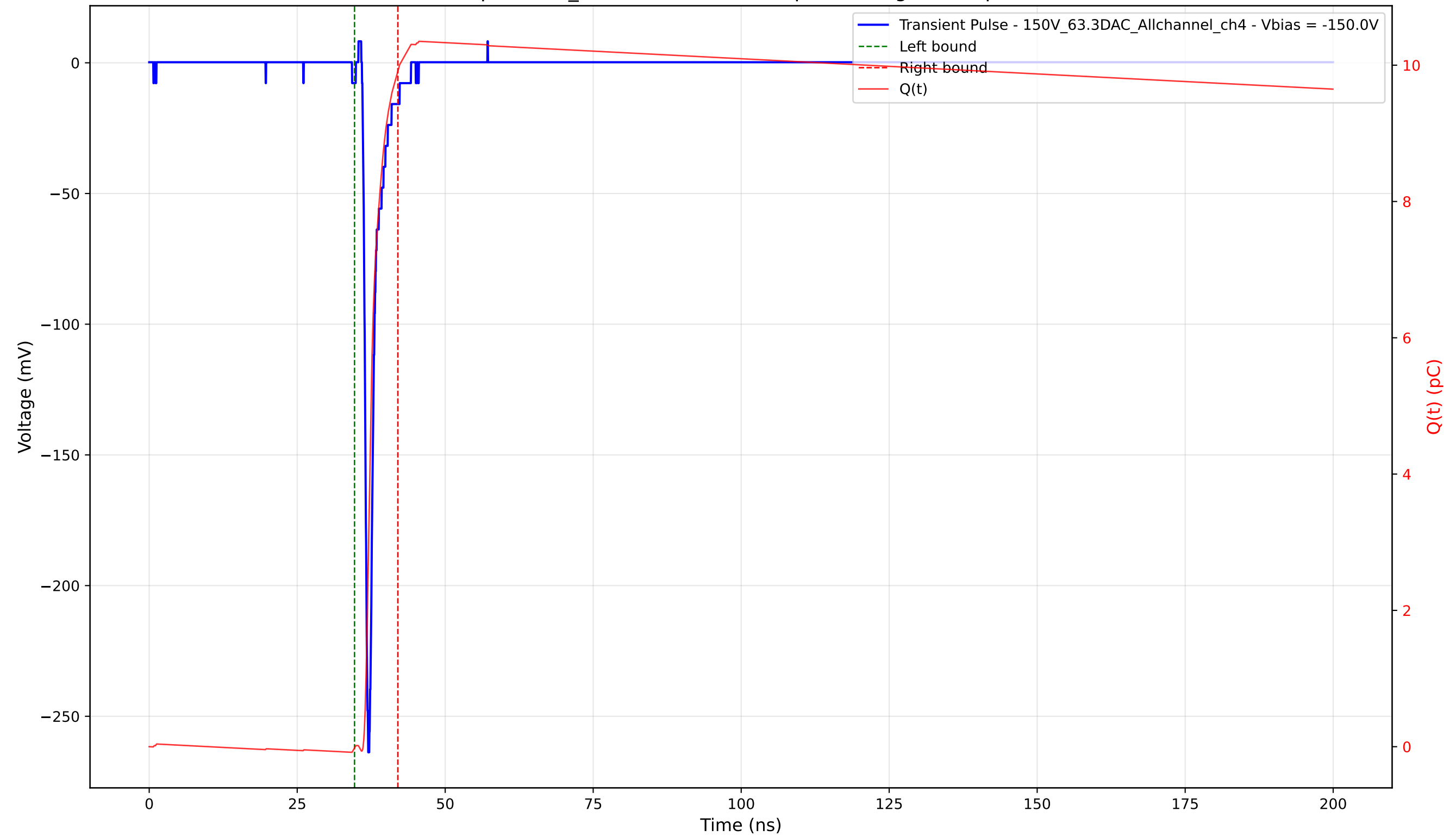
Transient Pulse - Sample: 1cm_42 - Position: 2485.0 \mu\text{m} - Charge: 9.93 pC - Rise Time: 0.74 ns
