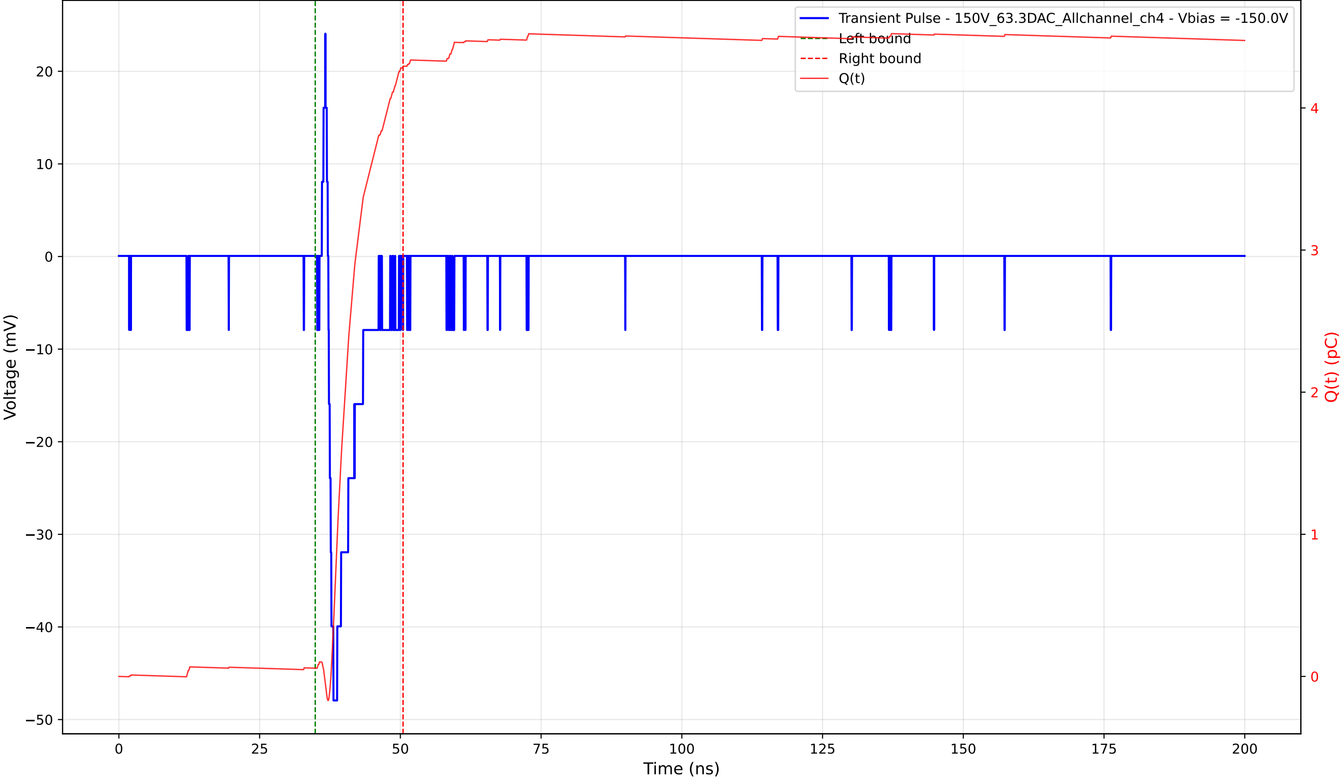
Transient Pulse - Sample: 1cm_42 - Position: 440.0 \mu\text{m} - Charge: 4.23 pC - Rise Time: 0.90 ns
