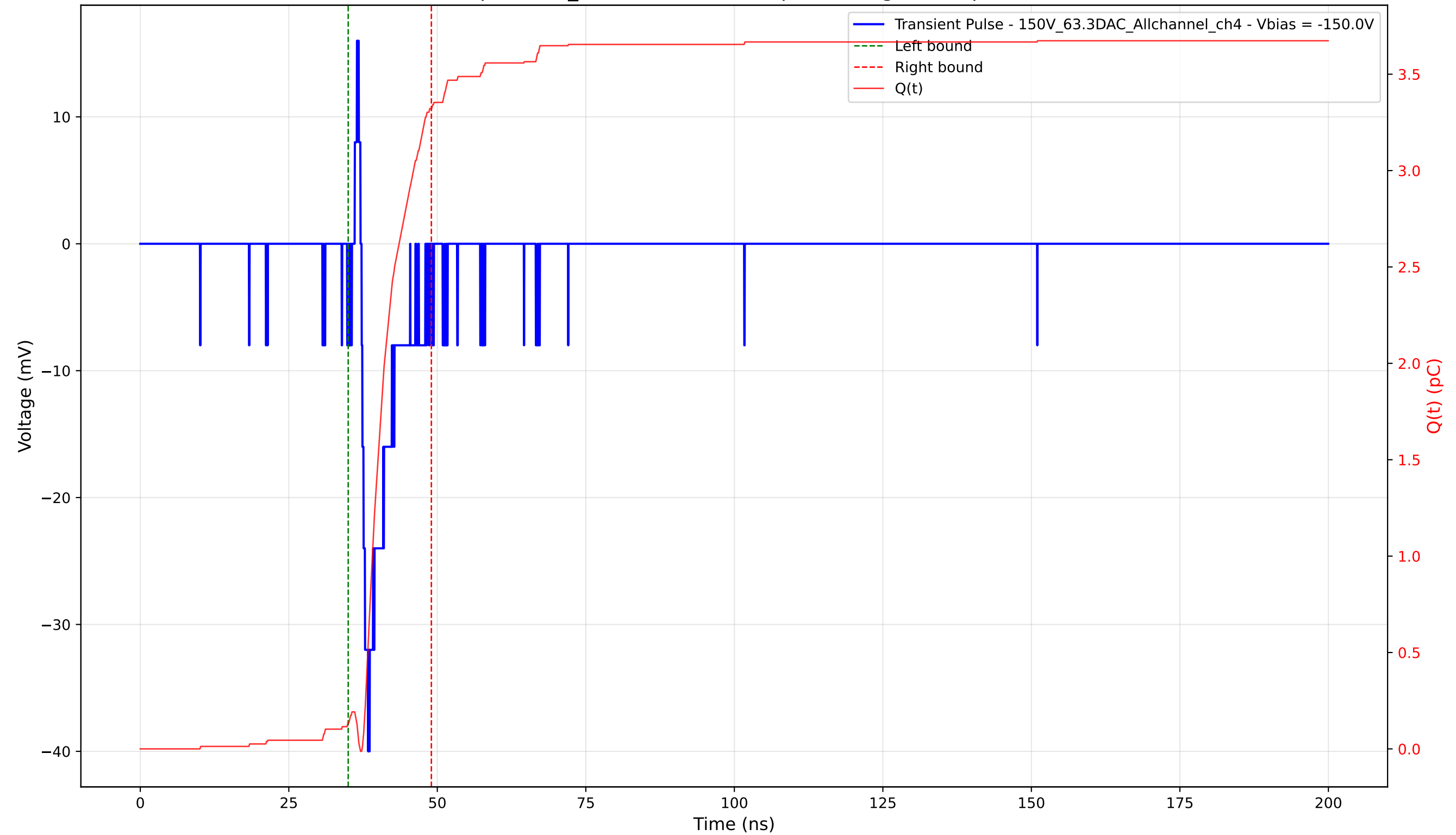
Transient Pulse - Sample: 1cm_42 - Position: 335.0 \mu\text{m} - Charge: 3.19 pC - Rise Time: 1.10 ns
