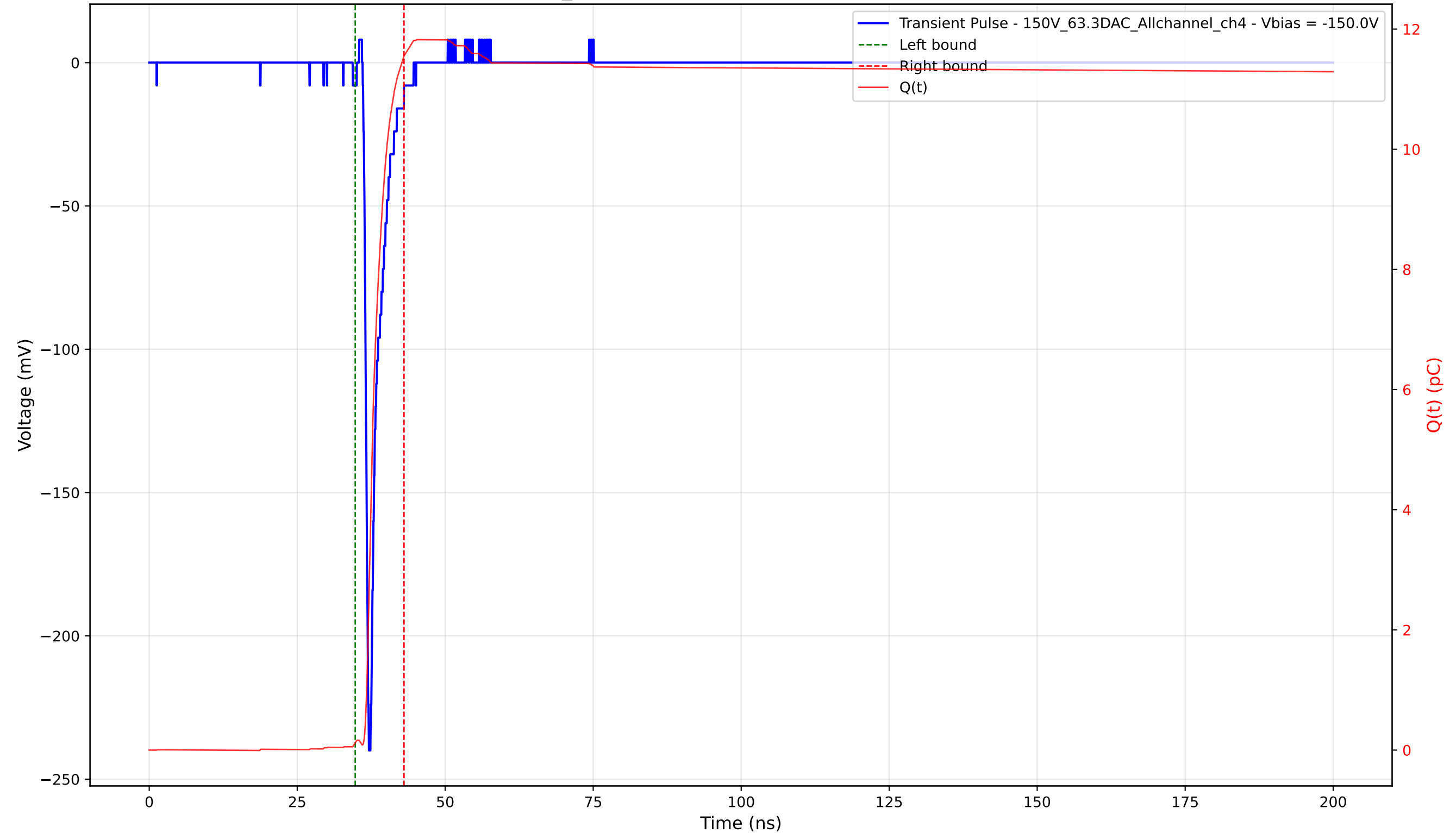
Transient Pulse - Sample: 1cm_42 - Position: 1470.0 \mu\text{m} - Charge: 11.43 pC - Rise Time: 0.76 ns
