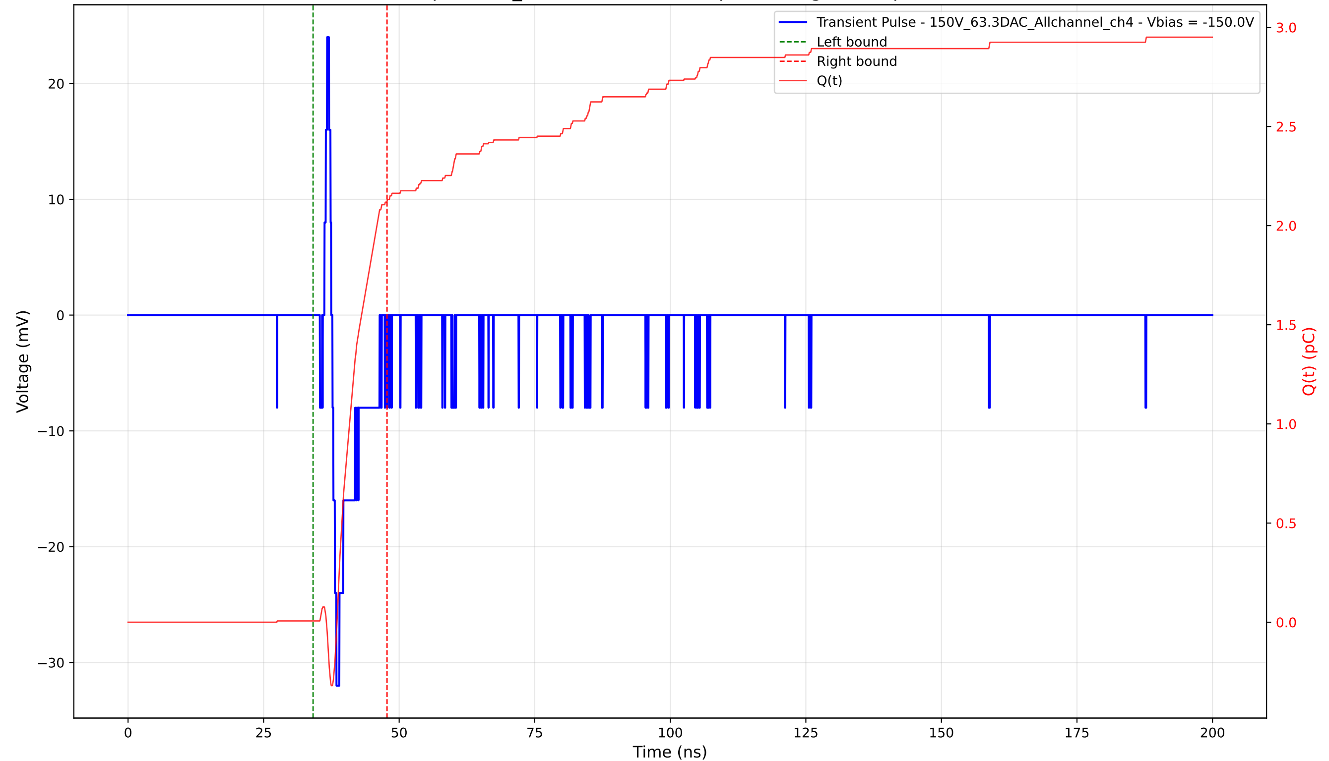
Transient Pulse - Sample: 1cm_42 - Position: 4545.0 \mu\text{m} - Charge: 2.12 pC - Rise Time: 0.74 ns
