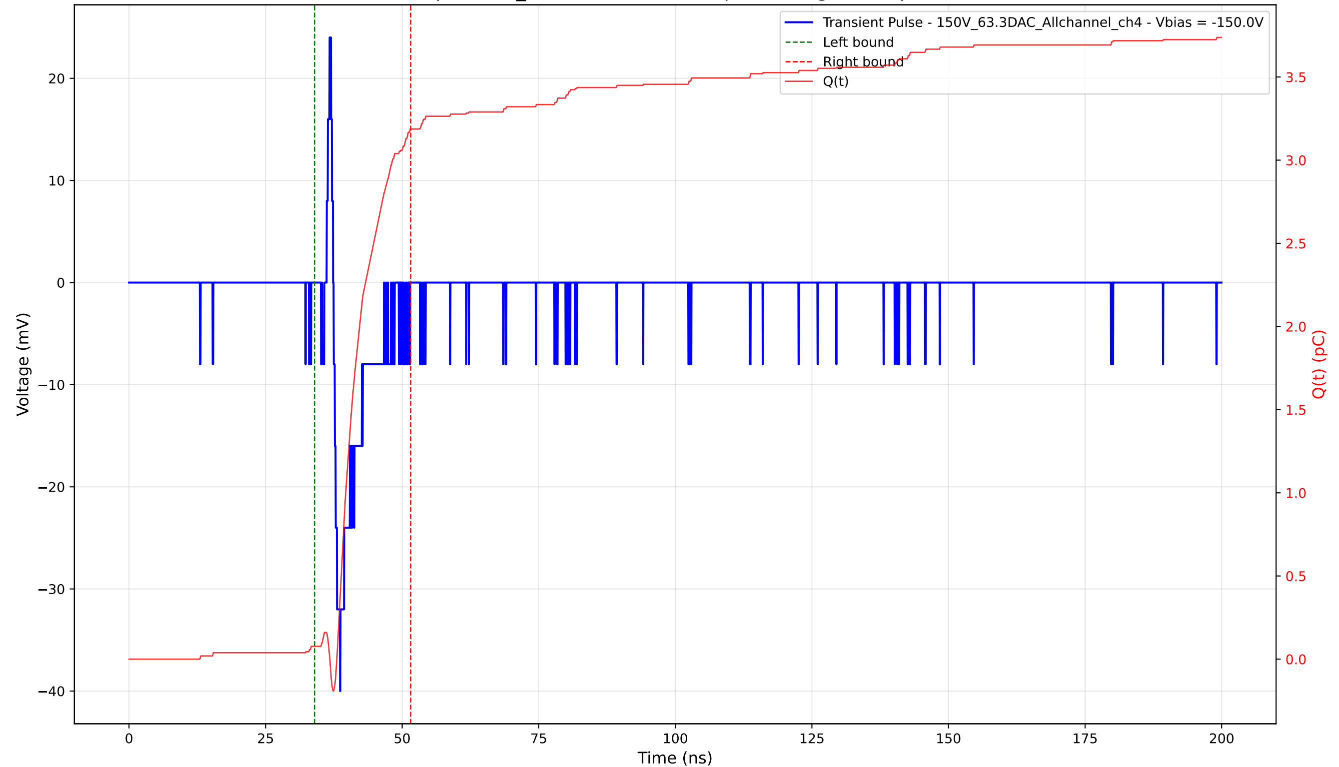
Transient Pulse - Sample: 1cm_42 - Position: 4810.0 \mu\text{m} - Charge: 3.11 pC - Rise Time: 1.18 ns
