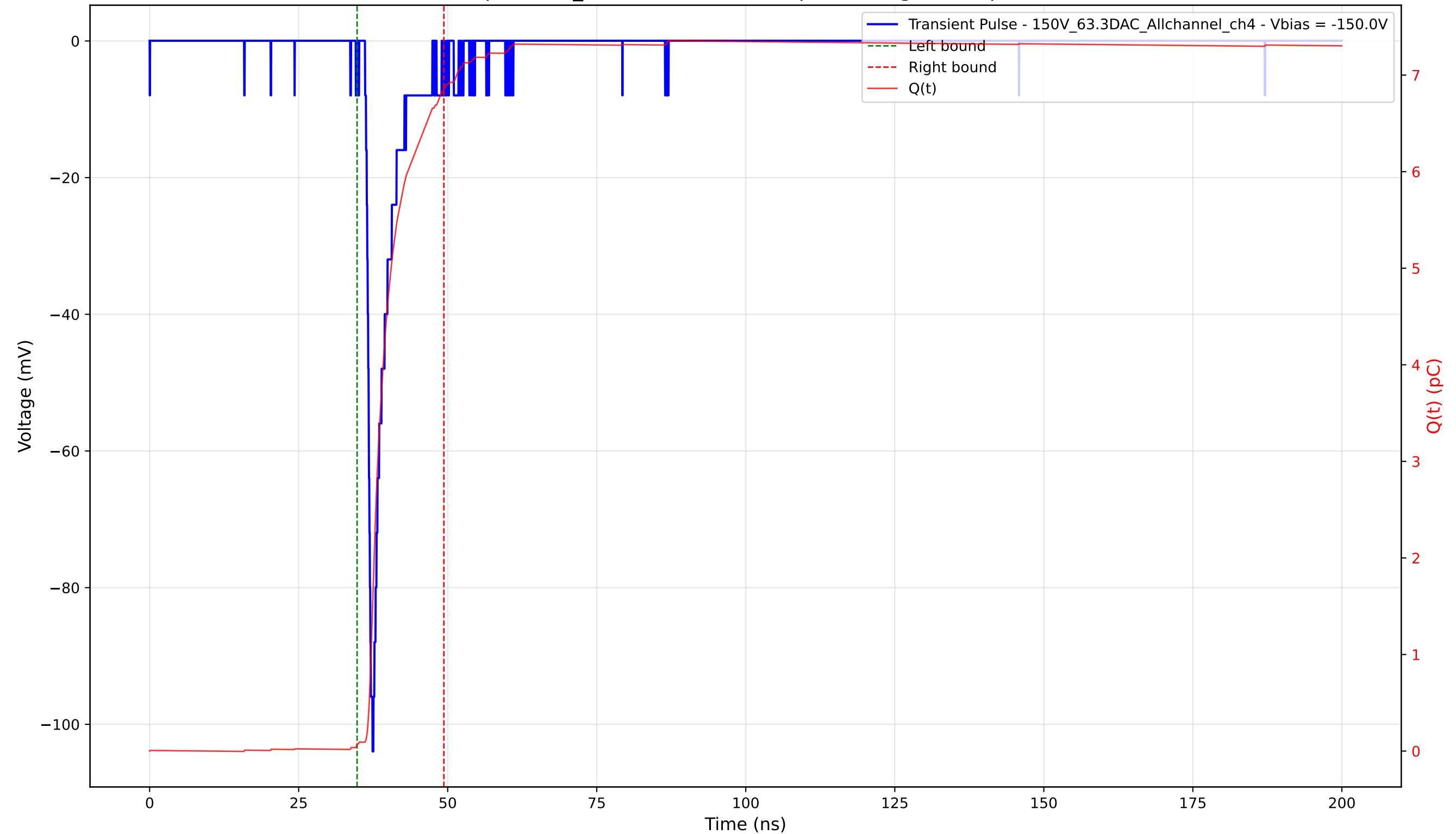
Transient Pulse - Sample: 1cm_42 - Position: 2895.0 \mu\text{m} - Charge: 6.79 pC - Rise Time: 0.83 ns
