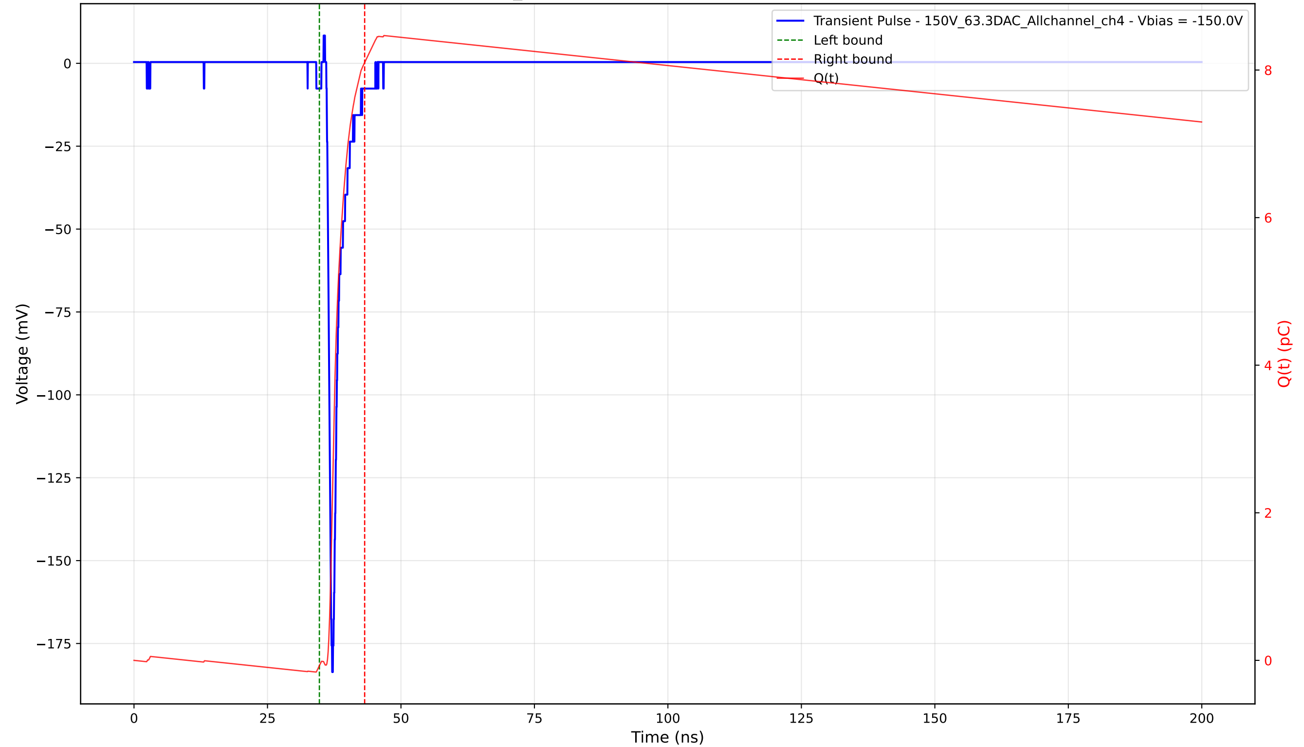
Transient Pulse - Sample: 1cm_42 - Position: 2600.0 \mu\text{m} - Charge: 8.17 pC - Rise Time: 0.79 ns
