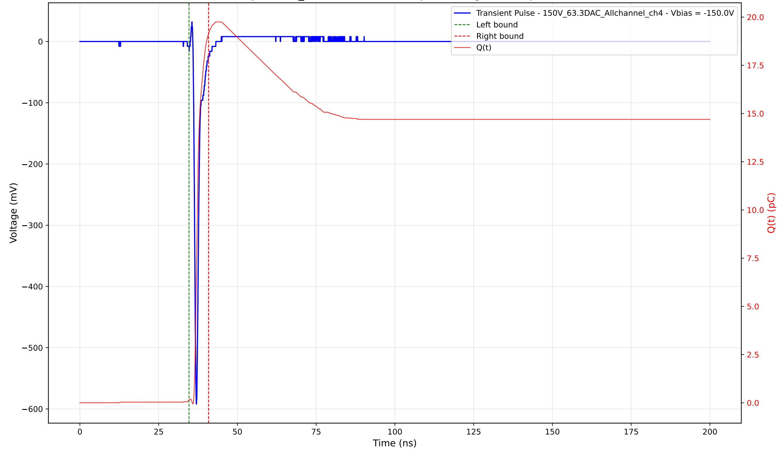
Transient Pulse - Sample: 1cm_42 - Position: 1860.0 \mu\text{m} - Charge: 19.01 pC - Rise Time: 0.72 ns
