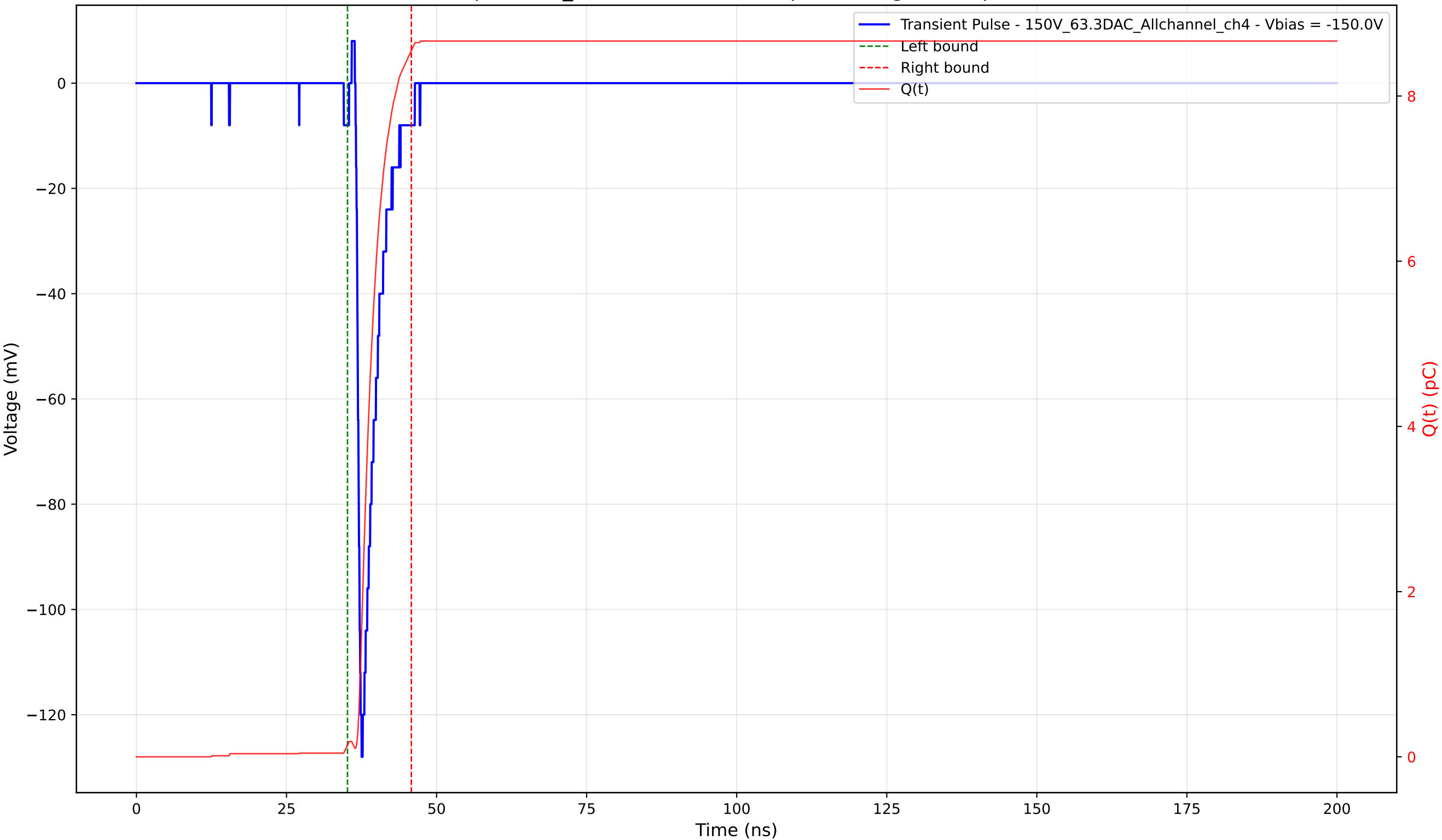
Transient Pulse - Sample: 1cm_42 - Position: 1105.0 \mu\text{m} - Charge: 8.41 pC - Rise Time: 0.78 ns
