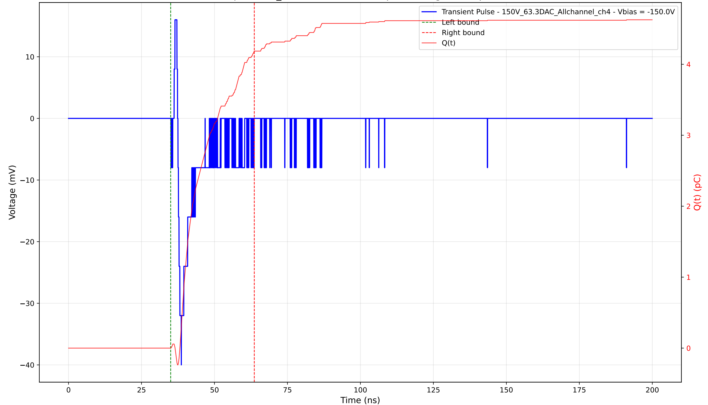
Transient Pulse - Sample: 1cm_42 - Position: 3575.0 \mu\text{m} - Charge: 4.19 pC - Rise Time: 1.14 ns
