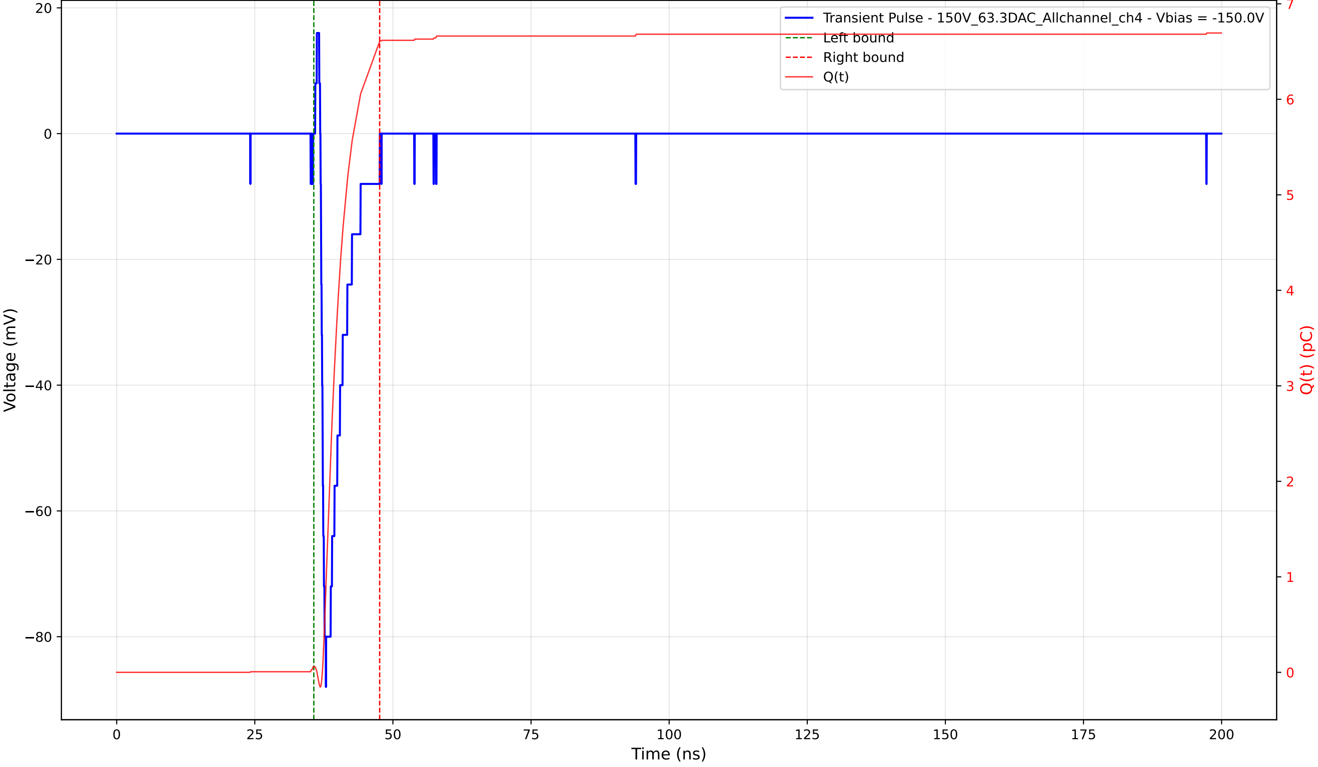
Transient Pulse - Sample: 1cm_42 - Position: 900.0 \mu\text{m} - Charge: 6.55 pC - Rise Time: 0.68 ns
