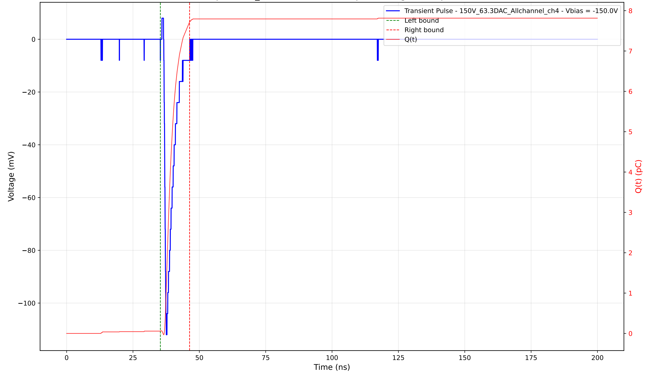
Transient Pulse - Sample: 1cm_42 - Position: 1050.0 \mu\text{m} - Charge: 7.66 pC - Rise Time: 0.70 ns
