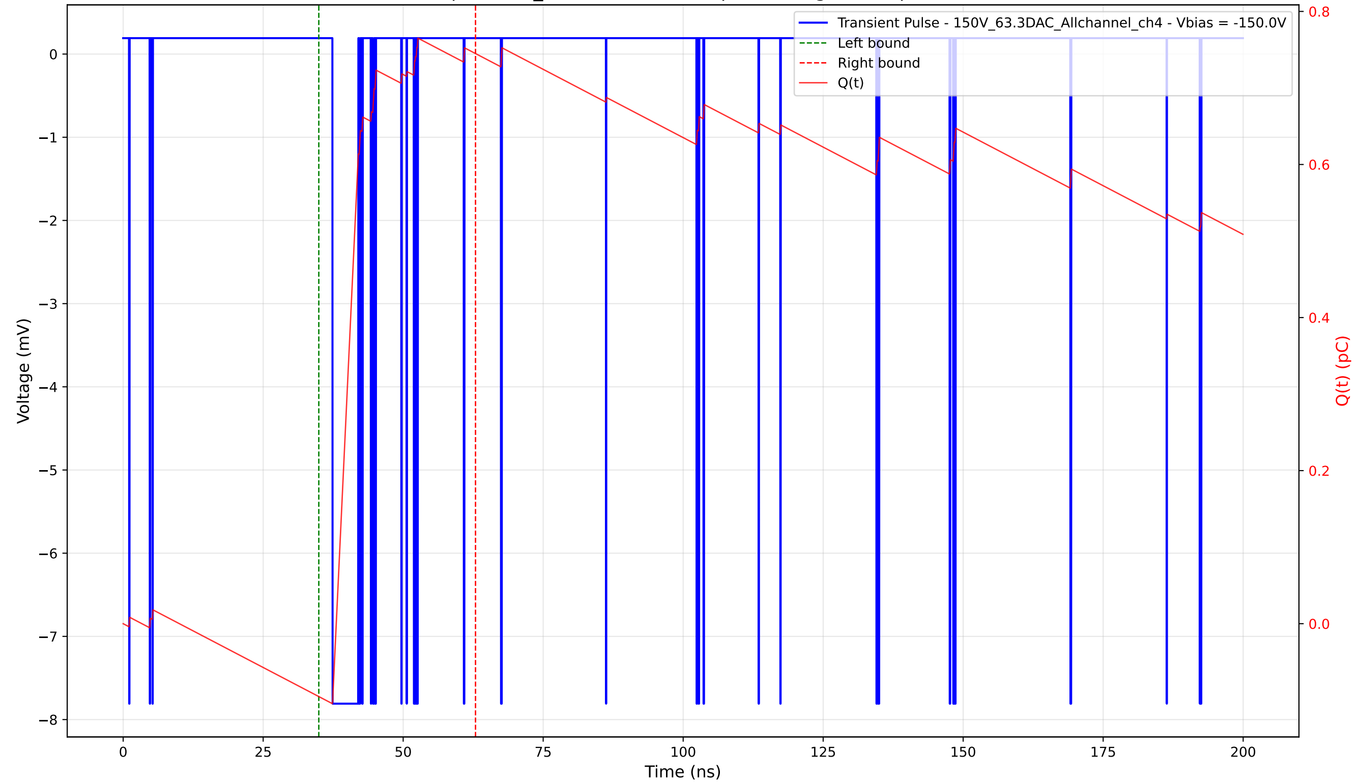
Transient Pulse - Sample: 1cm_42 - Position: 65.0 \mu\text{m} - Charge: 0.84 pC - Rise Time: 0.04 ns
