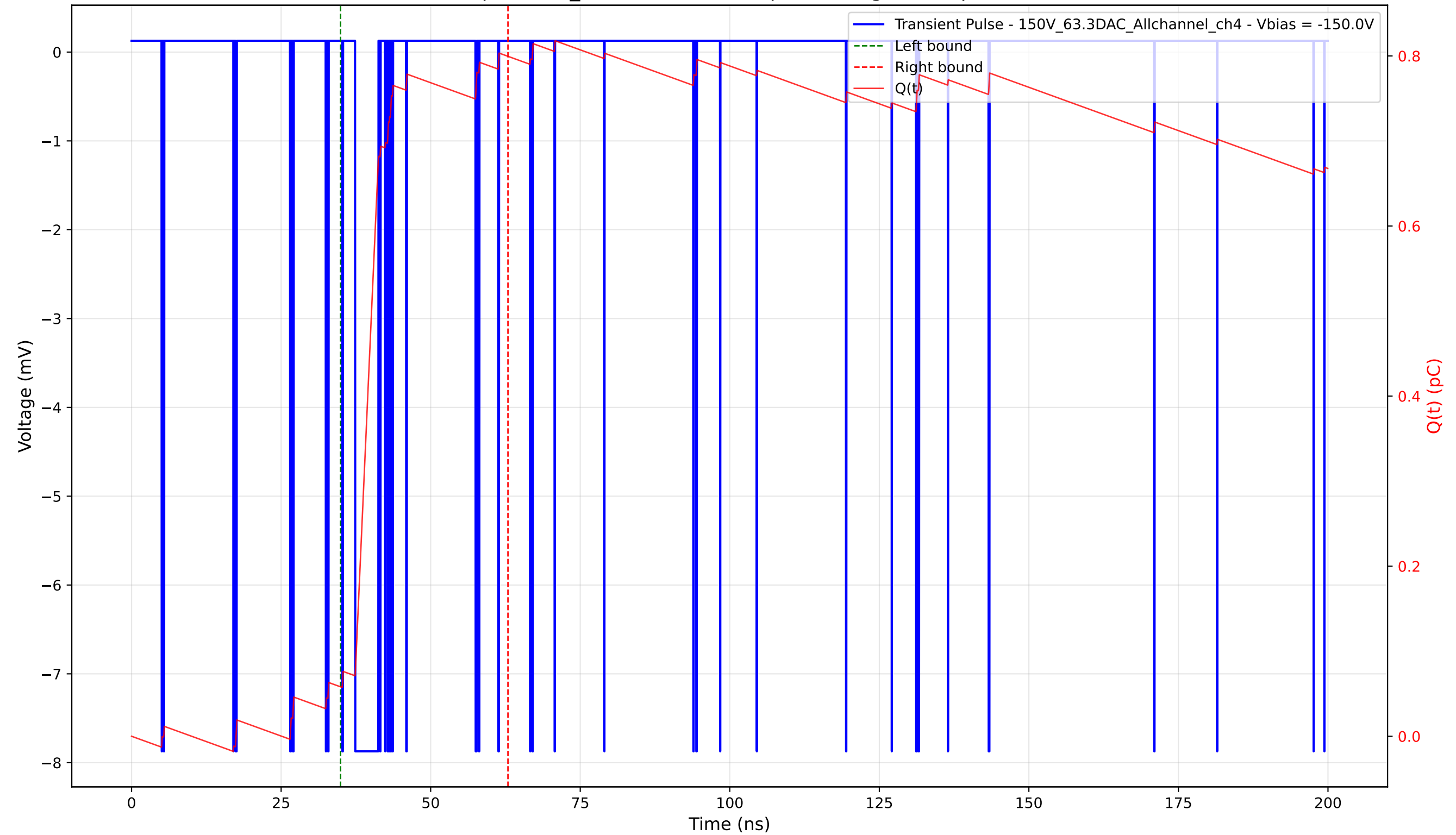
Transient Pulse - Sample: 1cm_42 - Position: 55.0 \mu\text{m} - Charge: 0.74 pC - Rise Time: 0.04 ns
