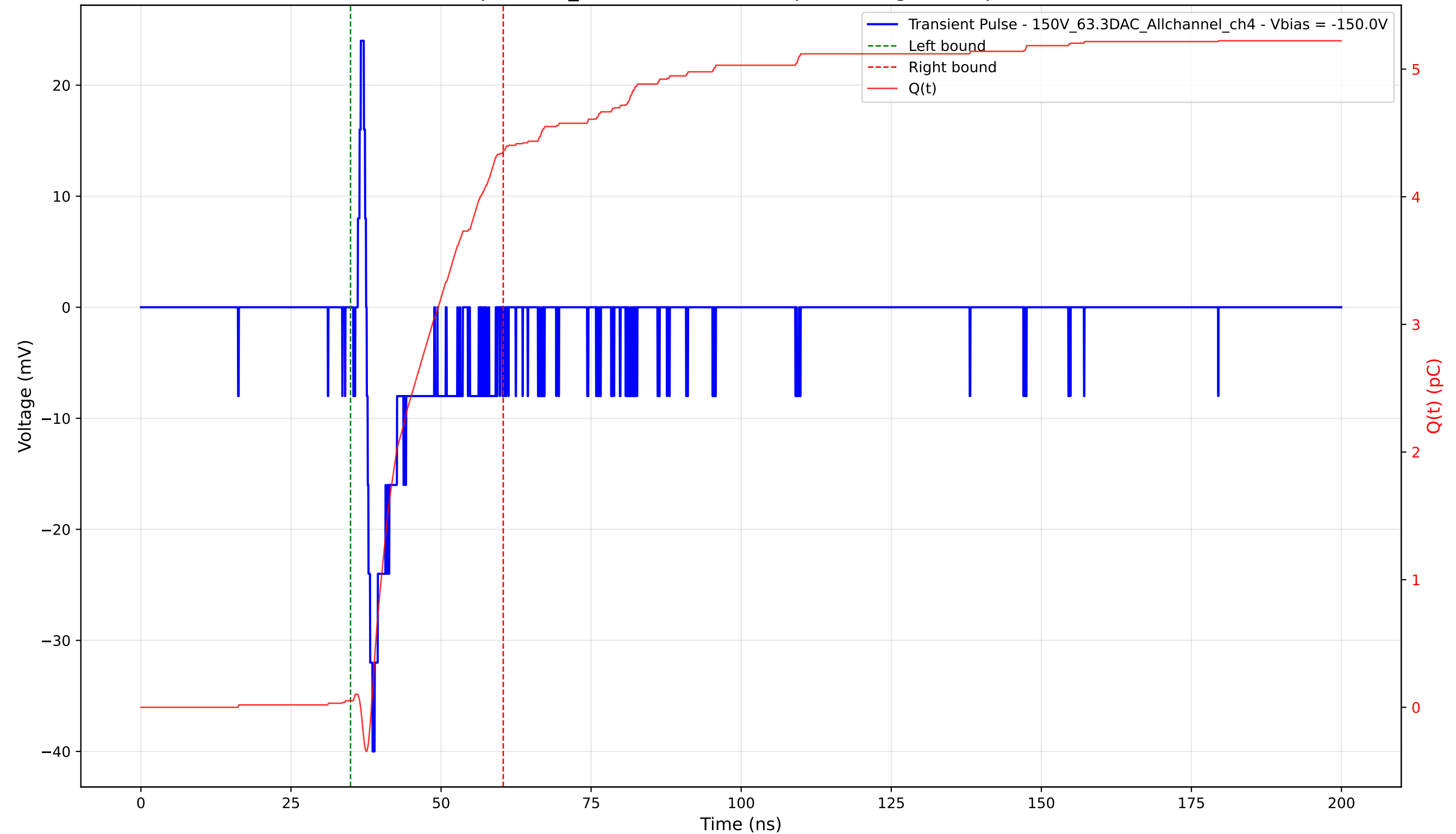
Transient Pulse - Sample: 1cm_42 - Position: 3705.0 \mu\text{m} - Charge: 4.31 pC - Rise Time: 0.98 ns
