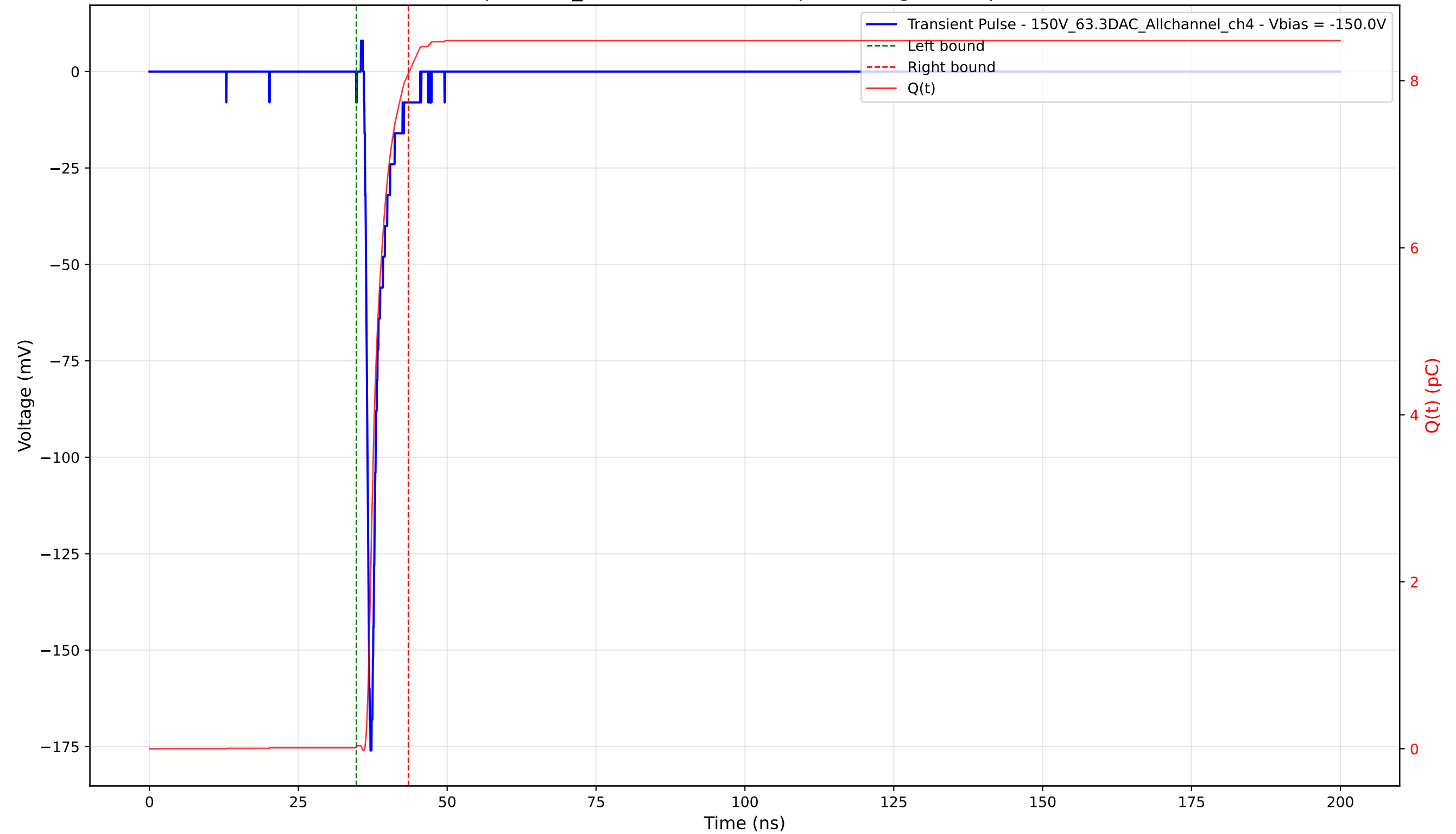
Transient Pulse - Sample: 1cm_42 - Position: 2620.0 \mu\text{m} - Charge: 8.06 pC - Rise Time: 0.75 ns
