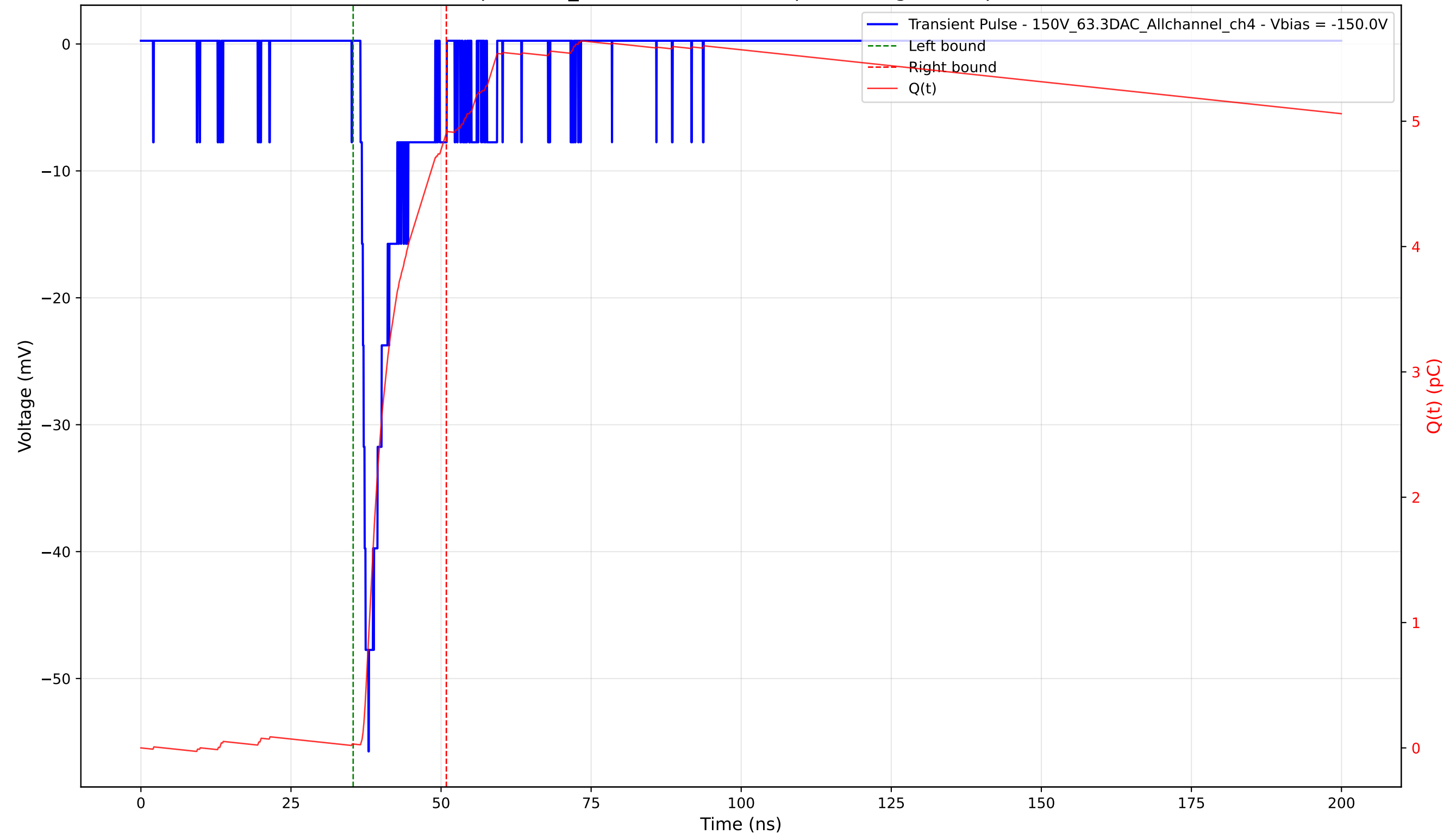
Transient Pulse - Sample: 1cm_42 - Position: 3110.0 \mu\text{m} - Charge: 4.88 pC - Rise Time: 1.33 ns
