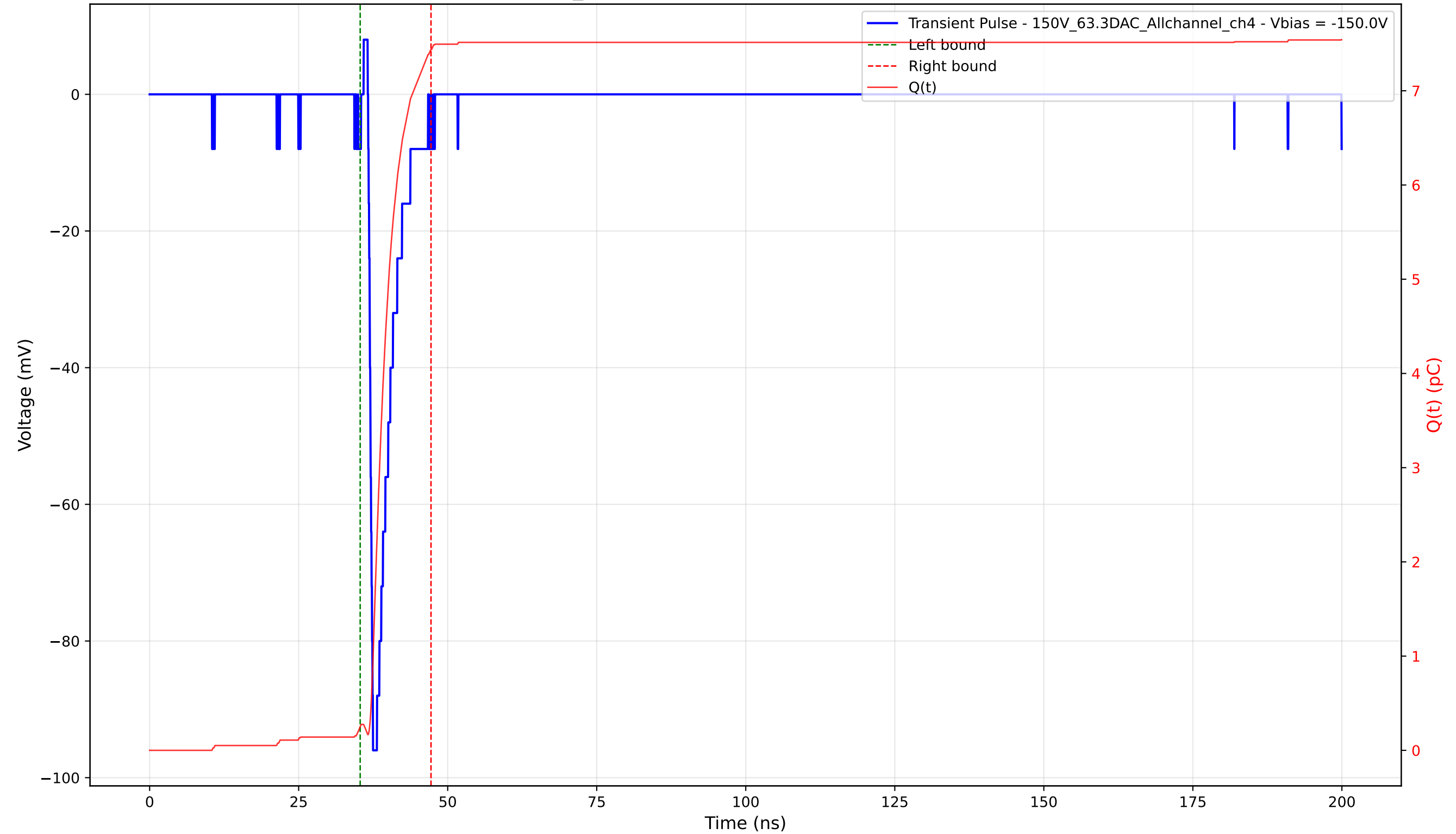
Transient Pulse - Sample: 1cm_42 - Position: 1015.0 \mu\text{m} - Charge: 7.18 pC - Rise Time: 0.67 ns
