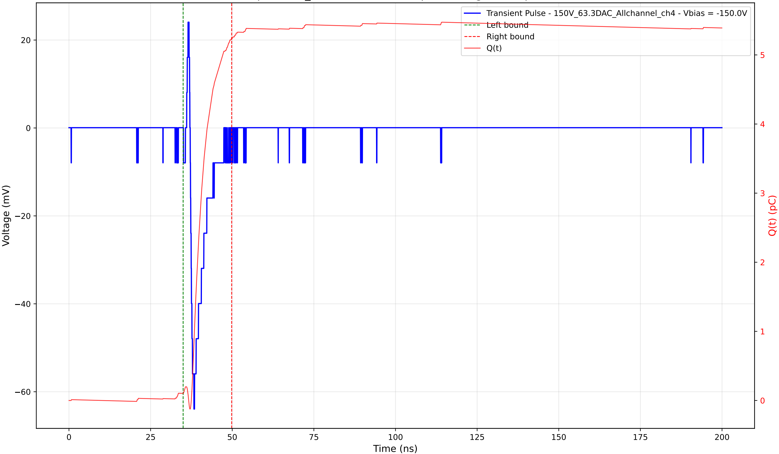
Transient Pulse - Sample: 1cm_42 - Position: 560.0 \mu\text{m} - Charge: 5.14 pC - Rise Time: 1.13 ns
