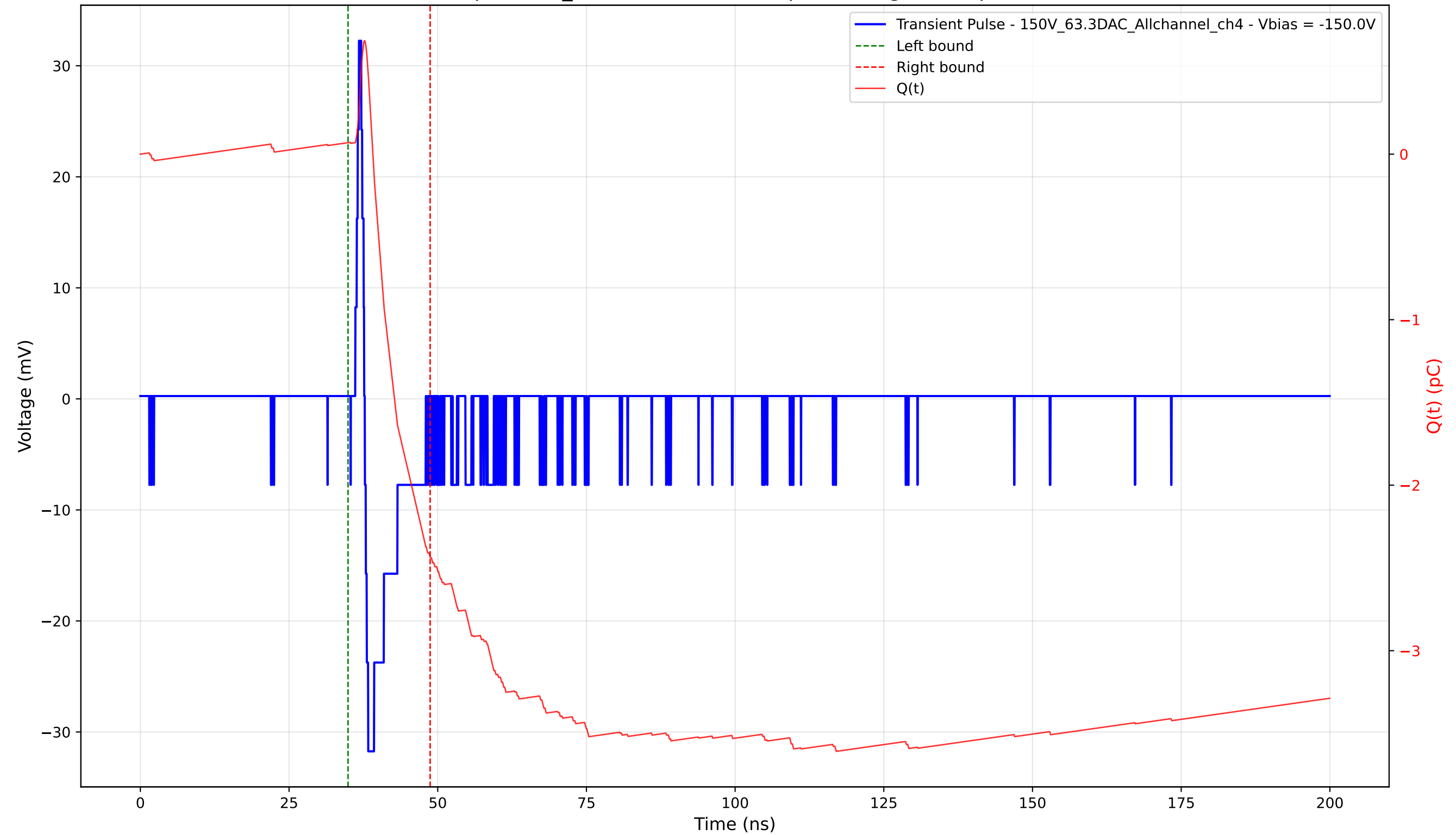
Transient Pulse - Sample: 1cm_42 - Position: 4255.0 \mu\text{m} - Charge: 2.51 pC - Rise Time: 0.63 ns
