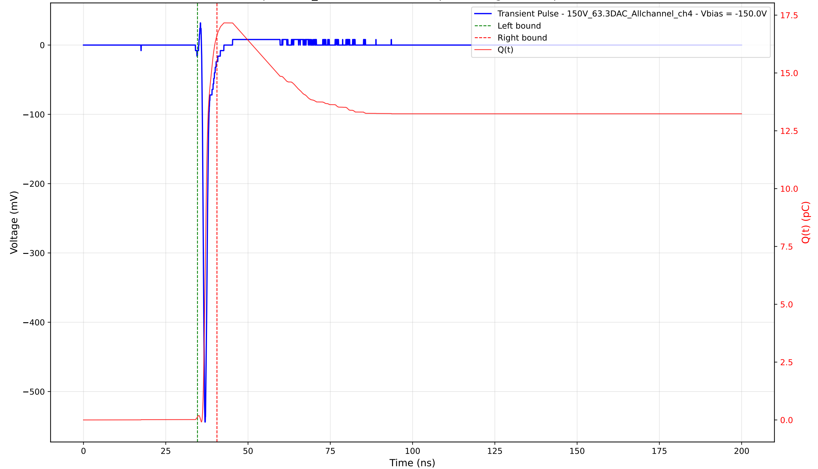
Transient Pulse - Sample: 1cm_42 - Position: 2145.0 \mu\text{m} - Charge: 16.49 pC - Rise Time: 0.71 ns
