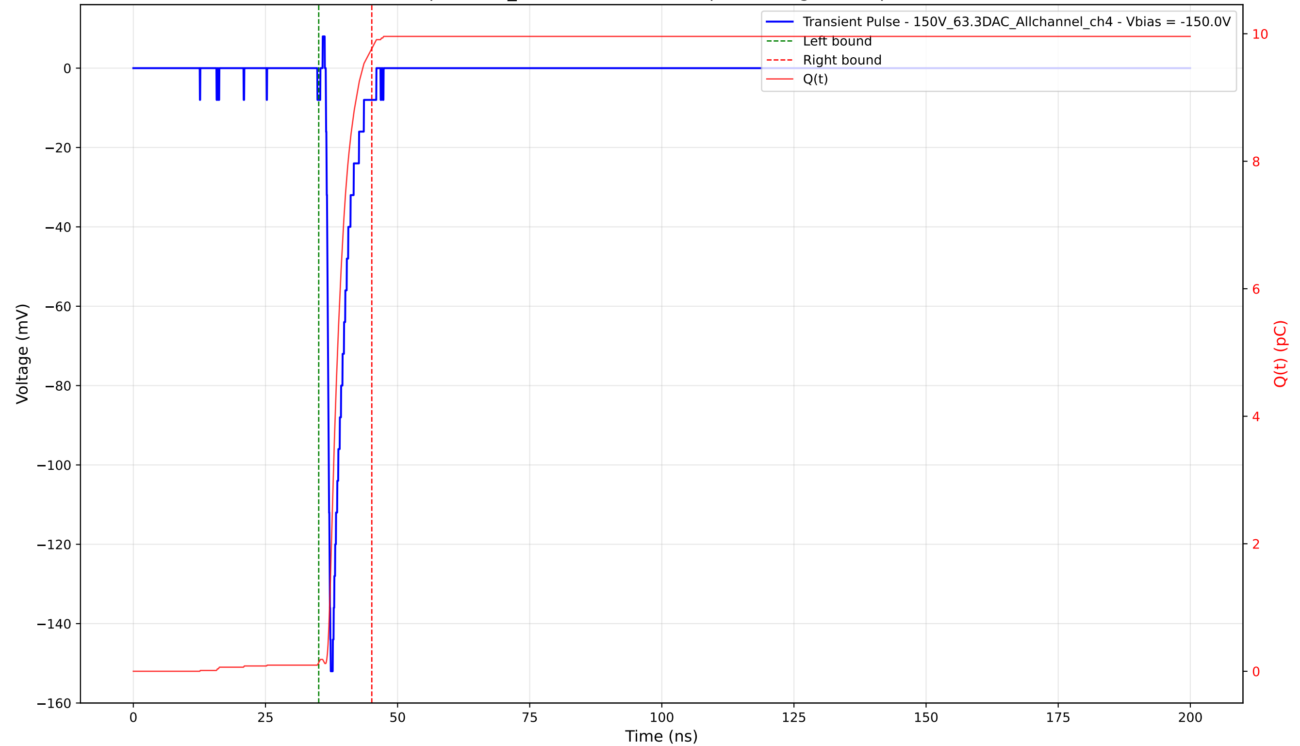
Transient Pulse - Sample: 1cm_42 - Position: 1170.0 \mu\text{m} - Charge: 9.63 pC - Rise Time: 0.80 ns
