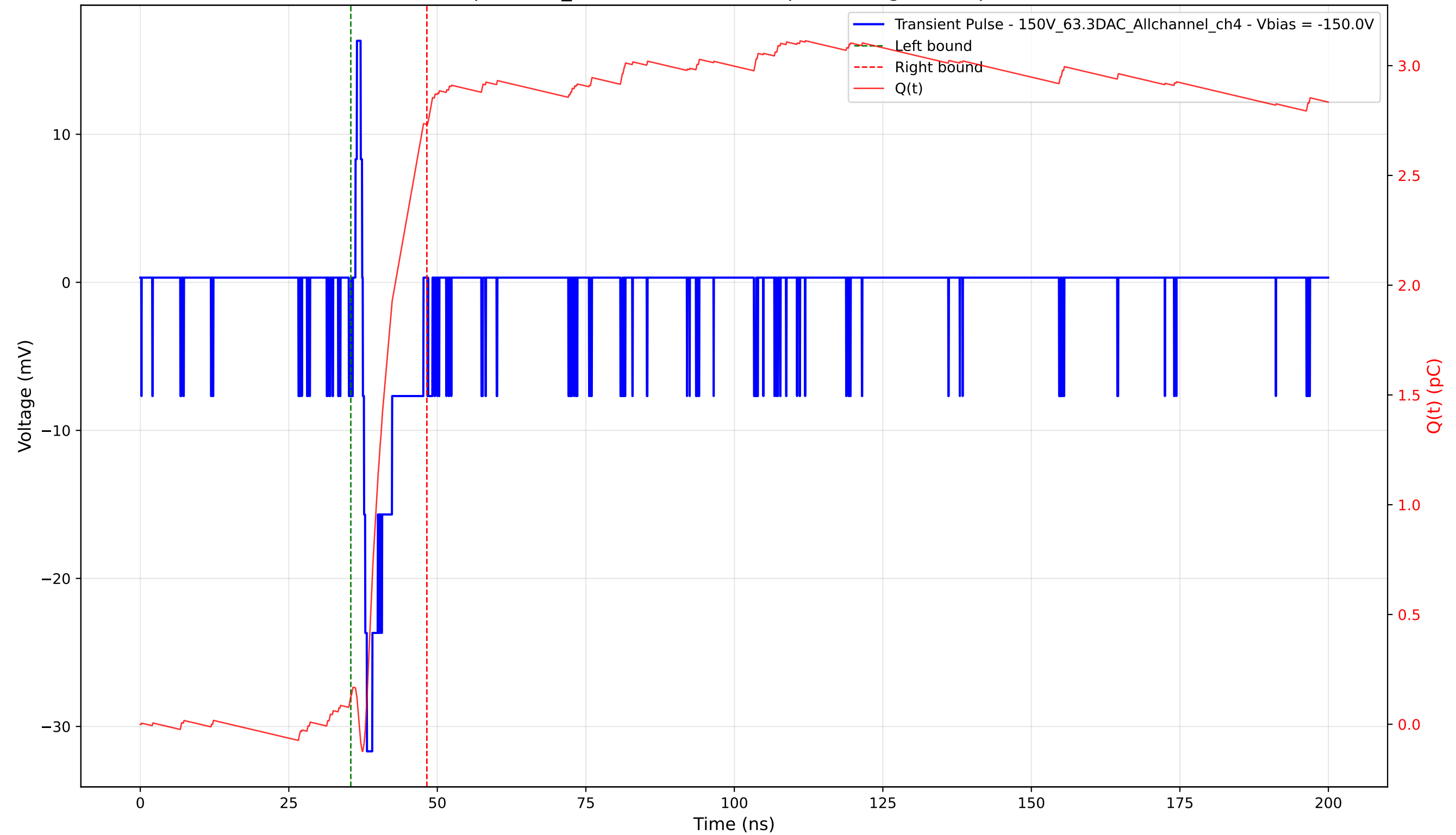
Transient Pulse - Sample: 1cm_42 - Position: 4880.0 \mu\text{m} - Charge: 2.60 pC - Rise Time: 0.70 ns
