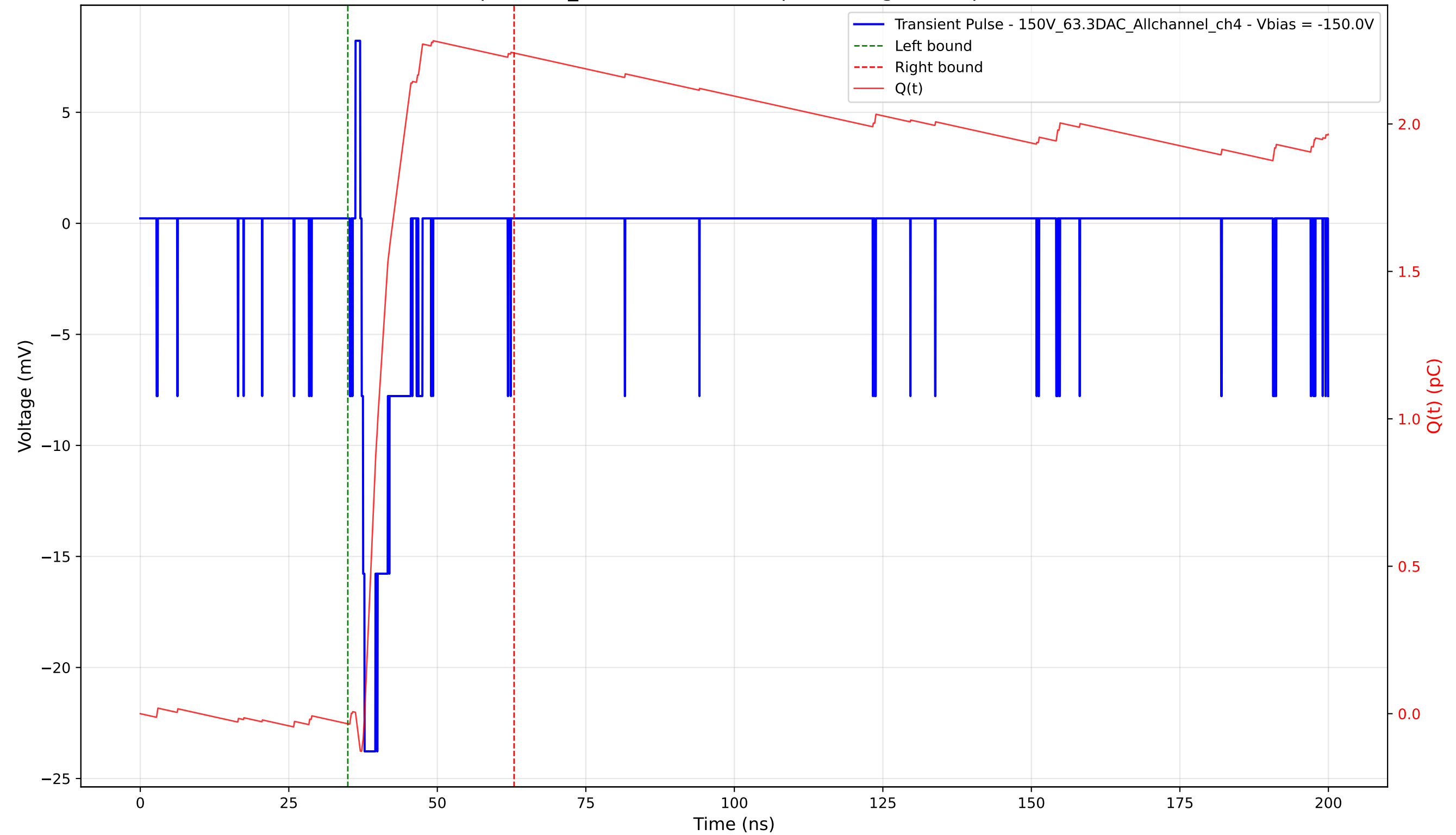
Transient Pulse - Sample: 1cm_42 - Position: 215.0 \mu\text{m} - Charge: 2.28 pC - Rise Time: 0.51 ns
