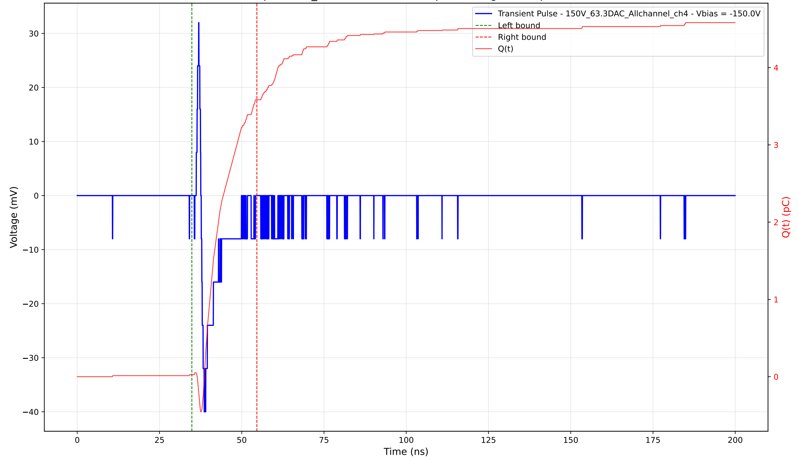
Transient Pulse - Sample: 1cm_42 - Position: 3825.0 \mu\text{m} - Charge: 3.56 pC - Rise Time: 0.90 ns
