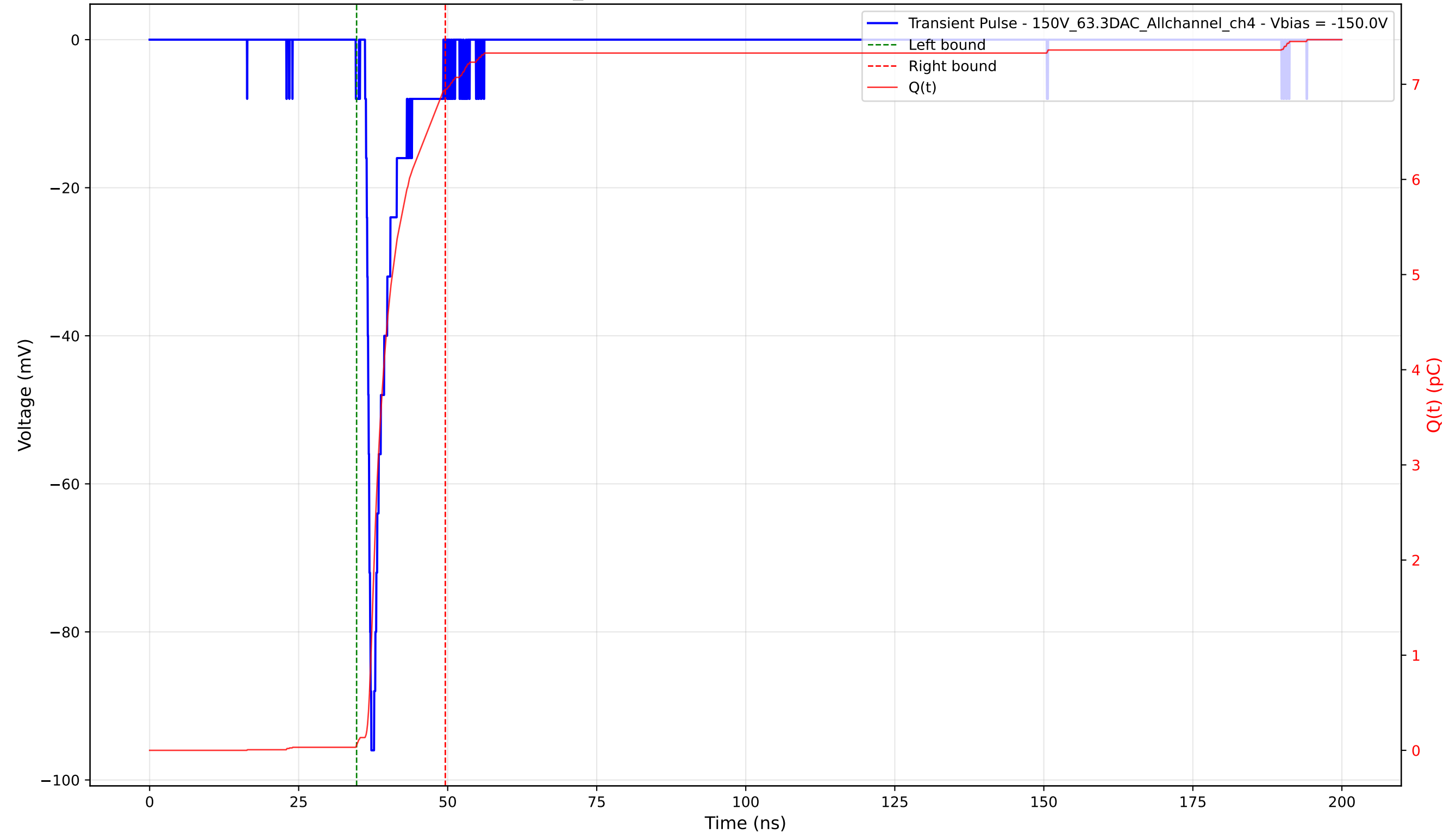
Transient Pulse - Sample: 1cm_42 - Position: 2900.0 \mu\text{m} - Charge: 6.90 pC - Rise Time: 0.79 ns
