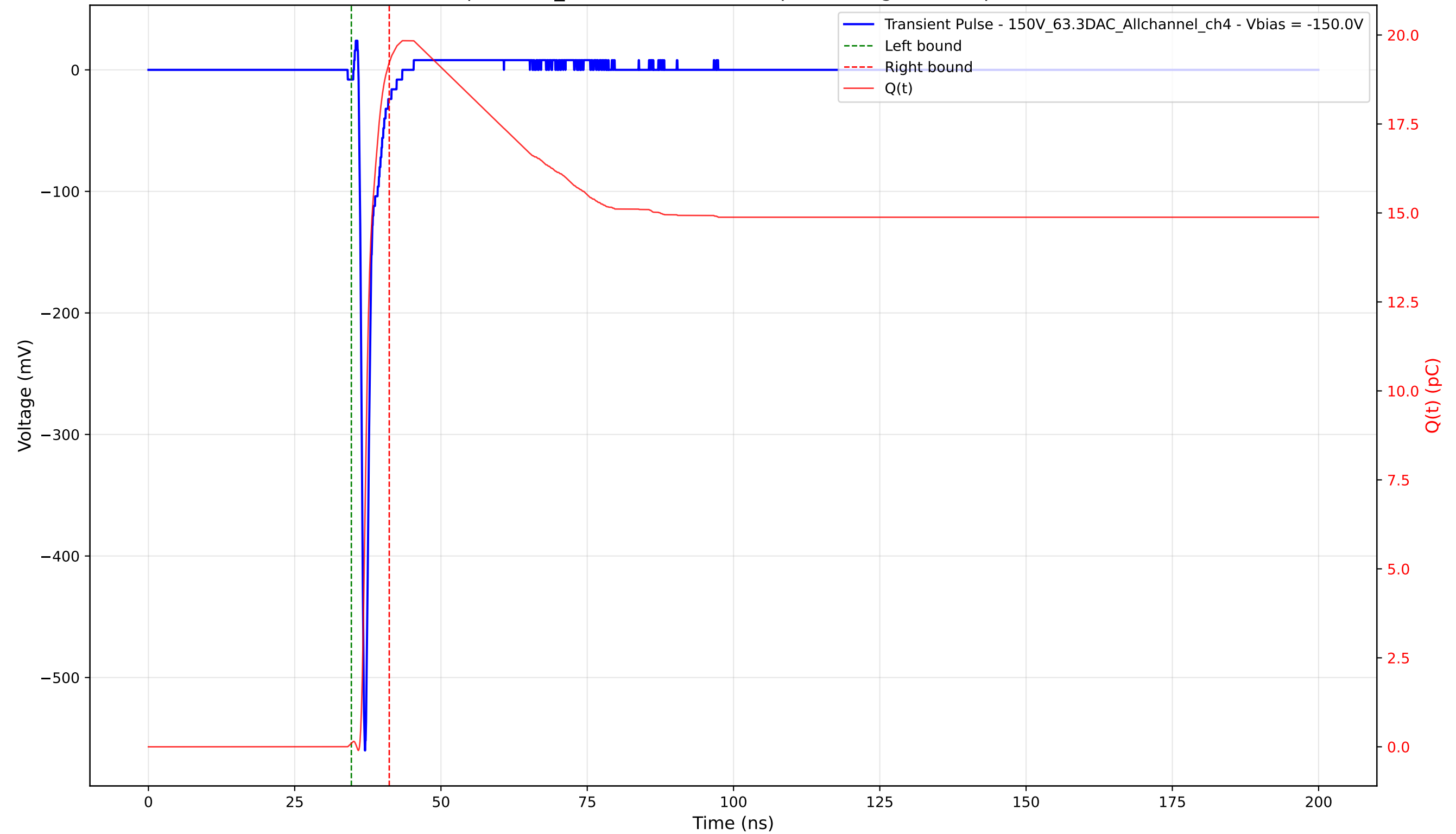
Transient Pulse - Sample: 1cm_42 - Position: 1730.0 \mu\text{m} - Charge: 19.12 pC - Rise Time: 0.72 ns
