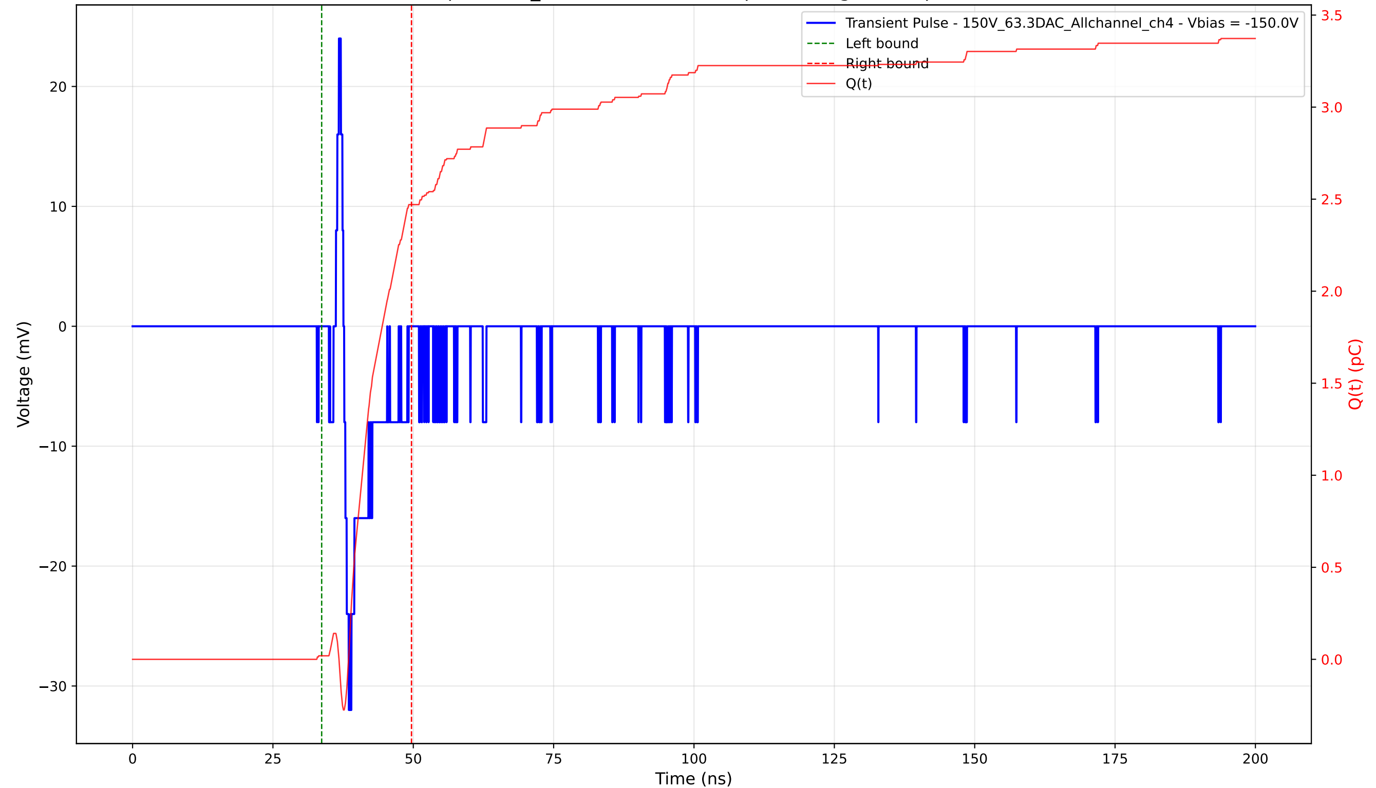
Transient Pulse - Sample: 1cm_42 - Position: 4510.0 \mu\text{m} - Charge: 2.45 pC - Rise Time: 0.82 ns
