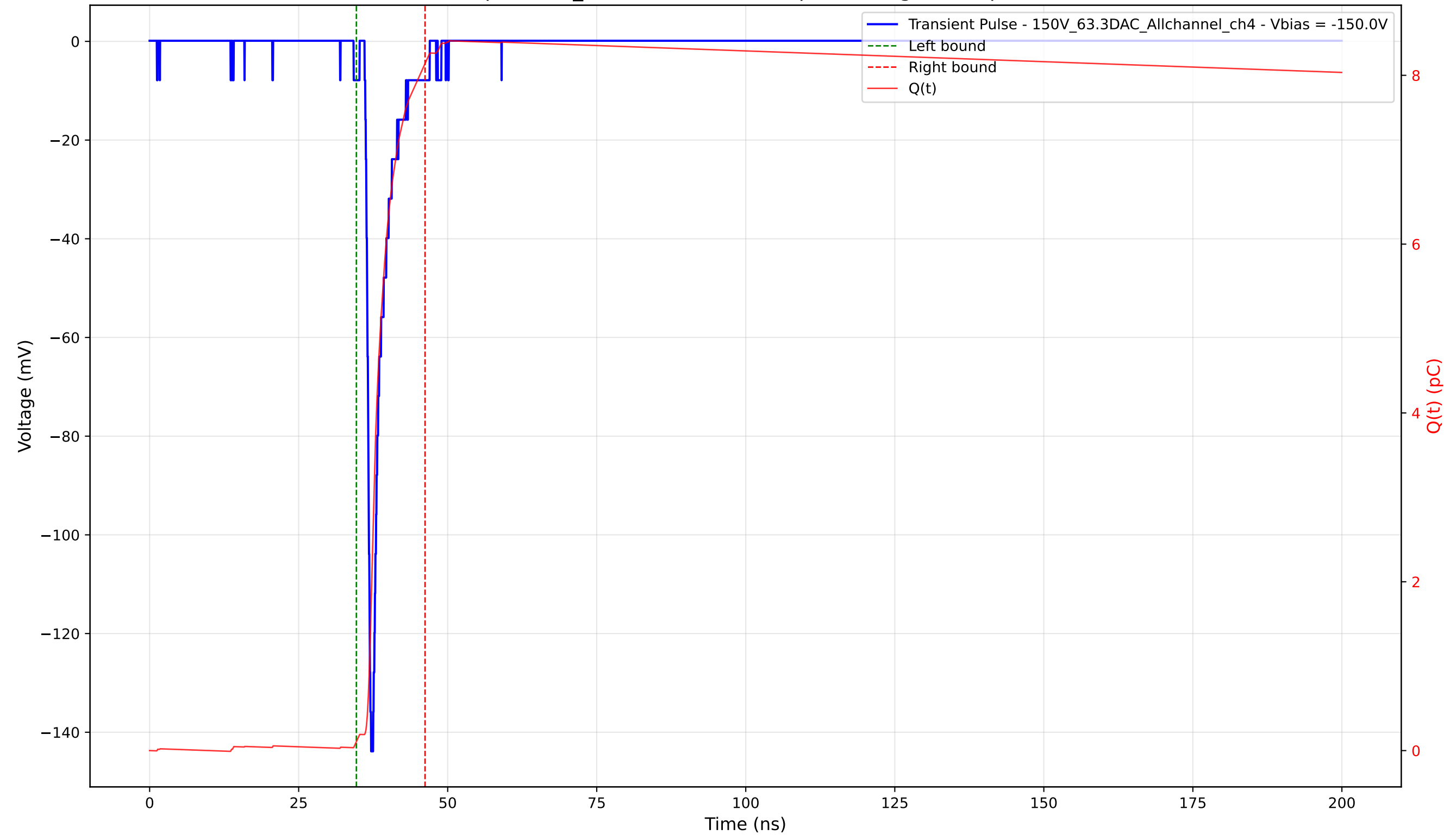
Transient Pulse - Sample: 1cm_42 - Position: 2715.0 \mu\text{m} - Charge: 8.03 pC - Rise Time: 0.85 ns
