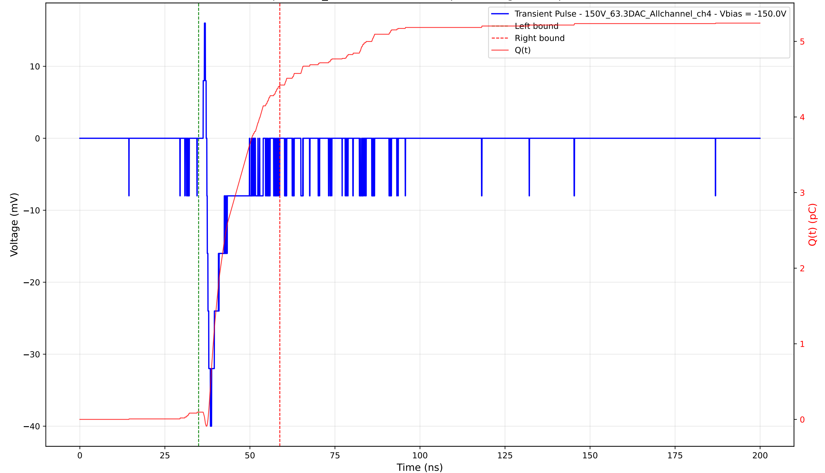
Transient Pulse - Sample: 1cm_42 - Position: 3480.0 \mu\text{m} - Charge: 4.33 pC - Rise Time: 1.06 ns
