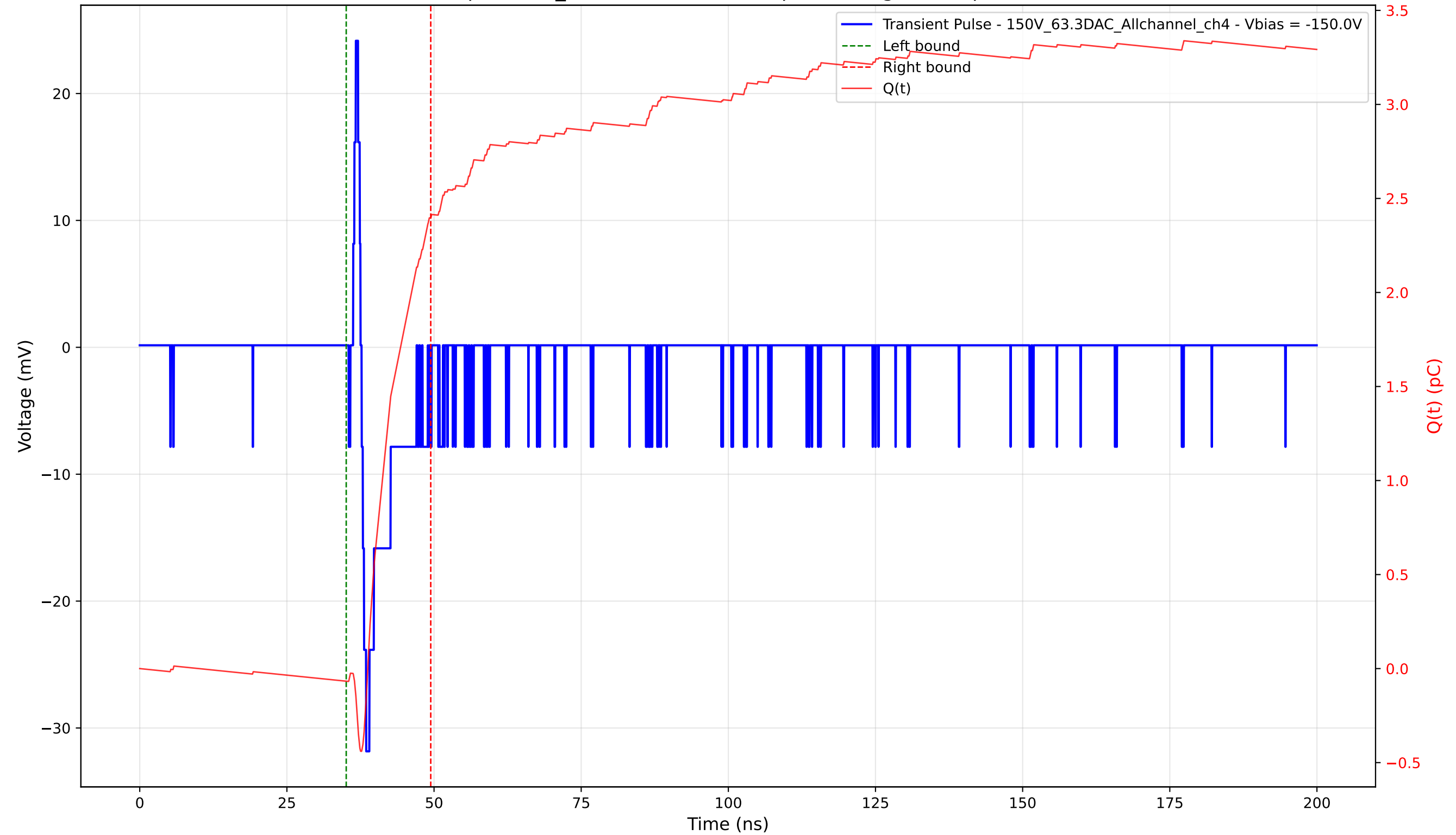
Transient Pulse - Sample: 1cm_42 - Position: 4505.0 \mu\text{m} - Charge: 2.46 pC - Rise Time: 0.78 ns
