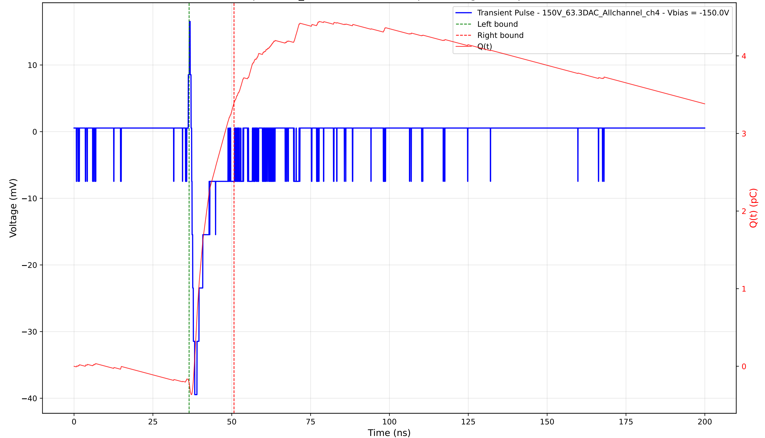
Transient Pulse - Sample: 1cm_42 - Position: 3450.0 \mu\text{m} - Charge: 3.61 pC - Rise Time: 0.98 ns
