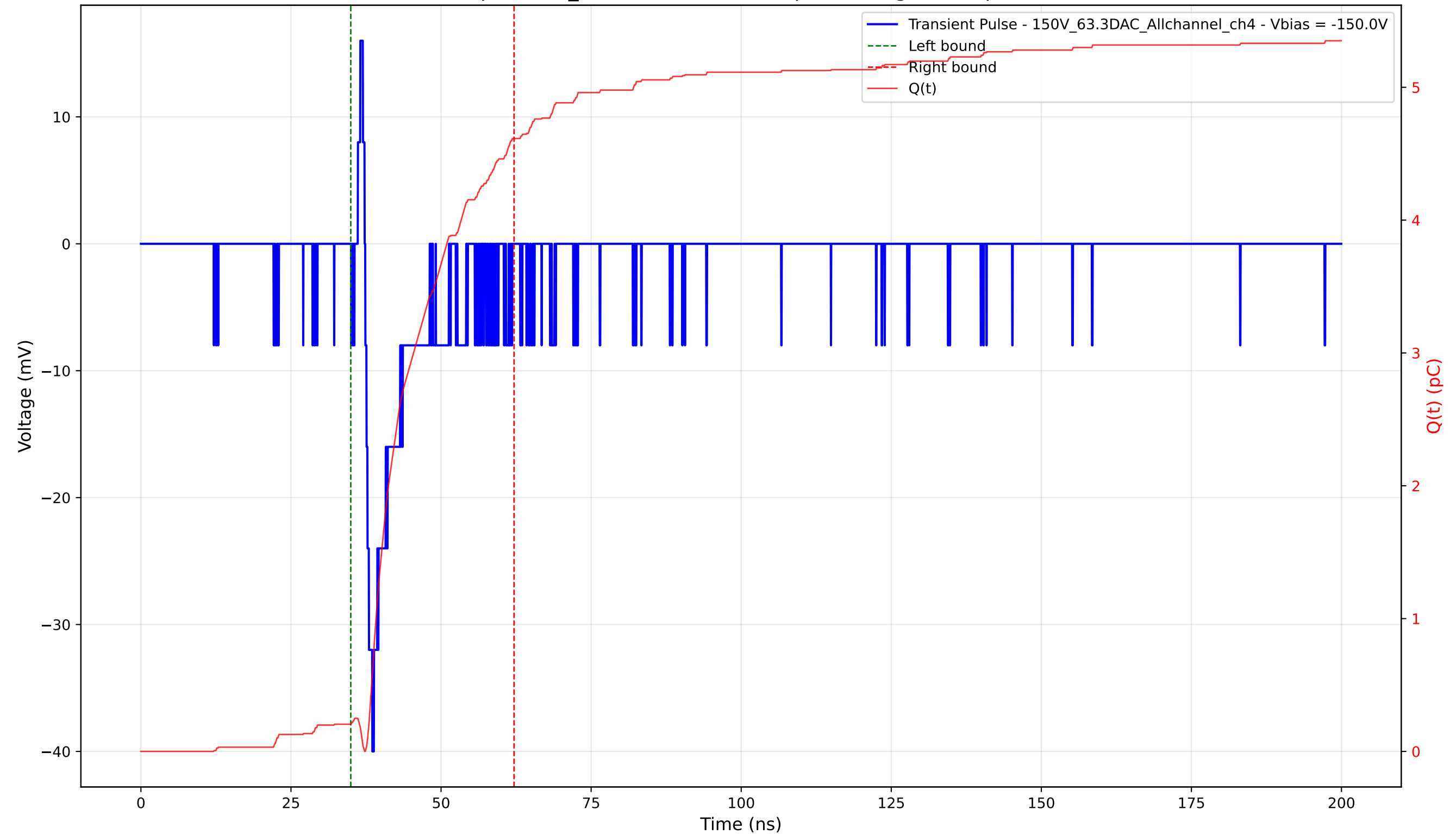
Transient Pulse - Sample: 1cm_42 - Position: 3510.0 \mu\text{m} - Charge: 4.41 pC - Rise Time: 1.18 ns
