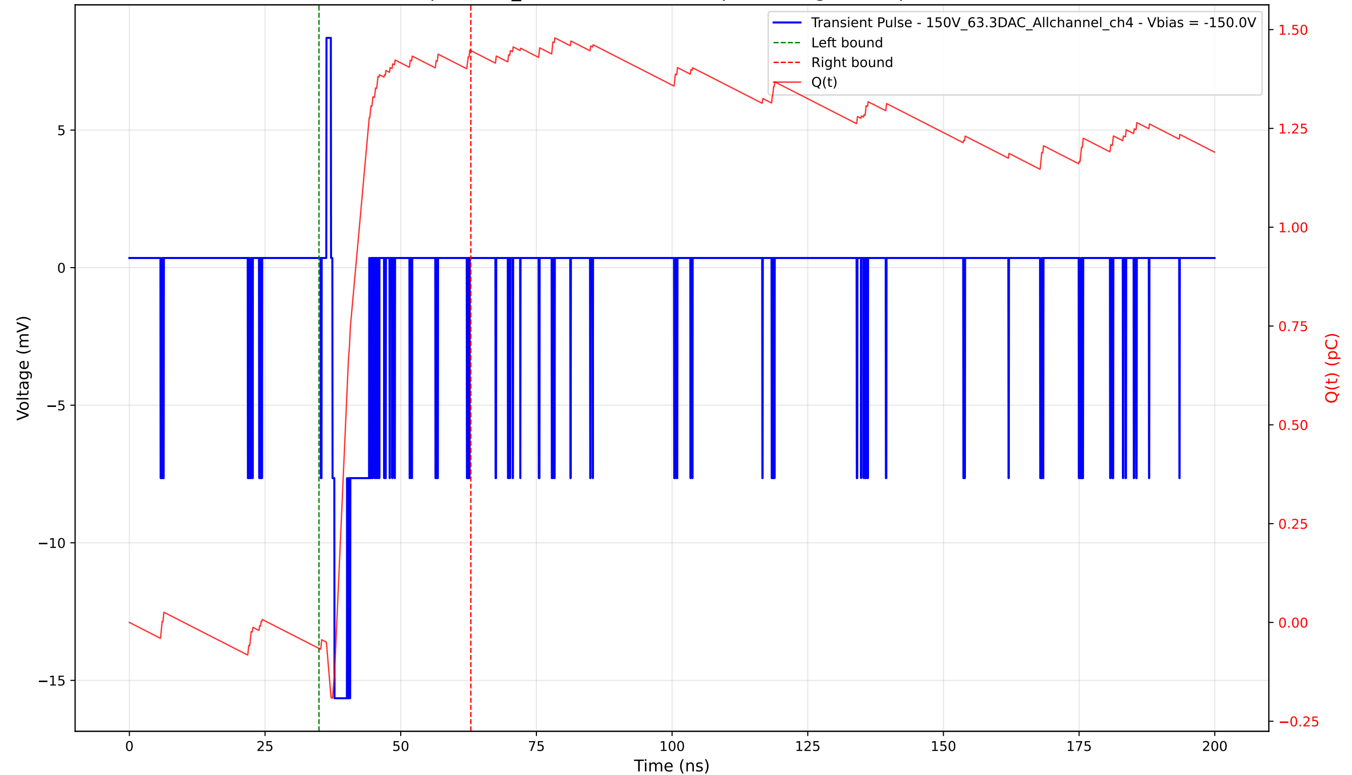
Transient Pulse - Sample: 1cm_42 - Position: 5030.0 \mu\text{m} - Charge: 1.51 pC - Rise Time: 0.39 ns
