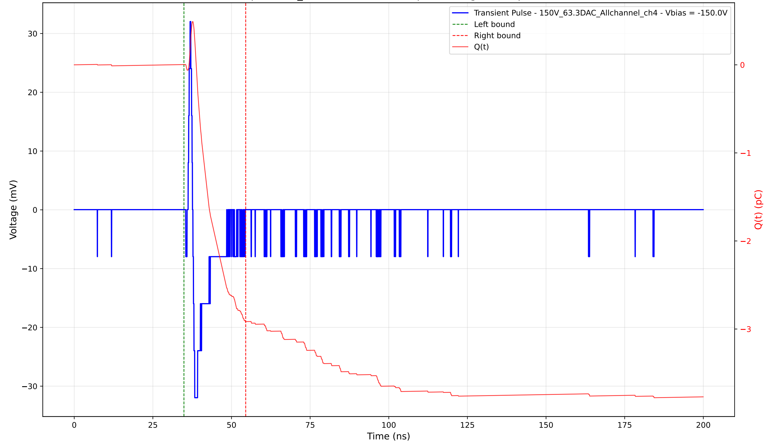
Transient Pulse - Sample: 1cm_42 - Position: 4360.0 \mu\text{m} - Charge: 2.92 pC - Rise Time: 0.62 ns
