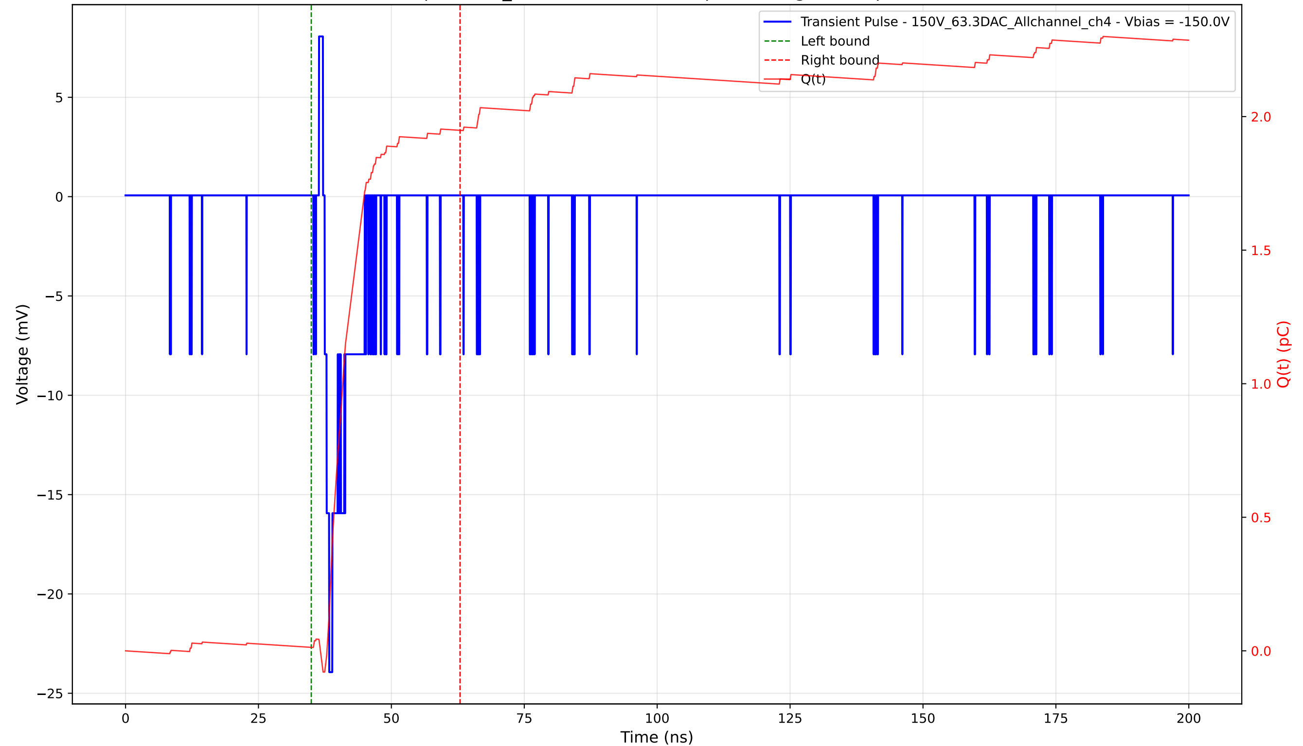
Transient Pulse - Sample: 1cm_42 - Position: 5010.0 \mu\text{m} - Charge: 1.94 pC - Rise Time: 0.87 ns
