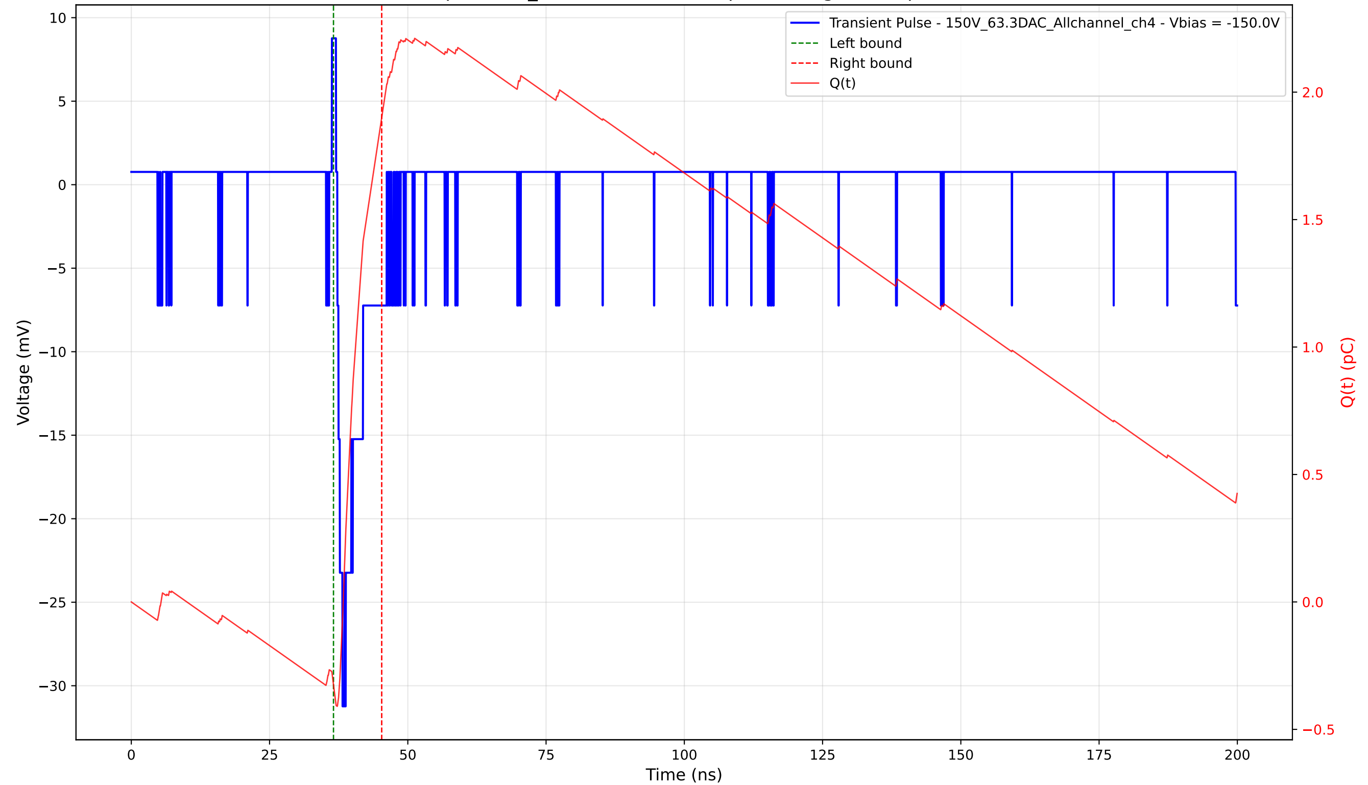
Transient Pulse - Sample: 1cm_42 - Position: 235.0 \mu\text{m} - Charge: 2.23 pC - Rise Time: 0.95 ns
