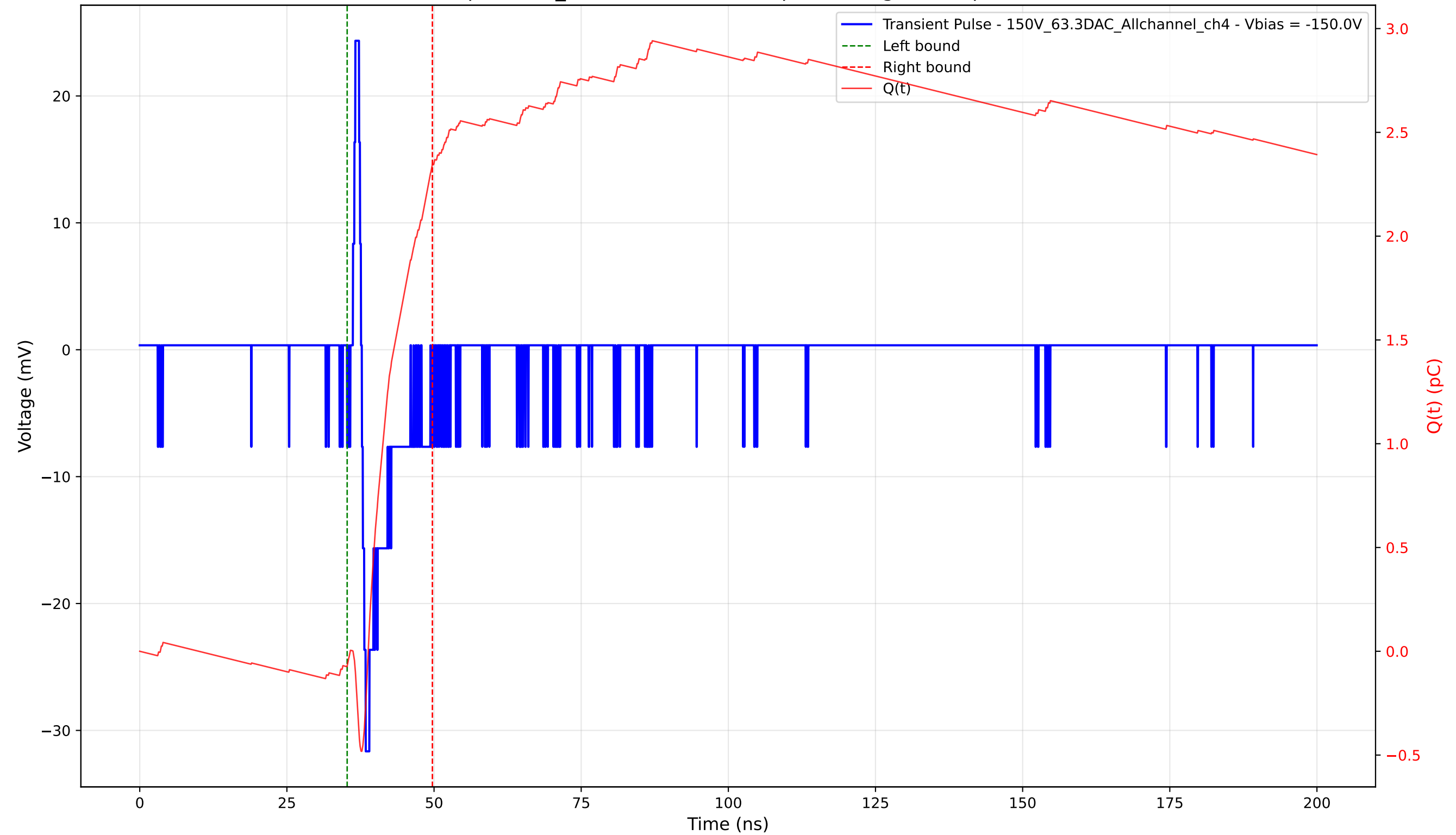
Transient Pulse - Sample: 1cm_42 - Position: 4430.0 \mu\text{m} - Charge: 2.42 pC - Rise Time: 0.66 ns
