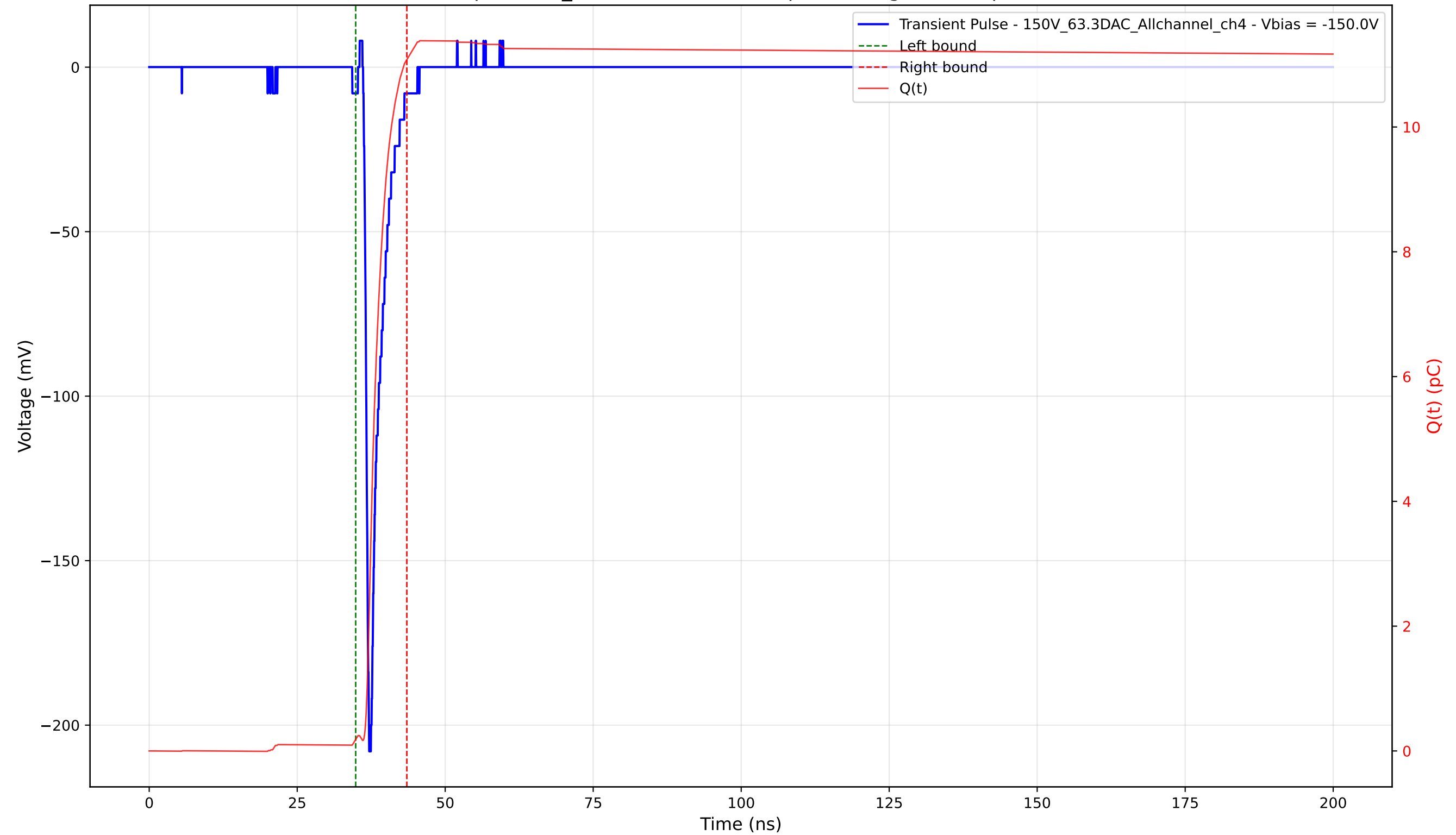
Transient Pulse - Sample: 1cm_42 - Position: 1415.0 \mu\text{m} - Charge: 10.89 pC - Rise Time: 0.79 ns
