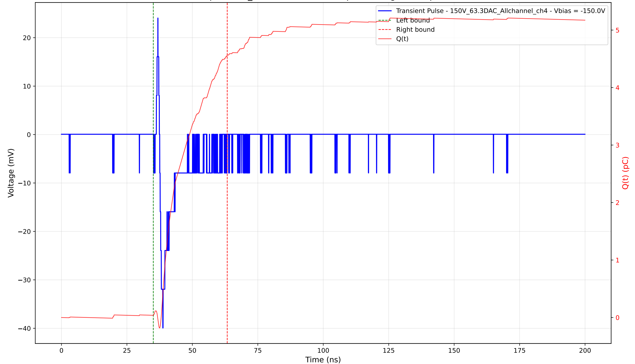
Transient Pulse - Sample: 1cm_42 - Position: 3605.0 \mu\text{m} - Charge: 4.53 pC - Rise Time: 1.18 ns
