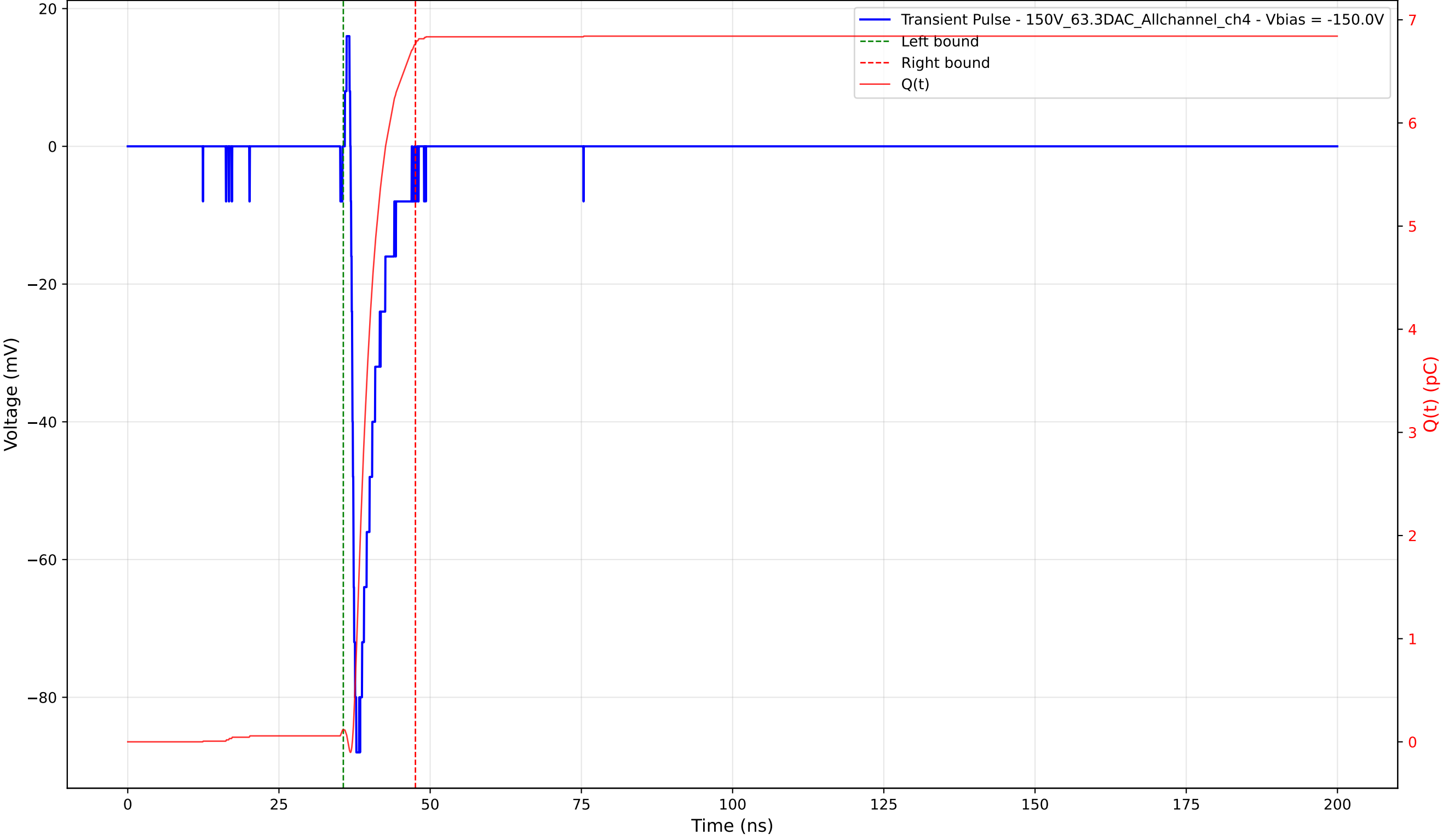
Transient Pulse - Sample: 1cm_42 - Position: 915.0 \mu\text{m} - Charge: 6.65 pC - Rise Time: 0.68 ns
