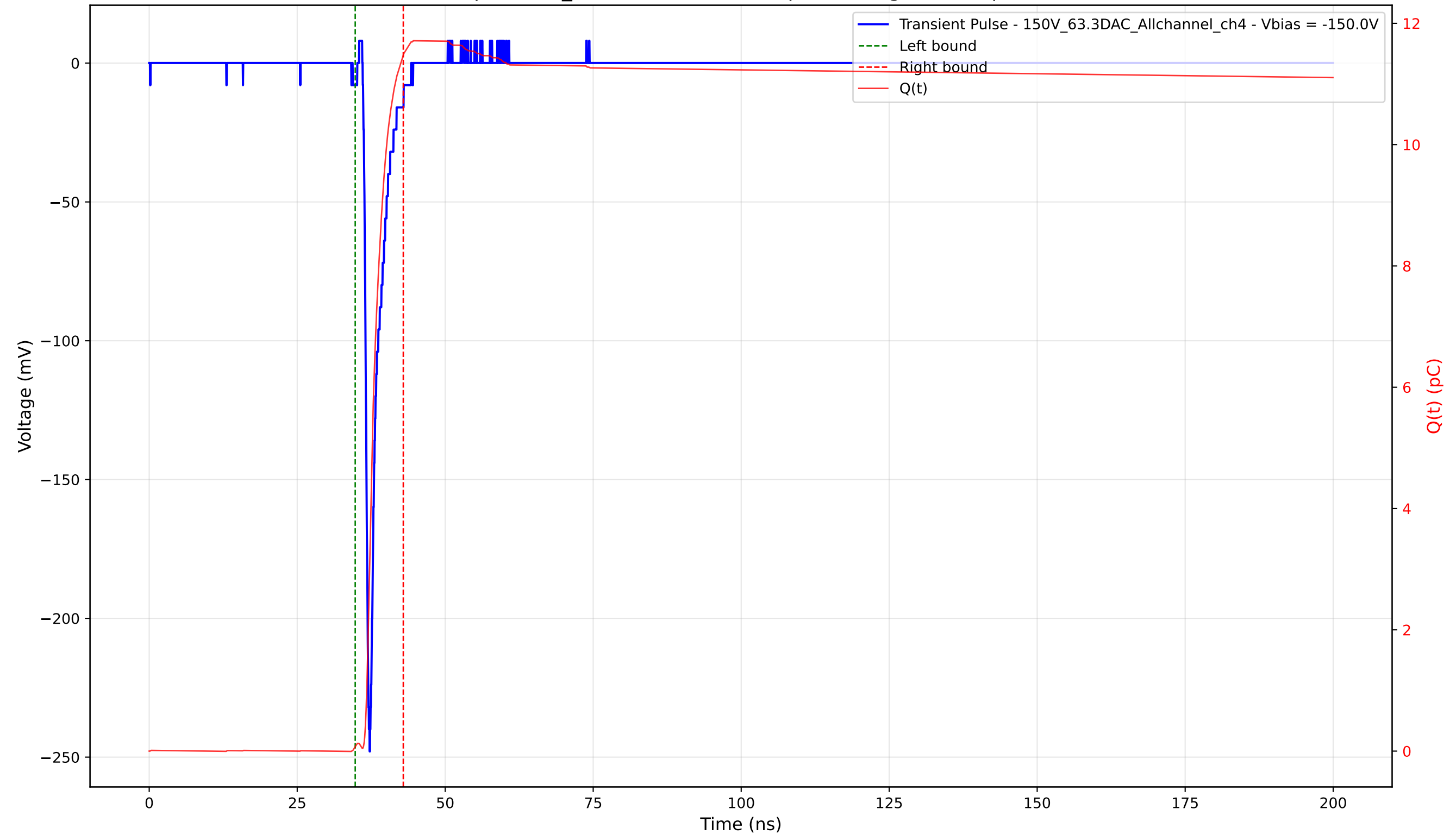
Transient Pulse - Sample: 1cm_42 - Position: 1480.0 \mu\text{m} - Charge: 11.40 pC - Rise Time: 0.75 ns
