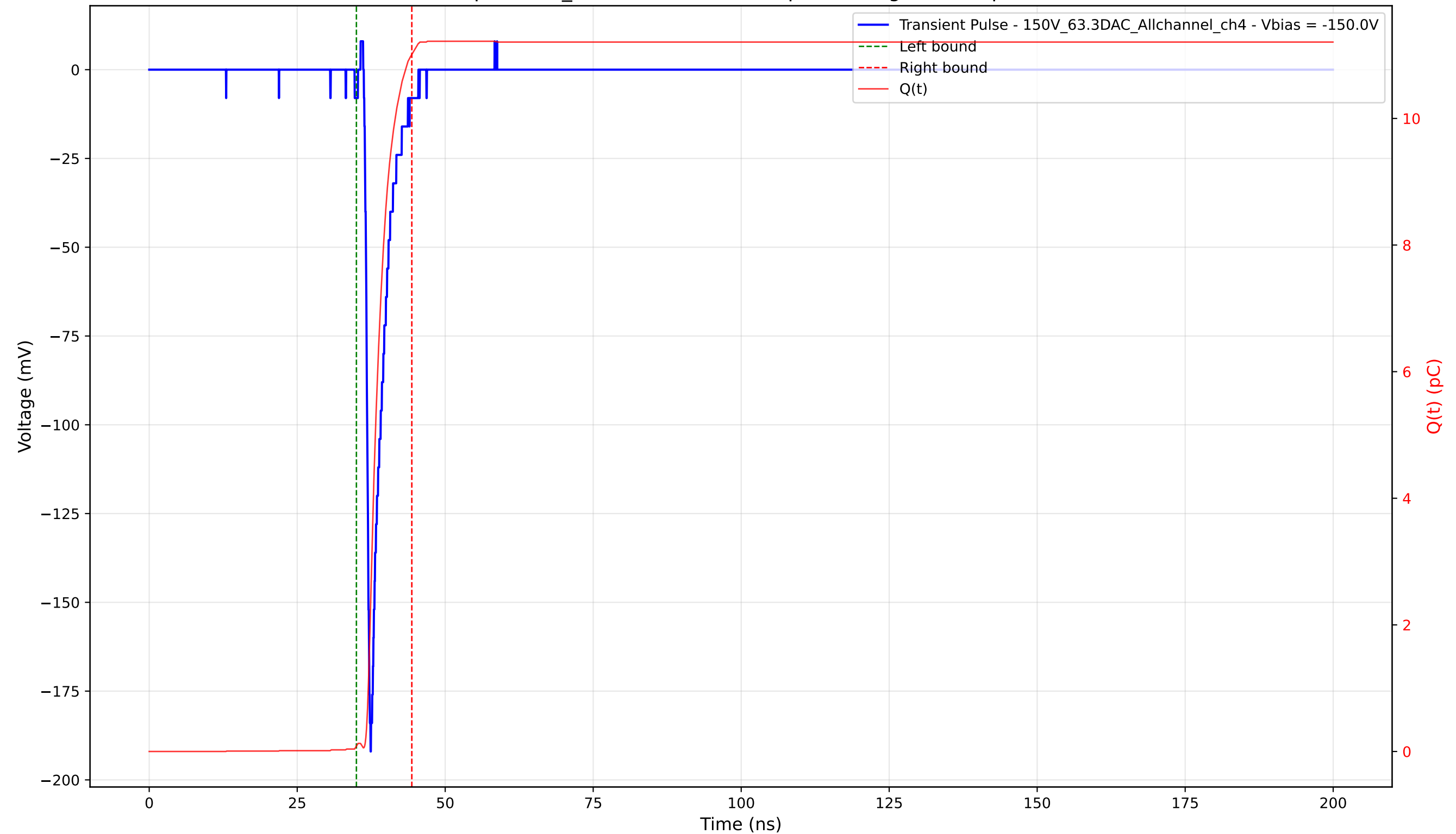
Transient Pulse - Sample: 1cm_42 - Position: 1290.0 \mu\text{m} - Charge: 10.92 pC - Rise Time: 0.78 ns
