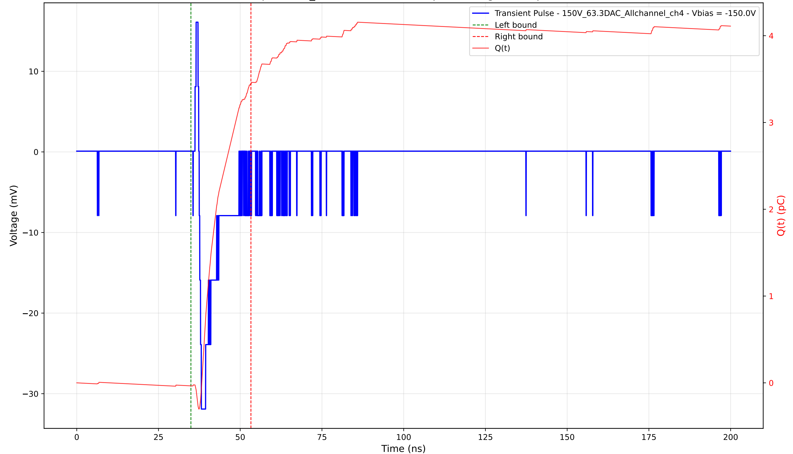
Transient Pulse - Sample: 1cm_42 - Position: 3560.0 \mu\text{m} - Charge: 3.48 pC - Rise Time: 0.66 ns
