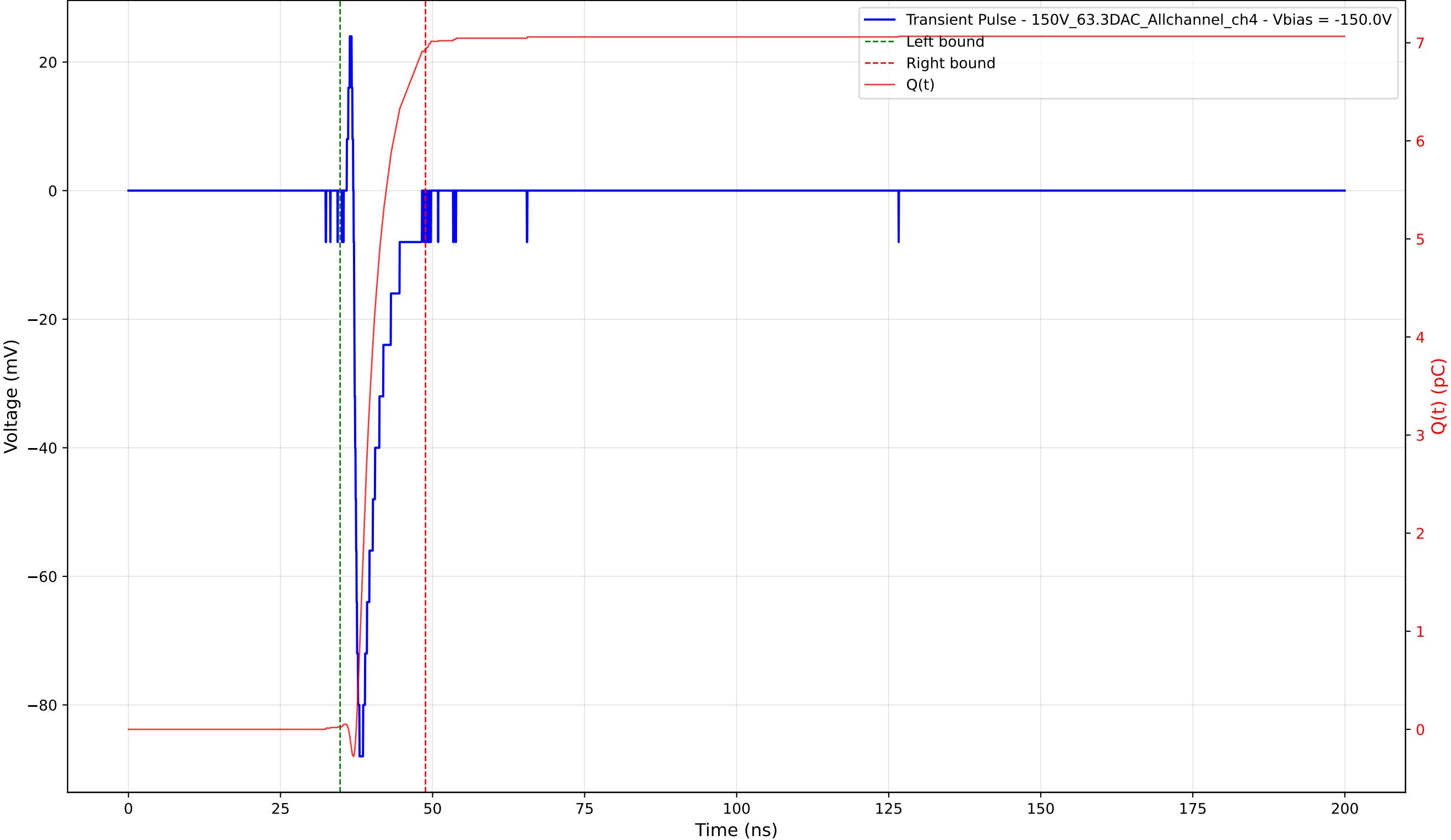
Transient Pulse - Sample: 1cm_42 - Position: 775.0 \mu\text{m} - Charge: 6.90 pC - Rise Time: 0.68 ns
