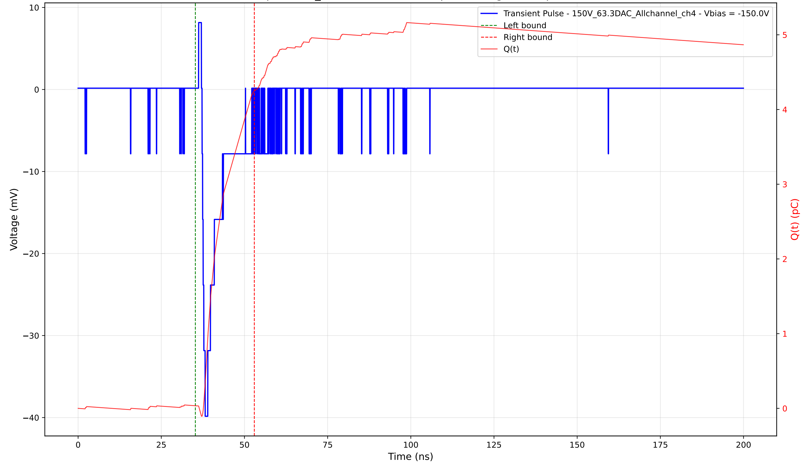
Transient Pulse - Sample: 1cm_42 - Position: 3440.0 \mu\text{m} - Charge: 4.22 pC - Rise Time: 0.94 ns
