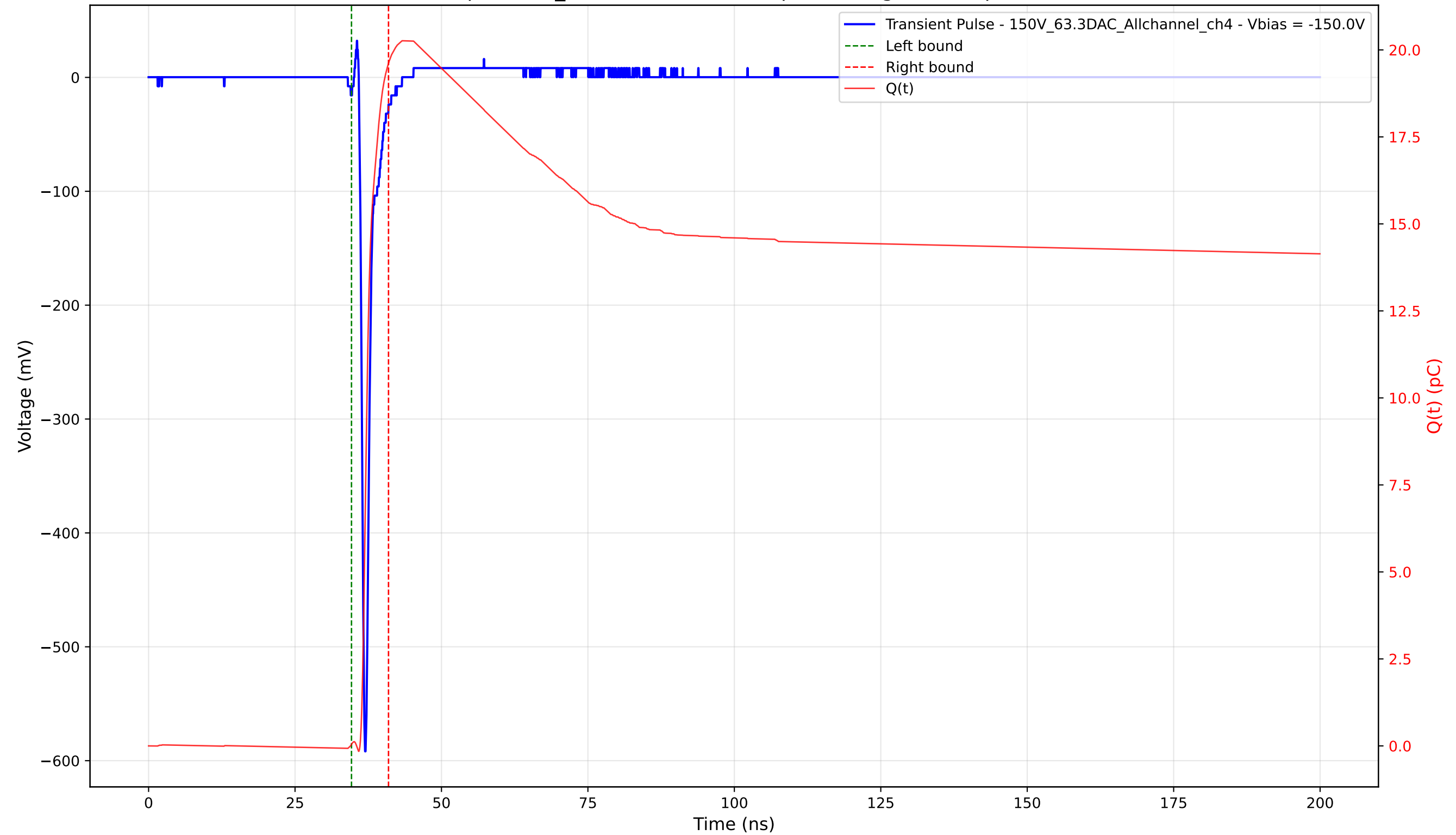
Transient Pulse - Sample: 1cm_42 - Position: 1805.0 \mu\text{m} - Charge: 19.58 pC - Rise Time: 0.71 ns
