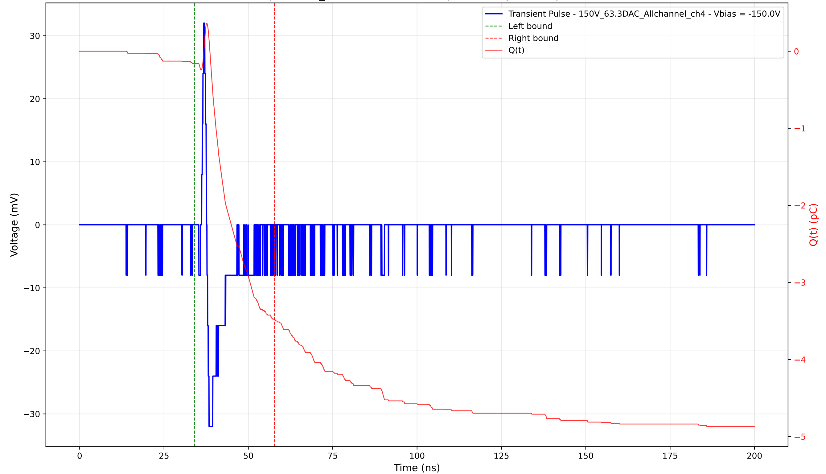
Transient Pulse - Sample: 1cm_42 - Position: 4310.0 \mu\text{m} - Charge: 3.33 pC - Rise Time: 0.58 ns
