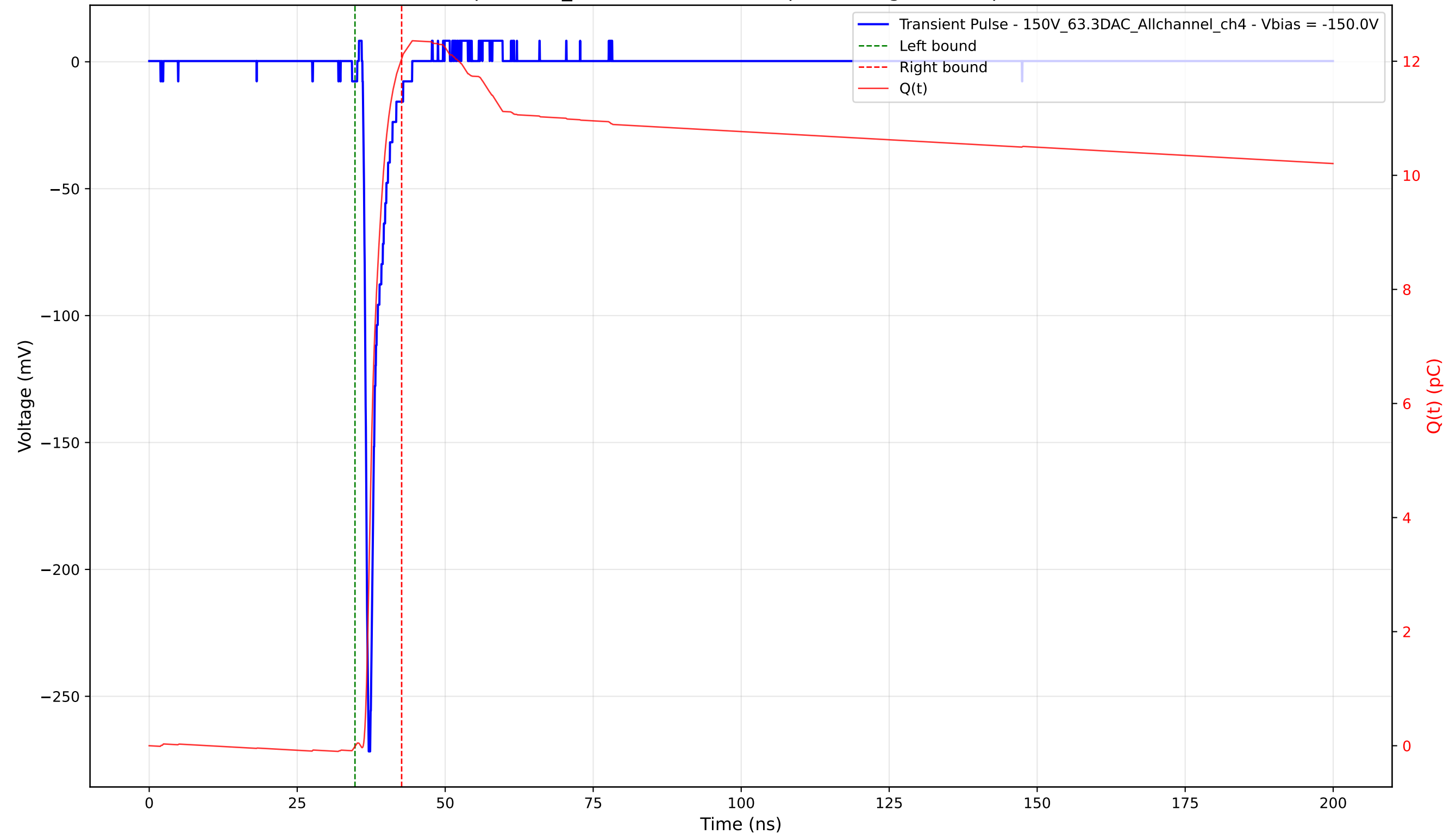
Transient Pulse - Sample: 1cm_42 - Position: 1515.0 \mu\text{m} - Charge: 12.05 pC - Rise Time: 0.77 ns
