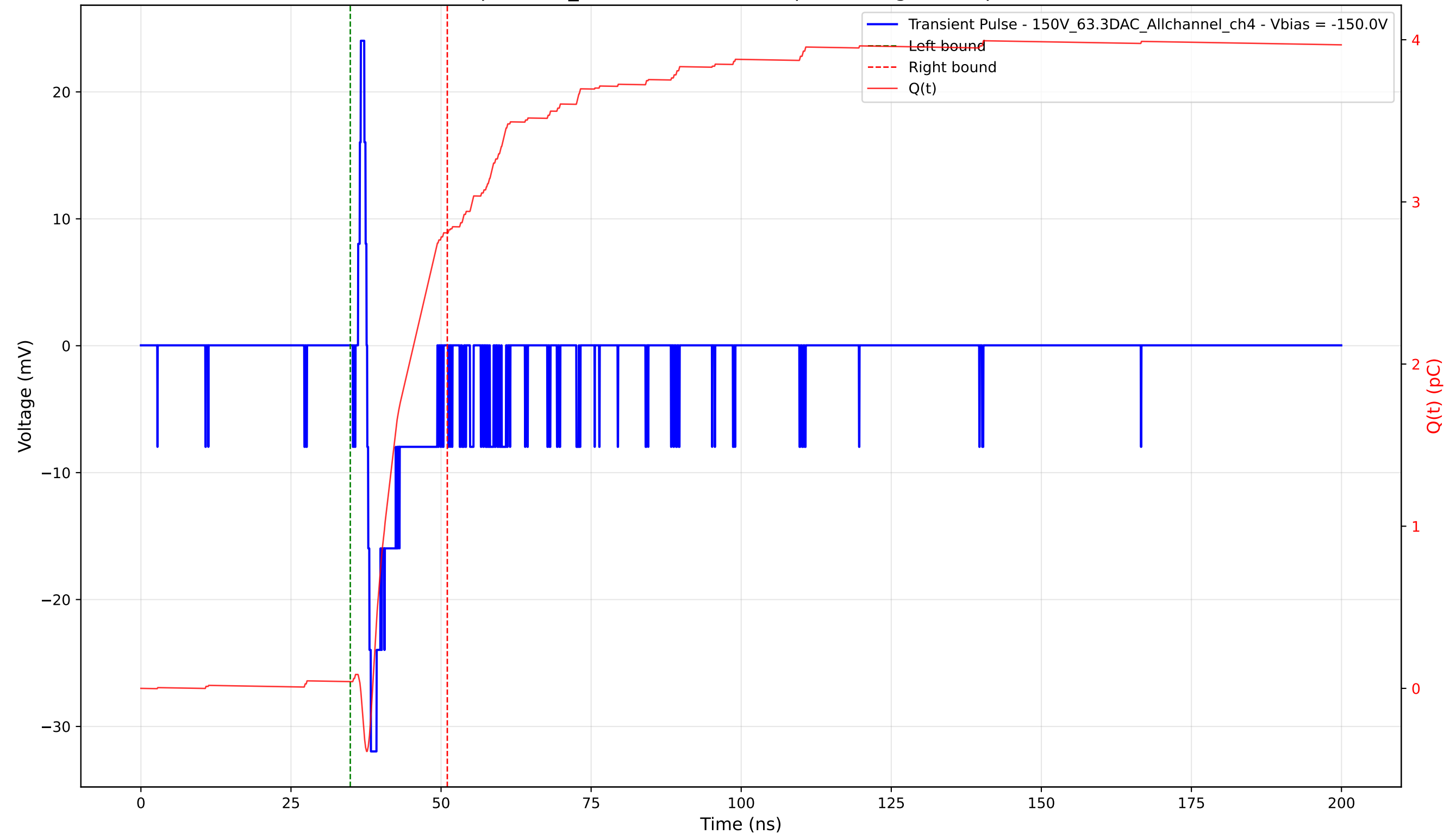
Transient Pulse - Sample: 1cm_42 - Position: 3920.0 \mu\text{m} - Charge: 2.77 pC - Rise Time: 0.62 ns
