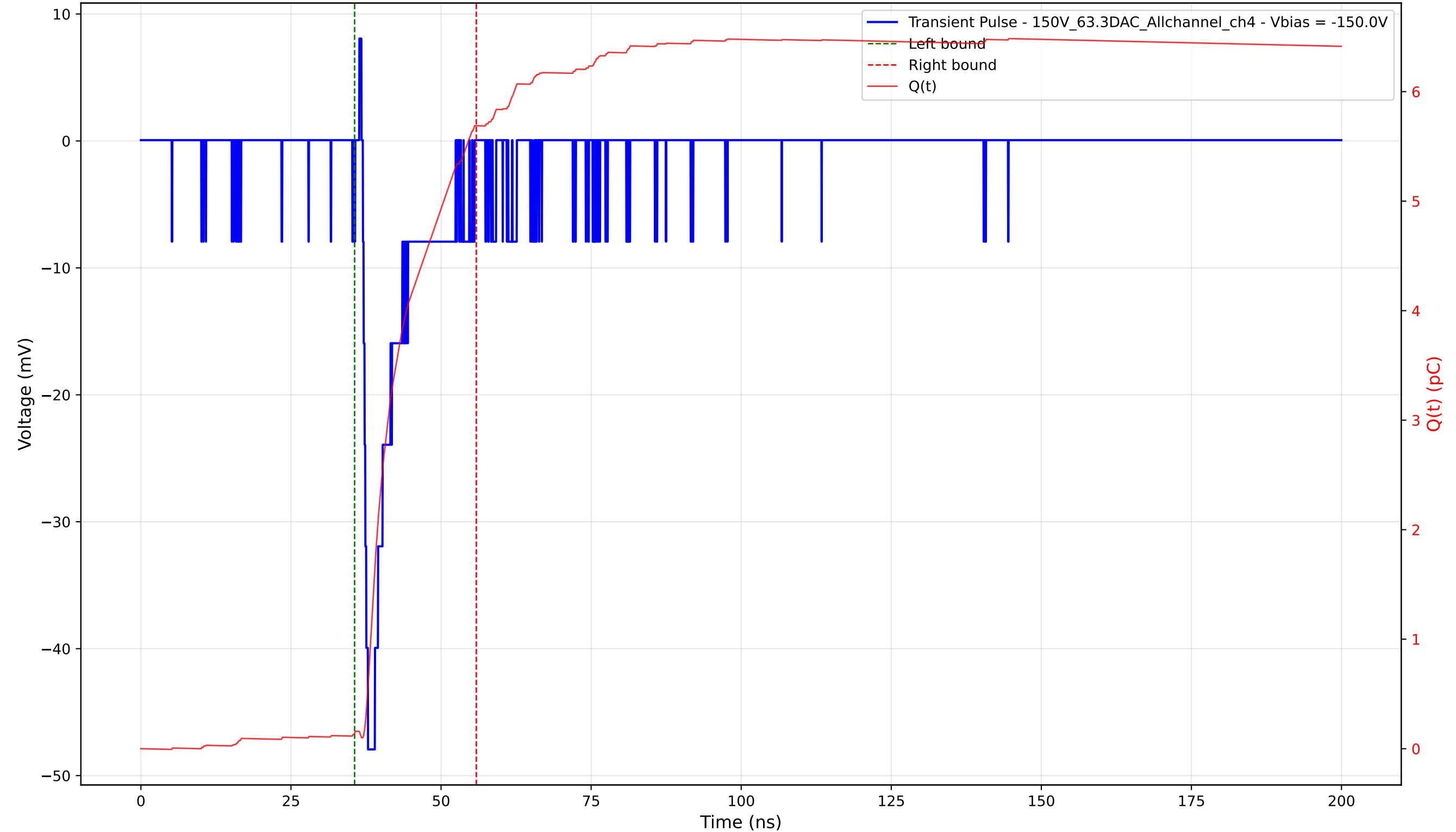
Transient Pulse - Sample: 1cm_42 - Position: 3240.0 \mu\text{m} - Charge: 5.55 pC - Rise Time: 0.86 ns
