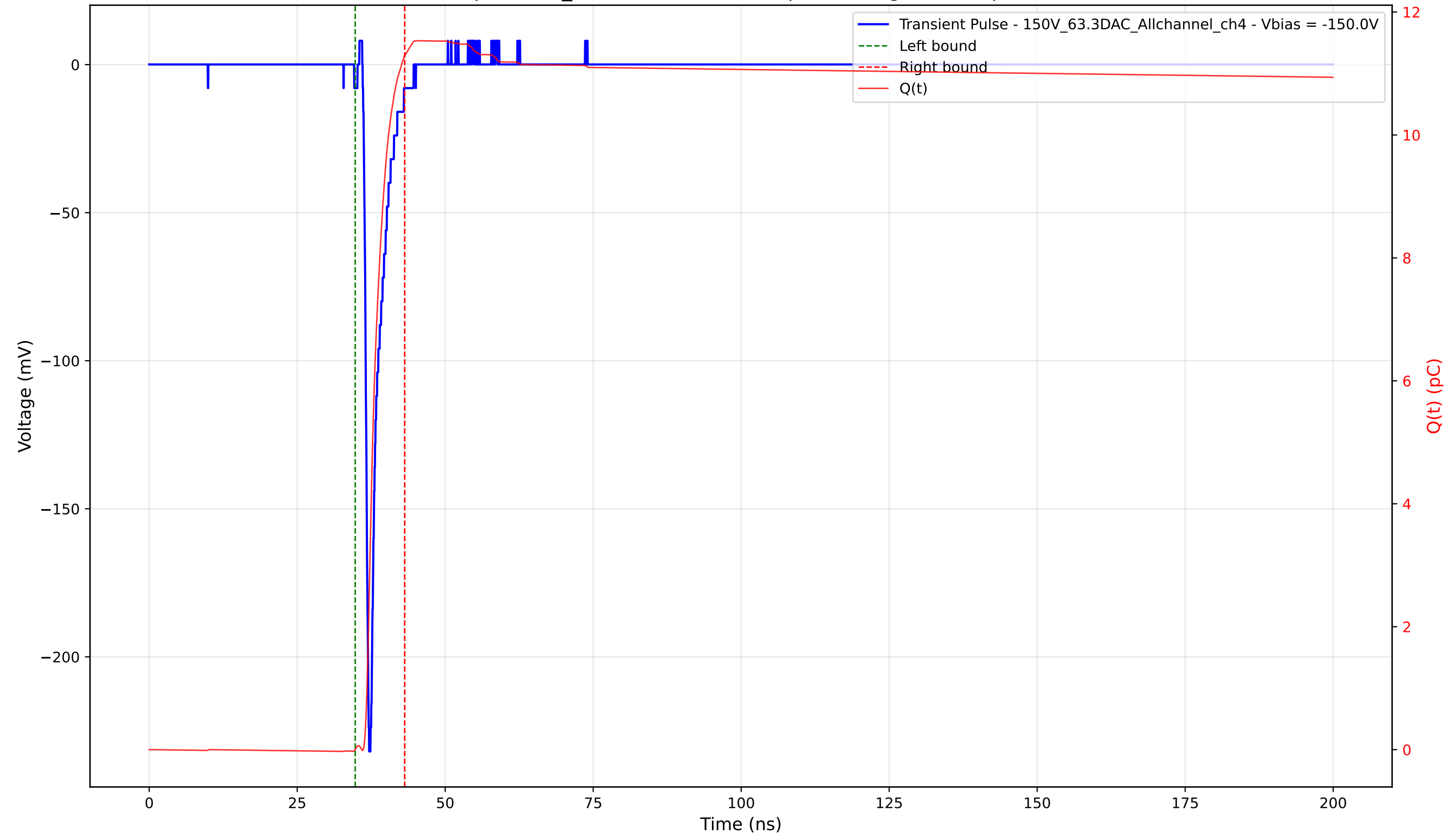
Transient Pulse - Sample: 1cm_42 - Position: 1460.0 \mu\text{m} - Charge: 11.29 pC - Rise Time: 0.77 ns
