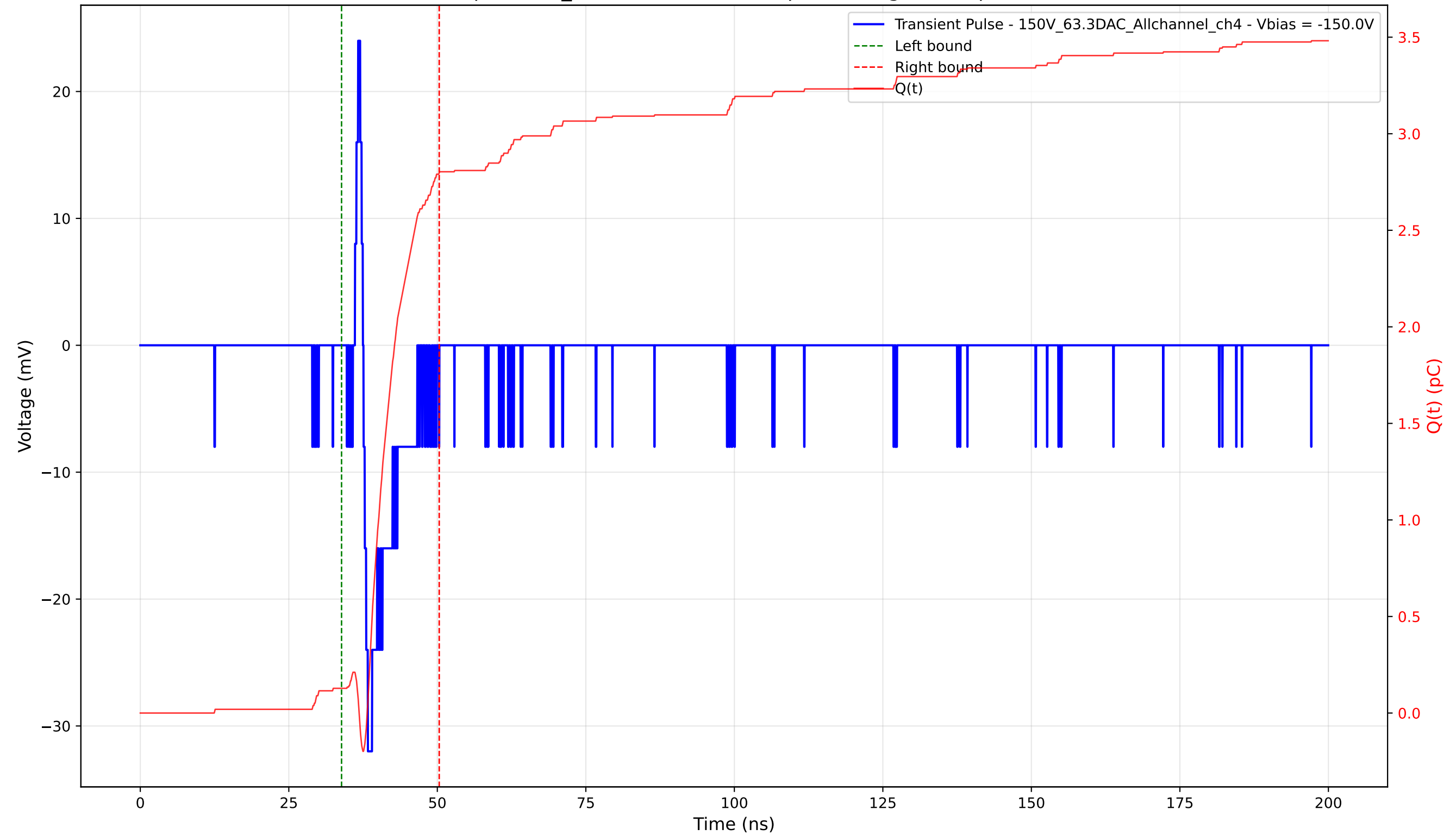
Transient Pulse - Sample: 1cm_42 - Position: 4640.0 \mu\text{m} - Charge: 2.67 pC - Rise Time: 0.74 ns
