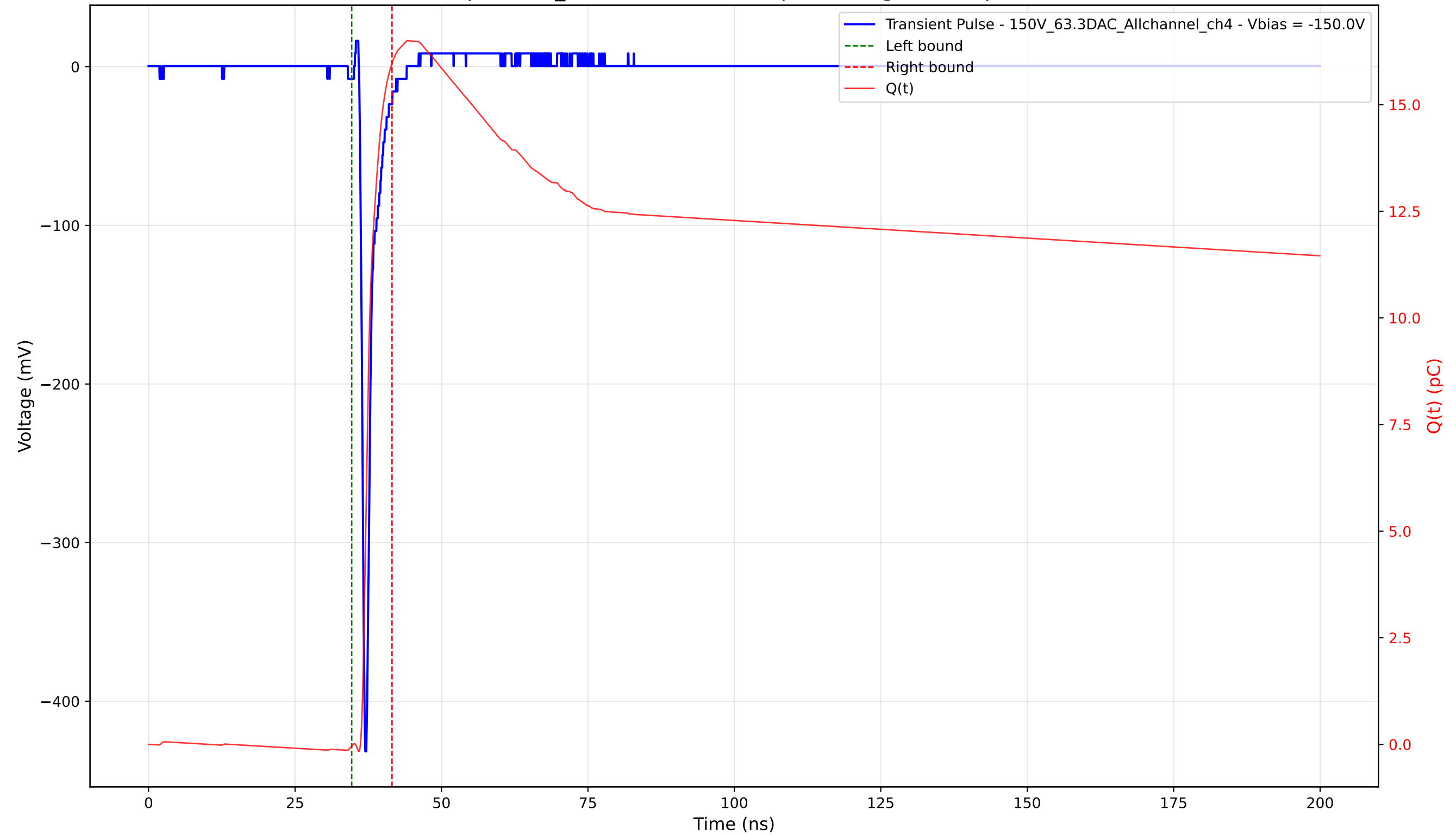
Transient Pulse - Sample: 1cm_42 - Position: 1645.0 \mu\text{m} - Charge: 16.02 pC - Rise Time: 0.70 ns
