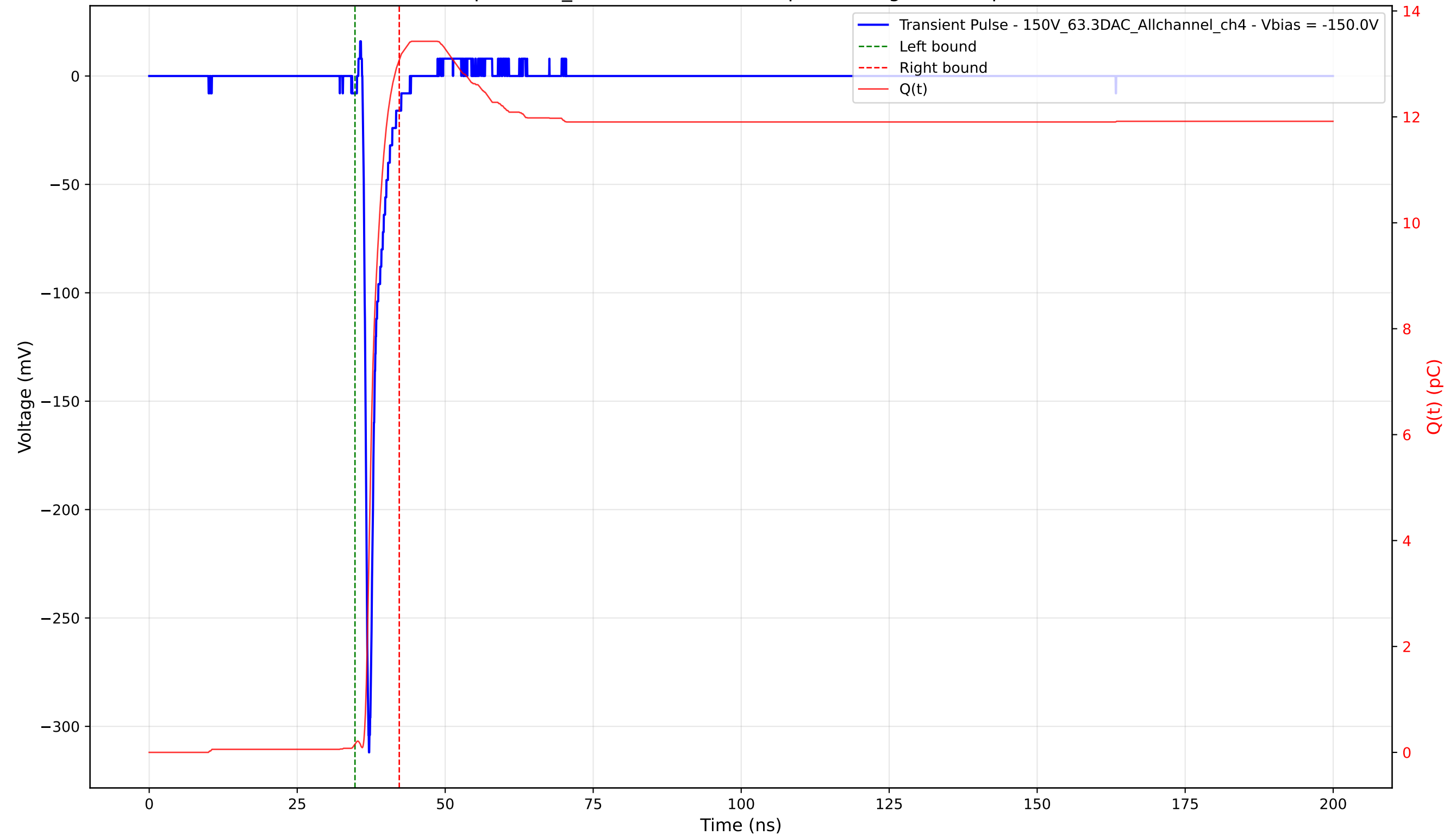
Transient Pulse - Sample: 1cm_42 - Position: 1550.0 \mu\text{m} - Charge: 12.92 pC - Rise Time: 0.77 ns
