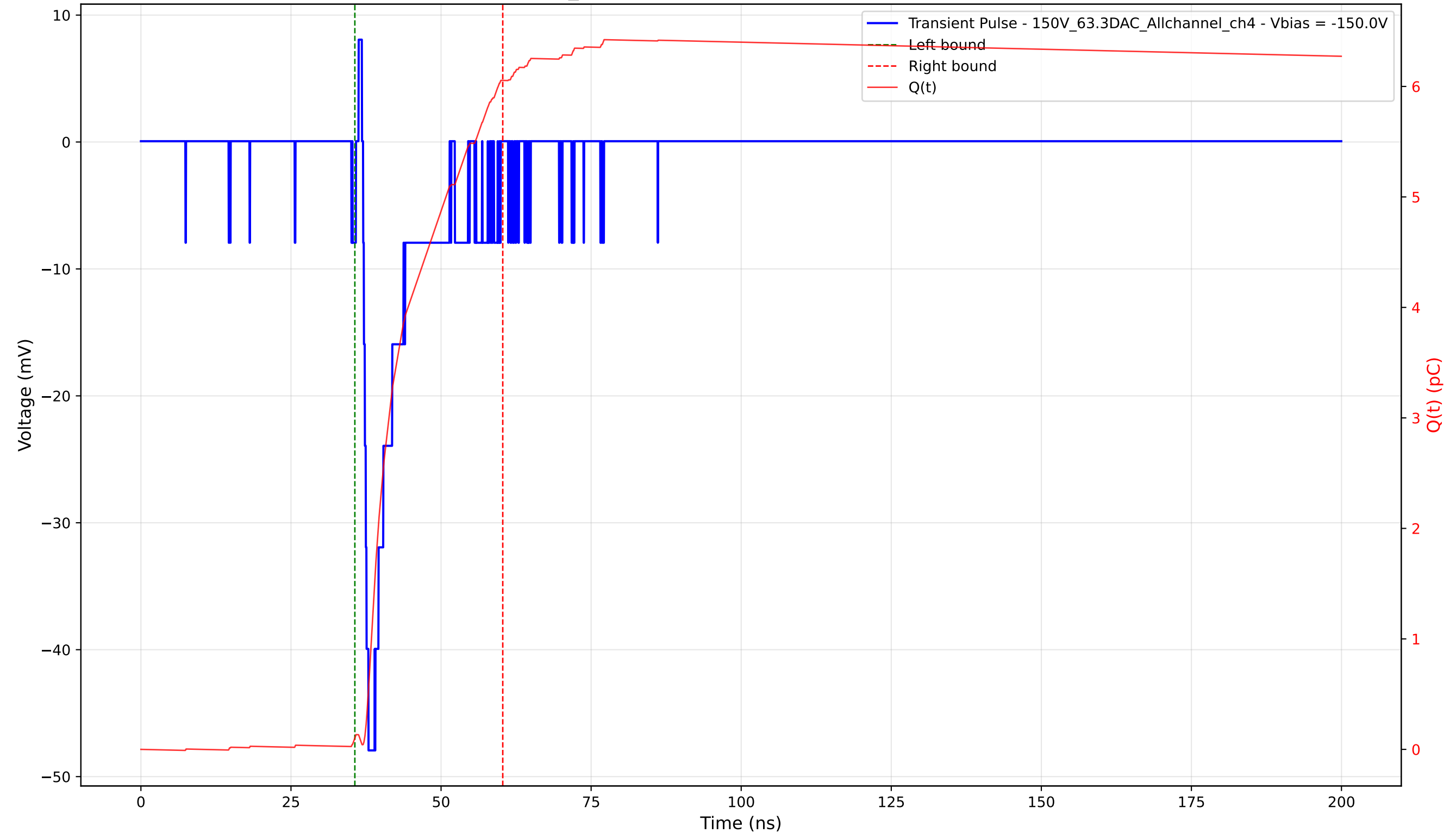
Transient Pulse - Sample: 1cm_42 - Position: 3285.0 \mu\text{m} - Charge: 5.95 pC - Rise Time: 0.90 ns
