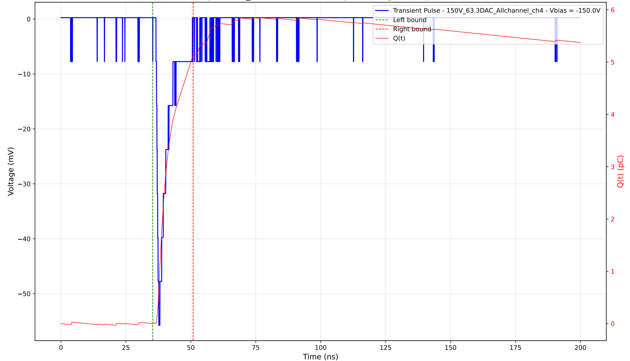
Transient Pulse - Sample: 1cm_42 - Position: 3105.0 \mu\text{m} - Charge: 5.13 pC - Rise Time: 1.09 ns
