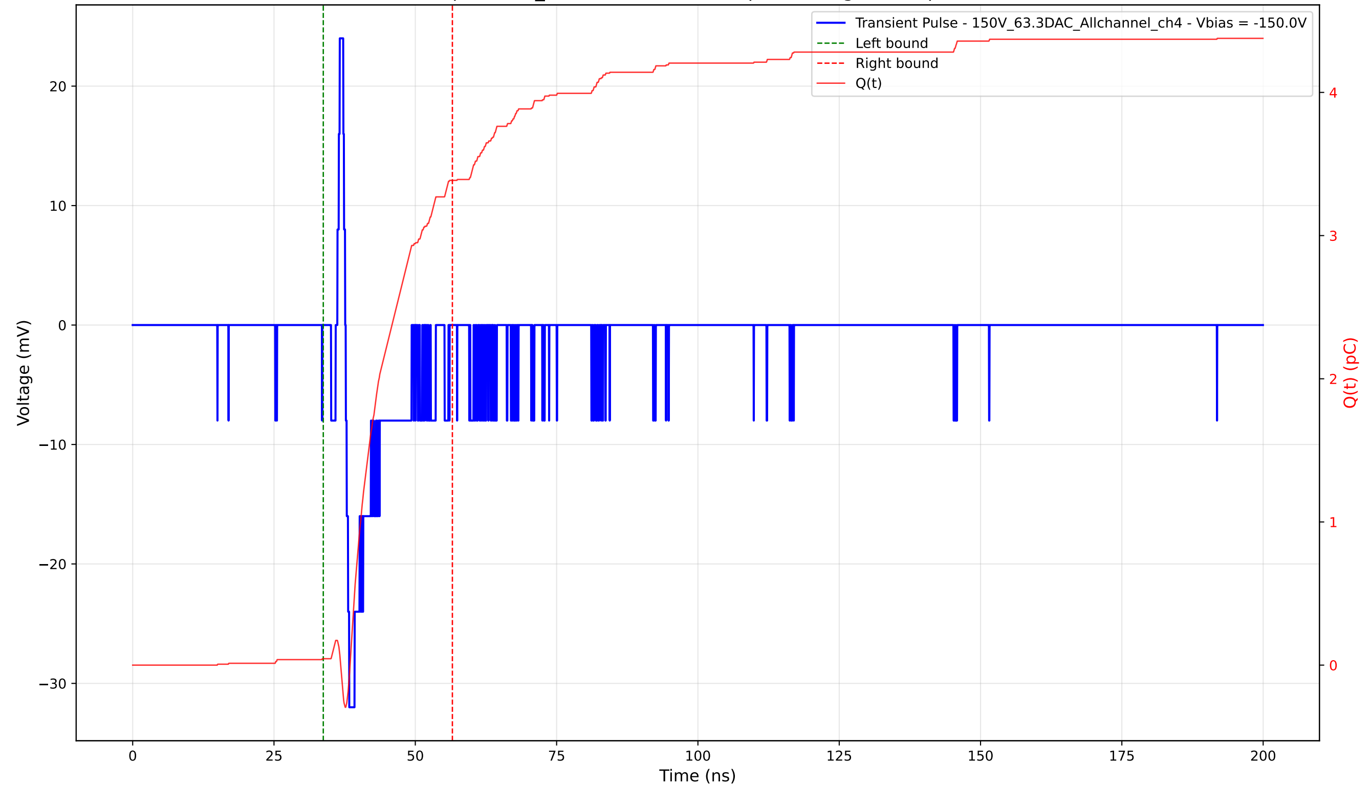
Transient Pulse - Sample: 1cm_42 - Position: 3905.0 \mu\text{m} - Charge: 3.34 pC - Rise Time: 0.62 ns
