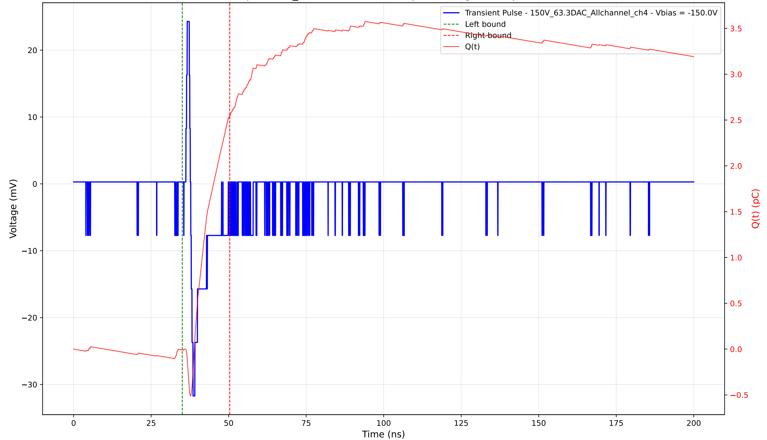
Transient Pulse - Sample: 1cm_42 - Position: 4130.0 \mu\text{m} - Charge: 2.56 pC - Rise Time: 0.74 ns
