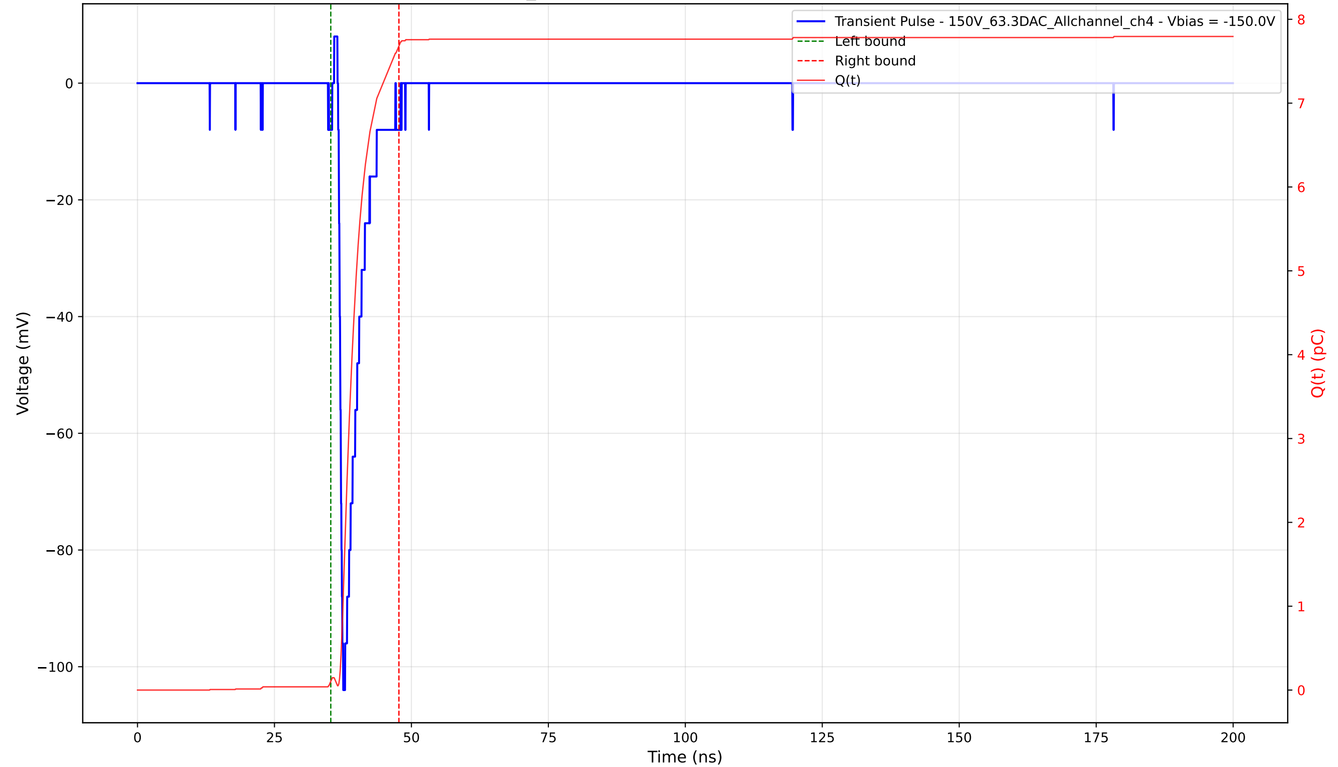
Transient Pulse - Sample: 1cm_42 - Position: 1030.0 \mu\text{m} - Charge: 7.58 pC - Rise Time: 0.67 ns
