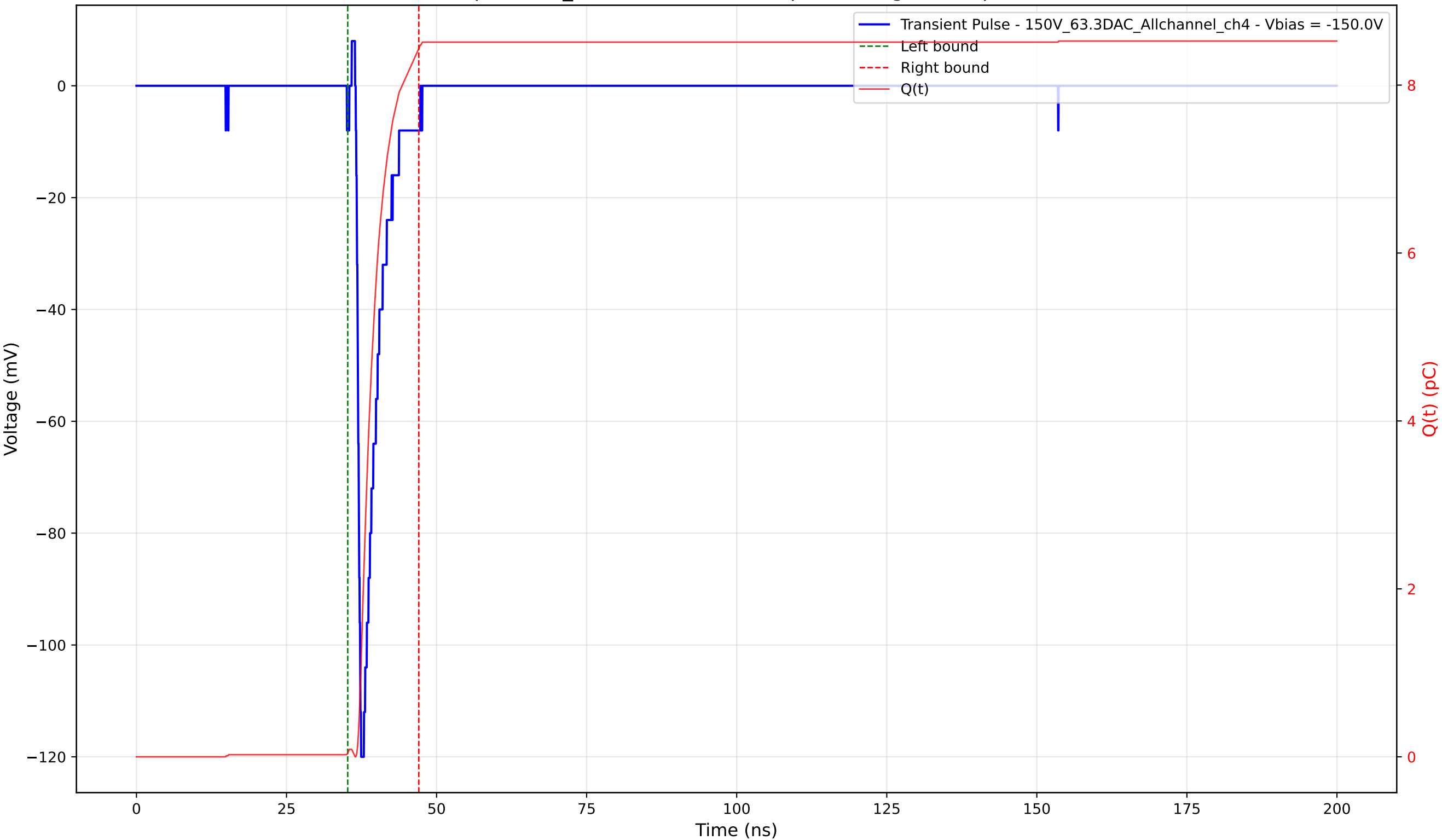
Transient Pulse - Sample: 1cm_42 - Position: 1090.0 \mu\text{m} - Charge: 8.39 pC - Rise Time: 0.70 ns
