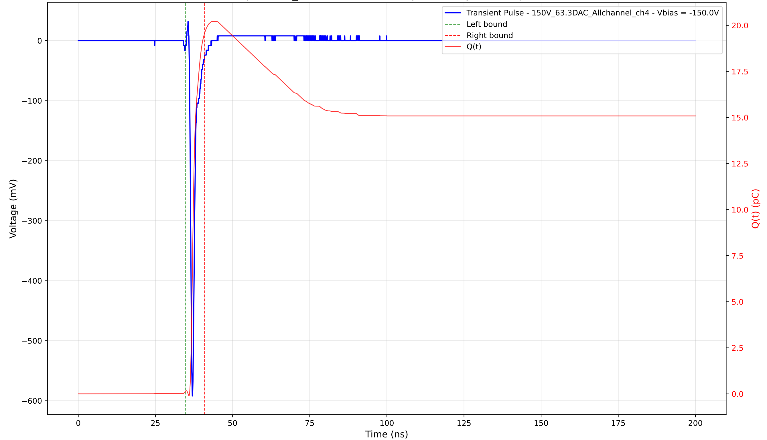
Transient Pulse - Sample: 1cm_42 - Position: 1815.0 \mu\text{m} - Charge: 19.50 pC - Rise Time: 0.66 ns
