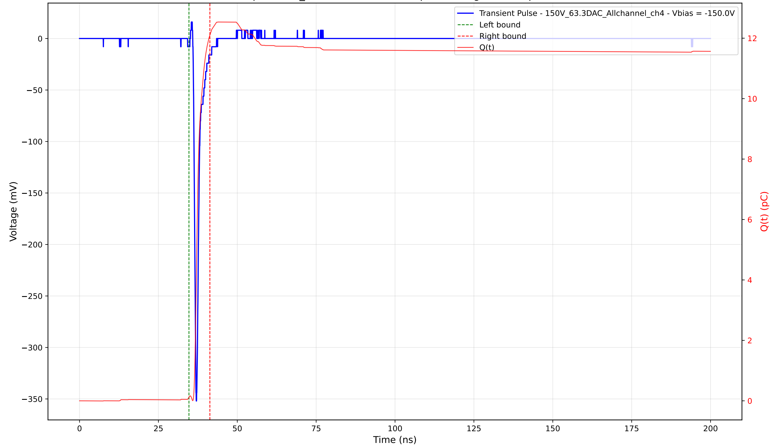
Transient Pulse - Sample: 1cm_42 - Position: 2410.0 \mu\text{m} - Charge: 11.99 pC - Rise Time: 0.72 ns
