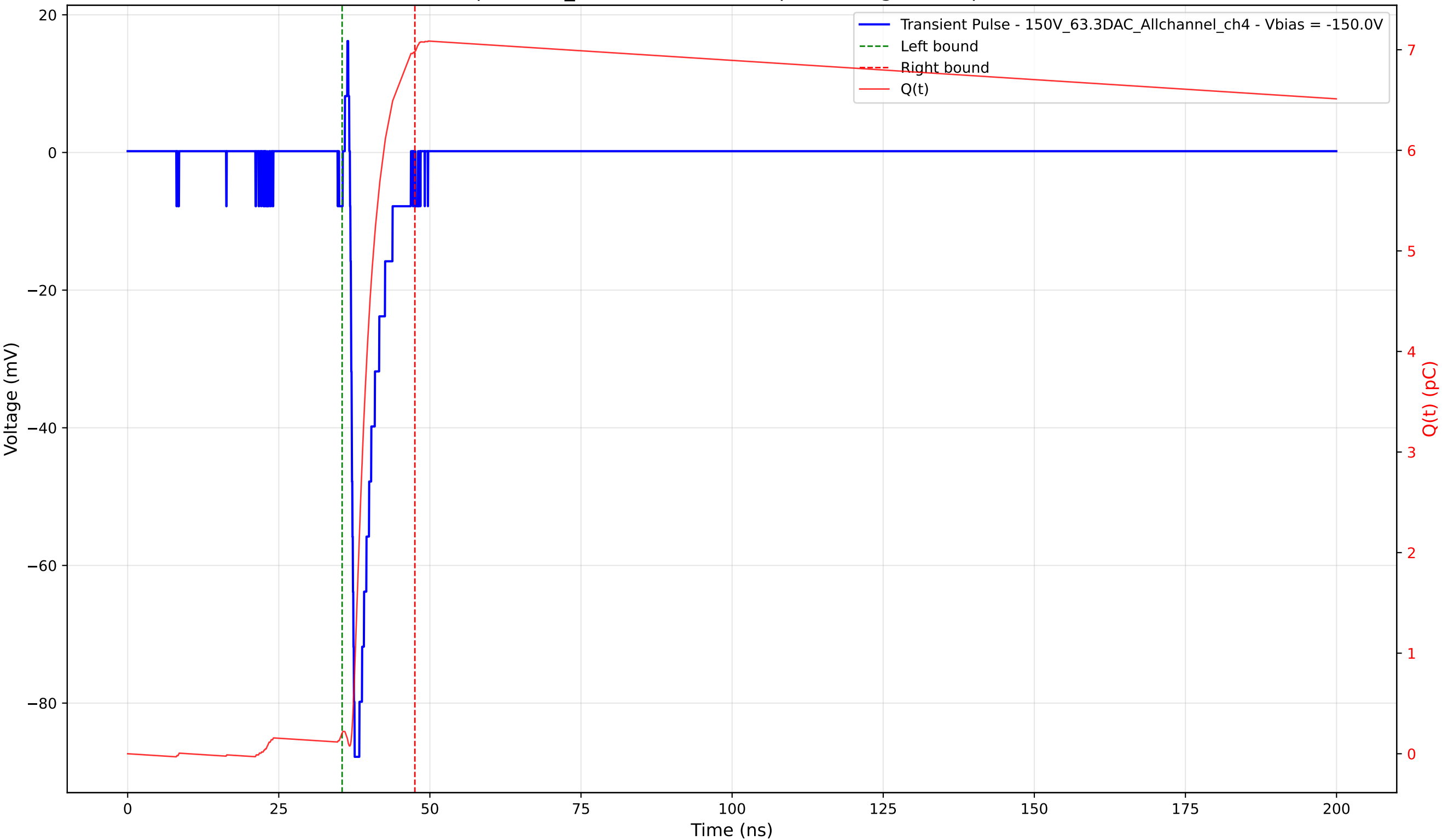
Transient Pulse - Sample: 1cm_42 - Position: 960.0 \mu\text{m} - Charge: 6.78 pC - Rise Time: 0.60 ns
