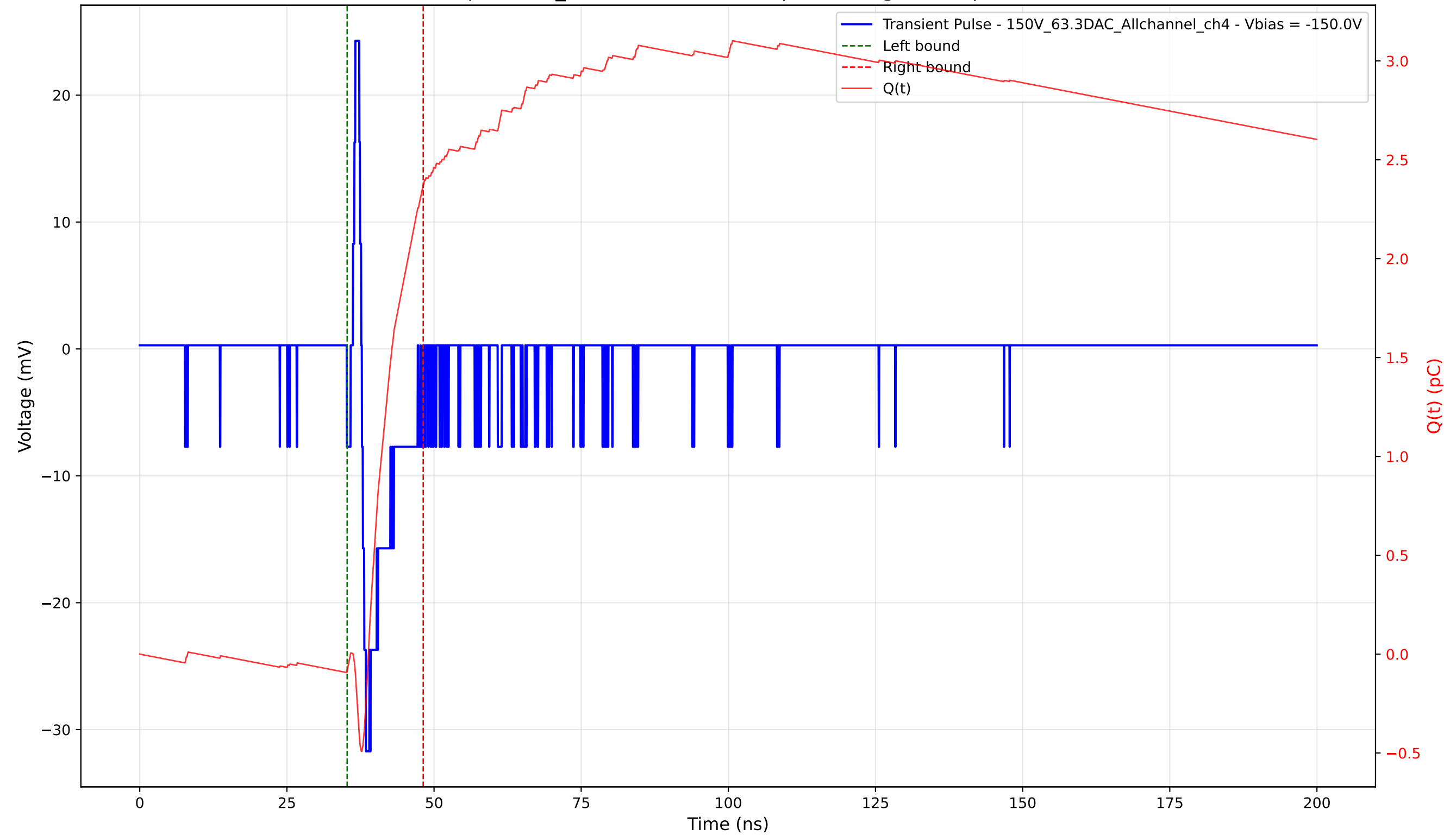
Transient Pulse - Sample: 1cm_42 - Position: 4100.0 \mu\text{m} - Charge: 2.46 pC - Rise Time: 0.70 ns
