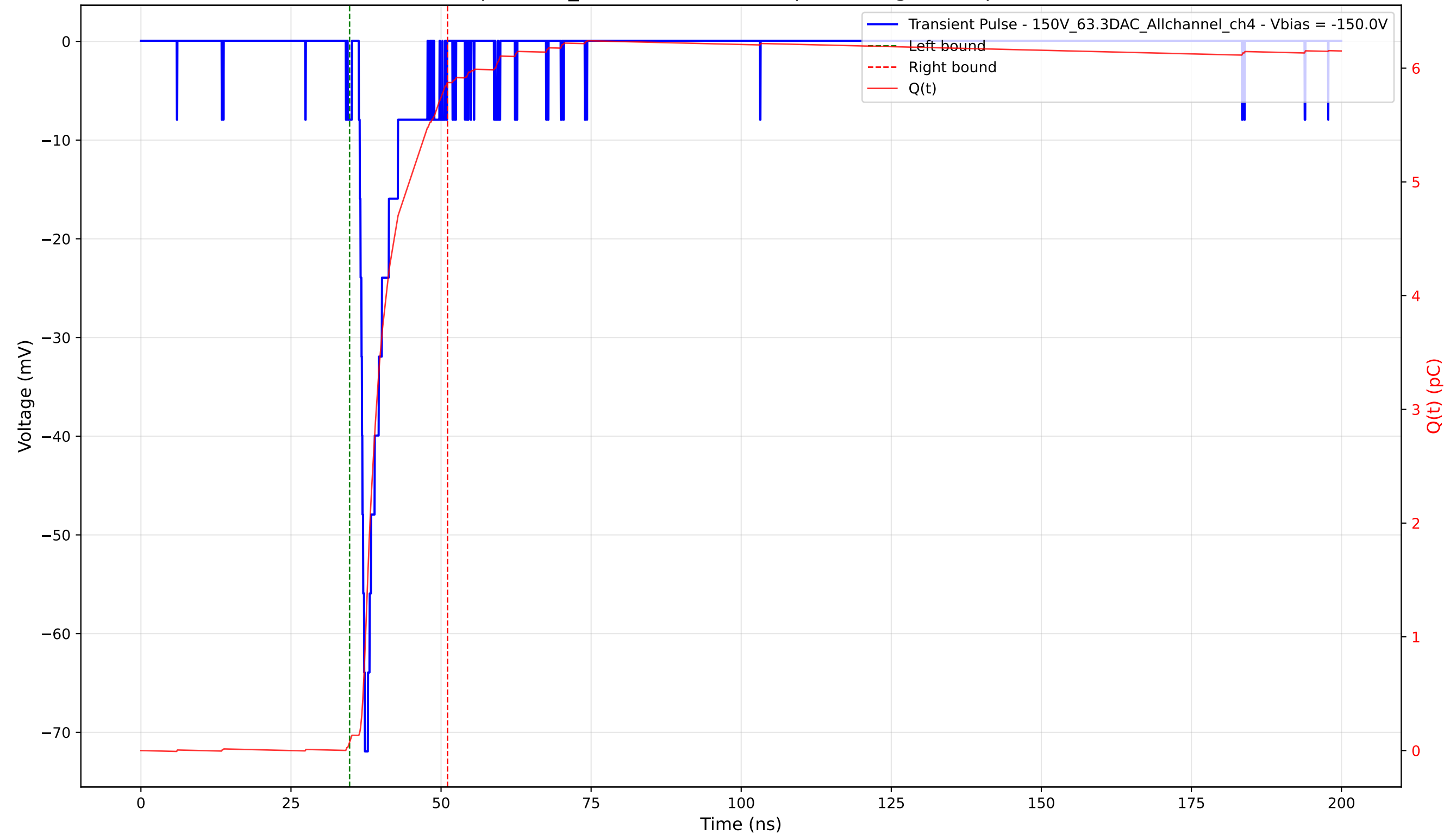
Transient Pulse - Sample: 1cm_42 - Position: 2990.0 \mu\text{m} - Charge: 5.80 pC - Rise Time: 1.00 ns
