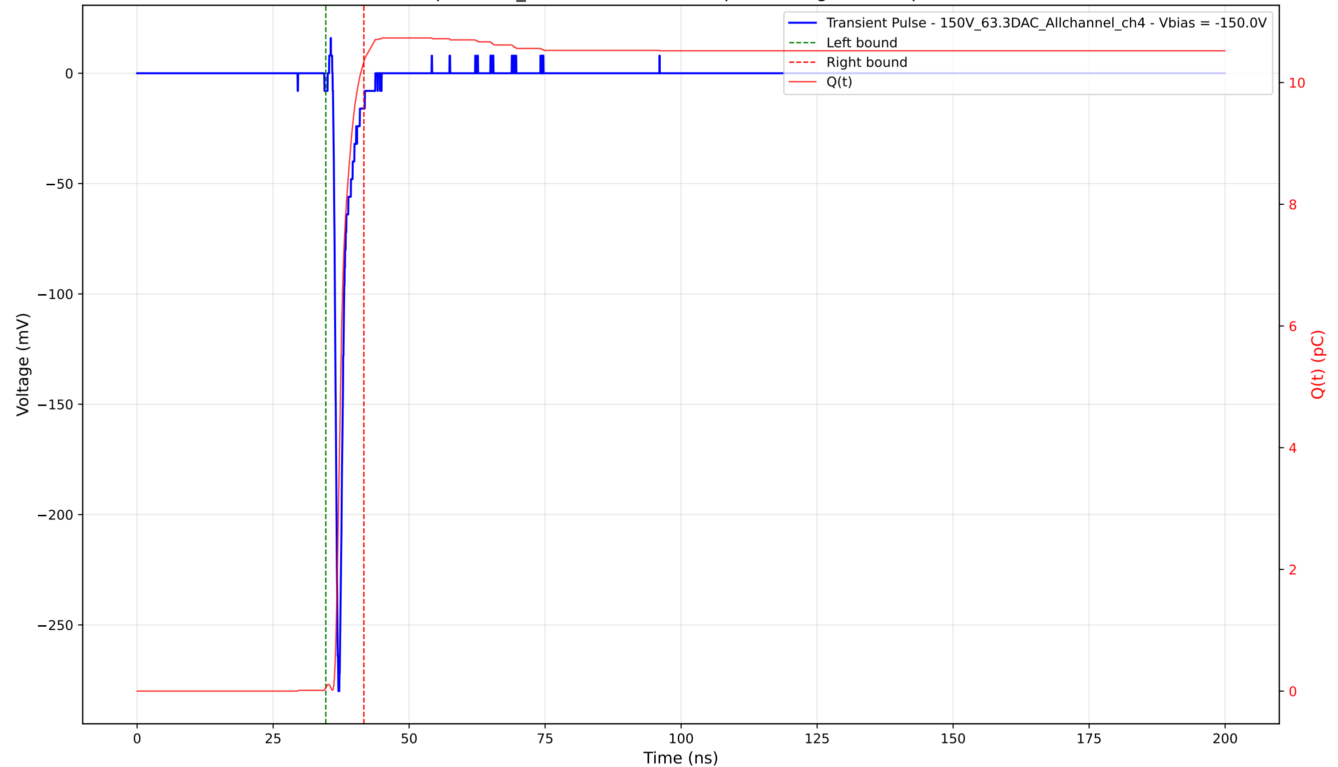
Transient Pulse - Sample: 1cm_42 - Position: 2470.0 \mu\text{m} - Charge: 10.29 pC - Rise Time: 0.72 ns
