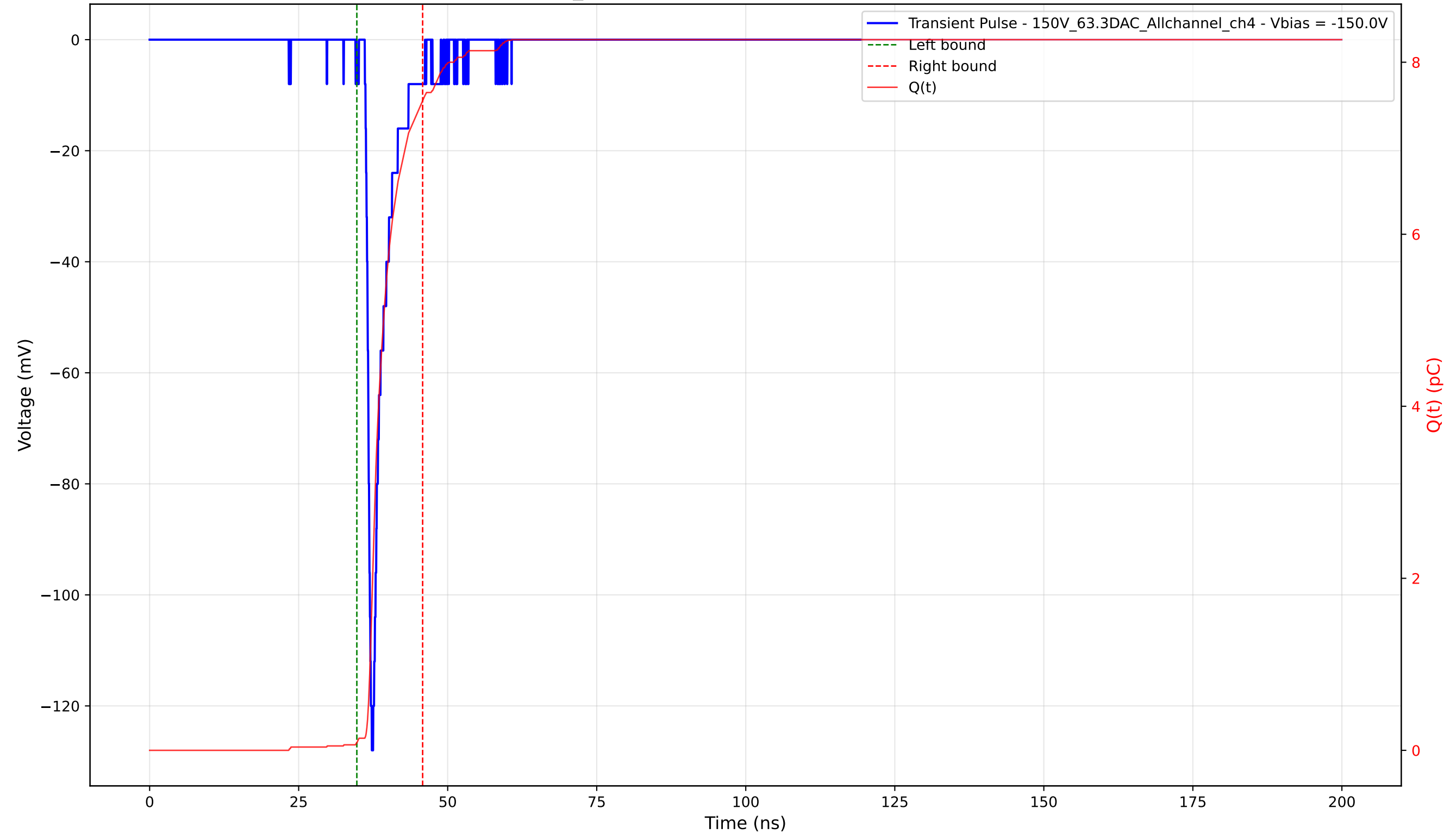
Transient Pulse - Sample: 1cm_42 - Position: 2820.0 \mu\text{m} - Charge: 7.47 pC - Rise Time: 0.90 ns
