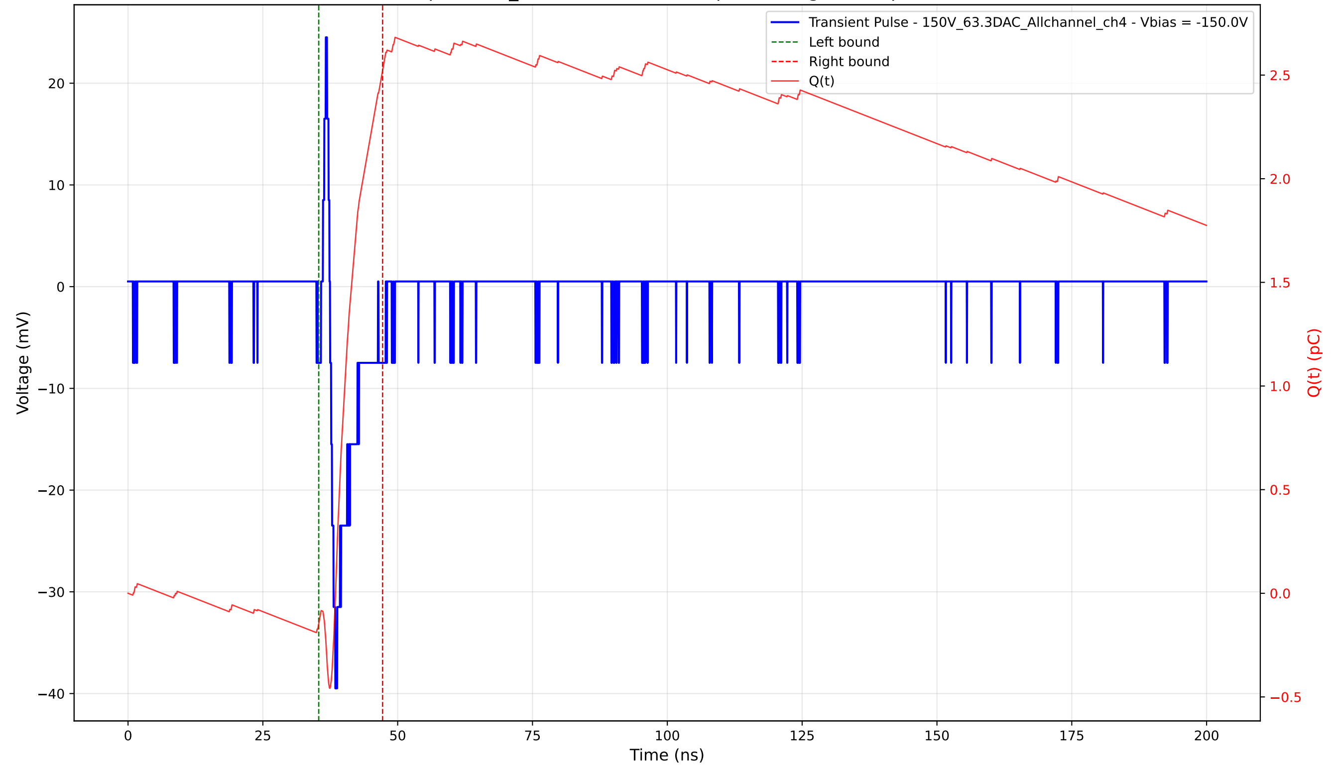
Transient Pulse - Sample: 1cm_42 - Position: 4820.0 \mu\text{m} - Charge: 2.67 pC - Rise Time: 0.98 ns
