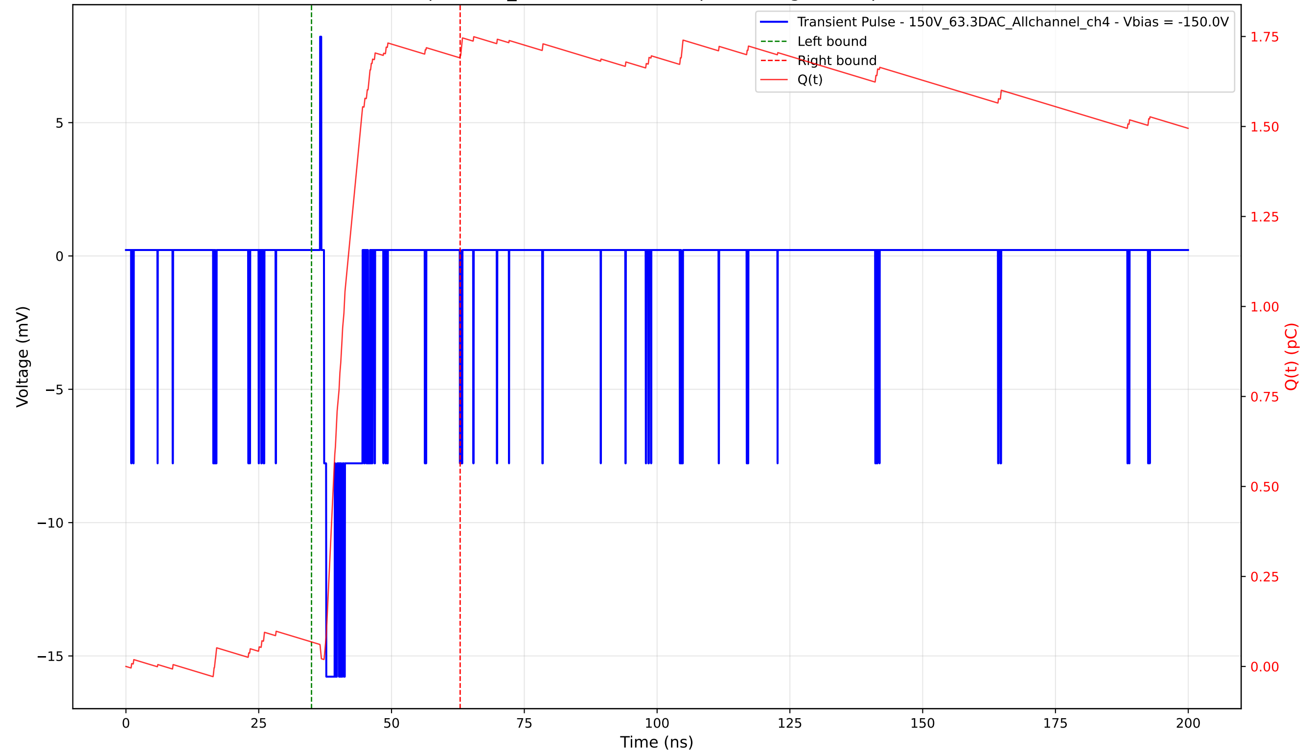
Transient Pulse - Sample: 1cm_42 - Position: 145.0 \mu\text{m} - Charge: 1.63 pC - Rise Time: 0.43 ns
