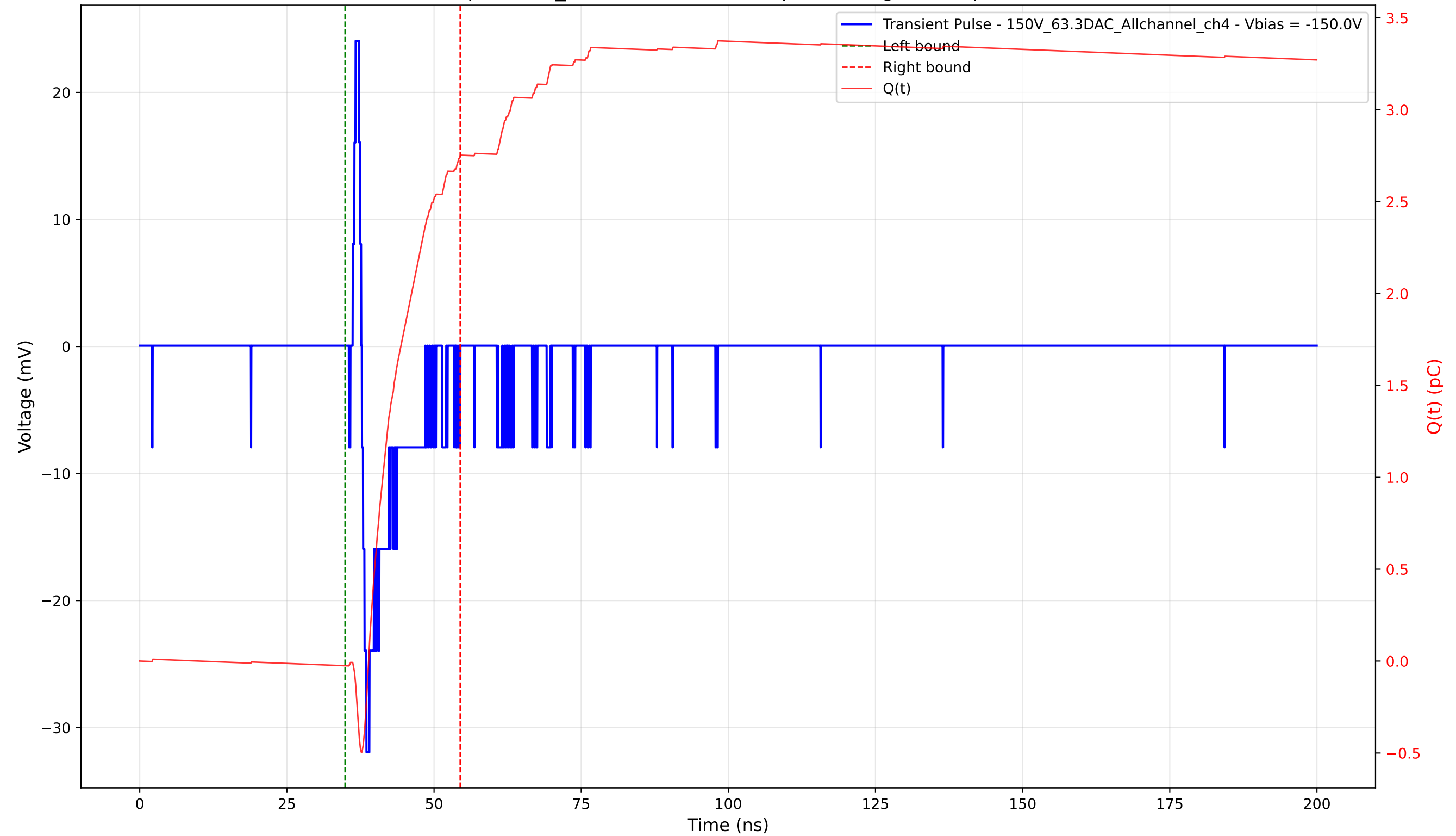
Transient Pulse - Sample: 1cm_42 - Position: 4070.0 \mu\text{m} - Charge: 2.78 pC - Rise Time: 0.78 ns
