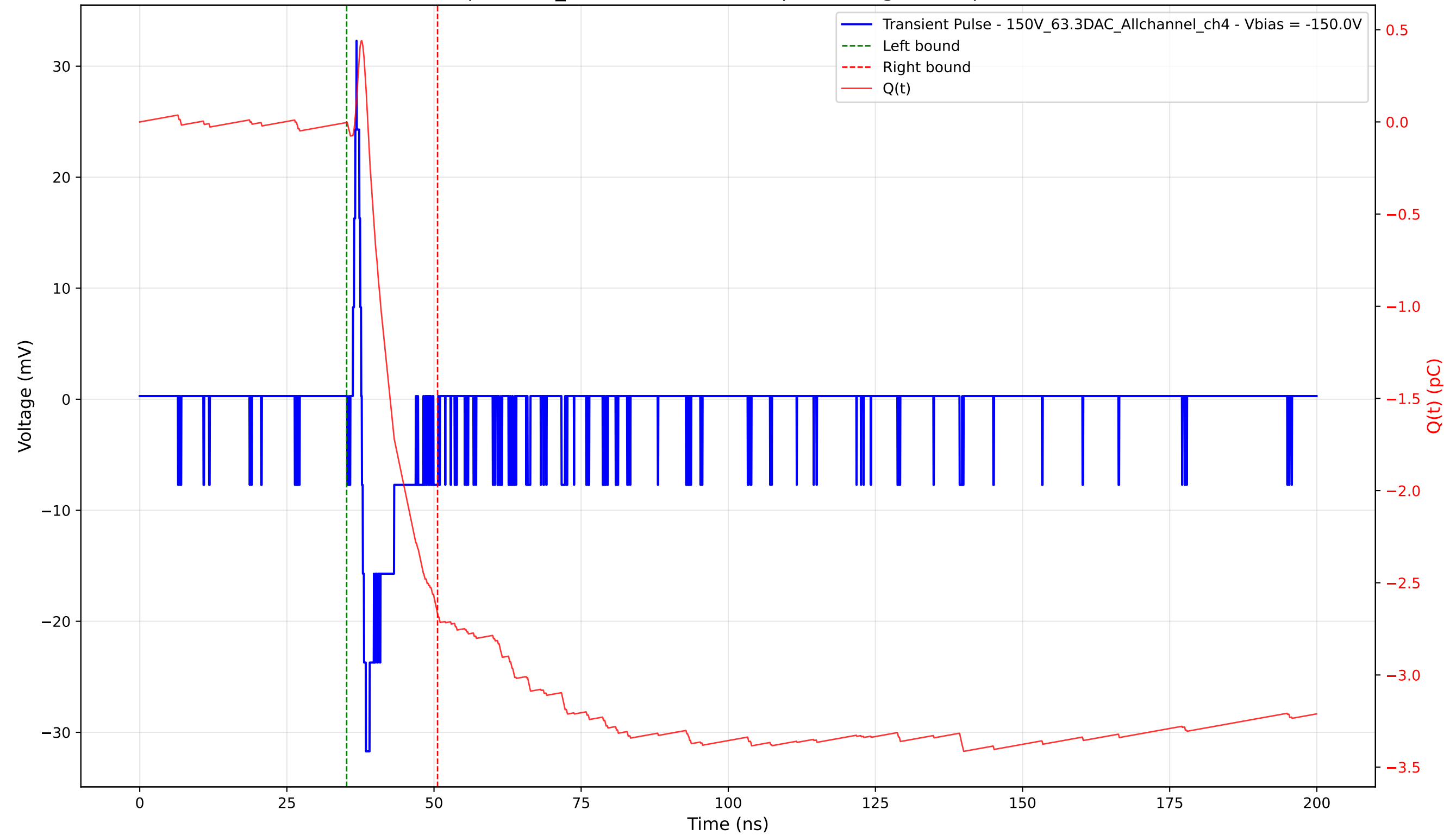
Transient Pulse - Sample: 1cm_42 - Position: 4405.0 \mu\text{m} - Charge: 2.67 pC - Rise Time: 0.63 ns
