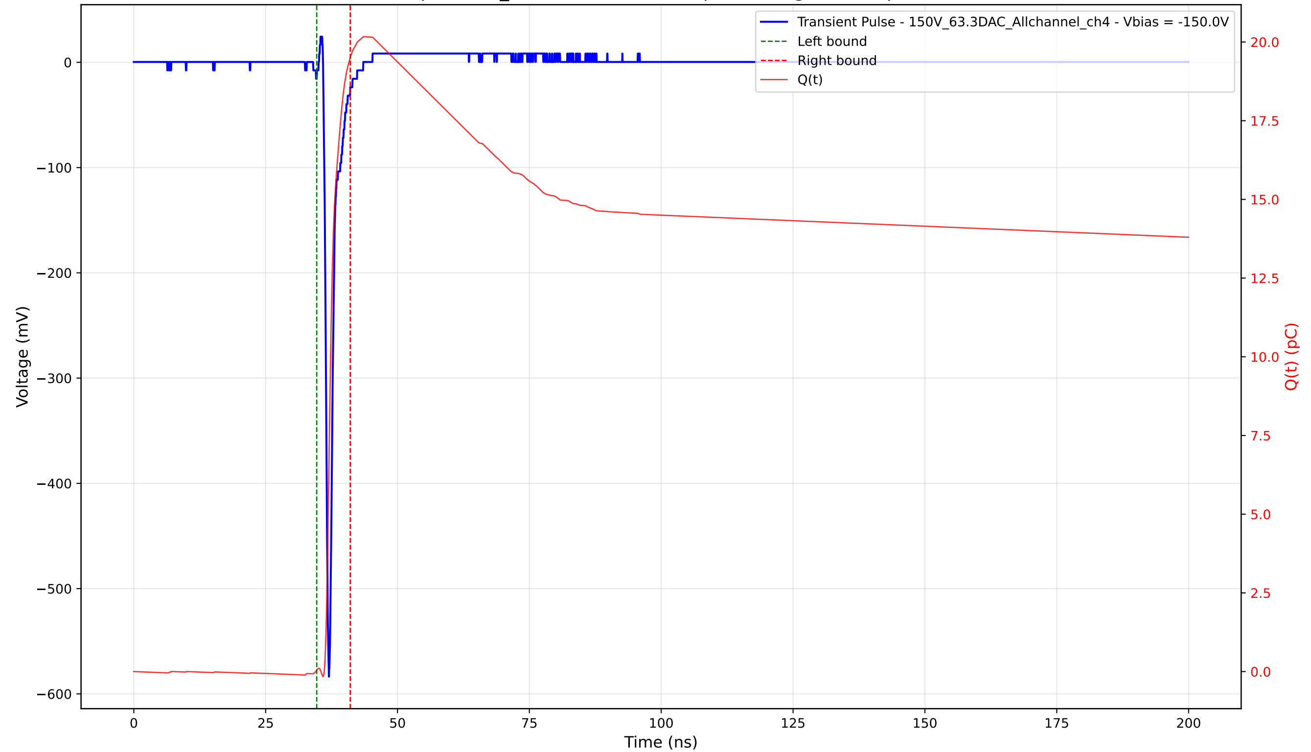
Transient Pulse - Sample: 1cm_42 - Position: 1755.0 \mu\text{m} - Charge: 19.47 pC - Rise Time: 0.70 ns
