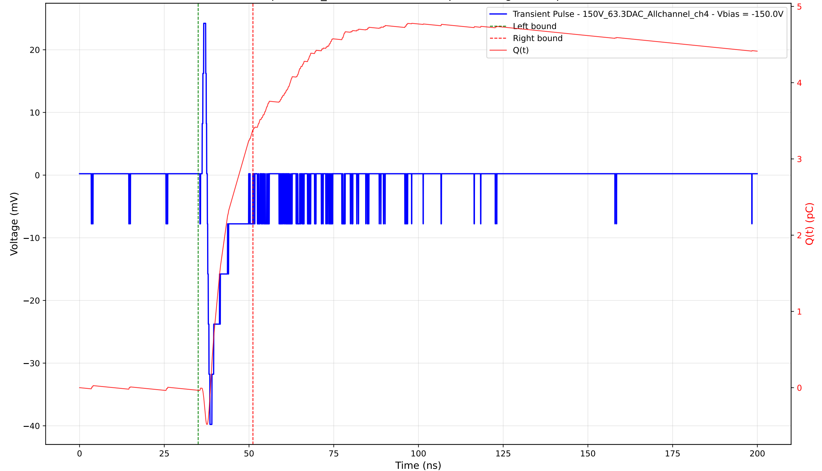
Transient Pulse - Sample: 1cm_42 - Position: 3790.0 \mu\text{m} - Charge: 3.42 pC - Rise Time: 0.78 ns
