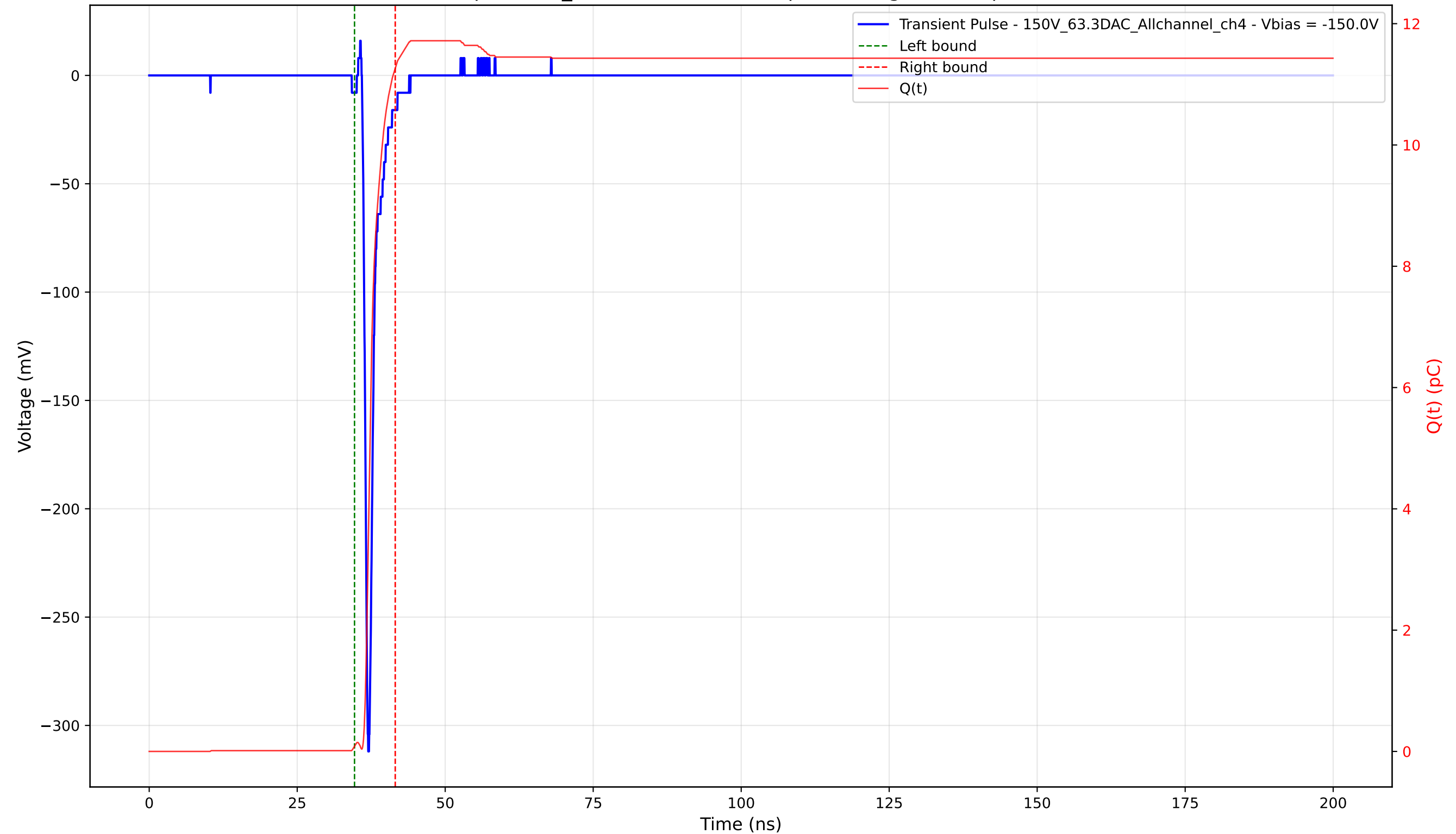
Transient Pulse - Sample: 1cm_42 - Position: 2445.0 \mu\text{m} - Charge: 11.18 pC - Rise Time: 0.73 ns
