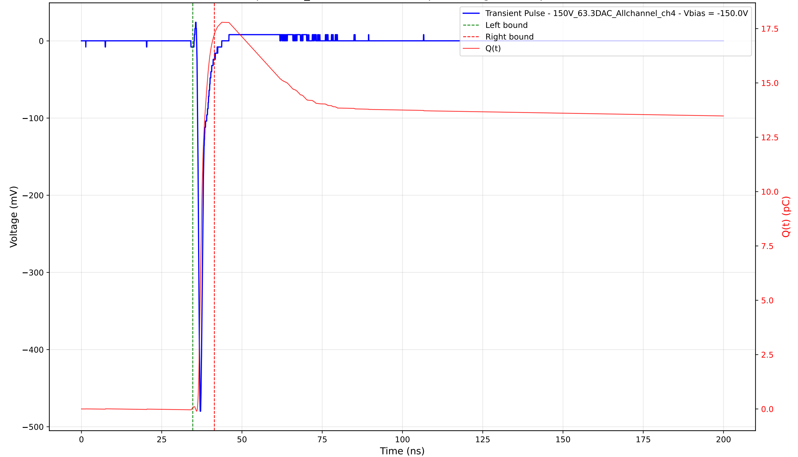
Transient Pulse - Sample: 1cm_42 - Position: 1675.0 \mu\text{m} - Charge: 17.19 pC - Rise Time: 0.74 ns
