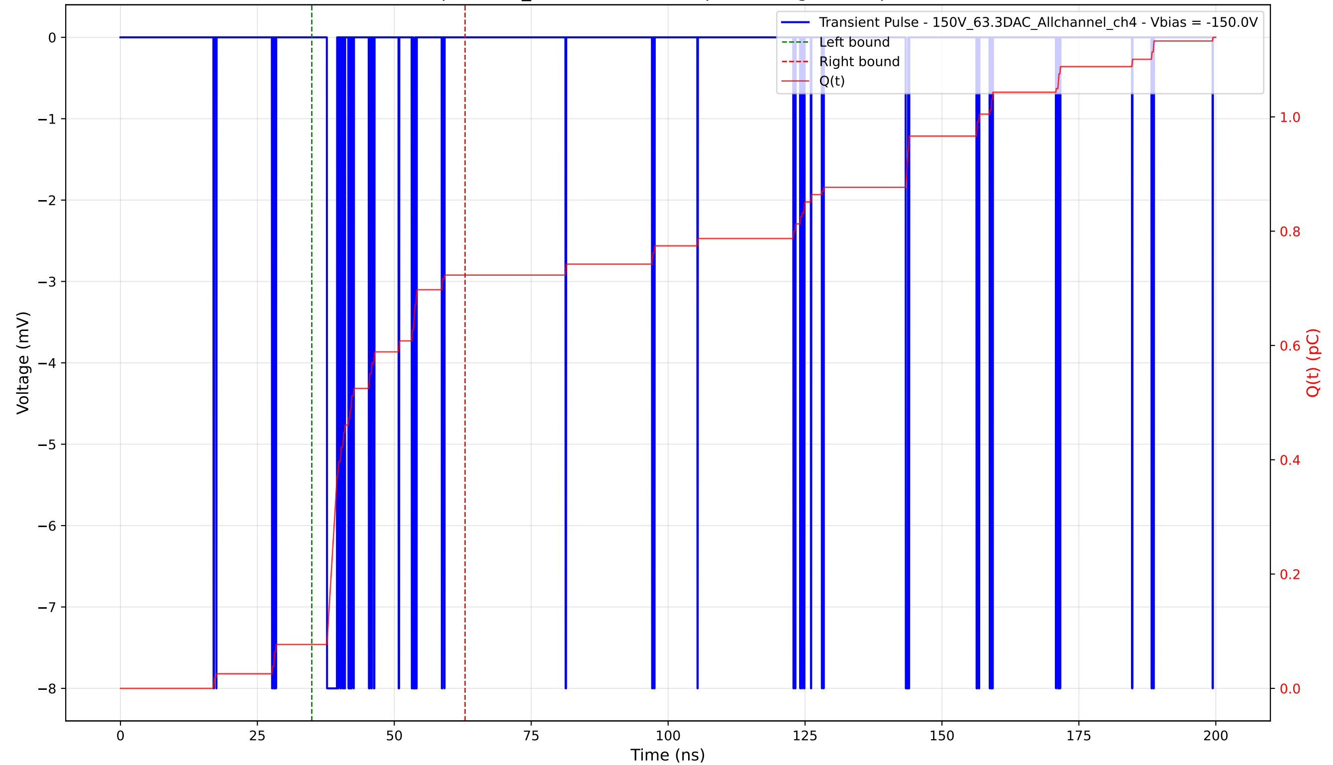
Transient Pulse - Sample: 1cm_42 - Position: 25.0 \mu\text{m} - Charge: 0.65 pC - Rise Time: 0.04 ns
