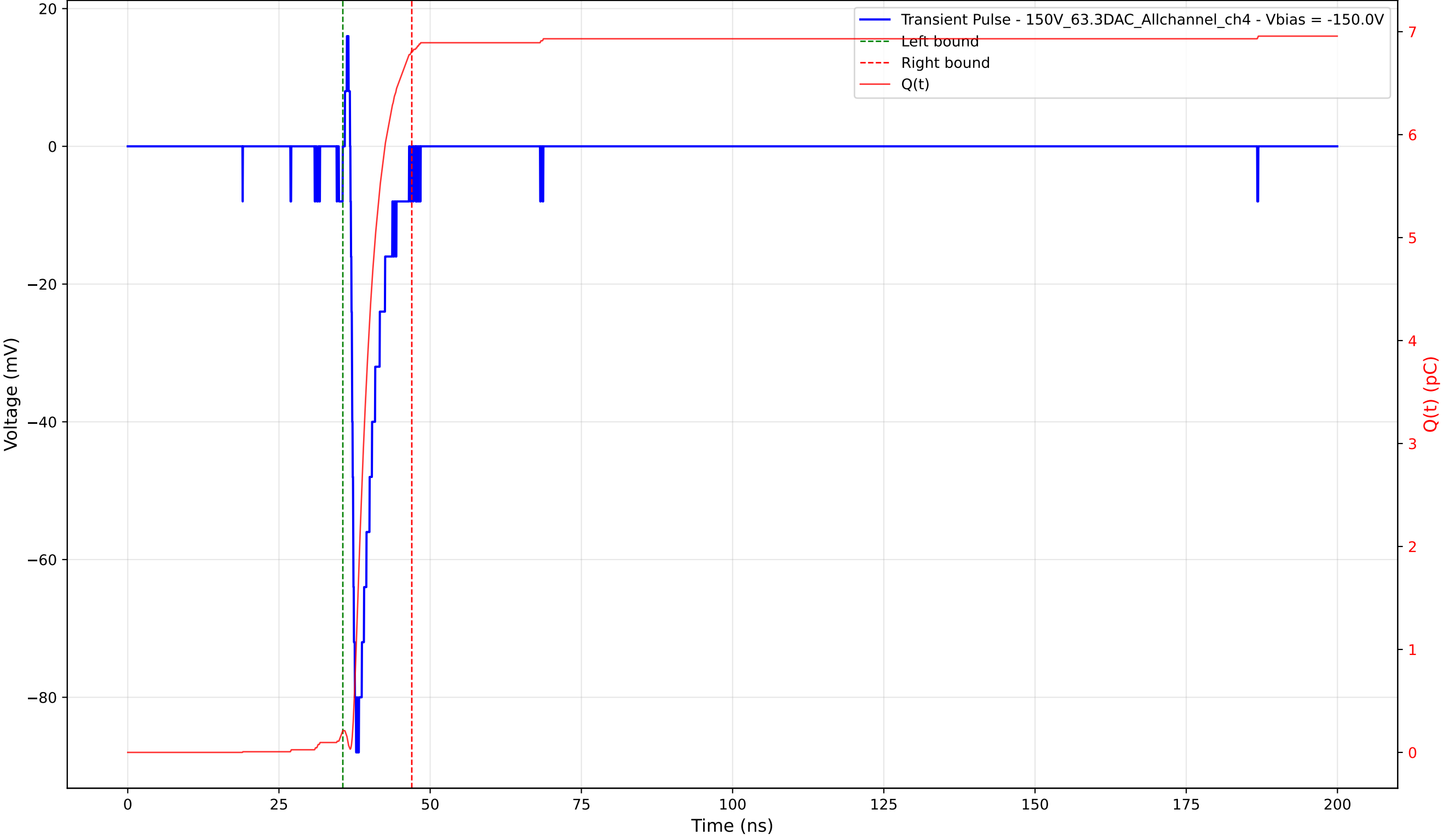
Transient Pulse - Sample: 1cm_42 - Position: 935.0 \mu\text{m} - Charge: 6.60 pC - Rise Time: 0.68 ns
