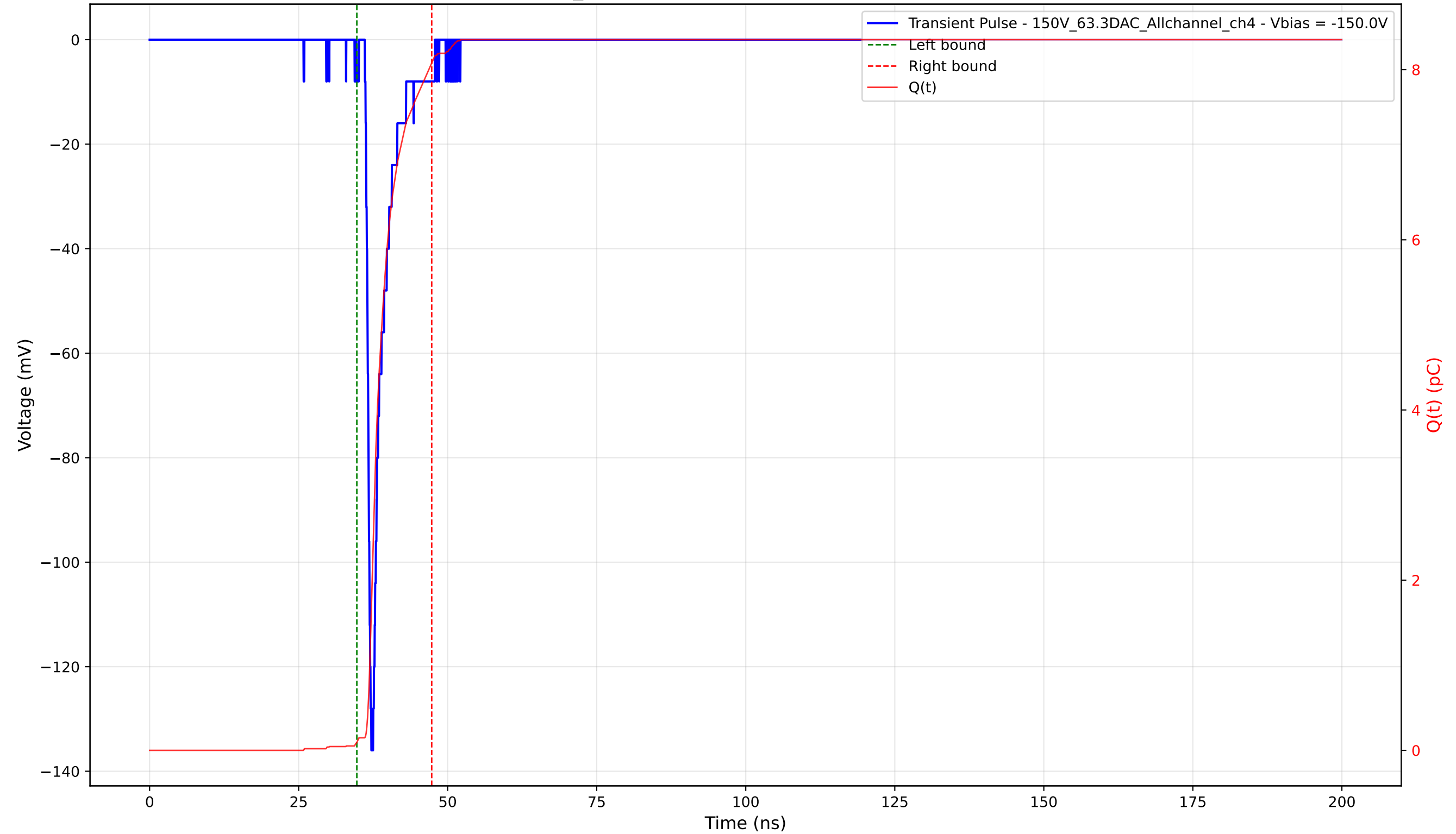
Transient Pulse - Sample: 1cm_42 - Position: 2770.0 \mu\text{m} - Charge: 7.99 pC - Rise Time: 0.85 ns
