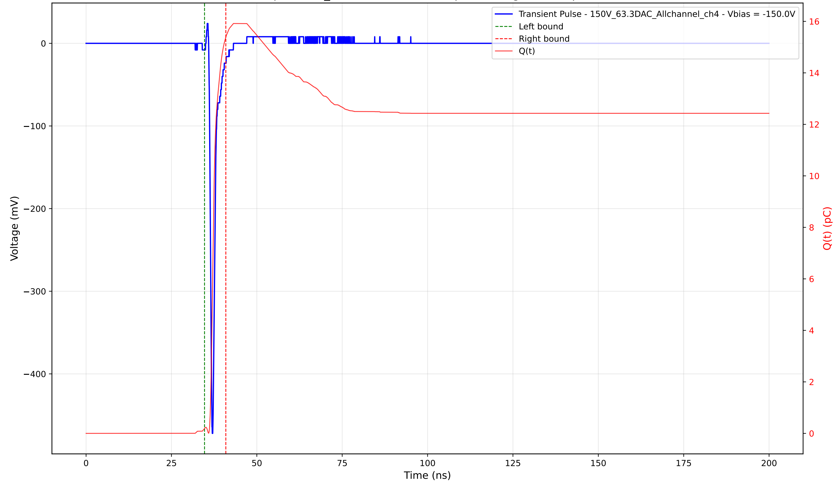
Transient Pulse - Sample: 1cm_42 - Position: 2300.0 \mu\text{m} - Charge: 15.20 pC - Rise Time: 0.69 ns
