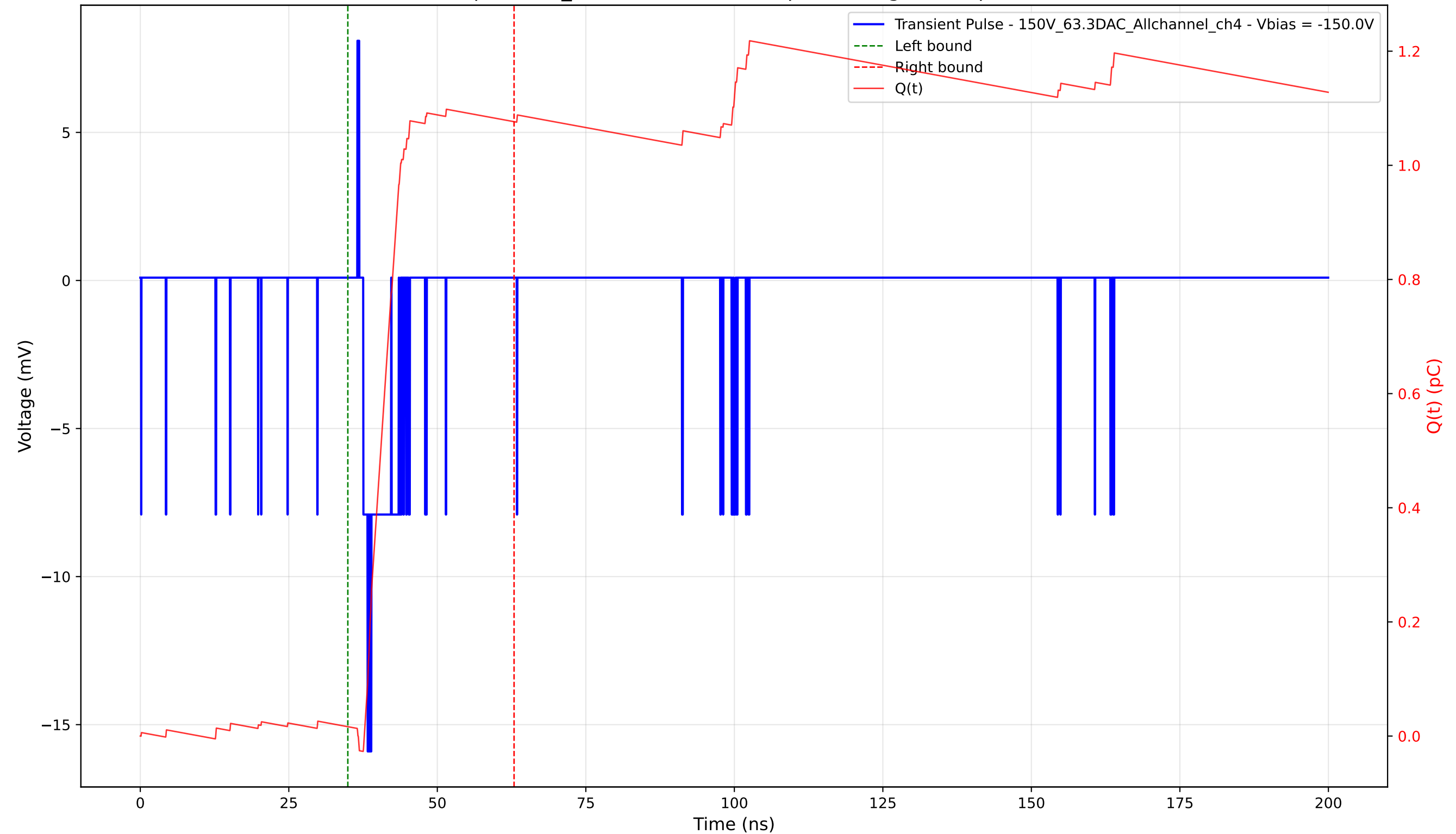
Transient Pulse - Sample: 1cm_42 - Position: 5095.0 \mu\text{m} - Charge: 1.06 pC - Rise Time: 0.75 ns
