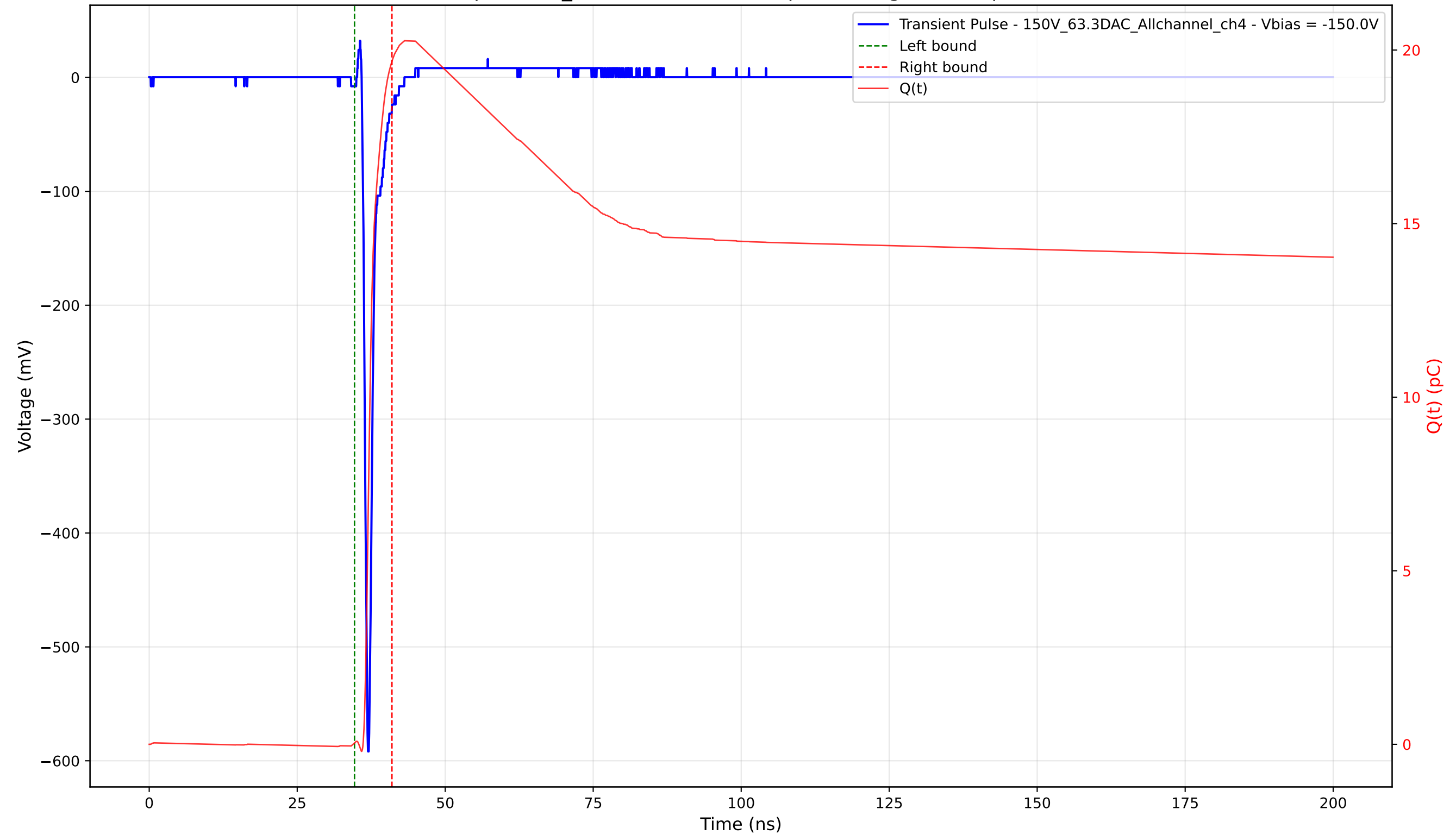
Transient Pulse - Sample: 1cm_42 - Position: 1800.0 \mu\text{m} - Charge: 19.64 pC - Rise Time: 0.70 ns
