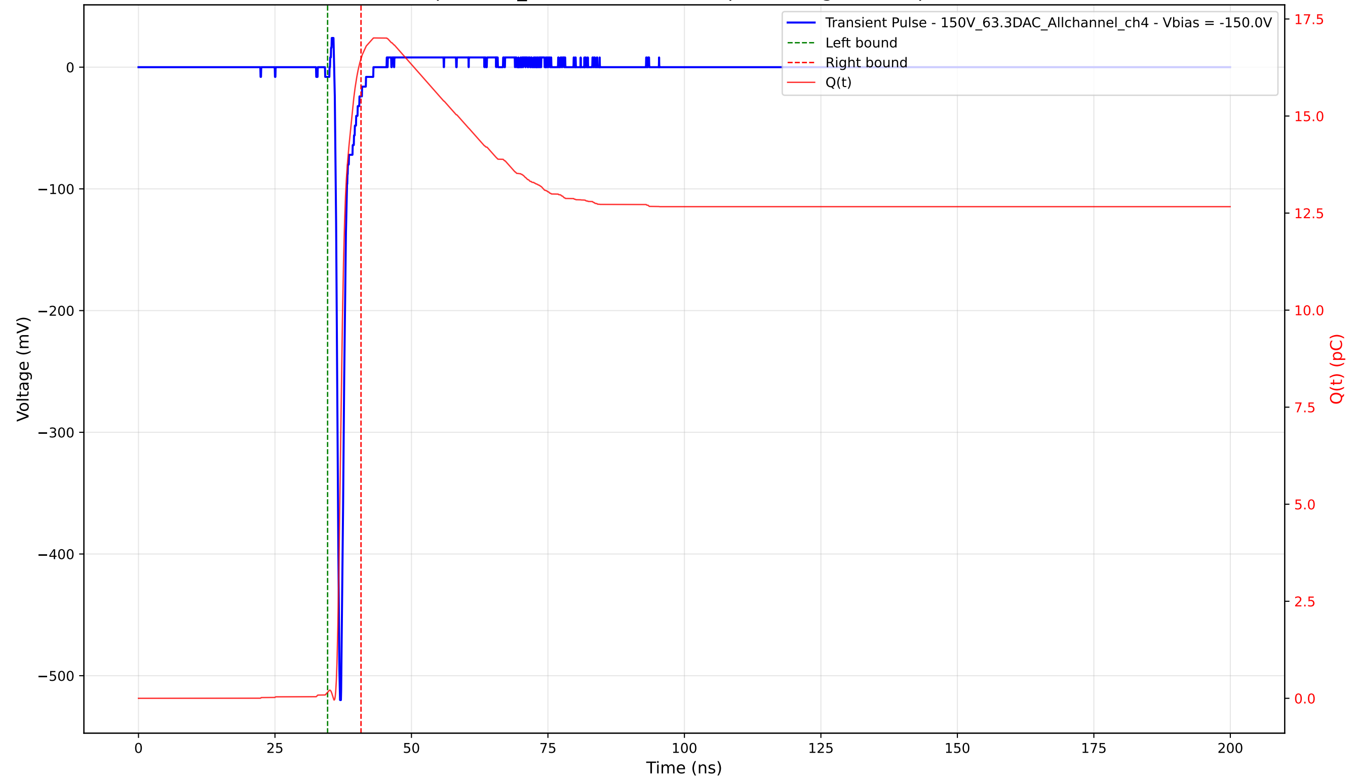
Transient Pulse - Sample: 1cm_42 - Position: 2215.0 \mu\text{m} - Charge: 16.32 pC - Rise Time: 0.70 ns
