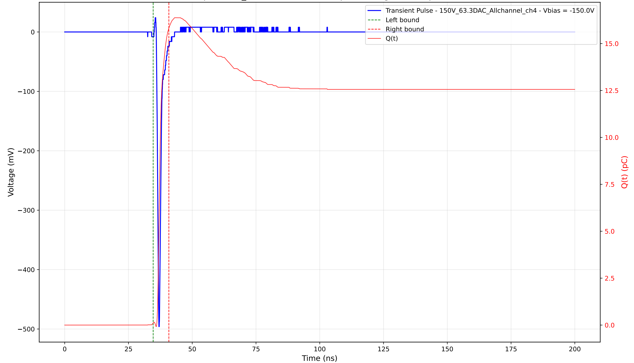
Transient Pulse - Sample: 1cm_42 - Position: 2275.0 \mu\text{m} - Charge: 15.72 pC - Rise Time: 0.73 ns
