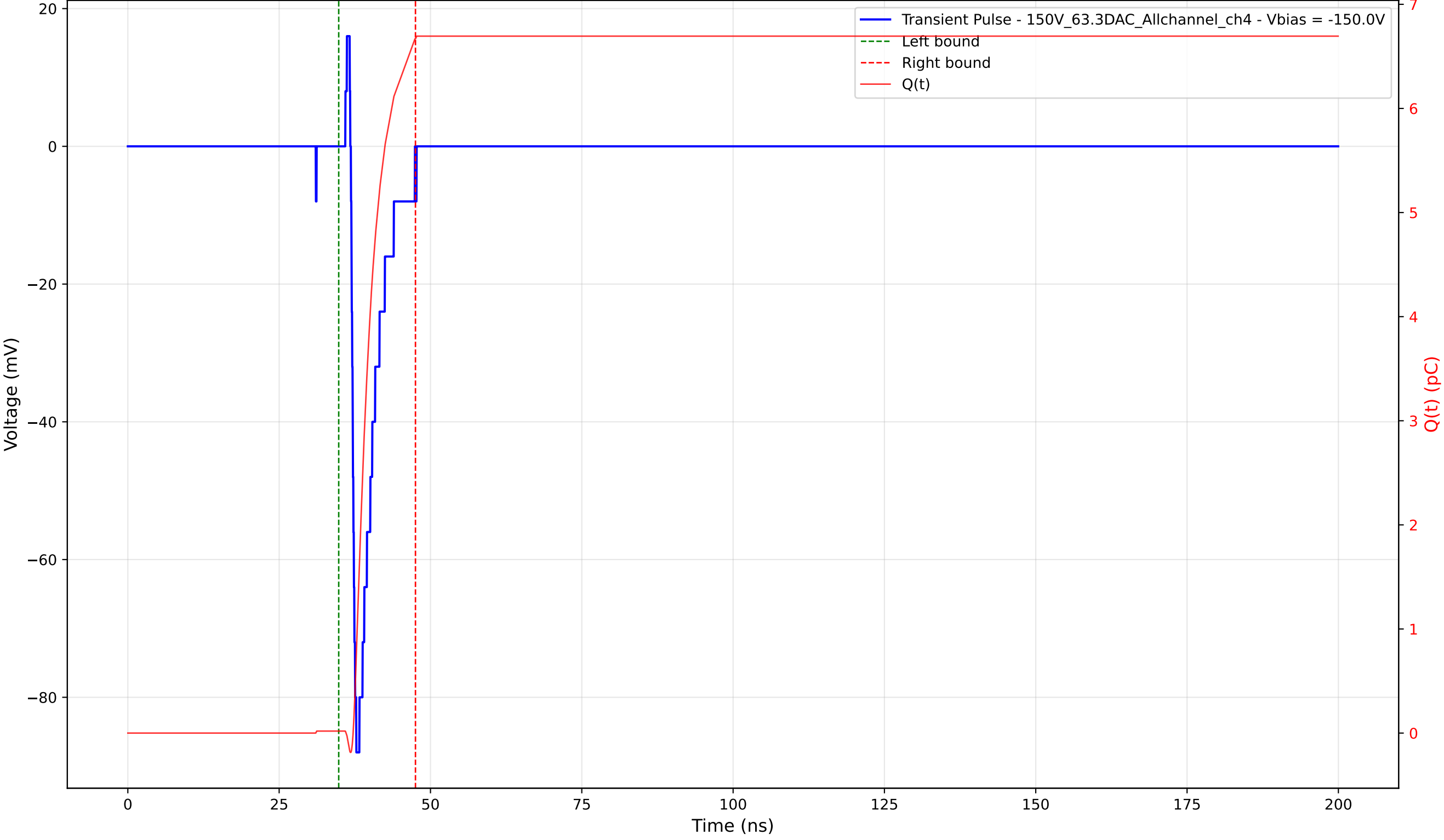
Transient Pulse - Sample: 1cm_42 - Position: 925.0 \mu\text{m} - Charge: 6.65 pC - Rise Time: 0.64 ns
