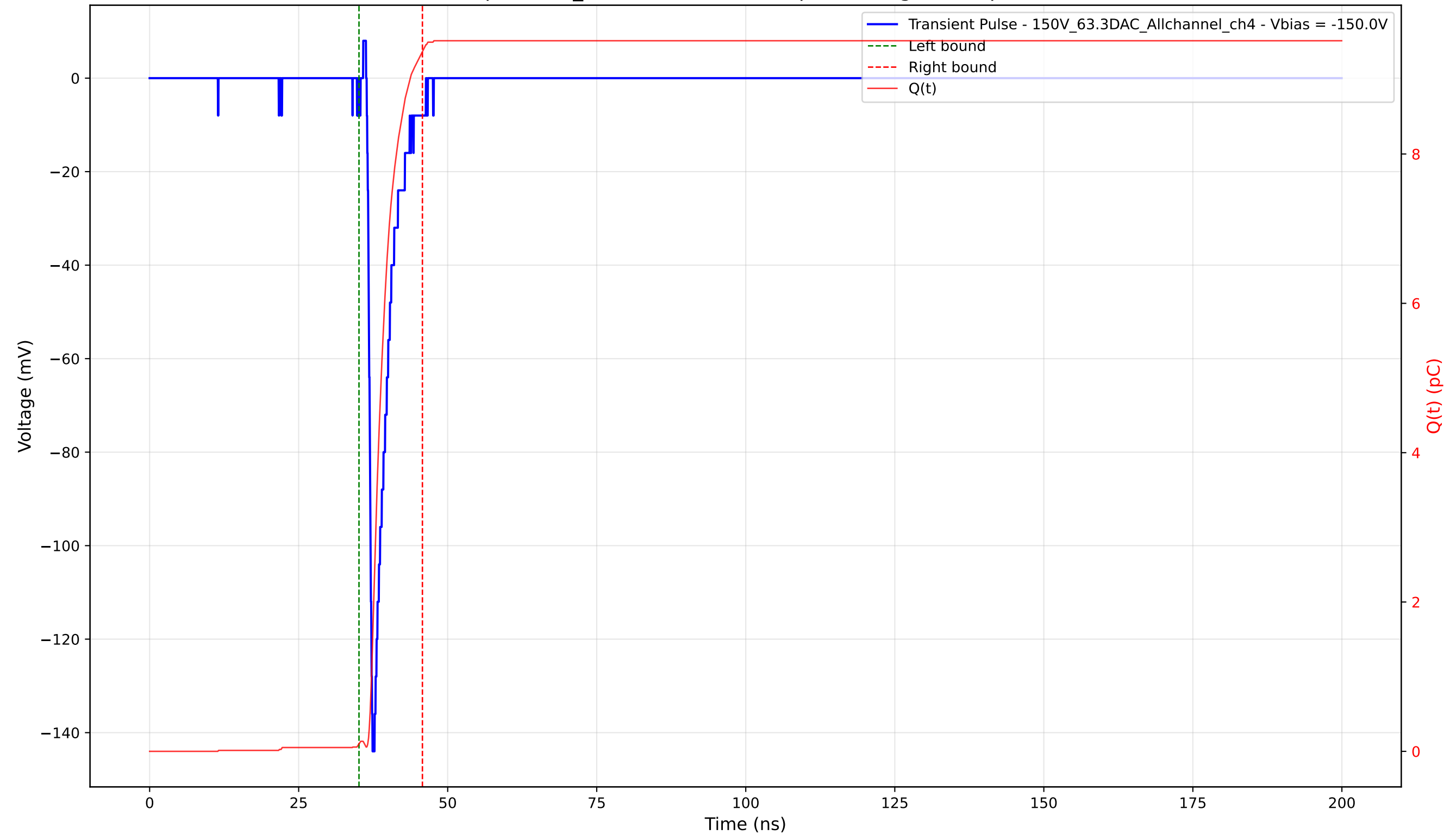
Transient Pulse - Sample: 1cm_42 - Position: 1145.0 \mu\text{m} - Charge: 9.27 pC - Rise Time: 0.81 ns
