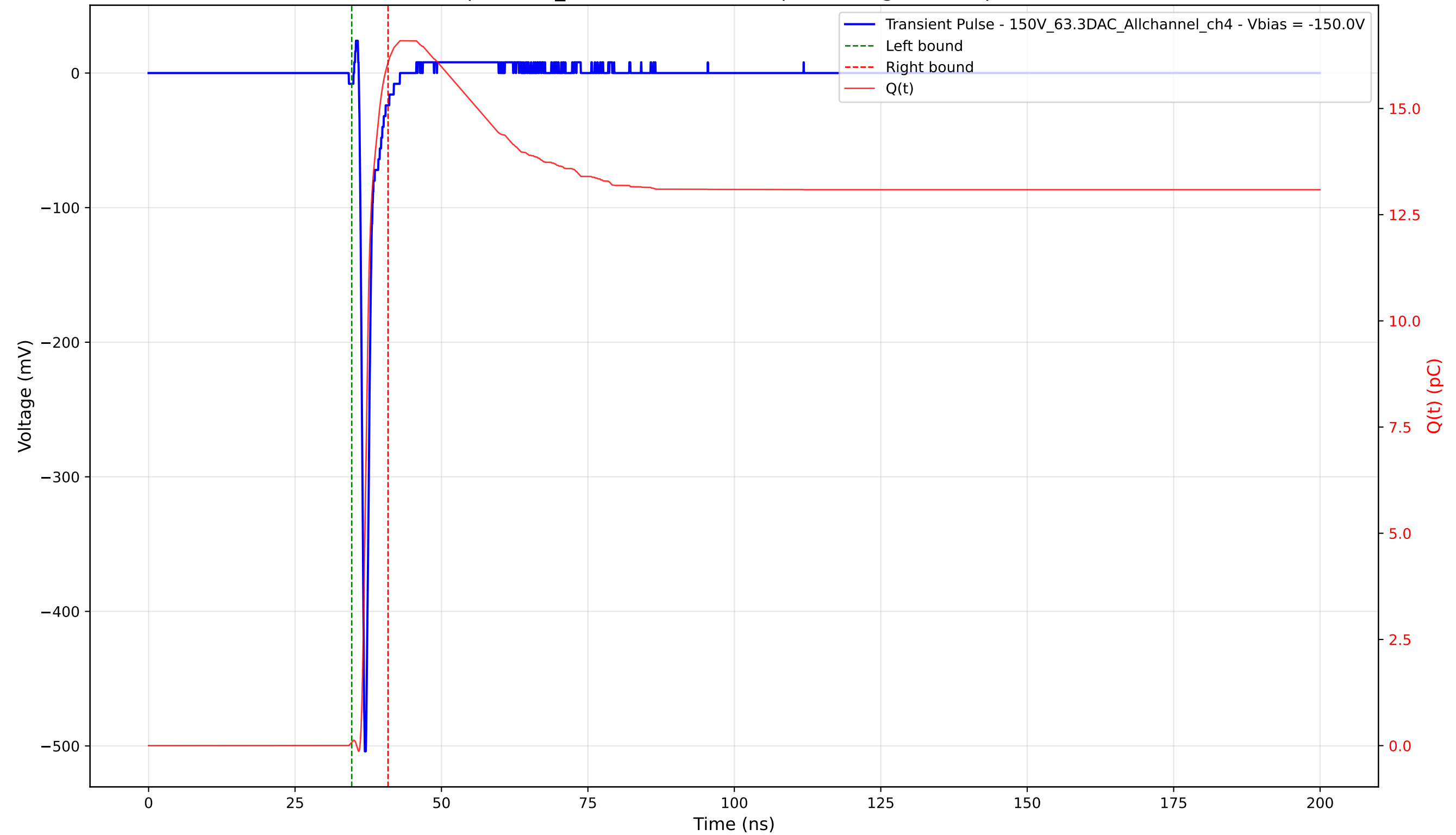
Transient Pulse - Sample: 1cm_42 - Position: 2245.0 \mu\text{m} - Charge: 16.00 pC - Rise Time: 0.71 ns
