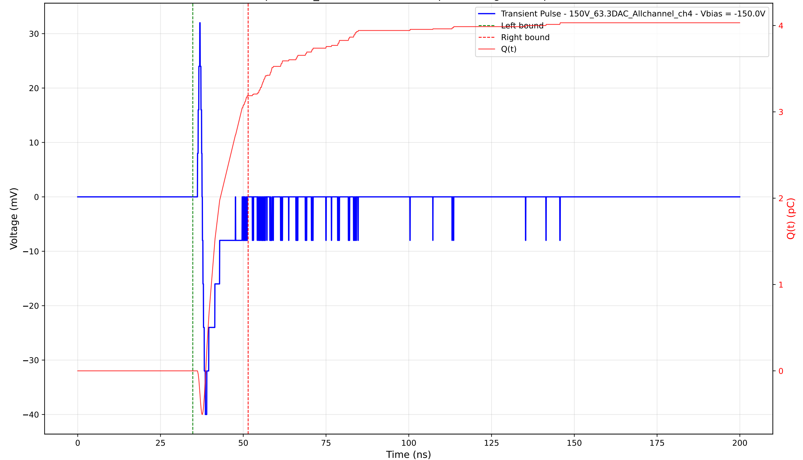
Transient Pulse - Sample: 1cm_42 - Position: 3820.0 \mu\text{m} - Charge: 3.19 pC - Rise Time: 0.90 ns
