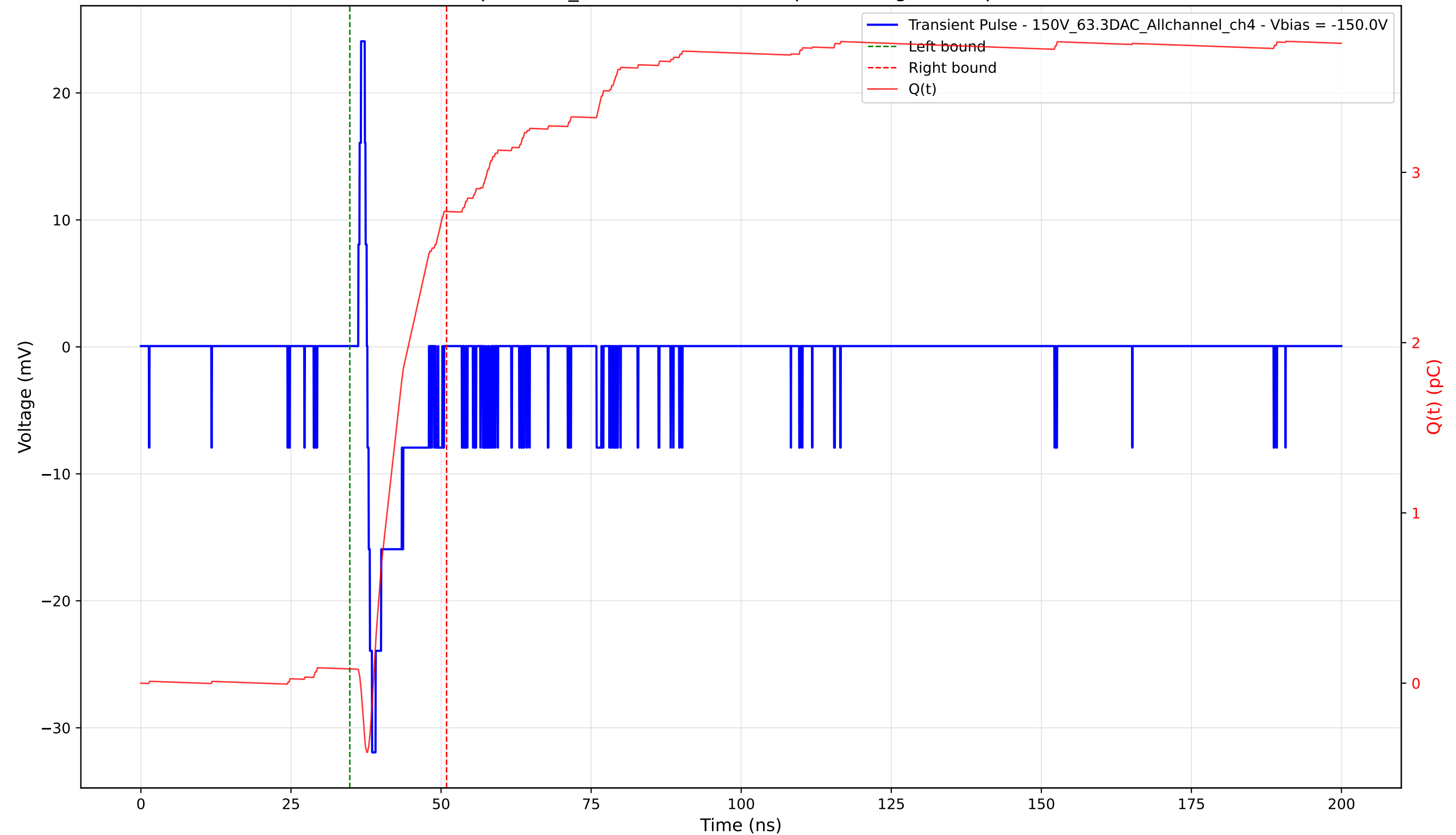
Transient Pulse - Sample: 1cm_42 - Position: 4095.0 \mu\text{m} - Charge: 2.69 pC - Rise Time: 0.78 ns
