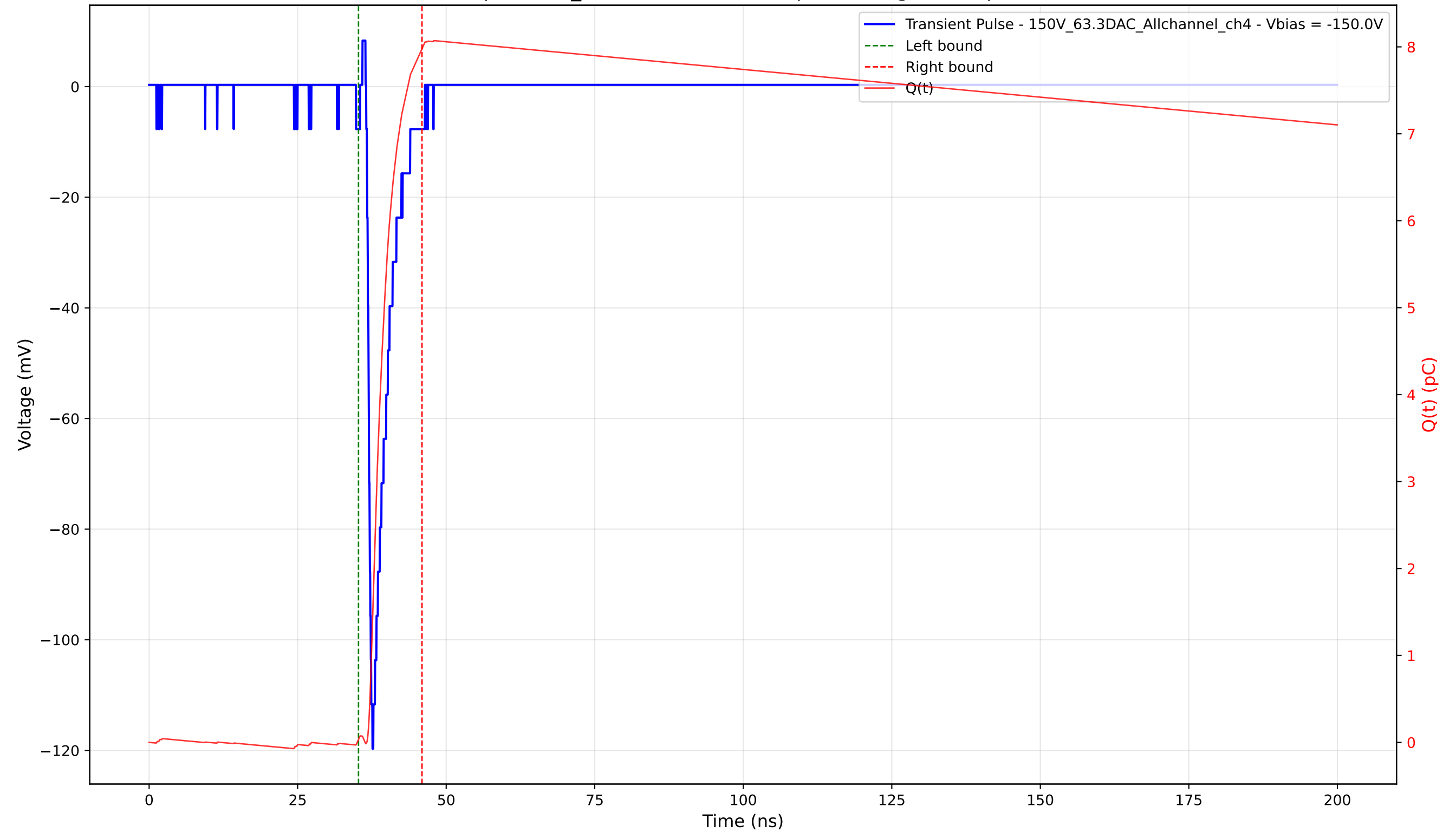
Transient Pulse - Sample: 1cm_42 - Position: 1075.0 \mu\text{m} - Charge: 7.94 pC - Rise Time: 0.74 ns
