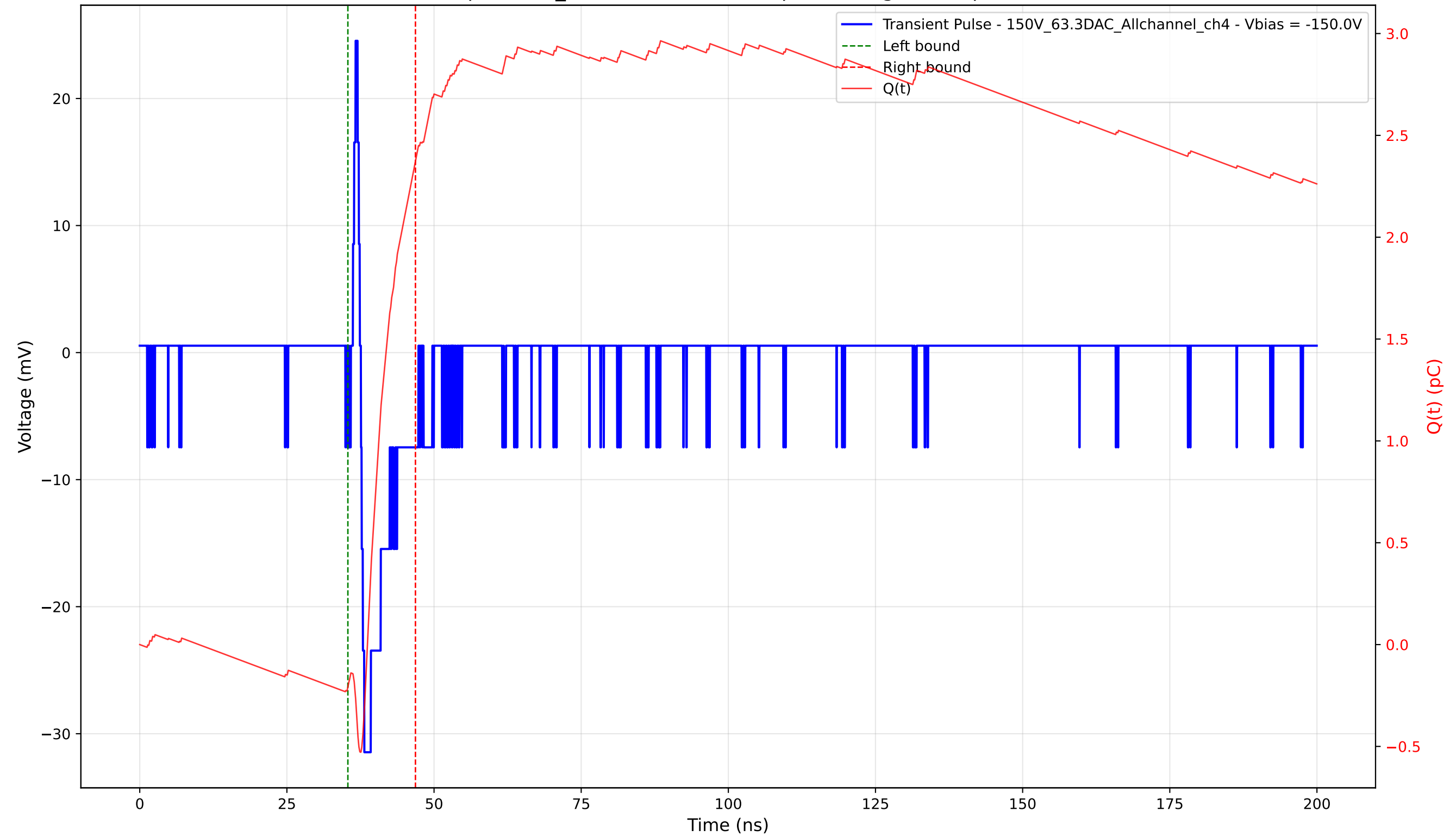
Transient Pulse - Sample: 1cm_42 - Position: 4730.0 \mu\text{m} - Charge: 2.58 pC - Rise Time: 0.58 ns
