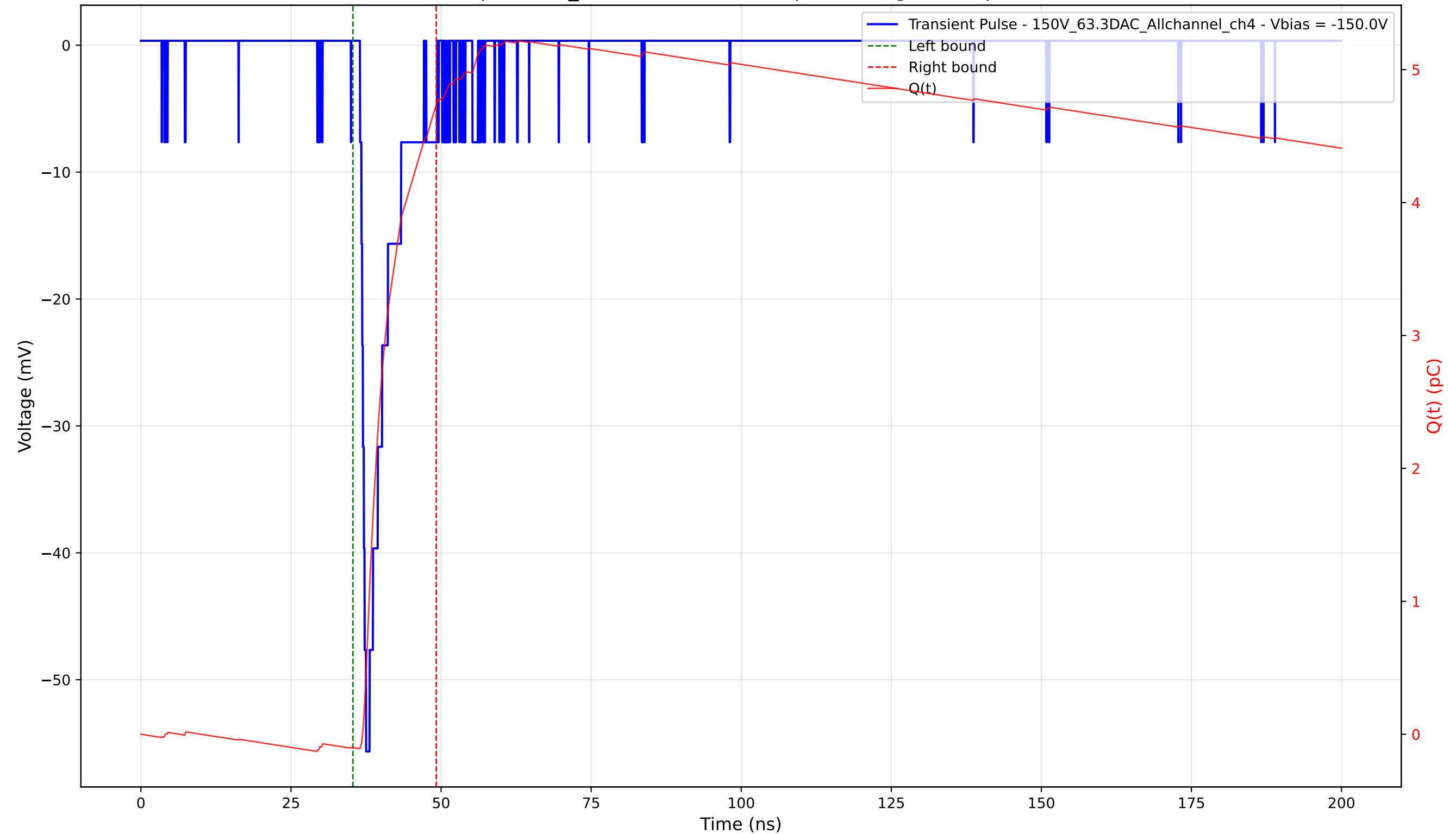
Transient Pulse - Sample: 1cm_42 - Position: 3075.0 \mu\text{m} - Charge: 4.84 pC - Rise Time: 1.01 ns
