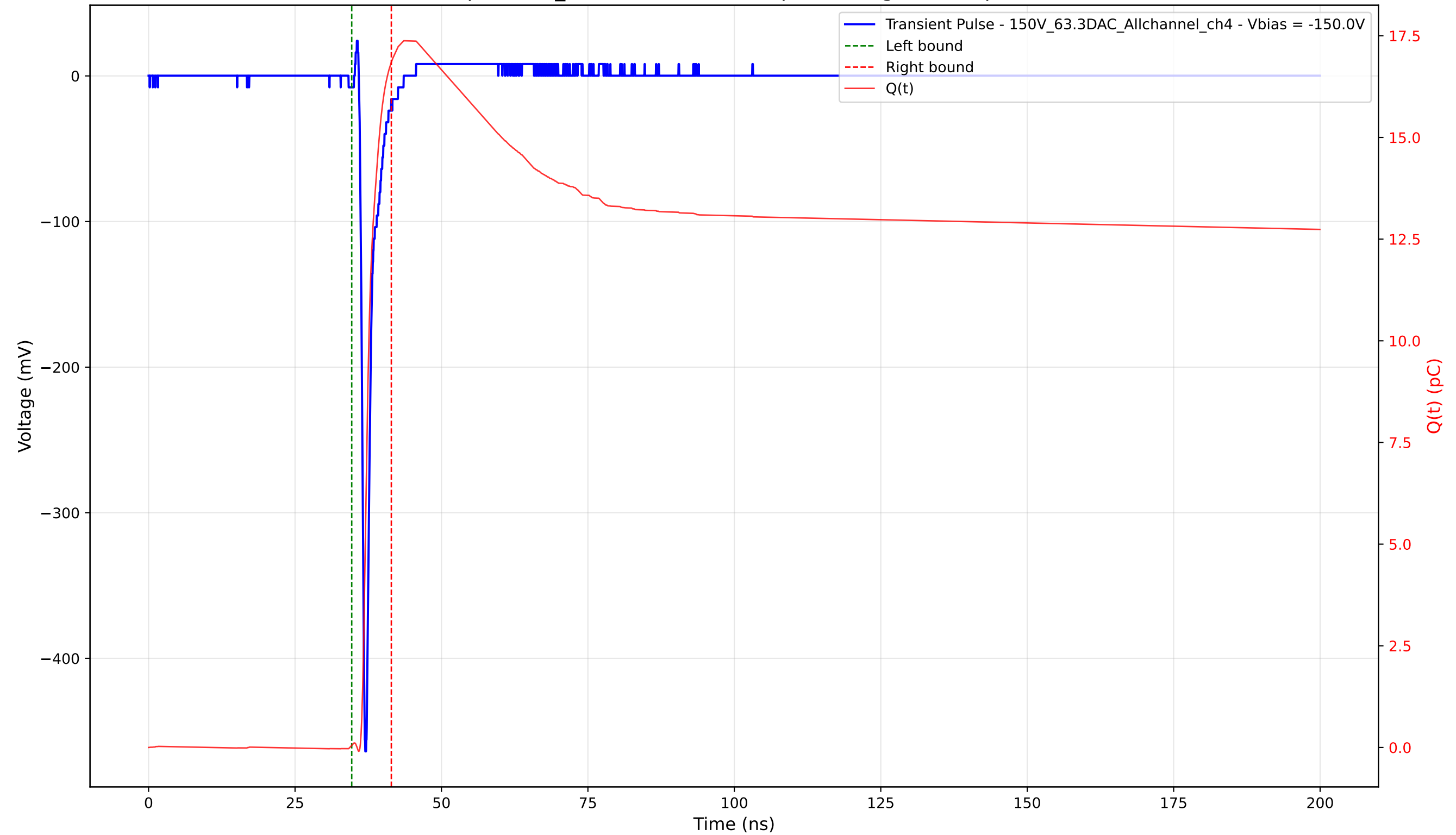
Transient Pulse - Sample: 1cm_42 - Position: 1670.0 \mu\text{m} - Charge: 16.80 pC - Rise Time: 0.69 ns
