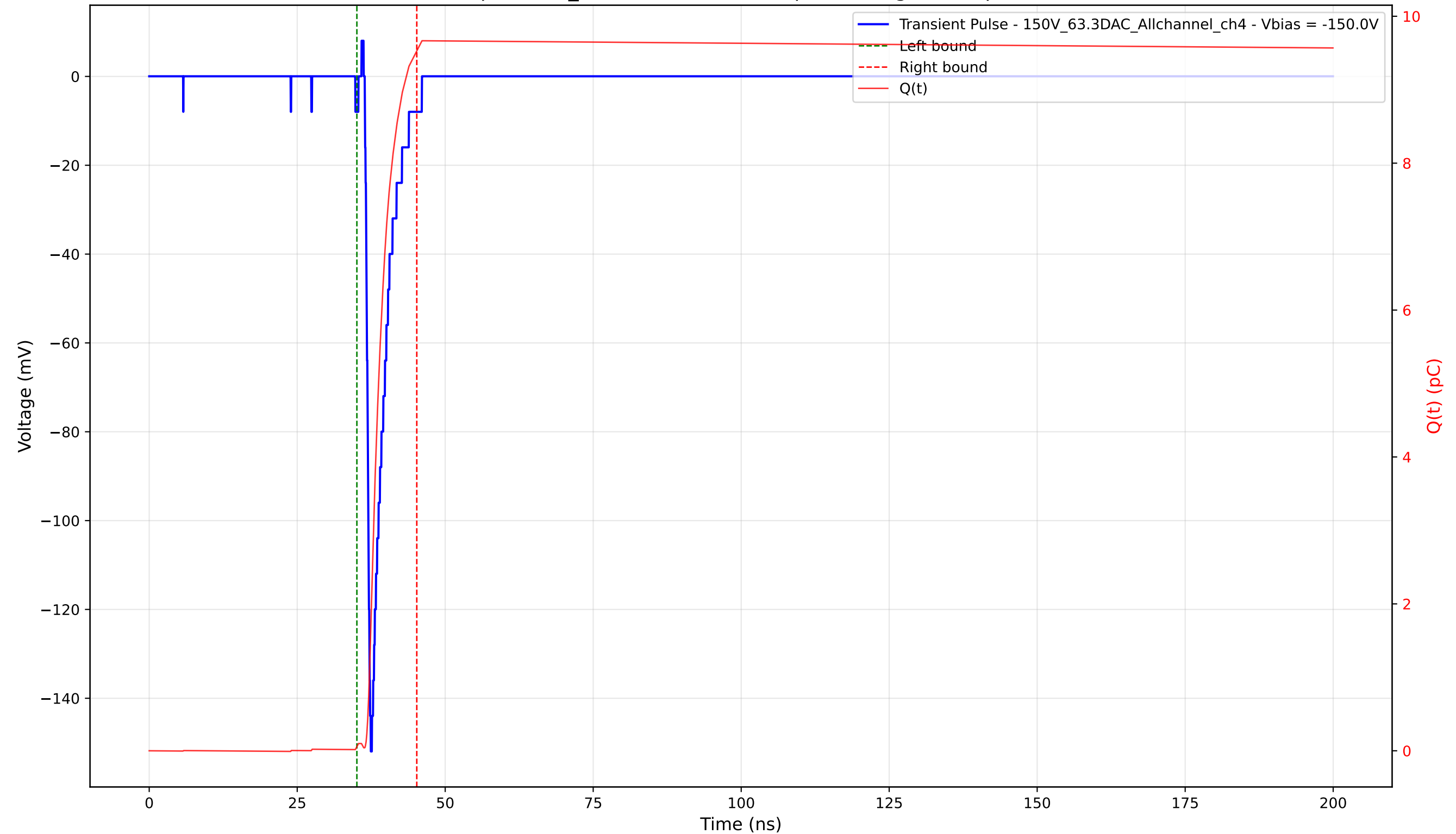
Transient Pulse - Sample: 1cm_42 - Position: 1160.0 \mu\text{m} - Charge: 9.47 pC - Rise Time: 0.84 ns
