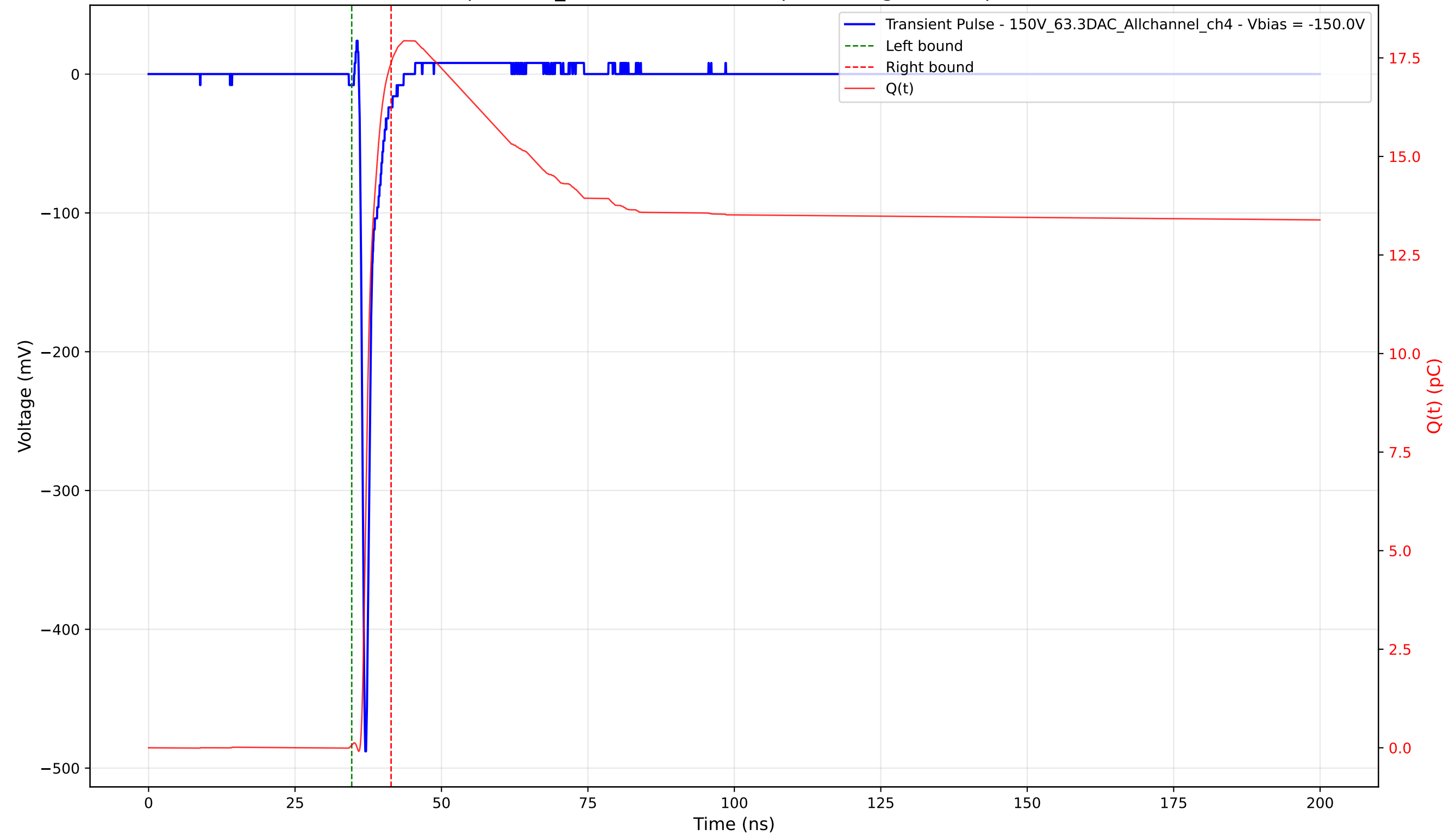
Transient Pulse - Sample: 1cm_42 - Position: 1680.0 \mu\text{m} - Charge: 17.31 pC - Rise Time: 0.74 ns
