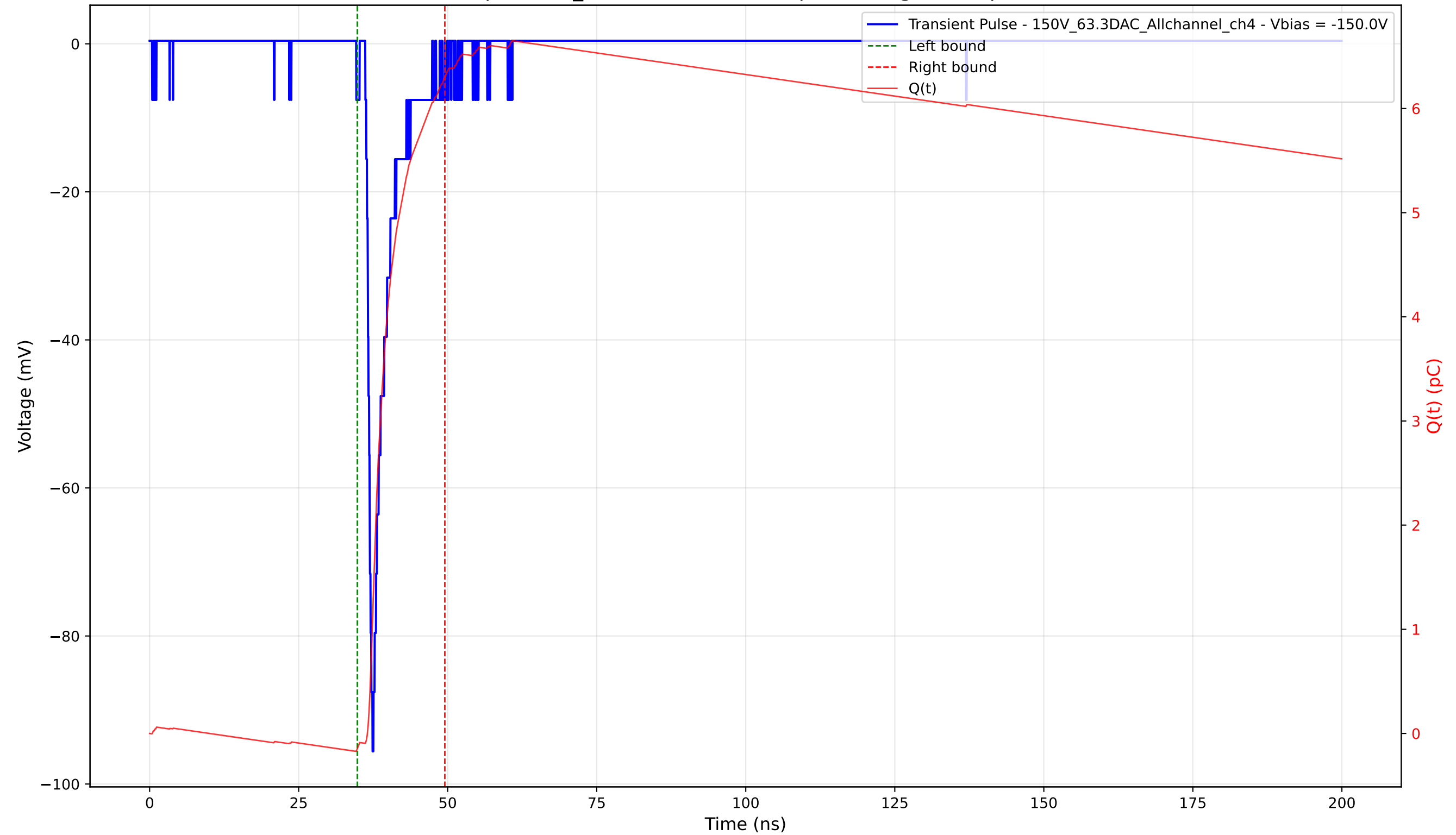
Transient Pulse - Sample: 1cm_42 - Position: 2920.0 \mu\text{m} - Charge: 6.44 pC - Rise Time: 0.87 ns
