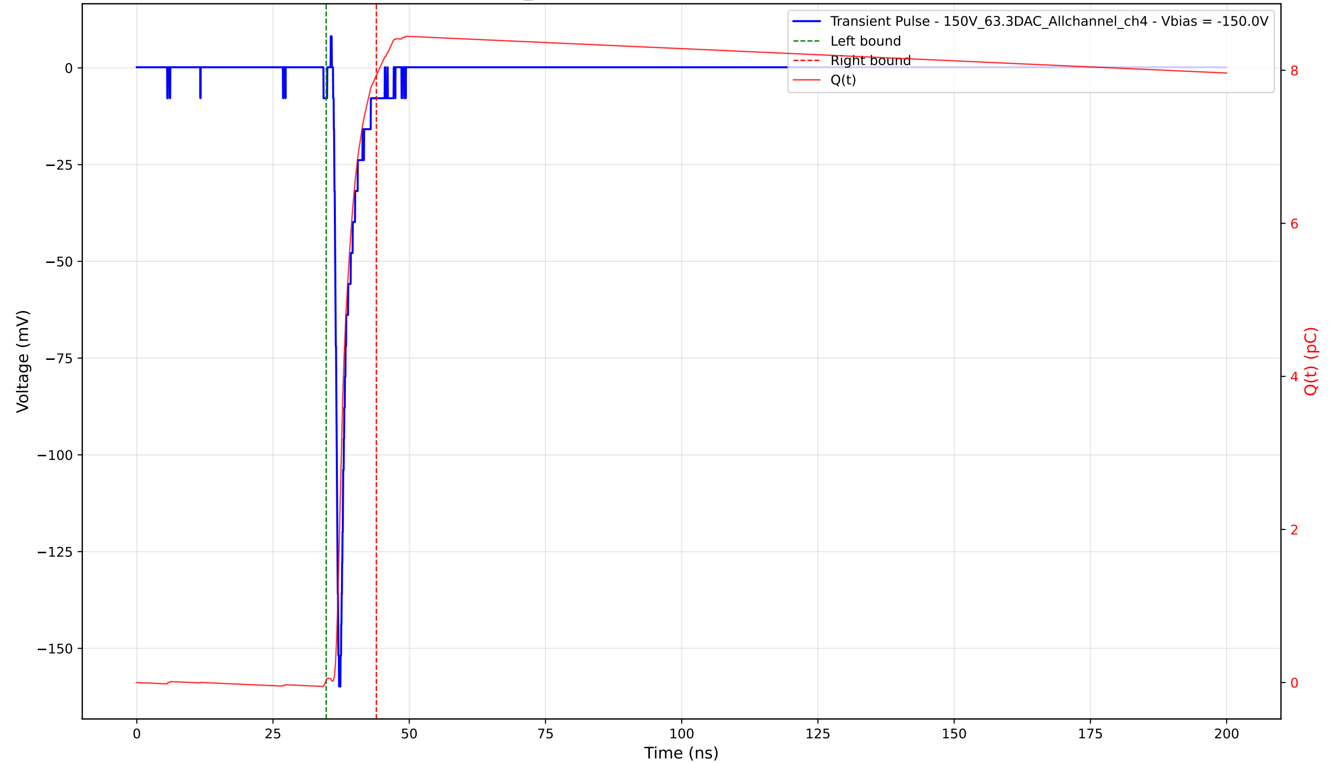
Transient Pulse - Sample: 1cm_42 - Position: 2660.0 \mu\text{m} - Charge: 7.91 pC - Rise Time: 0.80 ns
