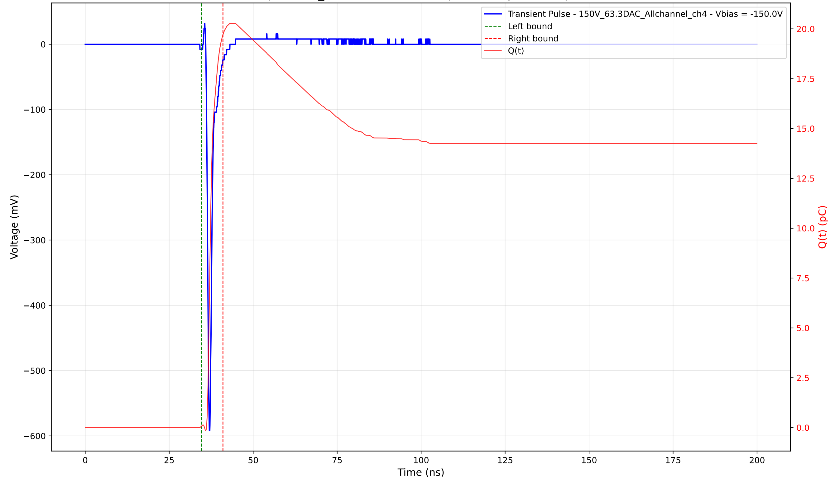
Transient Pulse - Sample: 1cm_42 - Position: 1795.0 \mu\text{m} - Charge: 19.62 pC - Rise Time: 0.72 ns
