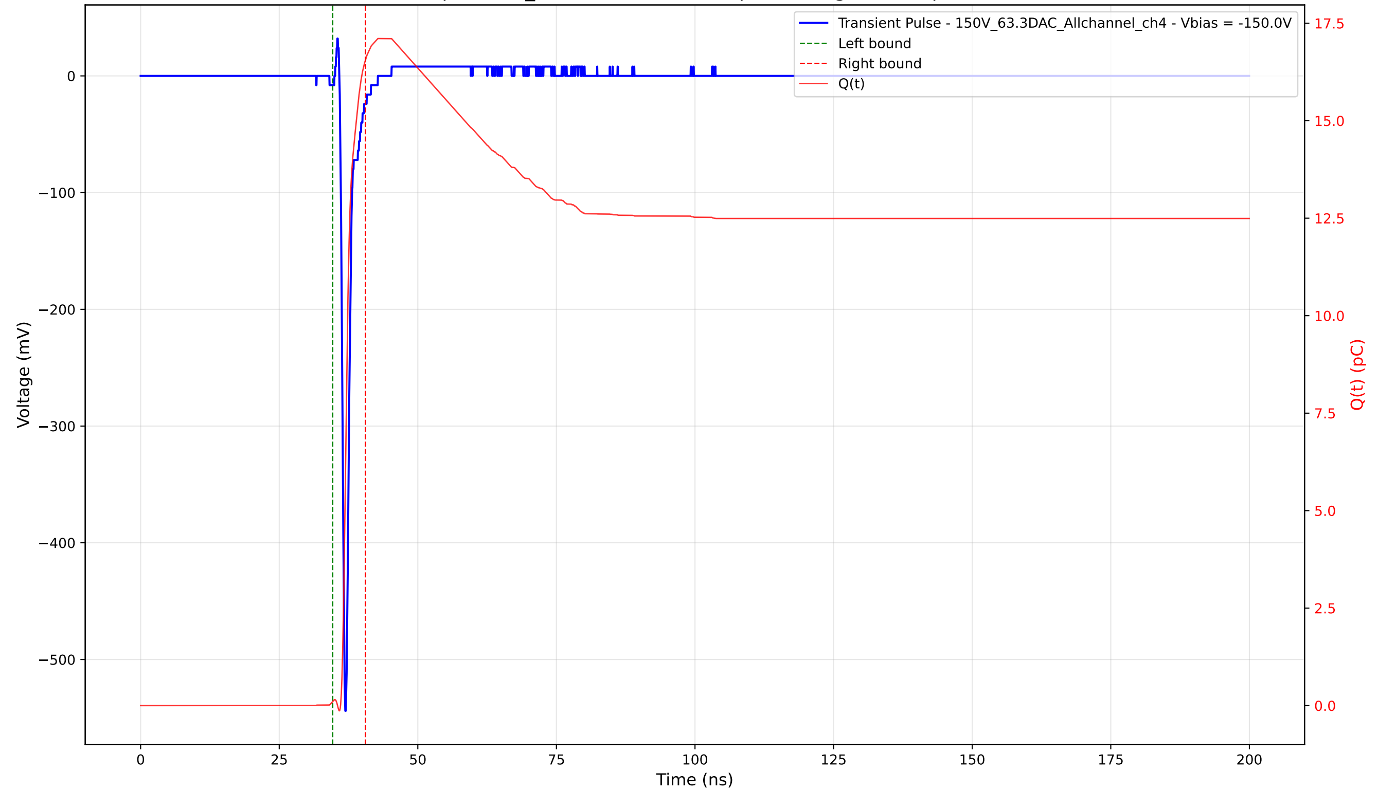
Transient Pulse - Sample: 1cm_42 - Position: 2155.0 \mu\text{m} - Charge: 16.45 pC - Rise Time: 0.71 ns
