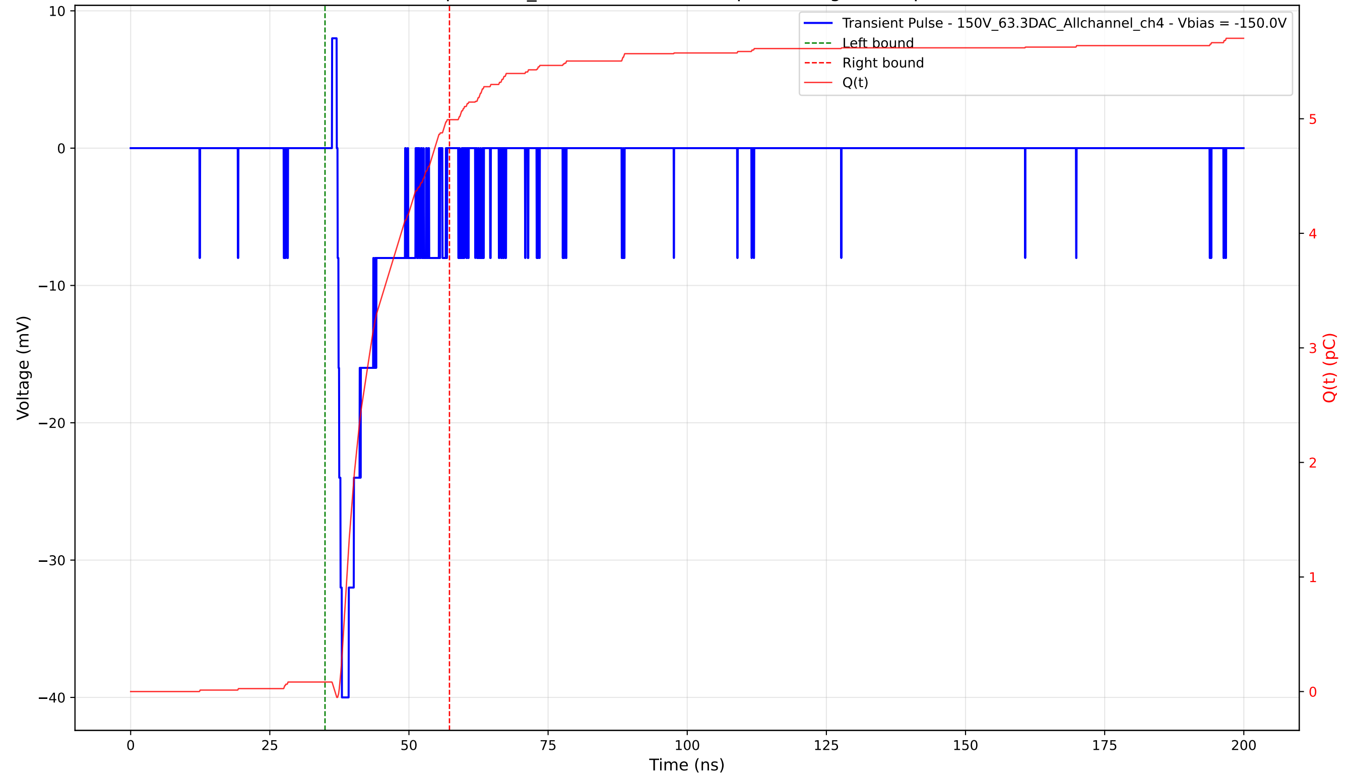
Transient Pulse - Sample: 1cm_42 - Position: 3395.0 \mu\text{m} - Charge: 4.91 pC - Rise Time: 0.78 ns
