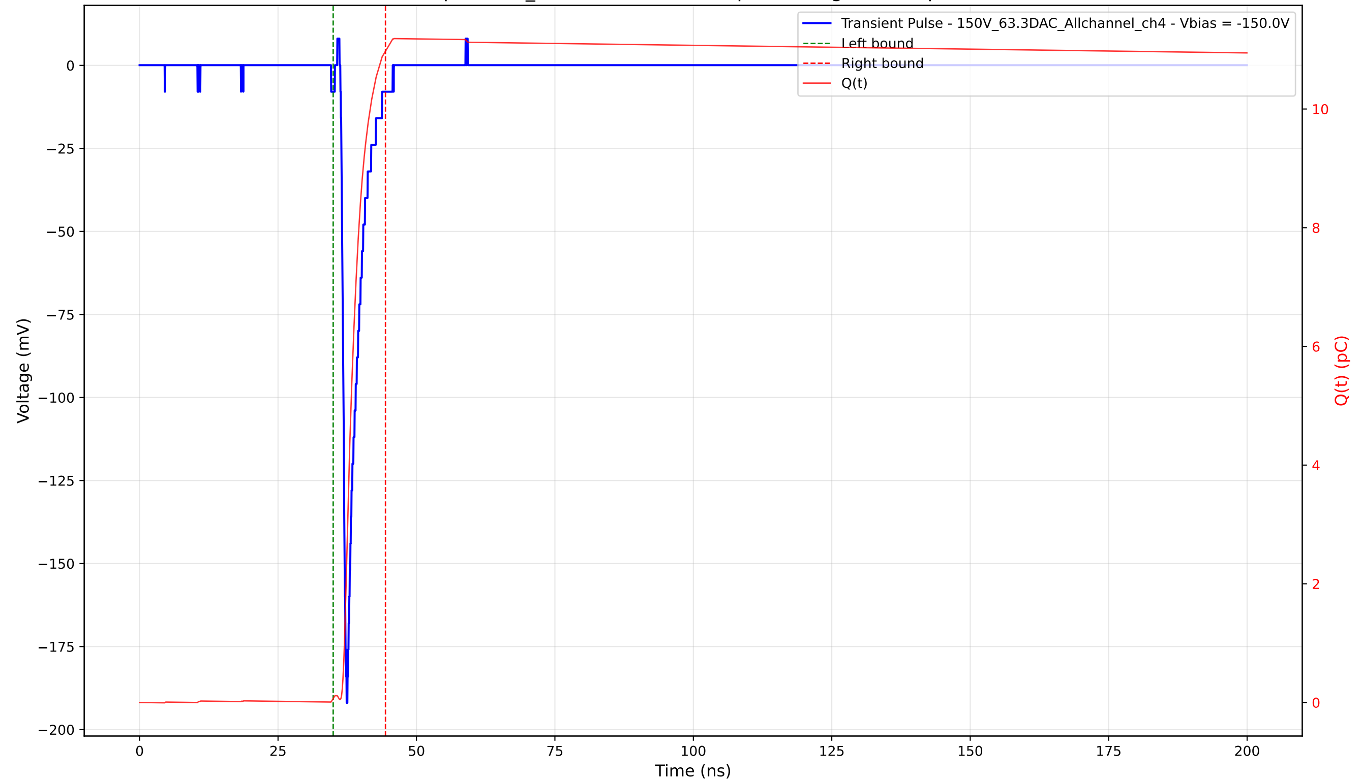
Transient Pulse - Sample: 1cm_42 - Position: 1300.0 \mu\text{m} - Charge: 10.91 pC - Rise Time: 0.78 ns
