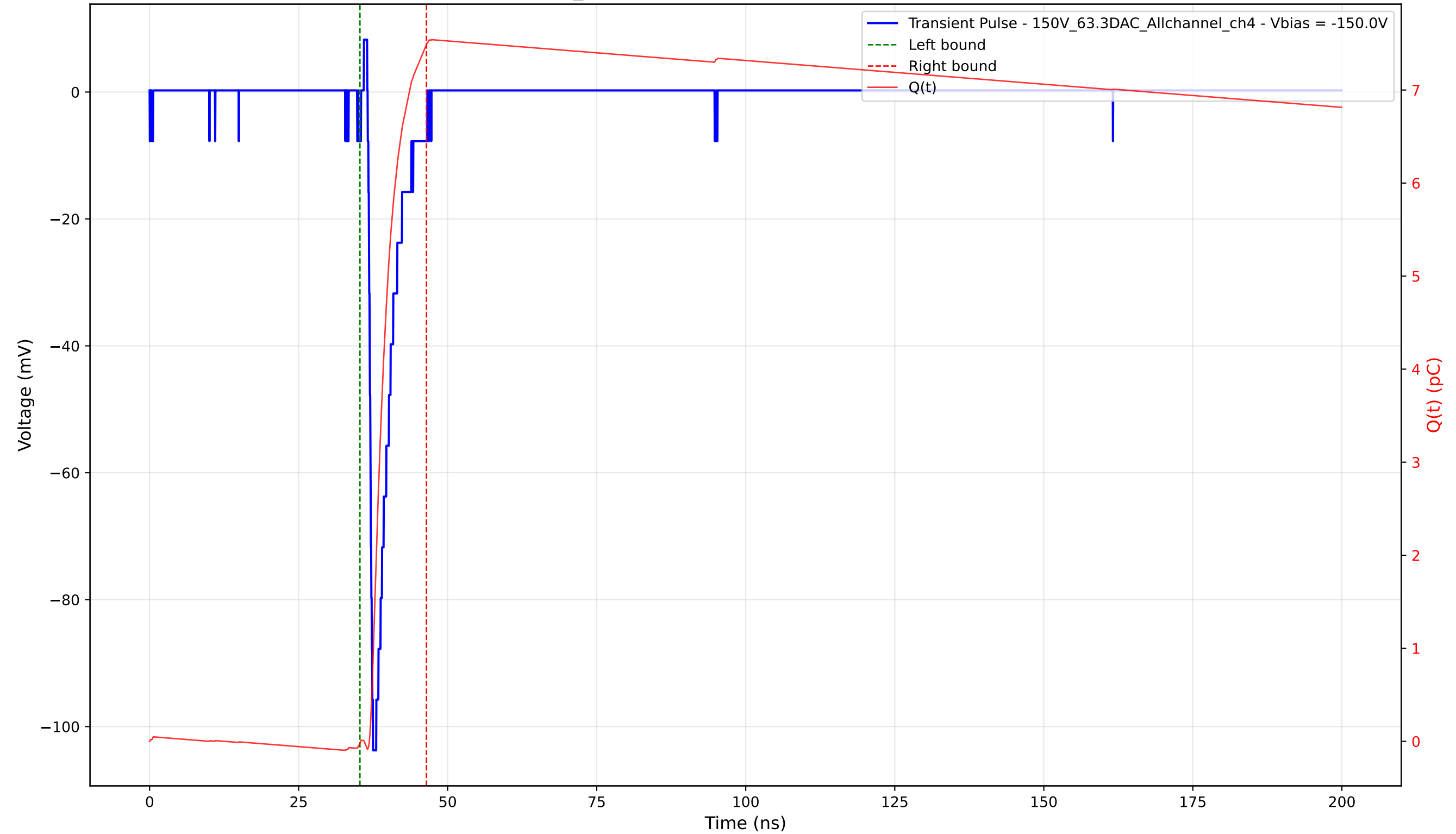
Transient Pulse - Sample: 1cm_42 - Position: 1045.0 \mu\text{m} - Charge: 7.51 pC - Rise Time: 0.67 ns
