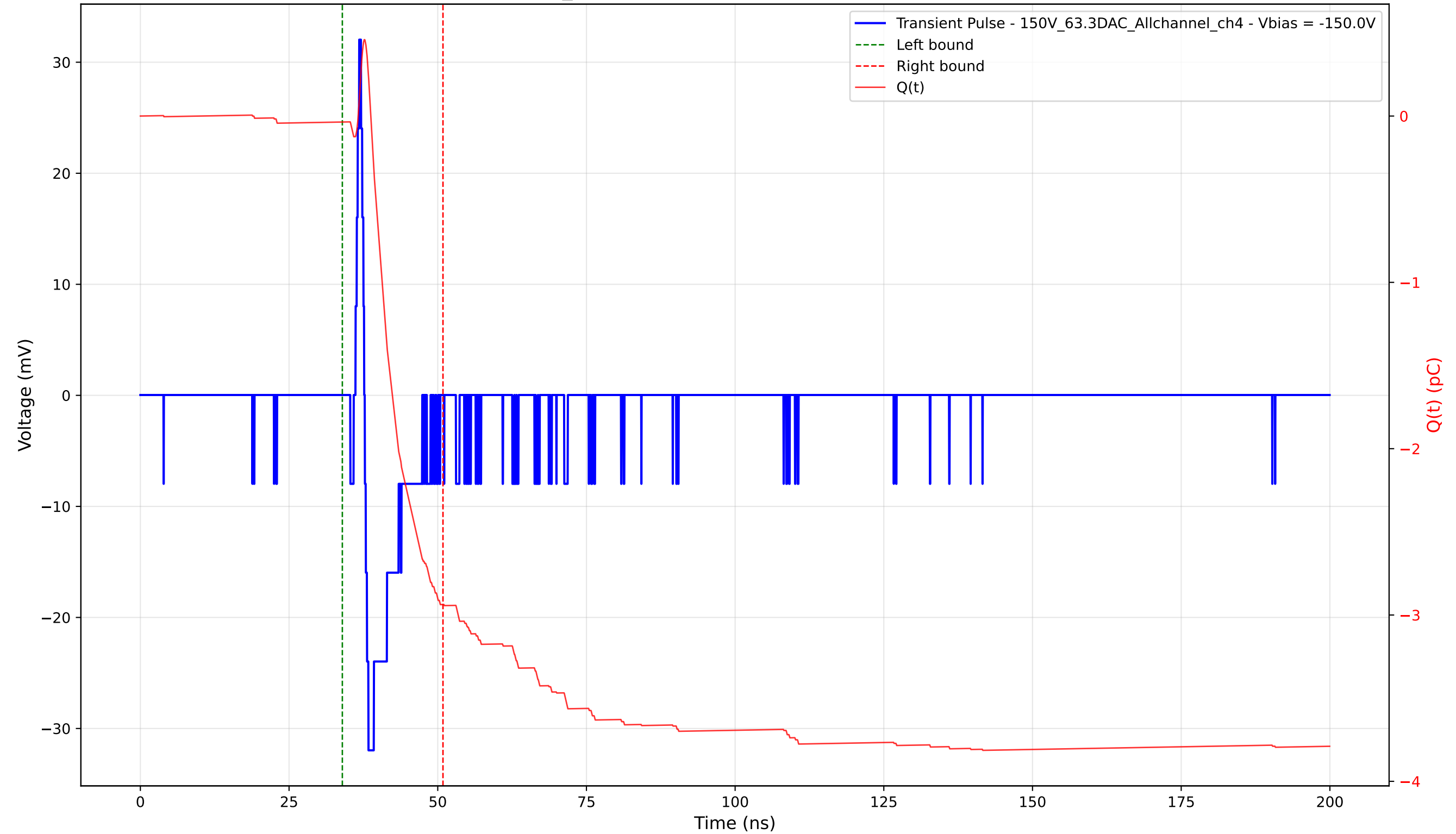
Transient Pulse - Sample: 1cm_42 - Position: 4345.0 \mu\text{m} - Charge: 2.90 pC - Rise Time: 0.62 ns
