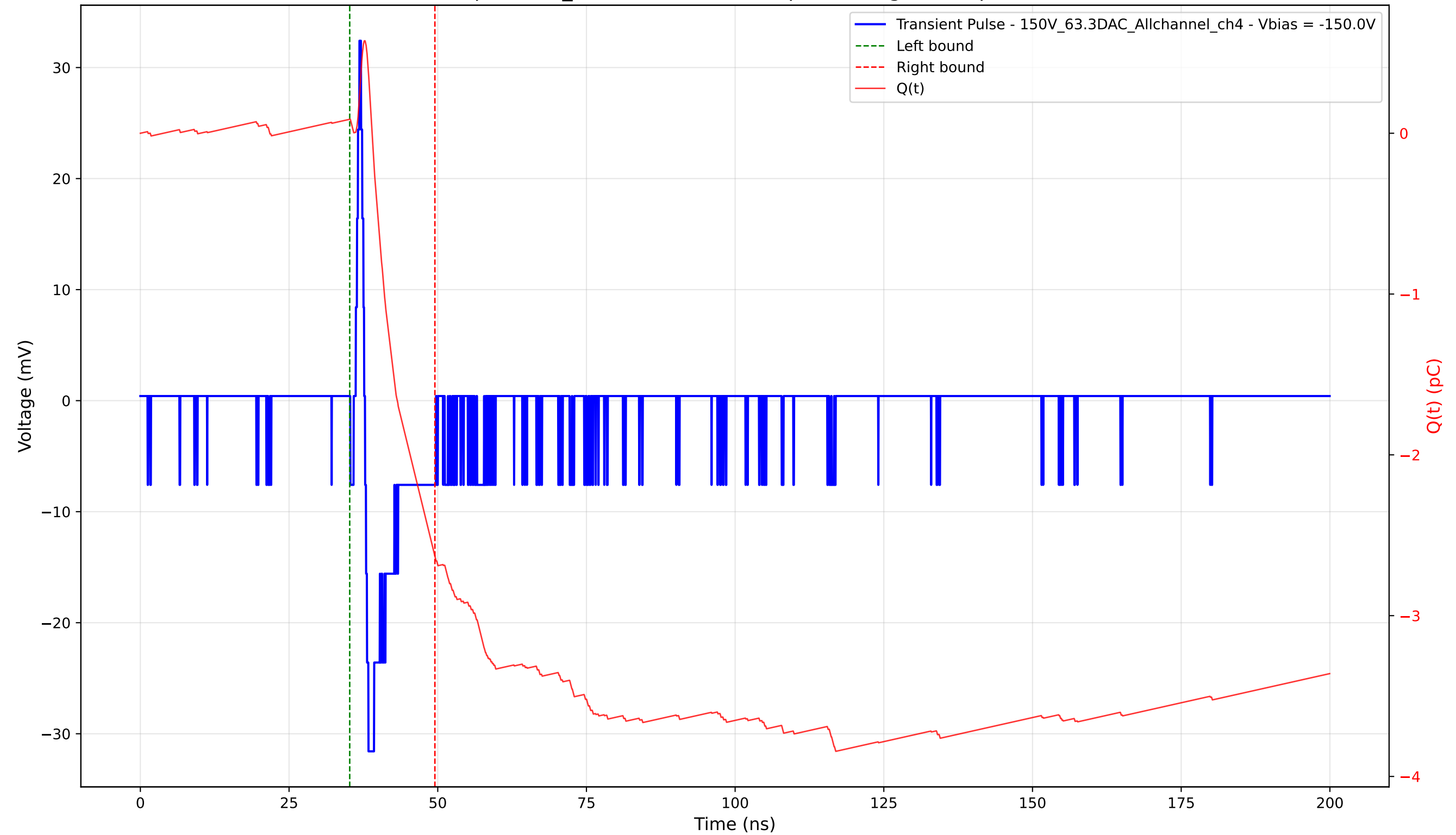
Transient Pulse - Sample: 1cm_42 - Position: 4240.0 \mu\text{m} - Charge: 2.72 pC - Rise Time: 0.63 ns
