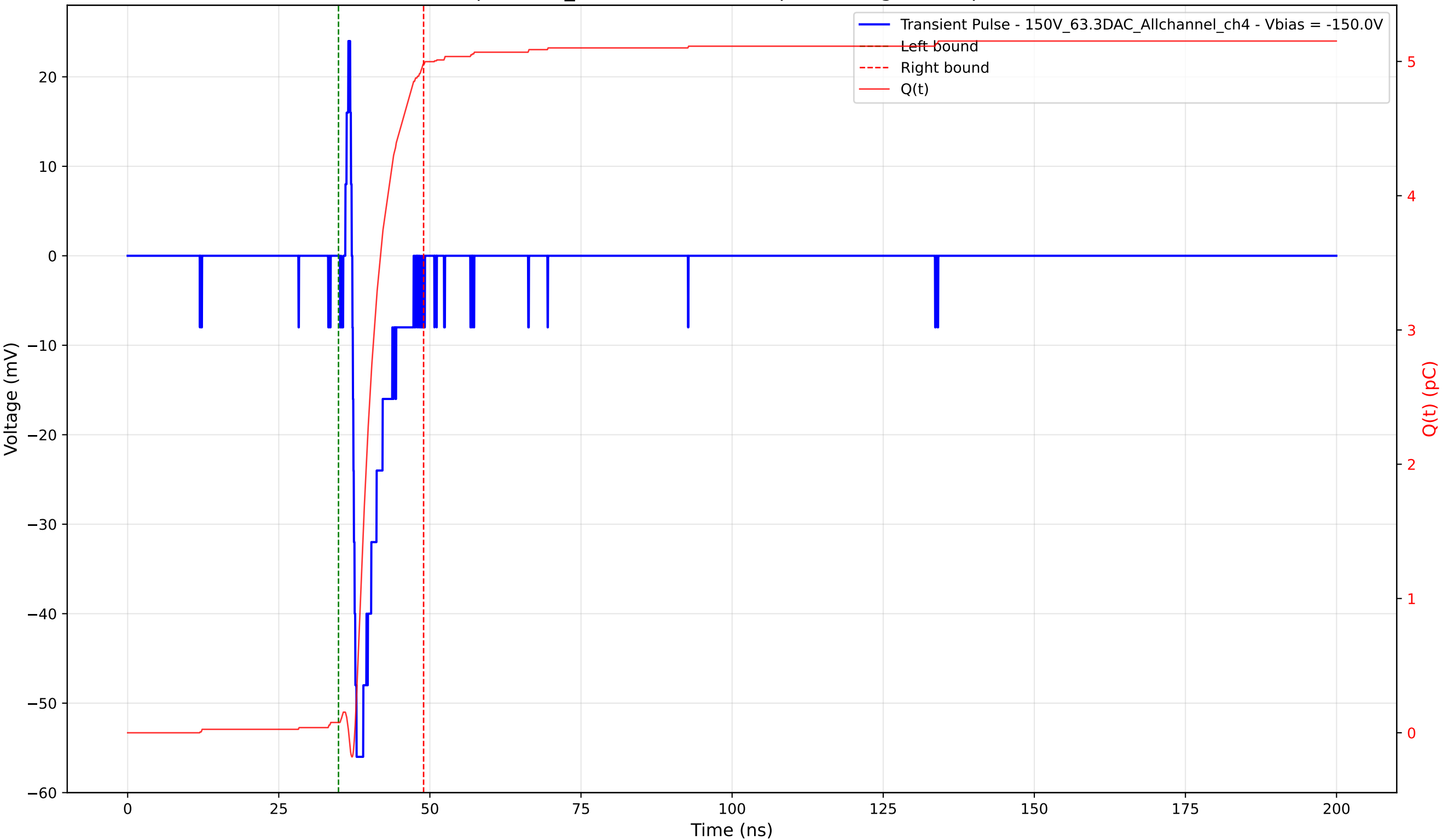
Transient Pulse - Sample: 1cm_42 - Position: 550.0 \mu\text{m} - Charge: 4.90 pC - Rise Time: 0.69 ns
