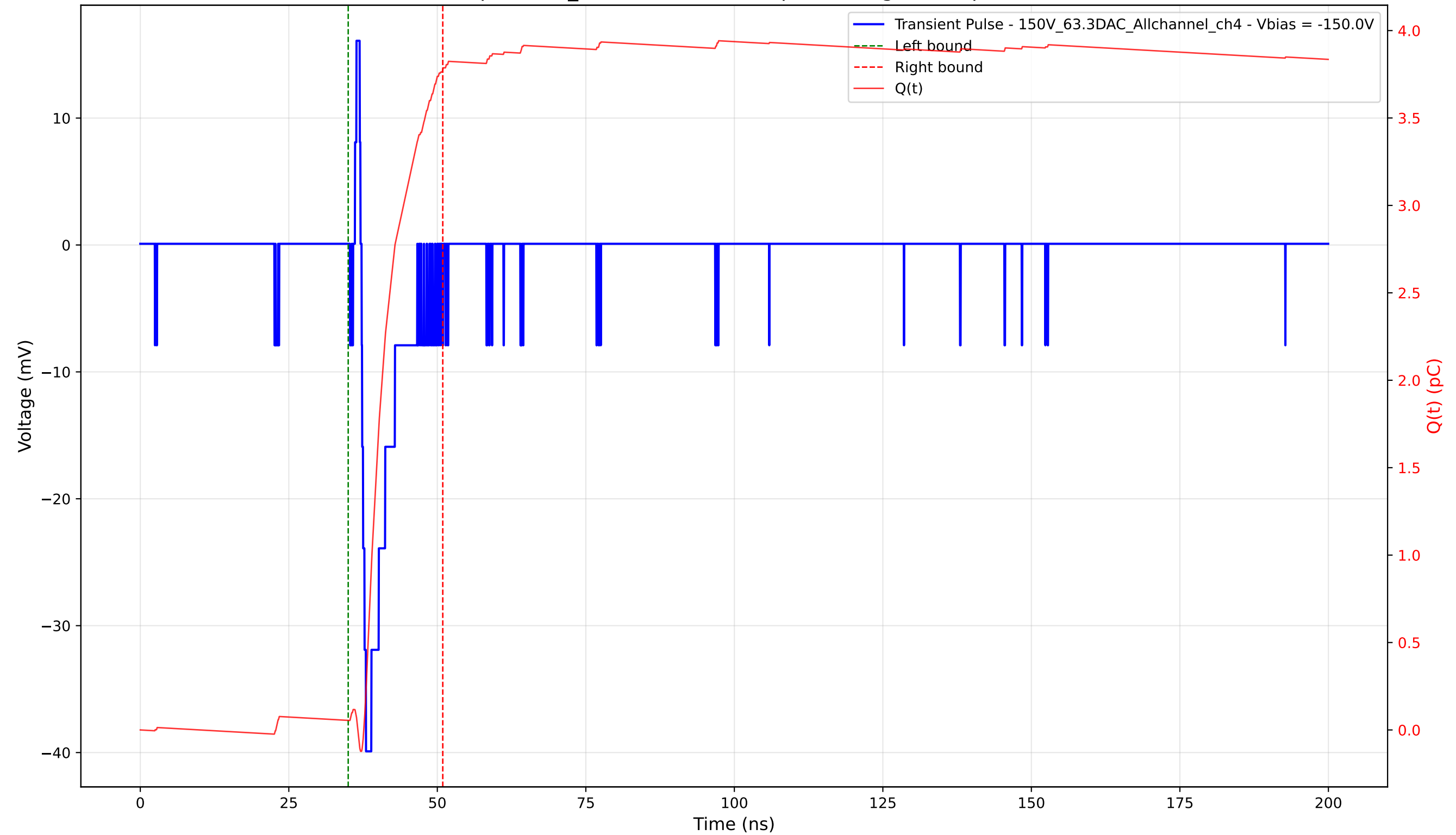
Transient Pulse - Sample: 1cm_42 - Position: 380.0 \mu\text{m} - Charge: 3.72 pC - Rise Time: 0.74 ns
