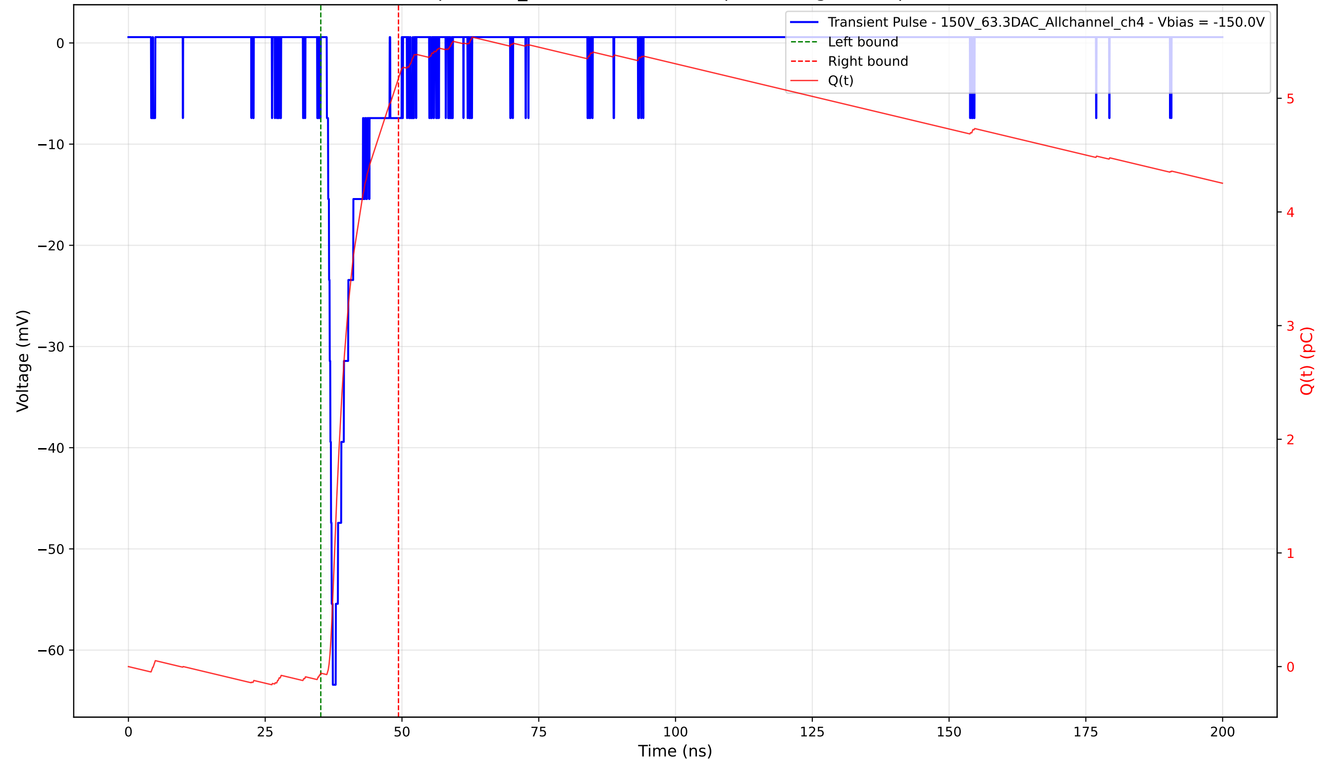
Transient Pulse - Sample: 1cm_42 - Position: 3010.0 \mu\text{m} - Charge: 5.24 pC - Rise Time: 1.09 ns
