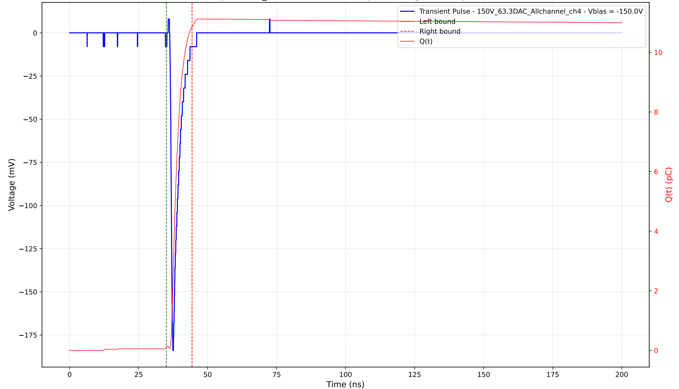
Transient Pulse - Sample: 1cm_42 - Position: 1240.0 \mu\text{m} - Charge: 10.75 pC - Rise Time: 0.75 ns
