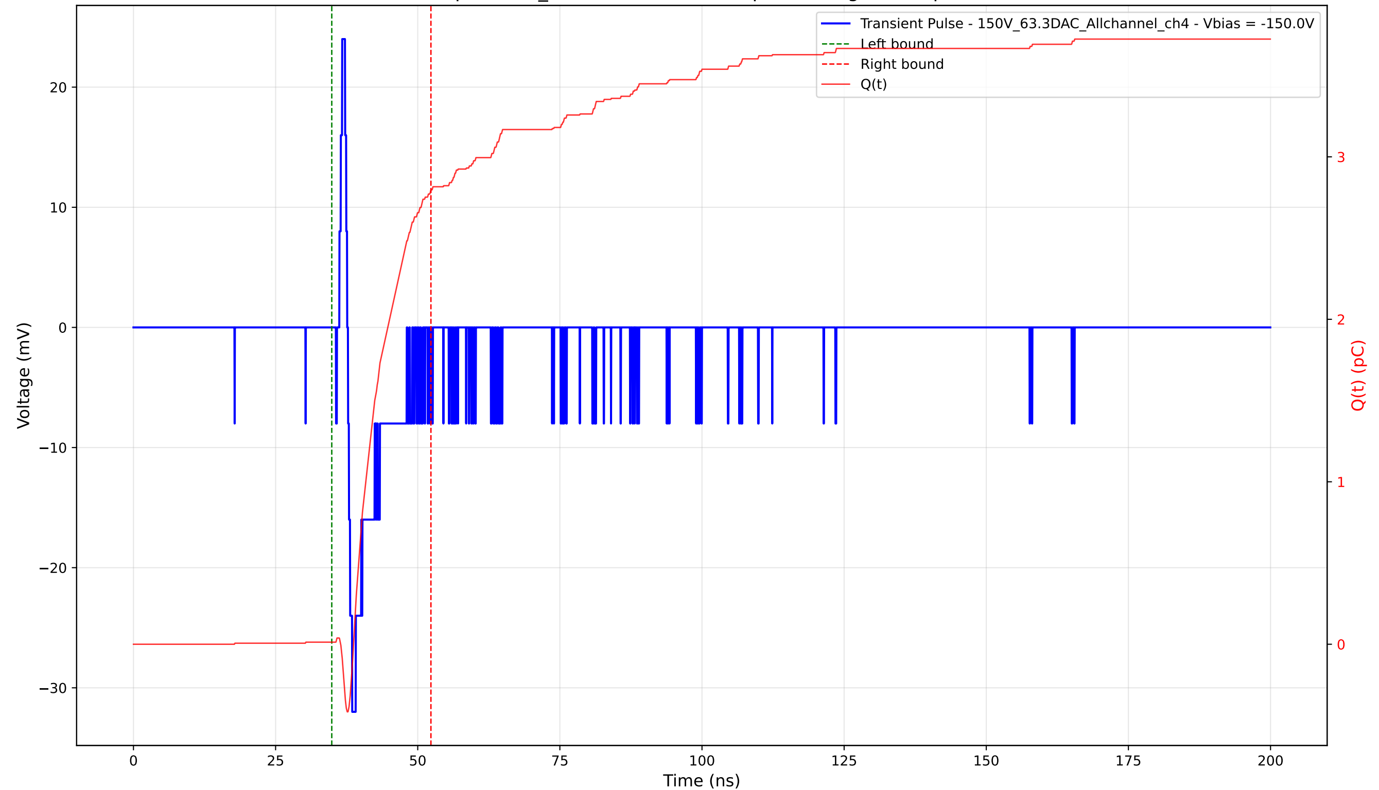
Transient Pulse - Sample: 1cm_42 - Position: 3965.0 \mu\text{m} - Charge: 2.78 pC - Rise Time: 0.74 ns
