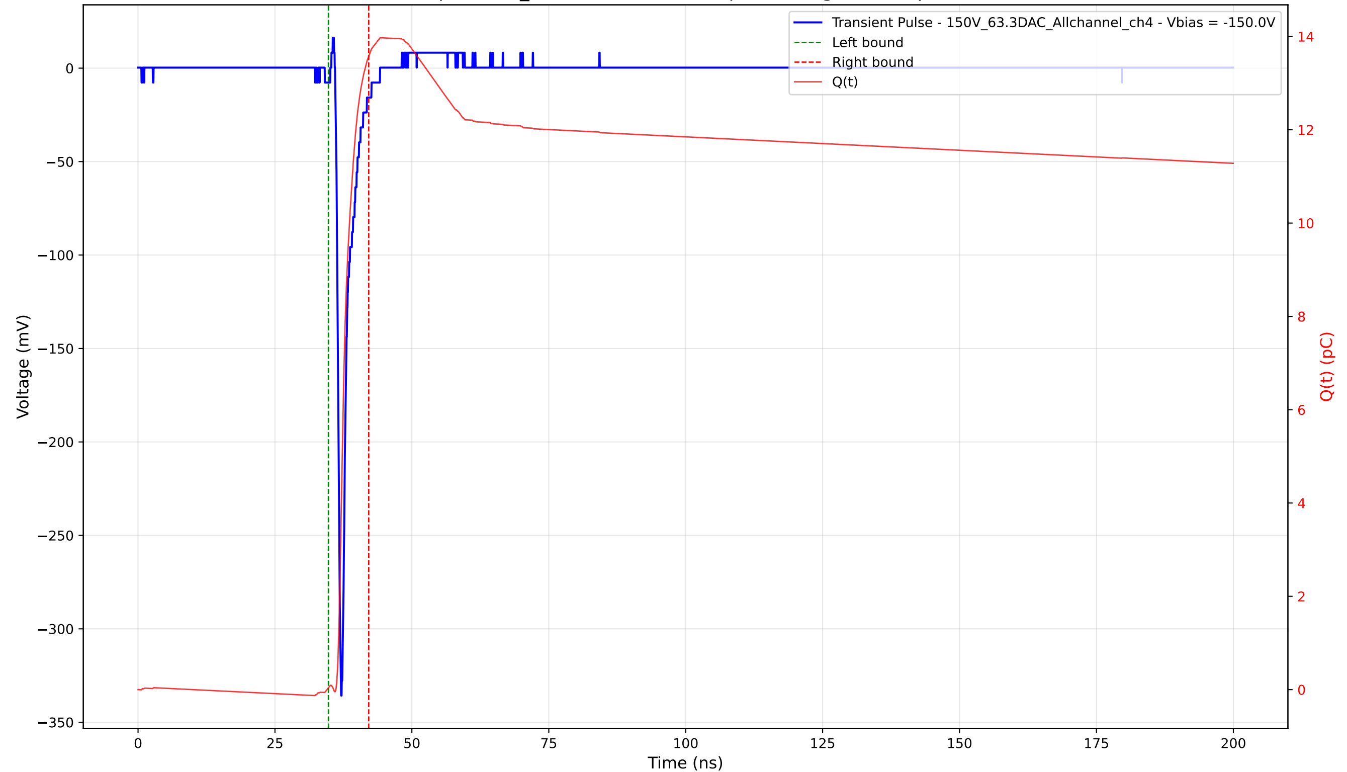
Transient Pulse - Sample: 1cm_42 - Position: 1570.0 \mu\text{m} - Charge: 13.54 pC - Rise Time: 0.78 ns
