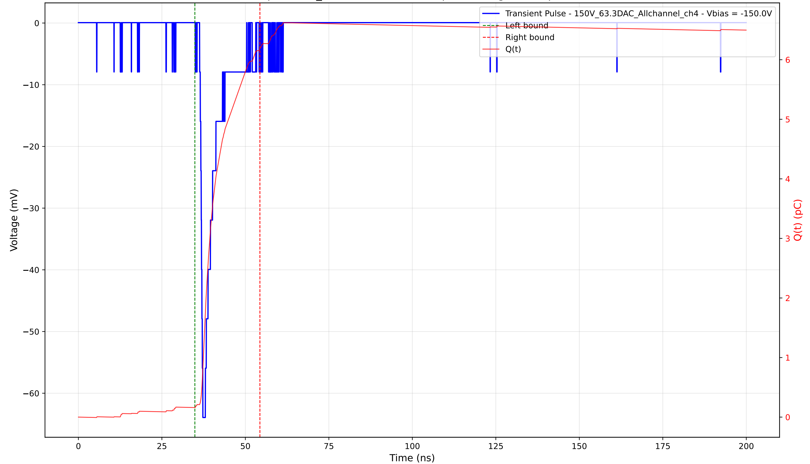
Transient Pulse - Sample: 1cm_42 - Position: 3005.0 \mu\text{m} - Charge: 6.03 pC - Rise Time: 0.97 ns
