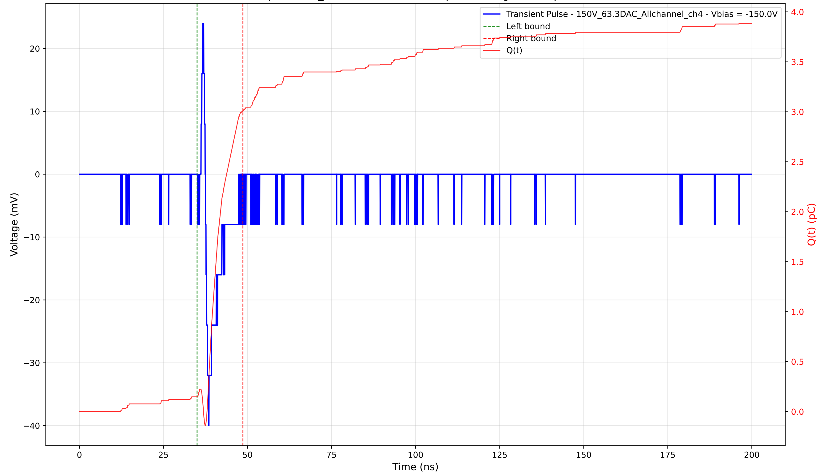
Transient Pulse - Sample: 1cm_42 - Position: 4780.0 \mu\text{m} - Charge: 2.86 pC - Rise Time: 0.94 ns
