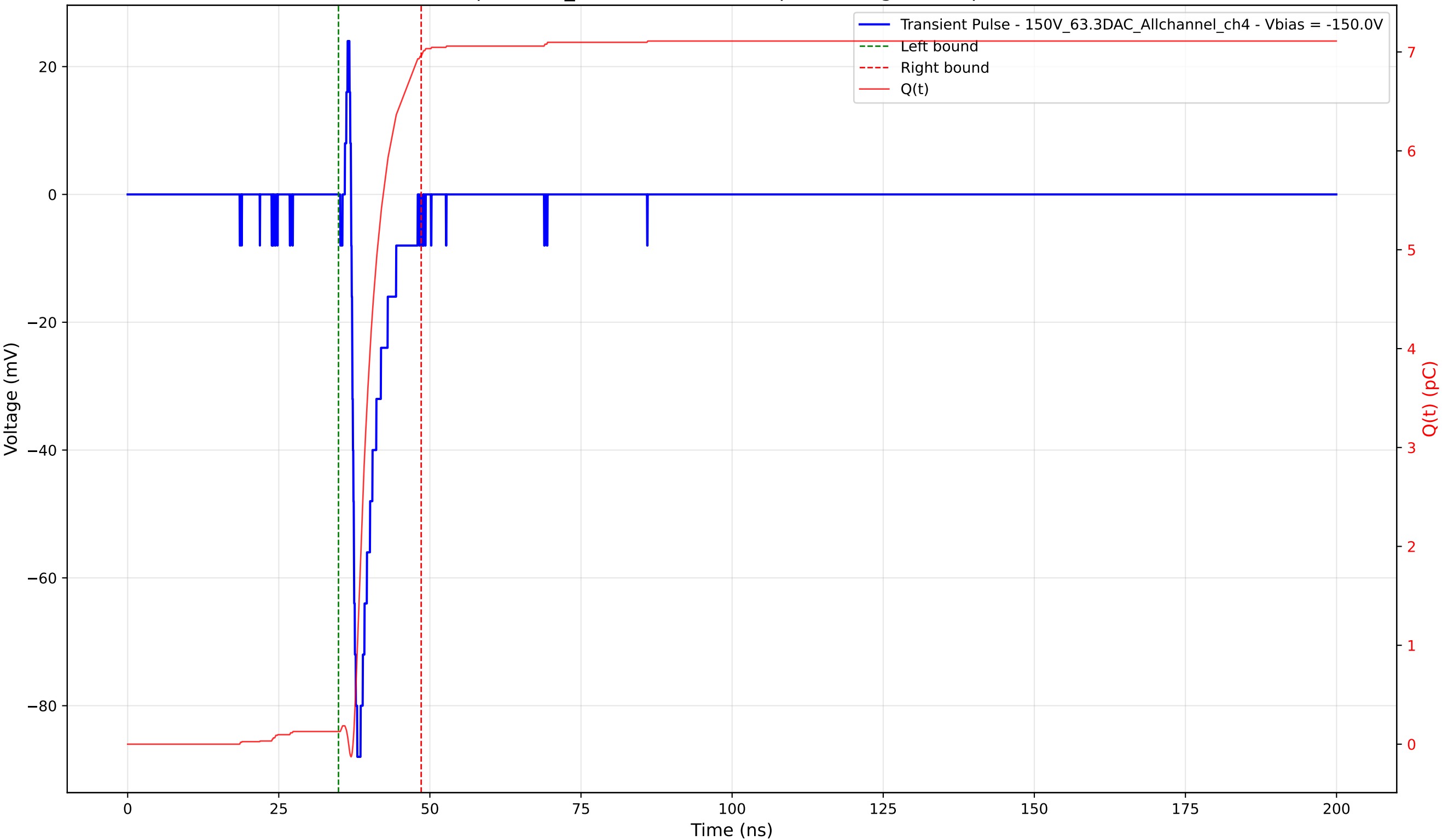
Transient Pulse - Sample: 1cm_42 - Position: 800.0 \mu\text{m} - Charge: 6.83 pC - Rise Time: 0.72 ns
