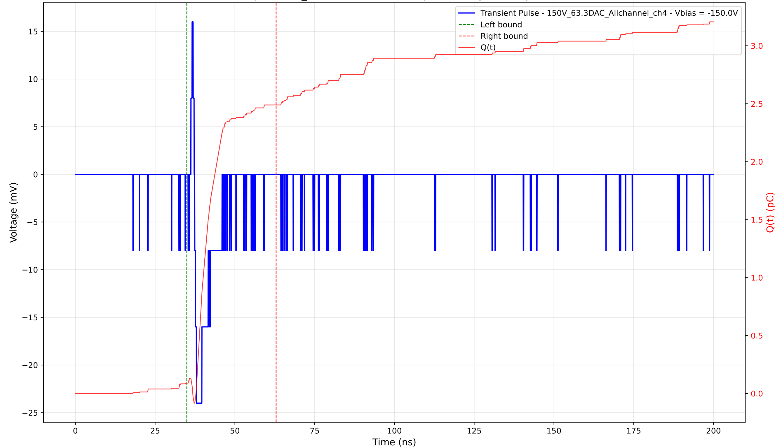
Transient Pulse - Sample: 1cm_42 - Position: 4960.0 \mu\text{m} - Charge: 2.40 pC - Rise Time: 0.55 ns
