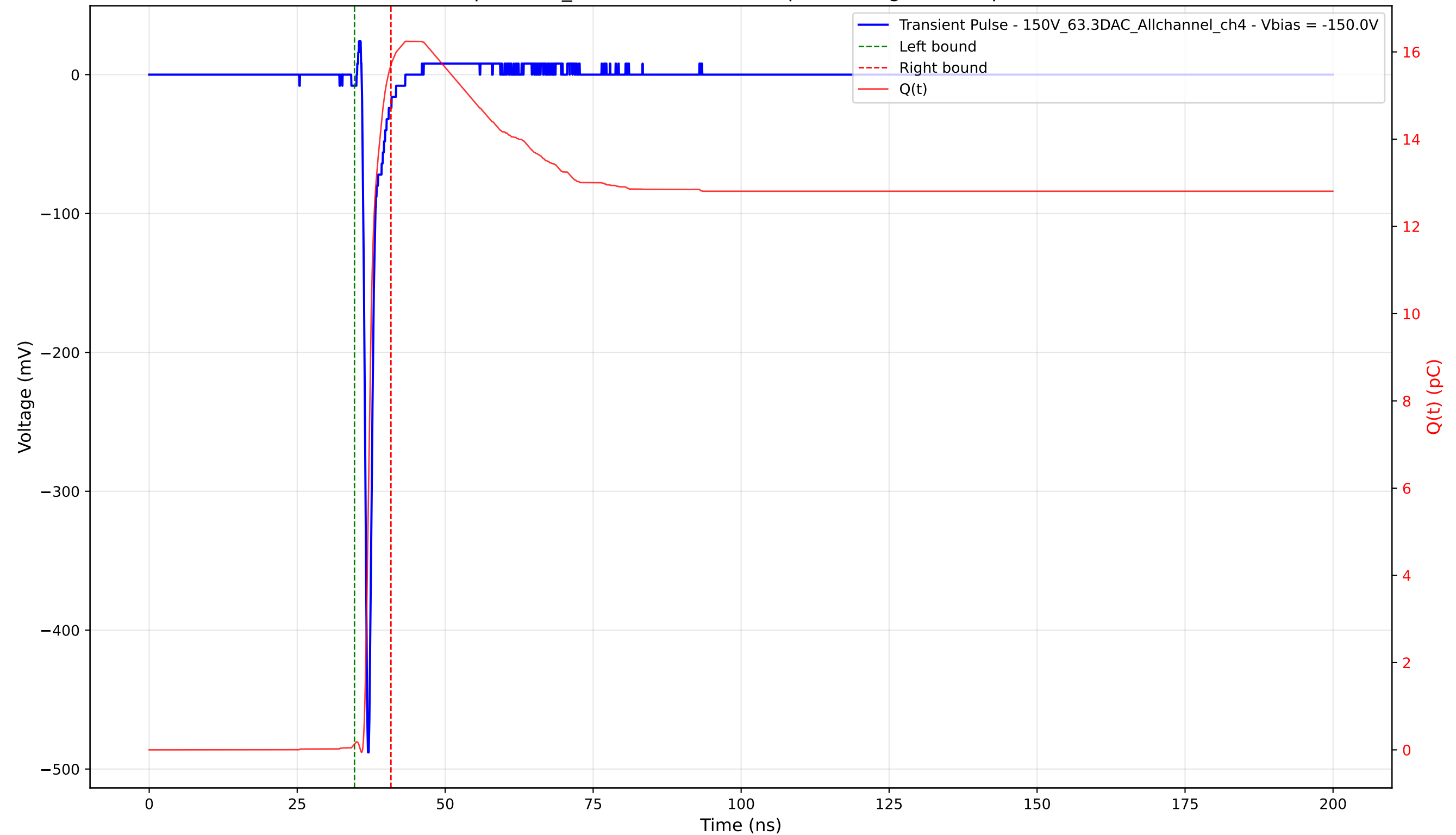
Transient Pulse - Sample: 1cm_42 - Position: 2290.0 \mu\text{m} - Charge: 15.57 pC - Rise Time: 0.72 ns
