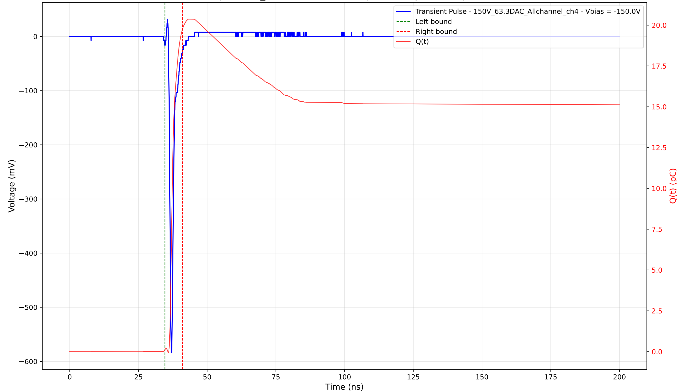
Transient Pulse - Sample: 1cm_42 - Position: 1770.0 \mu\text{m} - Charge: 19.67 pC - Rise Time: 0.73 ns
