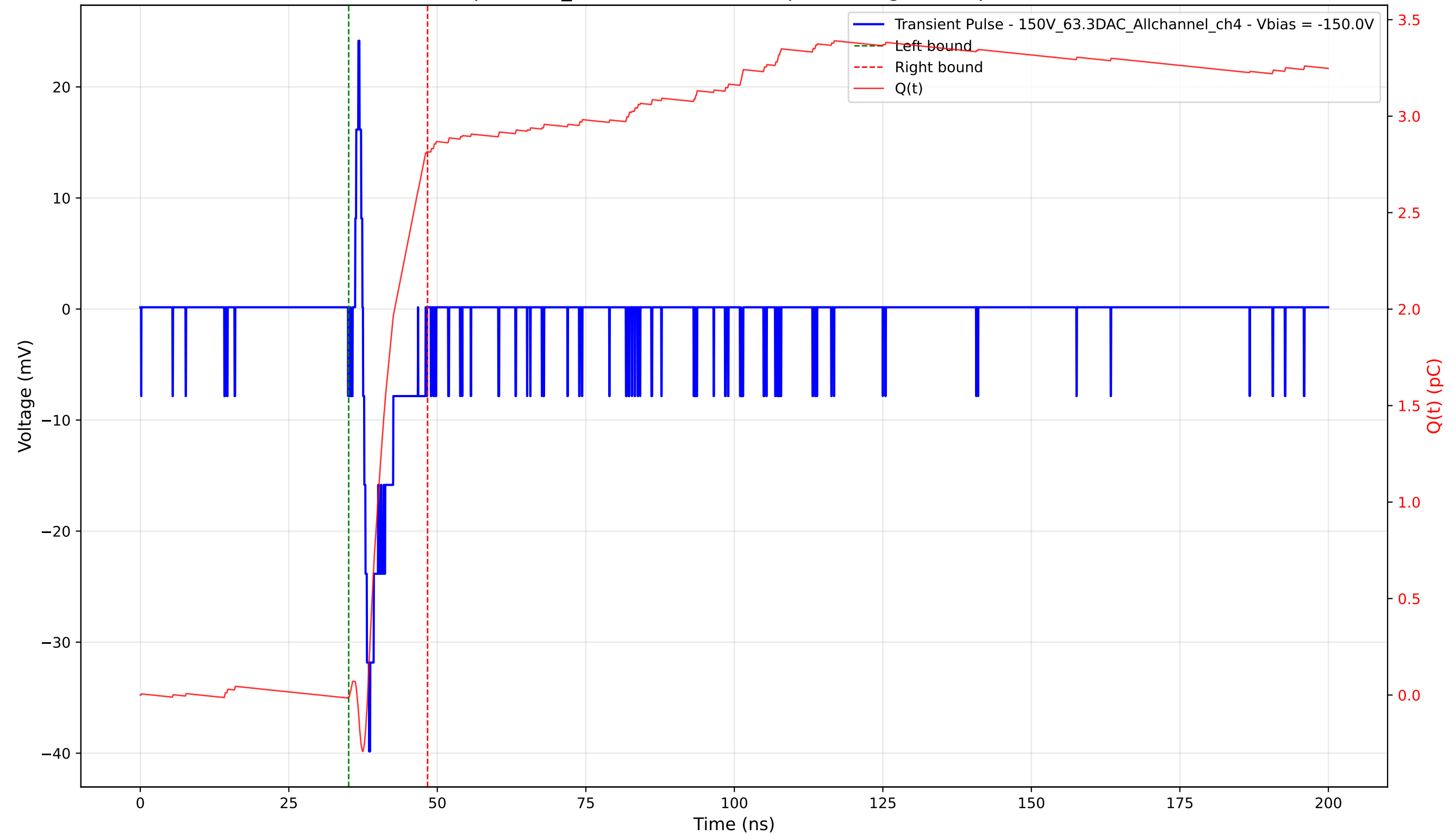
Transient Pulse - Sample: 1cm_42 - Position: 4735.0 \mu\text{m} - Charge: 2.82 pC - Rise Time: 1.02 ns
