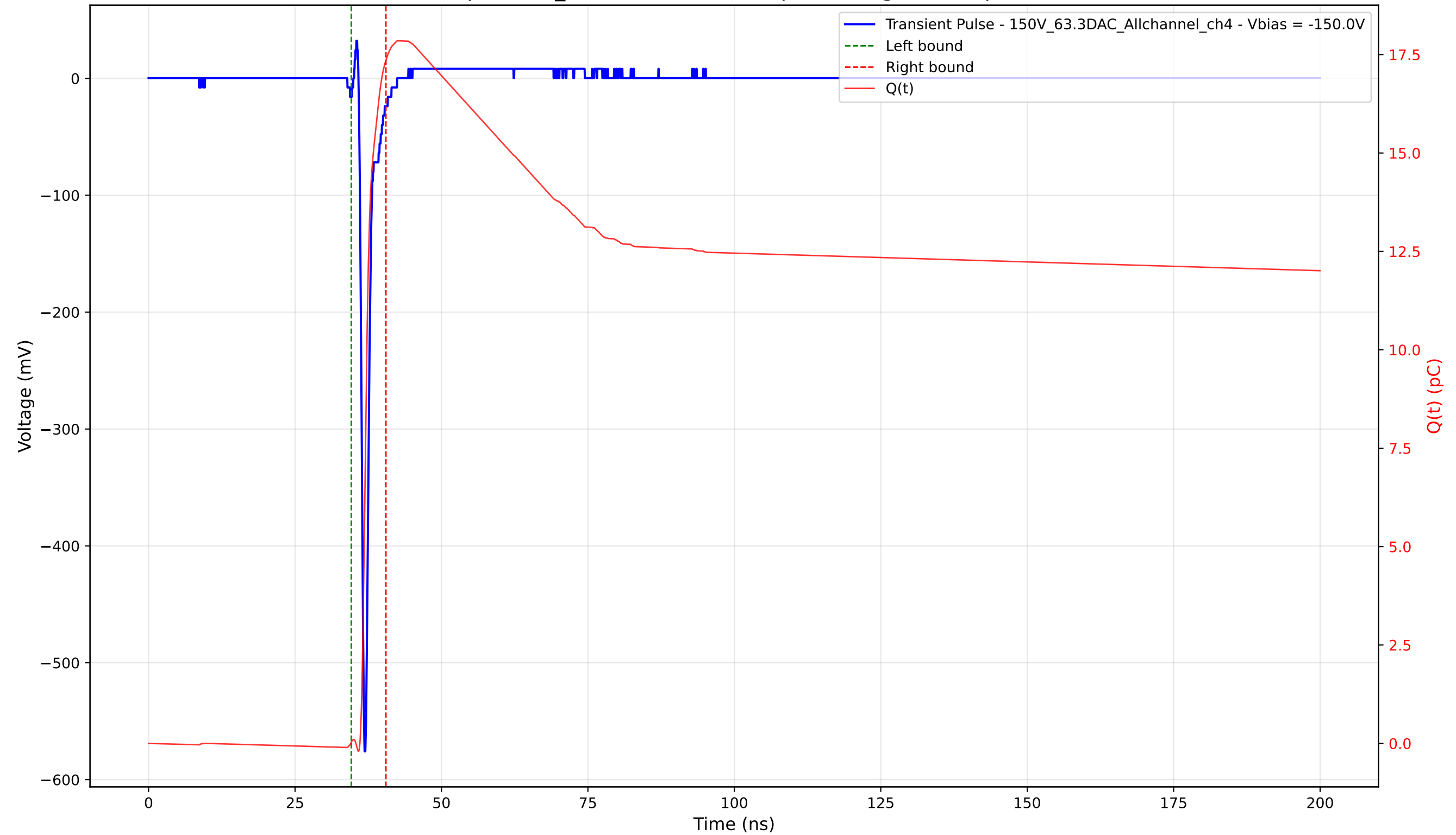
Transient Pulse - Sample: 1cm_42 - Position: 2055.0 \mu\text{m} - Charge: 17.33 pC - Rise Time: 0.69 ns
