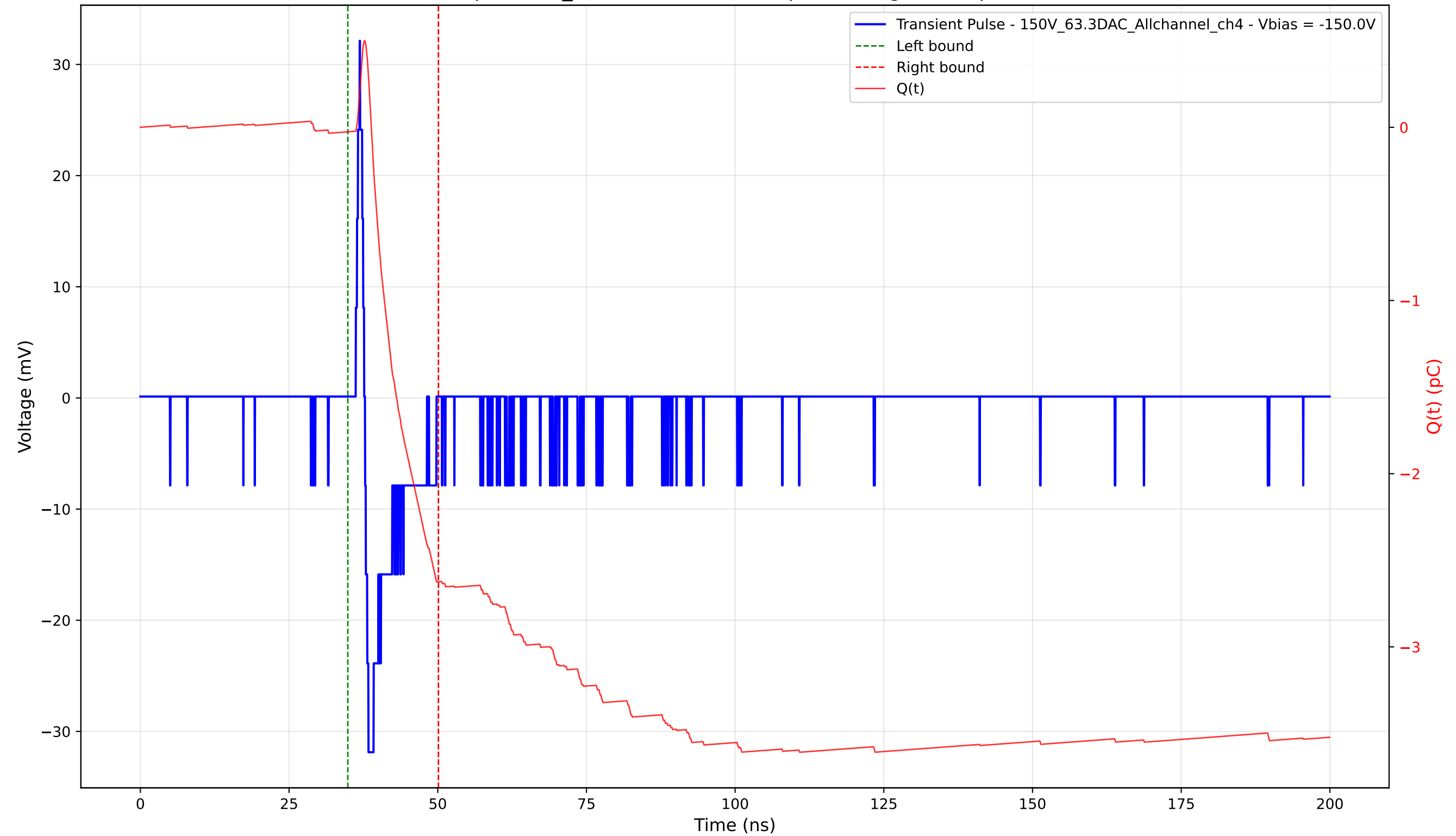
Transient Pulse - Sample: 1cm_42 - Position: 4365.0 \mu\text{m} - Charge: 2.60 pC - Rise Time: 0.66 ns
