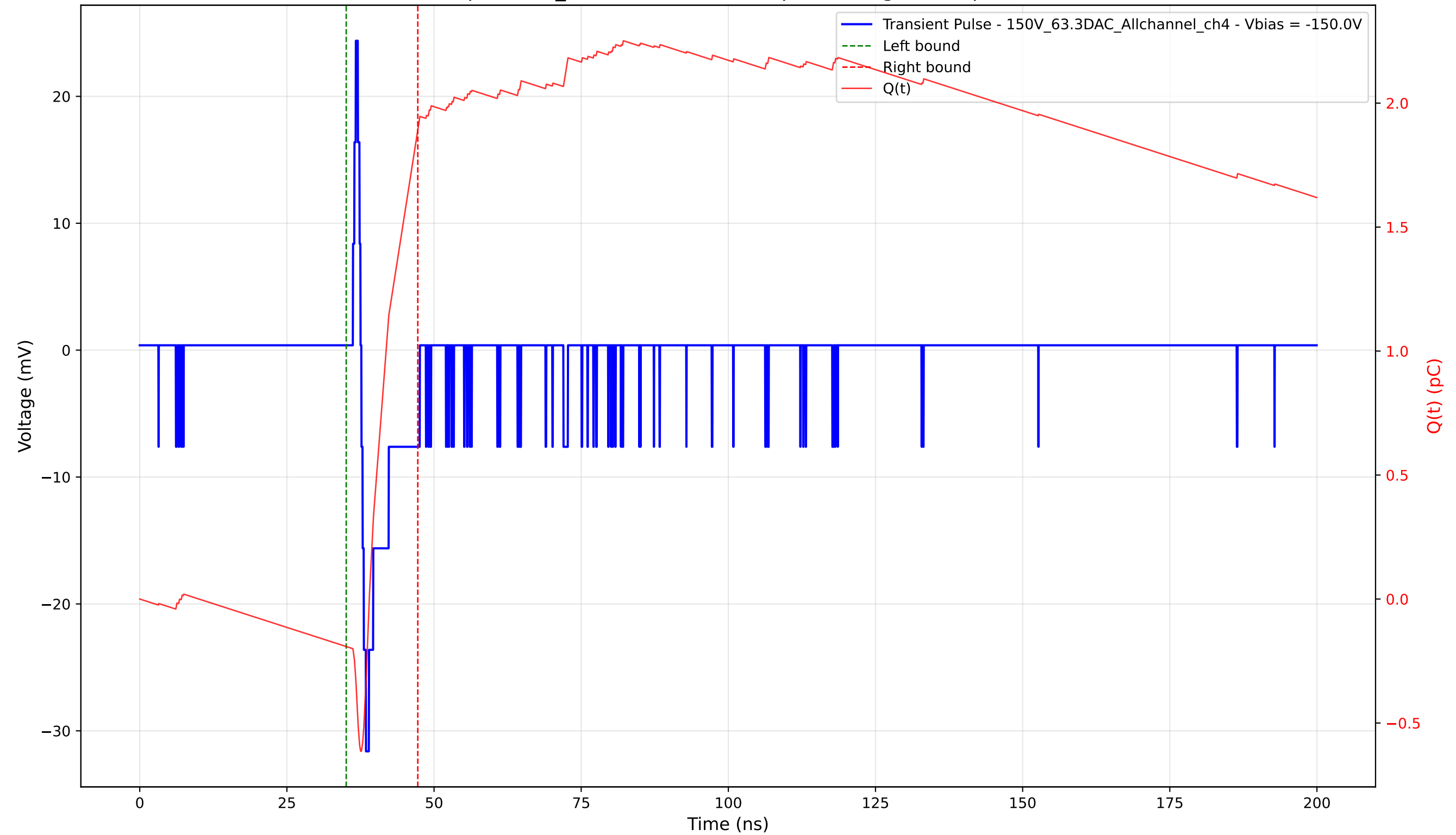
Transient Pulse - Sample: 1cm_42 - Position: 4560.0 \mu\text{m} - Charge: 2.09 pC - Rise Time: 0.78 ns
