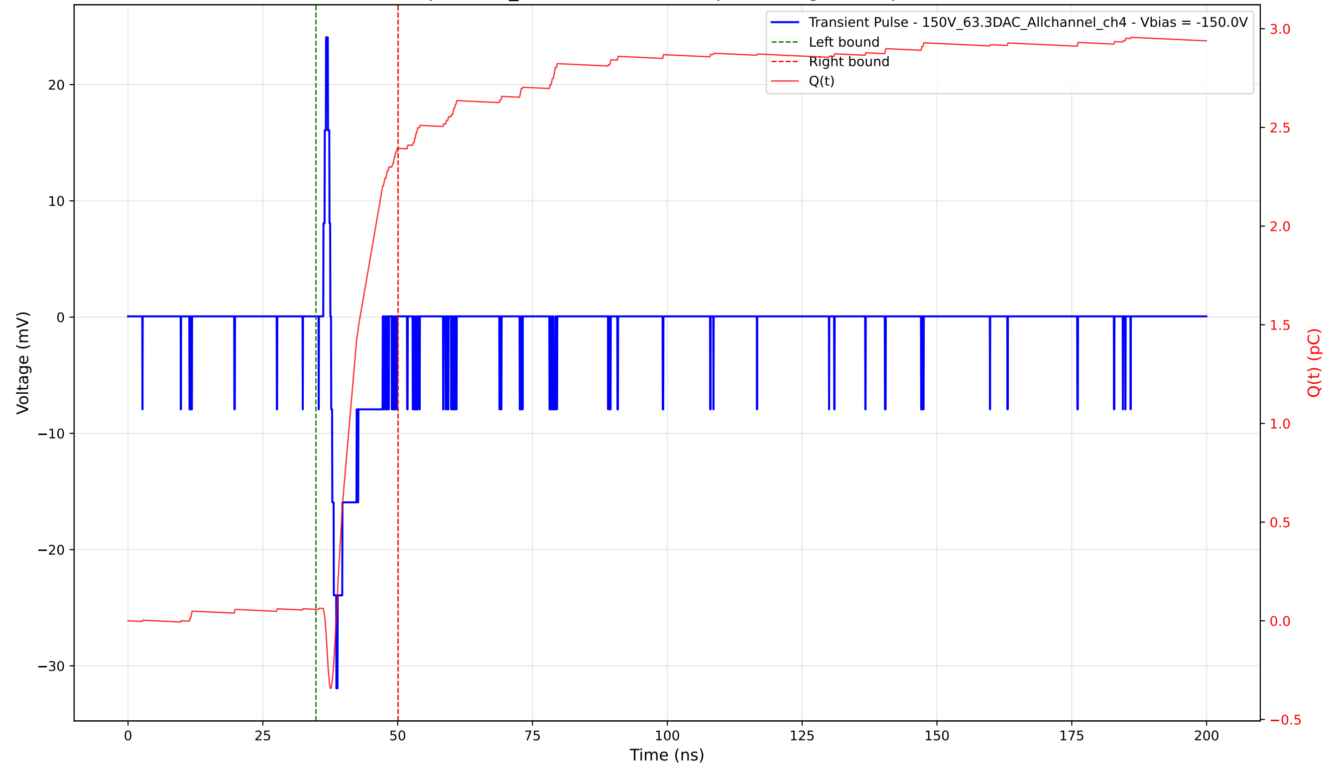
Transient Pulse - Sample: 1cm_42 - Position: 4540.0 \mu\text{m} - Charge: 2.34 pC - Rise Time: 0.98 ns
