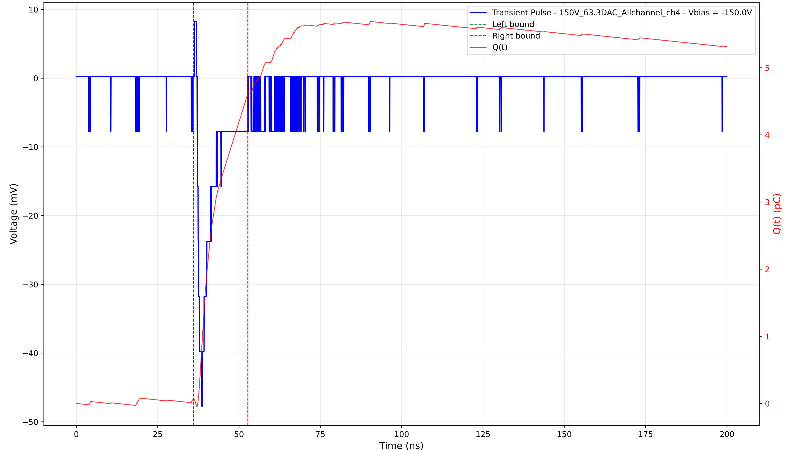
Transient Pulse - Sample: 1cm_42 - Position: 3360.0 \mu\text{m} - Charge: 4.54 pC - Rise Time: 1.42 ns
