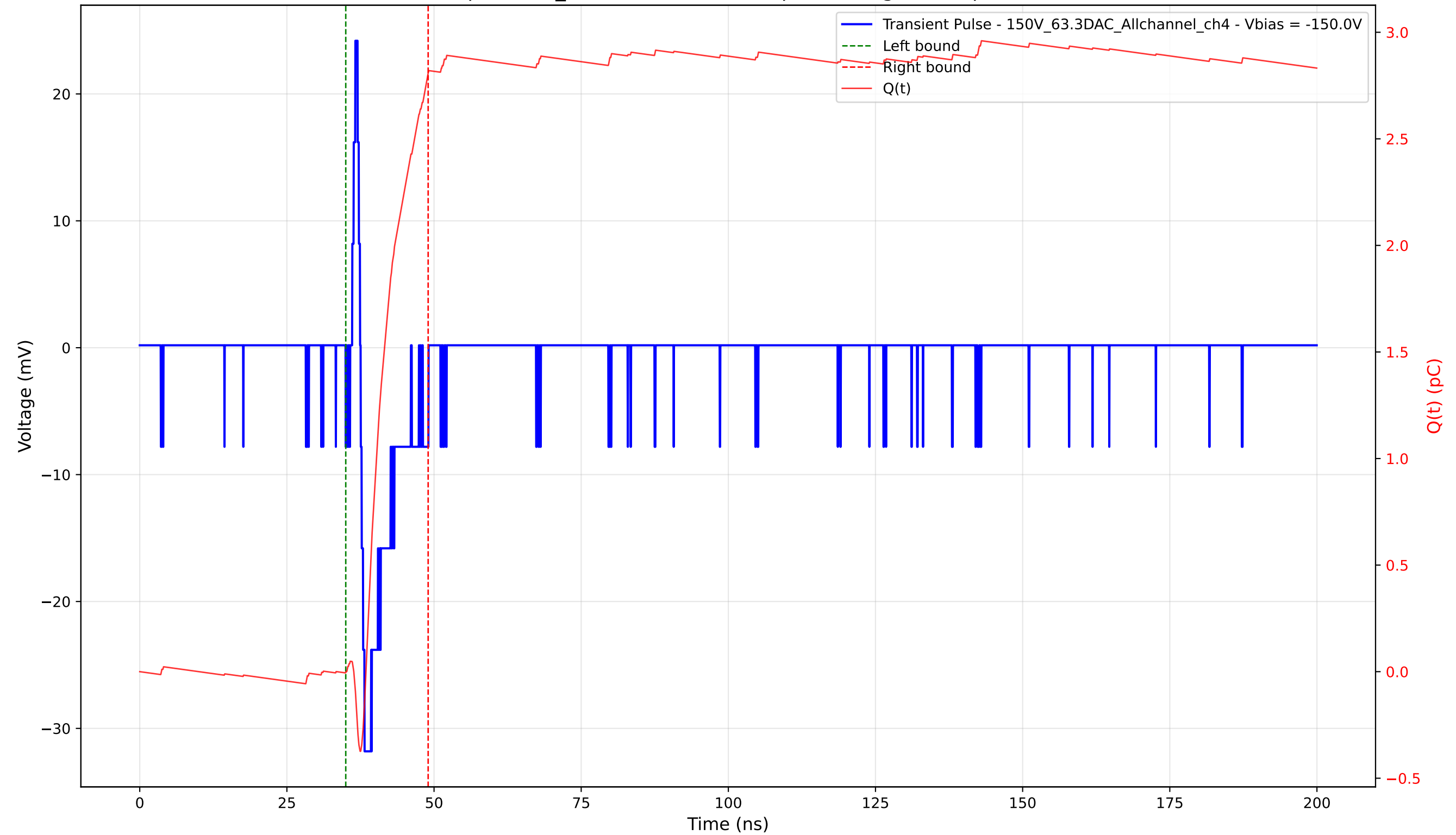
Transient Pulse - Sample: 1cm_42 - Position: 4710.0 \mu\text{m} - Charge: 2.81 pC - Rise Time: 0.66 ns
