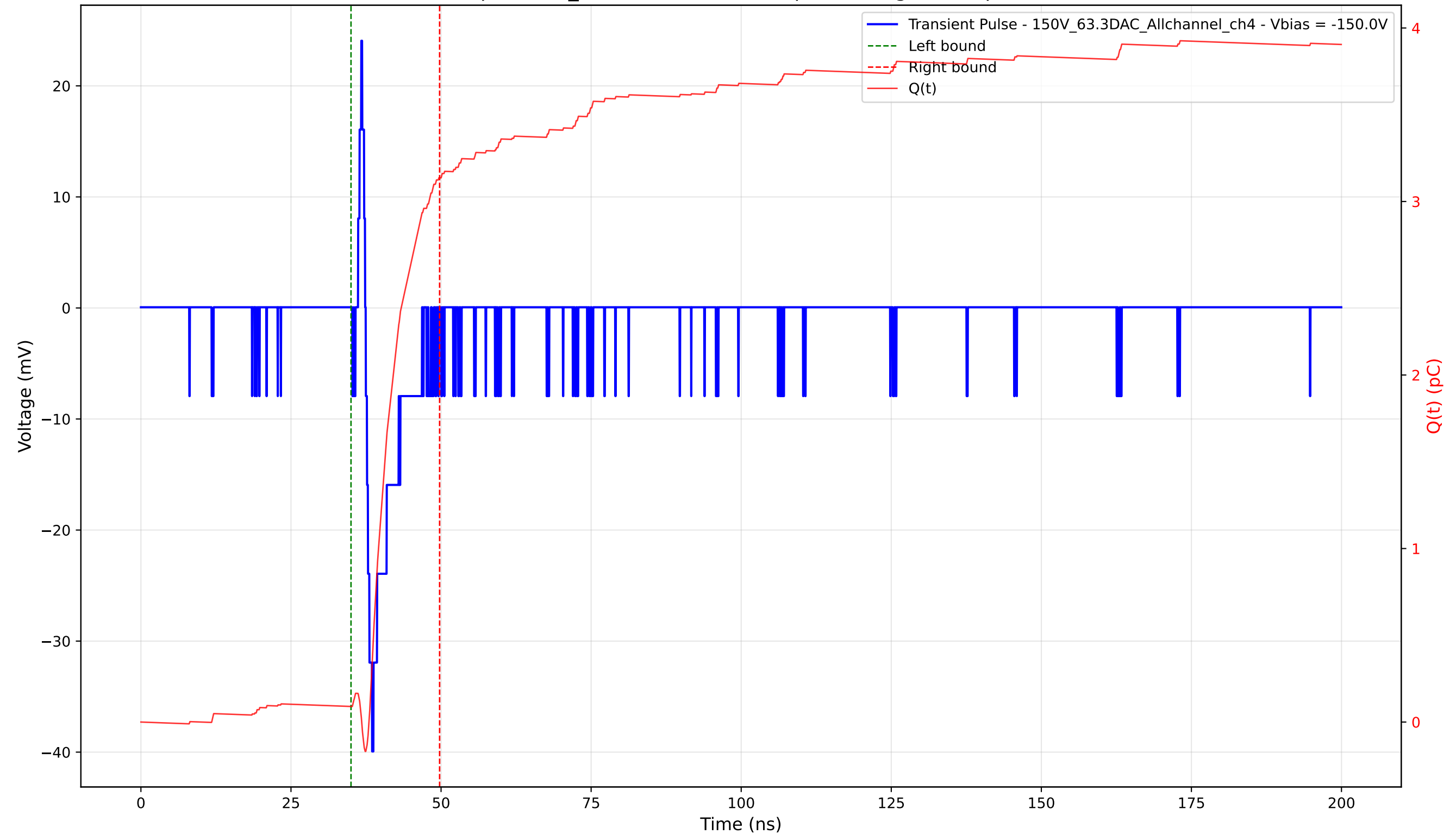
Transient Pulse - Sample: 1cm_42 - Position: 4800.0 \mu\text{m} - Charge: 3.05 pC - Rise Time: 1.06 ns
