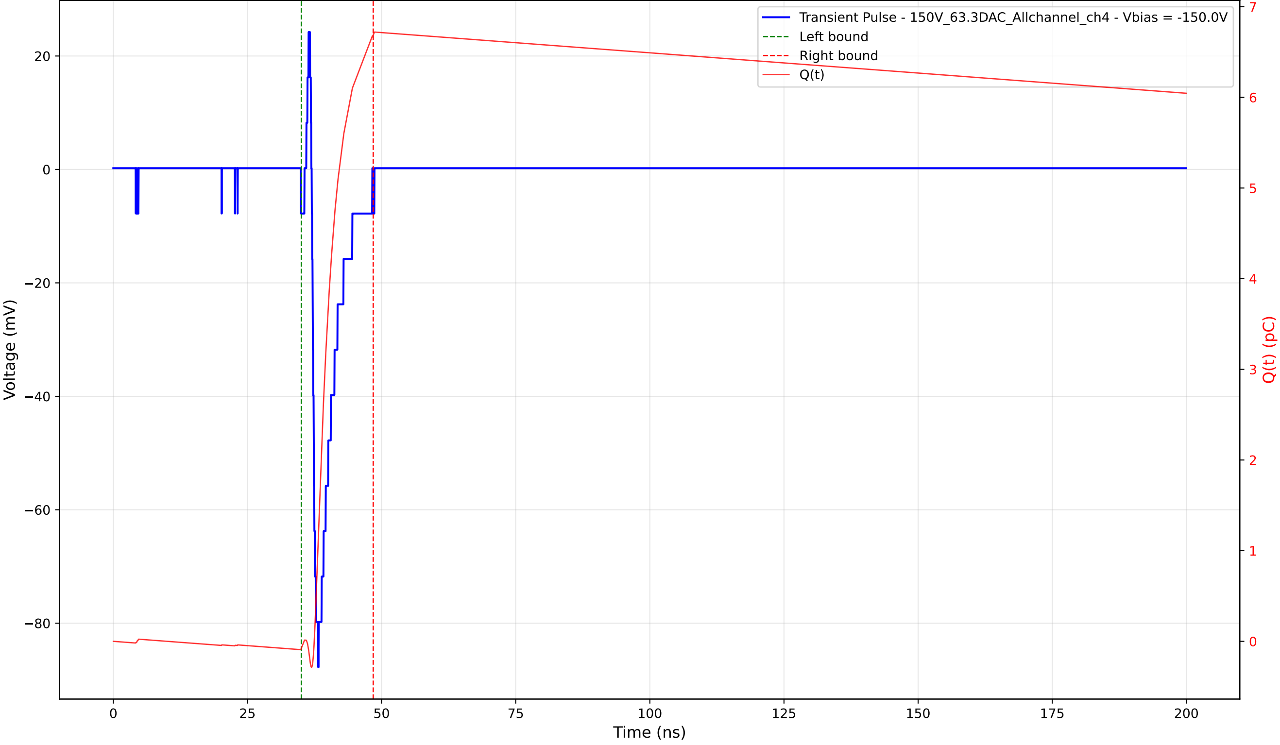
Transient Pulse - Sample: 1cm_42 - Position: 820.0 \mu\text{m} - Charge: 6.76 pC - Rise Time: 0.71 ns
