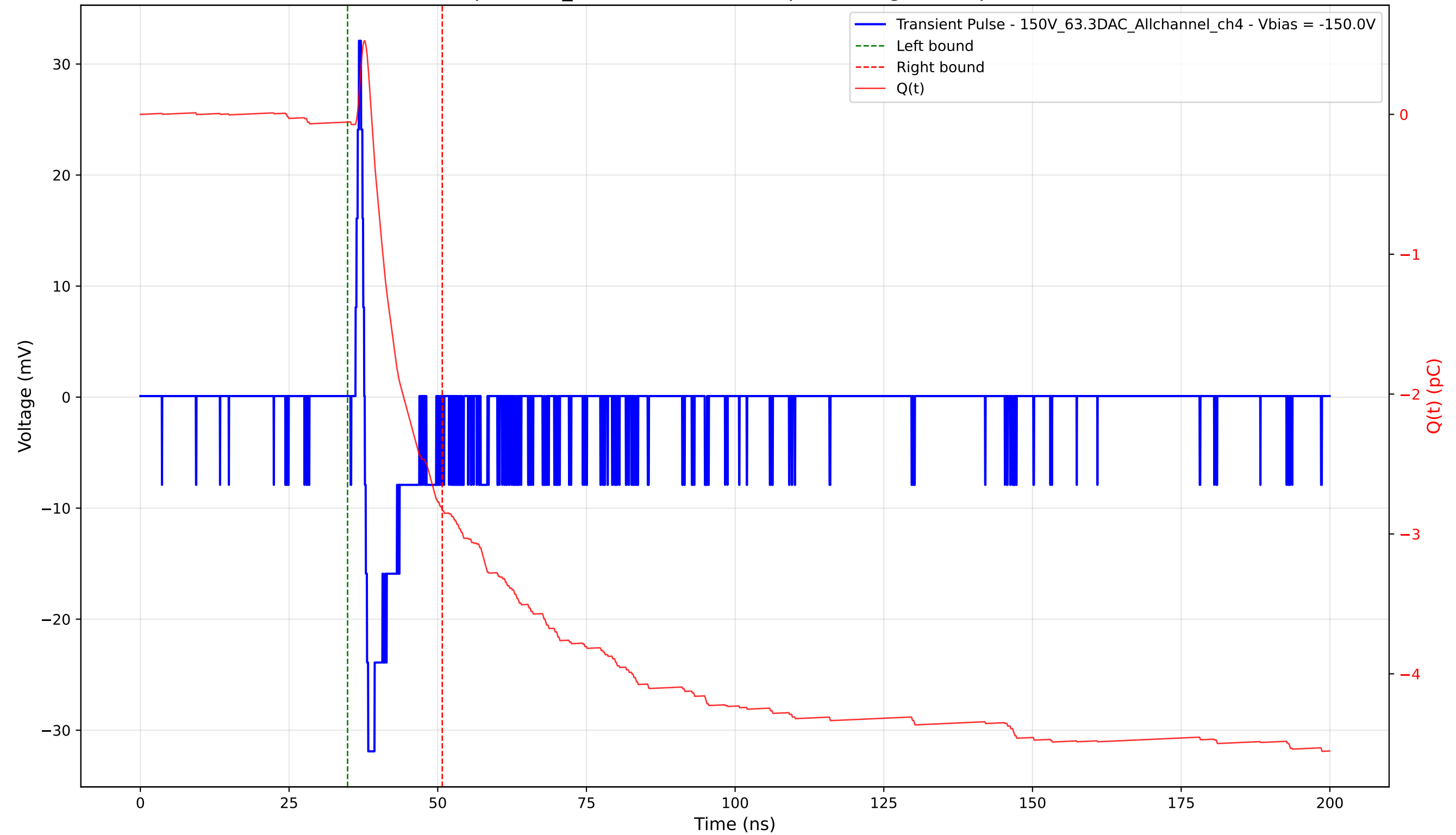
Transient Pulse - Sample: 1cm_42 - Position: 4245.0 \mu\text{m} - Charge: 2.78 pC - Rise Time: 0.58 ns
