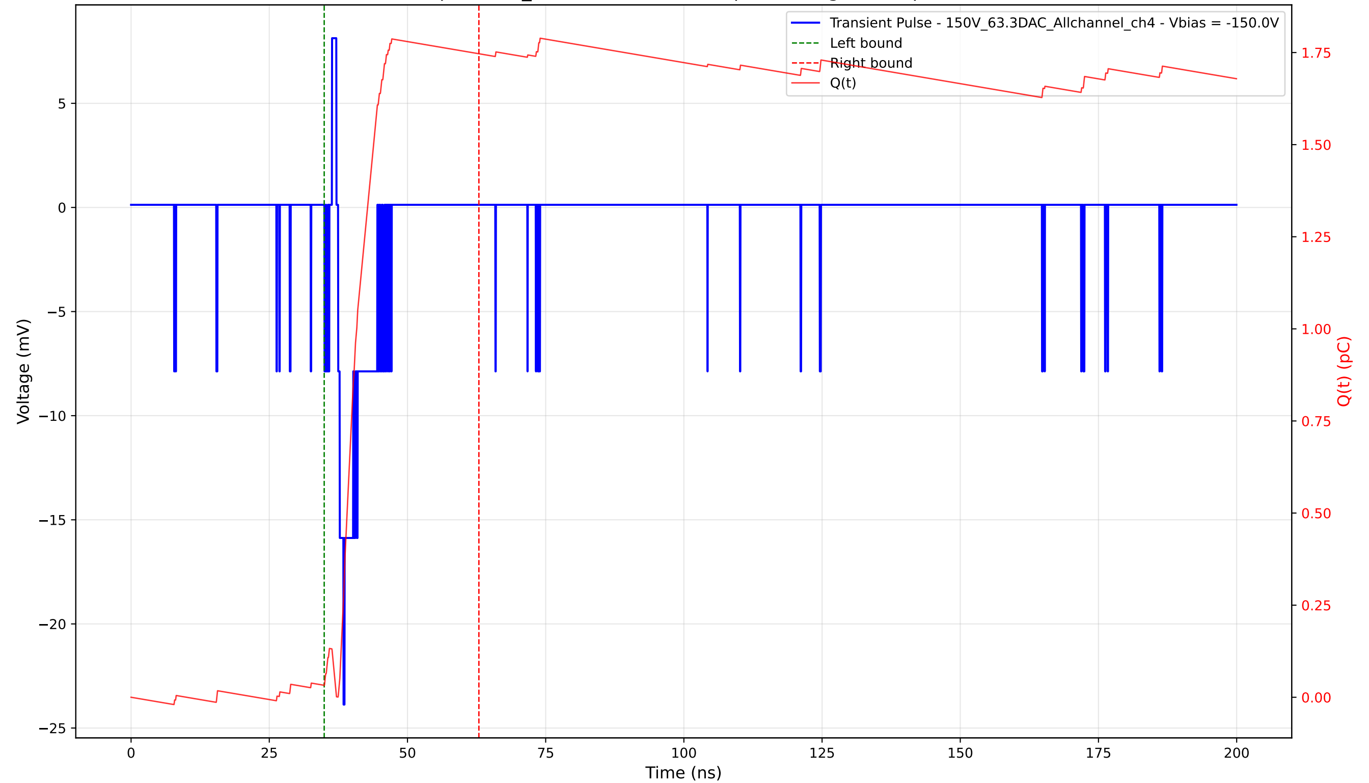
Transient Pulse - Sample: 1cm_42 - Position: 5015.0 \mu\text{m} - Charge: 1.71 pC - Rise Time: 0.99 ns
