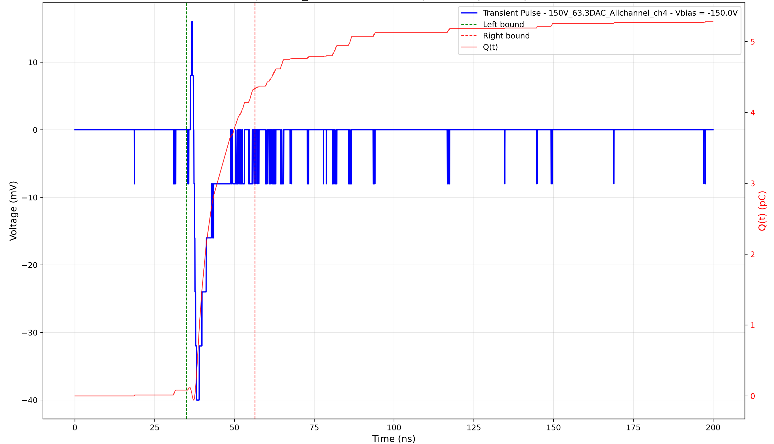
Transient Pulse - Sample: 1cm_42 - Position: 3445.0 \mu\text{m} - Charge: 4.26 pC - Rise Time: 0.86 ns
