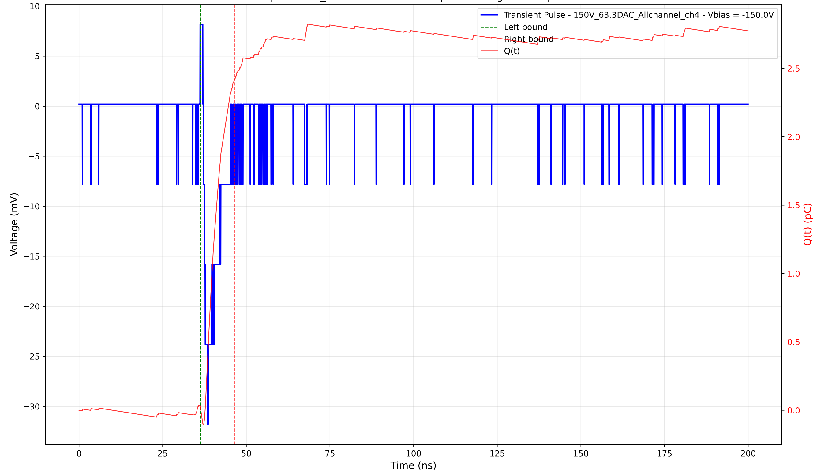
Transient Pulse - Sample: 1cm_42 - Position: 230.0 \mu\text{m} - Charge: 2.41 pC - Rise Time: 1.14 ns
