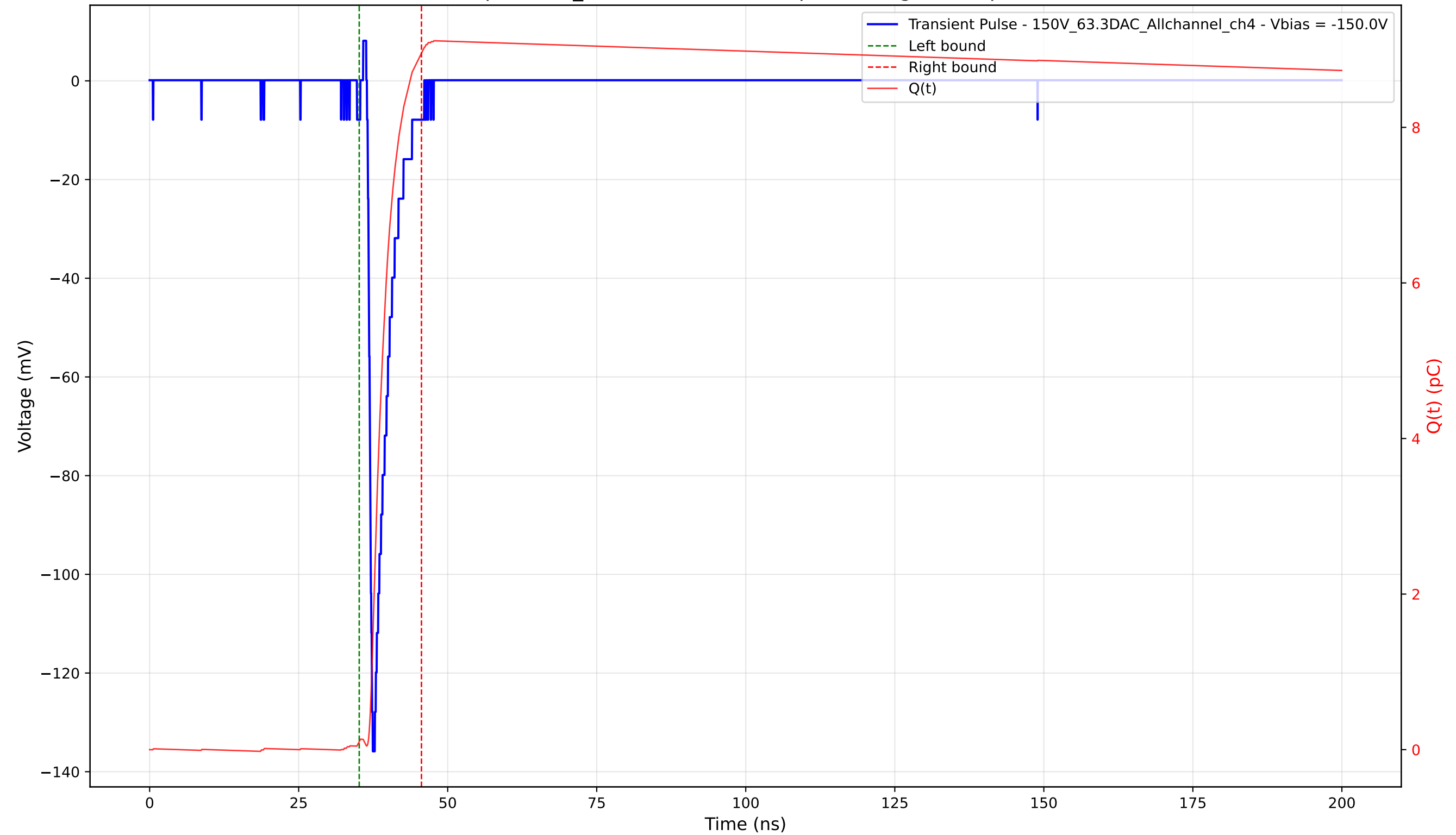
Transient Pulse - Sample: 1cm_42 - Position: 1125.0 \mu\text{m} - Charge: 8.85 pC - Rise Time: 0.73 ns
