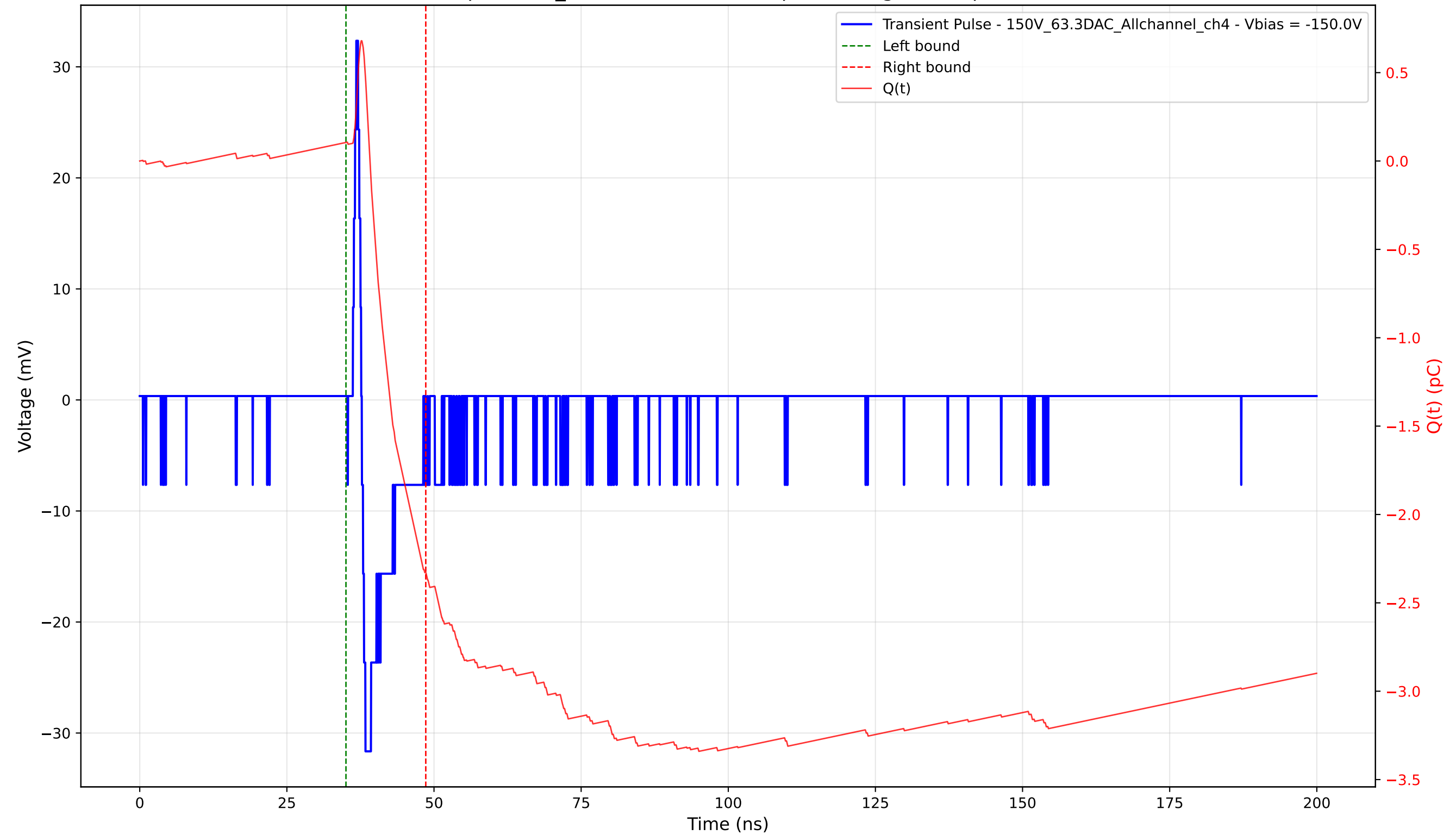
Transient Pulse - Sample: 1cm_42 - Position: 4340.0 \mu\text{m} - Charge: 2.43 pC - Rise Time: 0.59 ns
