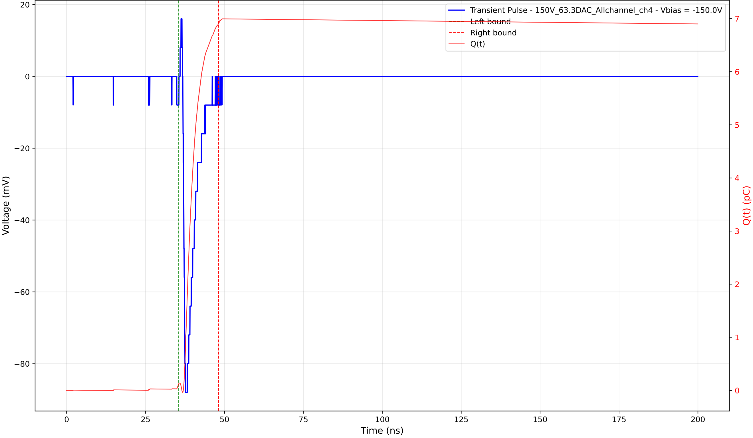
Transient Pulse - Sample: 1cm_42 - Position: 950.0 \mu\text{m} - Charge: 6.77 pC - Rise Time: 0.64 ns
