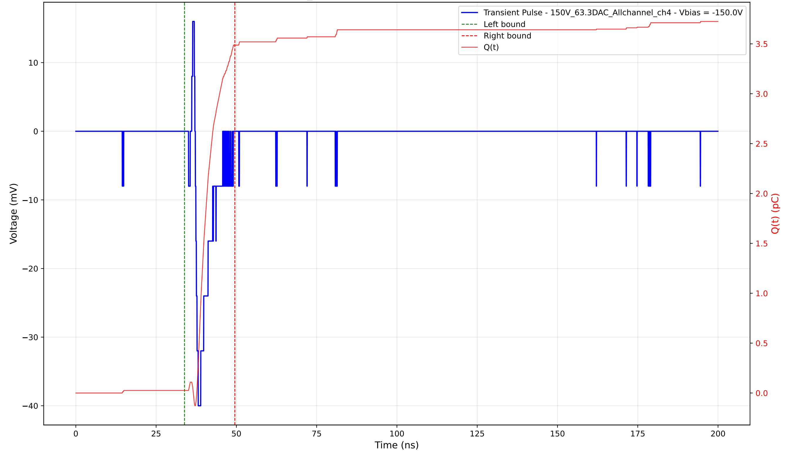
Transient Pulse - Sample: 1cm_42 - Position: 365.0 \mu\text{m} - Charge: 3.46 pC - Rise Time: 0.90 ns
