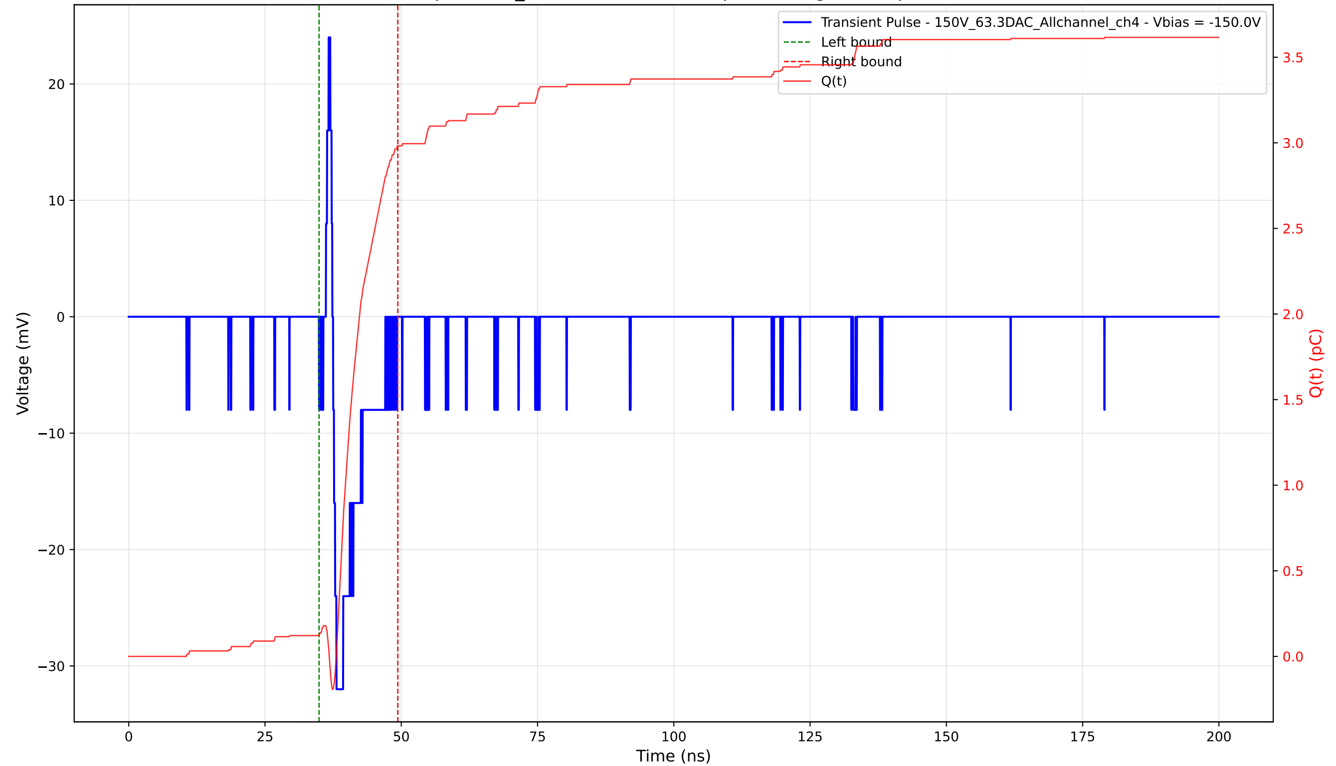
Transient Pulse - Sample: 1cm_42 - Position: 4765.0 \mu\text{m} - Charge: 2.86 pC - Rise Time: 0.62 ns
