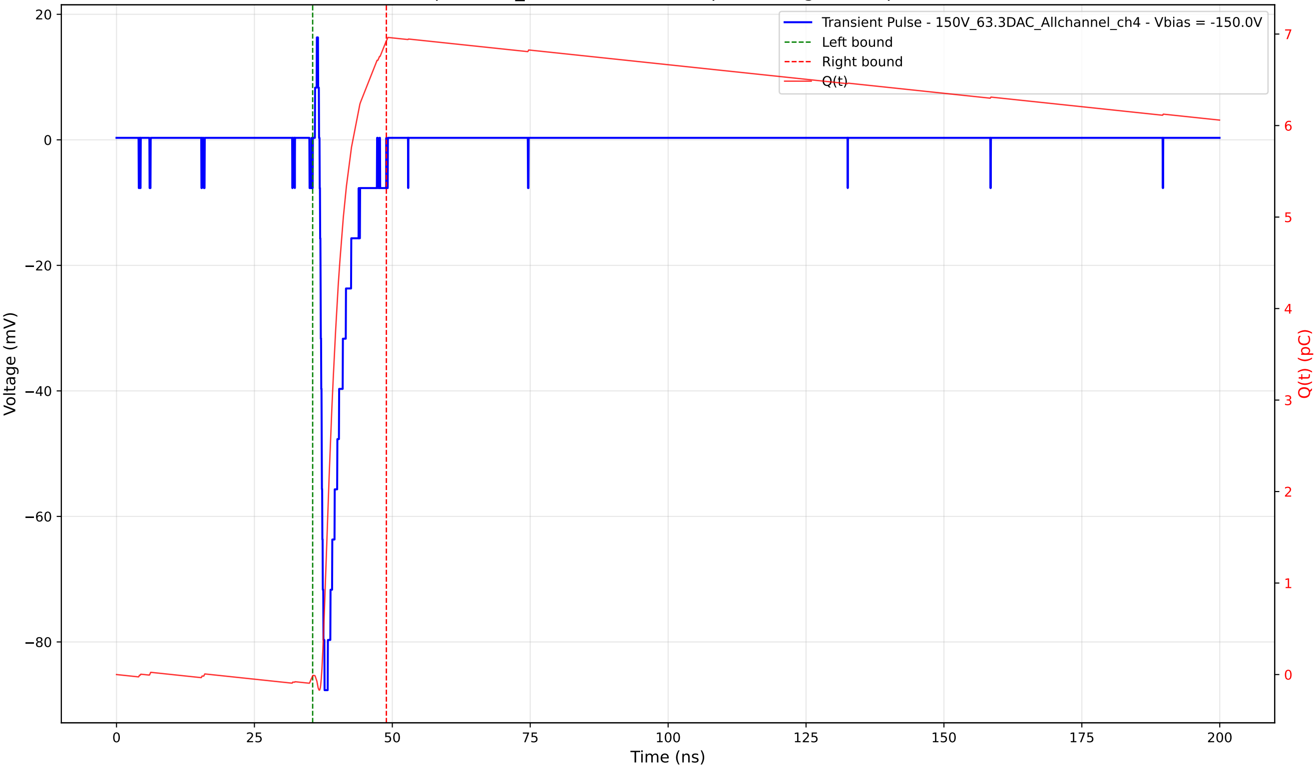
Transient Pulse - Sample: 1cm_42 - Position: 940.0 \mu\text{m} - Charge: 6.94 pC - Rise Time: 0.63 ns
