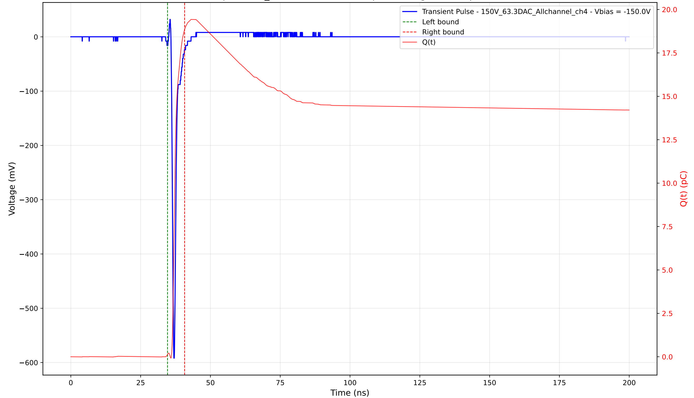
Transient Pulse - Sample: 1cm_42 - Position: 1905.0 \mu\text{m} - Charge: 18.71 pC - Rise Time: 0.70 ns
