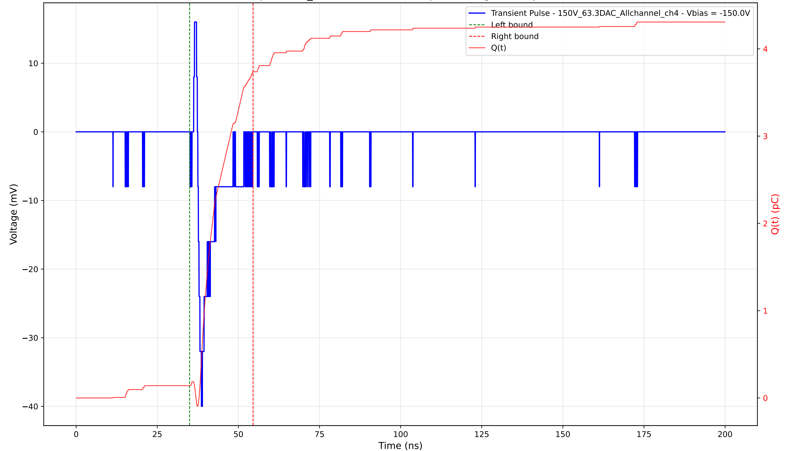
Transient Pulse - Sample: 1cm_42 - Position: 3570.0 \mu\text{m} - Charge: 3.60 pC - Rise Time: 1.10 ns
