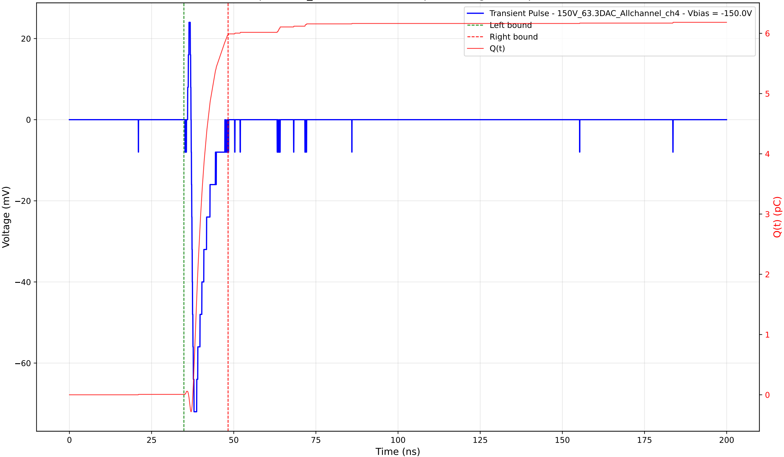
Transient Pulse - Sample: 1cm_42 - Position: 650.0 \mu\text{m} - Charge: 5.96 pC - Rise Time: 0.84 ns
