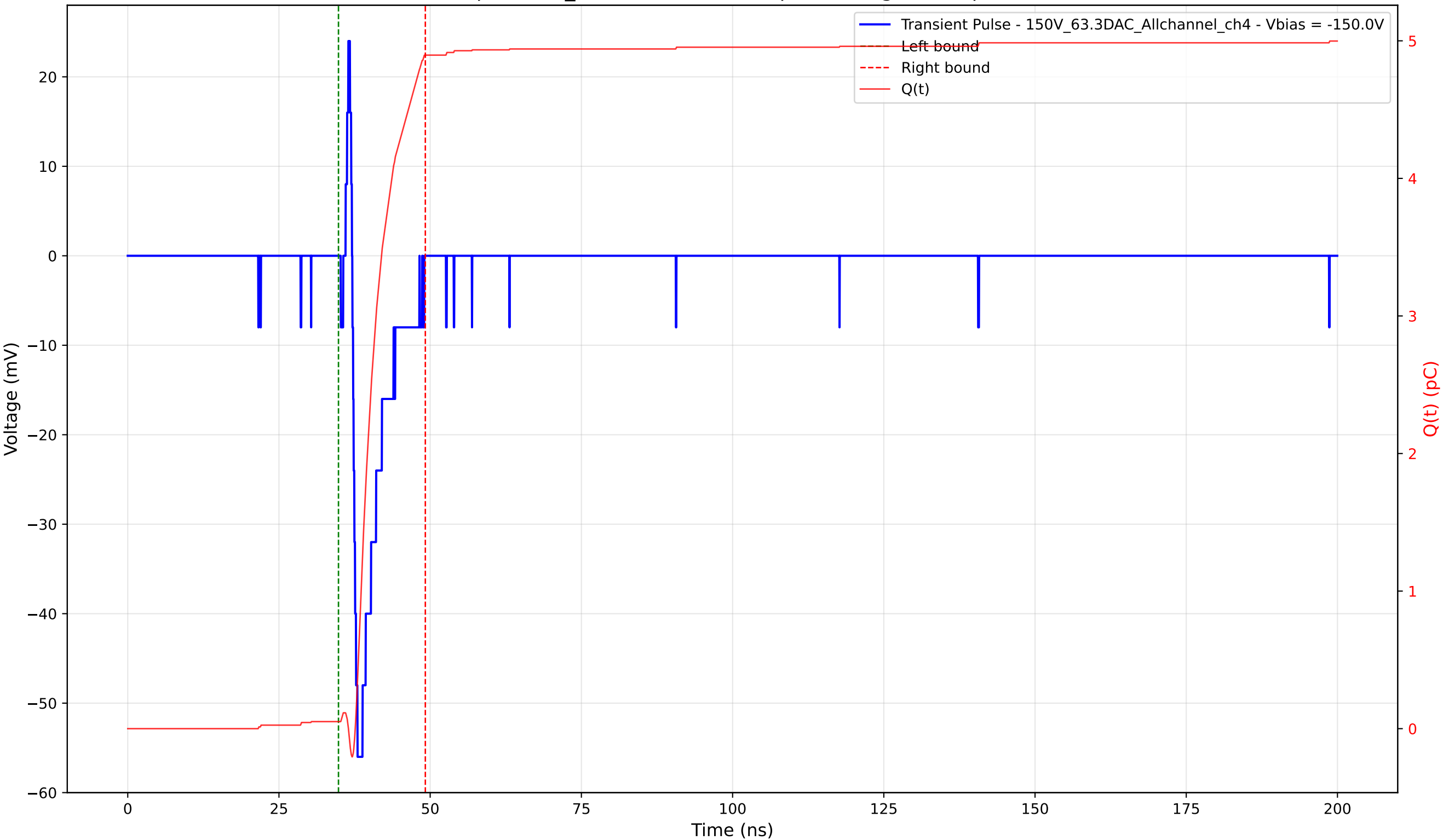
Transient Pulse - Sample: 1cm_42 - Position: 525.0 \mu\text{m} - Charge: 4.84 pC - Rise Time: 0.85 ns
