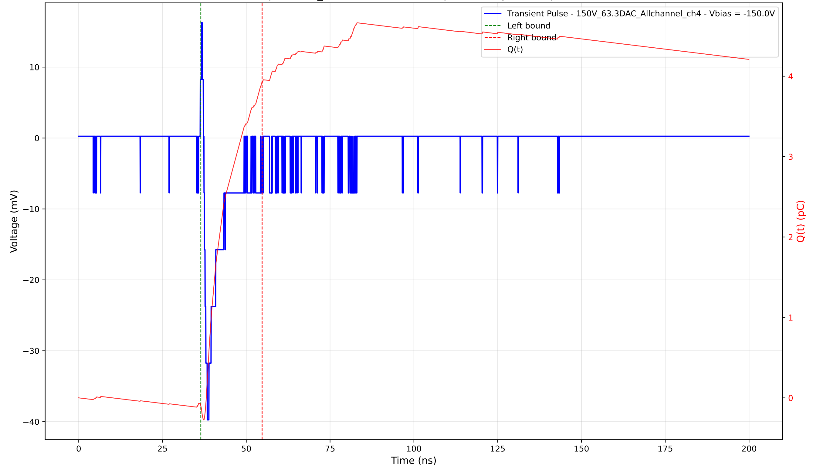
Transient Pulse - Sample: 1cm_42 - Position: 3475.0 \mu\text{m} - Charge: 4.03 pC - Rise Time: 0.98 ns
