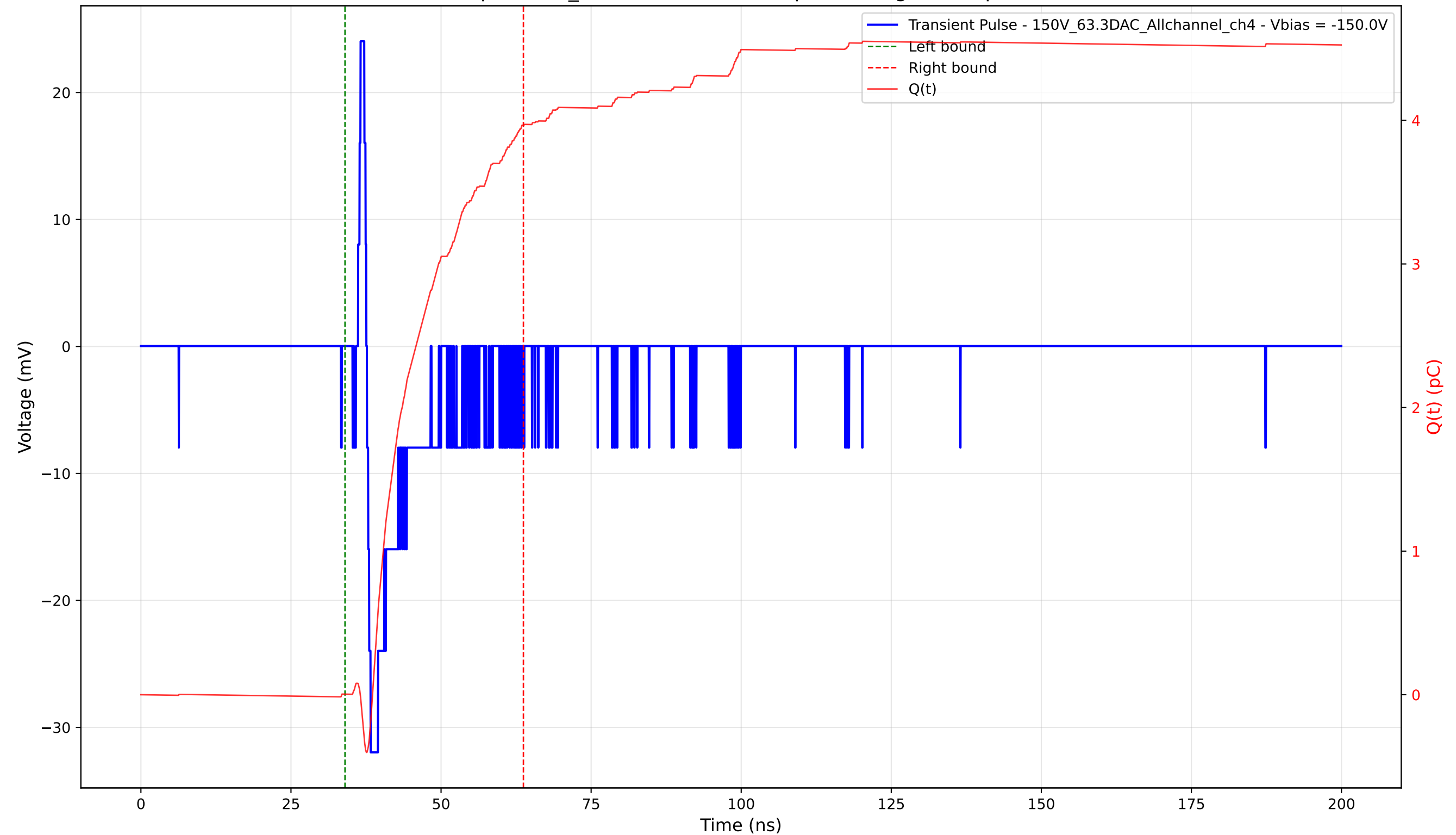
Transient Pulse - Sample: 1cm_42 - Position: 3860.0 \mu\text{m} - Charge: 3.96 pC - Rise Time: 0.62 ns
