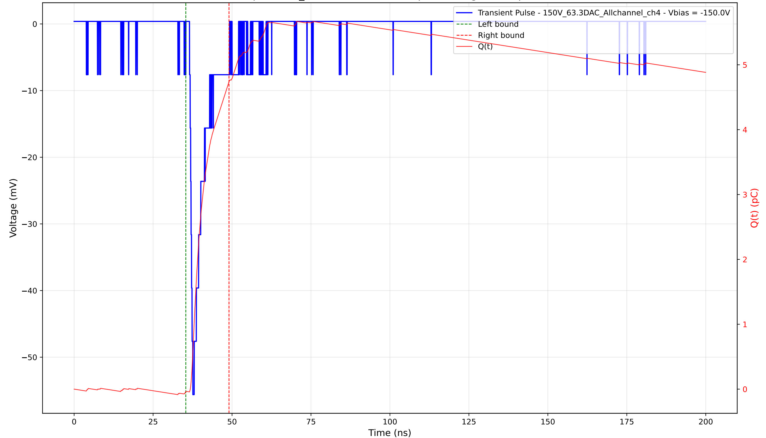
Transient Pulse - Sample: 1cm_42 - Position: 3090.0 \mu\text{m} - Charge: 4.78 pC - Rise Time: 1.05 ns
