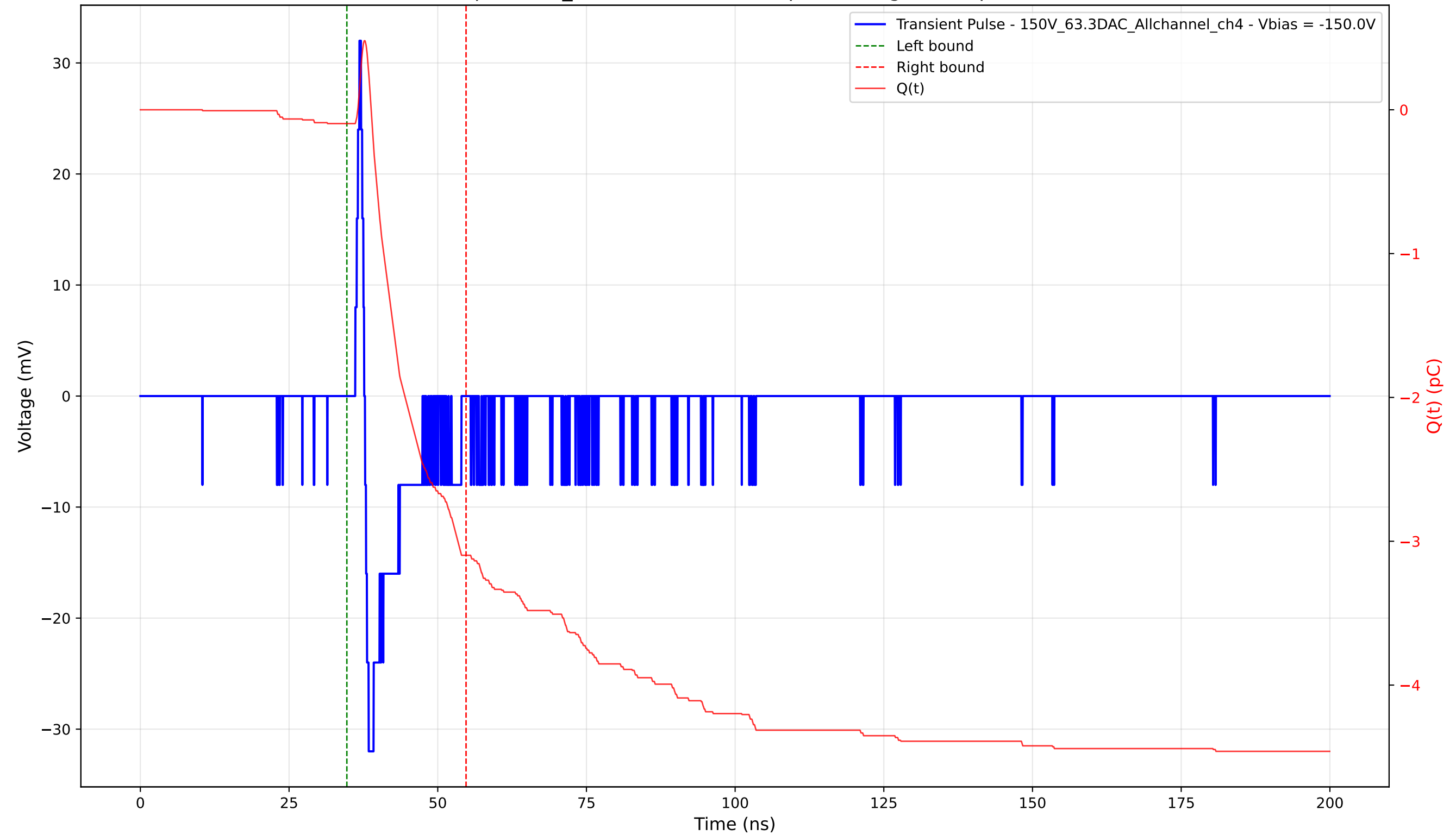
Transient Pulse - Sample: 1cm_42 - Position: 4180.0 \mu\text{m} - Charge: 3.00 pC - Rise Time: 0.70 ns
