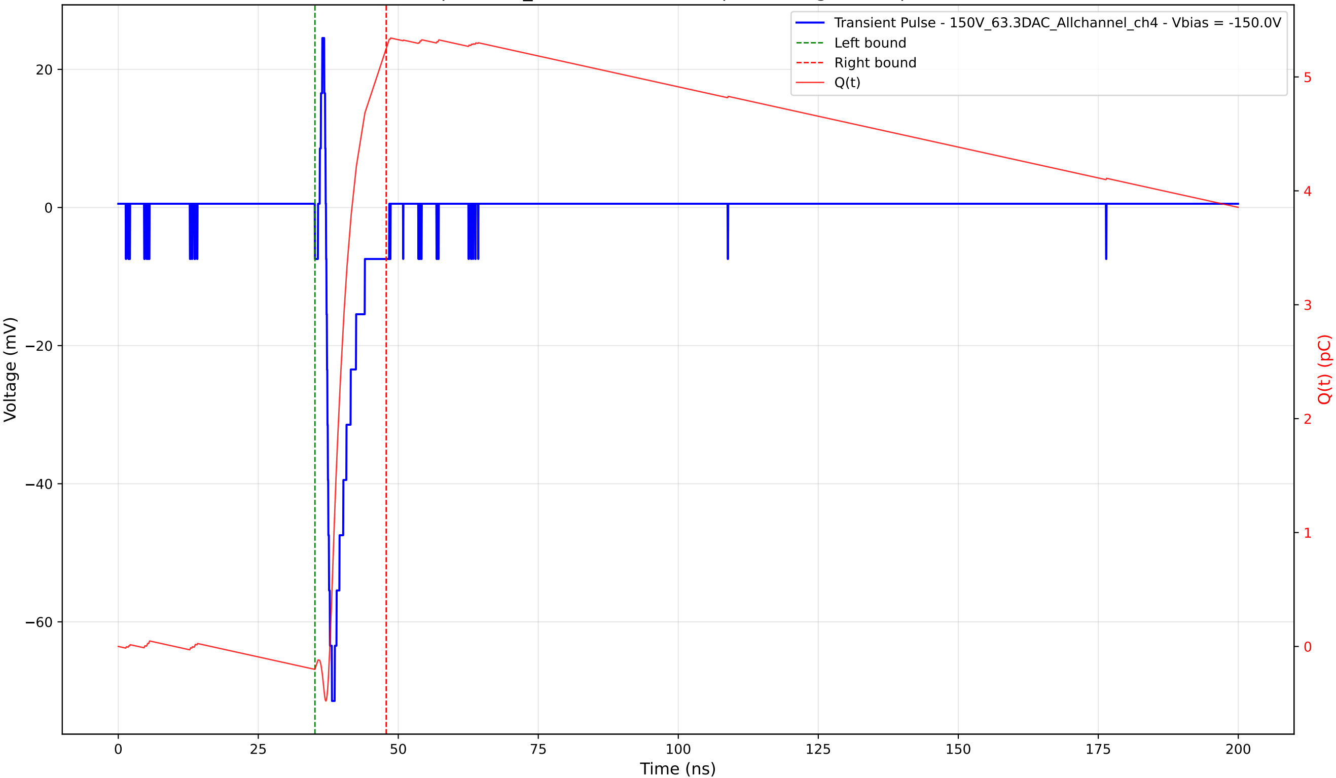
Transient Pulse - Sample: 1cm_42 - Position: 625.0 \mu\text{m} - Charge: 5.45 pC - Rise Time: 1.04 ns
