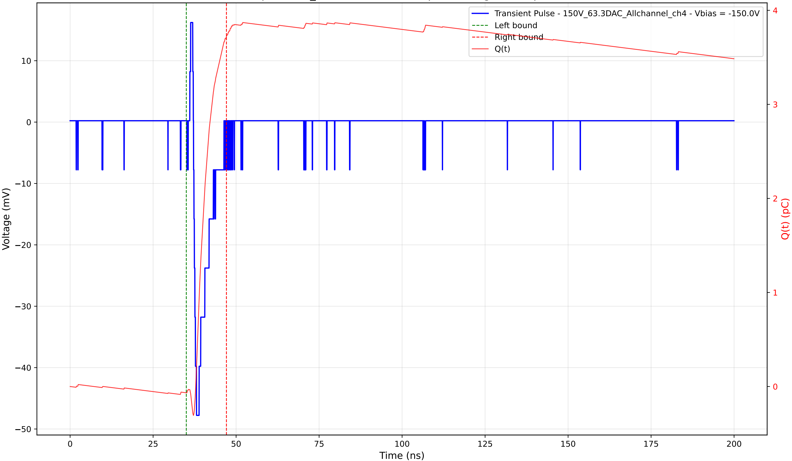
Transient Pulse - Sample: 1cm_42 - Position: 445.0 \mu\text{m} - Charge: 3.79 pC - Rise Time: 0.90 ns
