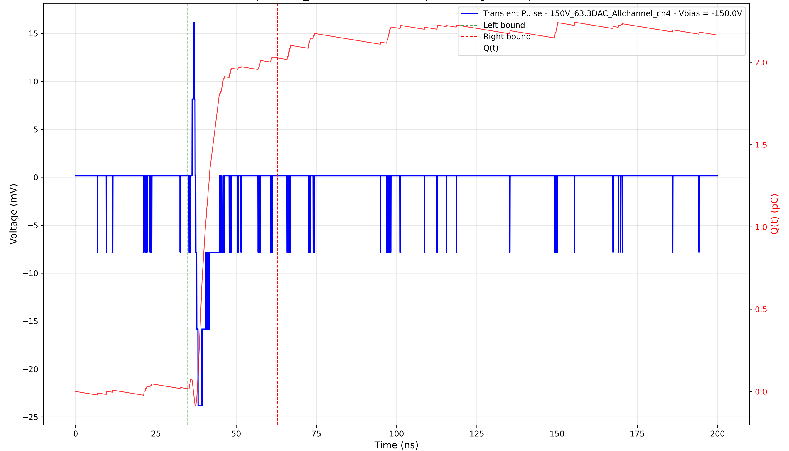
Transient Pulse - Sample: 1cm_42 - Position: 4980.0 \mu\text{m} - Charge: 2.01 pC - Rise Time: 0.71 ns
