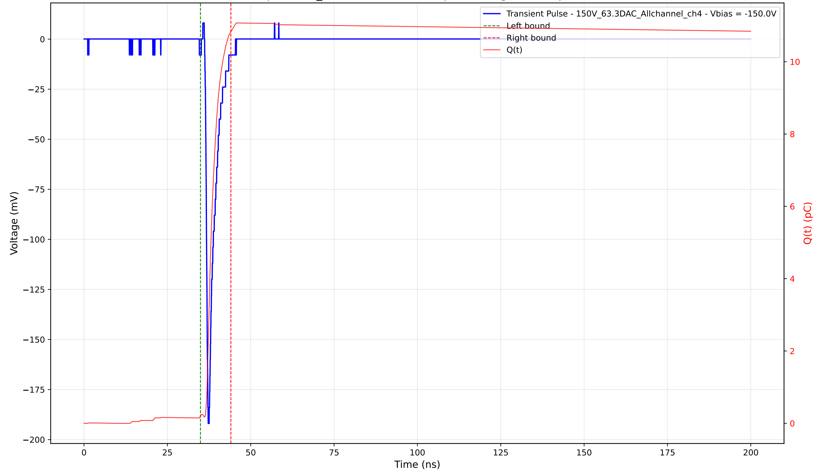
Transient Pulse - Sample: 1cm_42 - Position: 1370.0 \mu\text{m} - Charge: 10.63 pC - Rise Time: 0.77 ns
