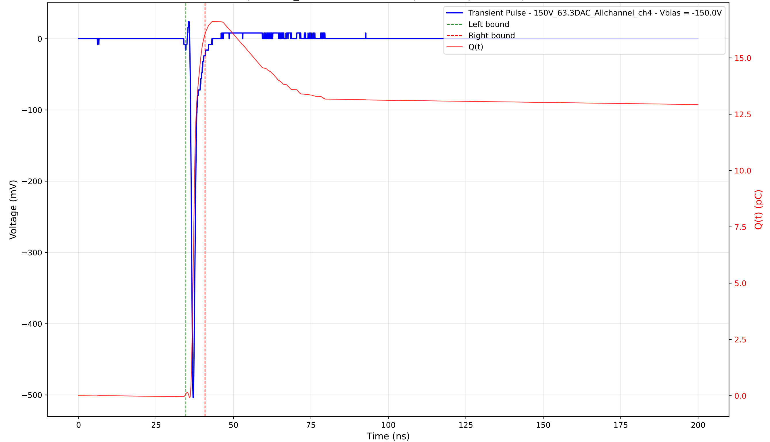
Transient Pulse - Sample: 1cm_42 - Position: 2260.0 \mu\text{m} - Charge: 15.97 pC - Rise Time: 0.71 ns
