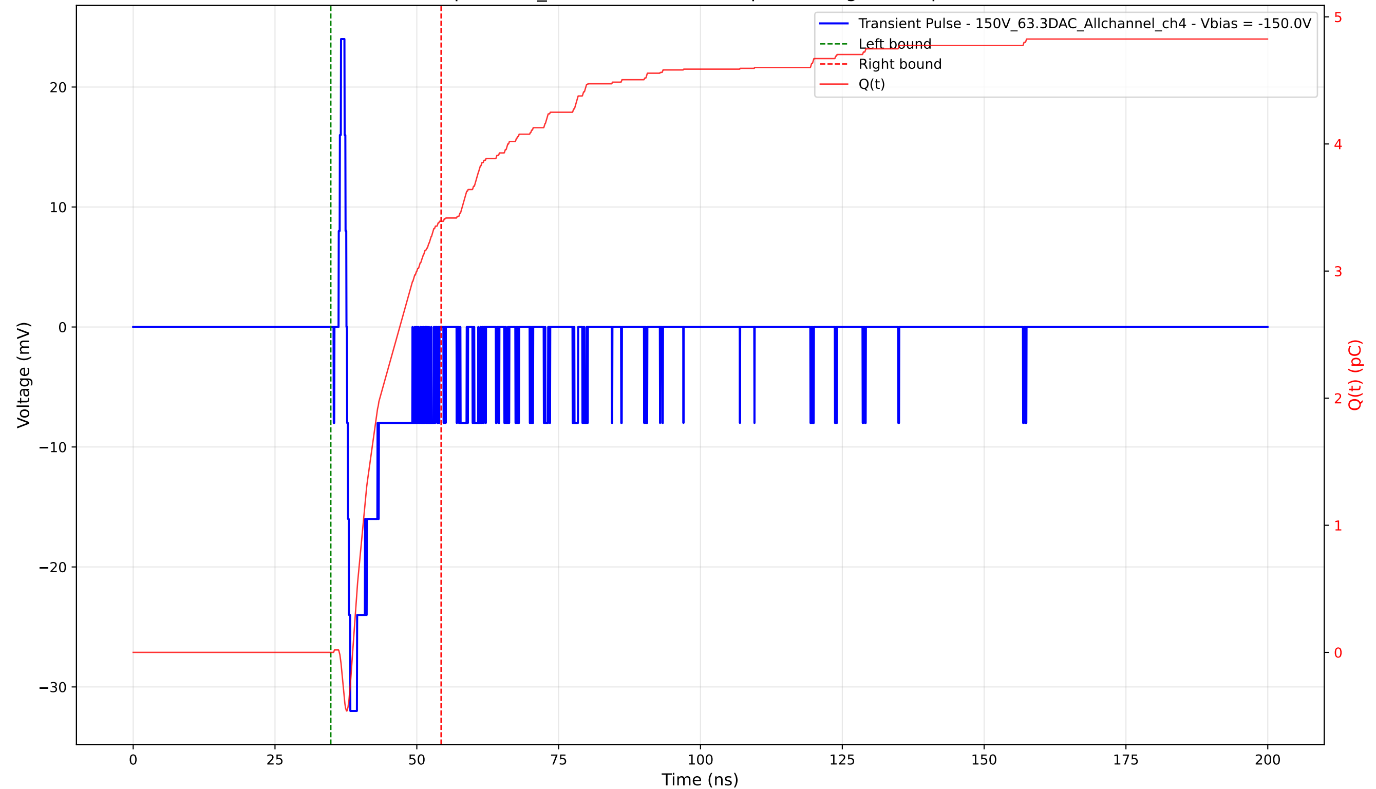
Transient Pulse - Sample: 1cm_42 - Position: 3870.0 \mu\text{m} - Charge: 3.39 pC - Rise Time: 0.58 ns
