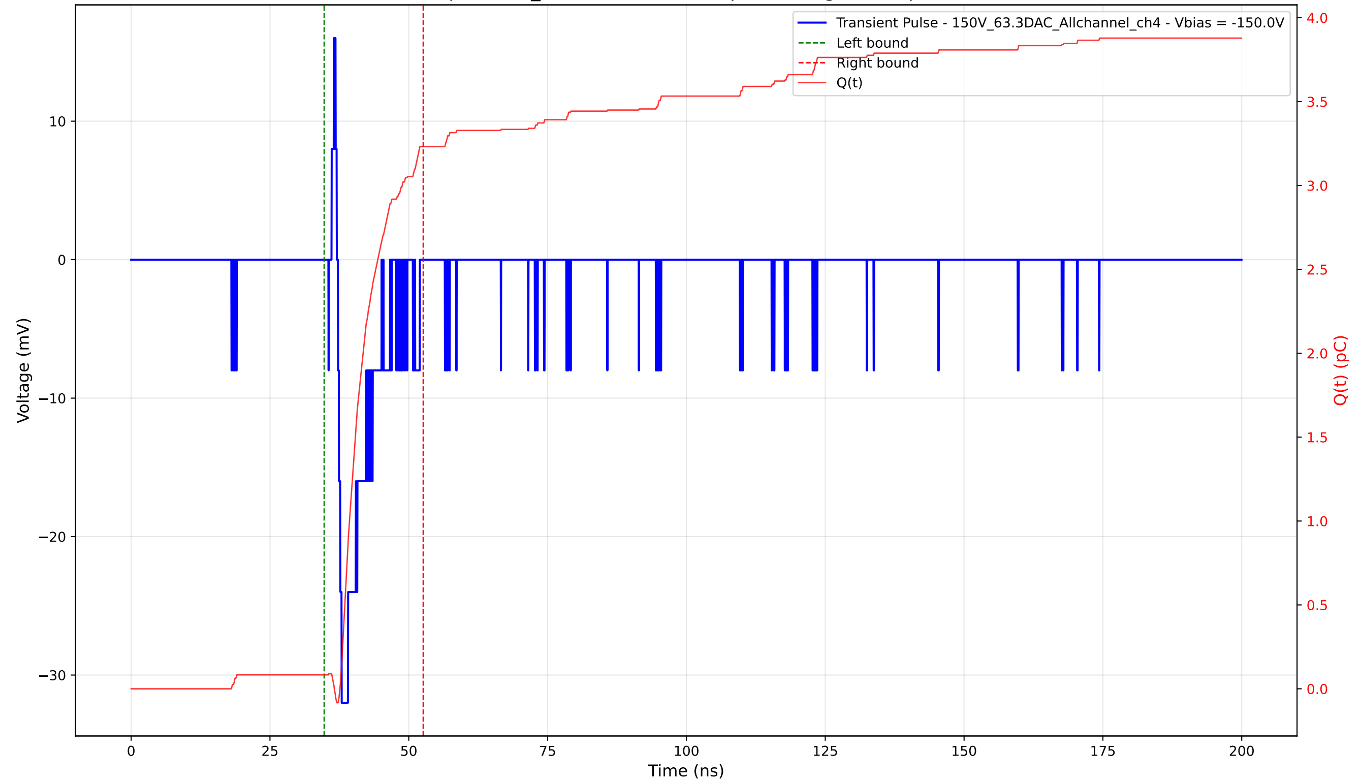
Transient Pulse - Sample: 1cm_42 - Position: 280.0 \mu\text{m} - Charge: 3.15 pC - Rise Time: 0.66 ns
