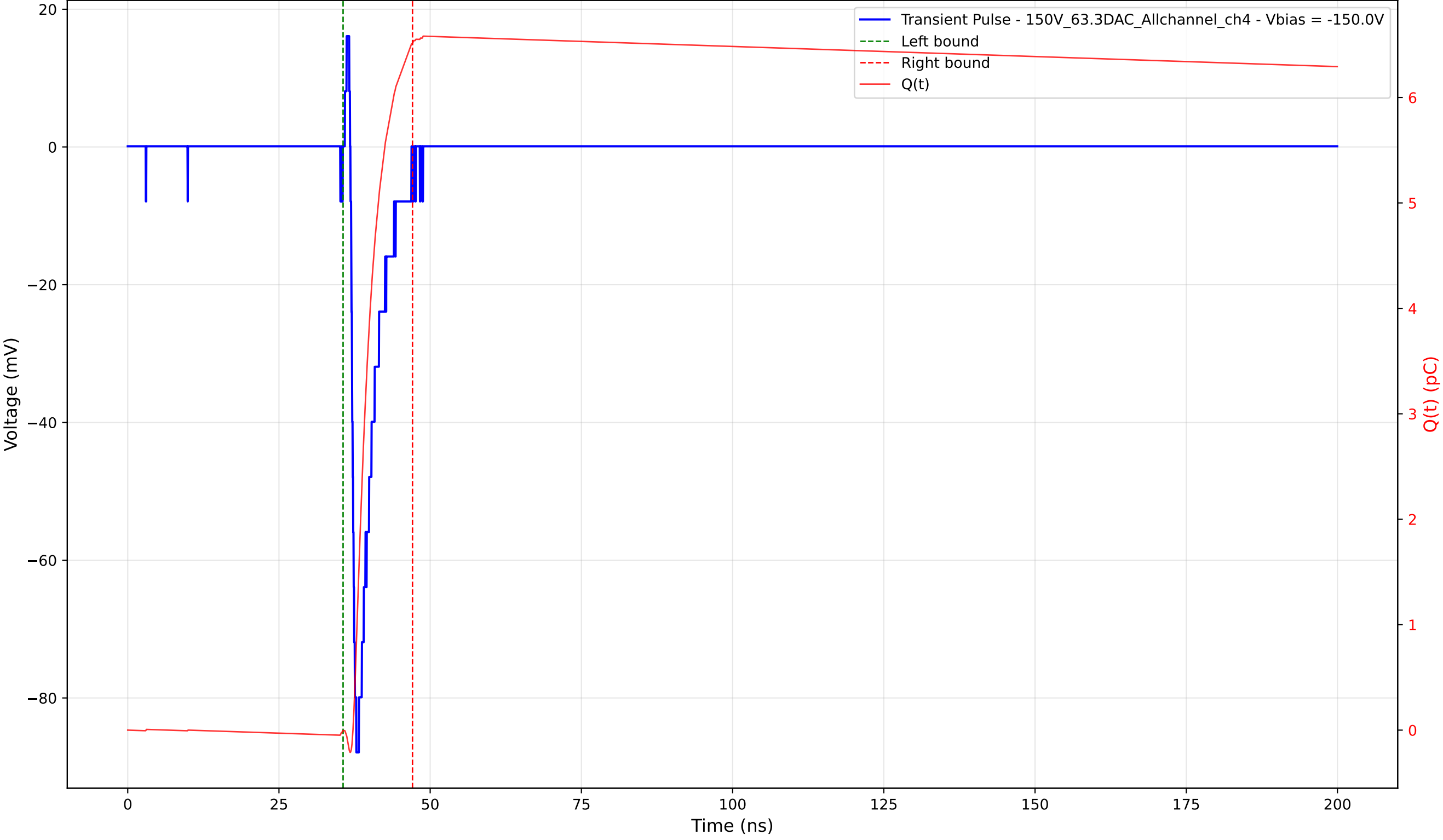
Transient Pulse - Sample: 1cm_42 - Position: 930.0 \mu\text{m} - Charge: 6.52 pC - Rise Time: 0.64 ns
