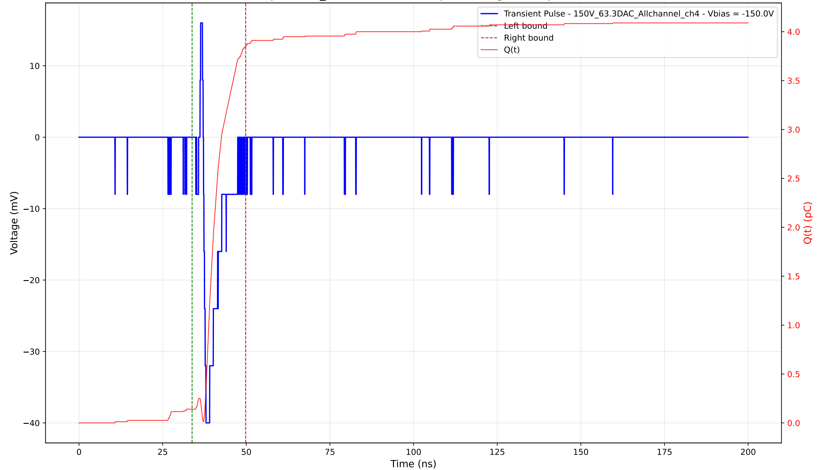
Transient Pulse - Sample: 1cm_42 - Position: 390.0 \mu\text{m} - Charge: 3.71 pC - Rise Time: 0.74 ns
