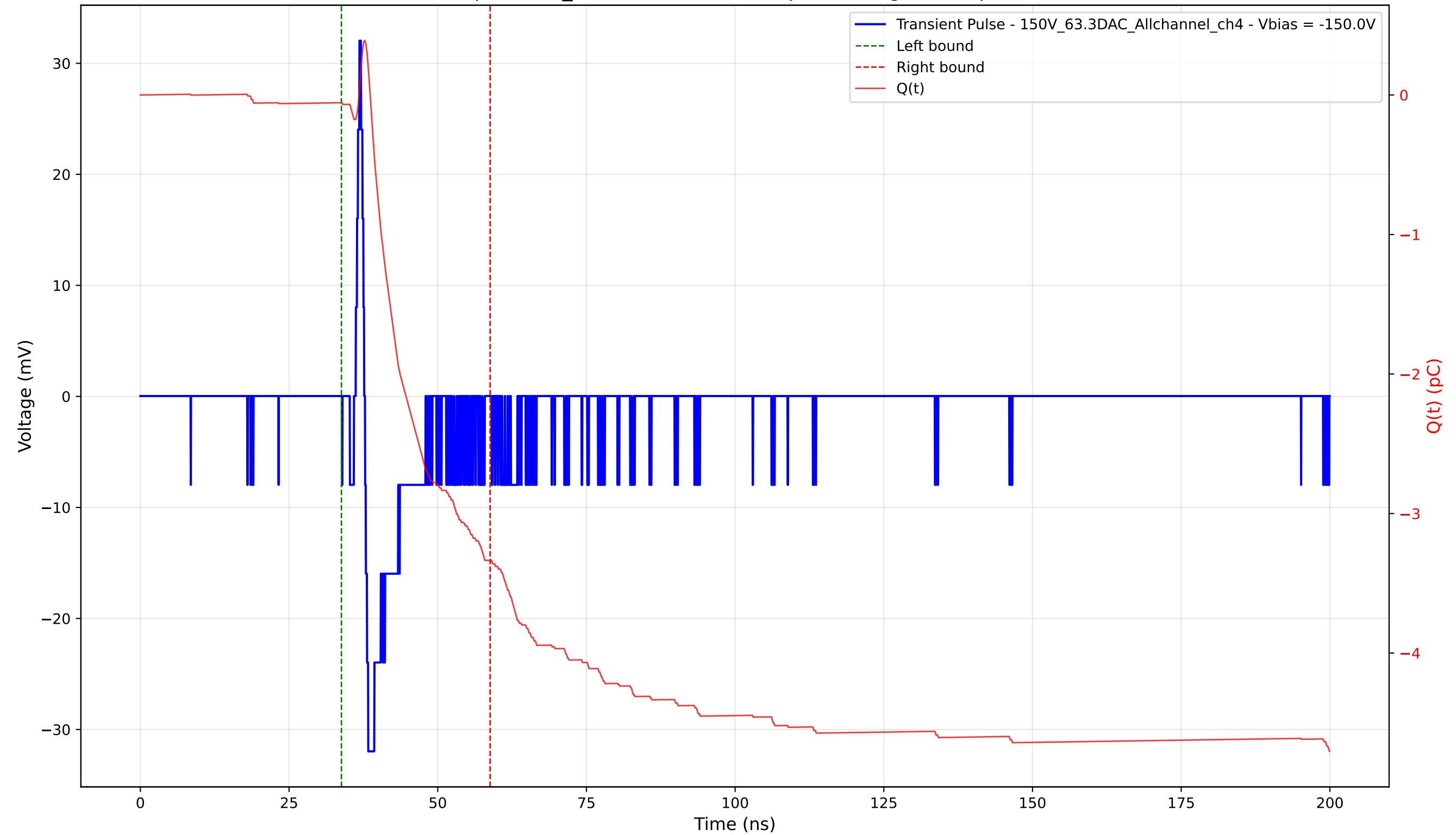
Transient Pulse - Sample: 1cm_42 - Position: 4215.0 \mu\text{m} - Charge: 3.28 pC - Rise Time: 0.62 ns
