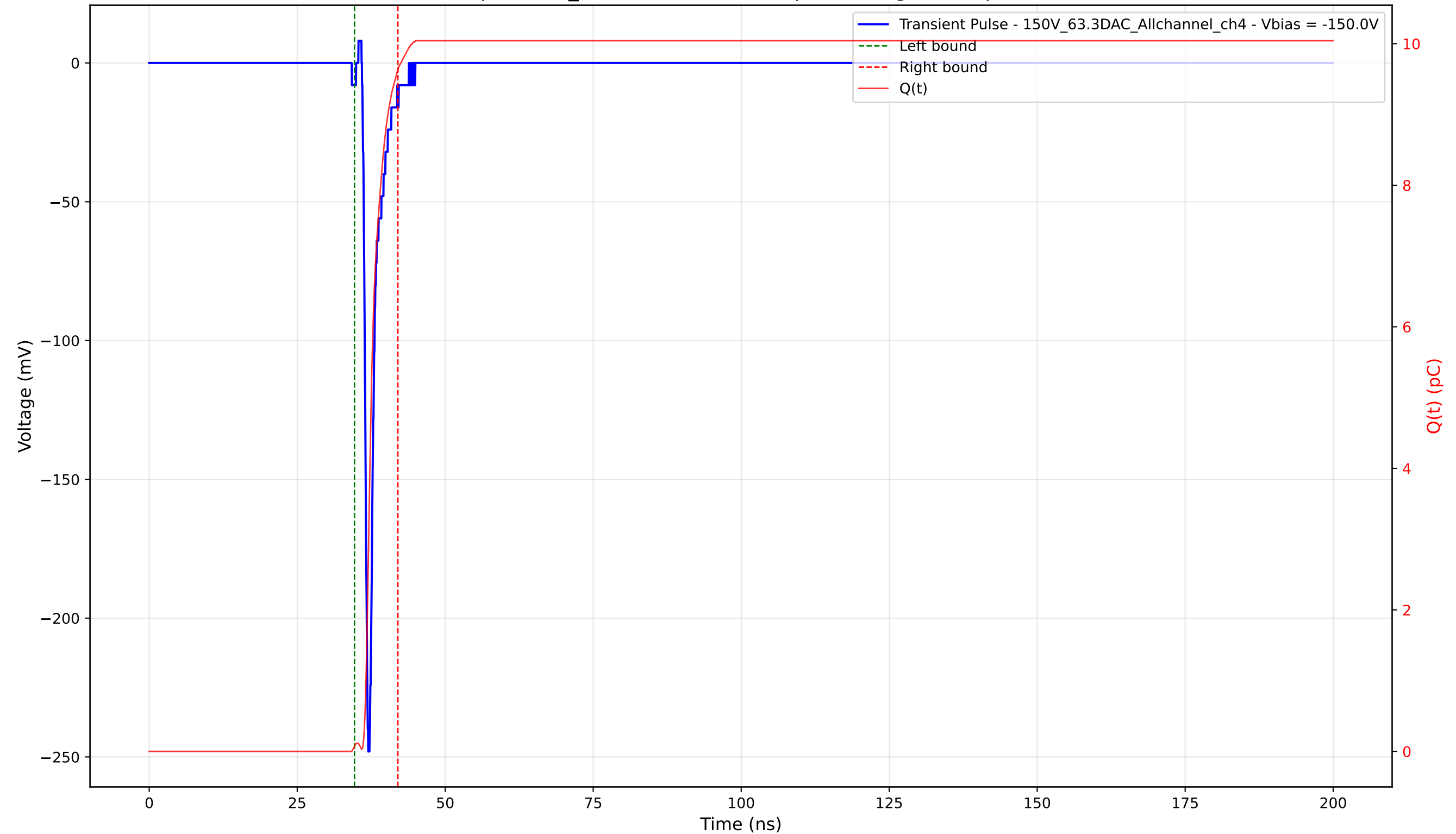
Transient Pulse - Sample: 1cm_42 - Position: 2500.0 \mu\text{m} - Charge: 9.55 pC - Rise Time: 0.75 ns
