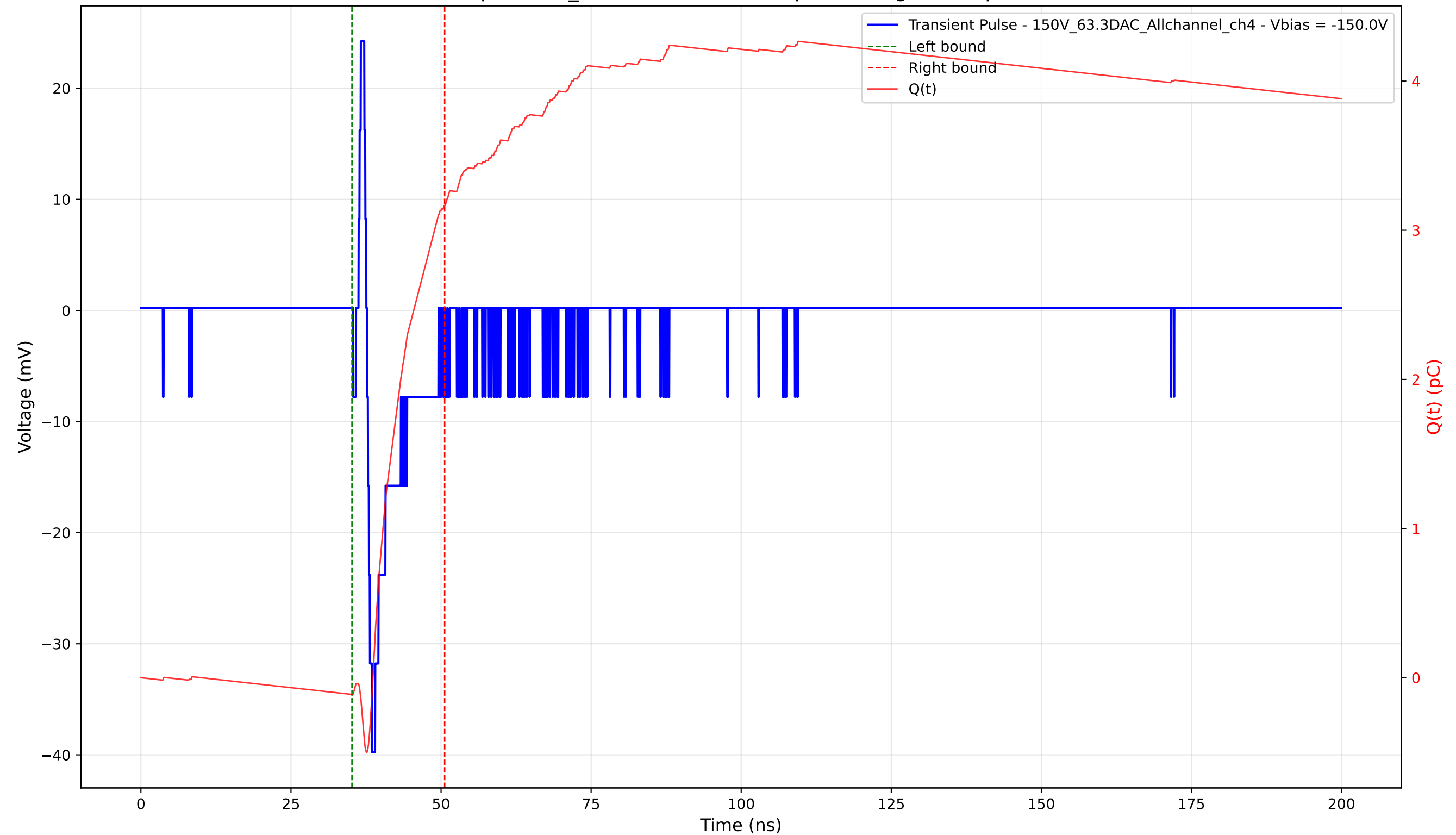
Transient Pulse - Sample: 1cm_42 - Position: 3745.0 \mu\text{m} - Charge: 3.28 pC - Rise Time: 0.86 ns
