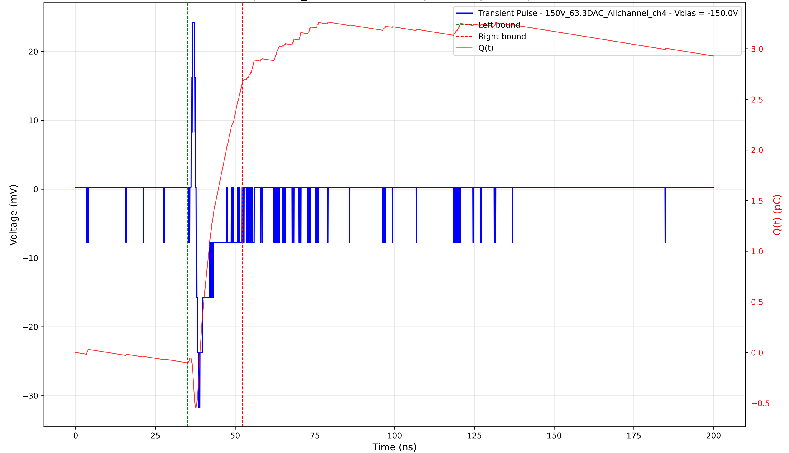
Transient Pulse - Sample: 1cm_42 - Position: 4045.0 \mu\text{m} - Charge: 2.77 pC - Rise Time: 0.78 ns
