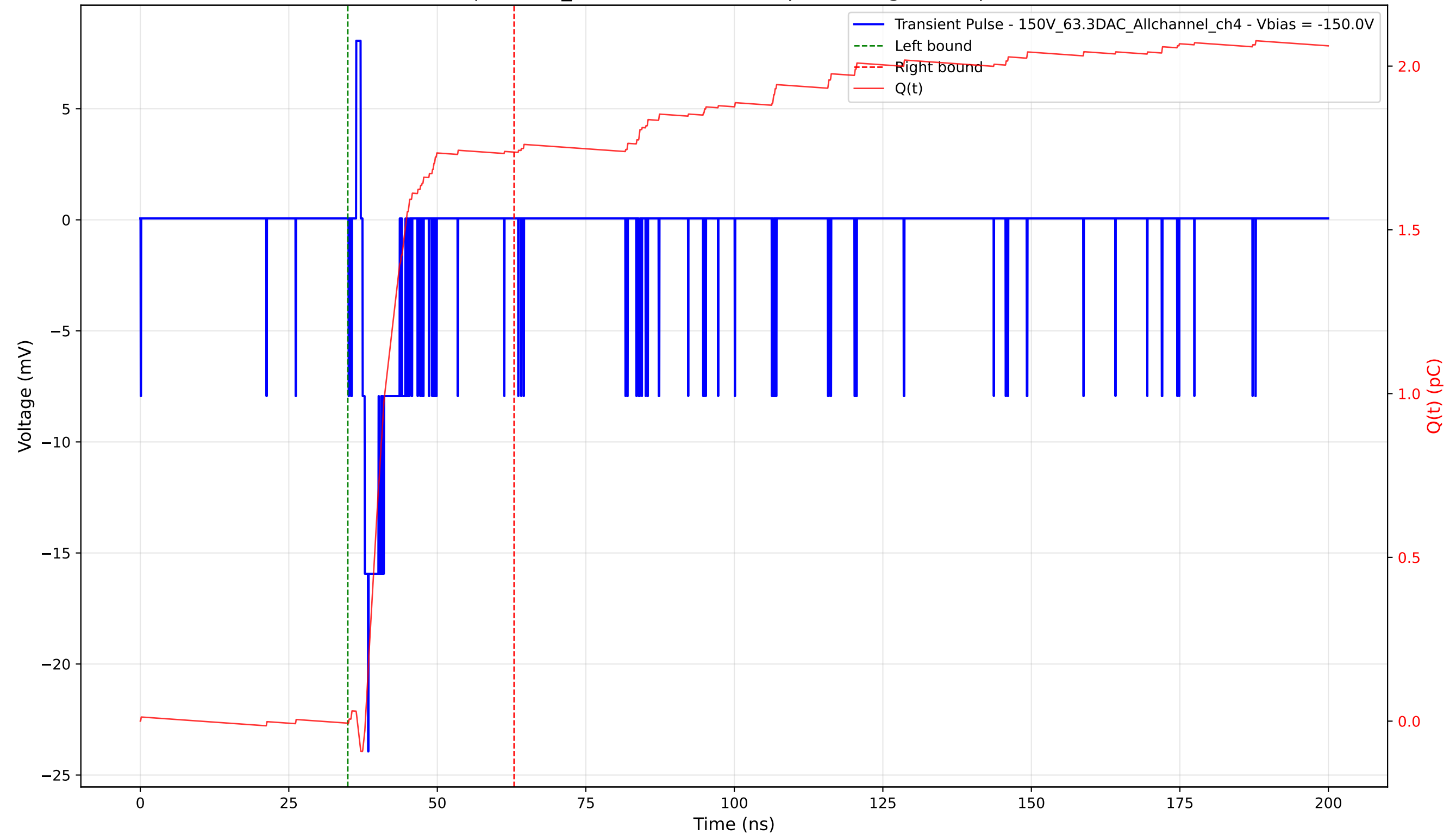
Transient Pulse - Sample: 1cm_42 - Position: 5025.0 \mu\text{m} - Charge: 1.74 pC - Rise Time: 0.95 ns
