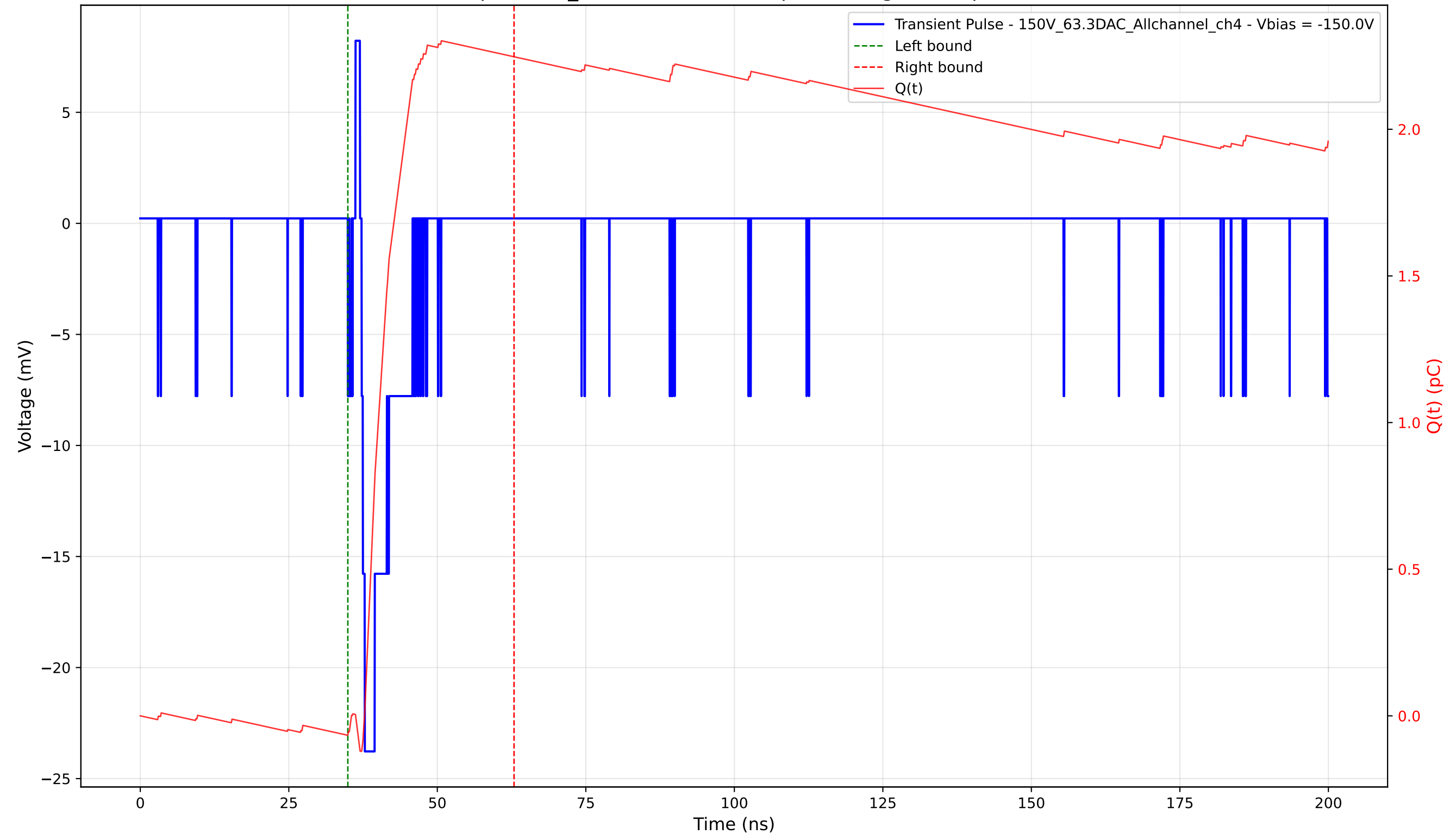
Transient Pulse - Sample: 1cm_42 - Position: 210.0 \mu\text{m} - Charge: 2.31 pC - Rise Time: 0.55 ns
