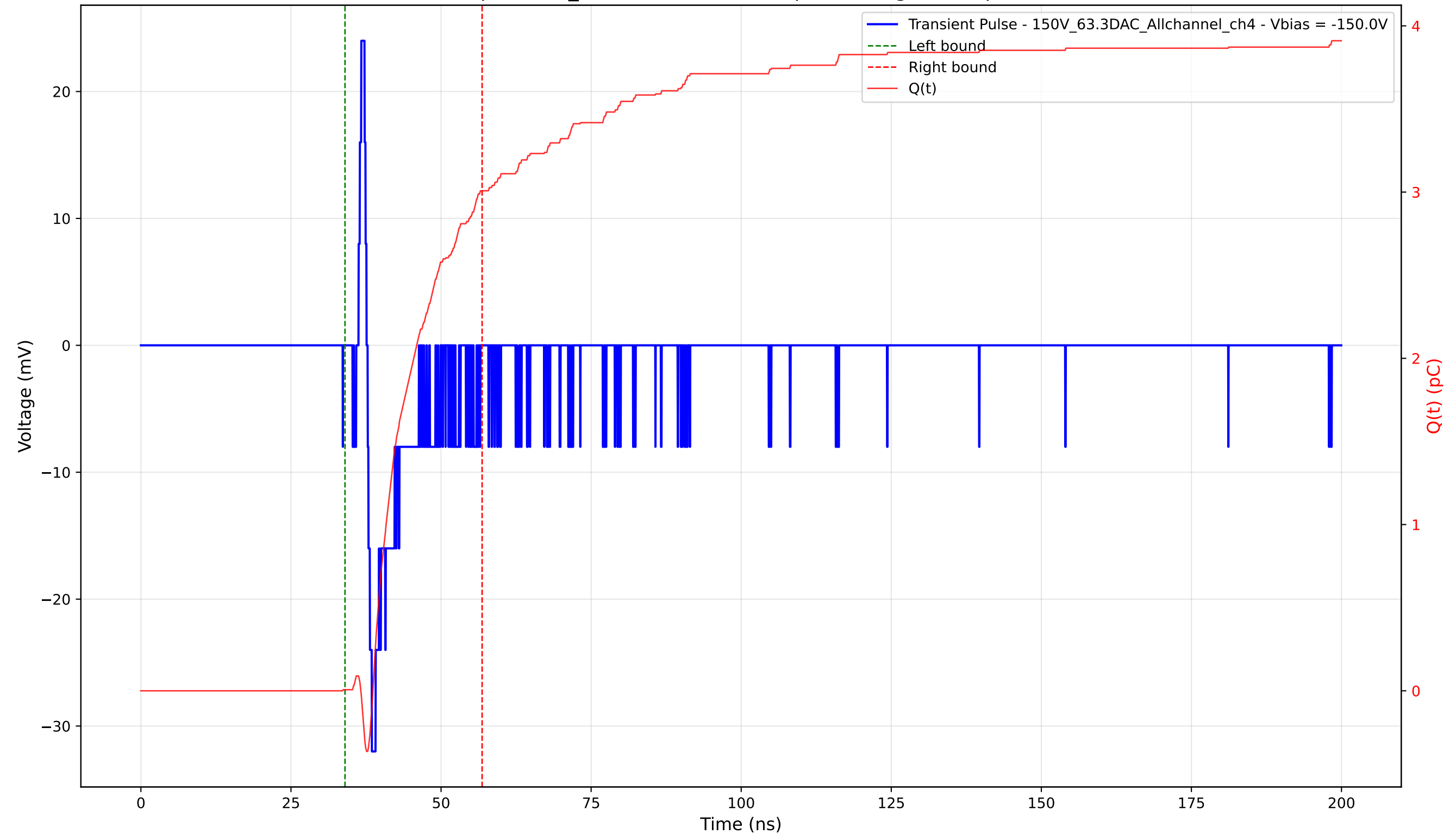
Transient Pulse - Sample: 1cm_42 - Position: 4015.0 \mu\text{m} - Charge: 3.00 pC - Rise Time: 0.70 ns
