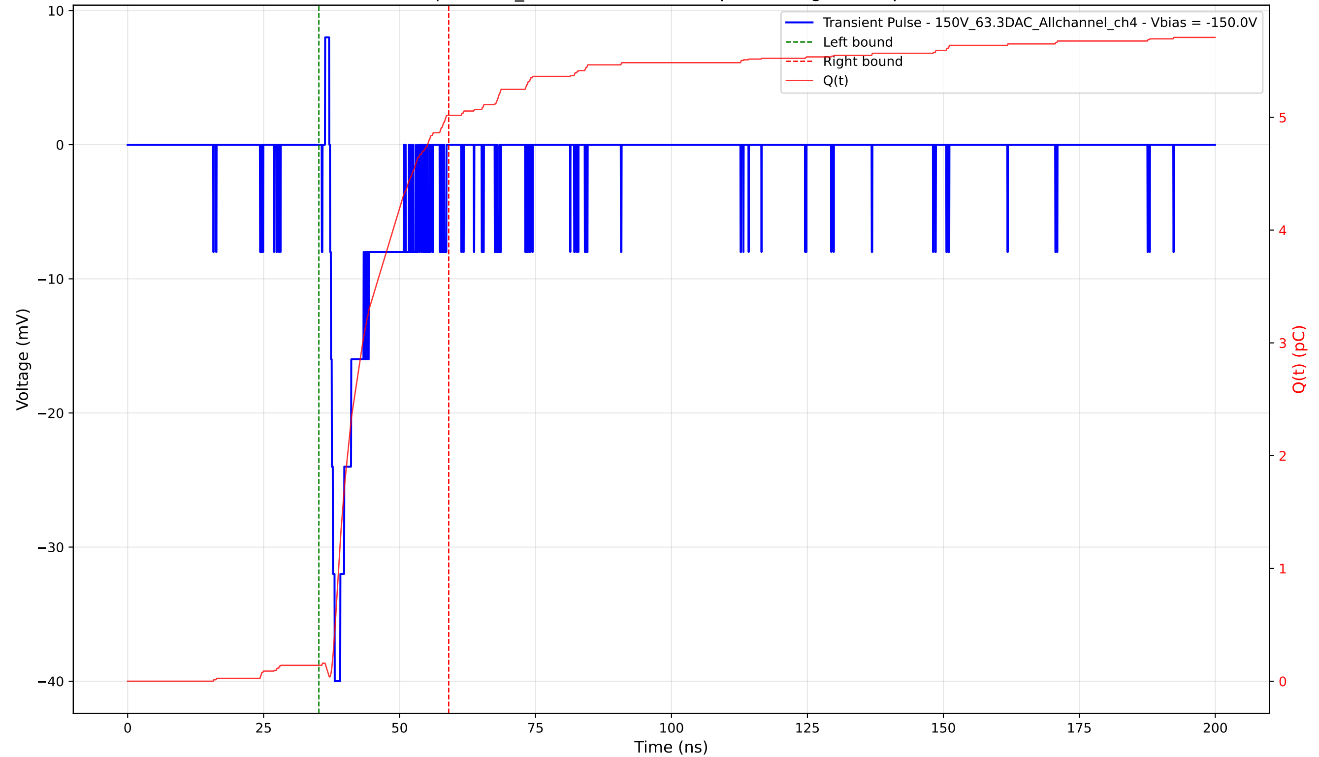
Transient Pulse - Sample: 1cm_42 - Position: 3420.0 \mu\text{m} - Charge: 4.88 pC - Rise Time: 0.86 ns
