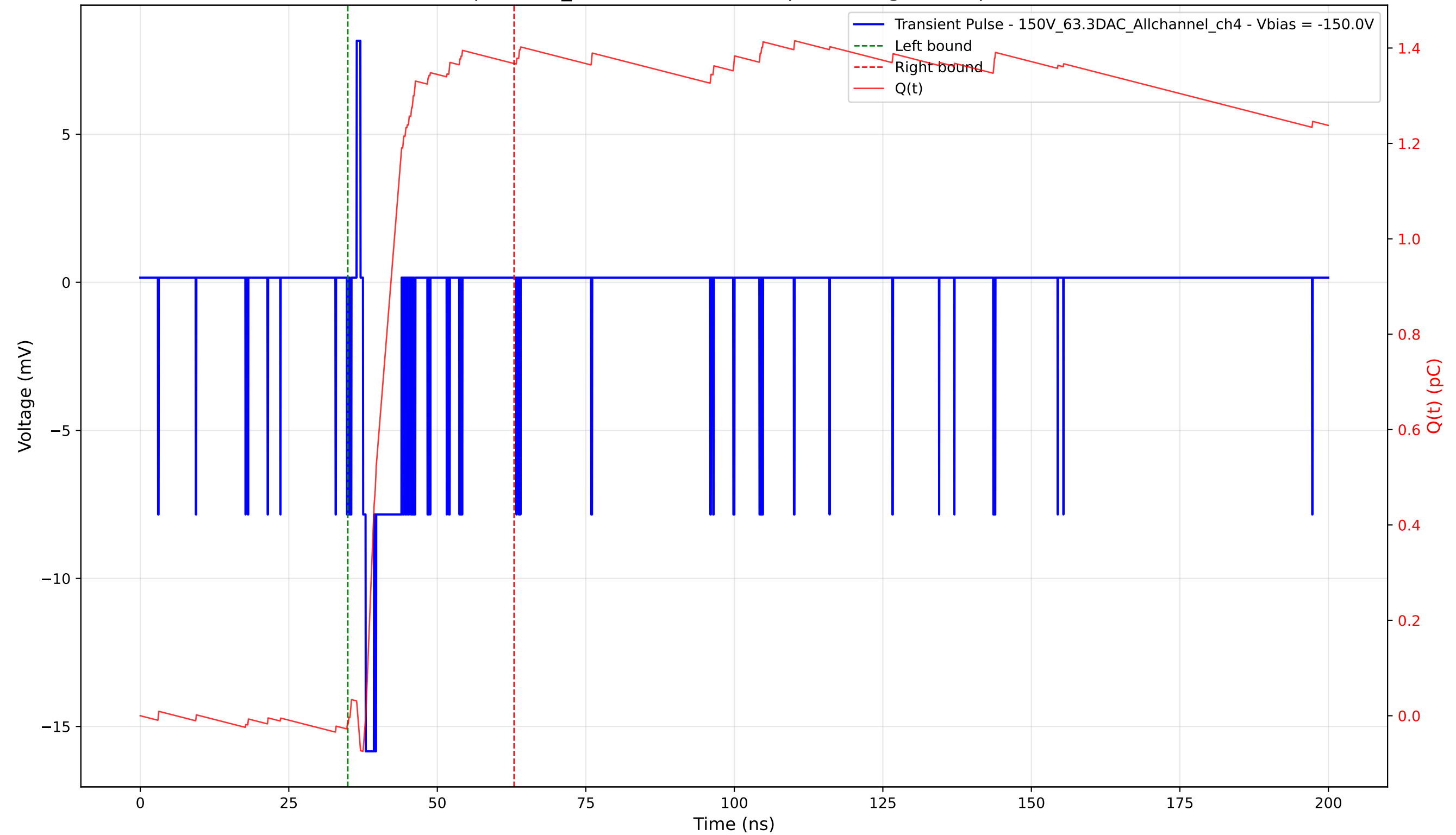
Transient Pulse - Sample: 1cm_42 - Position: 5060.0 \mu\text{m} - Charge: 1.38 pC - Rise Time: 0.47 ns
