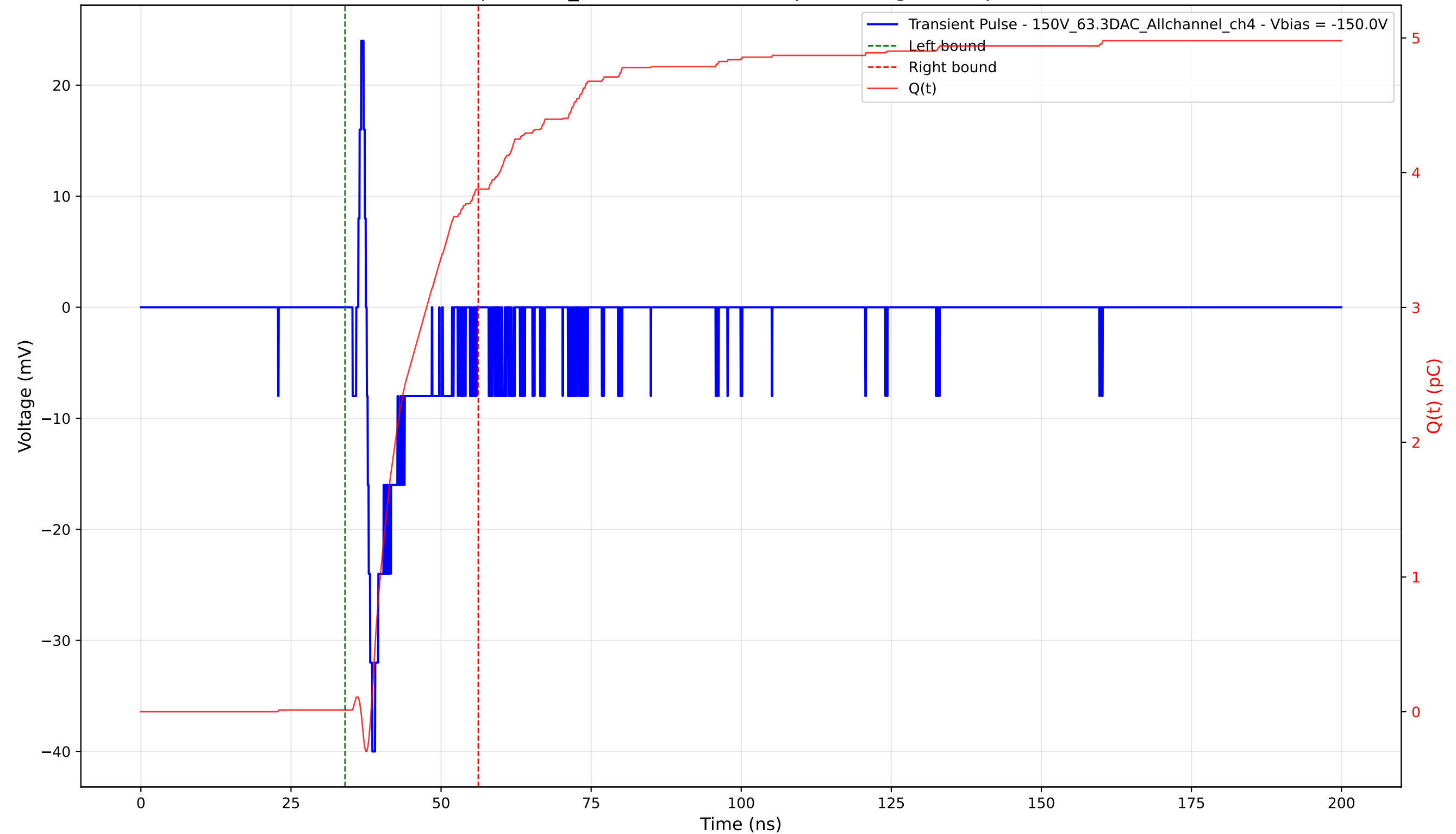
Transient Pulse - Sample: 1cm_42 - Position: 3690.0 \mu\text{m} - Charge: 3.87 pC - Rise Time: 0.94 ns
