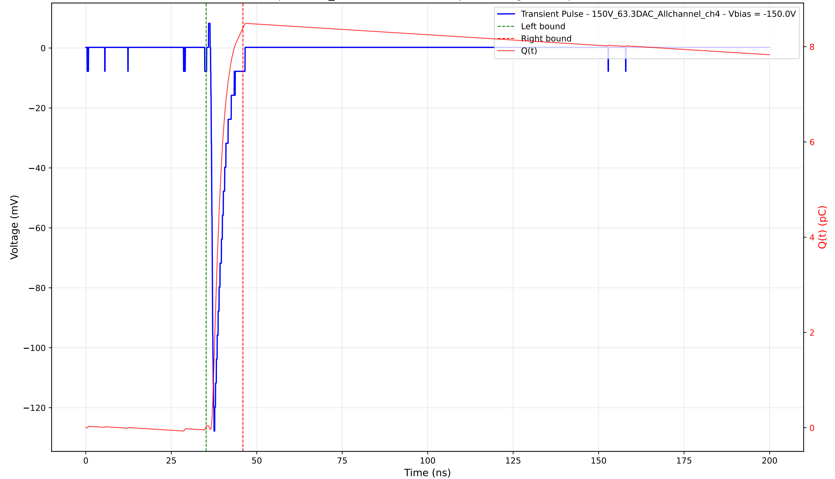
Transient Pulse - Sample: 1cm_42 - Position: 1100.0 \mu\text{m} - Charge: 8.37 pC - Rise Time: 0.77 ns
