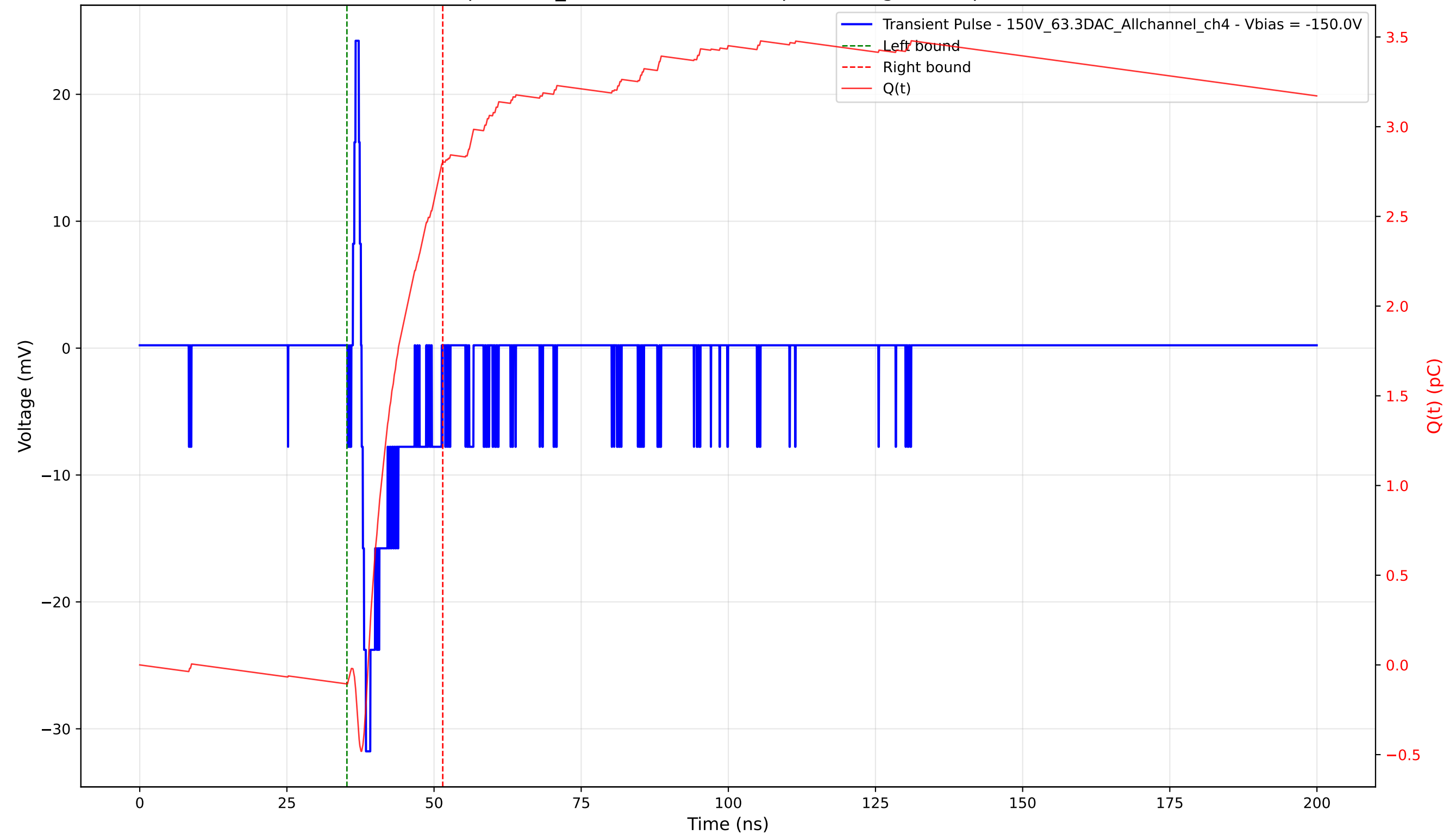
Transient Pulse - Sample: 1cm_42 - Position: 3970.0 \mu\text{m} - Charge: 2.91 pC - Rise Time: 0.74 ns
