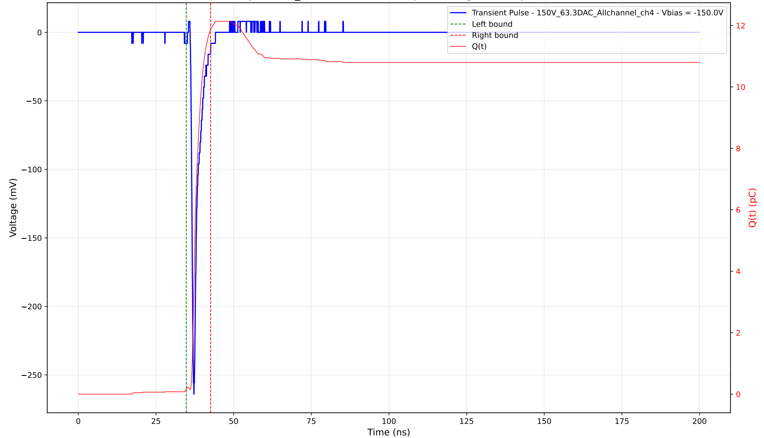
Transient Pulse - Sample: 1cm_42 - Position: 1500.0 \mu\text{m} - Charge: 11.72 pC - Rise Time: 0.75 ns
