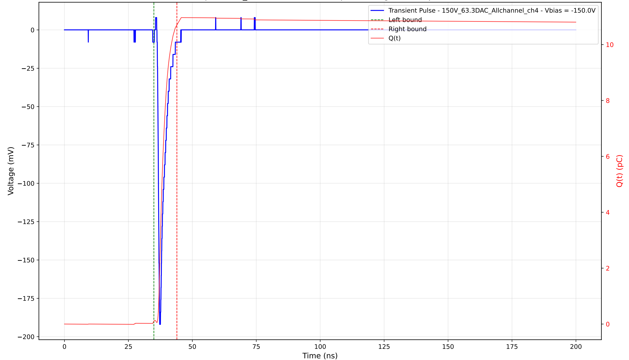
Transient Pulse - Sample: 1cm_42 - Position: 1365.0 \mu\text{m} - Charge: 10.61 pC - Rise Time: 0.77 ns
