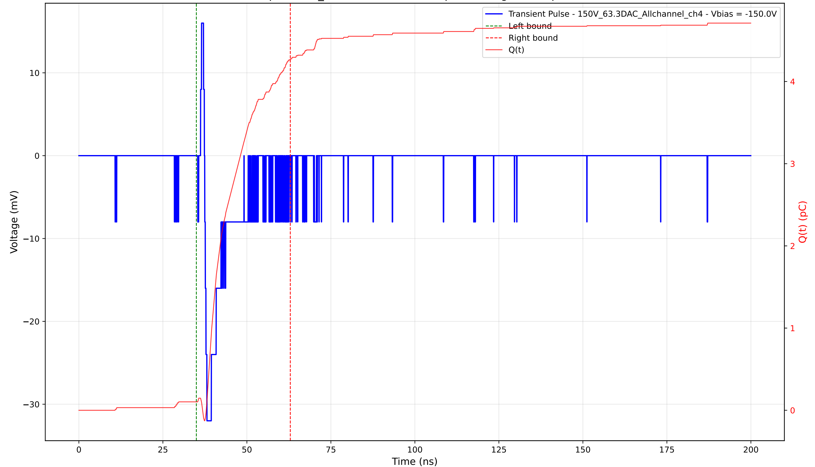
Transient Pulse - Sample: 1cm_42 - Position: 3555.0 \mu\text{m} - Charge: 4.17 pC - Rise Time: 0.66 ns
