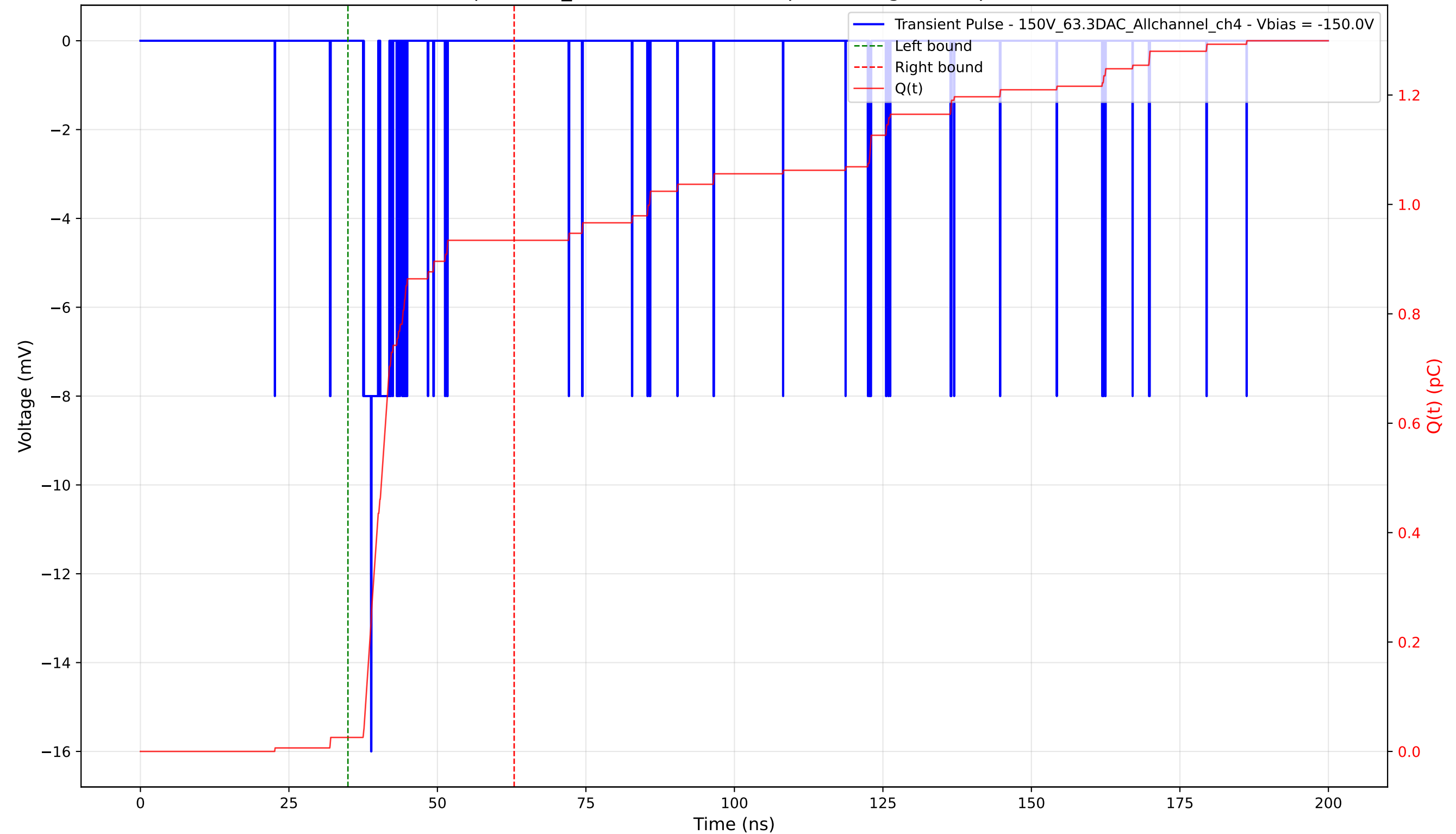
Transient Pulse - Sample: 1cm_42 - Position: 5125.0 \mu\text{m} - Charge: 0.91 pC - Rise Time: 1.23 ns
