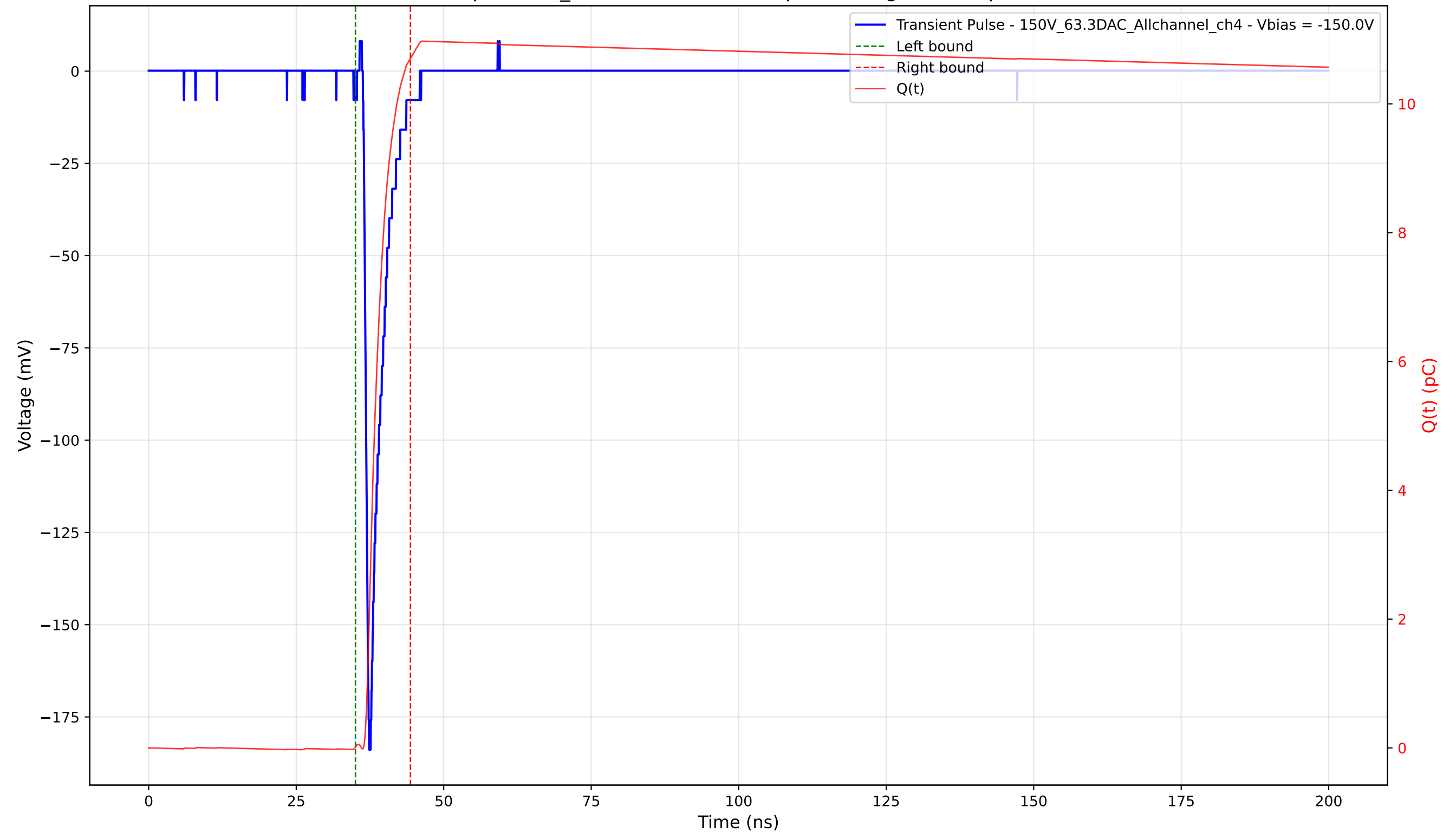
Transient Pulse - Sample: 1cm_42 - Position: 1245.0 \mu\text{m} - Charge: 10.70 pC - Rise Time: 0.75 ns
