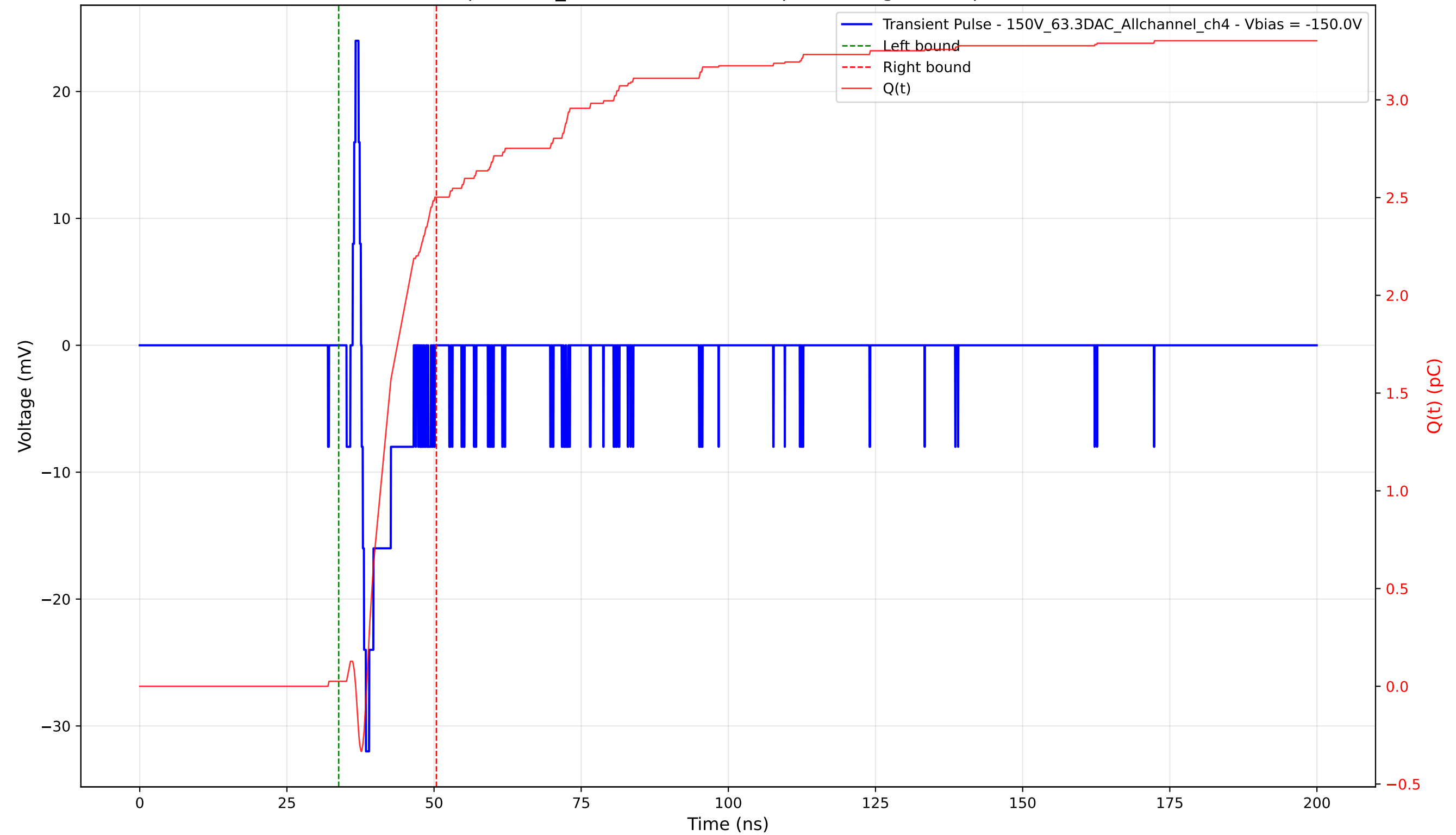
Transient Pulse - Sample: 1cm_42 - Position: 4480.0 \mu\text{m} - Charge: 2.48 pC - Rise Time: 0.74 ns
