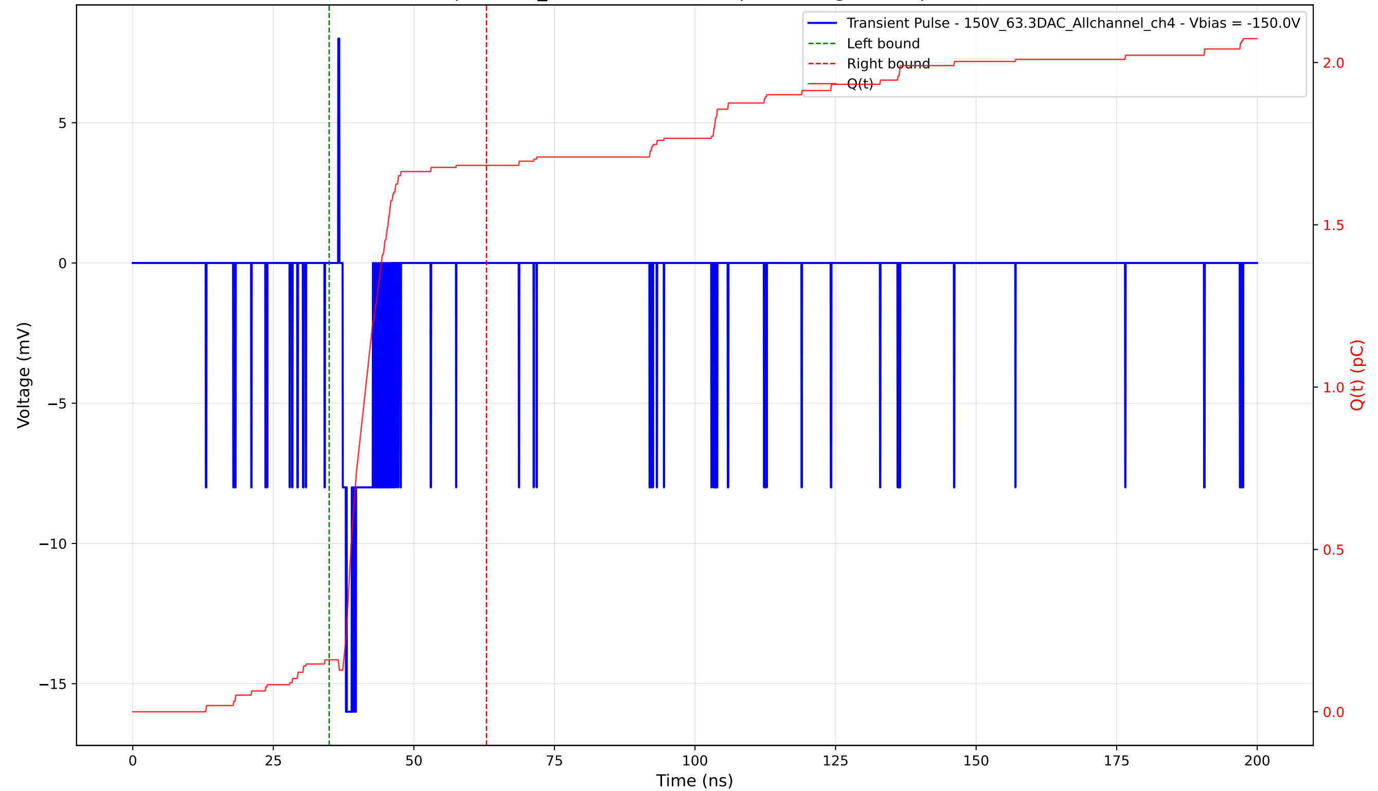
Transient Pulse - Sample: 1cm_42 - Position: 115.0 \mu\text{m} - Charge: 1.52 pC - Rise Time: 0.59 ns
