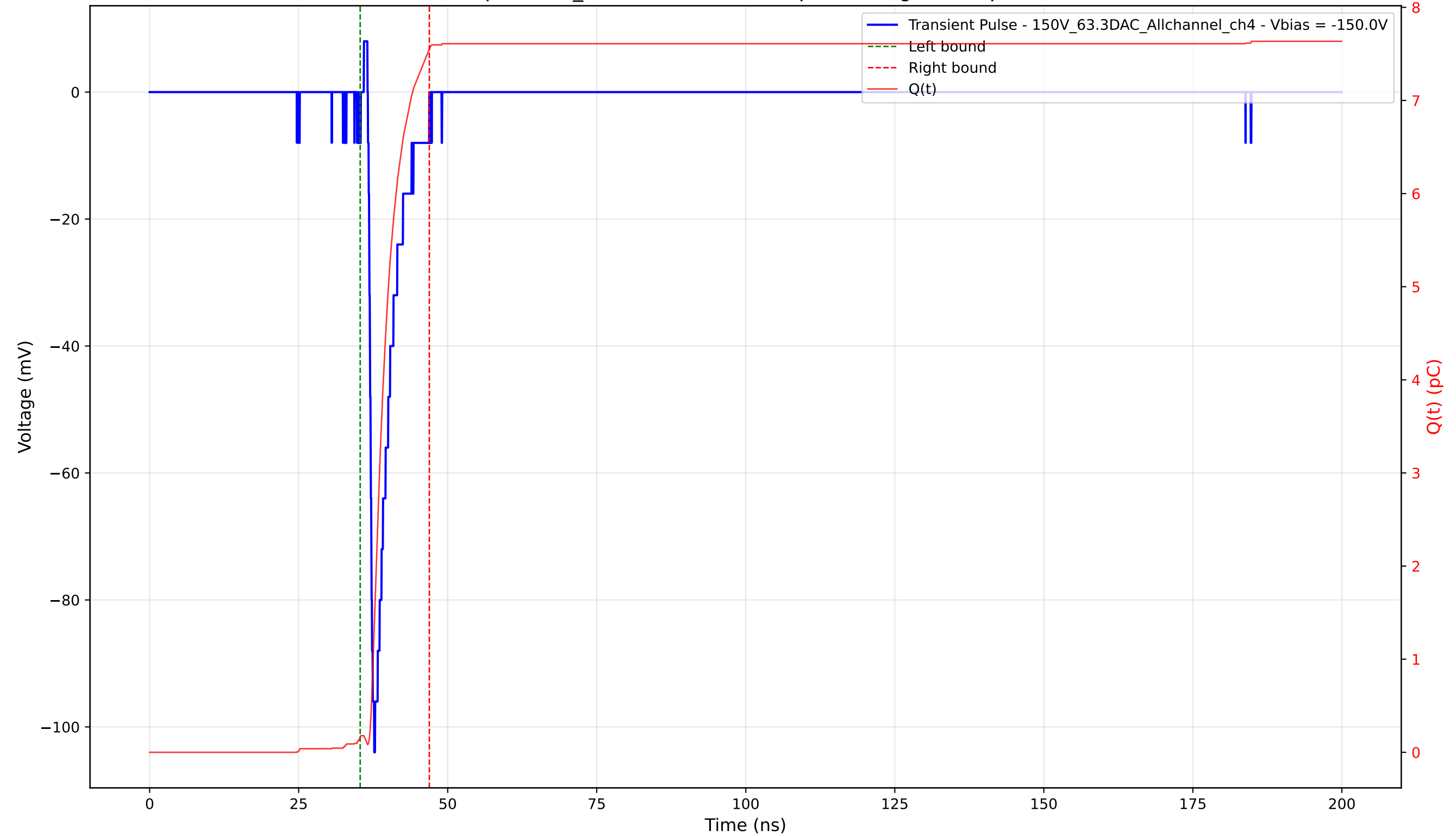
Transient Pulse - Sample: 1cm_42 - Position: 1020.0 \mu\text{m} - Charge: 7.39 pC - Rise Time: 0.71 ns
