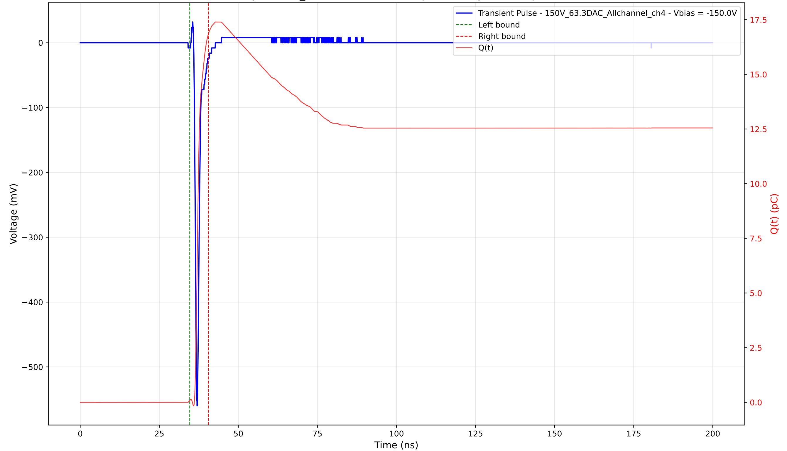
Transient Pulse - Sample: 1cm_42 - Position: 2130.0 \mu\text{m} - Charge: 16.77 pC - Rise Time: 0.66 ns
