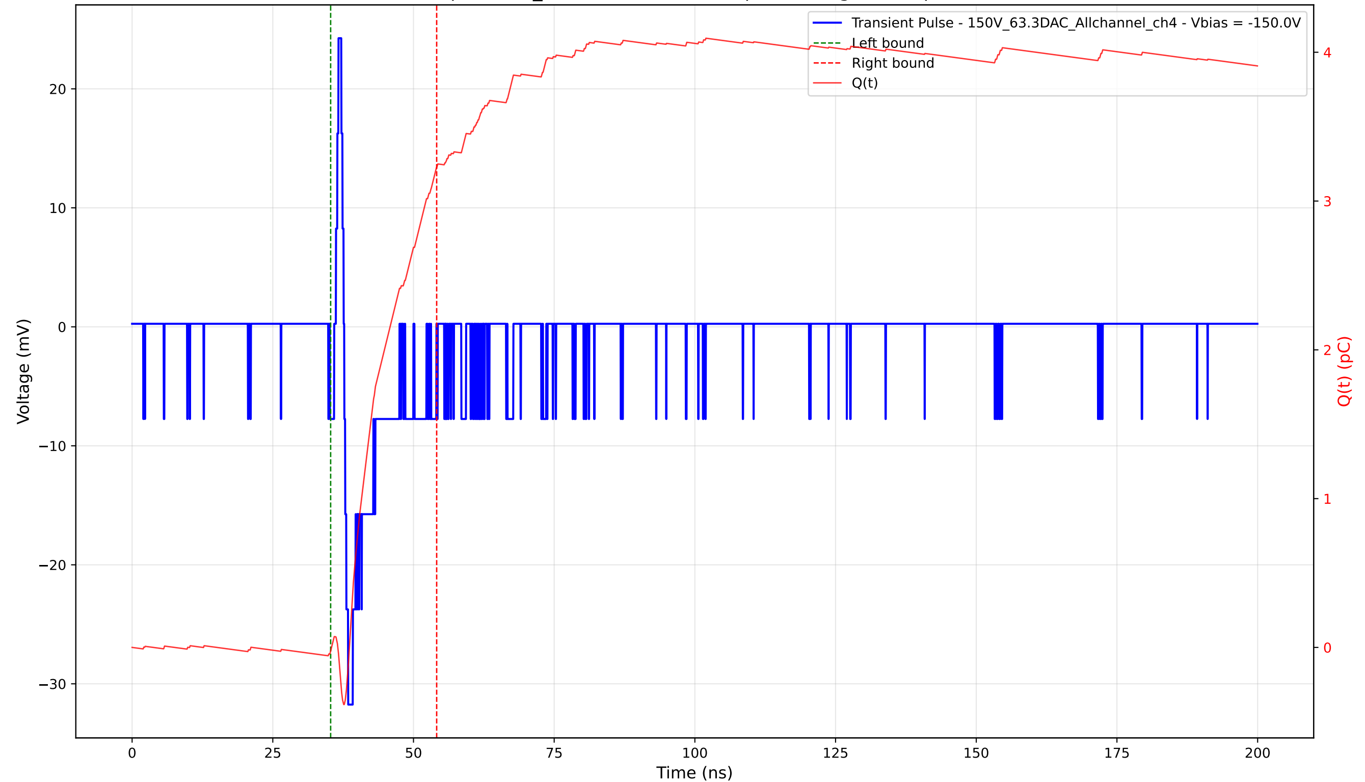
Transient Pulse - Sample: 1cm_42 - Position: 3935.0 \mu\text{m} - Charge: 3.25 pC - Rise Time: 0.70 ns
