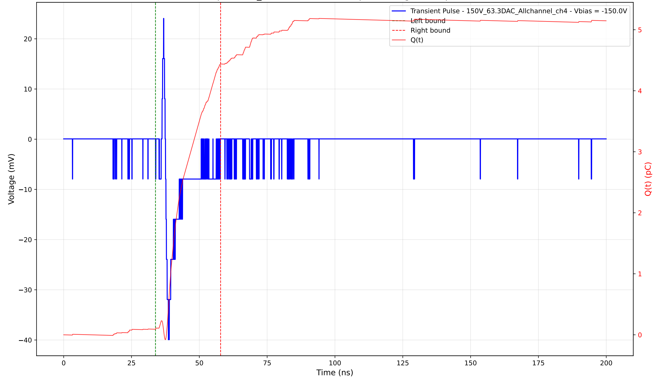
Transient Pulse - Sample: 1cm_42 - Position: 3595.0 \mu\text{m} - Charge: 4.35 pC - Rise Time: 1.06 ns
