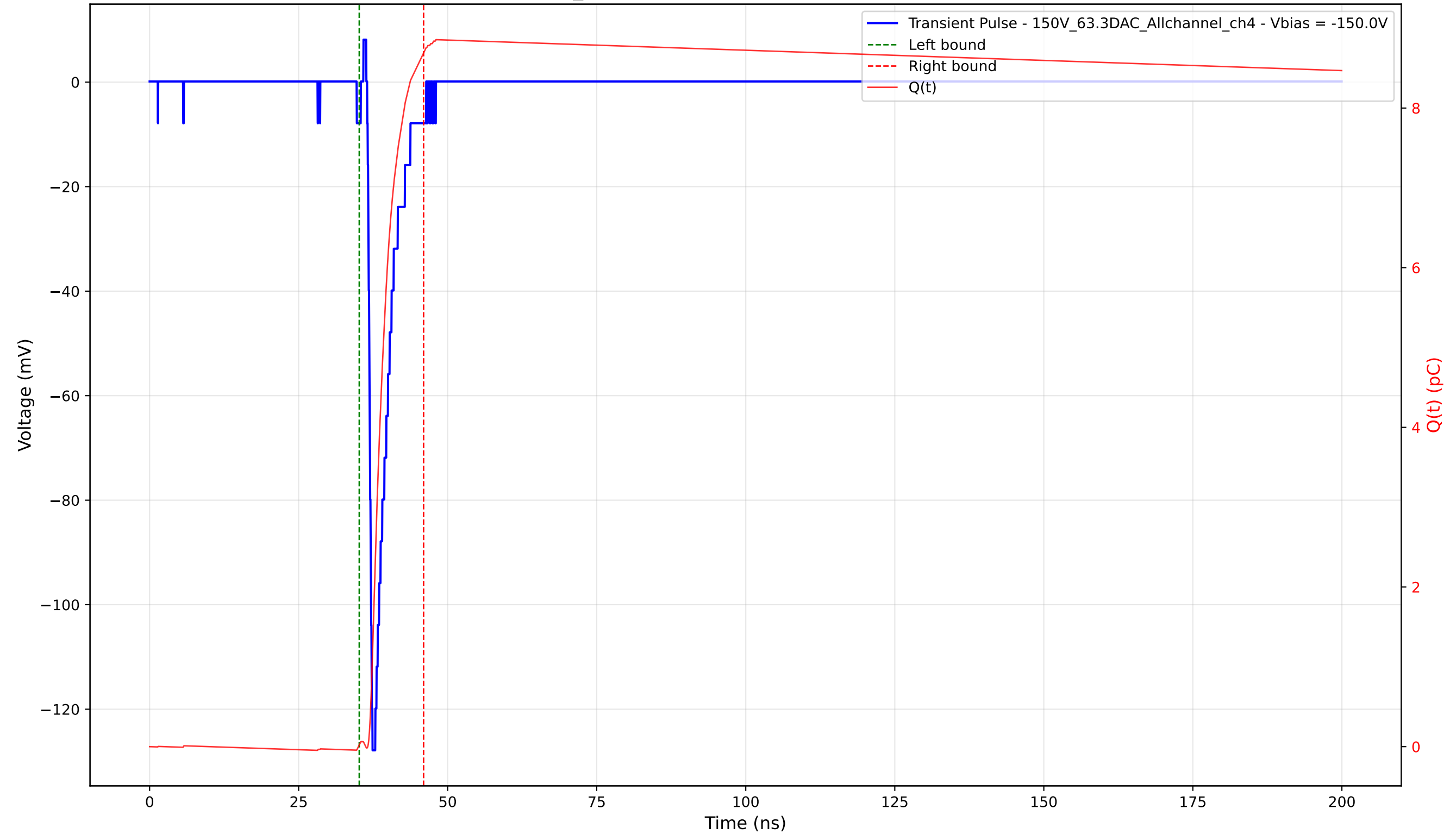
Transient Pulse - Sample: 1cm_42 - Position: 1110.0 \mu\text{m} - Charge: 8.67 pC - Rise Time: 0.70 ns
