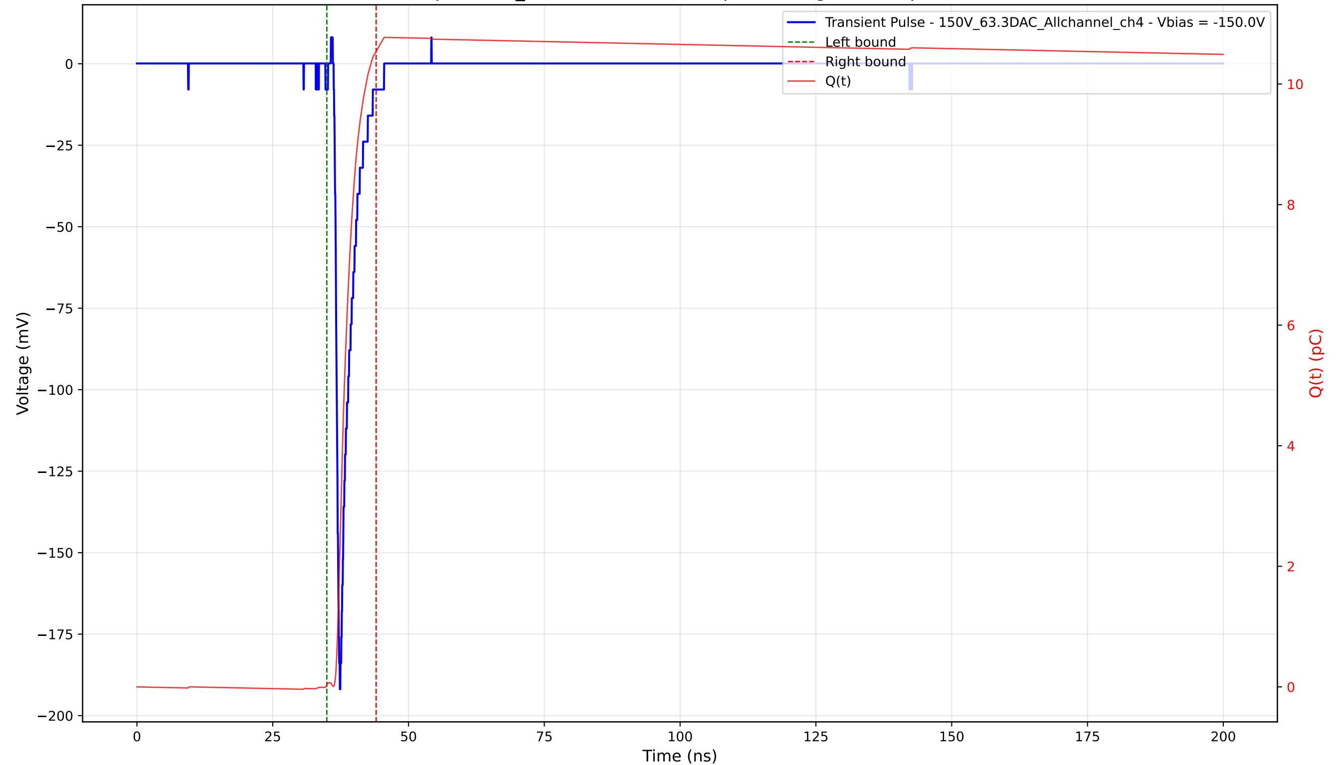
Transient Pulse - Sample: 1cm_42 - Position: 1350.0 \mu\text{m} - Charge: 10.51 pC - Rise Time: 0.78 ns
