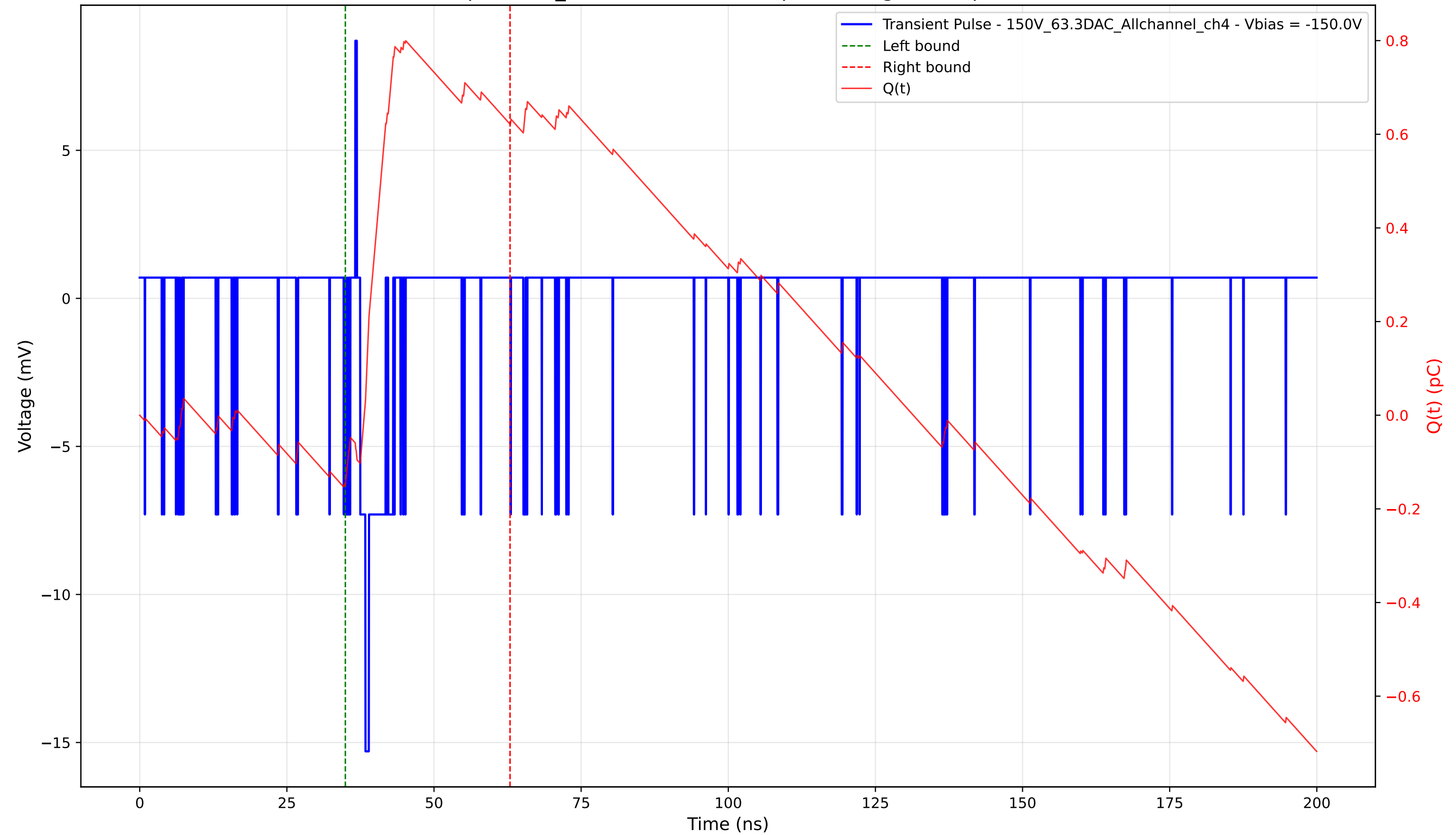
Transient Pulse - Sample: 1cm_42 - Position: 5110.0 \mu\text{m} - Charge: 0.77 pC - Rise Time: 0.91 ns
