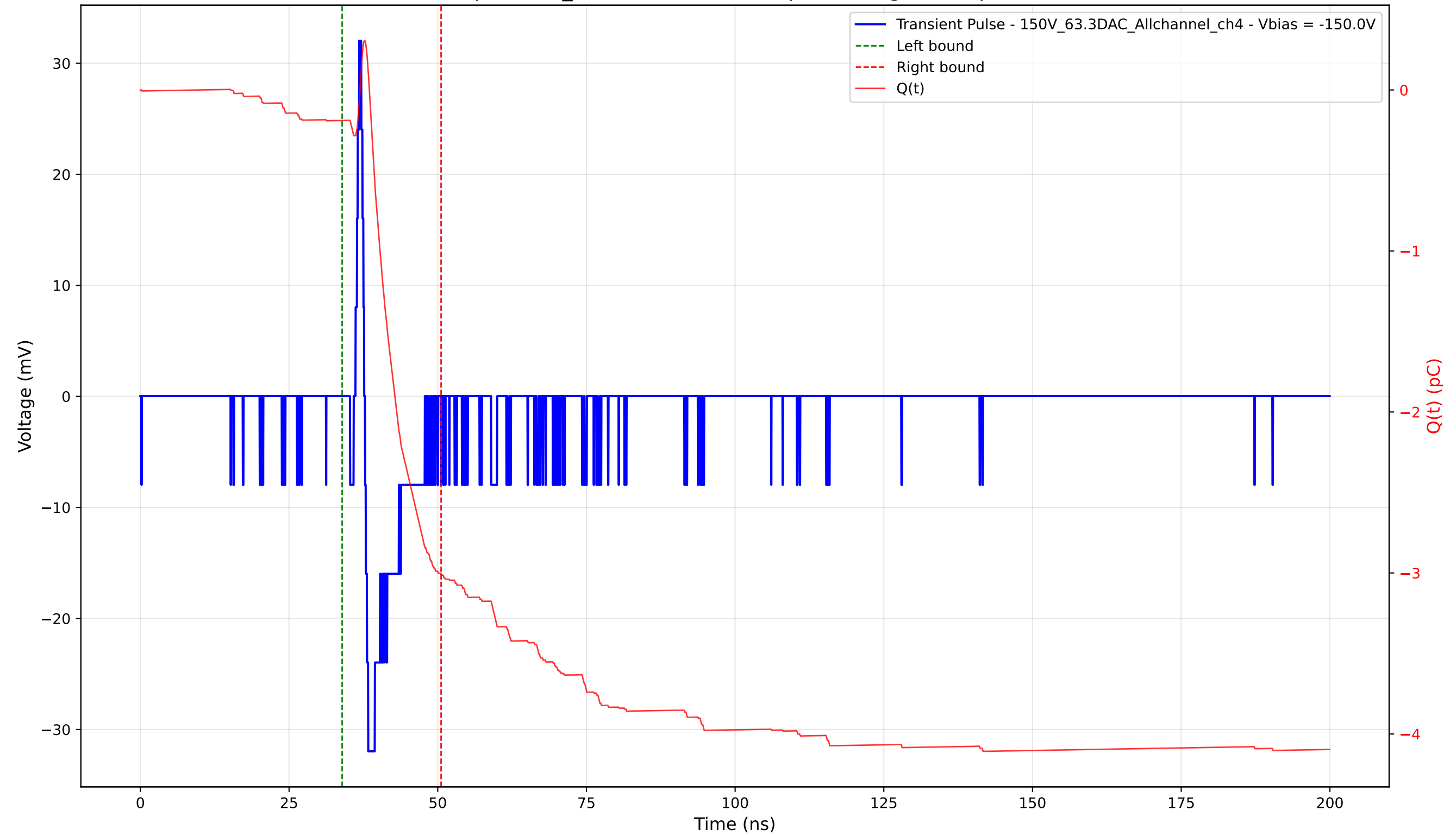
Transient Pulse - Sample: 1cm_42 - Position: 4260.0 \mu\text{m} - Charge: 2.81 pC - Rise Time: 0.62 ns
