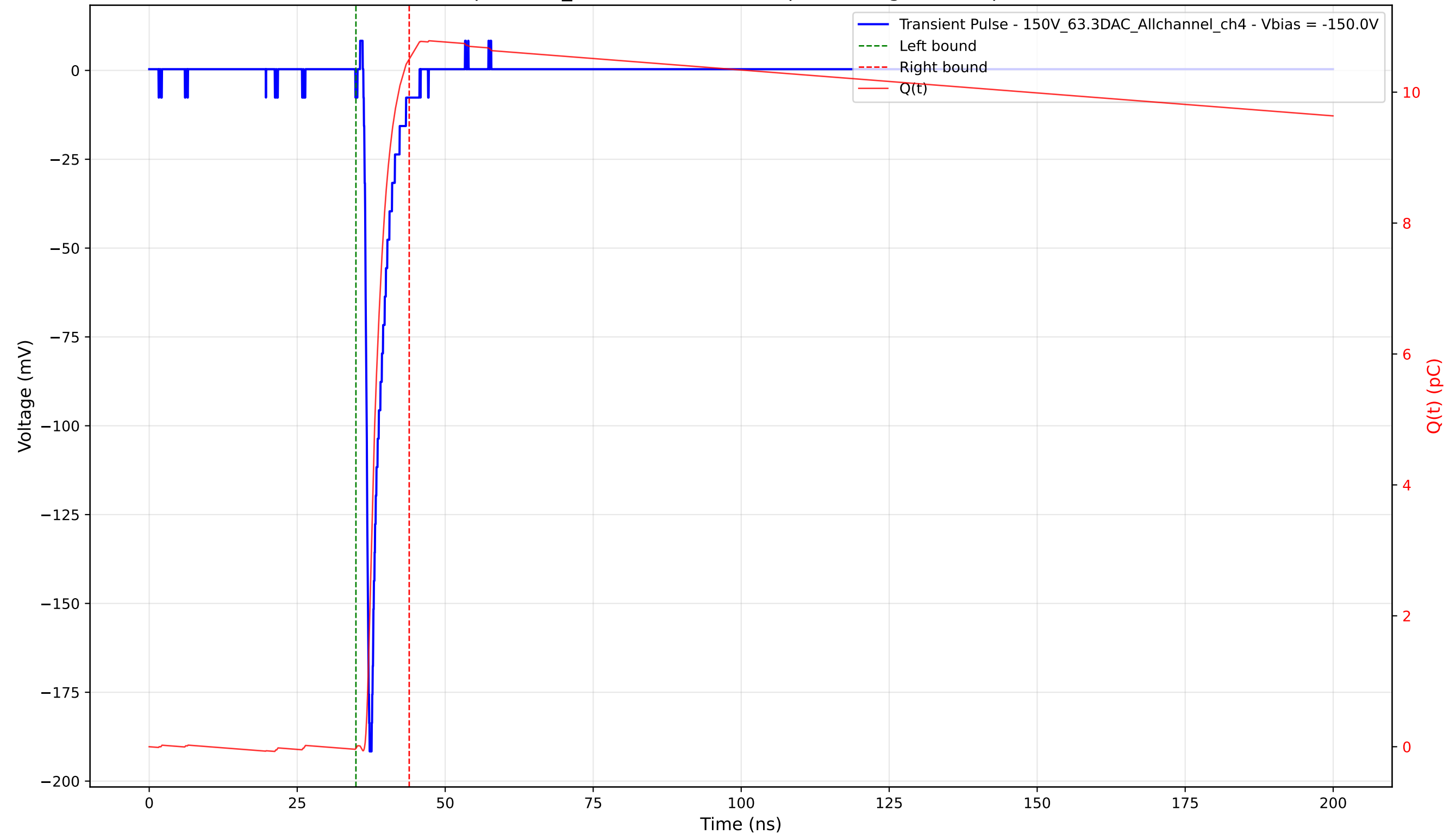
Transient Pulse - Sample: 1cm_42 - Position: 1380.0 \mu\text{m} - Charge: 10.53 pC - Rise Time: 0.74 ns
