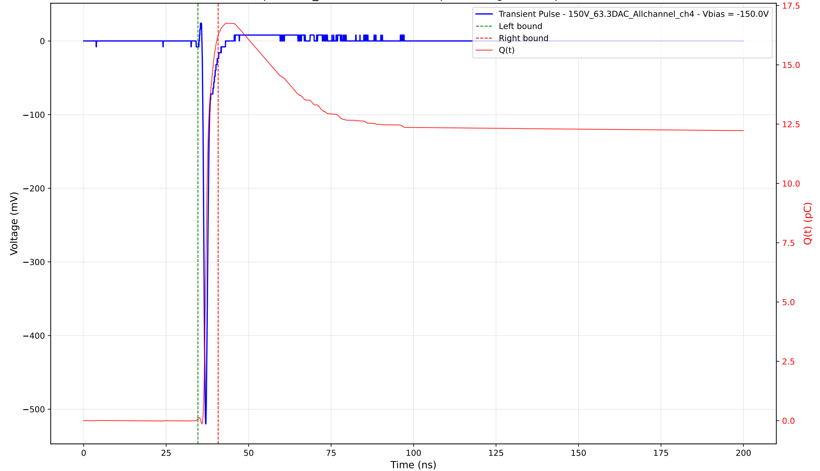
Transient Pulse - Sample: 1cm_42 - Position: 2210.0 \mu\text{m} - Charge: 16.15 pC - Rise Time: 0.72 ns
