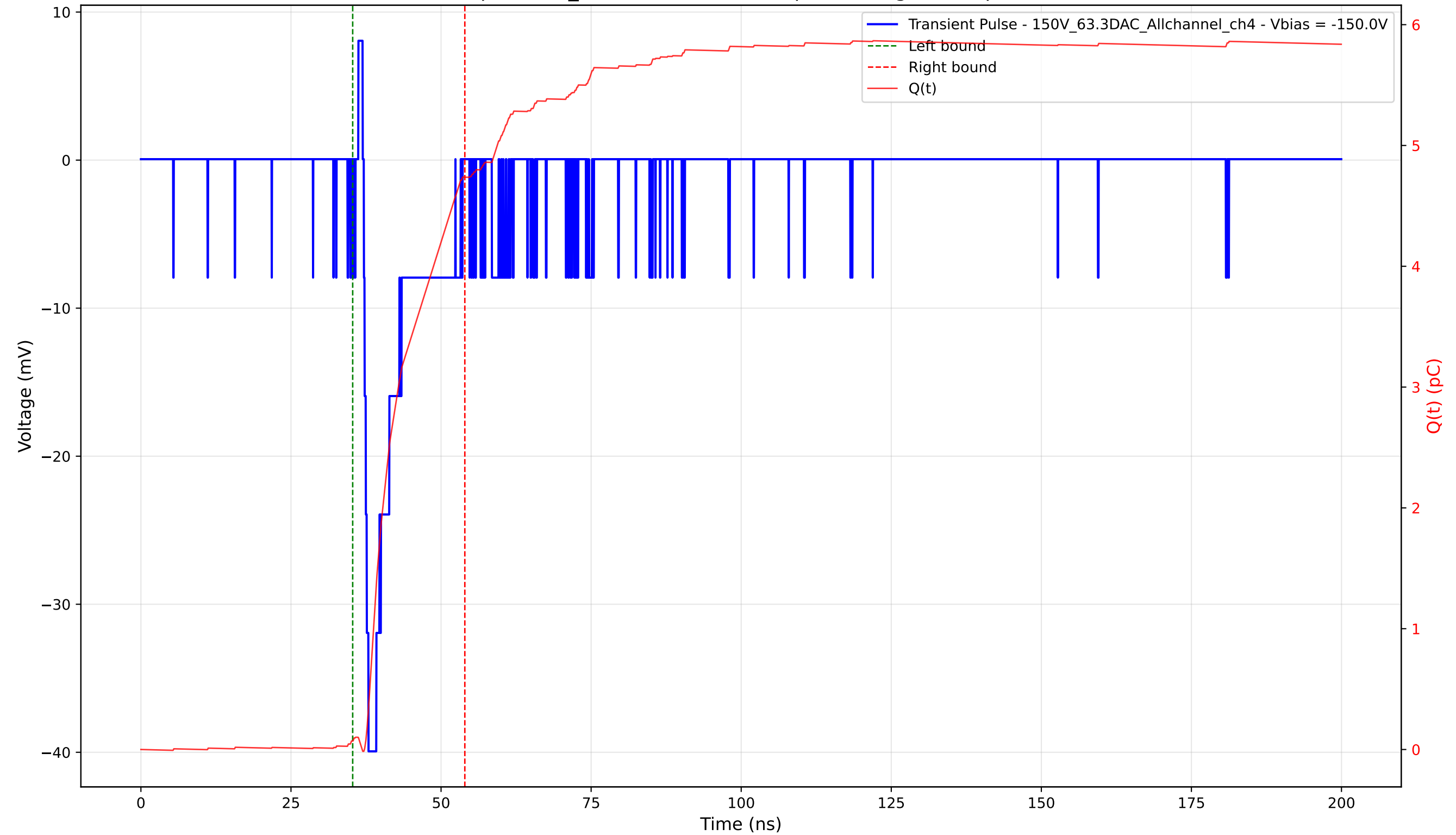
Transient Pulse - Sample: 1cm_42 - Position: 3370.0 \mu\text{m} - Charge: 4.67 pC - Rise Time: 0.78 ns
