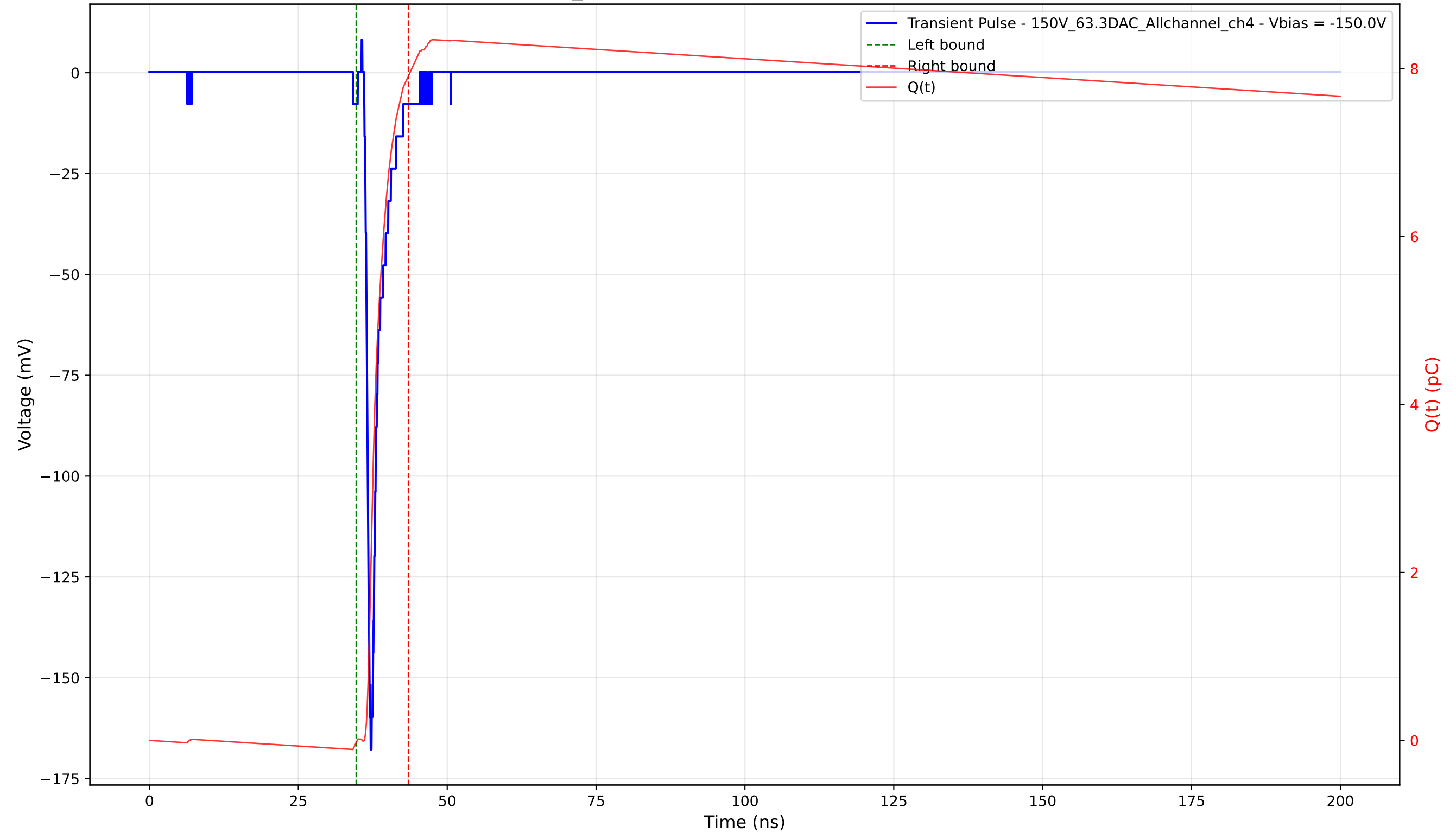
Transient Pulse - Sample: 1cm_42 - Position: 2645.0 \mu\text{m} - Charge: 7.94 pC - Rise Time: 0.79 ns
