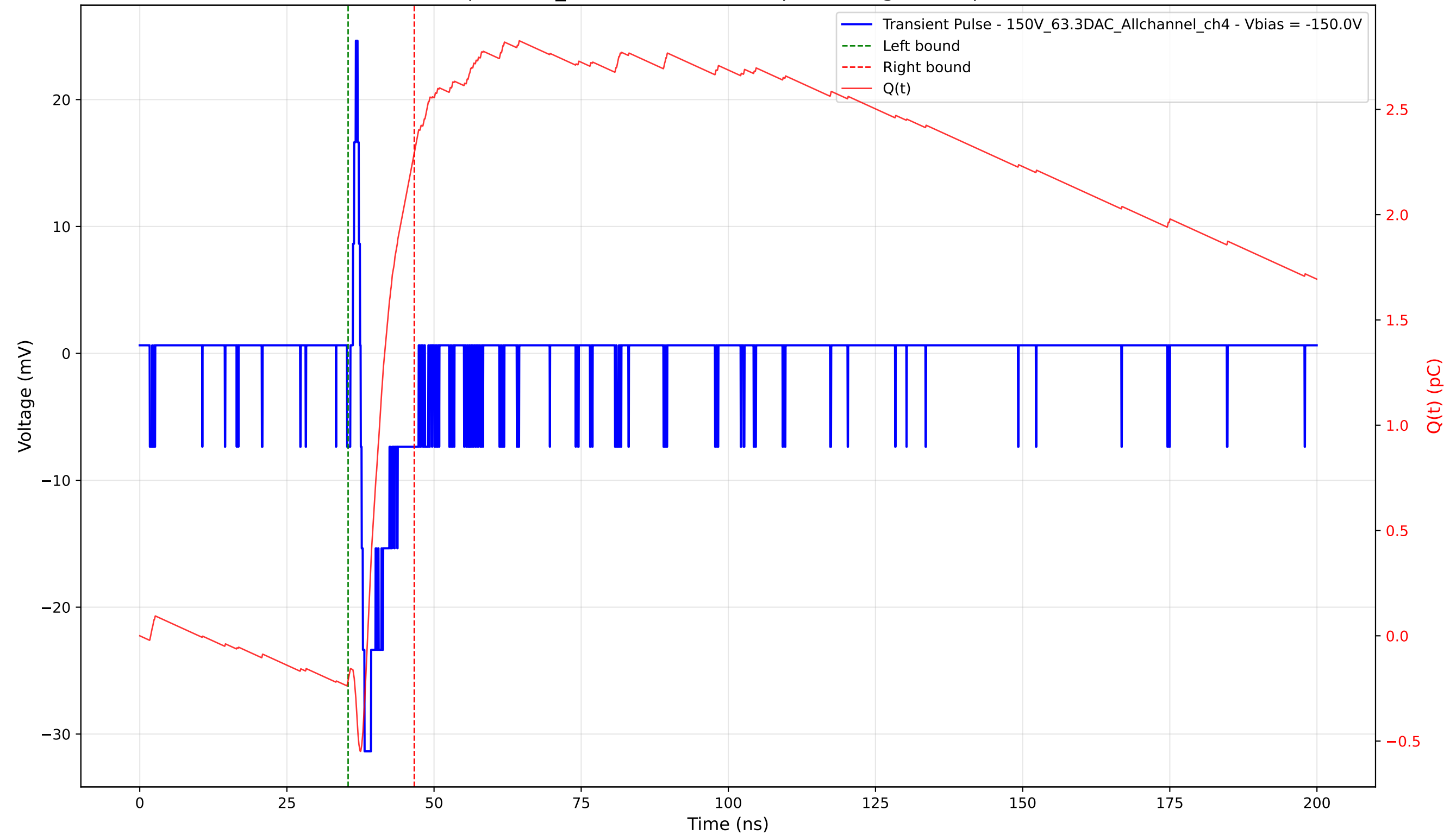
Transient Pulse - Sample: 1cm_42 - Position: 4720.0 \mu\text{m} - Charge: 2.51 pC - Rise Time: 0.67 ns
