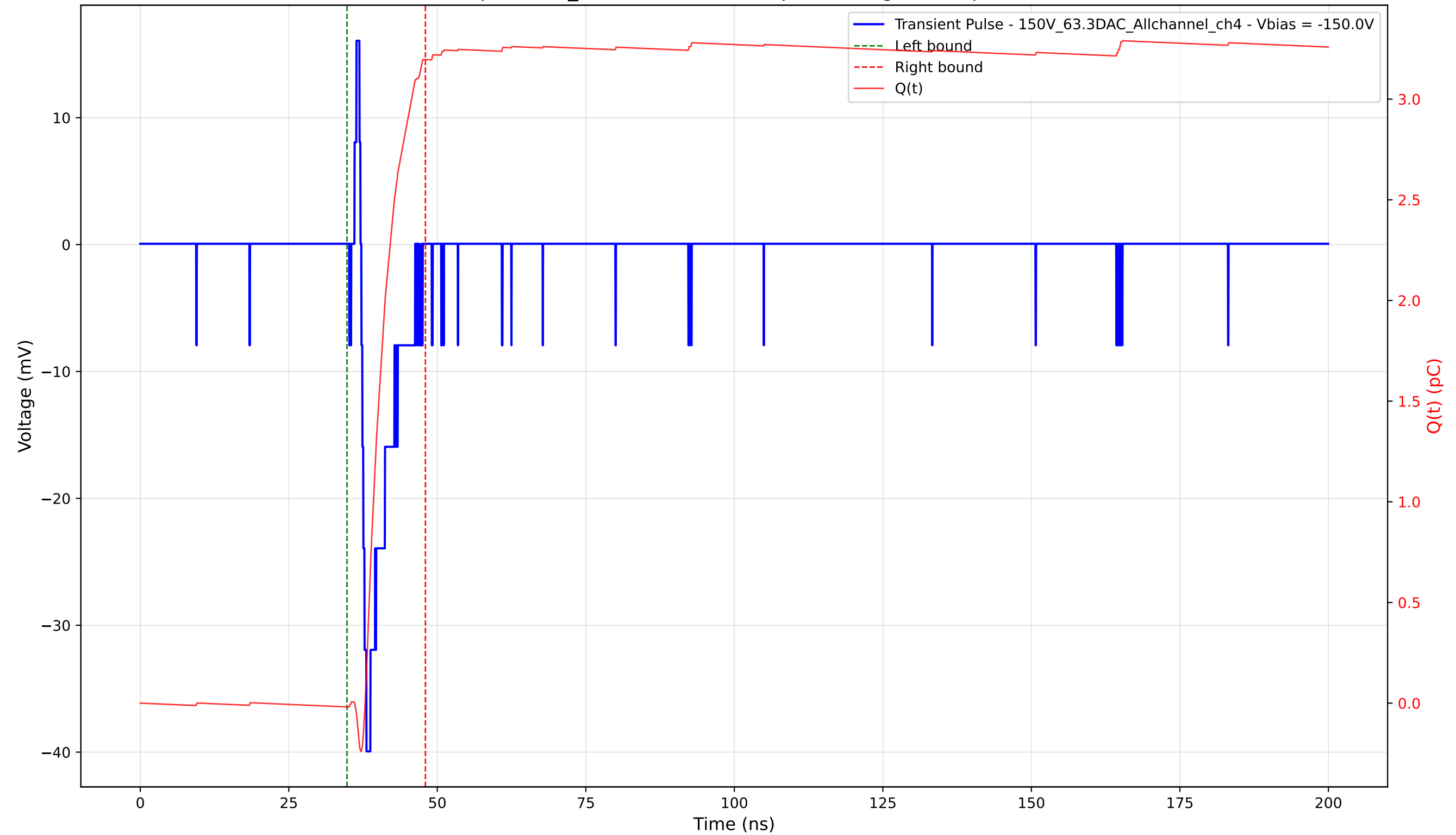
Transient Pulse - Sample: 1cm_42 - Position: 360.0 \mu\text{m} - Charge: 3.22 pC - Rise Time: 0.86 ns
