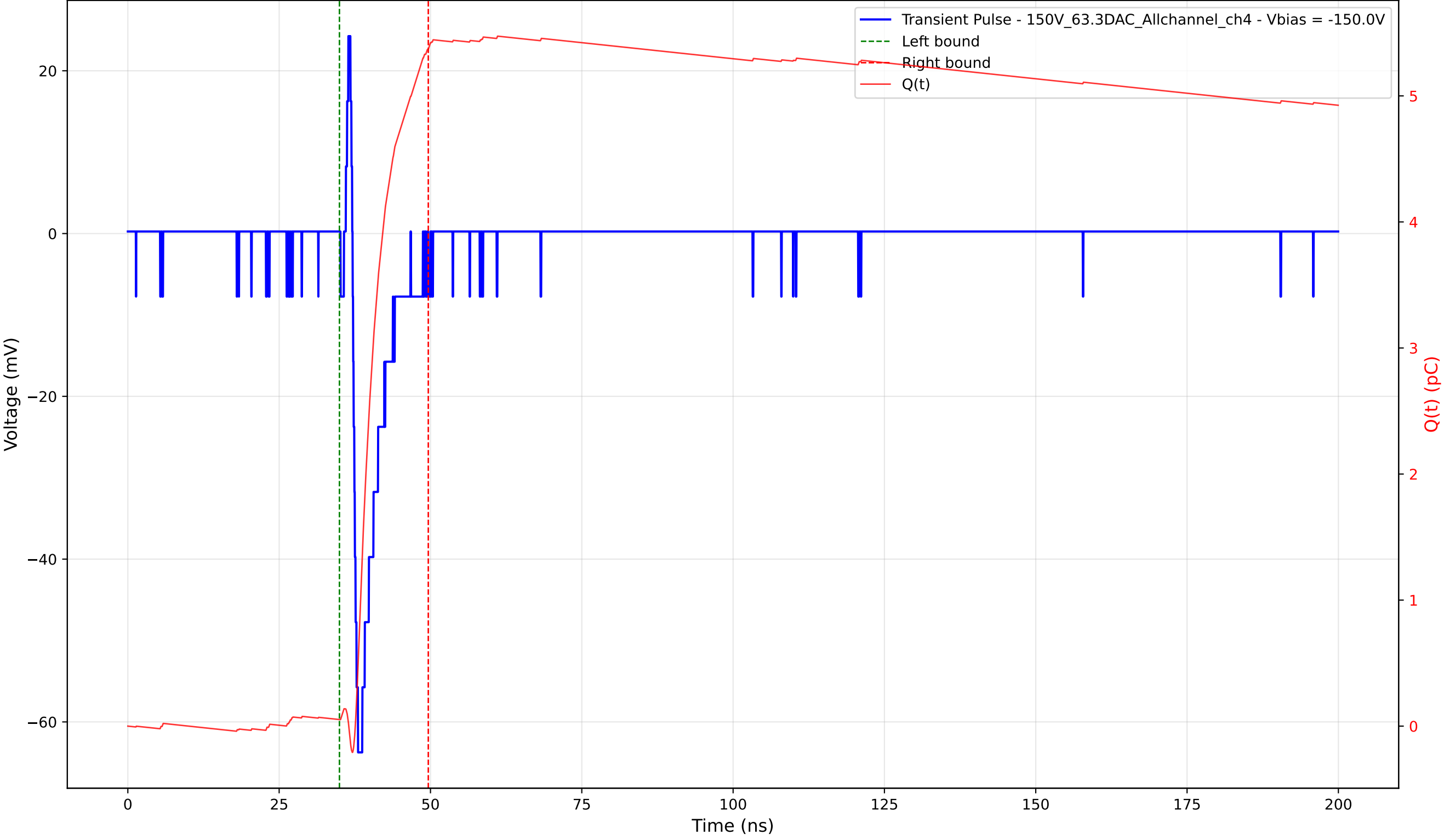
Transient Pulse - Sample: 1cm_42 - Position: 575.0 \mu\text{m} - Charge: 5.32 pC - Rise Time: 0.89 ns
