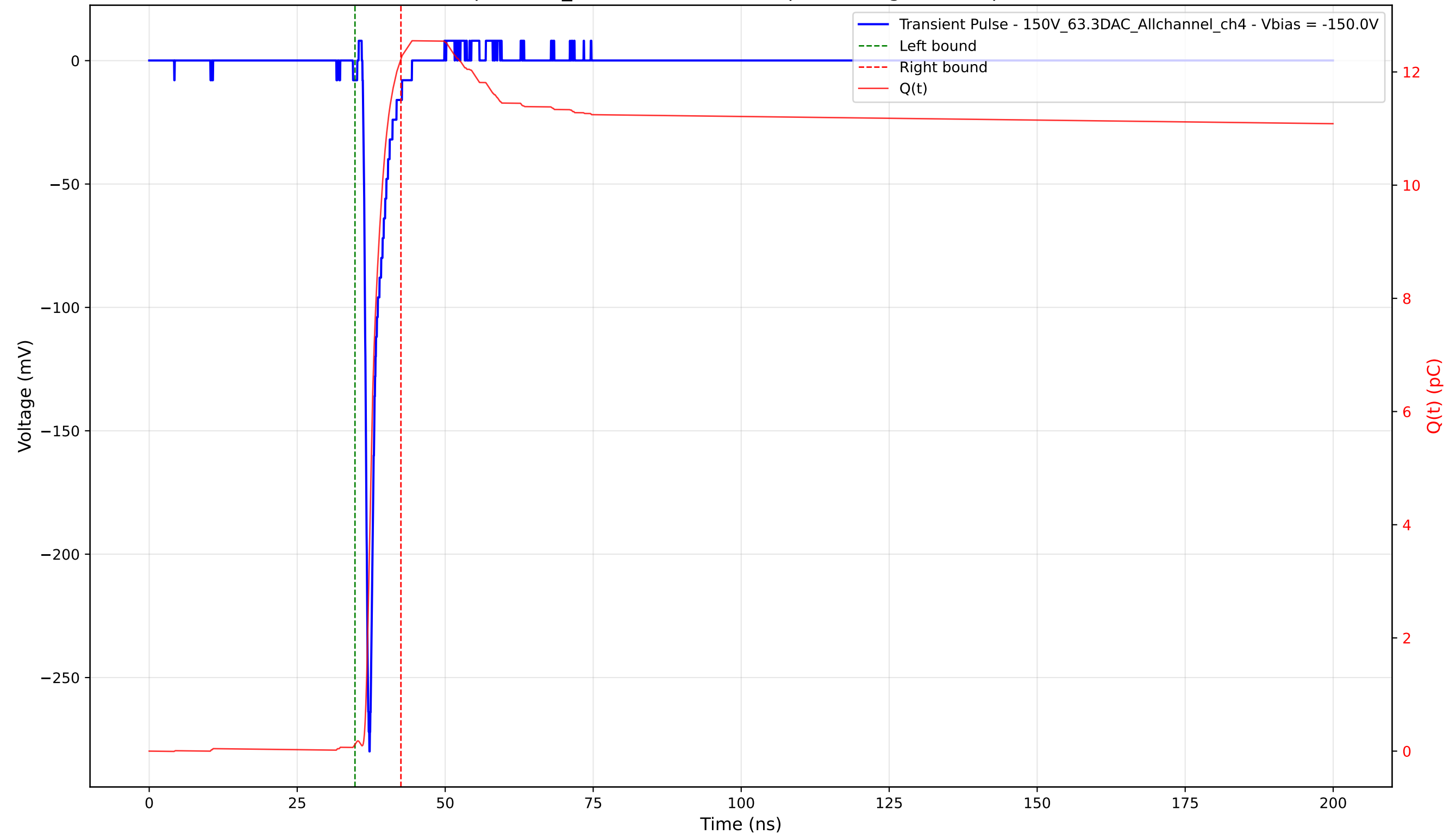
Transient Pulse - Sample: 1cm_42 - Position: 1520.0 \mu\text{m} - Charge: 12.11 pC - Rise Time: 0.76 ns
