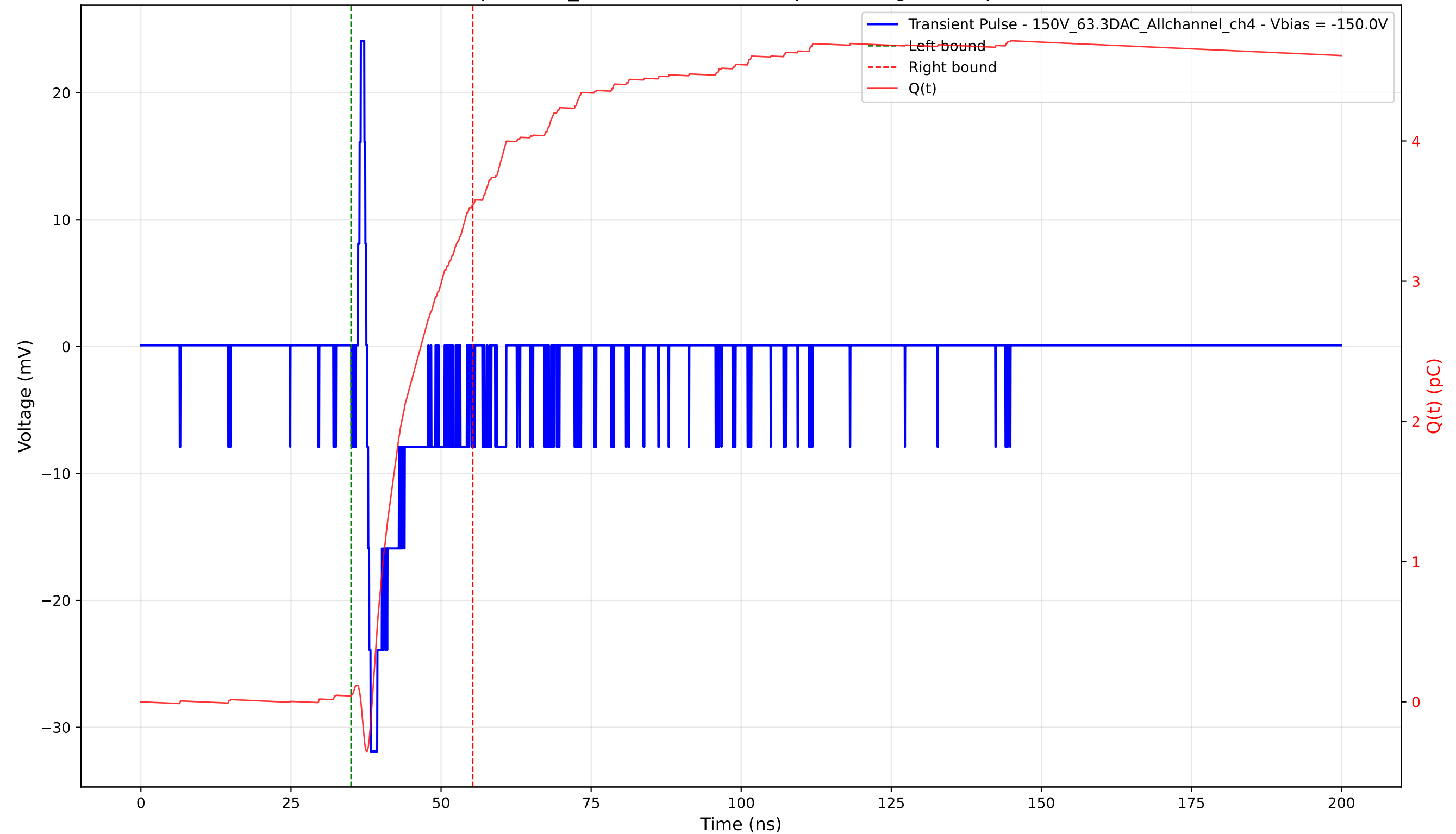
Transient Pulse - Sample: 1cm_42 - Position: 3880.0 \mu\text{m} - Charge: 3.51 pC - Rise Time: 0.58 ns
