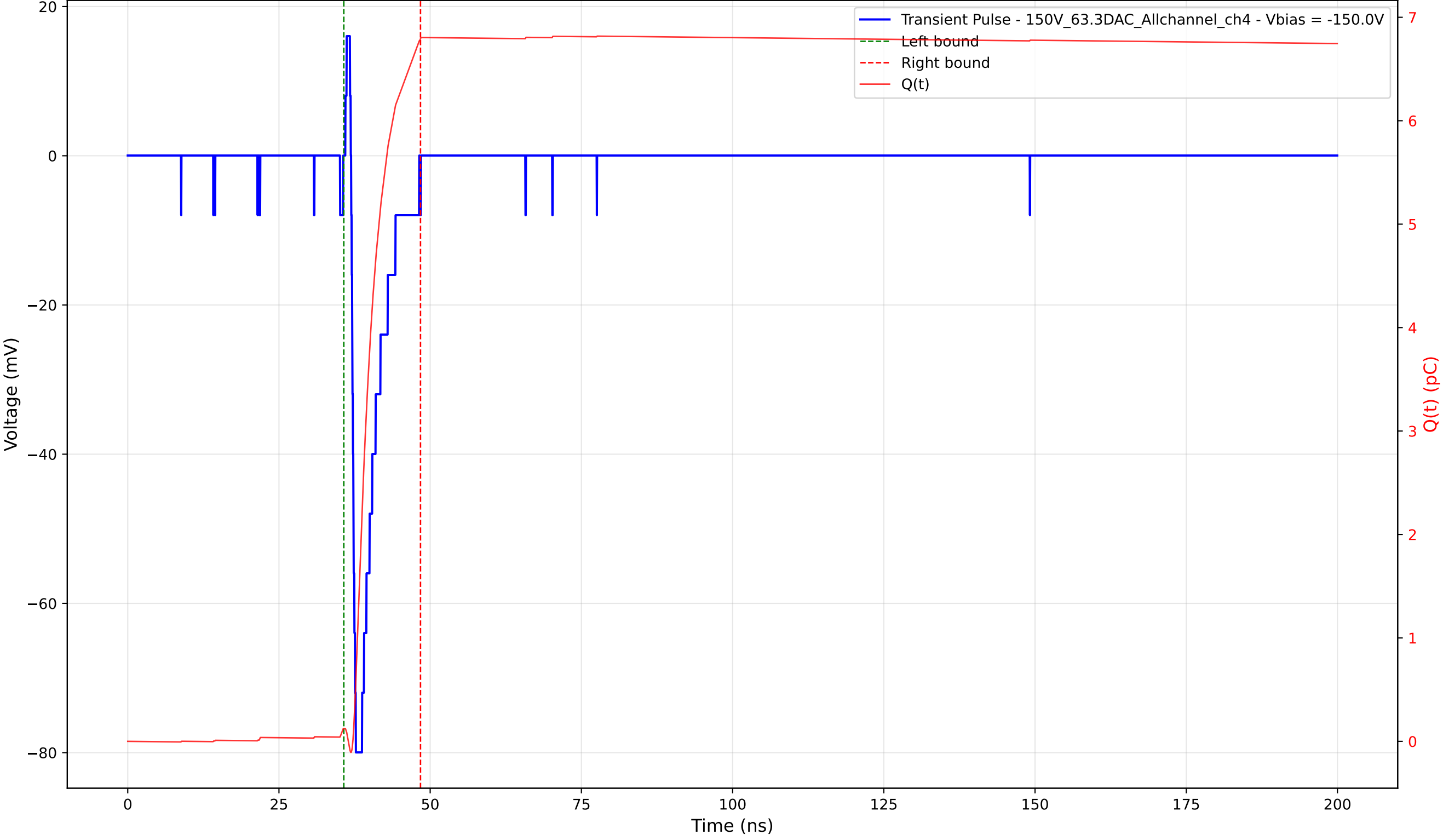
Transient Pulse - Sample: 1cm_42 - Position: 860.0 \mu\text{m} - Charge: 6.67 pC - Rise Time: 0.72 ns
