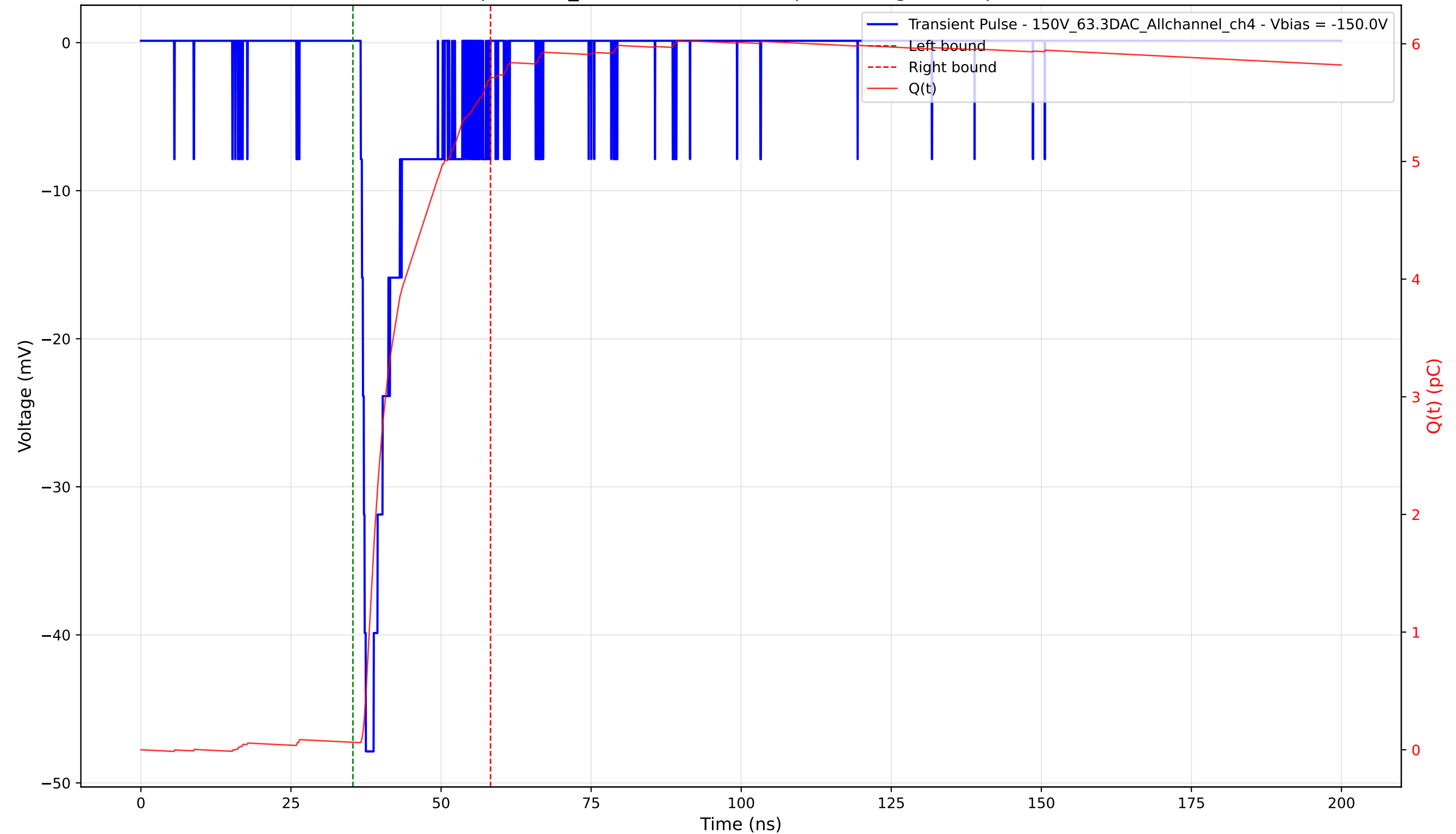
Transient Pulse - Sample: 1cm_42 - Position: 3120.0 \mu\text{m} - Charge: 5.65 pC - Rise Time: 0.86 ns
