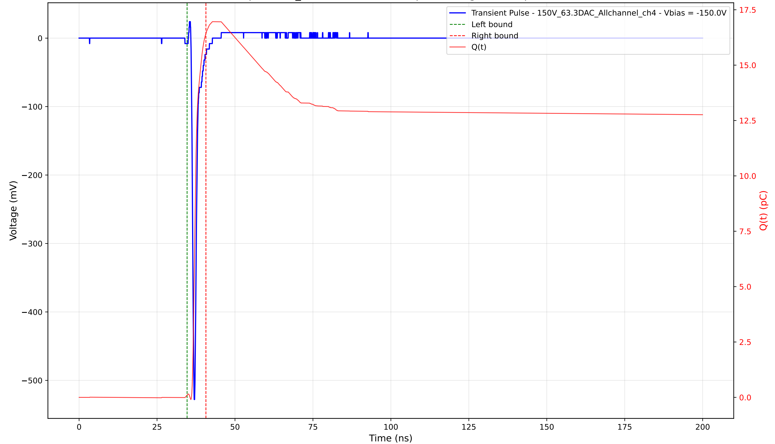
Transient Pulse - Sample: 1cm_42 - Position: 2200.0 \mu\text{m} - Charge: 16.33 pC - Rise Time: 0.72 ns
