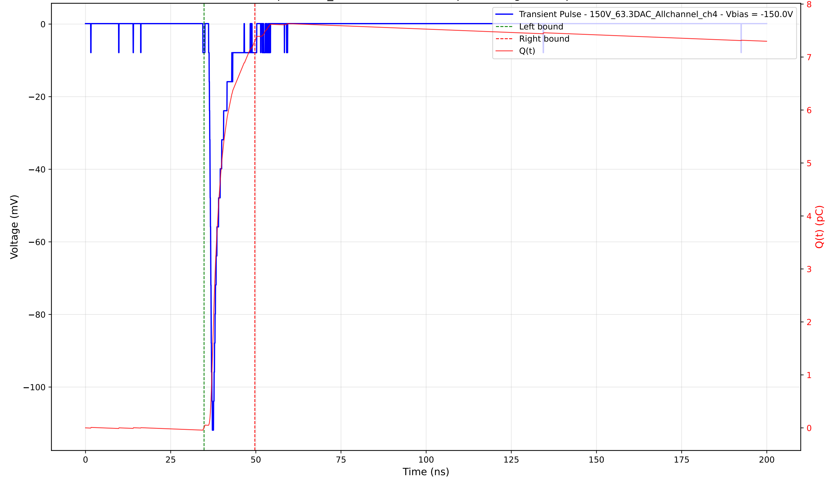
Transient Pulse - Sample: 1cm_42 - Position: 2865.0 \mu\text{m} - Charge: 7.30 pC - Rise Time: 0.82 ns
