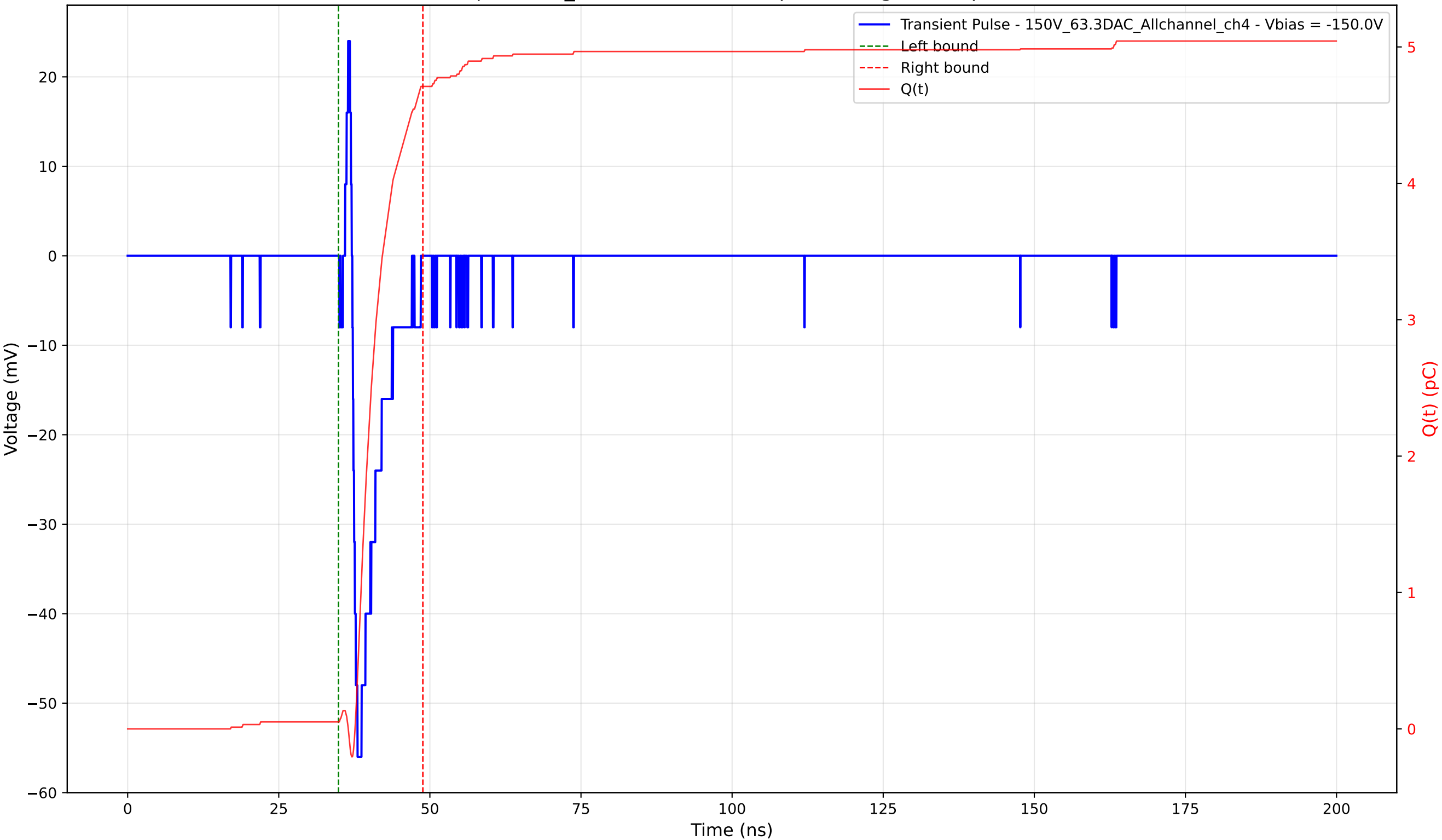
Transient Pulse - Sample: 1cm_42 - Position: 510.0 \mu\text{m} - Charge: 4.66 pC - Rise Time: 0.85 ns
