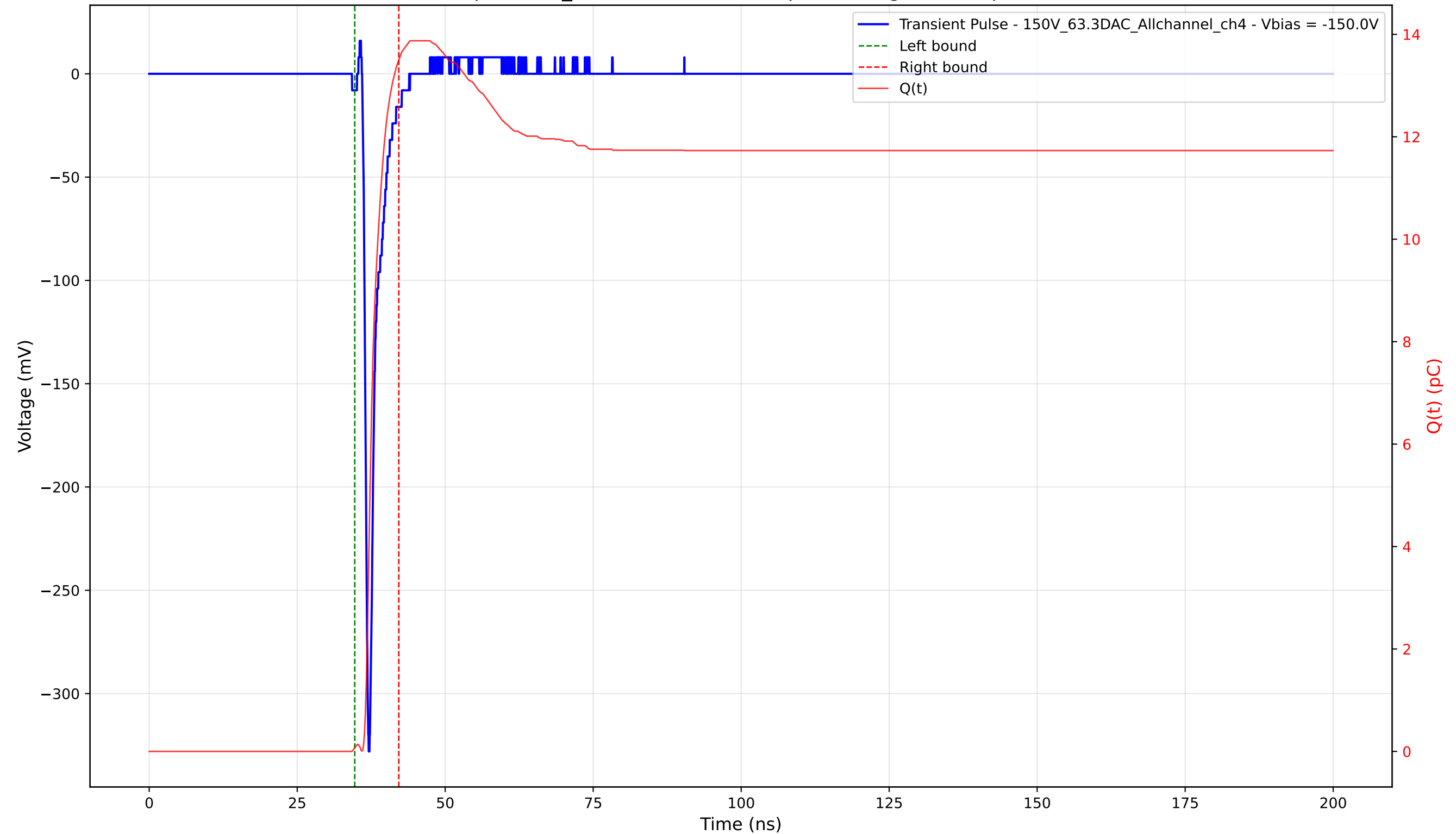
Transient Pulse - Sample: 1cm_42 - Position: 1565.0 \mu\text{m} - Charge: 13.42 pC - Rise Time: 0.75 ns
