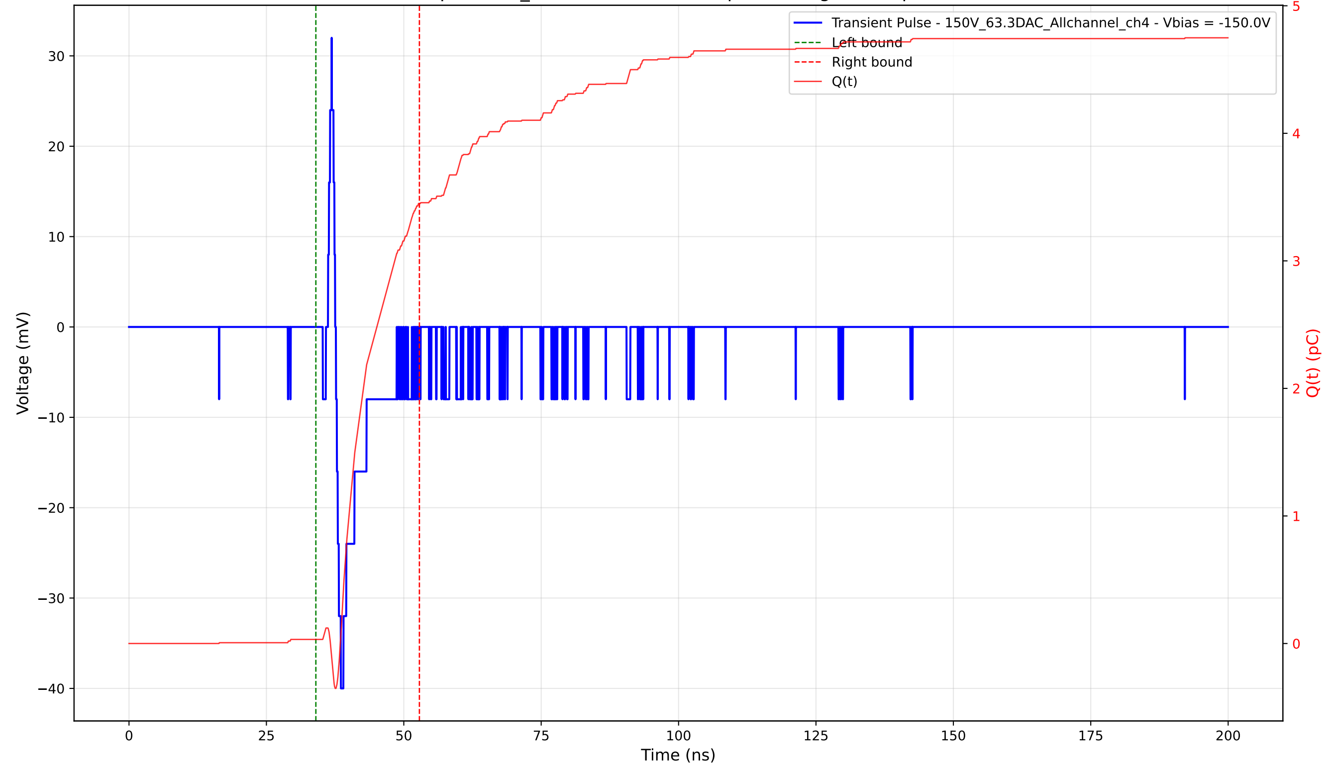
Transient Pulse - Sample: 1cm_42 - Position: 3795.0 \mu\text{m} - Charge: 3.42 pC - Rise Time: 0.90 ns
