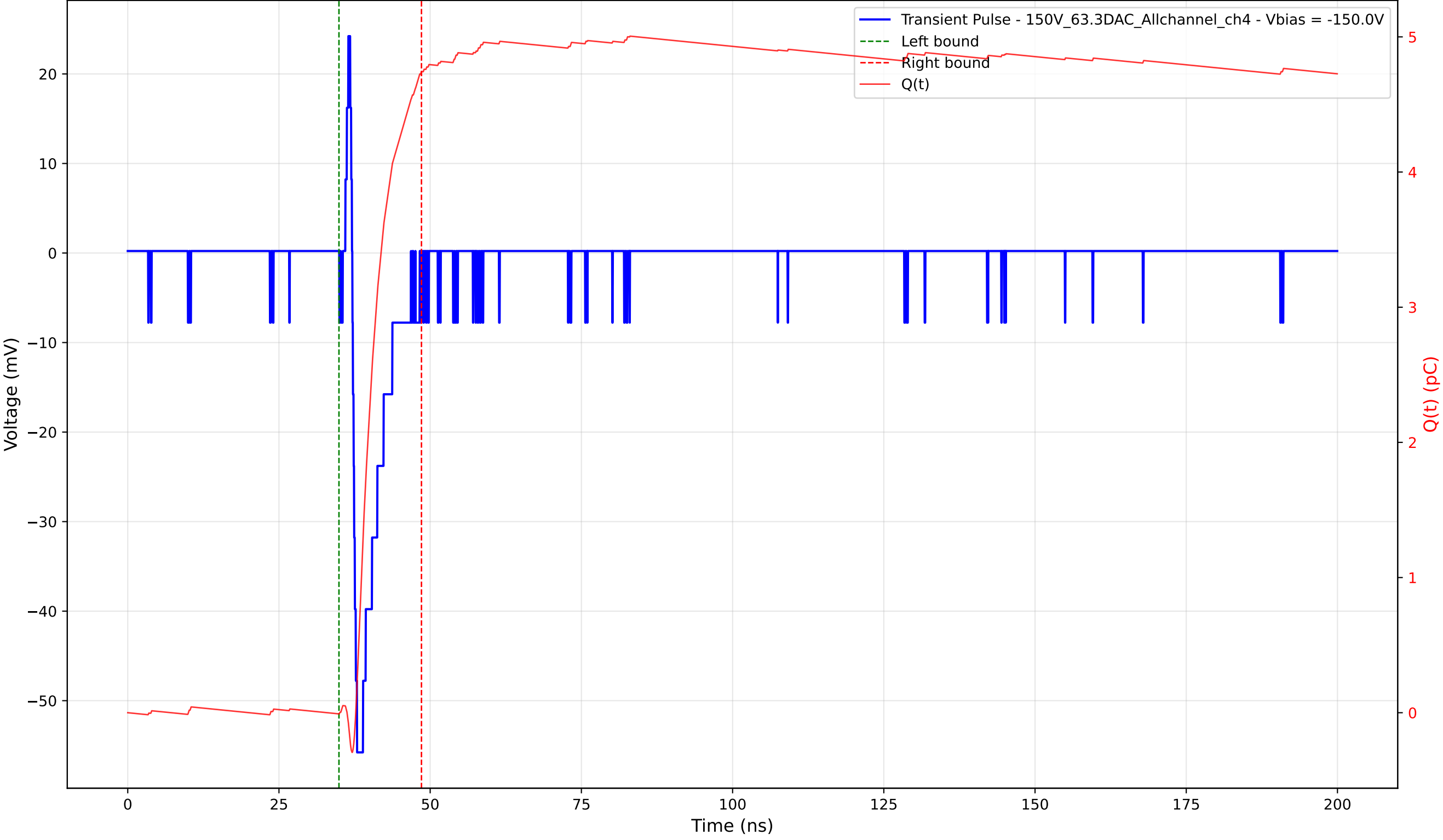
Transient Pulse - Sample: 1cm_42 - Position: 540.0 \mu\text{m} - Charge: 4.75 pC - Rise Time: 0.77 ns
