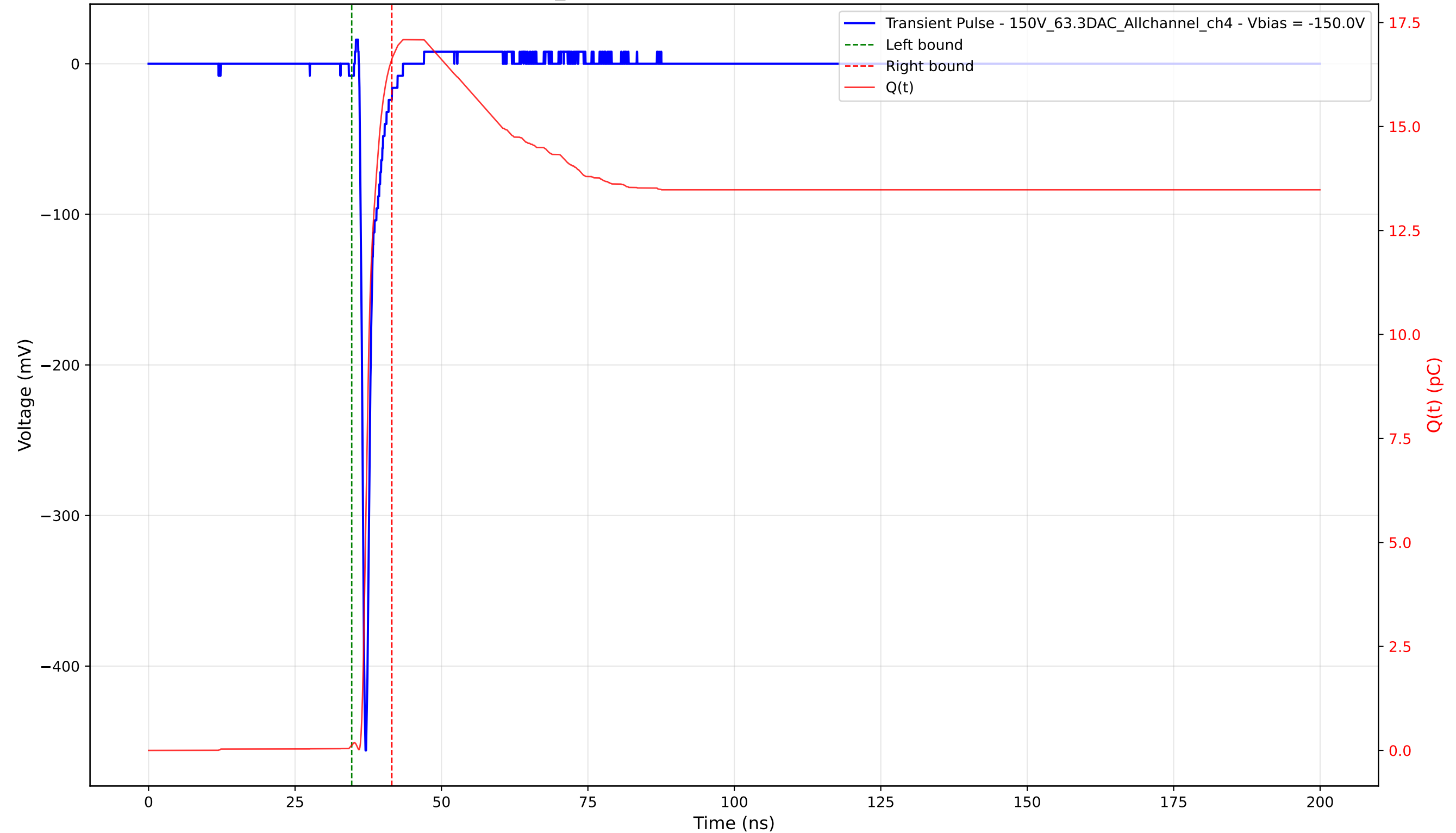
Transient Pulse - Sample: 1cm_42 - Position: 1660.0 \mu\text{m} - Charge: 16.50 pC - Rise Time: 0.72 ns
