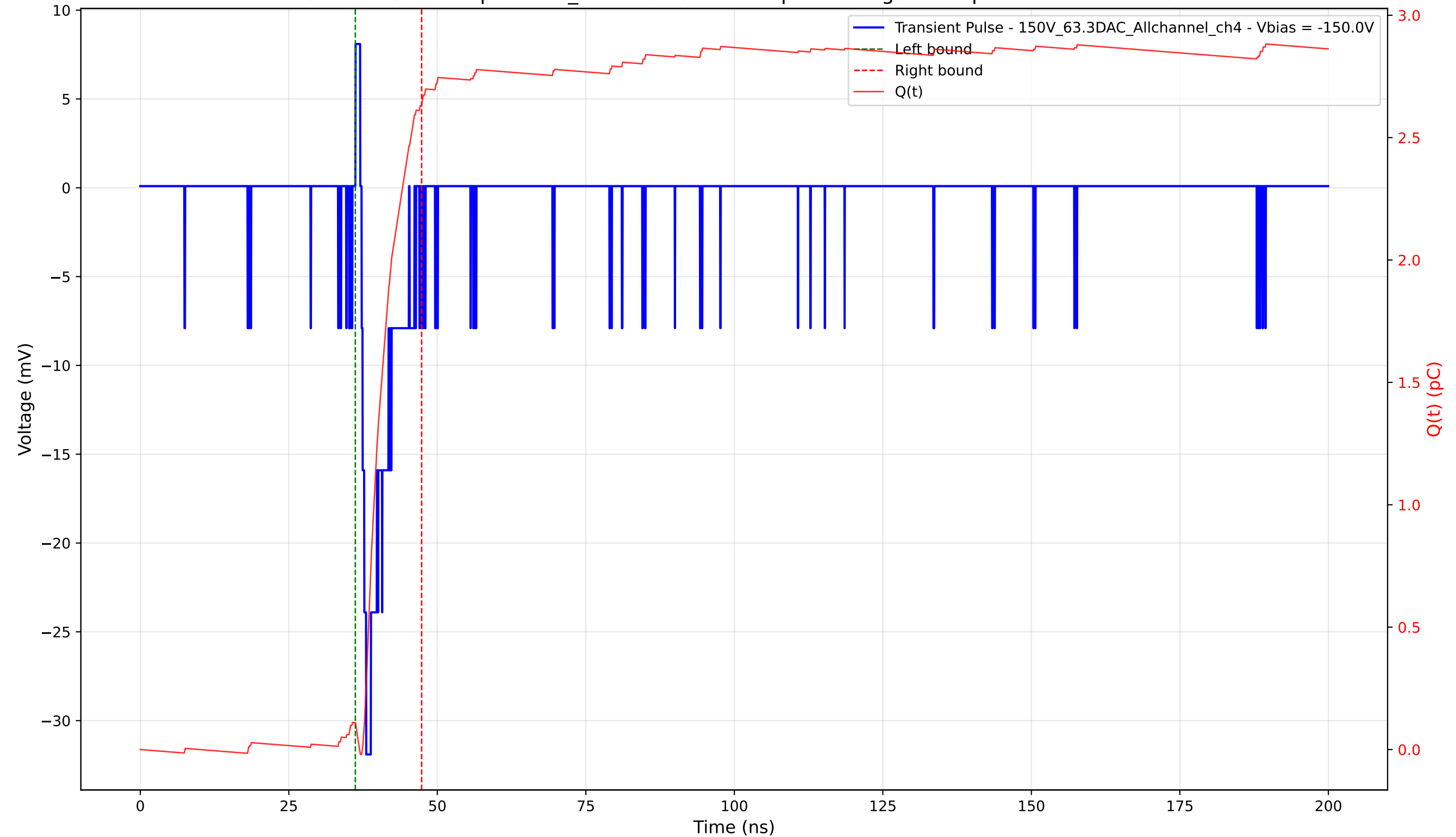
Transient Pulse - Sample: 1cm_42 - Position: 240.0 \mu\text{m} - Charge: 2.52 pC - Rise Time: 0.78 ns
