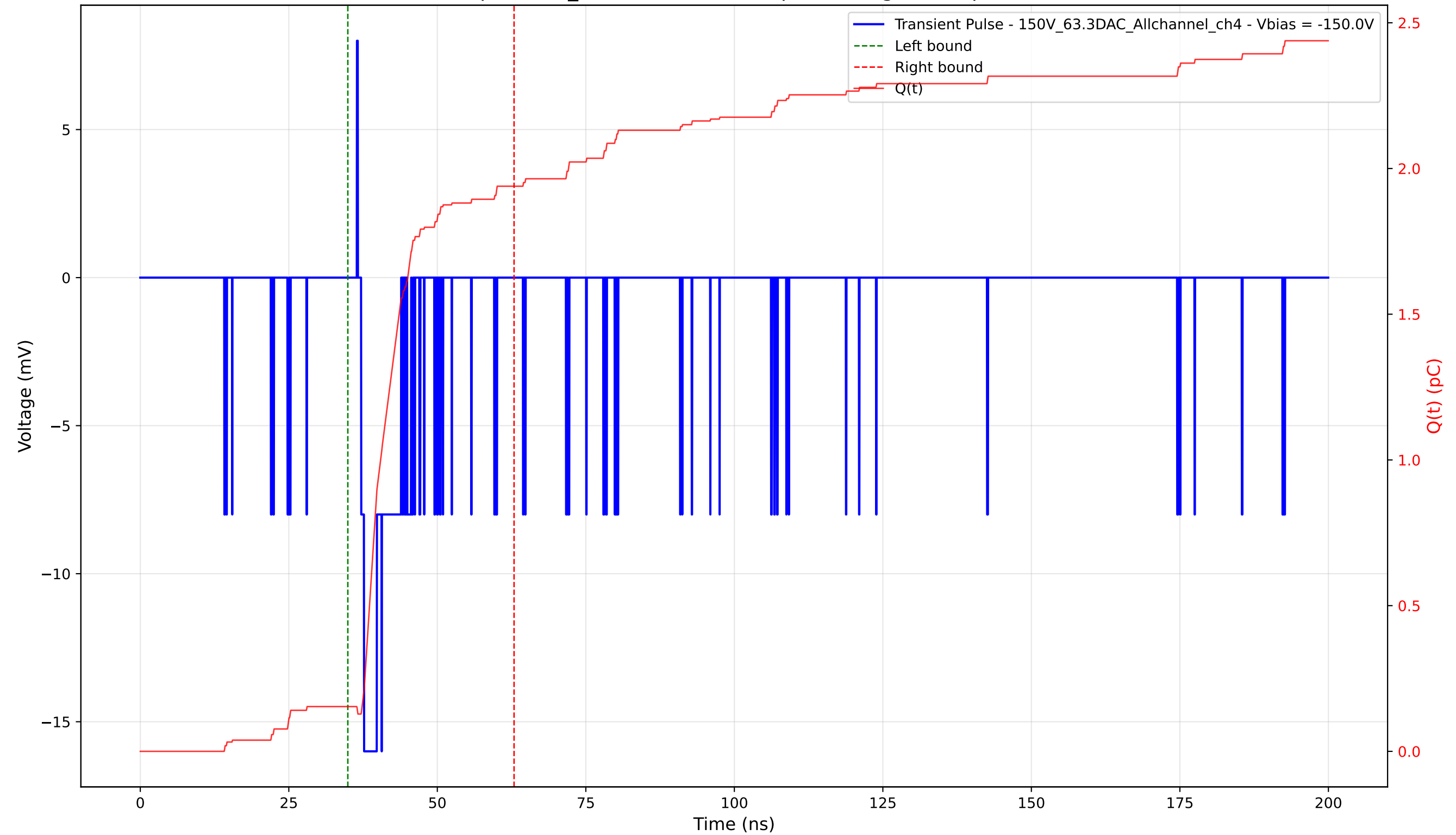
Transient Pulse - Sample: 1cm_42 - Position: 140.0 \mu\text{m} - Charge: 1.79 pC - Rise Time: 0.51 ns
