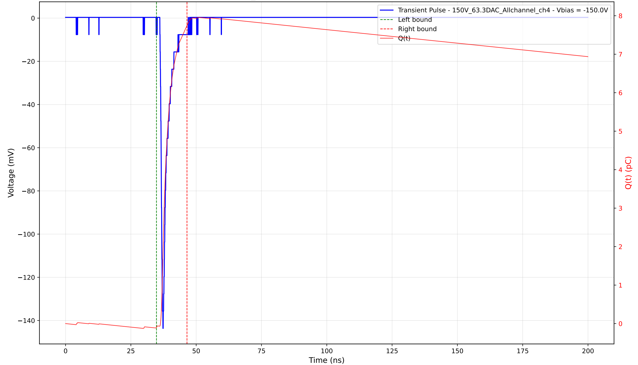
Transient Pulse - Sample: 1cm_42 - Position: 2740.0 \mu\text{m} - Charge: 7.84 pC - Rise Time: 0.89 ns
