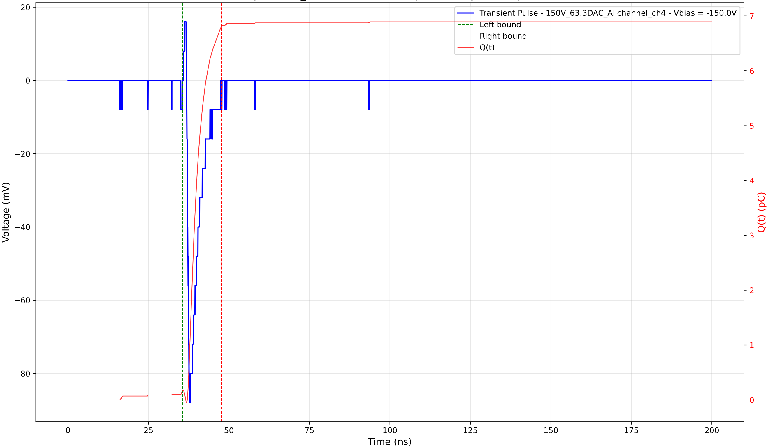
Transient Pulse - Sample: 1cm_42 - Position: 905.0 \mu\text{m} - Charge: 6.62 pC - Rise Time: 0.68 ns
