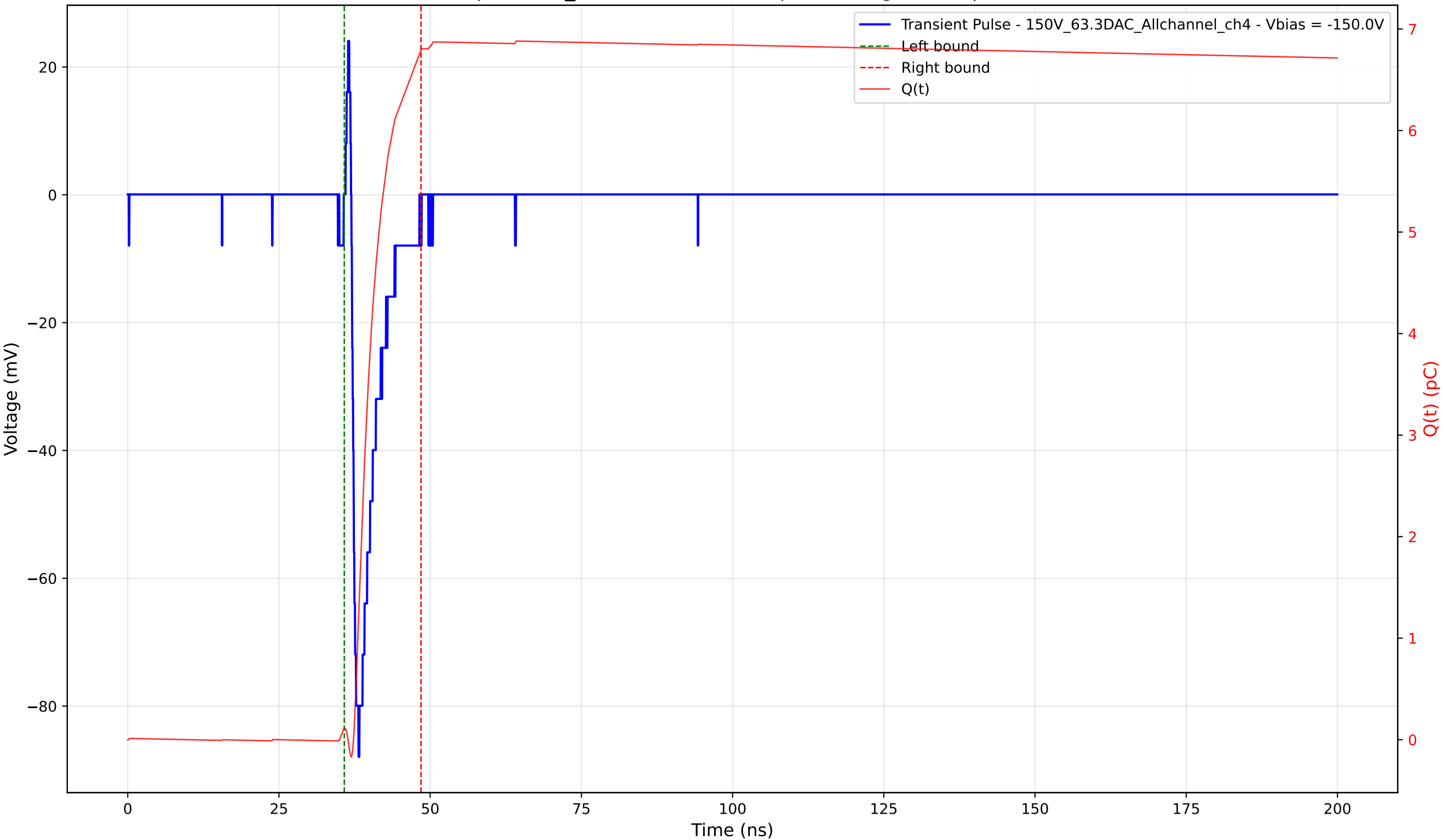
Transient Pulse - Sample: 1cm_42 - Position: 815.0 \mu\text{m} - Charge: 6.68 pC - Rise Time: 0.72 ns
