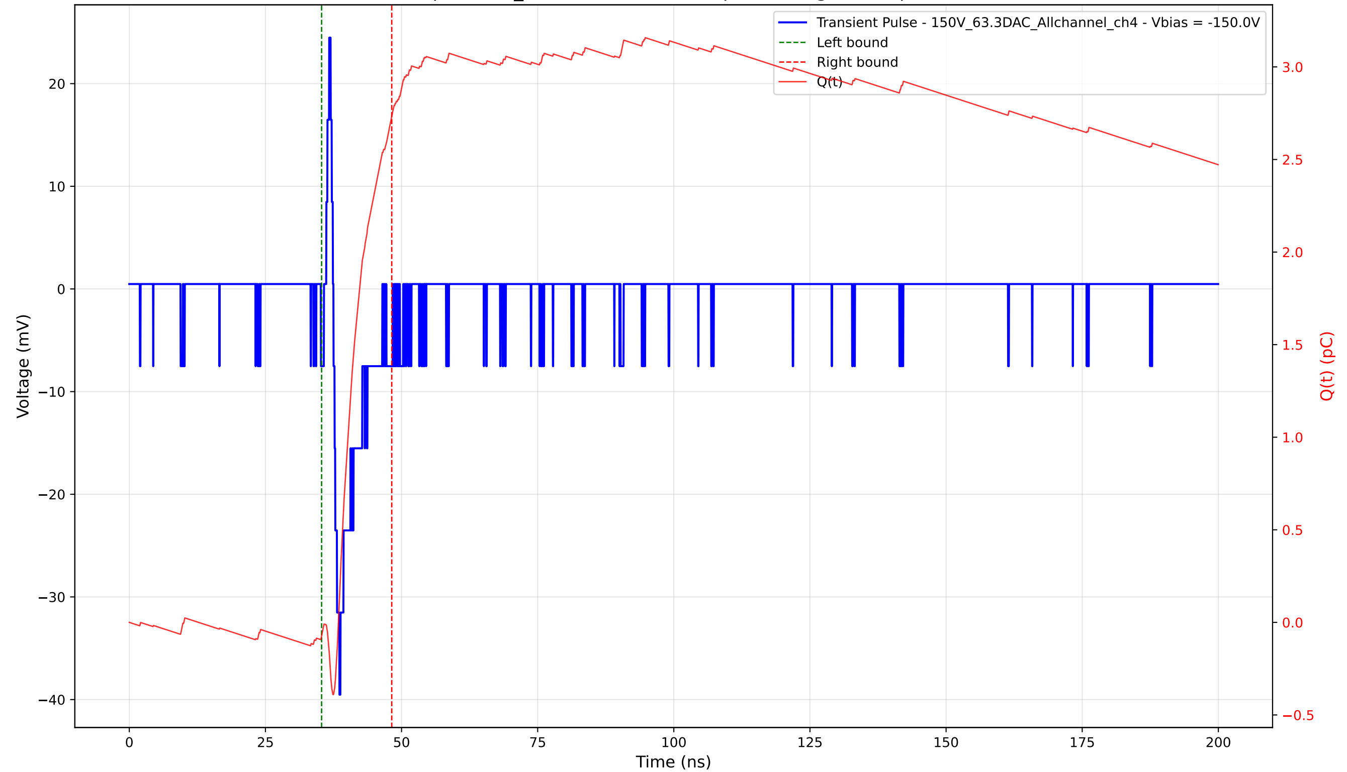
Transient Pulse - Sample: 1cm_42 - Position: 4775.0 \mu\text{m} - Charge: 2.81 pC - Rise Time: 1.10 ns
