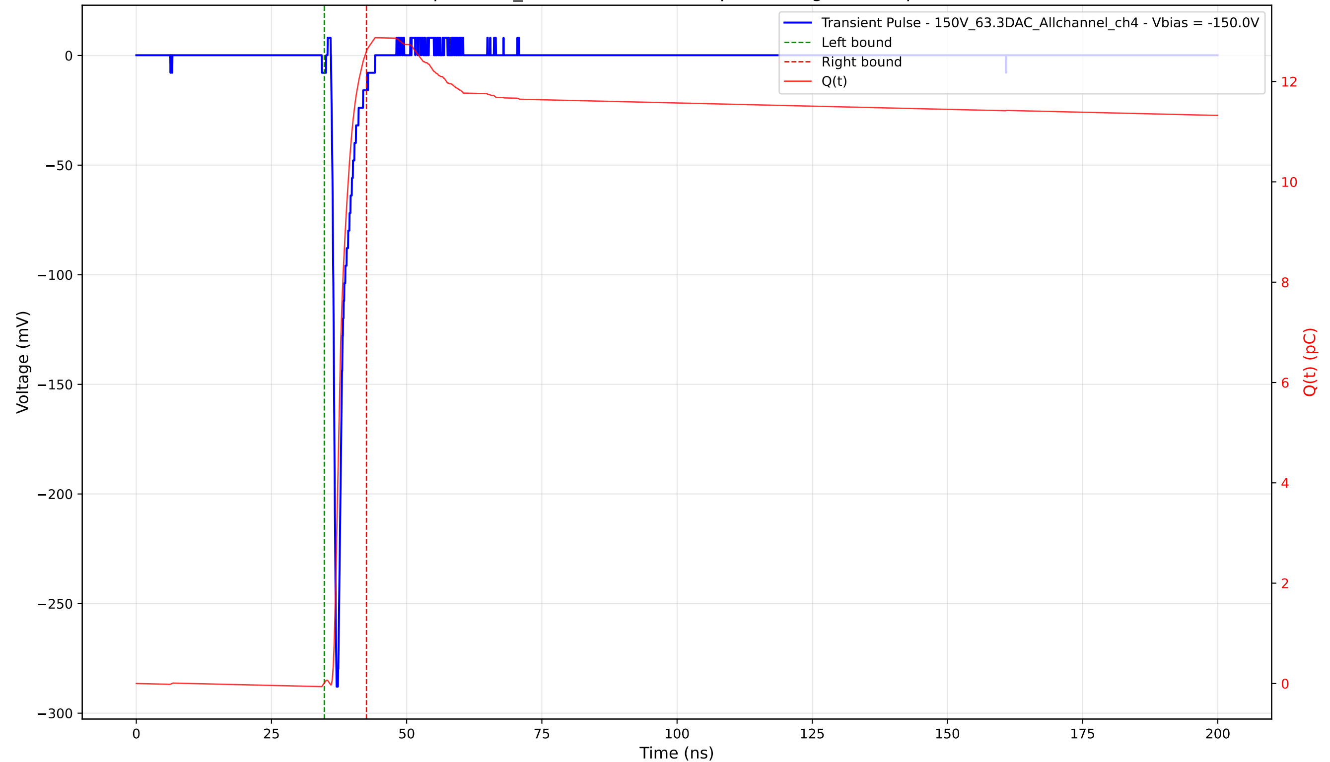
Transient Pulse - Sample: 1cm_42 - Position: 1535.0 \mu\text{m} - Charge: 12.59 pC - Rise Time: 0.75 ns
