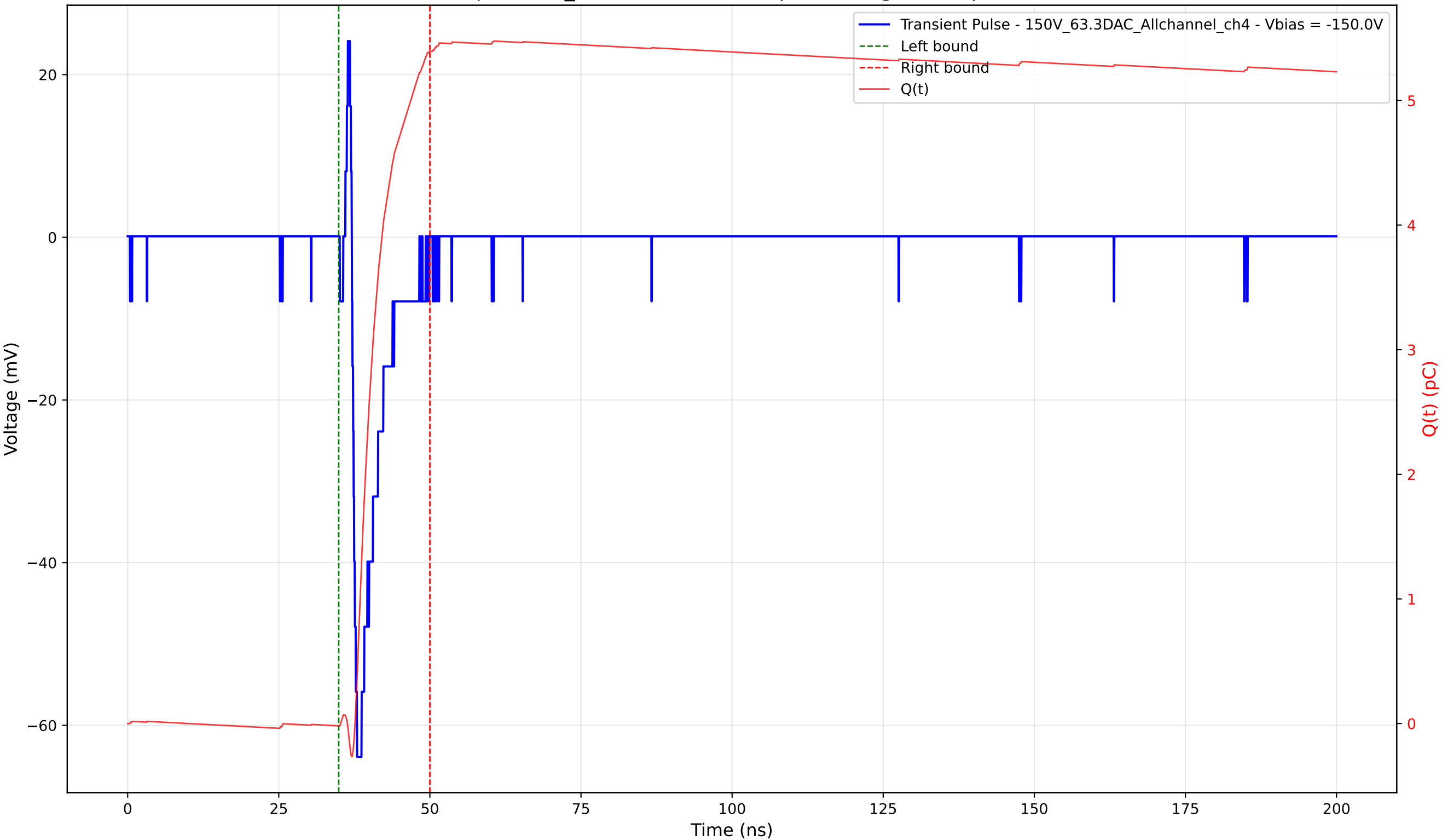
Transient Pulse - Sample: 1cm_42 - Position: 590.0 \mu\text{m} - Charge: 5.41 pC - Rise Time: 0.85 ns
