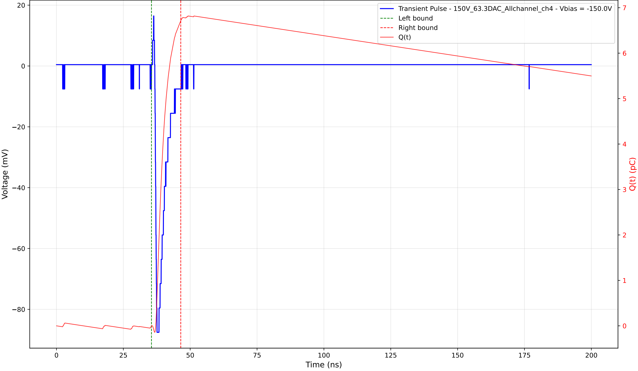
Transient Pulse - Sample: 1cm_42 - Position: 965.0 \mu\text{m} - Charge: 6.71 pC - Rise Time: 0.59 ns
