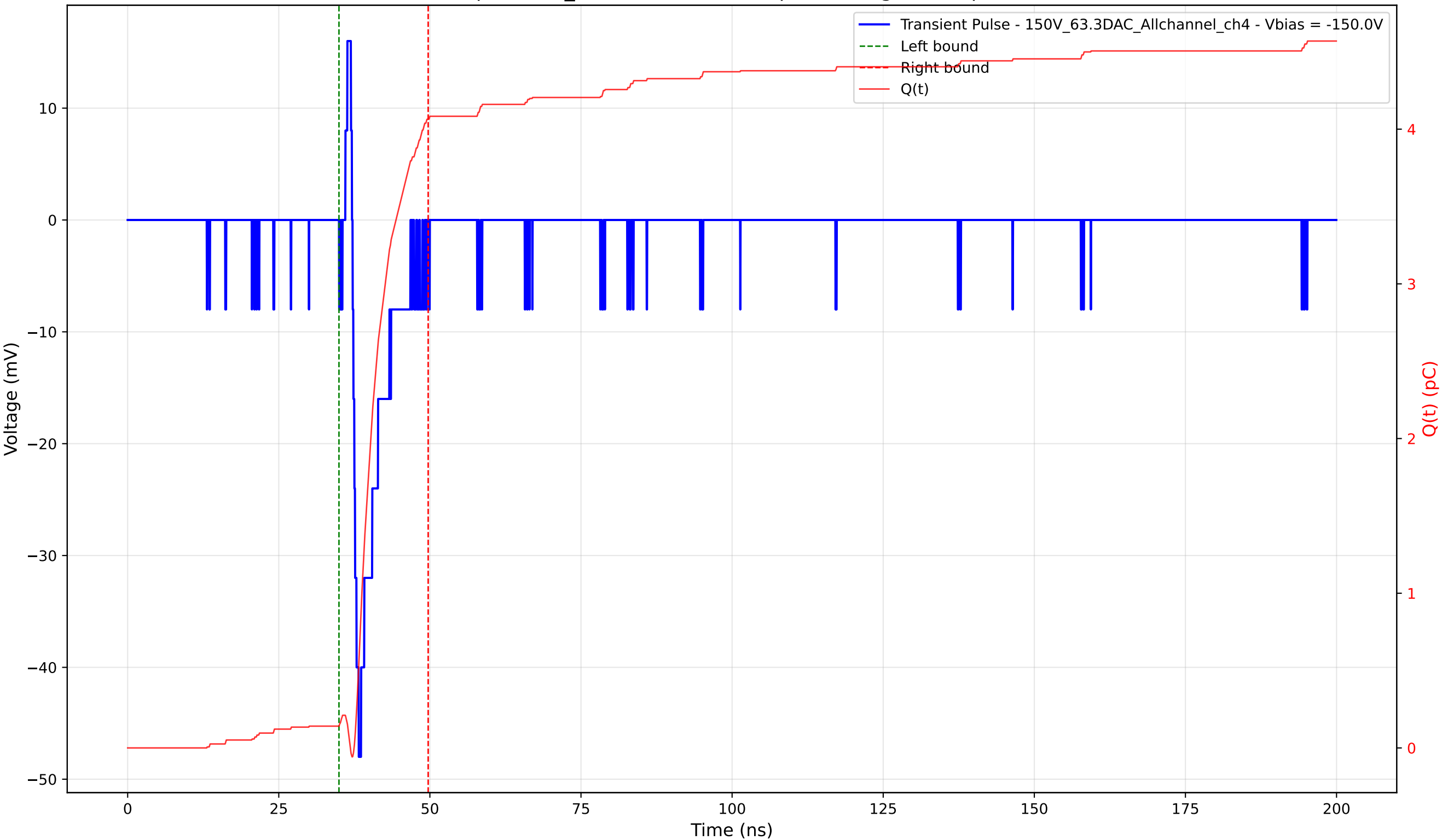
Transient Pulse - Sample: 1cm_42 - Position: 410.0 \mu\text{m} - Charge: 3.92 pC - Rise Time: 1.02 ns
