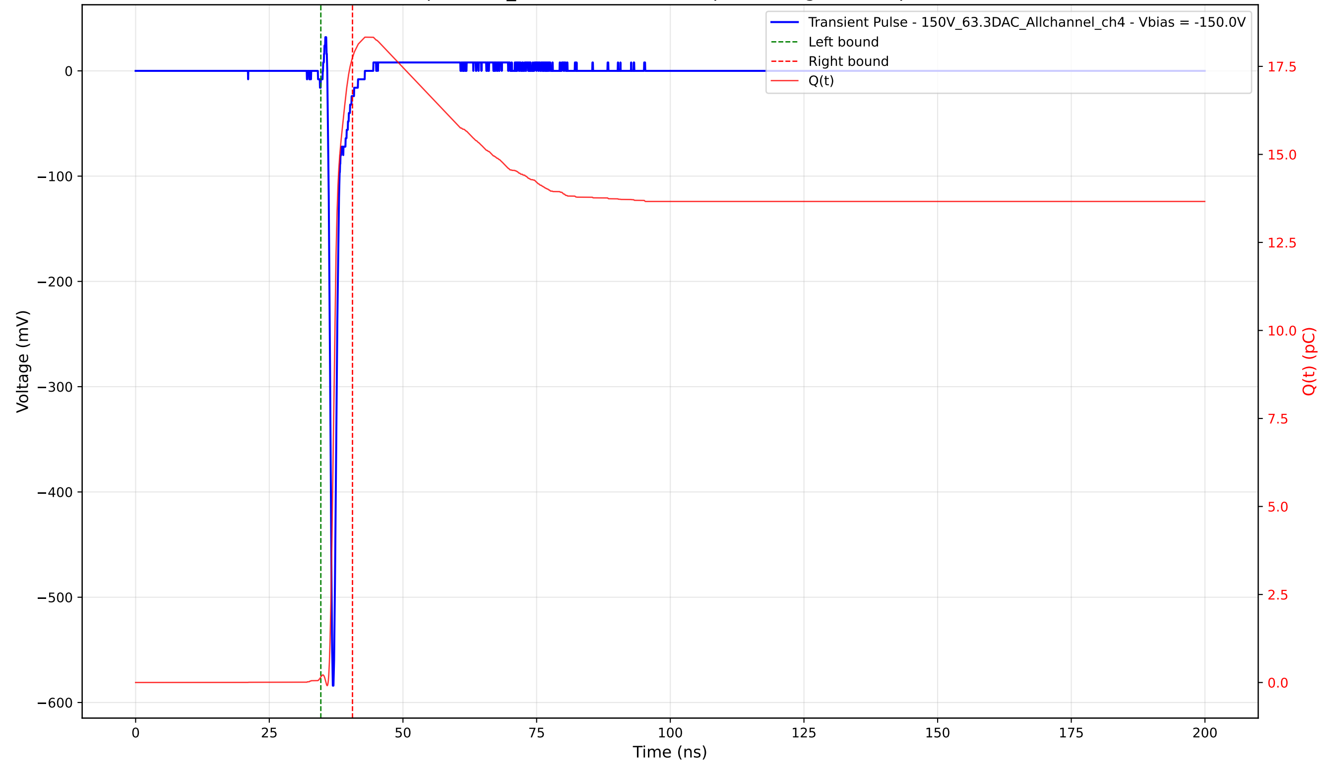
Transient Pulse - Sample: 1cm_42 - Position: 2065.0 \mu\text{m} - Charge: 17.59 pC - Rise Time: 0.71 ns
