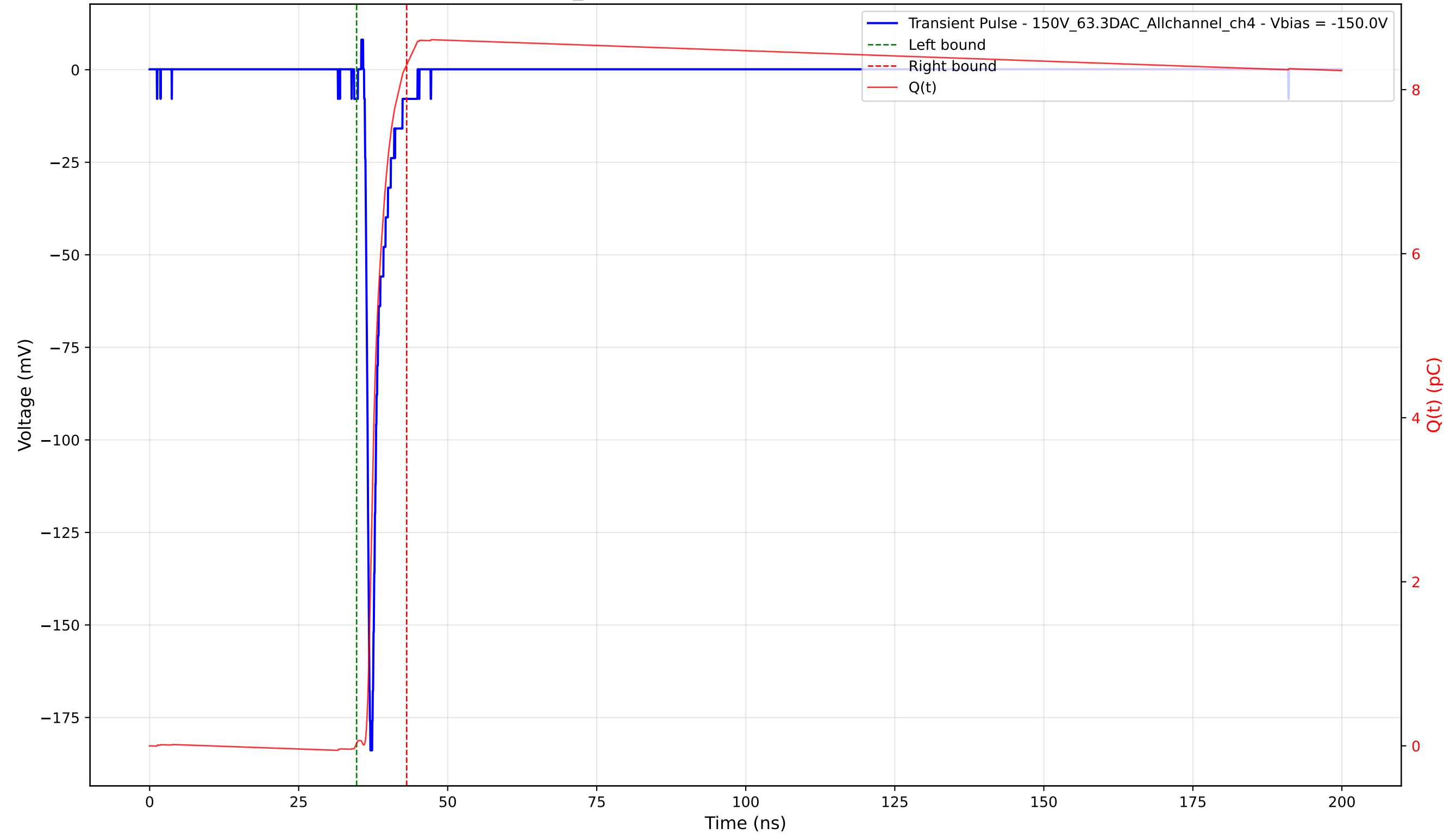
Transient Pulse - Sample: 1cm_42 - Position: 2595.0 \mu\text{m} - Charge: 8.27 pC - Rise Time: 0.75 ns
