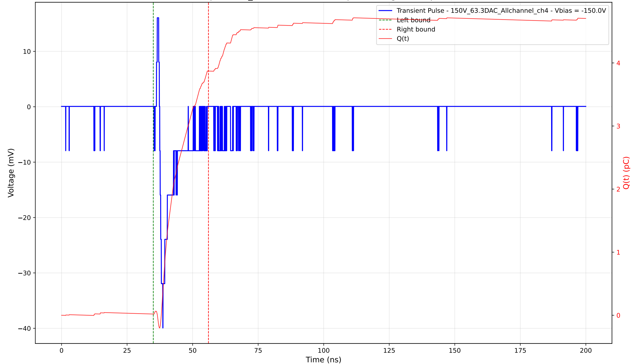
Transient Pulse - Sample: 1cm_42 - Position: 3545.0 \mu\text{m} - Charge: 3.85 pC - Rise Time: 1.18 ns
