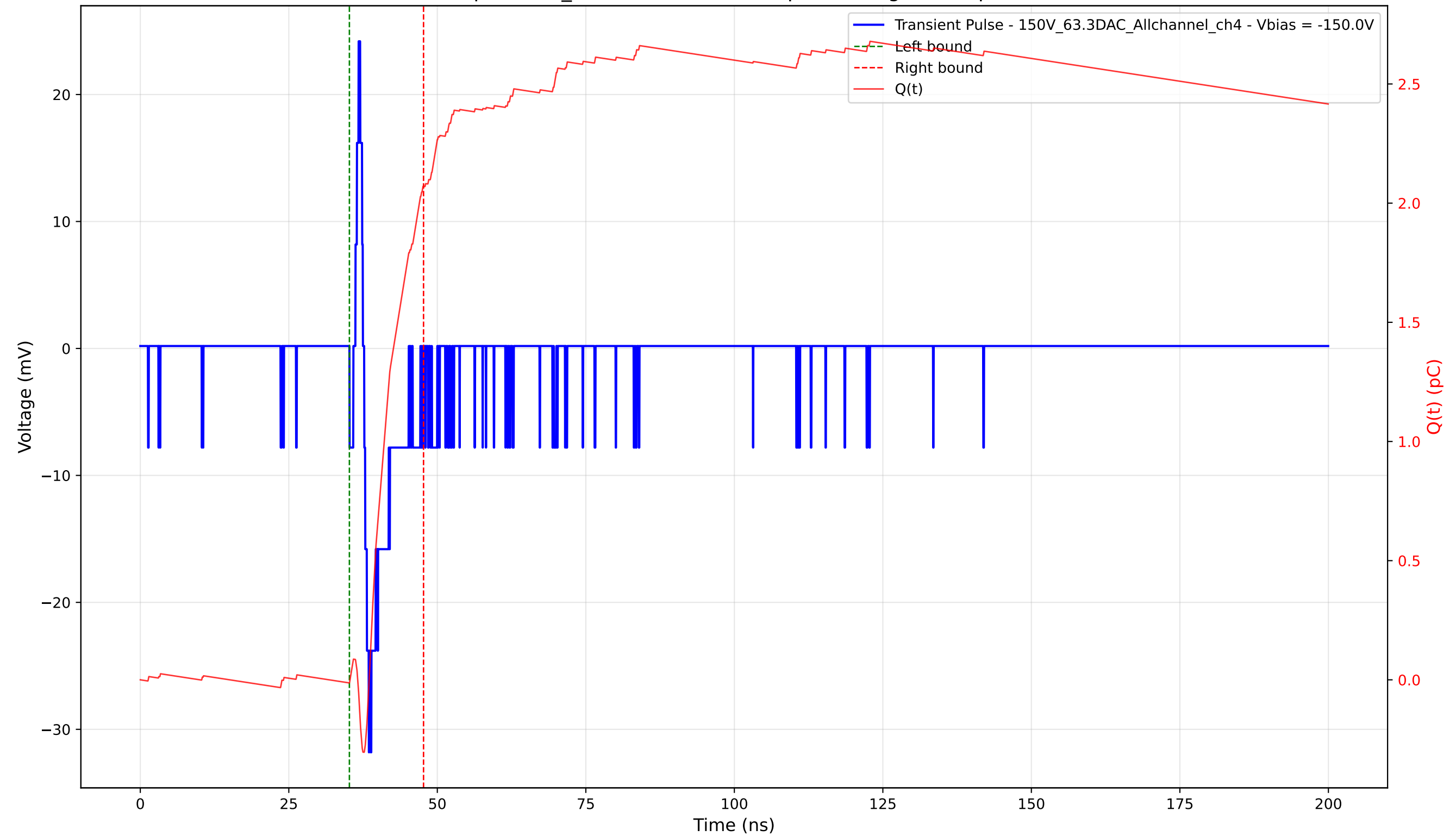
Transient Pulse - Sample: 1cm_42 - Position: 4555.0 \mu\text{m} - Charge: 2.08 pC - Rise Time: 0.78 ns
