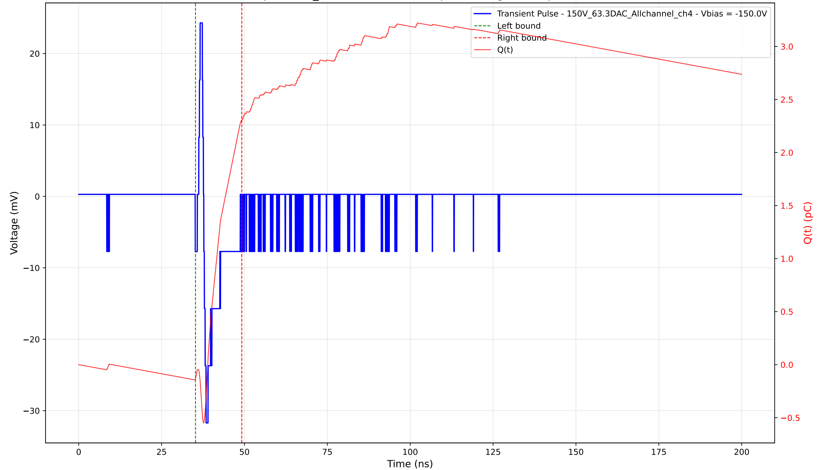
Transient Pulse - Sample: 1cm_42 - Position: 4110.0 \mu\text{m} - Charge: 2.43 pC - Rise Time: 0.70 ns
