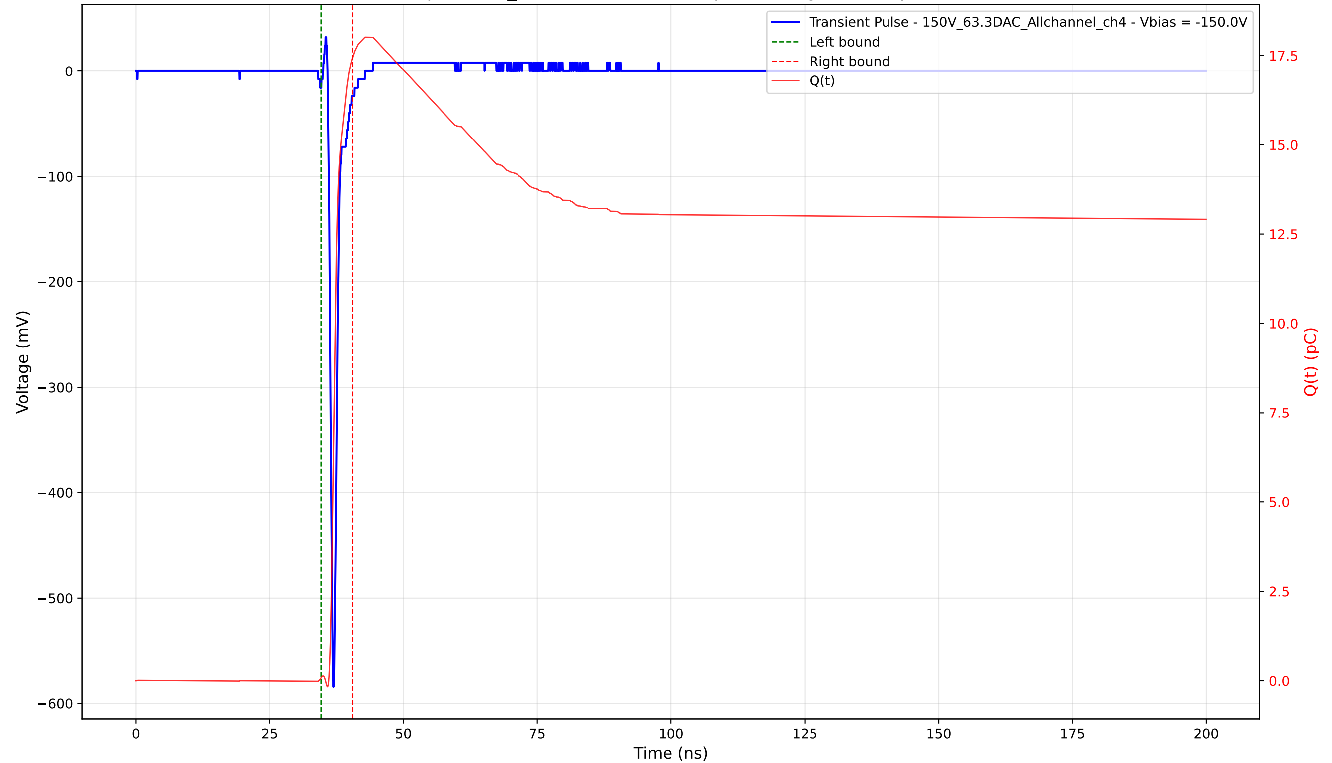
Transient Pulse - Sample: 1cm_42 - Position: 2080.0 \mu\text{m} - Charge: 17.37 pC - Rise Time: 0.71 ns
