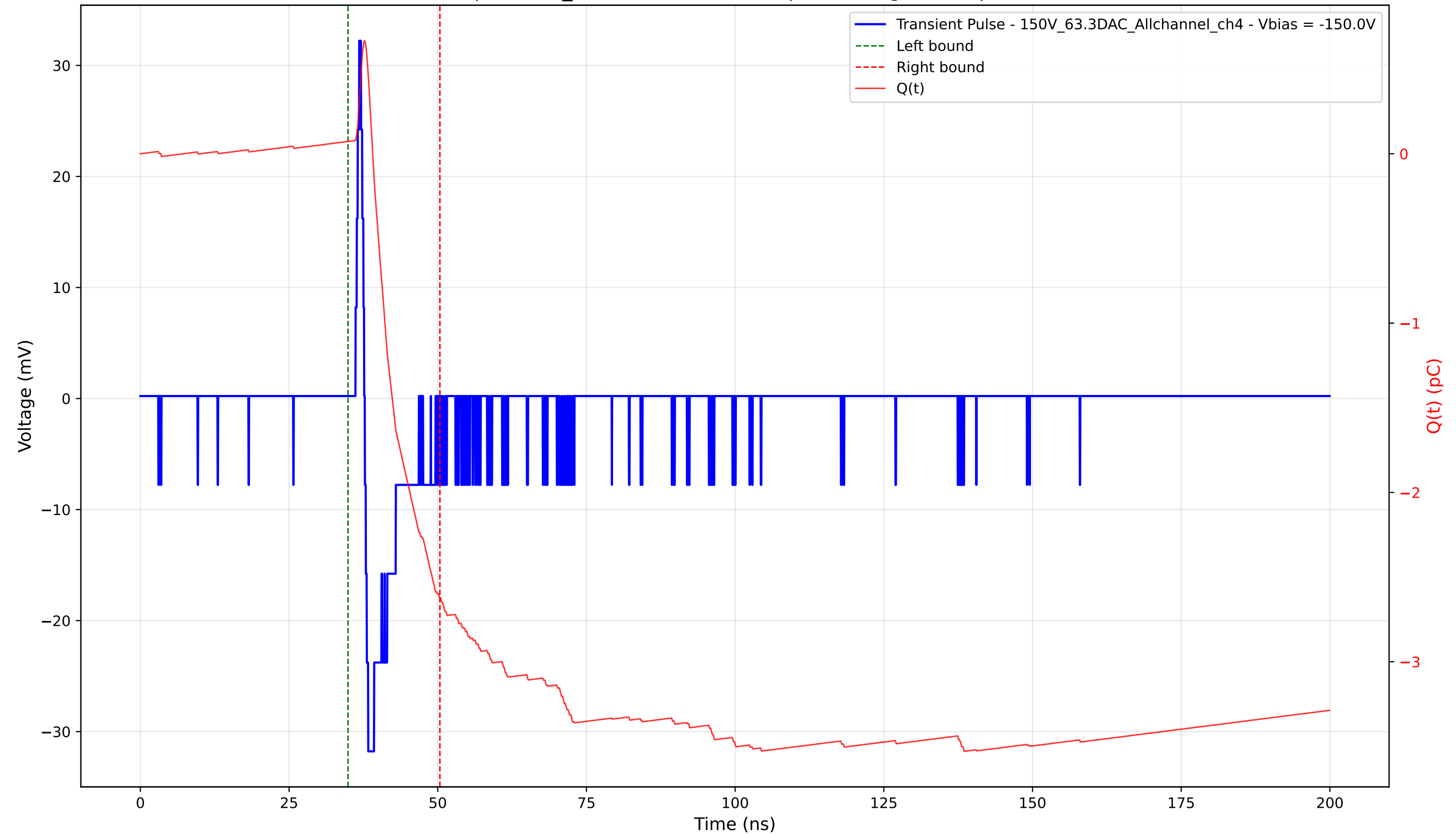
Transient Pulse - Sample: 1cm_42 - Position: 4325.0 \mu\text{m} - Charge: 2.70 pC - Rise Time: 0.63 ns
