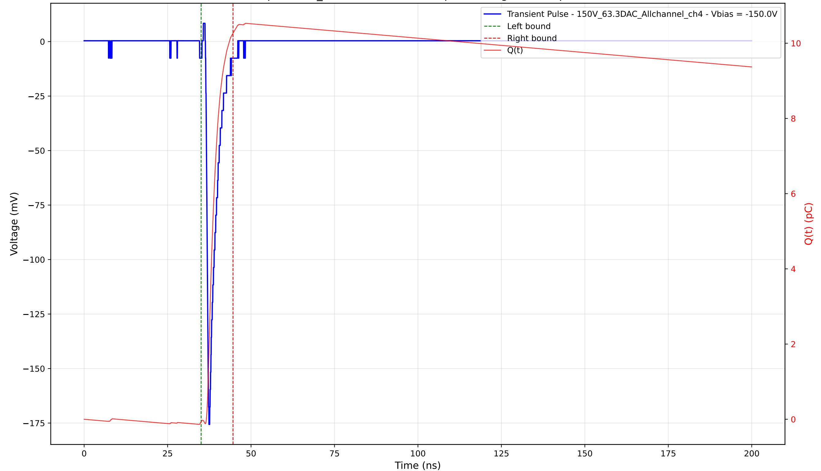
Transient Pulse - Sample: 1cm_42 - Position: 1225.0 \mu\text{m} - Charge: 10.33 pC - Rise Time: 0.75 ns
