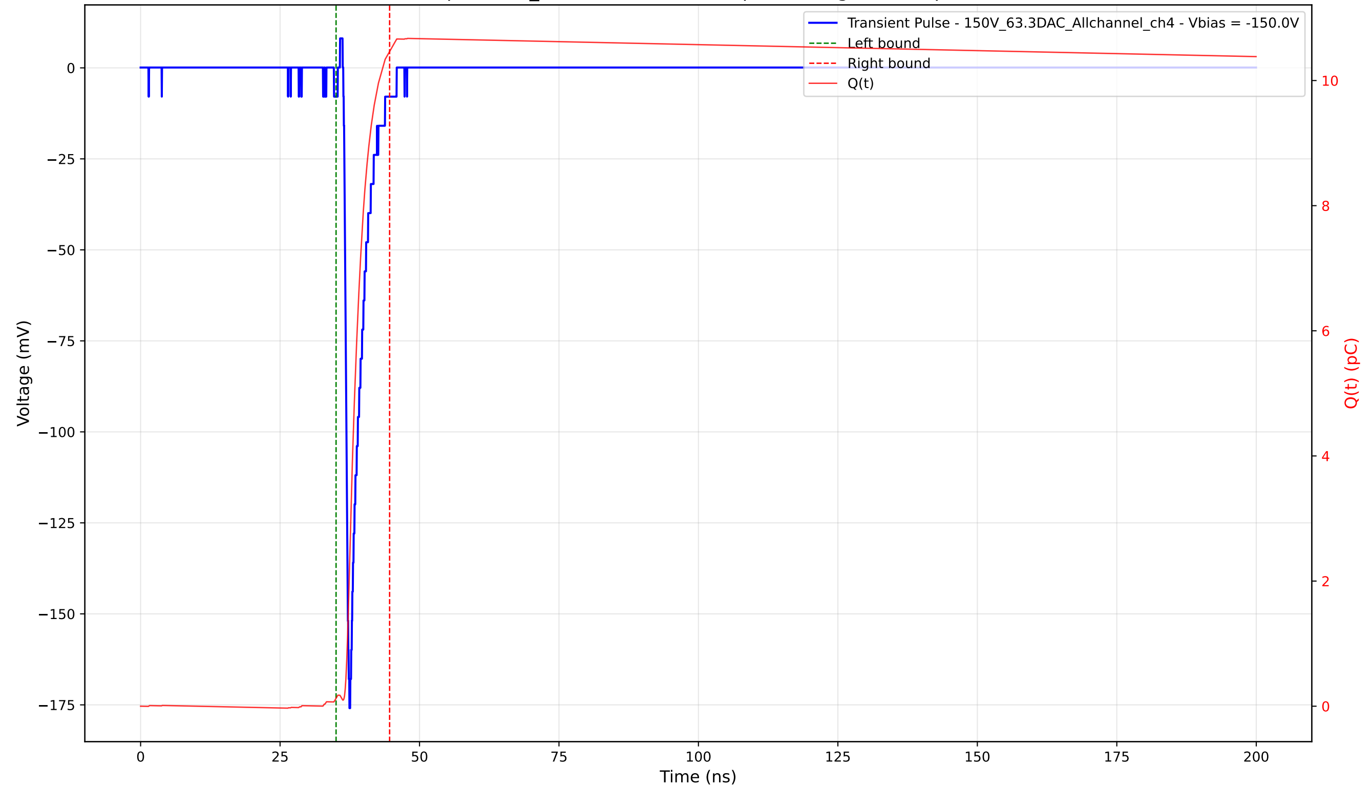
Transient Pulse - Sample: 1cm_42 - Position: 1215.0 \mu\text{m} - Charge: 10.34 pC - Rise Time: 0.75 ns
