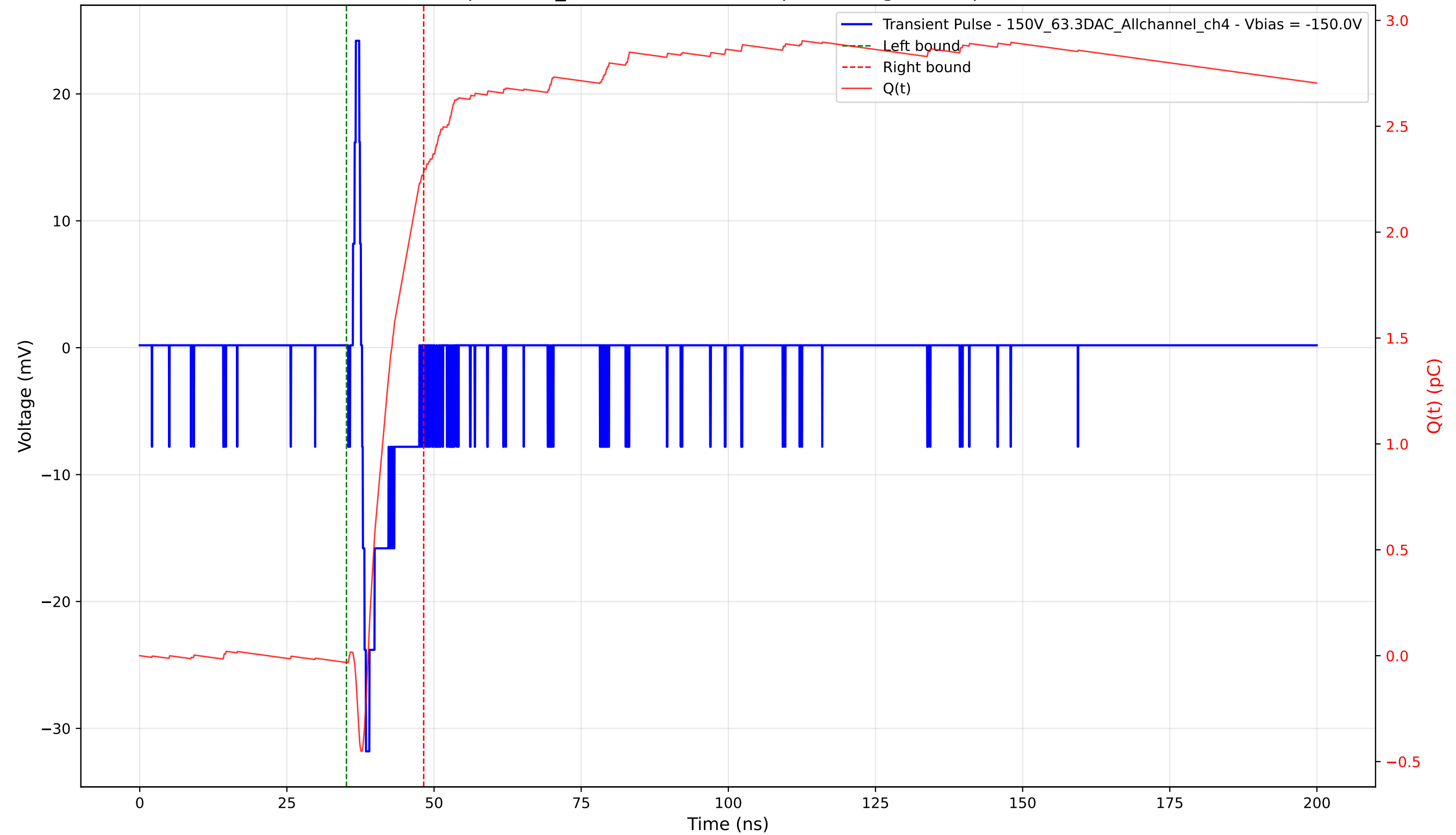
Transient Pulse - Sample: 1cm_42 - Position: 4030.0 \mu\text{m} - Charge: 2.31 pC - Rise Time: 0.66 ns
