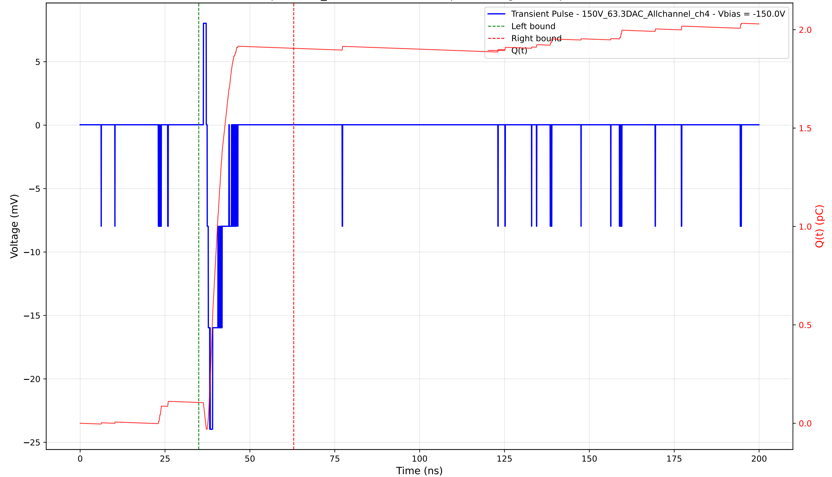
Transient Pulse - Sample: 1cm_42 - Position: 5000.0 \mu\text{m} - Charge: 1.80 pC - Rise Time: 0.79 ns
