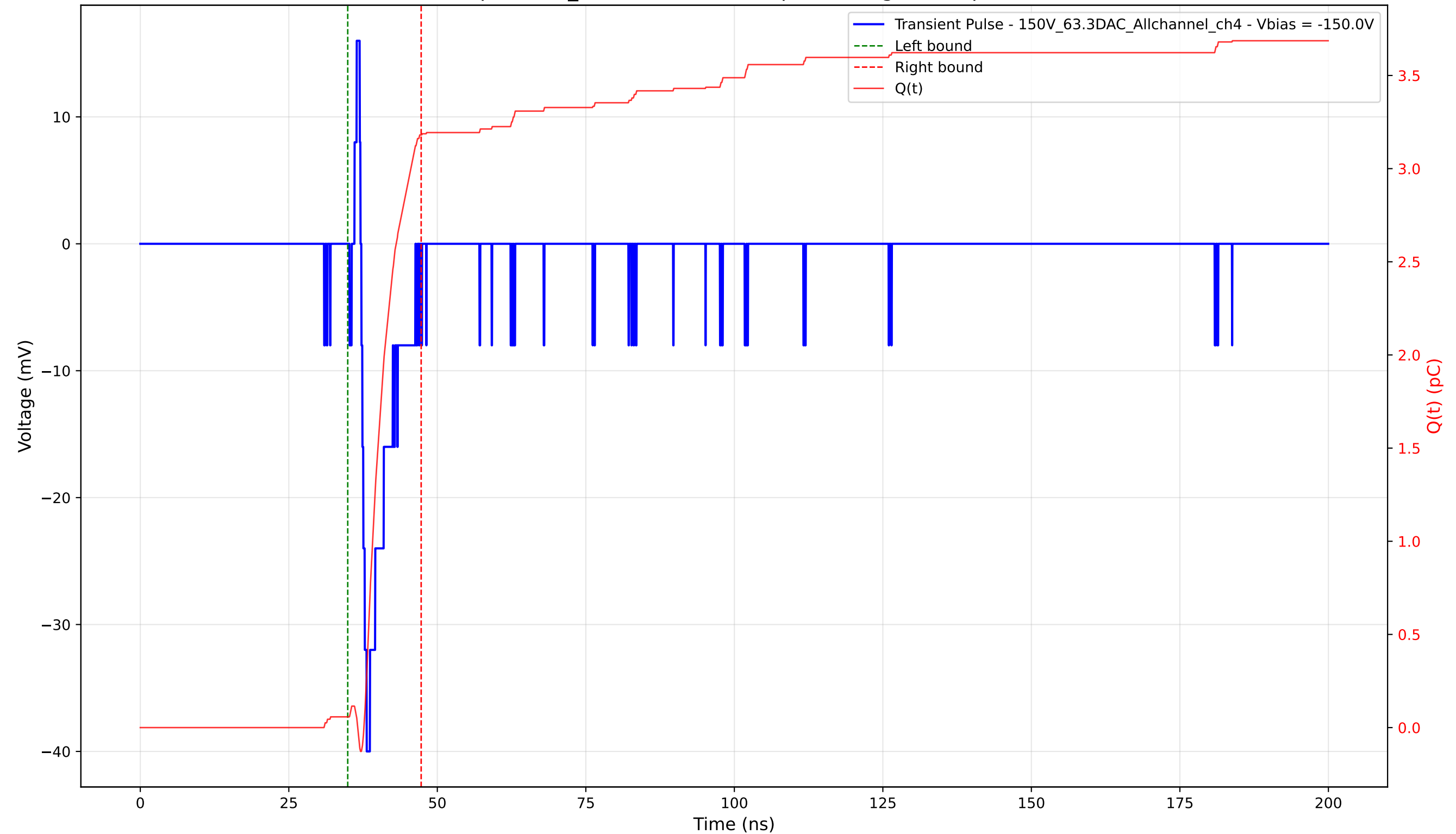
Transient Pulse - Sample: 1cm_42 - Position: 350.0 \mu\text{m} - Charge: 3.12 pC - Rise Time: 0.90 ns
