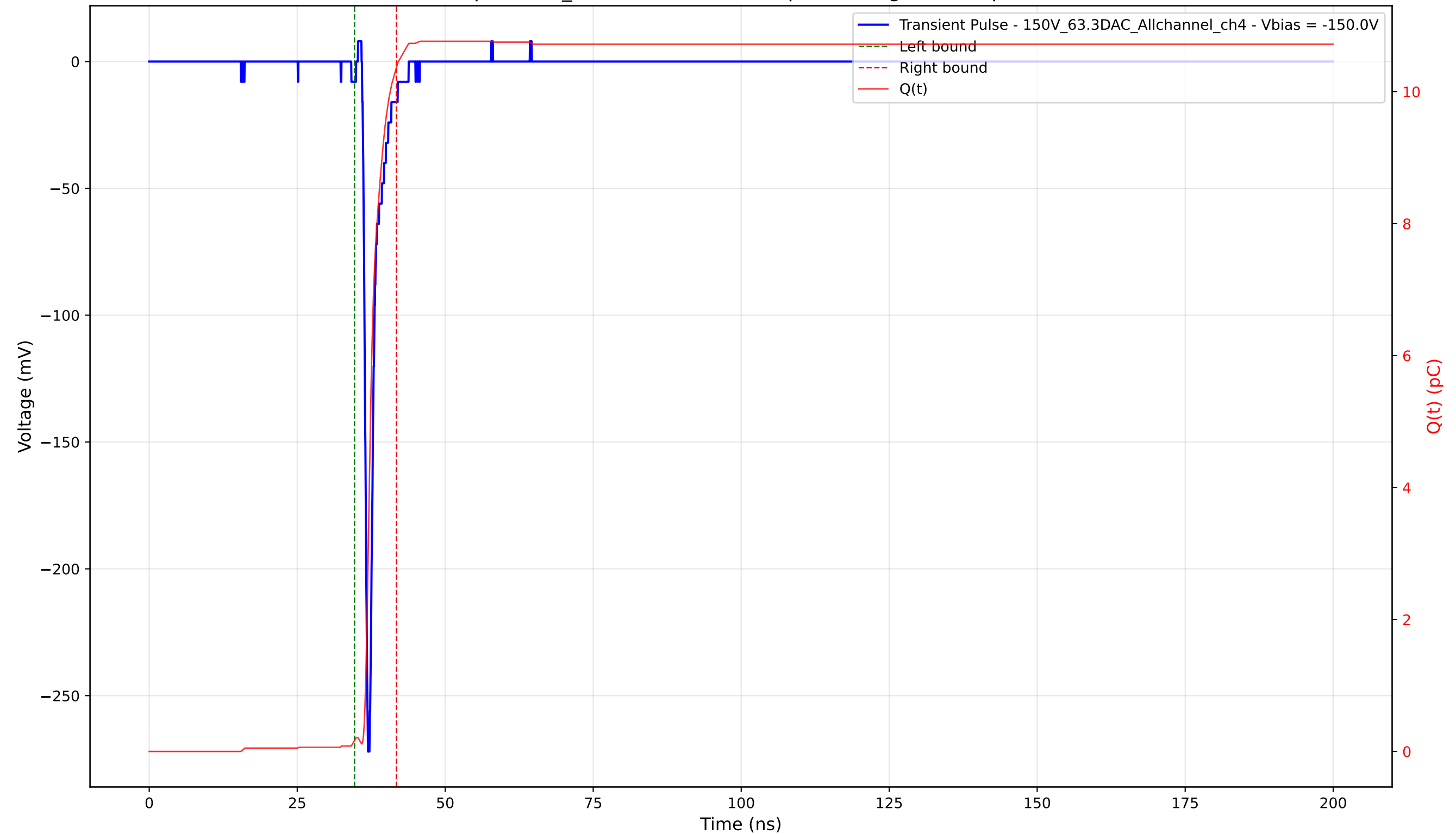
Transient Pulse - Sample: 1cm_42 - Position: 2475.0 \mu\text{m} - Charge: 10.20 pC - Rise Time: 0.73 ns
