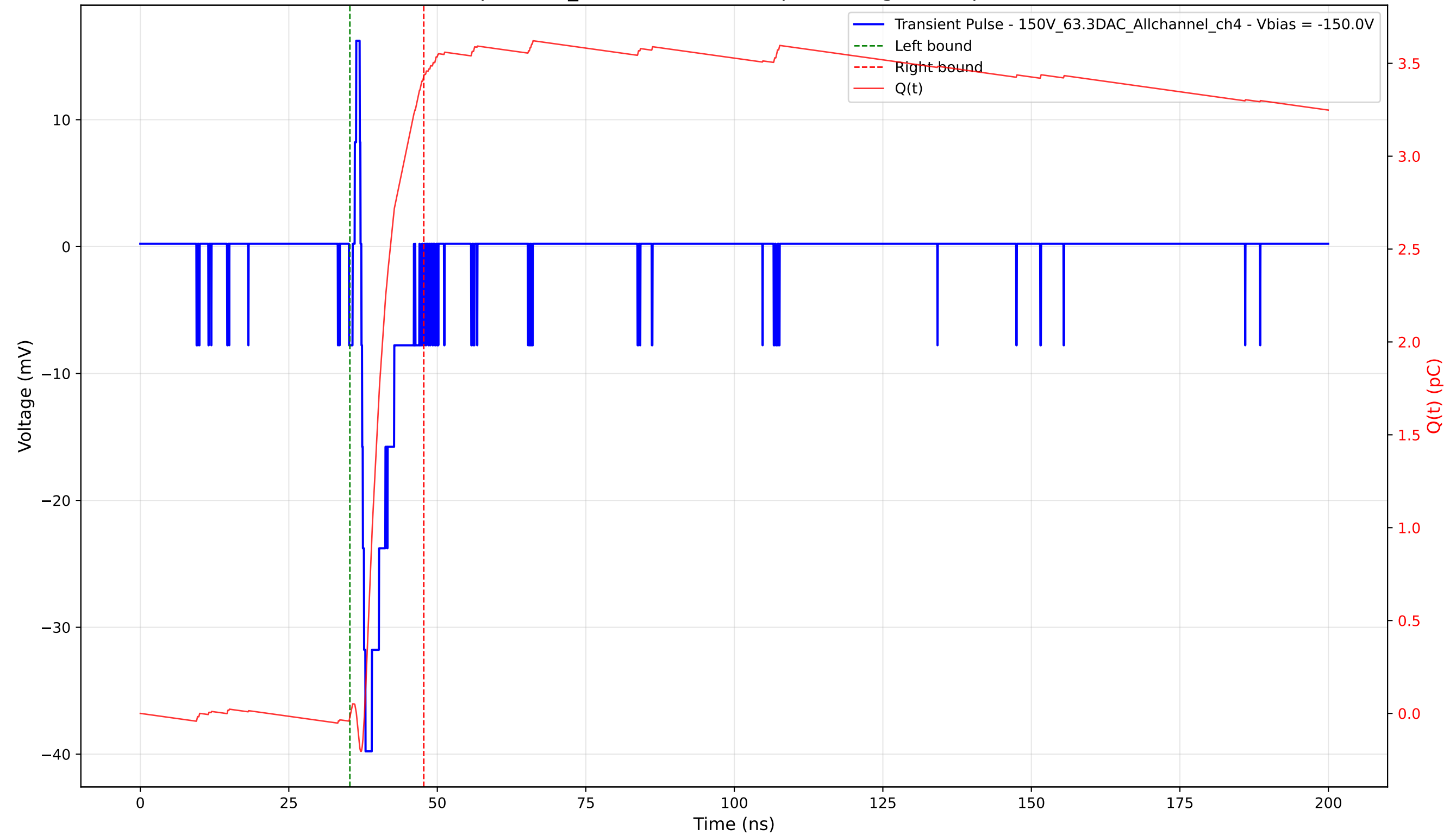
Transient Pulse - Sample: 1cm_42 - Position: 395.0 \mu\text{m} - Charge: 3.45 pC - Rise Time: 0.70 ns
