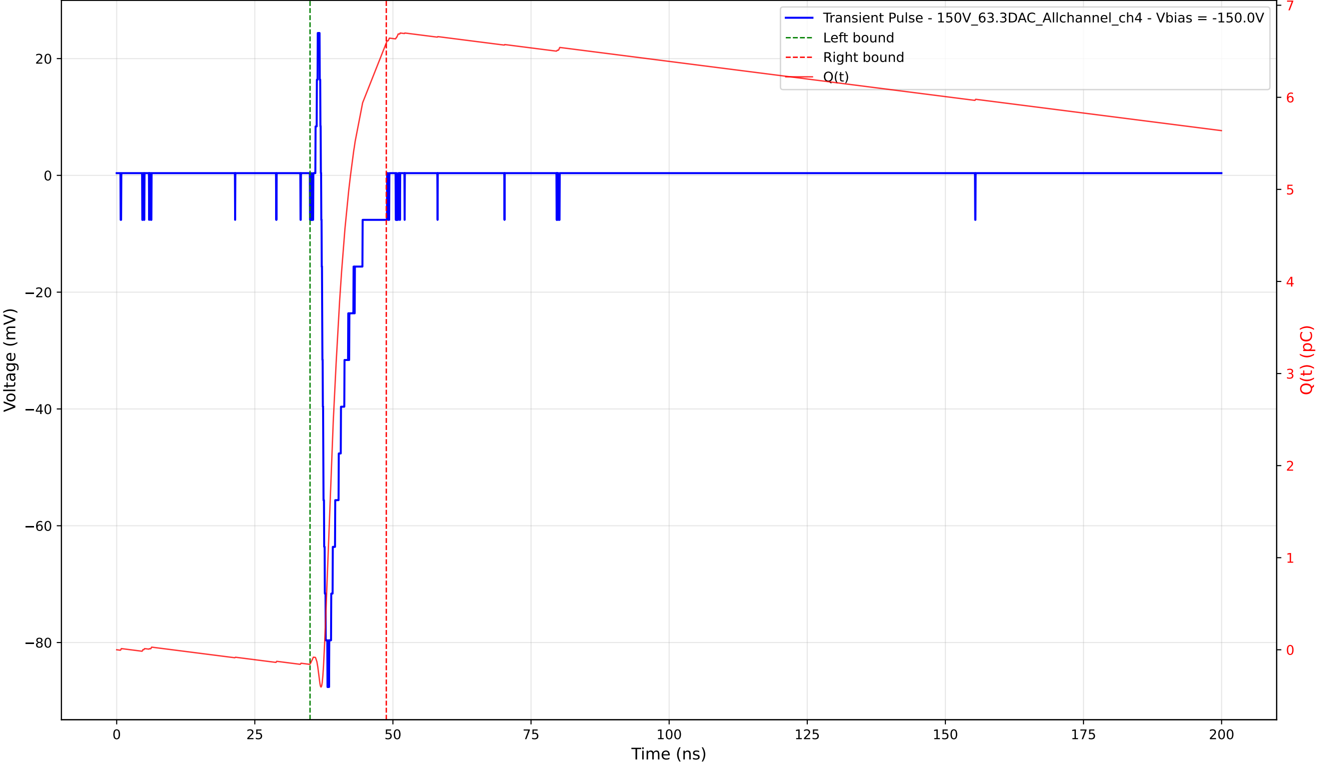
Transient Pulse - Sample: 1cm_42 - Position: 730.0 \mu\text{m} - Charge: 6.75 pC - Rise Time: 0.75 ns
