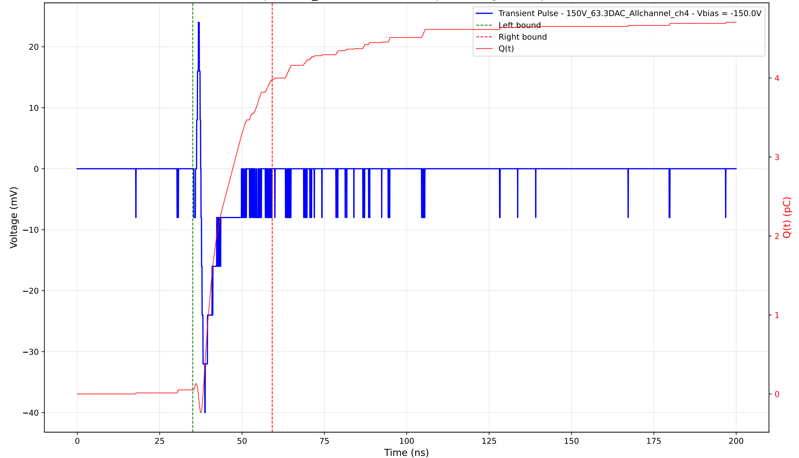
Transient Pulse - Sample: 1cm_42 - Position: 3625.0 \mu\text{m} - Charge: 3.94 pC - Rise Time: 1.18 ns
