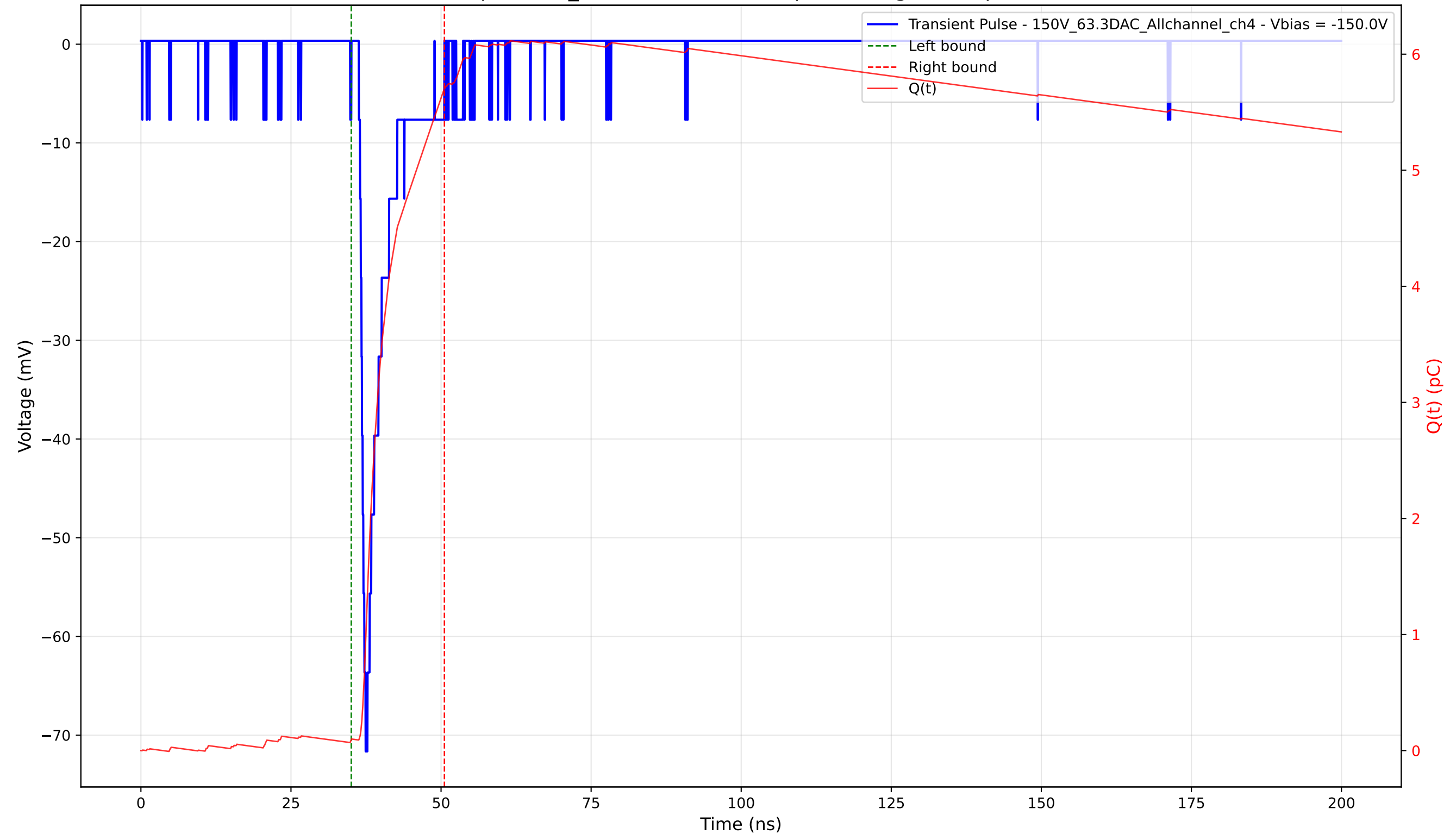
Transient Pulse - Sample: 1cm_42 - Position: 2995.0 \mu\text{m} - Charge: 5.61 pC - Rise Time: 1.12 ns
