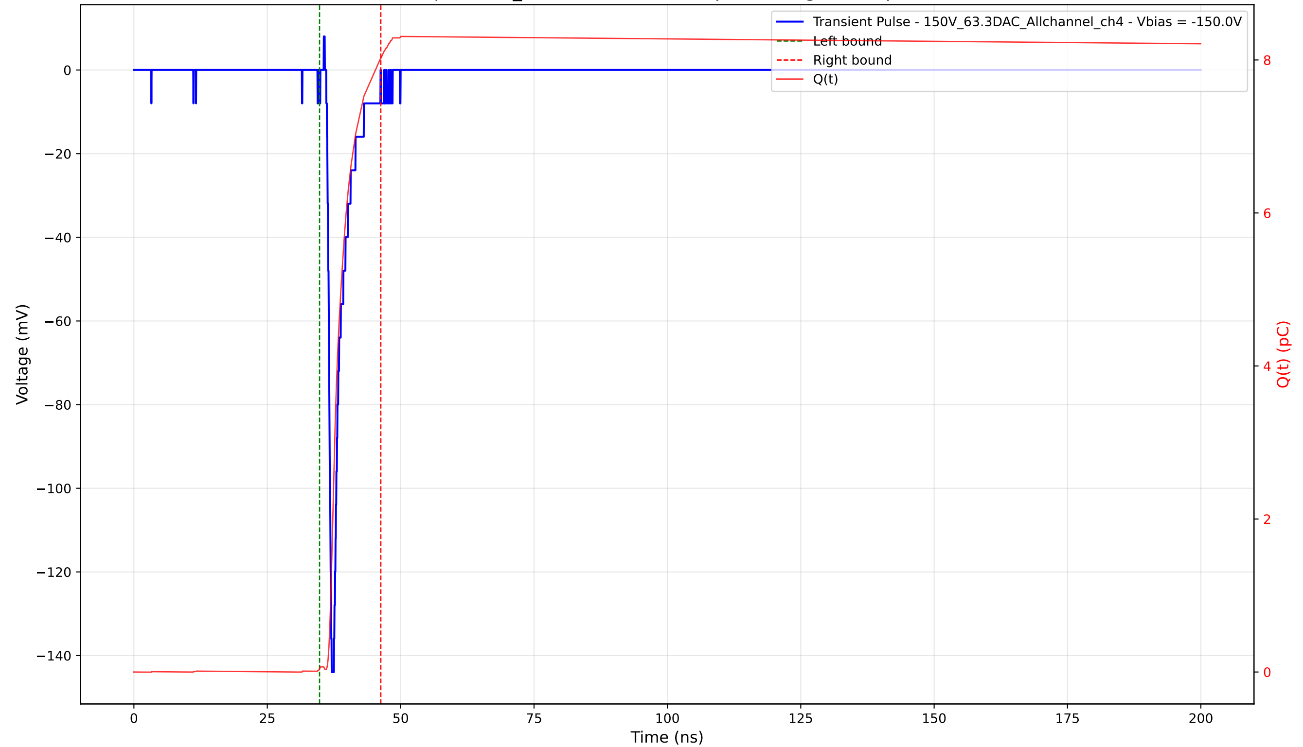
Transient Pulse - Sample: 1cm_42 - Position: 2700.0 \mu\text{m} - Charge: 7.98 pC - Rise Time: 0.81 ns
