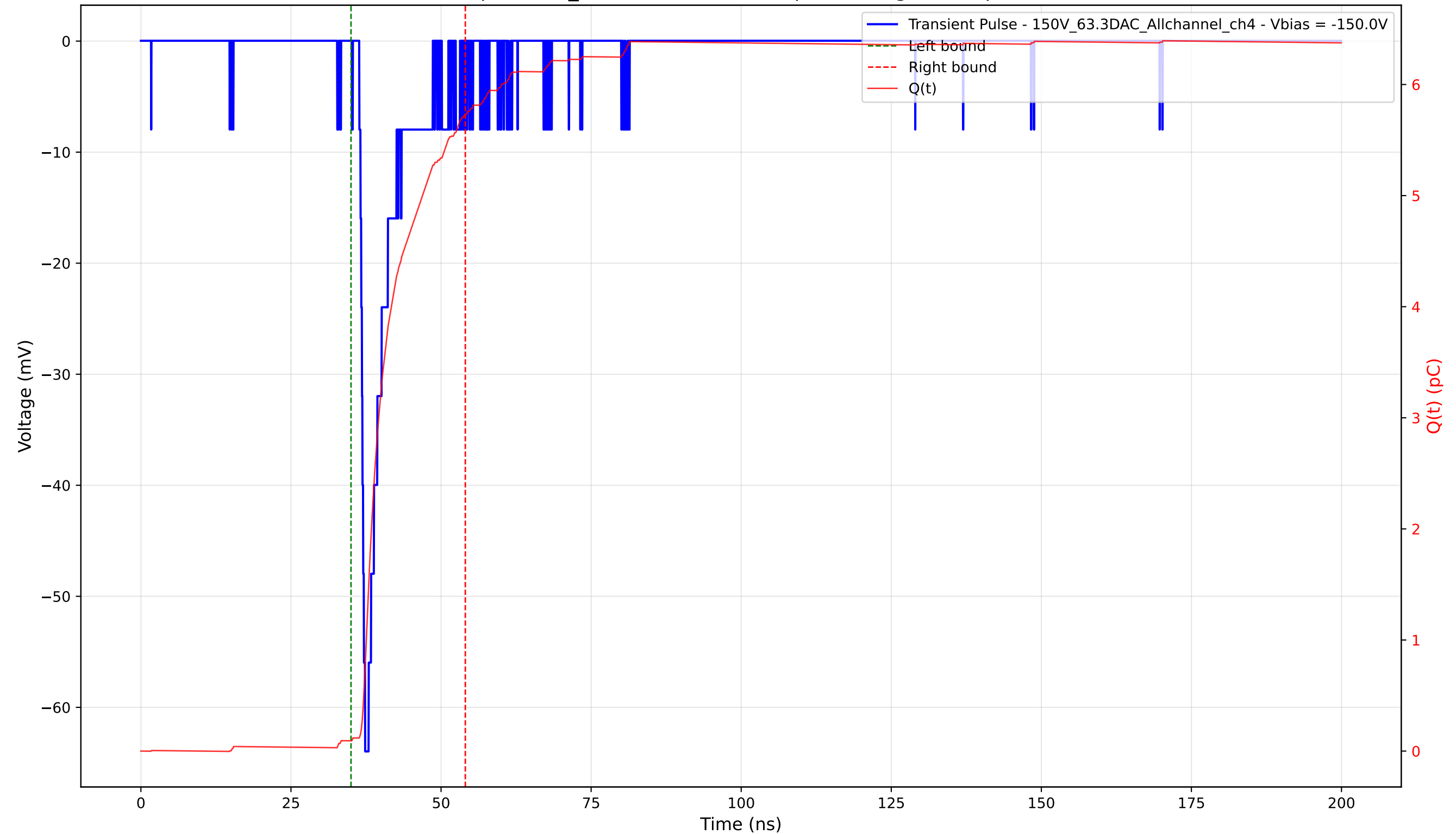
Transient Pulse - Sample: 1cm_42 - Position: 3015.0 \mu\text{m} - Charge: 5.64 pC - Rise Time: 0.97 ns
