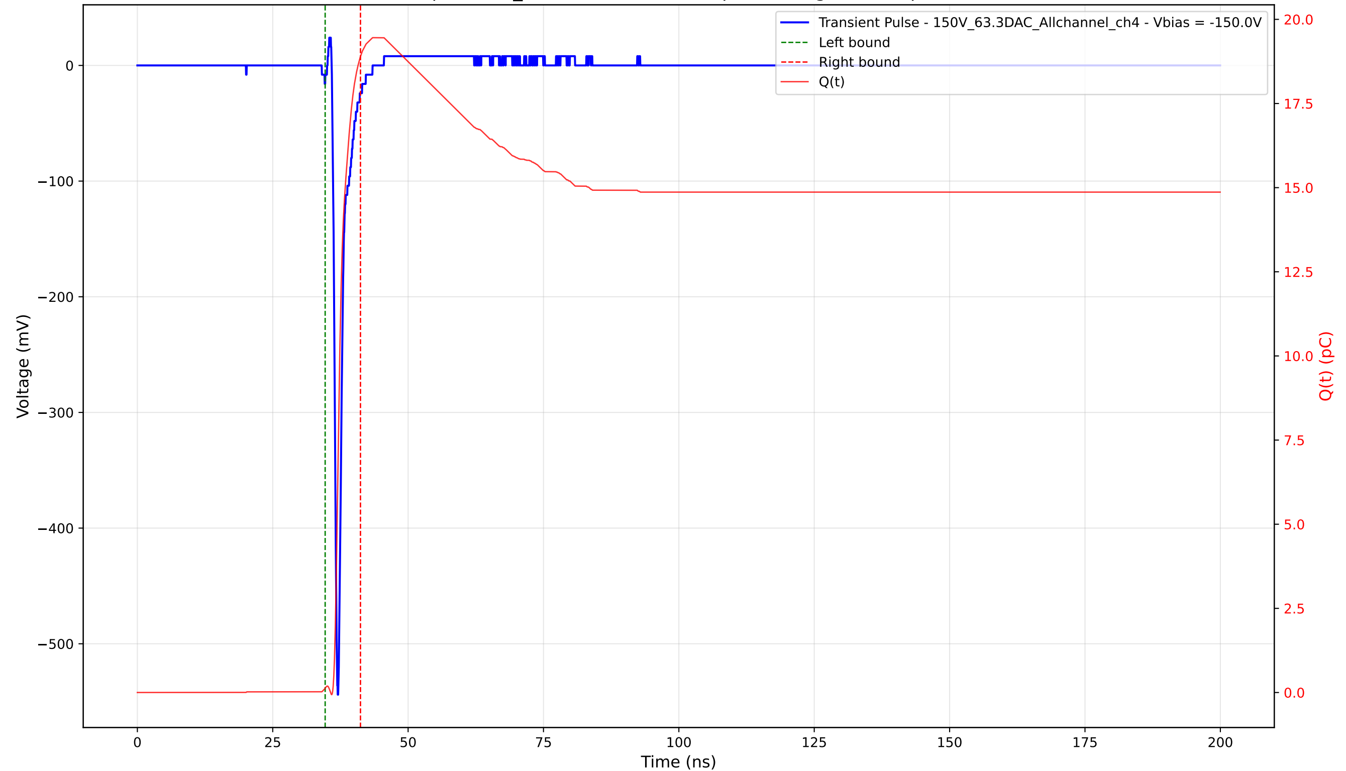
Transient Pulse - Sample: 1cm_42 - Position: 1720.0 \mu\text{m} - Charge: 18.76 pC - Rise Time: 0.73 ns
