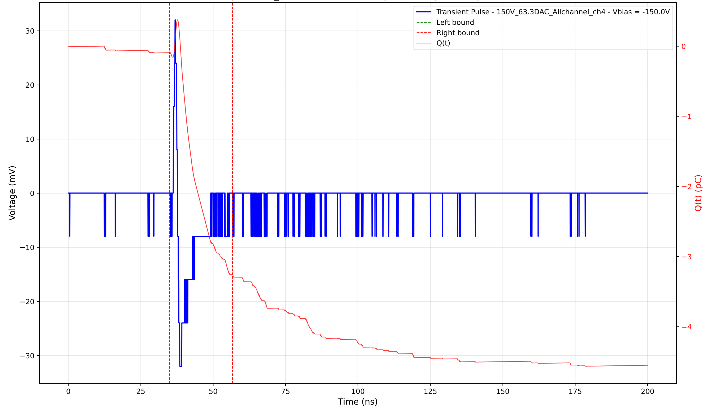
Transient Pulse - Sample: 1cm_42 - Position: 4170.0 \mu\text{m} - Charge: 3.16 pC - Rise Time: 0.62 ns
