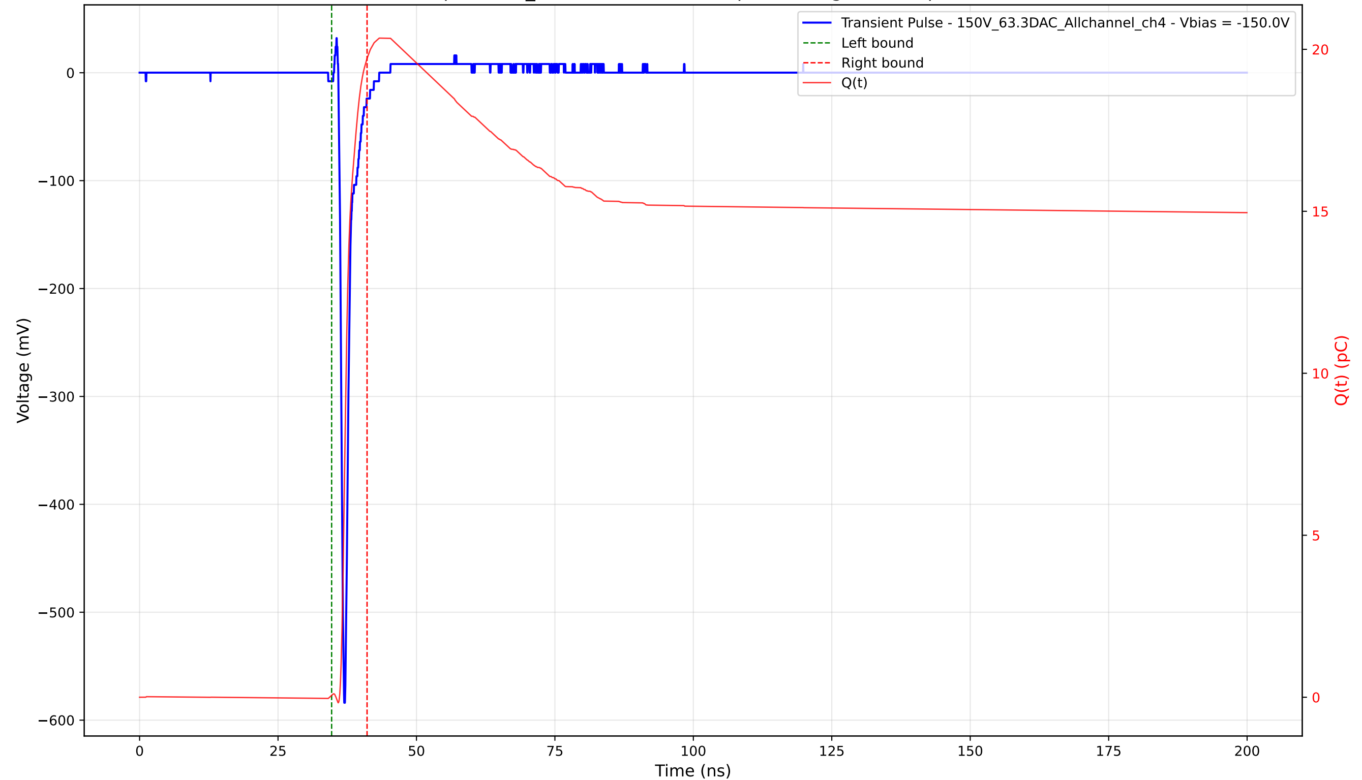
Transient Pulse - Sample: 1cm_42 - Position: 1775.0 \mu\text{m} - Charge: 19.66 pC - Rise Time: 0.71 ns
