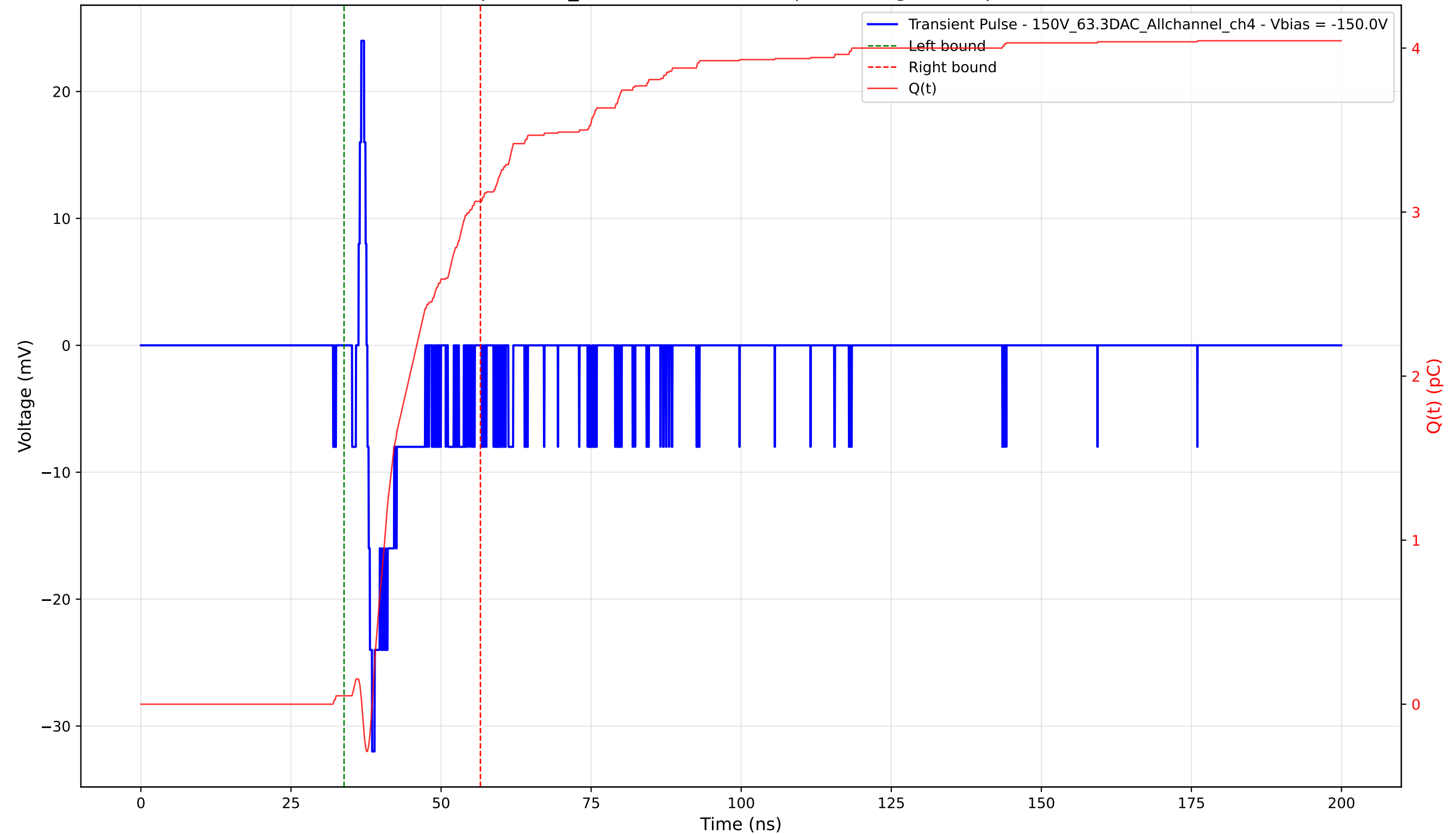
Transient Pulse - Sample: 1cm_42 - Position: 3990.0 \mu\text{m} - Charge: 3.01 pC - Rise Time: 0.78 ns
