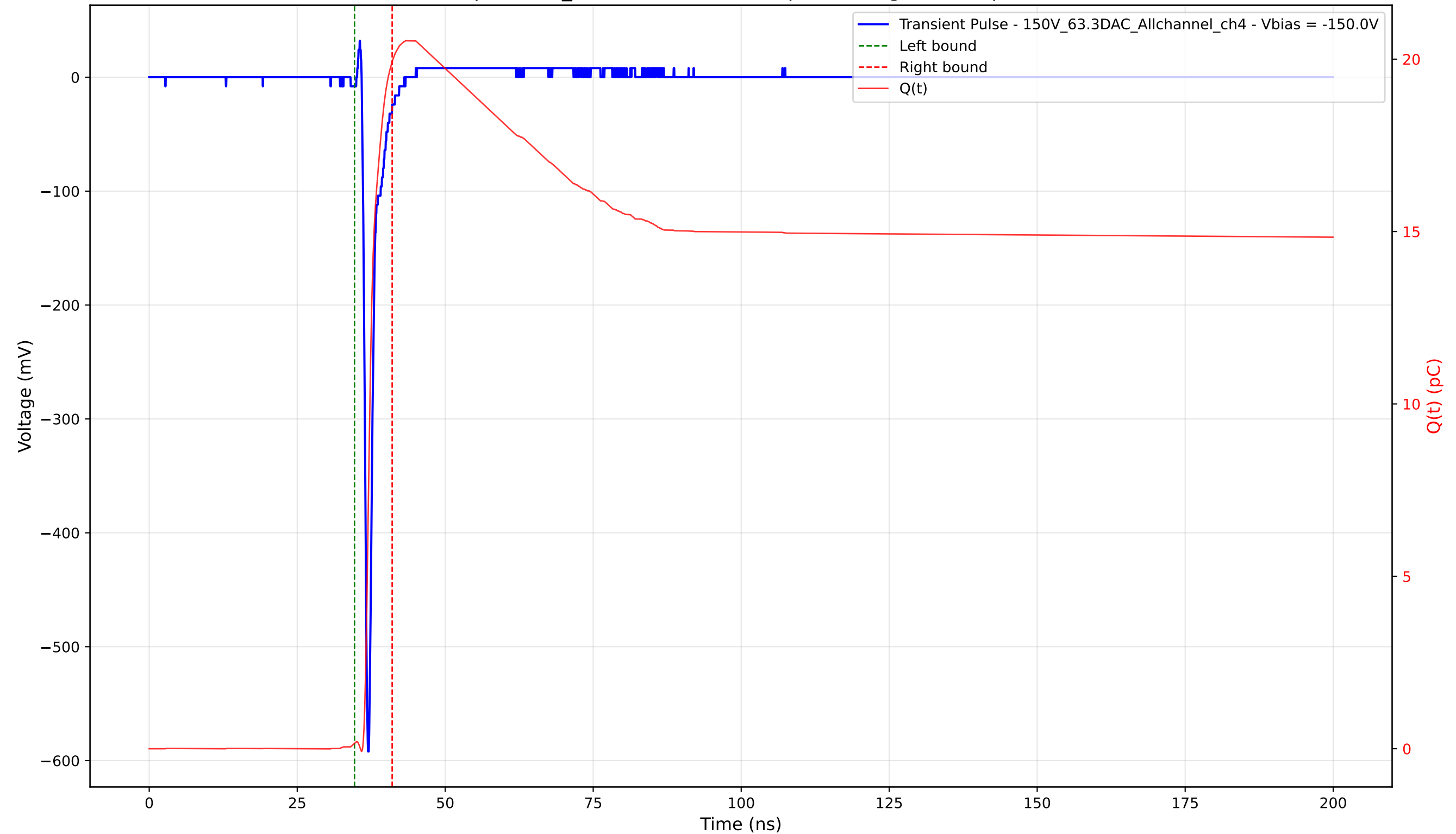
Transient Pulse - Sample: 1cm_42 - Position: 1790.0 \mu\text{m} - Charge: 19.77 pC - Rise Time: 0.66 ns
