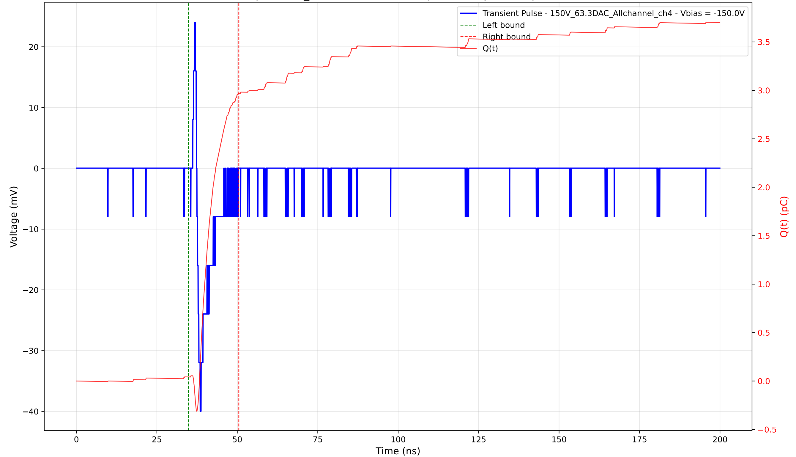
Transient Pulse - Sample: 1cm_42 - Position: 4805.0 \mu\text{m} - Charge: 2.93 pC - Rise Time: 1.02 ns
