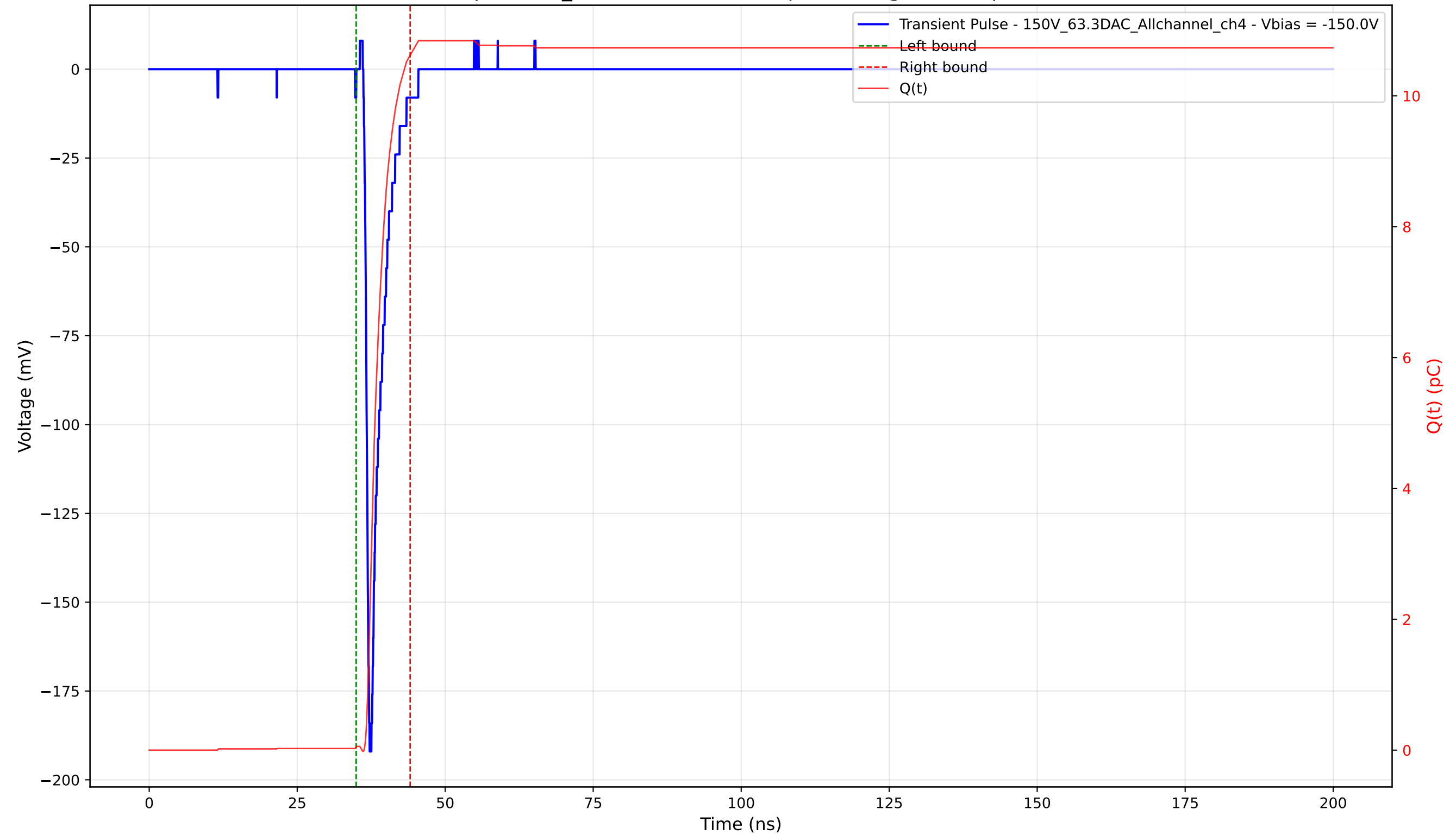
Transient Pulse - Sample: 1cm_42 - Position: 1375.0 \mu\text{m} - Charge: 10.57 pC - Rise Time: 0.77 ns
