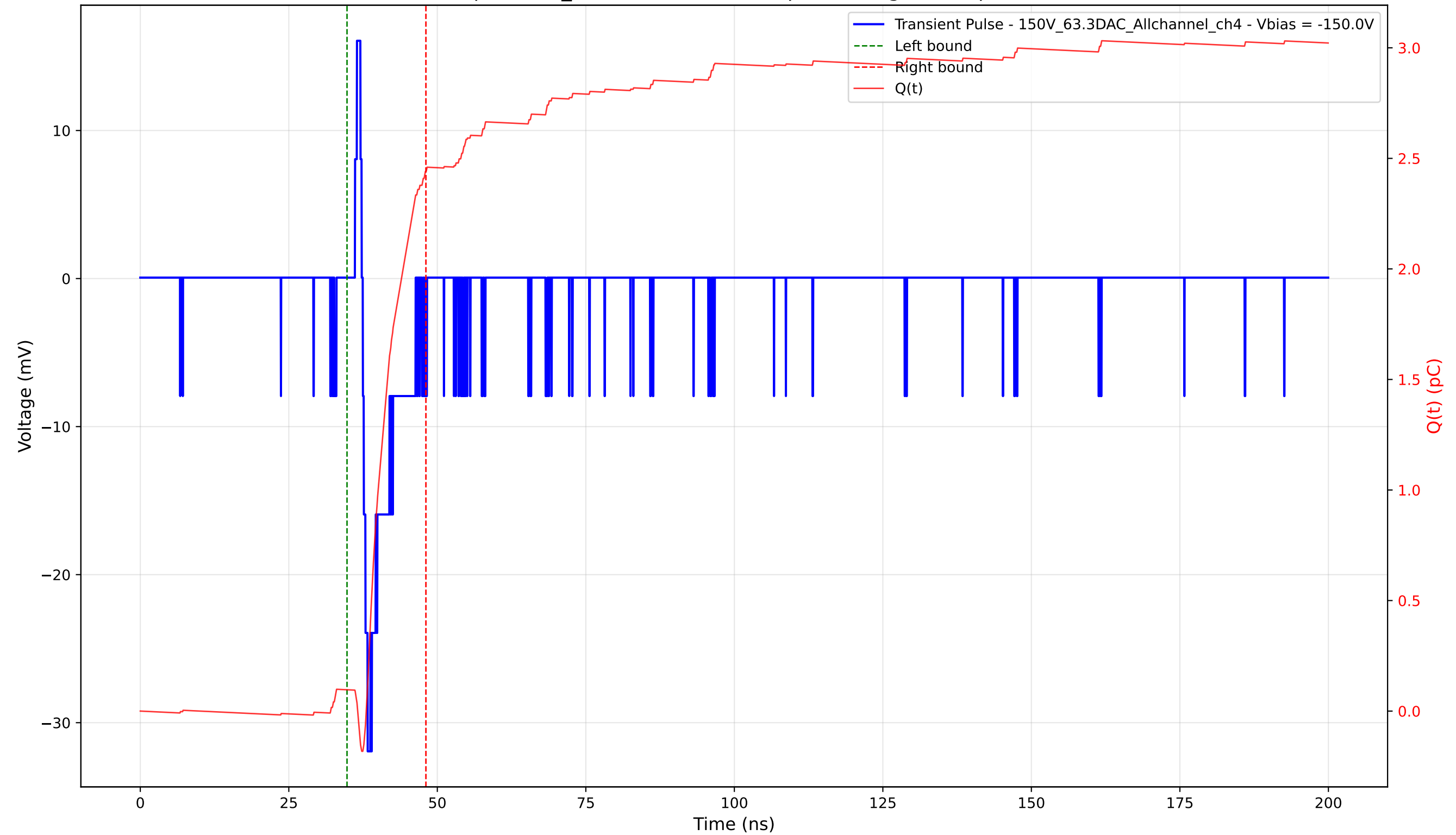
Transient Pulse - Sample: 1cm_42 - Position: 4925.0 \mu\text{m} - Charge: 2.34 pC - Rise Time: 0.82 ns
