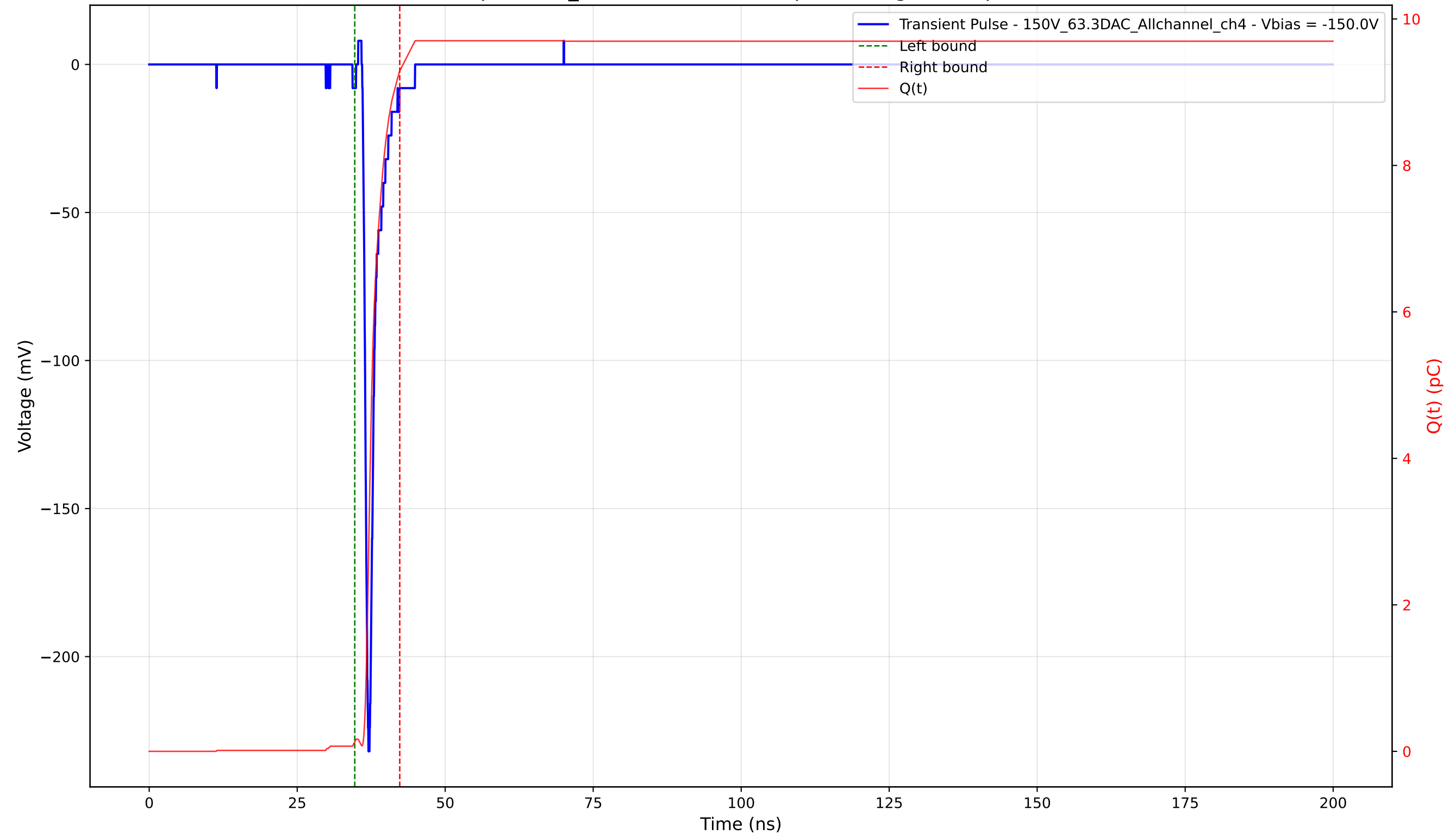
Transient Pulse - Sample: 1cm_42 - Position: 2520.0 \mu\text{m} - Charge: 9.16 pC - Rise Time: 0.77 ns
