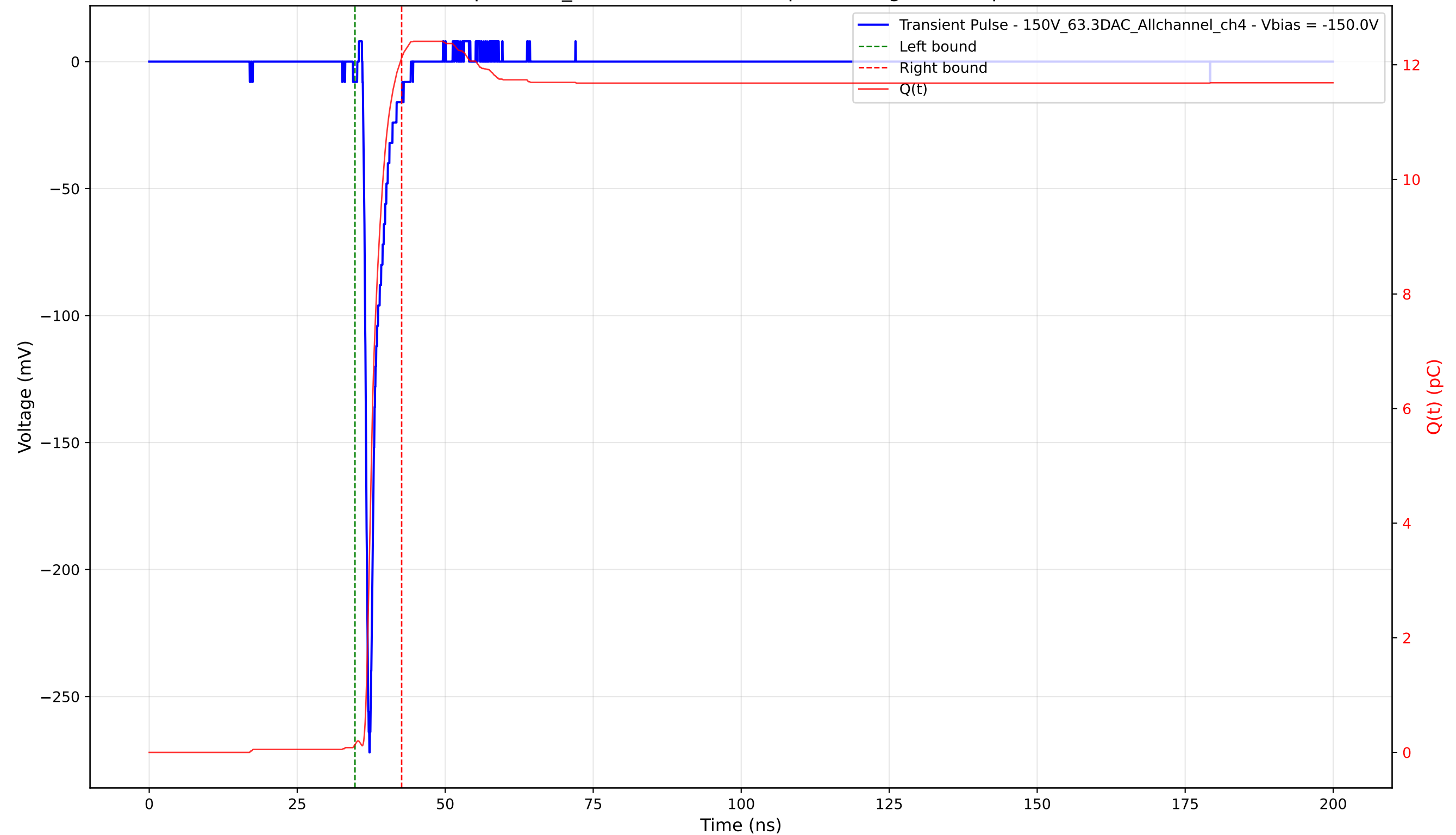
Transient Pulse - Sample: 1cm_42 - Position: 1510.0 \mu\text{m} - Charge: 11.98 pC - Rise Time: 0.77 ns
