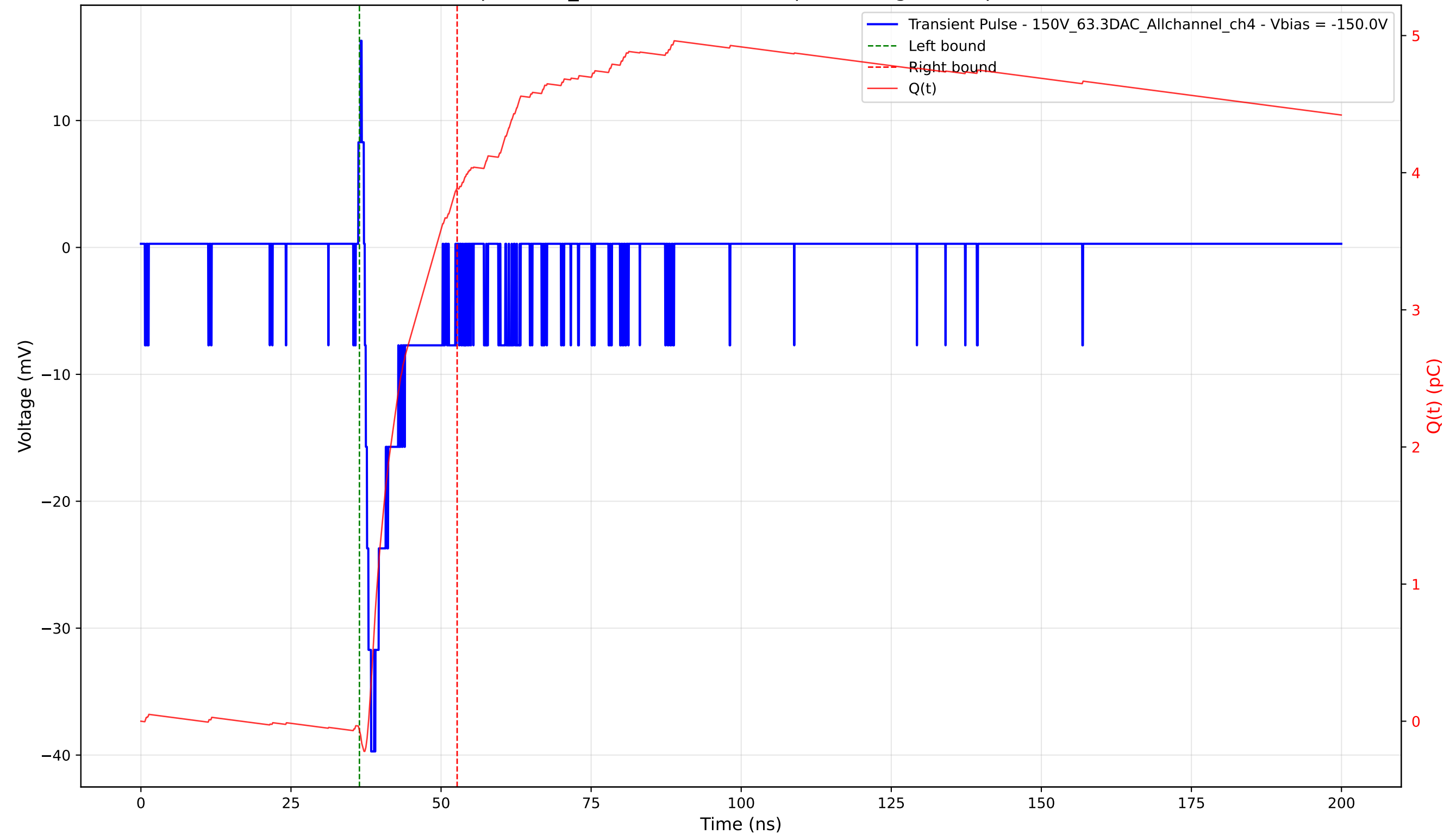
Transient Pulse - Sample: 1cm_42 - Position: 3470.0 \mu\text{m} - Charge: 3.95 pC - Rise Time: 1.06 ns
