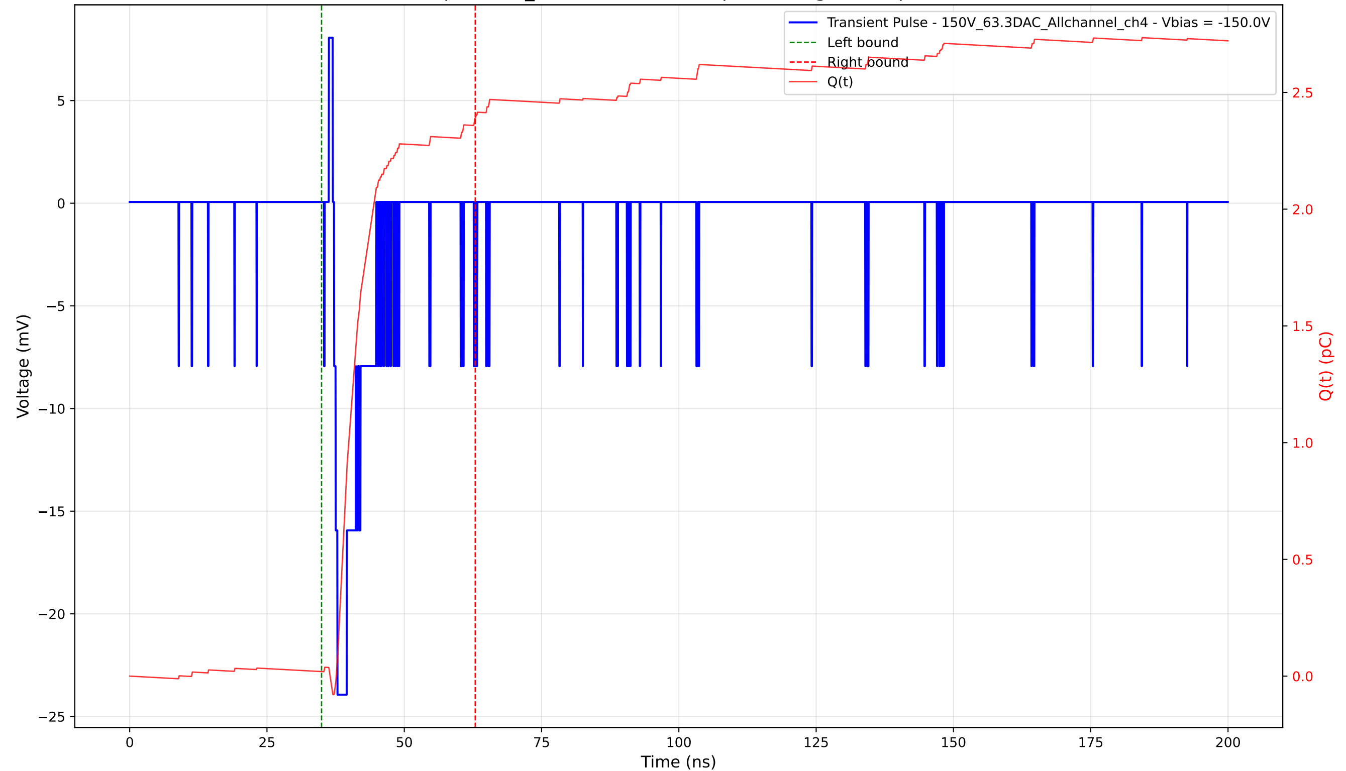
Transient Pulse - Sample: 1cm_42 - Position: 200.0 \mu\text{m} - Charge: 2.37 pC - Rise Time: 0.63 ns
