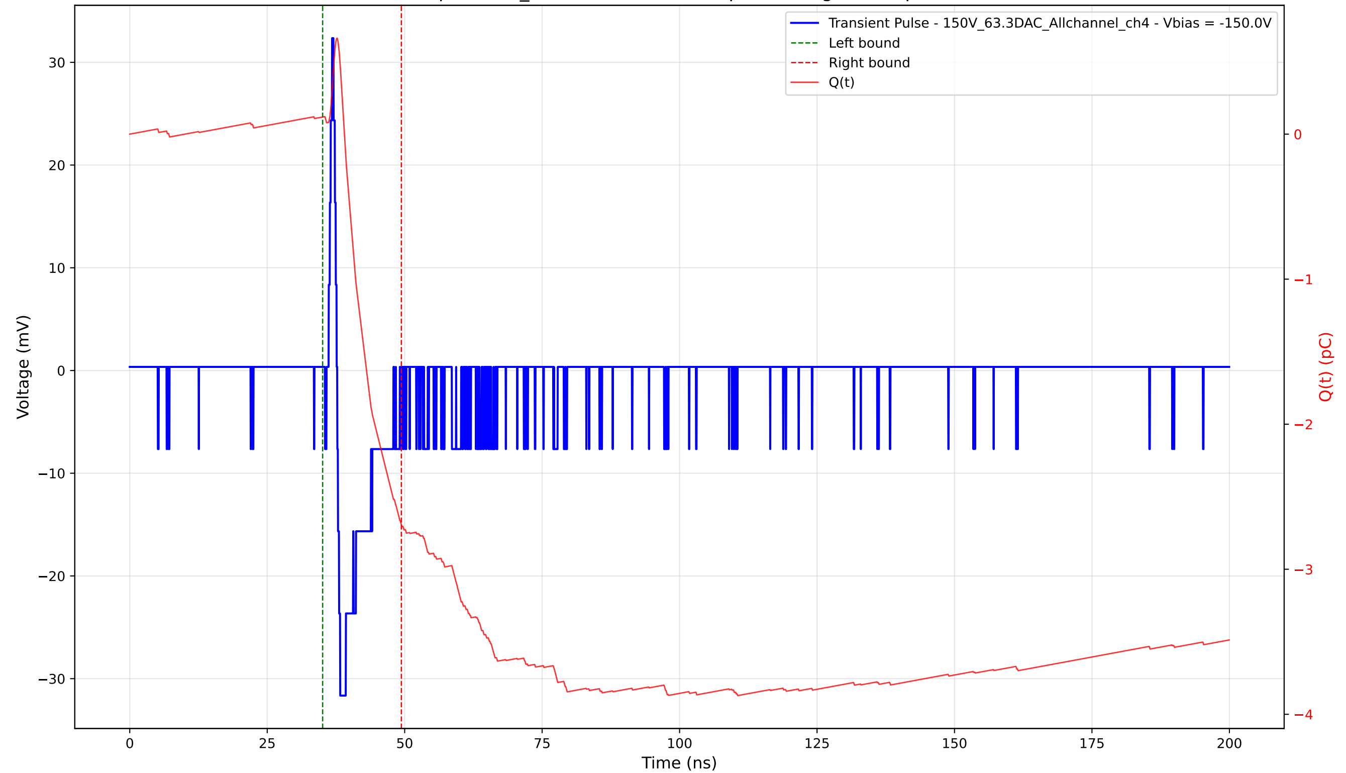
Transient Pulse - Sample: 1cm_42 - Position: 4320.0 \mu\text{m} - Charge: 2.81 pC - Rise Time: 0.63 ns
