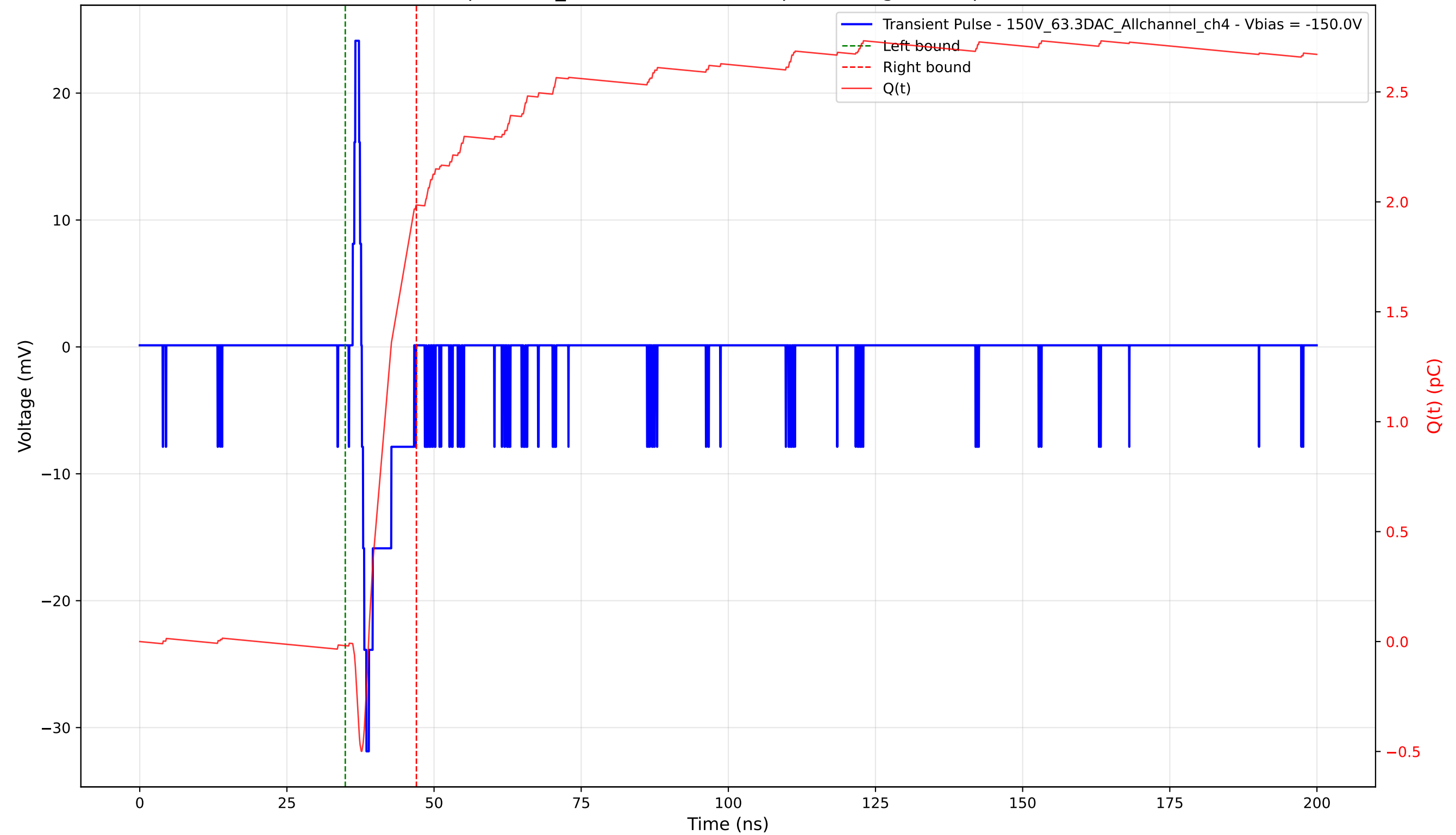
Transient Pulse - Sample: 1cm_42 - Position: 4450.0 \mu\text{m} - Charge: 2.00 pC - Rise Time: 0.78 ns
