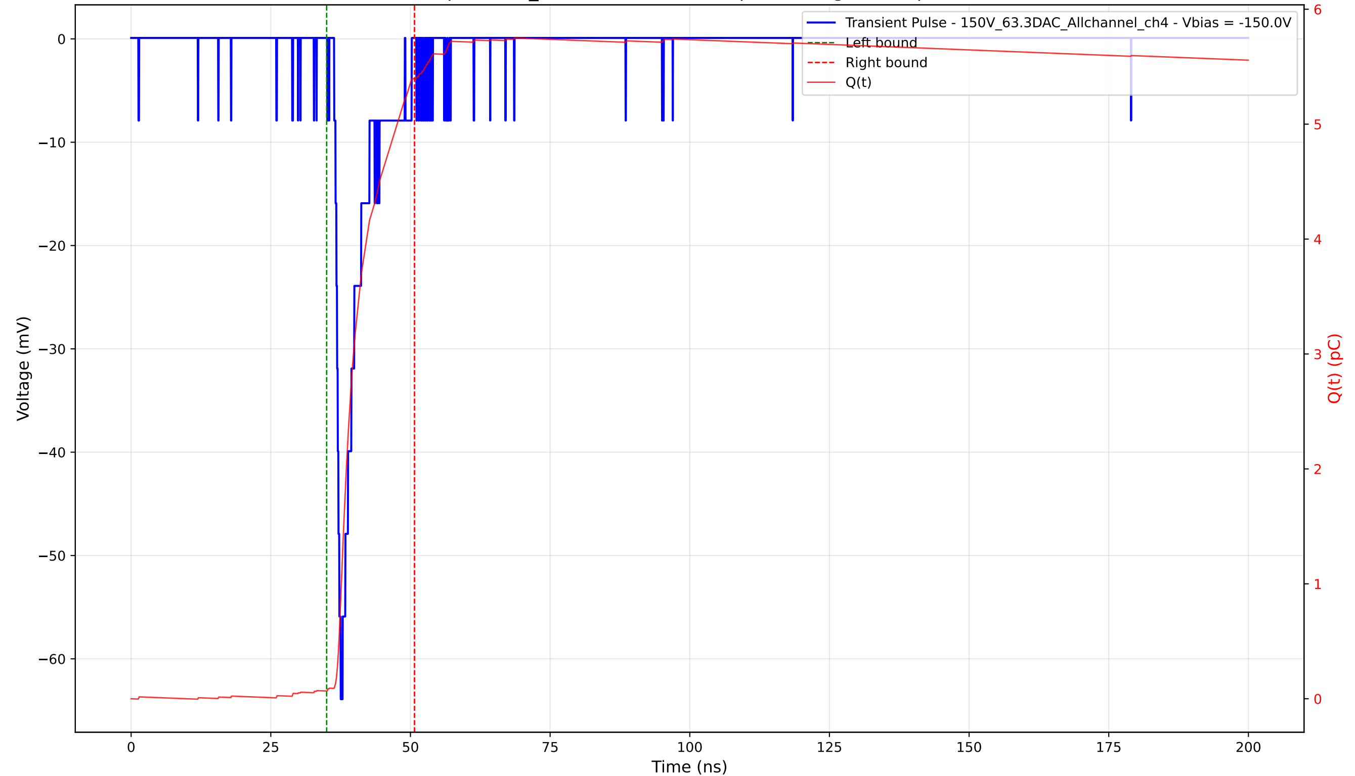
Transient Pulse - Sample: 1cm_42 - Position: 3030.0 \mu\text{m} - Charge: 5.33 pC - Rise Time: 1.17 ns
