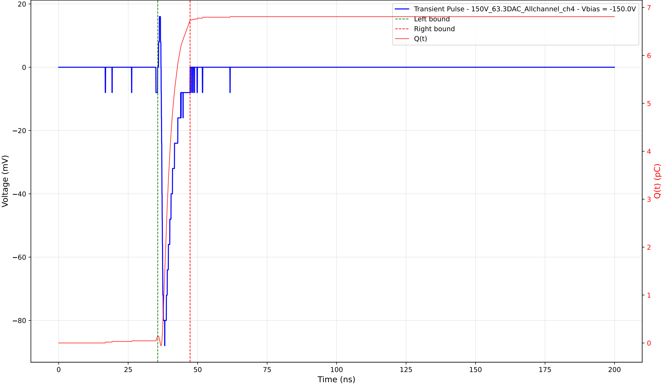
Transient Pulse - Sample: 1cm_42 - Position: 910.0 \mu\text{m} - Charge: 6.59 pC - Rise Time: 0.72 ns
