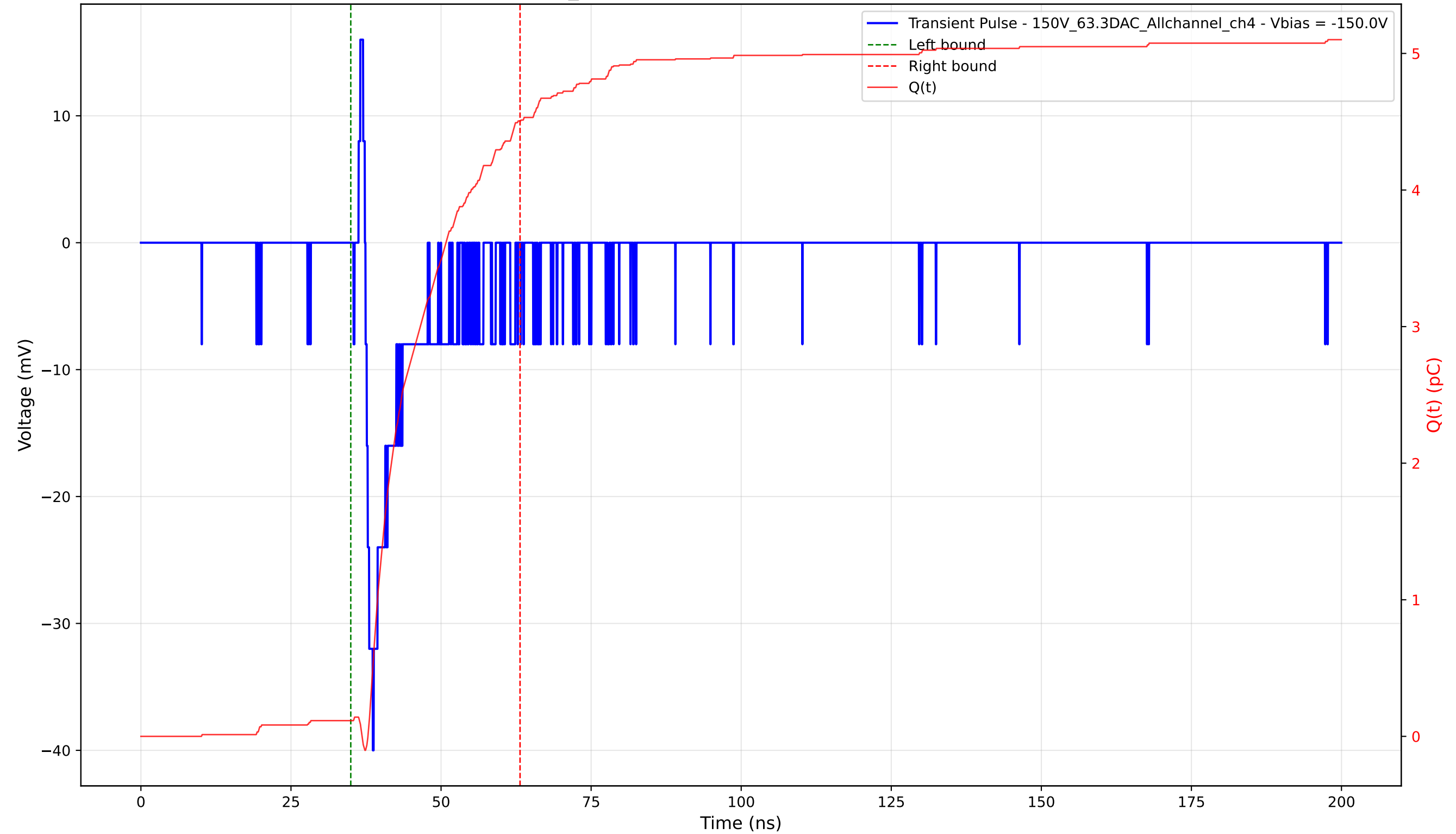
Transient Pulse - Sample: 1cm_42 - Position: 3535.0 \mu\text{m} - Charge: 4.39 pC - Rise Time: 1.22 ns
