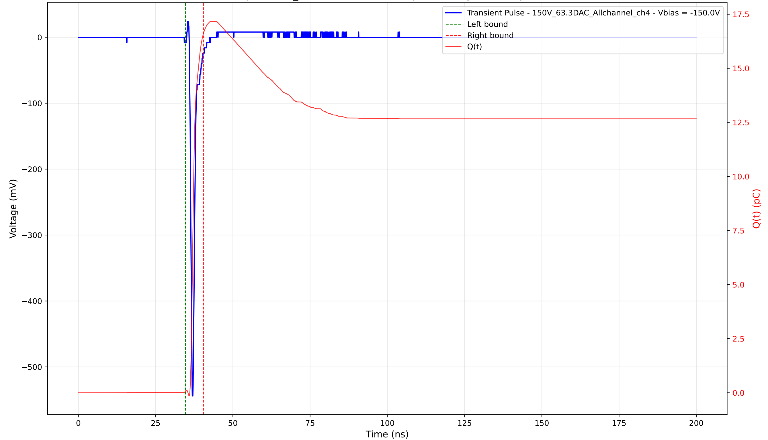
Transient Pulse - Sample: 1cm_42 - Position: 2140.0 \mu\text{m} - Charge: 16.58 pC - Rise Time: 0.71 ns
