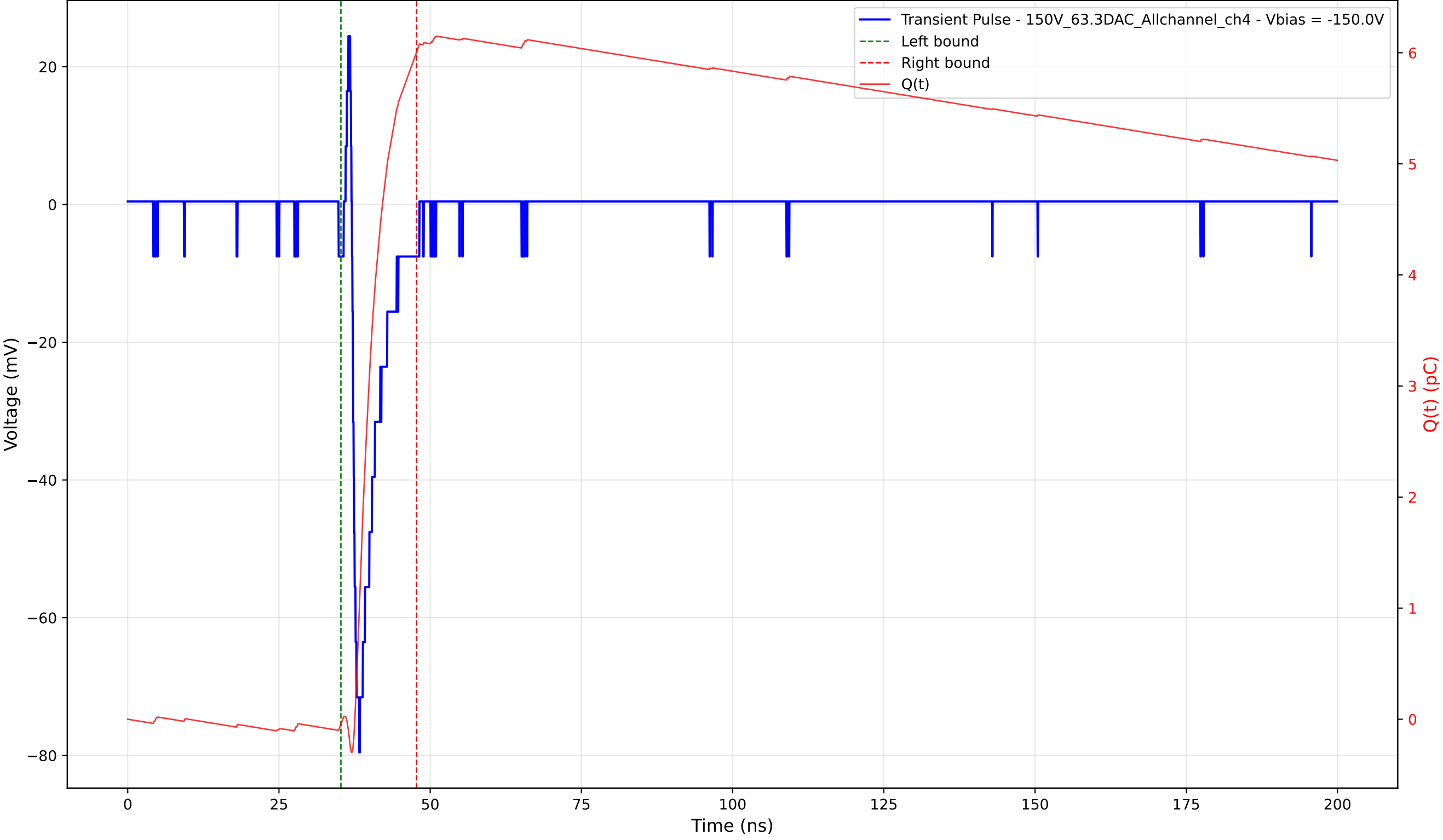
Transient Pulse - Sample: 1cm_42 - Position: 670.0 \mu\text{m} - Charge: 6.05 pC - Rise Time: 1.16 ns
