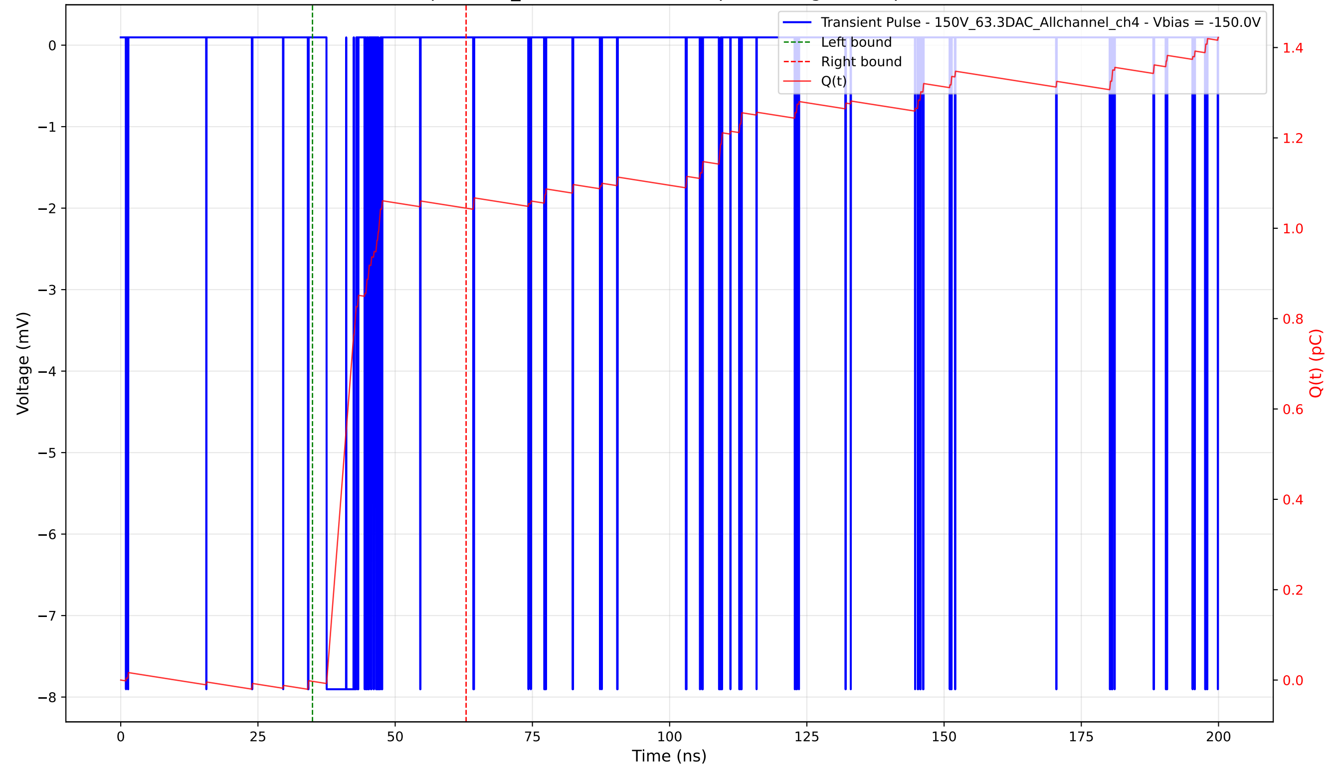
Transient Pulse - Sample: 1cm_42 - Position: 5145.0 \mu\text{m} - Charge: 1.05 pC - Rise Time: 0.04 ns
