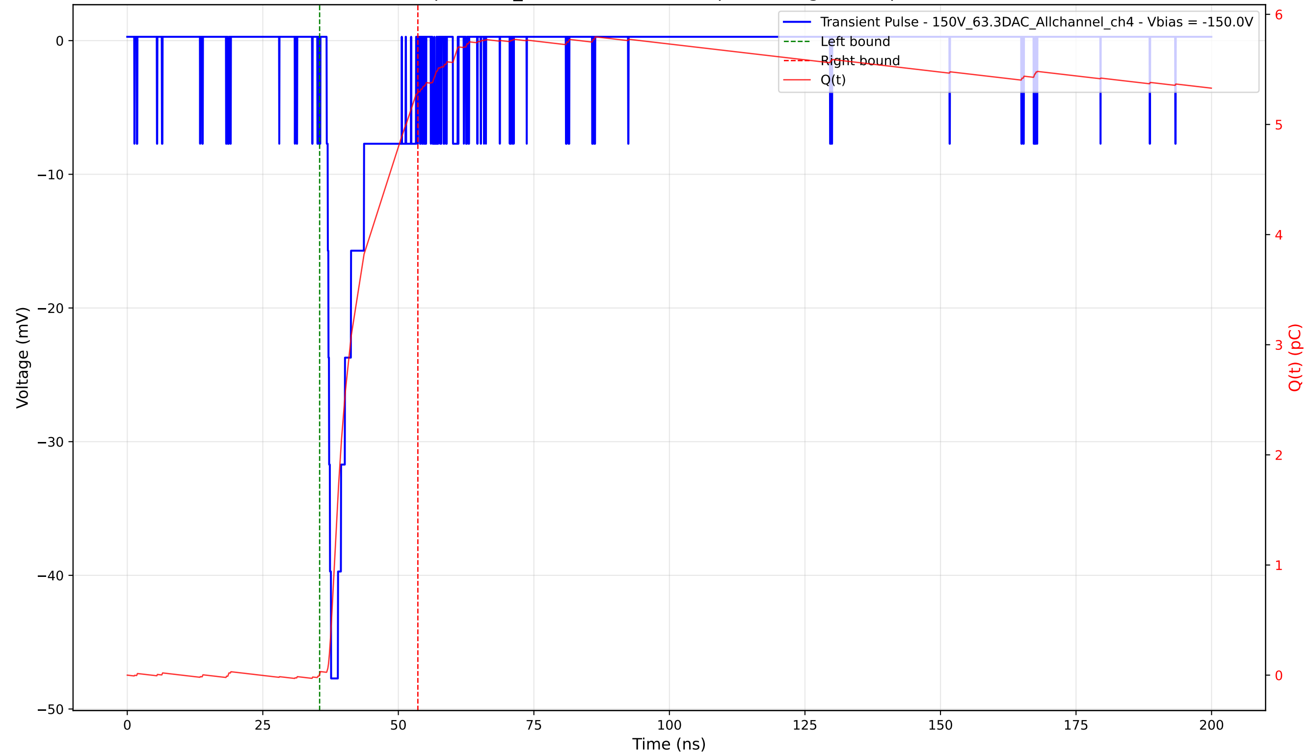
Transient Pulse - Sample: 1cm_42 - Position: 3155.0 \mu\text{m} - Charge: 5.28 pC - Rise Time: 0.82 ns
