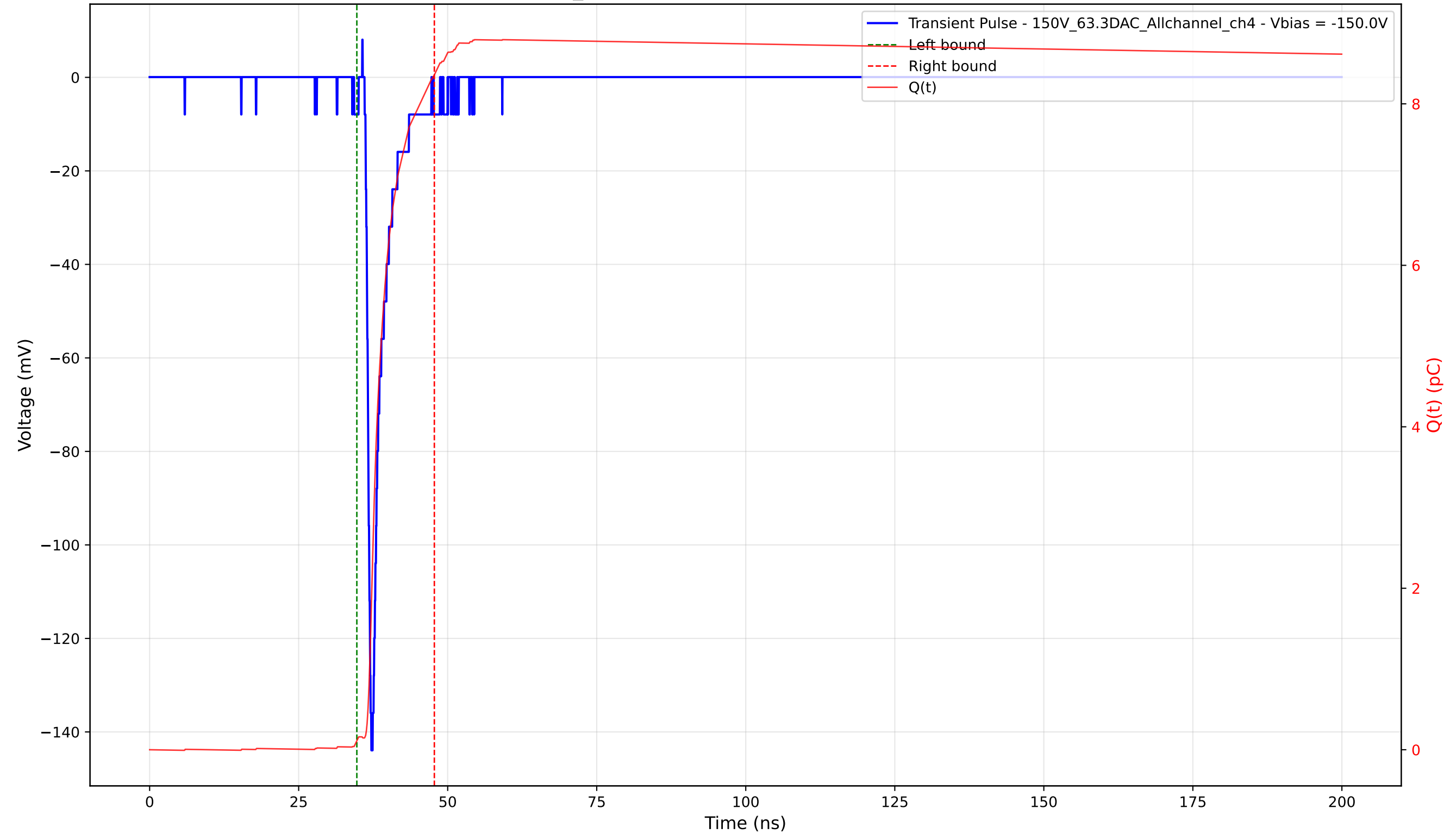
Transient Pulse - Sample: 1cm_42 - Position: 2735.0 \mu\text{m} - Charge: 8.25 pC - Rise Time: 0.85 ns
