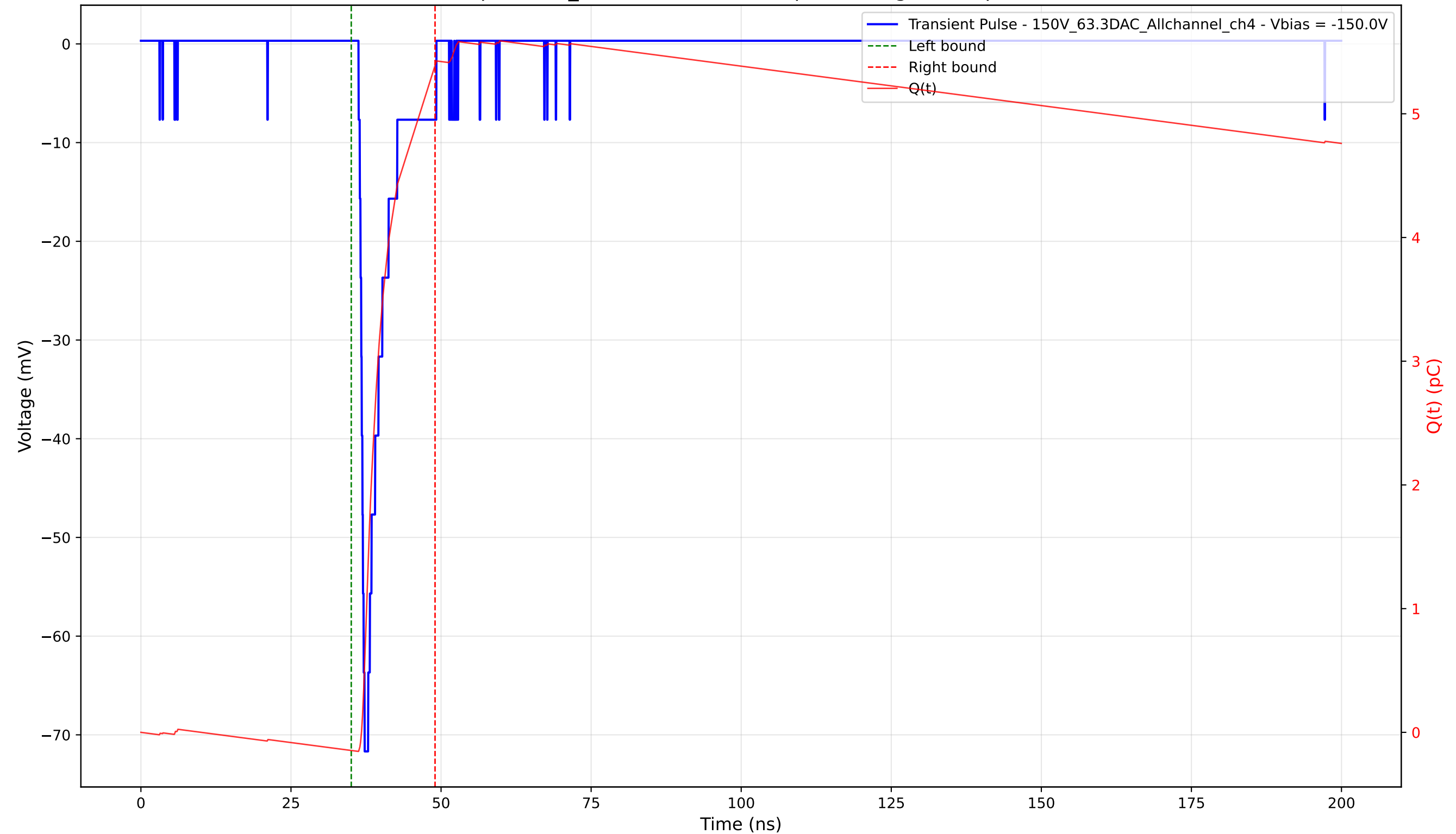
Transient Pulse - Sample: 1cm_42 - Position: 2980.0 \mu\text{m} - Charge: 5.54 pC - Rise Time: 1.00 ns
