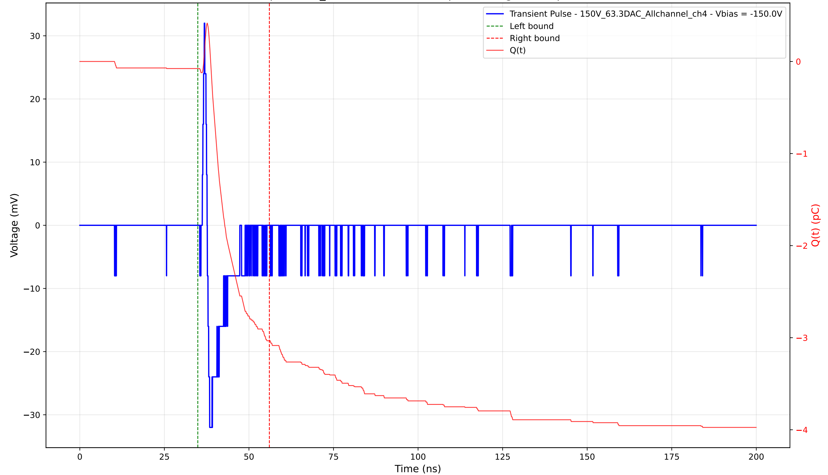
Transient Pulse - Sample: 1cm_42 - Position: 4355.0 \mu\text{m} - Charge: 2.96 pC - Rise Time: 0.58 ns
