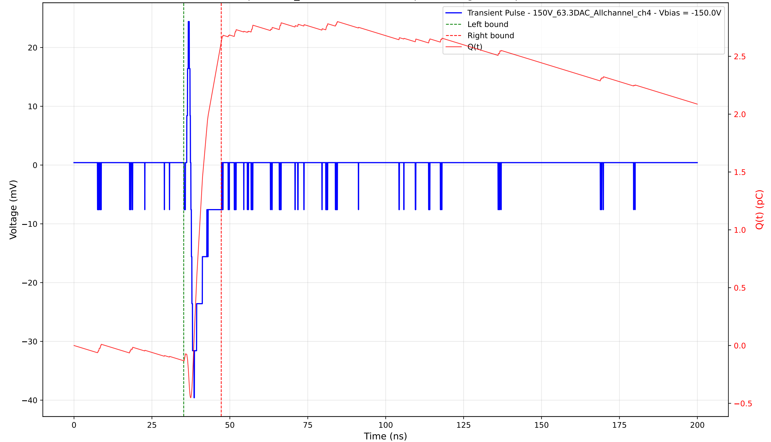
Transient Pulse - Sample: 1cm_42 - Position: 4790.0 \mu\text{m} - Charge: 2.76 pC - Rise Time: 1.02 ns
