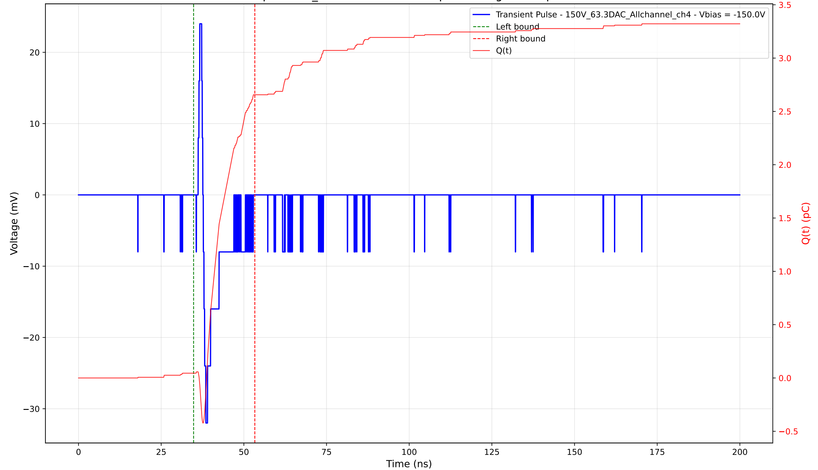
Transient Pulse - Sample: 1cm_42 - Position: 4075.0 \mu\text{m} - Charge: 2.61 pC - Rise Time: 0.78 ns
