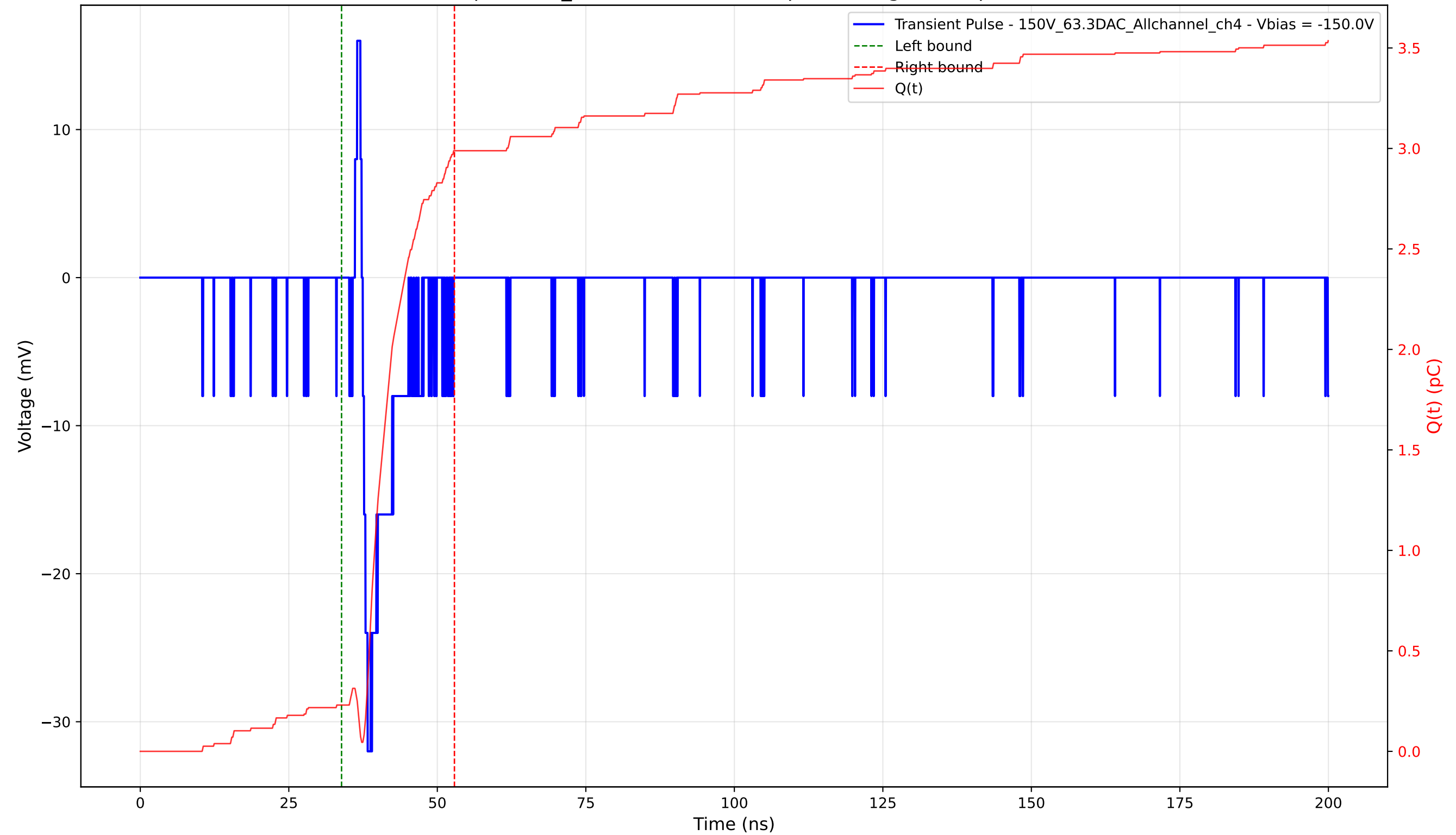
Transient Pulse - Sample: 1cm_42 - Position: 4915.0 \mu\text{m} - Charge: 2.76 pC - Rise Time: 0.82 ns
