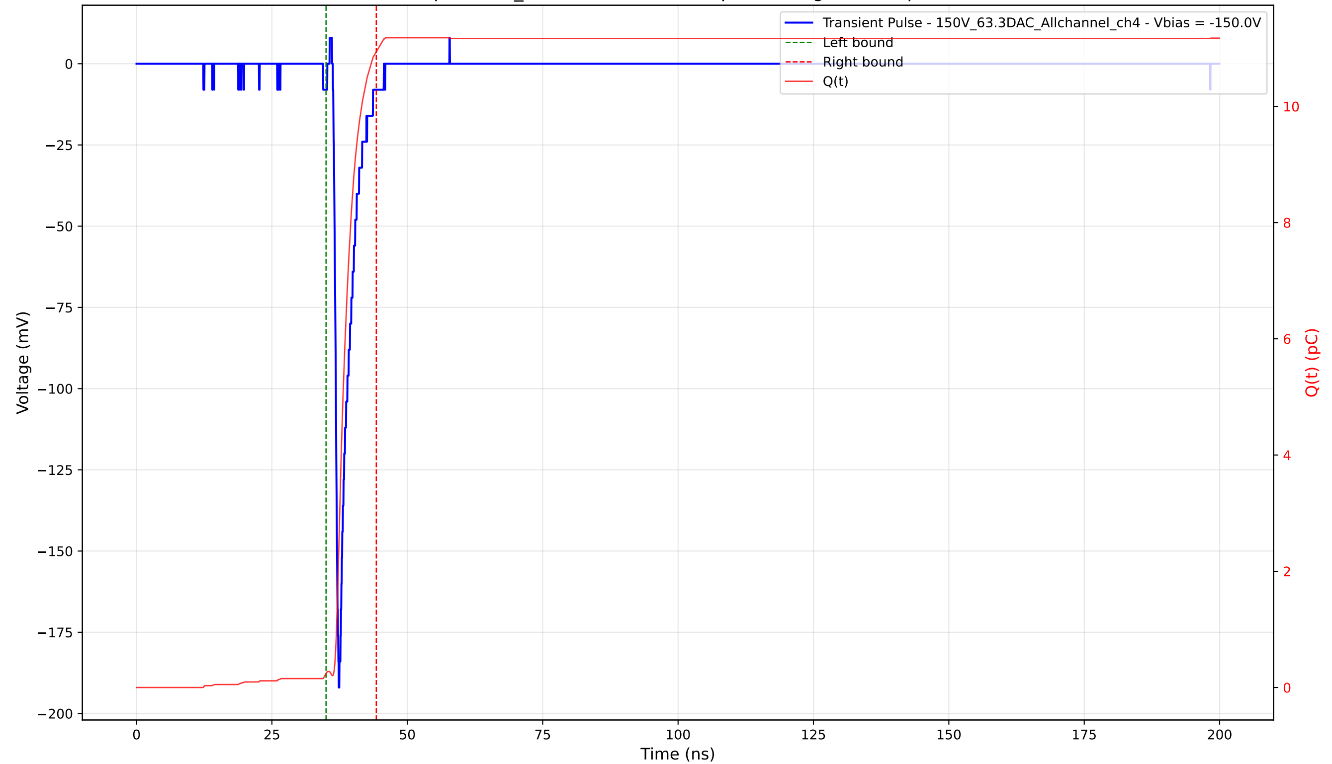
Transient Pulse - Sample: 1cm_42 - Position: 1325.0 \mu\text{m} - Charge: 10.70 pC - Rise Time: 0.82 ns
