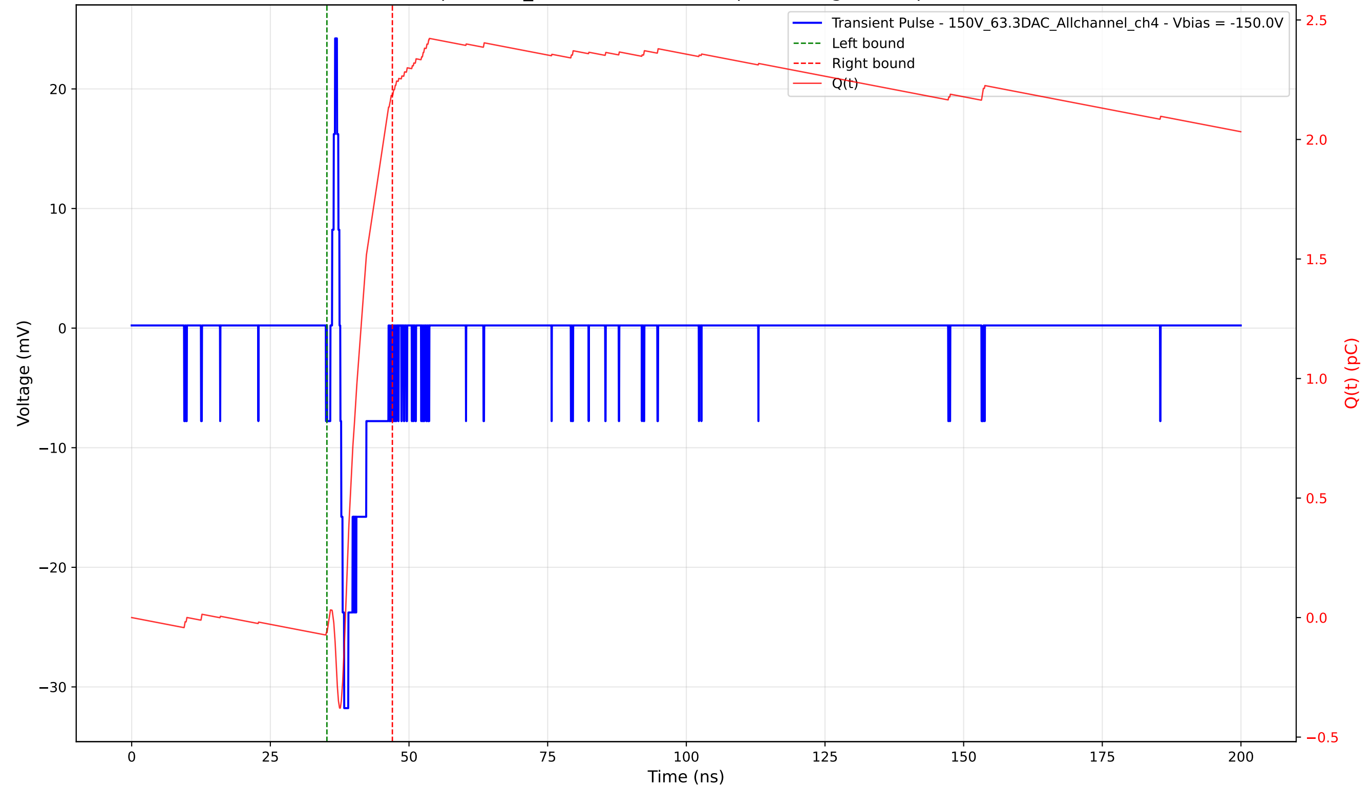
Transient Pulse - Sample: 1cm_42 - Position: 4615.0 \mu\text{m} - Charge: 2.24 pC - Rise Time: 0.70 ns
