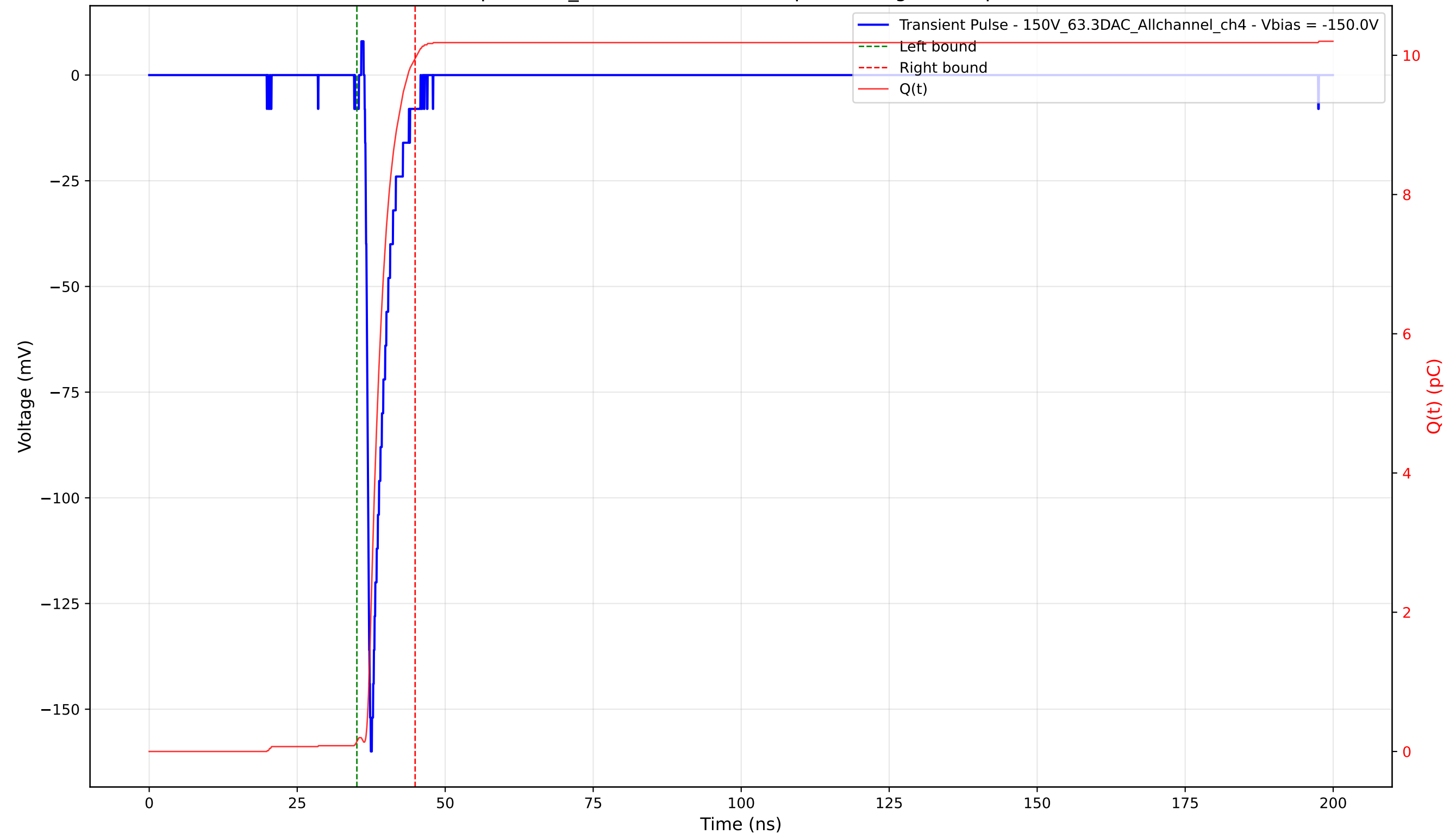
Transient Pulse - Sample: 1cm_42 - Position: 1180.0 \mu\text{m} - Charge: 9.81 pC - Rise Time: 0.72 ns
