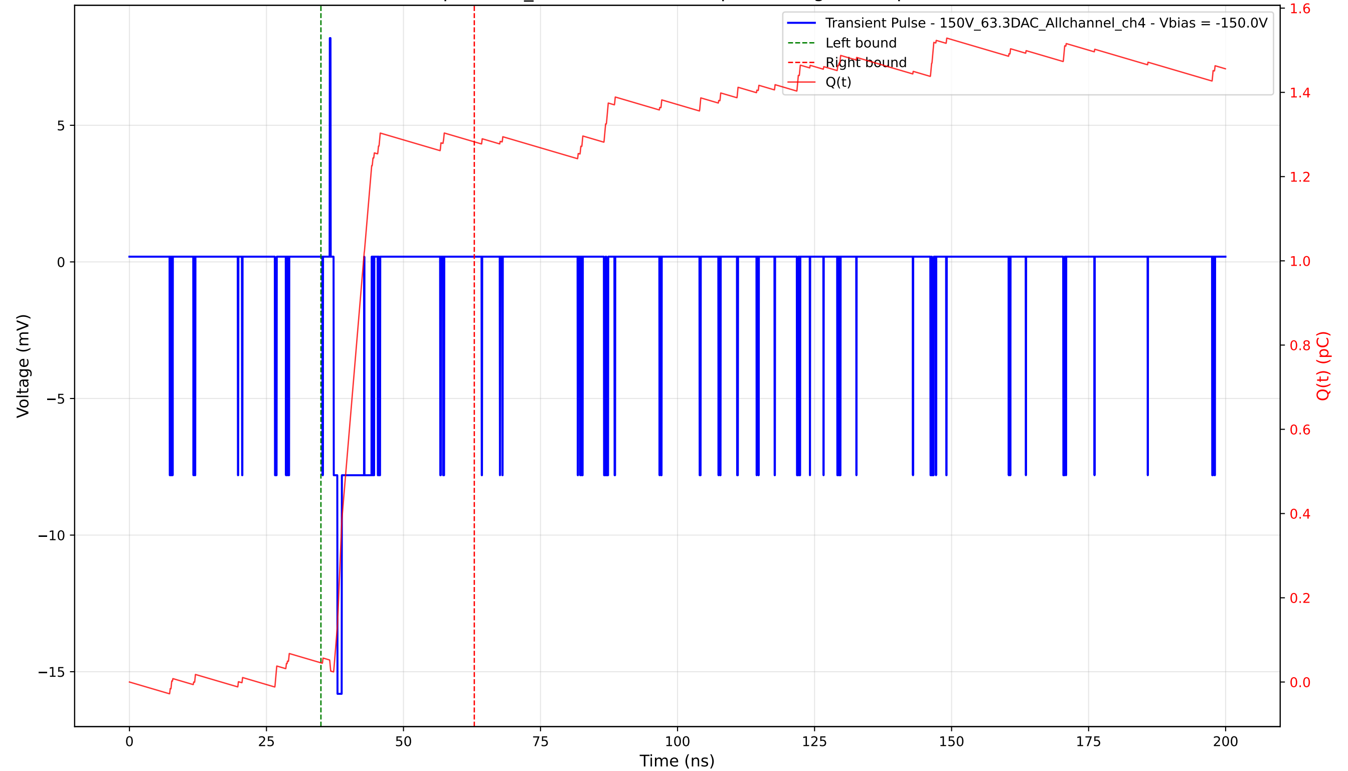
Transient Pulse - Sample: 1cm_42 - Position: 105.0 \mu\text{m} - Charge: 1.24 pC - Rise Time: 0.71 ns
