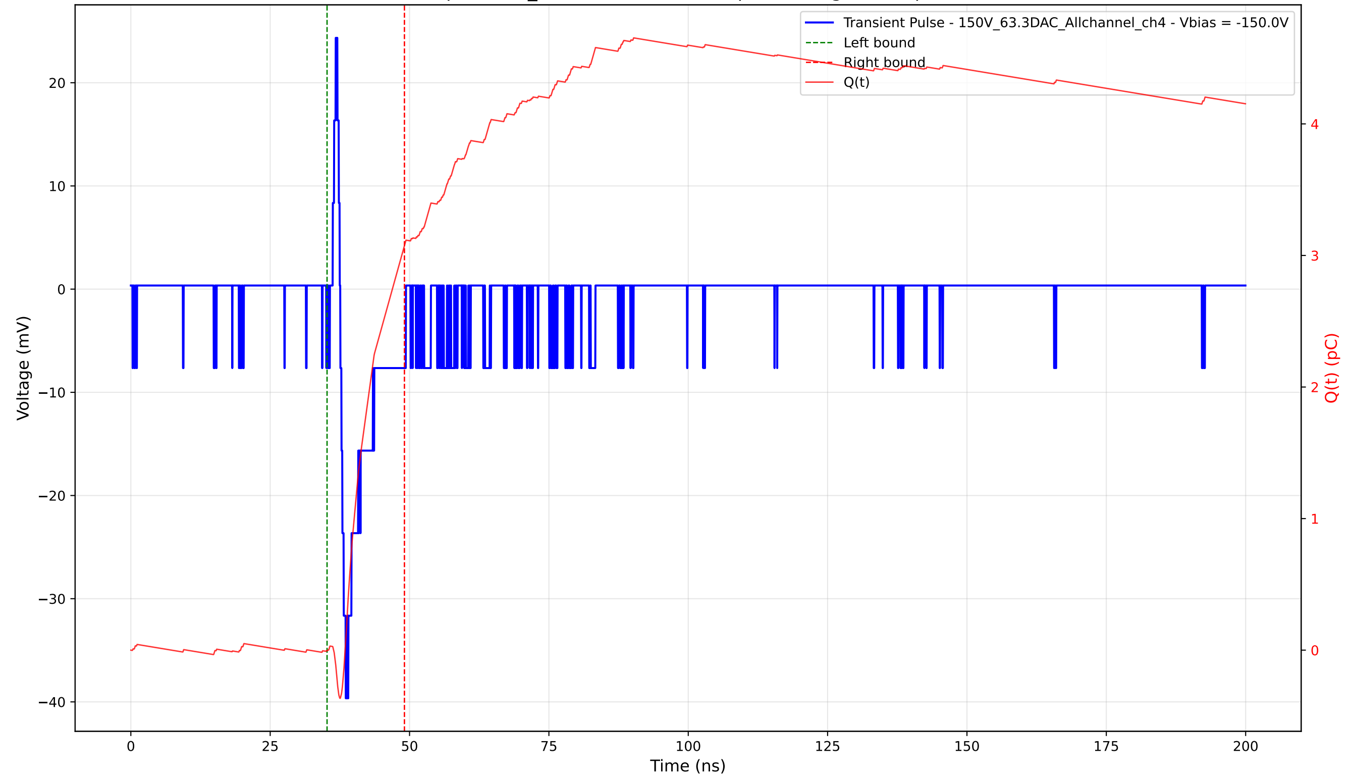
Transient Pulse - Sample: 1cm_42 - Position: 3660.0 \mu\text{m} - Charge: 3.08 pC - Rise Time: 0.98 ns
