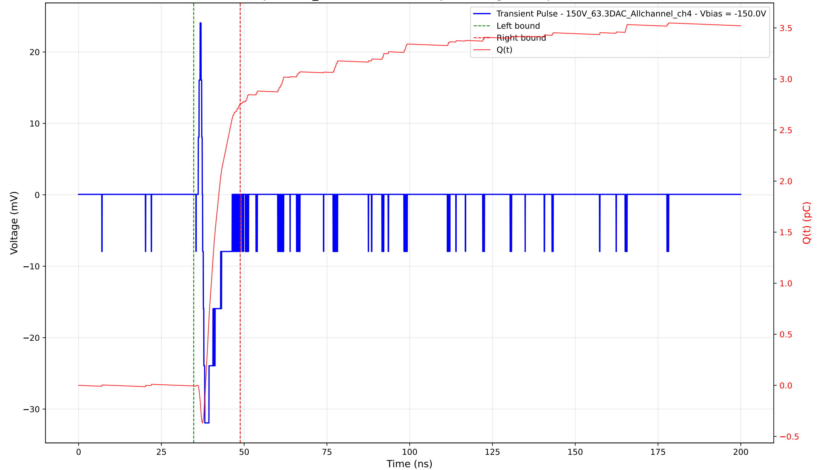
Transient Pulse - Sample: 1cm_42 - Position: 4770.0 \mu\text{m} - Charge: 2.76 pC - Rise Time: 0.66 ns
