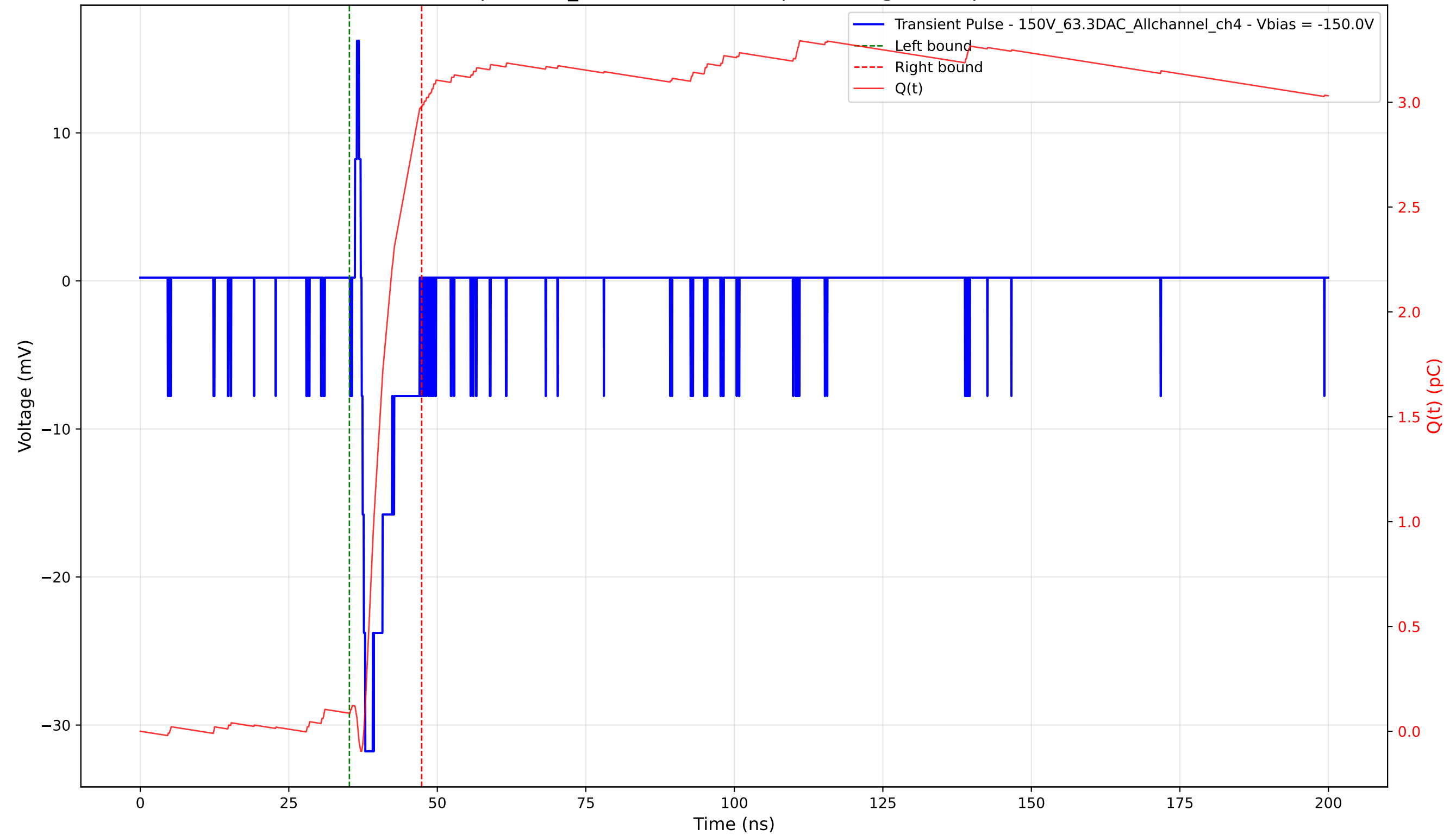
Transient Pulse - Sample: 1cm_42 - Position: 315.0 \mu\text{m} - Charge: 2.89 pC - Rise Time: 0.62 ns
