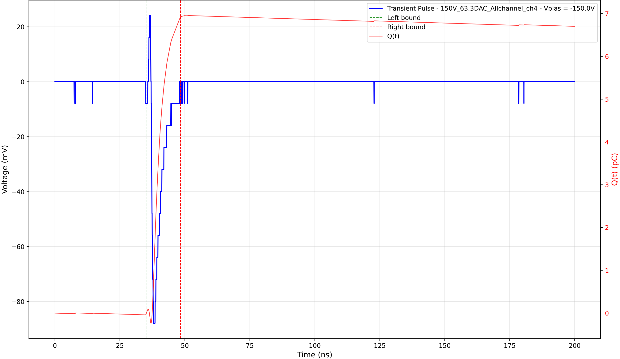
Transient Pulse - Sample: 1cm_42 - Position: 750.0 \mu\text{m} - Charge: 6.94 pC - Rise Time: 0.72 ns
