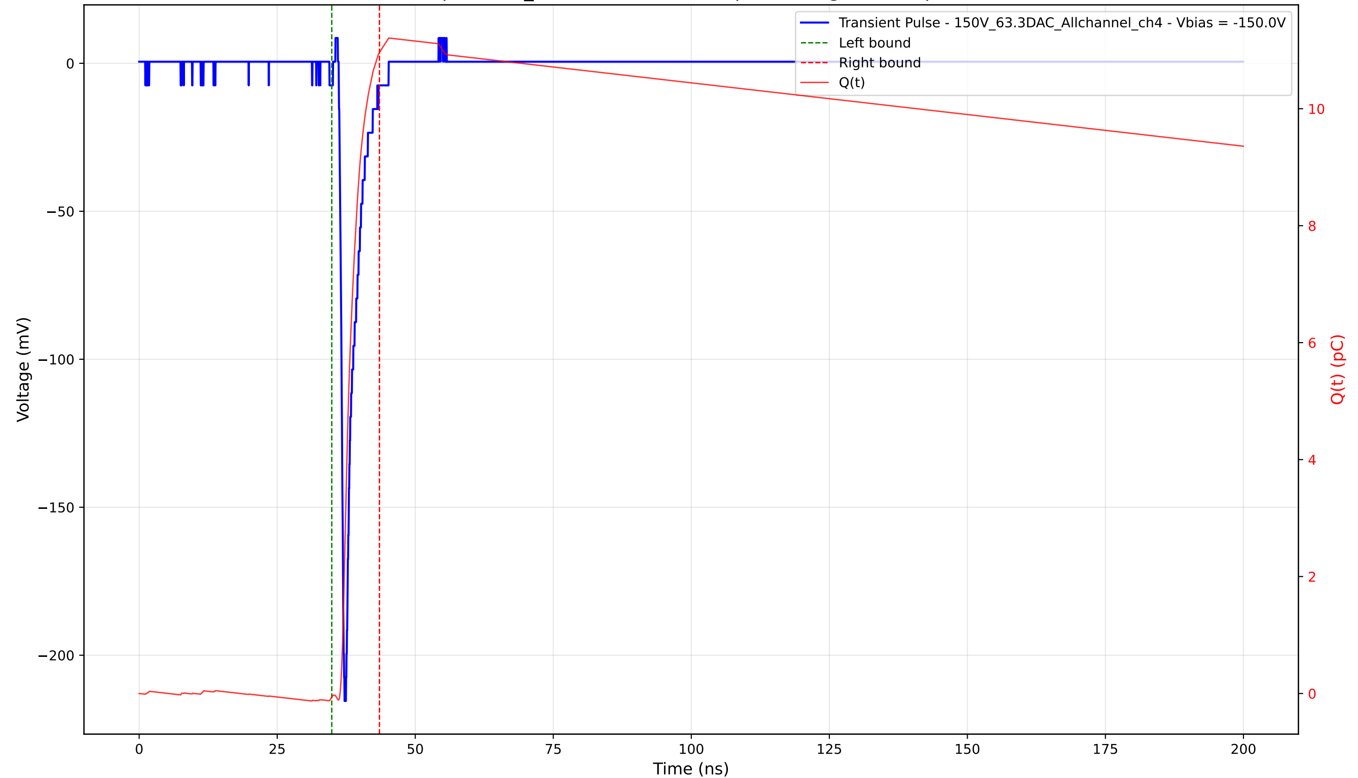
Transient Pulse - Sample: 1cm_42 - Position: 1430.0 \mu\text{m} - Charge: 11.02 pC - Rise Time: 0.77 ns
