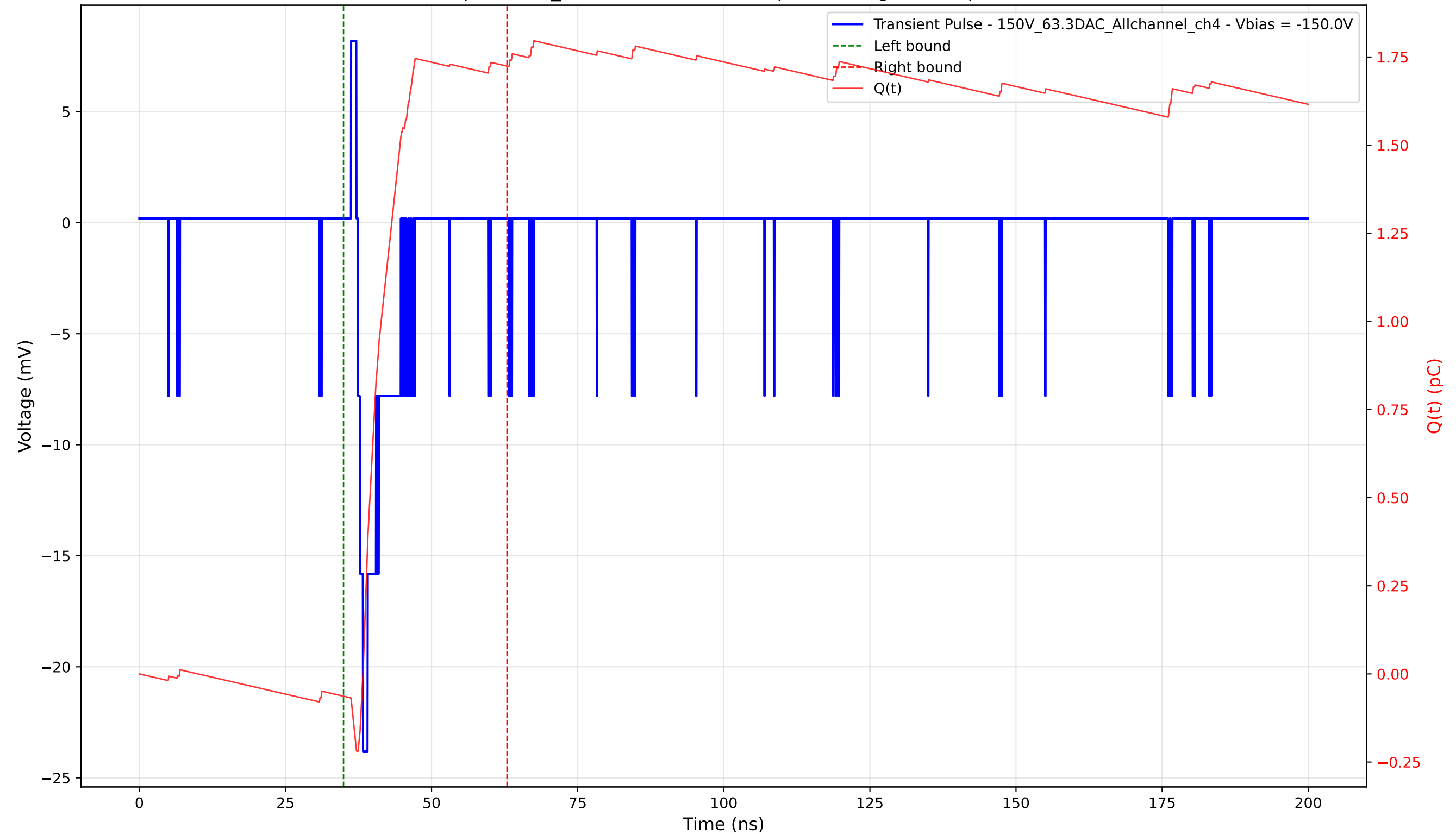
Transient Pulse - Sample: 1cm_42 - Position: 5005.0 \mu\text{m} - Charge: 1.79 pC - Rise Time: 0.87 ns
