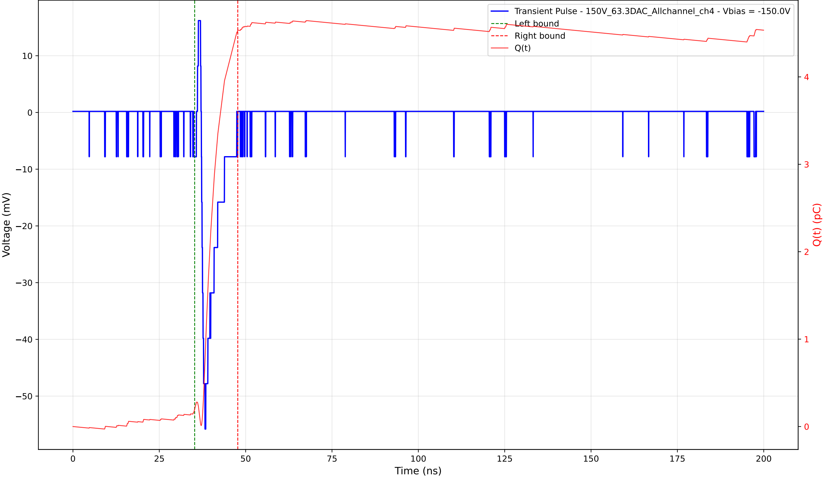
Transient Pulse - Sample: 1cm_42 - Position: 480.0 \mu\text{m} - Charge: 4.33 pC - Rise Time: 1.05 ns
