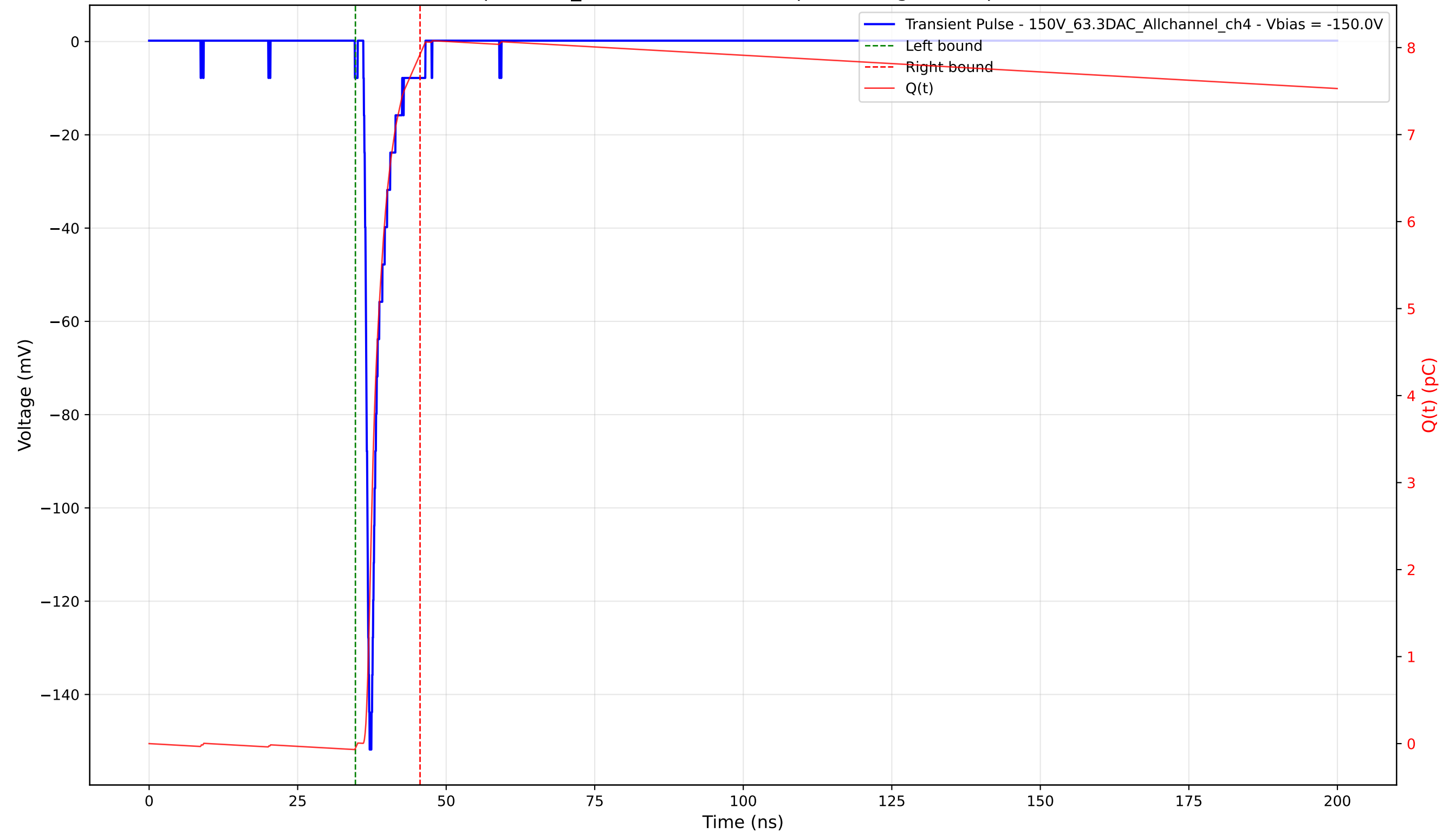
Transient Pulse - Sample: 1cm_42 - Position: 2685.0 \mu\text{m} - Charge: 7.98 pC - Rise Time: 0.88 ns
