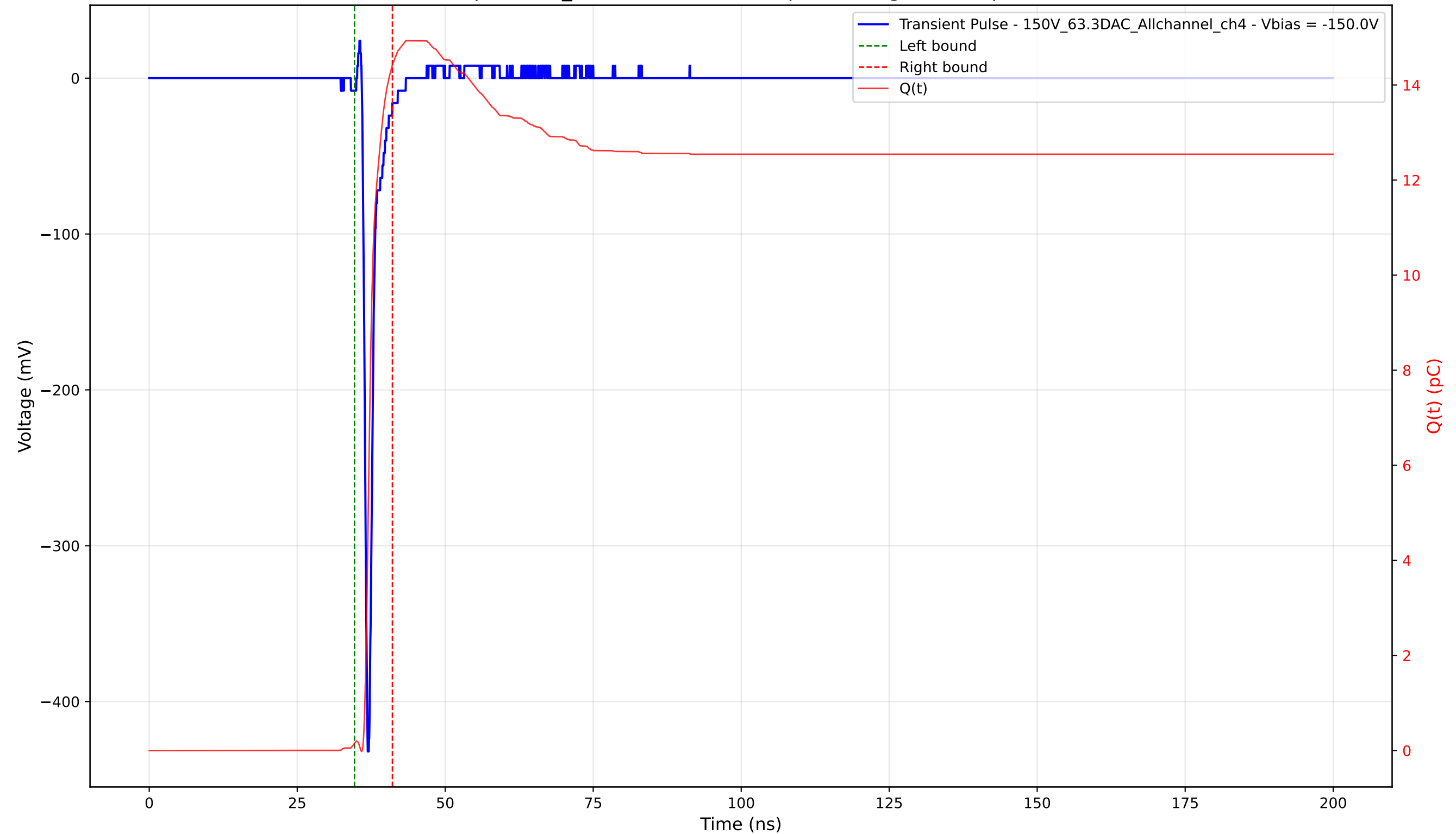
Transient Pulse - Sample: 1cm_42 - Position: 2345.0 \mu\text{m} - Charge: 14.28 pC - Rise Time: 0.70 ns
