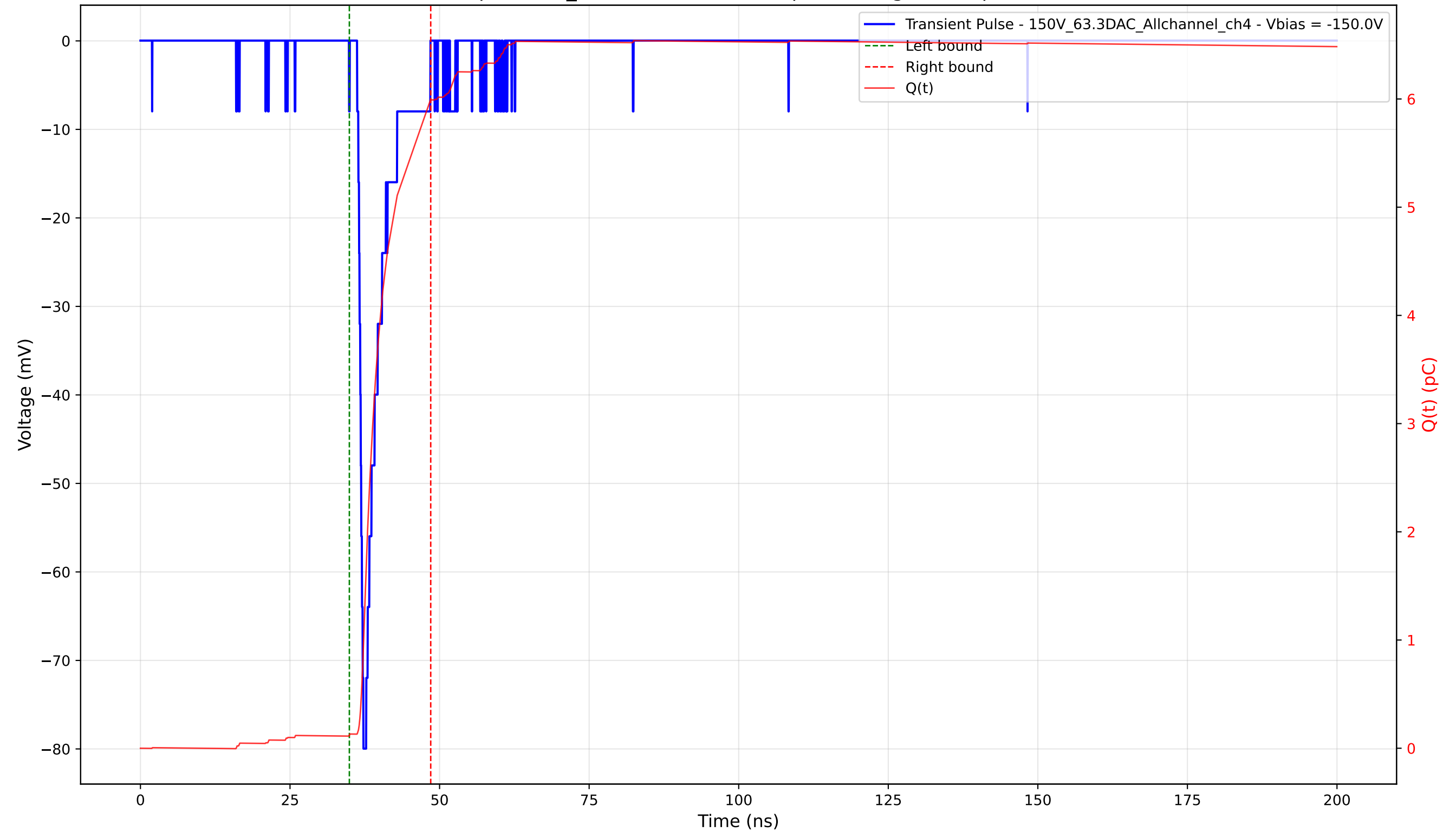
Transient Pulse - Sample: 1cm_42 - Position: 2960.0 \mu\text{m} - Charge: 5.87 pC - Rise Time: 0.88 ns
