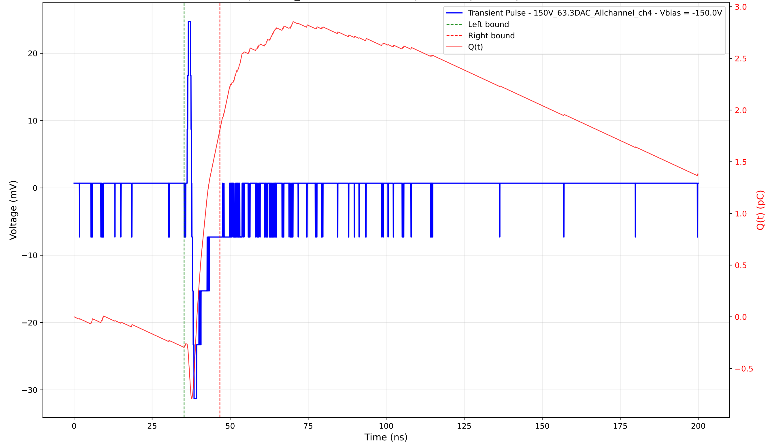
Transient Pulse - Sample: 1cm_42 - Position: 4155.0 \mu\text{m} - Charge: 2.11 pC - Rise Time: 0.71 ns
