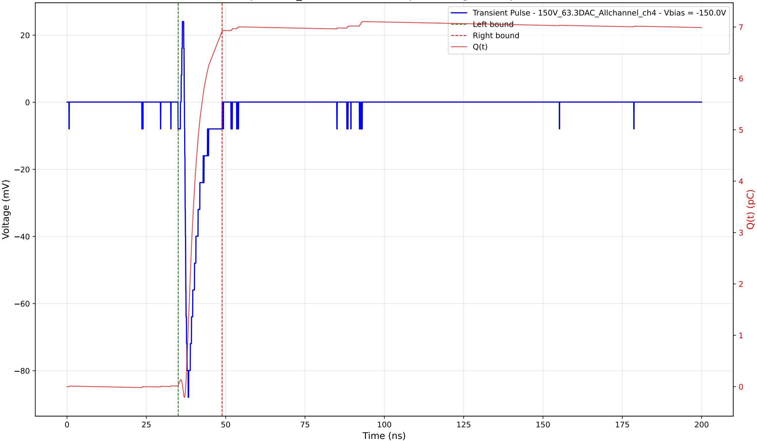
Transient Pulse - Sample: 1cm_42 - Position: 725.0 \mu\text{m} - Charge: 6.90 pC - Rise Time: 0.76 ns
