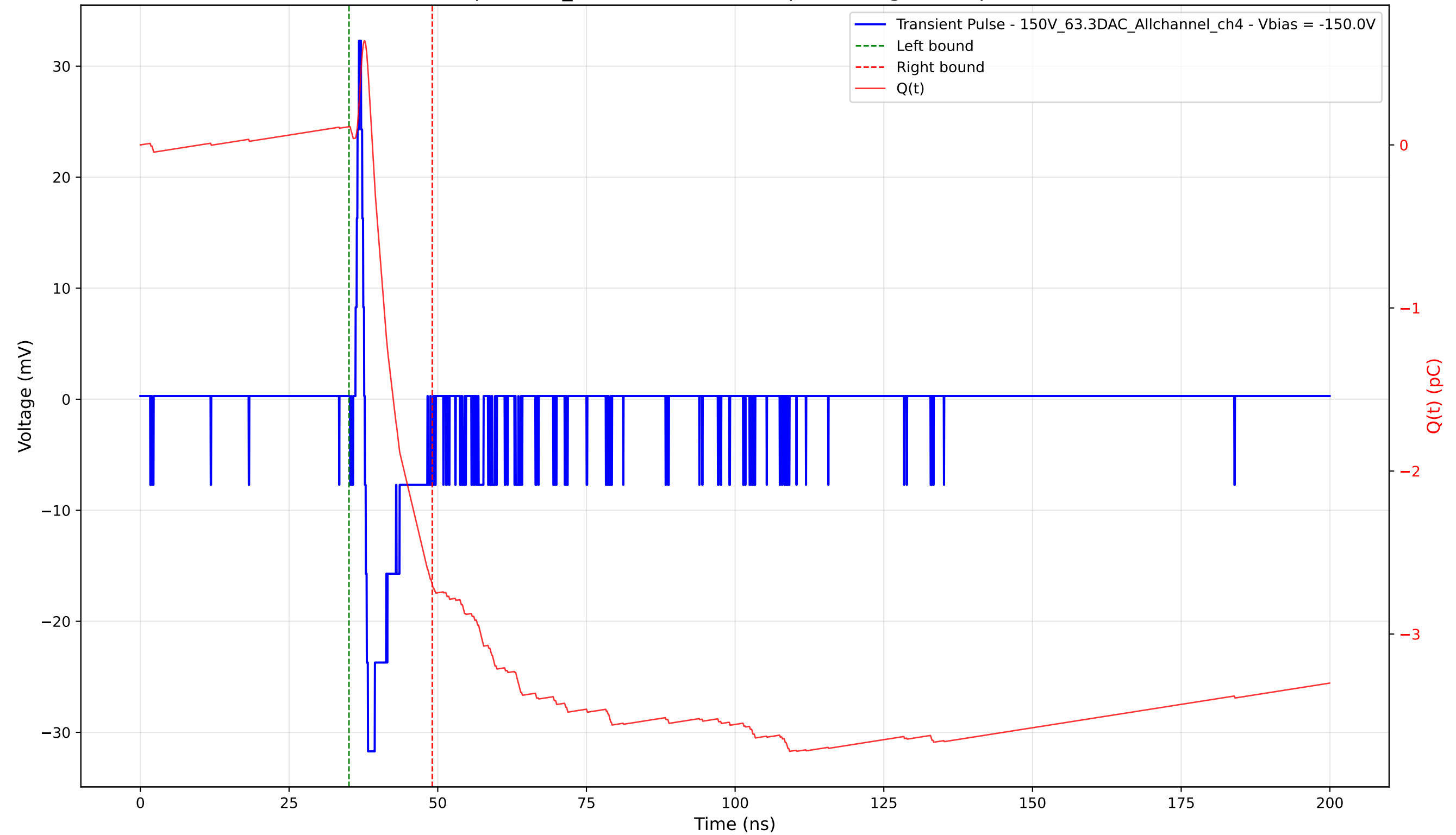
Transient Pulse - Sample: 1cm_42 - Position: 4315.0 \mu\text{m} - Charge: 2.81 pC - Rise Time: 0.59 ns
