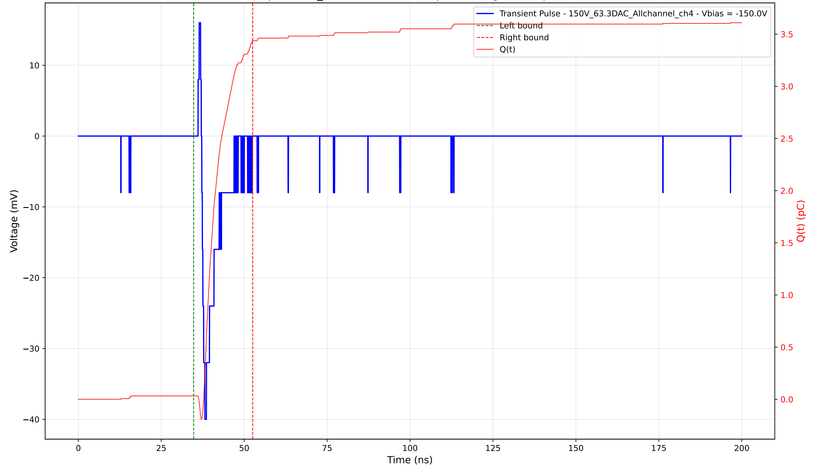
Transient Pulse - Sample: 1cm_42 - Position: 345.0 \mu\text{m} - Charge: 3.40 pC - Rise Time: 0.94 ns
