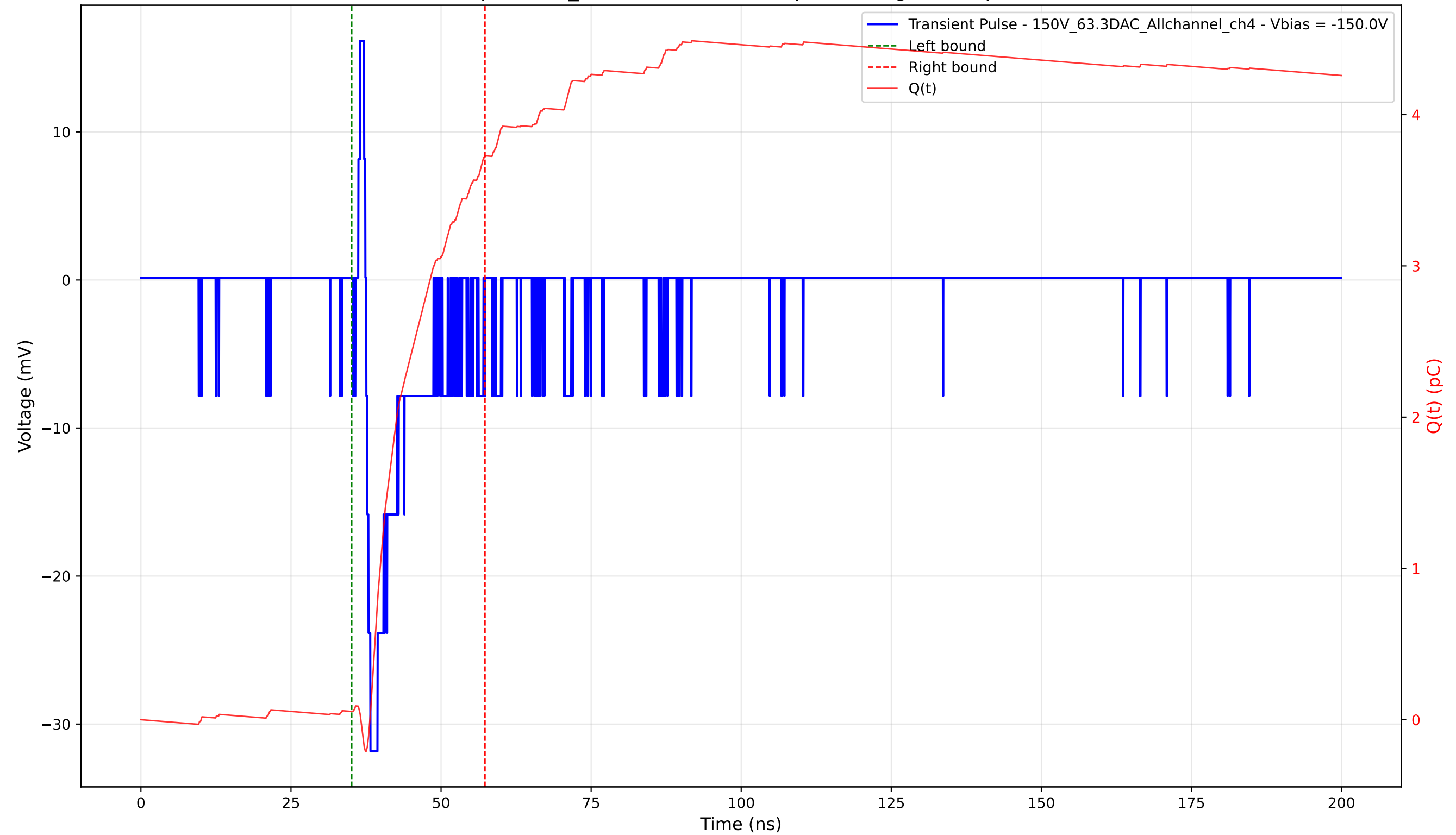
Transient Pulse - Sample: 1cm_42 - Position: 3590.0 \mu\text{m} - Charge: 3.67 pC - Rise Time: 0.70 ns
