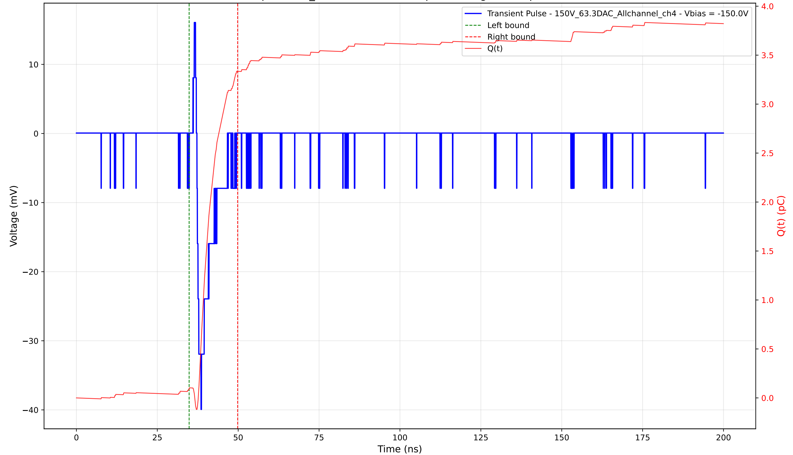
Transient Pulse - Sample: 1cm_42 - Position: 340.0 \mu\text{m} - Charge: 3.24 pC - Rise Time: 1.26 ns
