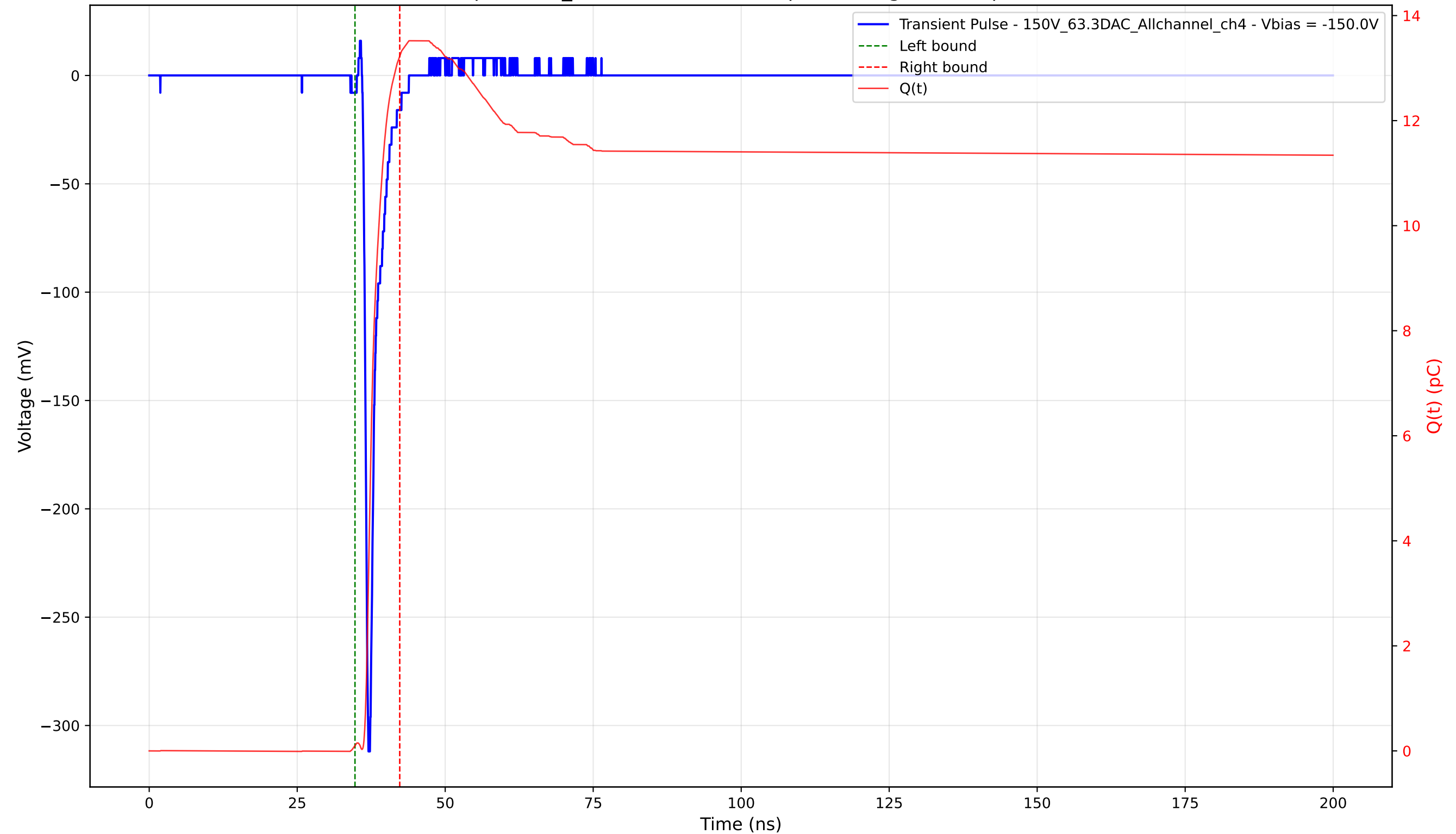
Transient Pulse - Sample: 1cm_42 - Position: 1555.0 \mu\text{m} - Charge: 13.12 pC - Rise Time: 0.73 ns
