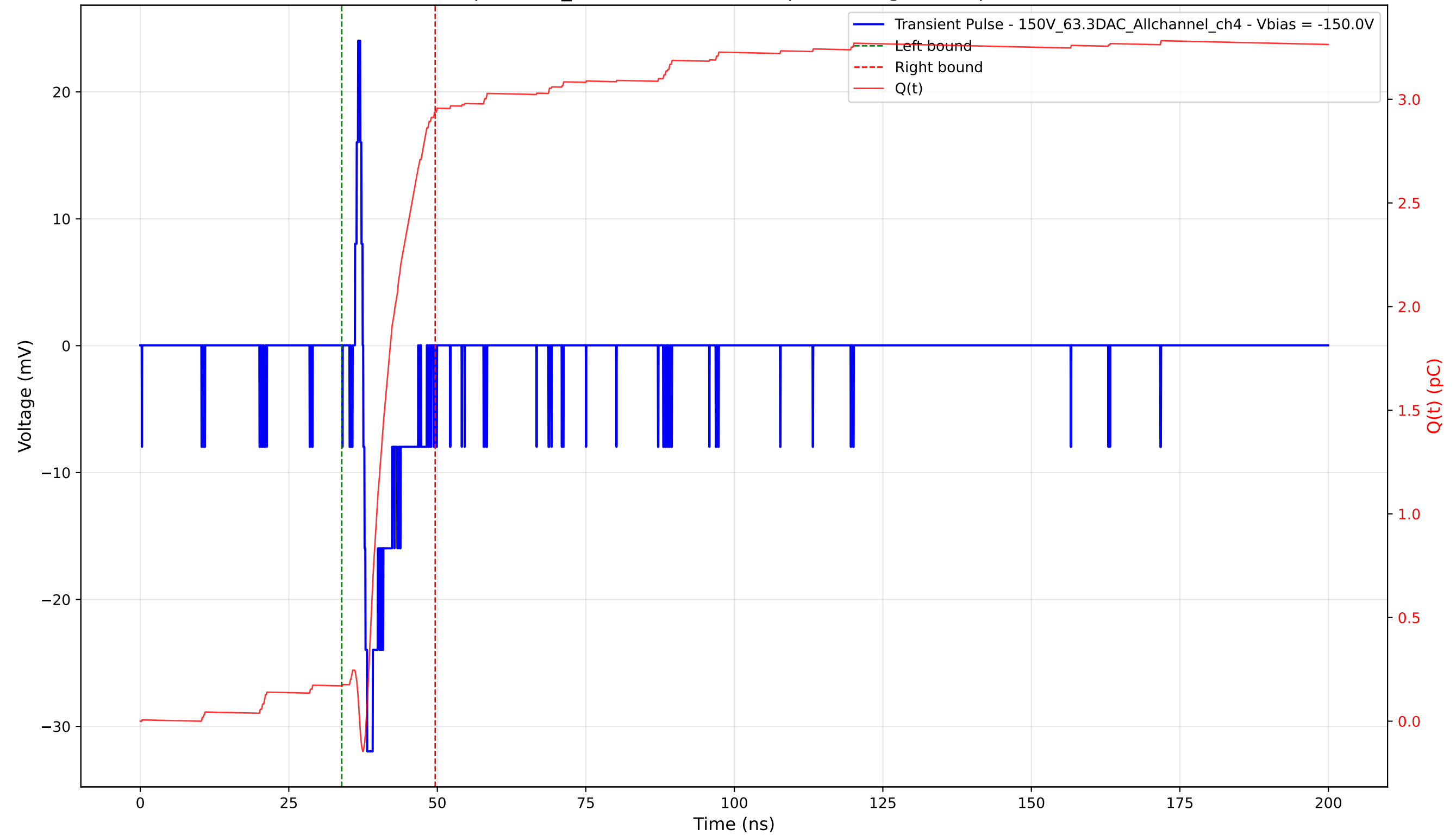
Transient Pulse - Sample: 1cm_42 - Position: 4695.0 \mu\text{m} - Charge: 2.77 pC - Rise Time: 0.66 ns
