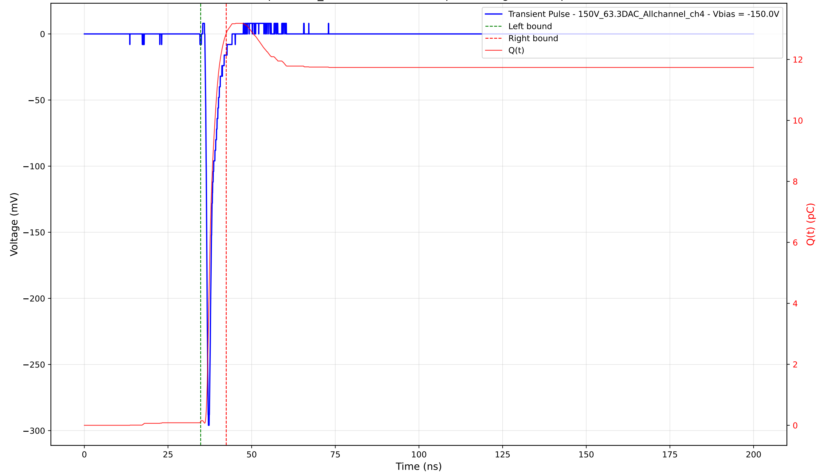
Transient Pulse - Sample: 1cm_42 - Position: 1540.0 \mu\text{m} - Charge: 12.73 pC - Rise Time: 0.74 ns
