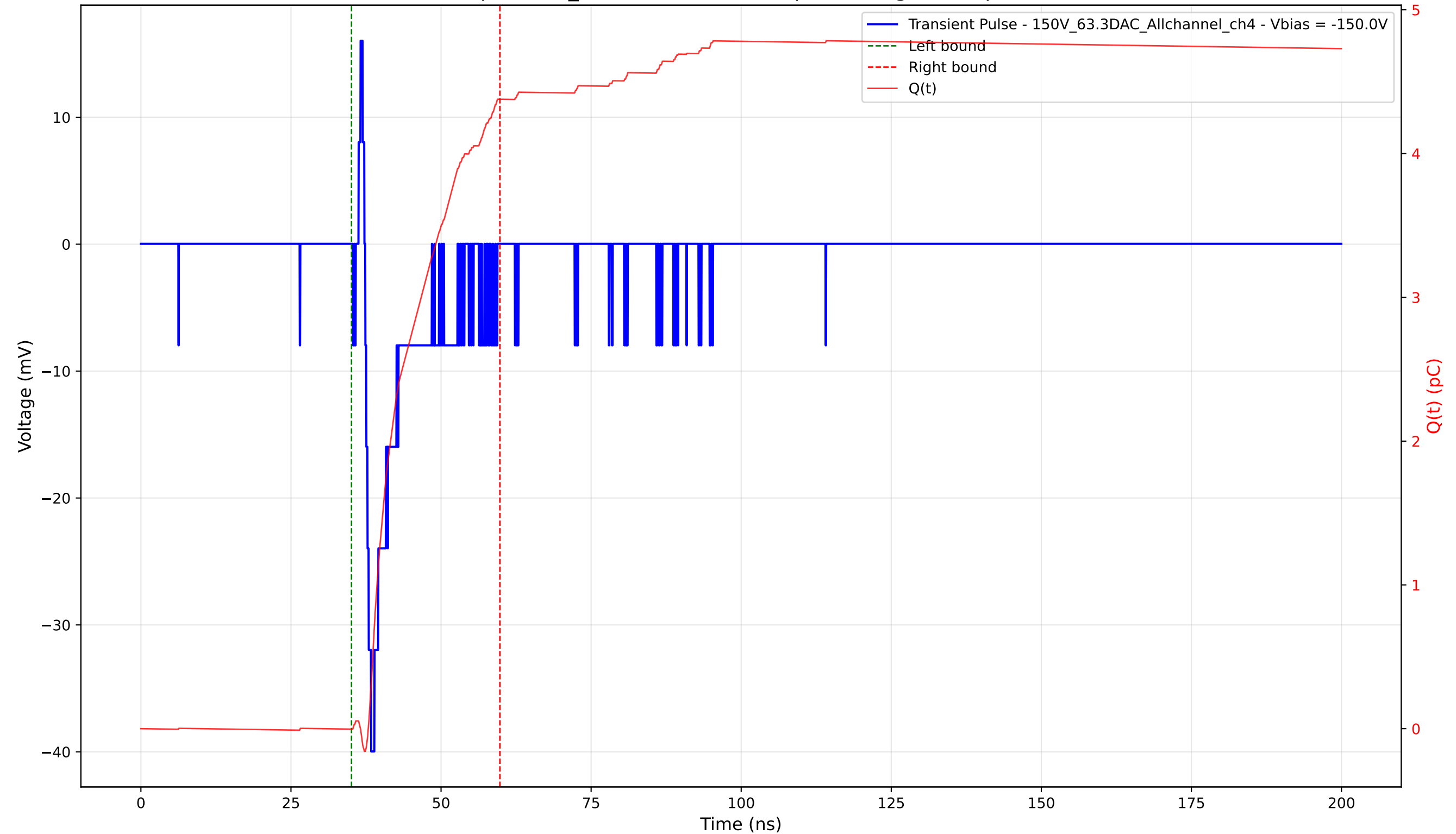
Transient Pulse - Sample: 1cm_42 - Position: 3495.0 \mu\text{m} - Charge: 4.38 pC - Rise Time: 0.98 ns
