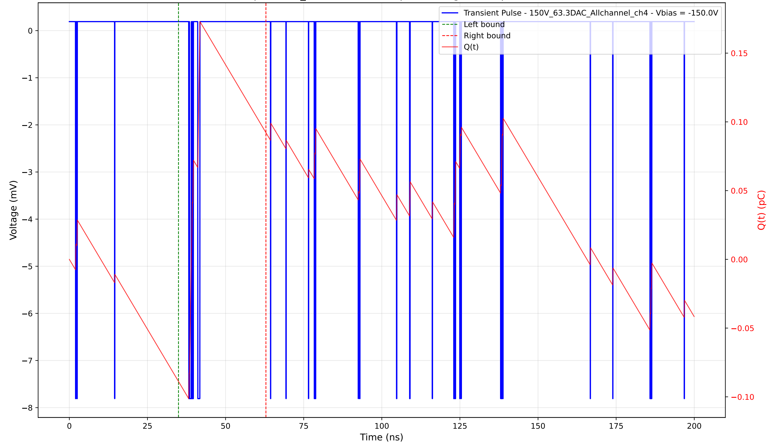
Transient Pulse - Sample: 1cm_42 - Position: 0.0 \mu\text{m} - Charge: 0.18 pC - Rise Time: 0.04 ns
