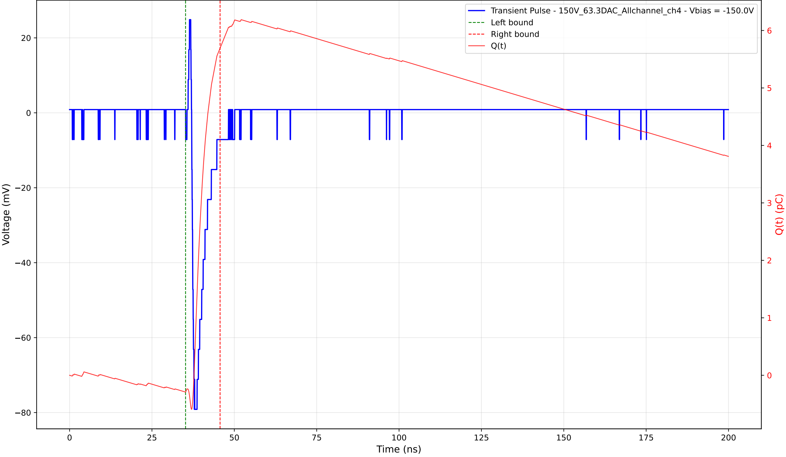
Transient Pulse - Sample: 1cm_42 - Position: 695.0 \mu\text{m} - Charge: 5.99 pC - Rise Time: 0.80 ns
