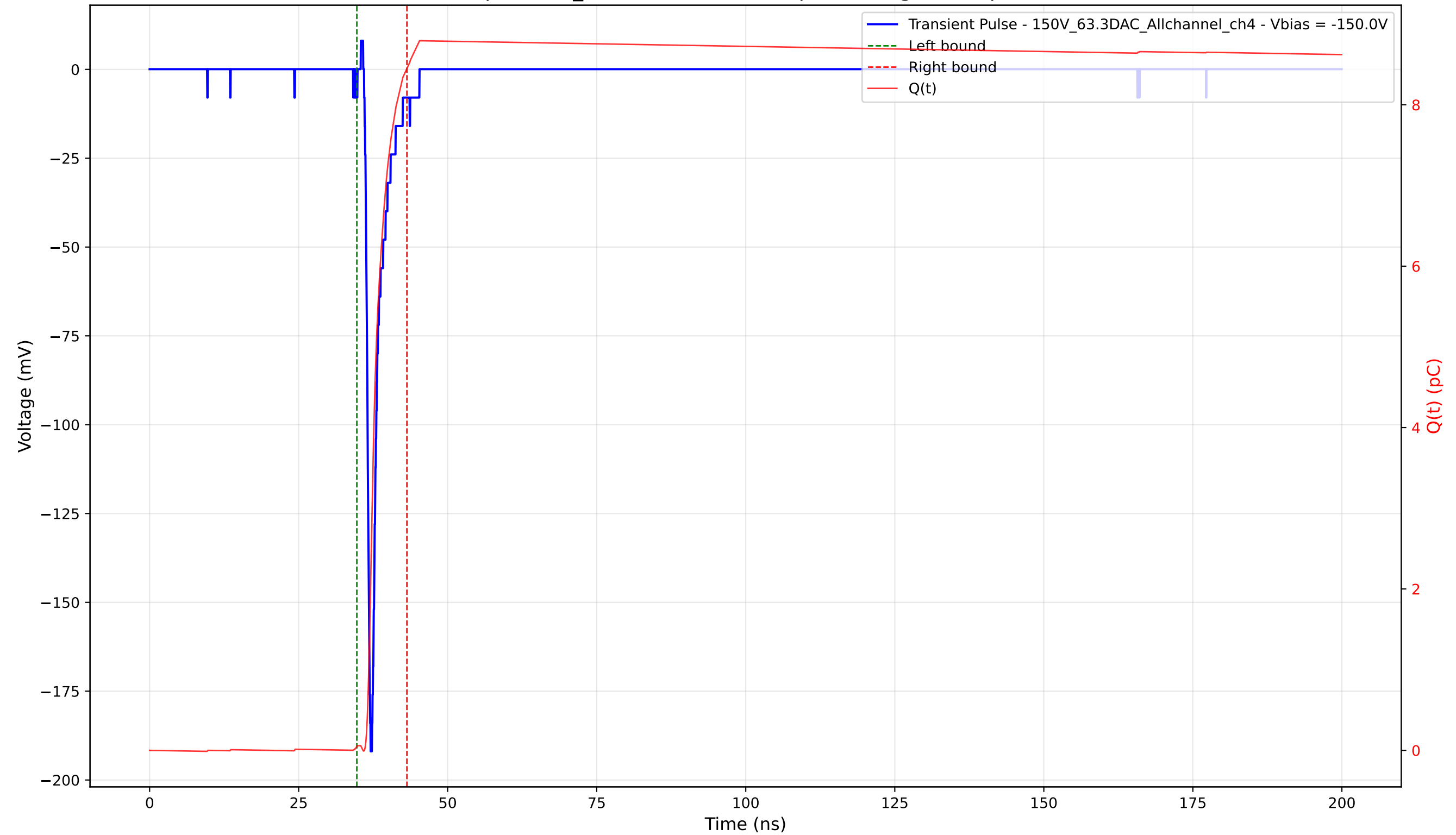
Transient Pulse - Sample: 1cm_42 - Position: 2585.0 \mu\text{m} - Charge: 8.40 pC - Rise Time: 0.78 ns
