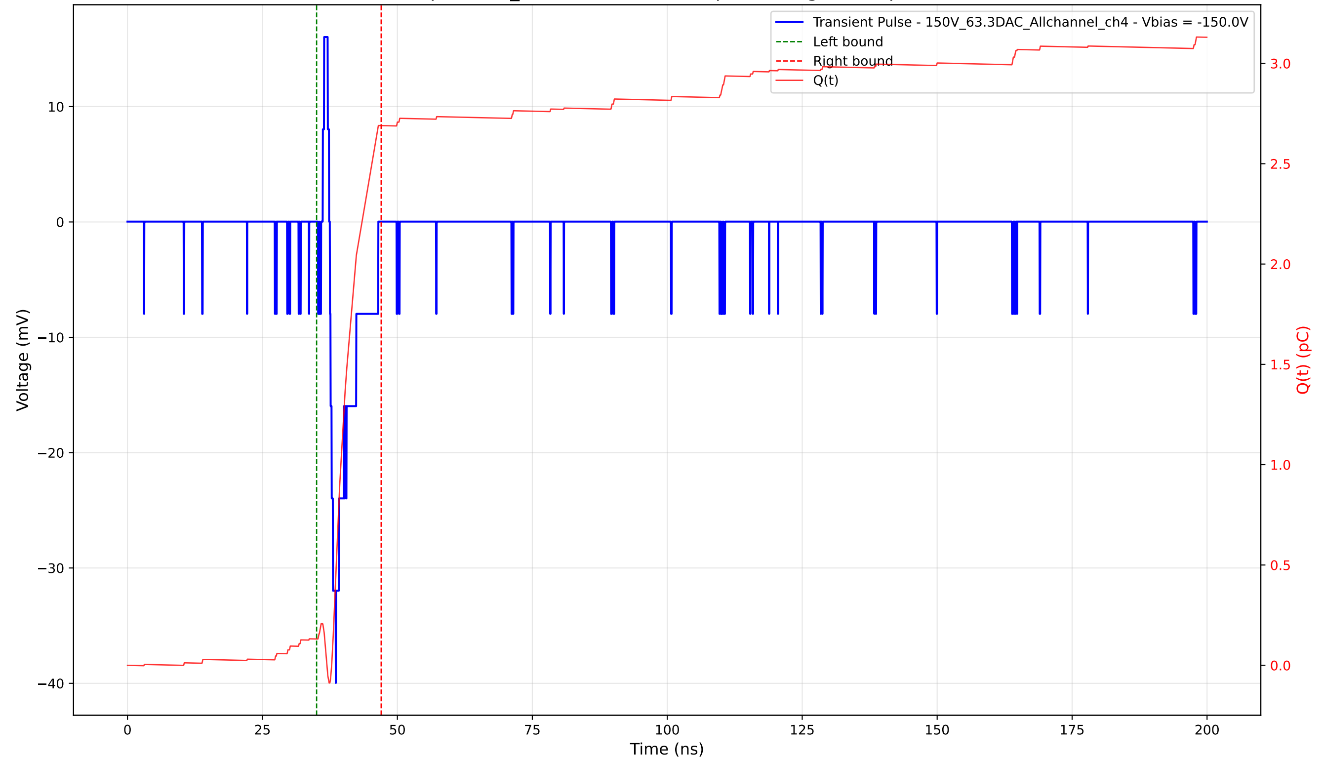
Transient Pulse - Sample: 1cm_42 - Position: 4865.0 \mu\text{m} - Charge: 2.56 pC - Rise Time: 1.10 ns
