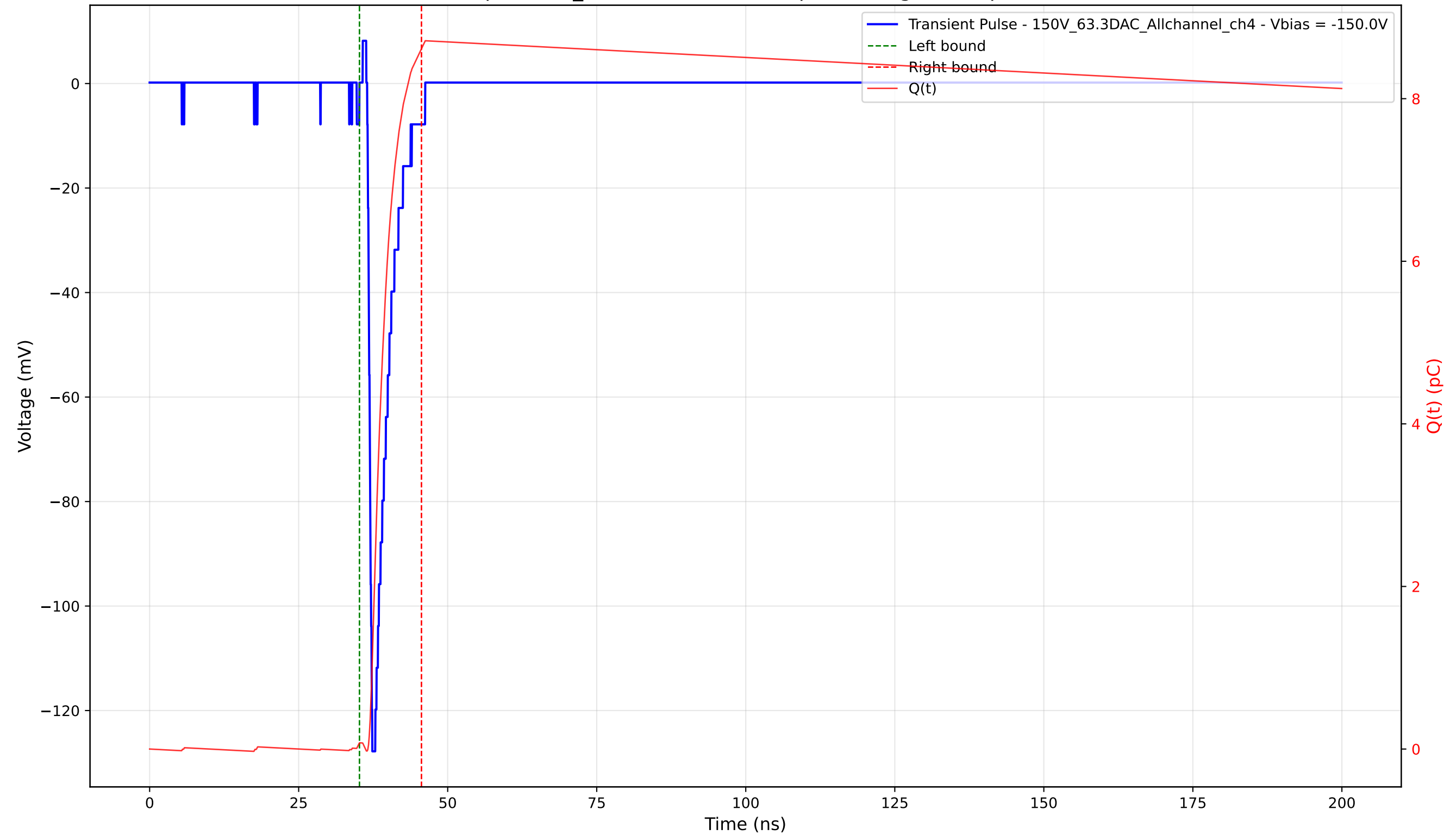
Transient Pulse - Sample: 1cm_42 - Position: 1120.0 \mu\text{m} - Charge: 8.54 pC - Rise Time: 0.70 ns
