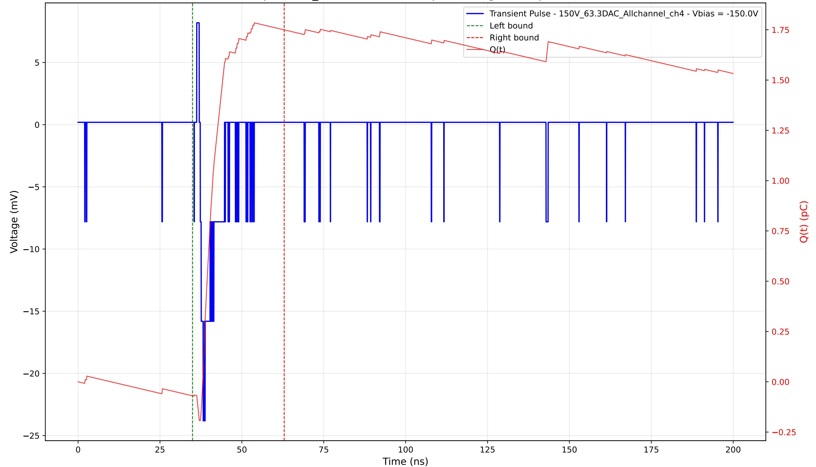
Transient Pulse - Sample: 1cm_42 - Position: 165.0 \mu\text{m} - Charge: 1.82 pC - Rise Time: 0.91 ns
