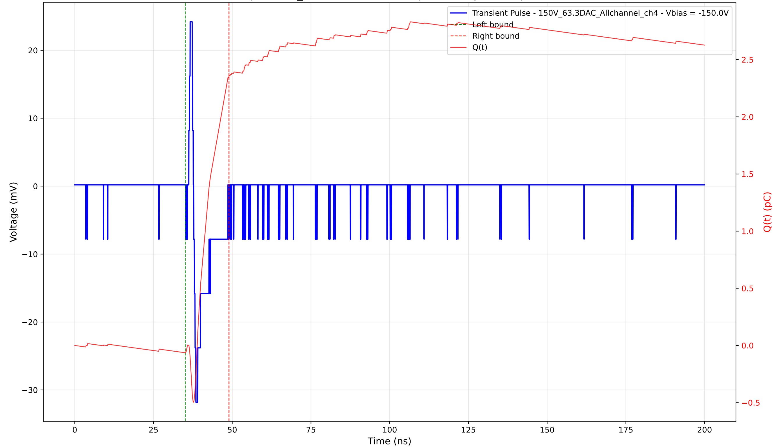
Transient Pulse - Sample: 1cm_42 - Position: 4105.0 \mu\text{m} - Charge: 2.42 pC - Rise Time: 0.70 ns
