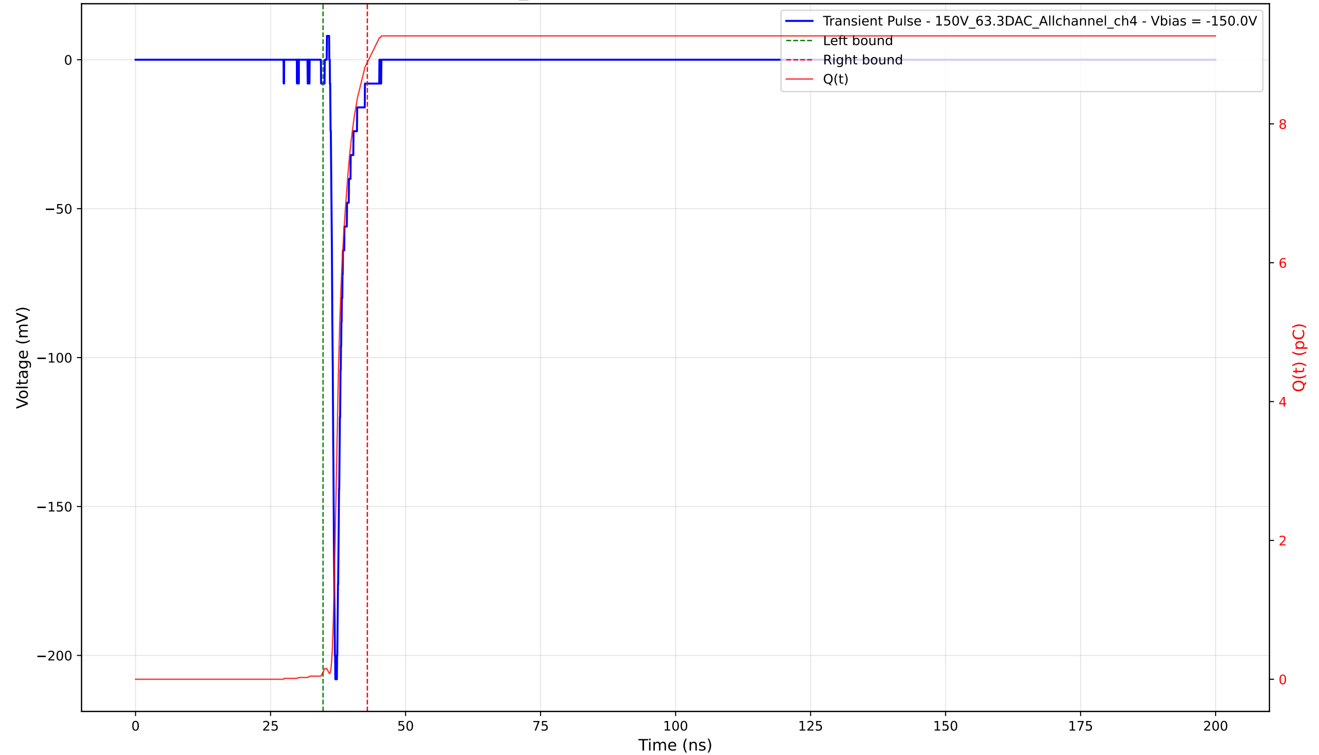
Transient Pulse - Sample: 1cm_42 - Position: 2550.0 \mu\text{m} - Charge: 8.78 pC - Rise Time: 0.75 ns
