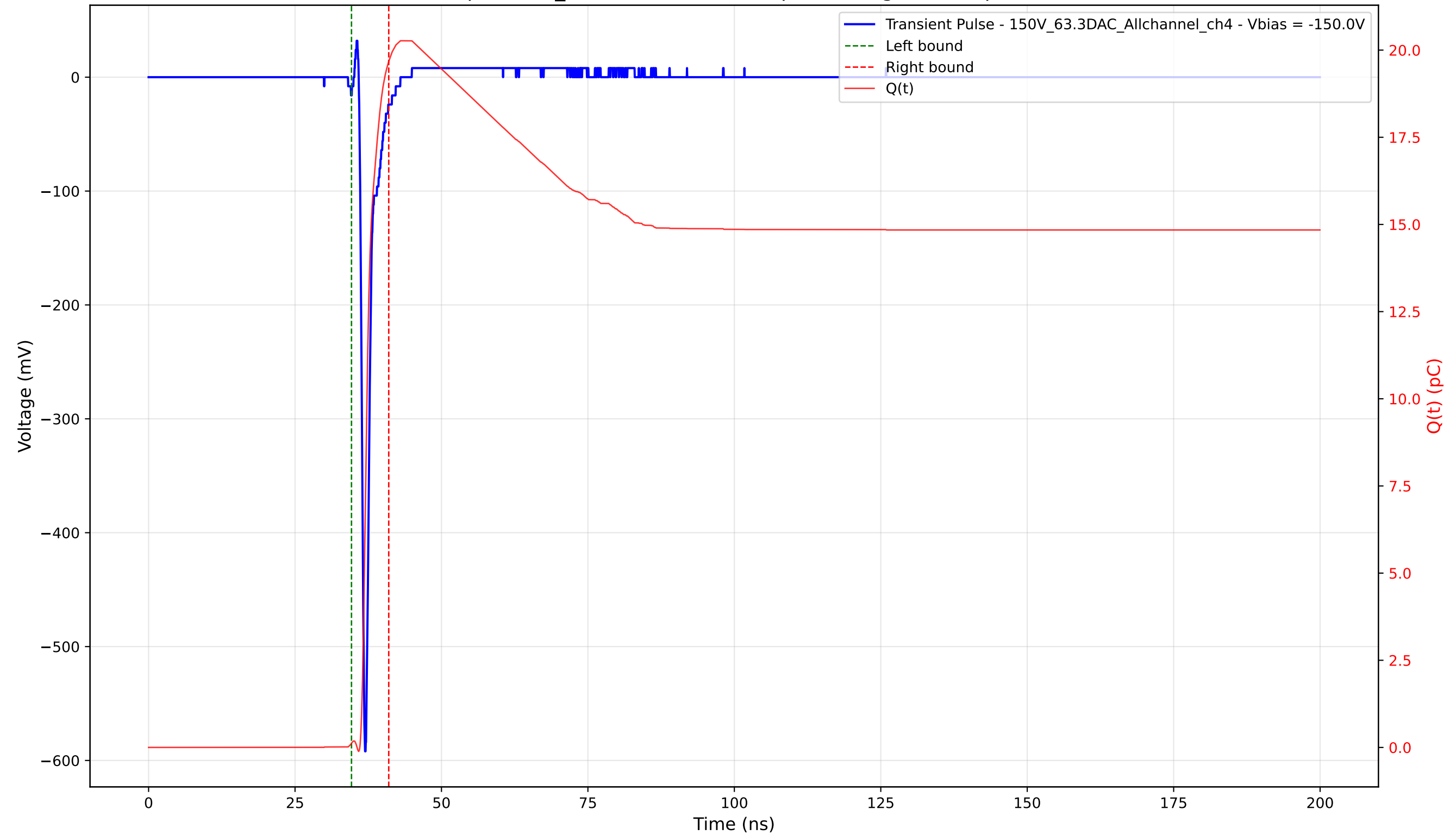
Transient Pulse - Sample: 1cm_42 - Position: 1810.0 \mu\text{m} - Charge: 19.56 pC - Rise Time: 0.71 ns
