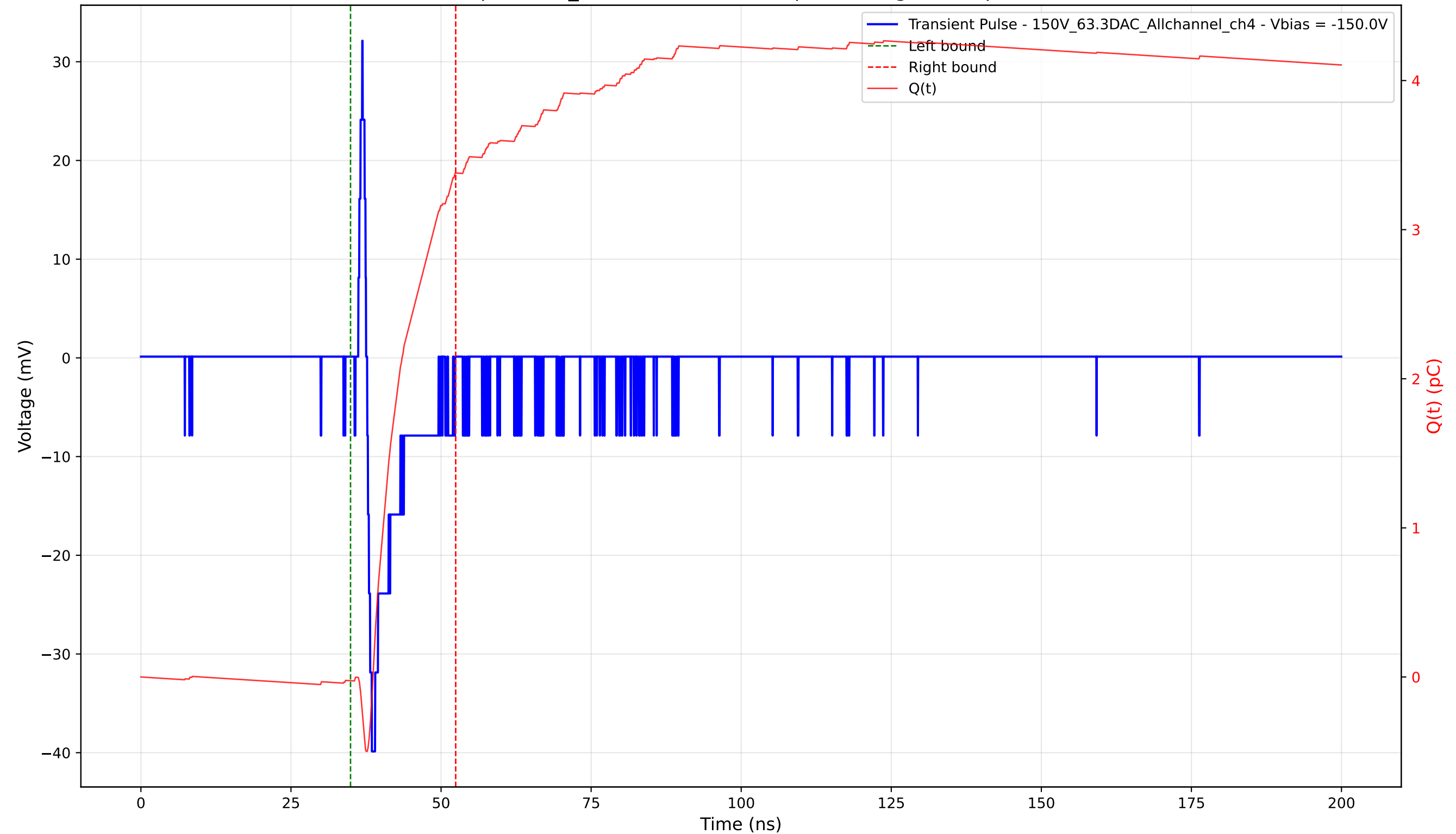
Transient Pulse - Sample: 1cm_42 - Position: 3775.0 \mu\text{m} - Charge: 3.40 pC - Rise Time: 0.78 ns
