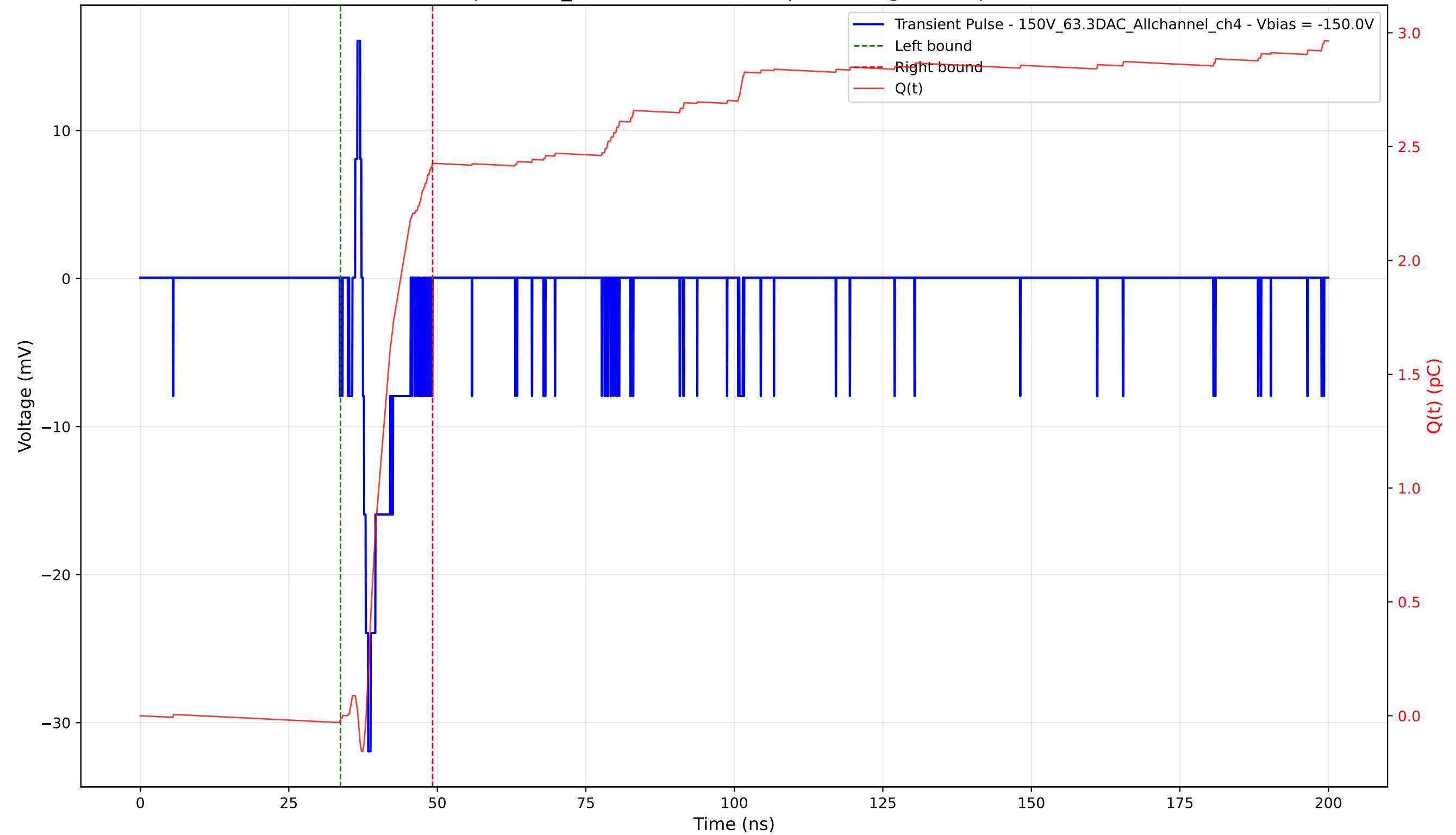
Transient Pulse - Sample: 1cm_42 - Position: 4930.0 \mu\text{m} - Charge: 2.44 pC - Rise Time: 0.90 ns
