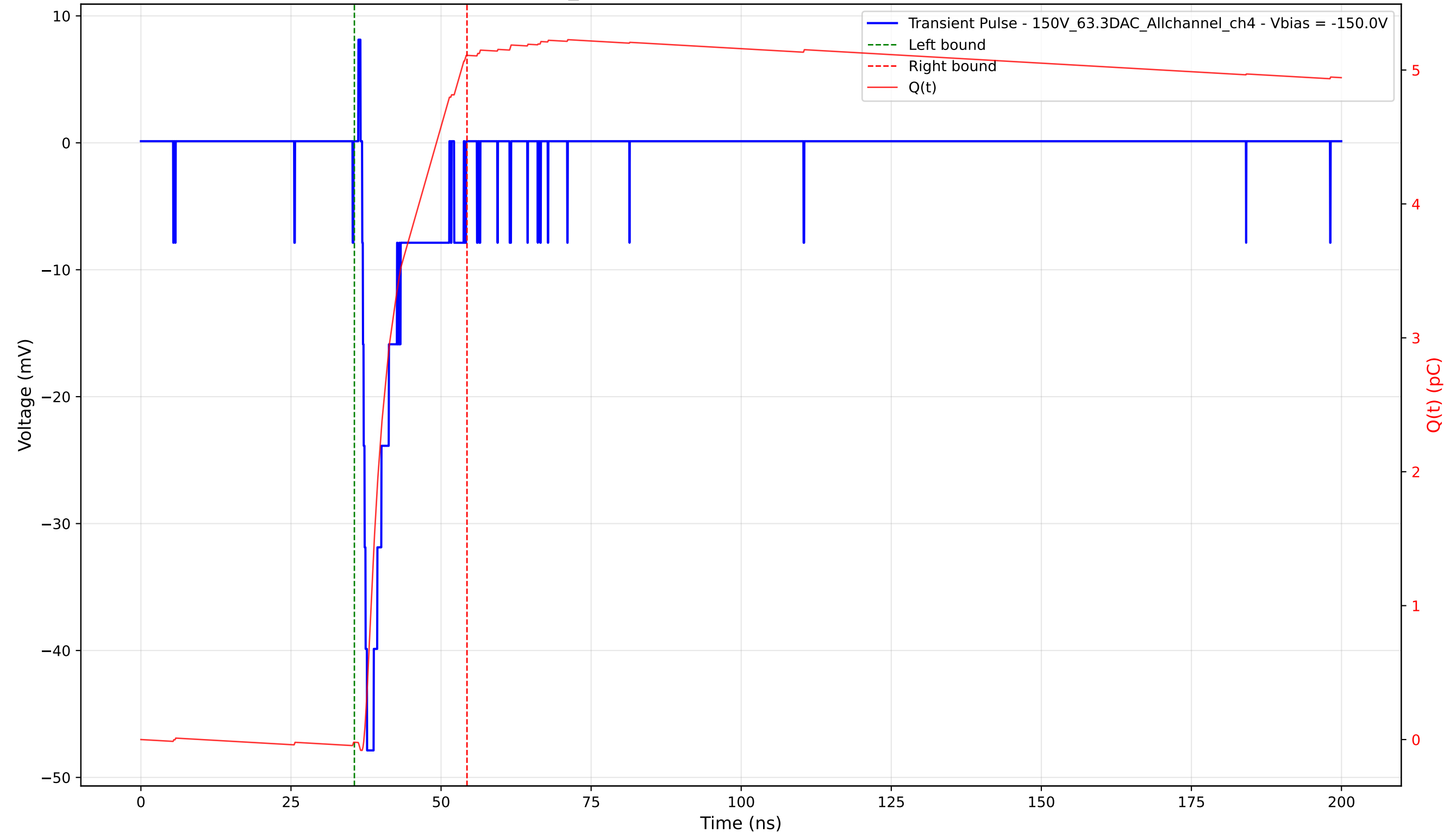
Transient Pulse - Sample: 1cm_42 - Position: 3165.0 \mu\text{m} - Charge: 5.13 pC - Rise Time: 0.82 ns
