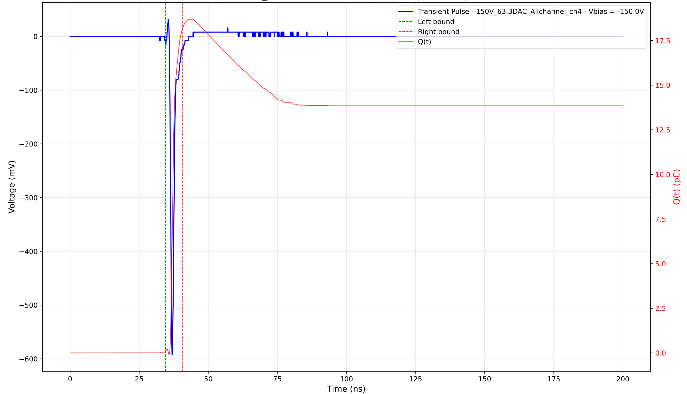
Transient Pulse - Sample: 1cm_42 - Position: 1985.0 \mu\text{m} - Charge: 17.99 pC - Rise Time: 0.71 ns
