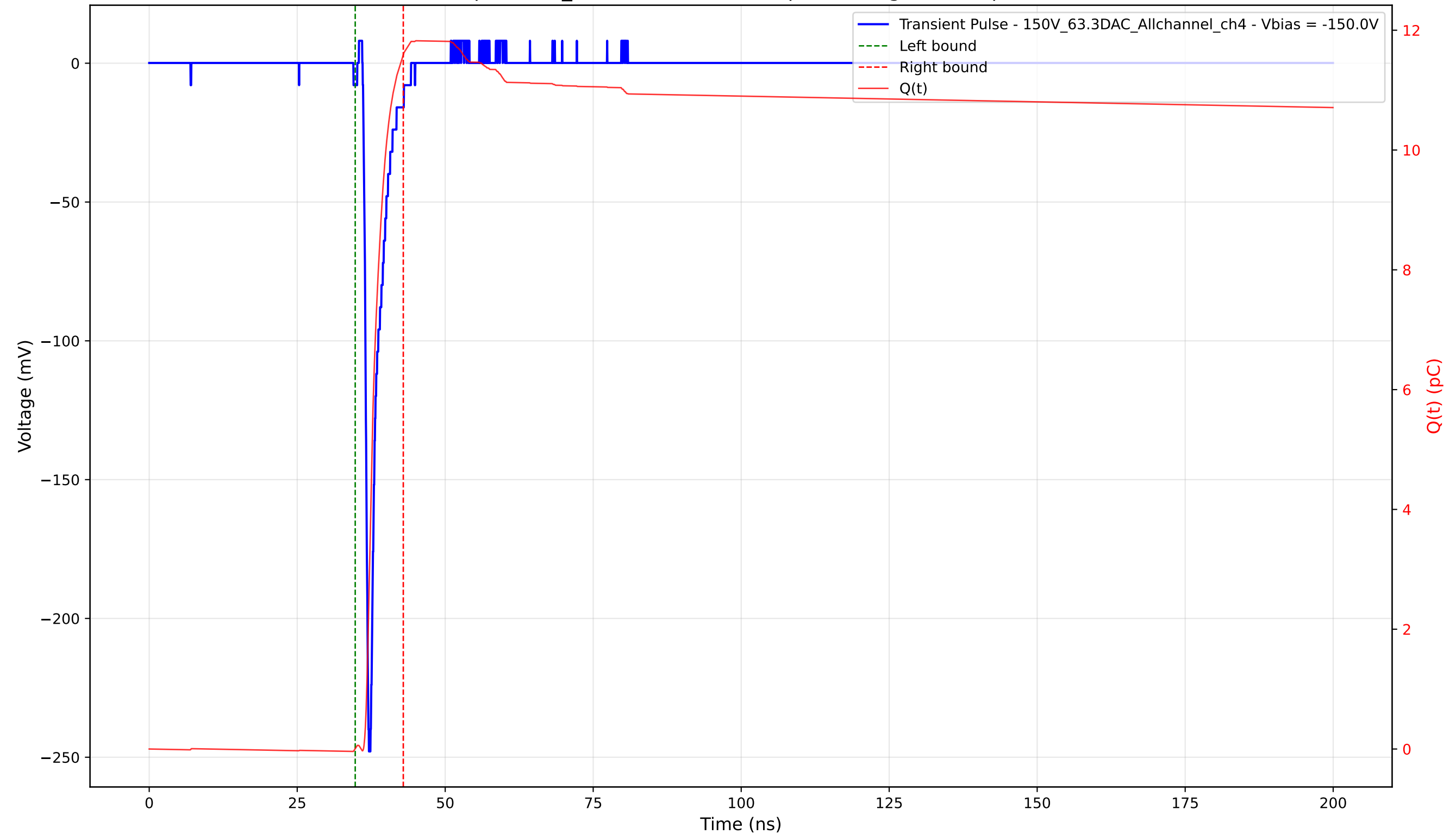
Transient Pulse - Sample: 1cm_42 - Position: 1485.0 \mu\text{m} - Charge: 11.58 pC - Rise Time: 0.75 ns
