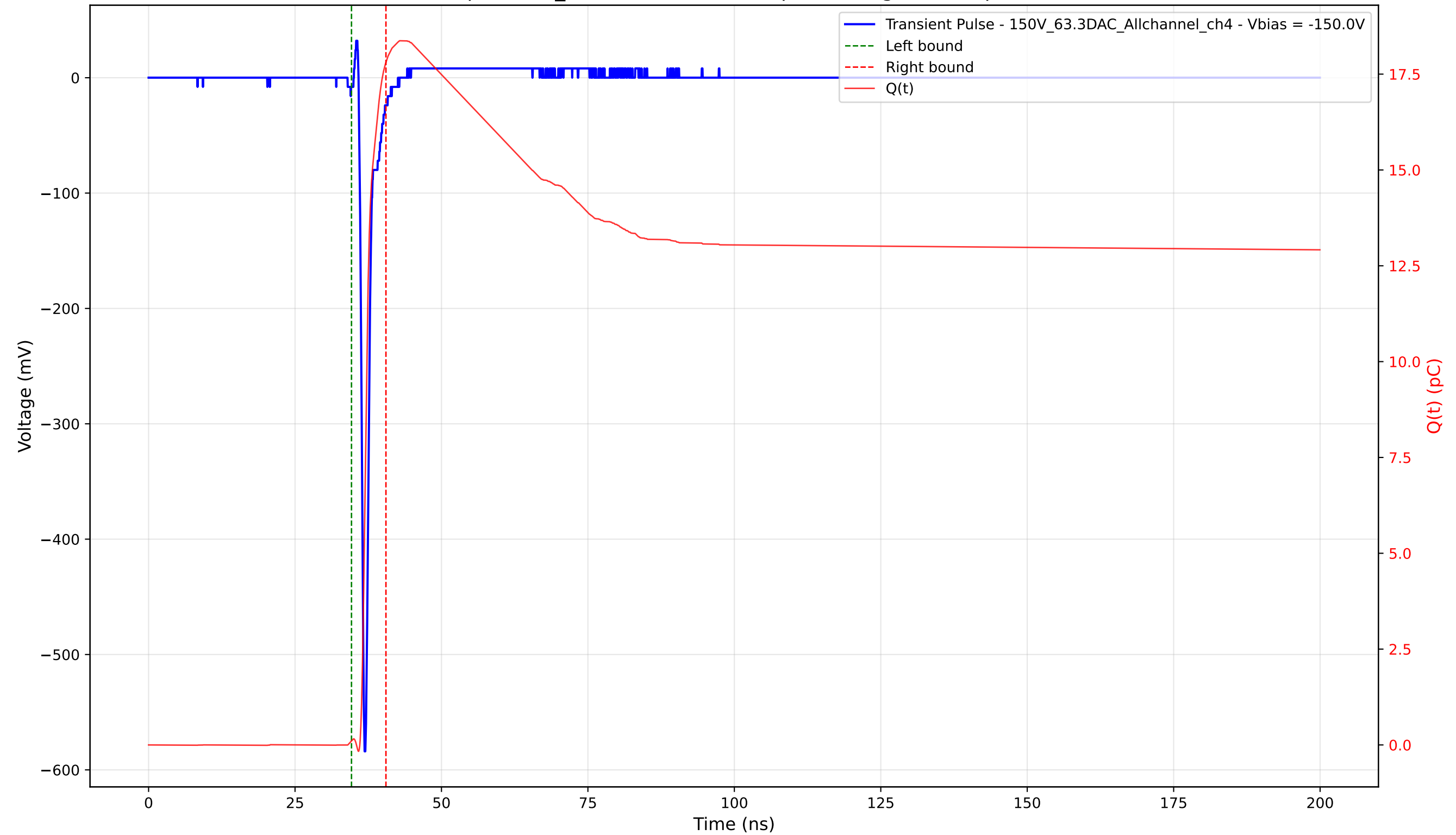
Transient Pulse - Sample: 1cm_42 - Position: 1995.0 \mu\text{m} - Charge: 17.70 pC - Rise Time: 0.71 ns
