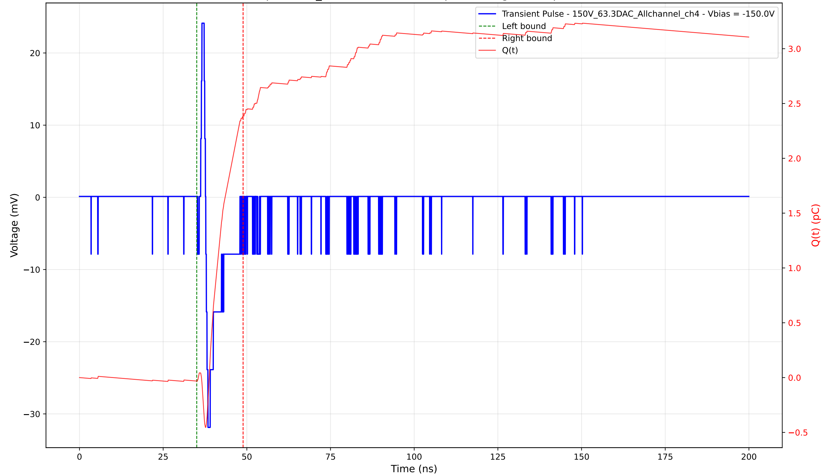
Transient Pulse - Sample: 1cm_42 - Position: 4400.0 \mu\text{m} - Charge: 2.42 pC - Rise Time: 0.66 ns
