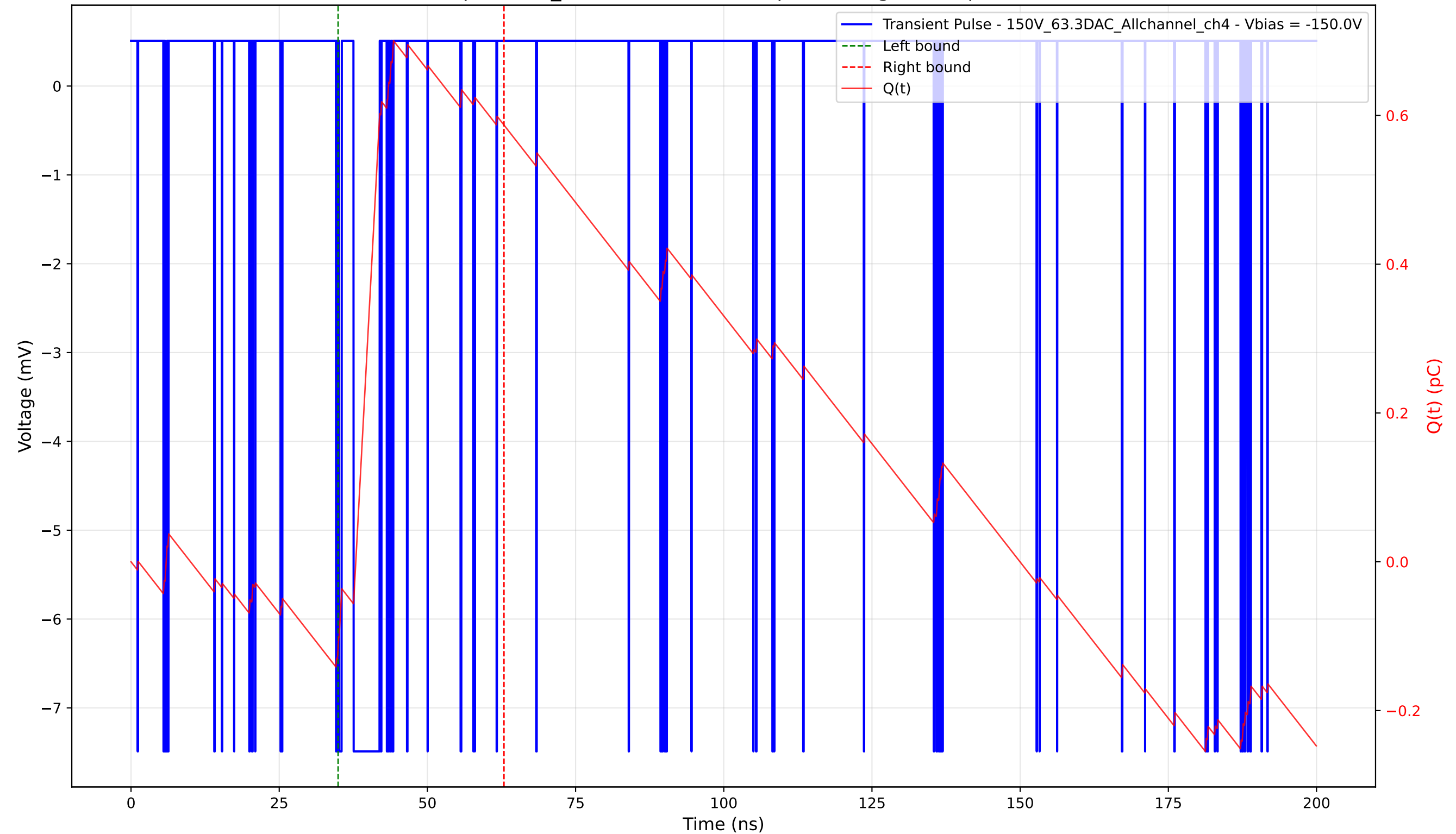
Transient Pulse - Sample: 1cm_42 - Position: 5130.0 \mu\text{m} - Charge: 0.70 pC - Rise Time: 0.04 ns
