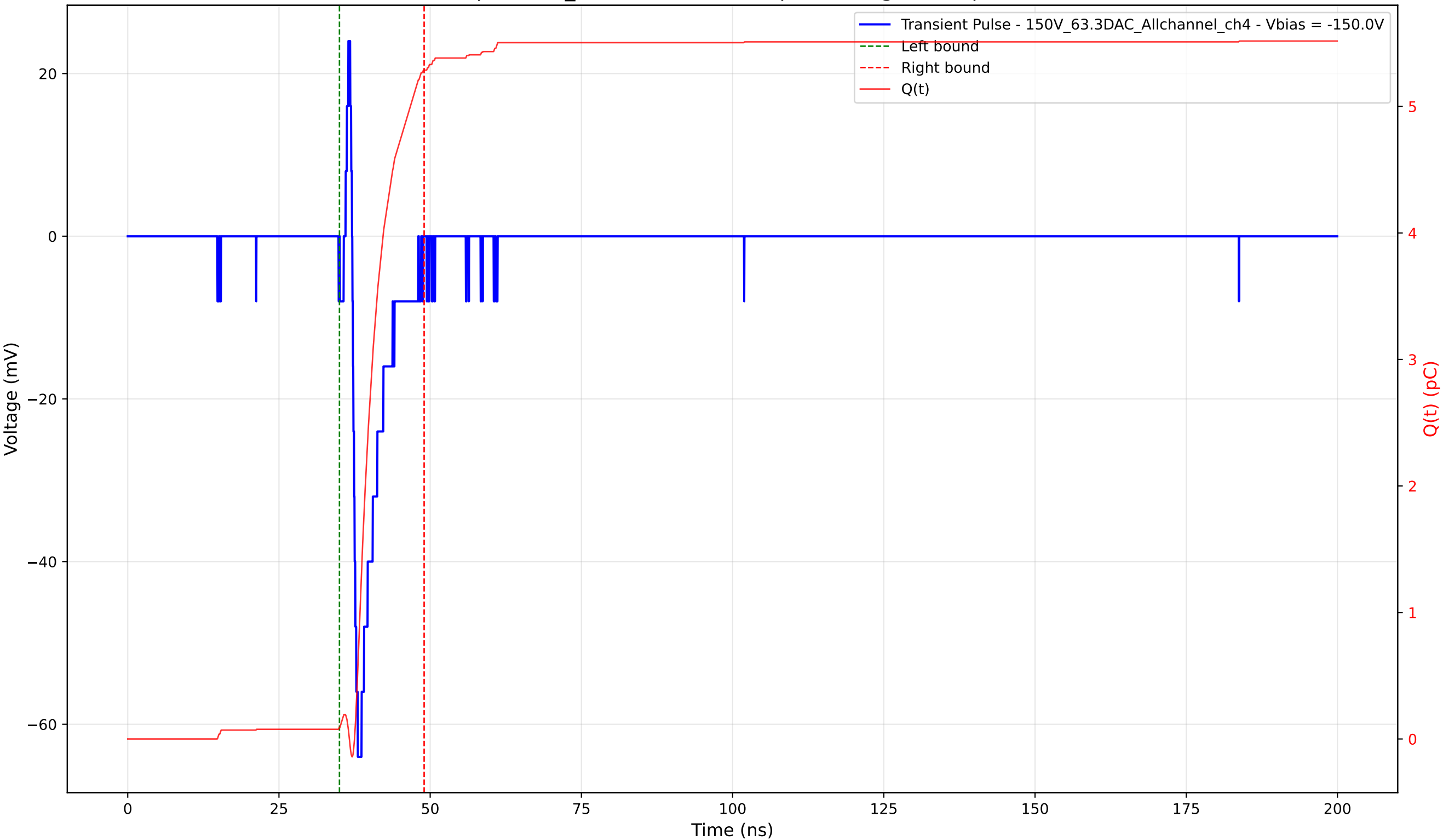
Transient Pulse - Sample: 1cm_42 - Position: 565.0 \mu\text{m} - Charge: 5.20 pC - Rise Time: 0.89 ns
