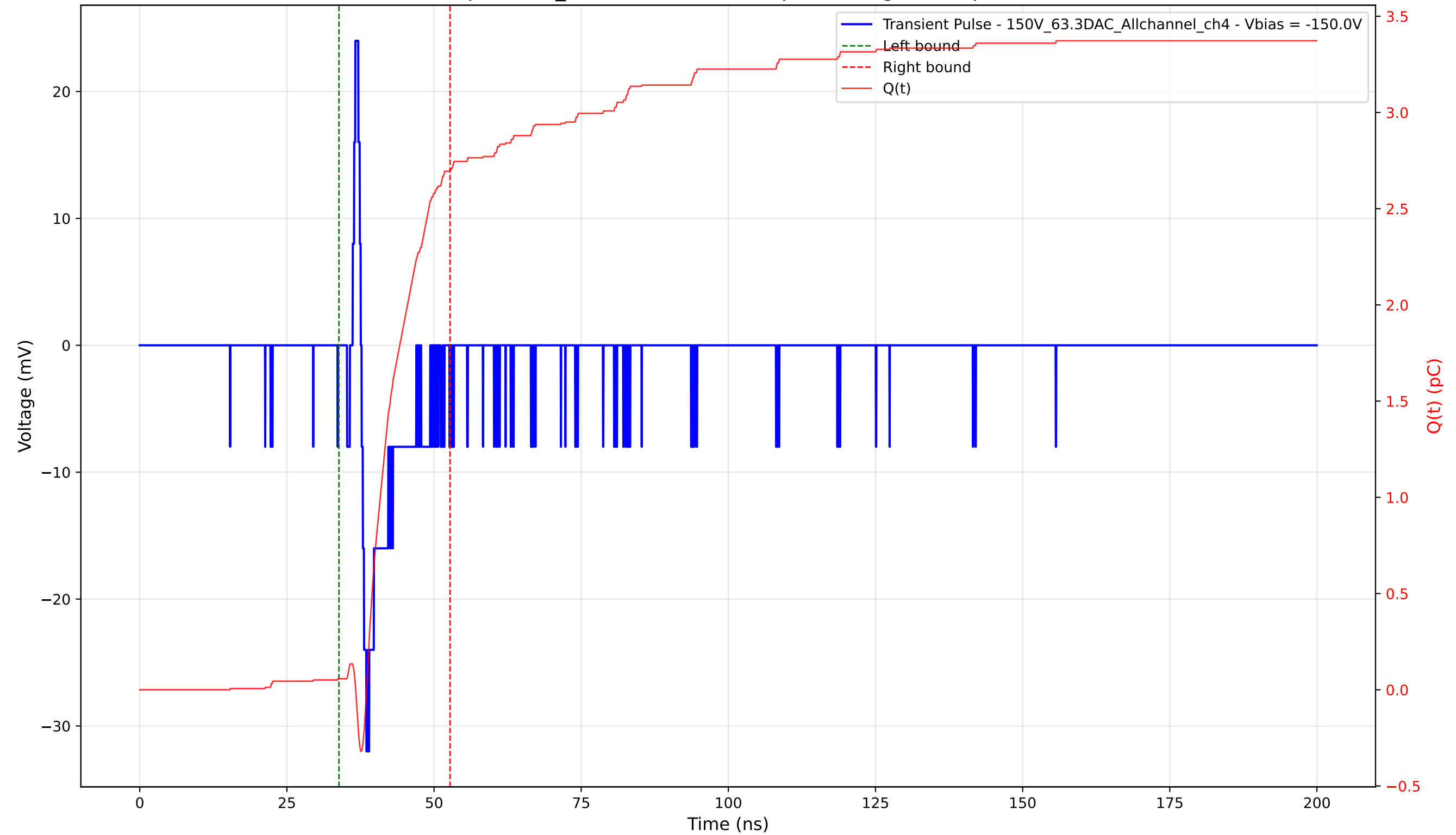
Transient Pulse - Sample: 1cm_42 - Position: 4490.0 \mu\text{m} - Charge: 2.64 pC - Rise Time: 0.82 ns
