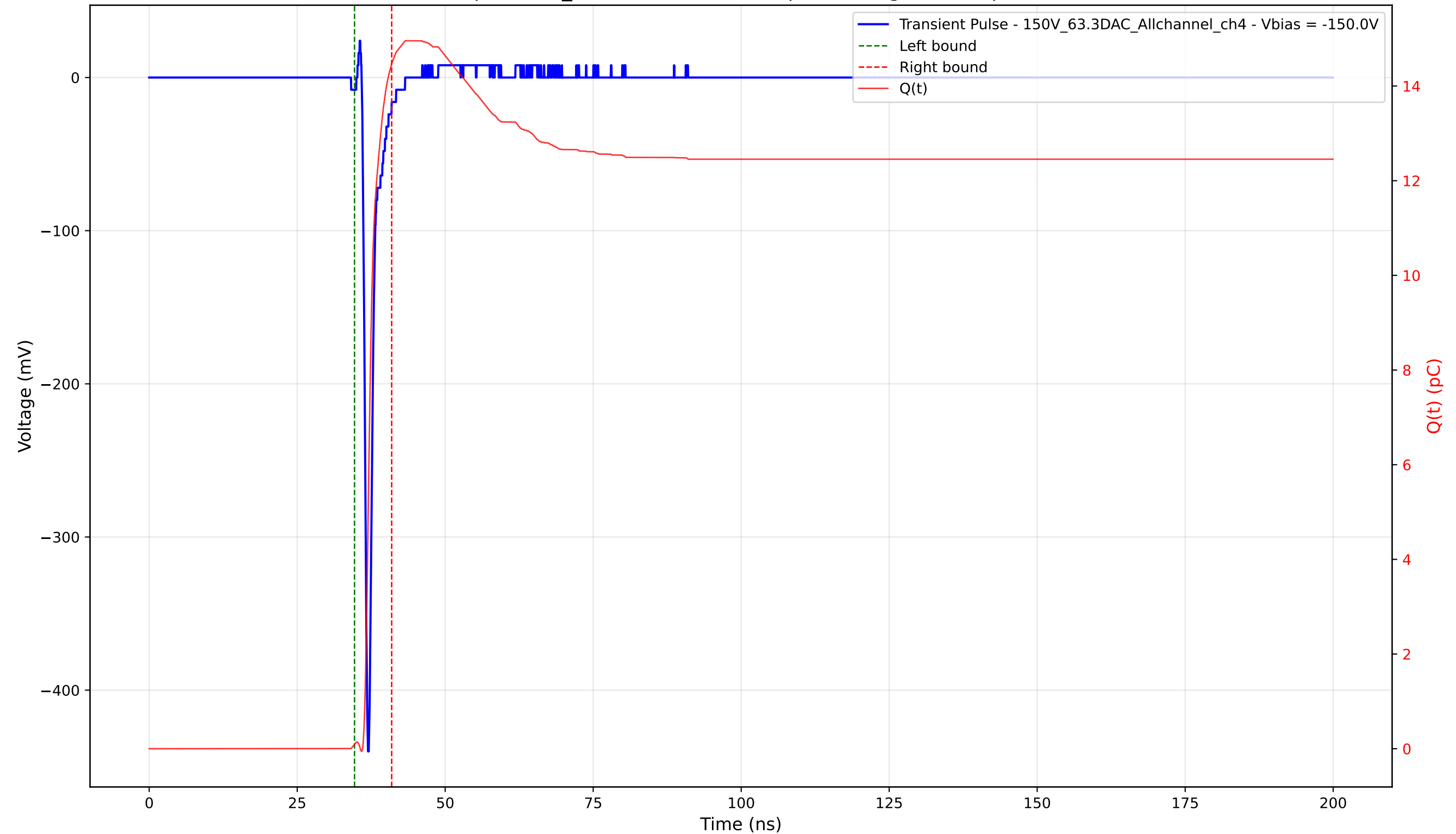
Transient Pulse - Sample: 1cm_42 - Position: 2335.0 \mu\text{m} - Charge: 14.38 pC - Rise Time: 0.69 ns
