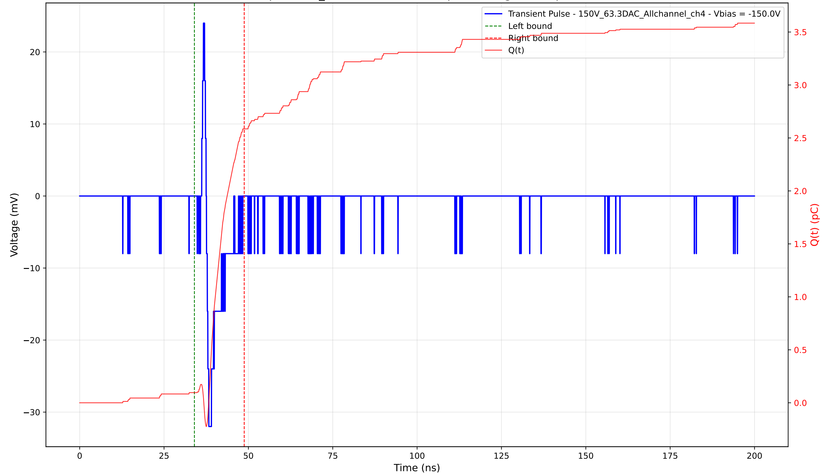
Transient Pulse - Sample: 1cm_42 - Position: 4635.0 \mu\text{m} - Charge: 2.49 pC - Rise Time: 0.70 ns
