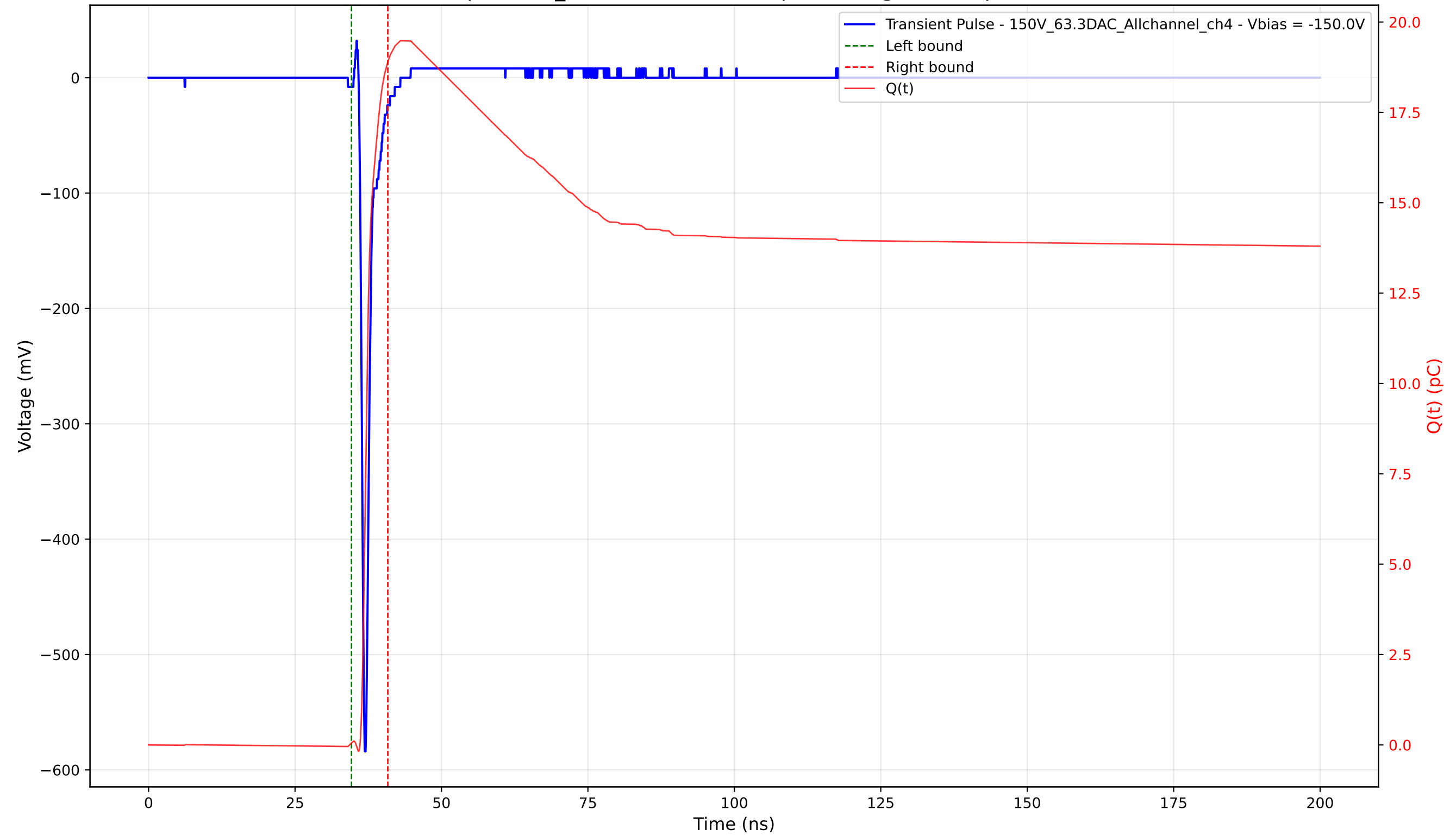
Transient Pulse - Sample: 1cm_42 - Position: 1865.0 \mu\text{m} - Charge: 18.84 pC - Rise Time: 0.71 ns
