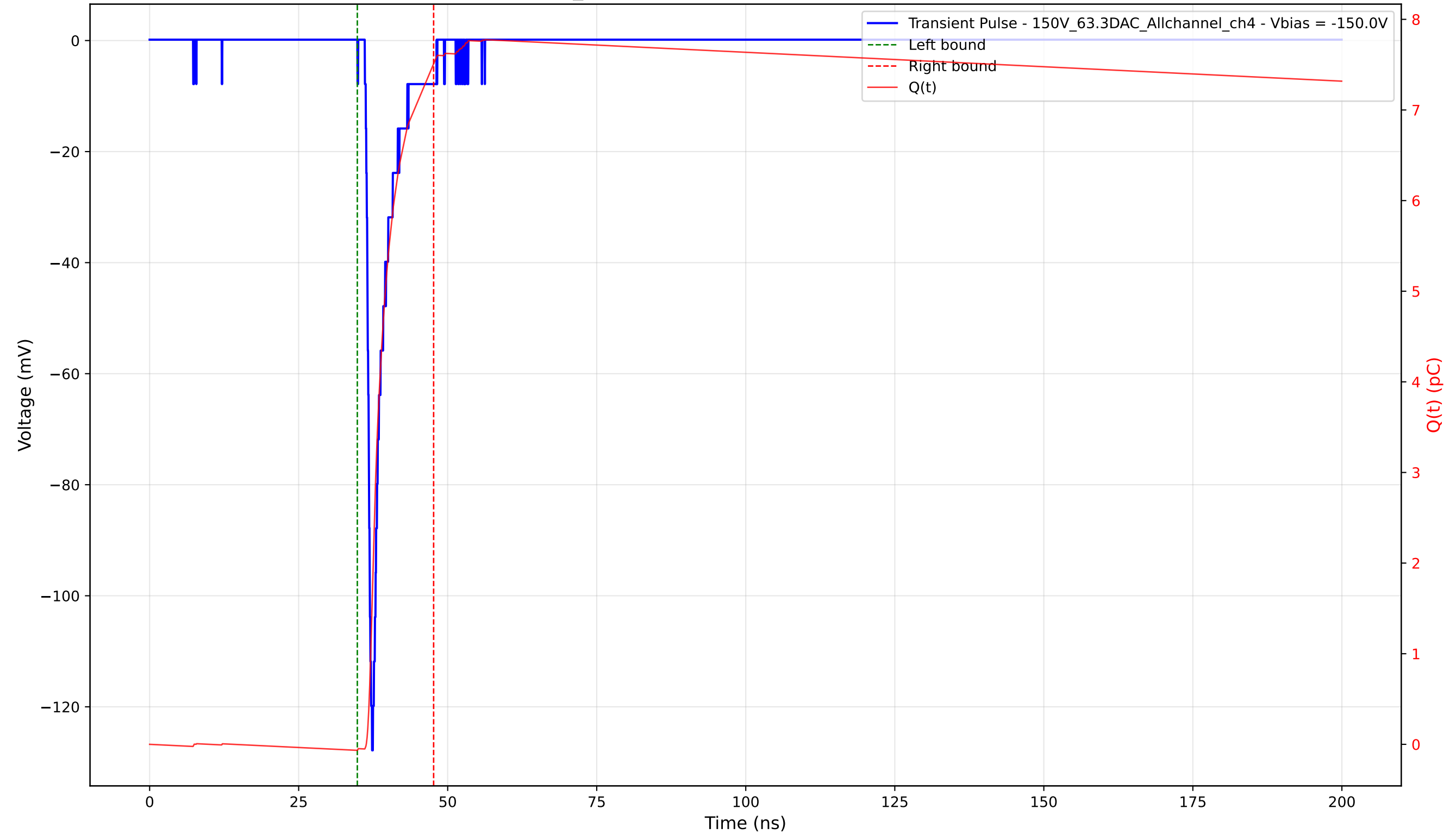
Transient Pulse - Sample: 1cm_42 - Position: 2830.0 \mu\text{m} - Charge: 7.58 pC - Rise Time: 0.90 ns
