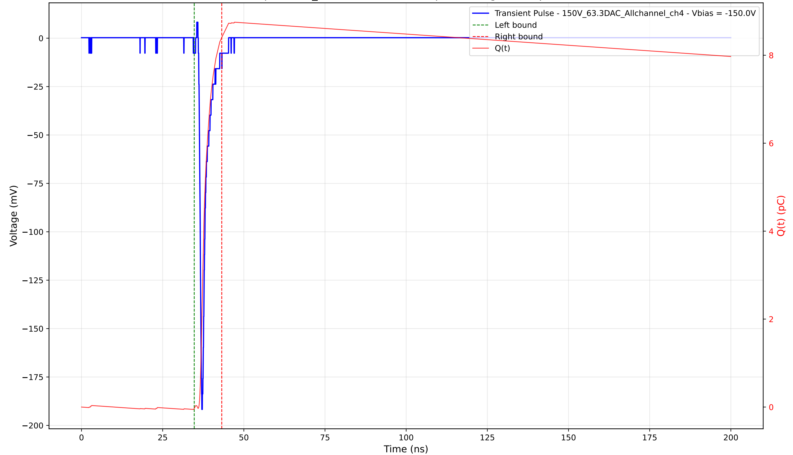
Transient Pulse - Sample: 1cm_42 - Position: 2590.0 \mu\text{m} - Charge: 8.43 pC - Rise Time: 0.78 ns
