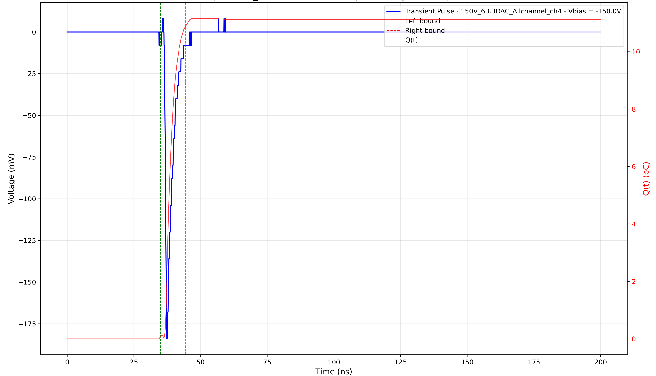
Transient Pulse - Sample: 1cm_42 - Position: 1305.0 \mu\text{m} - Charge: 10.81 pC - Rise Time: 0.74 ns
