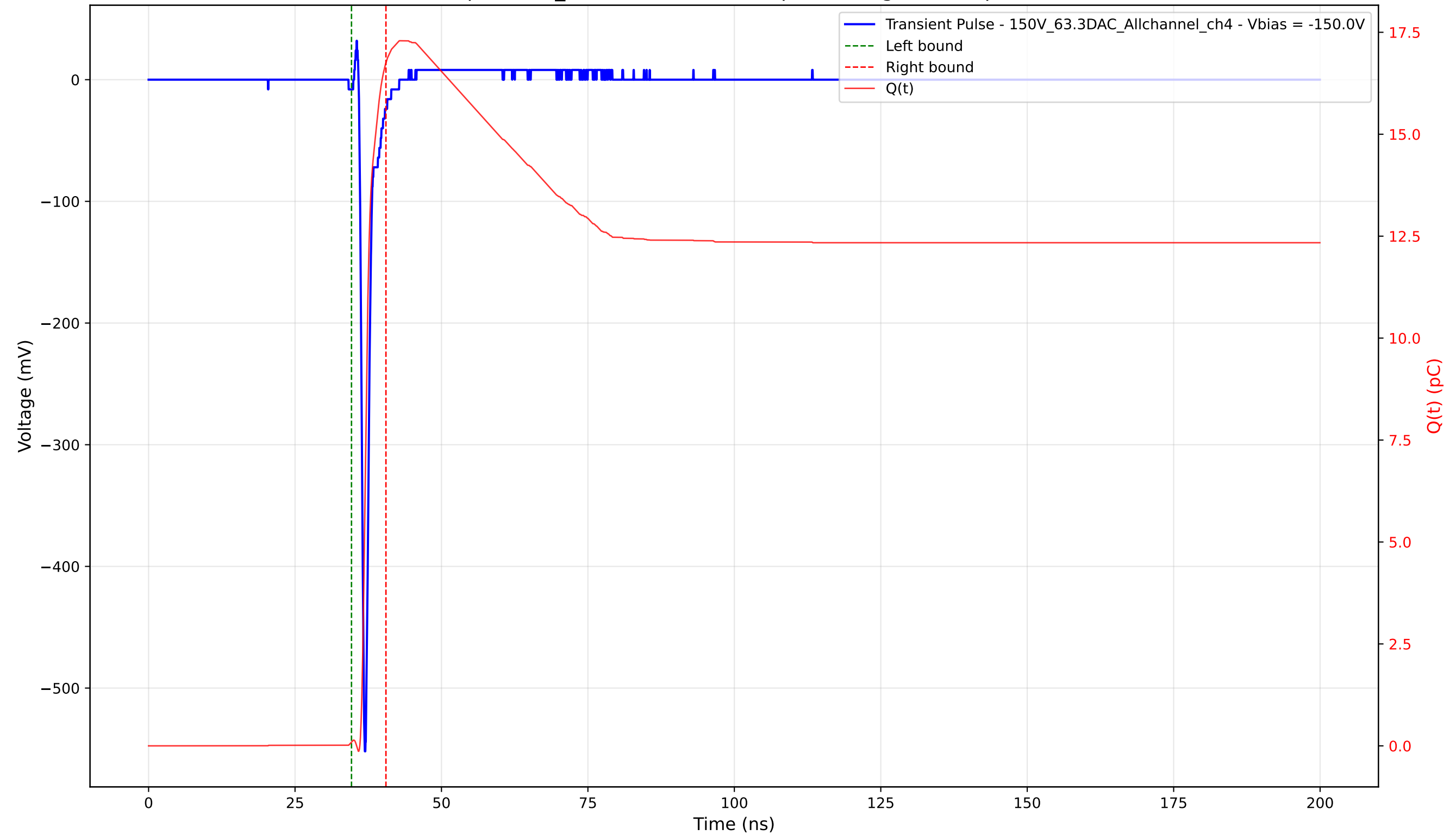
Transient Pulse - Sample: 1cm_42 - Position: 2135.0 \mu\text{m} - Charge: 16.66 pC - Rise Time: 0.70 ns
