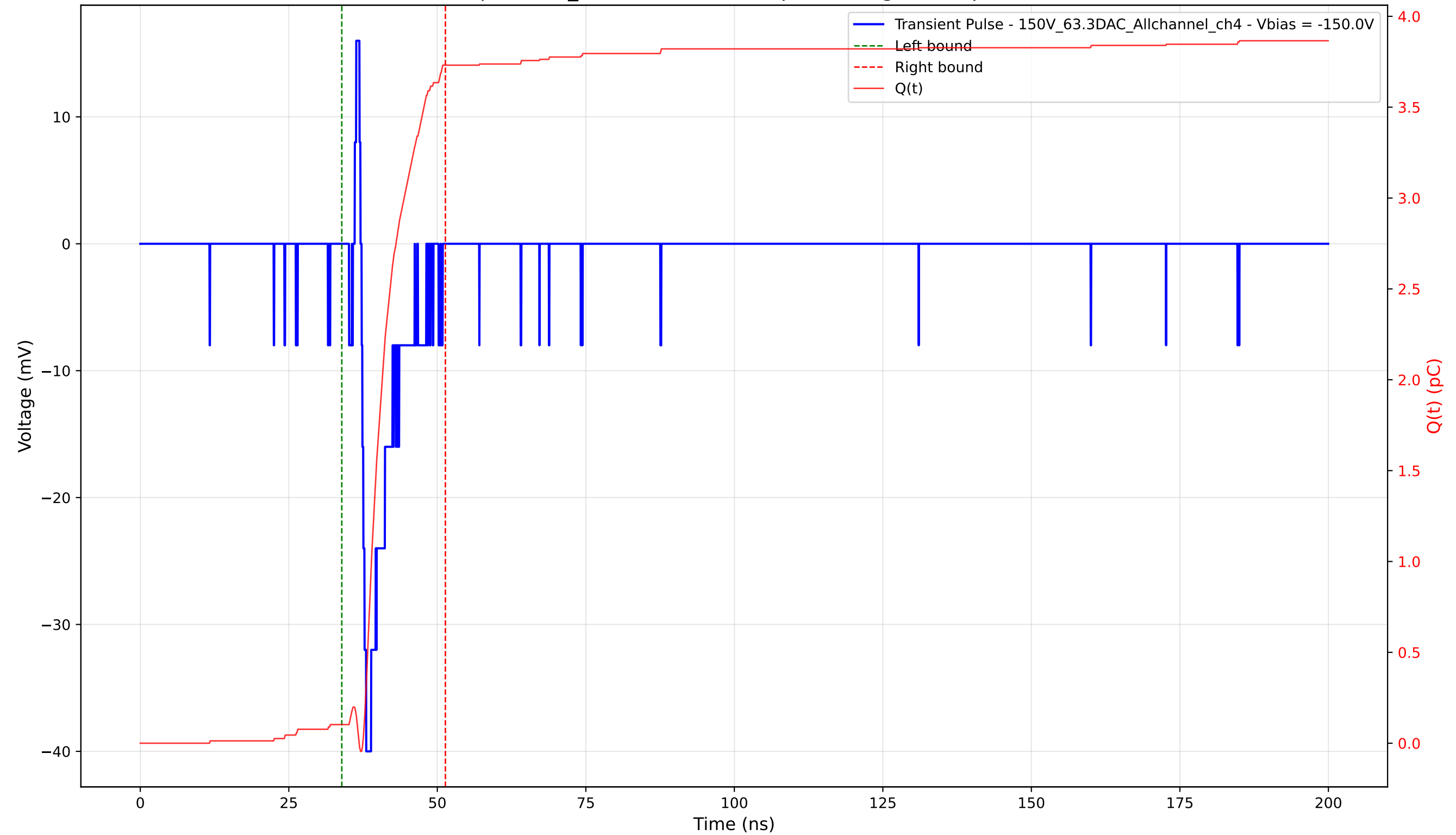
Transient Pulse - Sample: 1cm_42 - Position: 370.0 \mu\text{m} - Charge: 3.63 pC - Rise Time: 0.78 ns
