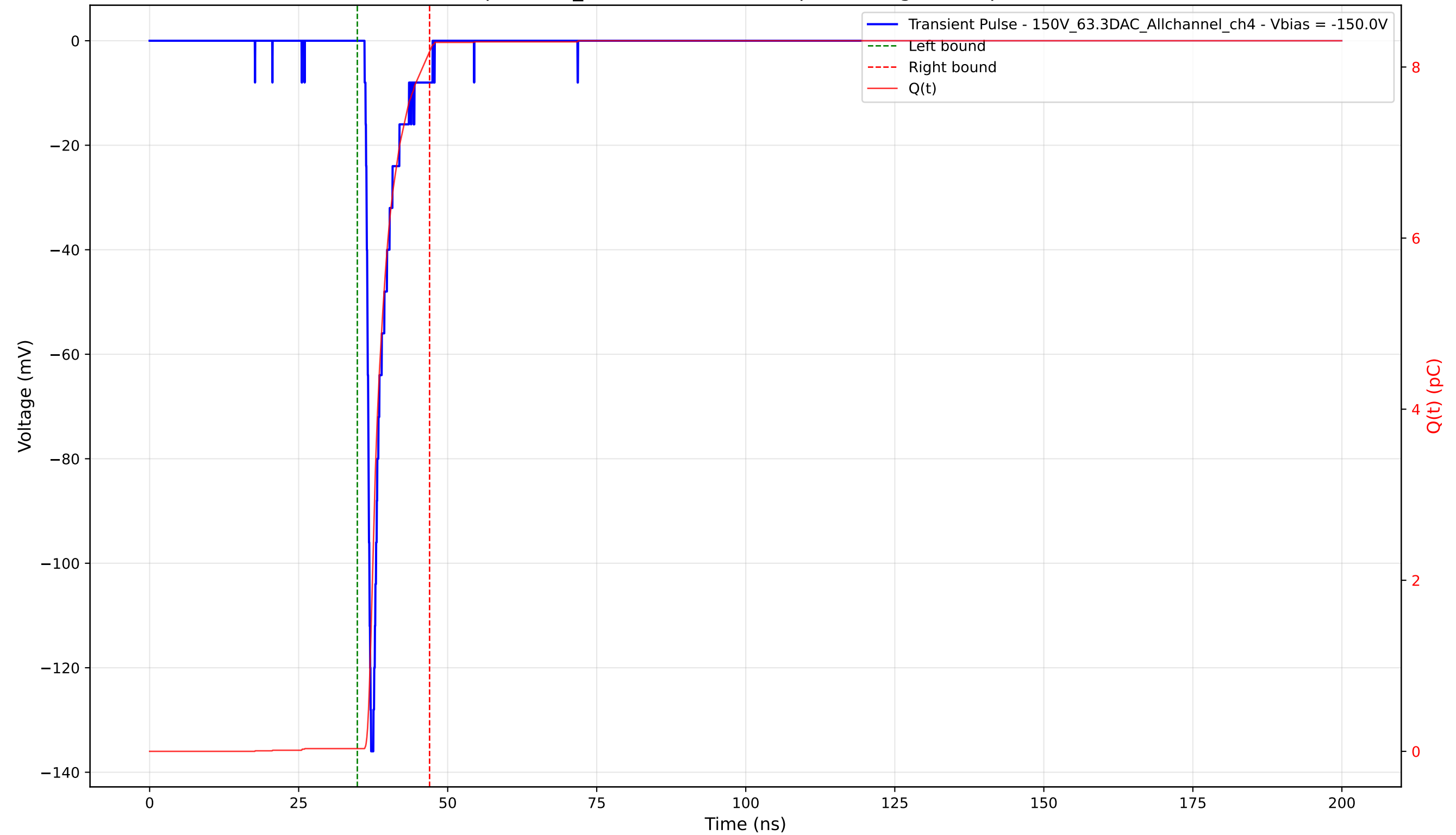
Transient Pulse - Sample: 1cm_42 - Position: 2775.0 \mu\text{m} - Charge: 8.15 pC - Rise Time: 0.85 ns
