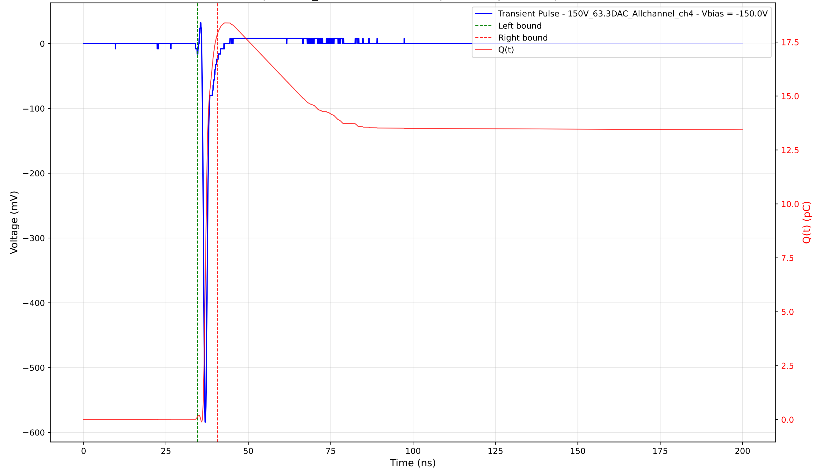
Transient Pulse - Sample: 1cm_42 - Position: 2015.0 \mu\text{m} - Charge: 17.71 pC - Rise Time: 0.69 ns
