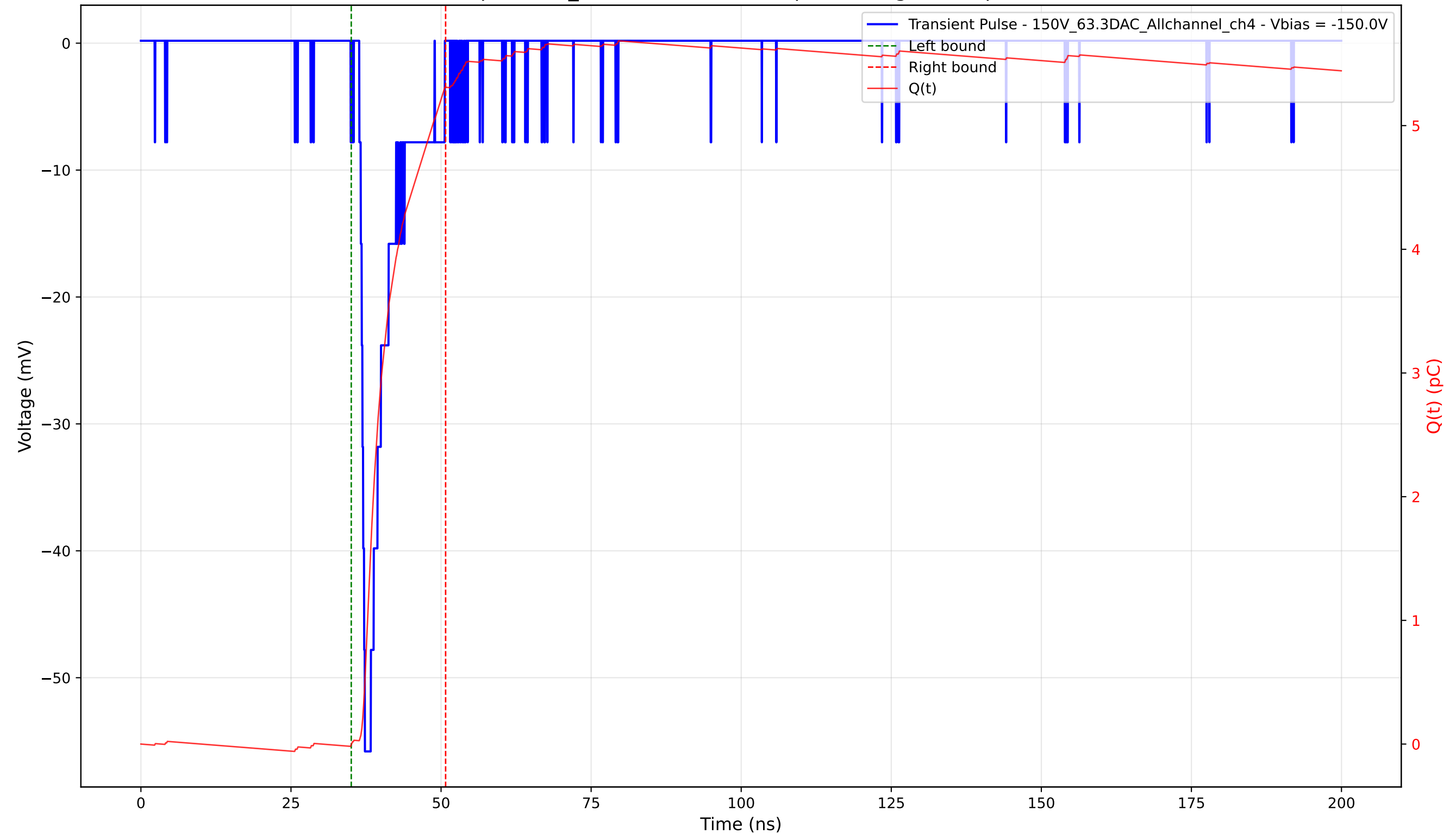
Transient Pulse - Sample: 1cm_42 - Position: 3045.0 \mu\text{m} - Charge: 5.31 pC - Rise Time: 0.93 ns
