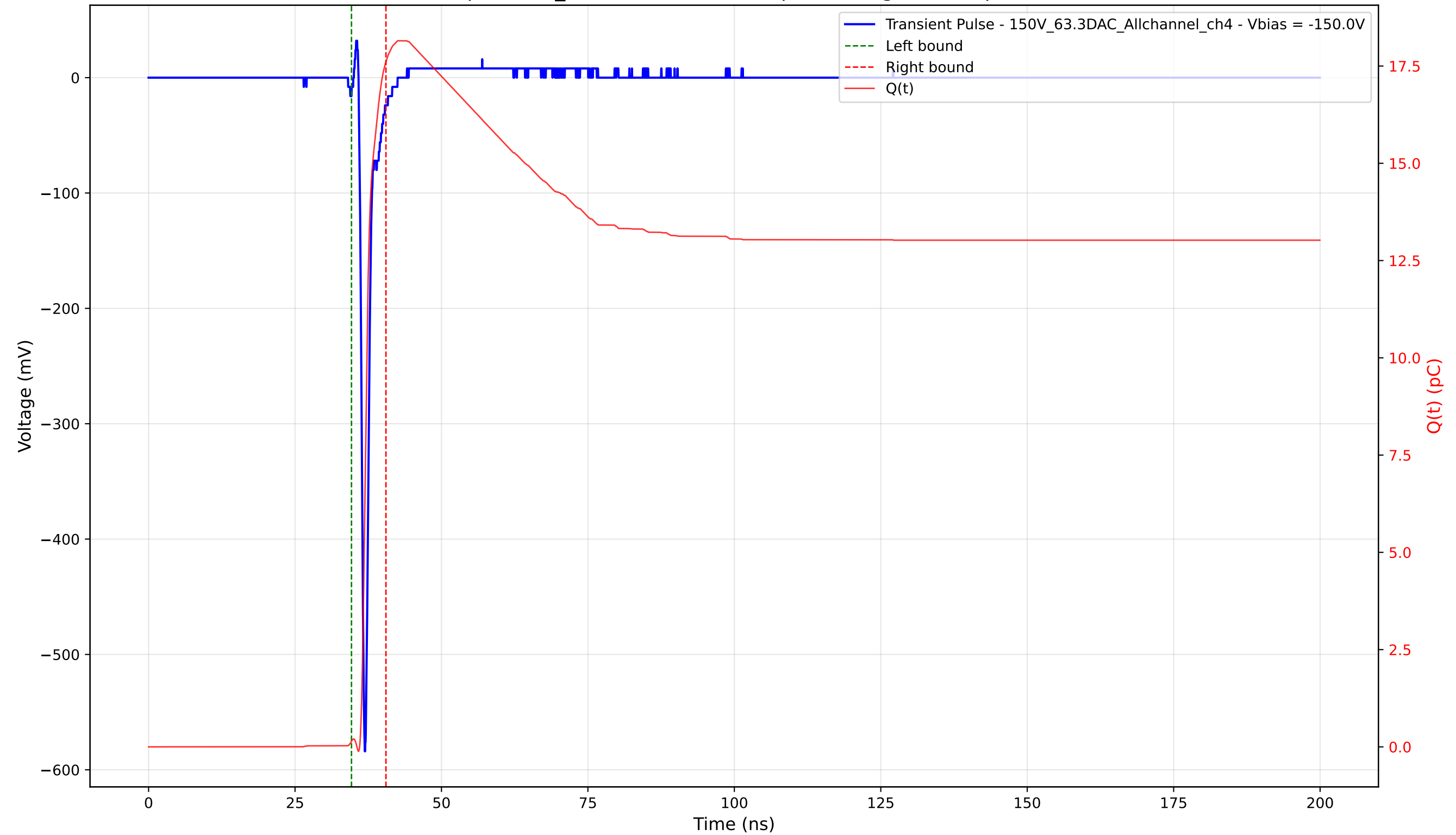
Transient Pulse - Sample: 1cm_42 - Position: 2045.0 \mu\text{m} - Charge: 17.46 pC - Rise Time: 0.71 ns
