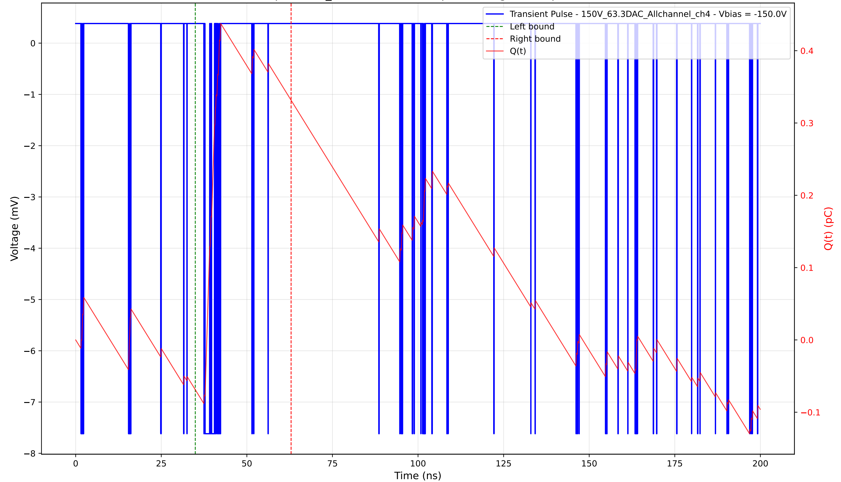
Transient Pulse - Sample: 1cm_42 - Position: 35.0 \mu\text{m} - Charge: 0.40 pC - Rise Time: 0.04 ns
