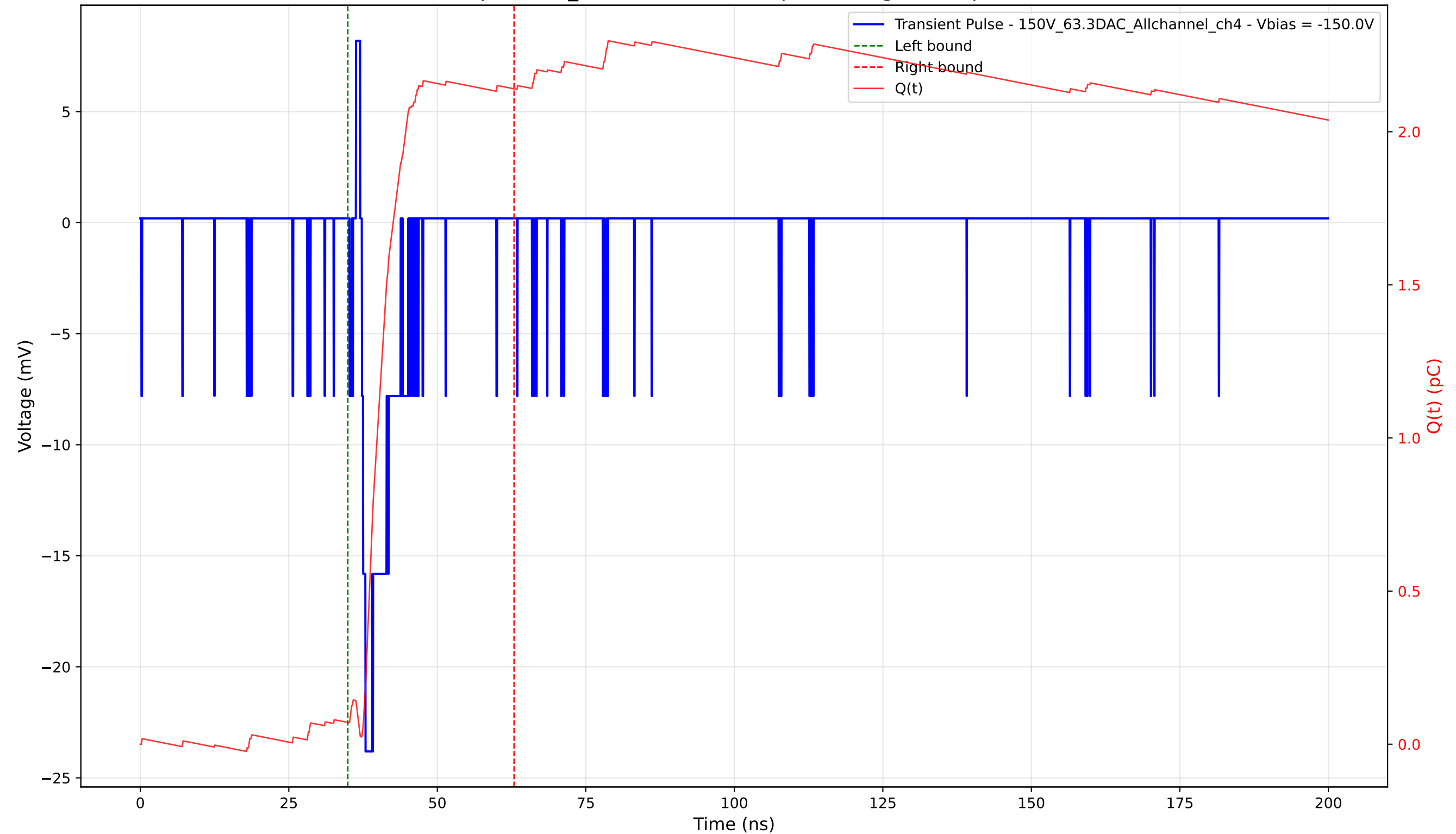
Transient Pulse - Sample: 1cm_42 - Position: 185.0 \mu\text{m} - Charge: 2.07 pC - Rise Time: 0.63 ns
