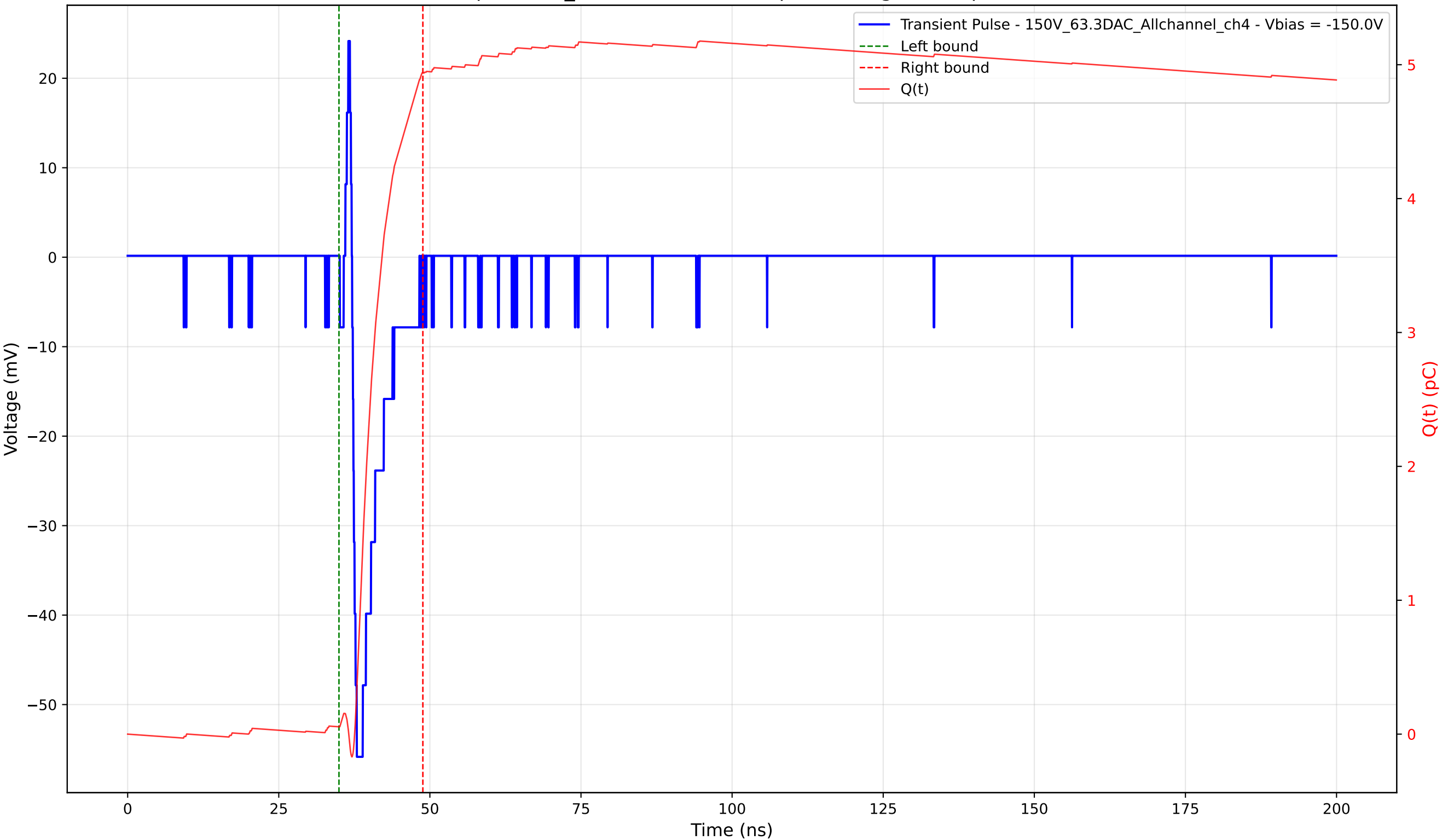
Transient Pulse - Sample: 1cm_42 - Position: 535.0 \mu\text{m} - Charge: 4.88 pC - Rise Time: 0.77 ns
