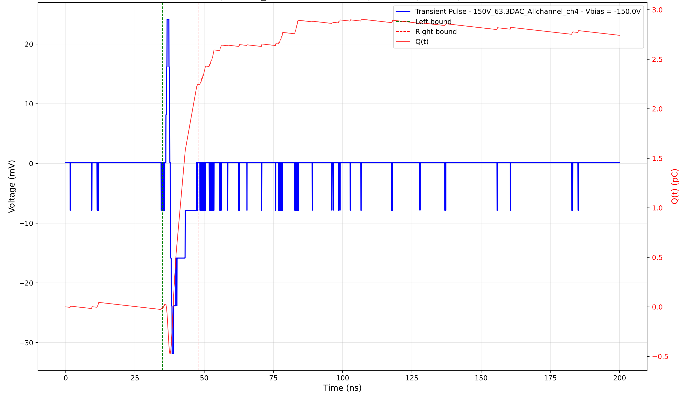
Transient Pulse - Sample: 1cm_42 - Position: 4435.0 \mu\text{m} - Charge: 2.26 pC - Rise Time: 0.66 ns
