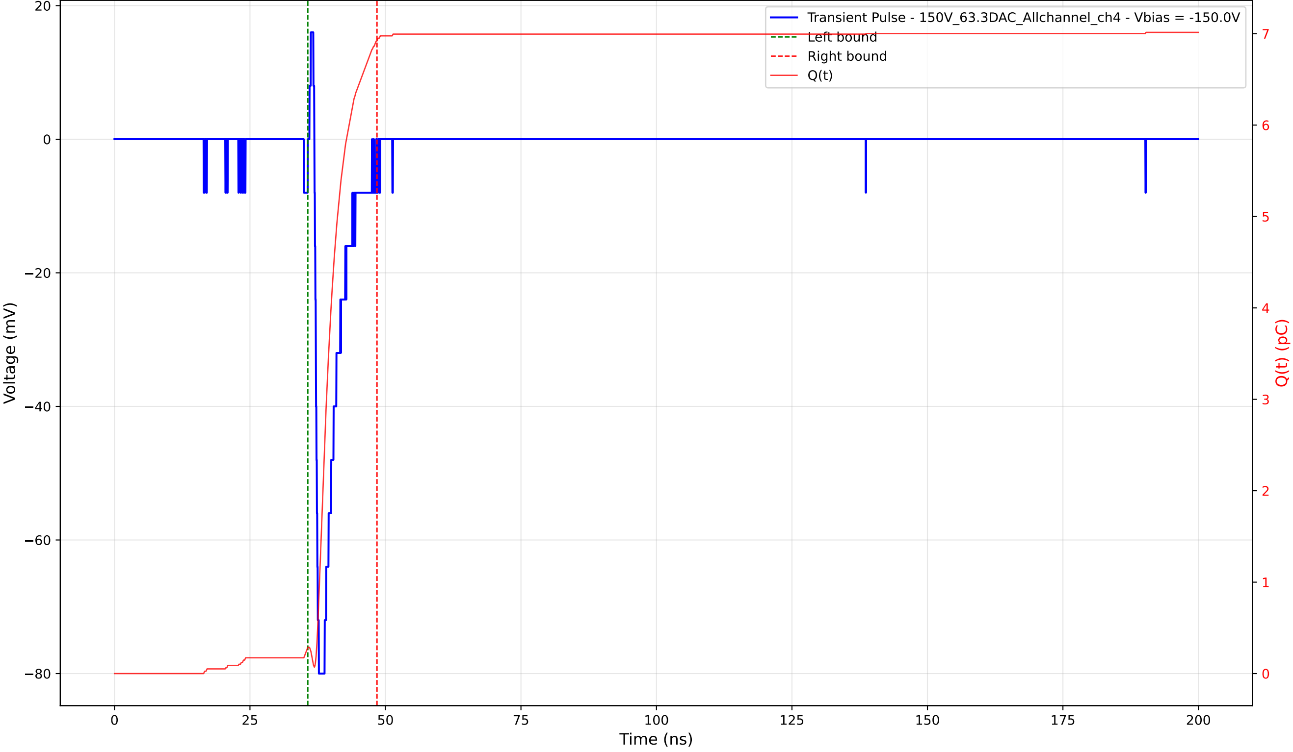
Transient Pulse - Sample: 1cm_42 - Position: 880.0 \mu\text{m} - Charge: 6.63 pC - Rise Time: 0.56 ns
