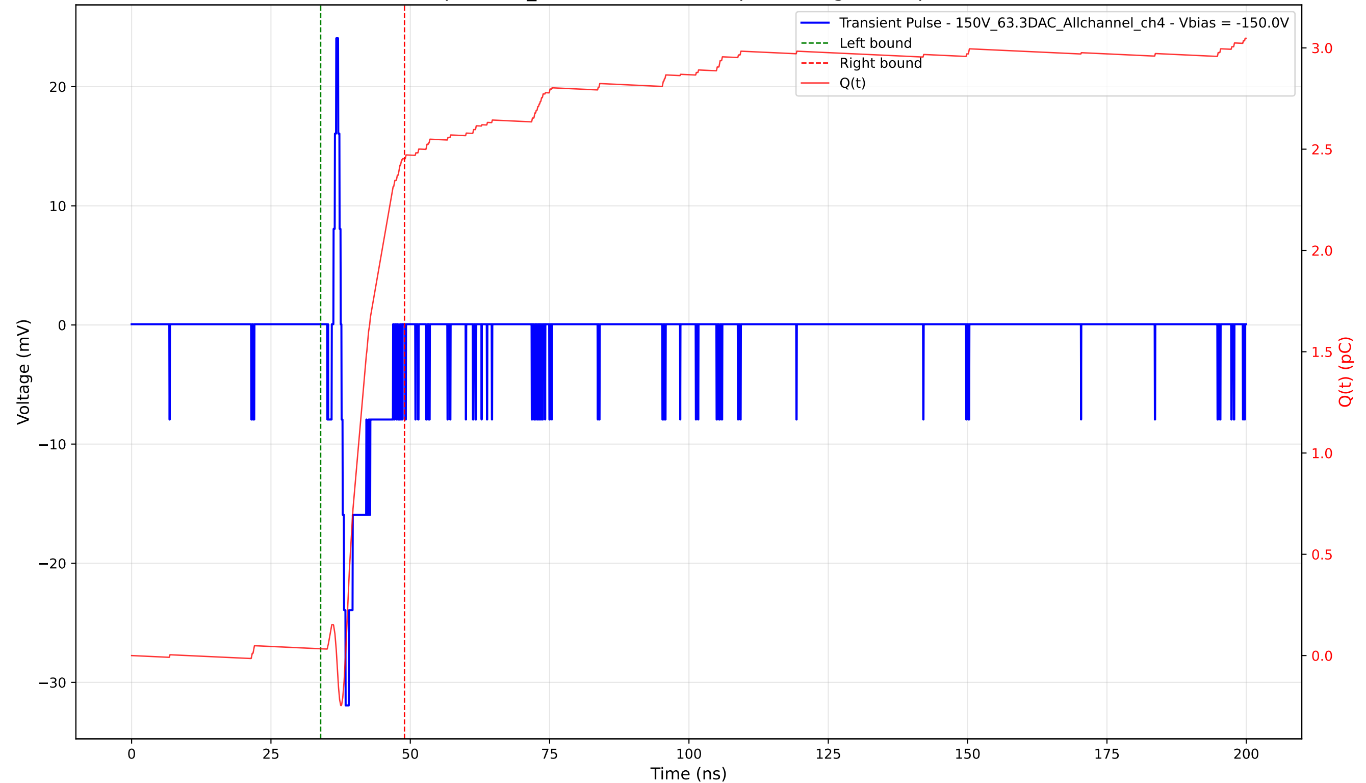
Transient Pulse - Sample: 1cm_42 - Position: 4575.0 \mu\text{m} - Charge: 2.42 pC - Rise Time: 0.74 ns
