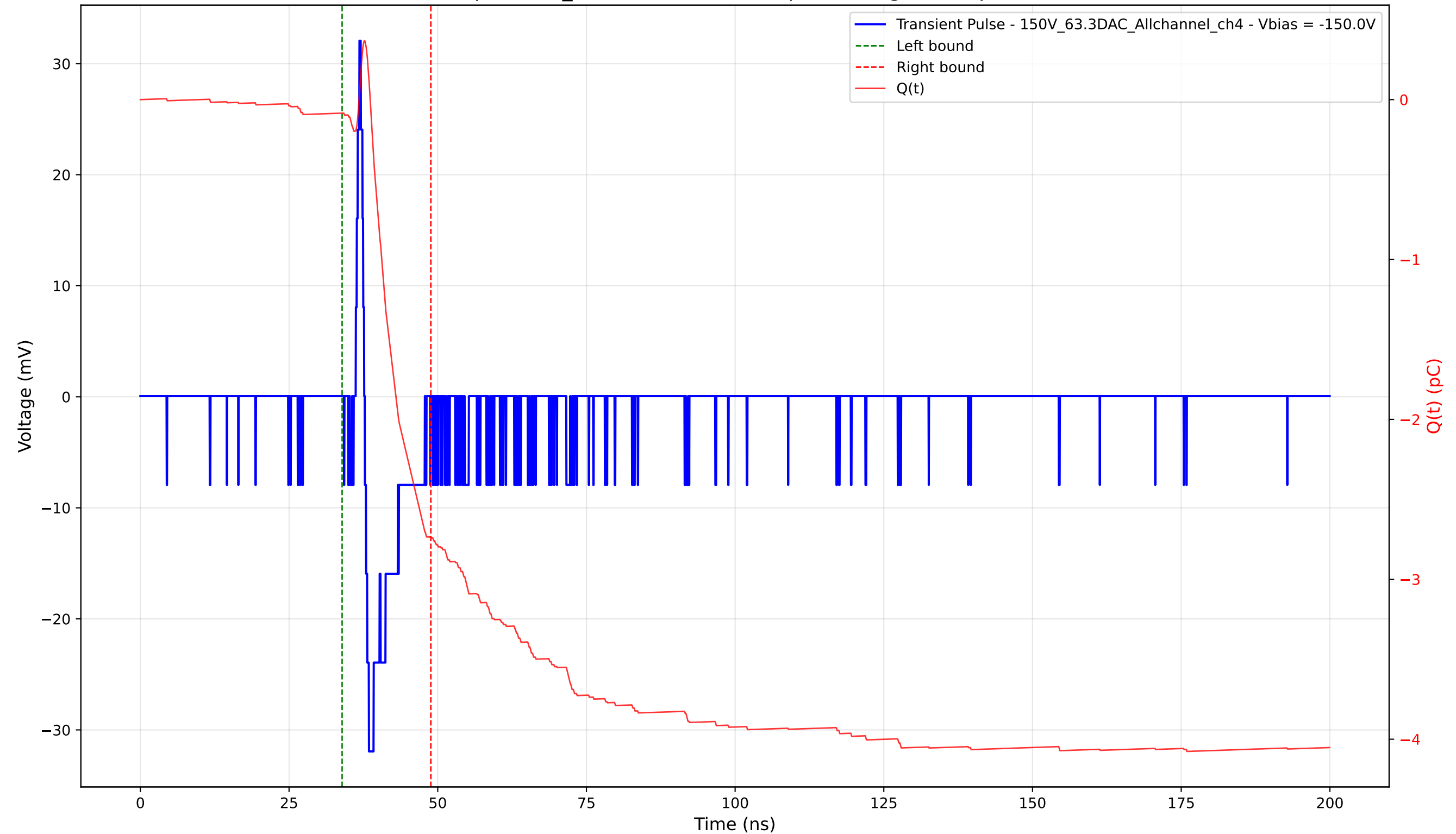
Transient Pulse - Sample: 1cm_42 - Position: 4195.0 \mu\text{m} - Charge: 2.66 pC - Rise Time: 0.62 ns
