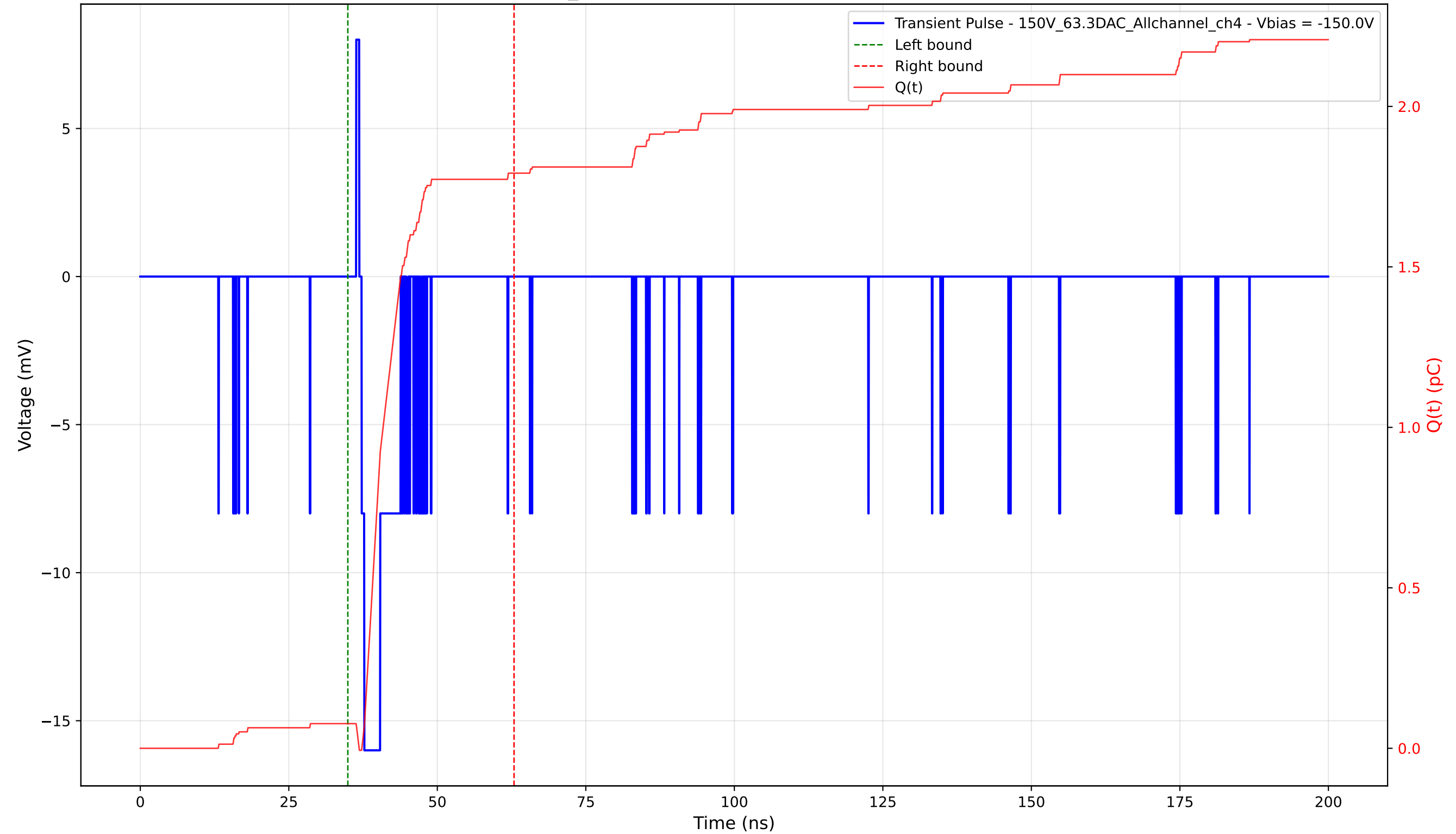
Transient Pulse - Sample: 1cm_42 - Position: 150.0 \mu\text{m} - Charge: 1.72 pC - Rise Time: 0.47 ns
