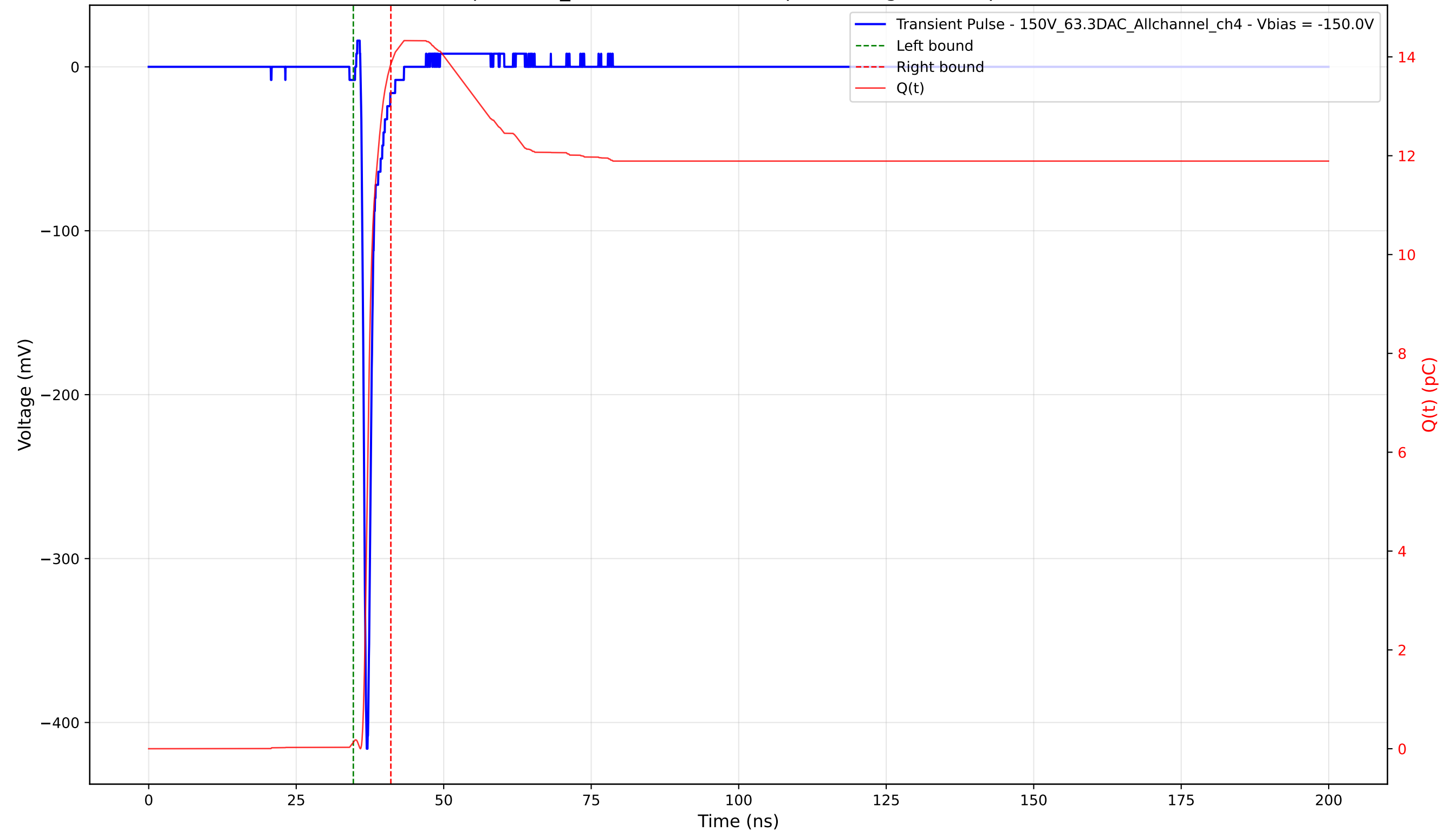
Transient Pulse - Sample: 1cm_42 - Position: 2360.0 \mu\text{m} - Charge: 13.72 pC - Rise Time: 0.69 ns
