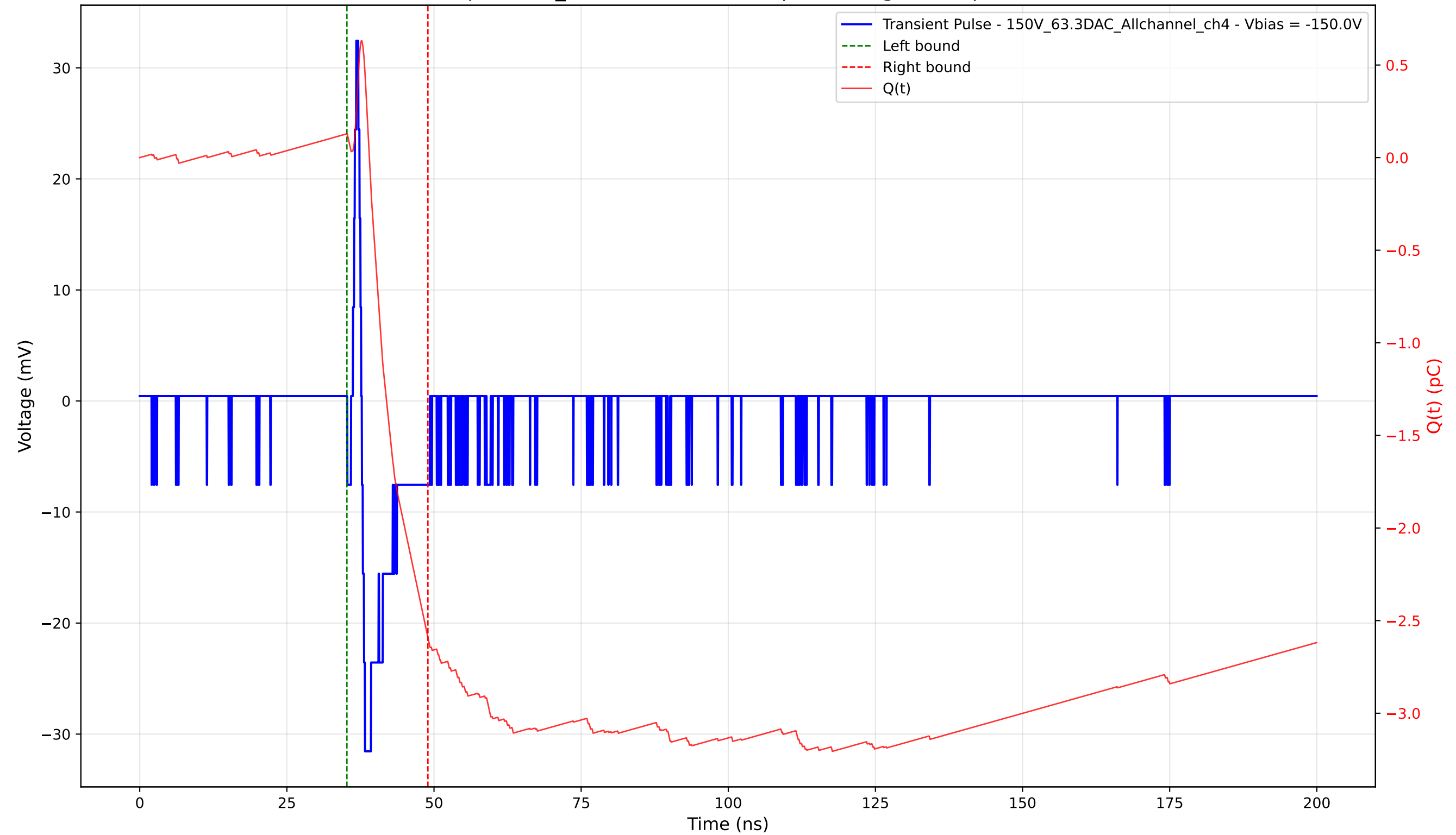
Transient Pulse - Sample: 1cm_42 - Position: 4265.0 \mu\text{m} - Charge: 2.72 pC - Rise Time: 0.59 ns
