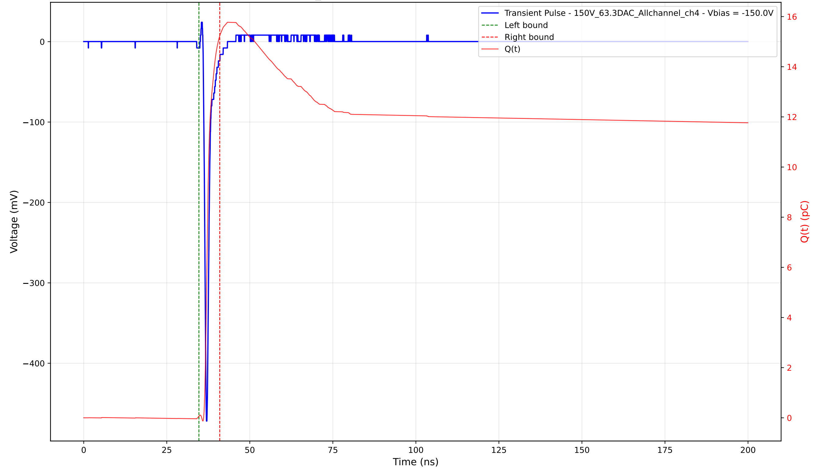
Transient Pulse - Sample: 1cm_42 - Position: 2315.0 \mu\text{m} - Charge: 15.18 pC - Rise Time: 0.72 ns
