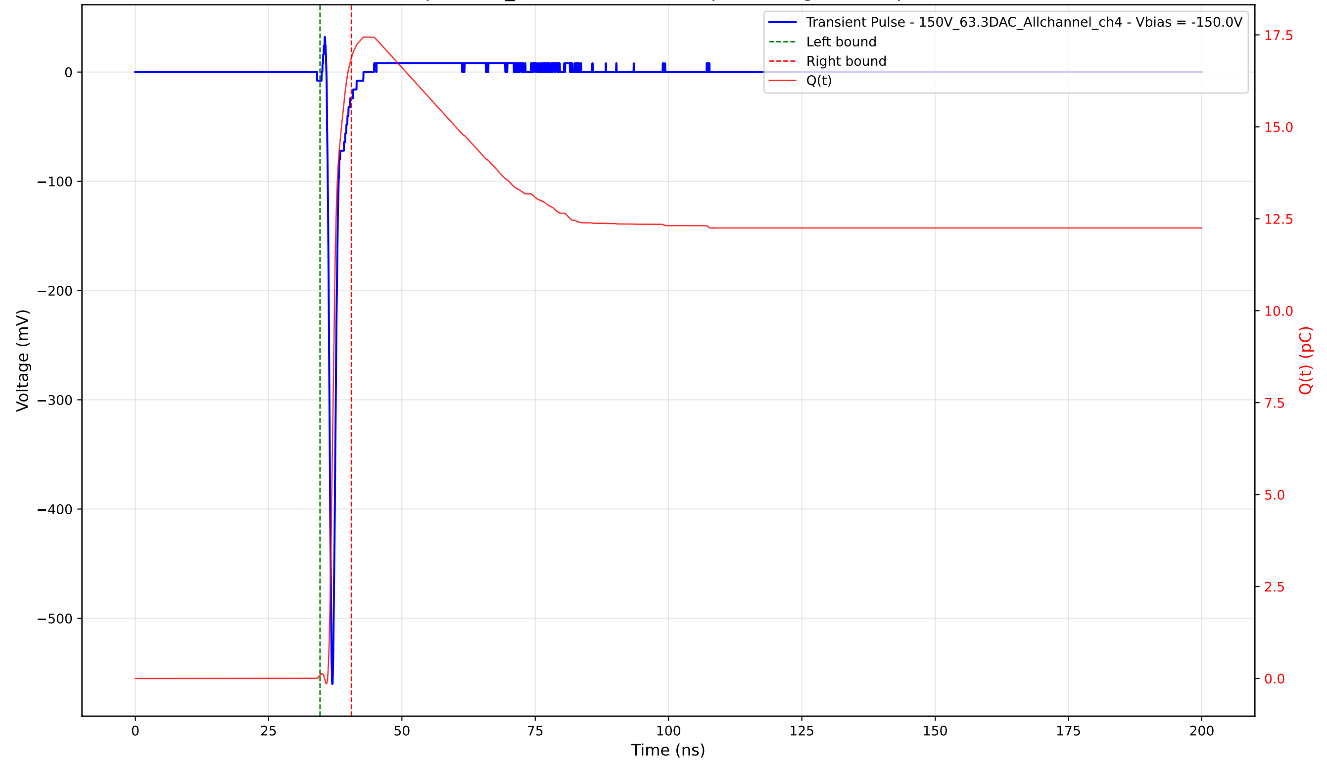
Transient Pulse - Sample: 1cm_42 - Position: 2120.0 \mu\text{m} - Charge: 16.78 pC - Rise Time: 0.70 ns
