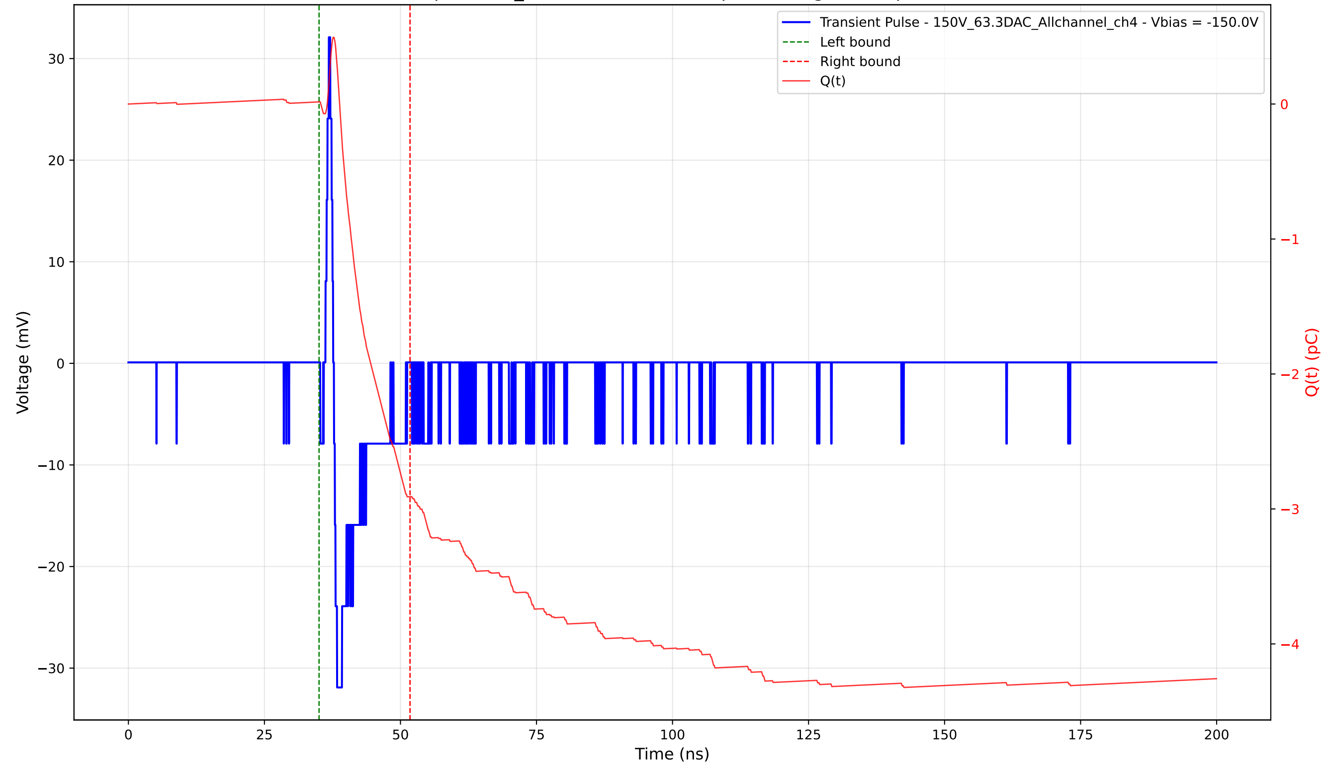
Transient Pulse - Sample: 1cm_42 - Position: 4225.0 \mu\text{m} - Charge: 2.92 pC - Rise Time: 0.62 ns
