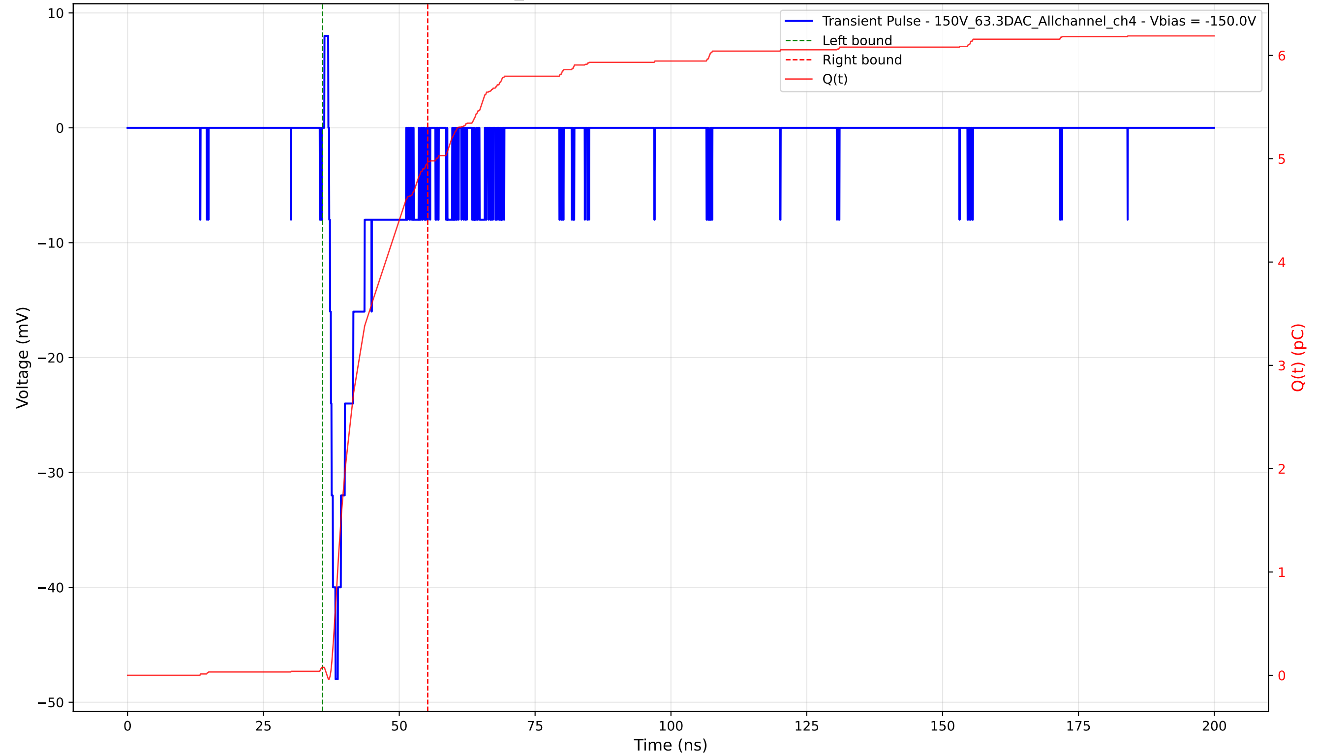
Transient Pulse - Sample: 1cm_42 - Position: 3350.0 \mu\text{m} - Charge: 4.89 pC - Rise Time: 1.18 ns
