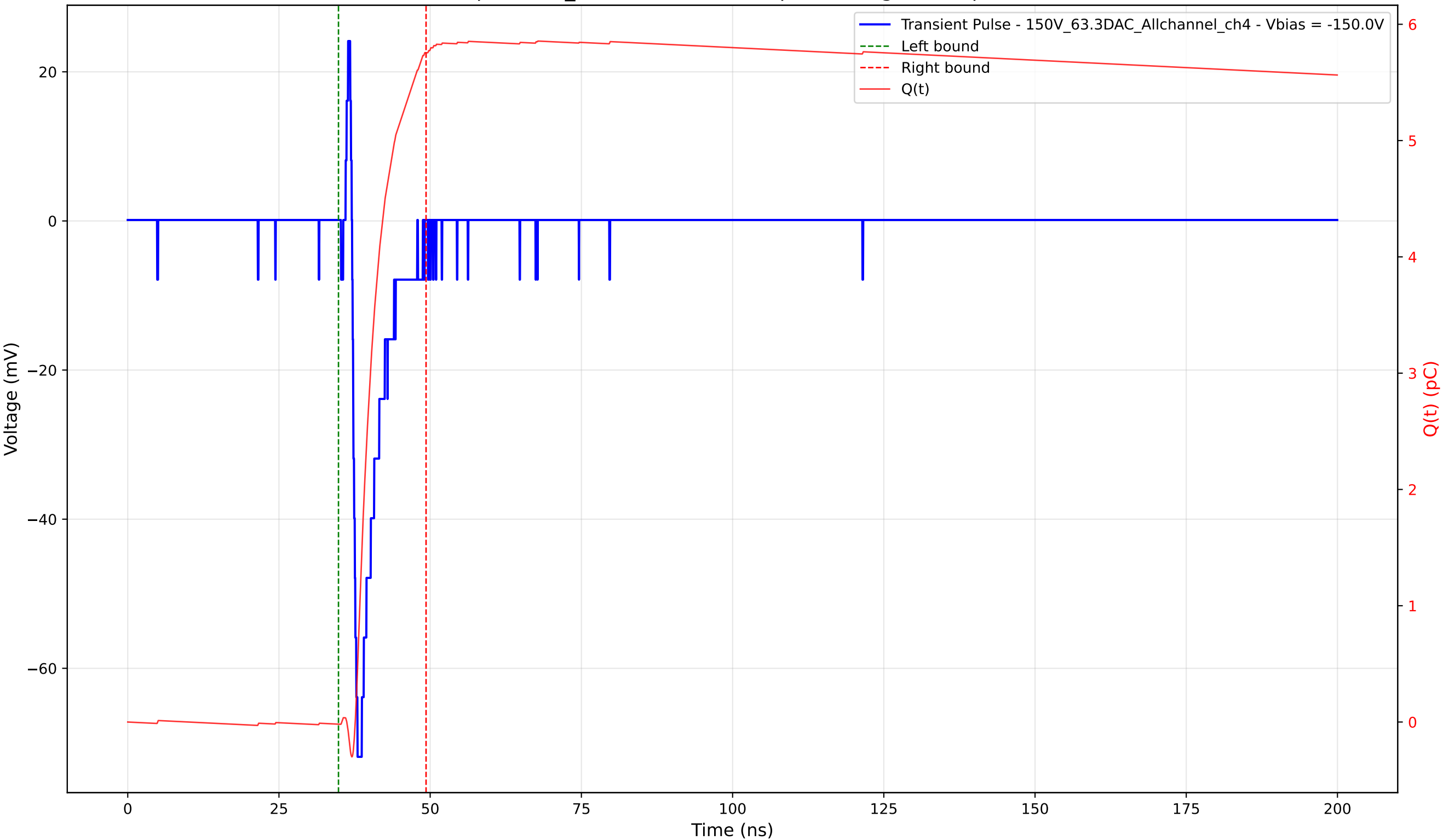
Transient Pulse - Sample: 1cm_42 - Position: 630.0 \mu\text{m} - Charge: 5.77 pC - Rise Time: 0.88 ns
