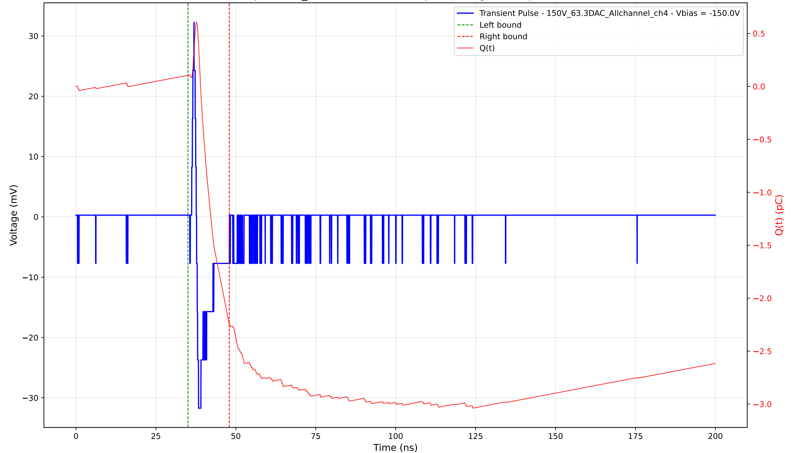
Transient Pulse - Sample: 1cm_42 - Position: 4380.0 \mu\text{m} - Charge: 2.35 pC - Rise Time: 0.71 ns
