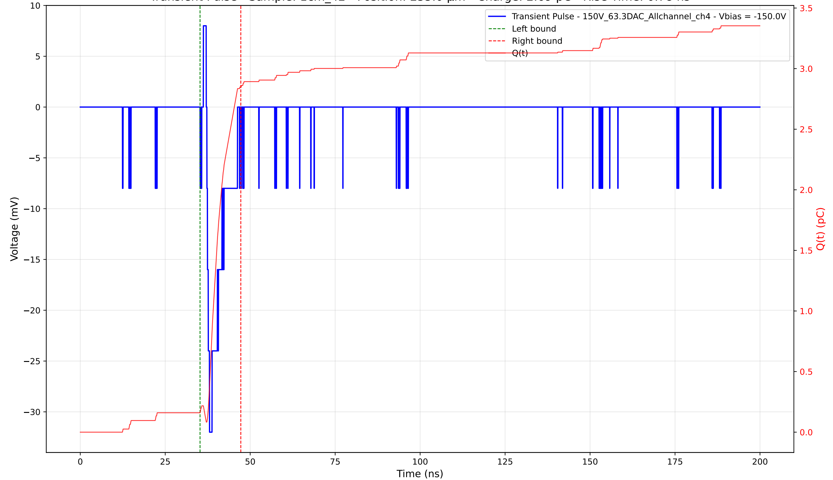
Transient Pulse - Sample: 1cm_42 - Position: 255.0 \mu\text{m} - Charge: 2.69 pC - Rise Time: 0.78 ns
