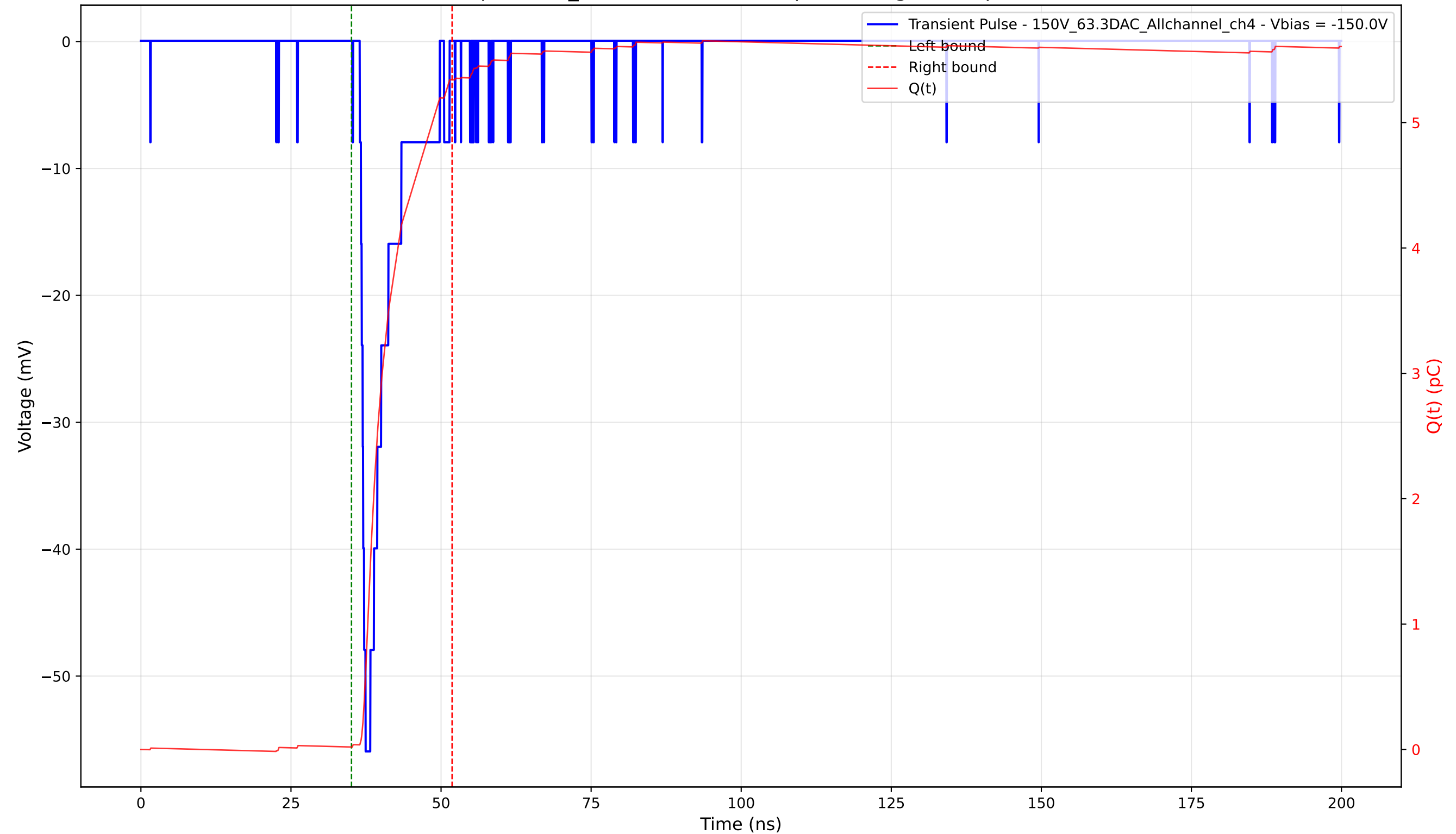
Transient Pulse - Sample: 1cm_42 - Position: 3055.0 \mu\text{m} - Charge: 5.32 pC - Rise Time: 0.97 ns
