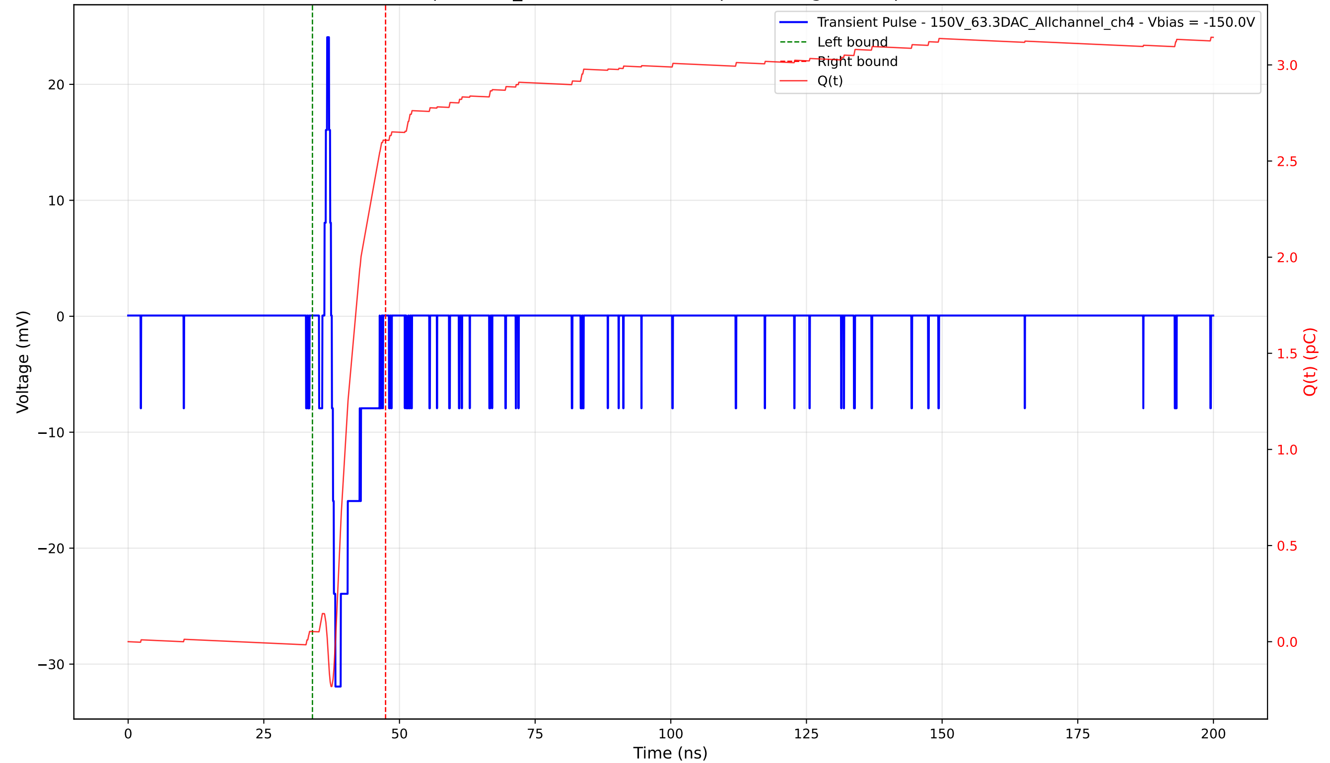
Transient Pulse - Sample: 1cm_42 - Position: 4705.0 \mu\text{m} - Charge: 2.56 pC - Rise Time: 0.66 ns
