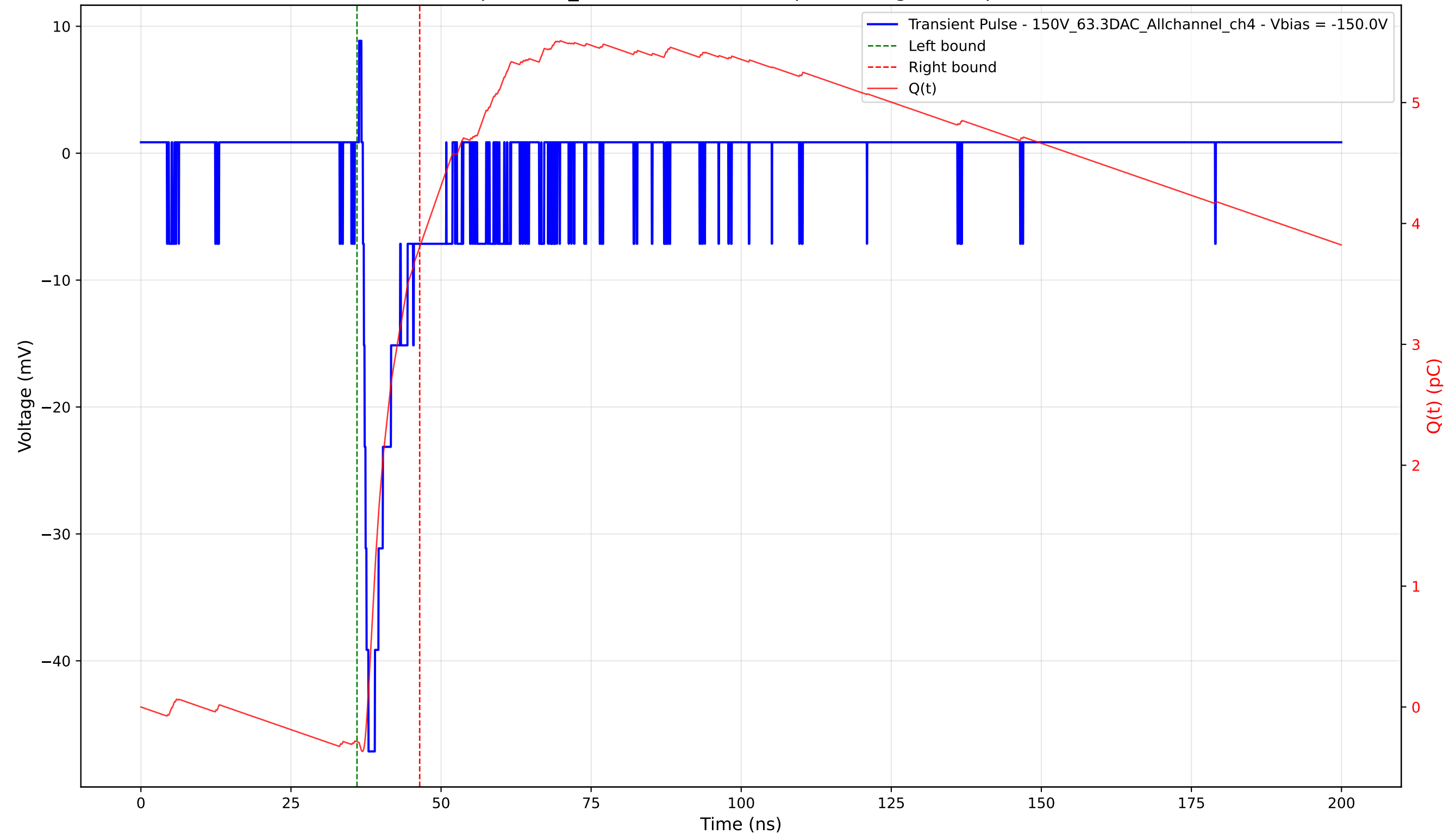
Transient Pulse - Sample: 1cm_42 - Position: 3245.0 \mu\text{m} - Charge: 4.09 pC - Rise Time: 0.94 ns
