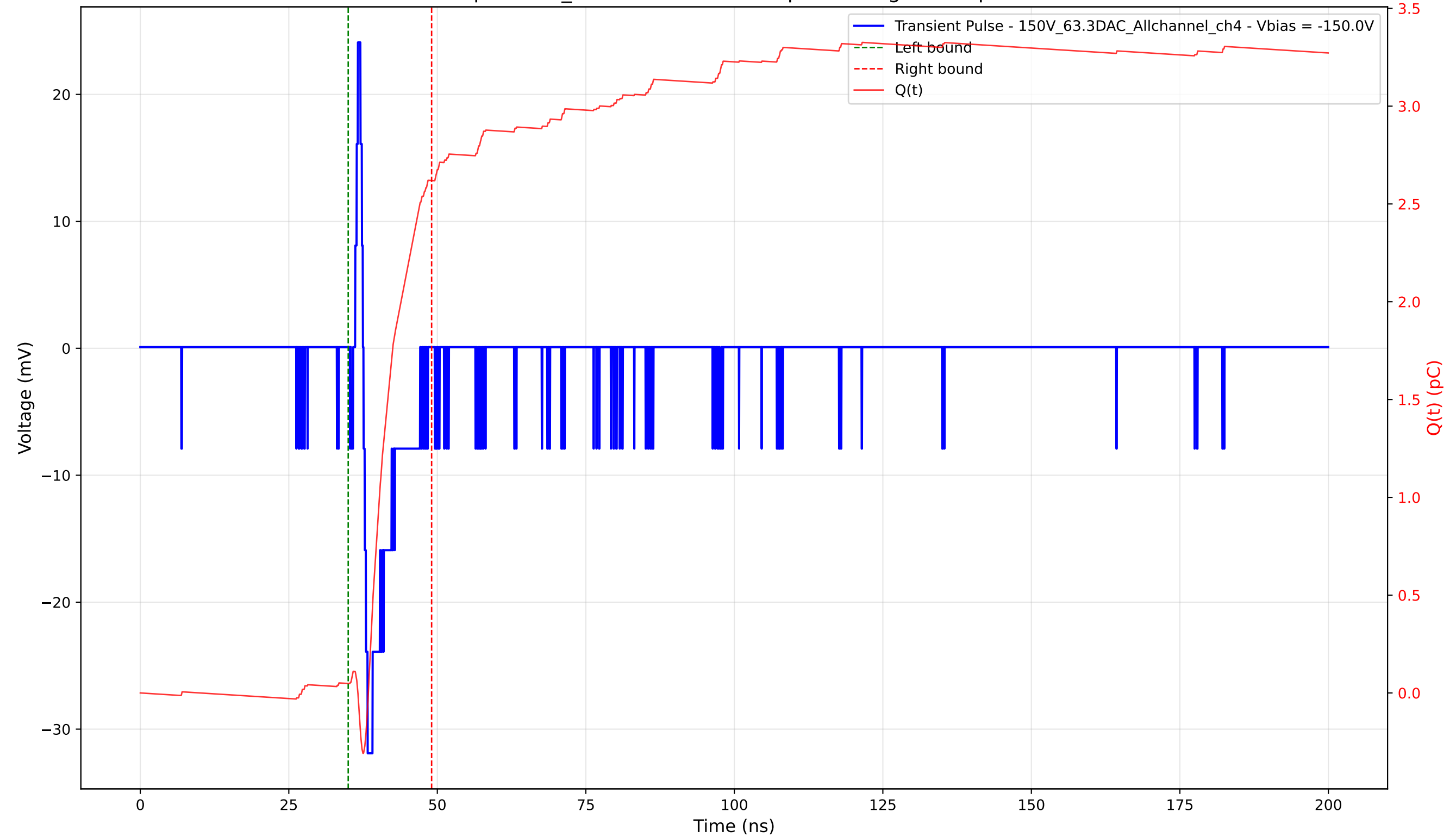
Transient Pulse - Sample: 1cm_42 - Position: 4670.0 \mu\text{m} - Charge: 2.57 pC - Rise Time: 0.70 ns
