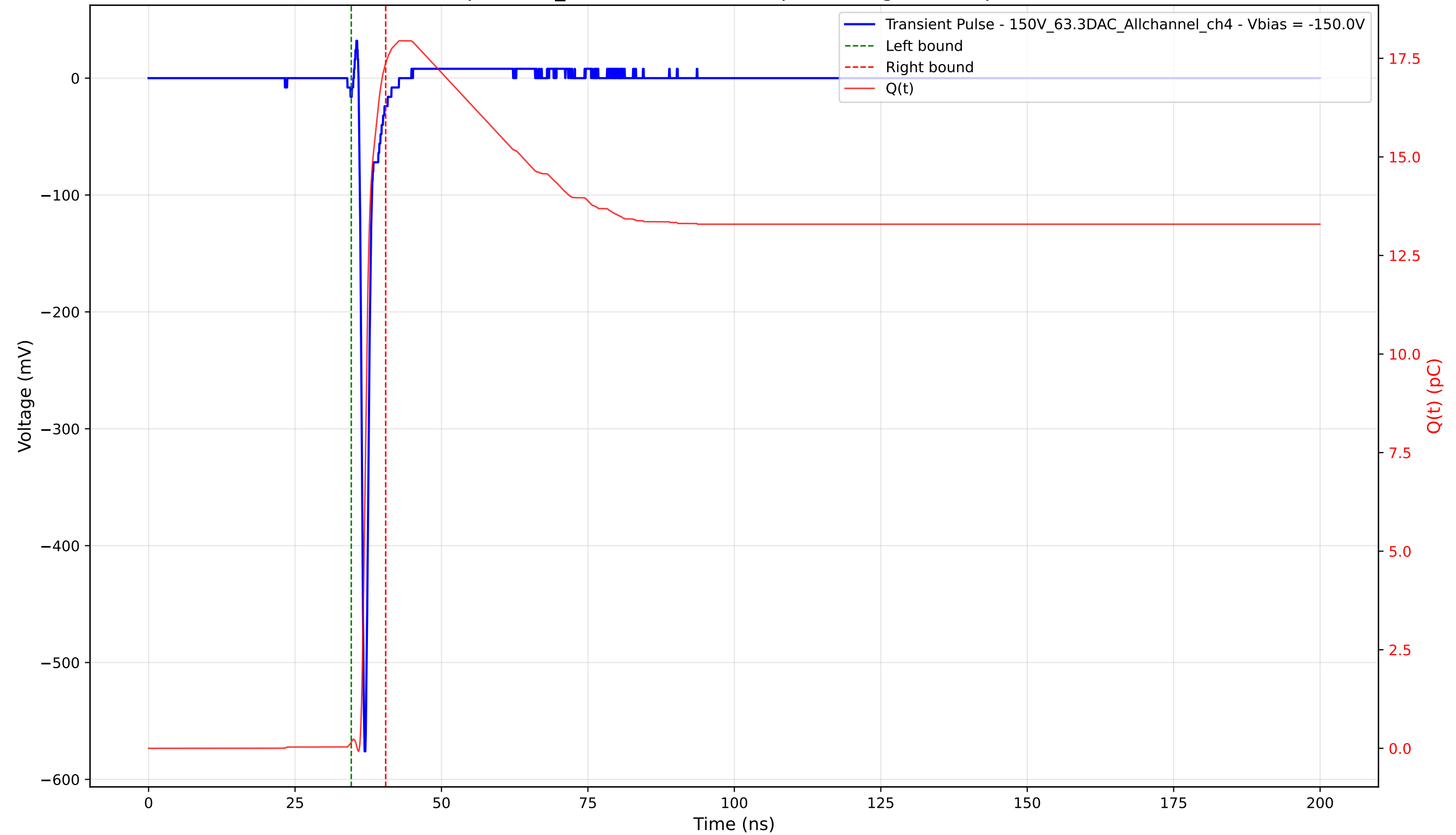
Transient Pulse - Sample: 1cm_42 - Position: 2075.0 \mu\text{m} - Charge: 17.21 pC - Rise Time: 0.69 ns
