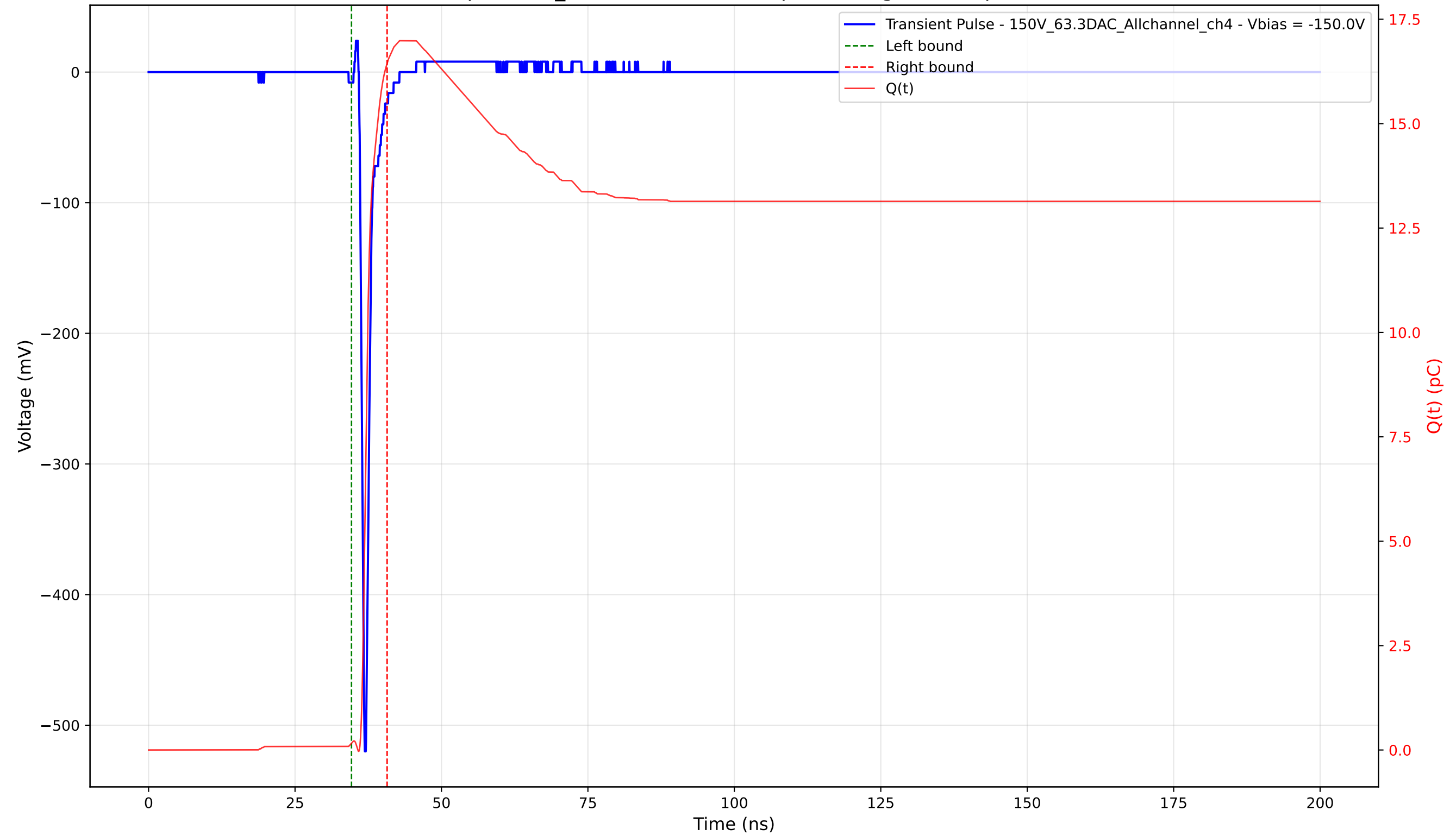
Transient Pulse - Sample: 1cm_42 - Position: 2220.0 \mu\text{m} - Charge: 16.28 pC - Rise Time: 0.70 ns
