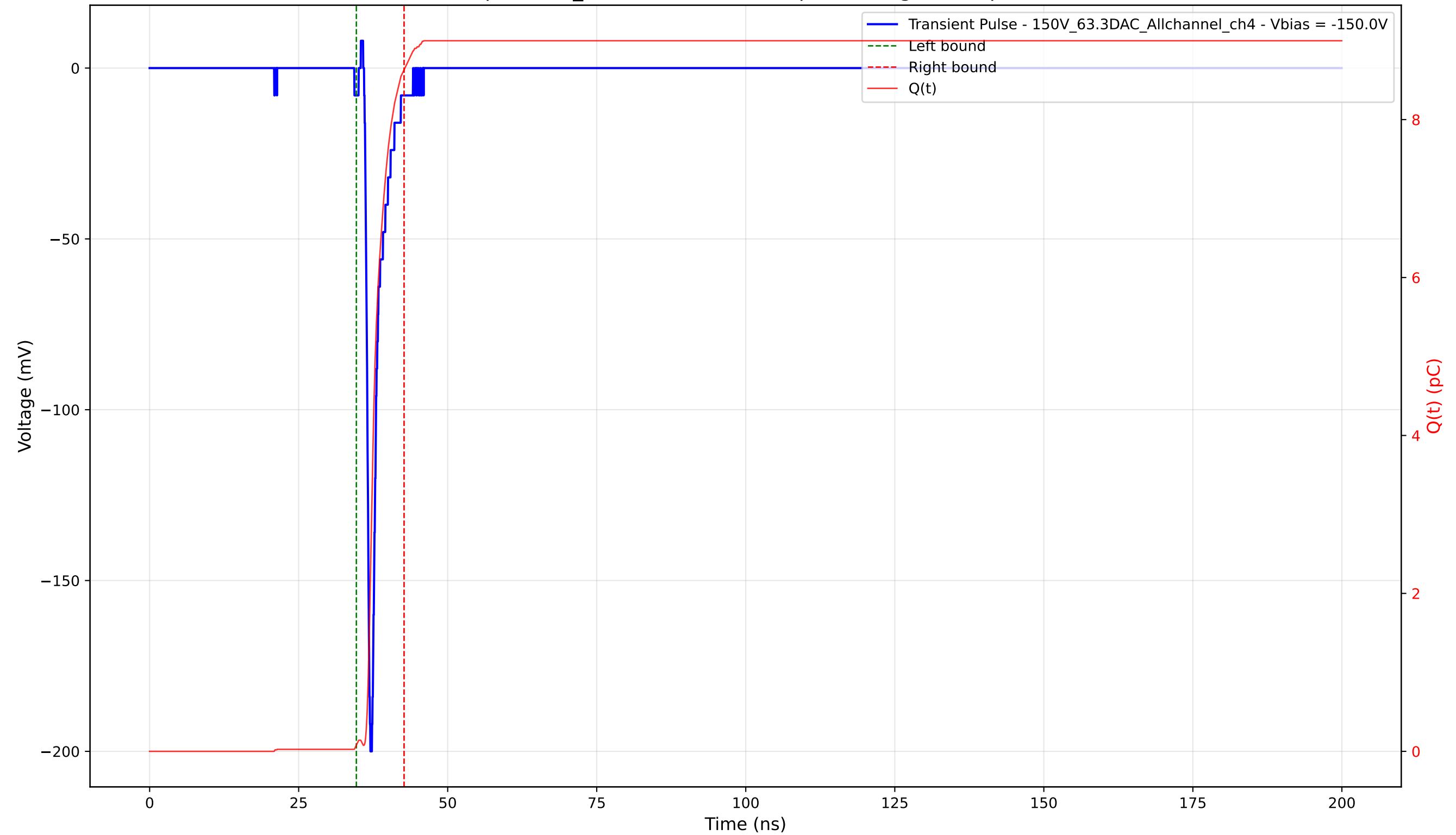
Transient Pulse - Sample: 1cm_42 - Position: 2565.0 \mu\text{m} - Charge: 8.55 pC - Rise Time: 0.74 ns
