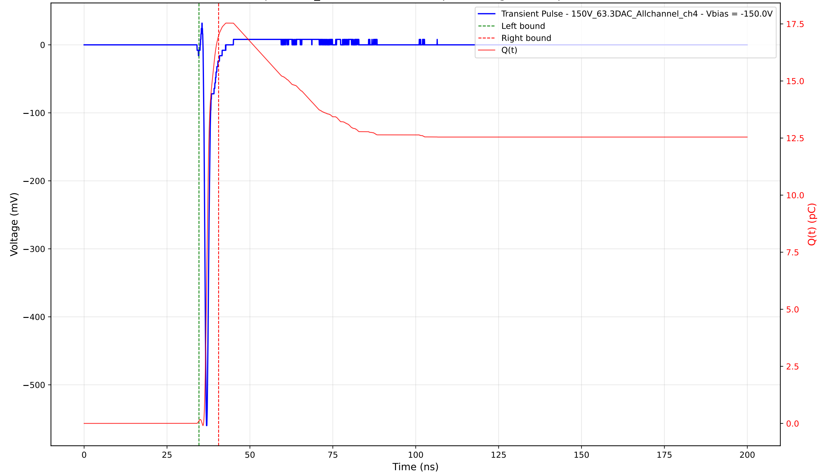
Transient Pulse - Sample: 1cm_42 - Position: 2125.0 \mu\text{m} - Charge: 16.86 pC - Rise Time: 0.70 ns
