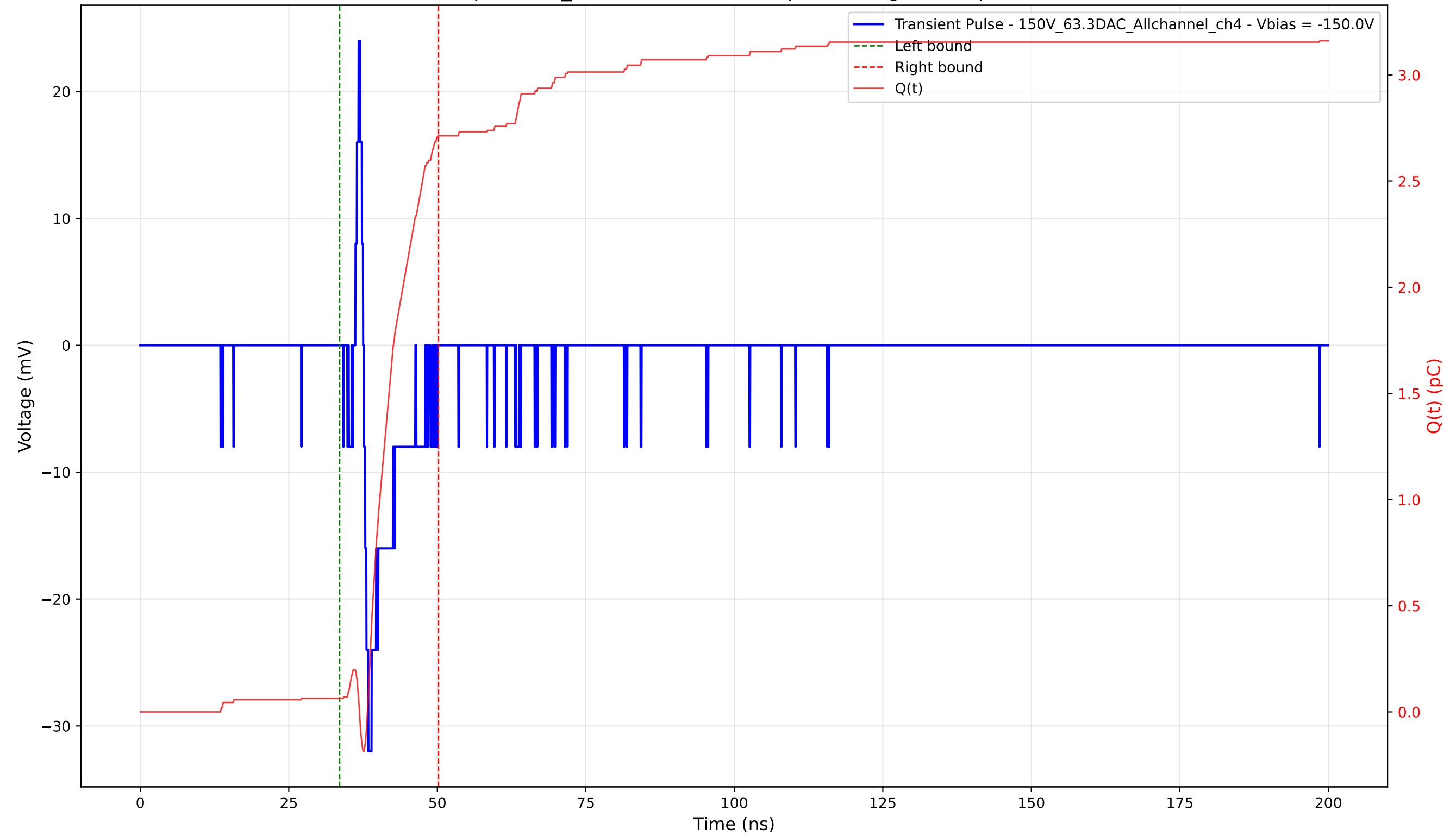
Transient Pulse - Sample: 1cm_42 - Position: 4565.0 \mu\text{m} - Charge: 2.65 pC - Rise Time: 0.74 ns
