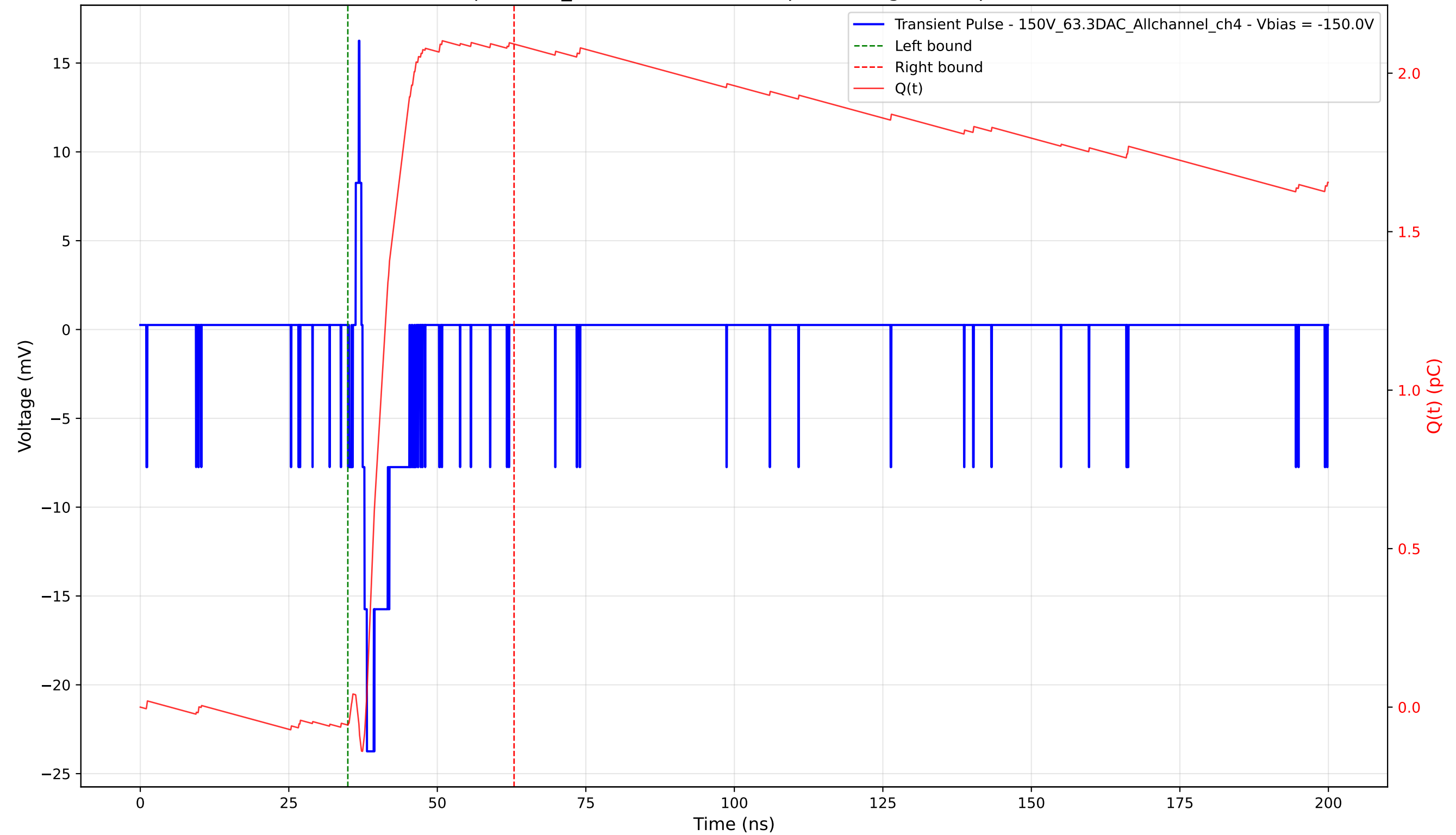
Transient Pulse - Sample: 1cm_42 - Position: 4975.0 \mu\text{m} - Charge: 2.15 pC - Rise Time: 0.75 ns
