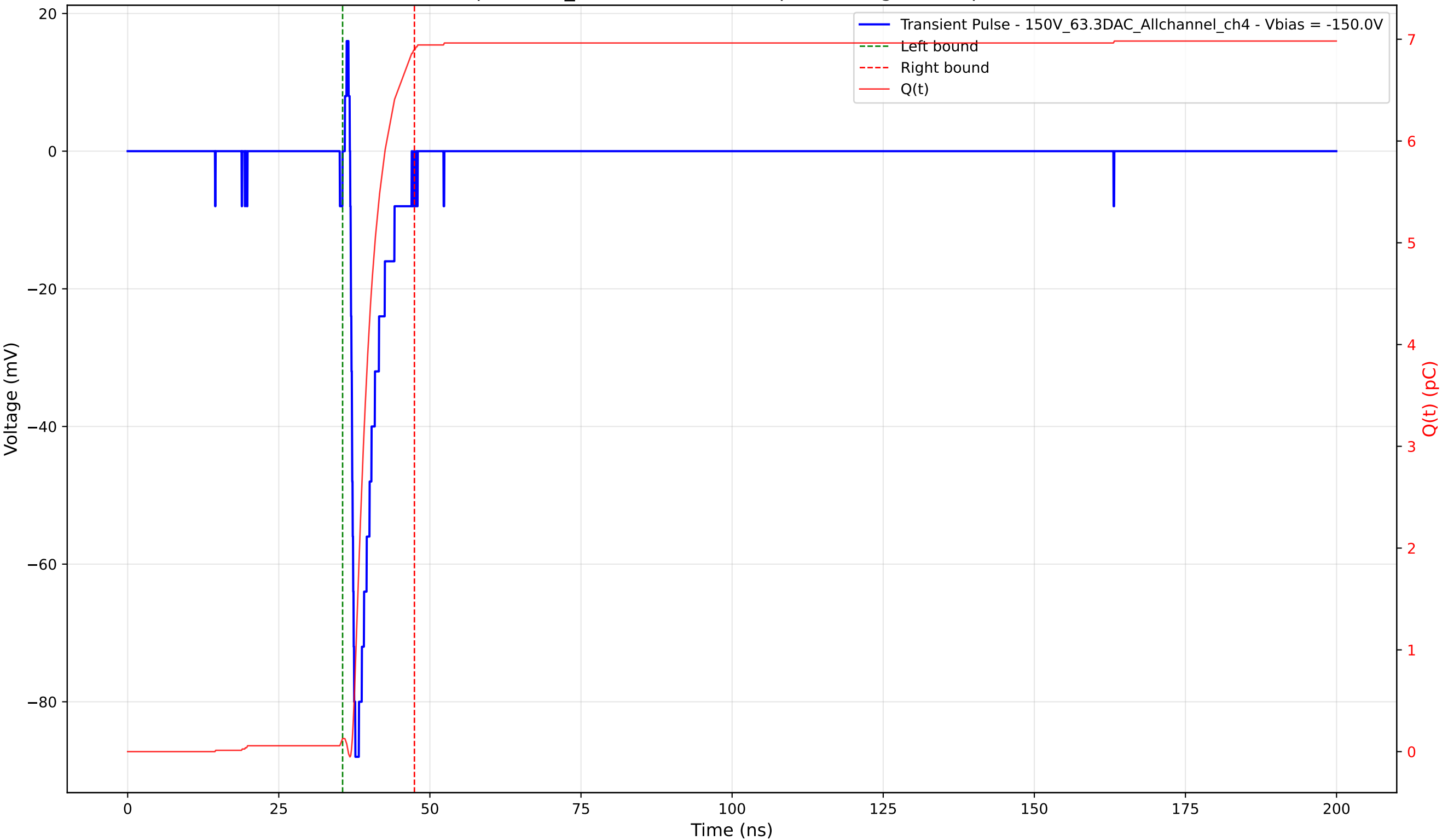
Transient Pulse - Sample: 1cm_42 - Position: 945.0 \mu\text{m} - Charge: 6.76 pC - Rise Time: 0.60 ns
