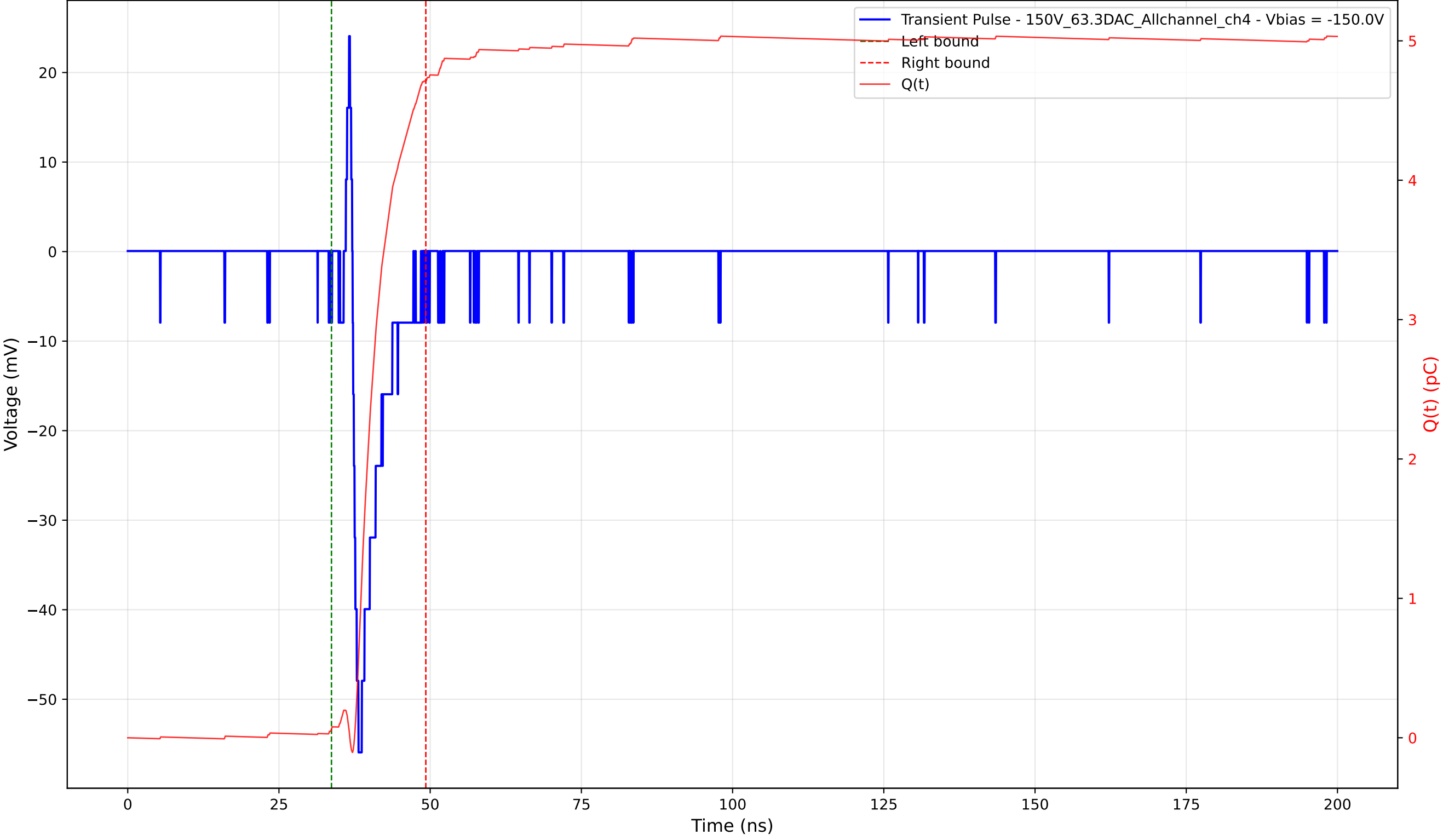
Transient Pulse - Sample: 1cm_42 - Position: 500.0 \mu\text{m} - Charge: 4.65 pC - Rise Time: 0.97 ns
