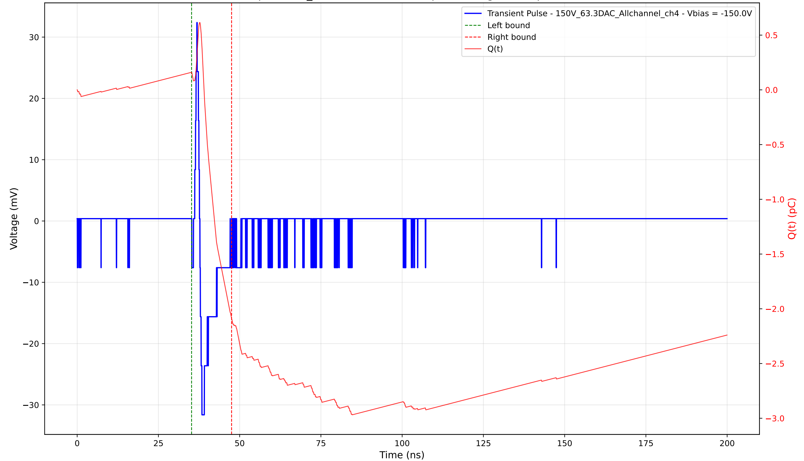
Transient Pulse - Sample: 1cm_42 - Position: 4150.0 \mu\text{m} - Charge: 2.25 pC - Rise Time: 0.71 ns
