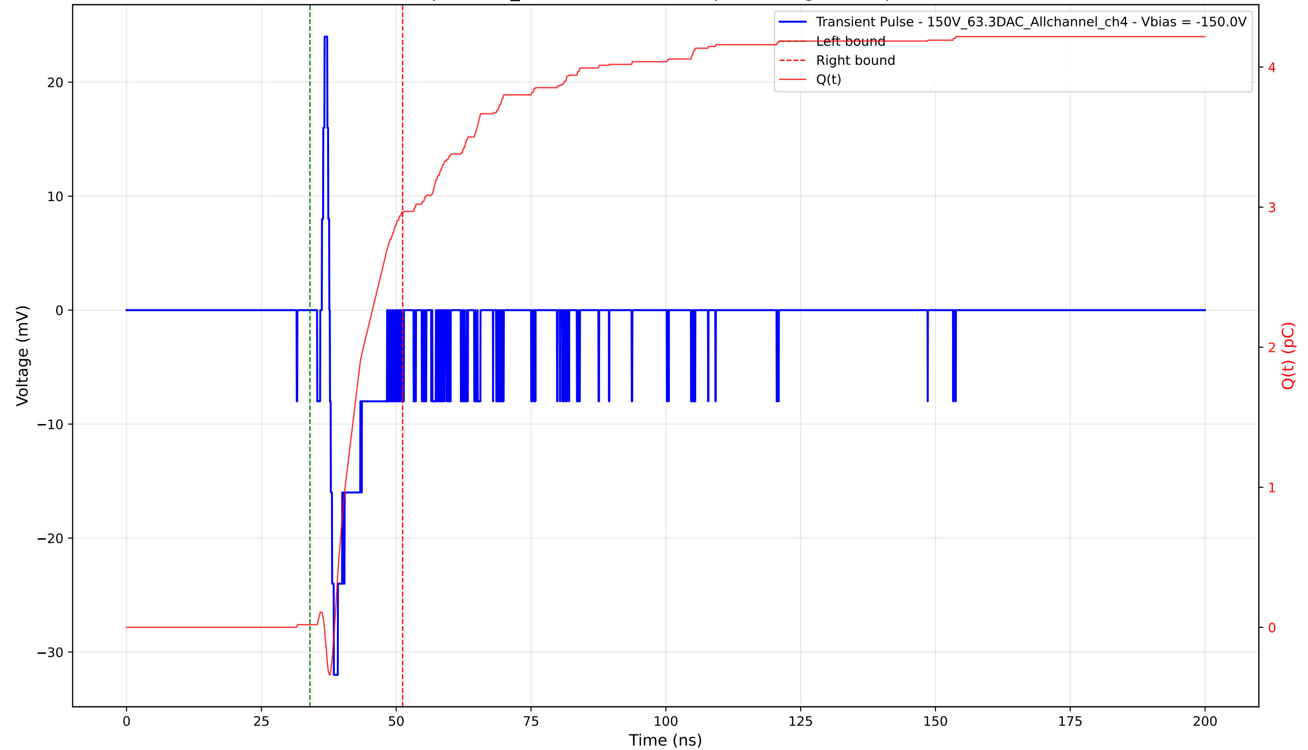
Transient Pulse - Sample: 1cm_42 - Position: 3945.0 \mu\text{m} - Charge: 2.94 pC - Rise Time: 0.74 ns
