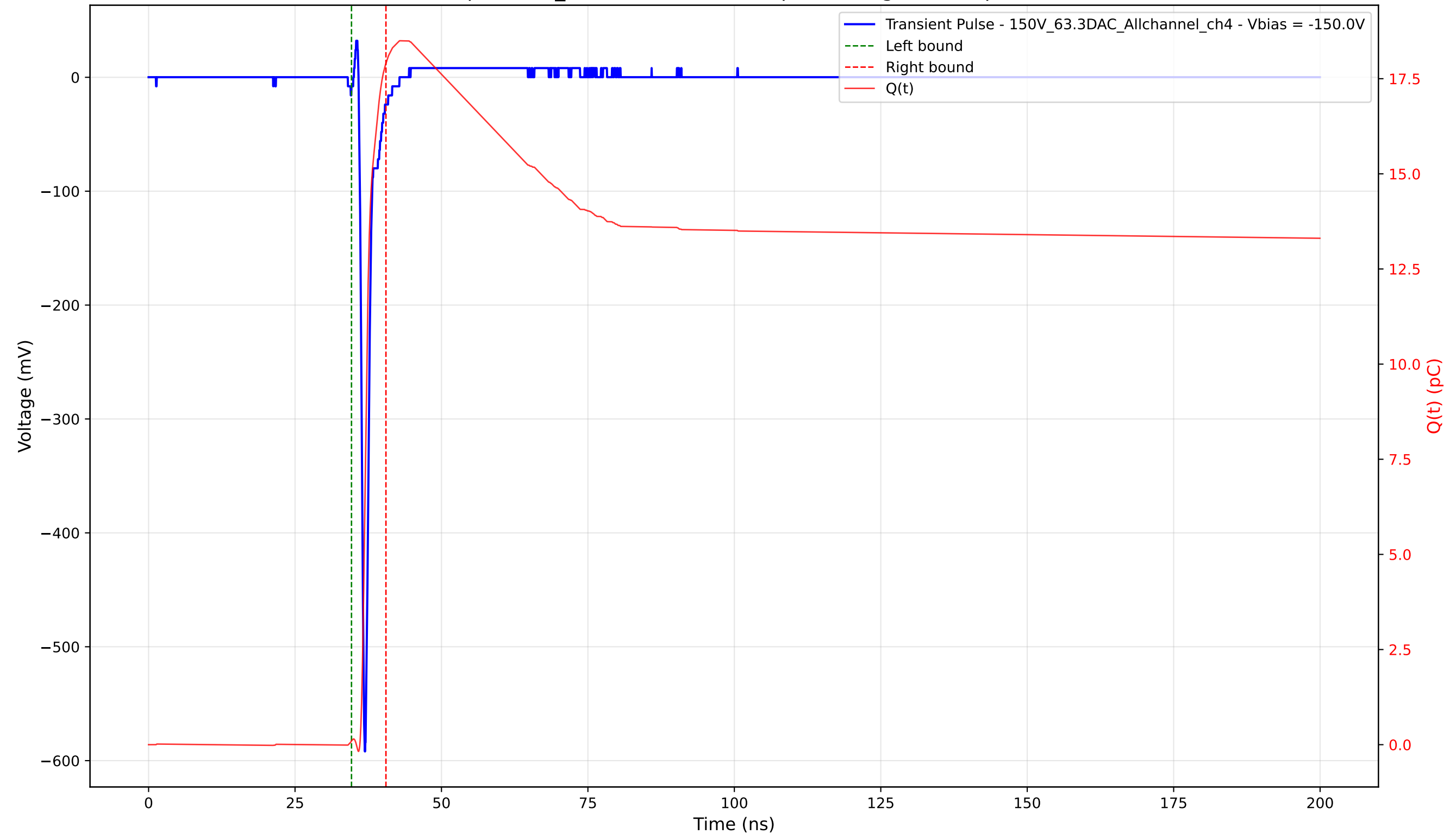
Transient Pulse - Sample: 1cm_42 - Position: 1990.0 \mu\text{m} - Charge: 17.80 pC - Rise Time: 0.70 ns
