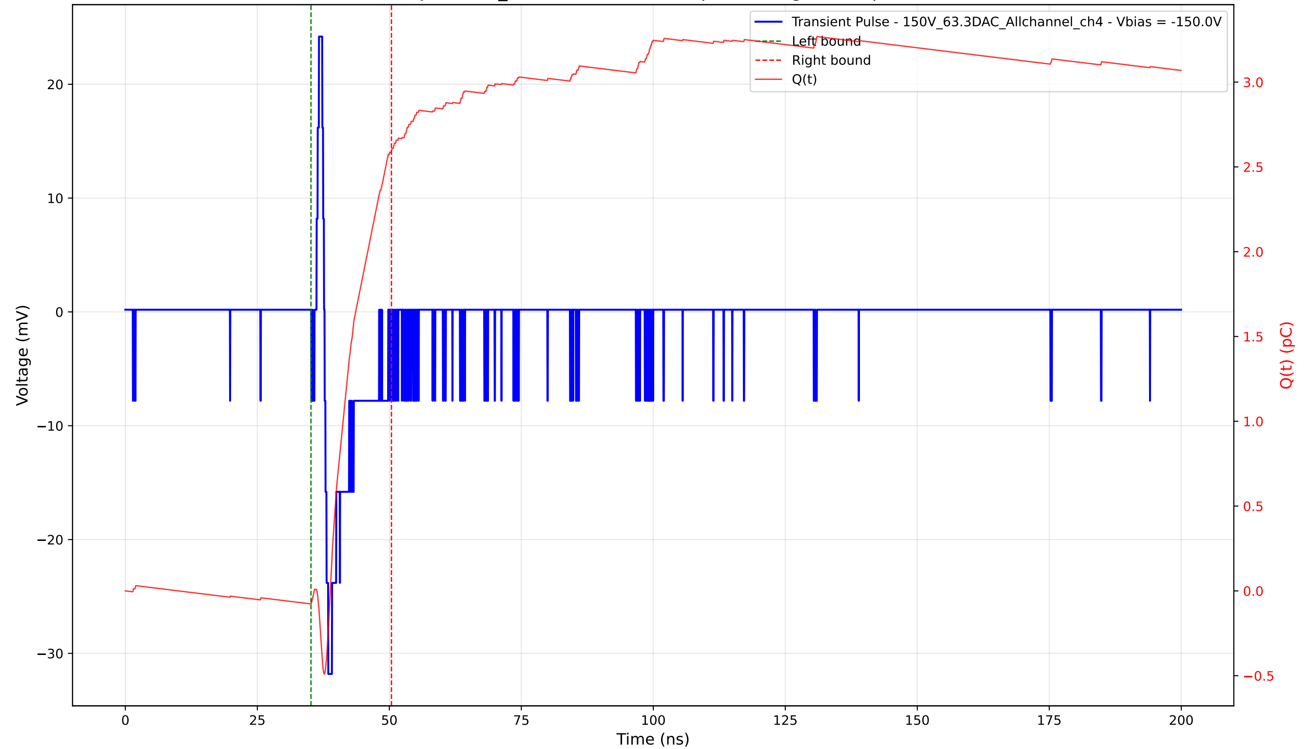
Transient Pulse - Sample: 1cm_42 - Position: 4115.0 \mu\text{m} - Charge: 2.67 pC - Rise Time: 0.70 ns
