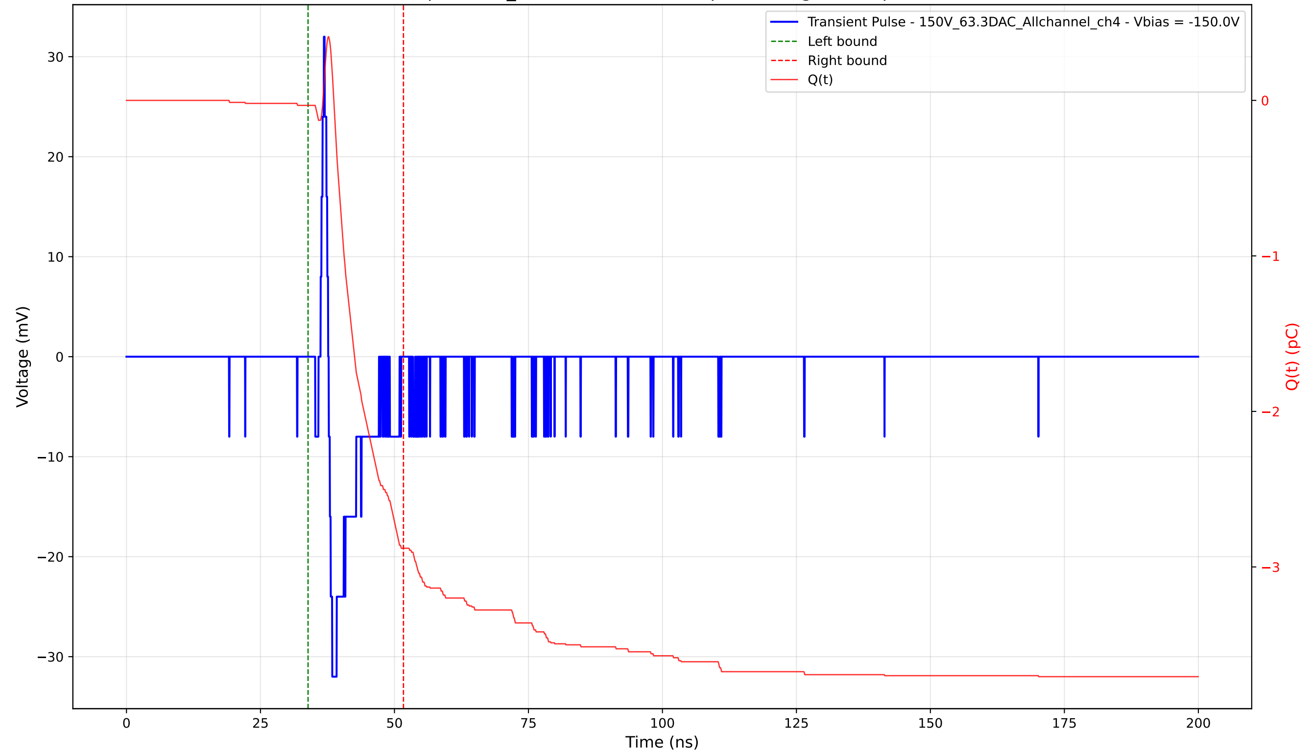
Transient Pulse - Sample: 1cm_42 - Position: 4370.0 \mu\text{m} - Charge: 2.85 pC - Rise Time: 0.62 ns
