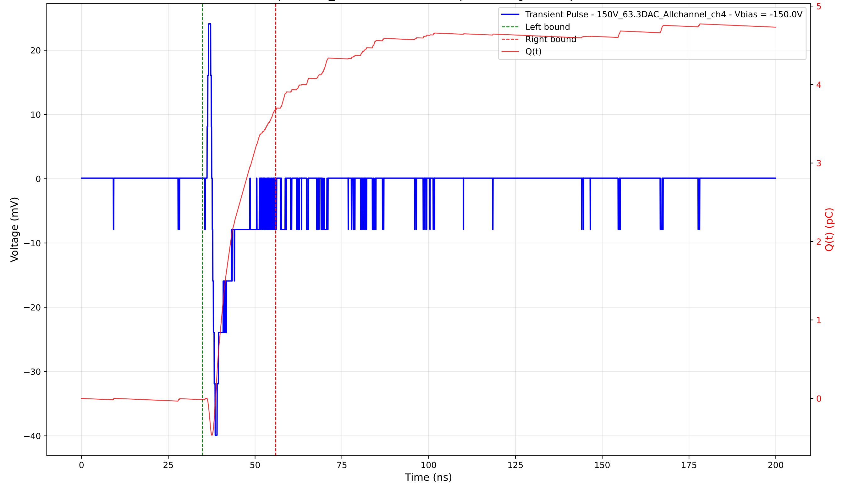
Transient Pulse - Sample: 1cm_42 - Position: 3725.0 \mu\text{m} - Charge: 3.70 pC - Rise Time: 0.86 ns
