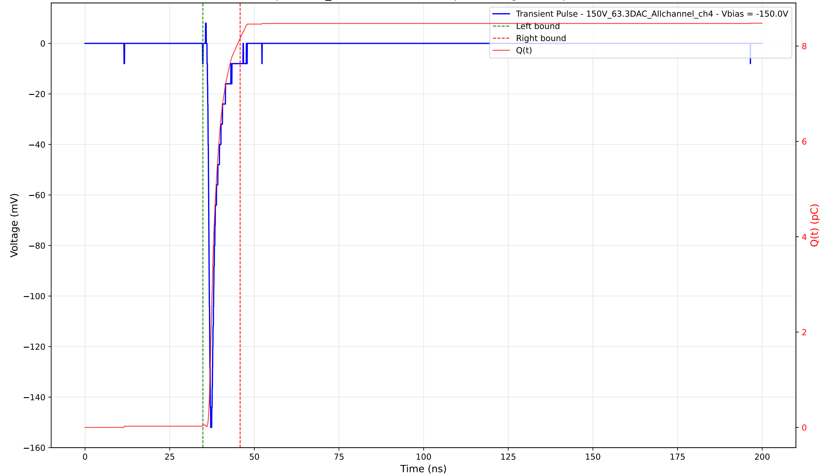
Transient Pulse - Sample: 1cm_42 - Position: 2680.0 \mu\text{m} - Charge: 8.12 pC - Rise Time: 0.84 ns
