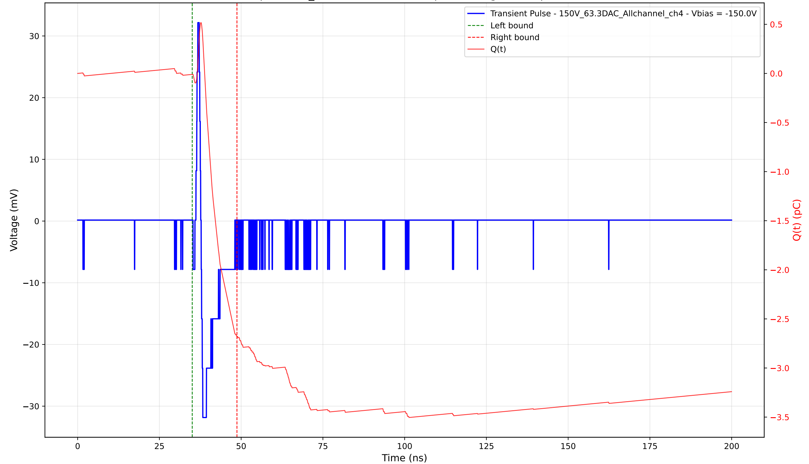
Transient Pulse - Sample: 1cm_42 - Position: 4285.0 \mu\text{m} - Charge: 2.67 pC - Rise Time: 0.58 ns
