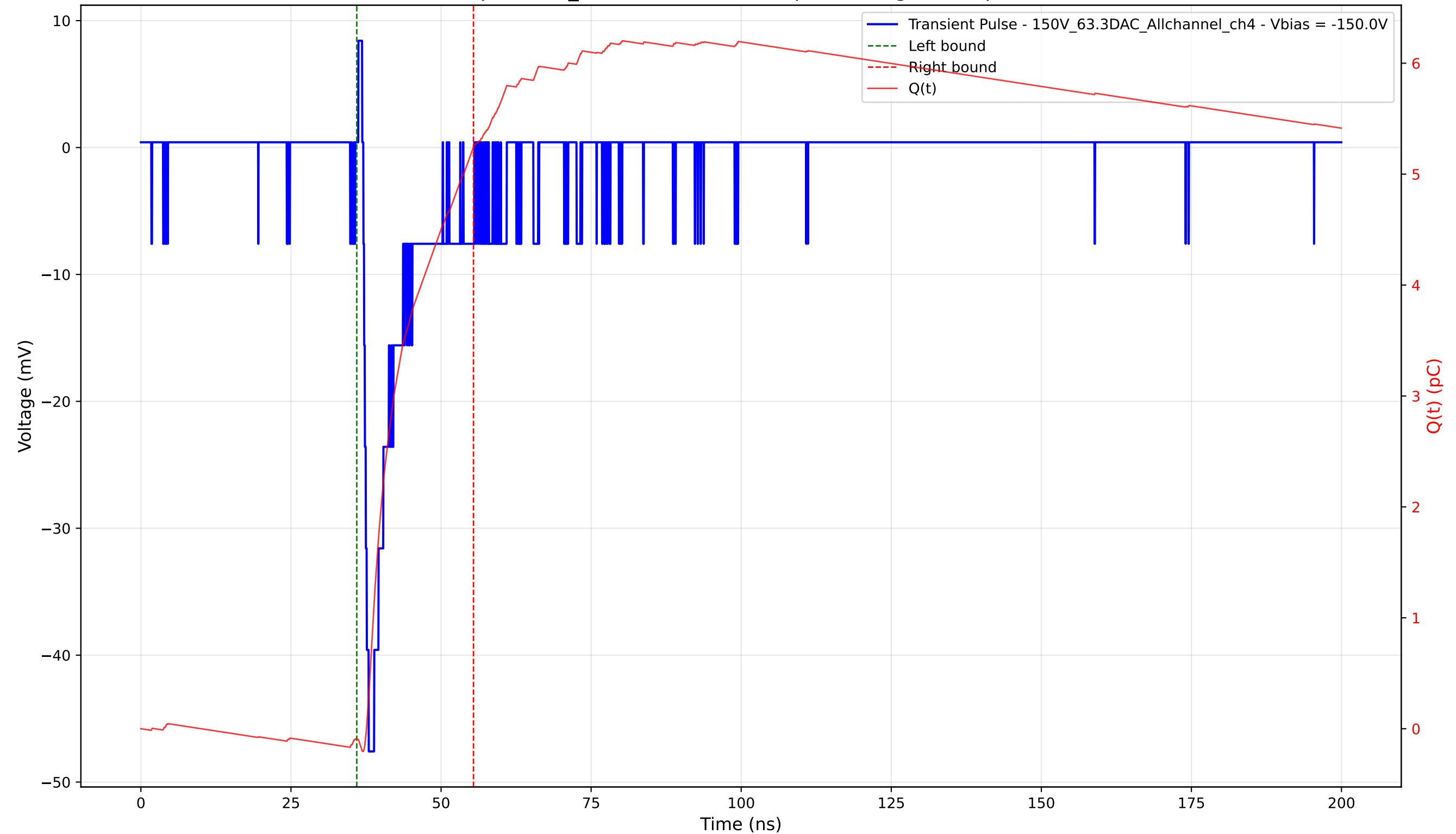
Transient Pulse - Sample: 1cm_42 - Position: 3290.0 \mu\text{m} - Charge: 5.34 pC - Rise Time: 0.90 ns
