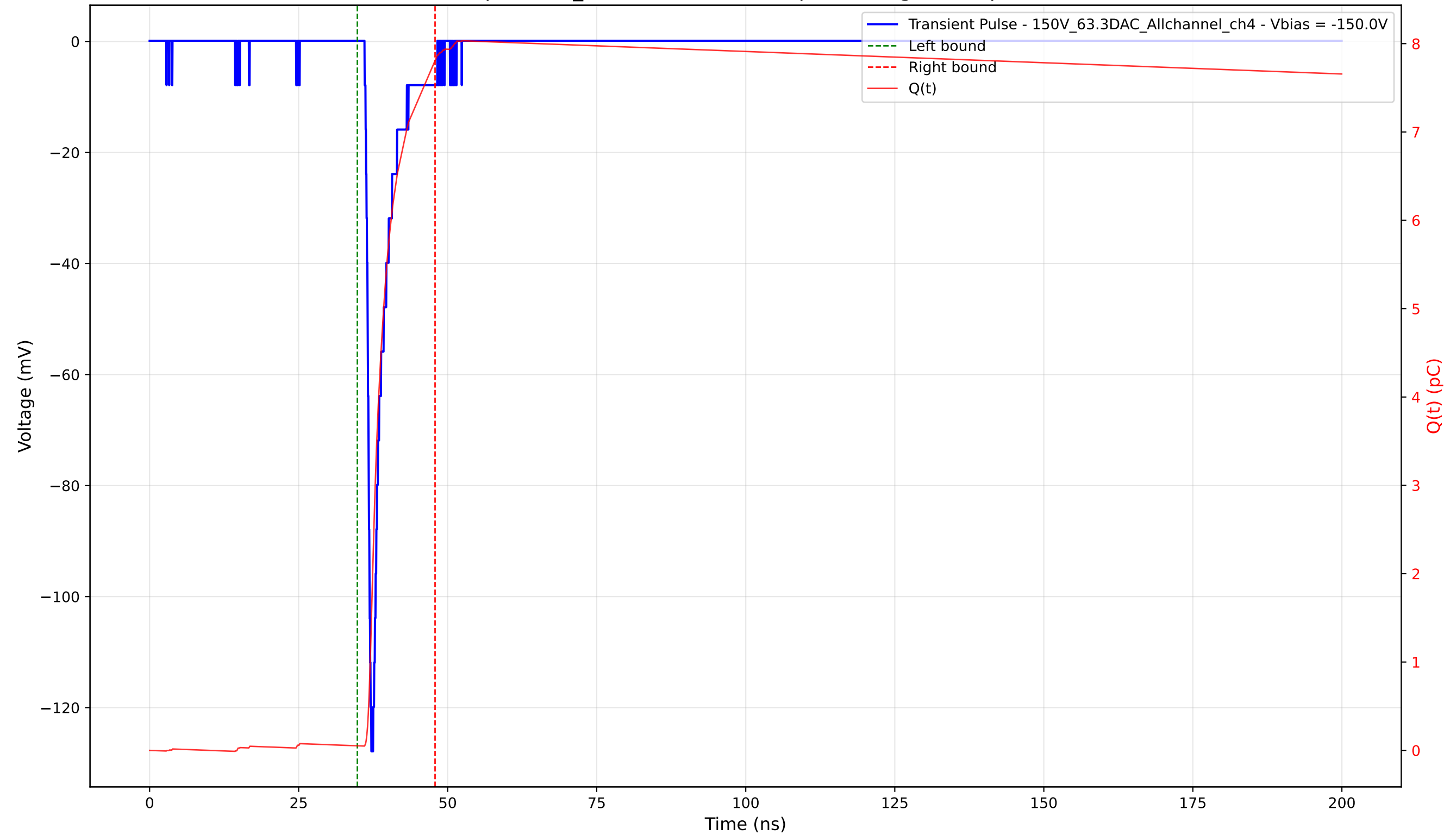
Transient Pulse - Sample: 1cm_42 - Position: 2815.0 \mu\text{m} - Charge: 7.76 pC - Rise Time: 0.86 ns
