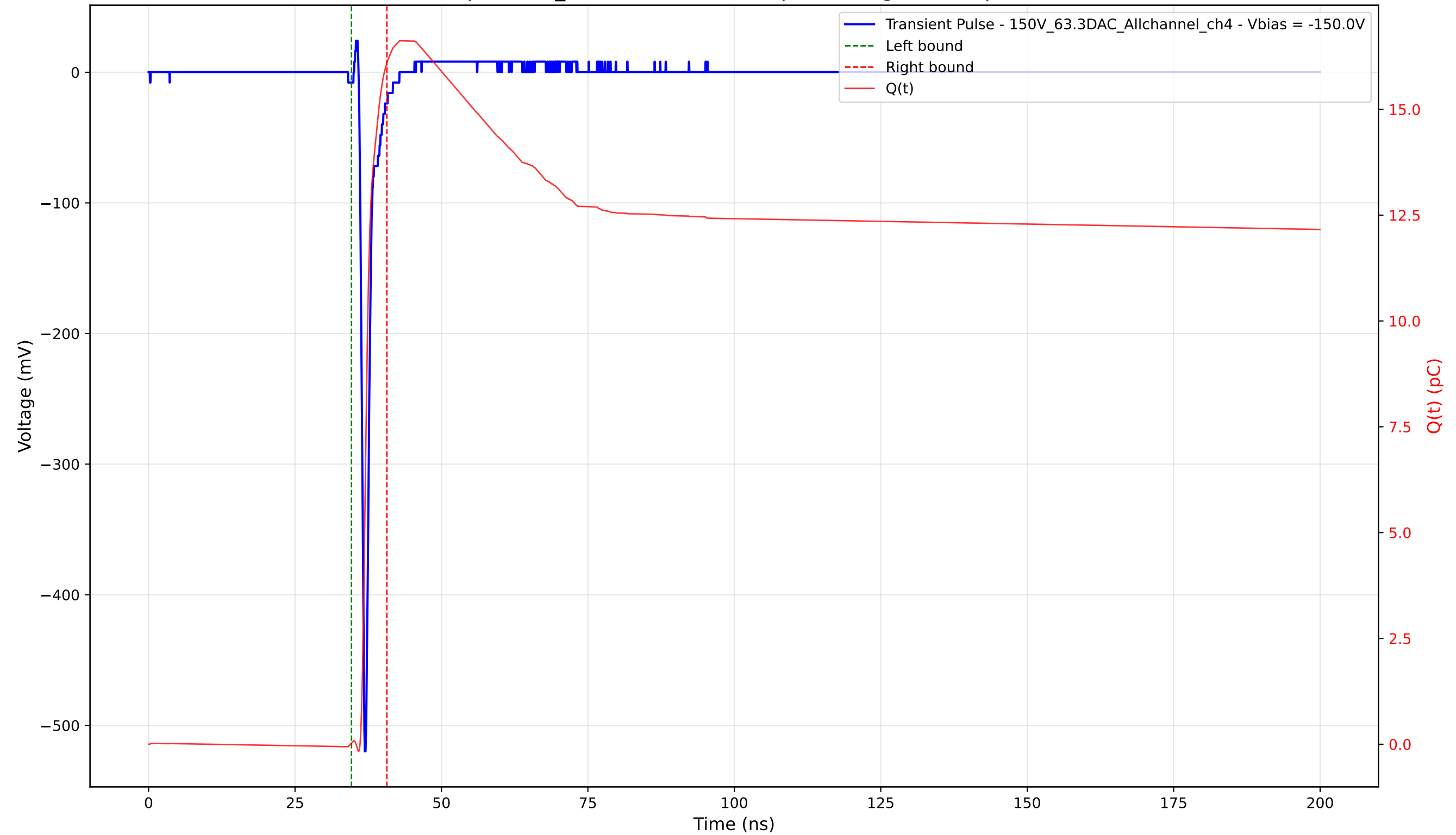
Transient Pulse - Sample: 1cm_42 - Position: 2185.0 \mu\text{m} - Charge: 16.07 pC - Rise Time: 0.70 ns
