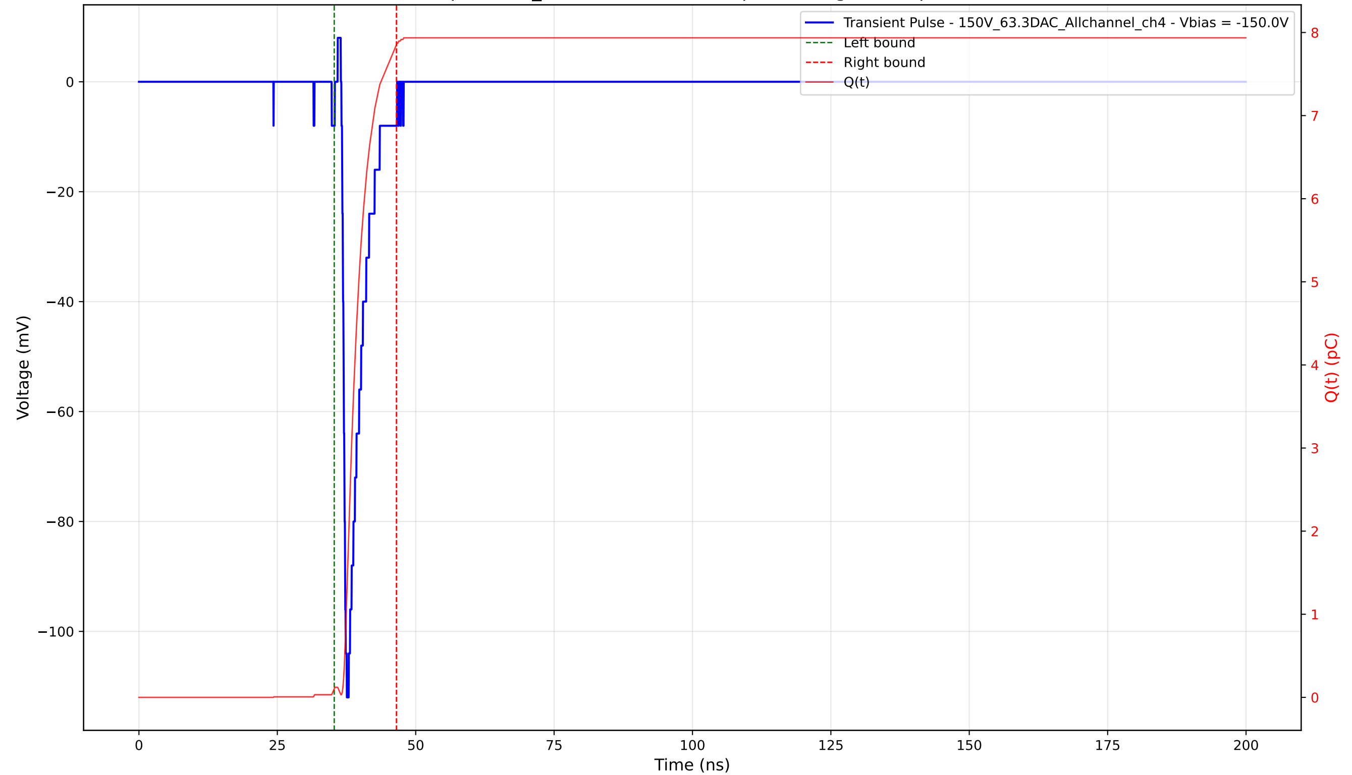
Transient Pulse - Sample: 1cm_42 - Position: 1055.0 \mu\text{m} - Charge: 7.75 pC - Rise Time: 0.66 ns
