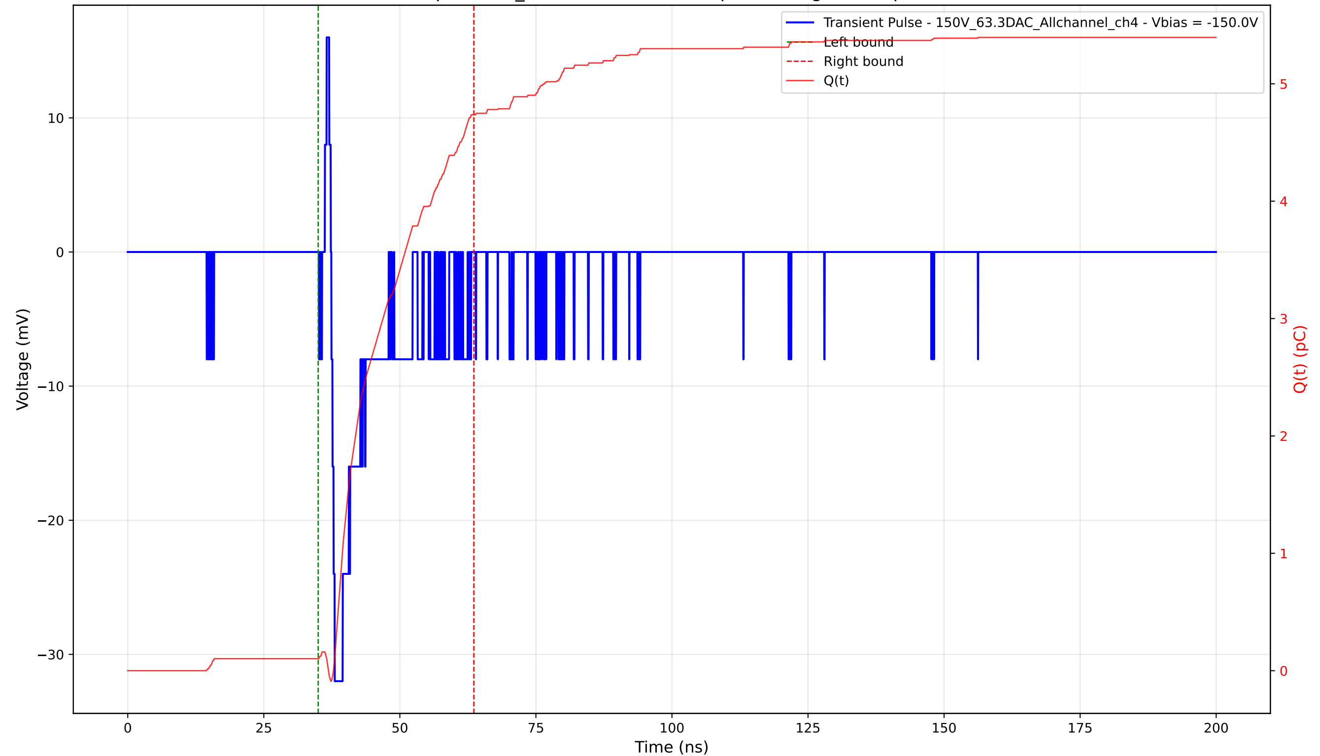
Transient Pulse - Sample: 1cm_42 - Position: 3540.0 \mu\text{m} - Charge: 4.63 pC - Rise Time: 0.62 ns
