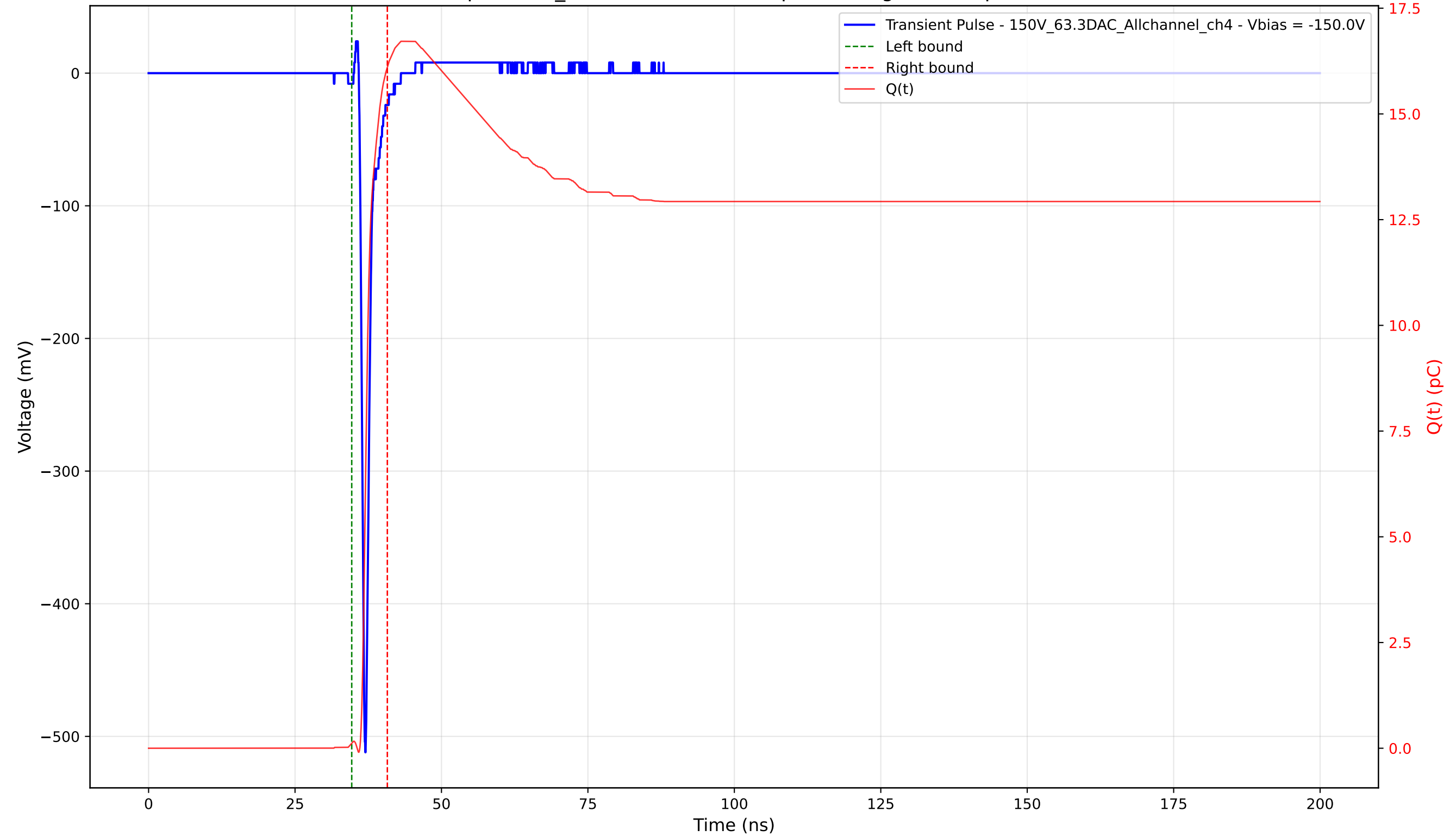
Transient Pulse - Sample: 1cm_42 - Position: 2255.0 \mu\text{m} - Charge: 15.99 pC - Rise Time: 0.72 ns
