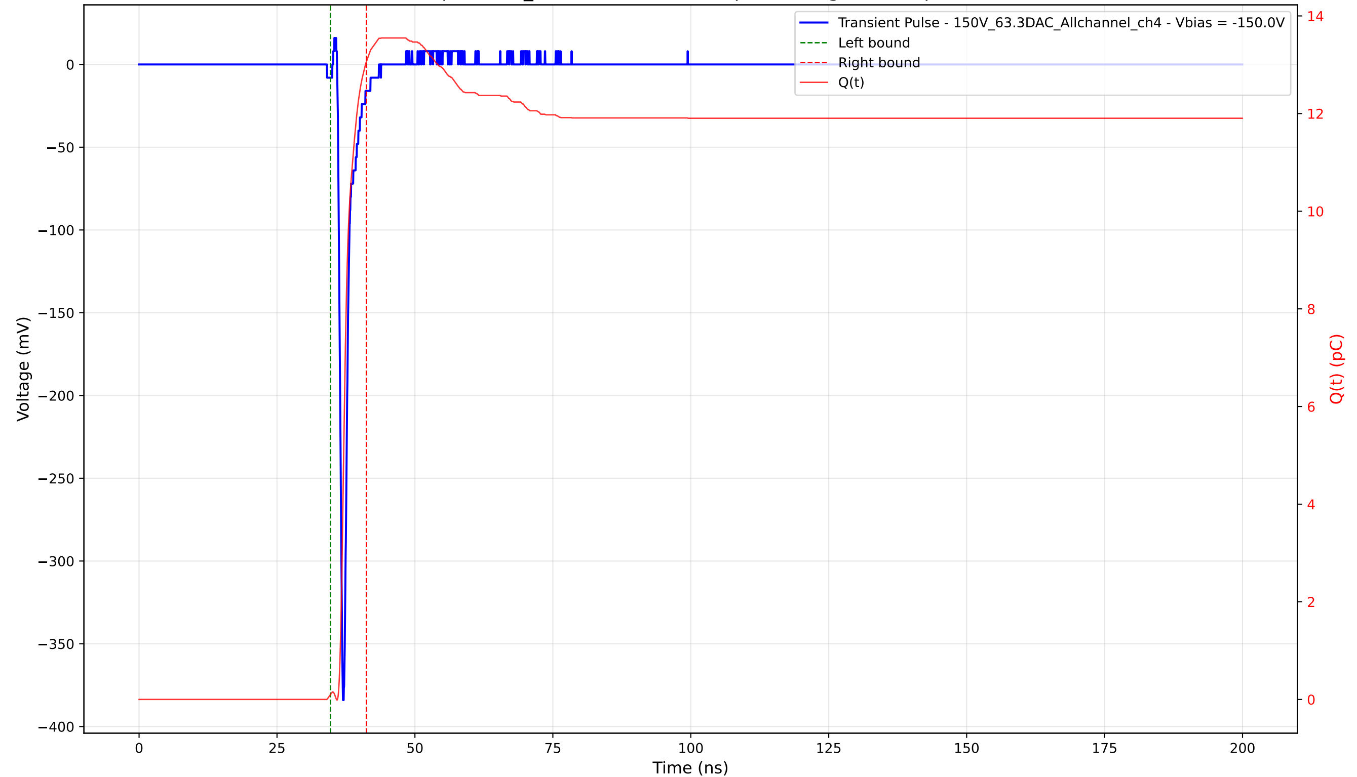
Transient Pulse - Sample: 1cm_42 - Position: 2385.0 \mu\text{m} - Charge: 12.96 pC - Rise Time: 0.71 ns
