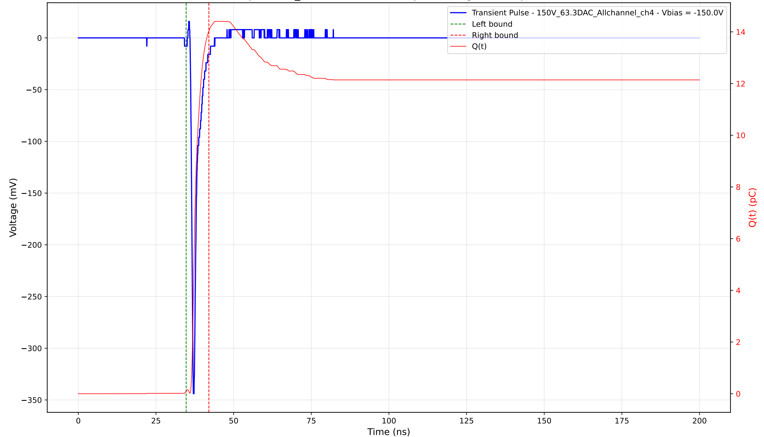
Transient Pulse - Sample: 1cm_42 - Position: 1580.0 \mu\text{m} - Charge: 13.93 pC - Rise Time: 0.74 ns
