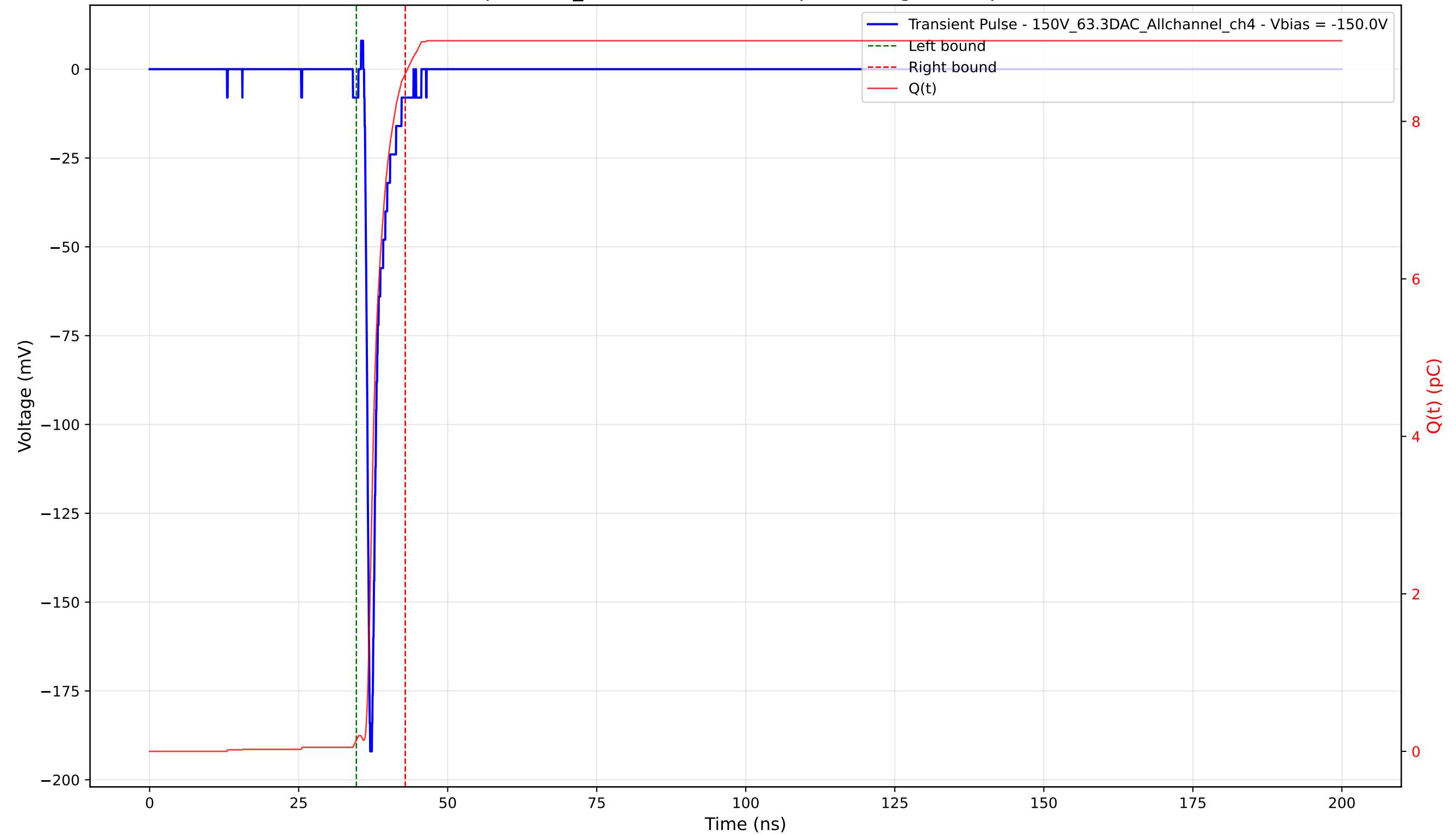
Transient Pulse - Sample: 1cm_42 - Position: 2575.0 \mu\text{m} - Charge: 8.46 pC - Rise Time: 0.73 ns
