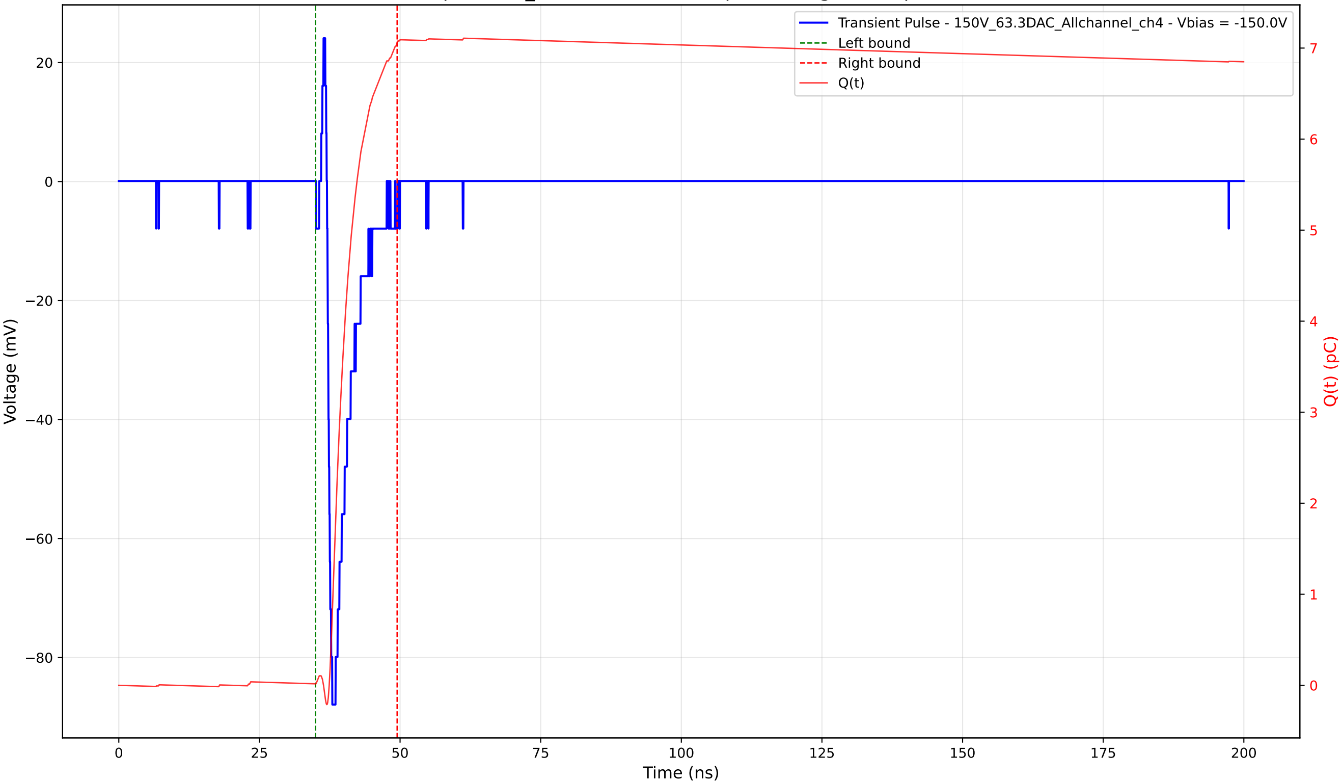
Transient Pulse - Sample: 1cm_42 - Position: 790.0 \mu\text{m} - Charge: 7.04 pC - Rise Time: 0.68 ns
