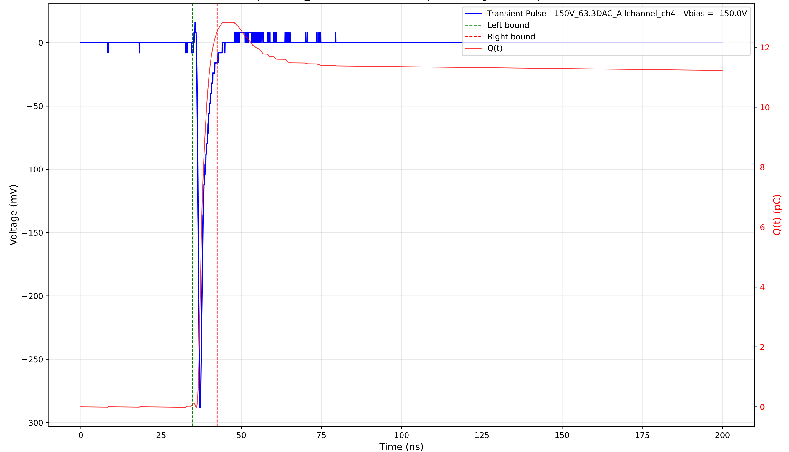
Transient Pulse - Sample: 1cm_42 - Position: 1530.0 \mu\text{m} - Charge: 12.45 pC - Rise Time: 0.71 ns
