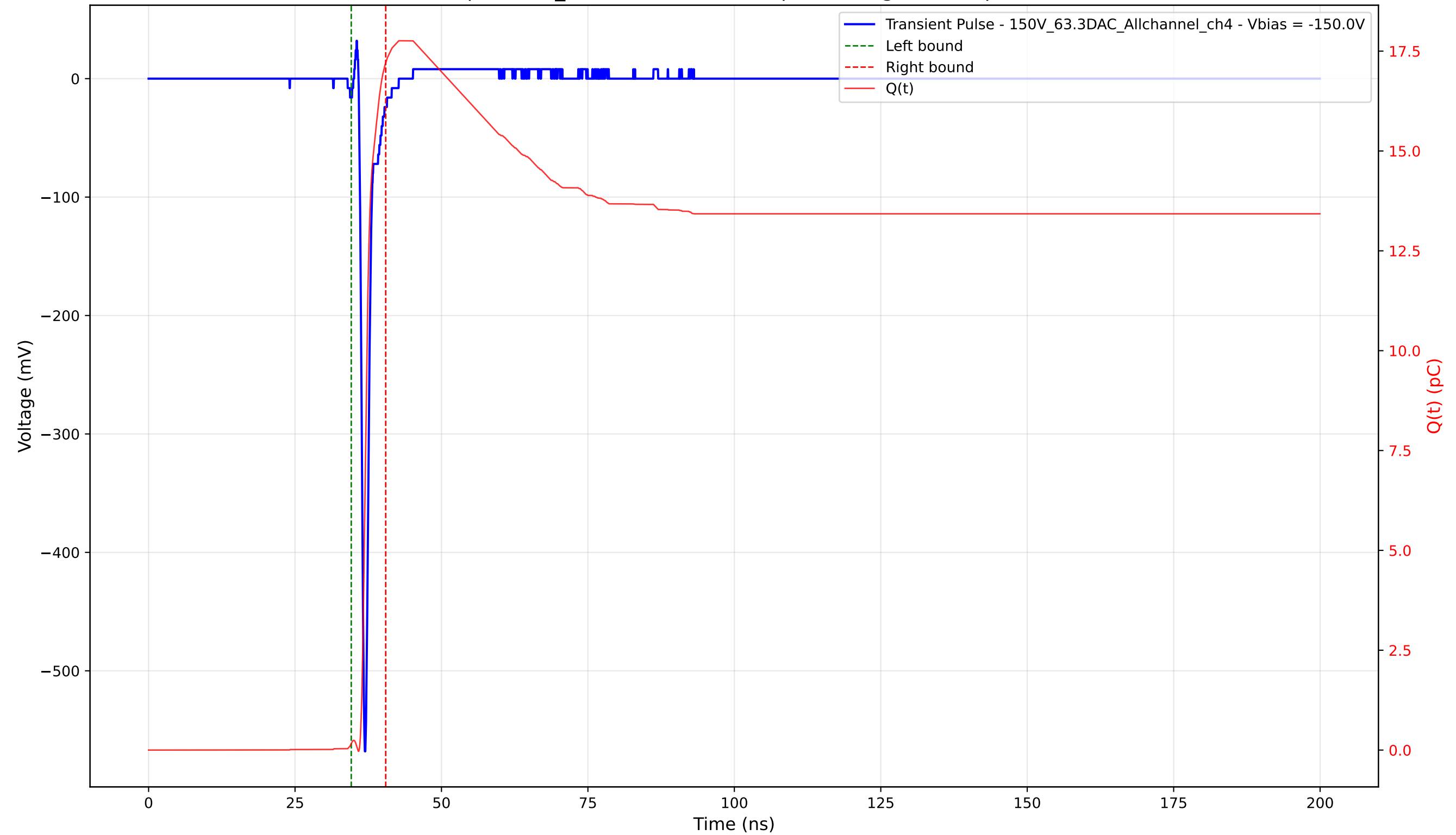
Transient Pulse - Sample: 1cm_42 - Position: 2100.0 \mu\text{m} - Charge: 17.04 pC - Rise Time: 0.72 ns
