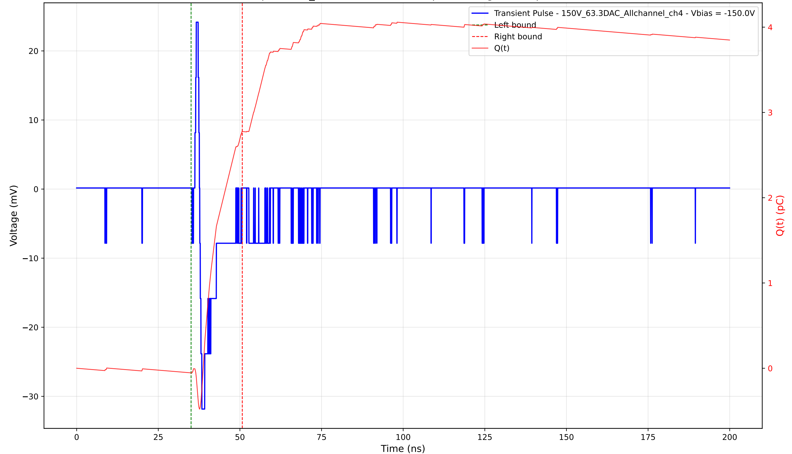
Transient Pulse - Sample: 1cm_42 - Position: 3890.0 \mu\text{m} - Charge: 2.83 pC - Rise Time: 0.66 ns
