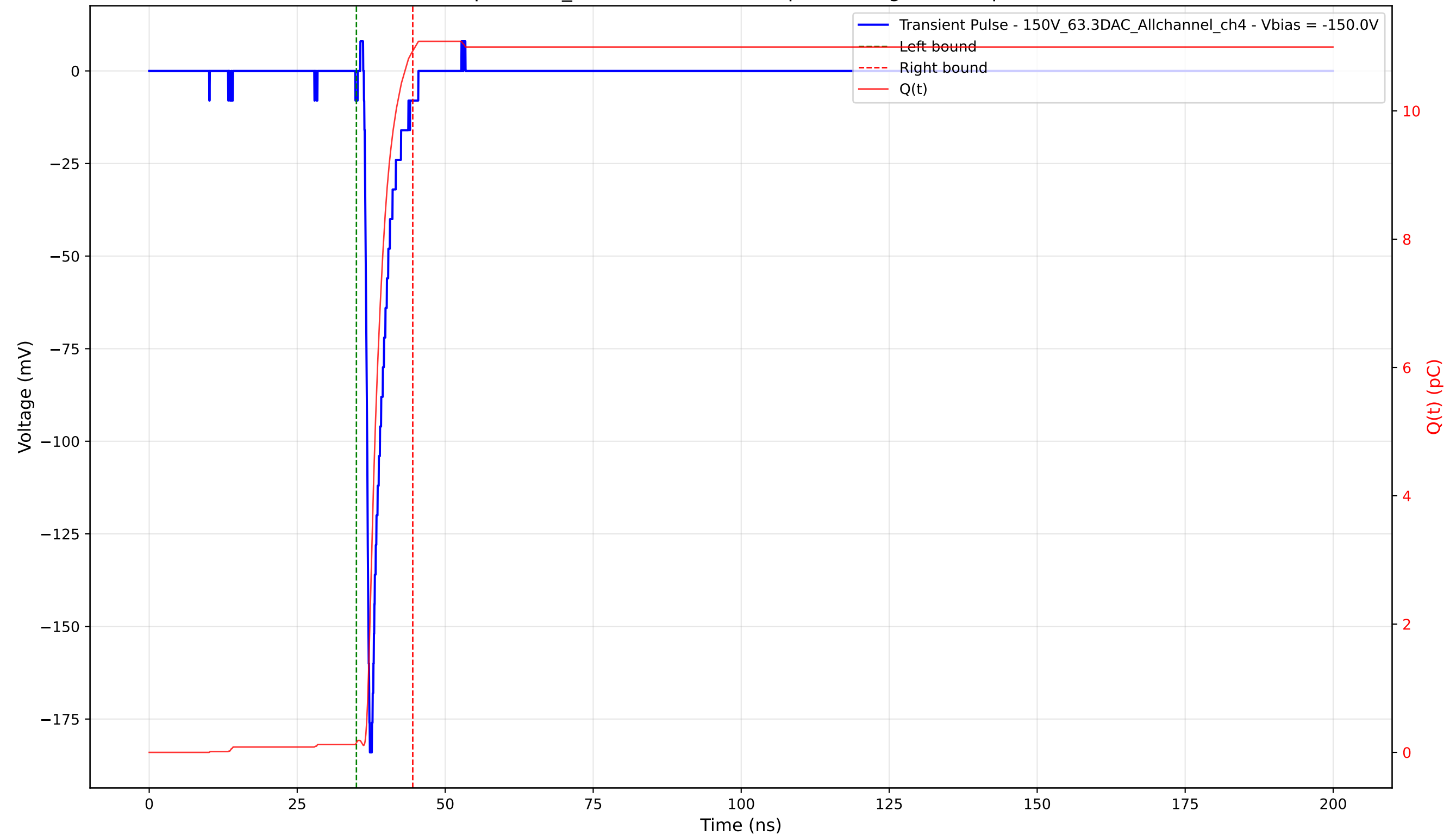
Transient Pulse - Sample: 1cm_42 - Position: 1315.0 \mu\text{m} - Charge: 10.78 pC - Rise Time: 0.74 ns
