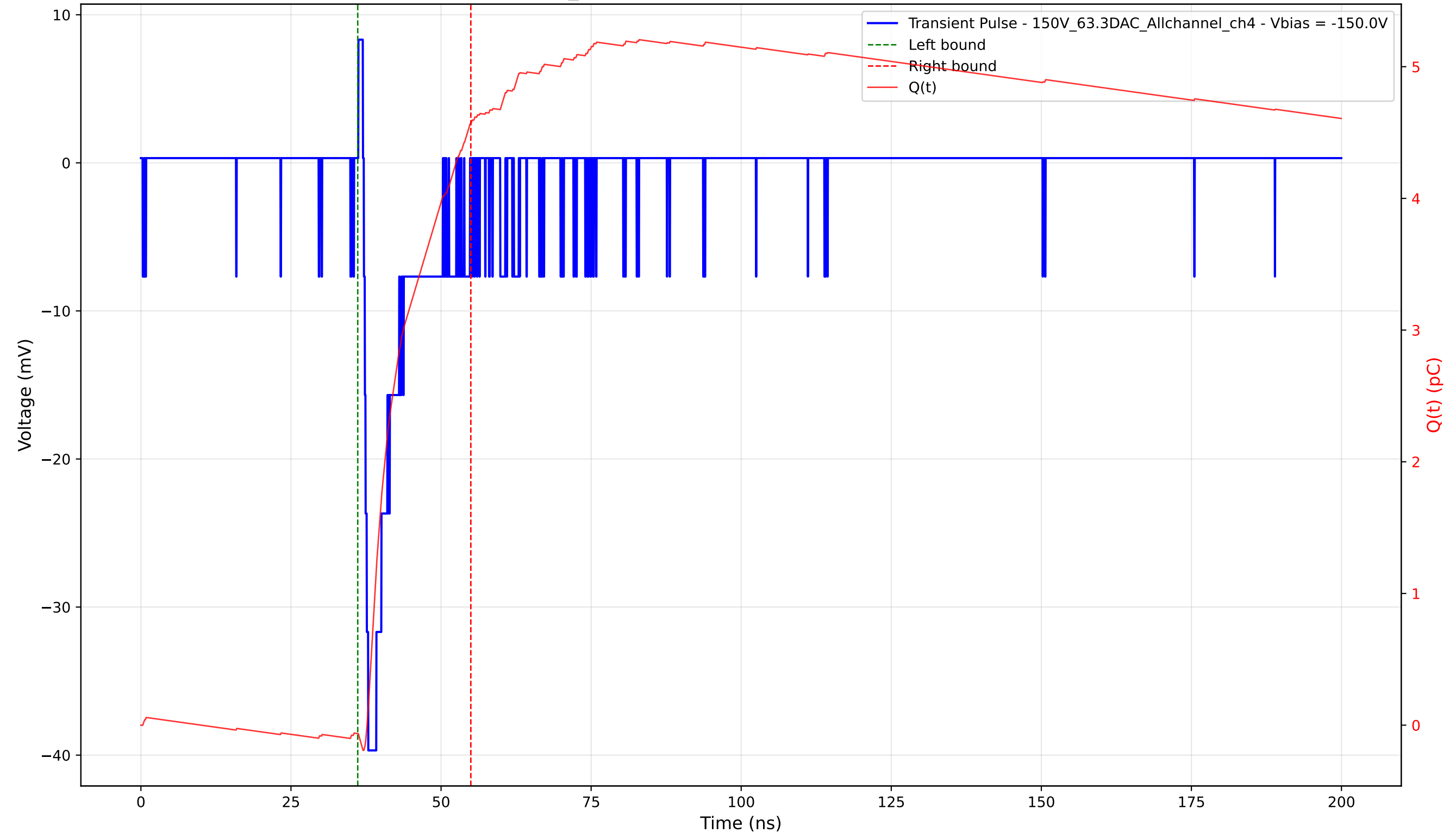
Transient Pulse - Sample: 1cm_42 - Position: 3380.0 \mu\text{m} - Charge: 4.63 pC - Rise Time: 0.74 ns
