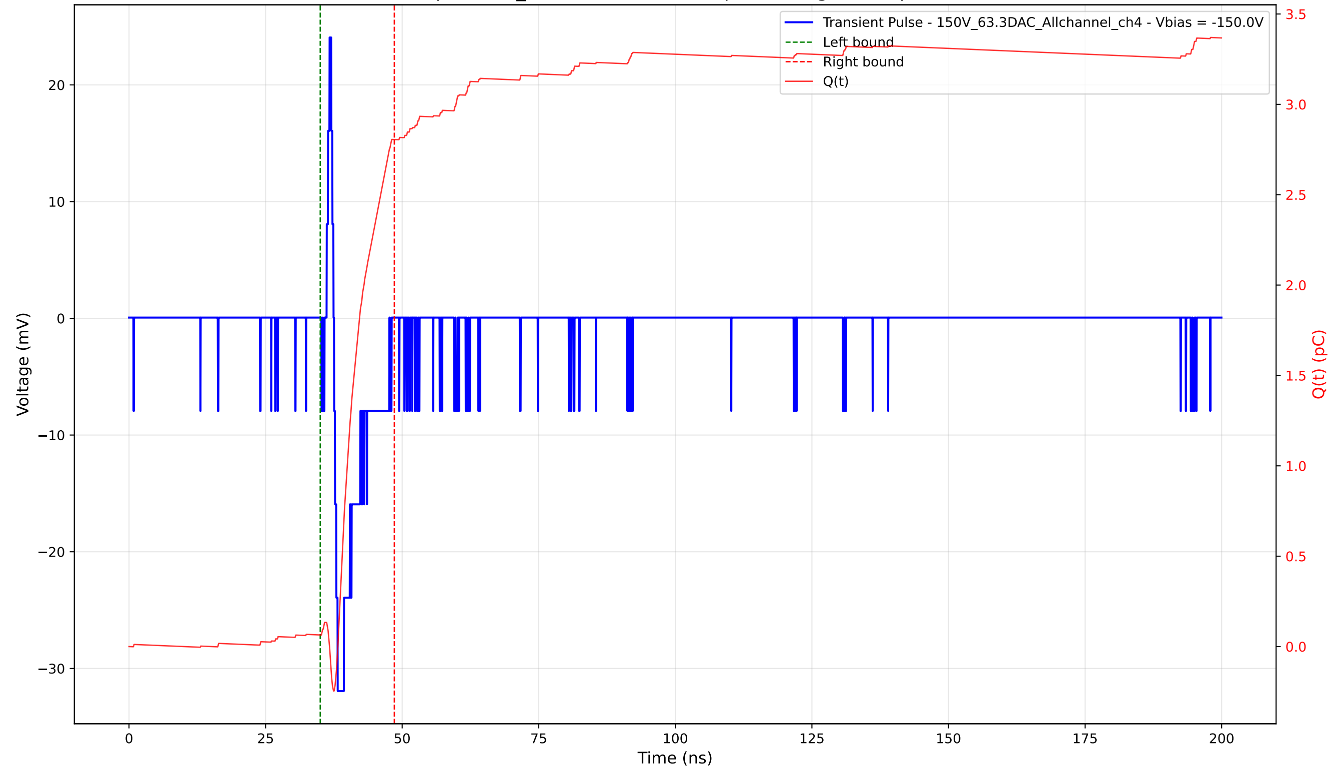
Transient Pulse - Sample: 1cm_42 - Position: 4700.0 \mu\text{m} - Charge: 2.74 pC - Rise Time: 0.66 ns
