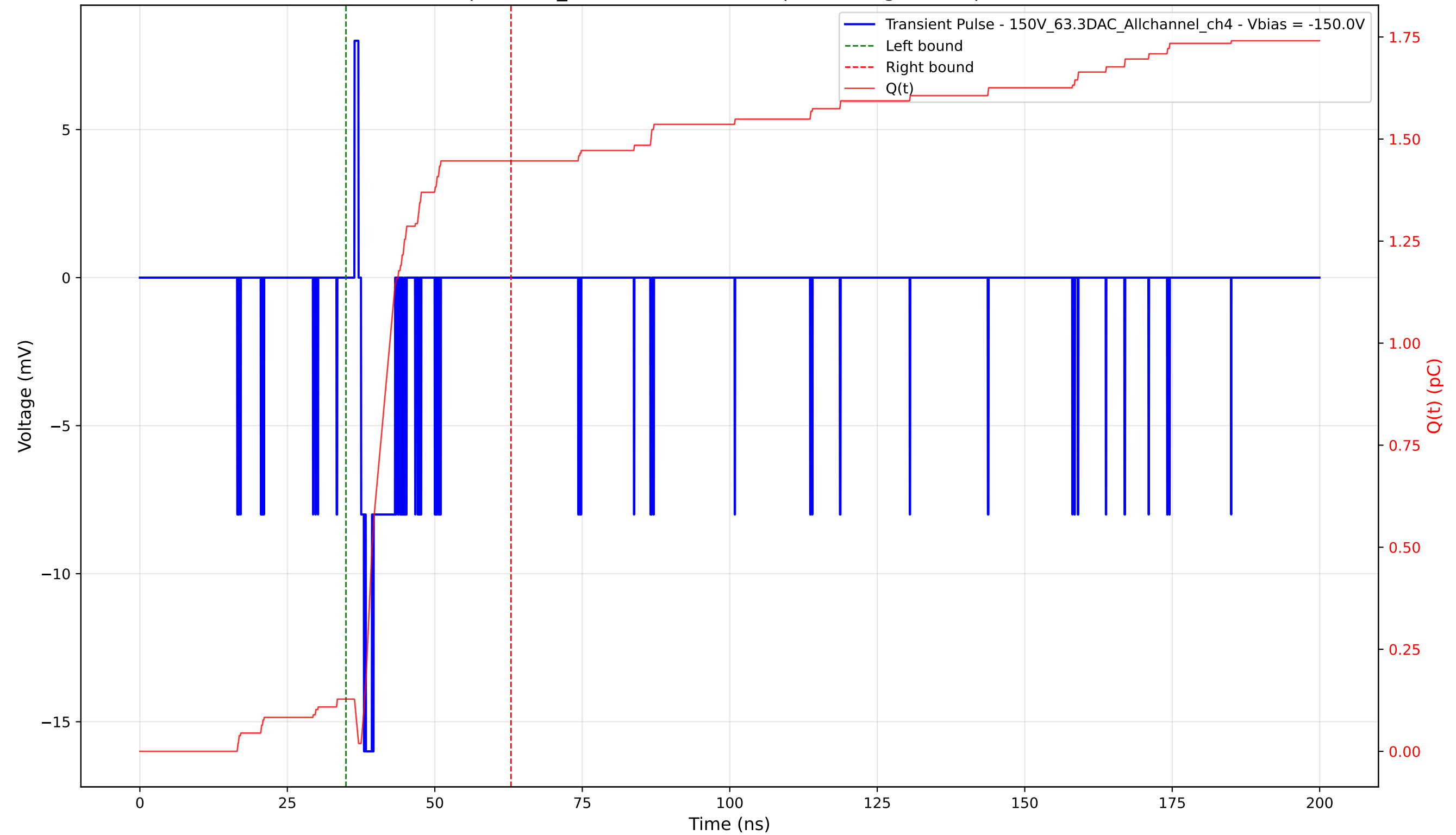
Transient Pulse - Sample: 1cm_42 - Position: 5075.0 \mu\text{m} - Charge: 1.32 pC - Rise Time: 0.51 ns
