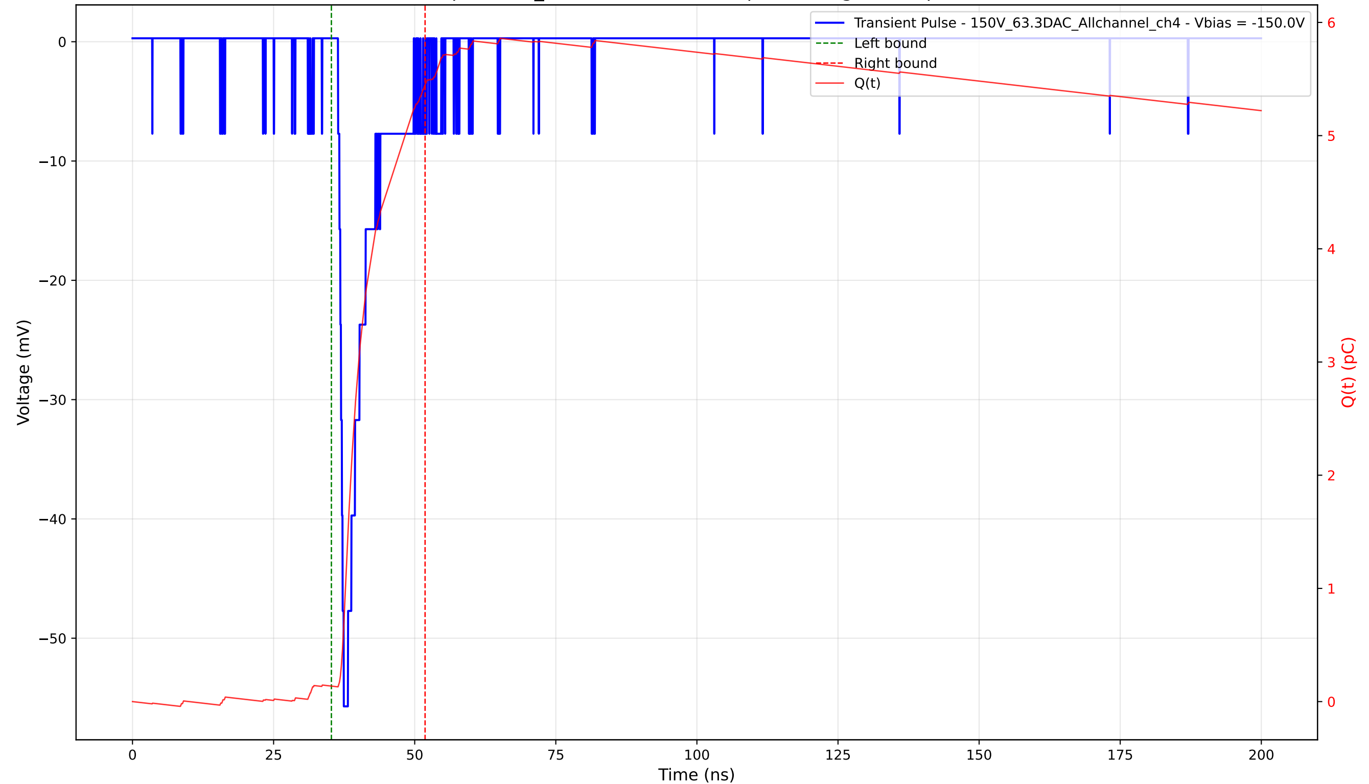
Transient Pulse - Sample: 1cm_42 - Position: 3065.0 \mu\text{m} - Charge: 5.32 pC - Rise Time: 1.01 ns
