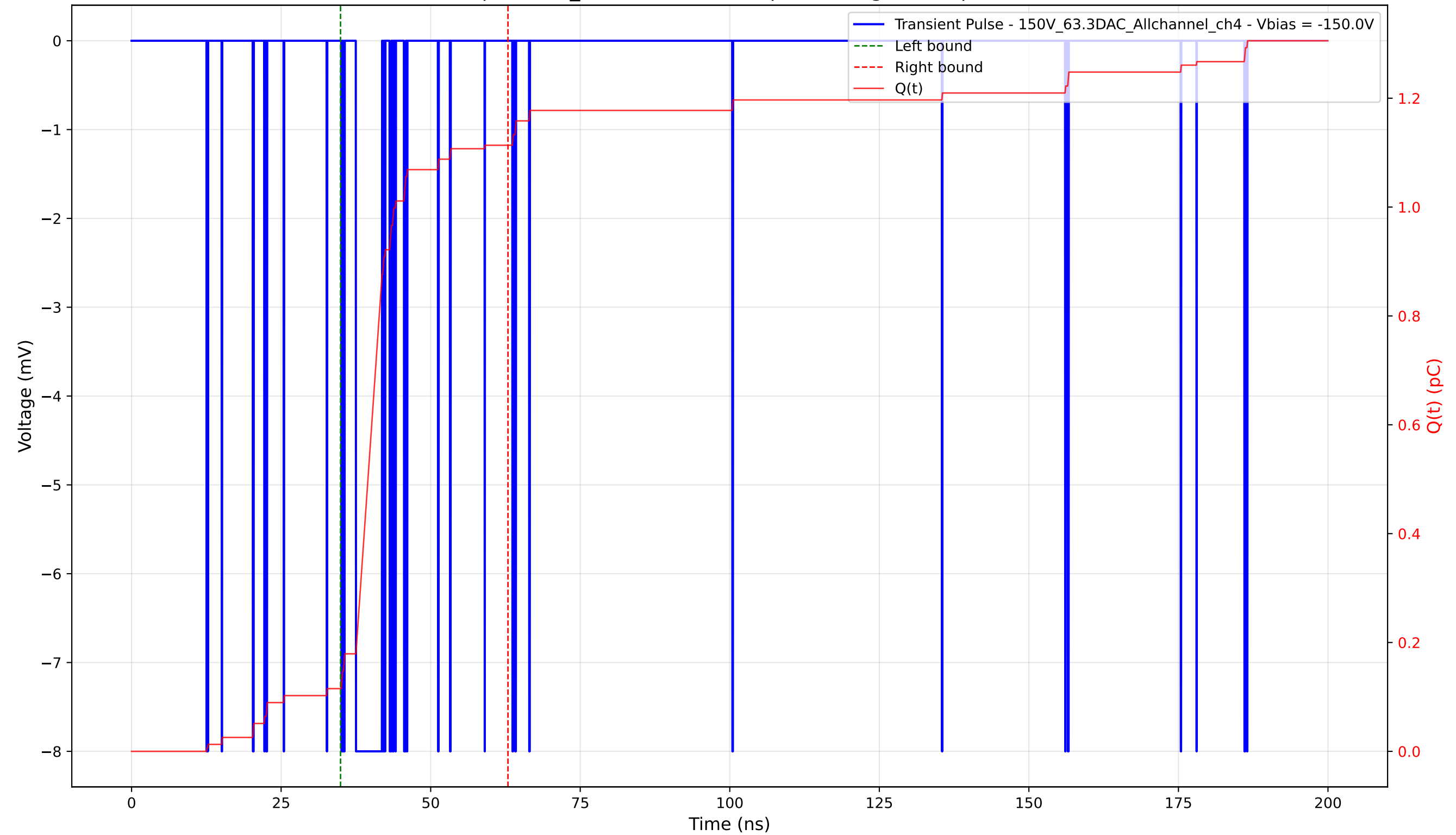
Transient Pulse - Sample: 1cm_42 - Position: 60.0 \mu\text{m} - Charge: 1.00 pC - Rise Time: 0.04 ns
