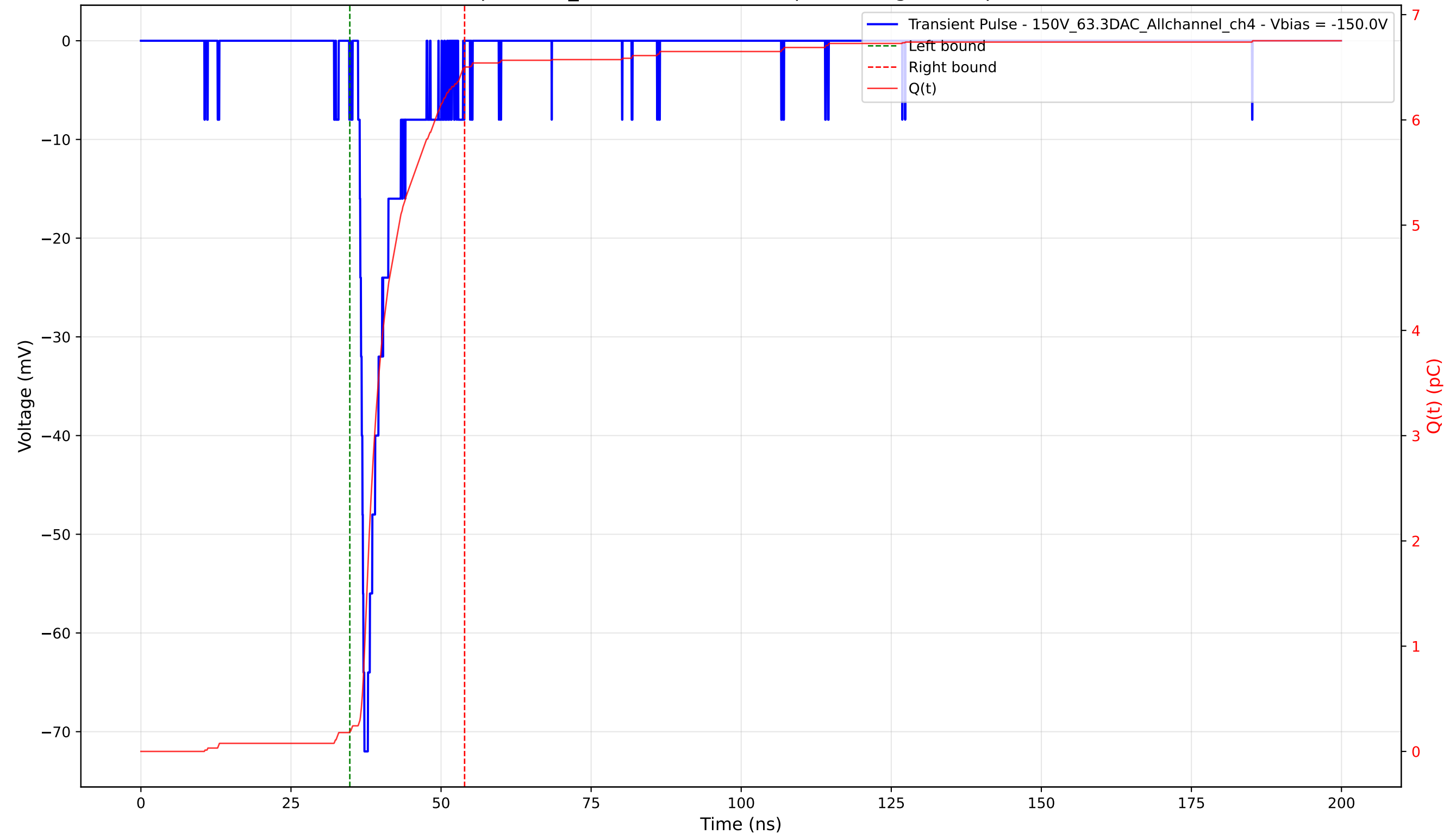
Transient Pulse - Sample: 1cm_42 - Position: 2970.0 \mu\text{m} - Charge: 6.31 pC - Rise Time: 1.04 ns
