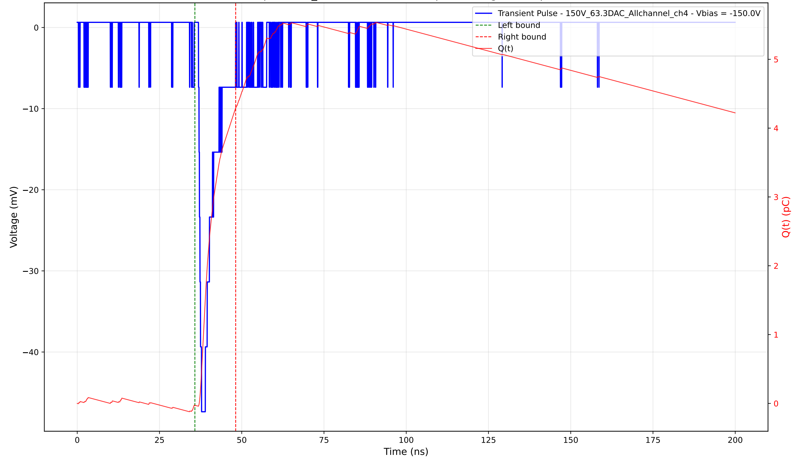
Transient Pulse - Sample: 1cm_42 - Position: 3180.0 \mu\text{m} - Charge: 4.32 pC - Rise Time: 0.94 ns
