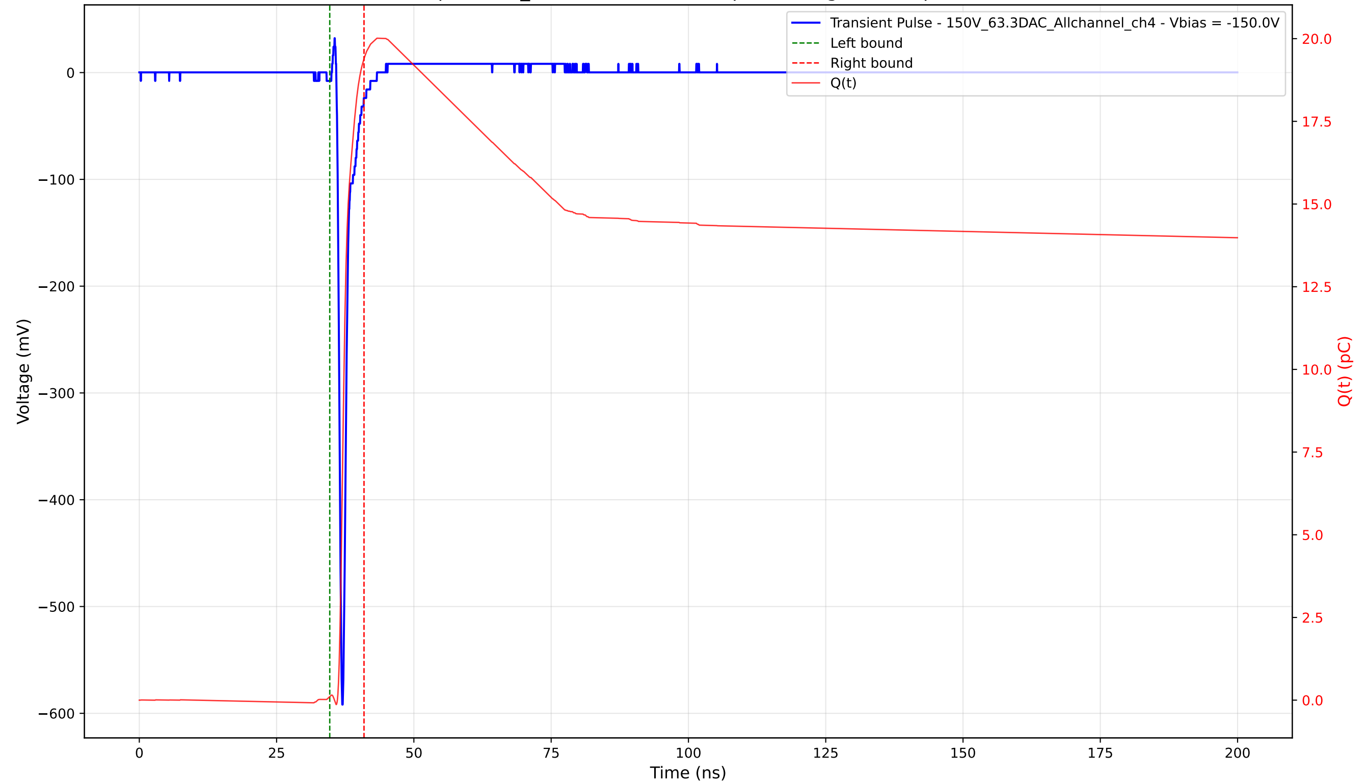
Transient Pulse - Sample: 1cm_42 - Position: 1825.0 \mu\text{m} - Charge: 19.29 pC - Rise Time: 0.71 ns
