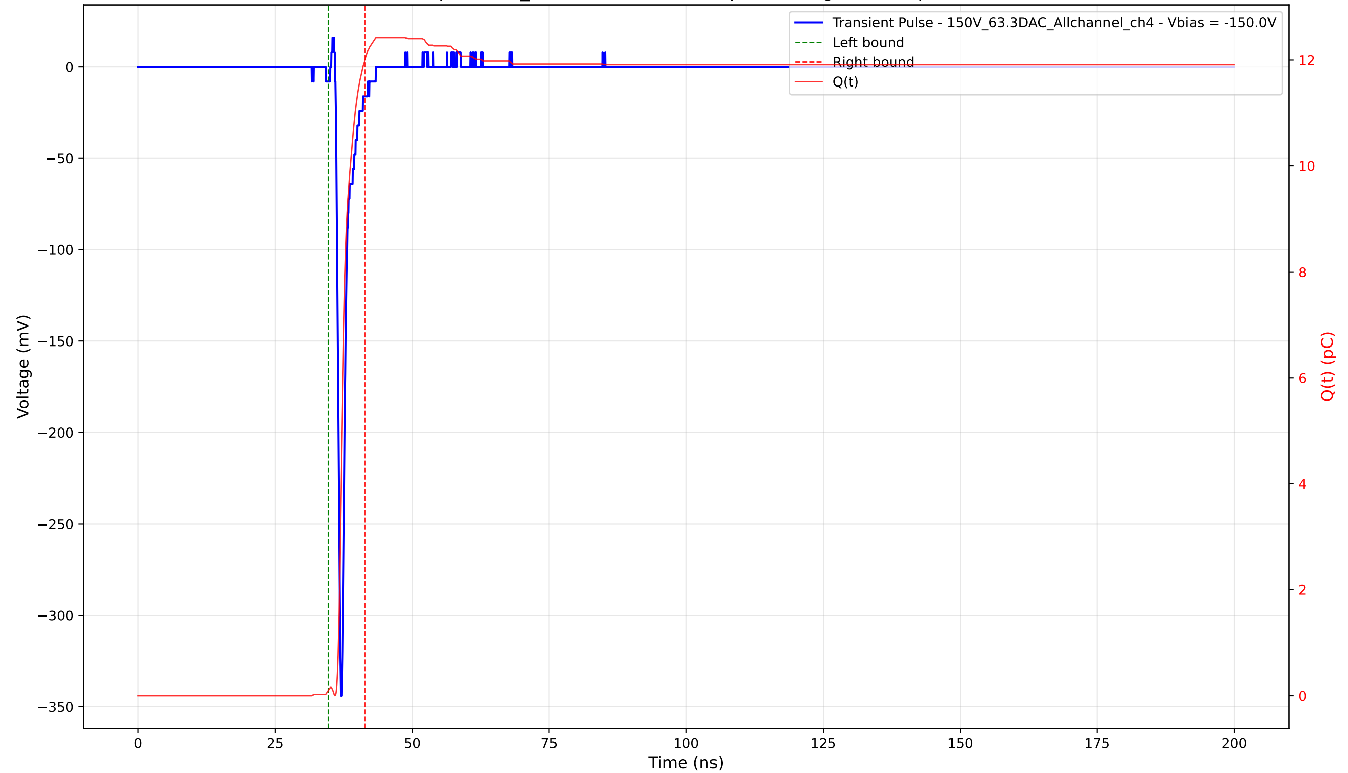
Transient Pulse - Sample: 1cm_42 - Position: 2415.0 \mu\text{m} - Charge: 11.91 pC - Rise Time: 0.70 ns
