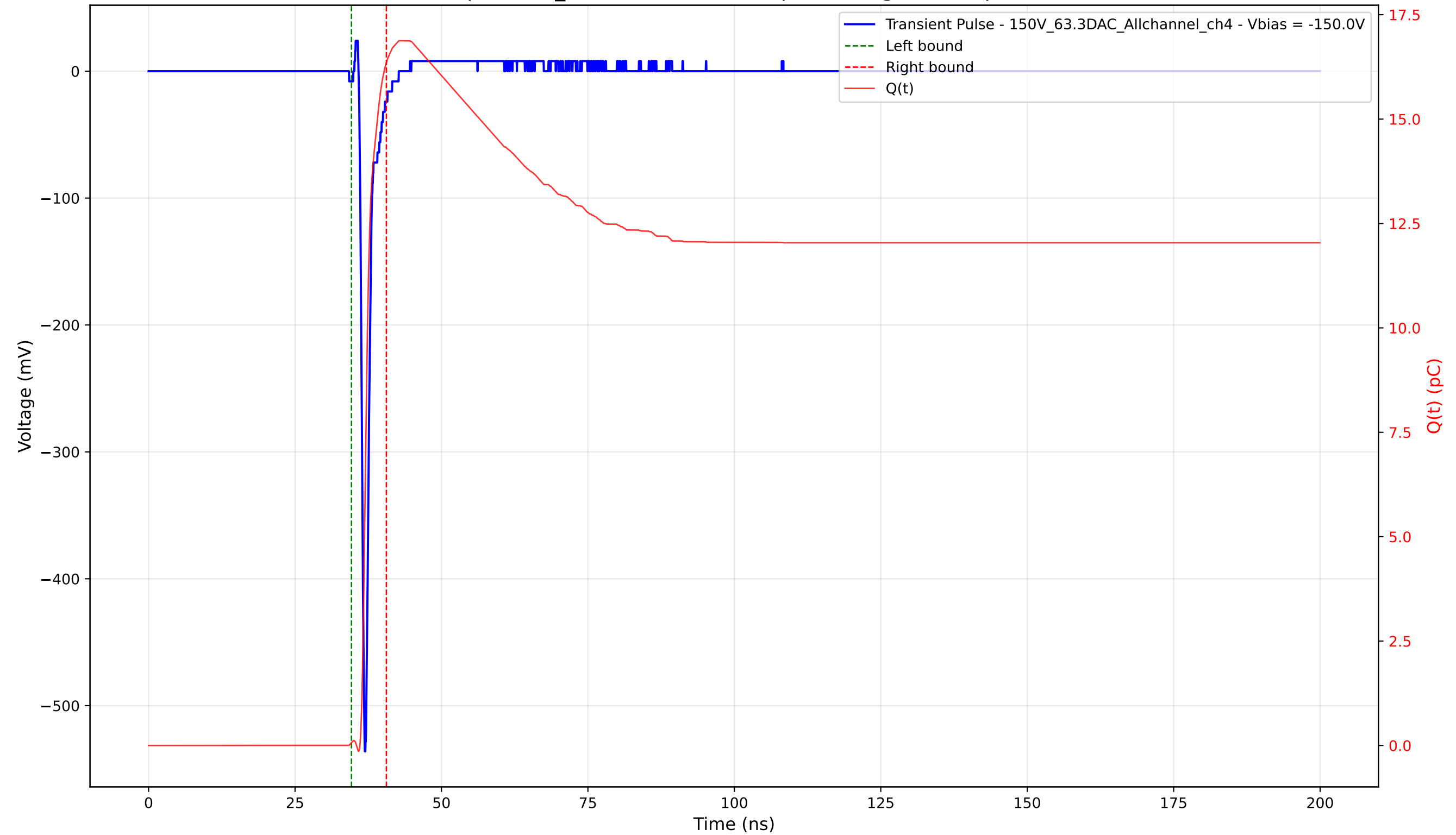
Transient Pulse - Sample: 1cm_42 - Position: 2165.0 \mu\text{m} - Charge: 16.29 pC - Rise Time: 0.71 ns
