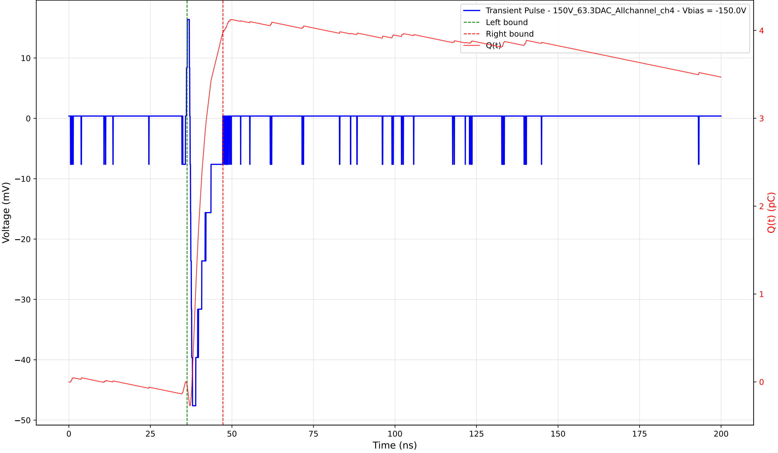
Transient Pulse - Sample: 1cm_42 - Position: 465.0 \mu\text{m} - Charge: 4.01 pC - Rise Time: 0.74 ns
