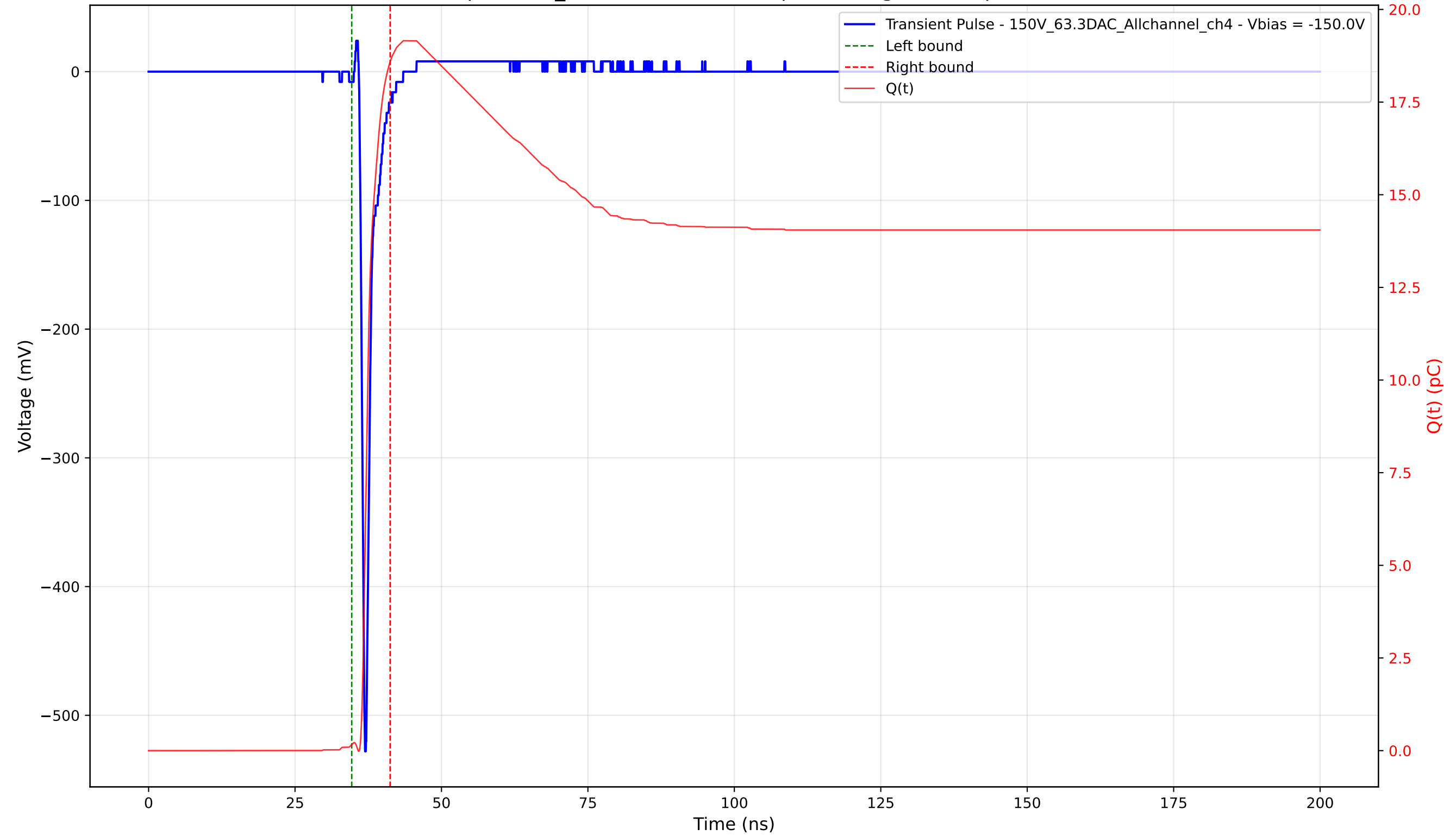
Transient Pulse - Sample: 1cm_42 - Position: 1705.0 \mu\text{m} - Charge: 18.43 pC - Rise Time: 0.74 ns
