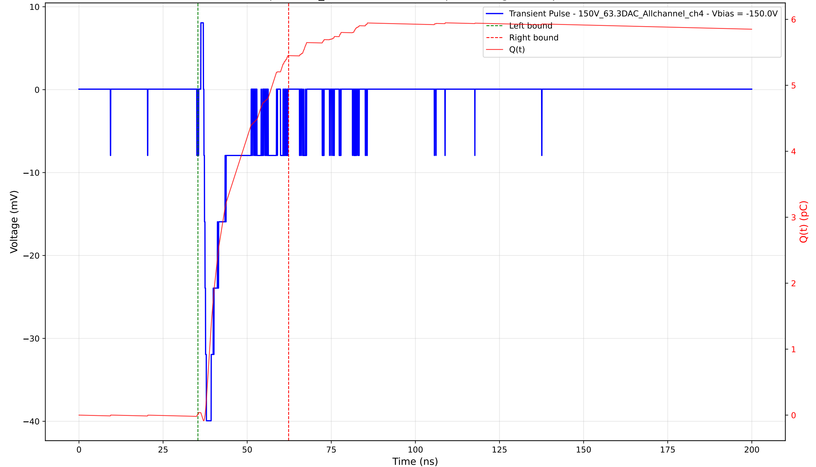
Transient Pulse - Sample: 1cm_42 - Position: 3375.0 \mu\text{m} - Charge: 5.44 pC - Rise Time: 0.74 ns
