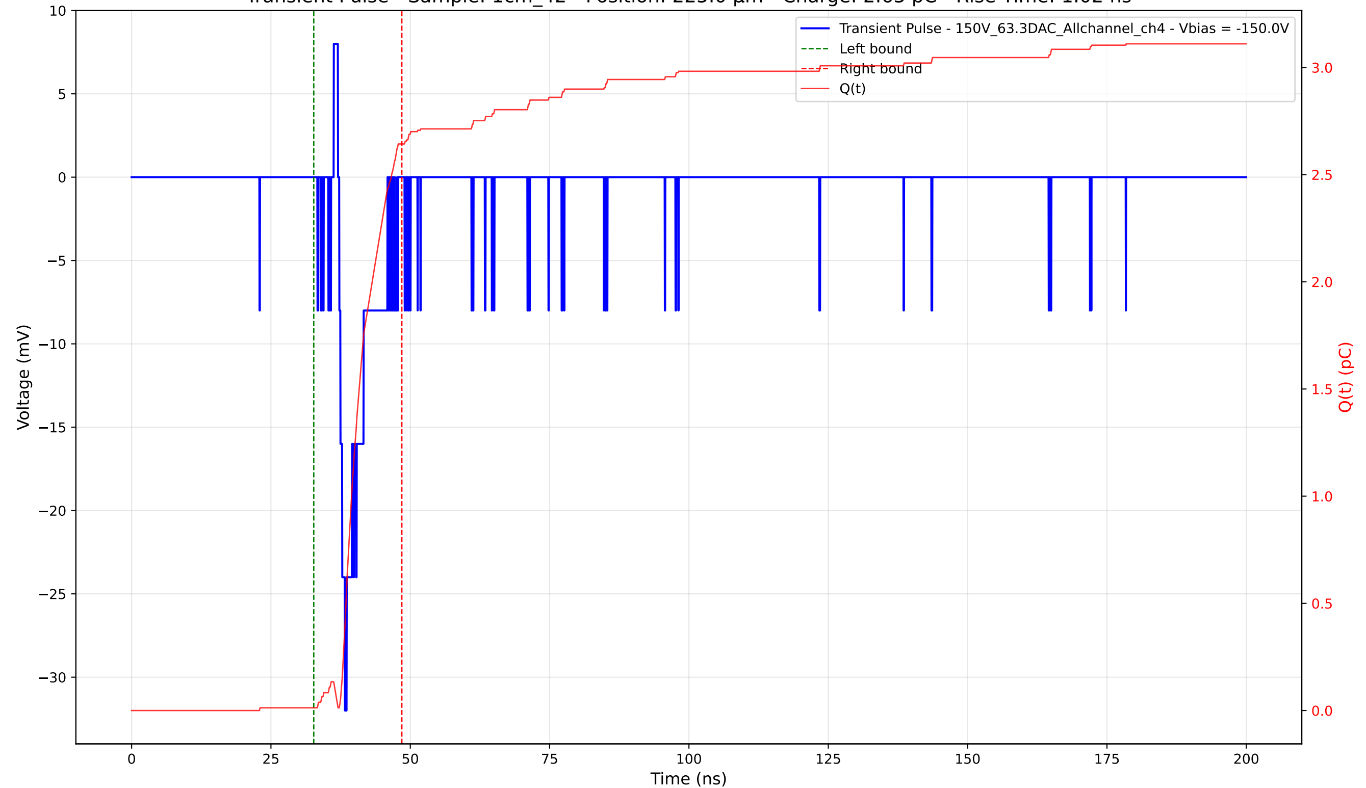
Transient Pulse - Sample: 1cm_42 - Position: 225.0 \mu\text{m} - Charge: 2.63 pC - Rise Time: 1.02 ns
