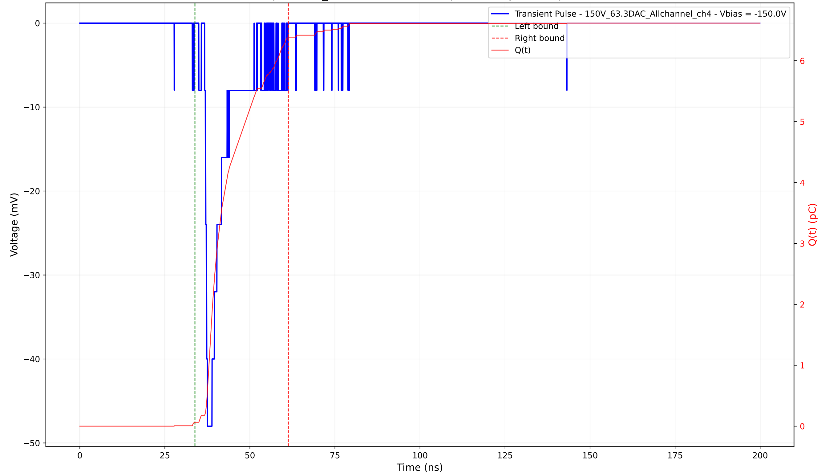
Transient Pulse - Sample: 1cm_42 - Position: 3140.0 \mu\text{m} - Charge: 6.32 pC - Rise Time: 0.82 ns
