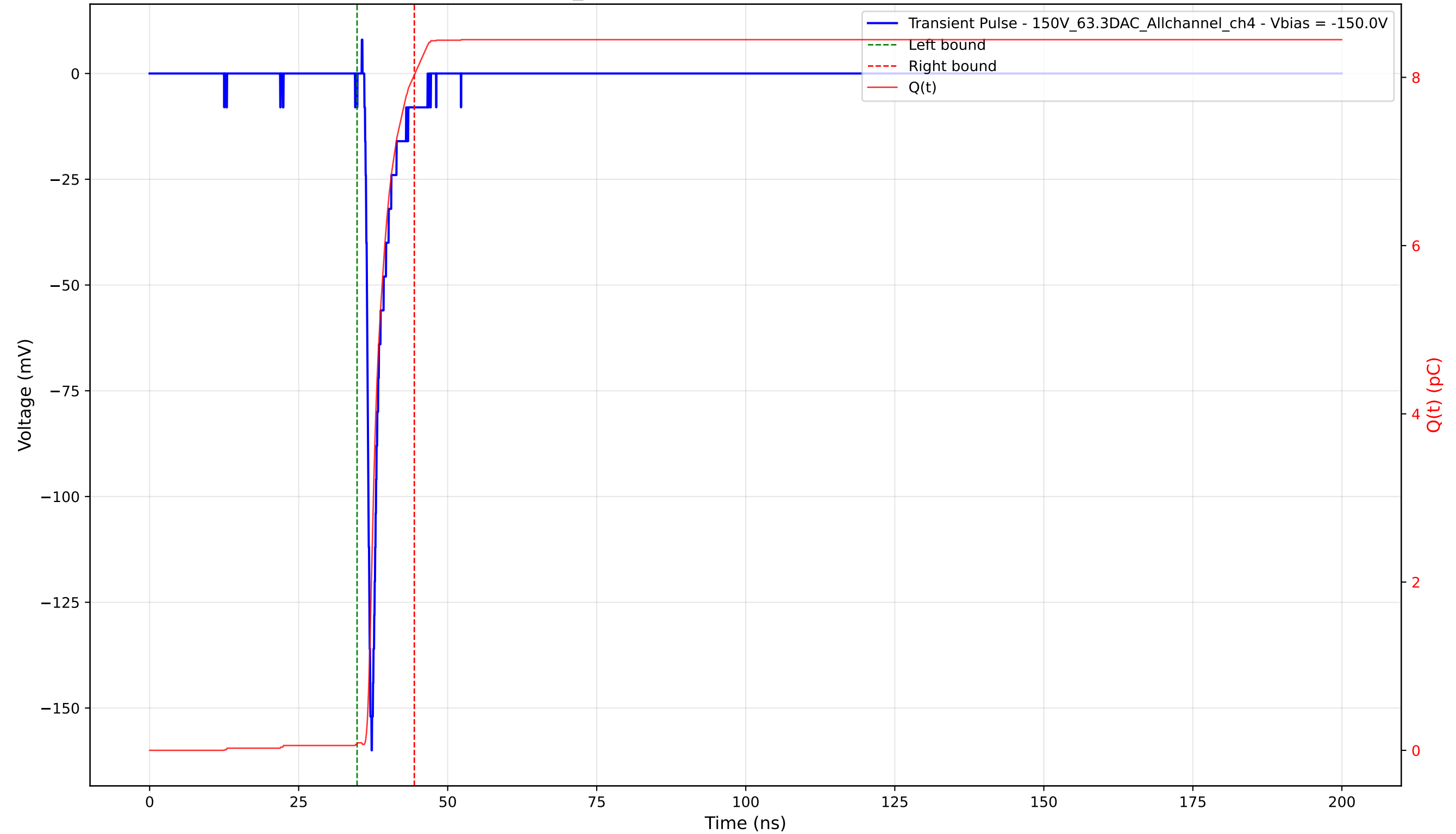
Transient Pulse - Sample: 1cm_42 - Position: 2675.0 \mu\text{m} - Charge: 7.95 pC - Rise Time: 0.80 ns
