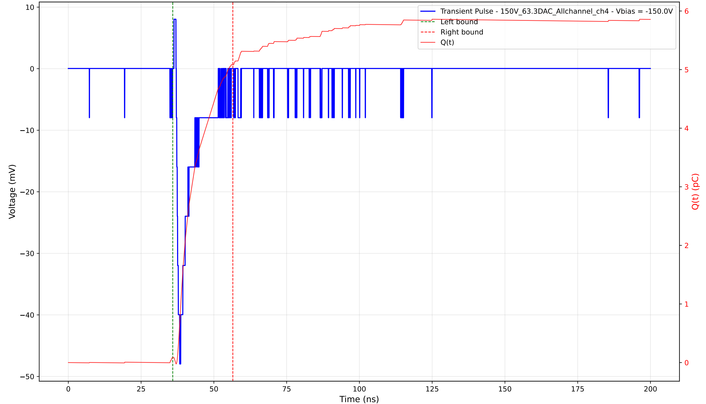
Transient Pulse - Sample: 1cm_42 - Position: 3355.0 \mu\text{m} - Charge: 5.00 pC - Rise Time: 1.18 ns
