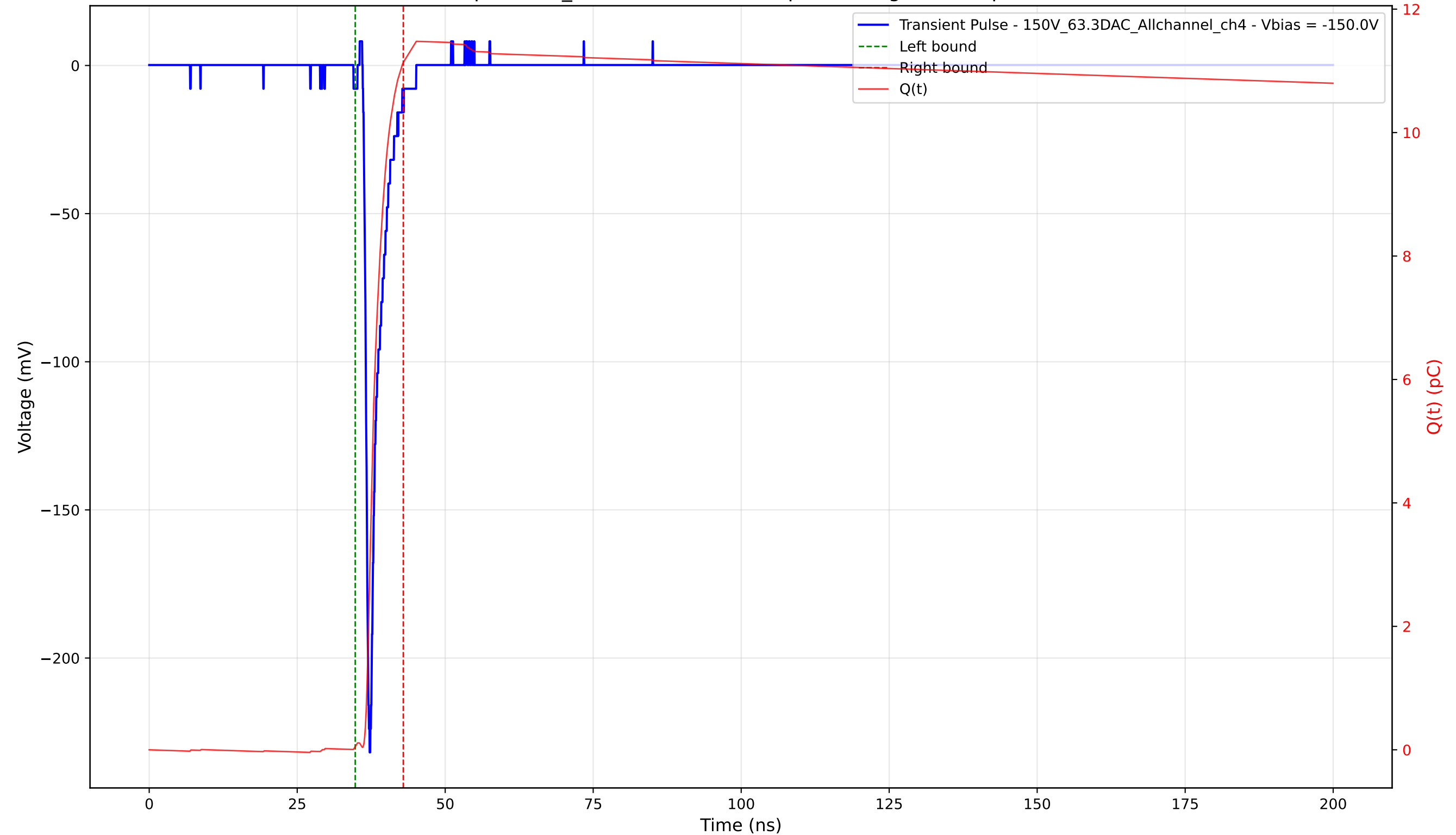
Transient Pulse - Sample: 1cm_42 - Position: 1455.0 \mu\text{m} - Charge: 11.08 pC - Rise Time: 0.80 ns
