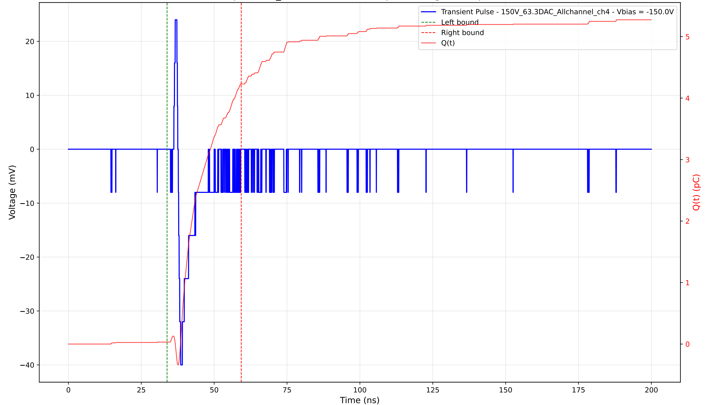
Transient Pulse - Sample: 1cm_42 - Position: 3755.0 \mu\text{m} - Charge: 4.20 pC - Rise Time: 0.82 ns
