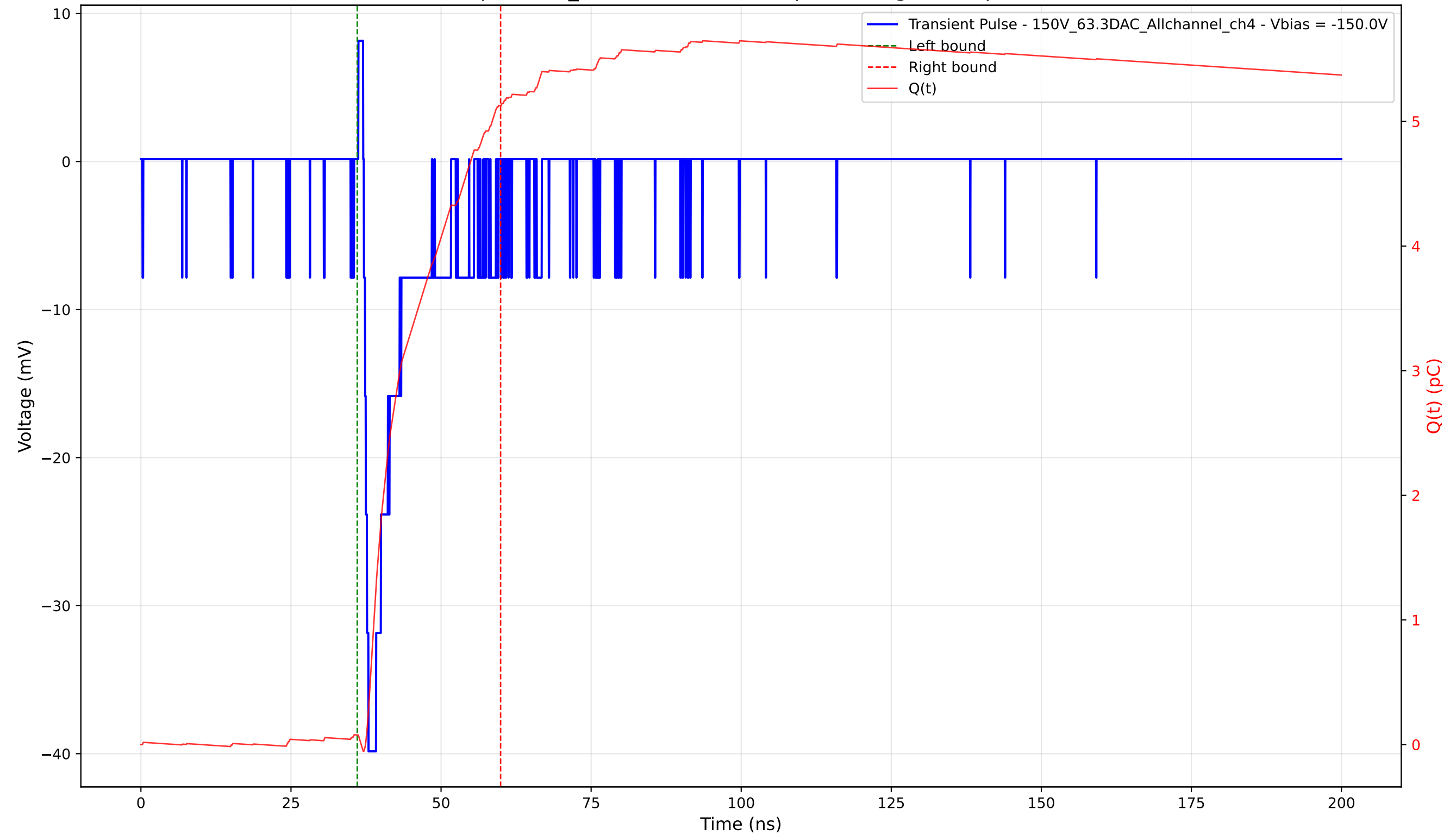
Transient Pulse - Sample: 1cm_42 - Position: 3390.0 \mu\text{m} - Charge: 5.05 pC - Rise Time: 0.78 ns
