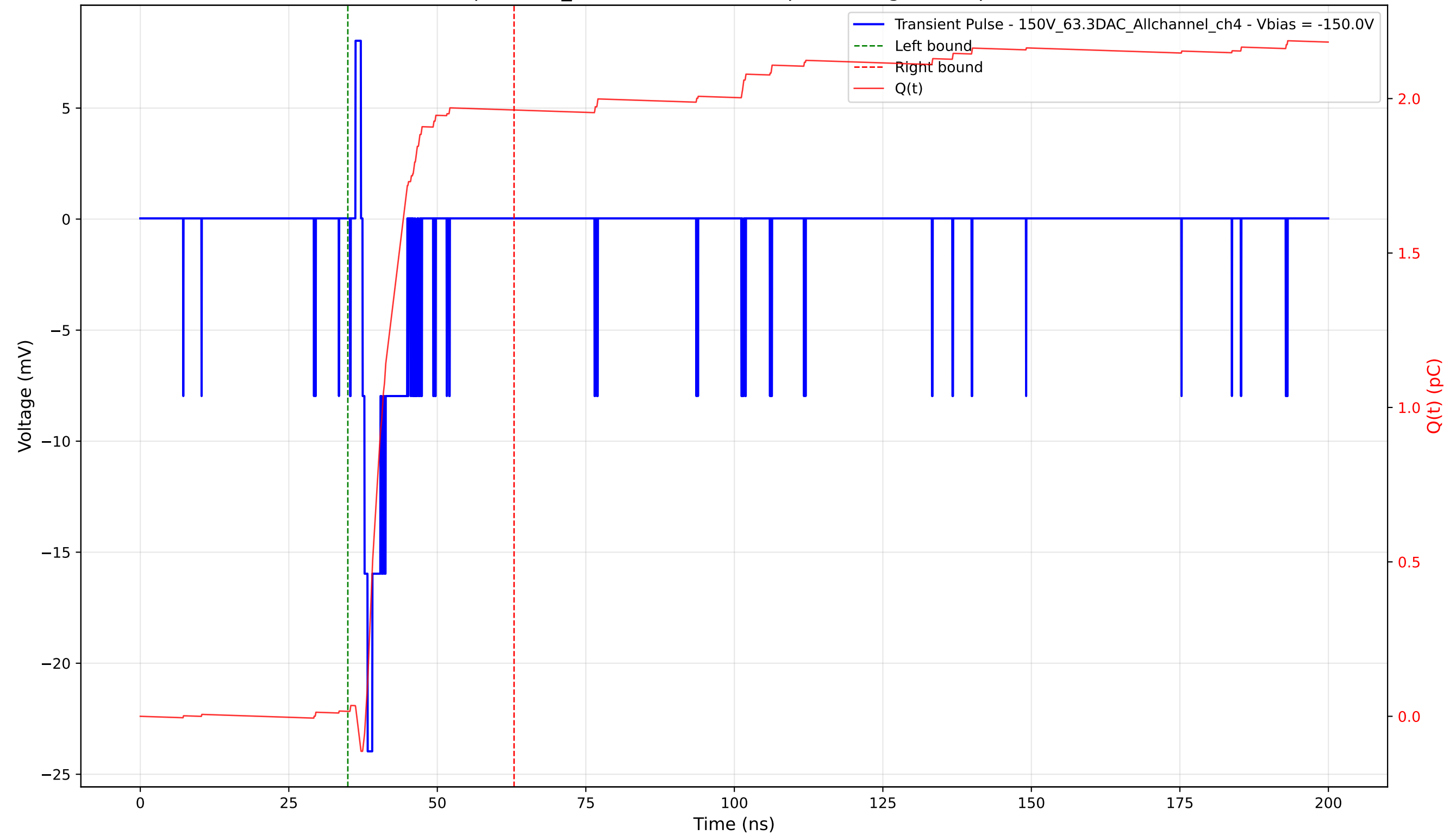
Transient Pulse - Sample: 1cm_42 - Position: 4995.0 \mu\text{m} - Charge: 1.95 pC - Rise Time: 0.87 ns
