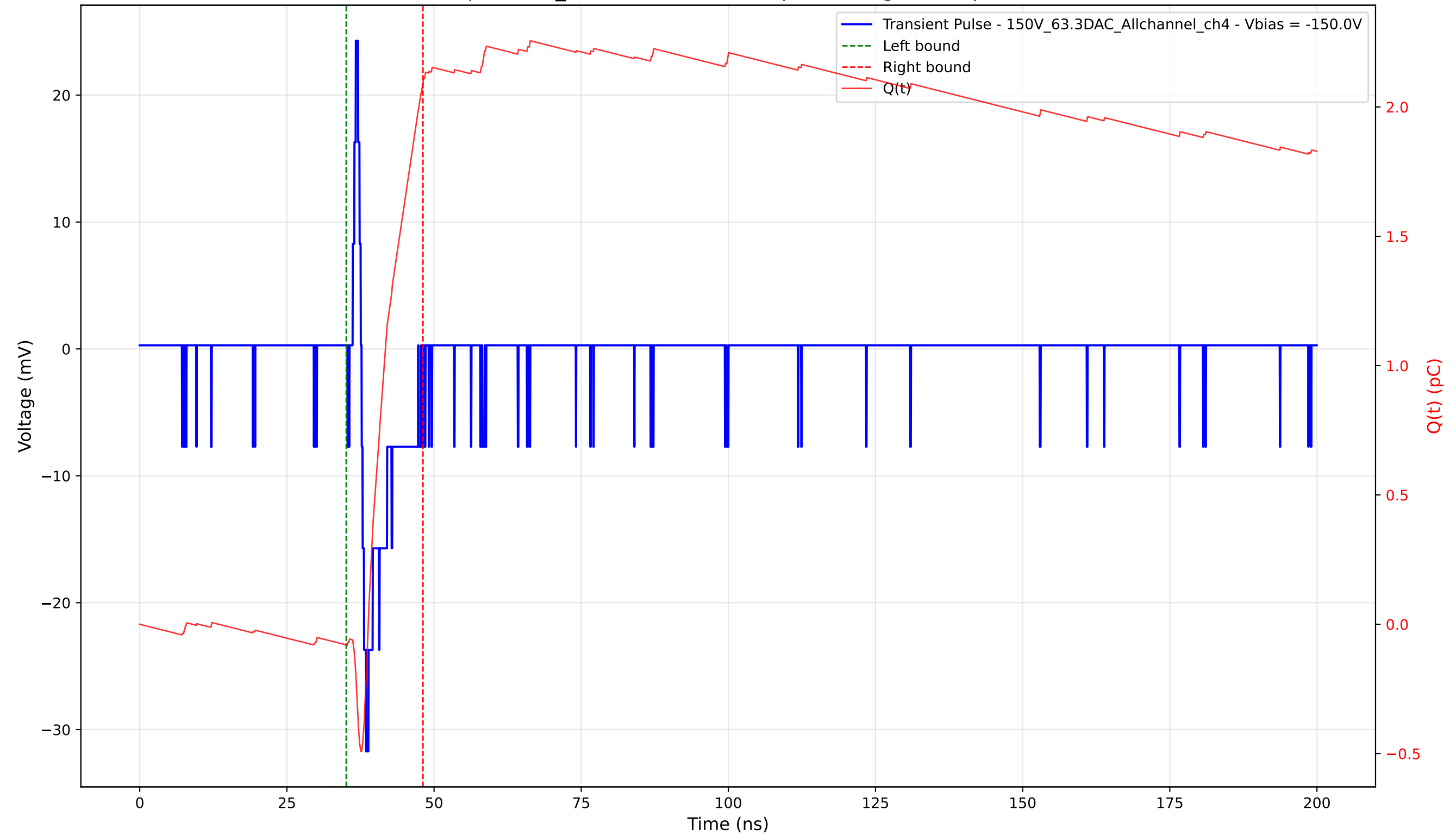
Transient Pulse - Sample: 1cm_42 - Position: 4520.0 \mu\text{m} - Charge: 2.17 pC - Rise Time: 0.78 ns
