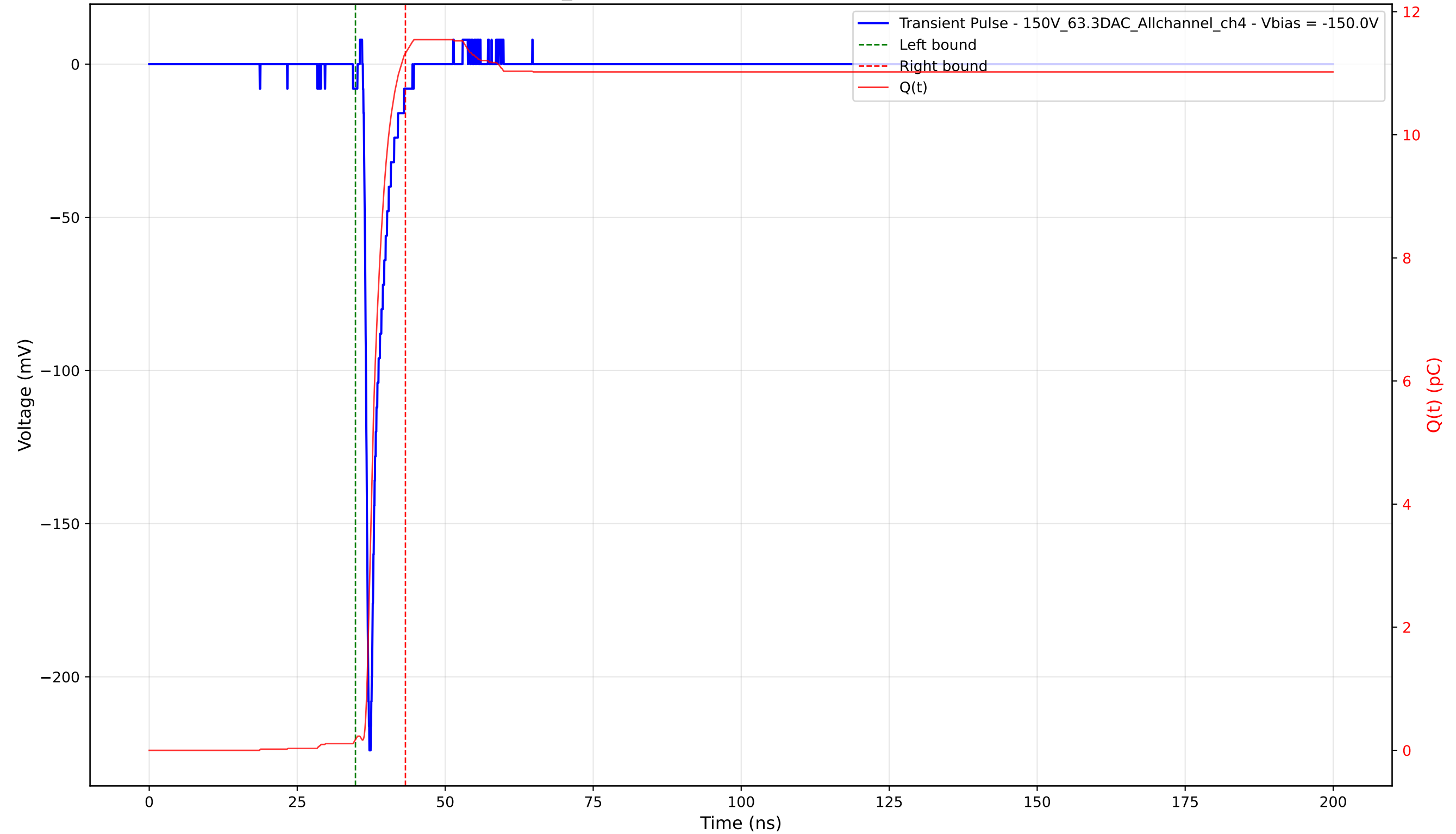
Transient Pulse - Sample: 1cm_42 - Position: 1440.0 \mu\text{m} - Charge: 11.15 pC - Rise Time: 0.77 ns
