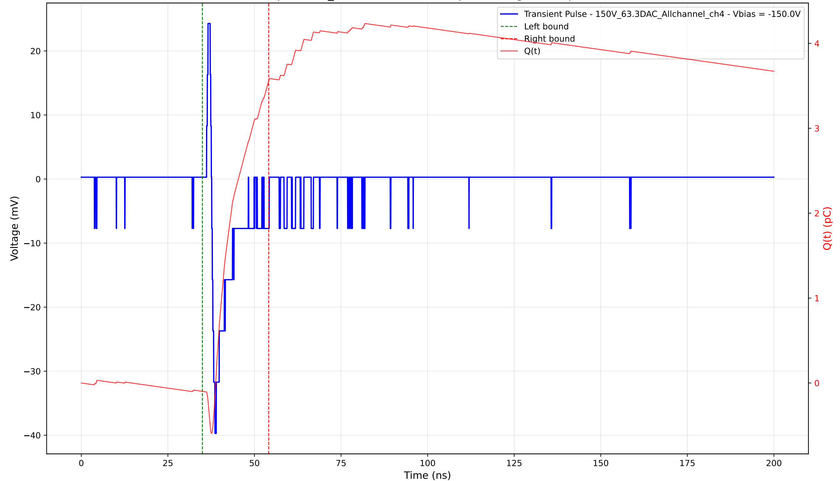
Transient Pulse - Sample: 1cm_42 - Position: 3780.0 \mu\text{m} - Charge: 3.66 pC - Rise Time: 0.94 ns
