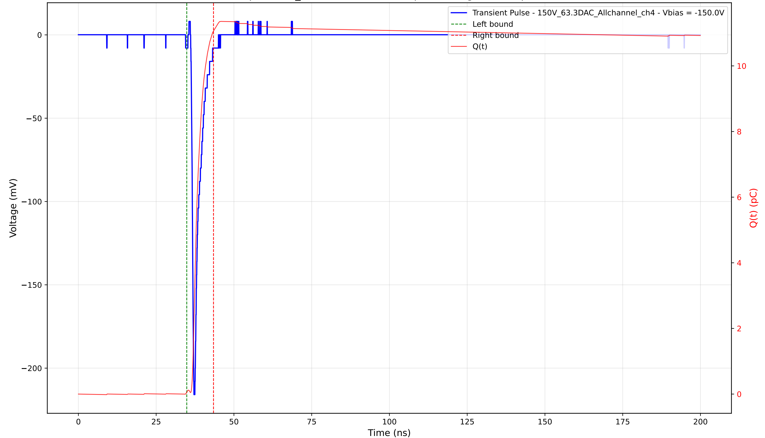
Transient Pulse - Sample: 1cm_42 - Position: 1435.0 \mu\text{m} - Charge: 11.00 pC - Rise Time: 0.74 ns
