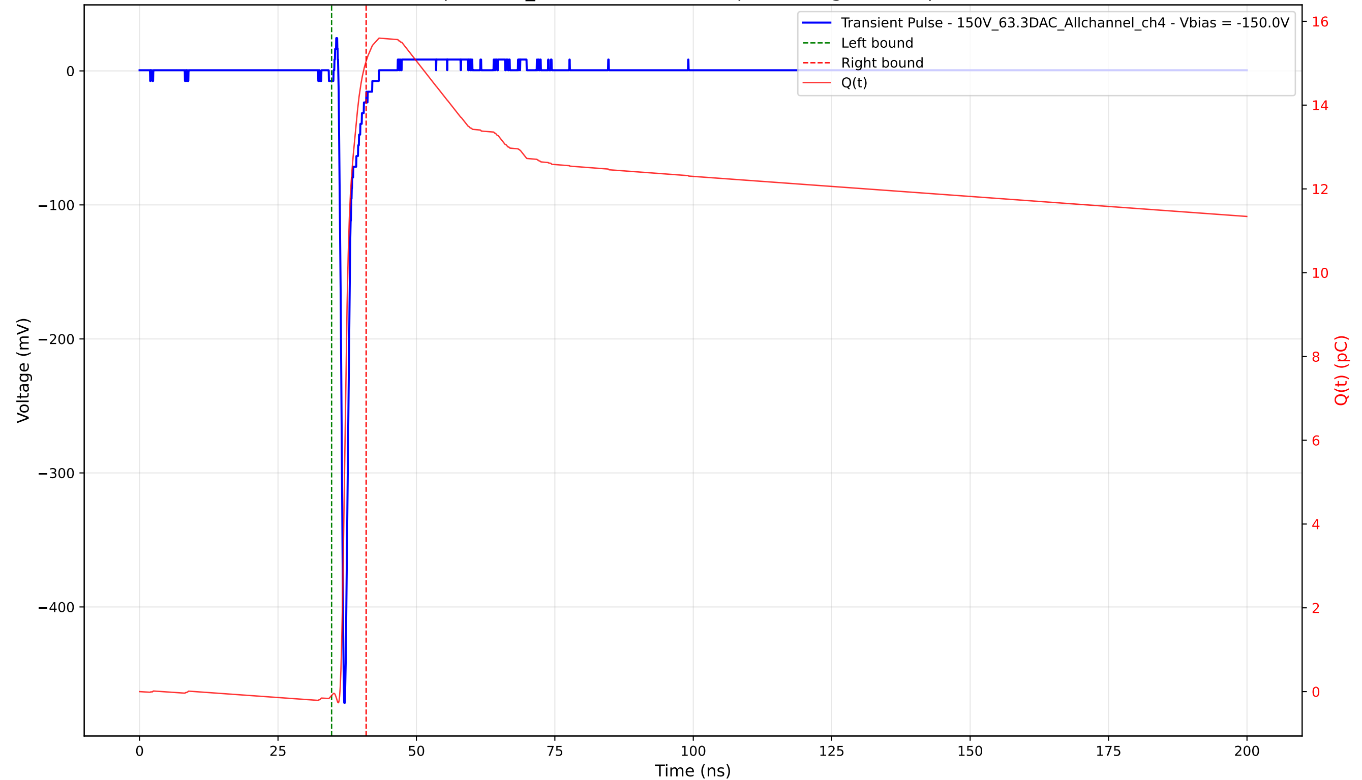
Transient Pulse - Sample: 1cm_42 - Position: 2310.0 \mu\text{m} - Charge: 15.15 pC - Rise Time: 0.72 ns
