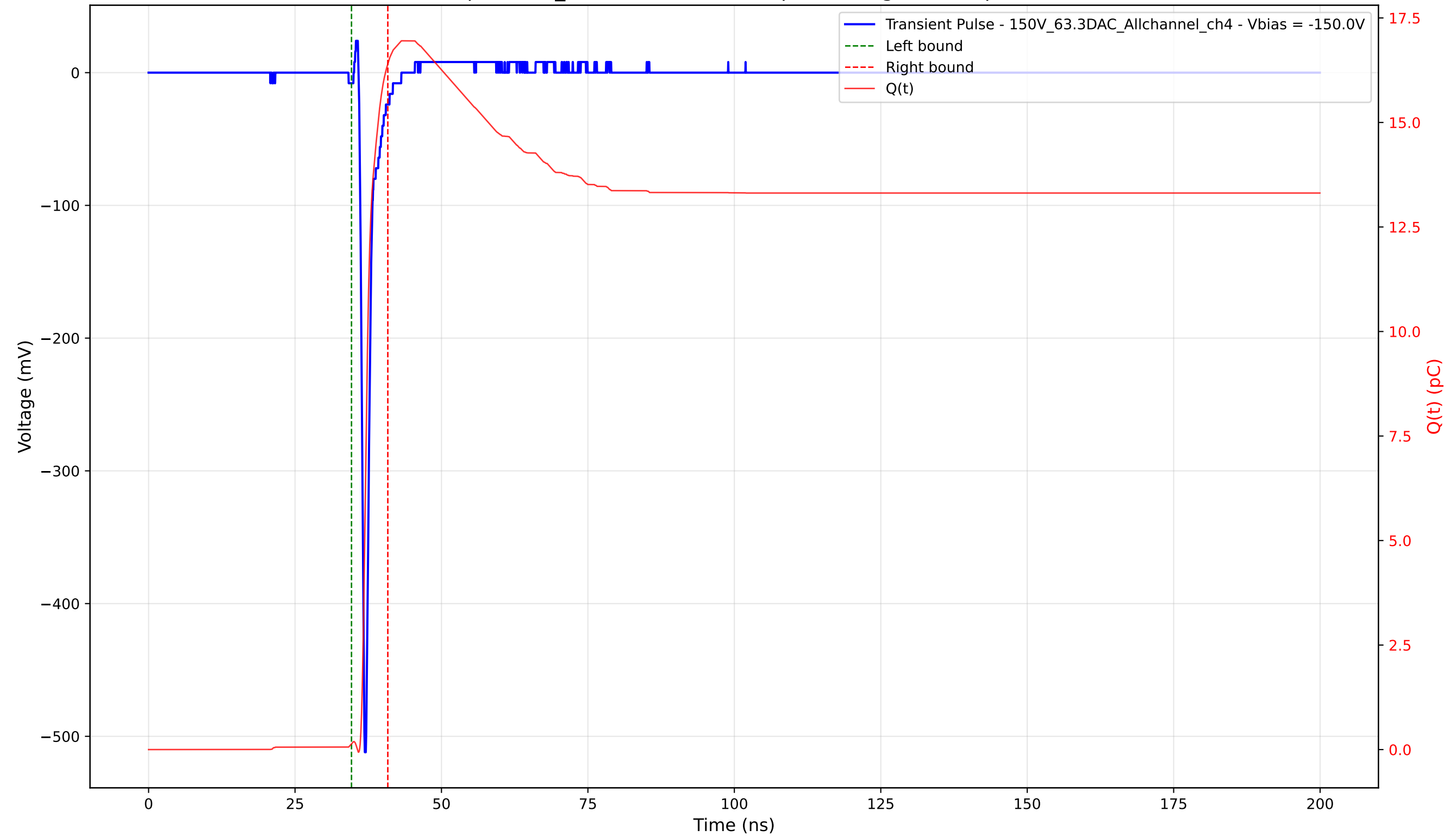
Transient Pulse - Sample: 1cm_42 - Position: 2250.0 \mu\text{m} - Charge: 16.26 pC - Rise Time: 0.70 ns
