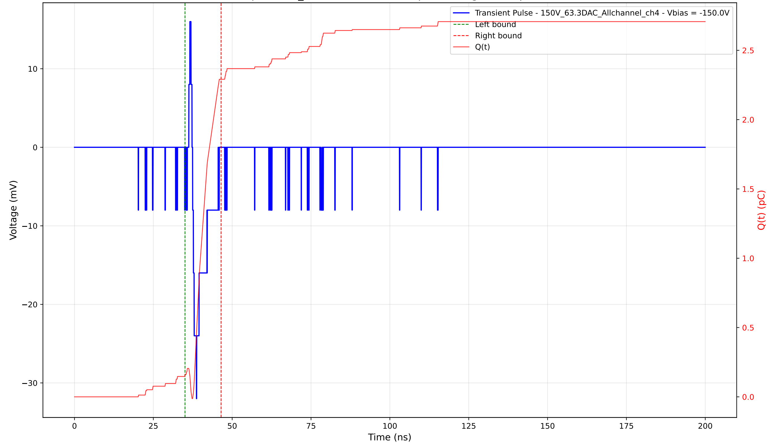
Transient Pulse - Sample: 1cm_42 - Position: 4935.0 \mu\text{m} - Charge: 2.13 pC - Rise Time: 1.22 ns
