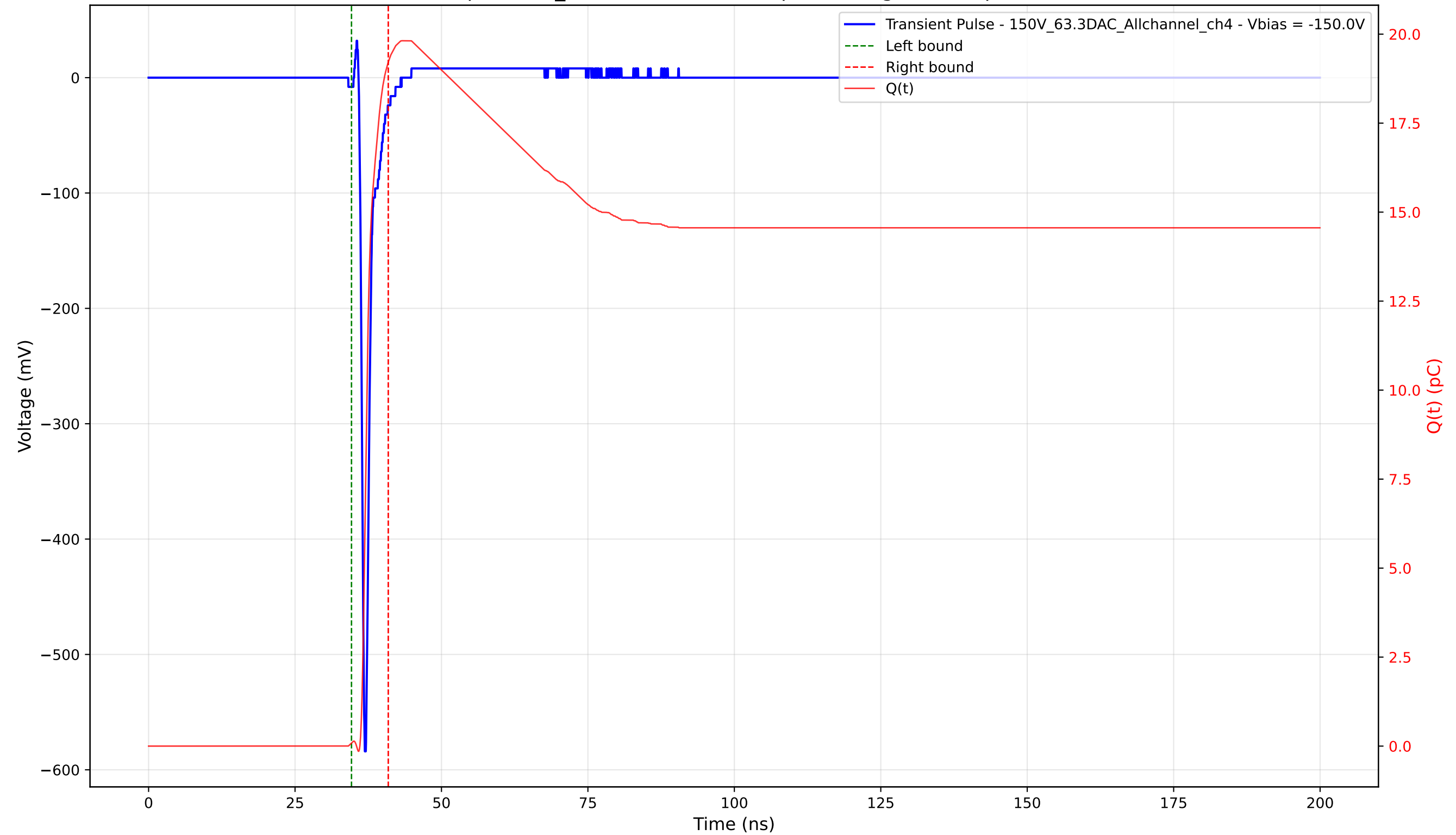
Transient Pulse - Sample: 1cm_42 - Position: 1840.0 \mu\text{m} - Charge: 19.13 pC - Rise Time: 0.71 ns
