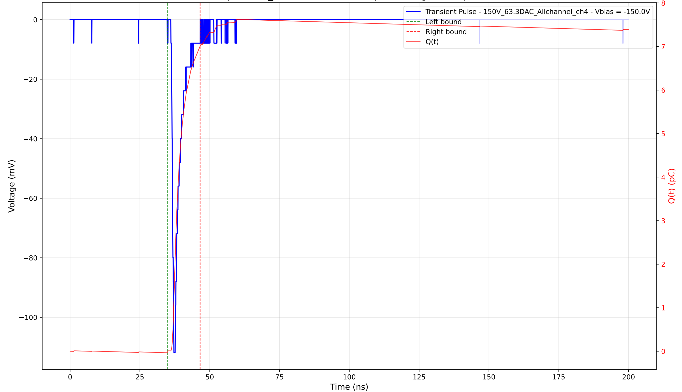
Transient Pulse - Sample: 1cm_42 - Position: 2860.0 \mu\text{m} - Charge: 7.04 pC - Rise Time: 0.82 ns
