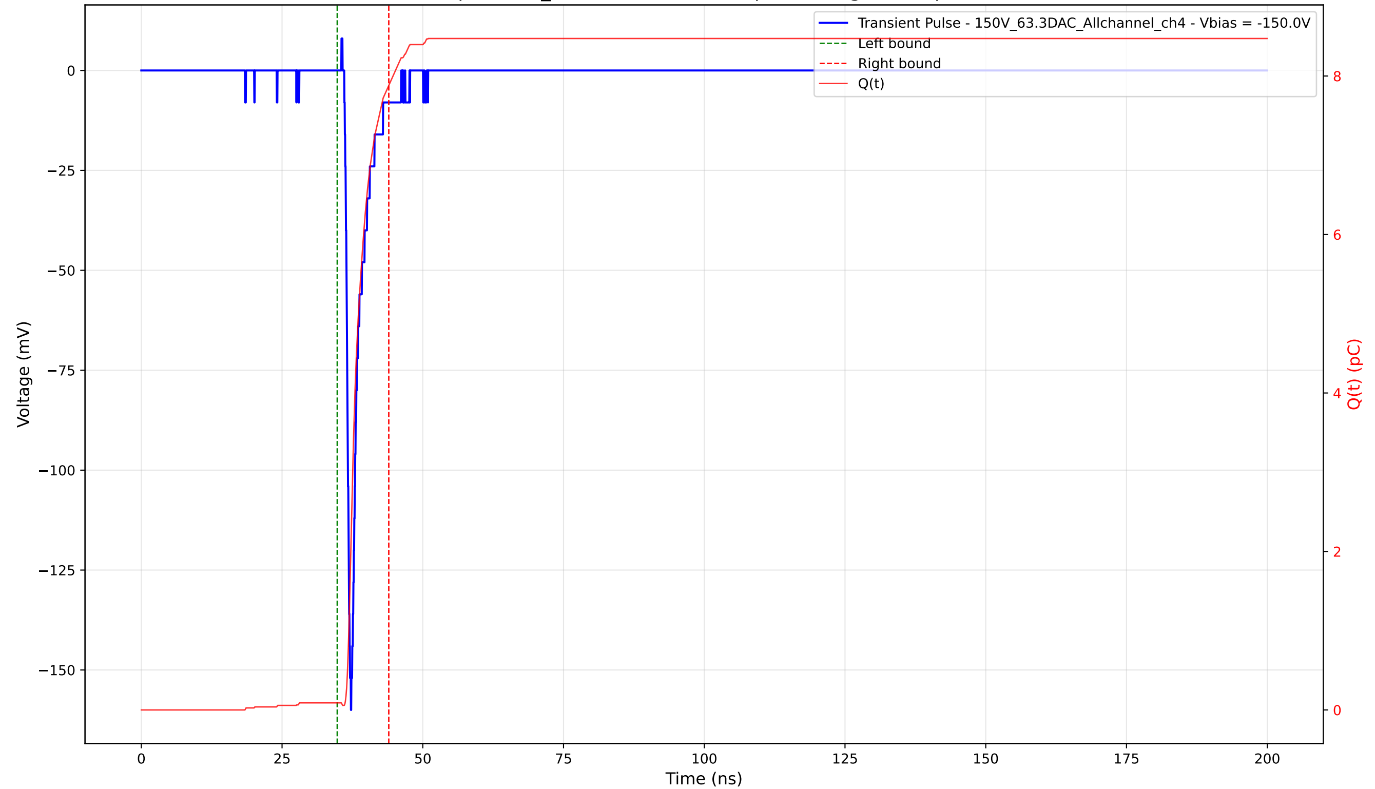
Transient Pulse - Sample: 1cm_42 - Position: 2670.0 \mu\text{m} - Charge: 7.79 pC - Rise Time: 0.80 ns
