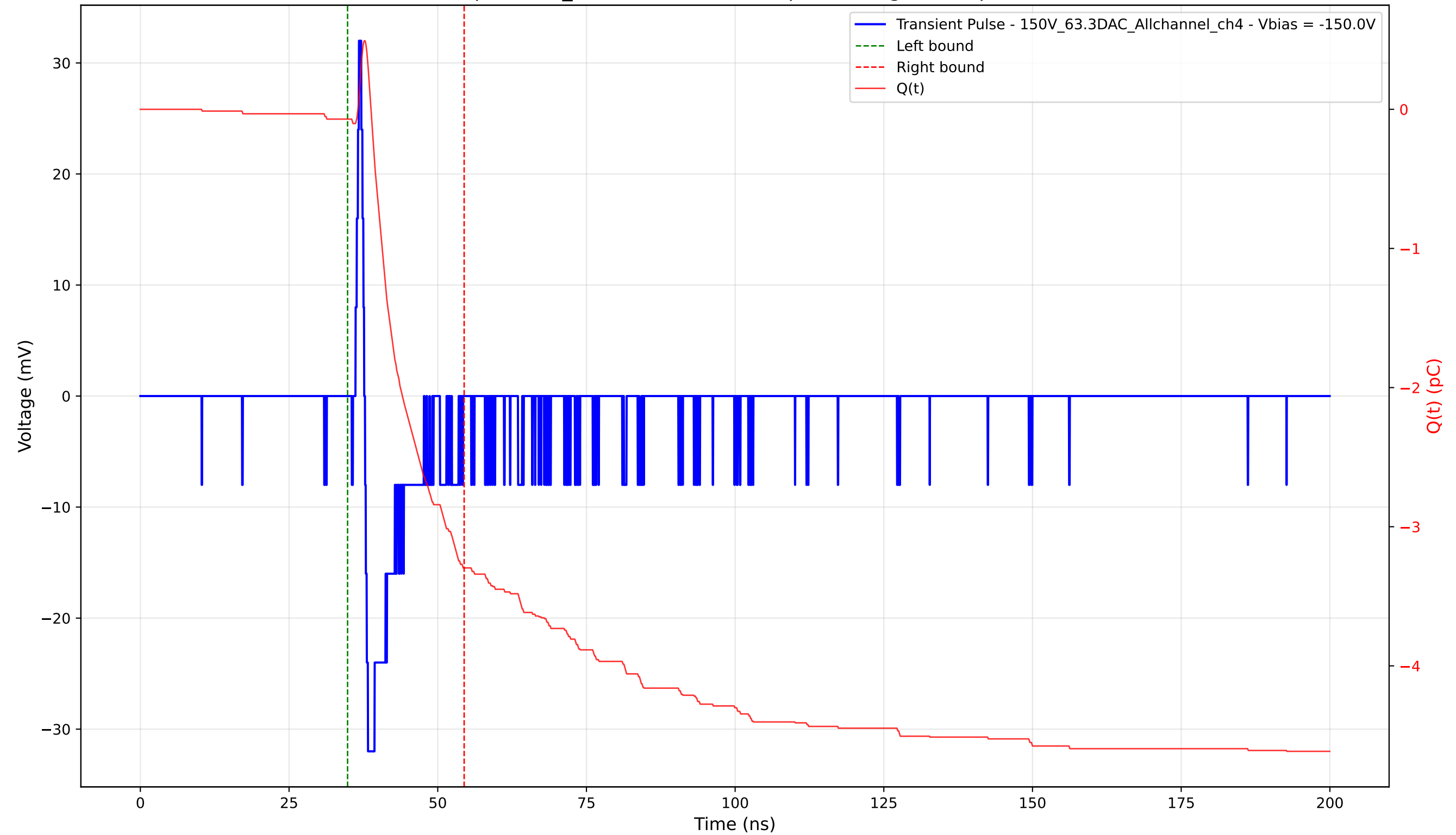
Transient Pulse - Sample: 1cm_42 - Position: 4295.0 \mu\text{m} - Charge: 3.23 pC - Rise Time: 0.58 ns
