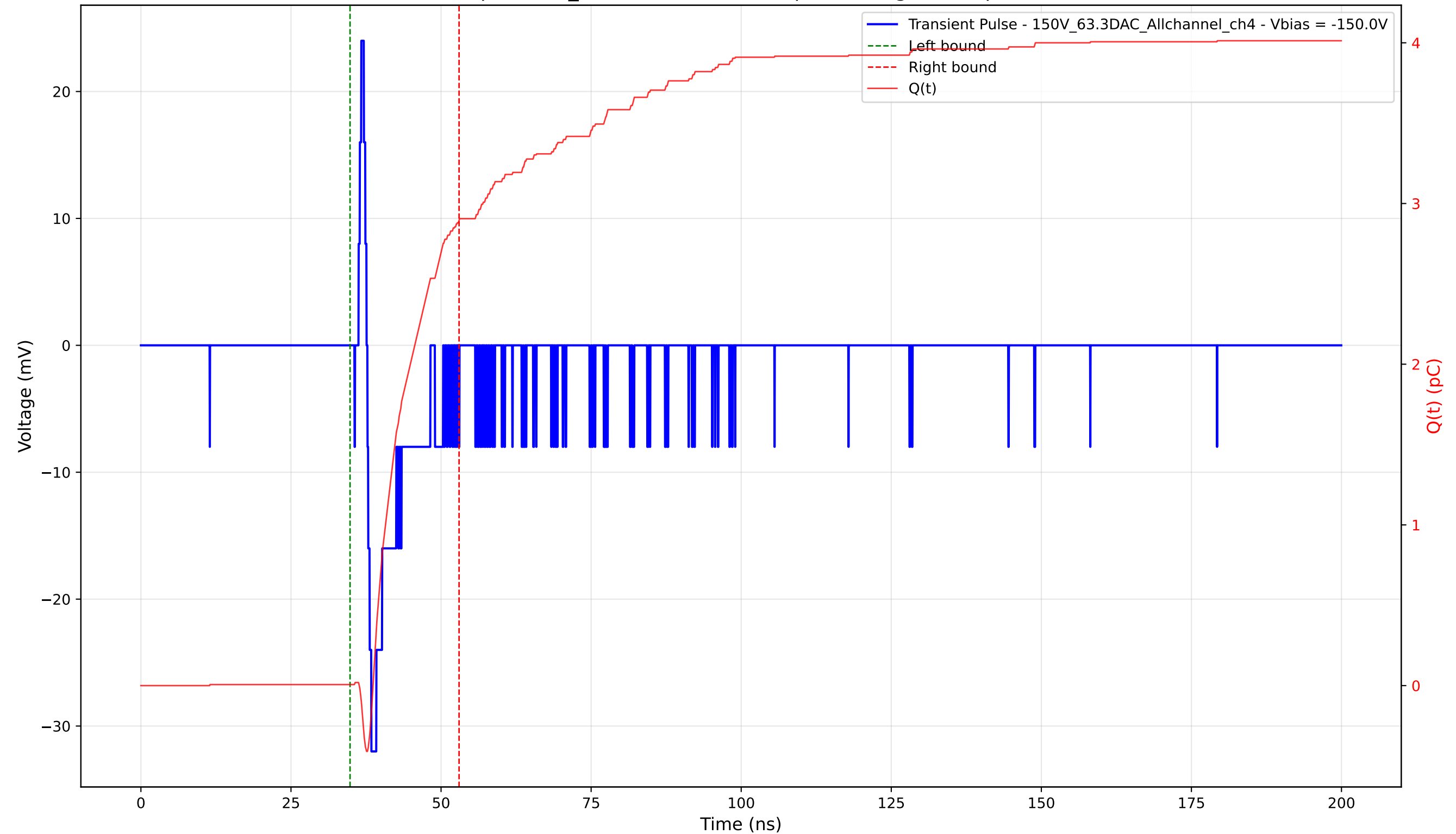
Transient Pulse - Sample: 1cm_42 - Position: 3955.0 \mu\text{m} - Charge: 2.89 pC - Rise Time: 0.66 ns
