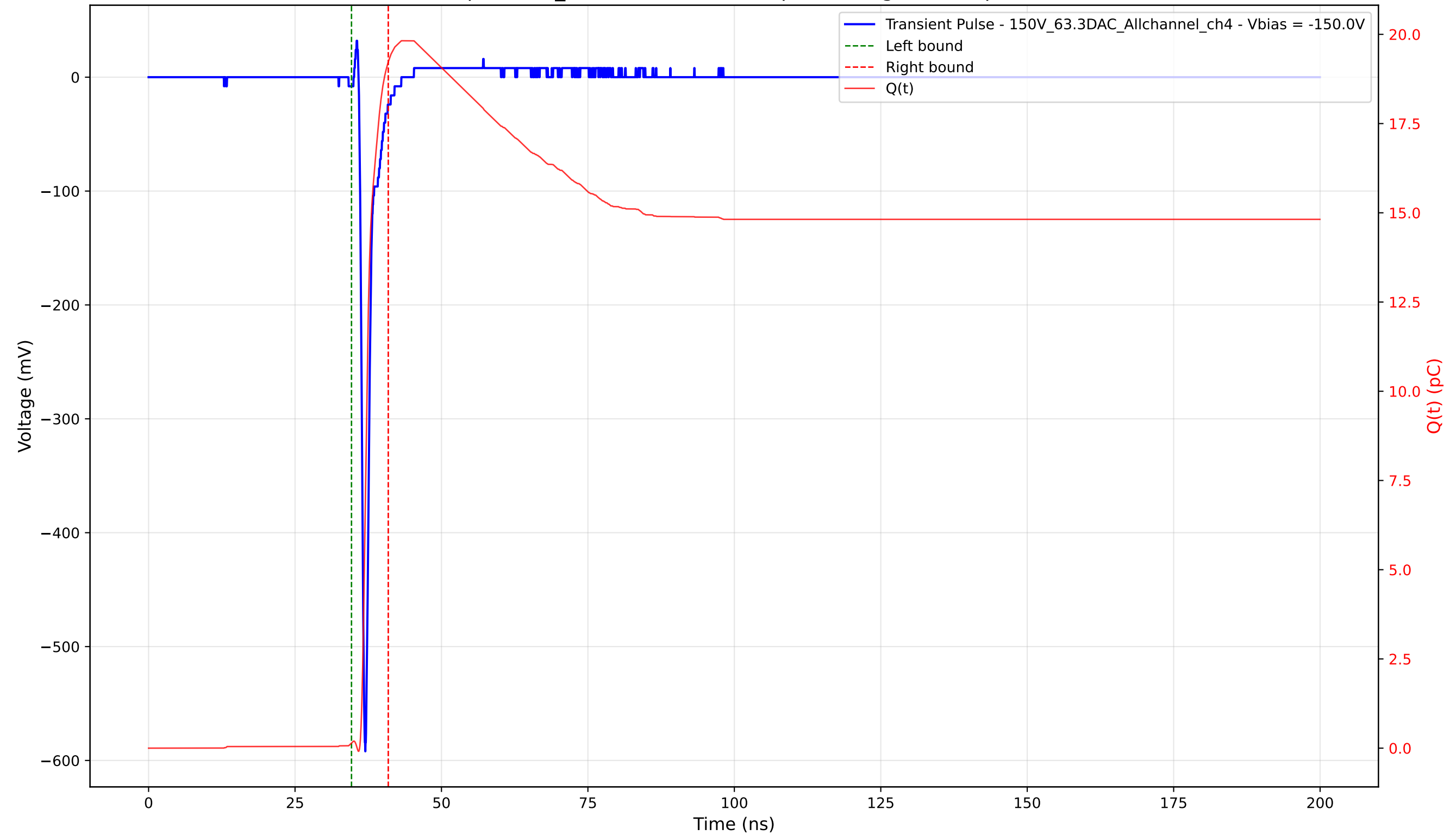
Transient Pulse - Sample: 1cm_42 - Position: 1845.0 \mu\text{m} - Charge: 19.08 pC - Rise Time: 0.72 ns
