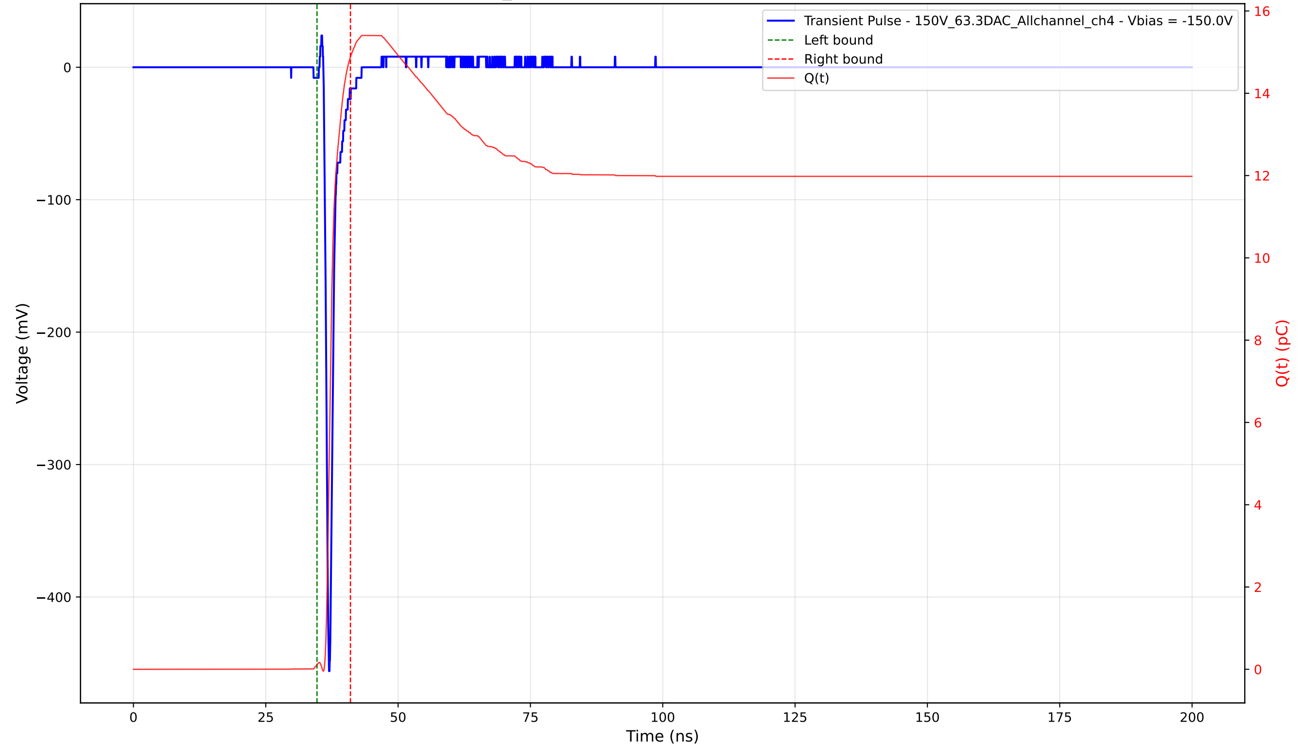
Transient Pulse - Sample: 1cm_42 - Position: 2330.0 \mu\text{m} - Charge: 14.77 pC - Rise Time: 0.68 ns
