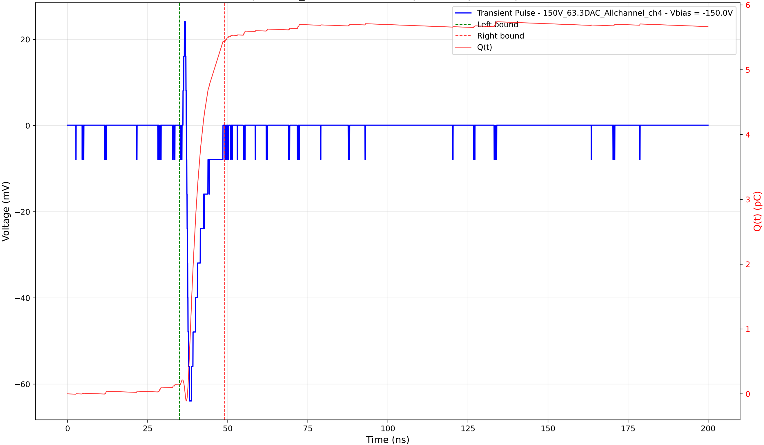
Transient Pulse - Sample: 1cm_42 - Position: 580.0 \mu\text{m} - Charge: 5.30 pC - Rise Time: 0.93 ns
