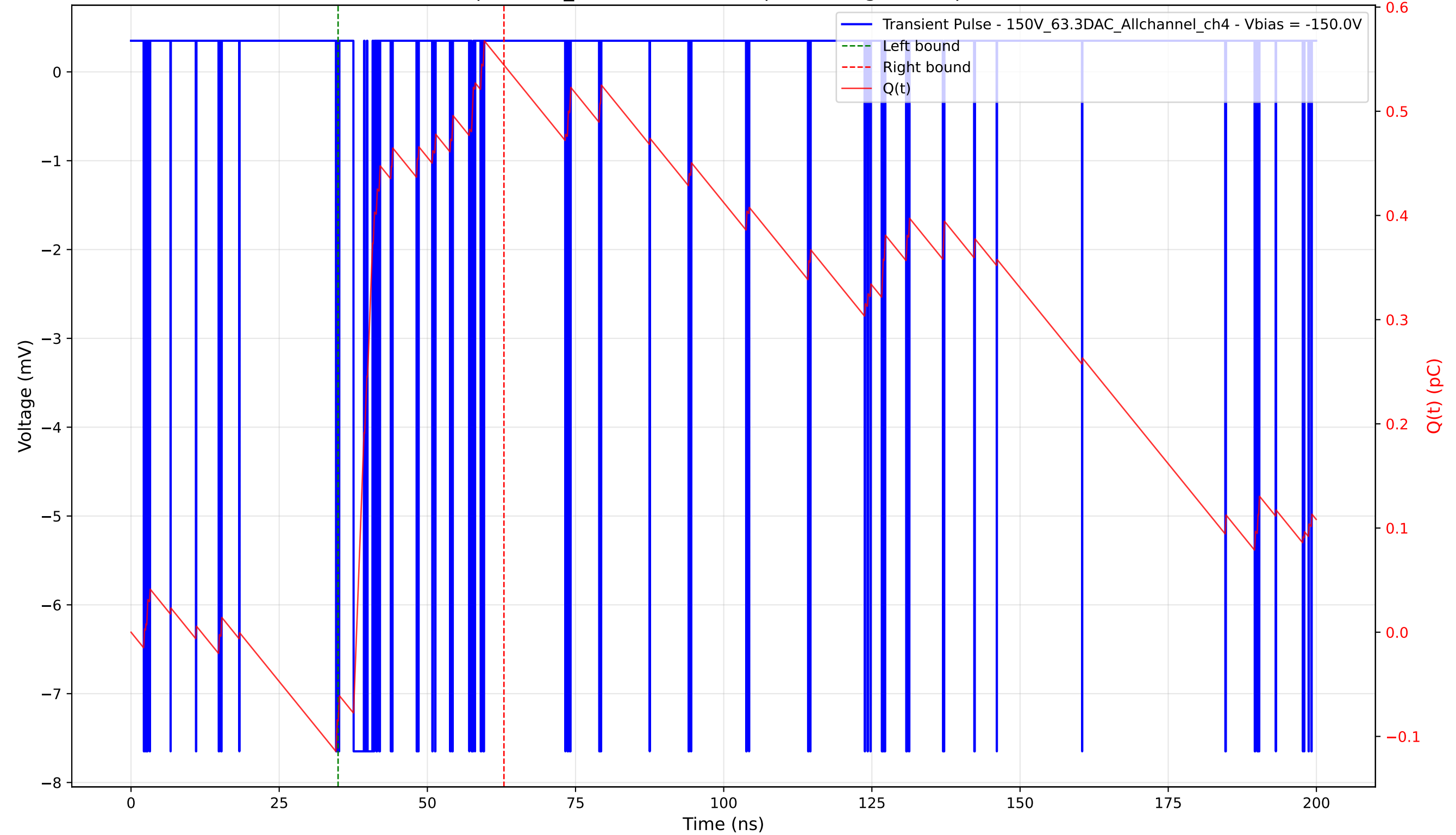
Transient Pulse - Sample: 1cm_42 - Position: 45.0 \mu\text{m} - Charge: 0.63 pC - Rise Time: 0.04 ns
