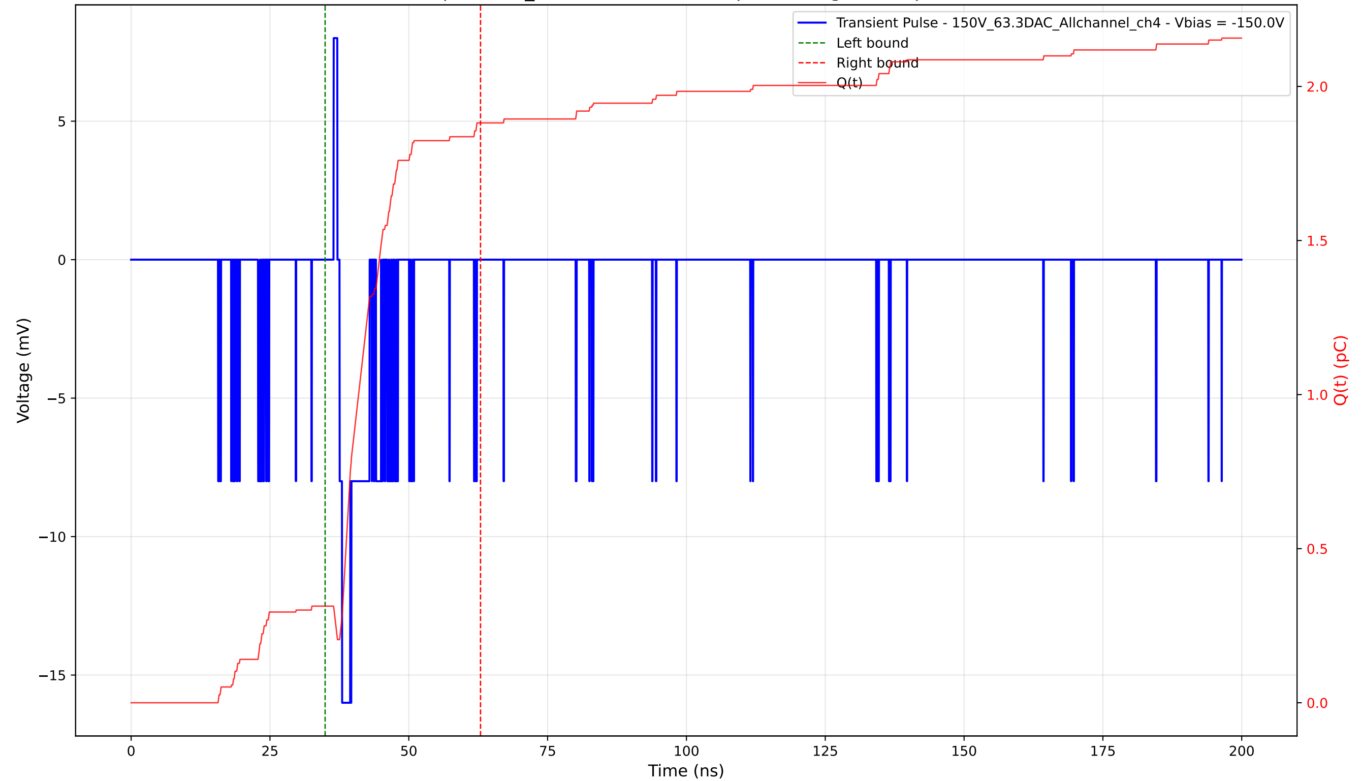
Transient Pulse - Sample: 1cm_42 - Position: 5050.0 \mu\text{m} - Charge: 1.57 pC - Rise Time: 0.47 ns
