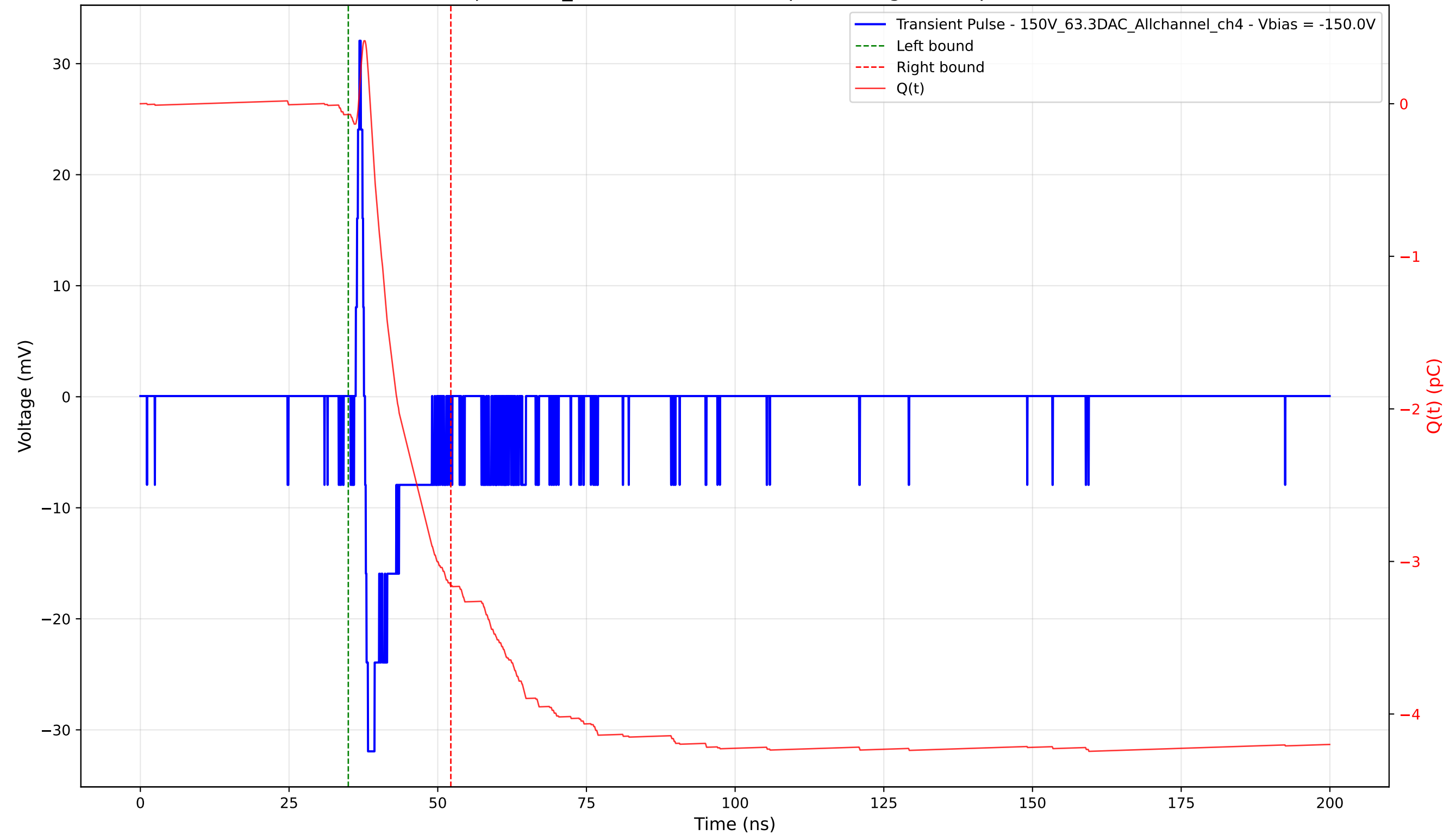
Transient Pulse - Sample: 1cm_42 - Position: 4290.0 \mu\text{m} - Charge: 3.09 pC - Rise Time: 0.62 ns
