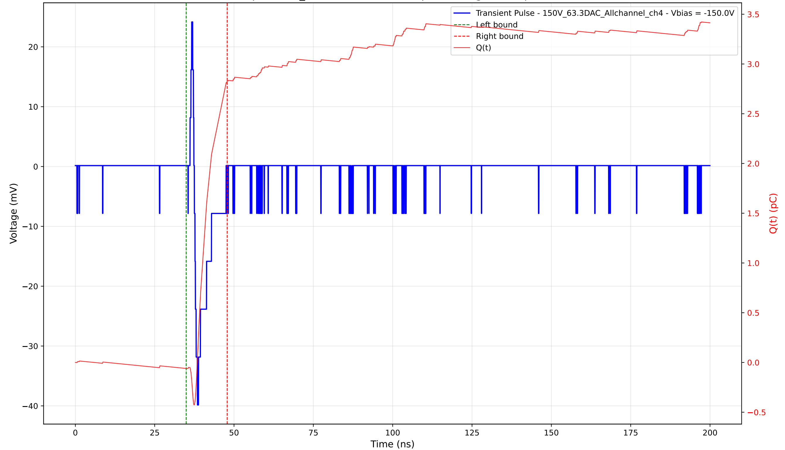
Transient Pulse - Sample: 1cm_42 - Position: 4785.0 \mu\text{m} - Charge: 2.89 pC - Rise Time: 0.98 ns
