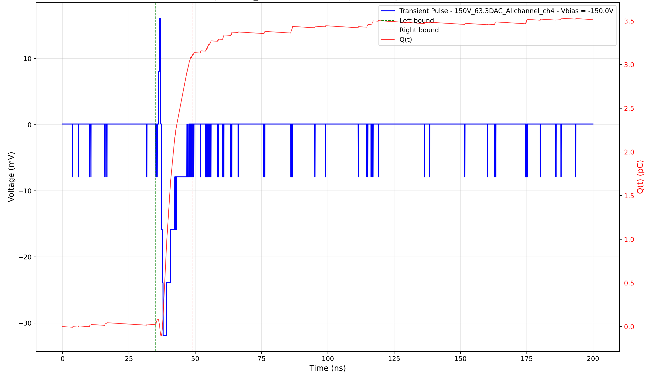
Transient Pulse - Sample: 1cm_42 - Position: 290.0 \mu\text{m} - Charge: 3.08 pC - Rise Time: 0.62 ns
