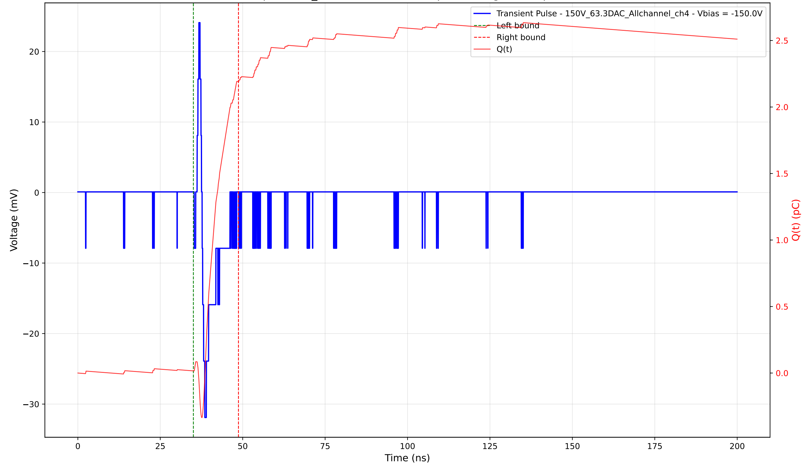
Transient Pulse - Sample: 1cm_42 - Position: 4535.0 \mu\text{m} - Charge: 2.18 pC - Rise Time: 0.82 ns
