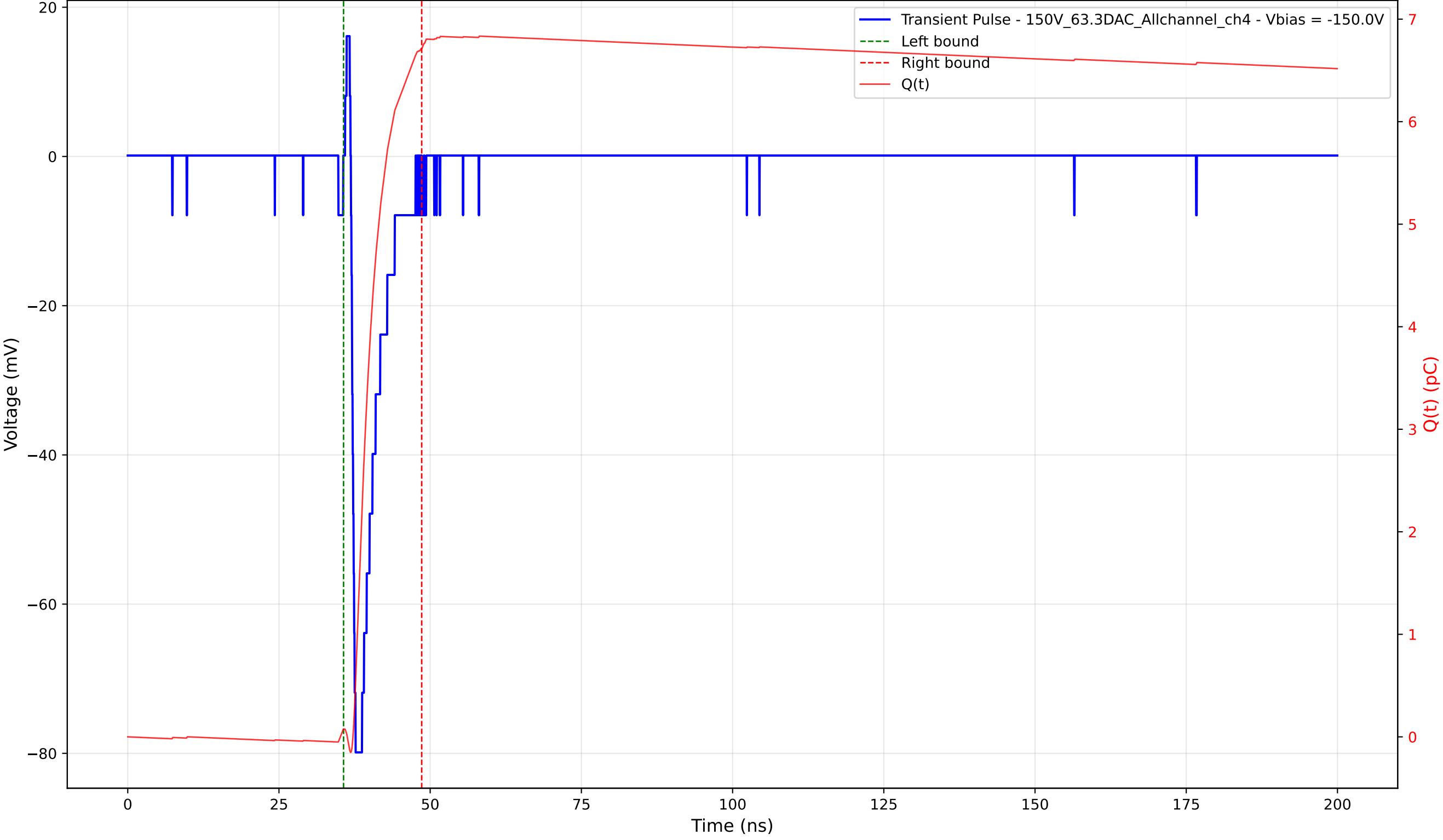
Transient Pulse - Sample: 1cm_42 - Position: 885.0 \mu\text{m} - Charge: 6.64 pC - Rise Time: 0.72 ns
