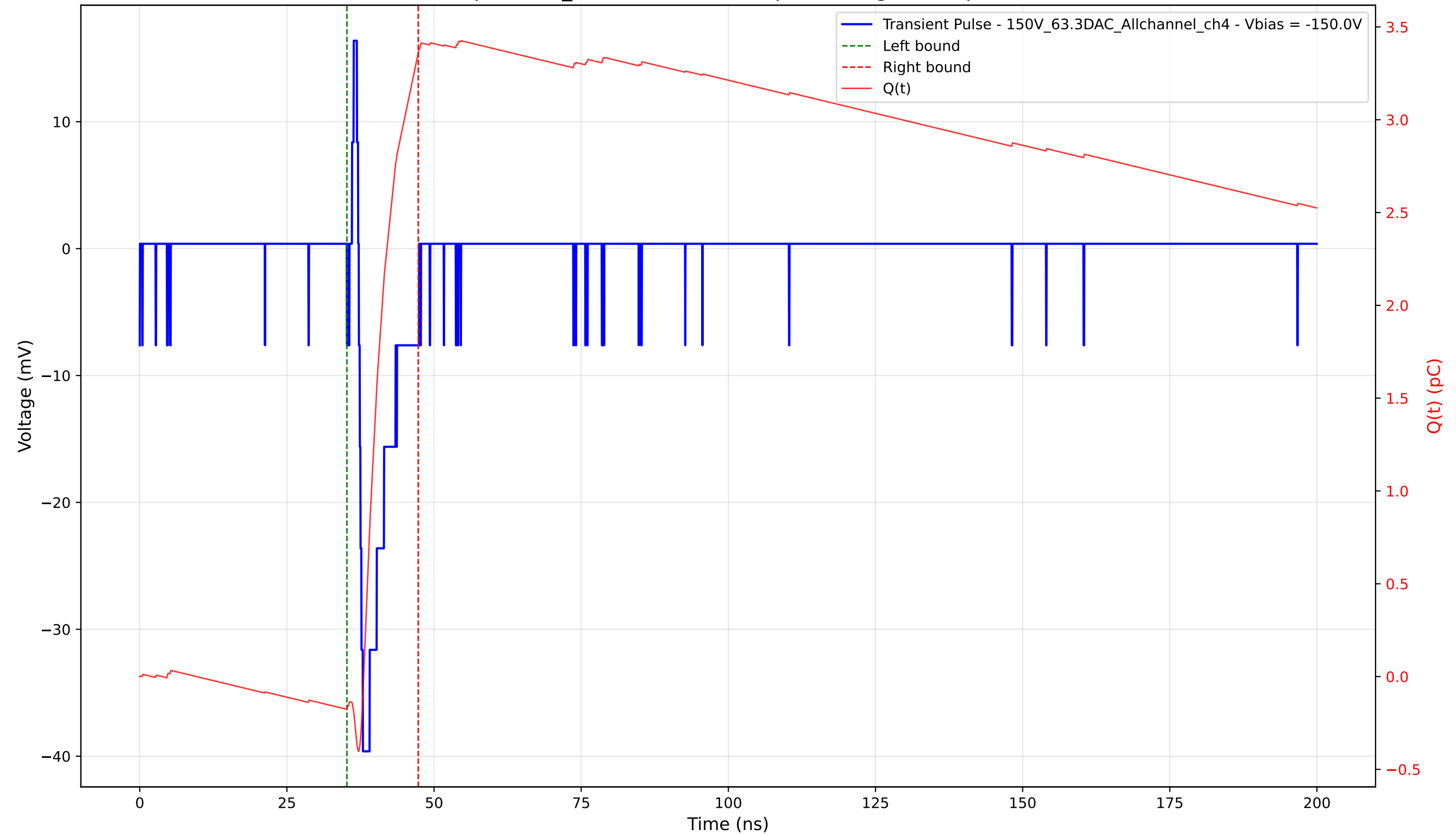
Transient Pulse - Sample: 1cm_42 - Position: 400.0 \mu\text{m} - Charge: 3.54 pC - Rise Time: 0.70 ns
