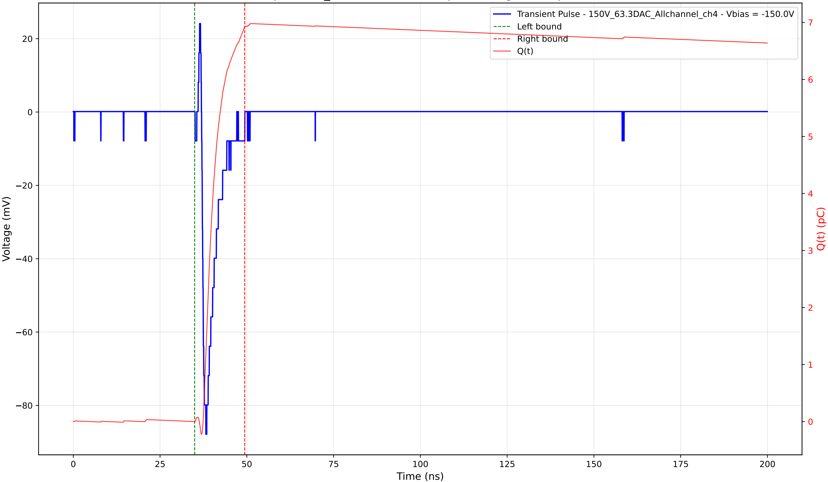
Transient Pulse - Sample: 1cm_42 - Position: 810.0 \mu\text{m} - Charge: 6.93 pC - Rise Time: 0.72 ns
