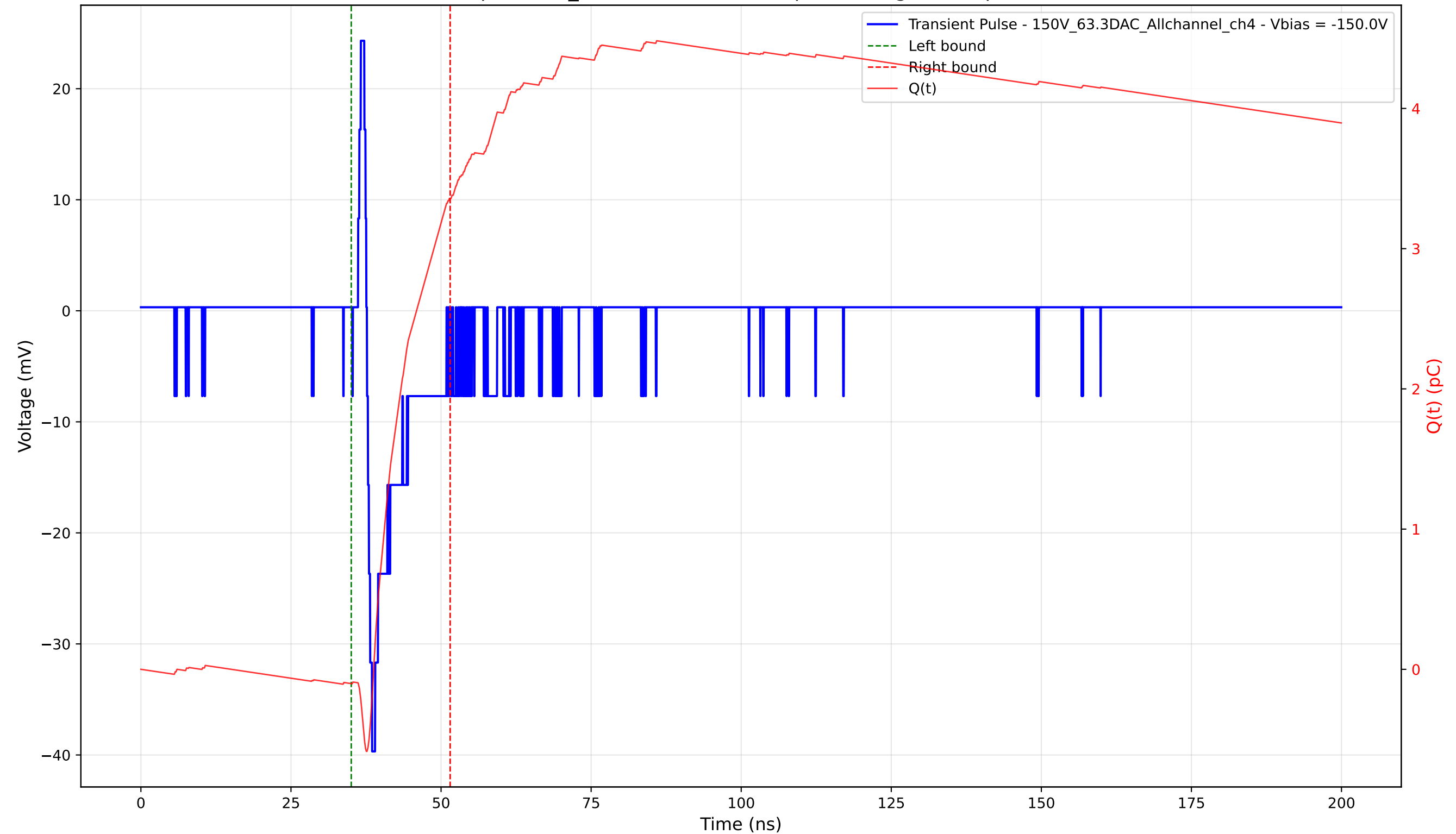
Transient Pulse - Sample: 1cm_42 - Position: 3770.0 \mu\text{m} - Charge: 3.46 pC - Rise Time: 0.86 ns
