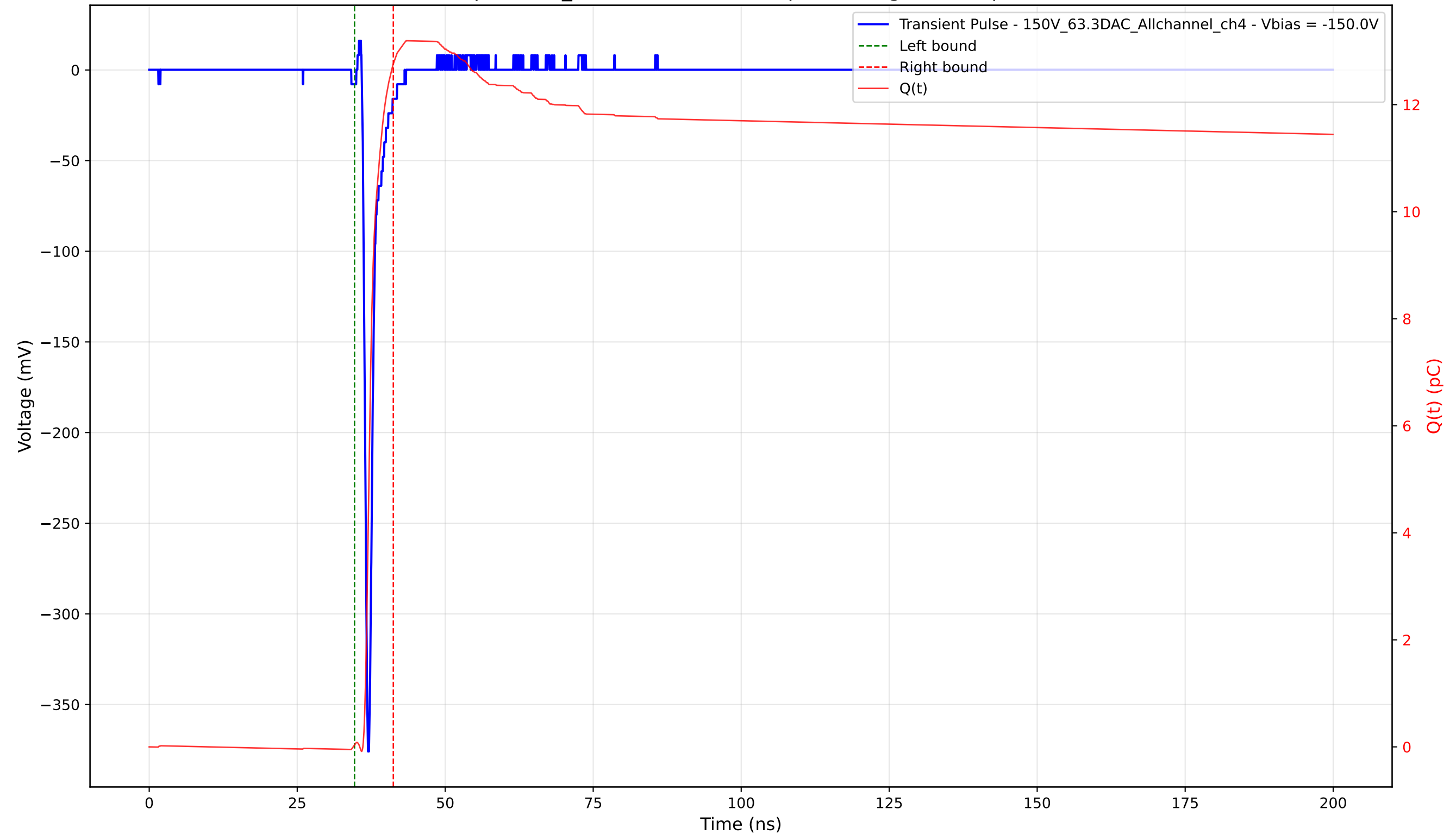
Transient Pulse - Sample: 1cm_42 - Position: 2390.0 \mu\text{m} - Charge: 12.73 pC - Rise Time: 0.70 ns
