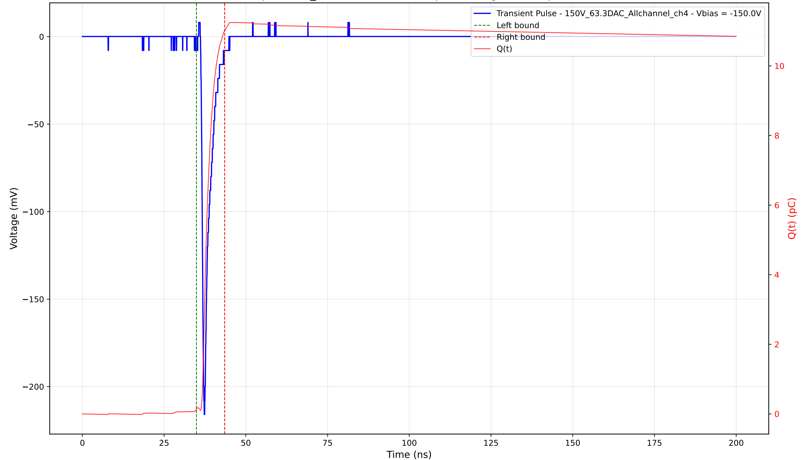
Transient Pulse - Sample: 1cm_42 - Position: 1420.0 \mu\text{m} - Charge: 10.88 pC - Rise Time: 0.81 ns
