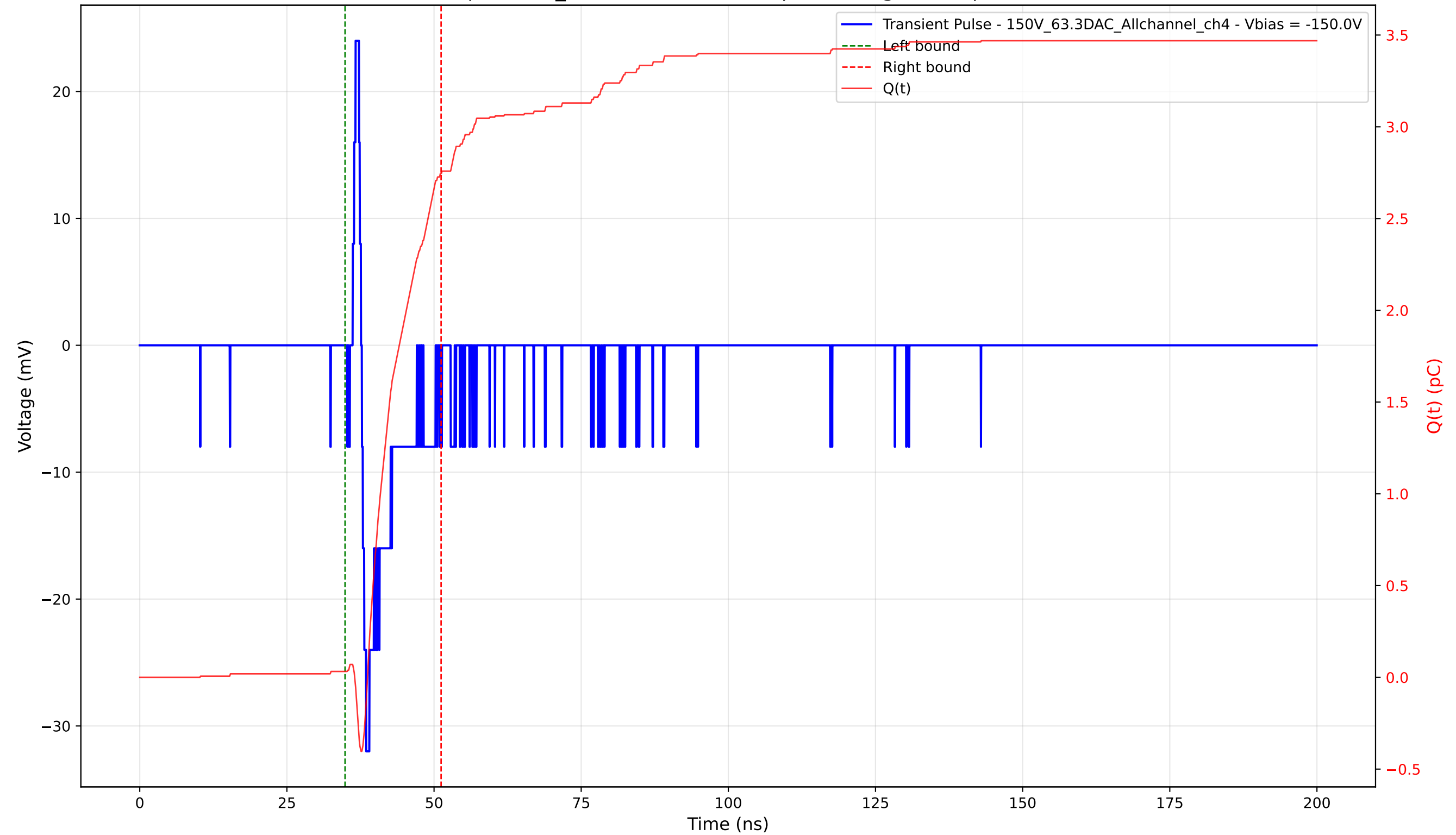
Transient Pulse - Sample: 1cm_42 - Position: 3985.0 \mu\text{m} - Charge: 2.71 pC - Rise Time: 0.74 ns
