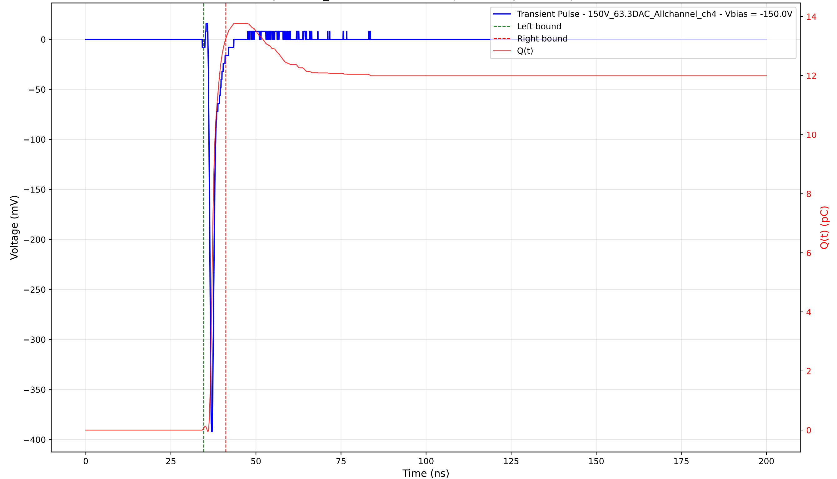
Transient Pulse - Sample: 1cm_42 - Position: 2375.0 \mu\text{m} - Charge: 13.19 pC - Rise Time: 0.72 ns
