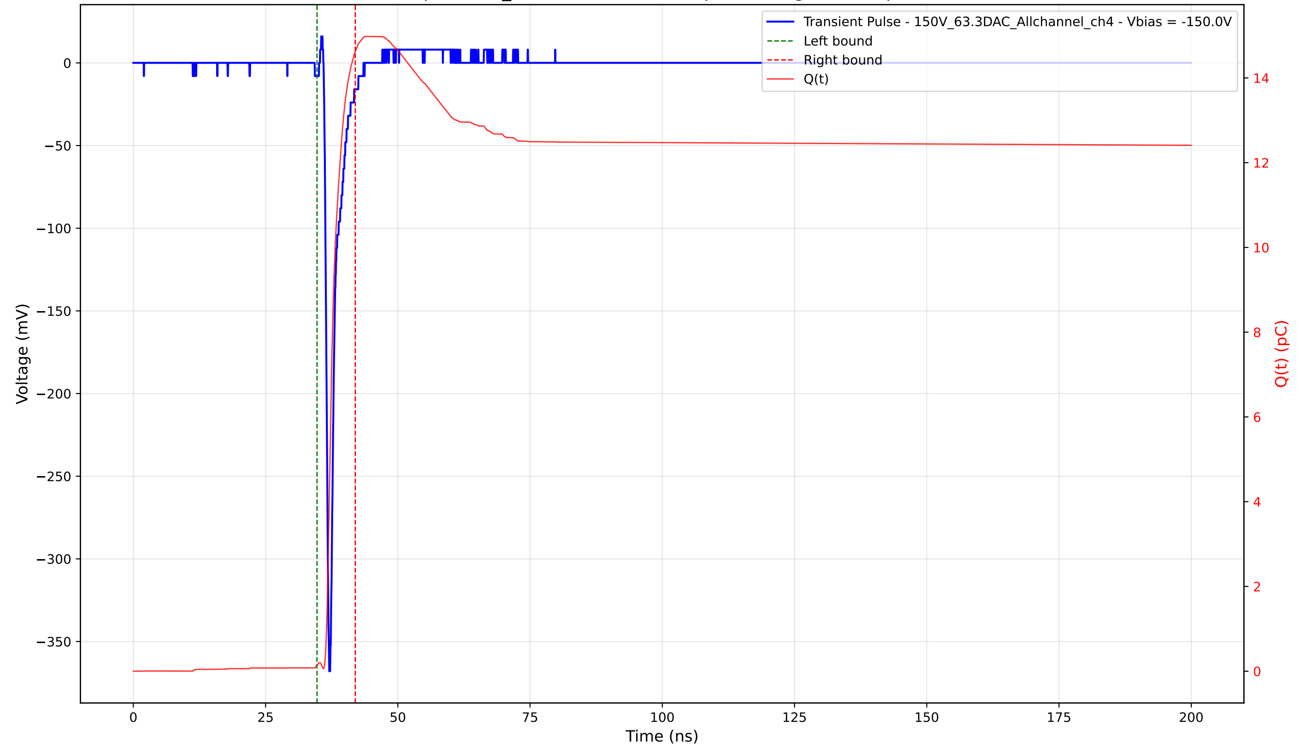
Transient Pulse - Sample: 1cm_42 - Position: 1595.0 \mu\text{m} - Charge: 14.48 pC - Rise Time: 0.74 ns
