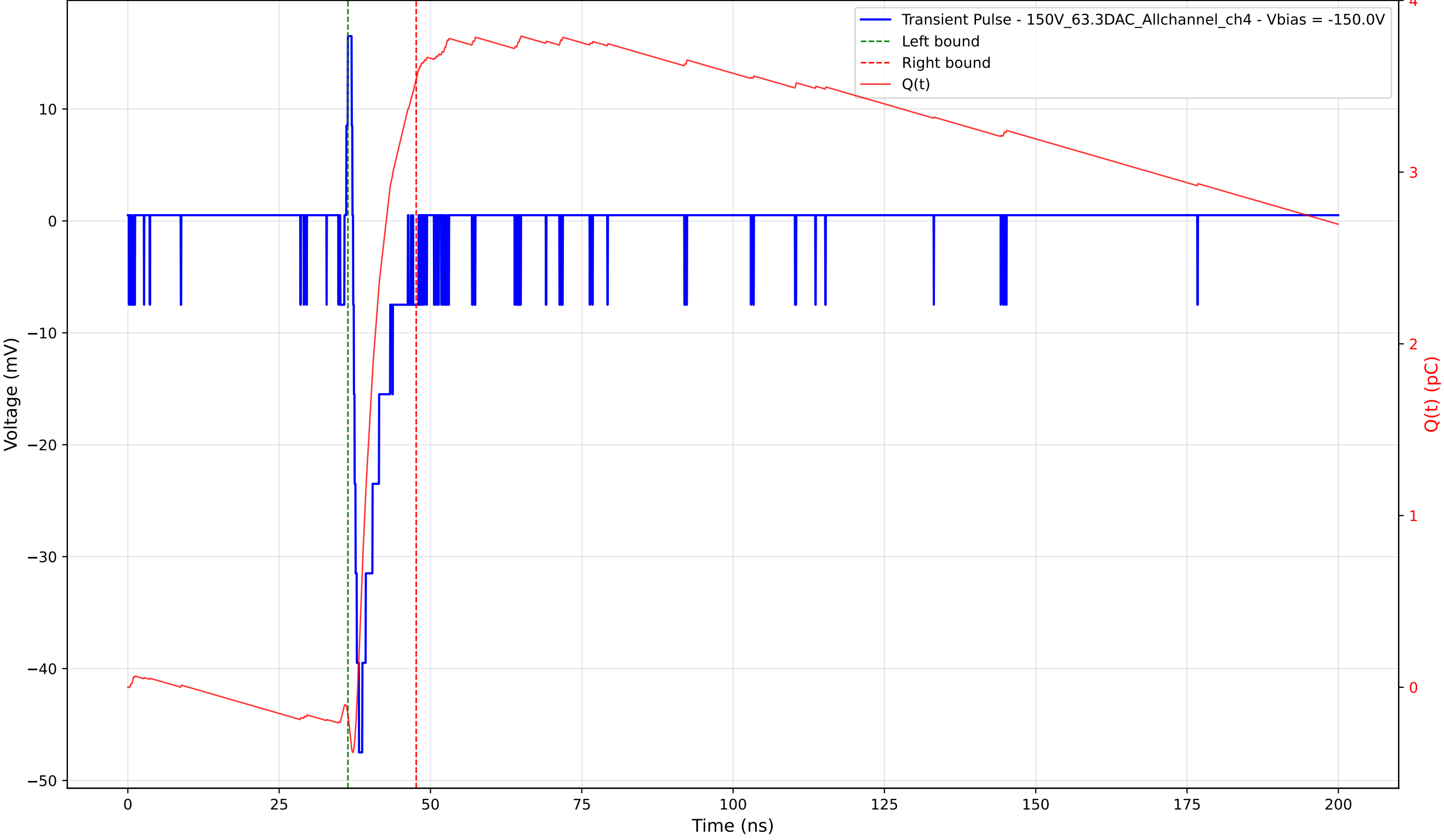
Transient Pulse - Sample: 1cm_42 - Position: 430.0 \mu\text{m} - Charge: 3.70 pC - Rise Time: 0.98 ns
