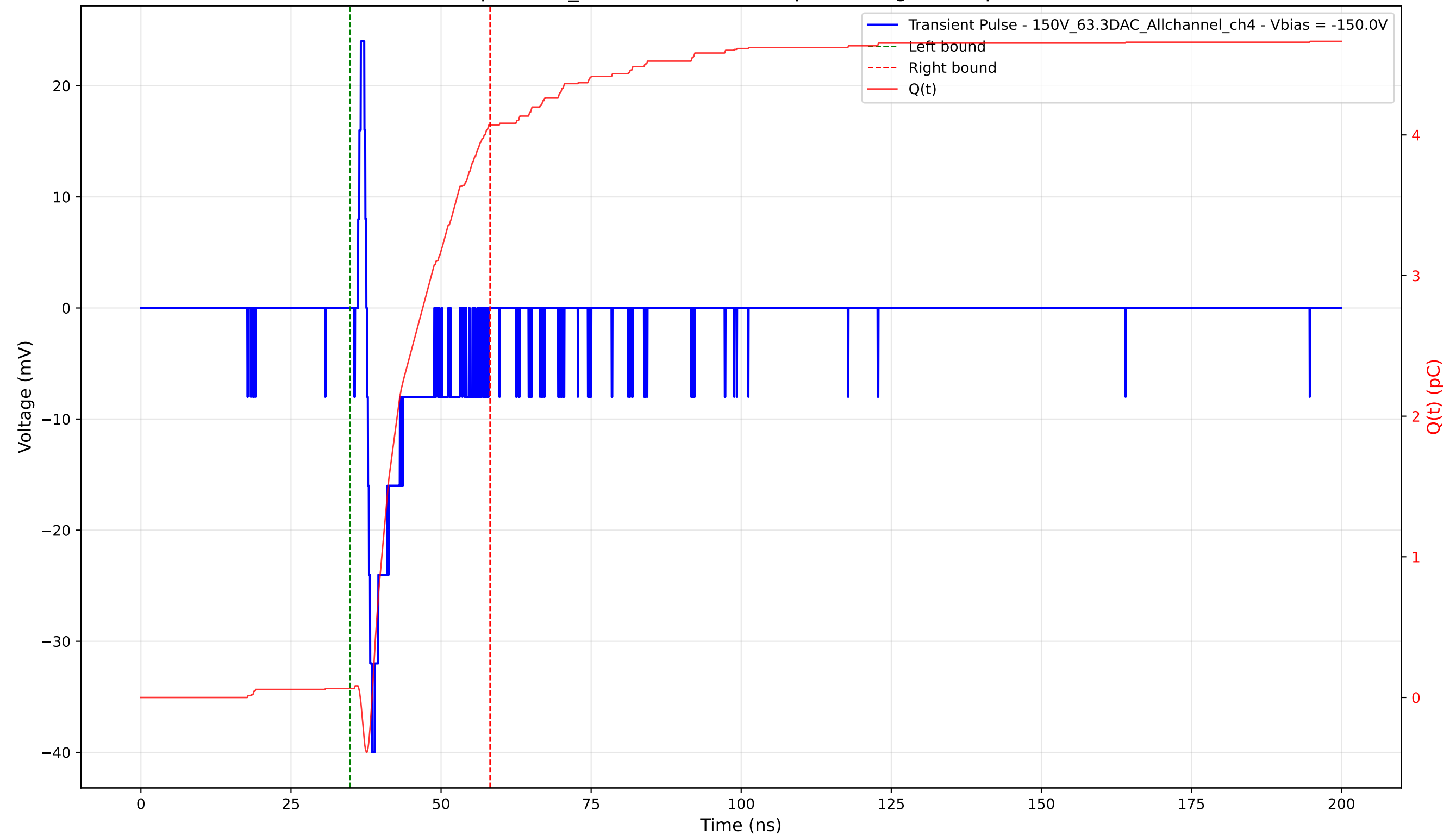
Transient Pulse - Sample: 1cm_42 - Position: 3740.0 \mu\text{m} - Charge: 4.01 pC - Rise Time: 0.86 ns
