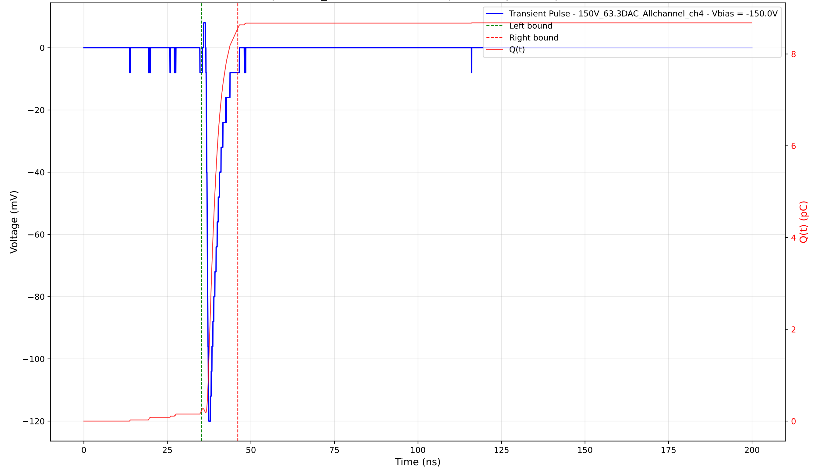
Transient Pulse - Sample: 1cm_42 - Position: 1095.0 \mu\text{m} - Charge: 8.33 pC - Rise Time: 0.66 ns
