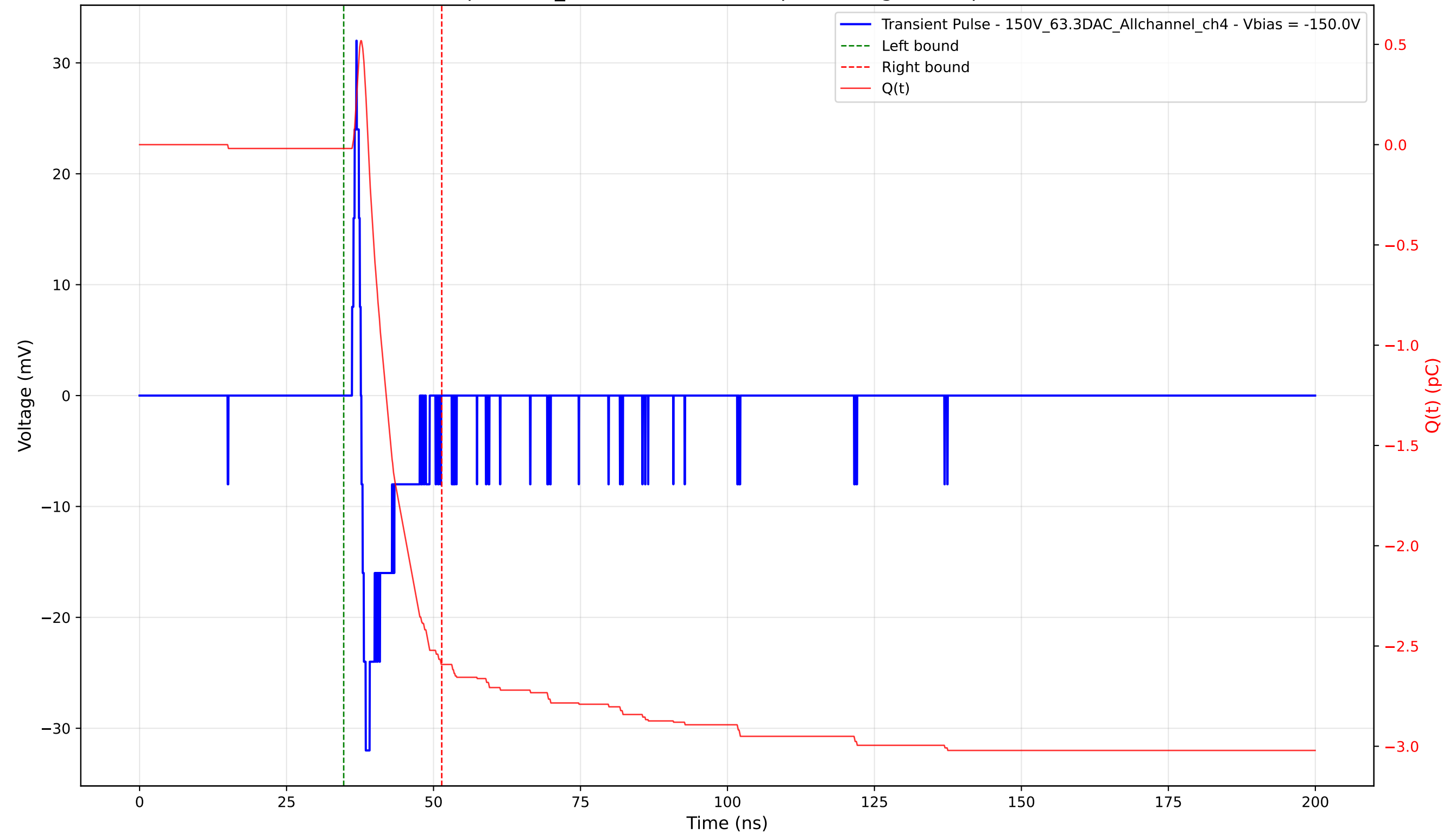
Transient Pulse - Sample: 1cm_42 - Position: 4390.0 \mu\text{m} - Charge: 2.57 pC - Rise Time: 0.74 ns
