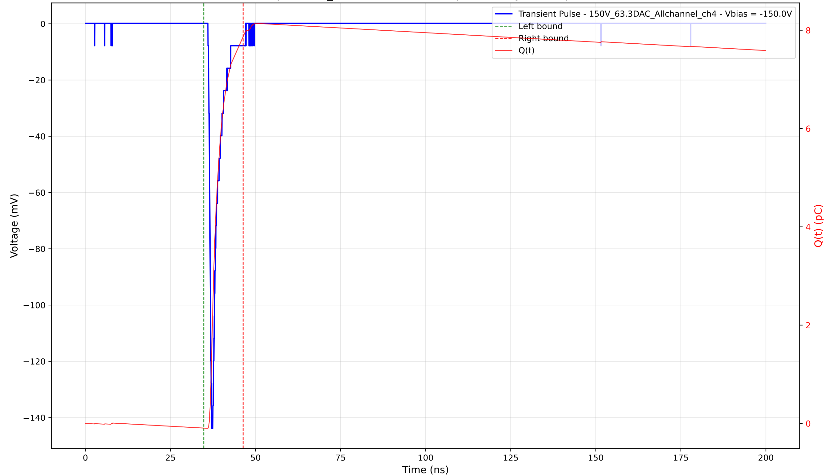
Transient Pulse - Sample: 1cm_42 - Position: 2705.0 \mu\text{m} - Charge: 7.97 pC - Rise Time: 0.85 ns
