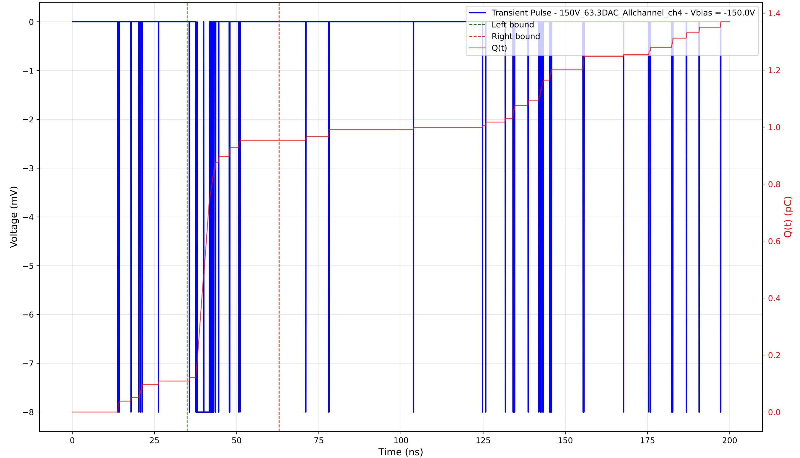
Transient Pulse - Sample: 1cm_42 - Position: 40.0 \mu\text{m} - Charge: 0.84 pC - Rise Time: 0.04 ns
