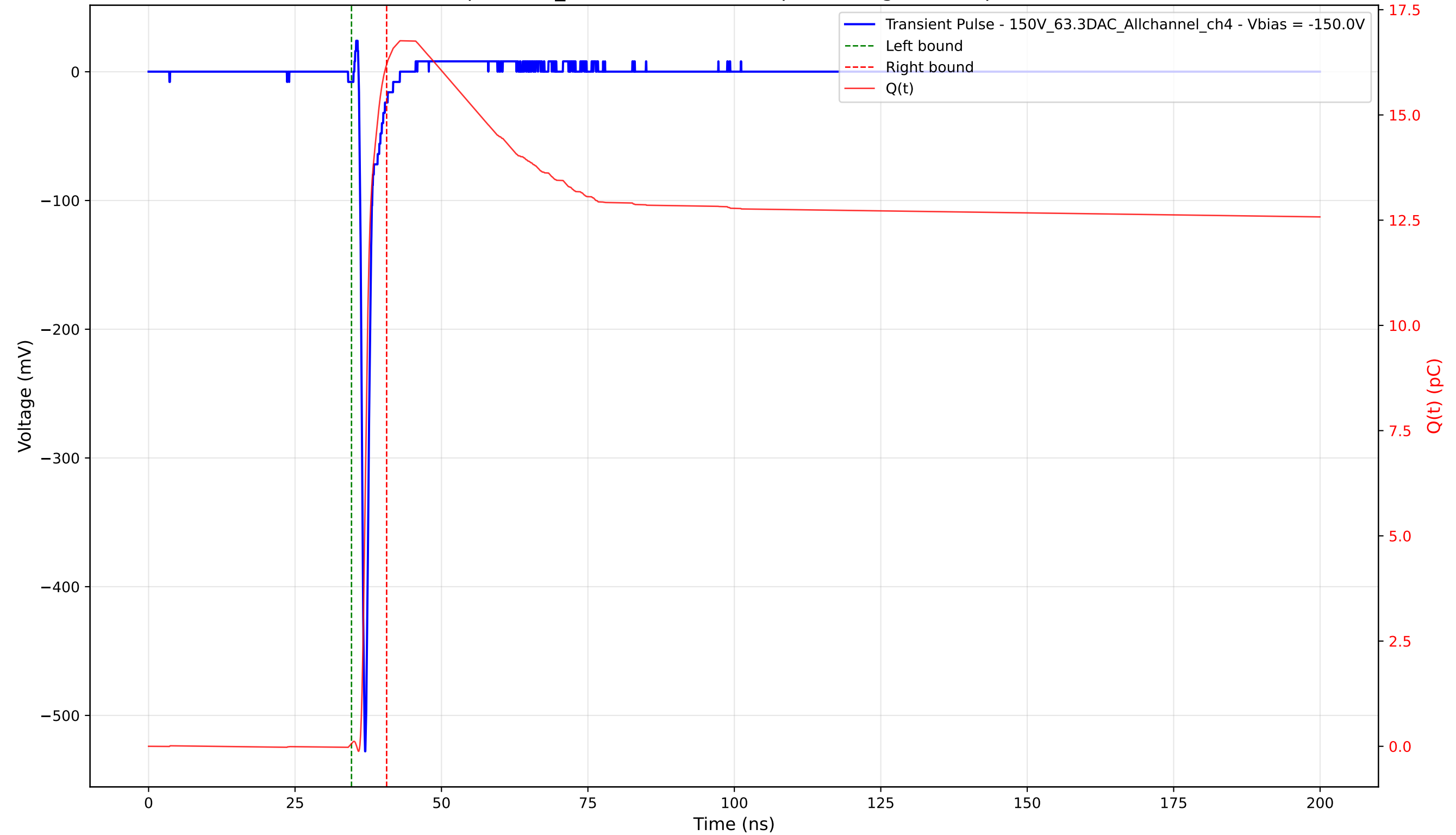
Transient Pulse - Sample: 1cm_42 - Position: 2195.0 \mu\text{m} - Charge: 16.14 pC - Rise Time: 0.72 ns
