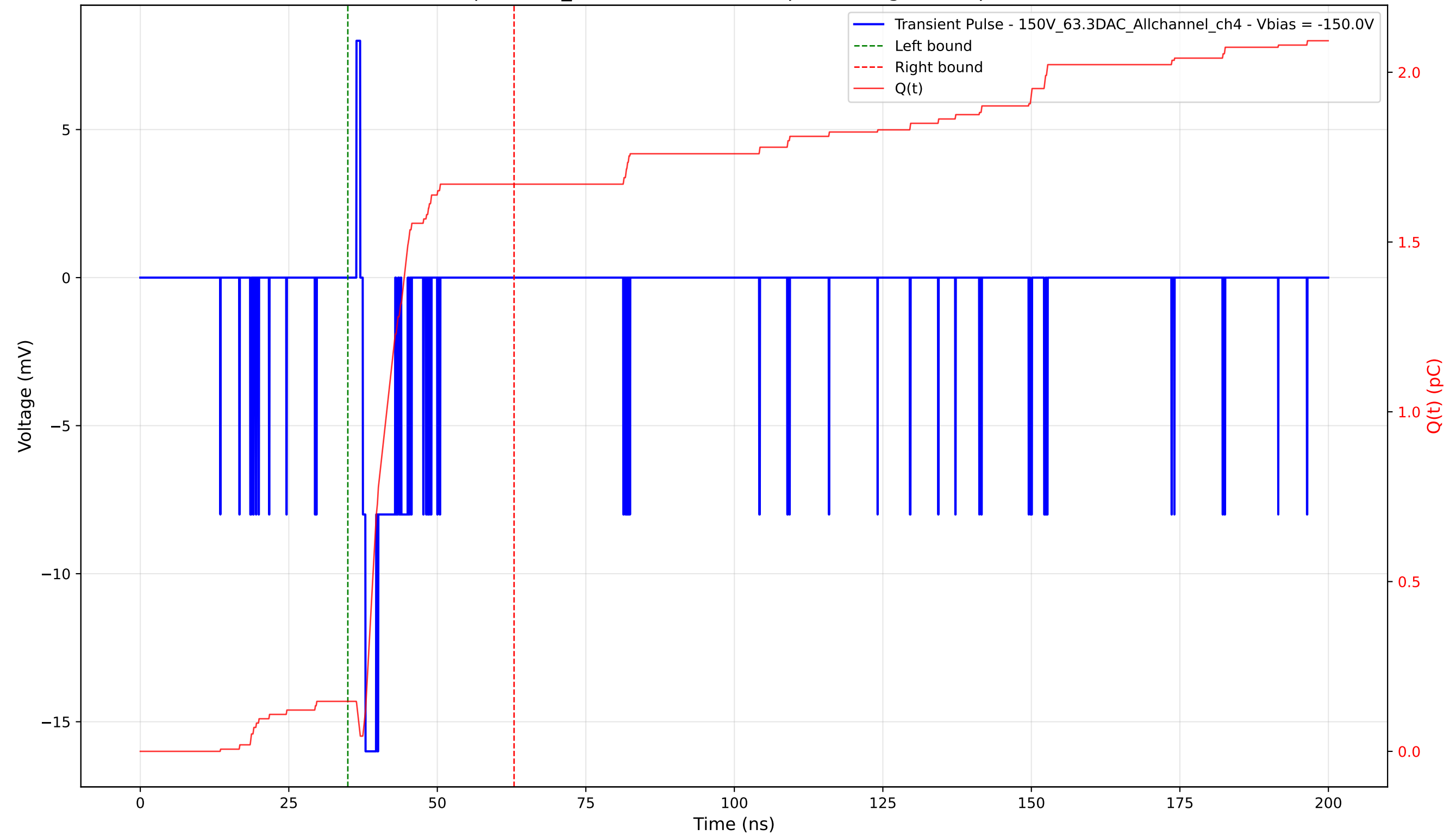
Transient Pulse - Sample: 1cm_42 - Position: 5040.0 \mu\text{m} - Charge: 1.52 pC - Rise Time: 0.47 ns
