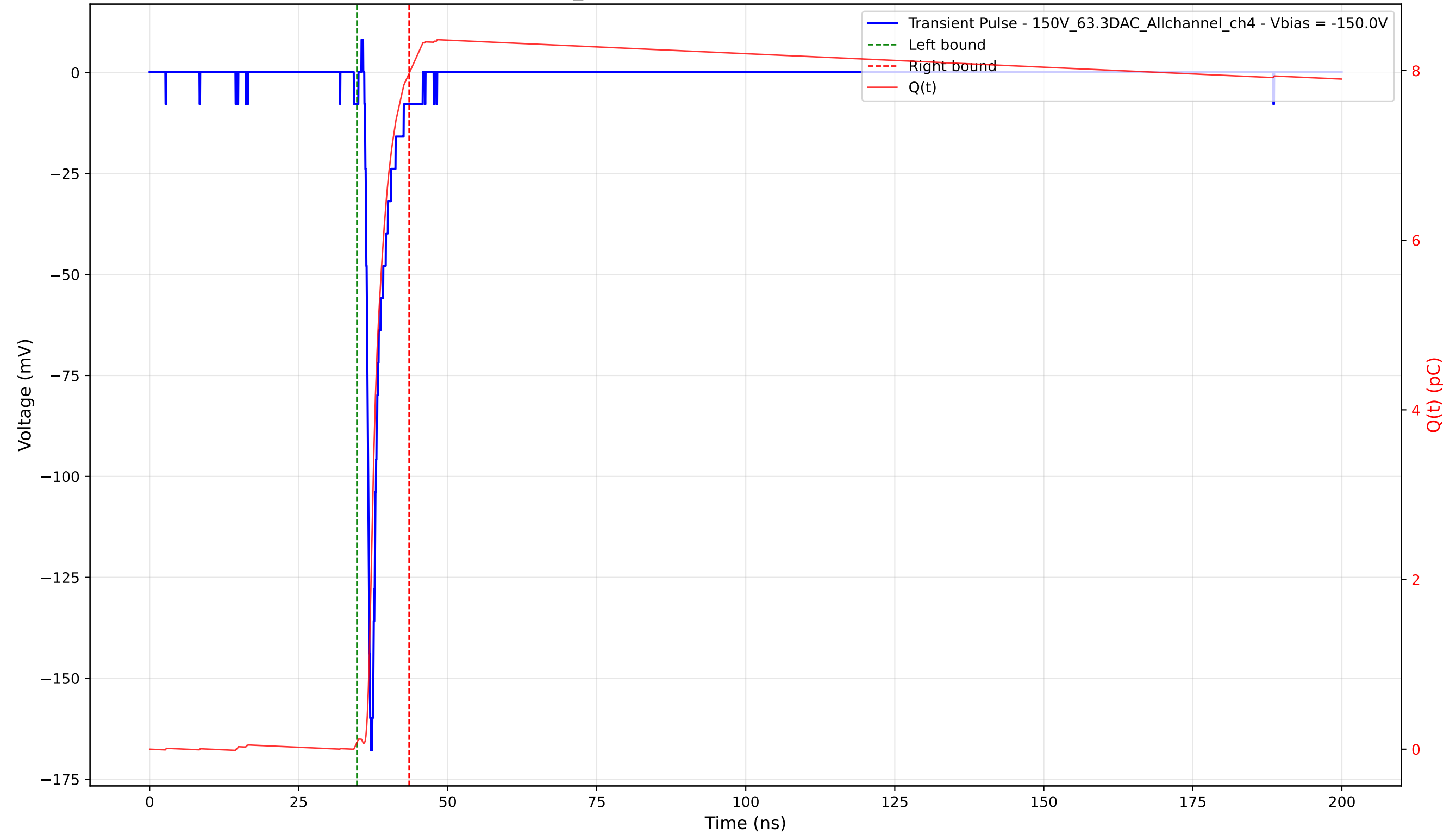
Transient Pulse - Sample: 1cm_42 - Position: 2635.0 \mu\text{m} - Charge: 7.89 pC - Rise Time: 0.79 ns
