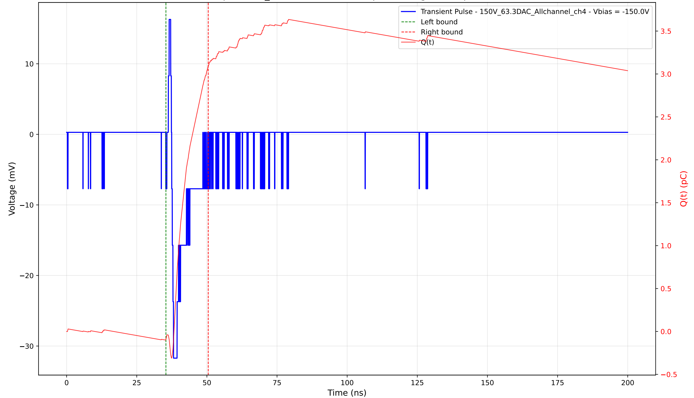
Transient Pulse - Sample: 1cm_42 - Position: 3550.0 \mu\text{m} - Charge: 3.19 pC - Rise Time: 0.66 ns
