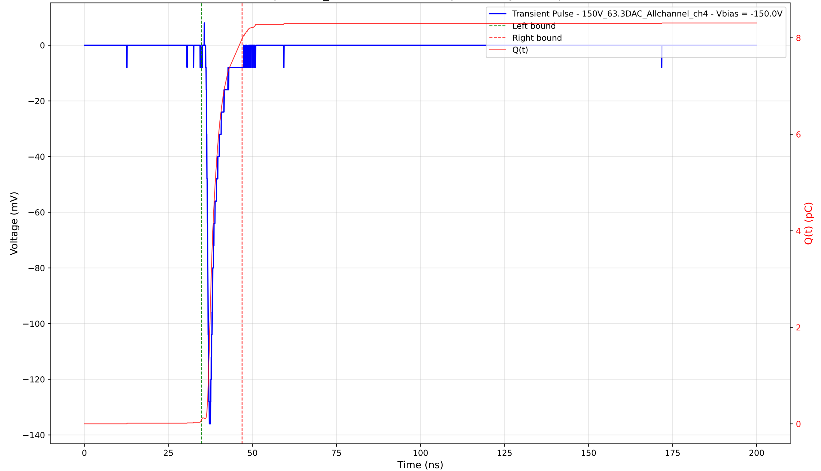
Transient Pulse - Sample: 1cm_42 - Position: 2750.0 \mu\text{m} - Charge: 7.92 pC - Rise Time: 0.81 ns
