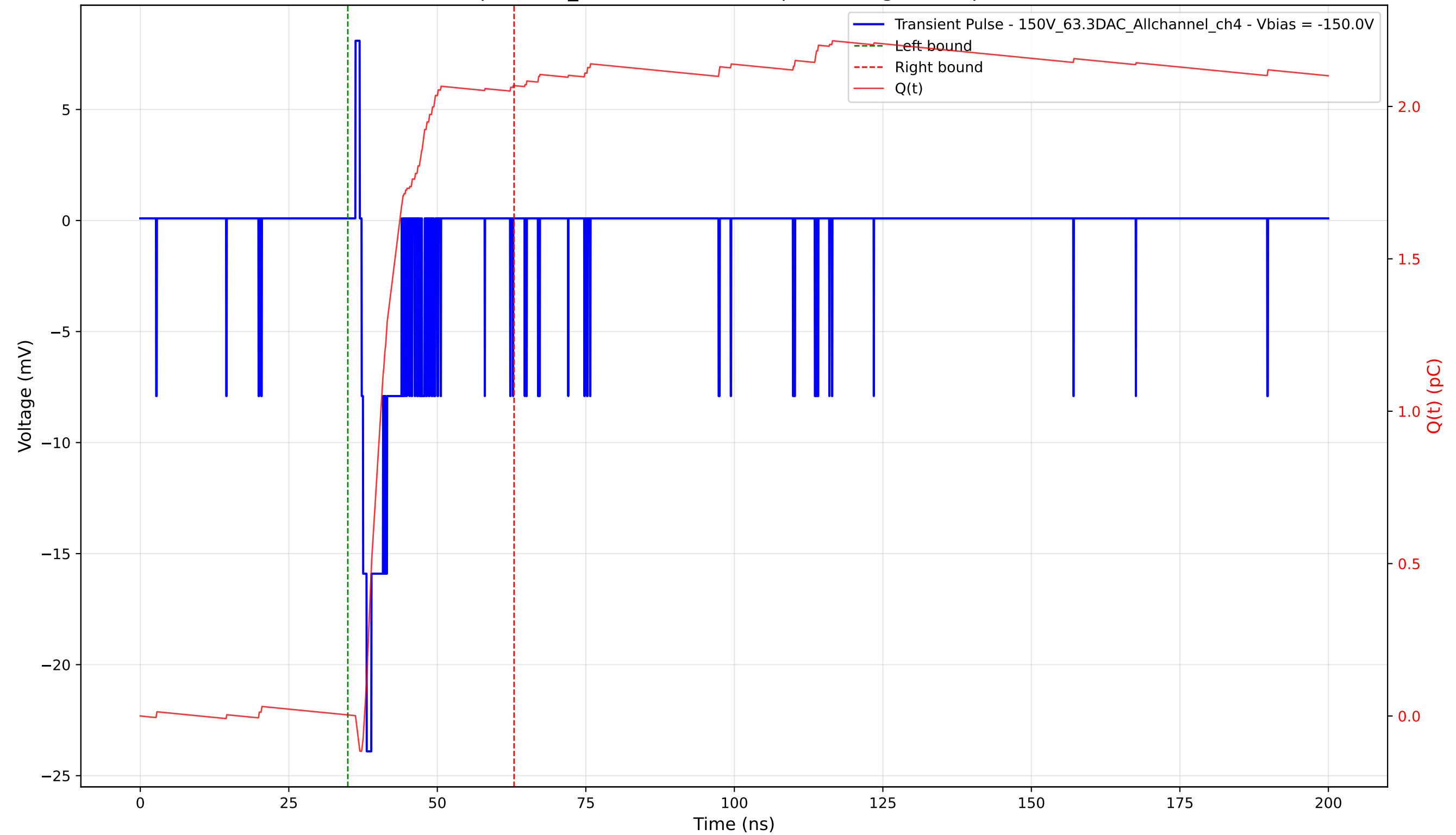
Transient Pulse - Sample: 1cm_42 - Position: 175.0 \mu\text{m} - Charge: 2.07 pC - Rise Time: 0.87 ns
