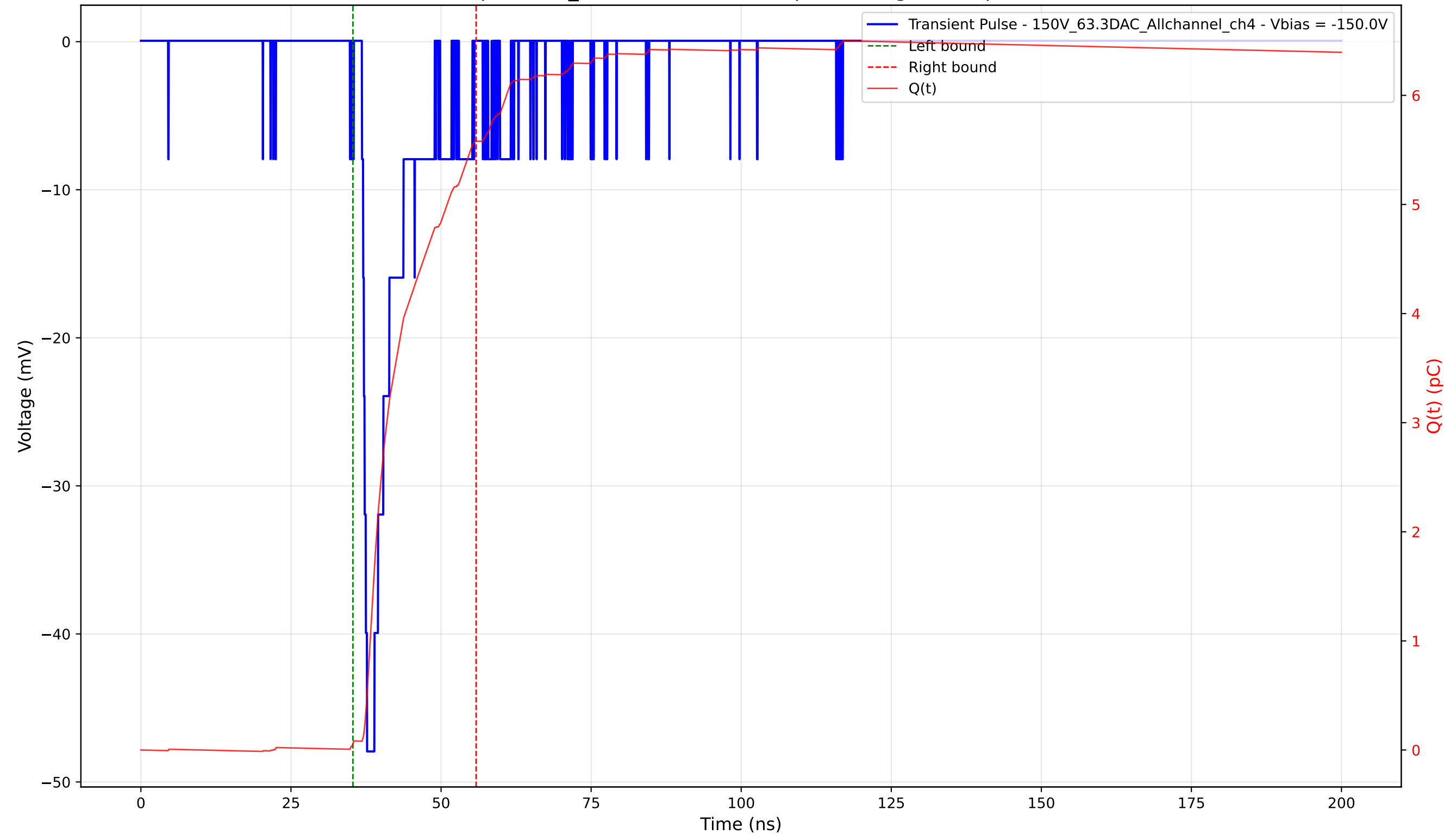
Transient Pulse - Sample: 1cm_42 - Position: 3175.0 \mu\text{m} - Charge: 5.52 pC - Rise Time: 0.86 ns
