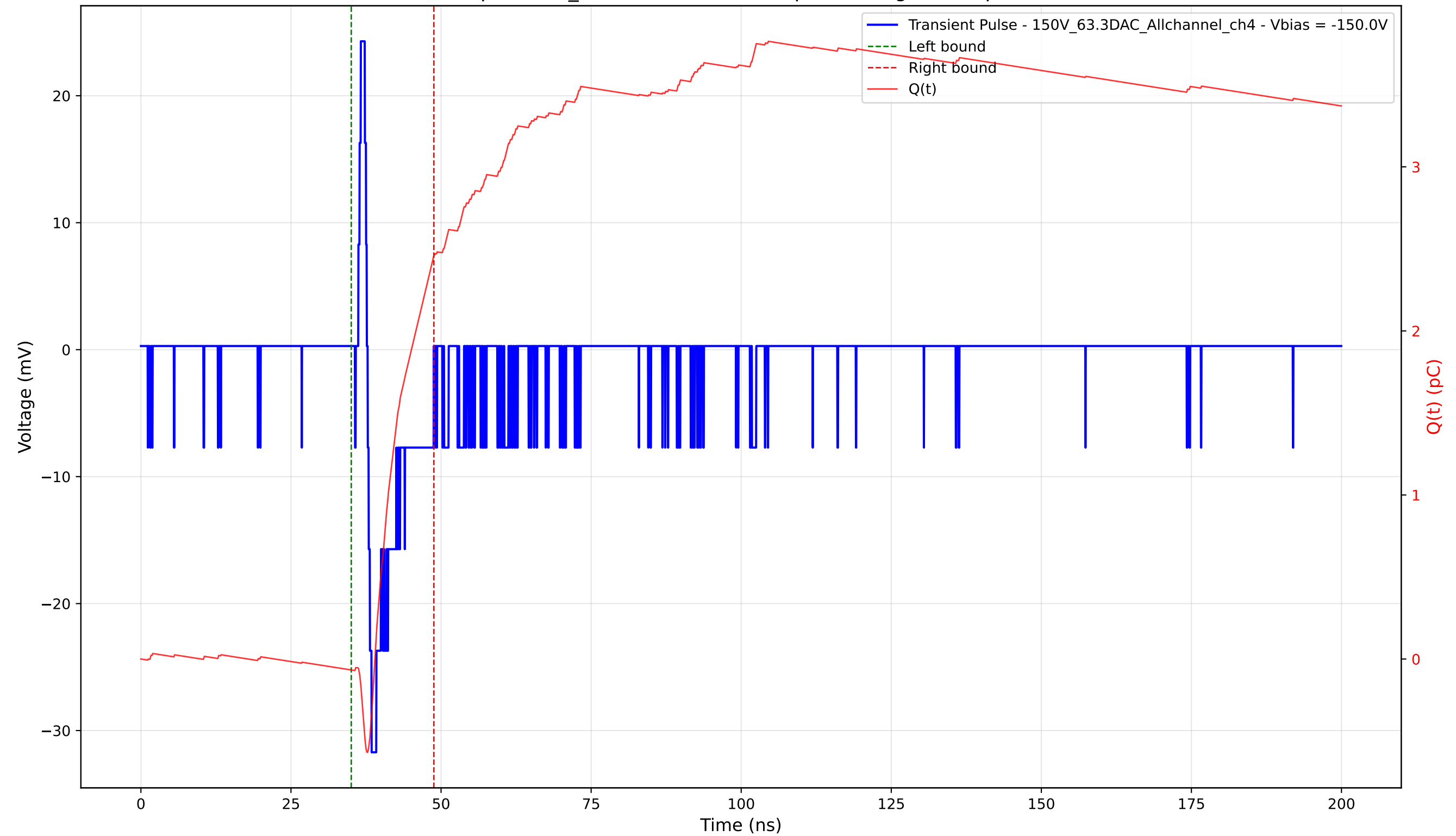
Transient Pulse - Sample: 1cm_42 - Position: 4140.0 \mu\text{m} - Charge: 2.53 pC - Rise Time: 0.66 ns
