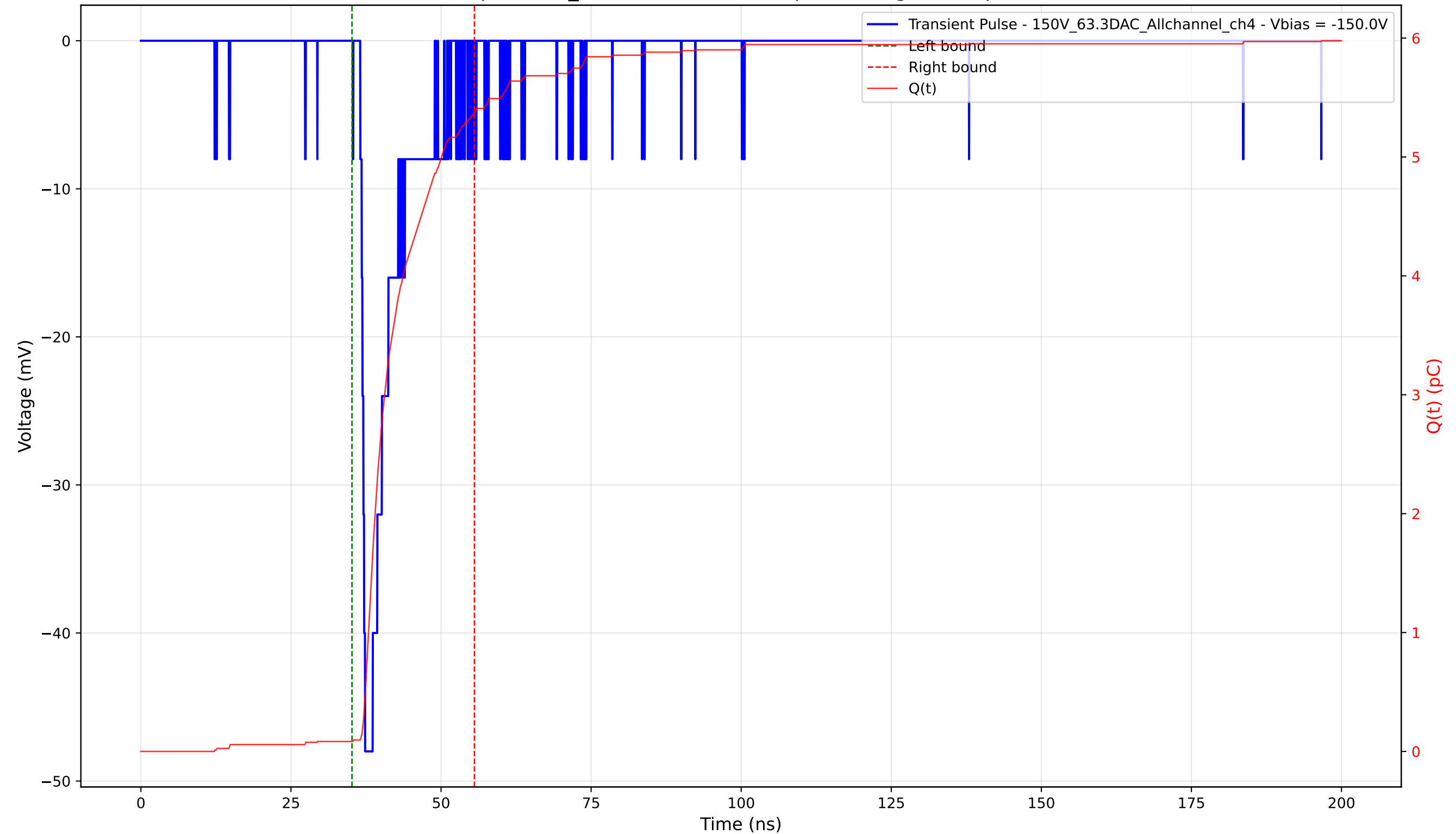
Transient Pulse - Sample: 1cm_42 - Position: 3100.0 \mu\text{m} - Charge: 5.29 pC - Rise Time: 0.82 ns
