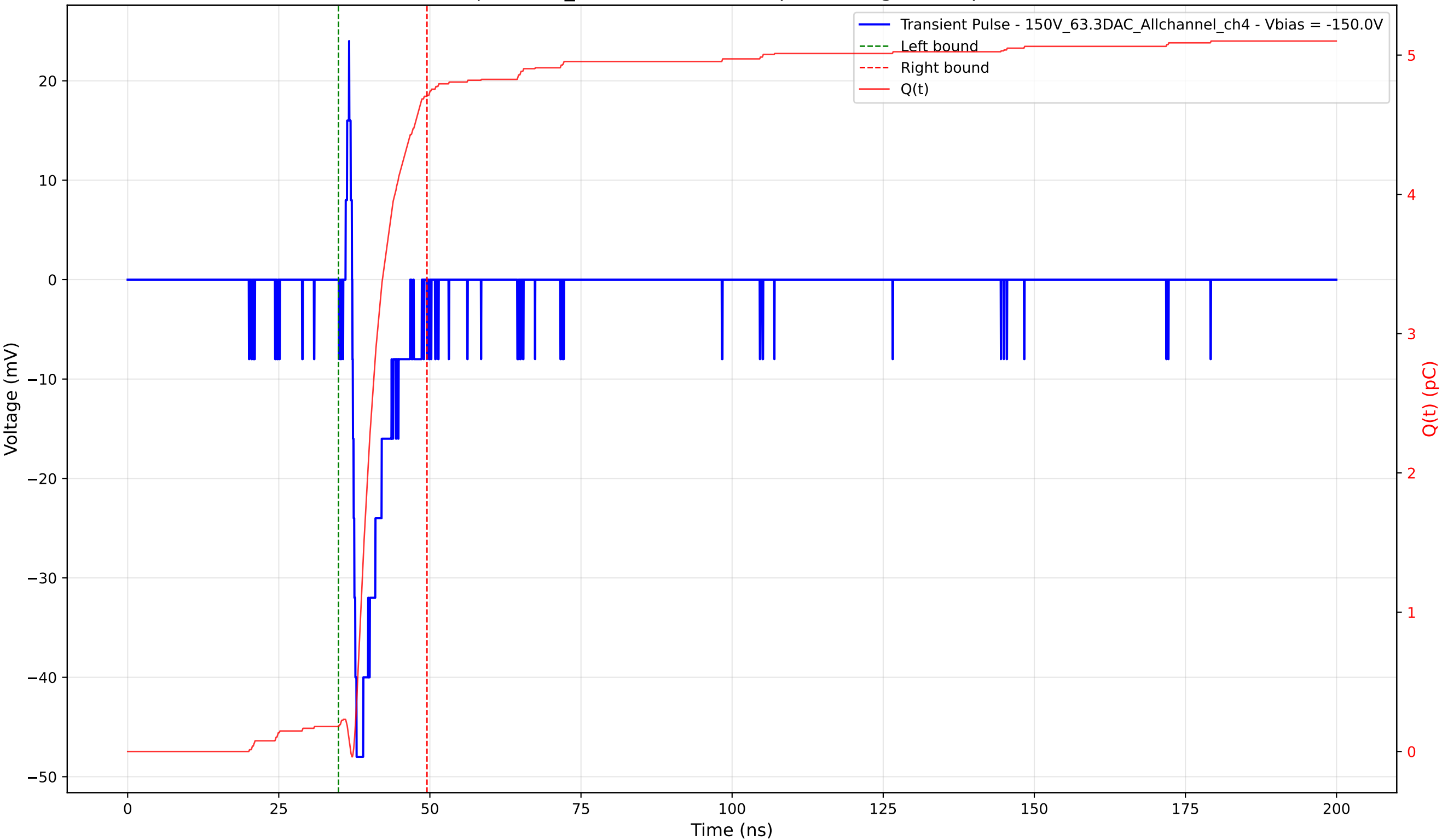
Transient Pulse - Sample: 1cm_42 - Position: 475.0 \mu\text{m} - Charge: 4.53 pC - Rise Time: 0.70 ns
