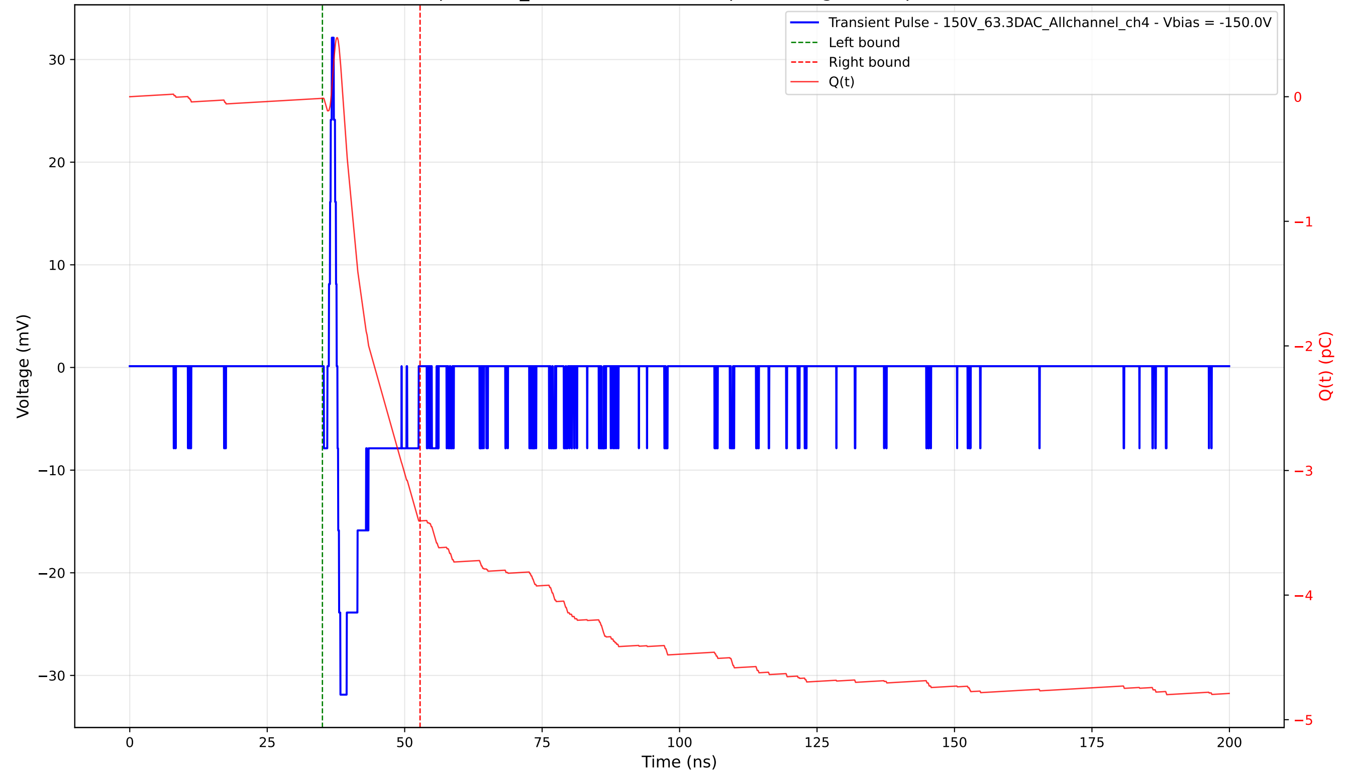
Transient Pulse - Sample: 1cm_42 - Position: 4305.0 \mu\text{m} - Charge: 3.39 pC - Rise Time: 0.54 ns
