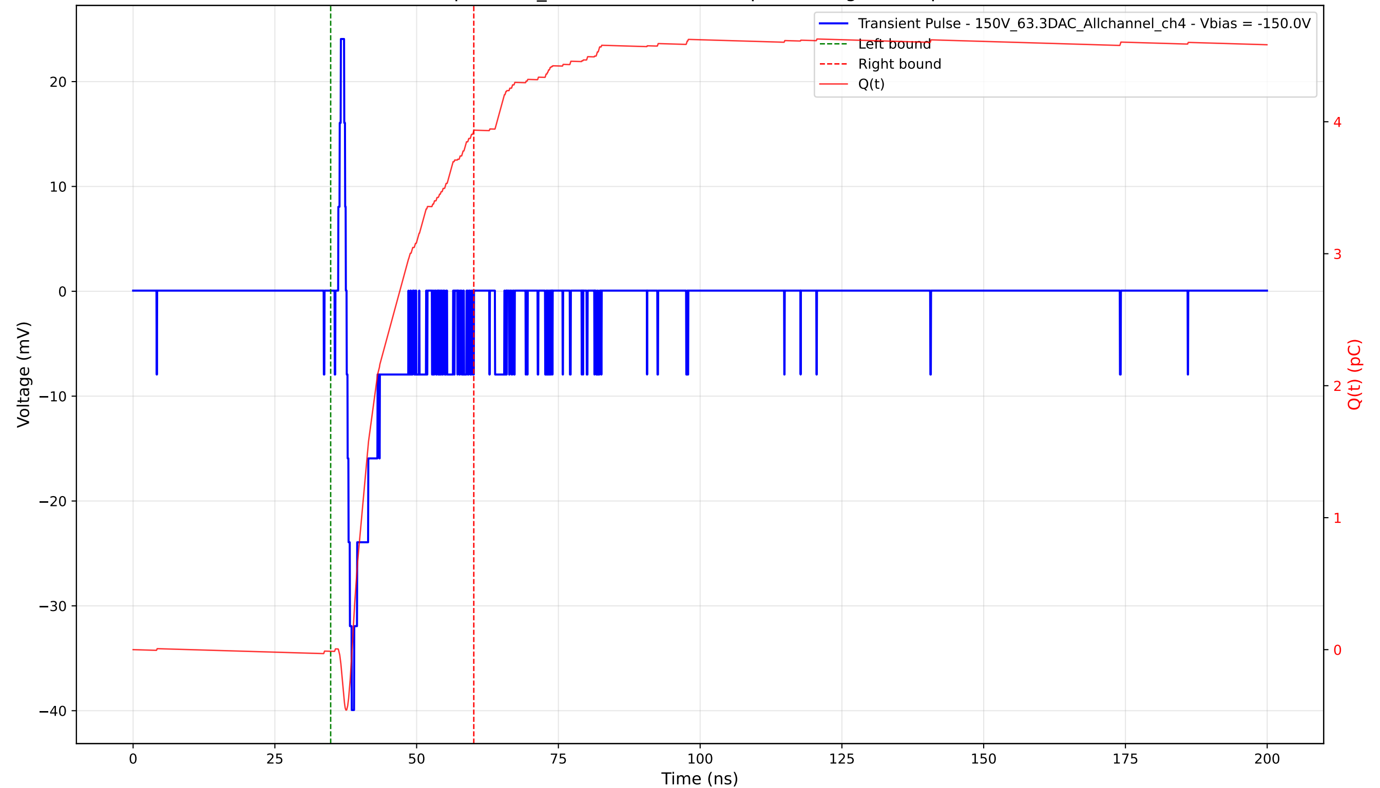
Transient Pulse - Sample: 1cm_42 - Position: 3765.0 \mu\text{m} - Charge: 3.95 pC - Rise Time: 0.90 ns
