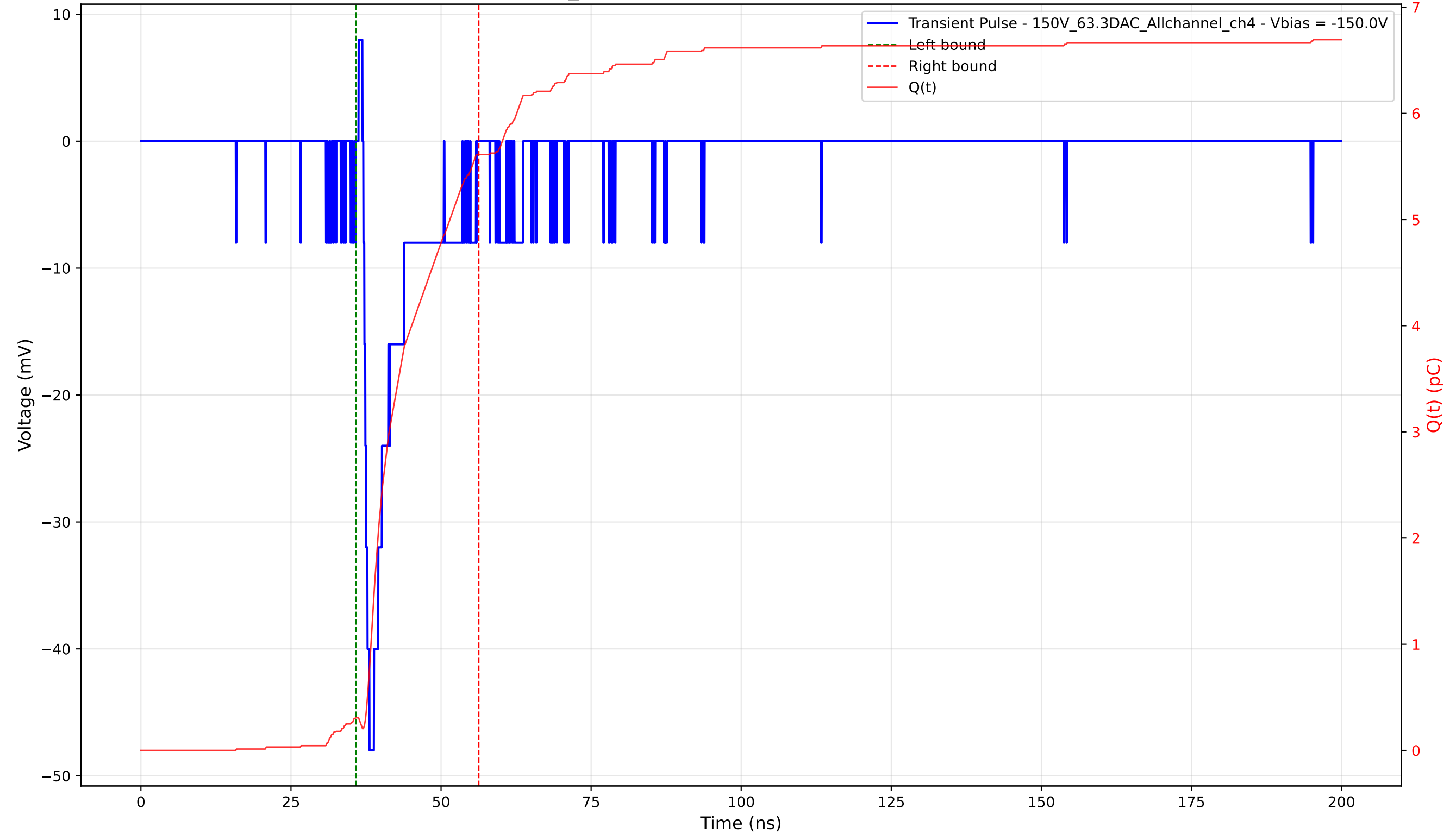
Transient Pulse - Sample: 1cm_42 - Position: 3335.0 \mu\text{m} - Charge: 5.31 pC - Rise Time: 1.02 ns
