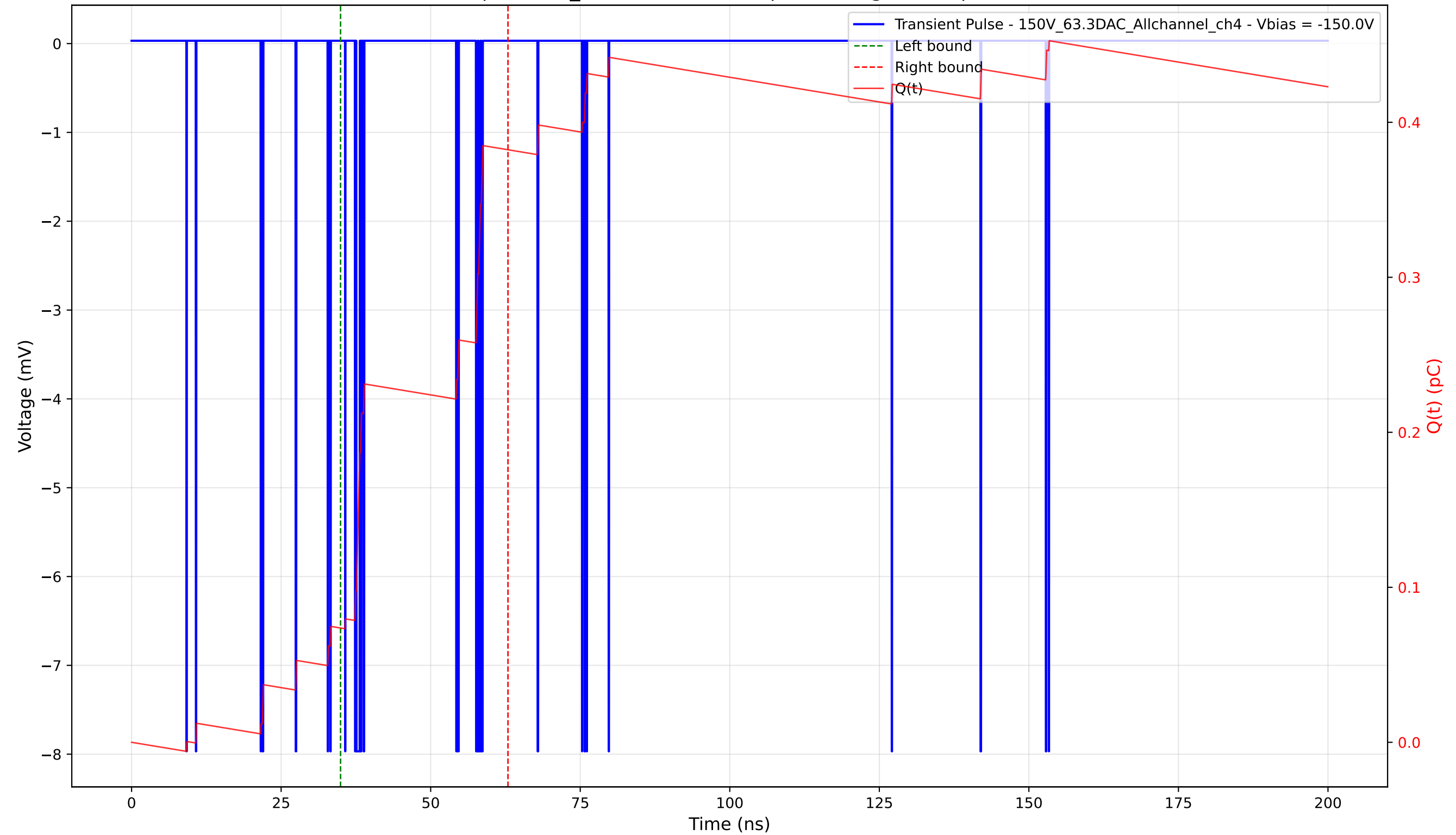
Transient Pulse - Sample: 1cm_42 - Position: 20.0 \mu\text{m} - Charge: 0.31 pC - Rise Time: 0.04 ns
