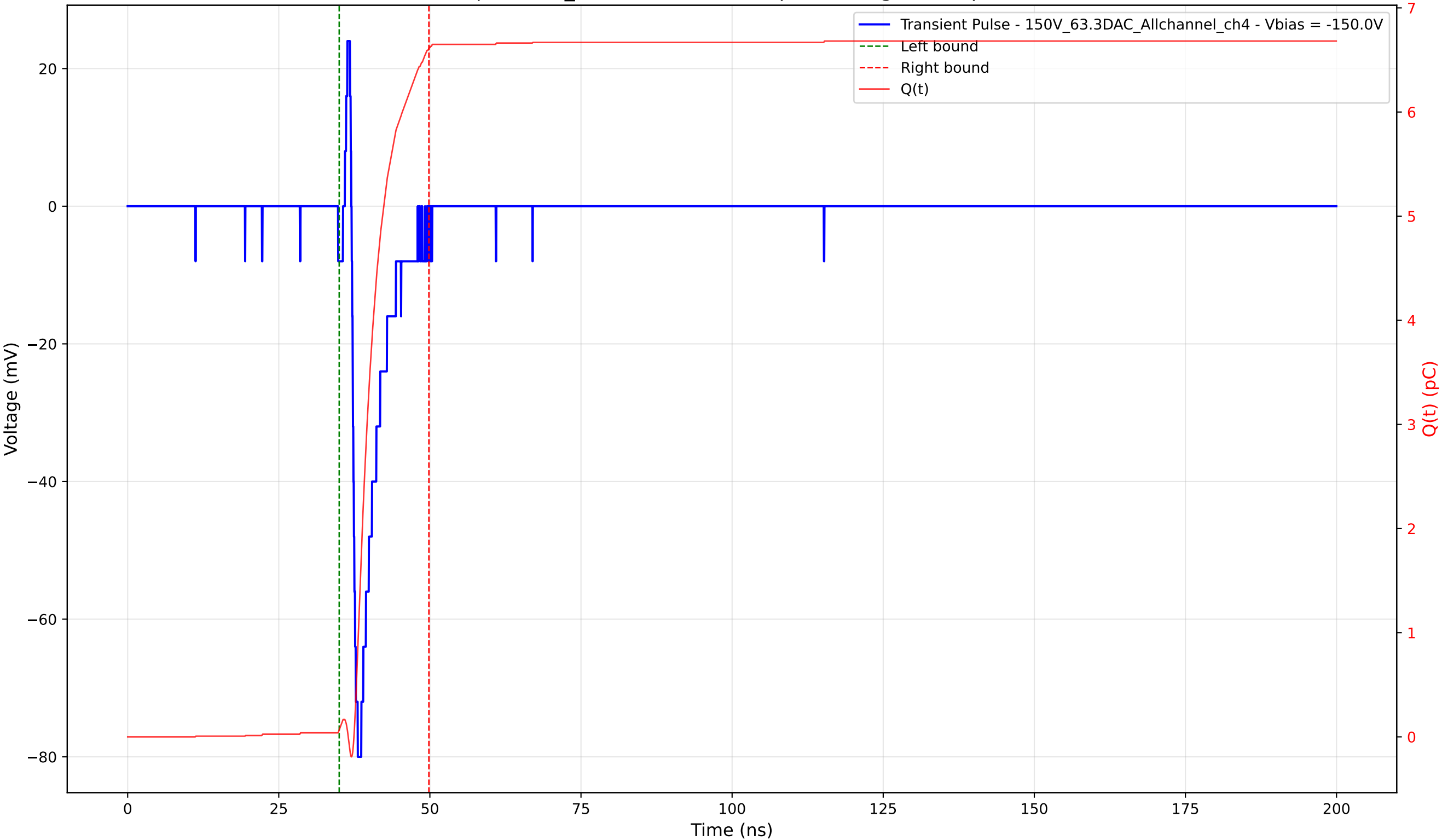
Transient Pulse - Sample: 1cm_42 - Position: 680.0 \mu\text{m} - Charge: 6.55 pC - Rise Time: 0.64 ns
