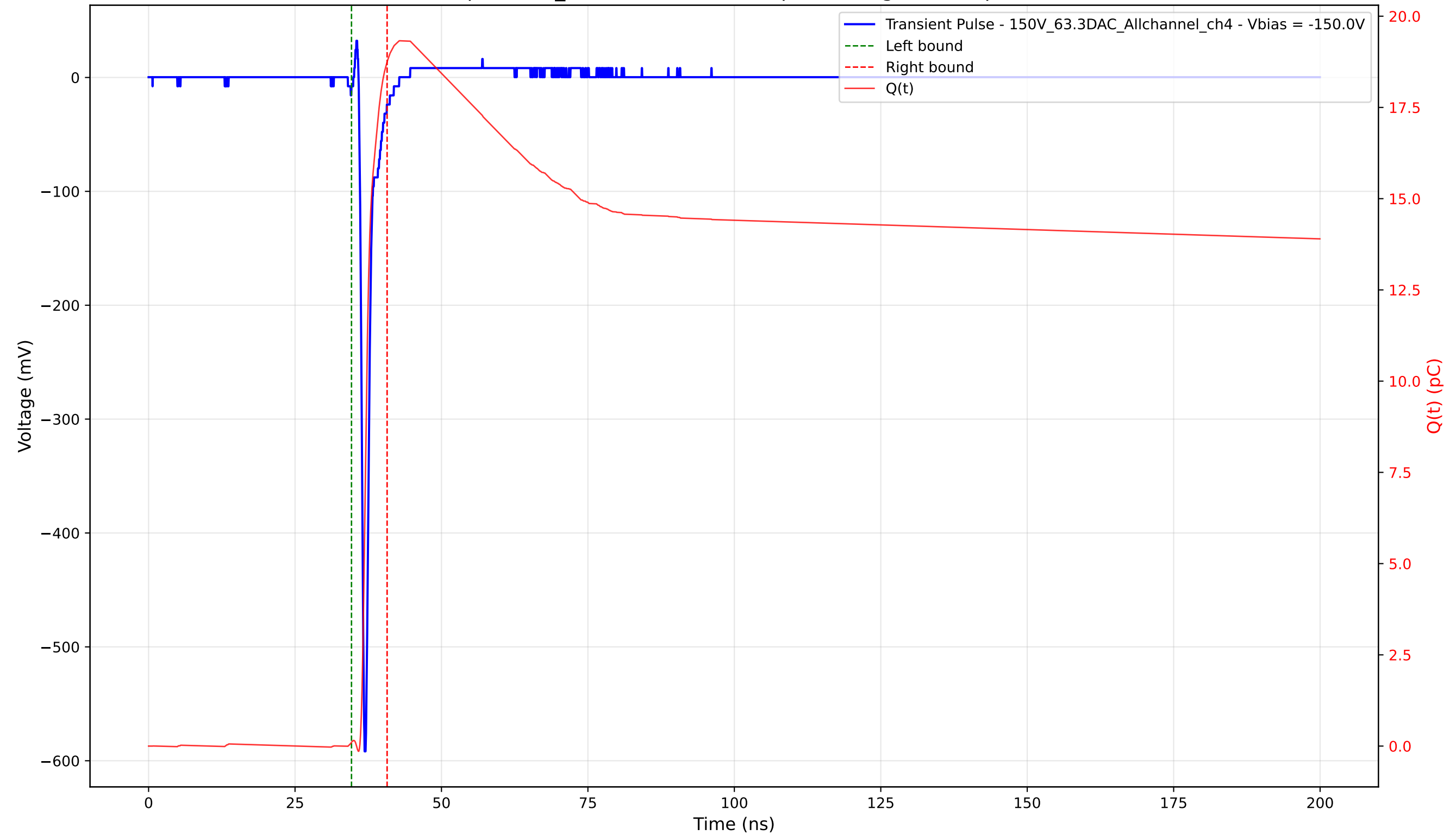
Transient Pulse - Sample: 1cm_42 - Position: 1900.0 \mu\text{m} - Charge: 18.64 pC - Rise Time: 0.70 ns
