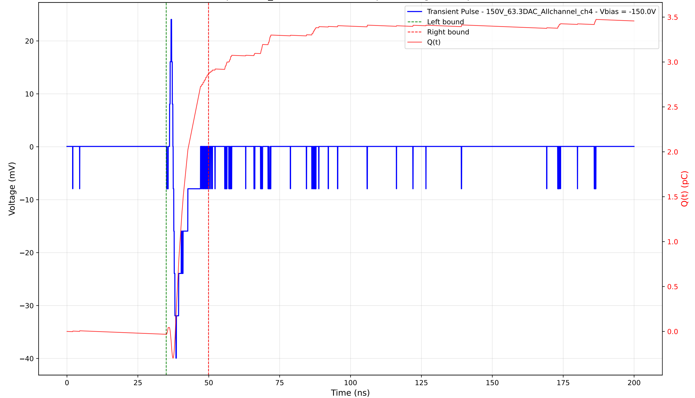
Transient Pulse - Sample: 1cm_42 - Position: 4850.0 \mu\text{m} - Charge: 2.91 pC - Rise Time: 0.98 ns
