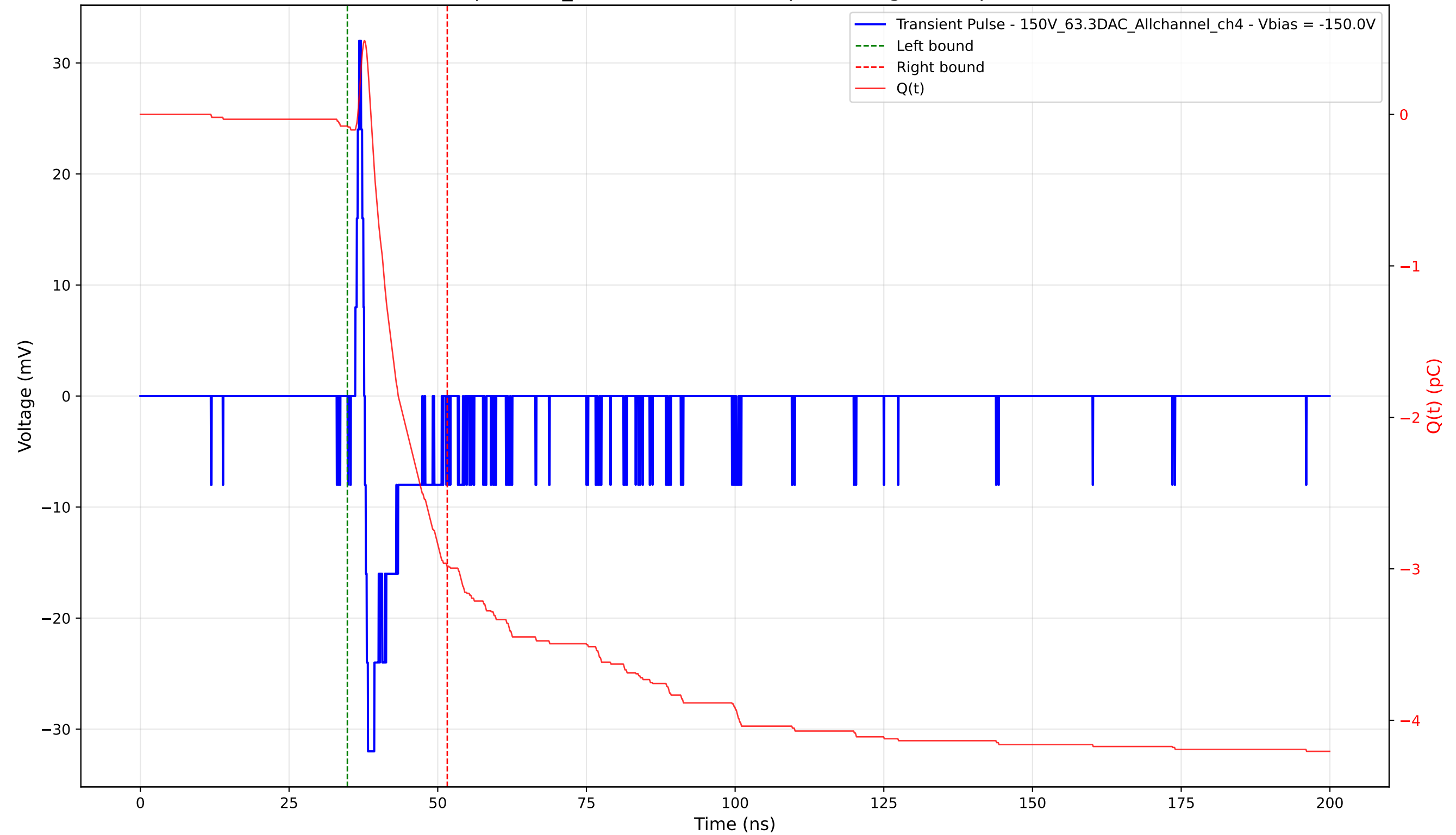
Transient Pulse - Sample: 1cm_42 - Position: 4220.0 \mu\text{m} - Charge: 2.91 pC - Rise Time: 0.66 ns
