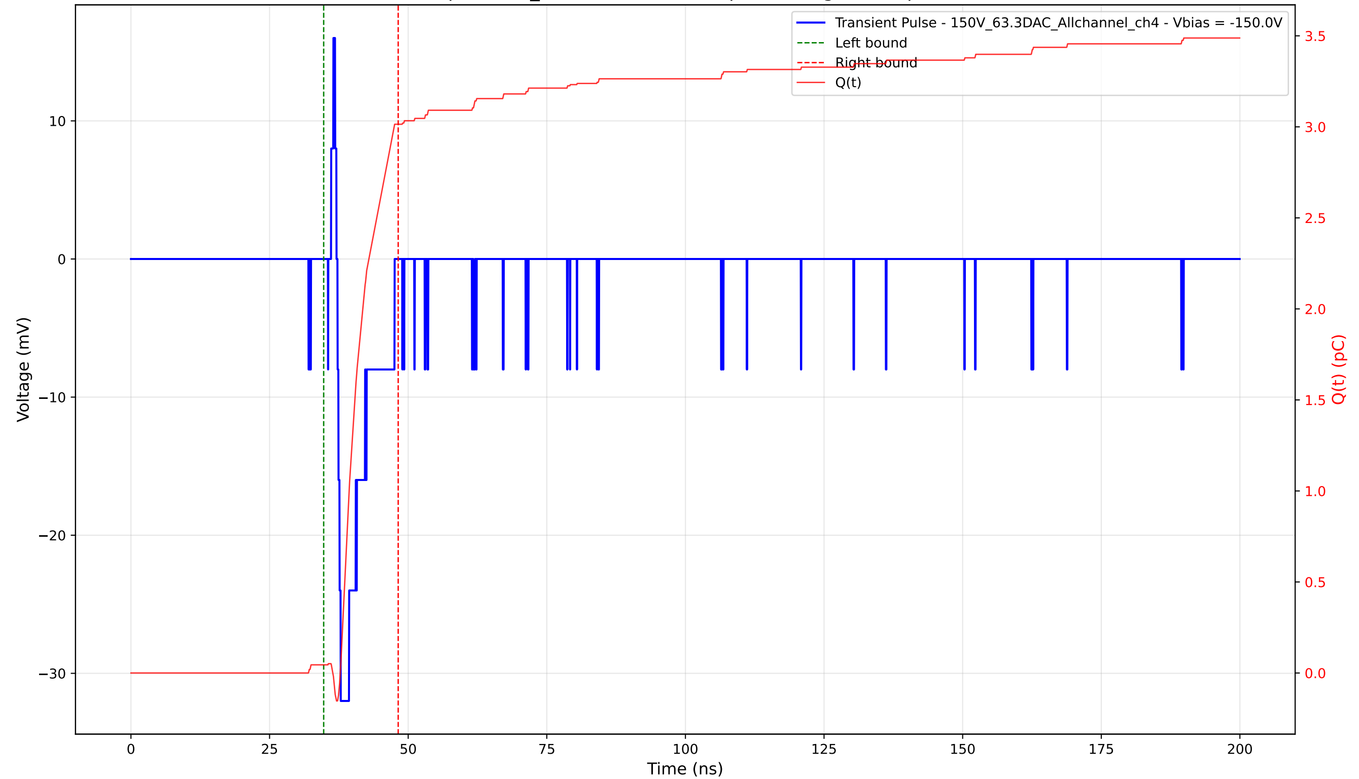
Transient Pulse - Sample: 1cm_42 - Position: 305.0 \mu\text{m} - Charge: 2.97 pC - Rise Time: 0.58 ns
