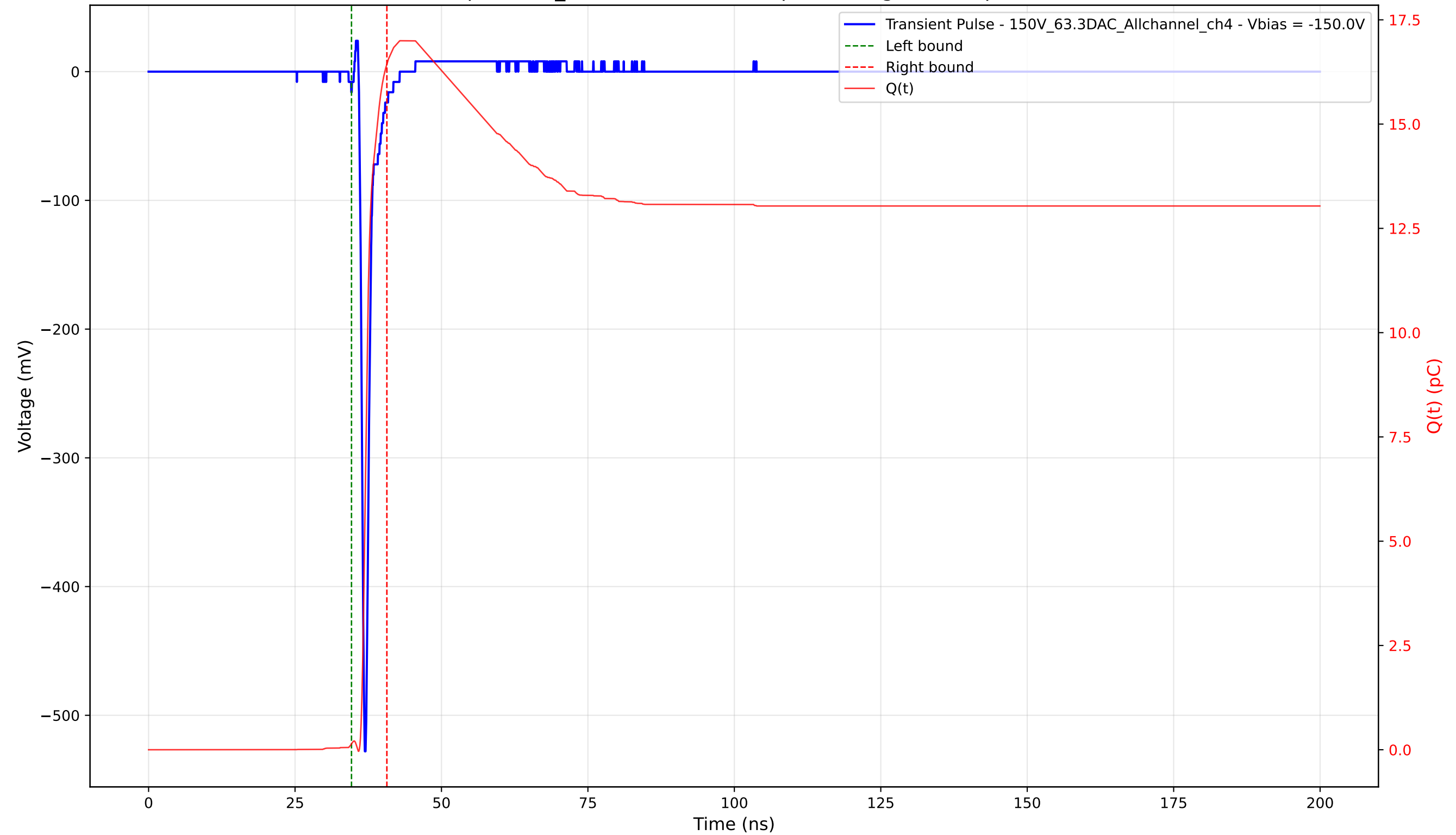
Transient Pulse - Sample: 1cm_42 - Position: 2180.0 \mu\text{m} - Charge: 16.30 pC - Rise Time: 0.72 ns
