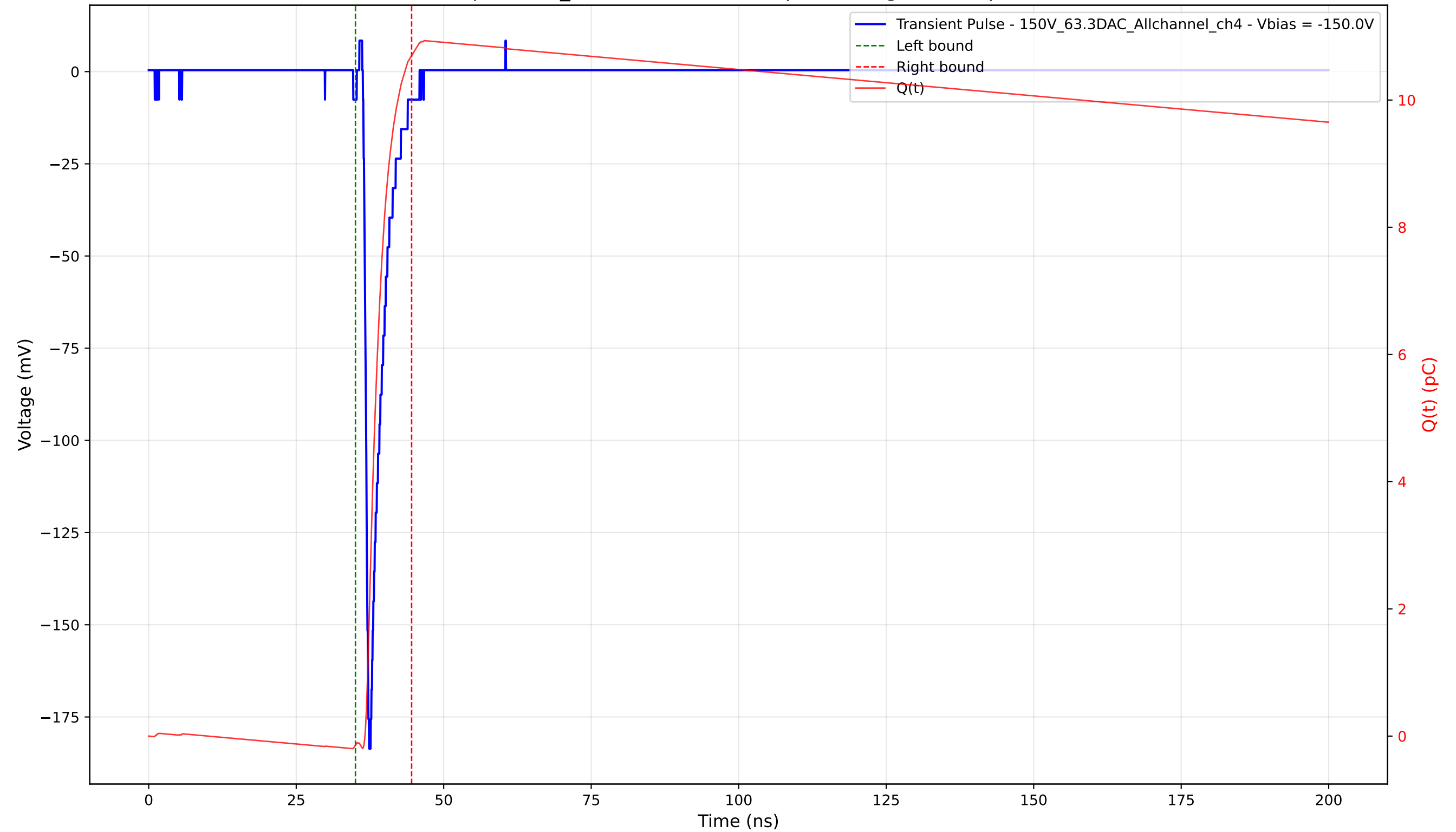
Transient Pulse - Sample: 1cm_42 - Position: 1255.0 \mu\text{m} - Charge: 10.84 pC - Rise Time: 0.77 ns
