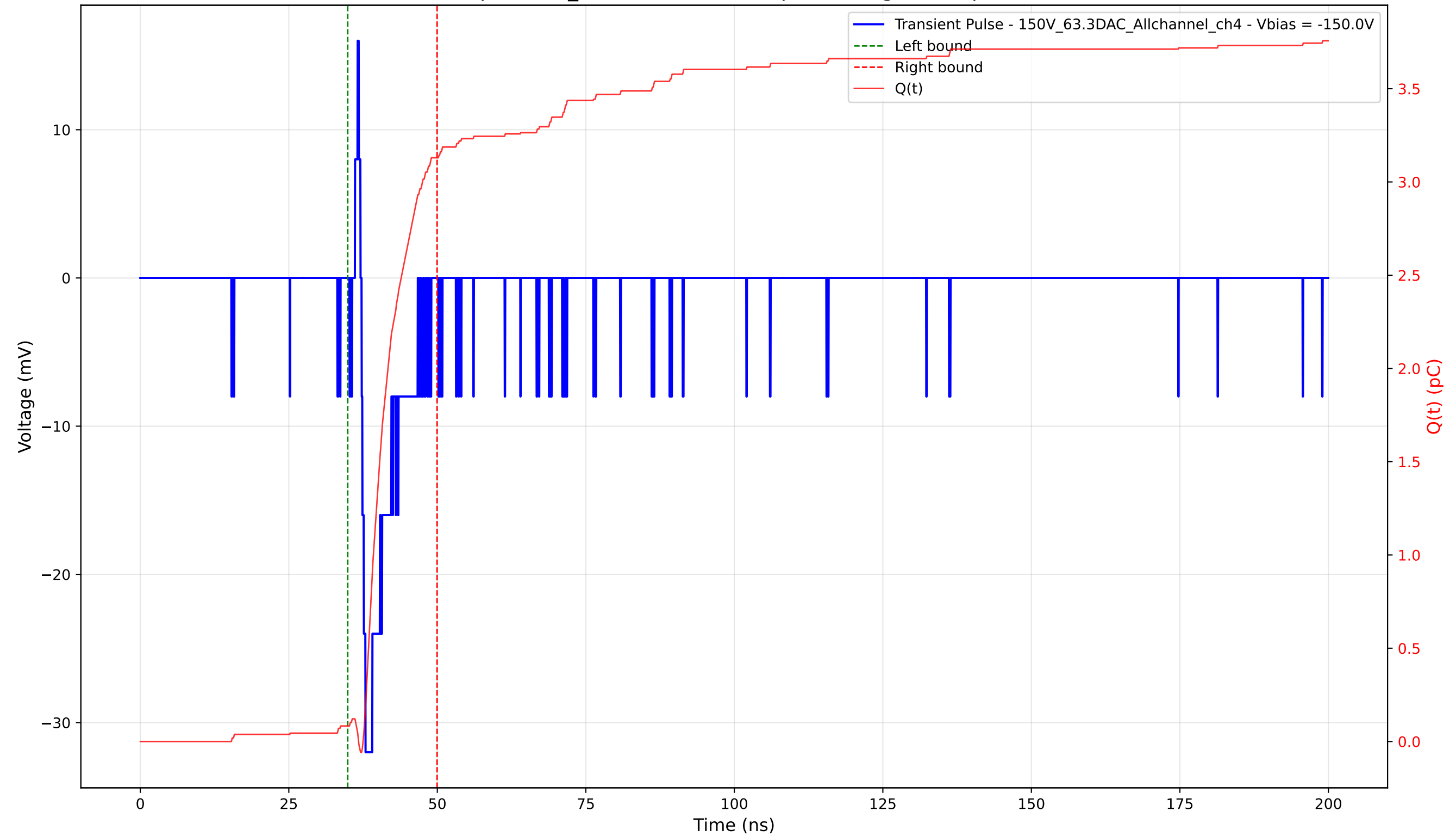
Transient Pulse - Sample: 1cm_42 - Position: 285.0 \mu\text{m} - Charge: 3.05 pC - Rise Time: 0.66 ns
