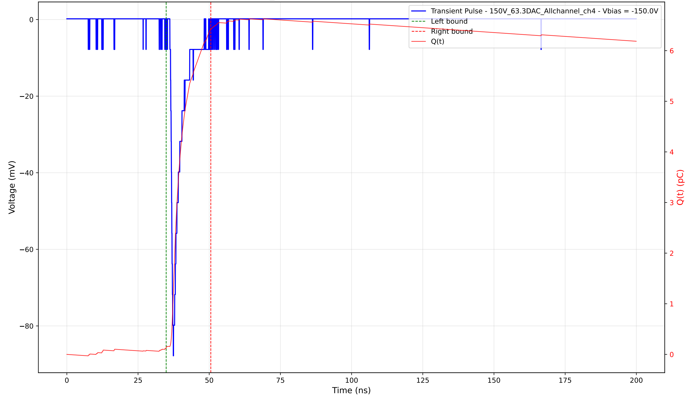
Transient Pulse - Sample: 1cm_42 - Position: 2945.0 \mu\text{m} - Charge: 6.30 pC - Rise Time: 0.80 ns
