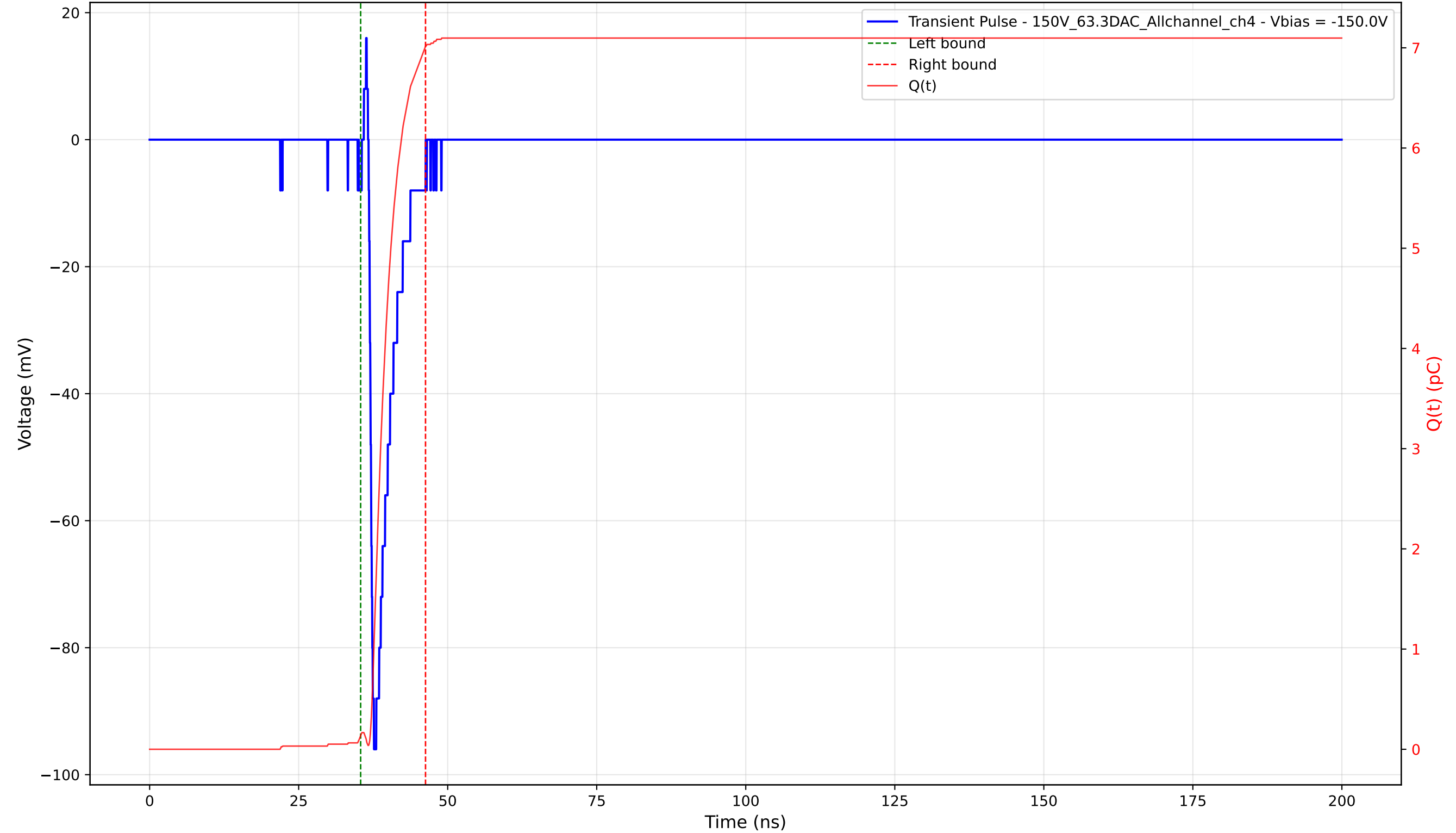
Transient Pulse - Sample: 1cm_42 - Position: 995.0 \mu\text{m} - Charge: 6.88 pC - Rise Time: 0.63 ns
