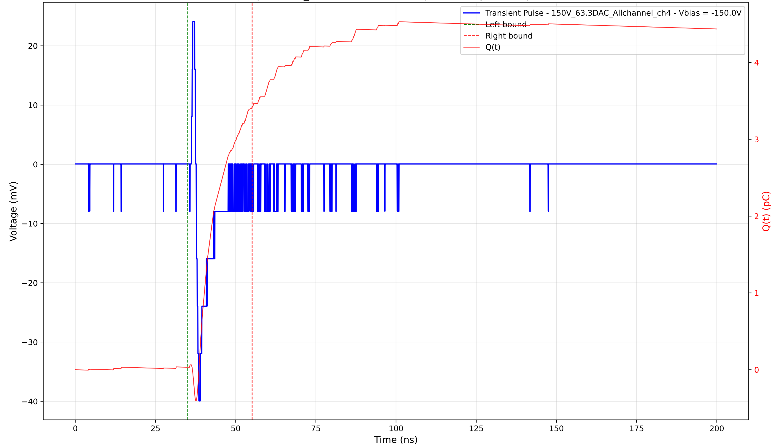
Transient Pulse - Sample: 1cm_42 - Position: 3830.0 \mu\text{m} - Charge: 3.39 pC - Rise Time: 0.86 ns
