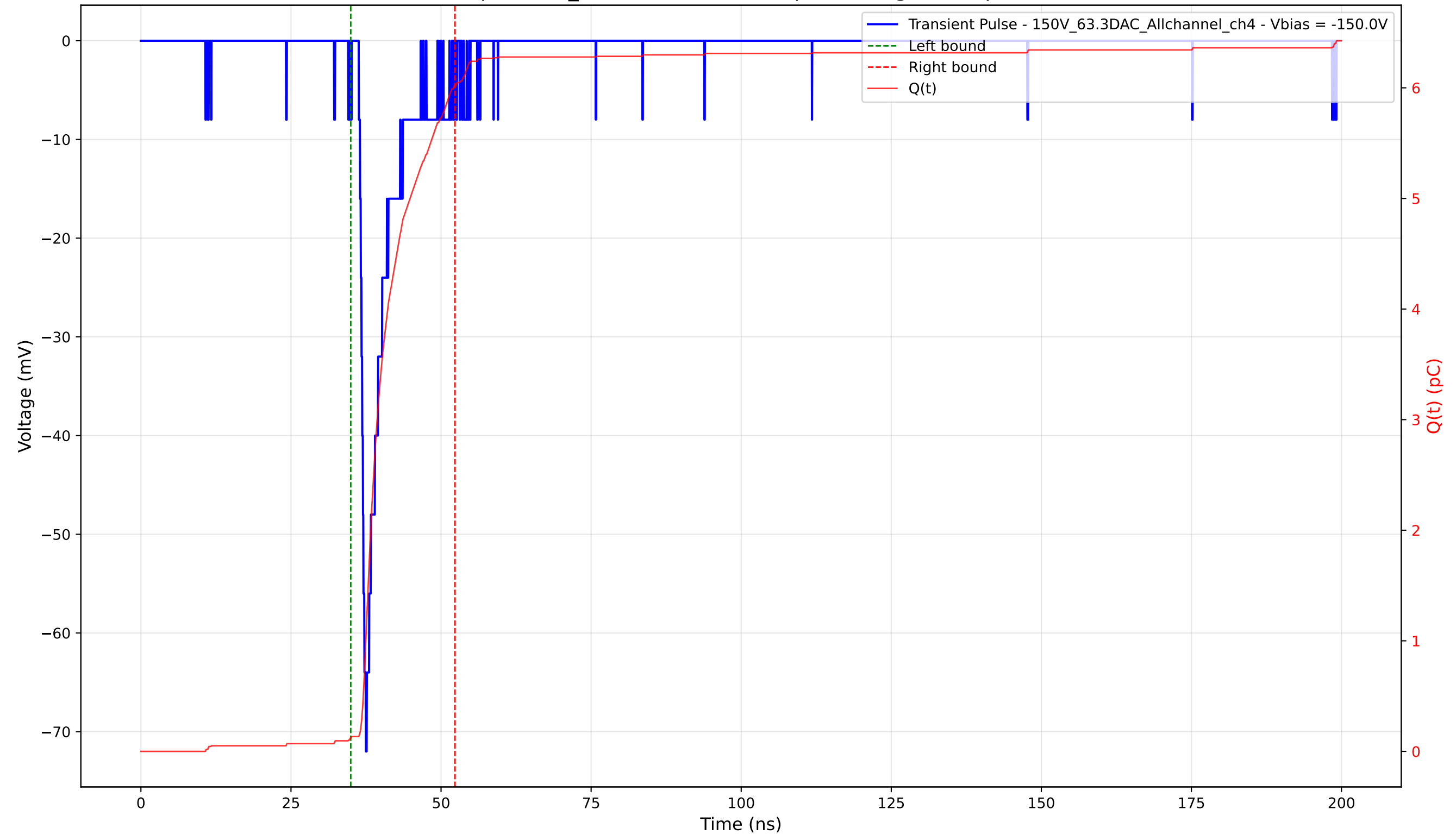
Transient Pulse - Sample: 1cm_42 - Position: 3000.0 \mu\text{m} - Charge: 5.90 pC - Rise Time: 1.16 ns
