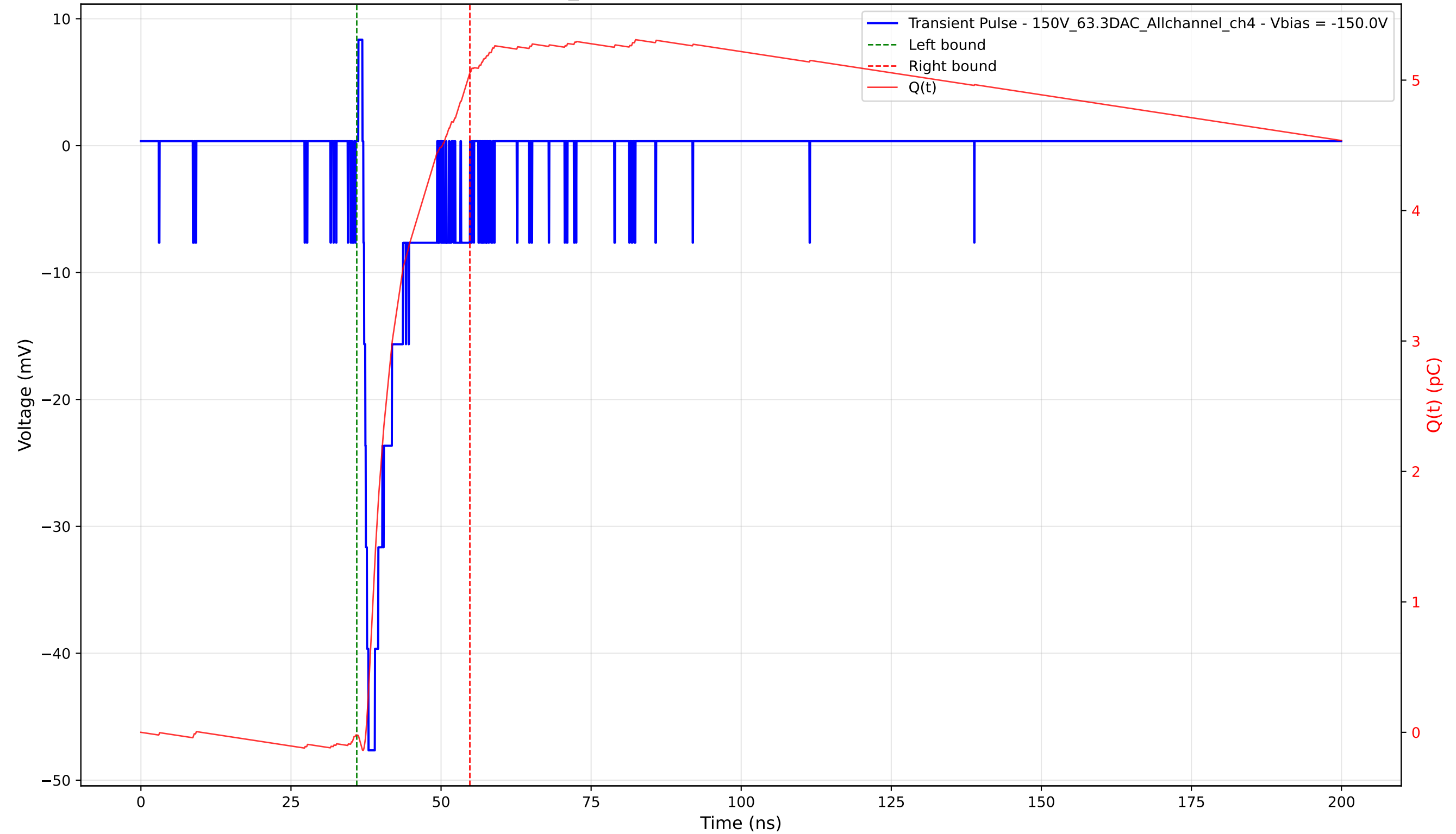
Transient Pulse - Sample: 1cm_42 - Position: 3315.0 \mu\text{m} - Charge: 5.08 pC - Rise Time: 0.86 ns
