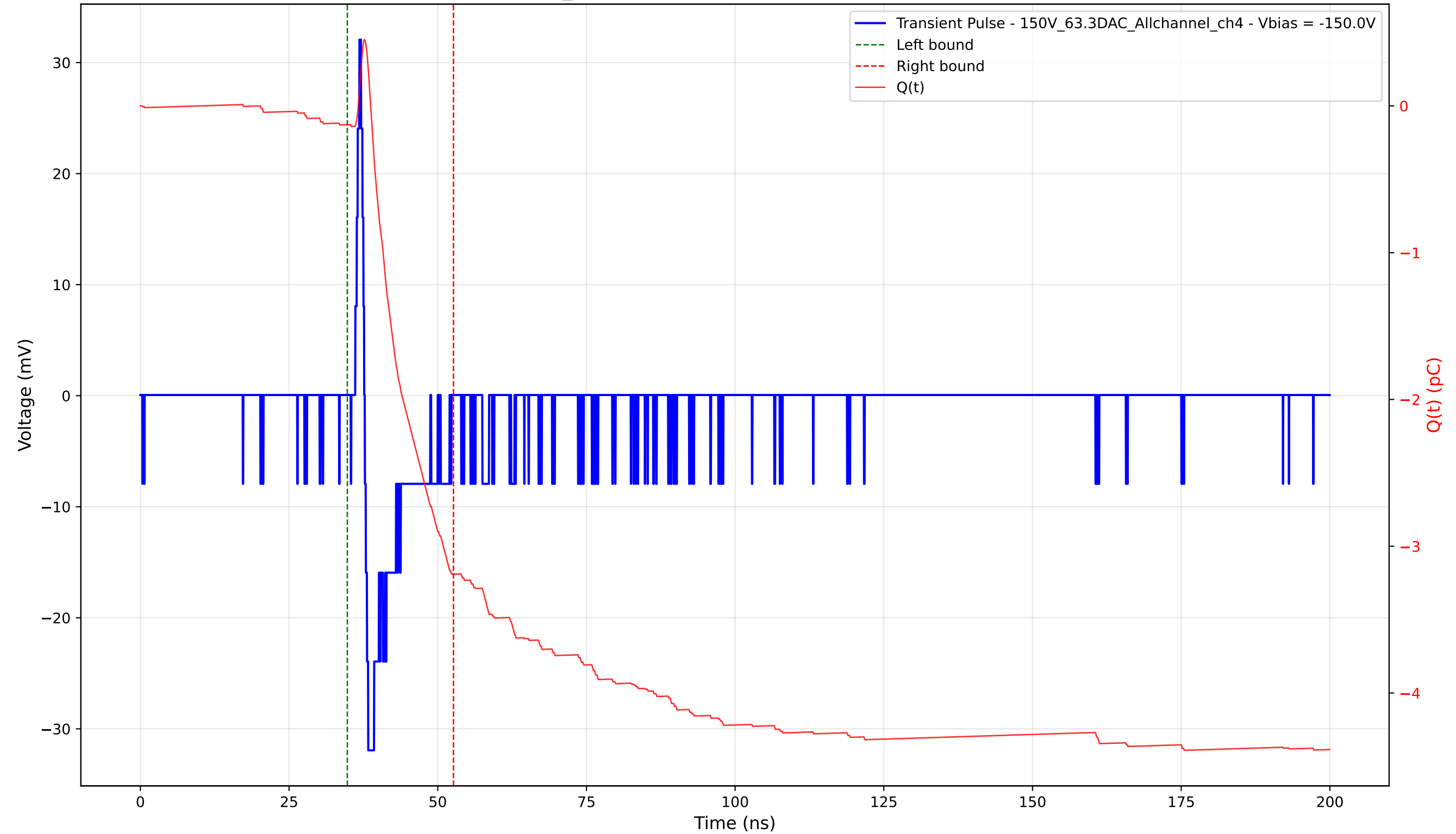
Transient Pulse - Sample: 1cm_42 - Position: 4230.0 \mu\text{m} - Charge: 3.06 pC - Rise Time: 0.70 ns
