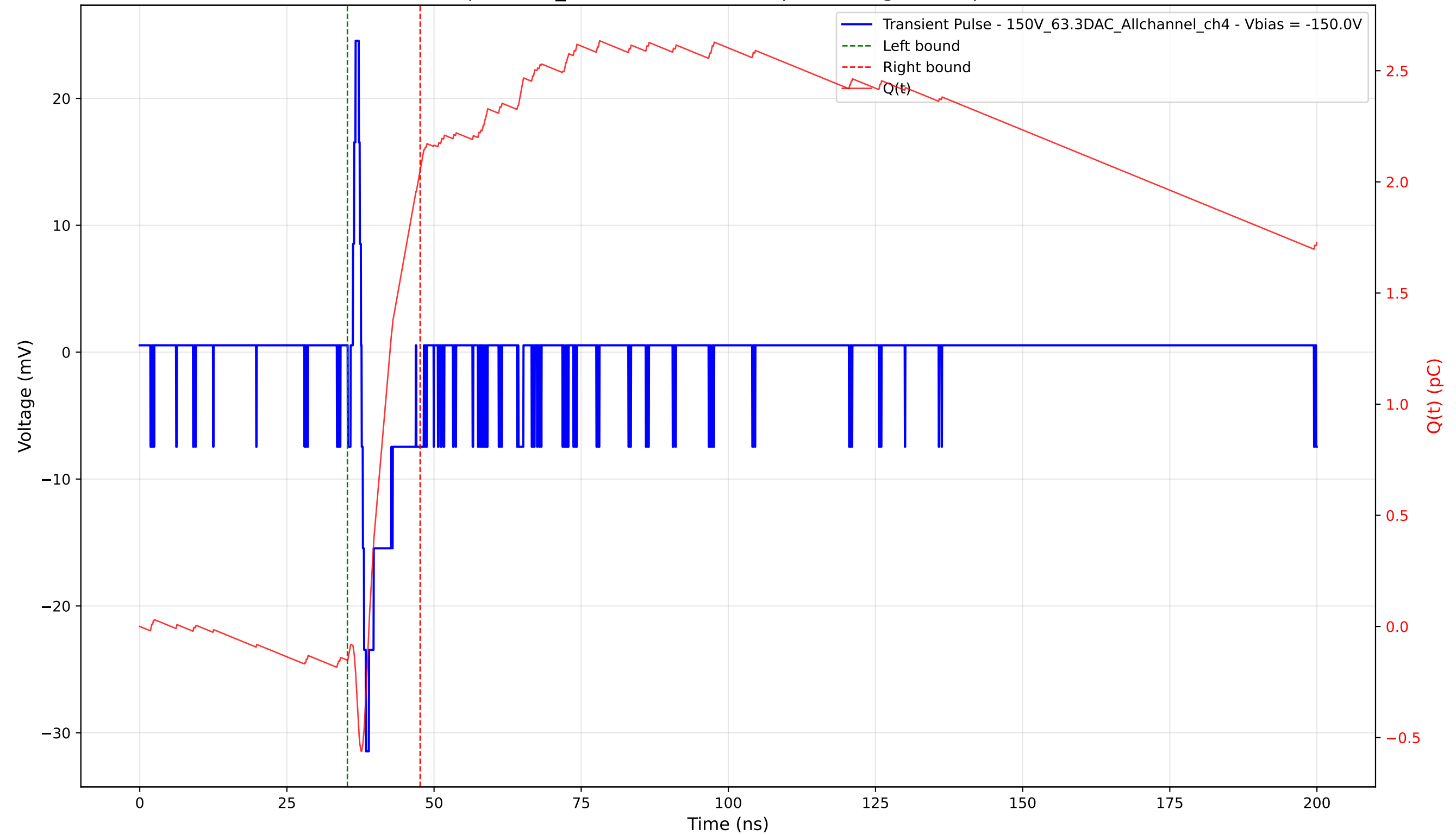
Transient Pulse - Sample: 1cm_42 - Position: 4470.0 \mu\text{m} - Charge: 2.21 pC - Rise Time: 0.74 ns
