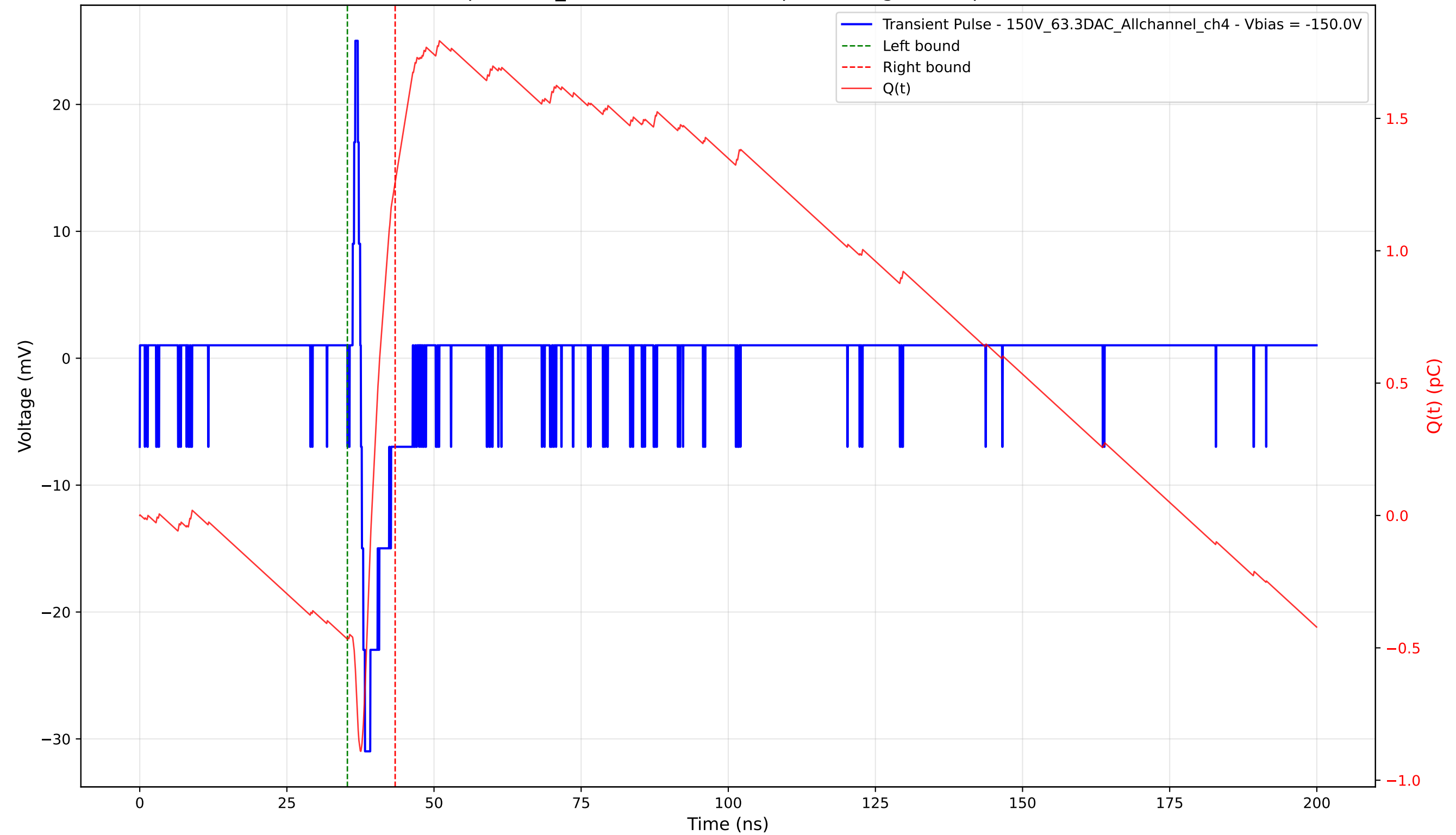
Transient Pulse - Sample: 1cm_42 - Position: 4675.0 \mu\text{m} - Charge: 1.73 pC - Rise Time: 0.71 ns
