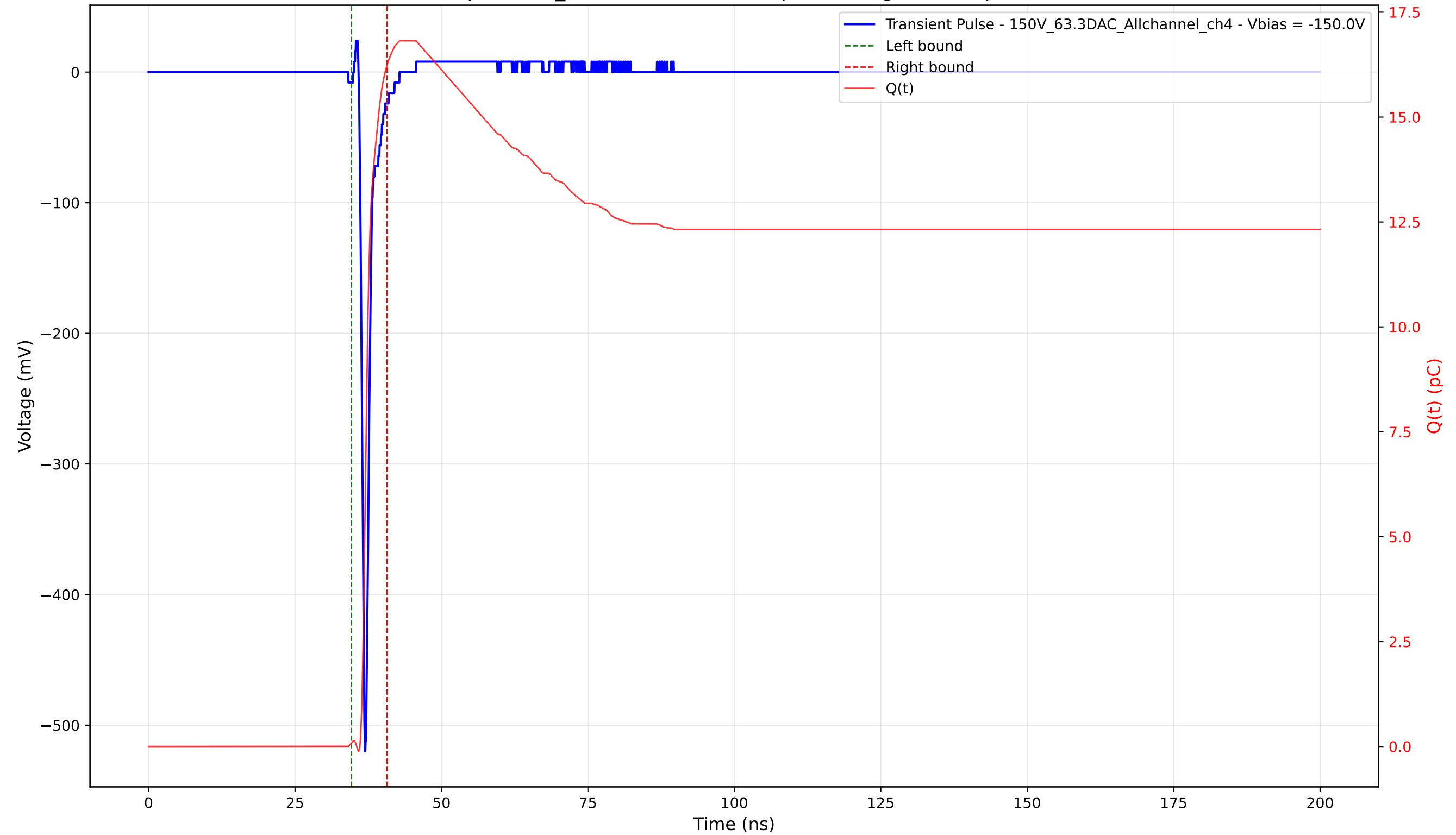
Transient Pulse - Sample: 1cm_42 - Position: 2225.0 \mu\text{m} - Charge: 16.15 pC - Rise Time: 0.72 ns
