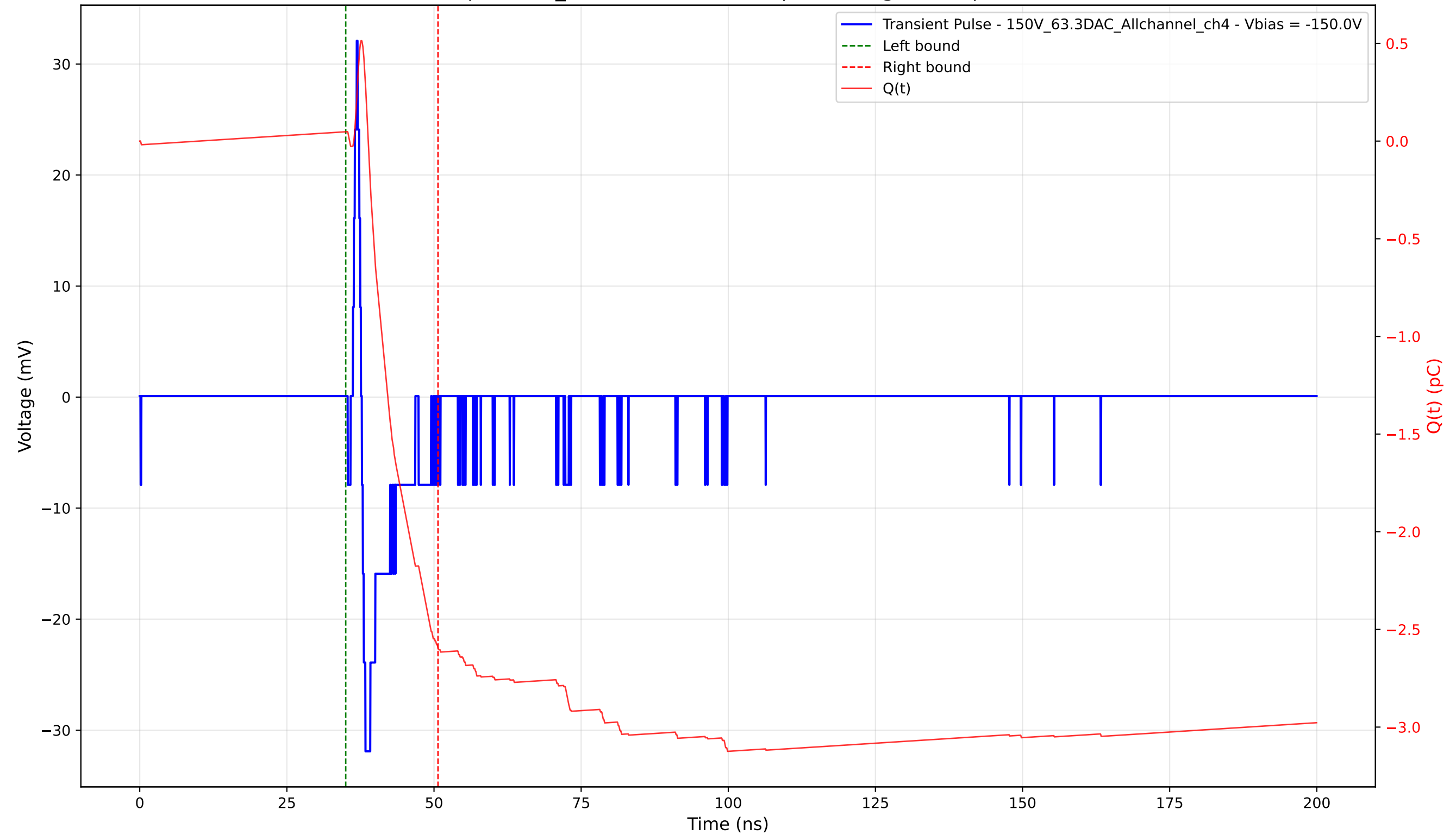
Transient Pulse - Sample: 1cm_42 - Position: 4375.0 \mu\text{m} - Charge: 2.64 pC - Rise Time: 0.66 ns
