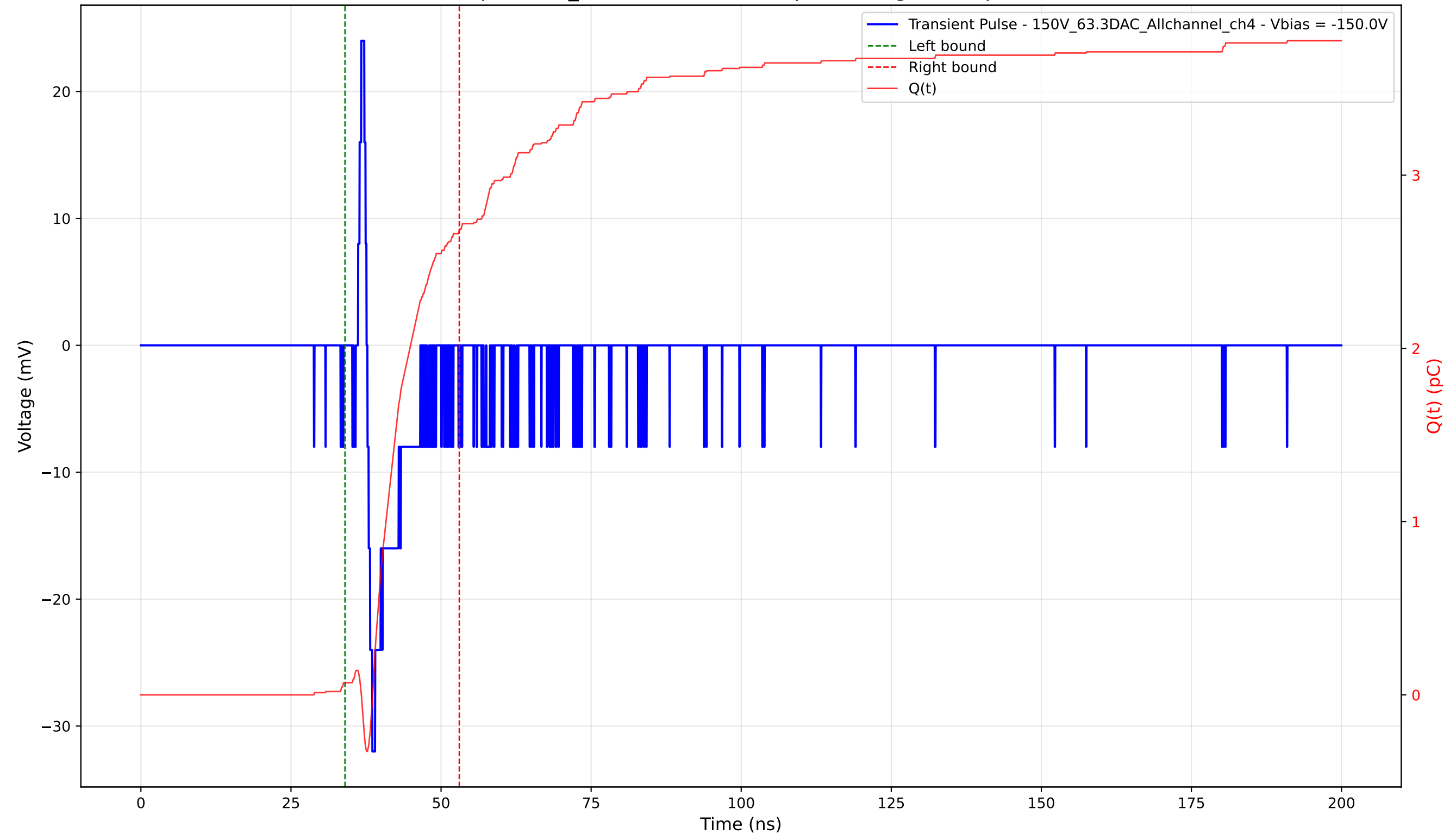
Transient Pulse - Sample: 1cm_42 - Position: 4035.0 \mu\text{m} - Charge: 2.61 pC - Rise Time: 0.82 ns
