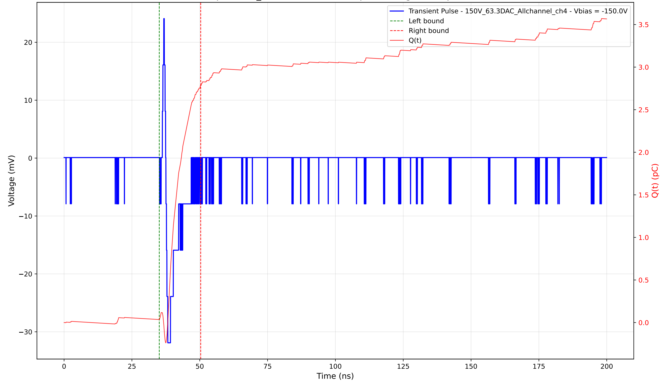
Transient Pulse - Sample: 1cm_42 - Position: 4685.0 \mu\text{m} - Charge: 2.75 pC - Rise Time: 0.70 ns
