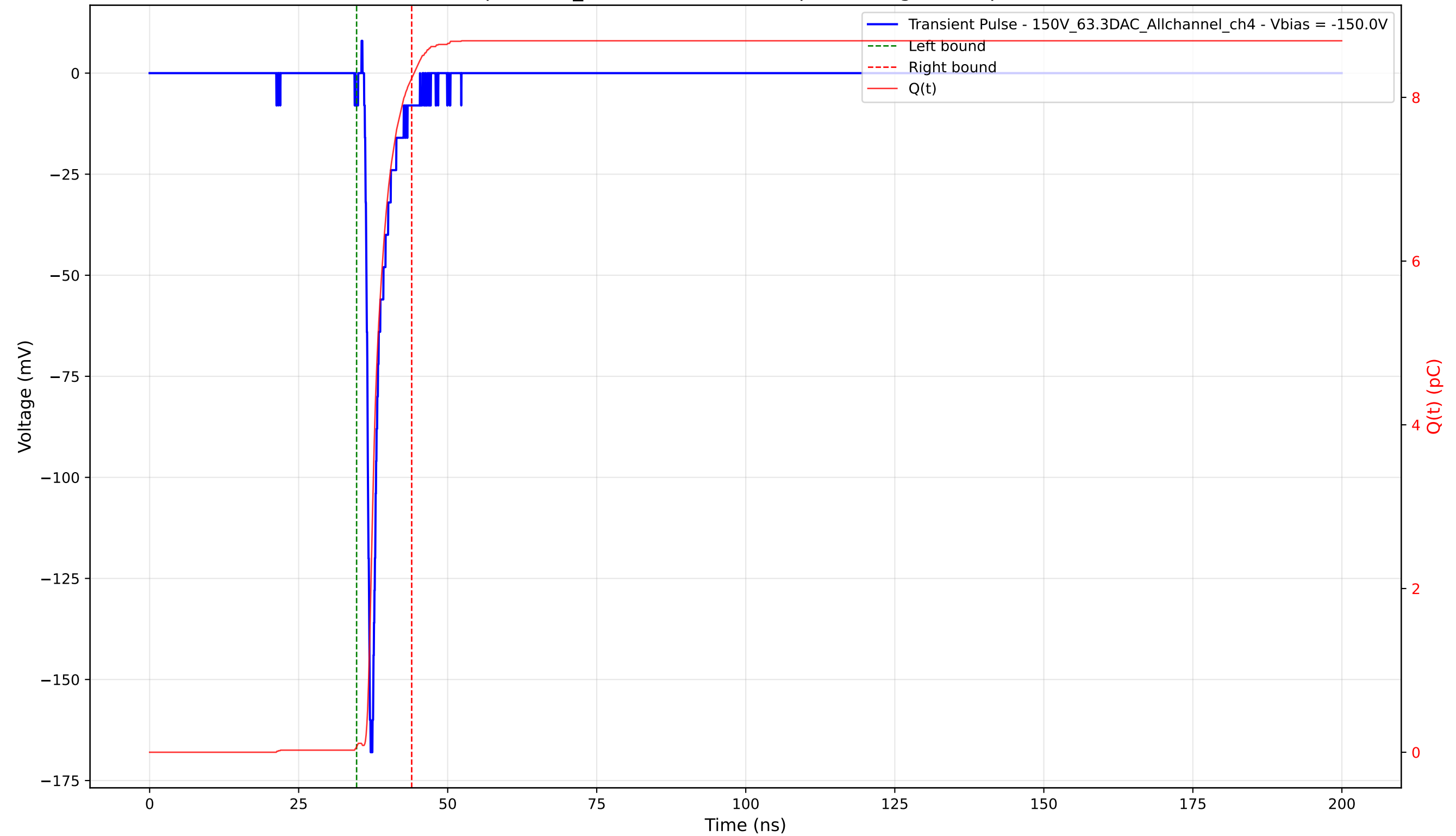
Transient Pulse - Sample: 1cm_42 - Position: 2630.0 \mu\text{m} - Charge: 8.17 pC - Rise Time: 0.75 ns
