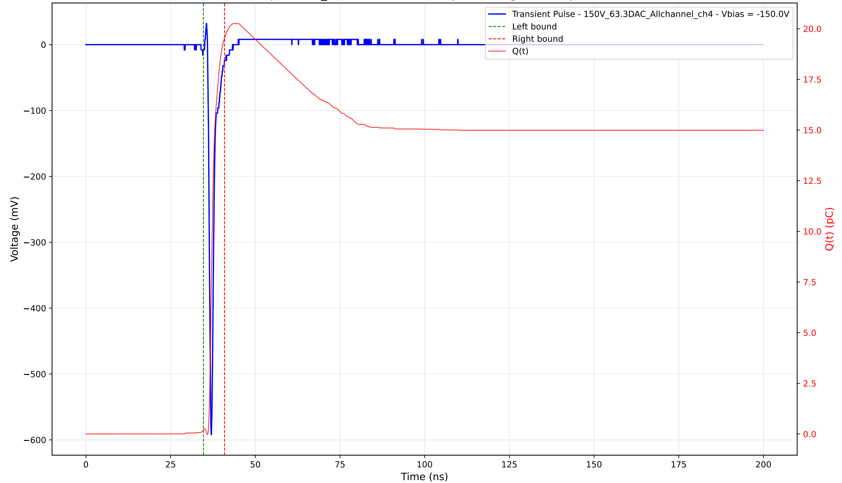
Transient Pulse - Sample: 1cm_42 - Position: 1820.0 \mu\text{m} - Charge: 19.35 pC - Rise Time: 0.72 ns
