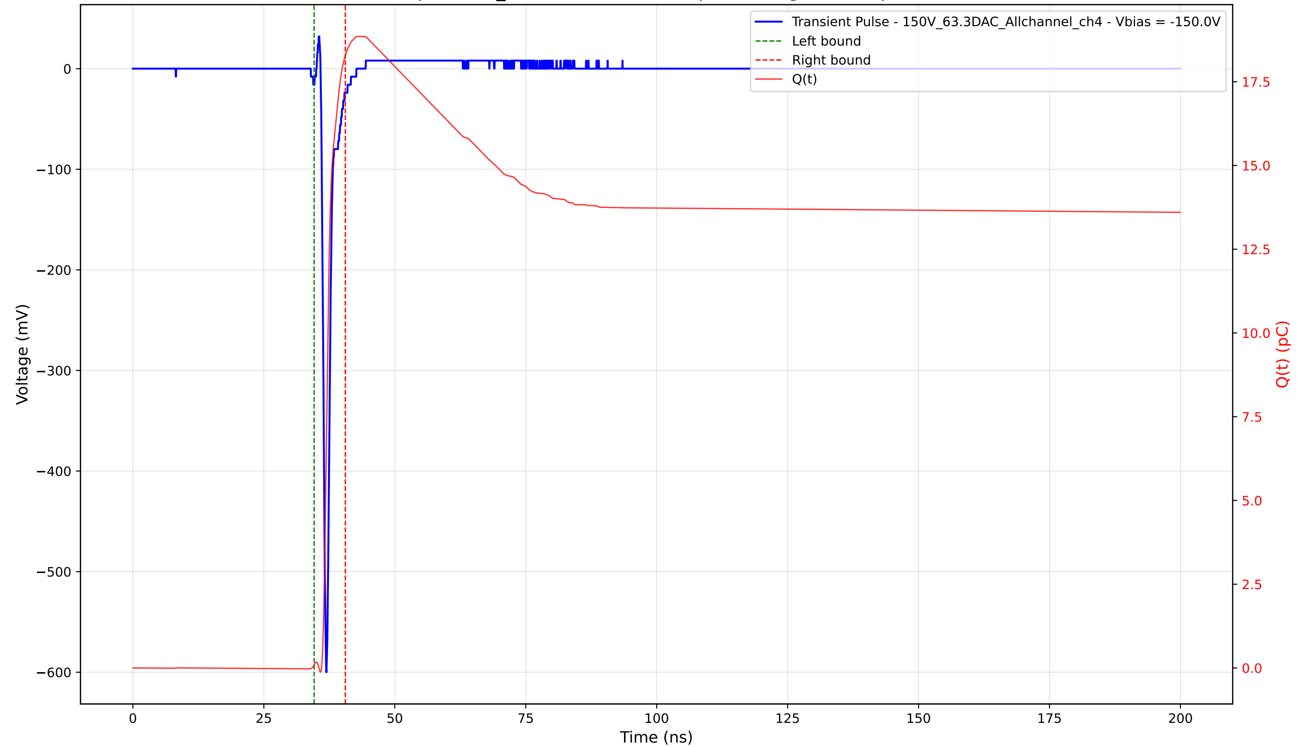
Transient Pulse - Sample: 1cm_42 - Position: 1965.0 \mu\text{m} - Charge: 18.18 pC - Rise Time: 0.72 ns
