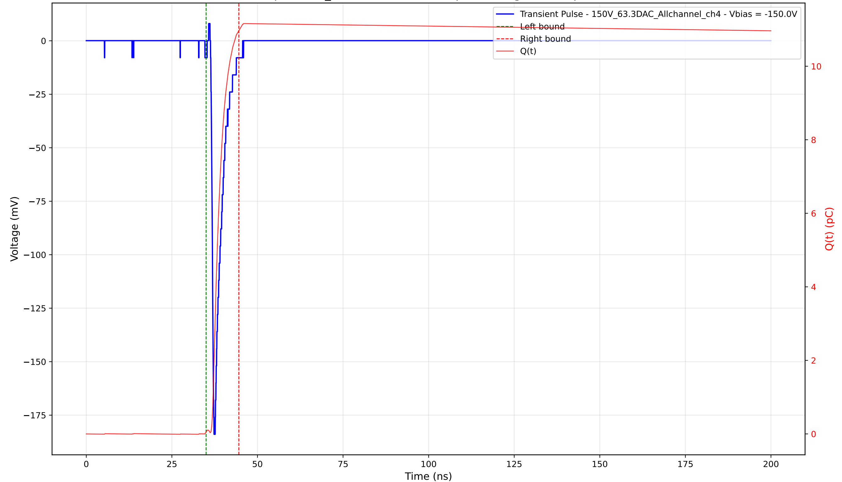
Transient Pulse - Sample: 1cm_42 - Position: 1265.0 \mu\text{m} - Charge: 10.91 pC - Rise Time: 0.75 ns
