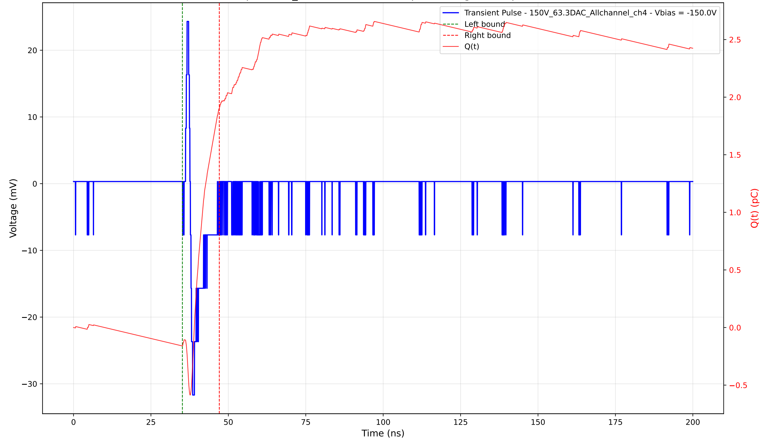
Transient Pulse - Sample: 1cm_42 - Position: 4455.0 \mu\text{m} - Charge: 2.06 pC - Rise Time: 0.74 ns
