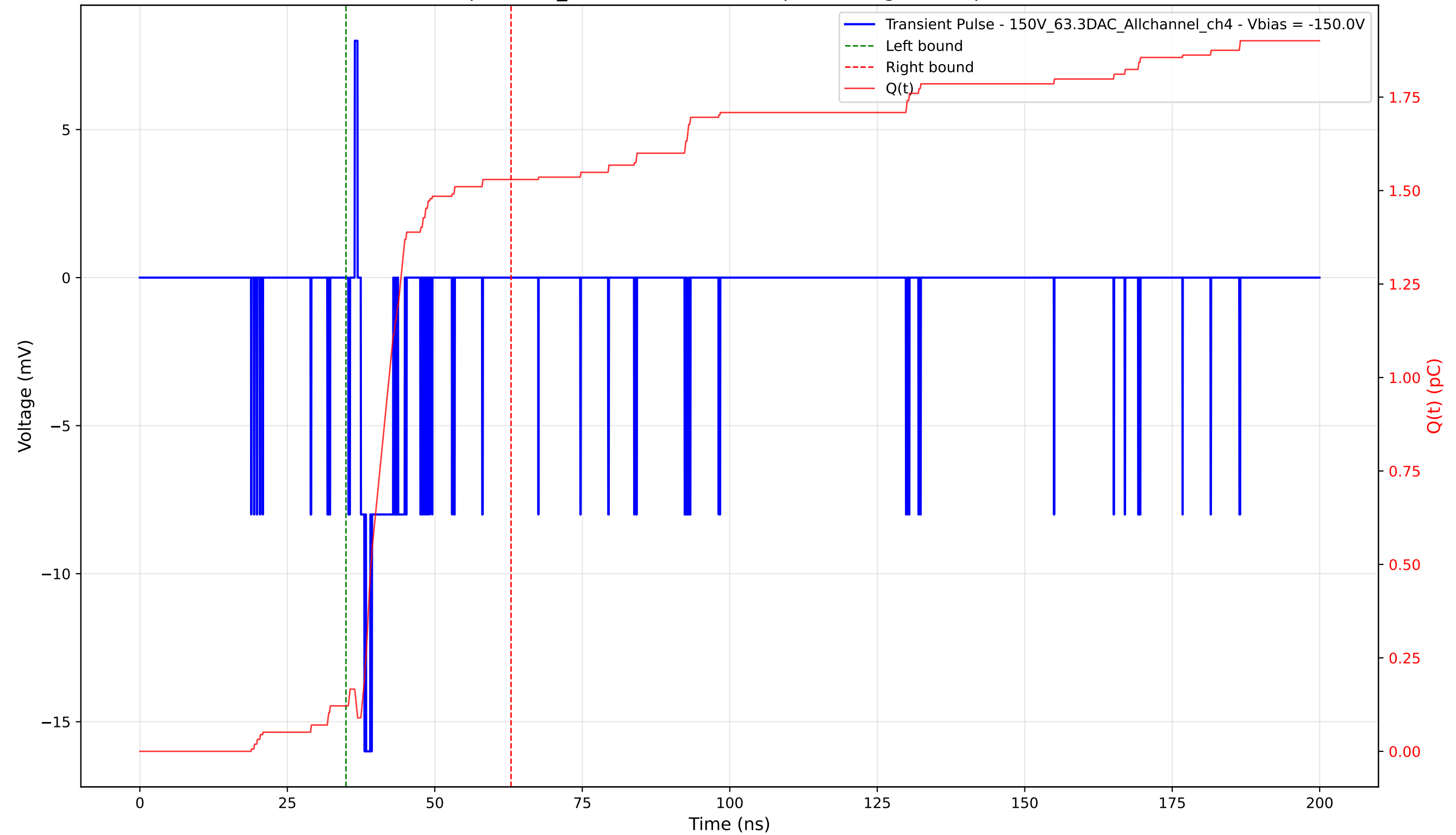
Transient Pulse - Sample: 1cm_42 - Position: 5085.0 \mu\text{m} - Charge: 1.41 pC - Rise Time: 0.63 ns
