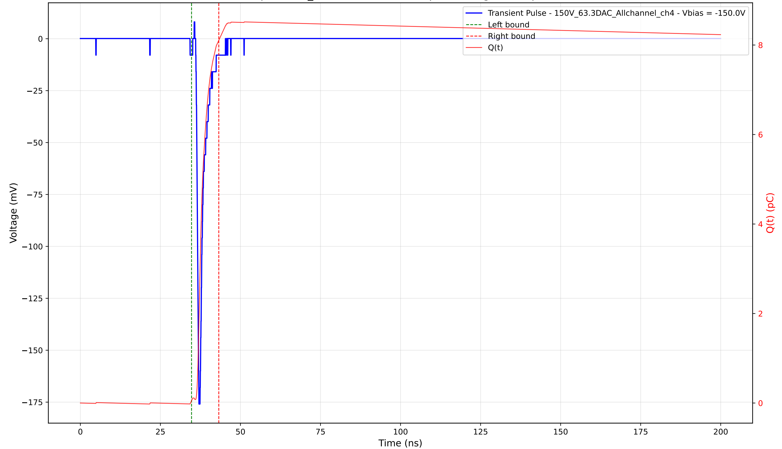
Transient Pulse - Sample: 1cm_42 - Position: 2610.0 \mu\text{m} - Charge: 8.05 pC - Rise Time: 0.75 ns
