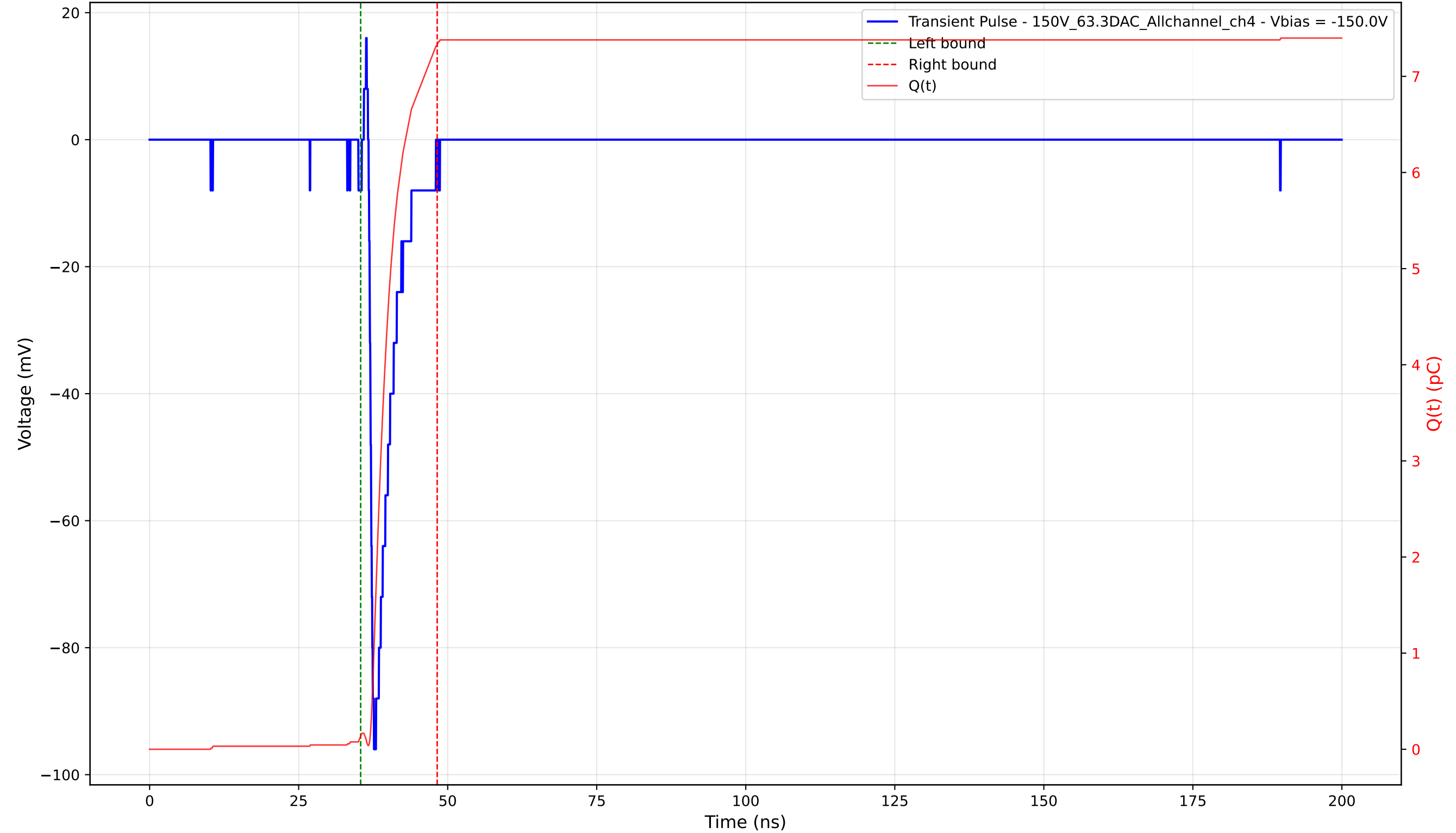
Transient Pulse - Sample: 1cm_42 - Position: 990.0 \mu\text{m} - Charge: 7.19 pC - Rise Time: 0.63 ns
