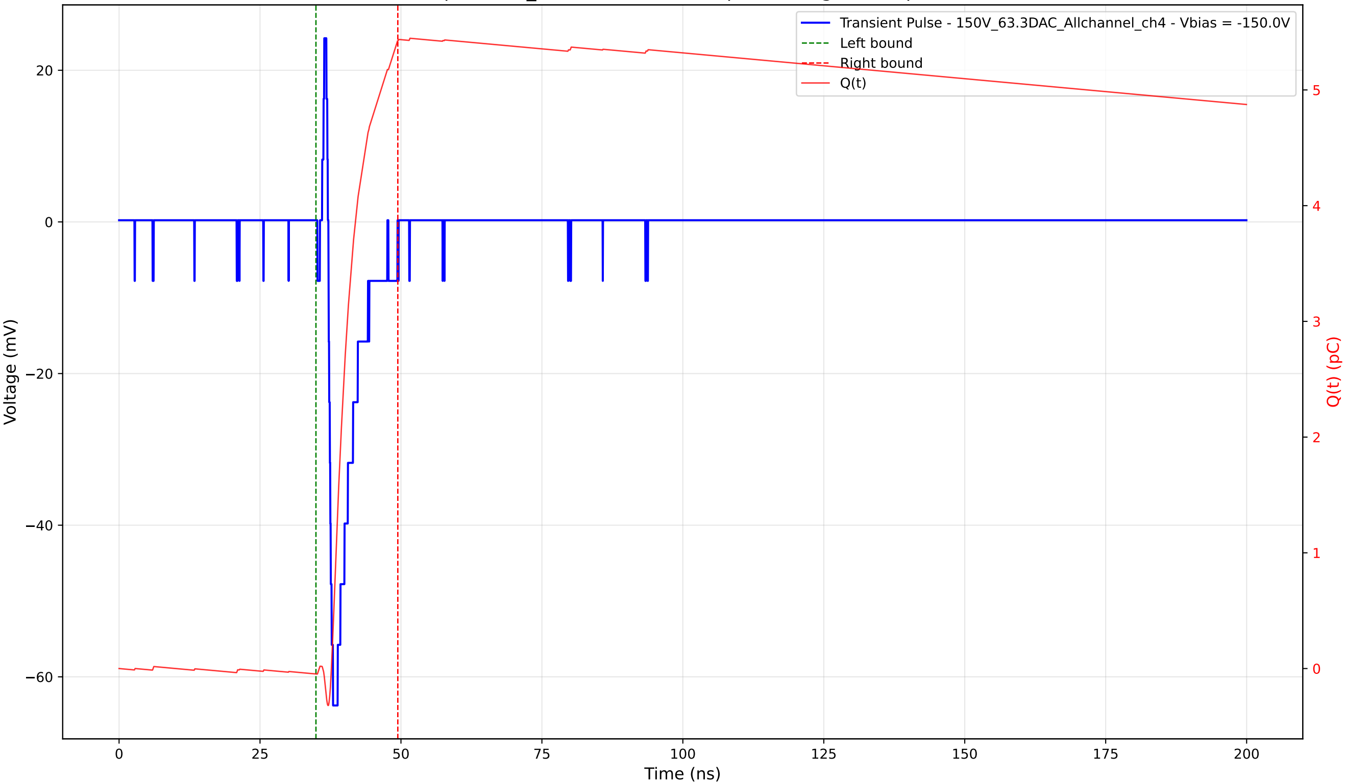
Transient Pulse - Sample: 1cm_42 - Position: 600.0 \mu\text{m} - Charge: 5.47 pC - Rise Time: 0.81 ns
