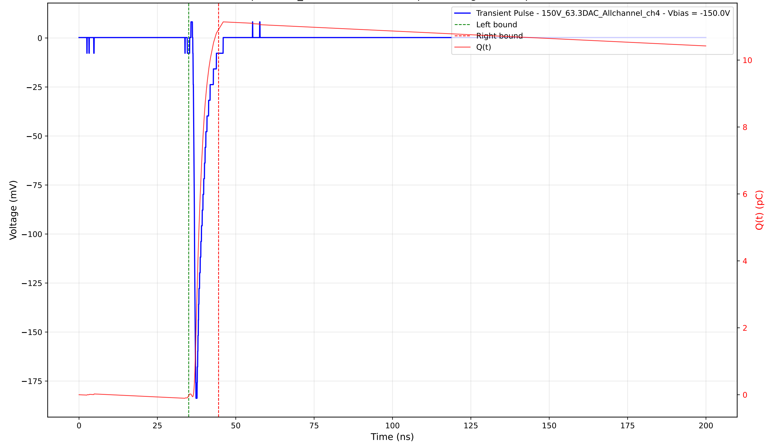
Transient Pulse - Sample: 1cm_42 - Position: 1260.0 \mu\text{m} - Charge: 10.94 pC - Rise Time: 0.75 ns
