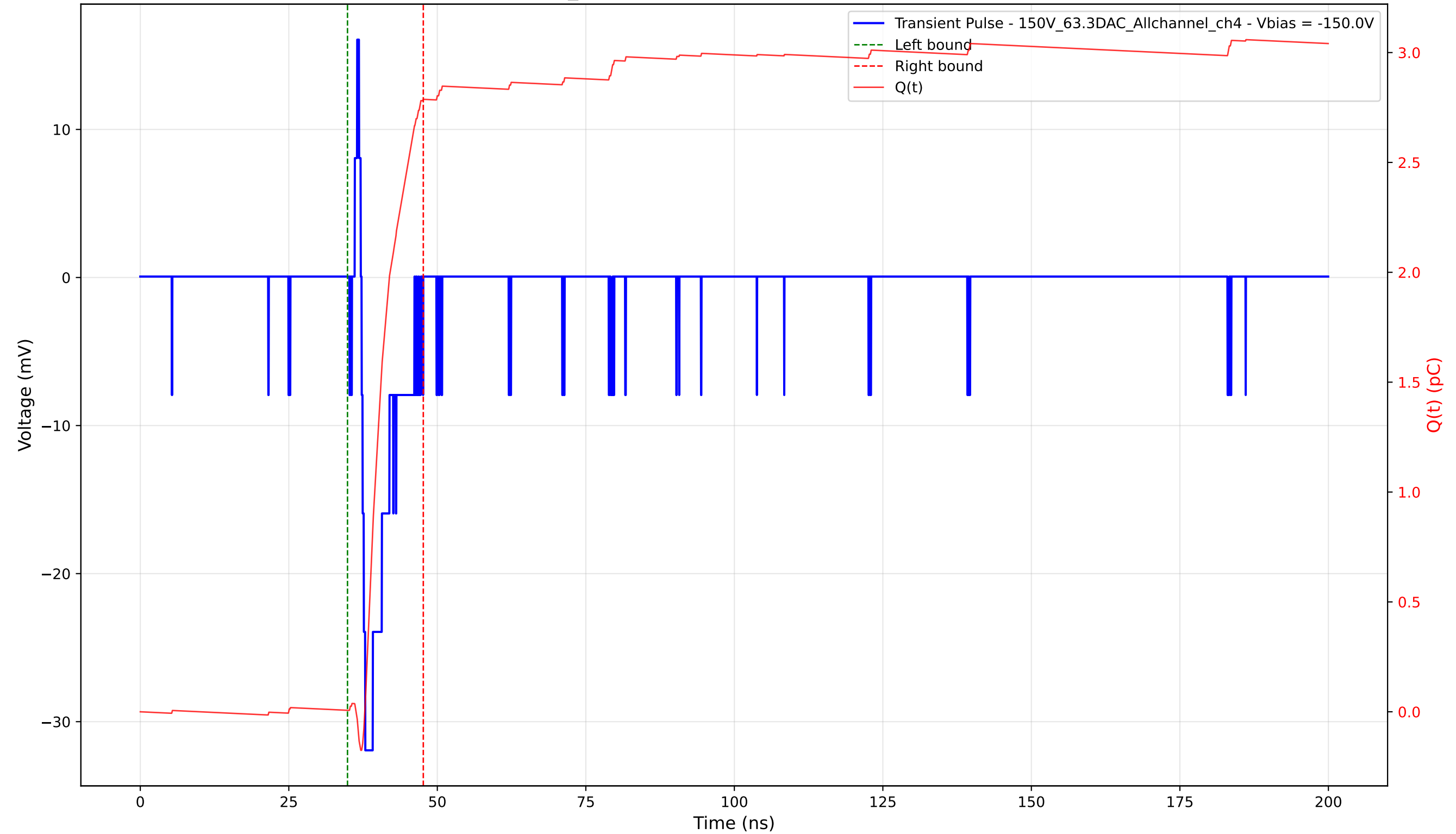
Transient Pulse - Sample: 1cm_42 - Position: 300.0 \mu\text{m} - Charge: 2.78 pC - Rise Time: 0.62 ns
