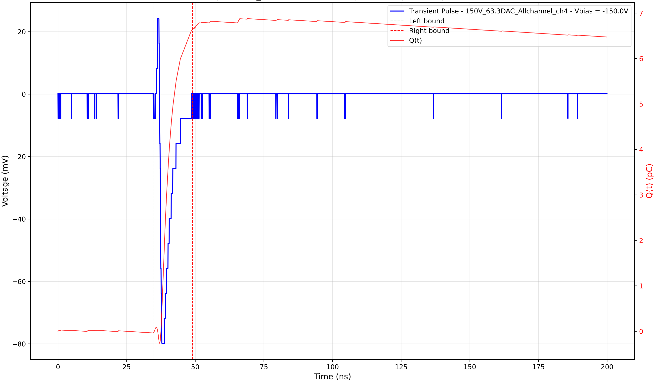
Transient Pulse - Sample: 1cm_42 - Position: 710.0 \mu\text{m} - Charge: 6.66 pC - Rise Time: 0.76 ns
