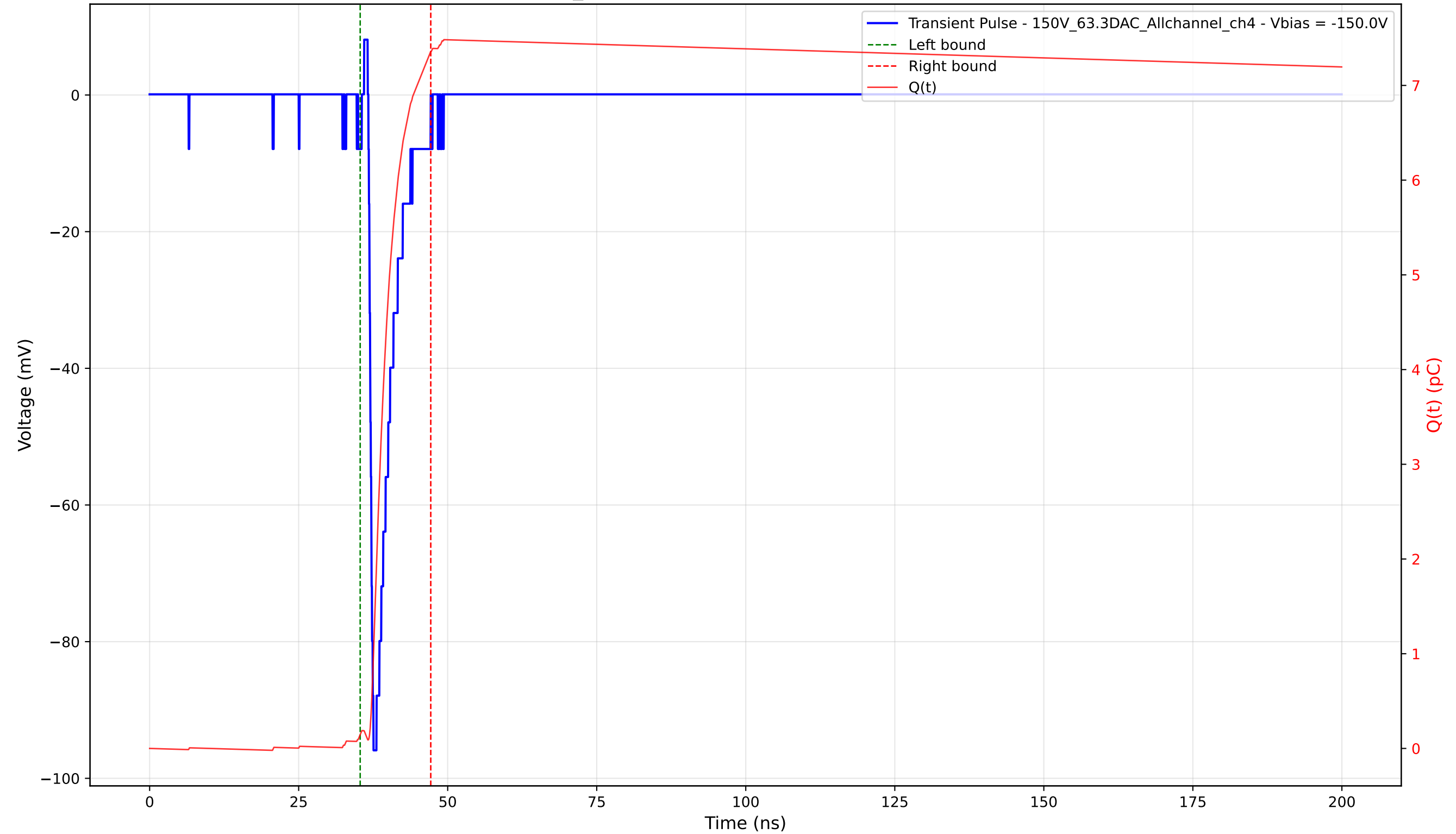
Transient Pulse - Sample: 1cm_42 - Position: 1000.0 \mu\text{m} - Charge: 7.21 pC - Rise Time: 0.67 ns
