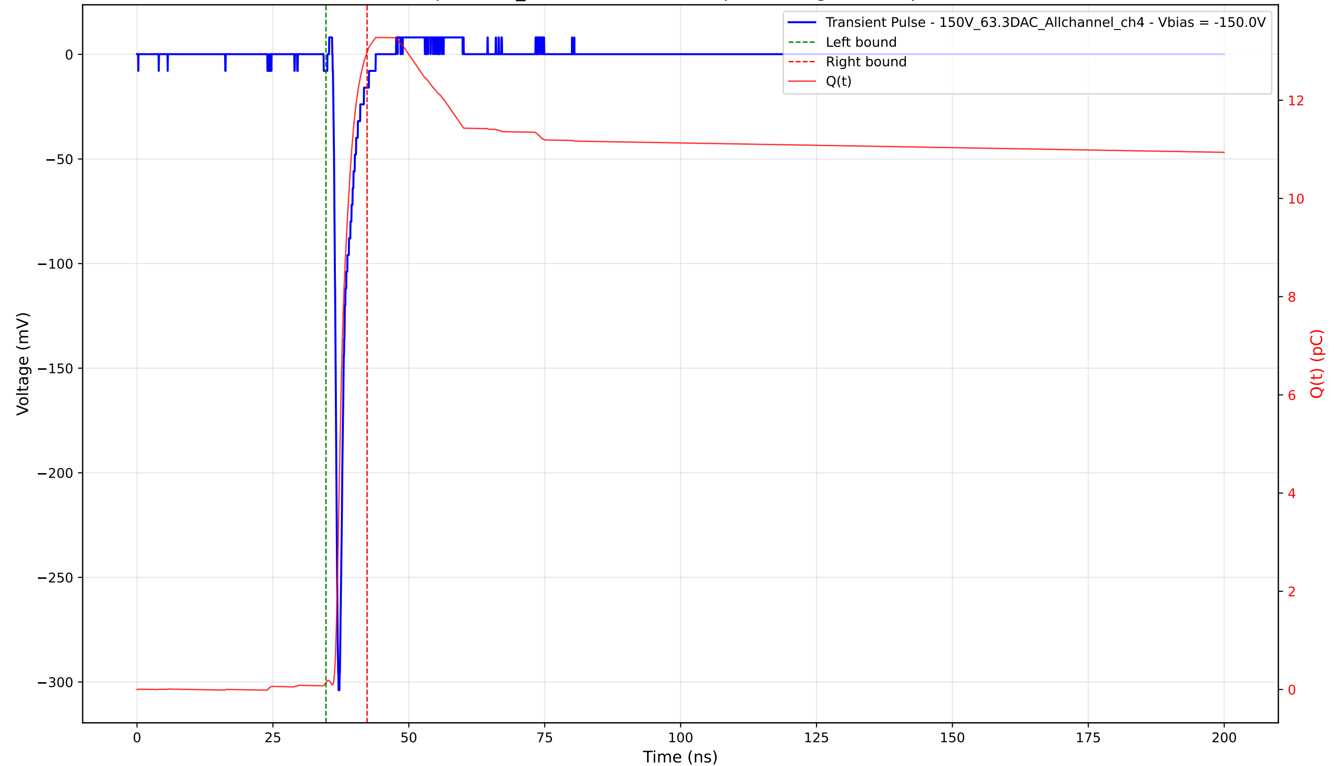
Transient Pulse - Sample: 1cm_42 - Position: 1545.0 \mu\text{m} - Charge: 12.83 pC - Rise Time: 0.74 ns
