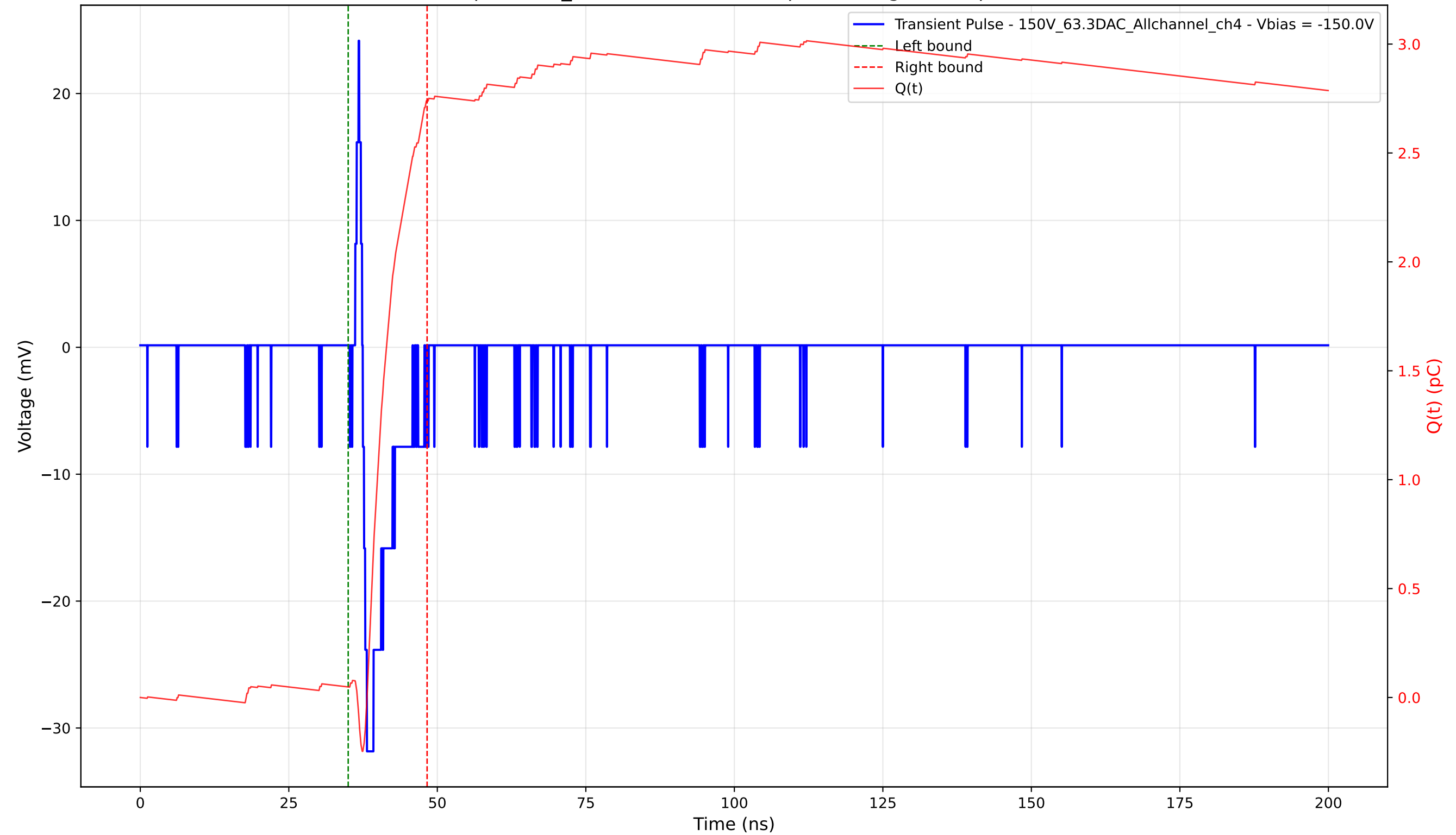
Transient Pulse - Sample: 1cm_42 - Position: 4855.0 \mu\text{m} - Charge: 2.69 pC - Rise Time: 0.70 ns
