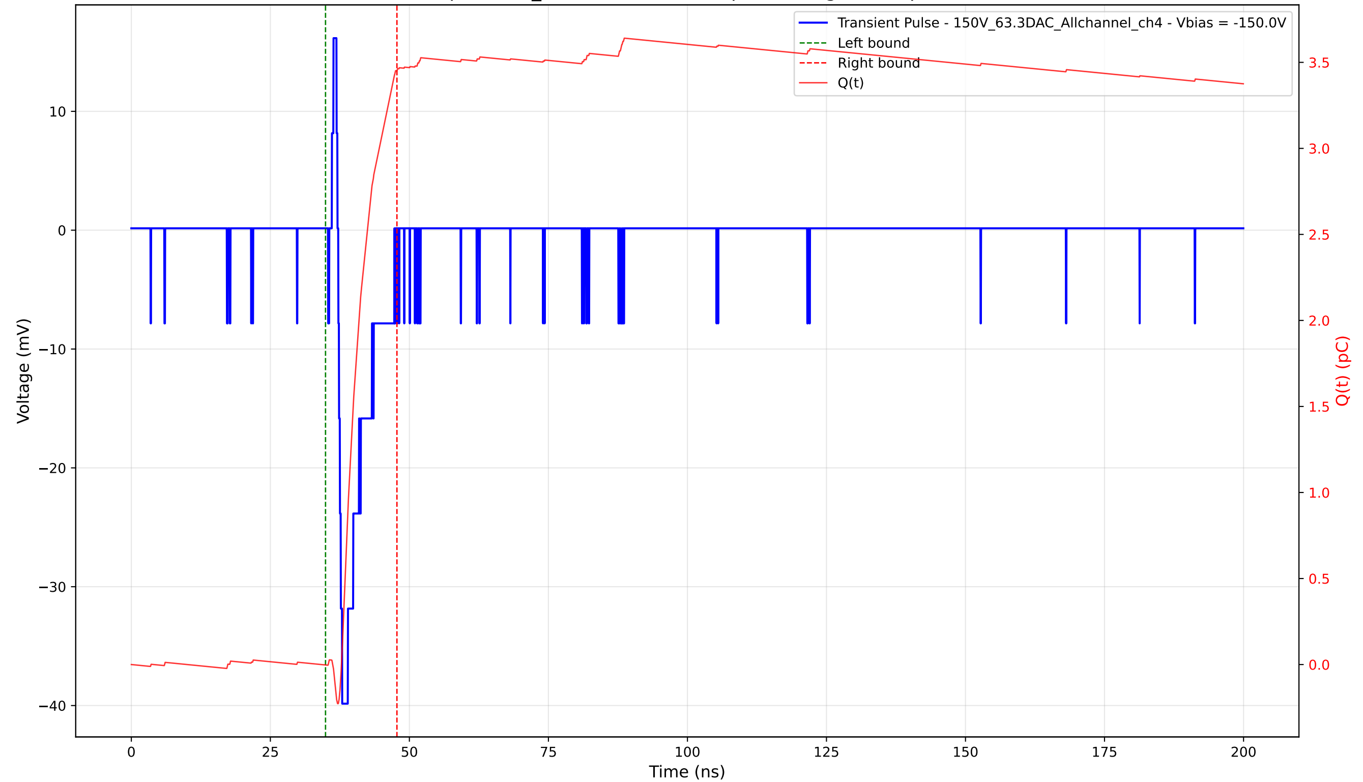
Transient Pulse - Sample: 1cm_42 - Position: 385.0 \mu\text{m} - Charge: 3.45 pC - Rise Time: 0.70 ns
