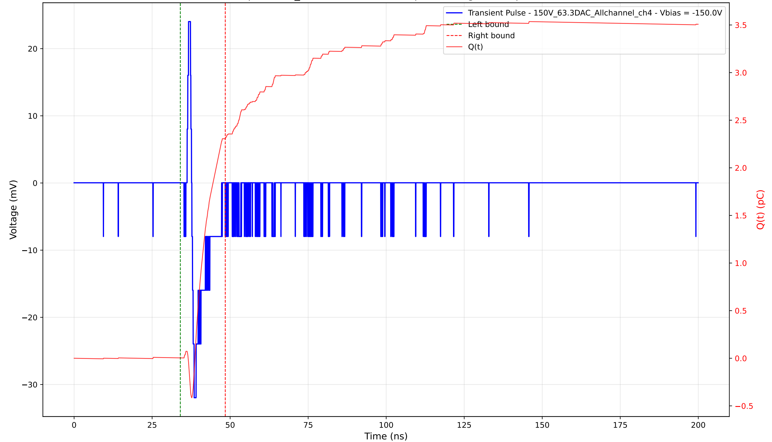
Transient Pulse - Sample: 1cm_42 - Position: 4080.0 \mu\text{m} - Charge: 2.30 pC - Rise Time: 0.74 ns
