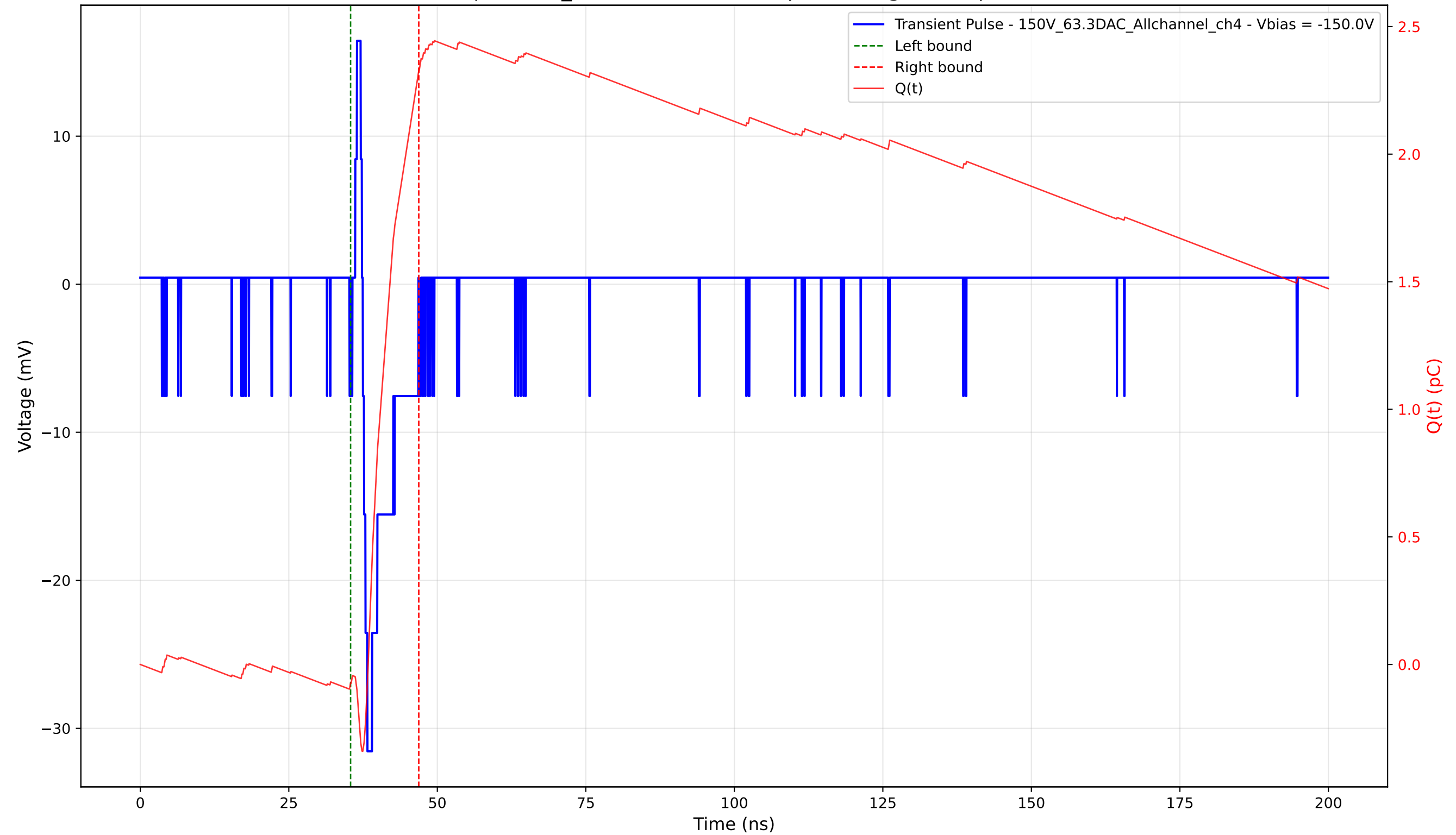
Transient Pulse - Sample: 1cm_42 - Position: 4910.0 \mu\text{m} - Charge: 2.39 pC - Rise Time: 0.78 ns
