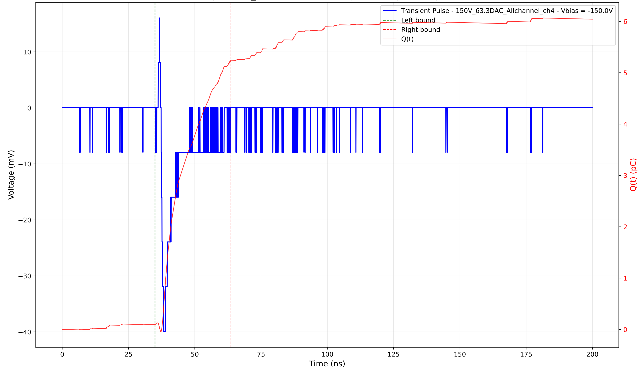
Transient Pulse - Sample: 1cm_42 - Position: 3455.0 \mu\text{m} - Charge: 5.15 pC - Rise Time: 0.98 ns
