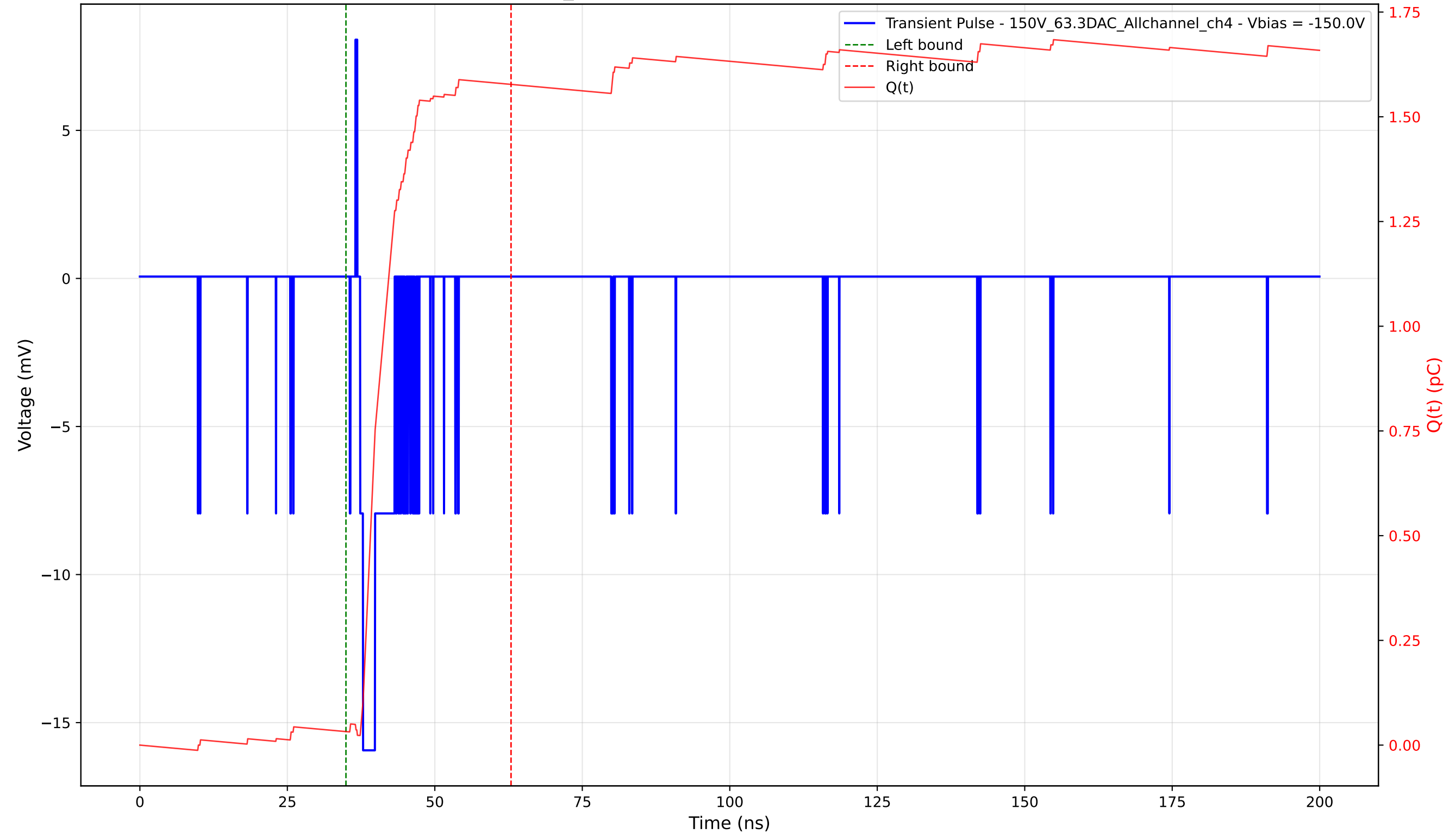
Transient Pulse - Sample: 1cm_42 - Position: 130.0 \mu\text{m} - Charge: 1.55 pC - Rise Time: 0.51 ns
