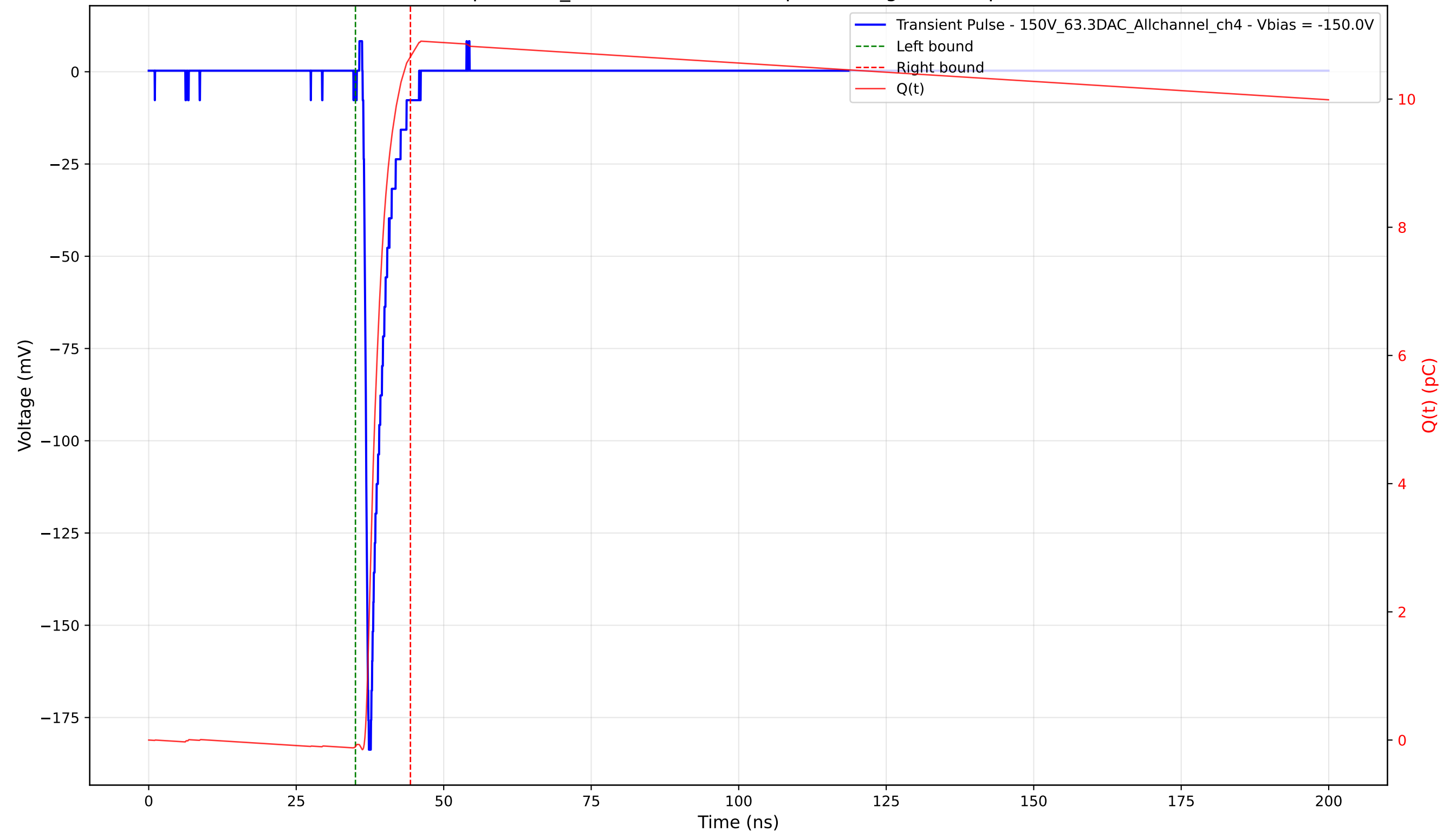
Transient Pulse - Sample: 1cm_42 - Position: 1280.0 \mu\text{m} - Charge: 10.76 pC - Rise Time: 0.75 ns
