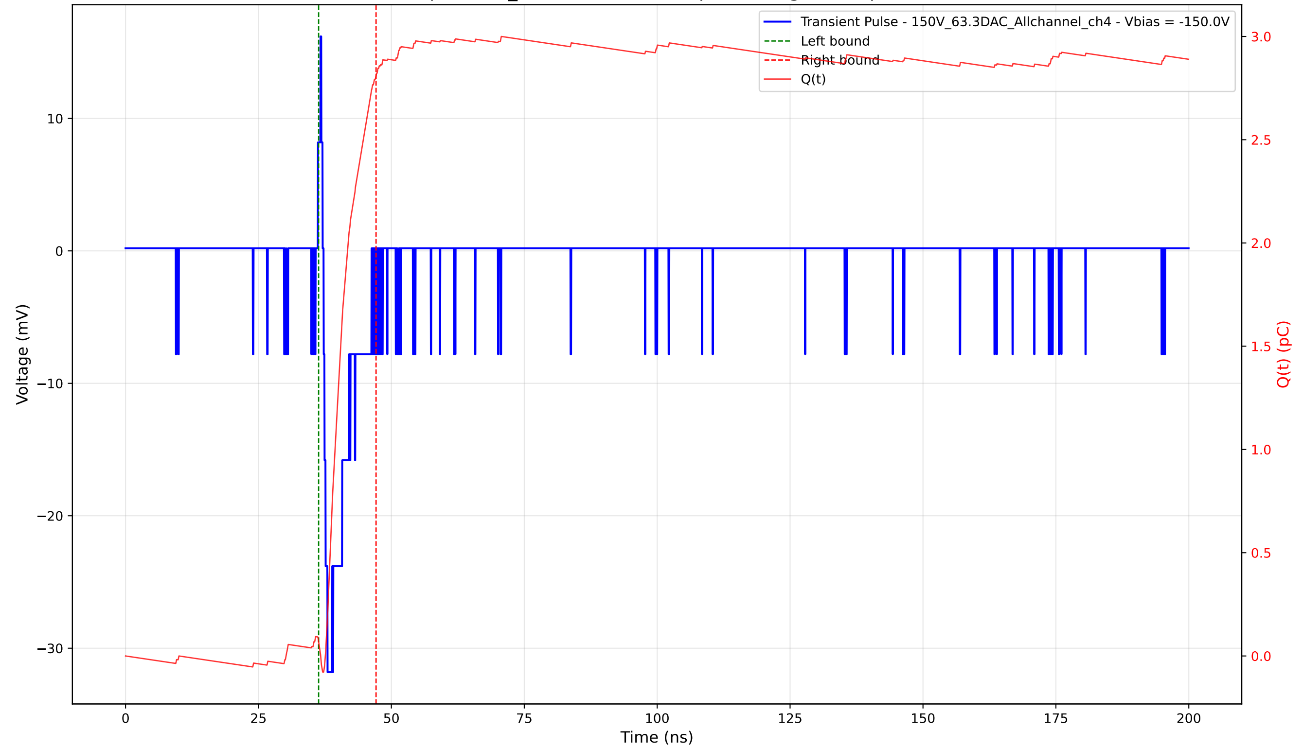
Transient Pulse - Sample: 1cm_42 - Position: 275.0 \mu\text{m} - Charge: 2.74 pC - Rise Time: 0.74 ns
