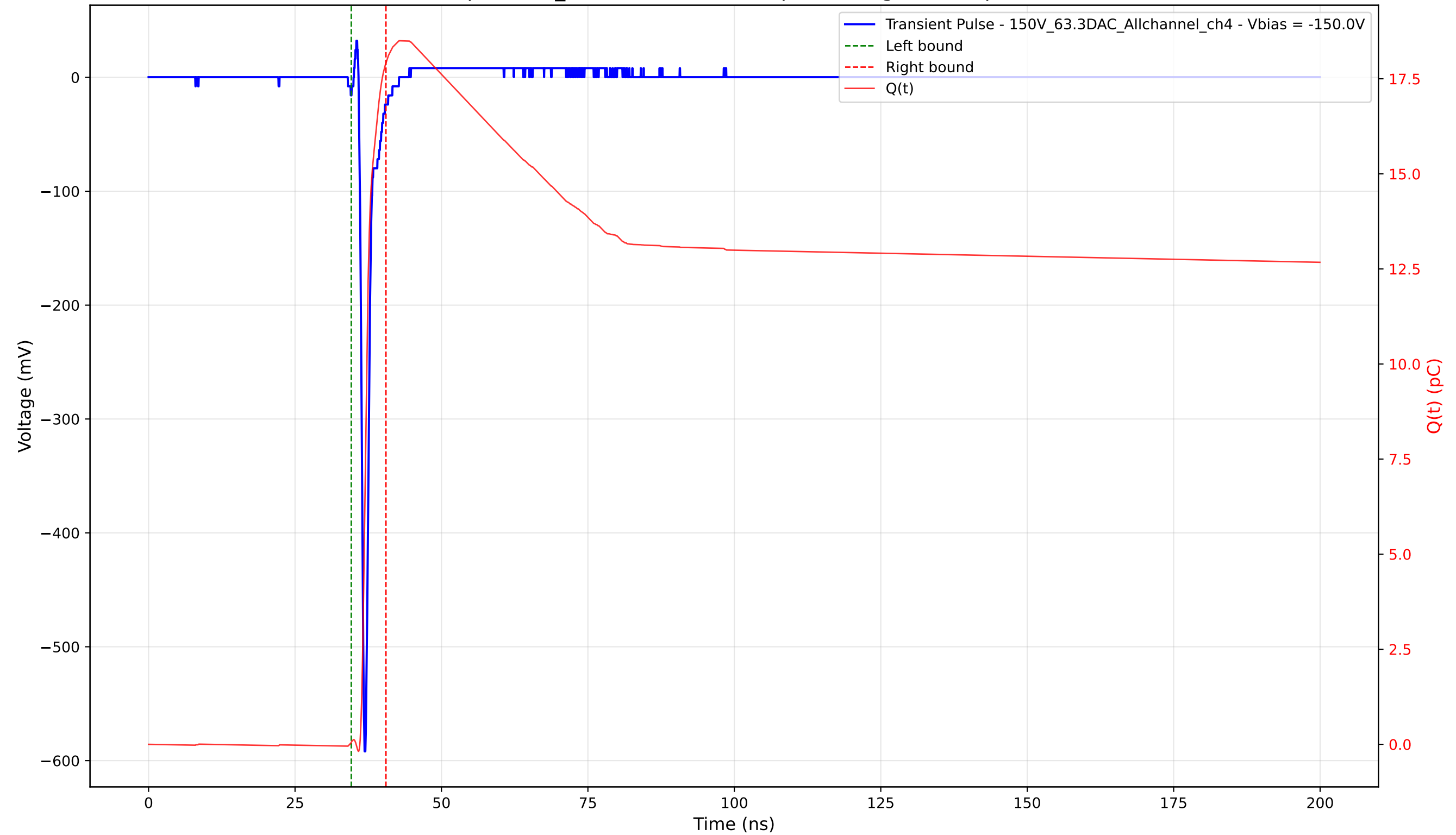
Transient Pulse - Sample: 1cm_42 - Position: 2005.0 \mu\text{m} - Charge: 17.86 pC - Rise Time: 0.71 ns
