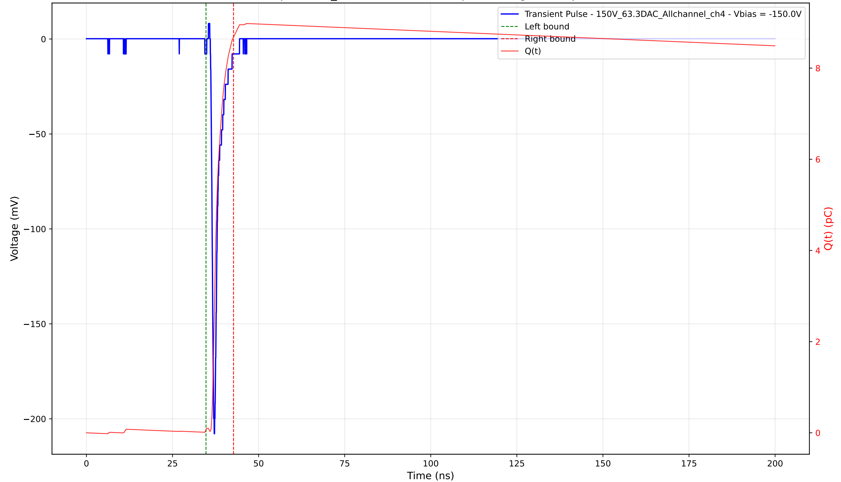
Transient Pulse - Sample: 1cm_42 - Position: 2560.0 \mu\text{m} - Charge: 8.61 pC - Rise Time: 0.75 ns
