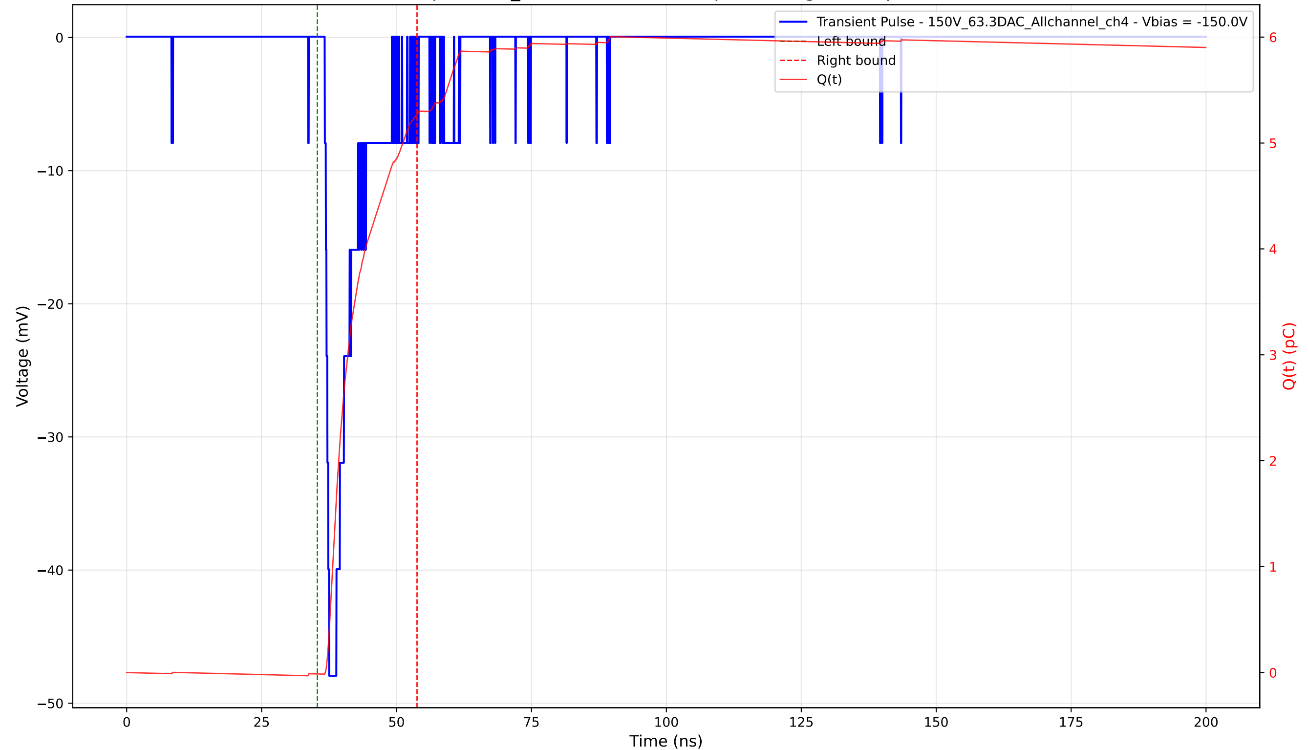
Transient Pulse - Sample: 1cm_42 - Position: 3135.0 \mu\text{m} - Charge: 5.29 pC - Rise Time: 0.82 ns
