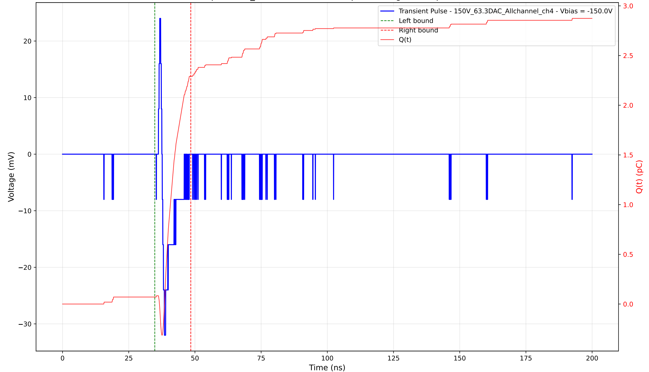
Transient Pulse - Sample: 1cm_42 - Position: 4580.0 \mu\text{m} - Charge: 2.22 pC - Rise Time: 0.82 ns
