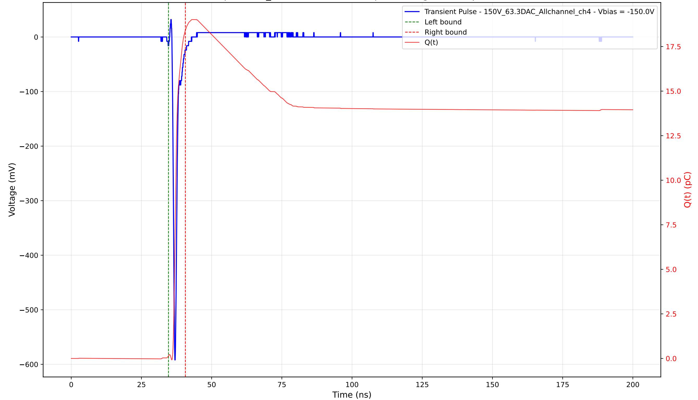
Transient Pulse - Sample: 1cm_42 - Position: 1940.0 \mu\text{m} - Charge: 18.26 pC - Rise Time: 0.70 ns
