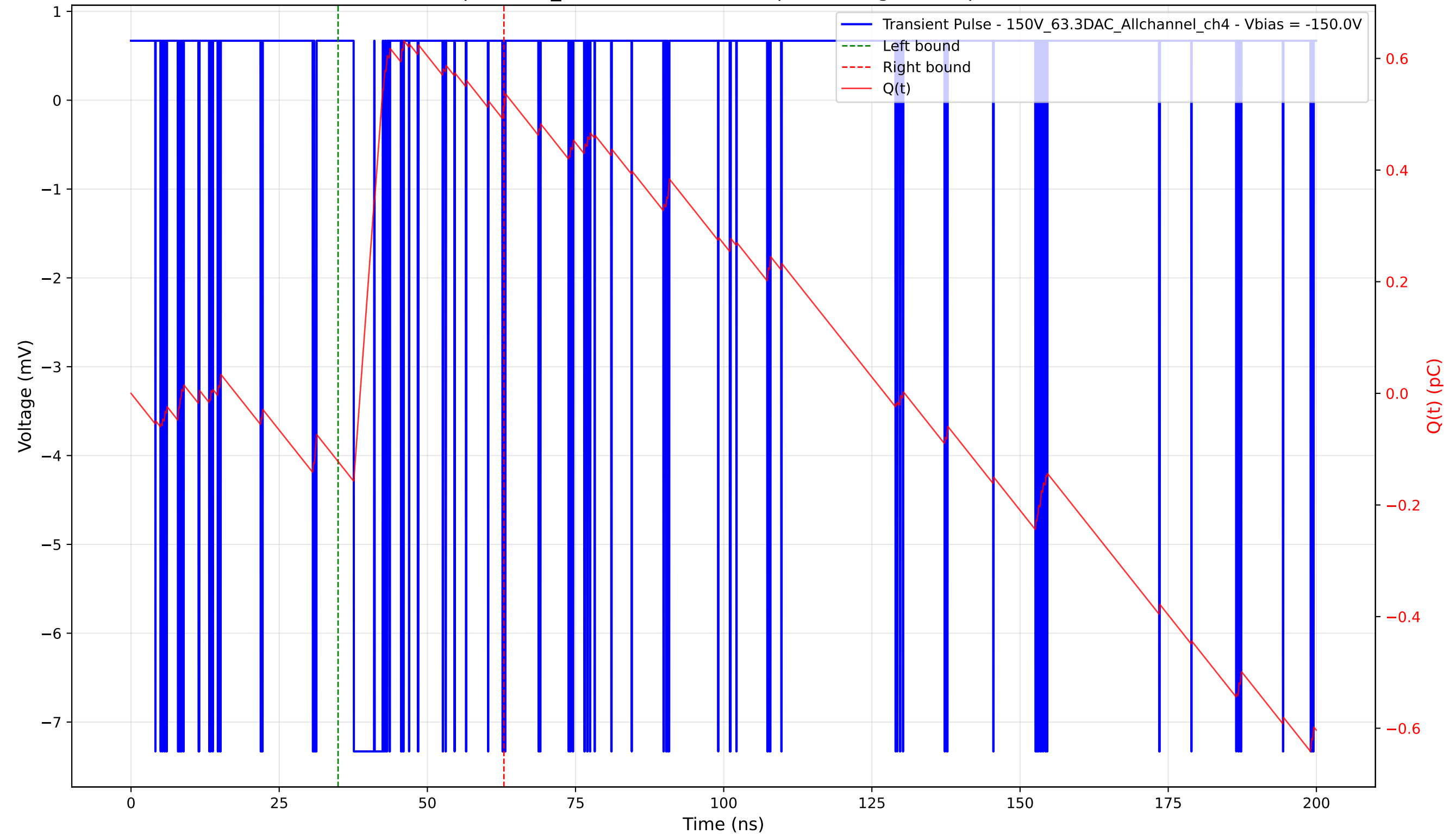
Transient Pulse - Sample: 1cm_42 - Position: 5120.0 \mu\text{m} - Charge: 0.64 pC - Rise Time: 0.04 ns
