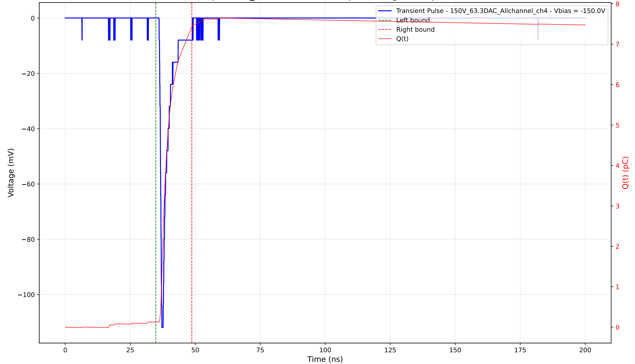
Transient Pulse - Sample: 1cm_42 - Position: 2855.0 \mu\text{m} - Charge: 7.31 pC - Rise Time: 0.78 ns
