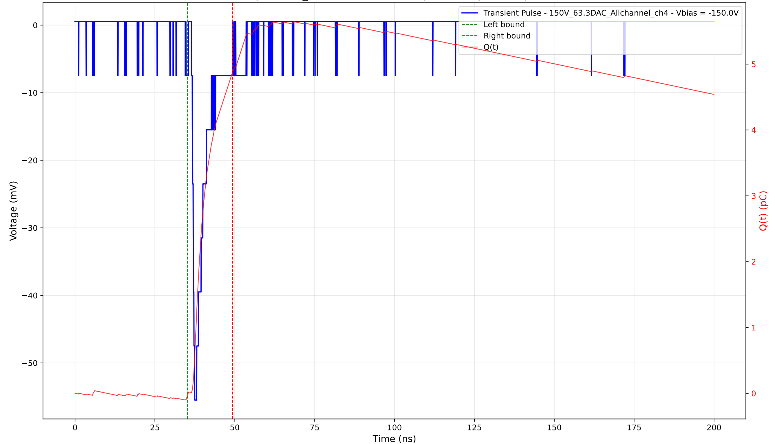
Transient Pulse - Sample: 1cm_42 - Position: 3070.0 \mu\text{m} - Charge: 4.90 pC - Rise Time: 1.01 ns
