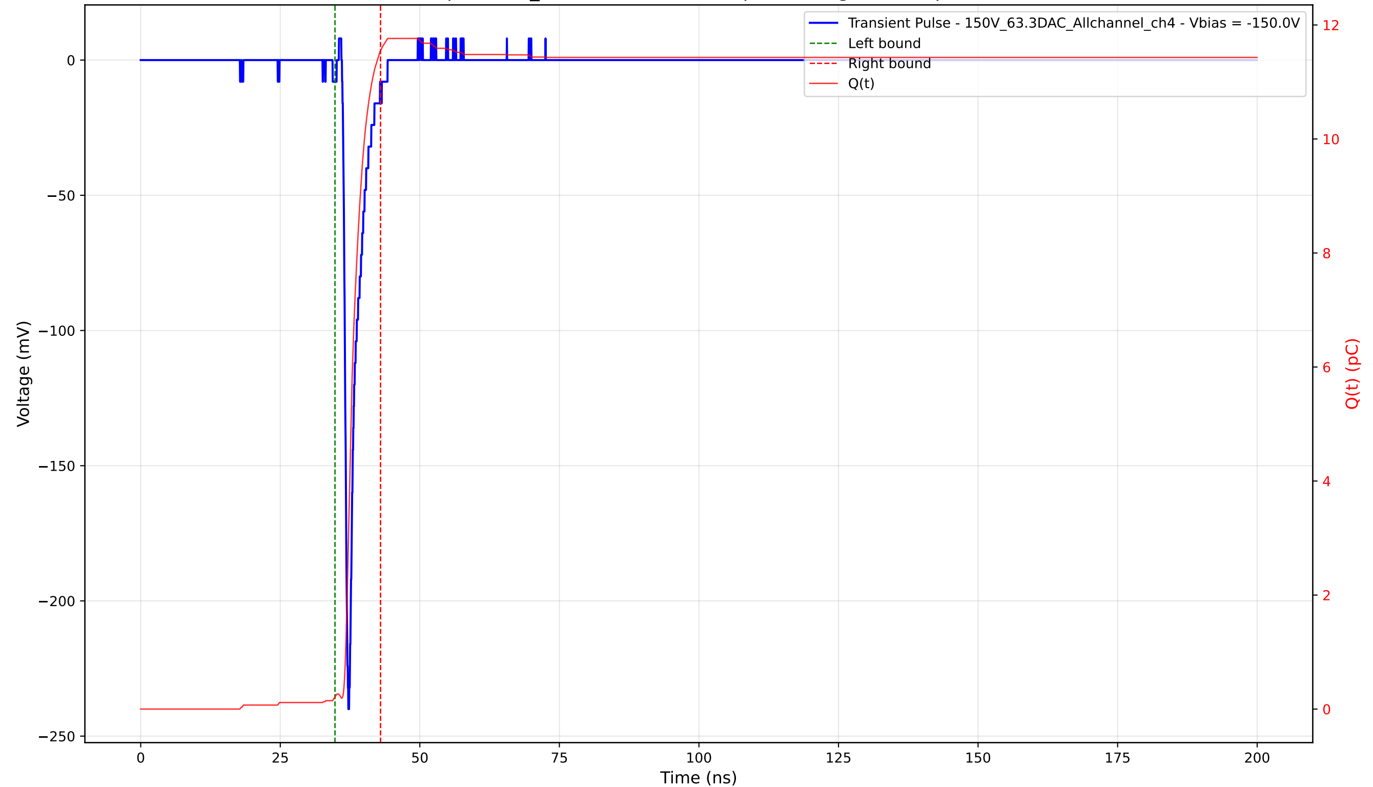
Transient Pulse - Sample: 1cm_42 - Position: 1465.0 \mu\text{m} - Charge: 11.33 pC - Rise Time: 0.76 ns
