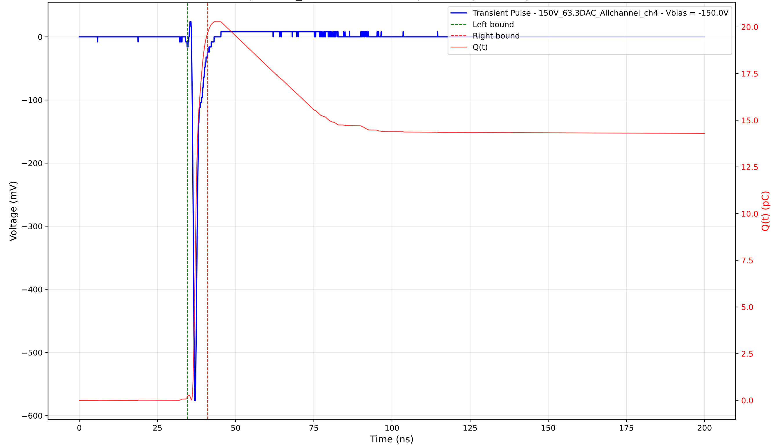
Transient Pulse - Sample: 1cm_42 - Position: 1760.0 \mu\text{m} - Charge: 19.50 pC - Rise Time: 0.73 ns
