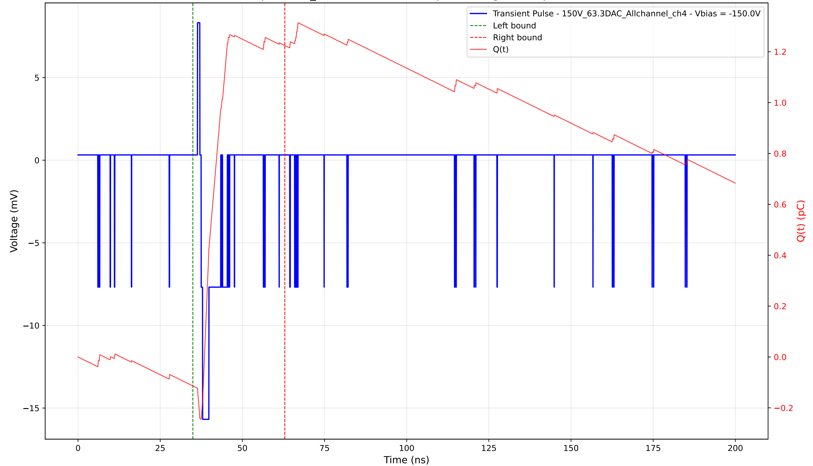
Transient Pulse - Sample: 1cm_42 - Position: 5035.0 \mu\text{m} - Charge: 1.34 pC - Rise Time: 0.47 ns
