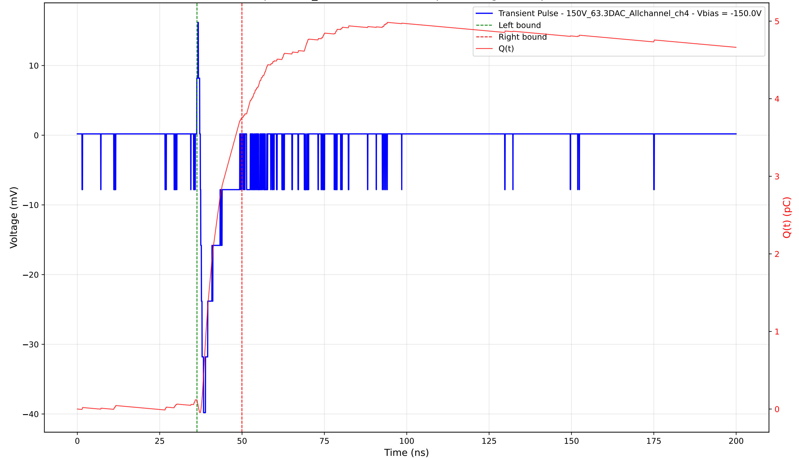
Transient Pulse - Sample: 1cm_42 - Position: 3460.0 \mu\text{m} - Charge: 3.65 pC - Rise Time: 0.98 ns
