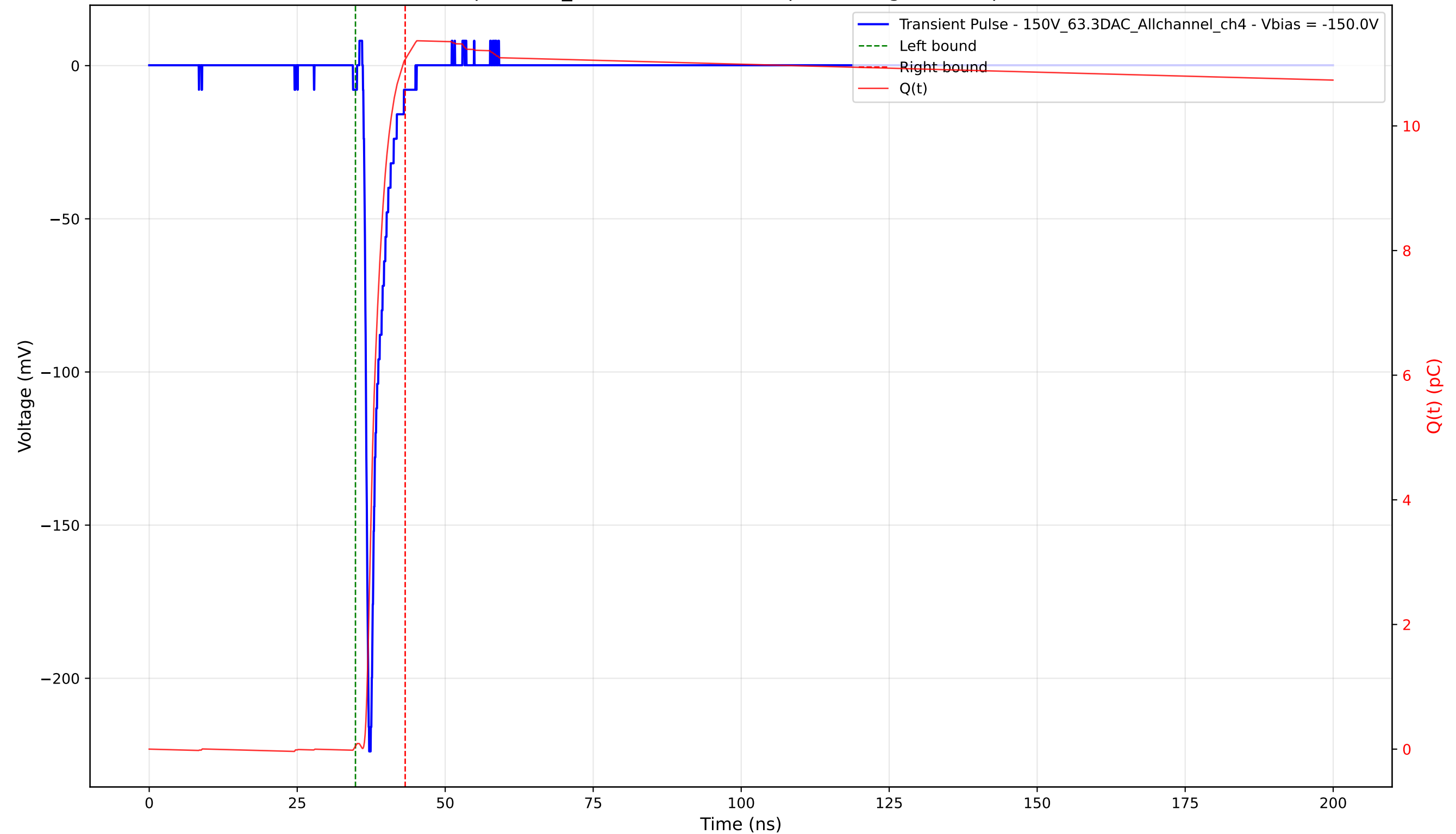
Transient Pulse - Sample: 1cm_42 - Position: 1450.0 \mu\text{m} - Charge: 11.02 pC - Rise Time: 0.78 ns
