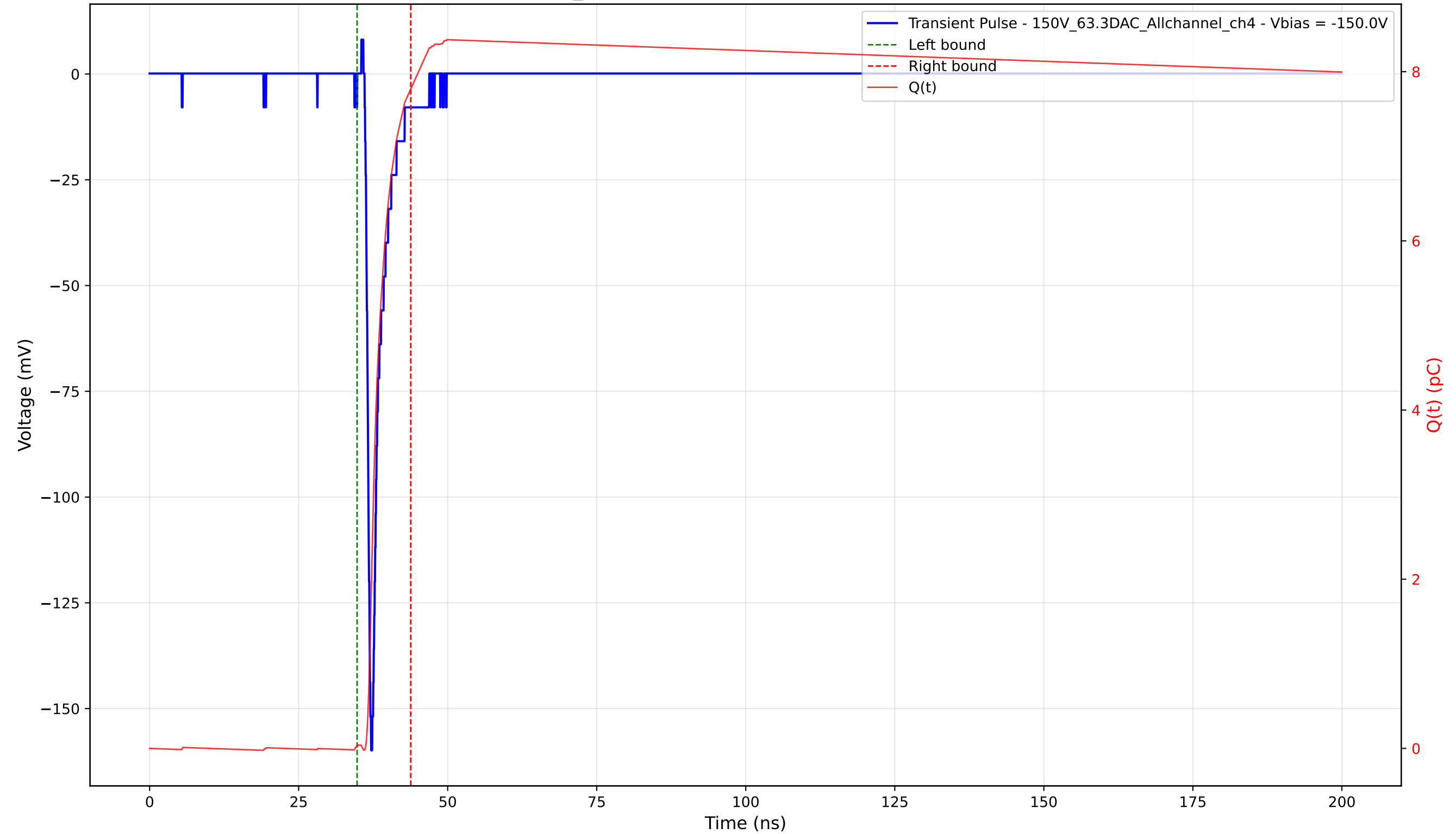
Transient Pulse - Sample: 1cm_42 - Position: 2665.0 \mu\text{m} - Charge: 7.76 pC - Rise Time: 0.84 ns
