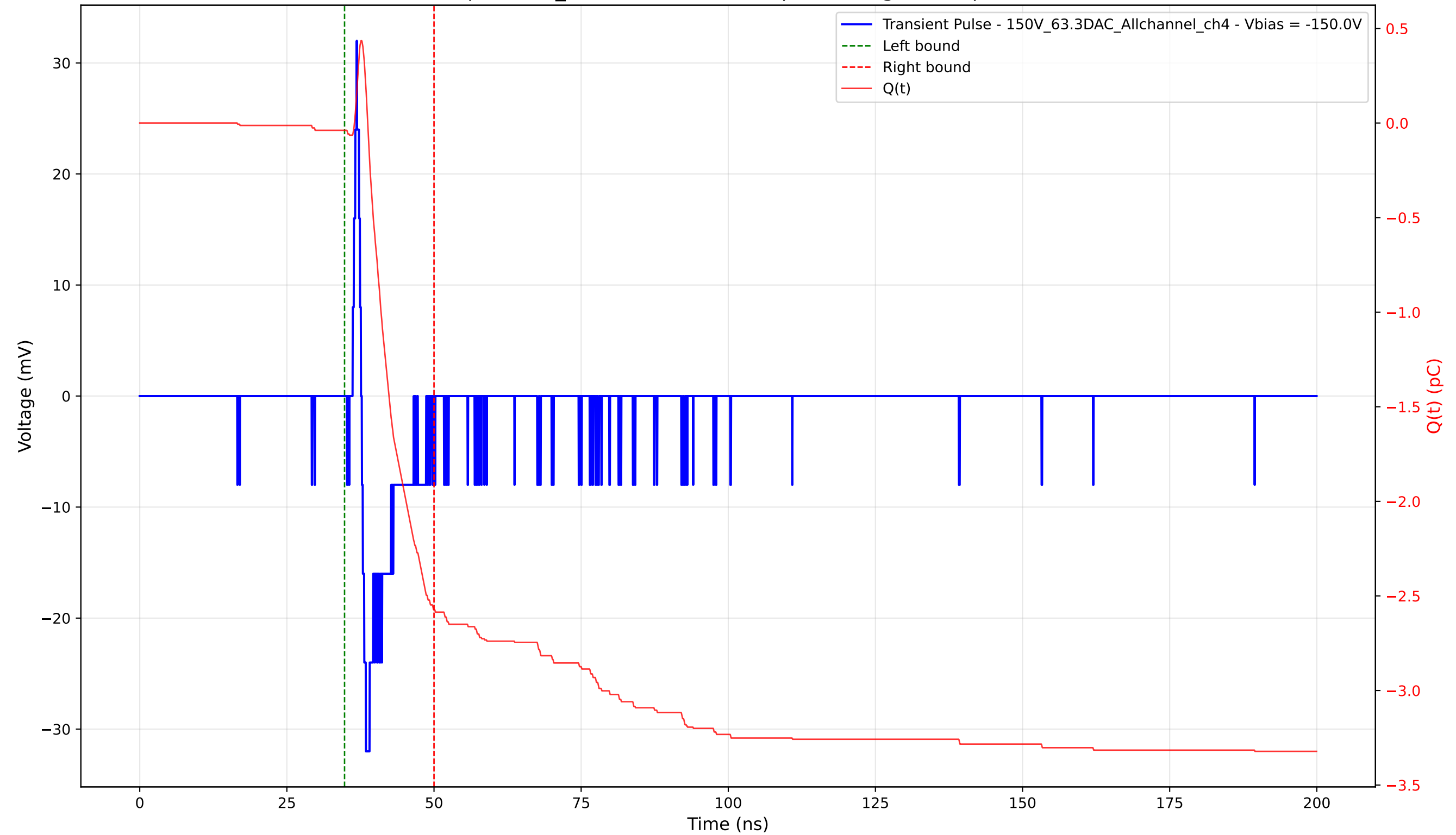
Transient Pulse - Sample: 1cm_42 - Position: 4425.0 \mu\text{m} - Charge: 2.53 pC - Rise Time: 0.70 ns
