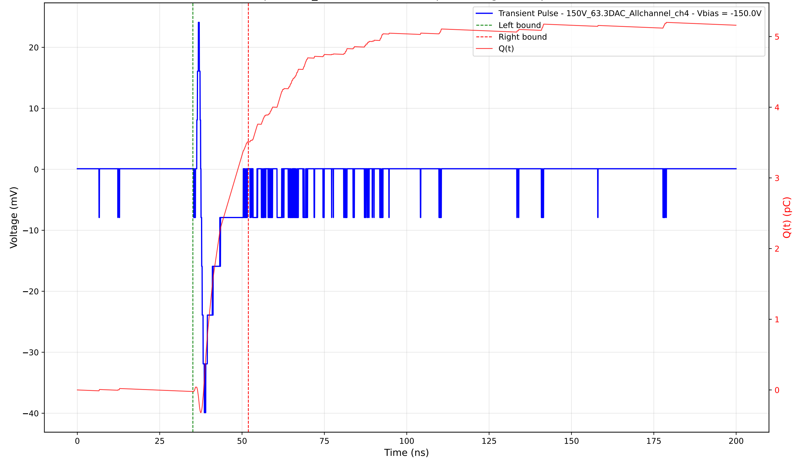
Transient Pulse - Sample: 1cm_42 - Position: 3650.0 \mu\text{m} - Charge: 3.53 pC - Rise Time: 1.02 ns
