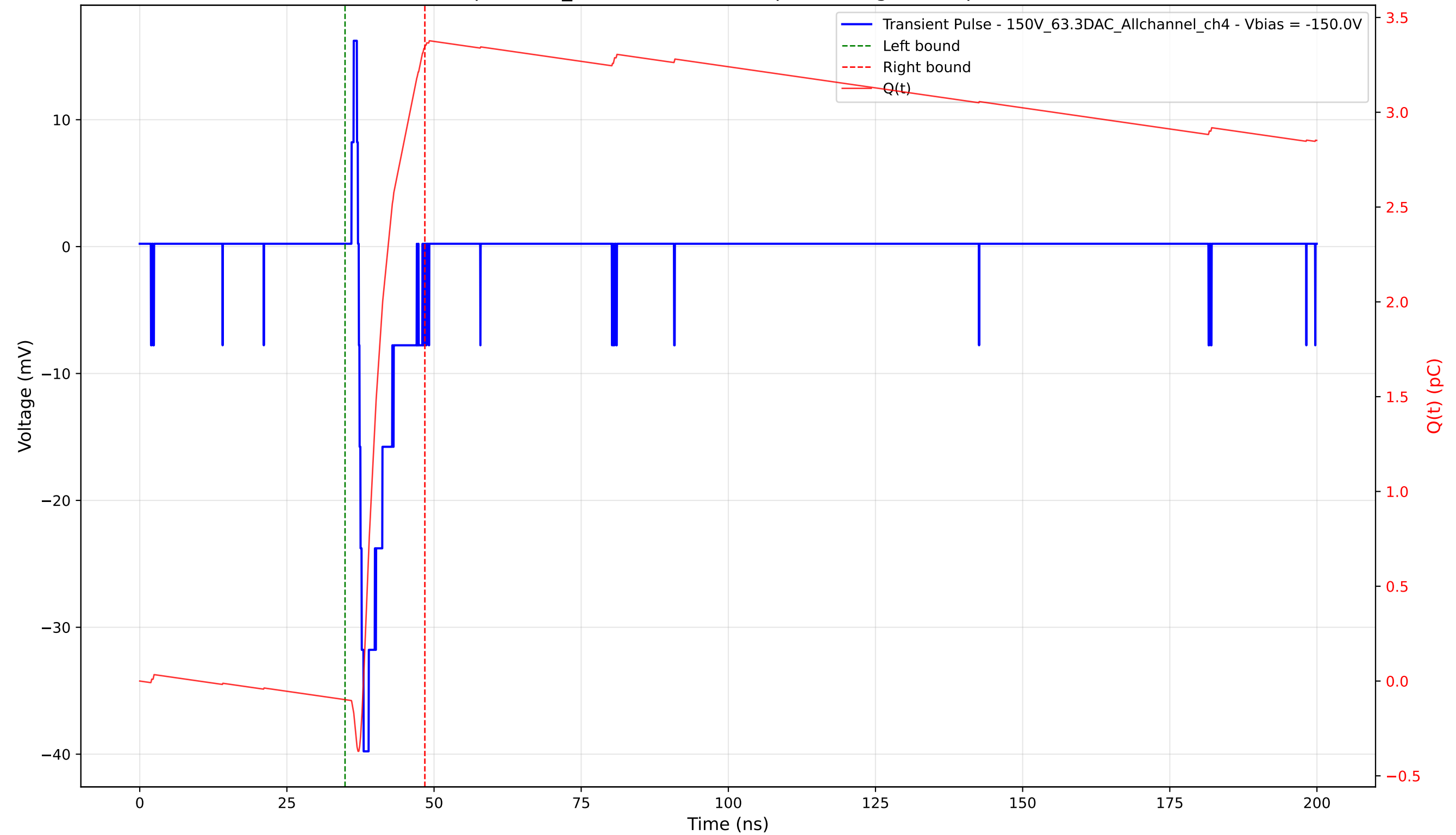
Transient Pulse - Sample: 1cm_42 - Position: 375.0 \mu\text{m} - Charge: 3.44 pC - Rise Time: 0.82 ns
