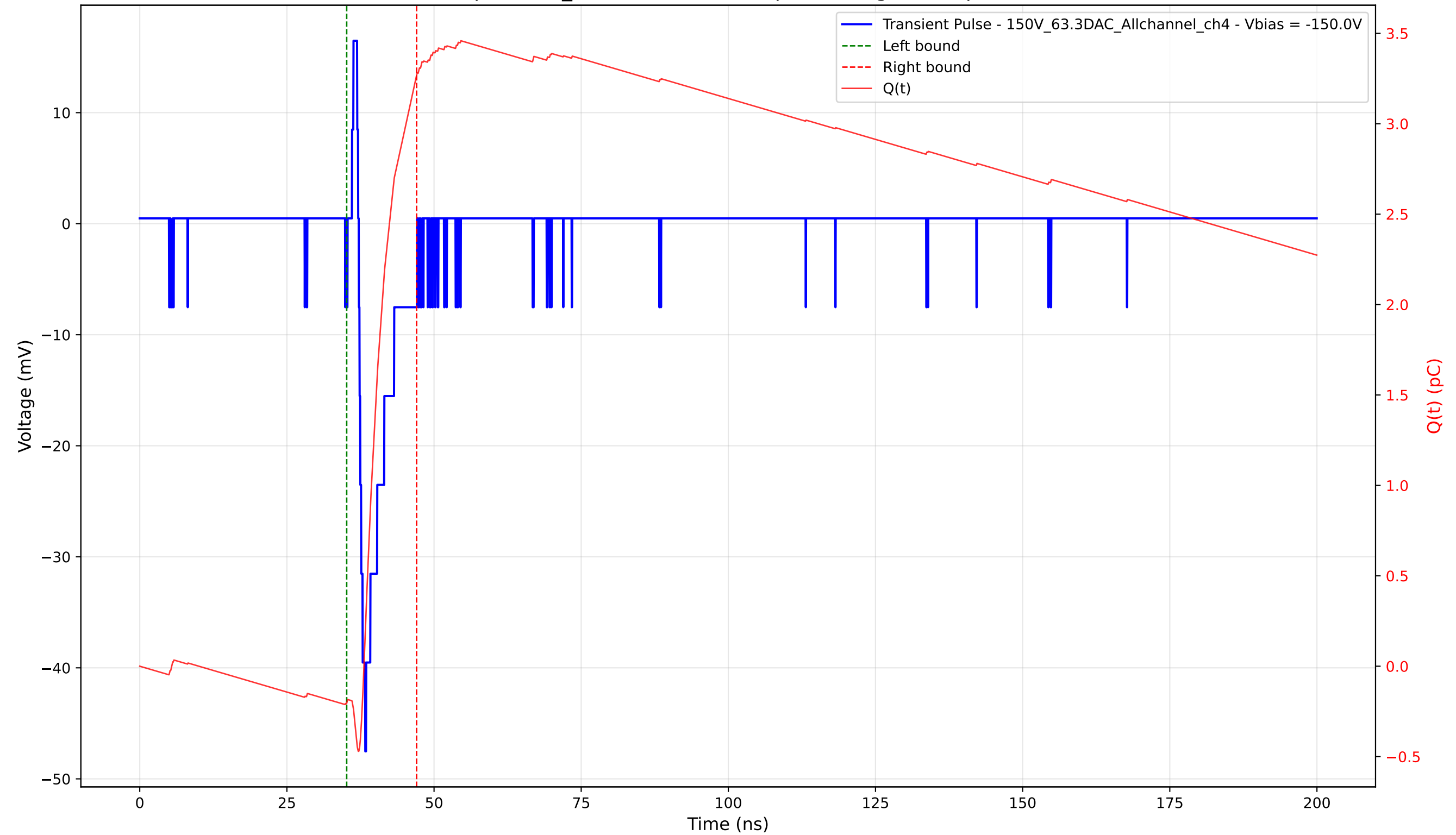
Transient Pulse - Sample: 1cm_42 - Position: 415.0 \mu\text{m} - Charge: 3.48 pC - Rise Time: 1.10 ns
