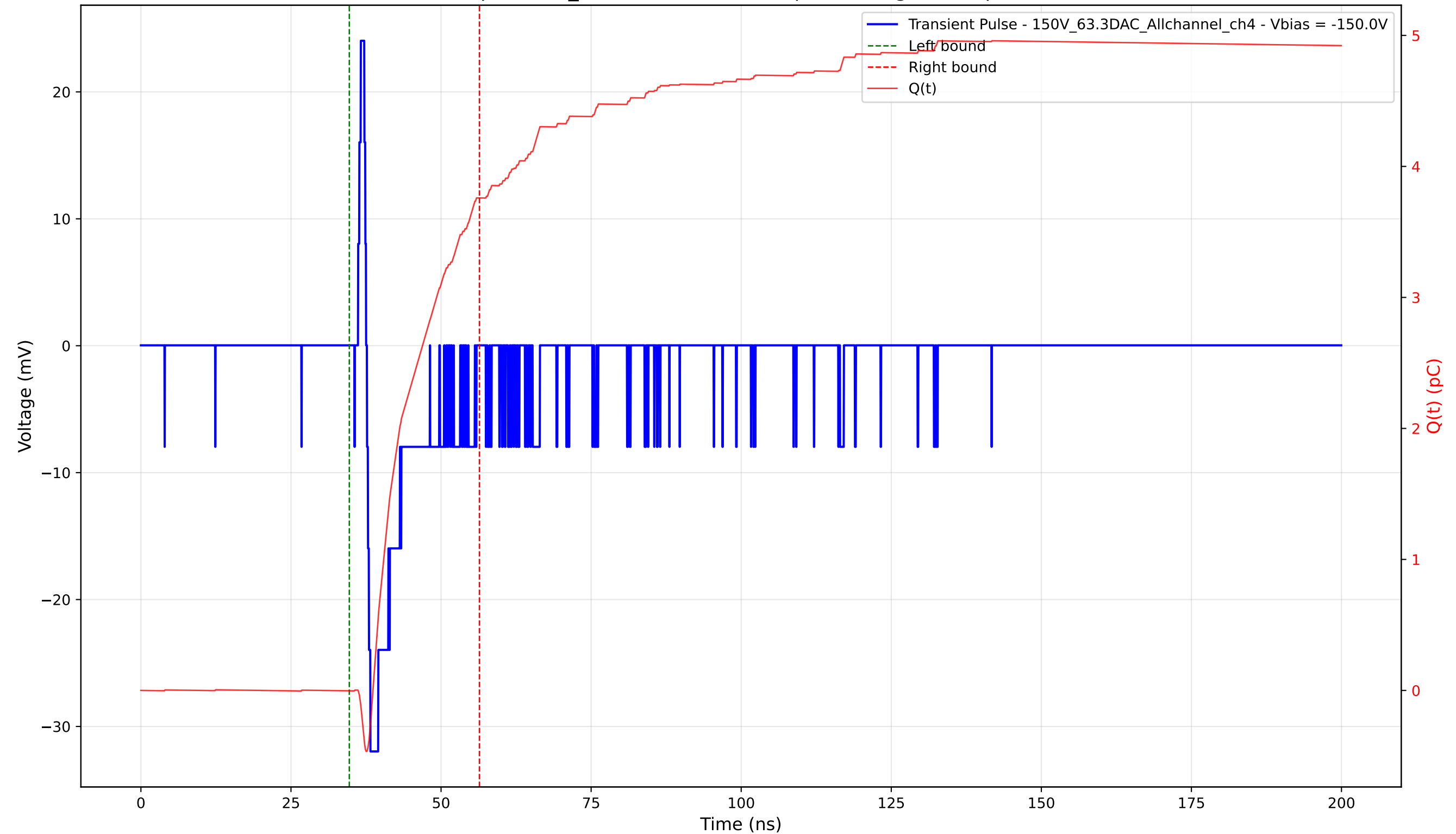
Transient Pulse - Sample: 1cm_42 - Position: 3840.0 \mu\text{m} - Charge: 3.76 pC - Rise Time: 0.58 ns
