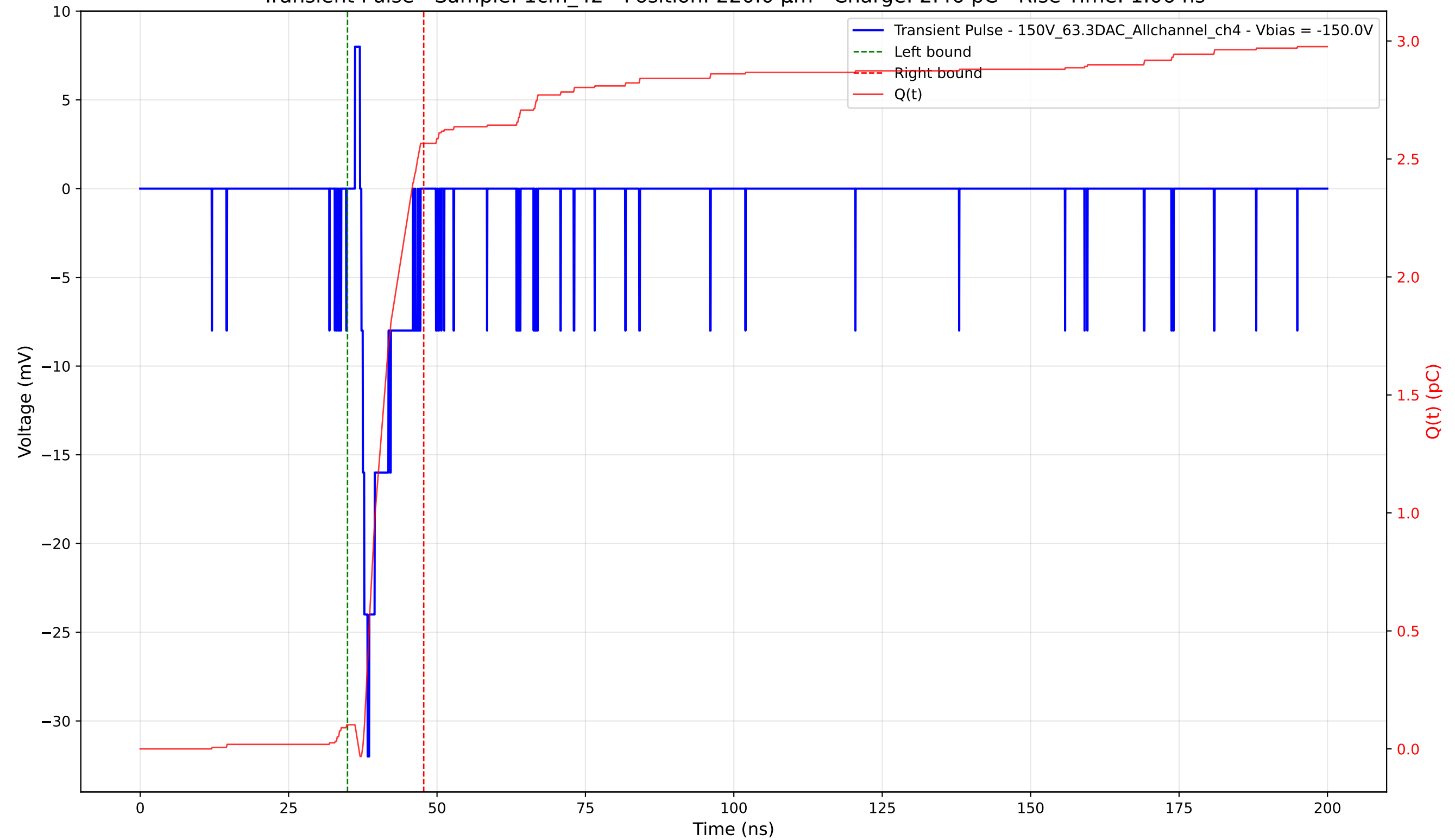
Transient Pulse - Sample: 1cm_42 - Position: 220.0 \mu\text{m} - Charge: 2.46 pC - Rise Time: 1.06 ns
