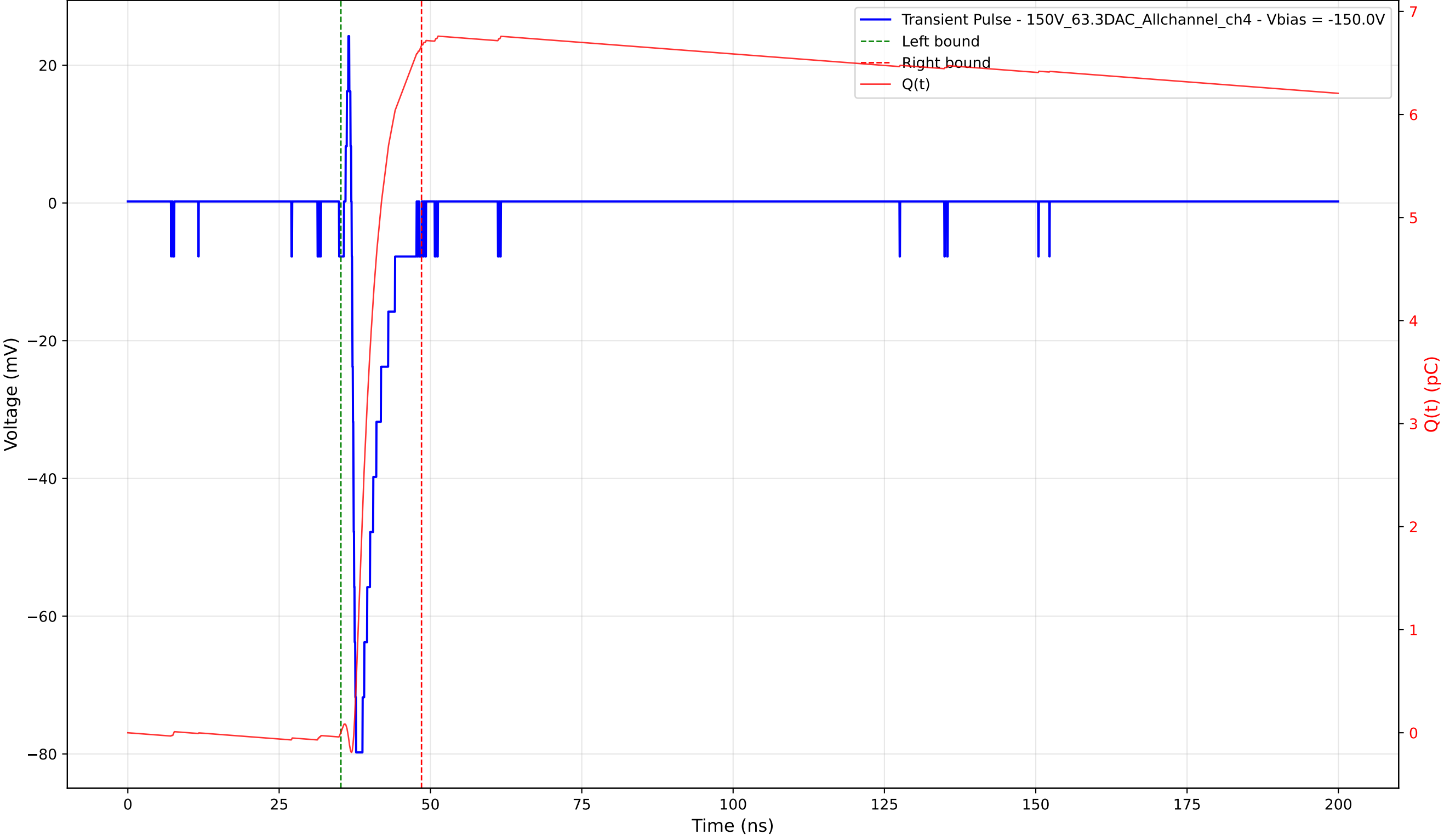
Transient Pulse - Sample: 1cm_42 - Position: 845.0 \mu\text{m} - Charge: 6.67 pC - Rise Time: 0.68 ns
