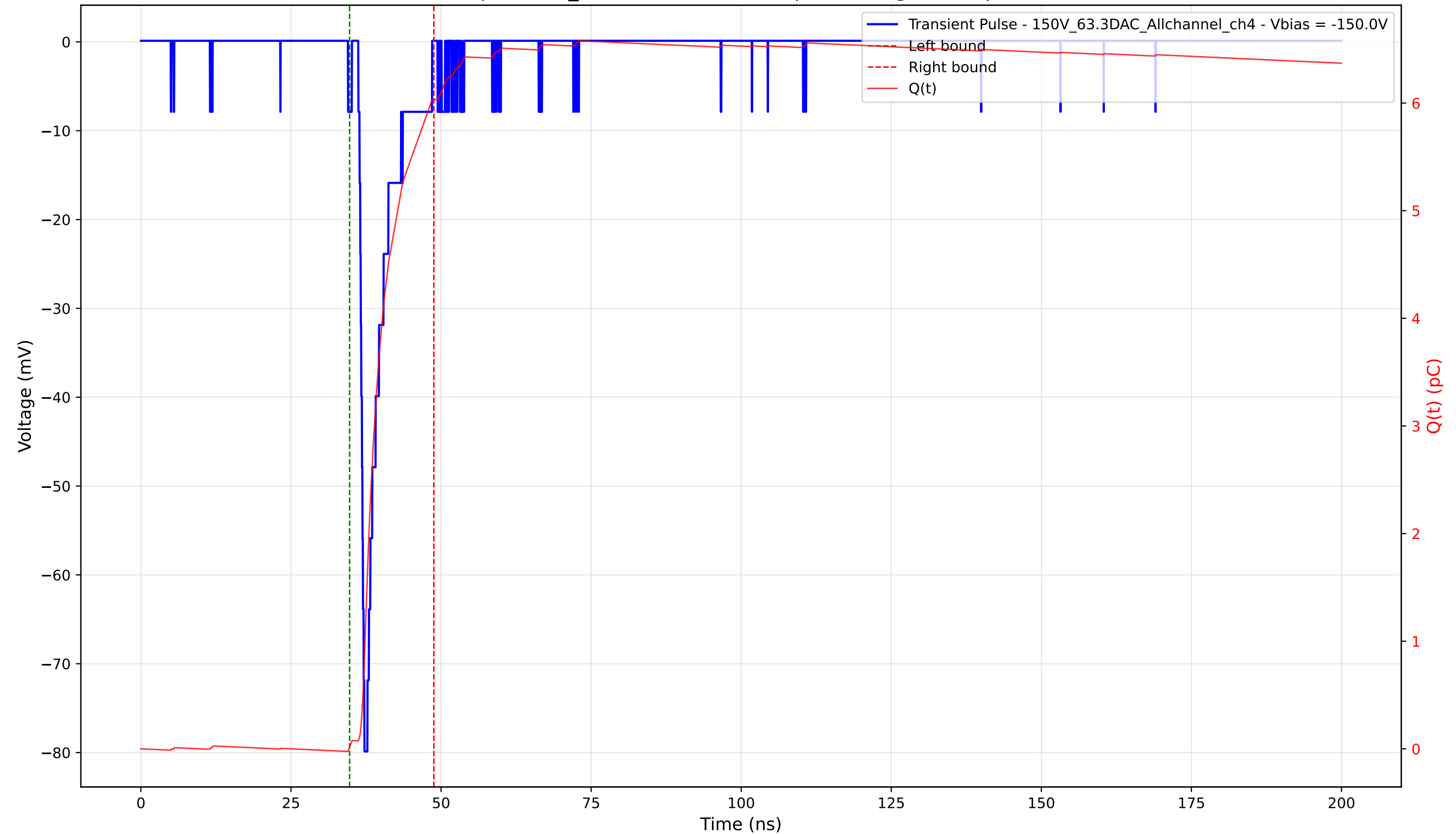
Transient Pulse - Sample: 1cm_42 - Position: 2955.0 \mu\text{m} - Charge: 6.02 pC - Rise Time: 0.84 ns
