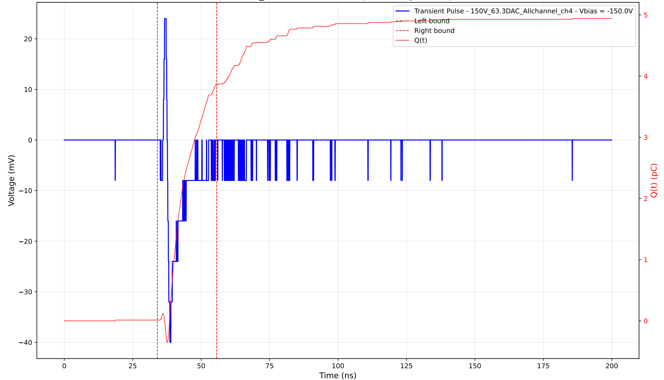
Transient Pulse - Sample: 1cm_42 - Position: 3815.0 \mu\text{m} - Charge: 3.85 pC - Rise Time: 0.90 ns
