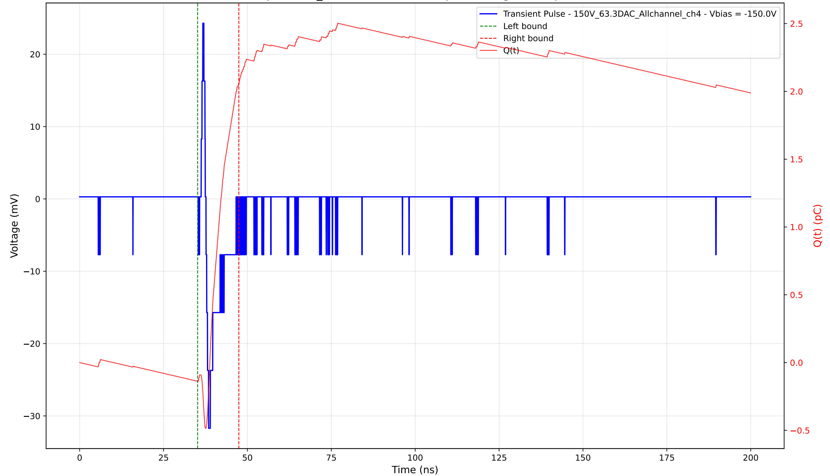
Transient Pulse - Sample: 1cm_42 - Position: 4570.0 \mu\text{m} - Charge: 2.20 pC - Rise Time: 0.78 ns
