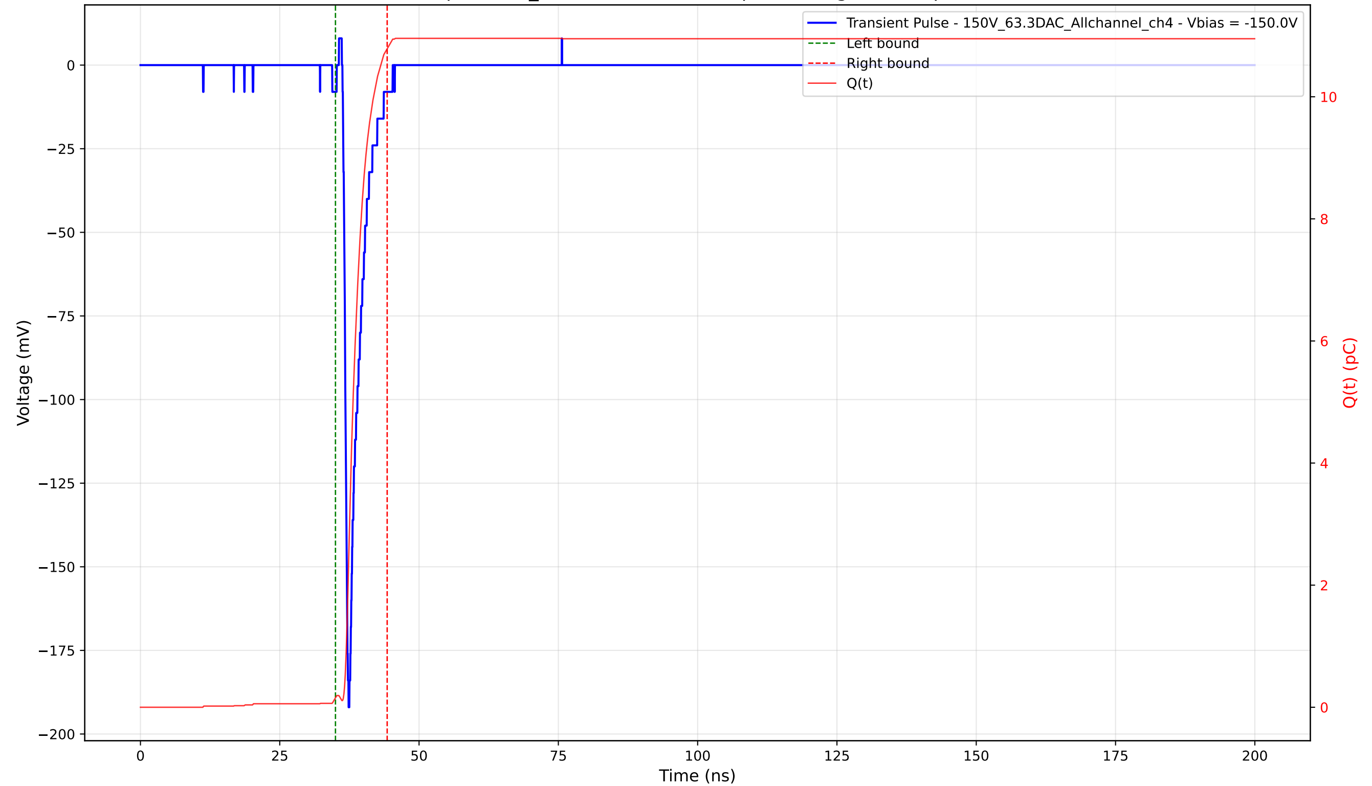
Transient Pulse - Sample: 1cm_42 - Position: 1340.0 \mu\text{m} - Charge: 10.63 pC - Rise Time: 0.78 ns
