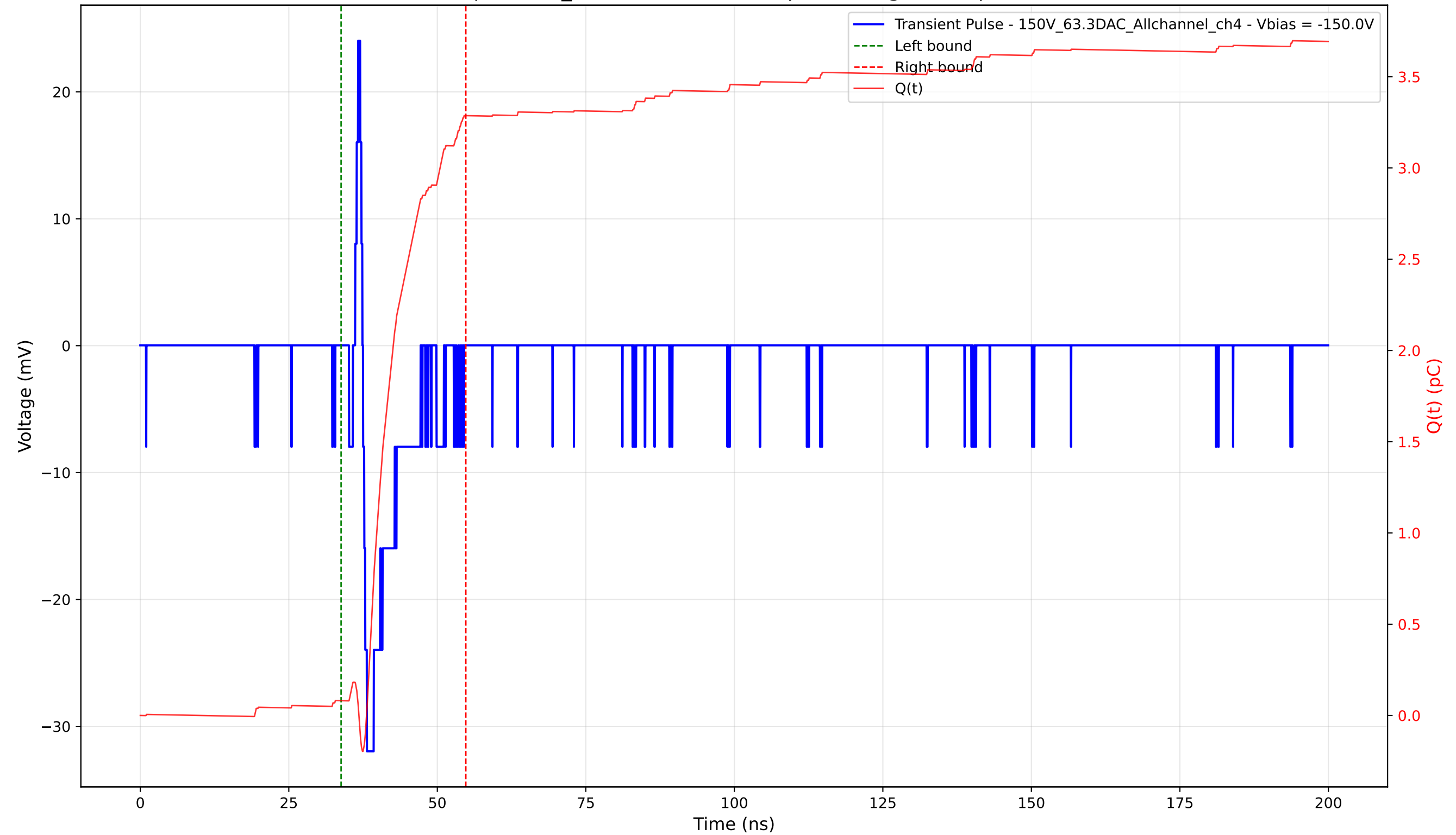
Transient Pulse - Sample: 1cm_42 - Position: 4750.0 \mu\text{m} - Charge: 3.21 pC - Rise Time: 0.66 ns
