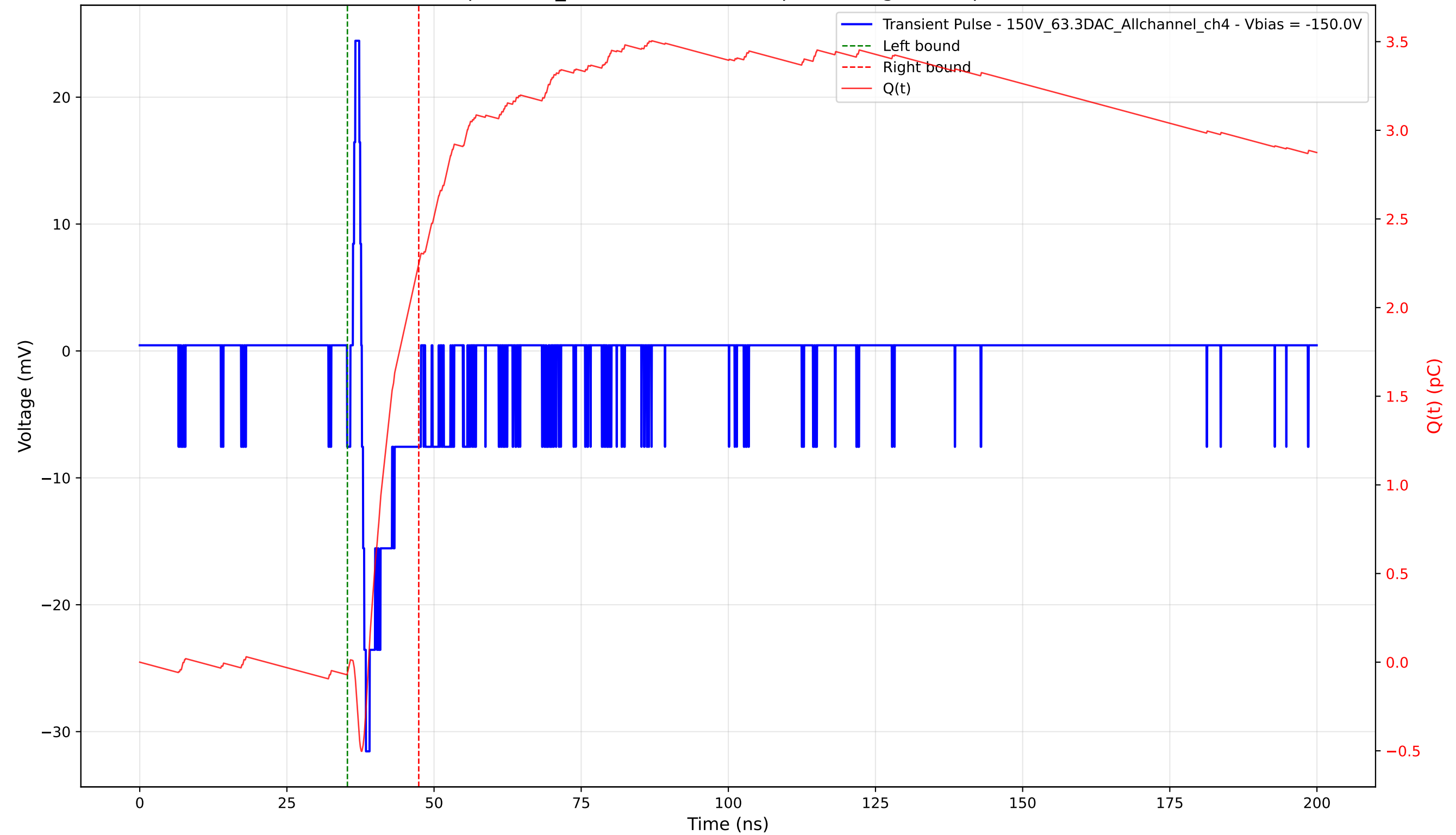
Transient Pulse - Sample: 1cm_42 - Position: 4120.0 \mu\text{m} - Charge: 2.31 pC - Rise Time: 0.70 ns
