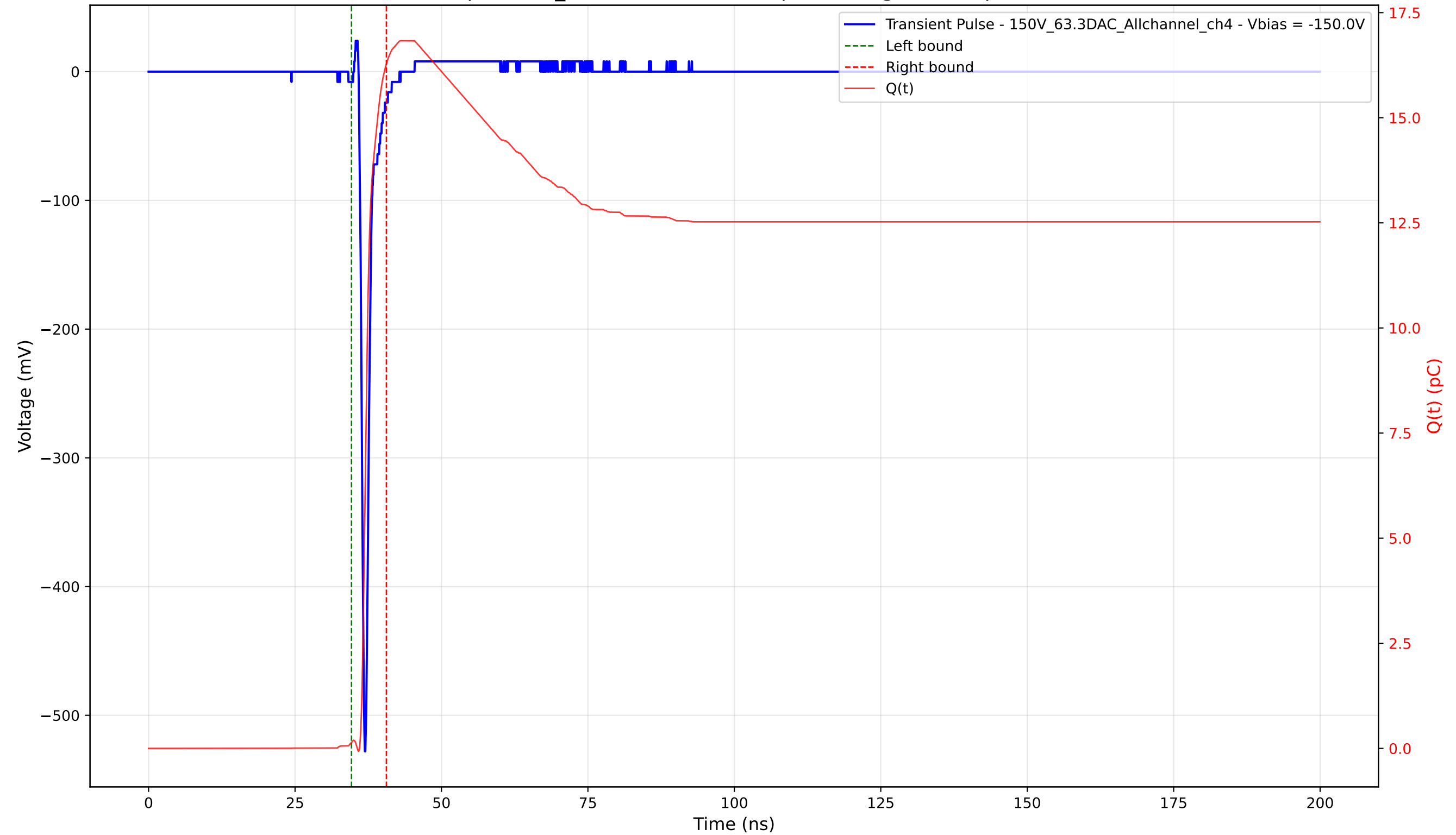
Transient Pulse - Sample: 1cm_42 - Position: 2170.0 \mu\text{m} - Charge: 16.14 pC - Rise Time: 0.72 ns
