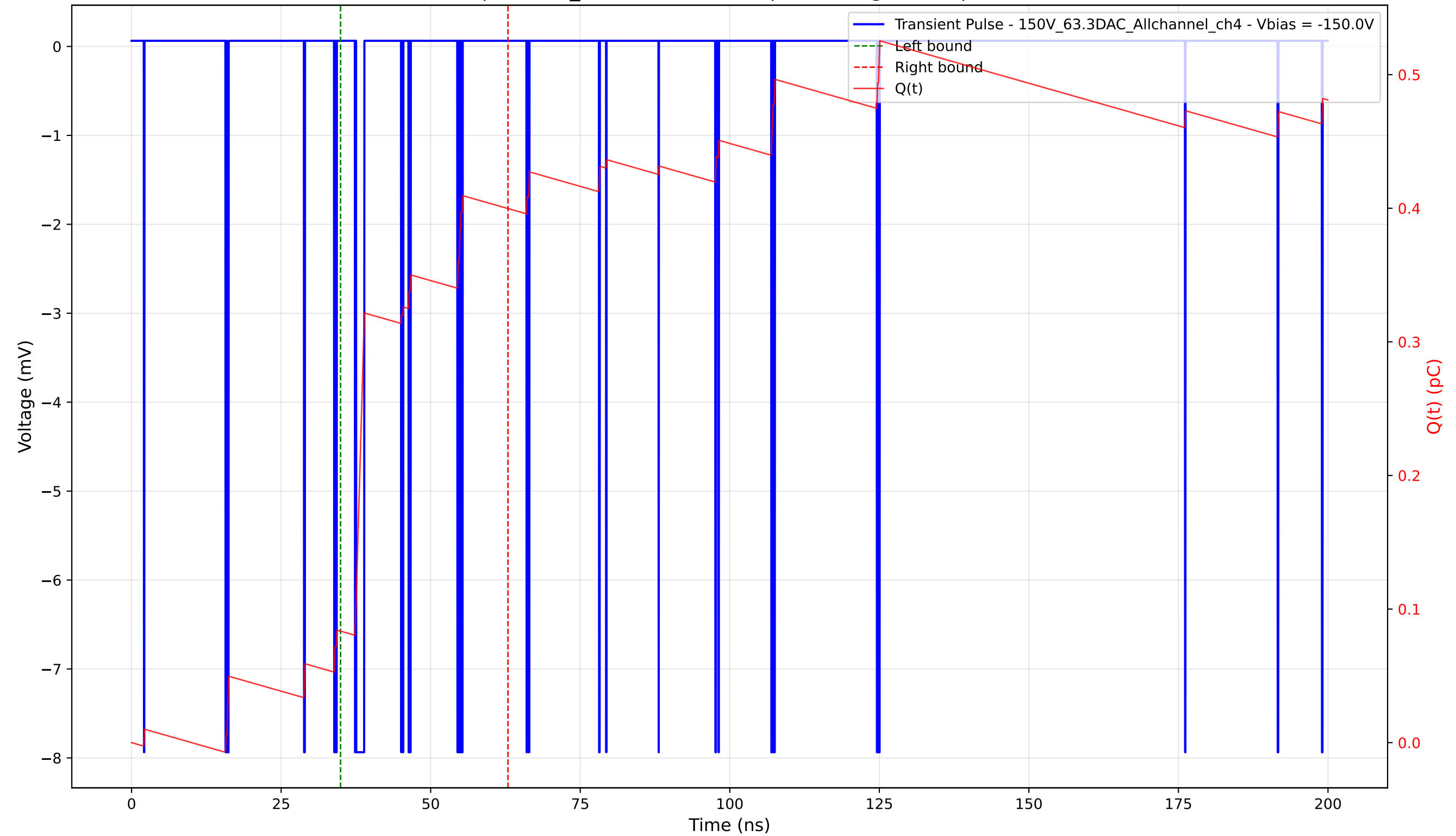
Transient Pulse - Sample: 1cm_42 - Position: 10.0 \mu\text{m} - Charge: 0.32 pC - Rise Time: 0.04 ns
