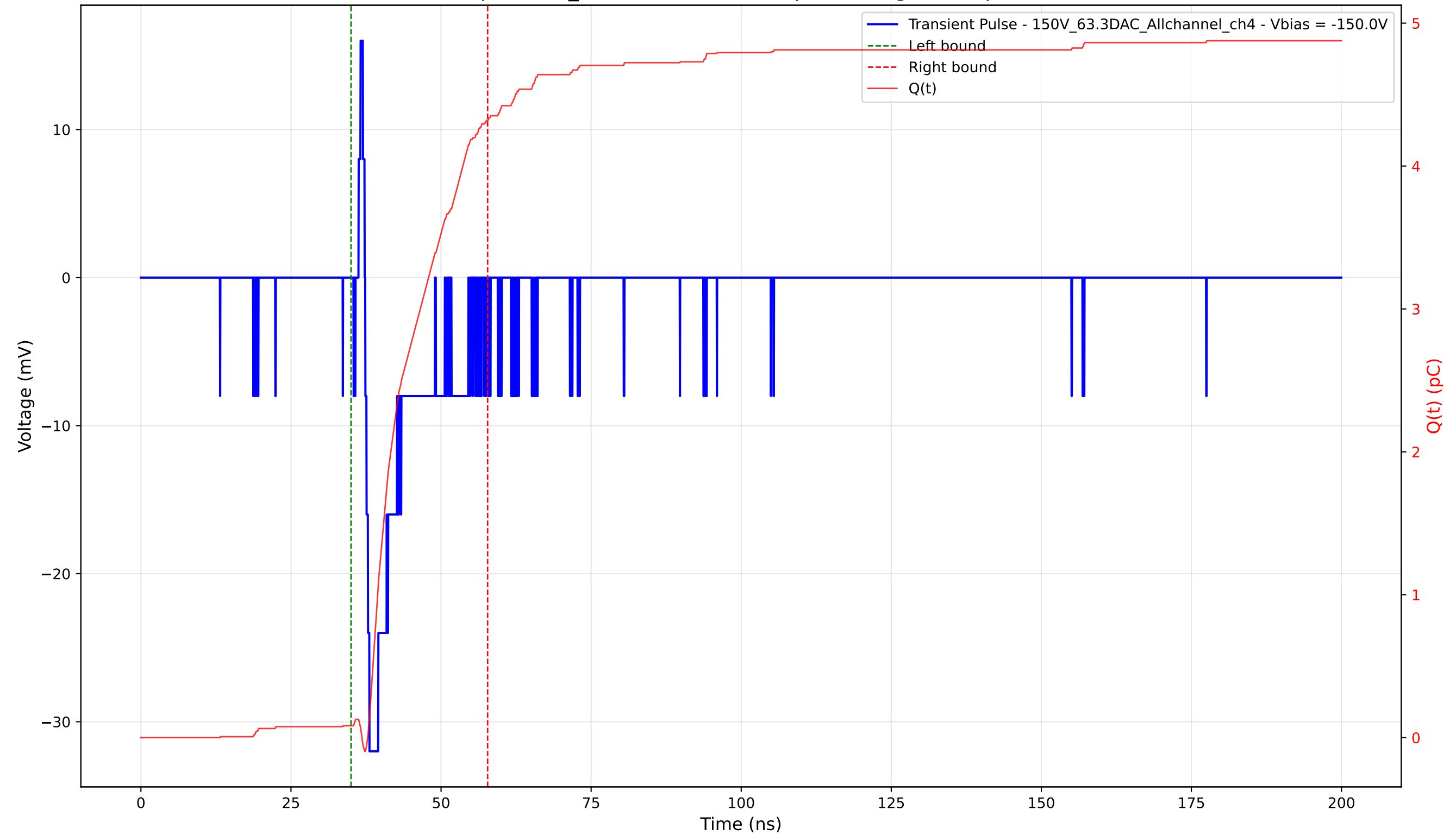
Transient Pulse - Sample: 1cm_42 - Position: 3515.0 \mu\text{m} - Charge: 4.24 pC - Rise Time: 0.70 ns
