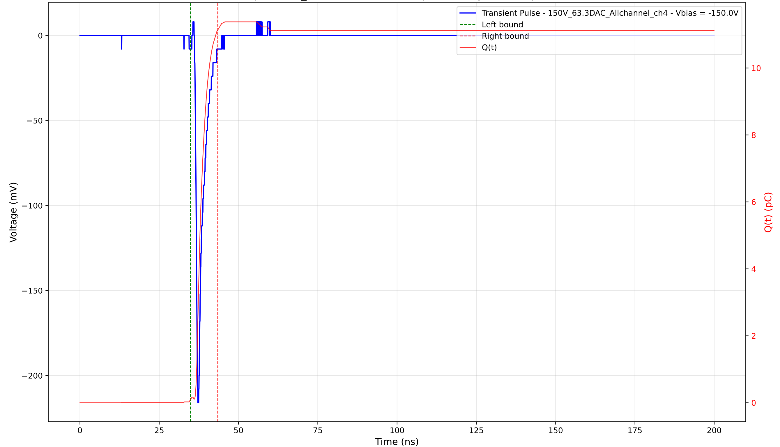
Transient Pulse - Sample: 1cm_42 - Position: 1425.0 \mu\text{m} - Charge: 11.05 pC - Rise Time: 0.78 ns
