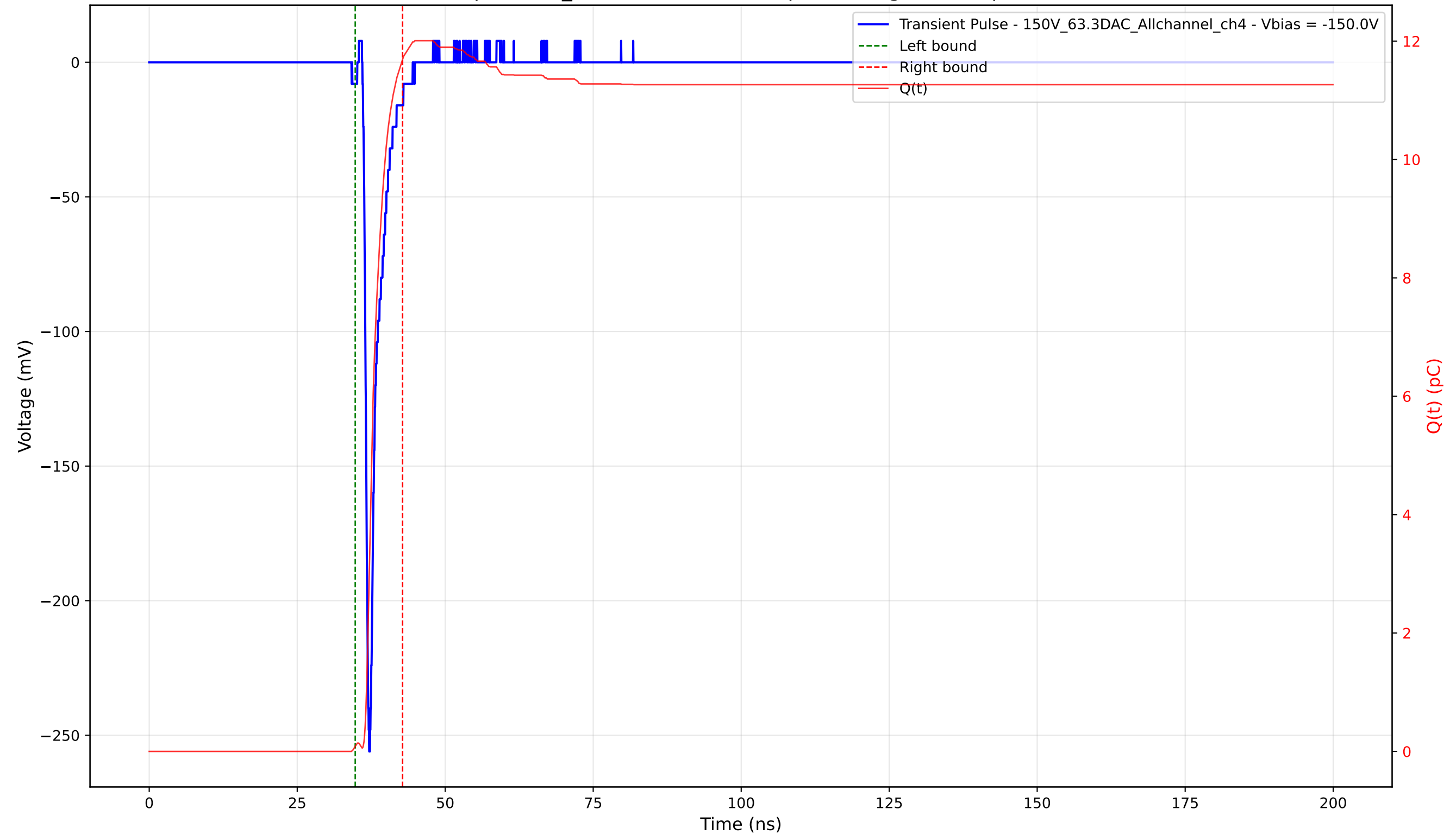
Transient Pulse - Sample: 1cm_42 - Position: 1495.0 \mu\text{m} - Charge: 11.61 pC - Rise Time: 0.74 ns
