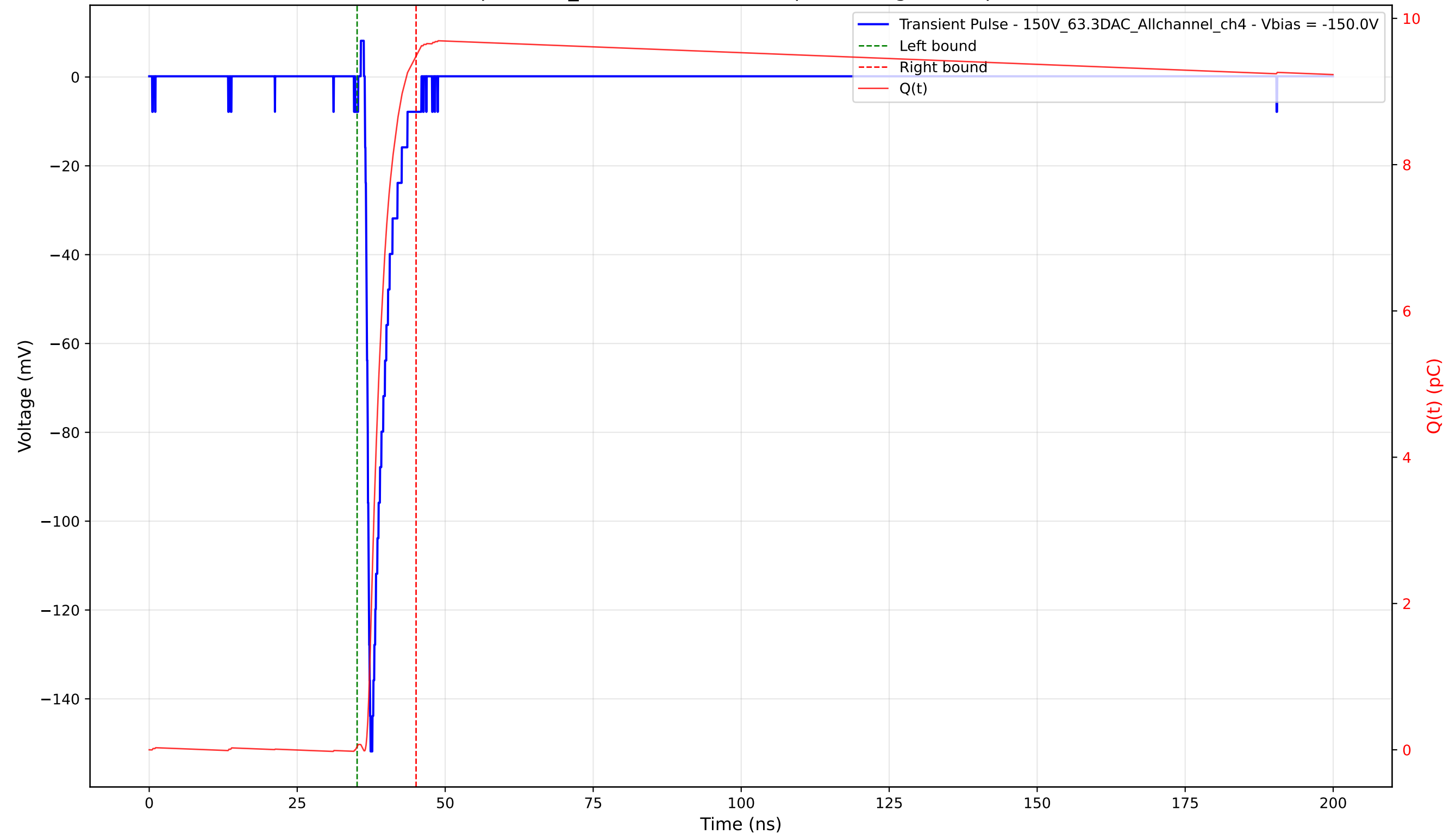
Transient Pulse - Sample: 1cm_42 - Position: 1165.0 \mu\text{m} - Charge: 9.44 pC - Rise Time: 0.84 ns
