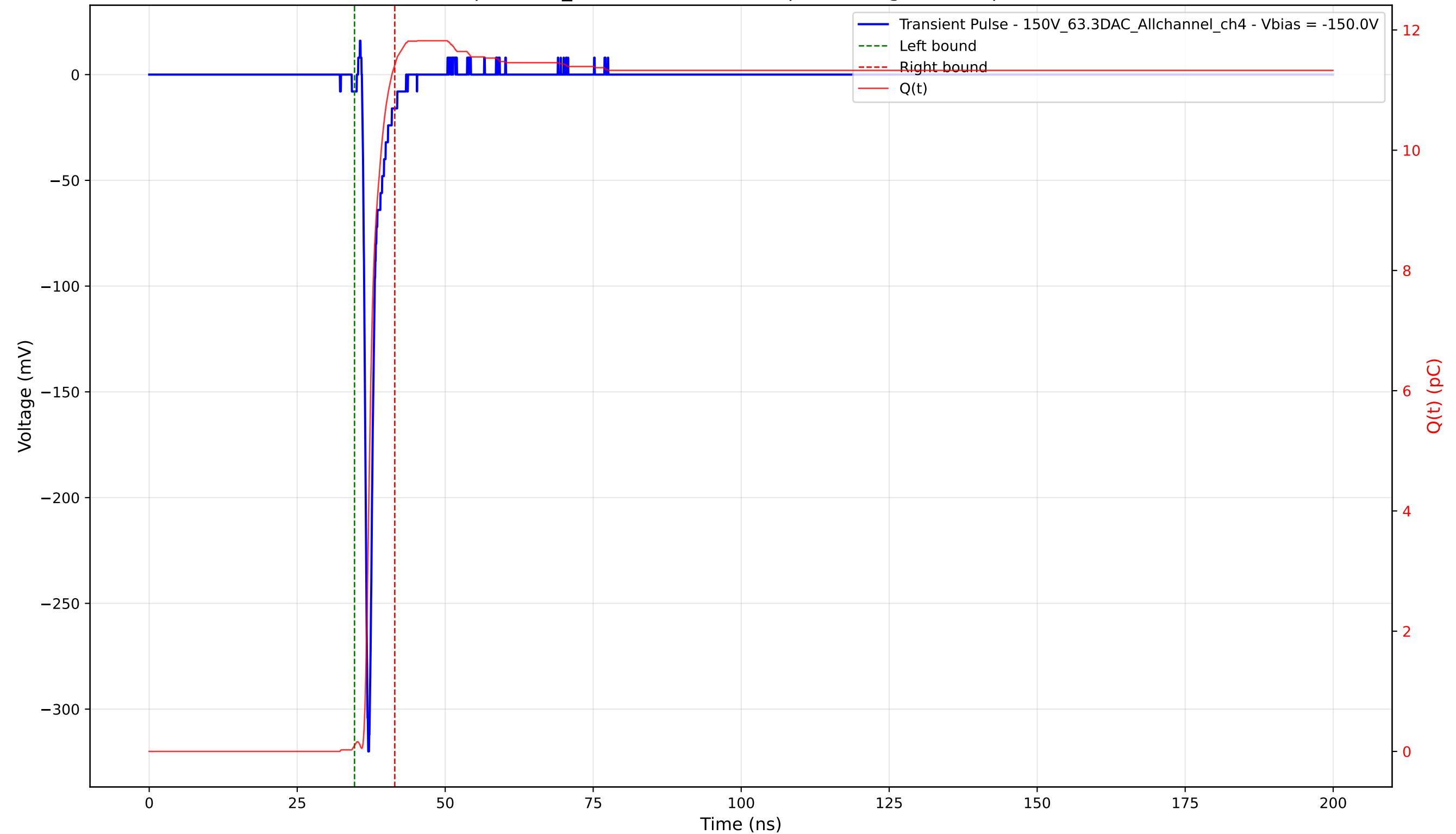
Transient Pulse - Sample: 1cm_42 - Position: 2435.0 \mu\text{m} - Charge: 11.32 pC - Rise Time: 0.72 ns
