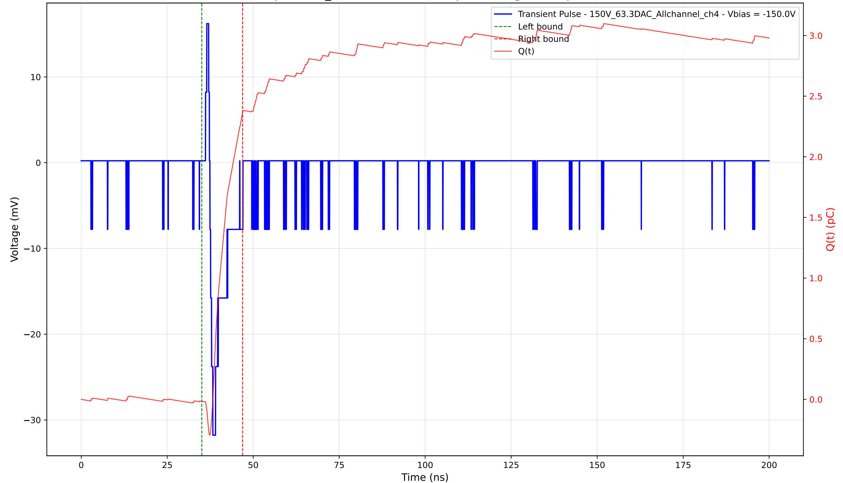
Transient Pulse - Sample: 1cm_42 - Position: 4920.0 \mu\text{m} - Charge: 2.38 pC - Rise Time: 0.86 ns
