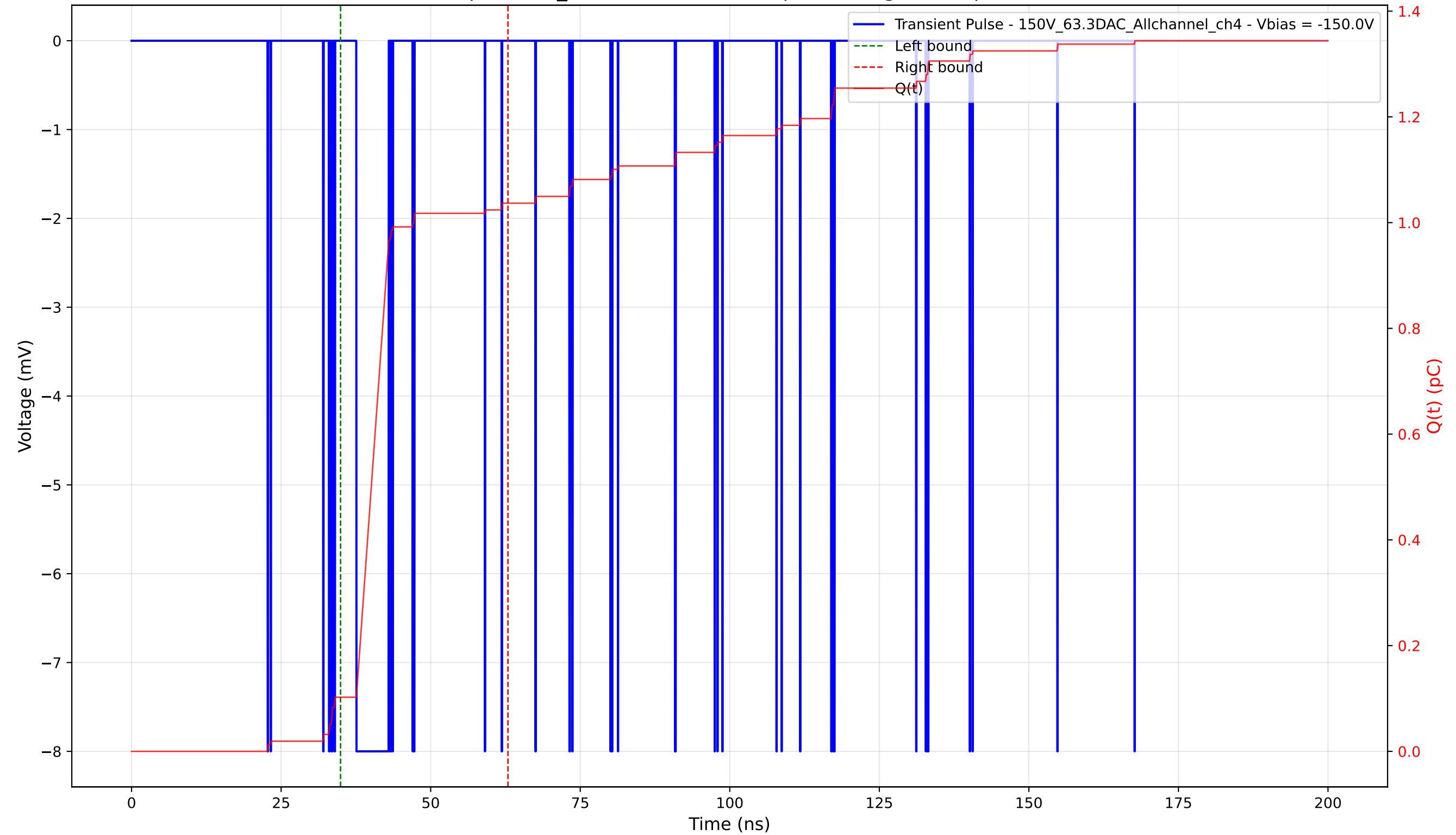
Transient Pulse - Sample: 1cm_42 - Position: 5135.0 \mu\text{m} - Charge: 0.93 pC - Rise Time: 0.04 ns
