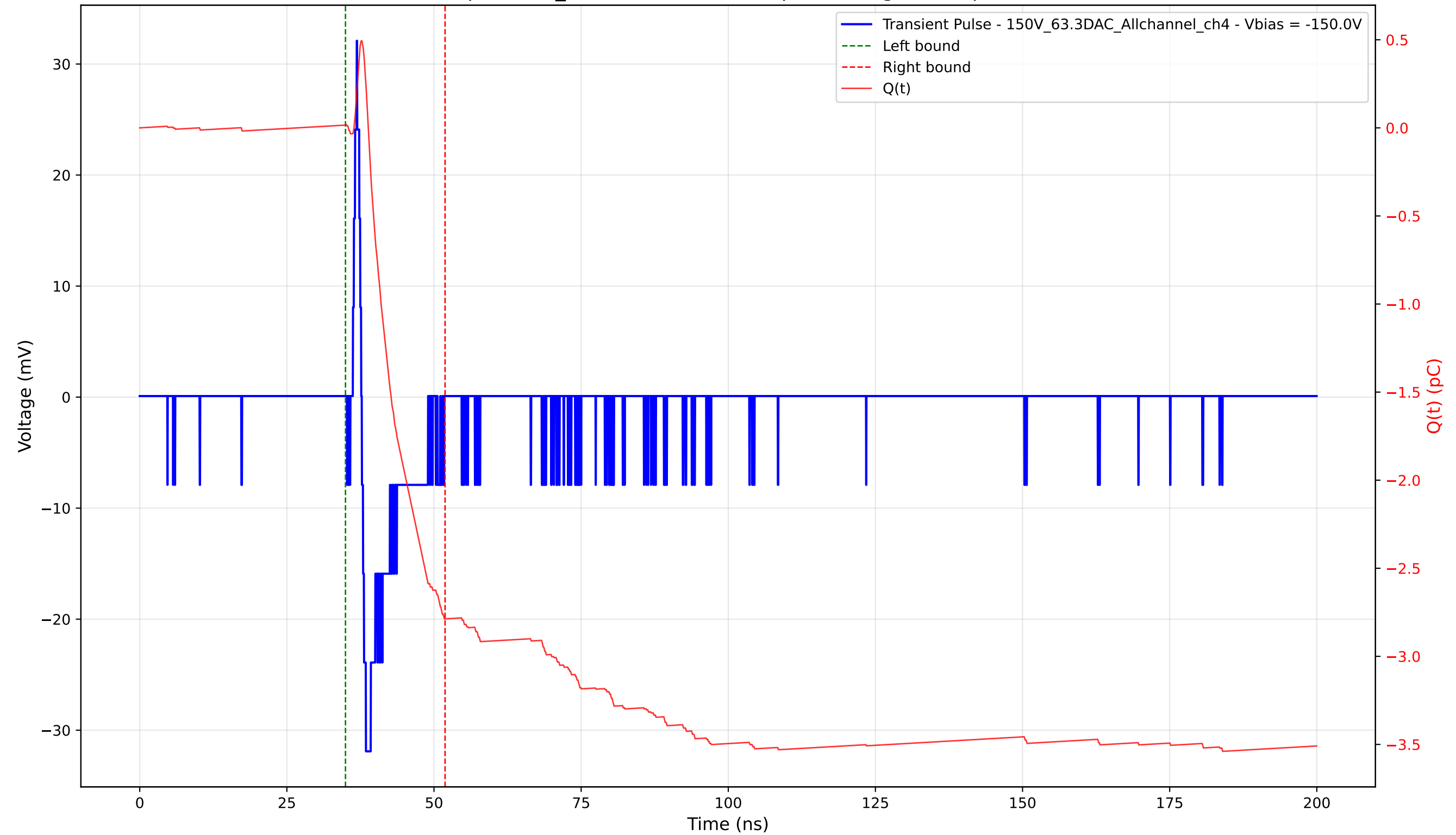
Transient Pulse - Sample: 1cm_42 - Position: 4190.0 \mu\text{m} - Charge: 2.80 pC - Rise Time: 0.66 ns
