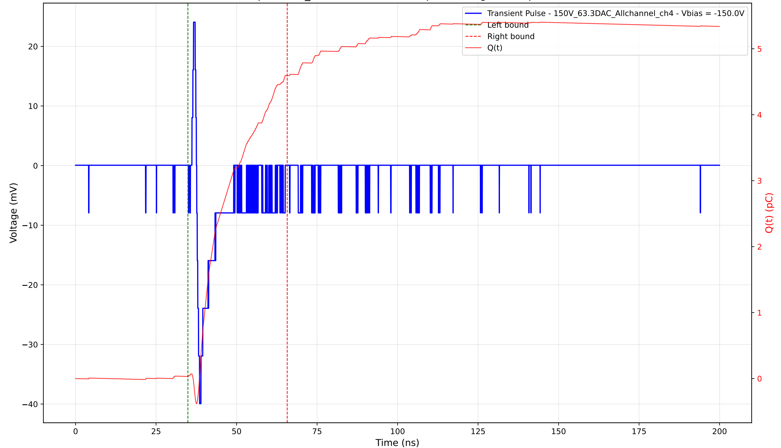
Transient Pulse - Sample: 1cm_42 - Position: 3700.0 \mu\text{m} - Charge: 4.56 pC - Rise Time: 0.90 ns
