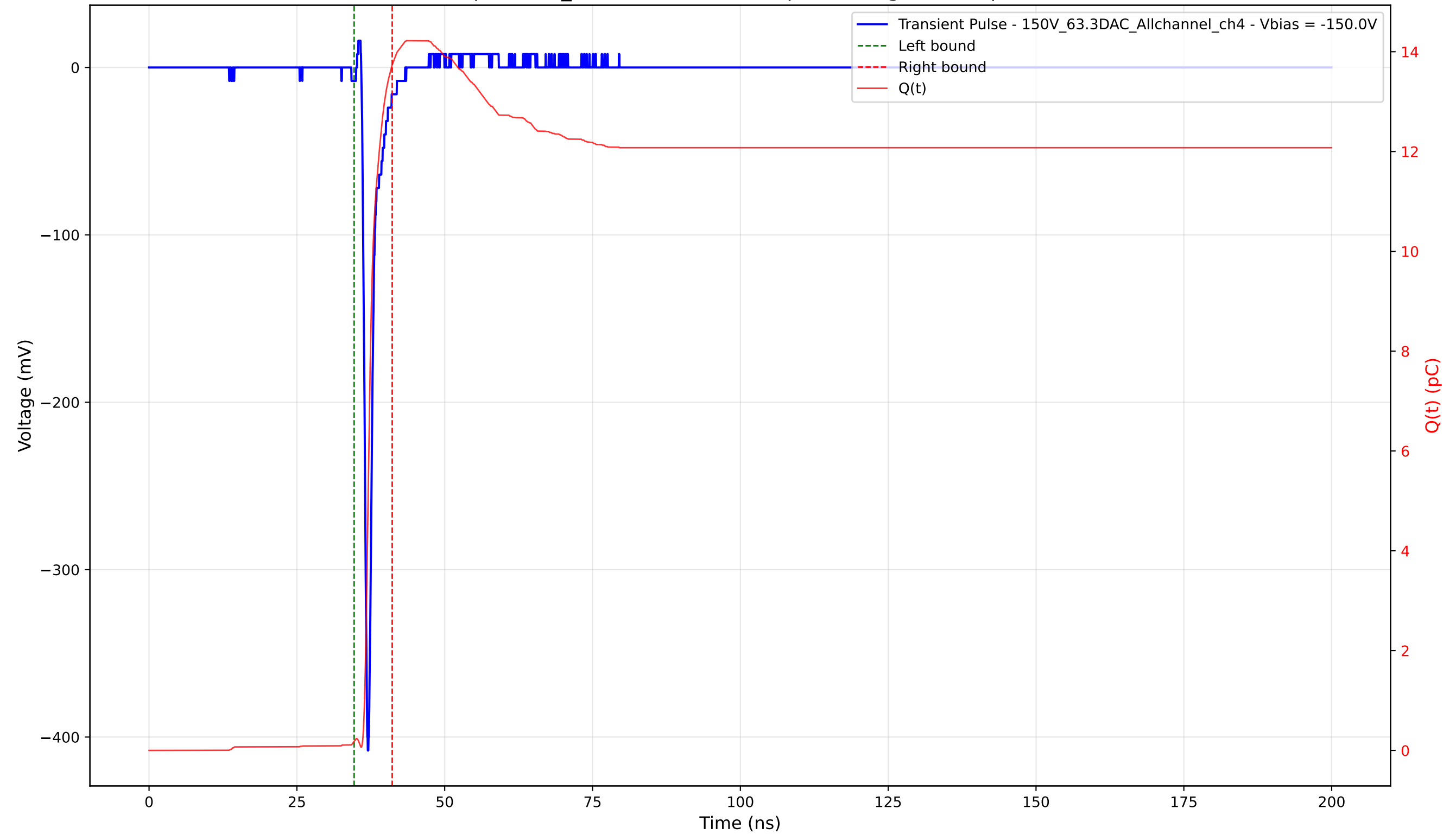
Transient Pulse - Sample: 1cm_42 - Position: 2365.0 \mu\text{m} - Charge: 13.55 pC - Rise Time: 0.74 ns
