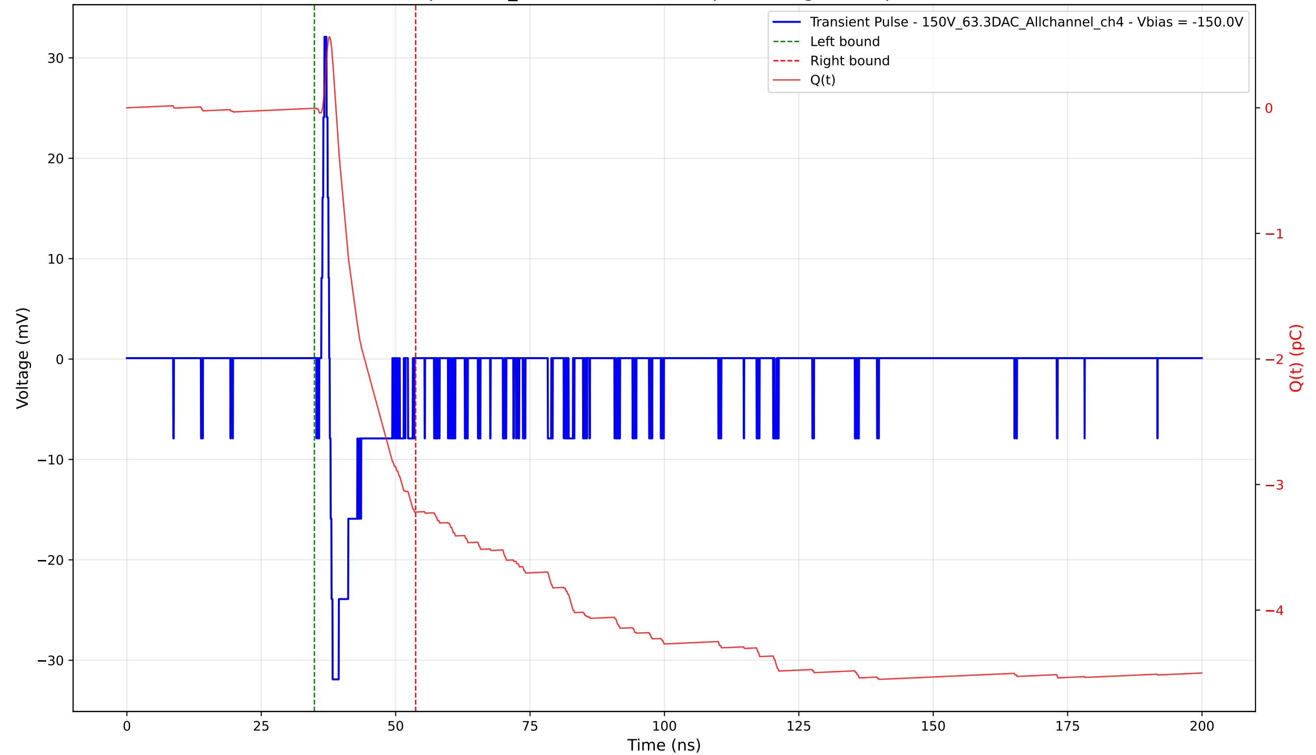
Transient Pulse - Sample: 1cm_42 - Position: 4270.0 \mu\text{m} - Charge: 3.22 pC - Rise Time: 0.58 ns
