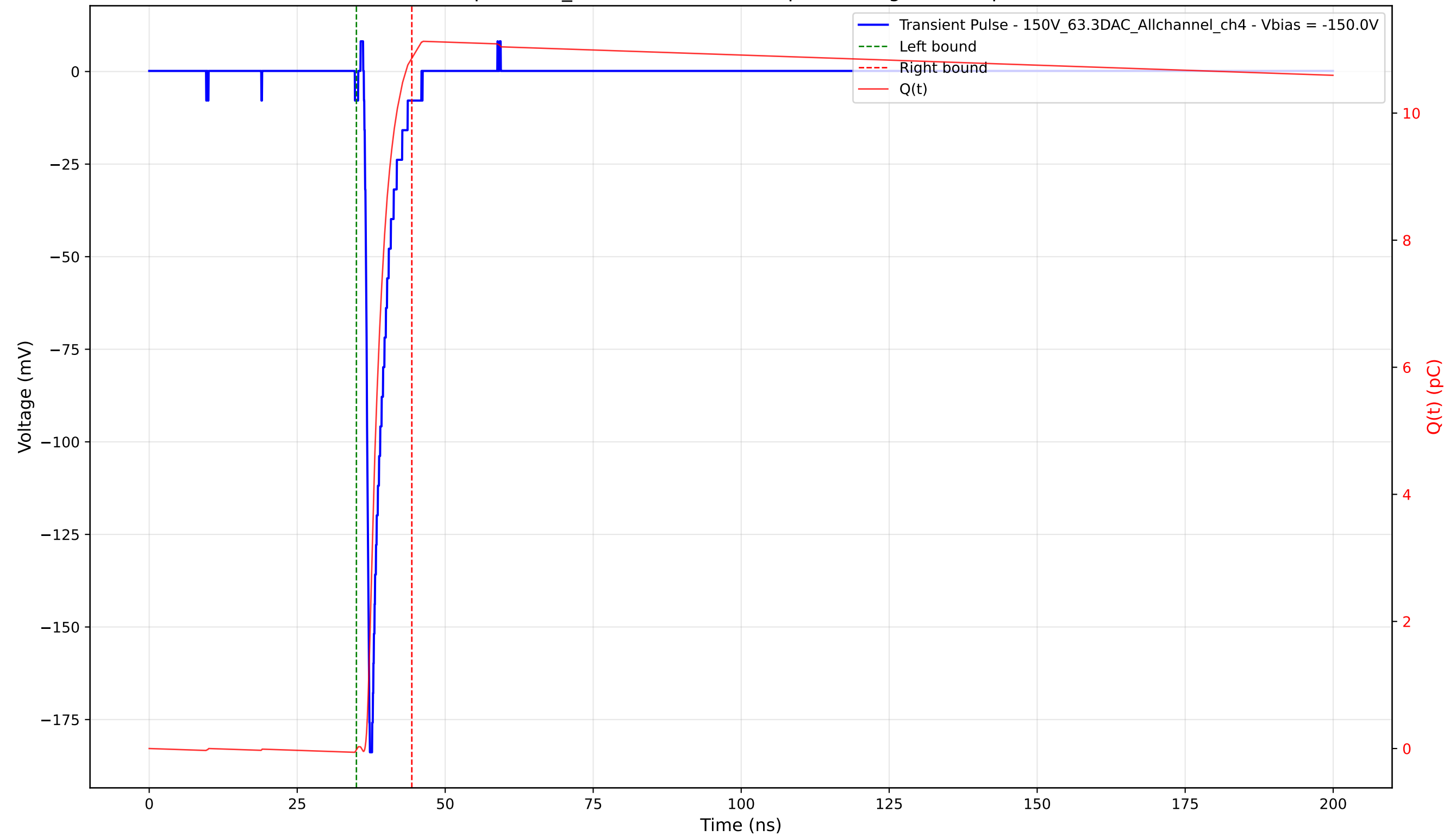
Transient Pulse - Sample: 1cm_42 - Position: 1285.0 \mu\text{m} - Charge: 10.88 pC - Rise Time: 0.74 ns
