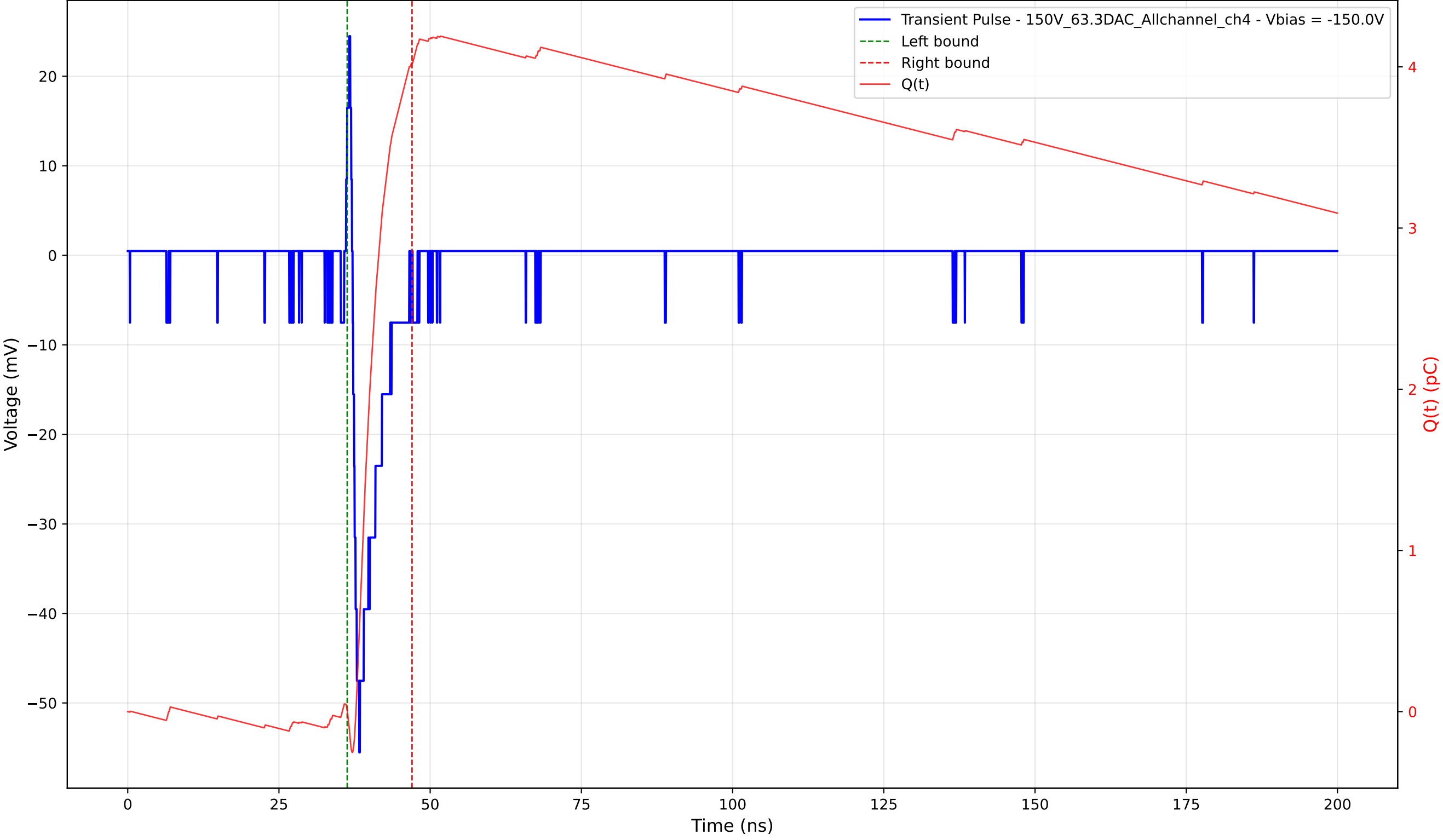
Transient Pulse - Sample: 1cm_42 - Position: 485.0 \mu\text{m} - Charge: 4.01 pC - Rise Time: 1.09 ns
