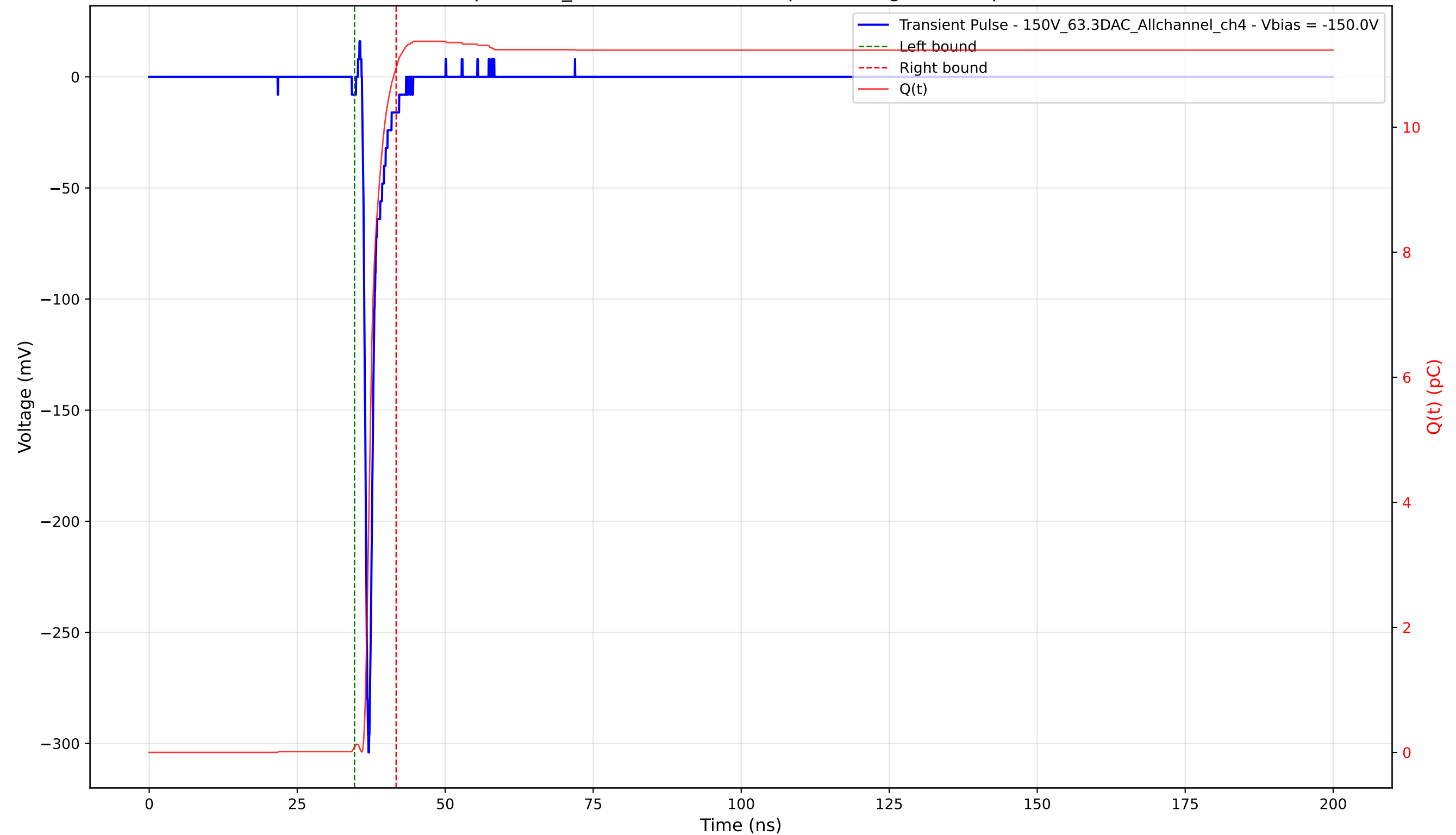
Transient Pulse - Sample: 1cm_42 - Position: 2450.0 \mu\text{m} - Charge: 10.86 pC - Rise Time: 0.77 ns
