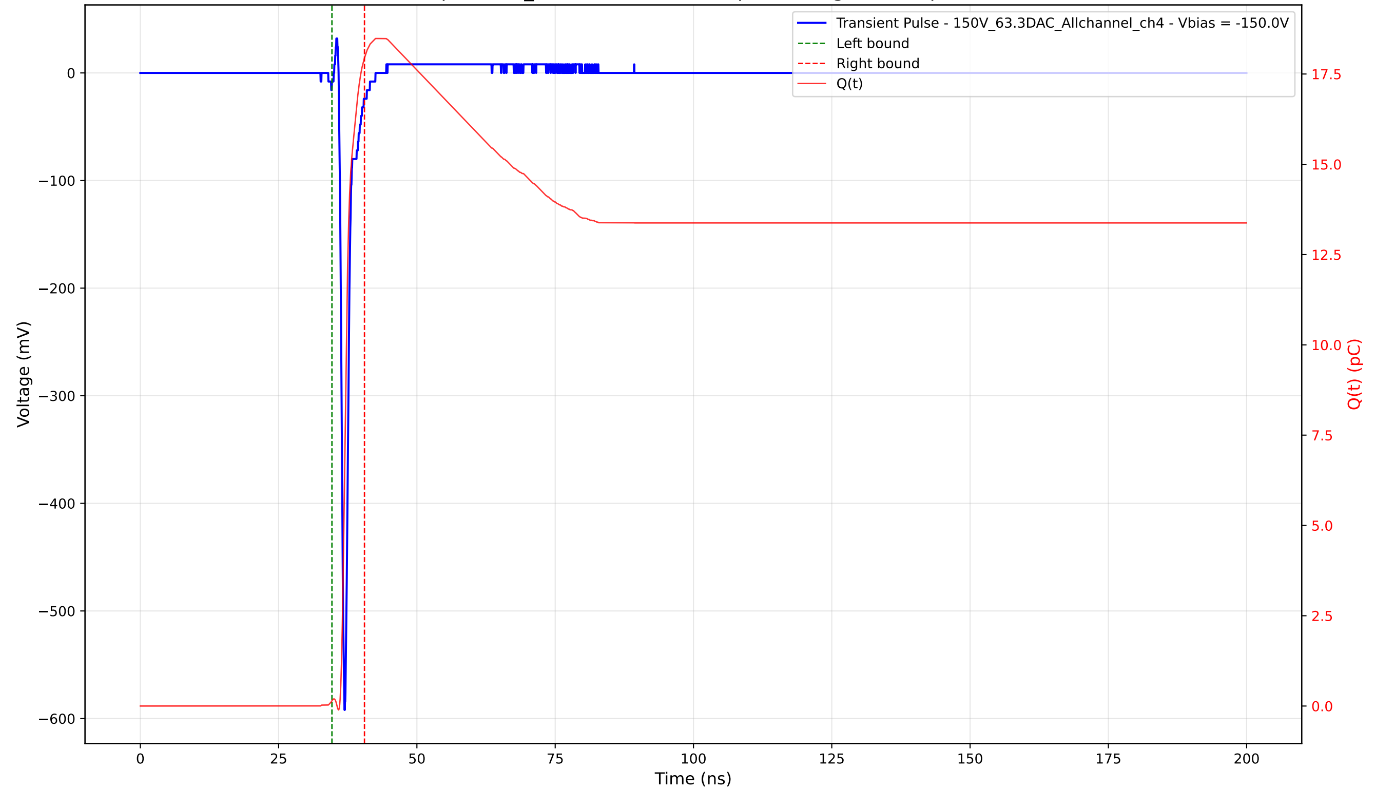
Transient Pulse - Sample: 1cm_42 - Position: 2010.0 \mu\text{m} - Charge: 17.79 pC - Rise Time: 0.71 ns
