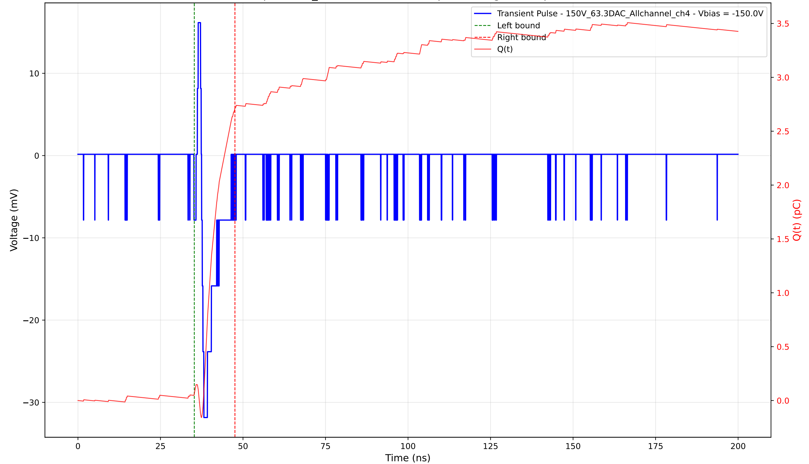
Transient Pulse - Sample: 1cm_42 - Position: 4875.0 \mu\text{m} - Charge: 2.65 pC - Rise Time: 0.70 ns
