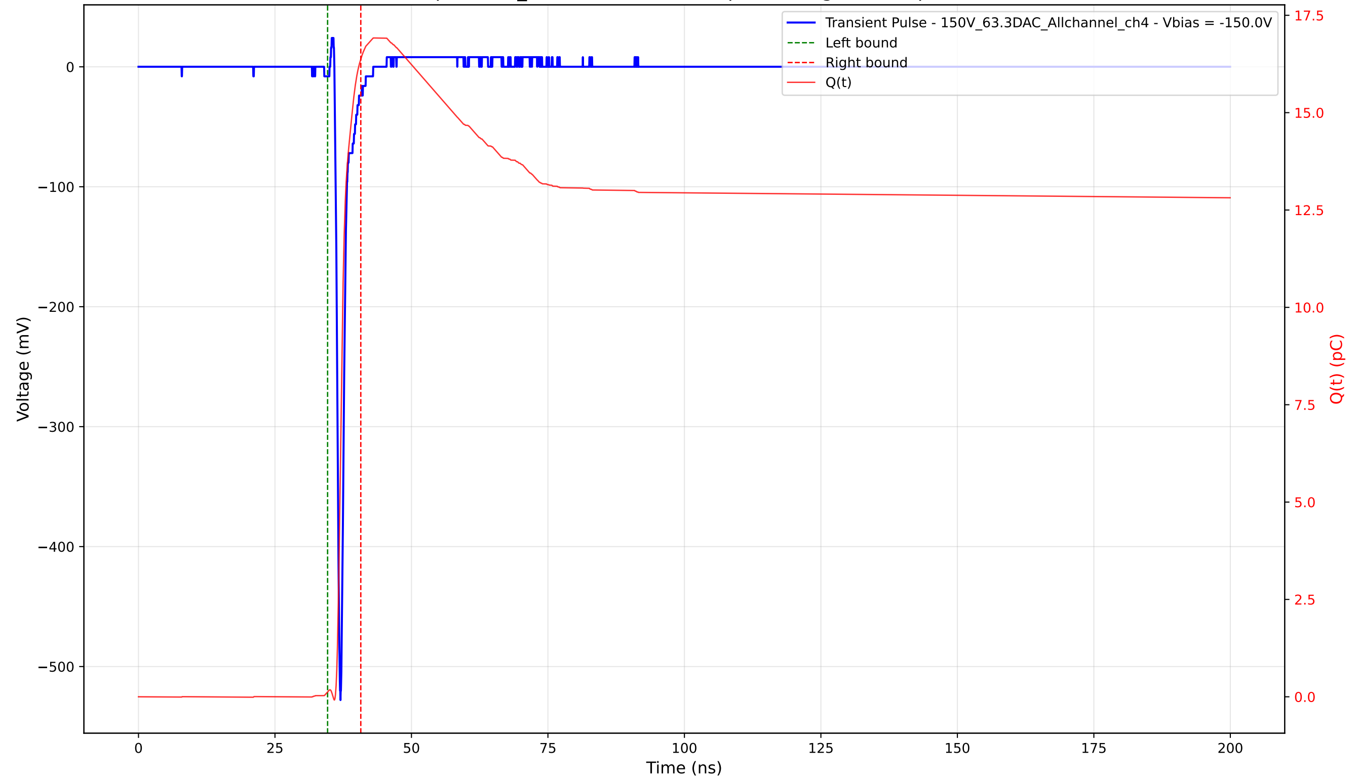
Transient Pulse - Sample: 1cm_42 - Position: 2205.0 \mu\text{m} - Charge: 16.25 pC - Rise Time: 0.74 ns
