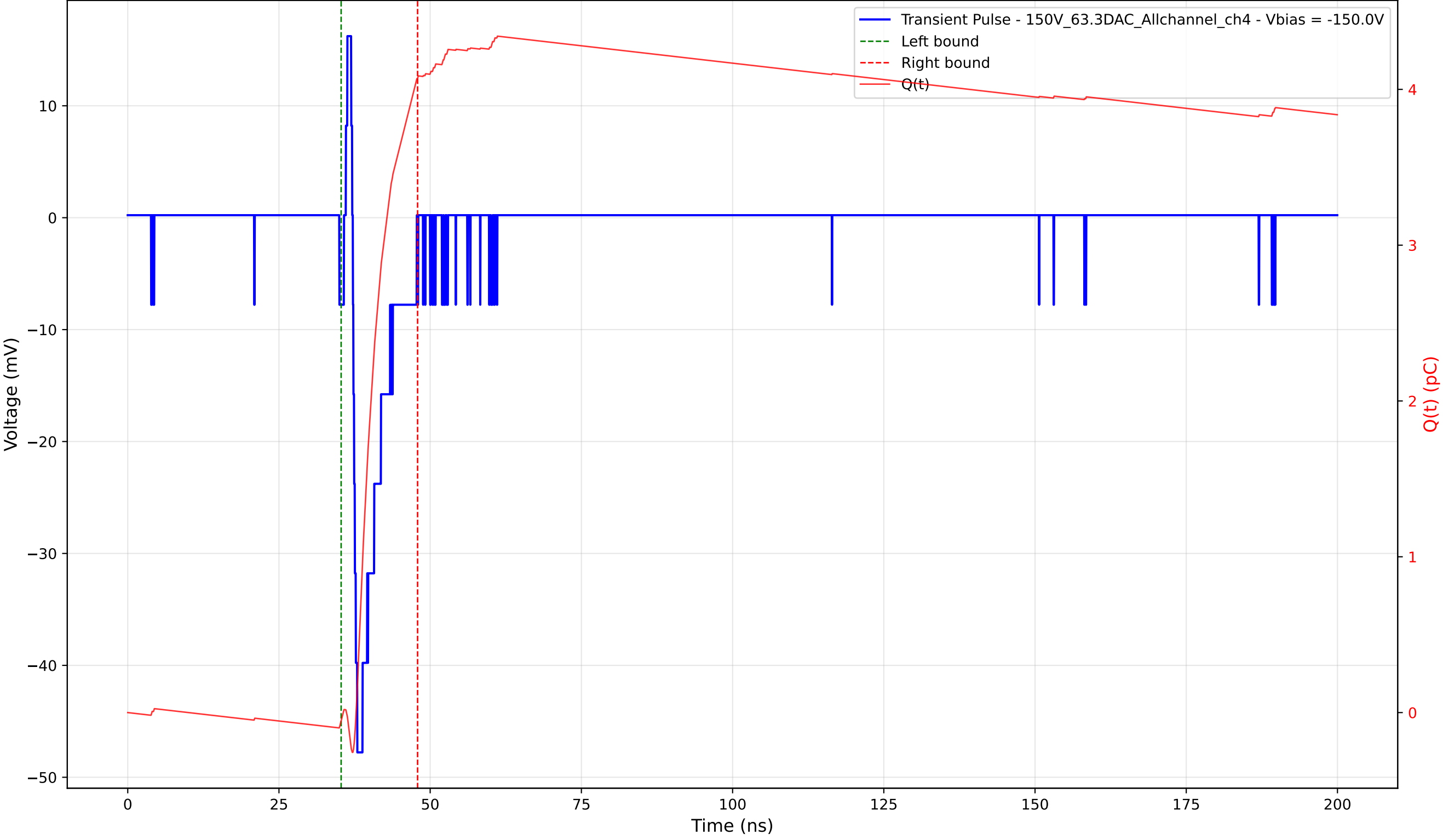
Transient Pulse - Sample: 1cm_42 - Position: 455.0 \mu\text{m} - Charge: 4.12 pC - Rise Time: 0.74 ns
