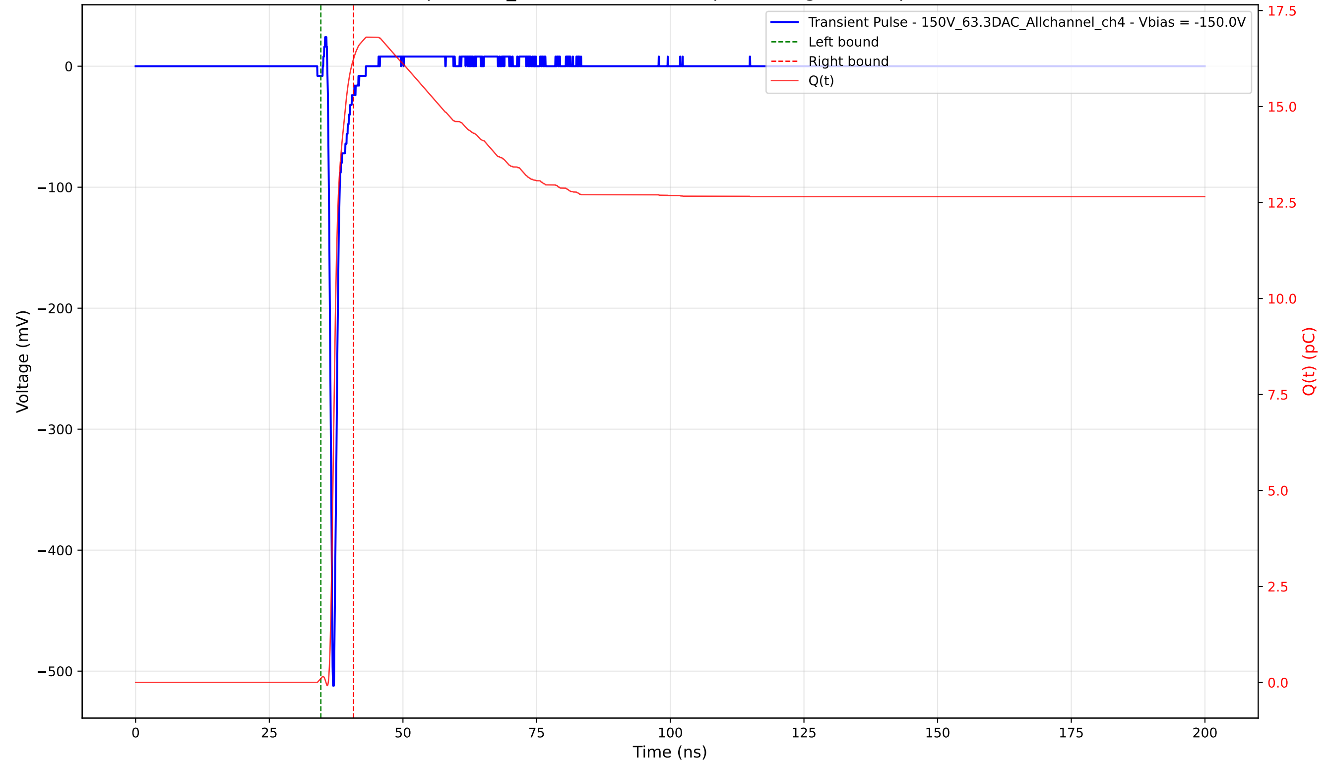
Transient Pulse - Sample: 1cm_42 - Position: 2230.0 \mu\text{m} - Charge: 16.14 pC - Rise Time: 0.71 ns
