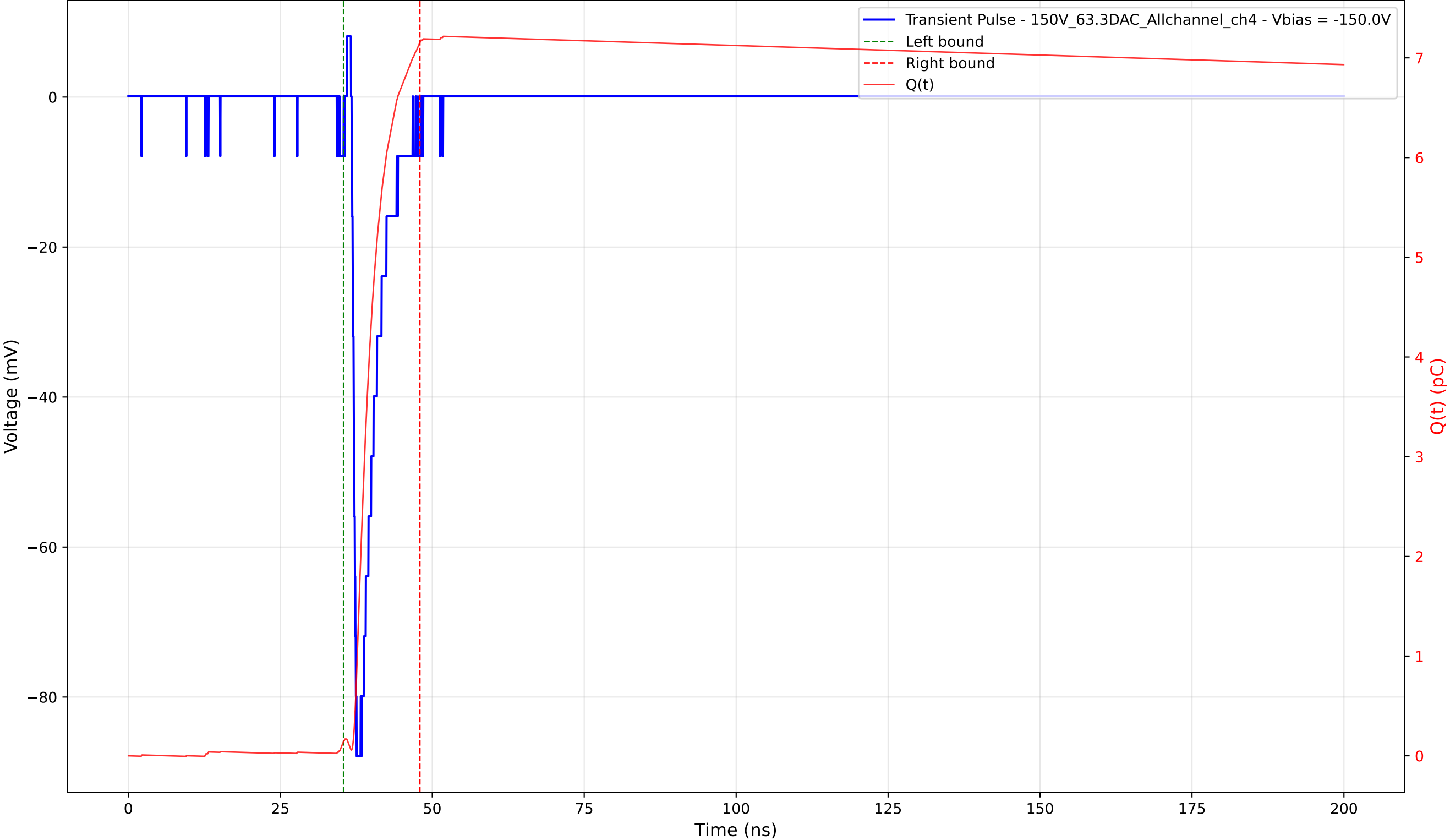
Transient Pulse - Sample: 1cm_42 - Position: 970.0 \mu\text{m} - Charge: 7.01 pC - Rise Time: 0.64 ns
