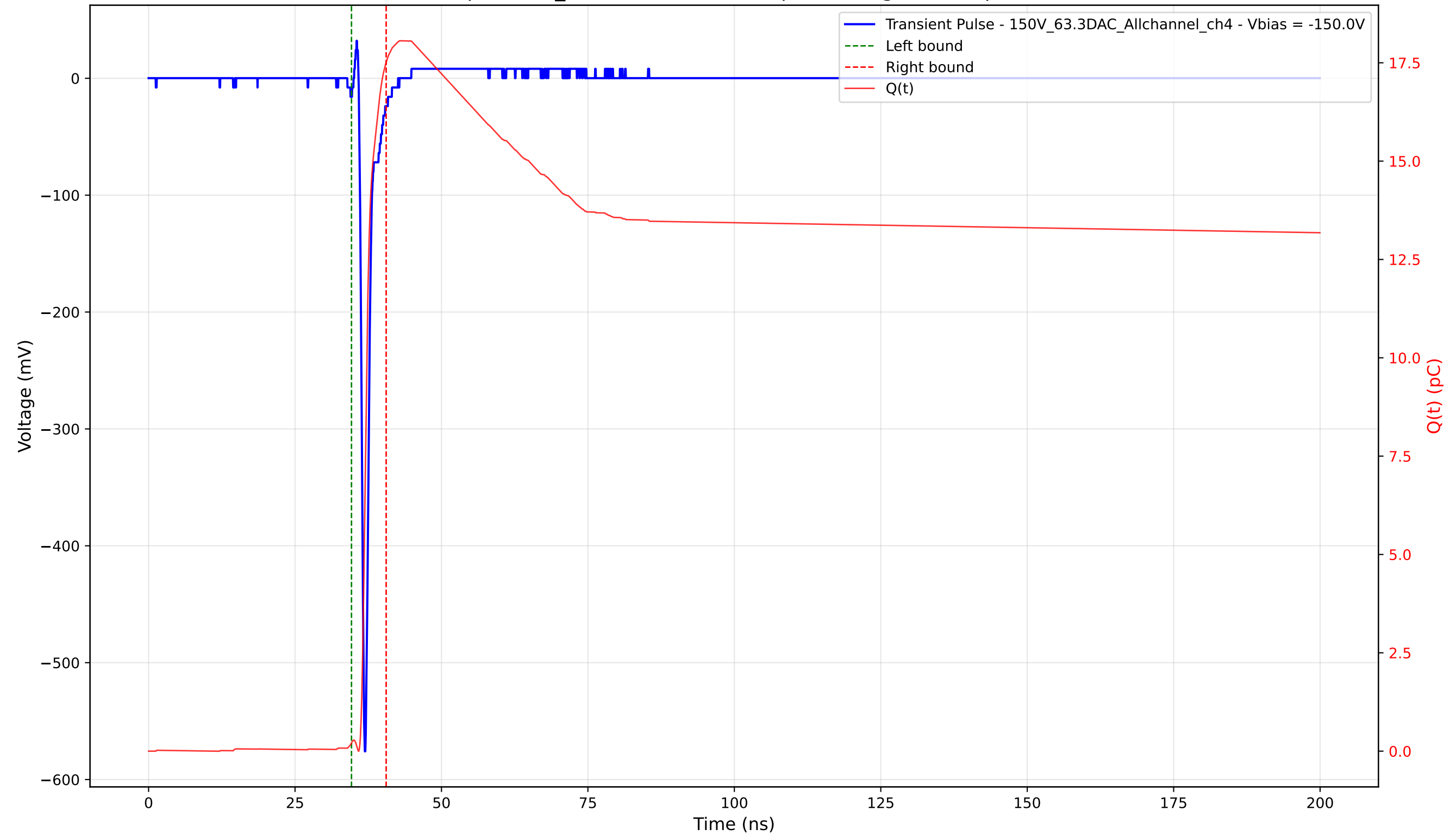
Transient Pulse - Sample: 1cm_42 - Position: 2095.0 \mu\text{m} - Charge: 17.30 pC - Rise Time: 0.71 ns
