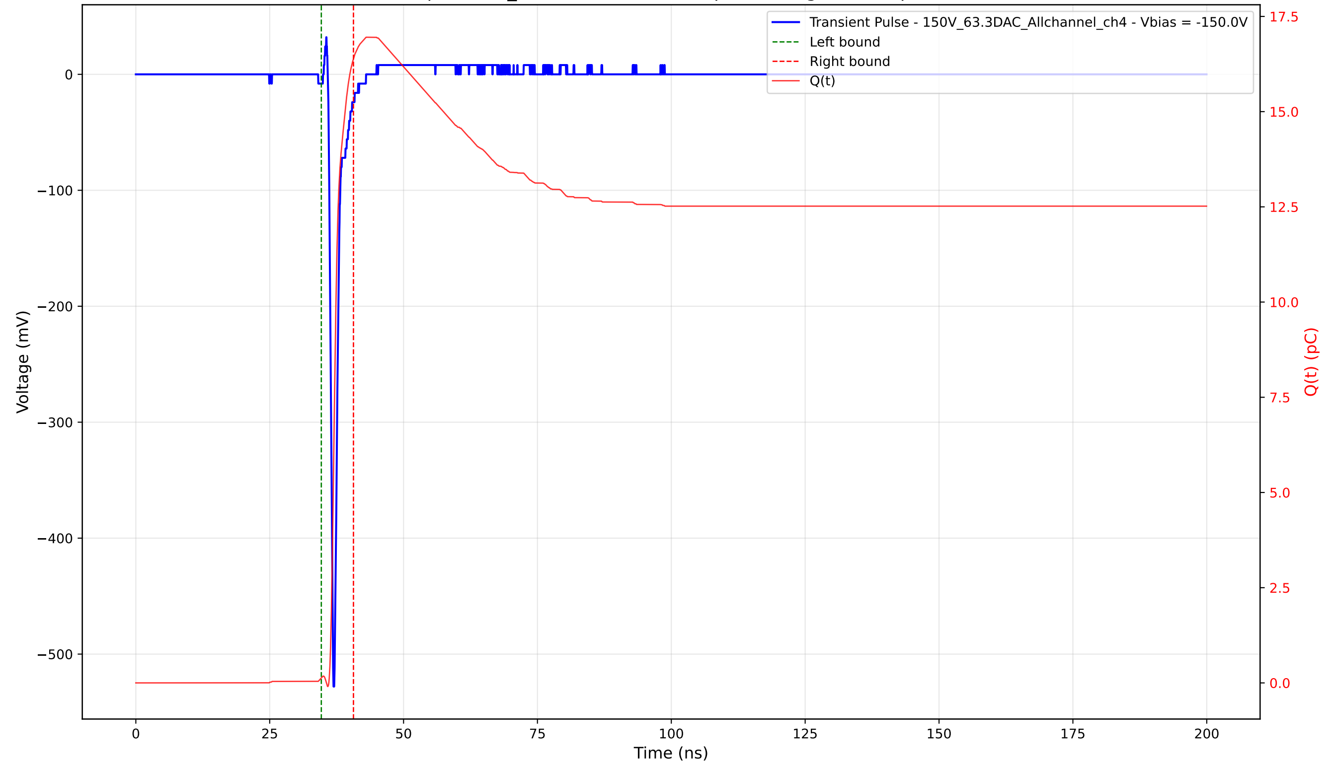
Transient Pulse - Sample: 1cm_42 - Position: 2190.0 \mu\text{m} - Charge: 16.26 pC - Rise Time: 0.70 ns
