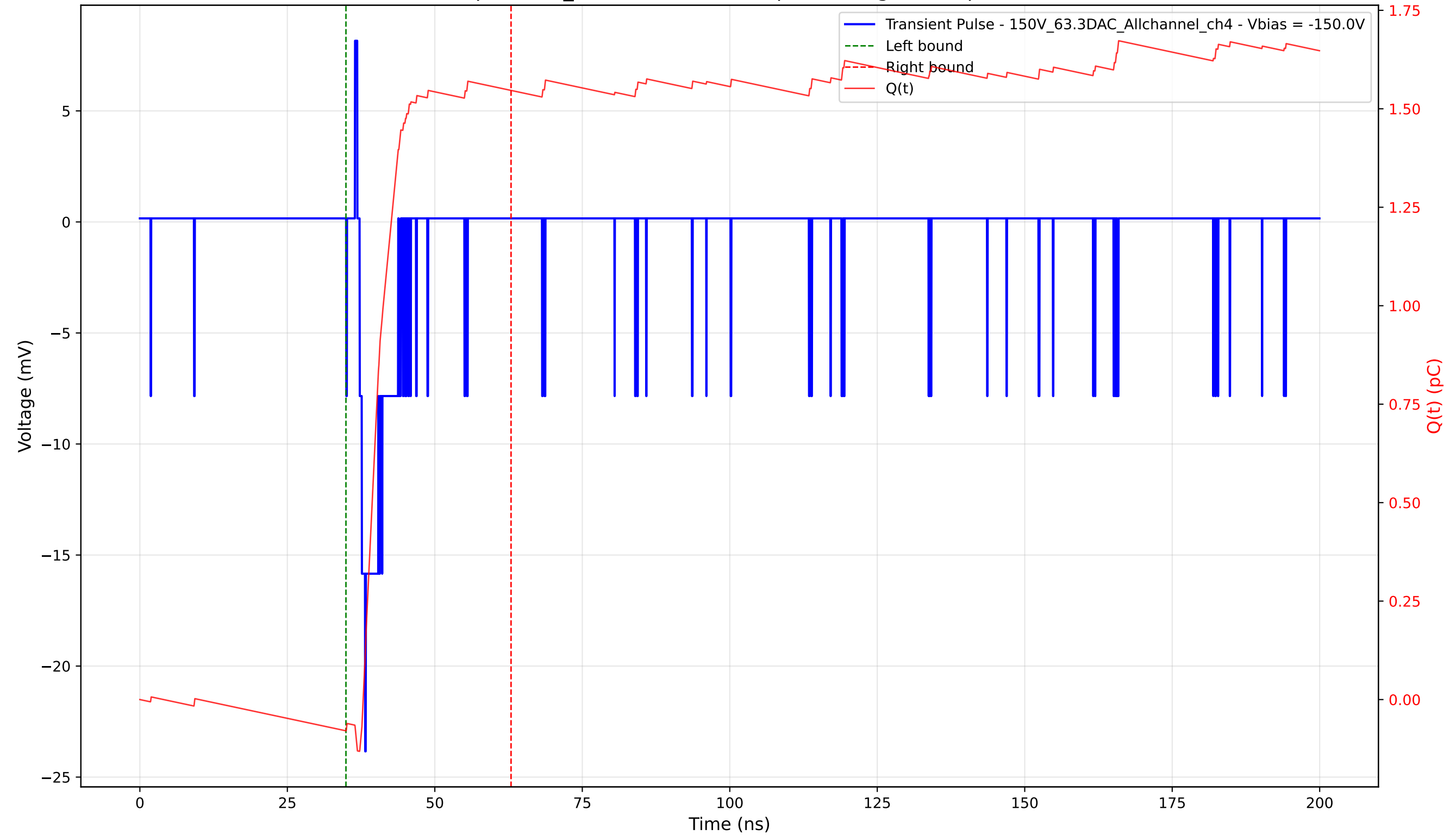
Transient Pulse - Sample: 1cm_42 - Position: 160.0 \mu\text{m} - Charge: 1.63 pC - Rise Time: 0.95 ns
