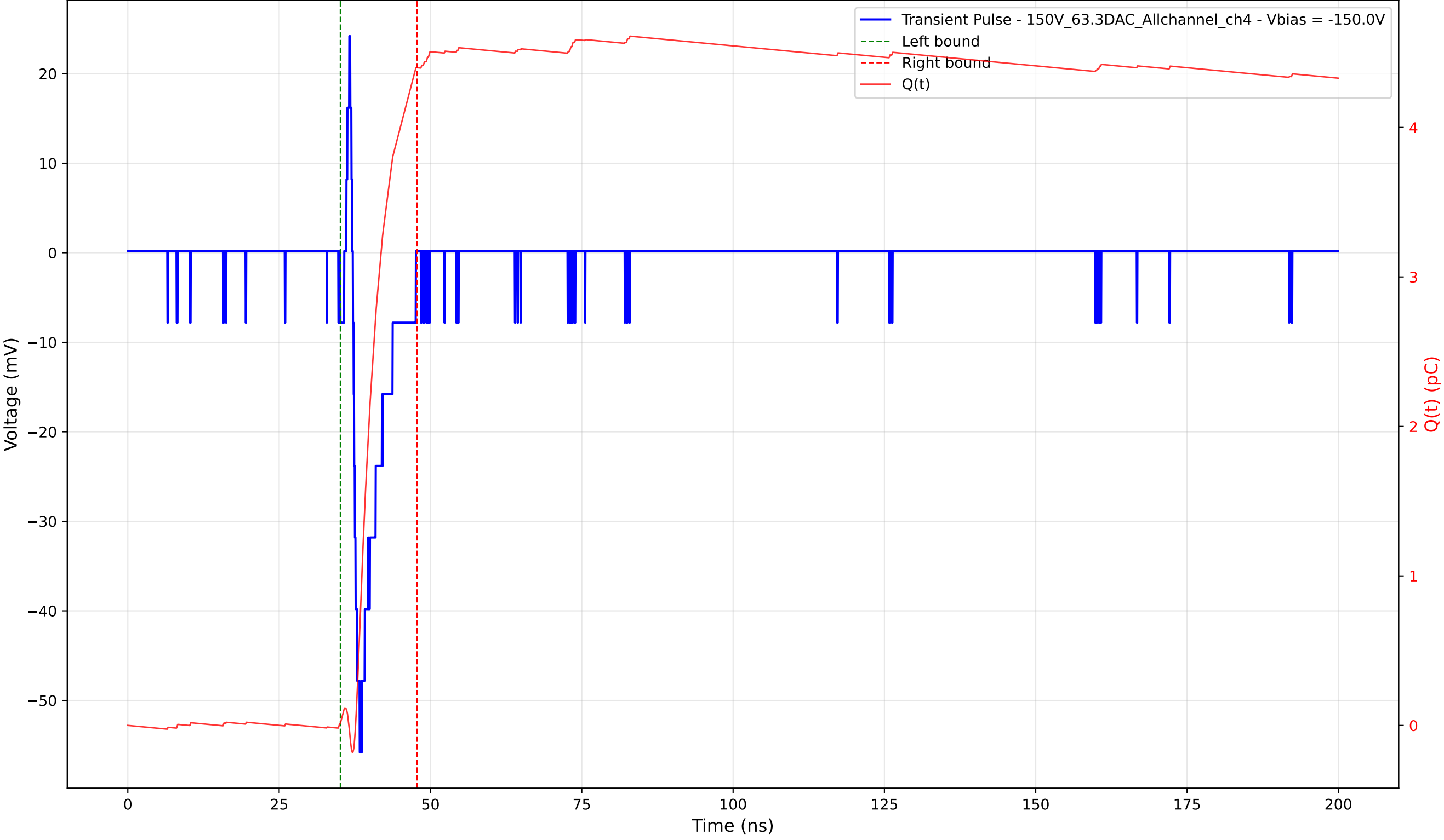
Transient Pulse - Sample: 1cm_42 - Position: 495.0 \mu\text{m} - Charge: 4.38 pC - Rise Time: 1.13 ns
