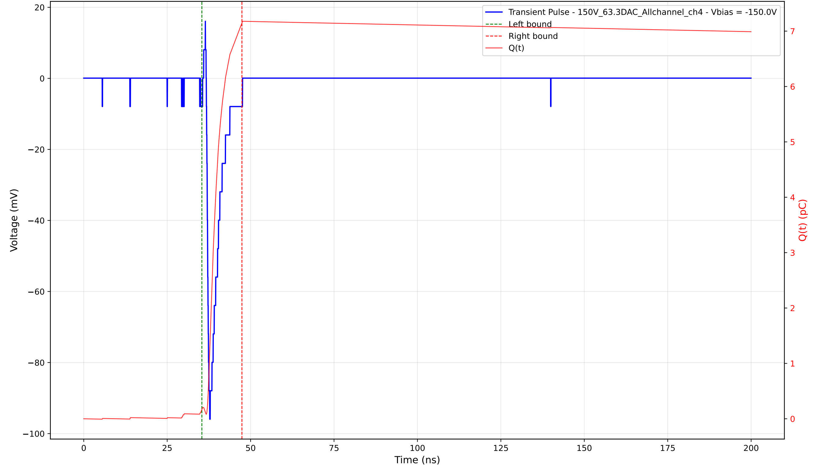
Transient Pulse - Sample: 1cm_42 - Position: 975.0 \mu\text{m} - Charge: 6.98 pC - Rise Time: 0.71 ns
