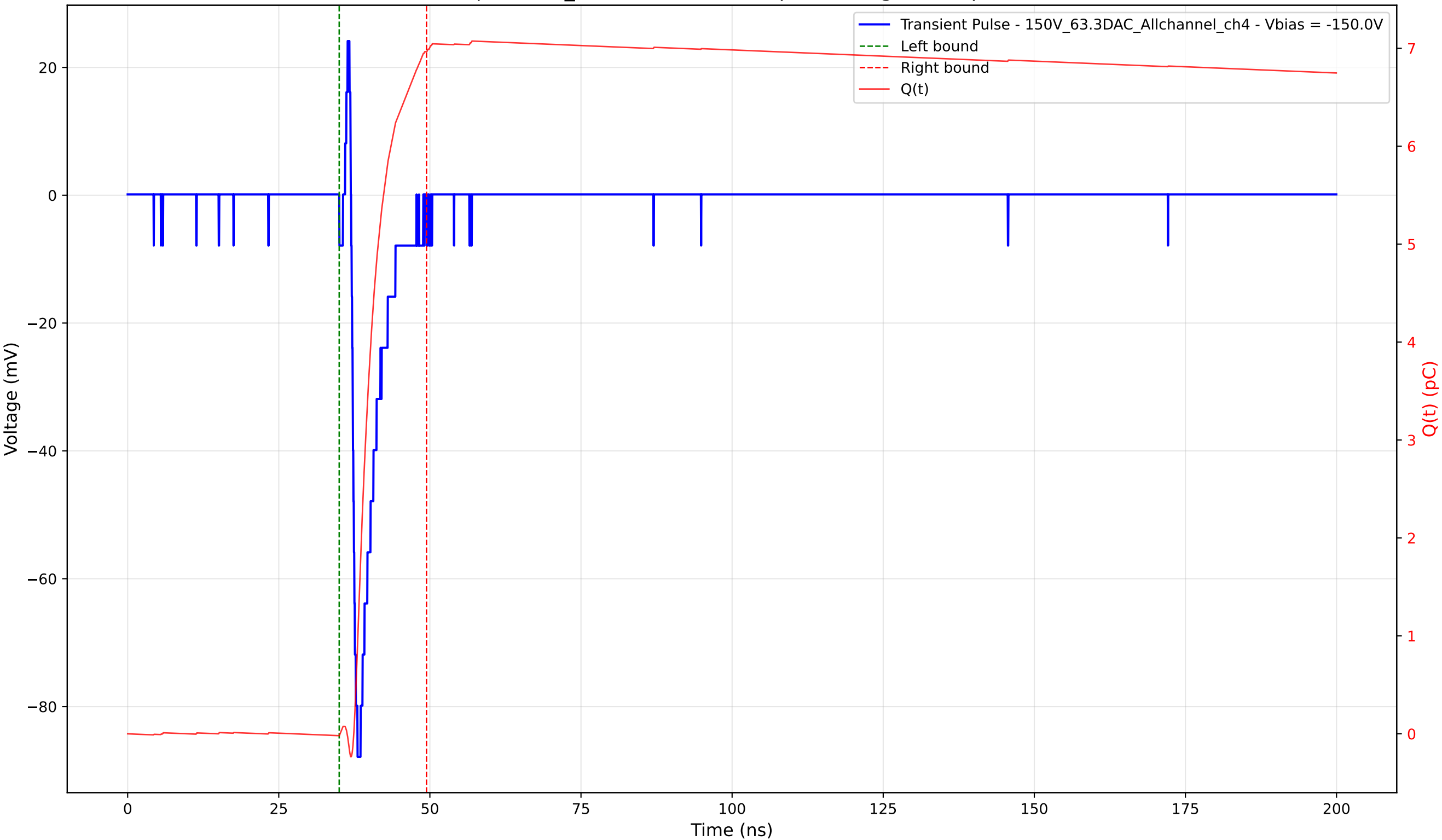
Transient Pulse - Sample: 1cm_42 - Position: 780.0 \mu\text{m} - Charge: 6.98 pC - Rise Time: 0.72 ns
