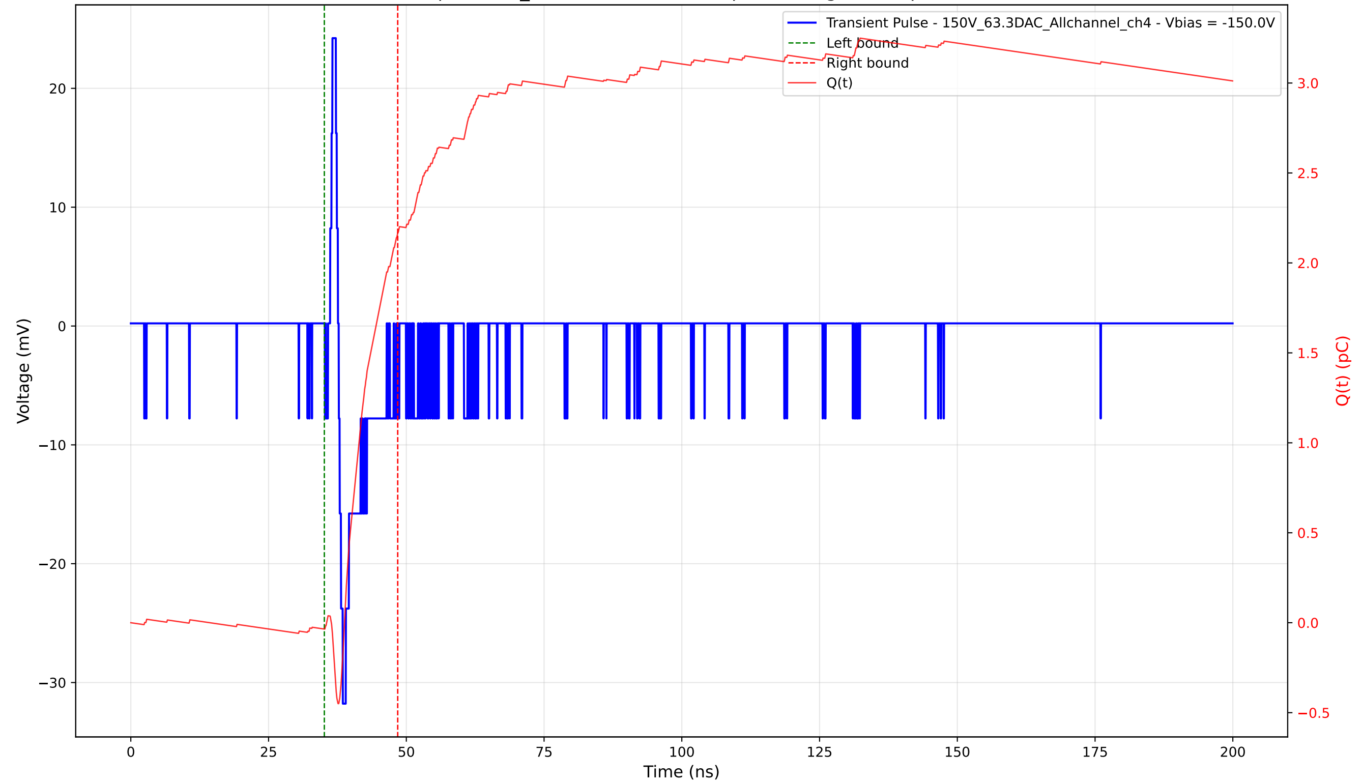
Transient Pulse - Sample: 1cm_42 - Position: 4485.0 \mu\text{m} - Charge: 2.20 pC - Rise Time: 0.74 ns
