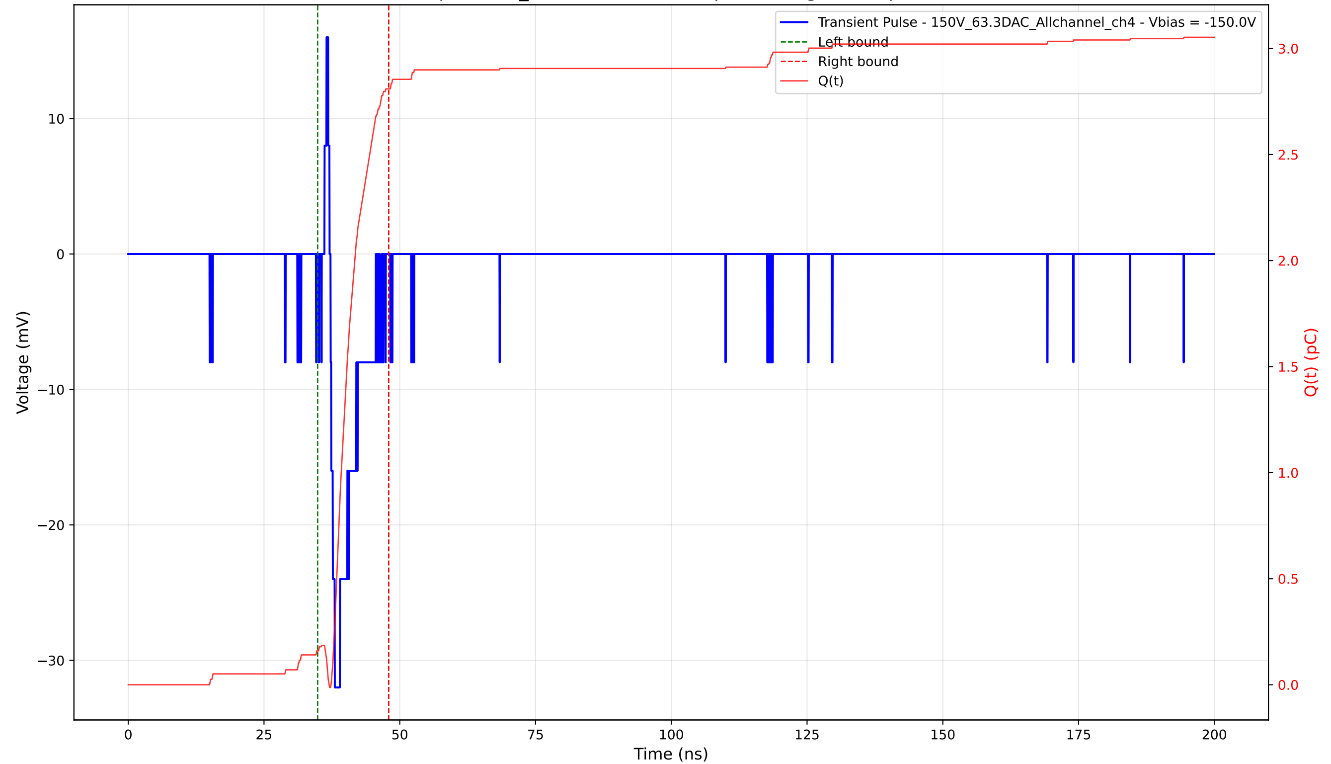
Transient Pulse - Sample: 1cm_42 - Position: 270.0 \mu\text{m} - Charge: 2.65 pC - Rise Time: 0.78 ns
