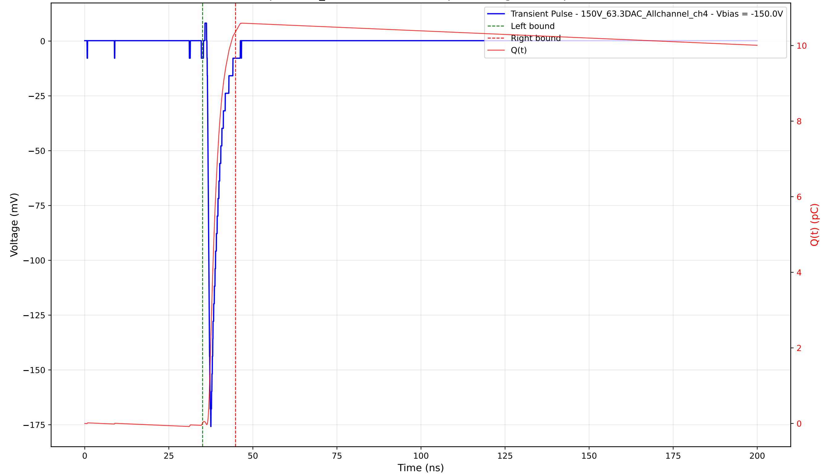
Transient Pulse - Sample: 1cm_42 - Position: 1210.0 \mu\text{m} - Charge: 10.36 pC - Rise Time: 0.75 ns
