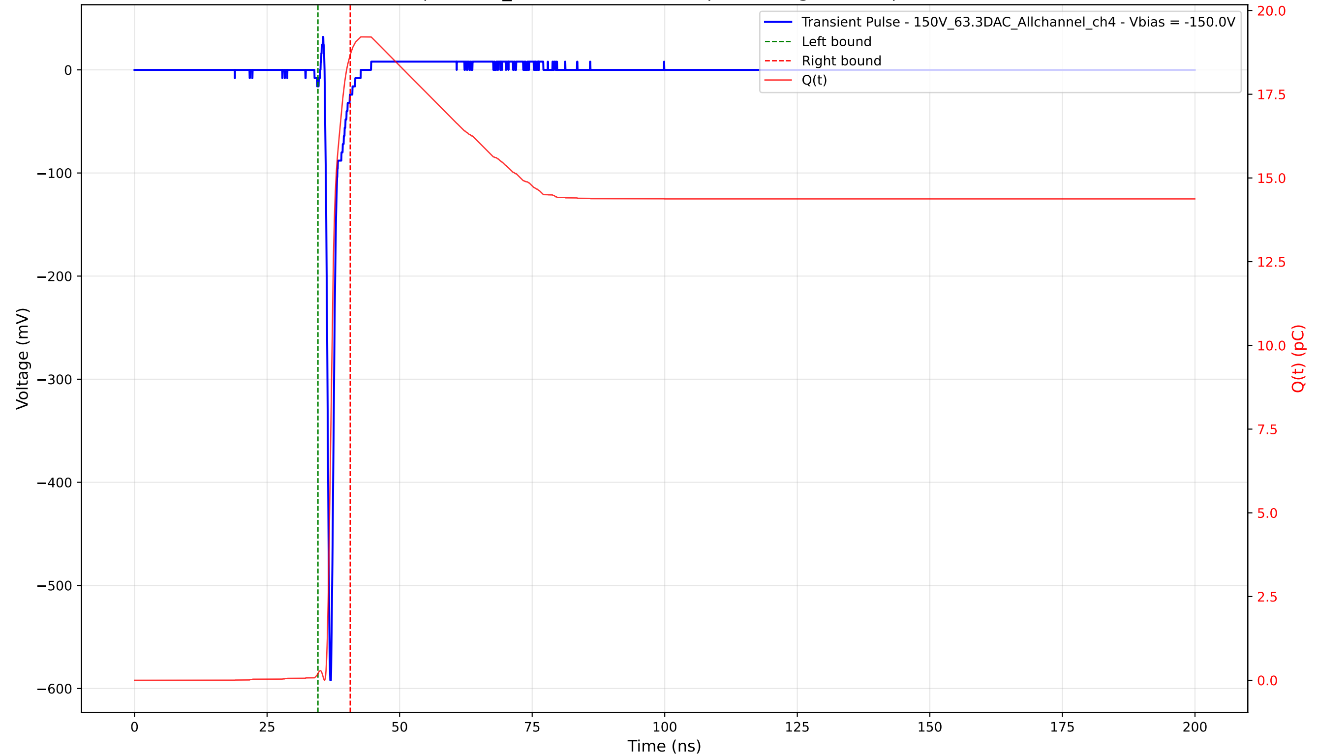
Transient Pulse - Sample: 1cm_42 - Position: 1925.0 \mu\text{m} - Charge: 18.47 pC - Rise Time: 0.70 ns
