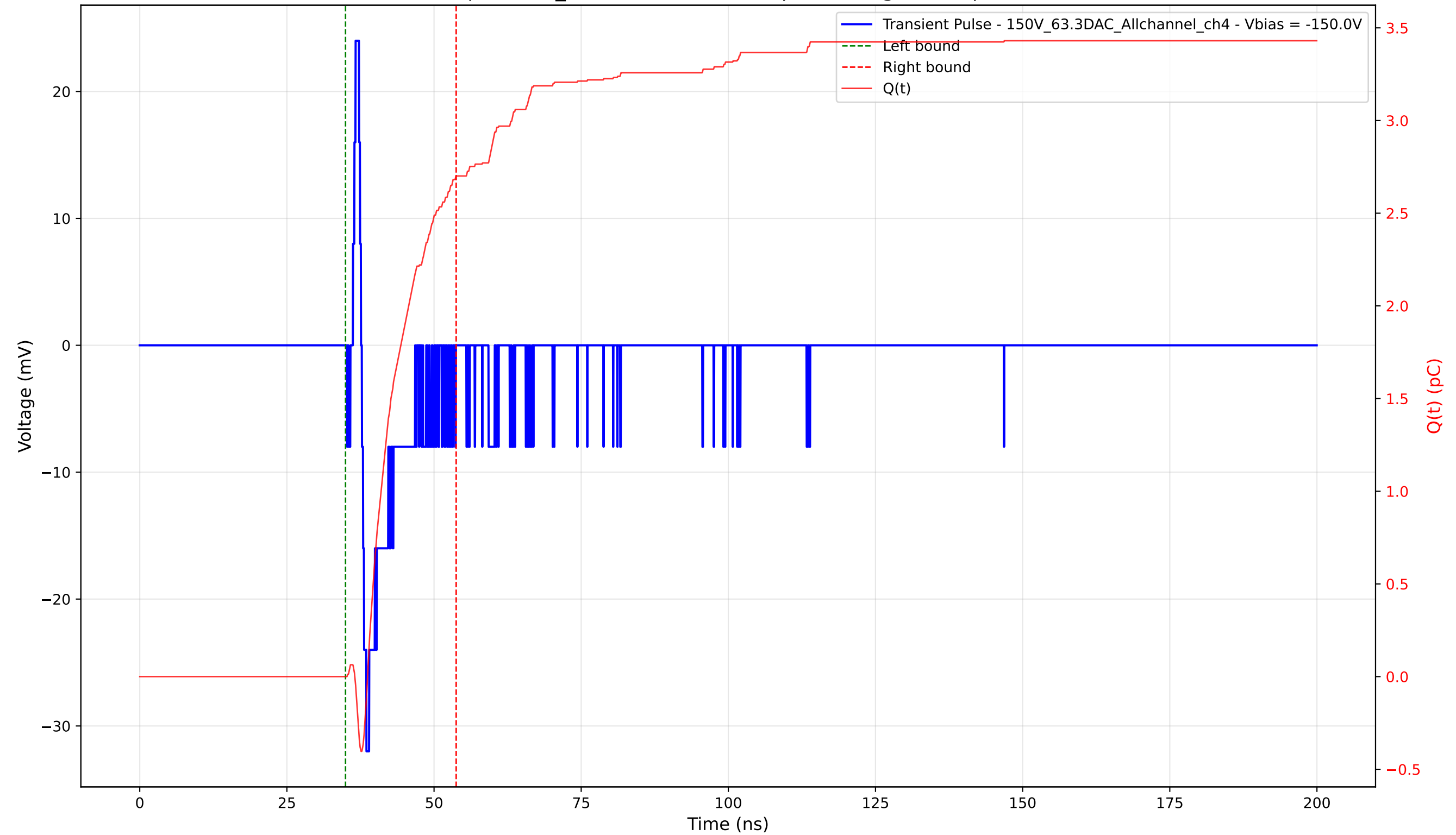
Transient Pulse - Sample: 1cm_42 - Position: 4005.0 \mu\text{m} - Charge: 2.70 pC - Rise Time: 0.78 ns
