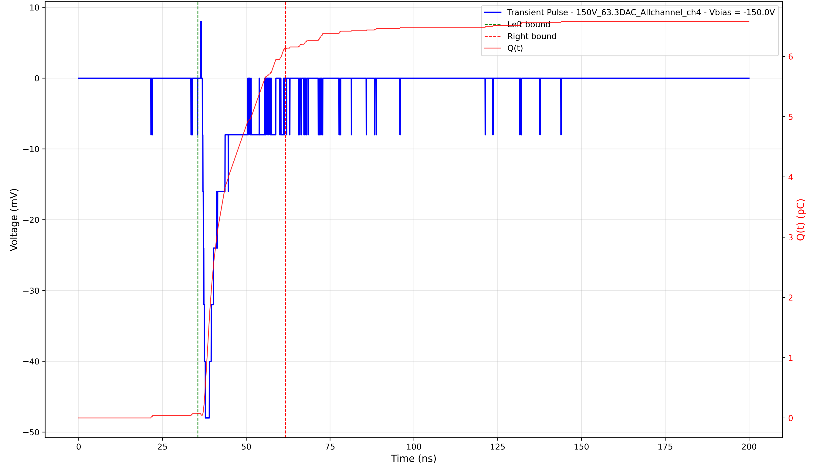
Transient Pulse - Sample: 1cm_42 - Position: 3200.0 \mu\text{m} - Charge: 6.05 pC - Rise Time: 0.90 ns
