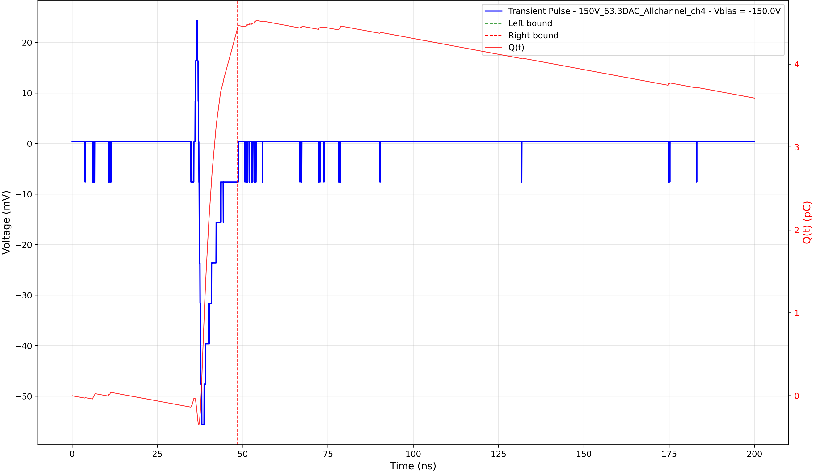
Transient Pulse - Sample: 1cm_42 - Position: 505.0 \mu\text{m} - Charge: 4.53 pC - Rise Time: 0.85 ns
