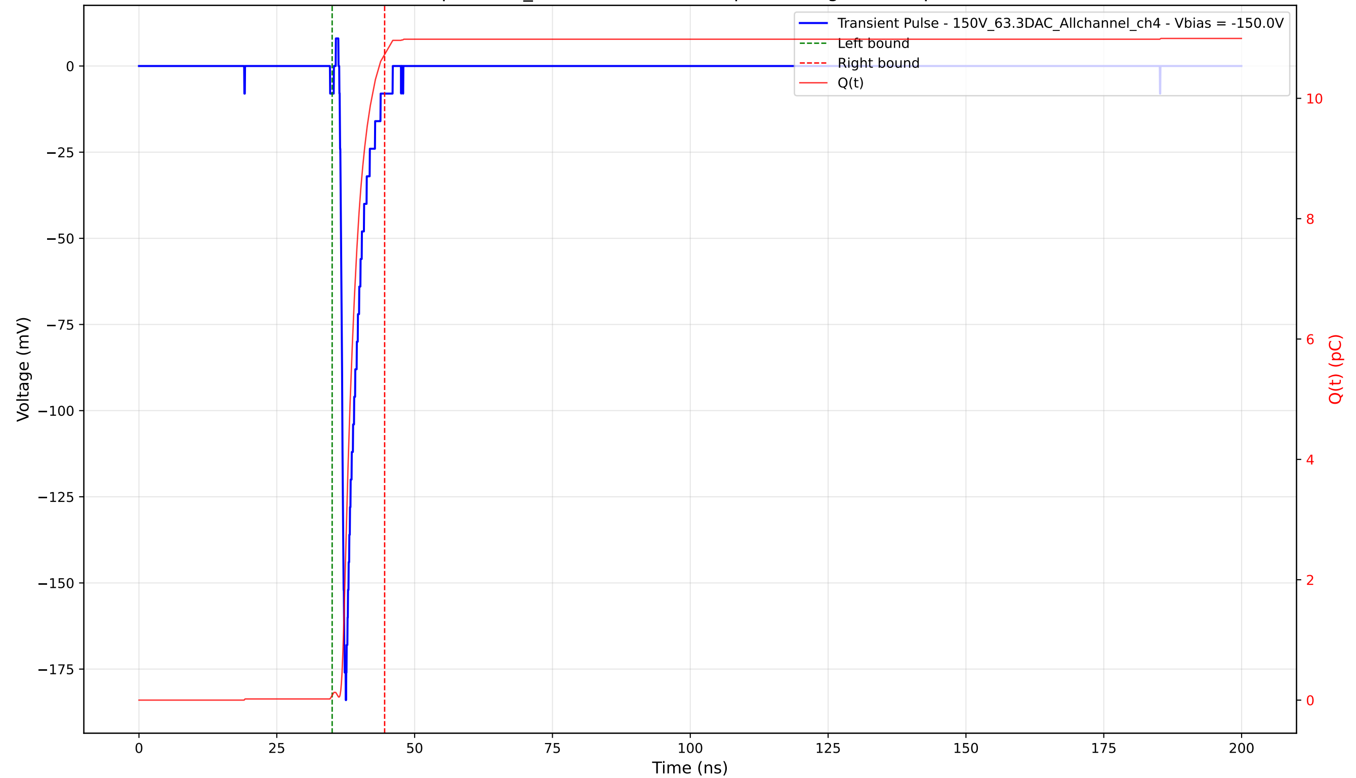
Transient Pulse - Sample: 1cm_42 - Position: 1230.0 \mu\text{m} - Charge: 10.65 pC - Rise Time: 0.79 ns
