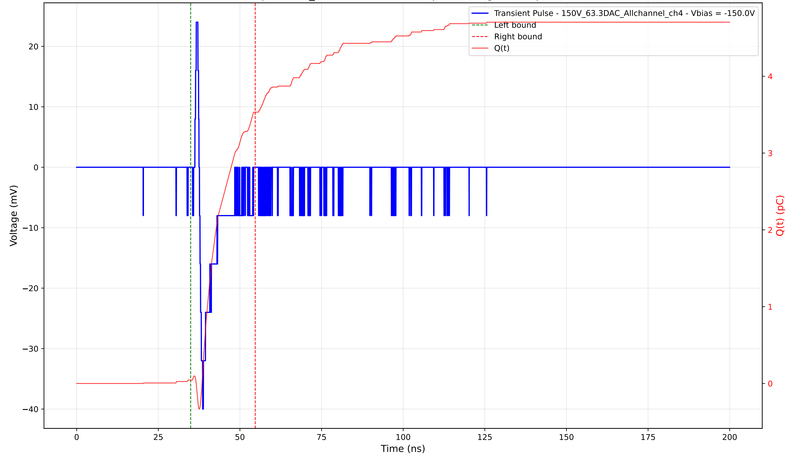
Transient Pulse - Sample: 1cm_42 - Position: 3675.0 \mu\text{m} - Charge: 3.49 pC - Rise Time: 0.98 ns
