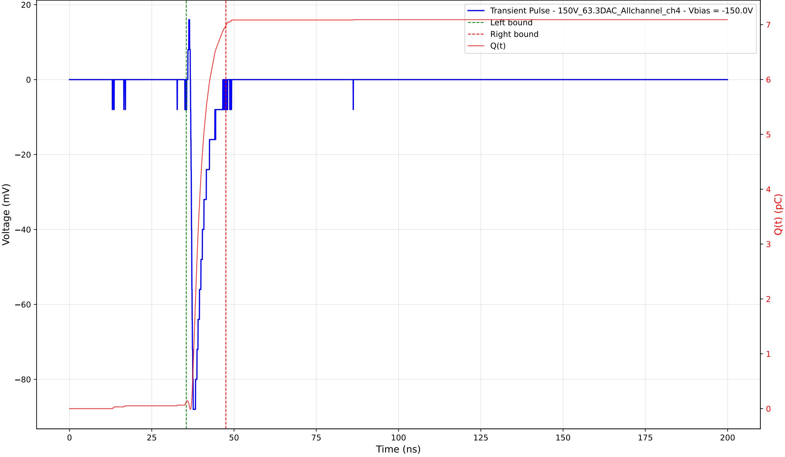
Transient Pulse - Sample: 1cm_42 - Position: 955.0 \mu\text{m} - Charge: 6.86 pC - Rise Time: 0.64 ns
