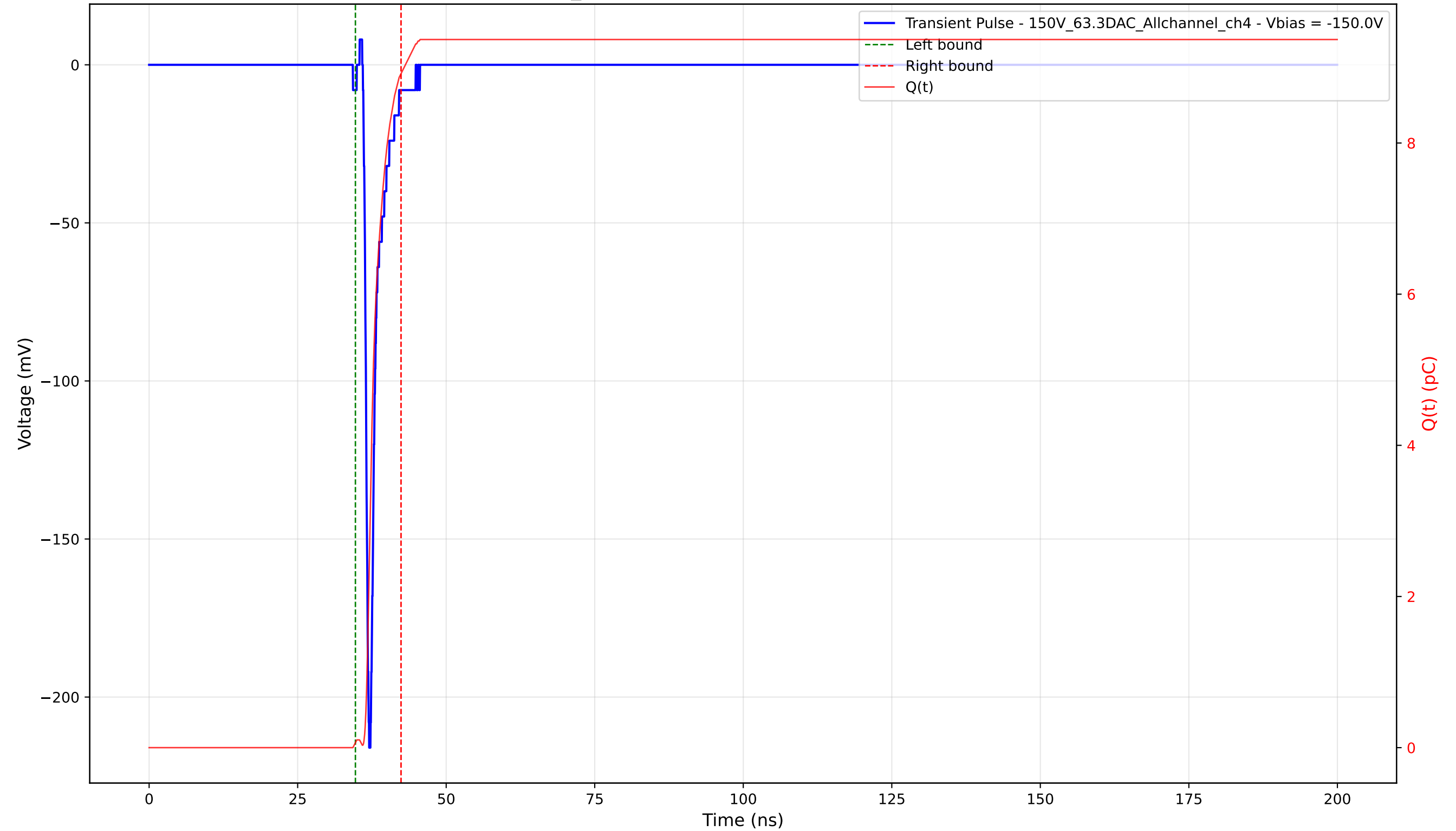
Transient Pulse - Sample: 1cm_42 - Position: 2540.0 \mu\text{m} - Charge: 8.85 pC - Rise Time: 0.78 ns
