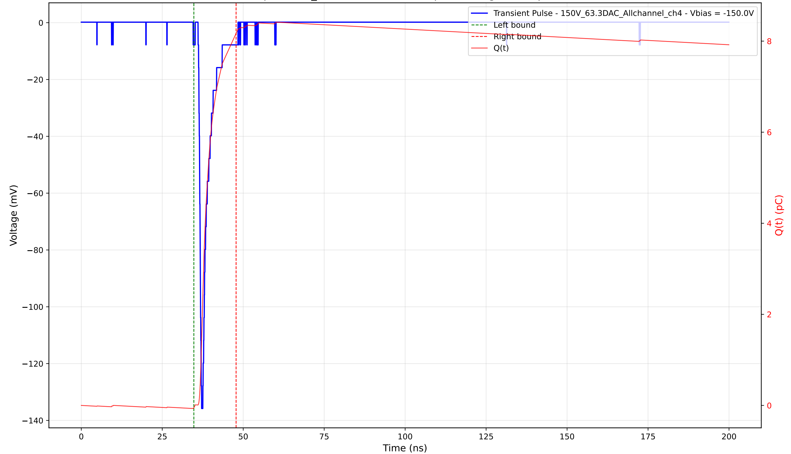
Transient Pulse - Sample: 1cm_42 - Position: 2760.0 \mu\text{m} - Charge: 8.23 pC - Rise Time: 0.81 ns
