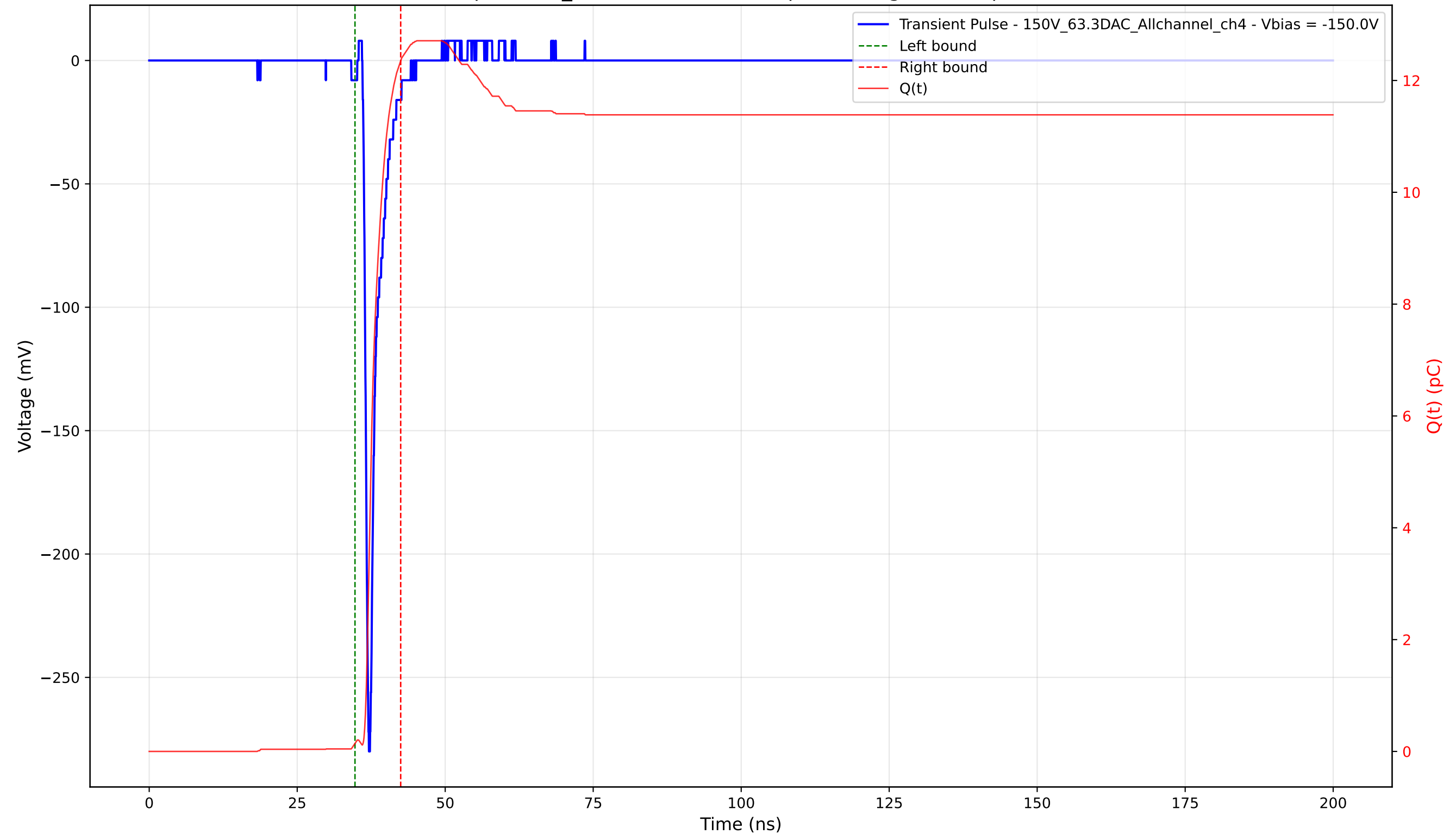
Transient Pulse - Sample: 1cm_42 - Position: 1525.0 \mu\text{m} - Charge: 12.21 pC - Rise Time: 0.76 ns
