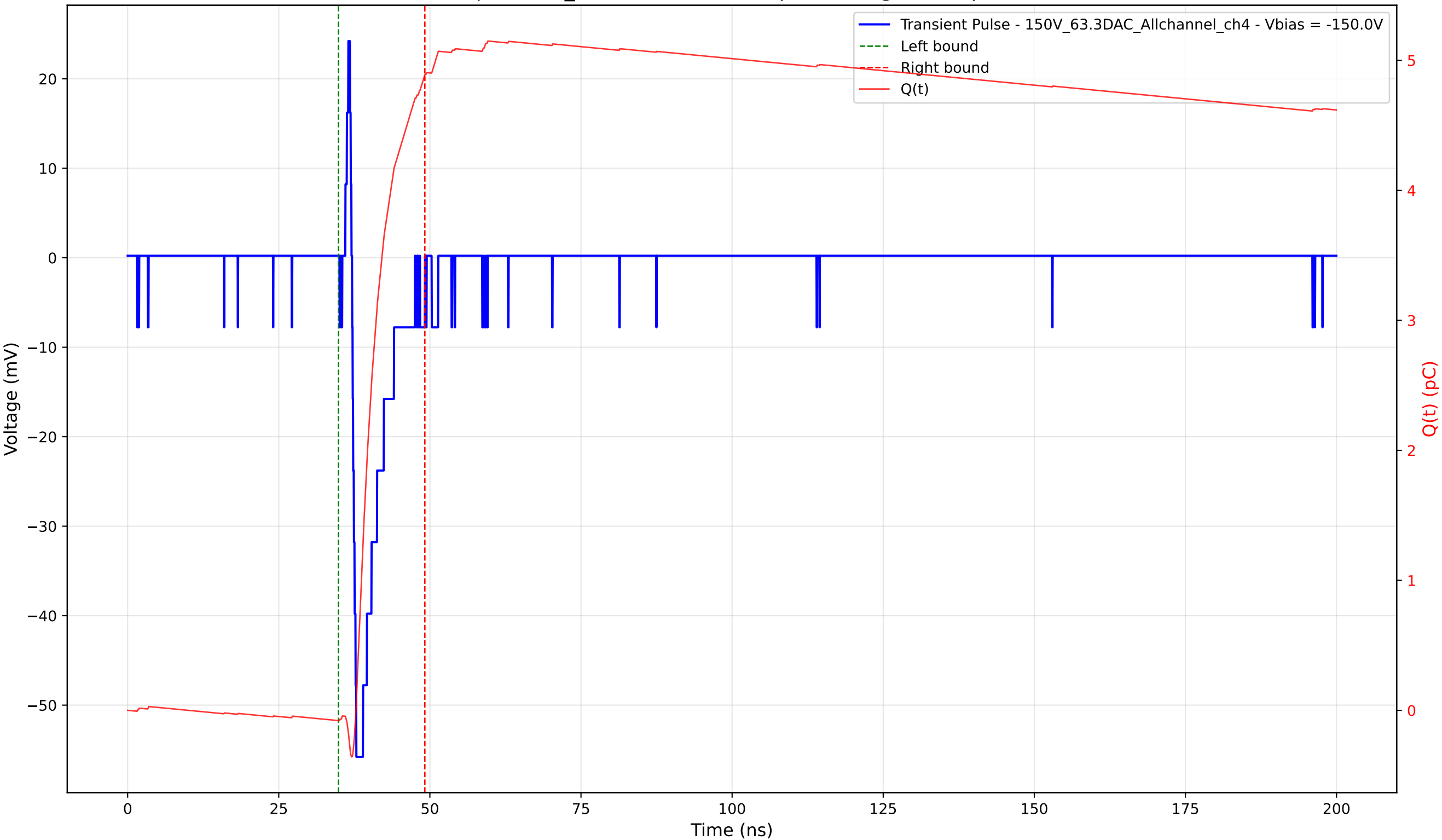
Transient Pulse - Sample: 1cm_42 - Position: 555.0 \mu\text{m} - Charge: 4.97 pC - Rise Time: 0.69 ns
