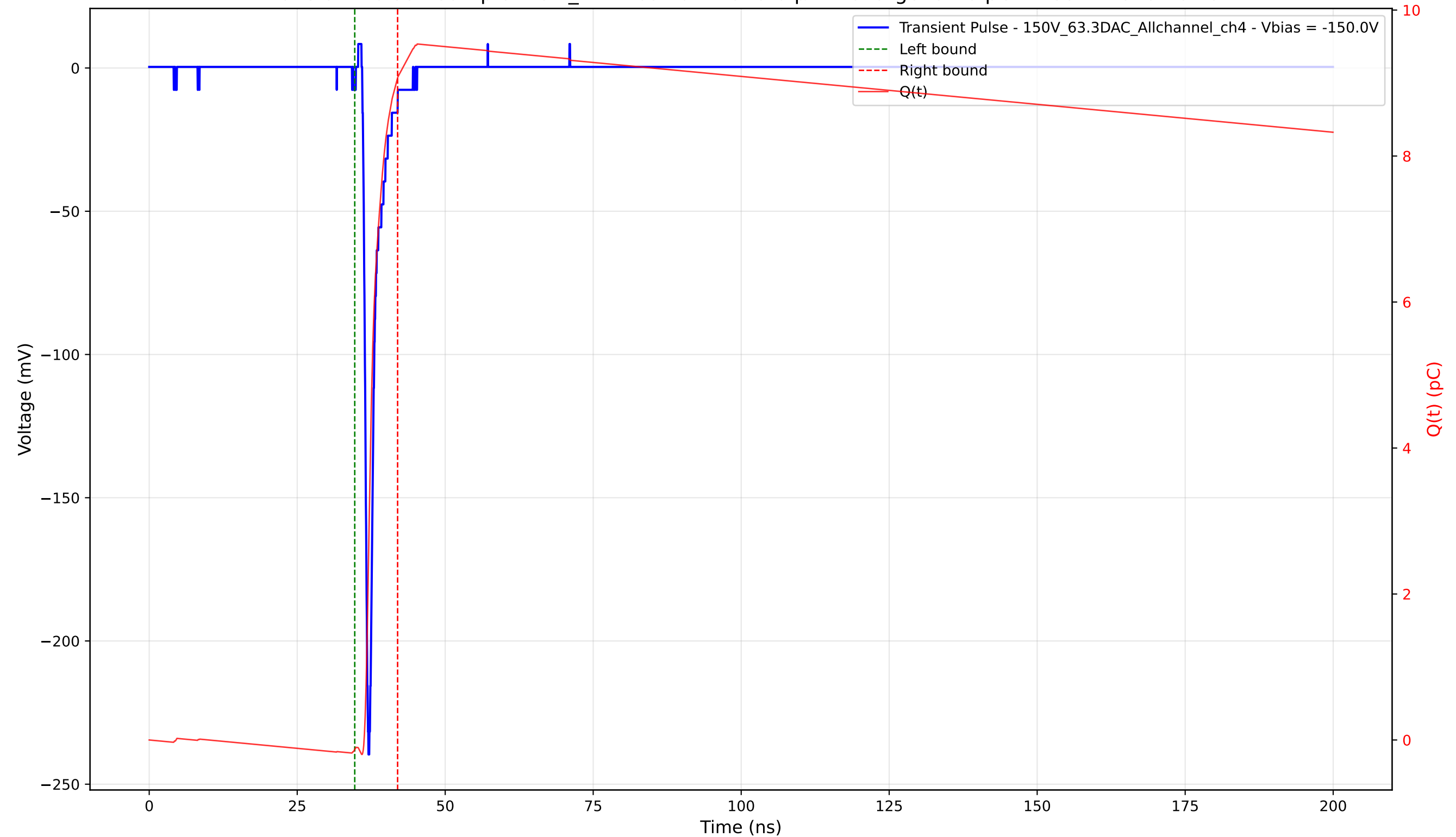
Transient Pulse - Sample: 1cm_42 - Position: 2515.0 \mu\text{m} - Charge: 9.20 pC - Rise Time: 0.76 ns
