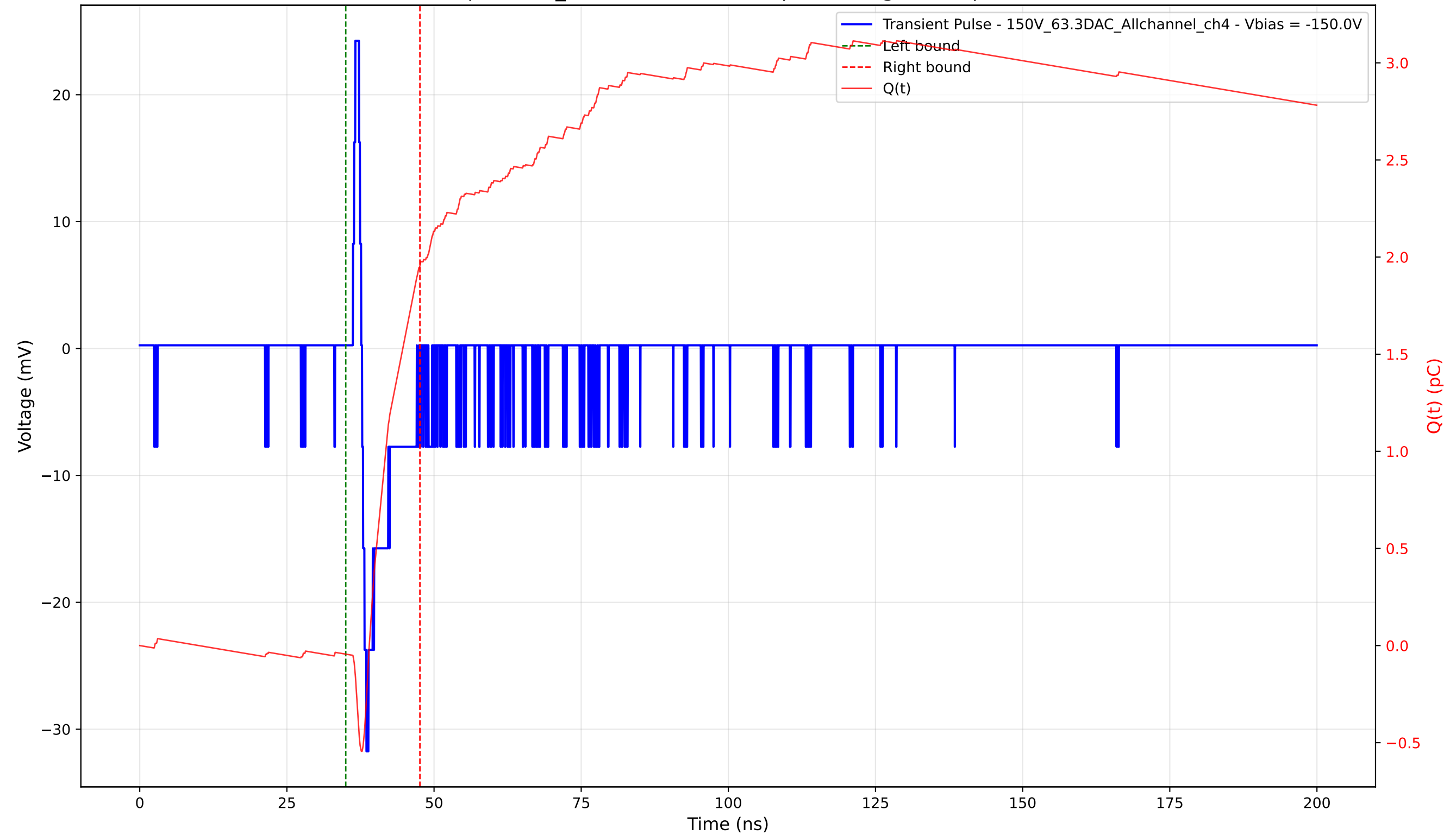
Transient Pulse - Sample: 1cm_42 - Position: 4065.0 \mu\text{m} - Charge: 2.00 pC - Rise Time: 0.74 ns
