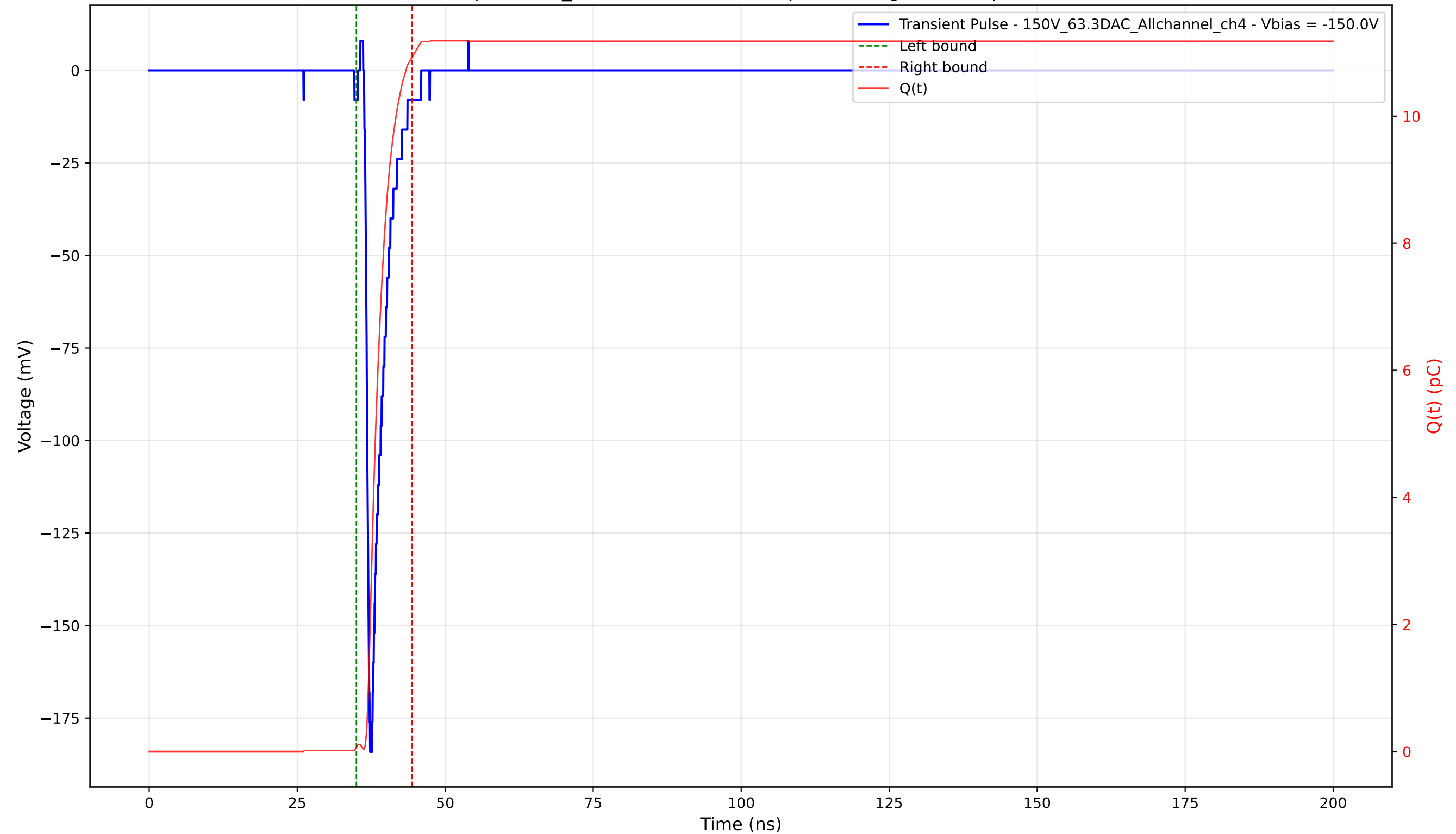
Transient Pulse - Sample: 1cm_42 - Position: 1275.0 \mu\text{m} - Charge: 10.85 pC - Rise Time: 0.75 ns
