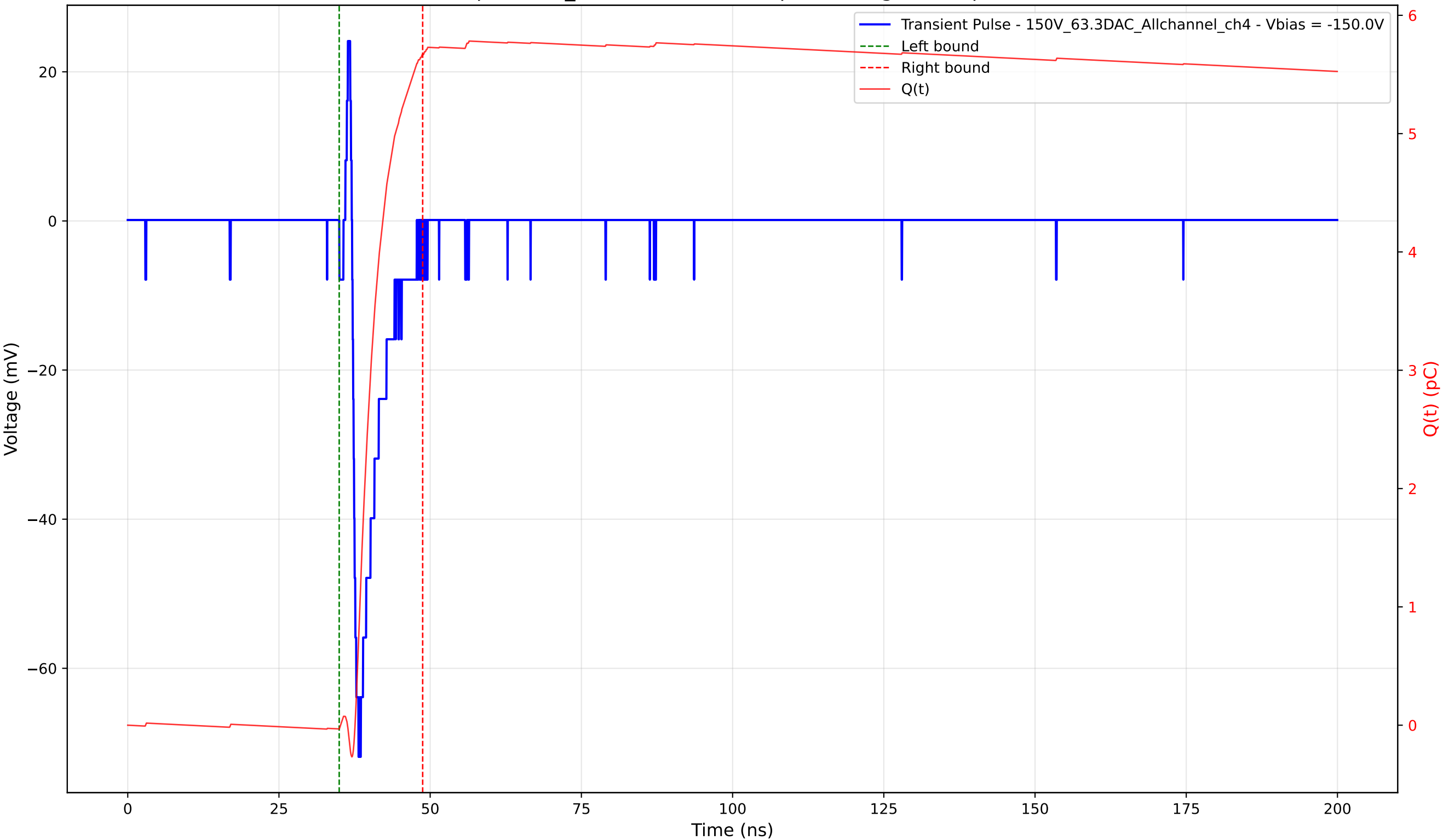
Transient Pulse - Sample: 1cm_42 - Position: 615.0 \mu\text{m} - Charge: 5.70 pC - Rise Time: 1.04 ns
