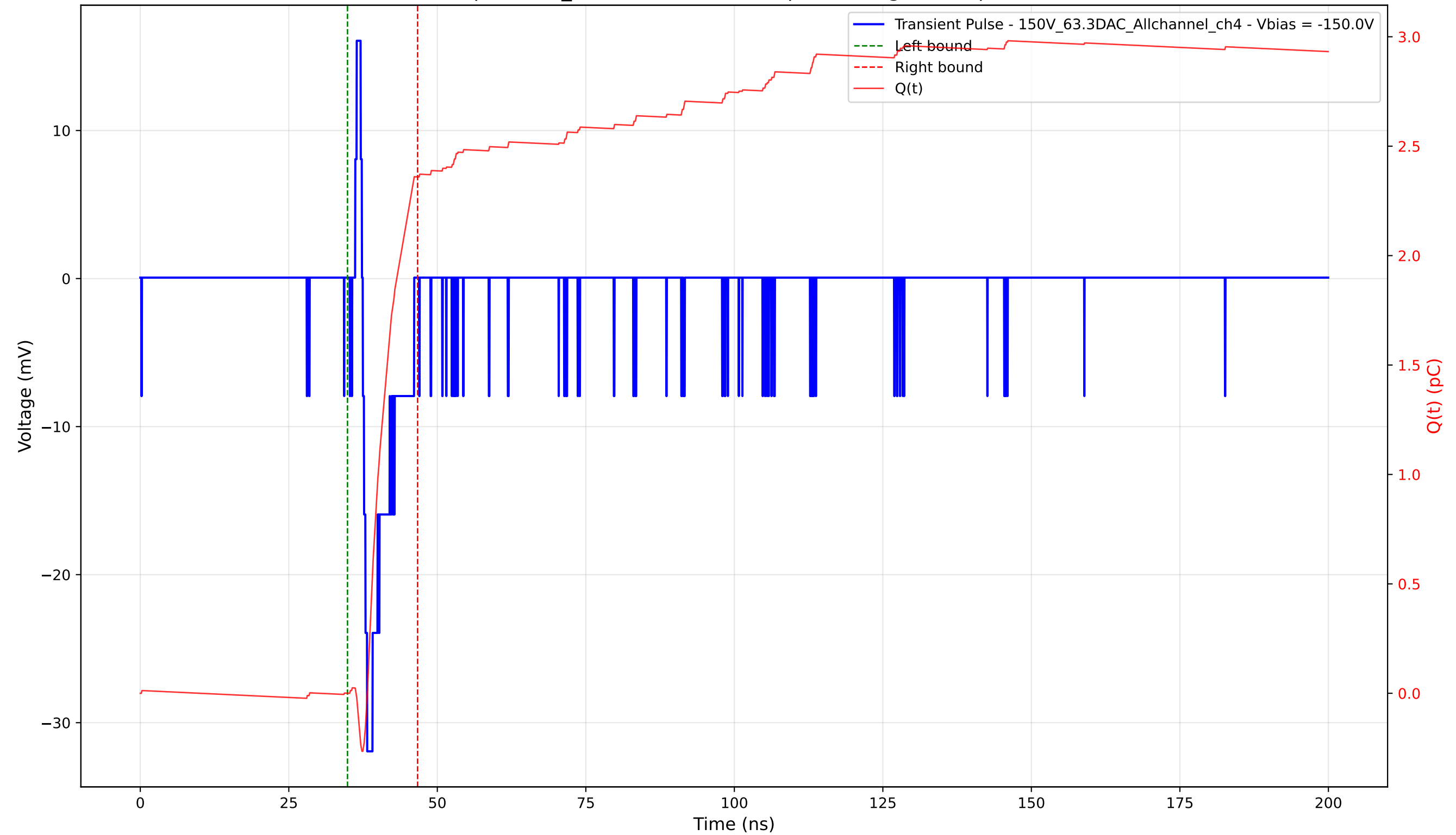
Transient Pulse - Sample: 1cm_42 - Position: 4900.0 \mu\text{m} - Charge: 2.36 pC - Rise Time: 0.74 ns
