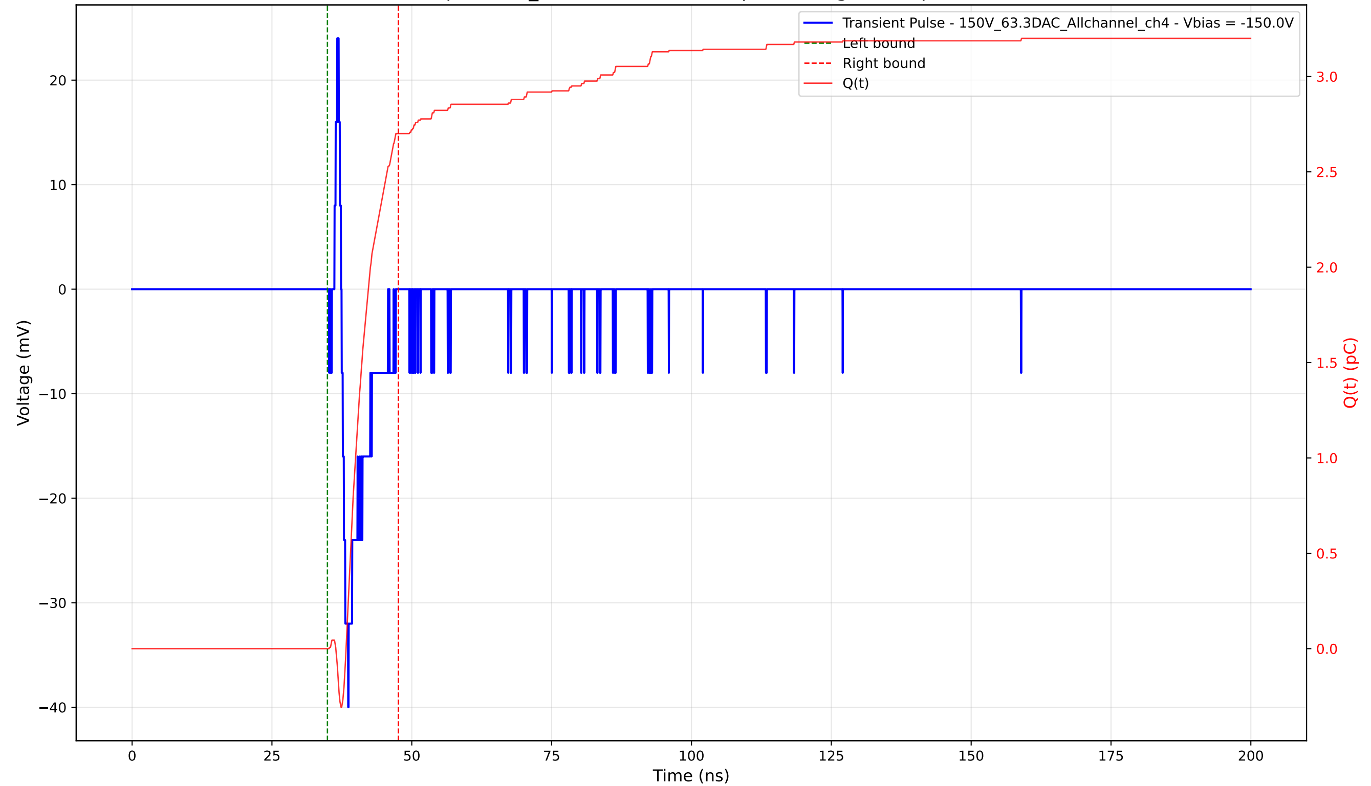
Transient Pulse - Sample: 1cm_42 - Position: 4830.0 \mu\text{m} - Charge: 2.70 pC - Rise Time: 1.18 ns
