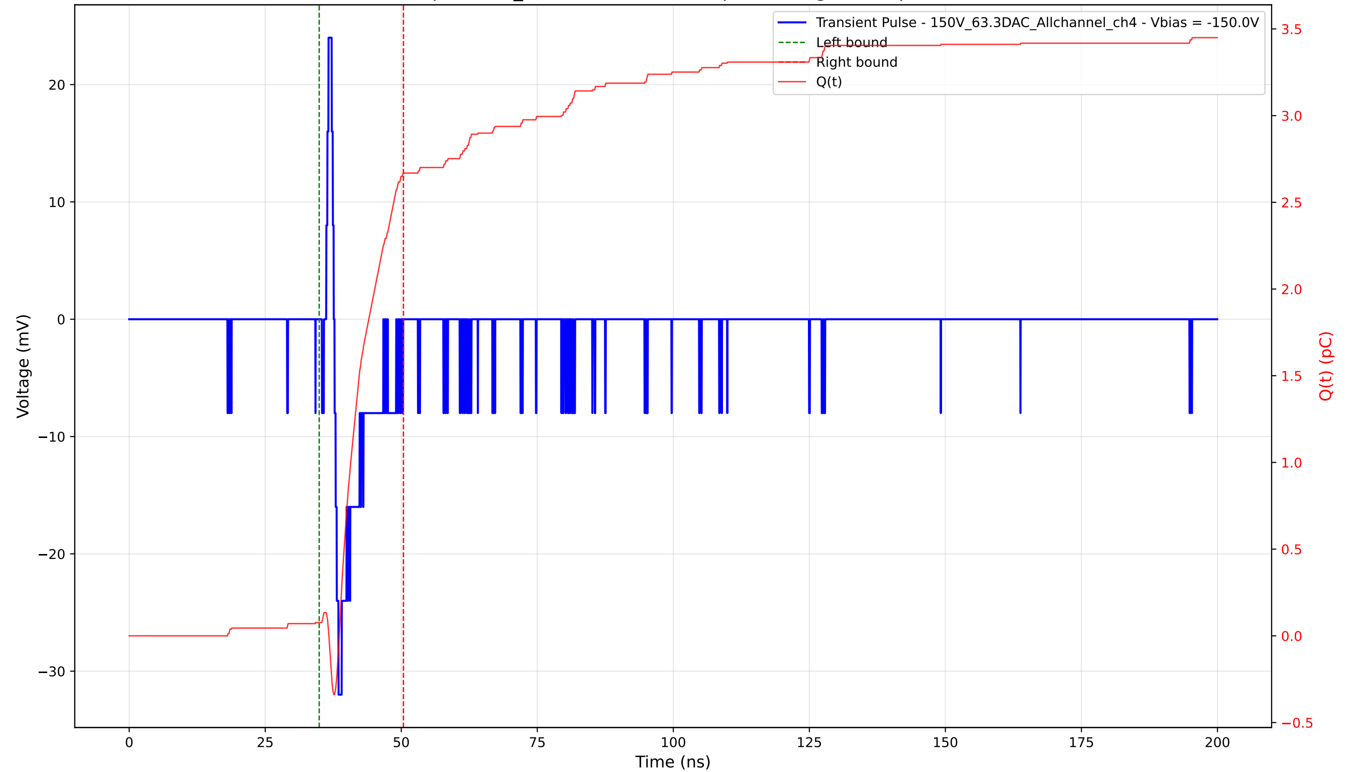
Transient Pulse - Sample: 1cm_42 - Position: 4440.0 \mu\text{m} - Charge: 2.59 pC - Rise Time: 0.74 ns
