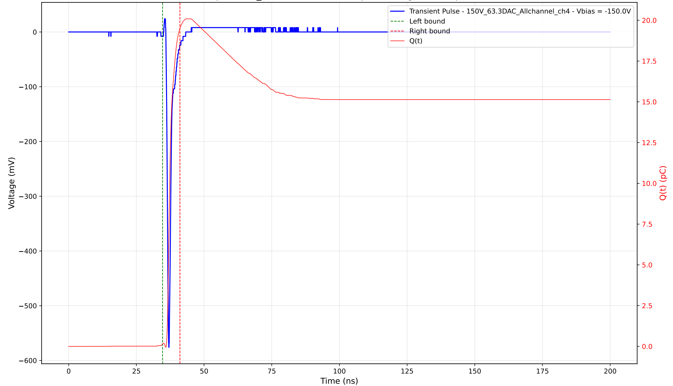
Transient Pulse - Sample: 1cm_42 - Position: 1750.0 \mu\text{m} - Charge: 19.36 pC - Rise Time: 0.73 ns
