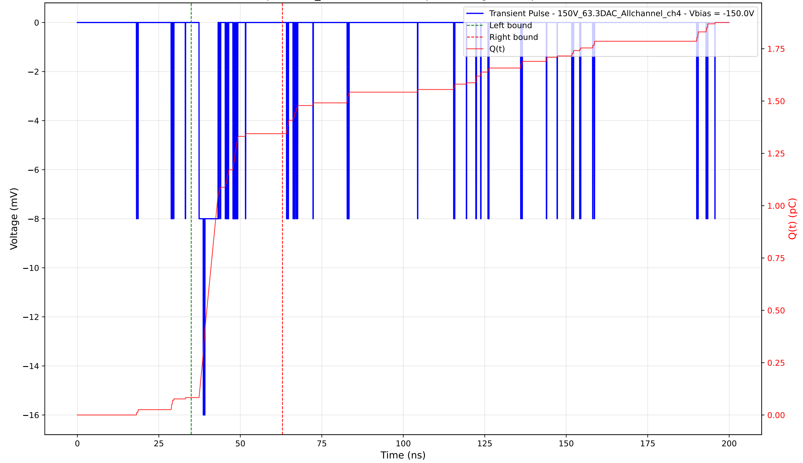
Transient Pulse - Sample: 1cm_42 - Position: 95.0 \mu\text{m} - Charge: 1.26 pC - Rise Time: 1.31 ns
