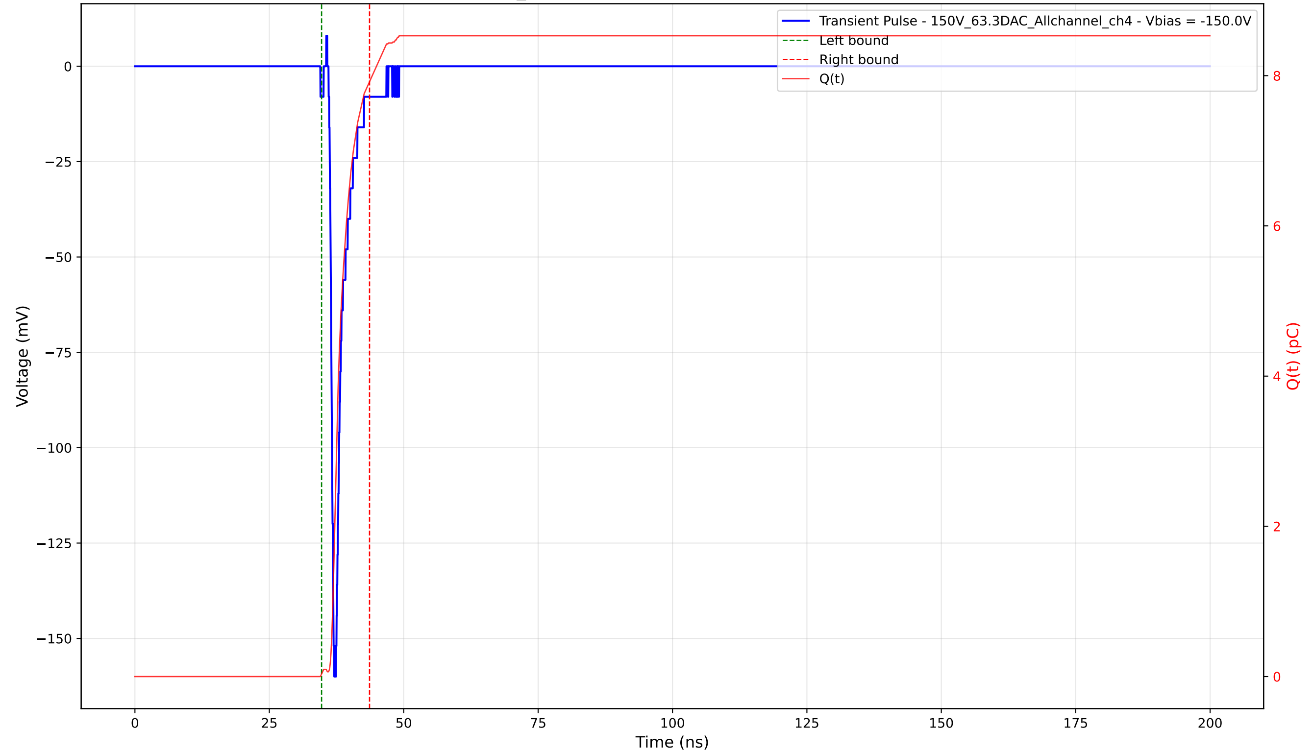
Transient Pulse - Sample: 1cm_42 - Position: 2650.0 \mu\text{m} - Charge: 7.88 pC - Rise Time: 0.72 ns
