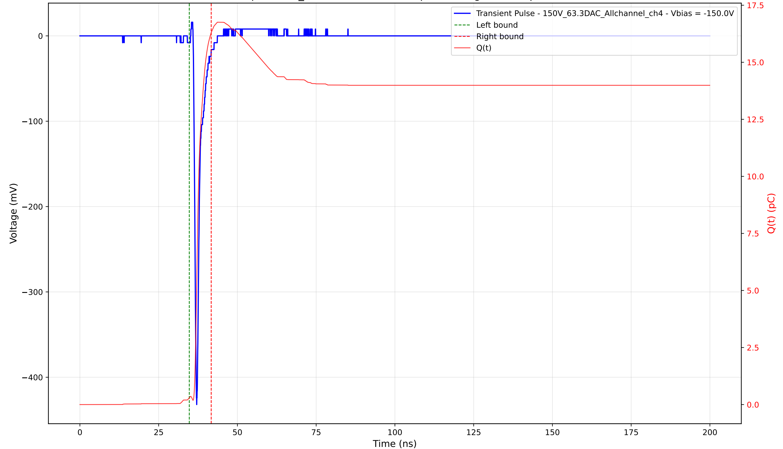
Transient Pulse - Sample: 1cm_42 - Position: 1640.0 \mu\text{m} - Charge: 16.00 pC - Rise Time: 0.73 ns
