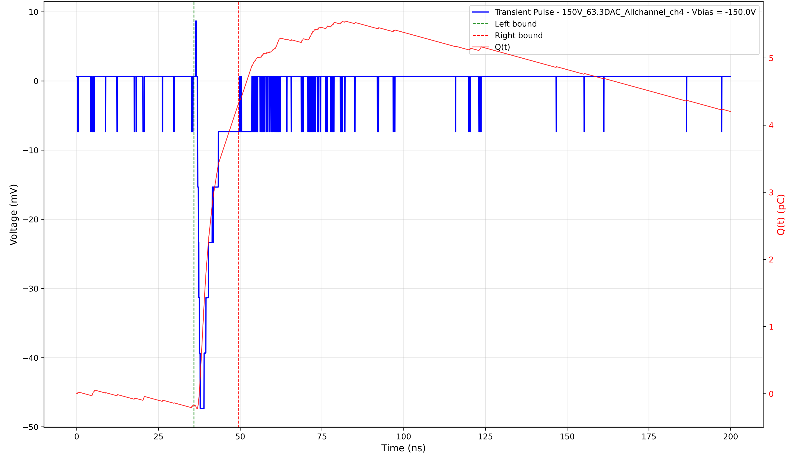
Transient Pulse - Sample: 1cm_42 - Position: 3195.0 \mu\text{m} - Charge: 4.49 pC - Rise Time: 0.86 ns
