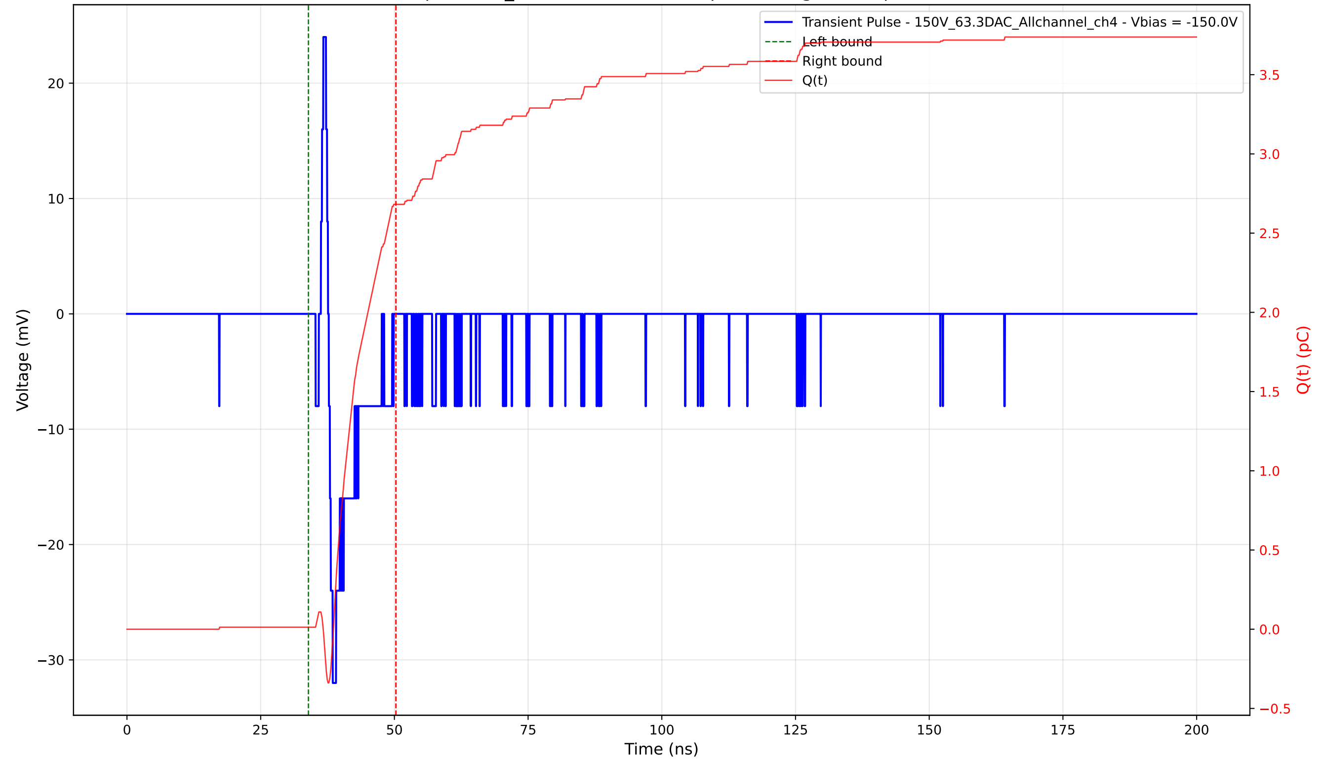
Transient Pulse - Sample: 1cm_42 - Position: 4040.0 \mu\text{m} - Charge: 2.67 pC - Rise Time: 0.74 ns
