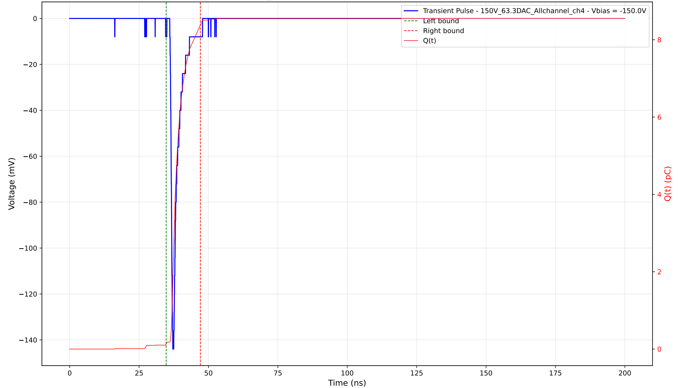
Transient Pulse - Sample: 1cm_42 - Position: 2720.0 \mu\text{m} - Charge: 8.24 pC - Rise Time: 0.85 ns
