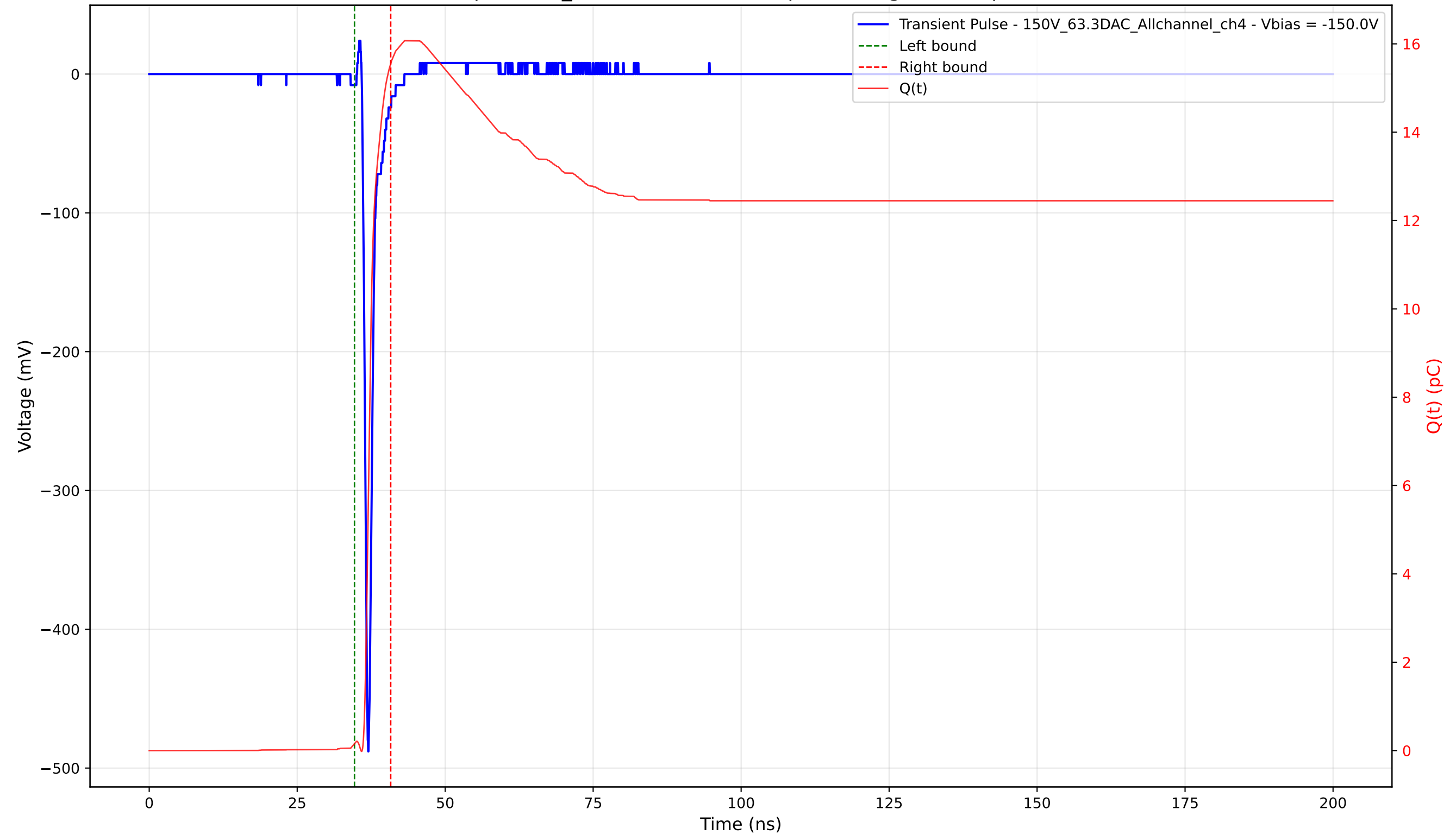
Transient Pulse - Sample: 1cm_42 - Position: 2285.0 \mu\text{m} - Charge: 15.40 pC - Rise Time: 0.69 ns
