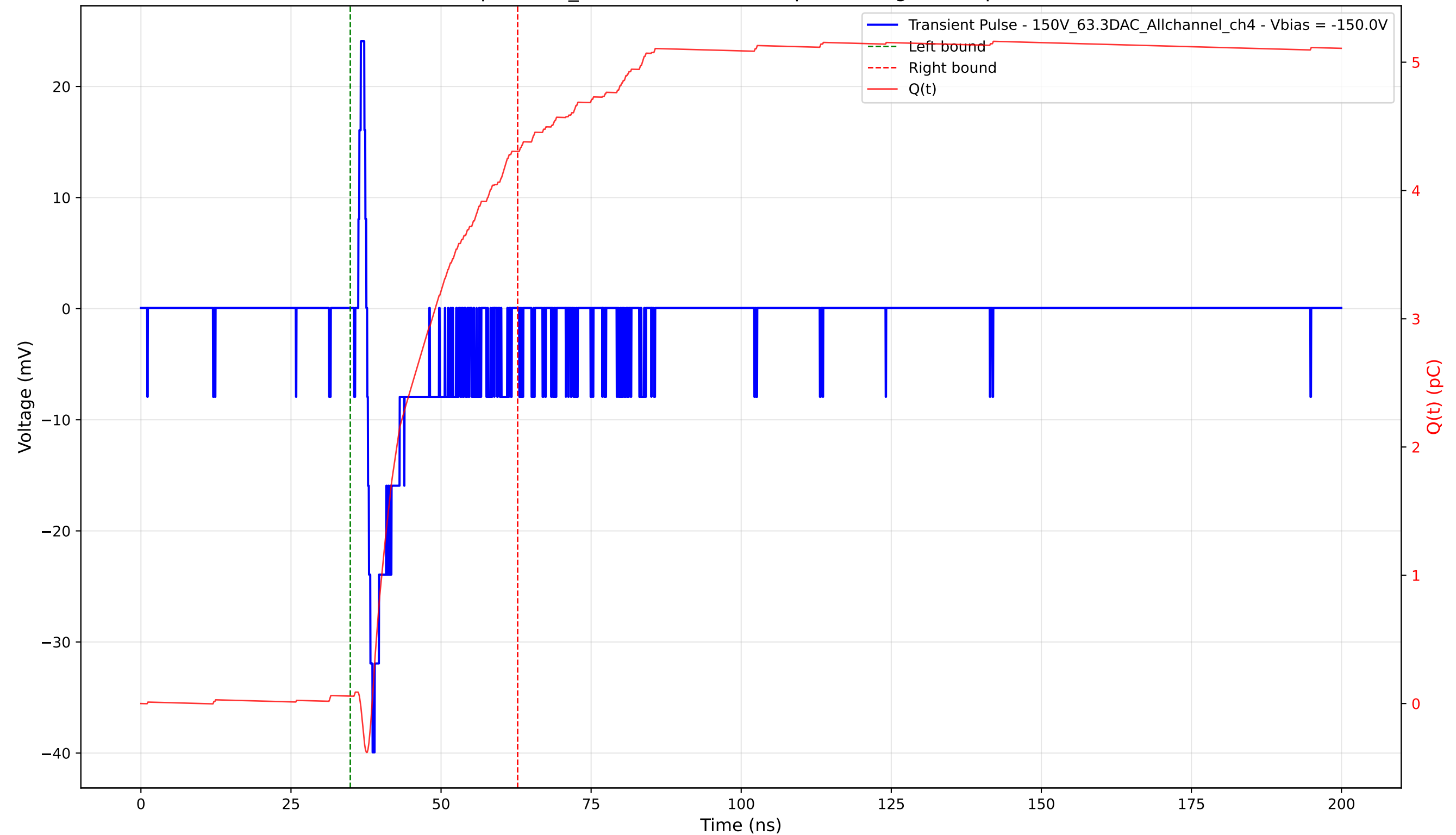
Transient Pulse - Sample: 1cm_42 - Position: 3785.0 \mu\text{m} - Charge: 4.25 pC - Rise Time: 0.90 ns
