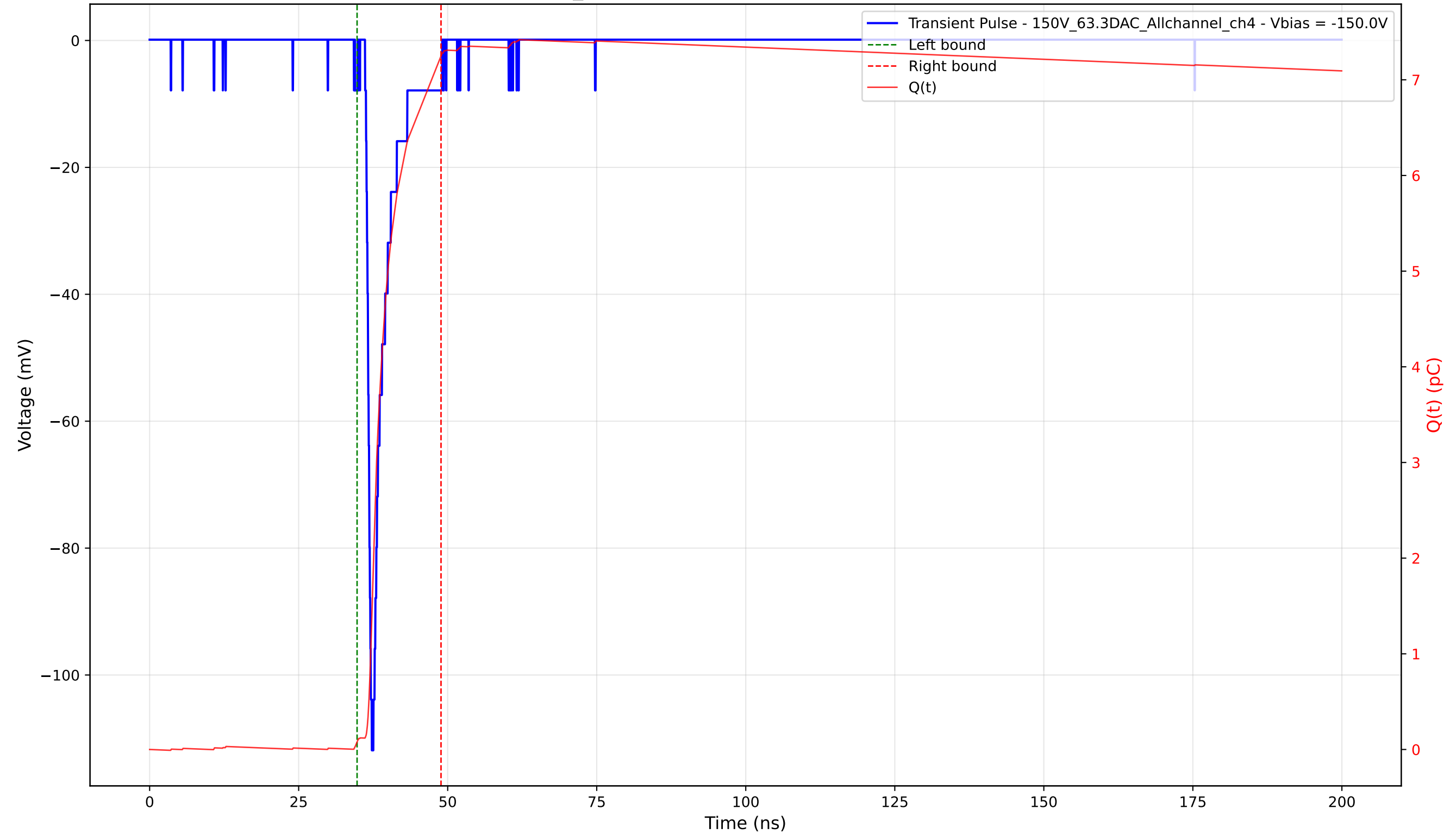
Transient Pulse - Sample: 1cm_42 - Position: 2870.0 \mu\text{m} - Charge: 7.17 pC - Rise Time: 0.82 ns
