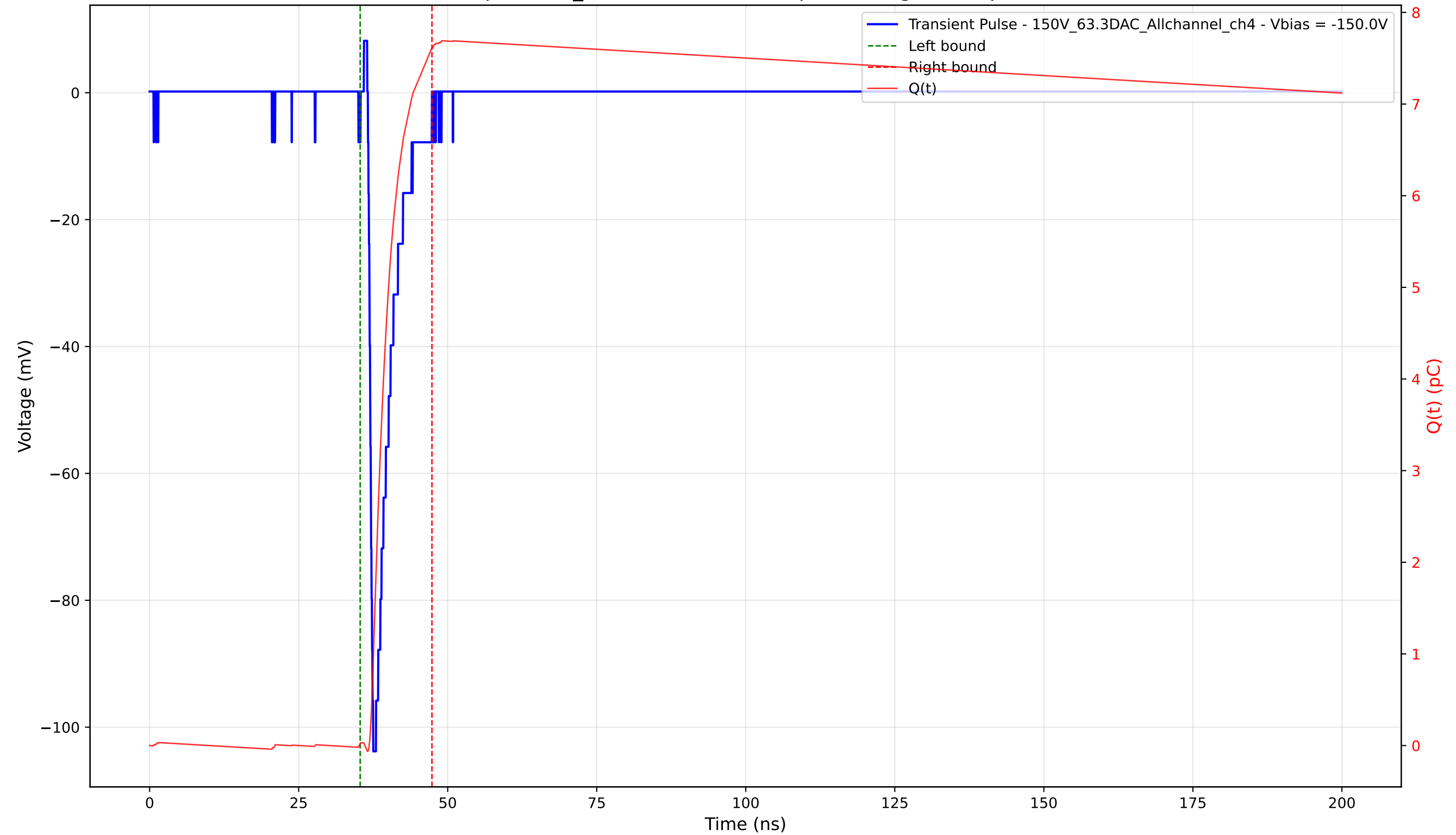
Transient Pulse - Sample: 1cm_42 - Position: 1035.0 \mu\text{m} - Charge: 7.59 pC - Rise Time: 0.71 ns
