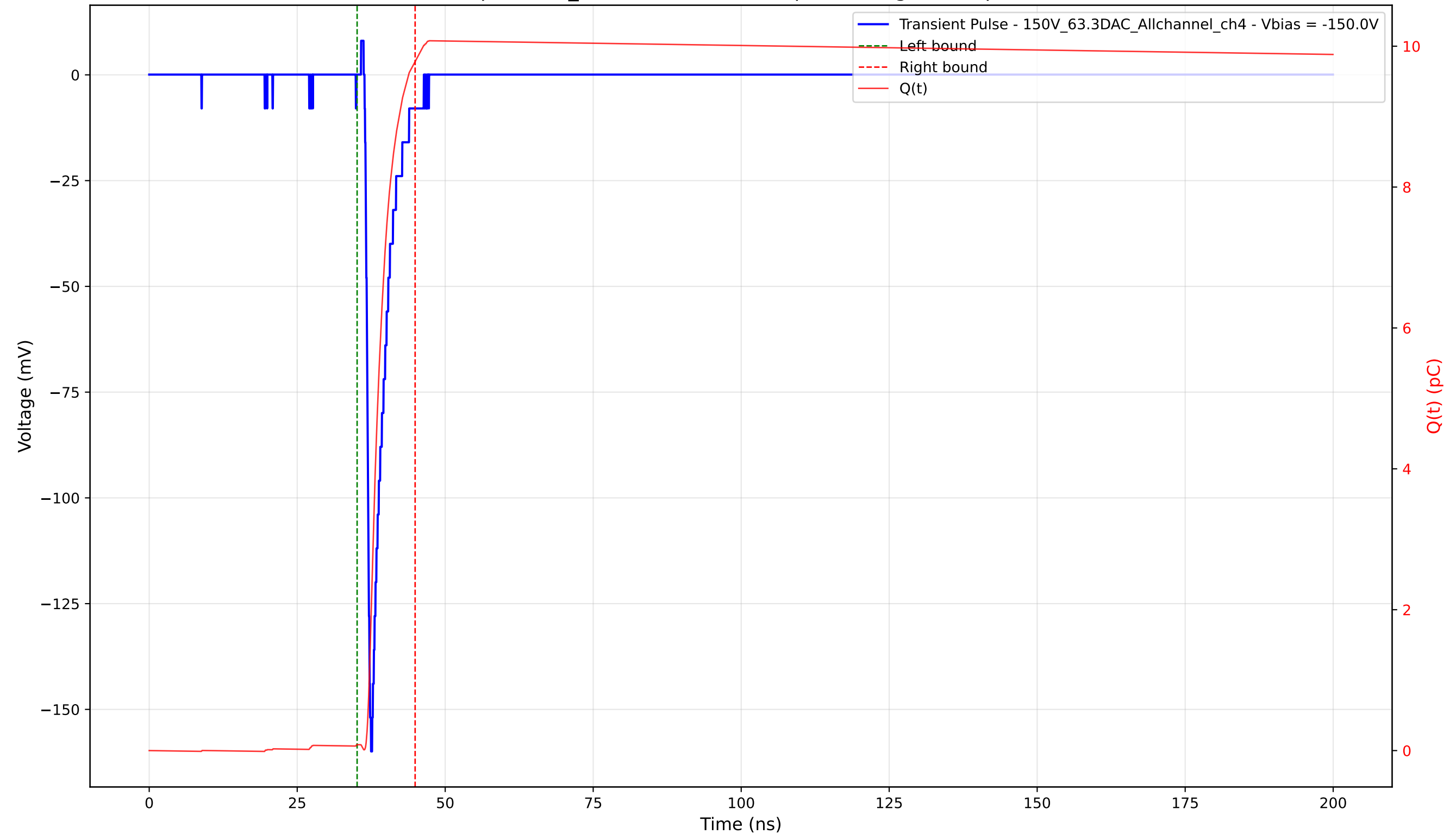
Transient Pulse - Sample: 1cm_42 - Position: 1175.0 \mu\text{m} - Charge: 9.70 pC - Rise Time: 0.80 ns
