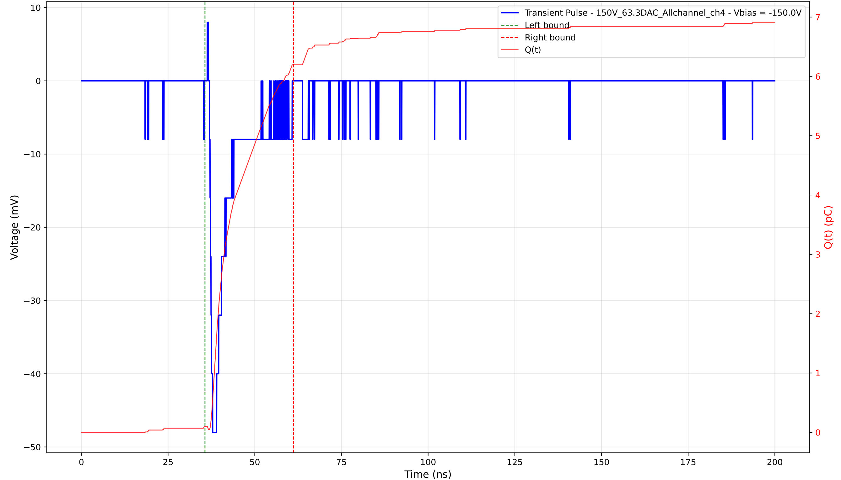
Transient Pulse - Sample: 1cm_42 - Position: 3220.0 \mu\text{m} - Charge: 6.09 pC - Rise Time: 0.94 ns
