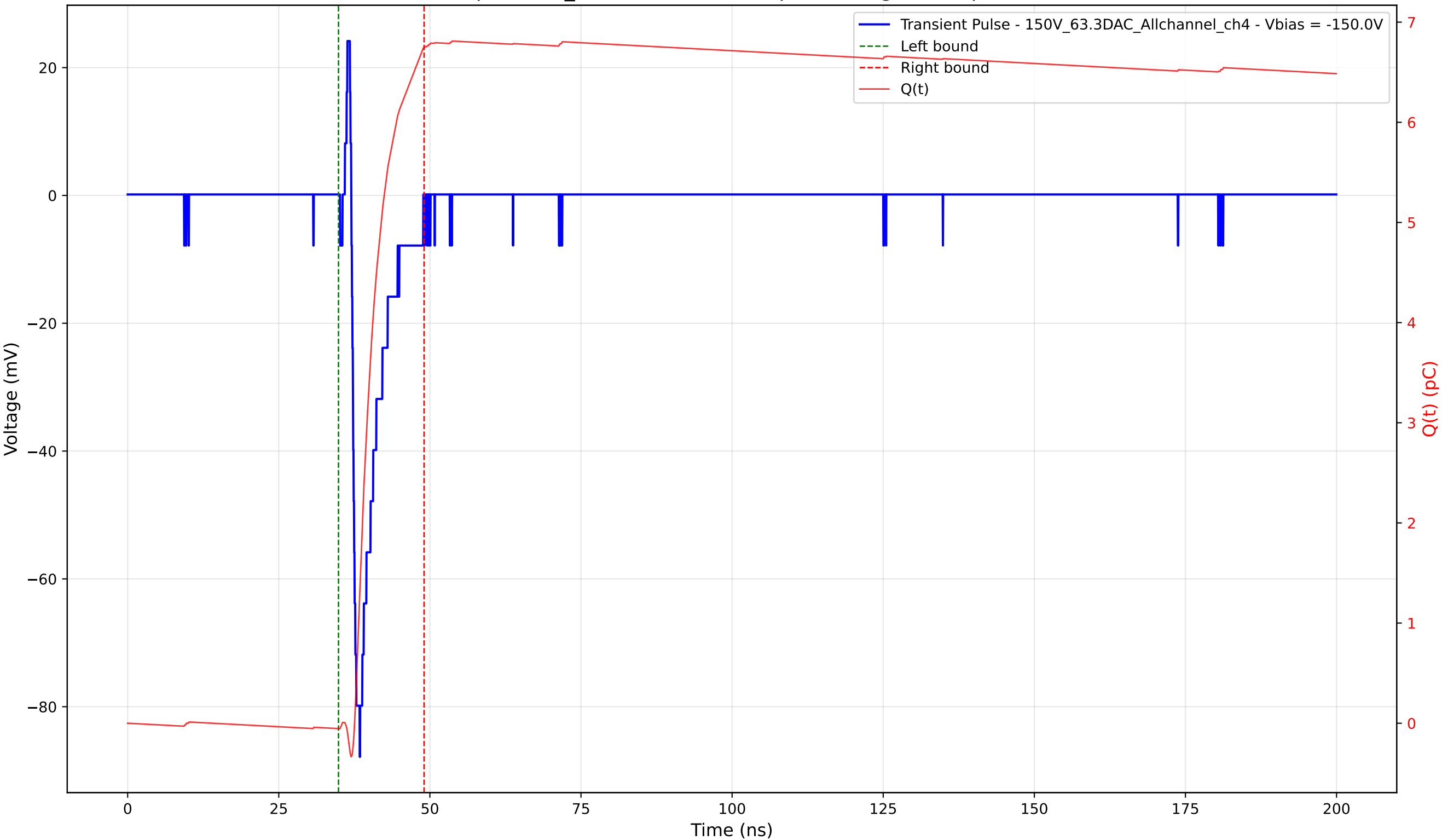
Transient Pulse - Sample: 1cm_42 - Position: 720.0 \mu\text{m} - Charge: 6.80 pC - Rise Time: 0.76 ns
