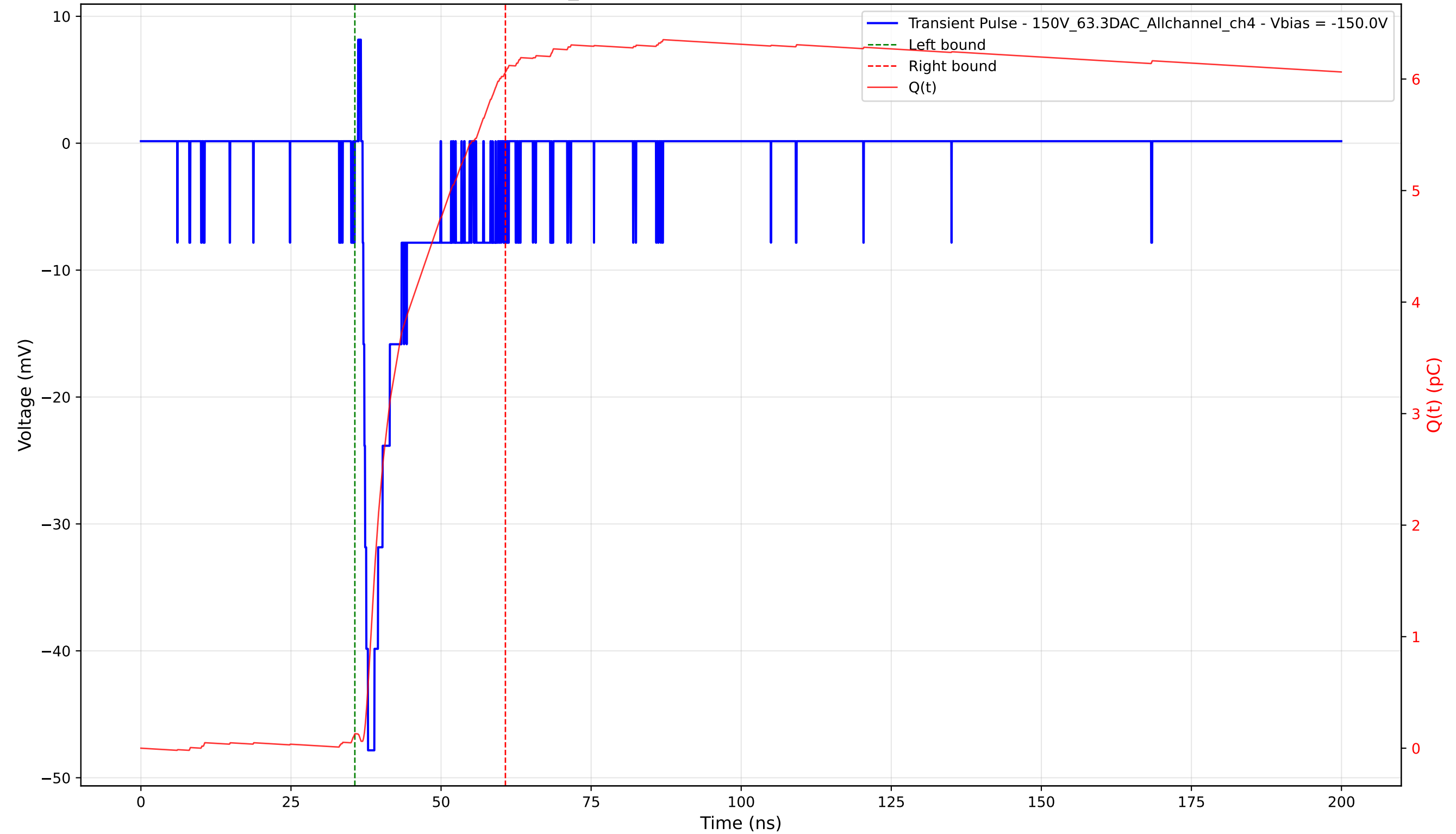
Transient Pulse - Sample: 1cm_42 - Position: 3205.0 \mu\text{m} - Charge: 5.93 pC - Rise Time: 0.90 ns
