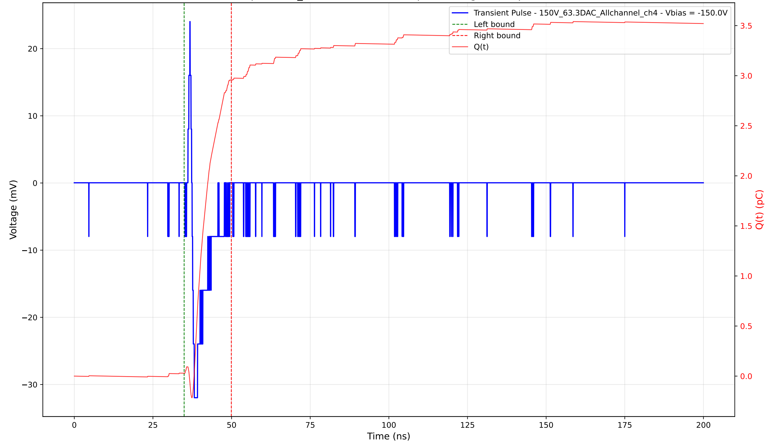
Transient Pulse - Sample: 1cm_42 - Position: 4870.0 \mu\text{m} - Charge: 2.93 pC - Rise Time: 0.70 ns
