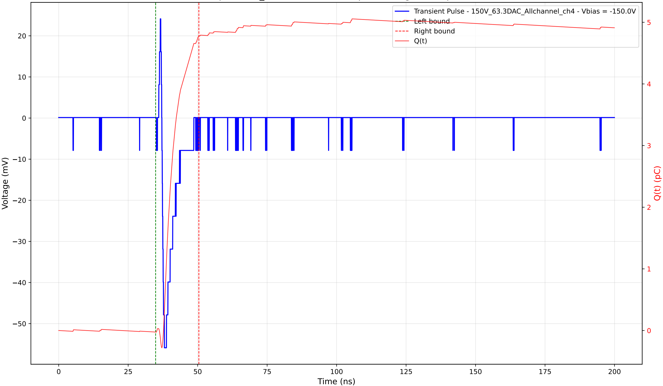
Transient Pulse - Sample: 1cm_42 - Position: 520.0 \mu\text{m} - Charge: 4.80 pC - Rise Time: 0.89 ns
