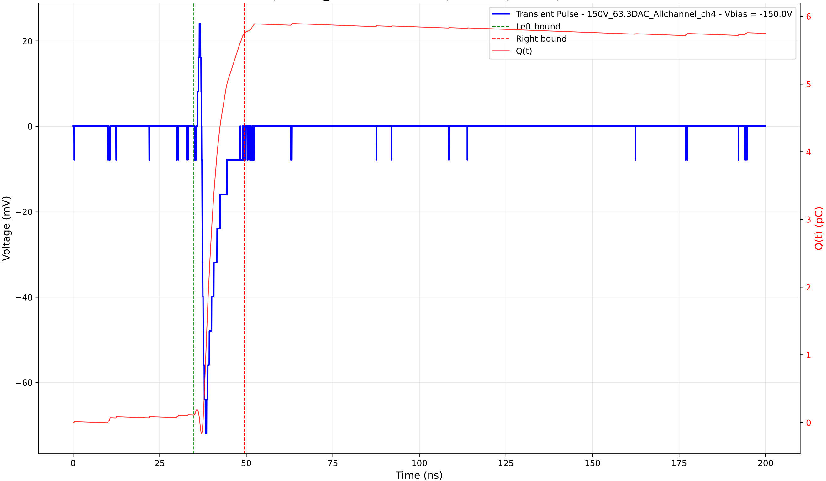
Transient Pulse - Sample: 1cm_42 - Position: 610.0 \mu\text{m} - Charge: 5.64 pC - Rise Time: 1.04 ns
