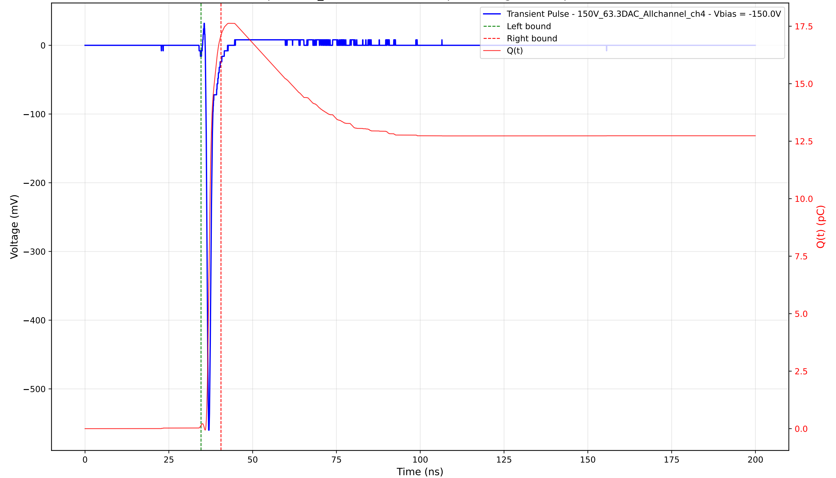
Transient Pulse - Sample: 1cm_42 - Position: 2110.0 \mu\text{m} - Charge: 16.96 pC - Rise Time: 0.71 ns
