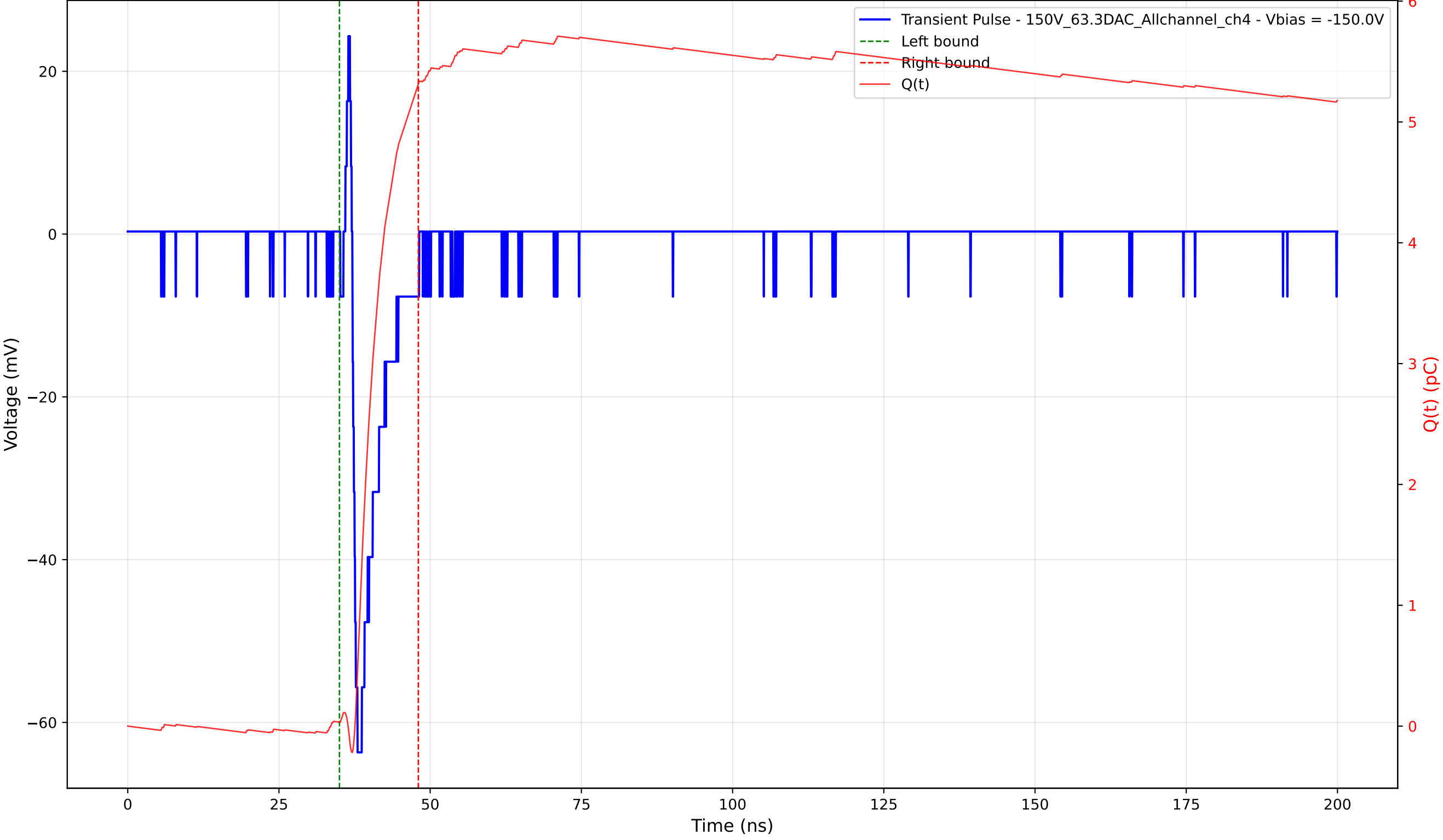
Transient Pulse - Sample: 1cm_42 - Position: 585.0 \mu\text{m} - Charge: 5.28 pC - Rise Time: 0.85 ns
