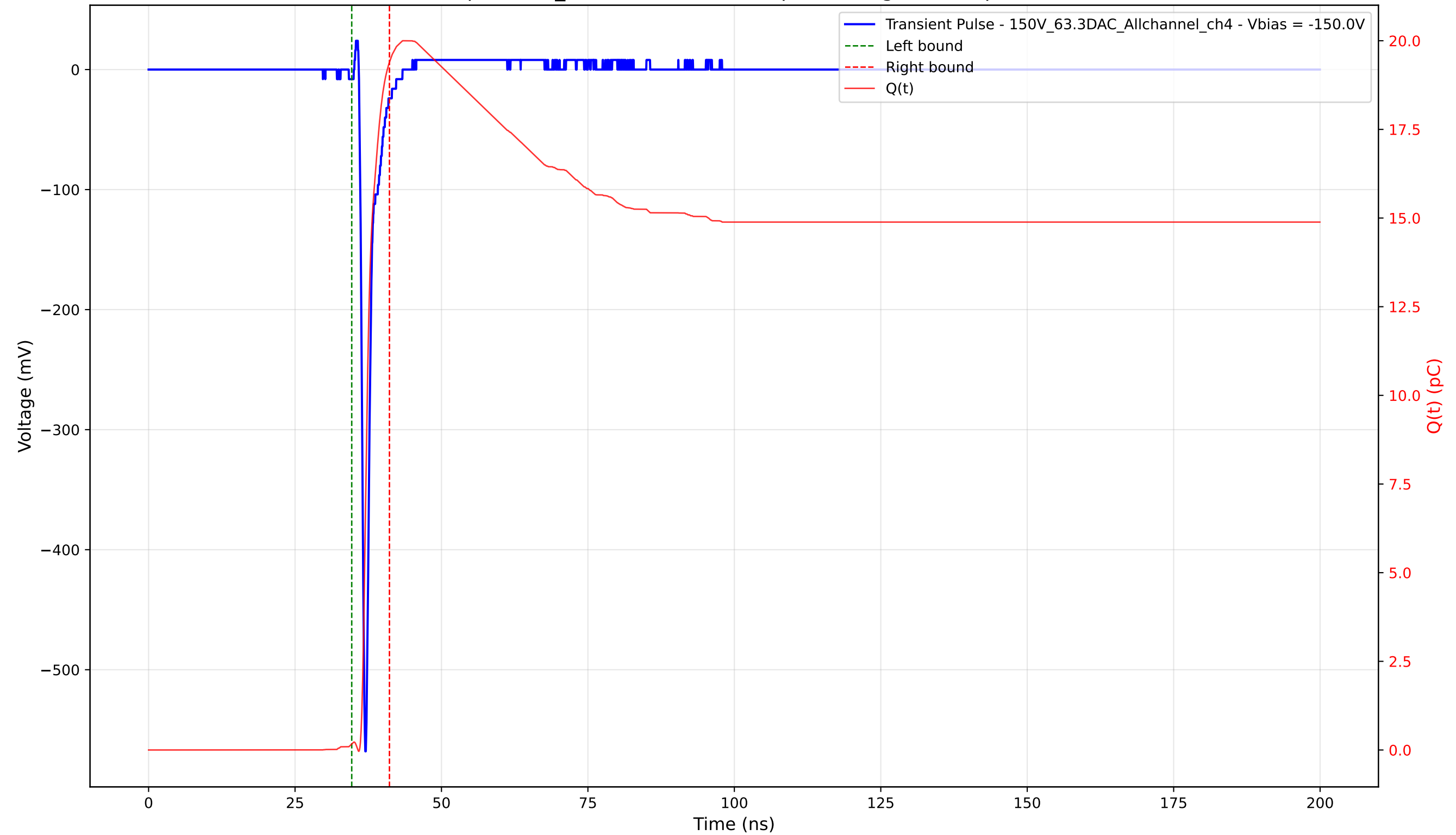
Transient Pulse - Sample: 1cm_42 - Position: 1740.0 \mu\text{m} - Charge: 19.23 pC - Rise Time: 0.74 ns
