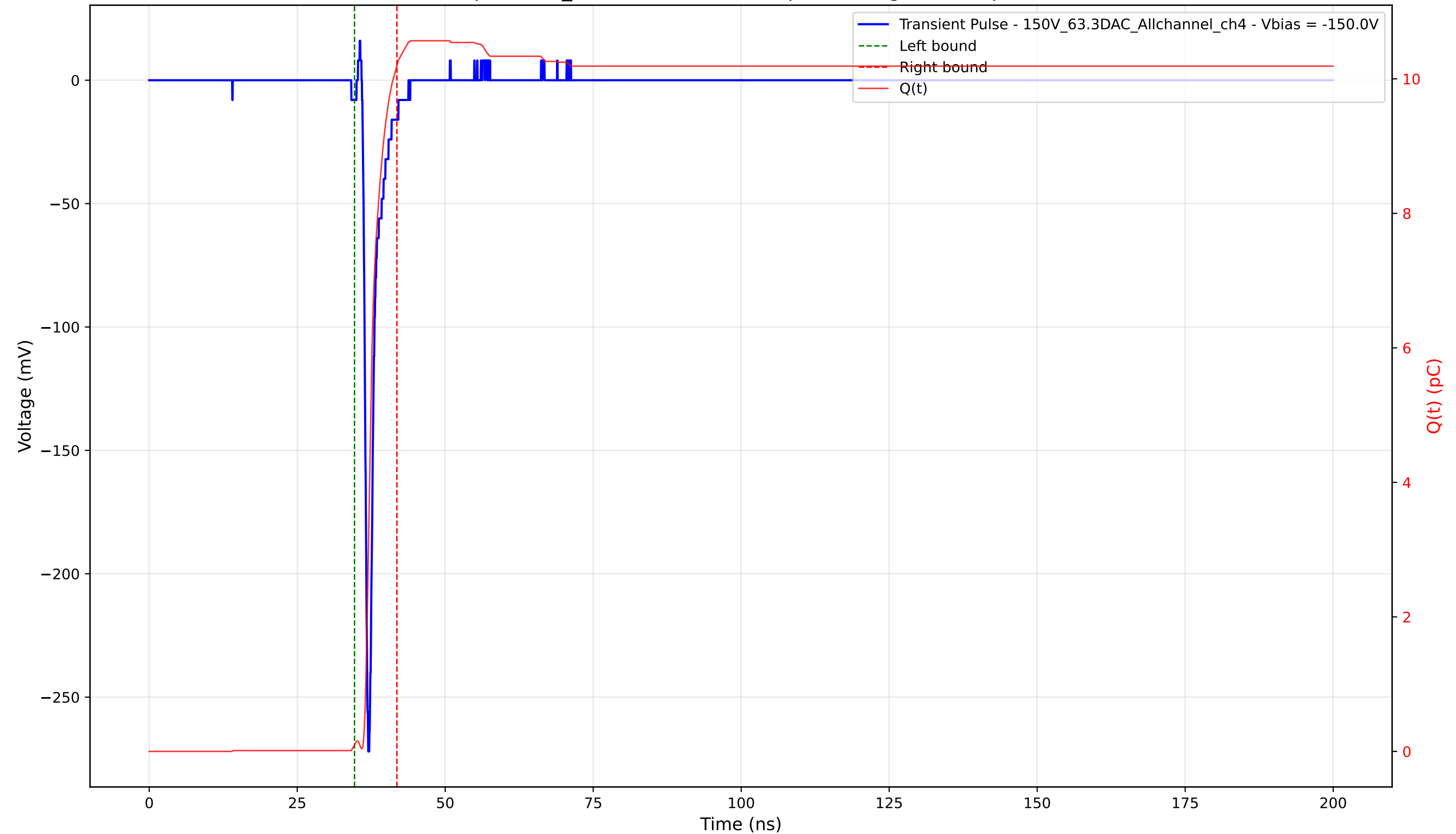
Transient Pulse - Sample: 1cm_42 - Position: 2480.0 \mu\text{m} - Charge: 10.10 pC - Rise Time: 0.73 ns
