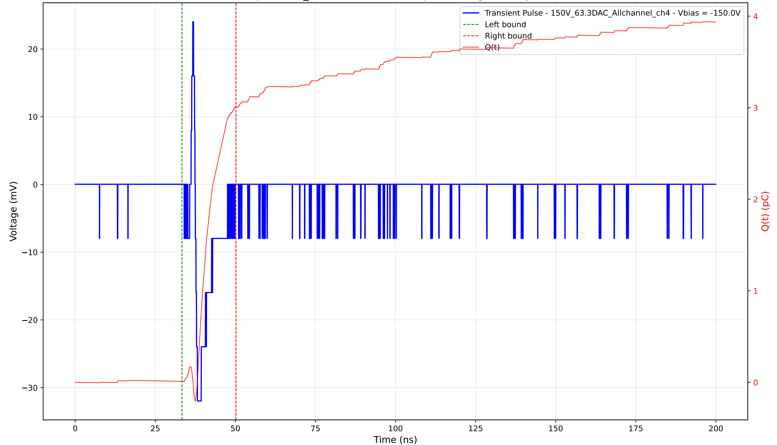
Transient Pulse - Sample: 1cm_42 - Position: 4725.0 \mu\text{m} - Charge: 3.00 pC - Rise Time: 0.66 ns
