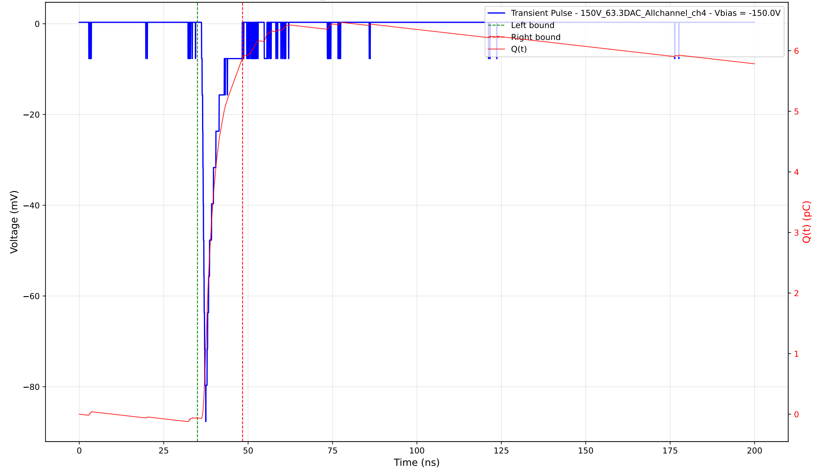
Transient Pulse - Sample: 1cm_42 - Position: 2950.0 \mu\text{m} - Charge: 5.94 pC - Rise Time: 0.83 ns
