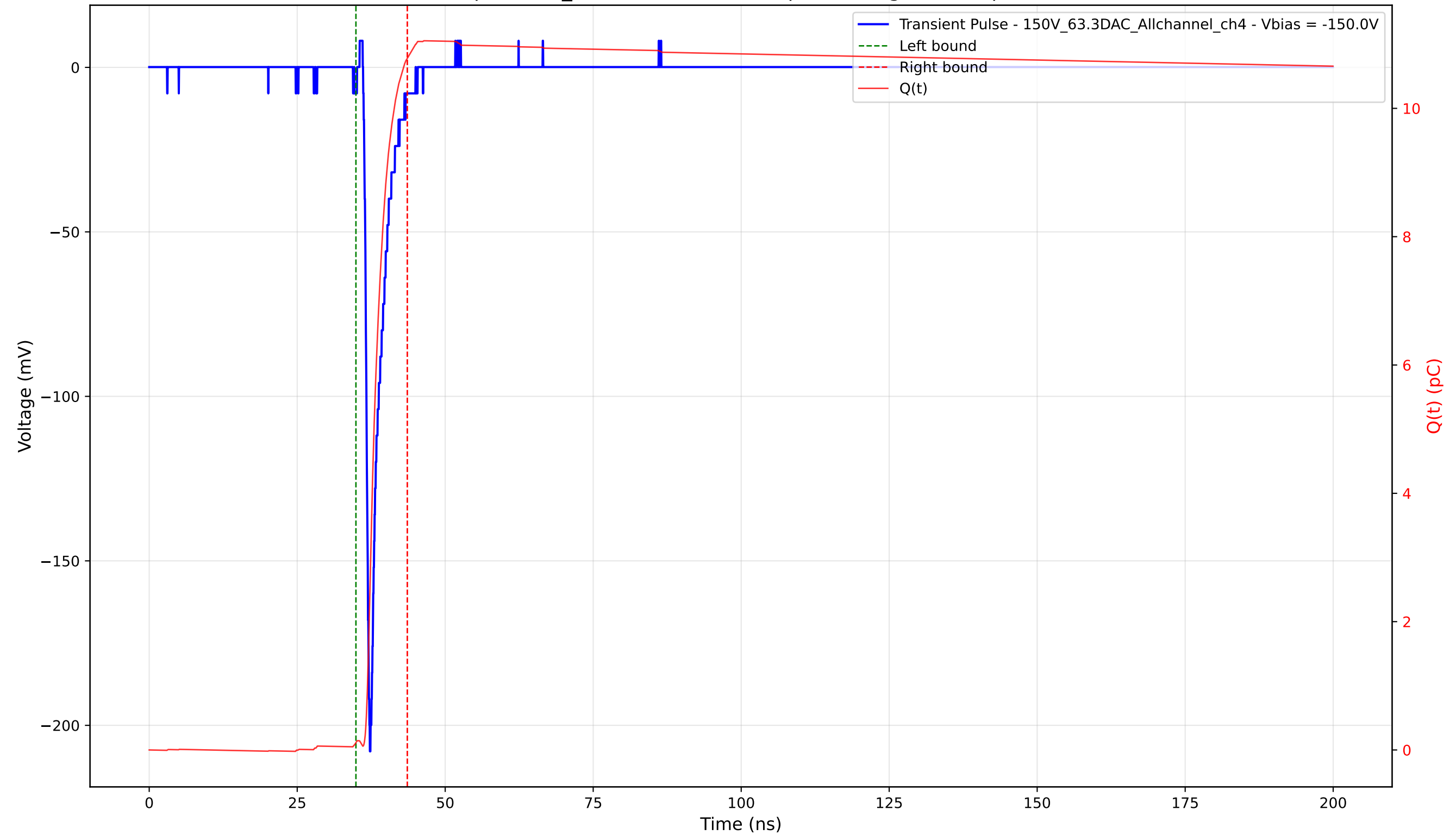
Transient Pulse - Sample: 1cm_42 - Position: 1400.0 \mu\text{m} - Charge: 10.67 pC - Rise Time: 0.82 ns
