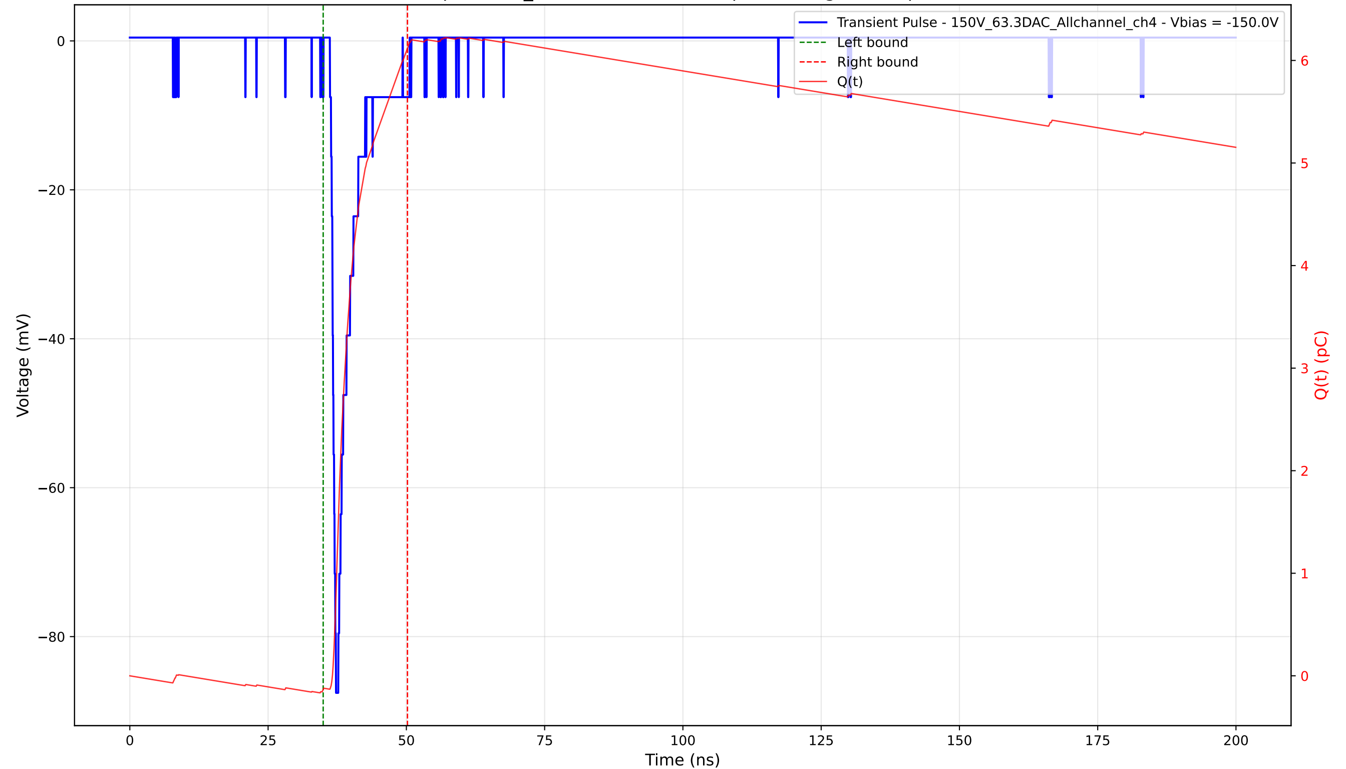
Transient Pulse - Sample: 1cm_42 - Position: 2935.0 \mu\text{m} - Charge: 6.25 pC - Rise Time: 0.79 ns
