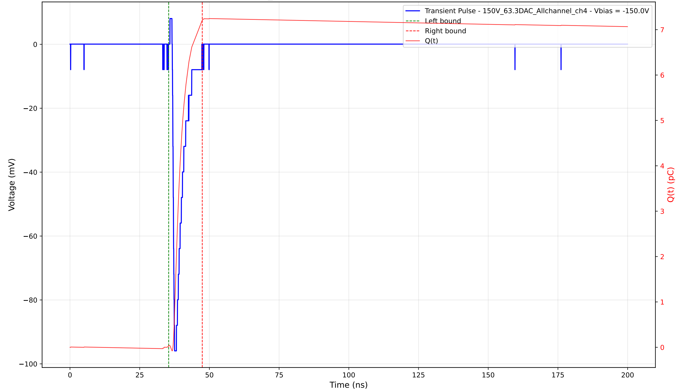
Transient Pulse - Sample: 1cm_42 - Position: 1010.0 \mu\text{m} - Charge: 7.17 pC - Rise Time: 0.63 ns
