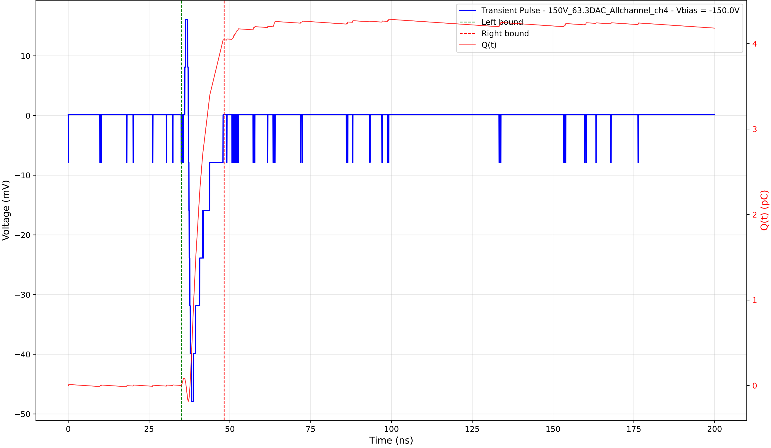
Transient Pulse - Sample: 1cm_42 - Position: 435.0 \mu\text{m} - Charge: 4.03 pC - Rise Time: 0.94 ns
