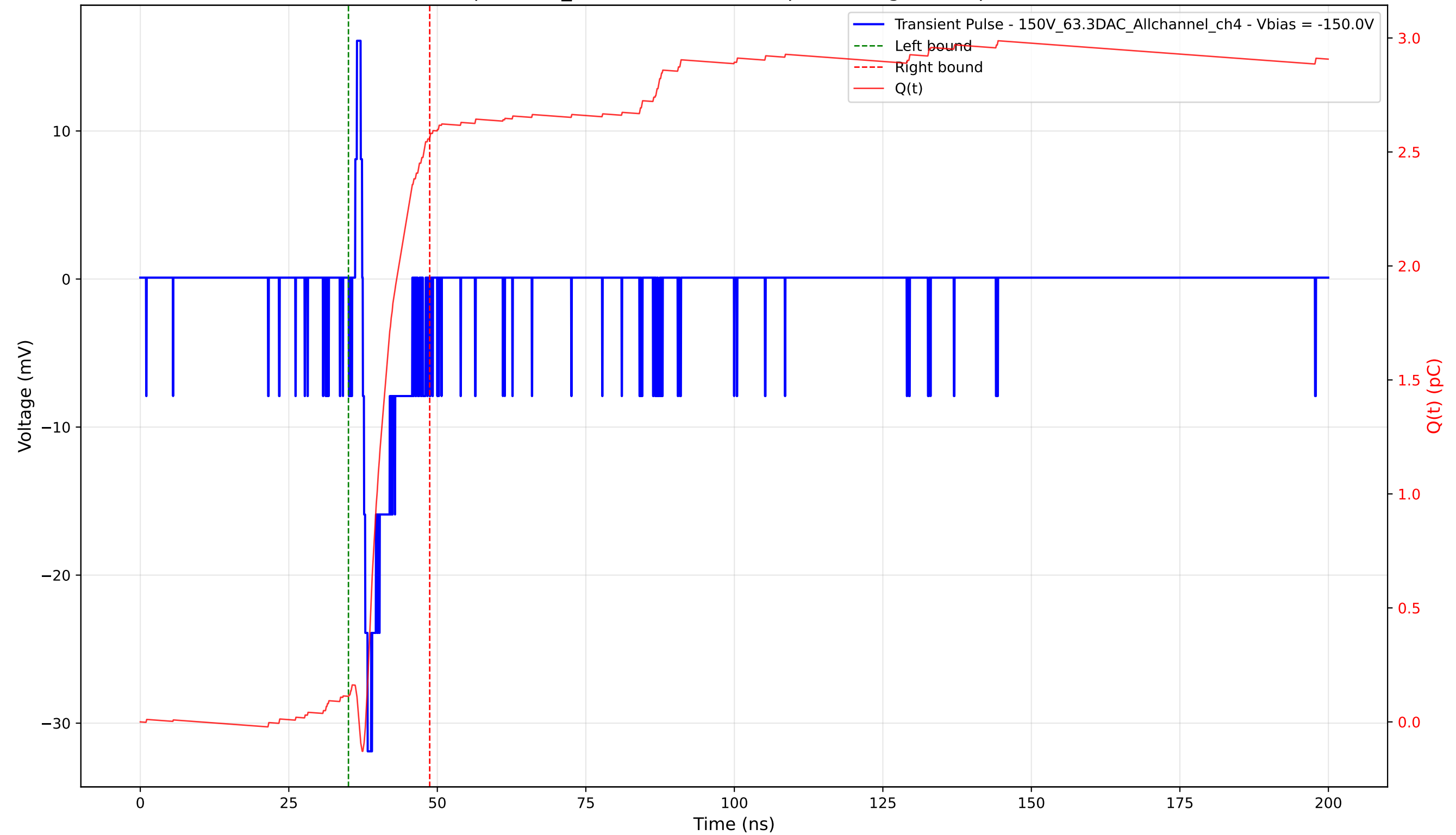
Transient Pulse - Sample: 1cm_42 - Position: 4905.0 \mu\text{m} - Charge: 2.45 pC - Rise Time: 0.82 ns
