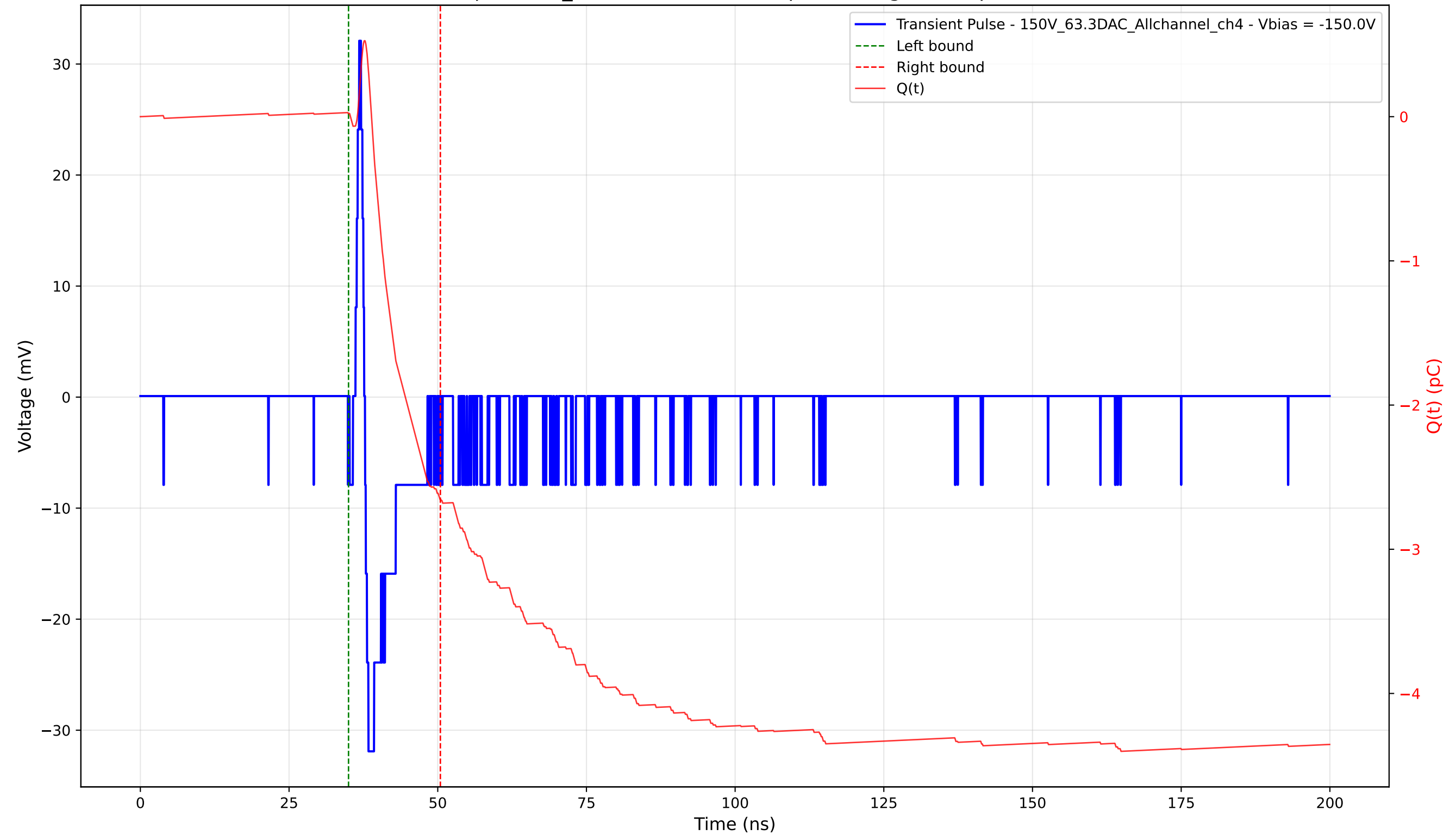
Transient Pulse - Sample: 1cm_42 - Position: 4335.0 \mu\text{m} - Charge: 2.68 pC - Rise Time: 0.62 ns
