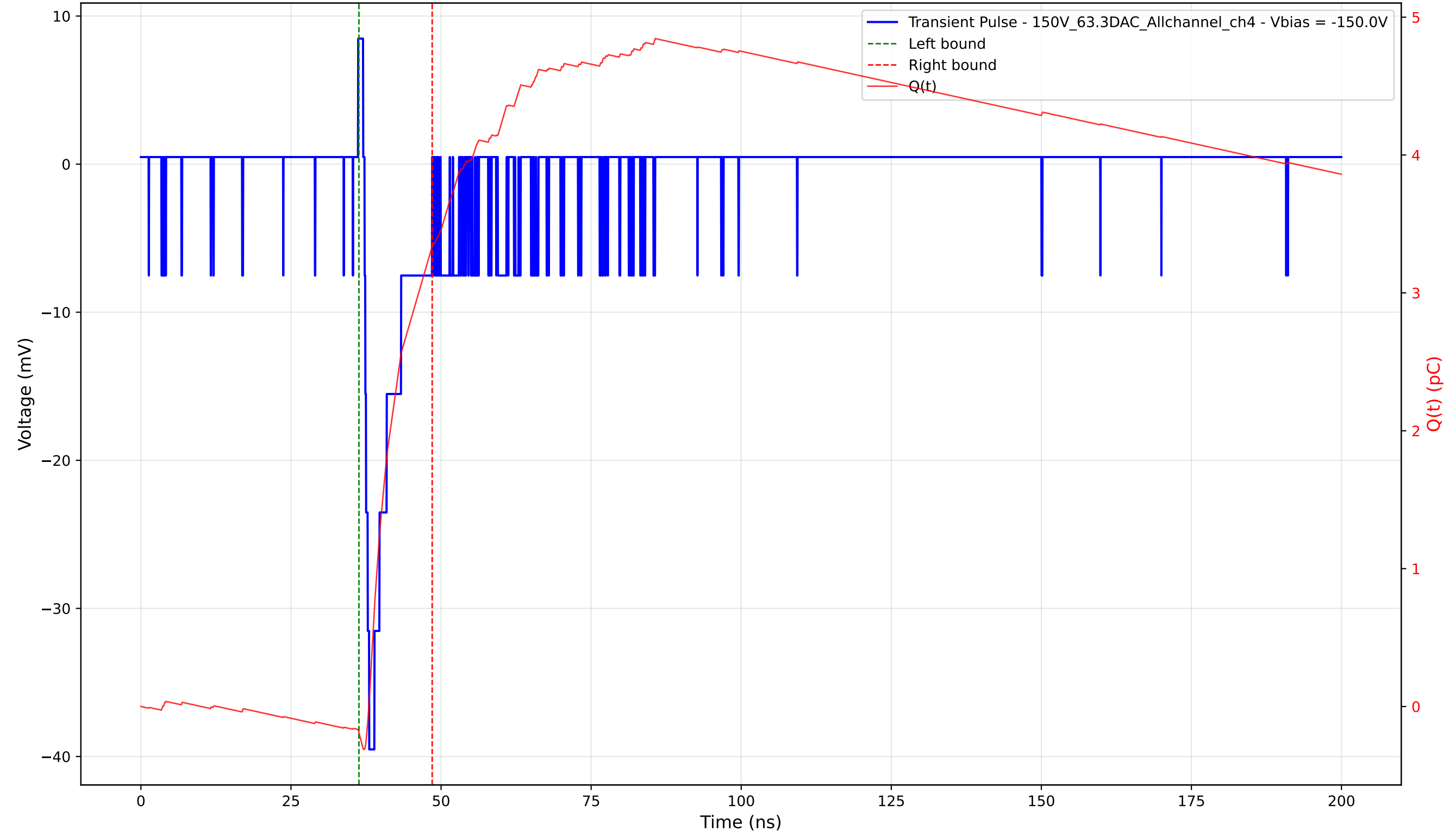
Transient Pulse - Sample: 1cm_42 - Position: 3435.0 \mu\text{m} - Charge: 3.53 pC - Rise Time: 0.78 ns
