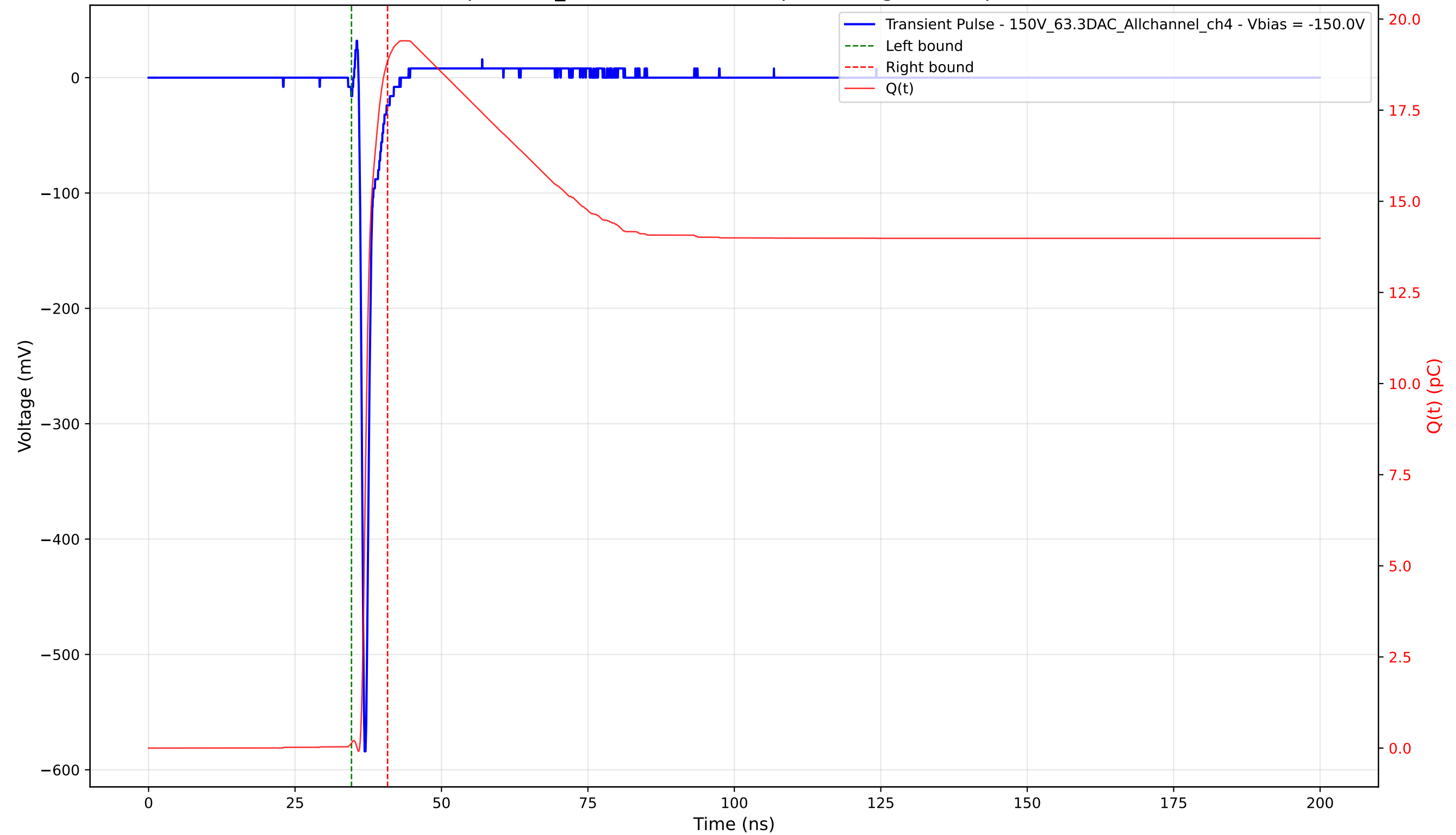
Transient Pulse - Sample: 1cm_42 - Position: 1880.0 \mu\text{m} - Charge: 18.70 pC - Rise Time: 0.70 ns
