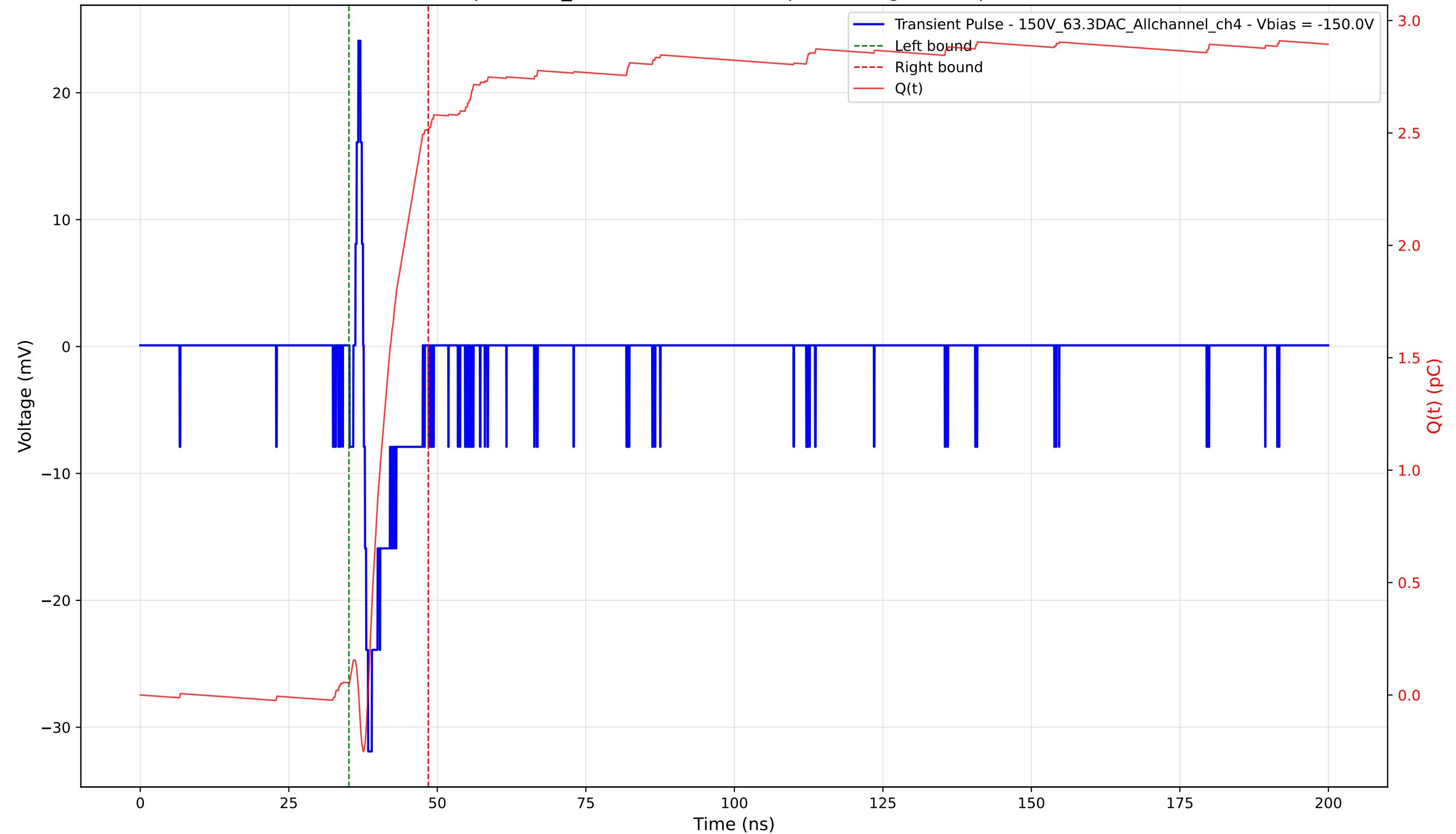
Transient Pulse - Sample: 1cm_42 - Position: 4620.0 \mu\text{m} - Charge: 2.46 pC - Rise Time: 0.74 ns
