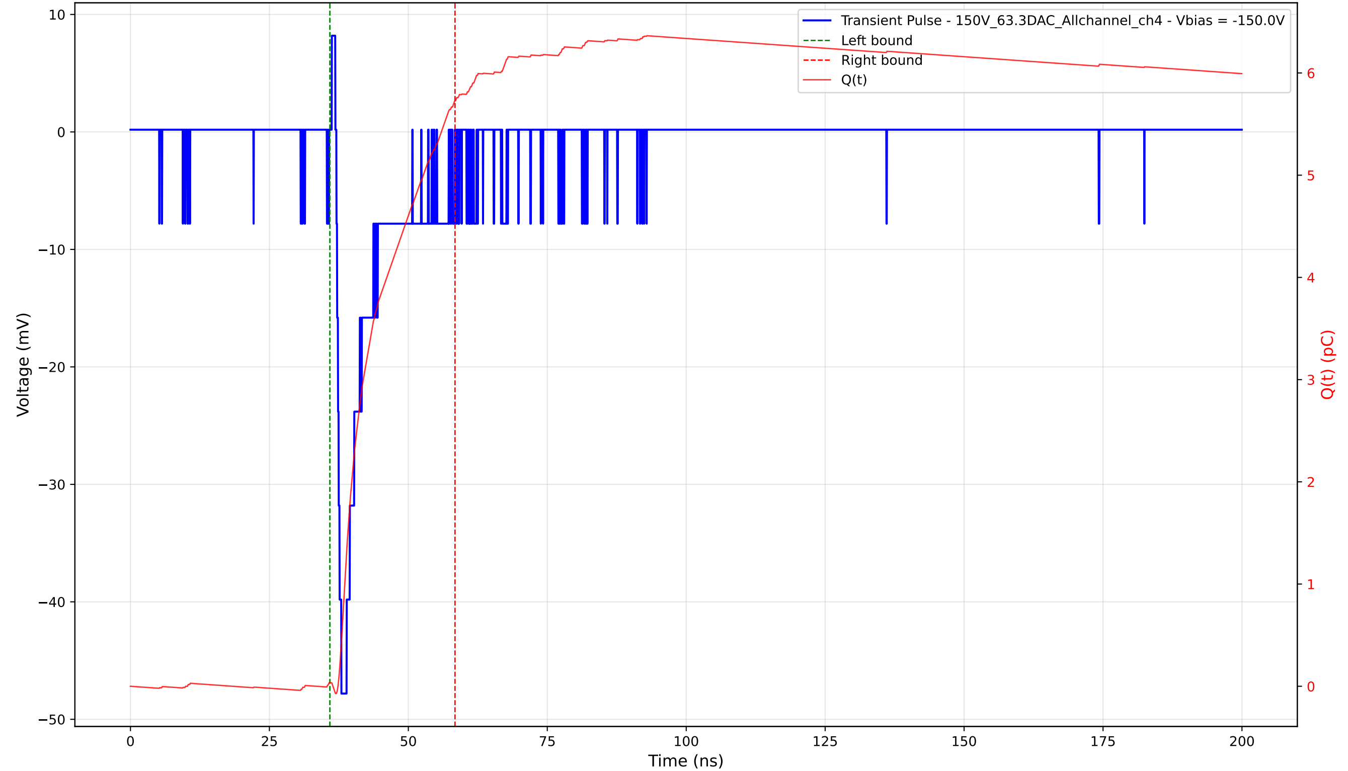
Transient Pulse - Sample: 1cm_42 - Position: 3310.0 \mu\text{m} - Charge: 5.69 pC - Rise Time: 0.90 ns
