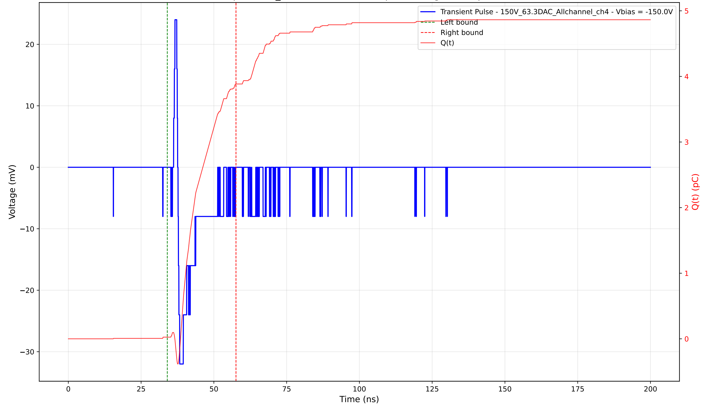
Transient Pulse - Sample: 1cm_42 - Position: 3855.0 \mu\text{m} - Charge: 3.86 pC - Rise Time: 0.58 ns
