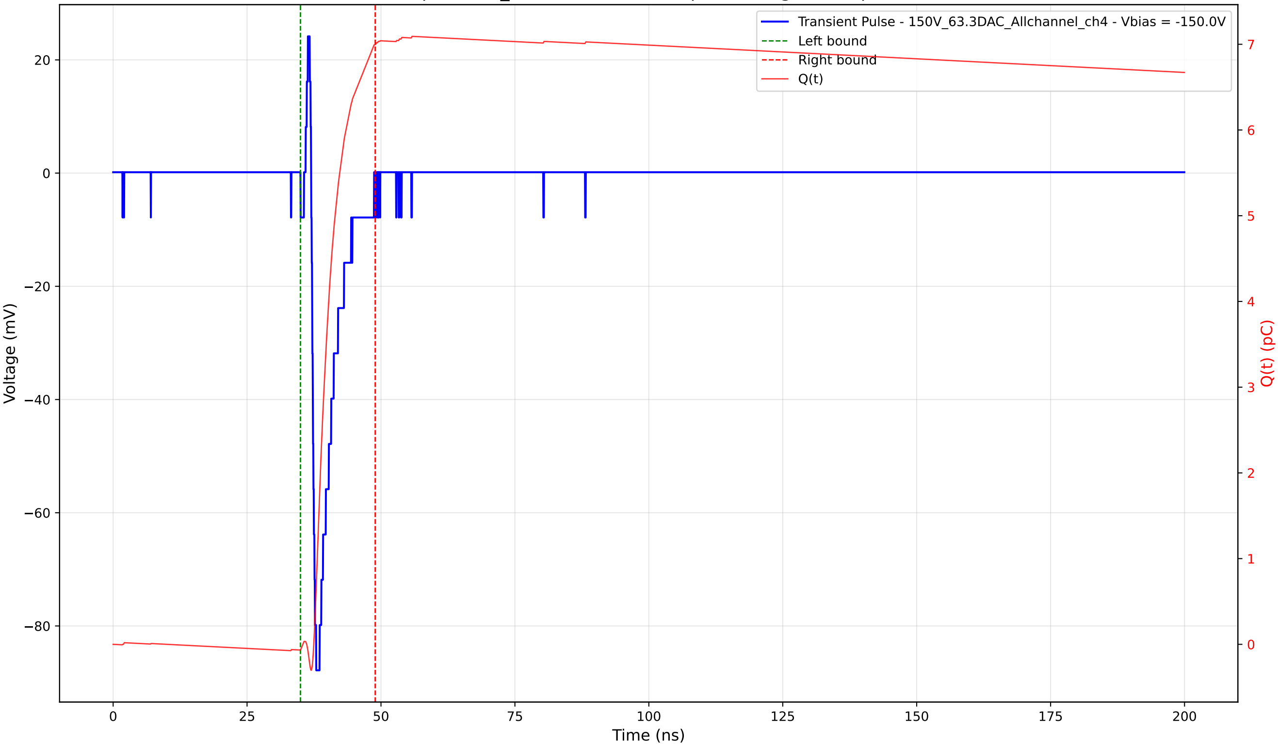
Transient Pulse - Sample: 1cm_42 - Position: 795.0 \mu\text{m} - Charge: 7.07 pC - Rise Time: 0.64 ns
