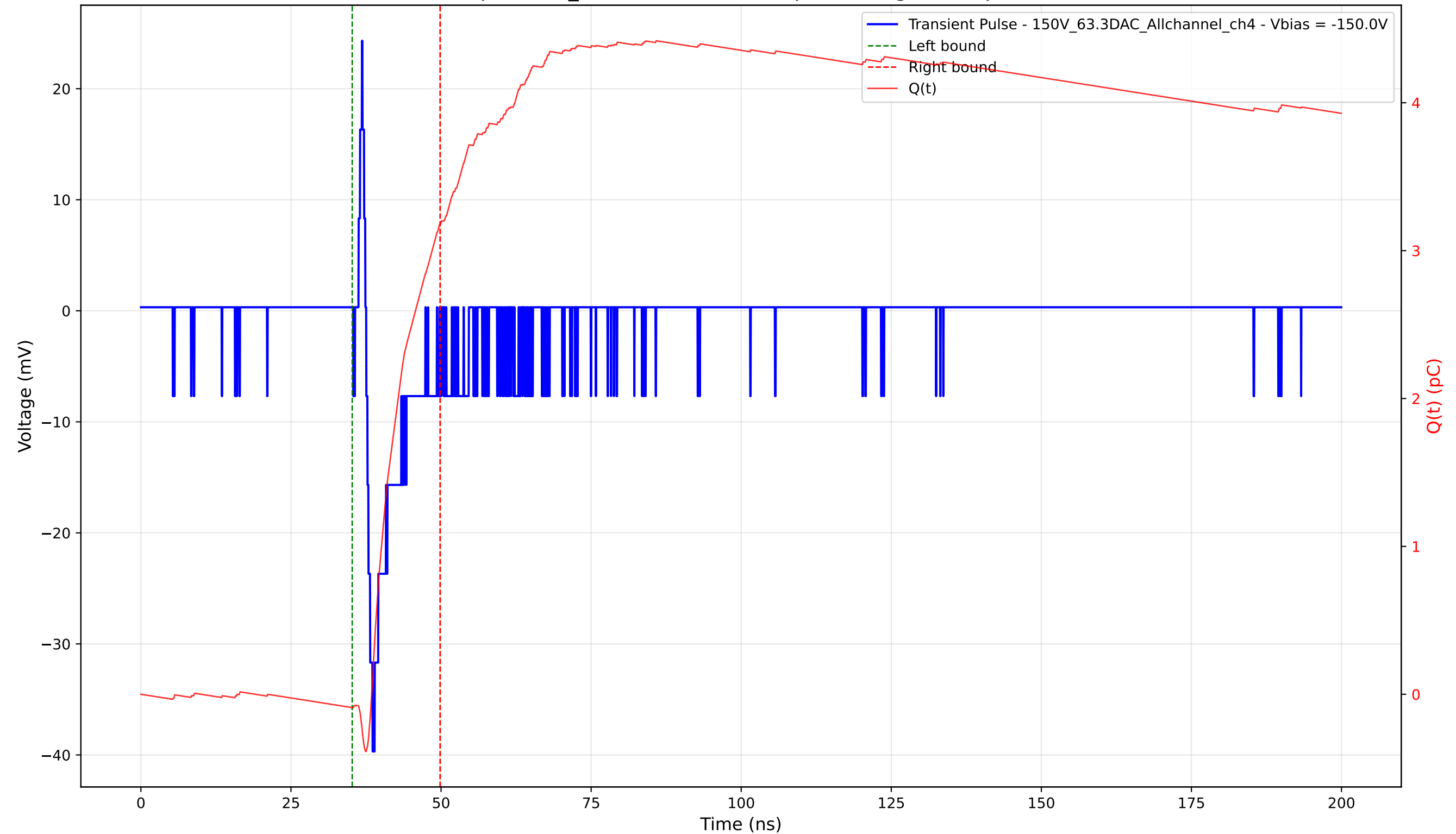
Transient Pulse - Sample: 1cm_42 - Position: 3615.0 \mu\text{m} - Charge: 3.27 pC - Rise Time: 1.06 ns
