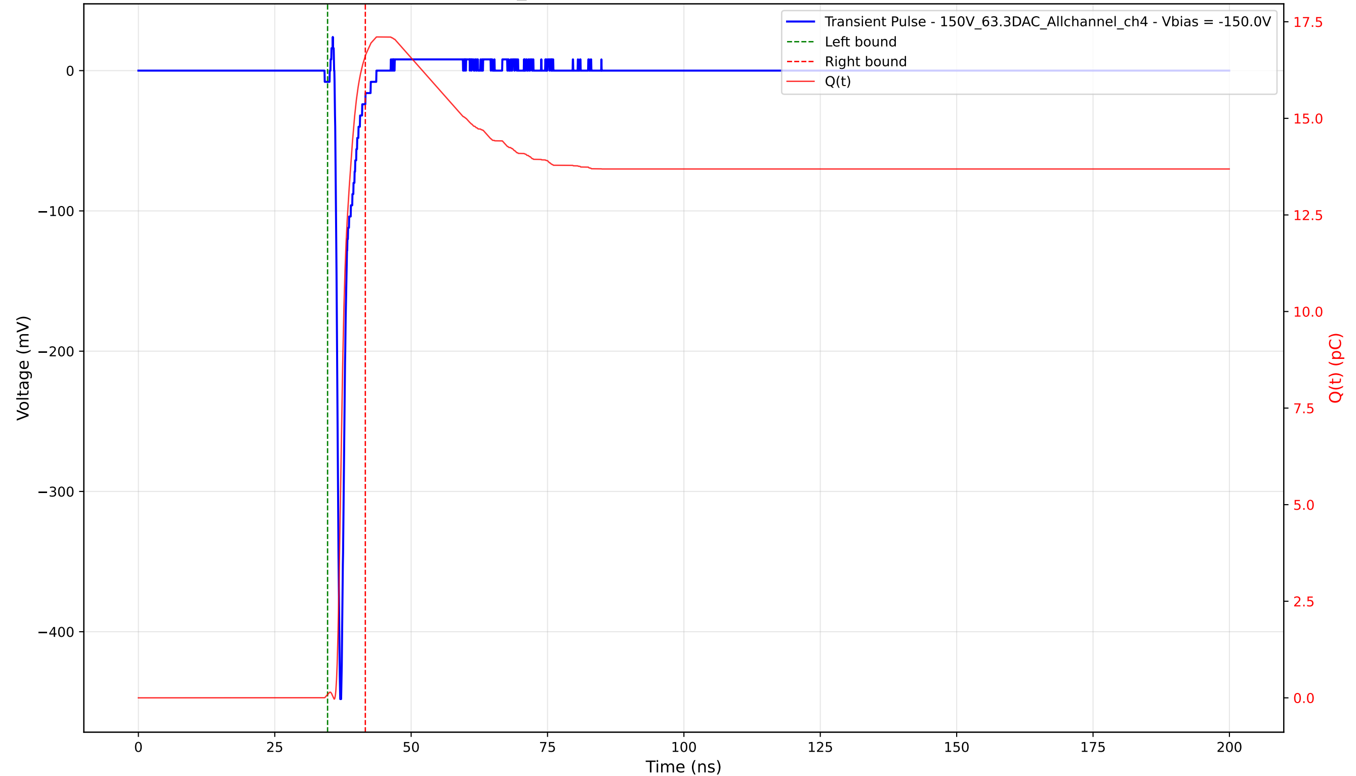
Transient Pulse - Sample: 1cm_42 - Position: 1655.0 \mu\text{m} - Charge: 16.54 pC - Rise Time: 0.74 ns
