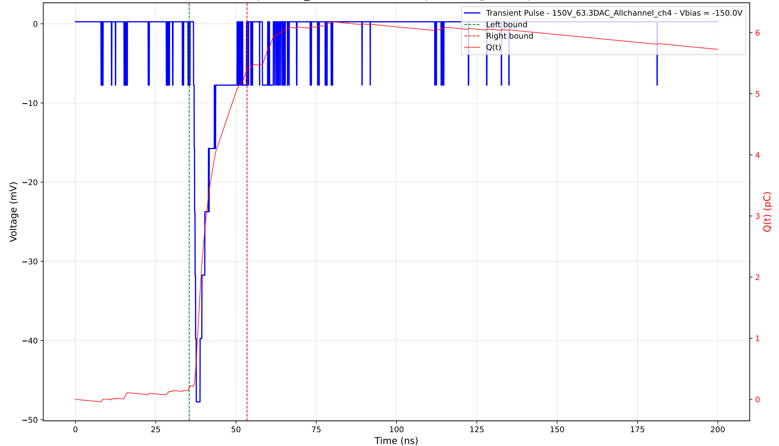
Transient Pulse - Sample: 1cm_42 - Position: 3160.0 \mu\text{m} - Charge: 5.20 pC - Rise Time: 0.86 ns
