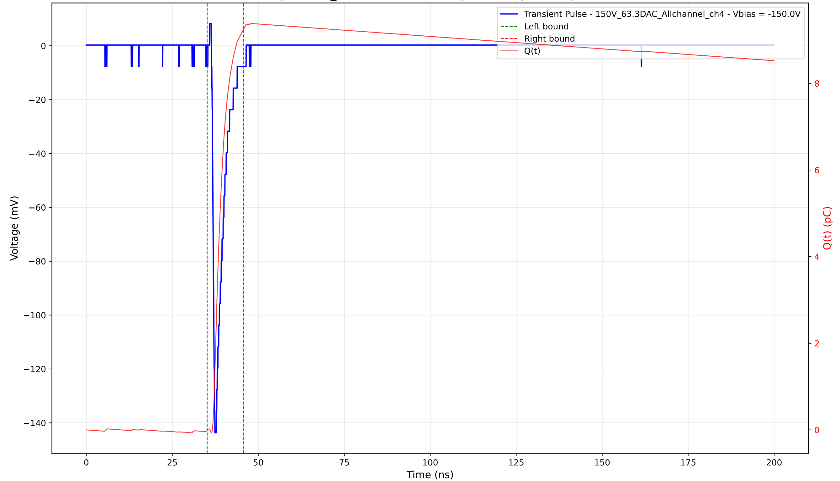
Transient Pulse - Sample: 1cm_42 - Position: 1155.0 \mu\text{m} - Charge: 9.25 pC - Rise Time: 0.77 ns
