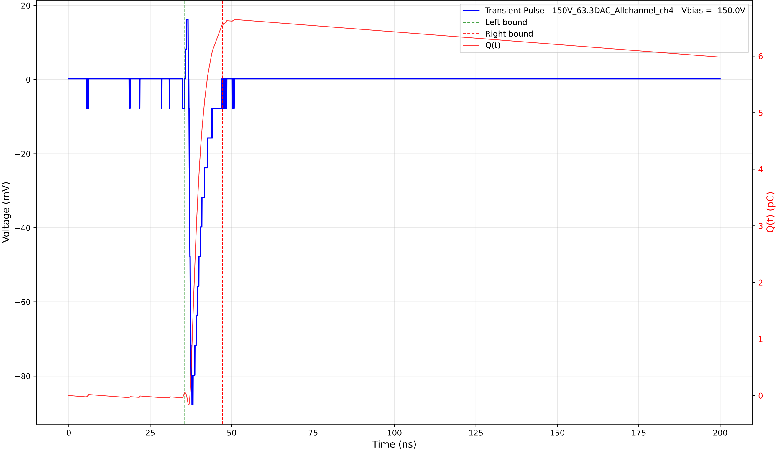
Transient Pulse - Sample: 1cm_42 - Position: 920.0 \mu\text{m} - Charge: 6.50 pC - Rise Time: 0.63 ns
