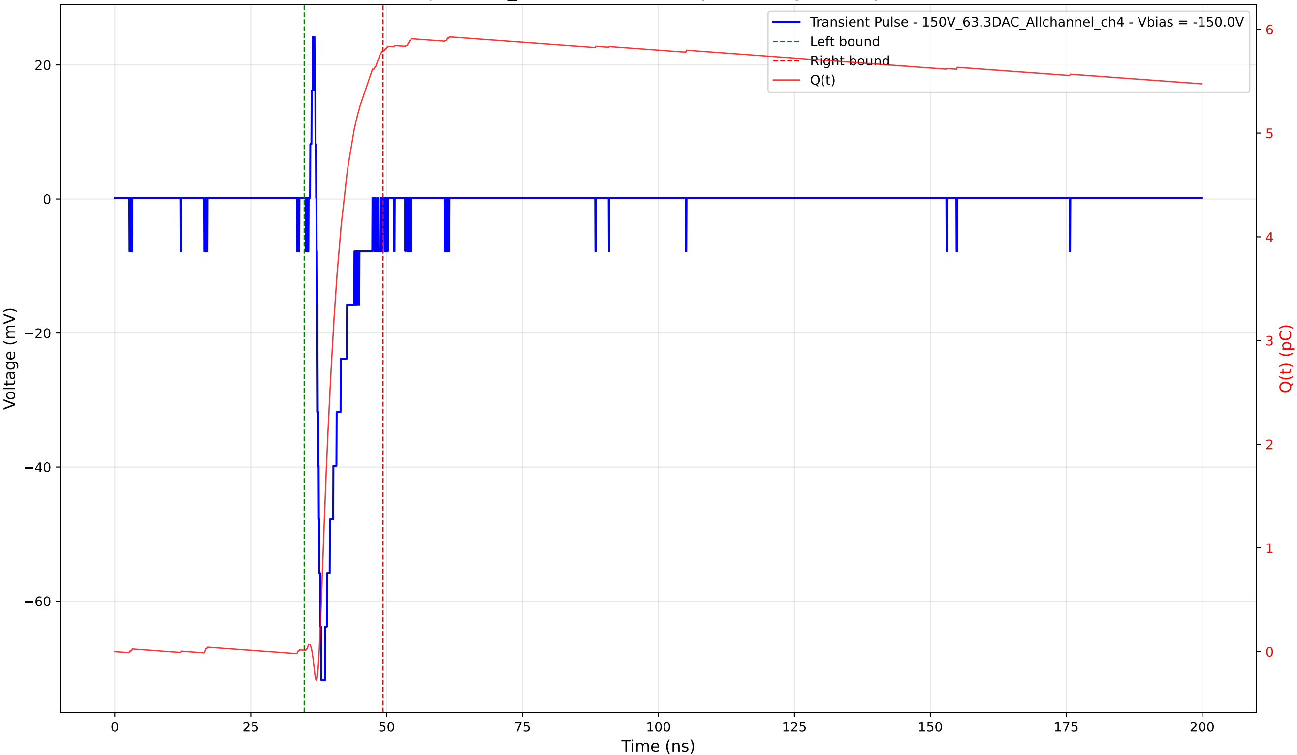
Transient Pulse - Sample: 1cm_42 - Position: 635.0 \mu\text{m} - Charge: 5.78 pC - Rise Time: 0.88 ns
