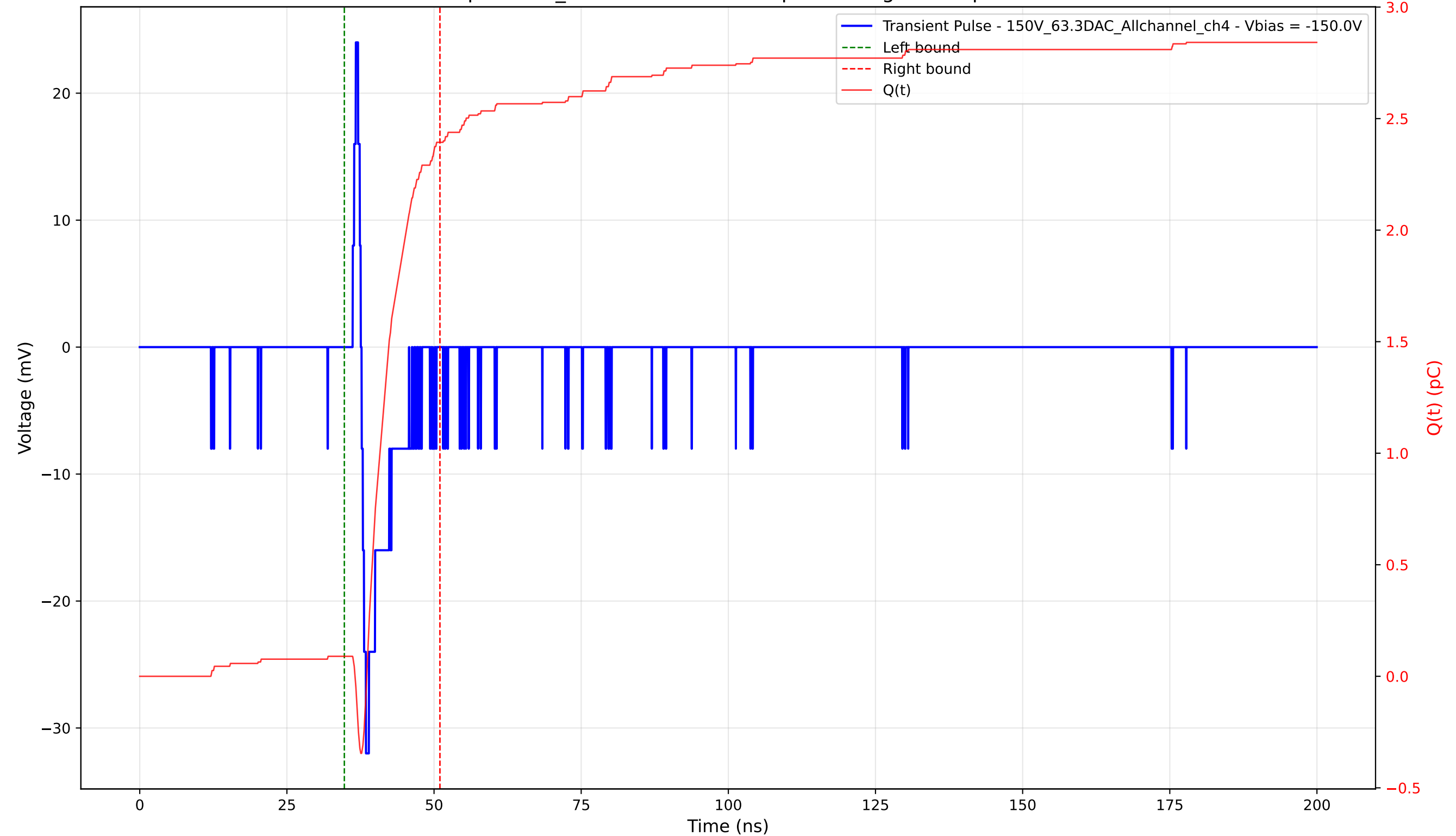
Transient Pulse - Sample: 1cm_42 - Position: 4530.0 \mu\text{m} - Charge: 2.30 pC - Rise Time: 0.74 ns
