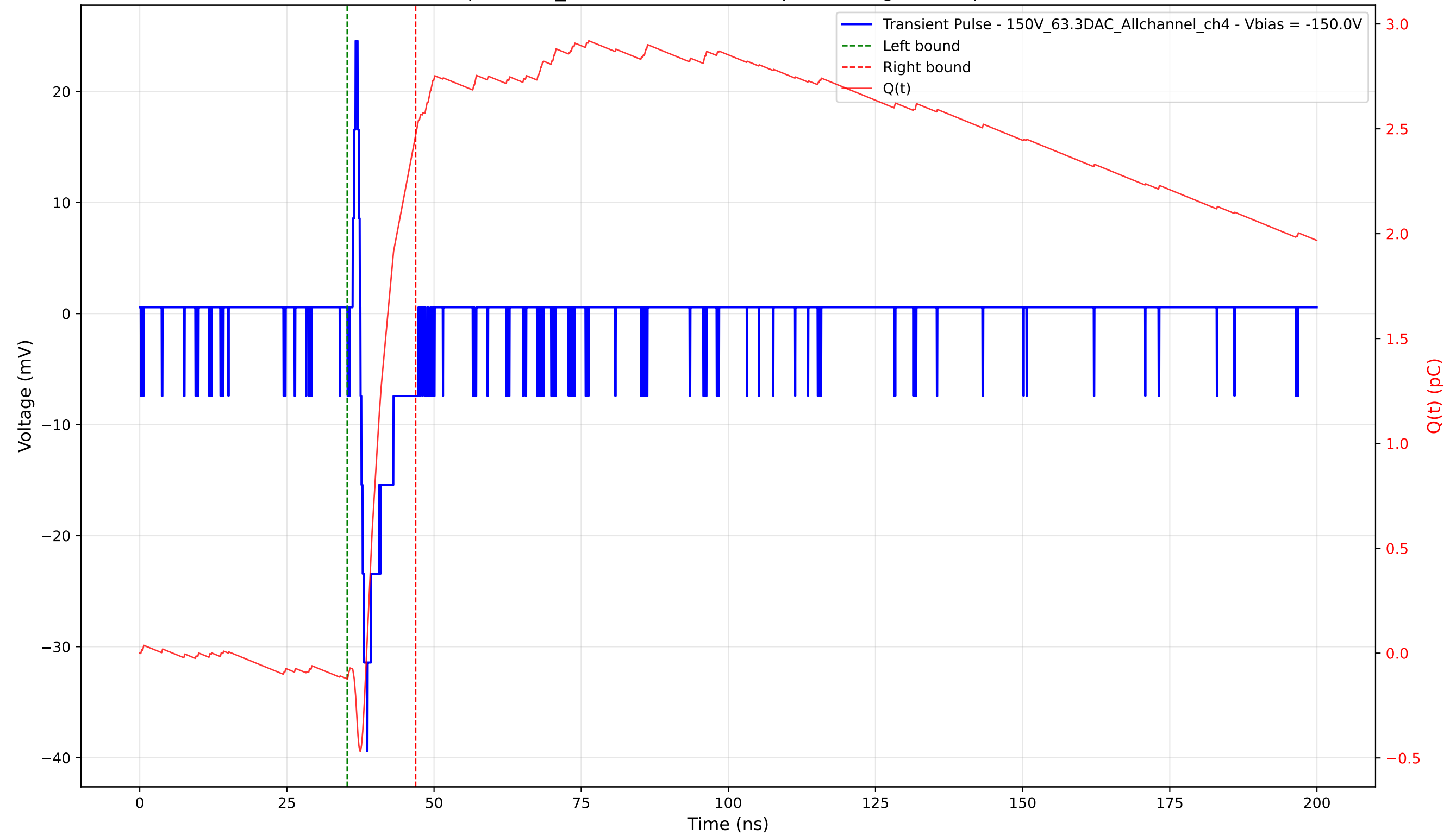
Transient Pulse - Sample: 1cm_42 - Position: 4740.0 \mu\text{m} - Charge: 2.60 pC - Rise Time: 1.14 ns
