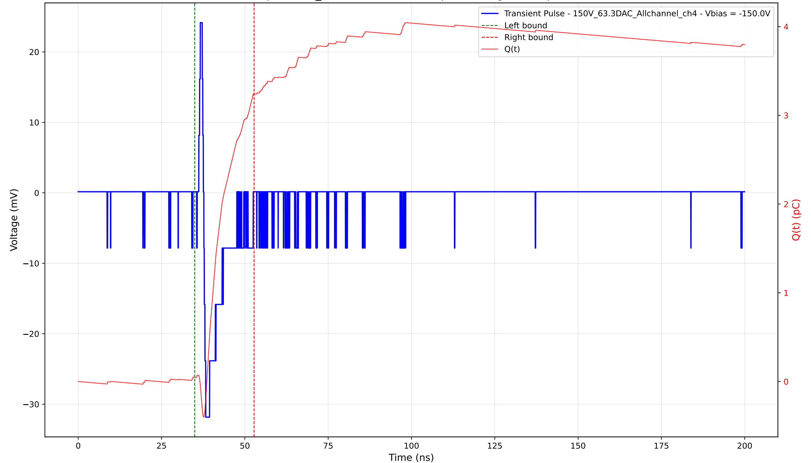
Transient Pulse - Sample: 1cm_42 - Position: 3865.0 \mu\text{m} - Charge: 3.19 pC - Rise Time: 0.58 ns
