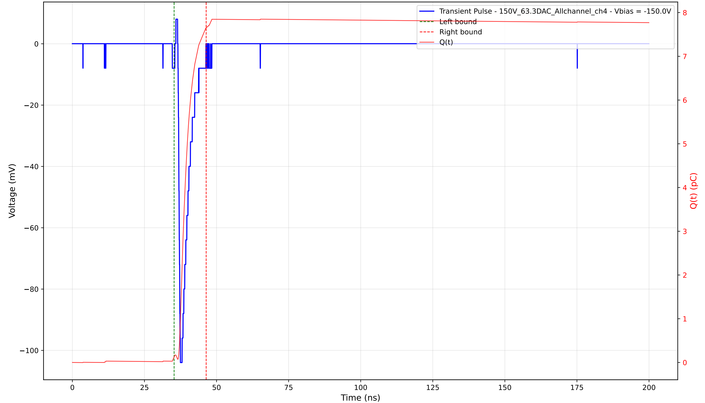
Transient Pulse - Sample: 1cm_42 - Position: 1040.0 \mu\text{m} - Charge: 7.52 pC - Rise Time: 0.67 ns
