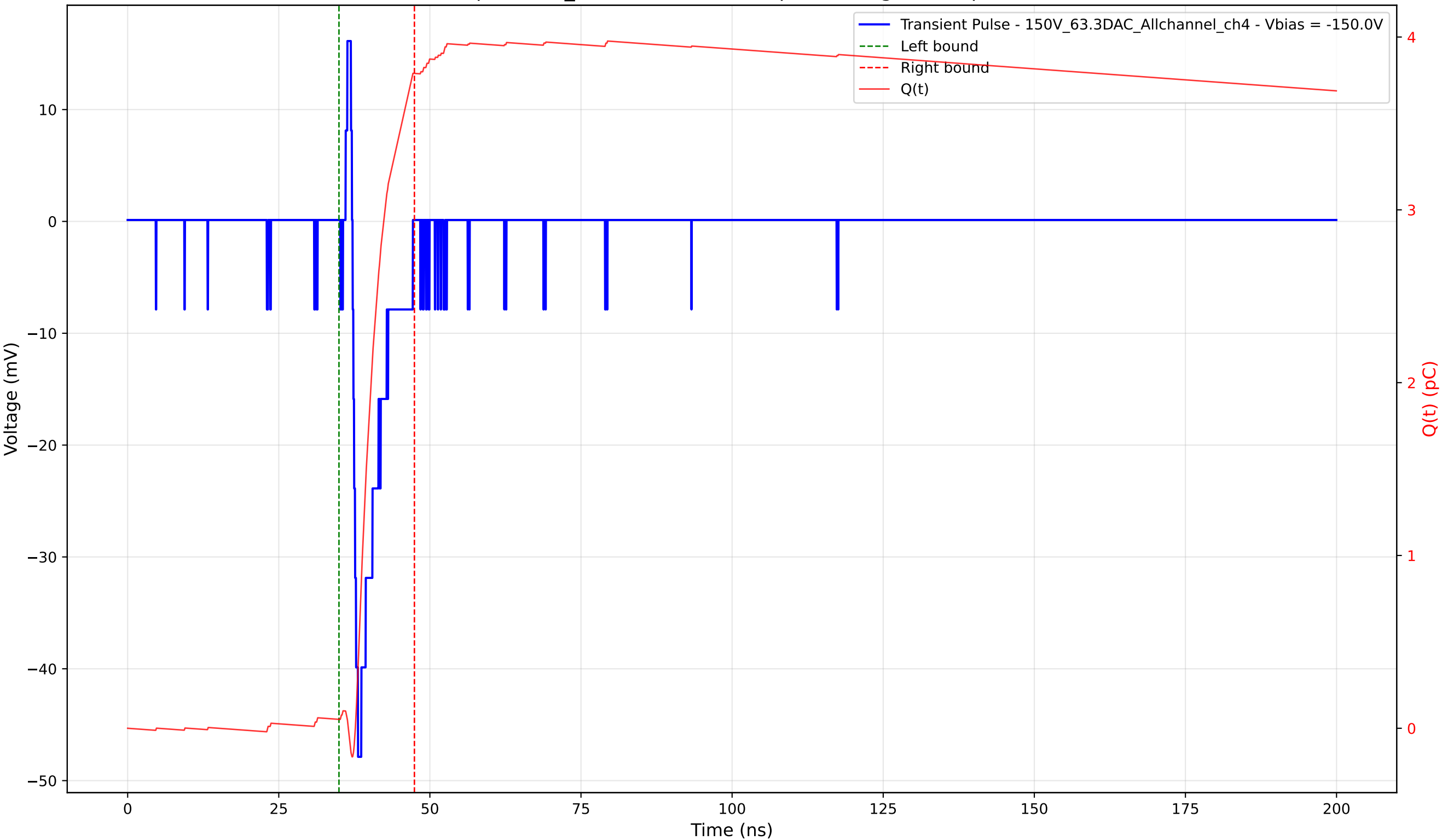
Transient Pulse - Sample: 1cm_42 - Position: 425.0 \mu\text{m} - Charge: 3.74 pC - Rise Time: 0.90 ns
