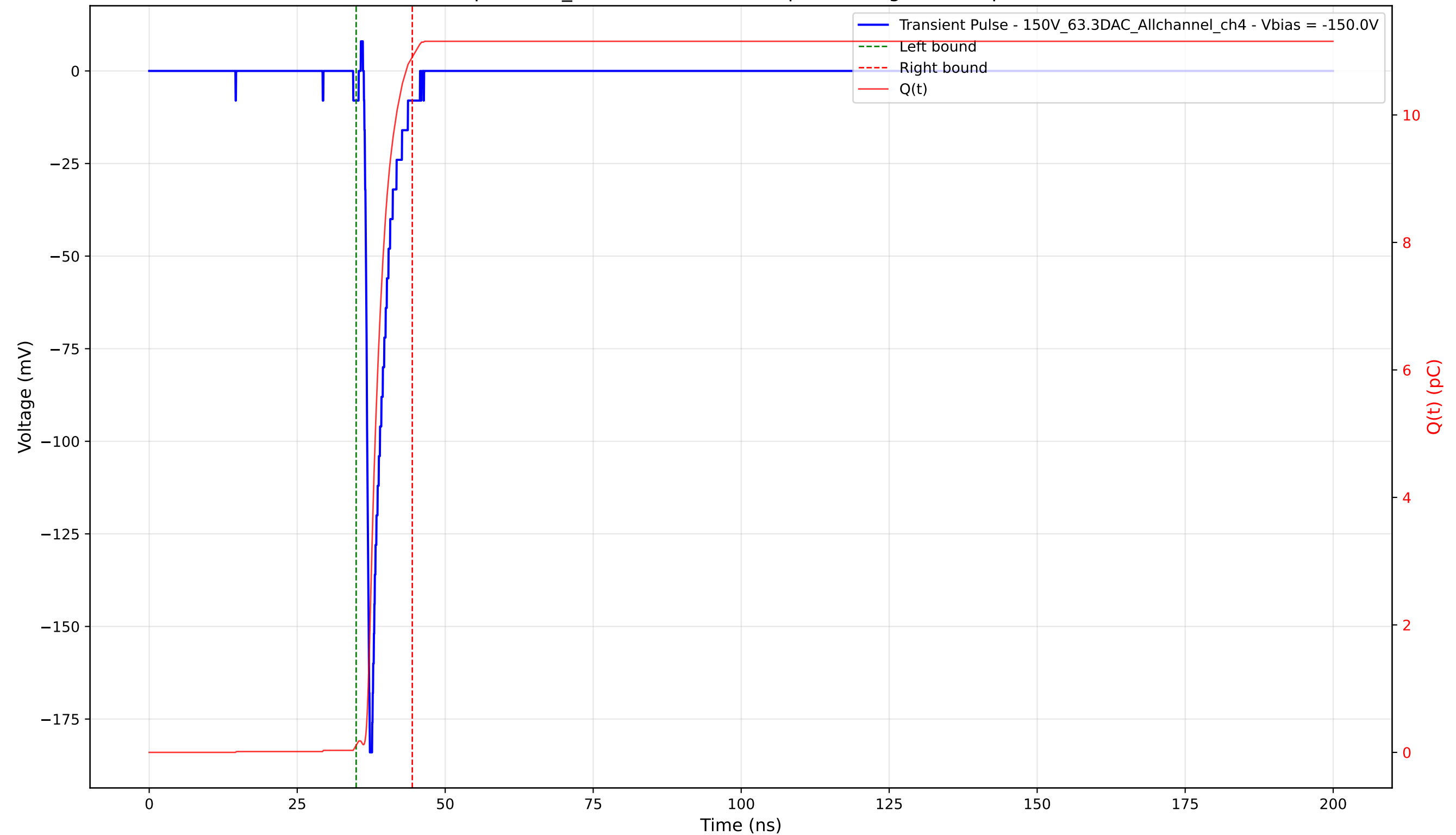
Transient Pulse - Sample: 1cm_42 - Position: 1295.0 \mu\text{m} - Charge: 10.80 pC - Rise Time: 0.75 ns
