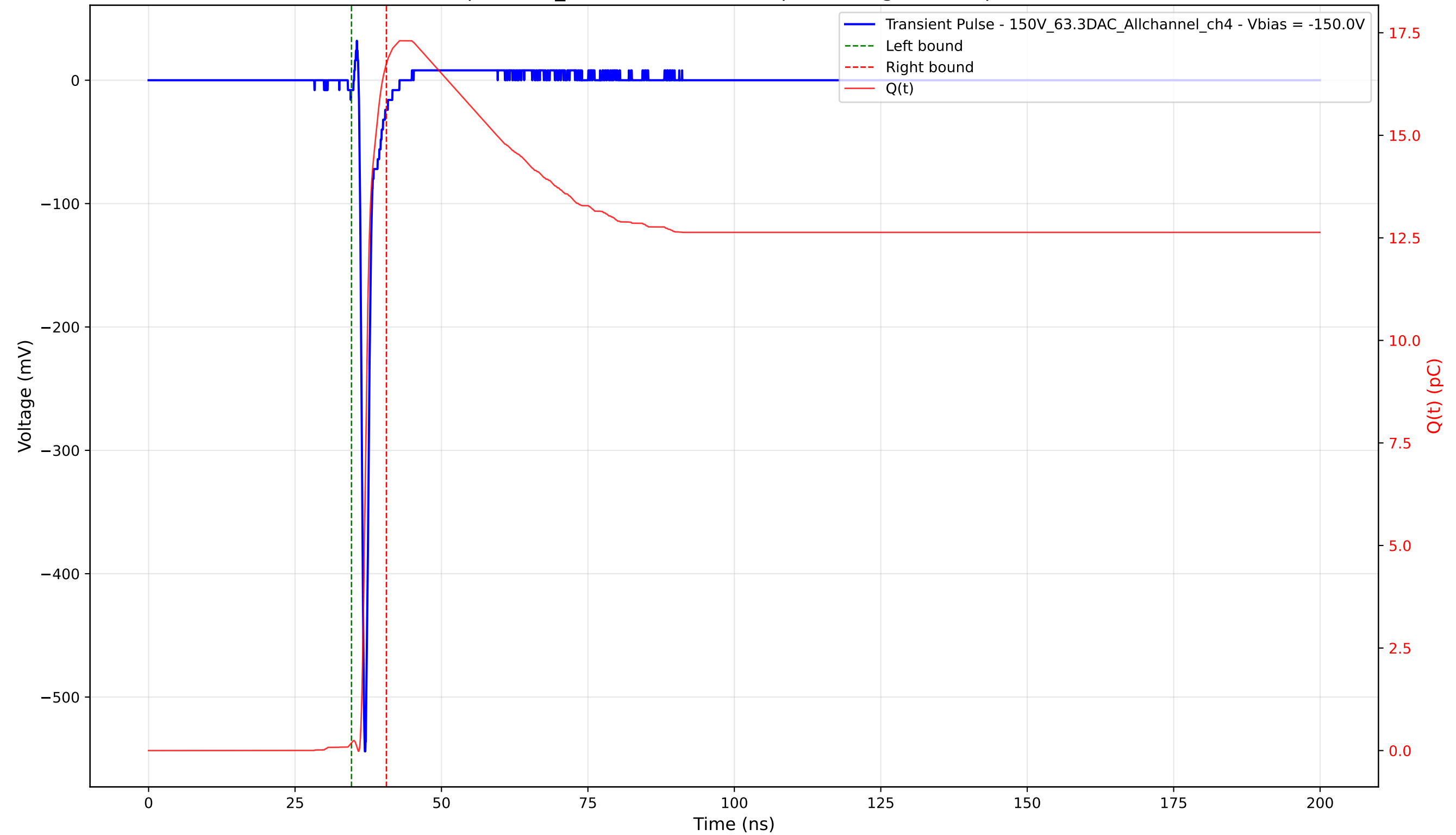
Transient Pulse - Sample: 1cm_42 - Position: 2150.0 \mu\text{m} - Charge: 16.56 pC - Rise Time: 0.71 ns
