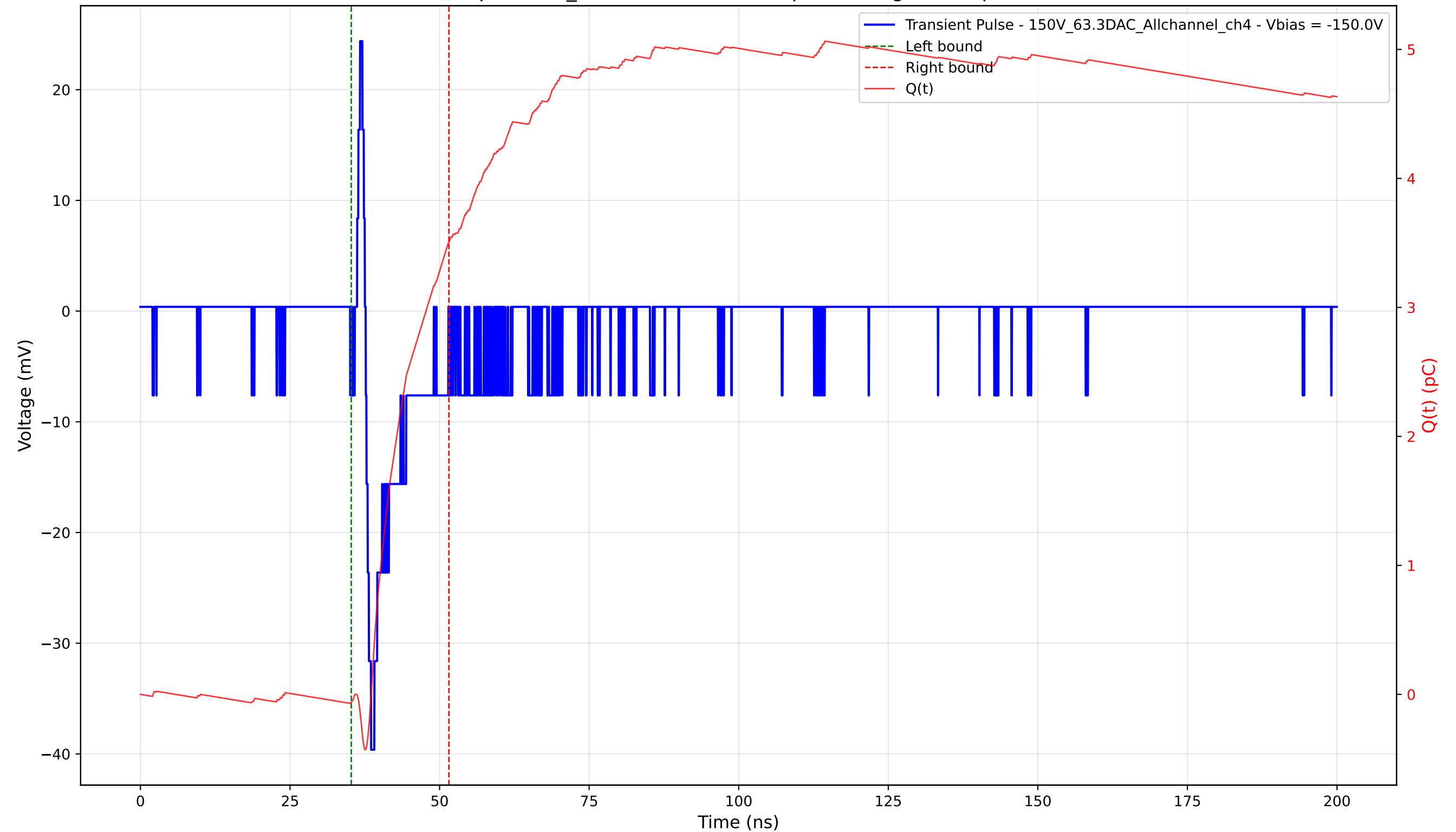
Transient Pulse - Sample: 1cm_42 - Position: 3695.0 \mu\text{m} - Charge: 3.57 pC - Rise Time: 0.90 ns
