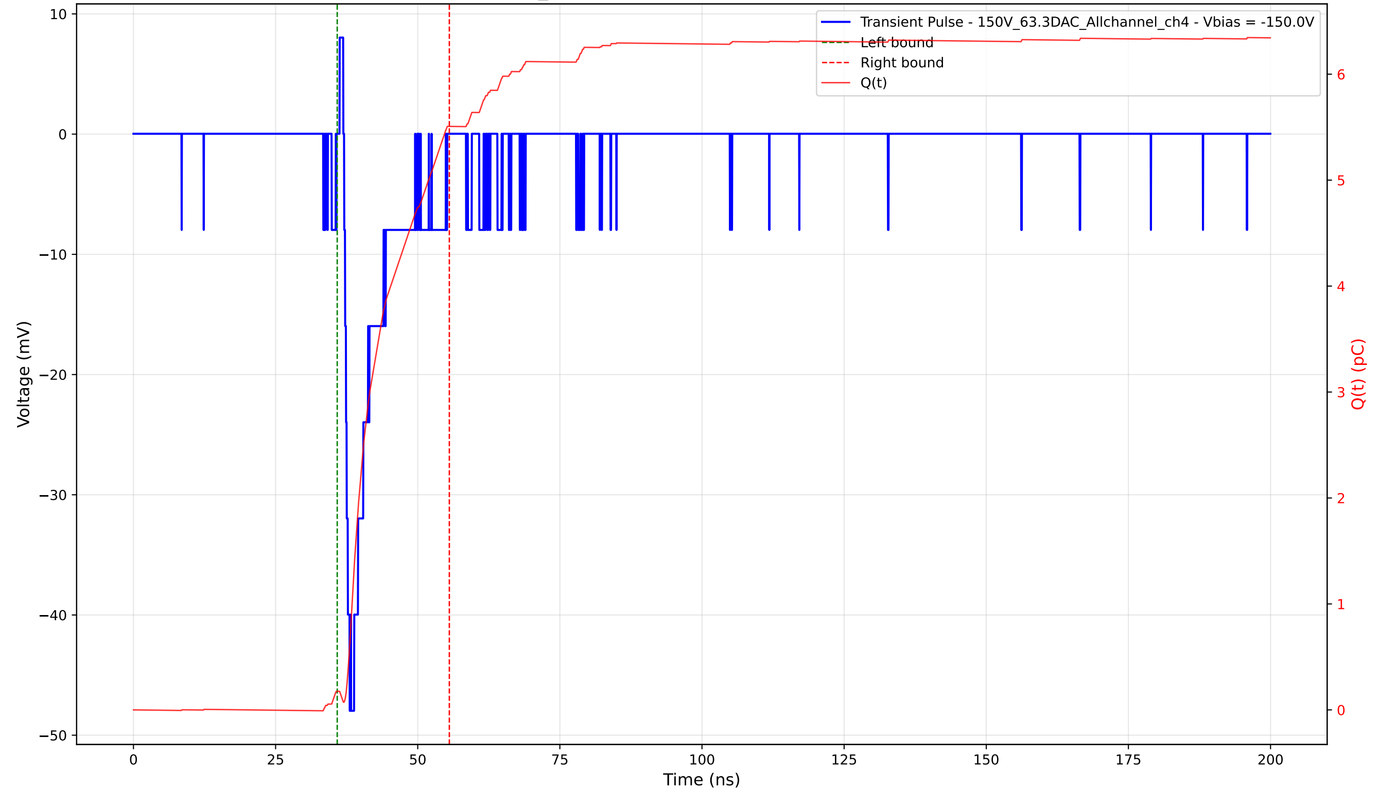
Transient Pulse - Sample: 1cm_42 - Position: 3330.0 \mu\text{m} - Charge: 5.33 pC - Rise Time: 0.98 ns
