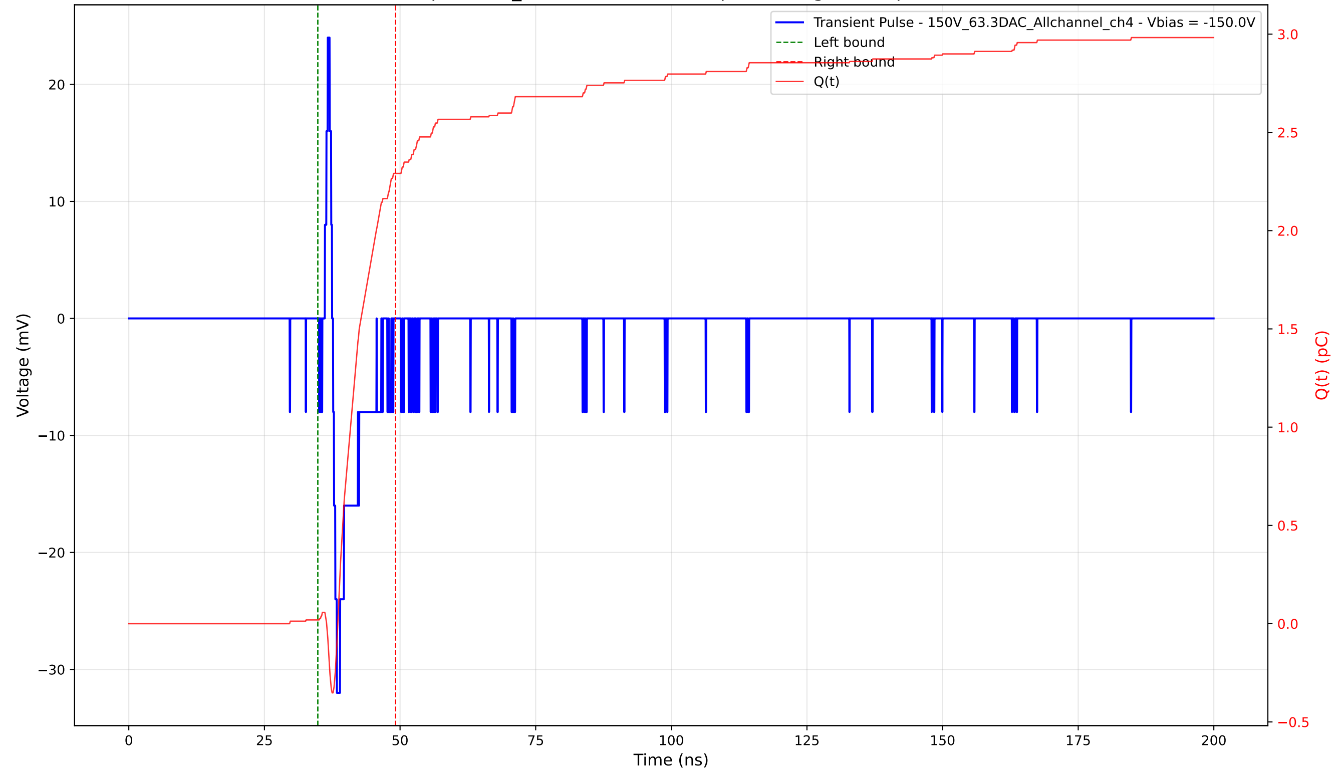
Transient Pulse - Sample: 1cm_42 - Position: 4595.0 \mu\text{m} - Charge: 2.27 pC - Rise Time: 0.70 ns
