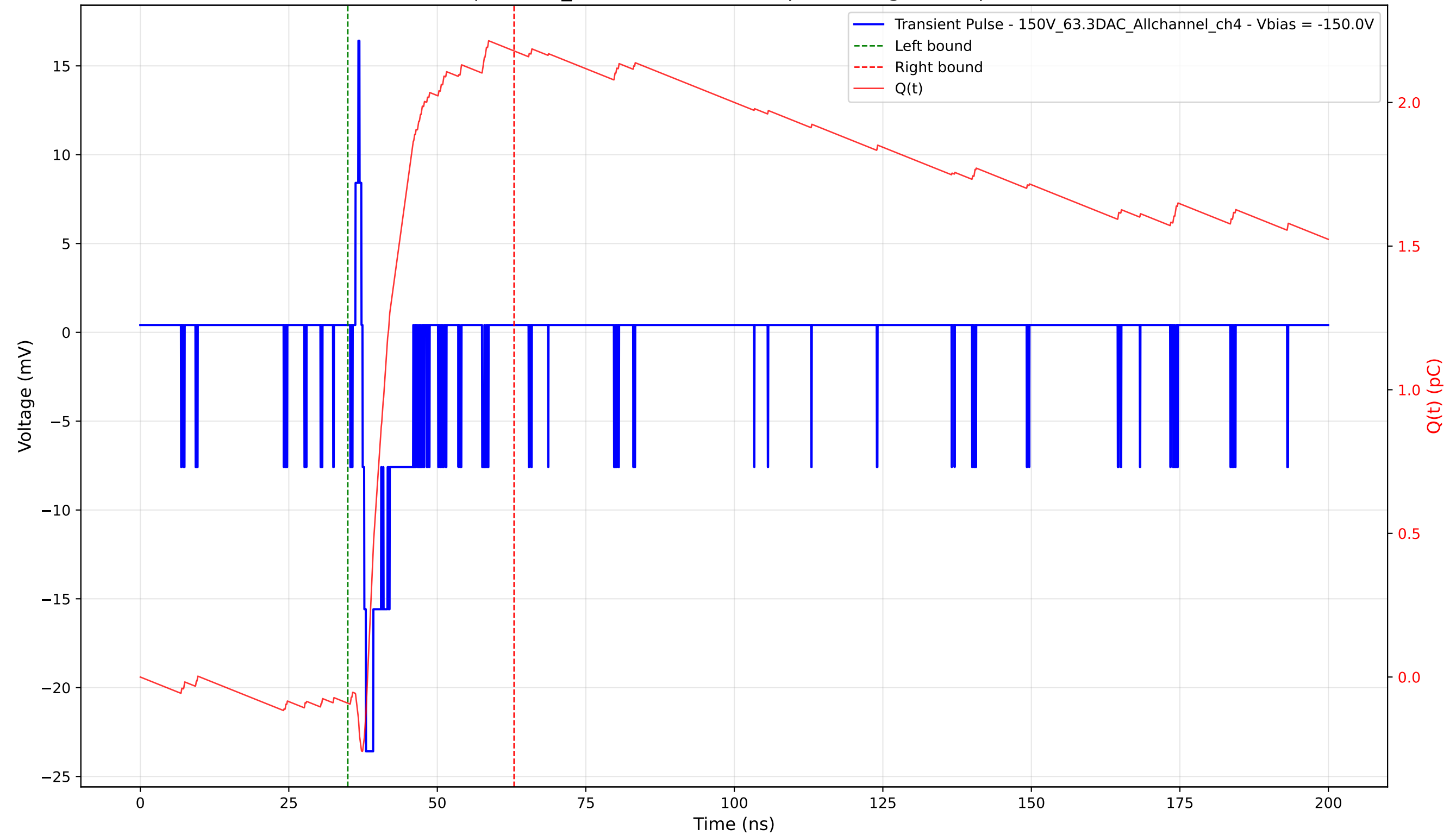
Transient Pulse - Sample: 1cm_42 - Position: 4970.0 \mu\text{m} - Charge: 2.27 pC - Rise Time: 0.59 ns
