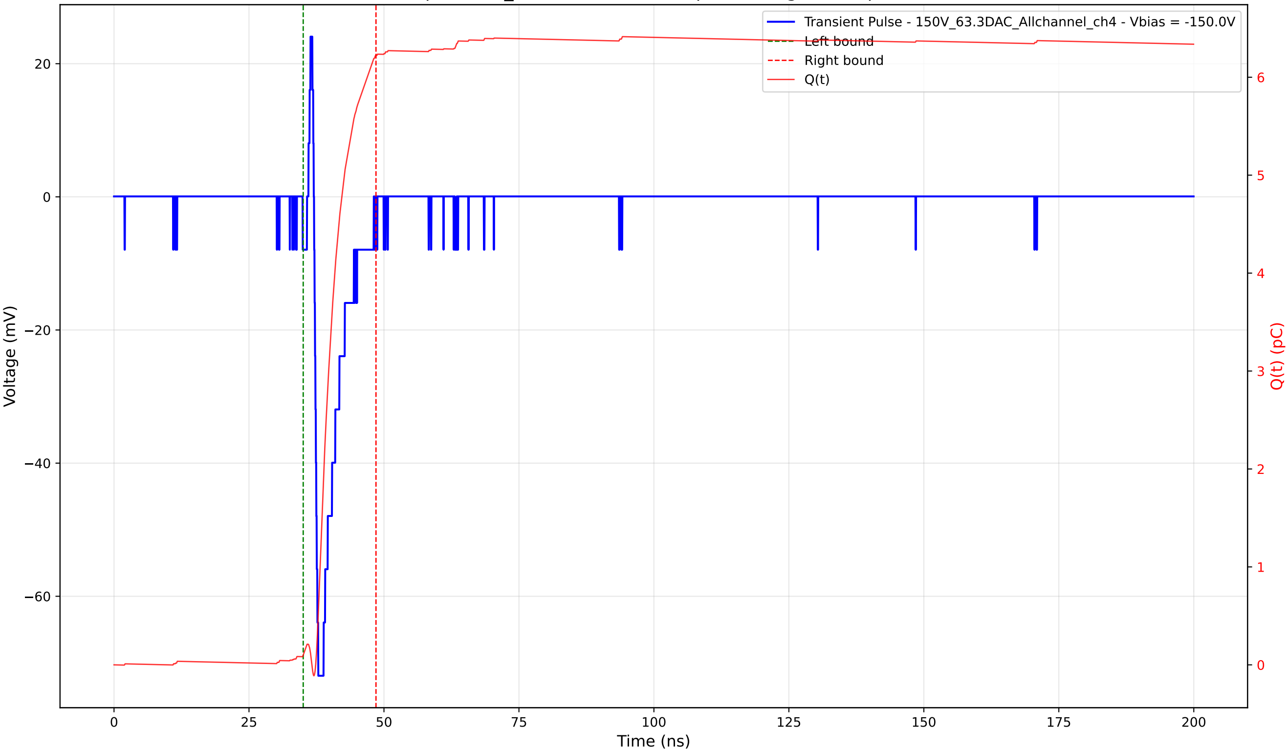
Transient Pulse - Sample: 1cm_42 - Position: 660.0 \mu\text{m} - Charge: 6.12 pC - Rise Time: 0.76 ns
