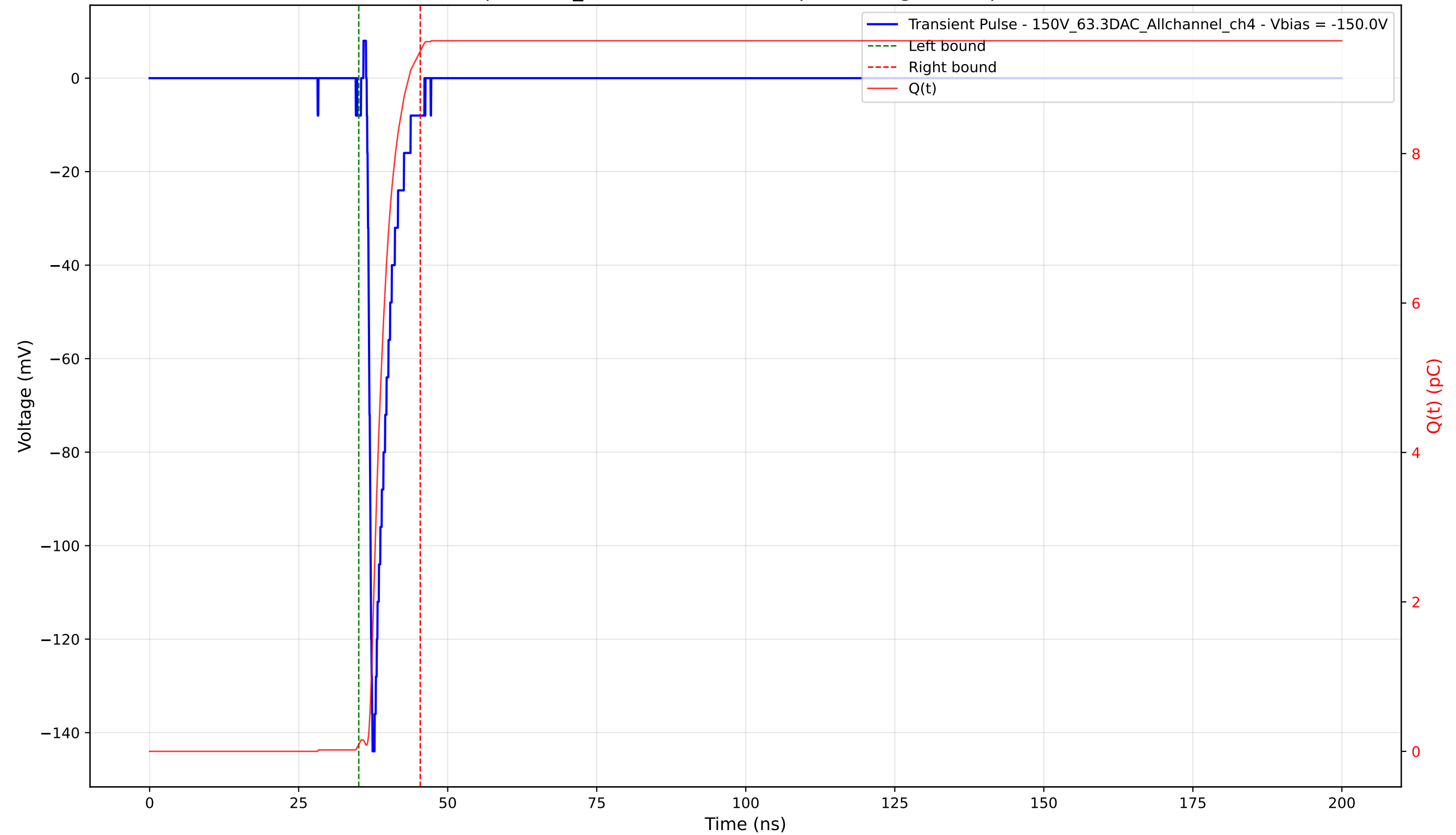
Transient Pulse - Sample: 1cm_42 - Position: 1150.0 \mu\text{m} - Charge: 9.28 pC - Rise Time: 0.81 ns
