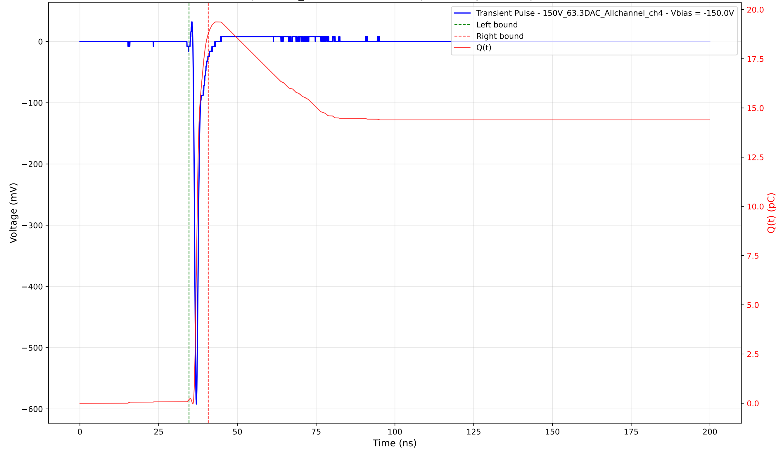
Transient Pulse - Sample: 1cm_42 - Position: 1890.0 \mu\text{m} - Charge: 18.57 pC - Rise Time: 0.72 ns
