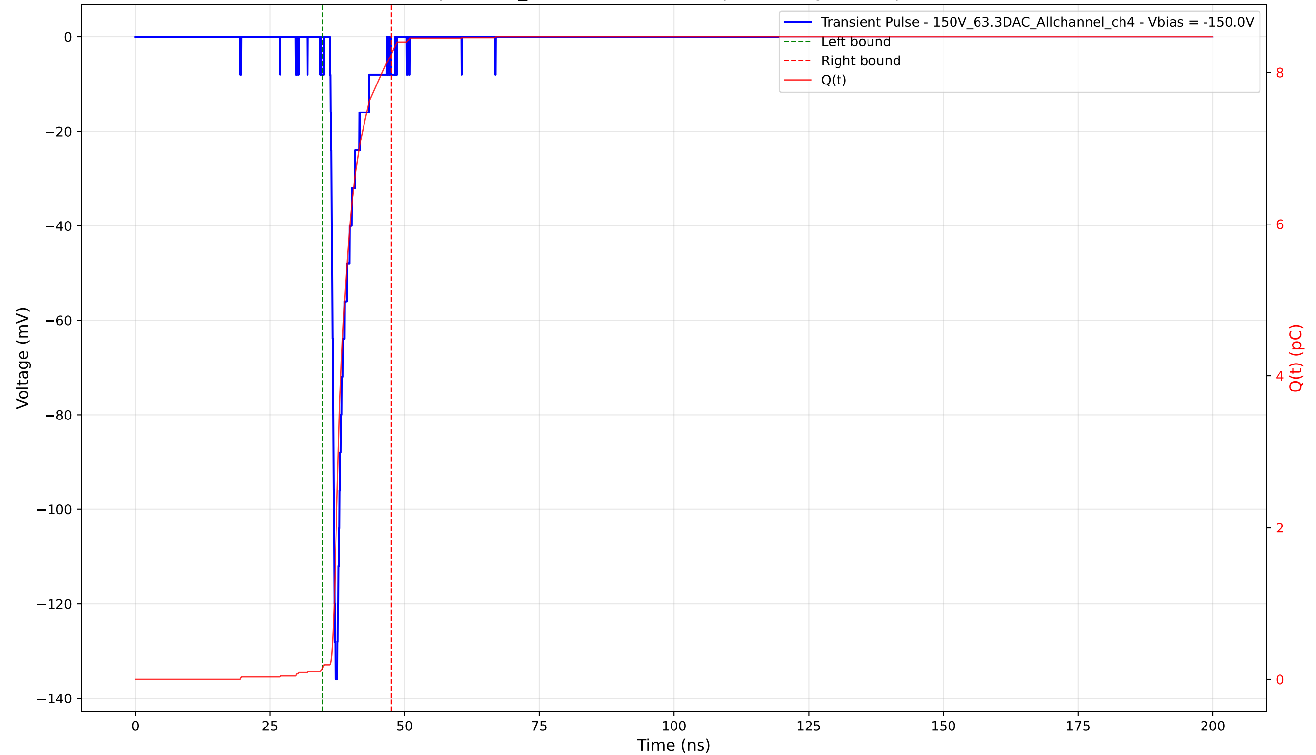
Transient Pulse - Sample: 1cm_42 - Position: 2755.0 \mu\text{m} - Charge: 8.08 pC - Rise Time: 0.81 ns
