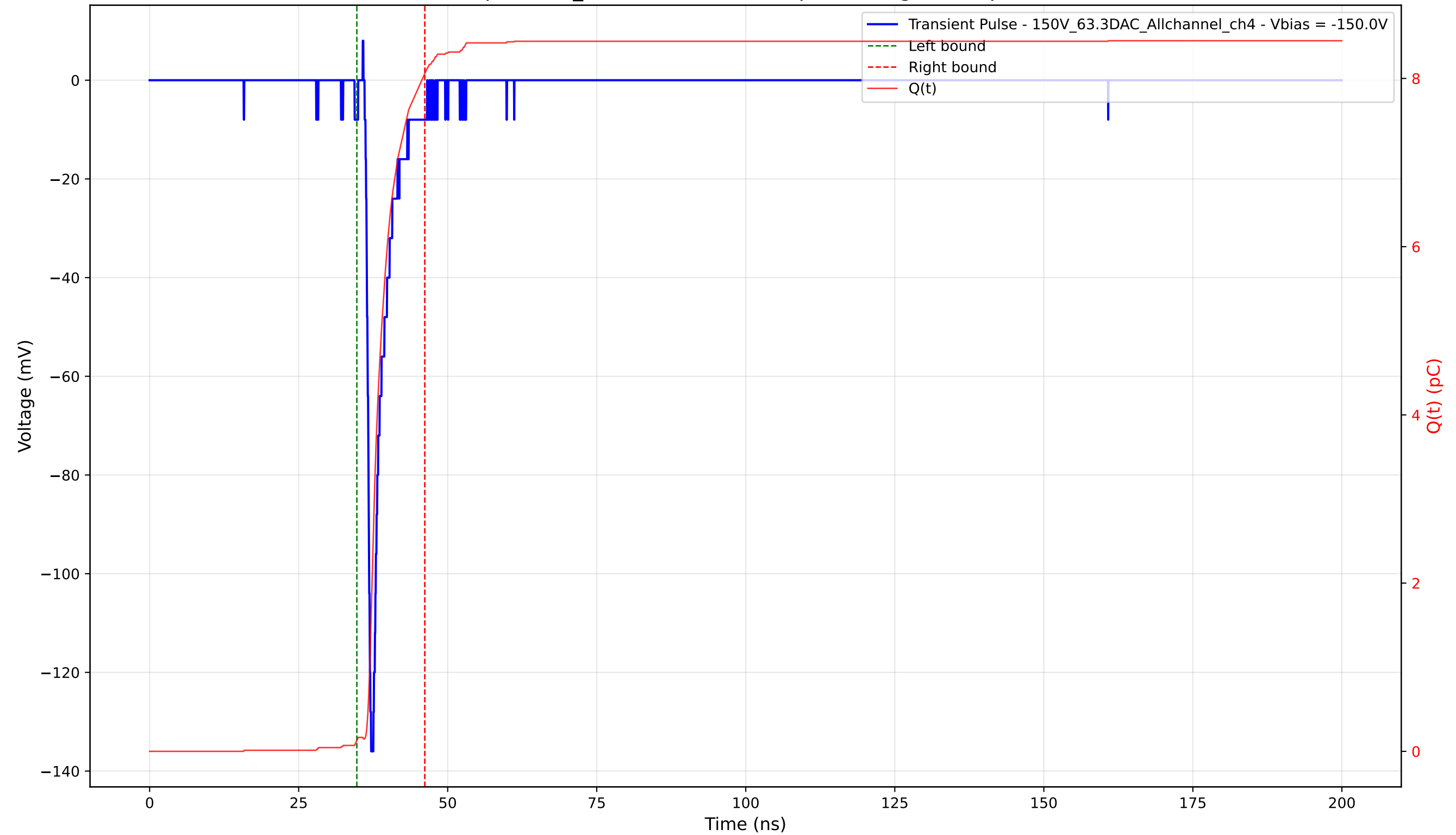
Transient Pulse - Sample: 1cm_42 - Position: 2765.0 \mu\text{m} - Charge: 7.93 pC - Rise Time: 0.81 ns
