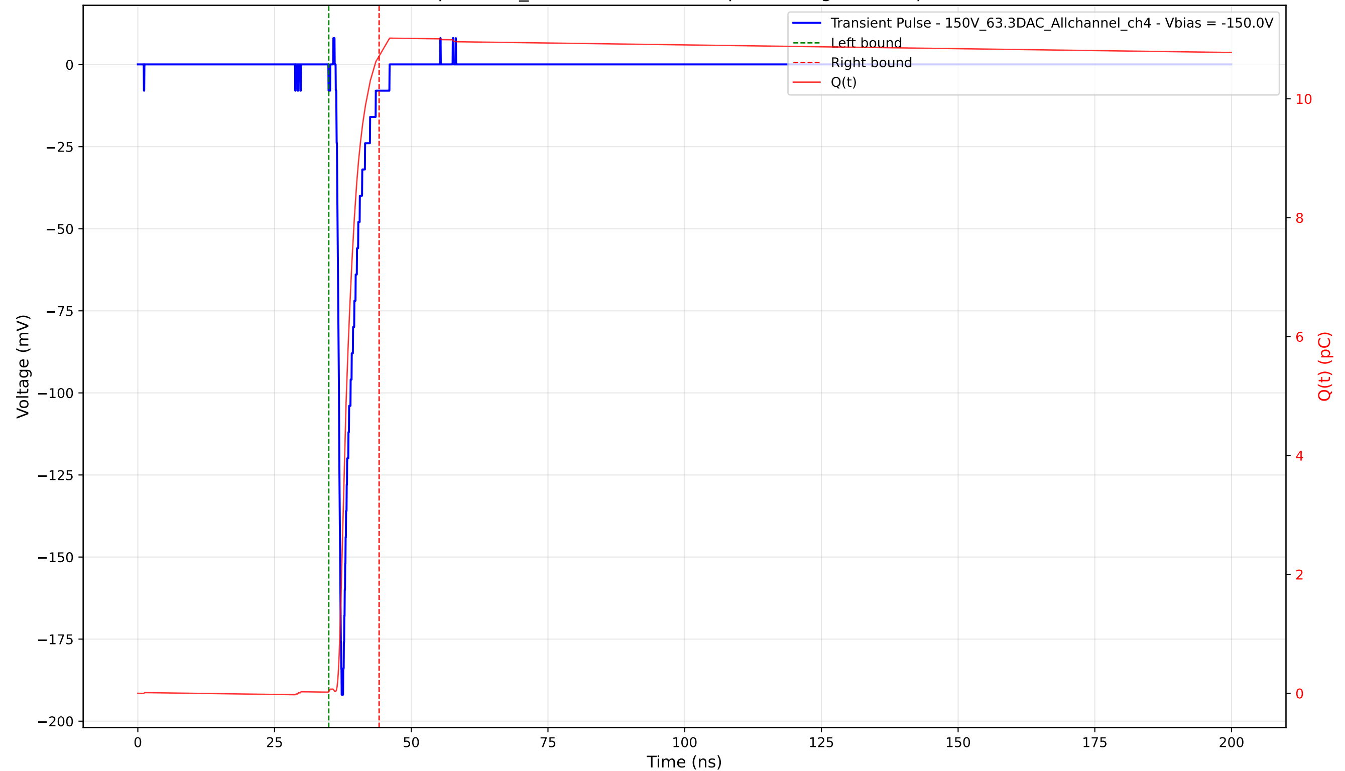
Transient Pulse - Sample: 1cm_42 - Position: 1360.0 \mu\text{m} - Charge: 10.69 pC - Rise Time: 0.78 ns
