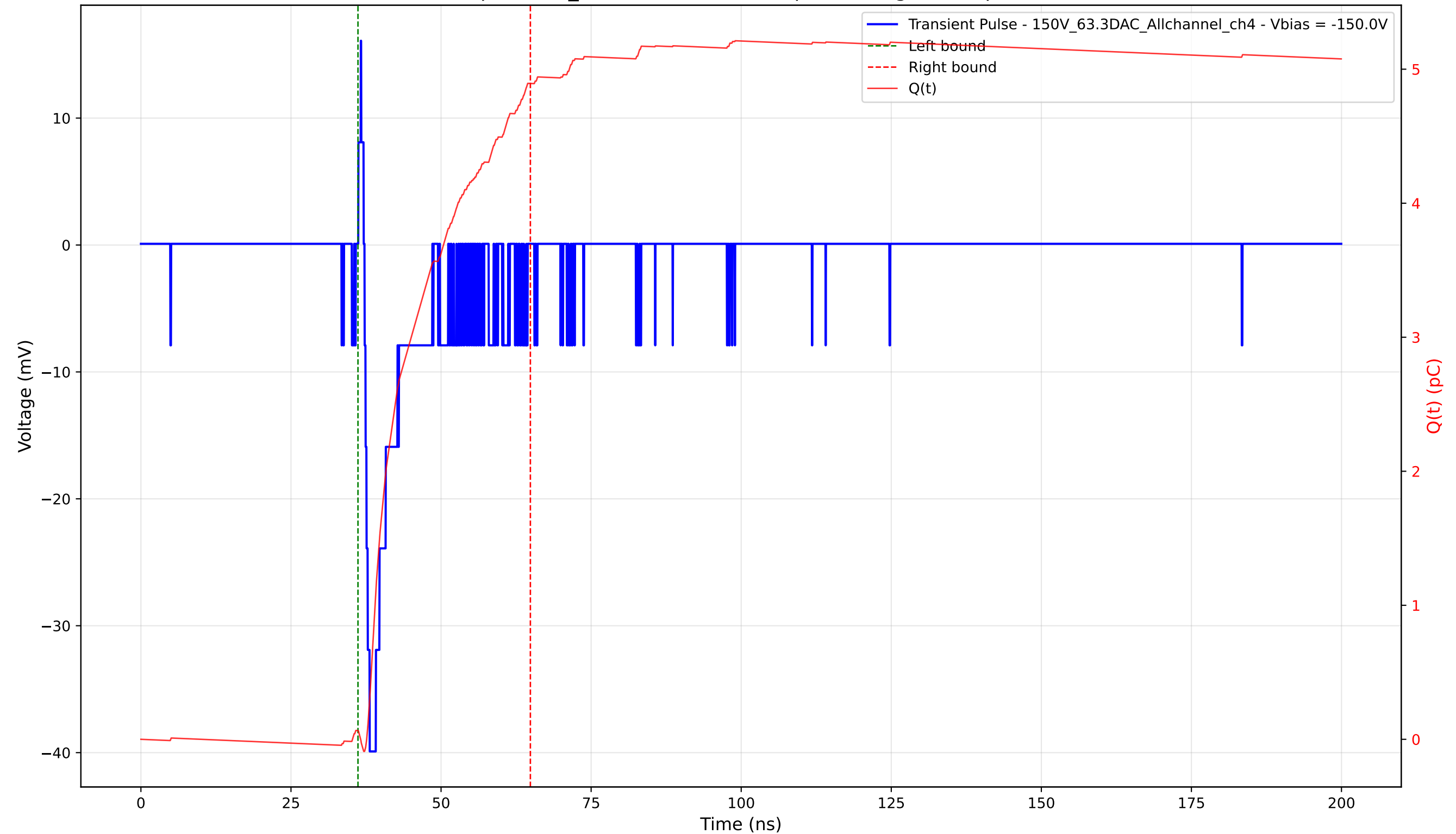
Transient Pulse - Sample: 1cm_42 - Position: 3430.0 \mu\text{m} - Charge: 4.83 pC - Rise Time: 0.86 ns
