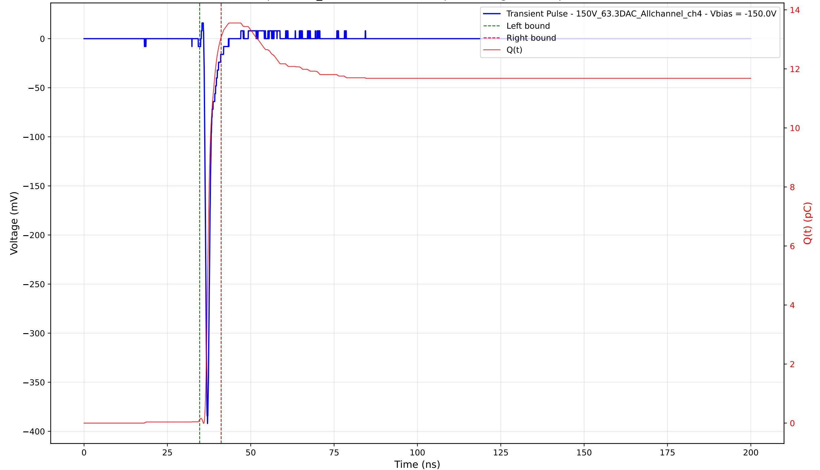
Transient Pulse - Sample: 1cm_42 - Position: 2380.0 \mu\text{m} - Charge: 12.96 pC - Rise Time: 0.71 ns
