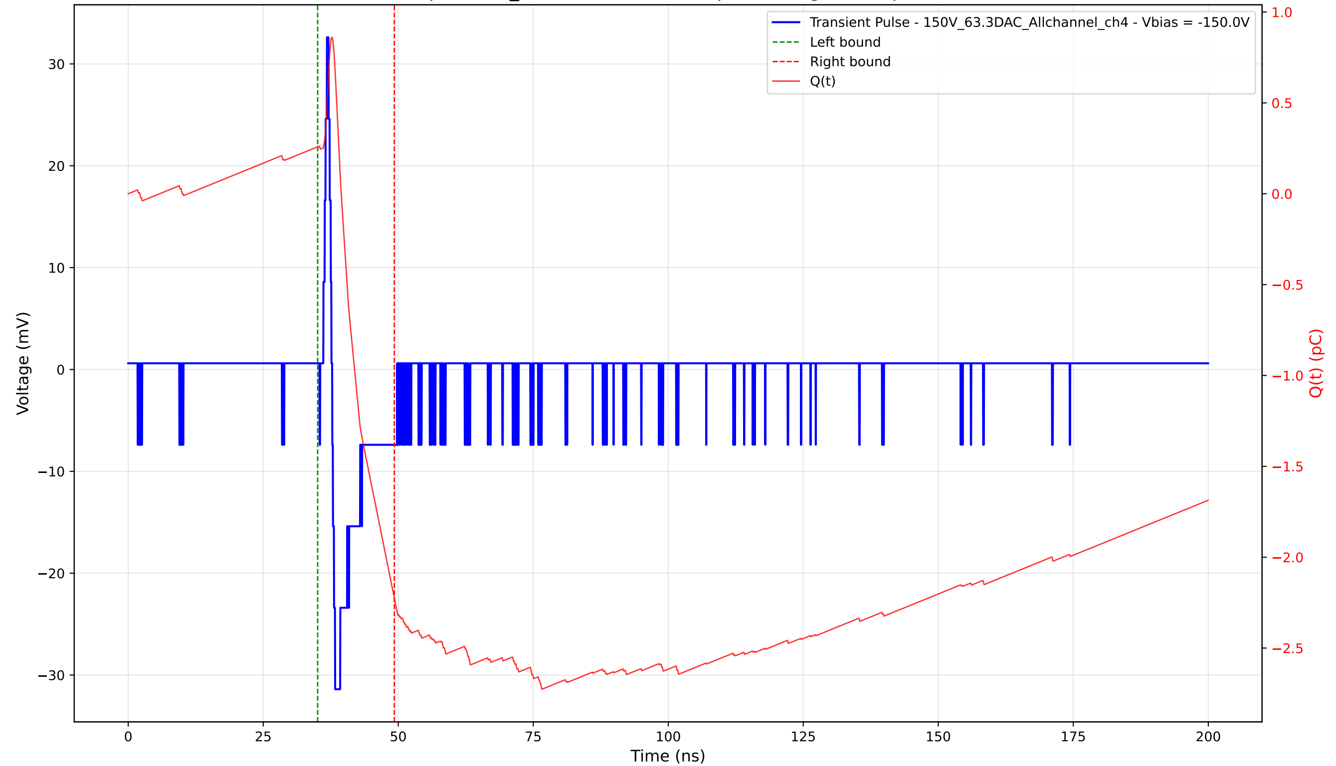
Transient Pulse - Sample: 1cm_42 - Position: 4200.0 \mu\text{m} - Charge: 2.49 pC - Rise Time: 0.67 ns
