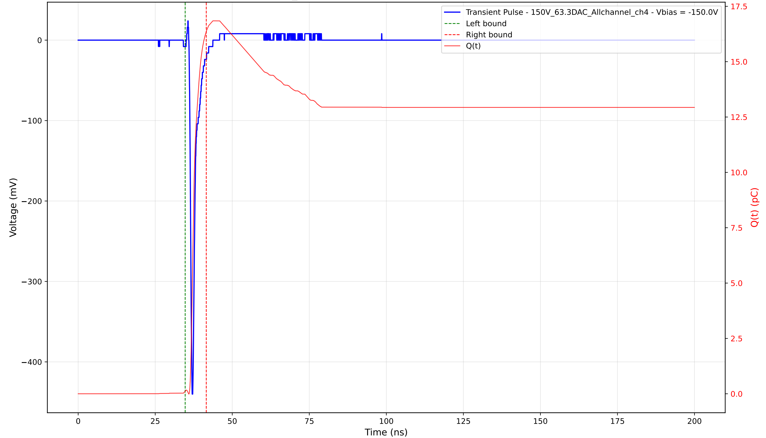
Transient Pulse - Sample: 1cm_42 - Position: 1650.0 \mu\text{m} - Charge: 16.24 pC - Rise Time: 0.74 ns
