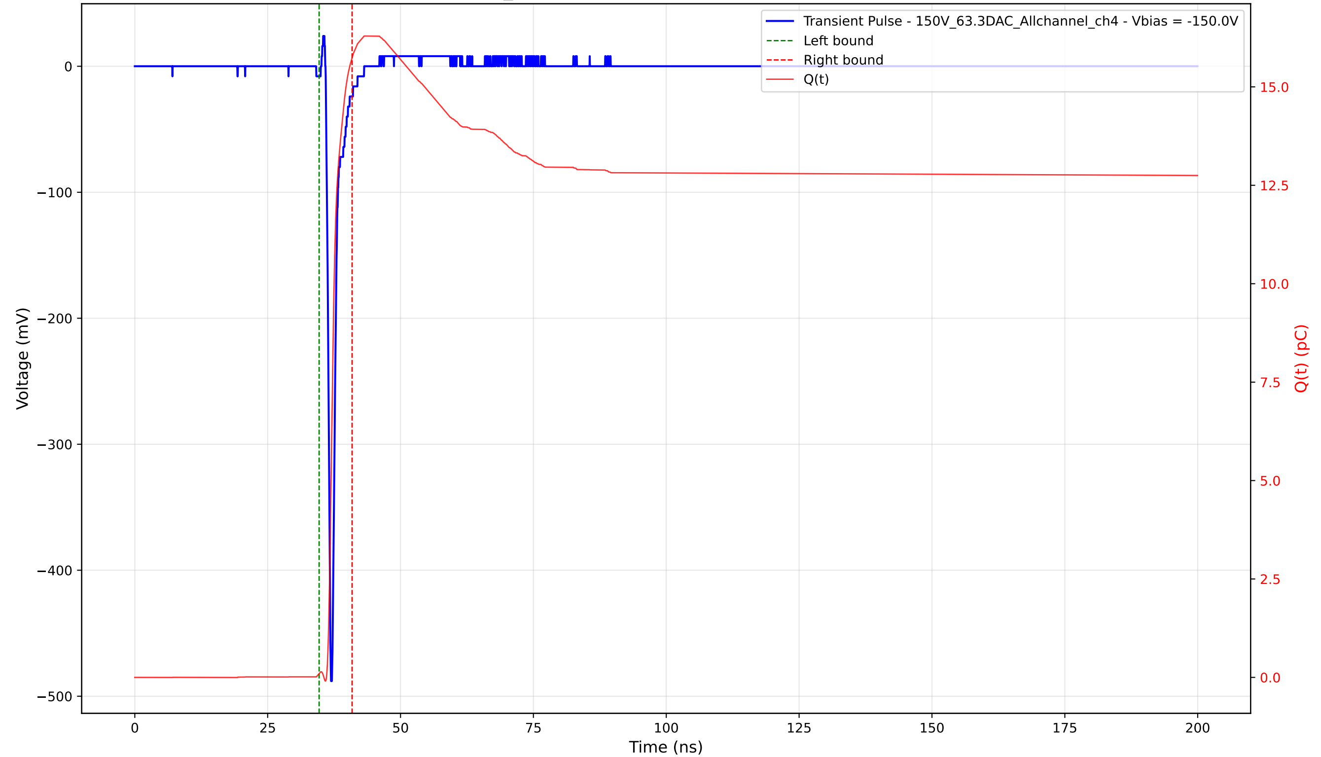
Transient Pulse - Sample: 1cm_42 - Position: 2280.0 \mu\text{m} - Charge: 15.64 pC - Rise Time: 0.72 ns
