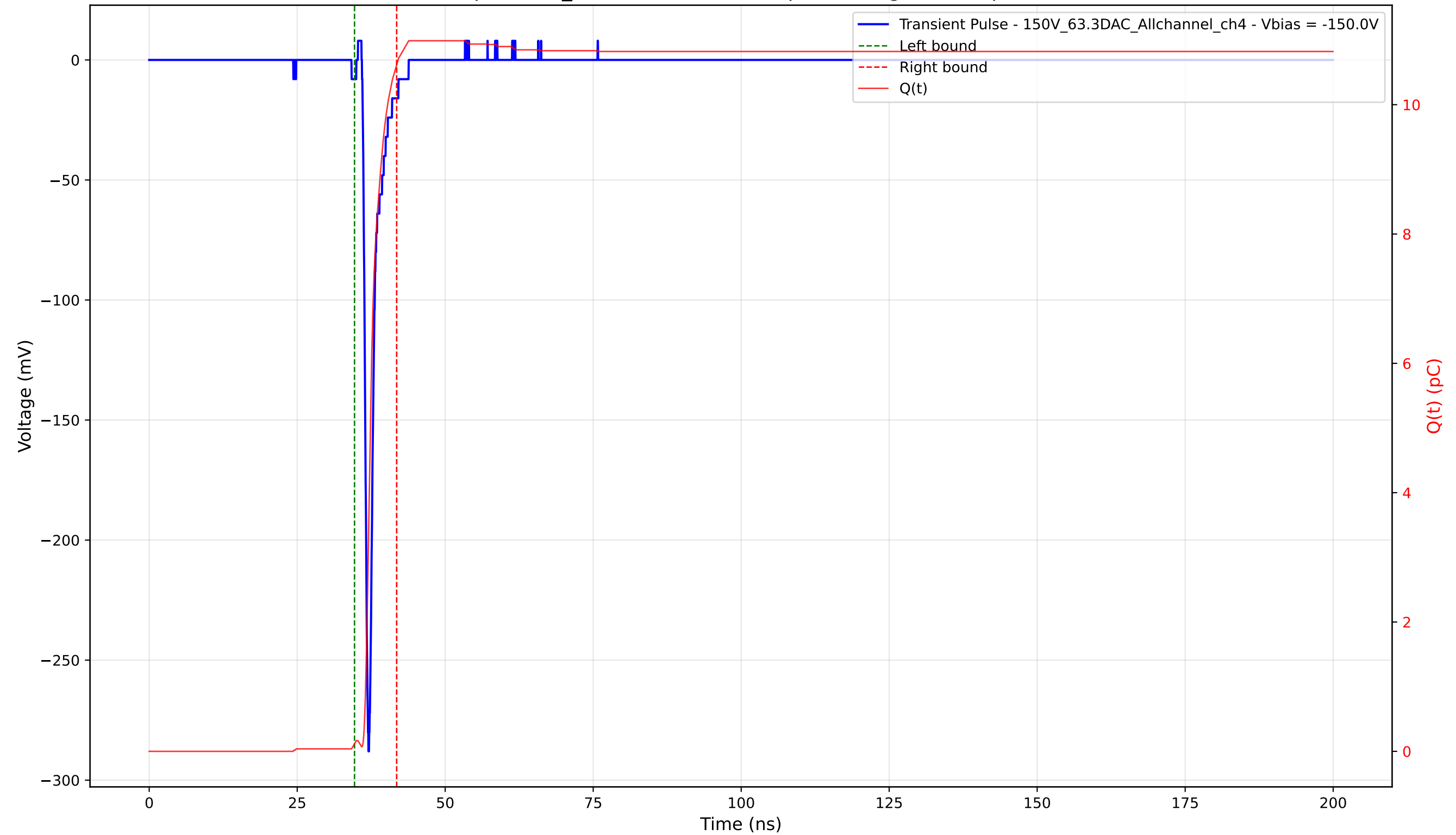
Transient Pulse - Sample: 1cm_42 - Position: 2465.0 \mu\text{m} - Charge: 10.50 pC - Rise Time: 0.75 ns
