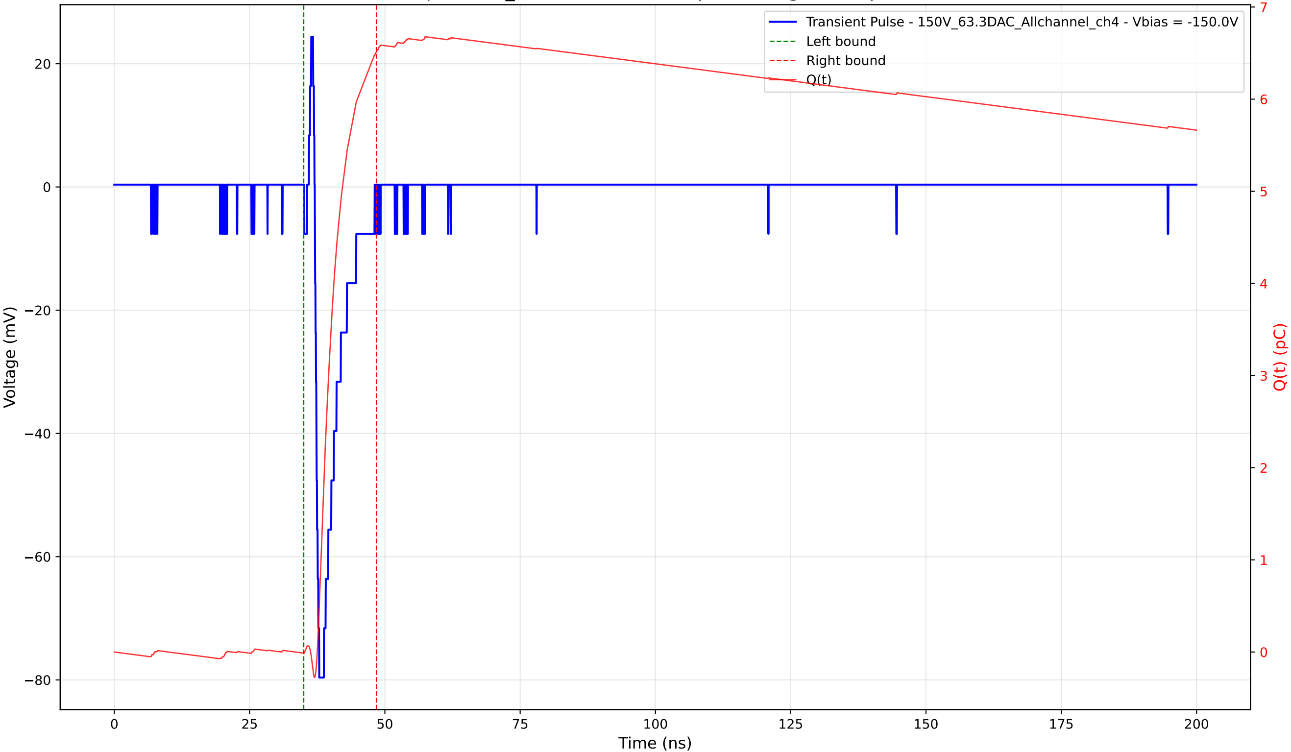
Transient Pulse - Sample: 1cm_42 - Position: 705.0 \mu\text{m} - Charge: 6.53 pC - Rise Time: 0.80 ns
