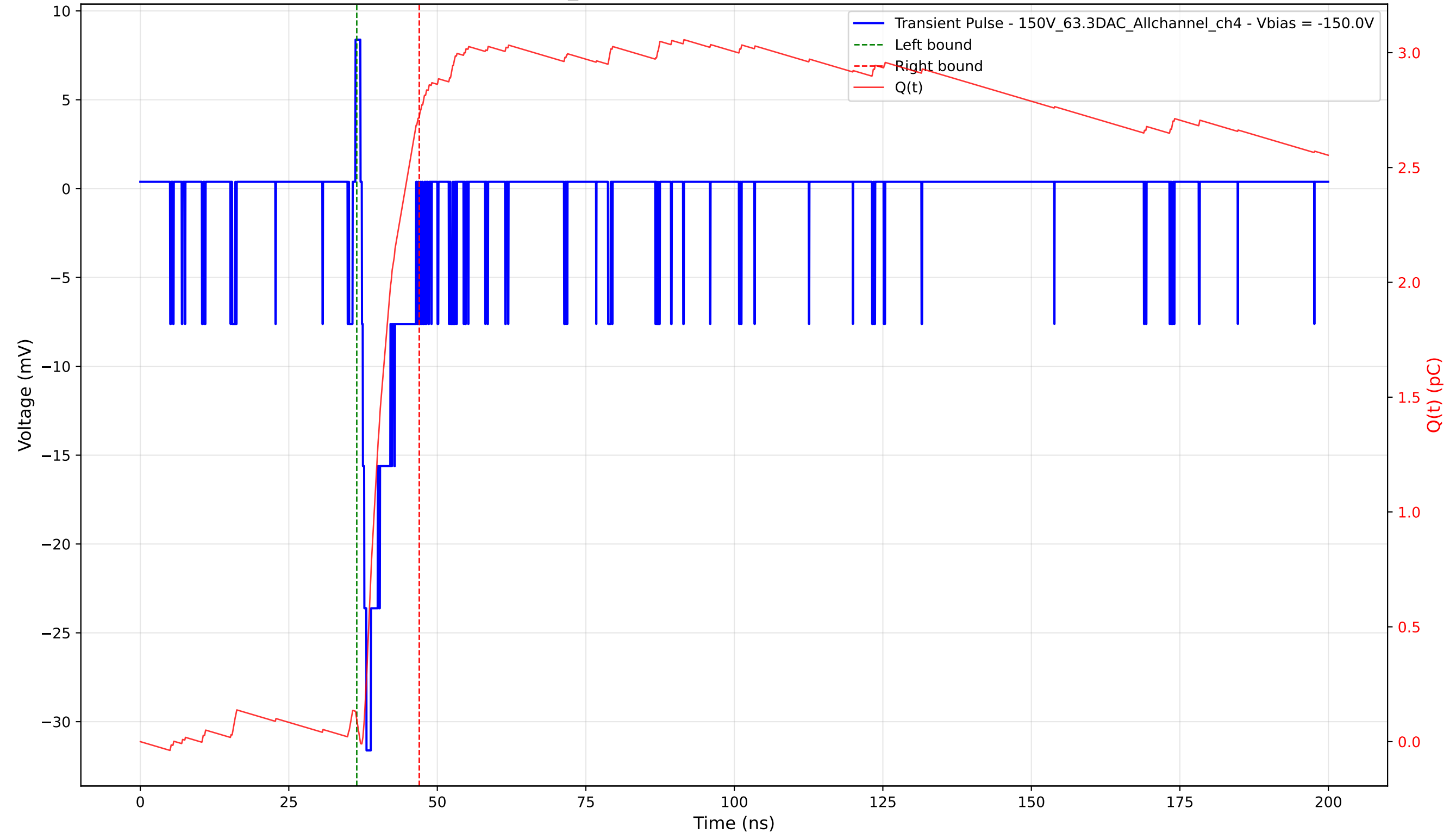
Transient Pulse - Sample: 1cm_42 - Position: 245.0 \mu\text{m} - Charge: 2.63 pC - Rise Time: 0.78 ns
