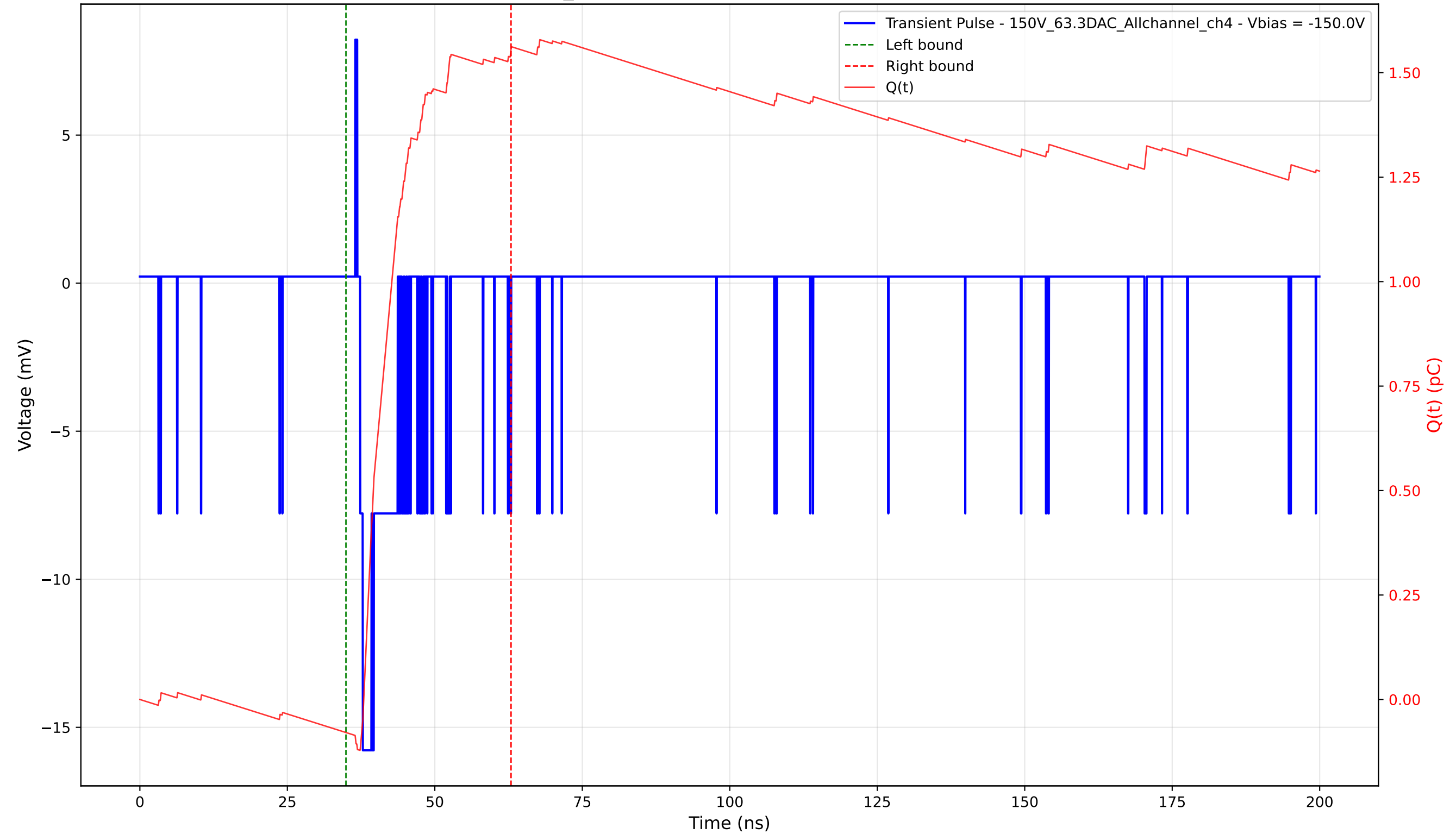
Transient Pulse - Sample: 1cm_42 - Position: 135.0 \mu\text{m} - Charge: 1.63 pC - Rise Time: 0.47 ns
