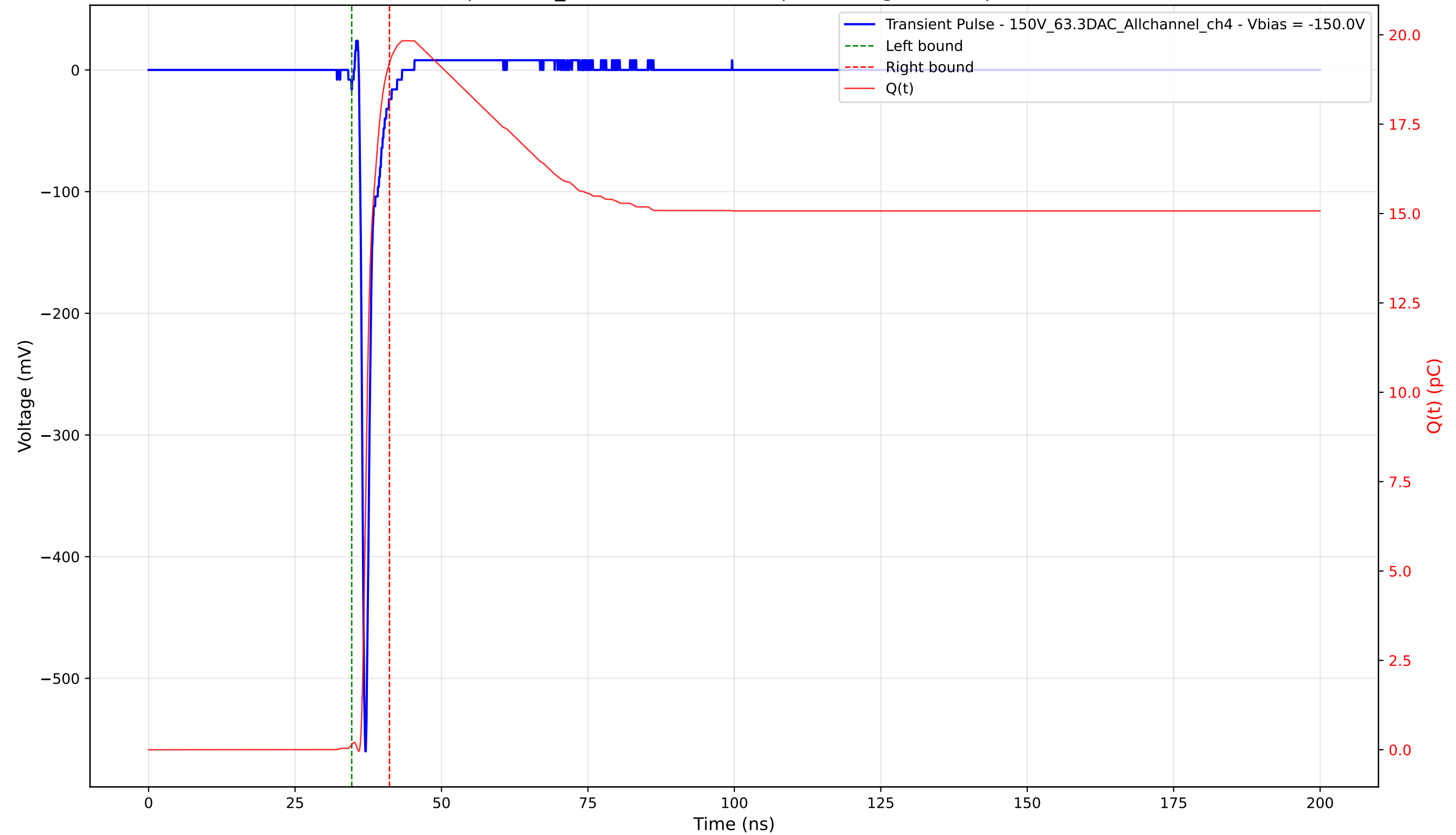
Transient Pulse - Sample: 1cm_42 - Position: 1735.0 \mu\text{m} - Charge: 19.08 pC - Rise Time: 0.70 ns
