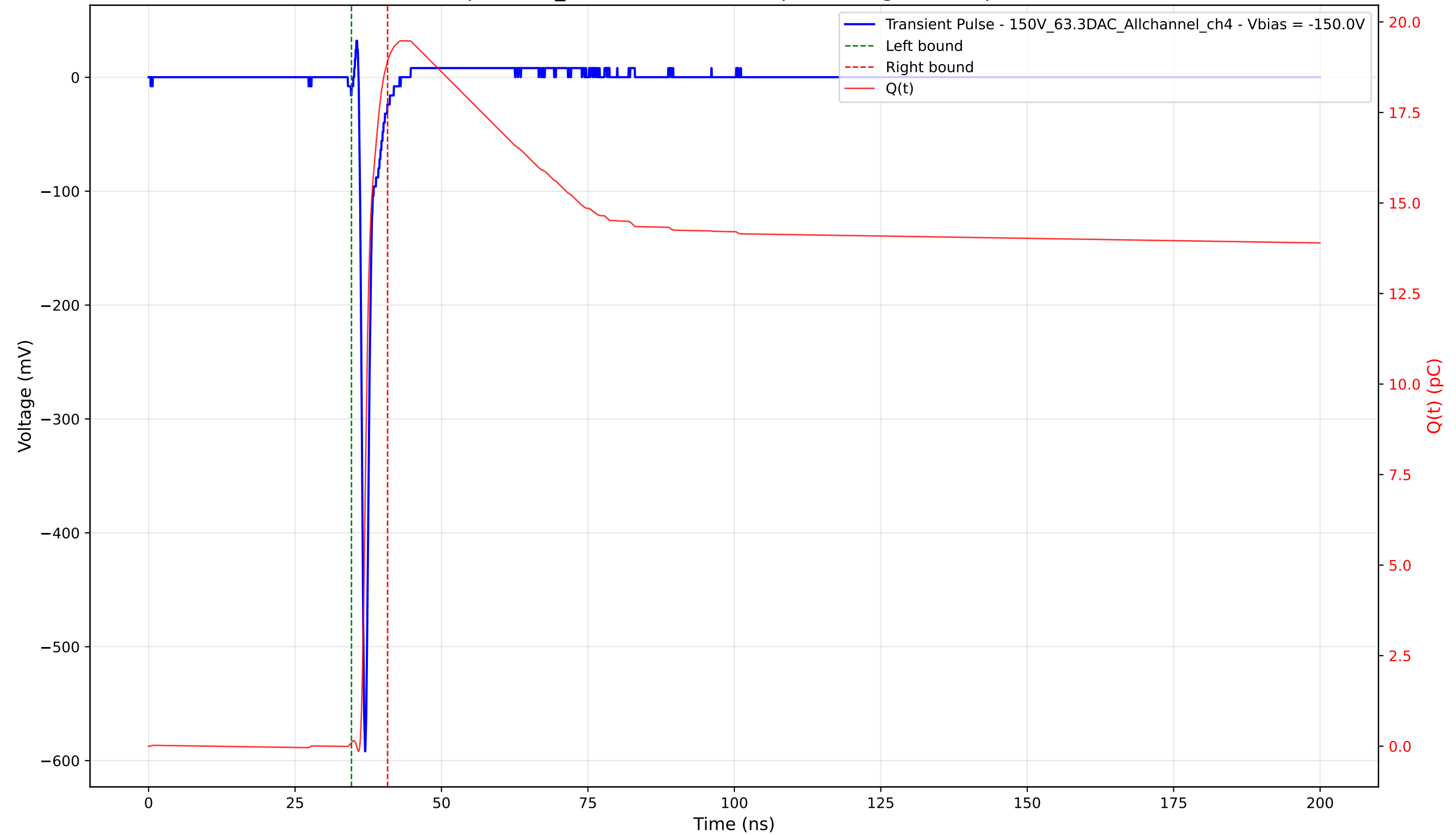
Transient Pulse - Sample: 1cm_42 - Position: 1870.0 \mu\text{m} - Charge: 18.82 pC - Rise Time: 0.71 ns
