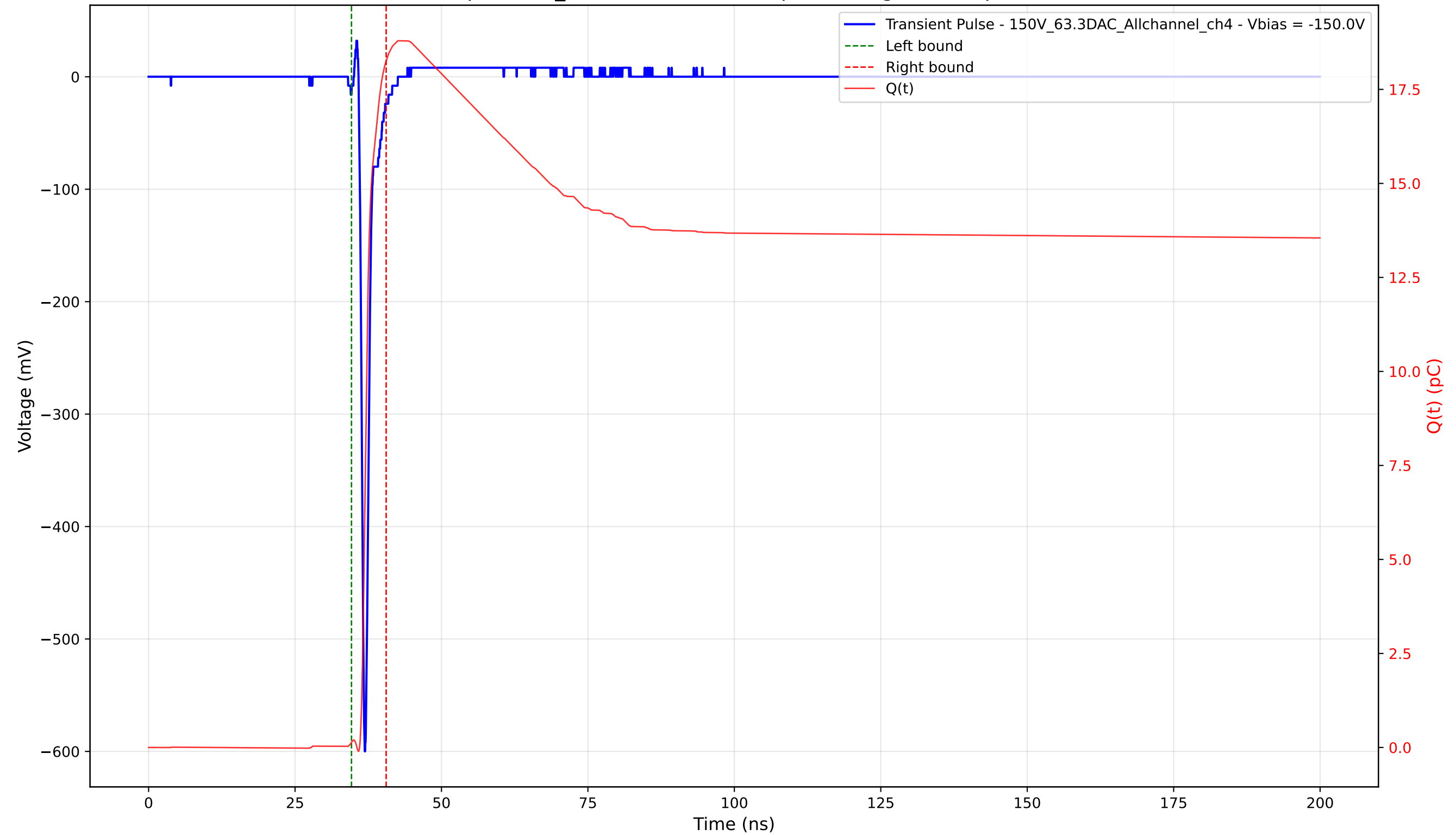
Transient Pulse - Sample: 1cm_42 - Position: 1975.0 \mu\text{m} - Charge: 18.11 pC - Rise Time: 0.70 ns
