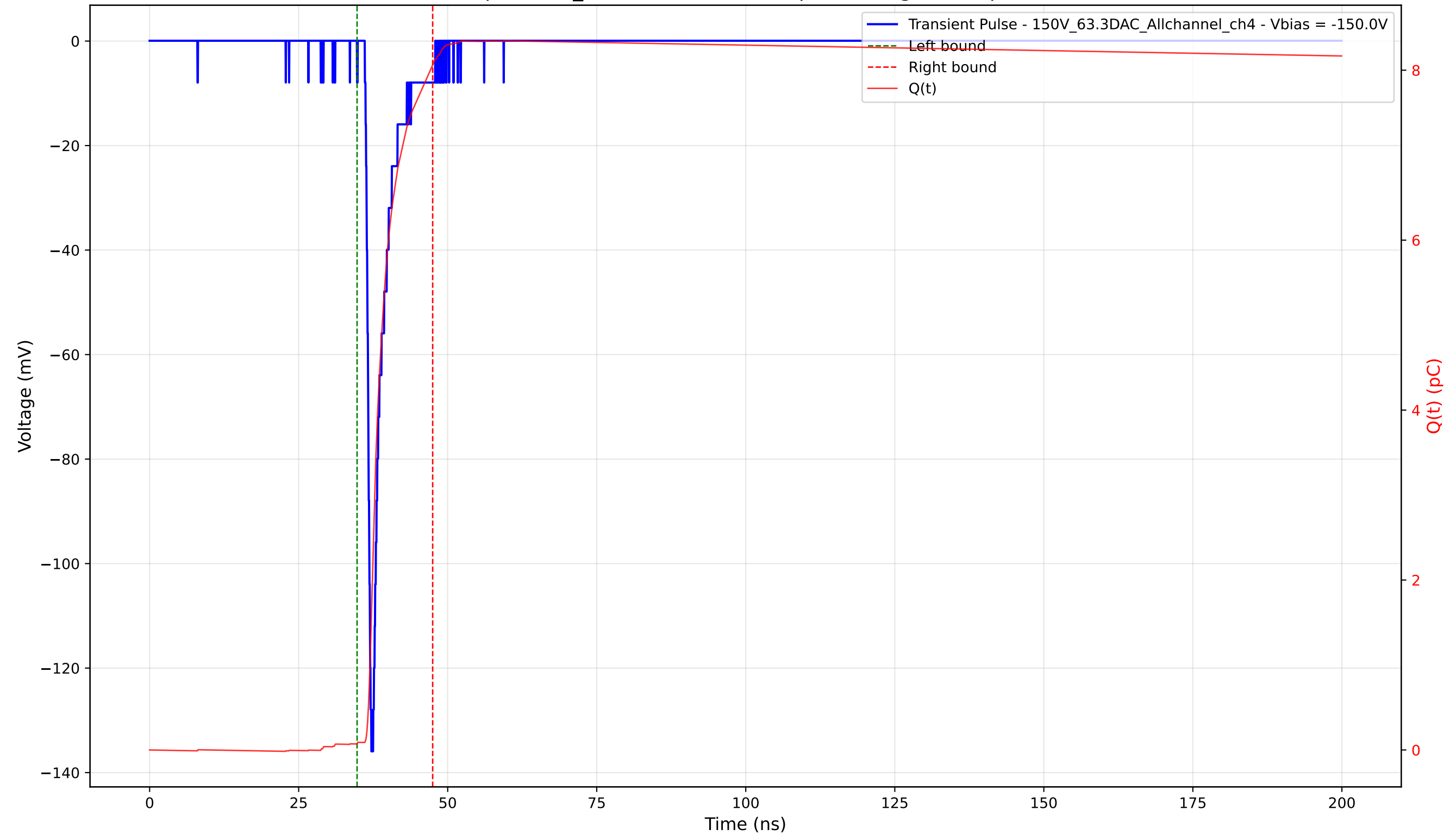
Transient Pulse - Sample: 1cm_42 - Position: 2785.0 \mu\text{m} - Charge: 7.99 pC - Rise Time: 0.85 ns
