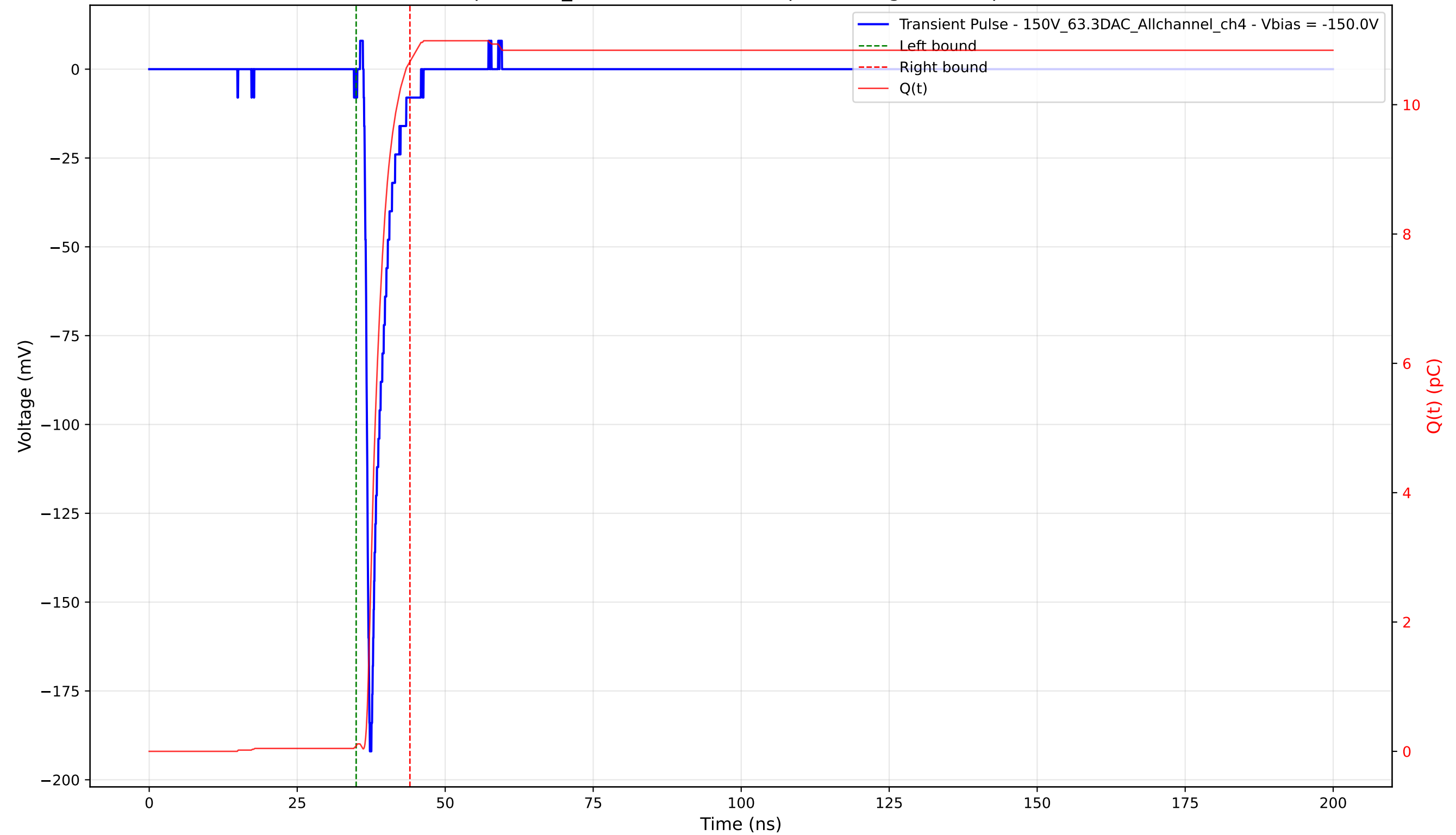
Transient Pulse - Sample: 1cm_42 - Position: 1355.0 \mu\text{m} - Charge: 10.58 pC - Rise Time: 0.77 ns
