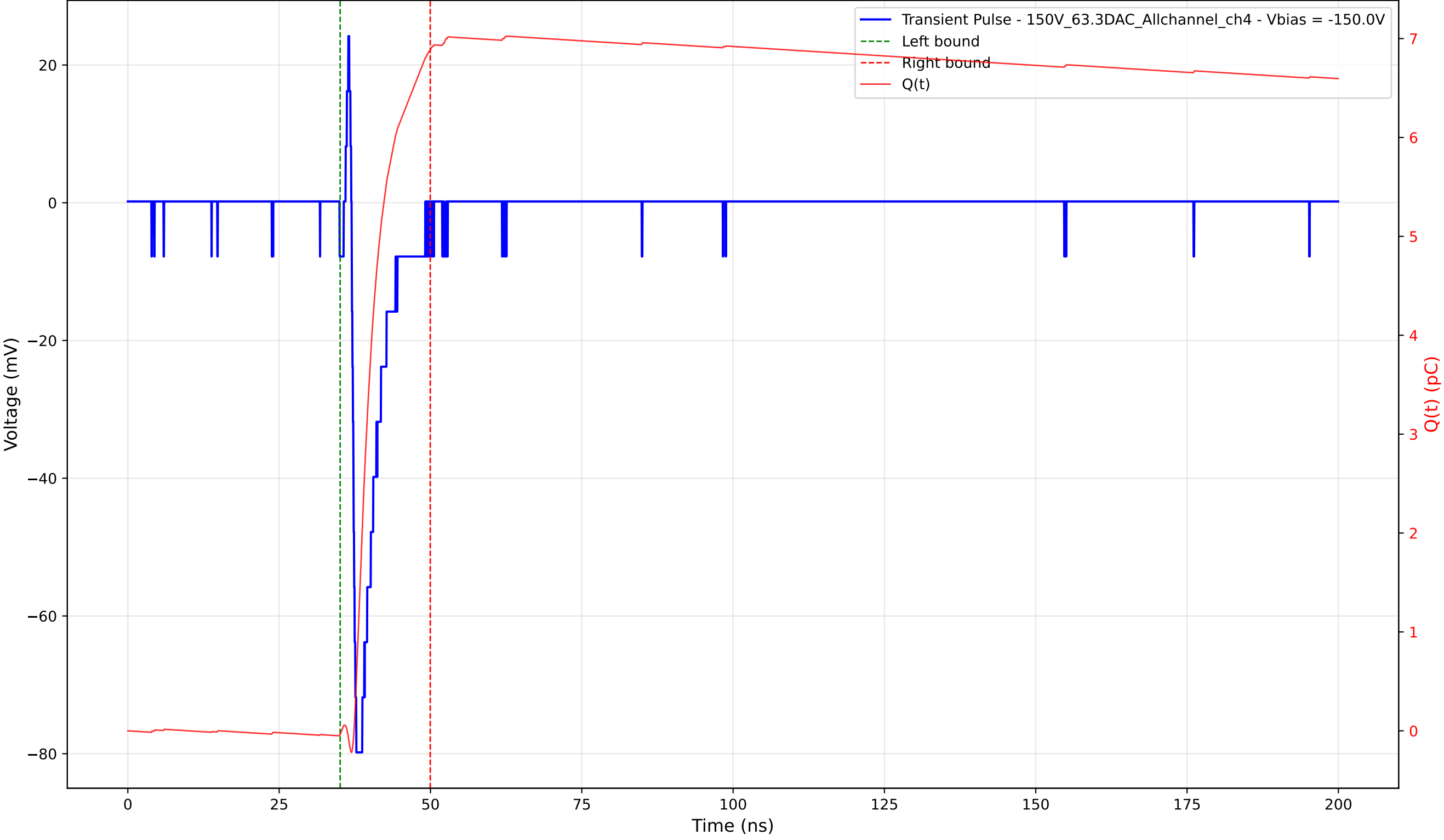
Transient Pulse - Sample: 1cm_42 - Position: 840.0 \mu\text{m} - Charge: 6.92 pC - Rise Time: 0.76 ns
