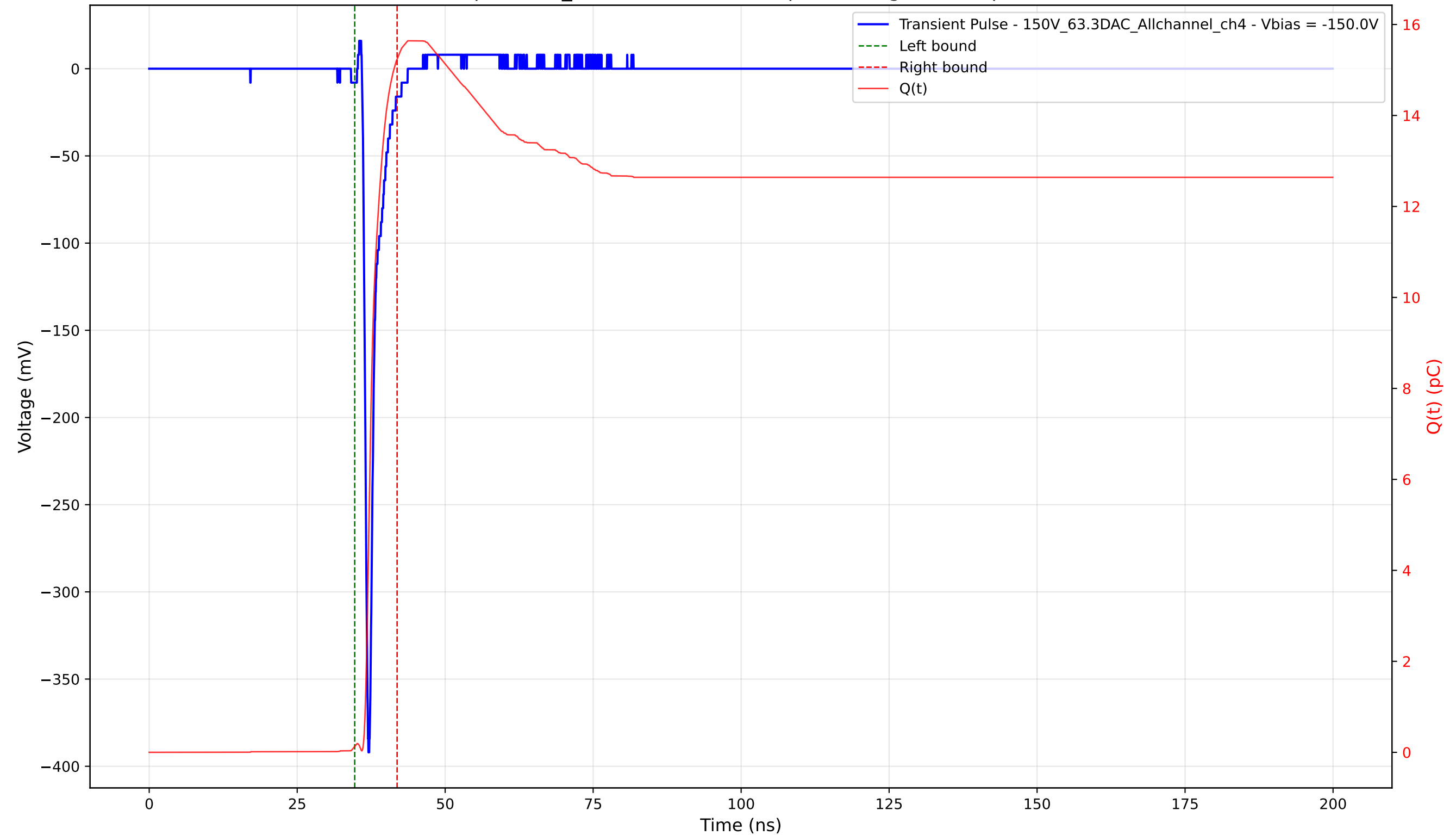
Transient Pulse - Sample: 1cm_42 - Position: 1615.0 \mu\text{m} - Charge: 15.11 pC - Rise Time: 0.73 ns
