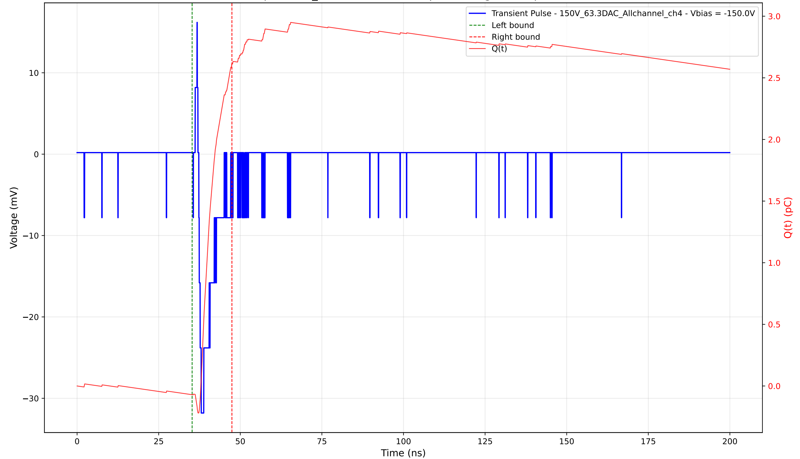
Transient Pulse - Sample: 1cm_42 - Position: 265.0 \mu\text{m} - Charge: 2.69 pC - Rise Time: 0.74 ns
