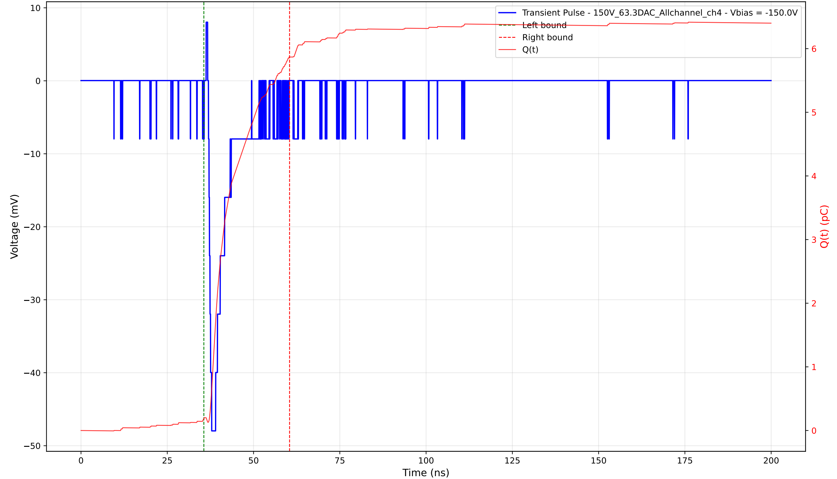
Transient Pulse - Sample: 1cm_42 - Position: 3230.0 \mu\text{m} - Charge: 5.68 pC - Rise Time: 0.94 ns
