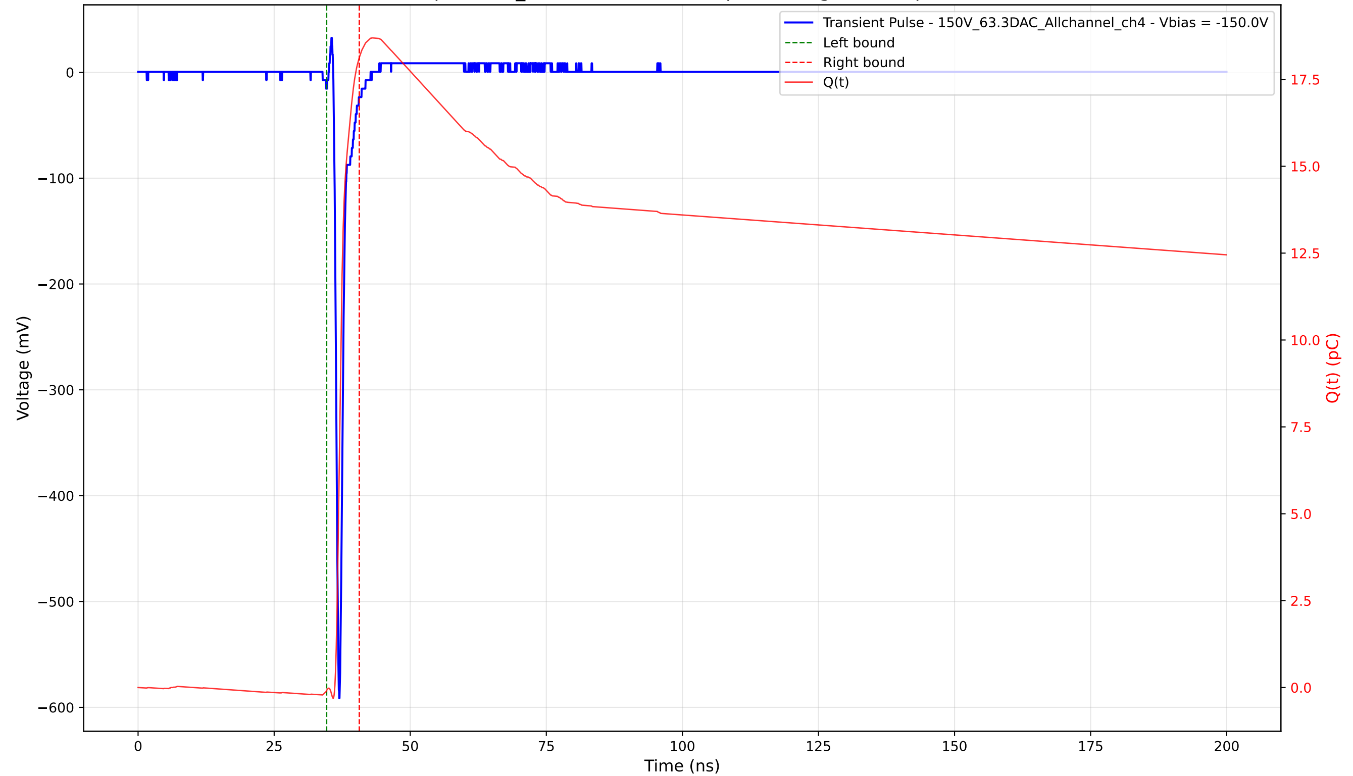
Transient Pulse - Sample: 1cm_42 - Position: 1930.0 \mu\text{m} - Charge: 18.21 pC - Rise Time: 0.72 ns
