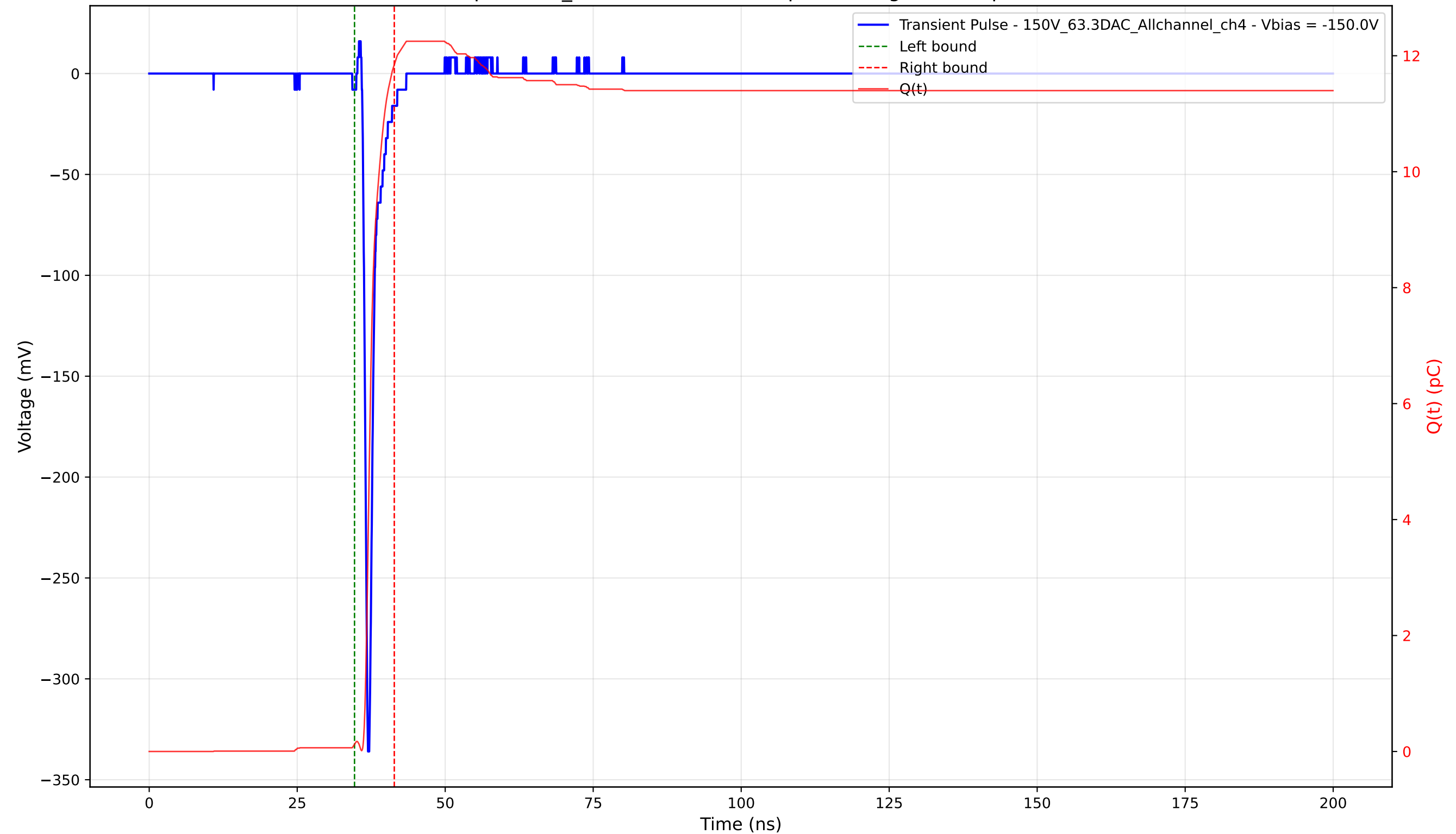
Transient Pulse - Sample: 1cm_42 - Position: 2420.0 \mu\text{m} - Charge: 11.72 pC - Rise Time: 0.71 ns
