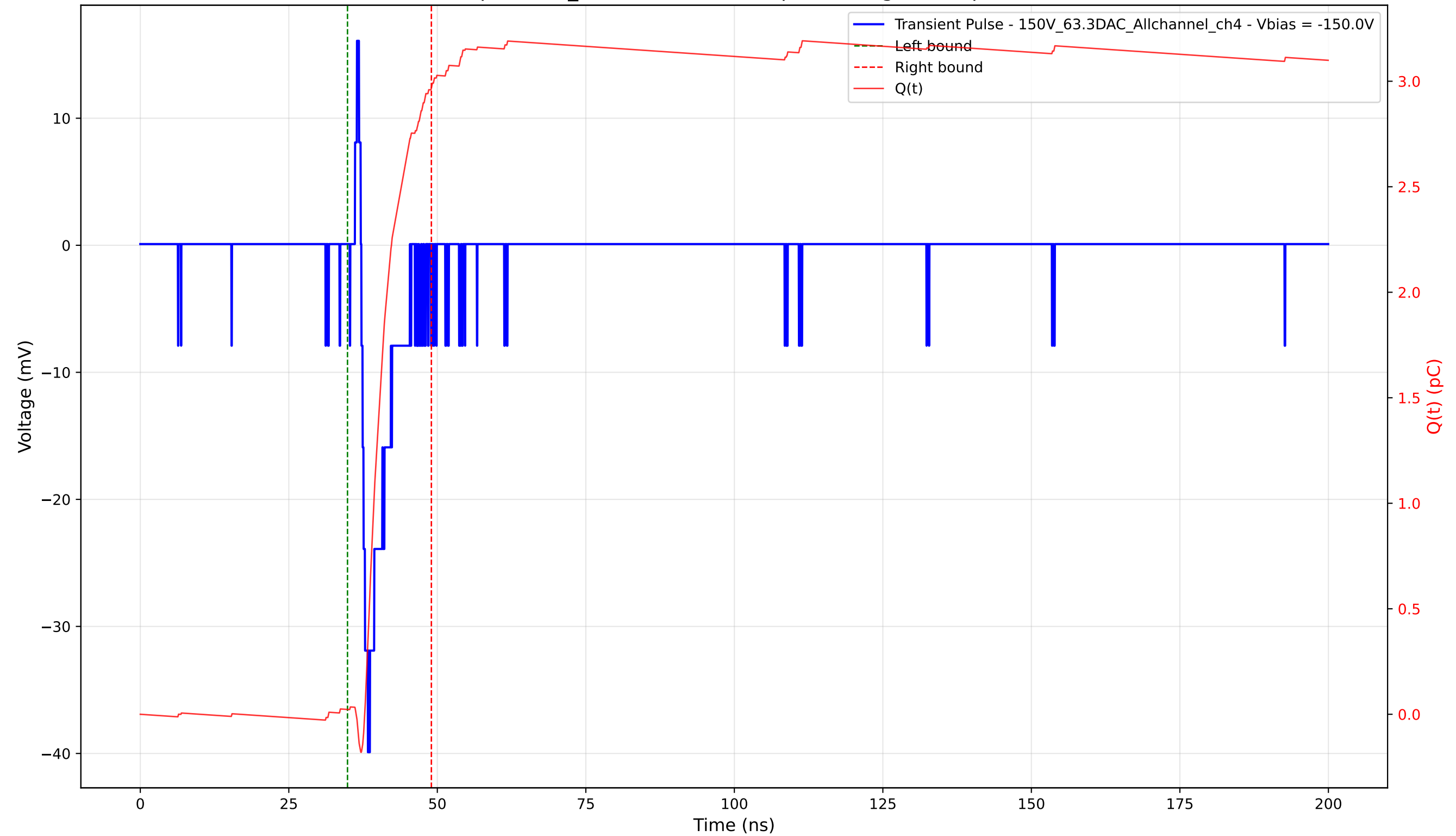
Transient Pulse - Sample: 1cm_42 - Position: 325.0 \mu\text{m} - Charge: 2.95 pC - Rise Time: 1.10 ns
