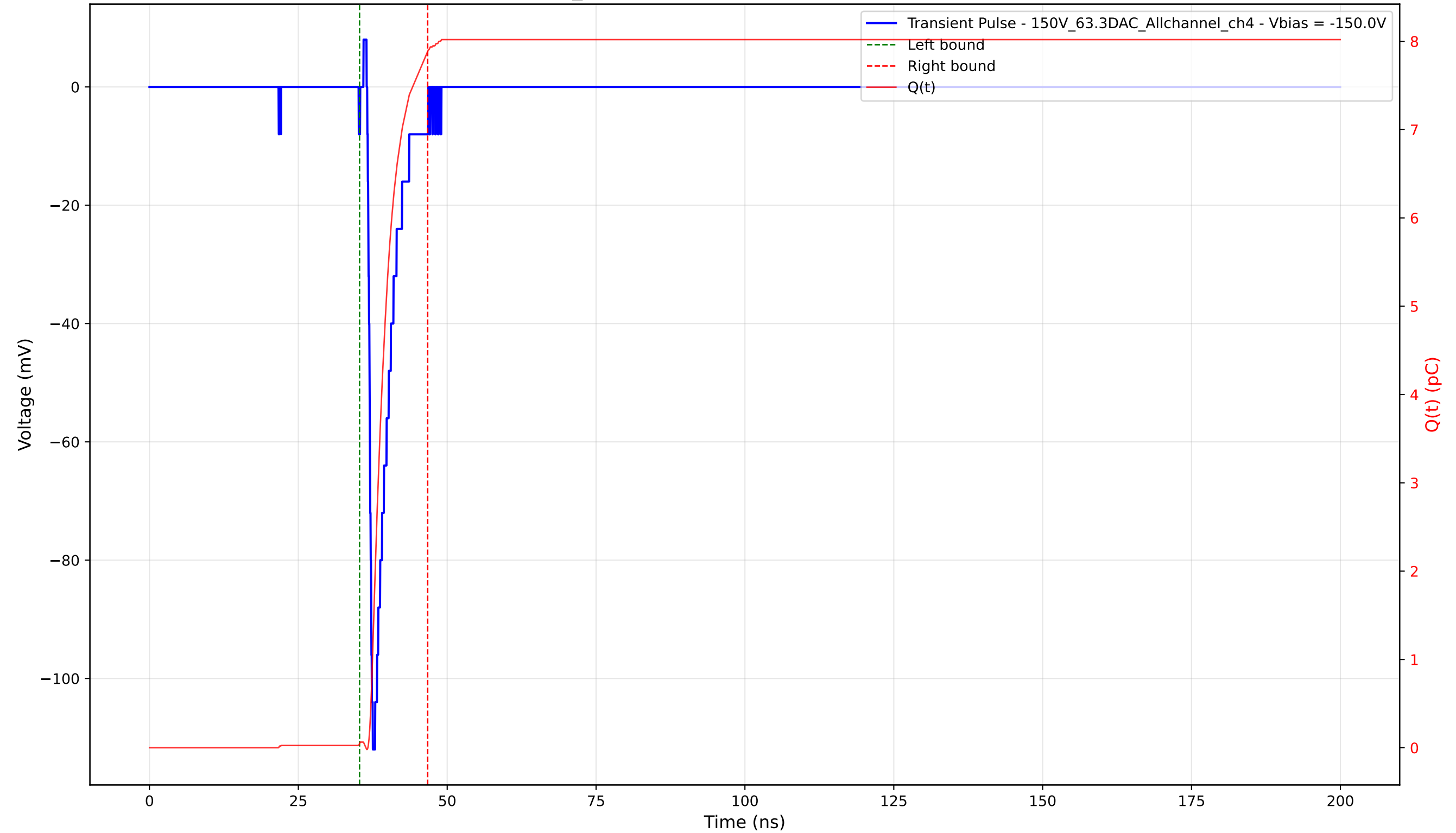
Transient Pulse - Sample: 1cm_42 - Position: 1060.0 \mu\text{m} - Charge: 7.84 pC - Rise Time: 0.70 ns
