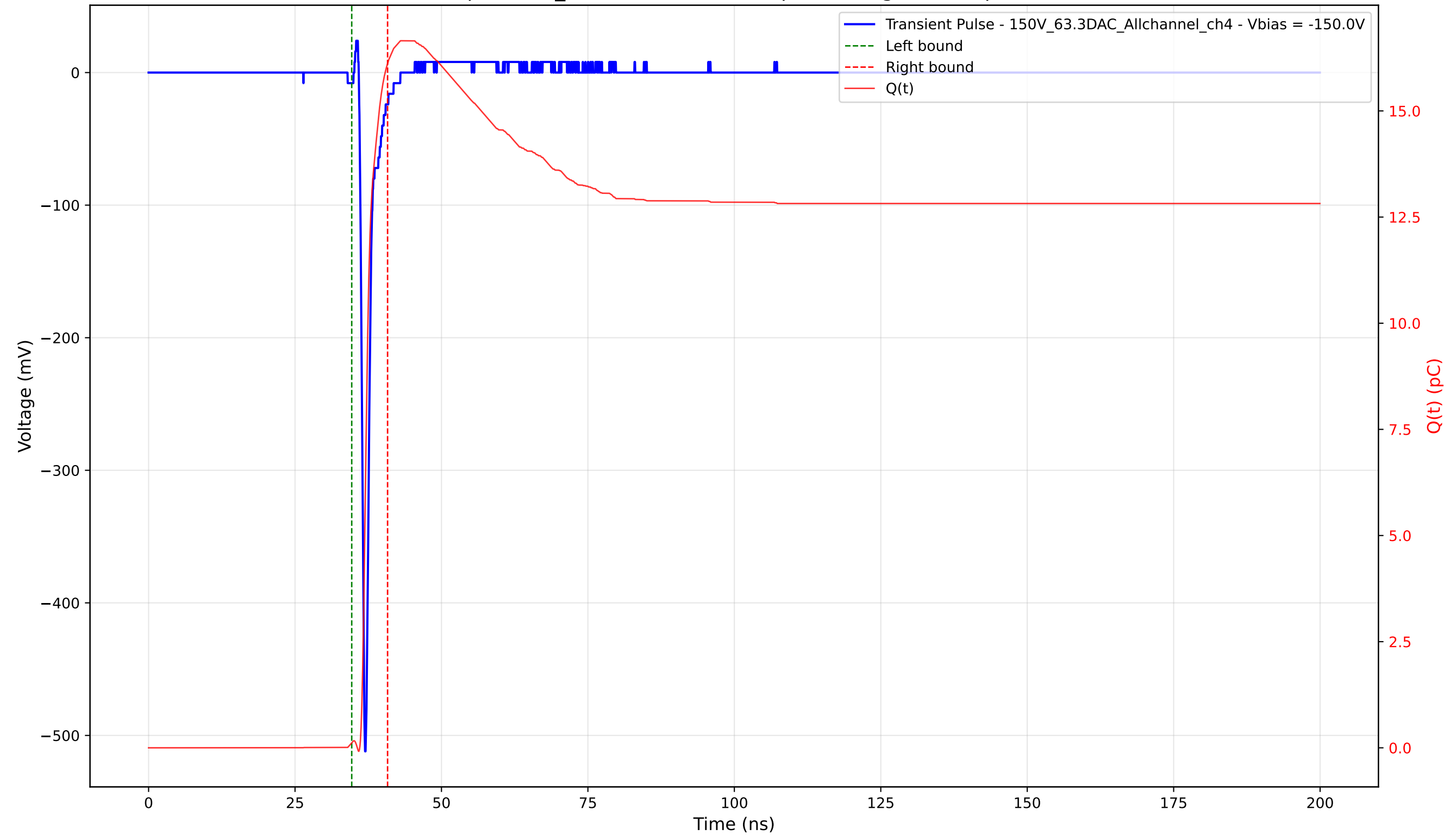
Transient Pulse - Sample: 1cm_42 - Position: 2240.0 \mu\text{m} - Charge: 16.00 pC - Rise Time: 0.72 ns
