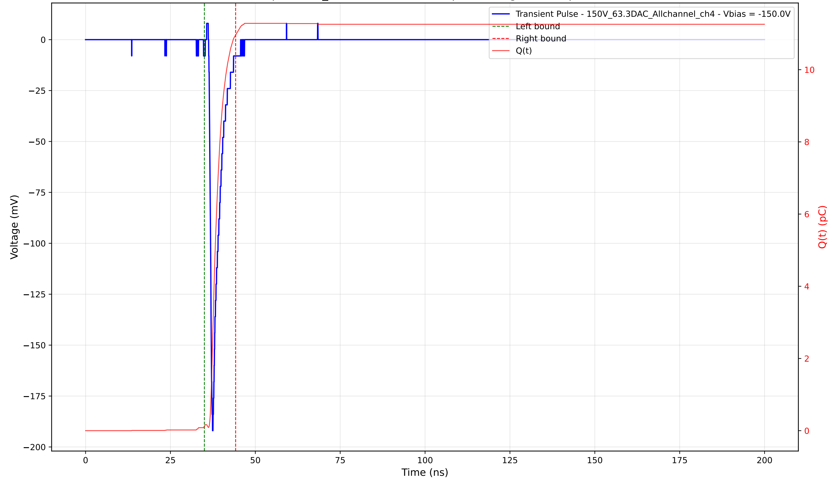
Transient Pulse - Sample: 1cm_42 - Position: 1310.0 \mu\text{m} - Charge: 10.84 pC - Rise Time: 0.78 ns
