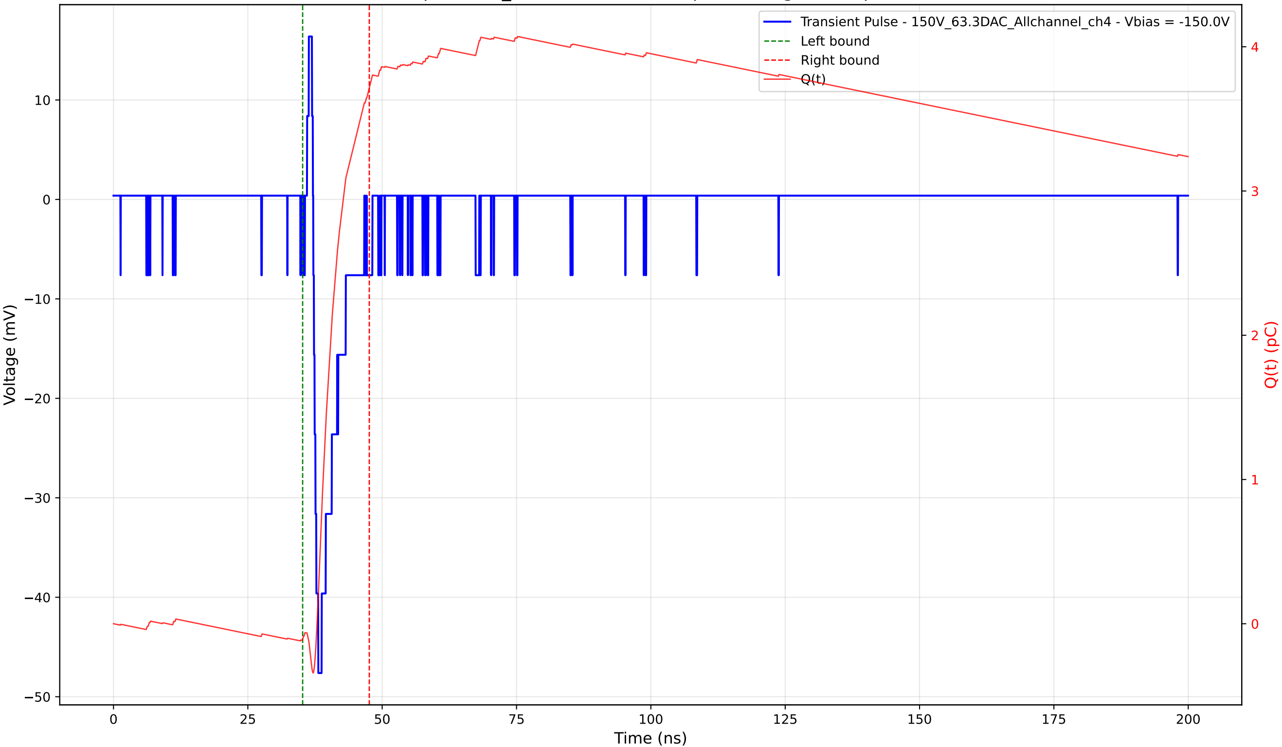
Transient Pulse - Sample: 1cm_42 - Position: 450.0 \mu\text{m} - Charge: 3.82 pC - Rise Time: 0.94 ns
