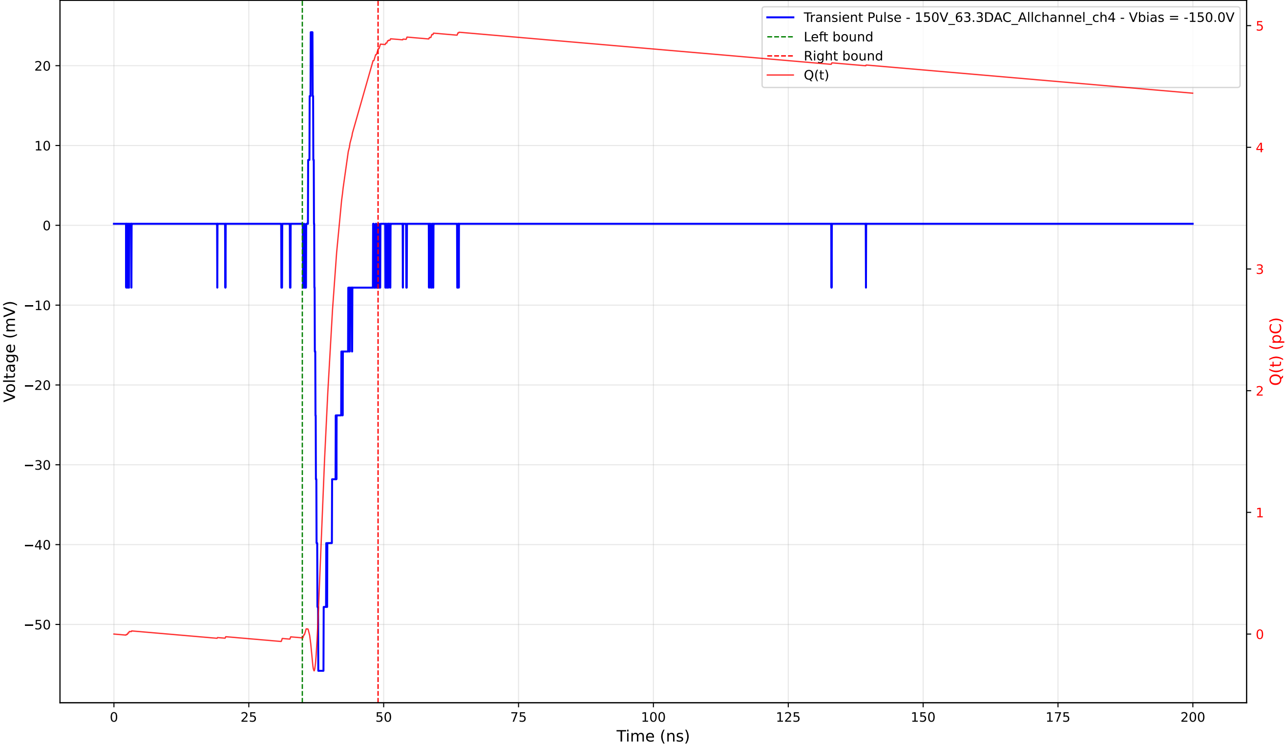
Transient Pulse - Sample: 1cm_42 - Position: 545.0 \mu\text{m} - Charge: 4.84 pC - Rise Time: 0.73 ns
