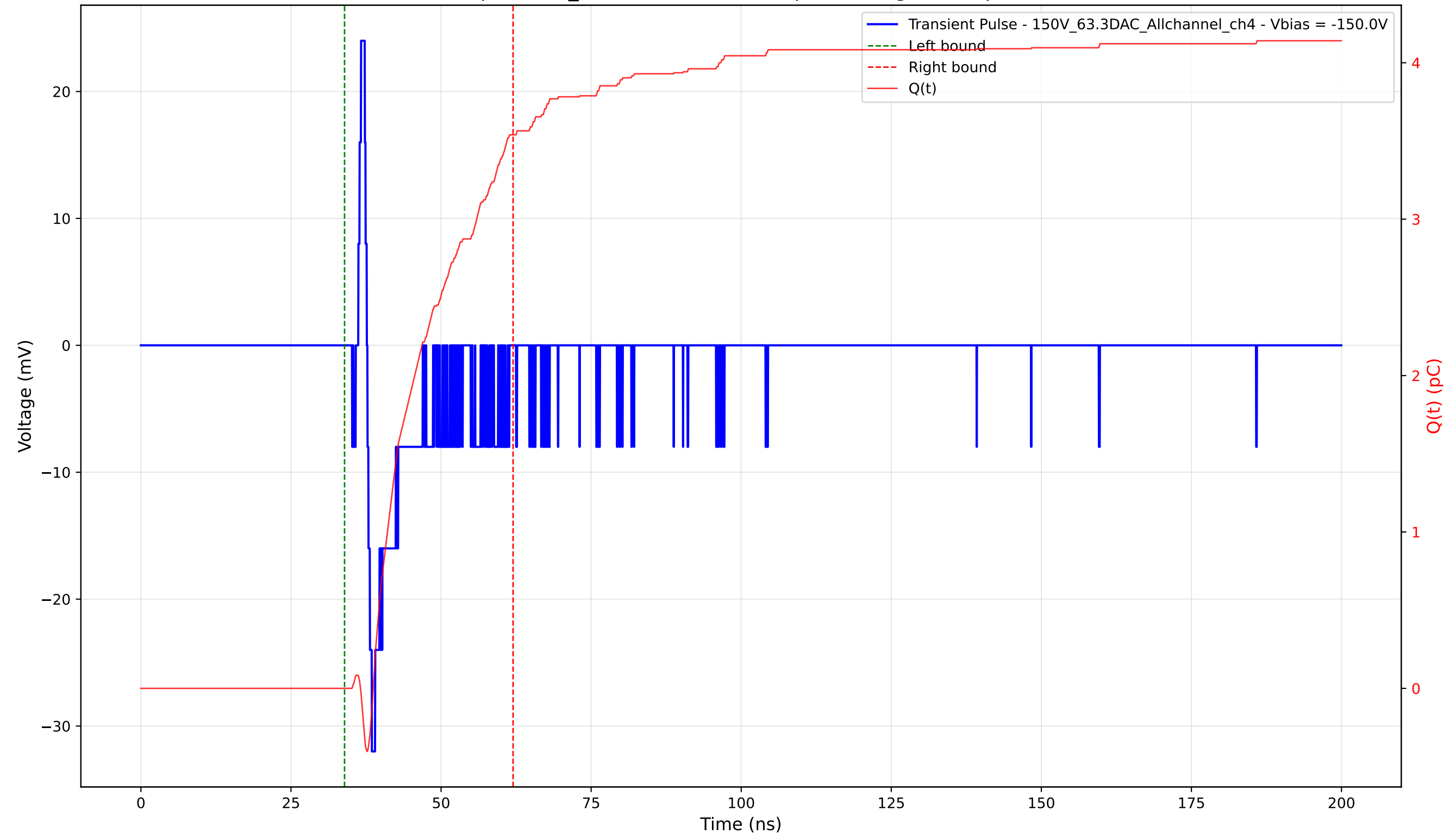
Transient Pulse - Sample: 1cm_42 - Position: 3980.0 \mu\text{m} - Charge: 3.54 pC - Rise Time: 0.74 ns
