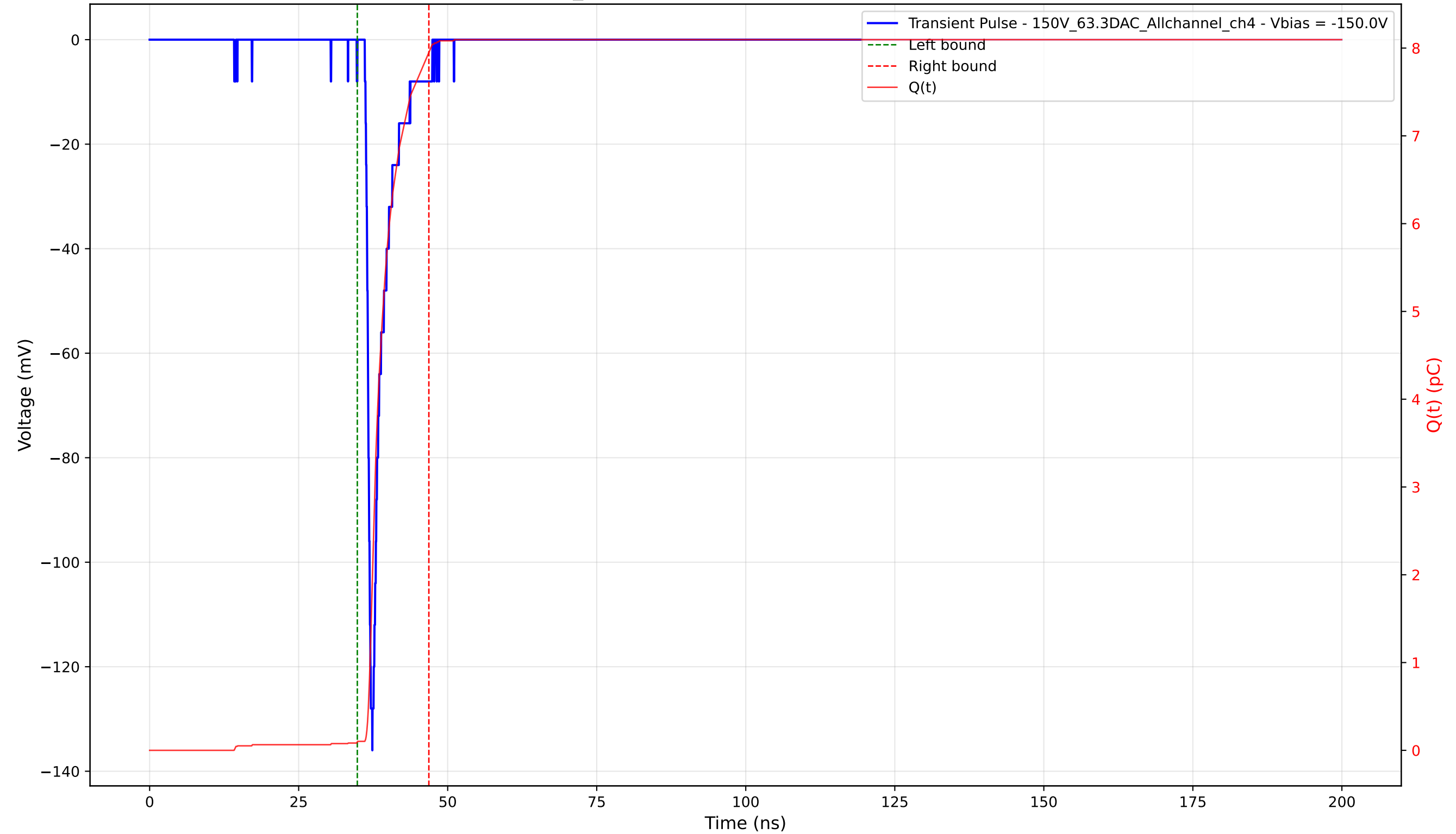
Transient Pulse - Sample: 1cm_42 - Position: 2795.0 \mu\text{m} - Charge: 7.85 pC - Rise Time: 0.89 ns
