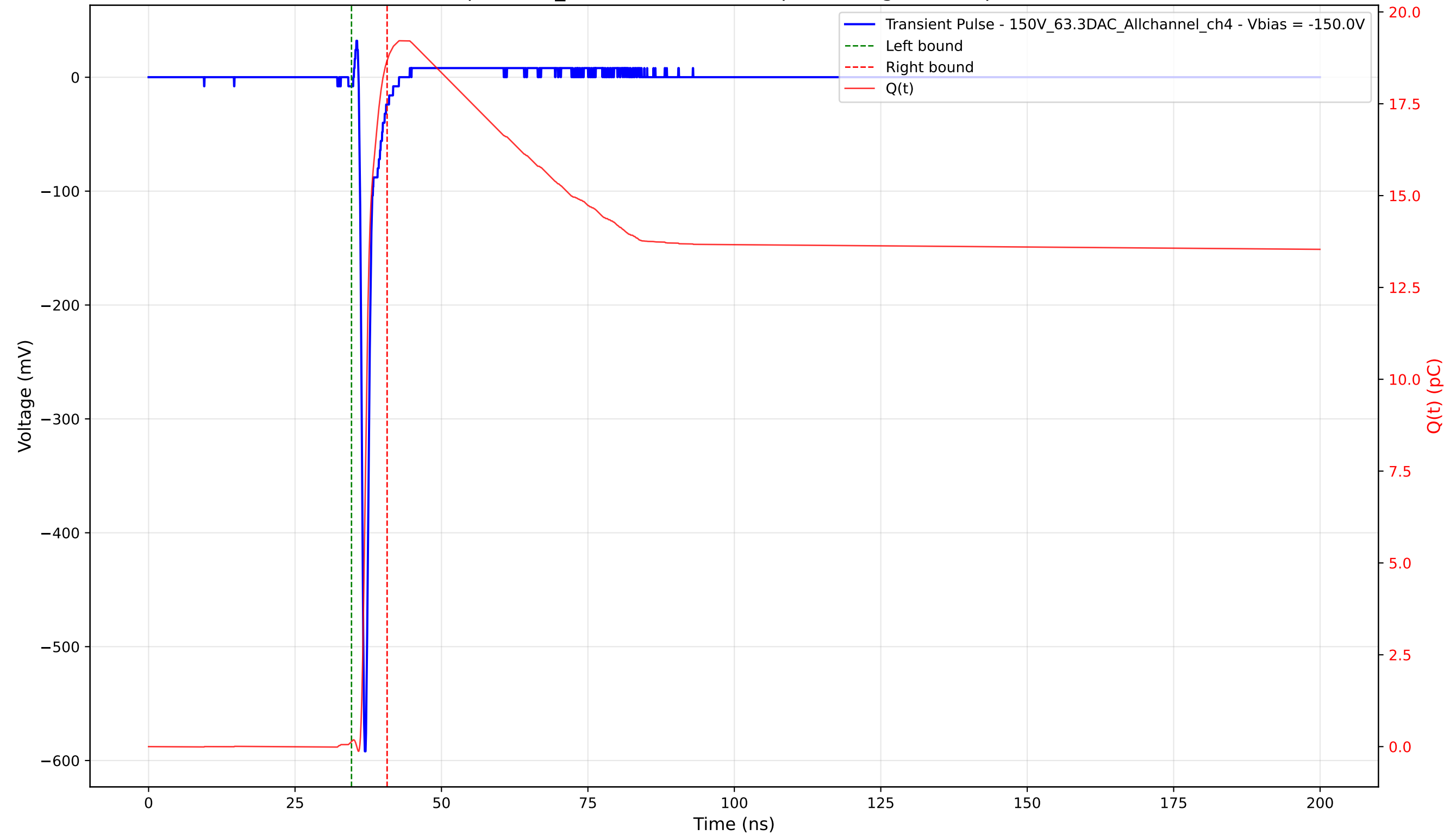
Transient Pulse - Sample: 1cm_42 - Position: 1910.0 \mu\text{m} - Charge: 18.54 pC - Rise Time: 0.70 ns
