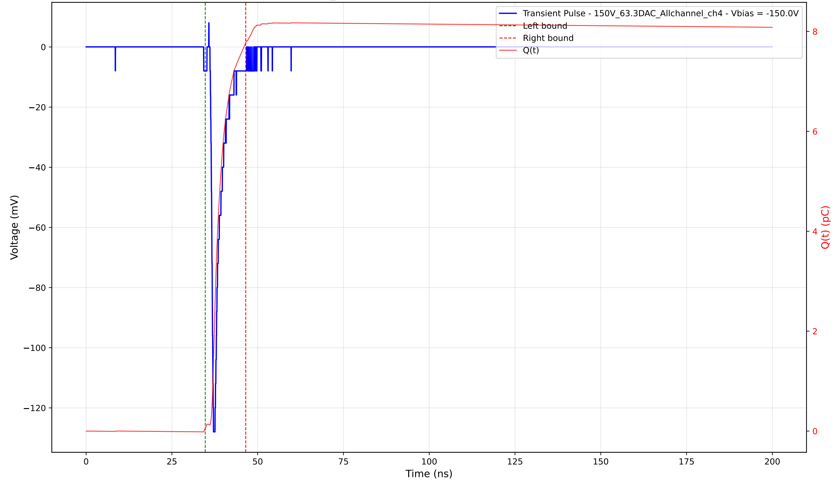
Transient Pulse - Sample: 1cm_42 - Position: 2790.0 \mu\text{m} - Charge: 7.72 pC - Rise Time: 0.82 ns
