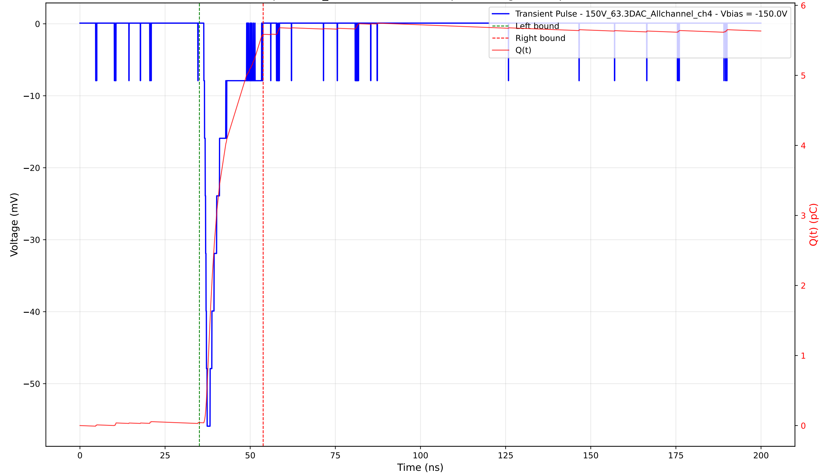
Transient Pulse - Sample: 1cm_42 - Position: 3040.0 \mu\text{m} - Charge: 5.55 pC - Rise Time: 0.97 ns
