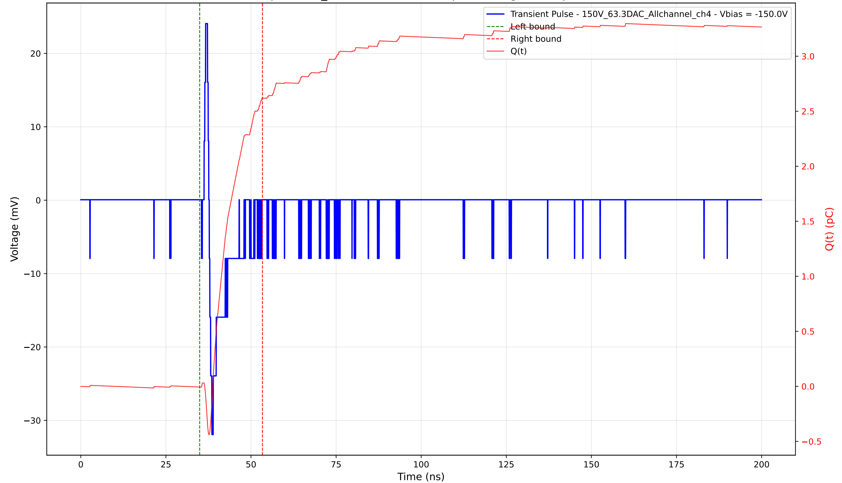
Transient Pulse - Sample: 1cm_42 - Position: 4445.0 \mu\text{m} - Charge: 2.63 pC - Rise Time: 0.78 ns
