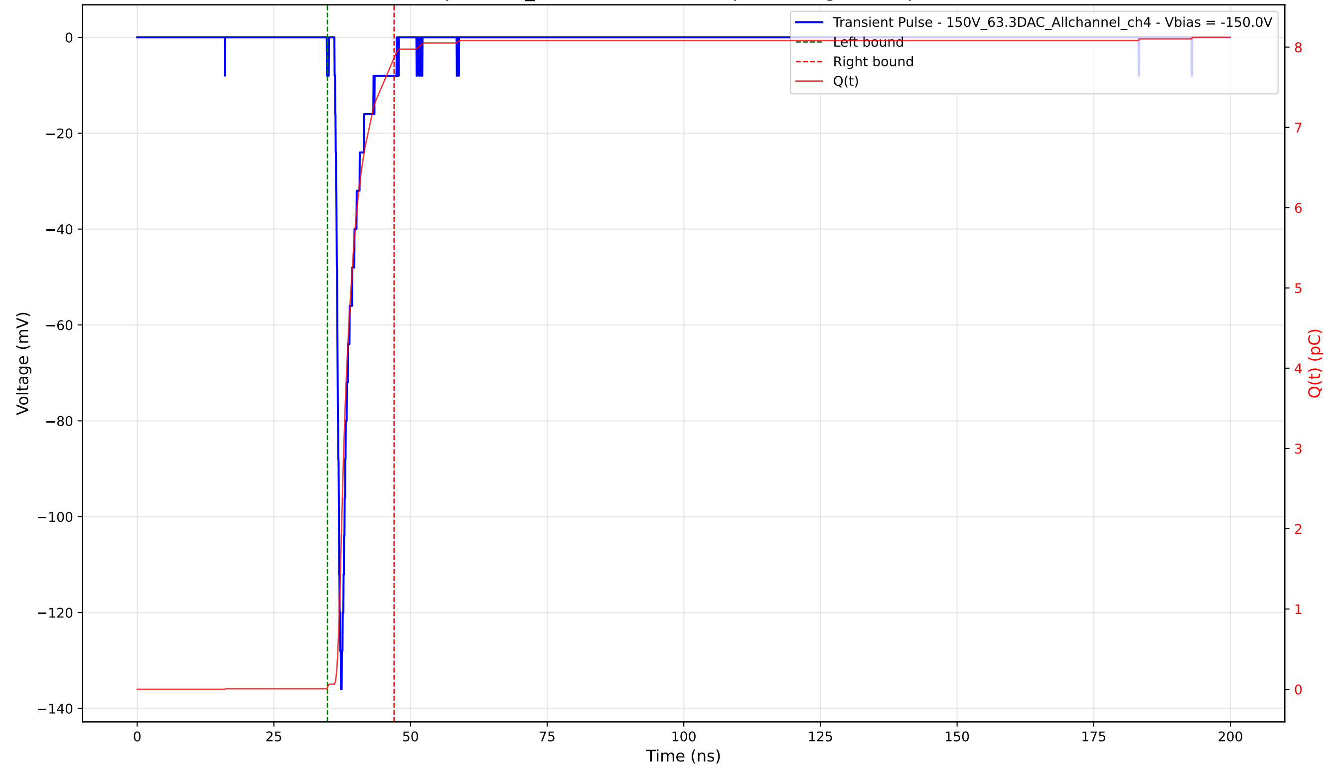
Transient Pulse - Sample: 1cm_42 - Position: 2800.0 \mu\text{m} - Charge: 7.85 pC - Rise Time: 0.93 ns
