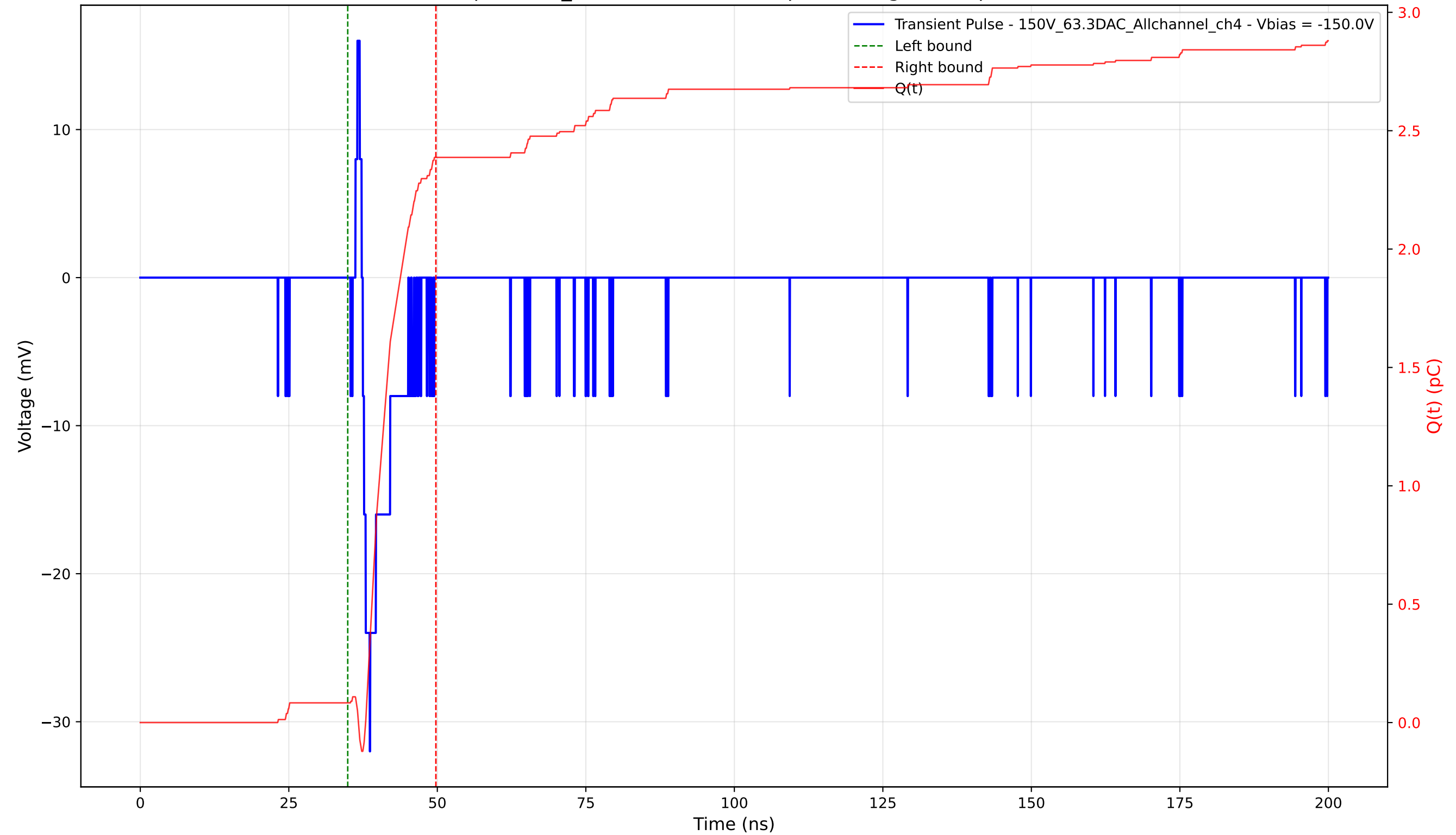
Transient Pulse - Sample: 1cm_42 - Position: 4950.0 \mu\text{m} - Charge: 2.30 pC - Rise Time: 1.18 ns
