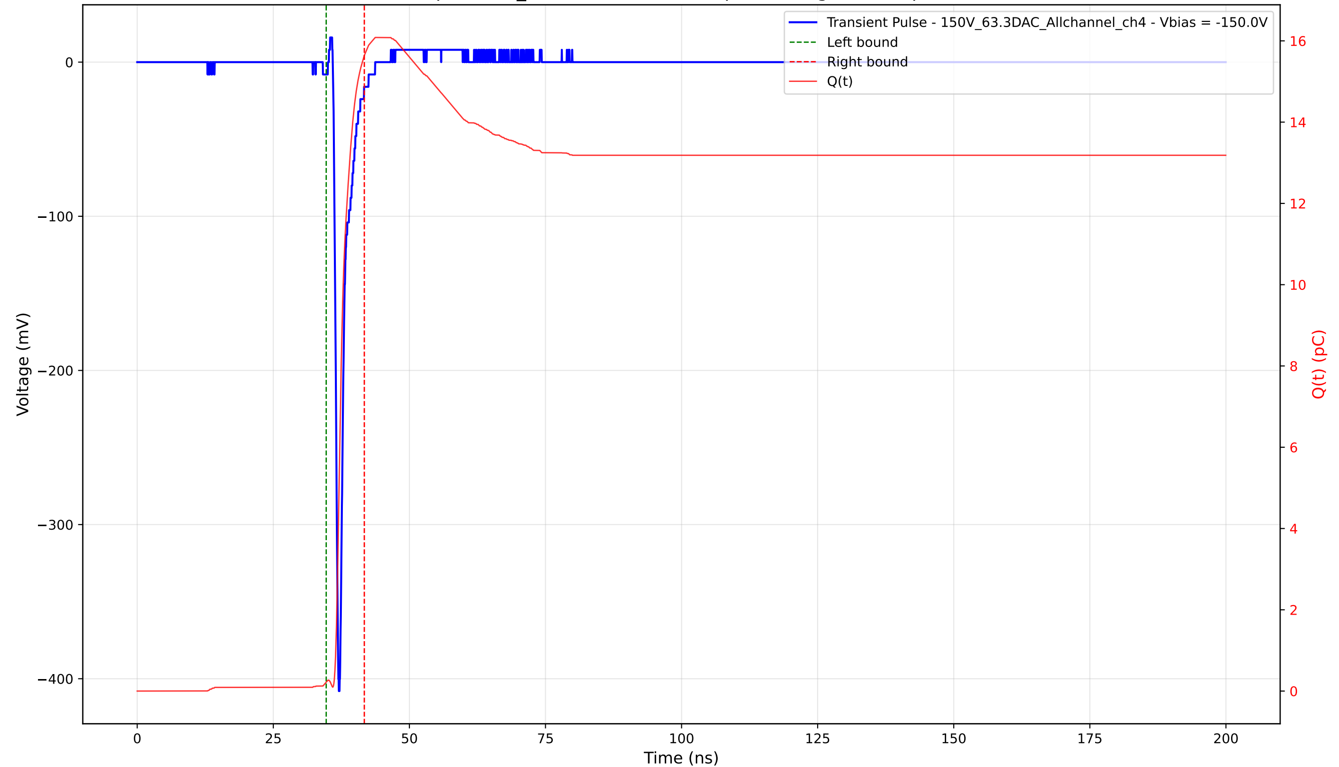
Transient Pulse - Sample: 1cm_42 - Position: 1625.0 \mu\text{m} - Charge: 15.42 pC - Rise Time: 0.74 ns
