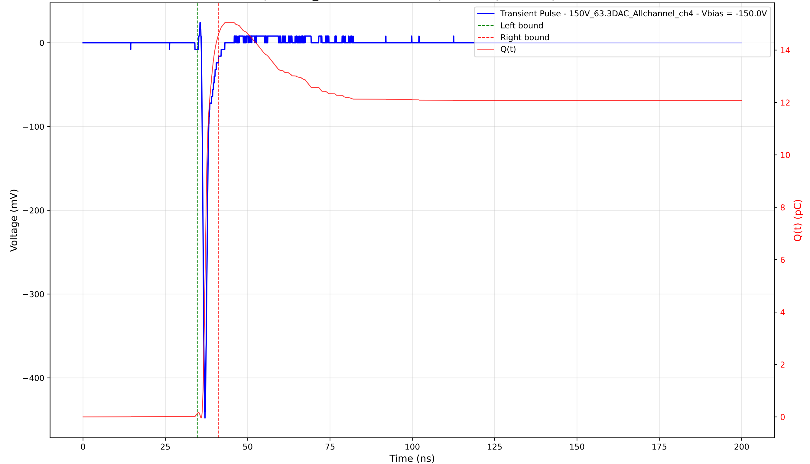
Transient Pulse - Sample: 1cm_42 - Position: 2340.0 \mu\text{m} - Charge: 14.44 pC - Rise Time: 0.72 ns
