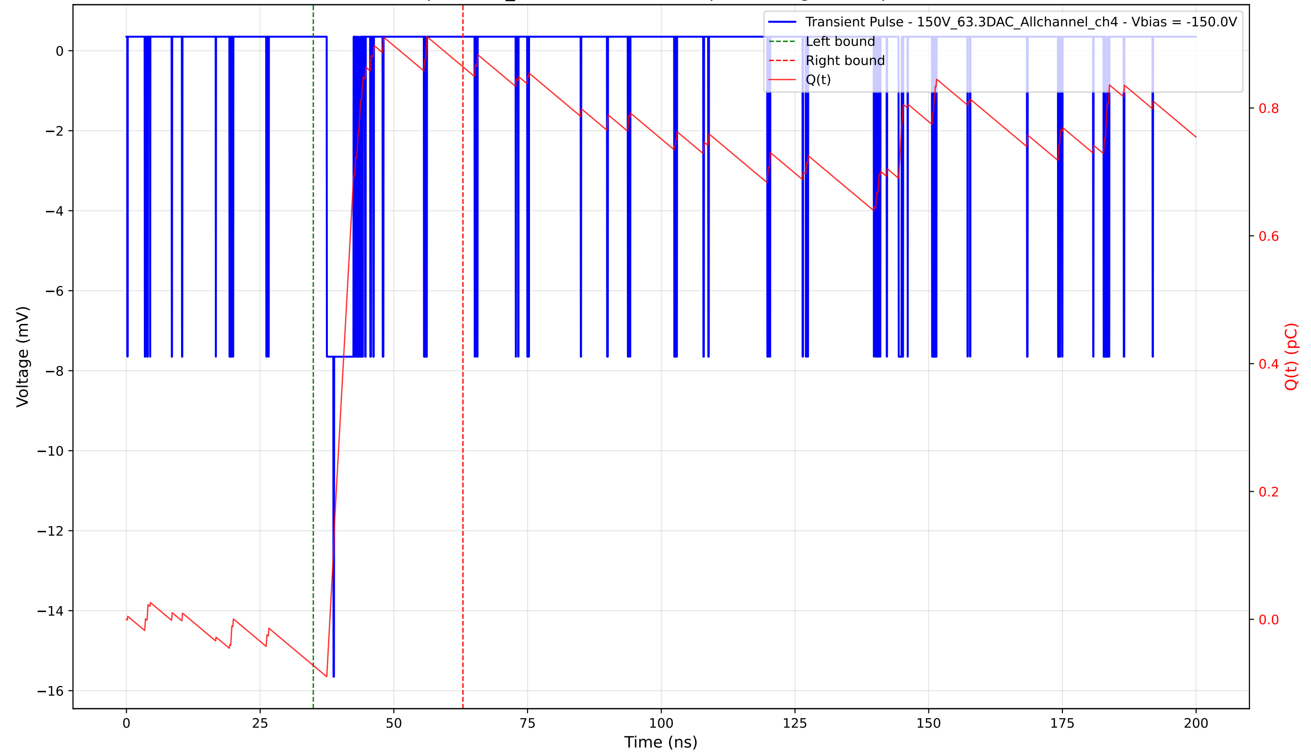
Transient Pulse - Sample: 1cm_42 - Position: 5115.0 \mu\text{m} - Charge: 0.94 pC - Rise Time: 1.27 ns
