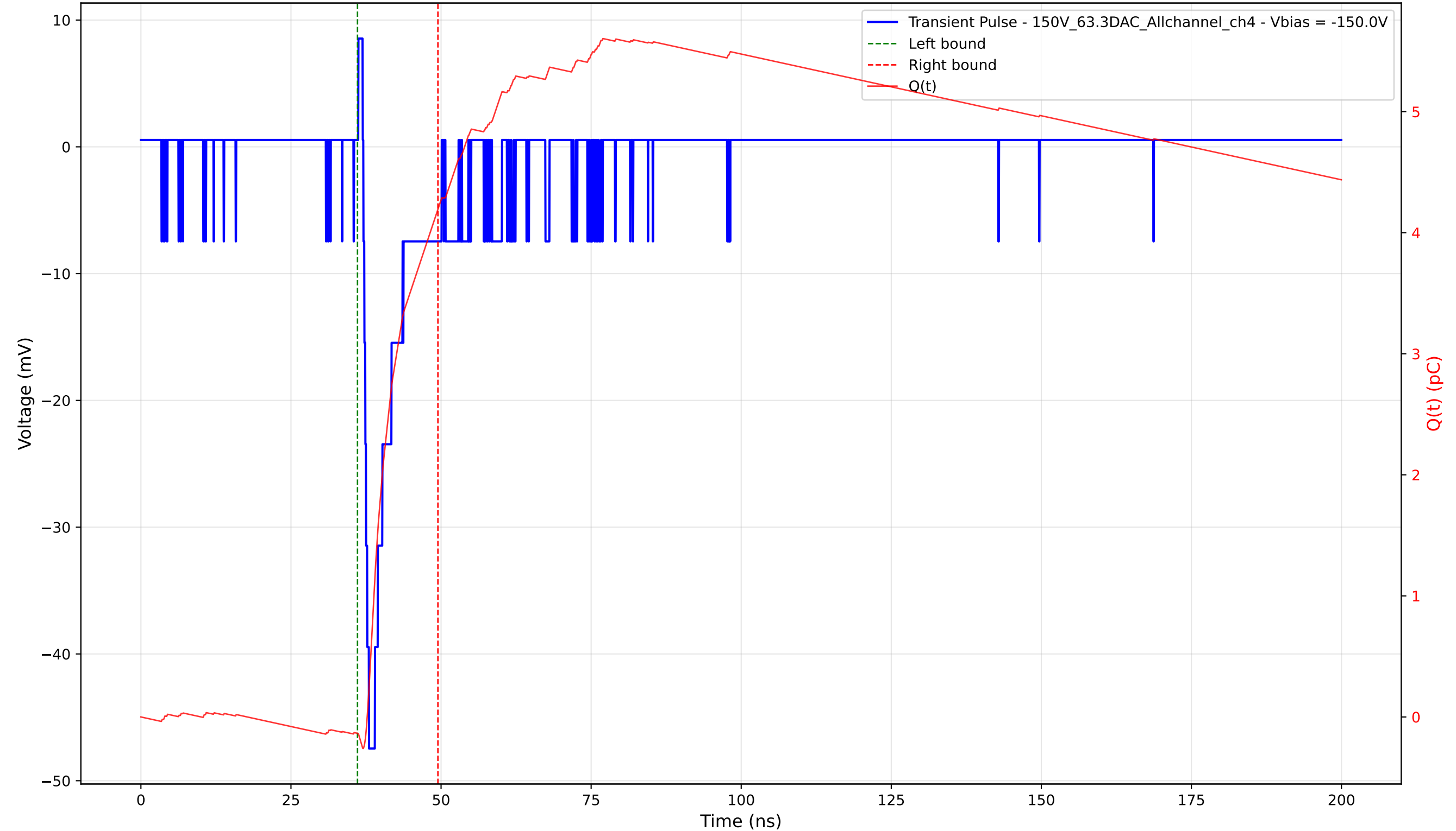
Transient Pulse - Sample: 1cm_42 - Position: 3325.0 \mu\text{m} - Charge: 4.33 pC - Rise Time: 0.94 ns
