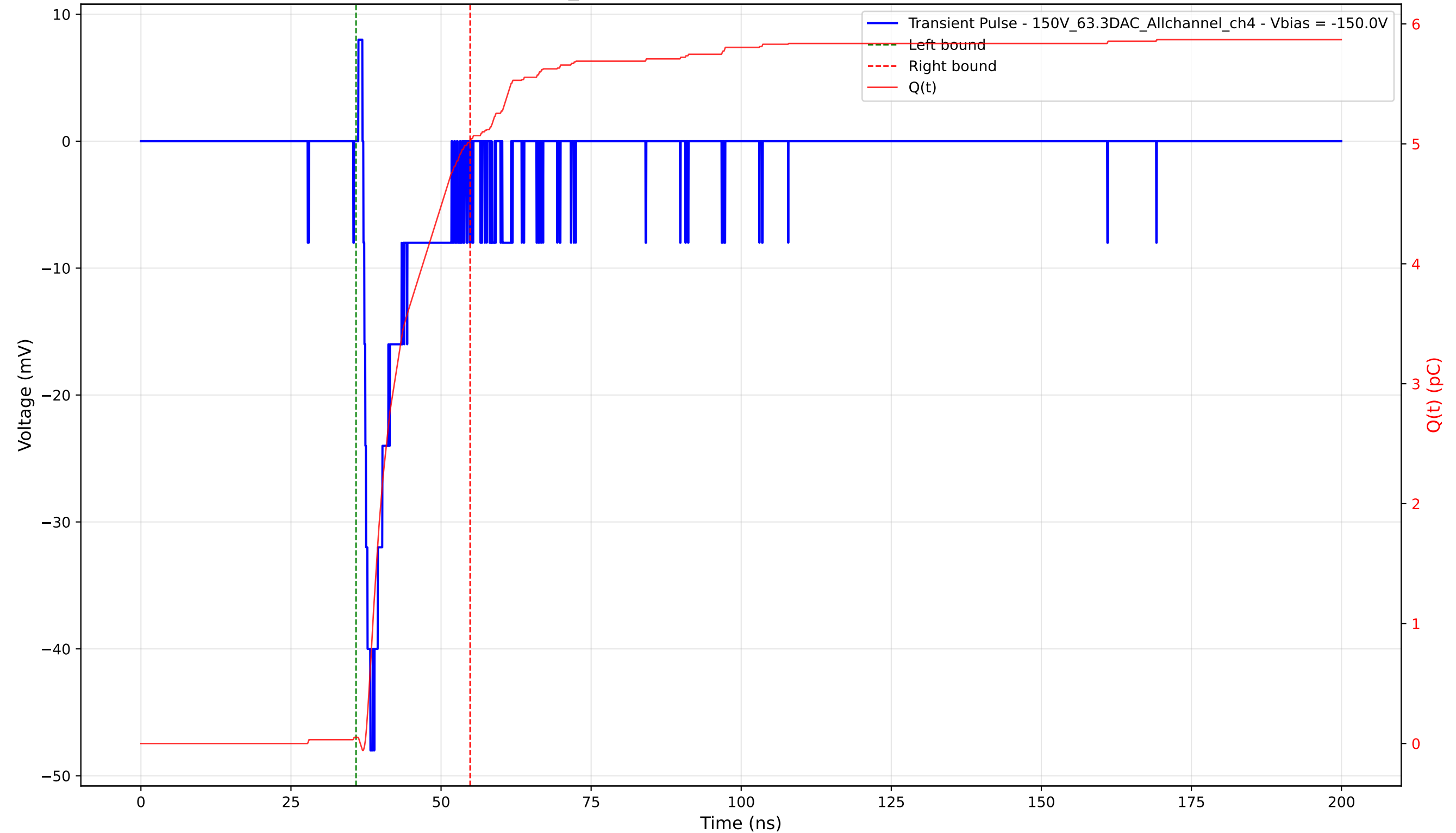
Transient Pulse - Sample: 1cm_42 - Position: 3340.0 \mu\text{m} - Charge: 4.97 pC - Rise Time: 1.18 ns
