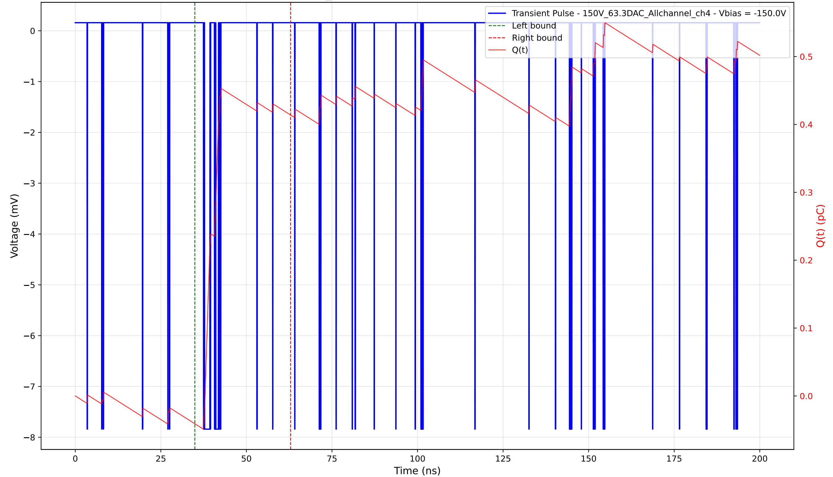
Transient Pulse - Sample: 1cm_42 - Position: 30.0 \mu\text{m} - Charge: 0.46 pC - Rise Time: 0.04 ns
