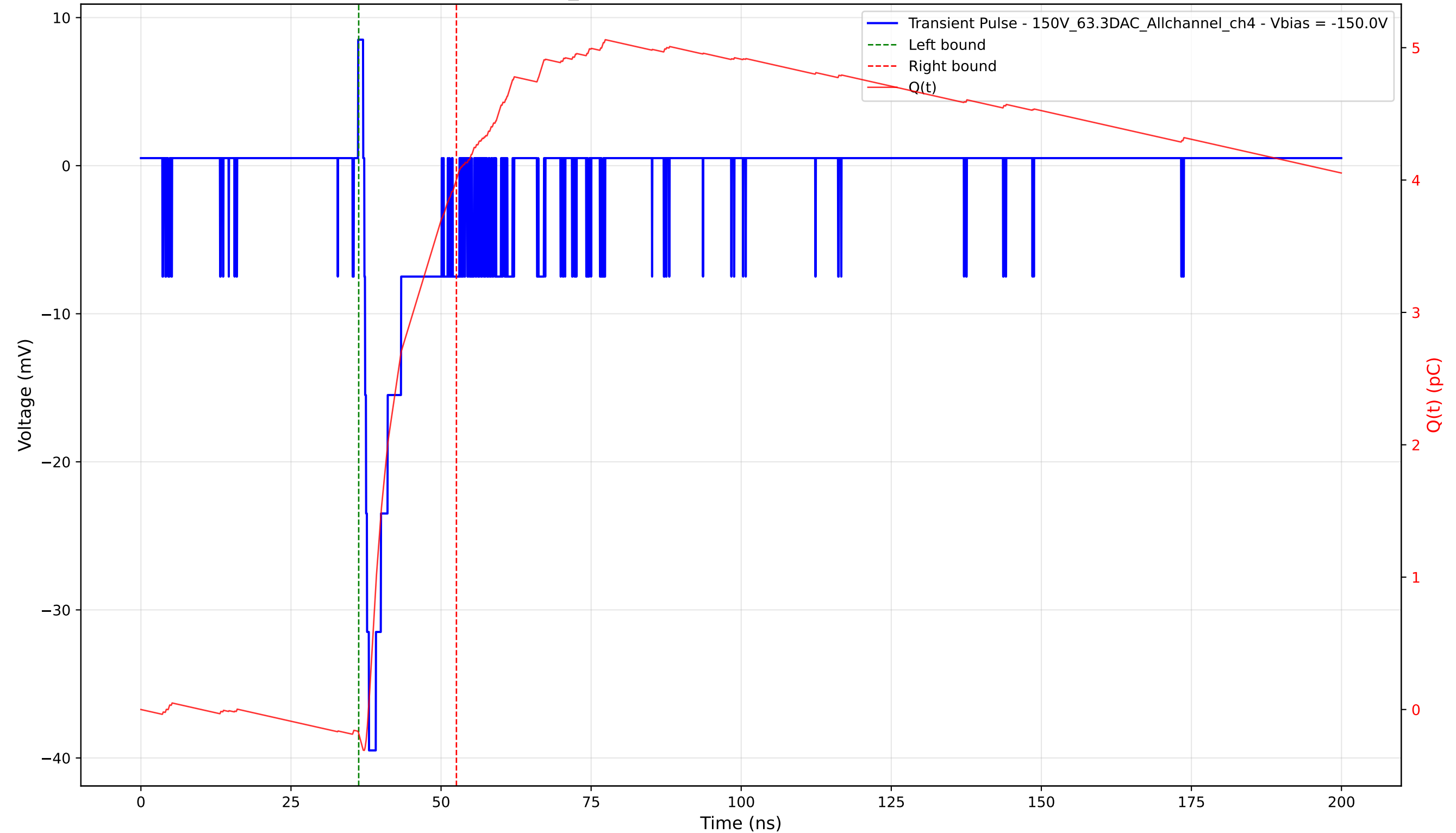
Transient Pulse - Sample: 1cm_42 - Position: 3405.0 \mu\text{m} - Charge: 4.19 pC - Rise Time: 0.78 ns
