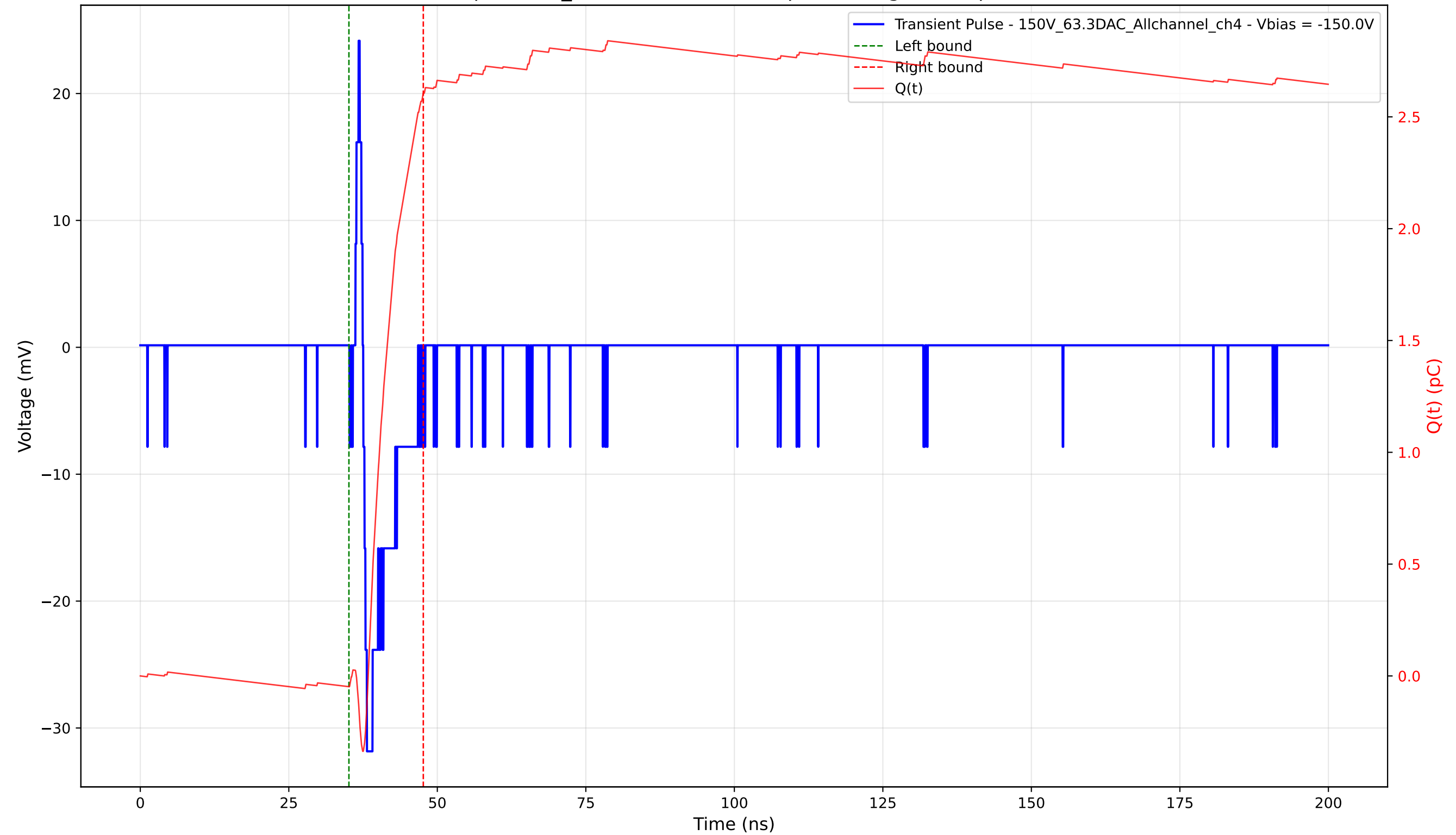
Transient Pulse - Sample: 1cm_42 - Position: 4715.0 \mu\text{m} - Charge: 2.65 pC - Rise Time: 0.62 ns
