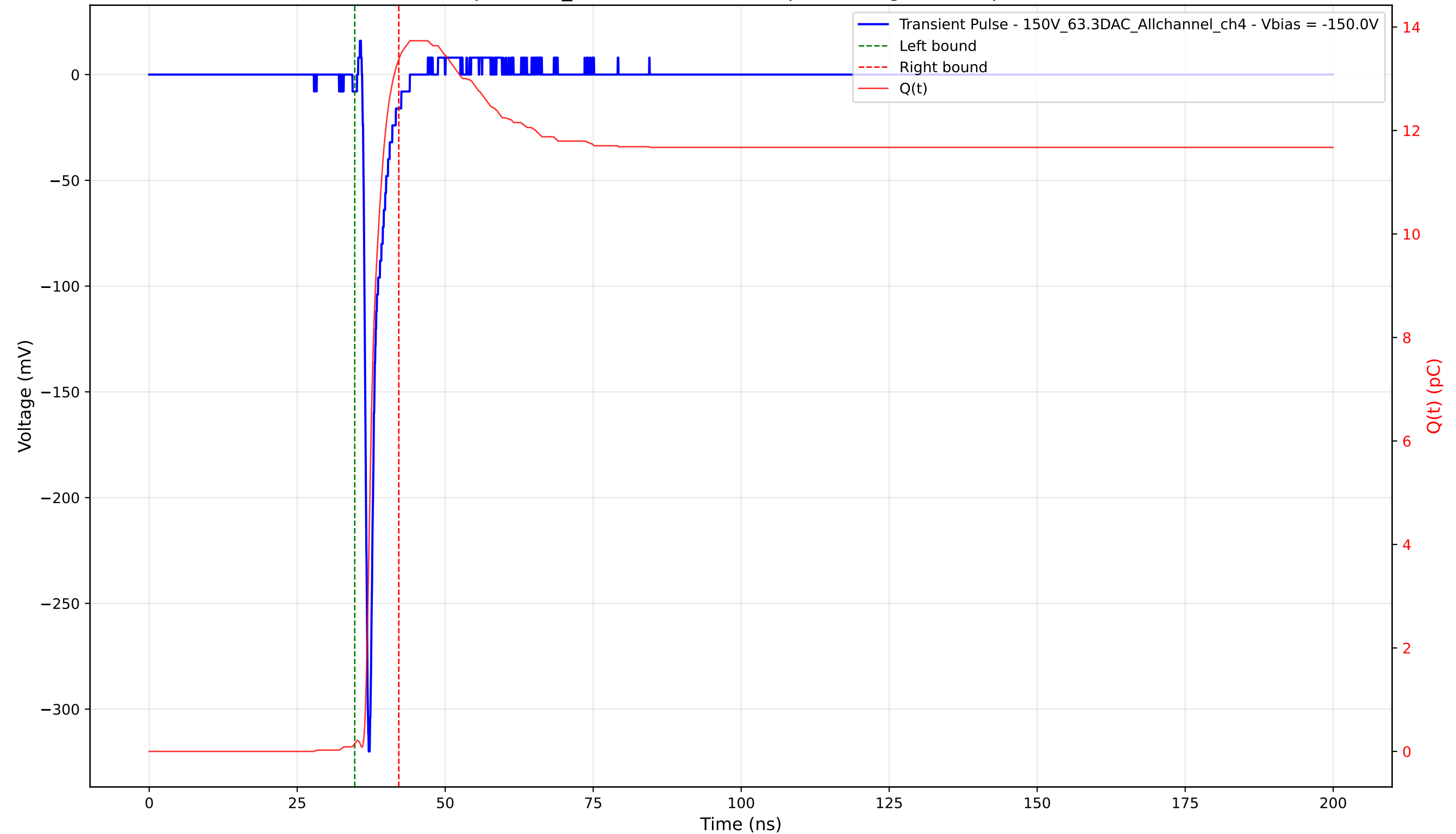
Transient Pulse - Sample: 1cm_42 - Position: 1560.0 \mu\text{m} - Charge: 13.22 pC - Rise Time: 0.74 ns
