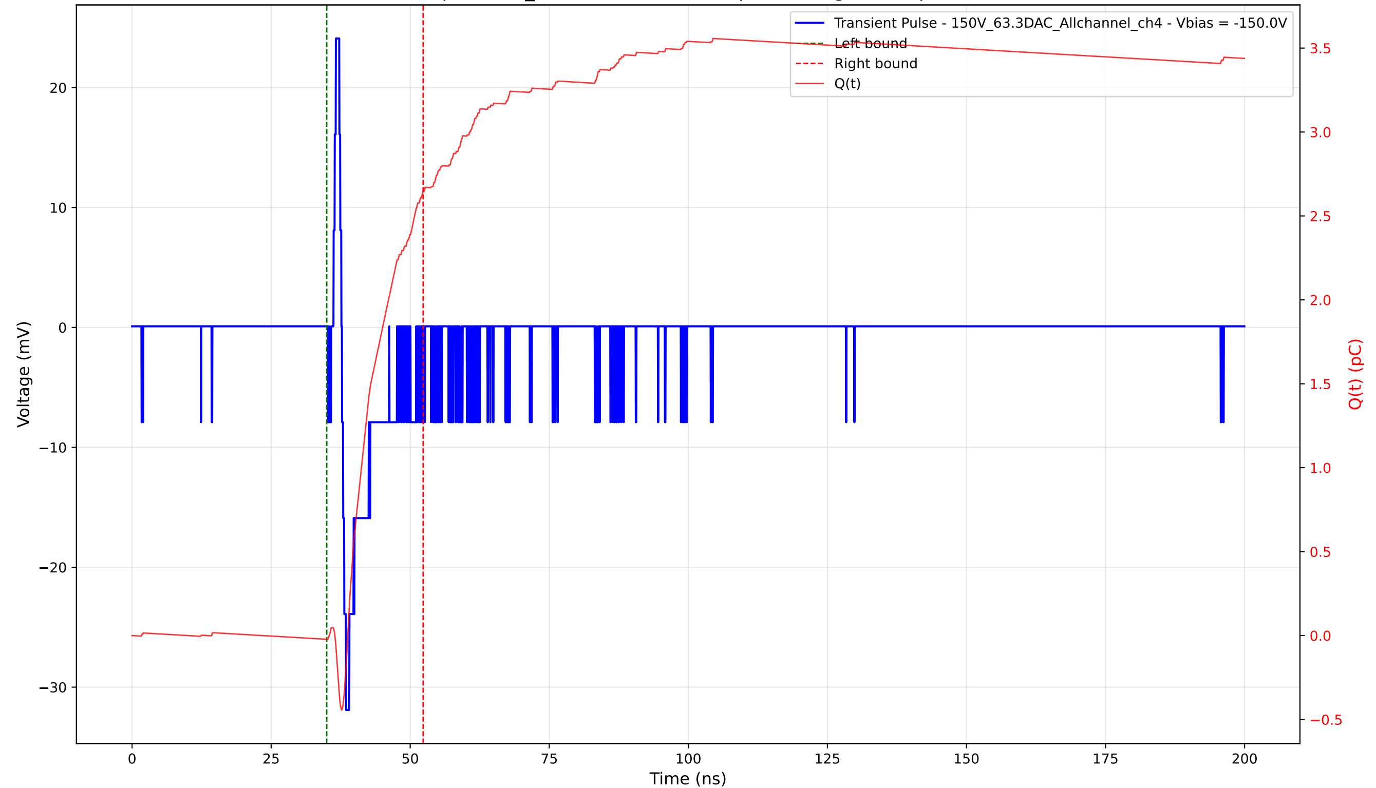
Transient Pulse - Sample: 1cm_42 - Position: 4085.0 \mu\text{m} - Charge: 2.67 pC - Rise Time: 0.74 ns
