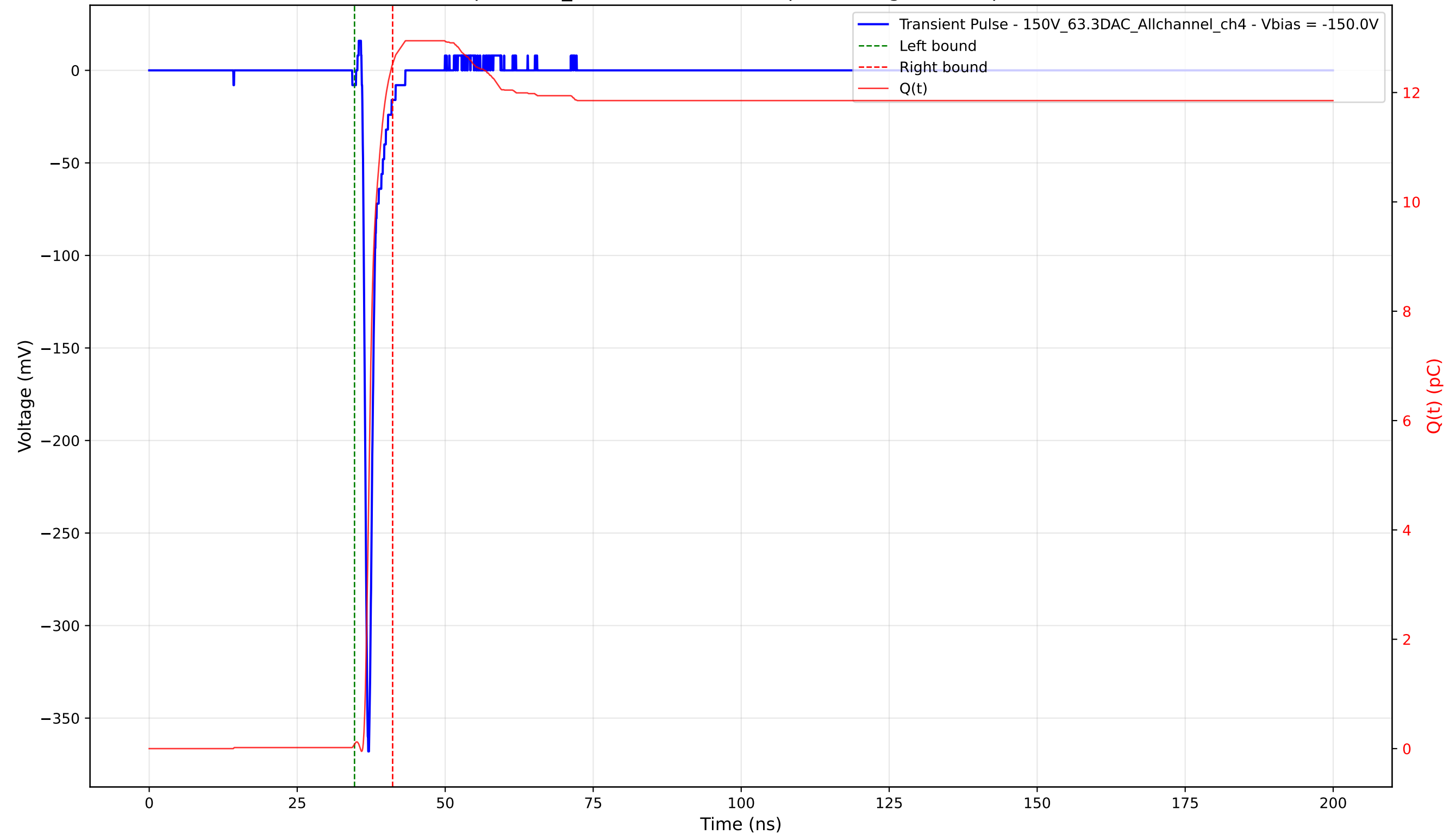
Transient Pulse - Sample: 1cm_42 - Position: 2395.0 \mu\text{m} - Charge: 12.44 pC - Rise Time: 0.71 ns
