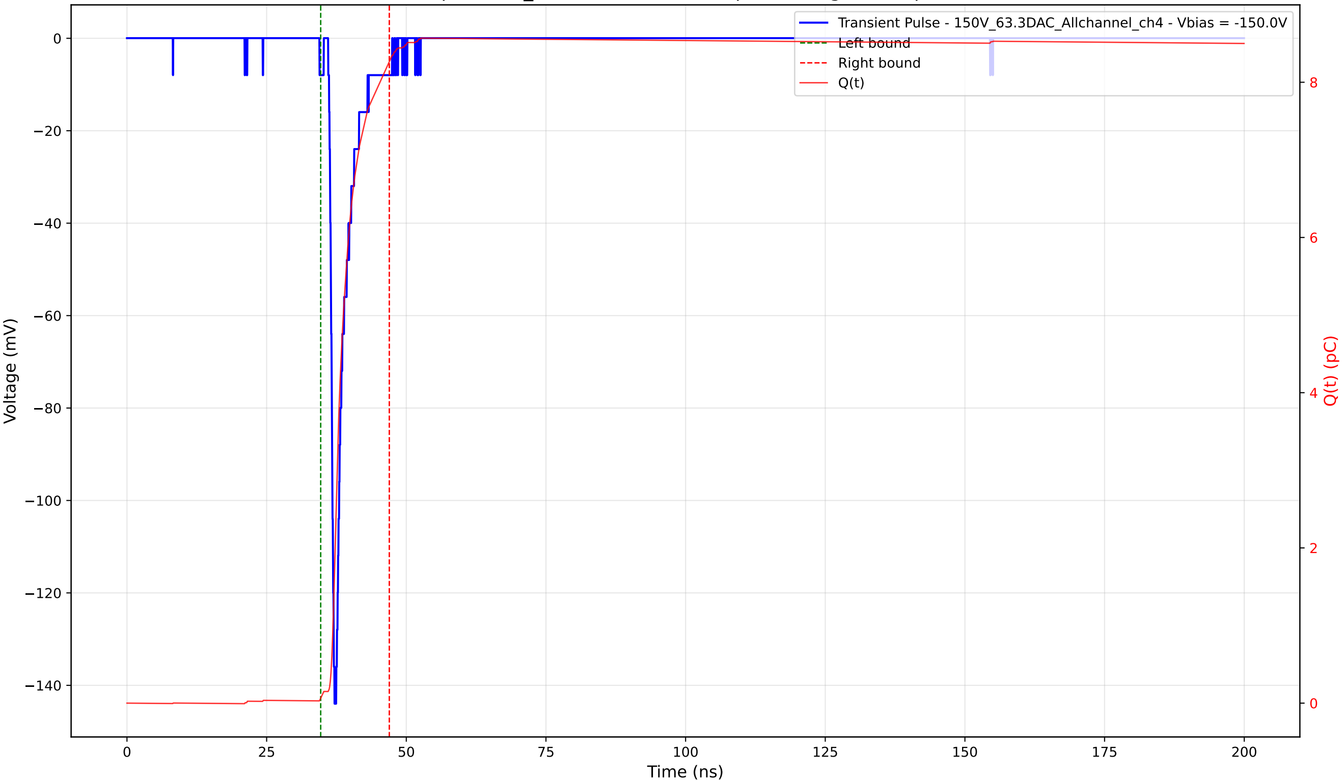
Transient Pulse - Sample: 1cm_42 - Position: 2725.0 \mu\text{m} - Charge: 8.20 pC - Rise Time: 0.85 ns
