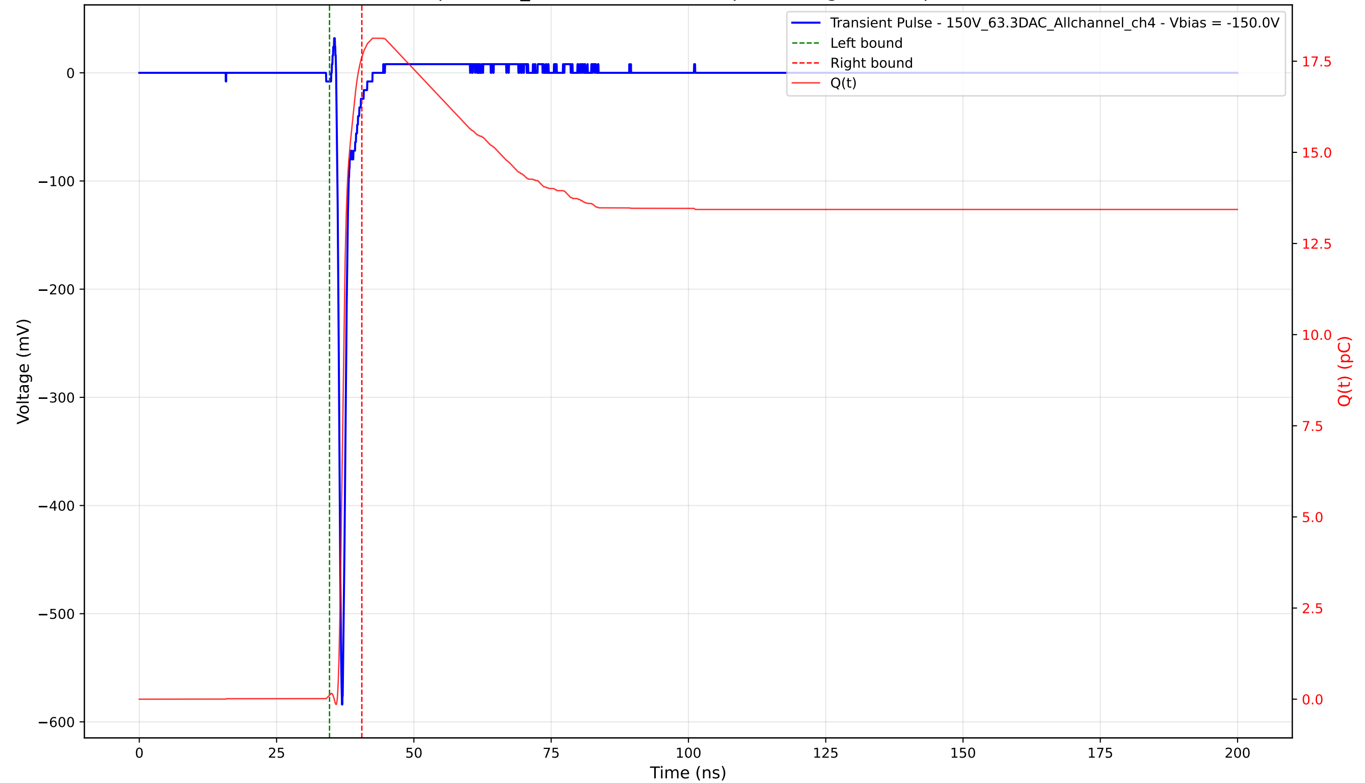
Transient Pulse - Sample: 1cm_42 - Position: 2030.0 \mu\text{m} - Charge: 17.50 pC - Rise Time: 0.71 ns
