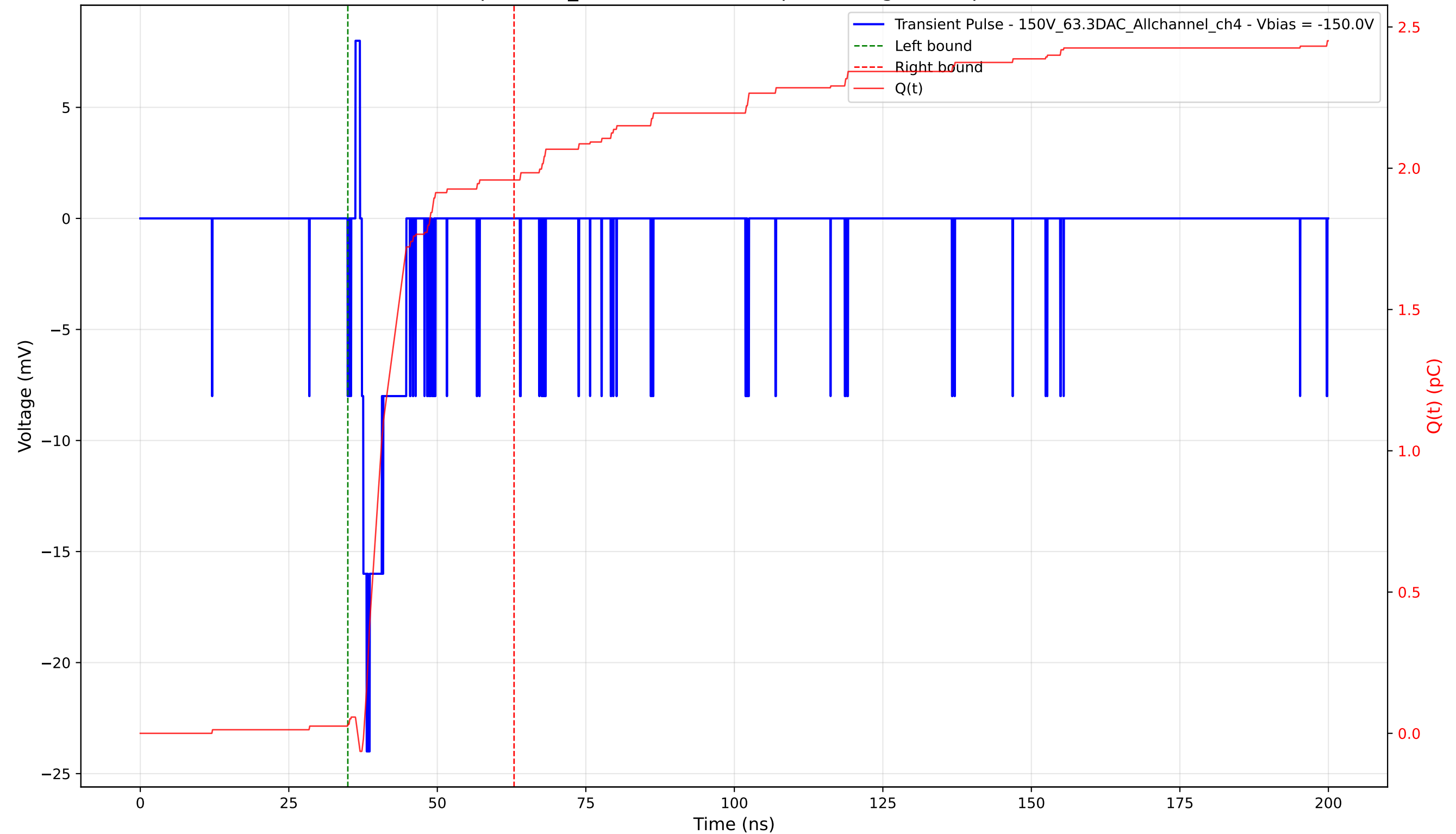
Transient Pulse - Sample: 1cm_42 - Position: 170.0 \mu\text{m} - Charge: 1.93 pC - Rise Time: 0.83 ns
