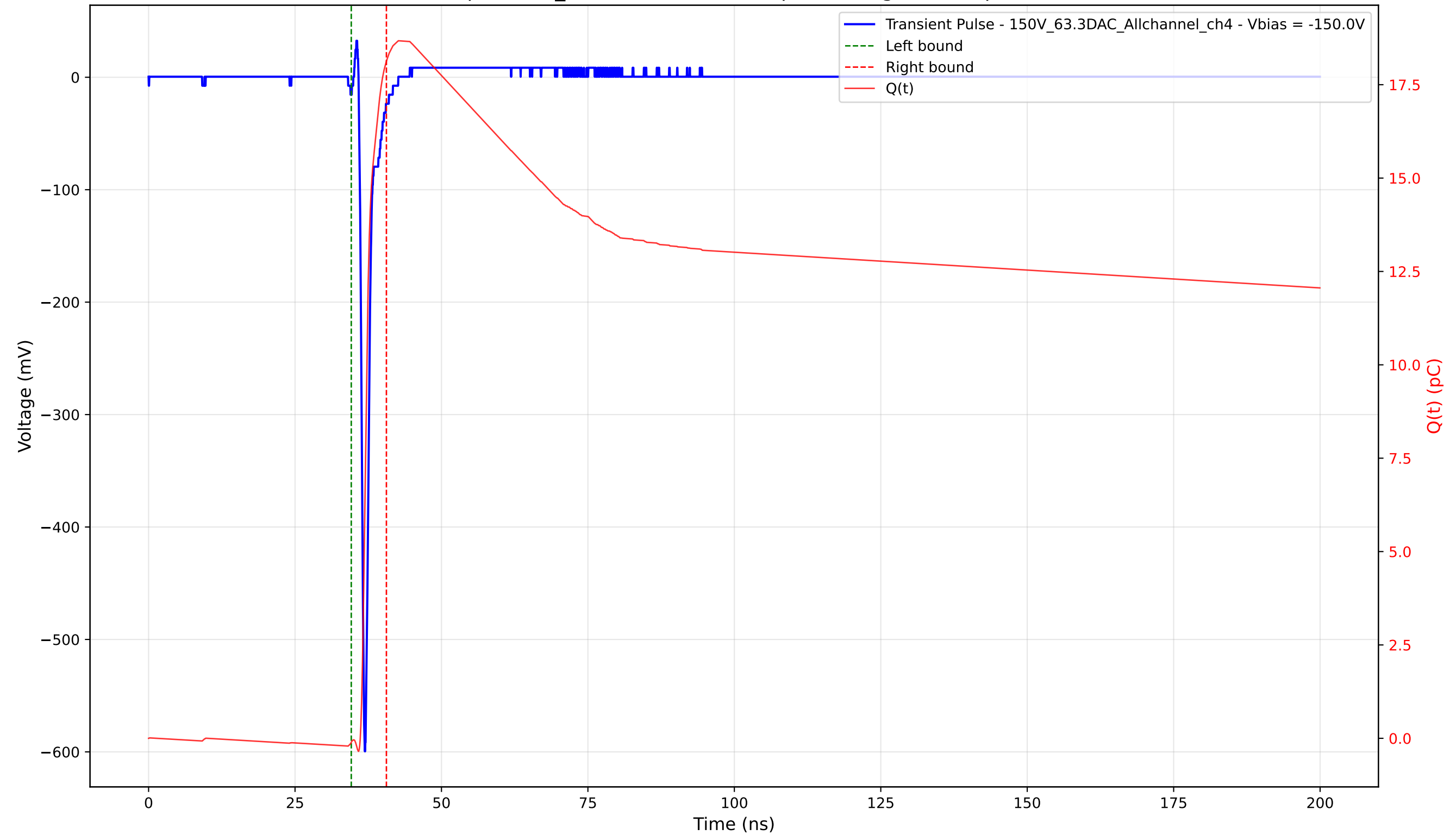
Transient Pulse - Sample: 1cm_42 - Position: 1945.0 \mu\text{m} - Charge: 18.24 pC - Rise Time: 0.72 ns
