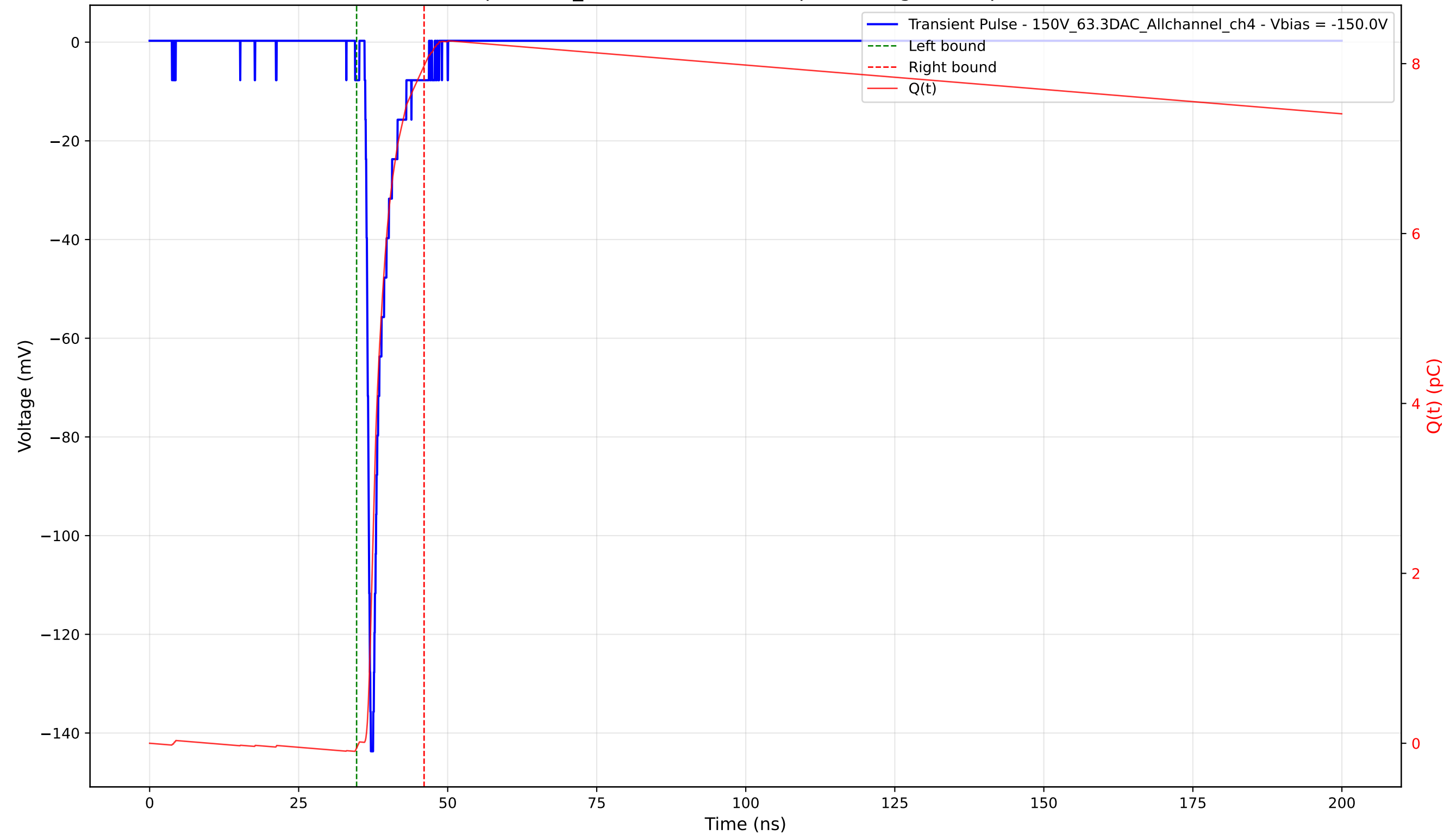
Transient Pulse - Sample: 1cm_42 - Position: 2710.0 \mu\text{m} - Charge: 8.03 pC - Rise Time: 0.85 ns
