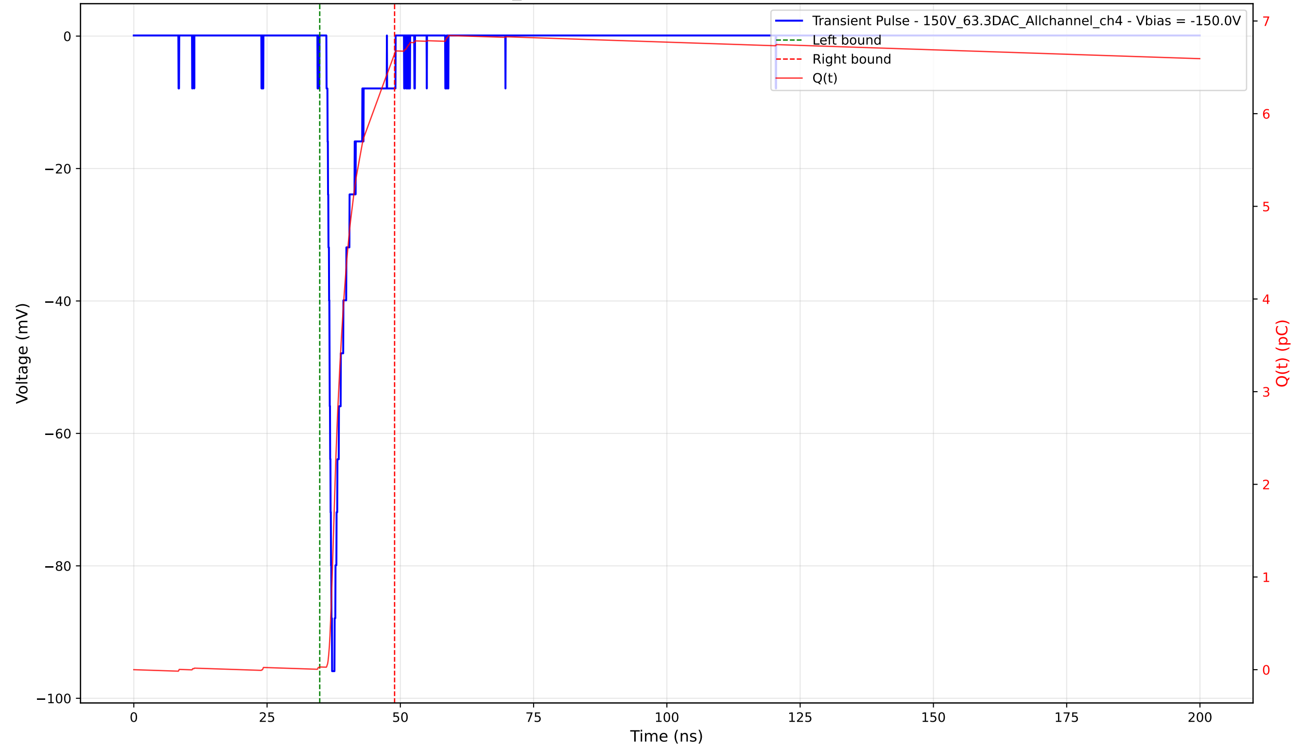
Transient Pulse - Sample: 1cm_42 - Position: 2905.0 \mu\text{m} - Charge: 6.62 pC - Rise Time: 0.75 ns
