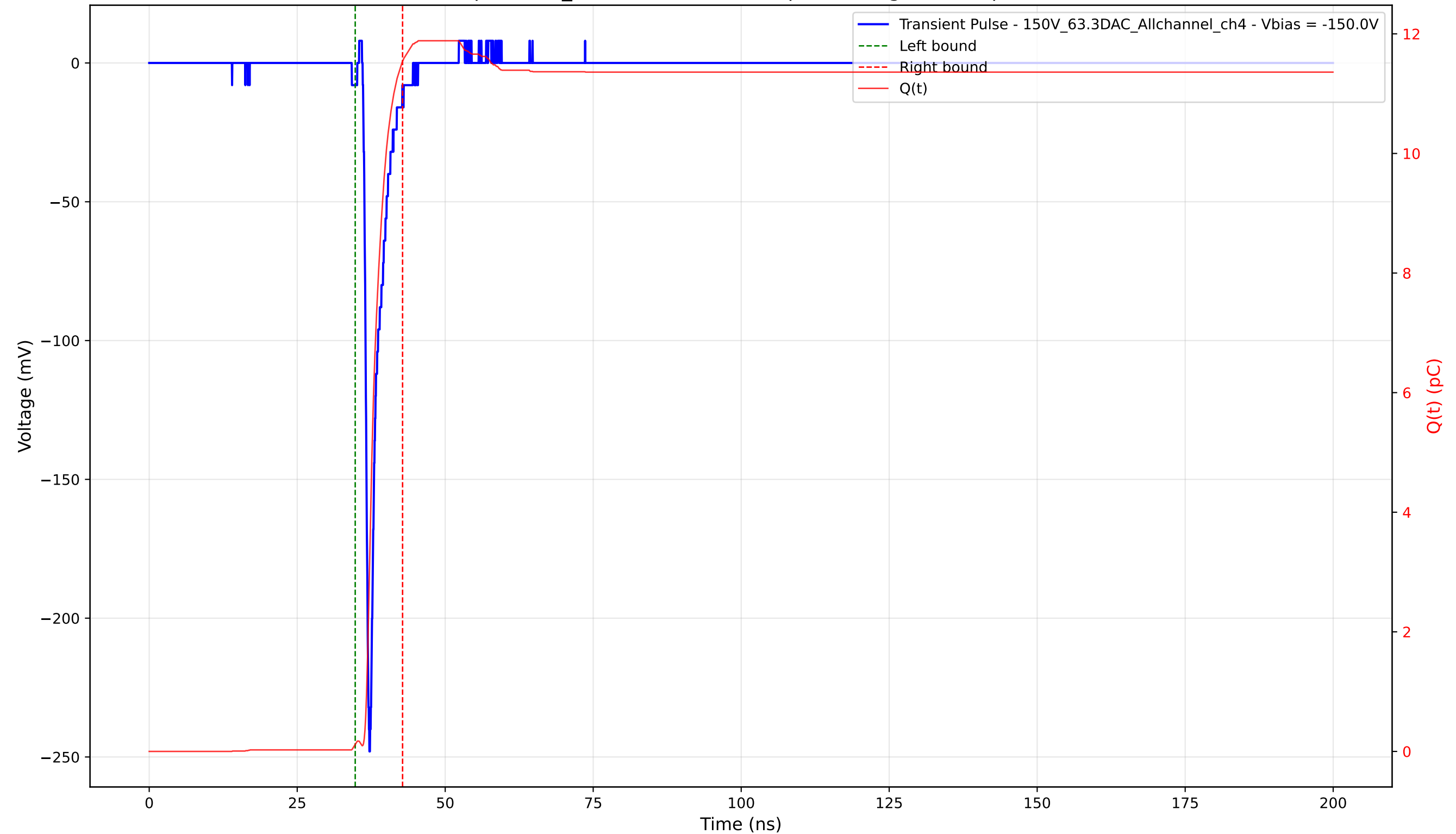
Transient Pulse - Sample: 1cm_42 - Position: 1475.0 \mu\text{m} - Charge: 11.42 pC - Rise Time: 0.79 ns
