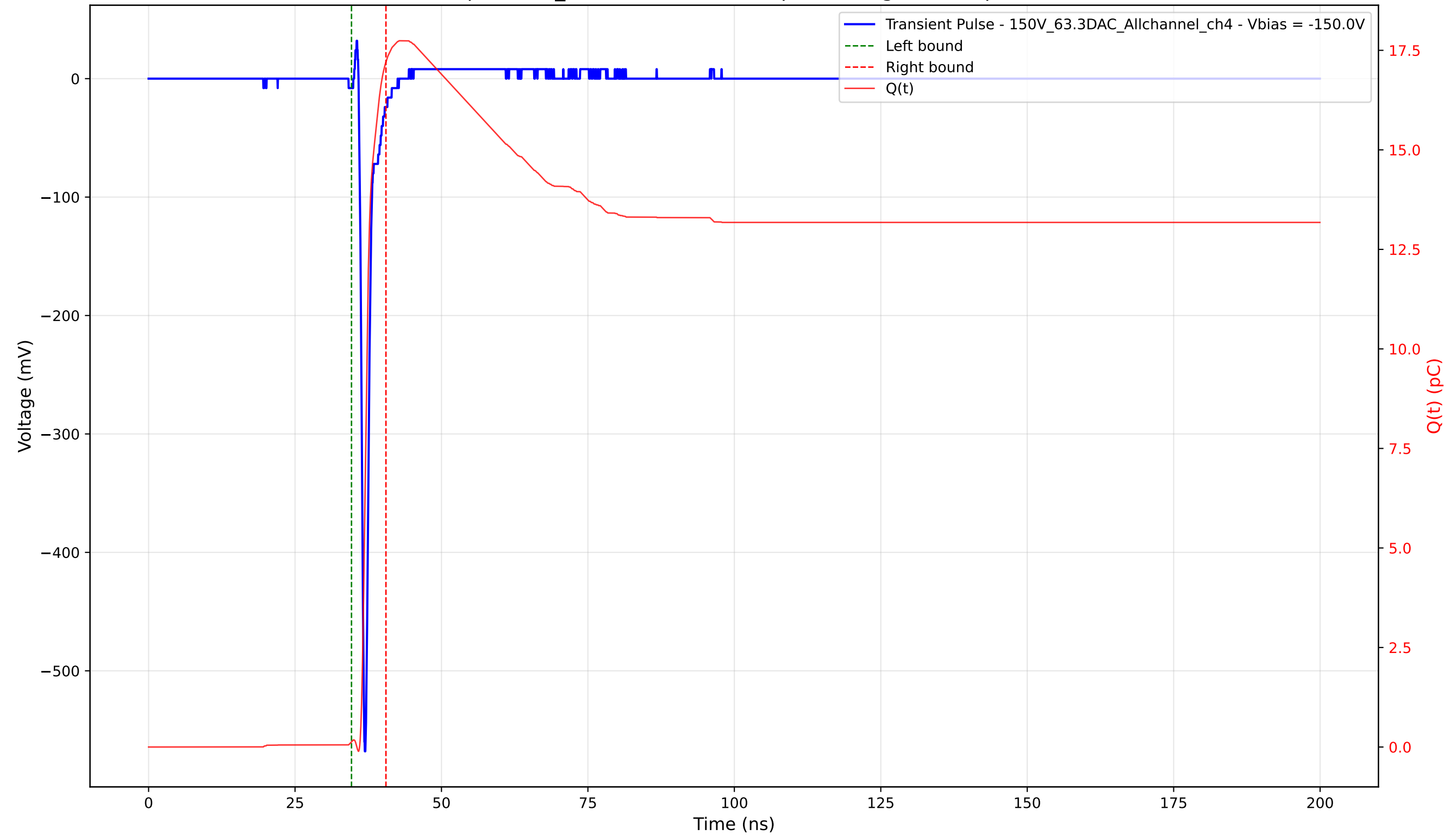
Transient Pulse - Sample: 1cm_42 - Position: 2105.0 \mu\text{m} - Charge: 17.08 pC - Rise Time: 0.72 ns
