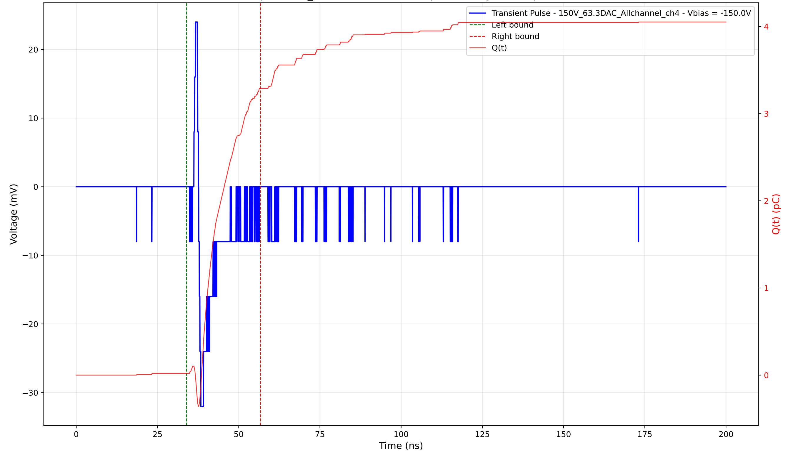
Transient Pulse - Sample: 1cm_42 - Position: 3925.0 \mu\text{m} - Charge: 3.27 pC - Rise Time: 0.66 ns
