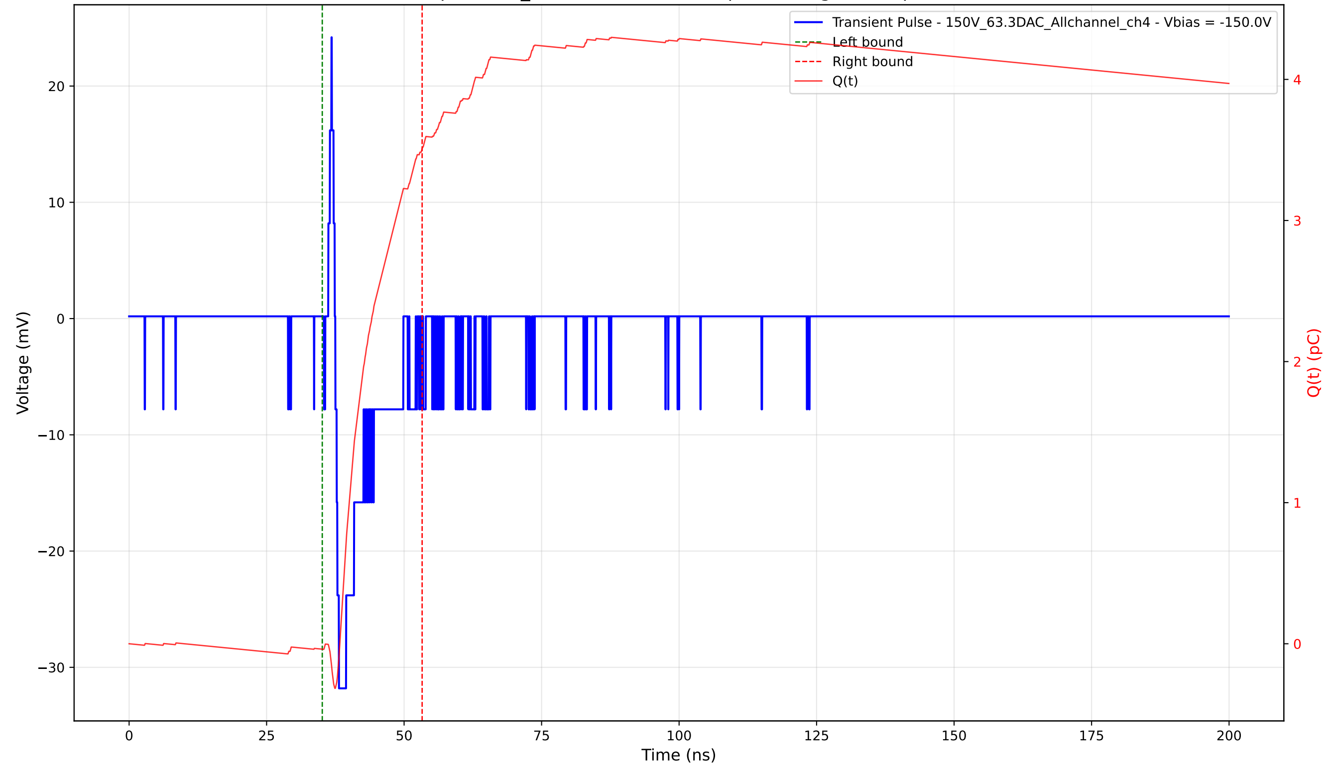
Transient Pulse - Sample: 1cm_42 - Position: 3610.0 \mu\text{m} - Charge: 3.55 pC - Rise Time: 0.66 ns
