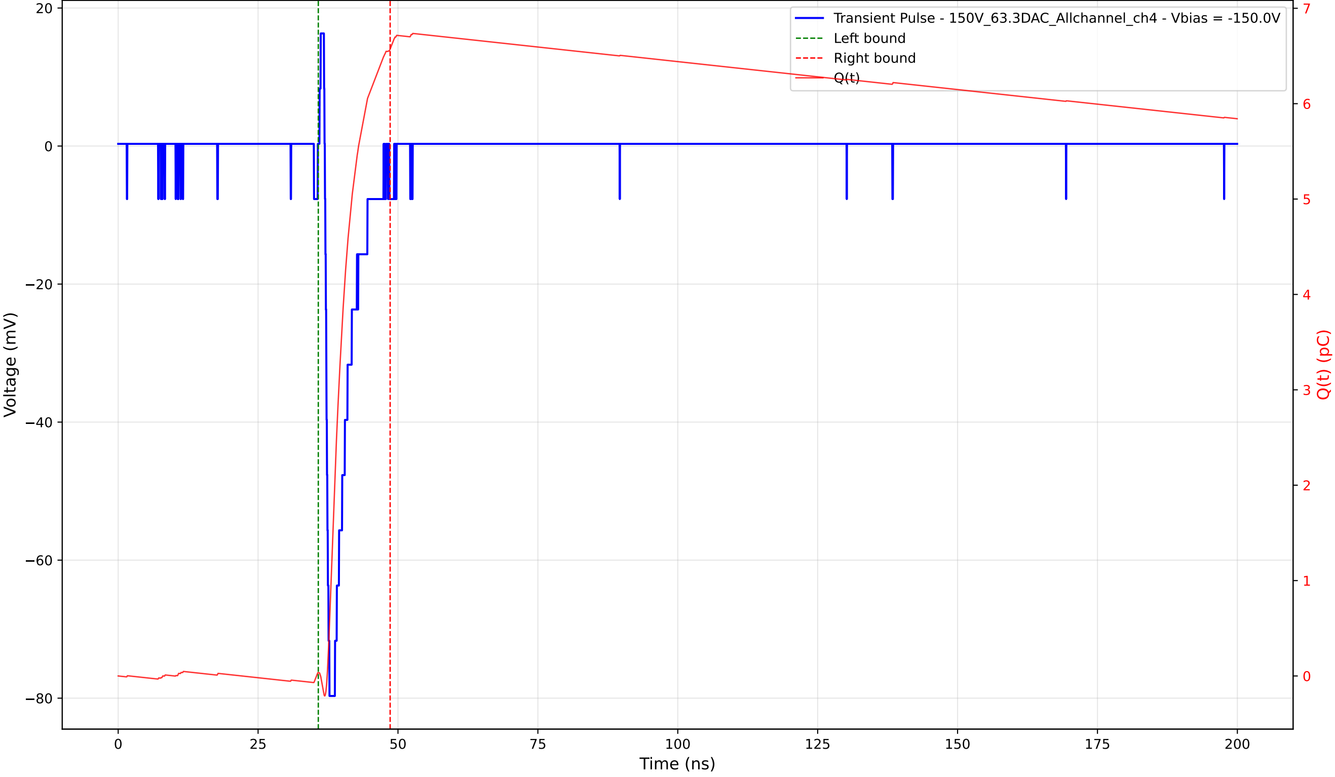
Transient Pulse - Sample: 1cm_42 - Position: 850.0 \mu\text{m} - Charge: 6.54 pC - Rise Time: 0.76 ns
