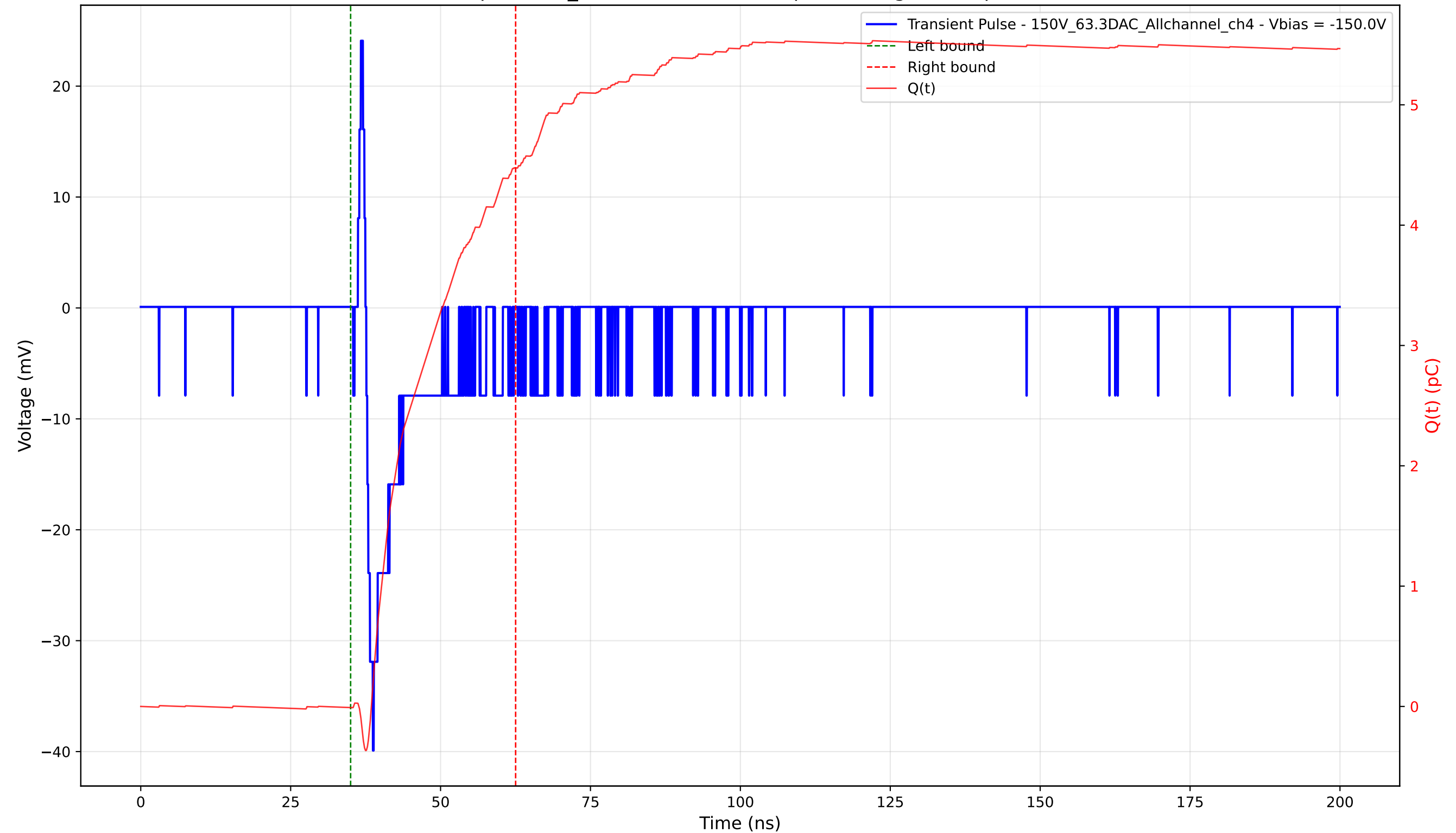
Transient Pulse - Sample: 1cm_42 - Position: 3670.0 \mu\text{m} - Charge: 4.48 pC - Rise Time: 1.10 ns
