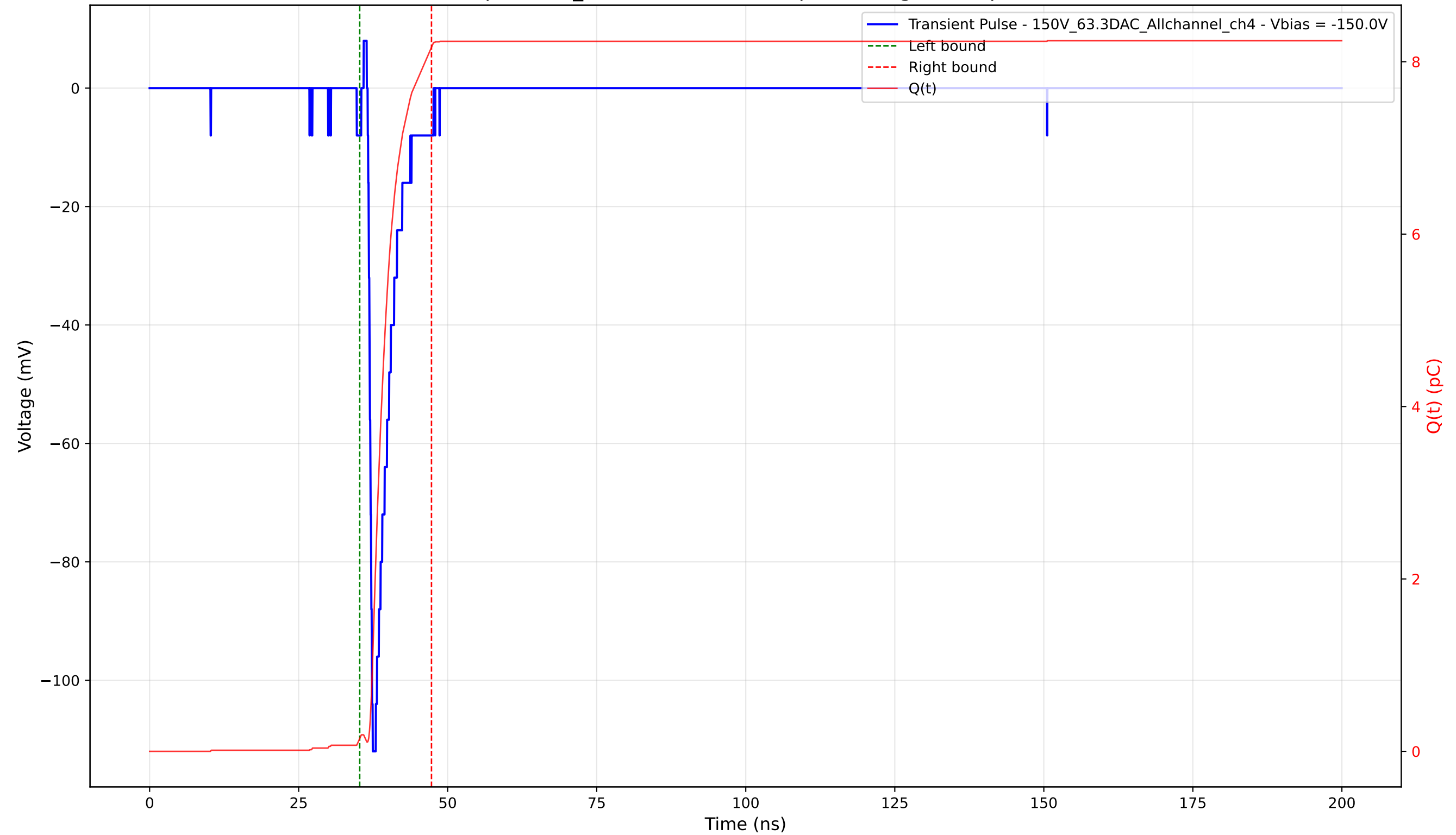
Transient Pulse - Sample: 1cm_42 - Position: 1065.0 \mu\text{m} - Charge: 8.02 pC - Rise Time: 0.66 ns
