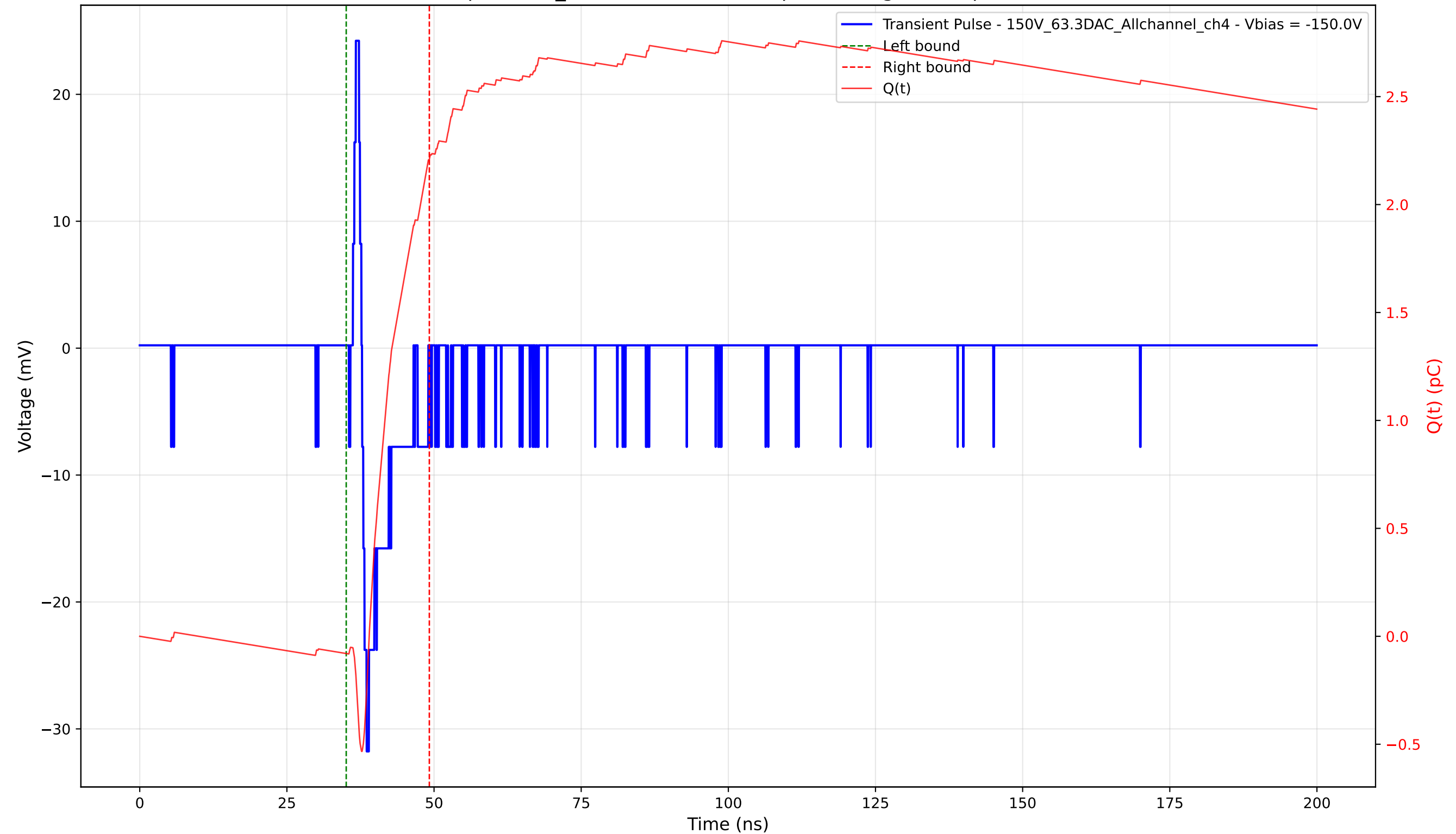
Transient Pulse - Sample: 1cm_42 - Position: 4025.0 \mu\text{m} - Charge: 2.29 pC - Rise Time: 0.78 ns
