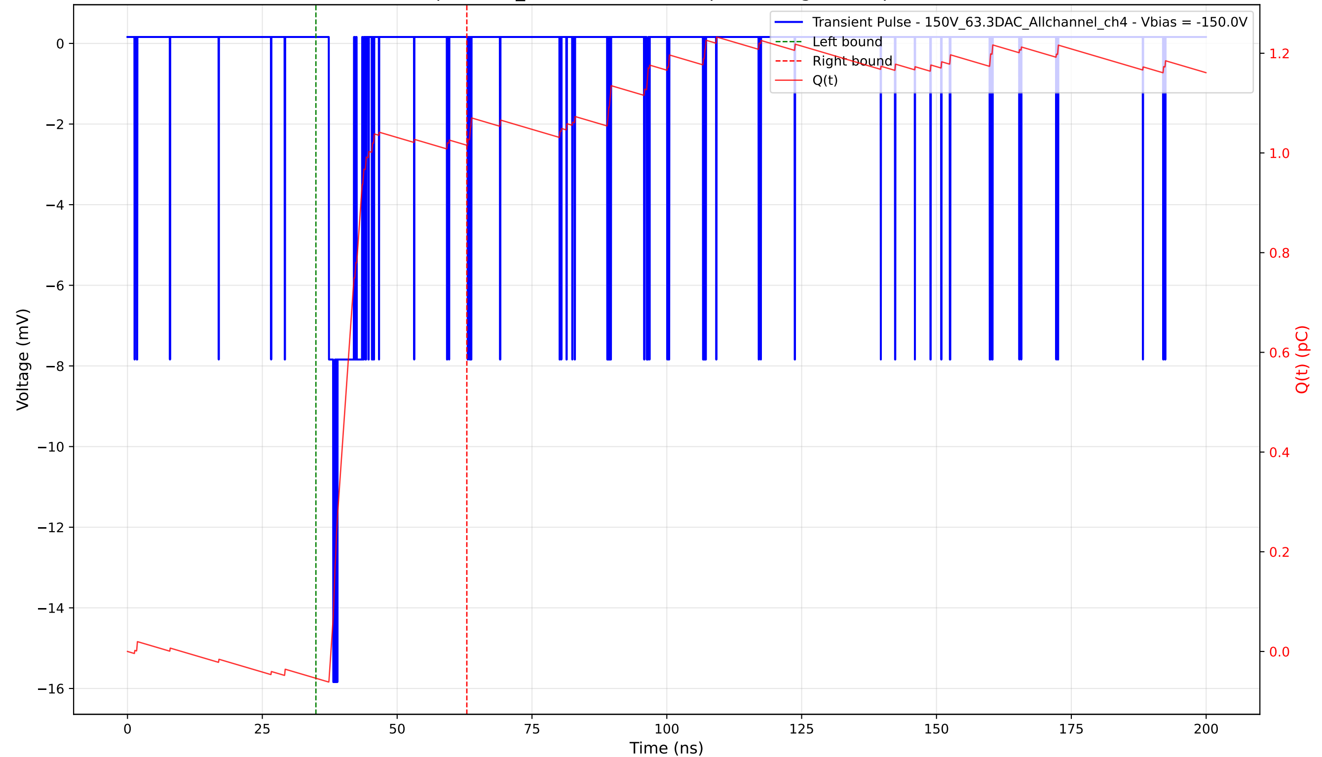
Transient Pulse - Sample: 1cm_42 - Position: 100.0 \mu\text{m} - Charge: 1.07 pC - Rise Time: 0.83 ns
