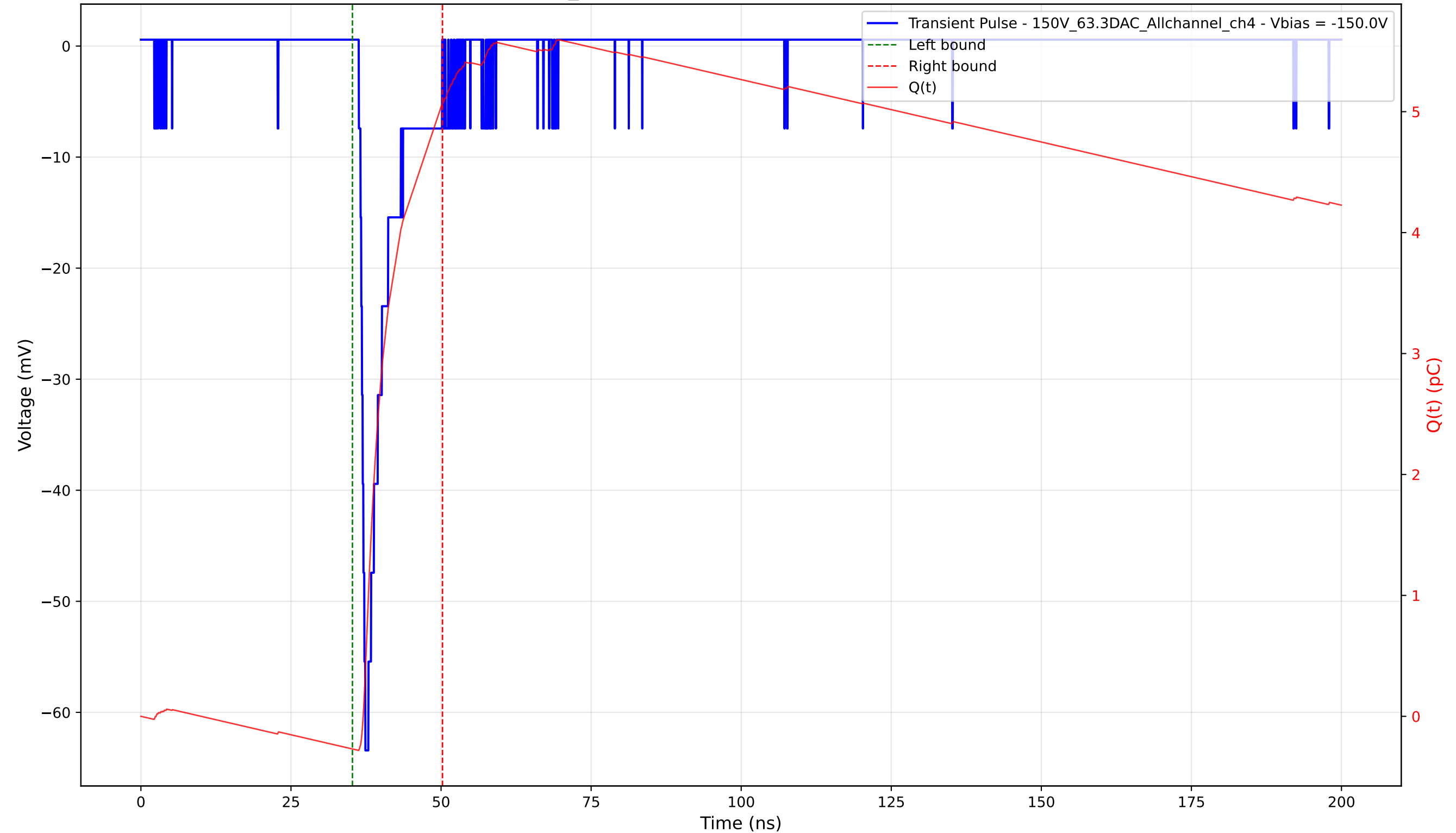
Transient Pulse - Sample: 1cm_42 - Position: 3025.0 \mu\text{m} - Charge: 5.34 pC - Rise Time: 1.09 ns
