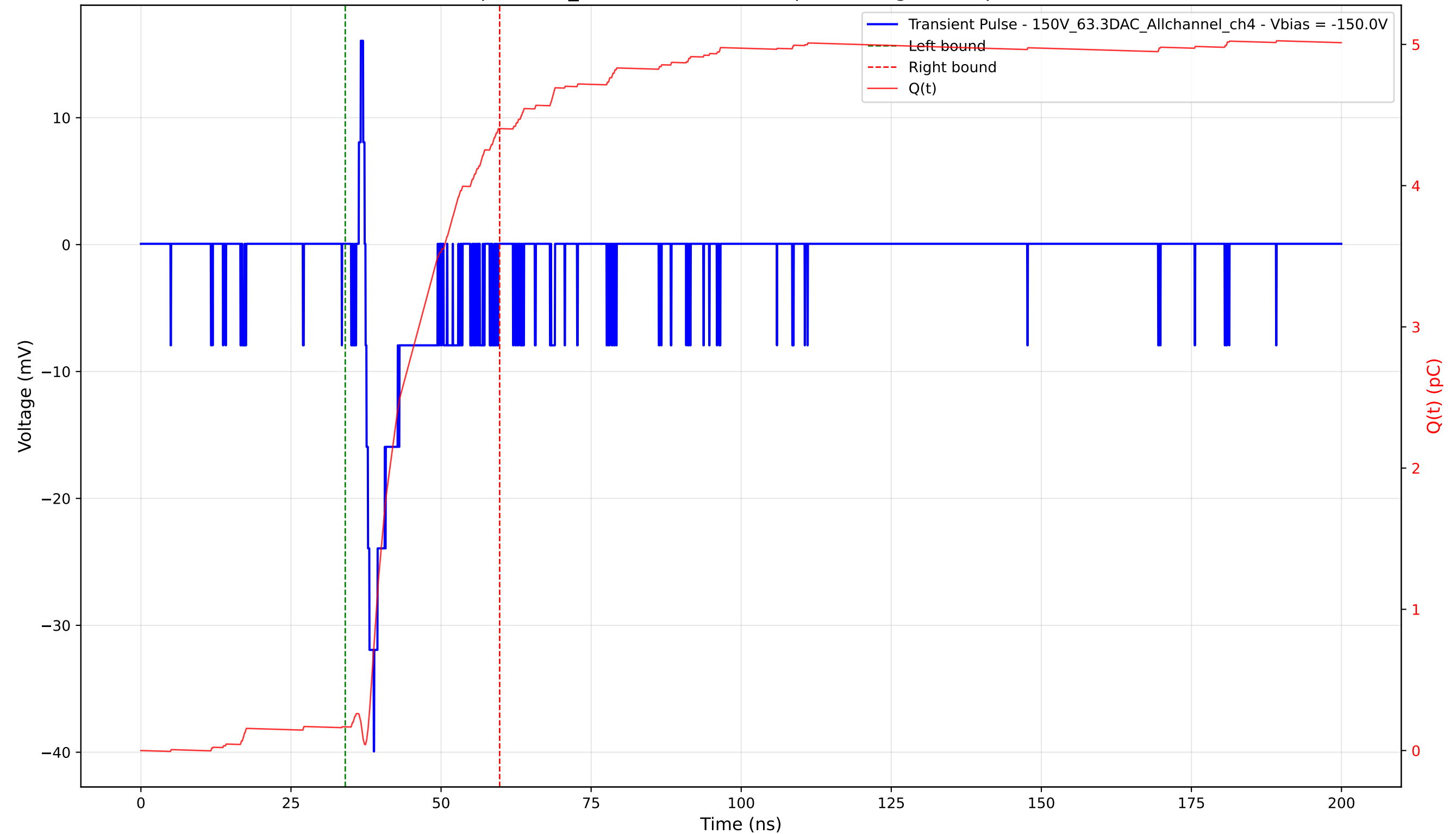
Transient Pulse - Sample: 1cm_42 - Position: 3520.0 \mu\text{m} - Charge: 4.24 pC - Rise Time: 1.38 ns
