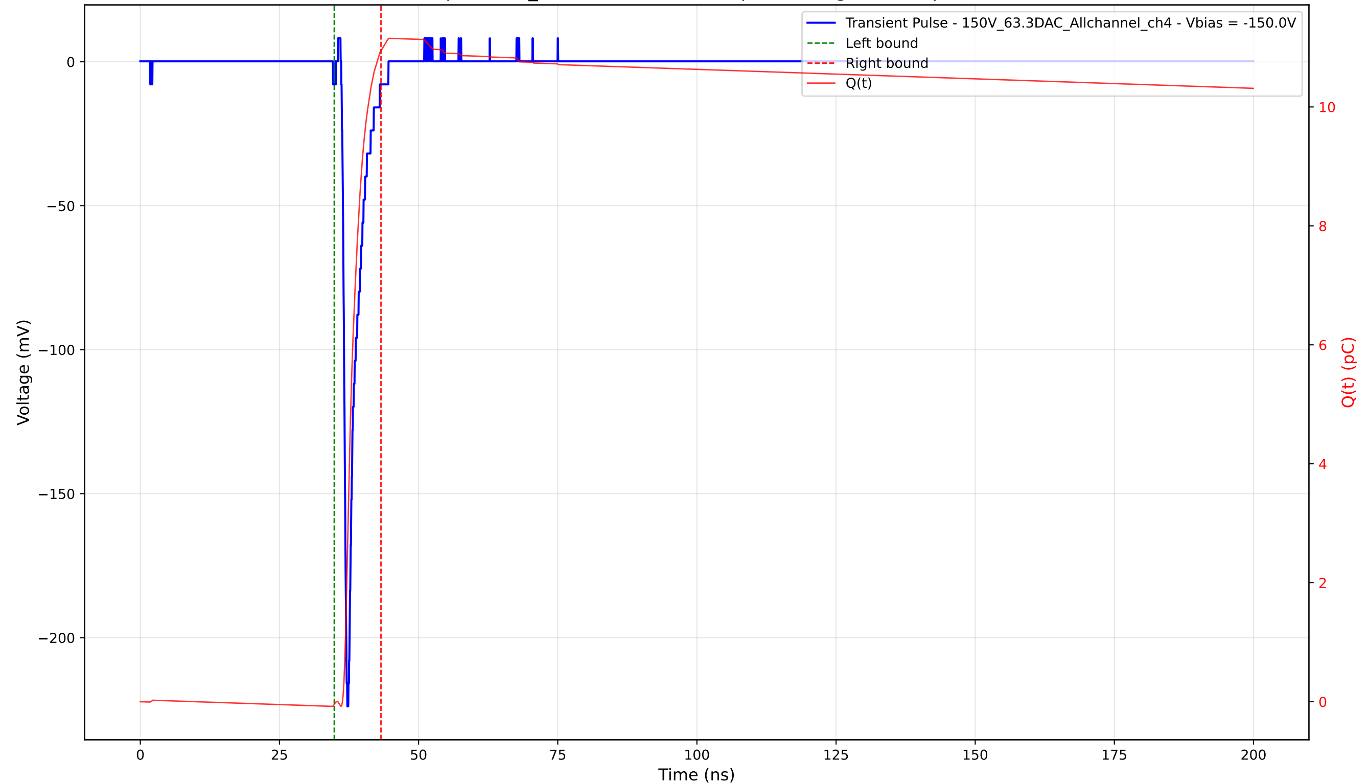
Transient Pulse - Sample: 1cm_42 - Position: 1445.0 \mu\text{m} - Charge: 10.99 pC - Rise Time: 0.78 ns
