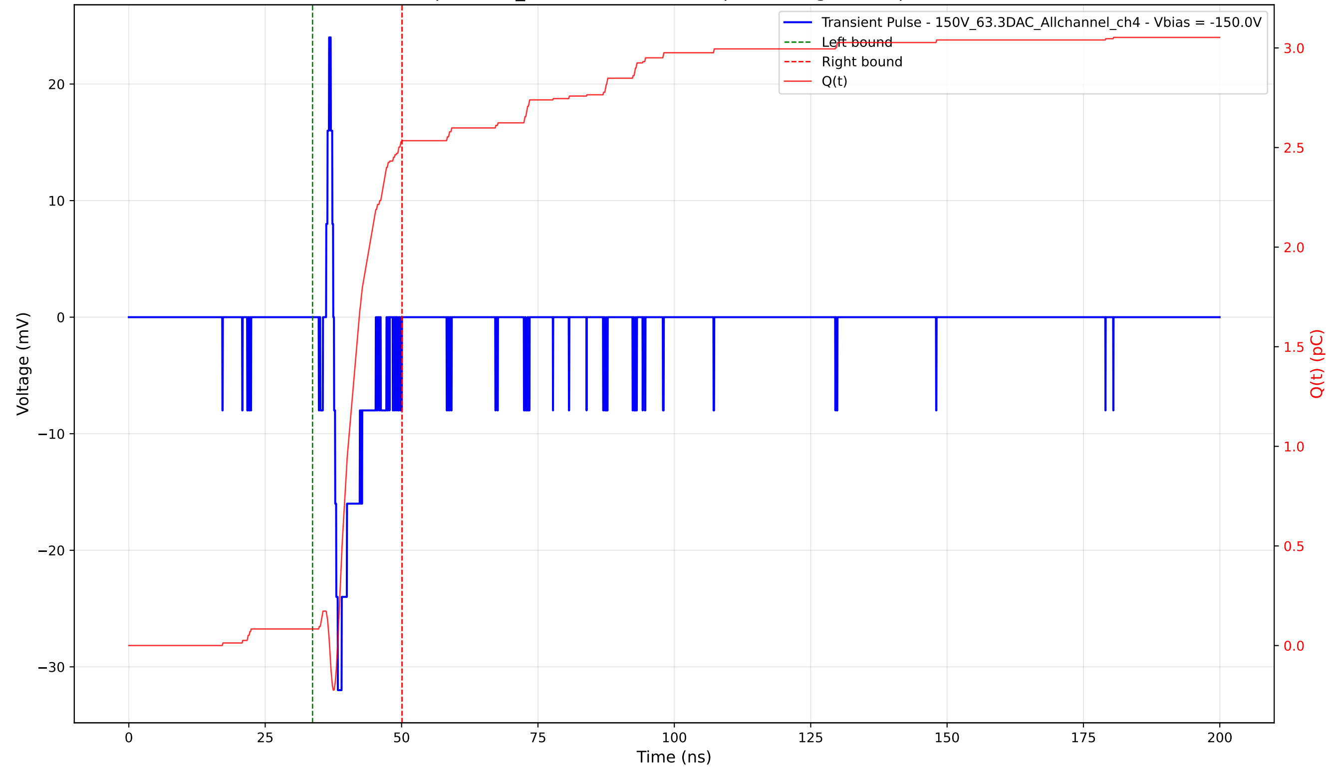
Transient Pulse - Sample: 1cm_42 - Position: 4610.0 \mu\text{m} - Charge: 2.45 pC - Rise Time: 0.70 ns
