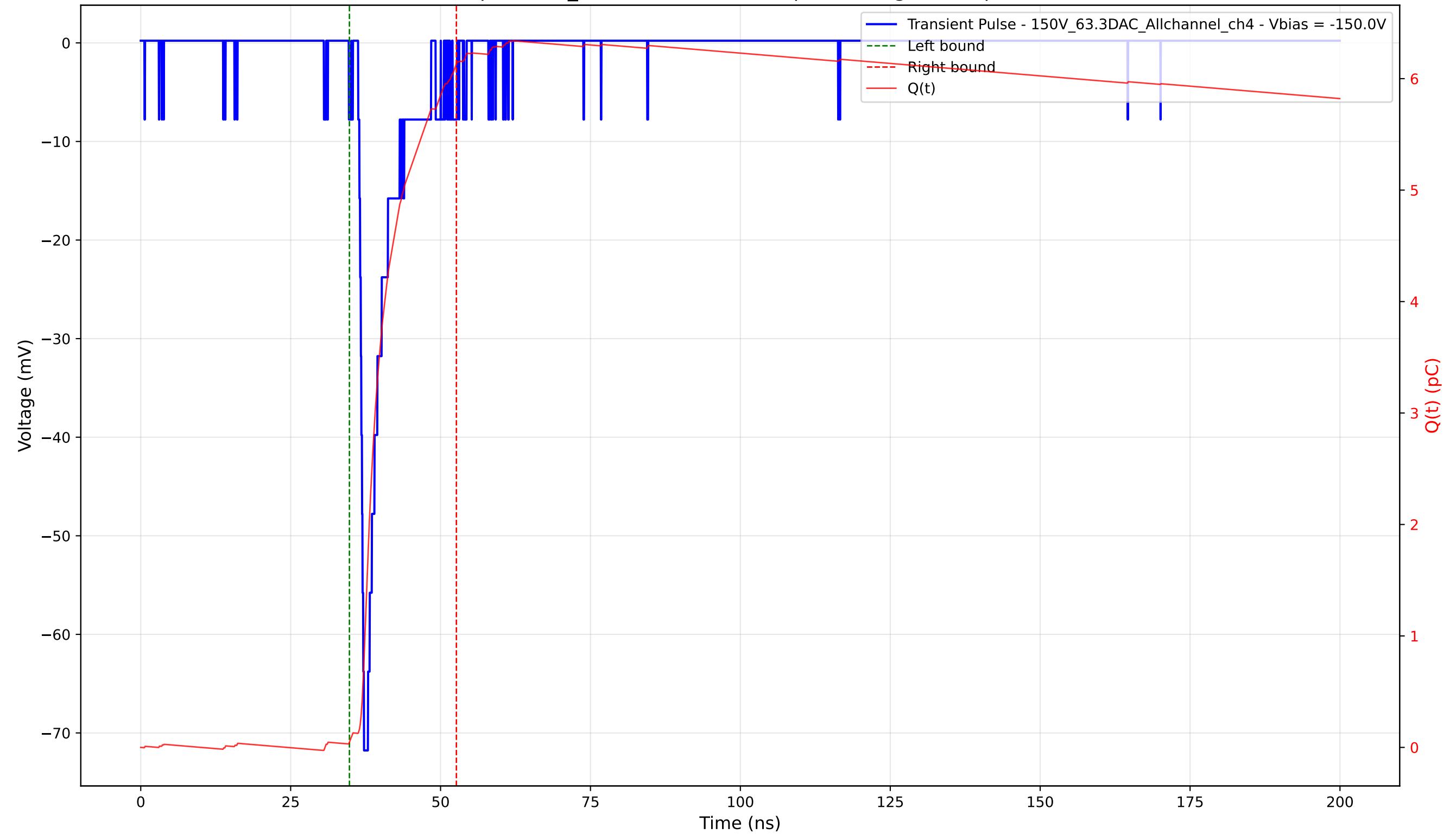
Transient Pulse - Sample: 1cm_42 - Position: 2975.0 \mu\text{m} - Charge: 6.09 pC - Rise Time: 0.96 ns
