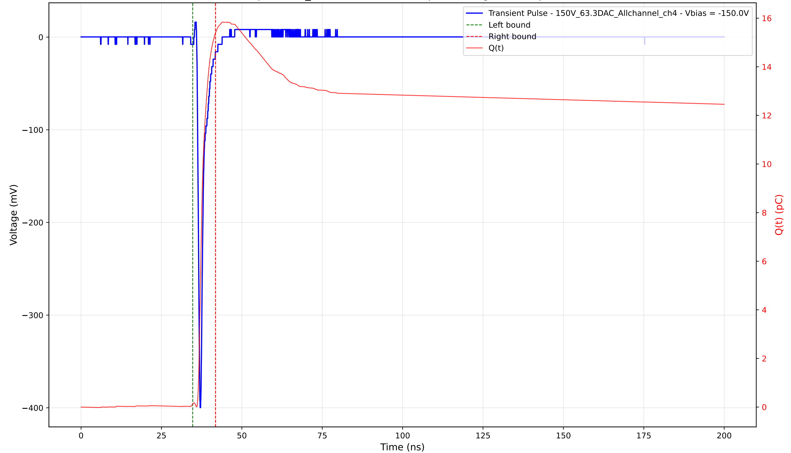
Transient Pulse - Sample: 1cm_42 - Position: 1620.0 \mu\text{m} - Charge: 15.28 pC - Rise Time: 0.76 ns
