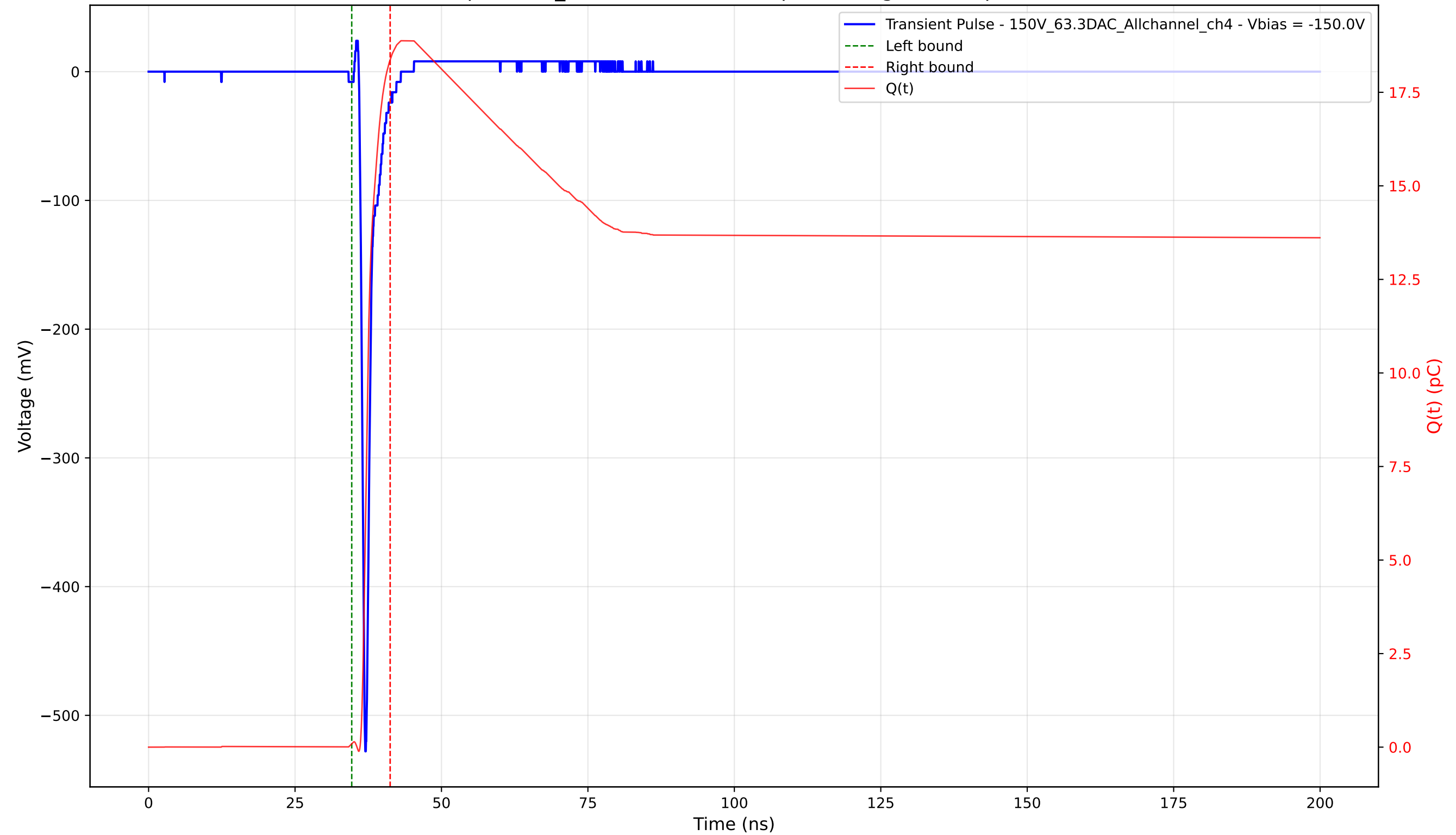
Transient Pulse - Sample: 1cm_42 - Position: 1710.0 \mu\text{m} - Charge: 18.28 pC - Rise Time: 0.72 ns
