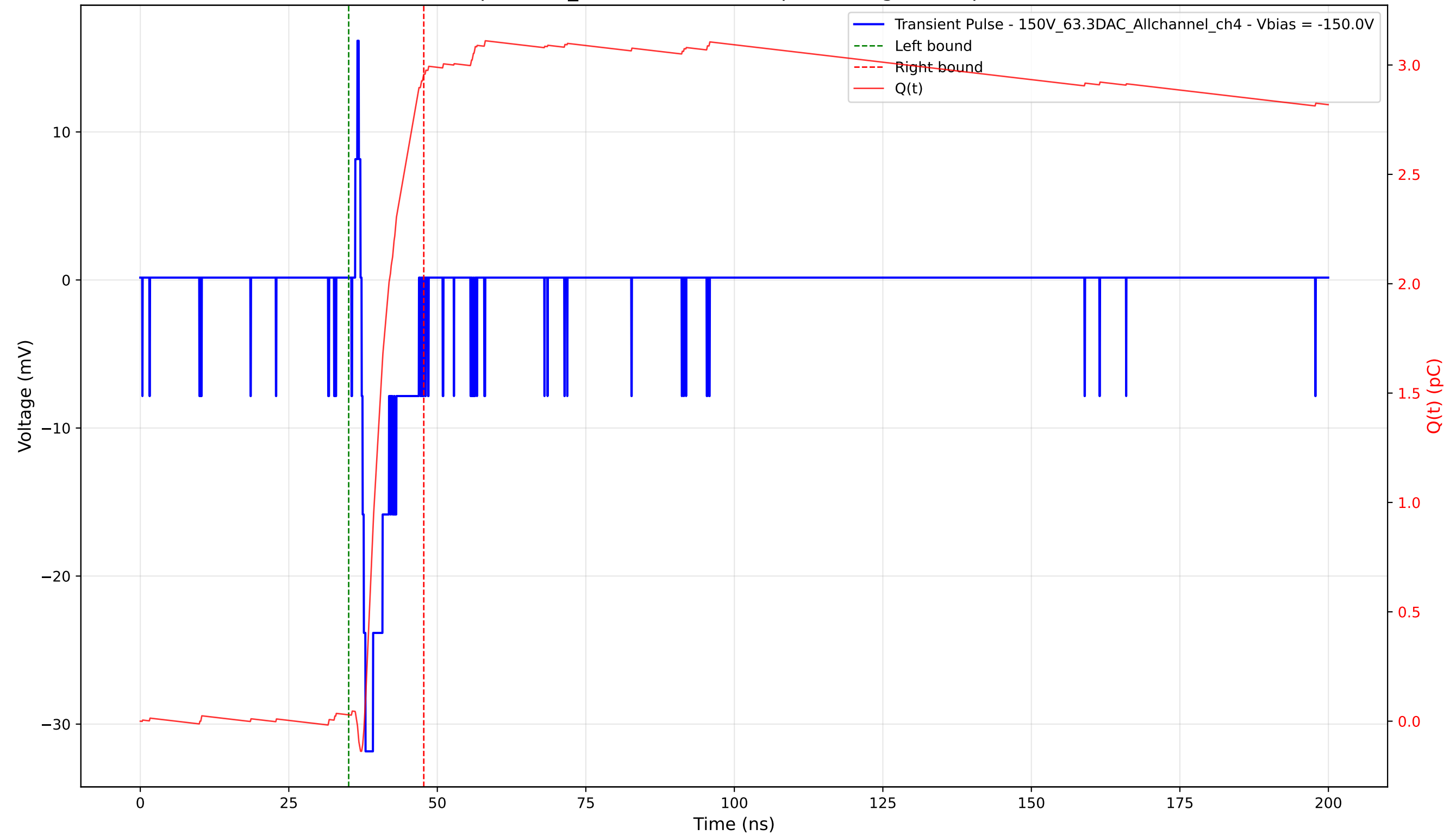
Transient Pulse - Sample: 1cm_42 - Position: 295.0 \mu\text{m} - Charge: 2.93 pC - Rise Time: 0.66 ns
