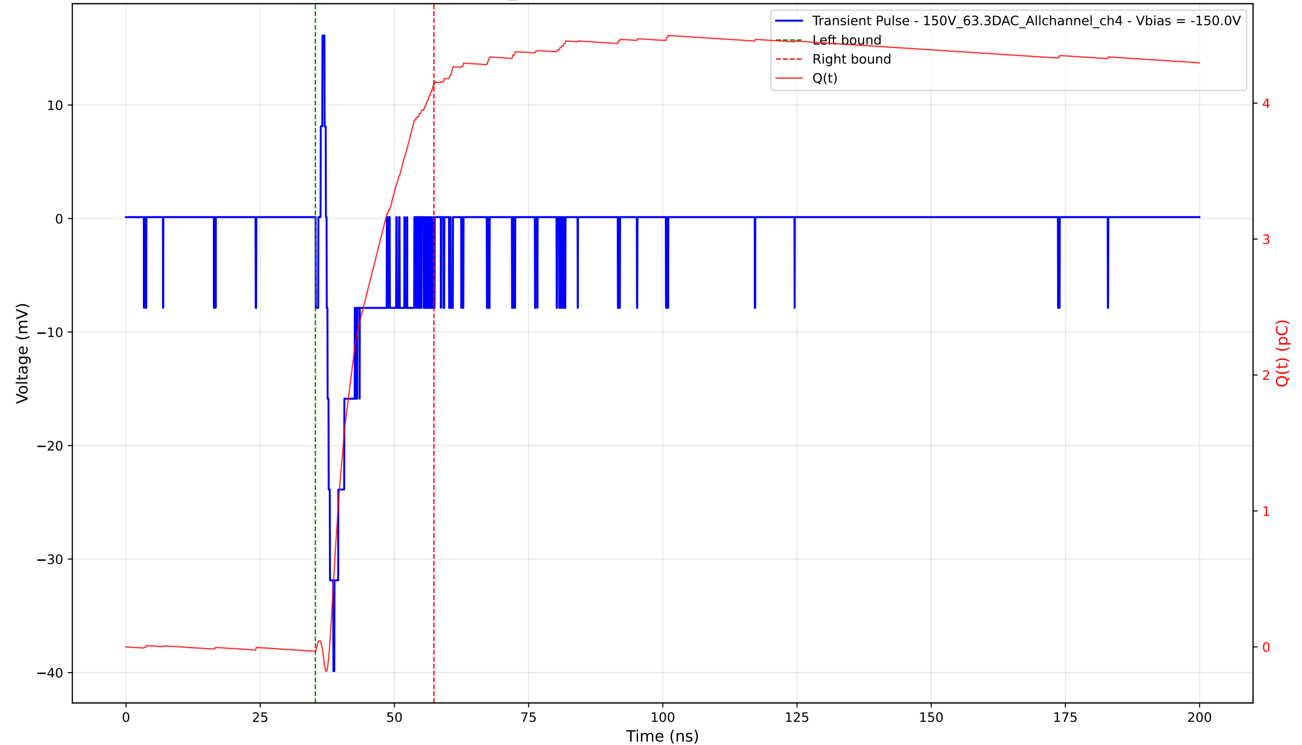
Transient Pulse - Sample: 1cm_42 - Position: 3505.0 \mu\text{m} - Charge: 4.16 pC - Rise Time: 1.26 ns
