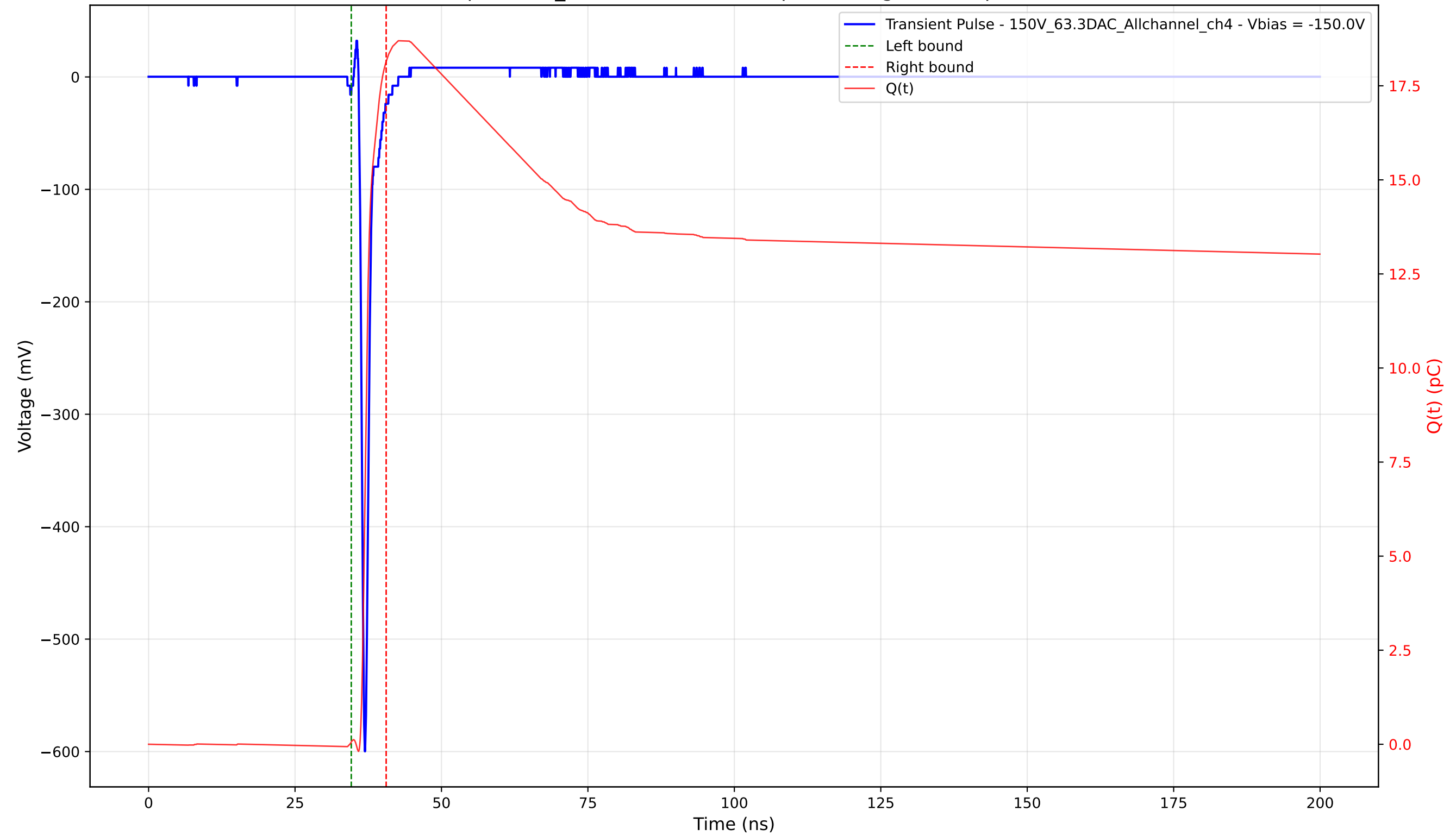
Transient Pulse - Sample: 1cm_42 - Position: 1970.0 \mu\text{m} - Charge: 18.08 pC - Rise Time: 0.72 ns
