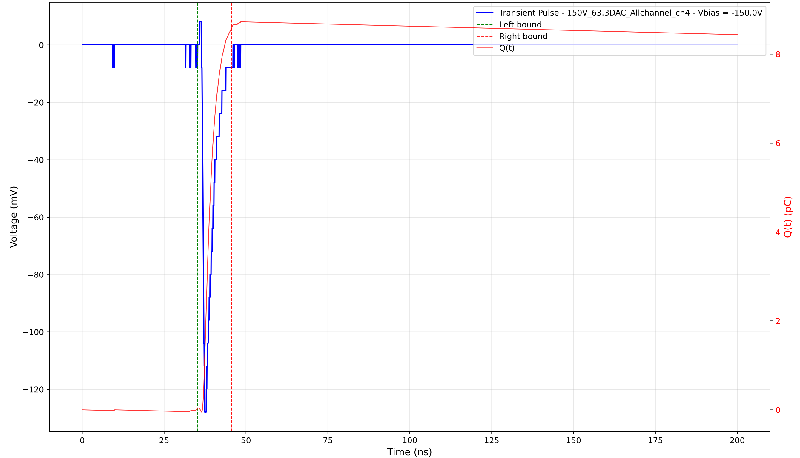
Transient Pulse - Sample: 1cm_42 - Position: 1115.0 \mu\text{m} - Charge: 8.54 pC - Rise Time: 0.74 ns
