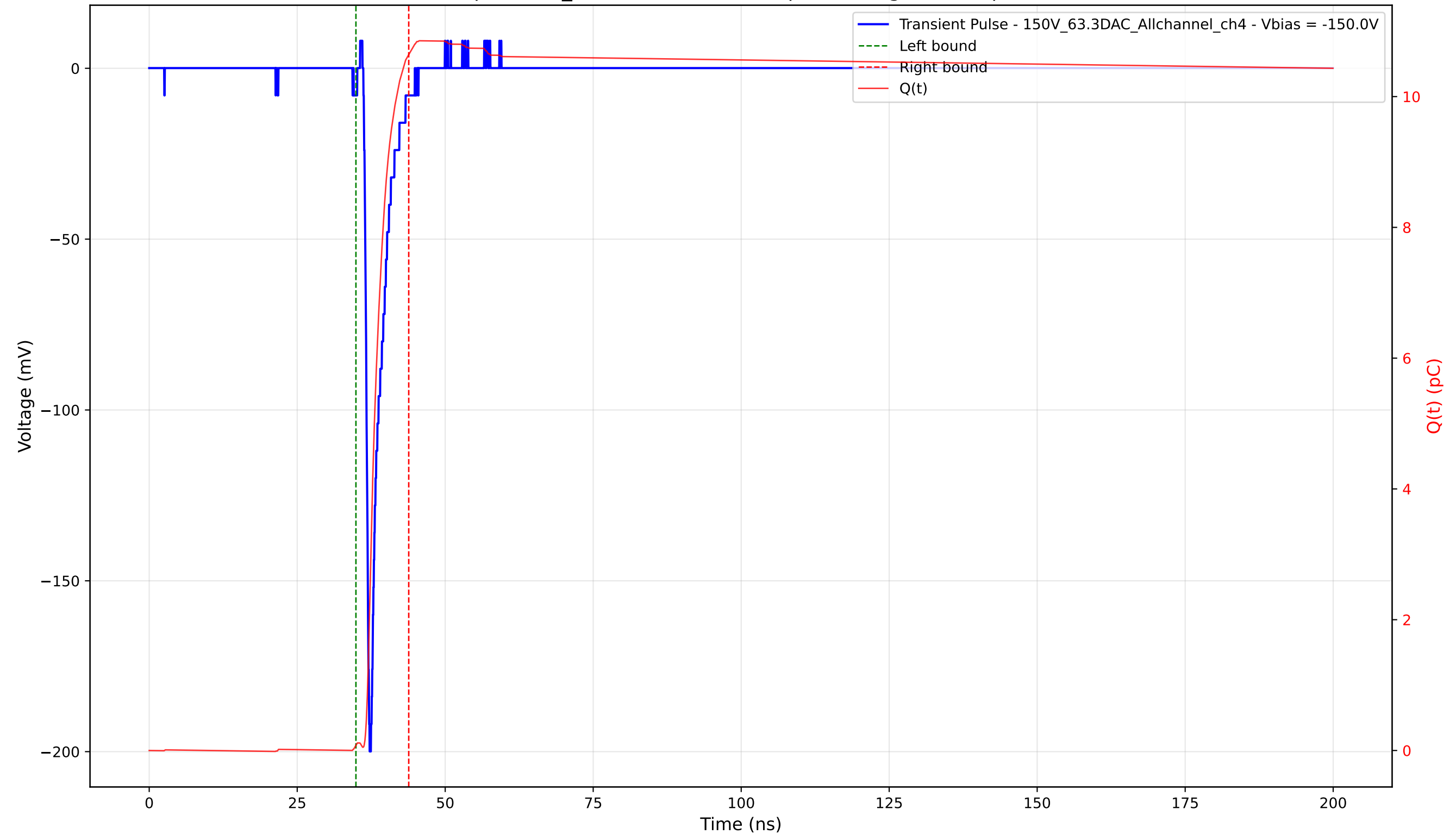
Transient Pulse - Sample: 1cm_42 - Position: 1390.0 \mu\text{m} - Charge: 10.56 pC - Rise Time: 0.80 ns
