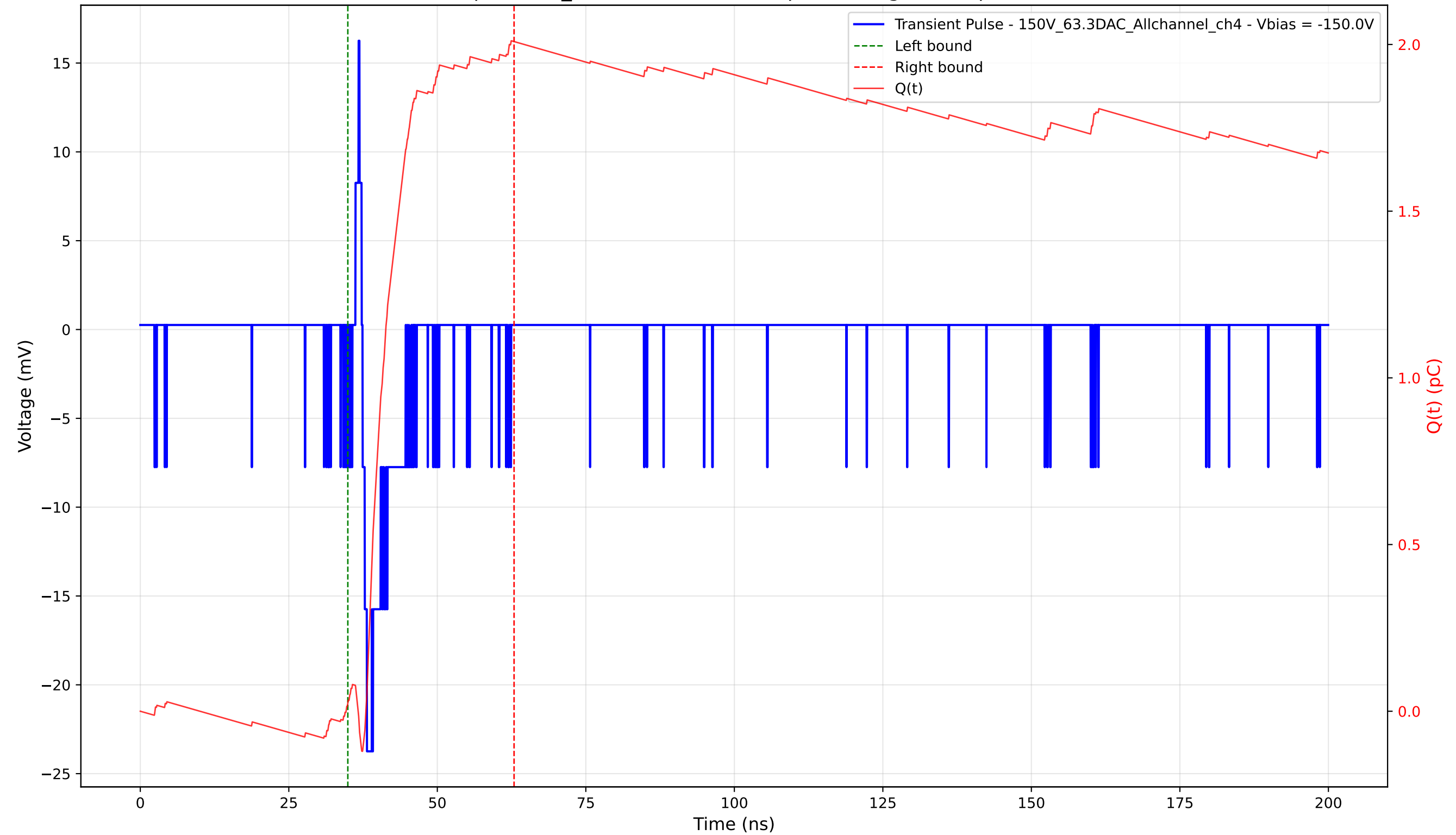
Transient Pulse - Sample: 1cm_42 - Position: 4985.0 \mu\text{m} - Charge: 1.98 pC - Rise Time: 0.75 ns
