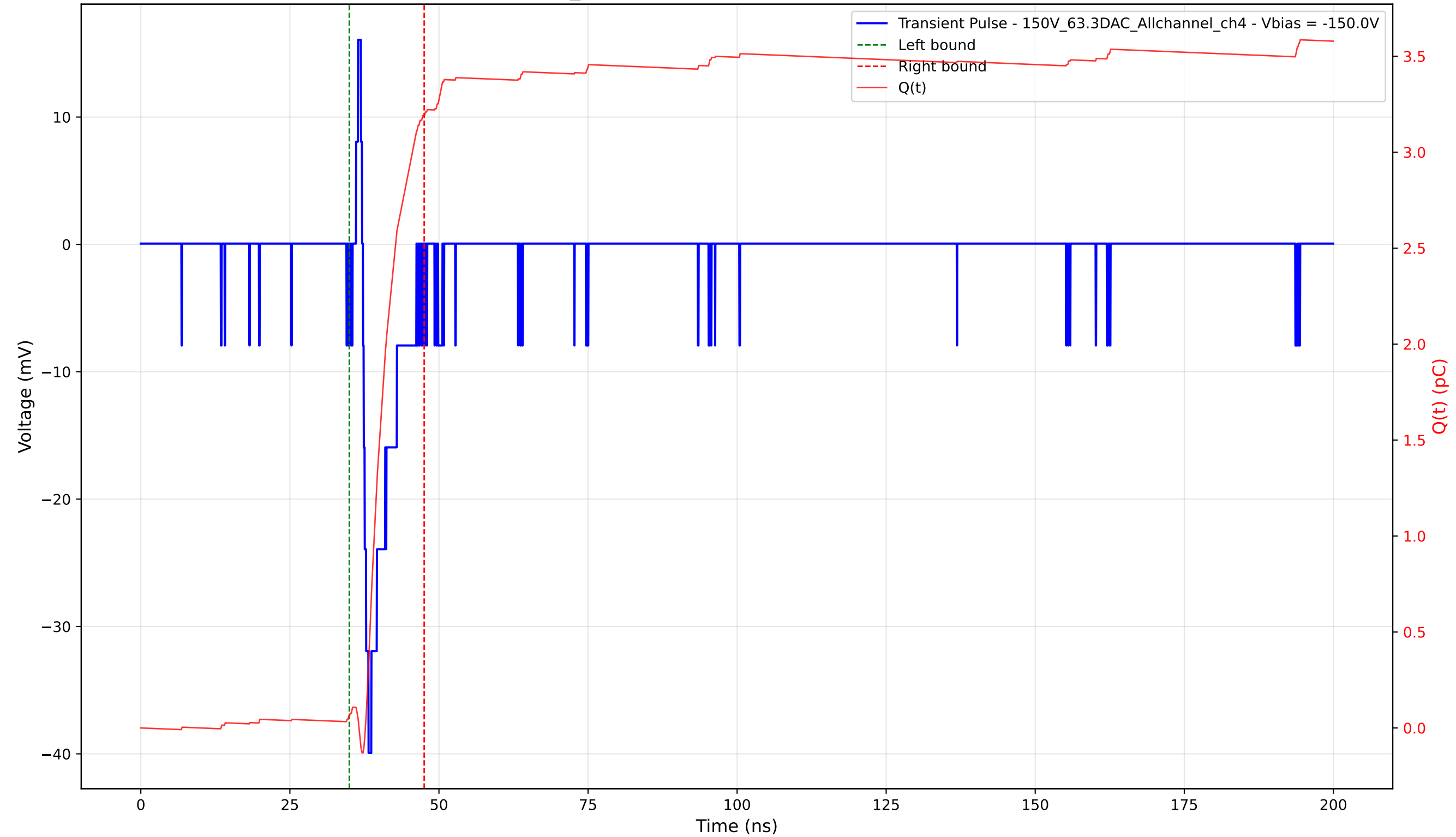
Transient Pulse - Sample: 1cm_42 - Position: 355.0 \mu\text{m} - Charge: 3.13 pC - Rise Time: 0.94 ns
