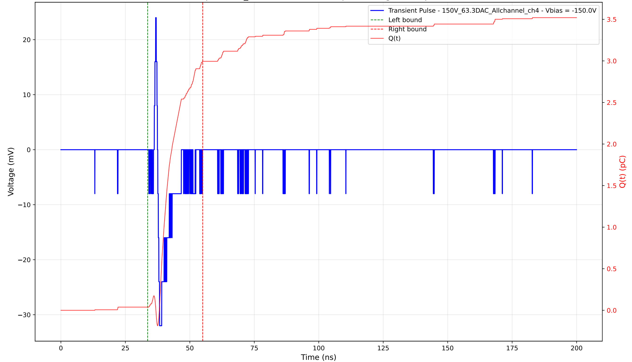
Transient Pulse - Sample: 1cm_42 - Position: 4665.0 \mu\text{m} - Charge: 2.96 pC - Rise Time: 0.70 ns
