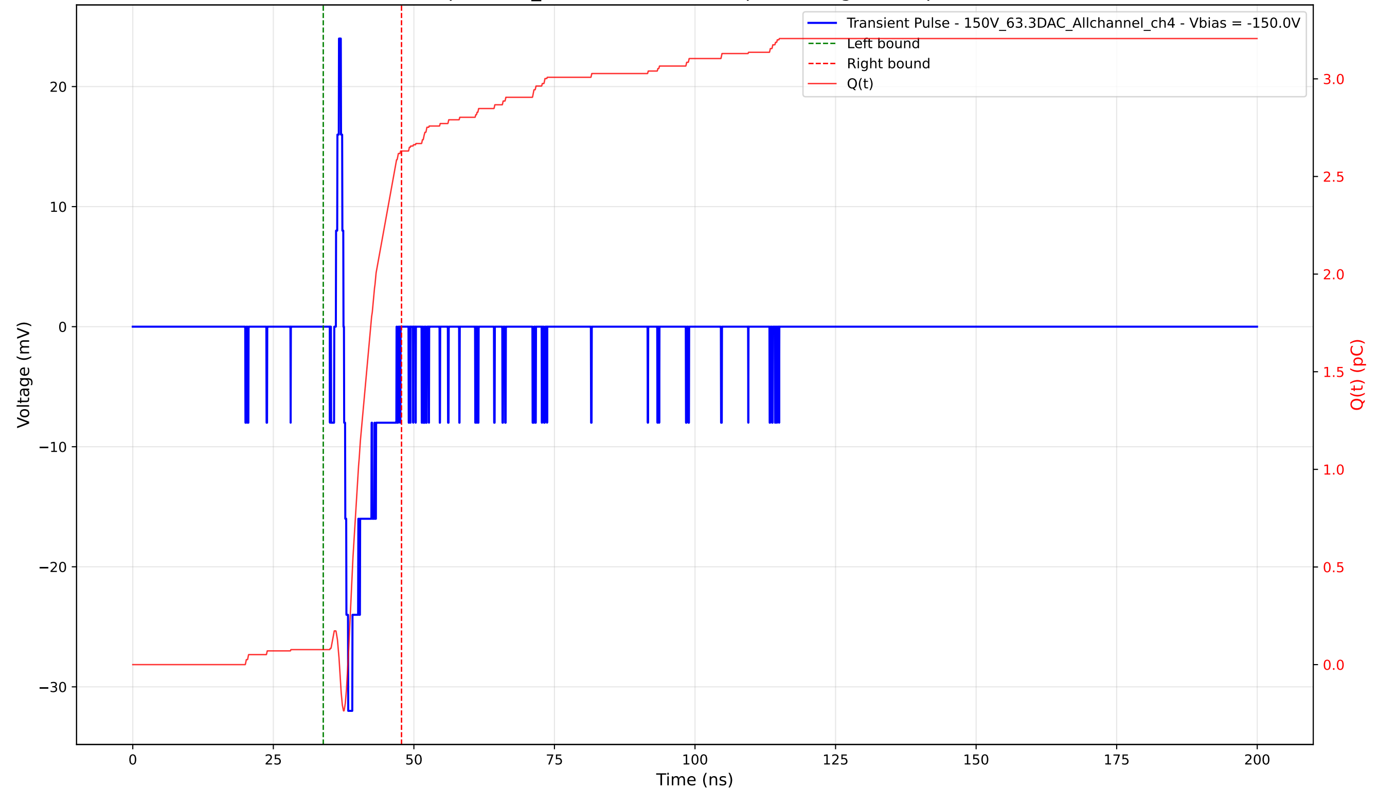
Transient Pulse - Sample: 1cm_42 - Position: 4650.0 \mu\text{m} - Charge: 2.55 pC - Rise Time: 0.74 ns
