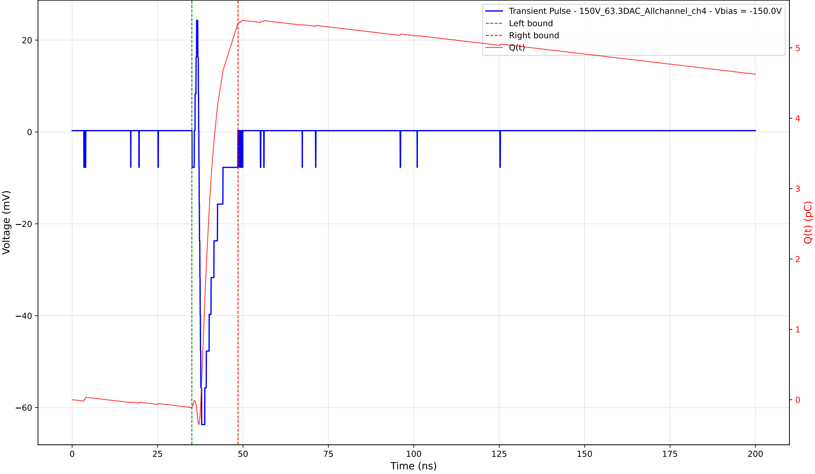
Transient Pulse - Sample: 1cm_42 - Position: 605.0 \mu\text{m} - Charge: 5.46 pC - Rise Time: 0.81 ns
