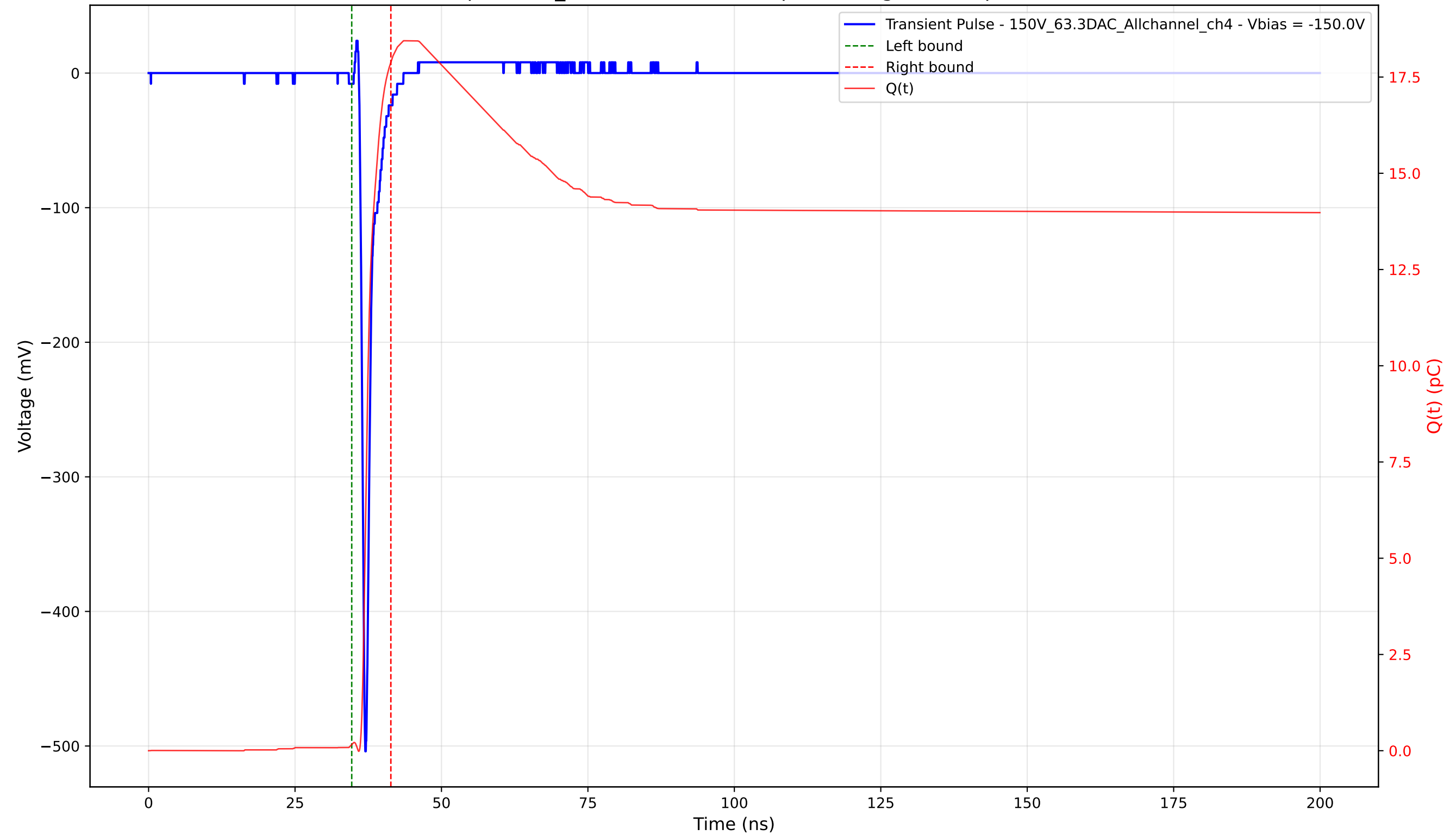
Transient Pulse - Sample: 1cm_42 - Position: 1690.0 \mu\text{m} - Charge: 17.72 pC - Rise Time: 0.75 ns
