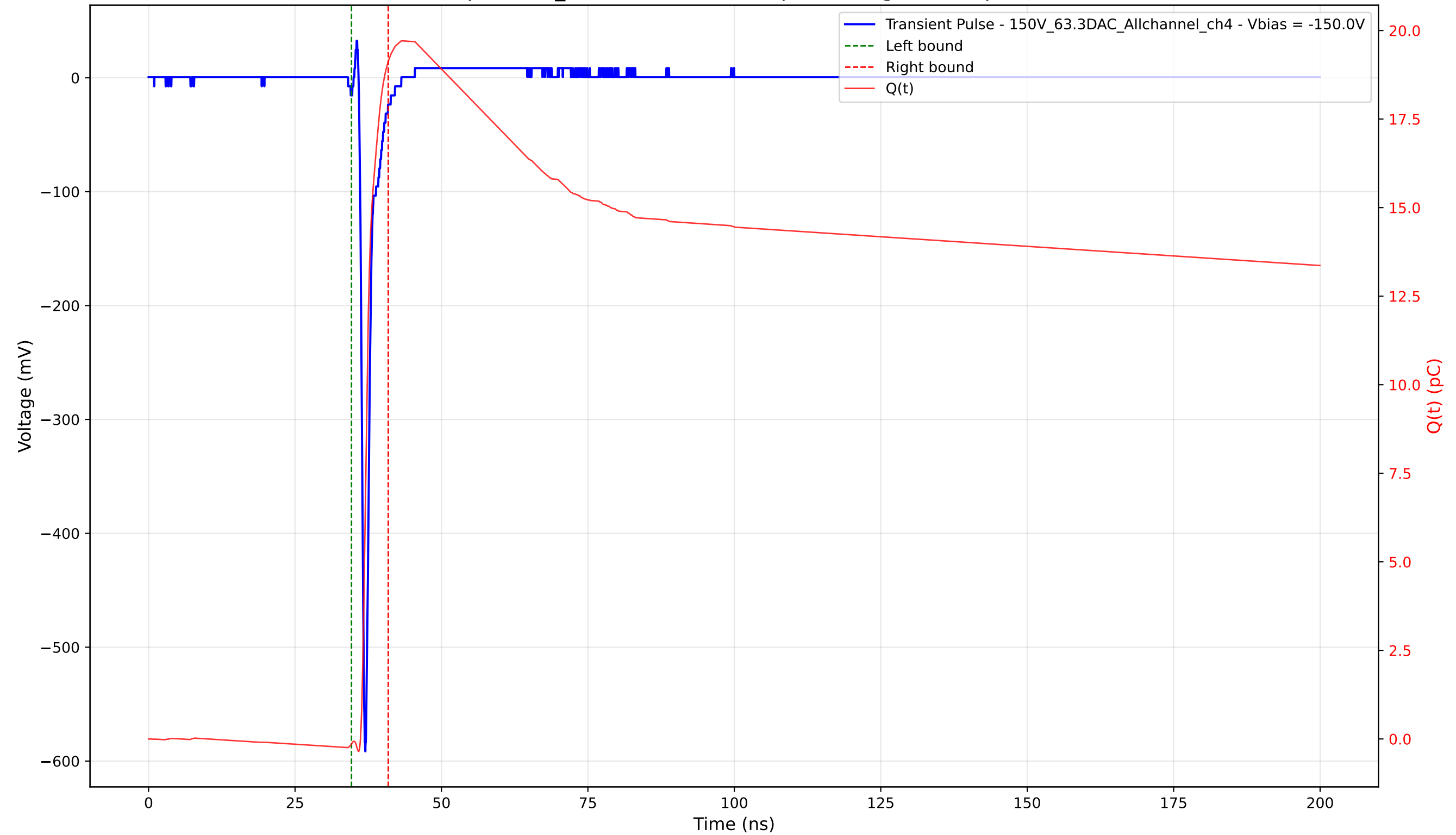
Transient Pulse - Sample: 1cm_42 - Position: 1830.0 \mu\text{m} - Charge: 19.27 pC - Rise Time: 0.72 ns
