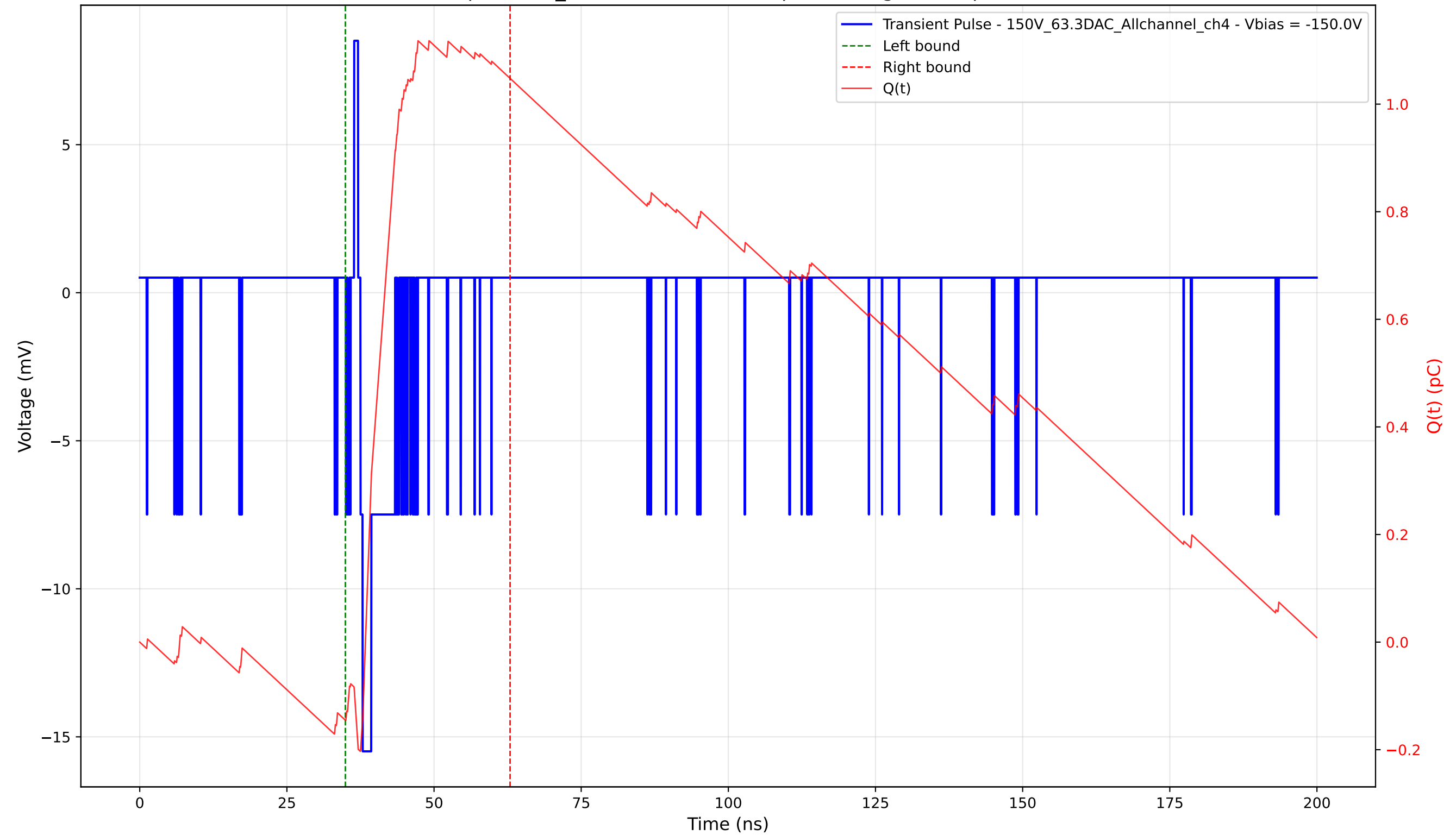
Transient Pulse - Sample: 1cm_42 - Position: 5045.0 \mu\text{m} - Charge: 1.19 pC - Rise Time: 0.39 ns
