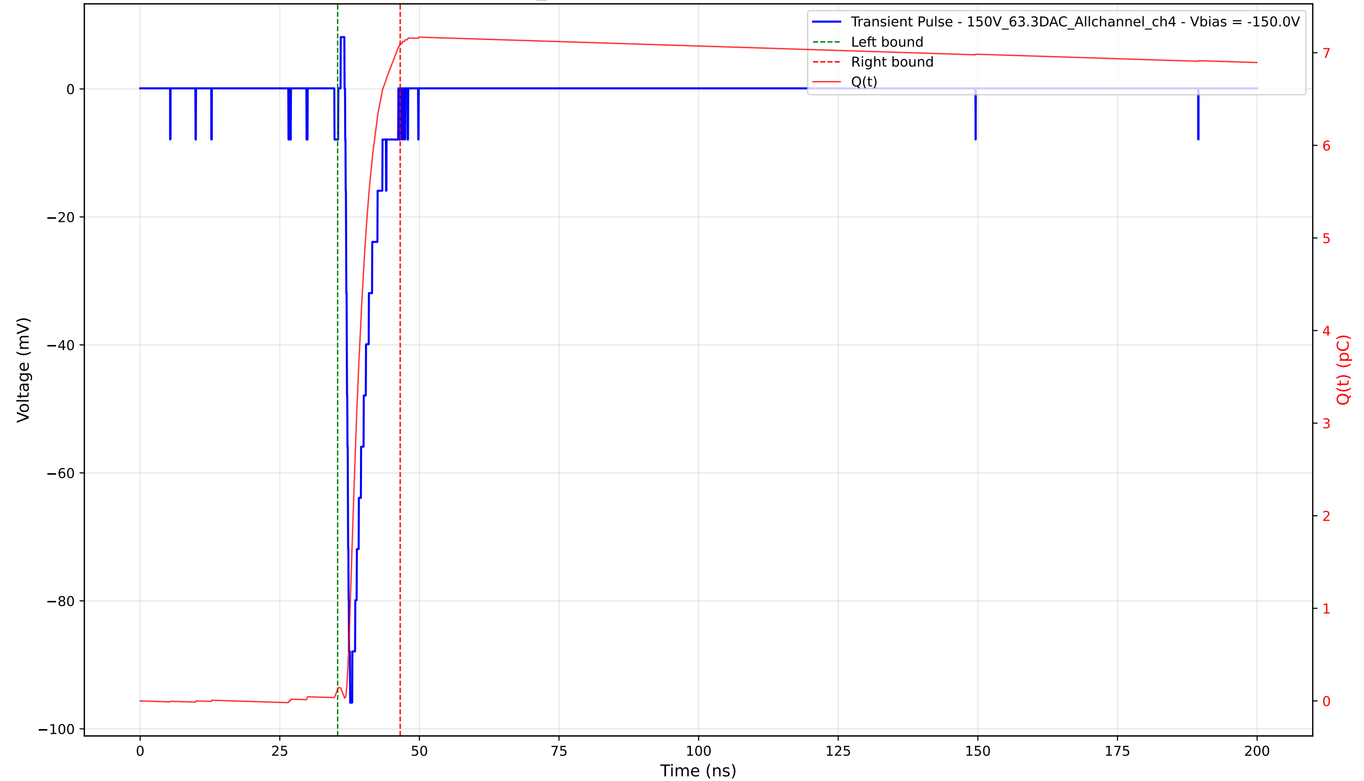
Transient Pulse - Sample: 1cm_42 - Position: 1005.0 \mu\text{m} - Charge: 6.97 pC - Rise Time: 0.63 ns
