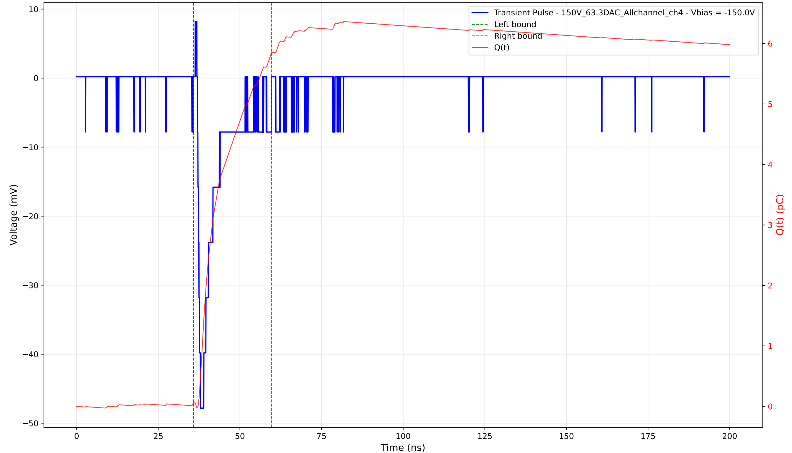
Transient Pulse - Sample: 1cm_42 - Position: 3265.0 \mu\text{m} - Charge: 5.79 pC - Rise Time: 0.90 ns
