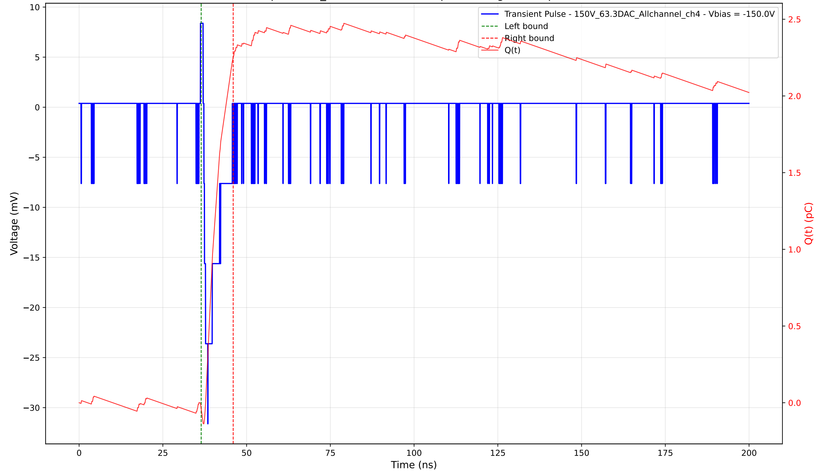
Transient Pulse - Sample: 1cm_42 - Position: 205.0 \mu\text{m} - Charge: 2.29 pC - Rise Time: 1.18 ns
