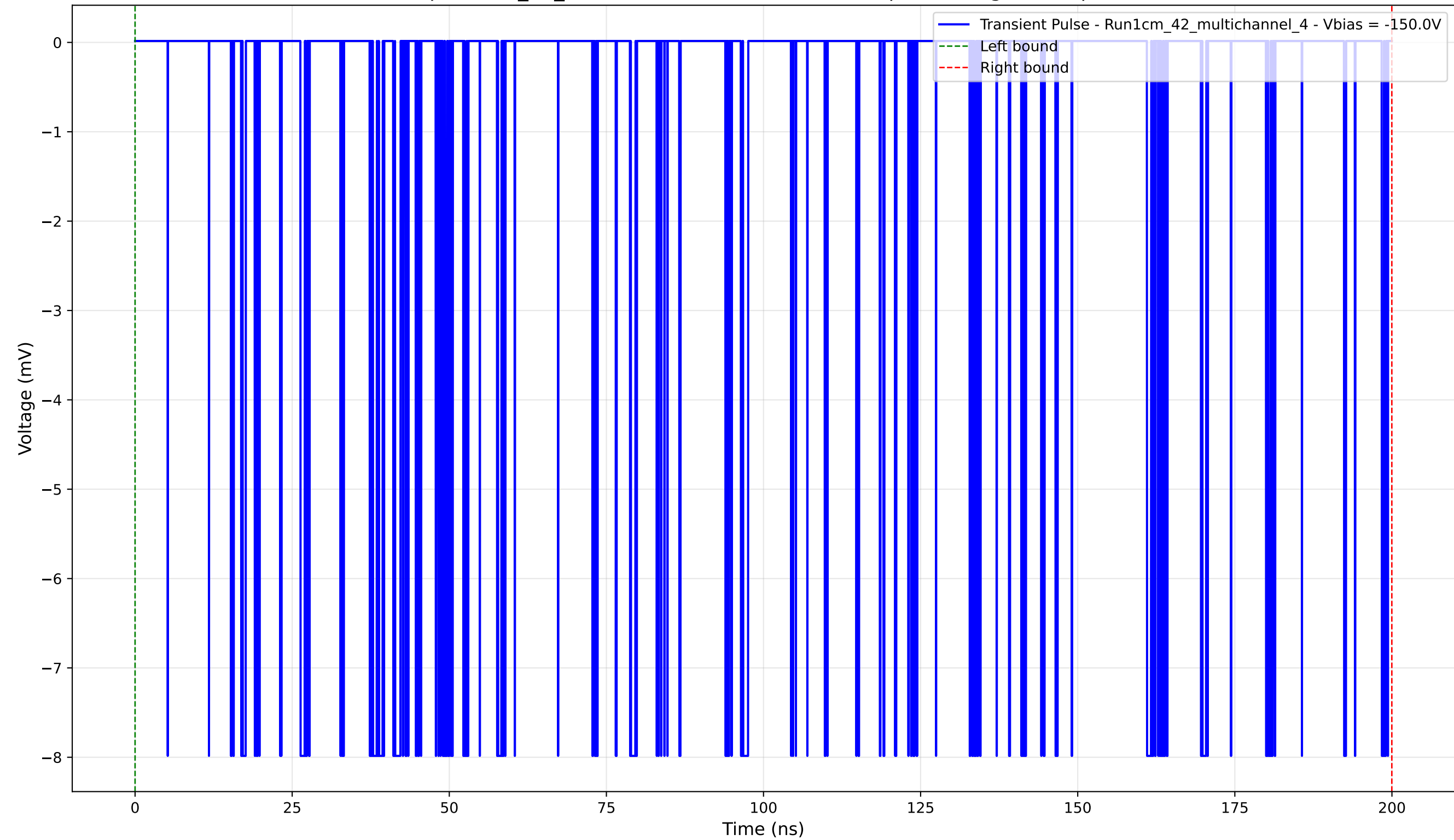
Transient Pulse - Sample: 1cm_42_multichannel - Position: 3890.0 \mu\text{m} - Charge: 3.09 pC - Rise Time: 0.02 ns
