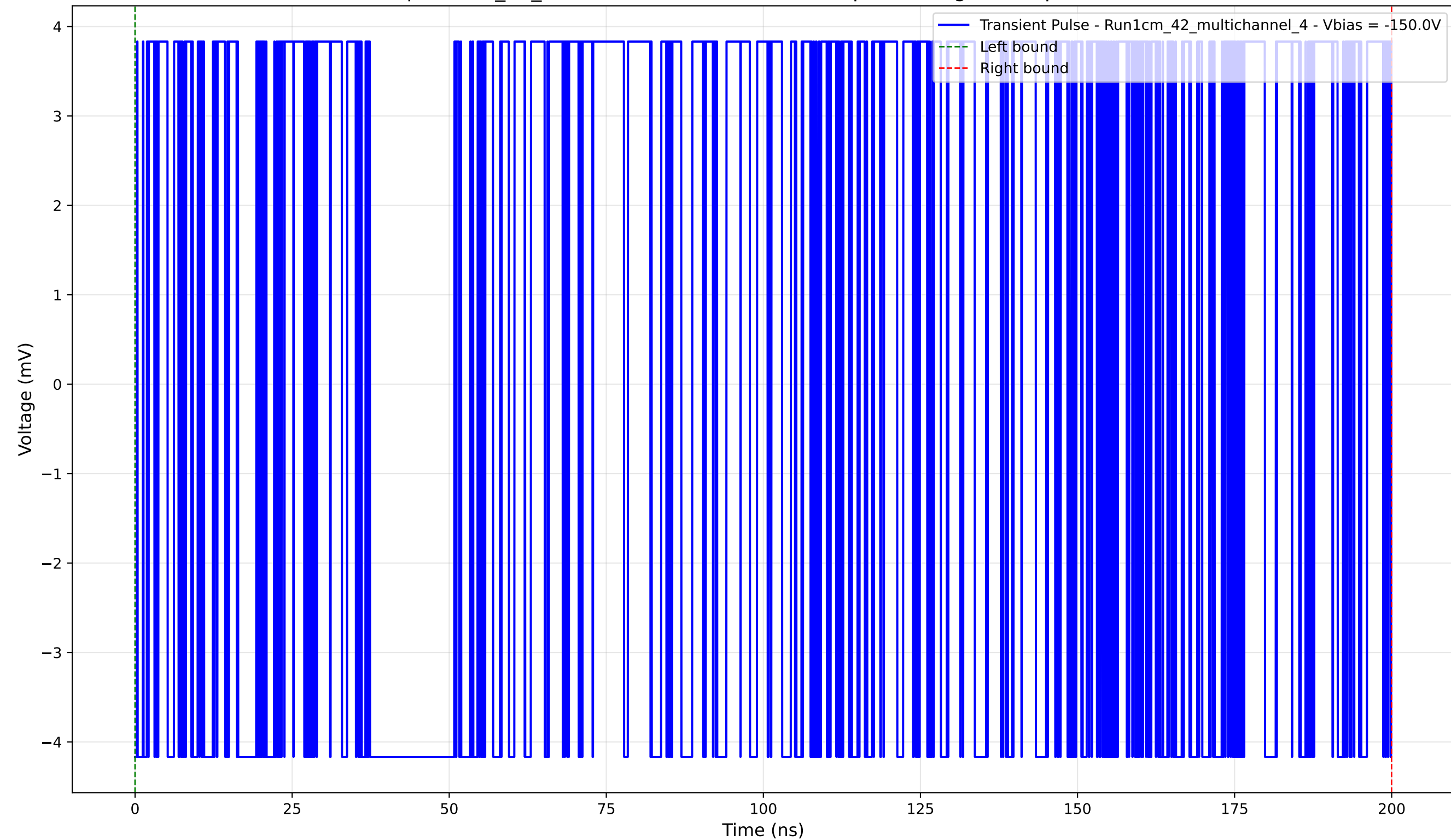
Transient Pulse - Sample: 1cm_42_multichannel - Position: 830.0 \mu\text{m} - Charge: 2.34 pC - Rise Time: 0.00 ns (N/A)
