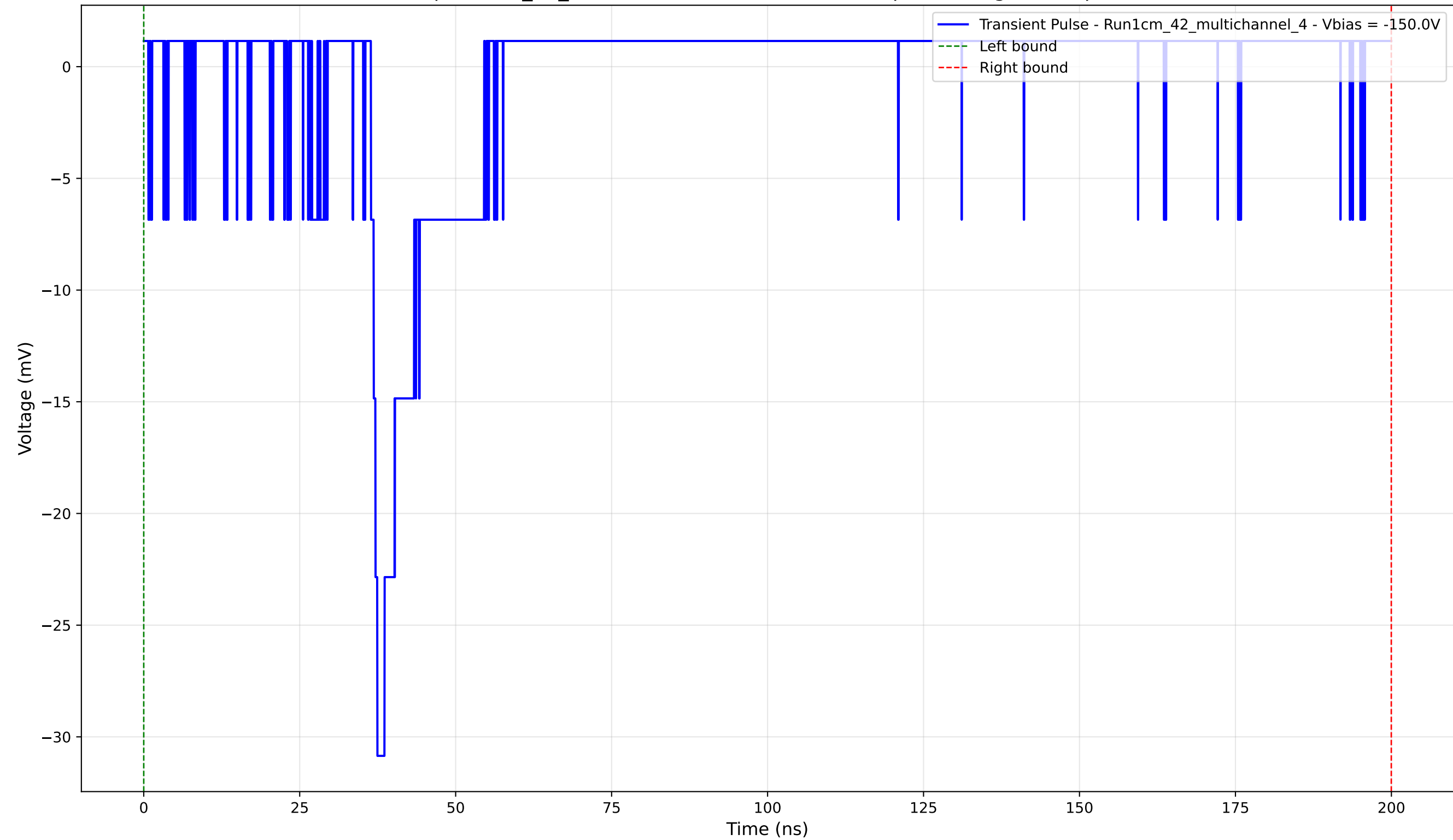
Transient Pulse - Sample: 1cm_42_multichannel - Position: 1555.0 \mu\text{m} - Charge: 1.28 pC - Rise Time: 1.03 ns
