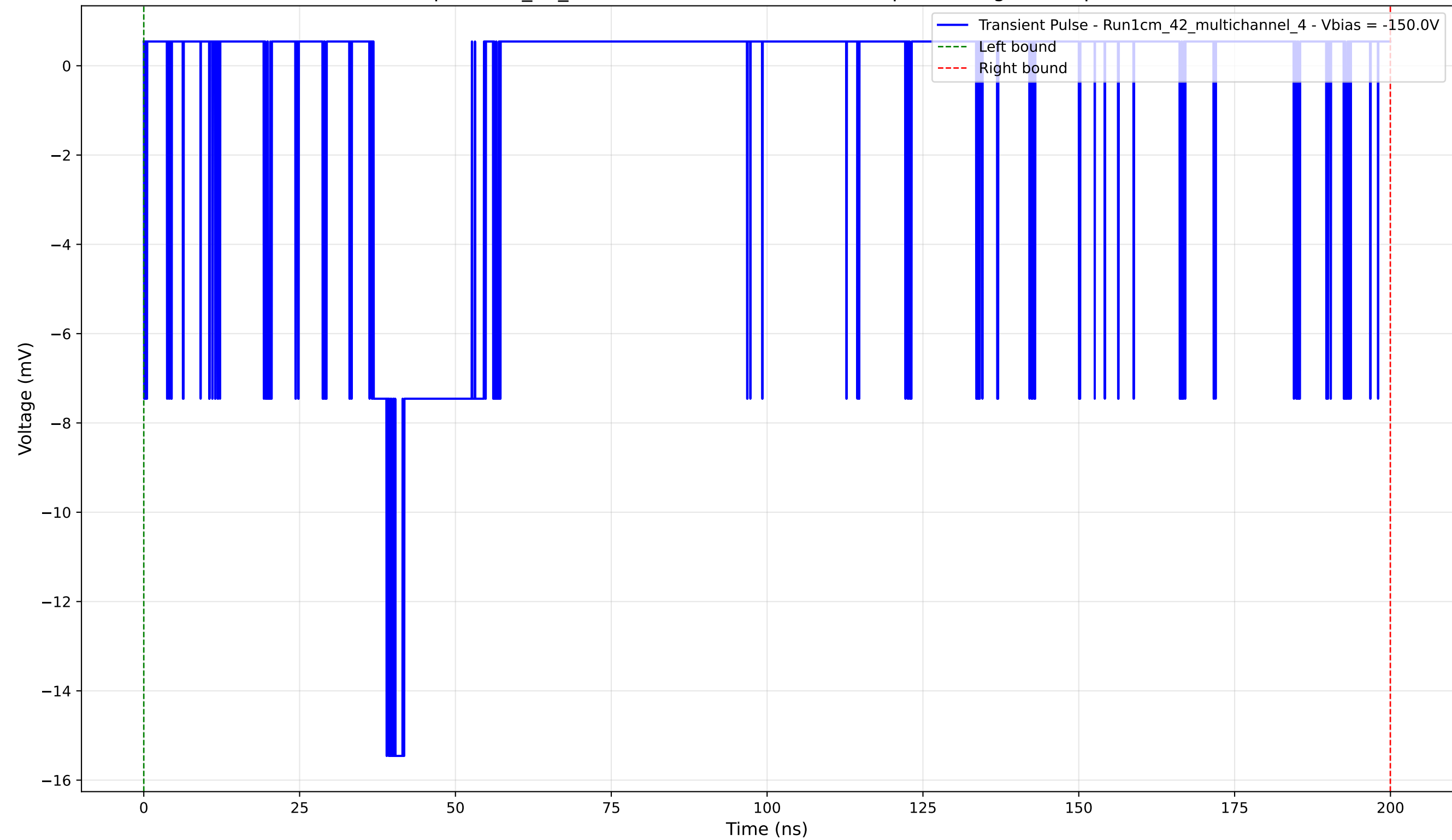
Transient Pulse - Sample: 1cm_42_multichannel - Position: 4465.0 \mu\text{m} - Charge: 2.37 pC - Rise Time: 2.08 ns
