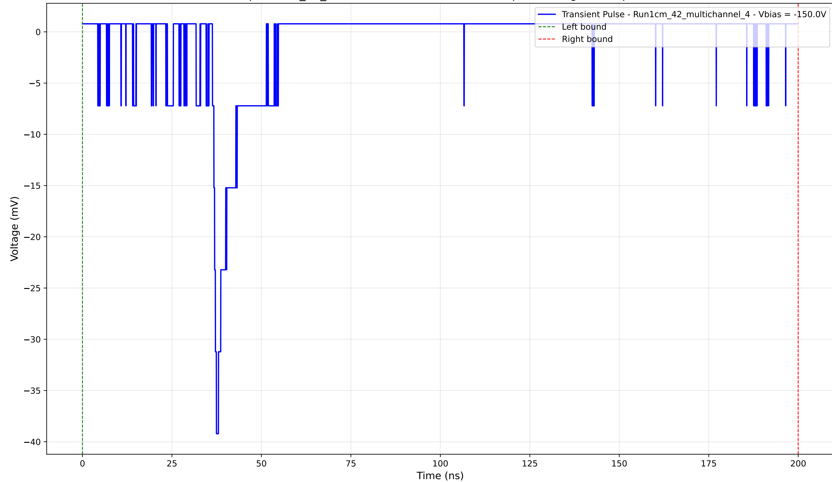
Transient Pulse - Sample: 1cm_42_multichannel - Position: 1700.0 \mu\text{m} - Charge: 2.94 pC - Rise Time: 1.11 ns
