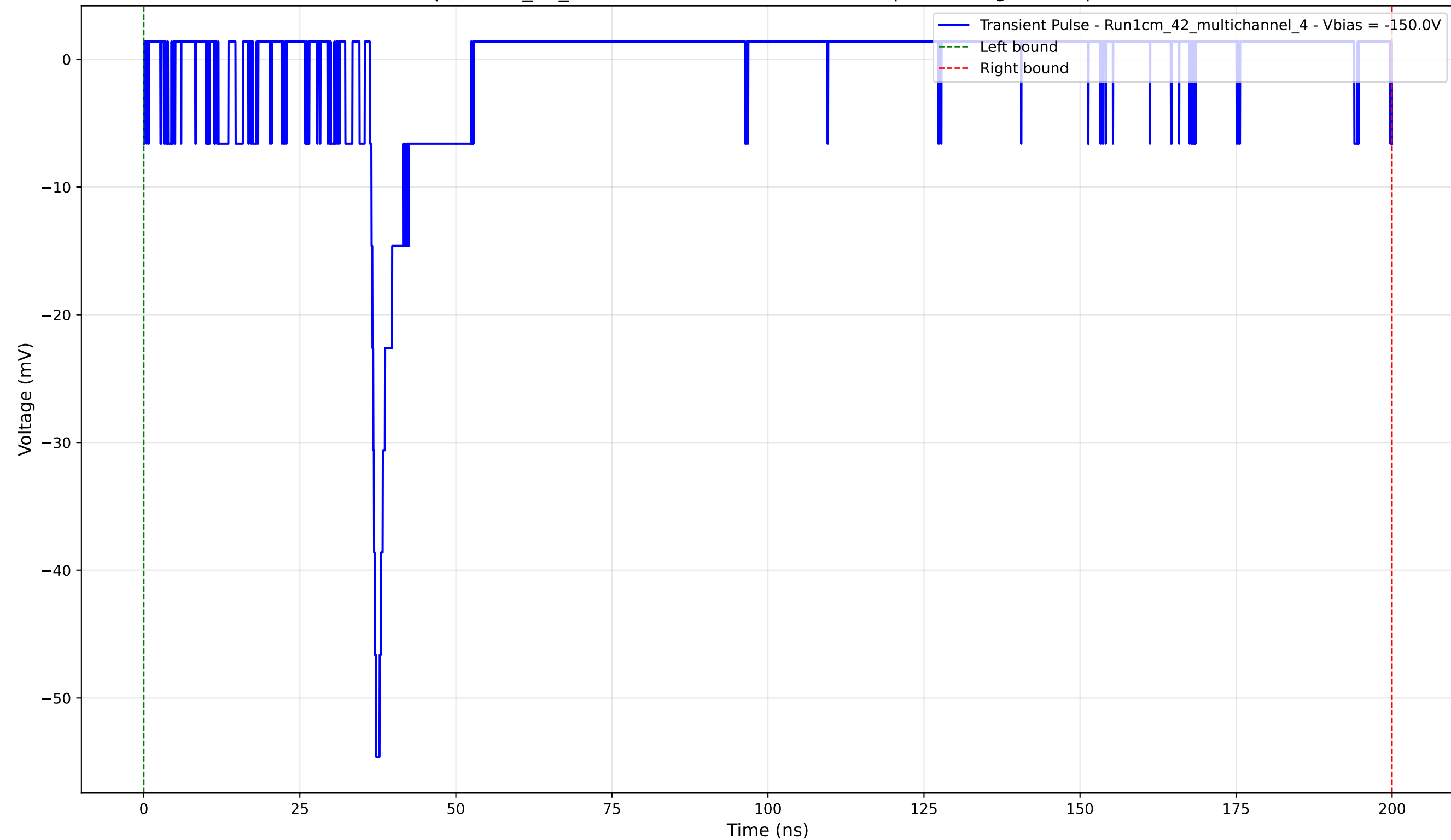
Transient Pulse - Sample: 1cm_42_multichannel - Position: 2740.0 \mu\text{m} - Charge: 1.39 pC - Rise Time: 0.98 ns
