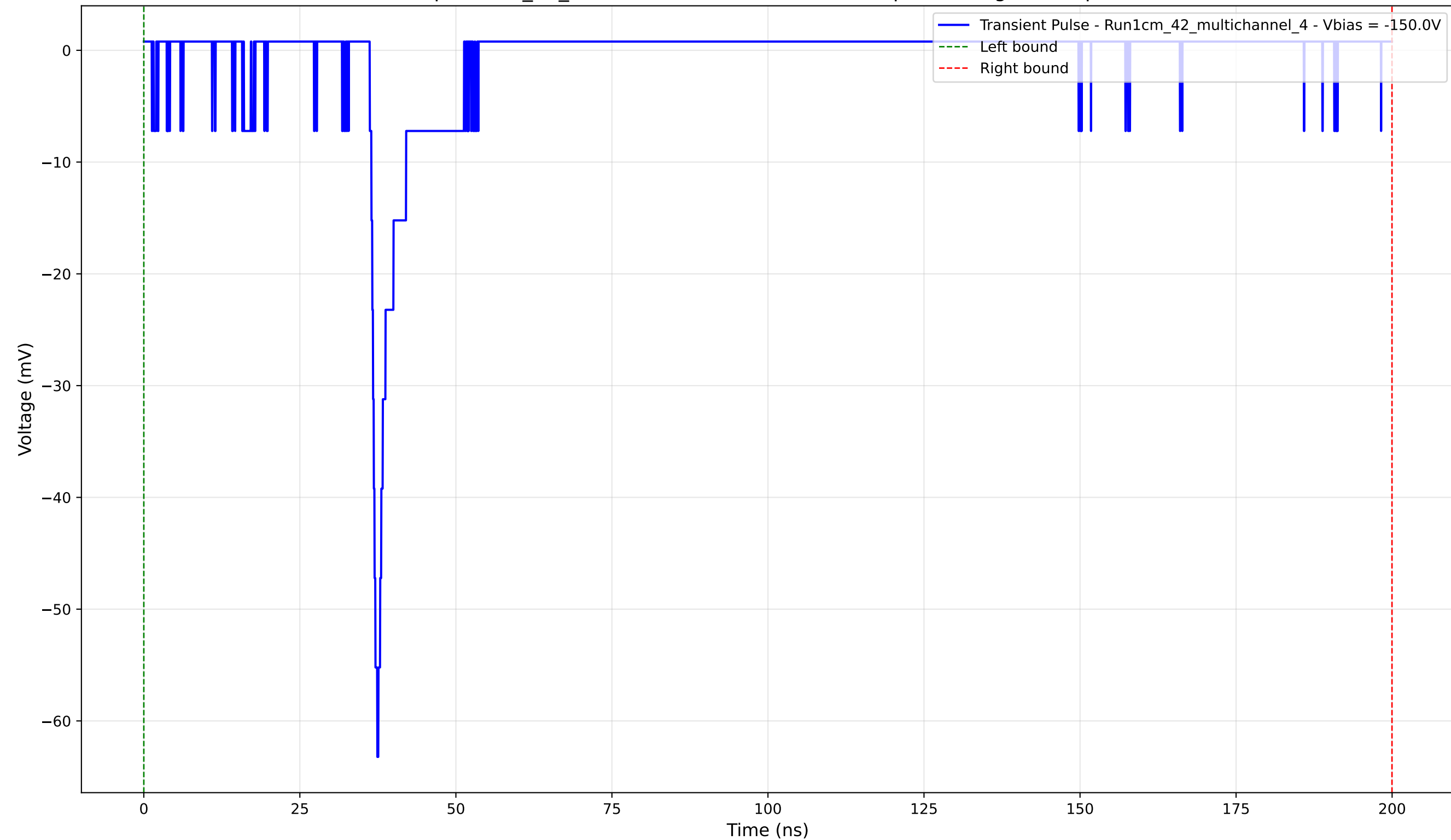
Transient Pulse - Sample: 1cm_42_multichannel - Position: 2060.0 \mu\text{m} - Charge: 2.66 pC - Rise Time: 1.20 ns
