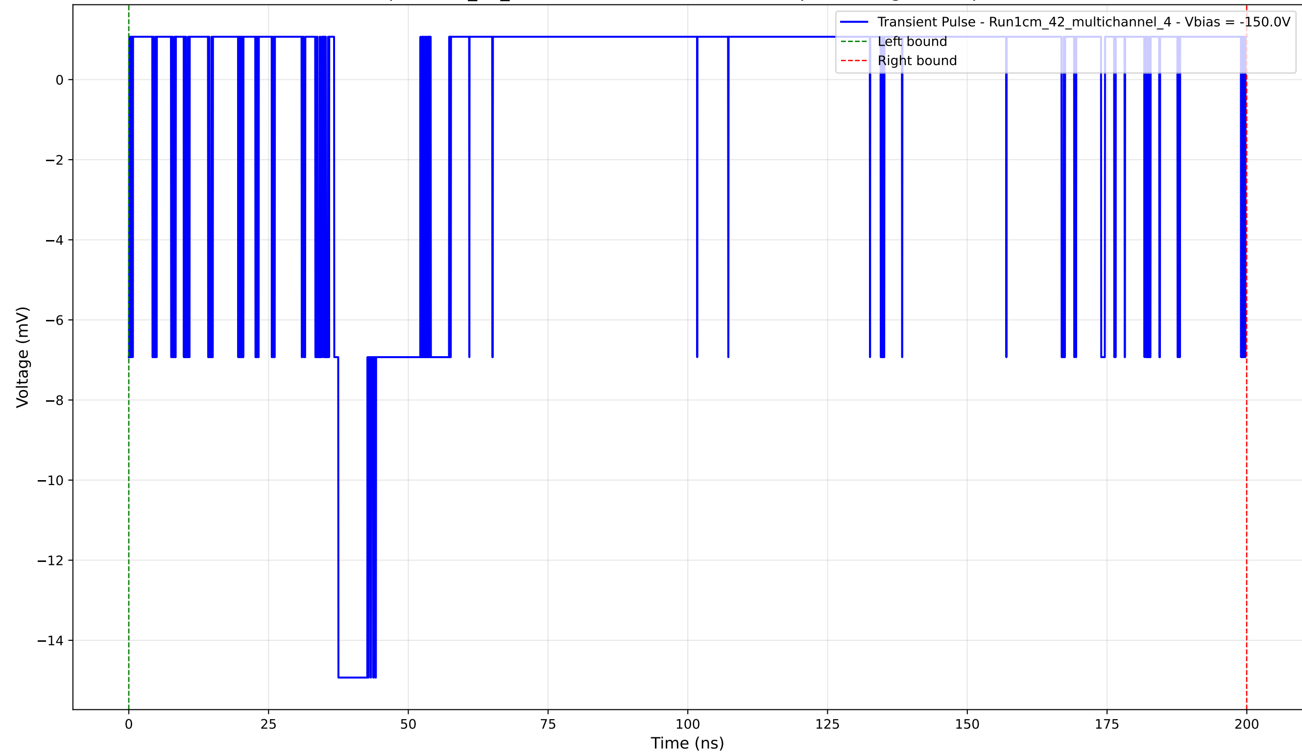
Transient Pulse - Sample: 1cm_42_multichannel - Position: 3655.0 \mu\text{m} - Charge: 1.26 pC - Rise Time: 0.76 ns
