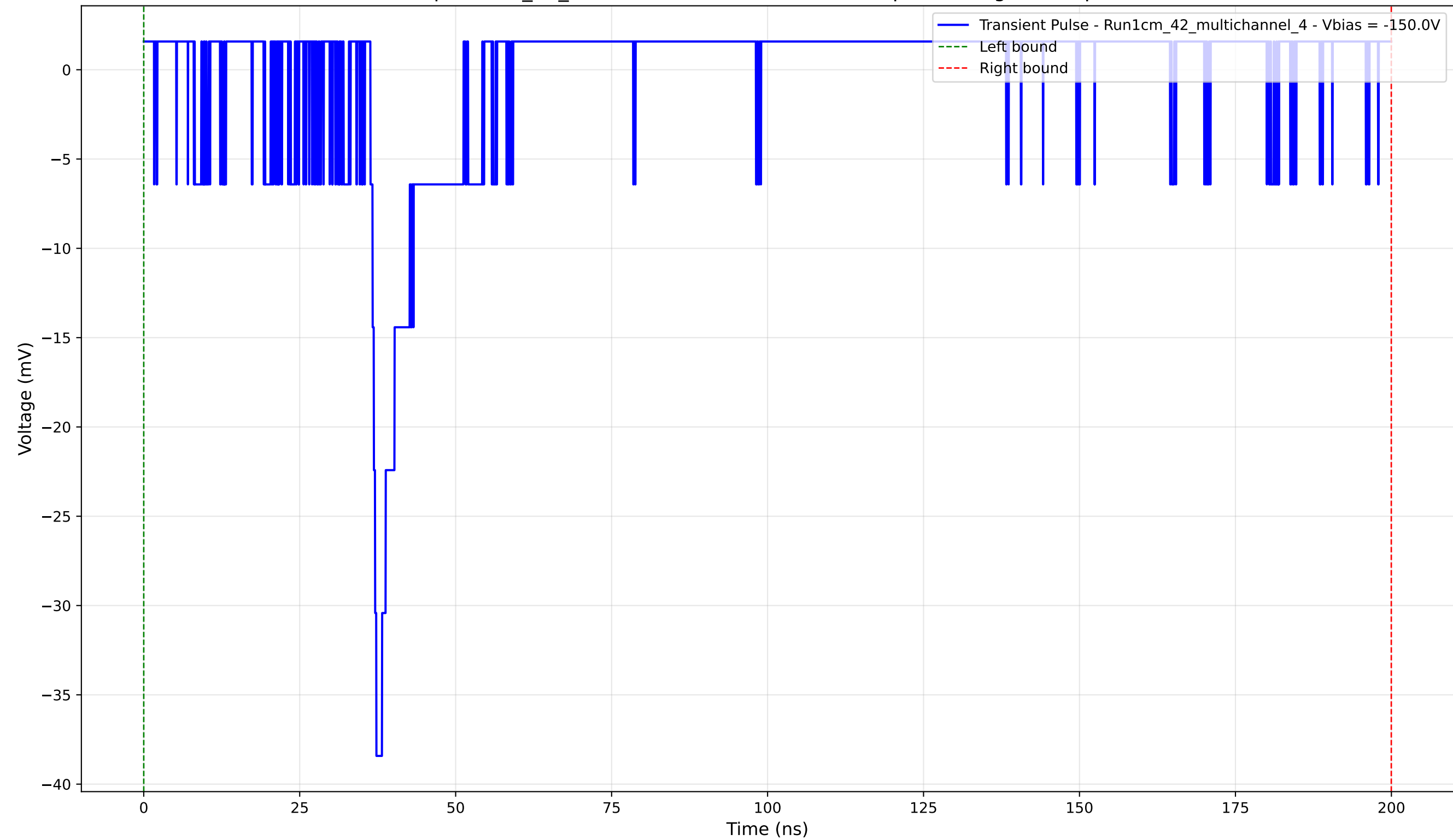
Transient Pulse - Sample: 1cm_42_multichannel - Position: 1745.0 \mu\text{m} - Charge: 0.87 pC - Rise Time: 0.95 ns
