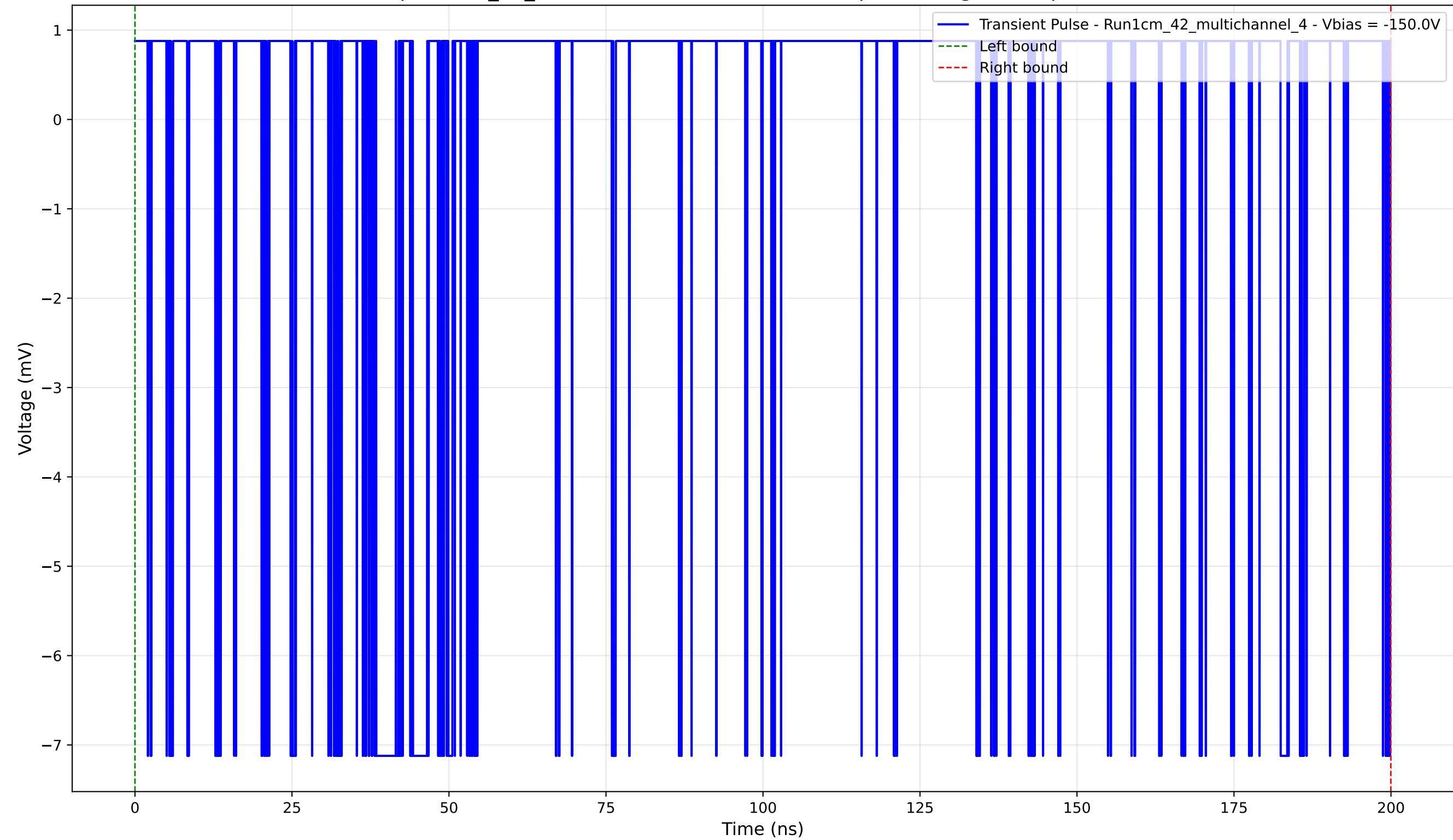
Transient Pulse - Sample: 1cm_42_multichannel - Position: 4875.0 \mu\text{m} - Charge: 0.02 pC - Rise Time: 0.00 ns (N/A)
