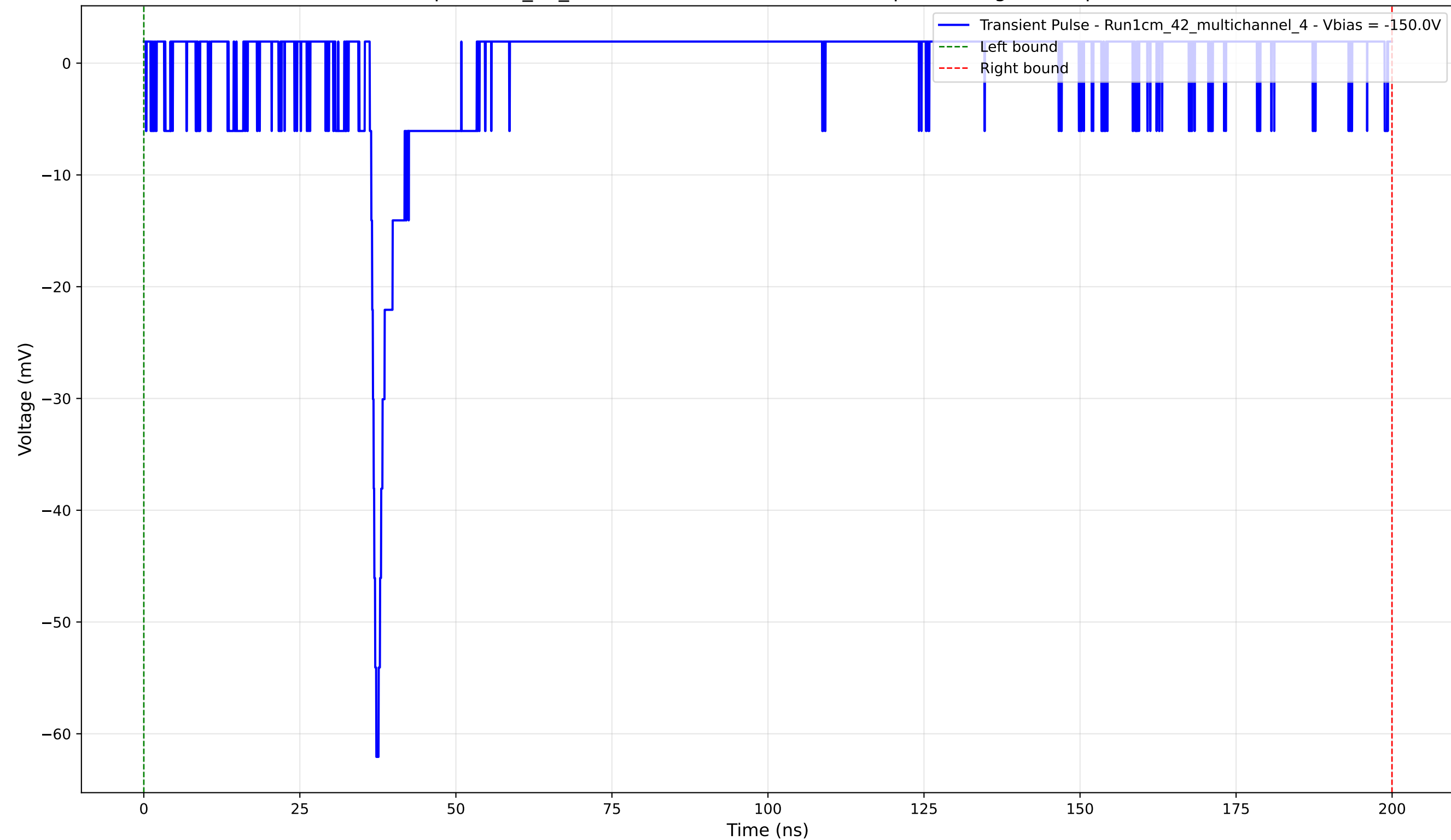
Transient Pulse - Sample: 1cm_42_multichannel - Position: 2080.0 \mu\text{m} - Charge: 0.19 pC - Rise Time: 0.82 ns
