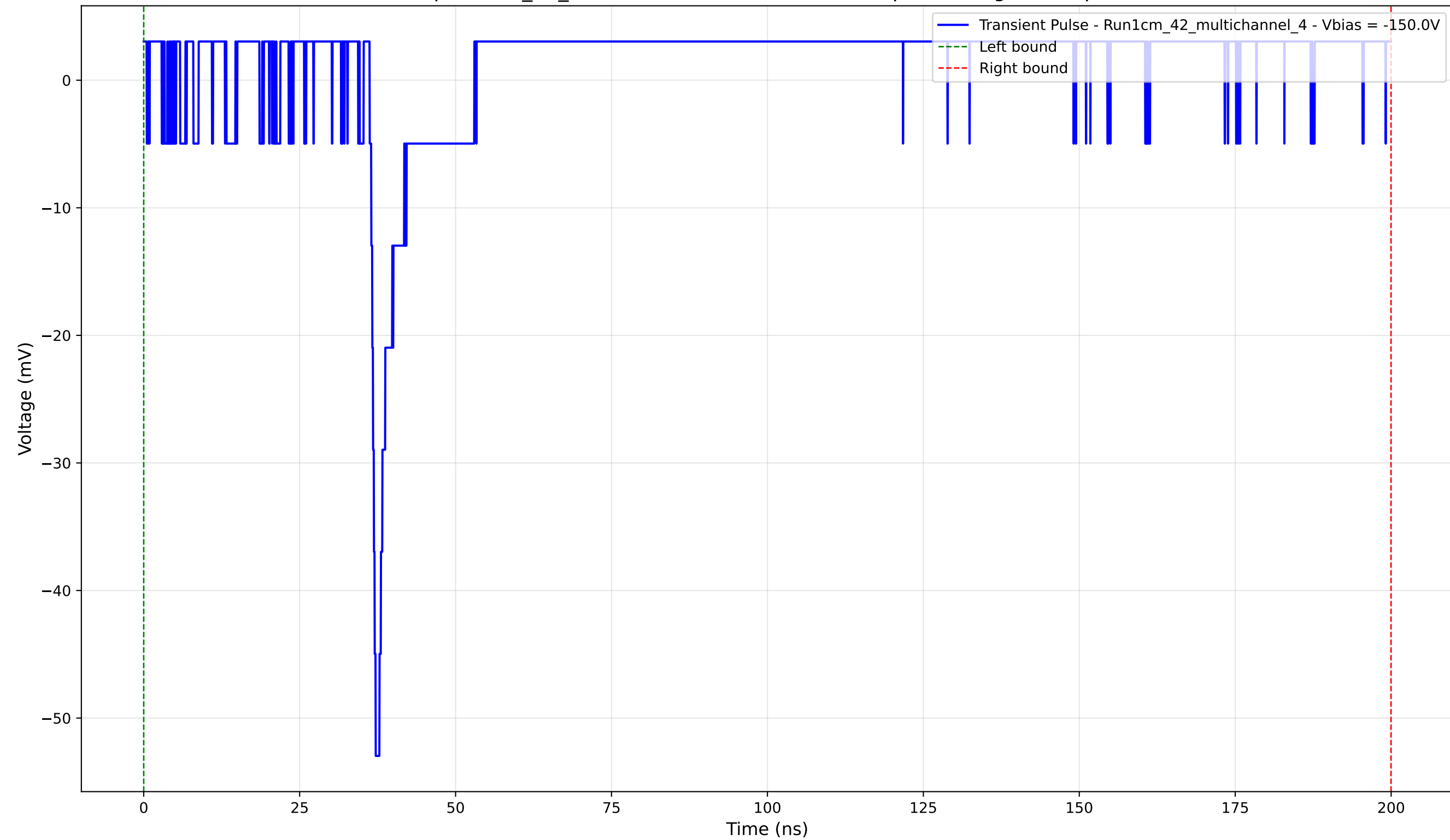
Transient Pulse - Sample: 1cm_42_multichannel - Position: 2010.0 \mu\text{m} - Charge: 5.33 pC - Rise Time: 0.72 ns
