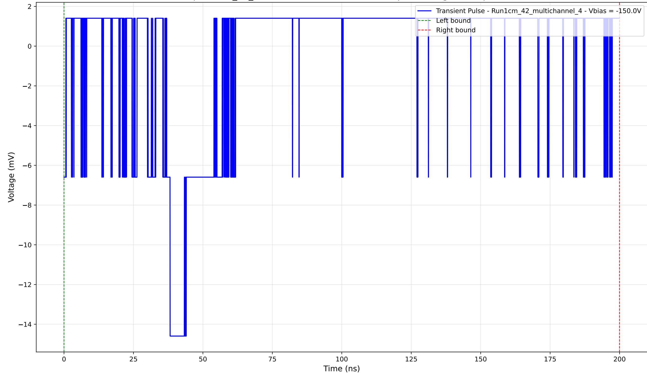
Transient Pulse - Sample: 1cm_42_multichannel - Position: 4300.0 \mu\text{m} - Charge: 0.57 pC - Rise Time: 1.24 ns
