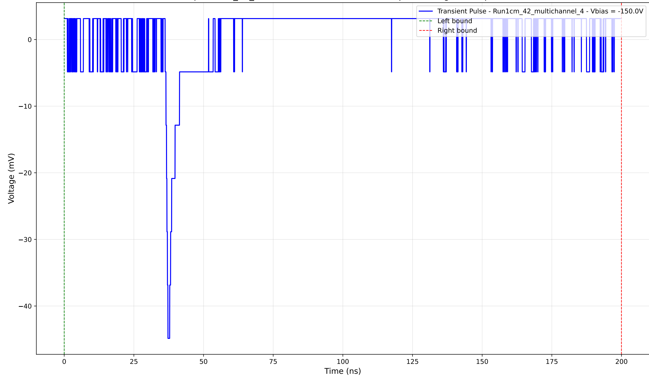
Transient Pulse - Sample: 1cm_42_multichannel - Position: 1950.0 \mu\text{m} - Charge: 4.28 pC - Rise Time: 1.00 ns
