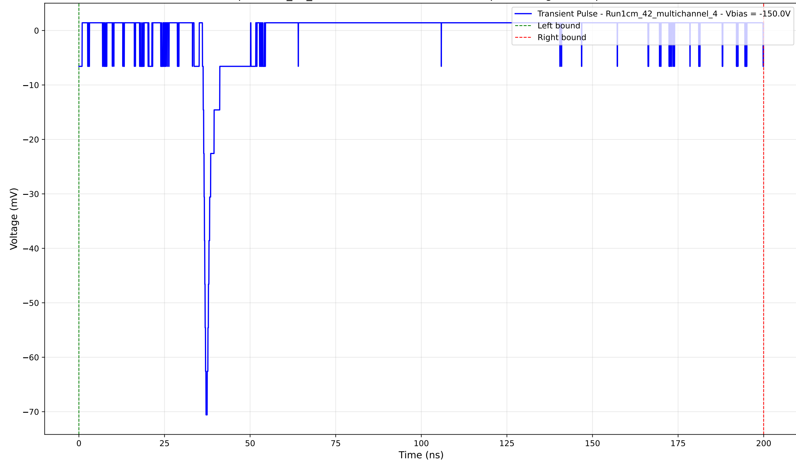
Transient Pulse - Sample: 1cm_42_multichannel - Position: 2555.0 \mu\text{m} - Charge: 0.87 pC - Rise Time: 0.84 ns
