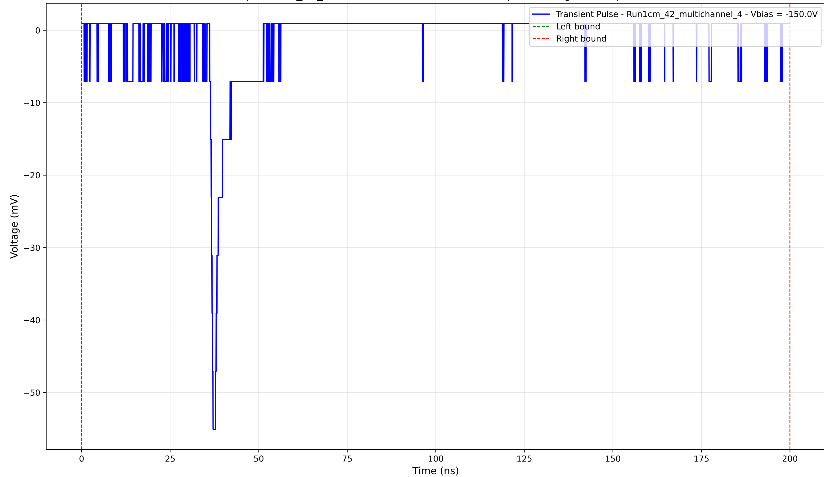
Transient Pulse - Sample: 1cm_42_multichannel - Position: 2695.0 \mu\text{m} - Charge: 3.05 pC - Rise Time: 0.93 ns
