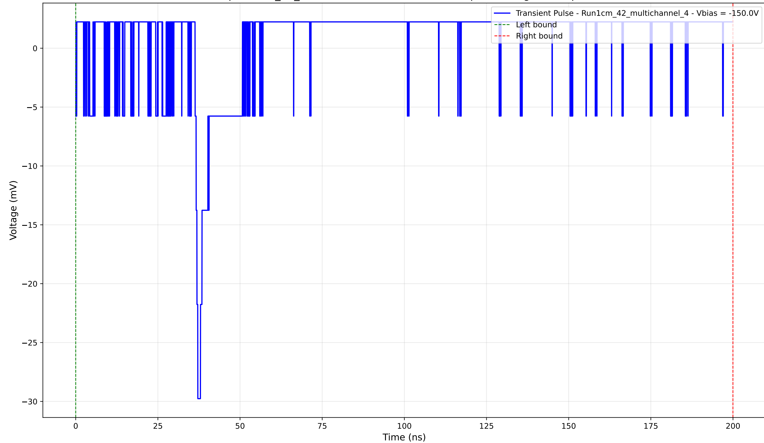
Transient Pulse - Sample: 1cm_42_multichannel - Position: 2835.0 \mu\text{m} - Charge: 3.48 pC - Rise Time: 0.84 ns
