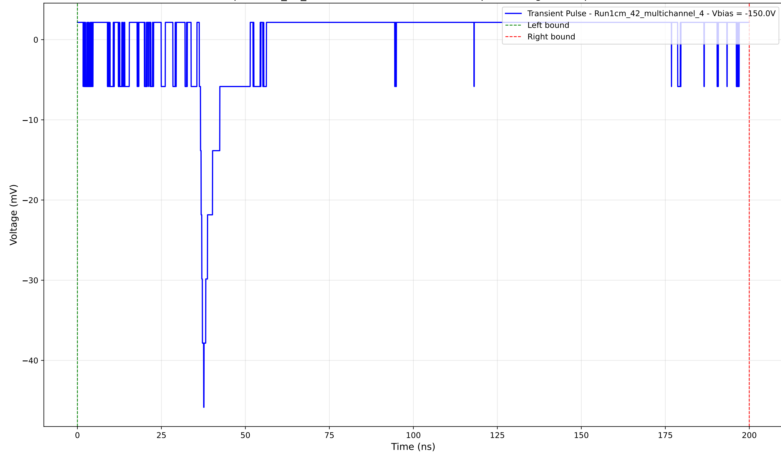
Transient Pulse - Sample: 1cm_42_multichannel - Position: 1795.0 \mu\text{m} - Charge: 1.45 pC - Rise Time: 1.31 ns
