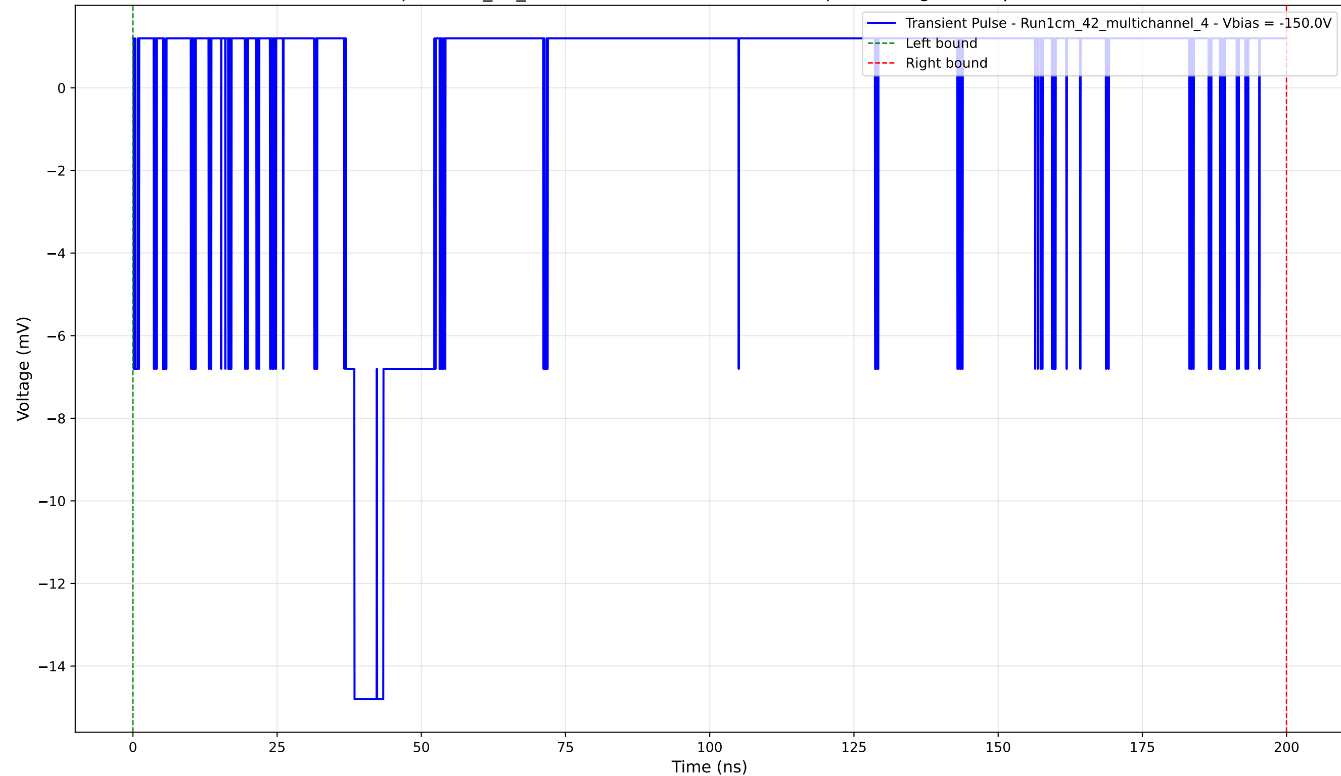
Transient Pulse - Sample: 1cm_42_multichannel - Position: 4225.0 \mu\text{m} - Charge: 0.12 pC - Rise Time: 1.50 ns
