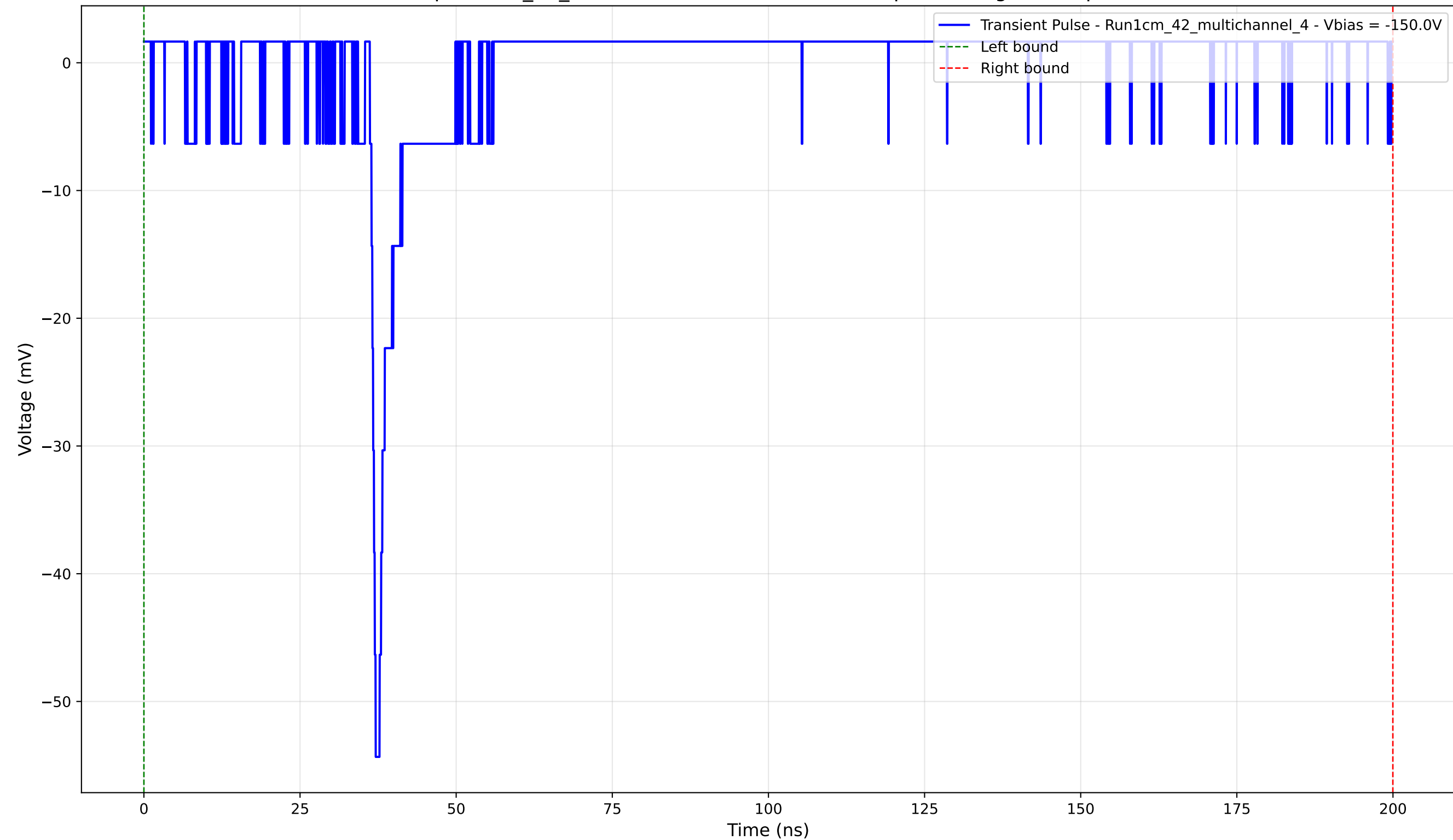
Transient Pulse - Sample: 1cm_42_multichannel - Position: 2705.0 \mu\text{m} - Charge: 0.00 pC - Rise Time: 0.92 ns
