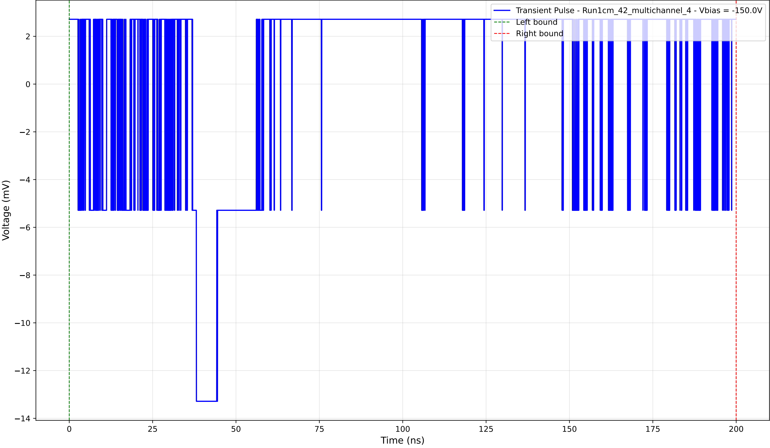
Transient Pulse - Sample: 1cm_42_multichannel - Position: 510.0 \mu\text{m} - Charge: 3.03 pC - Rise Time: 0.00 ns (N/A)
