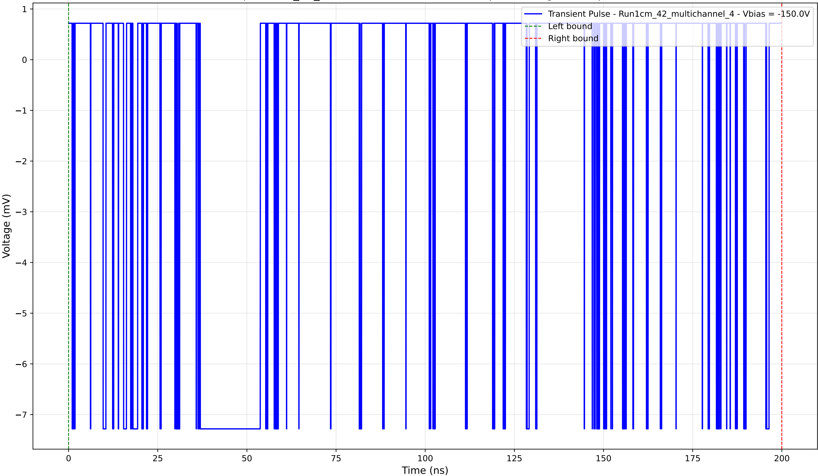
Transient Pulse - Sample: 1cm_42_multichannel - Position: 95.0 \mu\text{m} - Charge: 2.20 pC - Rise Time: 0.02 ns
