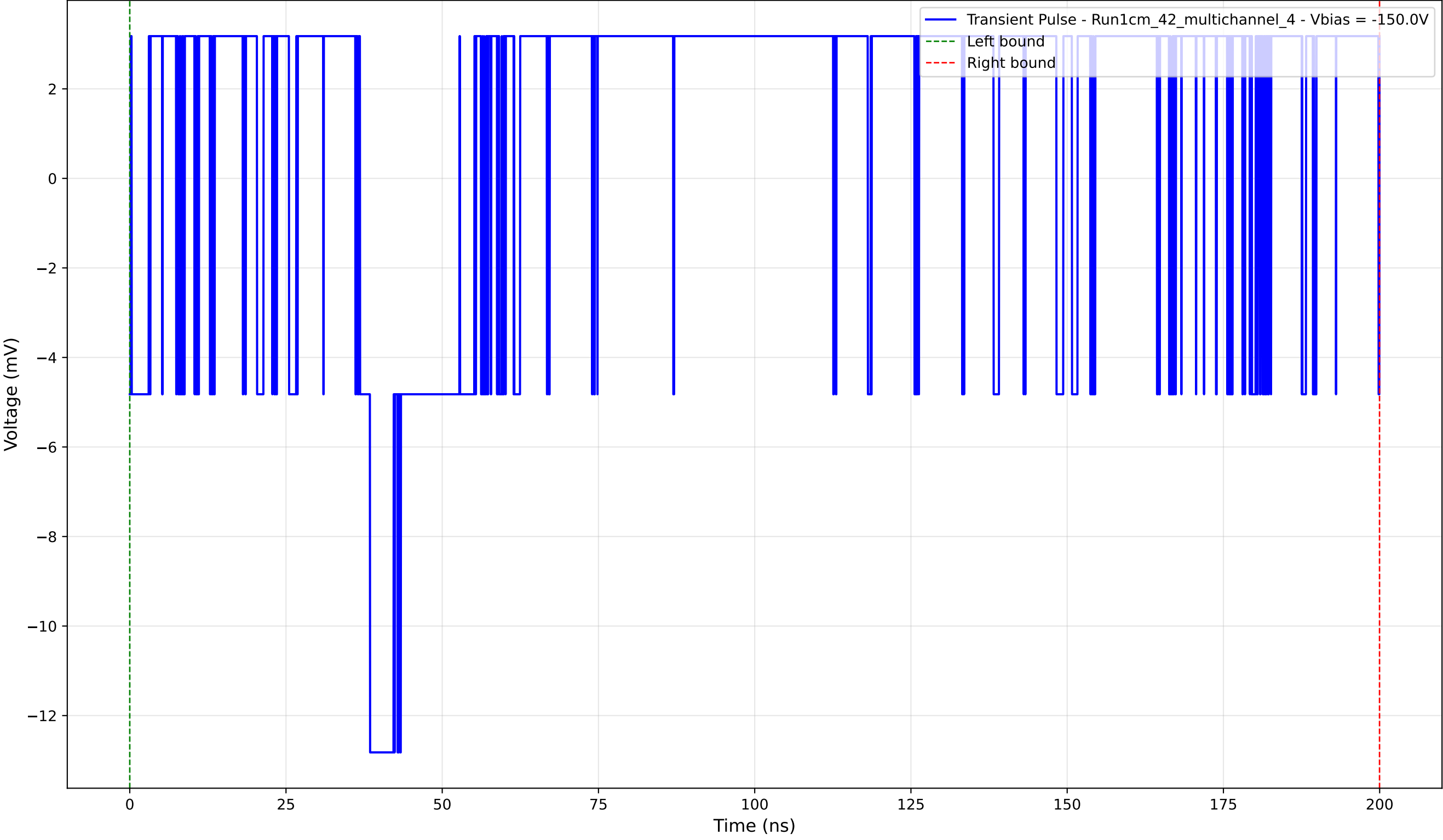
Transient Pulse - Sample: 1cm_42_multichannel - Position: 155.0 \mu\text{m} - Charge: 5.78 pC - Rise Time: 0.00 ns (N/A)
