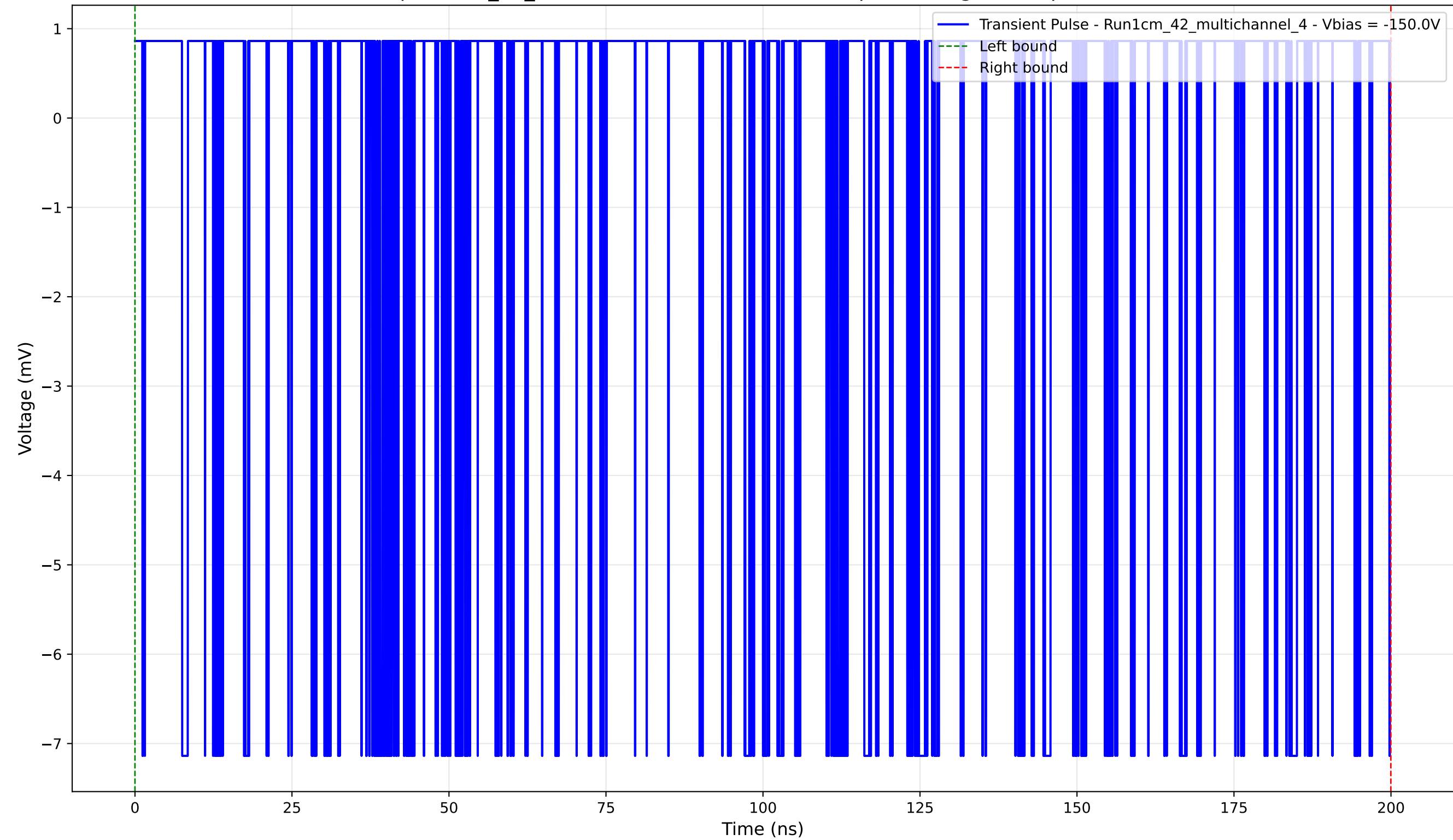
Transient Pulse - Sample: 1cm_42_multichannel - Position: 4385.0 \mu\text{m} - Charge: 1.49 pC - Rise Time: 0.00 ns (N/A)
