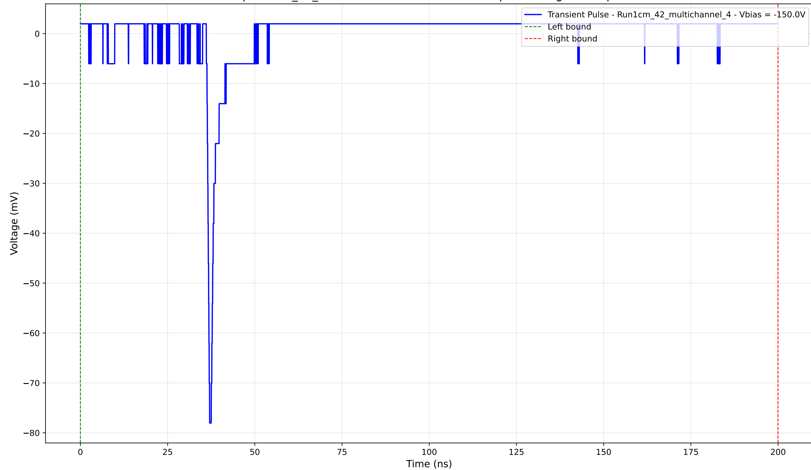
Transient Pulse - Sample: 1cm_42_multichannel - Position: 2245.0 \mu\text{m} - Charge: 1.35 pC - Rise Time: 0.76 ns
