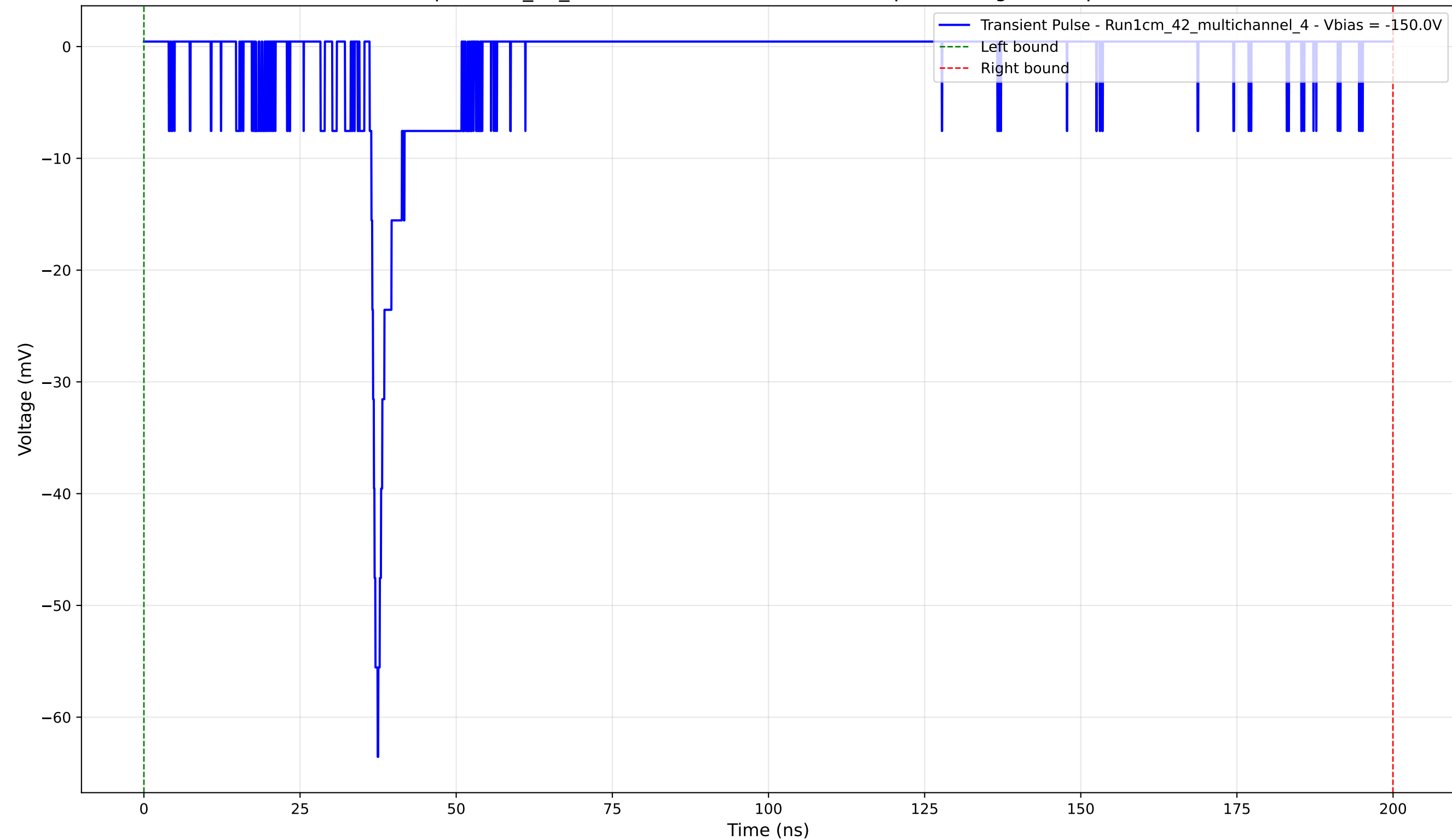
Transient Pulse - Sample: 1cm_42_multichannel - Position: 2670.0 \mu\text{m} - Charge: 4.59 pC - Rise Time: 1.28 ns
