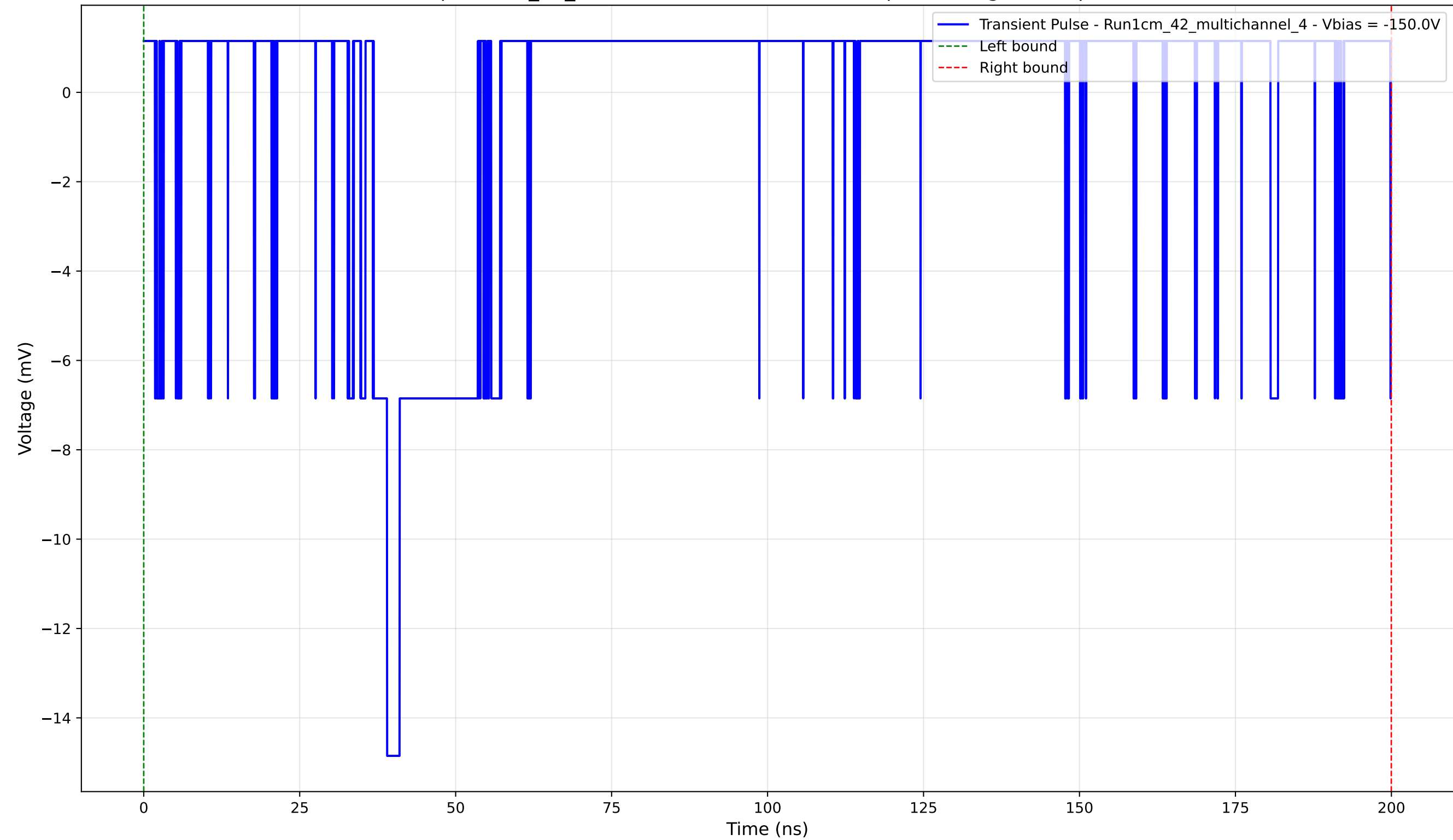
Transient Pulse - Sample: 1cm_42_multichannel - Position: 125.0 \mu\text{m} - Charge: 0.22 pC - Rise Time: 2.16 ns
