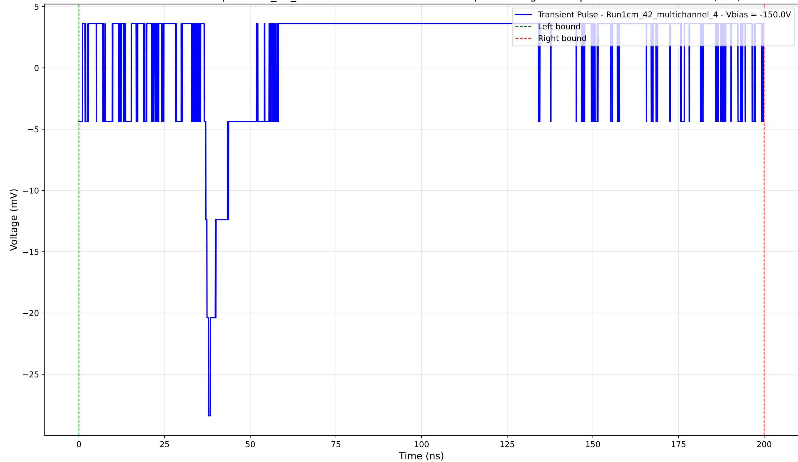
Transient Pulse - Sample: 1cm_42_multichannel - Position: 1445.0 \mu\text{m} - Charge: 6.48 pC - Rise Time: 0.00 ns (N/A)
