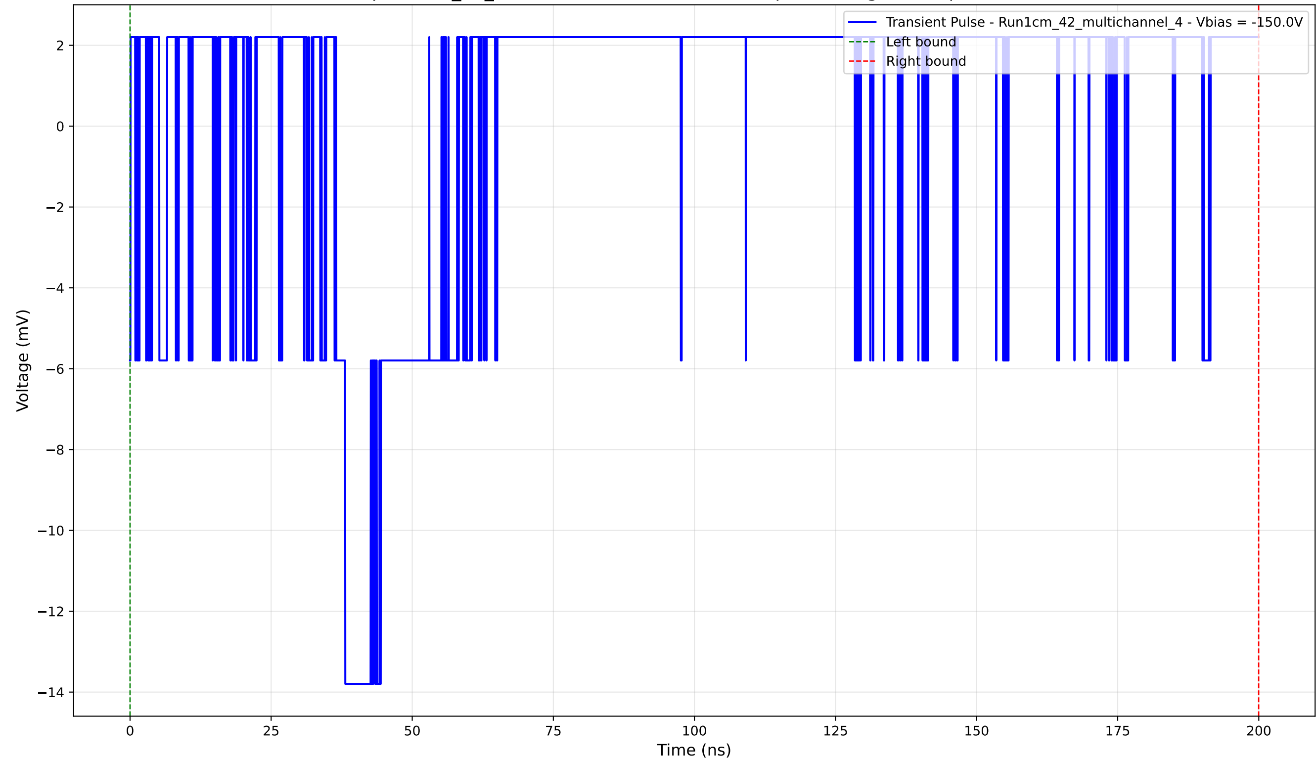
Transient Pulse - Sample: 1cm_42_multichannel - Position: 480.0 \mu\text{m} - Charge: 1.93 pC - Rise Time: 0.00 ns (N/A)
