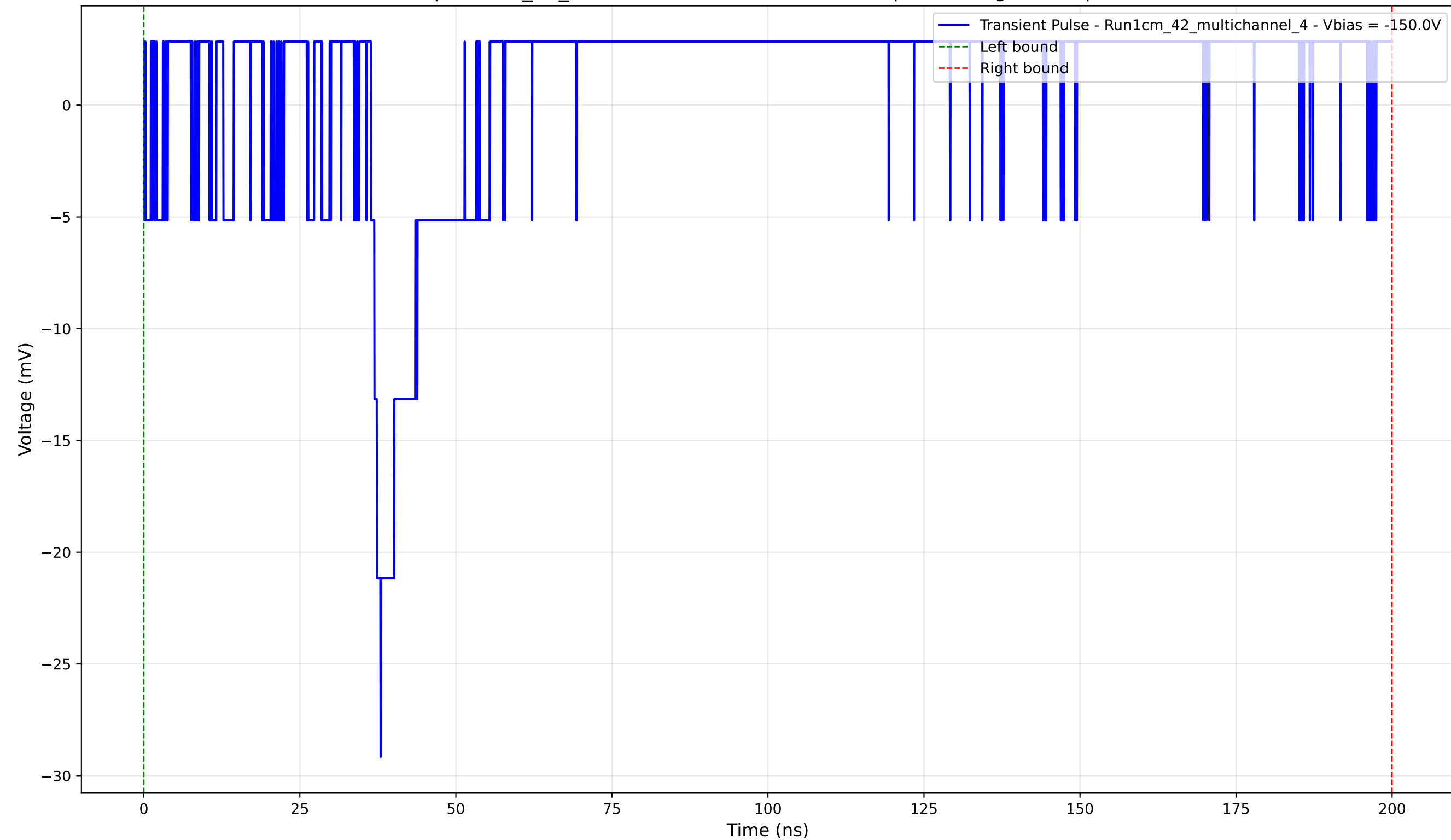
Transient Pulse - Sample: 1cm_42_multichannel - Position: 1450.0 \mu\text{m} - Charge: 4.32 pC - Rise Time: 1.54 ns
