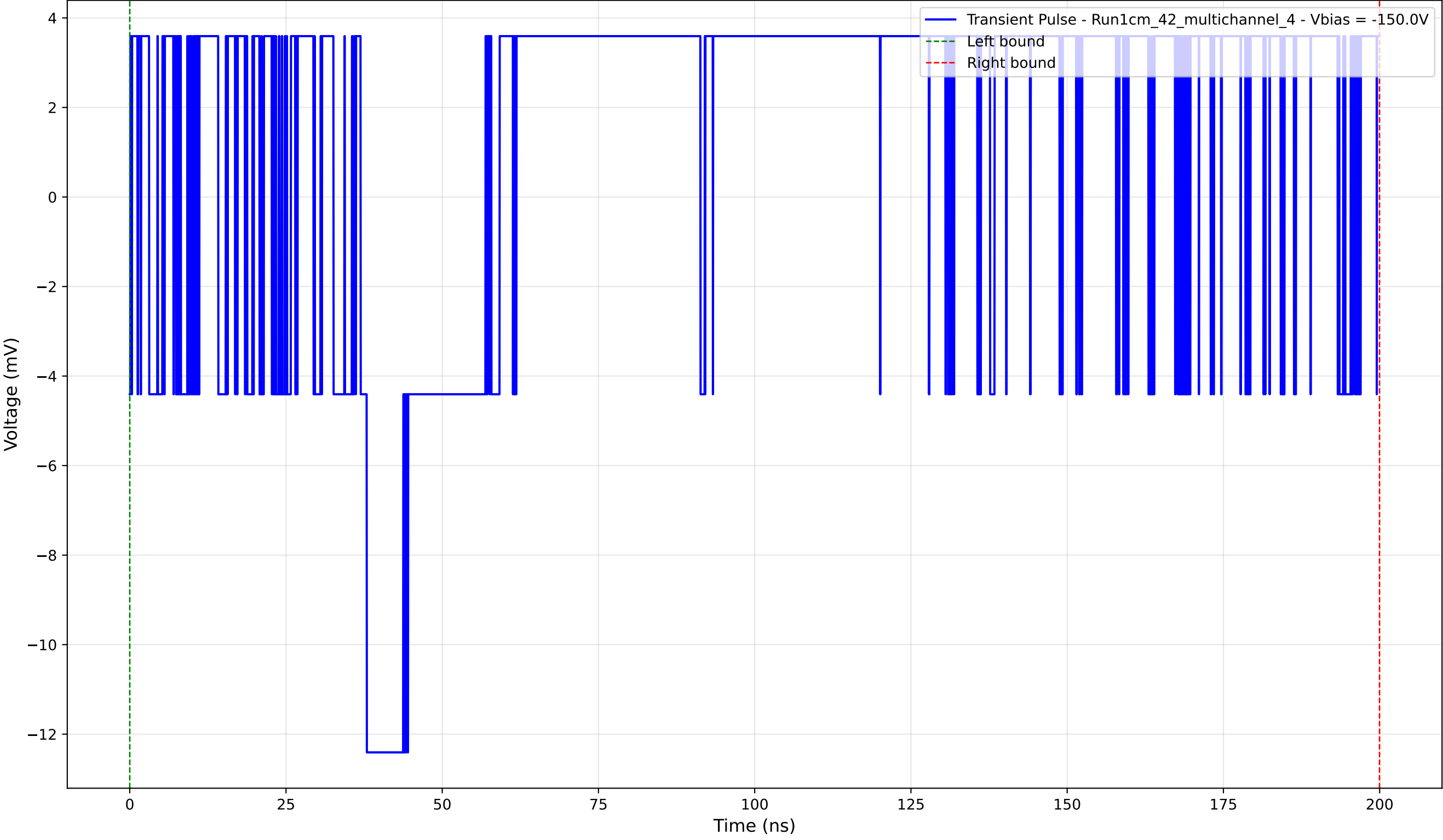
Transient Pulse - Sample: 1cm_42_multichannel - Position: 560.0 \mu\text{m} - Charge: 5.77 pC - Rise Time: 0.00 ns (N/A)
