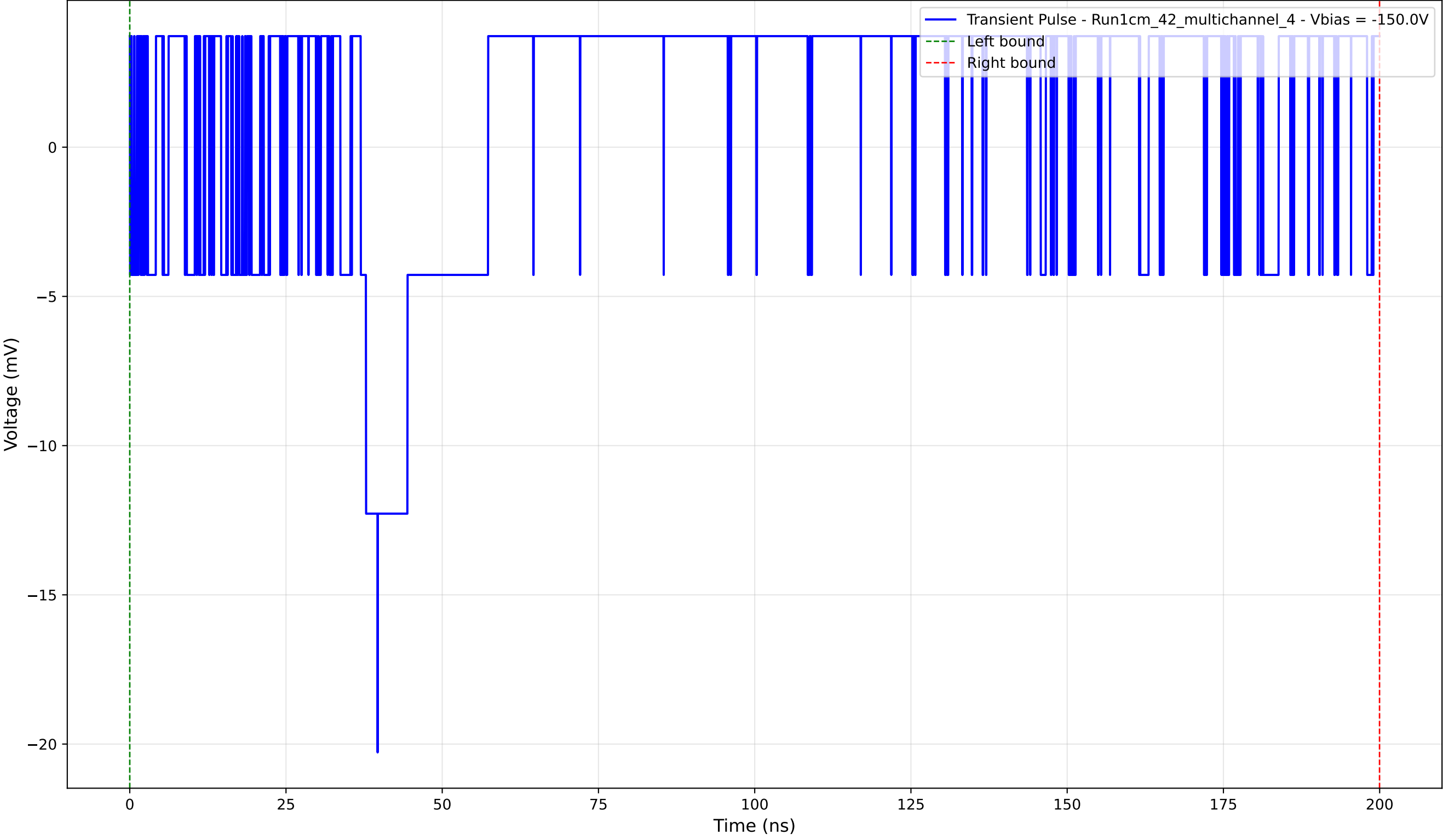
Transient Pulse - Sample: 1cm_42_multichannel - Position: 720.0 \mu\text{m} - Charge: 6.02 pC - Rise Time: 0.00 ns (N/A)
