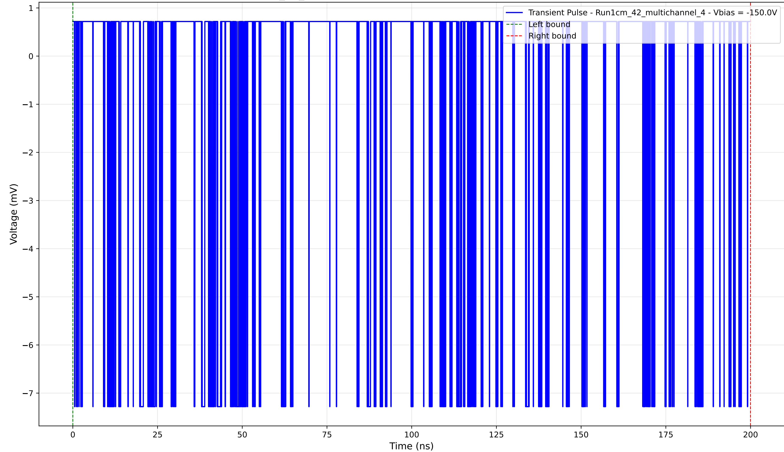
Transient Pulse - Sample: 1cm_42_multichannel - Position: 4395.0 \mu\text{m} - Charge: 2.24 pC - Rise Time: 0.02 ns
