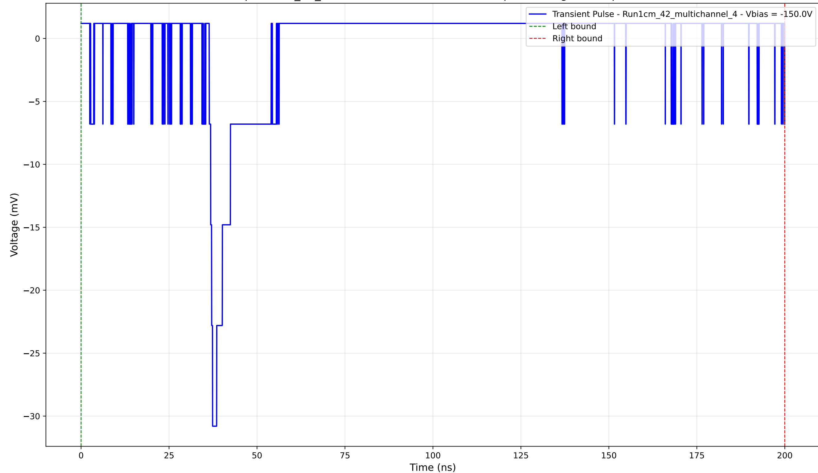
Transient Pulse - Sample: 1cm_42_multichannel - Position: 1575.0 \mu\text{m} - Charge: 0.90 pC - Rise Time: 0.95 ns
