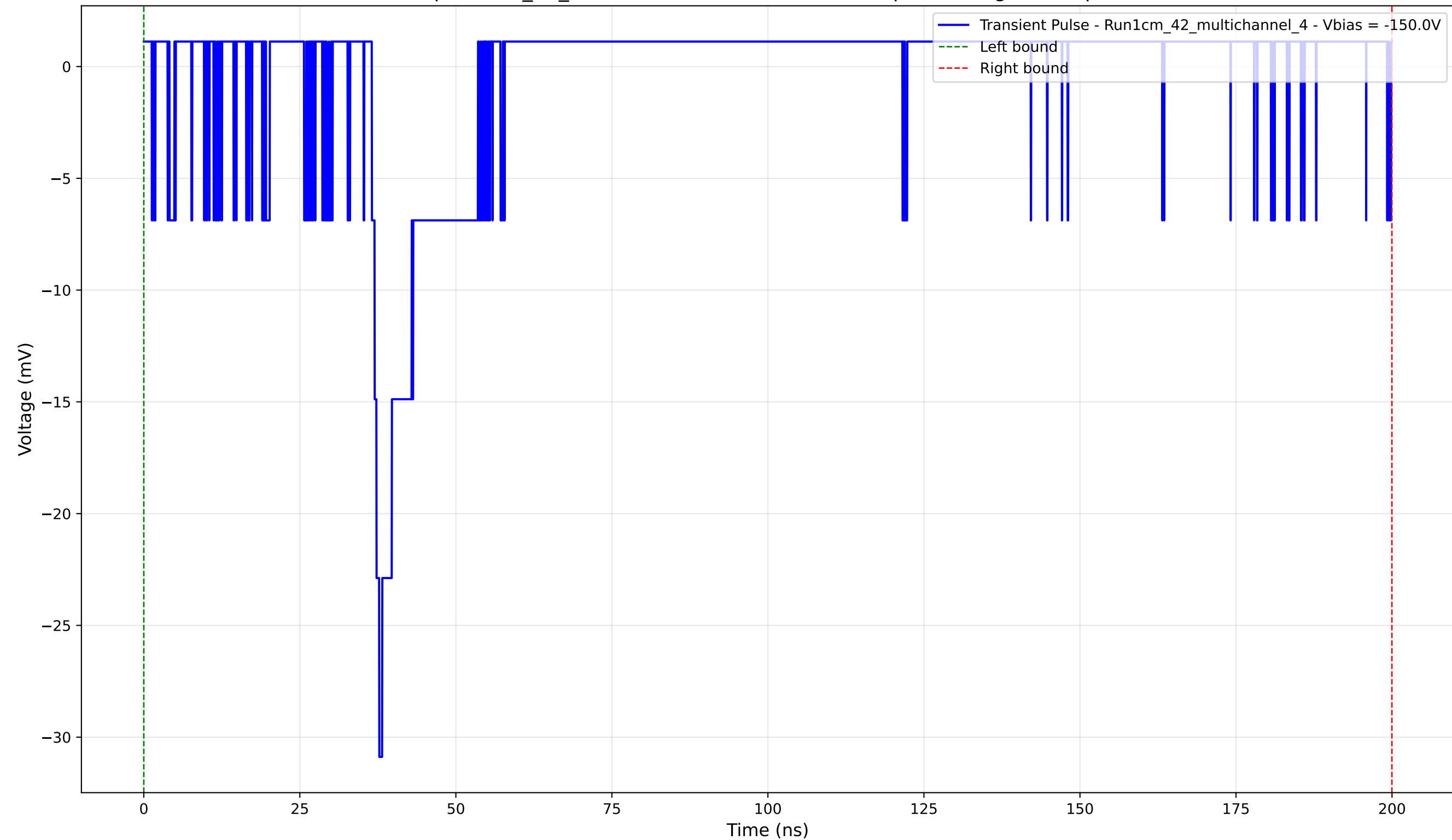
Transient Pulse - Sample: 1cm_42_multichannel - Position: 3255.0 \mu\text{m} - Charge: 1.30 pC - Rise Time: 1.19 ns
