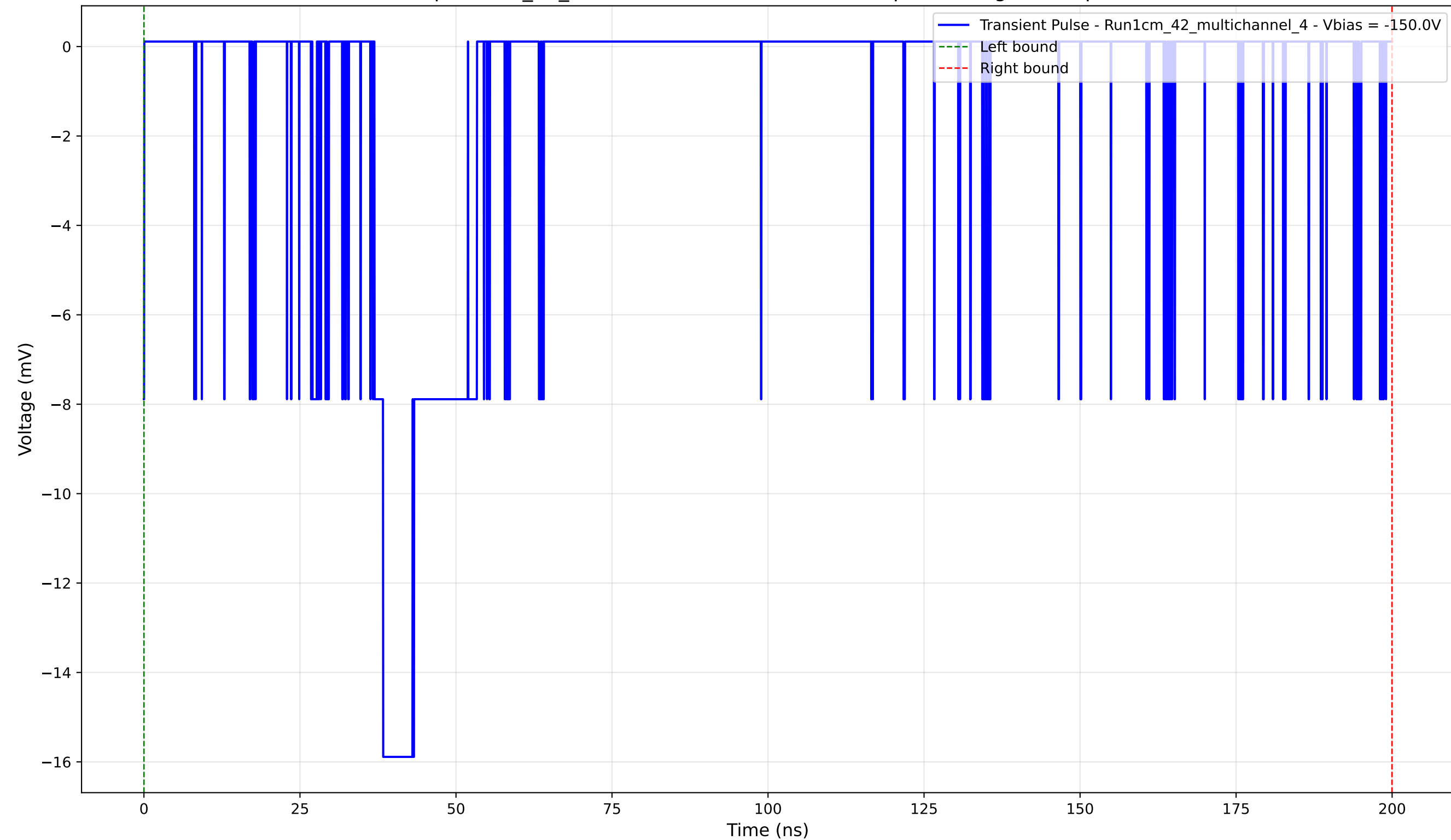
Transient Pulse - Sample: 1cm_42_multichannel - Position: 4490.0 \mu\text{m} - Charge: 4.42 pC - Rise Time: 1.40 ns
