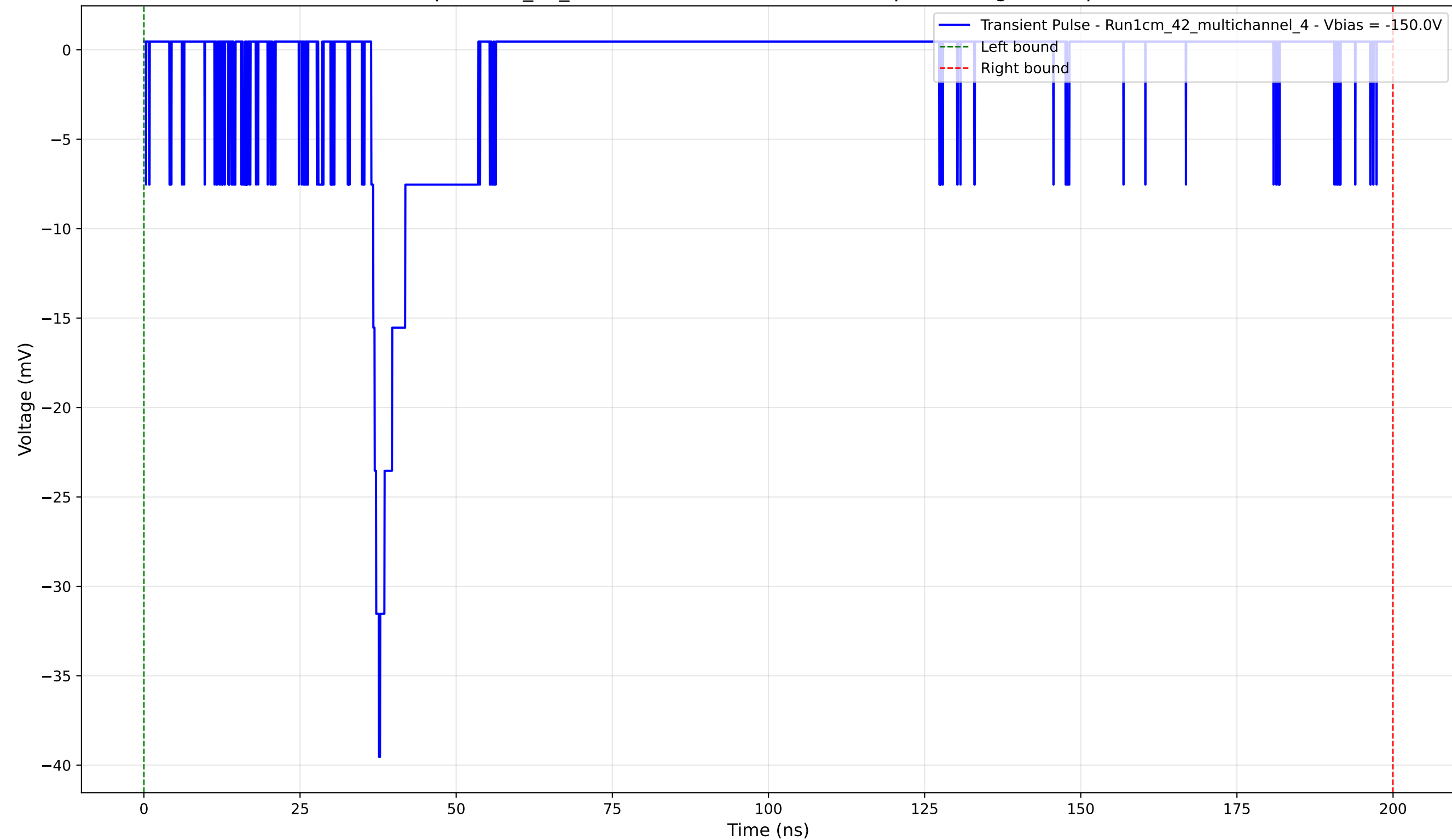
Transient Pulse - Sample: 1cm_42_multichannel - Position: 3035.0 \mu\text{m} - Charge: 3.81 pC - Rise Time: 1.23 ns
