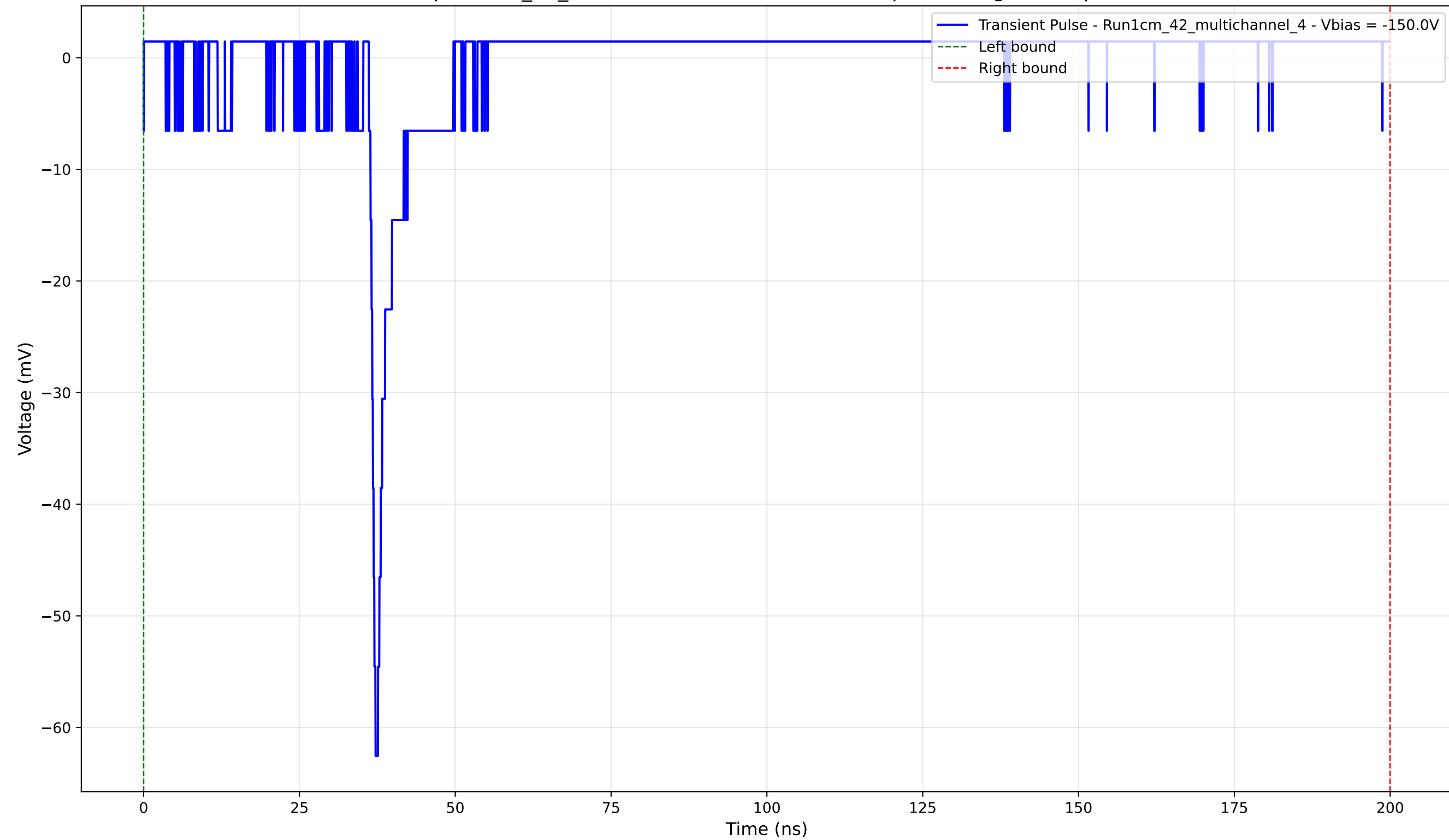
Transient Pulse - Sample: 1cm_42_multichannel - Position: 2095.0 \mu\text{m} - Charge: 0.58 pC - Rise Time: 1.06 ns
