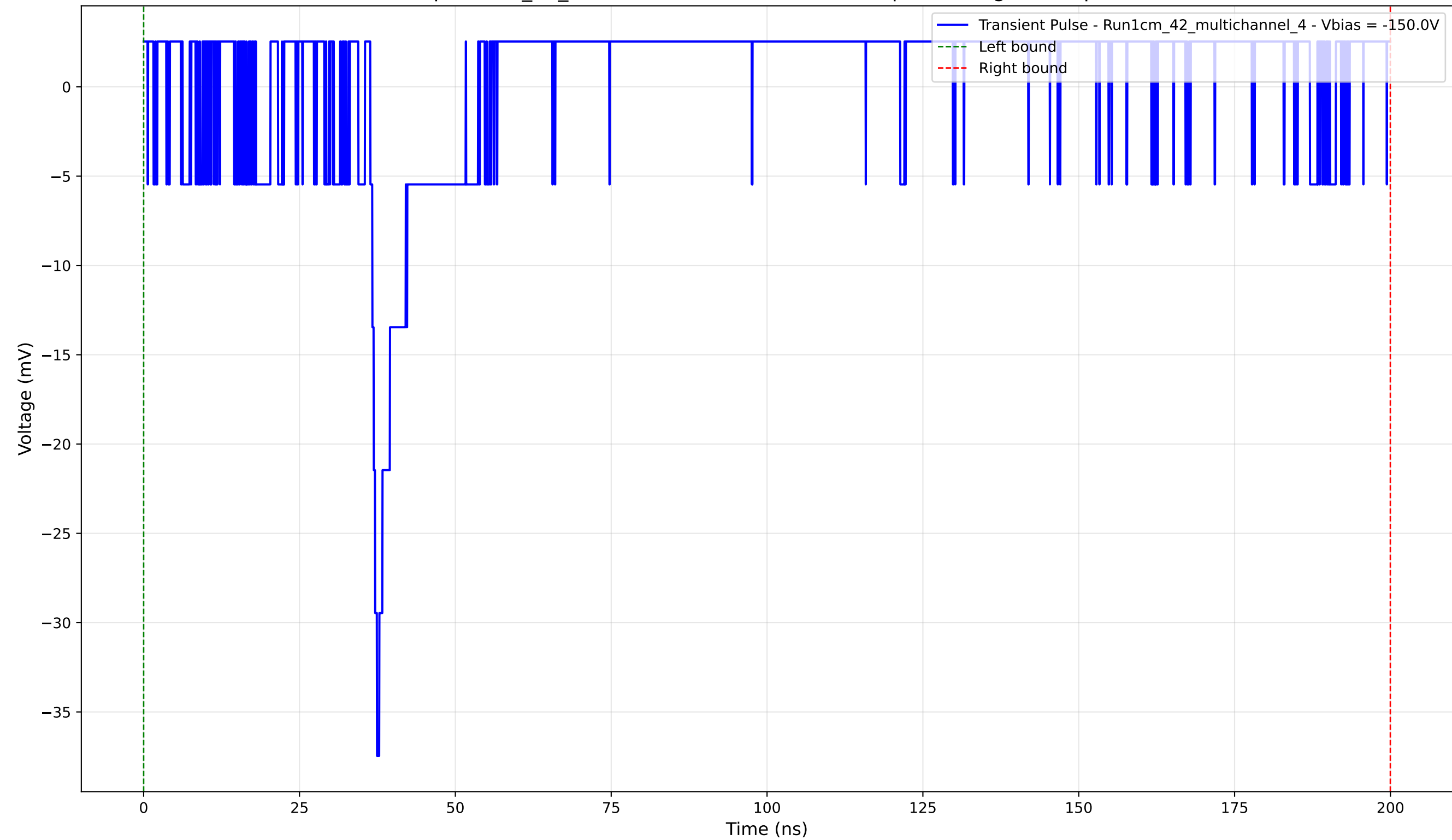
Transient Pulse - Sample: 1cm_42_multichannel - Position: 1815.0 \mu\text{m} - Charge: 2.22 pC - Rise Time: 1.07 ns
