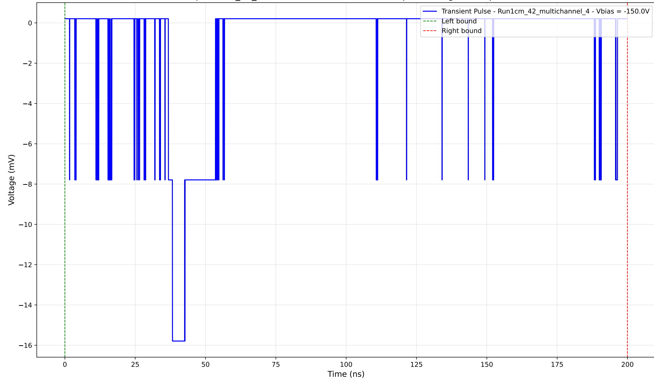
Transient Pulse - Sample: 1cm_42_multichannel - Position: 4100.0 \mu\text{m} - Charge: 3.50 pC - Rise Time: 1.46 ns
