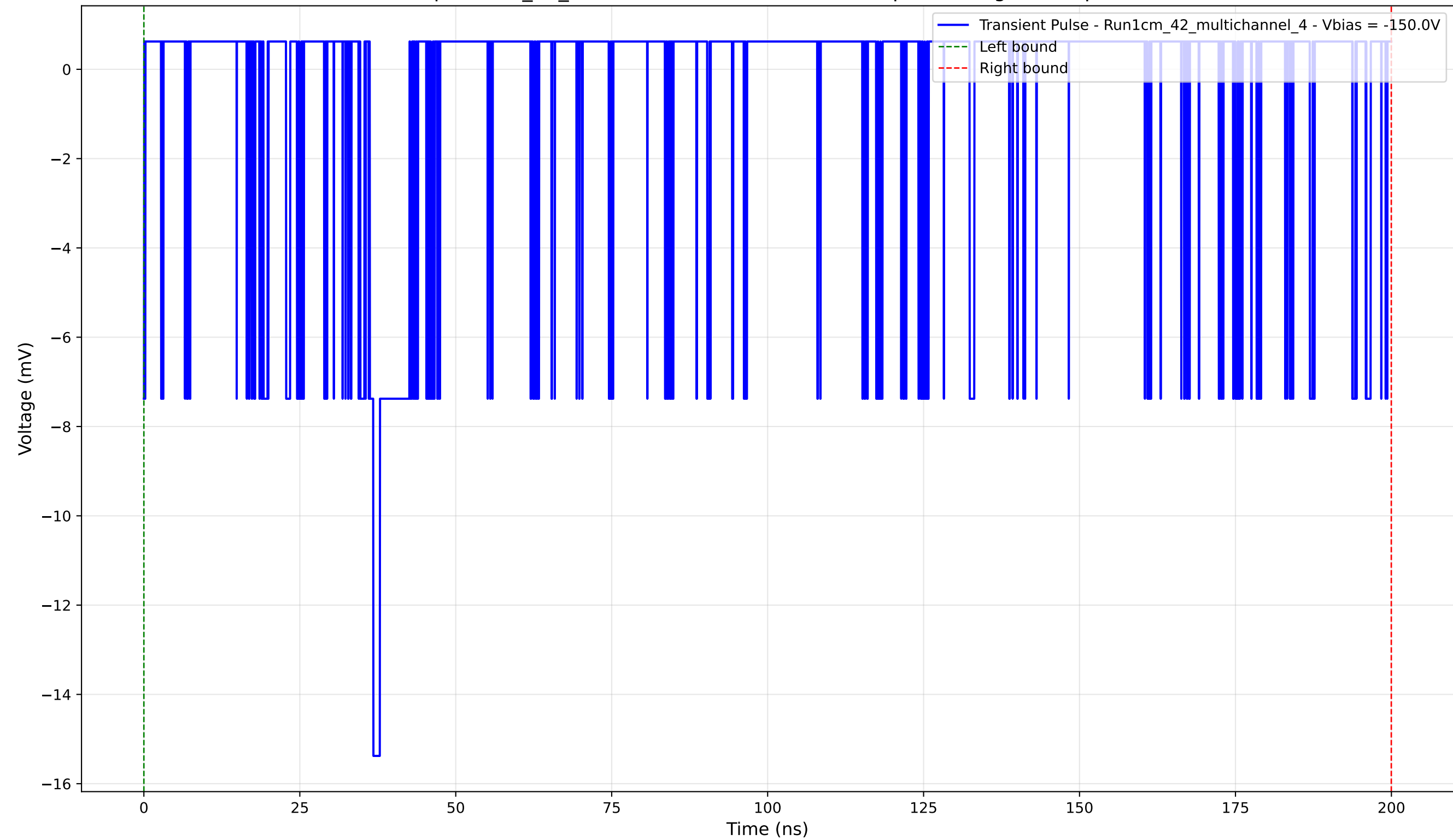
Transient Pulse - Sample: 1cm_42_multichannel - Position: 2350.0 \mu\text{m} - Charge: 1.91 pC - Rise Time: 0.58 ns
