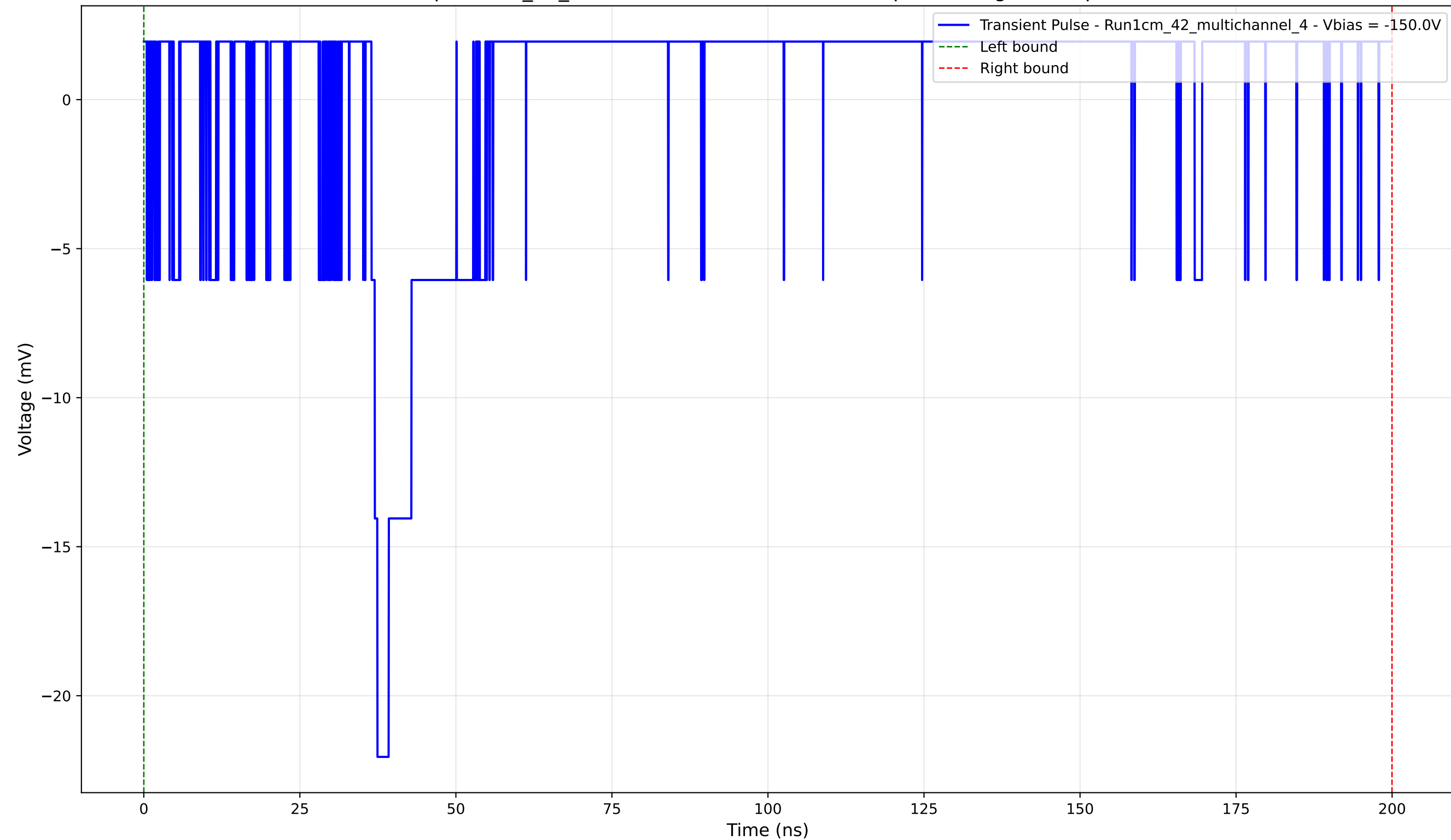
Transient Pulse - Sample: 1cm_42_multichannel - Position: 3315.0 \mu\text{m} - Charge: 1.84 pC - Rise Time: 0.96 ns
