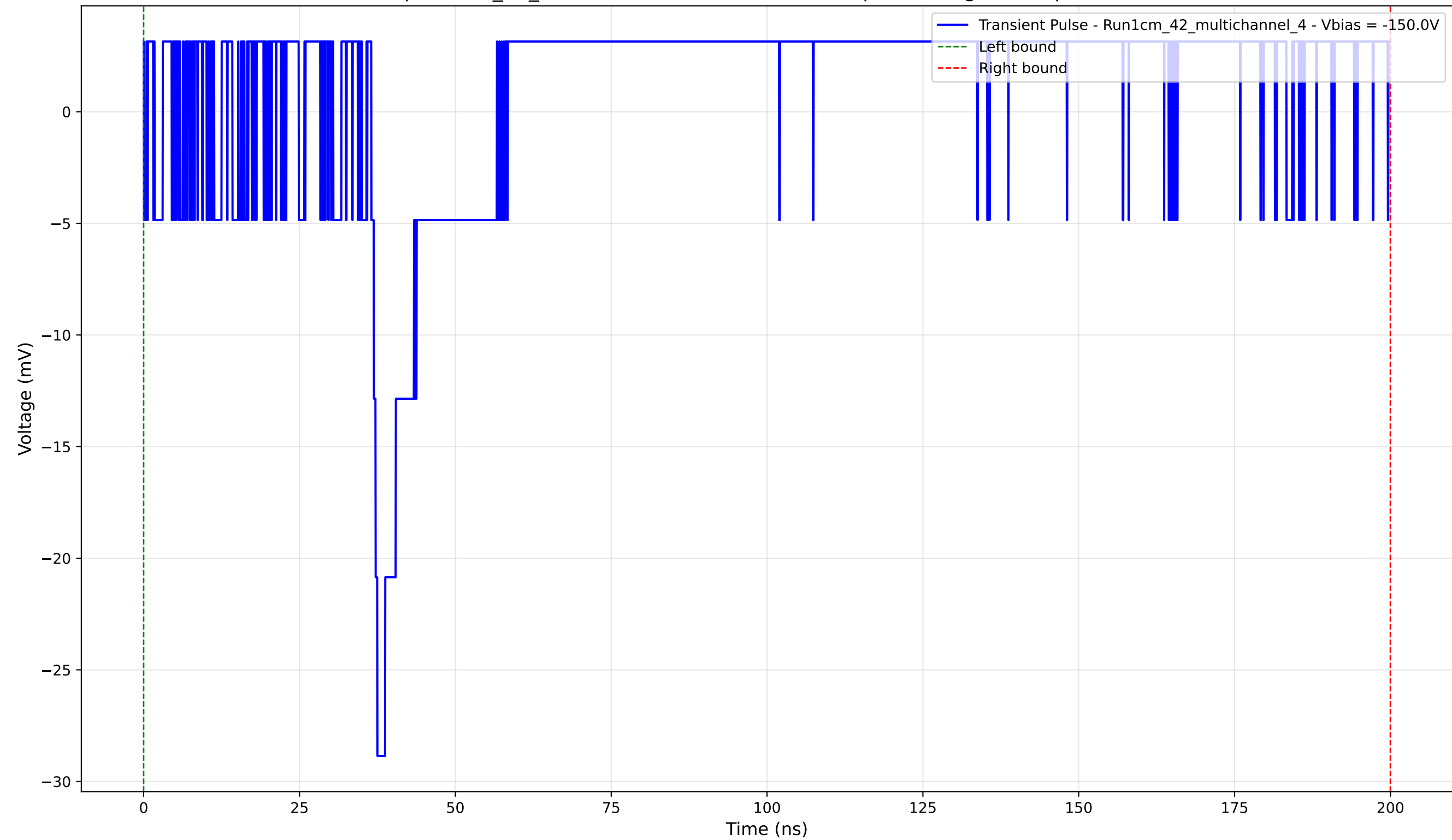
Transient Pulse - Sample: 1cm_42_multichannel - Position: 1505.0 \mu\text{m} - Charge: 4.60 pC - Rise Time: 0.00 ns (N/A)
