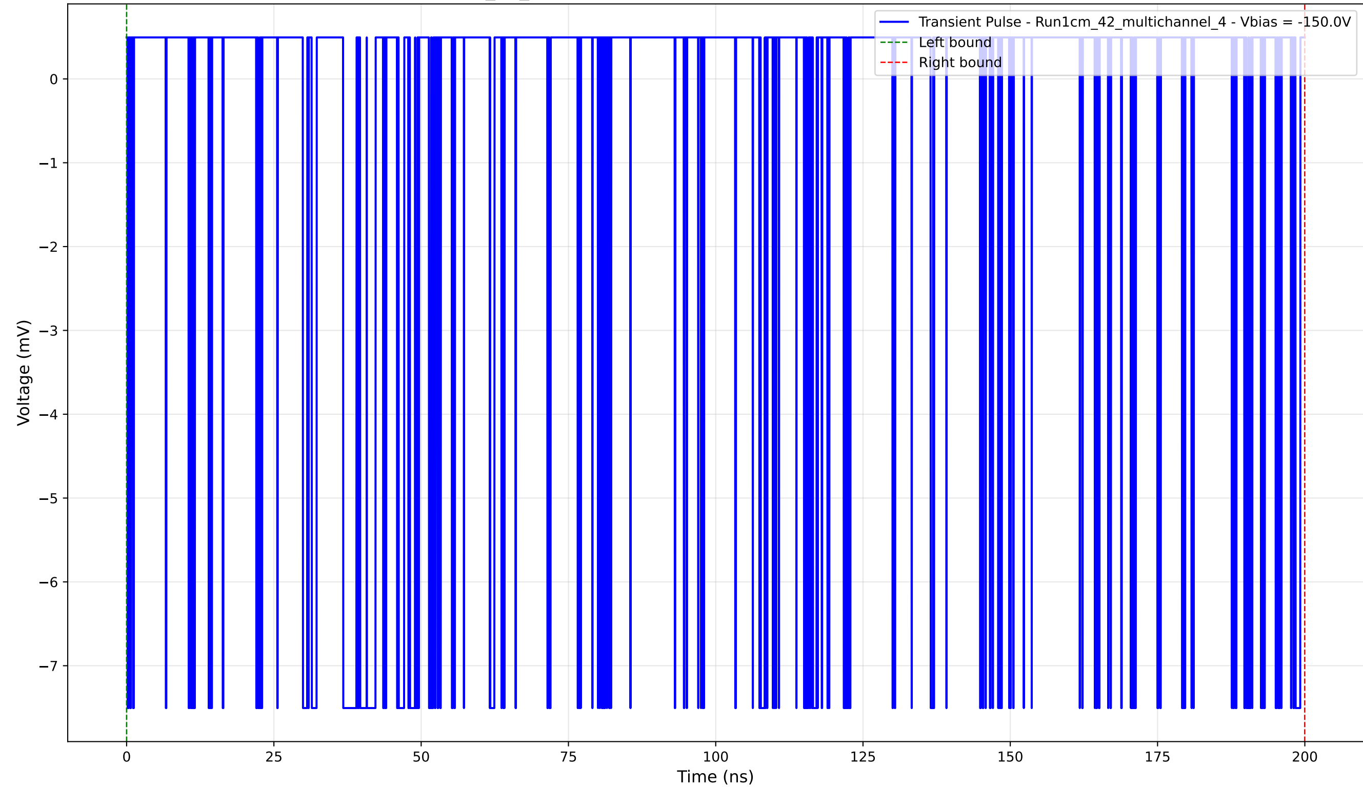
Transient Pulse - Sample: 1cm_42_multichannel - Position: 2905.0 \mu\text{m} - Charge: 2.29 pC - Rise Time: 0.02 ns
