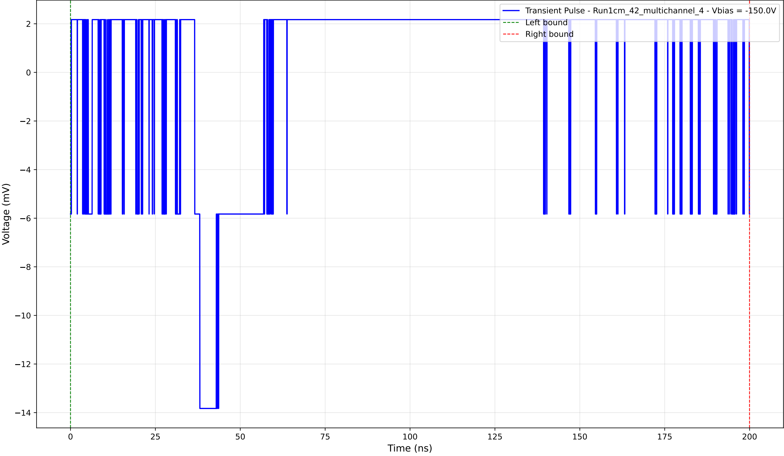
Transient Pulse - Sample: 1cm_42_multichannel - Position: 540.0 \mu\text{m} - Charge: 2.55 pC - Rise Time: 0.00 ns (N/A)
