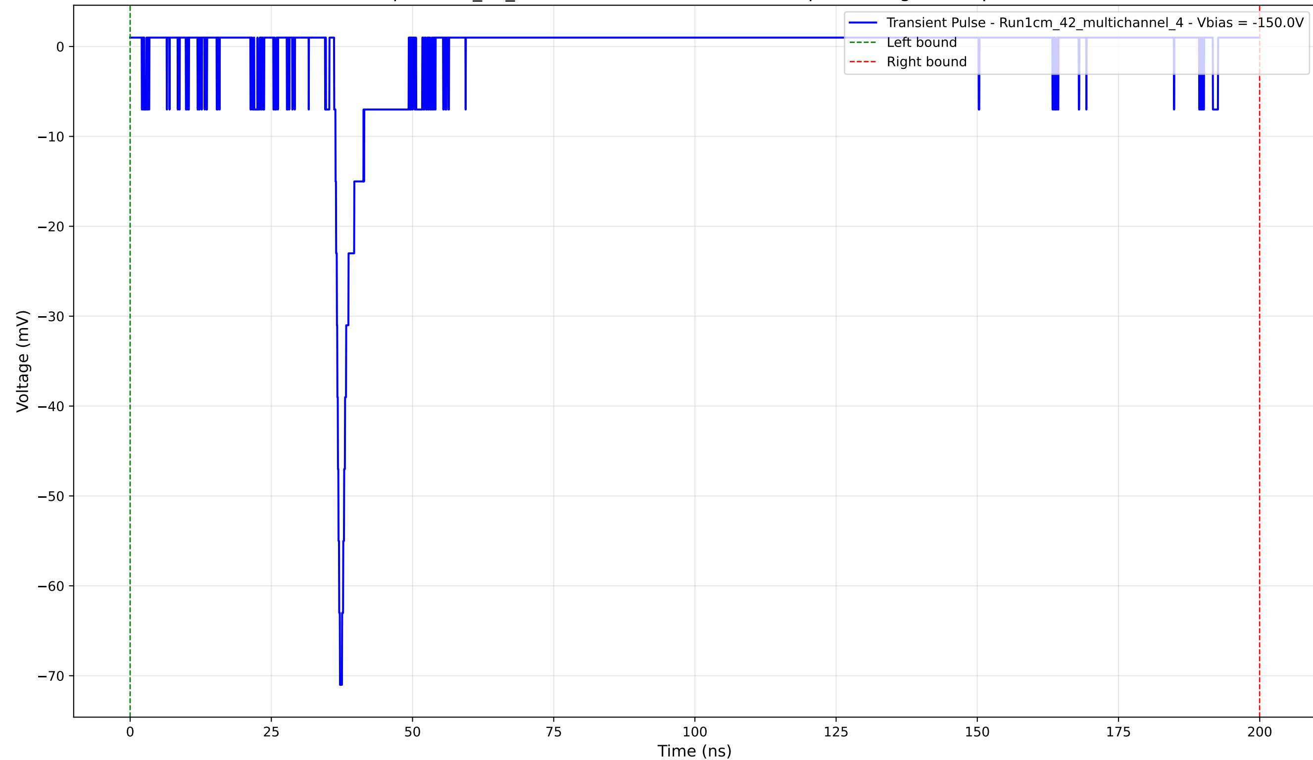
Transient Pulse - Sample: 1cm_42_multichannel - Position: 2170.0 \mu\text{m} - Charge: 2.30 pC - Rise Time: 0.80 ns
