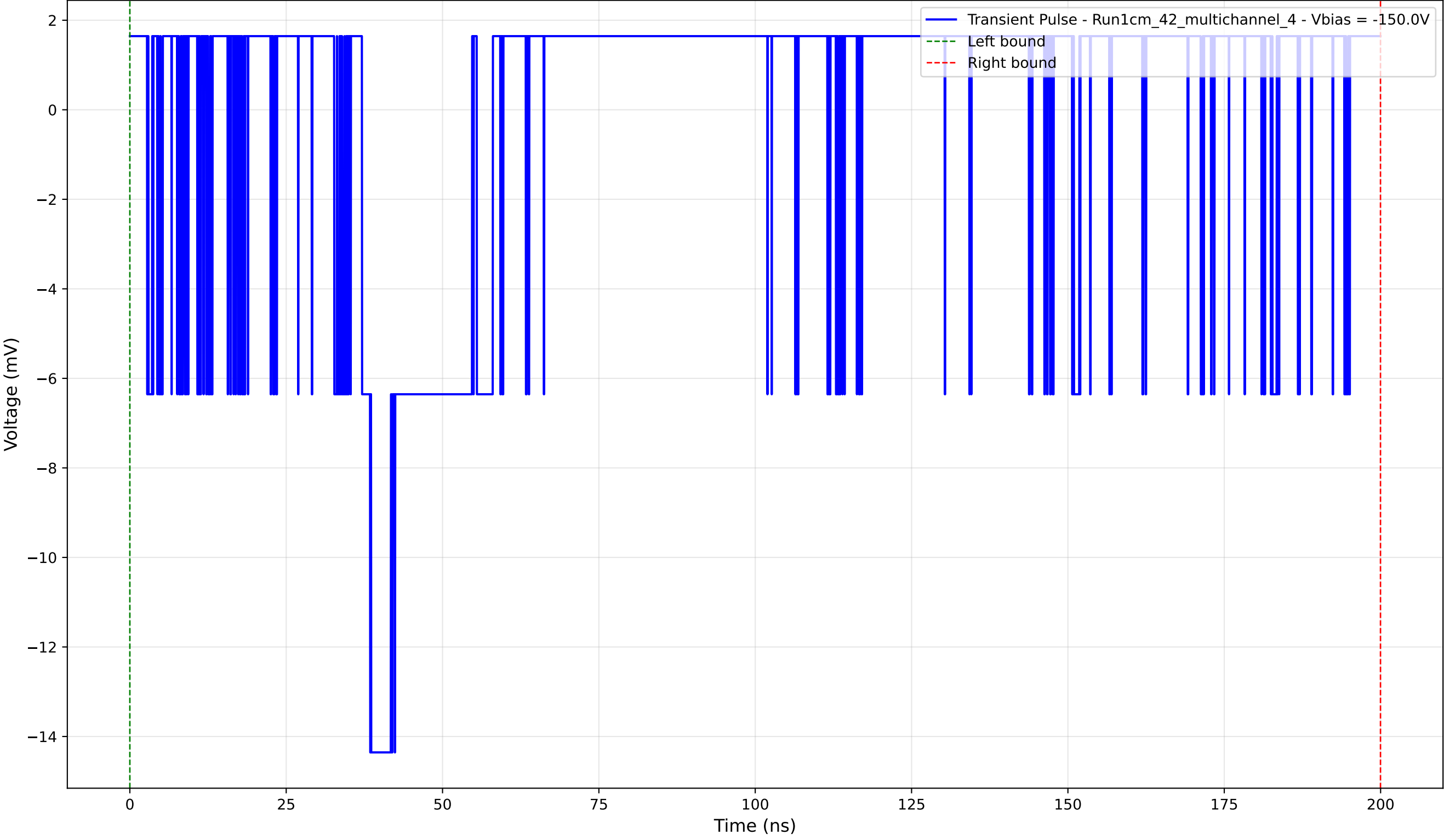
Transient Pulse - Sample: 1cm_42_multichannel - Position: 145.0 \mu\text{m} - Charge: 0.54 pC - Rise Time: 0.00 ns (N/A)
