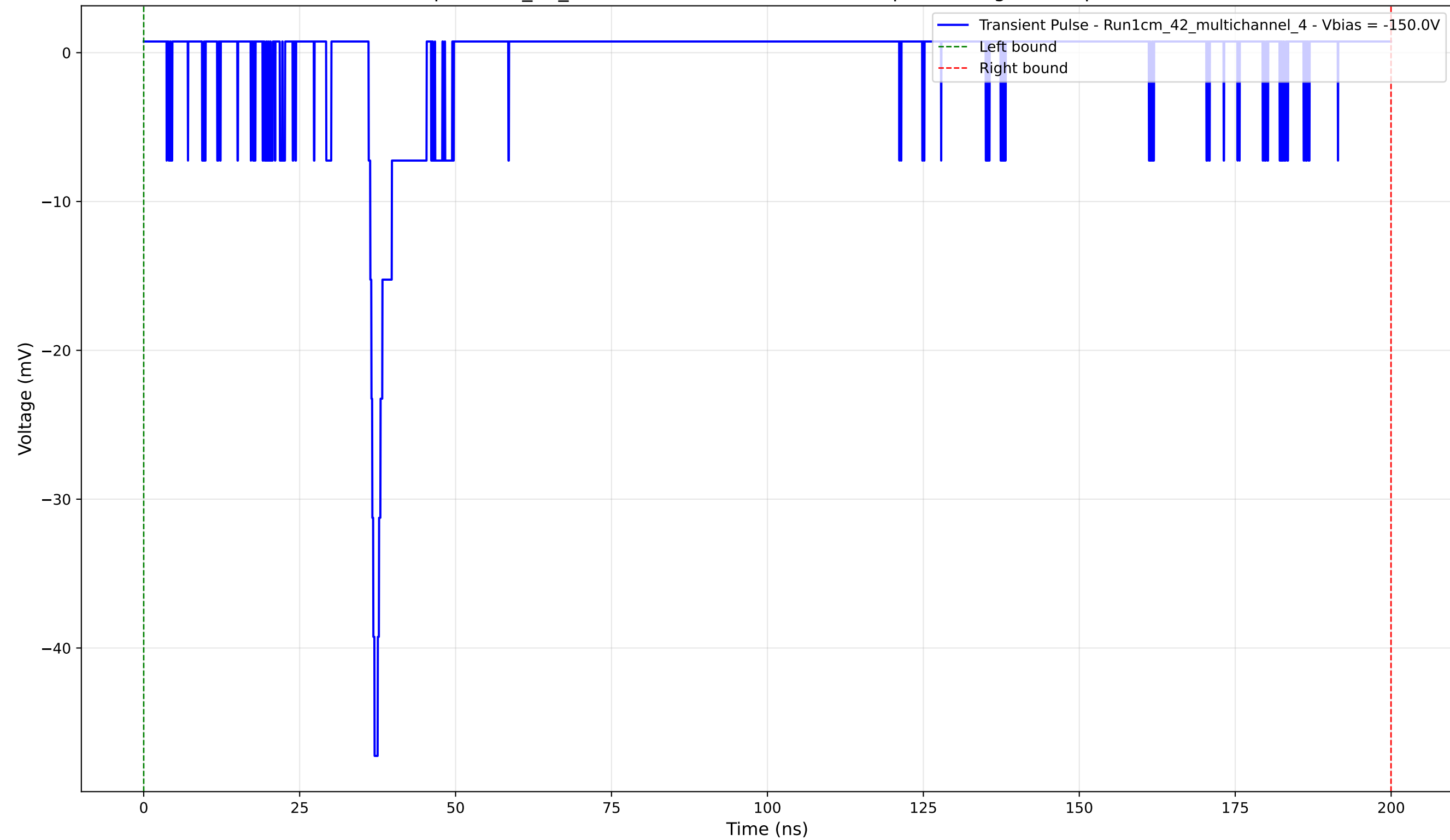
Transient Pulse - Sample: 1cm_42_multichannel - Position: 2440.0 \mu\text{m} - Charge: 1.66 pC - Rise Time: 0.95 ns
