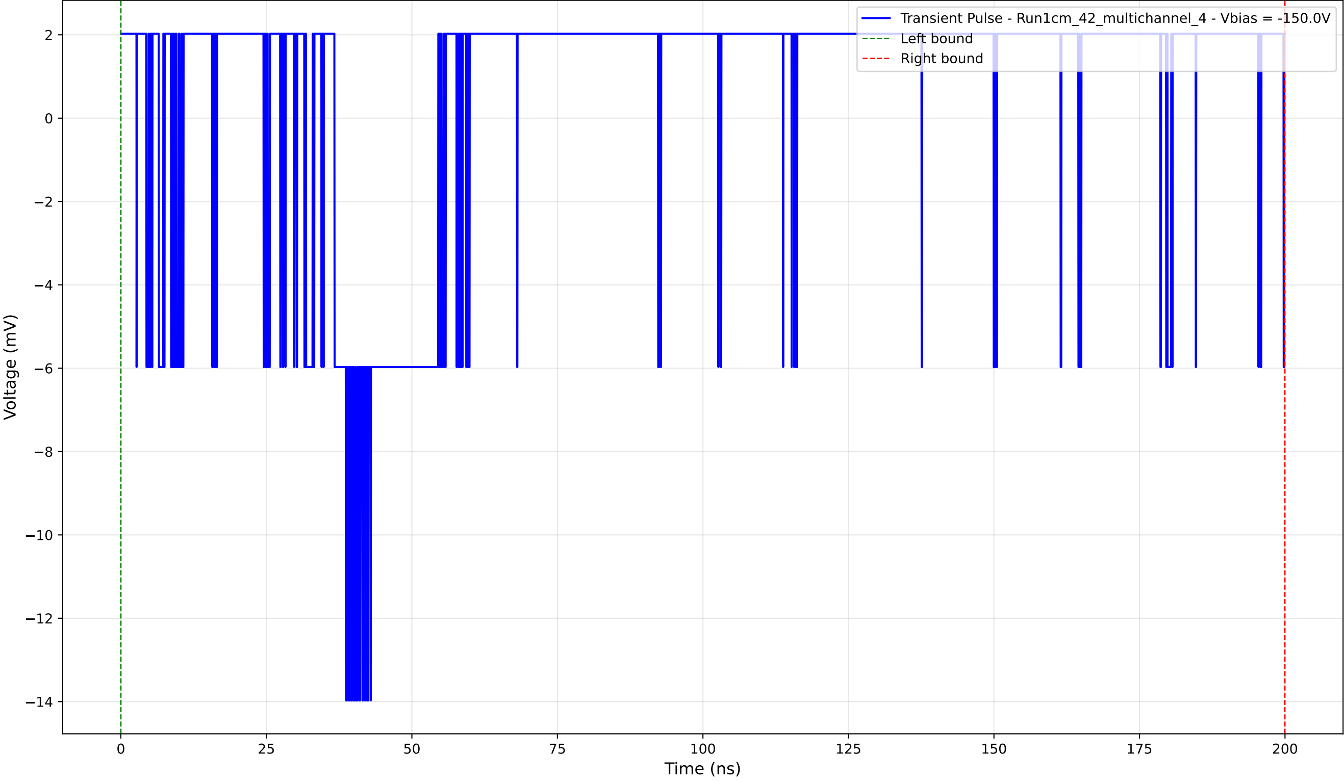
Transient Pulse - Sample: 1cm_42_multichannel - Position: 120.0 \mu\text{m} - Charge: 3.26 pC - Rise Time: 0.00 ns (N/A)
