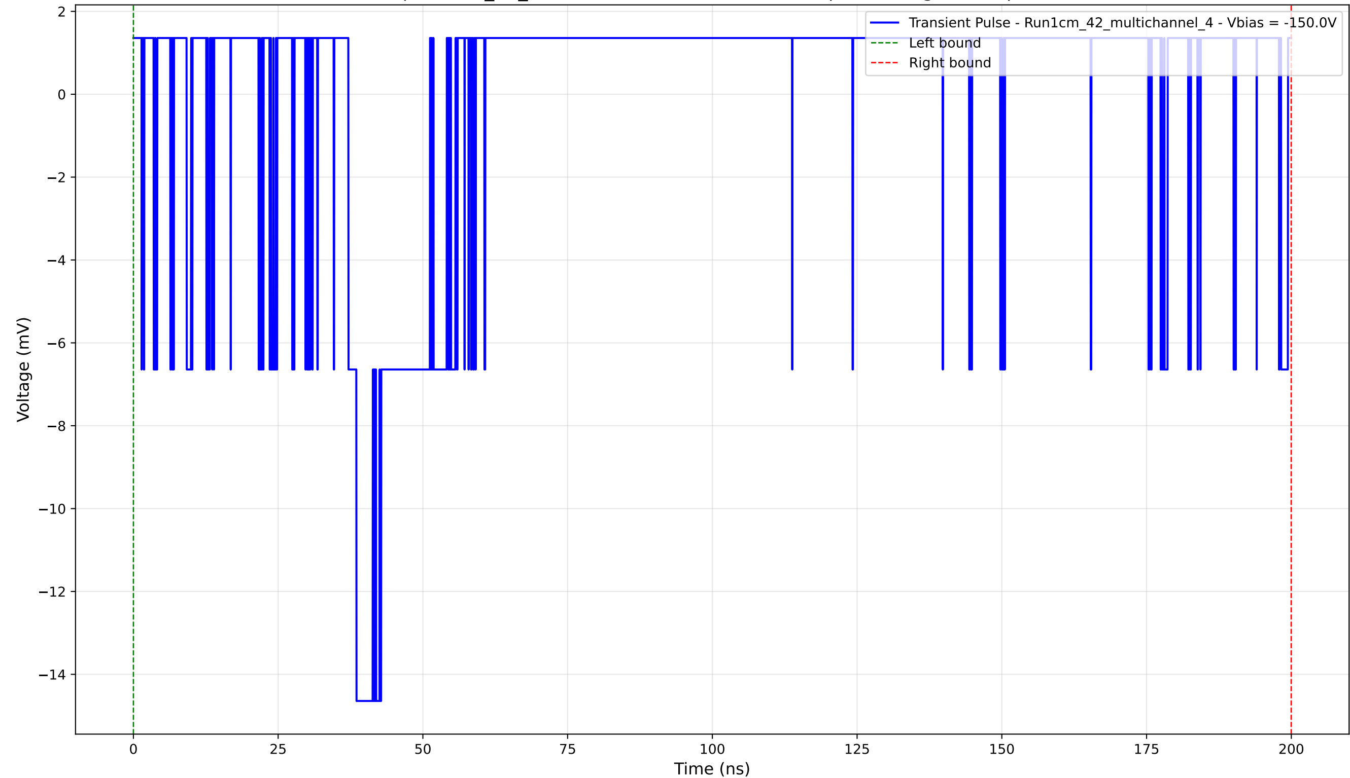
Transient Pulse - Sample: 1cm_42_multichannel - Position: 4730.0 \mu\text{m} - Charge: 0.39 pC - Rise Time: 1.40 ns
