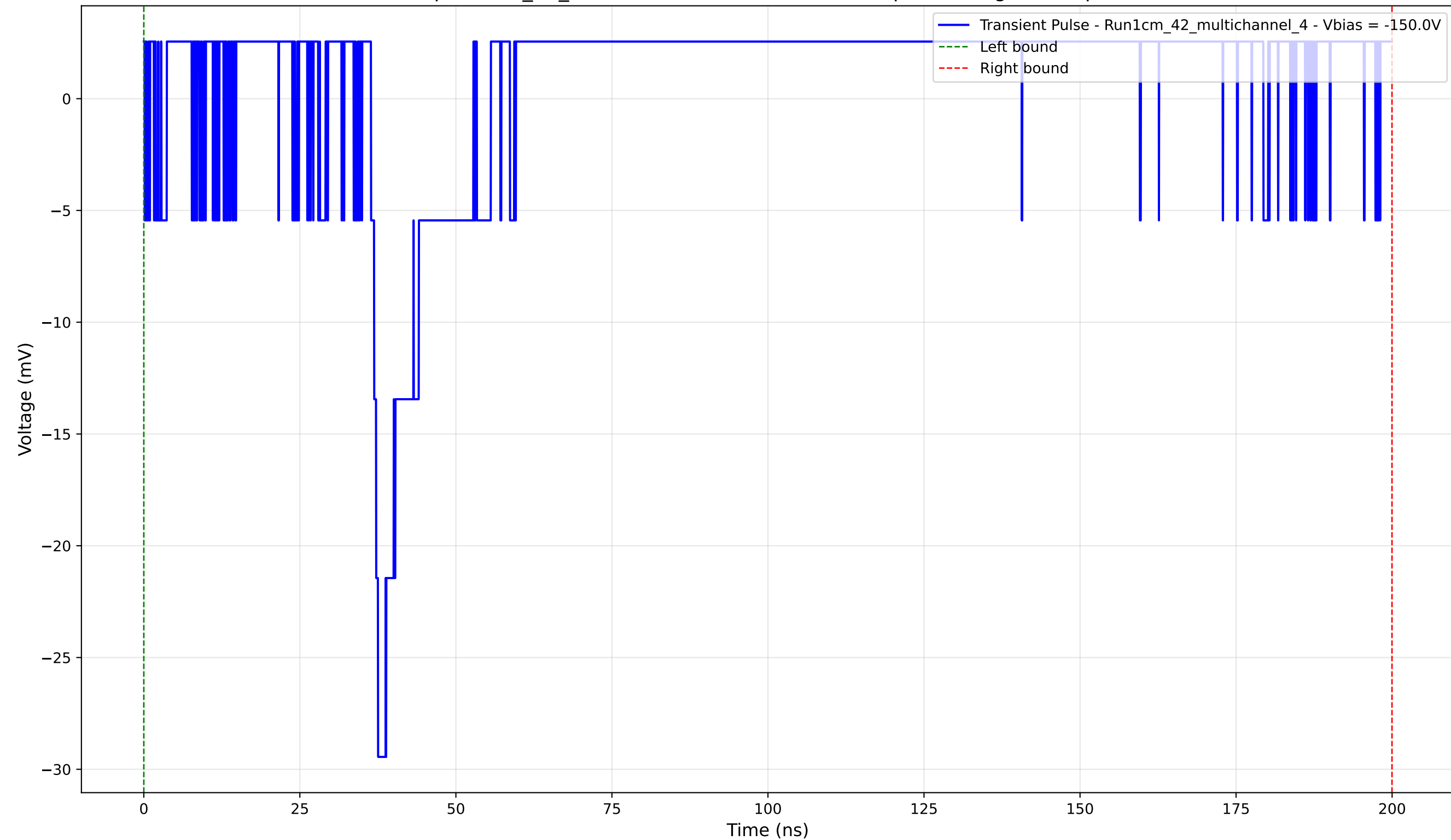
Transient Pulse - Sample: 1cm_42_multichannel - Position: 1500.0 \mu\text{m} - Charge: 3.56 pC - Rise Time: 1.14 ns
