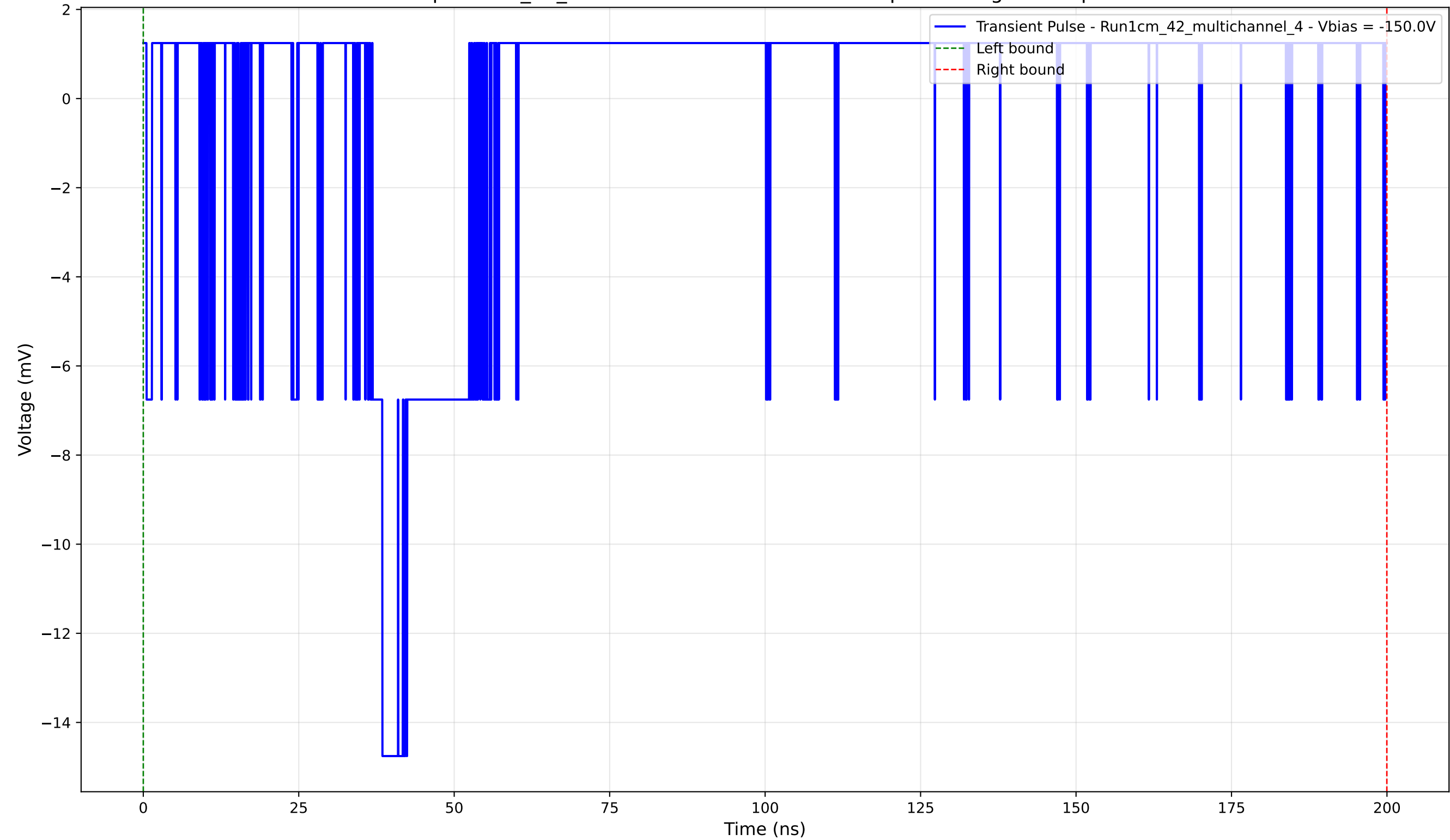
Transient Pulse - Sample: 1cm_42_multichannel - Position: 4775.0 \mu\text{m} - Charge: 0.02 pC - Rise Time: 1.58 ns
