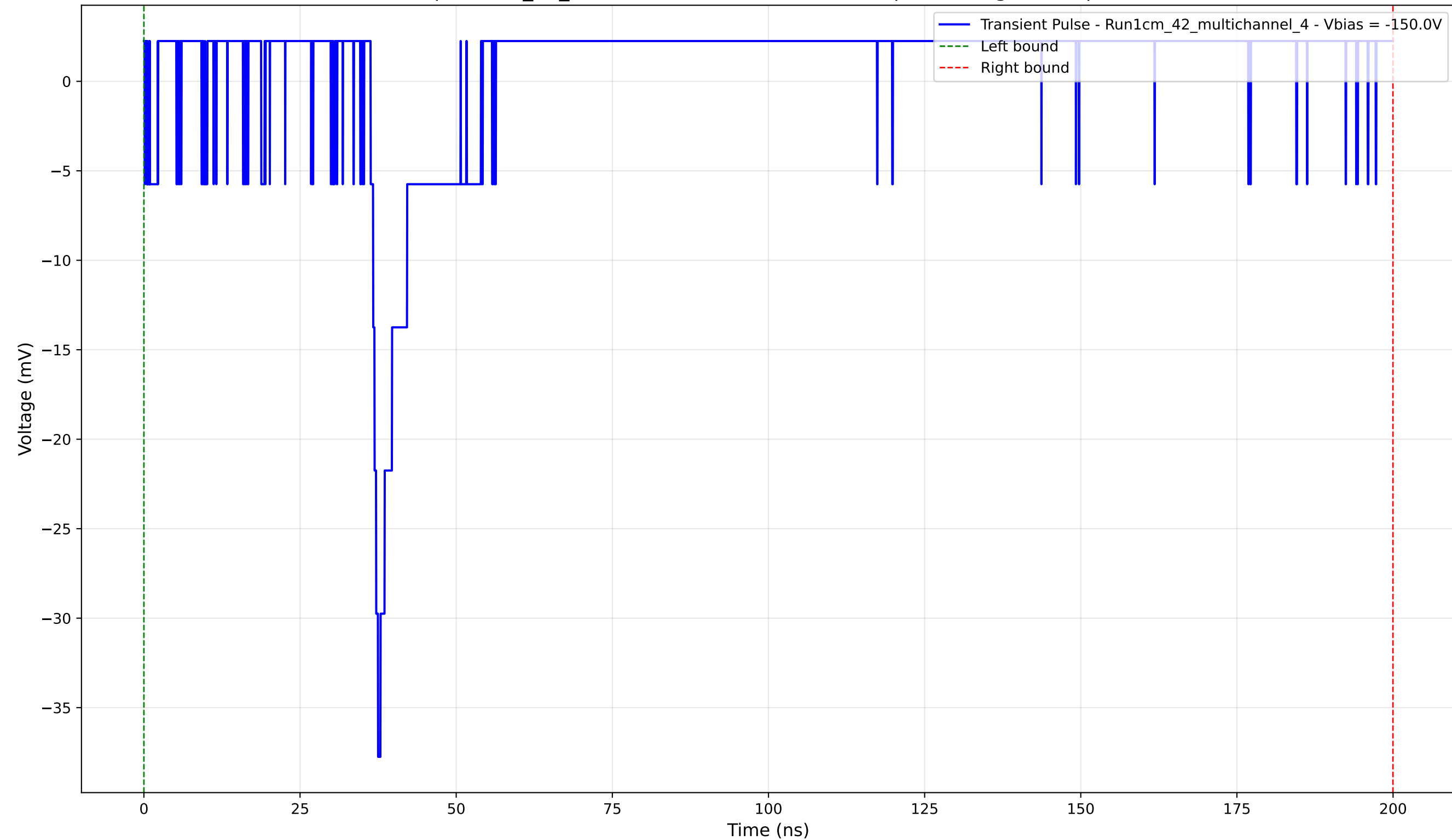
Transient Pulse - Sample: 1cm_42_multichannel - Position: 3050.0 \mu\text{m} - Charge: 3.54 pC - Rise Time: 1.19 ns
