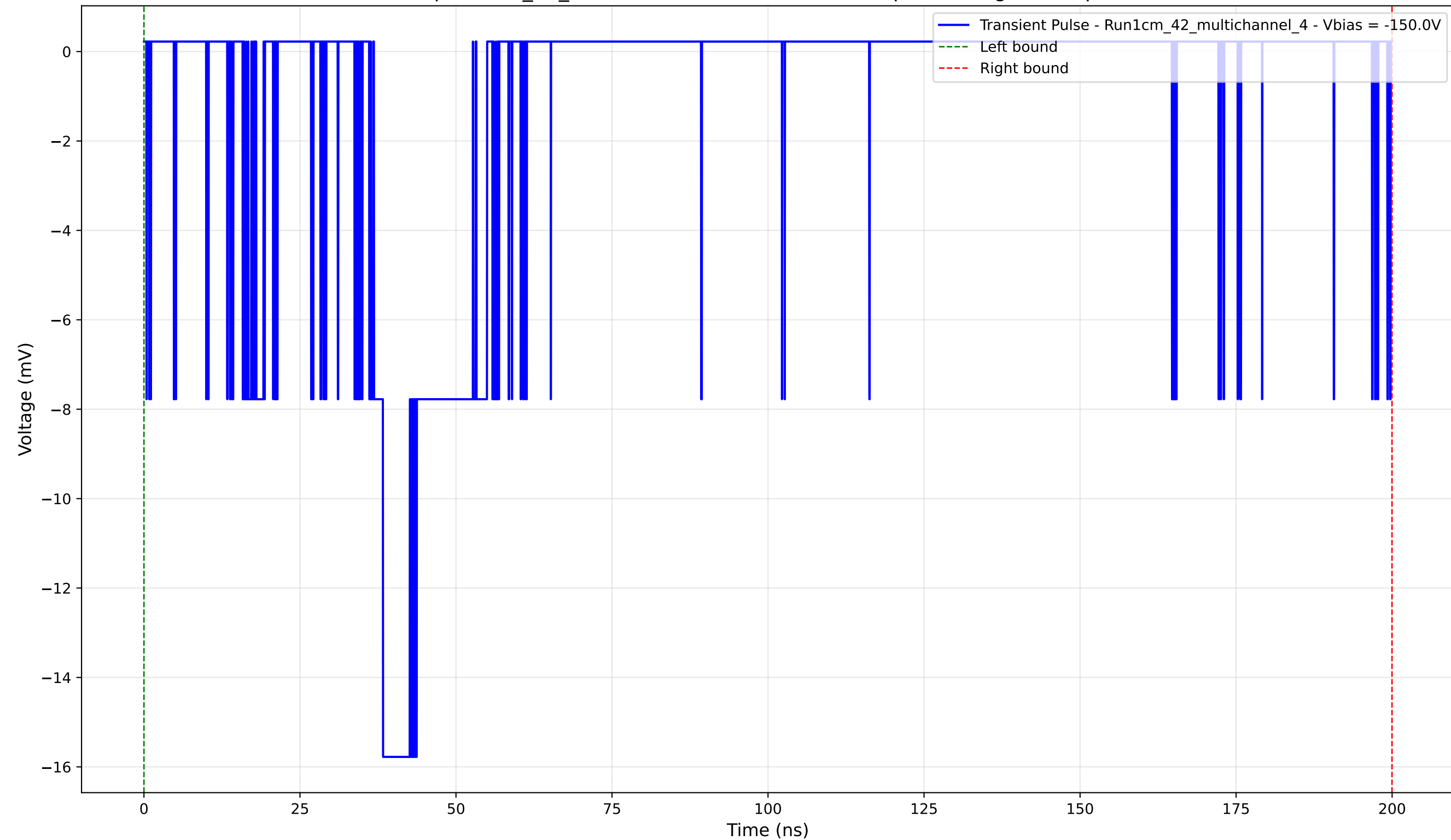
Transient Pulse - Sample: 1cm_42_multichannel - Position: 4285.0 \mu\text{m} - Charge: 4.17 pC - Rise Time: 1.46 ns
