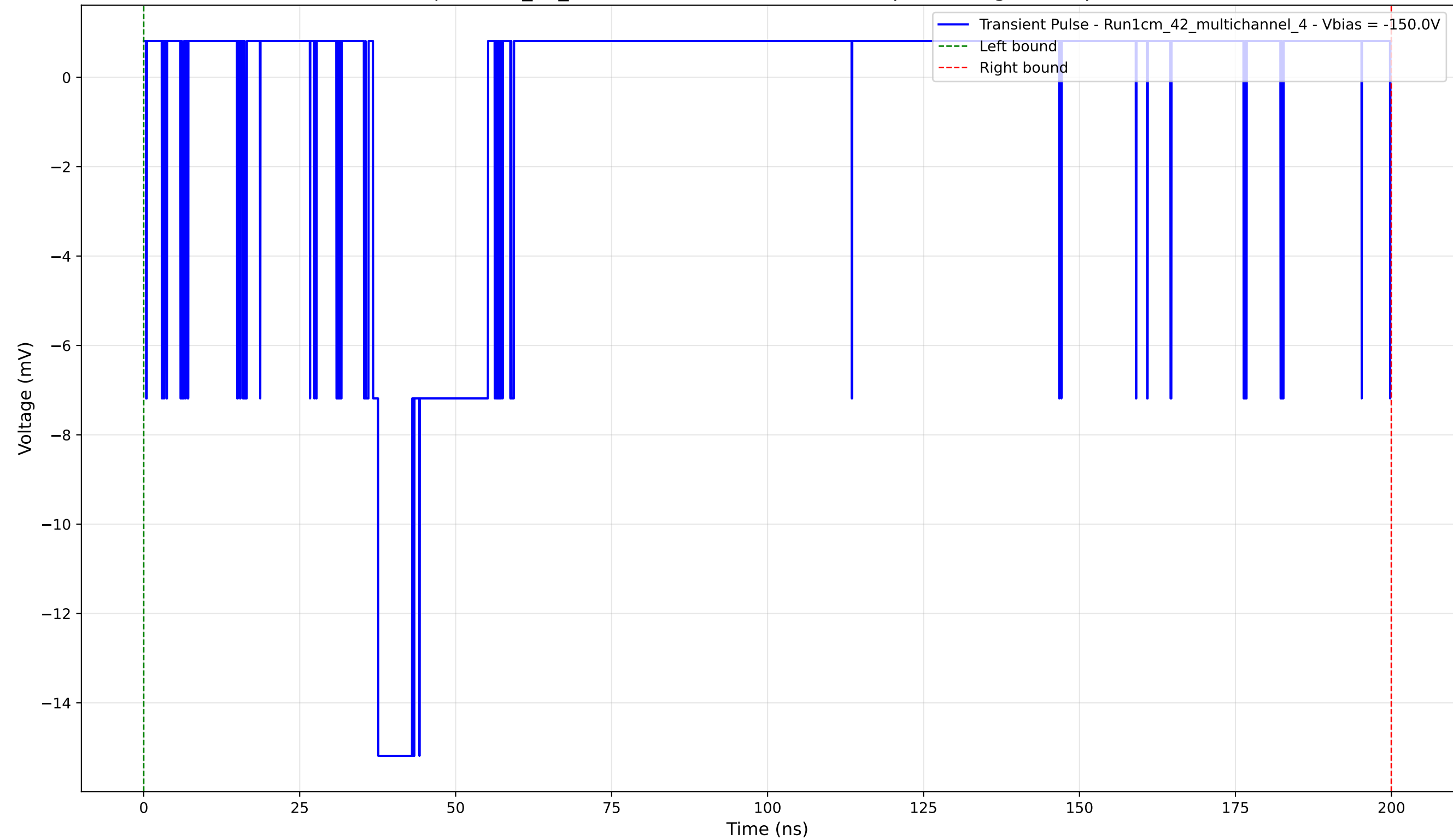
Transient Pulse - Sample: 1cm_42_multichannel - Position: 3785.0 \mu\text{m} - Charge: 1.49 pC - Rise Time: 0.84 ns
