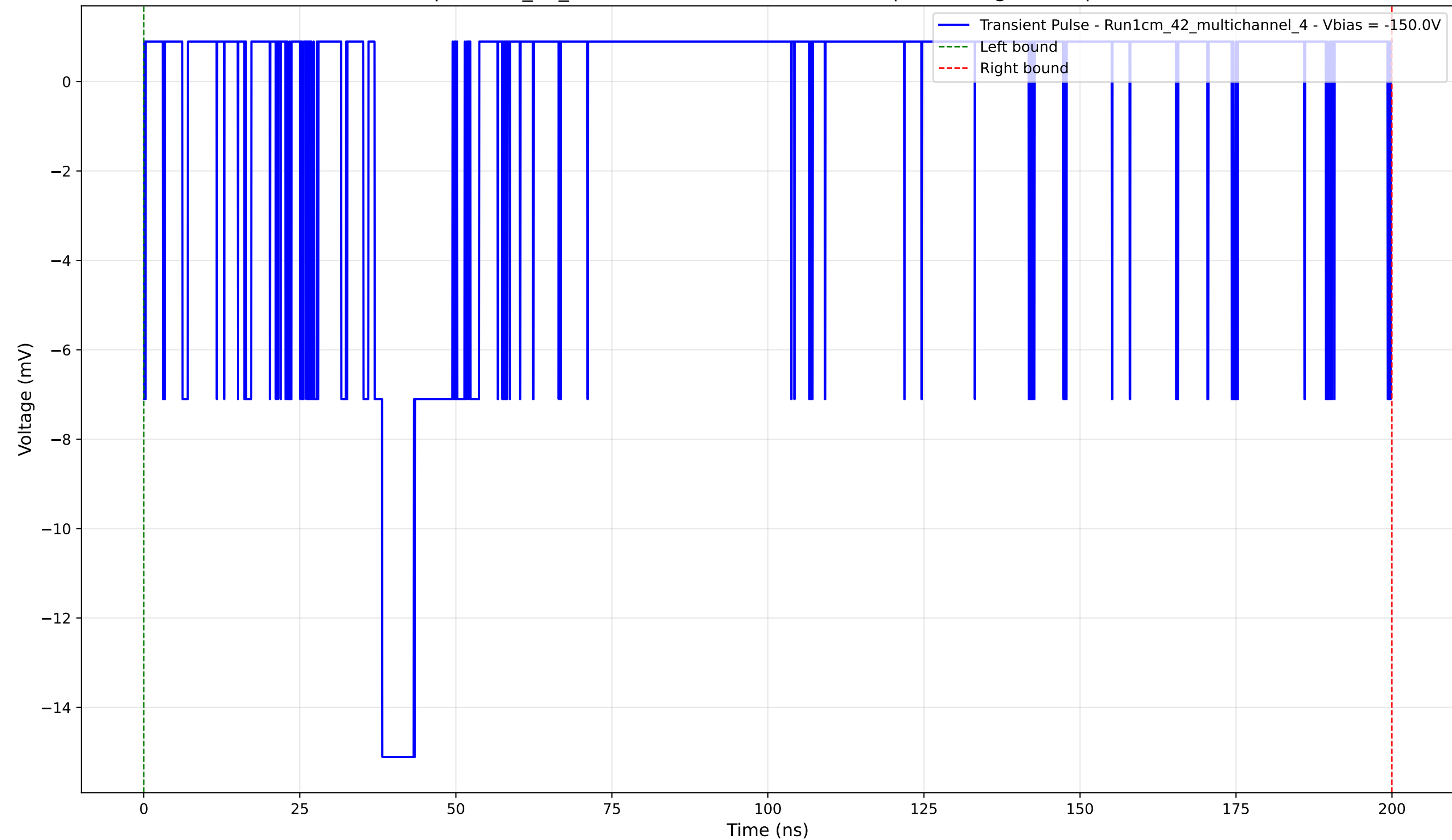
Transient Pulse - Sample: 1cm_42_multichannel - Position: 4530.0 \mu\text{m} - Charge: 1.52 pC - Rise Time: 1.24 ns
