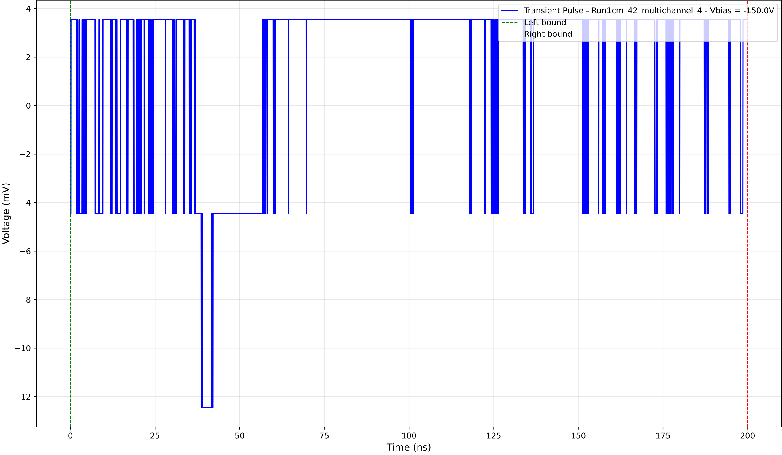
Transient Pulse - Sample: 1cm_42_multichannel - Position: 200.0 \mu\text{m} - Charge: 7.43 pC - Rise Time: 0.00 ns (N/A)
