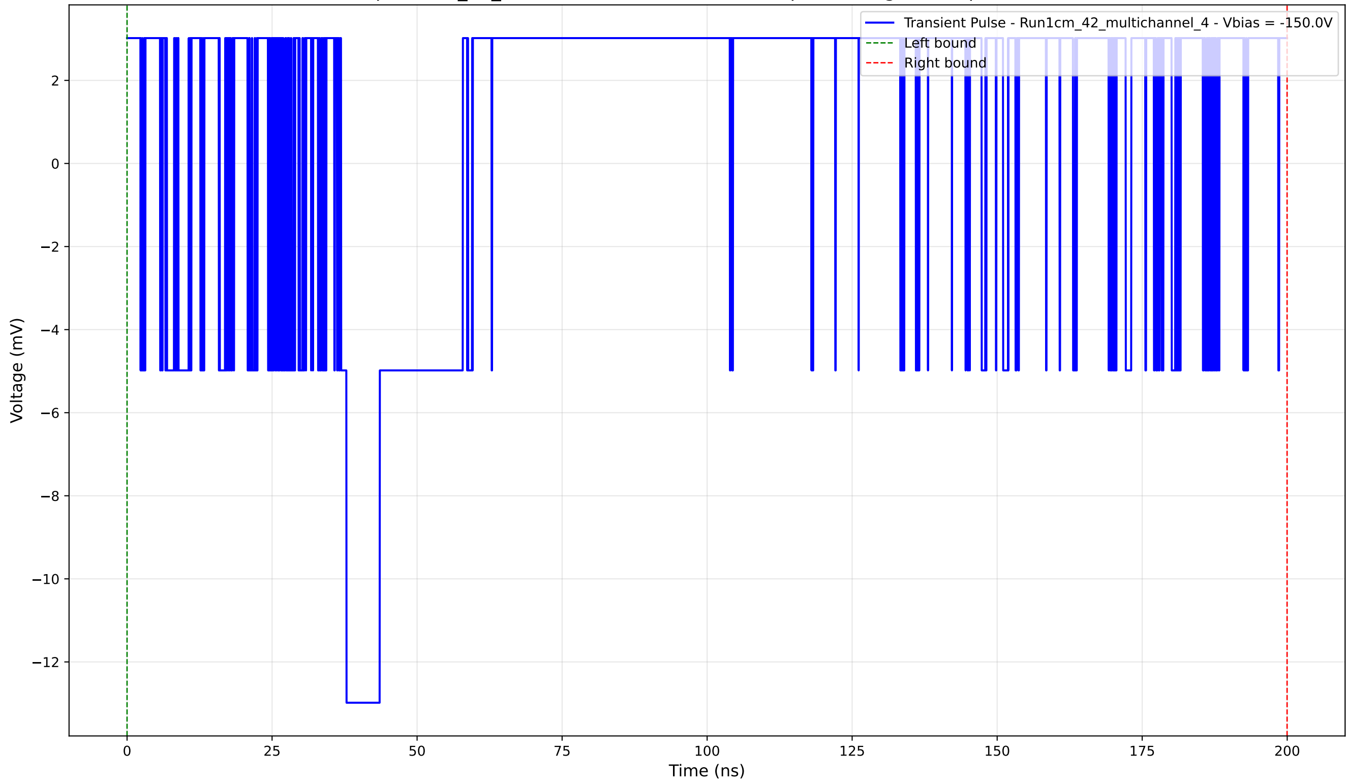
Transient Pulse - Sample: 1cm_42_multichannel - Position: 775.0 \mu\text{m} - Charge: 3.99 pC - Rise Time: 0.00 ns (N/A)
