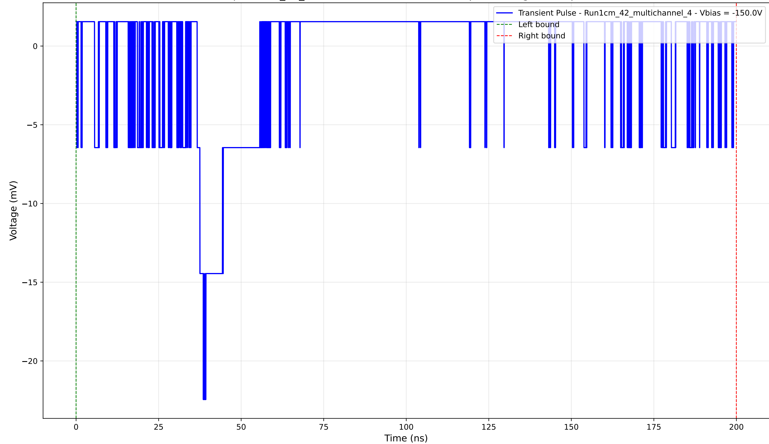
Transient Pulse - Sample: 1cm_42_multichannel - Position: 975.0 \mu\text{m} - Charge: 1.63 pC - Rise Time: 1.88 ns
