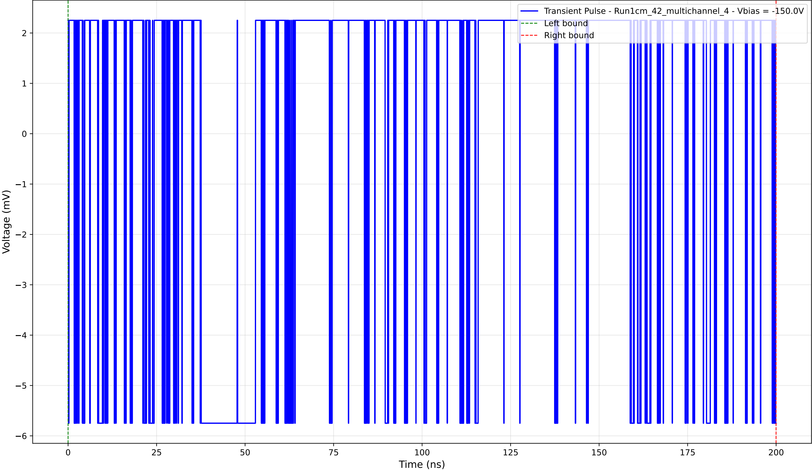
Transient Pulse - Sample: 1cm_42_multichannel - Position: 4360.0 \mu\text{m} - Charge: 2.72 pC - Rise Time: 0.00 ns (N/A)
