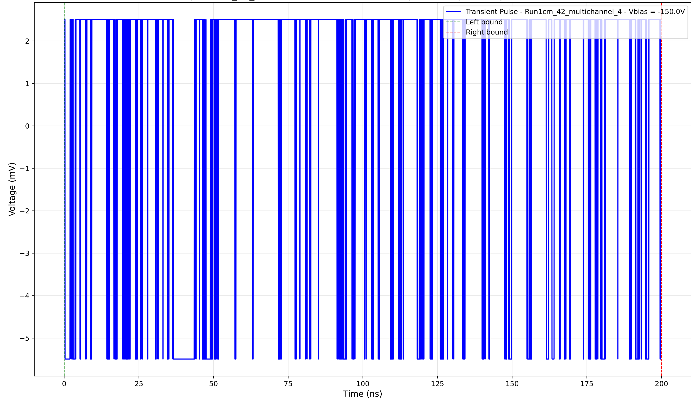
Transient Pulse - Sample: 1cm_42_multichannel - Position: 2925.0 \mu\text{m} - Charge: 4.00 pC - Rise Time: 0.00 ns (N/A)
