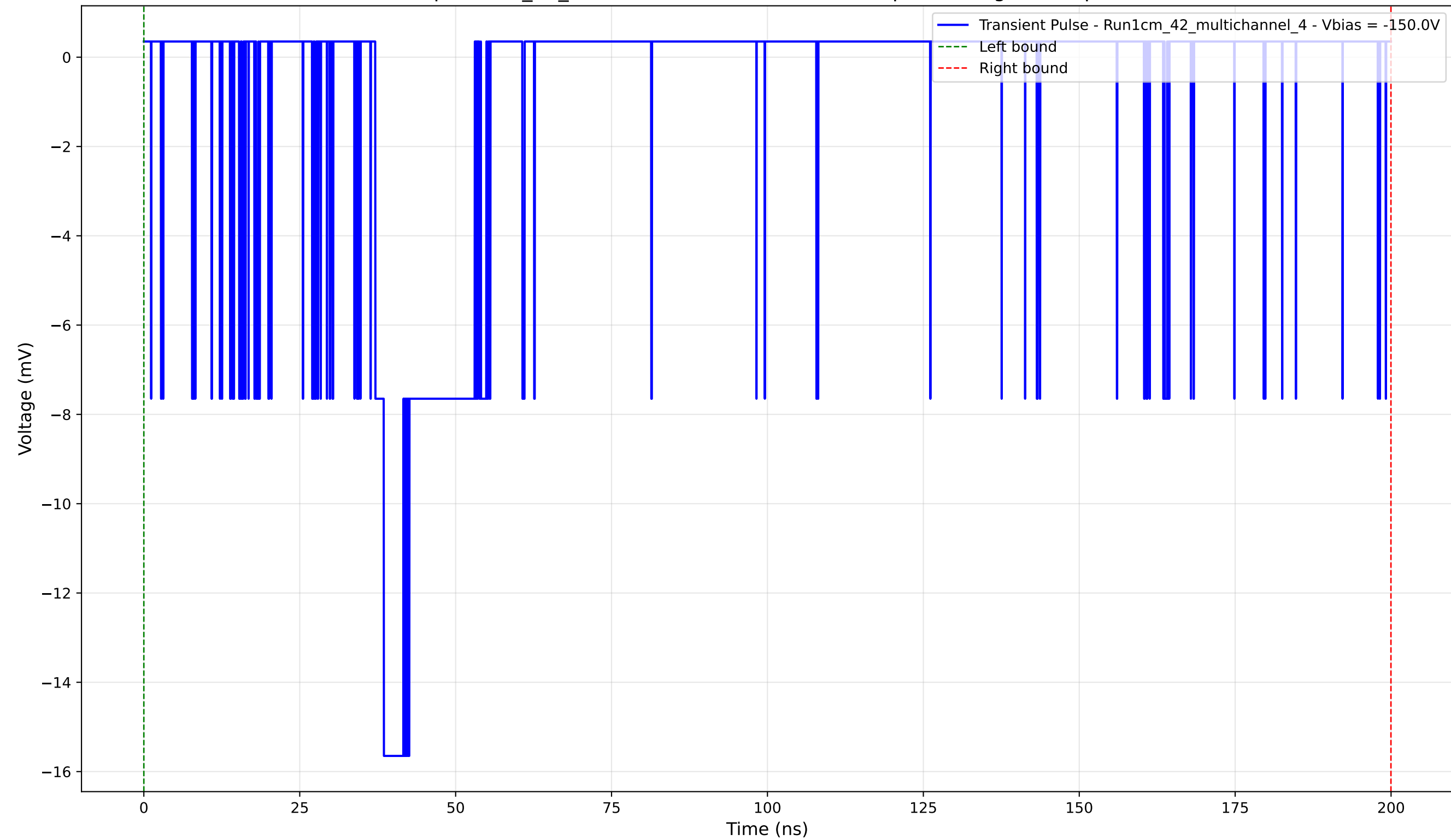
Transient Pulse - Sample: 1cm_42_multichannel - Position: 4665.0 \mu\text{m} - Charge: 3.11 pC - Rise Time: 1.38 ns
