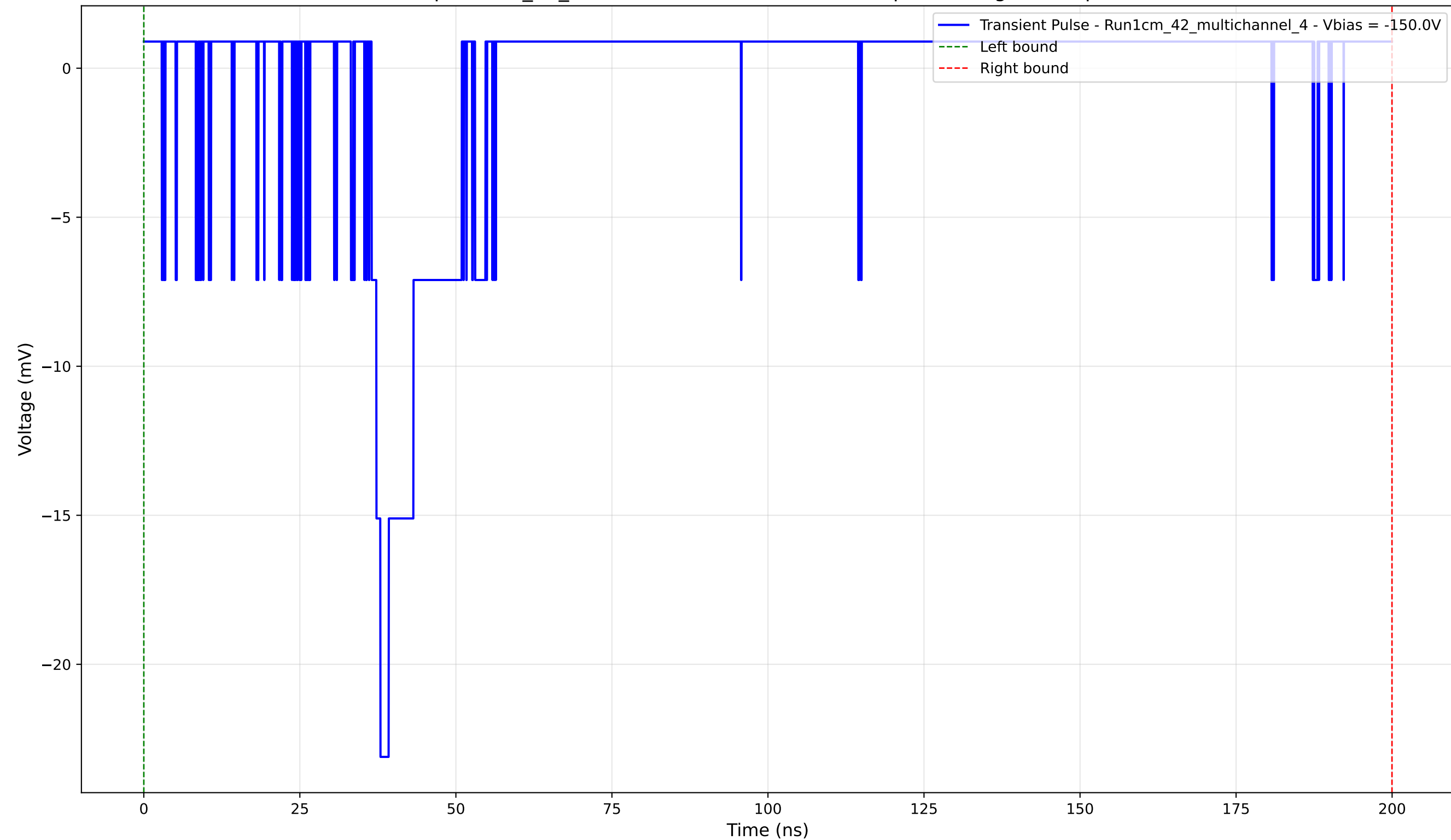
Transient Pulse - Sample: 1cm_42_multichannel - Position: 3525.0 \mu\text{m} - Charge: 1.12 pC - Rise Time: 1.42 ns
