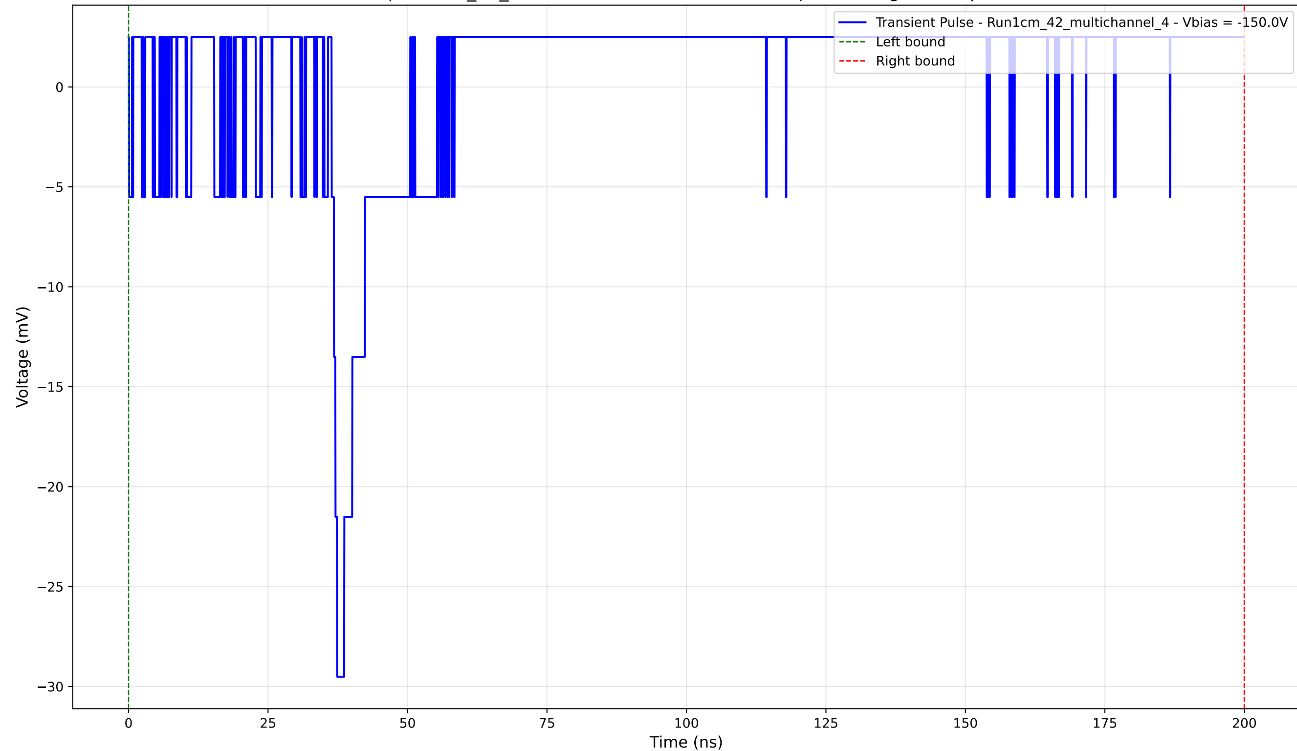
Transient Pulse - Sample: 1cm_42_multichannel - Position: 1585.0 \mu\text{m} - Charge: 3.53 pC - Rise Time: 1.00 ns
