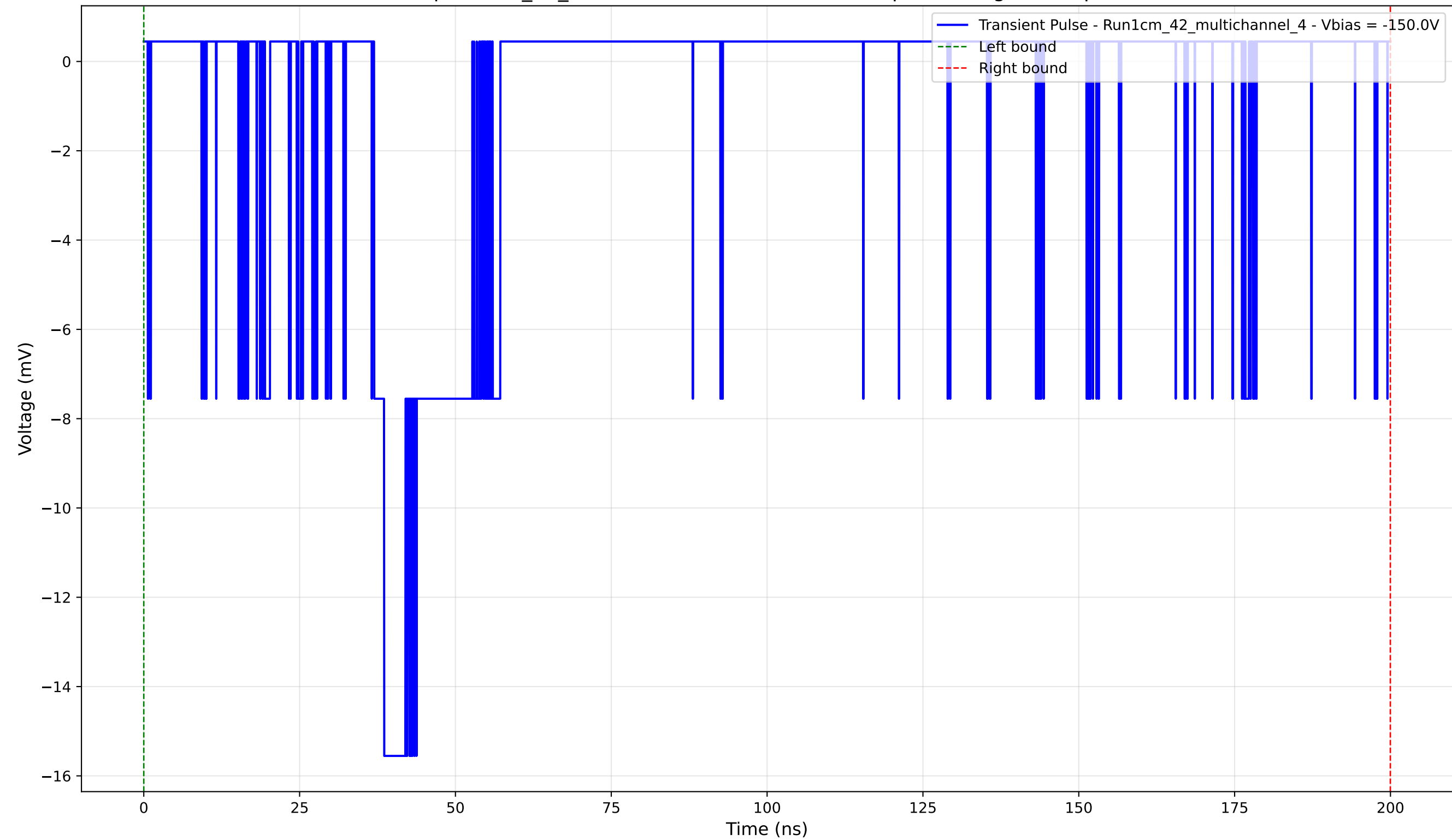
Transient Pulse - Sample: 1cm_42_multichannel - Position: 4705.0 \mu\text{m} - Charge: 3.31 pC - Rise Time: 1.62 ns
