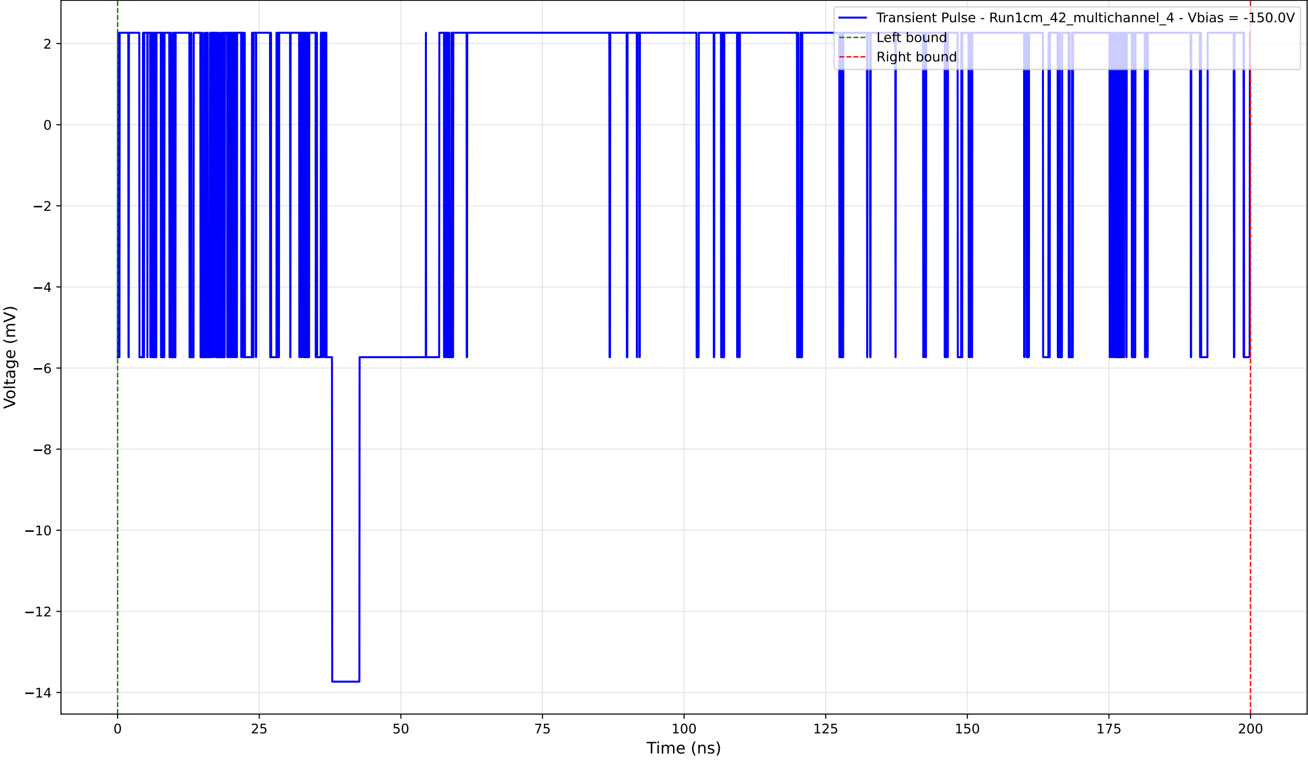
Transient Pulse - Sample: 1cm_42_multichannel - Position: 800.0 \mu\text{m} - Charge: 1.31 pC - Rise Time: 0.00 ns (N/A)
