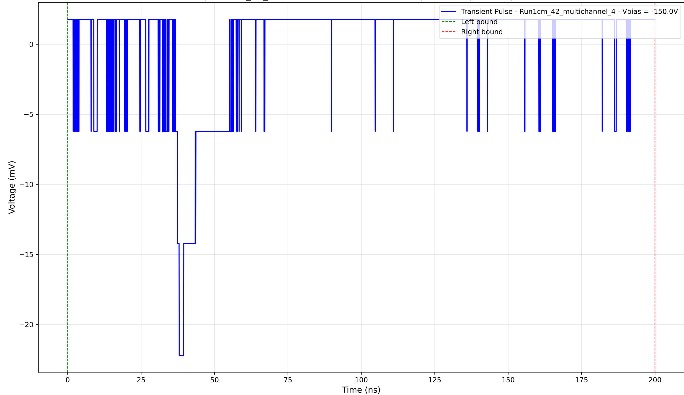
Transient Pulse - Sample: 1cm_42_multichannel - Position: 1145.0 \mu\text{m} - Charge: 0.96 pC - Rise Time: 1.30 ns
