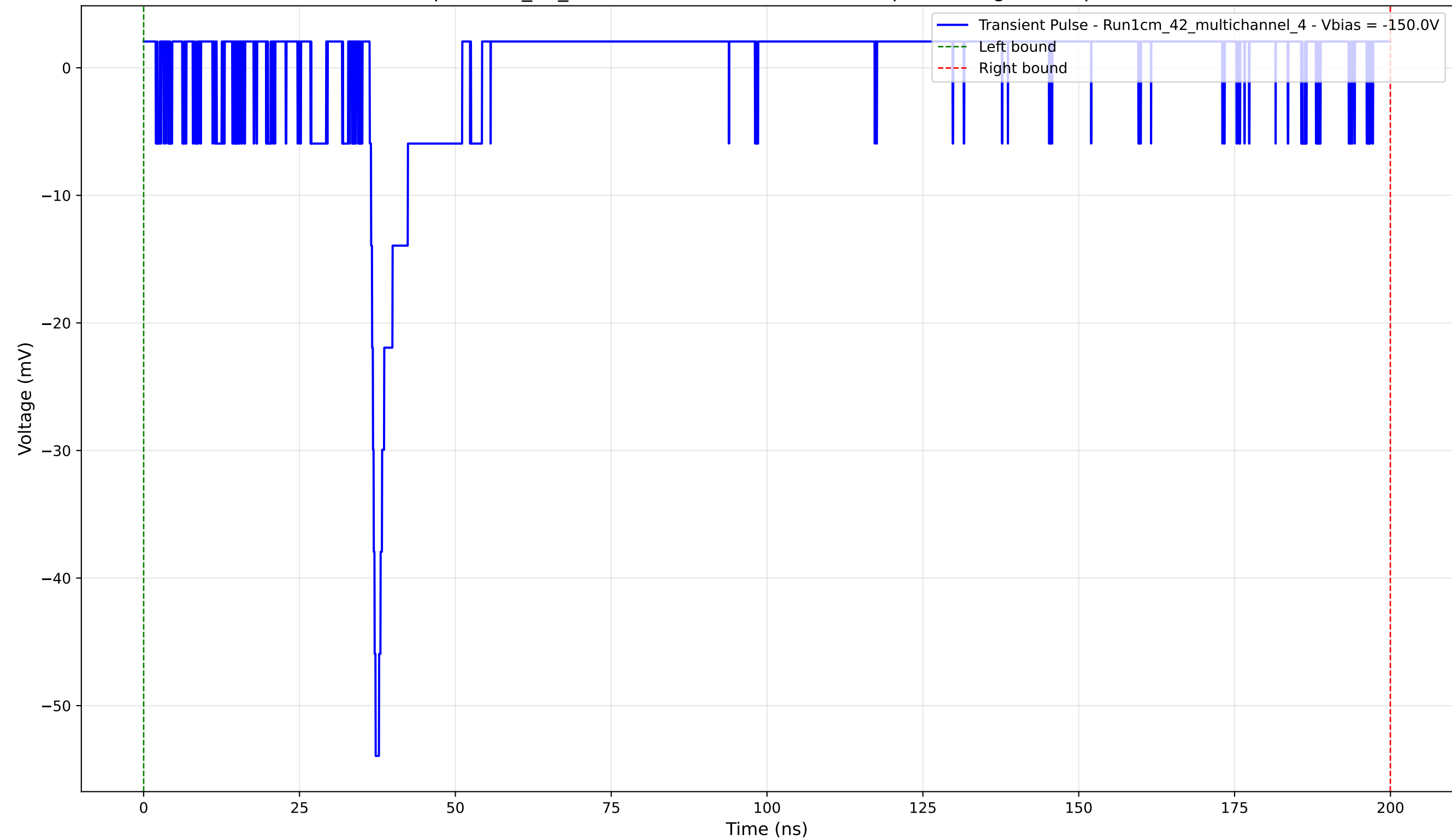
Transient Pulse - Sample: 1cm_42_multichannel - Position: 2760.0 \mu\text{m} - Charge: 0.98 pC - Rise Time: 0.94 ns
