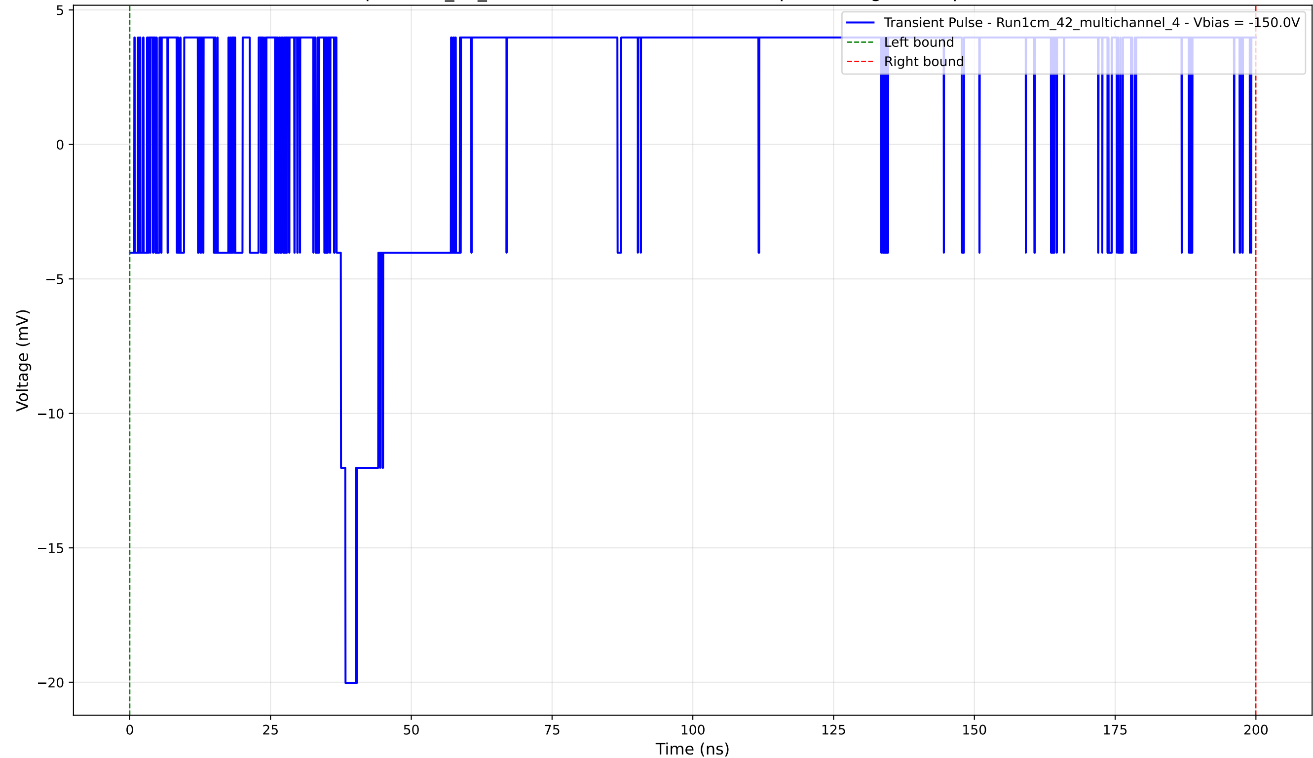
Transient Pulse - Sample: 1cm_42_multichannel - Position: 1000.0 \mu\text{m} - Charge: 7.80 pC - Rise Time: 0.00 ns (N/A)
