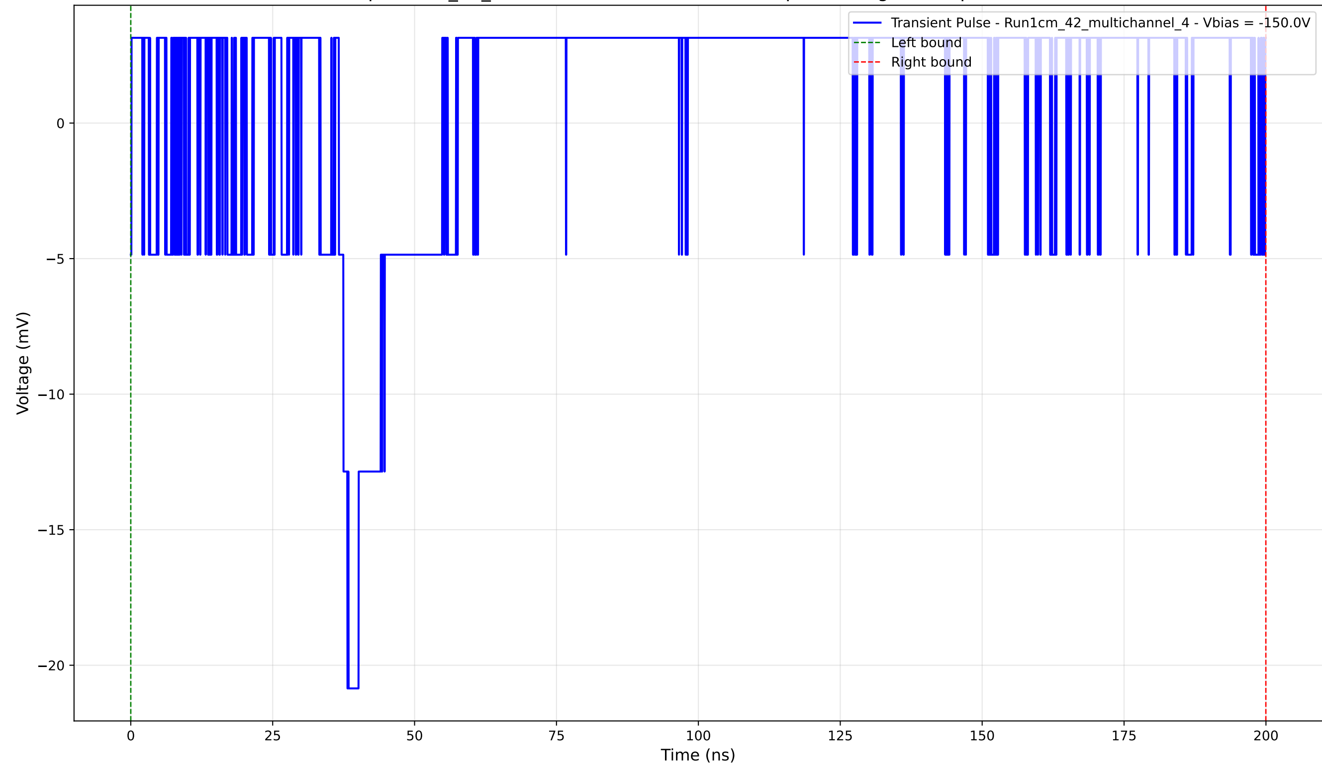
Transient Pulse - Sample: 1cm_42_multichannel - Position: 1055.0 \mu\text{m} - Charge: 4.28 pC - Rise Time: 0.00 ns (N/A)
