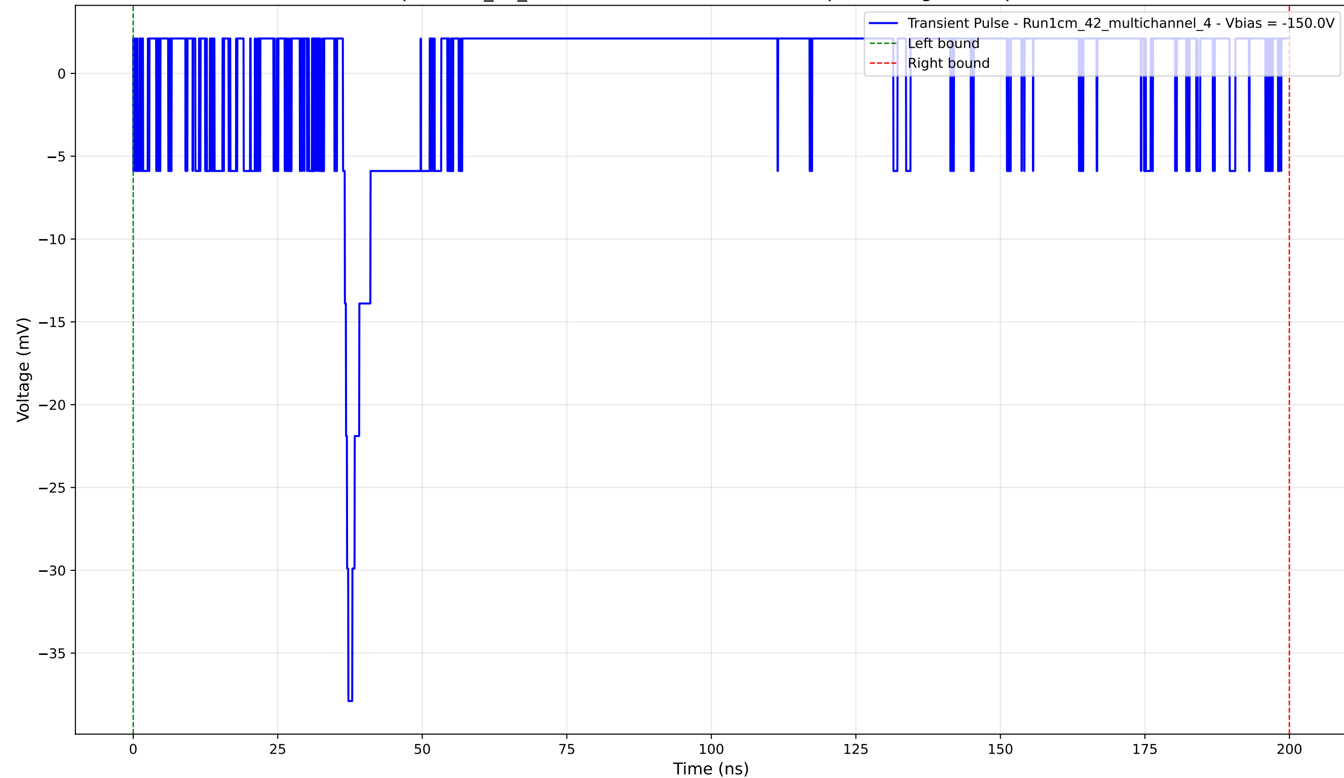
Transient Pulse - Sample: 1cm_42_multichannel - Position: 1940.0 \mu\text{m} - Charge: 0.71 pC - Rise Time: 0.93 ns
