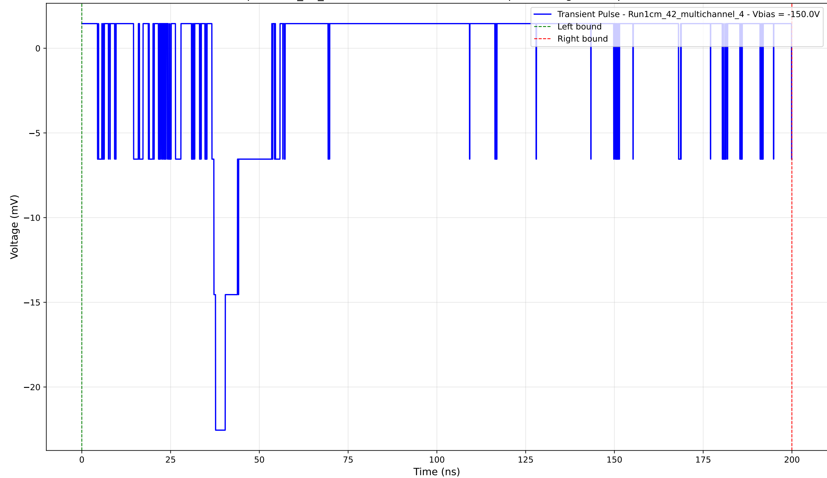
Transient Pulse - Sample: 1cm_42_multichannel - Position: 1240.0 \mu\text{m} - Charge: 1.01 pC - Rise Time: 1.04 ns
