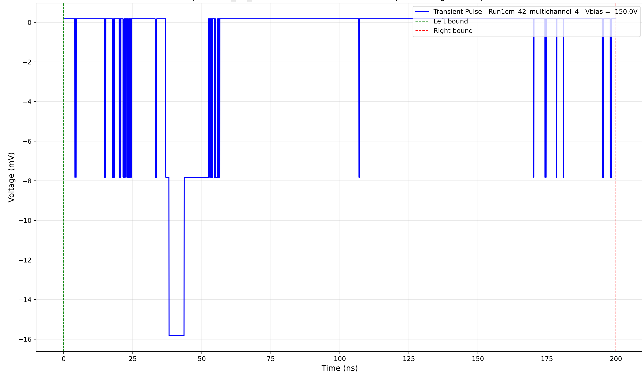
Transient Pulse - Sample: 1cm_42_multichannel - Position: 4045.0 \mu\text{m} - Charge: 3.59 pC - Rise Time: 1.20 ns
