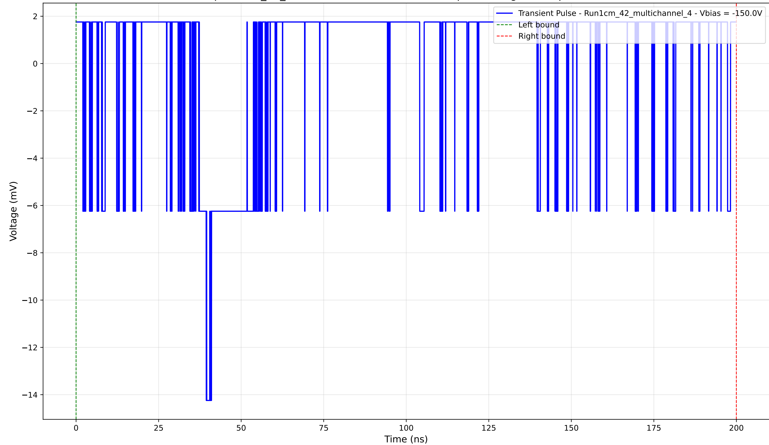
Transient Pulse - Sample: 1cm_42_multichannel - Position: 4345.0 \mu\text{m} - Charge: 1.48 pC - Rise Time: 0.00 ns (N/A)
