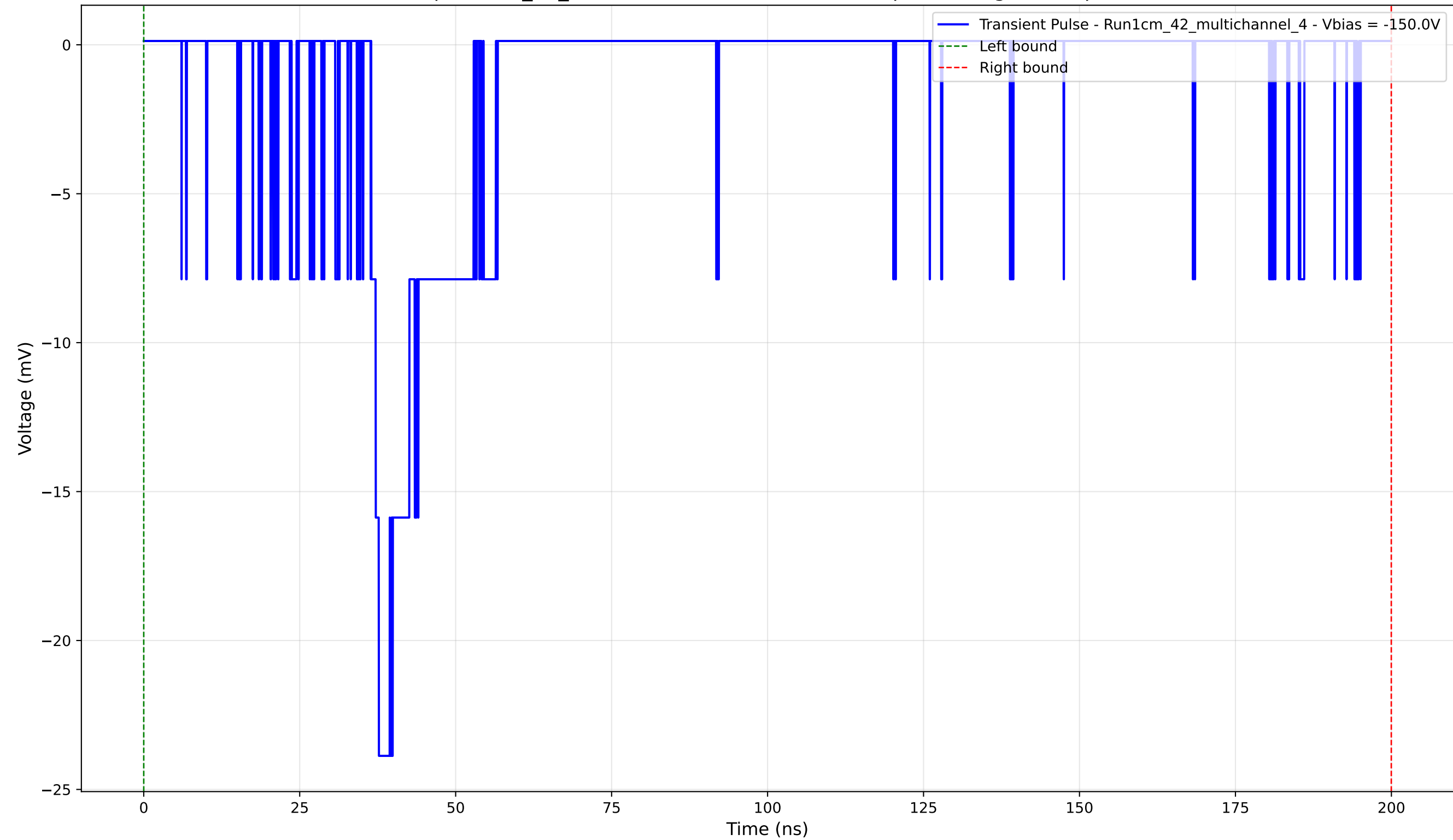
Transient Pulse - Sample: 1cm_42_multichannel - Position: 3490.0 \mu\text{m} - Charge: 4.98 pC - Rise Time: 1.21 ns
