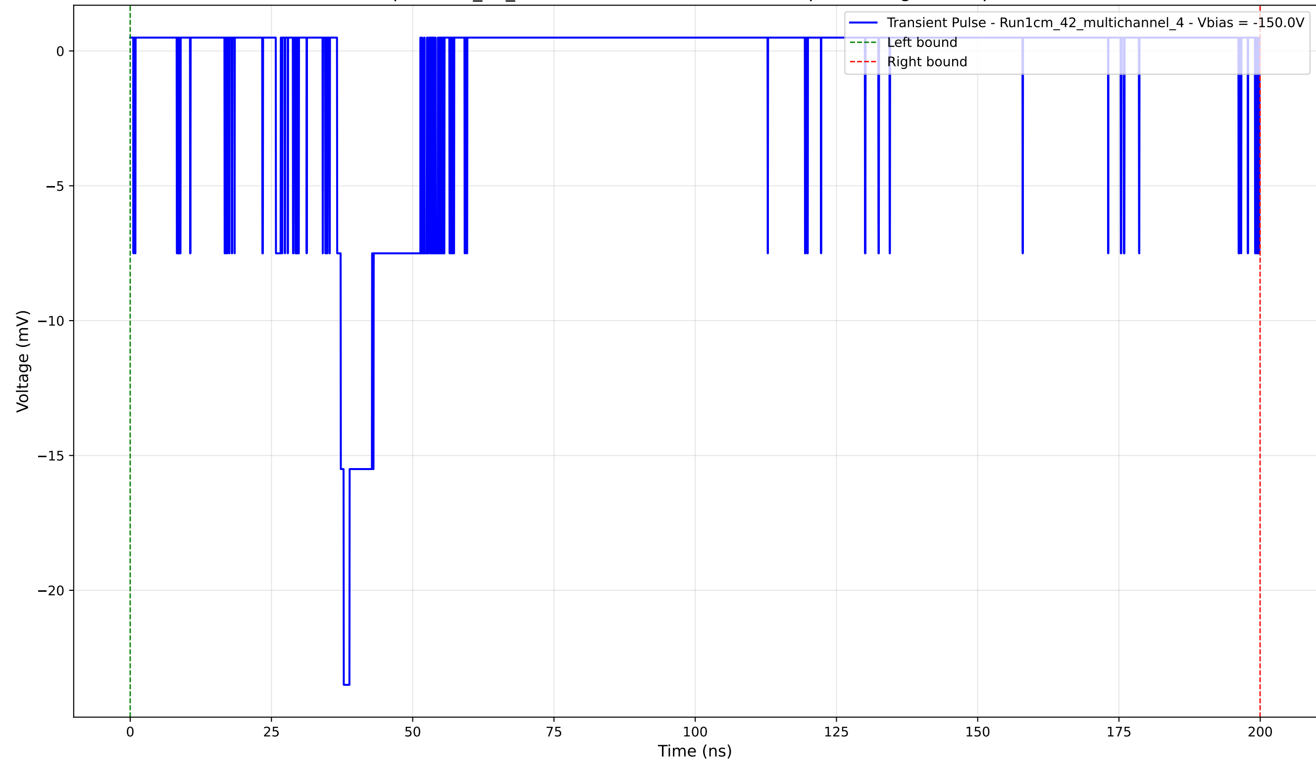
Transient Pulse - Sample: 1cm_42_multichannel - Position: 3530.0 \mu\text{m} - Charge: 2.76 pC - Rise Time: 1.17 ns
