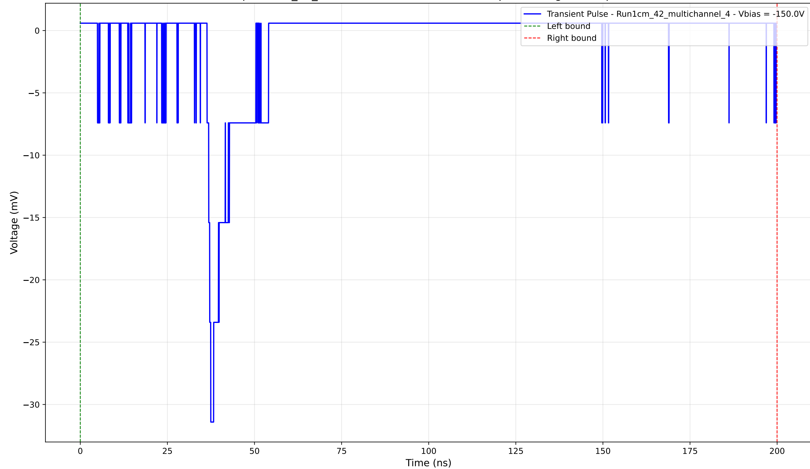
Transient Pulse - Sample: 1cm_42_multichannel - Position: 3180.0 \mu\text{m} - Charge: 2.45 pC - Rise Time: 1.07 ns
