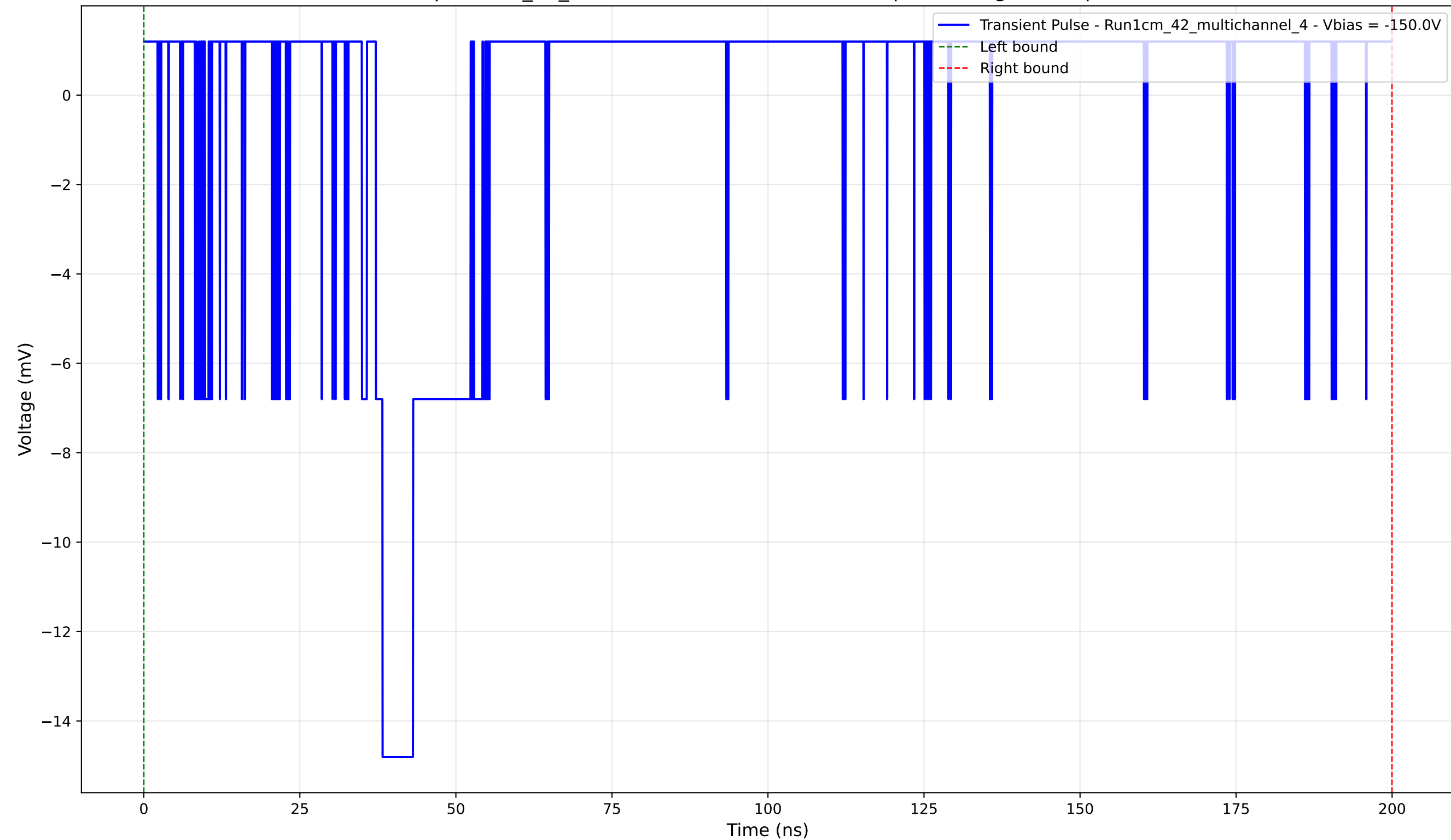
Transient Pulse - Sample: 1cm_42_multichannel - Position: 4310.0 \mu\text{m} - Charge: 0.07 pC - Rise Time: 1.08 ns
