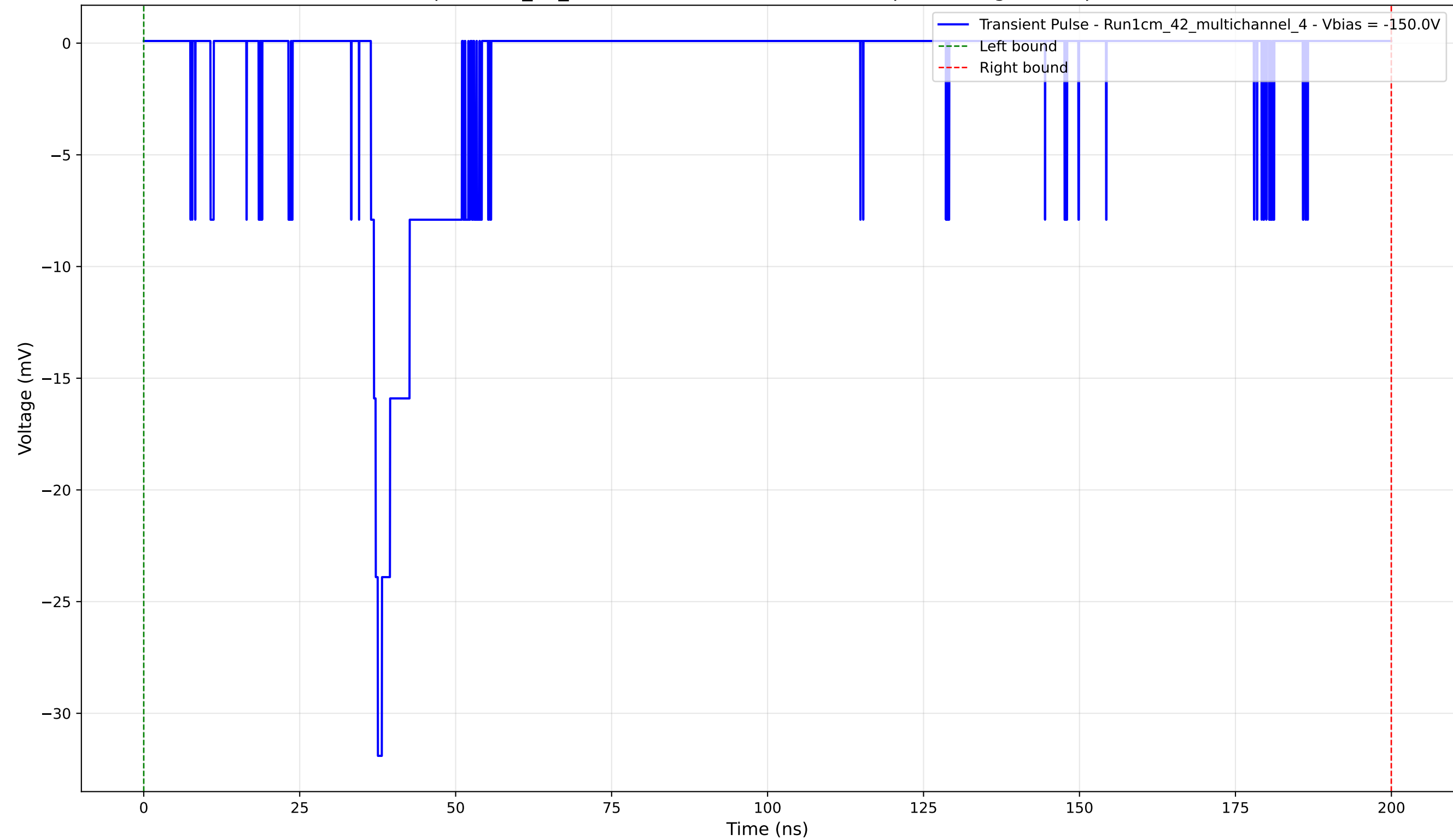
Transient Pulse - Sample: 1cm_42_multichannel - Position: 3205.0 \mu\text{m} - Charge: 4.34 pC - Rise Time: 1.11 ns
