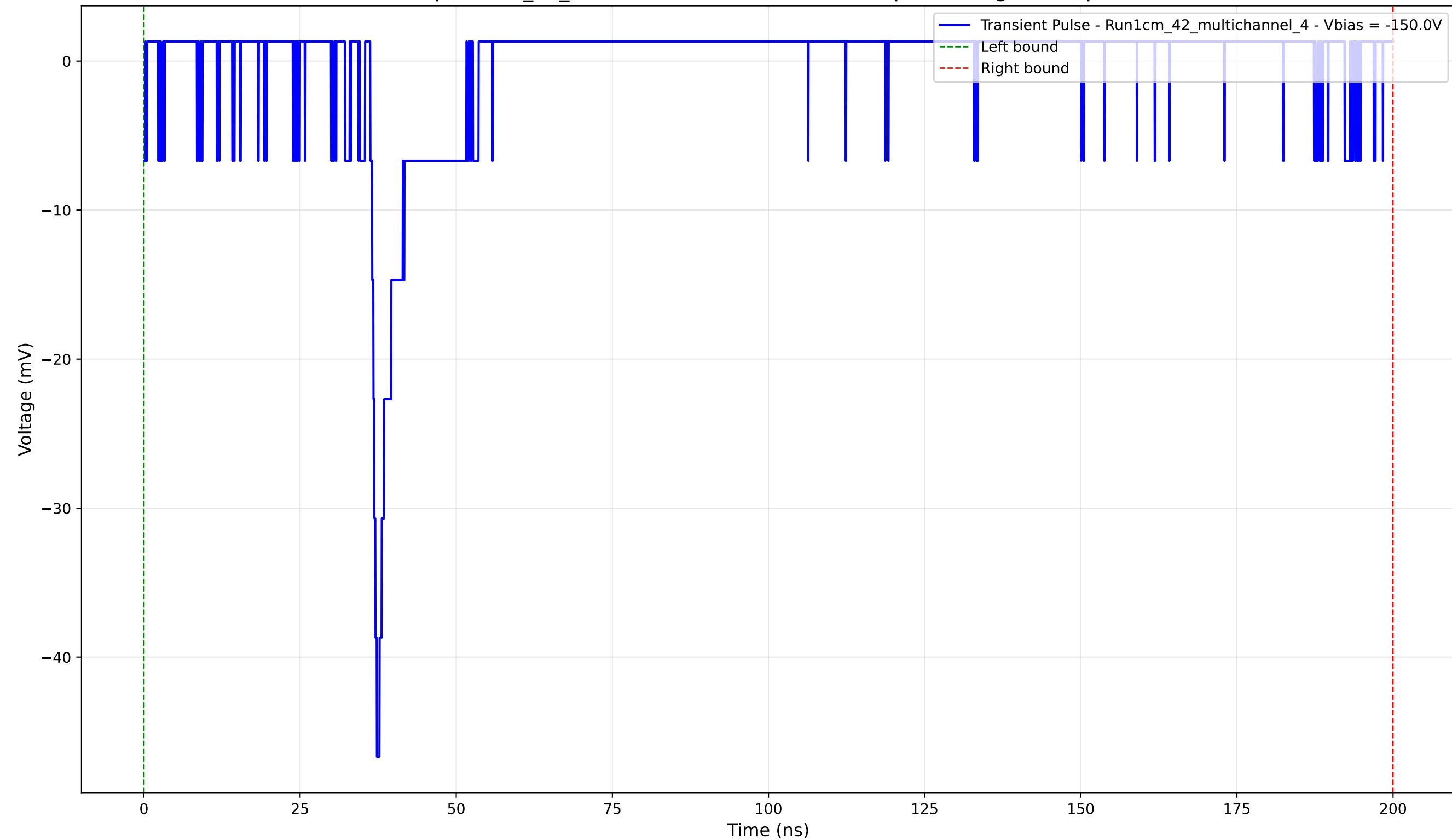
Transient Pulse - Sample: 1cm_42_multichannel - Position: 2815.0 \mu\text{m} - Charge: 0.67 pC - Rise Time: 1.05 ns
