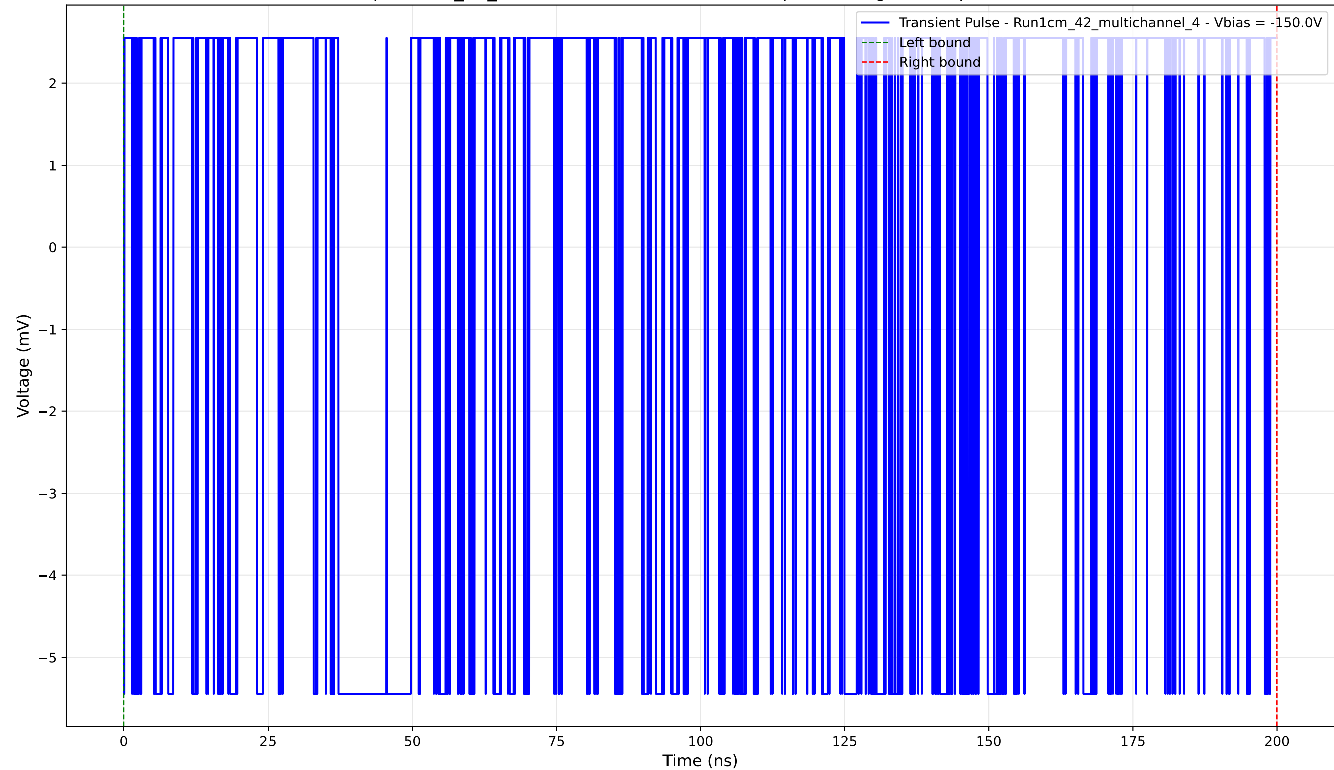
Transient Pulse - Sample: 1cm_42_multichannel - Position: 900.0 \mu\text{m} - Charge: 1.06 pC - Rise Time: 0.00 ns (N/A)
