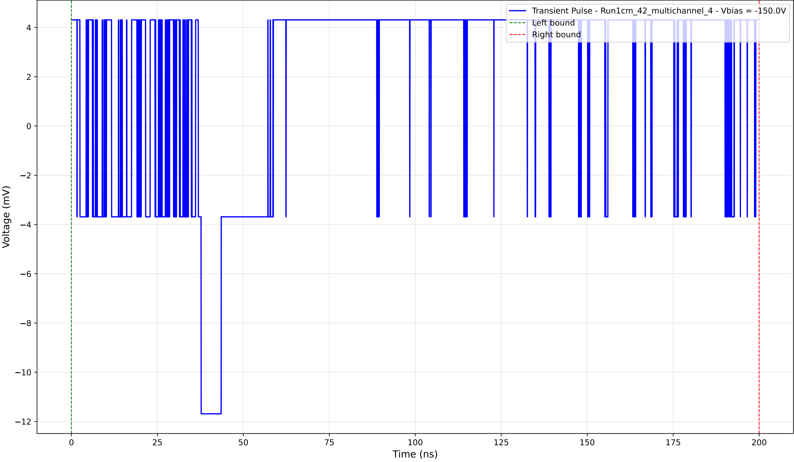
Transient Pulse - Sample: 1cm_42_multichannel - Position: 790.0 \mu\text{m} - Charge: 8.42 pC - Rise Time: 0.00 ns (N/A)
