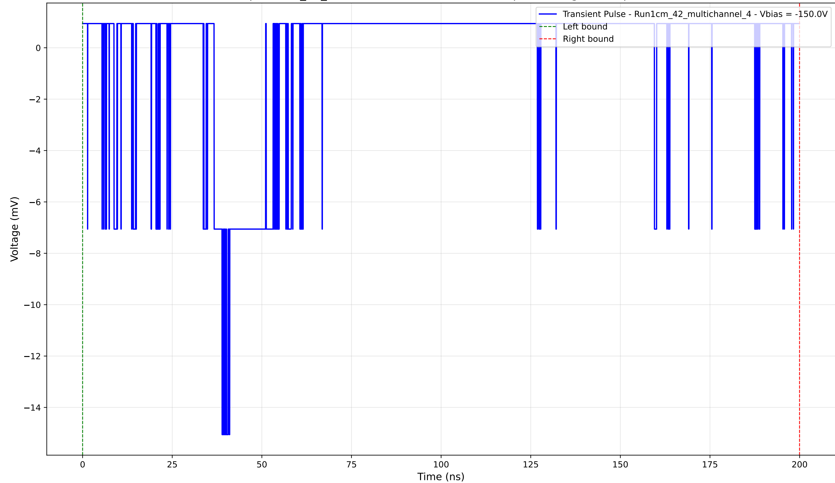
Transient Pulse - Sample: 1cm_42_multichannel - Position: 4815.0 \mu\text{m} - Charge: 0.55 pC - Rise Time: 2.24 ns
