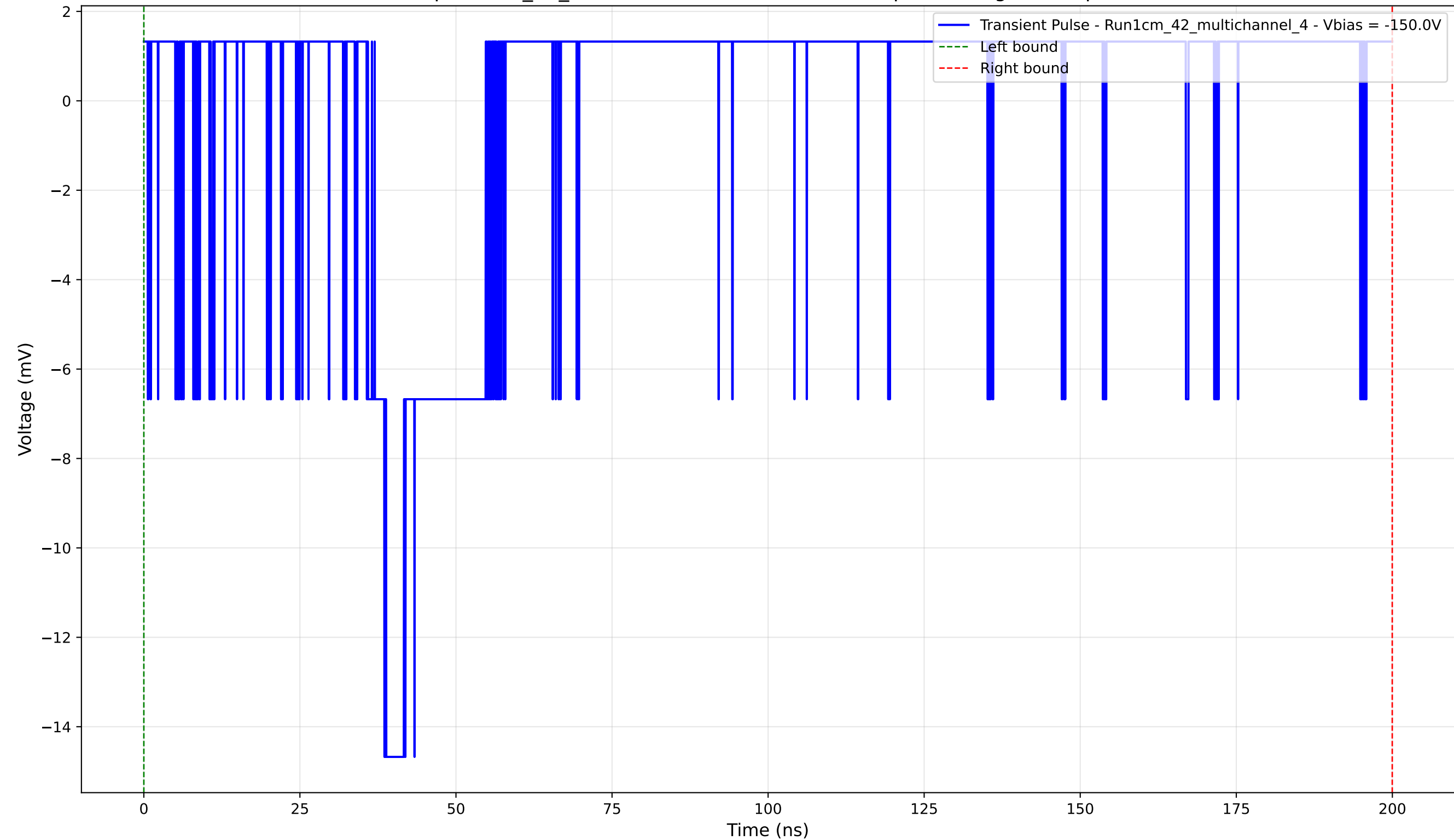
Transient Pulse - Sample: 1cm_42_multichannel - Position: 4725.0 \mu\text{m} - Charge: 0.25 pC - Rise Time: 1.54 ns
