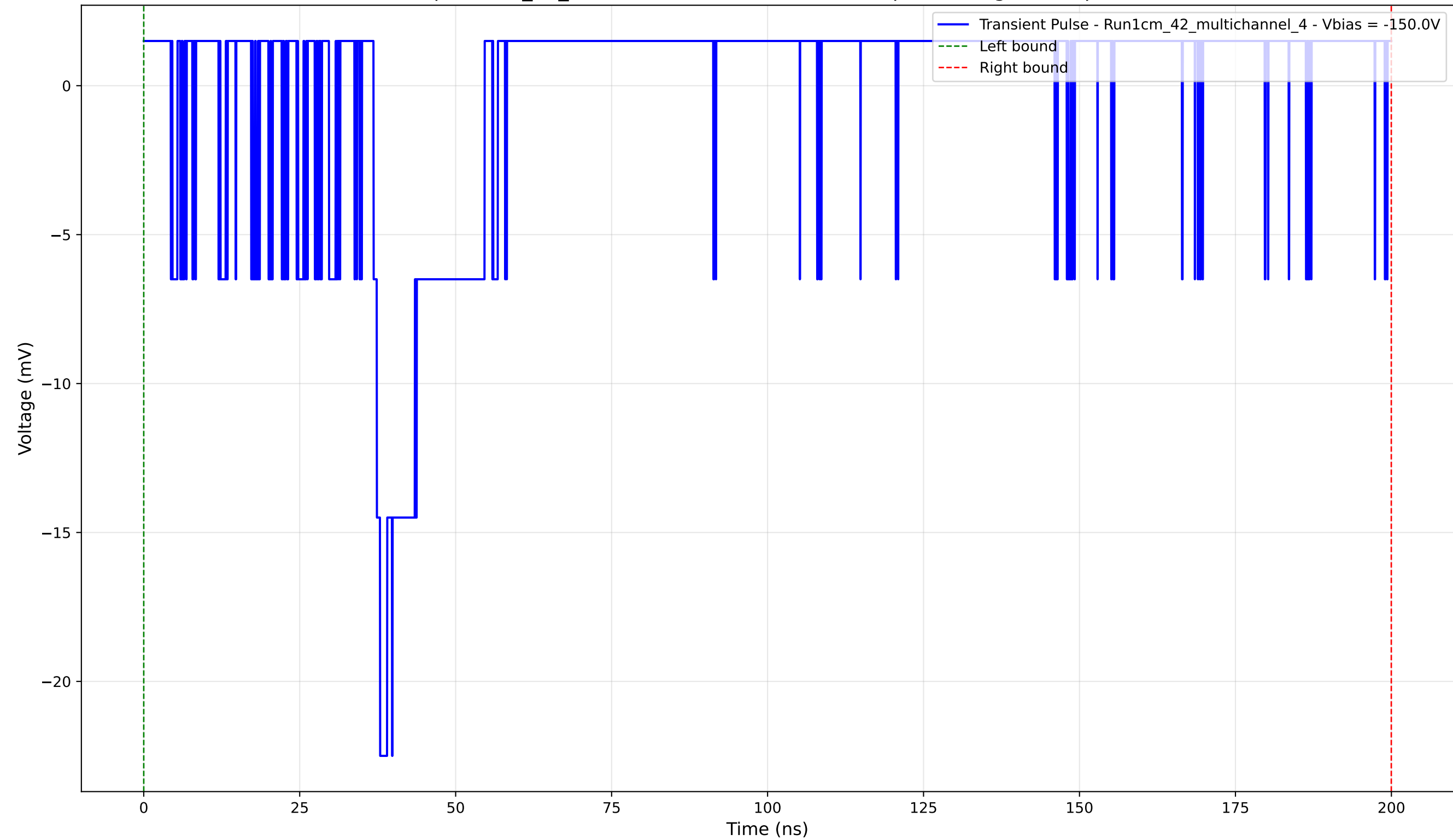
Transient Pulse - Sample: 1cm_42_multichannel - Position: 1120.0 \mu\text{m} - Charge: 0.21 pC - Rise Time: 1.06 ns
