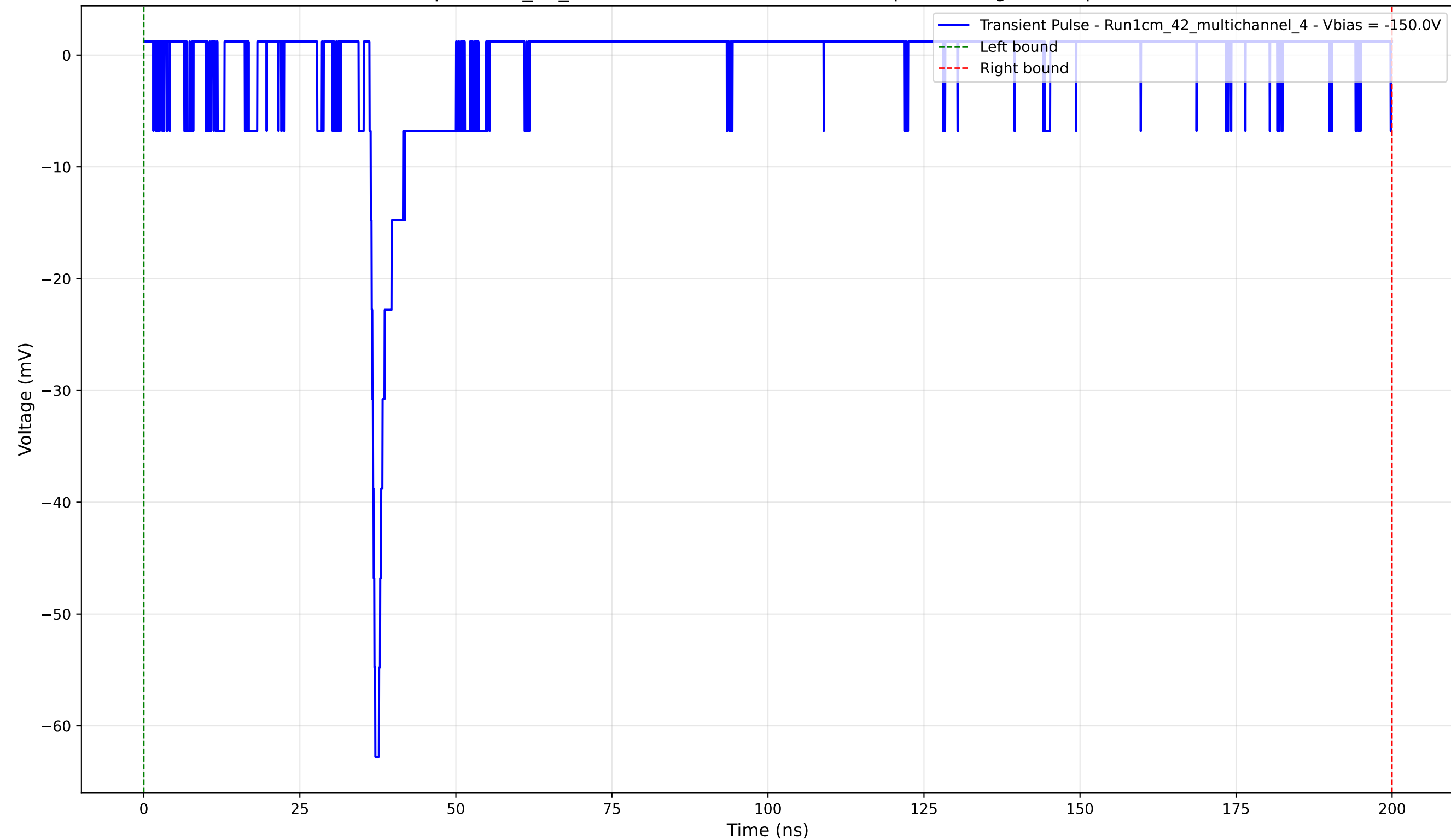
Transient Pulse - Sample: 1cm_42_multichannel - Position: 2160.0 \mu\text{m} - Charge: 2.20 pC - Rise Time: 0.92 ns
