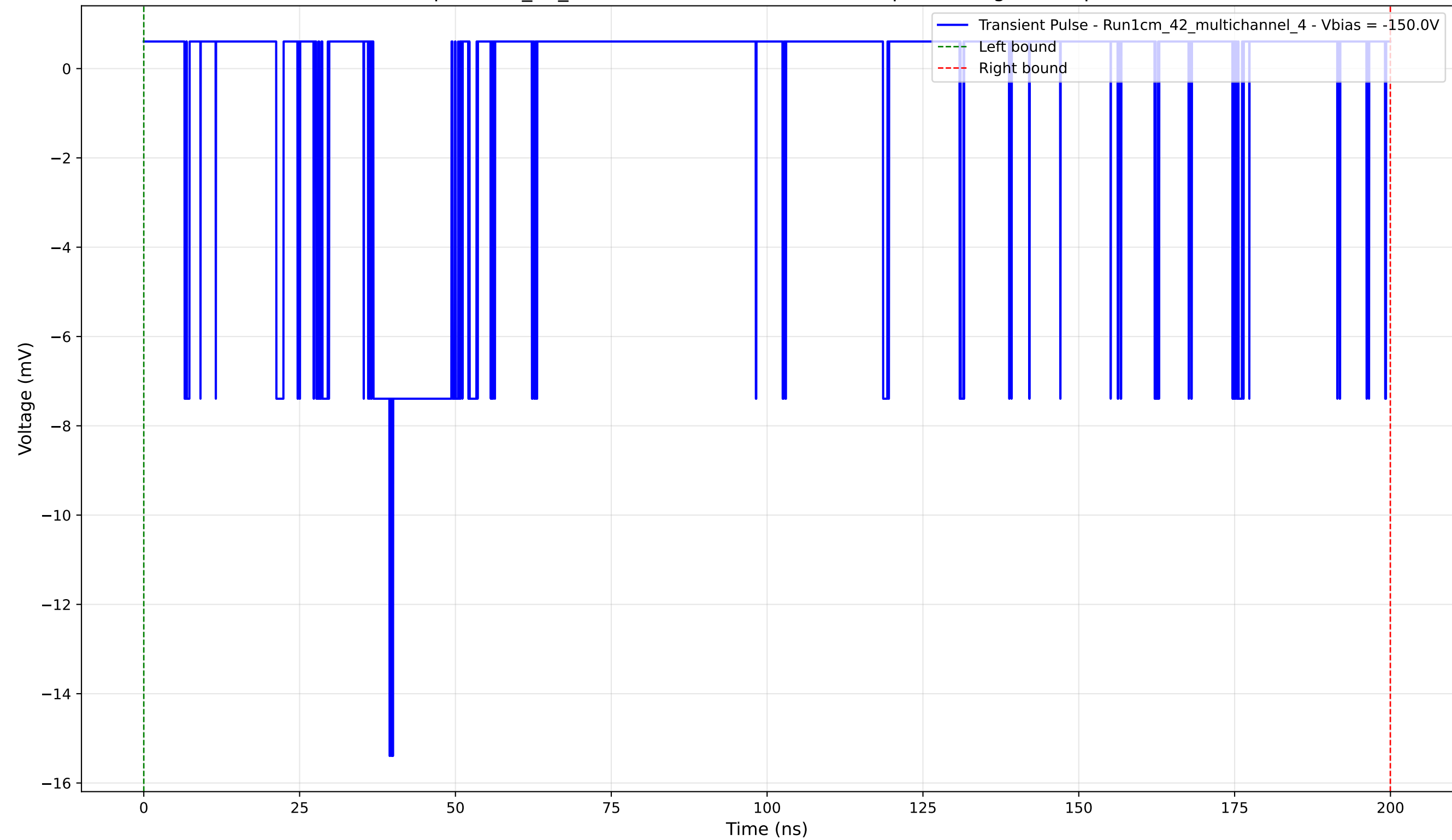
Transient Pulse - Sample: 1cm_42_multichannel - Position: 3850.0 \mu\text{m} - Charge: 1.52 pC - Rise Time: 2.60 ns
