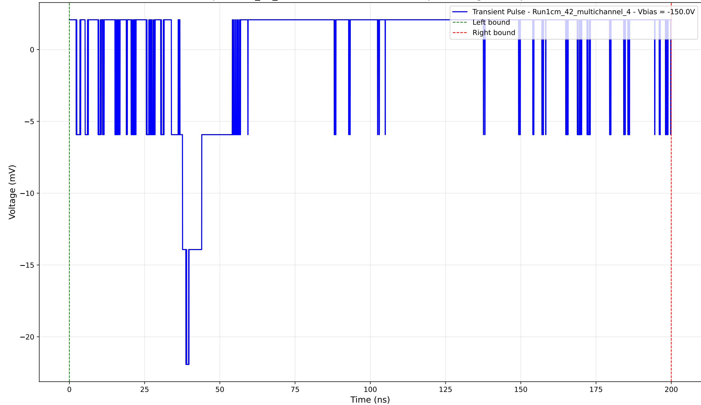
Transient Pulse - Sample: 1cm_42_multichannel - Position: 965.0 \mu\text{m} - Charge: 1.29 pC - Rise Time: 2.00 ns
