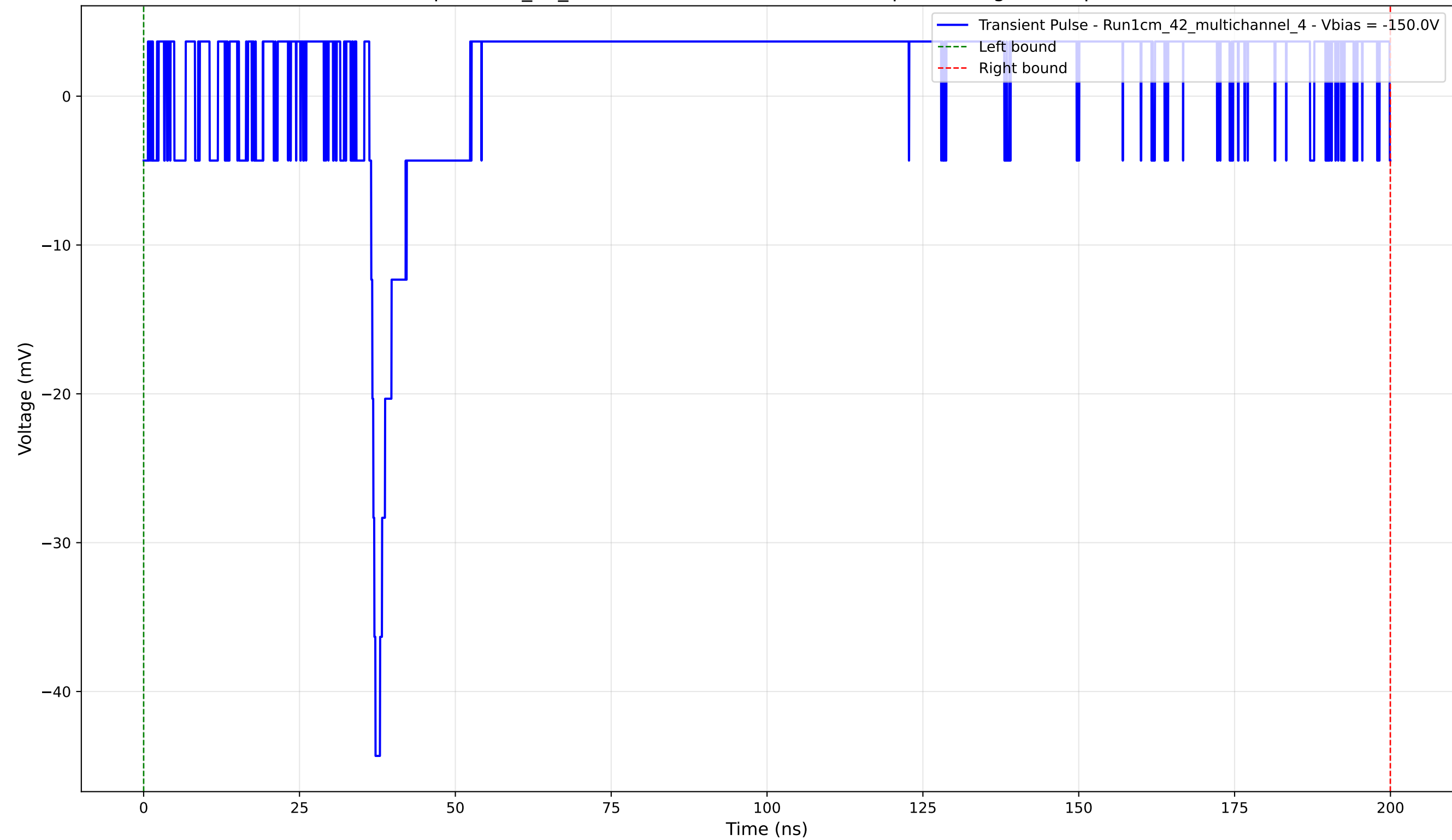
Transient Pulse - Sample: 1cm_42_multichannel - Position: 1955.0 \mu\text{m} - Charge: 6.89 pC - Rise Time: 0.70 ns
