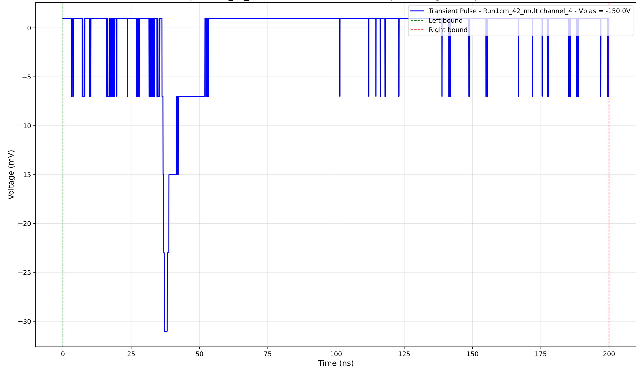
Transient Pulse - Sample: 1cm_42_multichannel - Position: 2955.0 \mu\text{m} - Charge: 1.23 pC - Rise Time: 0.89 ns
