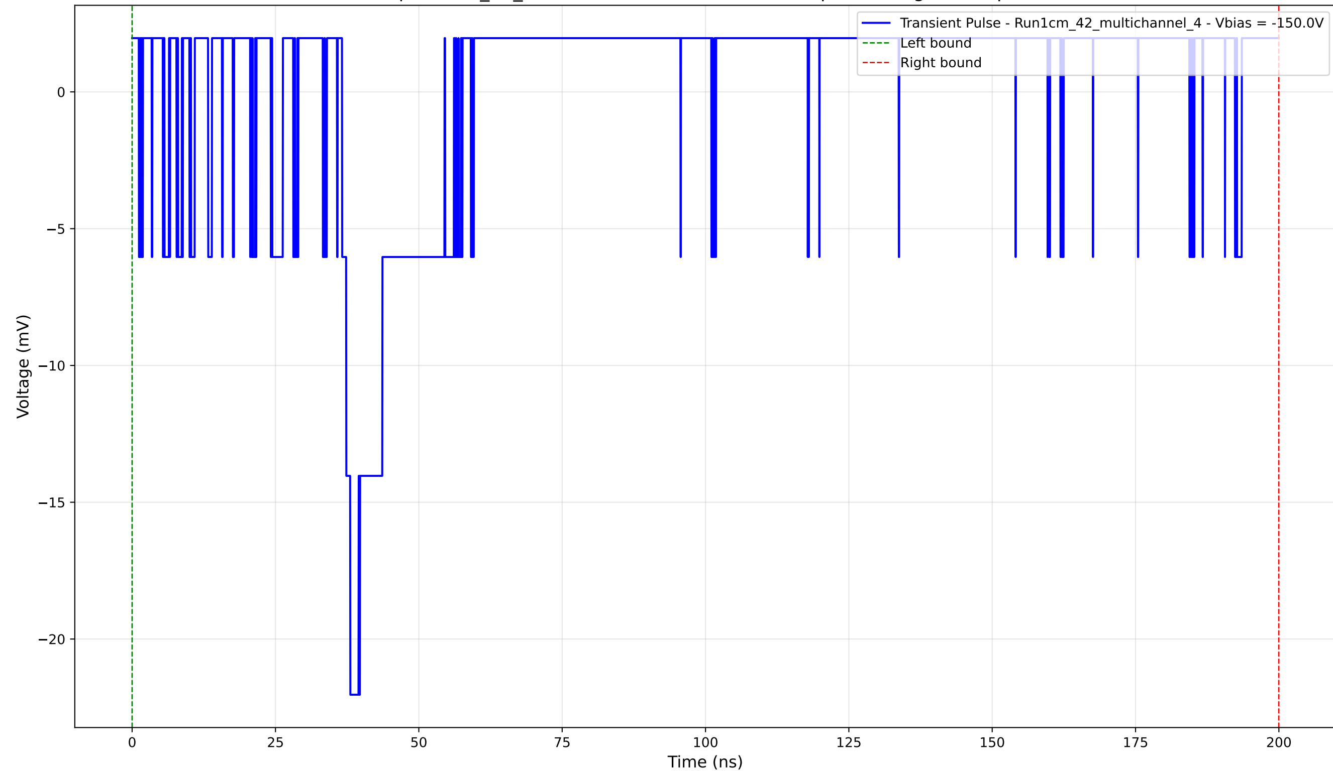
Transient Pulse - Sample: 1cm_42_multichannel - Position: 1130.0 \mu\text{m} - Charge: 1.43 pC - Rise Time: 1.44 ns
