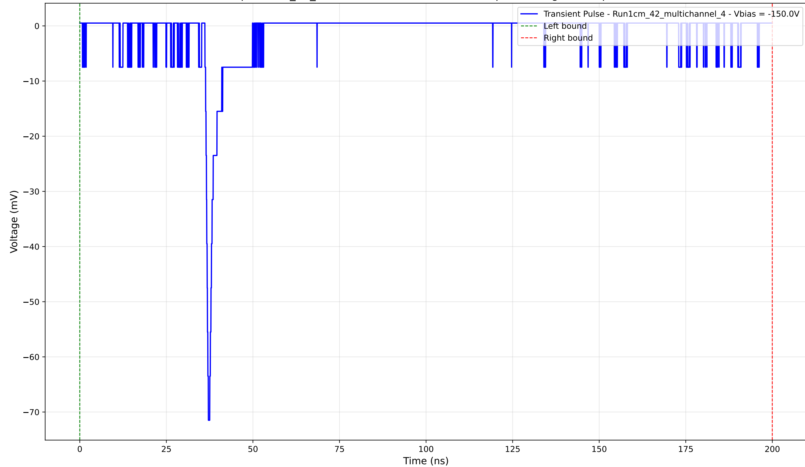
Transient Pulse - Sample: 1cm_42_multichannel - Position: 2195.0 \mu\text{m} - Charge: 4.73 pC - Rise Time: 0.98 ns
