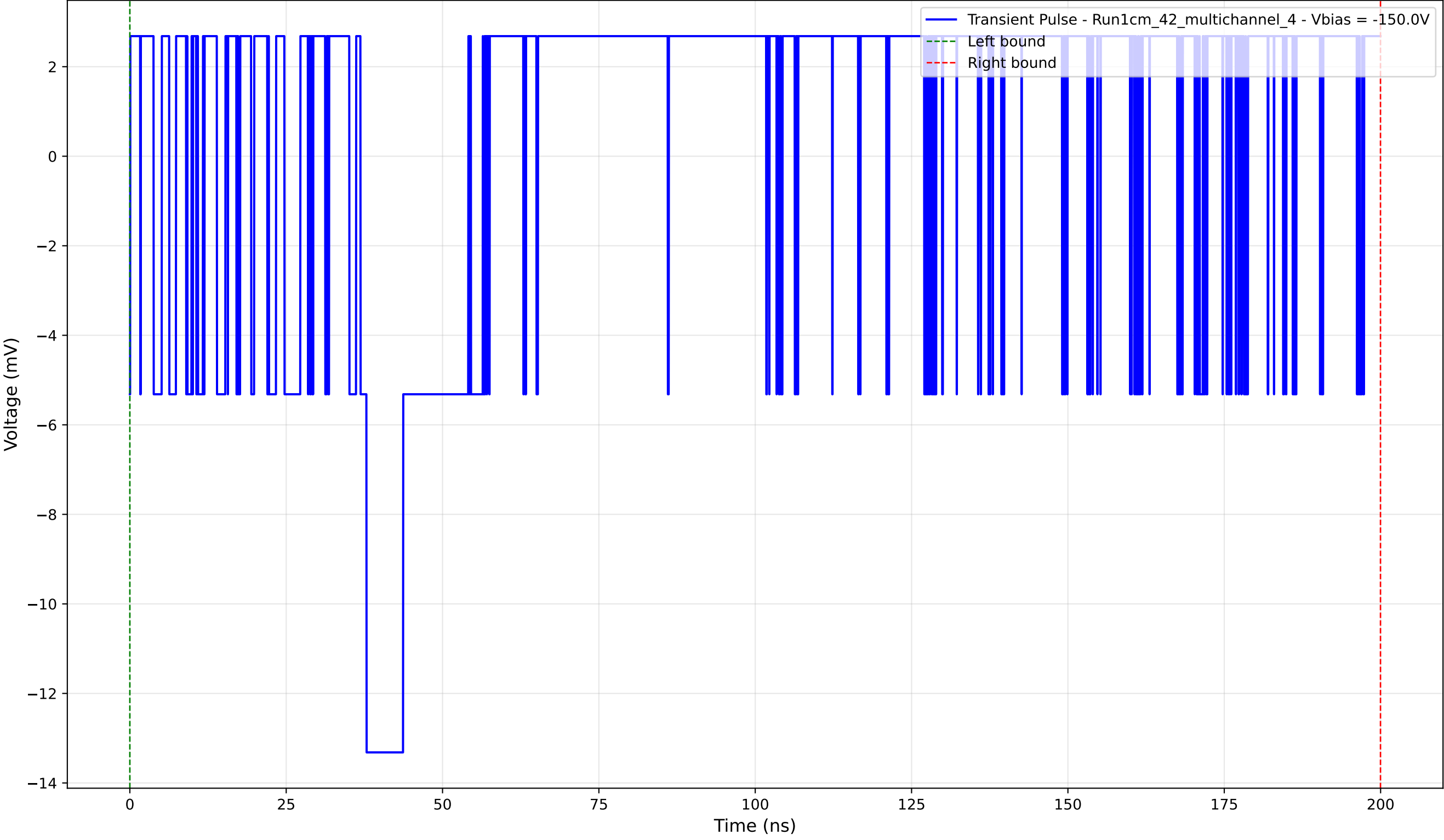
Transient Pulse - Sample: 1cm_42_multichannel - Position: 705.0 \mu\text{m} - Charge: 3.04 pC - Rise Time: 0.00 ns (N/A)
