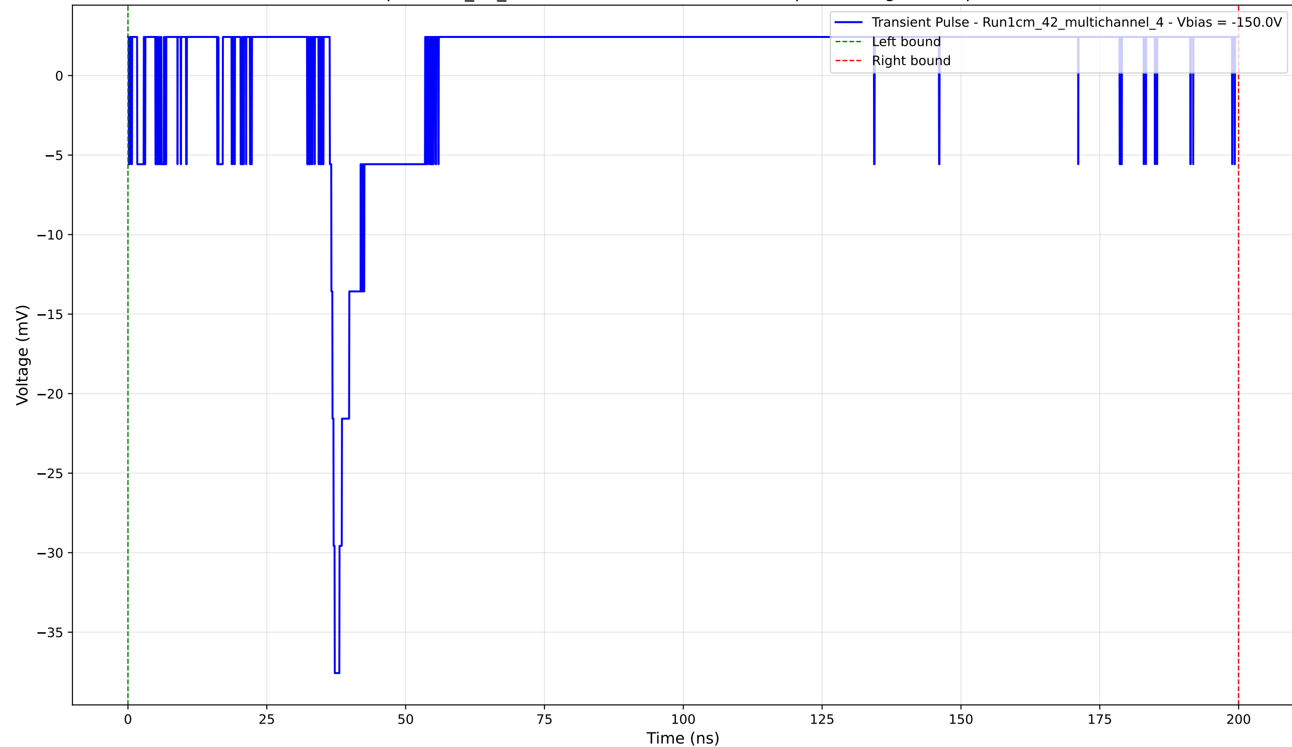
Transient Pulse - Sample: 1cm_42_multichannel - Position: 1805.0 \mu\text{m} - Charge: 3.88 pC - Rise Time: 0.89 ns
