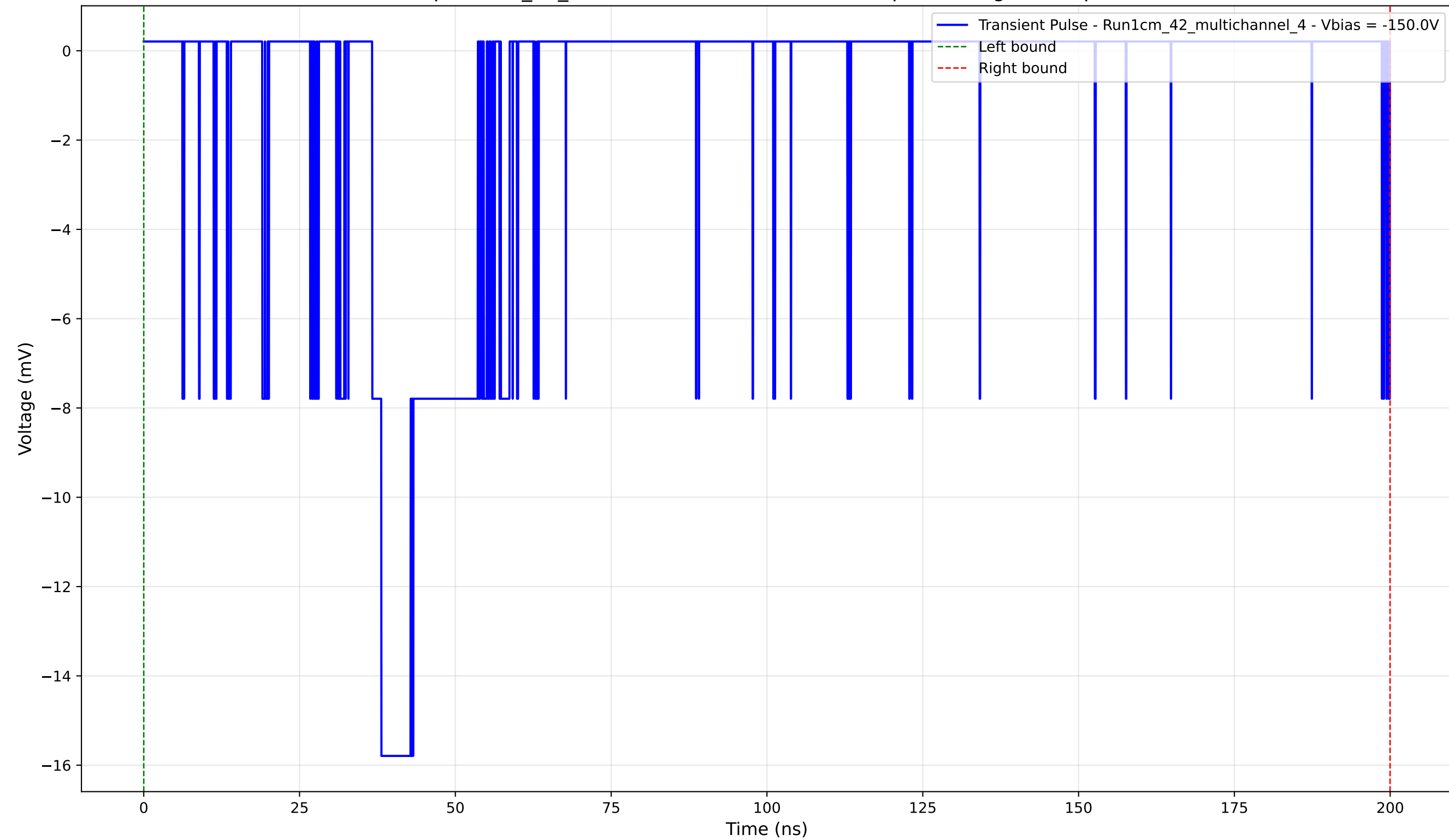
Transient Pulse - Sample: 1cm_42_multichannel - Position: 4125.0 \mu\text{m} - Charge: 4.19 pC - Rise Time: 1.48 ns
