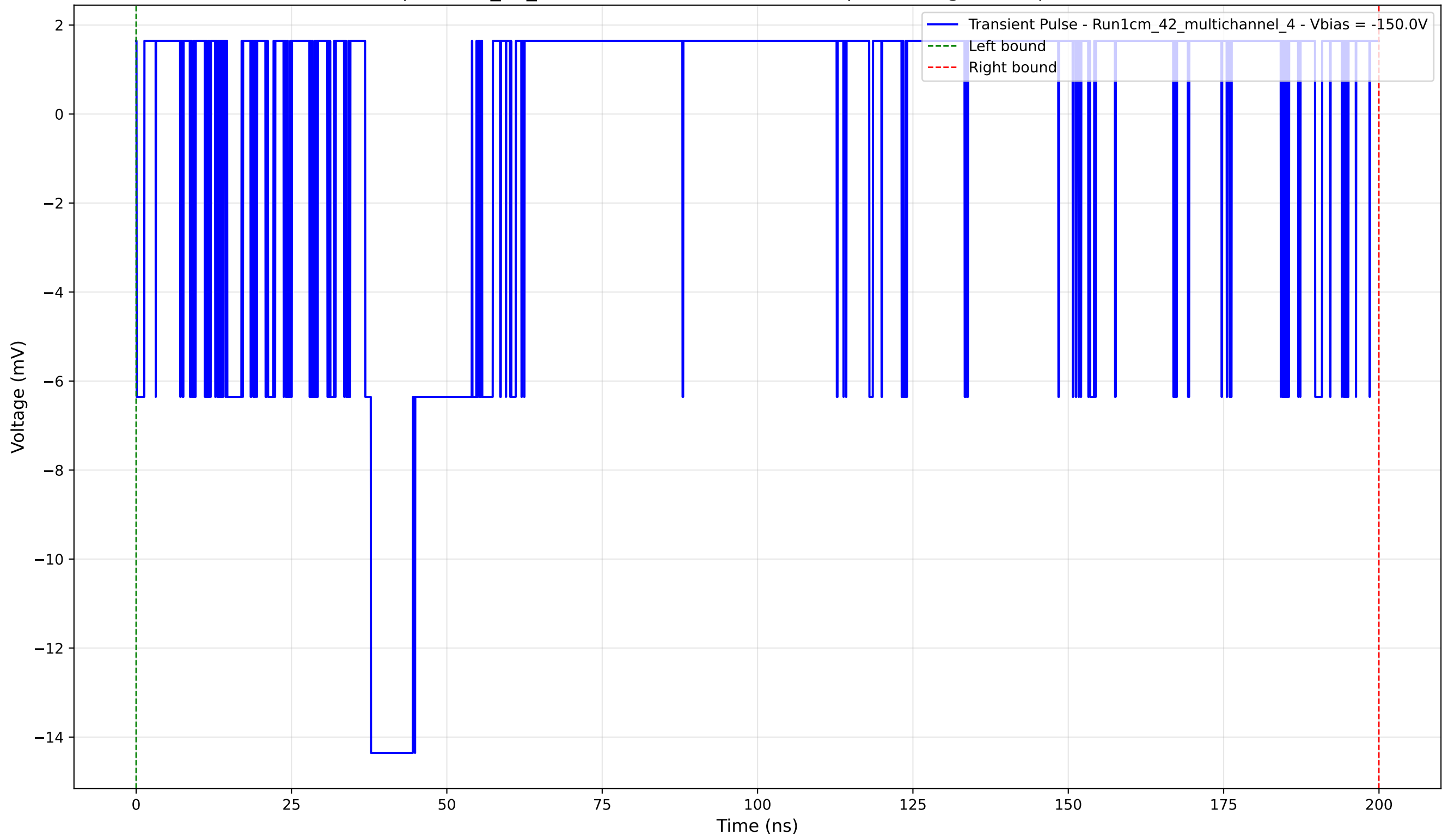
Transient Pulse - Sample: 1cm_42_multichannel - Position: 740.0 \mu\text{m} - Charge: 0.70 pC - Rise Time: 0.00 ns (N/A)
