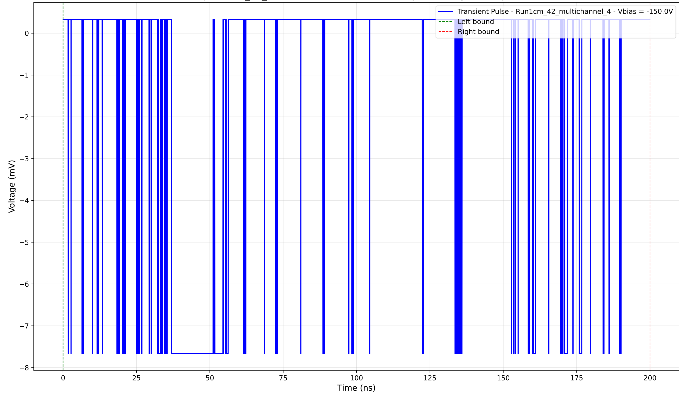
Transient Pulse - Sample: 1cm_42_multichannel - Position: 100.0 \mu\text{m} - Charge: 3.42 pC - Rise Time: 0.02 ns
