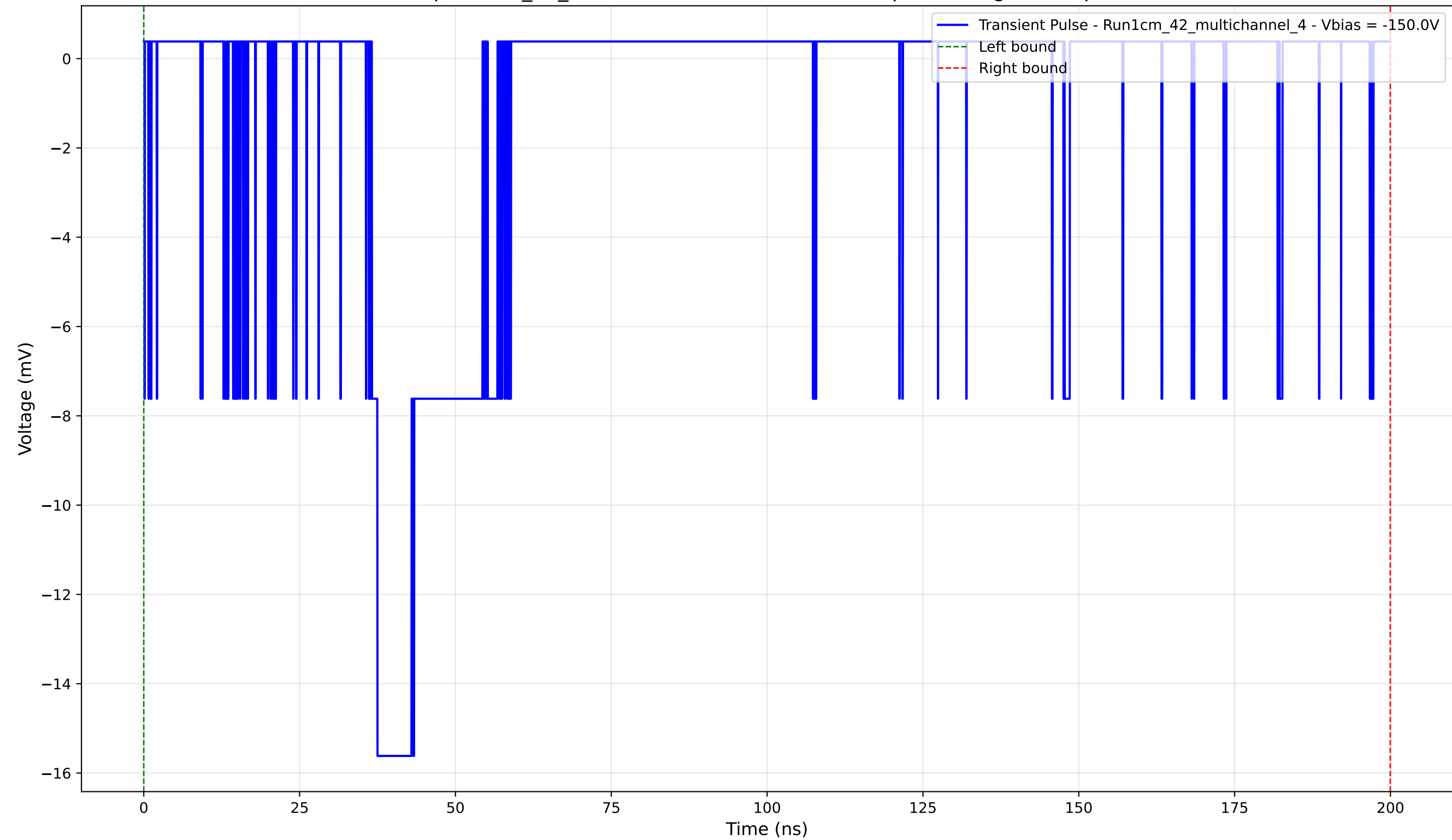
Transient Pulse - Sample: 1cm_42_multichannel - Position: 3620.0 \mu\text{m} - Charge: 3.70 pC - Rise Time: 0.90 ns
