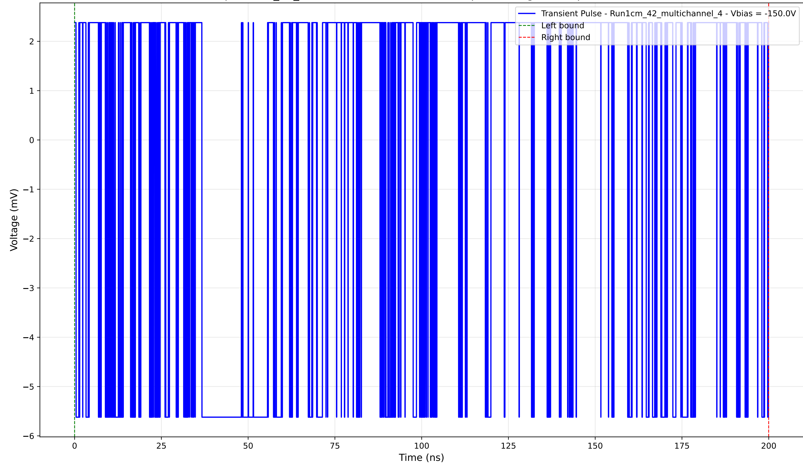
Transient Pulse - Sample: 1cm_42_multichannel - Position: 825.0 \mu\text{m} - Charge: 0.17 pC - Rise Time: 0.00 ns (N/A)
