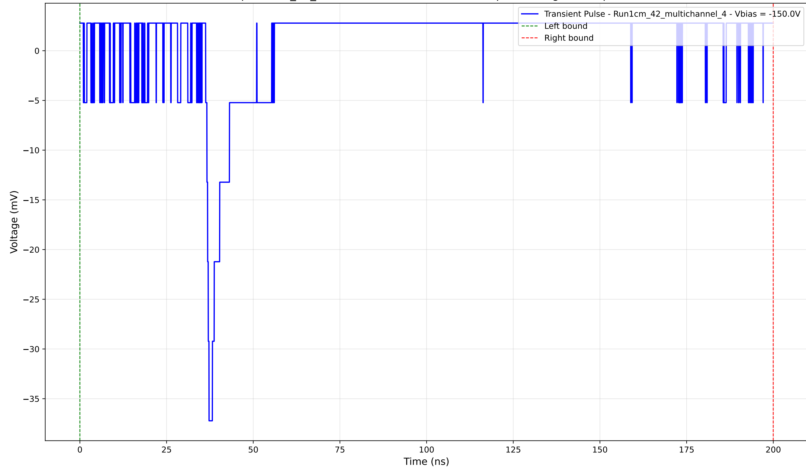
Transient Pulse - Sample: 1cm_42_multichannel - Position: 1755.0 \mu\text{m} - Charge: 3.94 pC - Rise Time: 0.97 ns
