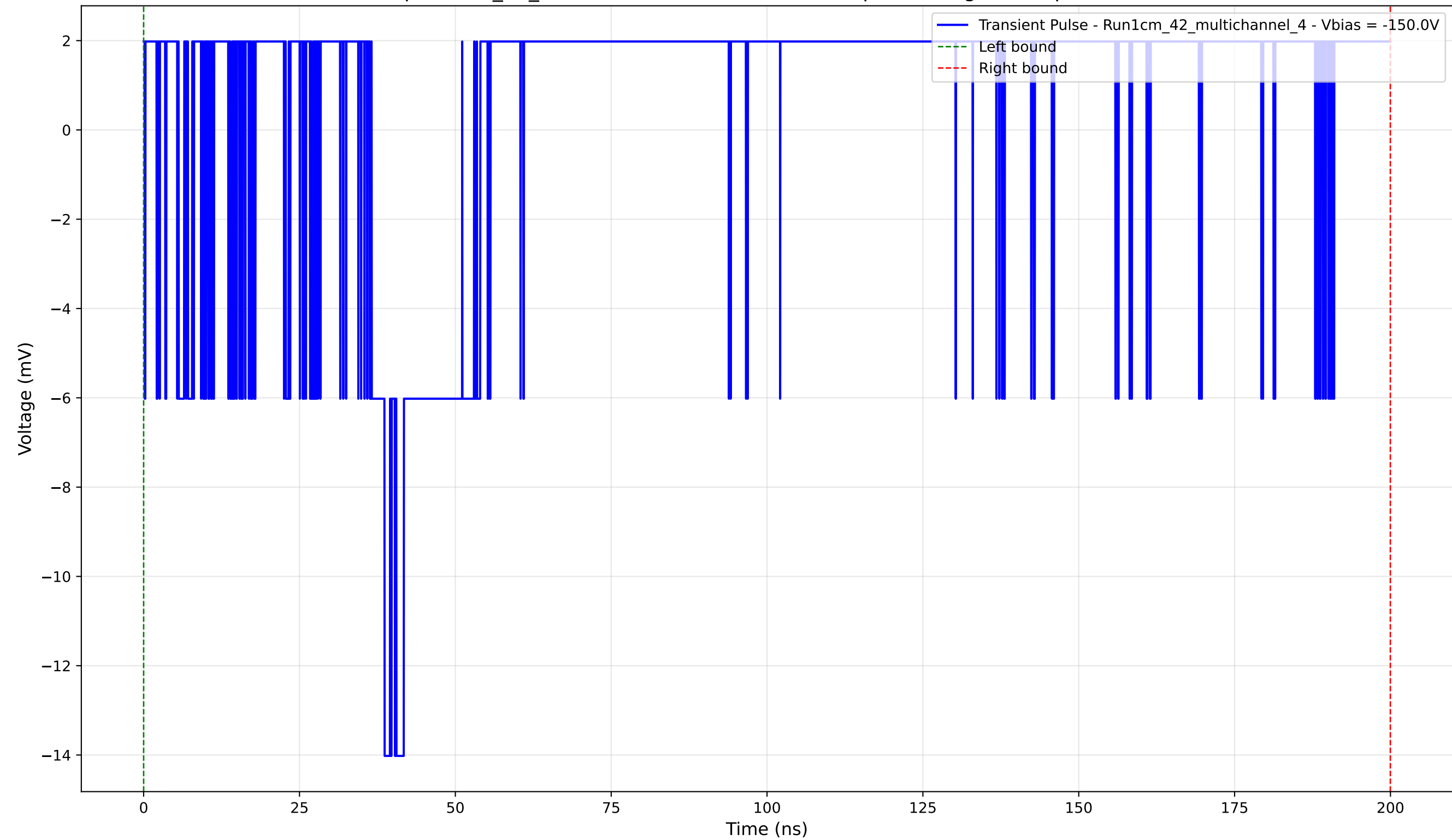
Transient Pulse - Sample: 1cm_42_multichannel - Position: 4820.0 \mu\text{m} - Charge: 3.26 pC - Rise Time: 0.00 ns (N/A)
