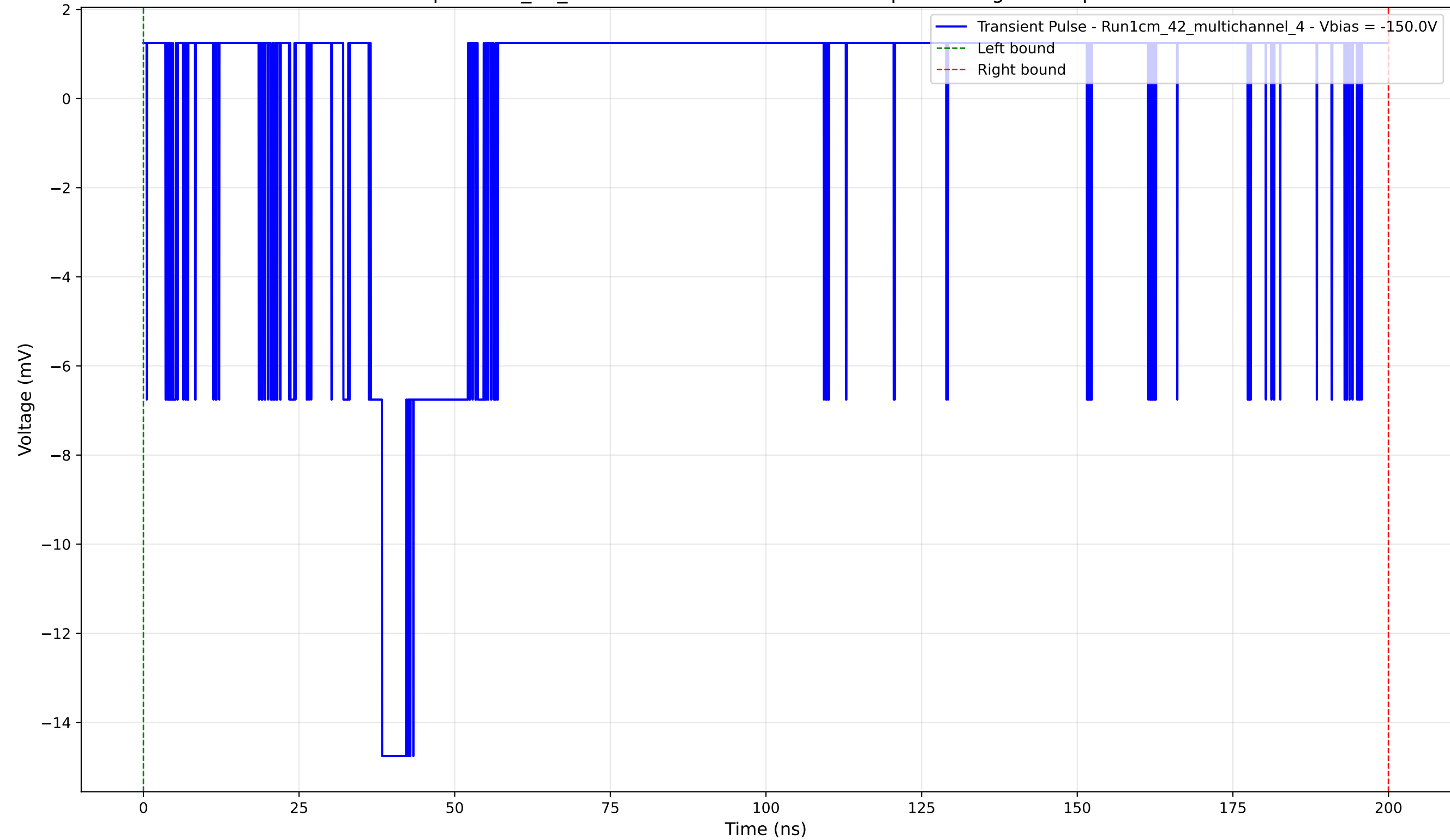
Transient Pulse - Sample: 1cm_42_multichannel - Position: 4575.0 \mu\text{m} - Charge: 0.05 pC - Rise Time: 1.82 ns
