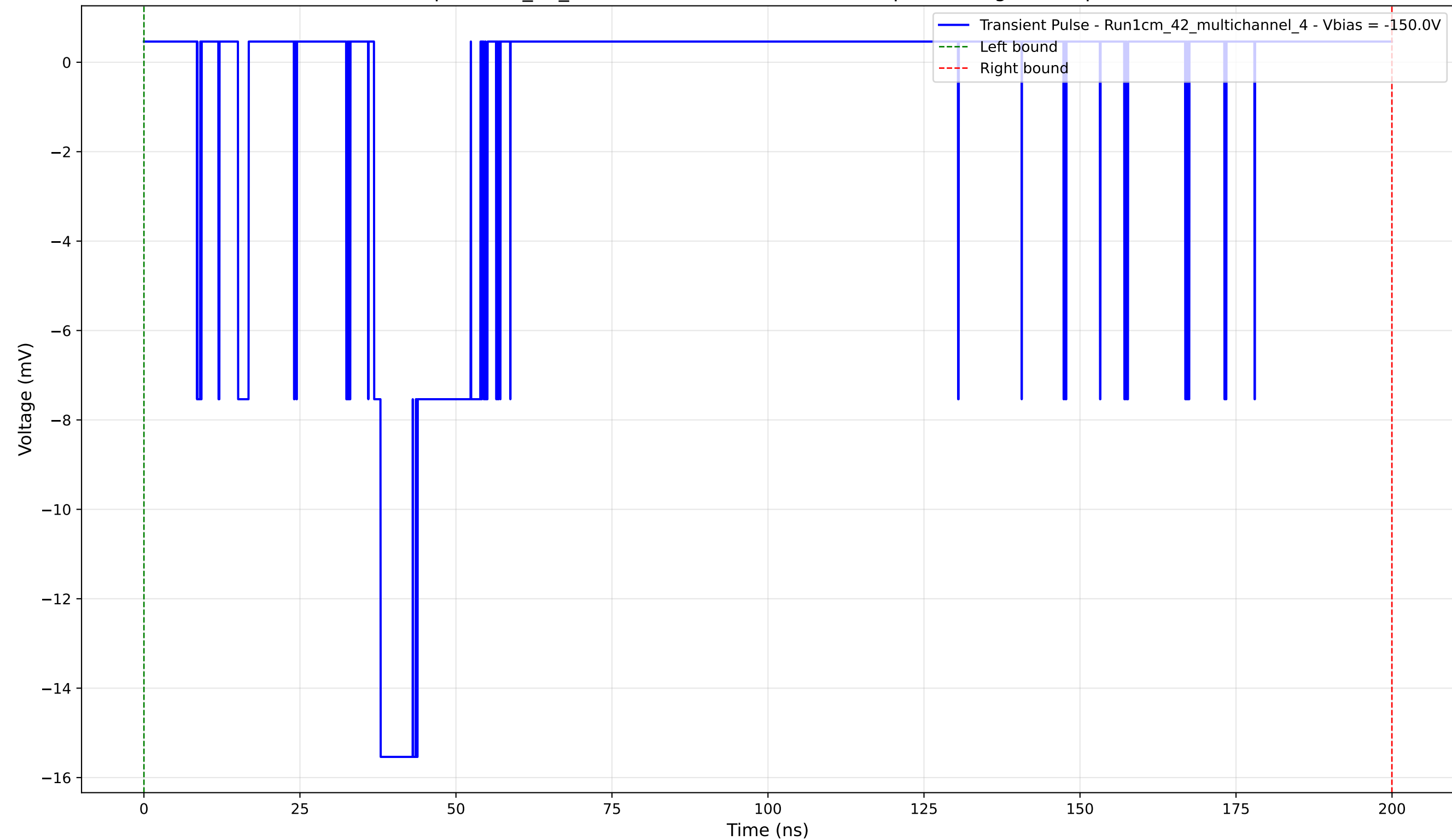
Transient Pulse - Sample: 1cm_42_multichannel - Position: 4005.0 \mu\text{m} - Charge: 2.69 pC - Rise Time: 1.06 ns
