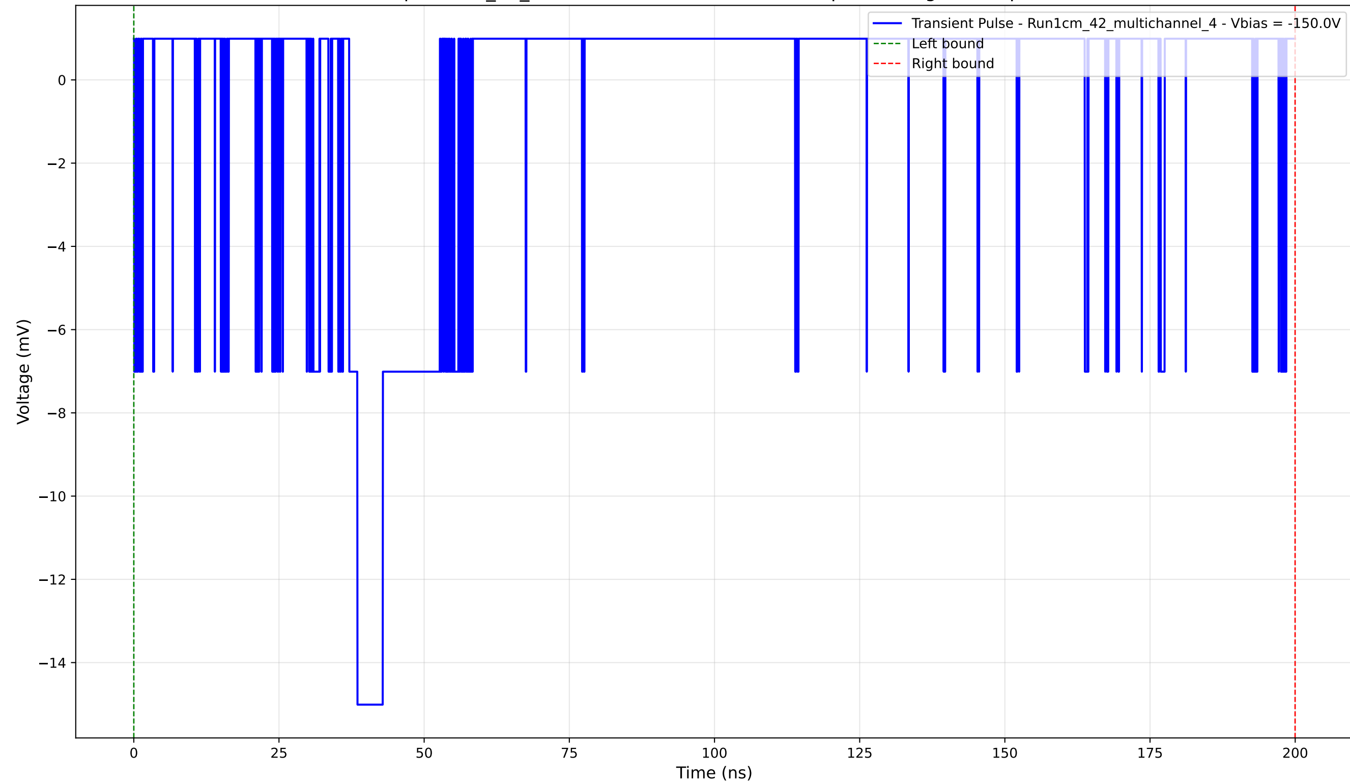
Transient Pulse - Sample: 1cm_42_multichannel - Position: 4315.0 \mu\text{m} - Charge: 1.56 pC - Rise Time: 1.42 ns
