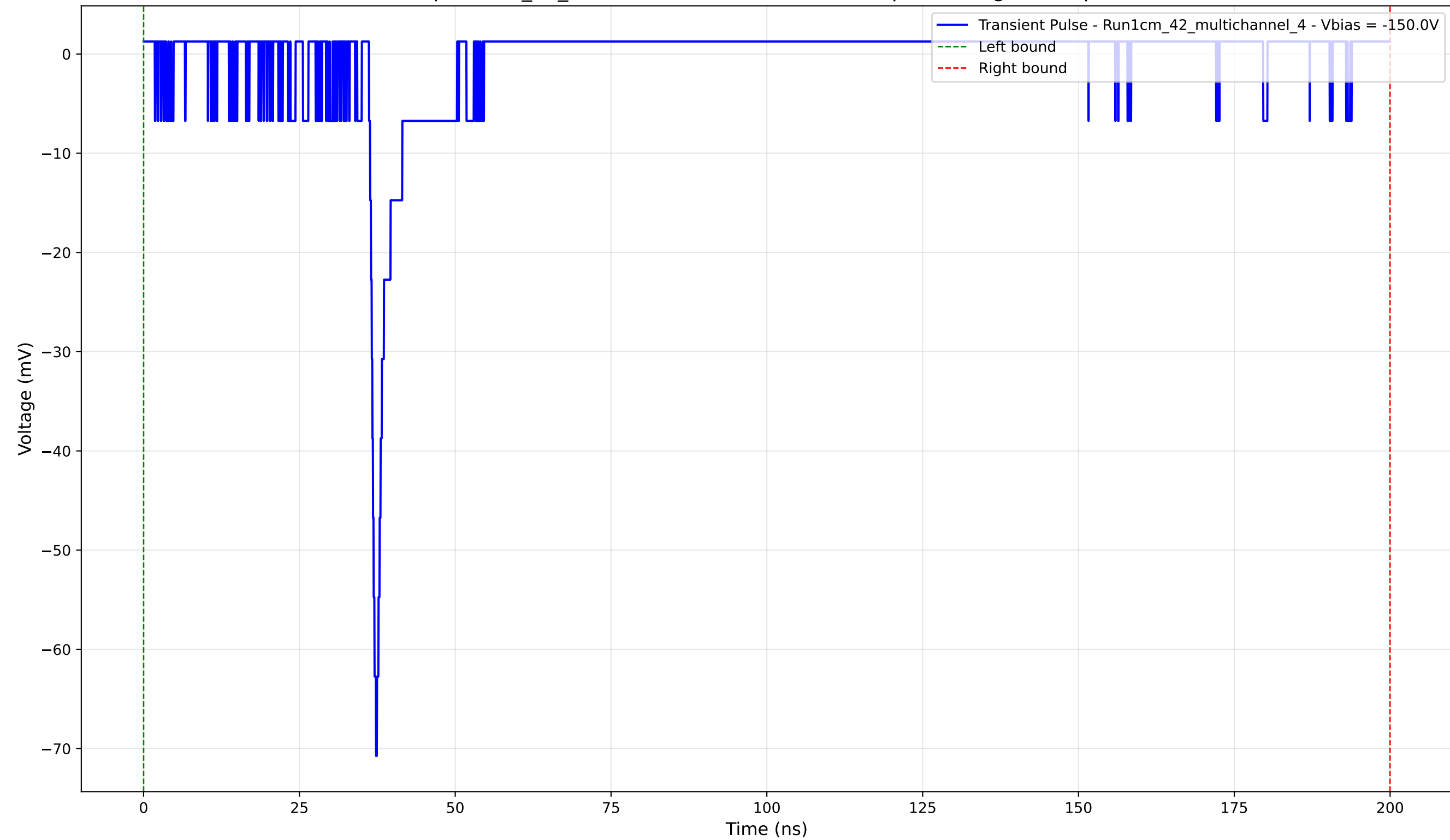
Transient Pulse - Sample: 1cm_42_multichannel - Position: 2165.0 \mu\text{m} - Charge: 1.80 pC - Rise Time: 0.96 ns
