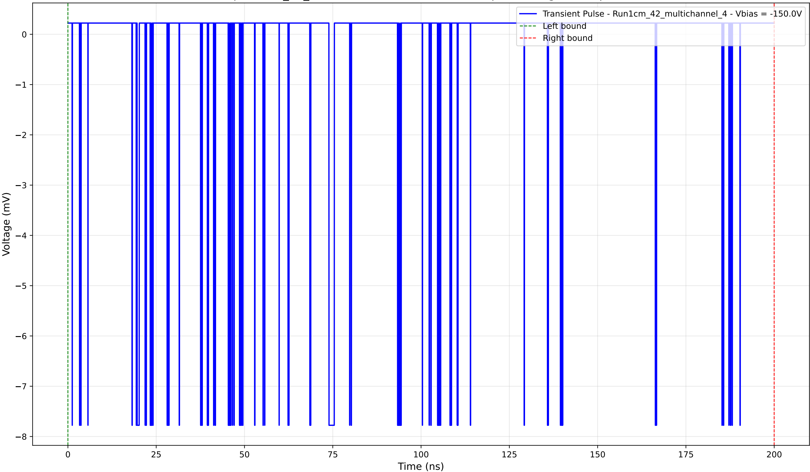
Transient Pulse - Sample: 1cm_42_multichannel - Position: 3915.0 \mu\text{m} - Charge: 0.58 pC - Rise Time: 0.02 ns
