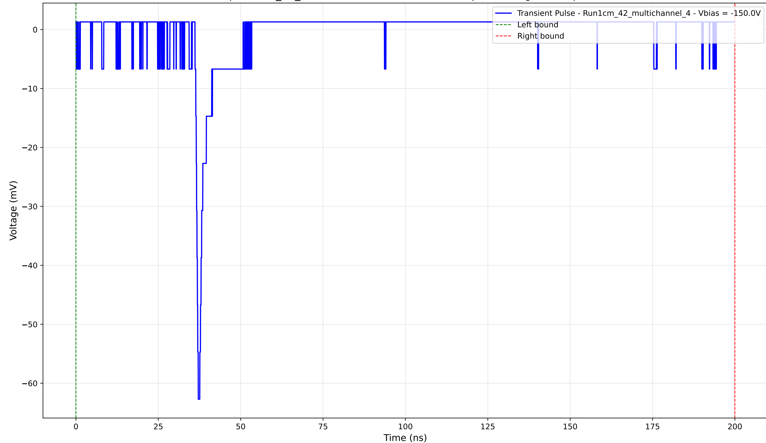
Transient Pulse - Sample: 1cm_42_multichannel - Position: 2610.0 \mu\text{m} - Charge: 0.87 pC - Rise Time: 0.98 ns
