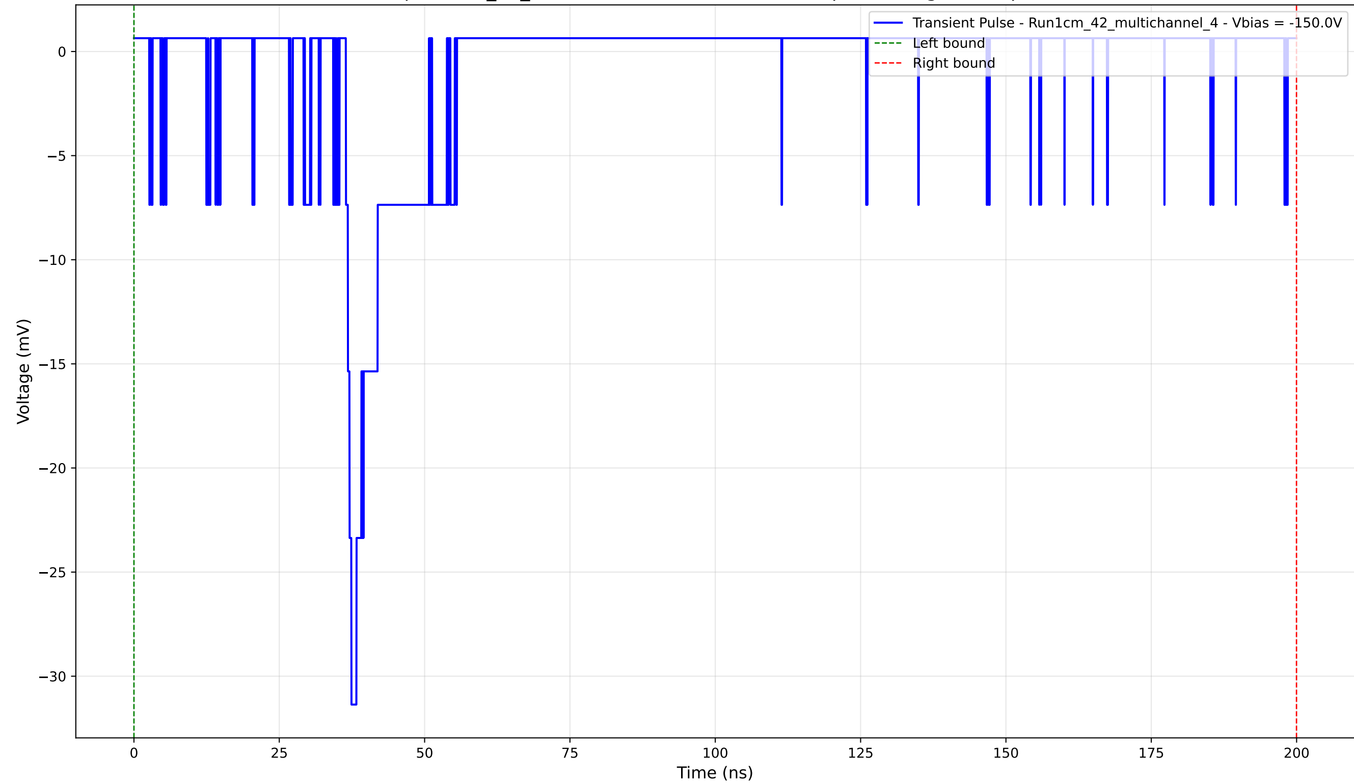
Transient Pulse - Sample: 1cm_42_multichannel - Position: 3120.0 \mu\text{m} - Charge: 2.65 pC - Rise Time: 0.95 ns
