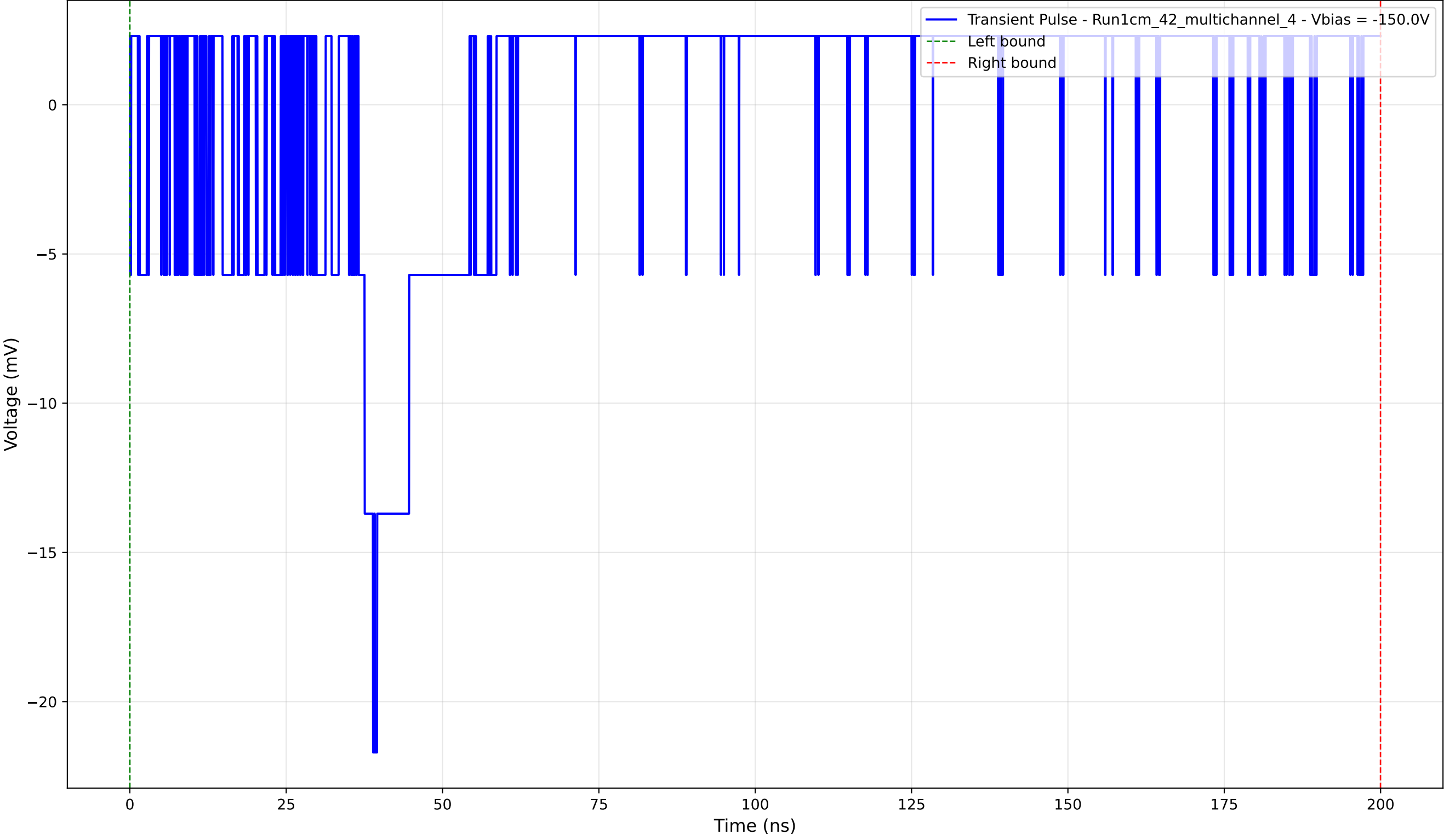
Transient Pulse - Sample: 1cm_42_multichannel - Position: 950.0 \mu\text{m} - Charge: 1.30 pC - Rise Time: 0.00 ns (N/A)
