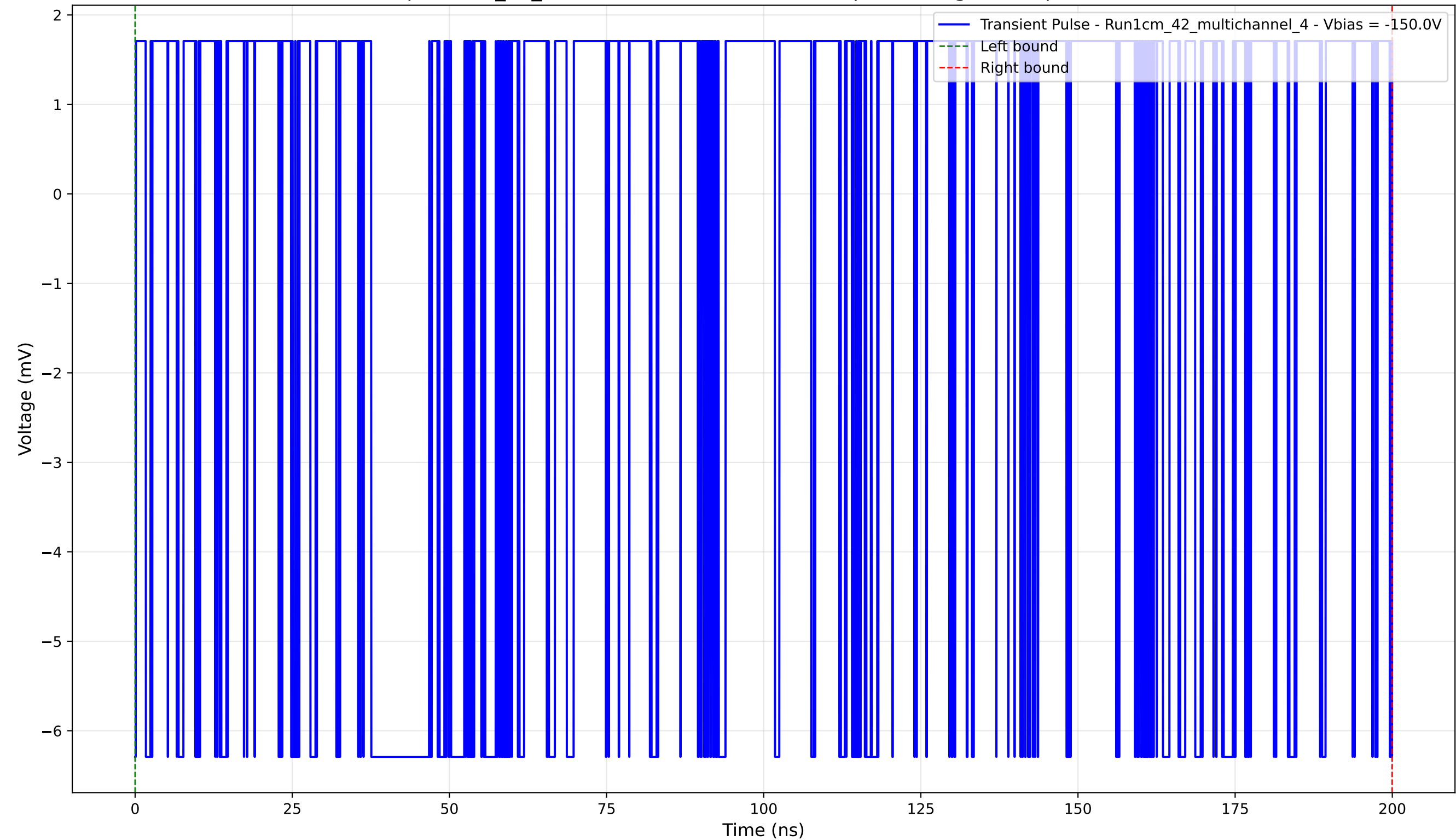
Transient Pulse - Sample: 1cm_42_multichannel - Position: 905.0 \mu\text{m} - Charge: 0.80 pC - Rise Time: 0.00 ns (N/A)
