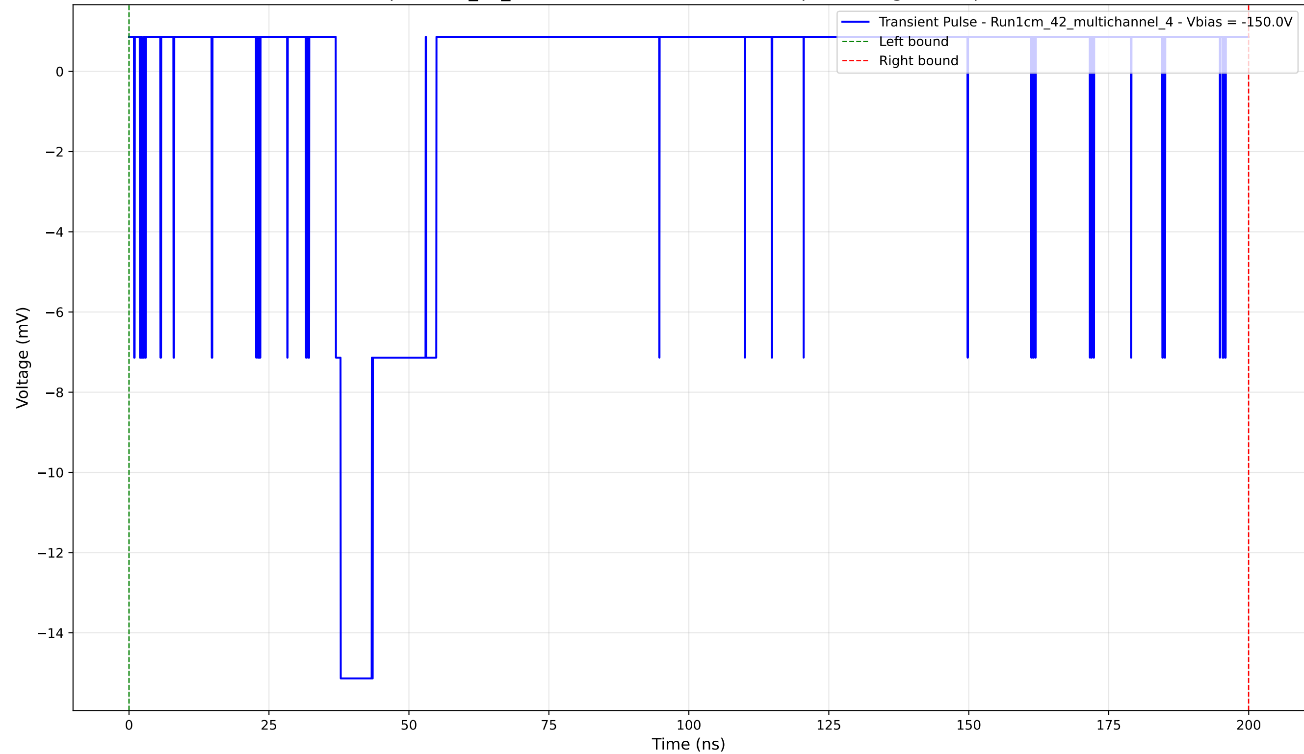
Transient Pulse - Sample: 1cm_42_multichannel - Position: 3820.0 \mu\text{m} - Charge: 0.86 pC - Rise Time: 0.88 ns
