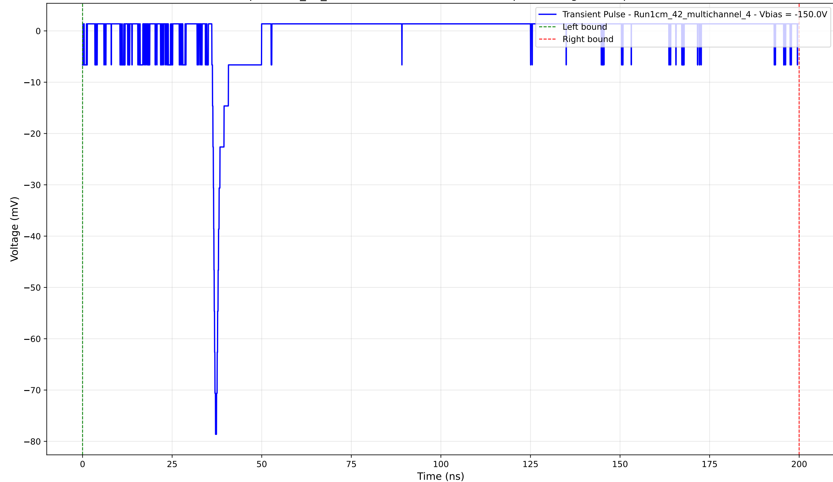
Transient Pulse - Sample: 1cm_42_multichannel - Position: 2310.0 \mu\text{m} - Charge: 0.98 pC - Rise Time: 0.86 ns
