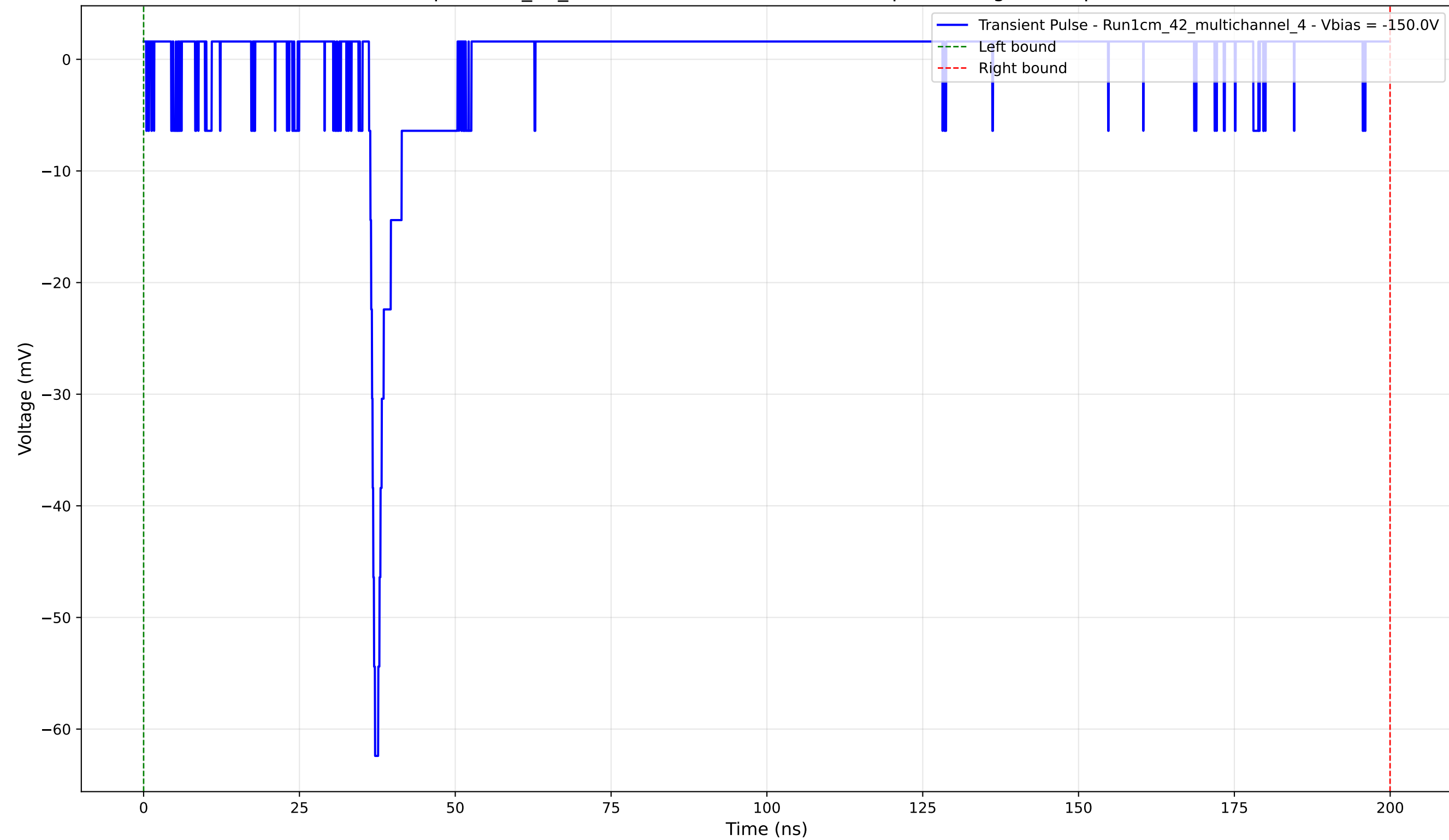
Transient Pulse - Sample: 1cm_42_multichannel - Position: 2145.0 \mu\text{m} - Charge: 0.23 pC - Rise Time: 0.96 ns
