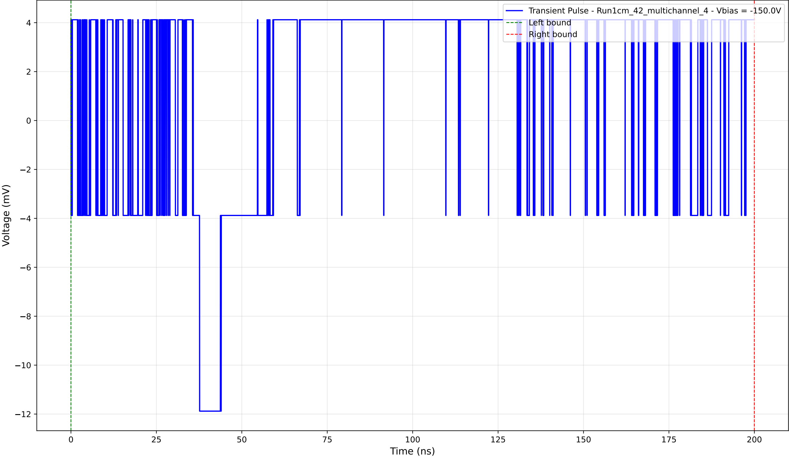
Transient Pulse - Sample: 1cm_42_multichannel - Position: 935.0 \mu\text{m} - Charge: 7.38 pC - Rise Time: 0.00 ns (N/A)
