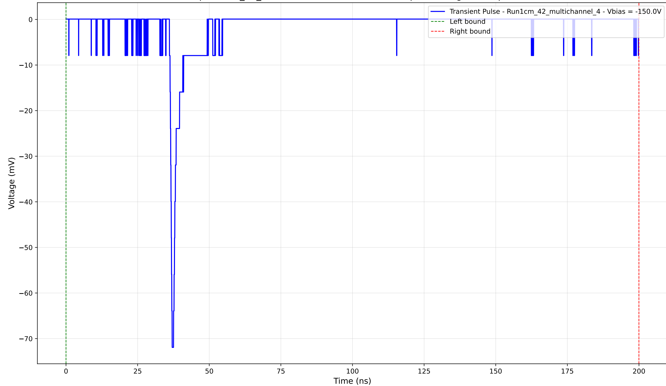
Transient Pulse - Sample: 1cm_42_multichannel - Position: 2550.0 \mu\text{m} - Charge: 5.31 pC - Rise Time: 0.94 ns
