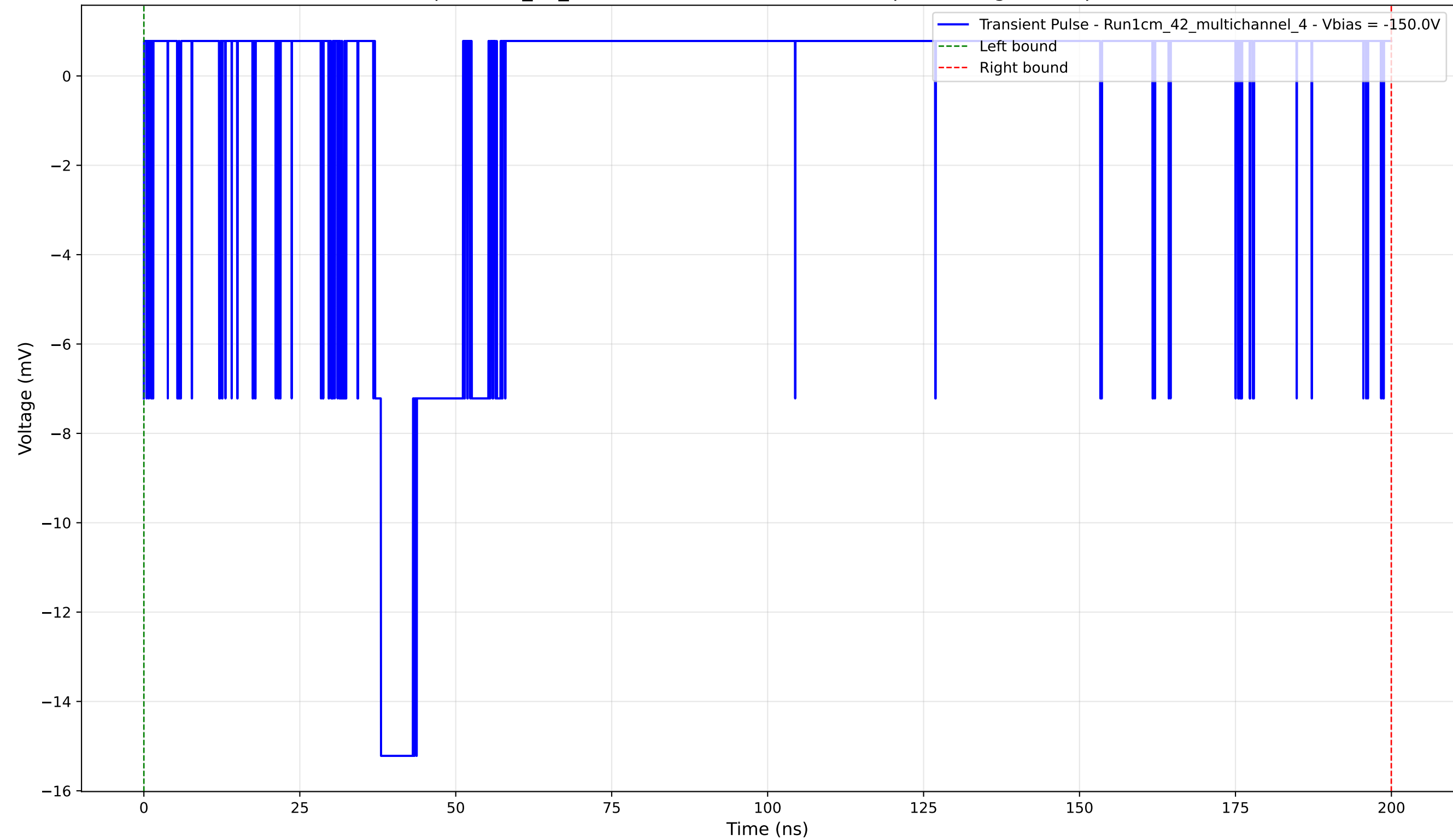
Transient Pulse - Sample: 1cm_42_multichannel - Position: 4010.0 \mu\text{m} - Charge: 1.53 pC - Rise Time: 0.96 ns
