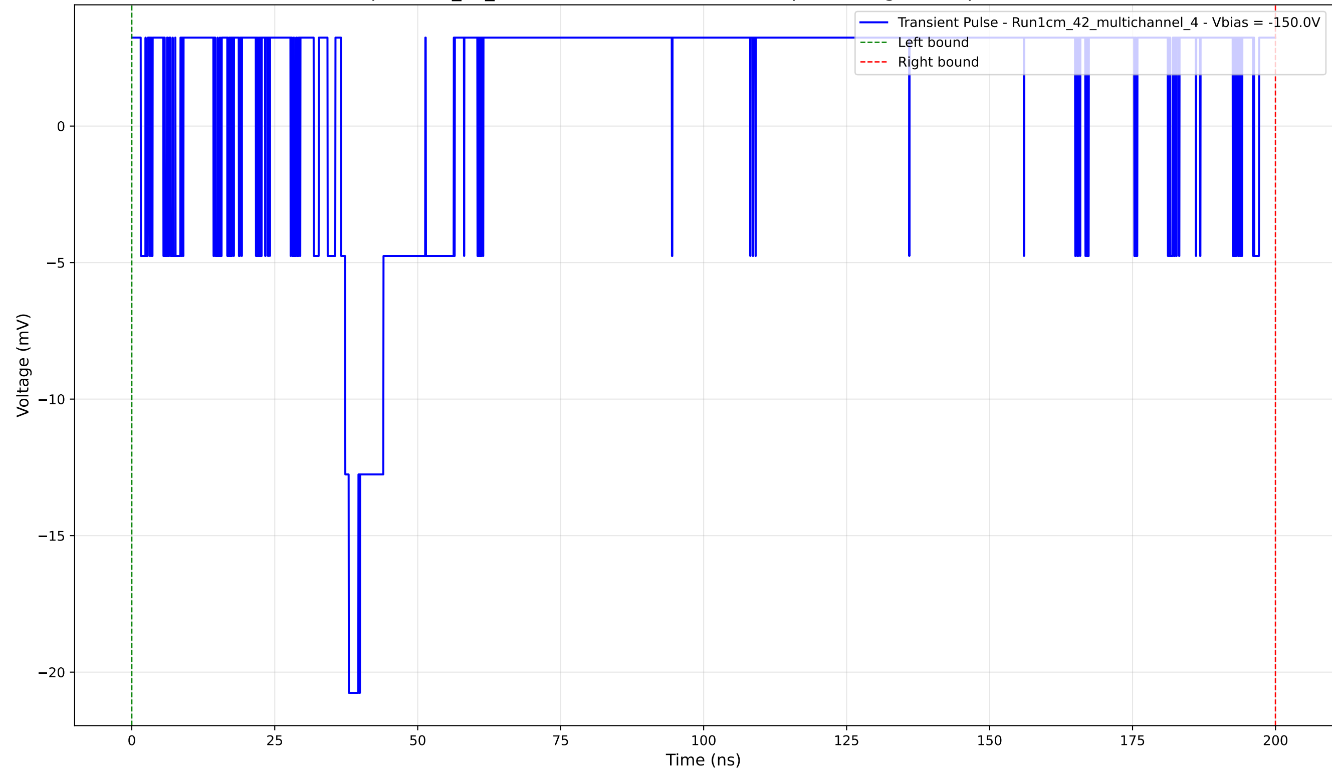
Transient Pulse - Sample: 1cm_42_multichannel - Position: 1095.0 \mu\text{m} - Charge: 6.07 pC - Rise Time: 0.00 ns (N/A)
