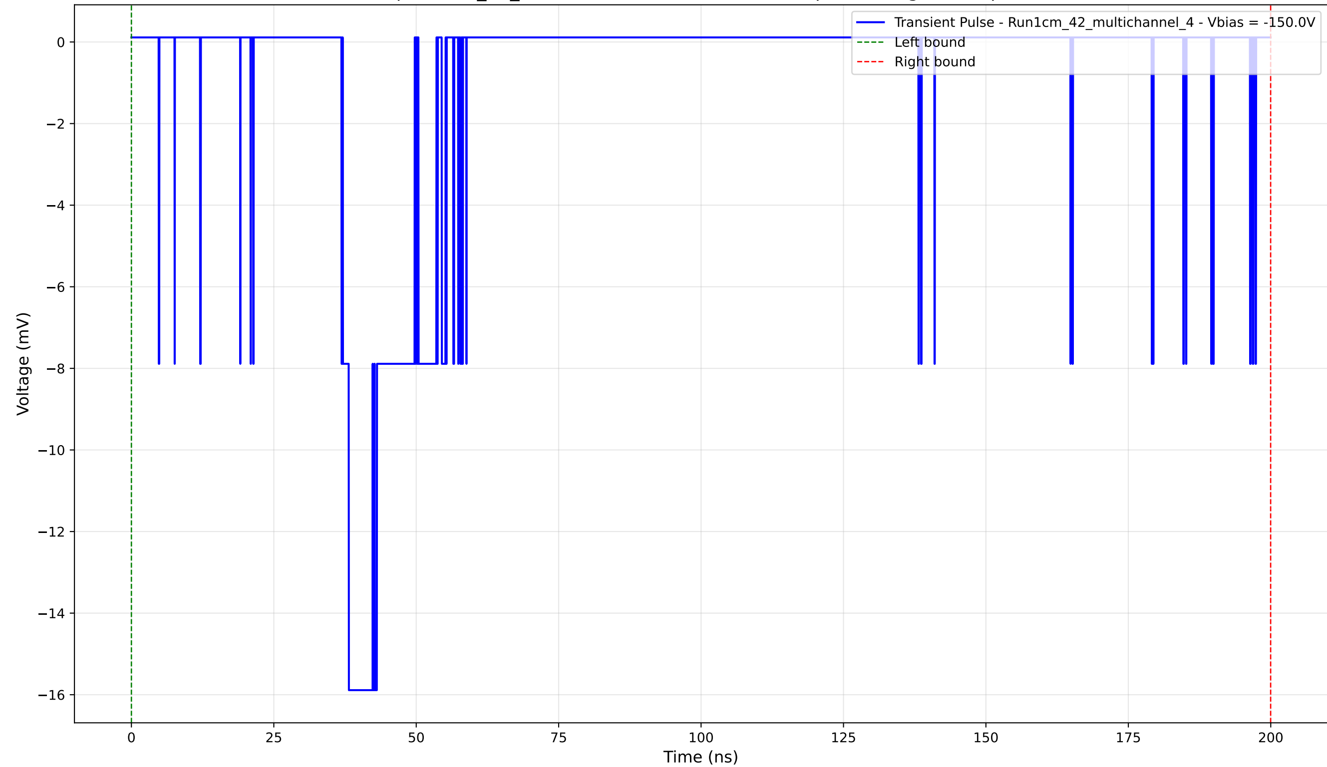
Transient Pulse - Sample: 1cm_42_multichannel - Position: 4060.0 \mu\text{m} - Charge: 3.42 pC - Rise Time: 1.06 ns
