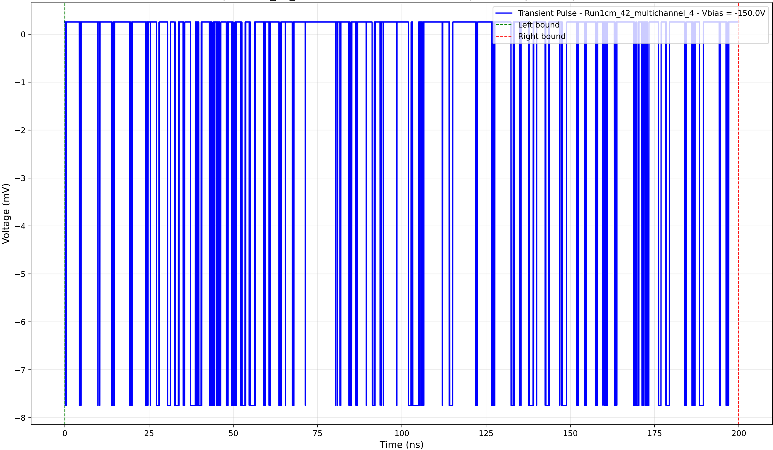
Transient Pulse - Sample: 1cm_42_multichannel - Position: 1875.0 \mu\text{m} - Charge: 4.63 pC - Rise Time: 0.02 ns
