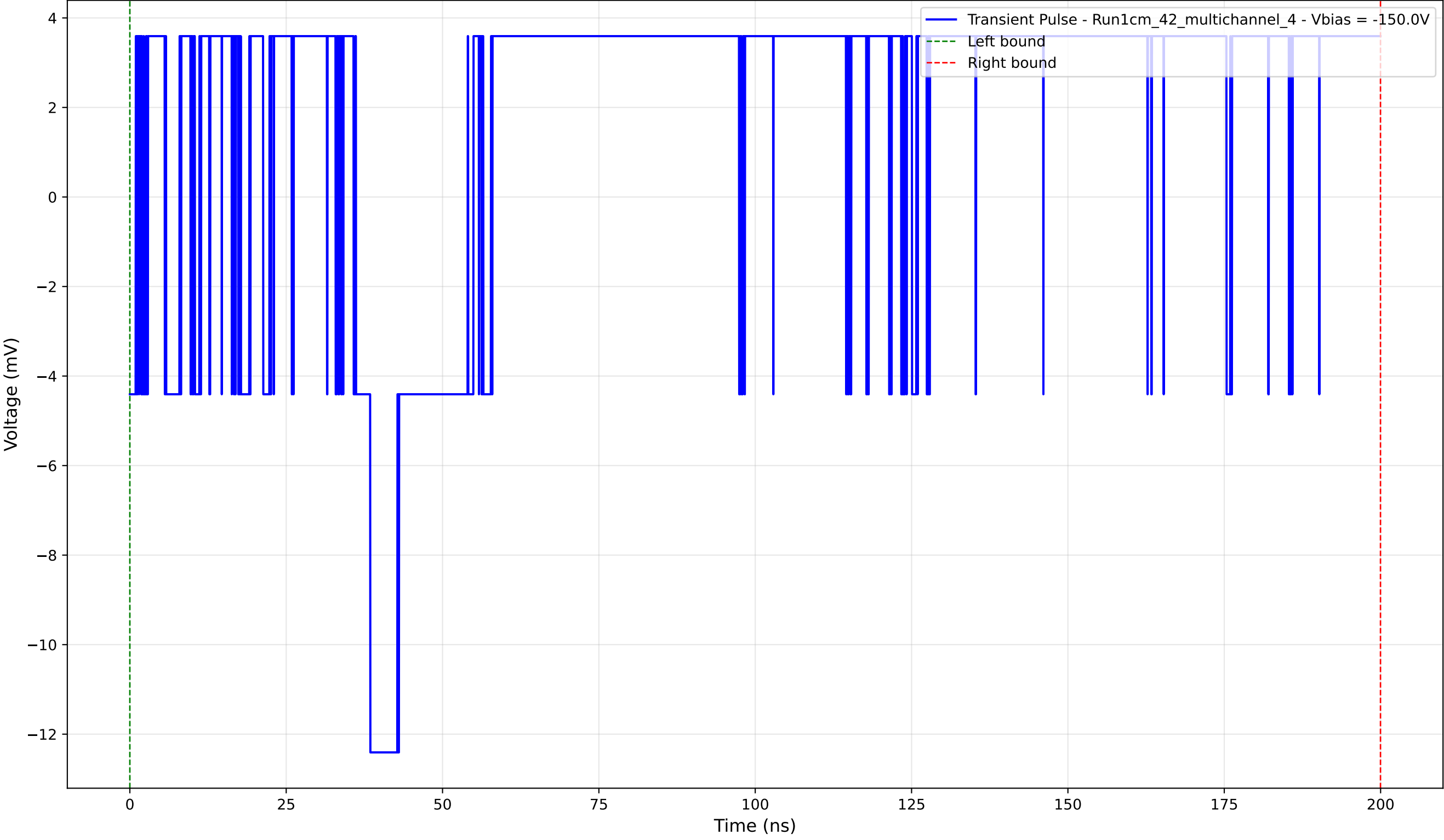
Transient Pulse - Sample: 1cm_42_multichannel - Position: 160.0 \mu\text{m} - Charge: 8.18 pC - Rise Time: 0.00 ns (N/A)
