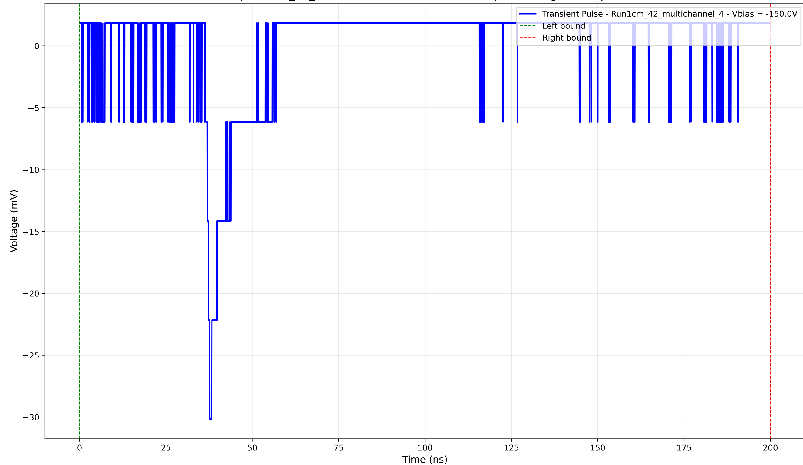
Transient Pulse - Sample: 1cm_42_multichannel - Position: 3275.0 \mu\text{m} - Charge: 1.09 pC - Rise Time: 1.19 ns
