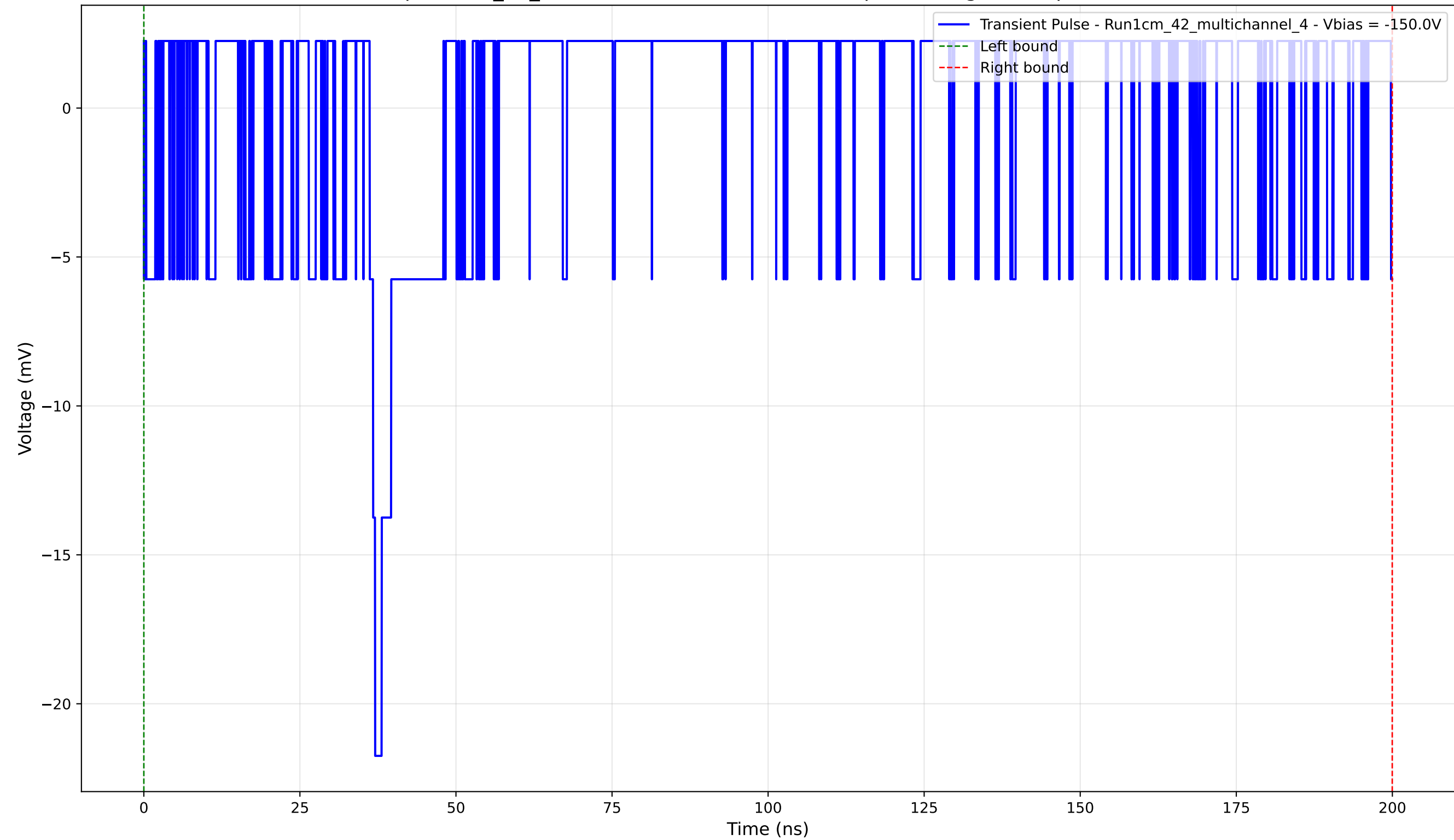
Transient Pulse - Sample: 1cm_42_multichannel - Position: 1930.0 \mu\text{m} - Charge: 1.64 pC - Rise Time: 0.00 ns (N/A)
