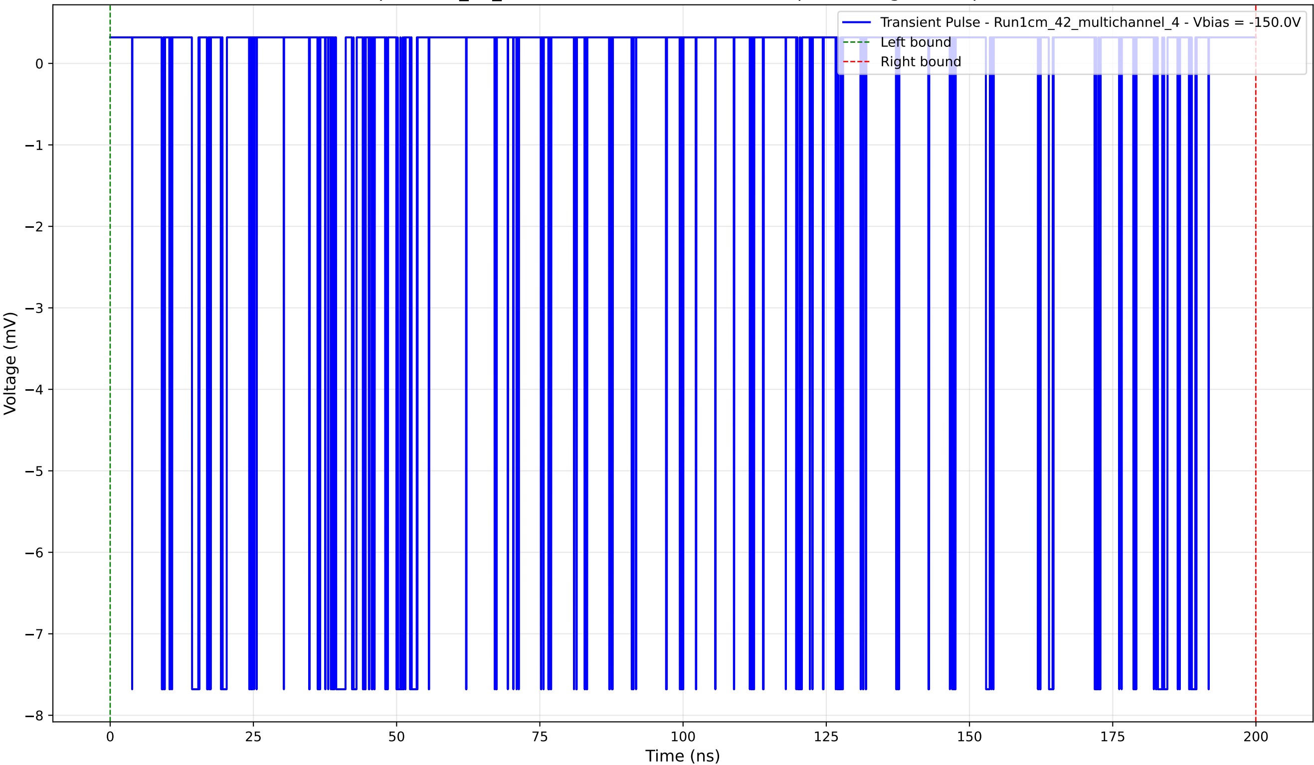
Transient Pulse - Sample: 1cm_42_multichannel - Position: 3920.0 \mu\text{m} - Charge: 2.19 pC - Rise Time: 0.02 ns
