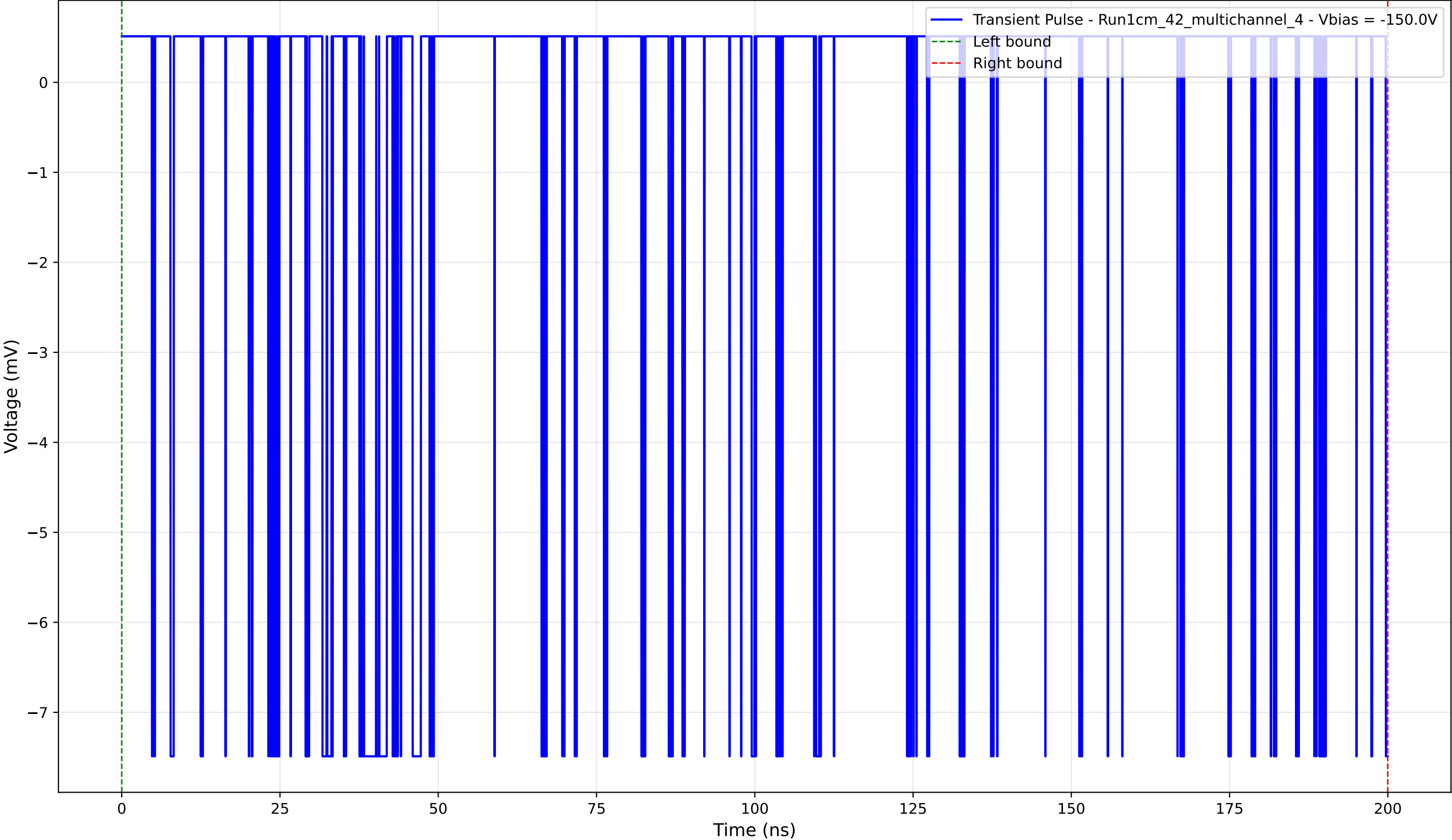
Transient Pulse - Sample: 1cm_42_multichannel - Position: 3930.0 \mu\text{m} - Charge: 1.06 pC - Rise Time: 0.02 ns
