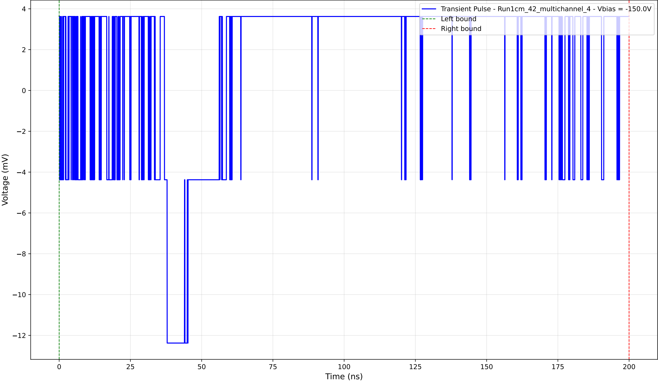
Transient Pulse - Sample: 1cm_42_multichannel - Position: 670.0 \mu\text{m} - Charge: 6.88 pC - Rise Time: 0.00 ns (N/A)
