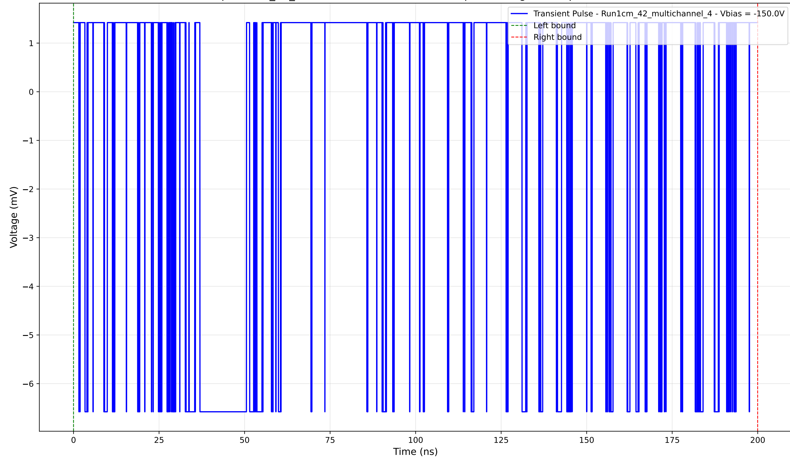
Transient Pulse - Sample: 1cm_42_multichannel - Position: 105.0 \mu\text{m} - Charge: 1.10 pC - Rise Time: 0.00 ns (N/A)
