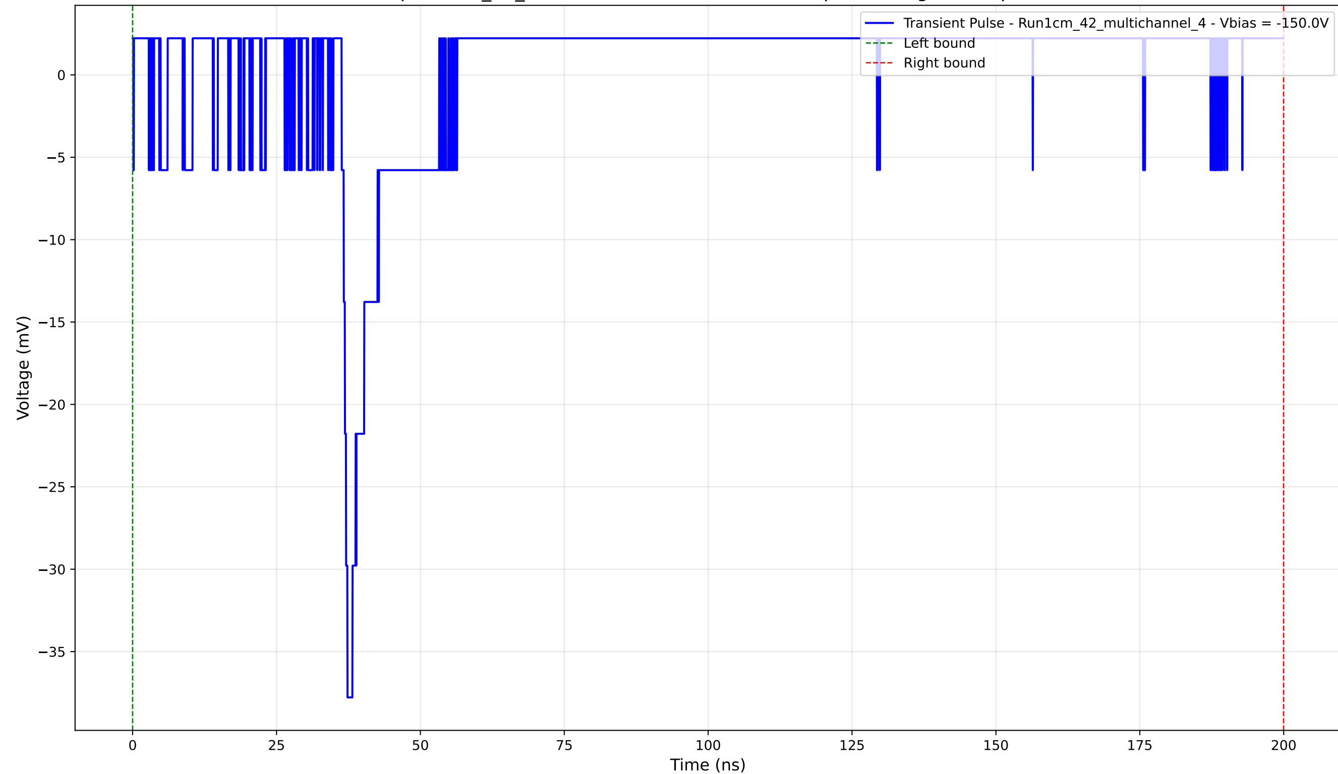
Transient Pulse - Sample: 1cm_42_multichannel - Position: 1740.0 \mu\text{m} - Charge: 2.26 pC - Rise Time: 1.01 ns
