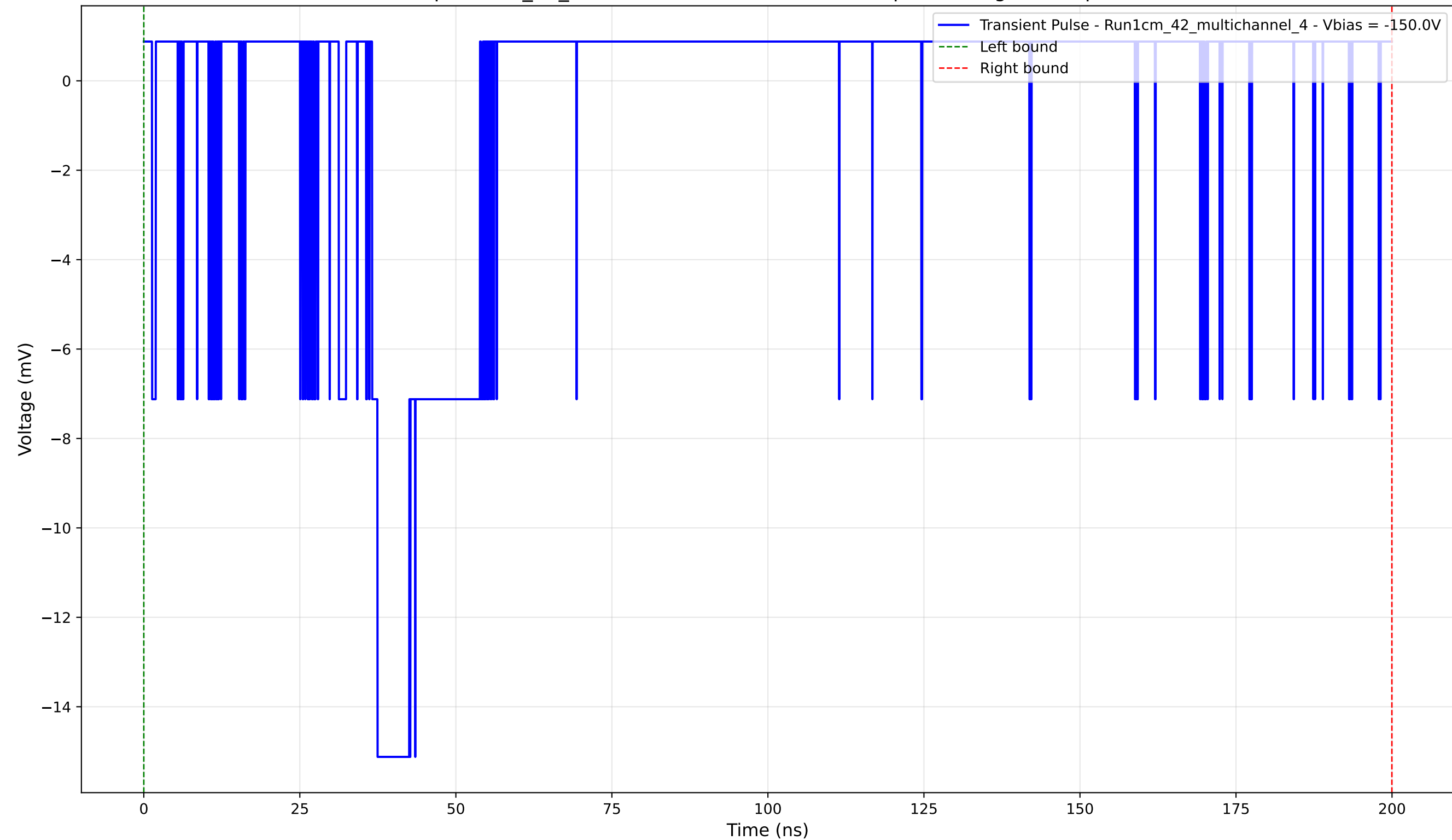
Transient Pulse - Sample: 1cm_42_multichannel - Position: 3700.0 \mu\text{m} - Charge: 1.44 pC - Rise Time: 0.88 ns
