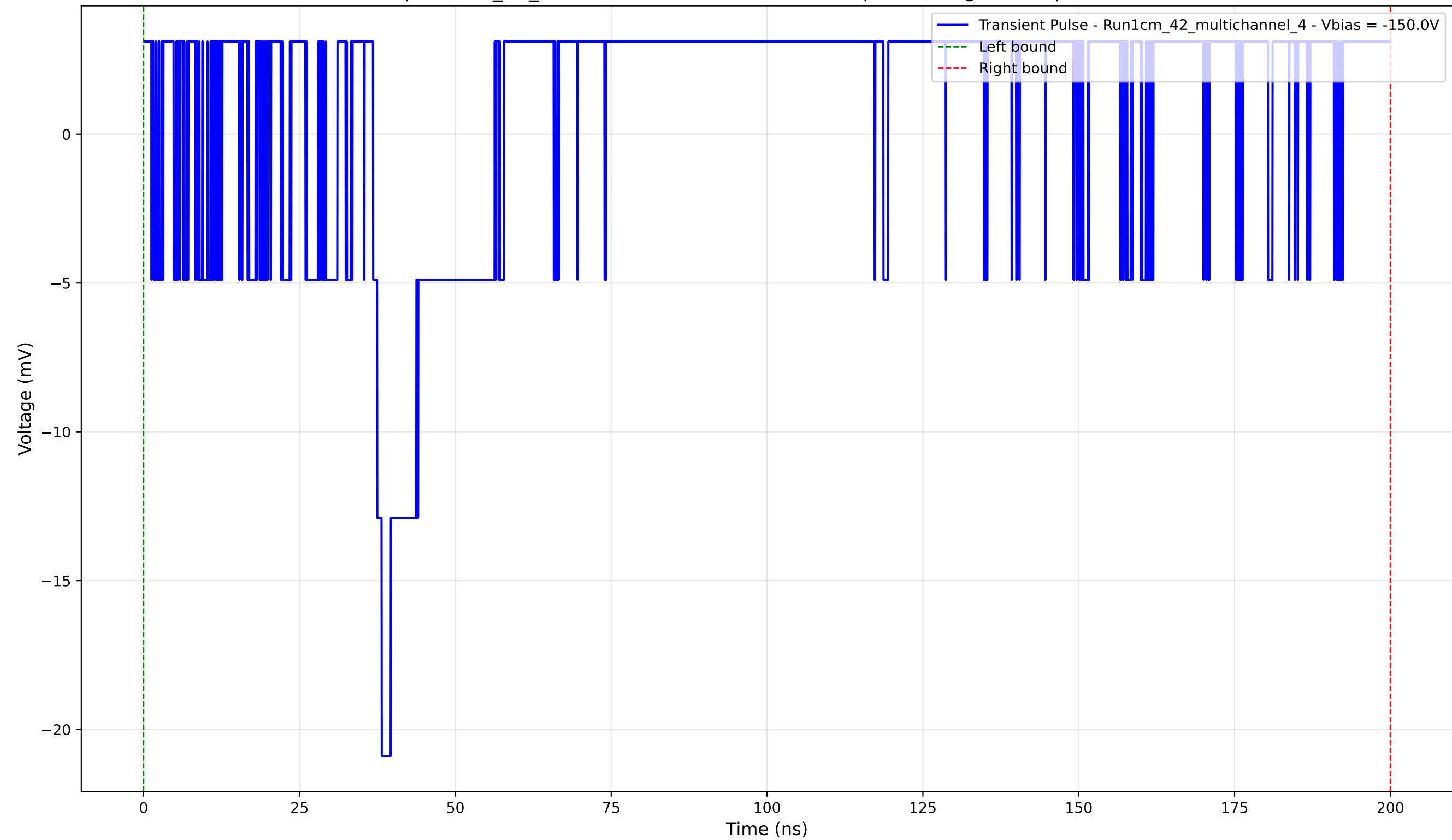
Transient Pulse - Sample: 1cm_42_multichannel - Position: 1050.0 \mu\text{m} - Charge: 4.19 pC - Rise Time: 0.00 ns (N/A)
