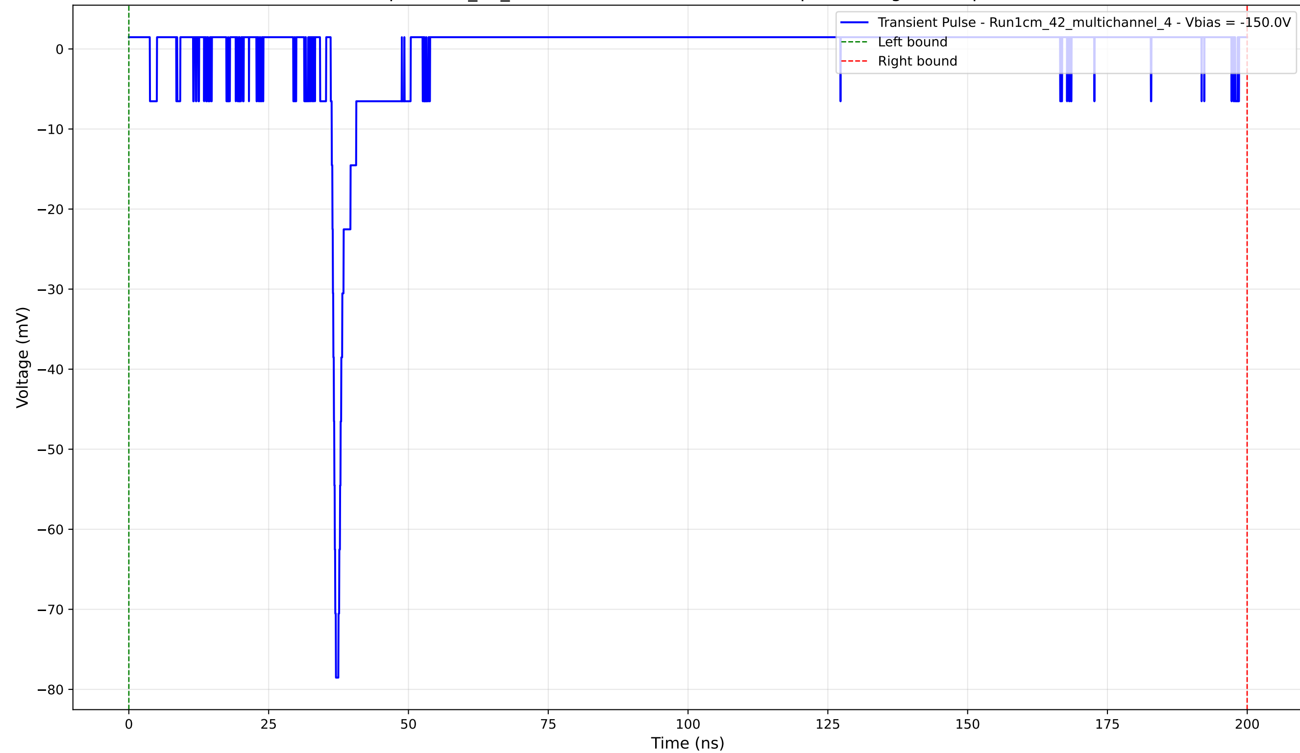
Transient Pulse - Sample: 1cm_42_multichannel - Position: 2290.0 \mu\text{m} - Charge: 0.43 pC - Rise Time: 0.76 ns
