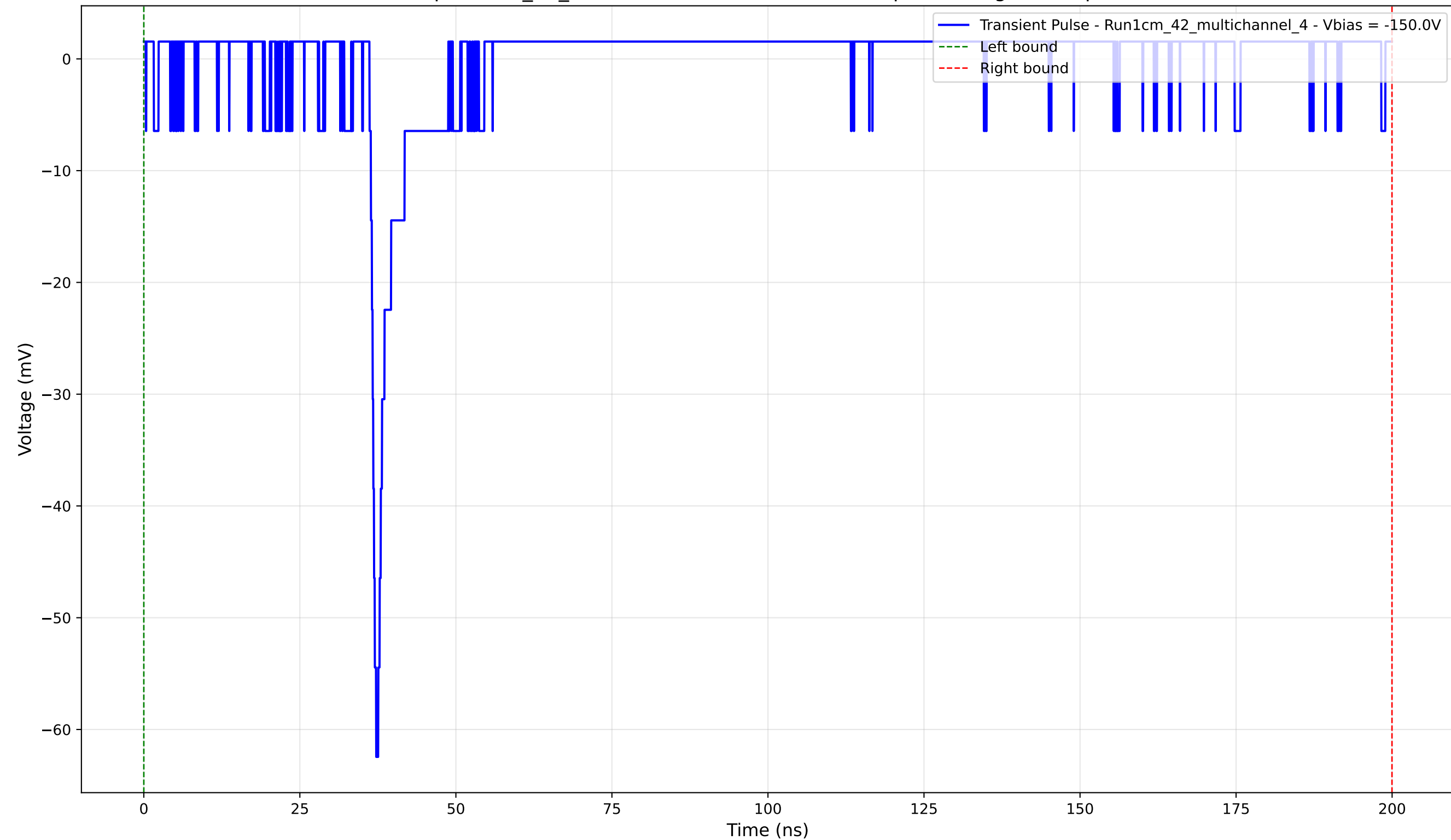
Transient Pulse - Sample: 1cm_42_multichannel - Position: 2135.0 \mu\text{m} - Charge: 0.59 pC - Rise Time: 1.06 ns
