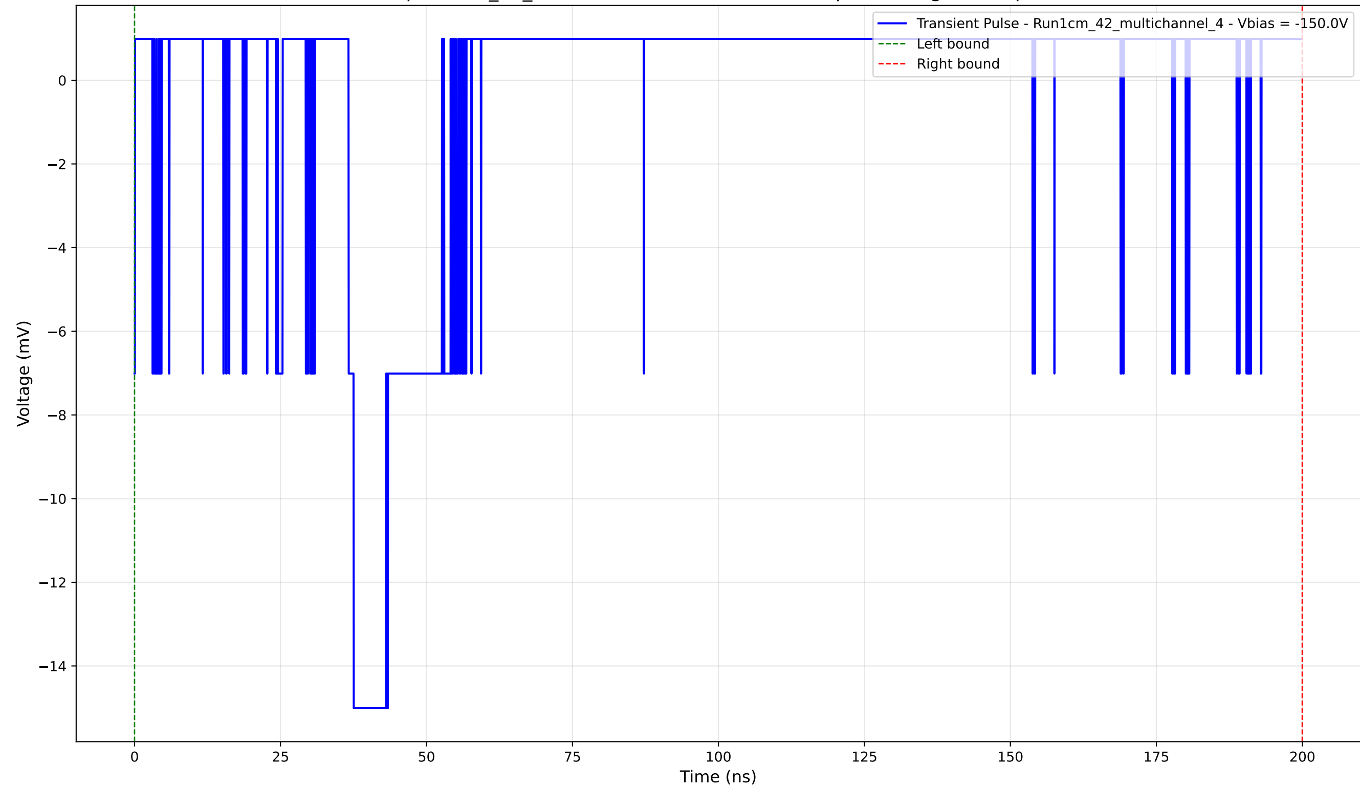
Transient Pulse - Sample: 1cm_42_multichannel - Position: 3710.0 \mu\text{m} - Charge: 0.90 pC - Rise Time: 0.88 ns
