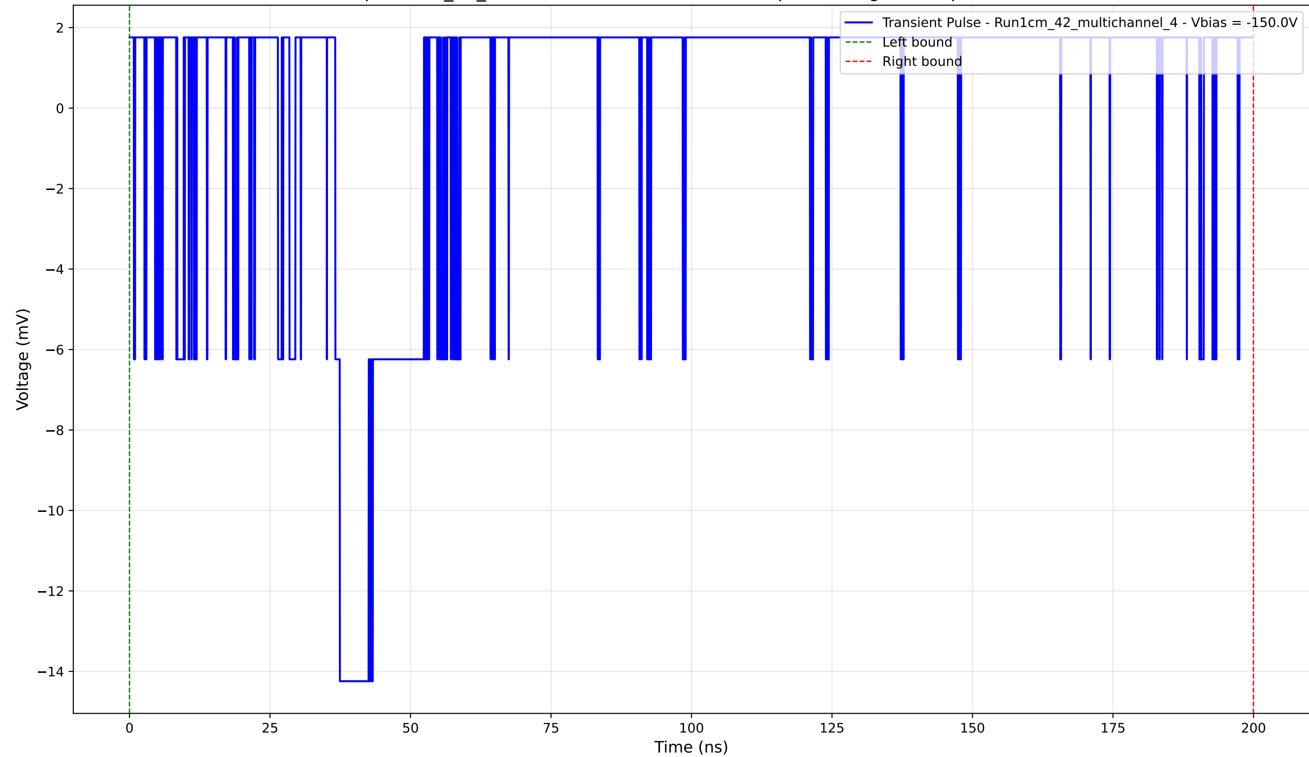
Transient Pulse - Sample: 1cm_42_multichannel - Position: 3645.0 \mu\text{m} - Charge: 1.53 pC - Rise Time: 0.00 ns (N/A)
