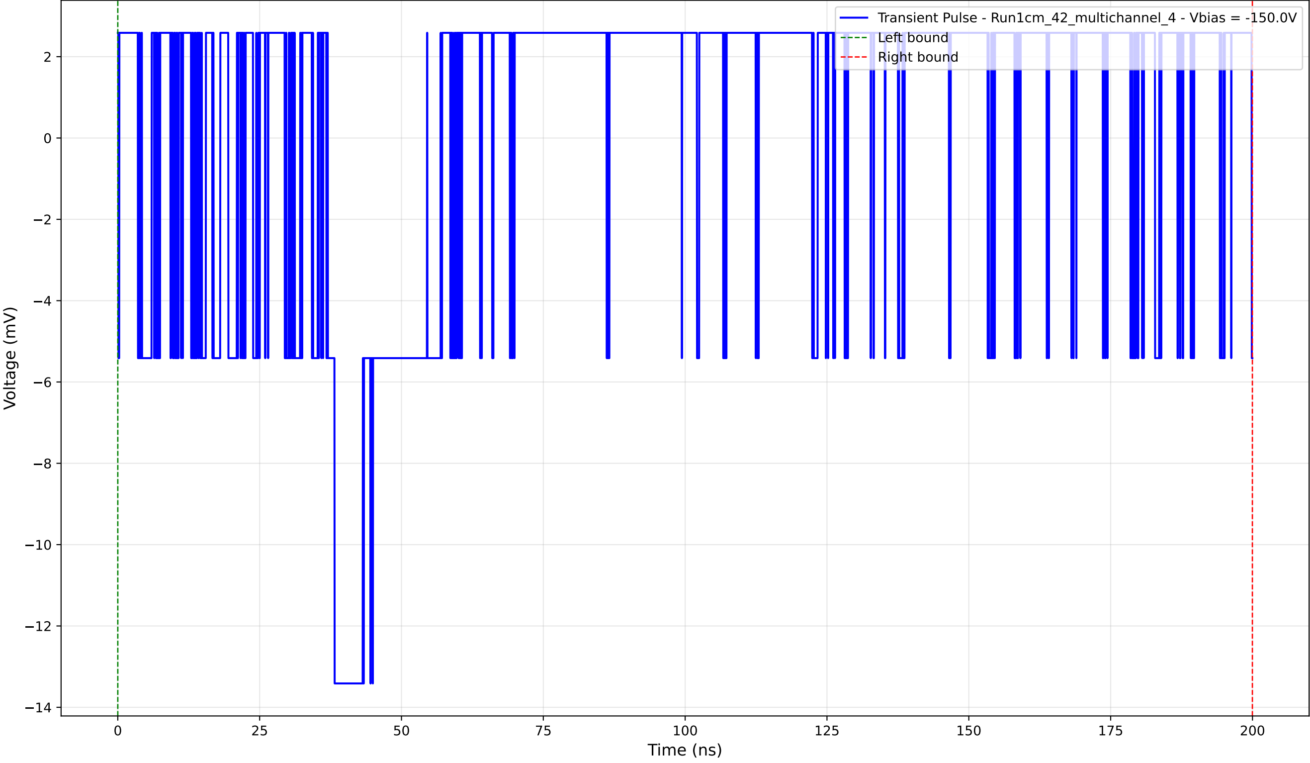
Transient Pulse - Sample: 1cm_42_multichannel - Position: 515.0 \mu\text{m} - Charge: 2.30 pC - Rise Time: 0.00 ns (N/A)
