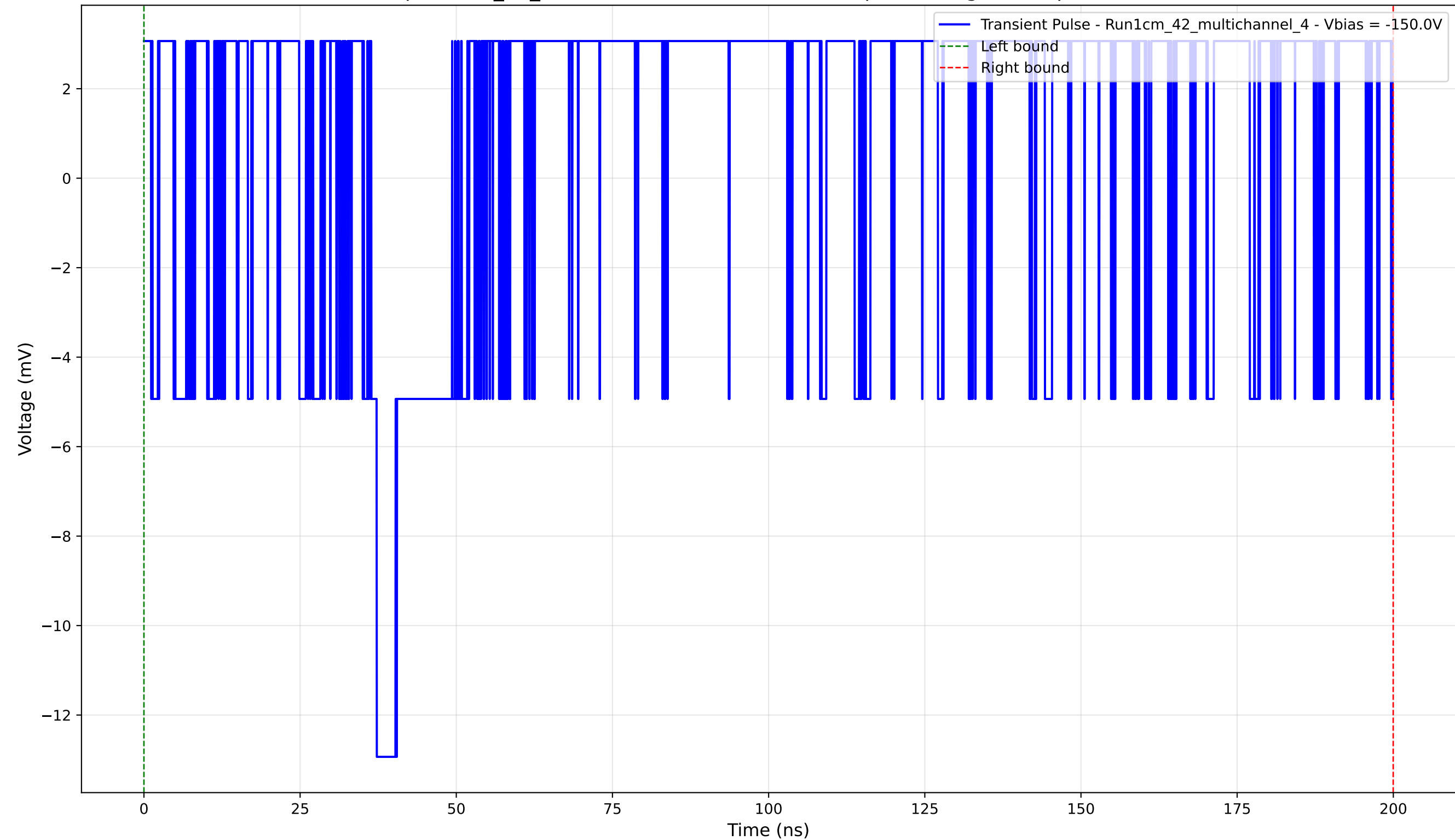
Transient Pulse - Sample: 1cm_42_multichannel - Position: 1425.0 \mu\text{m} - Charge: 4.52 pC - Rise Time: 0.00 ns (N/A)
