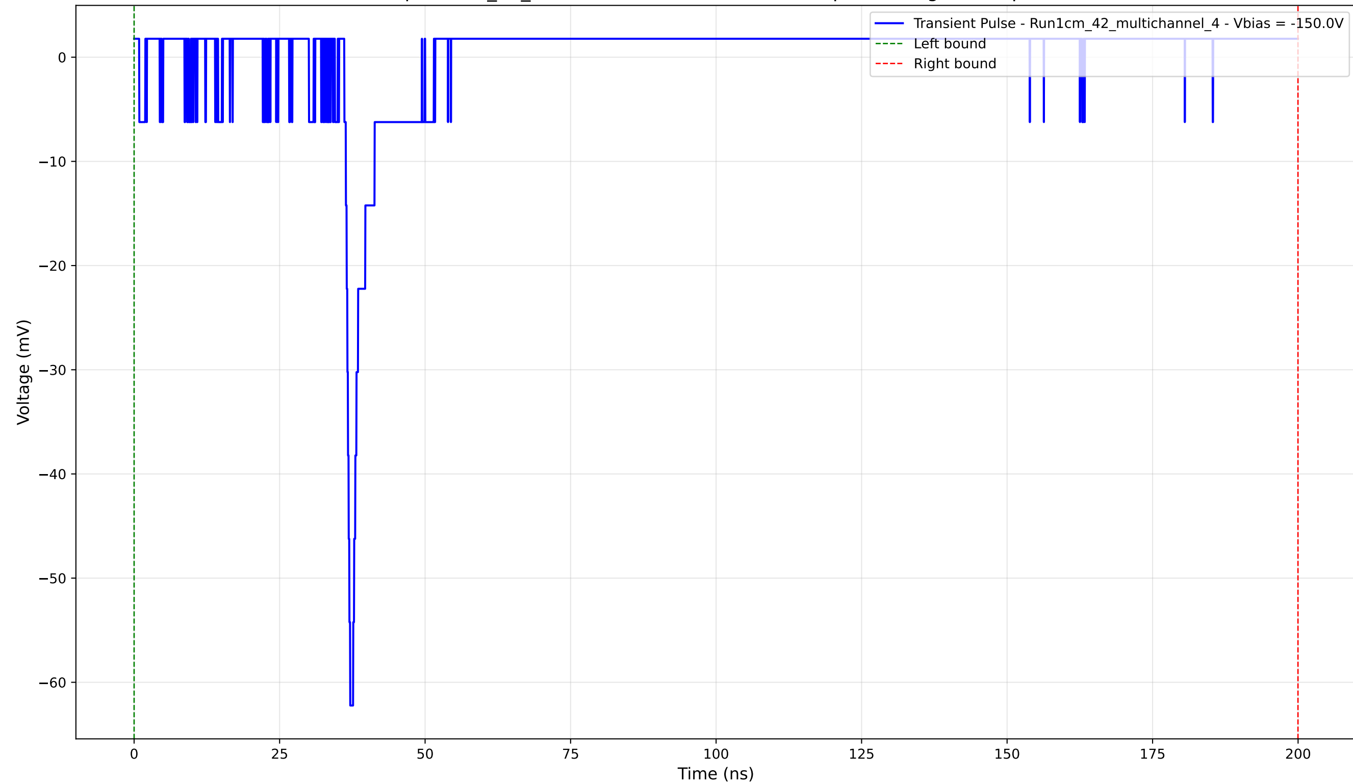
Transient Pulse - Sample: 1cm_42_multichannel - Position: 2155.0 \mu\text{m} - Charge: 1.13 pC - Rise Time: 1.00 ns
