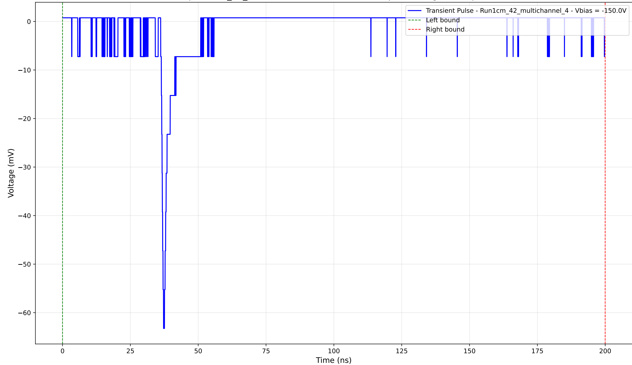
Transient Pulse - Sample: 1cm_42_multichannel - Position: 2105.0 \mu\text{m} - Charge: 3.27 pC - Rise Time: 1.04 ns
