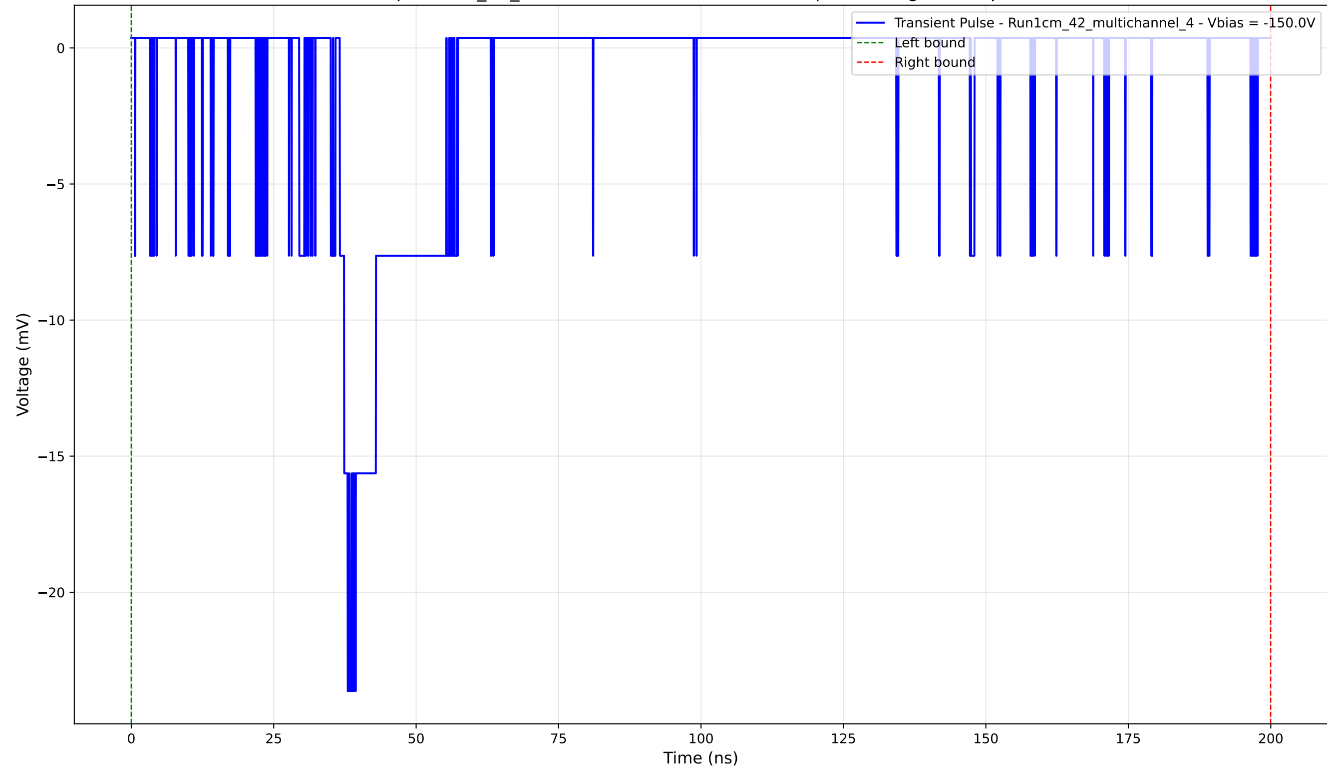
Transient Pulse - Sample: 1cm_42_multichannel - Position: 3545.0 \mu\text{m} - Charge: 4.03 pC - Rise Time: 1.39 ns
