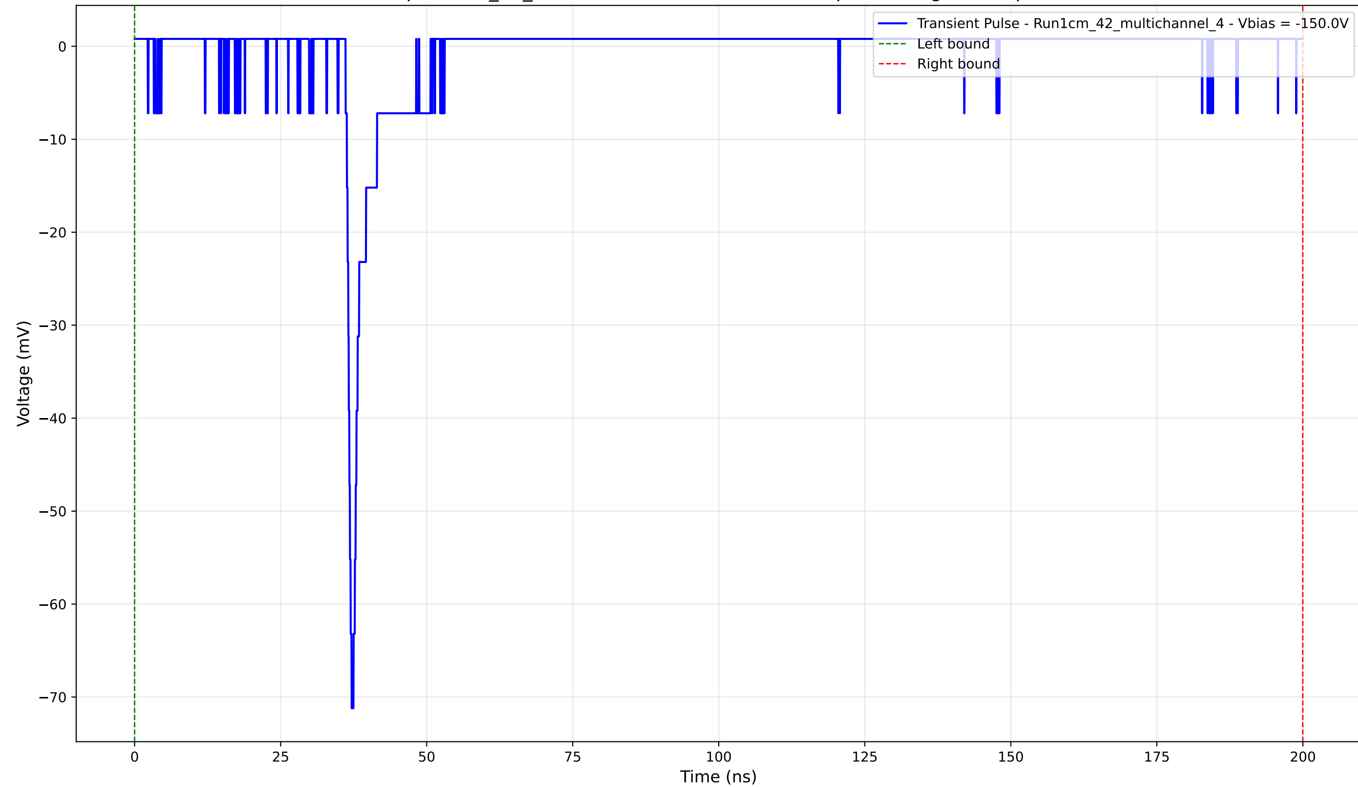
Transient Pulse - Sample: 1cm_42_multichannel - Position: 2570.0 \mu\text{m} - Charge: 2.44 pC - Rise Time: 1.02 ns
