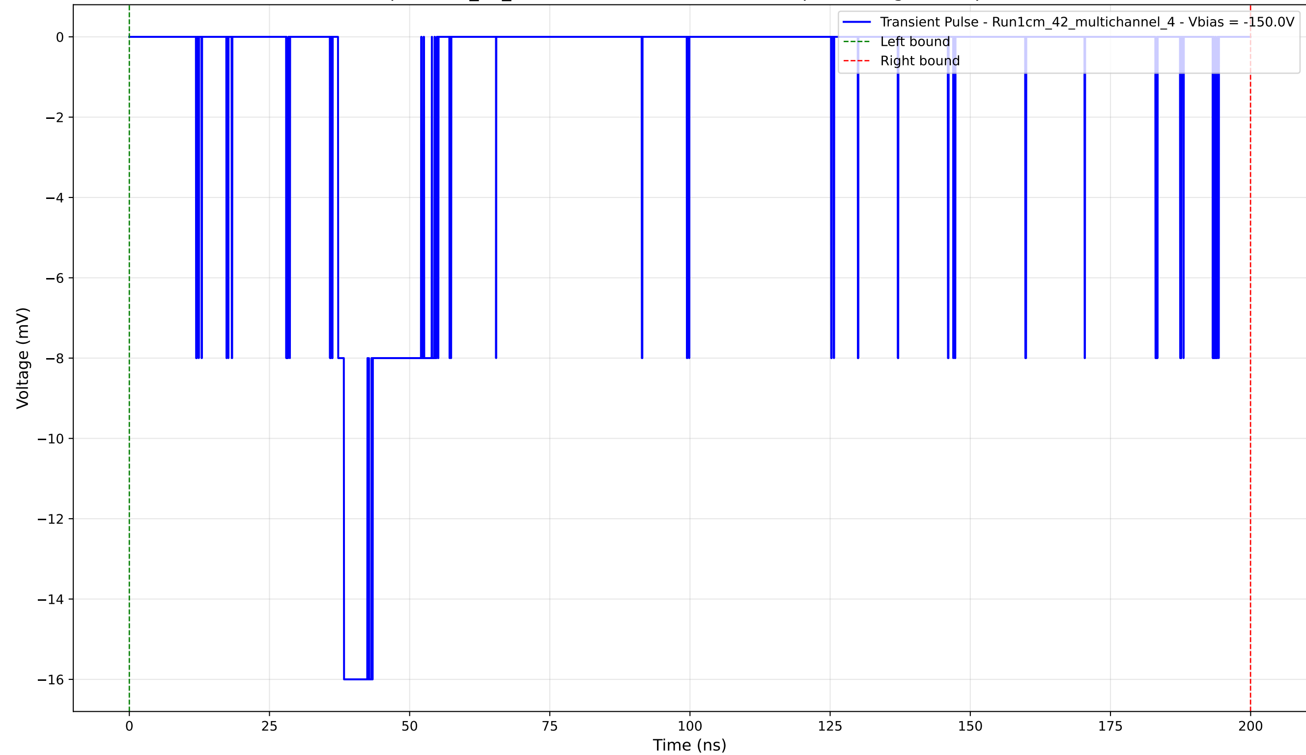
Transient Pulse - Sample: 1cm_42_multichannel - Position: 4250.0 \mu\text{m} - Charge: 4.07 pC - Rise Time: 1.06 ns
