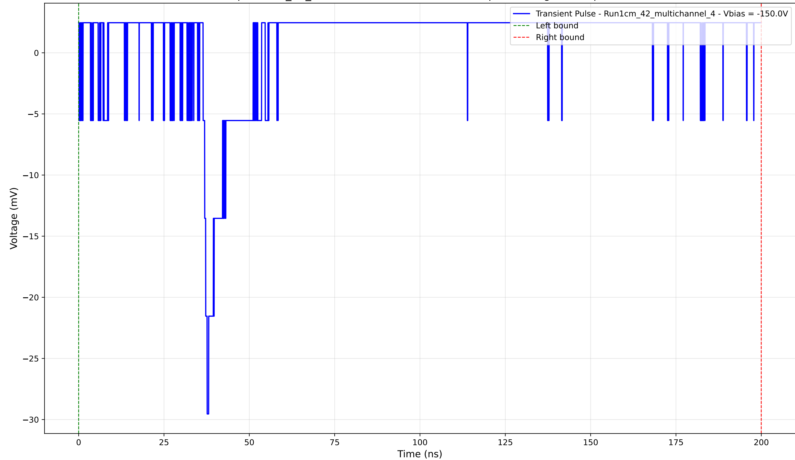
Transient Pulse - Sample: 1cm_42_multichannel - Position: 3235.0 \mu\text{m} - Charge: 4.39 pC - Rise Time: 1.20 ns
