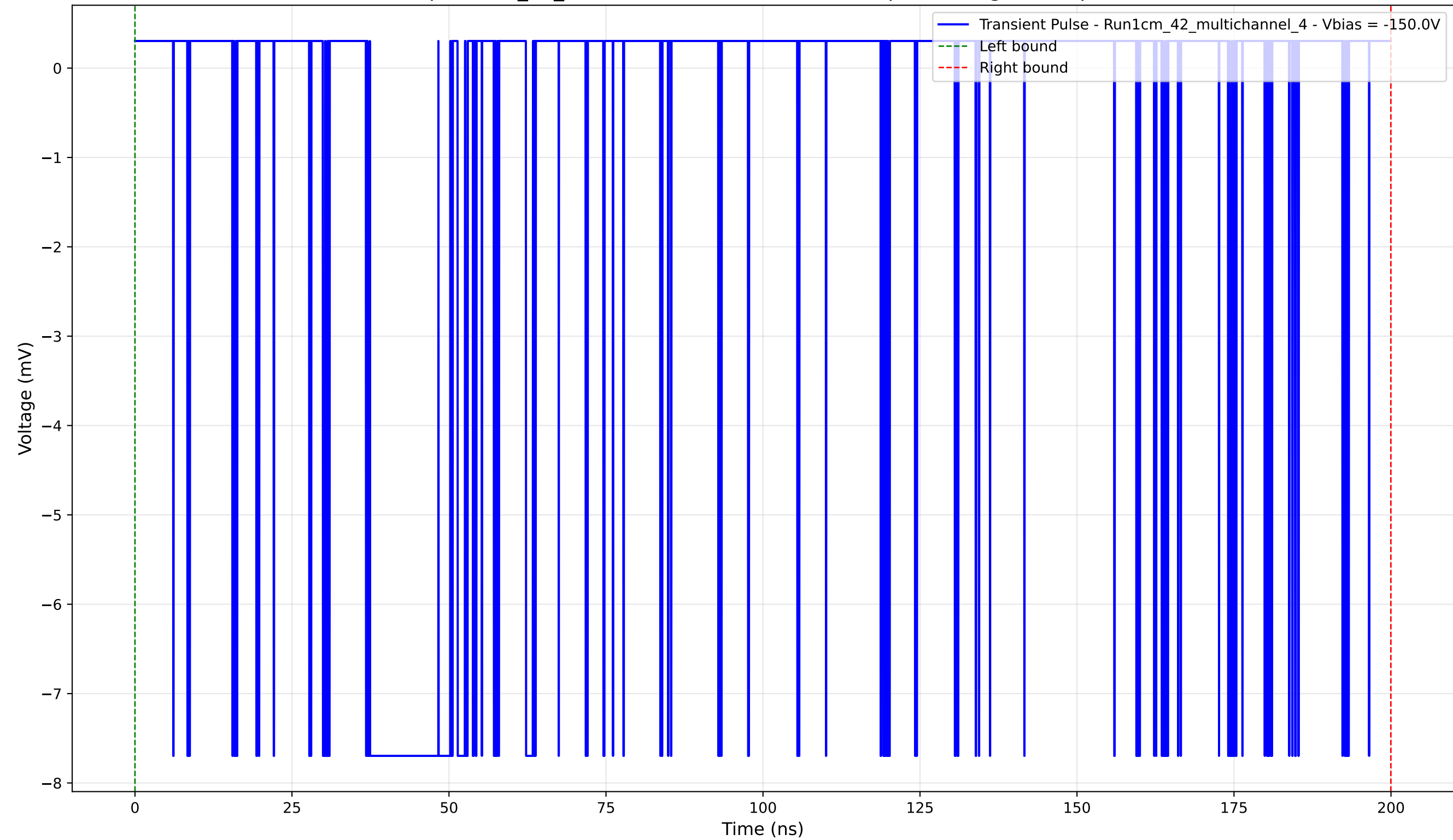
Transient Pulse - Sample: 1cm_42_multichannel - Position: 4860.0 \mu\text{m} - Charge: 2.92 pC - Rise Time: 0.02 ns
