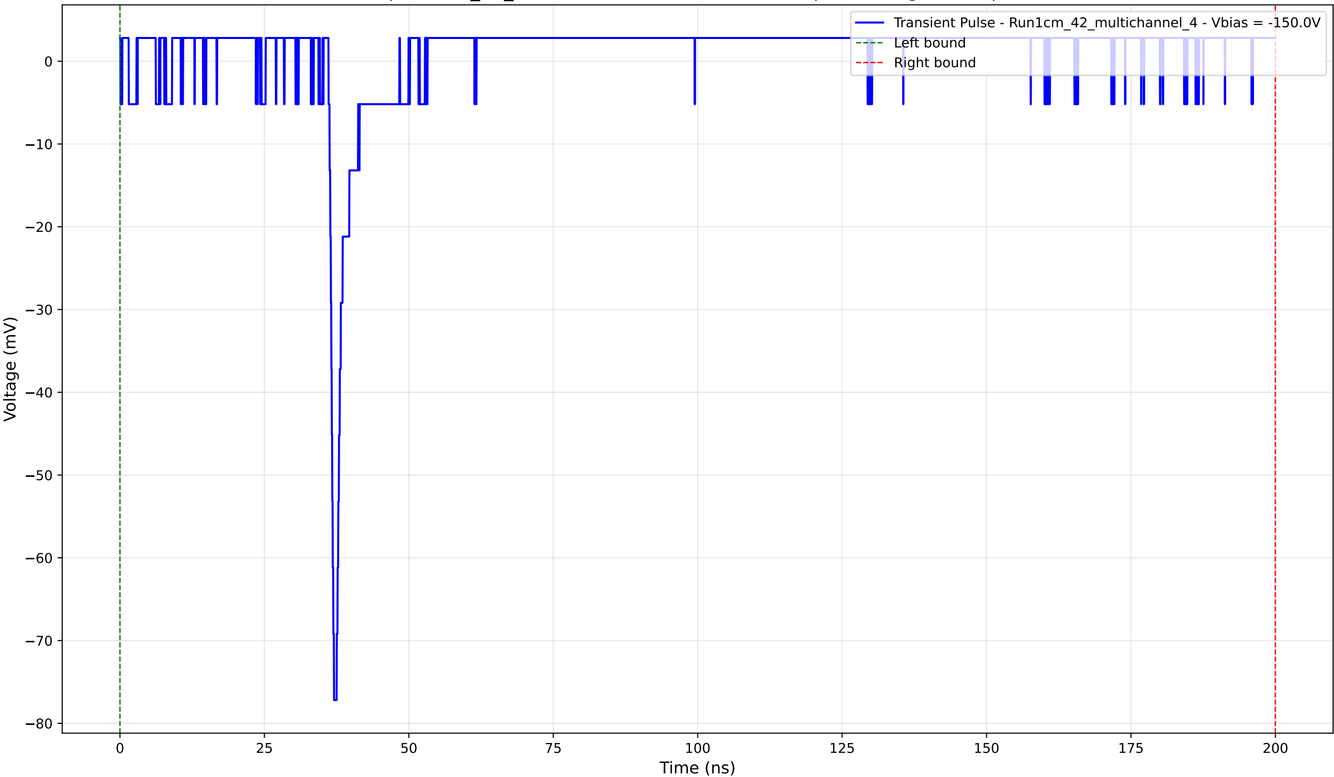
Transient Pulse - Sample: 1cm_42_multichannel - Position: 2270.0 \mu\text{m} - Charge: 4.55 pC - Rise Time: 0.77 ns
