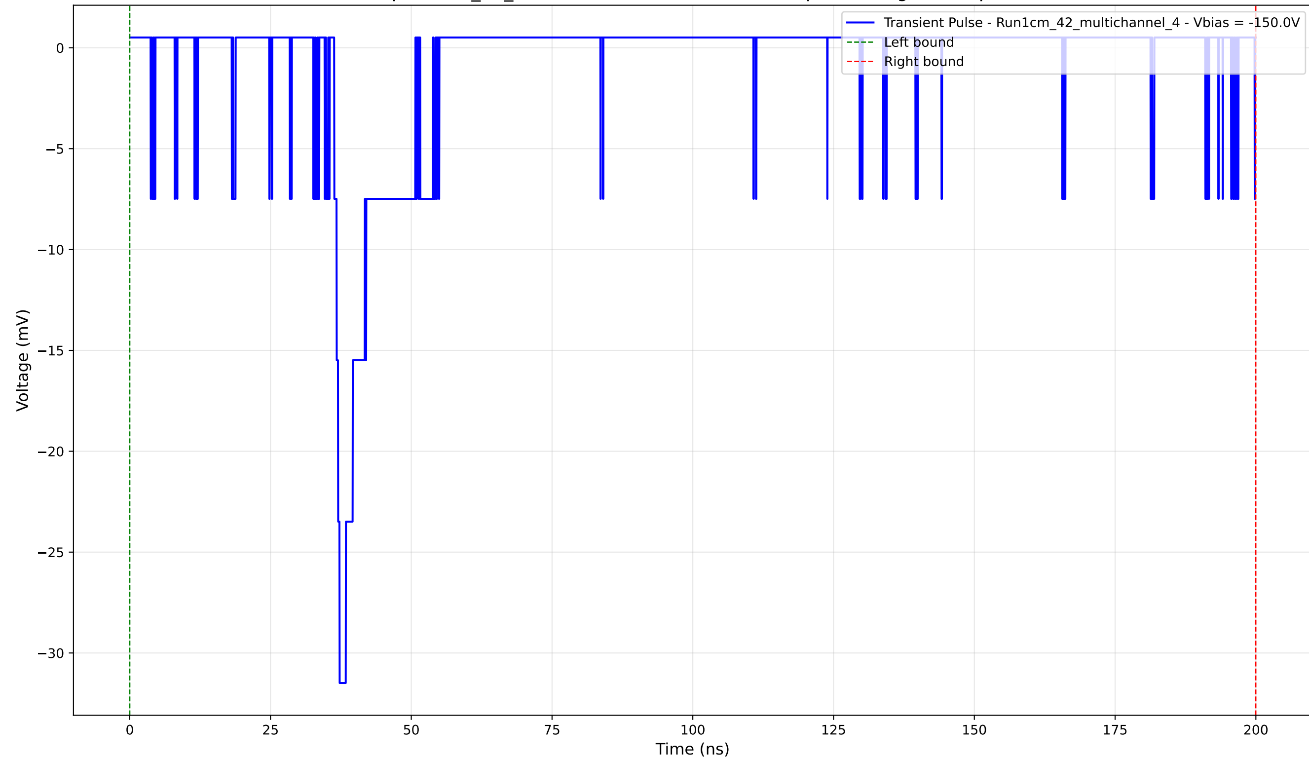
Transient Pulse - Sample: 1cm_42_multichannel - Position: 3075.0 \mu\text{m} - Charge: 3.18 pC - Rise Time: 0.95 ns
