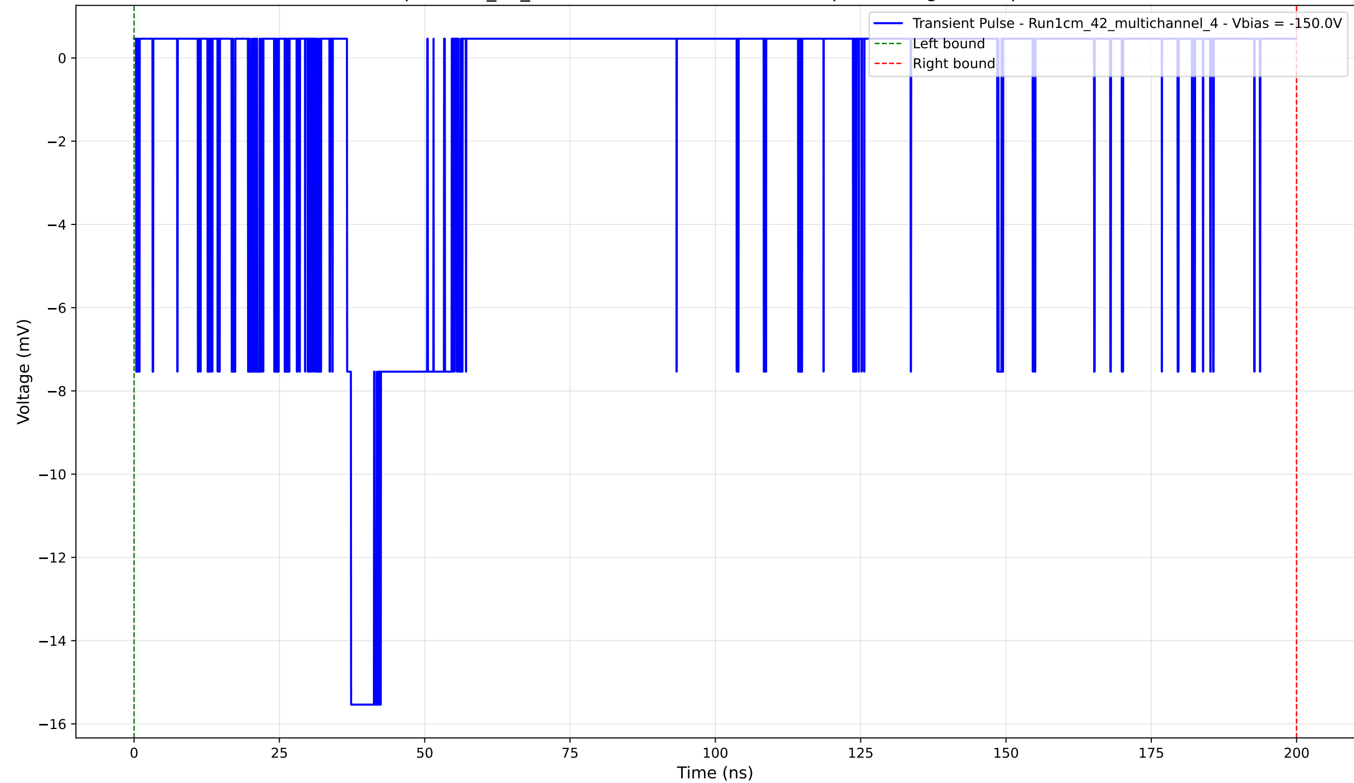
Transient Pulse - Sample: 1cm_42_multichannel - Position: 3460.0 \mu\text{m} - Charge: 3.33 pC - Rise Time: 0.70 ns
