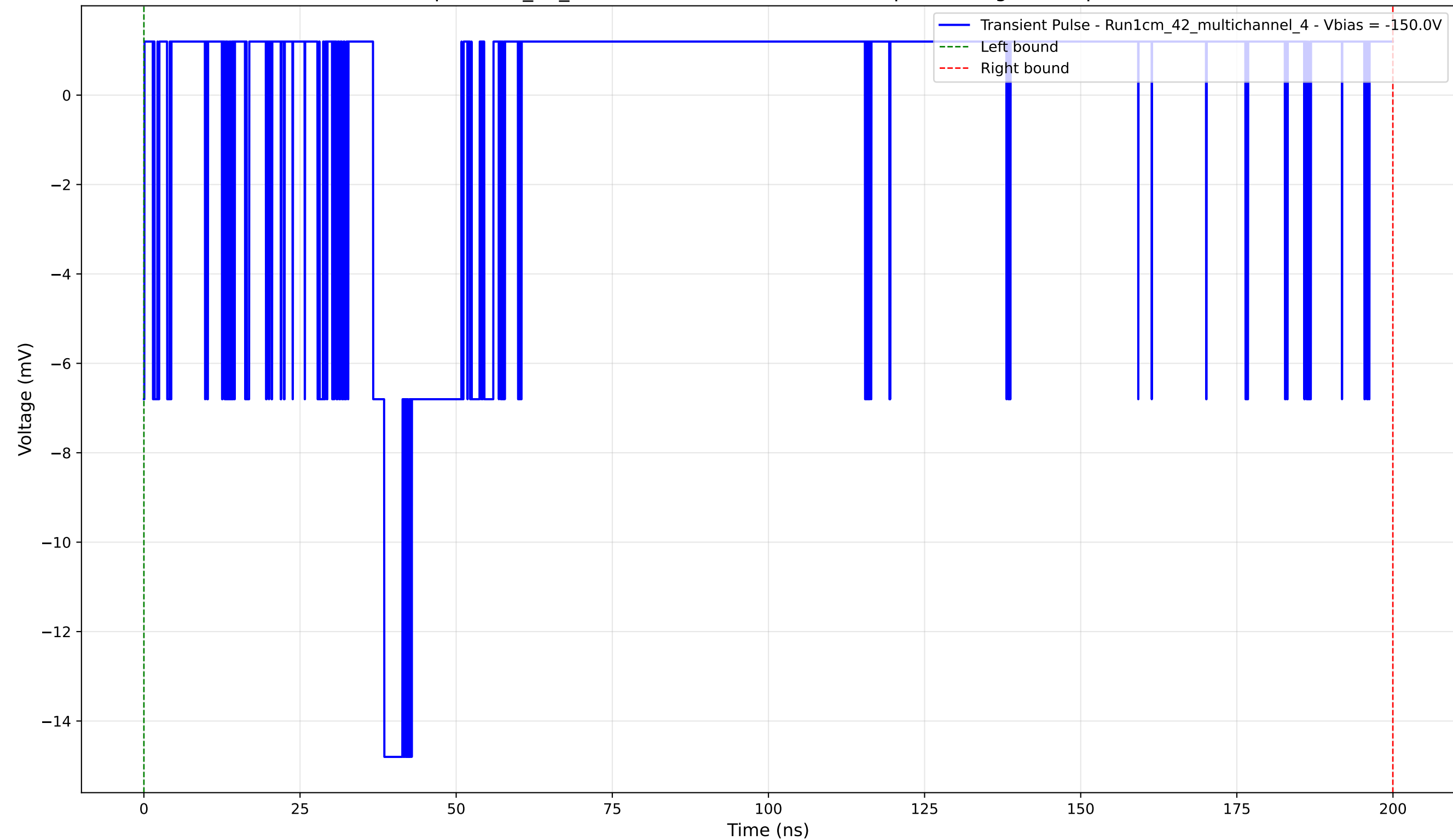
Transient Pulse - Sample: 1cm_42_multichannel - Position: 4735.0 \mu\text{m} - Charge: 0.09 pC - Rise Time: 1.80 ns
