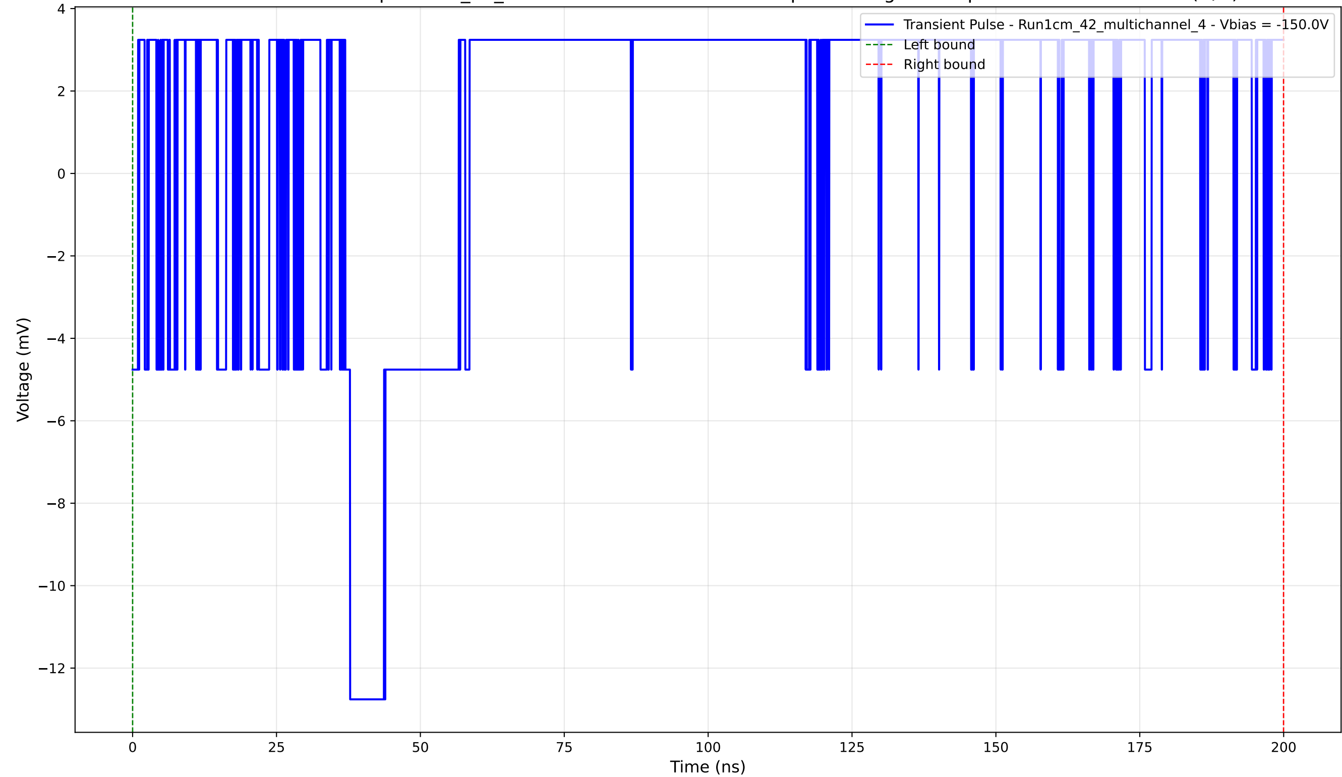
Transient Pulse - Sample: 1cm_42_multichannel - Position: 650.0 \mu\text{m} - Charge: 5.65 pC - Rise Time: 0.00 ns (N/A)
