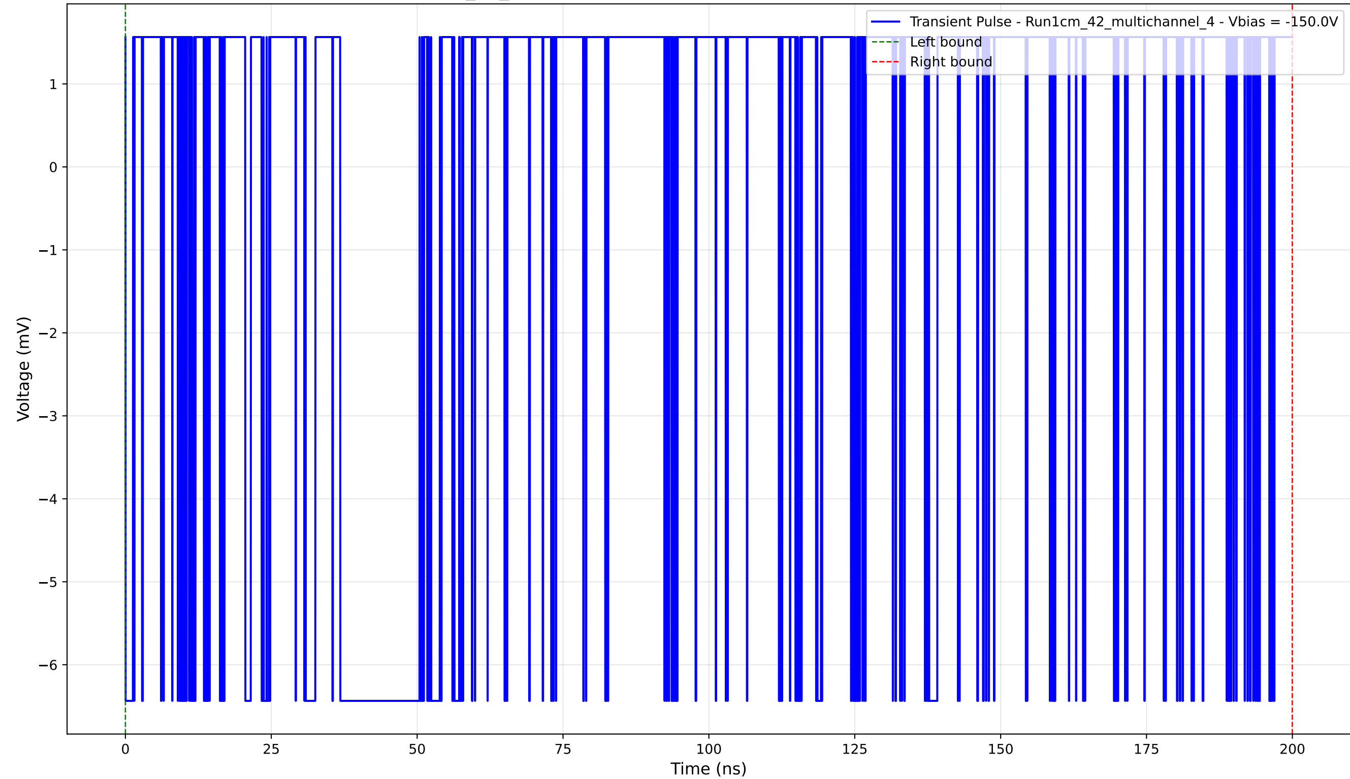
Transient Pulse - Sample: 1cm_42_multichannel - Position: 90.0 \mu\text{m} - Charge: 0.03 pC - Rise Time: 0.00 ns (N/A)
