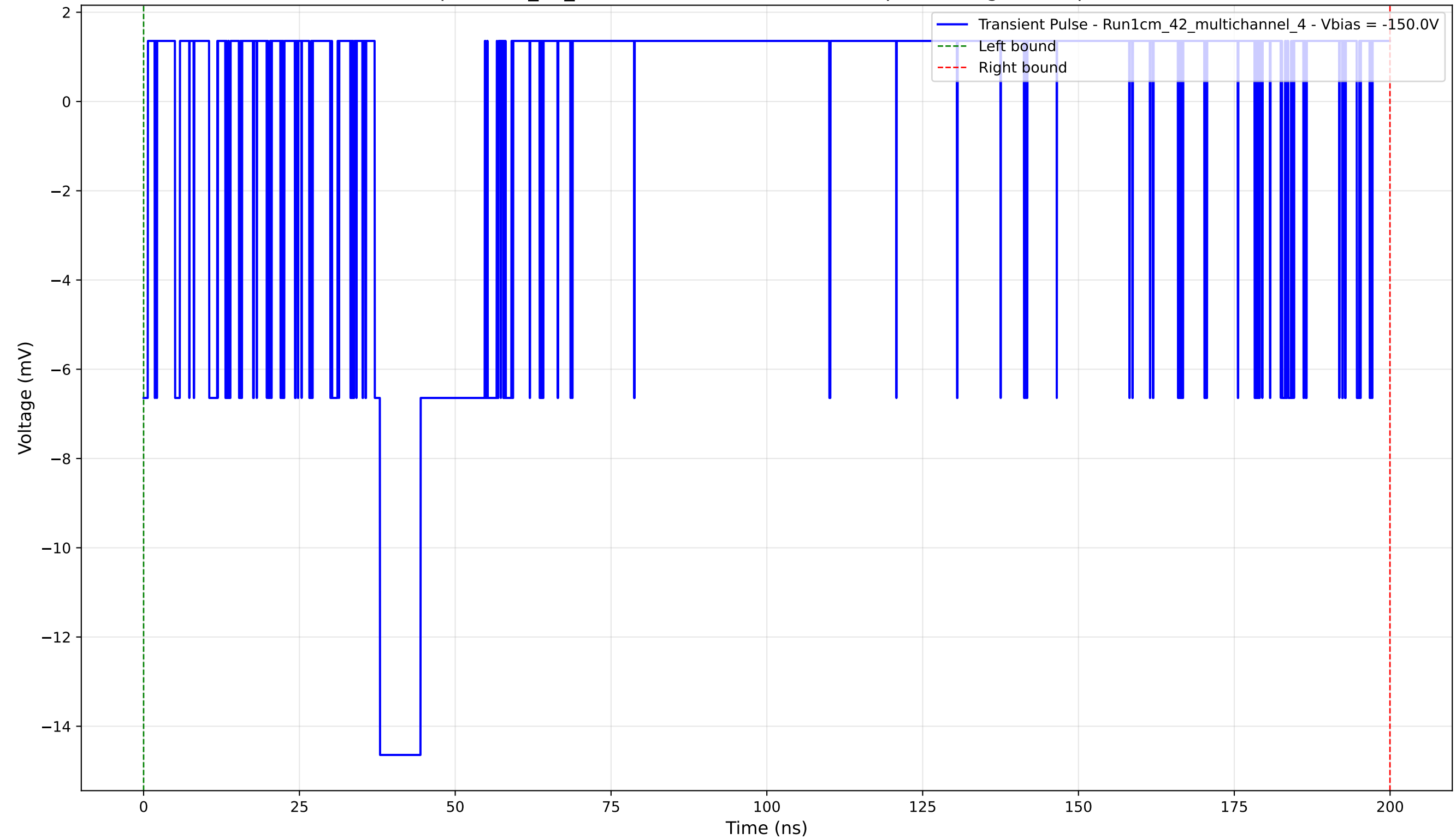
Transient Pulse - Sample: 1cm_42_multichannel - Position: 640.0 \mu\text{m} - Charge: 1.11 pC - Rise Time: 0.86 ns
