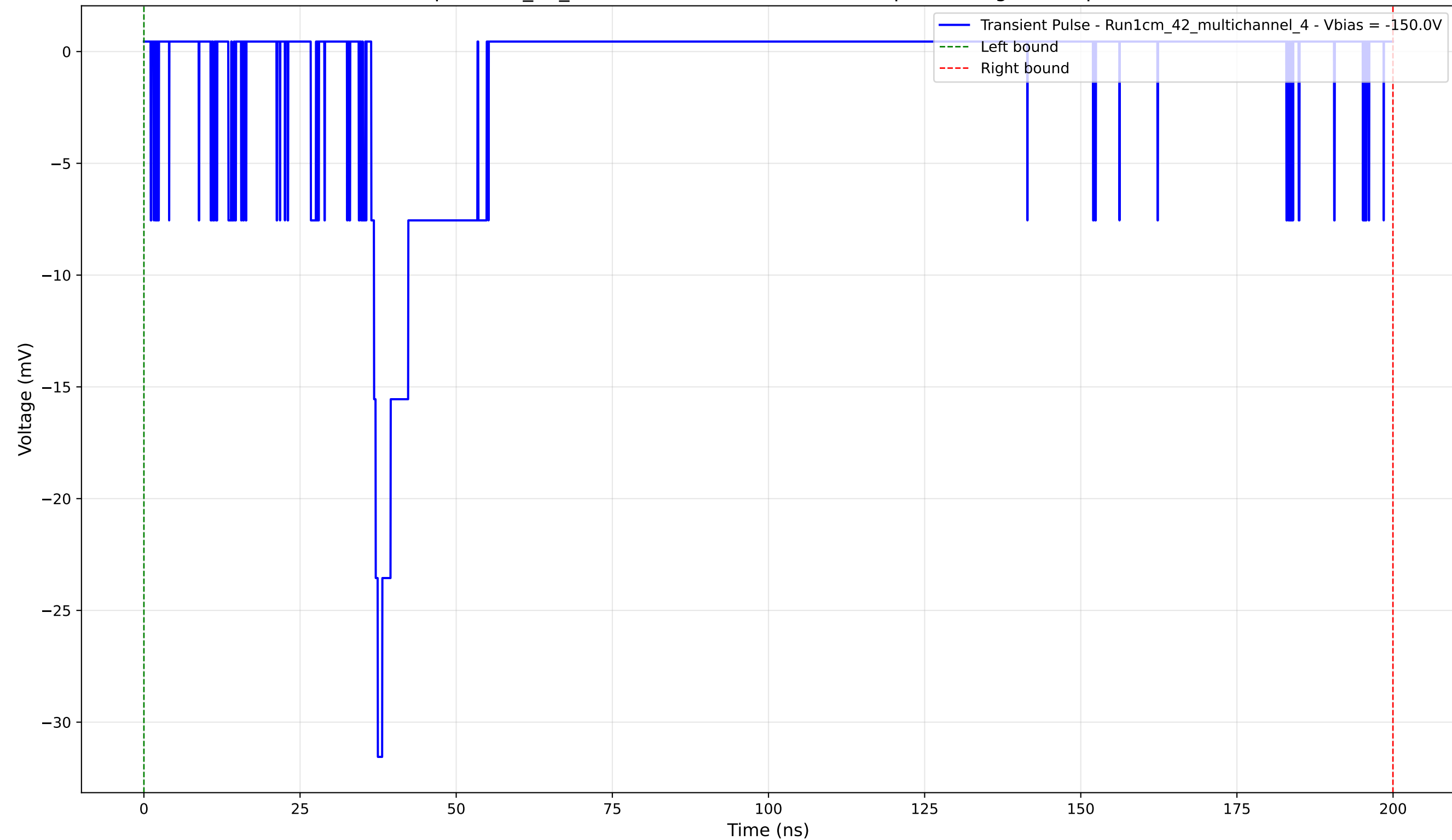
Transient Pulse - Sample: 1cm_42_multichannel - Position: 3160.0 \mu\text{m} - Charge: 3.54 pC - Rise Time: 1.05 ns
