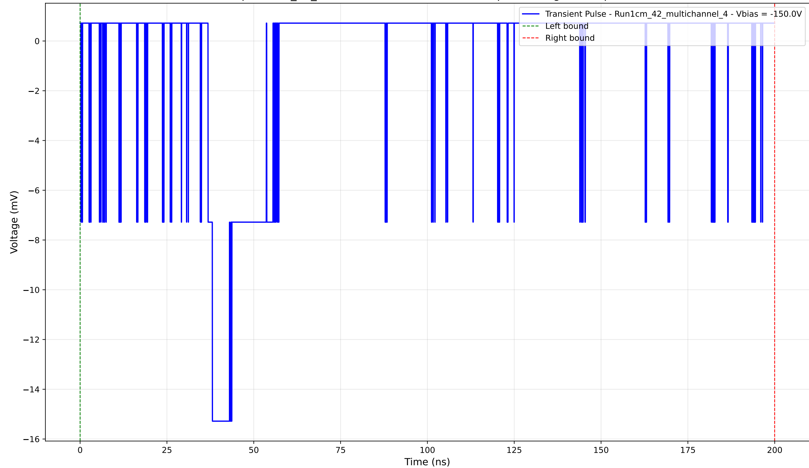
Transient Pulse - Sample: 1cm_42_multichannel - Position: 4115.0 \mu\text{m} - Charge: 2.06 pC - Rise Time: 1.26 ns
