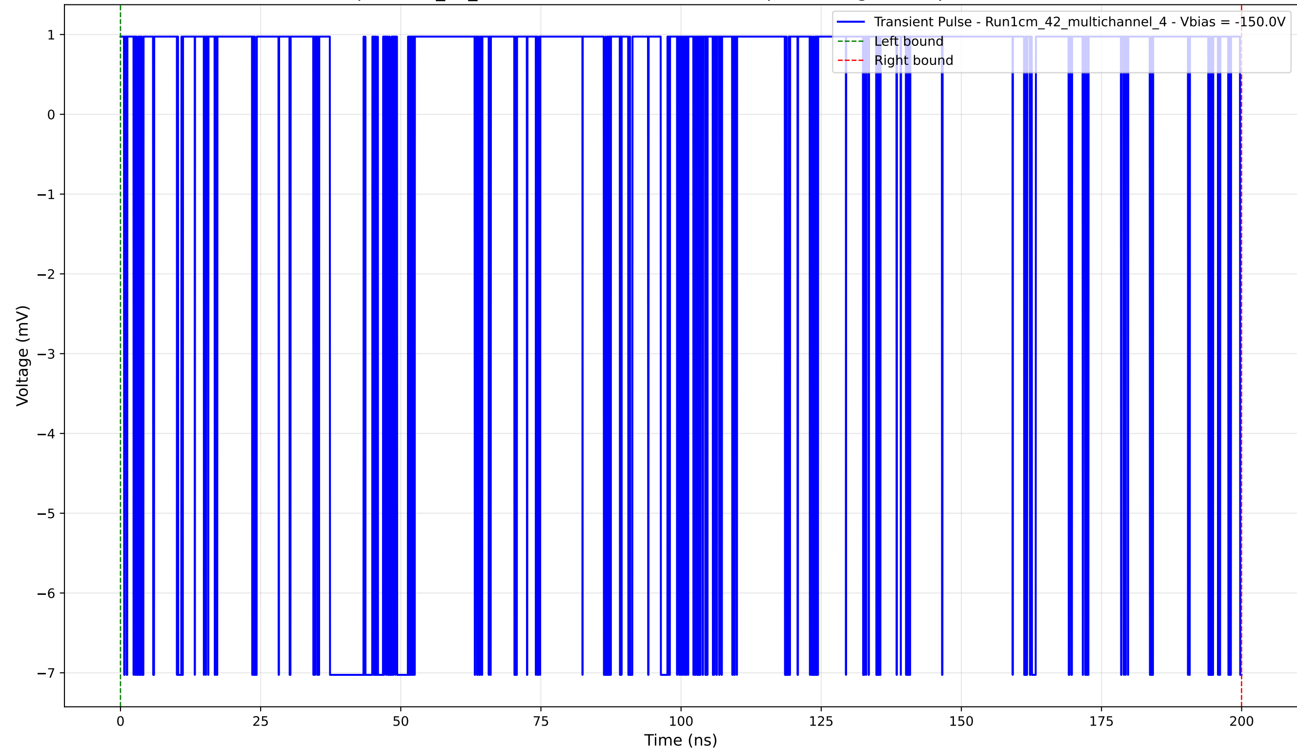
Transient Pulse - Sample: 1cm_42_multichannel - Position: 4870.0 \mu\text{m} - Charge: 0.81 pC - Rise Time: 0.00 ns (N/A)
