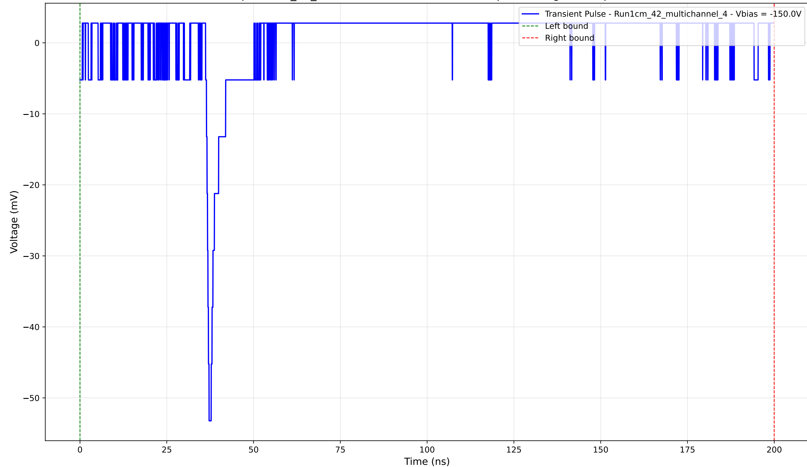
Transient Pulse - Sample: 1cm_42_multichannel - Position: 2020.0 \mu\text{m} - Charge: 3.77 pC - Rise Time: 0.76 ns
