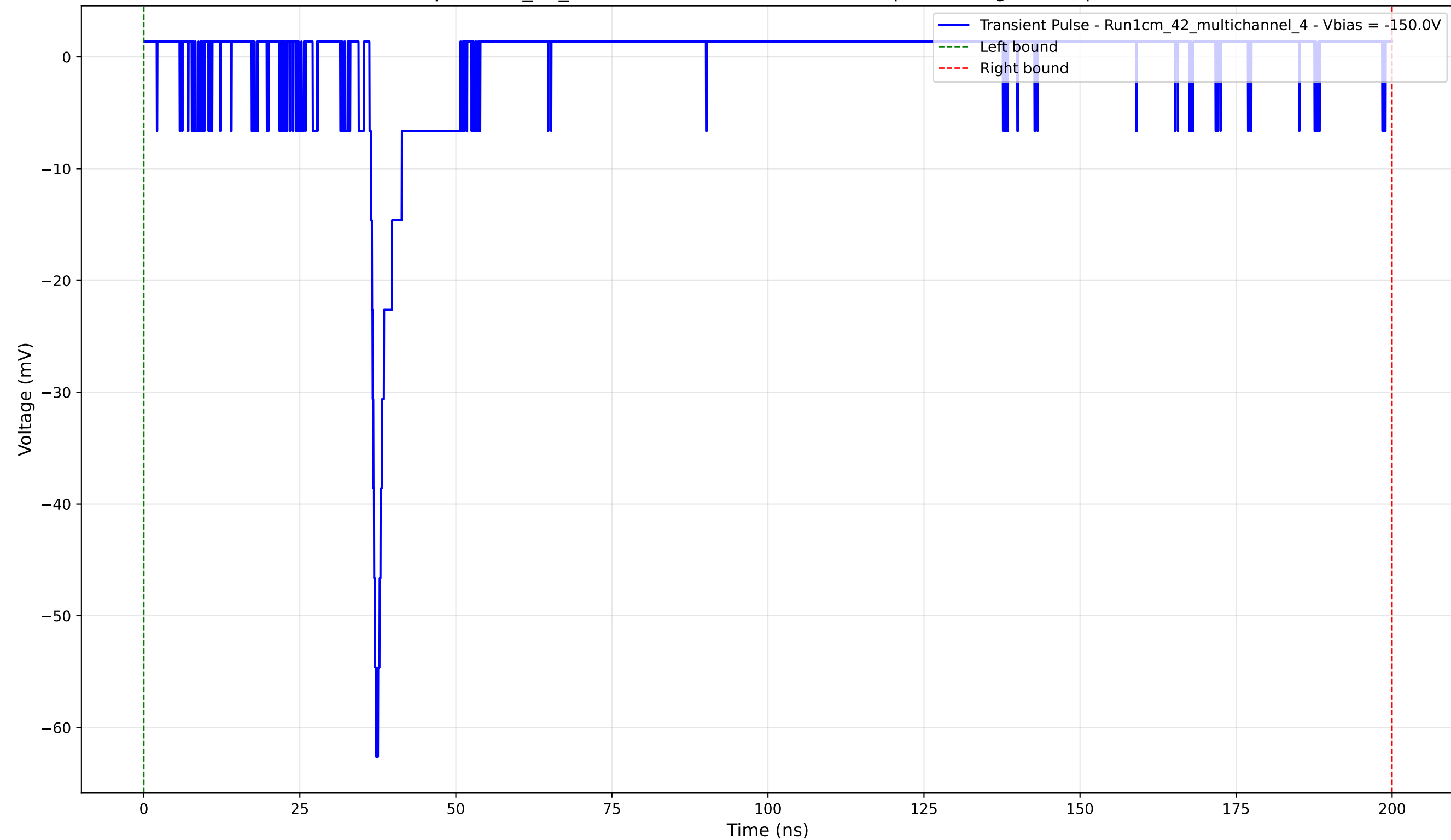
Transient Pulse - Sample: 1cm_42_multichannel - Position: 2650.0 \mu\text{m} - Charge: 0.79 pC - Rise Time: 1.06 ns
