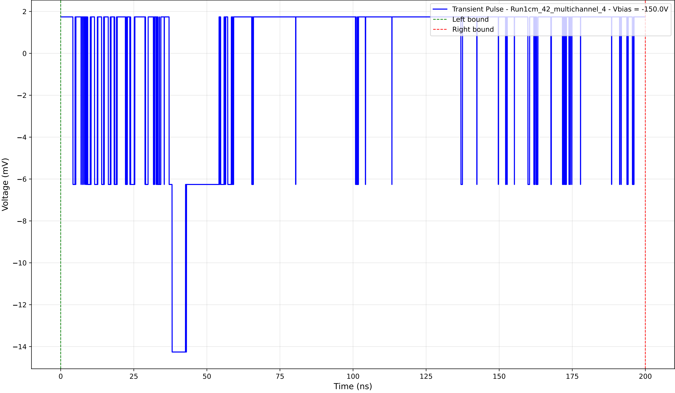
Transient Pulse - Sample: 1cm_42_multichannel - Position: 445.0 \mu\text{m} - Charge: 0.46 pC - Rise Time: 0.00 ns (N/A)
