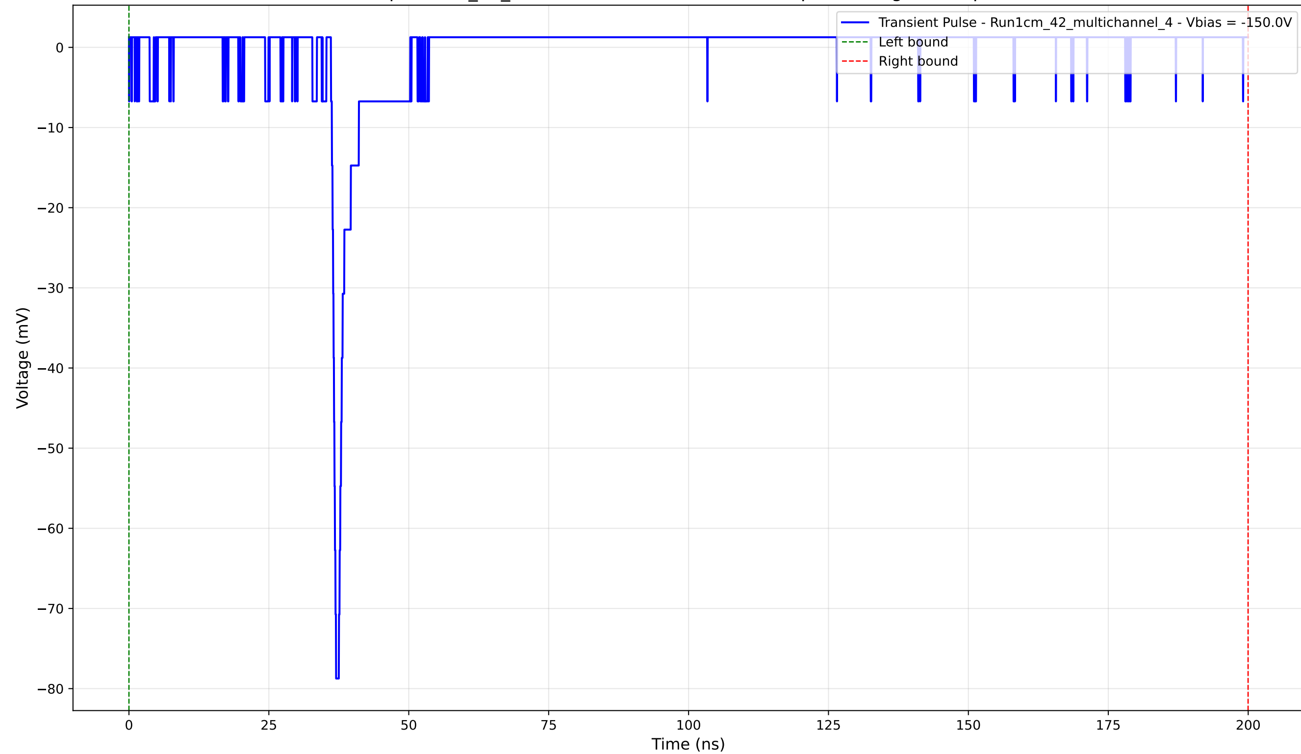
Transient Pulse - Sample: 1cm_42_multichannel - Position: 2485.0 \mu\text{m} - Charge: 1.26 pC - Rise Time: 0.76 ns
