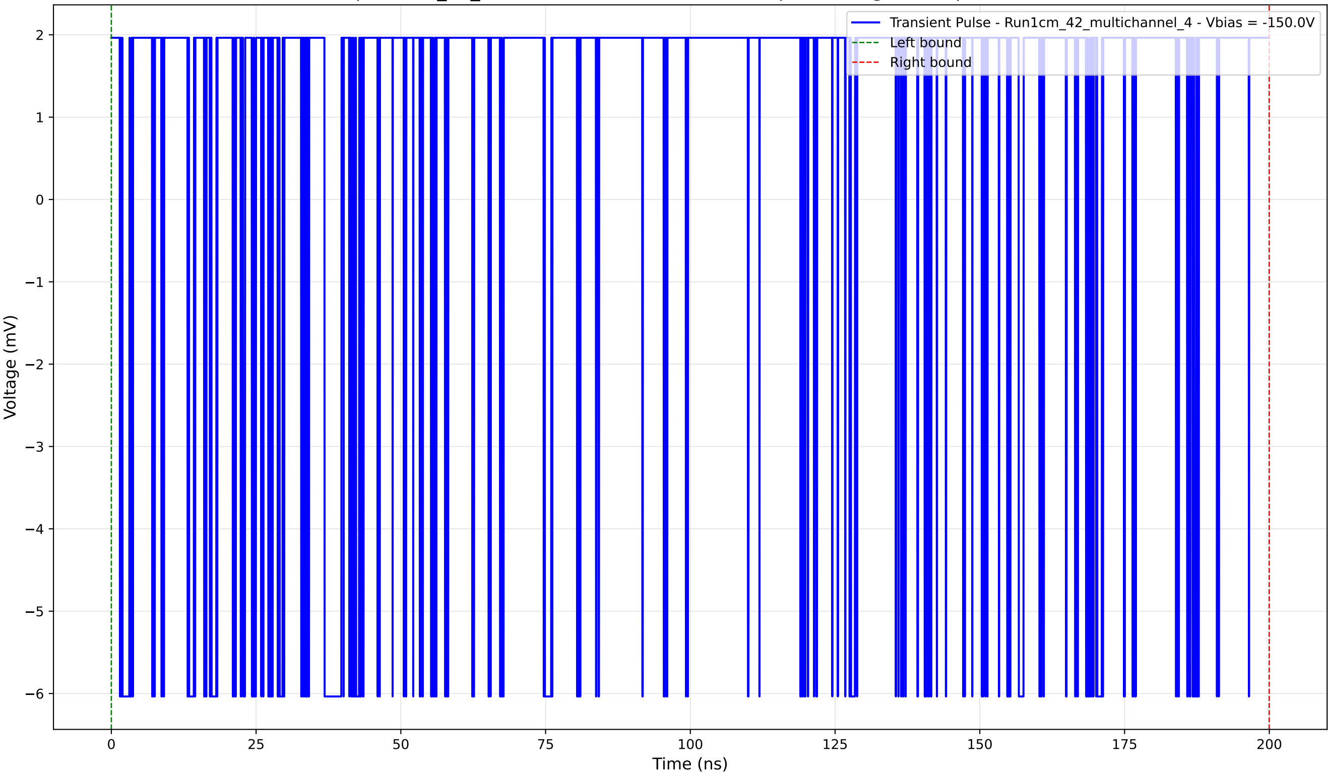
Transient Pulse - Sample: 1cm_42_multichannel - Position: 2890.0 \mu\text{m} - Charge: 3.69 pC - Rise Time: 0.00 ns (N/A)
