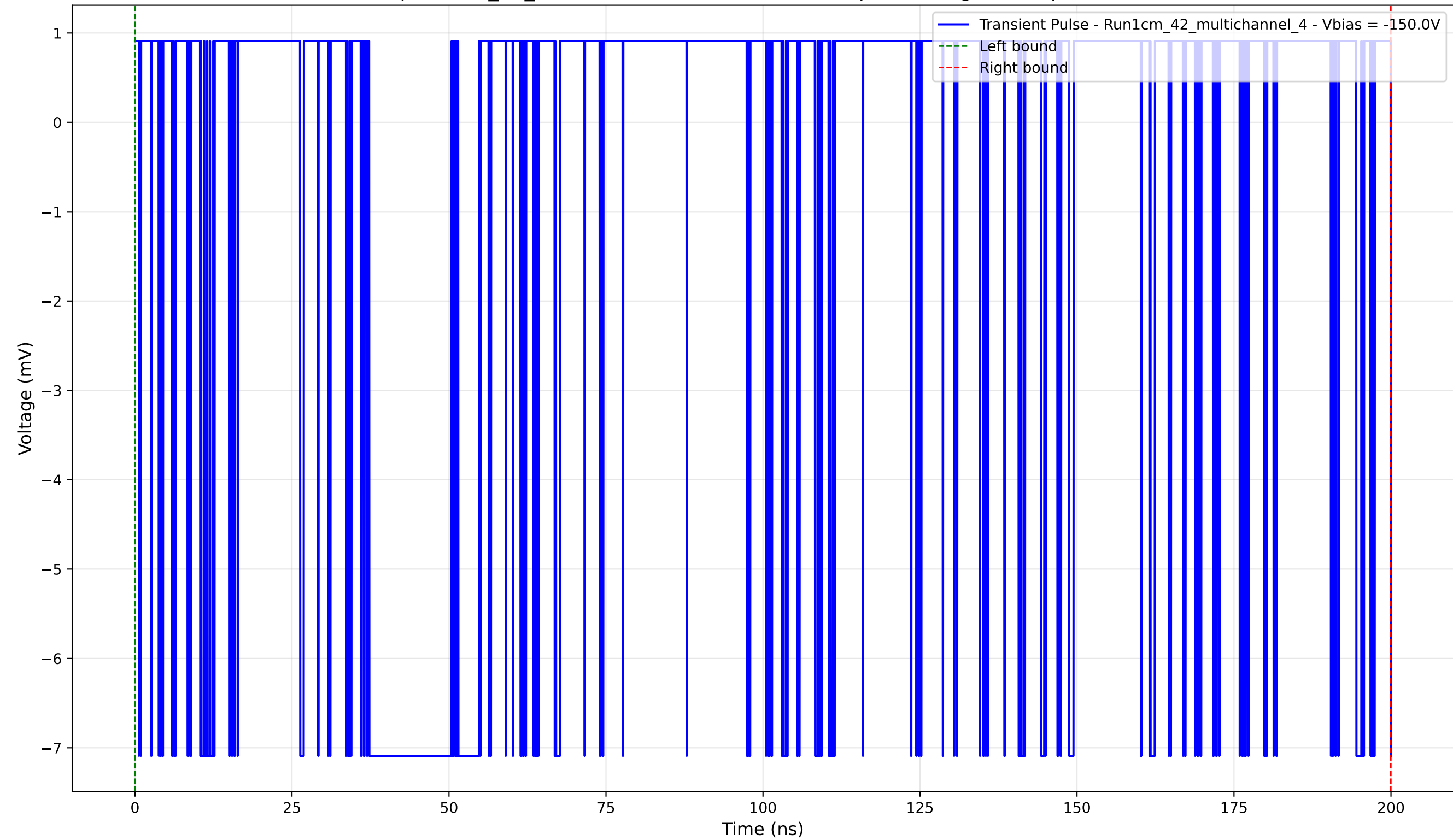
Transient Pulse - Sample: 1cm_42_multichannel - Position: 4355.0 \mu\text{m} - Charge: 2.08 pC - Rise Time: 0.00 ns (N/A)
