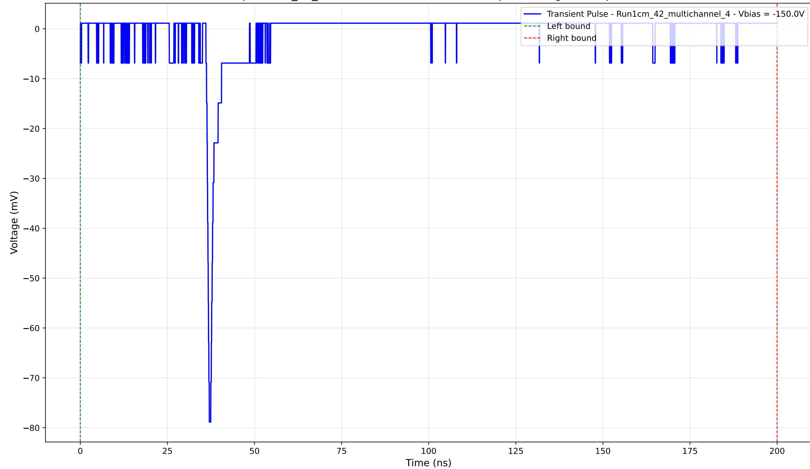
Transient Pulse - Sample: 1cm_42_multichannel - Position: 2465.0 \mu\text{m} - Charge: 2.04 pC - Rise Time: 0.80 ns
