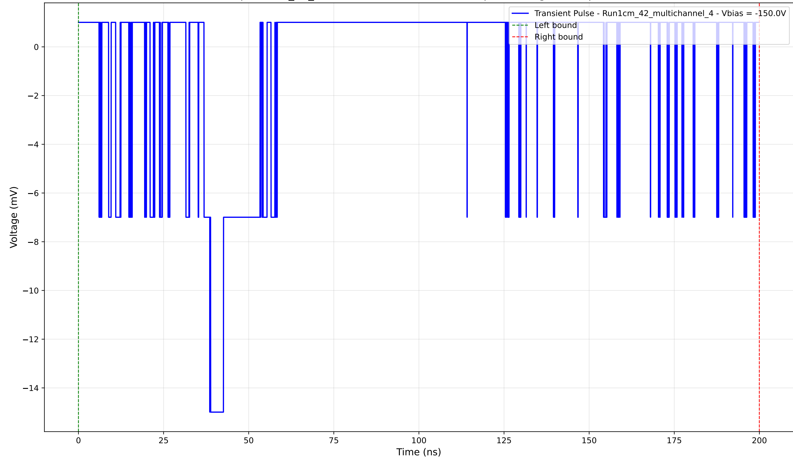
Transient Pulse - Sample: 1cm_42_multichannel - Position: 215.0 \mu\text{m} - Charge: 1.74 pC - Rise Time: 1.74 ns
