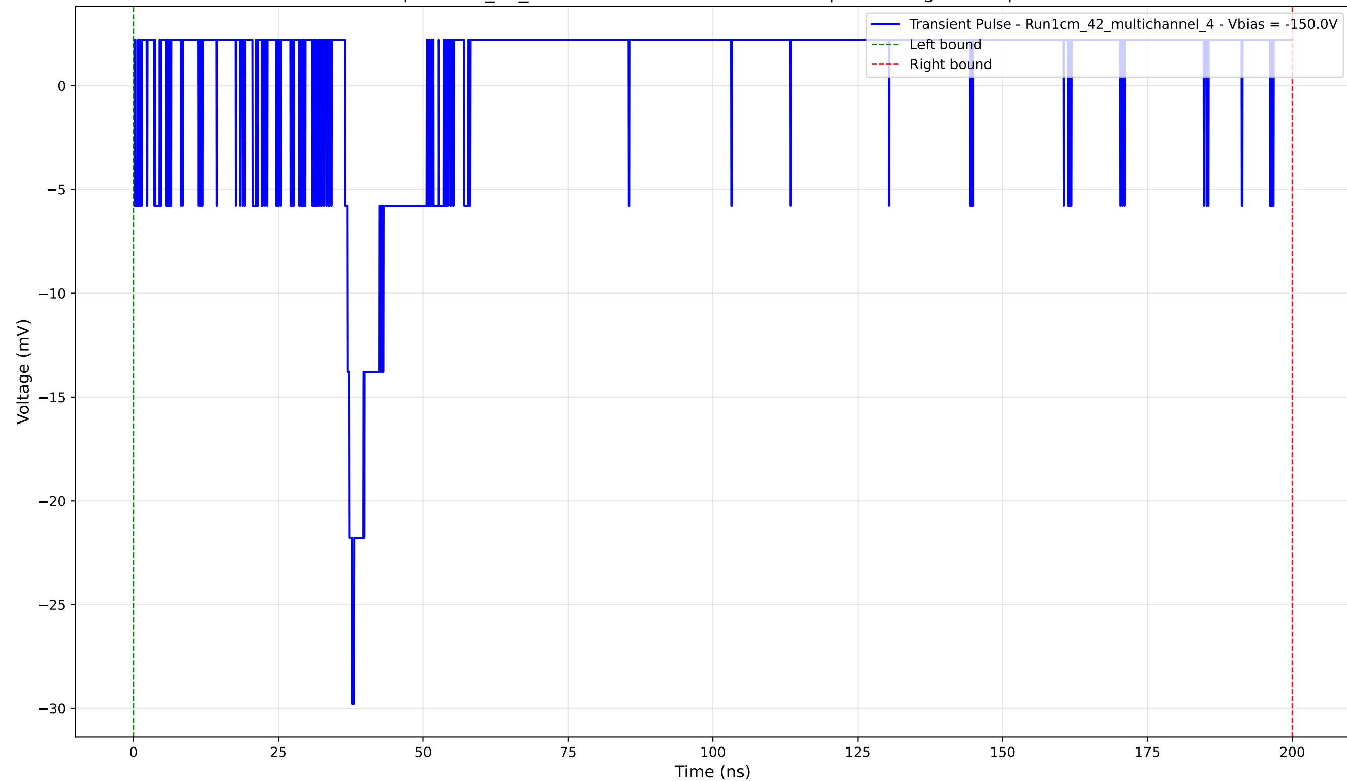
Transient Pulse - Sample: 1cm_42_multichannel - Position: 3240.0 \mu\text{m} - Charge: 3.07 pC - Rise Time: 1.28 ns
