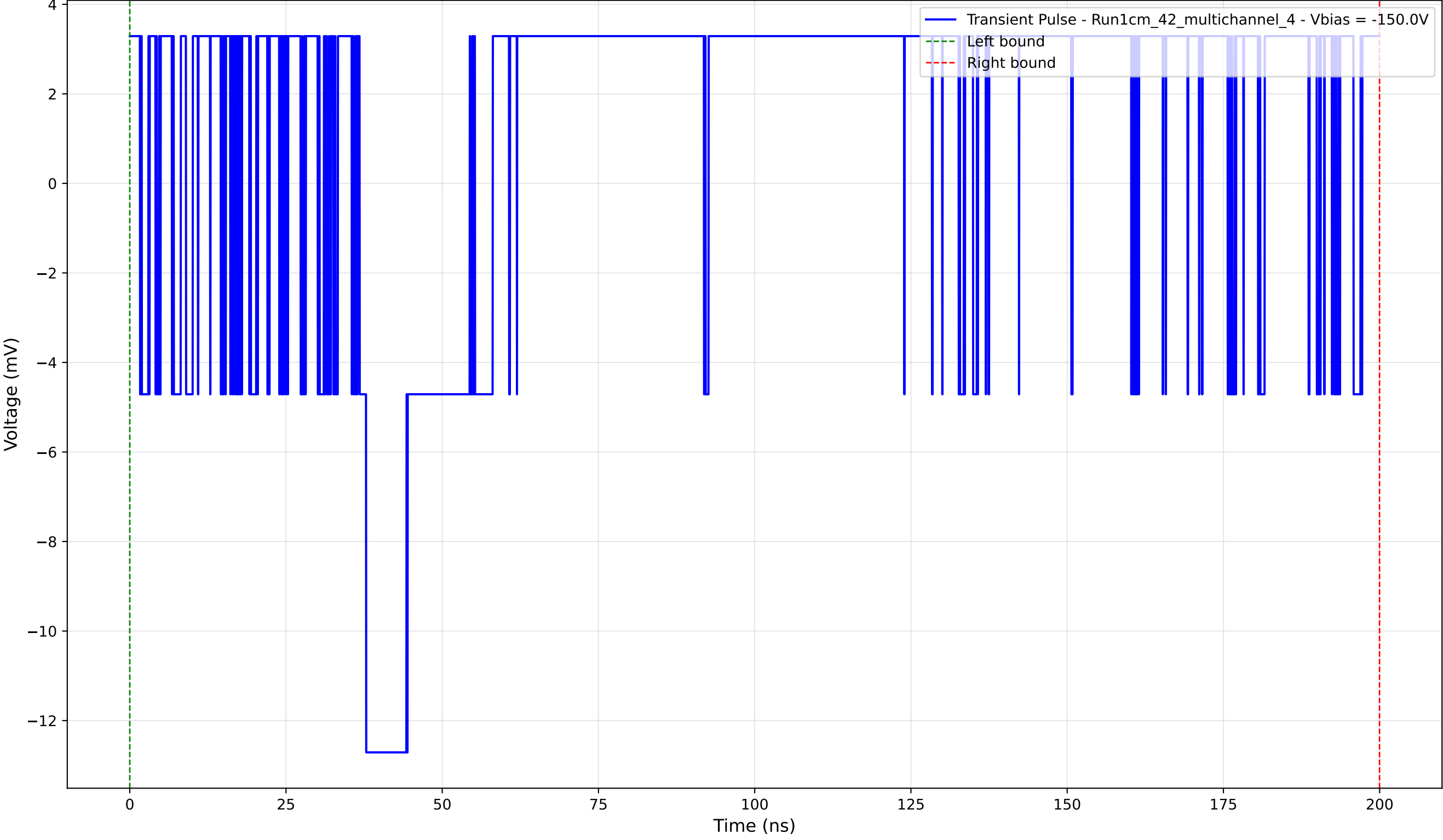
Transient Pulse - Sample: 1cm_42_multichannel - Position: 605.0 \mu\text{m} - Charge: 5.69 pC - Rise Time: 0.00 ns (N/A)
