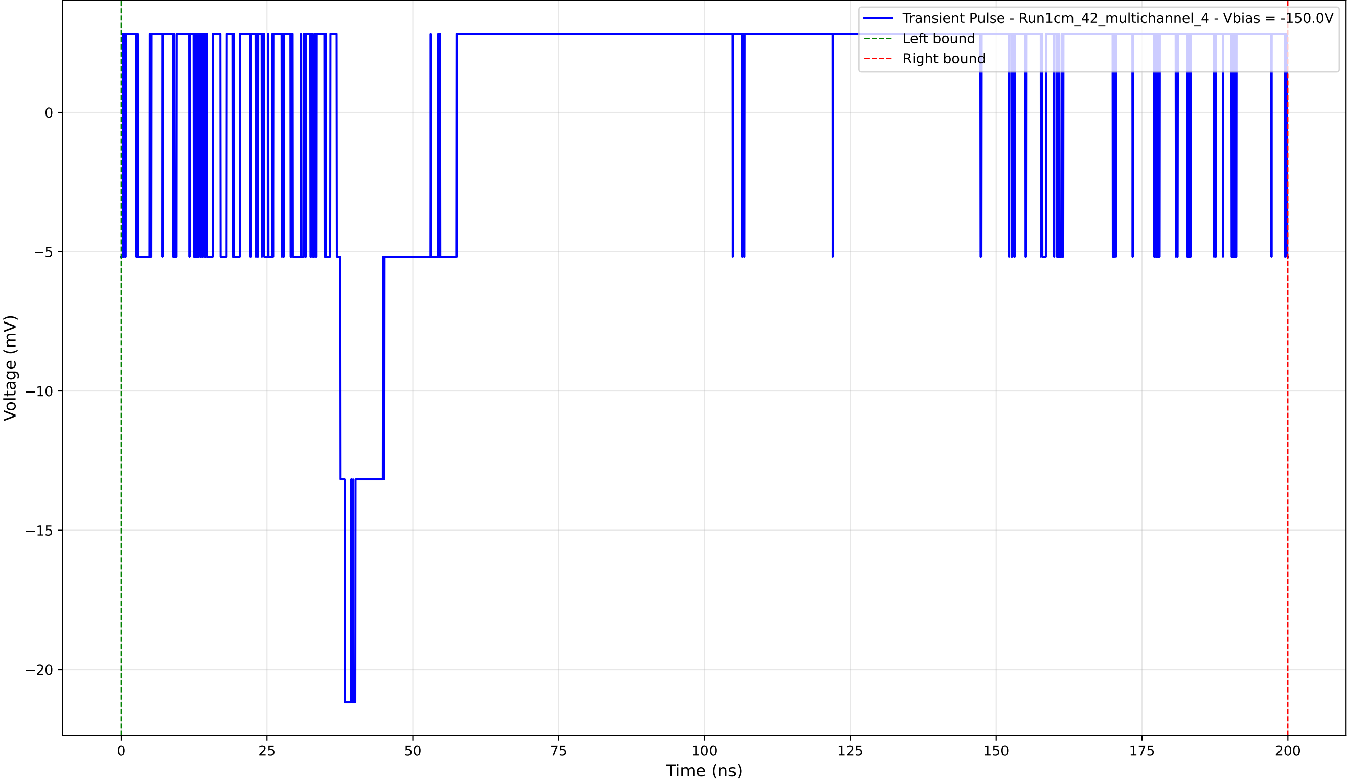
Transient Pulse - Sample: 1cm_42_multichannel - Position: 985.0 \mu\text{m} - Charge: 3.66 pC - Rise Time: 0.00 ns (N/A)
