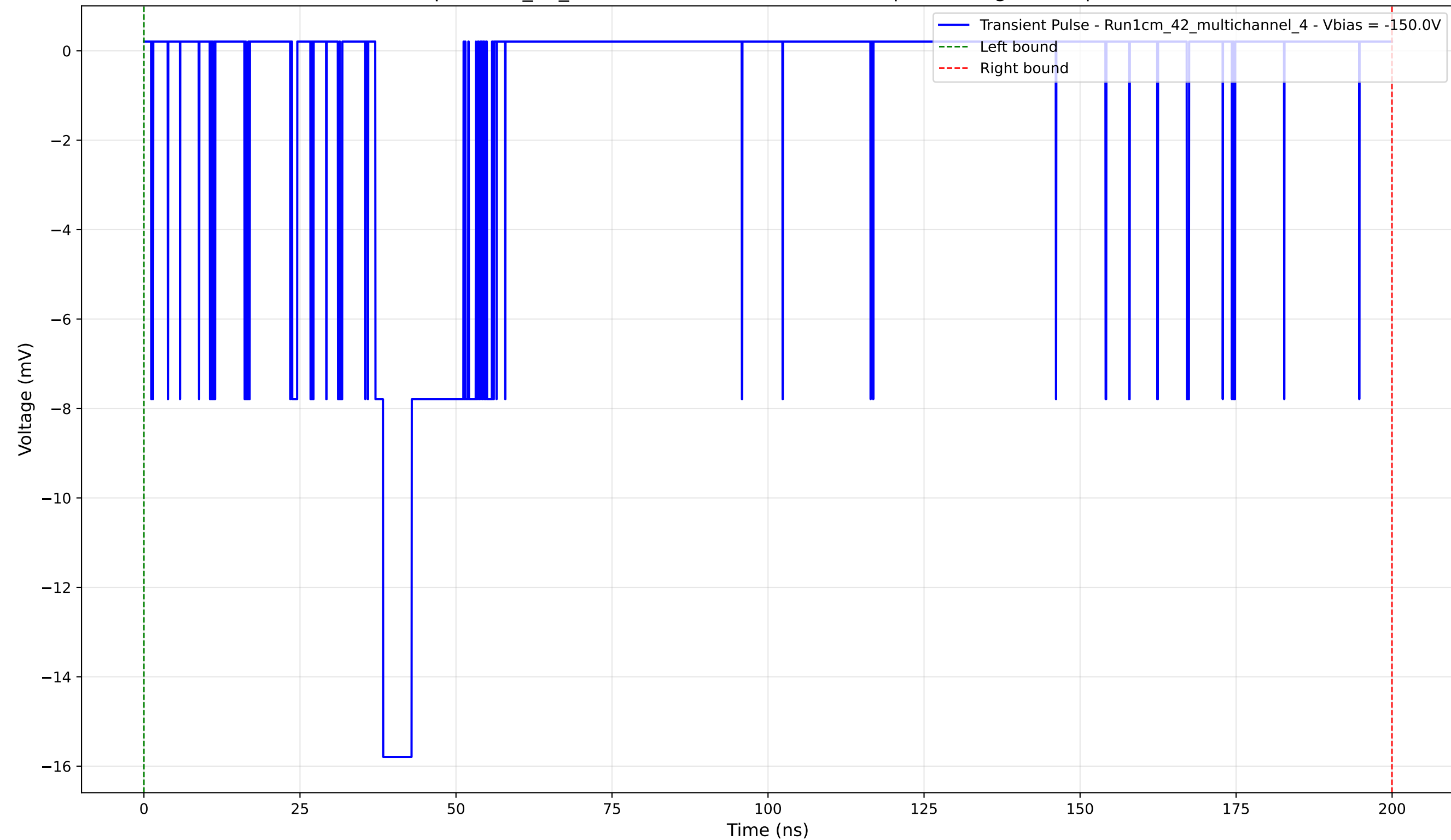
Transient Pulse - Sample: 1cm_42_multichannel - Position: 4220.0 \mu\text{m} - Charge: 3.48 pC - Rise Time: 1.26 ns
