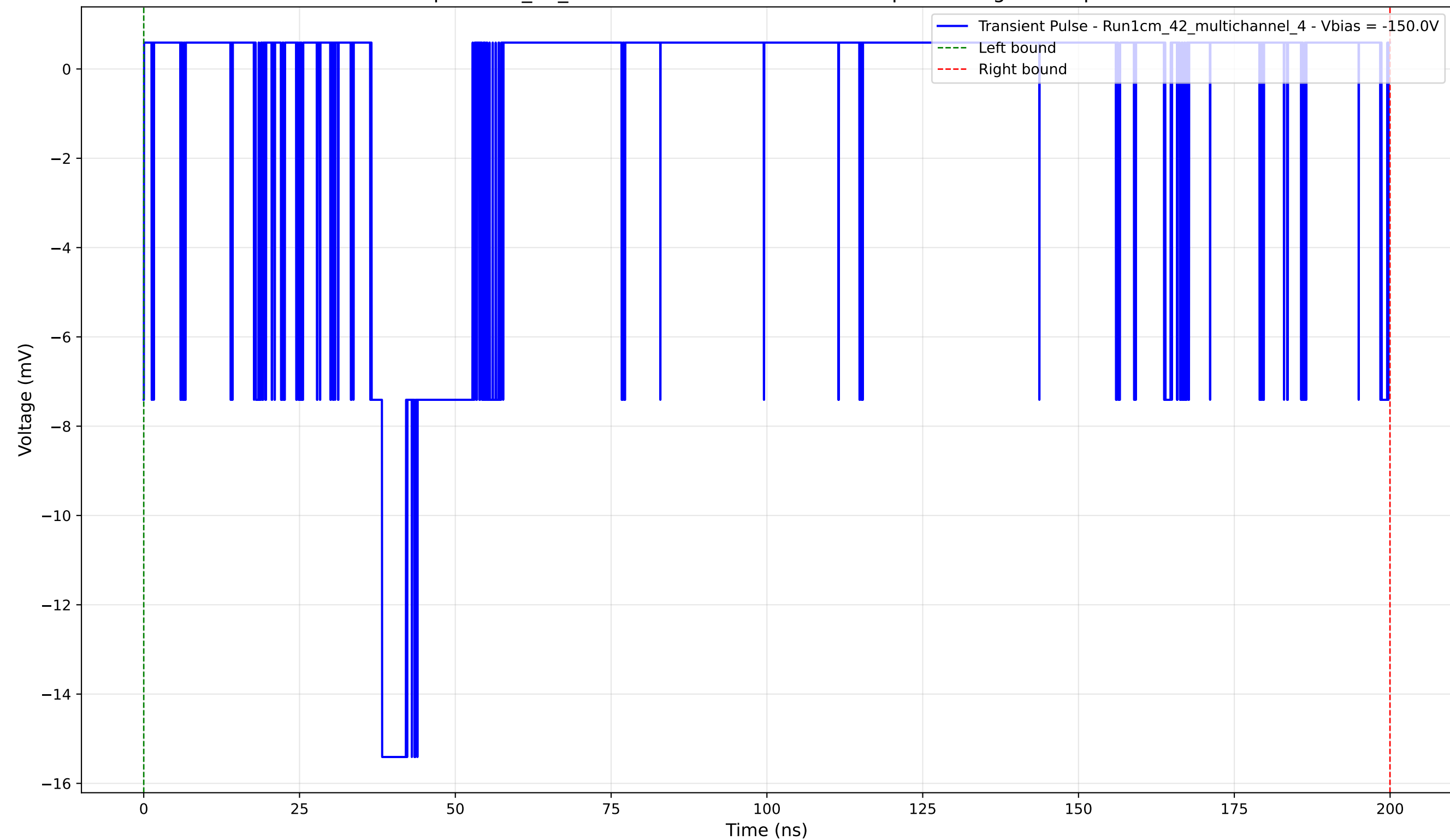
Transient Pulse - Sample: 1cm_42_multichannel - Position: 4320.0 \mu\text{m} - Charge: 2.96 pC - Rise Time: 1.70 ns
