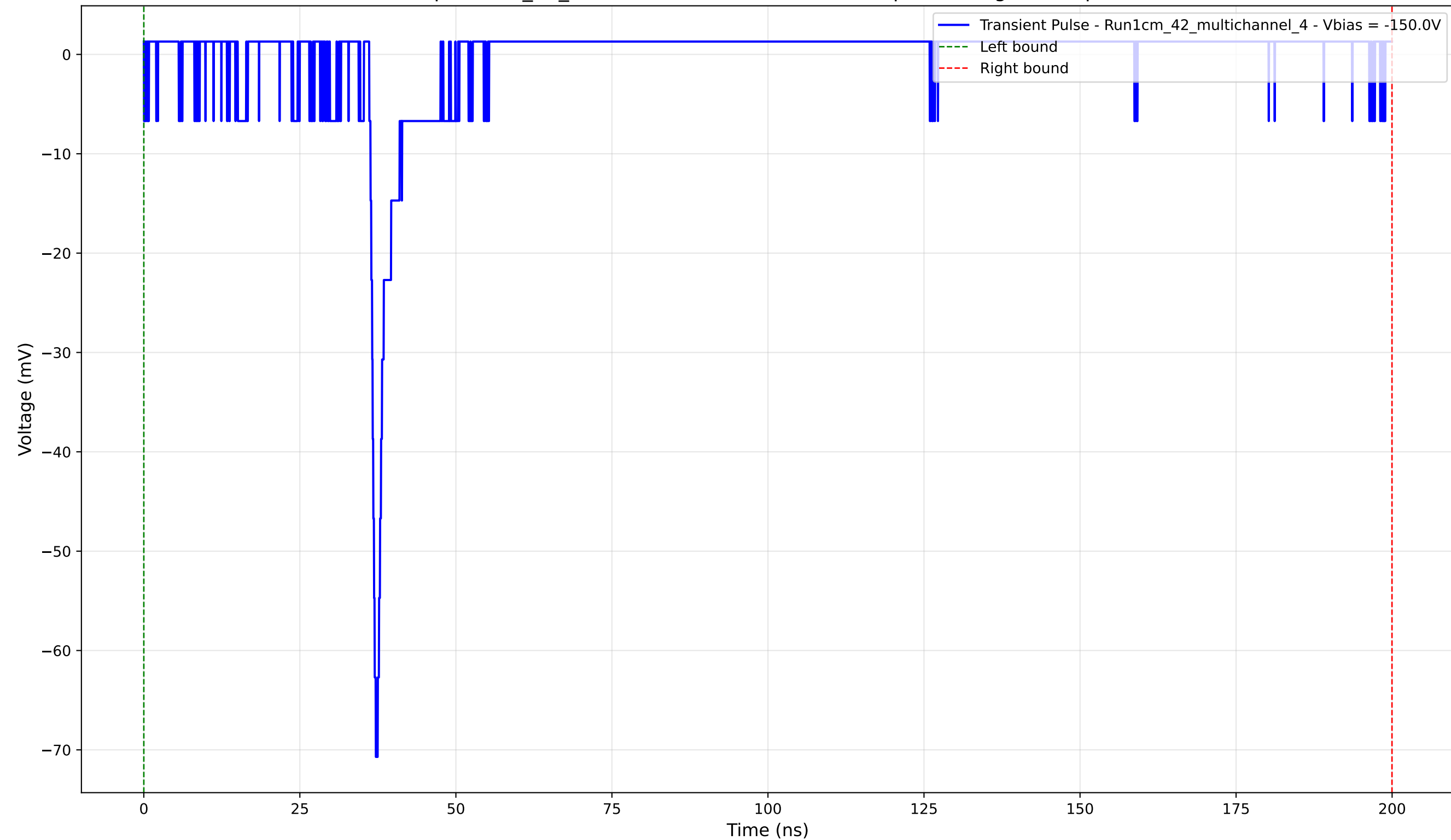
Transient Pulse - Sample: 1cm_42_multichannel - Position: 2580.0 \mu\text{m} - Charge: 1.21 pC - Rise Time: 0.86 ns
