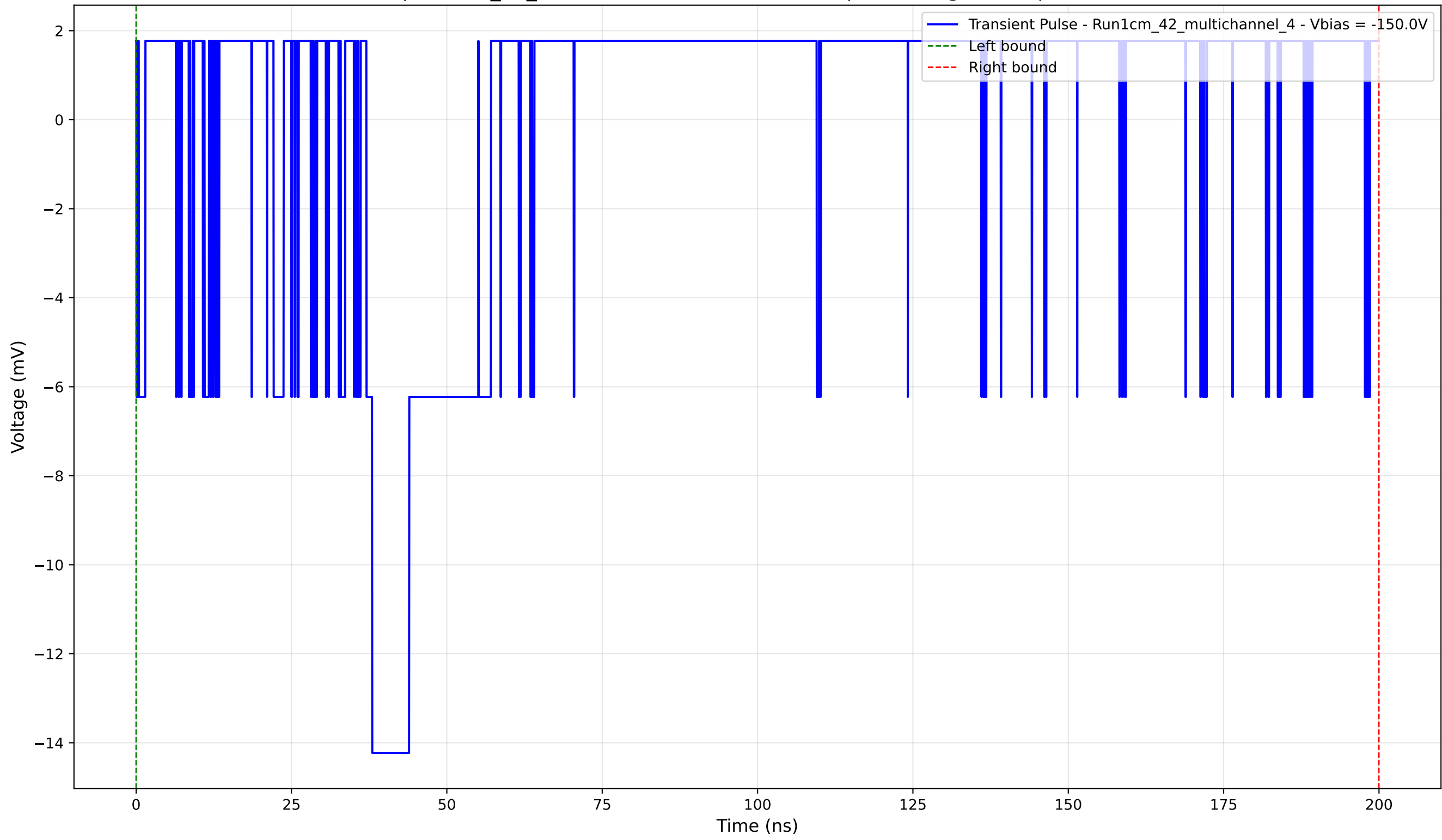
Transient Pulse - Sample: 1cm_42_multichannel - Position: 500.0 \mu\text{m} - Charge: 0.81 pC - Rise Time: 0.00 ns (N/A)
