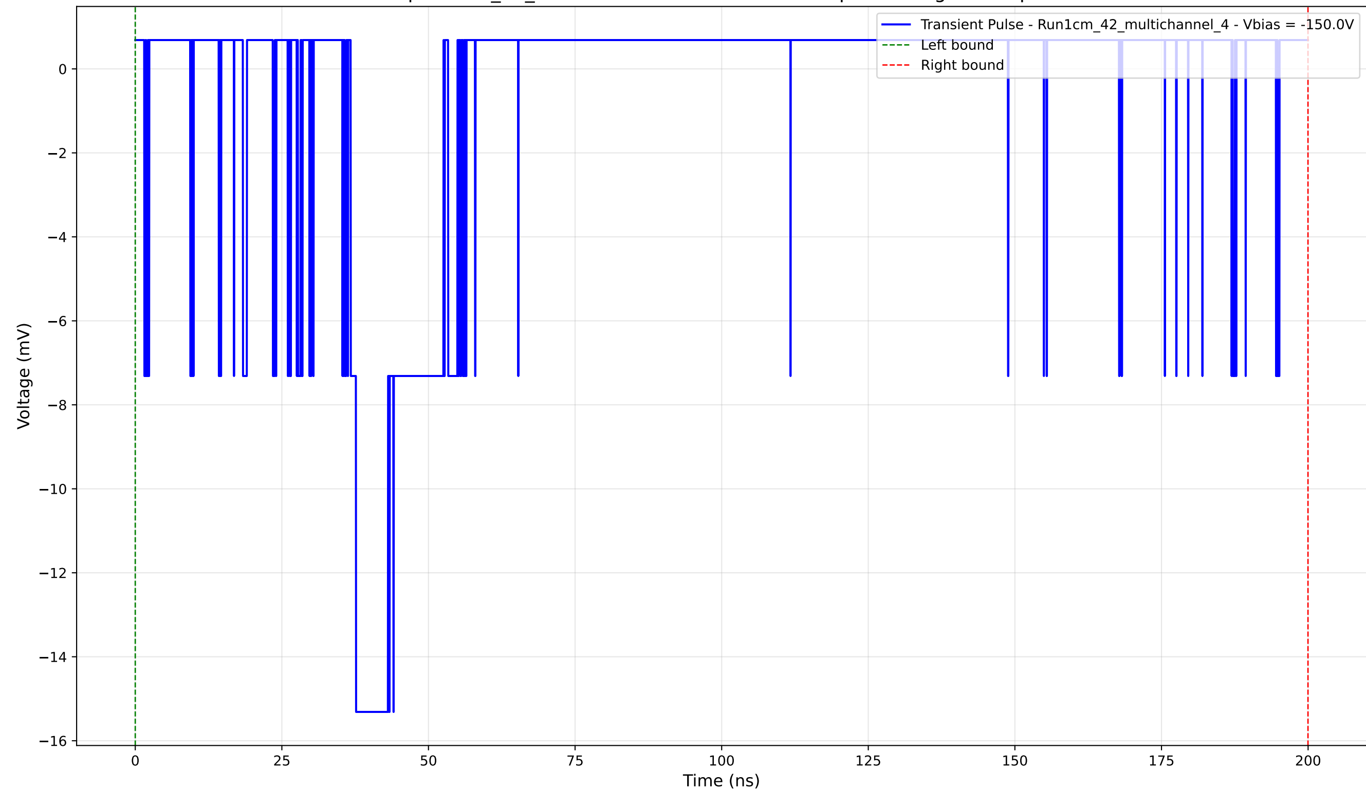
Transient Pulse - Sample: 1cm_42_multichannel - Position: 3765.0 \mu\text{m} - Charge: 1.94 pC - Rise Time: 0.92 ns
