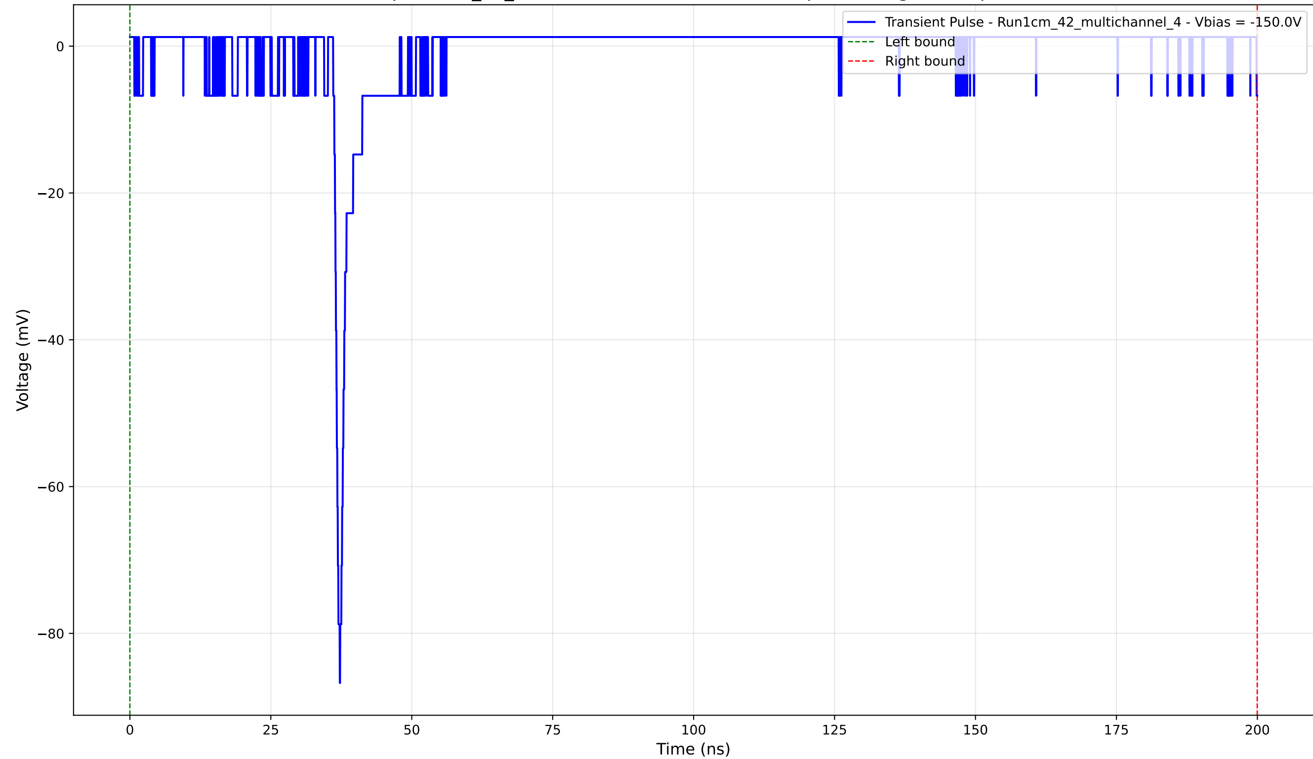
Transient Pulse - Sample: 1cm_42_multichannel - Position: 2475.0 \mu\text{m} - Charge: 2.11 pC - Rise Time: 0.74 ns
