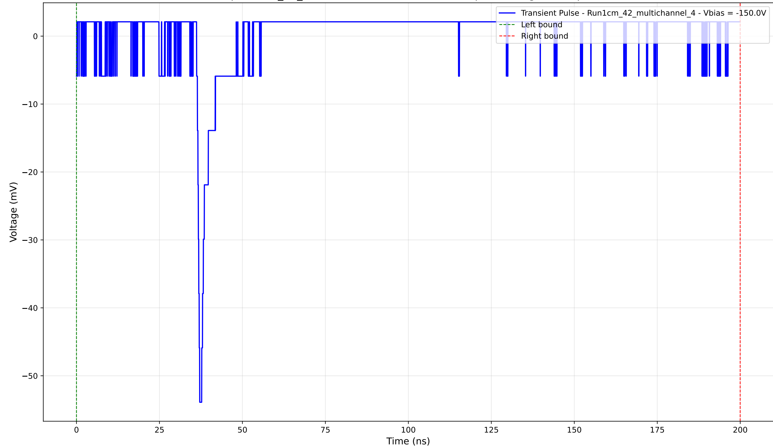
Transient Pulse - Sample: 1cm_42_multichannel - Position: 2710.0 \mu\text{m} - Charge: 1.77 pC - Rise Time: 0.92 ns
