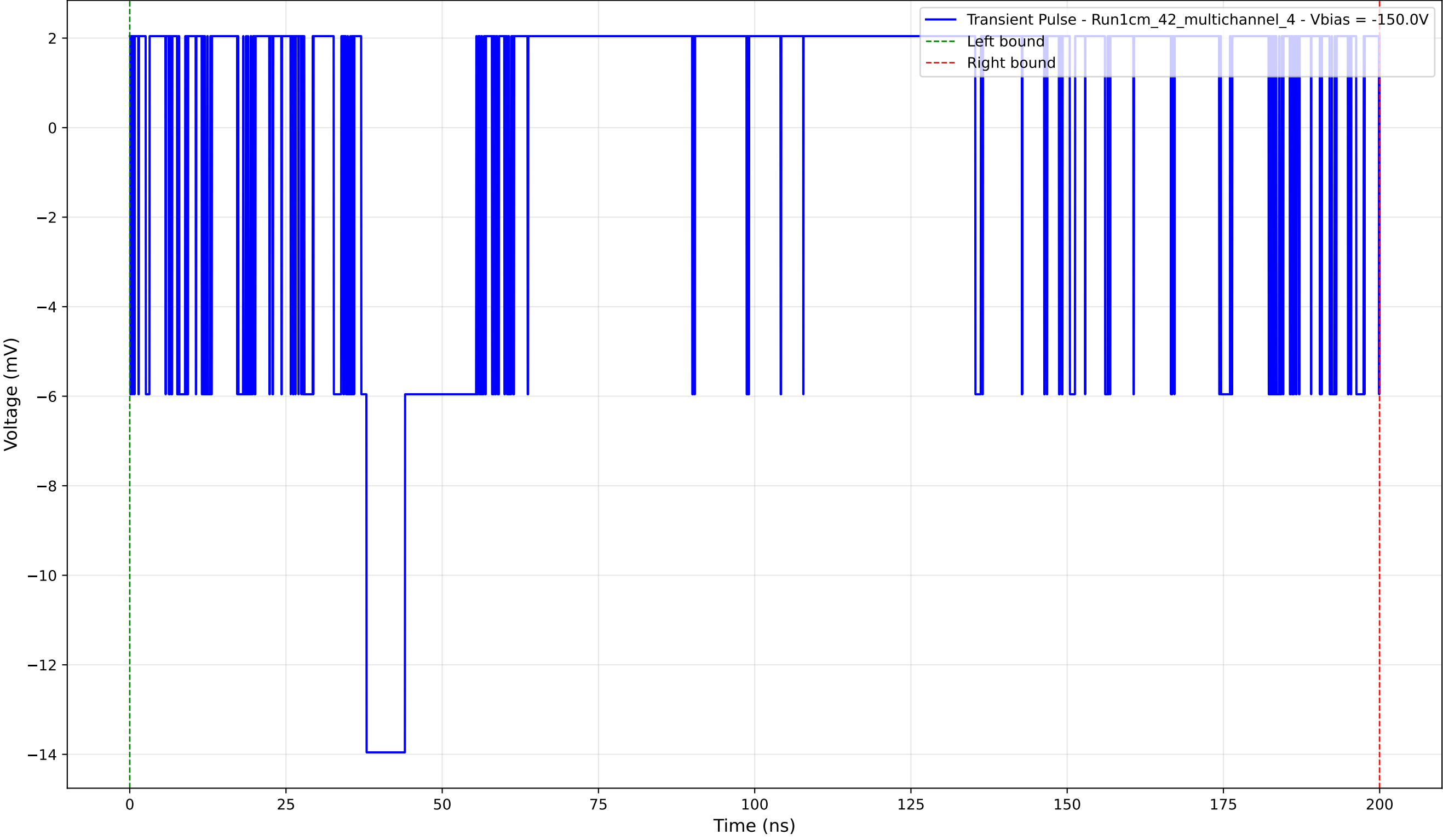
Transient Pulse - Sample: 1cm_42_multichannel - Position: 585.0 \mu\text{m} - Charge: 0.60 pC - Rise Time: 0.00 ns (N/A)
