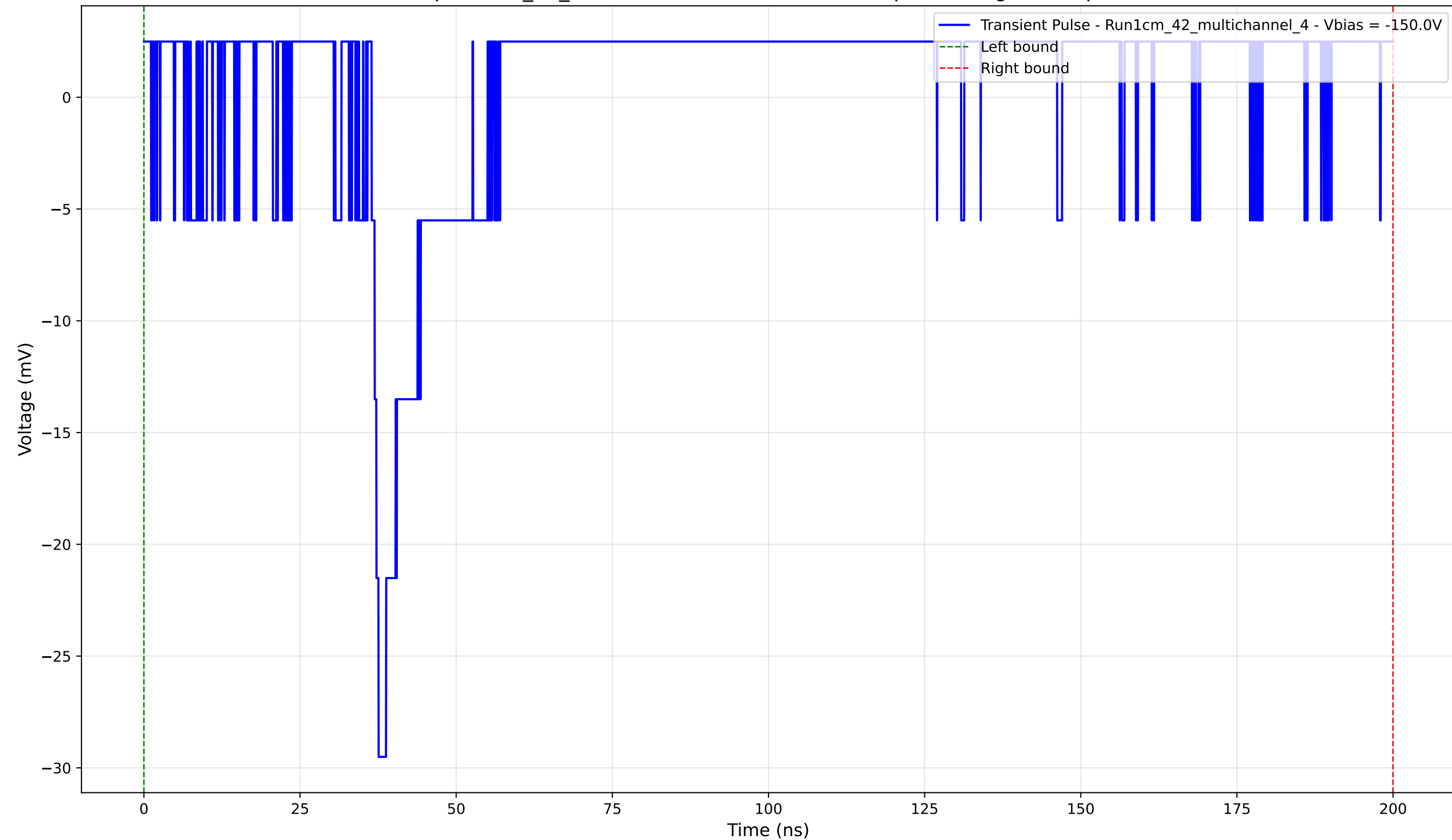
Transient Pulse - Sample: 1cm_42_multichannel - Position: 1485.0 \mu\text{m} - Charge: 2.93 pC - Rise Time: 1.12 ns
