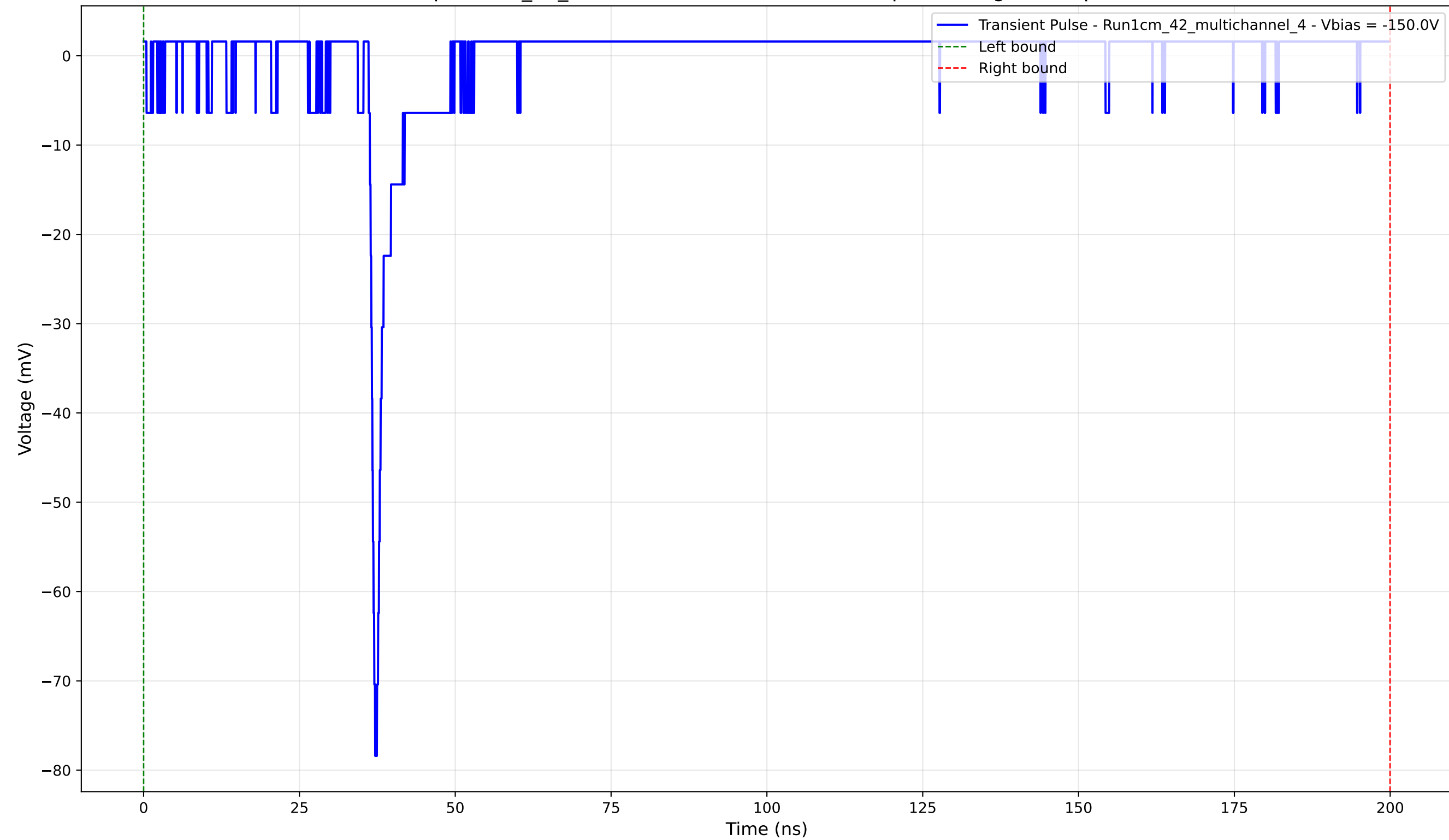
Transient Pulse - Sample: 1cm_42_multichannel - Position: 2535.0 \mu\text{m} - Charge: 0.16 pC - Rise Time: 0.86 ns
