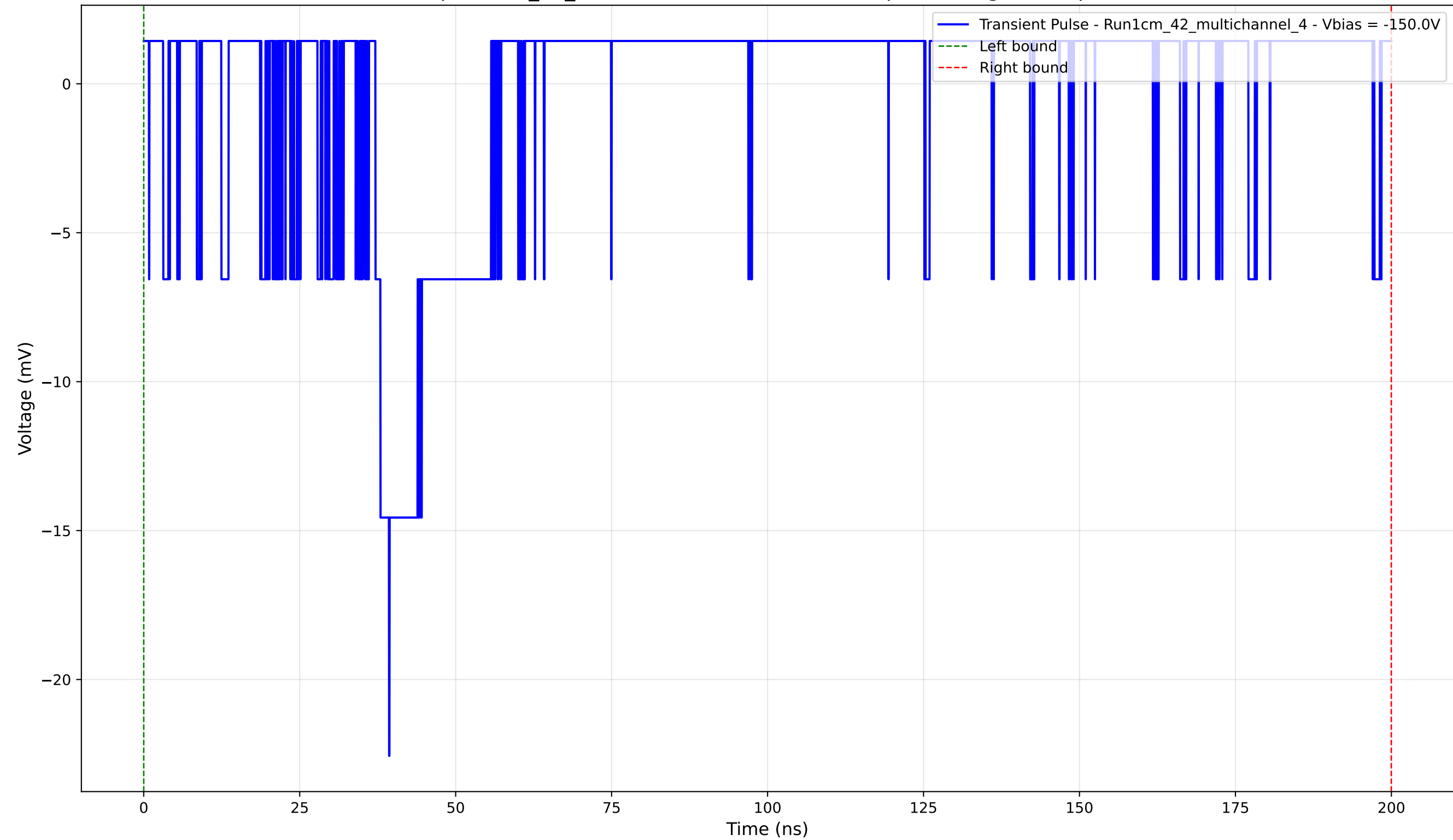
Transient Pulse - Sample: 1cm_42_multichannel - Position: 675.0 \mu\text{m} - Charge: 0.96 pC - Rise Time: 2.20 ns
