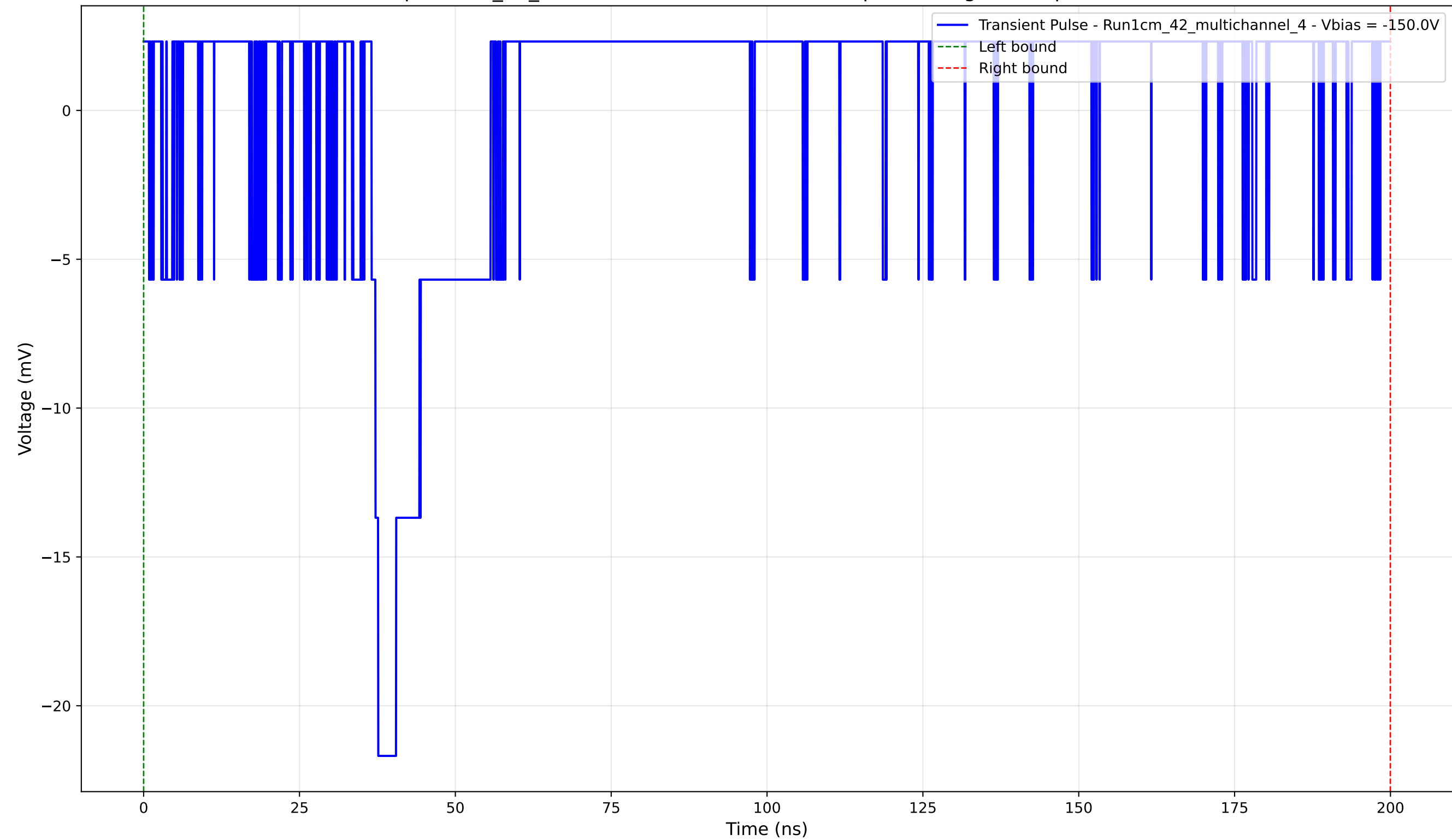
Transient Pulse - Sample: 1cm_42_multichannel - Position: 1255.0 \mu\text{m} - Charge: 1.92 pC - Rise Time: 0.00 ns (N/A)
