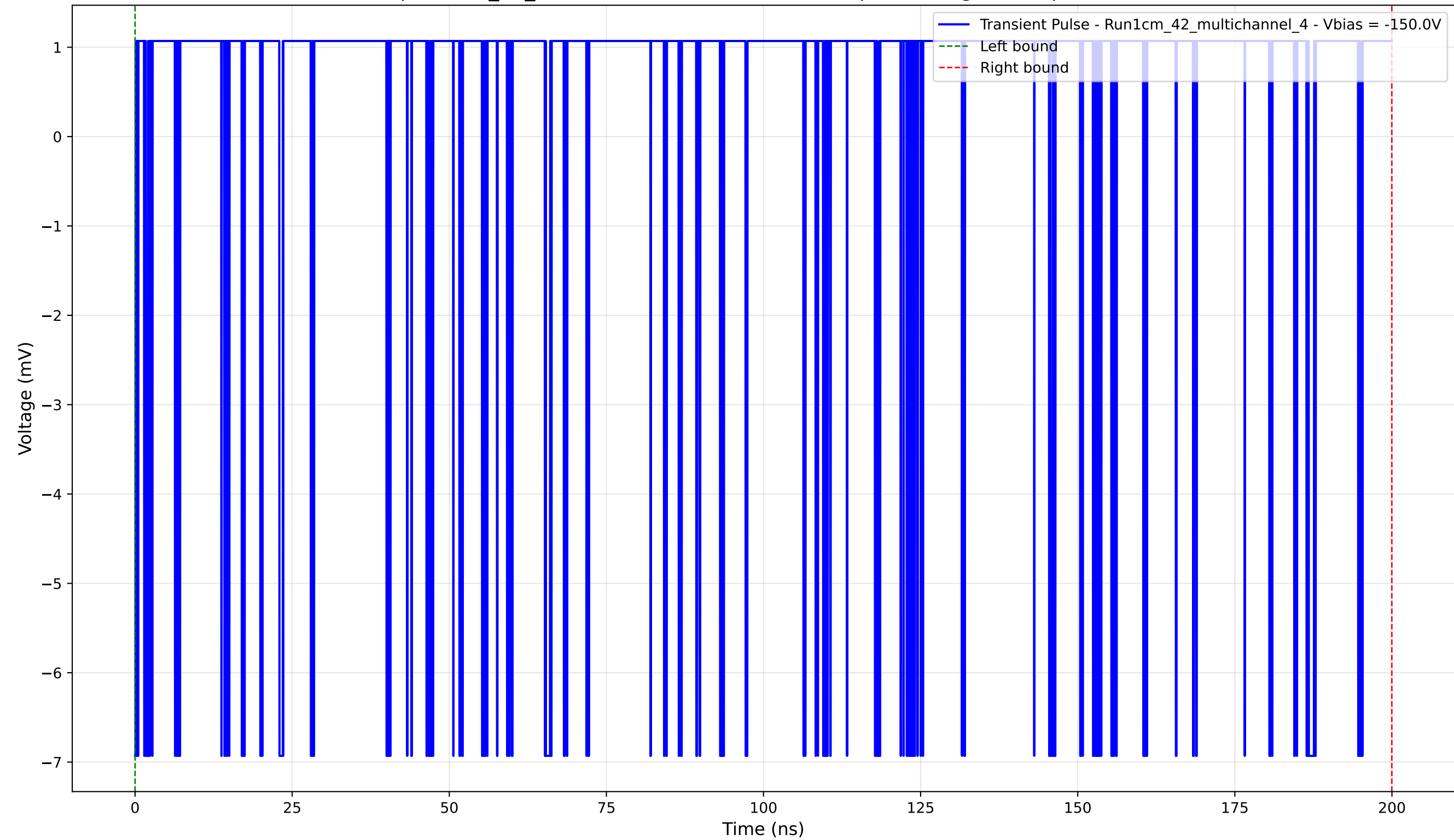
Transient Pulse - Sample: 1cm_42_multichannel - Position: 3905.0 \mu\text{m} - Charge: 1.73 pC - Rise Time: 0.00 ns (N/A)
