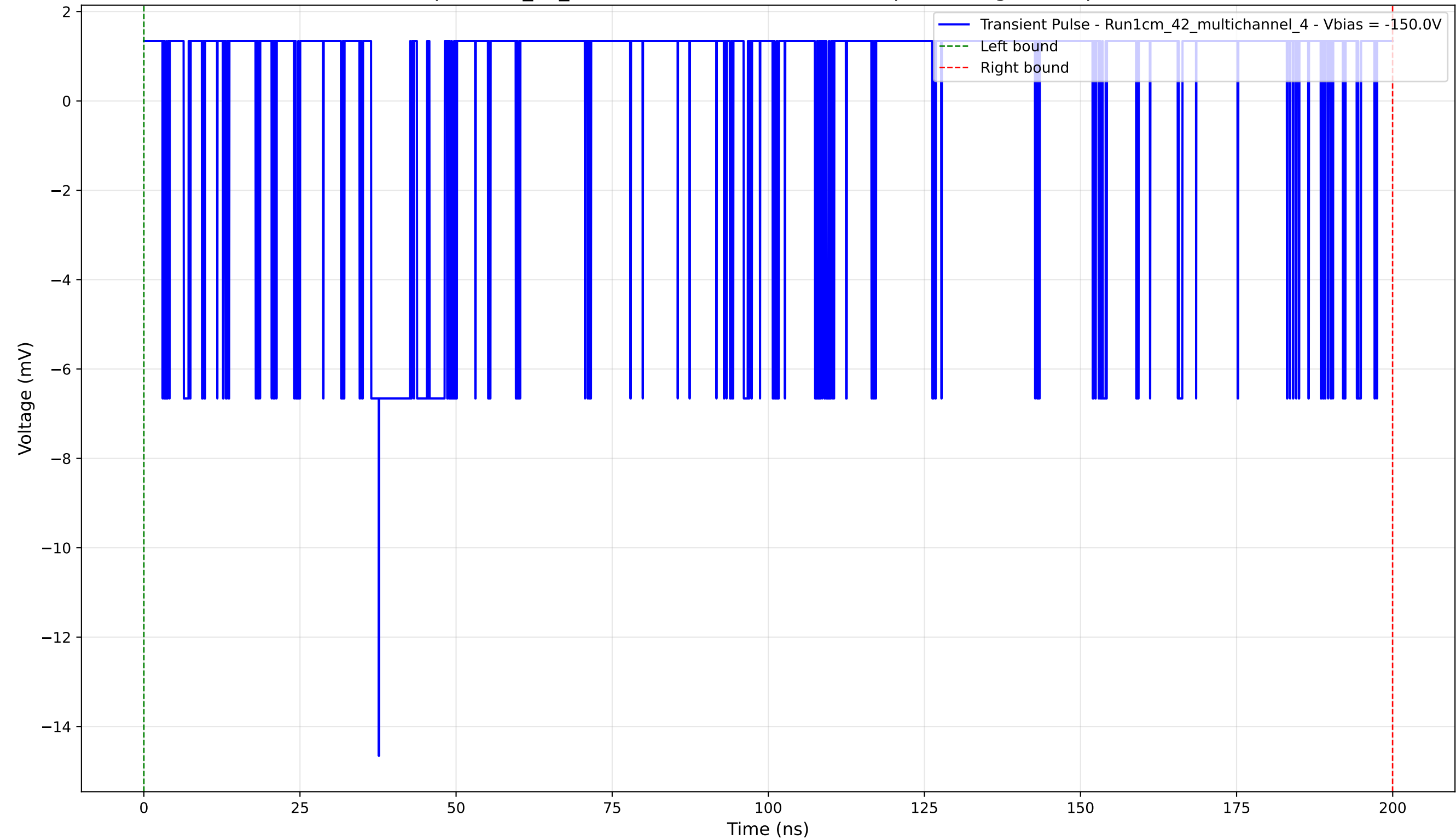
Transient Pulse - Sample: 1cm_42_multichannel - Position: 2855.0 \mu\text{m} - Charge: 1.13 pC - Rise Time: 1.26 ns
