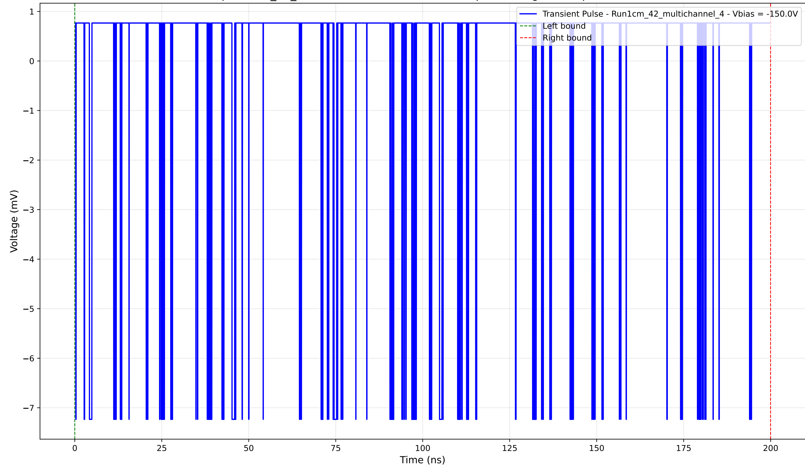
Transient Pulse - Sample: 1cm_42_multichannel - Position: 3900.0 \mu\text{m} - Charge: 0.54 pC - Rise Time: 0.00 ns (N/A)
