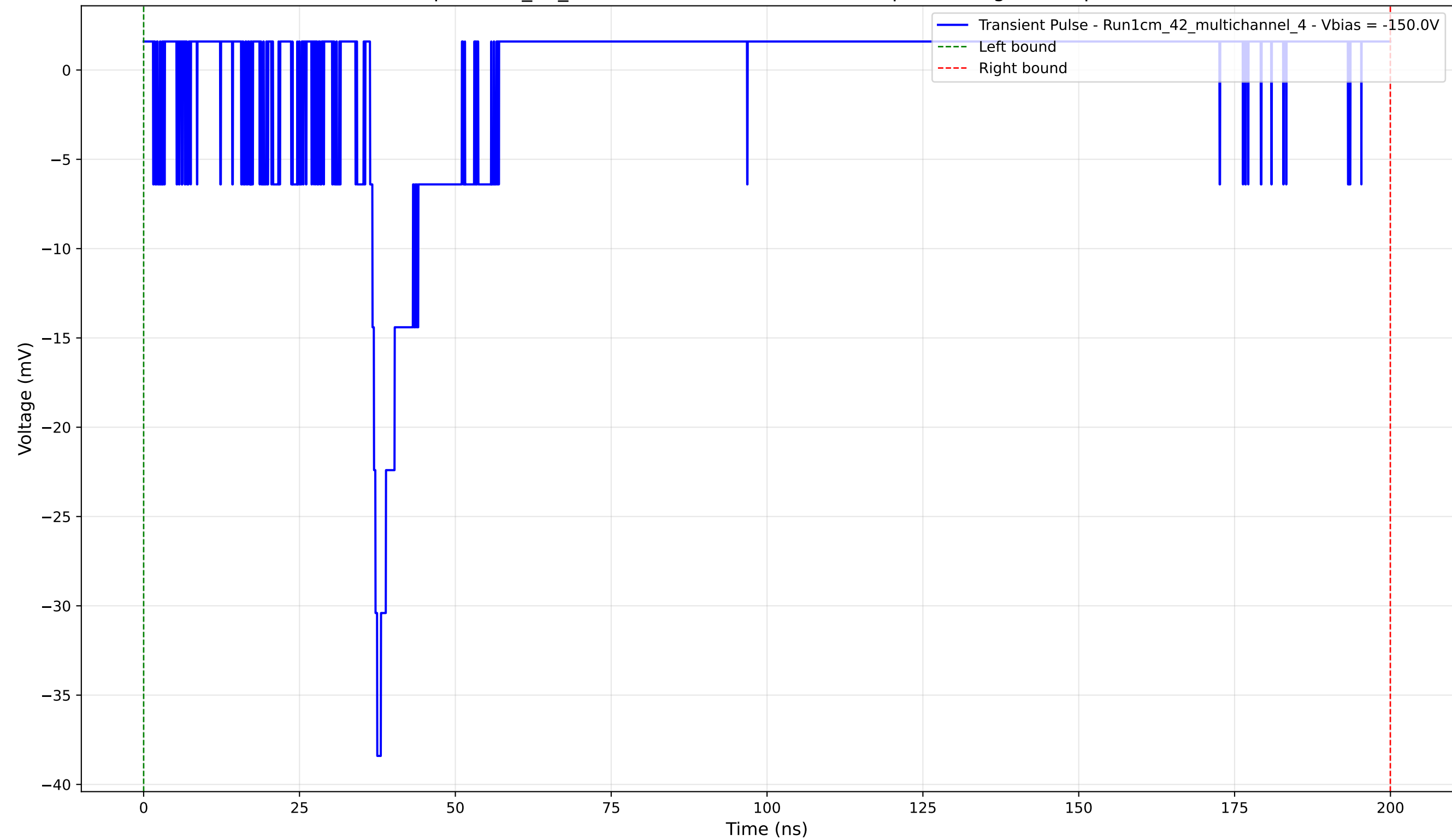
Transient Pulse - Sample: 1cm_42_multichannel - Position: 1685.0 \mu\text{m} - Charge: 0.60 pC - Rise Time: 1.15 ns
