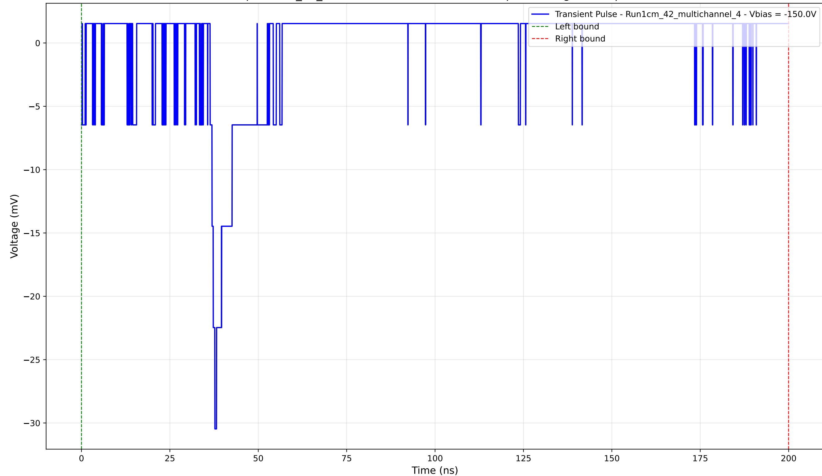
Transient Pulse - Sample: 1cm_42_multichannel - Position: 3245.0 \mu\text{m} - Charge: 0.48 pC - Rise Time: 1.35 ns
