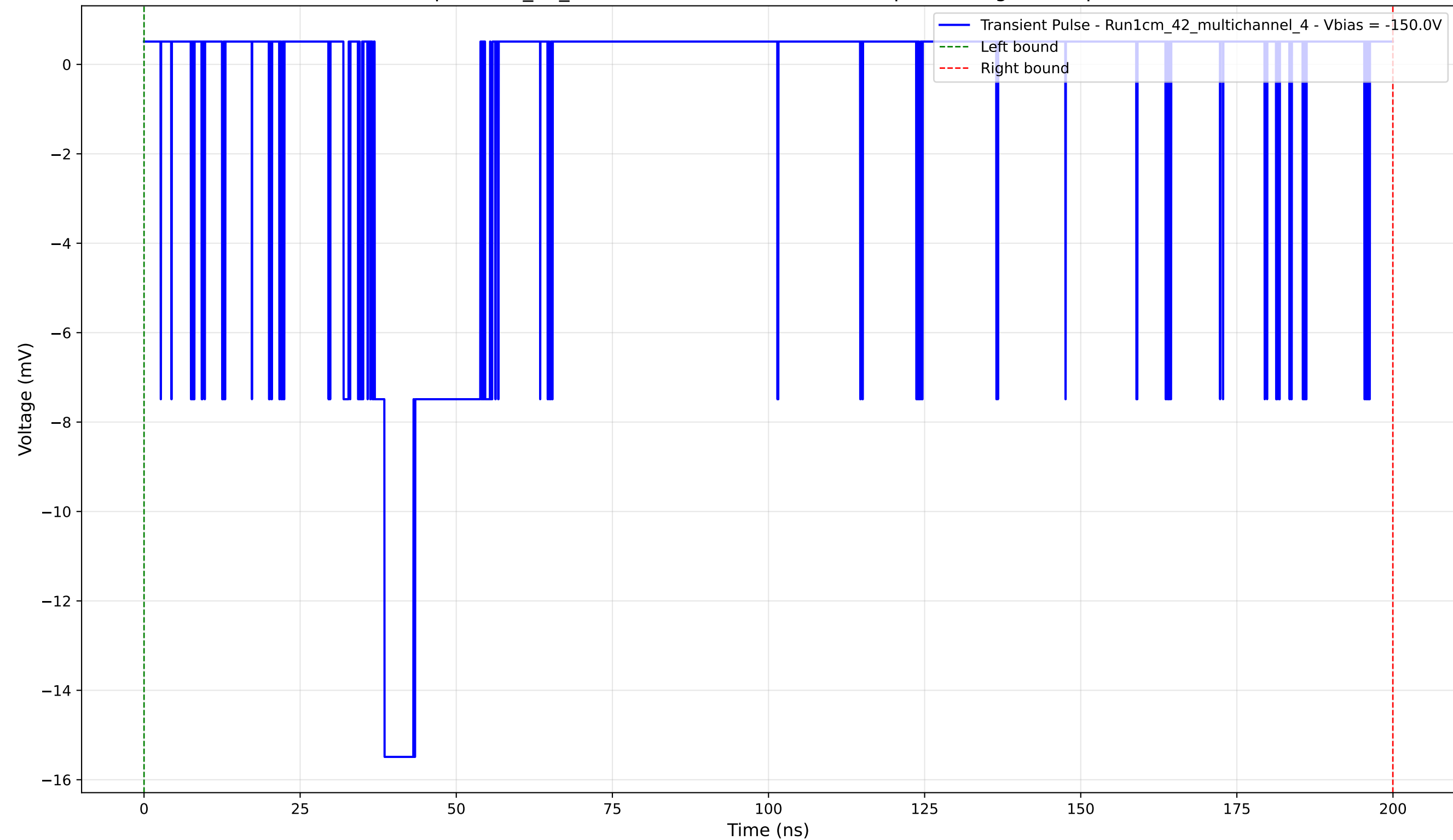
Transient Pulse - Sample: 1cm_42_multichannel - Position: 4595.0 \mu\text{m} - Charge: 2.84 pC - Rise Time: 1.58 ns
