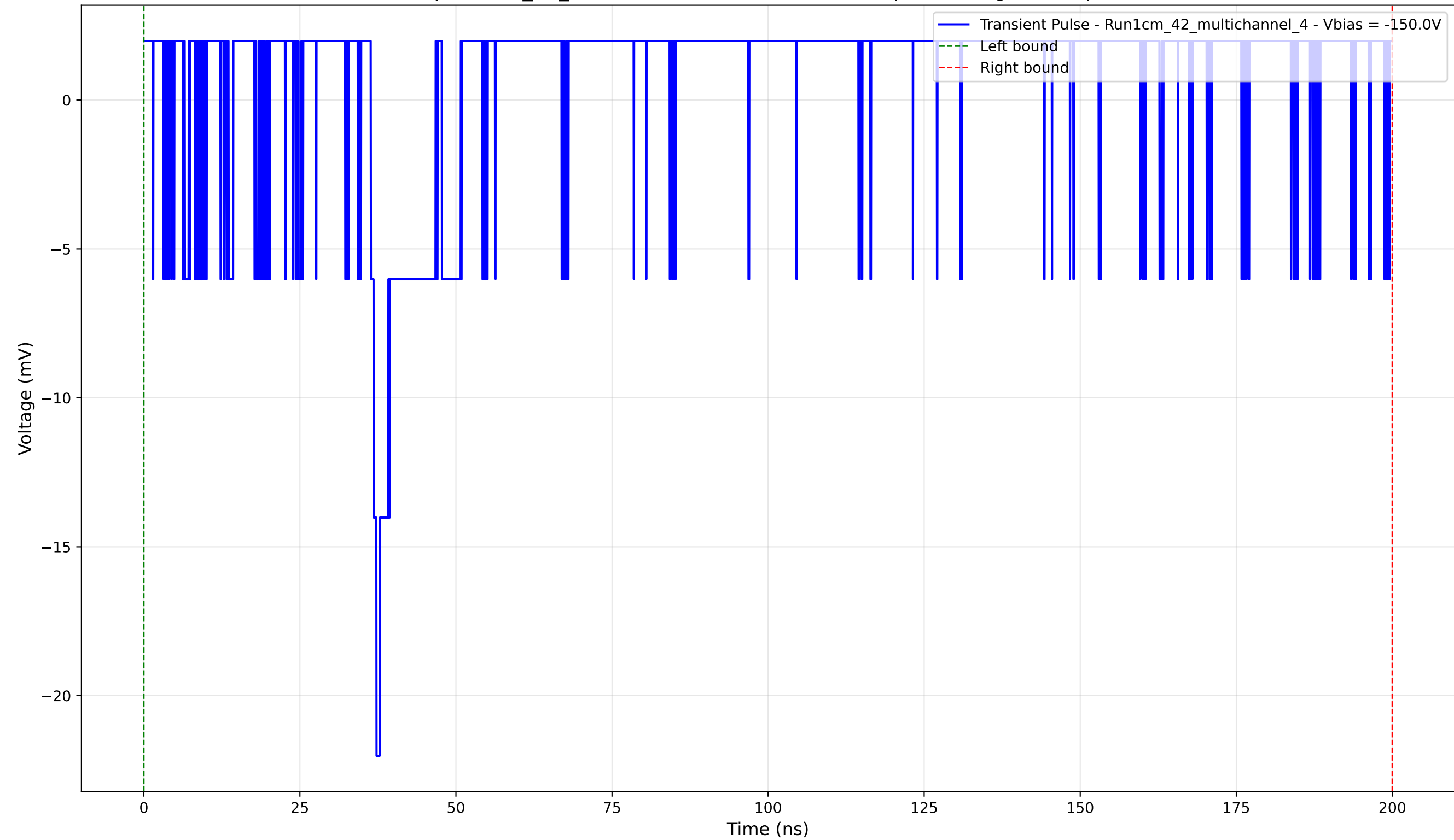
Transient Pulse - Sample: 1cm_42_multichannel - Position: 2845.0 \mu\text{m} - Charge: 3.10 pC - Rise Time: 0.92 ns
