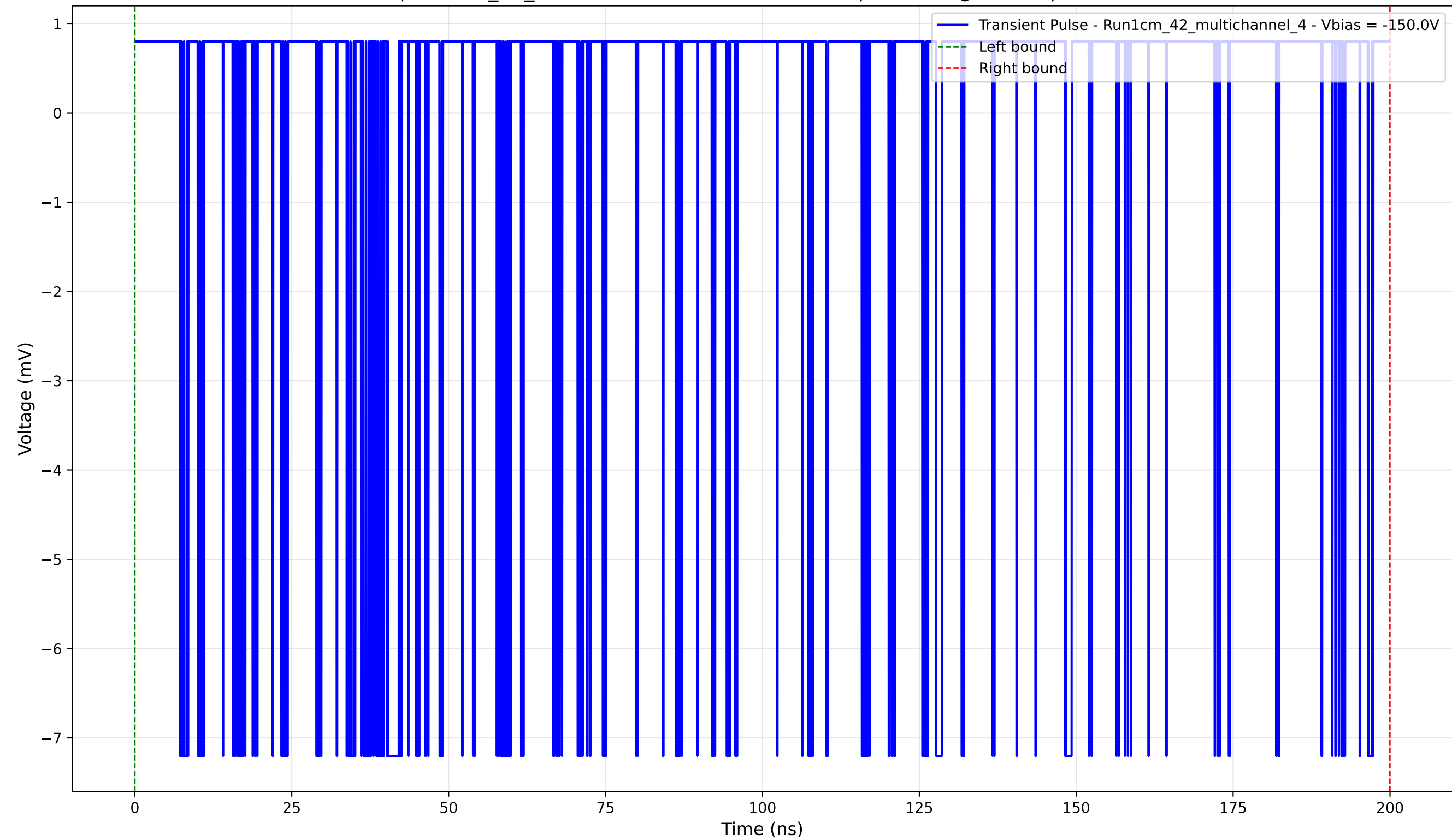
Transient Pulse - Sample: 1cm_42_multichannel - Position: 3380.0 \mu\text{m} - Charge: 0.57 pC - Rise Time: 0.00 ns (N/A)
