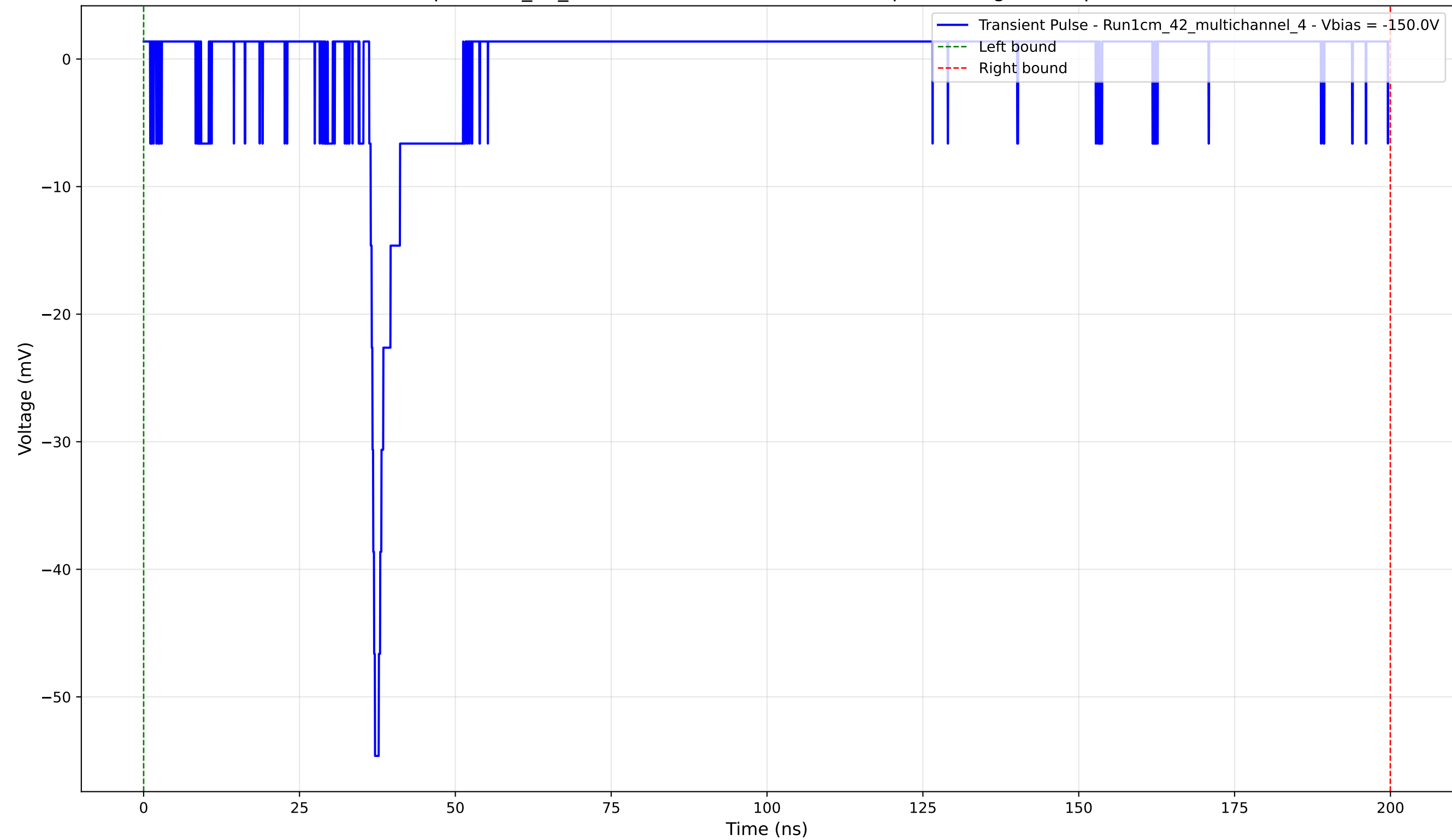
Transient Pulse - Sample: 1cm_42_multichannel - Position: 2680.0 \mu\text{m} - Charge: 0.23 pC - Rise Time: 0.92 ns
