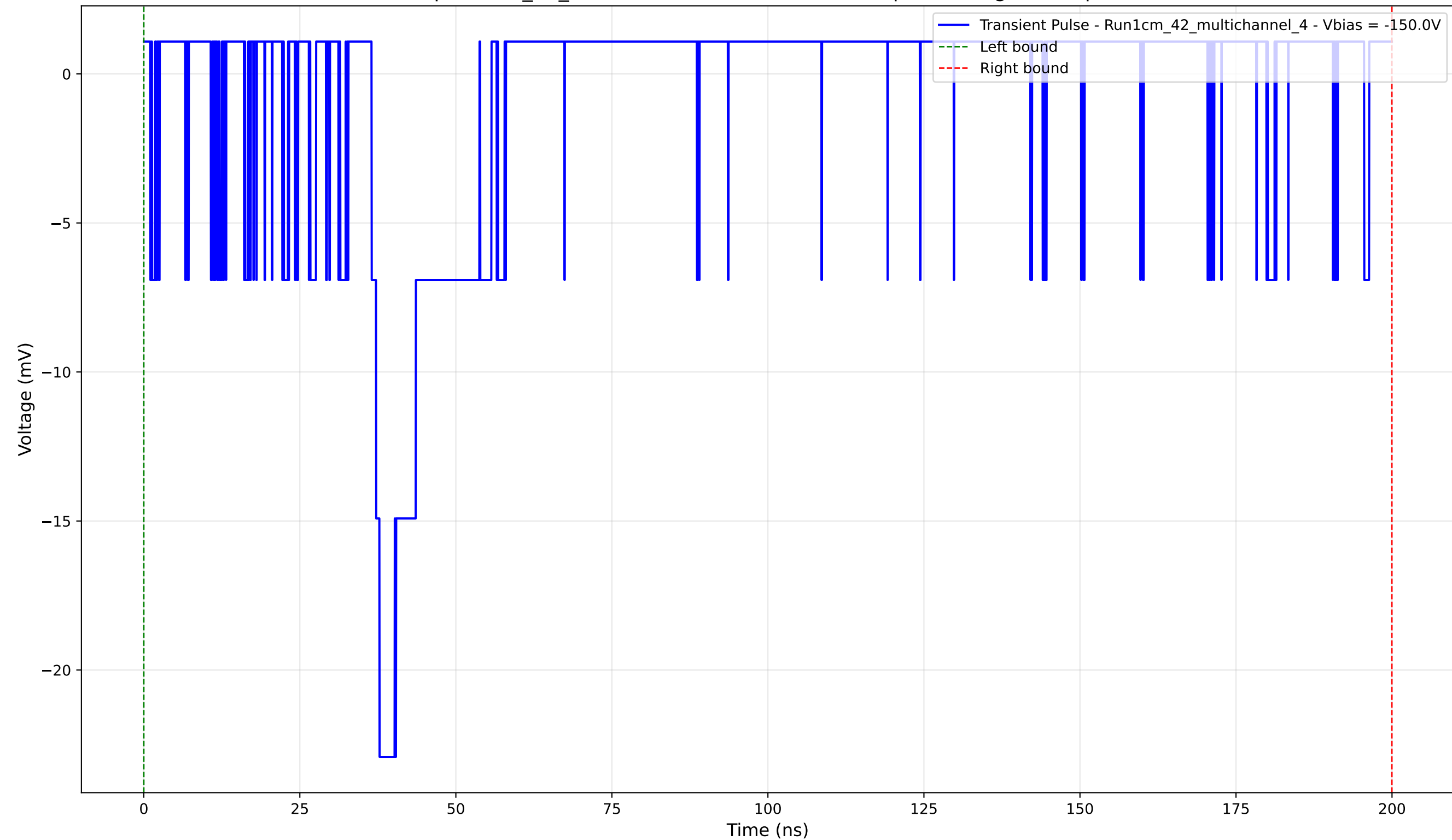
Transient Pulse - Sample: 1cm_42_multichannel - Position: 1200.0 \mu\text{m} - Charge: 2.24 pC - Rise Time: 1.28 ns
