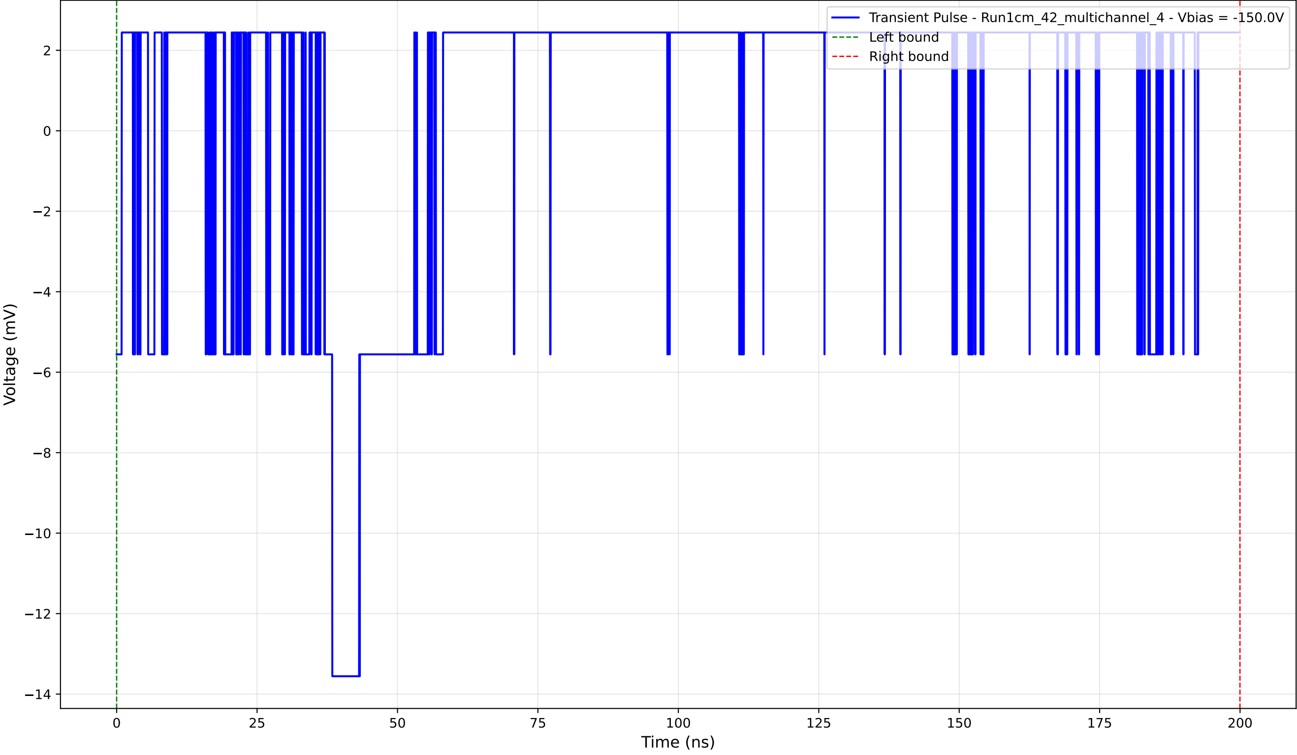
Transient Pulse - Sample: 1cm_42_multichannel - Position: 450.0 \mu\text{m} - Charge: 3.30 pC - Rise Time: 0.00 ns (N/A)
