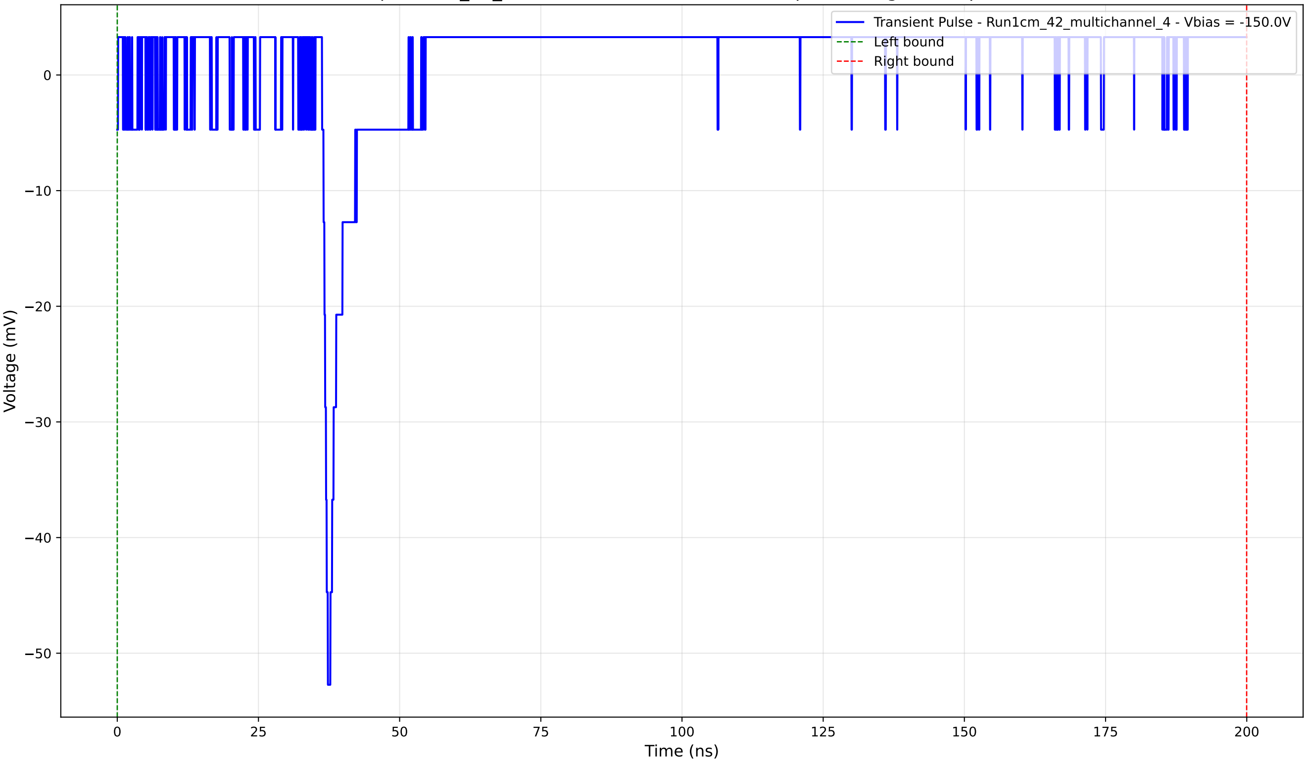
Transient Pulse - Sample: 1cm_42_multichannel - Position: 1970.0 \mu\text{m} - Charge: 5.63 pC - Rise Time: 0.78 ns
