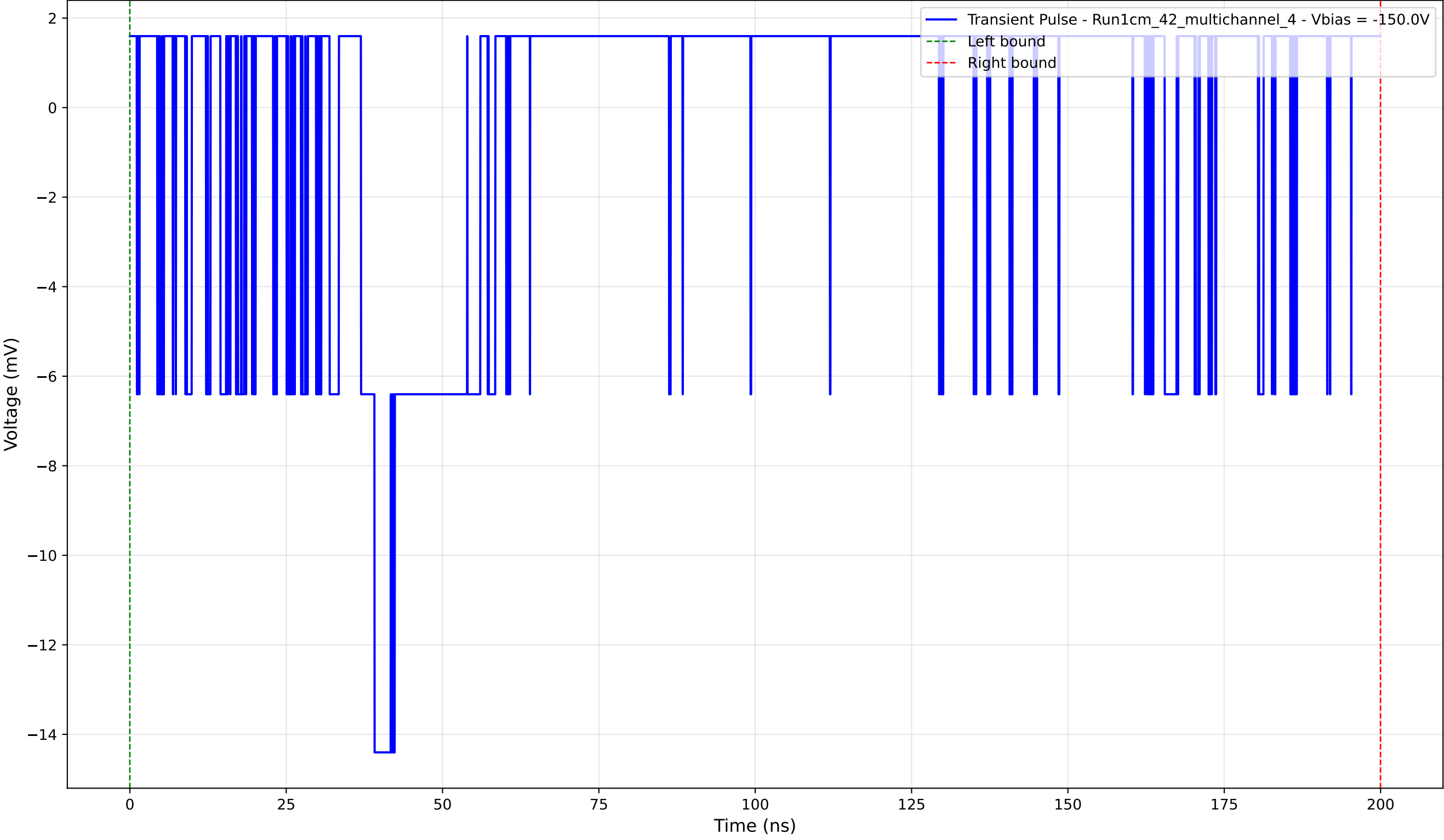
Transient Pulse - Sample: 1cm_42_multichannel - Position: 175.0 \mu\text{m} - Charge: 0.24 pC - Rise Time: 0.00 ns (N/A)
