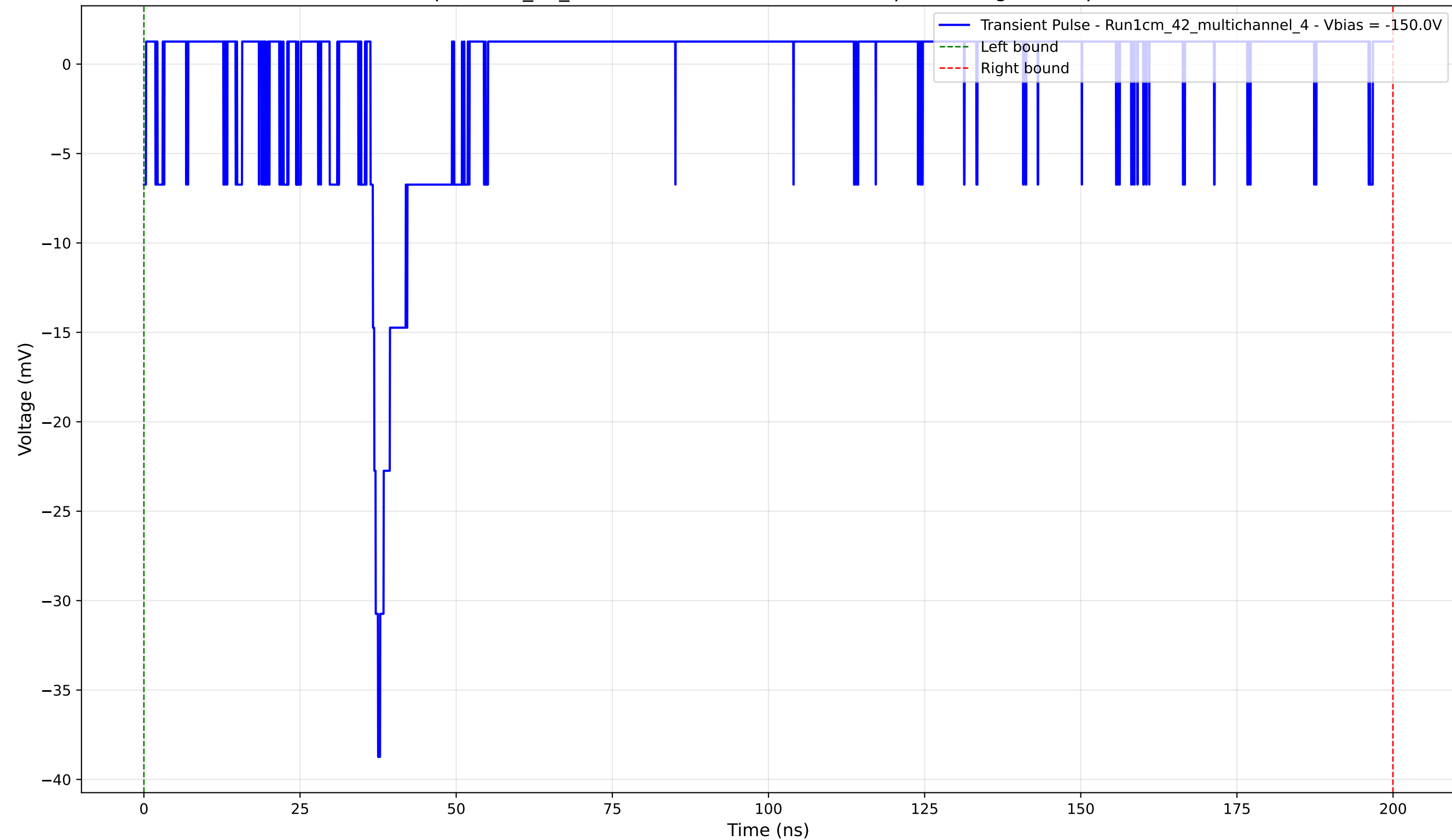
Transient Pulse - Sample: 1cm_42_multichannel - Position: 2965.0 \mu\text{m} - Charge: 0.85 pC - Rise Time: 1.21 ns
