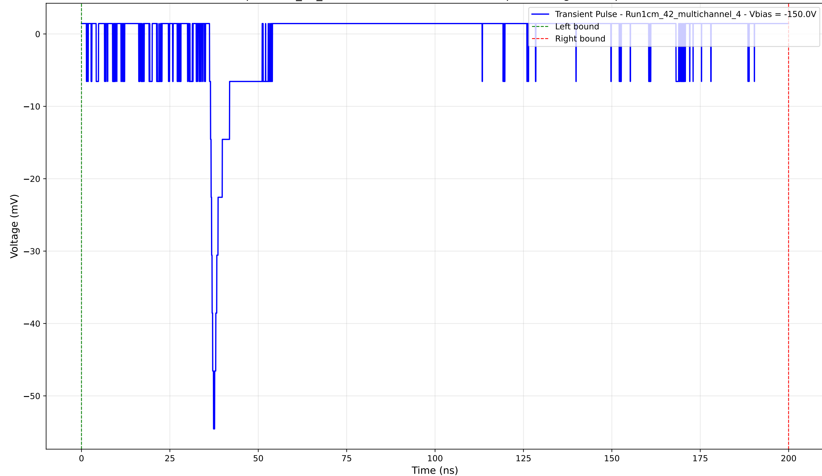
Transient Pulse - Sample: 1cm_42_multichannel - Position: 2790.0 \mu\text{m} - Charge: 0.82 pC - Rise Time: 1.12 ns
