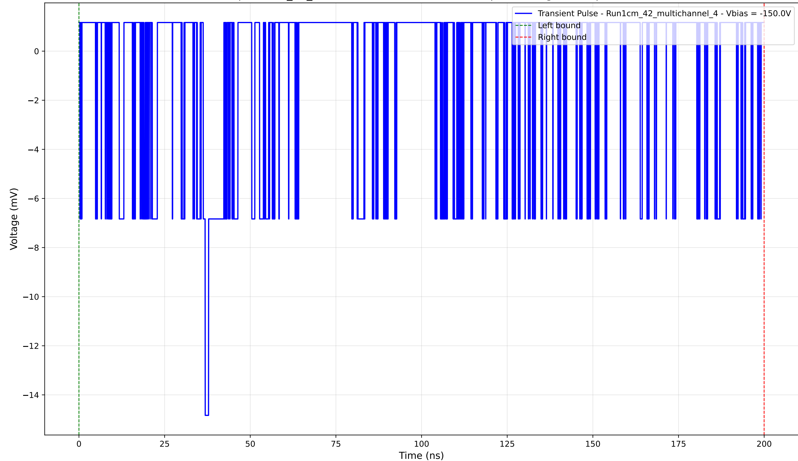
Transient Pulse - Sample: 1cm_42_multichannel - Position: 2420.0 \mu\text{m} - Charge: 1.87 pC - Rise Time: 0.58 ns
