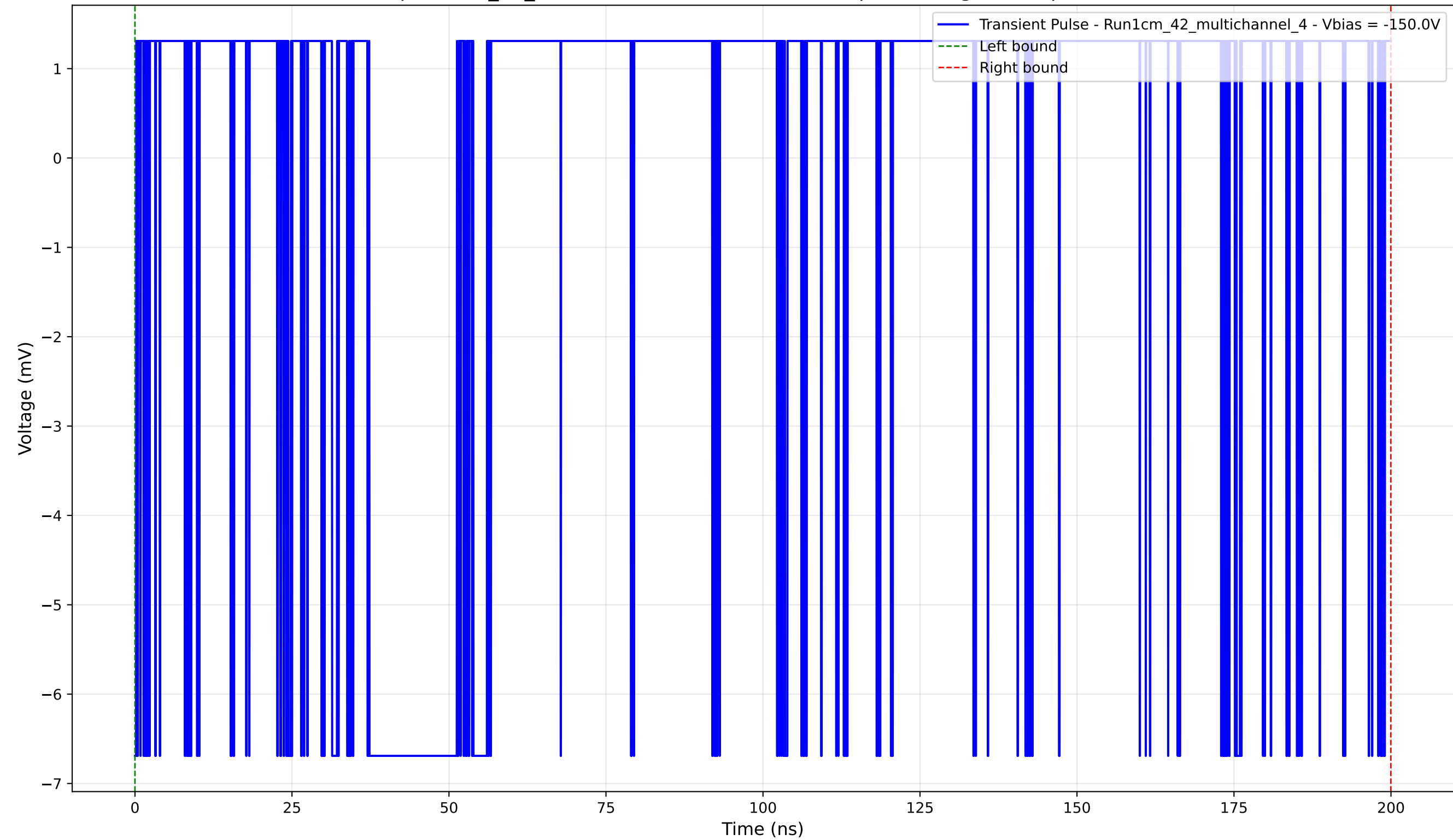
Transient Pulse - Sample: 1cm_42_multichannel - Position: 4455.0 \mu\text{m} - Charge: 0.32 pC - Rise Time: 0.00 ns (N/A)
