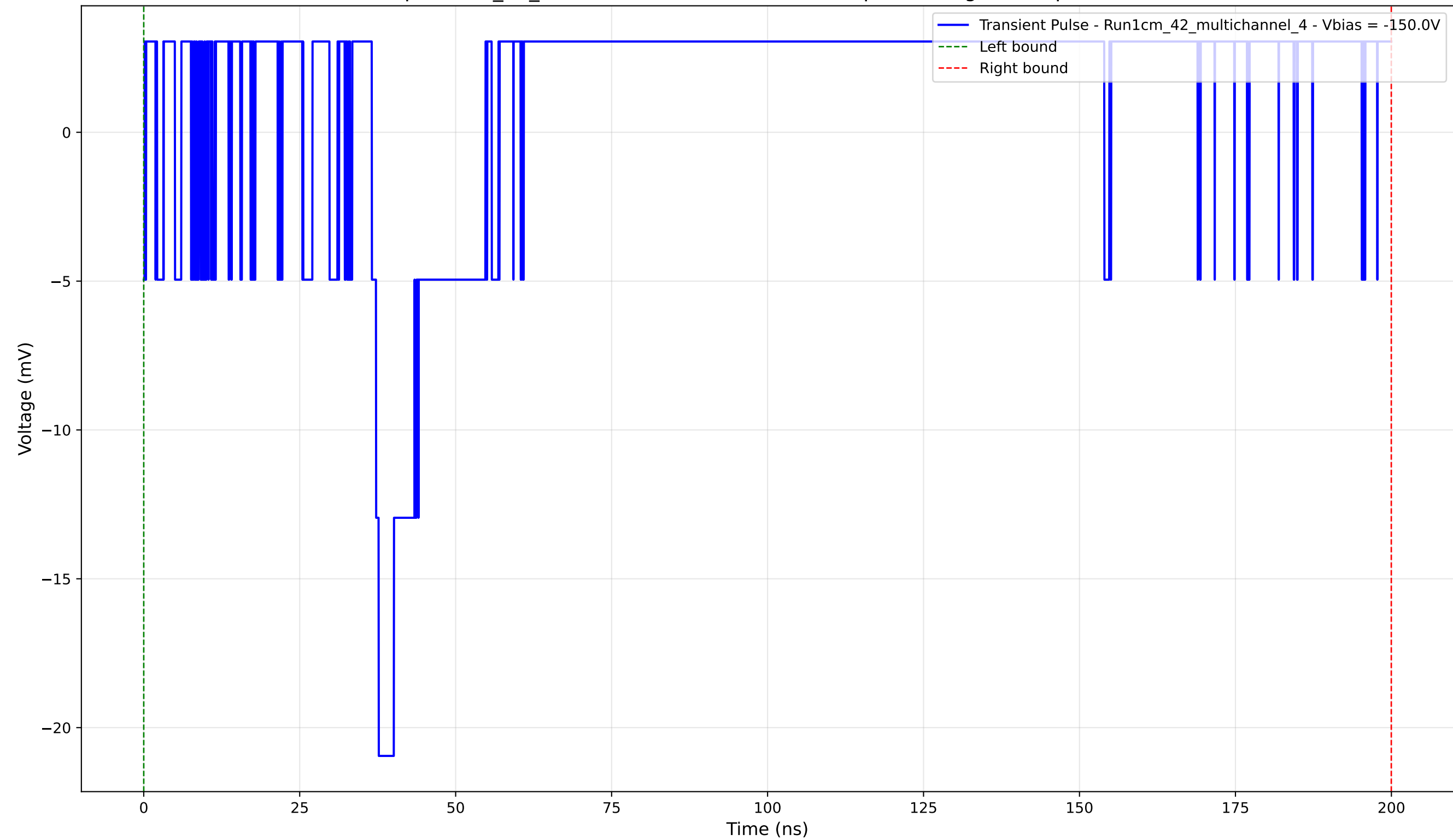
Transient Pulse - Sample: 1cm_42_multichannel - Position: 1250.0 \mu\text{m} - Charge: 5.68 pC - Rise Time: 0.00 ns (N/A)
