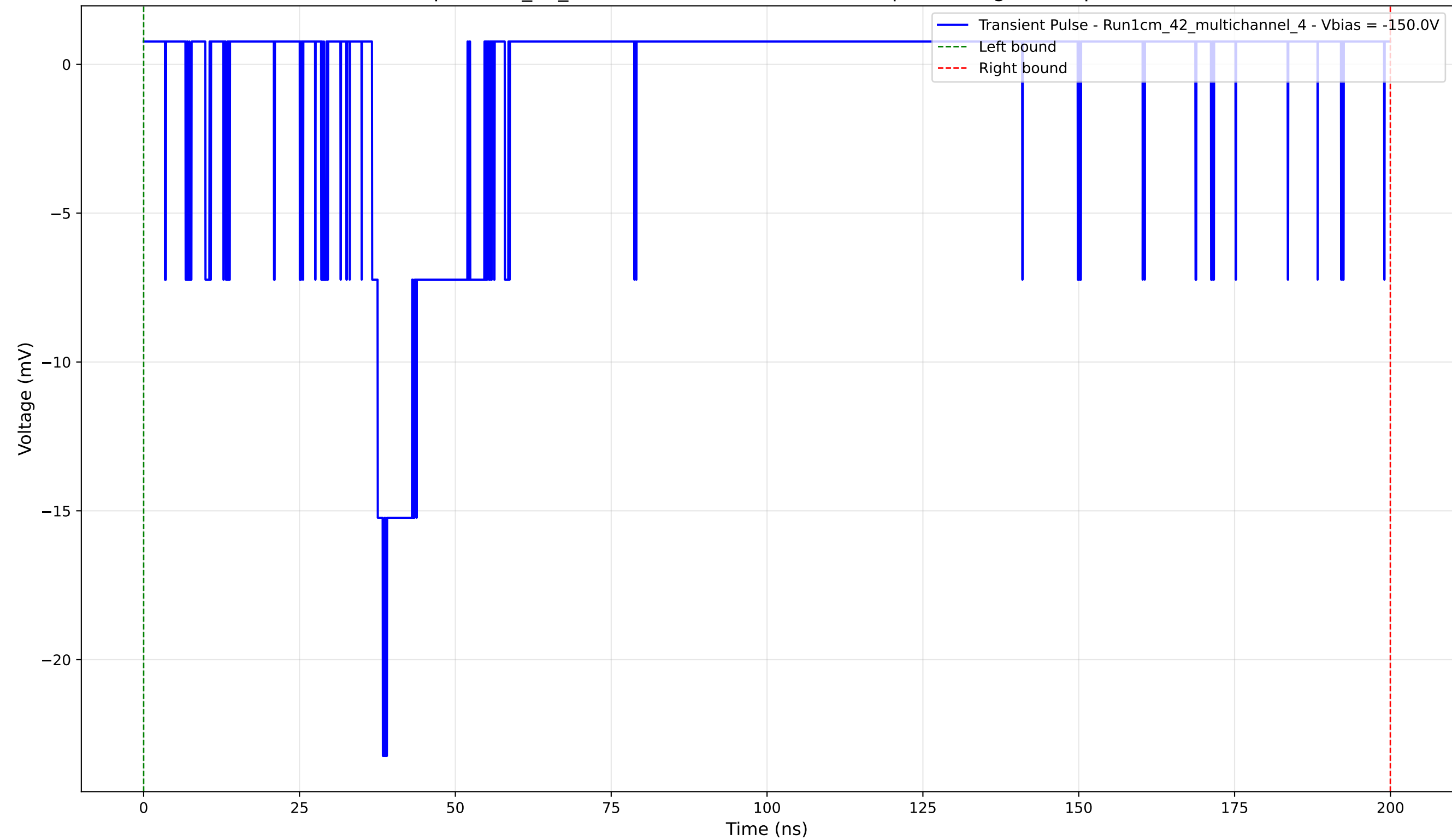
Transient Pulse - Sample: 1cm_42_multichannel - Position: 3670.0 \mu\text{m} - Charge: 1.85 pC - Rise Time: 1.74 ns
