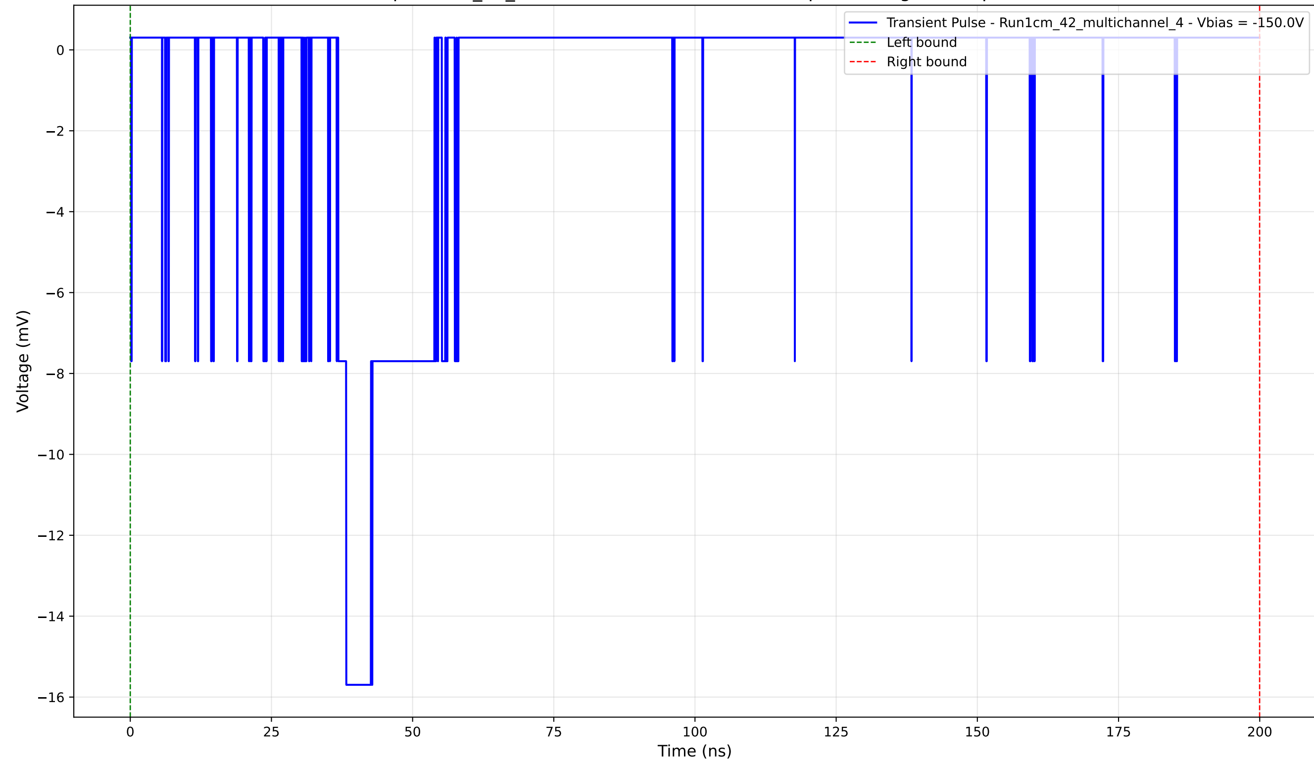
Transient Pulse - Sample: 1cm_42_multichannel - Position: 4150.0 \mu\text{m} - Charge: 3.11 pC - Rise Time: 1.42 ns
