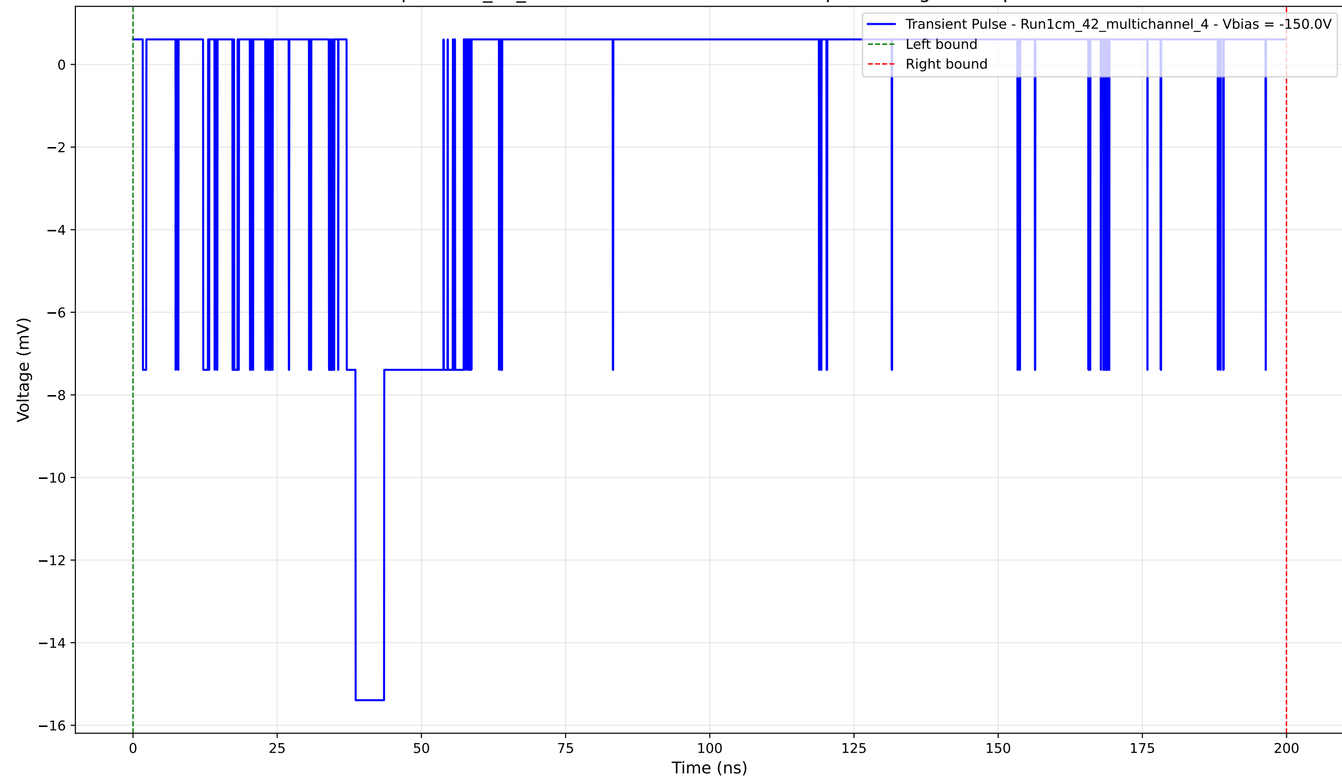
Transient Pulse - Sample: 1cm_42_multichannel - Position: 4710.0 \mu\text{m} - Charge: 2.67 pC - Rise Time: 1.56 ns
