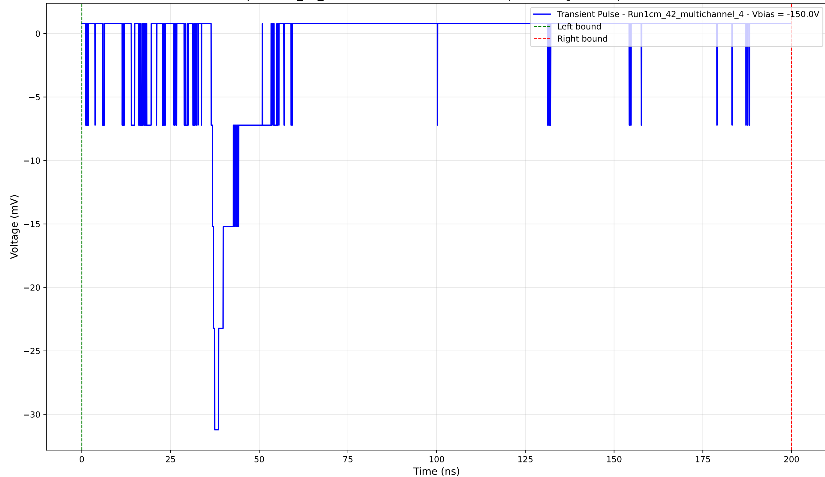
Transient Pulse - Sample: 1cm_42_multichannel - Position: 1560.0 \mu\text{m} - Charge: 2.83 pC - Rise Time: 0.99 ns
