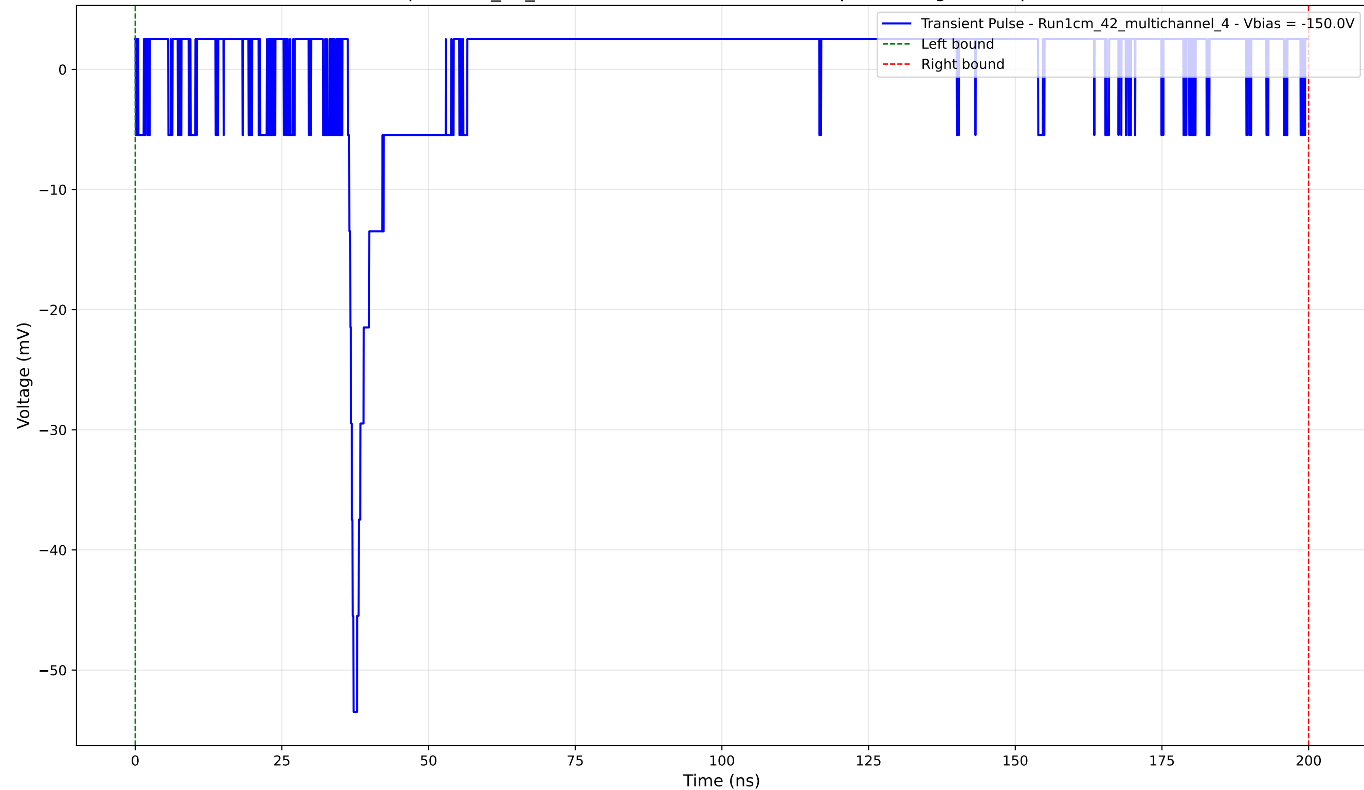
Transient Pulse - Sample: 1cm_42_multichannel - Position: 1985.0 \mu\text{m} - Charge: 2.41 pC - Rise Time: 0.94 ns
