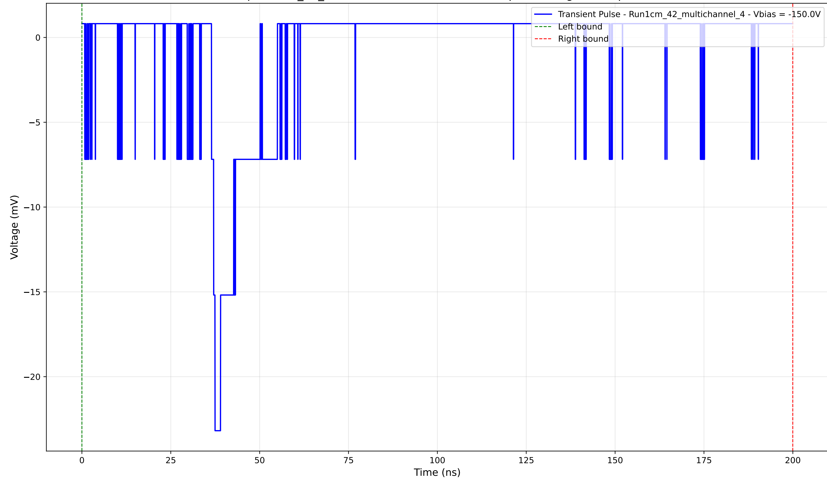
Transient Pulse - Sample: 1cm_42_multichannel - Position: 3320.0 \mu\text{m} - Charge: 2.11 pC - Rise Time: 1.00 ns
