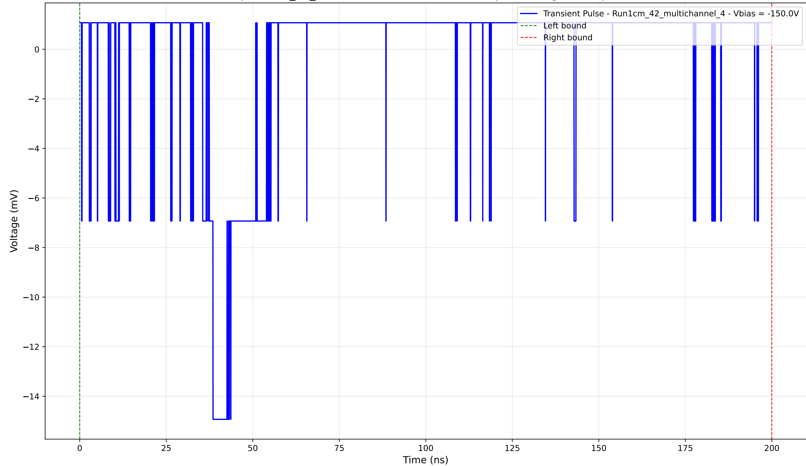
Transient Pulse - Sample: 1cm_42_multichannel - Position: 4525.0 \mu\text{m} - Charge: 0.33 pC - Rise Time: 1.08 ns
