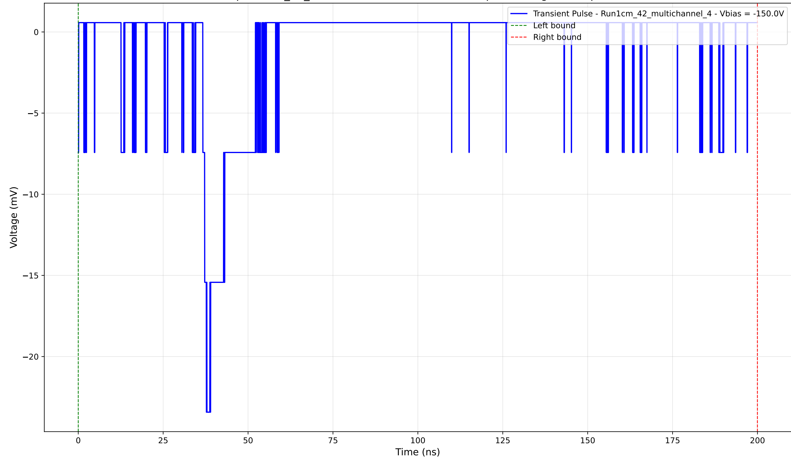
Transient Pulse - Sample: 1cm_42_multichannel - Position: 3485.0 \mu\text{m} - Charge: 2.92 pC - Rise Time: 1.05 ns
