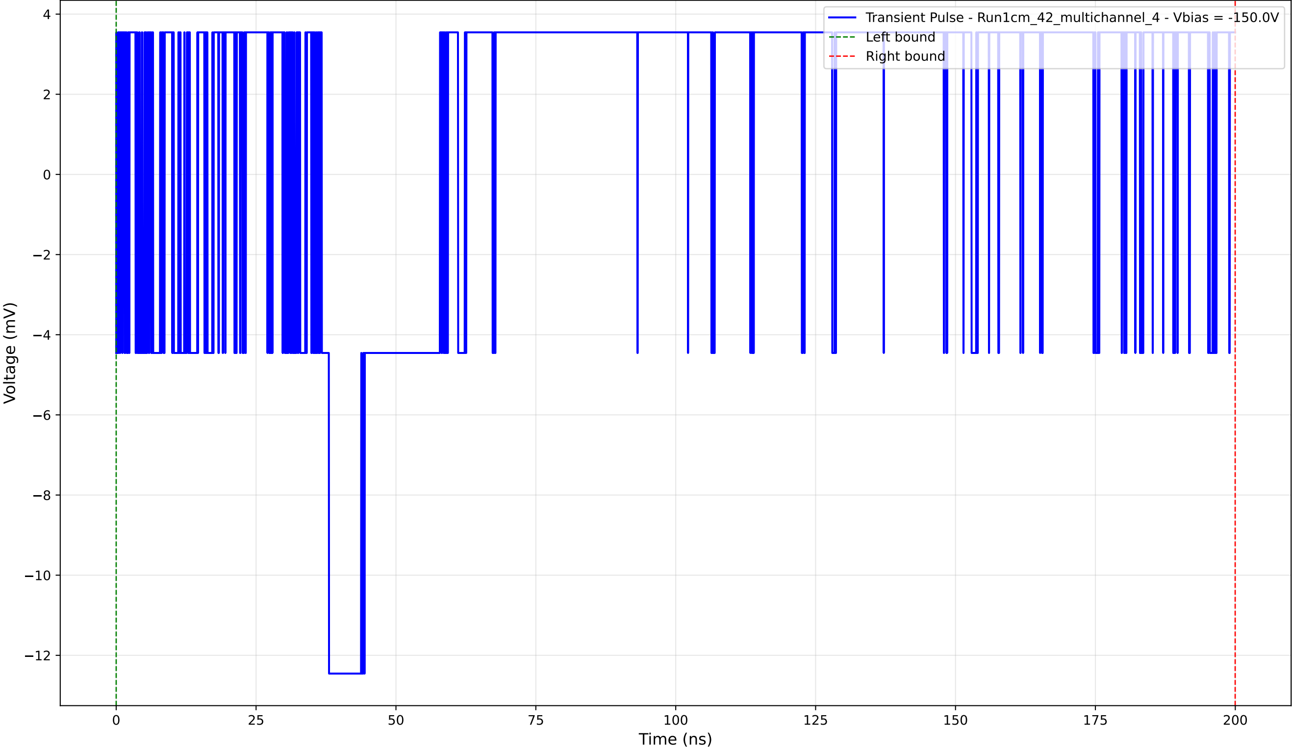
Transient Pulse - Sample: 1cm_42_multichannel - Position: 575.0 \mu\text{m} - Charge: 6.10 pC - Rise Time: 0.00 ns (N/A)
