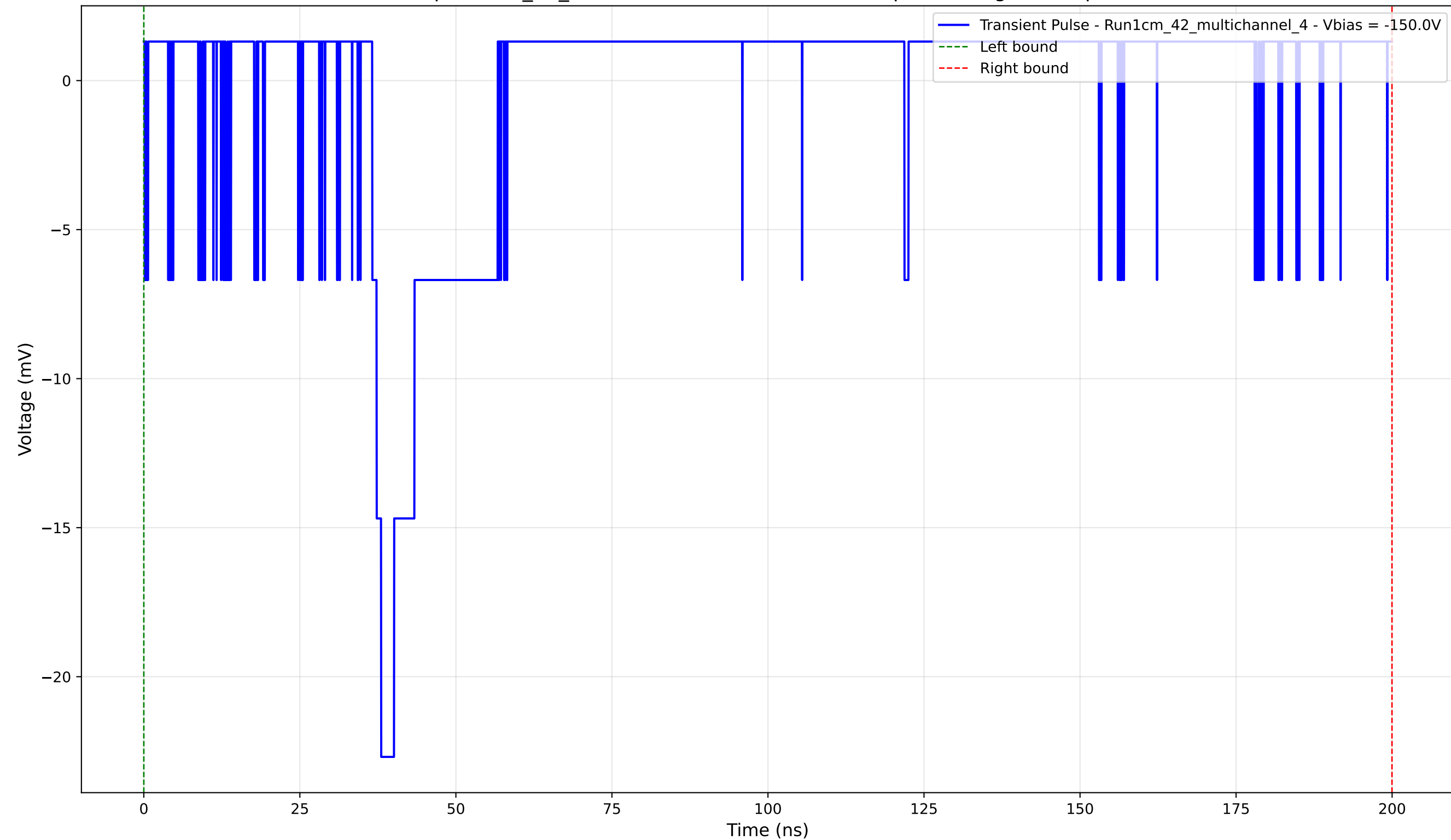
Transient Pulse - Sample: 1cm_42_multichannel - Position: 1150.0 \mu\text{m} - Charge: 0.59 pC - Rise Time: 1.44 ns
