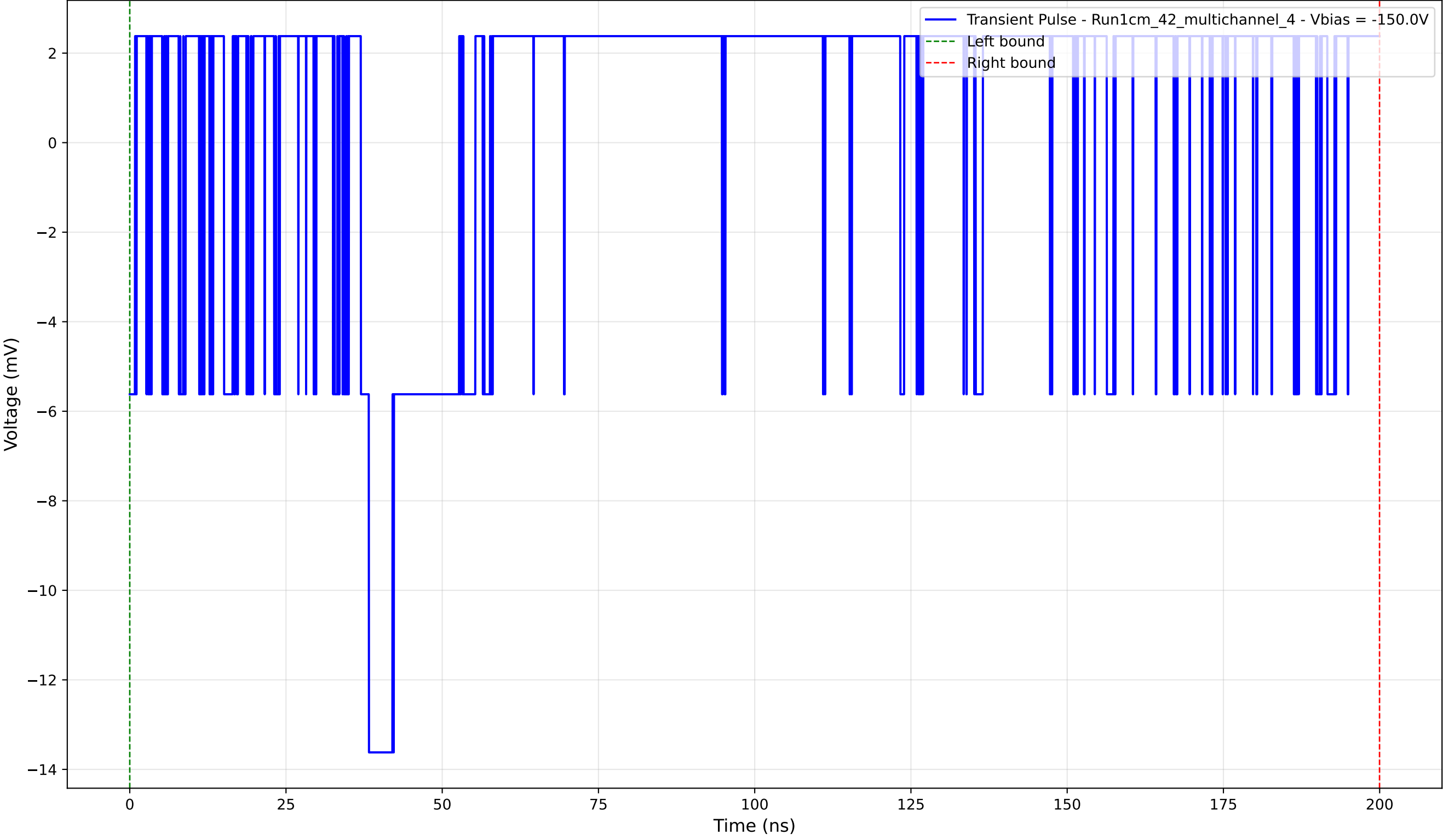
Transient Pulse - Sample: 1cm_42_multichannel - Position: 170.0 \mu\text{m} - Charge: 2.93 pC - Rise Time: 0.00 ns (N/A)
