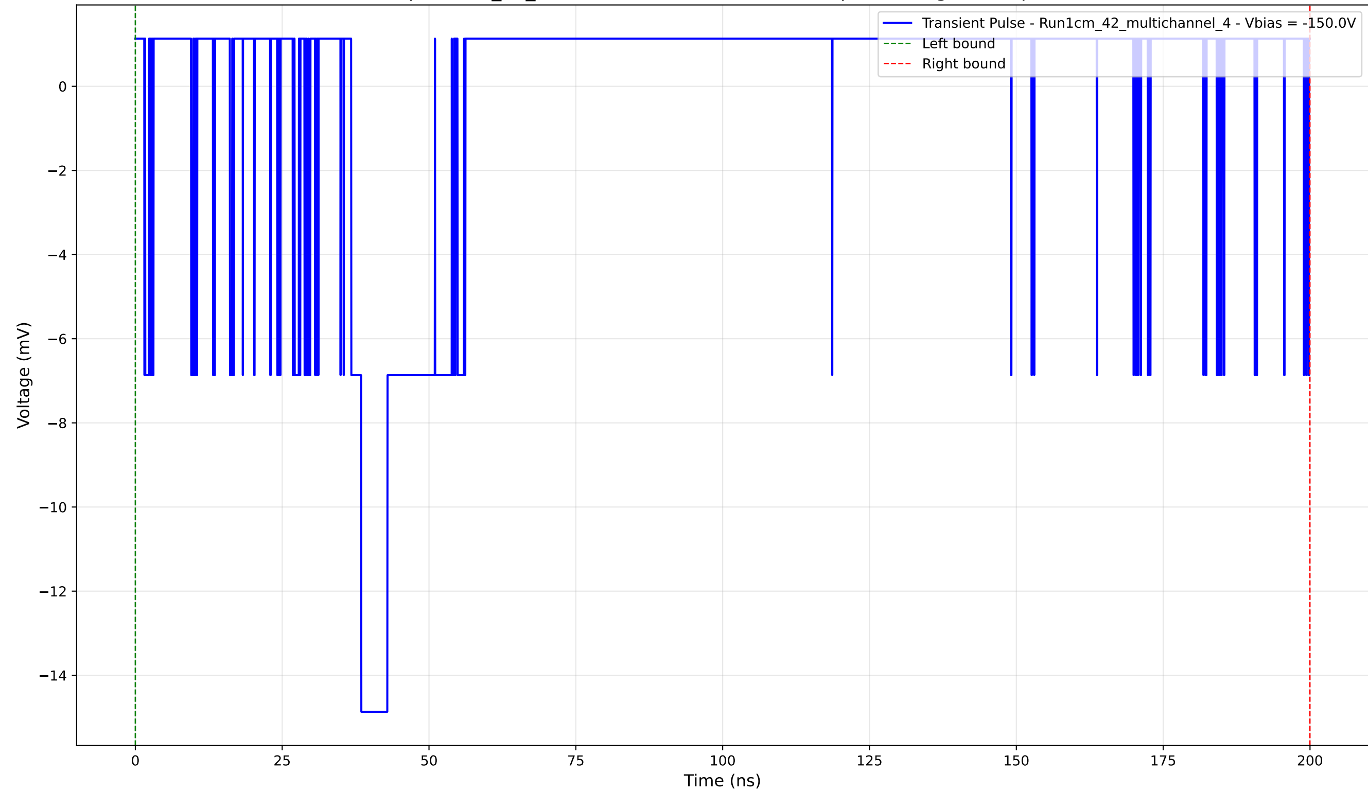
Transient Pulse - Sample: 1cm_42_multichannel - Position: 4560.0 \mu\text{m} - Charge: 0.36 pC - Rise Time: 1.72 ns
