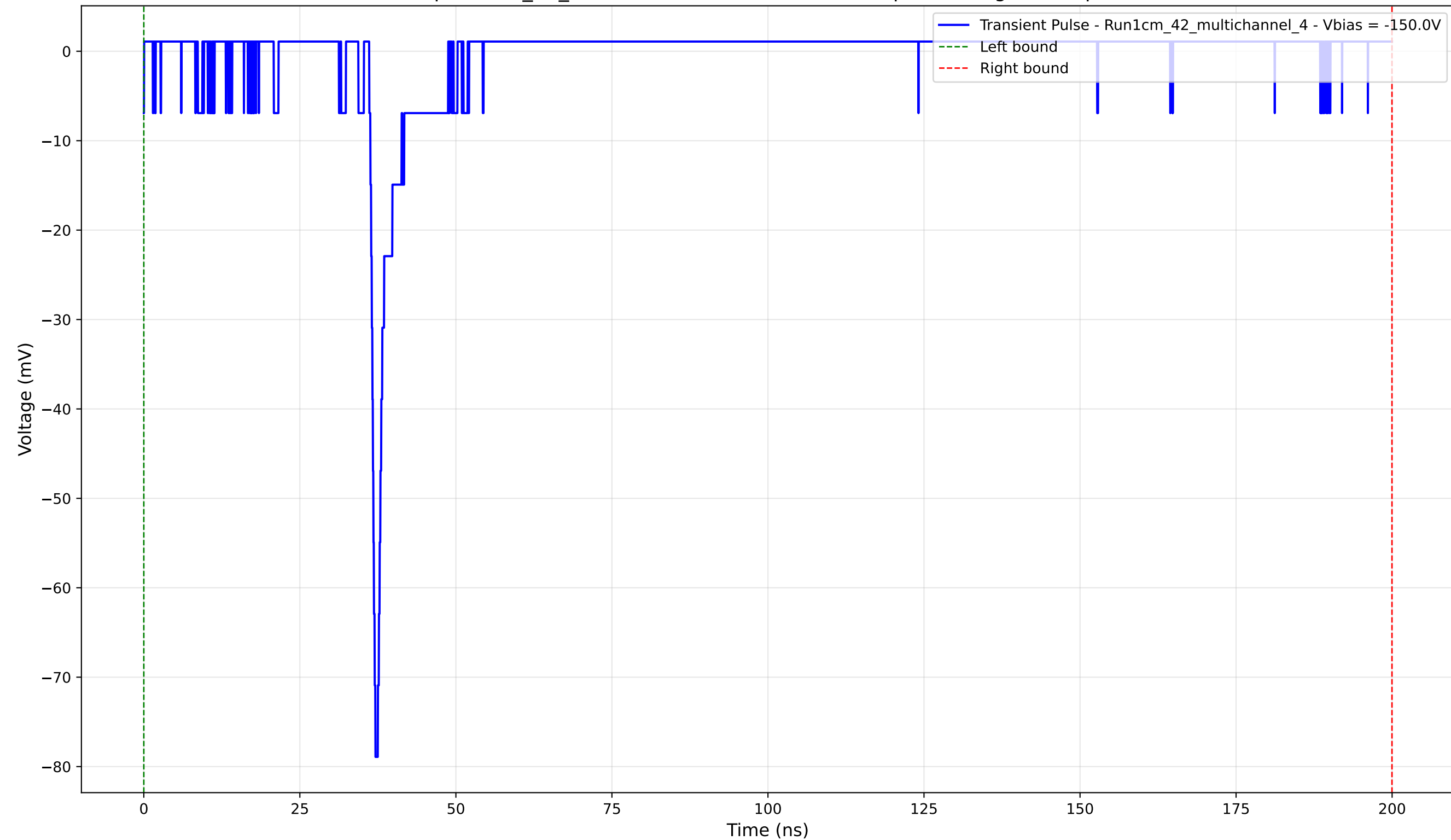
Transient Pulse - Sample: 1cm_42_multichannel - Position: 2230.0 \mu\text{m} - Charge: 1.77 pC - Rise Time: 0.82 ns
