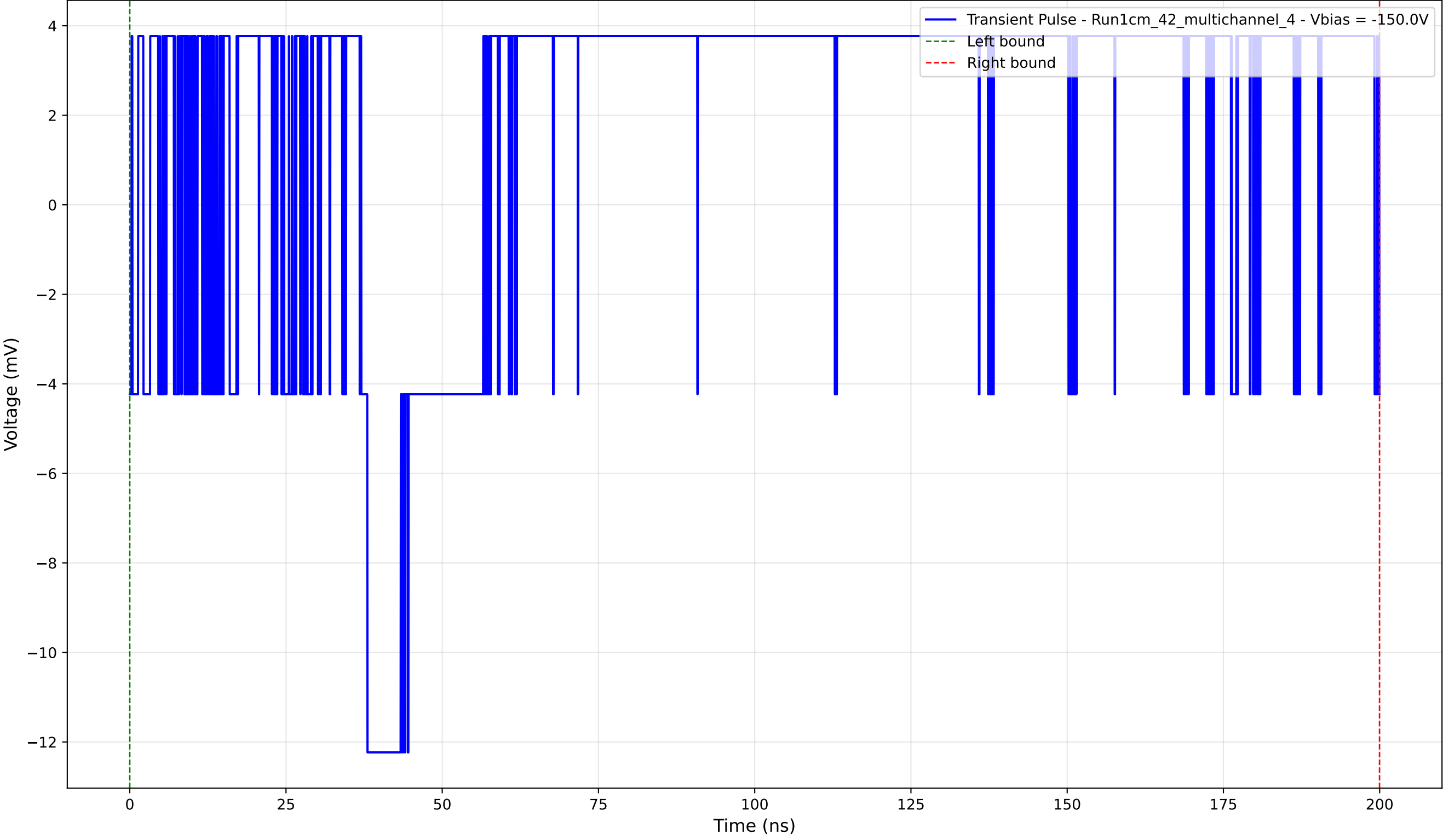
Transient Pulse - Sample: 1cm_42_multichannel - Position: 550.0 \mu\text{m} - Charge: 7.89 pC - Rise Time: 0.00 ns (N/A)
