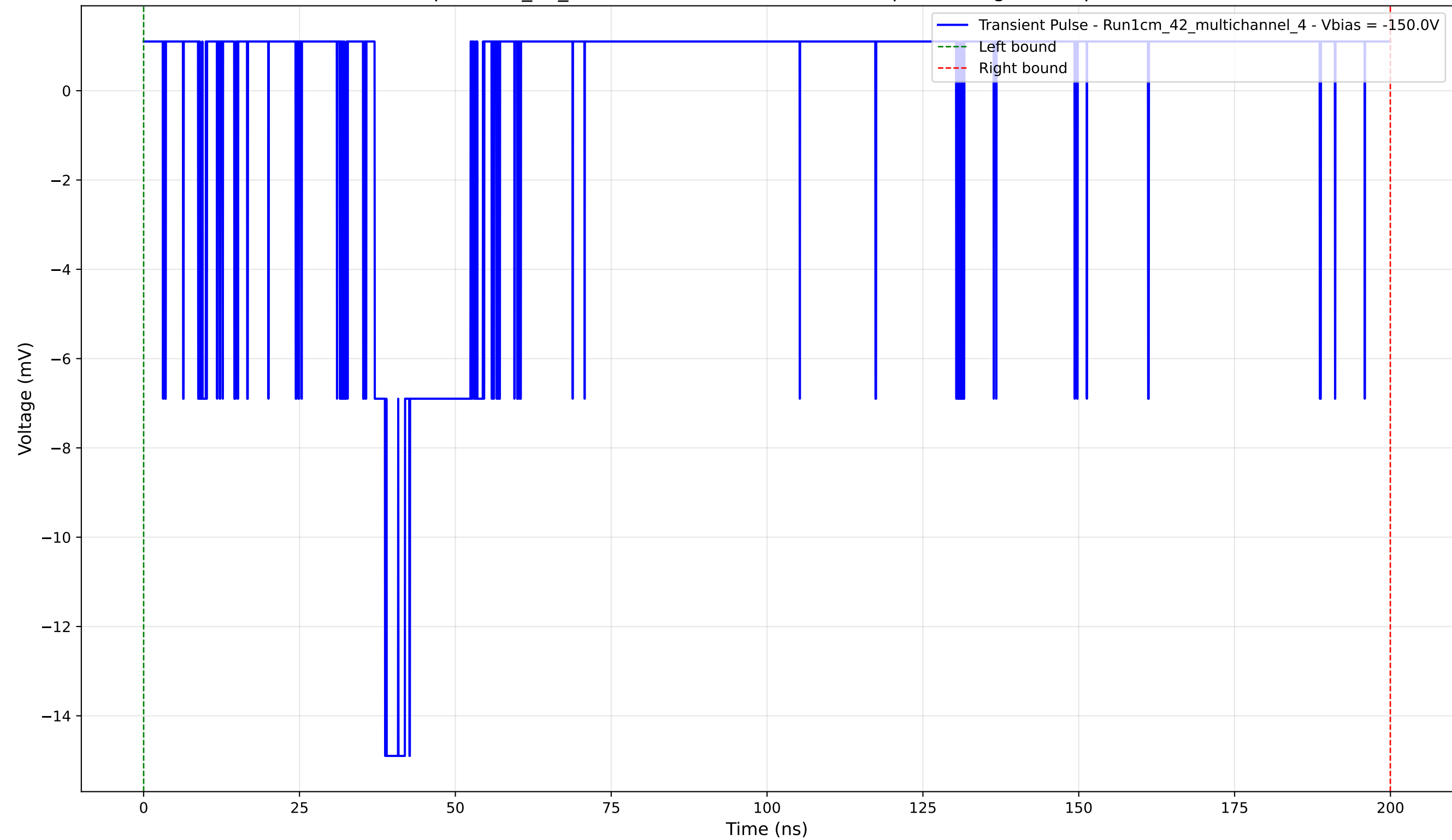
Transient Pulse - Sample: 1cm_42_multichannel - Position: 4805.0 \mu\text{m} - Charge: 0.20 pC - Rise Time: 1.68 ns
