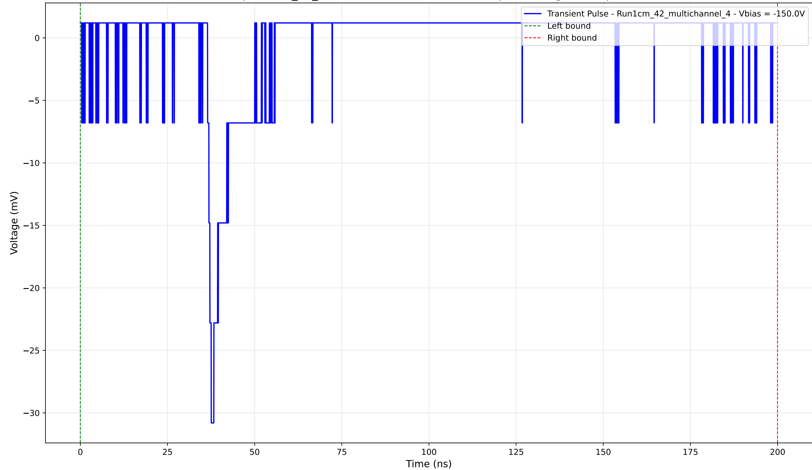
Transient Pulse - Sample: 1cm_42_multichannel - Position: 3185.0 \mu\text{m} - Charge: 0.44 pC - Rise Time: 1.05 ns
