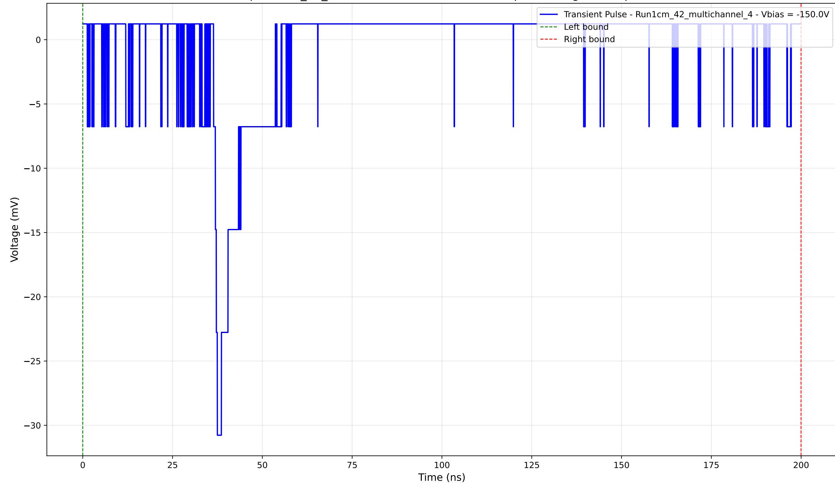
Transient Pulse - Sample: 1cm_42_multichannel - Position: 1520.0 \mu\text{m} - Charge: 1.60 pC - Rise Time: 1.05 ns
