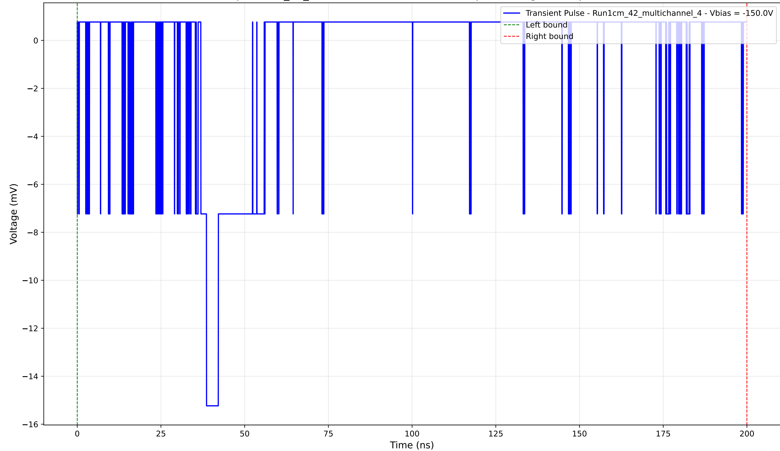
Transient Pulse - Sample: 1cm_42_multichannel - Position: 150.0 \mu\text{m} - Charge: 2.23 pC - Rise Time: 1.70 ns
