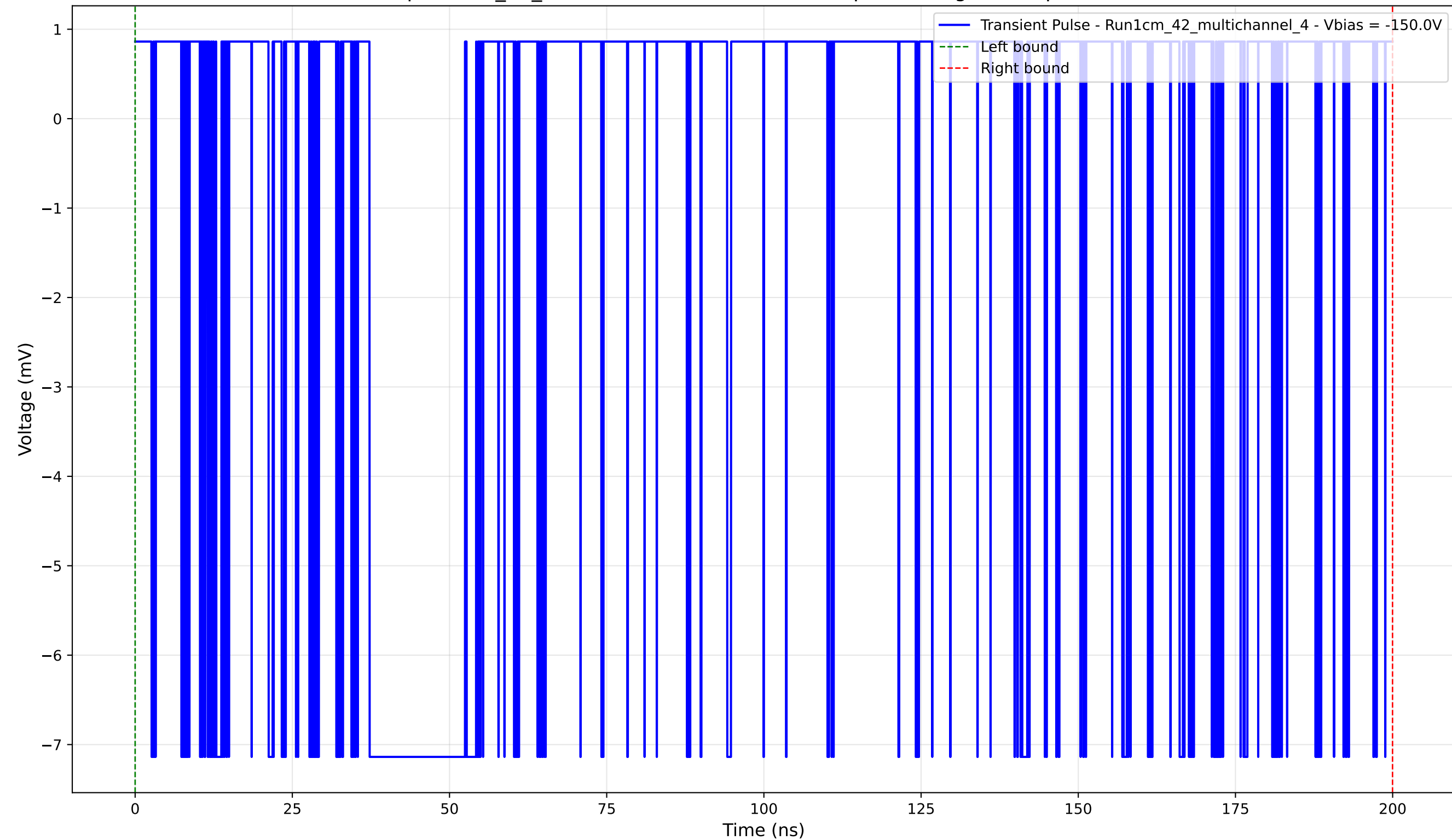
Transient Pulse - Sample: 1cm_42_multichannel - Position: 820.0 \mu\text{m} - Charge: 2.63 pC - Rise Time: 0.00 ns (N/A)
