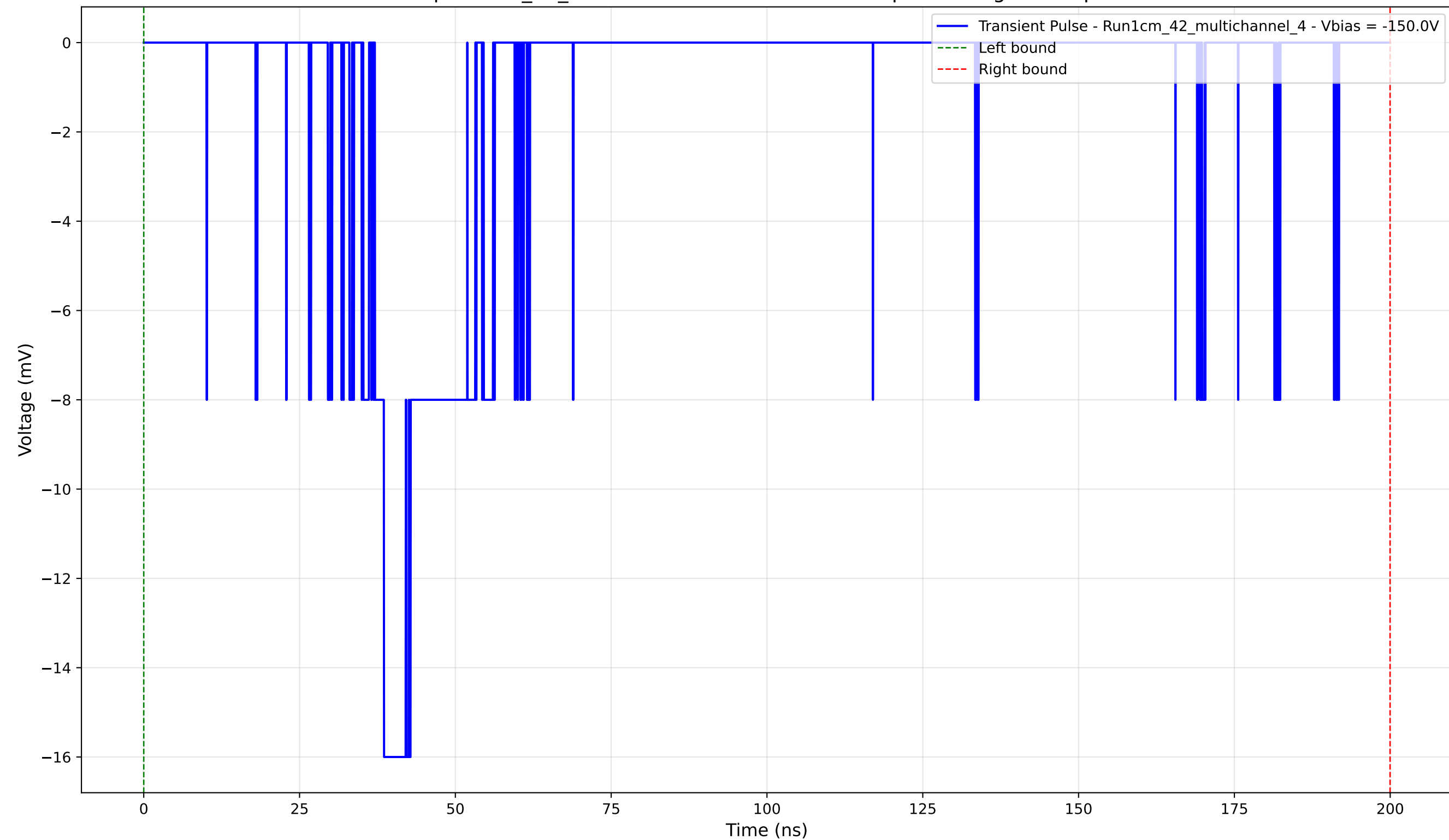
Transient Pulse - Sample: 1cm_42_multichannel - Position: 4770.0 \mu\text{m} - Charge: 4.52 pC - Rise Time: 1.46 ns
