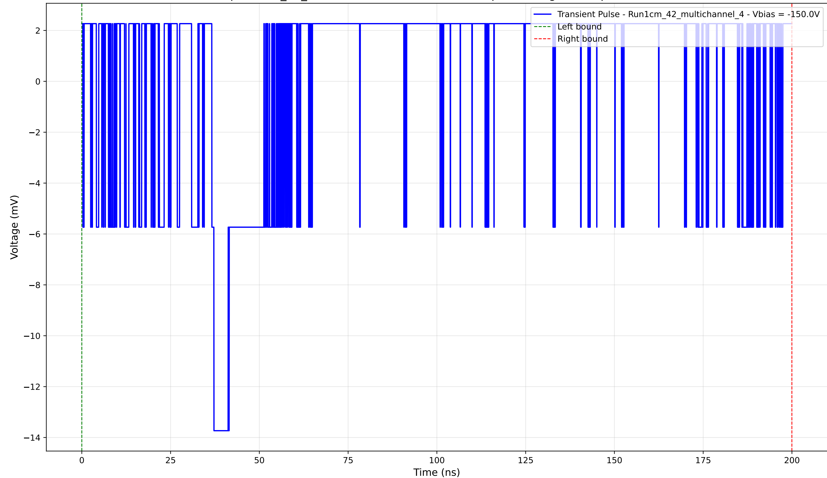
Transient Pulse - Sample: 1cm_42_multichannel - Position: 1430.0 \mu\text{m} - Charge: 1.81 pC - Rise Time: 0.00 ns (N/A)
