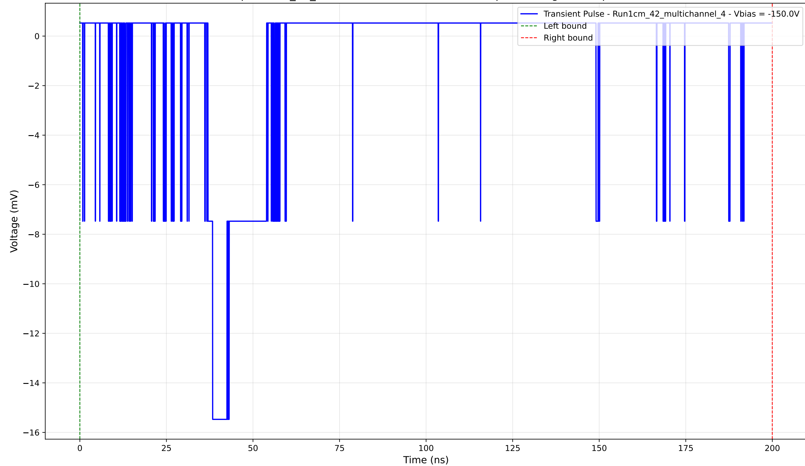
Transient Pulse - Sample: 1cm_42_multichannel - Position: 4200.0 \mu\text{m} - Charge: 2.57 pC - Rise Time: 1.36 ns
