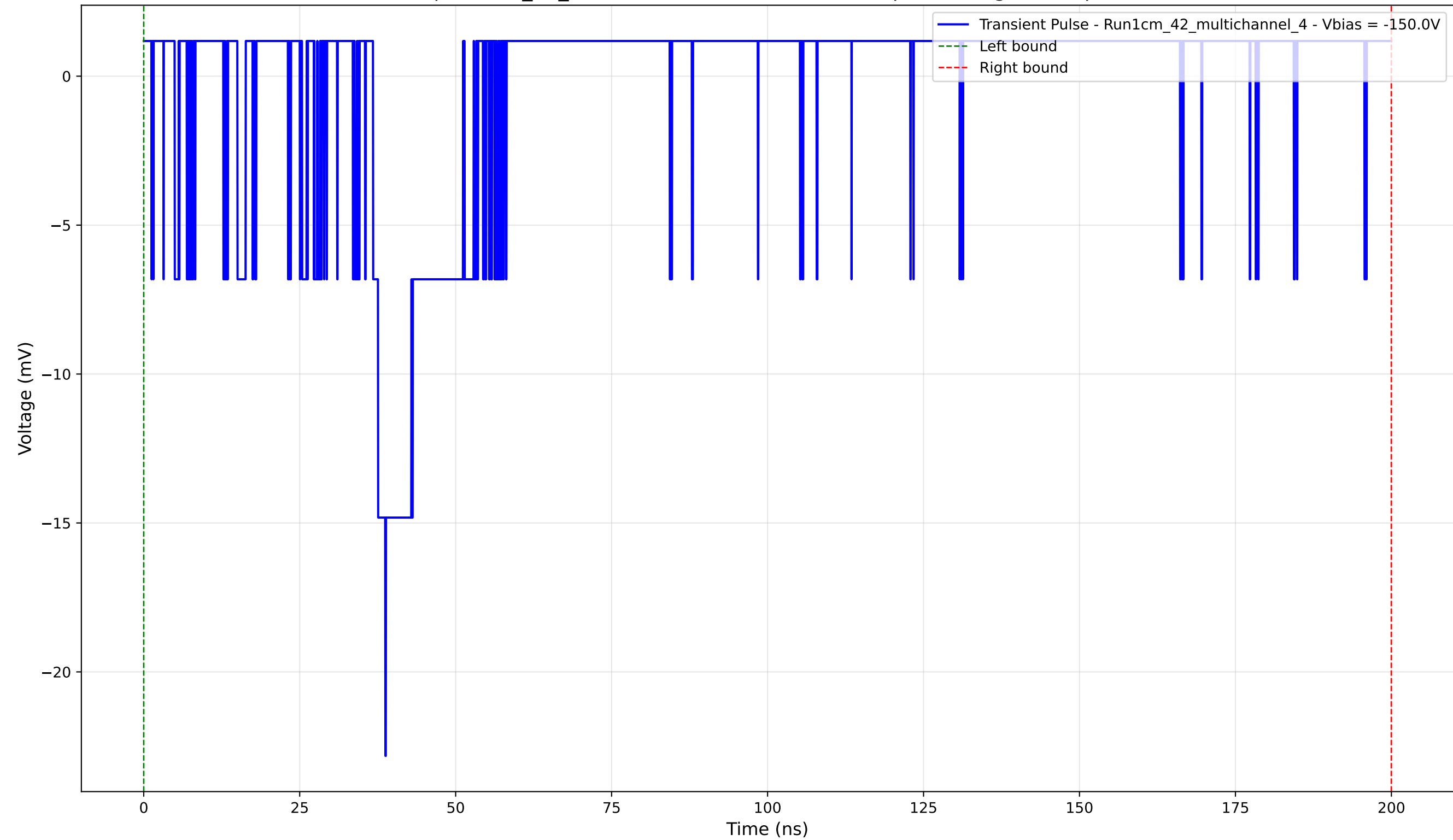
Transient Pulse - Sample: 1cm_42_multichannel - Position: 3695.0 \mu\text{m} - Charge: 0.52 pC - Rise Time: 1.98 ns
