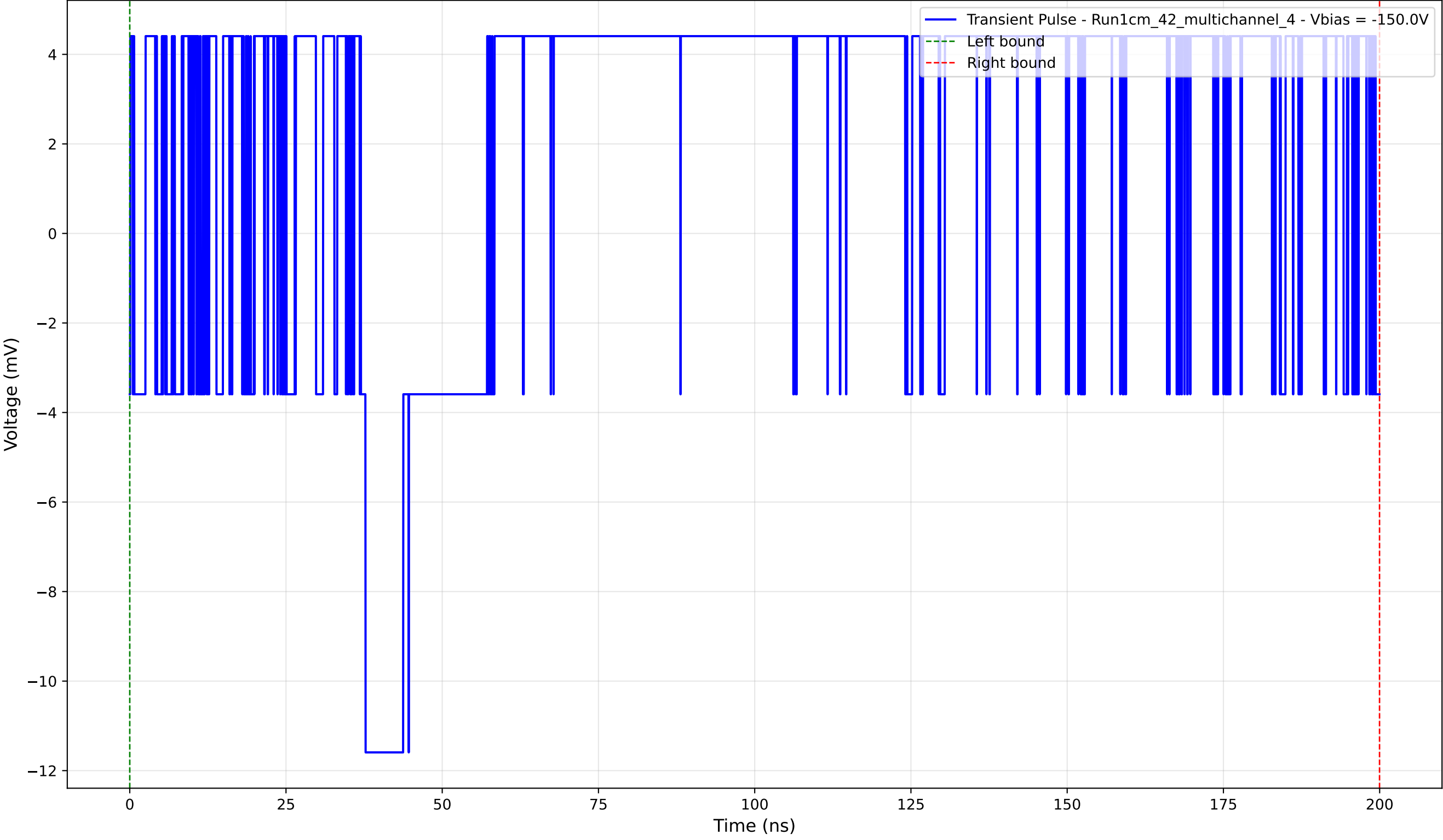
Transient Pulse - Sample: 1cm_42_multichannel - Position: 715.0 \mu\text{m} - Charge: 9.32 pC - Rise Time: 0.00 ns (N/A)
