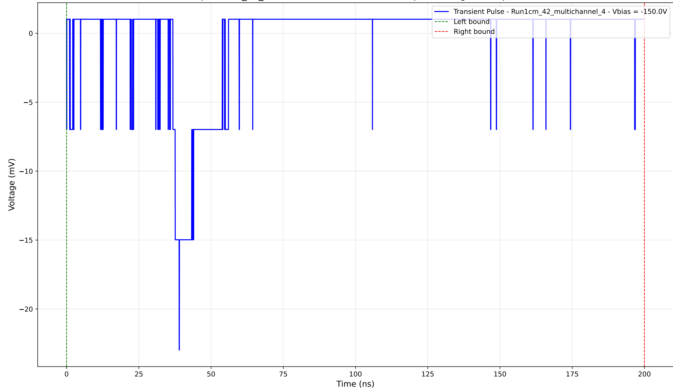
Transient Pulse - Sample: 1cm_42_multichannel - Position: 3790.0 \mu\text{m} - Charge: 0.46 pC - Rise Time: 2.18 ns
