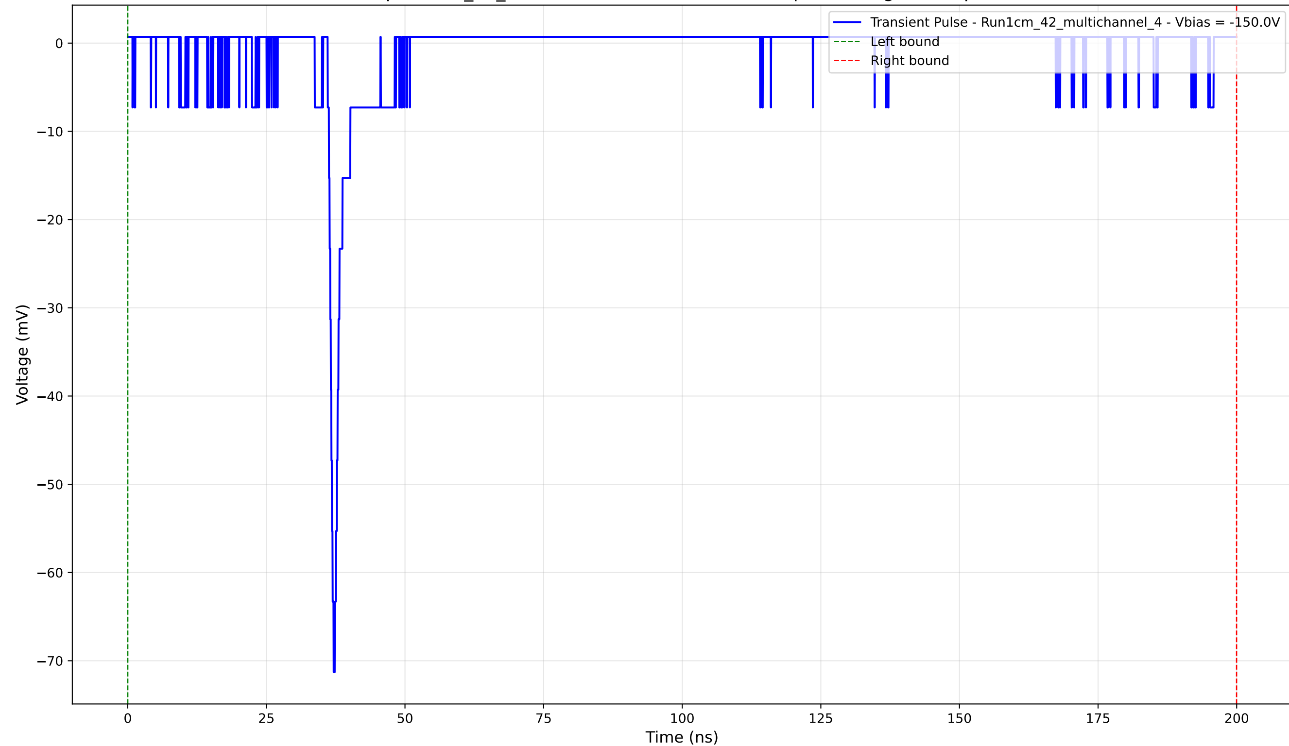
Transient Pulse - Sample: 1cm_42_multichannel - Position: 2320.0 \mu\text{m} - Charge: 2.68 pC - Rise Time: 1.06 ns
