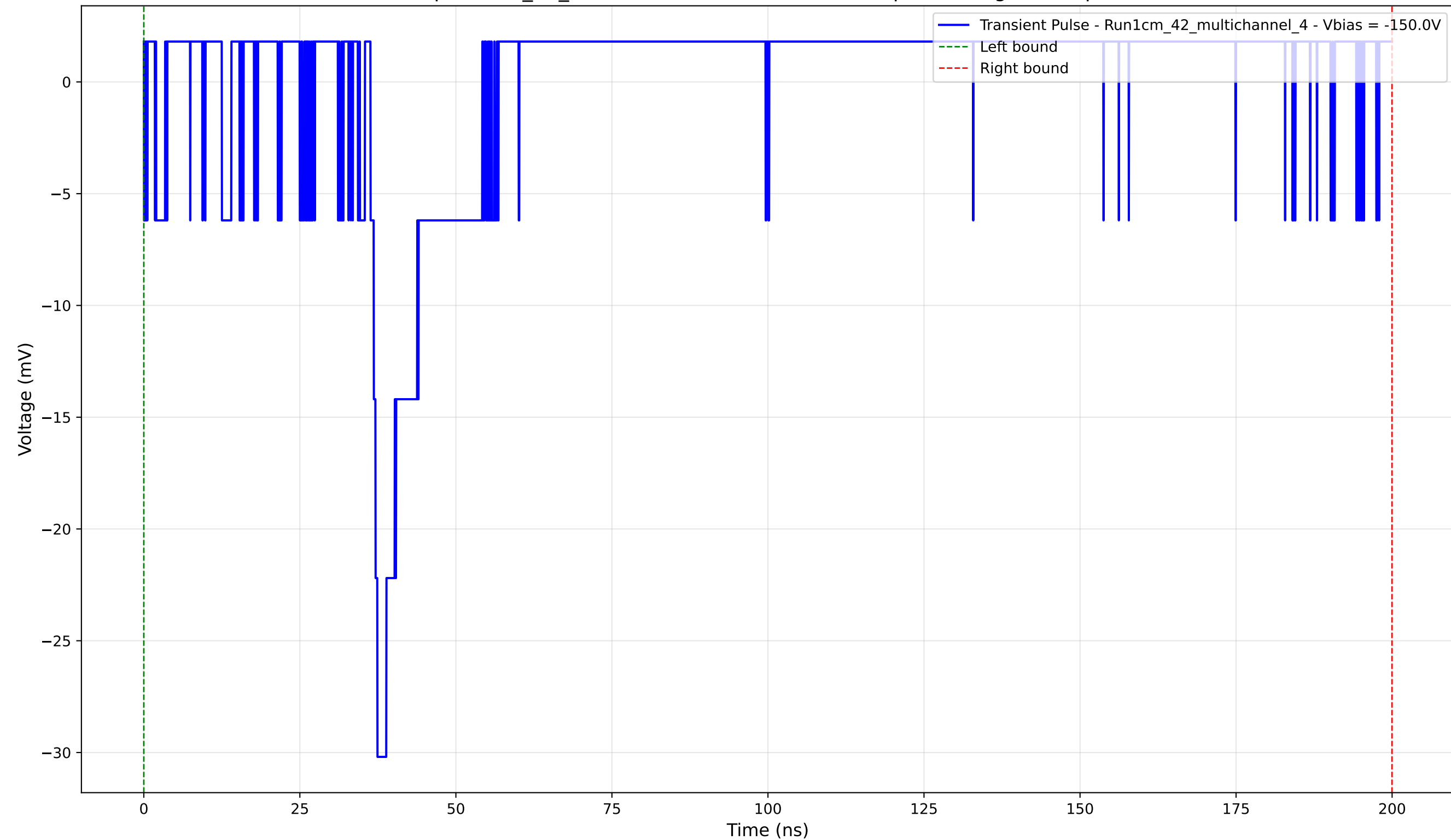
Transient Pulse - Sample: 1cm_42_multichannel - Position: 1535.0 \mu\text{m} - Charge: 0.52 pC - Rise Time: 1.11 ns
