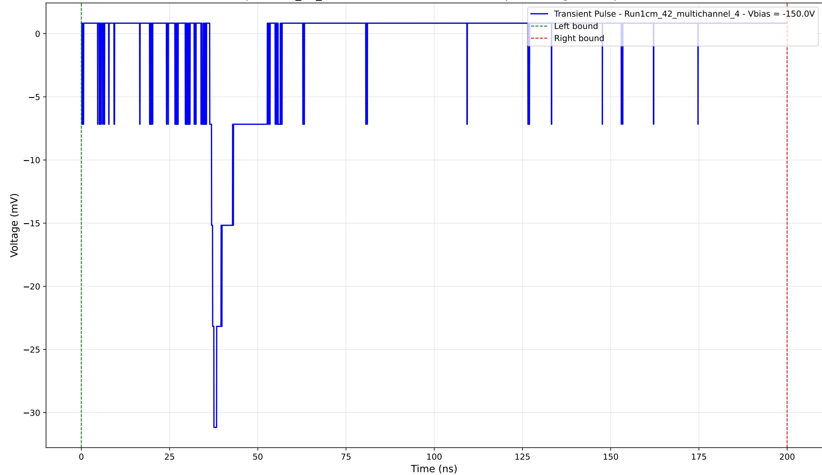
Transient Pulse - Sample: 1cm_42_multichannel - Position: 3220.0 \mu\text{m} - Charge: 1.88 pC - Rise Time: 1.19 ns
