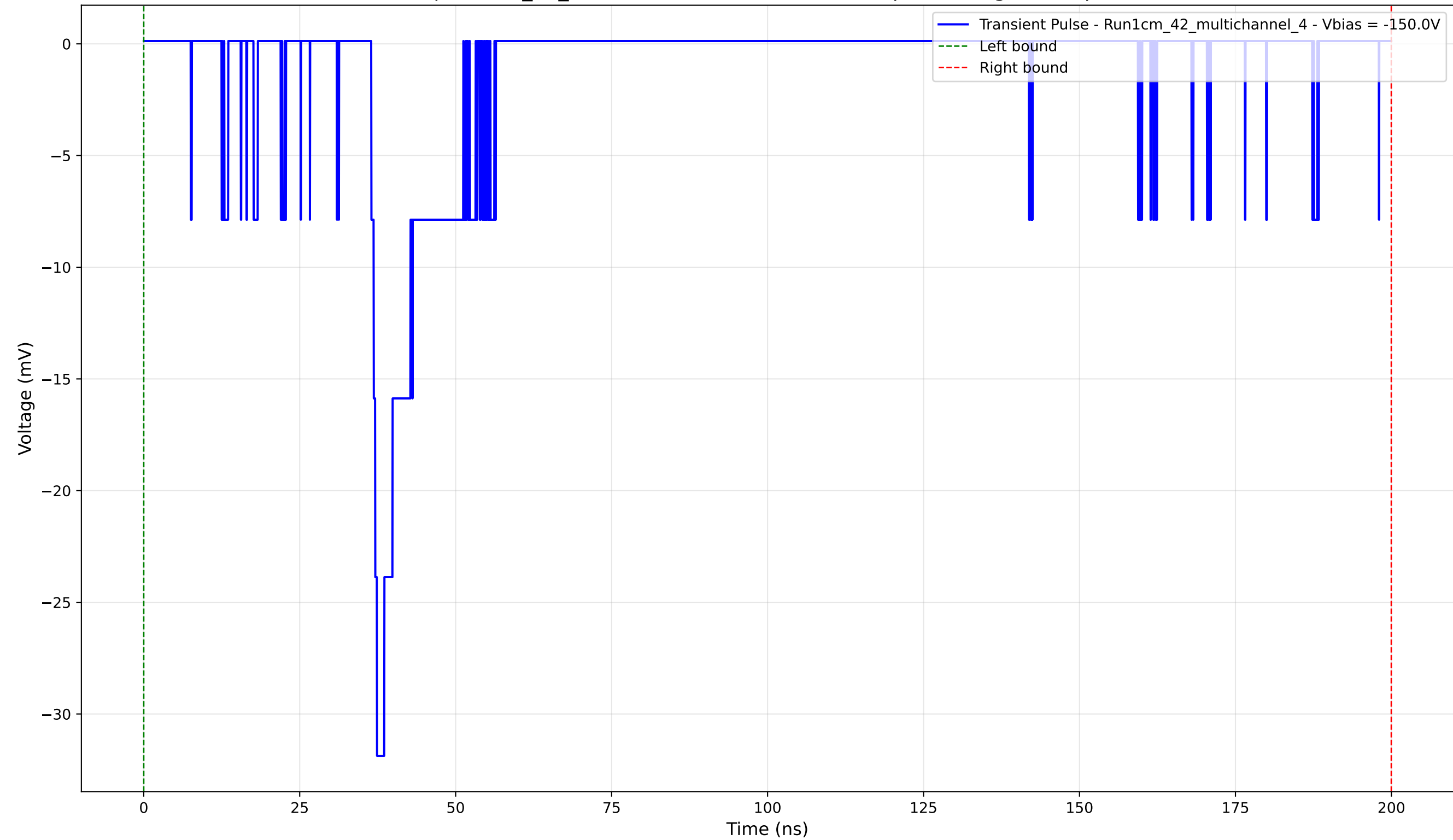
Transient Pulse - Sample: 1cm_42_multichannel - Position: 1610.0 \mu\text{m} - Charge: 4.88 pC - Rise Time: 0.91 ns
