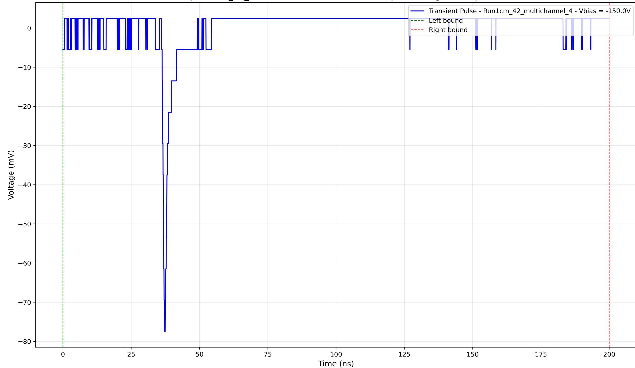
Transient Pulse - Sample: 1cm_42_multichannel - Position: 2210.0 \mu\text{m} - Charge: 2.94 pC - Rise Time: 0.93 ns
