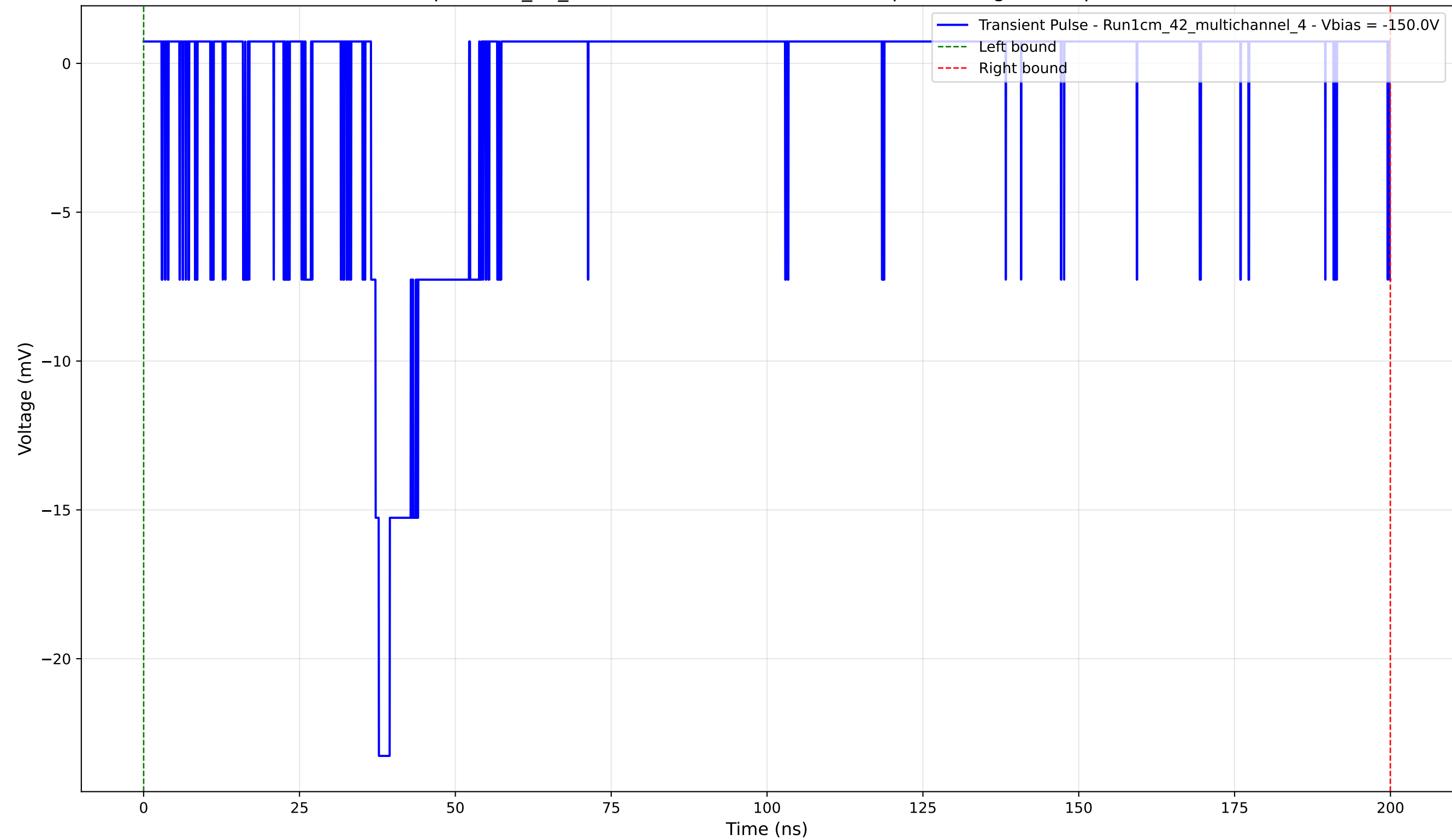
Transient Pulse - Sample: 1cm_42_multichannel - Position: 3495.0 \mu\text{m} - Charge: 2.37 pC - Rise Time: 1.26 ns
