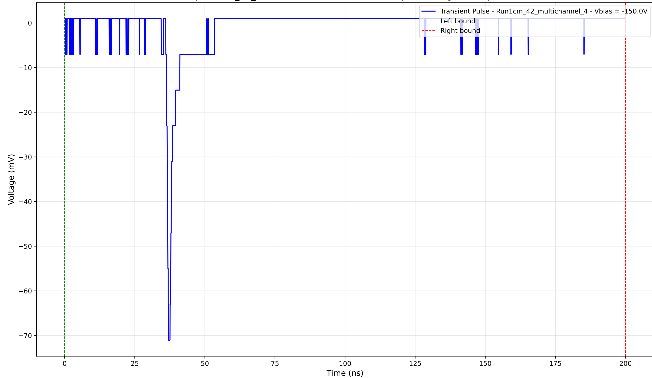
Transient Pulse - Sample: 1cm_42_multichannel - Position: 2220.0 \mu\text{m} - Charge: 2.27 pC - Rise Time: 0.78 ns
