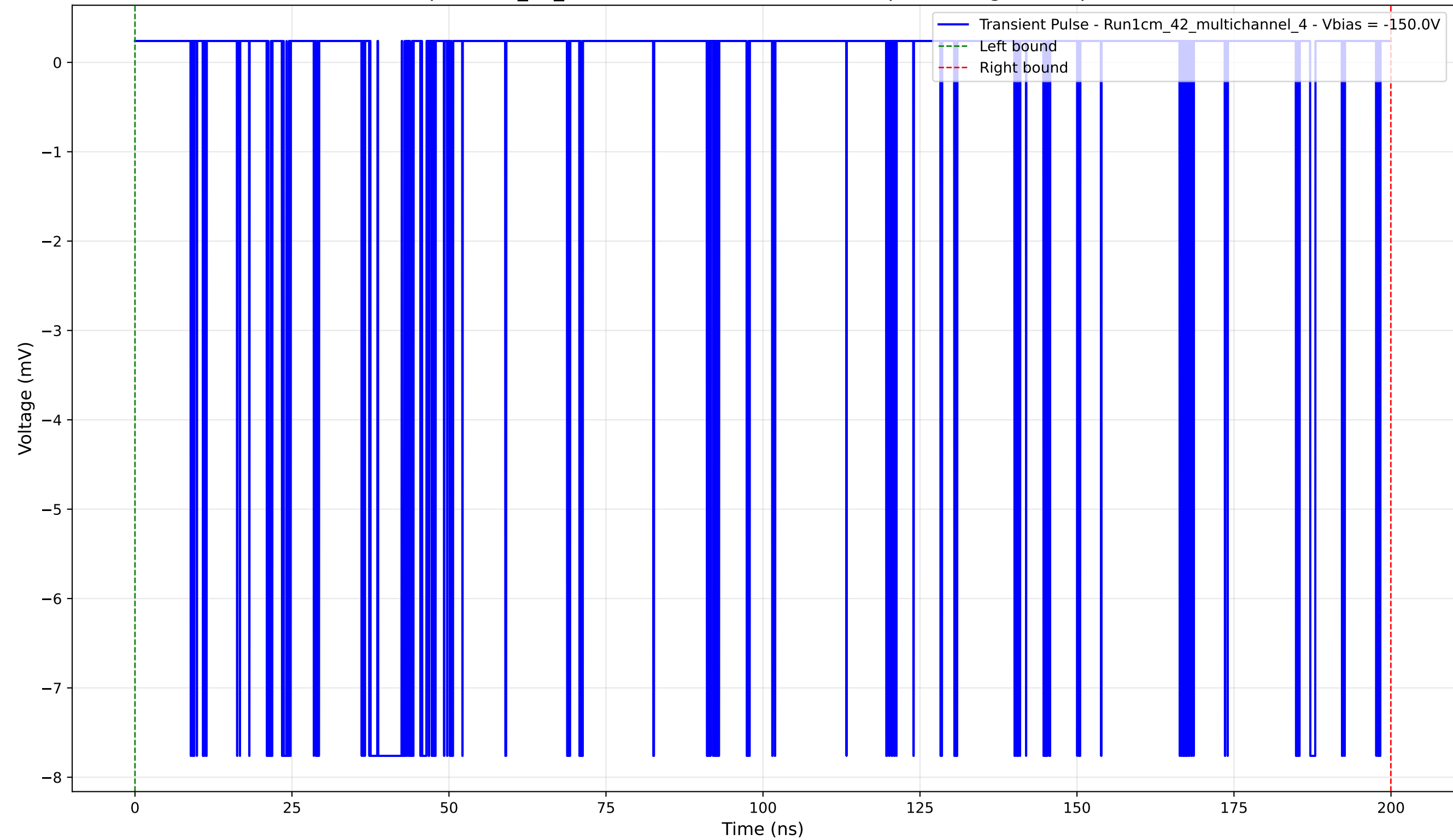
Transient Pulse - Sample: 1cm_42_multichannel - Position: 3875.0 \mu\text{m} - Charge: 2.06 pC - Rise Time: 0.02 ns
