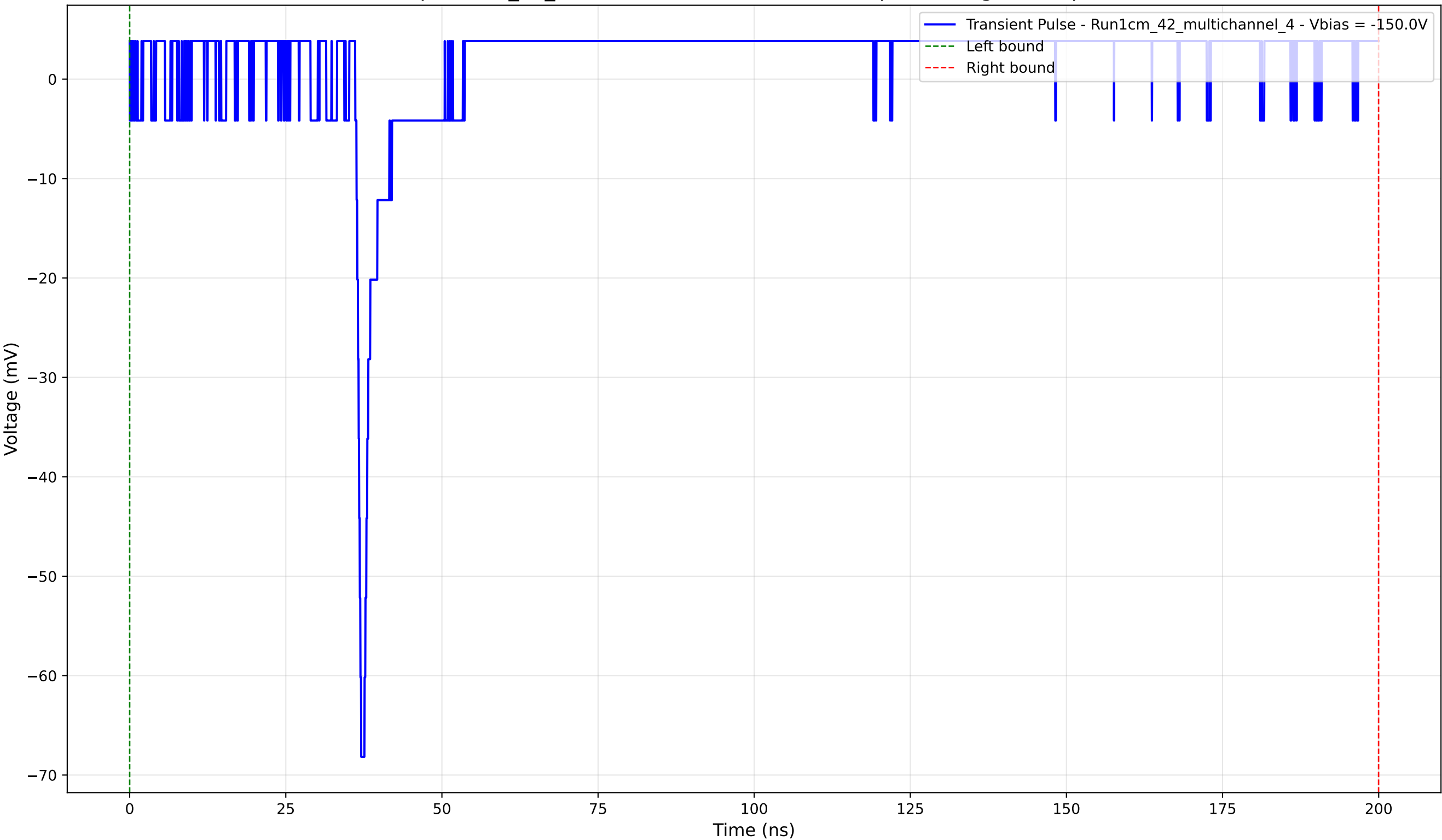
Transient Pulse - Sample: 1cm_42_multichannel - Position: 2200.0 \mu\text{m} - Charge: 7.71 pC - Rise Time: 0.75 ns
