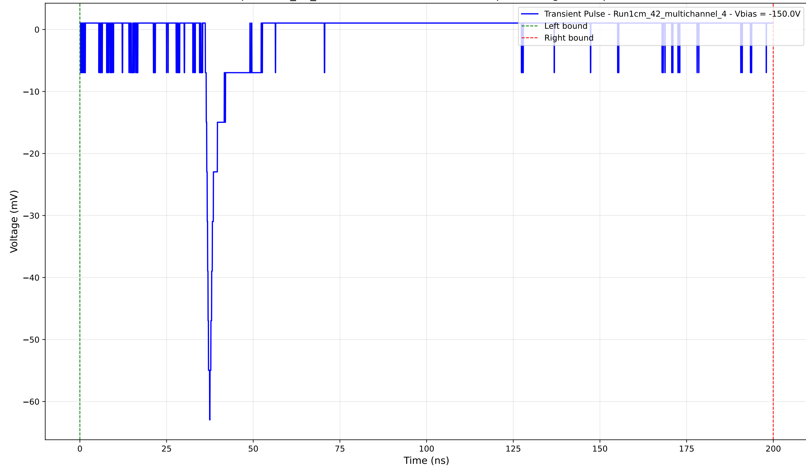
Transient Pulse - Sample: 1cm_42_multichannel - Position: 2690.0 \mu\text{m} - Charge: 1.61 pC - Rise Time: 1.24 ns
