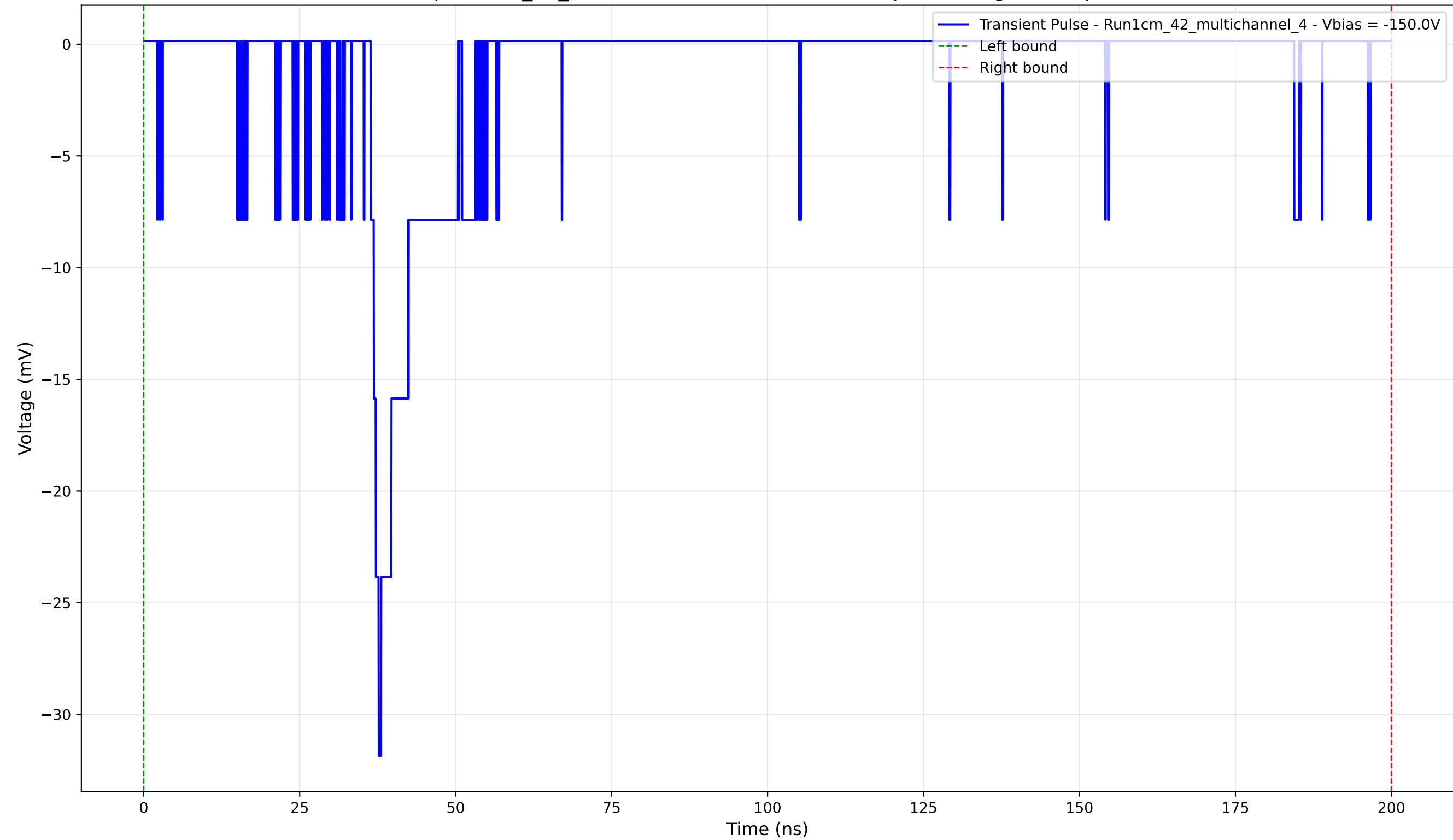
Transient Pulse - Sample: 1cm_42_multichannel - Position: 3210.0 \mu\text{m} - Charge: 4.50 pC - Rise Time: 1.29 ns
