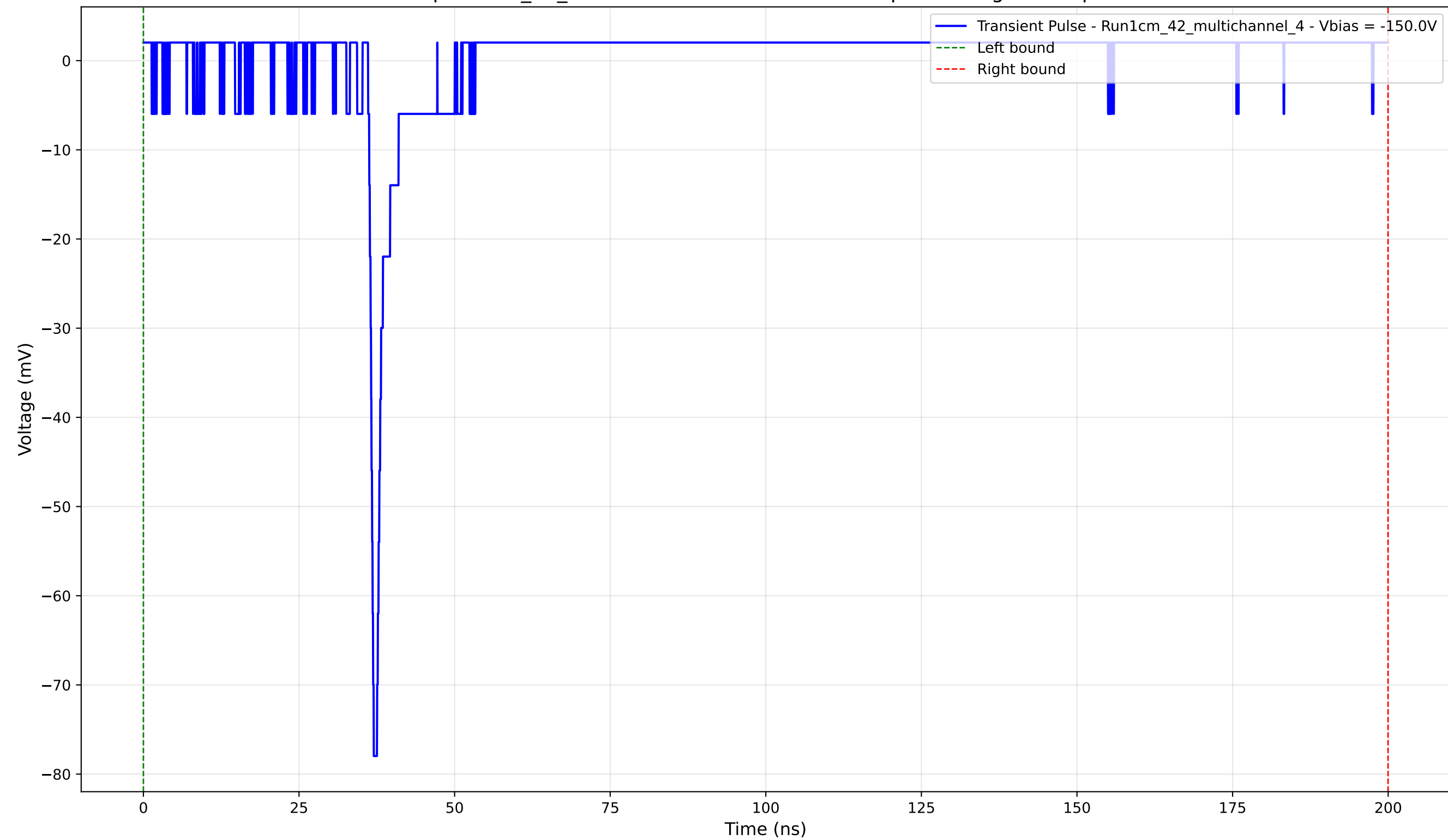
Transient Pulse - Sample: 1cm_42_multichannel - Position: 2490.0 \mu\text{m} - Charge: 1.57 pC - Rise Time: 0.74 ns
