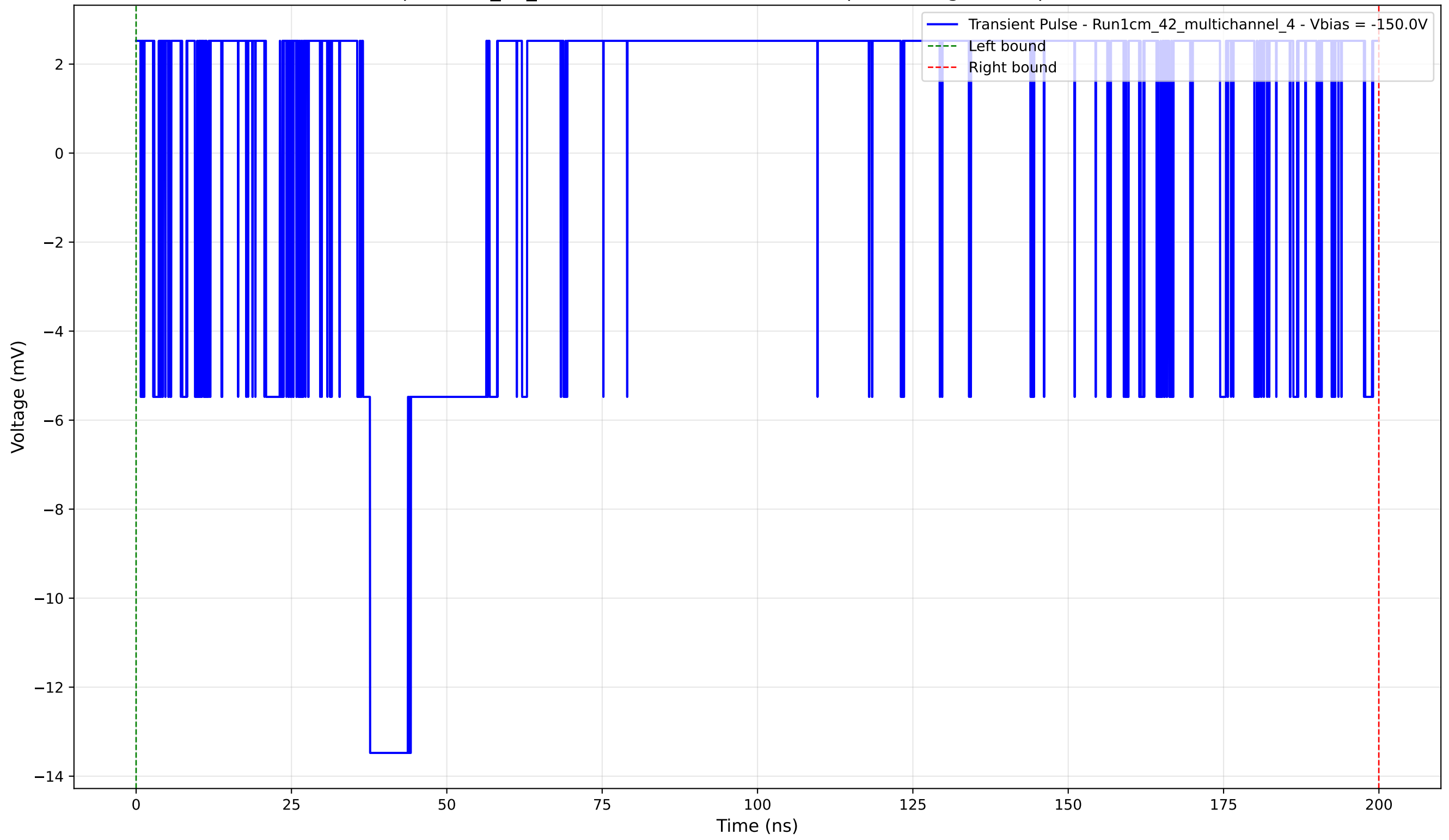
Transient Pulse - Sample: 1cm_42_multichannel - Position: 940.0 \mu\text{m} - Charge: 2.21 pC - Rise Time: 0.00 ns (N/A)
