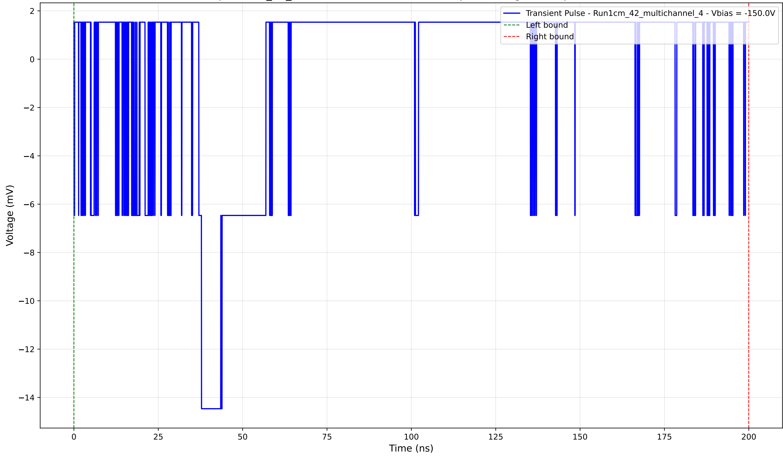
Transient Pulse - Sample: 1cm_42_multichannel - Position: 695.0 \mu\text{m} - Charge: 0.32 pC - Rise Time: 0.00 ns (N/A)
