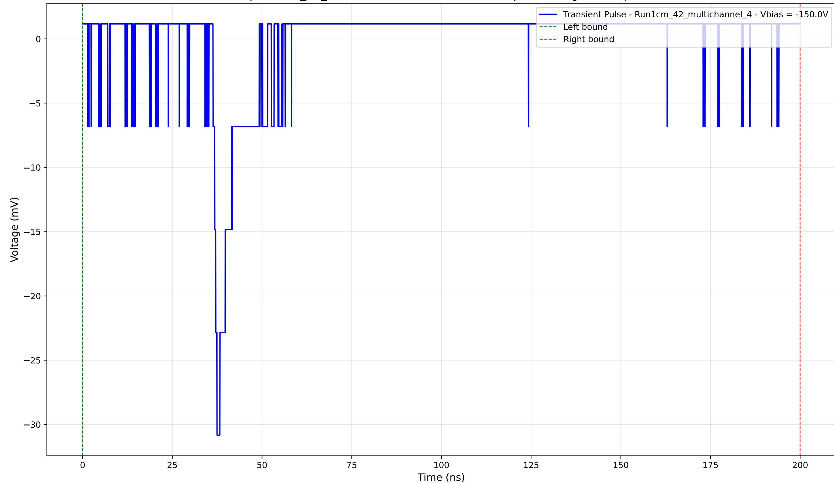
Transient Pulse - Sample: 1cm_42_multichannel - Position: 3125.0 \mu\text{m} - Charge: 0.14 pC - Rise Time: 1.11 ns
