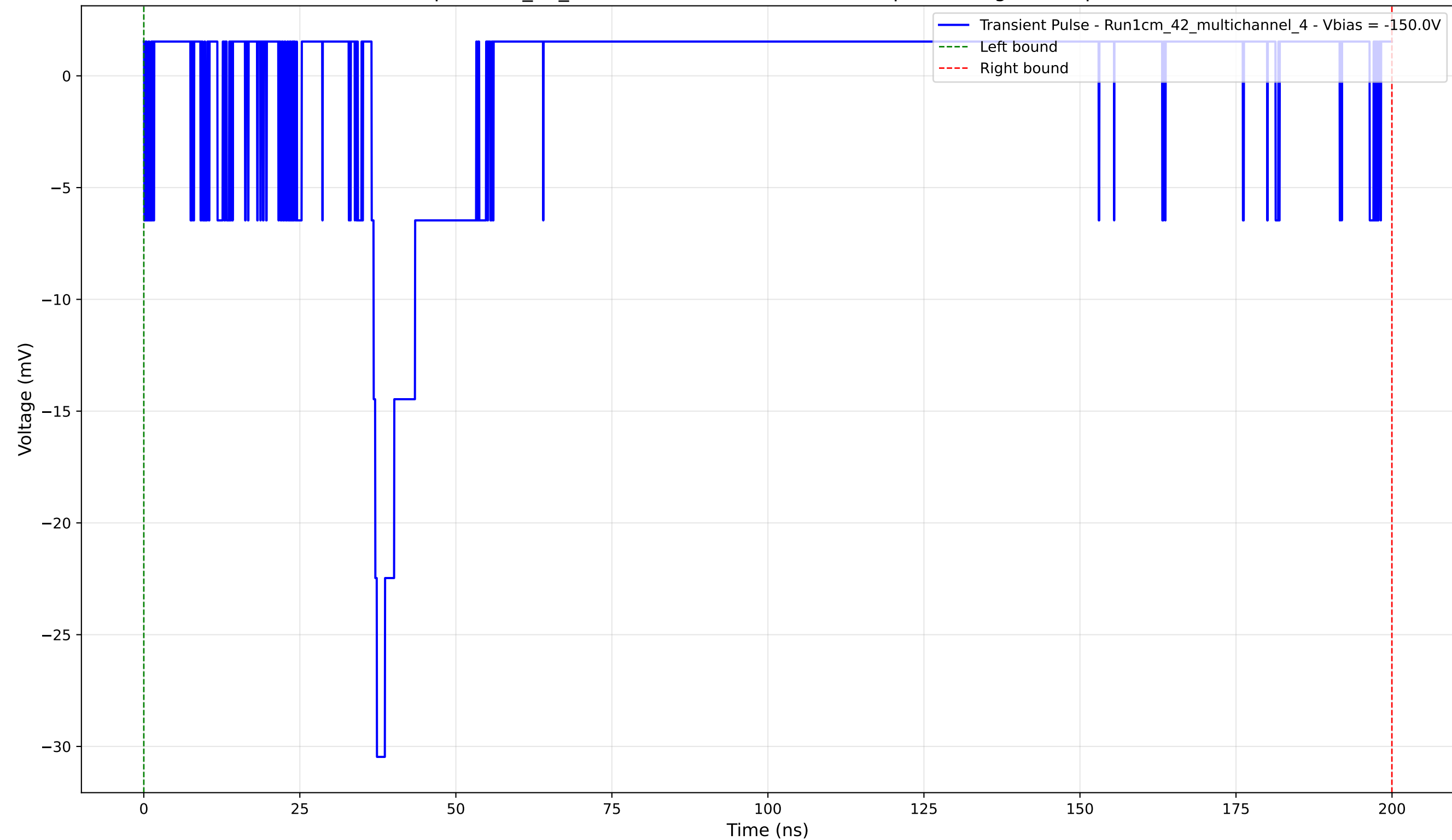
Transient Pulse - Sample: 1cm_42_multichannel - Position: 1615.0 \mu\text{m} - Charge: 0.27 pC - Rise Time: 0.85 ns
