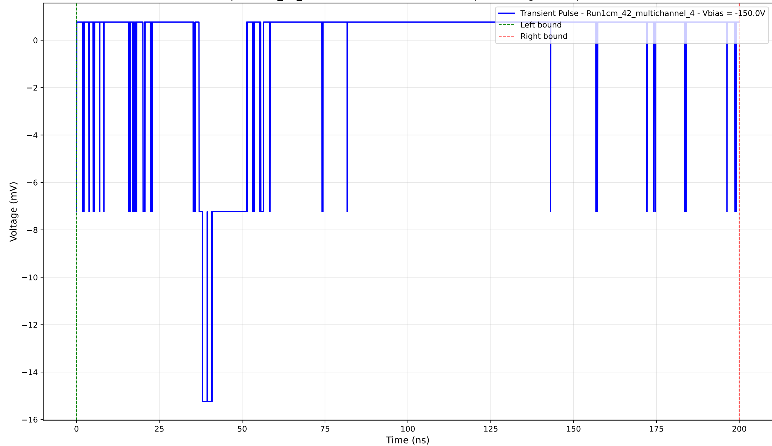
Transient Pulse - Sample: 1cm_42_multichannel - Position: 3845.0 \mu\text{m} - Charge: 0.62 pC - Rise Time: 1.08 ns
