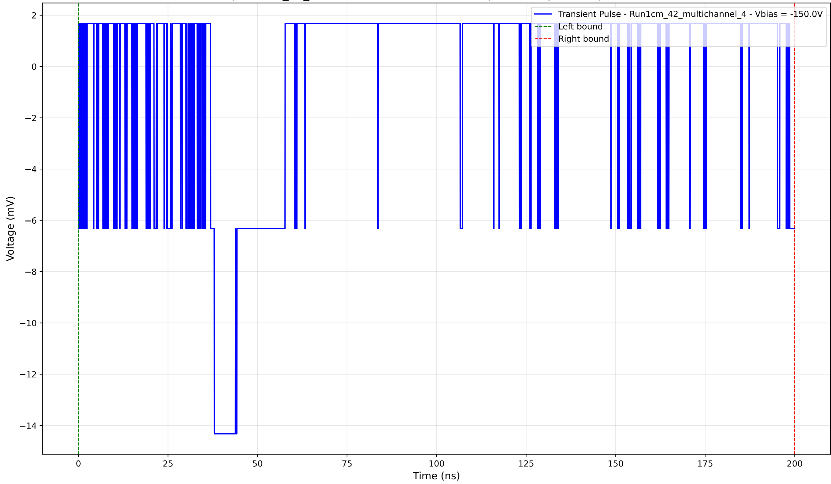
Transient Pulse - Sample: 1cm_42_multichannel - Position: 660.0 \mu\text{m} - Charge: 0.33 pC - Rise Time: 0.00 ns (N/A)
