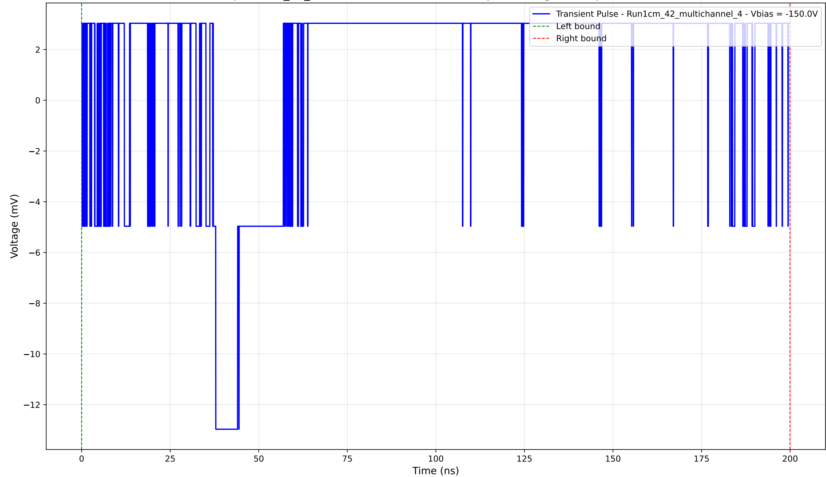
Transient Pulse - Sample: 1cm_42_multichannel - Position: 700.0 \mu\text{m} - Charge: 5.44 pC - Rise Time: 0.00 ns (N/A)
