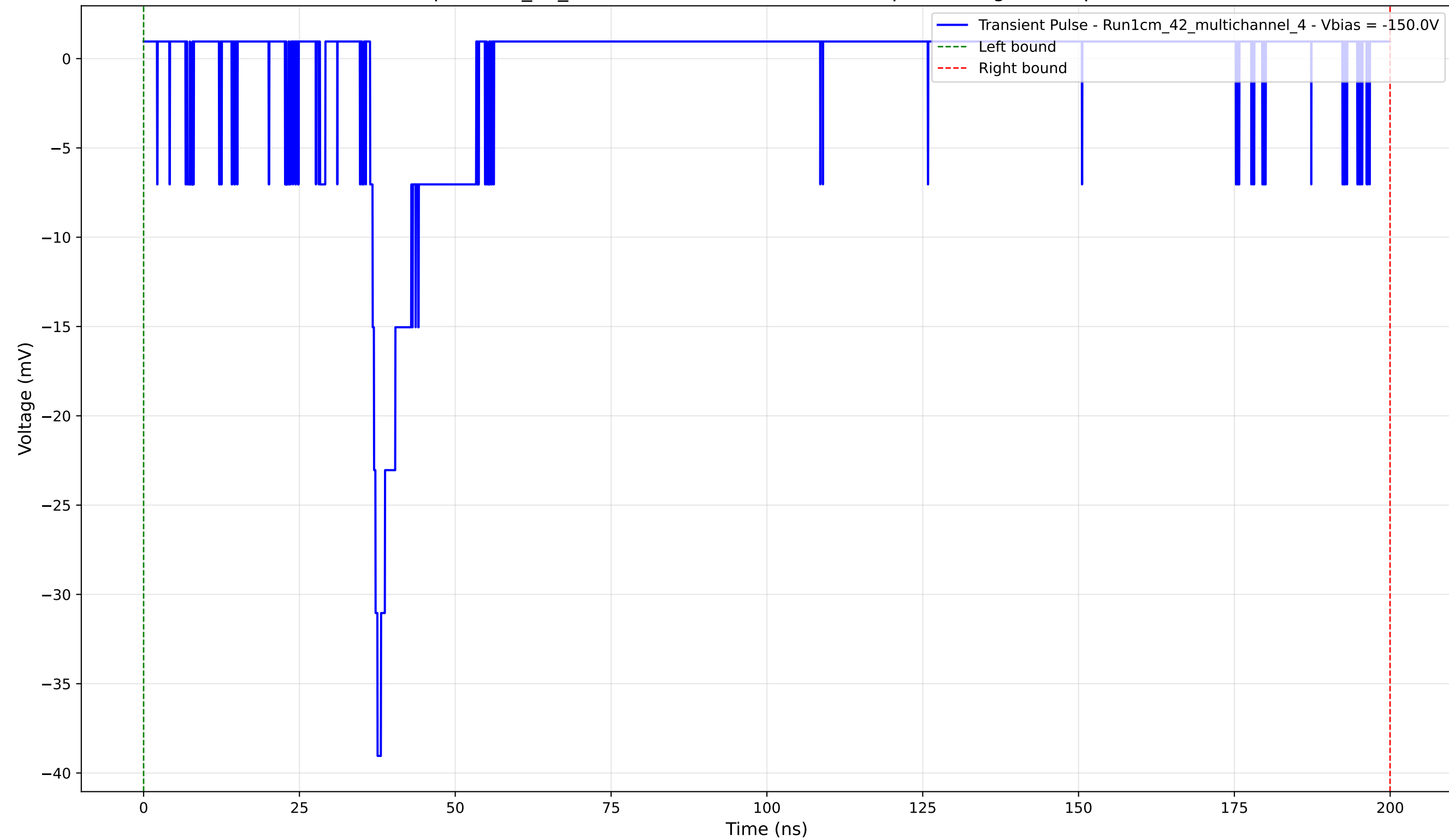
Transient Pulse - Sample: 1cm_42_multichannel - Position: 1660.0 \mu\text{m} - Charge: 2.01 pC - Rise Time: 1.19 ns
