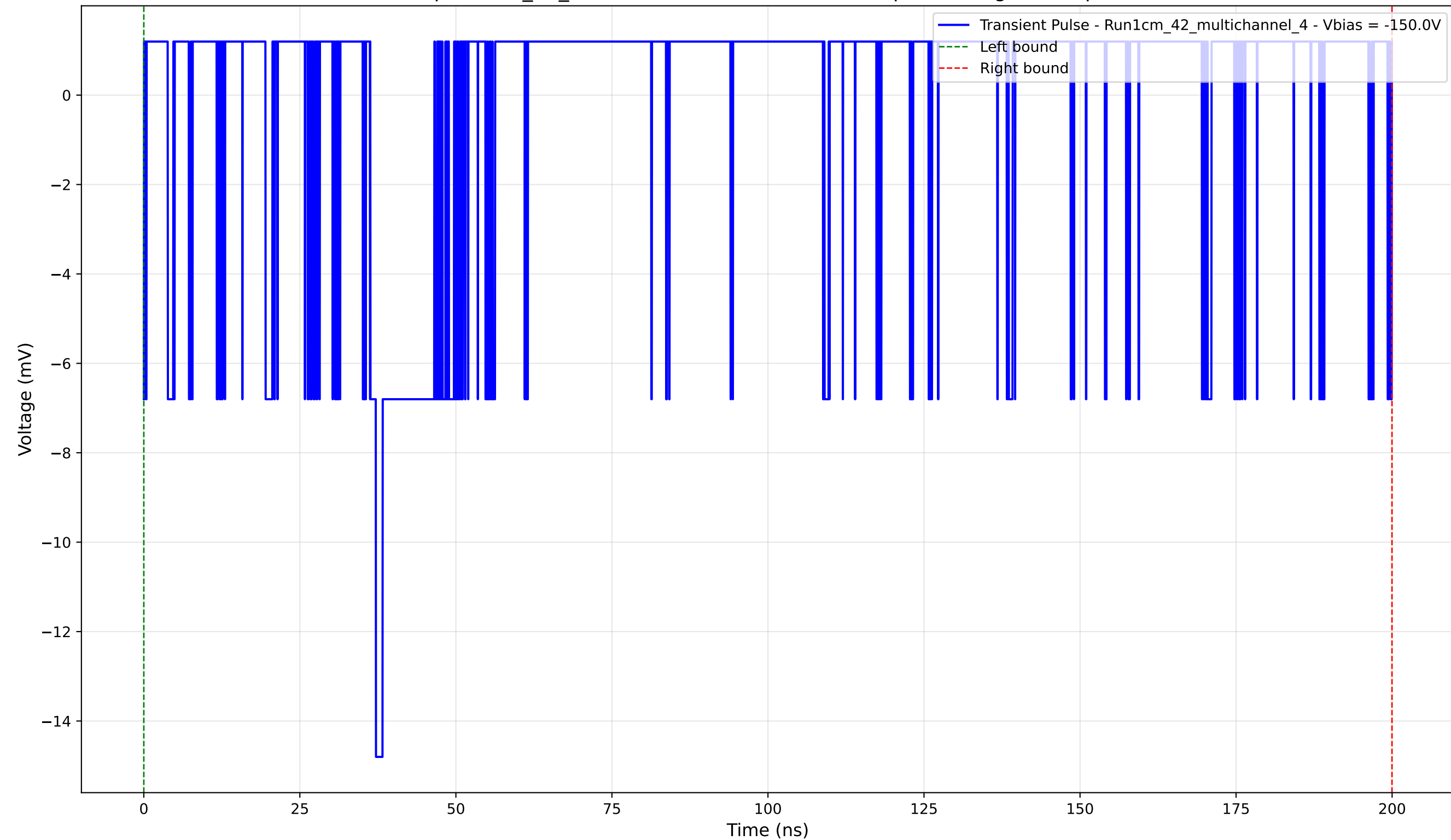
Transient Pulse - Sample: 1cm_42_multichannel - Position: 2935.0 \mu\text{m} - Charge: 0.21 pC - Rise Time: 0.90 ns
