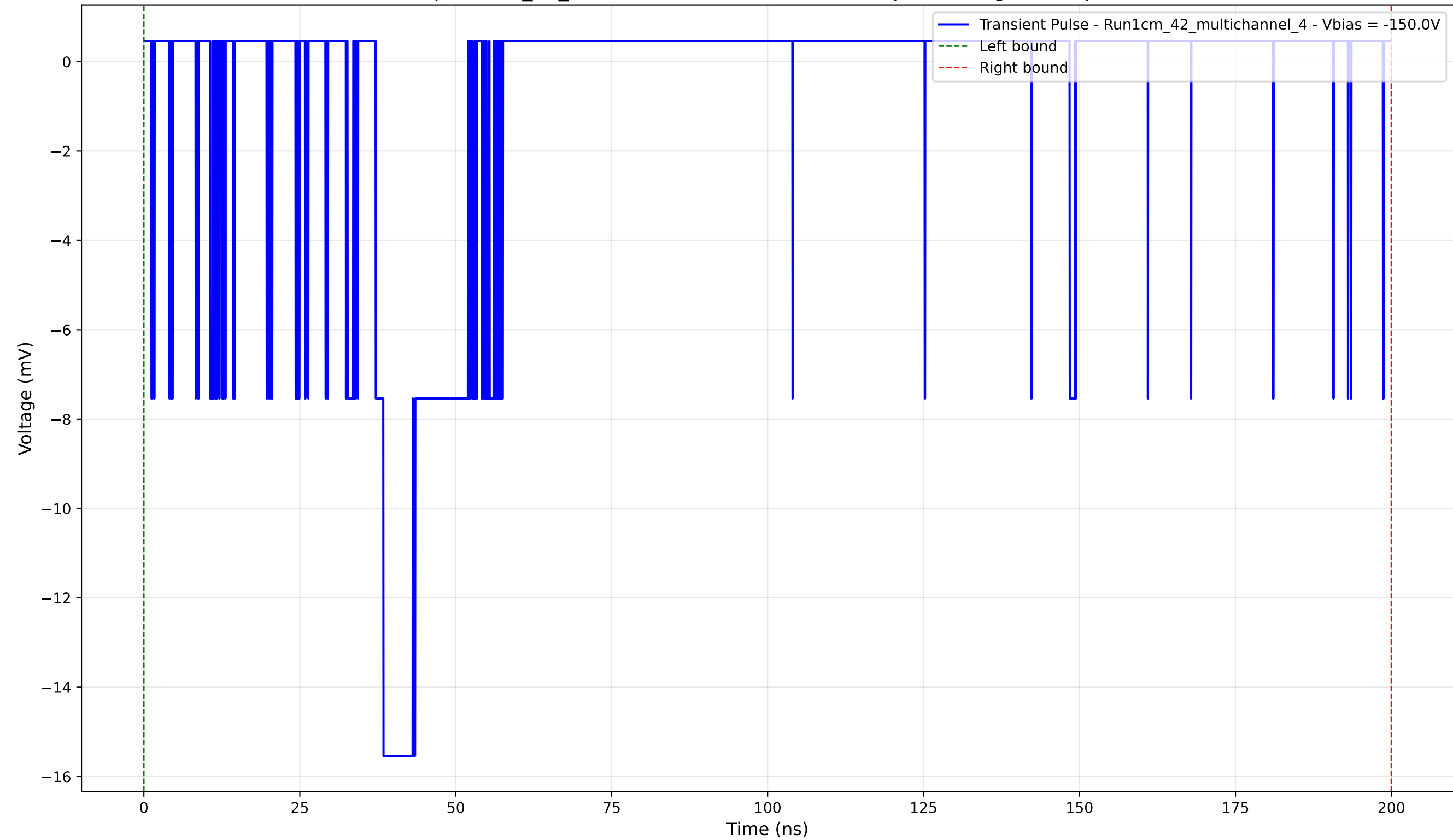
Transient Pulse - Sample: 1cm_42_multichannel - Position: 4615.0 \mu\text{m} - Charge: 2.80 pC - Rise Time: 1.26 ns
