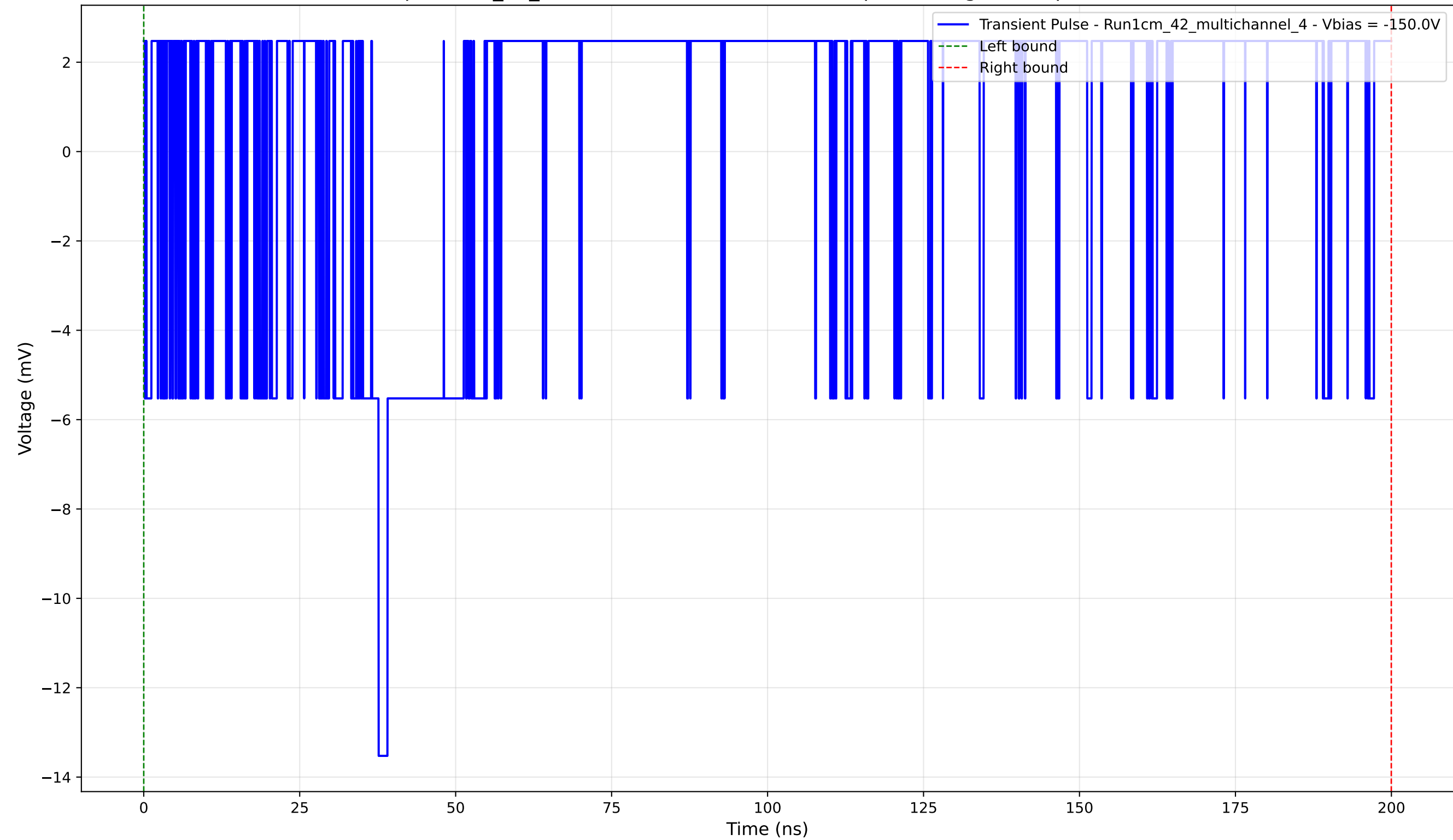
Transient Pulse - Sample: 1cm_42_multichannel - Position: 1420.0 \mu\text{m} - Charge: 3.15 pC - Rise Time: 0.00 ns (N/A)
