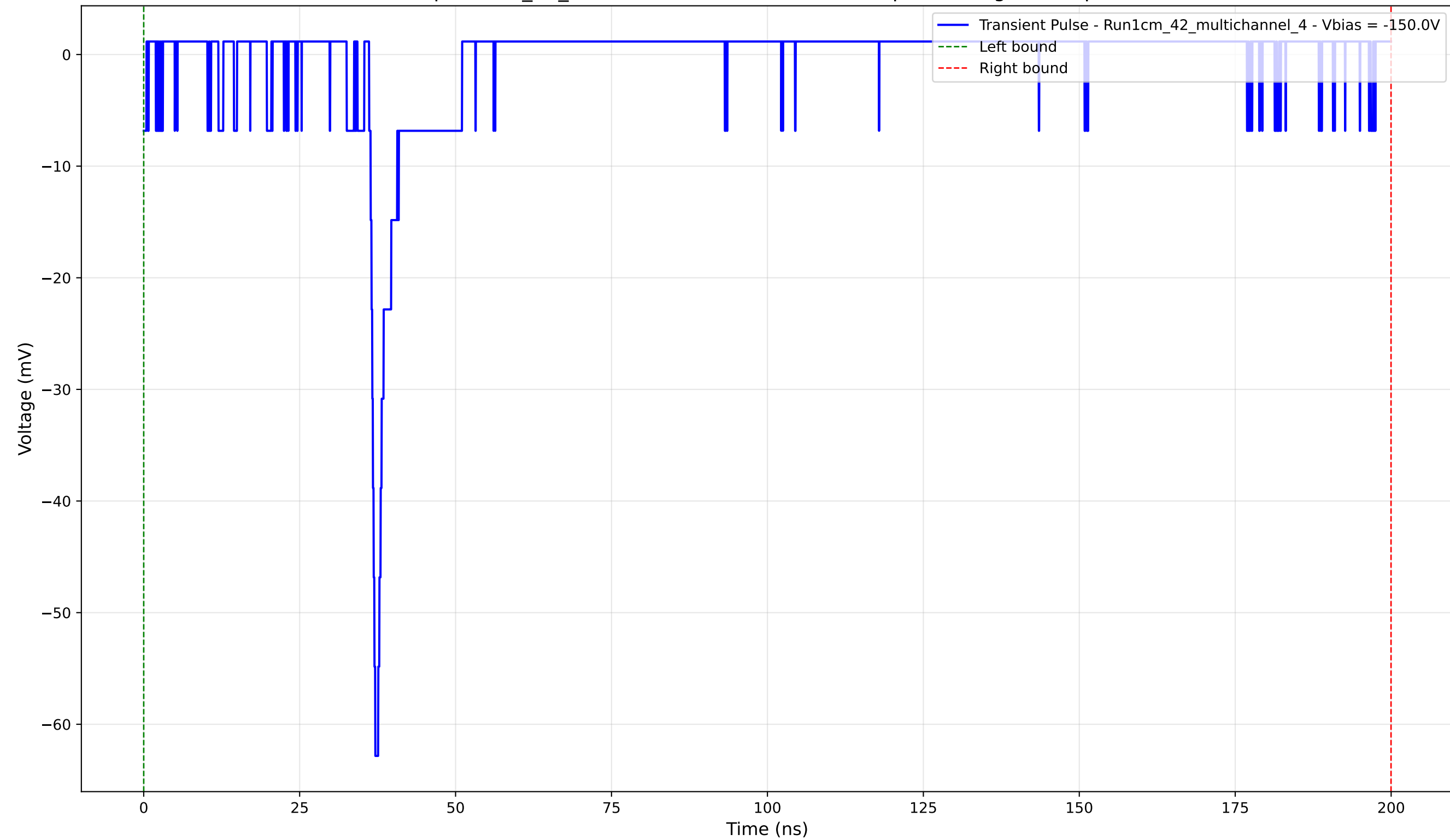
Transient Pulse - Sample: 1cm_42_multichannel - Position: 2615.0 \mu\text{m} - Charge: 1.57 pC - Rise Time: 0.98 ns
