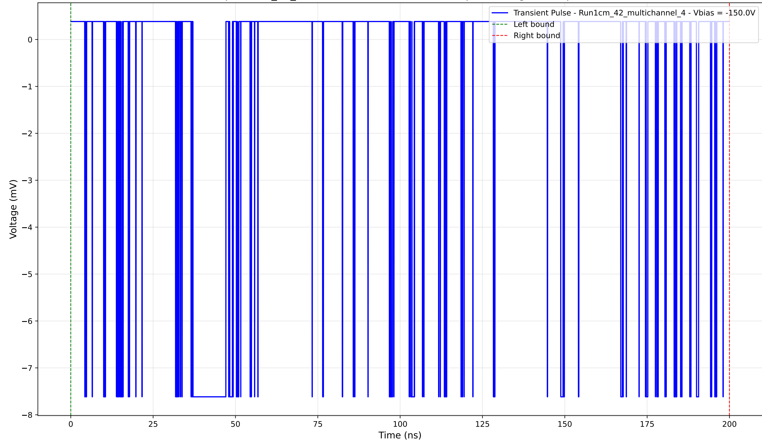
Transient Pulse - Sample: 1cm_42_multichannel - Position: 3865.0 \mu\text{m} - Charge: 2.47 pC - Rise Time: 0.02 ns
