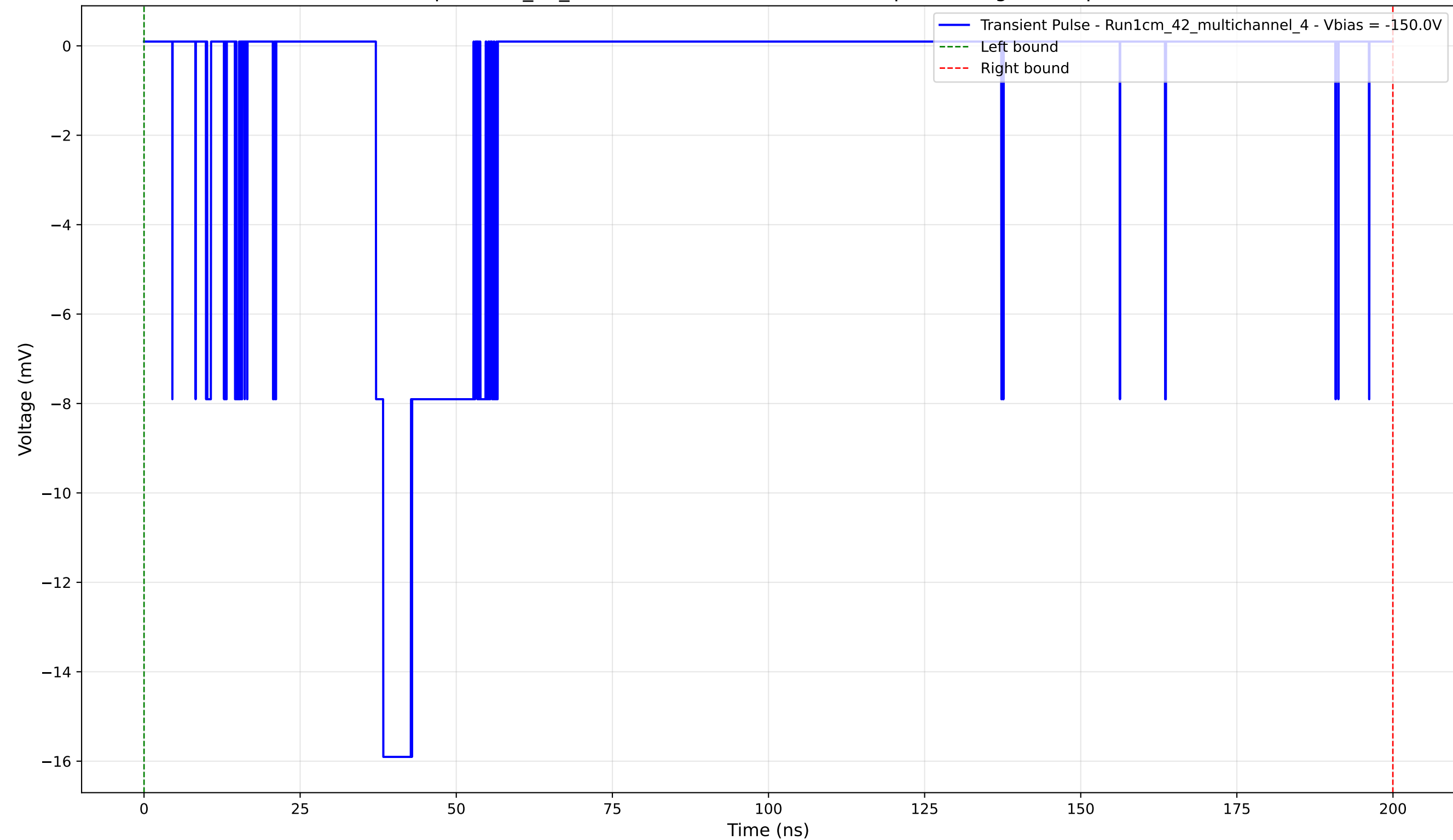
Transient Pulse - Sample: 1cm_42_multichannel - Position: 4195.0 \mu\text{m} - Charge: 3.67 pC - Rise Time: 1.18 ns
