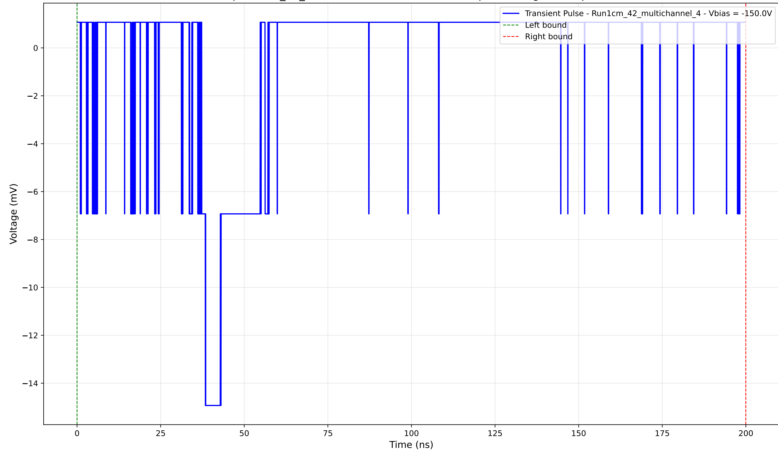
Transient Pulse - Sample: 1cm_42_multichannel - Position: 4245.0 \mu\text{m} - Charge: 0.36 pC - Rise Time: 1.10 ns
