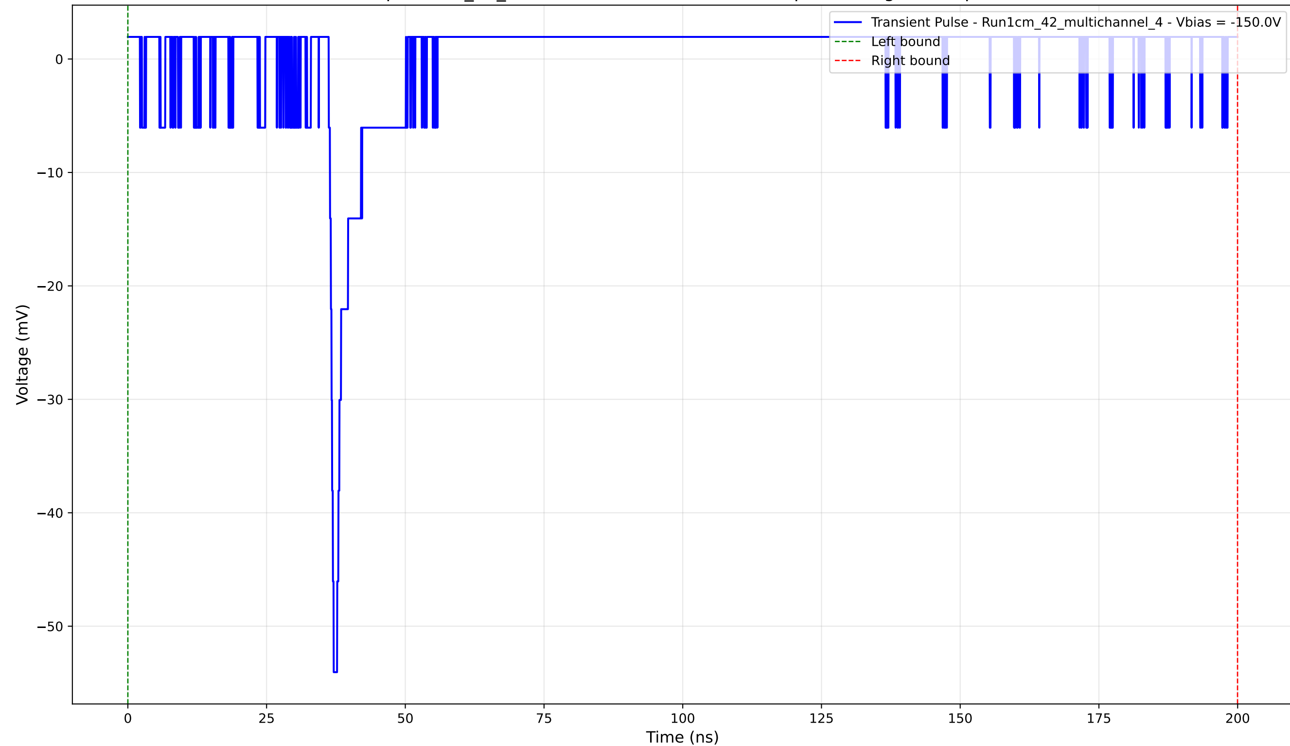
Transient Pulse - Sample: 1cm_42_multichannel - Position: 2665.0 \mu\text{m} - Charge: 1.25 pC - Rise Time: 0.88 ns
