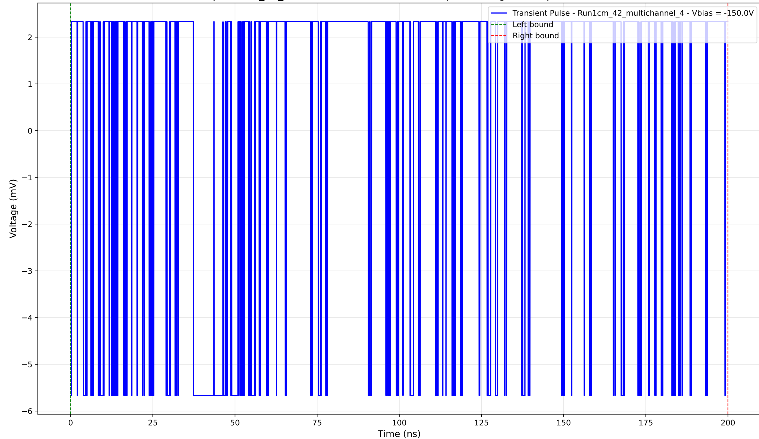
Transient Pulse - Sample: 1cm_42_multichannel - Position: 405.0 \mu\text{m} - Charge: 3.31 pC - Rise Time: 0.00 ns (N/A)
