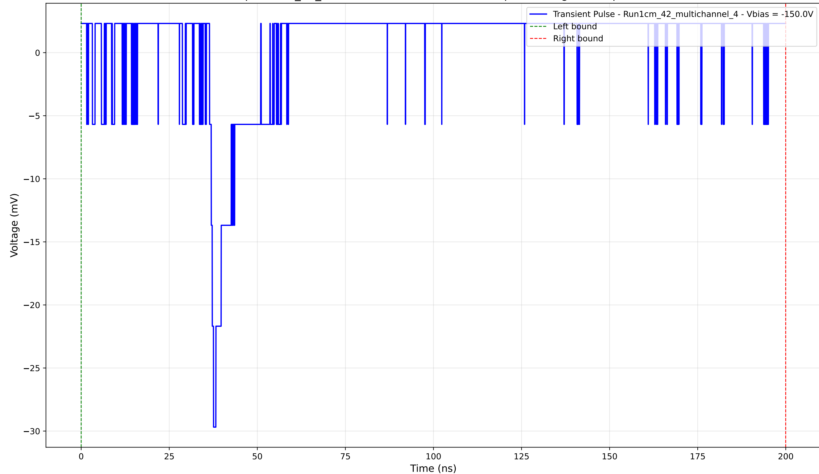
Transient Pulse - Sample: 1cm_42_multichannel - Position: 3225.0 \mu\text{m} - Charge: 3.16 pC - Rise Time: 1.14 ns
