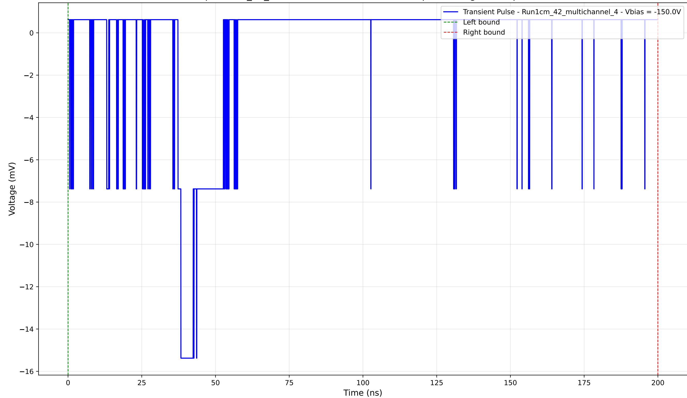
Transient Pulse - Sample: 1cm_42_multichannel - Position: 4165.0 \mu\text{m} - Charge: 1.72 pC - Rise Time: 1.00 ns
