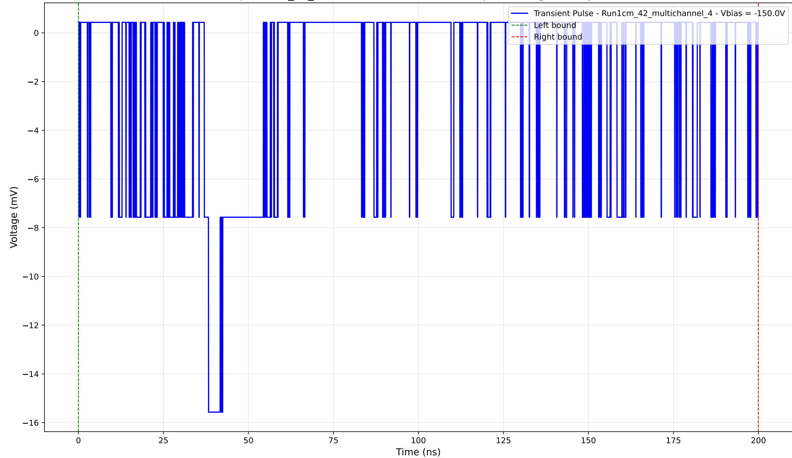
Transient Pulse - Sample: 1cm_42_multichannel - Position: 180.0 \mu\text{m} - Charge: 6.91 pC - Rise Time: 1.26 ns
