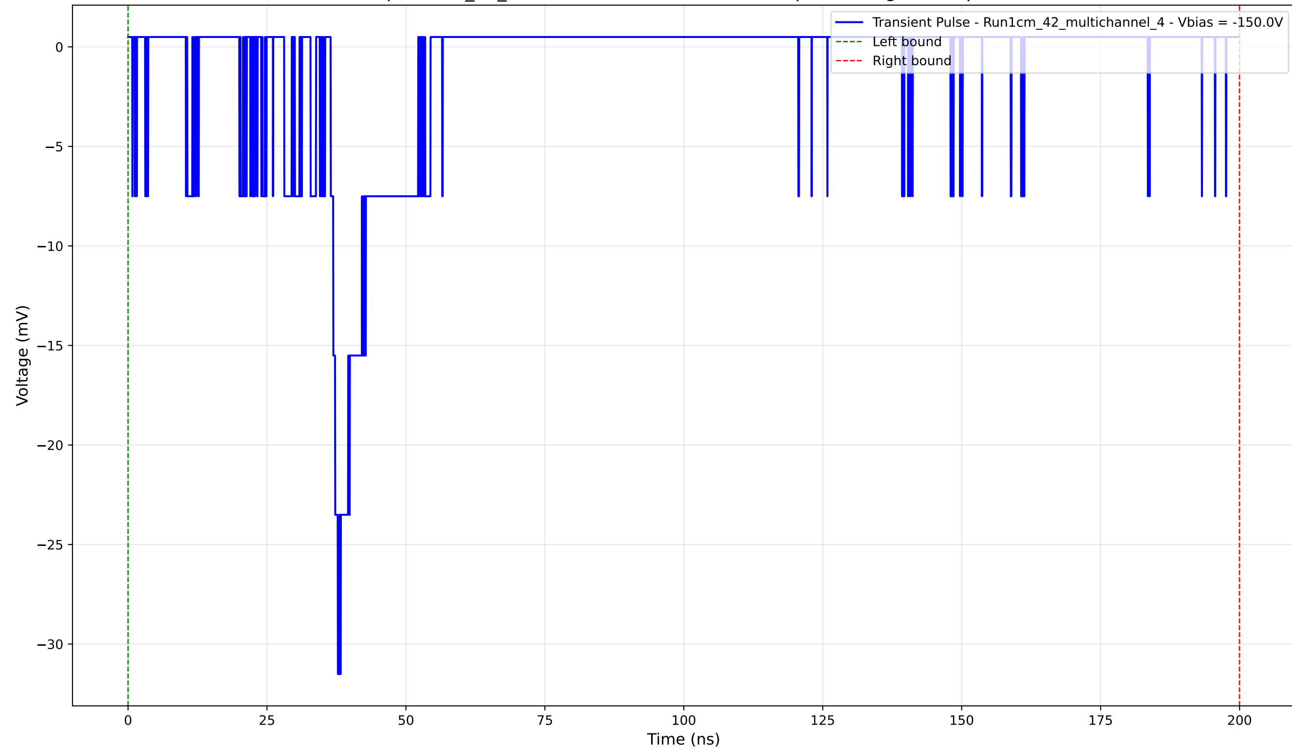
Transient Pulse - Sample: 1cm_42_multichannel - Position: 3270.0 \mu\text{m} - Charge: 3.85 pC - Rise Time: 1.29 ns
