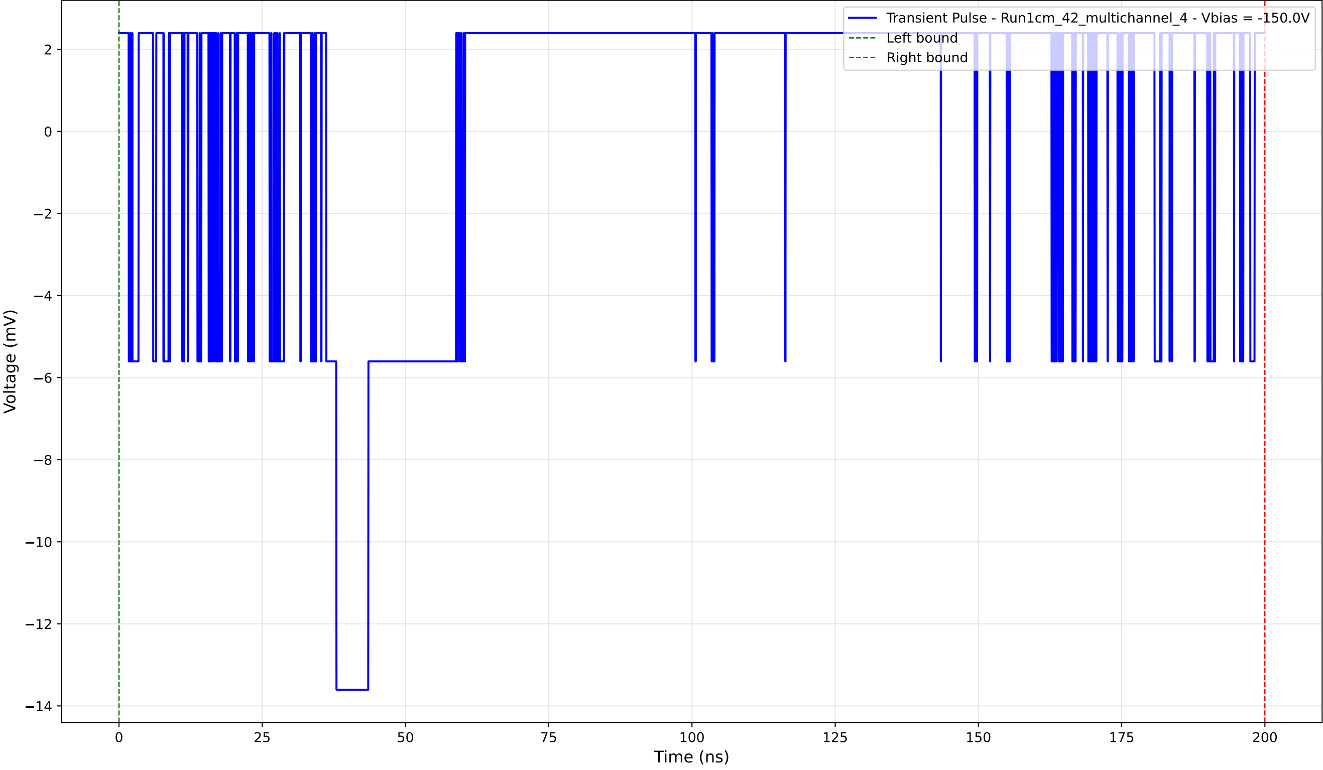
Transient Pulse - Sample: 1cm_42_multichannel - Position: 600.0 \mu\text{m} - Charge: 2.29 pC - Rise Time: 0.00 ns (N/A)
