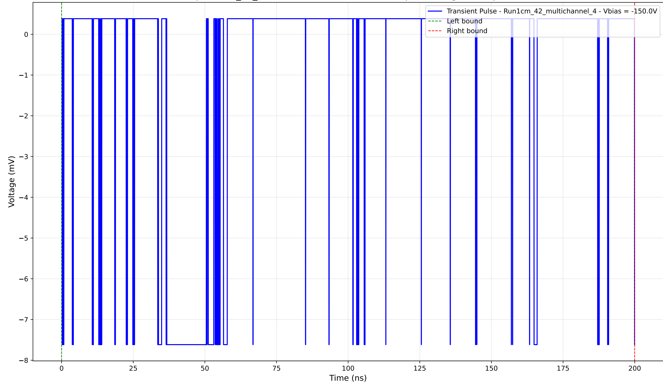
Transient Pulse - Sample: 1cm_42_multichannel - Position: 4845.0 \mu\text{m} - Charge: 2.46 pC - Rise Time: 0.02 ns
