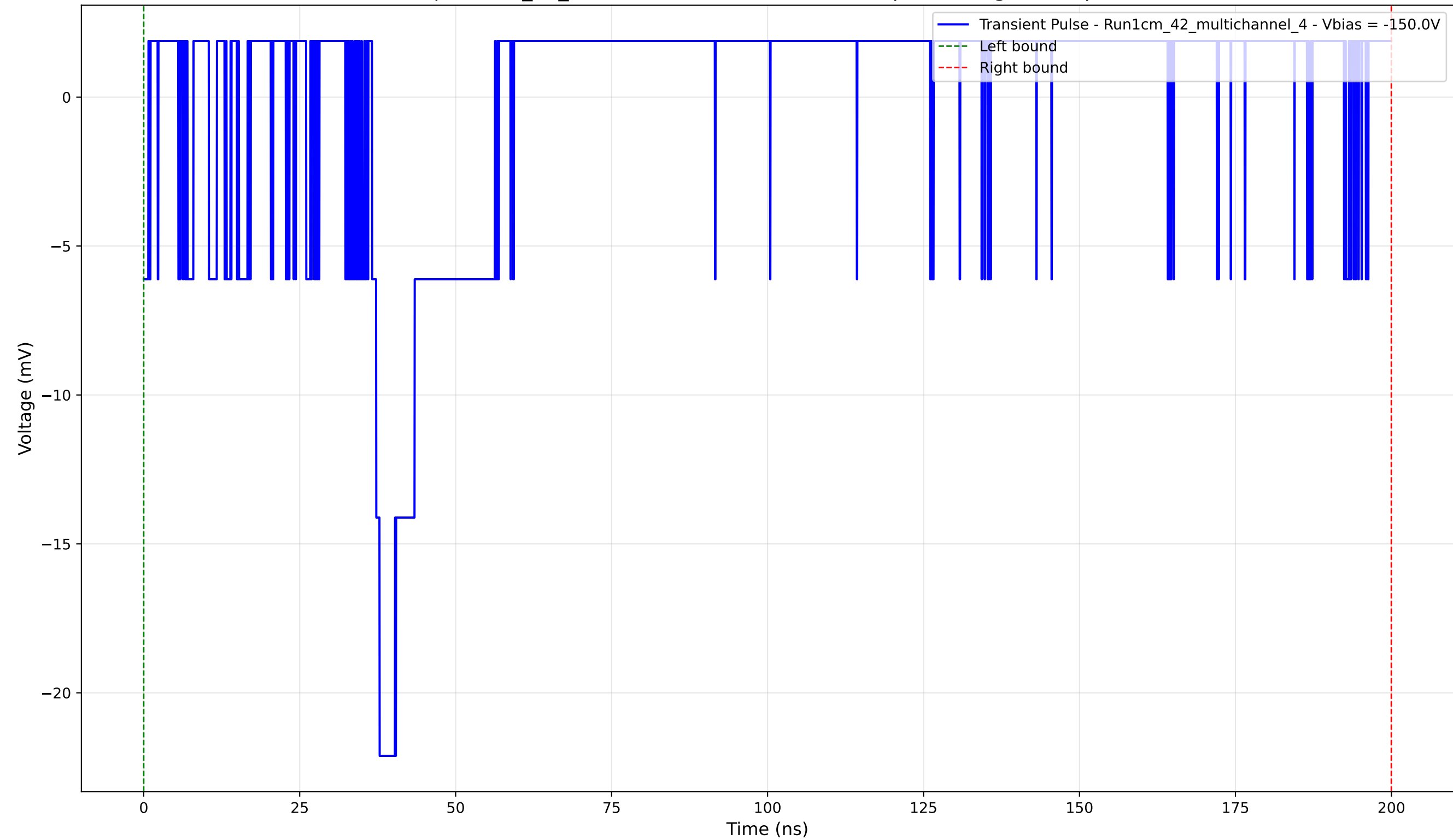
Transient Pulse - Sample: 1cm_42_multichannel - Position: 1185.0 \mu\text{m} - Charge: 0.72 pC - Rise Time: 1.22 ns
