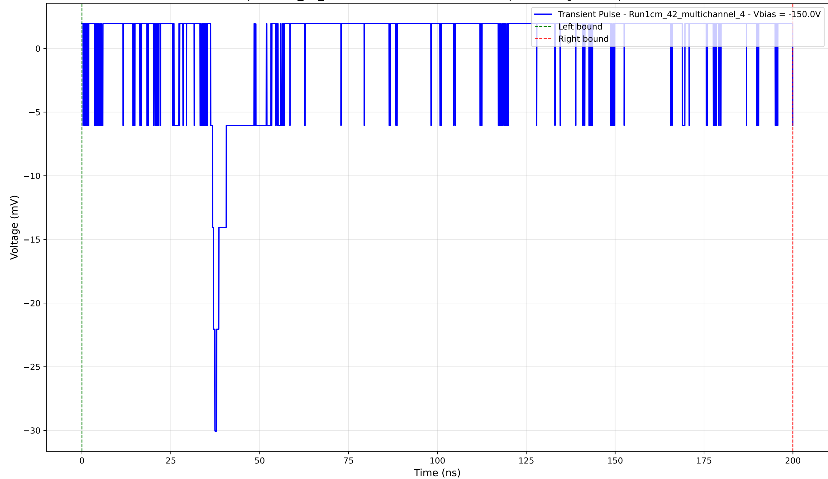
Transient Pulse - Sample: 1cm_42_multichannel - Position: 1825.0 \mu\text{m} - Charge: 1.64 pC - Rise Time: 1.21 ns
