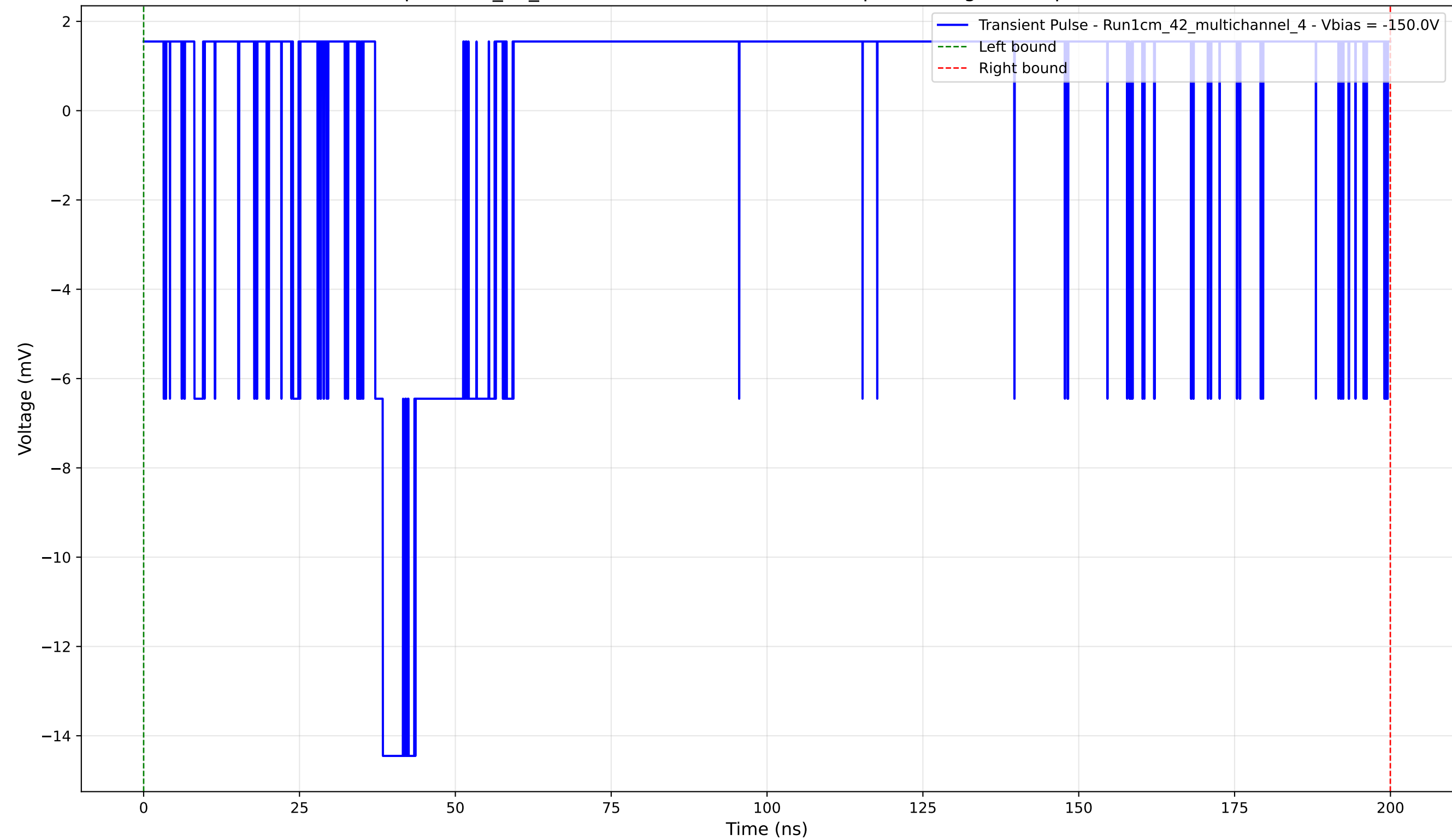
Transient Pulse - Sample: 1cm_42_multichannel - Position: 4565.0 \mu\text{m} - Charge: 0.95 pC - Rise Time: 0.00 ns (N/A)
