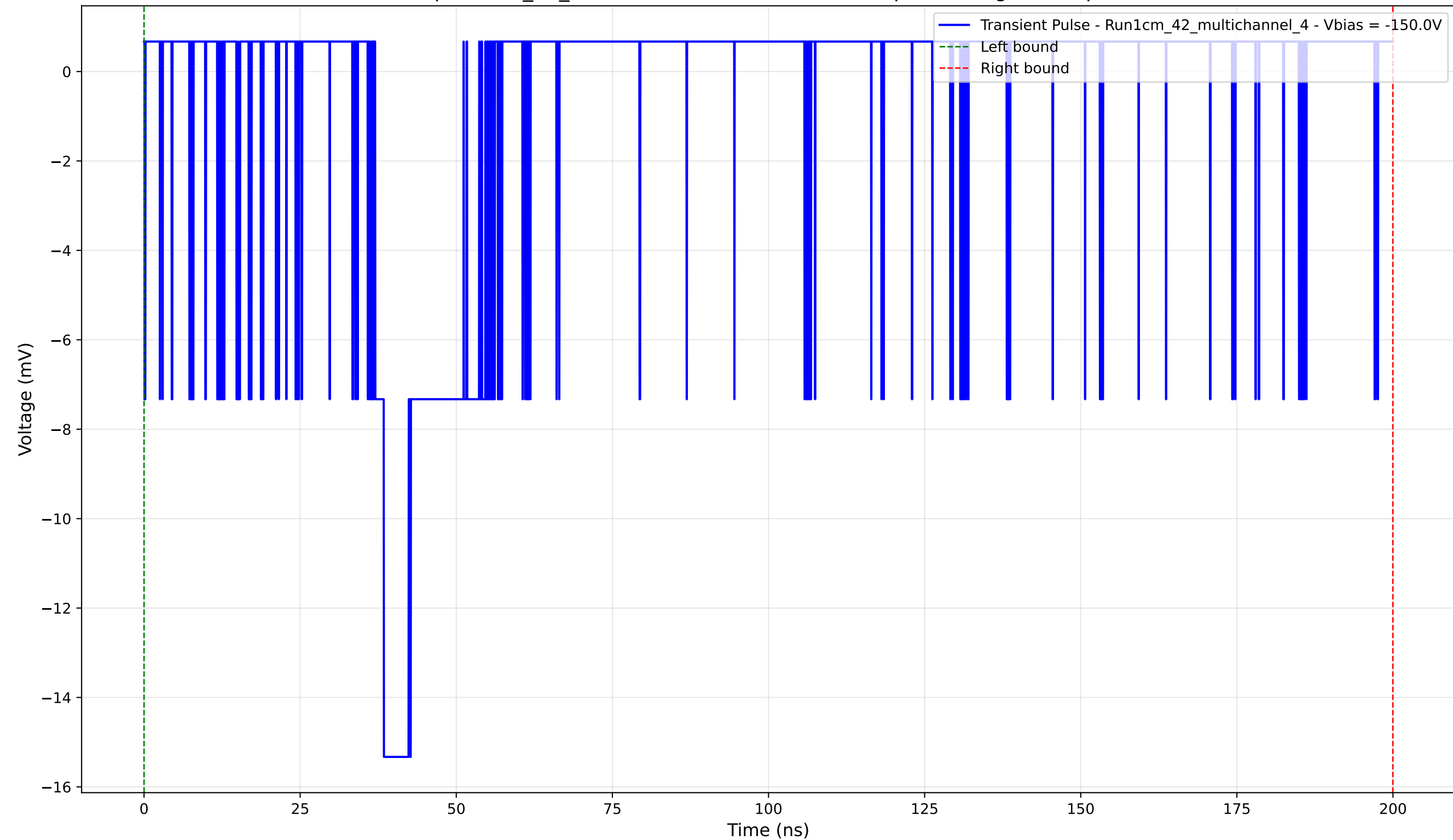
Transient Pulse - Sample: 1cm_42_multichannel - Position: 4605.0 \mu\text{m} - Charge: 2.32 pC - Rise Time: 1.40 ns
