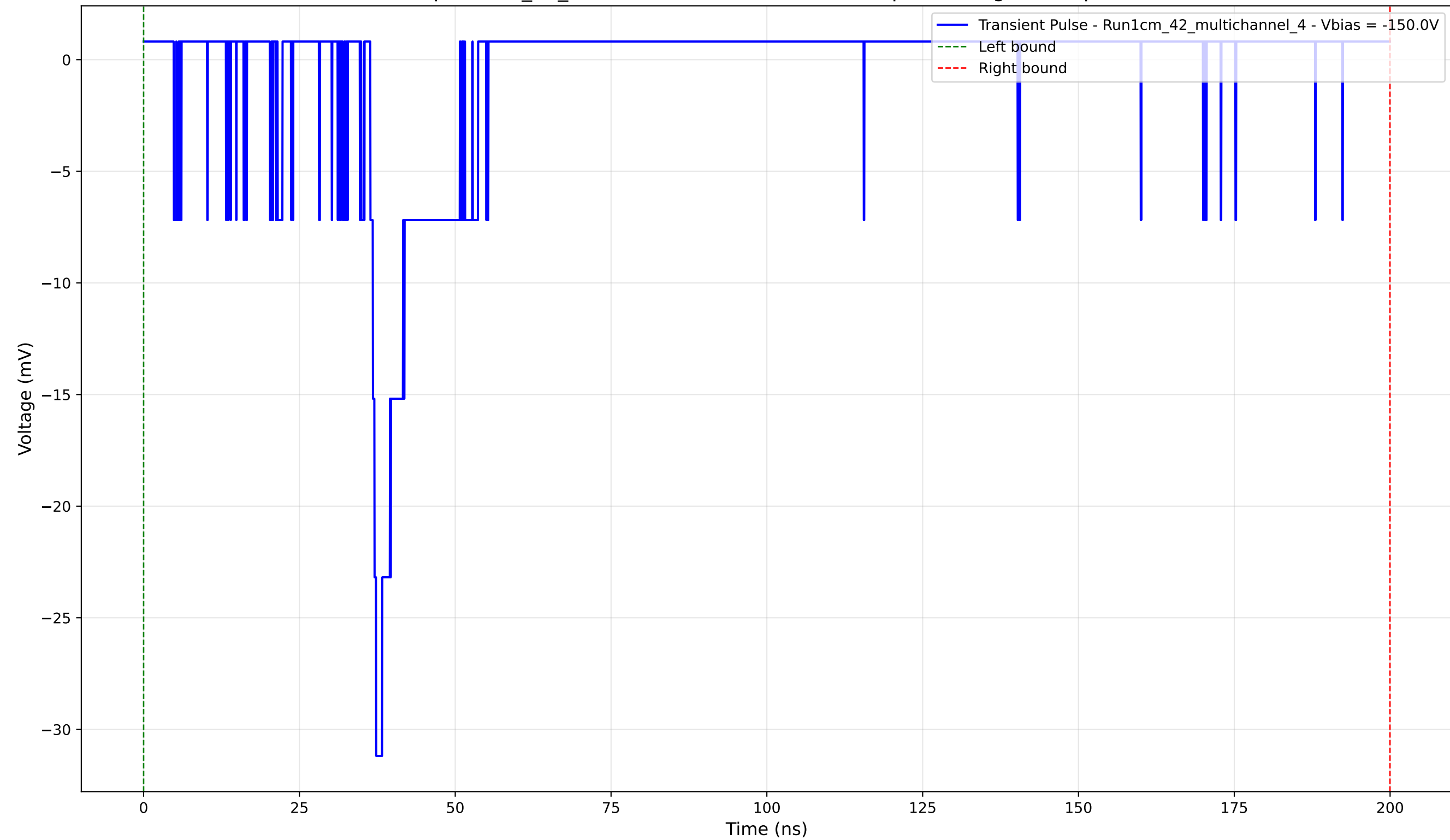
Transient Pulse - Sample: 1cm_42_multichannel - Position: 3100.0 \mu\text{m} - Charge: 1.69 pC - Rise Time: 0.93 ns
