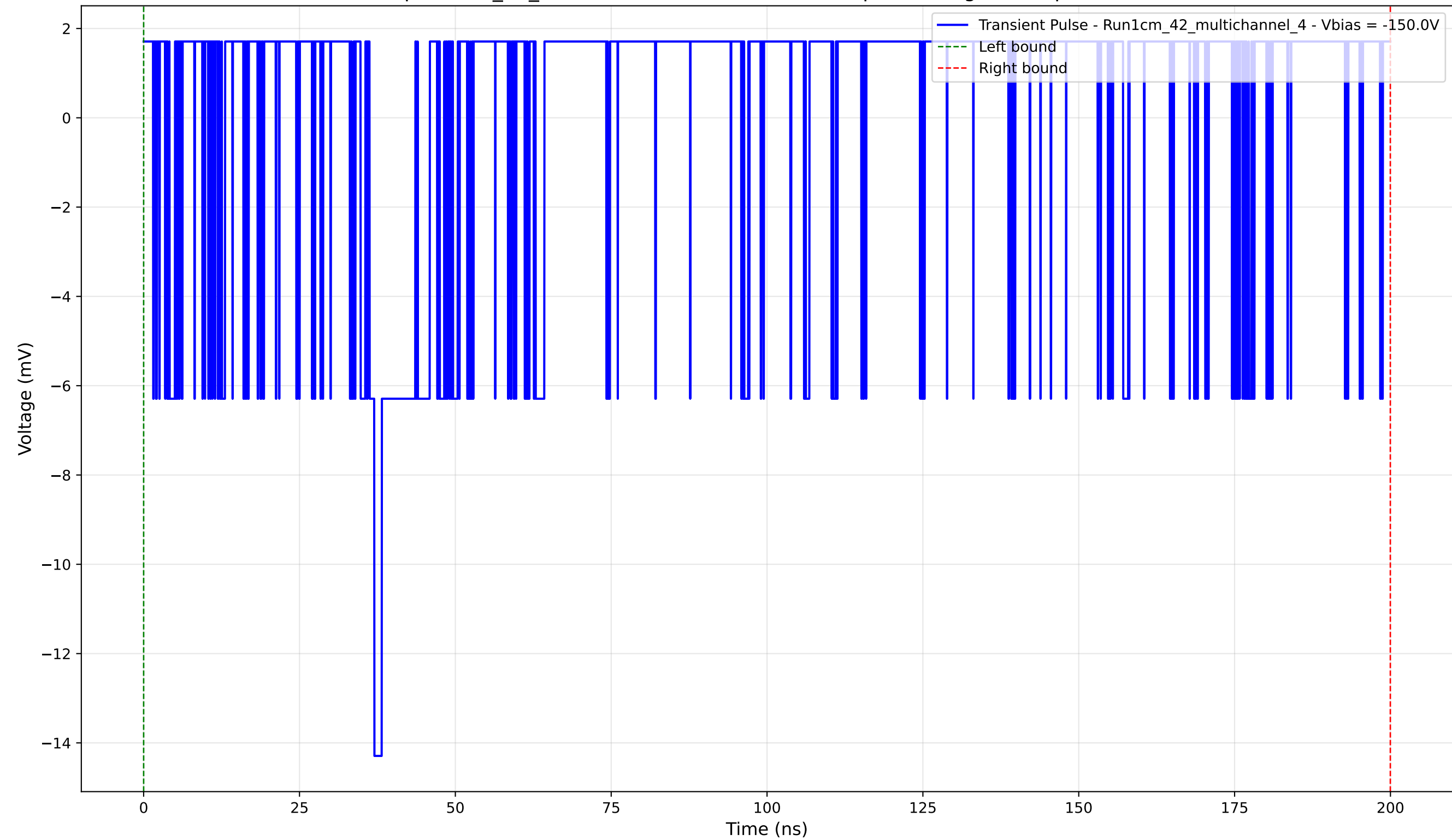
Transient Pulse - Sample: 1cm_42_multichannel - Position: 2850.0 \mu\text{m} - Charge: 1.34 pC - Rise Time: 0.00 ns (N/A)
