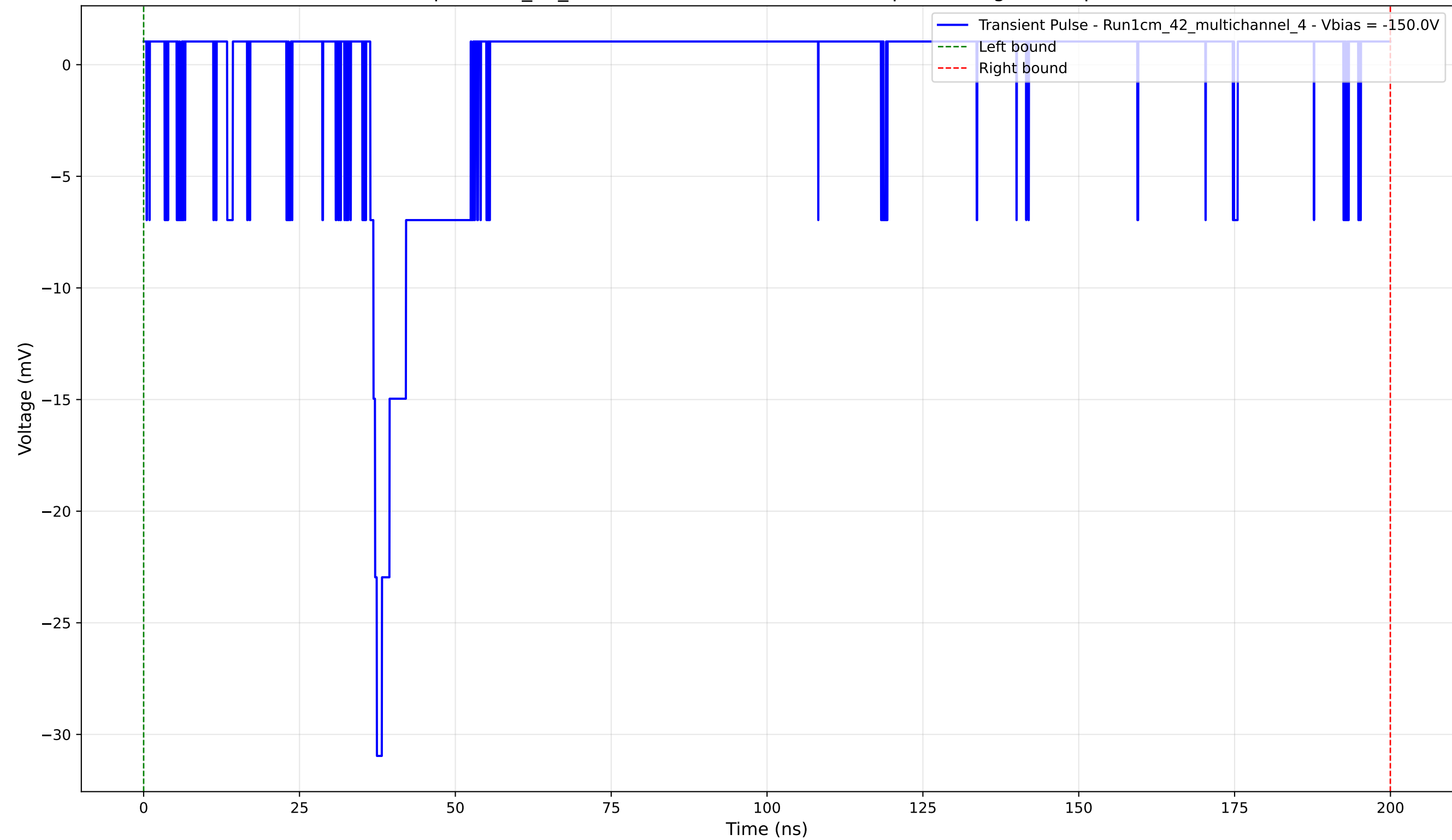
Transient Pulse - Sample: 1cm_42_multichannel - Position: 3115.0 \mu\text{m} - Charge: 1.09 pC - Rise Time: 1.05 ns
