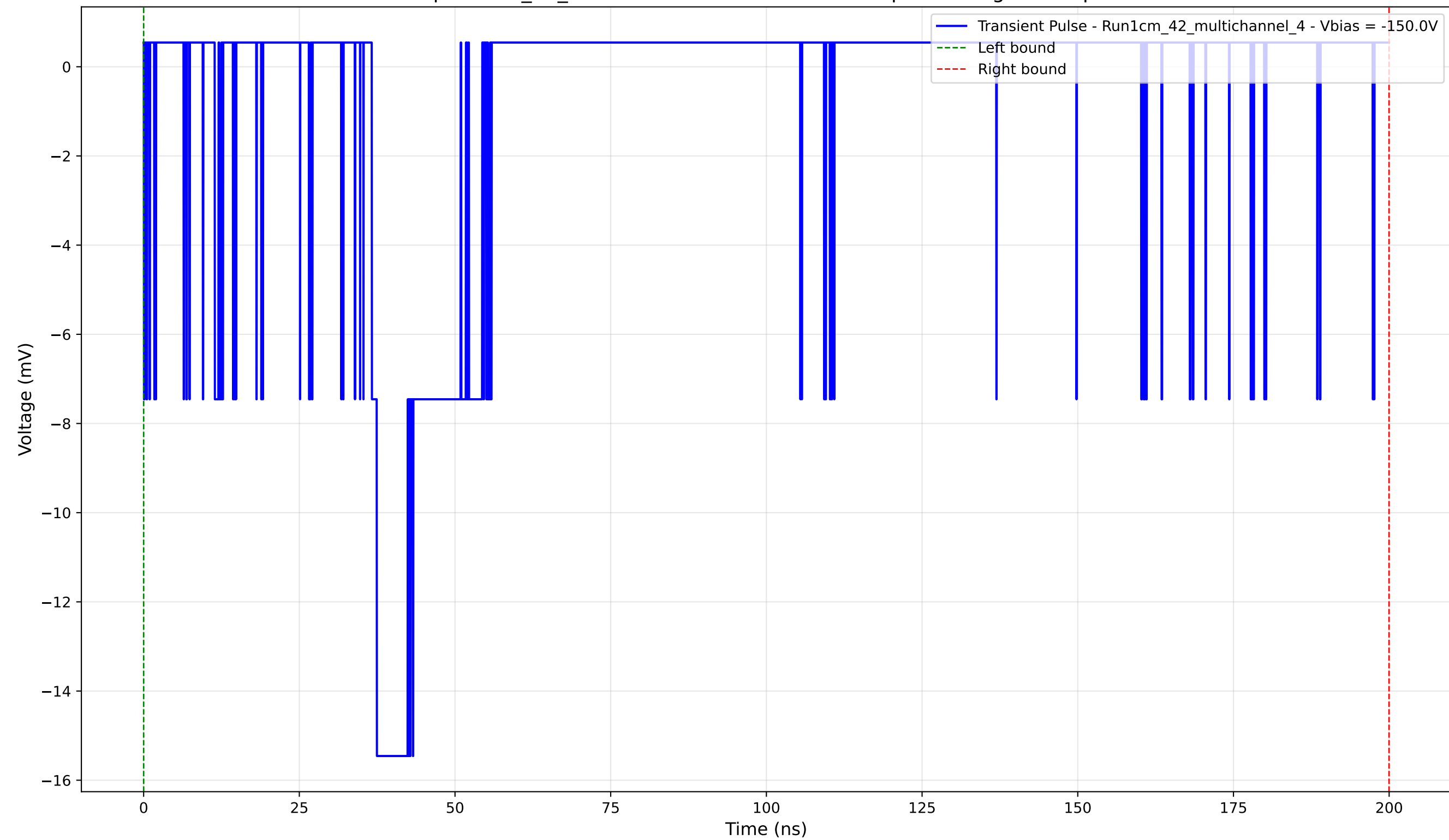
Transient Pulse - Sample: 1cm_42_multichannel - Position: 3640.0 \mu\text{m} - Charge: 2.35 pC - Rise Time: 0.82 ns
