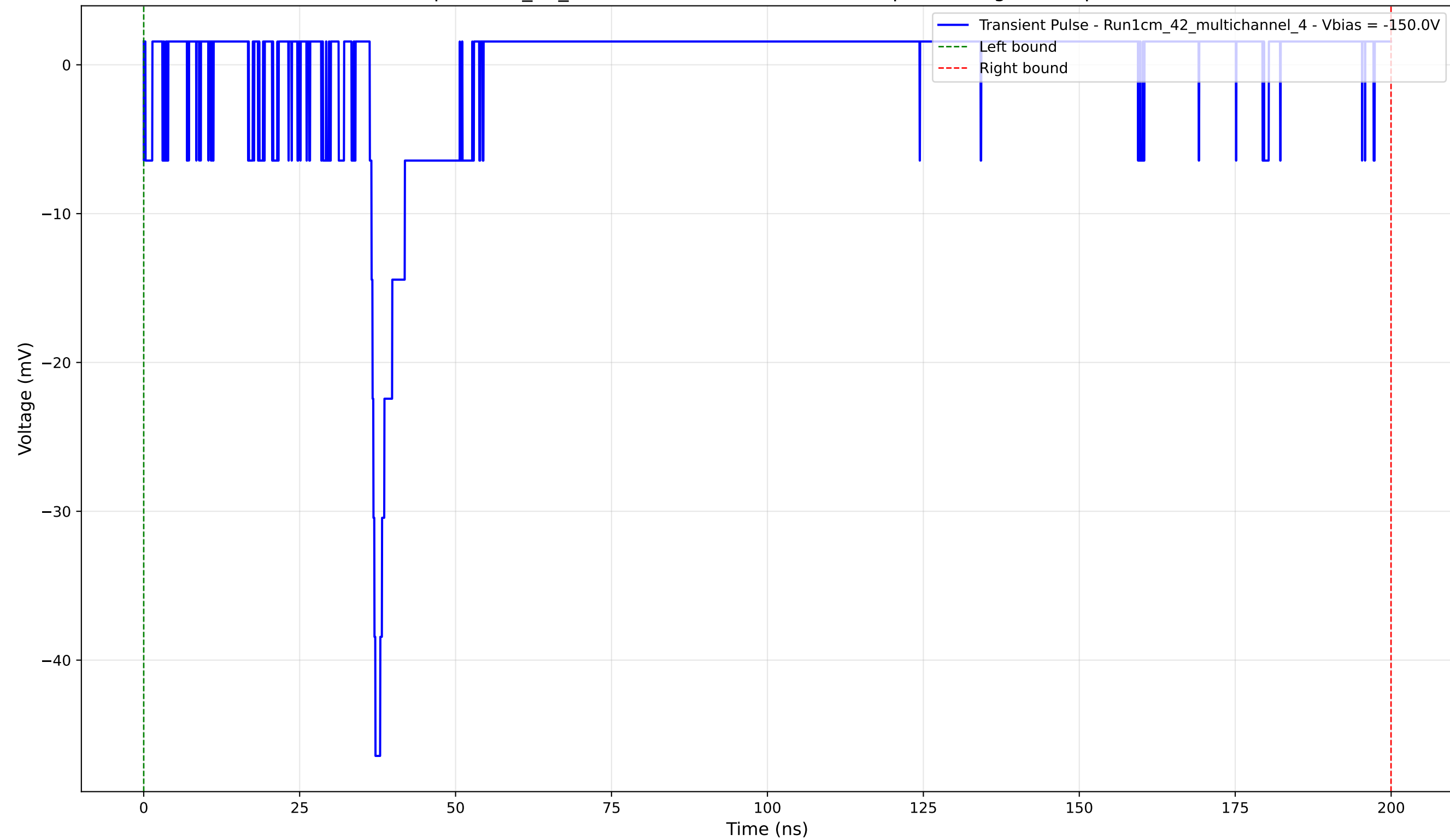
Transient Pulse - Sample: 1cm_42_multichannel - Position: 2805.0 \mu\text{m} - Charge: 0.00 pC - Rise Time: 0.91 ns
