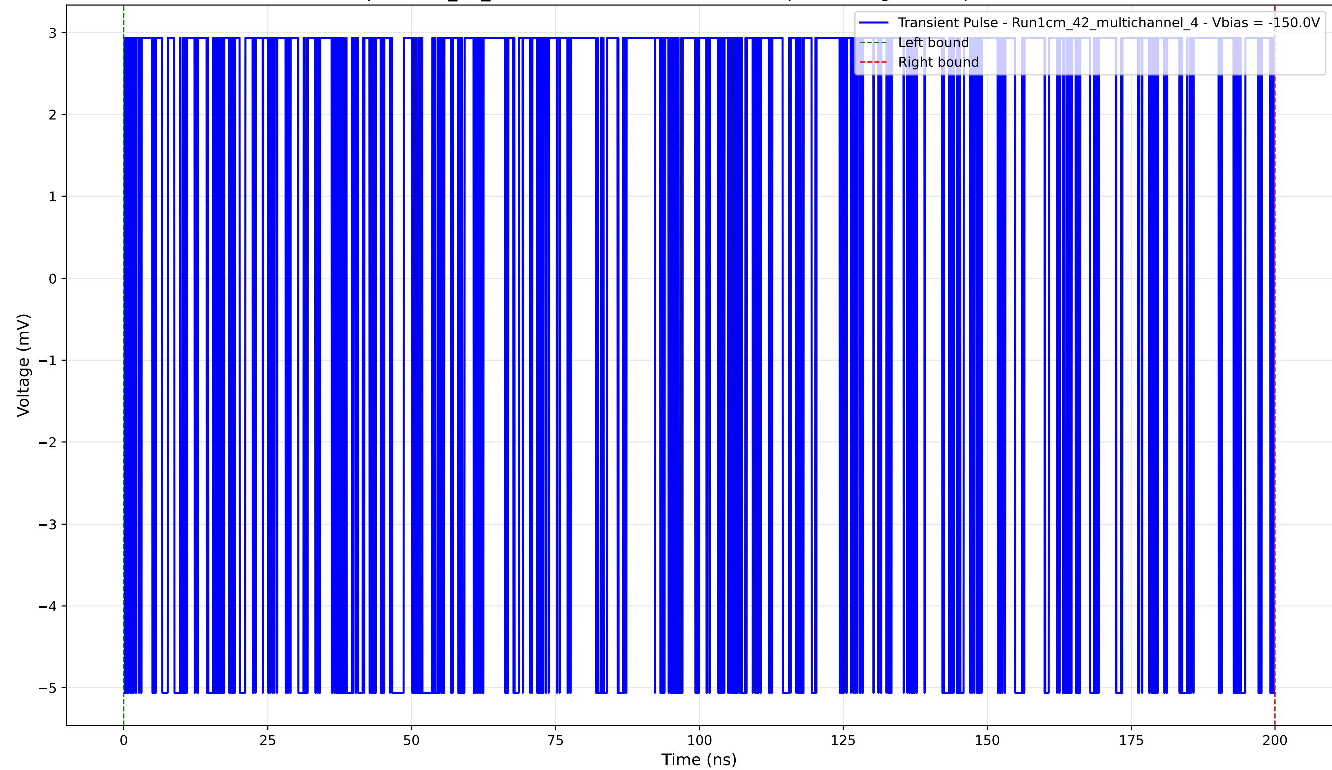
Transient Pulse - Sample: 1cm_42_multichannel - Position: 1385.0 \mu\text{m} - Charge: 2.63 pC - Rise Time: 0.00 ns (N/A)
