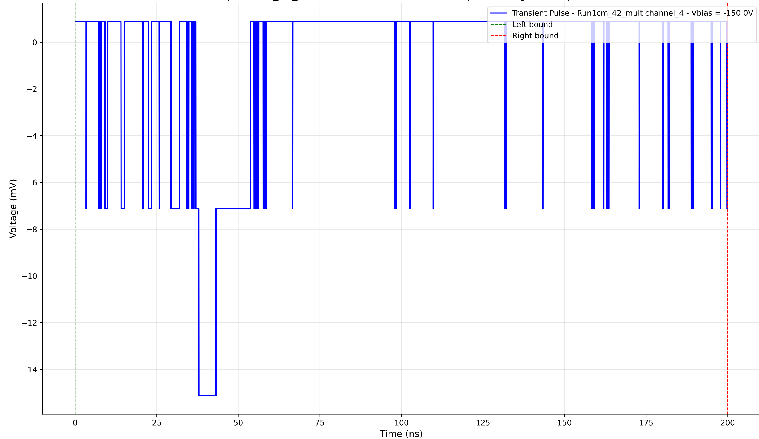
Transient Pulse - Sample: 1cm_42_multichannel - Position: 4015.0 \mu\text{m} - Charge: 1.54 pC - Rise Time: 0.90 ns
