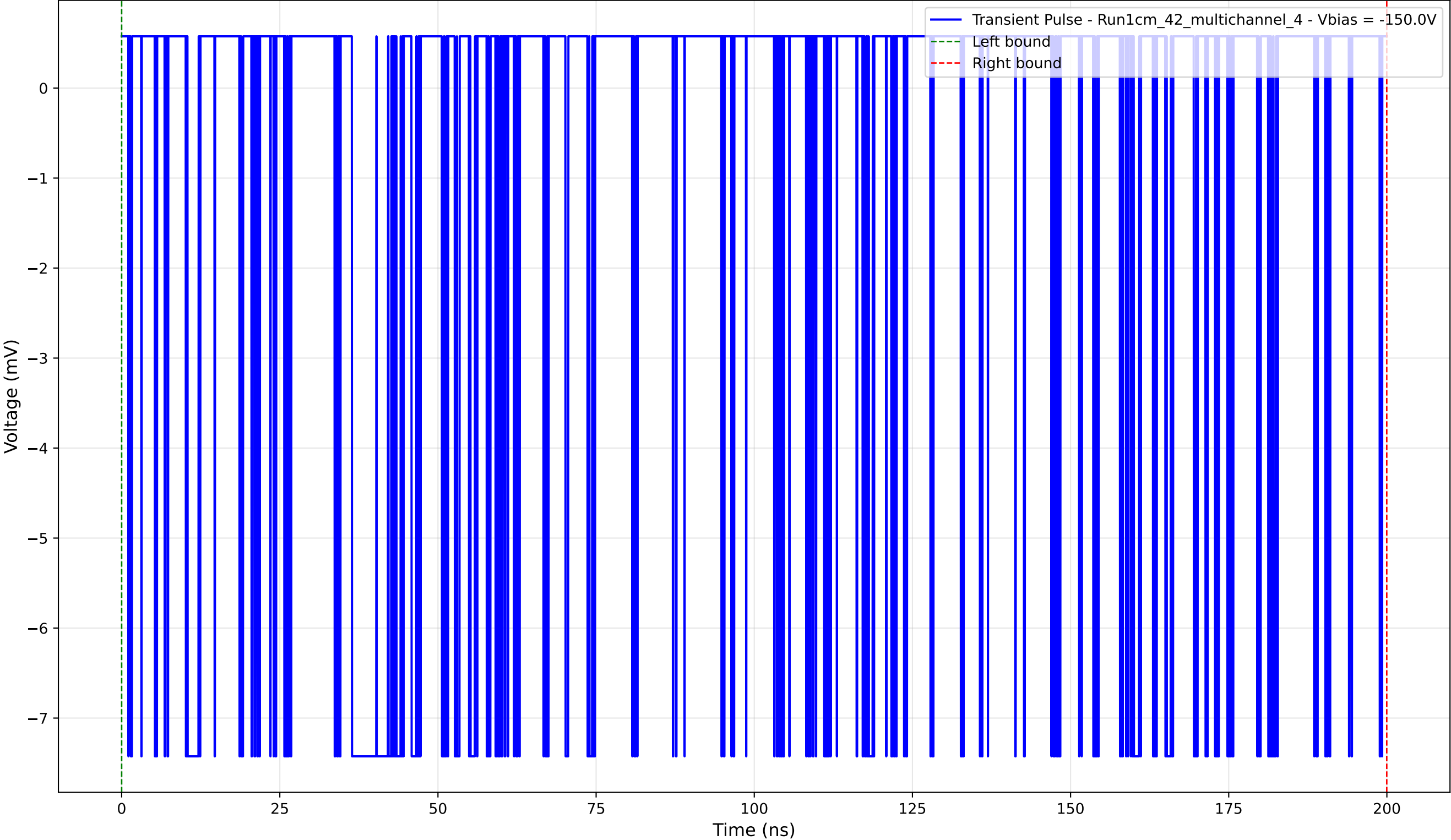
Transient Pulse - Sample: 1cm_42_multichannel - Position: 2865.0 \mu\text{m} - Charge: 2.94 pC - Rise Time: 0.02 ns
