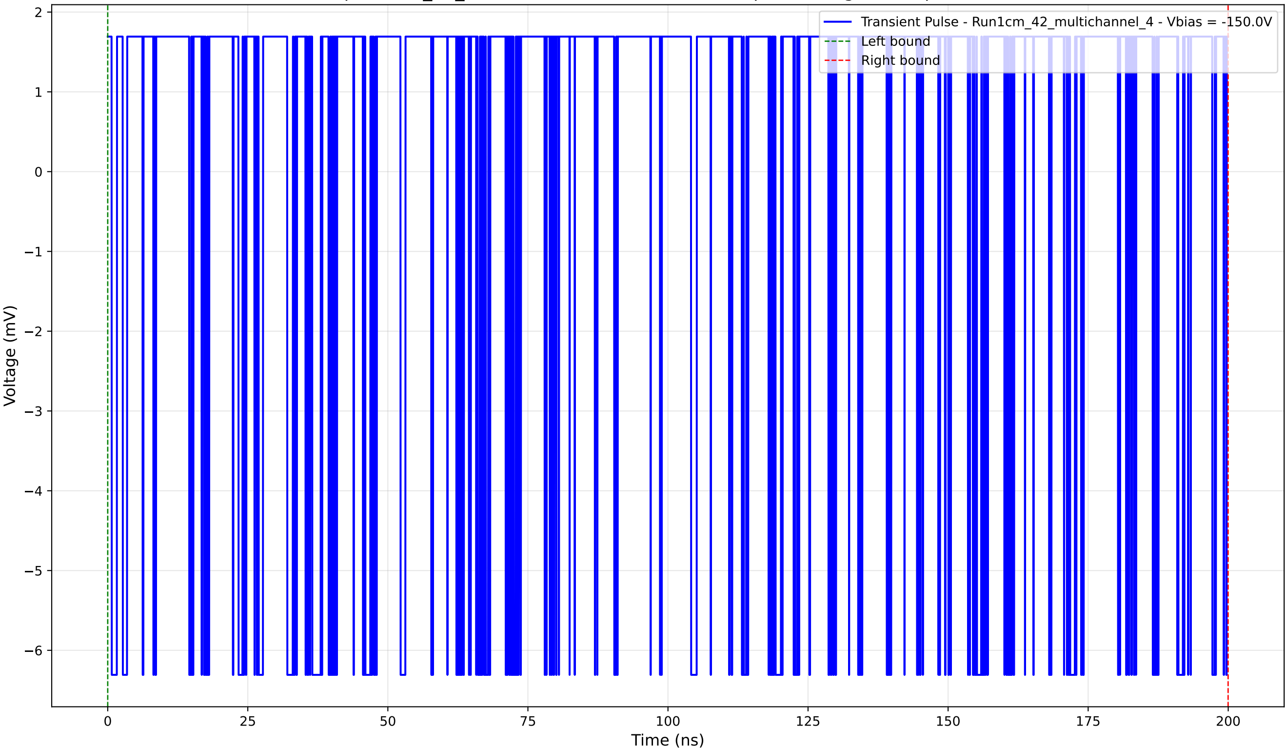
Transient Pulse - Sample: 1cm_42_multichannel - Position: 2375.0 \mu\text{m} - Charge: 1.37 pC - Rise Time: 0.00 ns (N/A)
