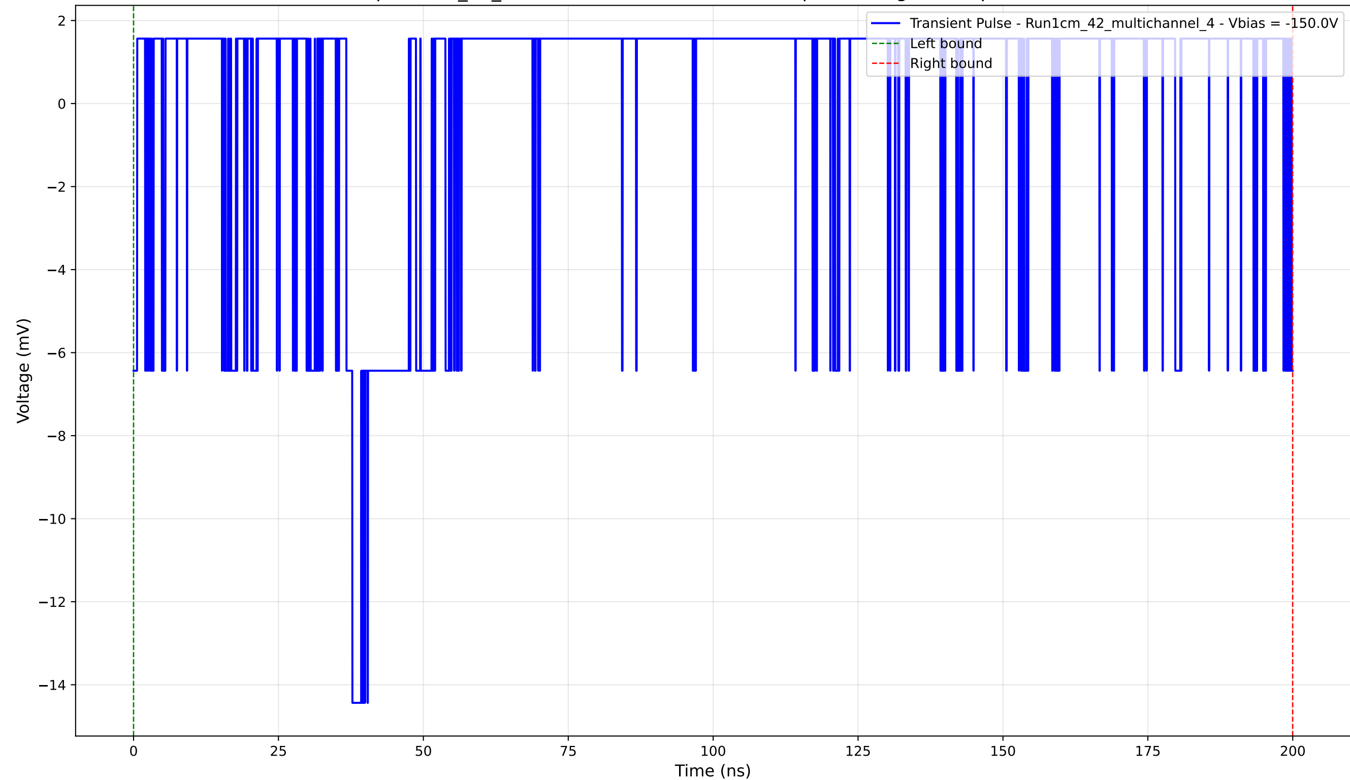
Transient Pulse - Sample: 1cm_42_multichannel - Position: 3450.0 \mu\text{m} - Charge: 0.85 pC - Rise Time: 0.00 ns (N/A)
