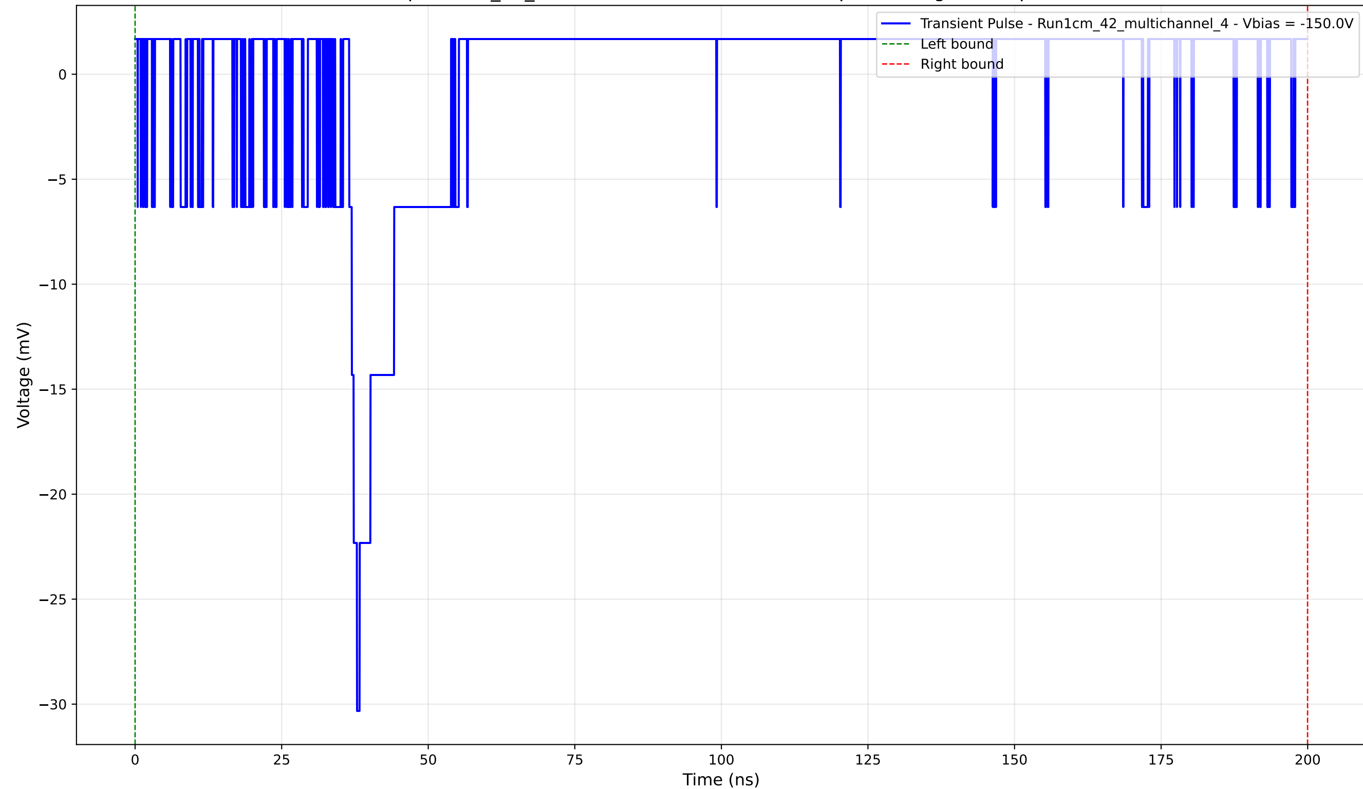
Transient Pulse - Sample: 1cm_42_multichannel - Position: 1455.0 \mu\text{m} - Charge: 0.10 pC - Rise Time: 1.33 ns
