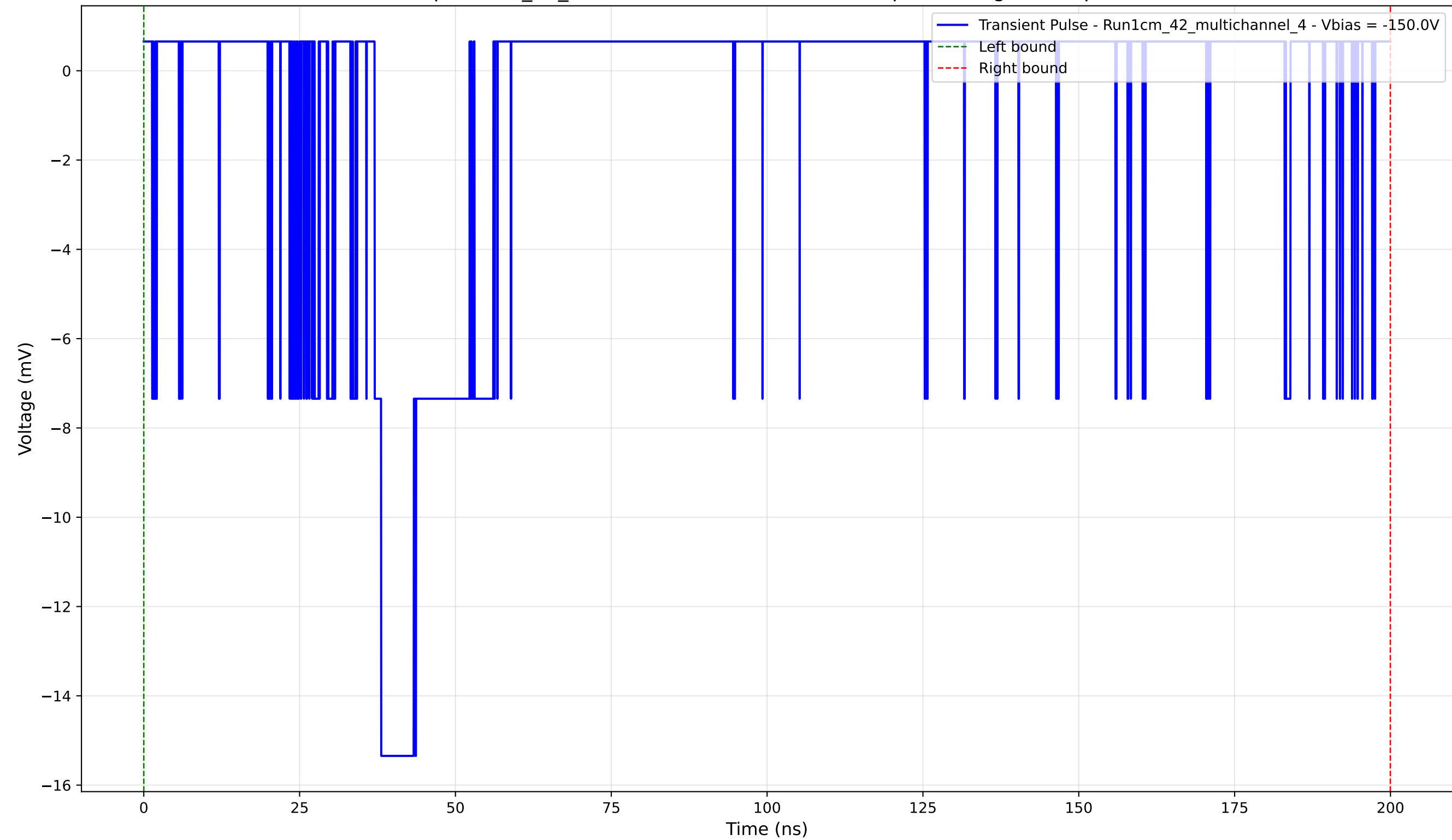
Transient Pulse - Sample: 1cm_42_multichannel - Position: 4120.0 \mu\text{m} - Charge: 2.69 pC - Rise Time: 1.06 ns
