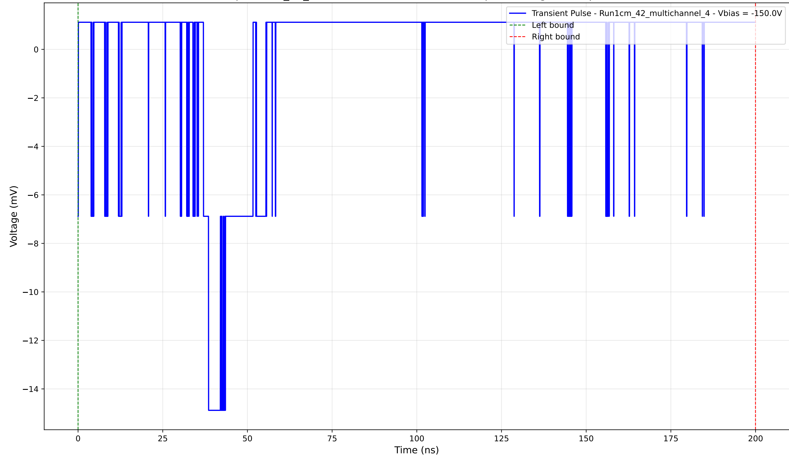
Transient Pulse - Sample: 1cm_42_multichannel - Position: 4750.0 \mu\text{m} - Charge: 0.11 pC - Rise Time: 1.52 ns
