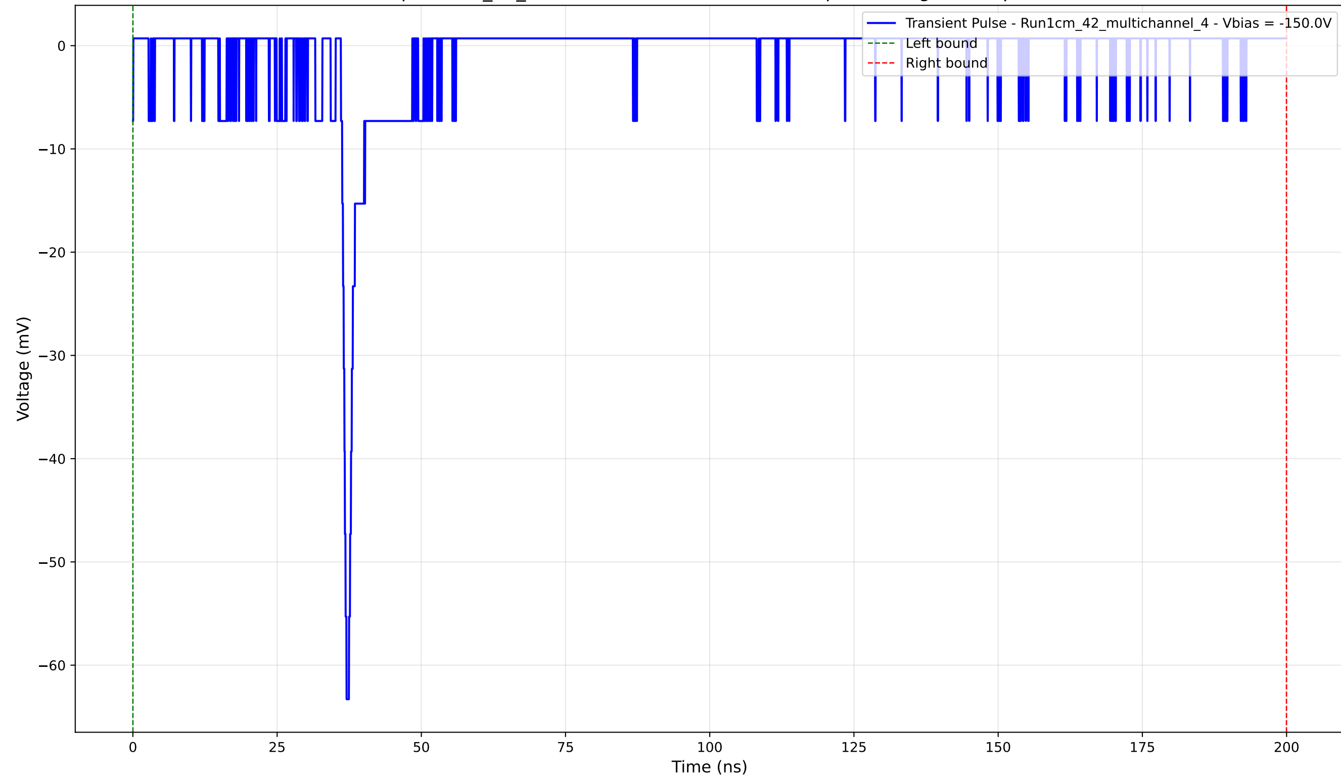
Transient Pulse - Sample: 1cm_42_multichannel - Position: 2325.0 \mu\text{m} - Charge: 3.43 pC - Rise Time: 0.96 ns
