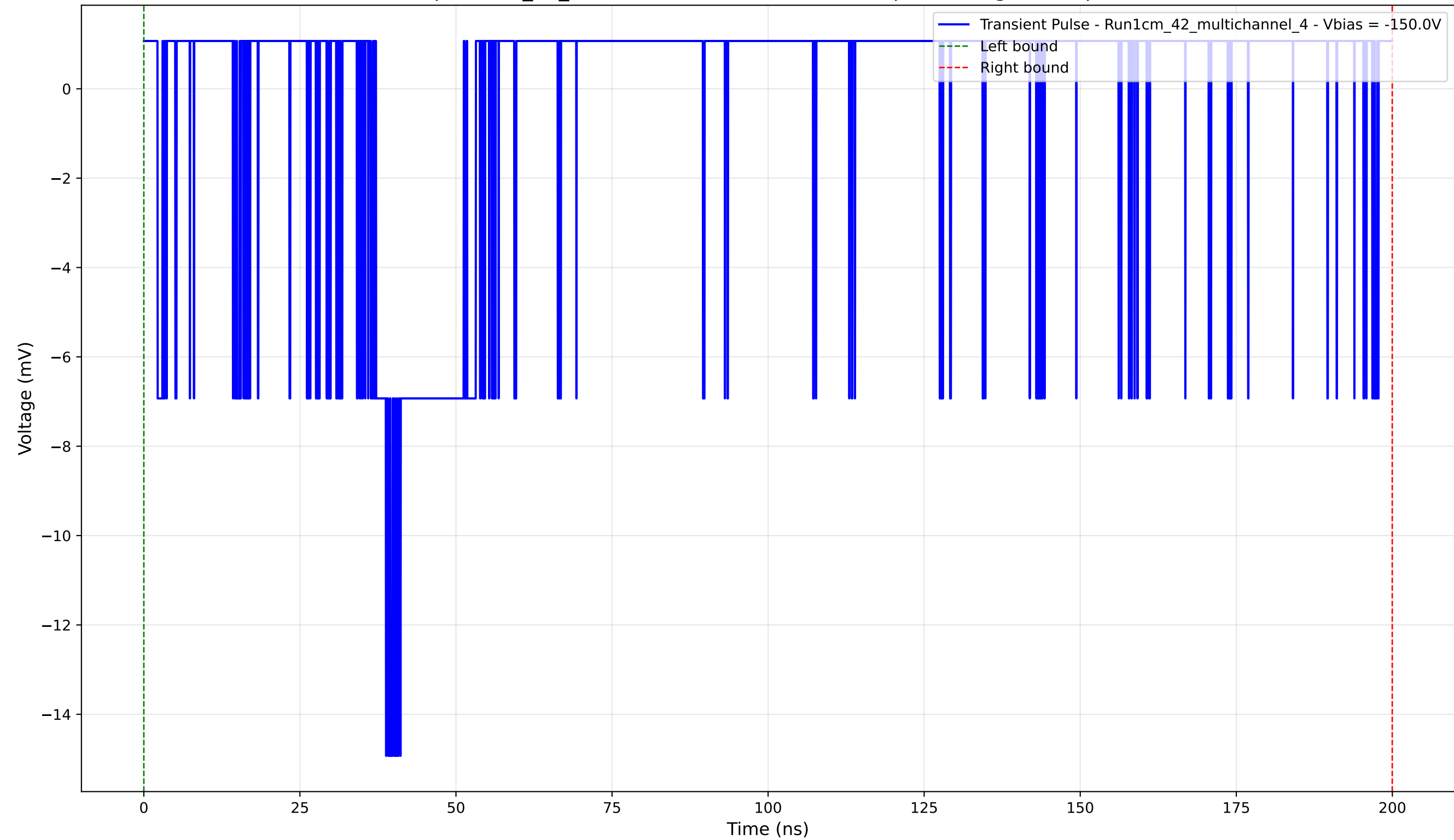
Transient Pulse - Sample: 1cm_42_multichannel - Position: 4460.0 \mu\text{m} - Charge: 0.29 pC - Rise Time: 1.60 ns
