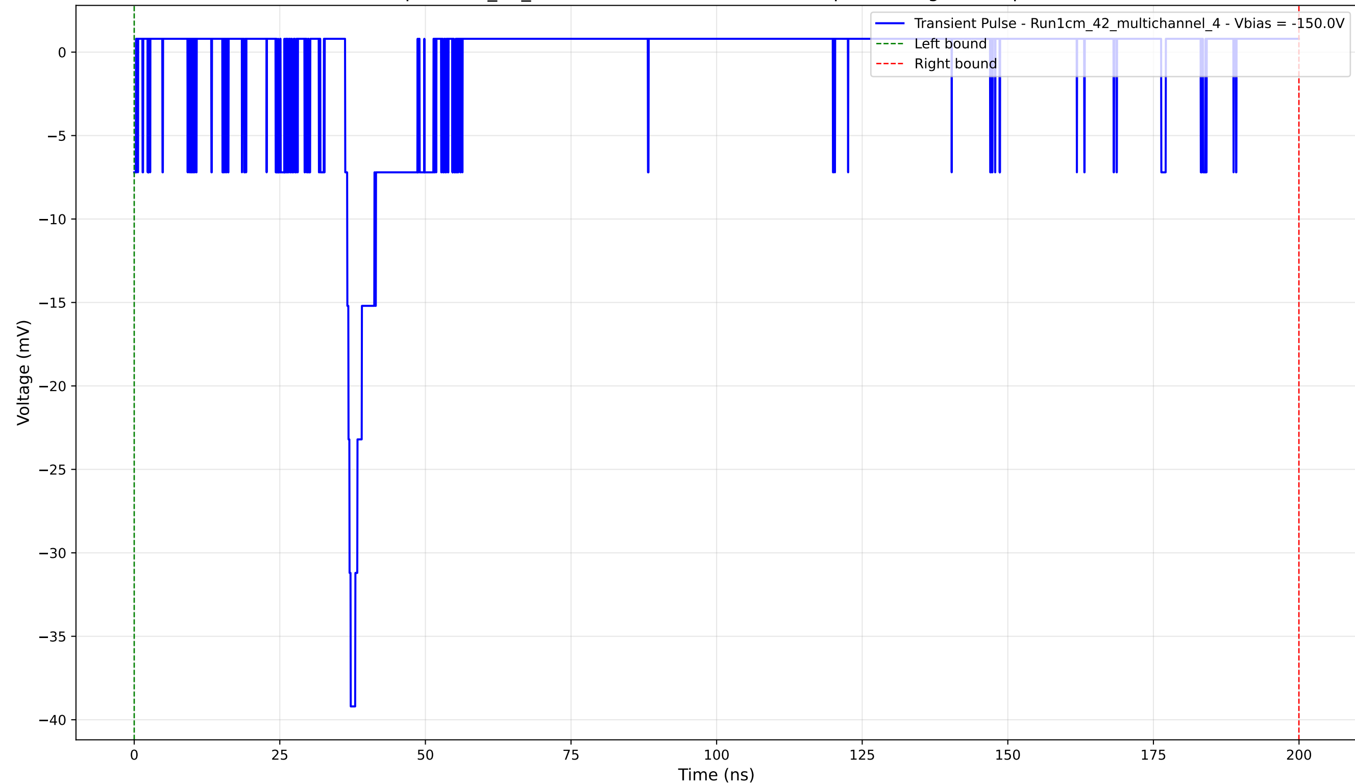
Transient Pulse - Sample: 1cm_42_multichannel - Position: 2825.0 \mu\text{m} - Charge: 2.30 pC - Rise Time: 0.95 ns
