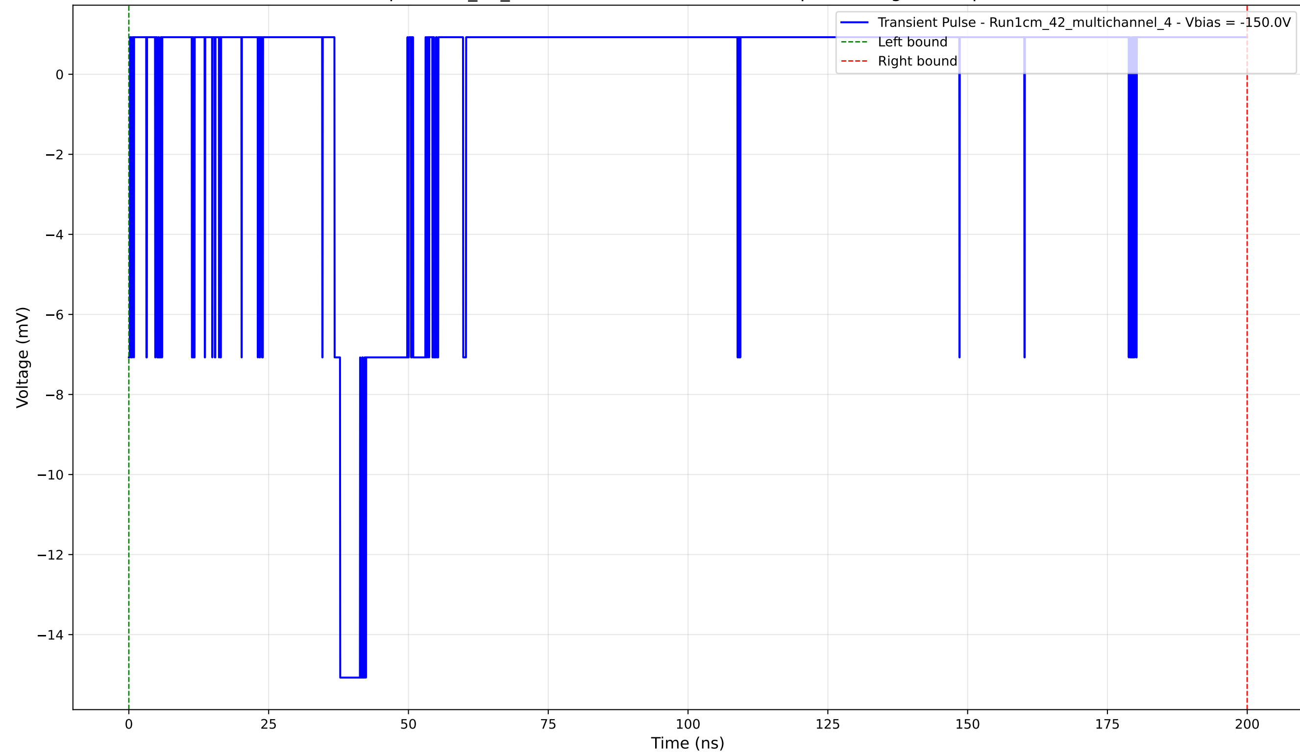
Transient Pulse - Sample: 1cm_42_multichannel - Position: 3835.0 \mu\text{m} - Charge: 0.23 pC - Rise Time: 1.02 ns
