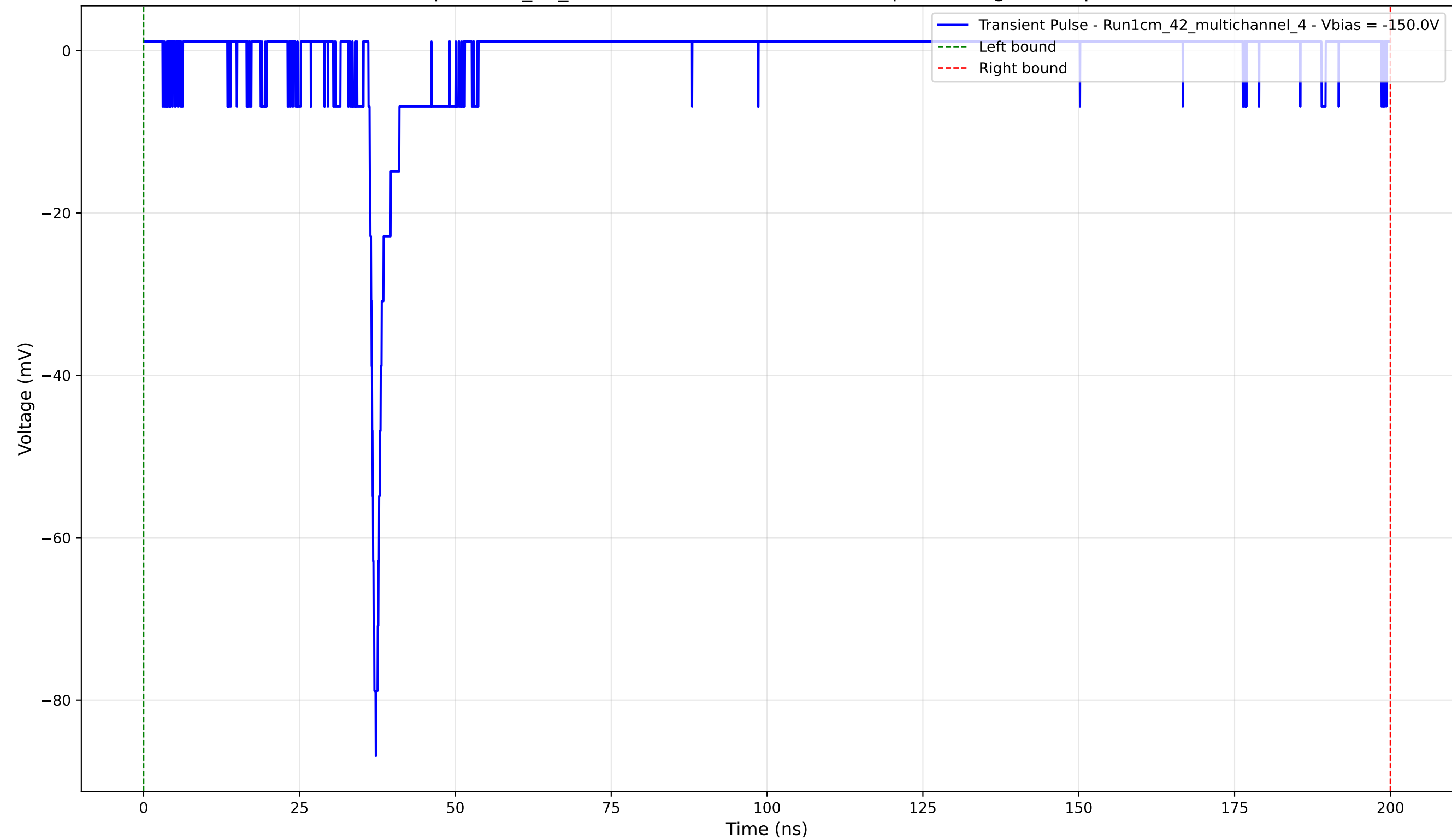
Transient Pulse - Sample: 1cm_42_multichannel - Position: 2480.0 \mu\text{m} - Charge: 2.14 pC - Rise Time: 0.76 ns
