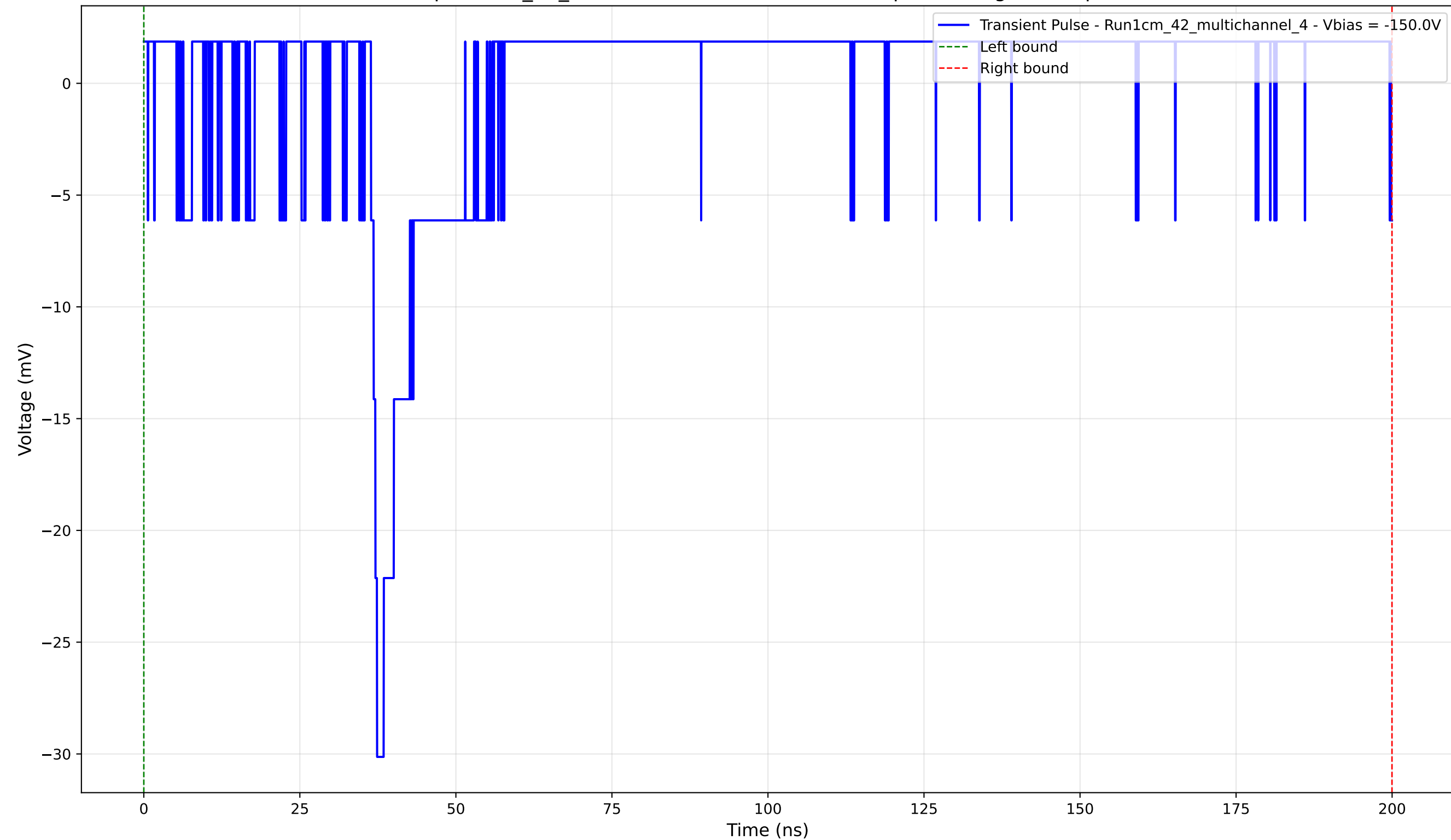
Transient Pulse - Sample: 1cm_42_multichannel - Position: 1600.0 \mu\text{m} - Charge: 1.15 pC - Rise Time: 0.97 ns
