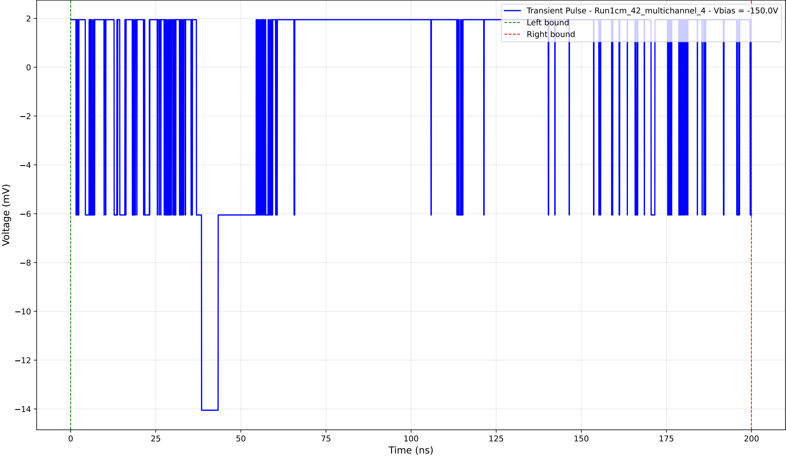
Transient Pulse - Sample: 1cm_42_multichannel - Position: 440.0 \mu\text{m} - Charge: 0.90 pC - Rise Time: 0.00 ns (N/A)
