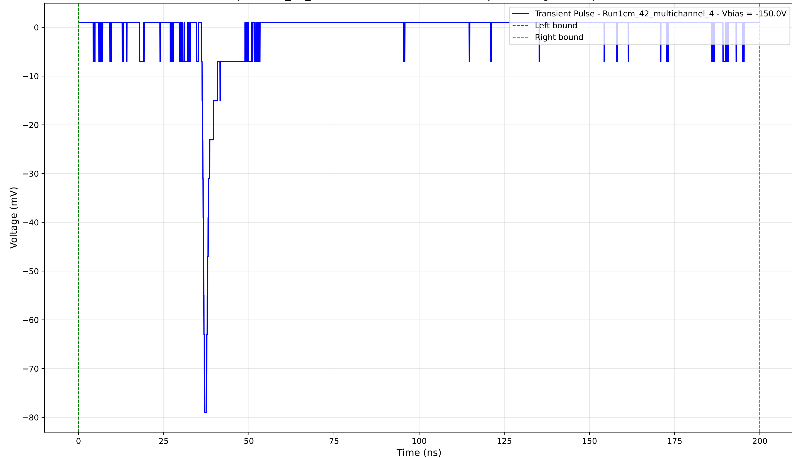
Transient Pulse - Sample: 1cm_42_multichannel - Position: 2495.0 \mu\text{m} - Charge: 2.64 pC - Rise Time: 0.78 ns
