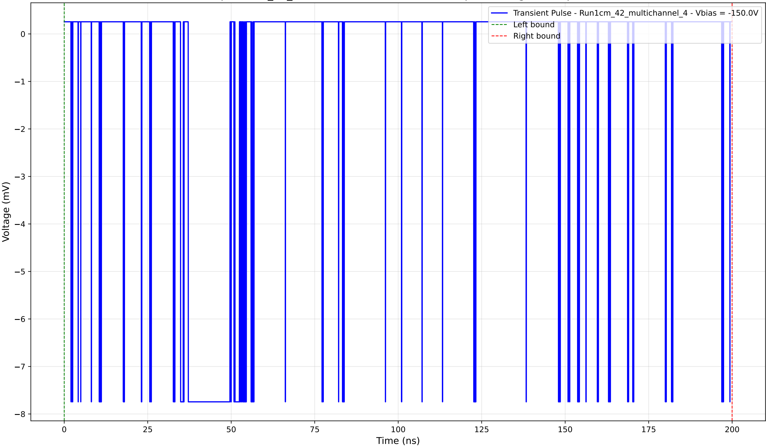
Transient Pulse - Sample: 1cm_42_multichannel - Position: 3855.0 \mu\text{m} - Charge: 2.52 pC - Rise Time: 0.02 ns
