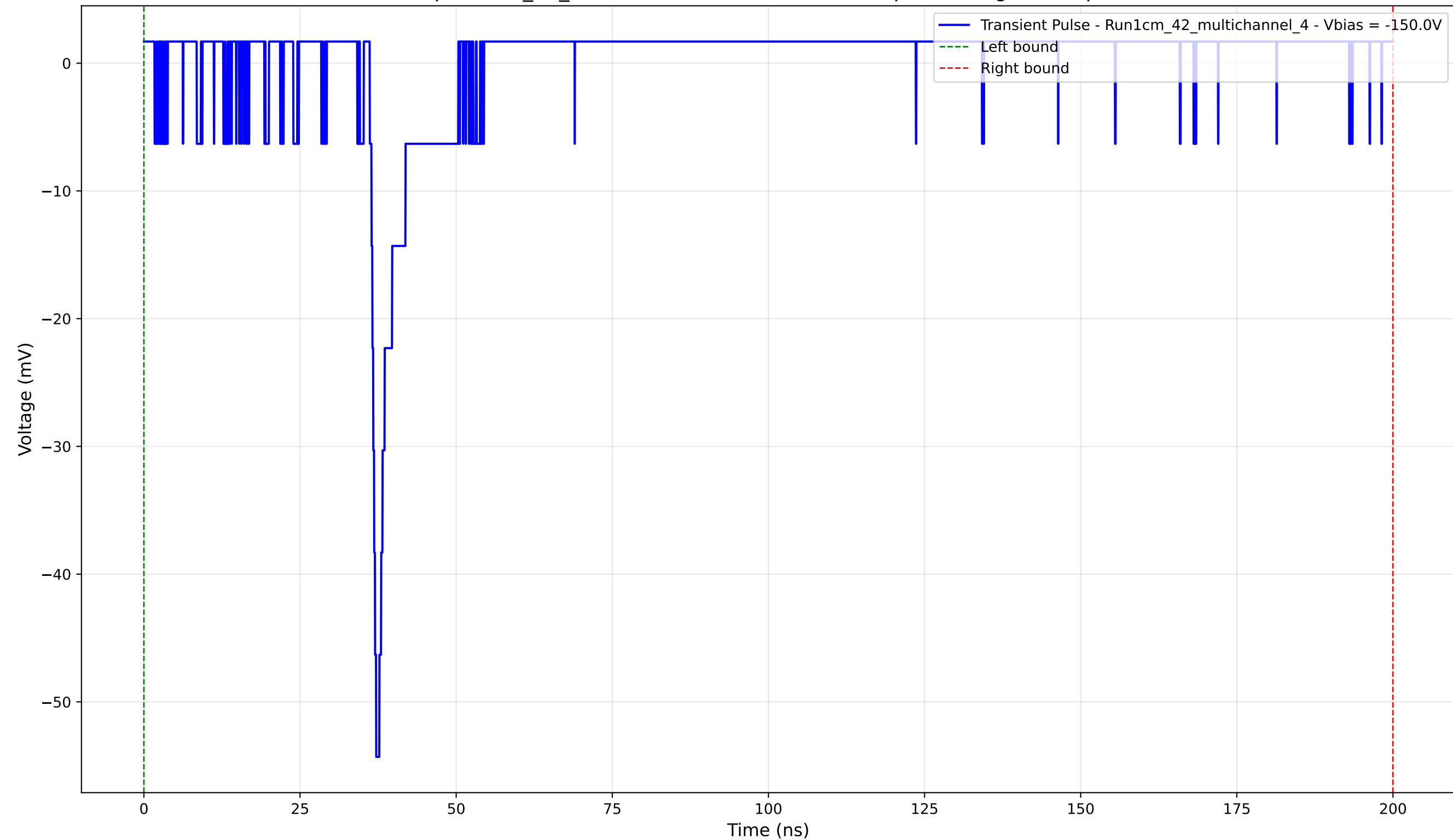
Transient Pulse - Sample: 1cm_42_multichannel - Position: 2720.0 \mu\text{m} - Charge: 0.79 pC - Rise Time: 1.02 ns
