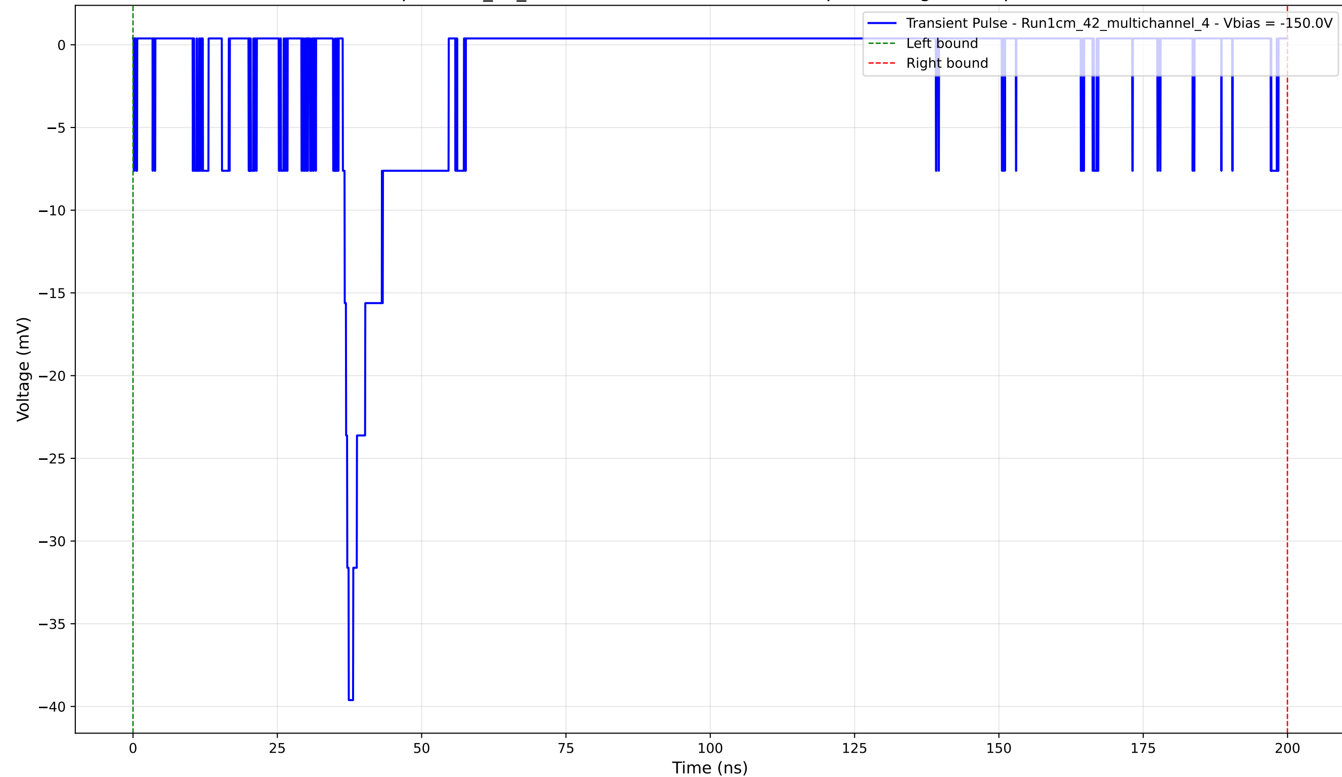
Transient Pulse - Sample: 1cm_42_multichannel - Position: 1725.0 \mu\text{m} - Charge: 5.41 pC - Rise Time: 1.03 ns
