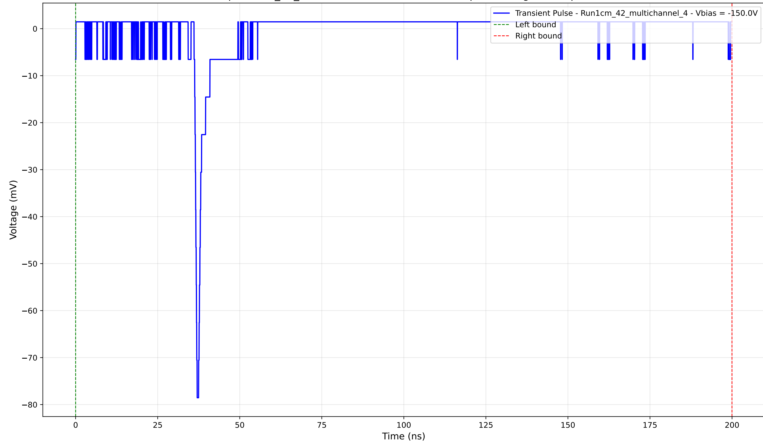
Transient Pulse - Sample: 1cm_42_multichannel - Position: 2470.0 \mu\text{m} - Charge: 0.65 pC - Rise Time: 0.76 ns
