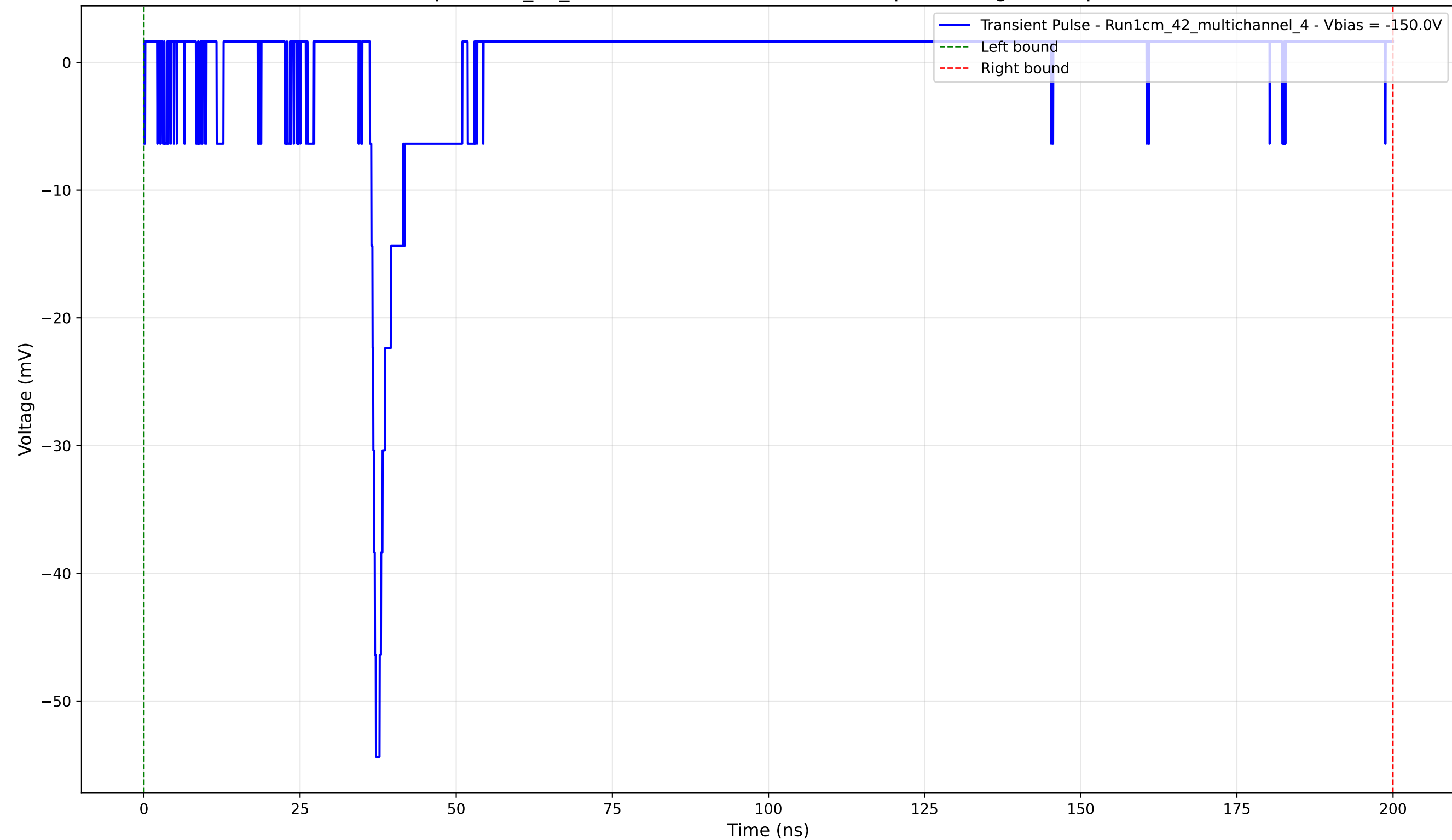
Transient Pulse - Sample: 1cm_42_multichannel - Position: 2070.0 \mu\text{m} - Charge: 0.79 pC - Rise Time: 0.96 ns
