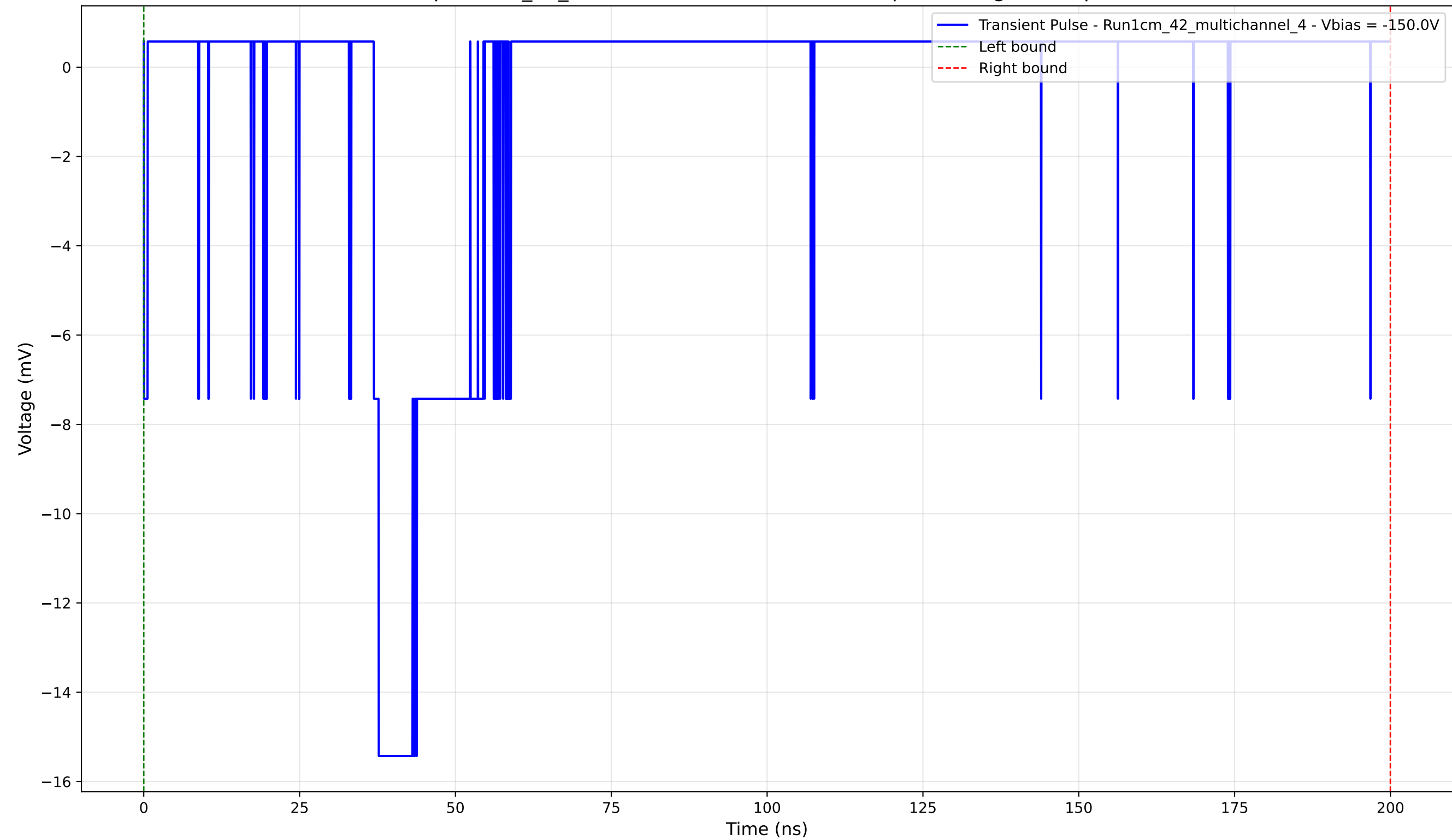
Transient Pulse - Sample: 1cm_42_multichannel - Position: 3805.0 \mu\text{m} - Charge: 1.99 pC - Rise Time: 0.80 ns
