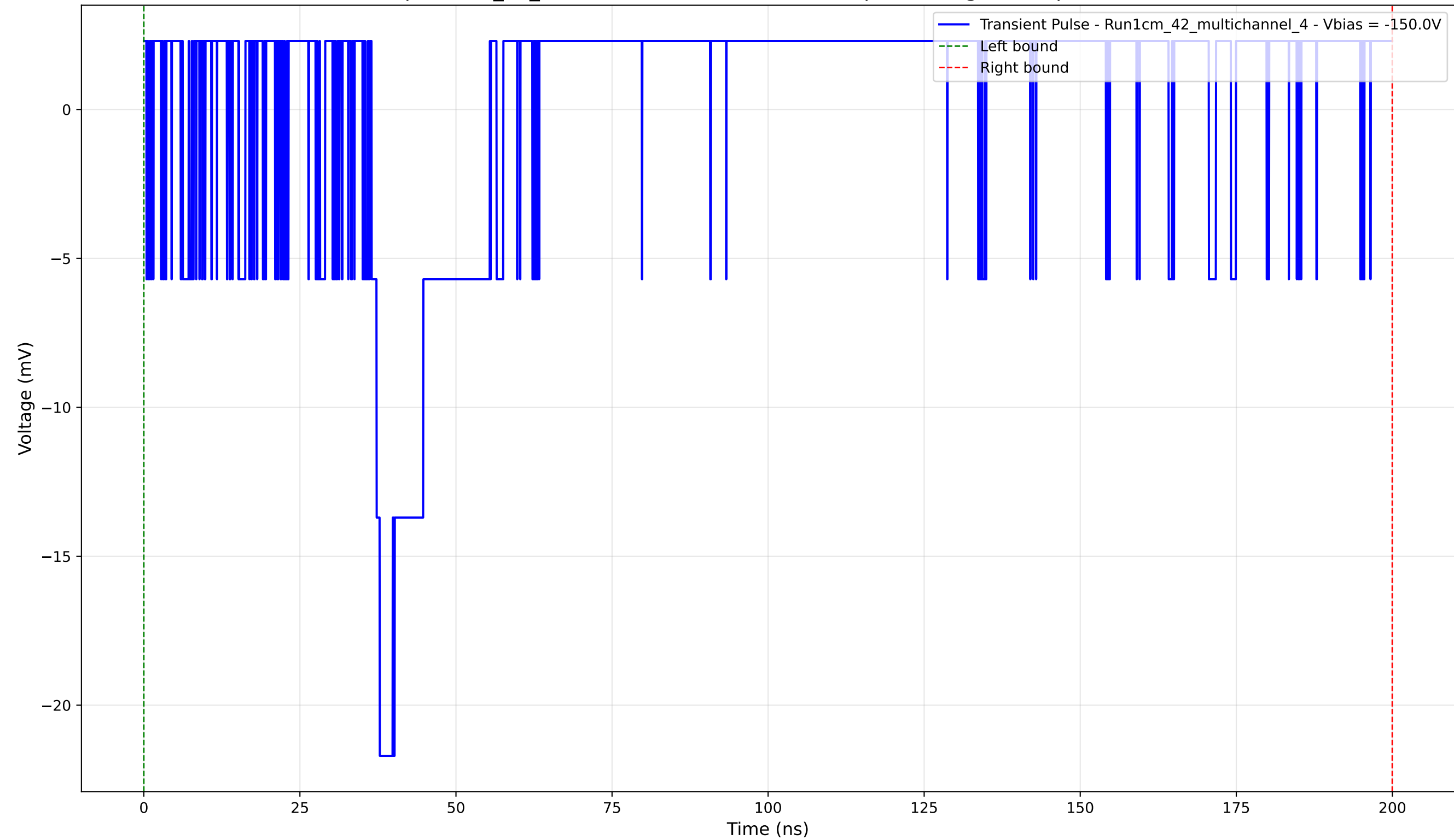
Transient Pulse - Sample: 1cm_42_multichannel - Position: 1160.0 \mu\text{m} - Charge: 1.96 pC - Rise Time: 0.00 ns (N/A)
