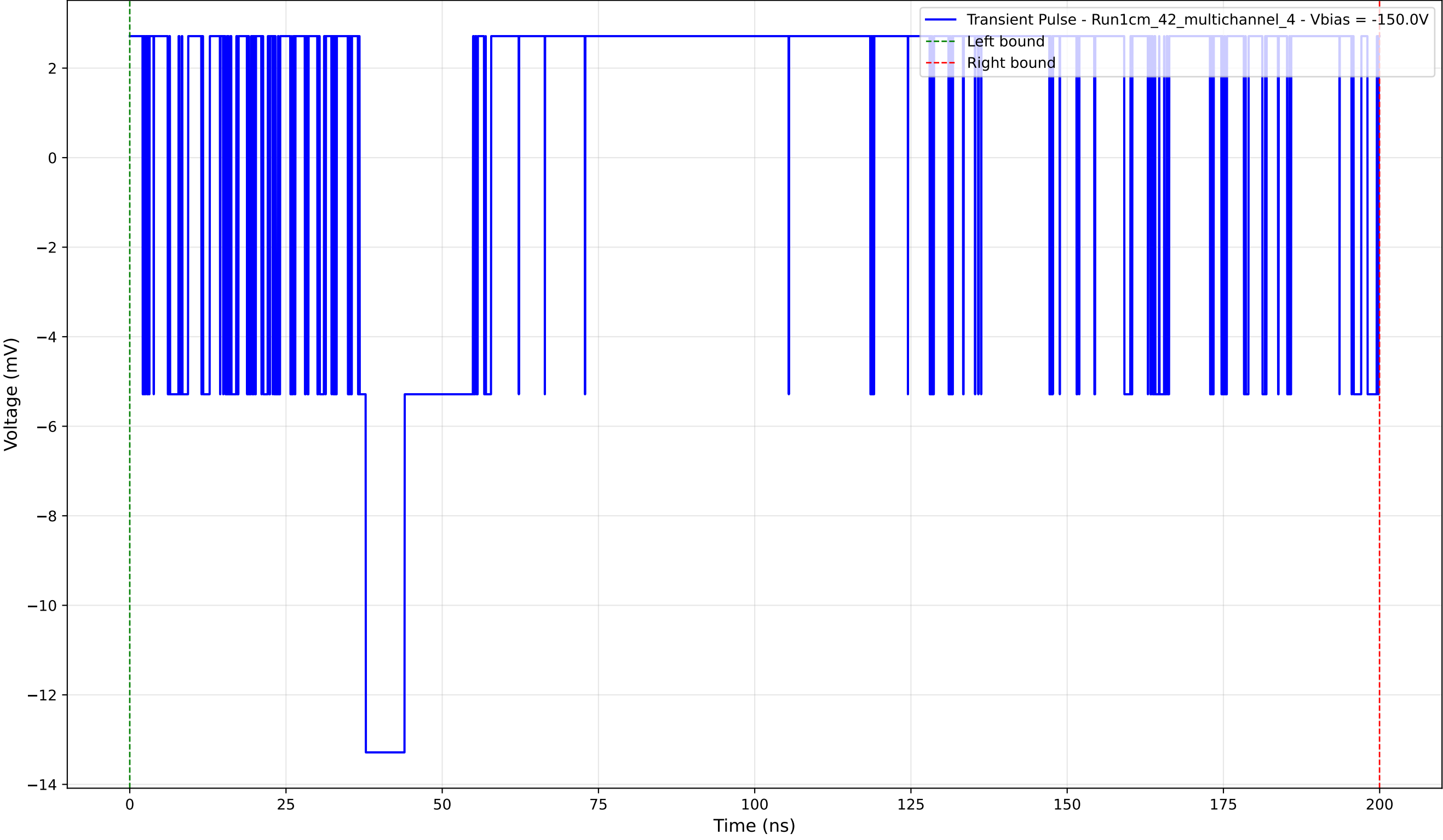
Transient Pulse - Sample: 1cm_42_multichannel - Position: 795.0 \mu\text{m} - Charge: 2.99 pC - Rise Time: 0.00 ns (N/A)
