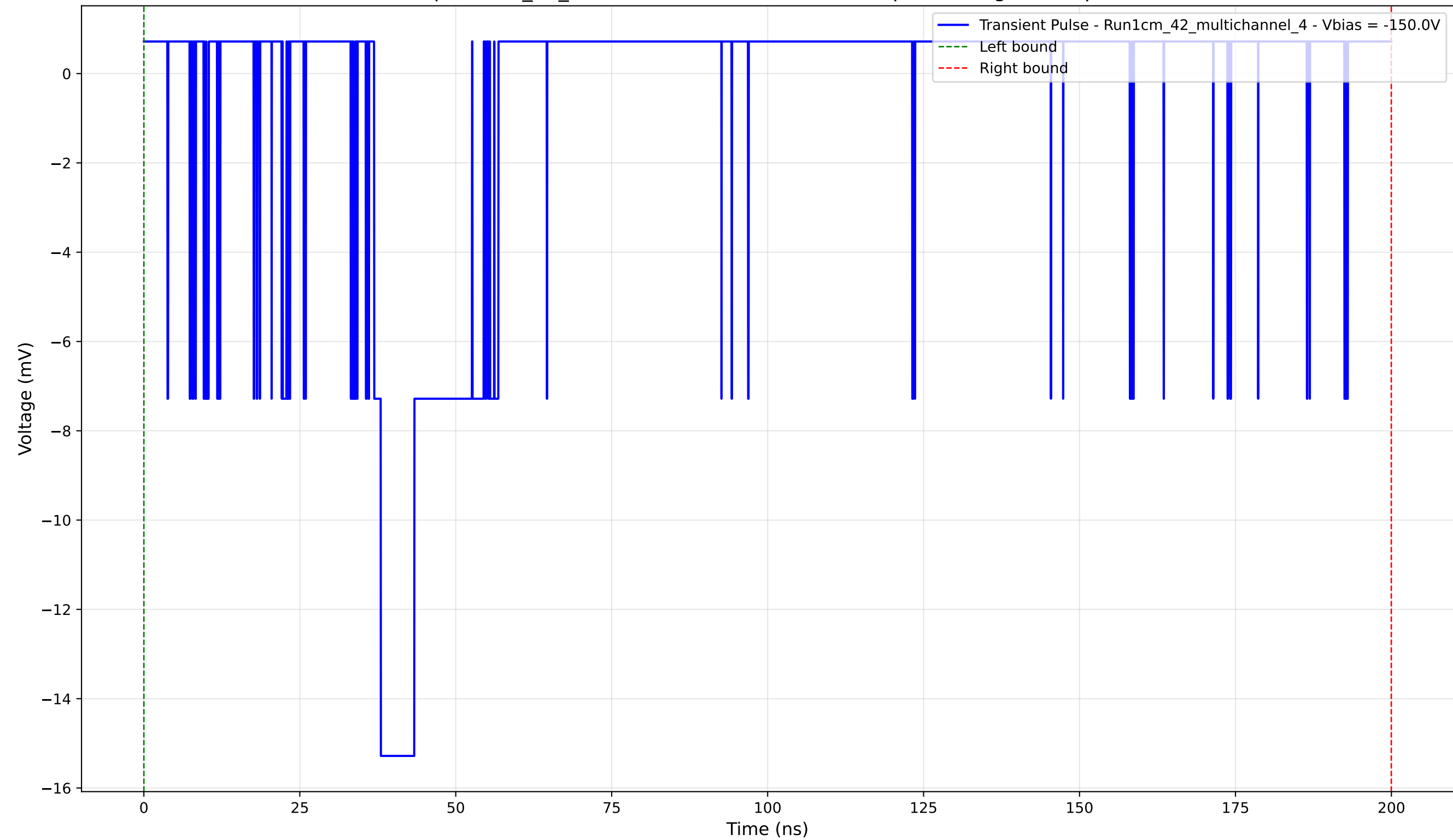
Transient Pulse - Sample: 1cm_42_multichannel - Position: 4075.0 \mu\text{m} - Charge: 2.02 pC - Rise Time: 1.08 ns
