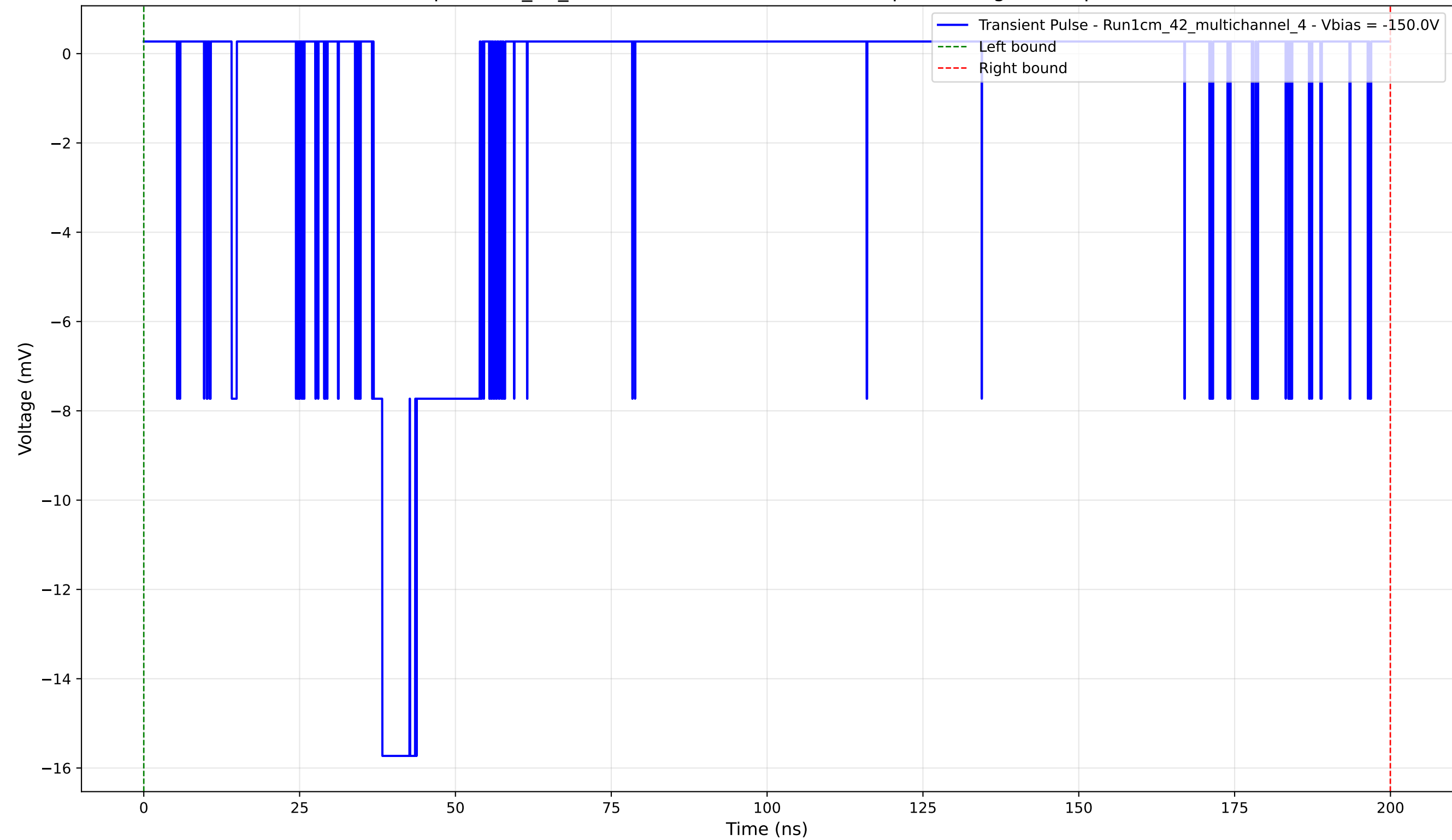
Transient Pulse - Sample: 1cm_42_multichannel - Position: 4110.0 \mu\text{m} - Charge: 3.72 pC - Rise Time: 1.40 ns
