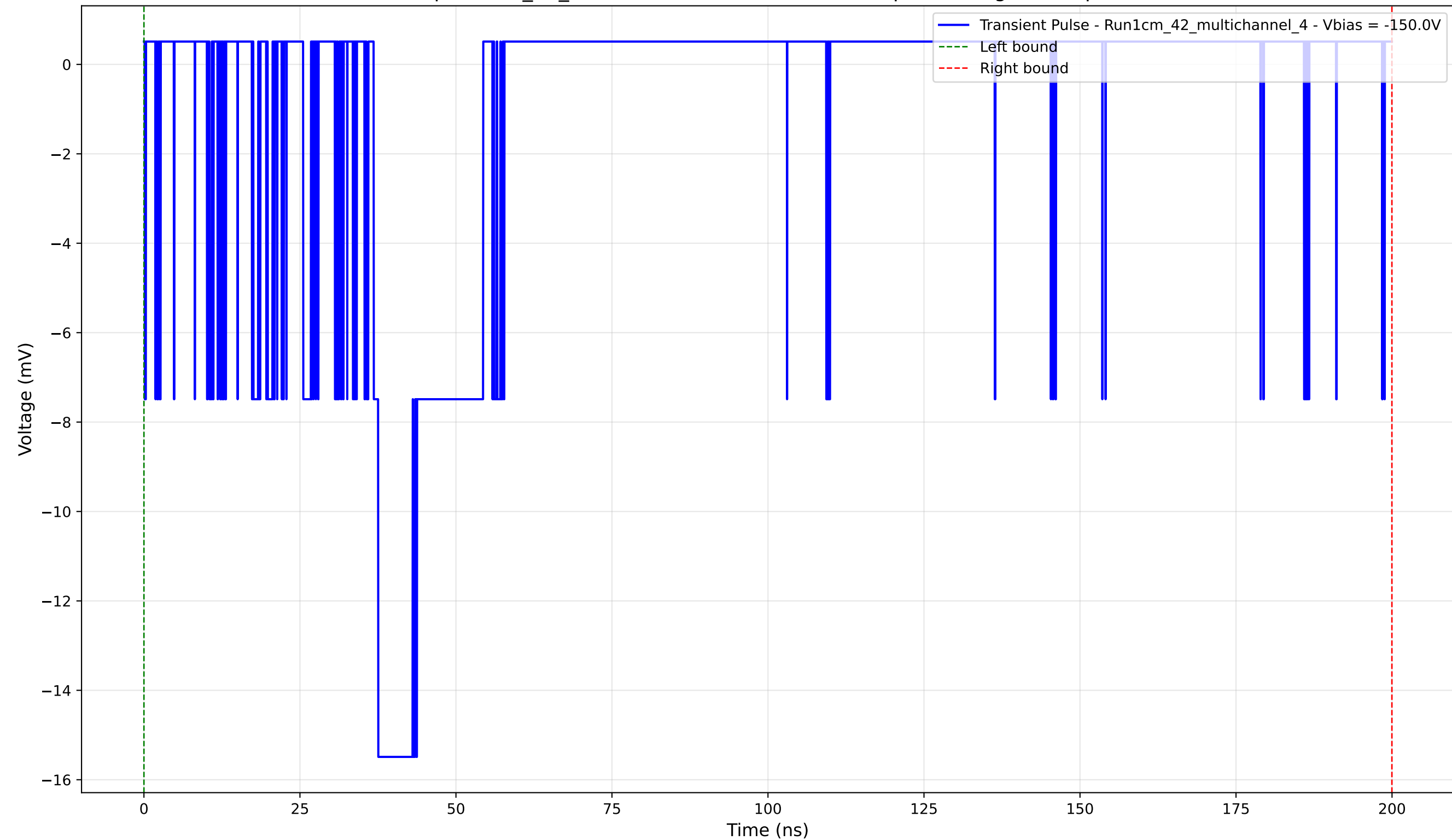
Transient Pulse - Sample: 1cm_42_multichannel - Position: 3755.0 \mu\text{m} - Charge: 3.33 pC - Rise Time: 0.74 ns
