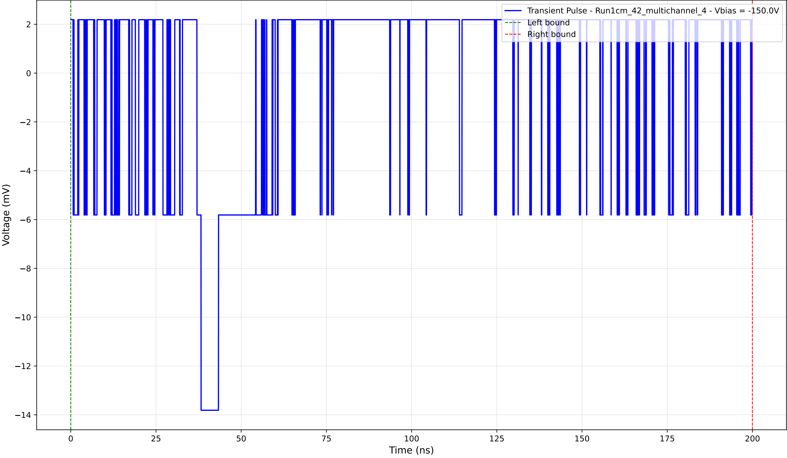
Transient Pulse - Sample: 1cm_42_multichannel - Position: 250.0 \mu\text{m} - Charge: 0.65 pC - Rise Time: 0.00 ns (N/A)
