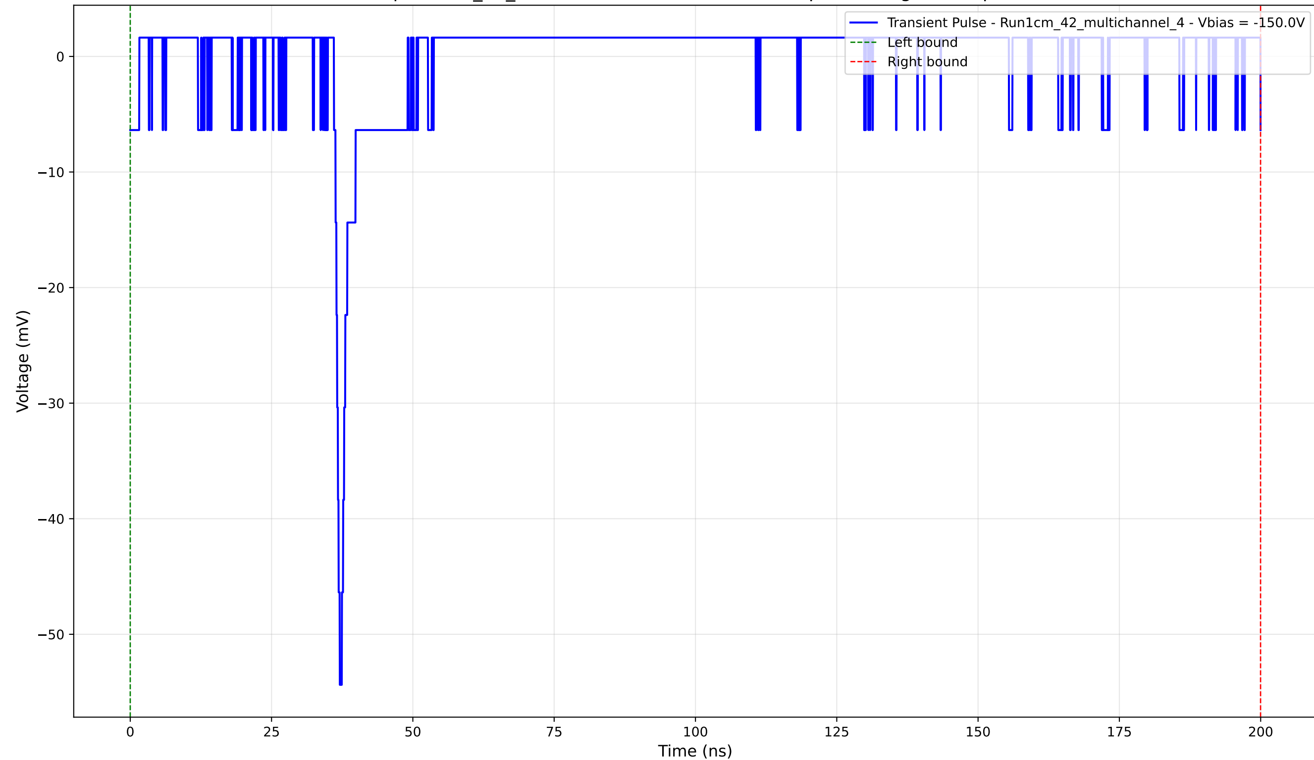
Transient Pulse - Sample: 1cm_42_multichannel - Position: 2330.0 \mu\text{m} - Charge: 0.53 pC - Rise Time: 1.02 ns
