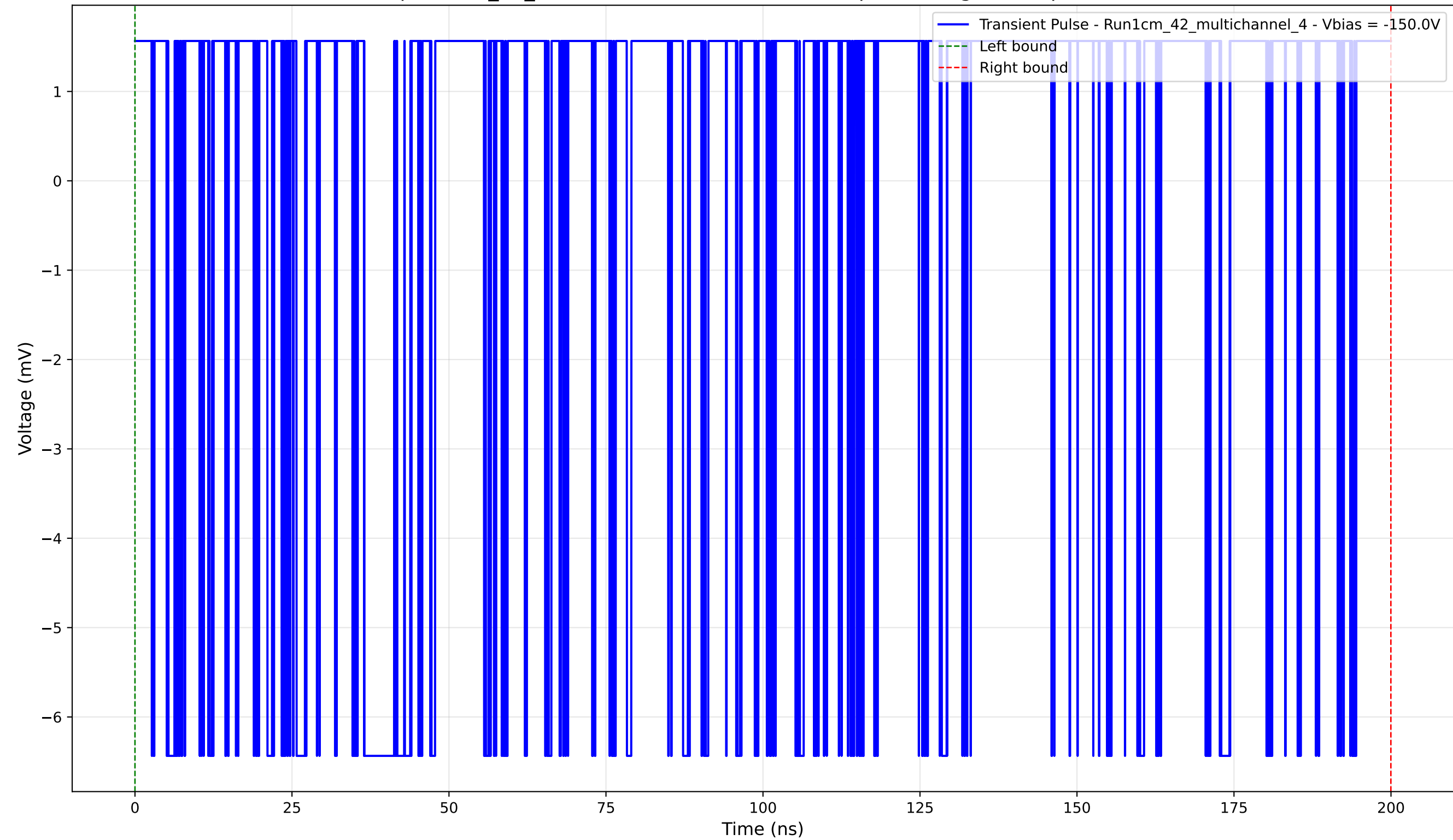
Transient Pulse - Sample: 1cm_42_multichannel - Position: 2860.0 \mu\text{m} - Charge: 0.66 pC - Rise Time: 0.00 ns (N/A)
