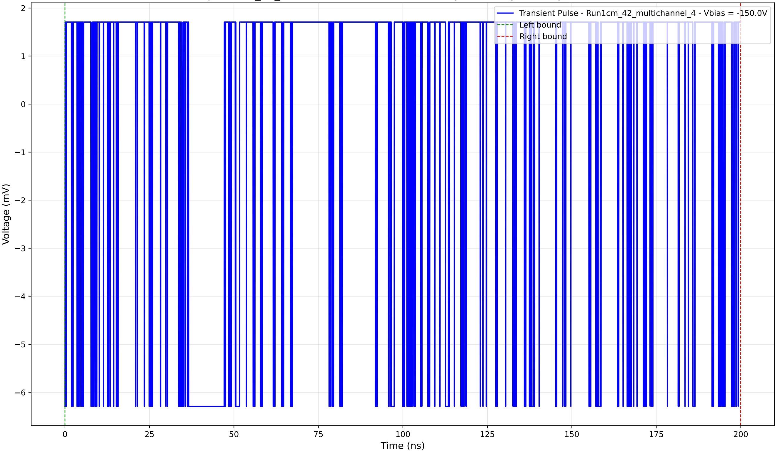
Transient Pulse - Sample: 1cm_42_multichannel - Position: 3360.0 \mu\text{m} - Charge: 1.35 pC - Rise Time: 0.00 ns (N/A)
