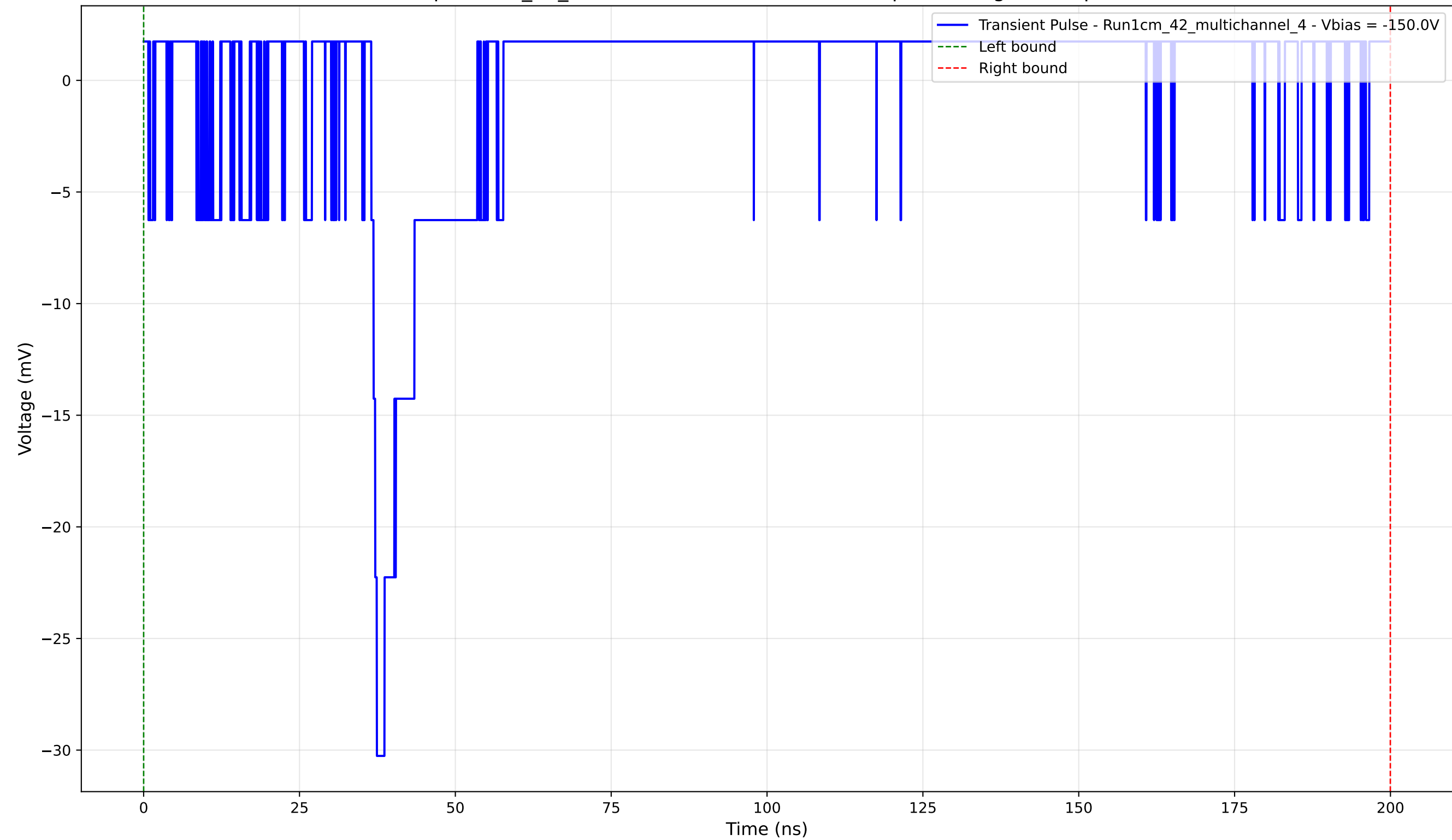
Transient Pulse - Sample: 1cm_42_multichannel - Position: 1545.0 \mu\text{m} - Charge: 0.06 pC - Rise Time: 0.89 ns
