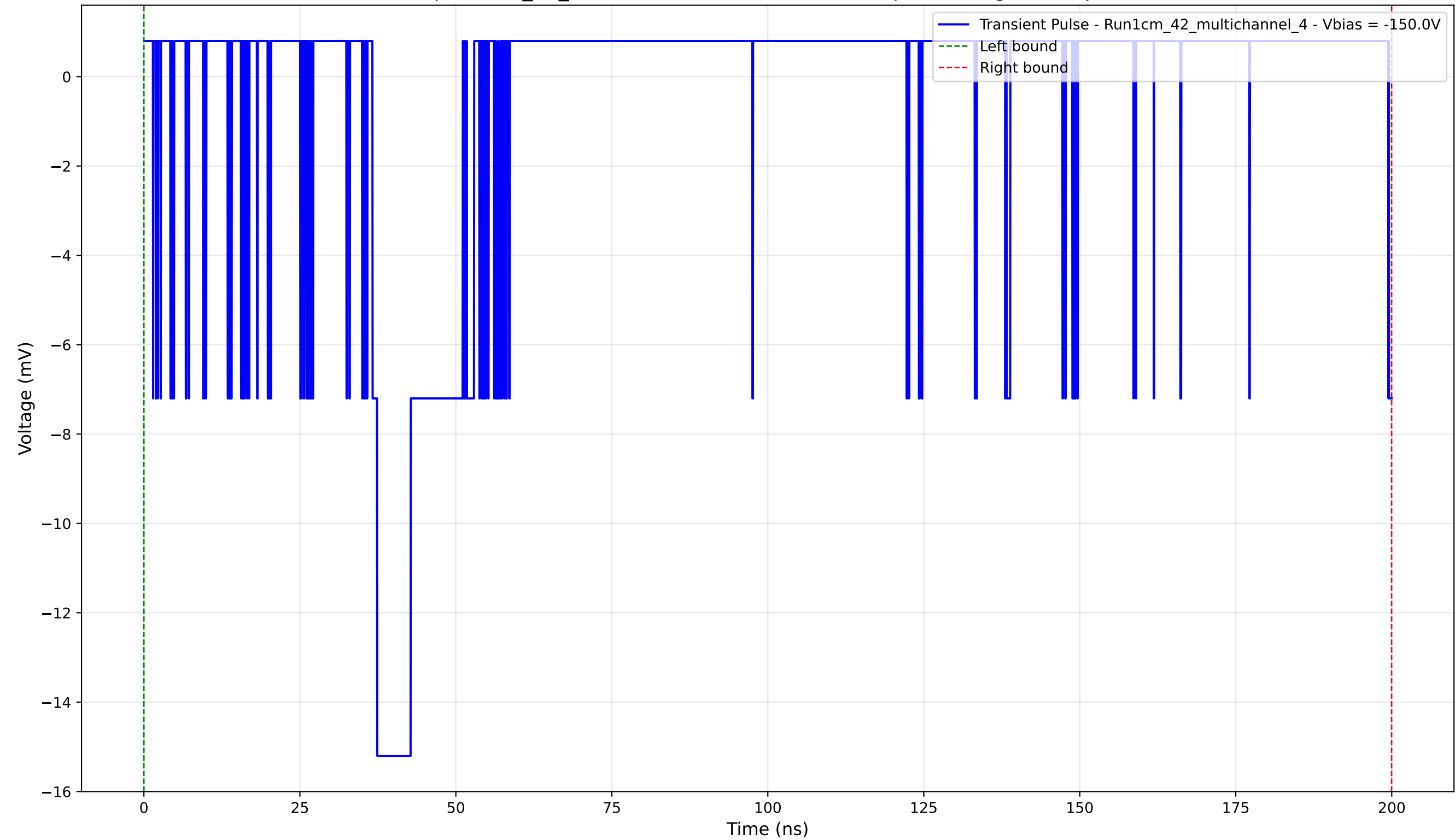
Transient Pulse - Sample: 1cm_42_multichannel - Position: 3595.0 \mu\text{m} - Charge: 1.61 pC - Rise Time: 0.76 ns
