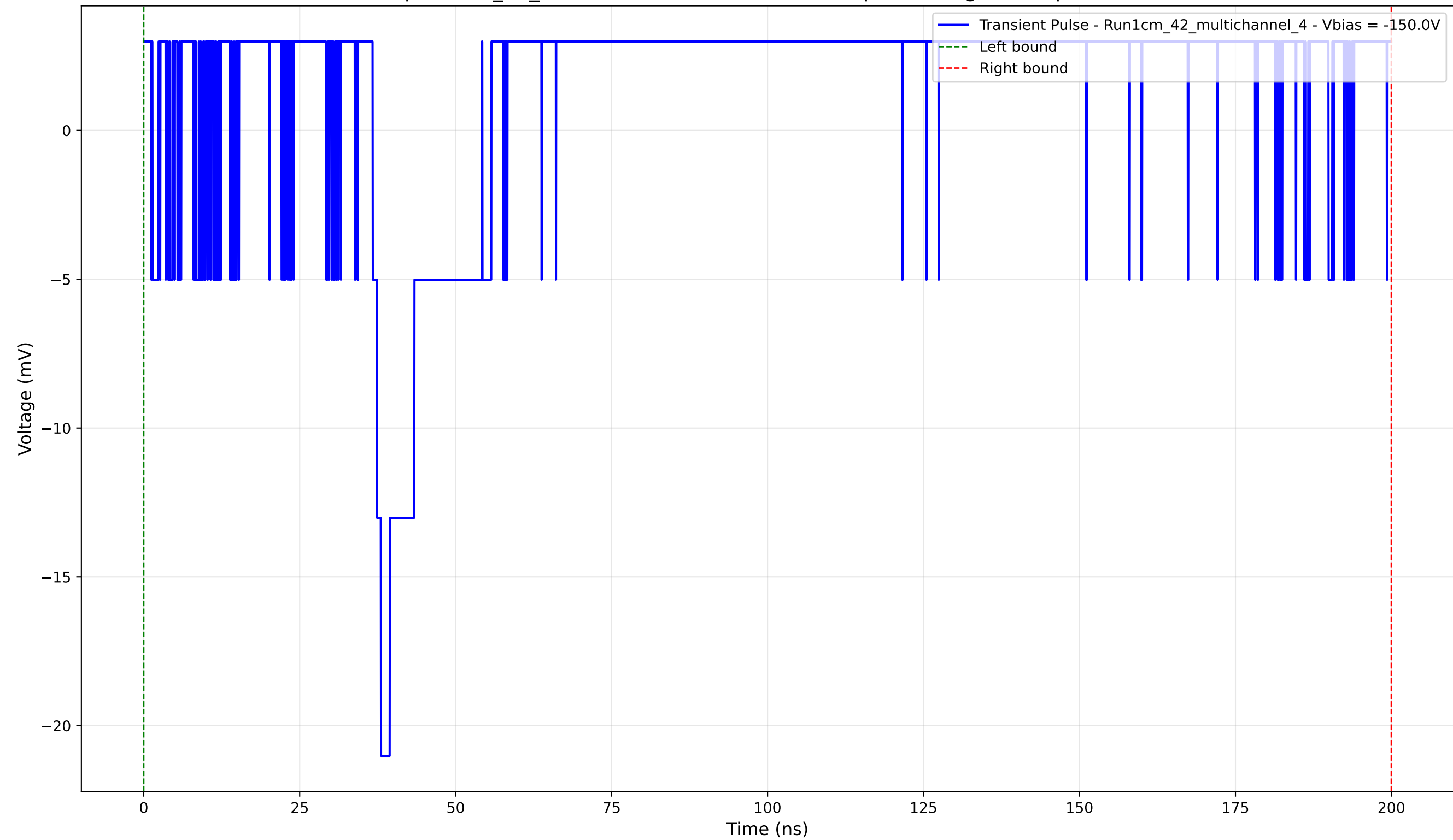
Transient Pulse - Sample: 1cm_42_multichannel - Position: 1140.0 \mu\text{m} - Charge: 5.82 pC - Rise Time: 0.00 ns (N/A)
