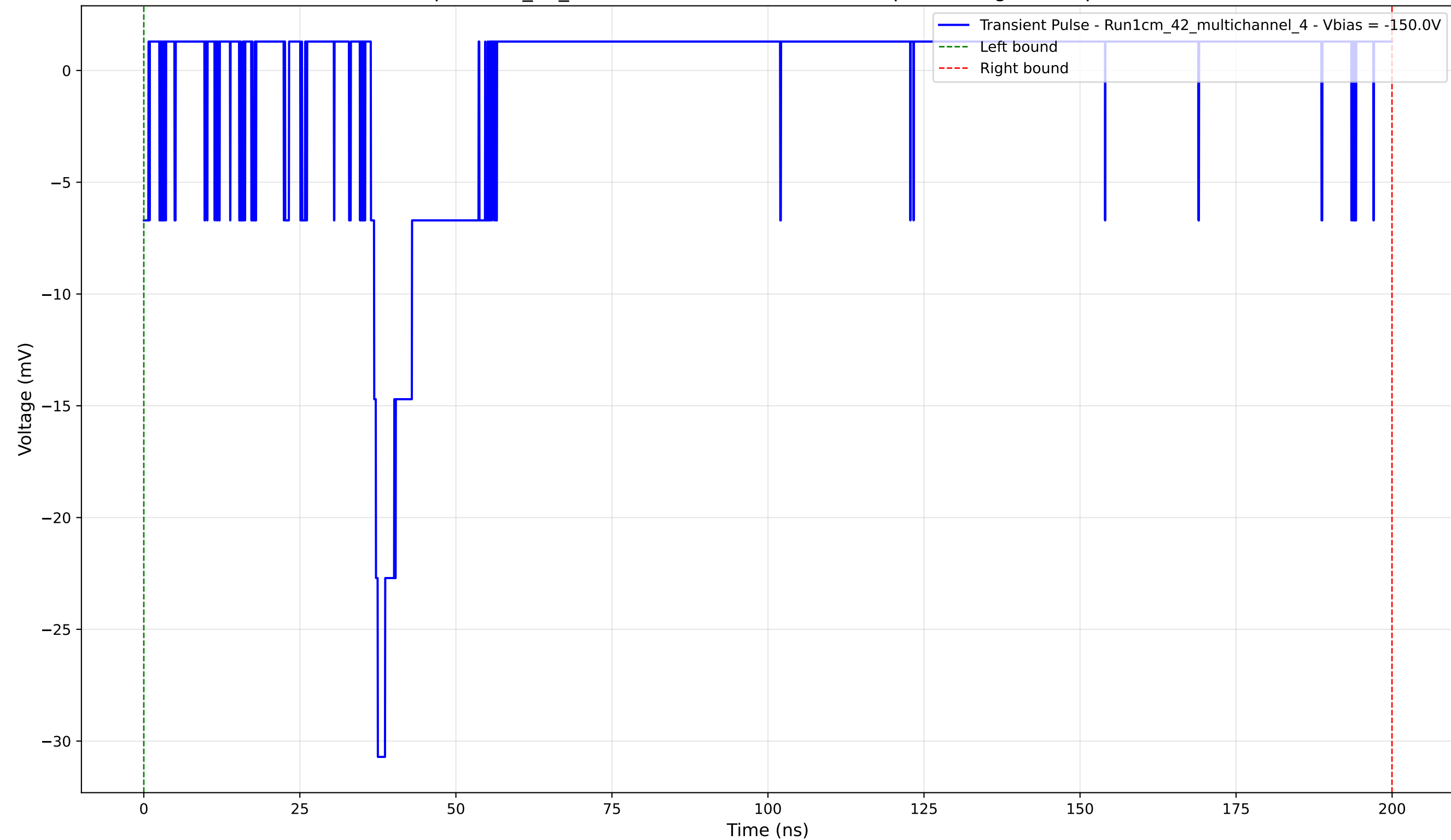
Transient Pulse - Sample: 1cm_42_multichannel - Position: 1530.0 \mu\text{m} - Charge: 0.54 pC - Rise Time: 1.11 ns
