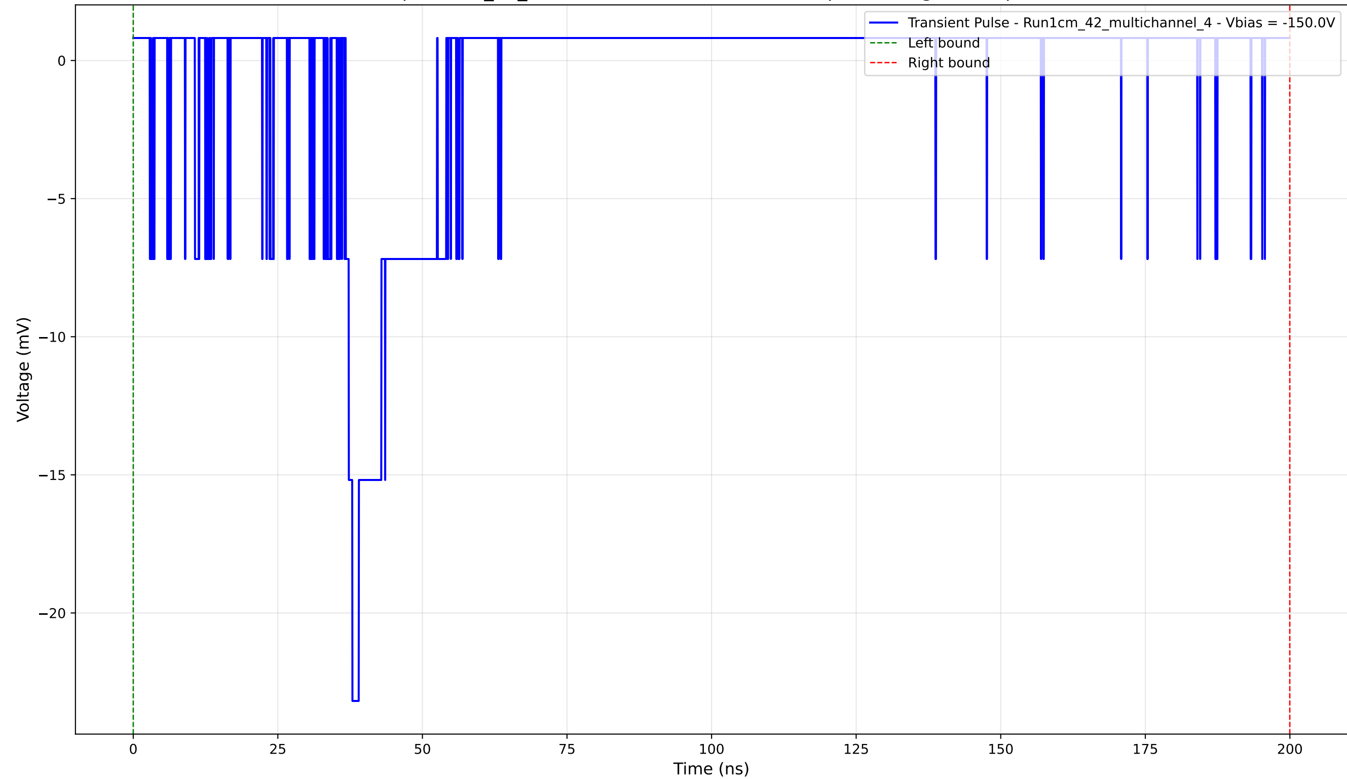
Transient Pulse - Sample: 1cm_42_multichannel - Position: 3535.0 \mu\text{m} - Charge: 1.77 pC - Rise Time: 1.16 ns
