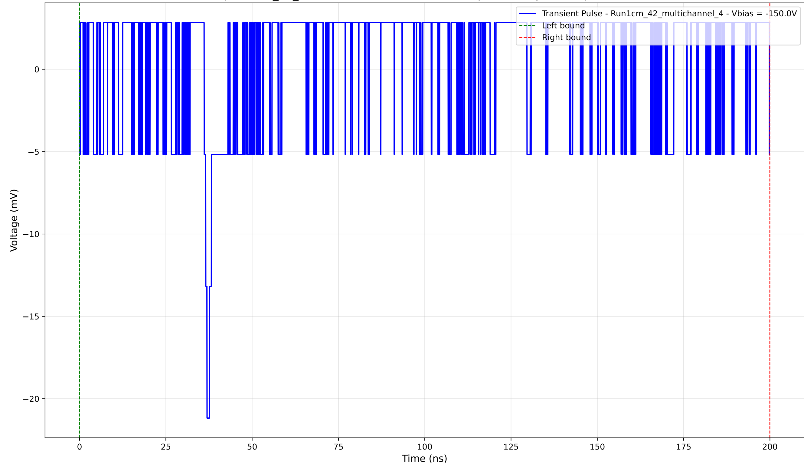
Transient Pulse - Sample: 1cm_42_multichannel - Position: 2345.0 \mu\text{m} - Charge: 3.22 pC - Rise Time: 0.00 ns (N/A)
