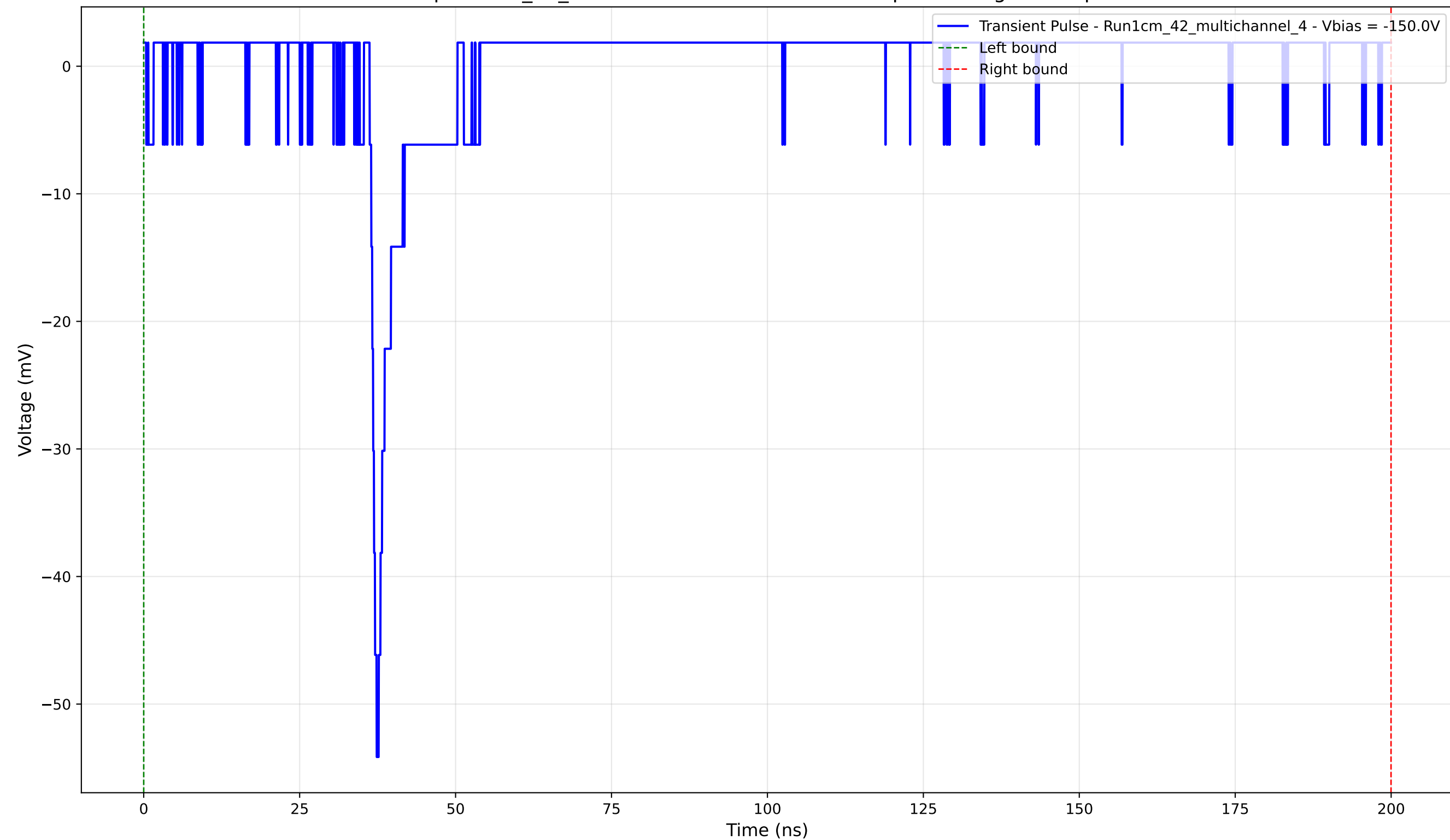
Transient Pulse - Sample: 1cm_42_multichannel - Position: 2770.0 \mu\text{m} - Charge: 1.20 pC - Rise Time: 1.12 ns
