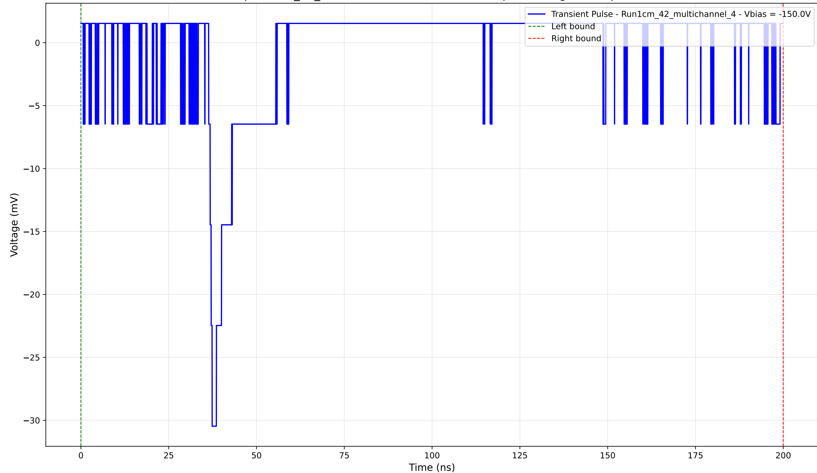
Transient Pulse - Sample: 1cm_42_multichannel - Position: 1590.0 \mu\text{m} - Charge: 1.00 pC - Rise Time: 0.99 ns
