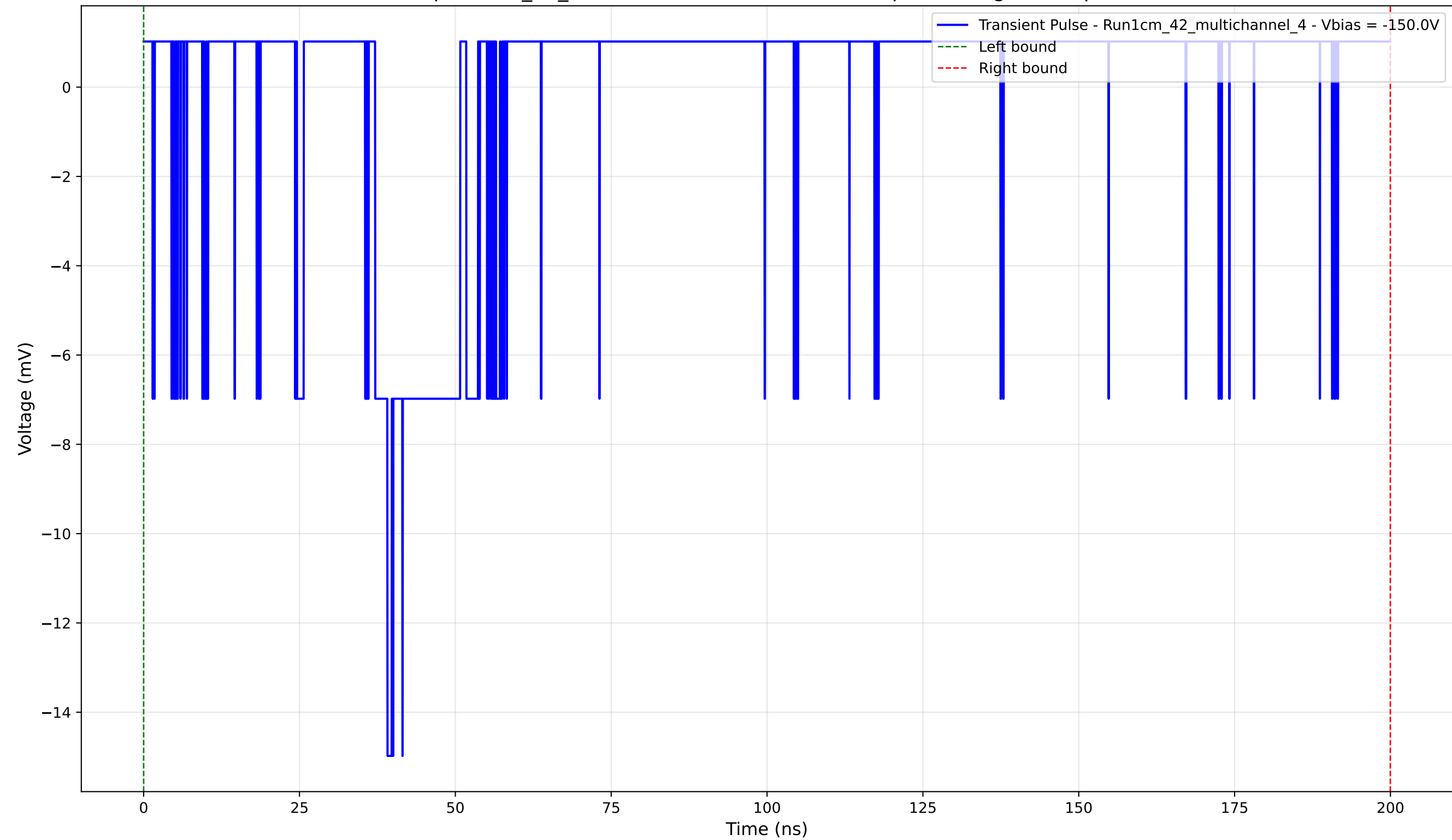
Transient Pulse - Sample: 1cm_42_multichannel - Position: 3960.0 \mu\text{m} - Charge: 0.32 pC - Rise Time: 1.98 ns
