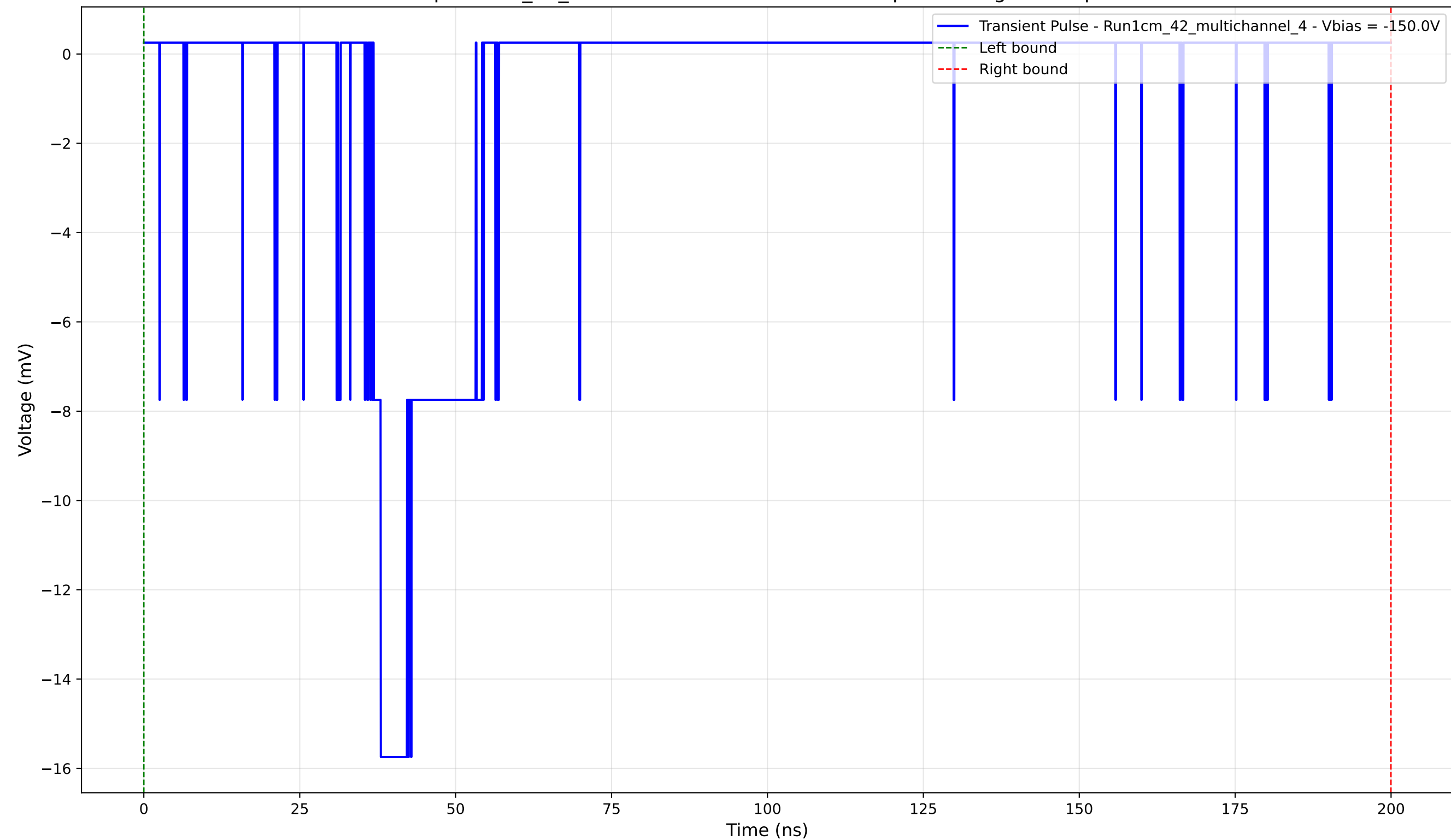
Transient Pulse - Sample: 1cm_42_multichannel - Position: 3830.0 \mu\text{m} - Charge: 3.01 pC - Rise Time: 1.14 ns
