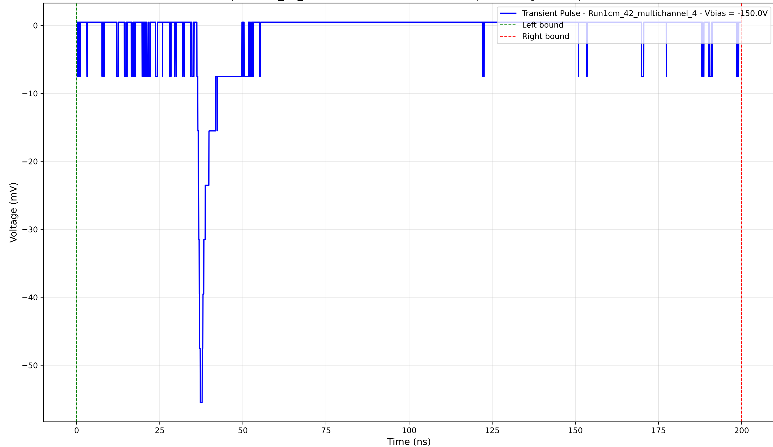
Transient Pulse - Sample: 1cm_42_multichannel - Position: 2735.0 \mu\text{m} - Charge: 4.16 pC - Rise Time: 0.99 ns
