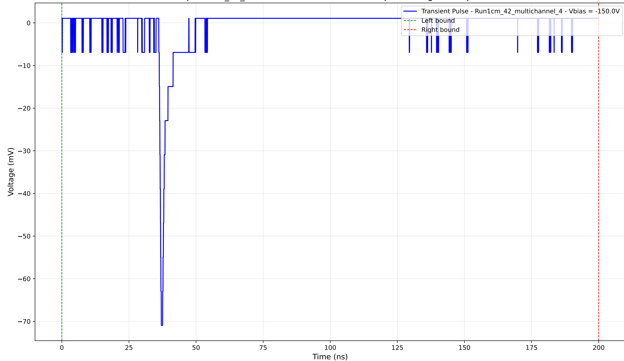
Transient Pulse - Sample: 1cm_42_multichannel - Position: 2530.0 \mu\text{m} - Charge: 1.65 pC - Rise Time: 0.76 ns
