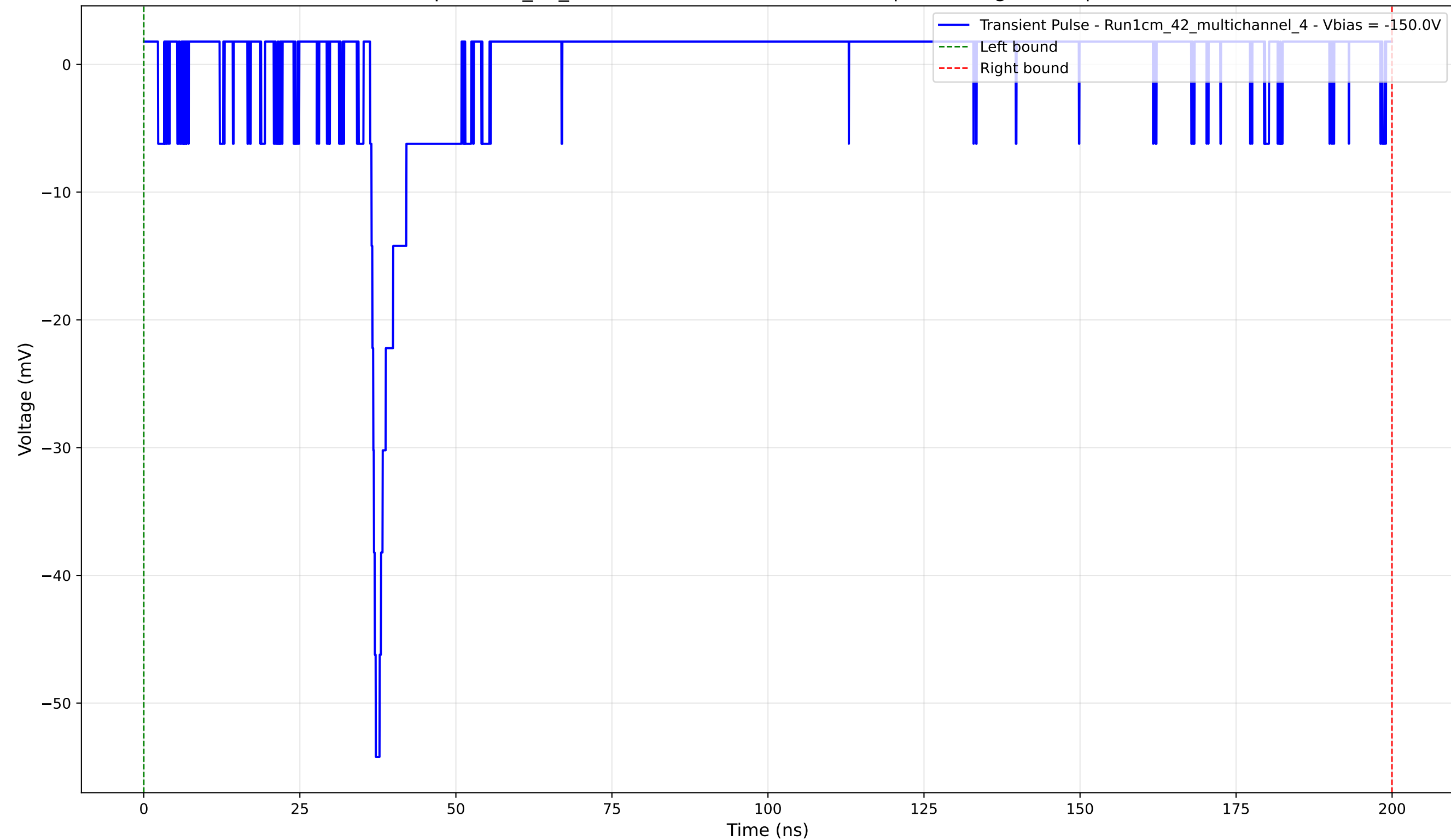
Transient Pulse - Sample: 1cm_42_multichannel - Position: 2745.0 \mu\text{m} - Charge: 0.45 pC - Rise Time: 0.90 ns
