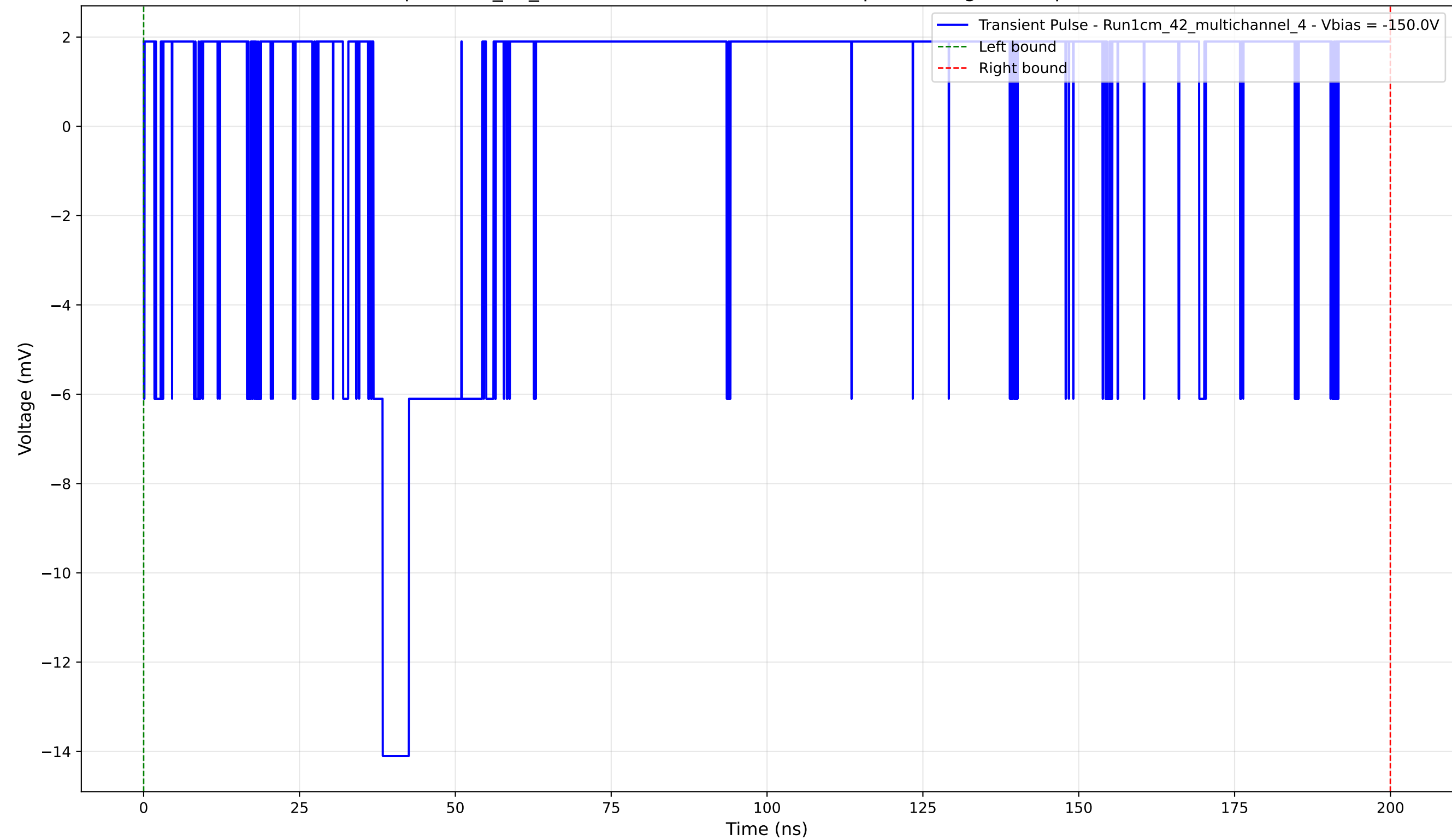
Transient Pulse - Sample: 1cm_42_multichannel - Position: 4760.0 \mu\text{m} - Charge: 2.09 pC - Rise Time: 0.00 ns (N/A)
