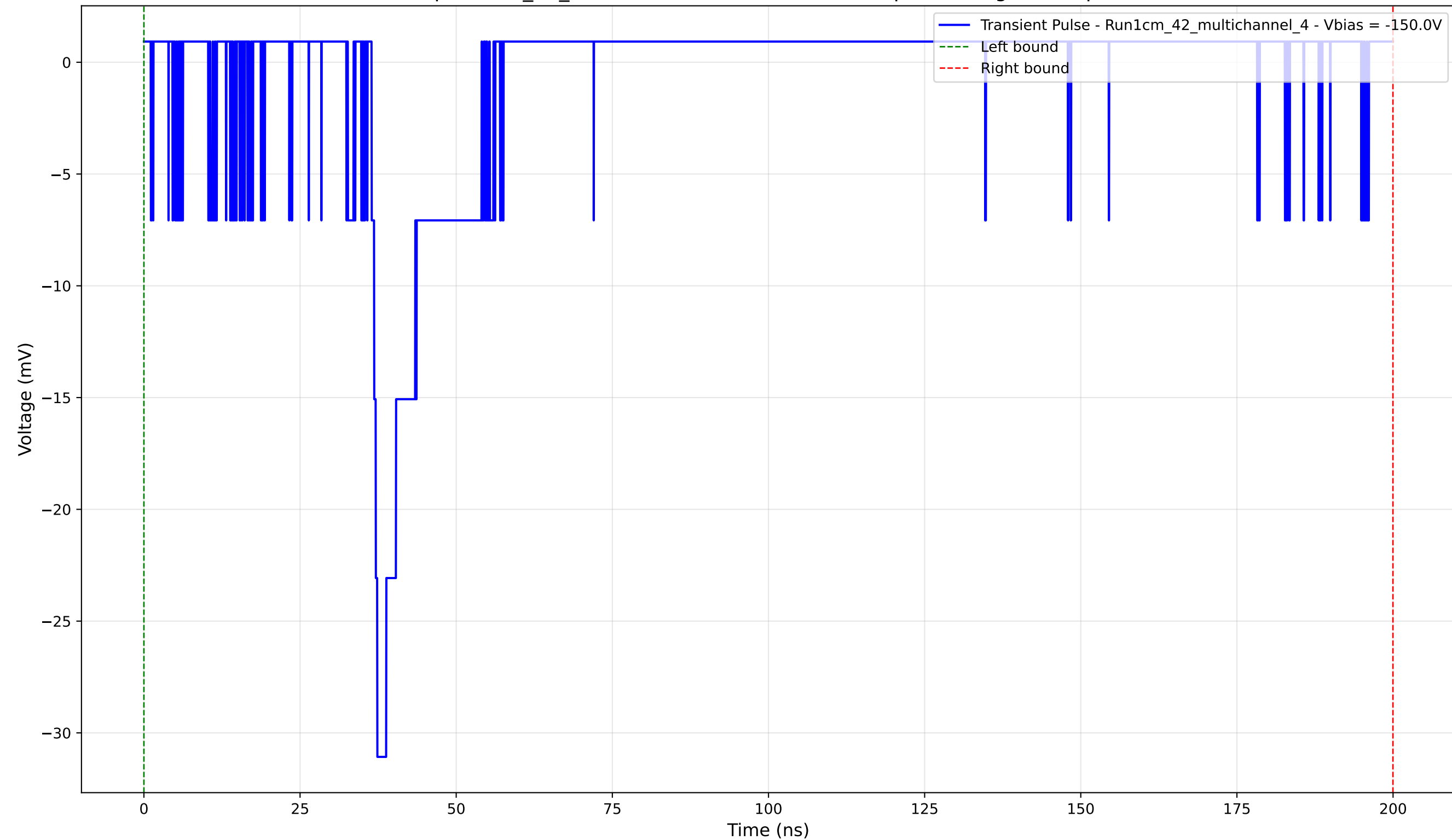
Transient Pulse - Sample: 1cm_42_multichannel - Position: 1540.0 \mu\text{m} - Charge: 2.50 pC - Rise Time: 0.91 ns
