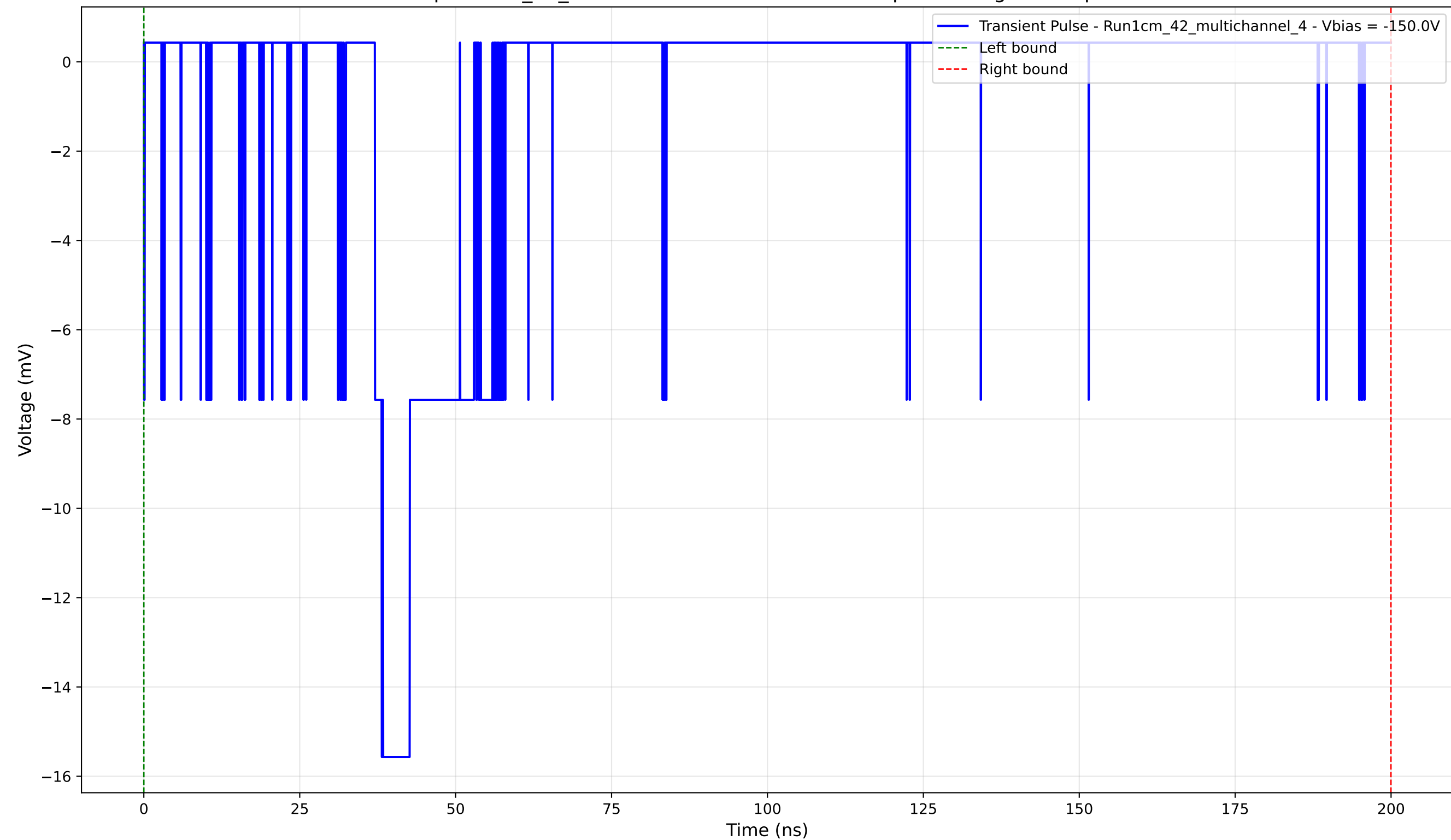
Transient Pulse - Sample: 1cm_42_multichannel - Position: 4265.0 \mu\text{m} - Charge: 2.75 pC - Rise Time: 1.10 ns
