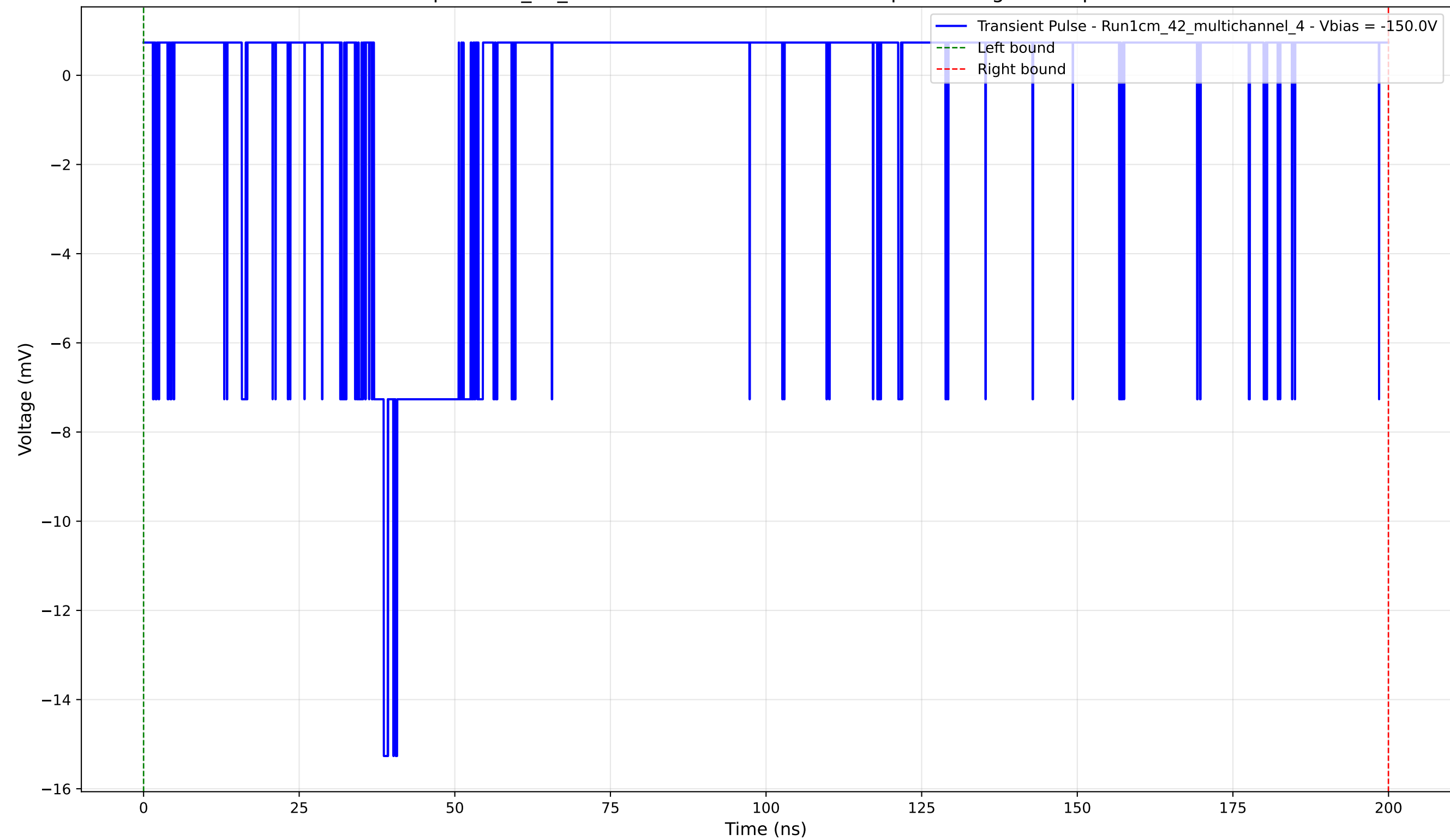
Transient Pulse - Sample: 1cm_42_multichannel - Position: 4825.0 \mu\text{m} - Charge: 1.22 pC - Rise Time: 1.58 ns
