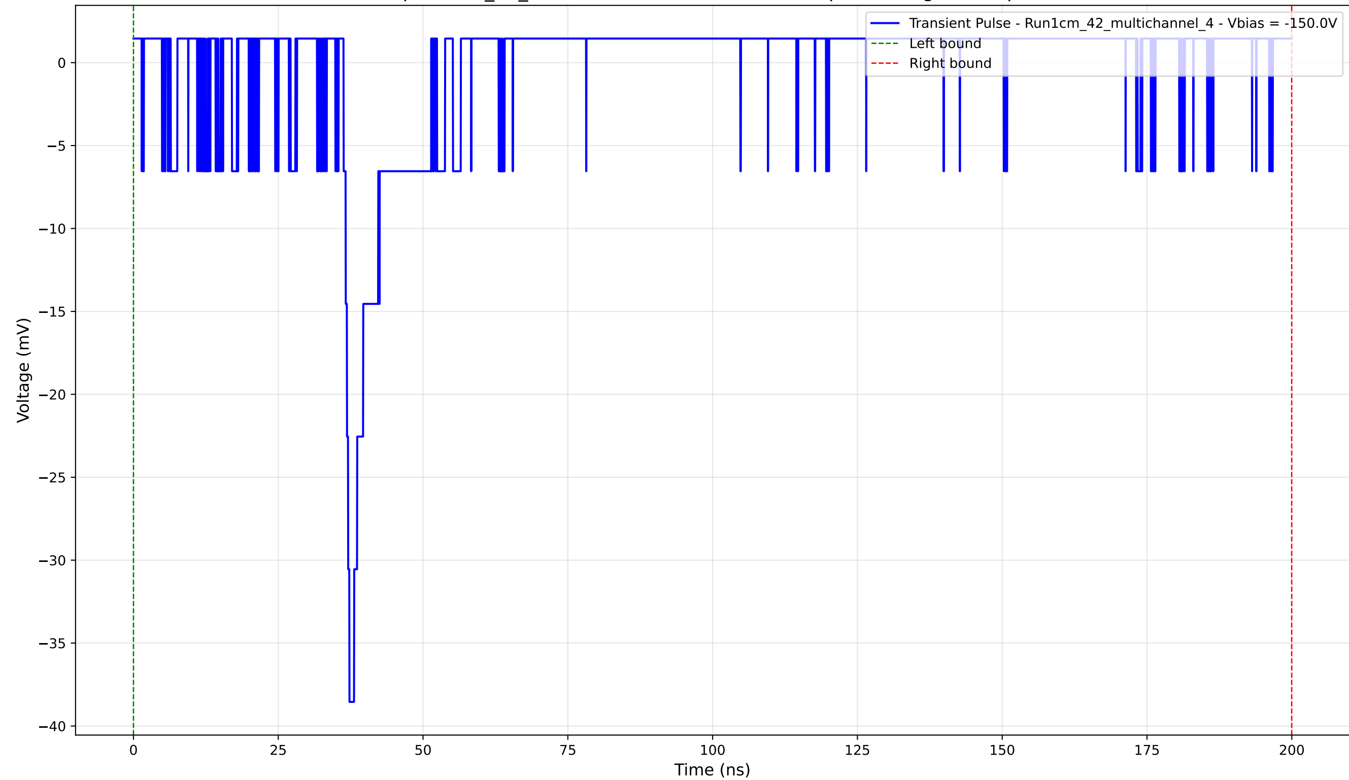
Transient Pulse - Sample: 1cm_42_multichannel - Position: 2990.0 \mu\text{m} - Charge: 0.99 pC - Rise Time: 1.01 ns
