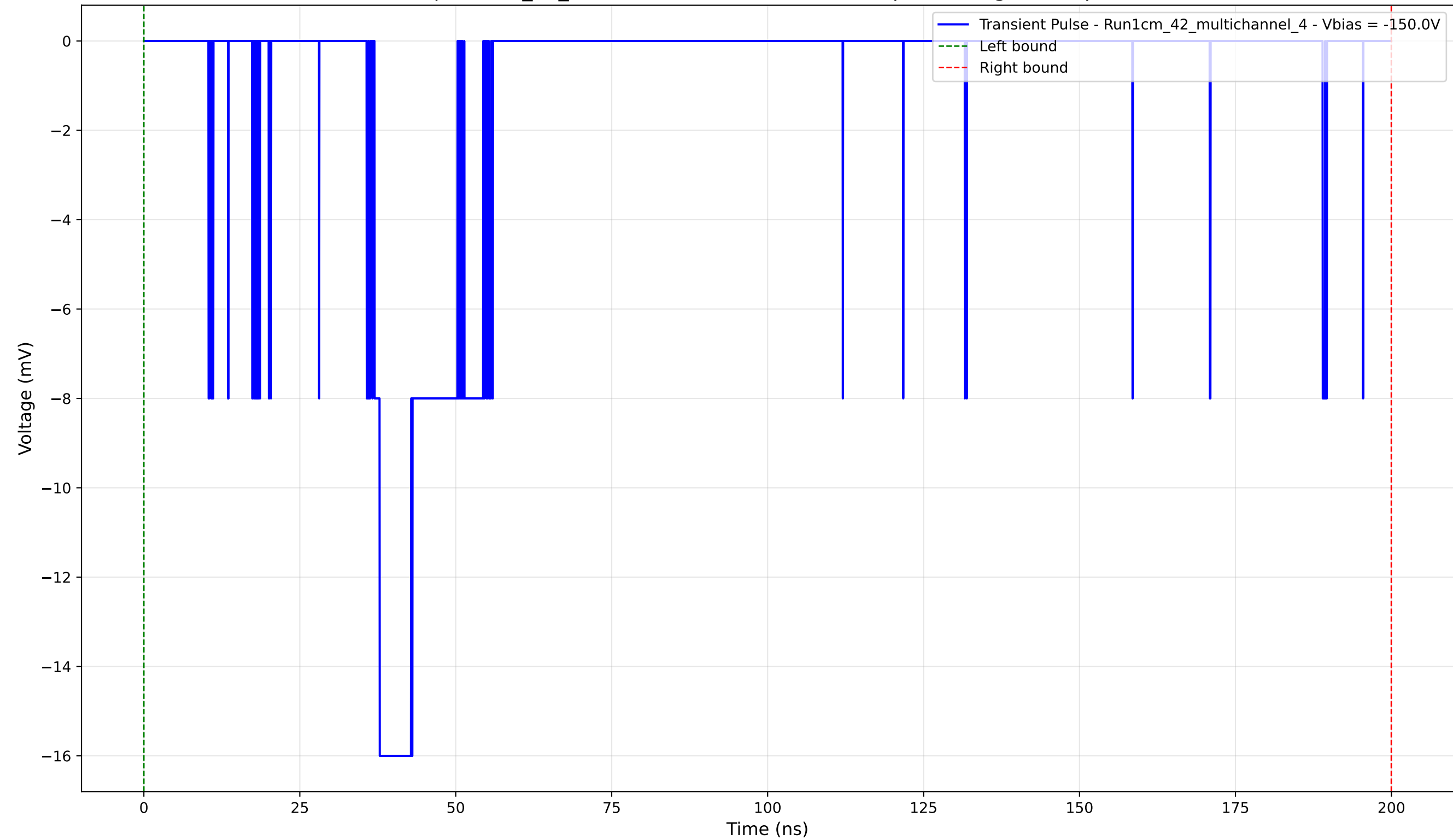
Transient Pulse - Sample: 1cm_42_multichannel - Position: 3825.0 \mu\text{m} - Charge: 4.07 pC - Rise Time: 0.84 ns
