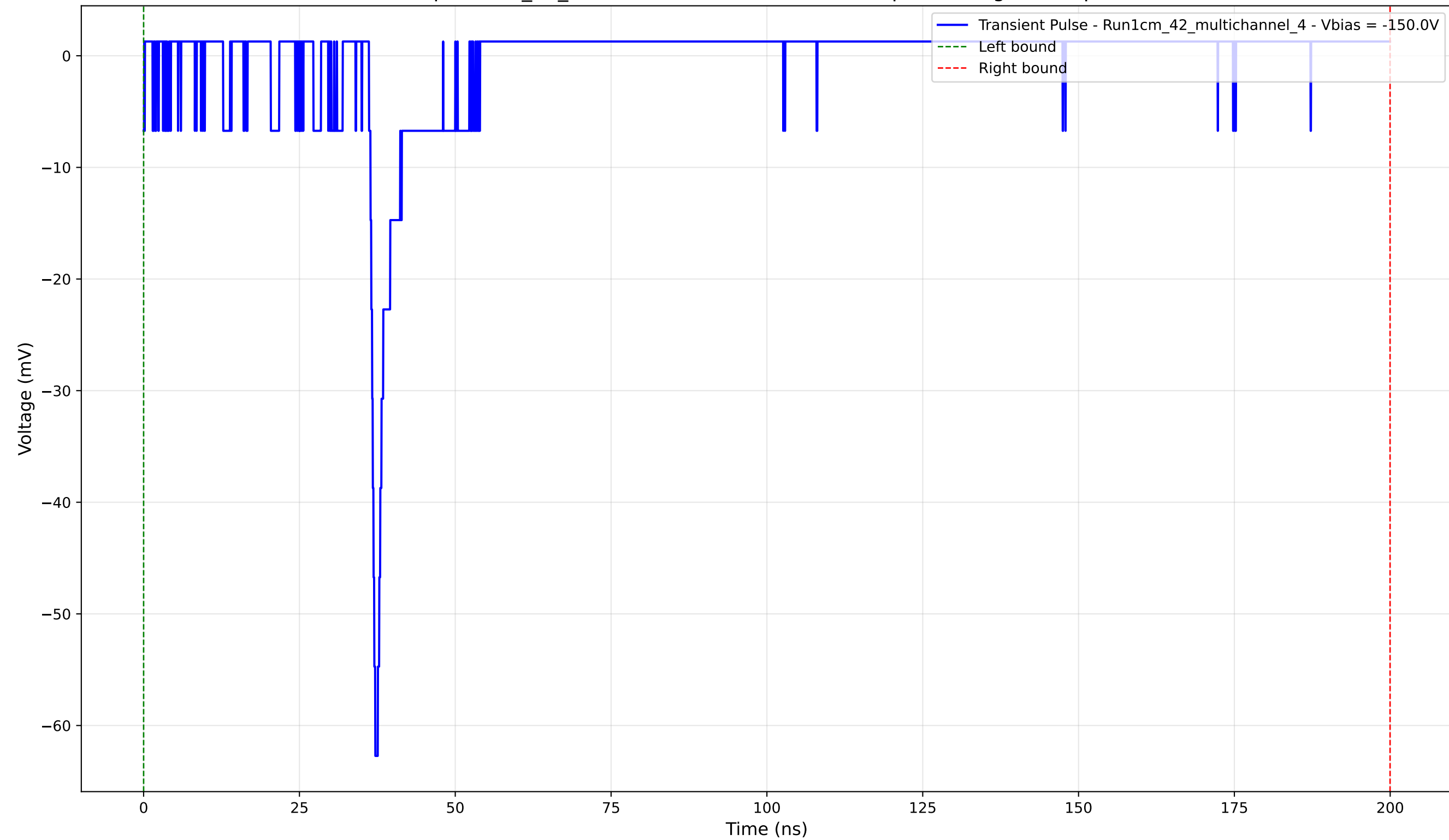
Transient Pulse - Sample: 1cm_42_multichannel - Position: 2635.0 \mu\text{m} - Charge: 1.28 pC - Rise Time: 1.00 ns
