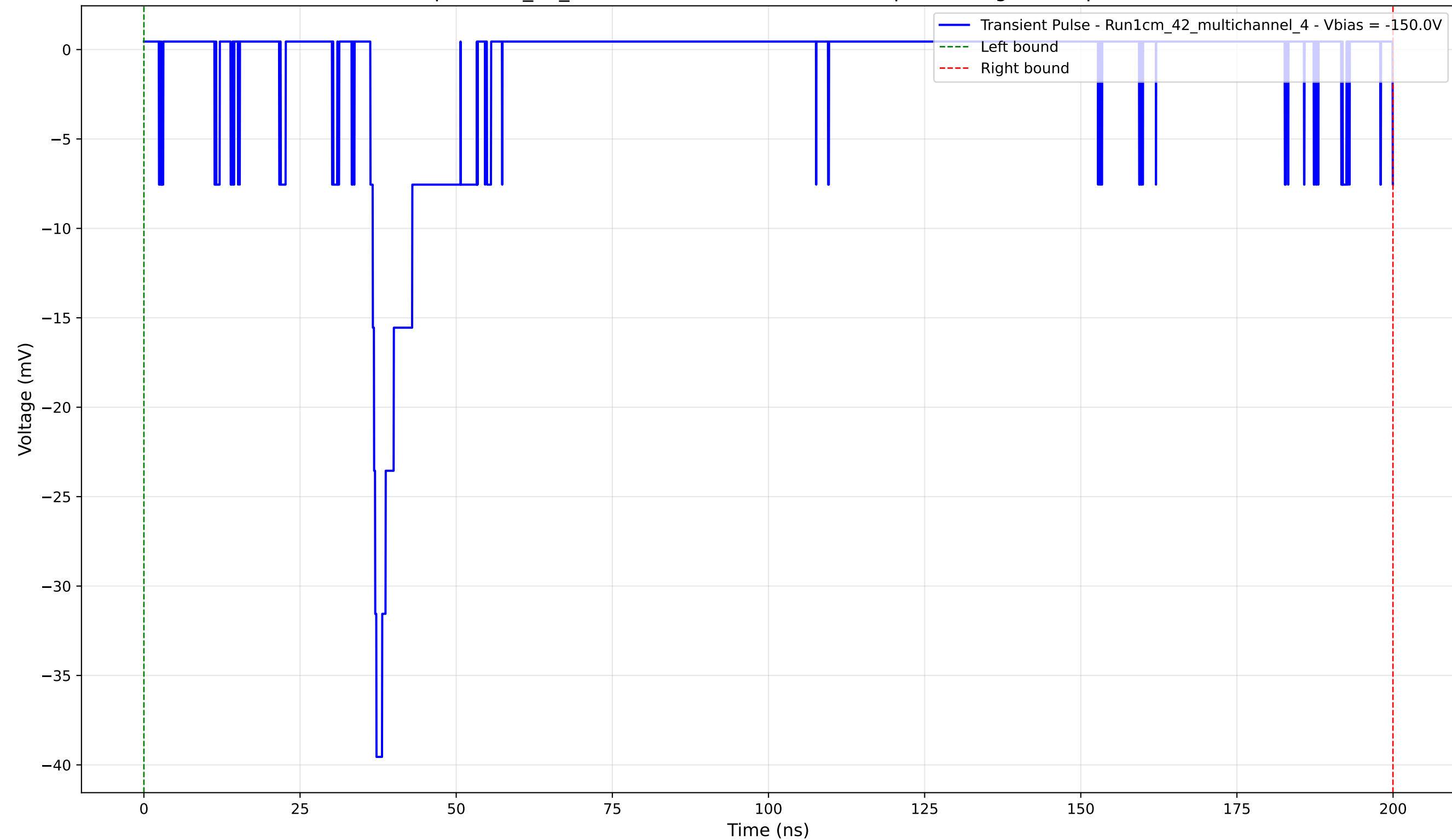
Transient Pulse - Sample: 1cm_42_multichannel - Position: 1790.0 \mu\text{m} - Charge: 4.02 pC - Rise Time: 0.97 ns
