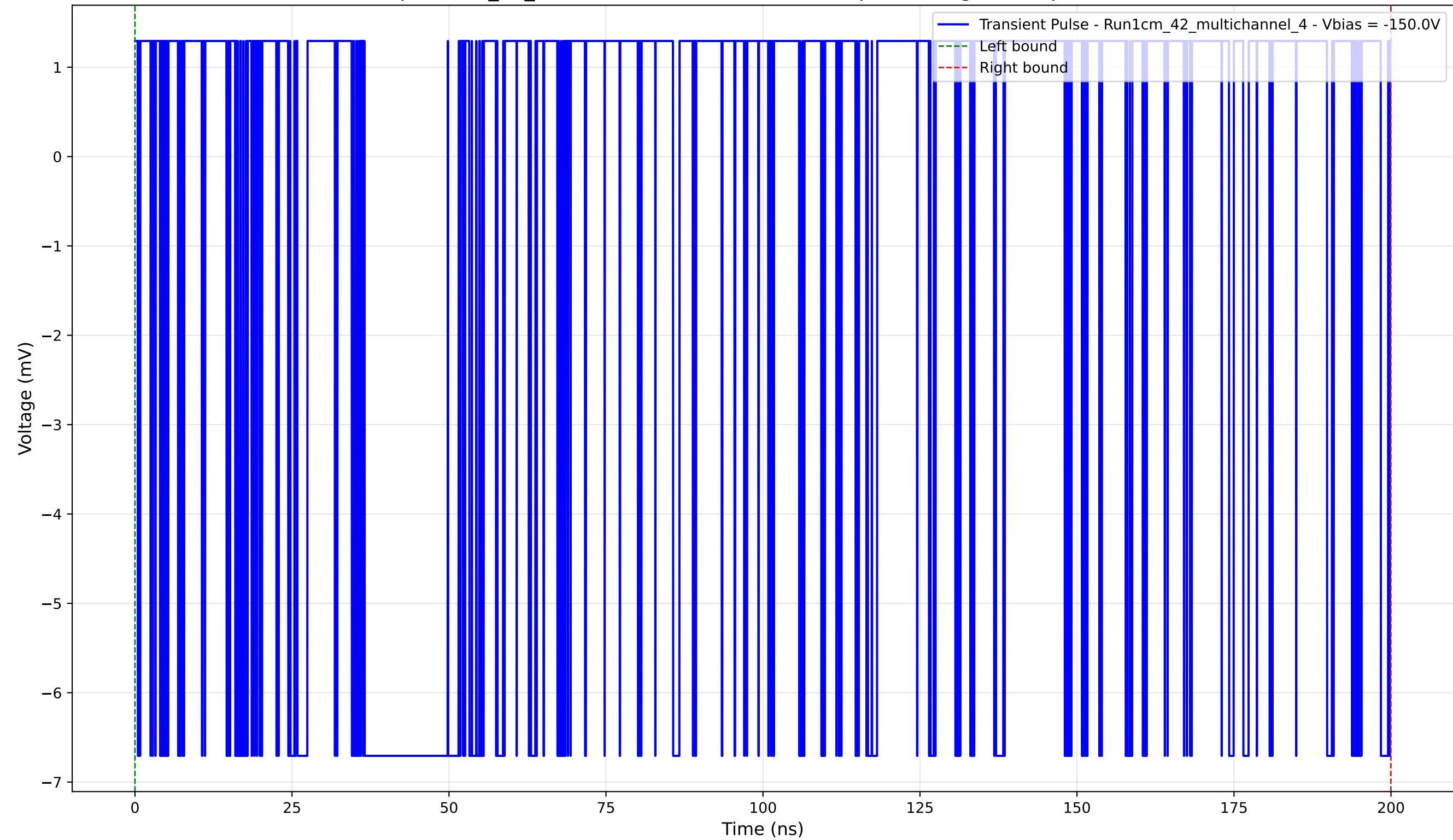
Transient Pulse - Sample: 1cm_42_multichannel - Position: 1415.0 \mu\text{m} - Charge: 2.13 pC - Rise Time: 0.00 ns (N/A)
