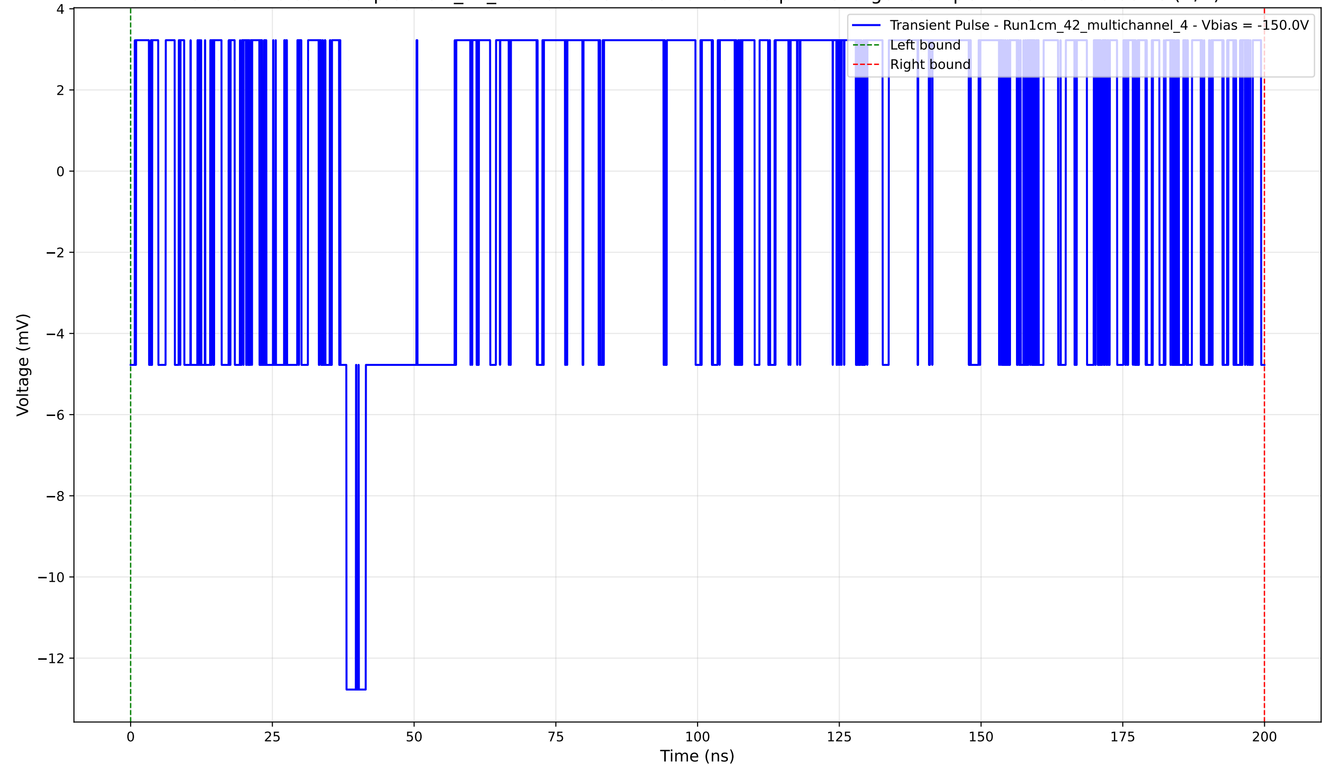
Transient Pulse - Sample: 1cm_42_multichannel - Position: 920.0 \mu\text{m} - Charge: 0.62 pC - Rise Time: 0.00 ns (N/A)
