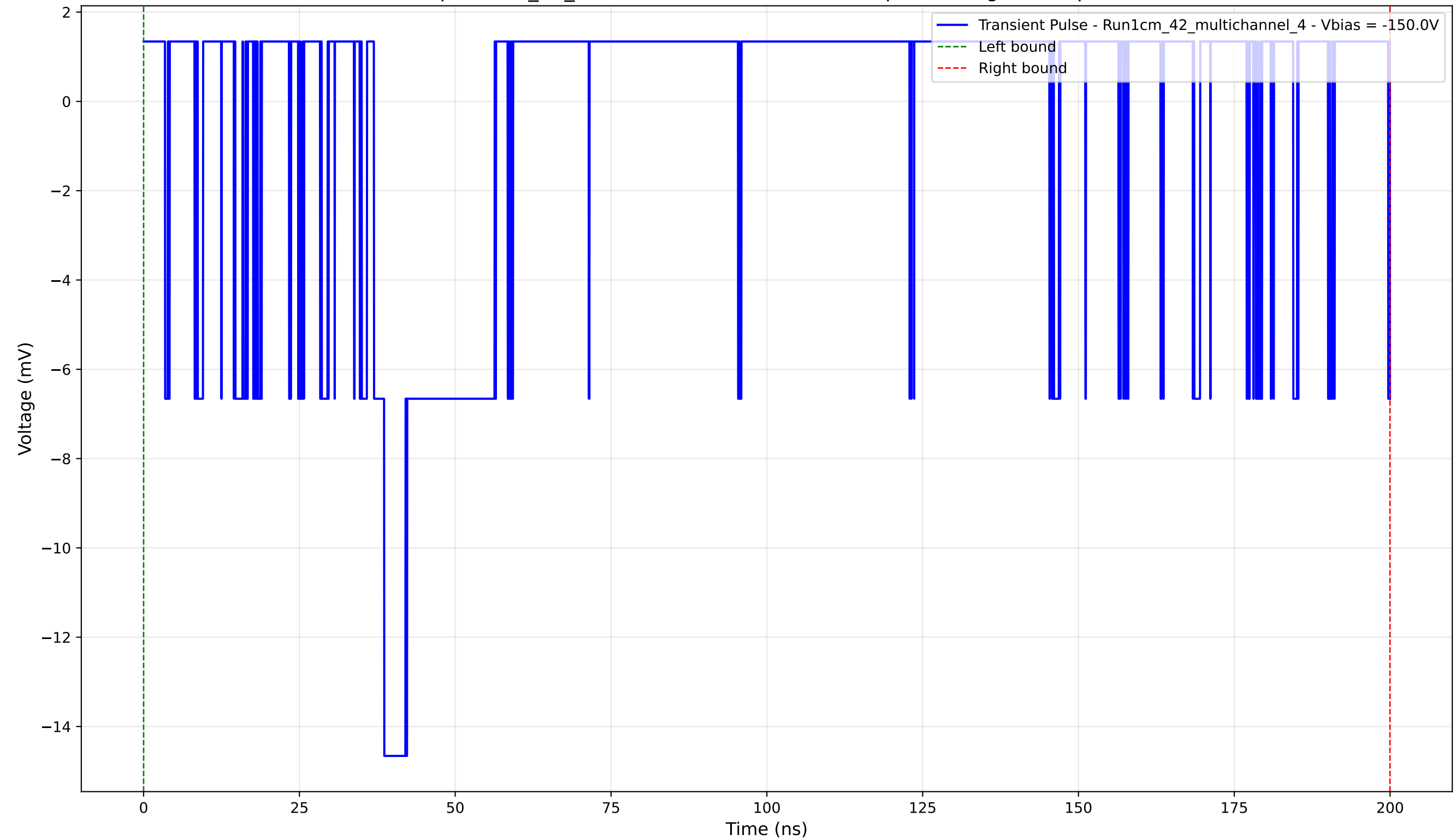
Transient Pulse - Sample: 1cm_42_multichannel - Position: 165.0 \mu\text{m} - Charge: 0.61 pC - Rise Time: 1.66 ns
