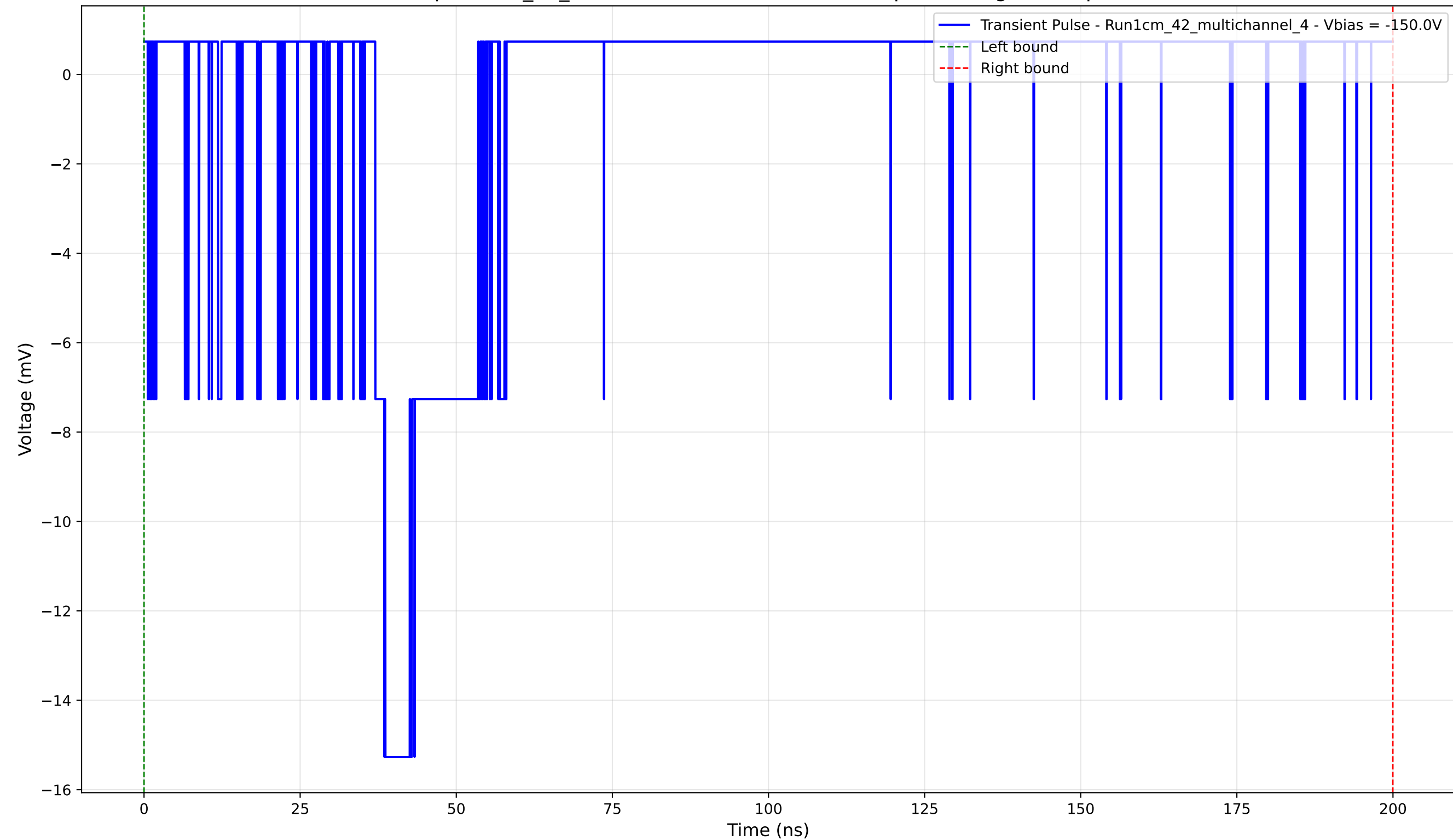
Transient Pulse - Sample: 1cm_42_multichannel - Position: 4600.0 \mu\text{m} - Charge: 1.81 pC - Rise Time: 1.48 ns
