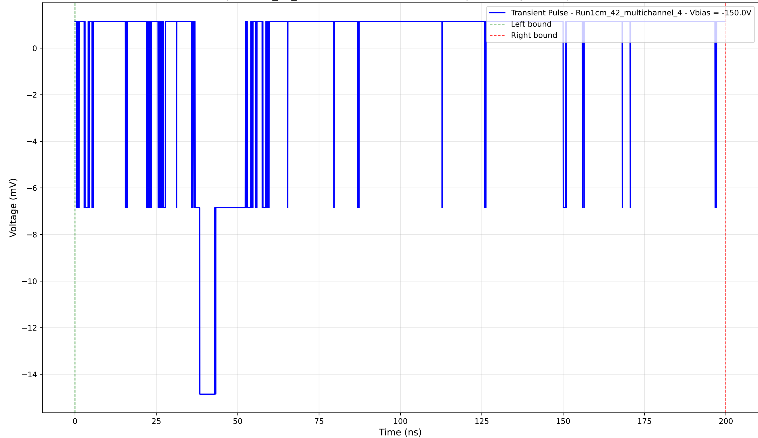
Transient Pulse - Sample: 1cm_42_multichannel - Position: 4240.0 \mu\text{m} - Charge: 0.10 pC - Rise Time: 1.48 ns
