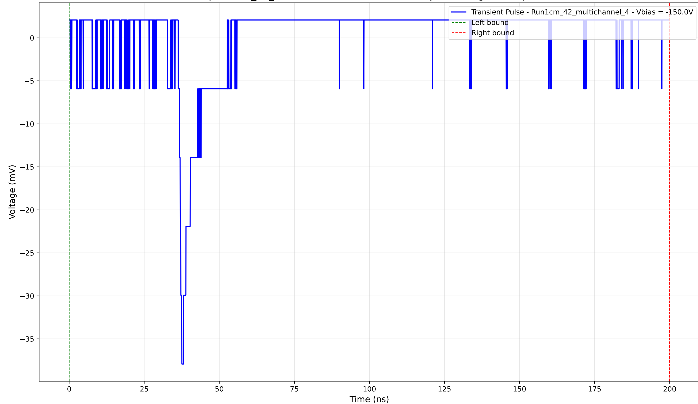
Transient Pulse - Sample: 1cm_42_multichannel - Position: 1680.0 \mu\text{m} - Charge: 1.68 pC - Rise Time: 1.23 ns
