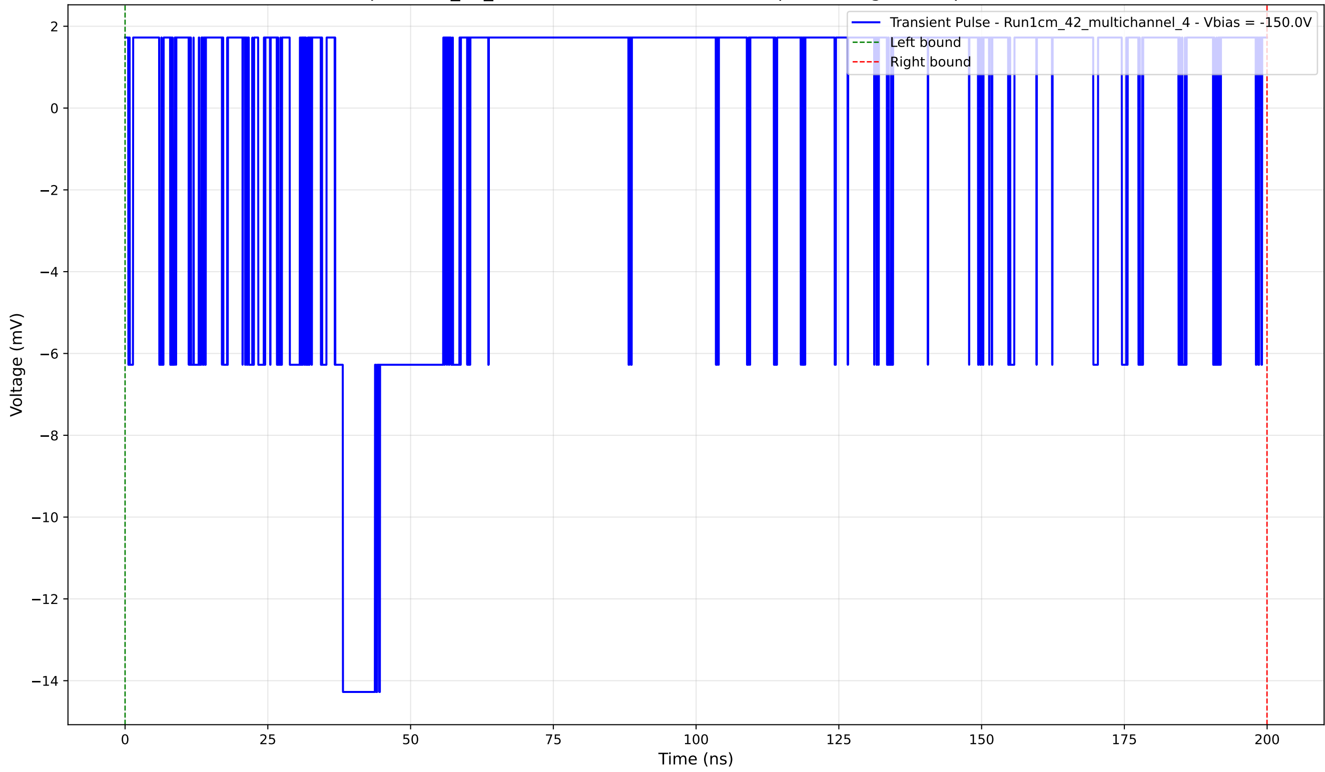
Transient Pulse - Sample: 1cm_42_multichannel - Position: 545.0 \mu\text{m} - Charge: 0.91 pC - Rise Time: 0.00 ns (N/A)
