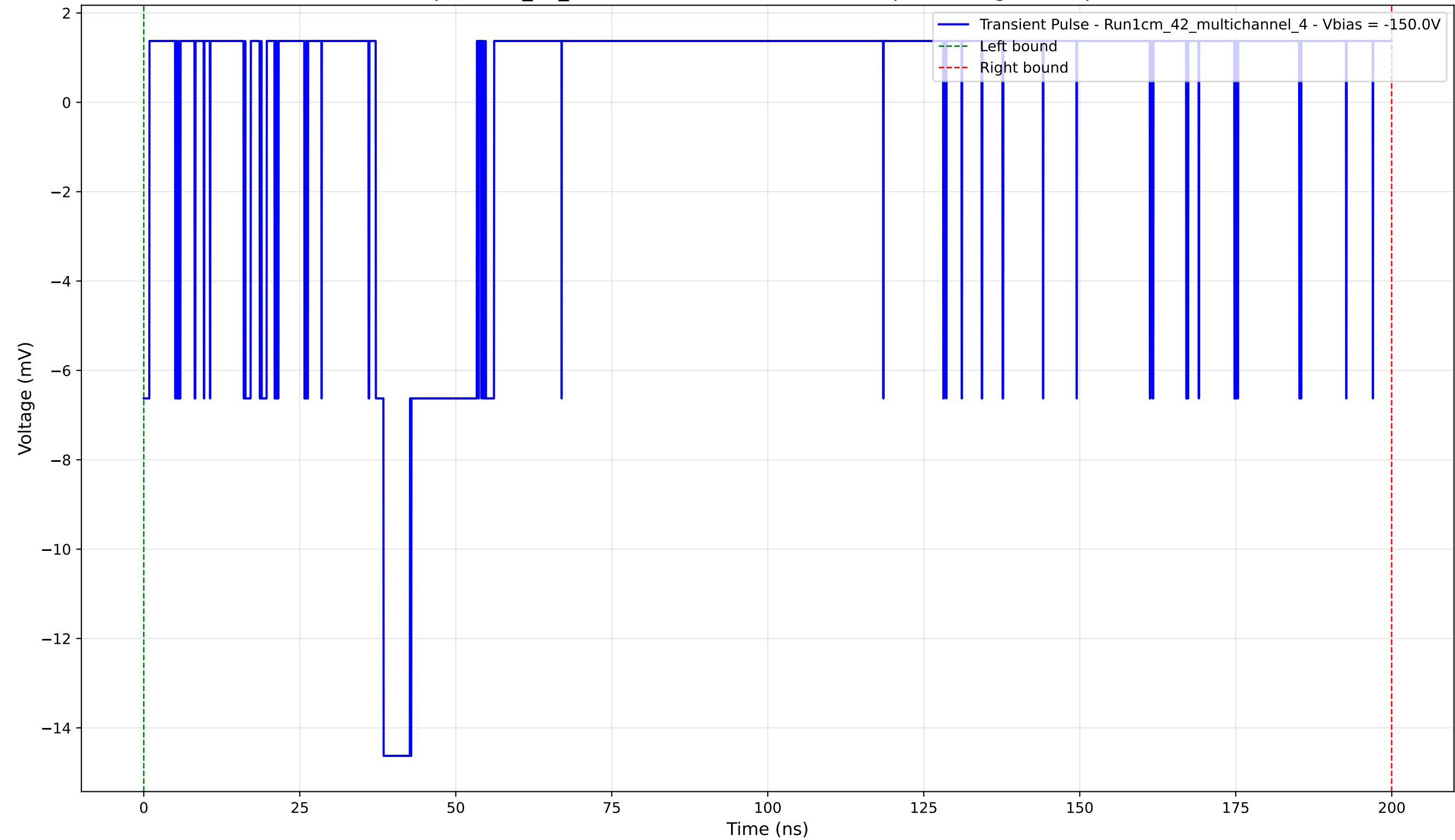
Transient Pulse - Sample: 1cm_42_multichannel - Position: 4230.0 \mu\text{m} - Charge: 0.88 pC - Rise Time: 1.26 ns
