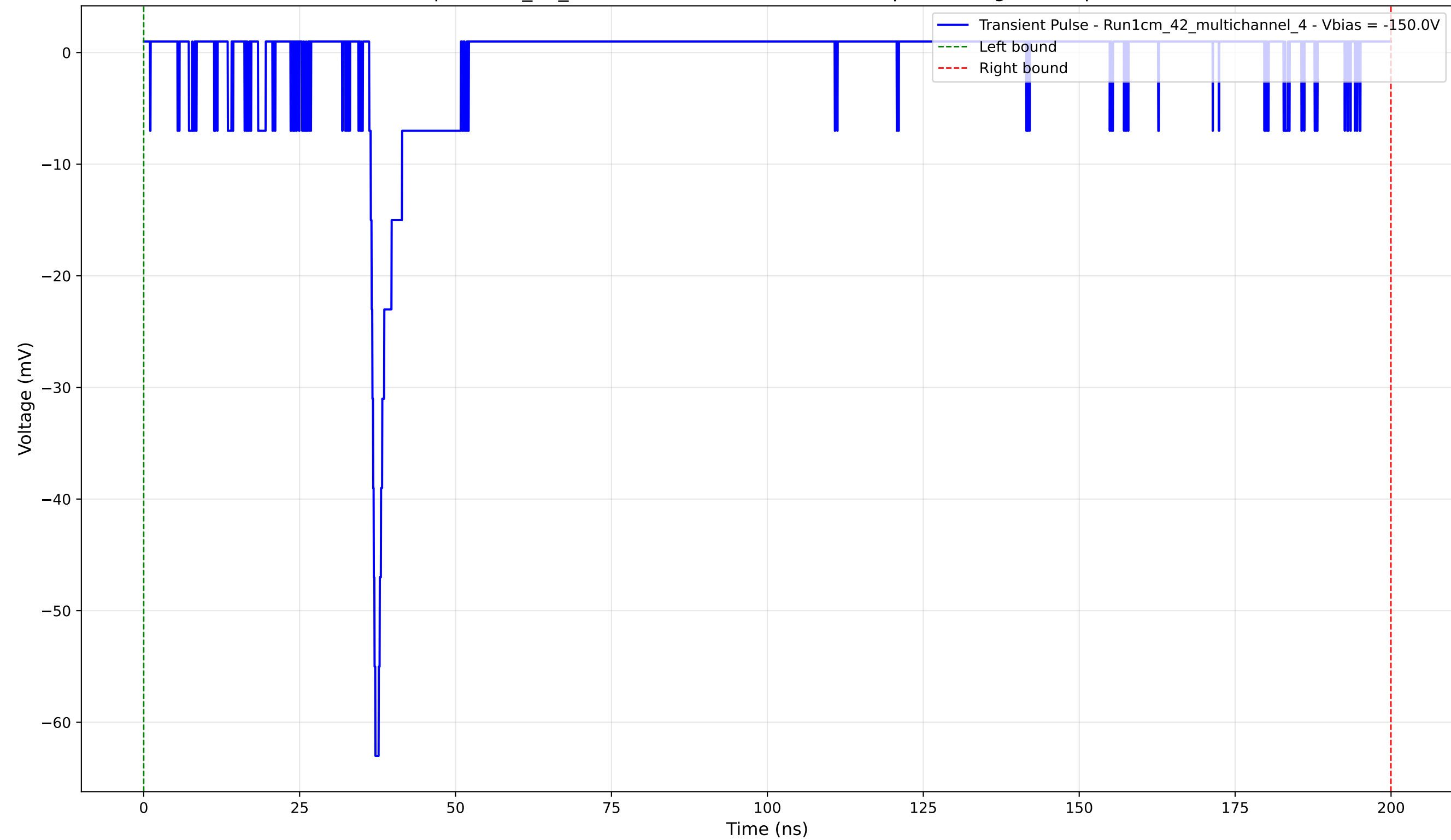
Transient Pulse - Sample: 1cm_42_multichannel - Position: 2125.0 \mu\text{m} - Charge: 2.35 pC - Rise Time: 0.98 ns
