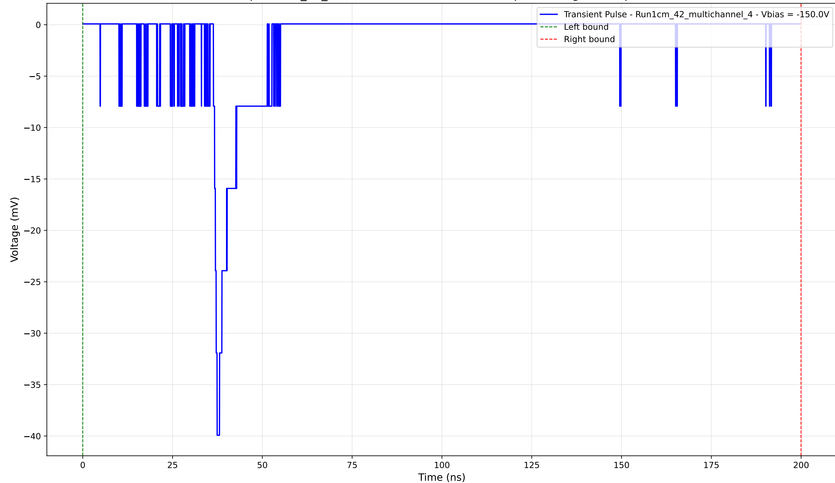
Transient Pulse - Sample: 1cm_42_multichannel - Position: 1705.0 \mu\text{m} - Charge: 5.35 pC - Rise Time: 1.03 ns
