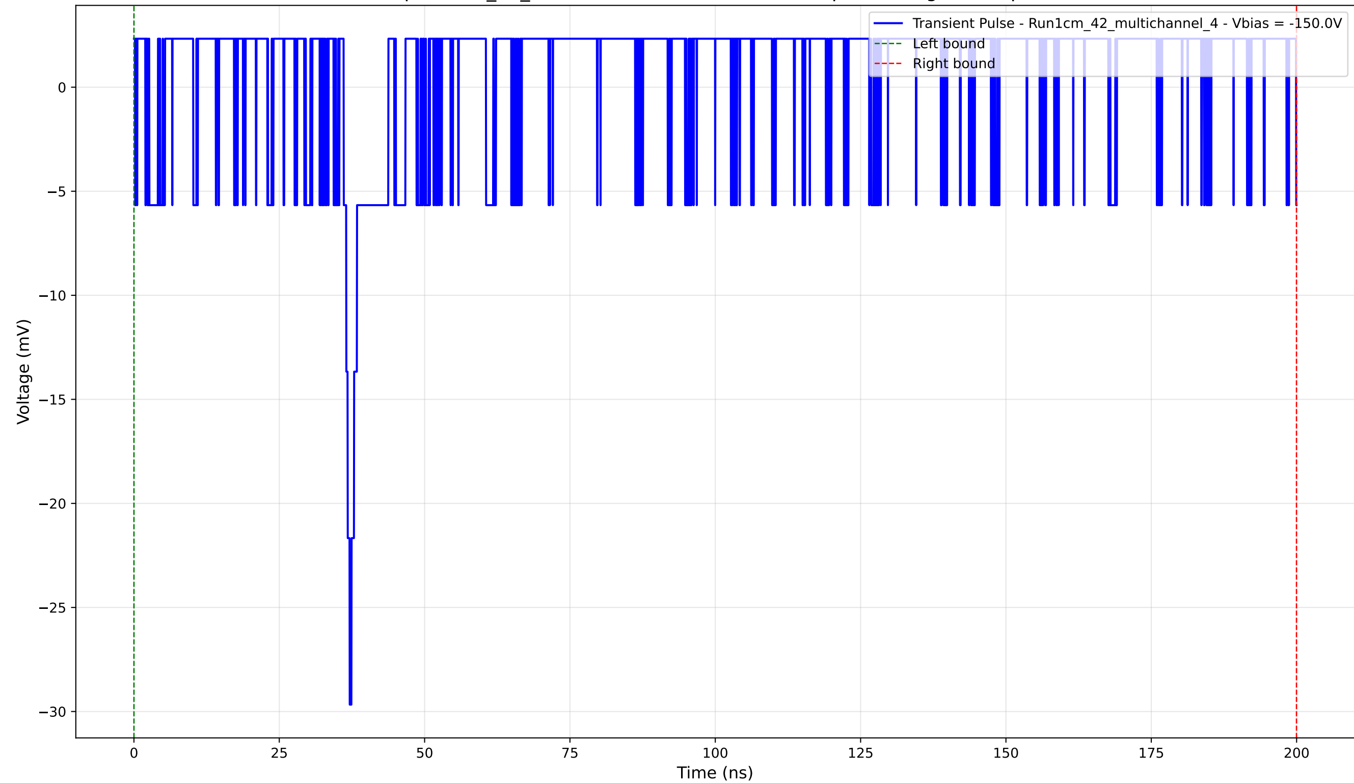
Transient Pulse - Sample: 1cm_42_multichannel - Position: 2430.0 \mu\text{m} - Charge: 3.06 pC - Rise Time: 1.04 ns
