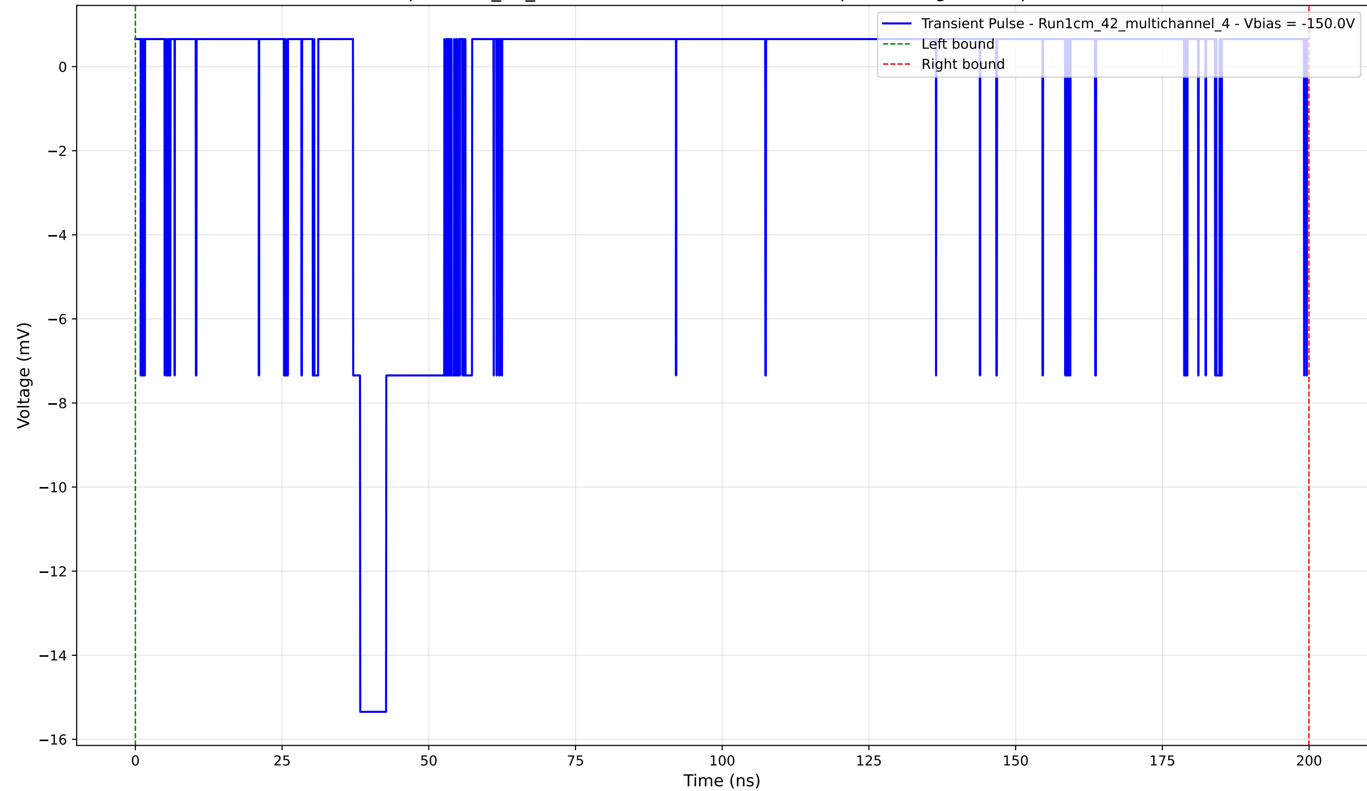
Transient Pulse - Sample: 1cm_42_multichannel - Position: 4215.0 \mu\text{m} - Charge: 1.96 pC - Rise Time: 1.22 ns
