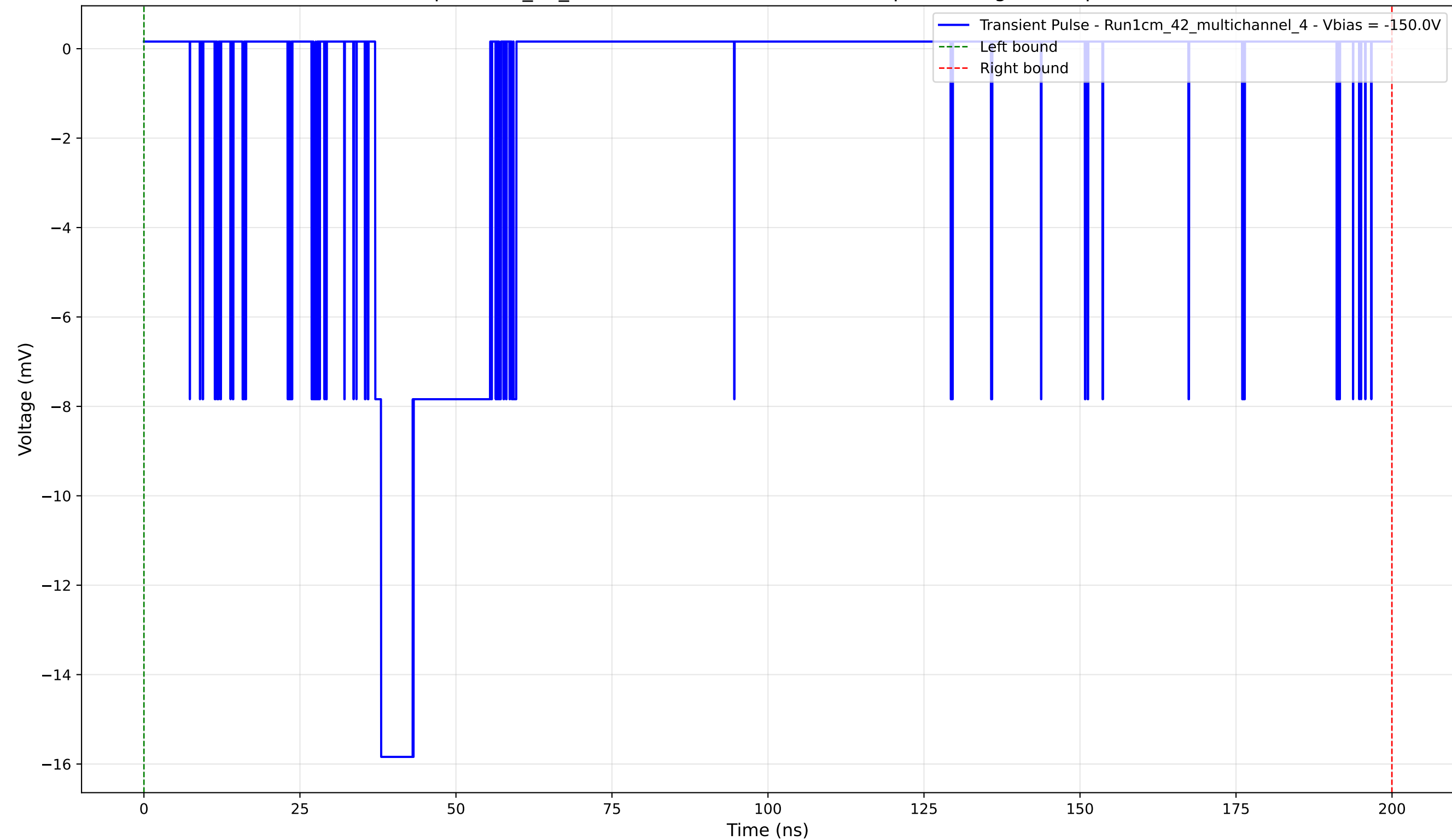
Transient Pulse - Sample: 1cm_42_multichannel - Position: 3995.0 \mu\text{m} - Charge: 4.21 pC - Rise Time: 0.96 ns
