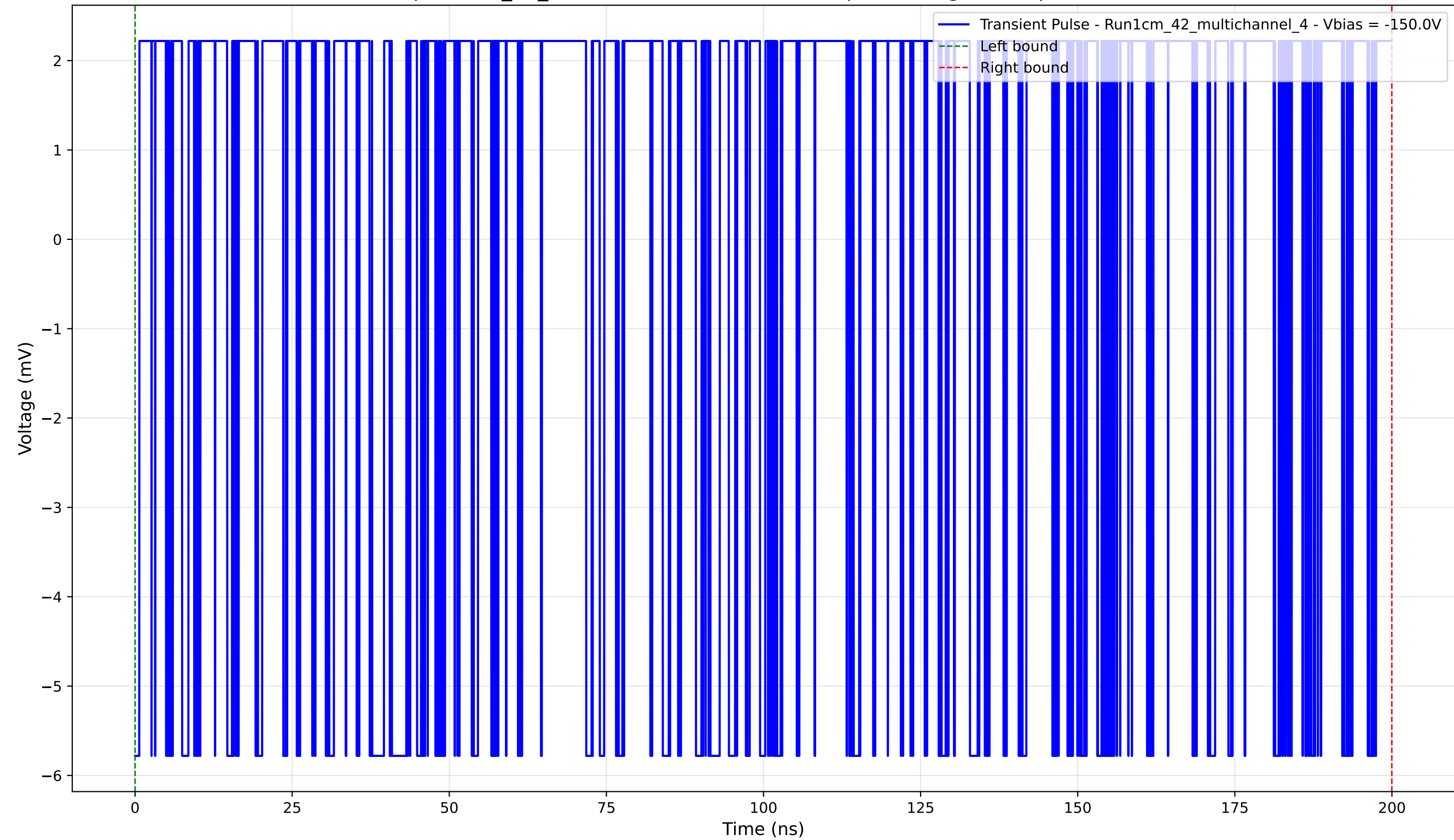
Transient Pulse - Sample: 1cm_42_multichannel - Position: 65.0 \mu\text{m} - Charge: 1.44 pC - Rise Time: 0.00 ns (N/A)
