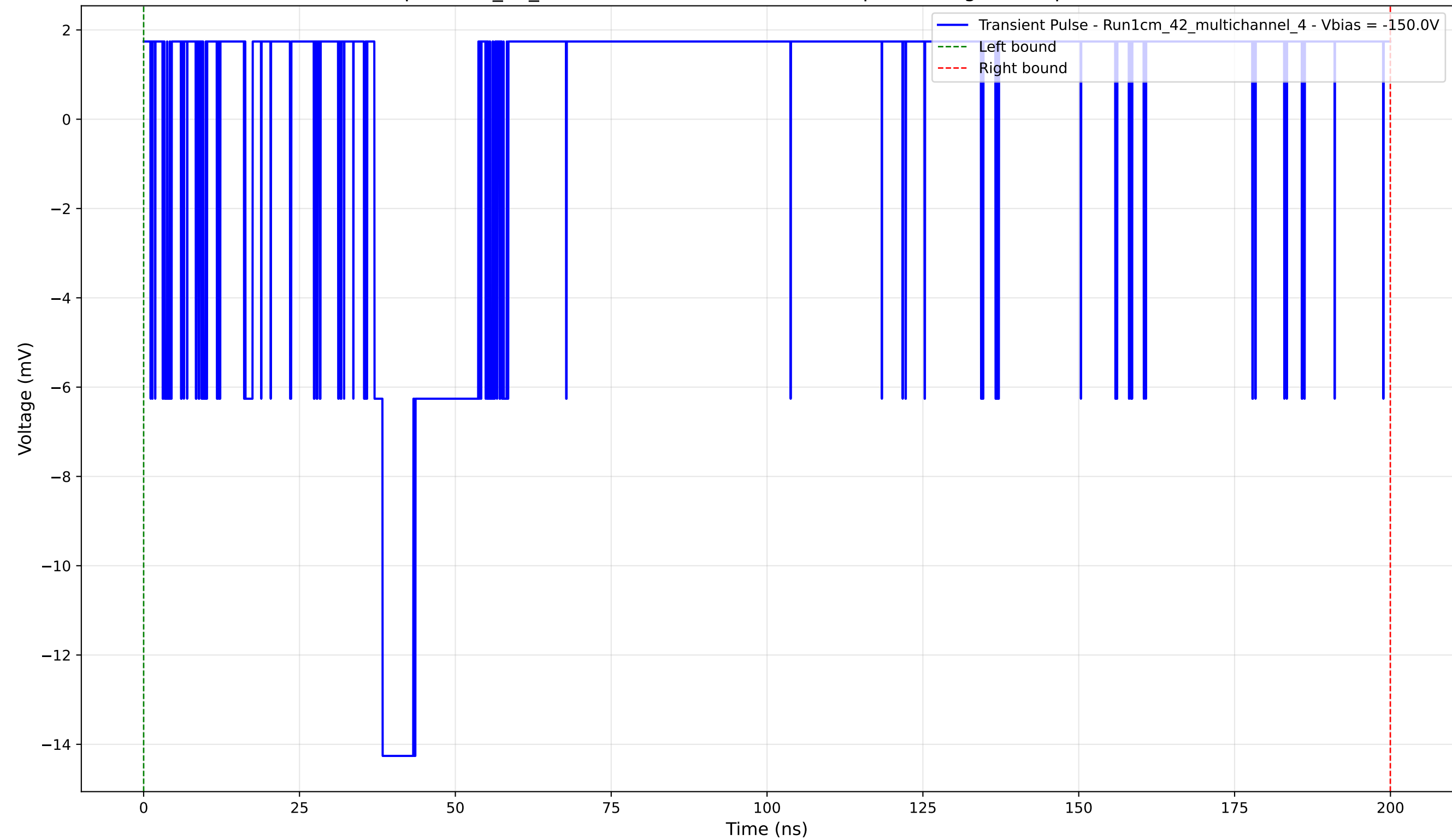
Transient Pulse - Sample: 1cm_42_multichannel - Position: 4290.0 \mu\text{m} - Charge: 1.92 pC - Rise Time: 0.00 ns (N/A)
