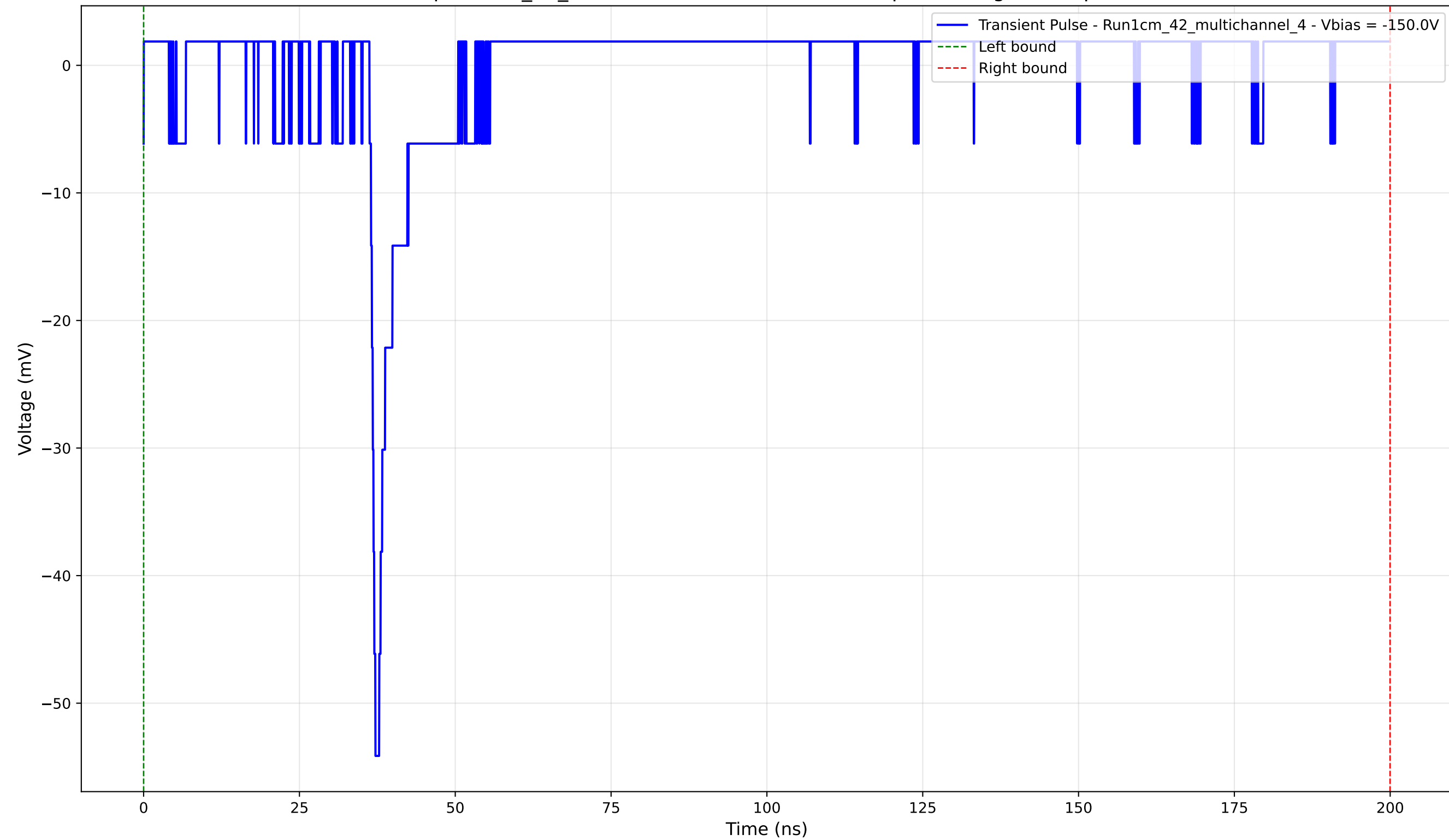
Transient Pulse - Sample: 1cm_42_multichannel - Position: 2005.0 \mu\text{m} - Charge: 0.52 pC - Rise Time: 0.94 ns
