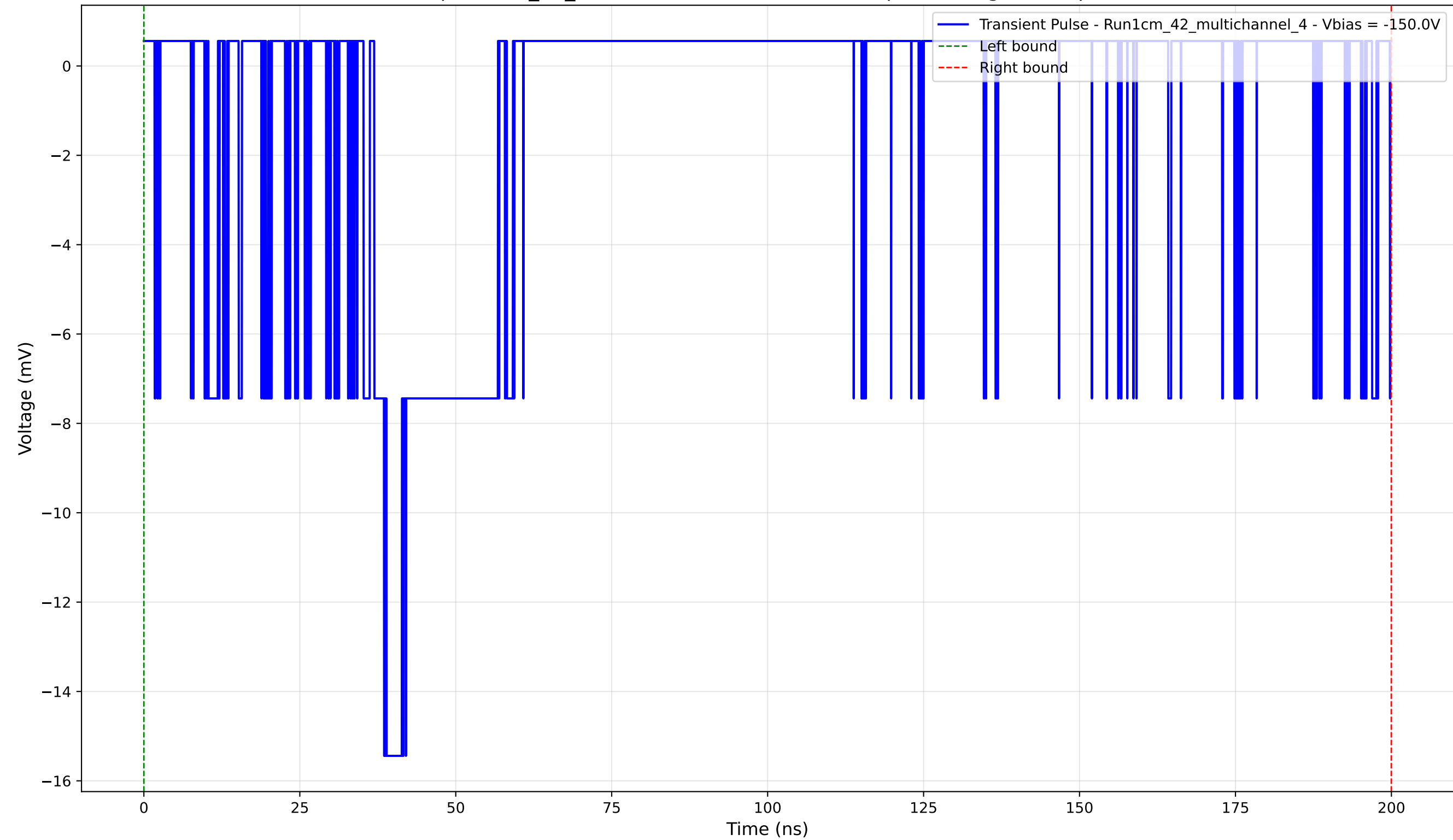
Transient Pulse - Sample: 1cm_42_multichannel - Position: 240.0 \mu\text{m} - Charge: 3.80 pC - Rise Time: 1.58 ns
