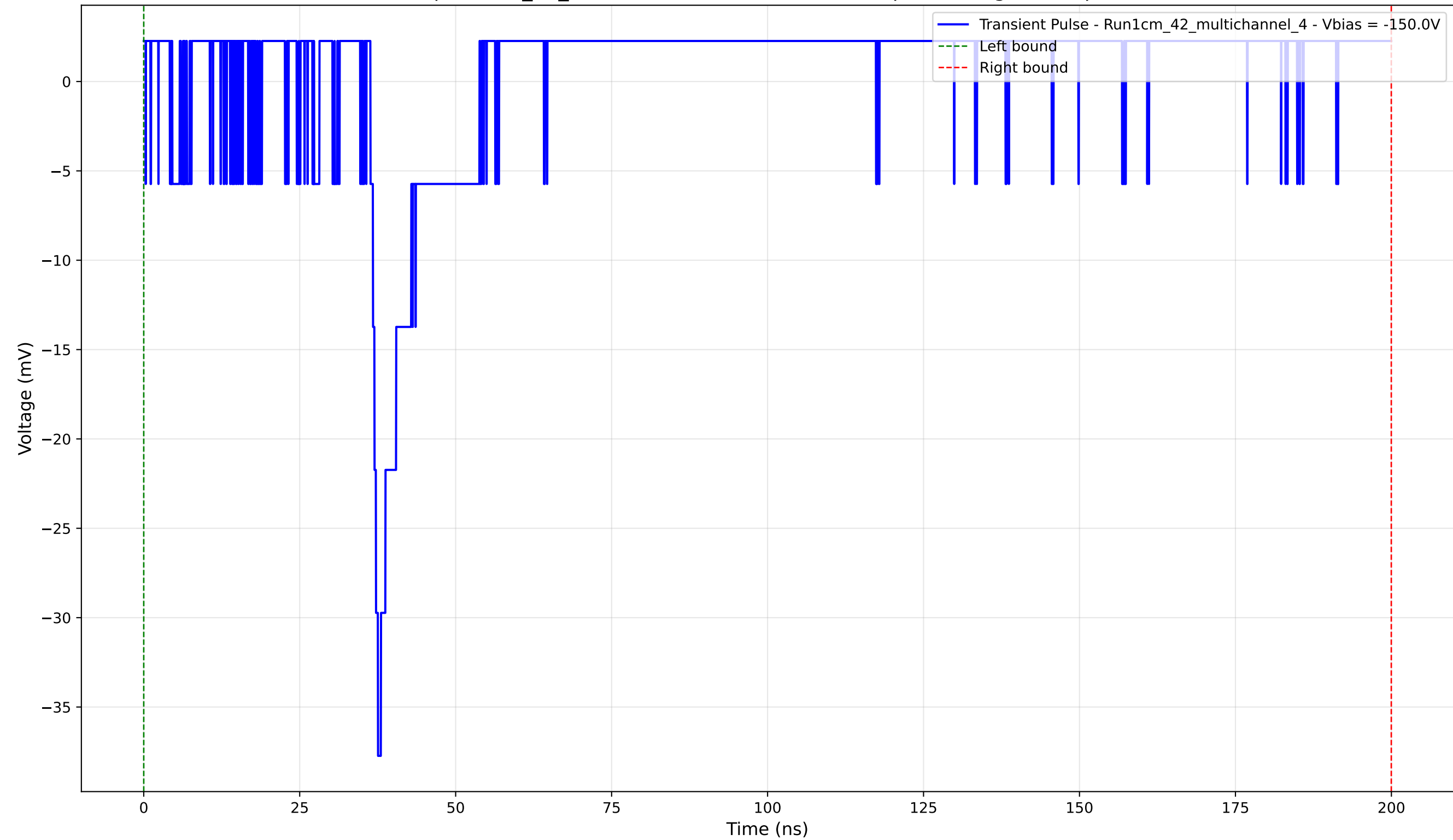
Transient Pulse - Sample: 1cm_42_multichannel - Position: 1670.0 \mu\text{m} - Charge: 2.47 pC - Rise Time: 1.21 ns
