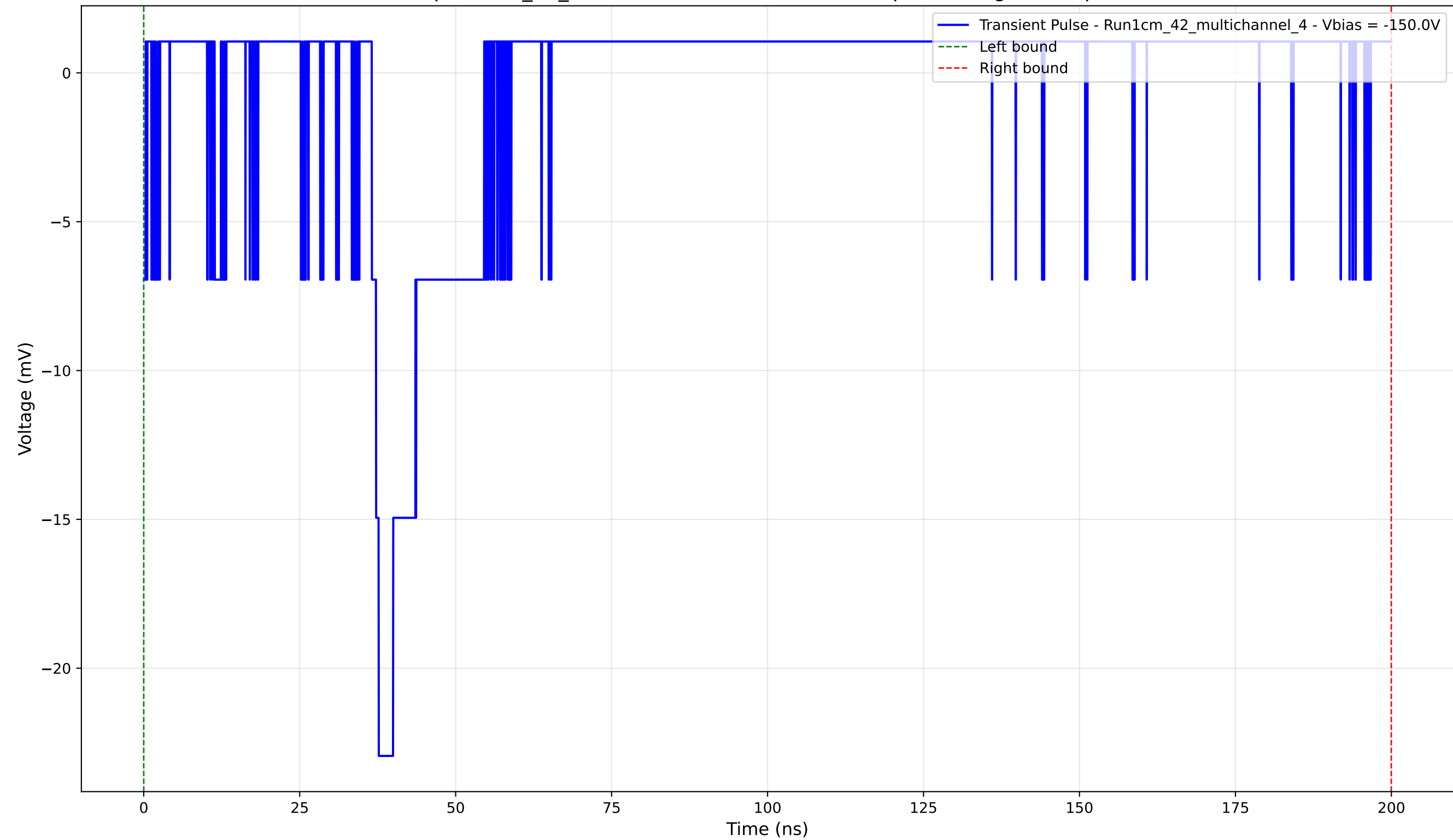
Transient Pulse - Sample: 1cm_42_multichannel - Position: 1230.0 \mu\text{m} - Charge: 1.59 pC - Rise Time: 1.12 ns
