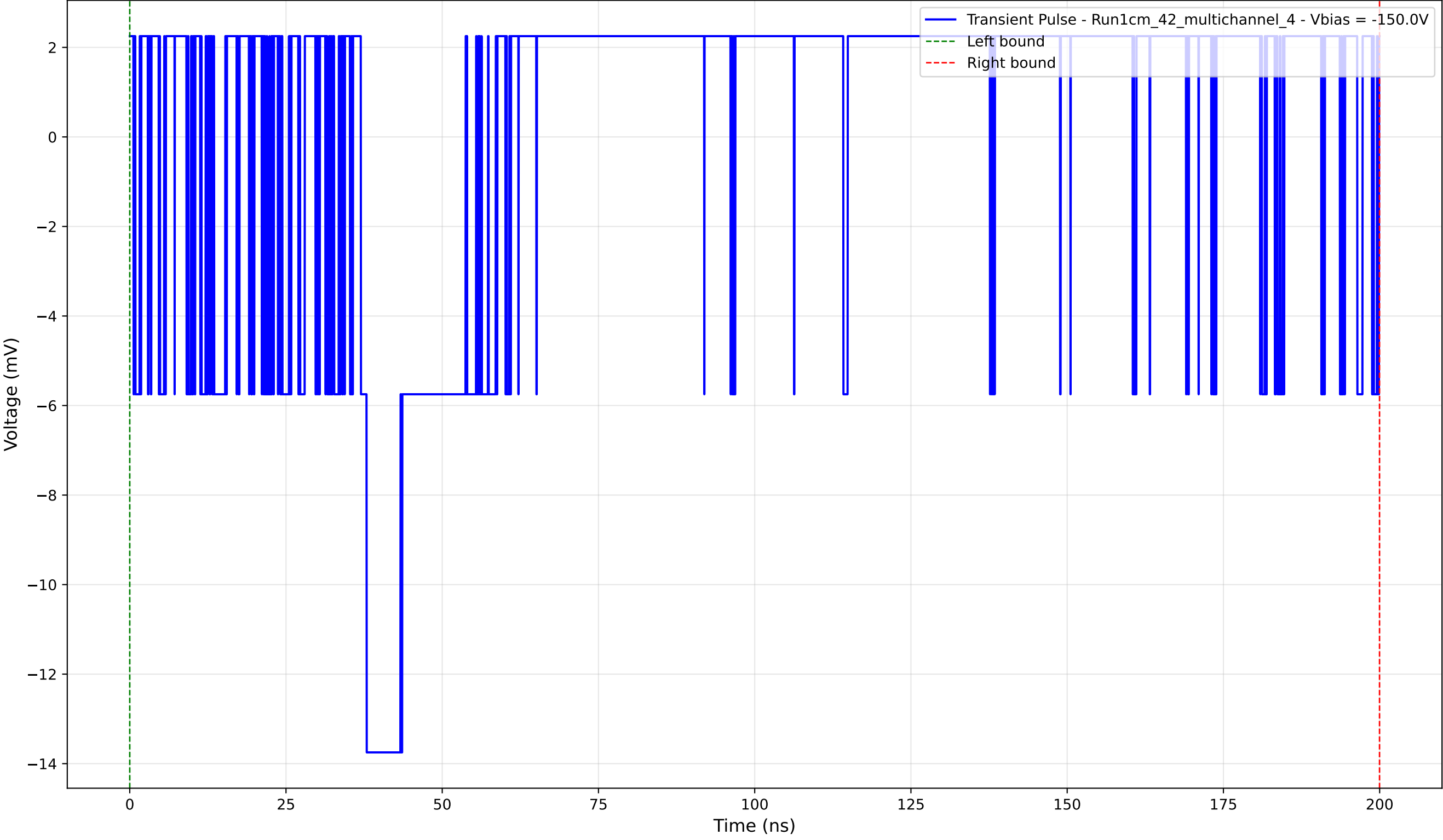
Transient Pulse - Sample: 1cm_42_multichannel - Position: 615.0 \mu\text{m} - Charge: 1.36 pC - Rise Time: 0.00 ns (N/A)
