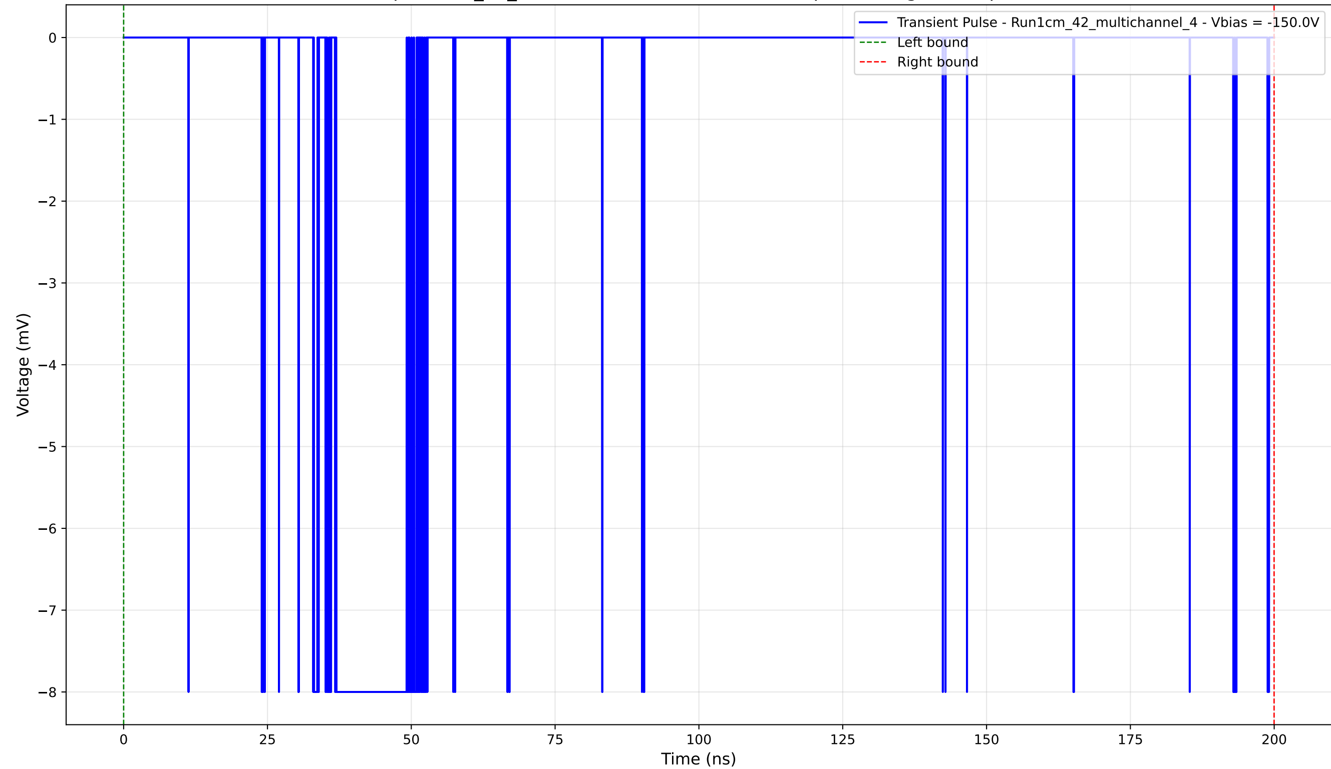
Transient Pulse - Sample: 1cm_42_multichannel - Position: 3955.0 \mu\text{m} - Charge: 2.86 pC - Rise Time: 0.02 ns
