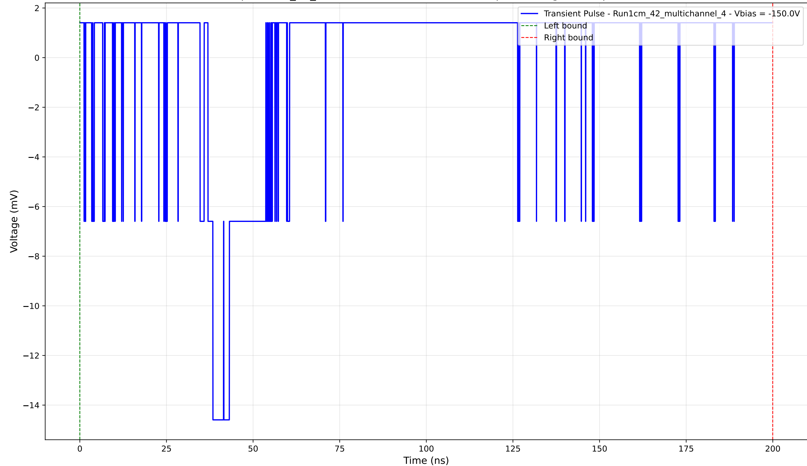
Transient Pulse - Sample: 1cm_42_multichannel - Position: 4155.0 \mu\text{m} - Charge: 0.85 pC - Rise Time: 1.44 ns
