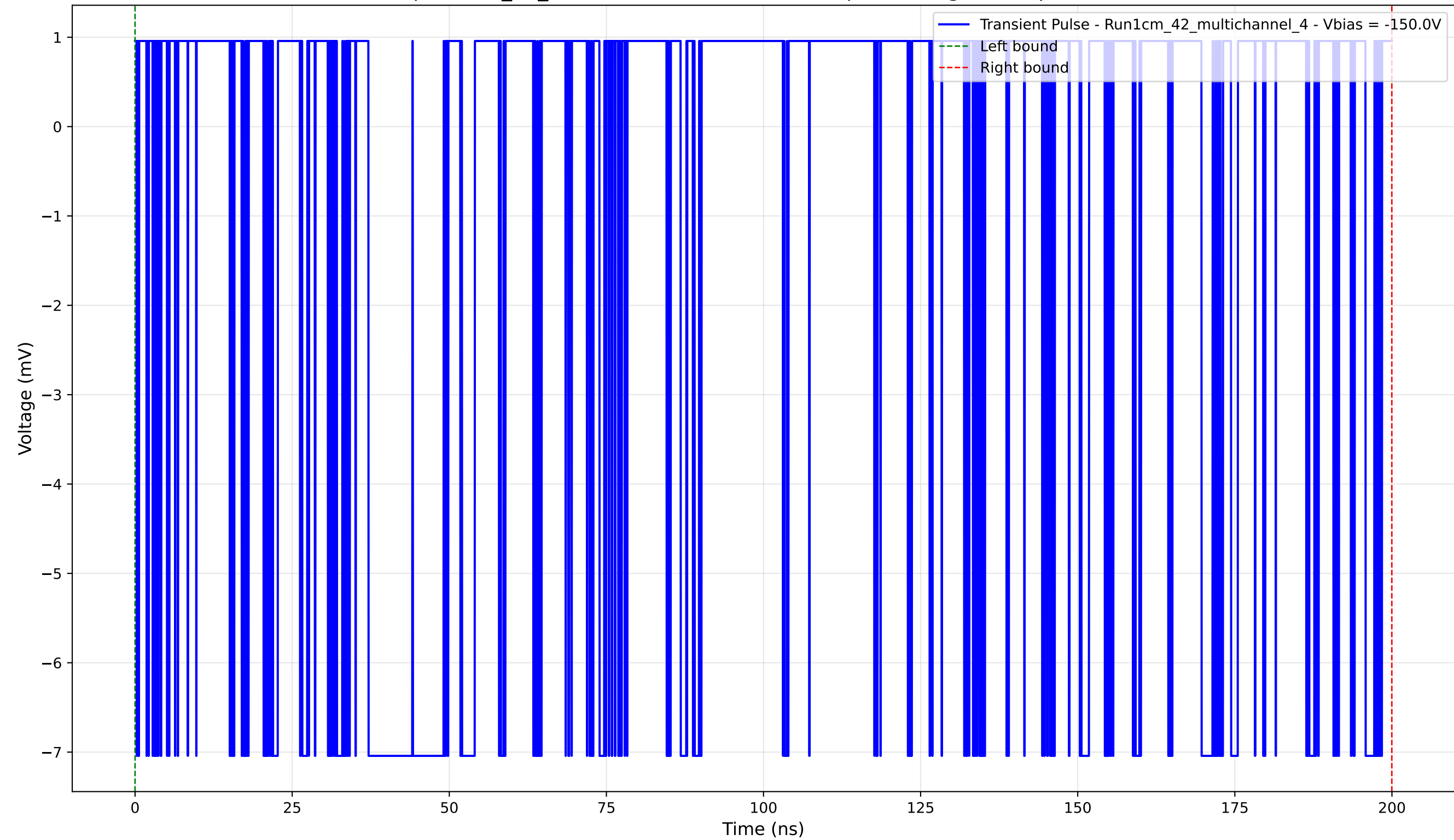
Transient Pulse - Sample: 1cm_42_multichannel - Position: 80.0 \mu\text{m} - Charge: 3.19 pC - Rise Time: 0.00 ns (N/A)
