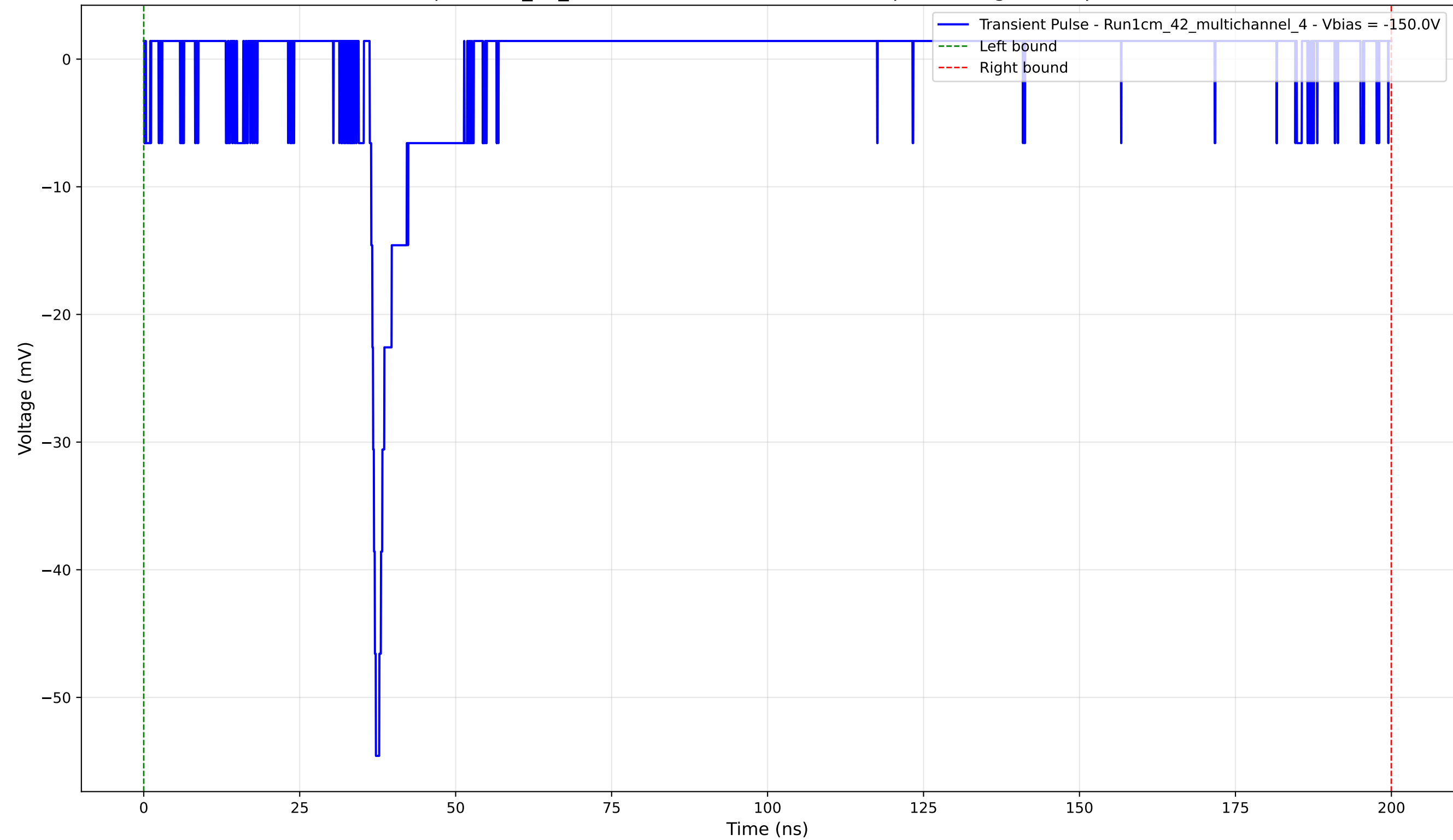
Transient Pulse - Sample: 1cm_42_multichannel - Position: 2755.0 \mu\text{m} - Charge: 0.75 pC - Rise Time: 0.98 ns
