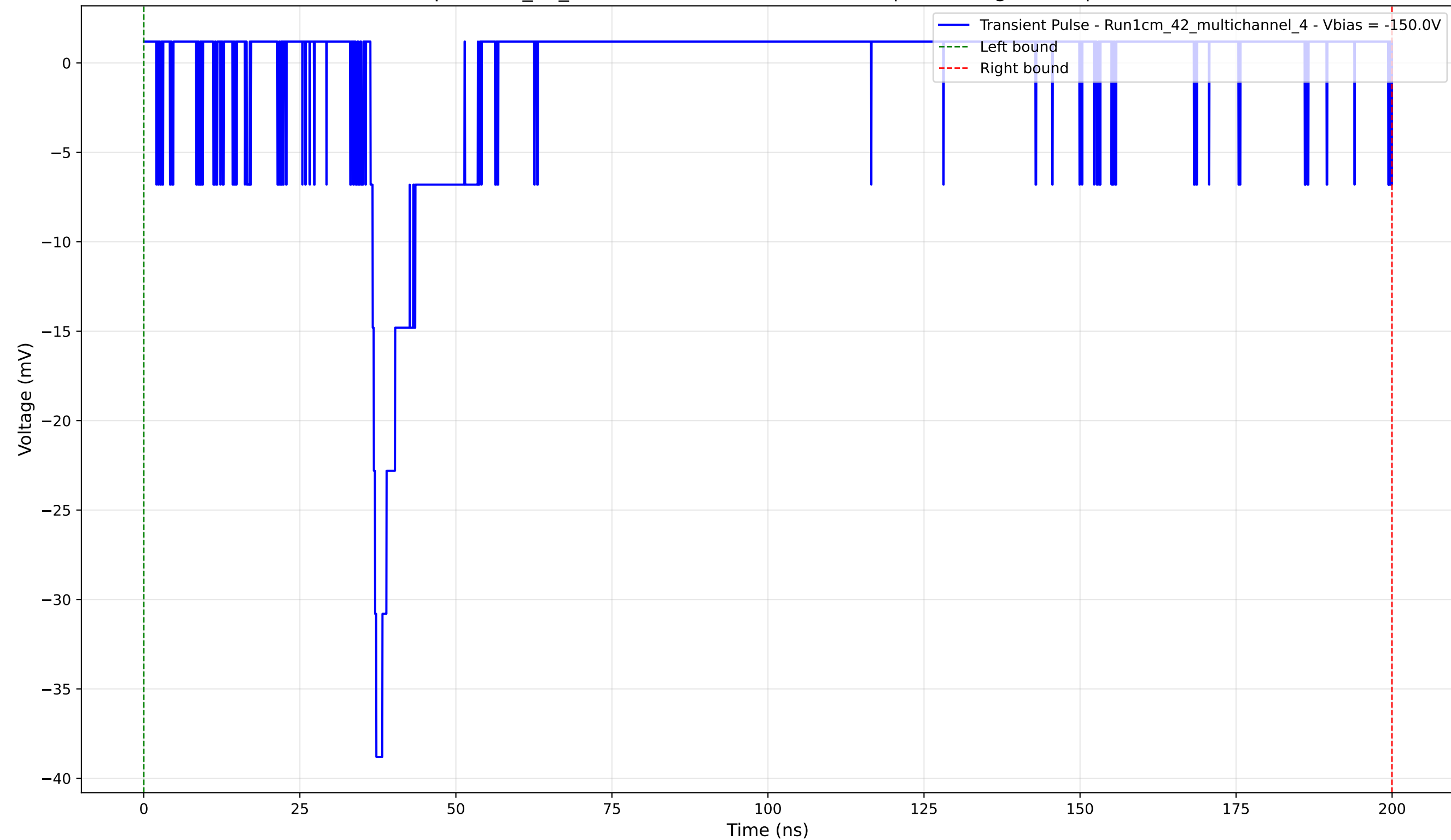
Transient Pulse - Sample: 1cm_42_multichannel - Position: 1760.0 \mu\text{m} - Charge: 1.47 pC - Rise Time: 0.93 ns
