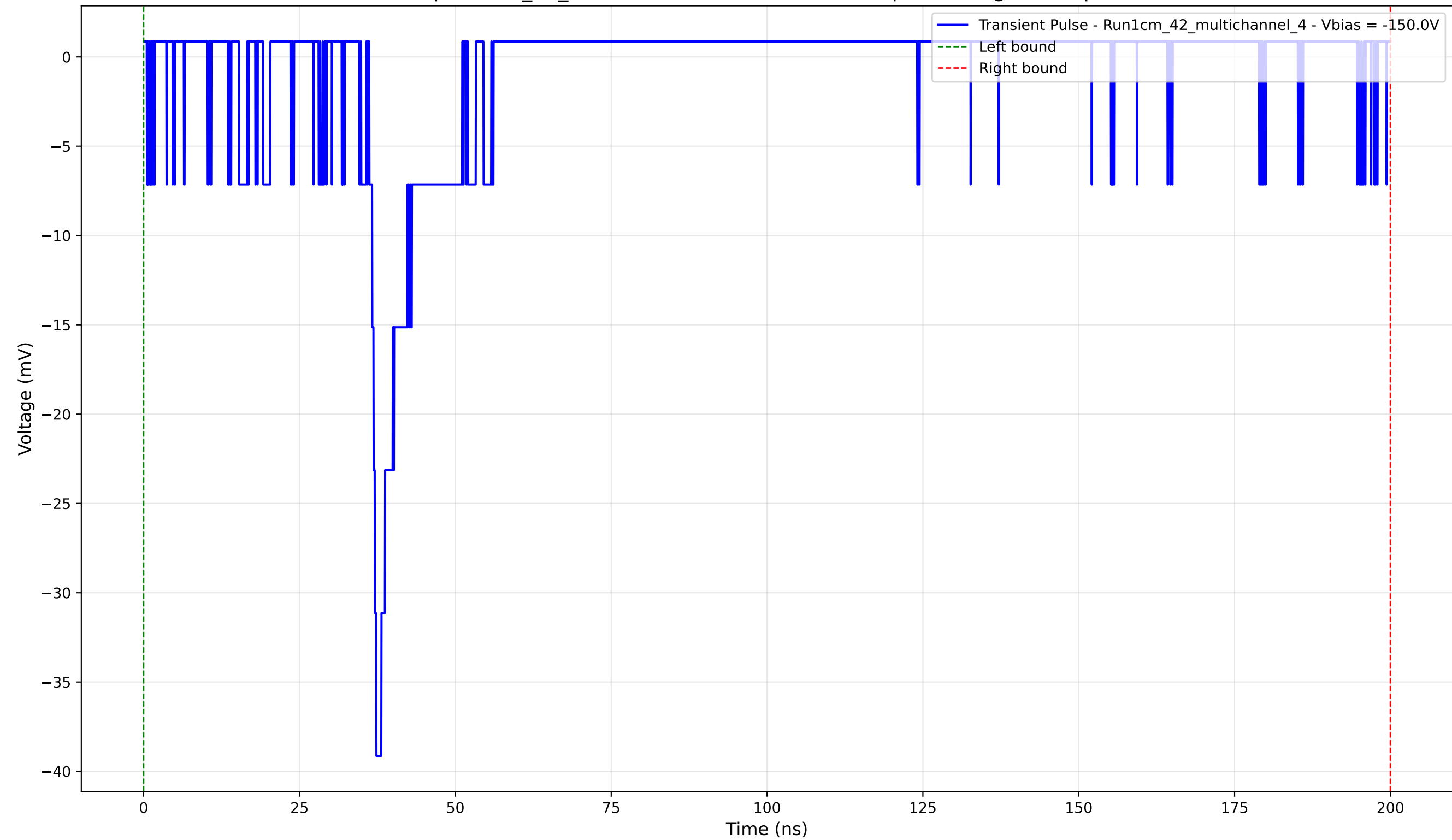
Transient Pulse - Sample: 1cm_42_multichannel - Position: 3000.0 \mu\text{m} - Charge: 2.89 pC - Rise Time: 1.13 ns
