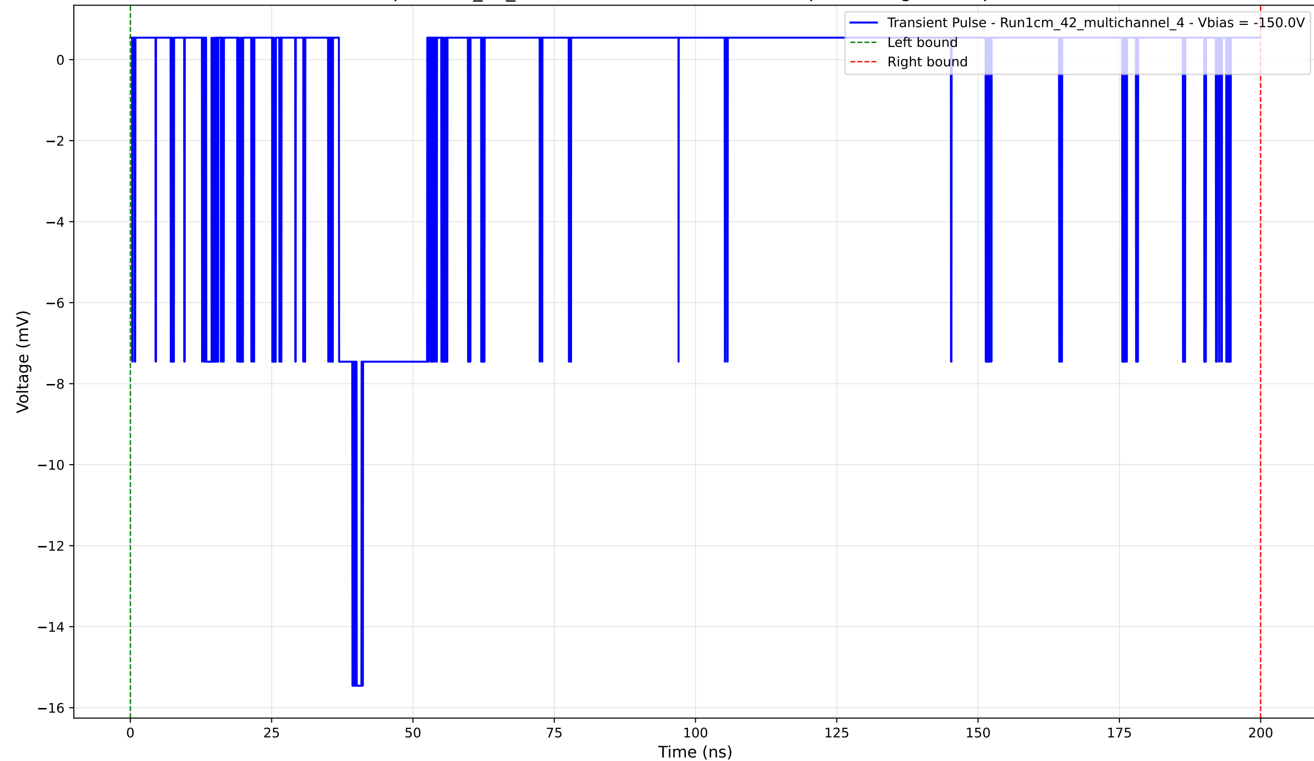
Transient Pulse - Sample: 1cm_42_multichannel - Position: 4810.0 \mu\text{m} - Charge: 2.10 pC - Rise Time: 2.38 ns
