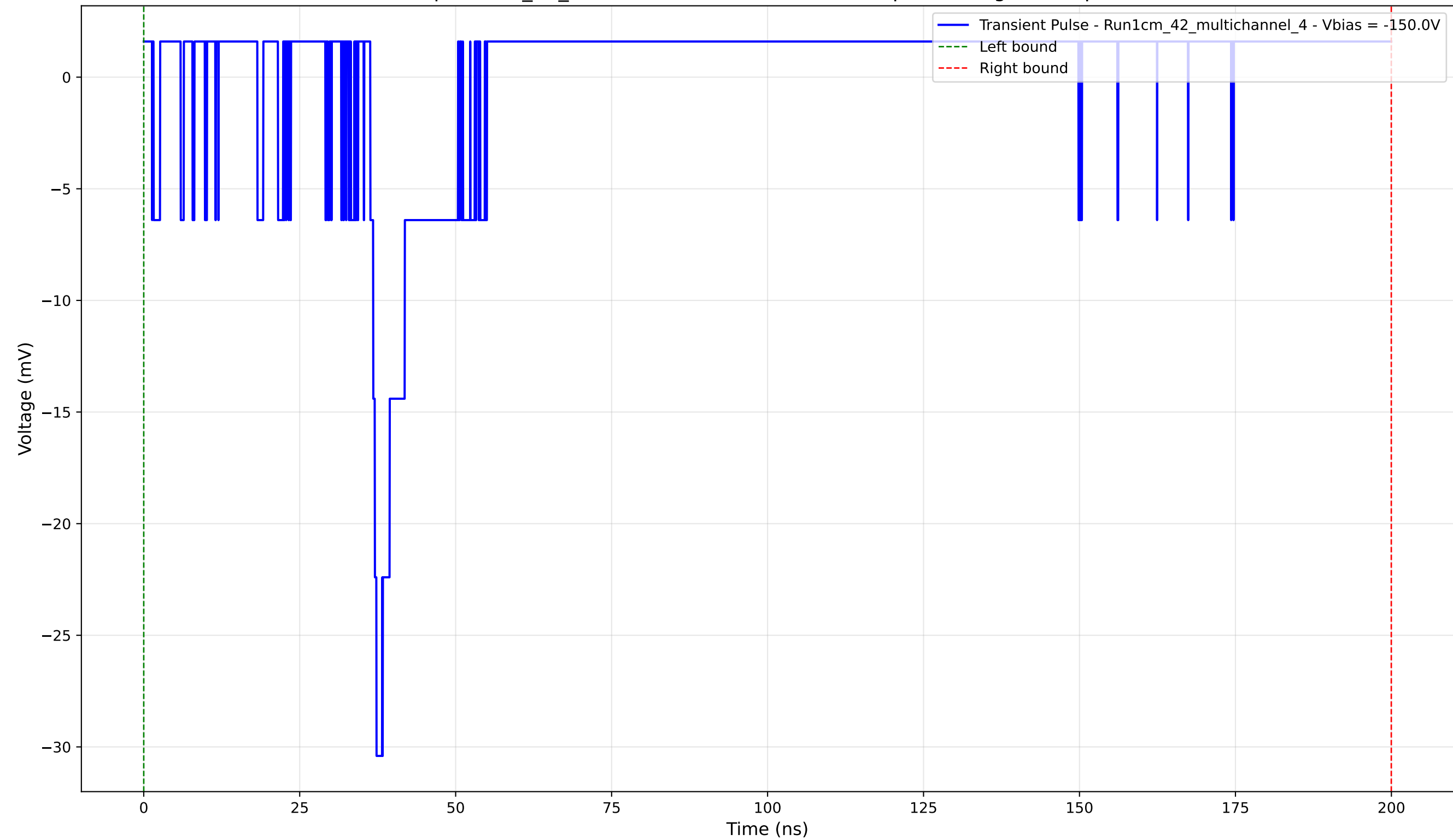
Transient Pulse - Sample: 1cm_42_multichannel - Position: 3080.0 \mu\text{m} - Charge: 1.17 pC - Rise Time: 0.99 ns
