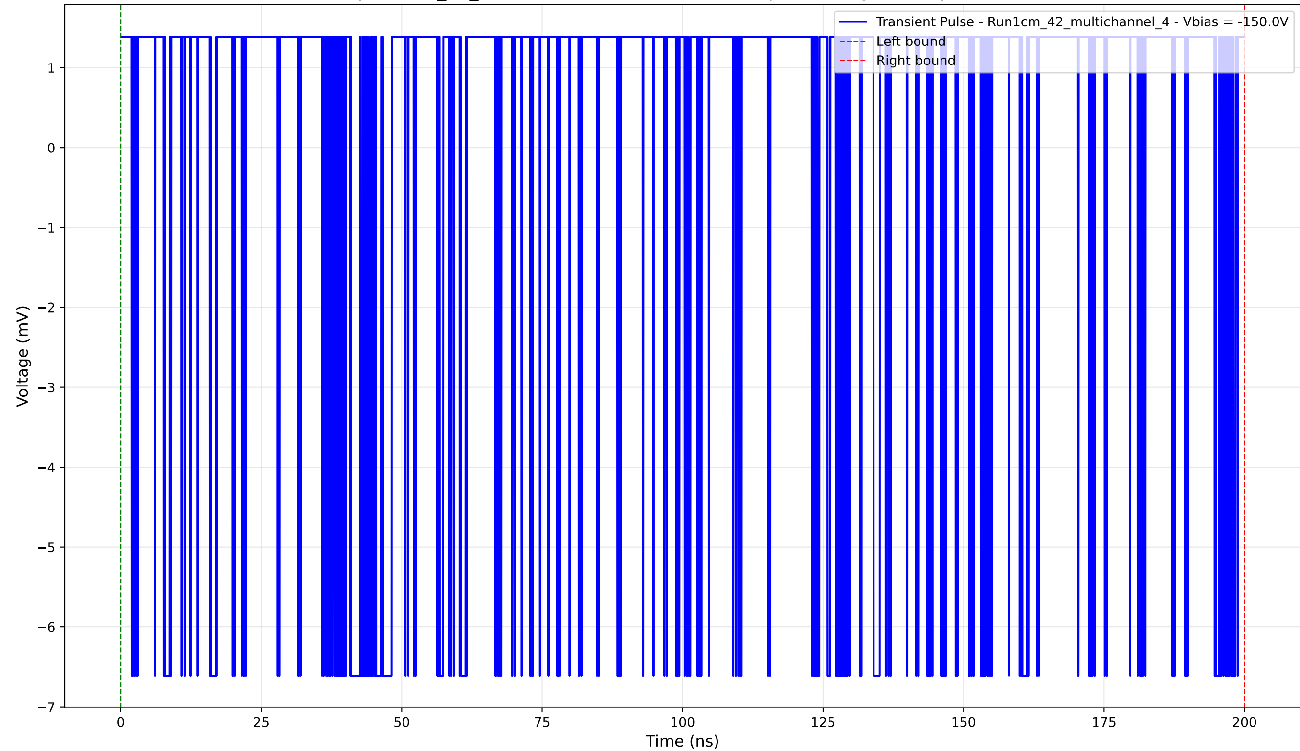
Transient Pulse - Sample: 1cm_42_multichannel - Position: 4380.0 \mu\text{m} - Charge: 0.19 pC - Rise Time: 0.00 ns (N/A)
