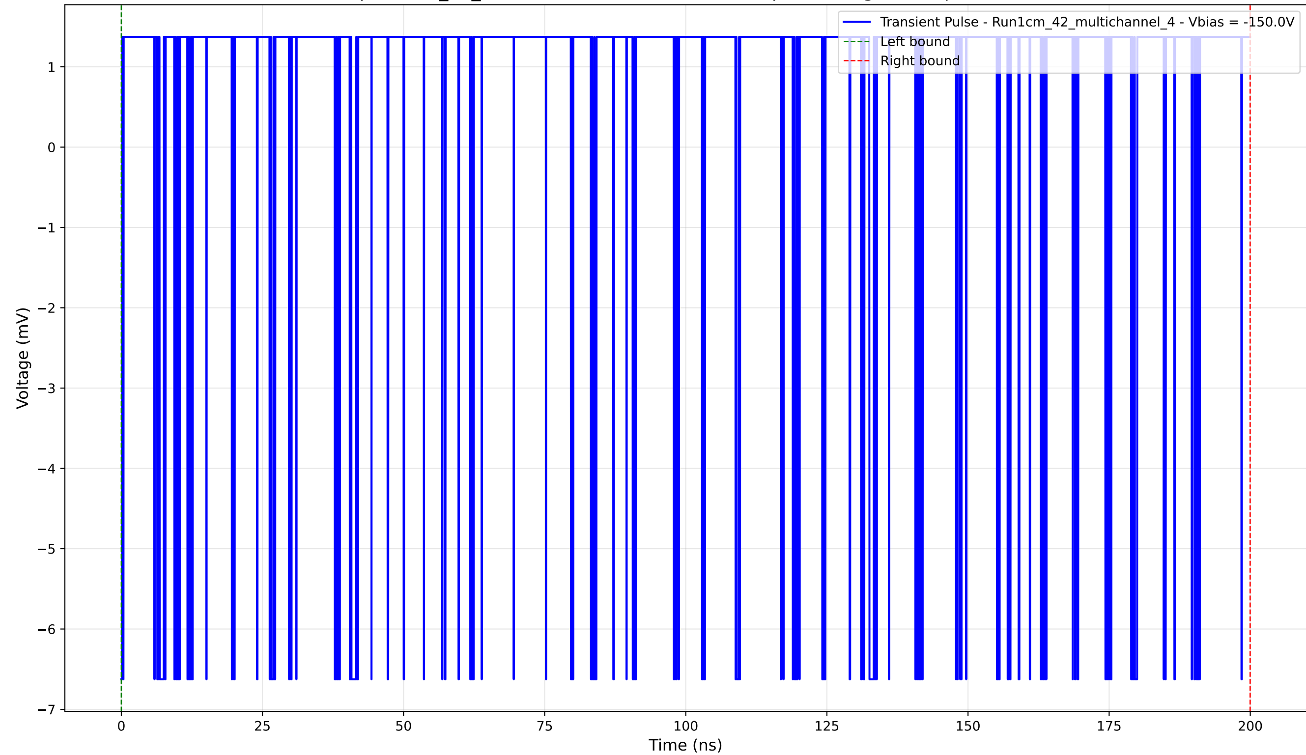
Transient Pulse - Sample: 1cm_42_multichannel - Position: 3910.0 \mu\text{m} - Charge: 2.68 pC - Rise Time: 0.00 ns (N/A)
