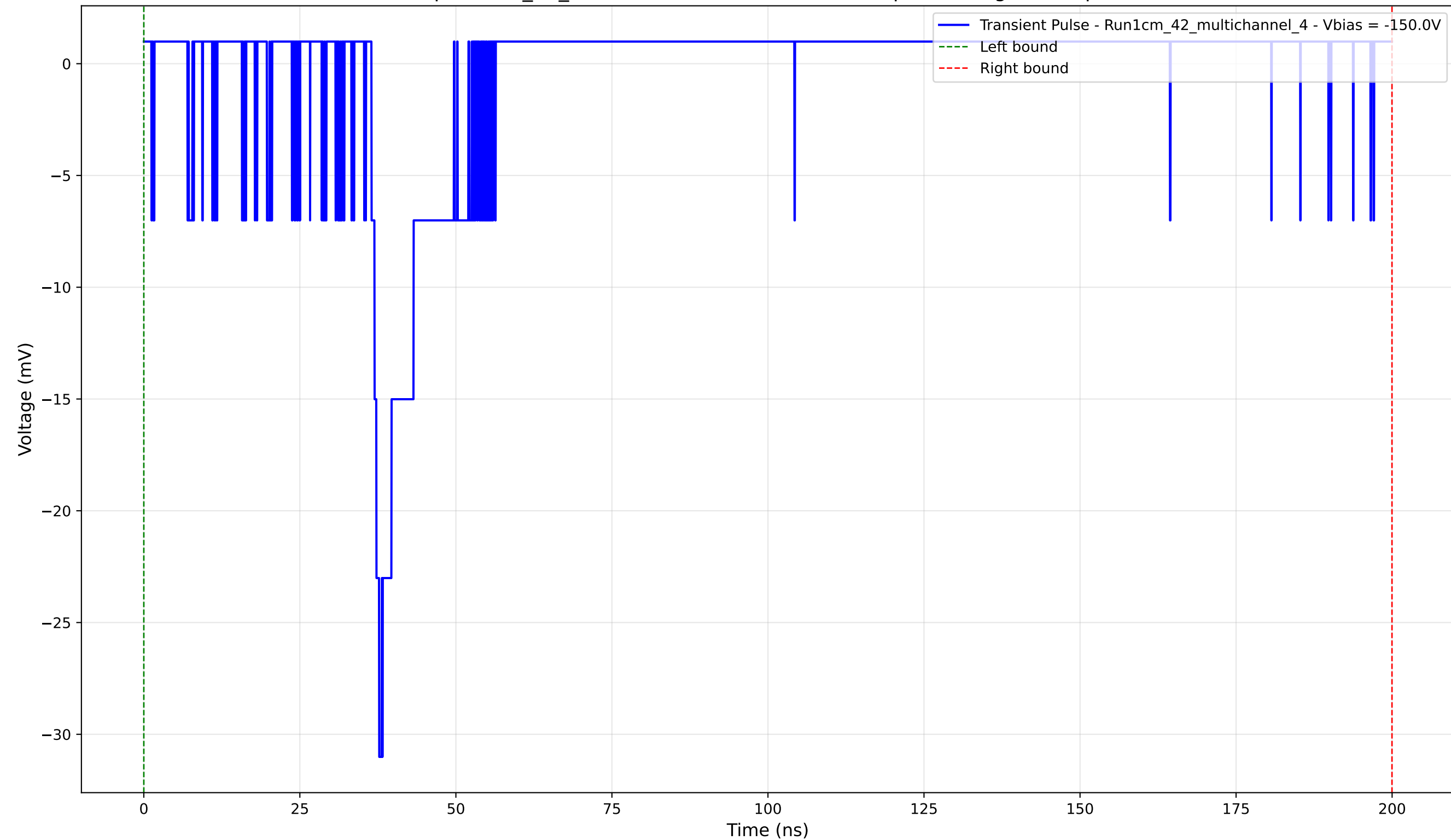
Transient Pulse - Sample: 1cm_42_multichannel - Position: 3250.0 \mu\text{m} - Charge: 1.22 pC - Rise Time: 1.23 ns
