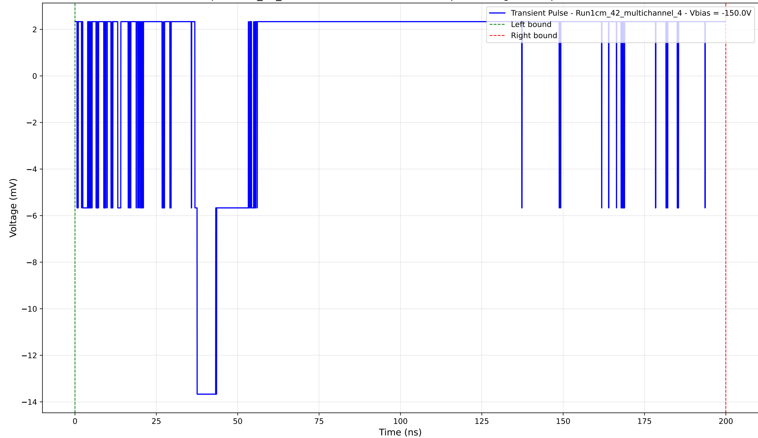
Transient Pulse - Sample: 1cm_42_multichannel - Position: 3675.0 \mu\text{m} - Charge: 4.21 pC - Rise Time: 0.00 ns (N/A)
