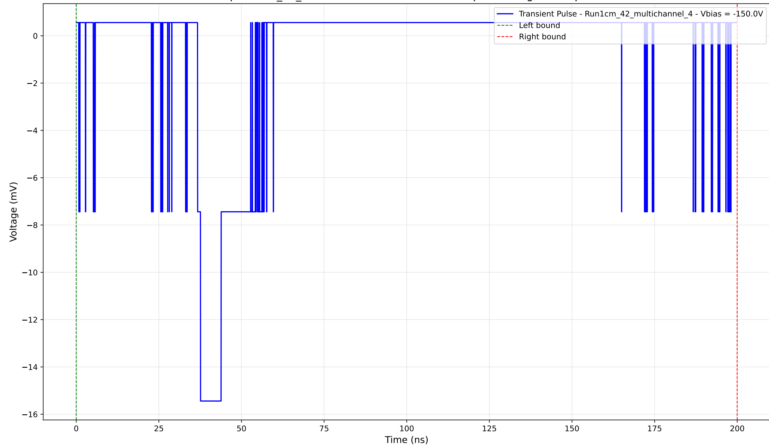
Transient Pulse - Sample: 1cm_42_multichannel - Position: 3775.0 \mu\text{m} - Charge: 2.48 pC - Rise Time: 0.90 ns
