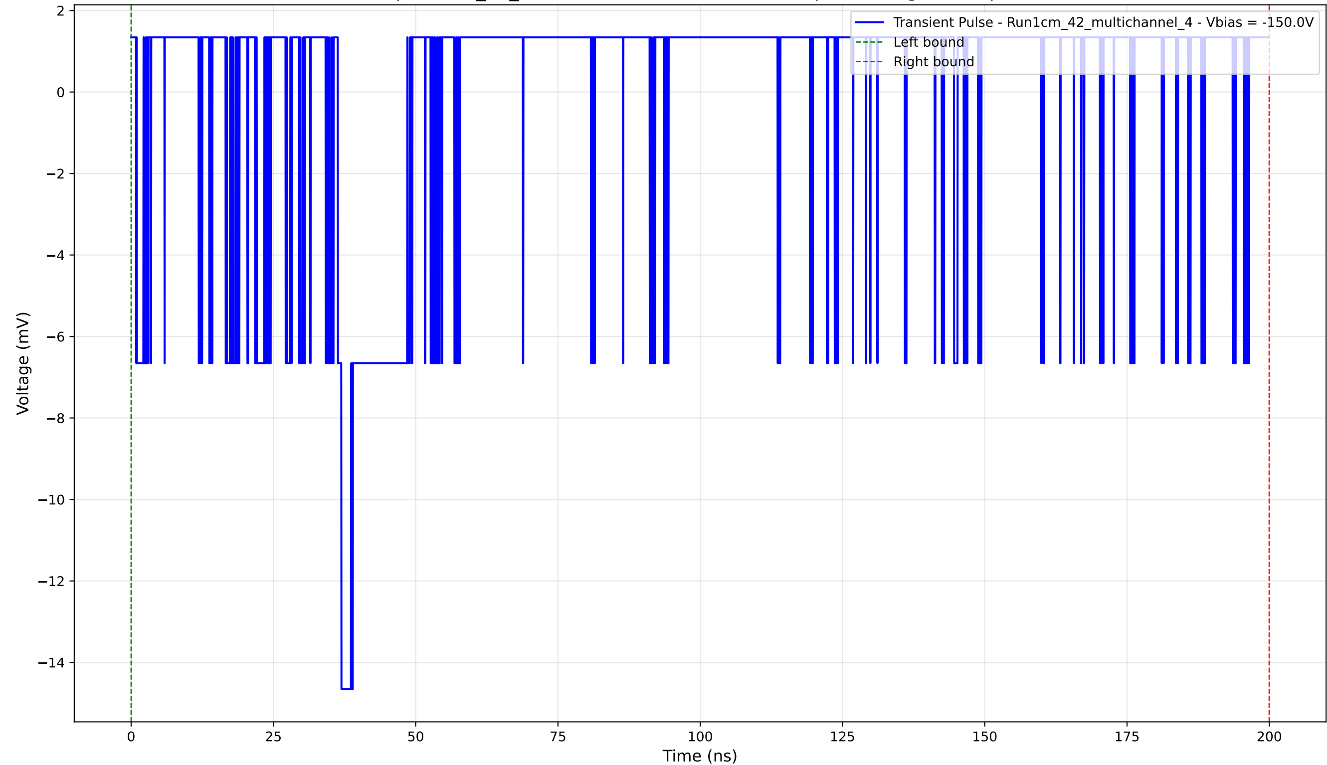
Transient Pulse - Sample: 1cm_42_multichannel - Position: 2940.0 \mu\text{m} - Charge: 0.24 pC - Rise Time: 0.64 ns
