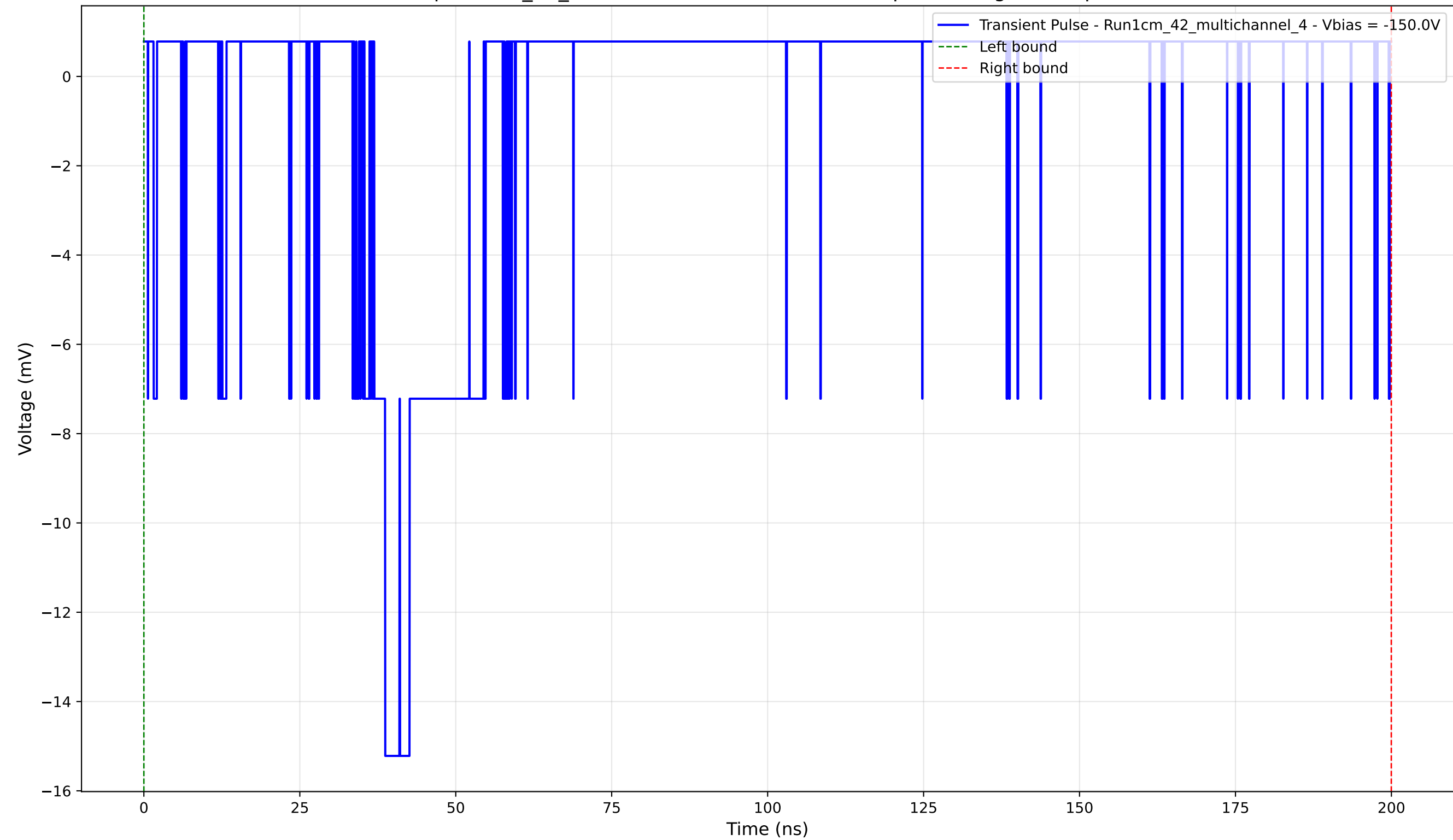
Transient Pulse - Sample: 1cm_42_multichannel - Position: 4640.0 \mu\text{m} - Charge: 1.52 pC - Rise Time: 1.76 ns
