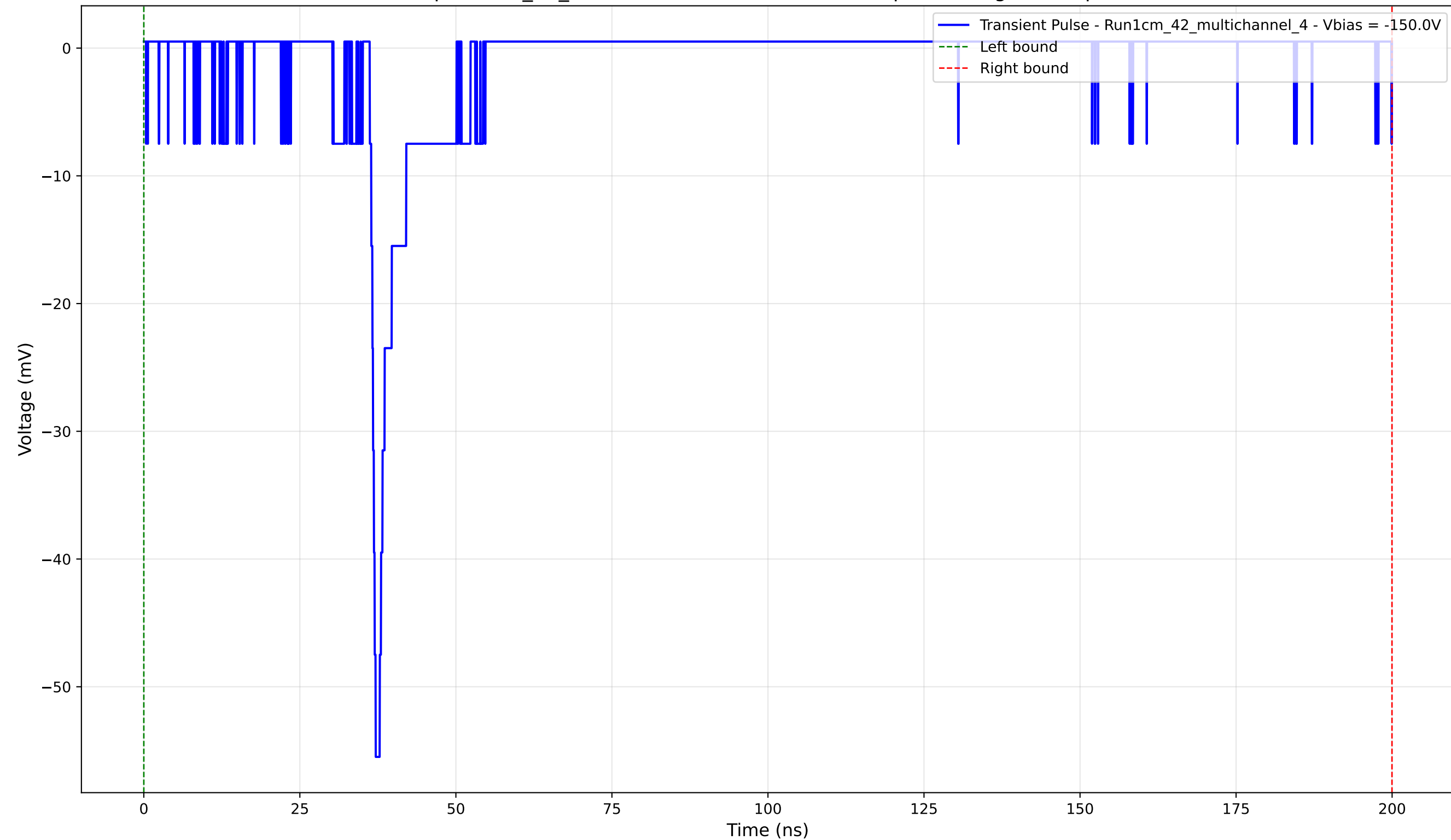
Transient Pulse - Sample: 1cm_42_multichannel - Position: 2055.0 \mu\text{m} - Charge: 4.00 pC - Rise Time: 0.95 ns
