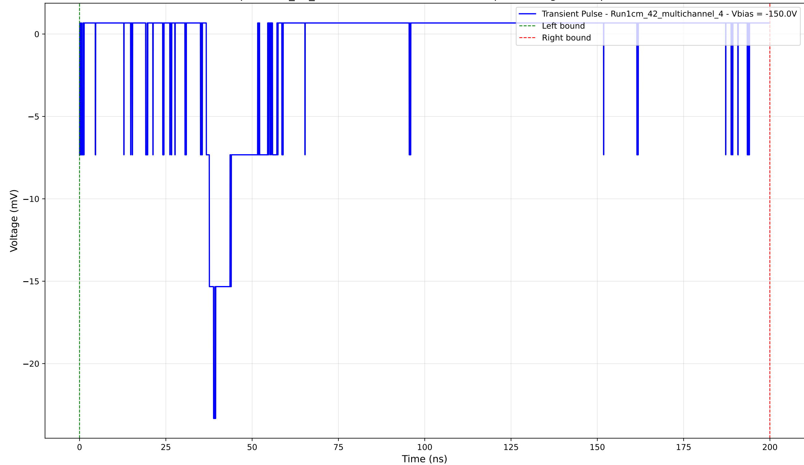
Transient Pulse - Sample: 1cm_42_multichannel - Position: 3740.0 \mu\text{m} - Charge: 2.12 pC - Rise Time: 2.12 ns
