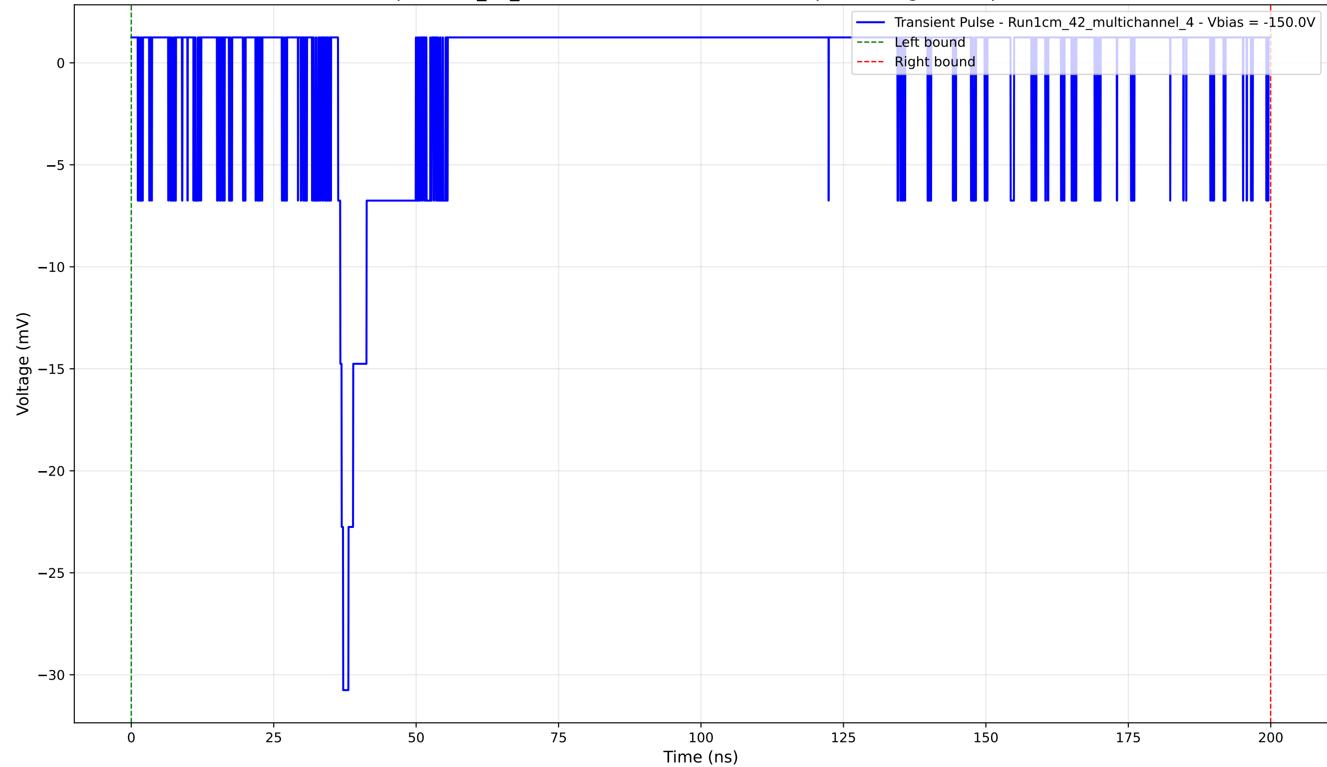
Transient Pulse - Sample: 1cm_42_multichannel - Position: 1820.0 \mu\text{m} - Charge: 1.13 pC - Rise Time: 0.89 ns
