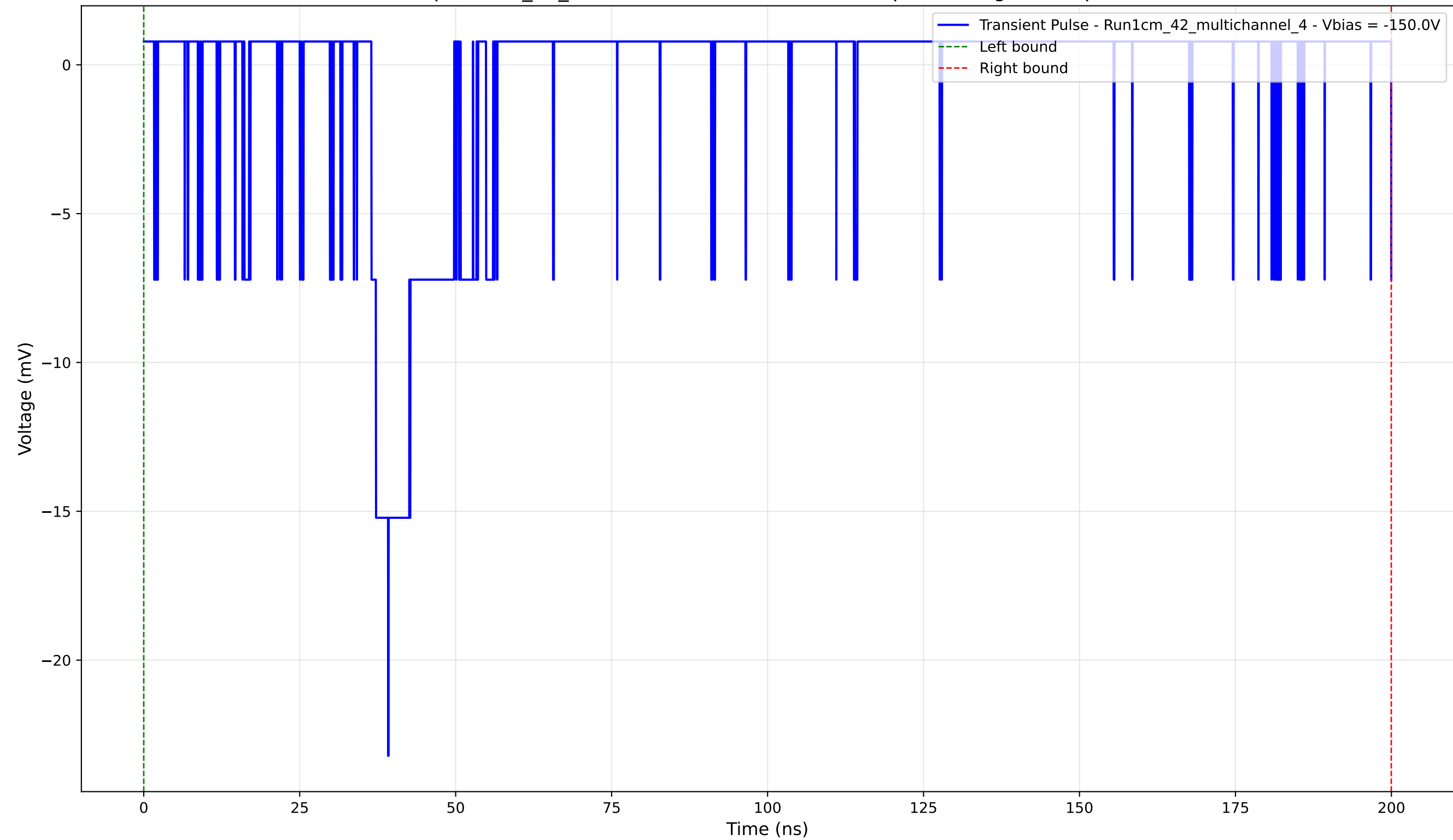
Transient Pulse - Sample: 1cm_42_multichannel - Position: 3470.0 \mu\text{m} - Charge: 1.64 pC - Rise Time: 2.70 ns
