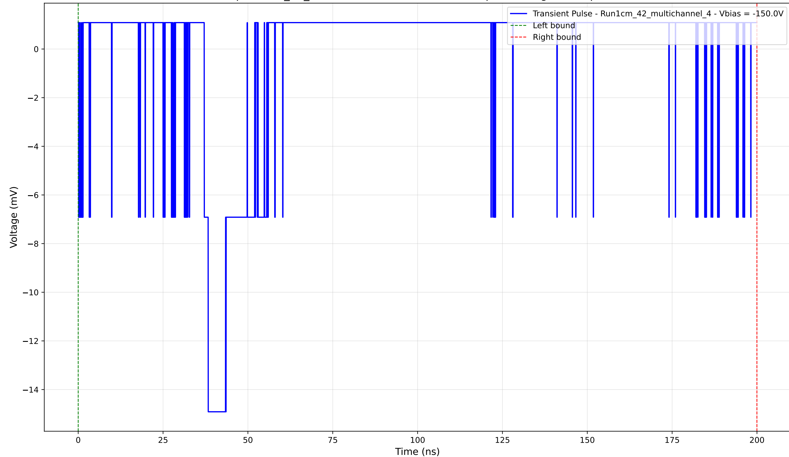
Transient Pulse - Sample: 1cm_42_multichannel - Position: 4205.0 \mu\text{m} - Charge: 0.37 pC - Rise Time: 1.18 ns
