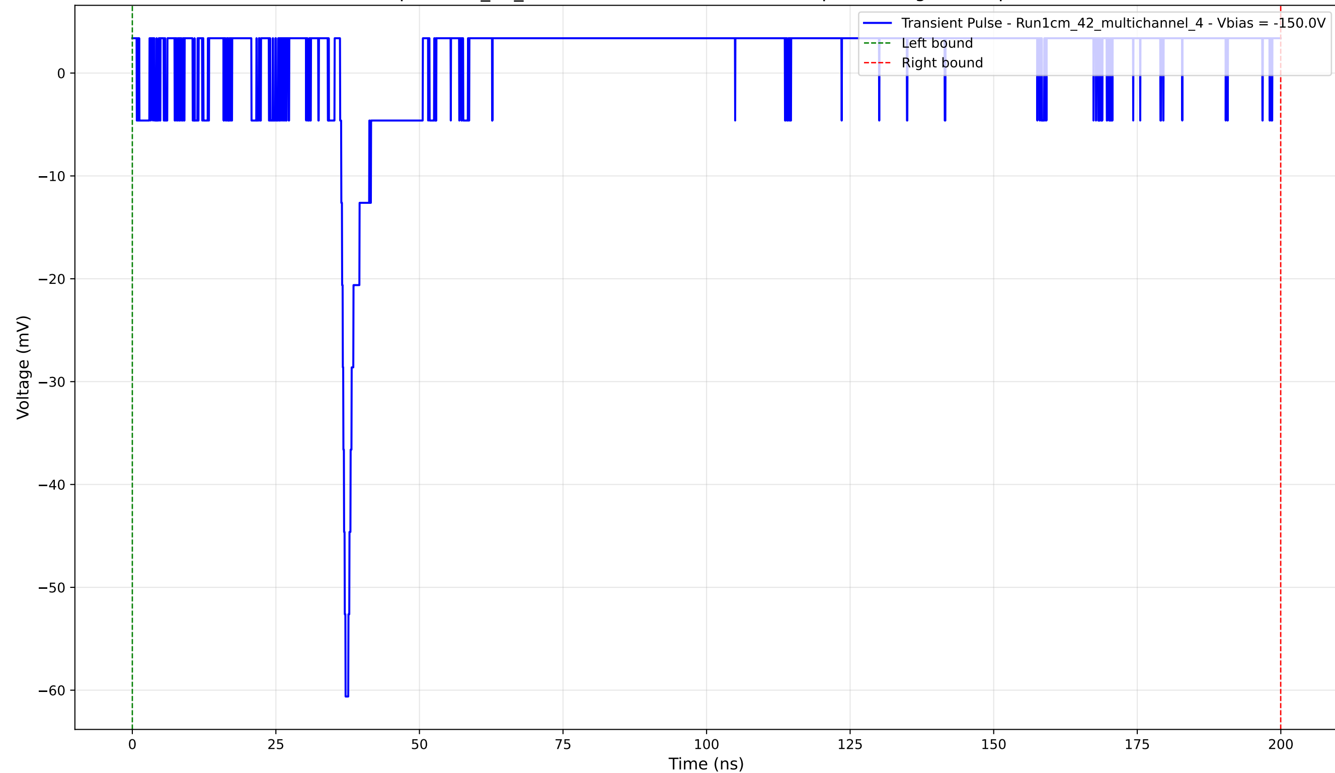
Transient Pulse - Sample: 1cm_42_multichannel - Position: 2620.0 \mu\text{m} - Charge: 6.21 pC - Rise Time: 0.76 ns
