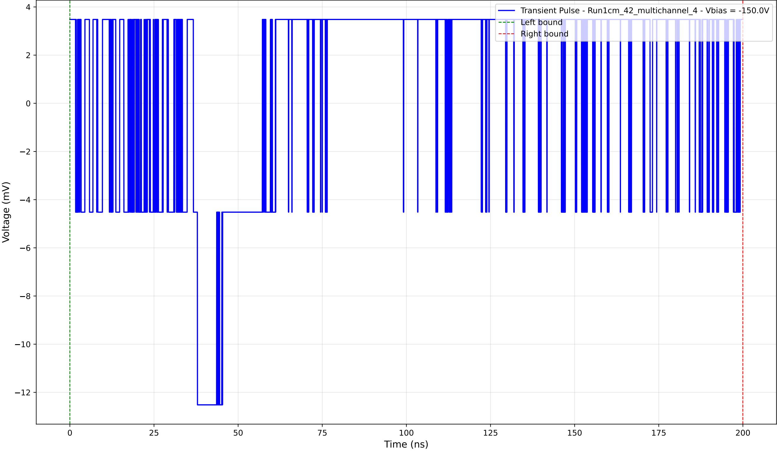
Transient Pulse - Sample: 1cm_42_multichannel - Position: 760.0 \mu\text{m} - Charge: 4.34 pC - Rise Time: 0.00 ns (N/A)
