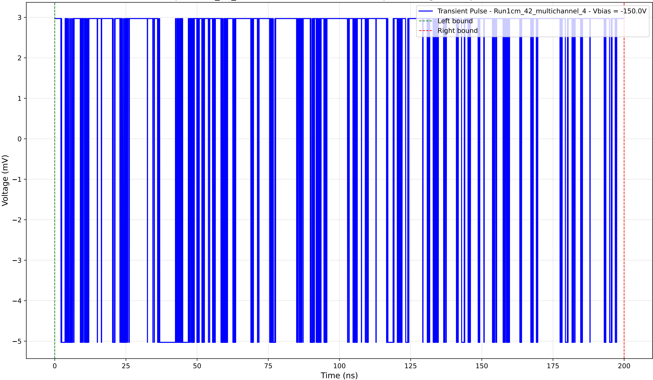
Transient Pulse - Sample: 1cm_42_multichannel - Position: 3425.0 \mu\text{m} - Charge: 5.10 pC - Rise Time: 0.00 ns (N/A)
