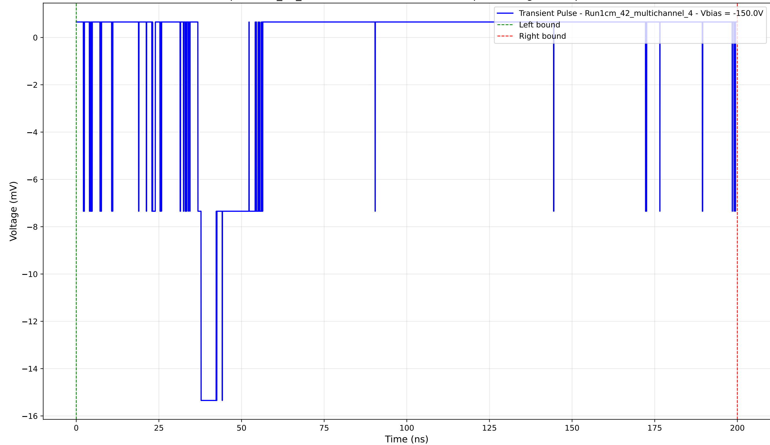
Transient Pulse - Sample: 1cm_42_multichannel - Position: 3815.0 \mu\text{m} - Charge: 1.76 pC - Rise Time: 0.98 ns
