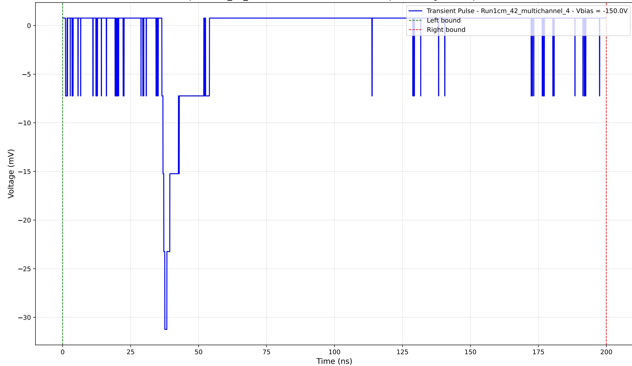
Transient Pulse - Sample: 1cm_42_multichannel - Position: 3200.0 \mu\text{m} - Charge: 1.85 pC - Rise Time: 1.09 ns
