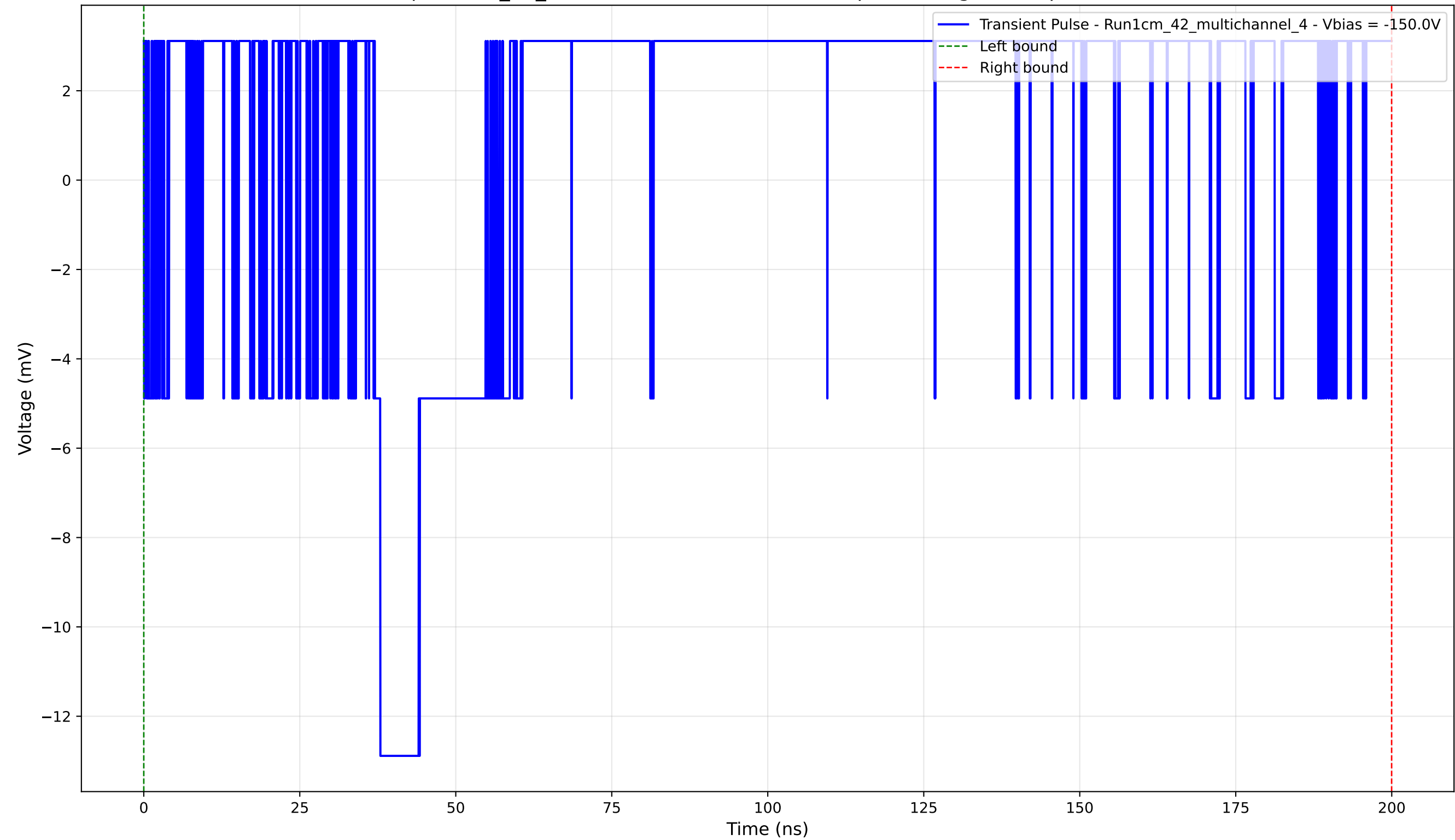
Transient Pulse - Sample: 1cm_42_multichannel - Position: 630.0 \mu\text{m} - Charge: 4.86 pC - Rise Time: 0.00 ns (N/A)
