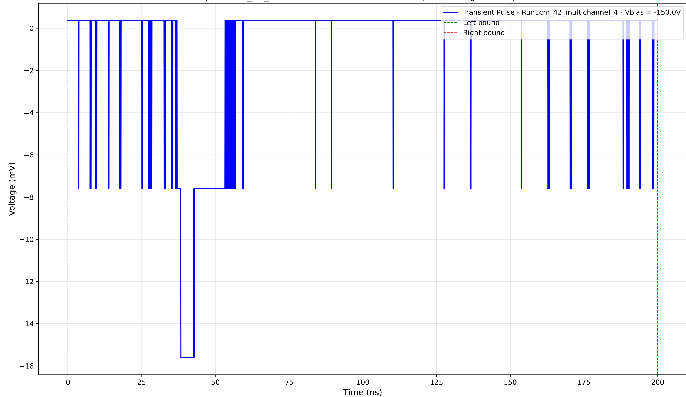
Transient Pulse - Sample: 1cm_42_multichannel - Position: 4275.0 \mu\text{m} - Charge: 2.69 pC - Rise Time: 1.36 ns
