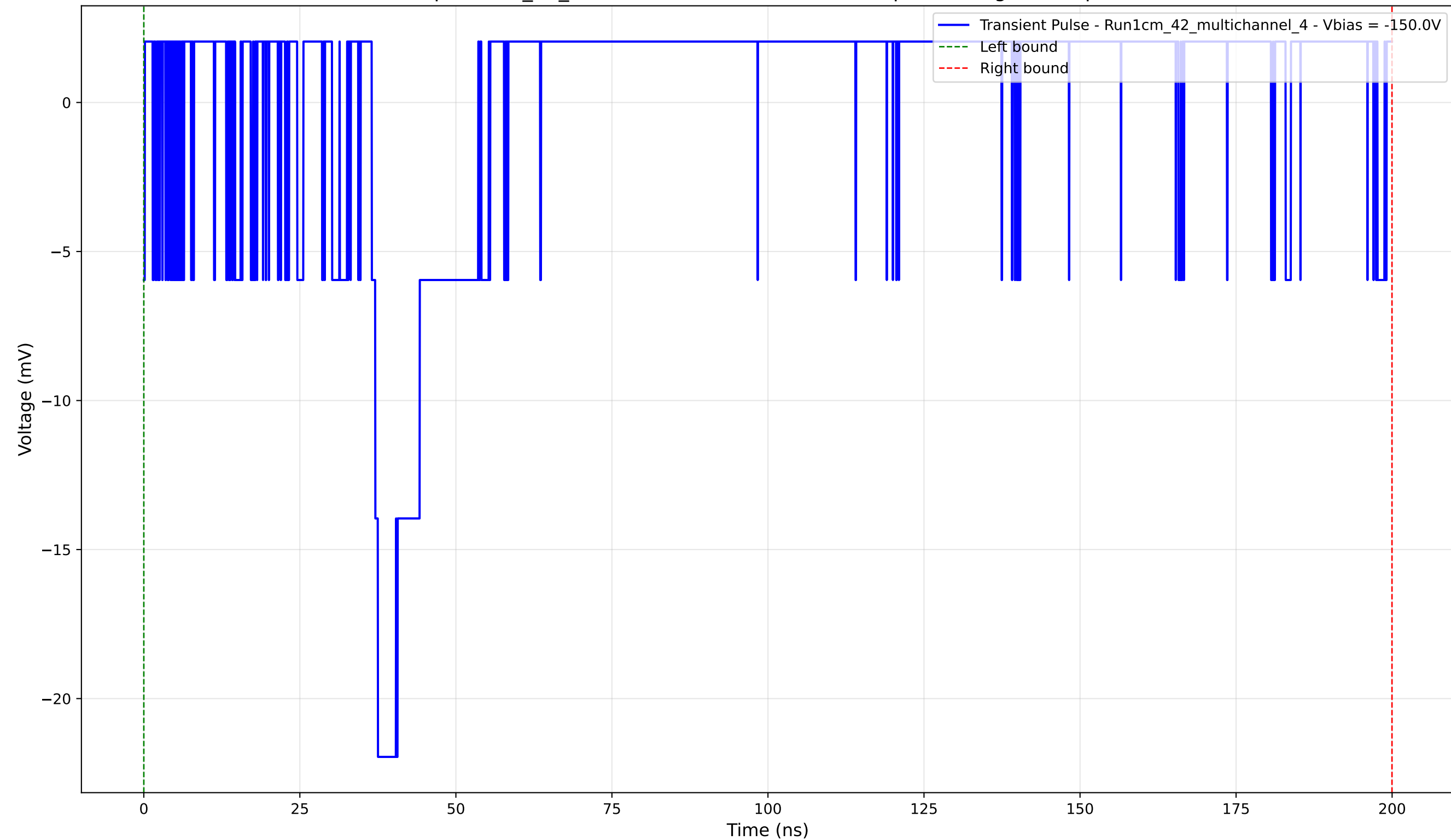
Transient Pulse - Sample: 1cm_42_multichannel - Position: 1285.0 \mu\text{m} - Charge: 1.08 pC - Rise Time: 1.00 ns
