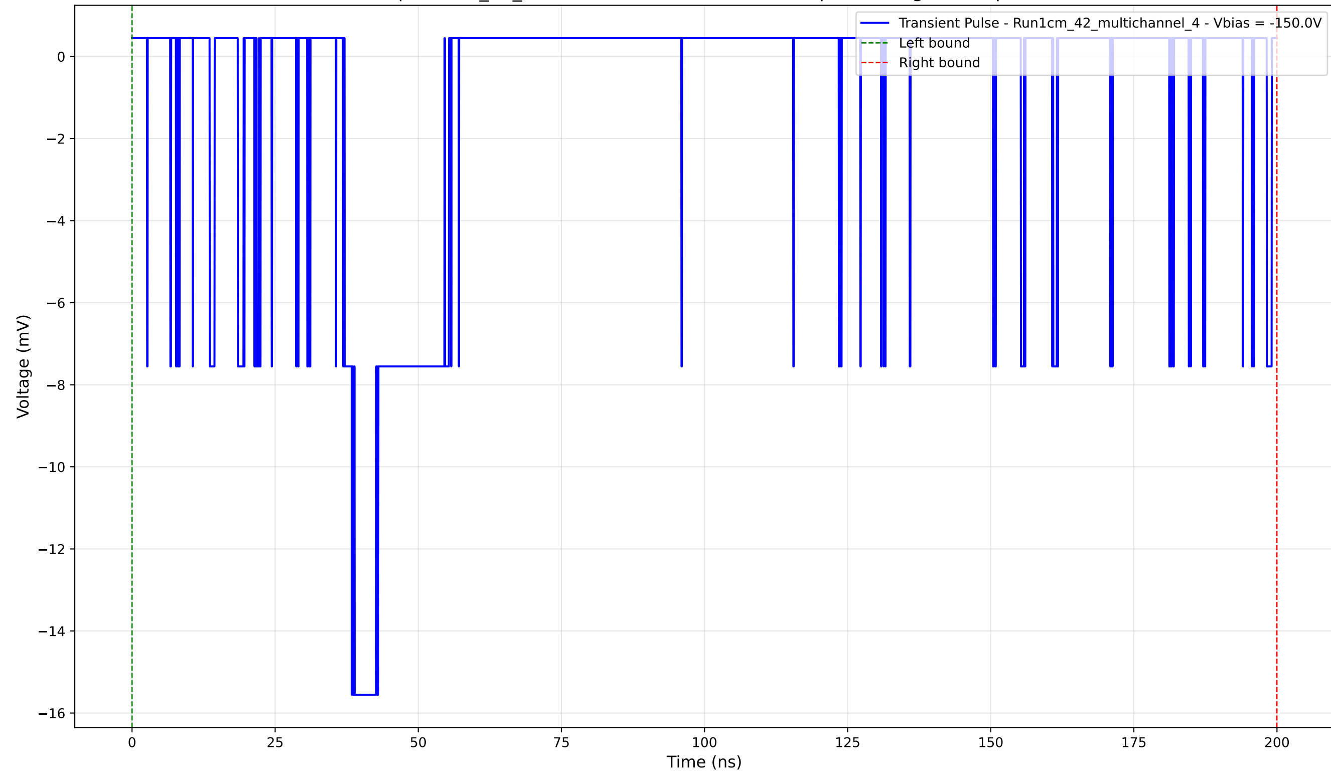
Transient Pulse - Sample: 1cm_42_multichannel - Position: 4700.0 \mu\text{m} - Charge: 3.13 pC - Rise Time: 1.28 ns
