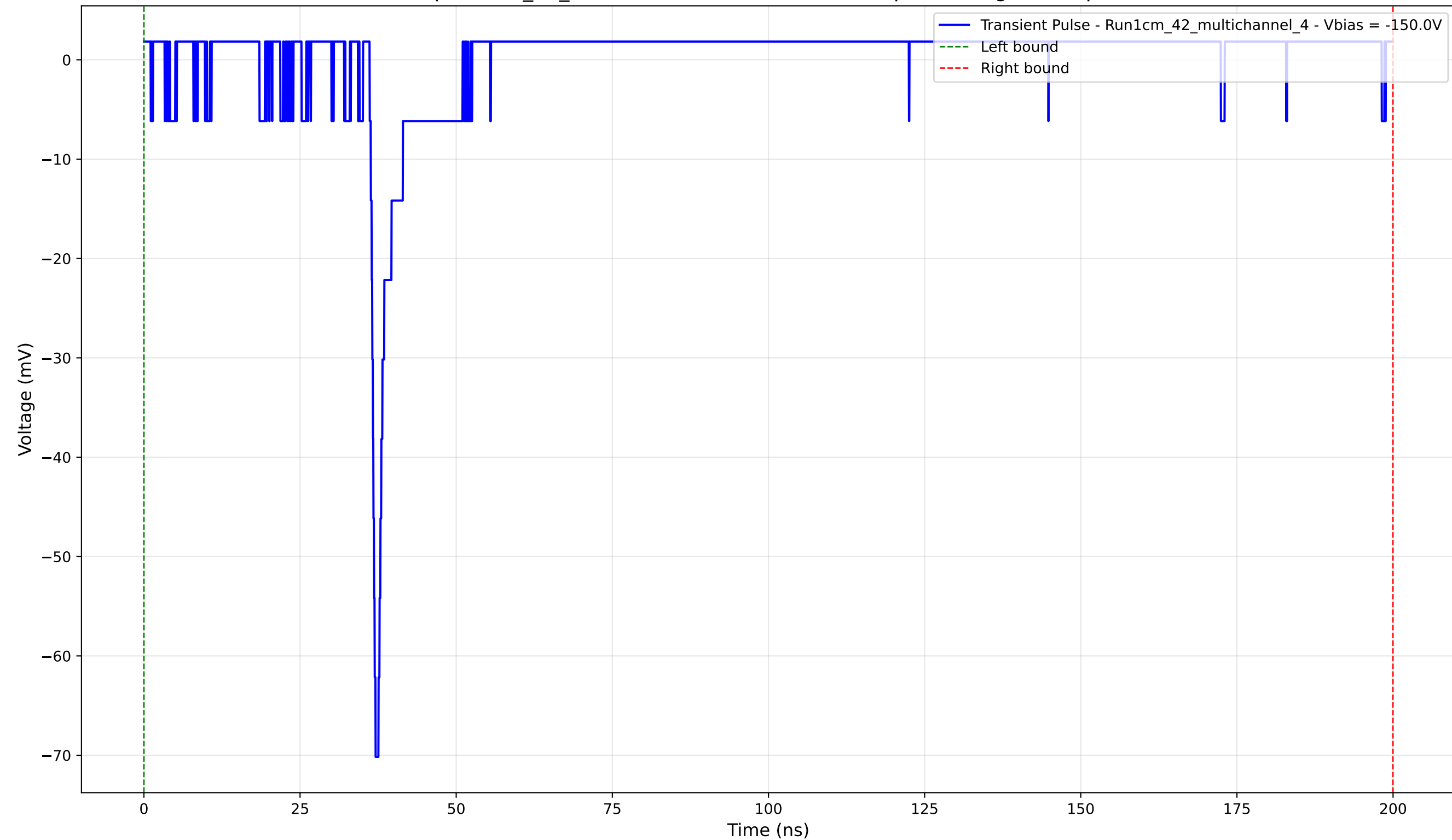
Transient Pulse - Sample: 1cm_42_multichannel - Position: 2565.0 \mu\text{m} - Charge: 0.81 pC - Rise Time: 0.78 ns
