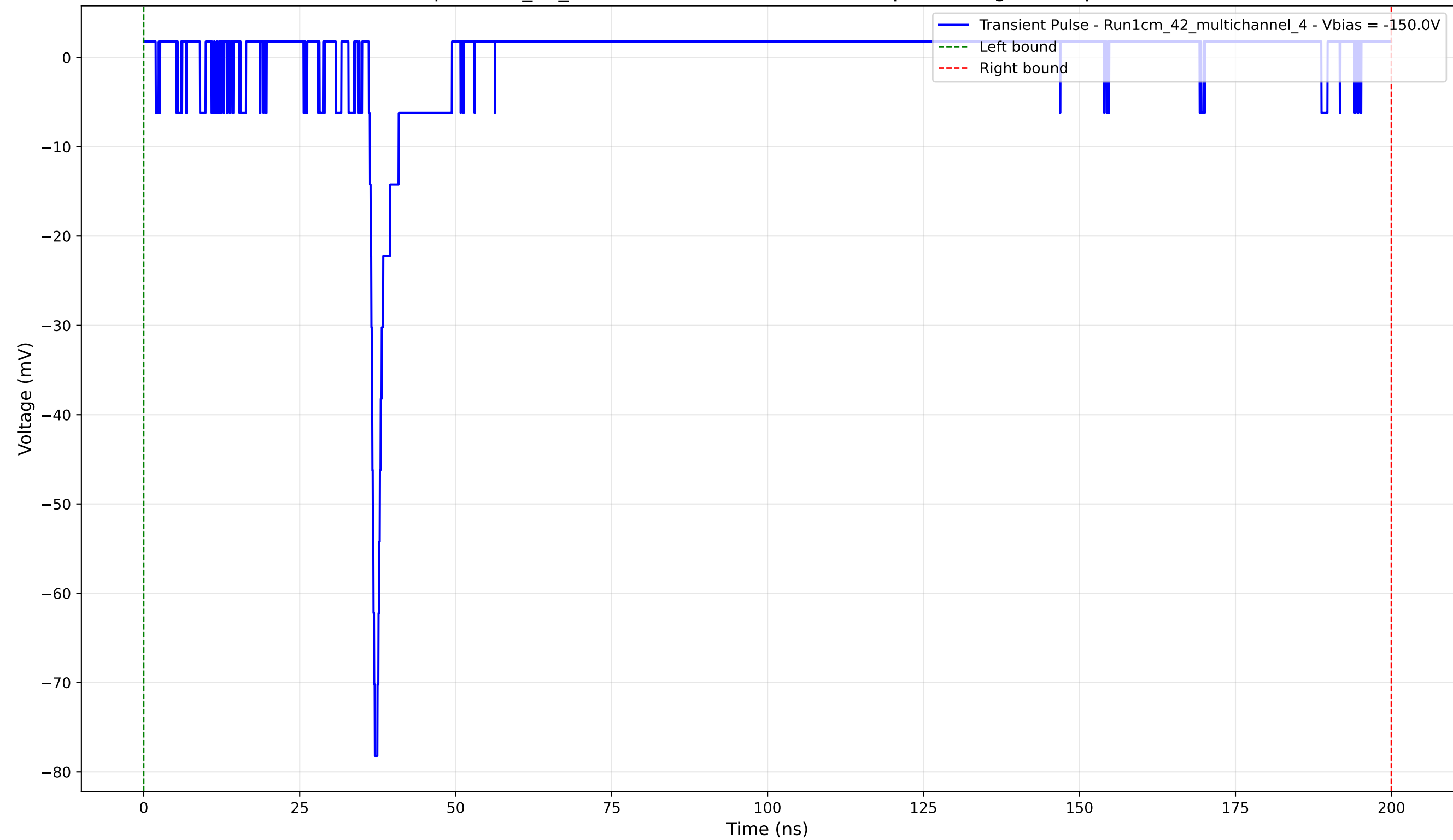
Transient Pulse - Sample: 1cm_42_multichannel - Position: 2300.0 \mu\text{m} - Charge: 0.72 pC - Rise Time: 0.80 ns
