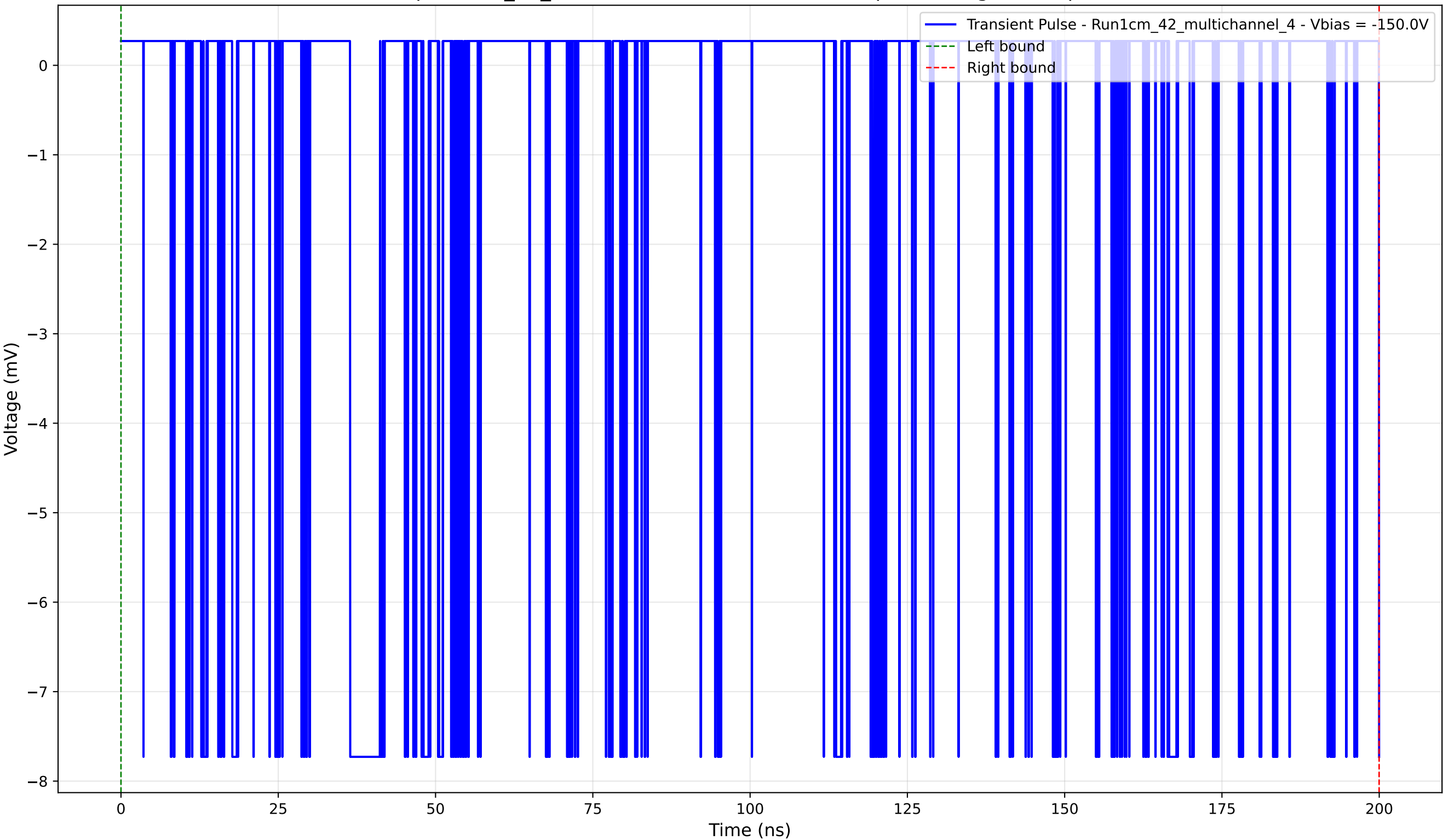
Transient Pulse - Sample: 1cm_42_multichannel - Position: 1880.0 \mu\text{m} - Charge: 3.33 pC - Rise Time: 0.02 ns
