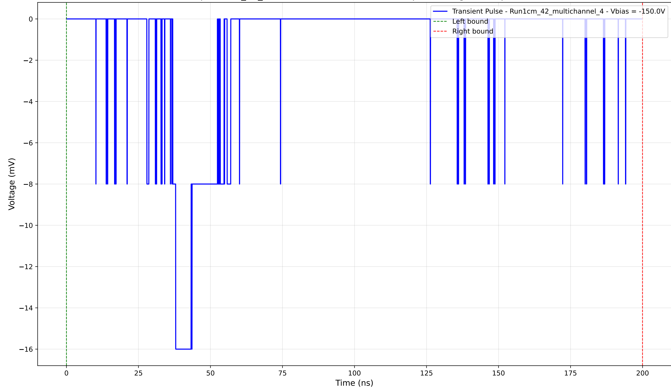
Transient Pulse - Sample: 1cm_42_multichannel - Position: 3985.0 \mu\text{m} - Charge: 4.42 pC - Rise Time: 1.02 ns
