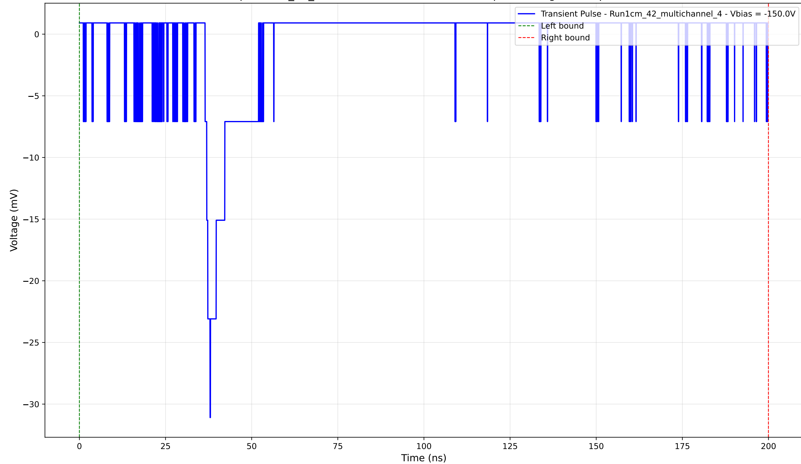
Transient Pulse - Sample: 1cm_42_multichannel - Position: 3260.0 \mu\text{m} - Charge: 1.77 pC - Rise Time: 1.45 ns
