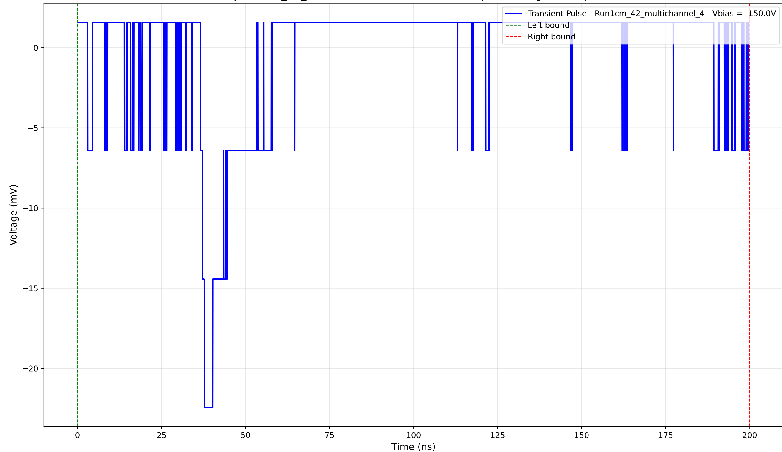
Transient Pulse - Sample: 1cm_42_multichannel - Position: 1235.0 \mu\text{m} - Charge: 0.48 pC - Rise Time: 1.12 ns
