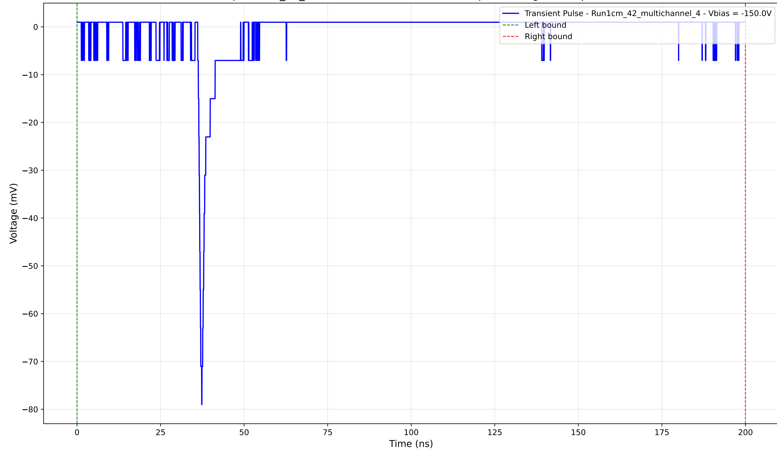
Transient Pulse - Sample: 1cm_42_multichannel - Position: 2215.0 \mu\text{m} - Charge: 2.56 pC - Rise Time: 1.02 ns
