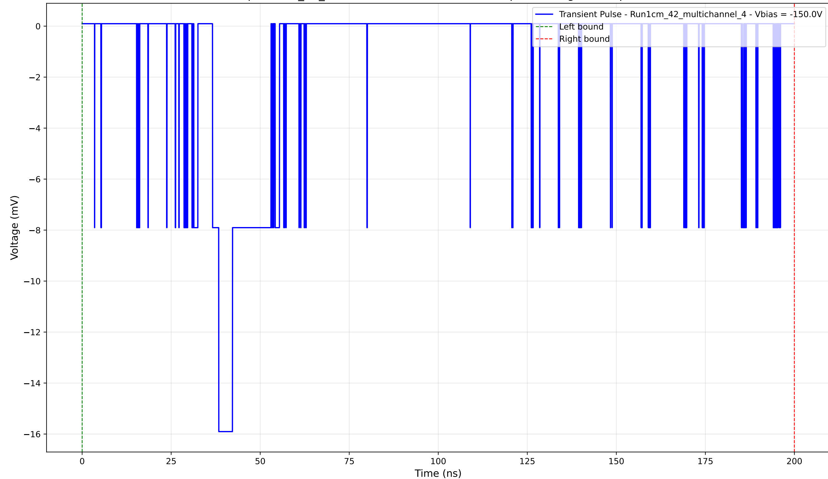
Transient Pulse - Sample: 1cm_42_multichannel - Position: 4720.0 \mu\text{m} - Charge: 4.47 pC - Rise Time: 1.76 ns
