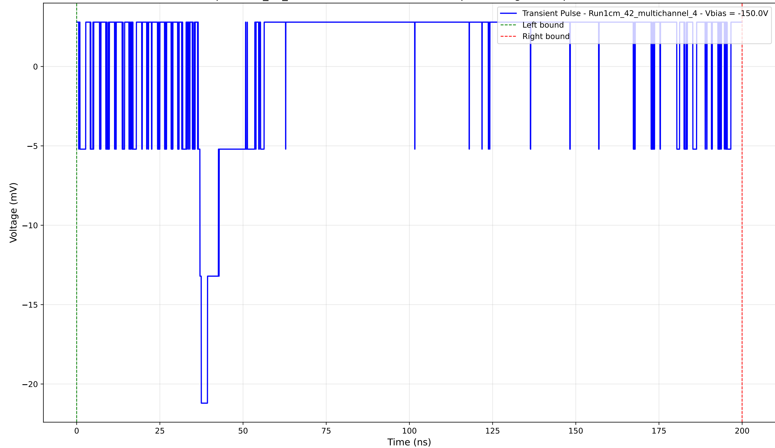
Transient Pulse - Sample: 1cm_42_multichannel - Position: 1440.0 \mu\text{m} - Charge: 4.45 pC - Rise Time: 0.00 ns (N/A)
