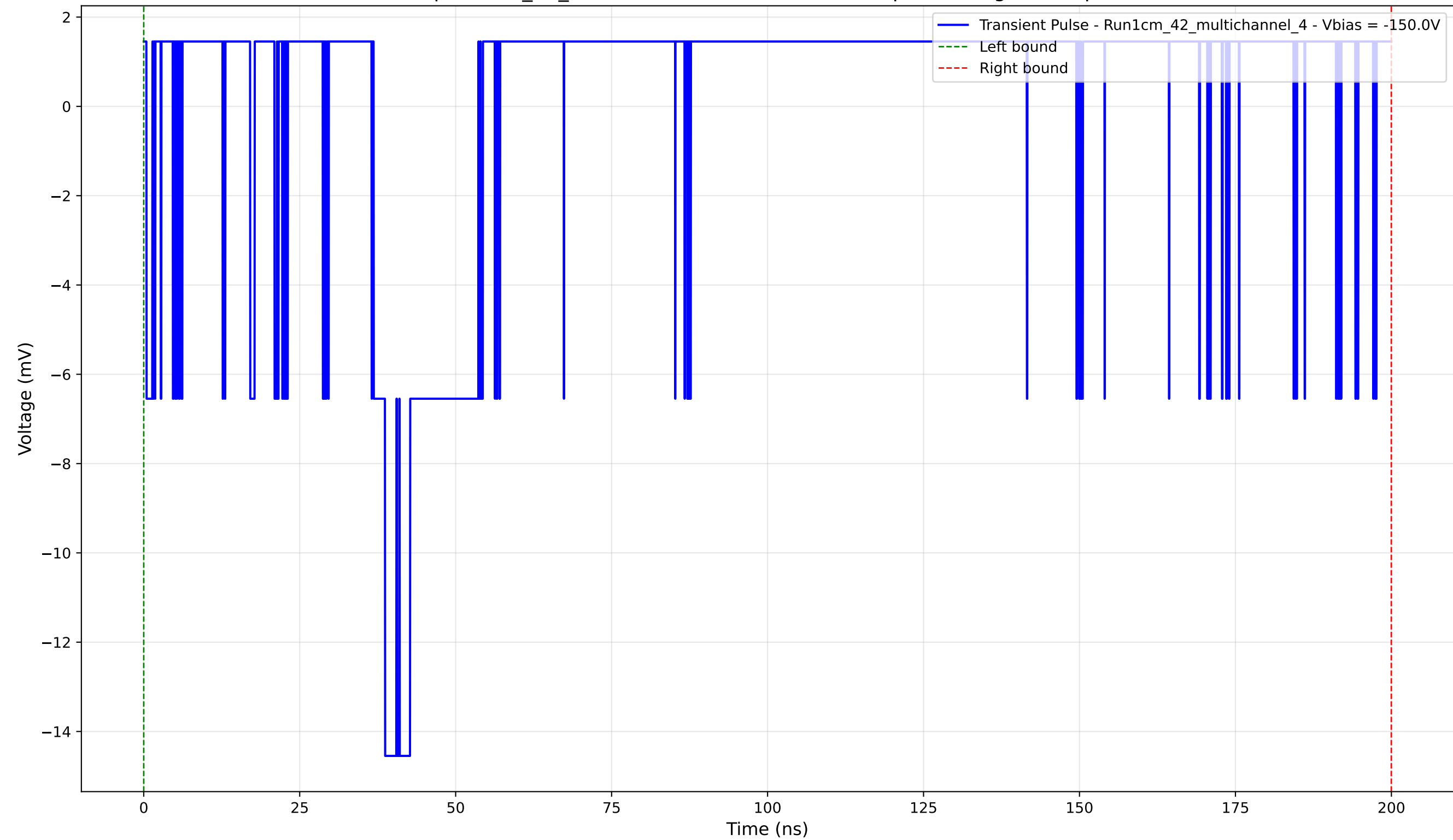
Transient Pulse - Sample: 1cm_42_multichannel - Position: 4790.0 \mu\text{m} - Charge: 1.21 pC - Rise Time: 1.84 ns
