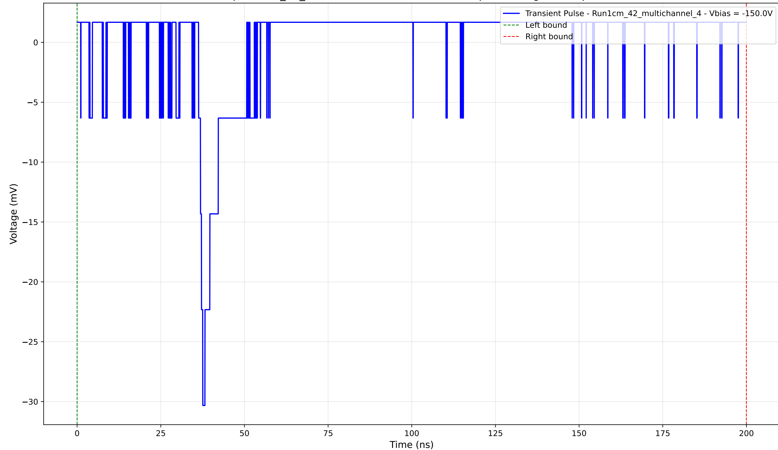
Transient Pulse - Sample: 1cm_42_multichannel - Position: 3170.0 \mu\text{m} - Charge: 1.45 pC - Rise Time: 1.25 ns
