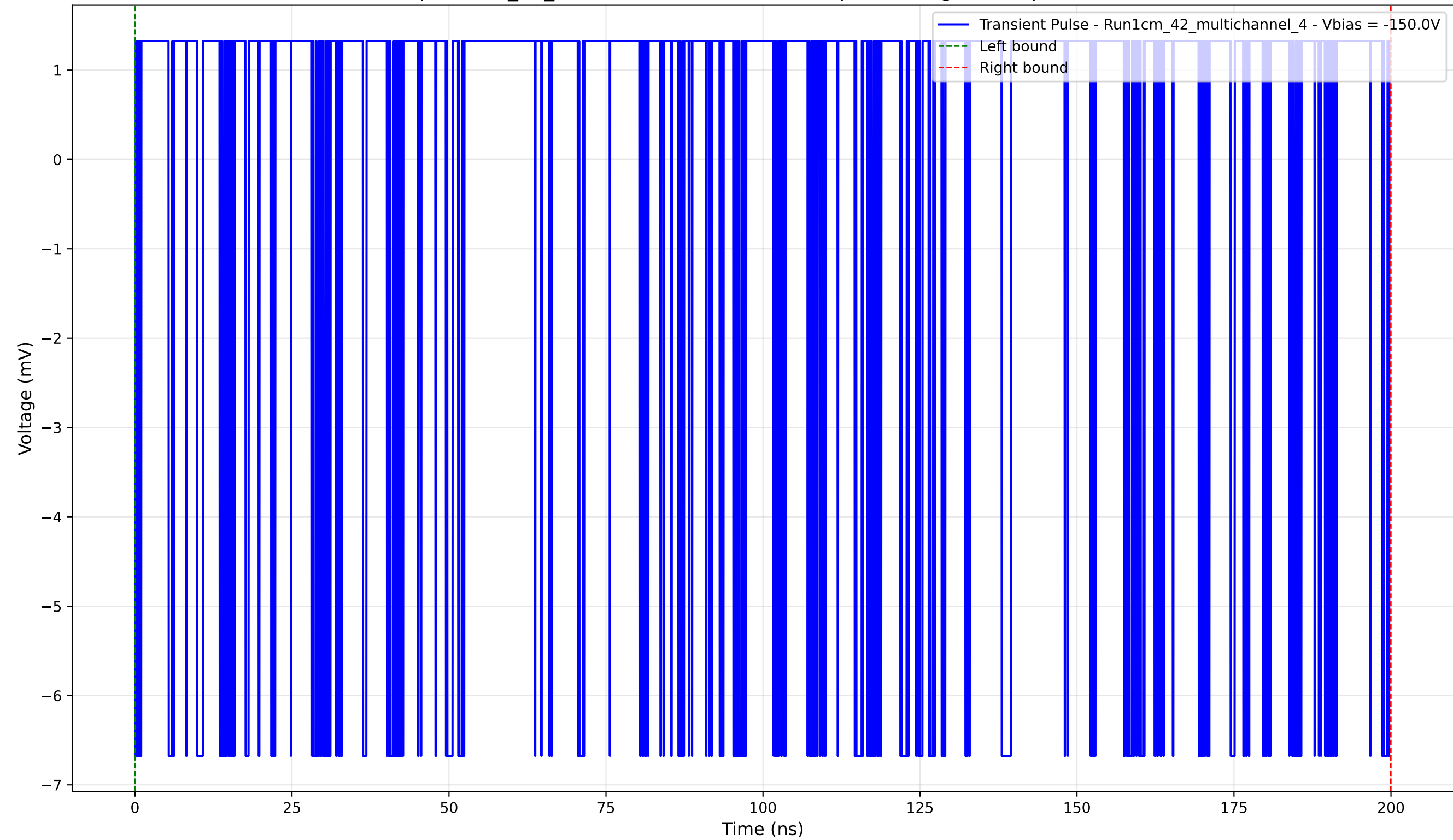
Transient Pulse - Sample: 1cm_42_multichannel - Position: 5.0 \mu\text{m} - Charge: 0.36 pC - Rise Time: 0.00 ns (N/A)
