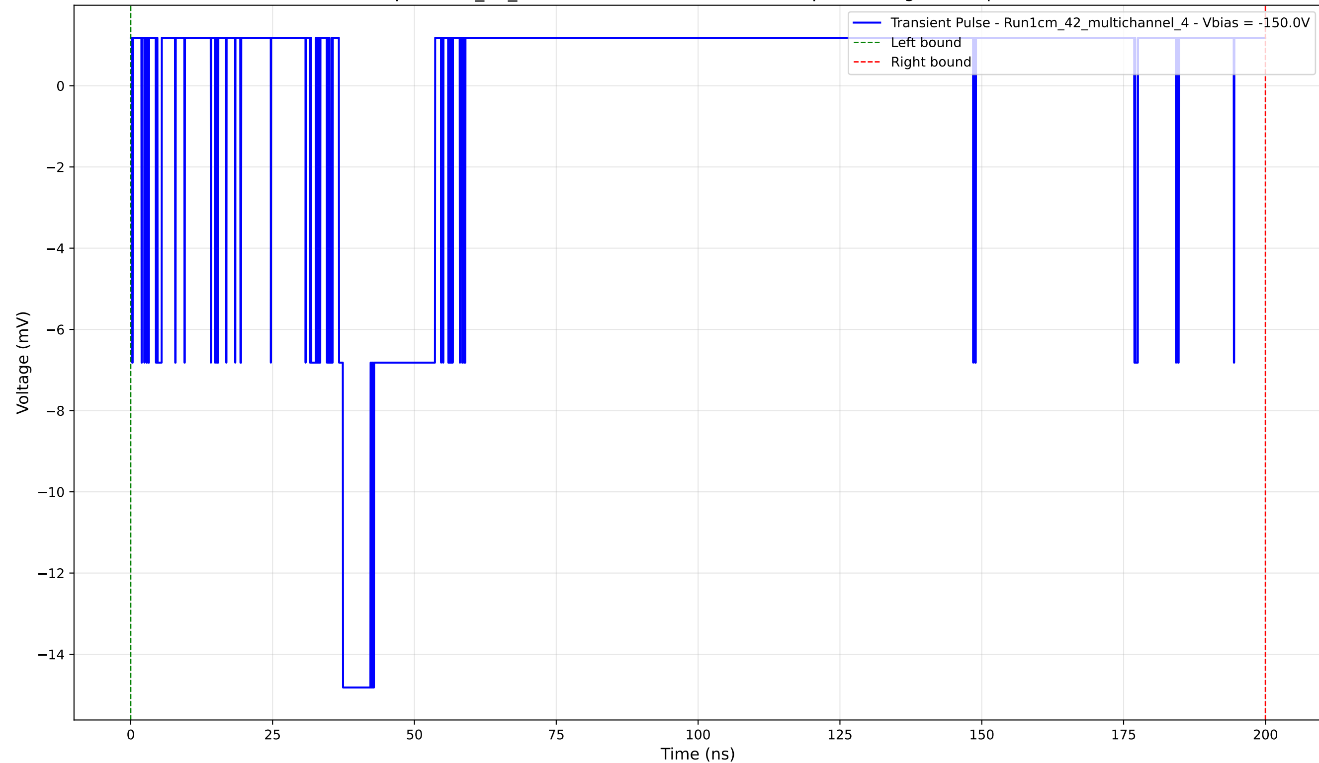
Transient Pulse - Sample: 1cm_42_multichannel - Position: 3605.0 \mu\text{m} - Charge: 0.19 pC - Rise Time: 0.72 ns
