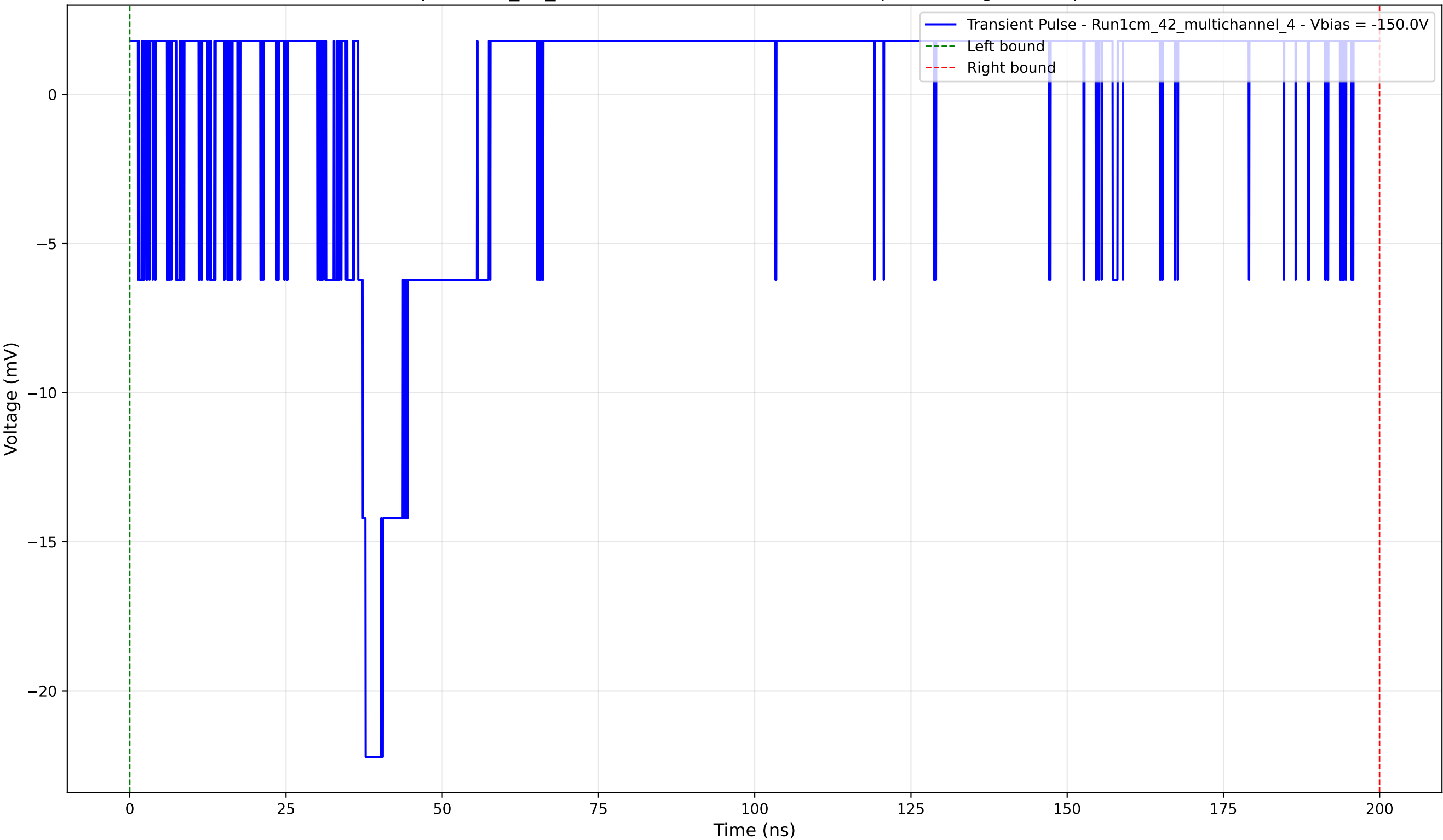
Transient Pulse - Sample: 1cm_42_multichannel - Position: 1220.0 \mu\text{m} - Charge: 0.27 pC - Rise Time: 1.20 ns
