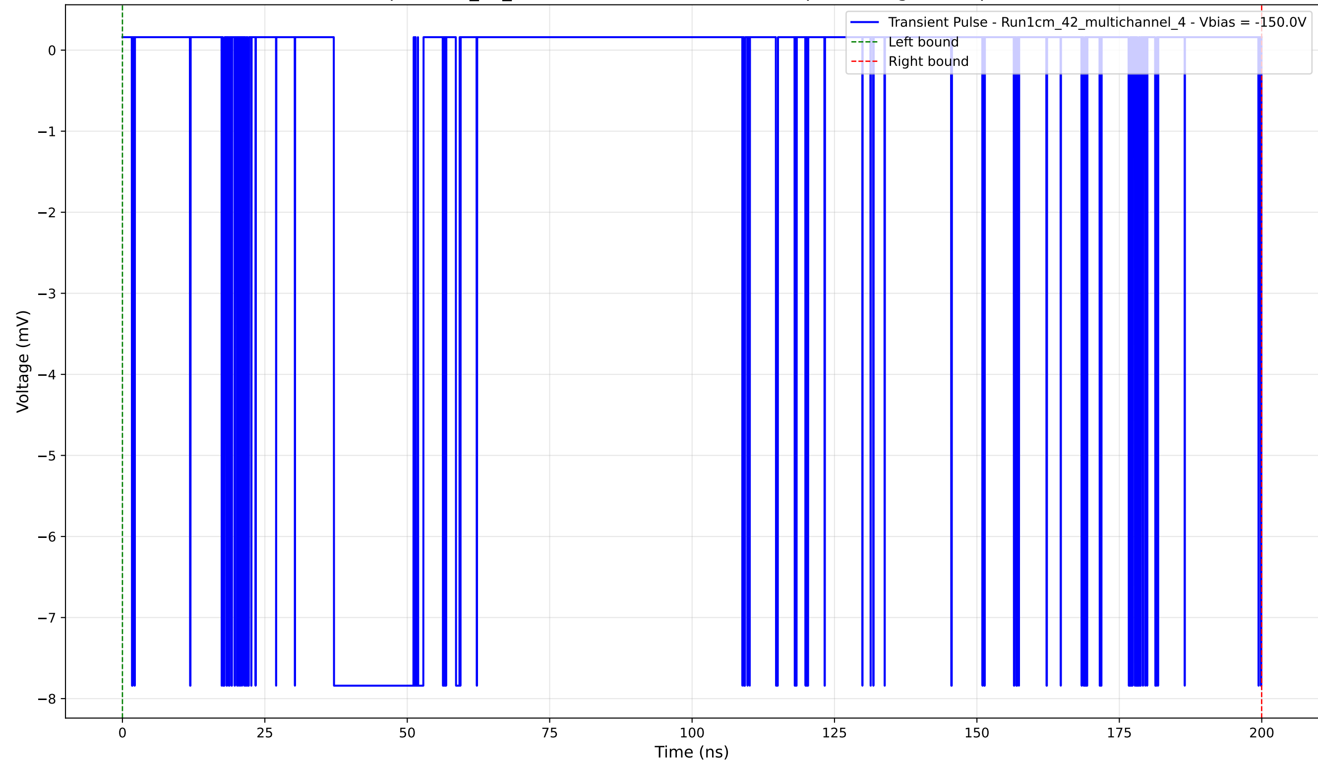
Transient Pulse - Sample: 1cm_42_multichannel - Position: 4855.0 \mu\text{m} - Charge: 3.01 pC - Rise Time: 0.02 ns
