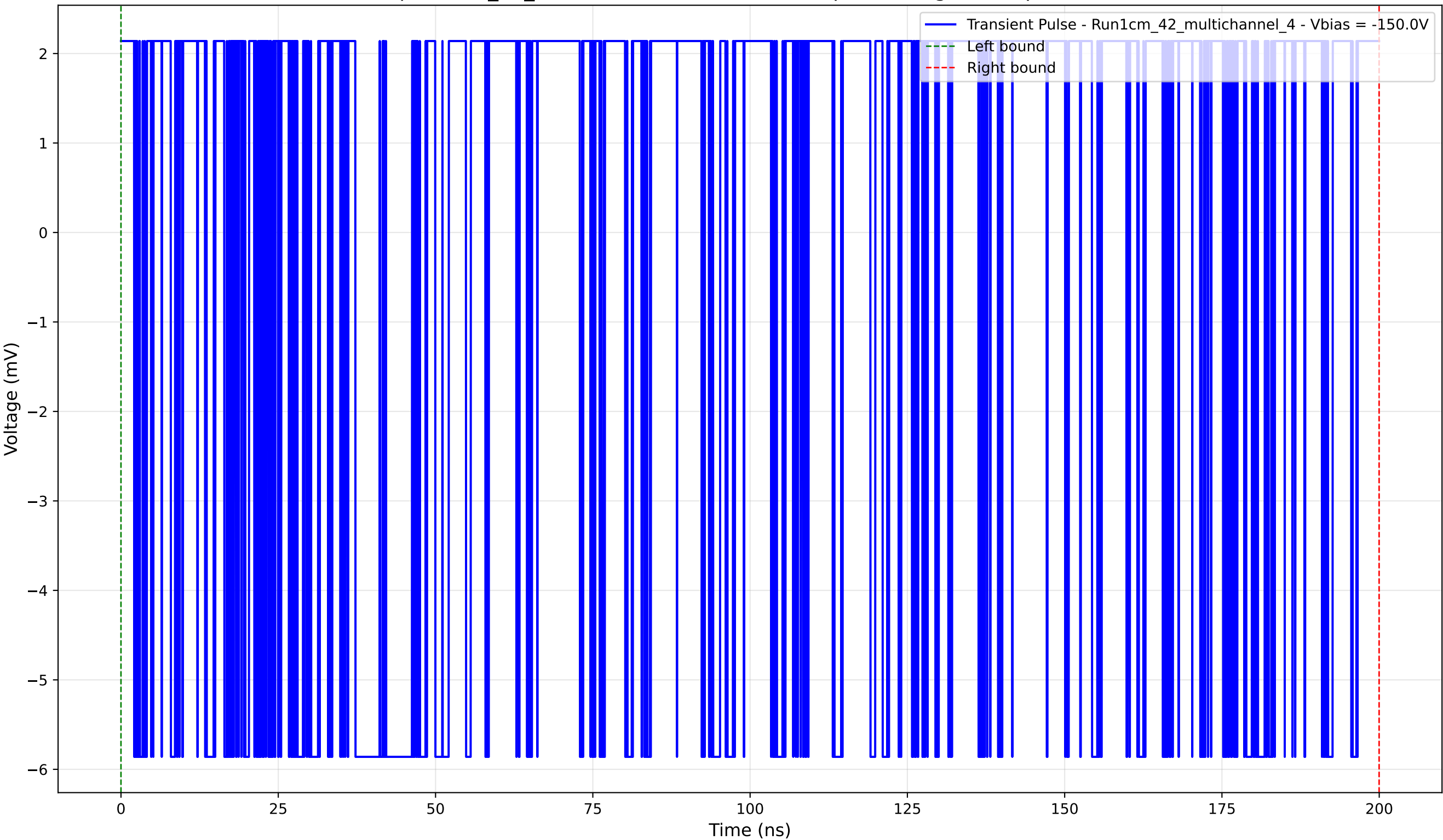
Transient Pulse - Sample: 1cm_42_multichannel - Position: 75.0 \mu\text{m} - Charge: 0.07 pC - Rise Time: 0.00 ns (N/A)
