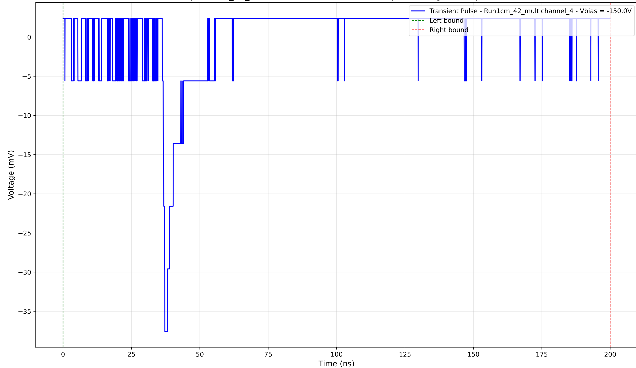
Transient Pulse - Sample: 1cm_42_multichannel - Position: 1765.0 \mu\text{m} - Charge: 2.30 pC - Rise Time: 0.97 ns
