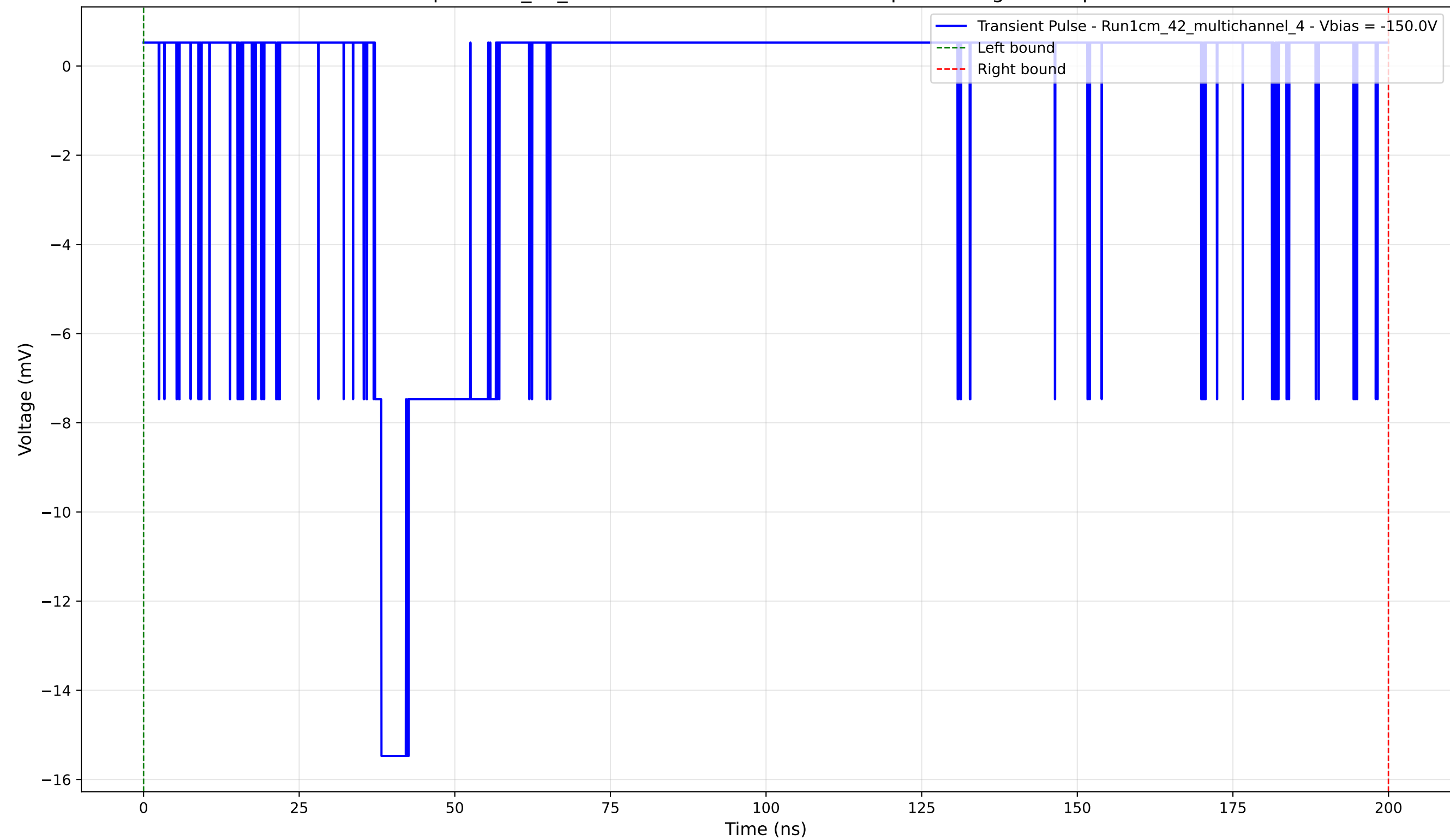
Transient Pulse - Sample: 1cm_42_multichannel - Position: 4105.0 \mu\text{m} - Charge: 2.56 pC - Rise Time: 1.04 ns
