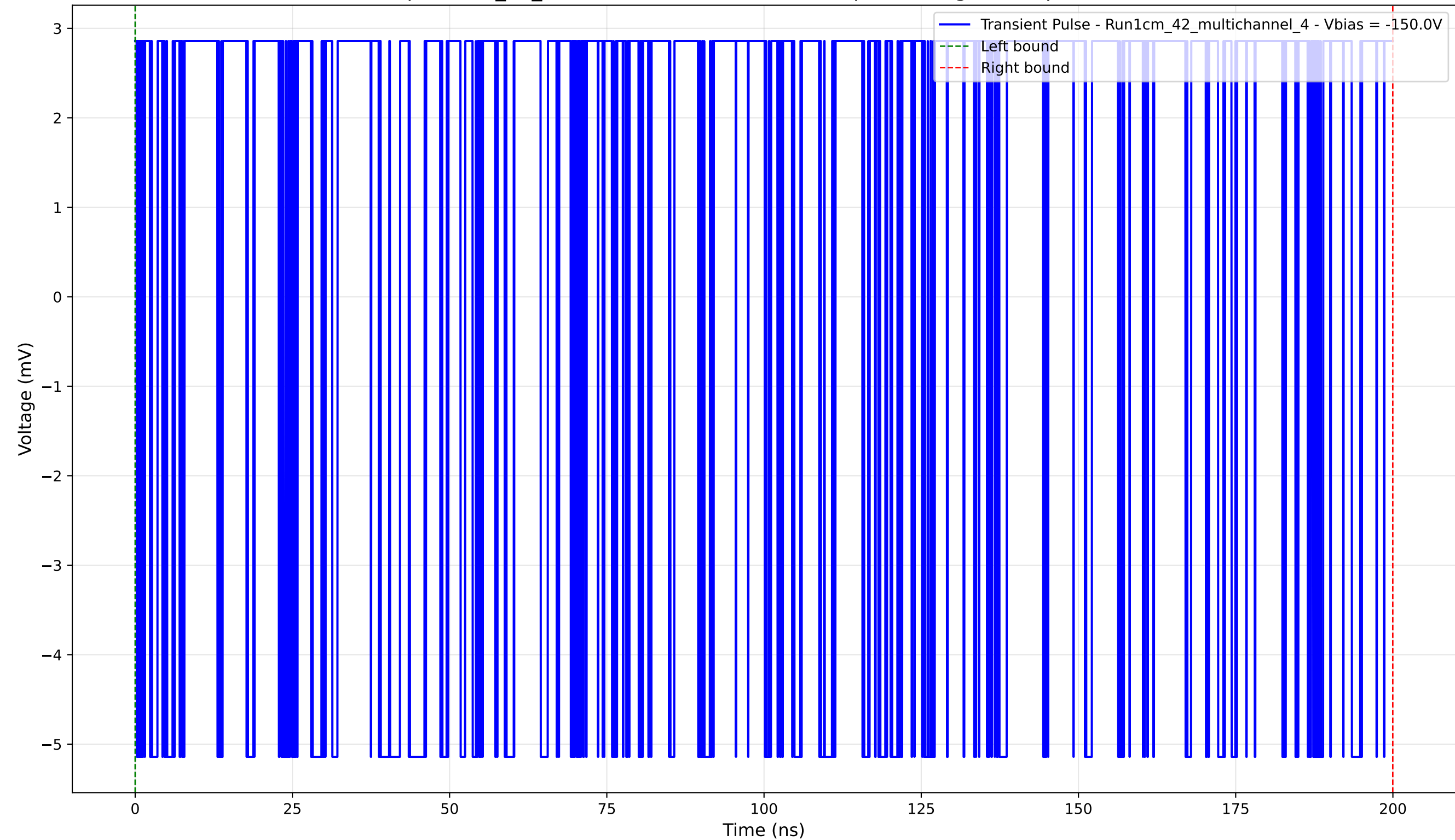
Transient Pulse - Sample: 1cm_42_multichannel - Position: 365.0 \mu\text{m} - Charge: 3.75 pC - Rise Time: 0.00 ns (N/A)
