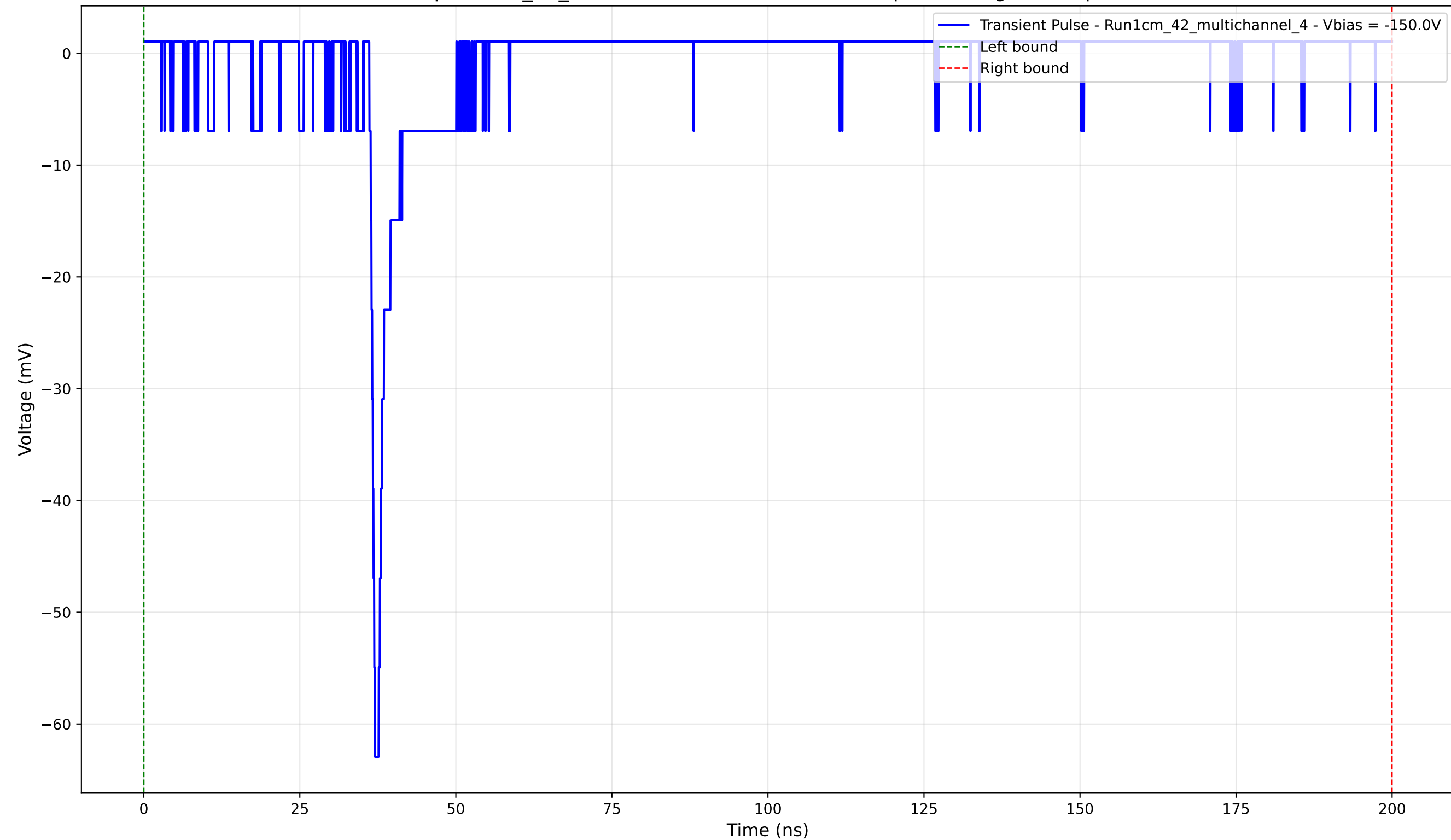
Transient Pulse - Sample: 1cm_42_multichannel - Position: 2590.0 \mu\text{m} - Charge: 2.08 pC - Rise Time: 0.90 ns
