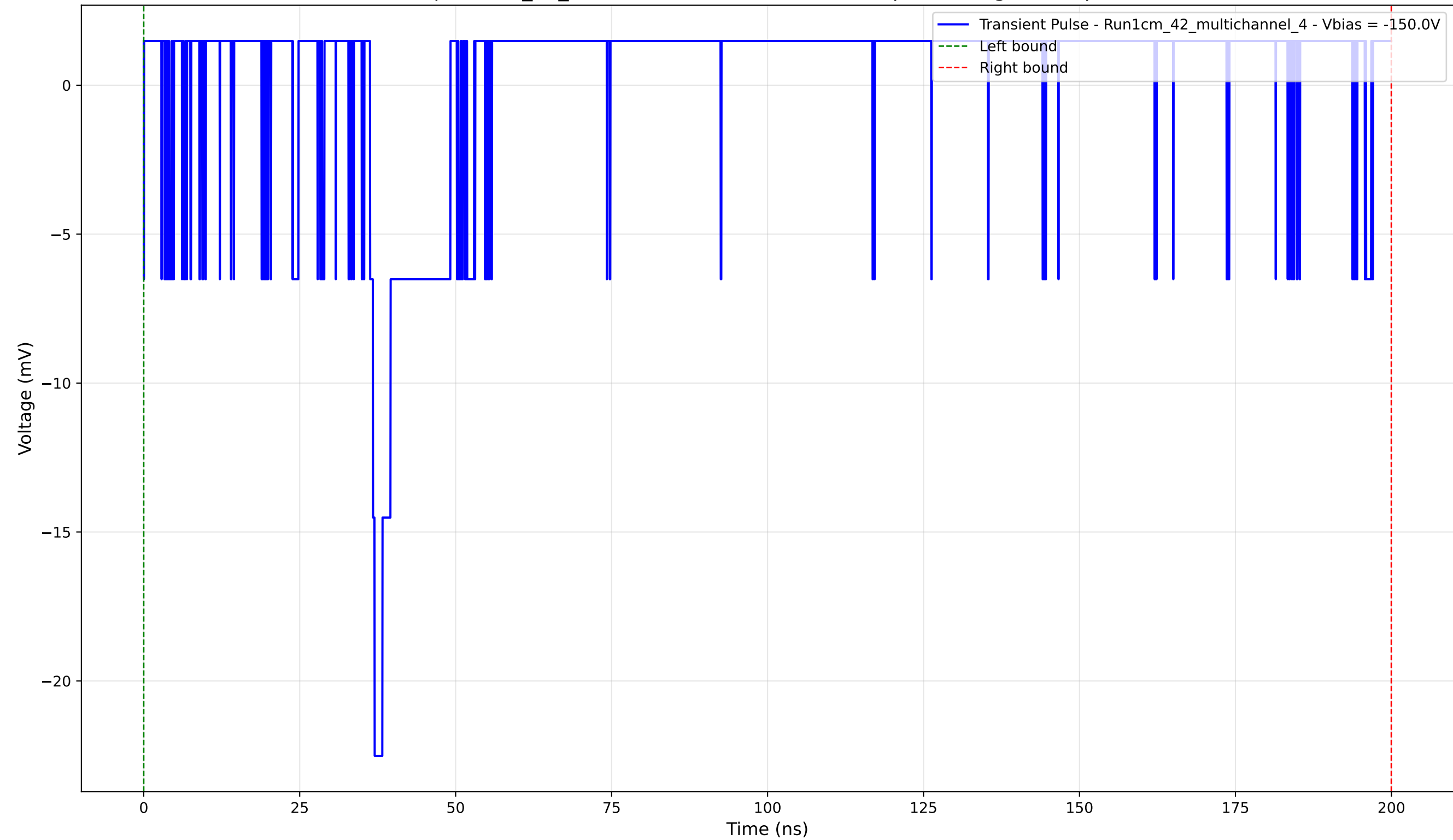
Transient Pulse - Sample: 1cm_42_multichannel - Position: 2840.0 \mu\text{m} - Charge: 1.53 pC - Rise Time: 0.74 ns
