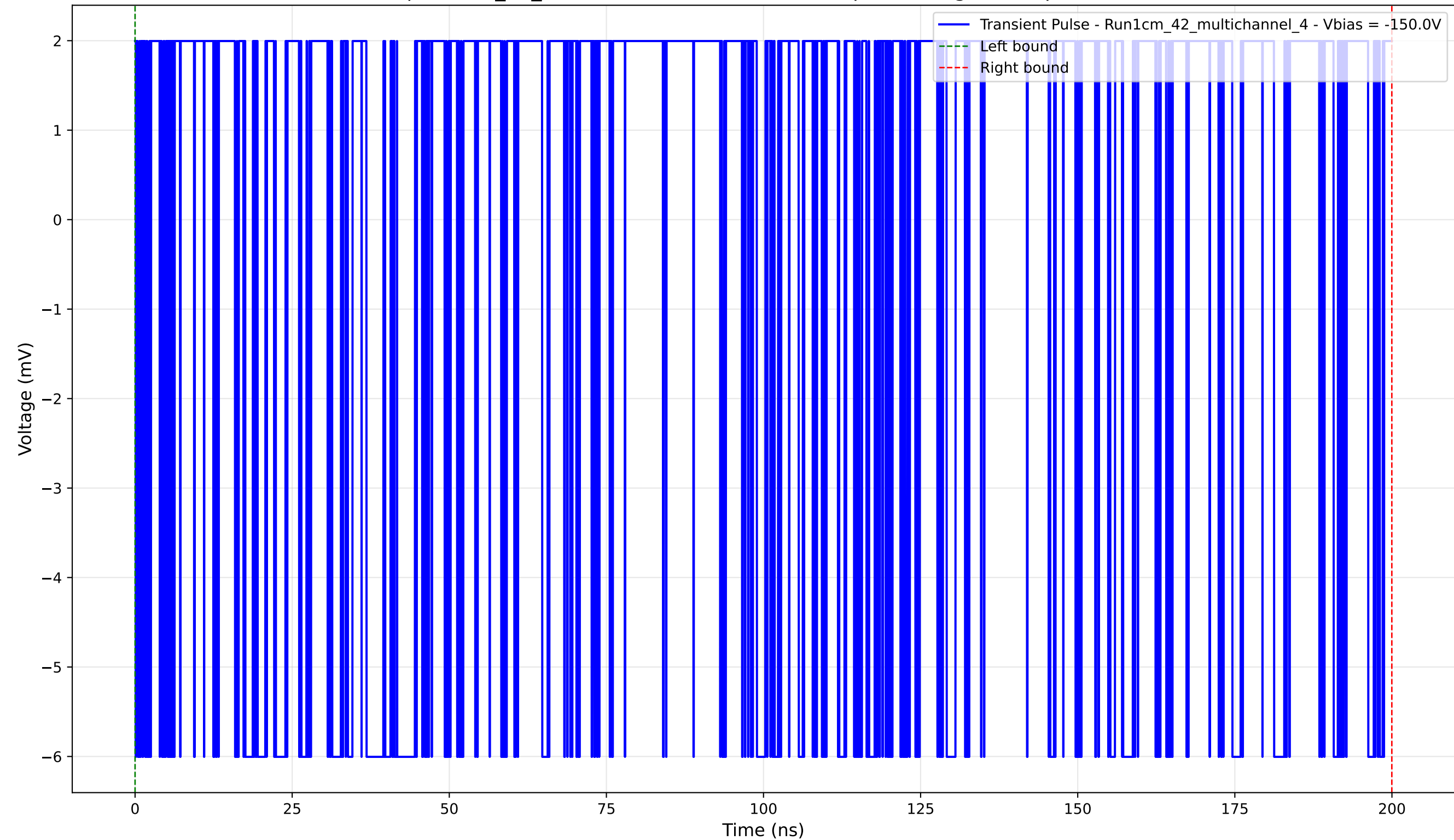
Transient Pulse - Sample: 1cm_42_multichannel - Position: 385.0 \mu\text{m} - Charge: 0.38 pC - Rise Time: 0.00 ns (N/A)
