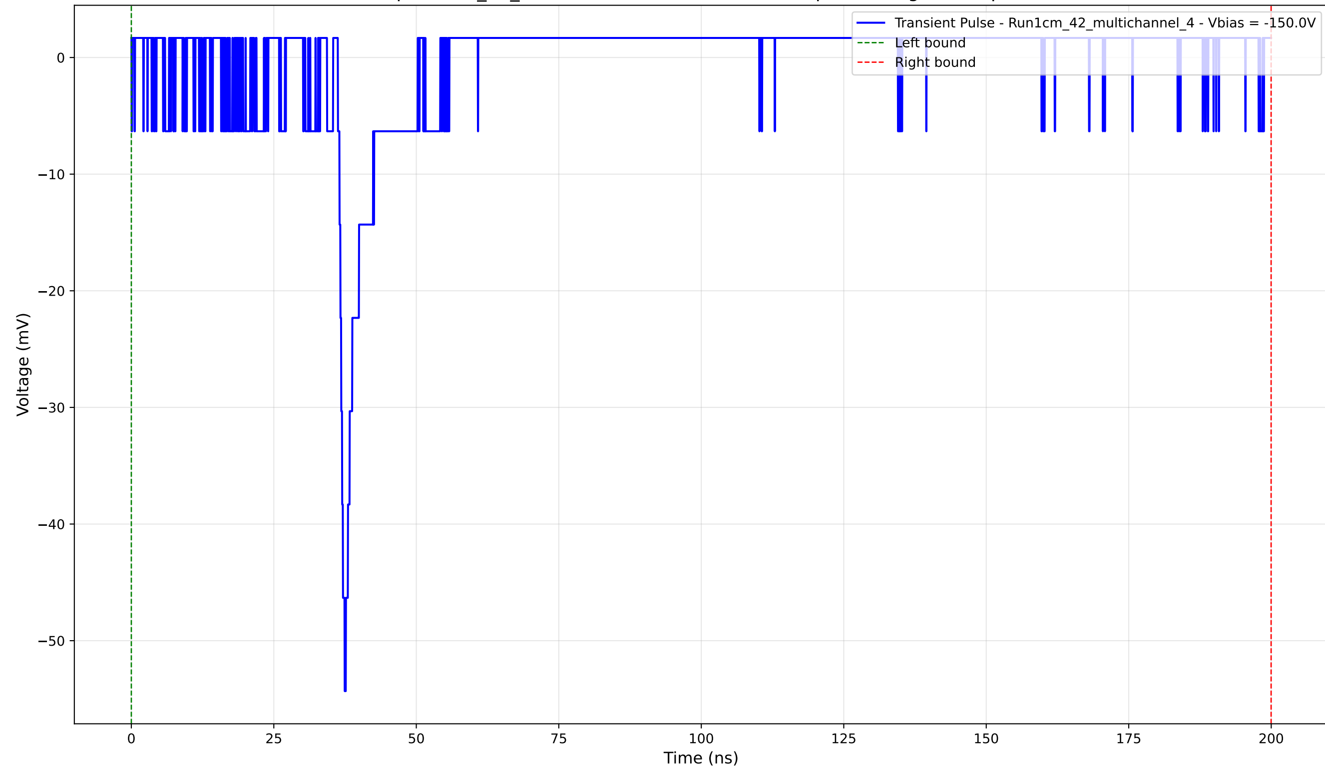
Transient Pulse - Sample: 1cm_42_multichannel - Position: 1960.0 \mu\text{m} - Charge: 0.80 pC - Rise Time: 1.18 ns
