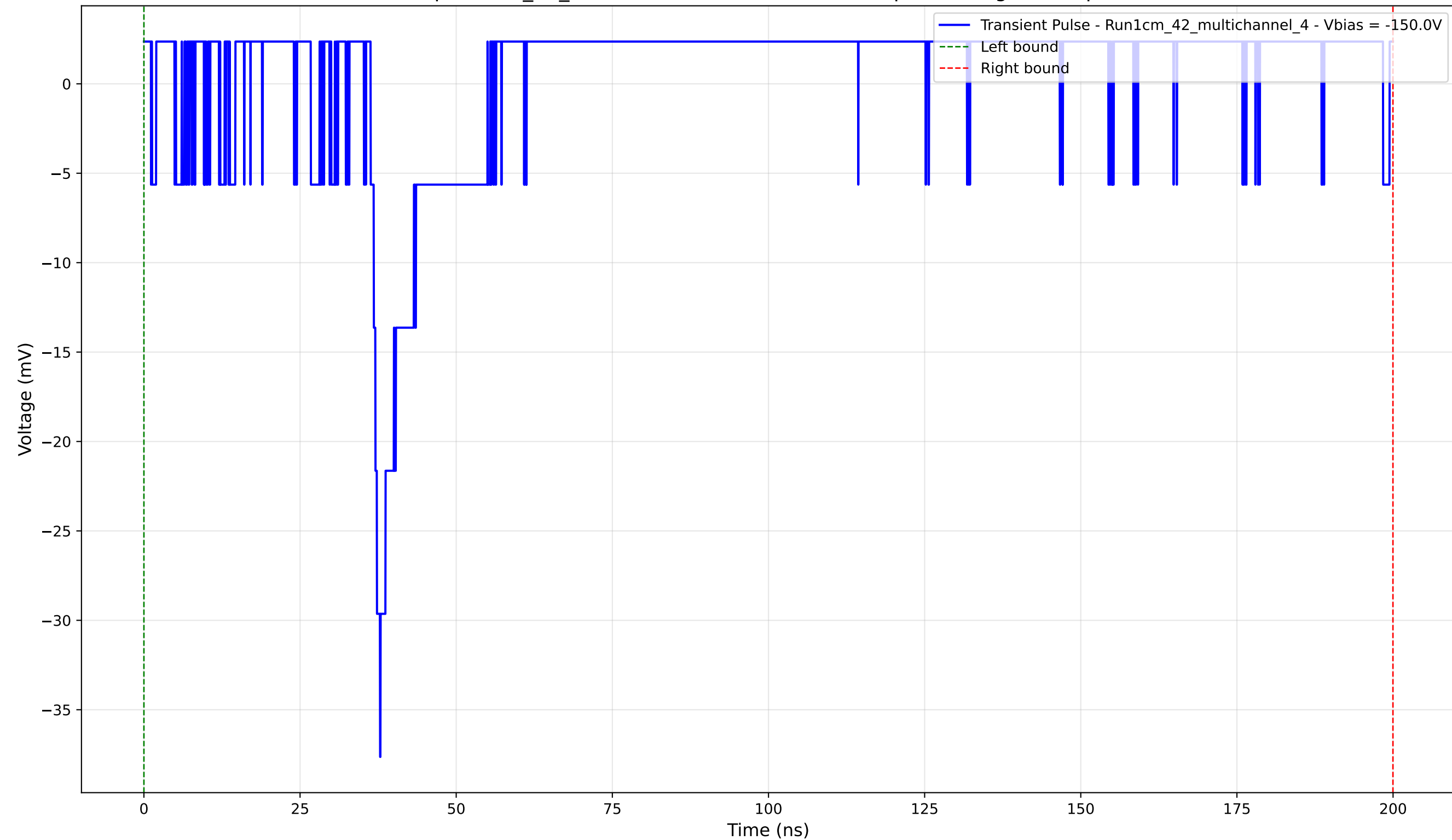
Transient Pulse - Sample: 1cm_42_multichannel - Position: 1625.0 \mu\text{m} - Charge: 2.48 pC - Rise Time: 1.51 ns
