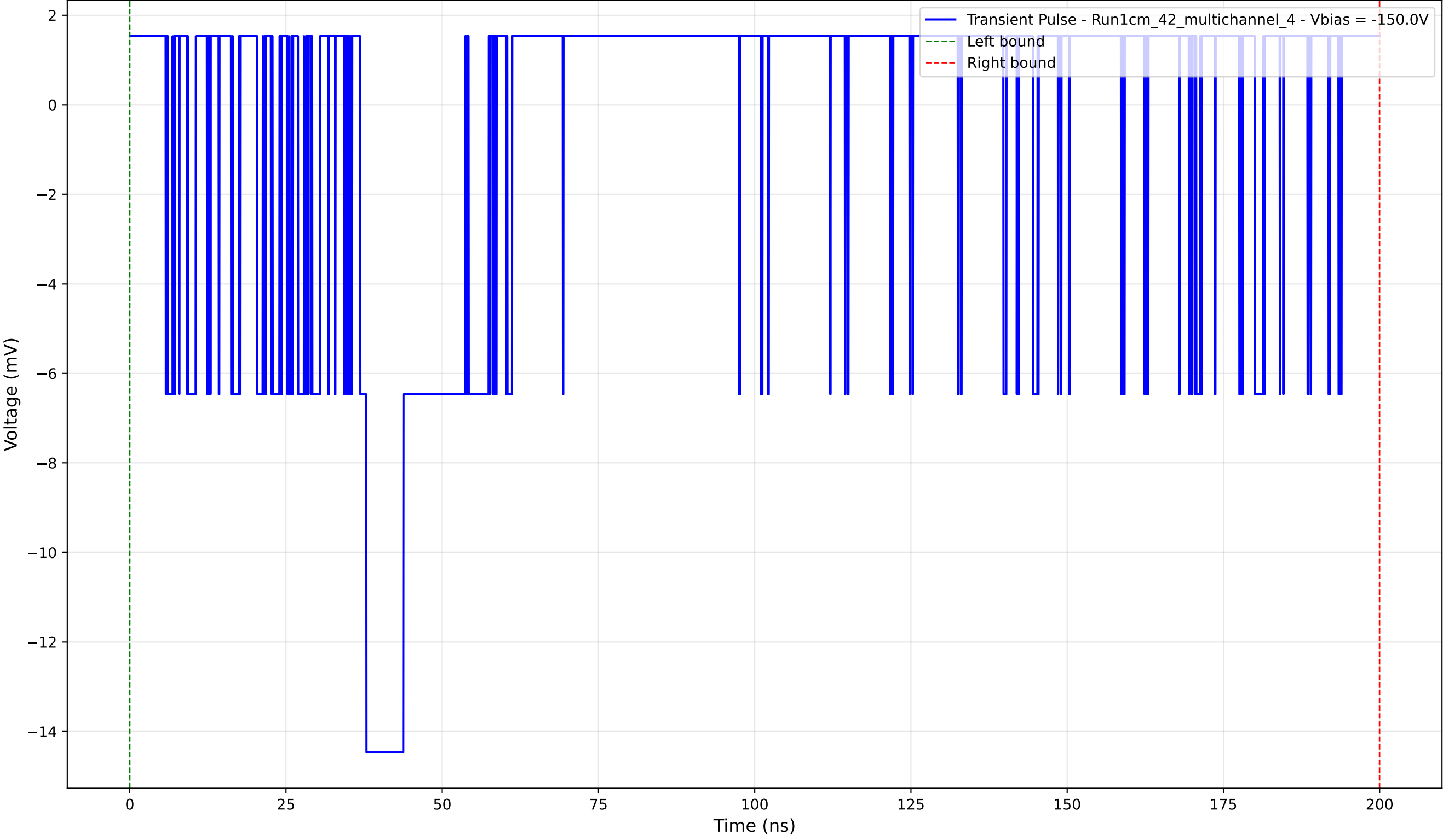
Transient Pulse - Sample: 1cm_42_multichannel - Position: 580.0 \mu\text{m} - Charge: 1.13 pC - Rise Time: 0.00 ns (N/A)
