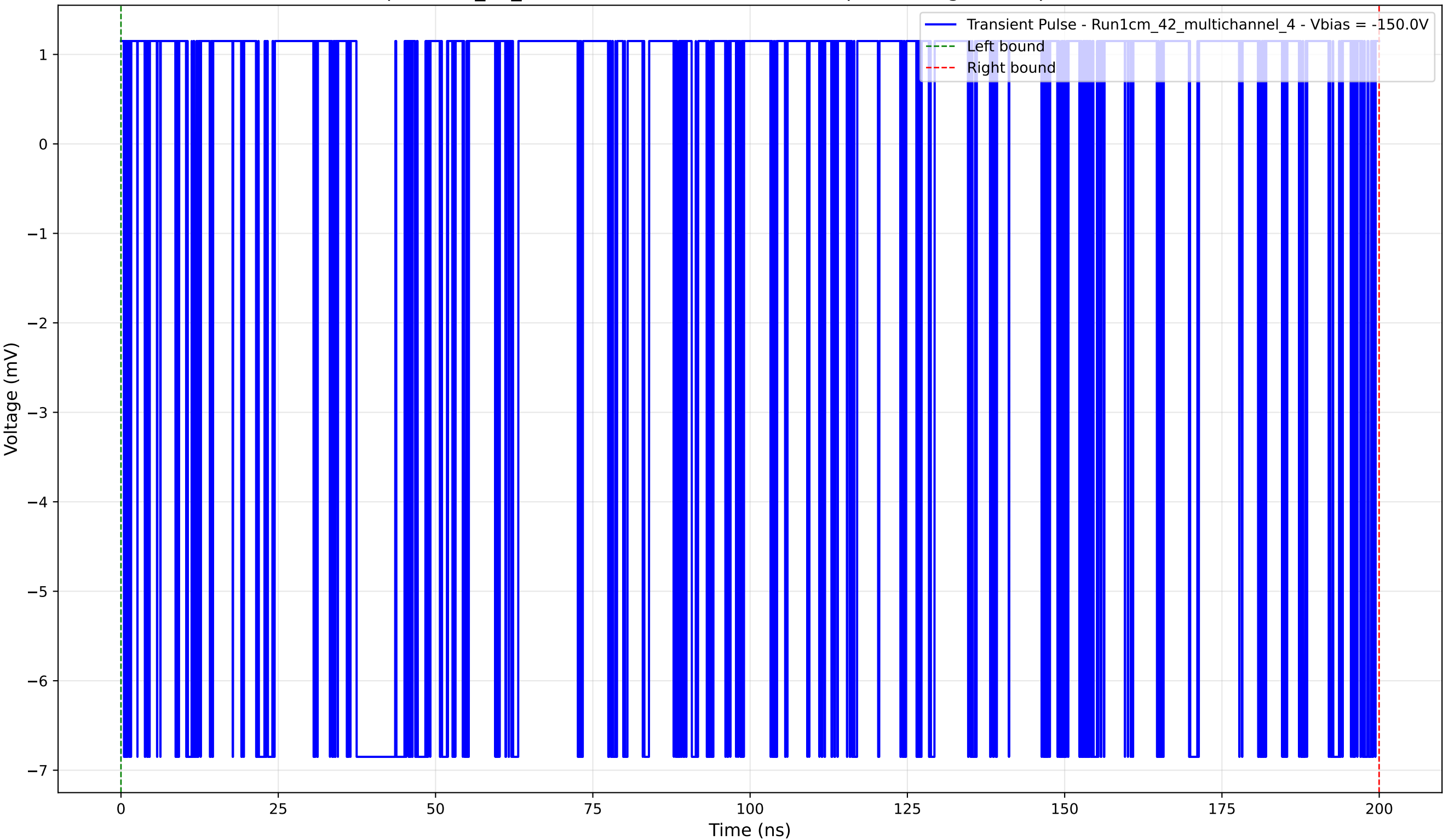
Transient Pulse - Sample: 1cm_42_multichannel - Position: 4435.0 \mu\text{m} - Charge: 2.51 pC - Rise Time: 0.00 ns (N/A)
