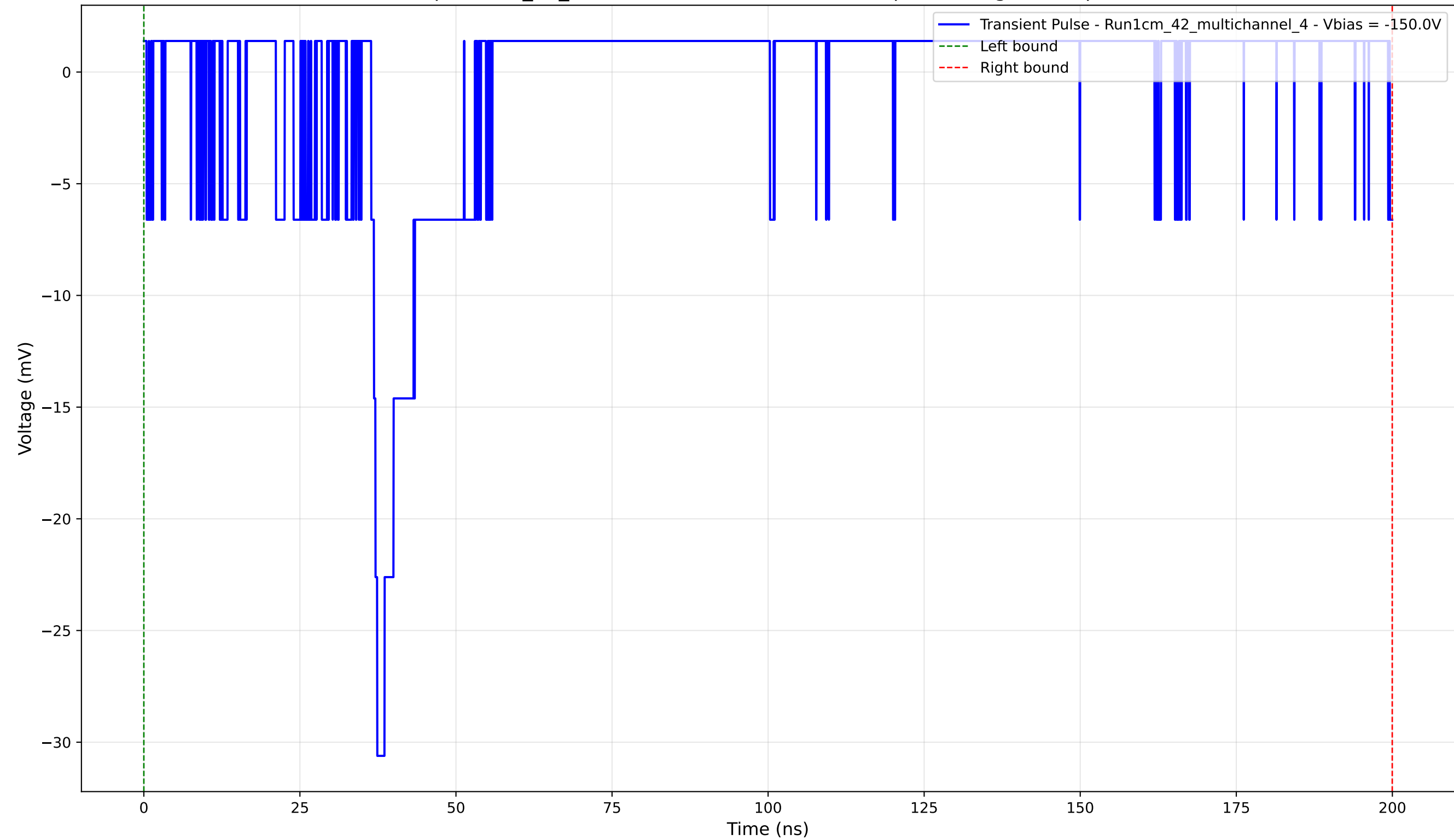
Transient Pulse - Sample: 1cm_42_multichannel - Position: 1595.0 \mu\text{m} - Charge: 1.30 pC - Rise Time: 0.97 ns
