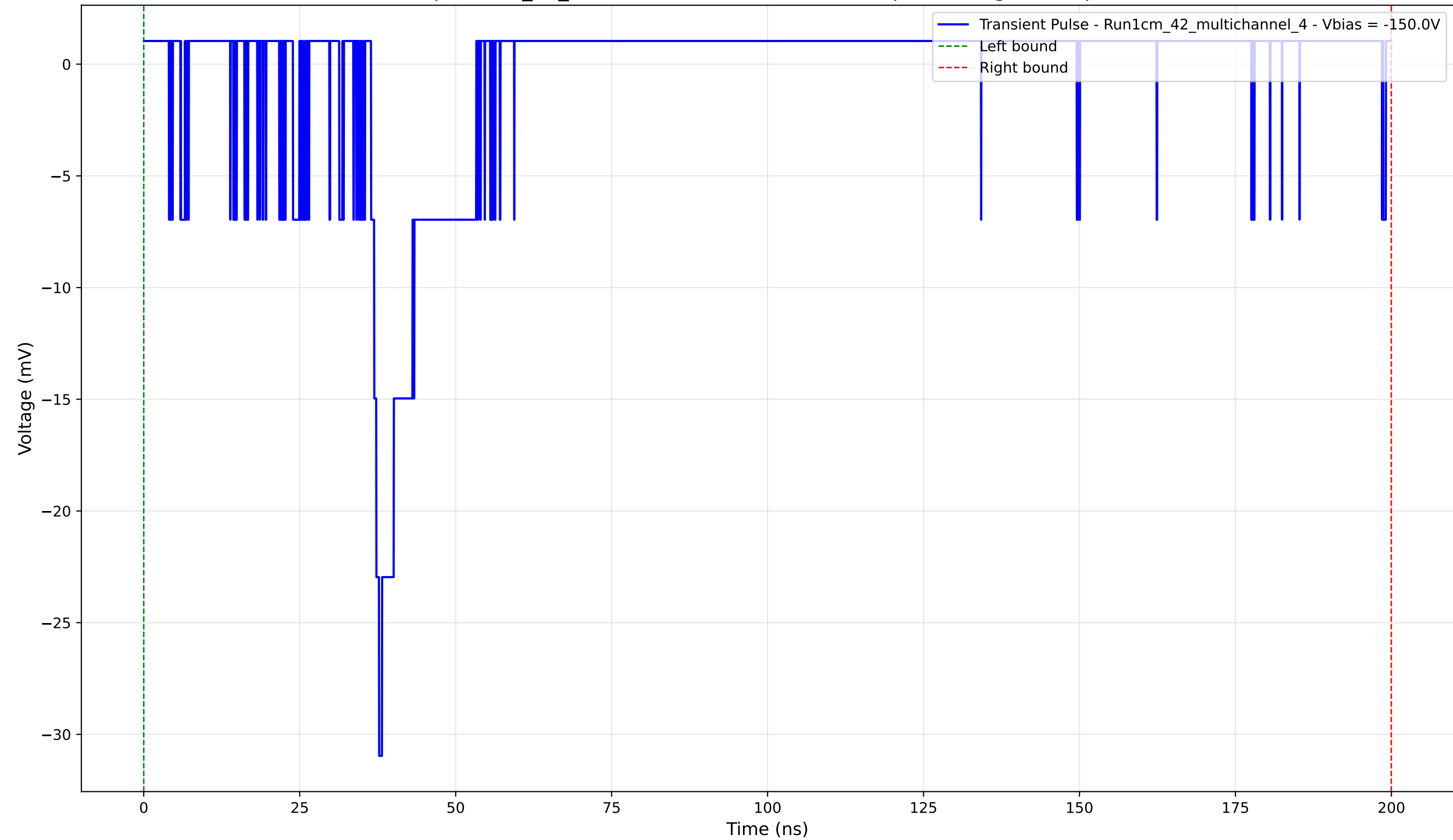
Transient Pulse - Sample: 1cm_42_multichannel - Position: 3290.0 \mu\text{m} - Charge: 1.41 pC - Rise Time: 1.29 ns
