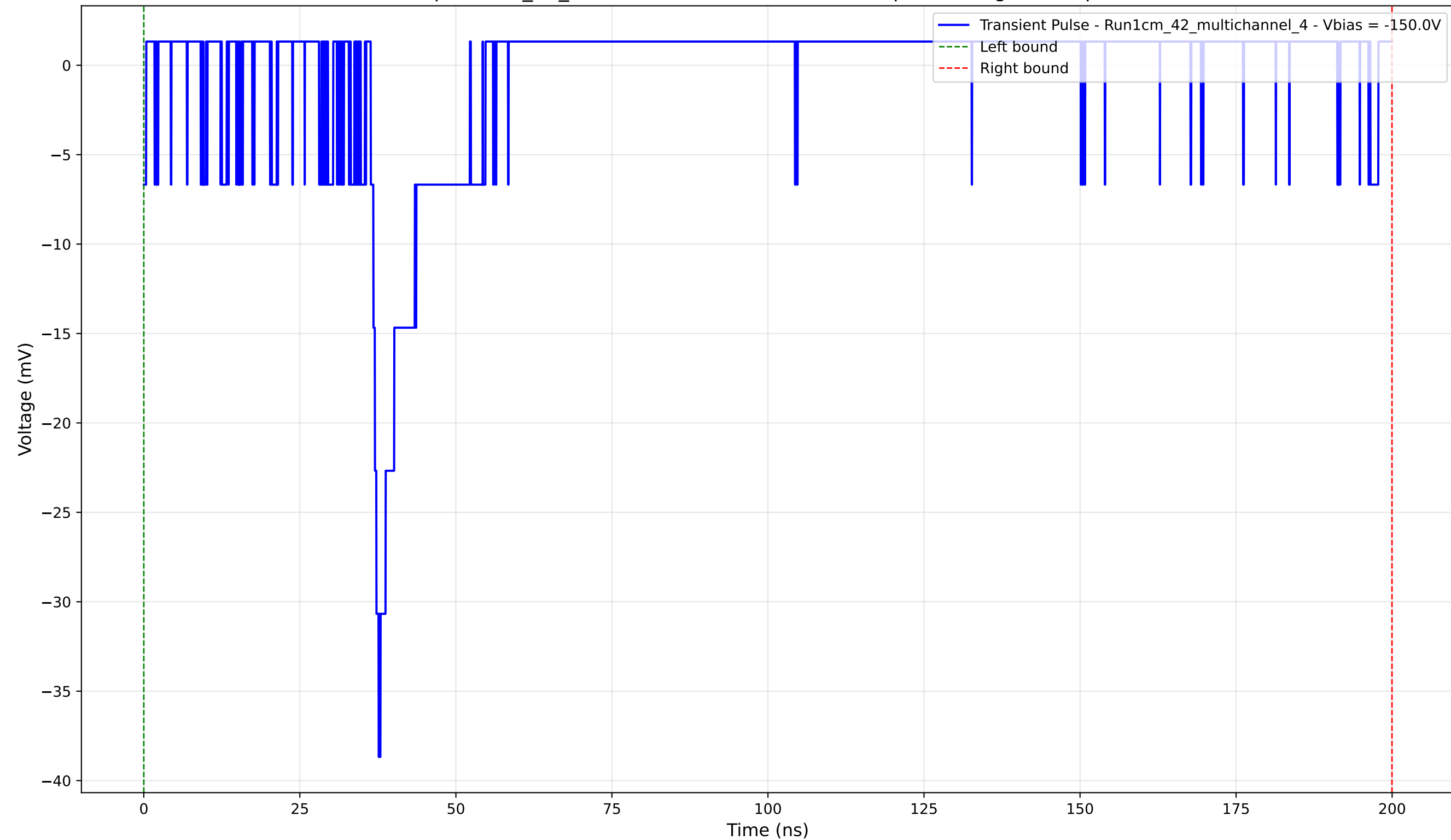
Transient Pulse - Sample: 1cm_42_multichannel - Position: 1655.0 \mu\text{m} - Charge: 1.44 pC - Rise Time: 1.27 ns
