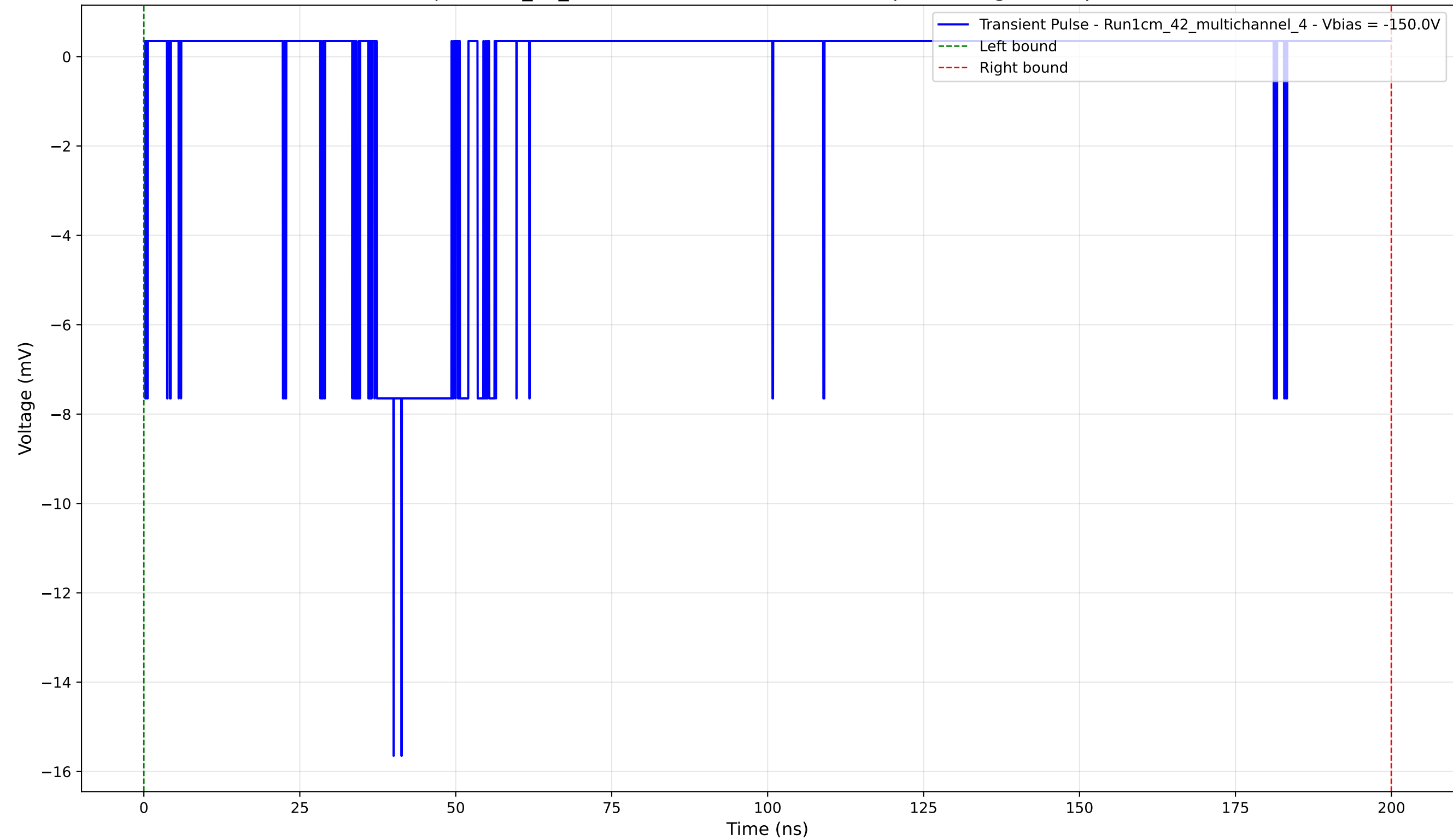
Transient Pulse - Sample: 1cm_42_multichannel - Position: 4830.0 \mu\text{m} - Charge: 1.67 pC - Rise Time: 2.70 ns
