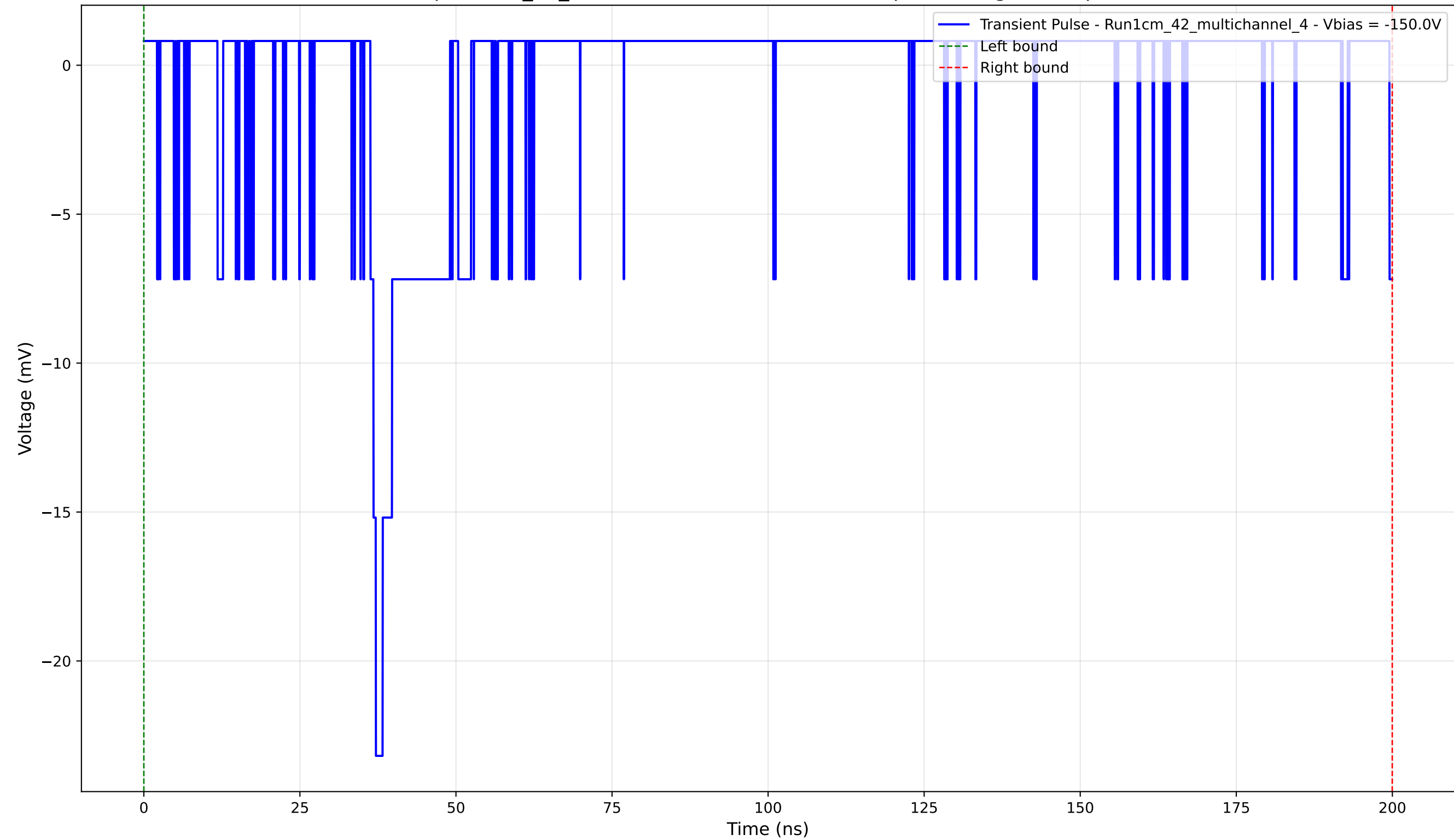
Transient Pulse - Sample: 1cm_42_multichannel - Position: 1830.0 \mu\text{m} - Charge: 1.43 pC - Rise Time: 0.88 ns
