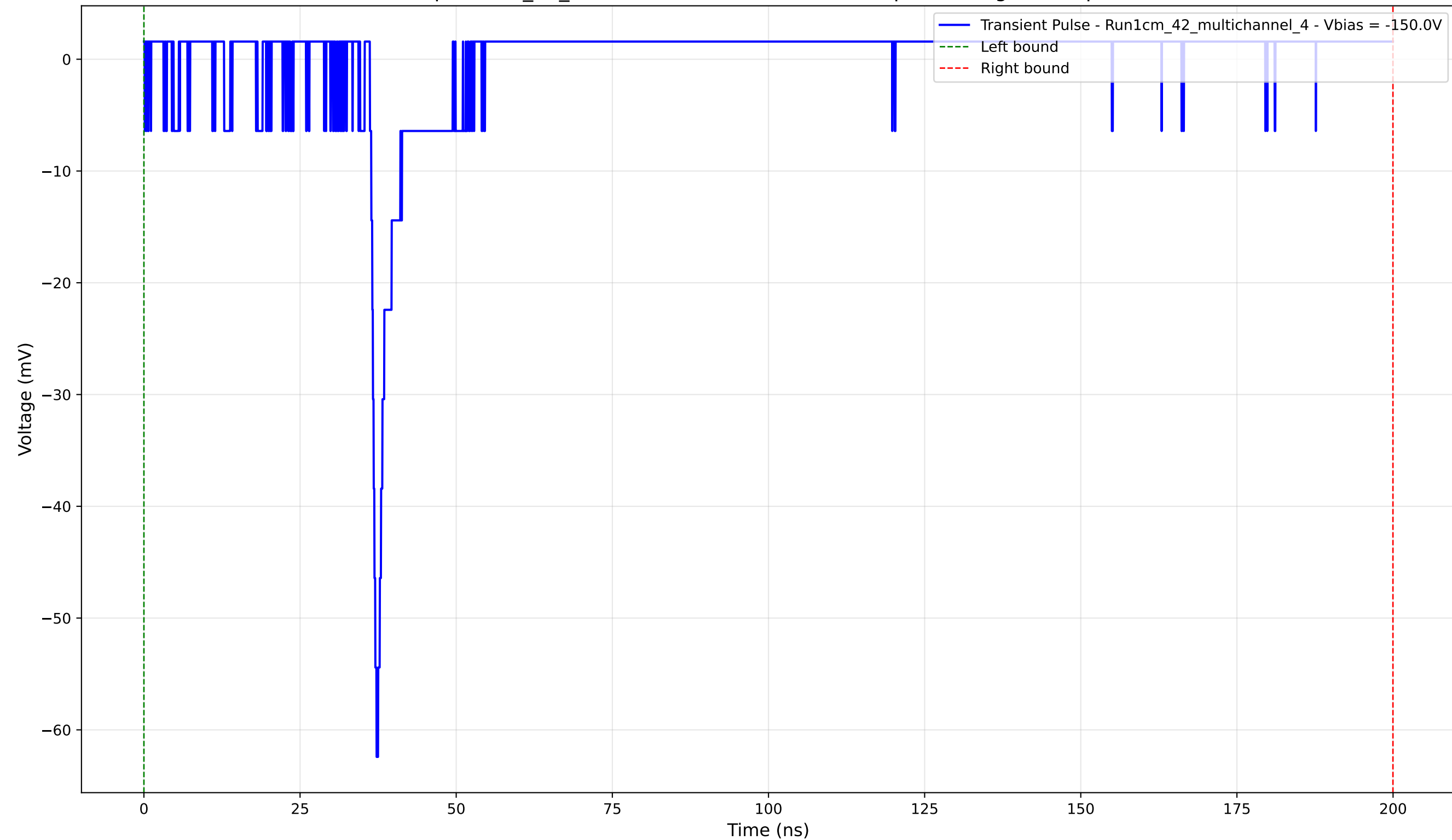
Transient Pulse - Sample: 1cm_42_multichannel - Position: 2660.0 \mu\text{m} - Charge: 0.26 pC - Rise Time: 1.06 ns
