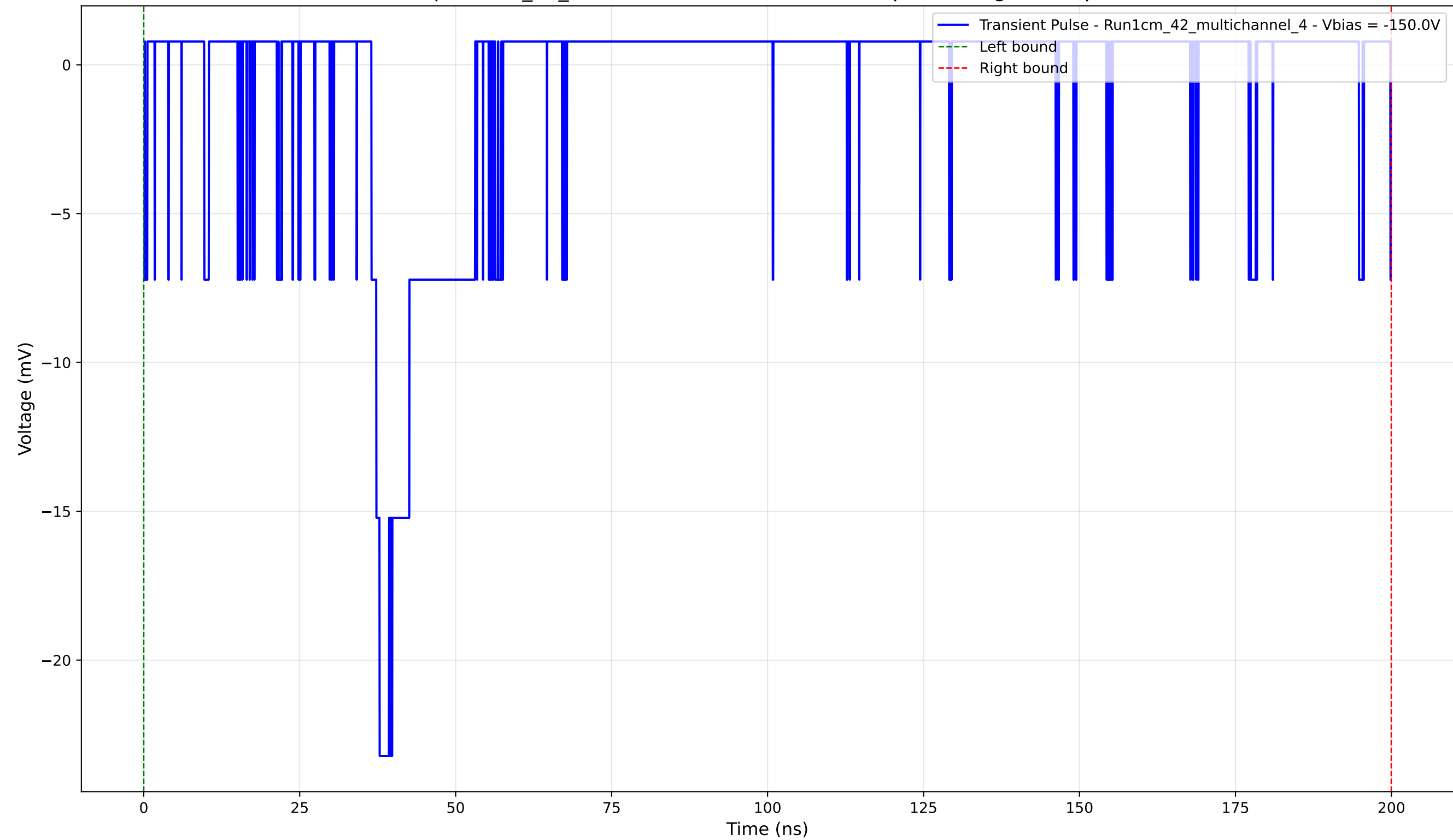
Transient Pulse - Sample: 1cm_42_multichannel - Position: 3510.0 \mu\text{m} - Charge: 2.15 pC - Rise Time: 1.32 ns
