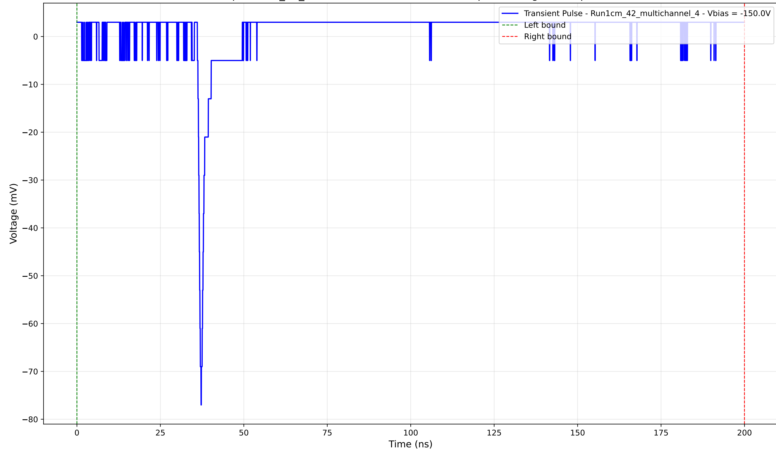
Transient Pulse - Sample: 1cm_42_multichannel - Position: 2455.0 \mu\text{m} - Charge: 5.79 pC - Rise Time: 0.93 ns
