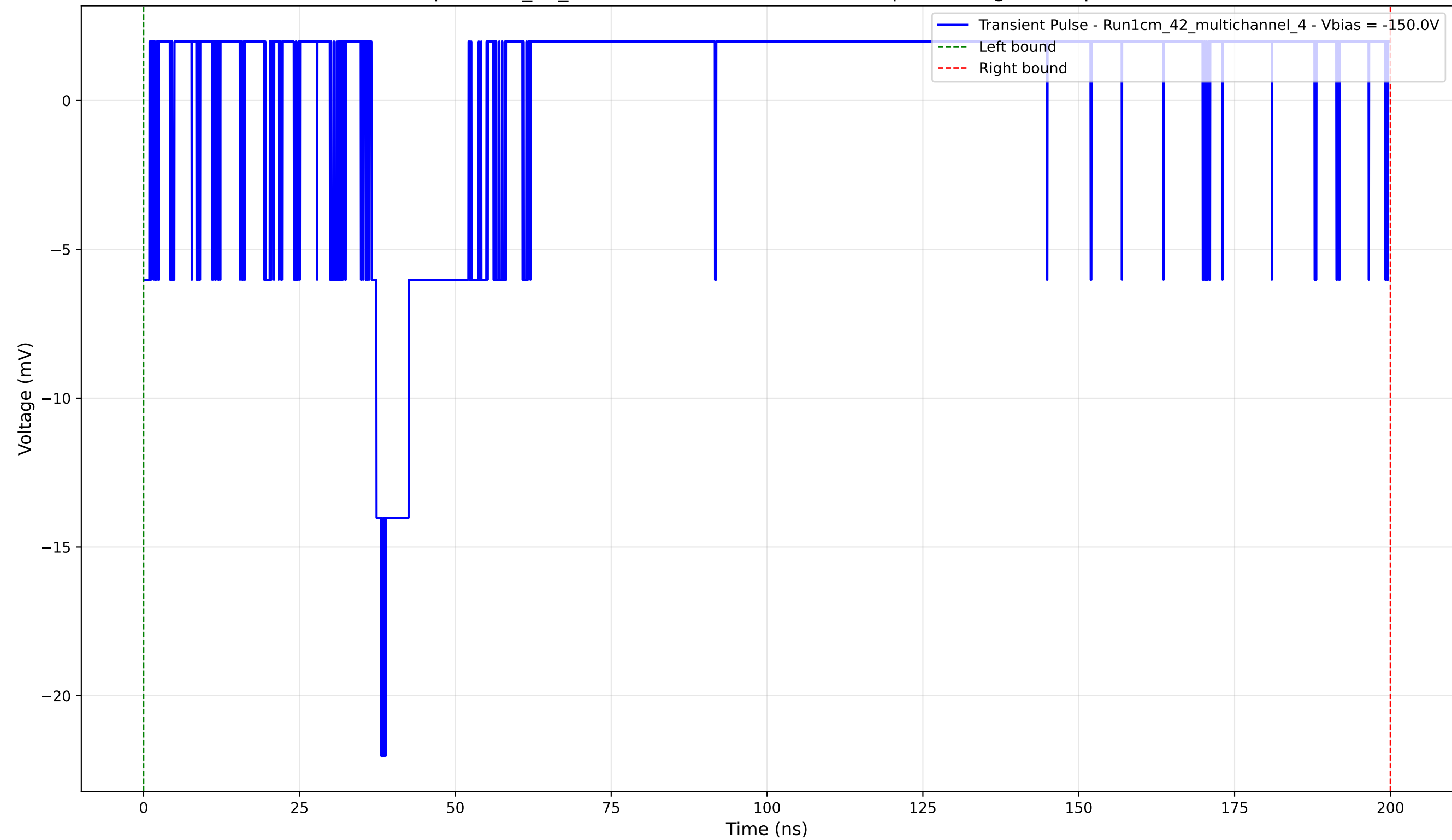
Transient Pulse - Sample: 1cm_42_multichannel - Position: 3585.0 \mu\text{m} - Charge: 2.30 pC - Rise Time: 1.56 ns
