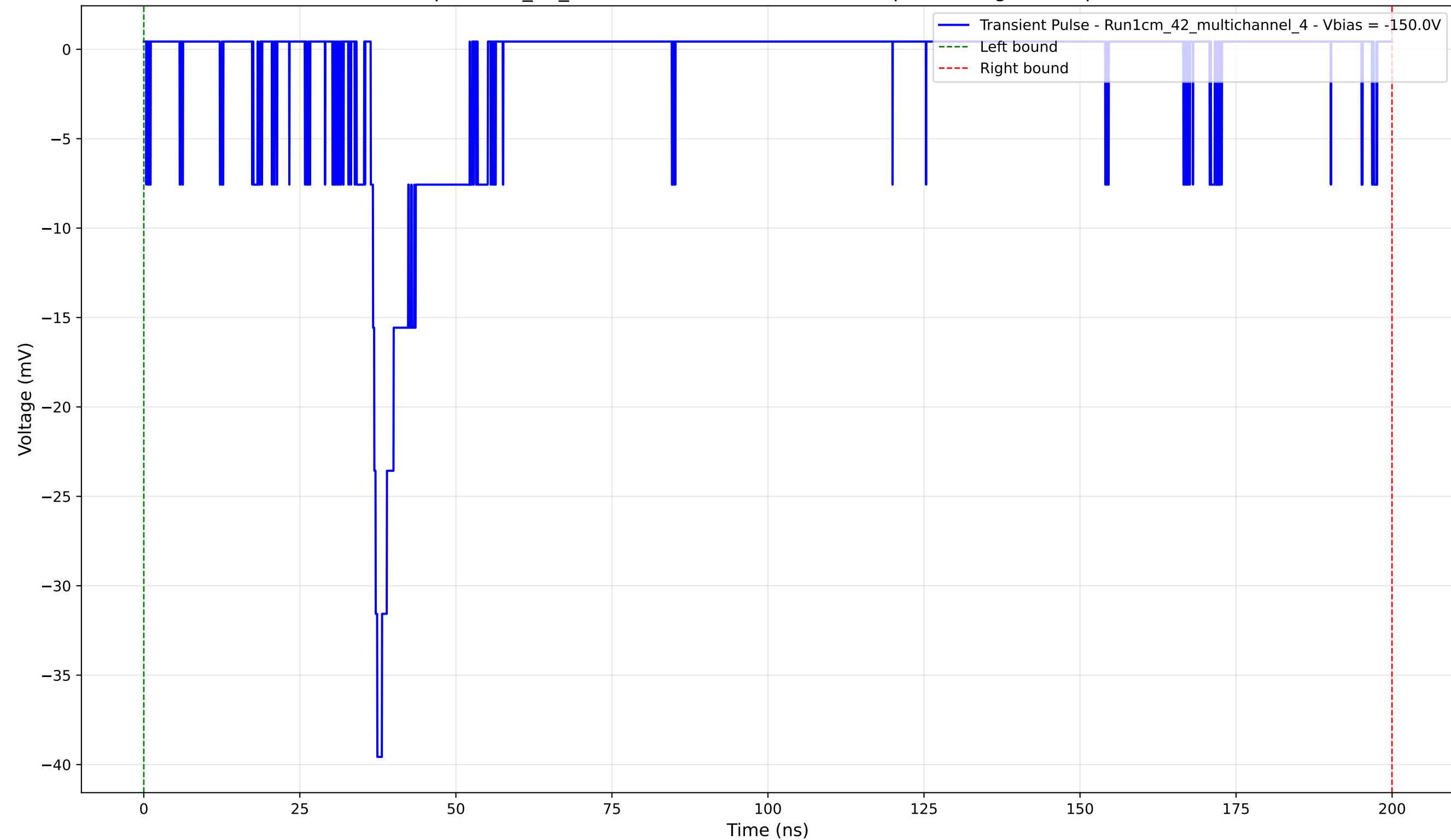
Transient Pulse - Sample: 1cm_42_multichannel - Position: 1720.0 \mu\text{m} - Charge: 4.62 pC - Rise Time: 1.05 ns
