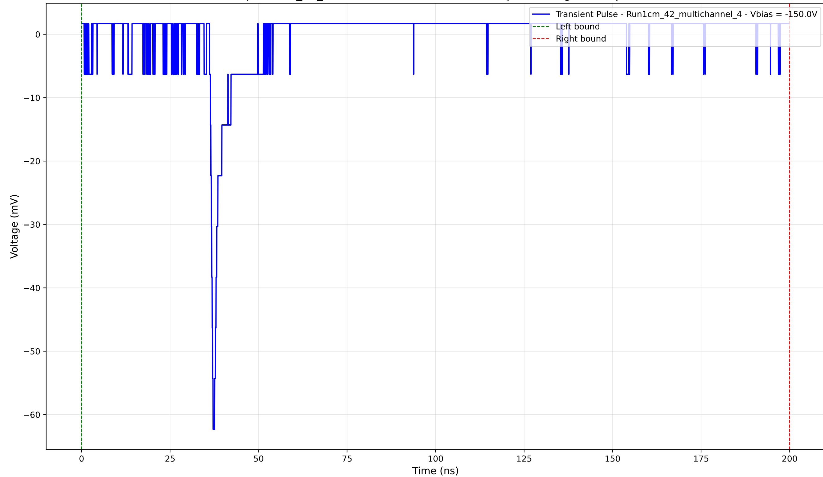
Transient Pulse - Sample: 1cm_42_multichannel - Position: 2640.0 \mu\text{m} - Charge: 0.27 pC - Rise Time: 1.00 ns
