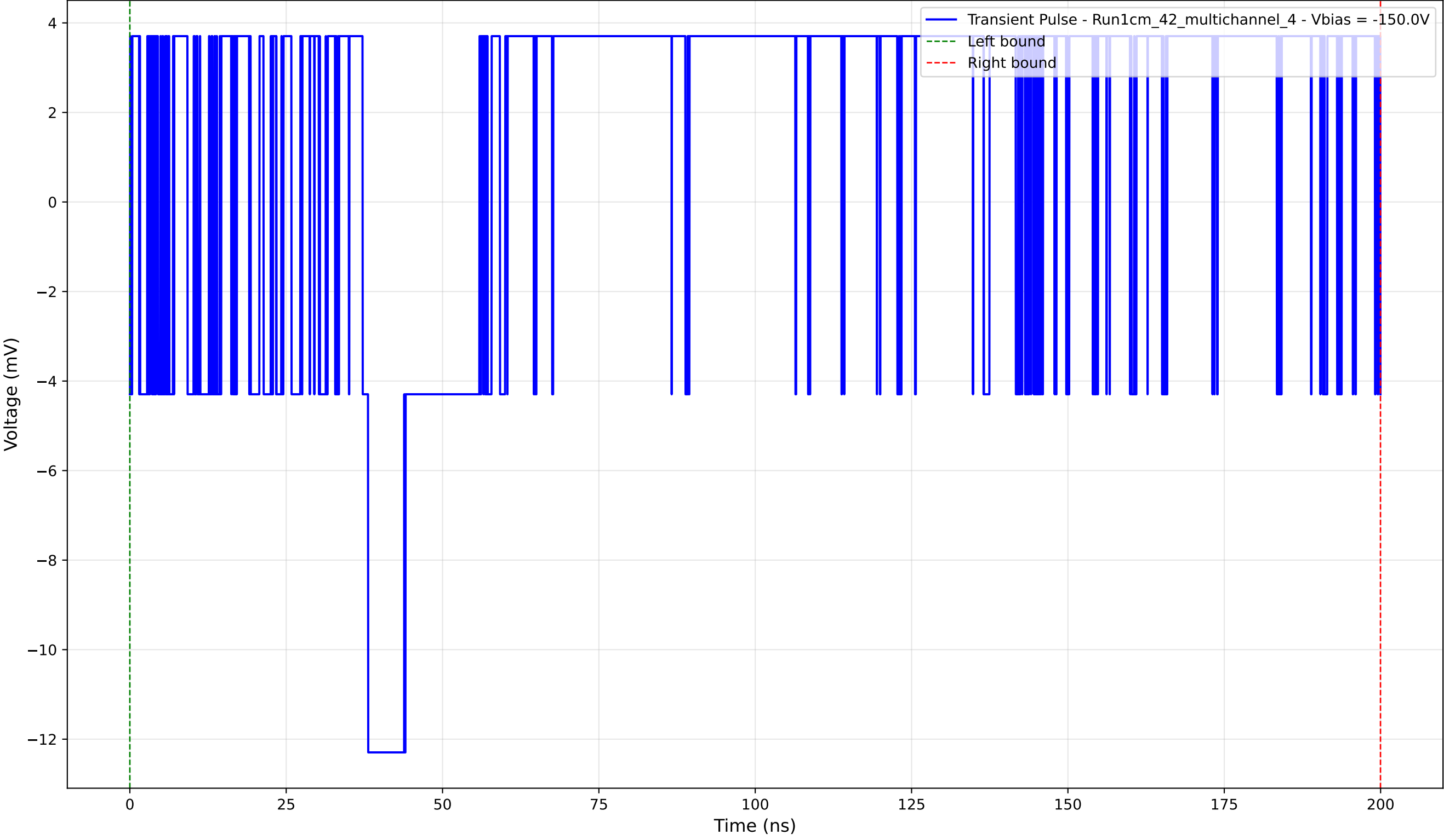
Transient Pulse - Sample: 1cm_42_multichannel - Position: 505.0 \mu\text{m} - Charge: 6.51 pC - Rise Time: 0.00 ns (N/A)
