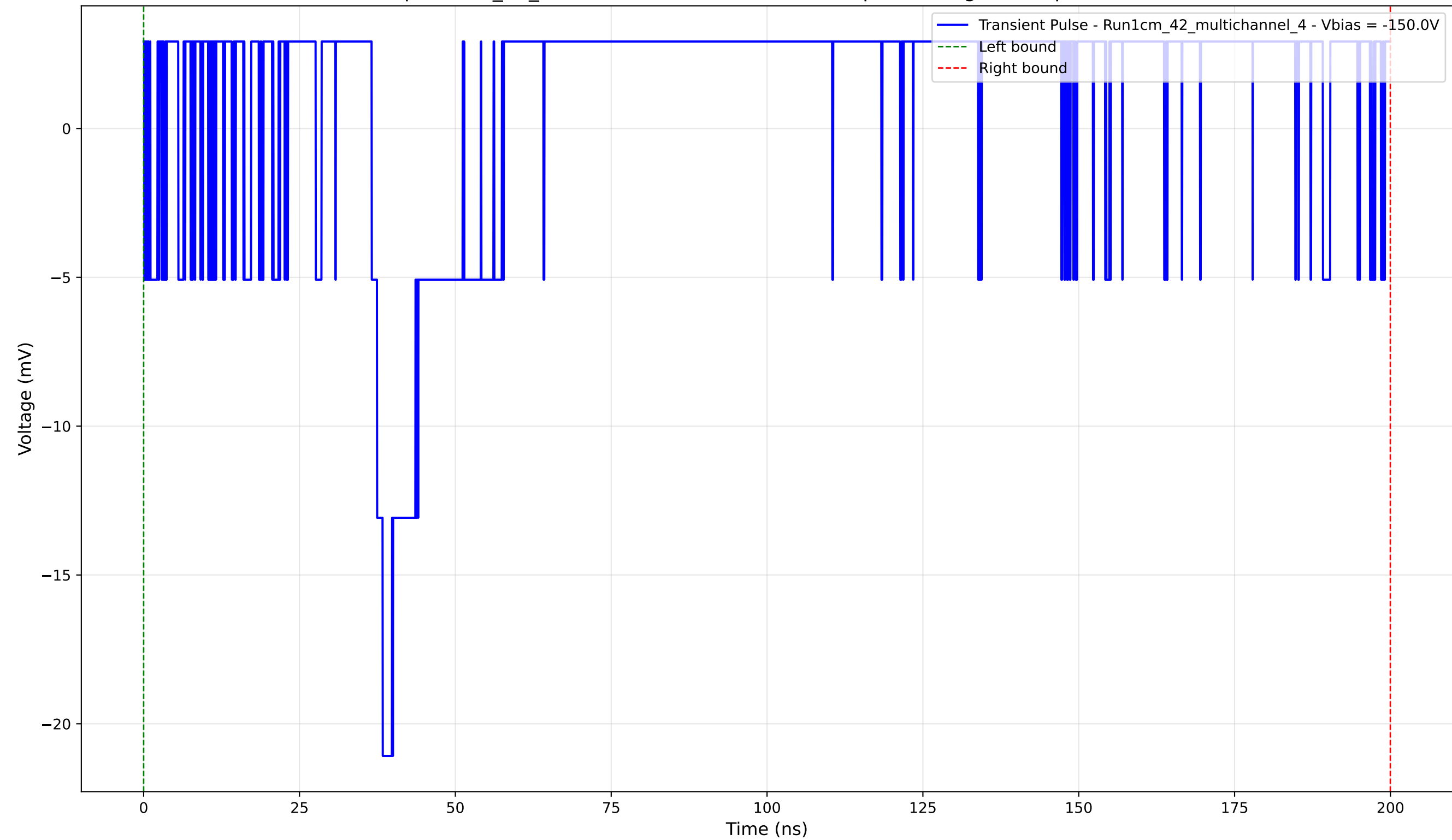
Transient Pulse - Sample: 1cm_42_multichannel - Position: 1040.0 \mu\text{m} - Charge: 4.68 pC - Rise Time: 0.00 ns (N/A)
