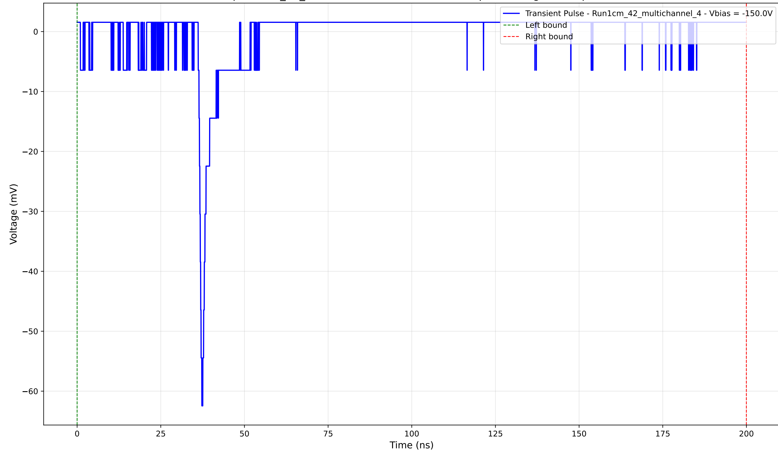
Transient Pulse - Sample: 1cm_42_multichannel - Position: 2675.0 \mu\text{m} - Charge: 0.29 pC - Rise Time: 1.08 ns
