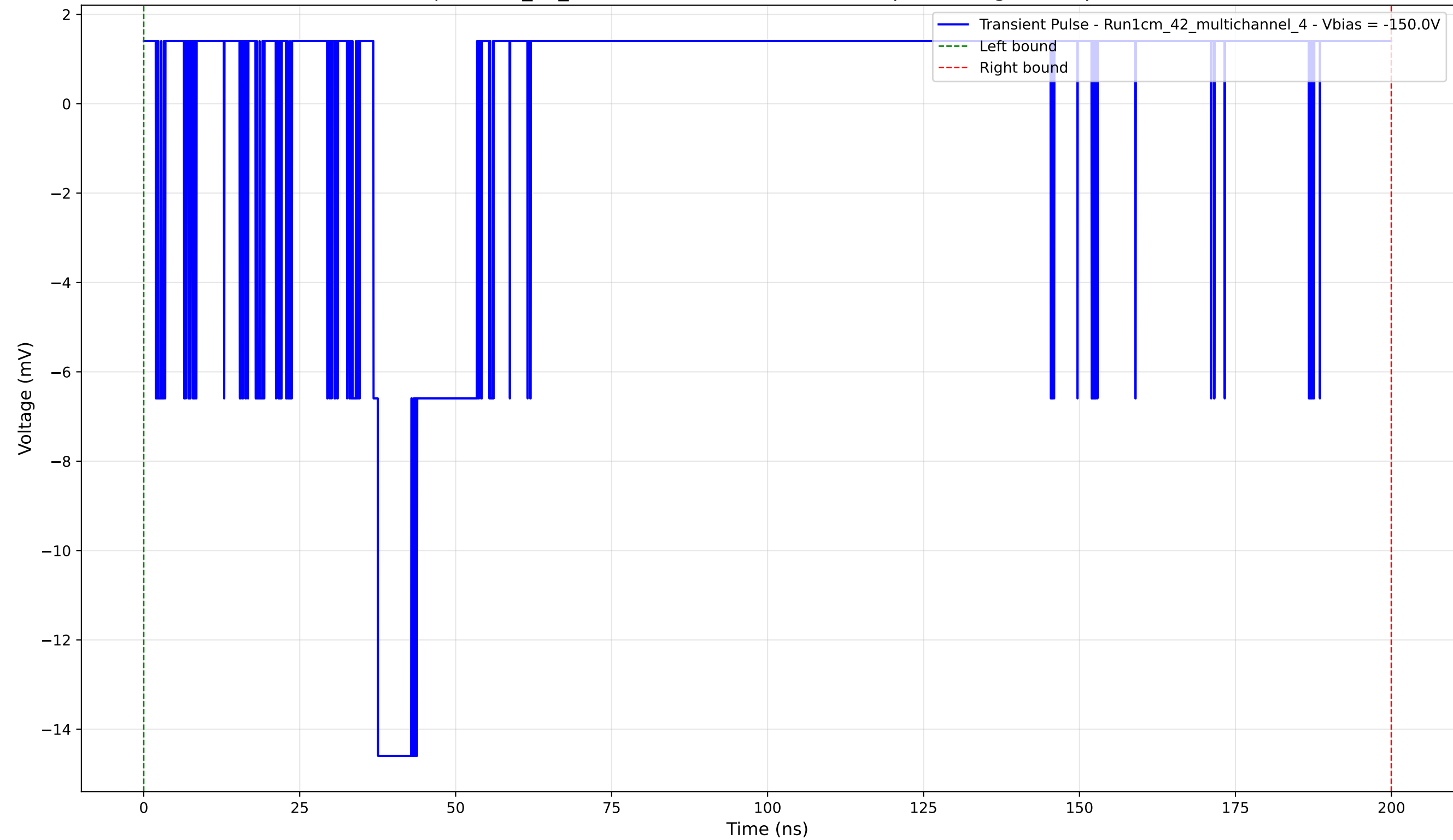
Transient Pulse - Sample: 1cm_42_multichannel - Position: 3730.0 \mu\text{m} - Charge: 0.58 pC - Rise Time: 0.74 ns
