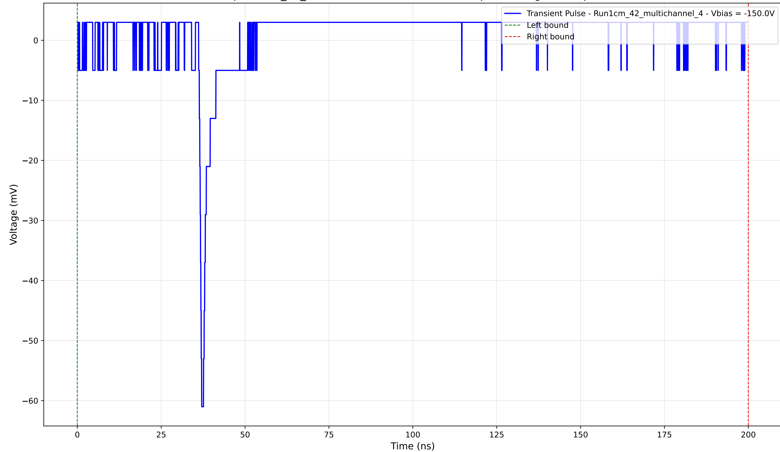
Transient Pulse - Sample: 1cm_42_multichannel - Position: 2600.0 \mu\text{m} - Charge: 5.18 pC - Rise Time: 0.72 ns
