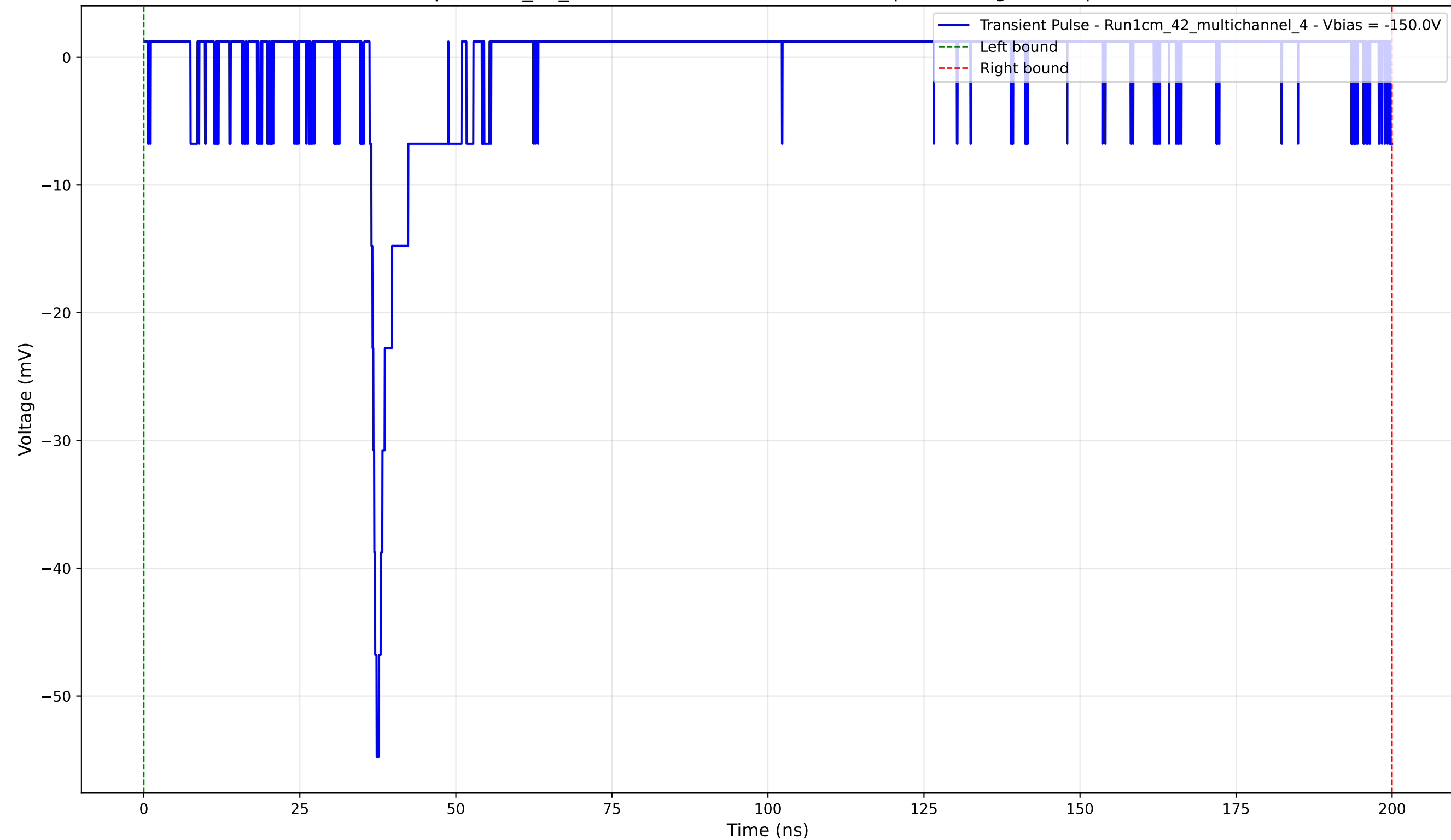
Transient Pulse - Sample: 1cm_42_multichannel - Position: 2765.0 \mu\text{m} - Charge: 1.64 pC - Rise Time: 1.12 ns
