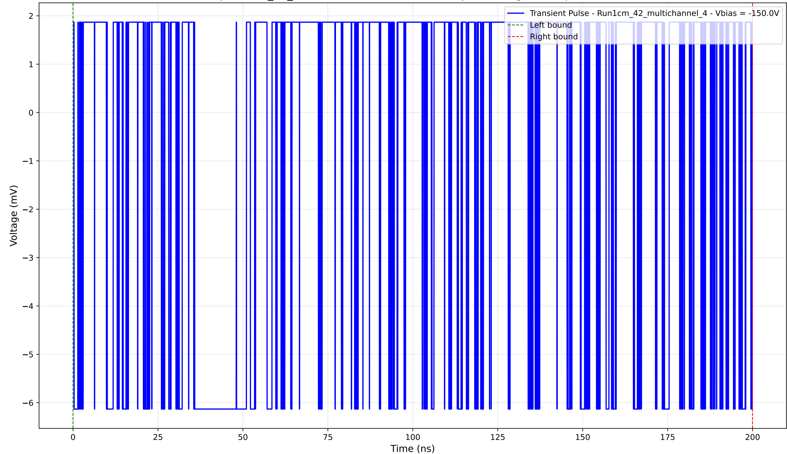
Transient Pulse - Sample: 1cm_42_multichannel - Position: 315.0 \mu\text{m} - Charge: 0.99 pC - Rise Time: 0.00 ns (N/A)
