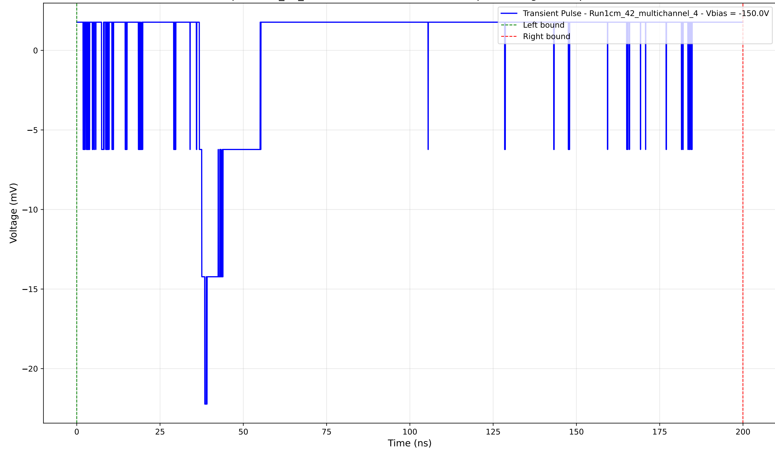
Transient Pulse - Sample: 1cm_42_multichannel - Position: 3715.0 \mu\text{m} - Charge: 2.15 pC - Rise Time: 1.64 ns
