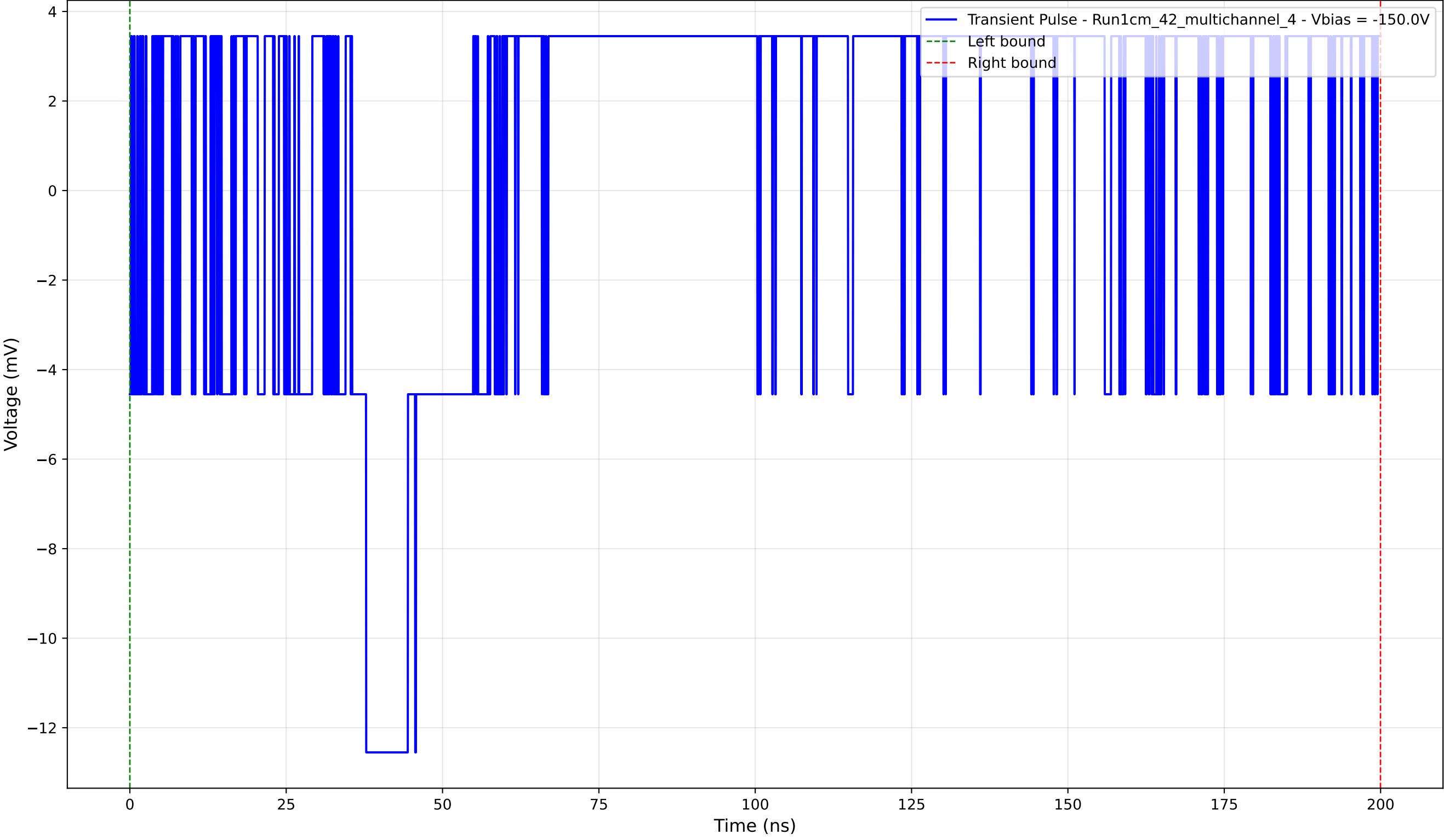
Transient Pulse - Sample: 1cm_42_multichannel - Position: 750.0 \mu\text{m} - Charge: 4.44 pC - Rise Time: 0.00 ns (N/A)
