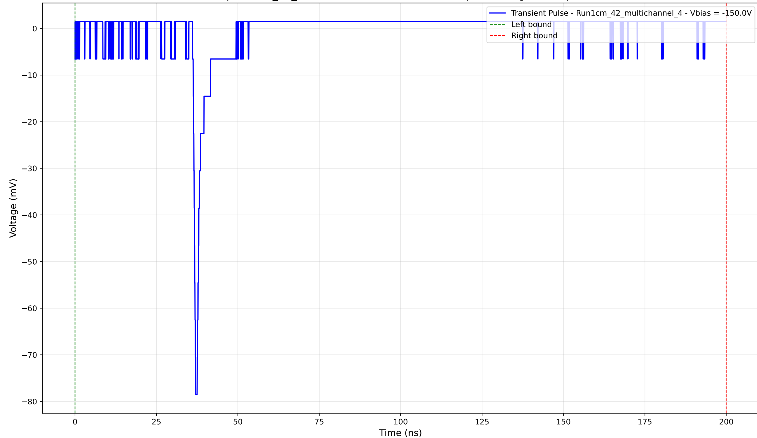
Transient Pulse - Sample: 1cm_42_multichannel - Position: 2505.0 \mu\text{m} - Charge: 0.69 pC - Rise Time: 0.80 ns
