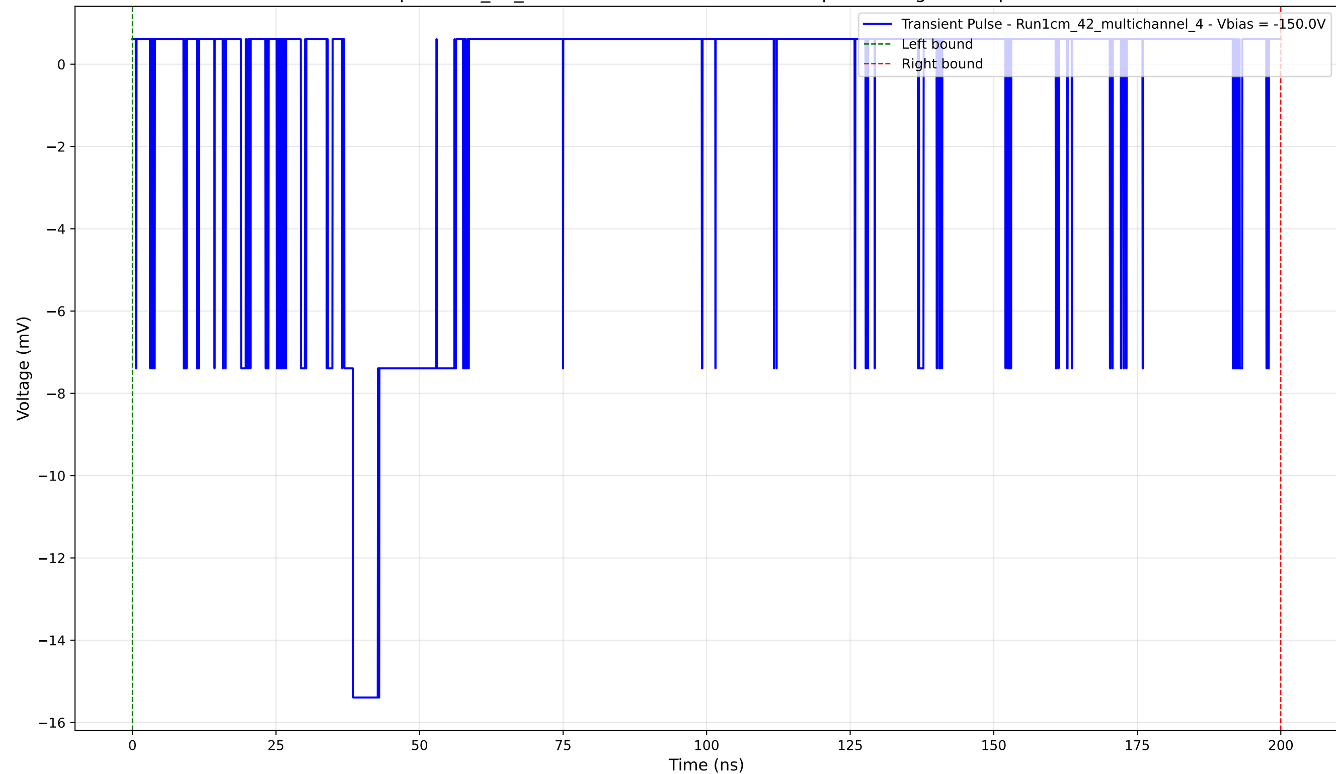
Transient Pulse - Sample: 1cm_42_multichannel - Position: 4270.0 \mu\text{m} - Charge: 3.02 pC - Rise Time: 1.54 ns
