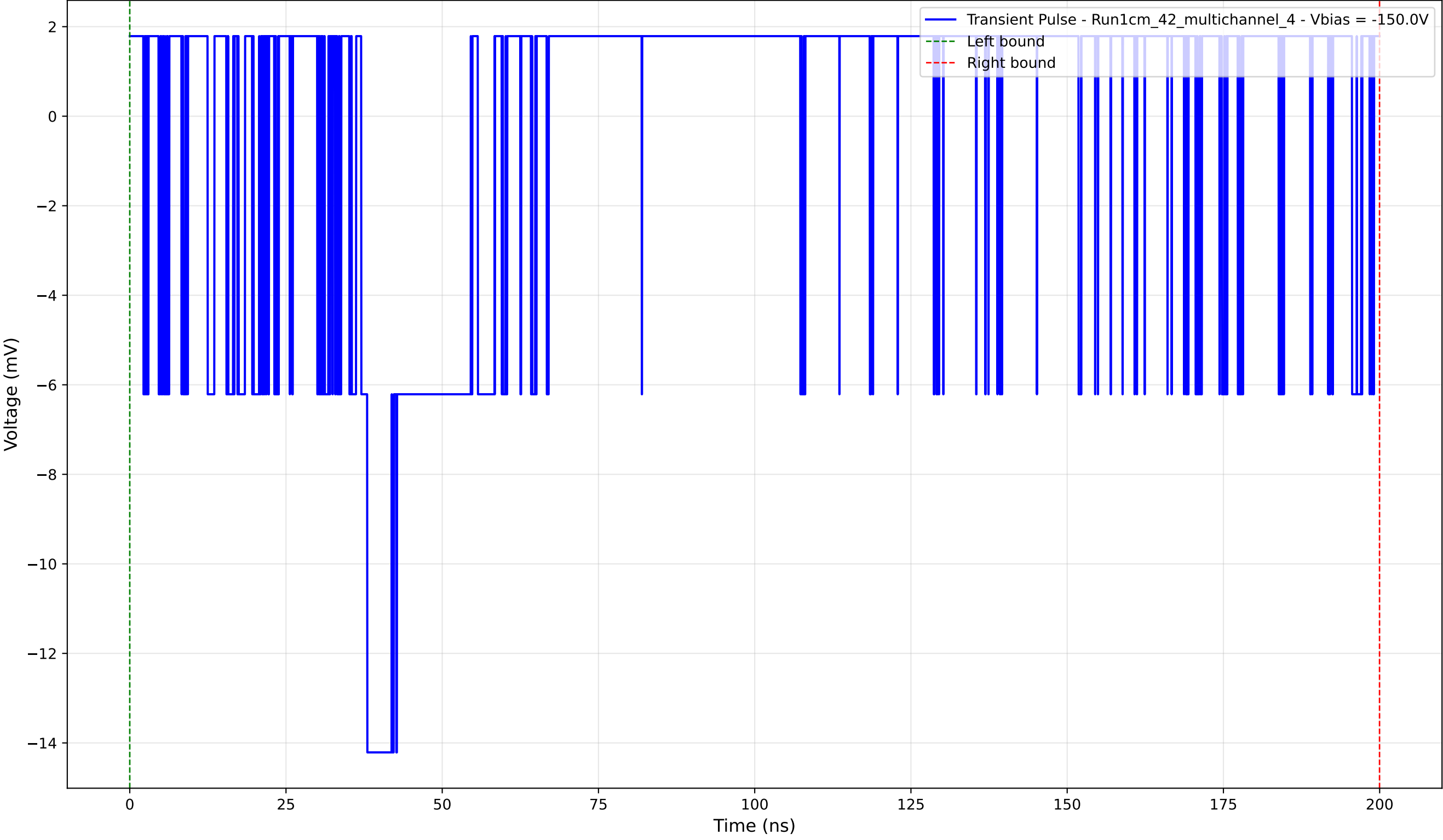
Transient Pulse - Sample: 1cm_42_multichannel - Position: 805.0 \mu\text{m} - Charge: 0.06 pC - Rise Time: 0.00 ns (N/A)
