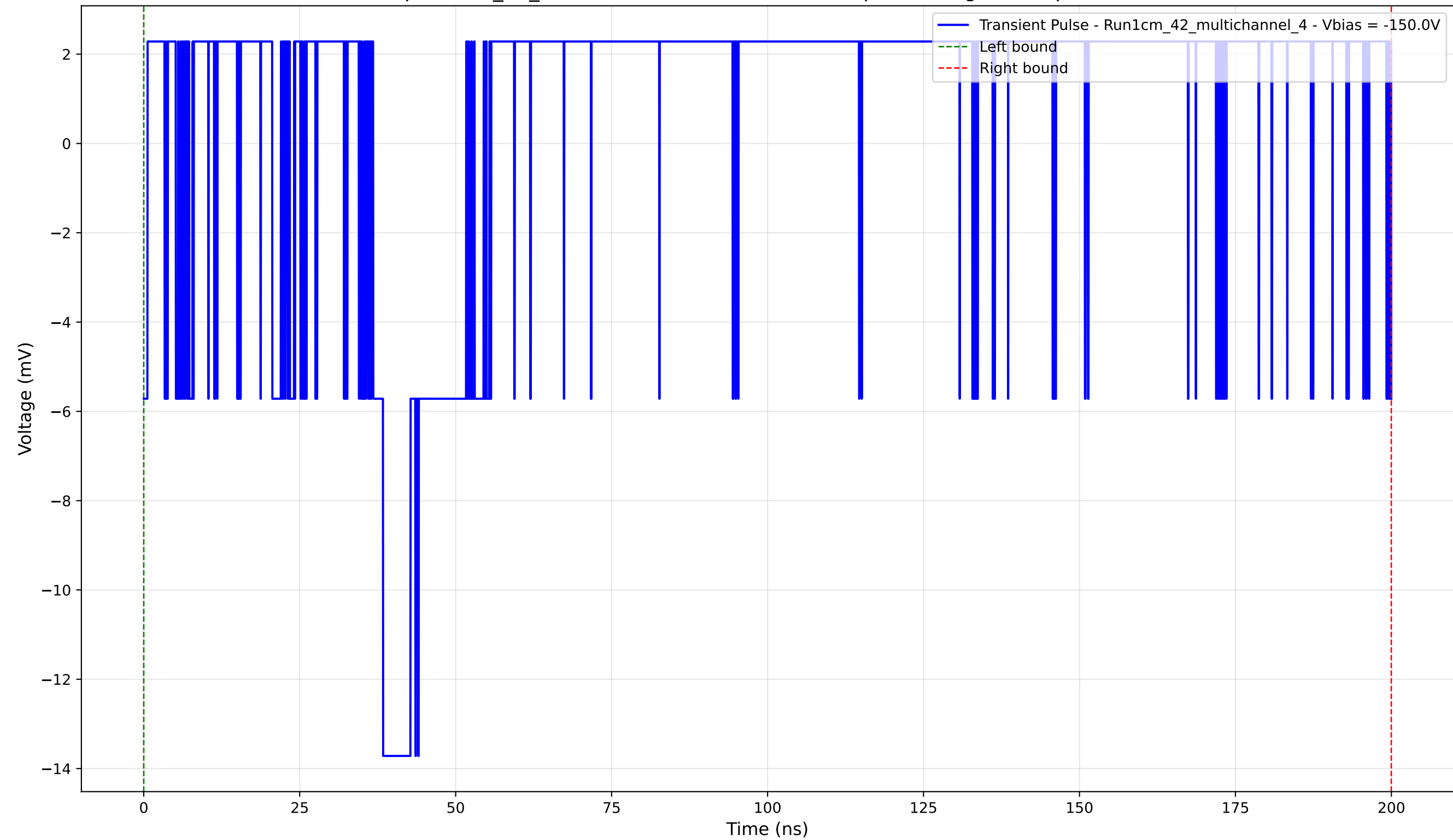
Transient Pulse - Sample: 1cm_42_multichannel - Position: 4305.0 \mu\text{m} - Charge: 3.58 pC - Rise Time: 0.00 ns (N/A)
