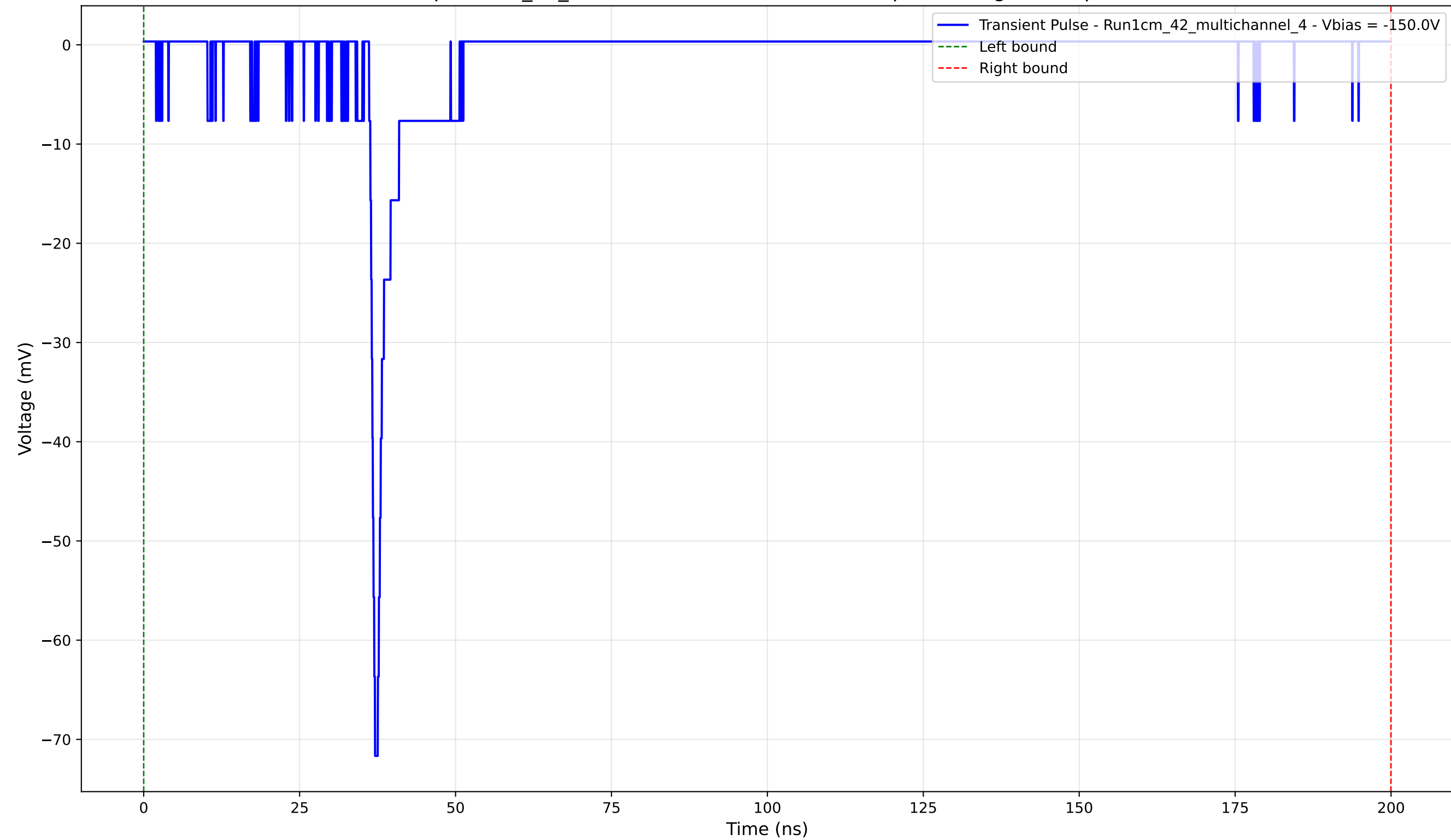
Transient Pulse - Sample: 1cm_42_multichannel - Position: 2560.0 \mu\text{m} - Charge: 4.27 pC - Rise Time: 0.94 ns
