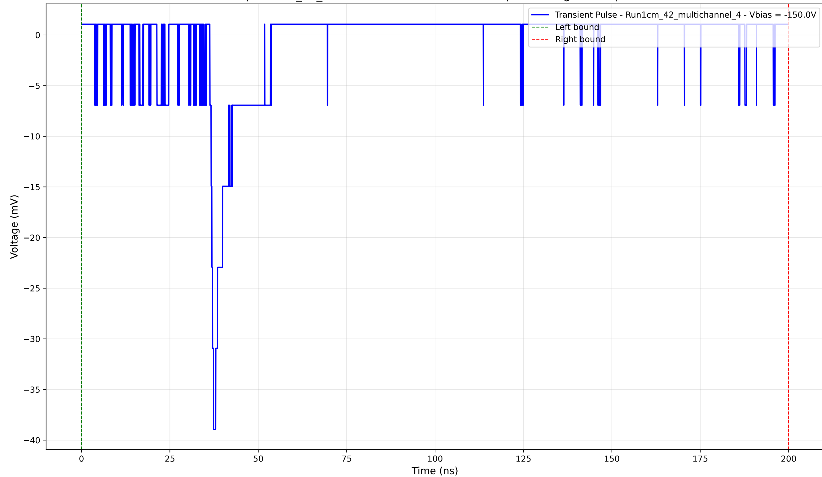
Transient Pulse - Sample: 1cm_42_multichannel - Position: 2975.0 \mu\text{m} - Charge: 1.98 pC - Rise Time: 1.03 ns
