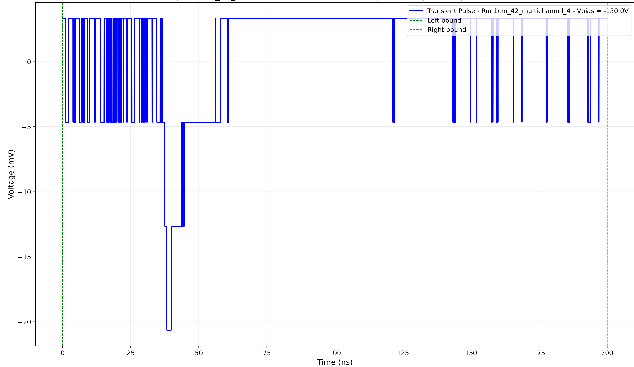
Transient Pulse - Sample: 1cm_42_multichannel - Position: 1025.0 \mu\text{m} - Charge: 6.05 pC - Rise Time: 0.00 ns (N/A)
