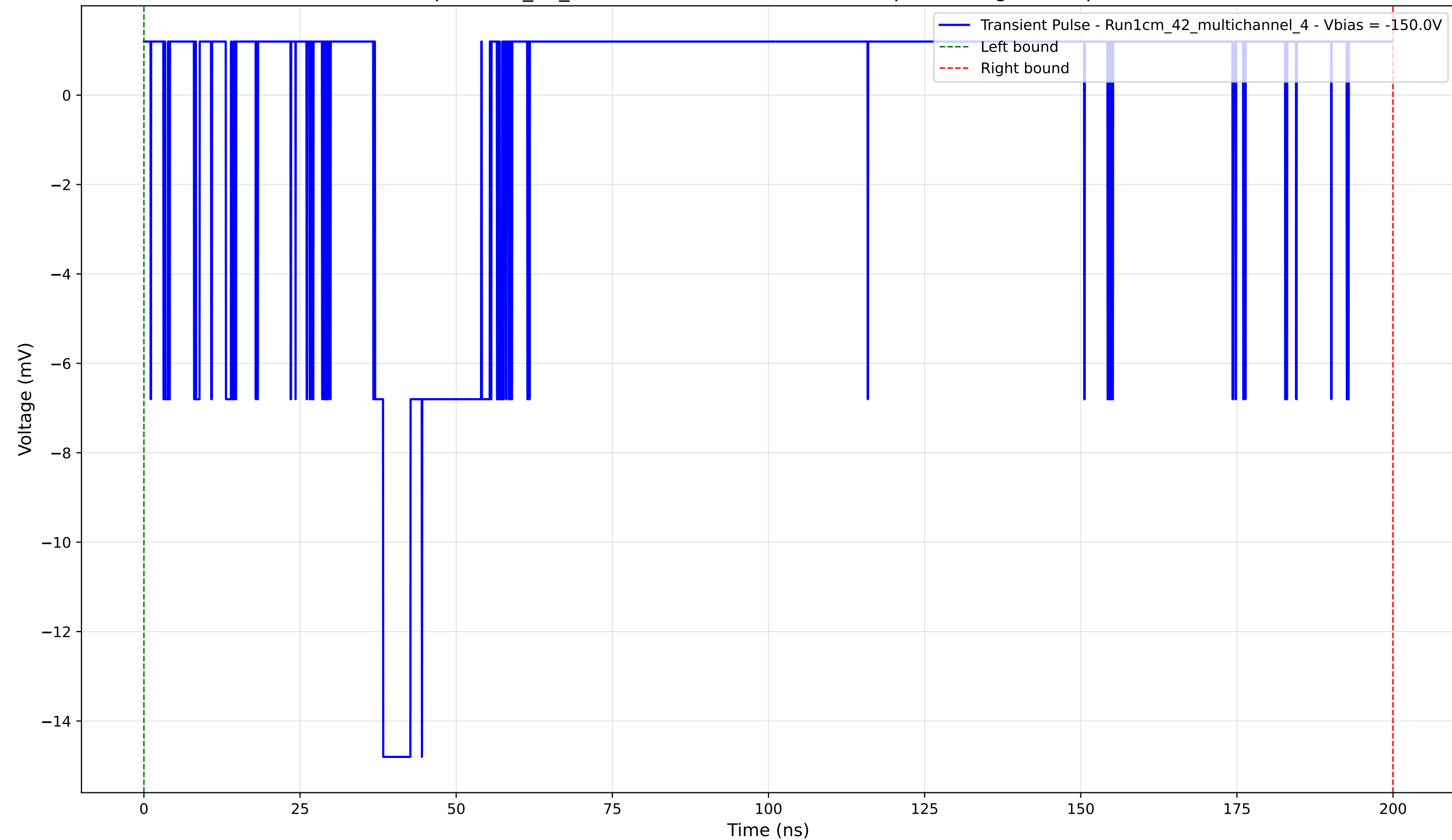
Transient Pulse - Sample: 1cm_42_multichannel - Position: 4210.0 \mu\text{m} - Charge: 0.02 pC - Rise Time: 1.32 ns
