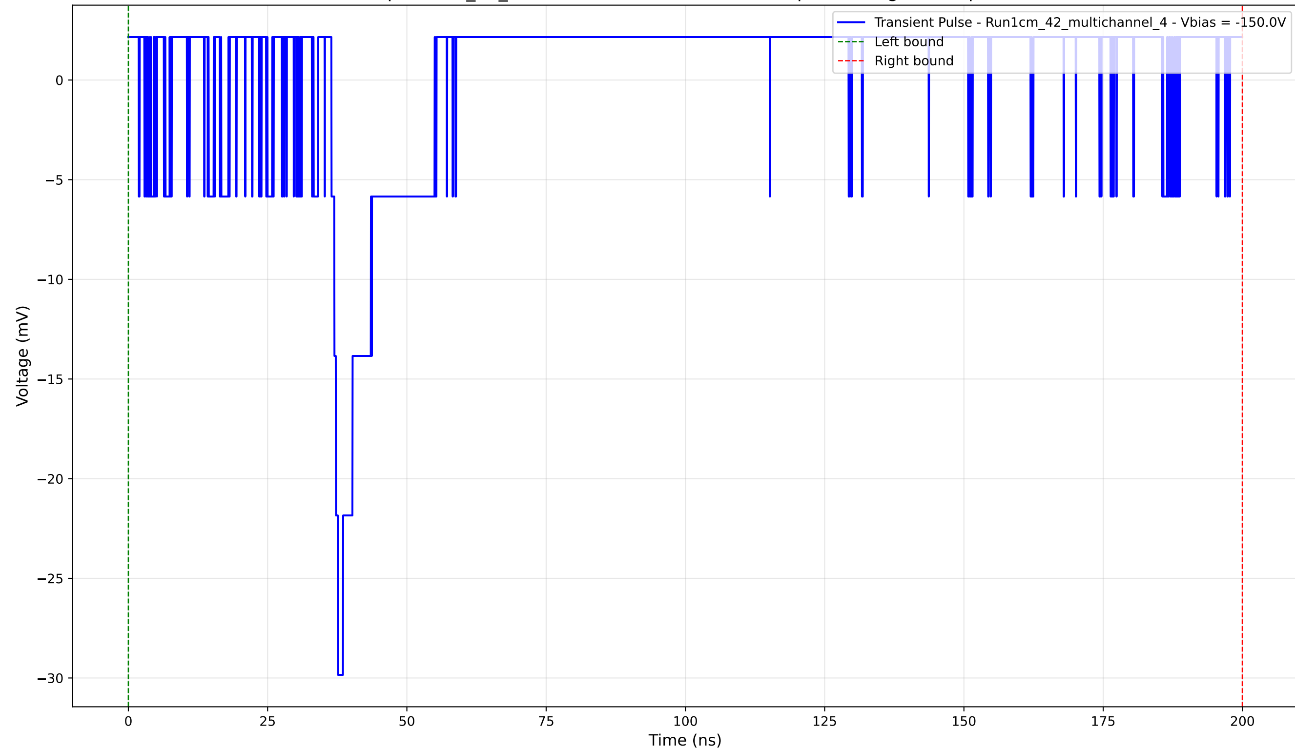
Transient Pulse - Sample: 1cm_42_multichannel - Position: 1465.0 \mu\text{m} - Charge: 1.65 pC - Rise Time: 1.18 ns
