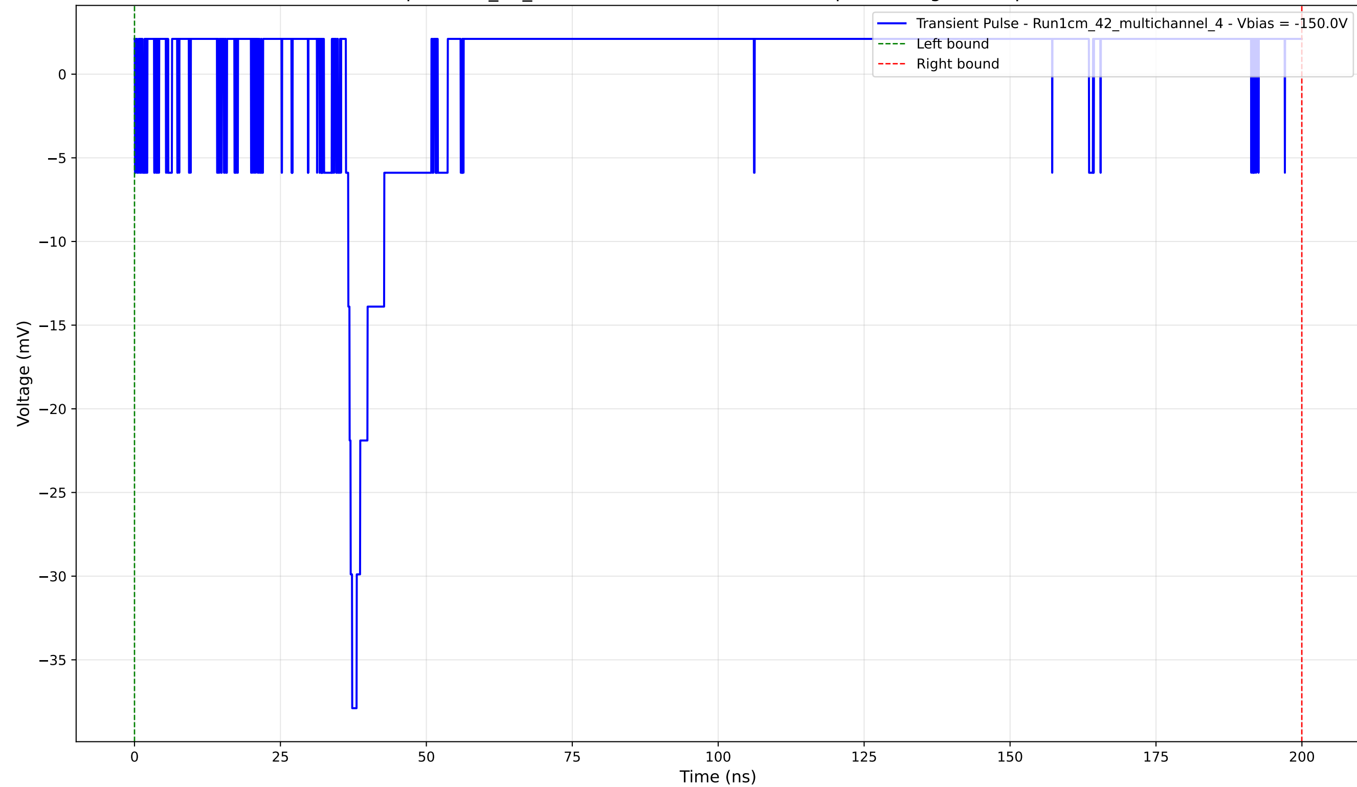
Transient Pulse - Sample: 1cm_42_multichannel - Position: 2980.0 \mu\text{m} - Charge: 2.44 pC - Rise Time: 1.07 ns
