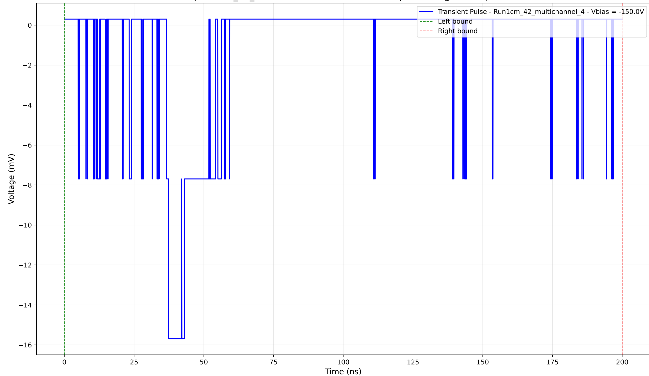
Transient Pulse - Sample: 1cm_42_multichannel - Position: 3600.0 \mu\text{m} - Charge: 3.72 pC - Rise Time: 0.72 ns
