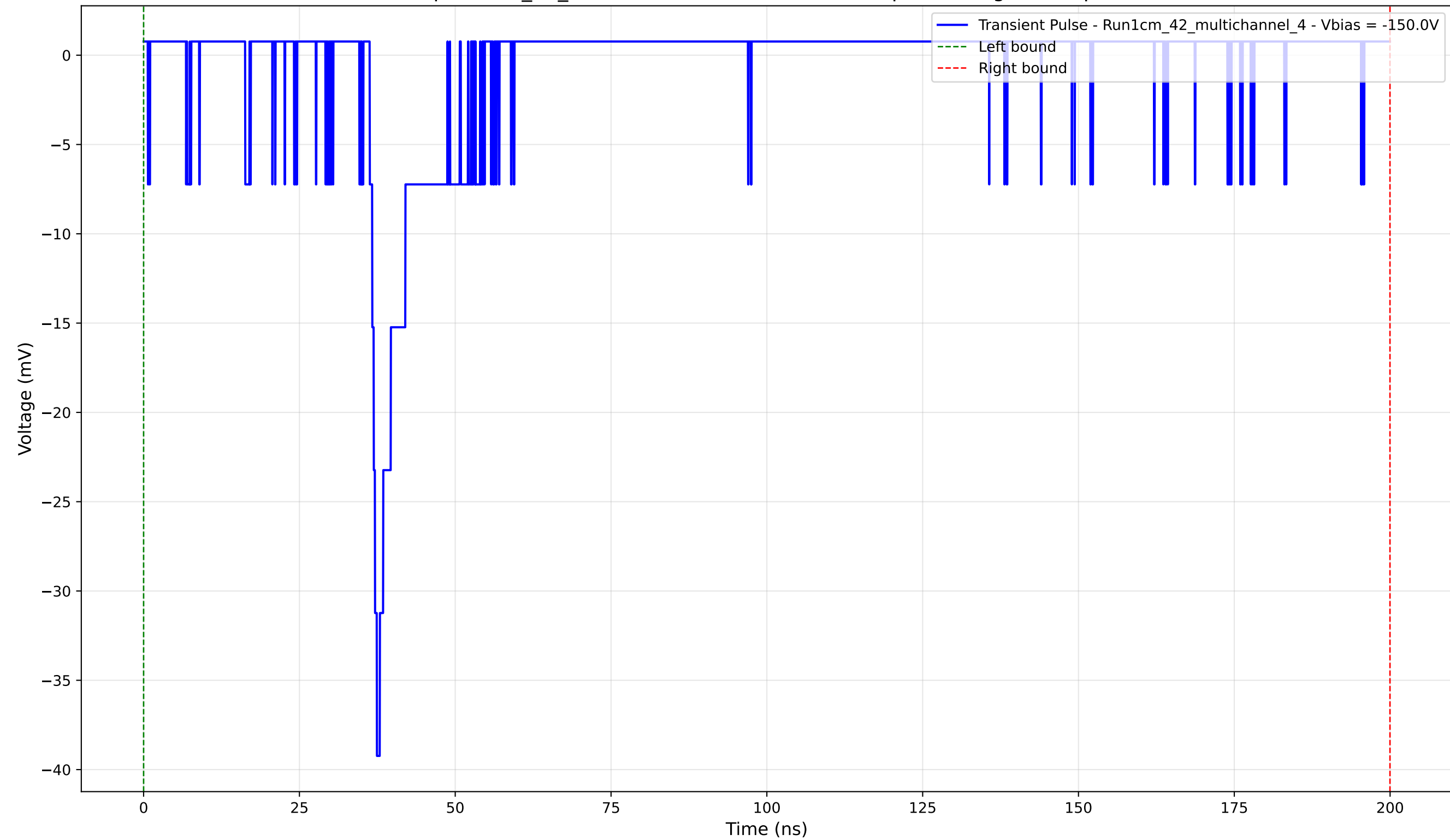
Transient Pulse - Sample: 1cm_42_multichannel - Position: 3020.0 \mu\text{m} - Charge: 2.39 pC - Rise Time: 1.15 ns
