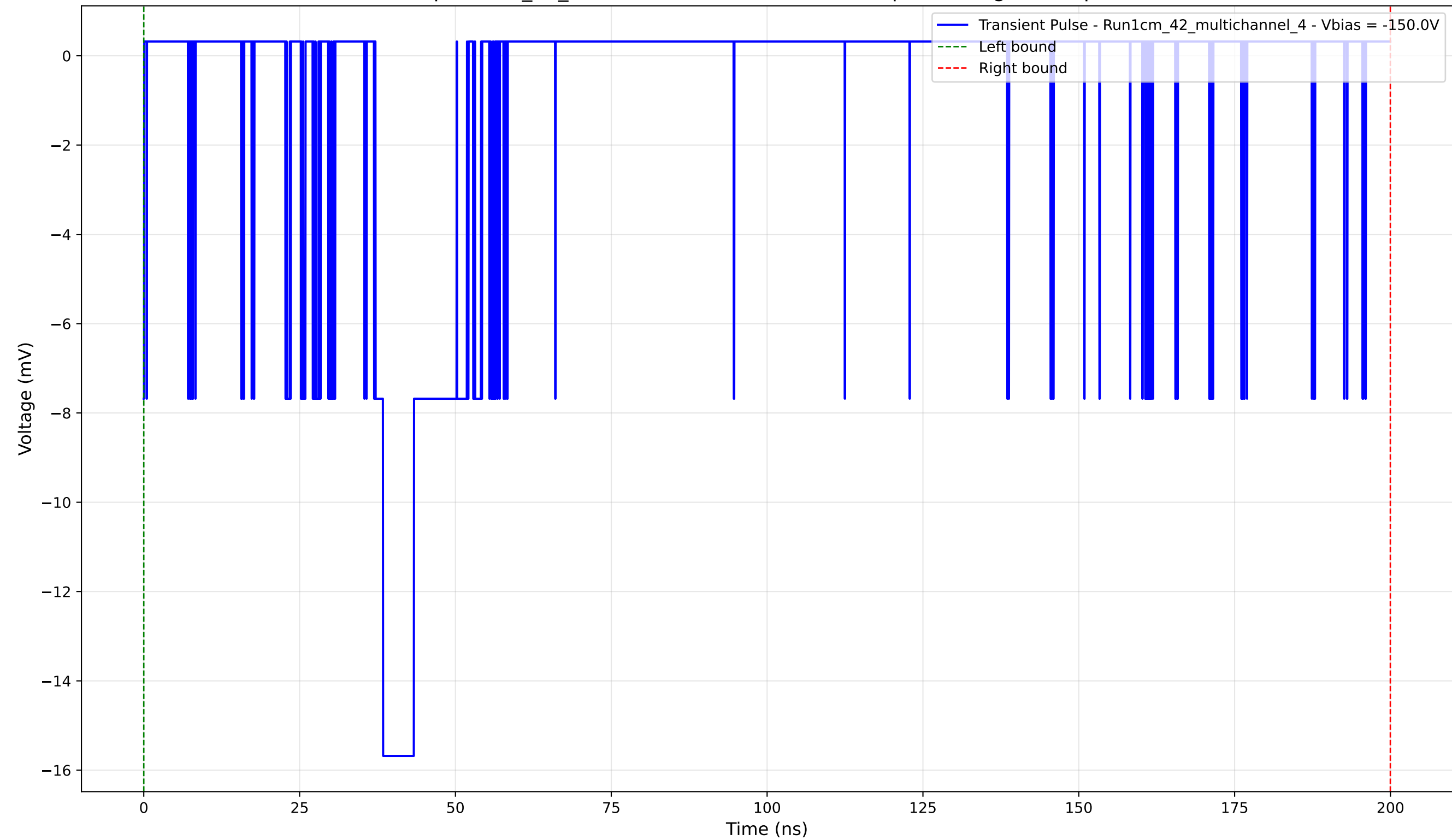
Transient Pulse - Sample: 1cm_42_multichannel - Position: 4535.0 \mu\text{m} - Charge: 3.36 pC - Rise Time: 1.22 ns
