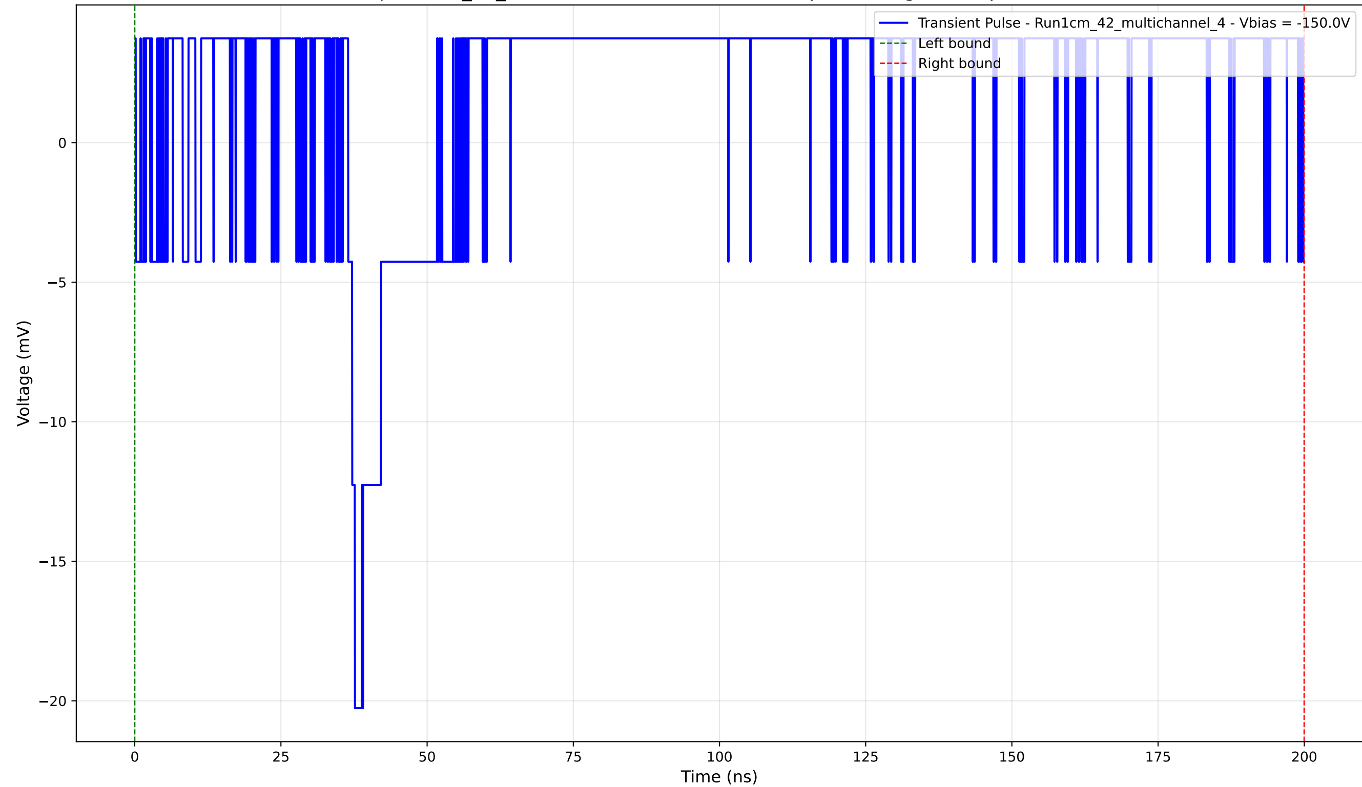
Transient Pulse - Sample: 1cm_42_multichannel - Position: 1435.0 \mu\text{m} - Charge: 8.05 pC - Rise Time: 0.00 ns (N/A)
