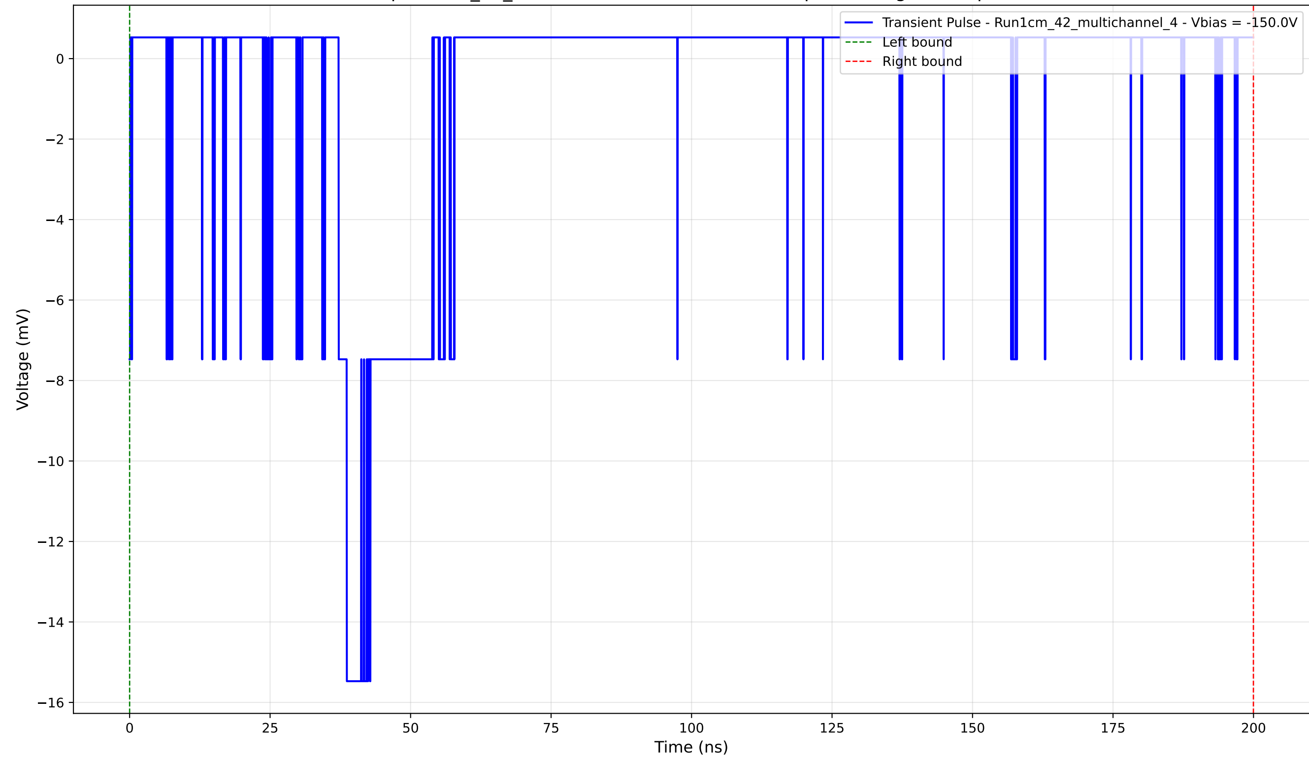
Transient Pulse - Sample: 1cm_42_multichannel - Position: 4715.0 \mu\text{m} - Charge: 2.43 pC - Rise Time: 1.46 ns
