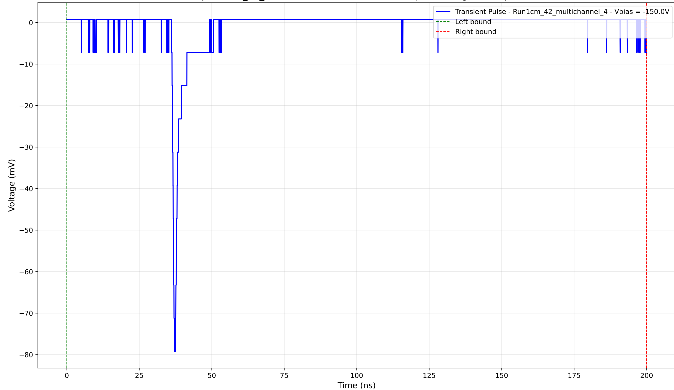
Transient Pulse - Sample: 1cm_42_multichannel - Position: 2510.0 \mu\text{m} - Charge: 2.43 pC - Rise Time: 0.82 ns
