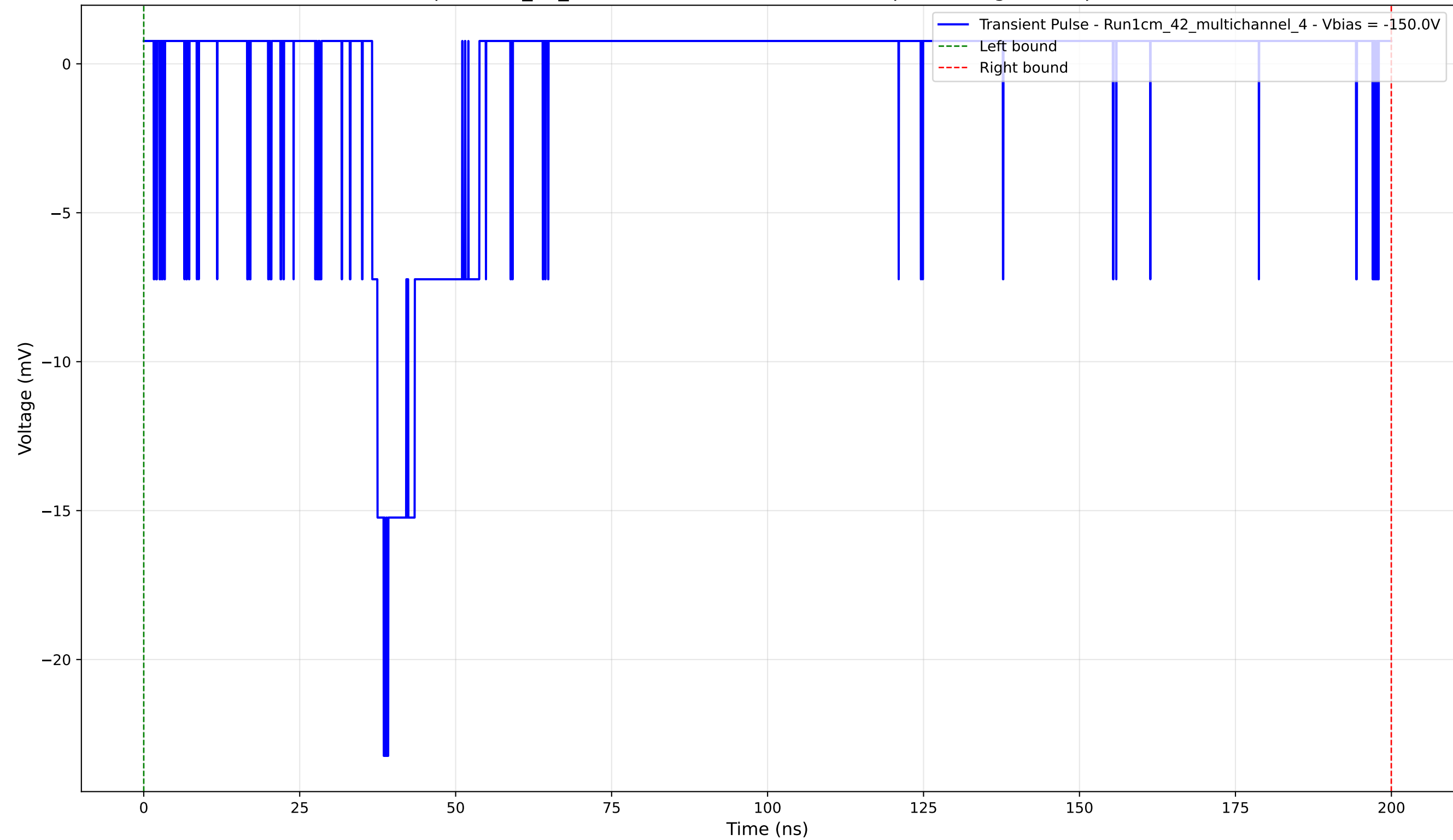
Transient Pulse - Sample: 1cm_42_multichannel - Position: 3615.0 \mu\text{m} - Charge: 1.35 pC - Rise Time: 1.86 ns
