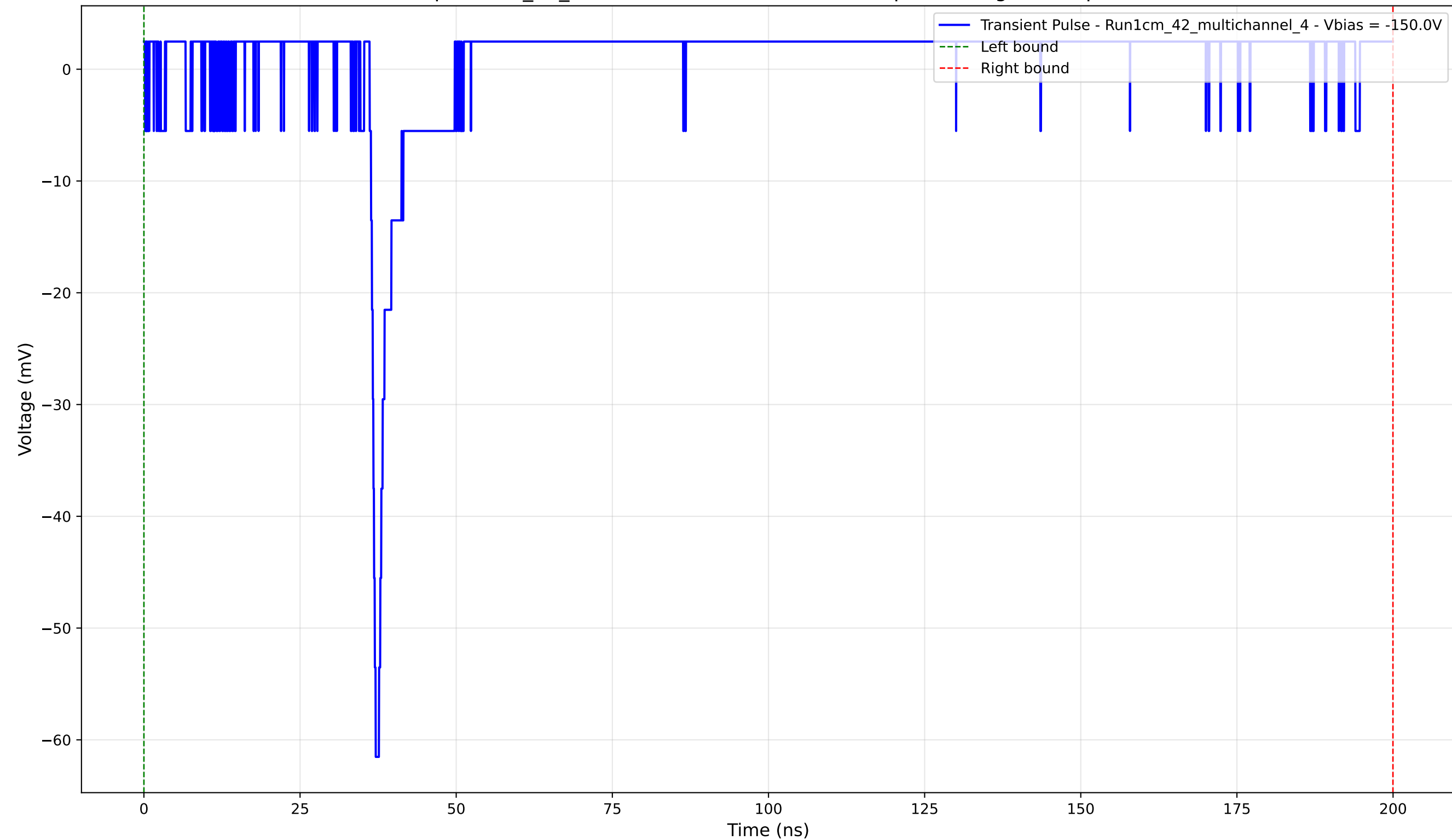
Transient Pulse - Sample: 1cm_42_multichannel - Position: 2625.0 \mu\text{m} - Charge: 3.79 pC - Rise Time: 0.76 ns
