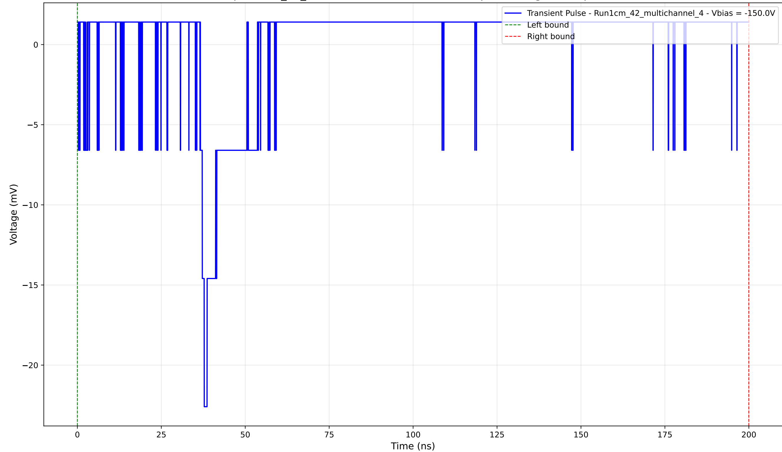
Transient Pulse - Sample: 1cm_42_multichannel - Position: 3335.0 \mu\text{m} - Charge: 1.26 pC - Rise Time: 1.16 ns
