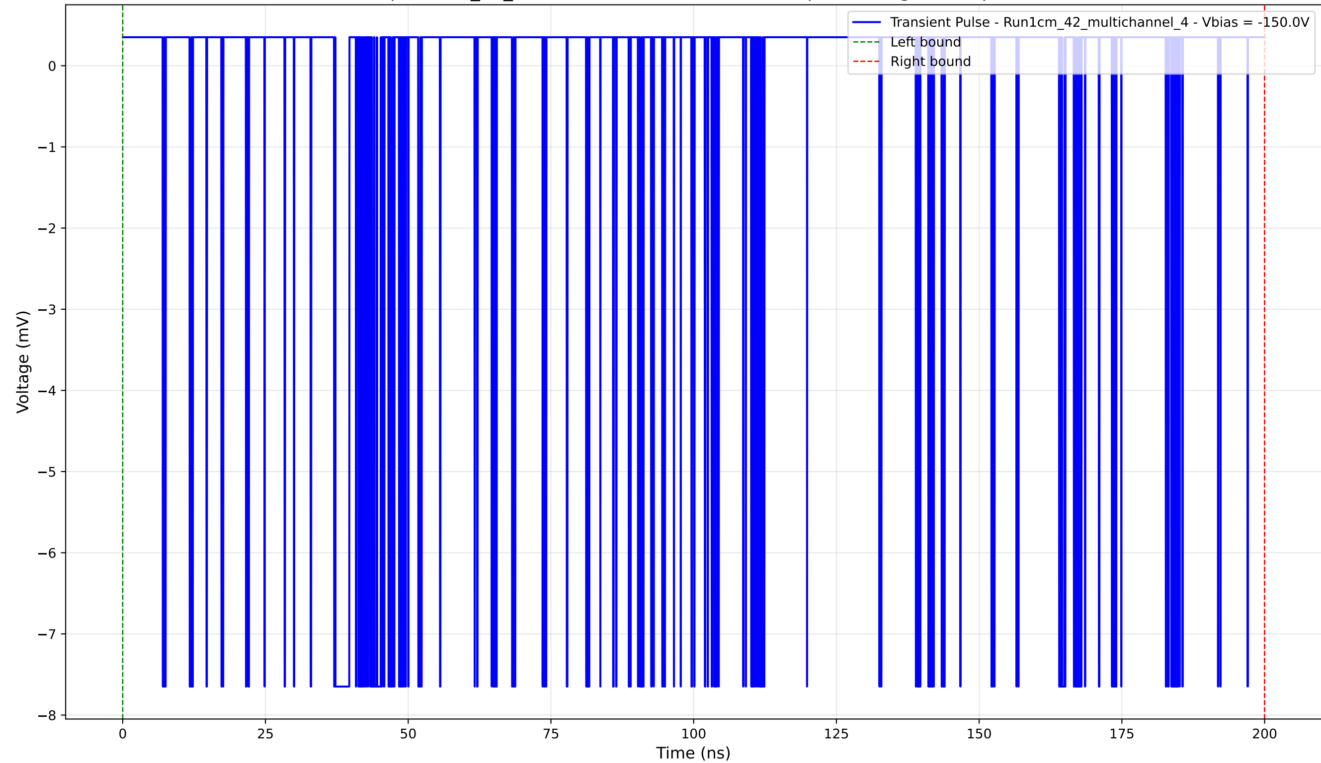
Transient Pulse - Sample: 1cm_42_multichannel - Position: 3375.0 \mu\text{m} - Charge: 1.73 pC - Rise Time: 0.02 ns
