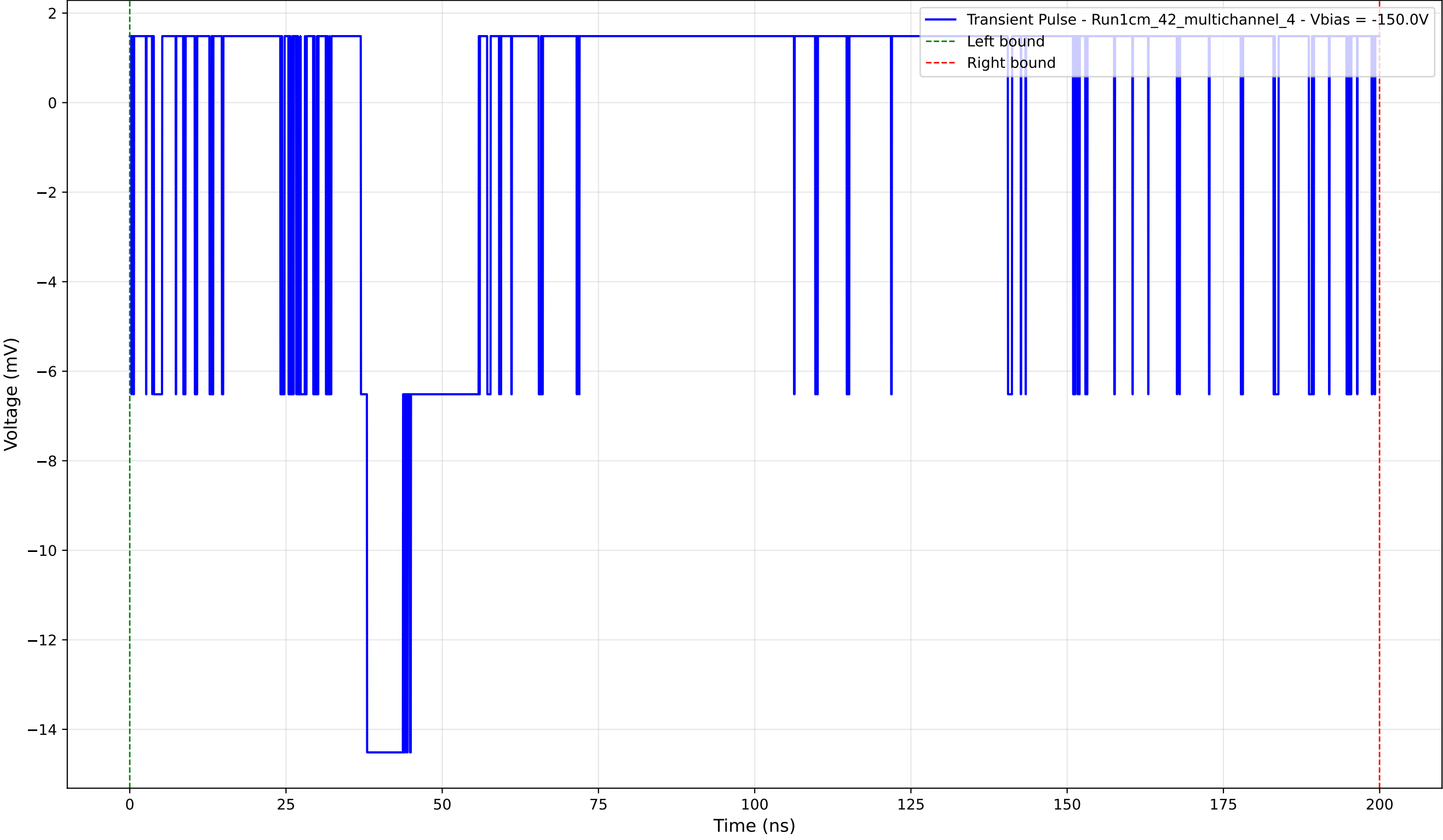
Transient Pulse - Sample: 1cm_42_multichannel - Position: 595.0 \mu\text{m} - Charge: 0.13 pC - Rise Time: 0.00 ns (N/A)
