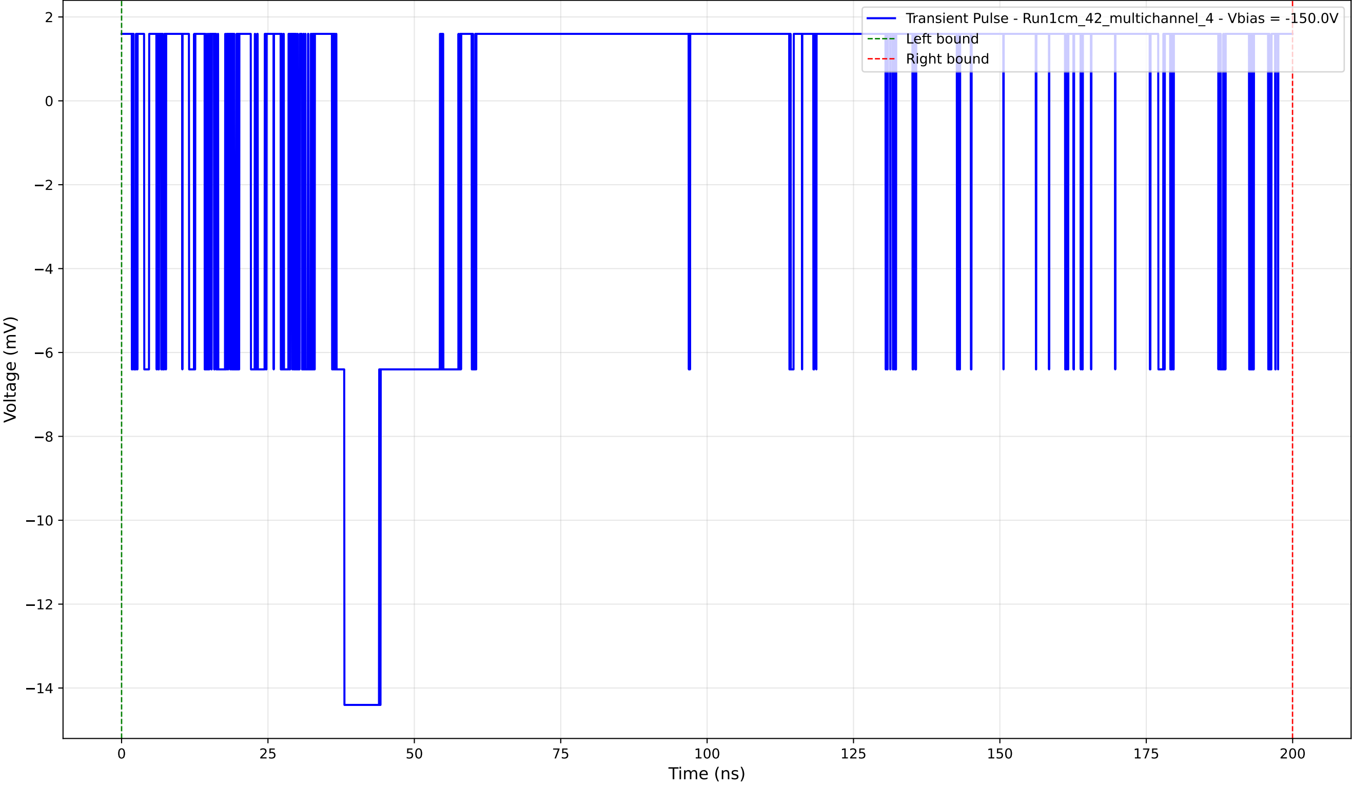
Transient Pulse - Sample: 1cm_42_multichannel - Position: 530.0 \mu\text{m} - Charge: 1.00 pC - Rise Time: 0.00 ns (N/A)
