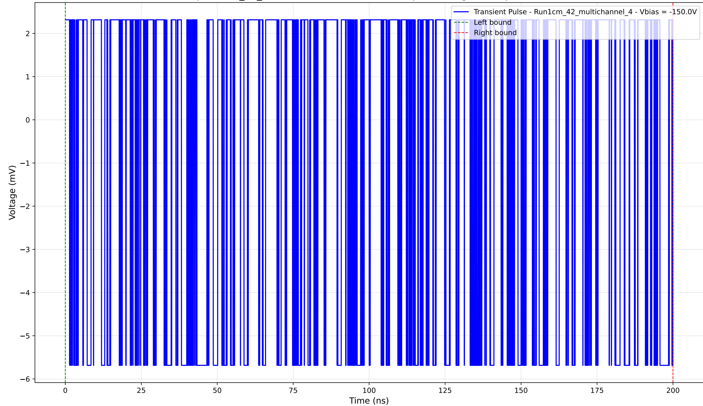
Transient Pulse - Sample: 1cm_42_multichannel - Position: 340.0 \mu\text{m} - Charge: 0.97 pC - Rise Time: 0.00 ns (N/A)
