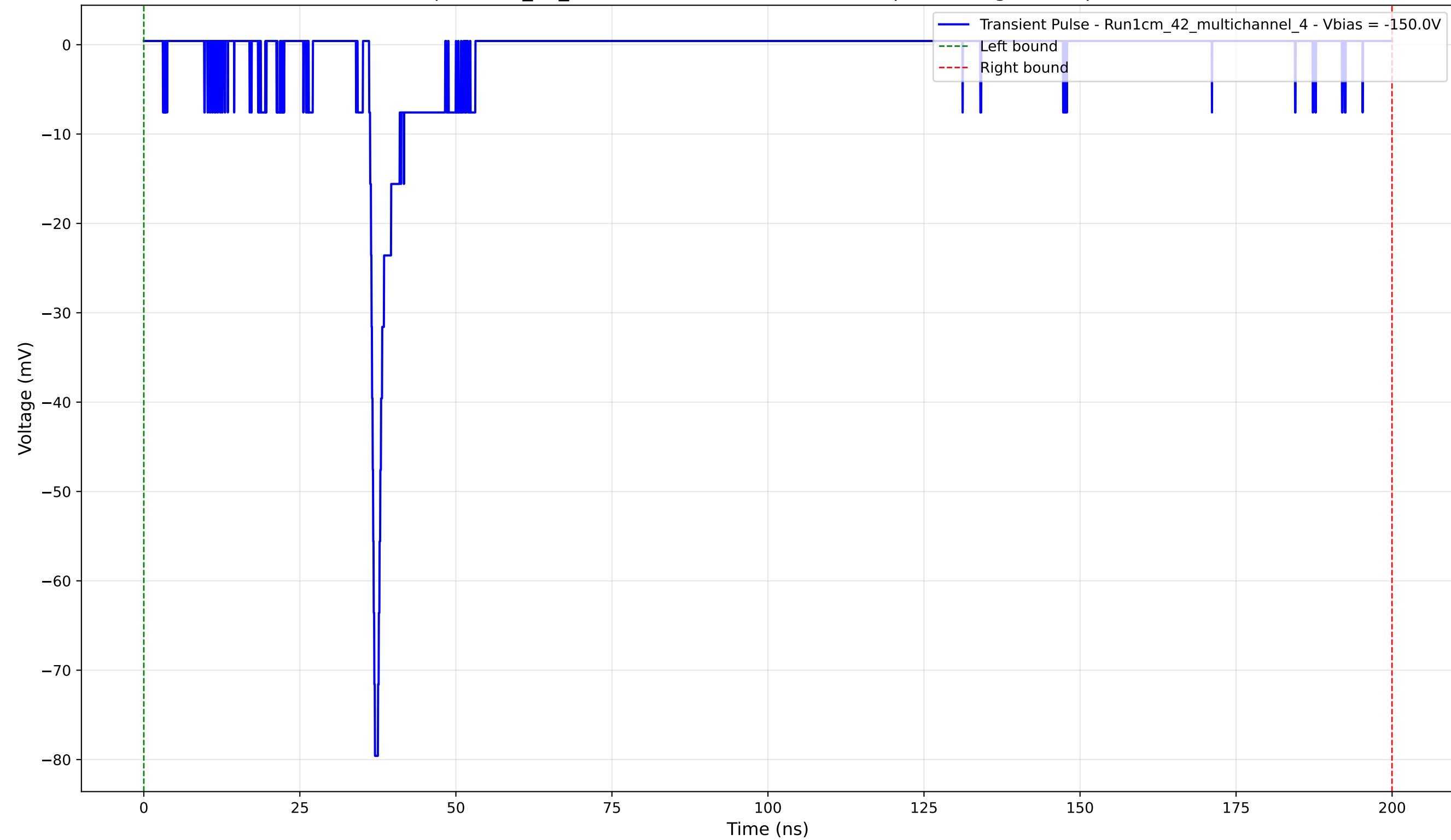
Transient Pulse - Sample: 1cm_42_multichannel - Position: 2280.0 \mu\text{m} - Charge: 4.54 pC - Rise Time: 0.78 ns
