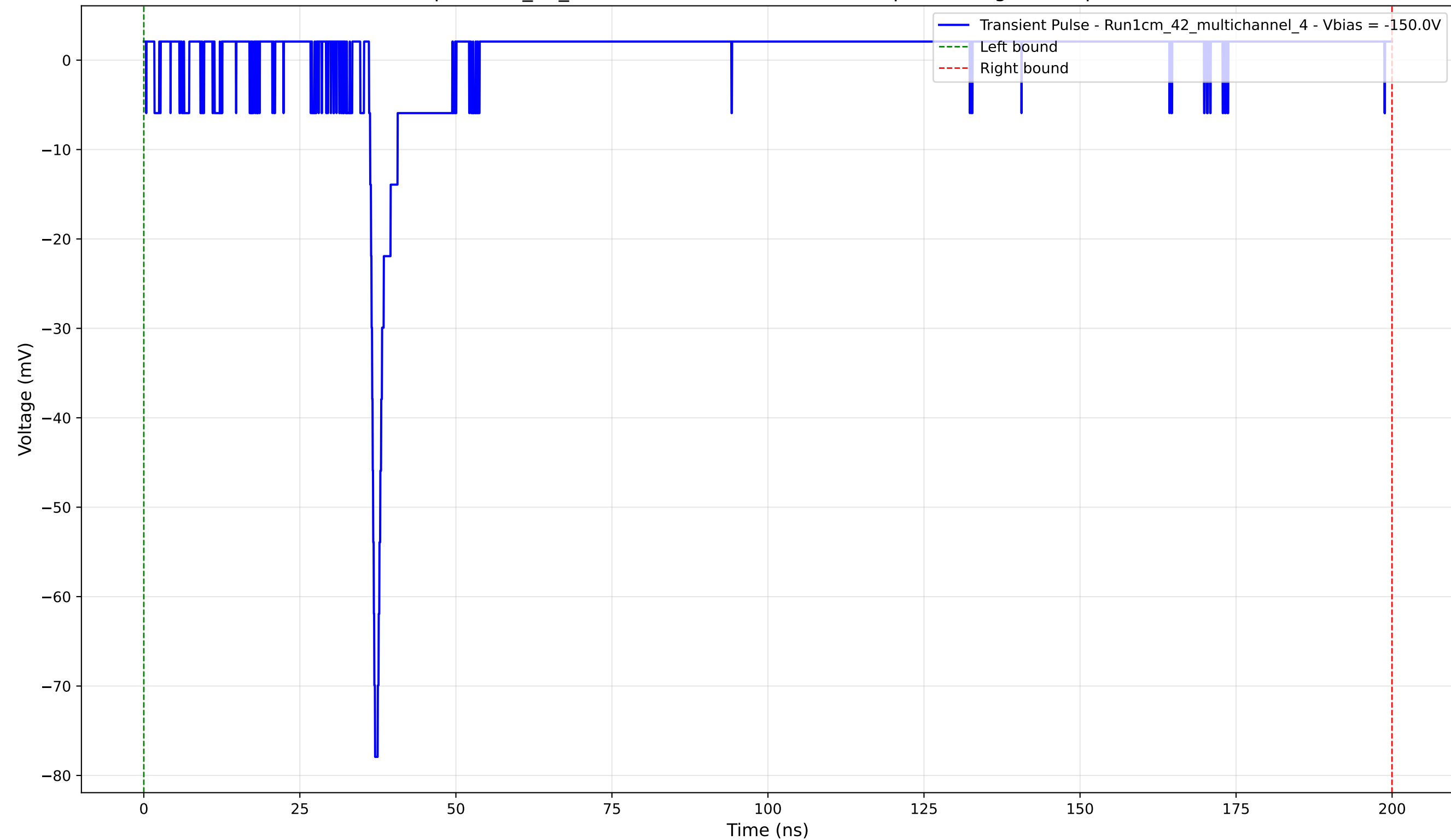
Transient Pulse - Sample: 1cm_42_multichannel - Position: 2285.0 \mu\text{m} - Charge: 1.91 pC - Rise Time: 0.80 ns
