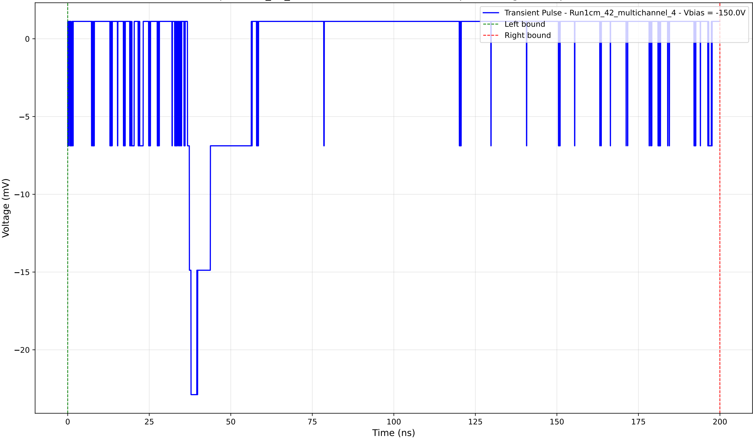
Transient Pulse - Sample: 1cm_42_multichannel - Position: 1165.0 \mu\text{m} - Charge: 1.84 pC - Rise Time: 1.10 ns
