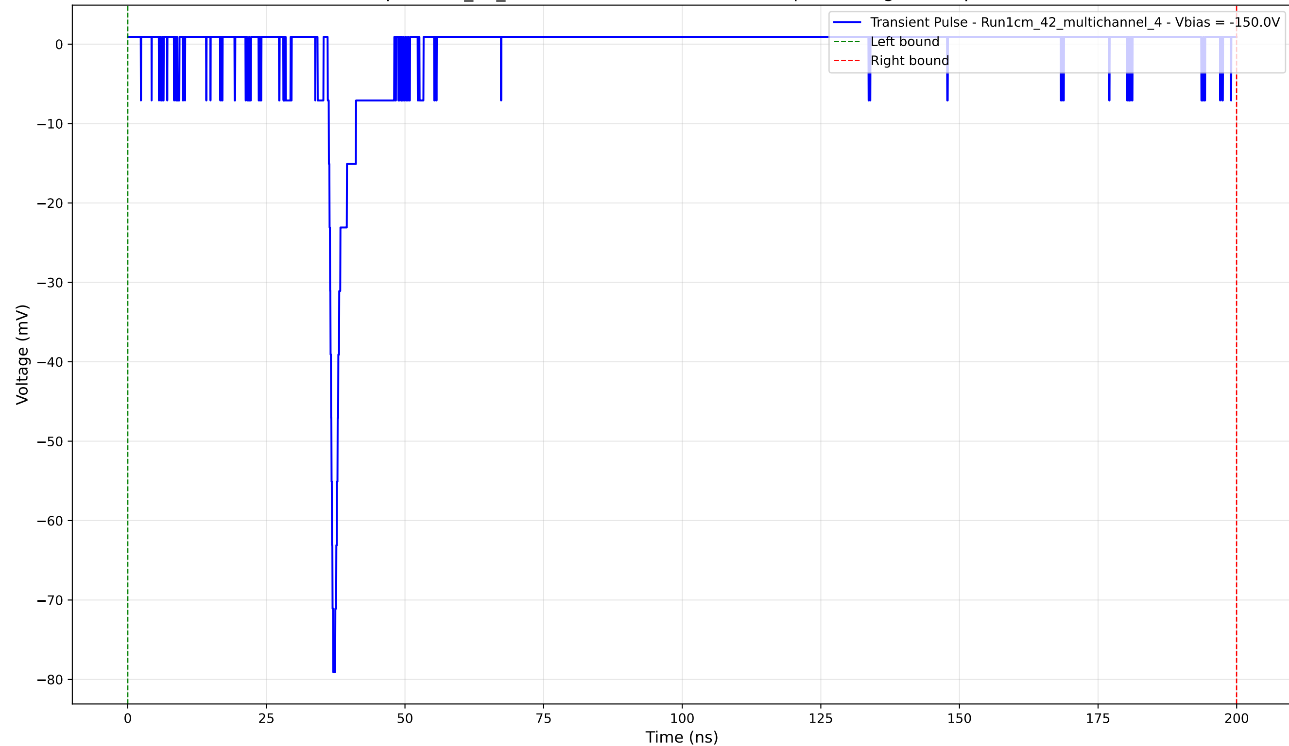
Transient Pulse - Sample: 1cm_42_multichannel - Position: 2305.0 \mu\text{m} - Charge: 2.25 pC - Rise Time: 0.80 ns
