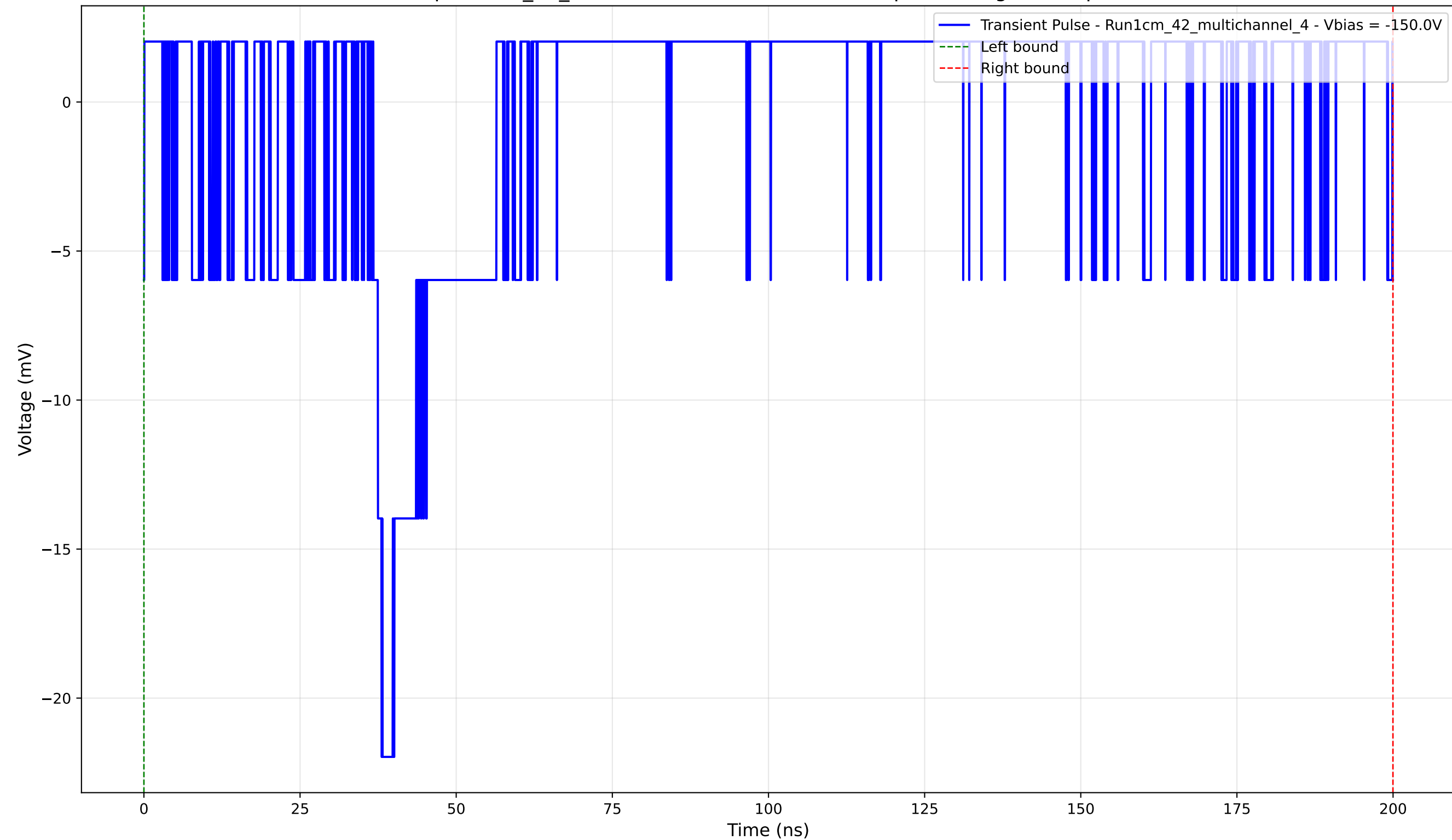
Transient Pulse - Sample: 1cm_42_multichannel - Position: 1045.0 \mu\text{m} - Charge: 0.53 pC - Rise Time: 1.32 ns
