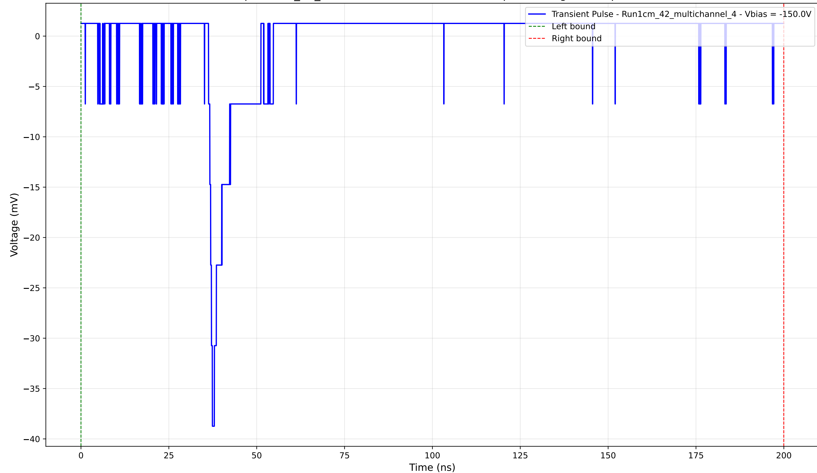
Transient Pulse - Sample: 1cm_42_multichannel - Position: 3025.0 \mu\text{m} - Charge: 0.16 pC - Rise Time: 1.09 ns
