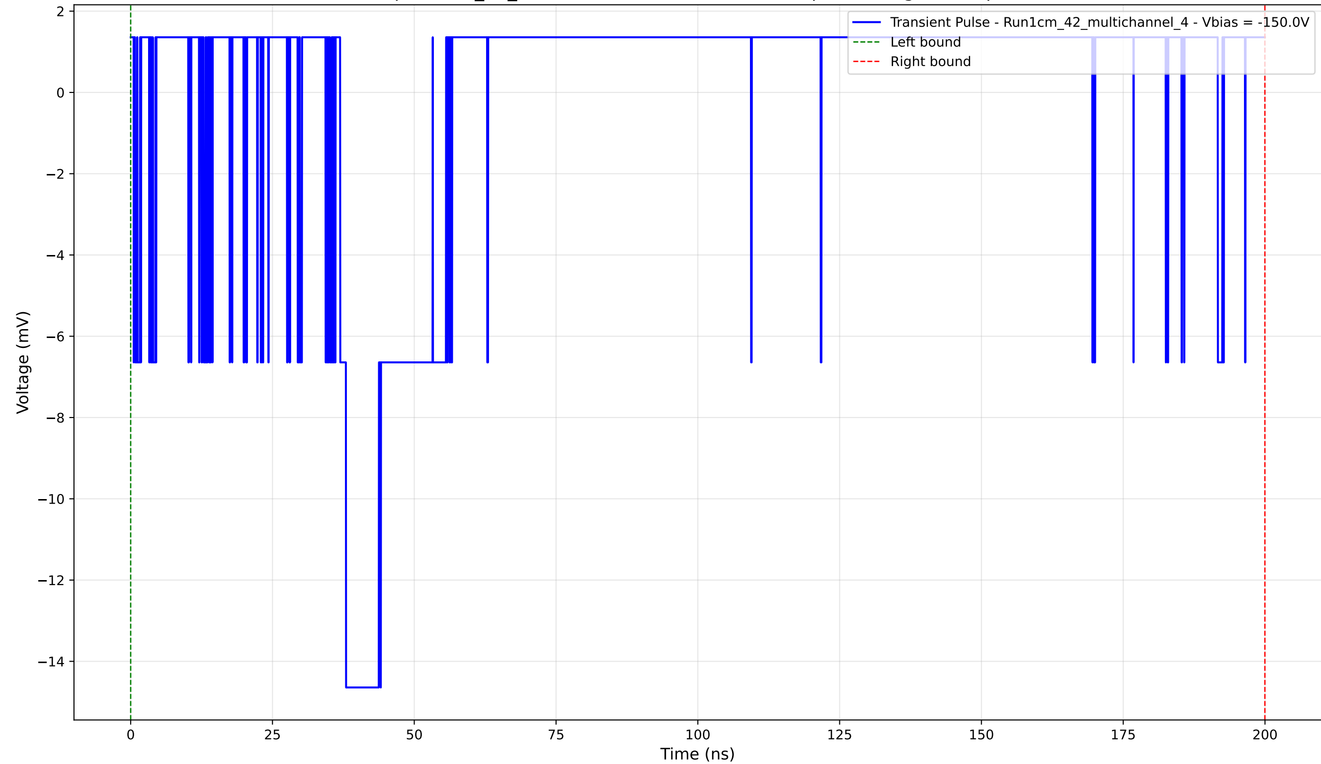
Transient Pulse - Sample: 1cm_42_multichannel - Position: 4055.0 \mu\text{m} - Charge: 0.26 pC - Rise Time: 1.04 ns
