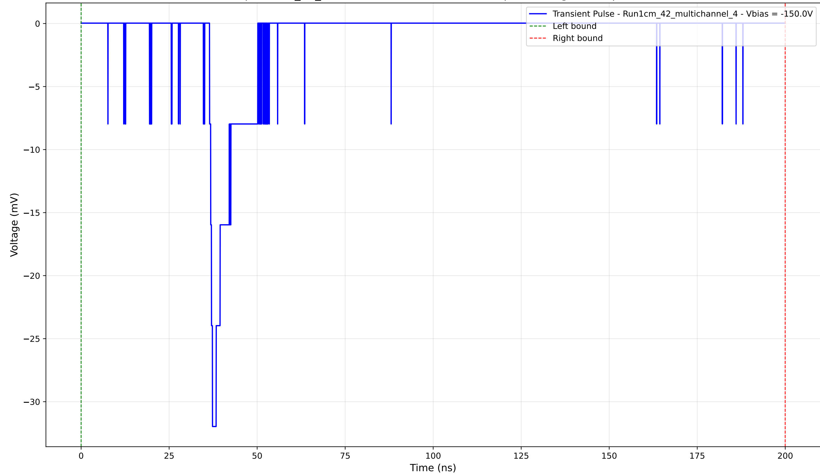
Transient Pulse - Sample: 1cm_42_multichannel - Position: 3085.0 \mu\text{m} - Charge: 3.90 pC - Rise Time: 0.83 ns
