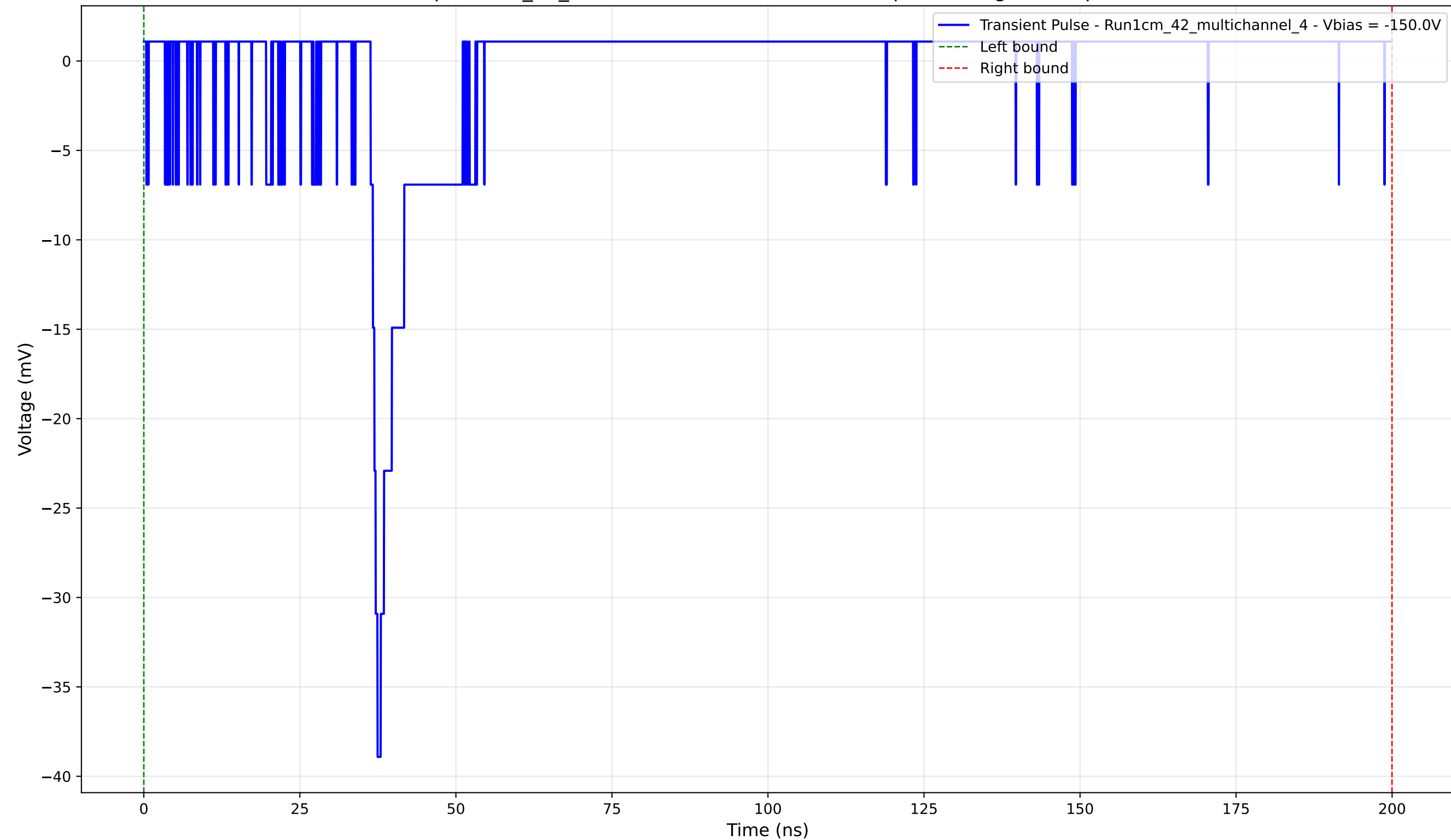
Transient Pulse - Sample: 1cm_42_multichannel - Position: 3015.0 \mu\text{m} - Charge: 0.83 pC - Rise Time: 1.11 ns
