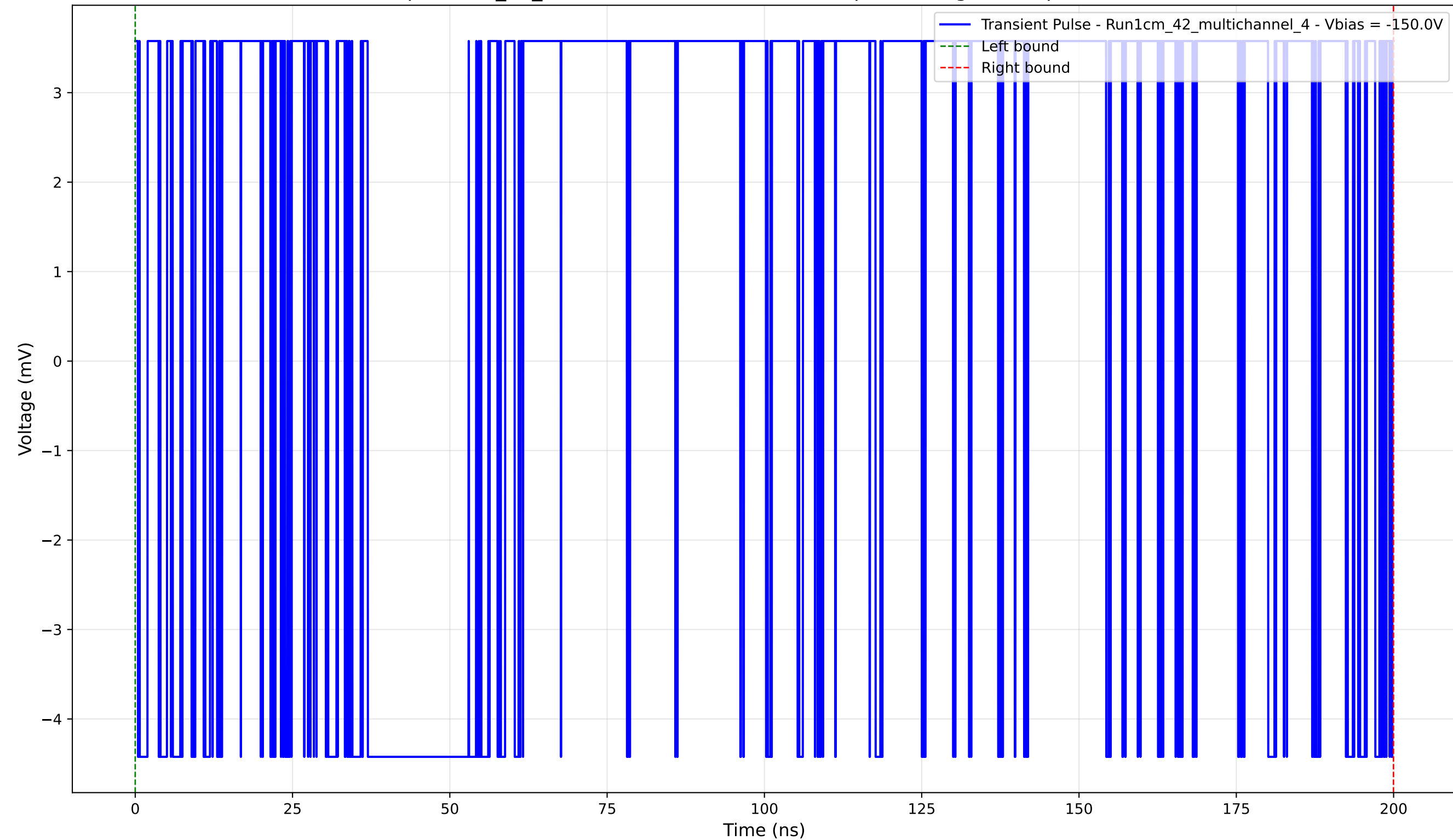
Transient Pulse - Sample: 1cm_42_multichannel - Position: 305.0 \mu\text{m} - Charge: 6.86 pC - Rise Time: 0.00 ns (N/A)
