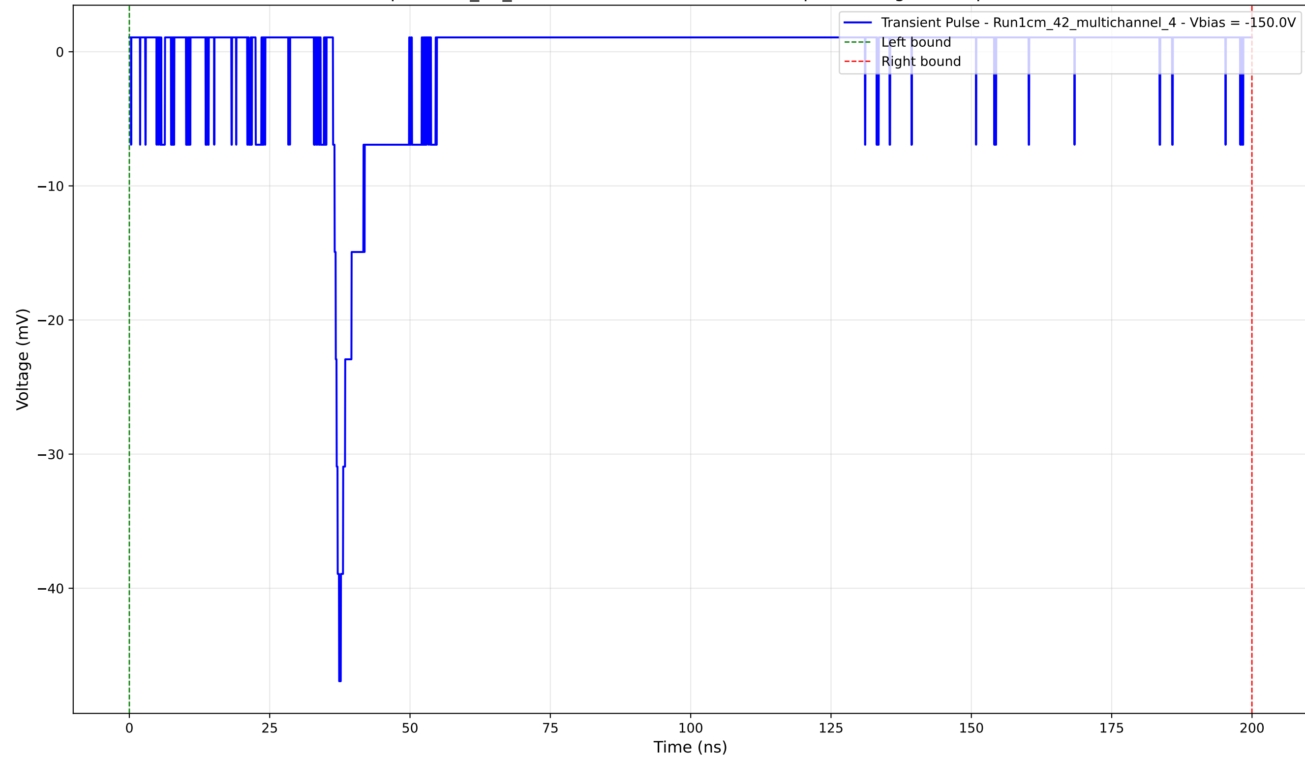
Transient Pulse - Sample: 1cm_42_multichannel - Position: 2820.0 \mu\text{m} - Charge: 1.24 pC - Rise Time: 1.09 ns
