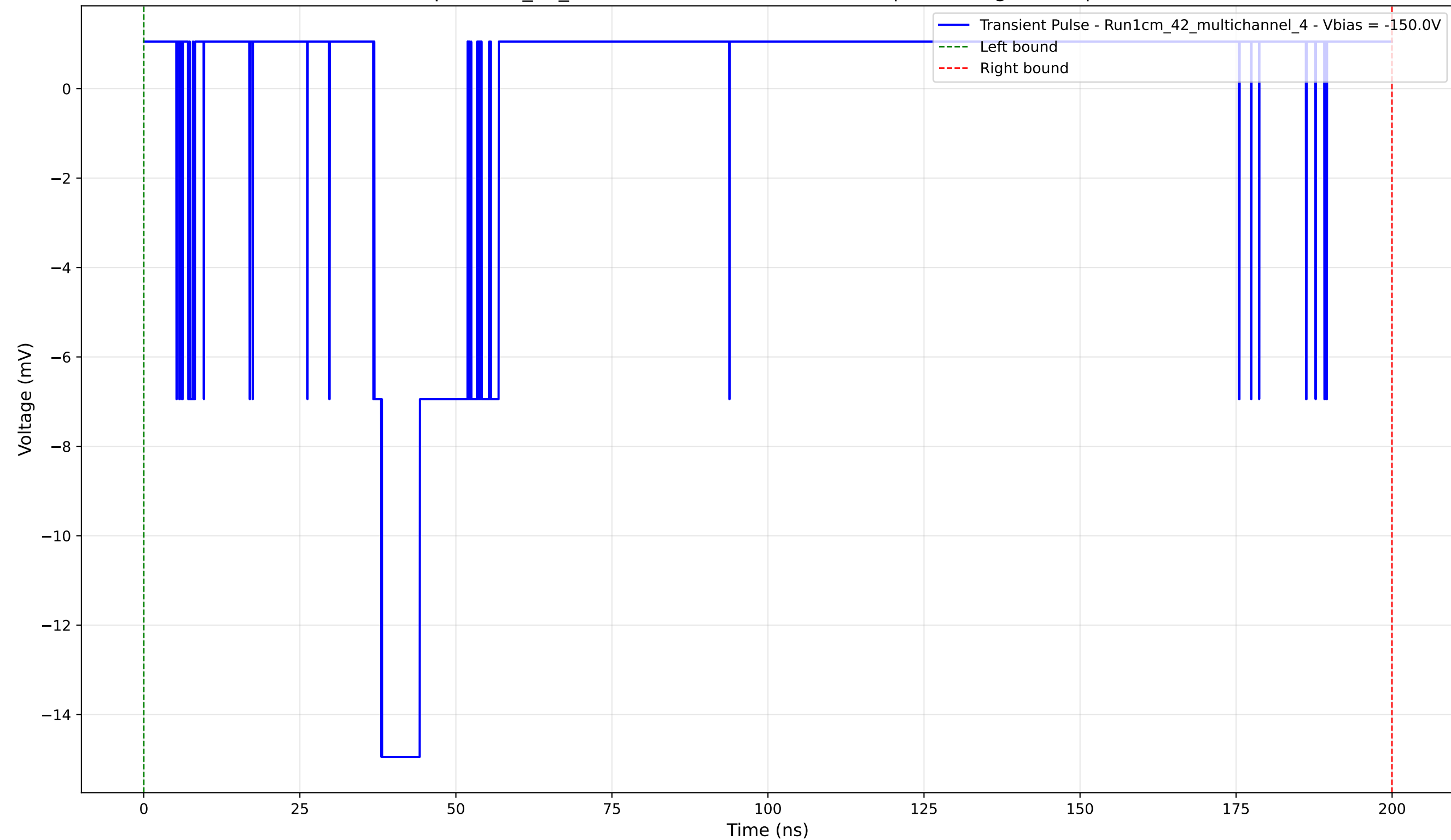
Transient Pulse - Sample: 1cm_42_multichannel - Position: 4030.0 \mu\text{m} - Charge: 0.18 pC - Rise Time: 1.12 ns
