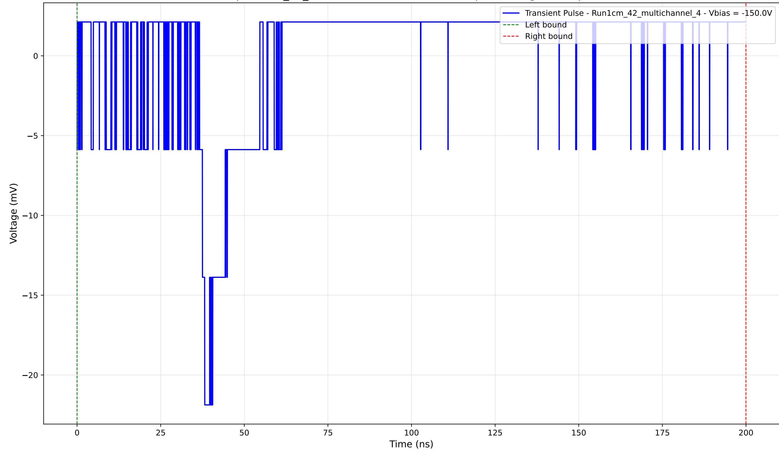
Transient Pulse - Sample: 1cm_42_multichannel - Position: 990.0 \mu\text{m} - Charge: 1.78 pC - Rise Time: 1.56 ns
