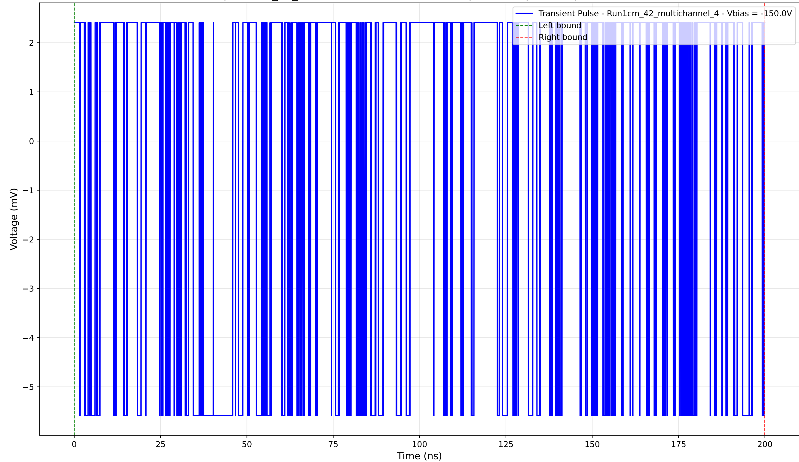
Transient Pulse - Sample: 1cm_42_multichannel - Position: 335.0 \mu\text{m} - Charge: 0.28 pC - Rise Time: 0.00 ns (N/A)
