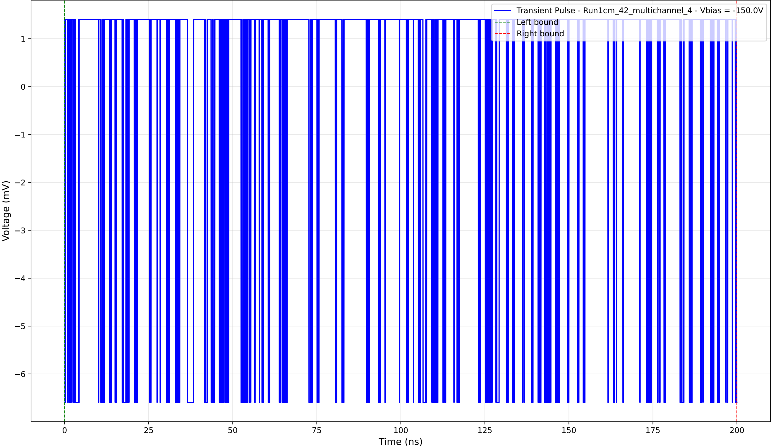
Transient Pulse - Sample: 1cm_42_multichannel - Position: 2895.0 \mu\text{m} - Charge: 0.75 pC - Rise Time: 0.00 ns (N/A)
