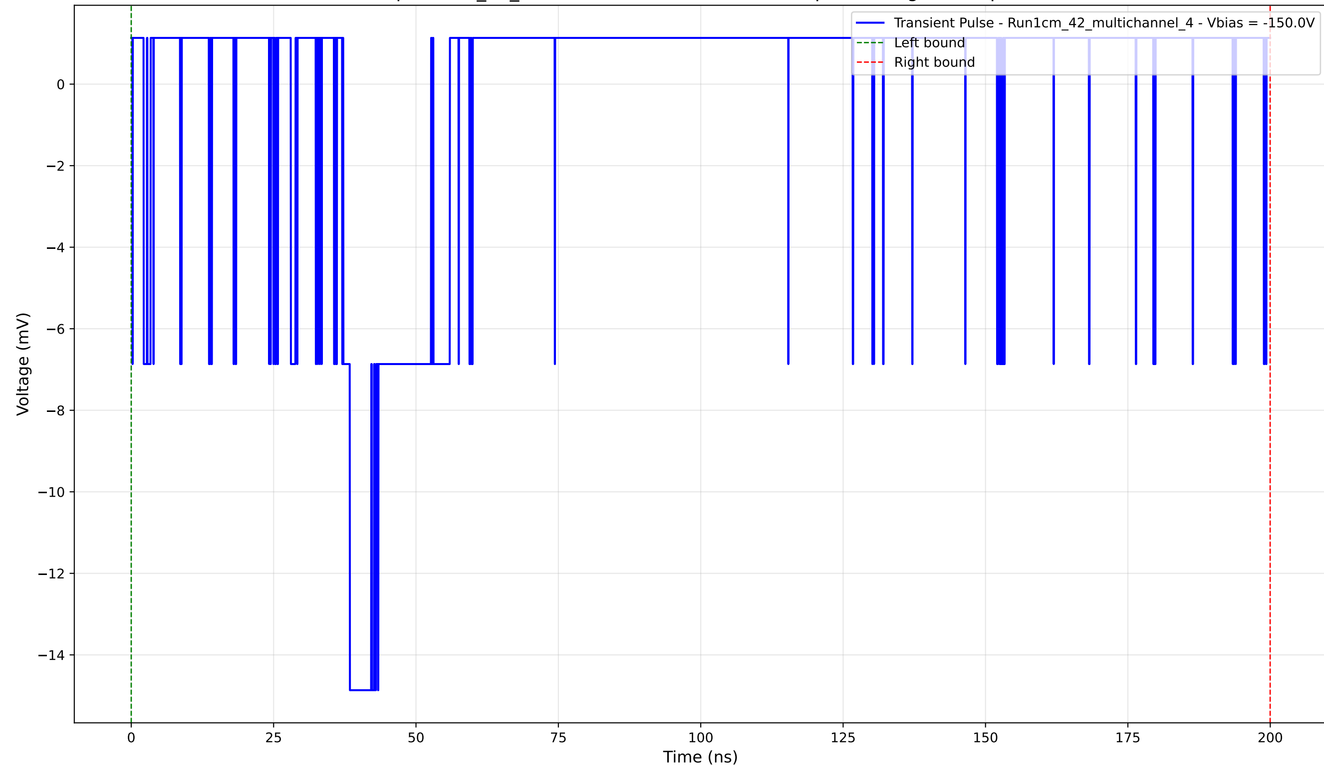
Transient Pulse - Sample: 1cm_42_multichannel - Position: 4185.0 \mu\text{m} - Charge: 0.22 pC - Rise Time: 1.16 ns
