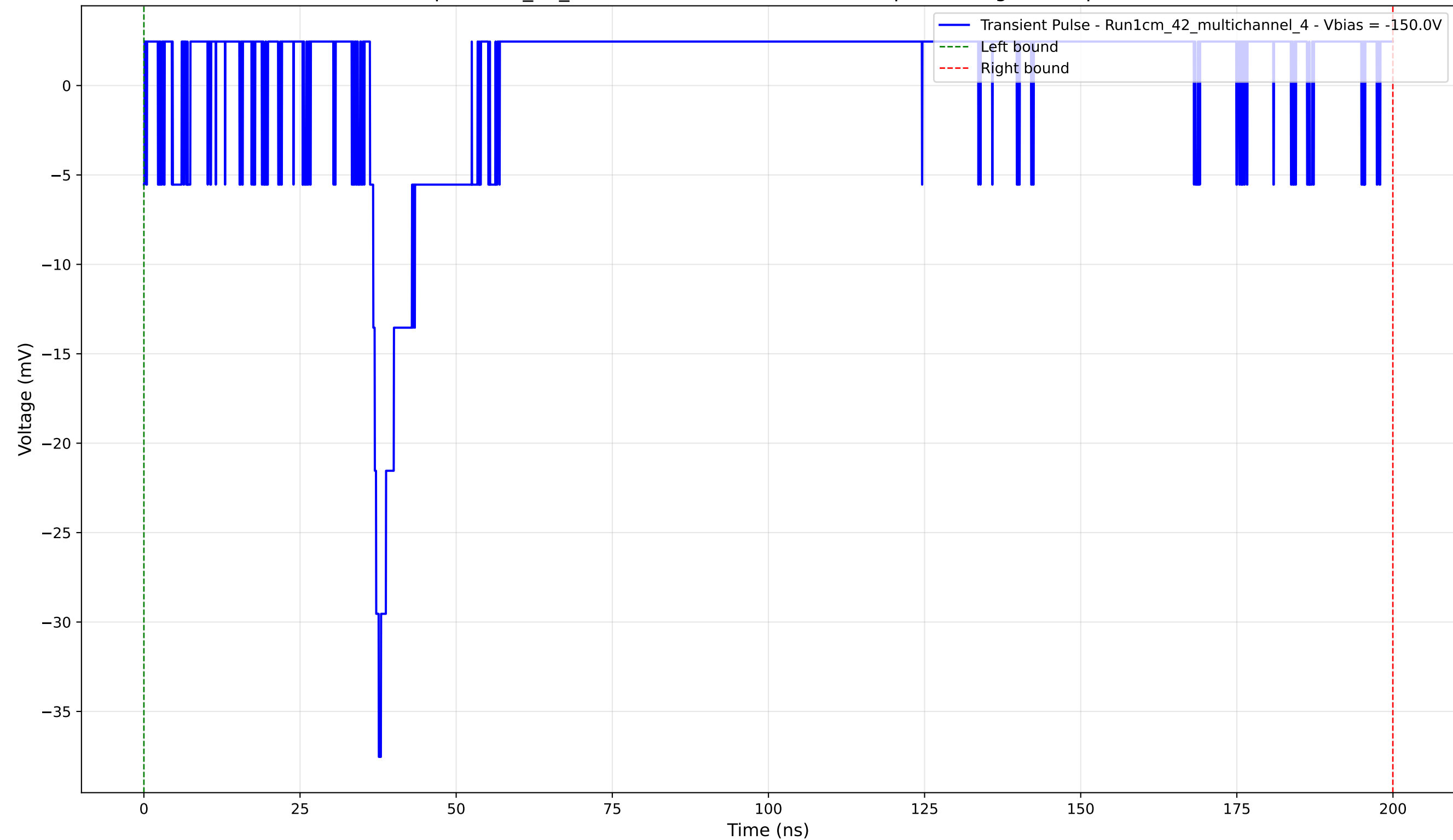
Transient Pulse - Sample: 1cm_42_multichannel - Position: 1675.0 \mu\text{m} - Charge: 3.12 pC - Rise Time: 1.41 ns
