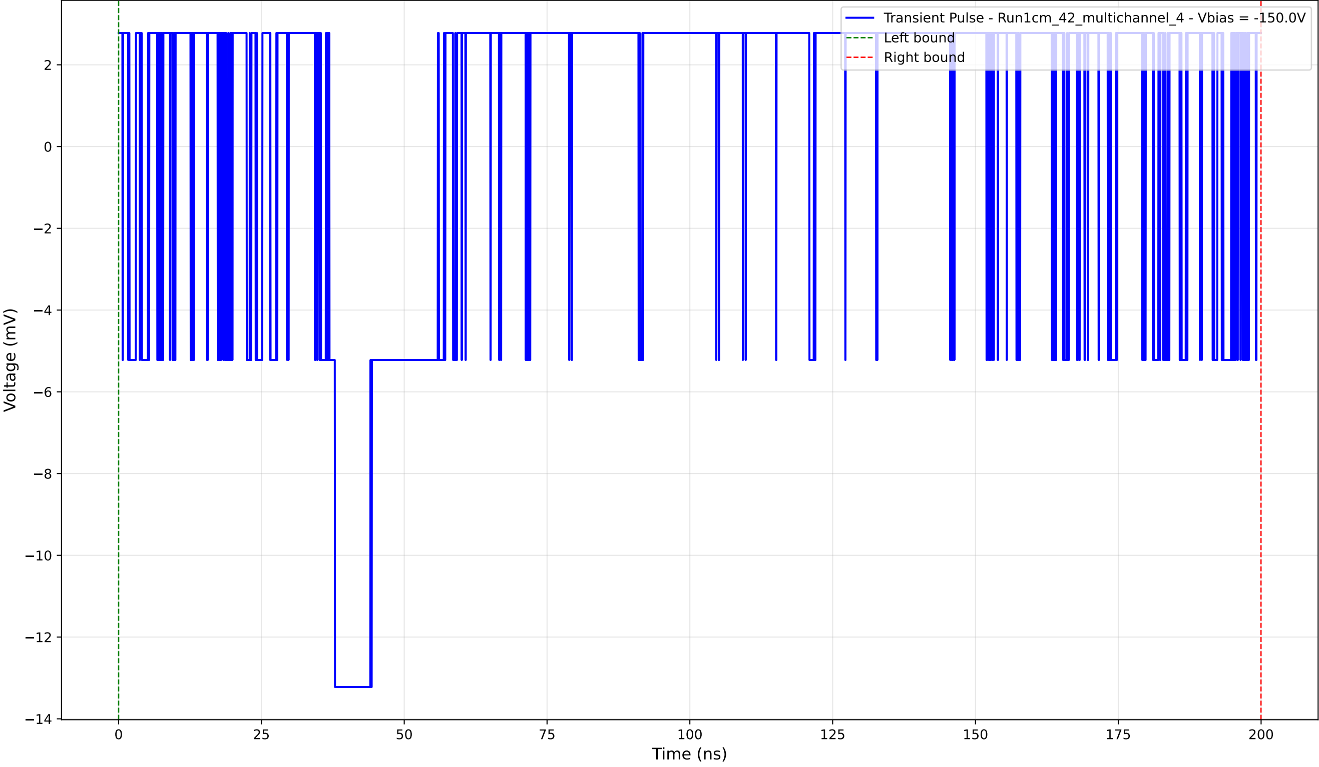
Transient Pulse - Sample: 1cm_42_multichannel - Position: 685.0 \mu\text{m} - Charge: 2.94 pC - Rise Time: 0.00 ns (N/A)
