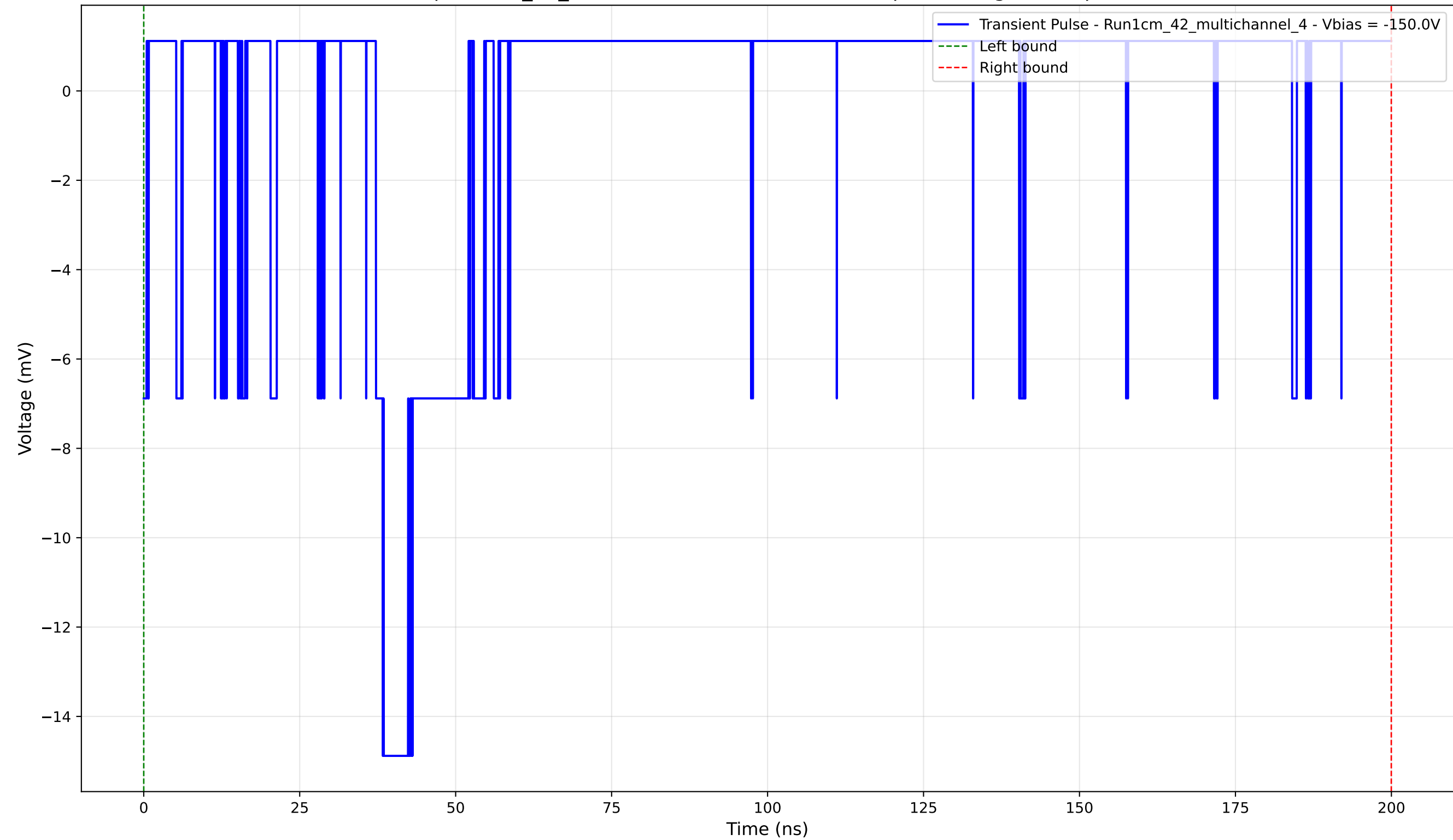
Transient Pulse - Sample: 1cm_42_multichannel - Position: 4235.0 \mu\text{m} - Charge: 0.18 pC - Rise Time: 1.10 ns
