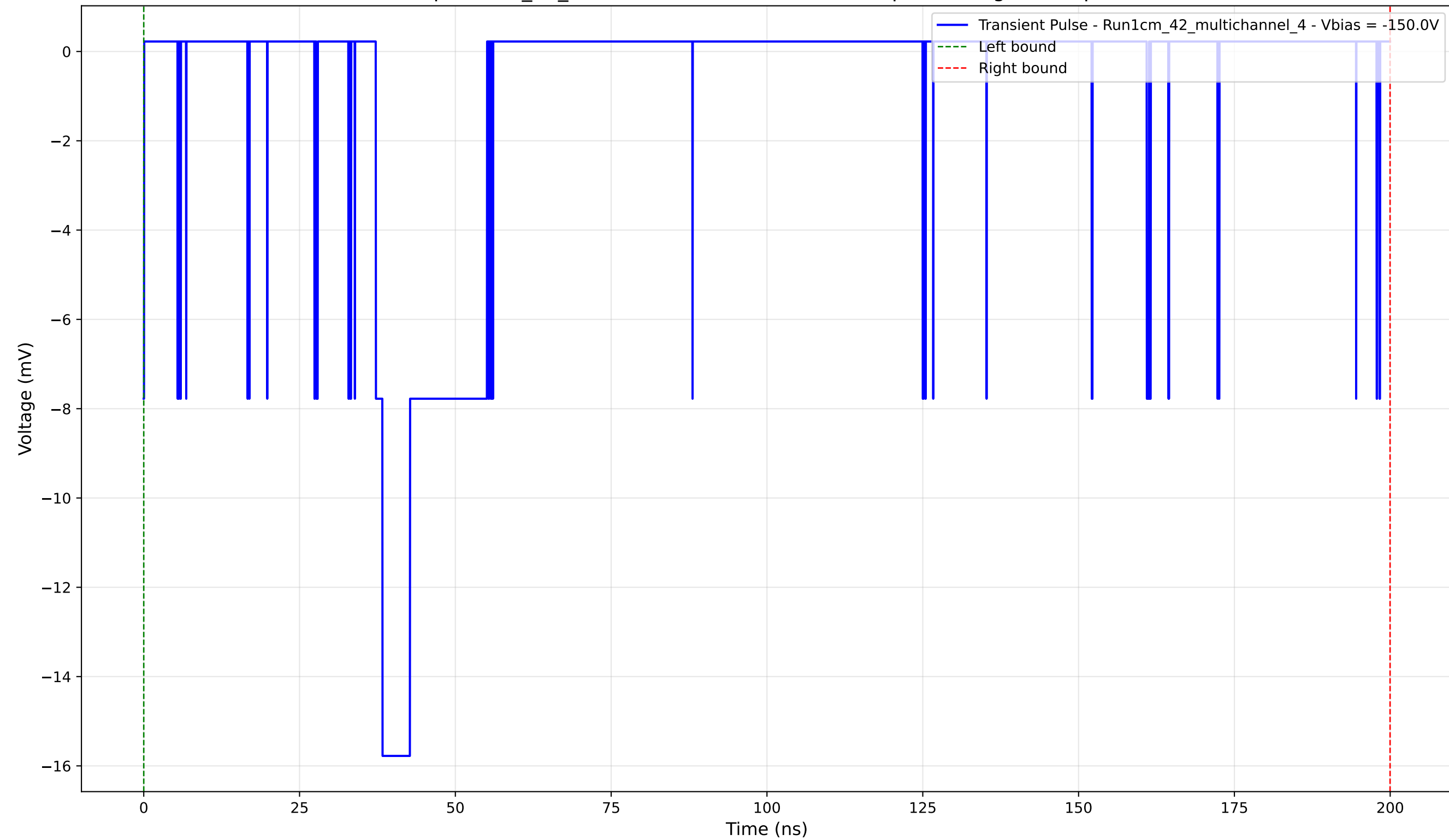
Transient Pulse - Sample: 1cm_42_multichannel - Position: 4140.0 \mu\text{m} - Charge: 3.10 pC - Rise Time: 1.08 ns
