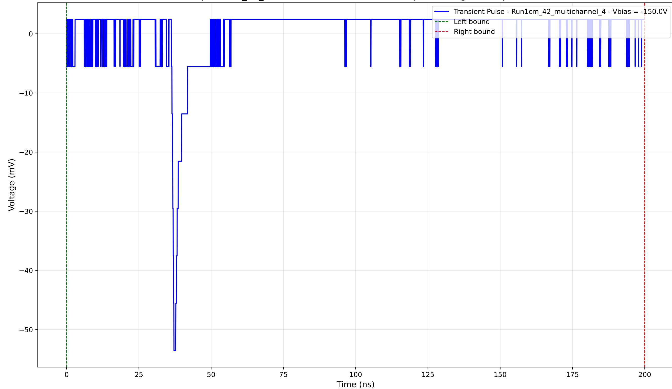
Transient Pulse - Sample: 1cm_42_multichannel - Position: 2725.0 \mu\text{m} - Charge: 2.83 pC - Rise Time: 0.92 ns
