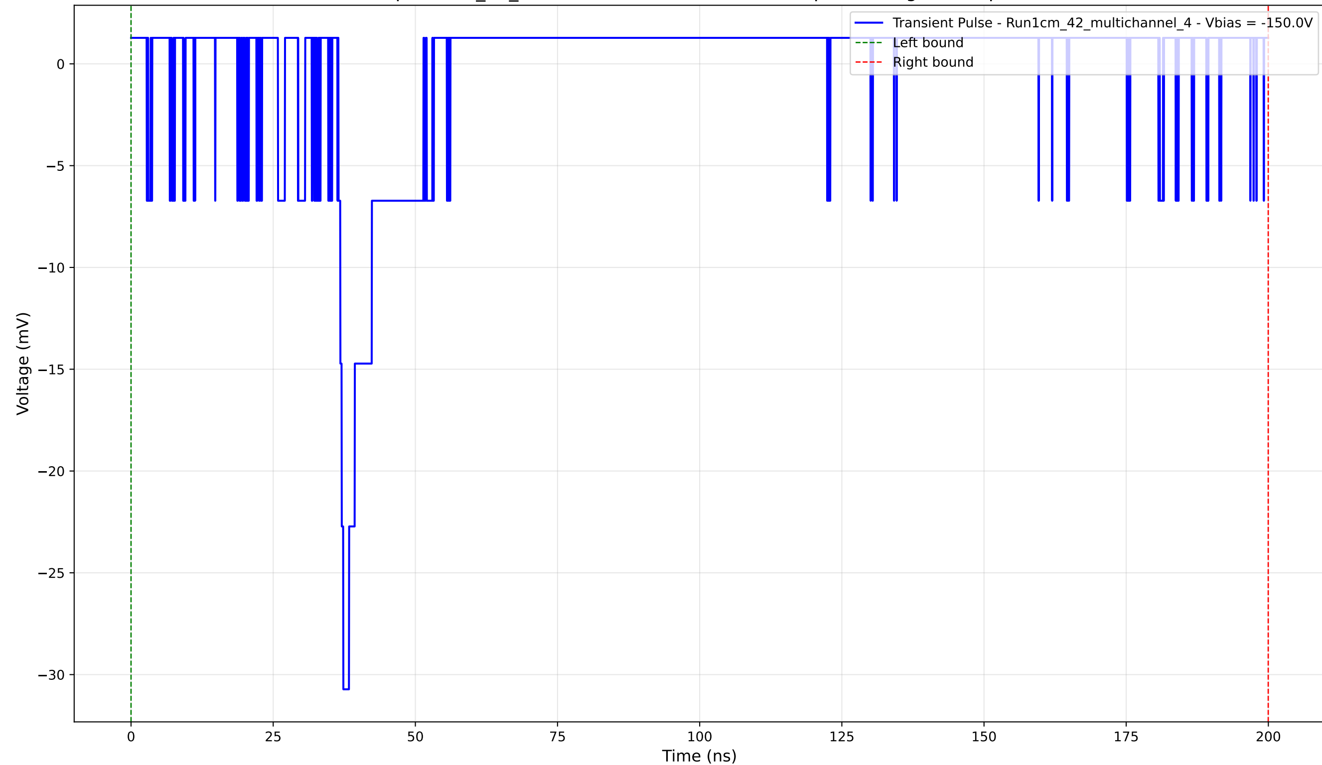
Transient Pulse - Sample: 1cm_42_multichannel - Position: 3110.0 \mu\text{m} - Charge: 0.63 pC - Rise Time: 0.85 ns
