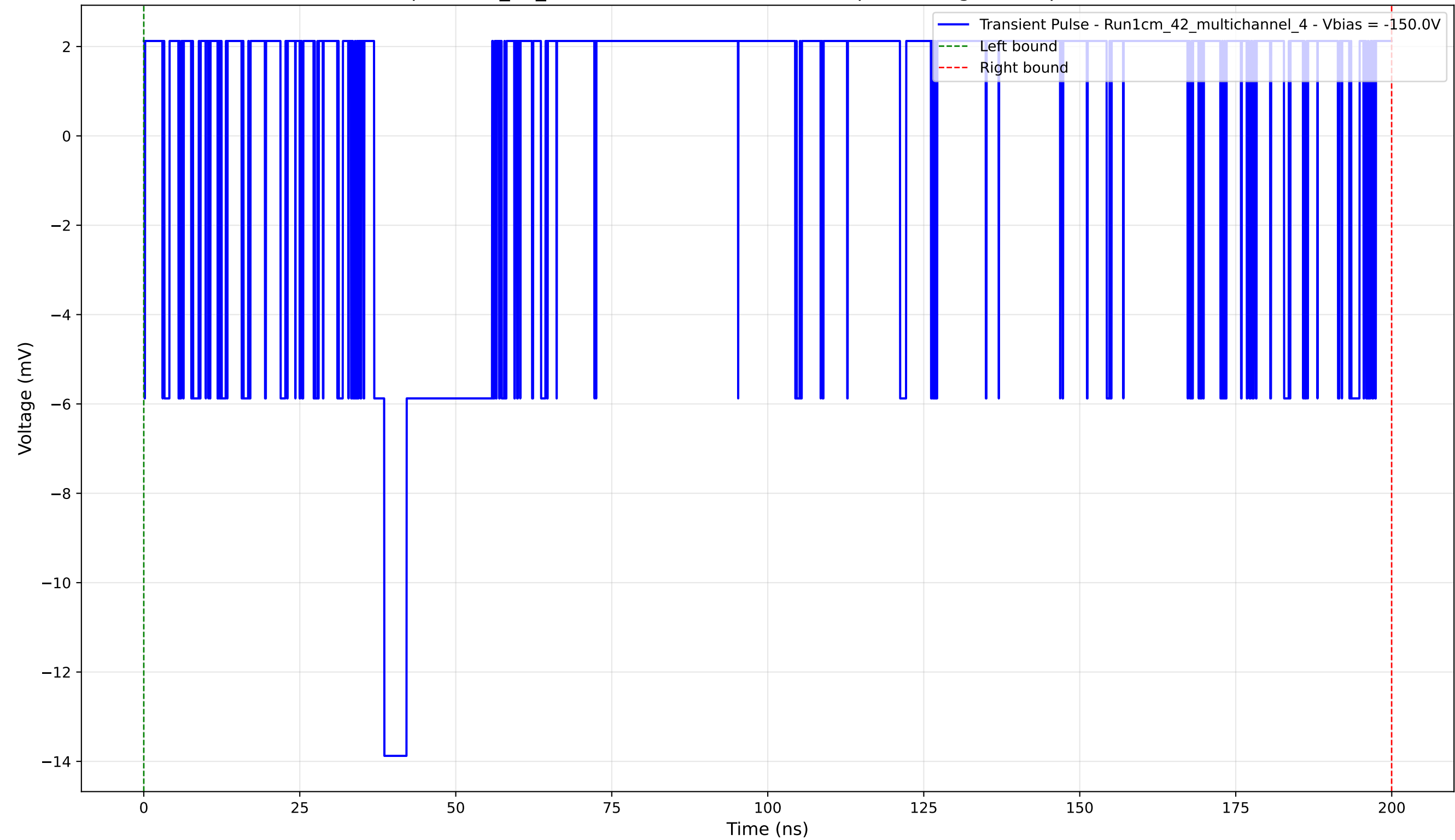
Transient Pulse - Sample: 1cm_42_multichannel - Position: 205.0 \mu\text{m} - Charge: 1.39 pC - Rise Time: 0.00 ns (N/A)
