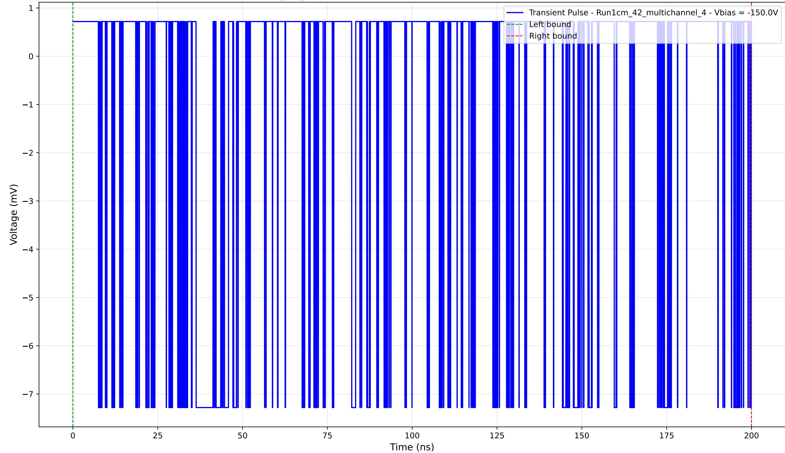
Transient Pulse - Sample: 1cm_42_multichannel - Position: 2415.0 \mu\text{m} - Charge: 2.88 pC - Rise Time: 0.02 ns
