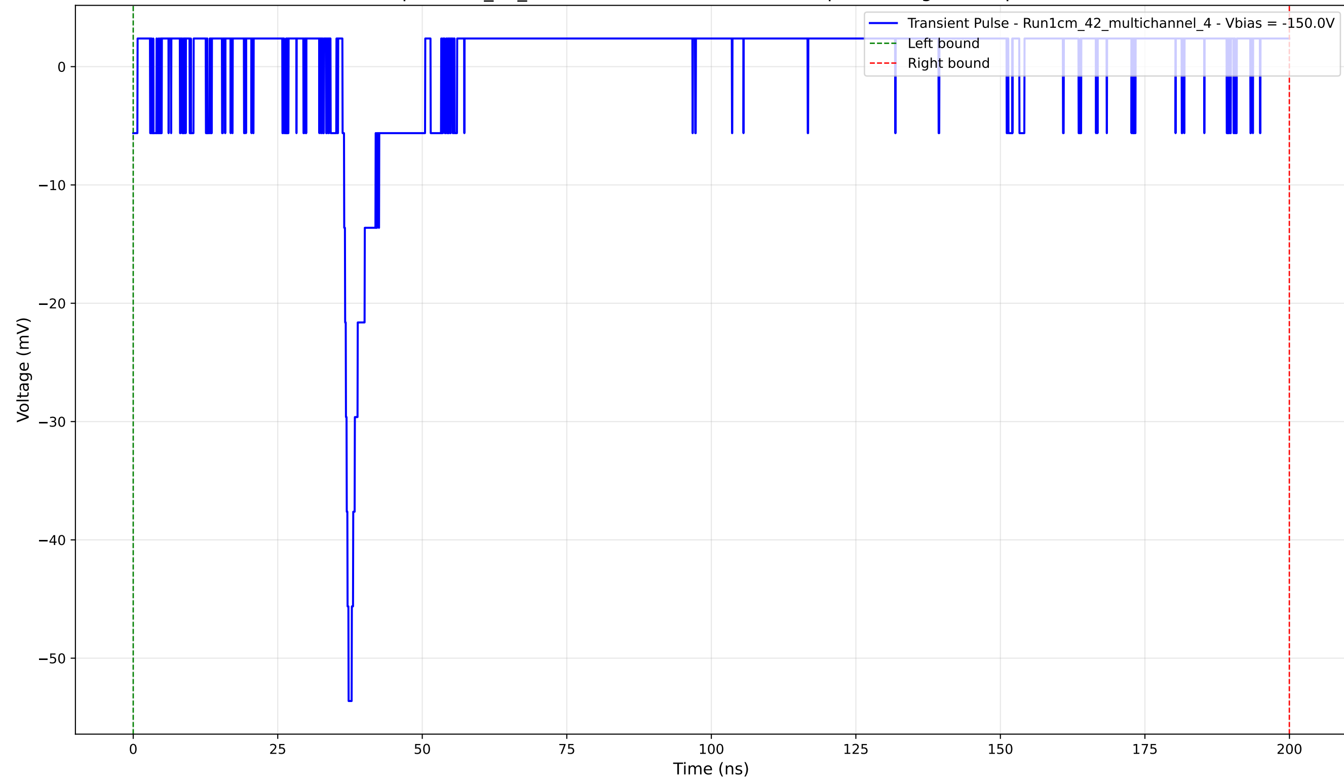
Transient Pulse - Sample: 1cm_42_multichannel - Position: 1980.0 \mu\text{m} - Charge: 2.57 pC - Rise Time: 1.04 ns
