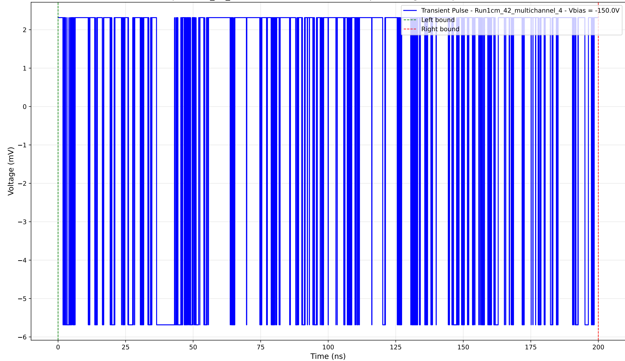
Transient Pulse - Sample: 1cm_42_multichannel - Position: 1910.0 \mu\text{m} - Charge: 1.52 pC - Rise Time: 0.00 ns (N/A)
