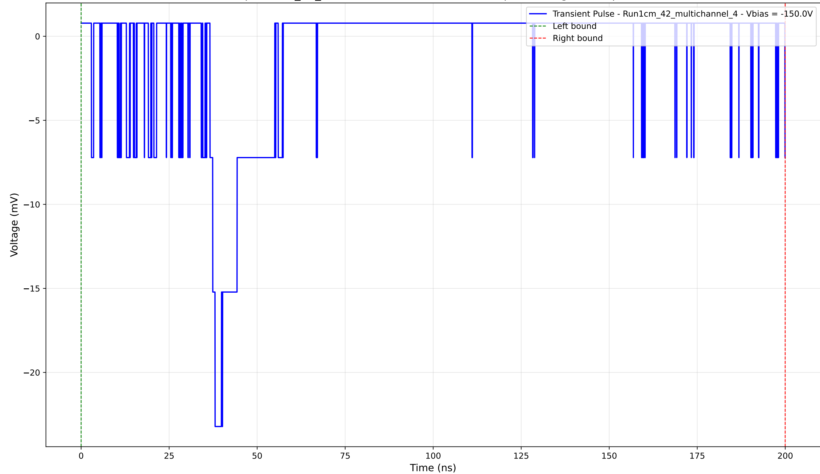
Transient Pulse - Sample: 1cm_42_multichannel - Position: 1110.0 \mu\text{m} - Charge: 3.11 pC - Rise Time: 1.46 ns
