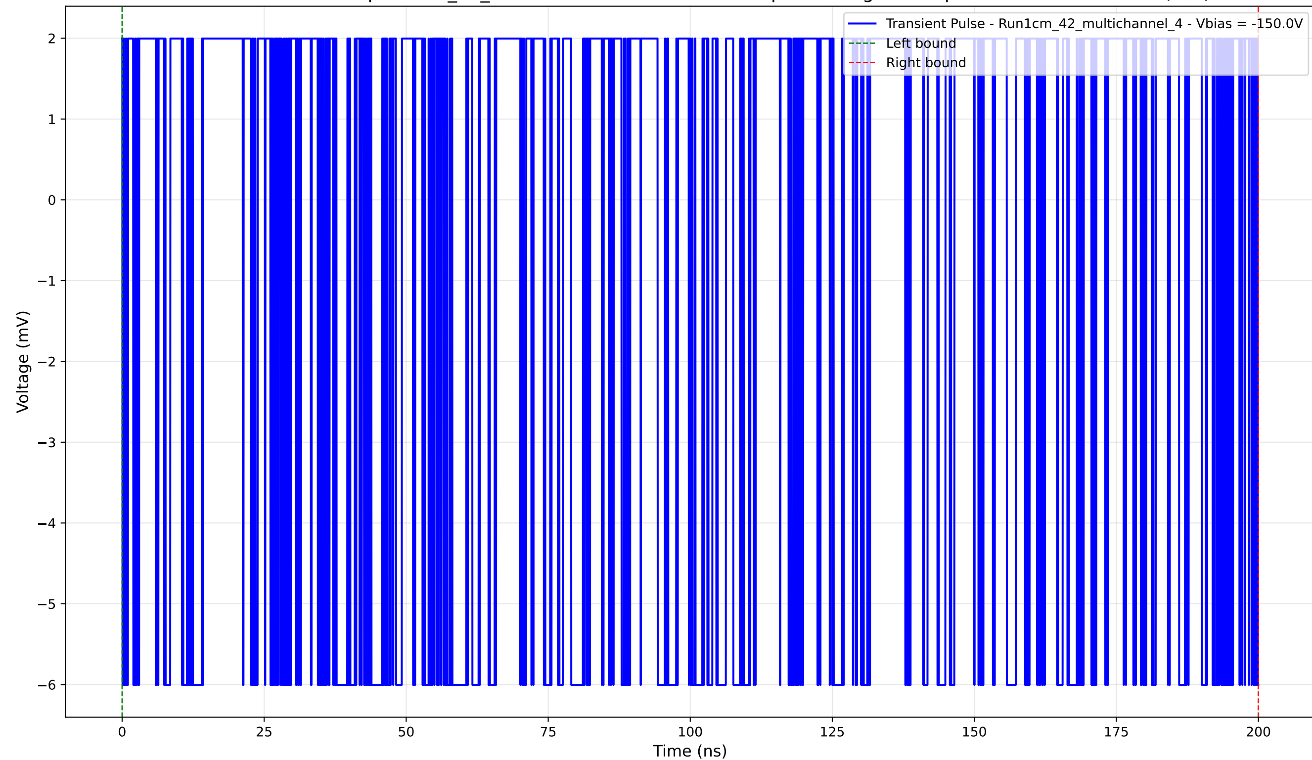
Transient Pulse - Sample: 1cm_42_multichannel - Position: 860.0 \mu\text{m} - Charge: 2.50 pC - Rise Time: 0.00 ns (N/A)
