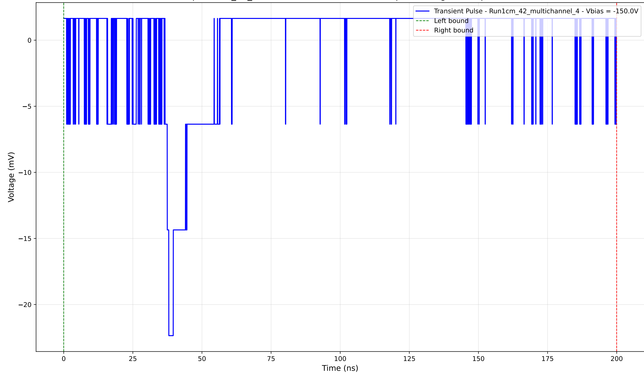
Transient Pulse - Sample: 1cm_42_multichannel - Position: 1070.0 \mu\text{m} - Charge: 0.03 pC - Rise Time: 1.38 ns
