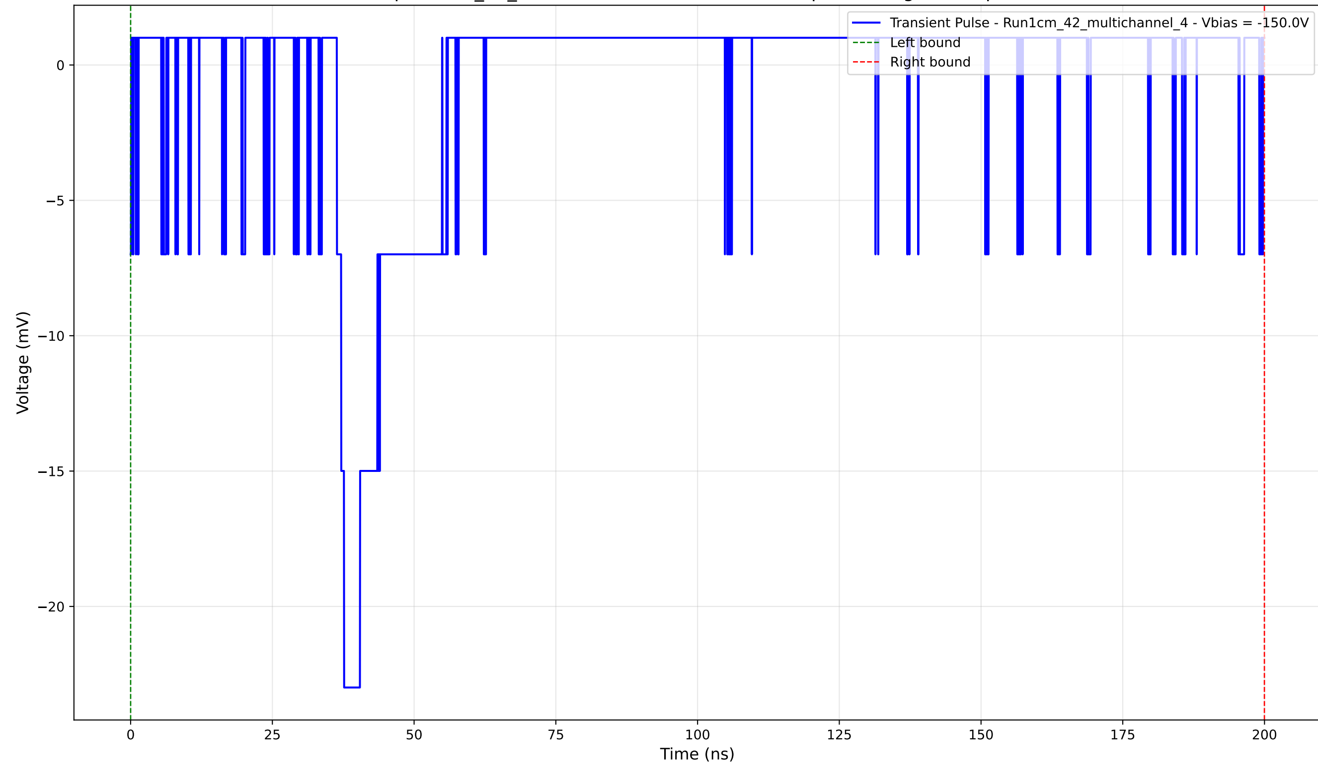
Transient Pulse - Sample: 1cm_42_multichannel - Position: 1265.0 \mu\text{m} - Charge: 2.17 pC - Rise Time: 1.28 ns
