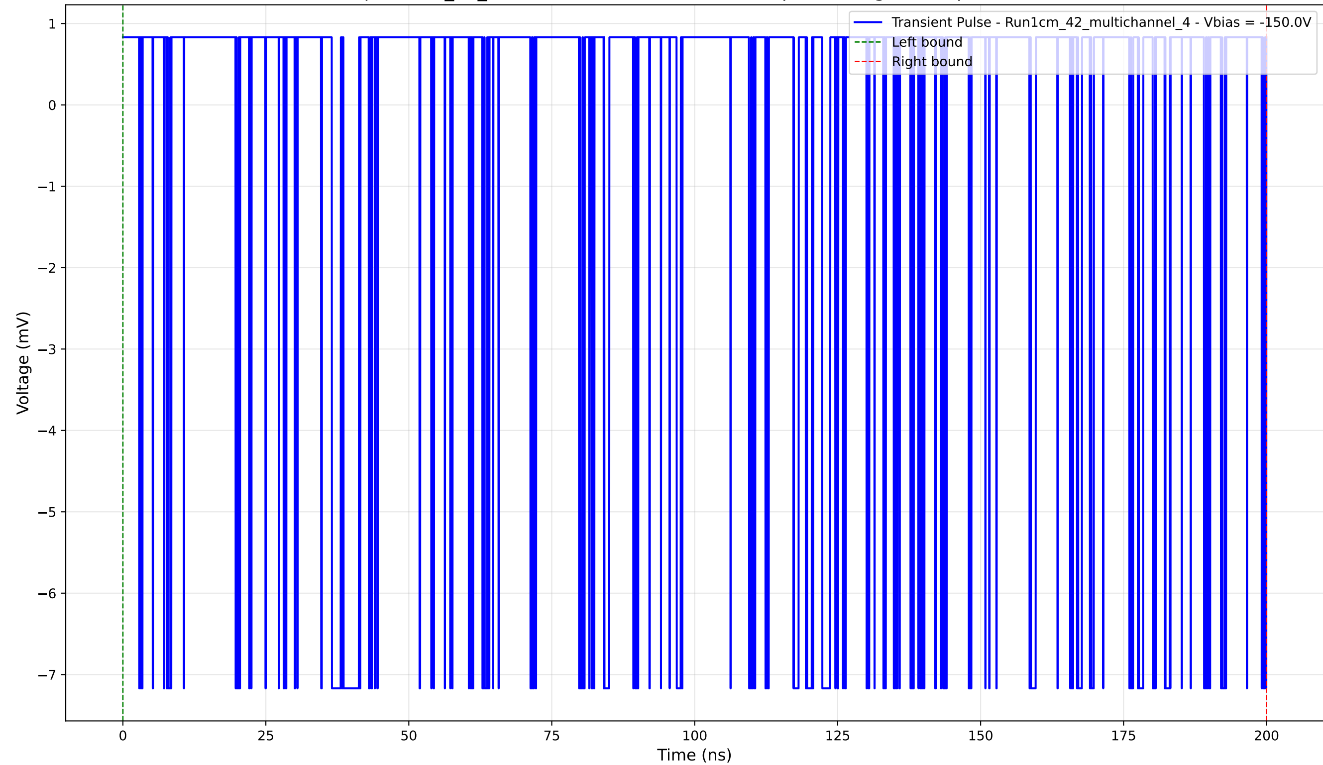
Transient Pulse - Sample: 1cm_42_multichannel - Position: 2910.0 \mu\text{m} - Charge: 1.32 pC - Rise Time: 0.00 ns (N/A)
