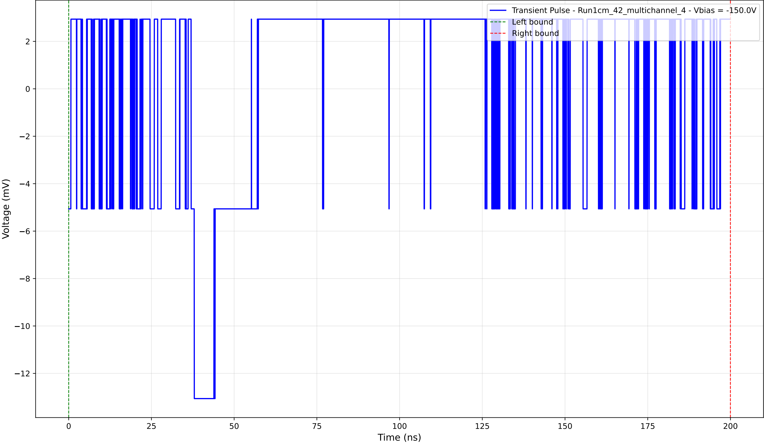
Transient Pulse - Sample: 1cm_42_multichannel - Position: 525.0 \mu\text{m} - Charge: 3.55 pC - Rise Time: 0.00 ns (N/A)
