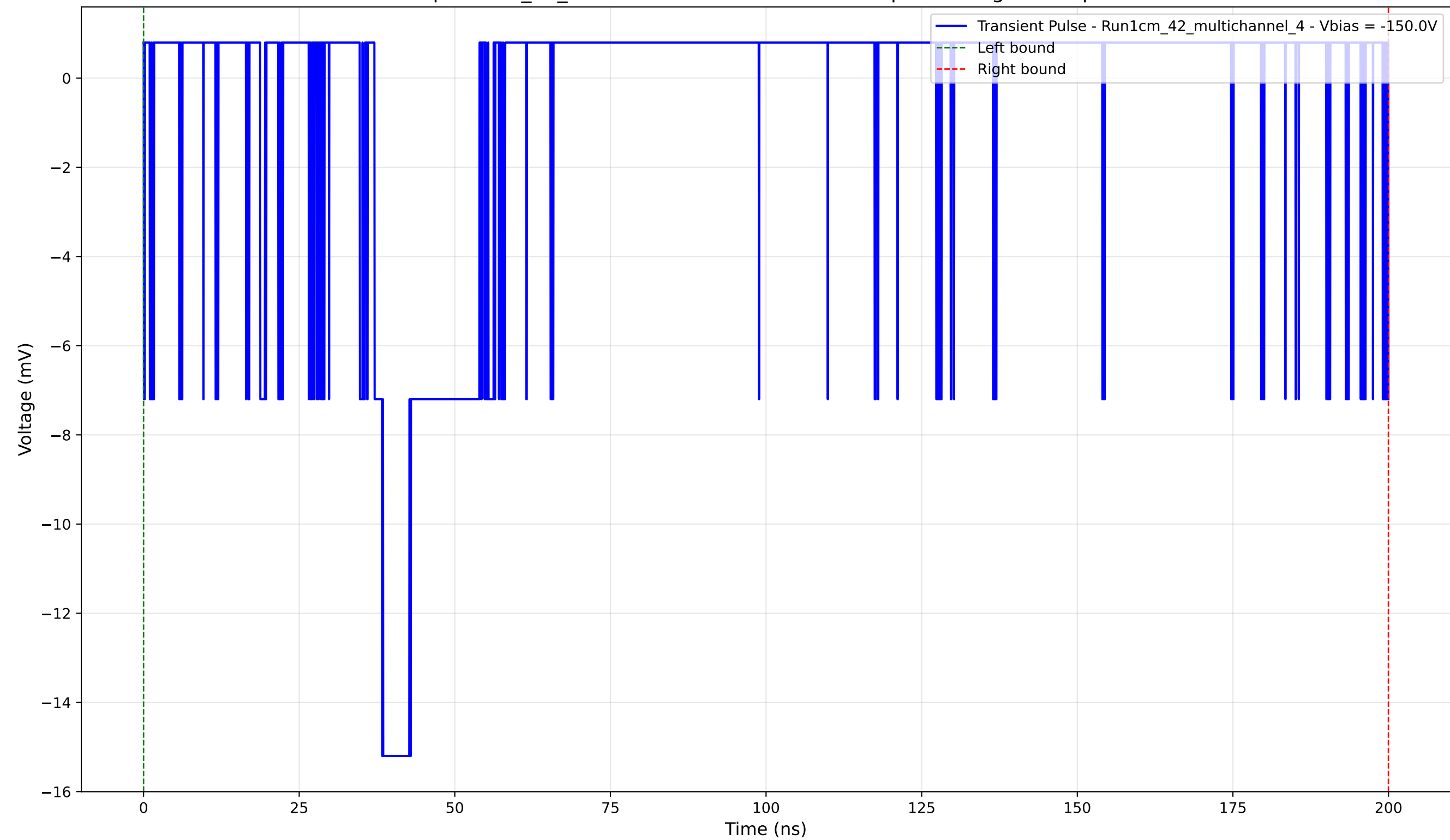
Transient Pulse - Sample: 1cm_42_multichannel - Position: 4505.0 \mu\text{m} - Charge: 1.94 pC - Rise Time: 1.24 ns
