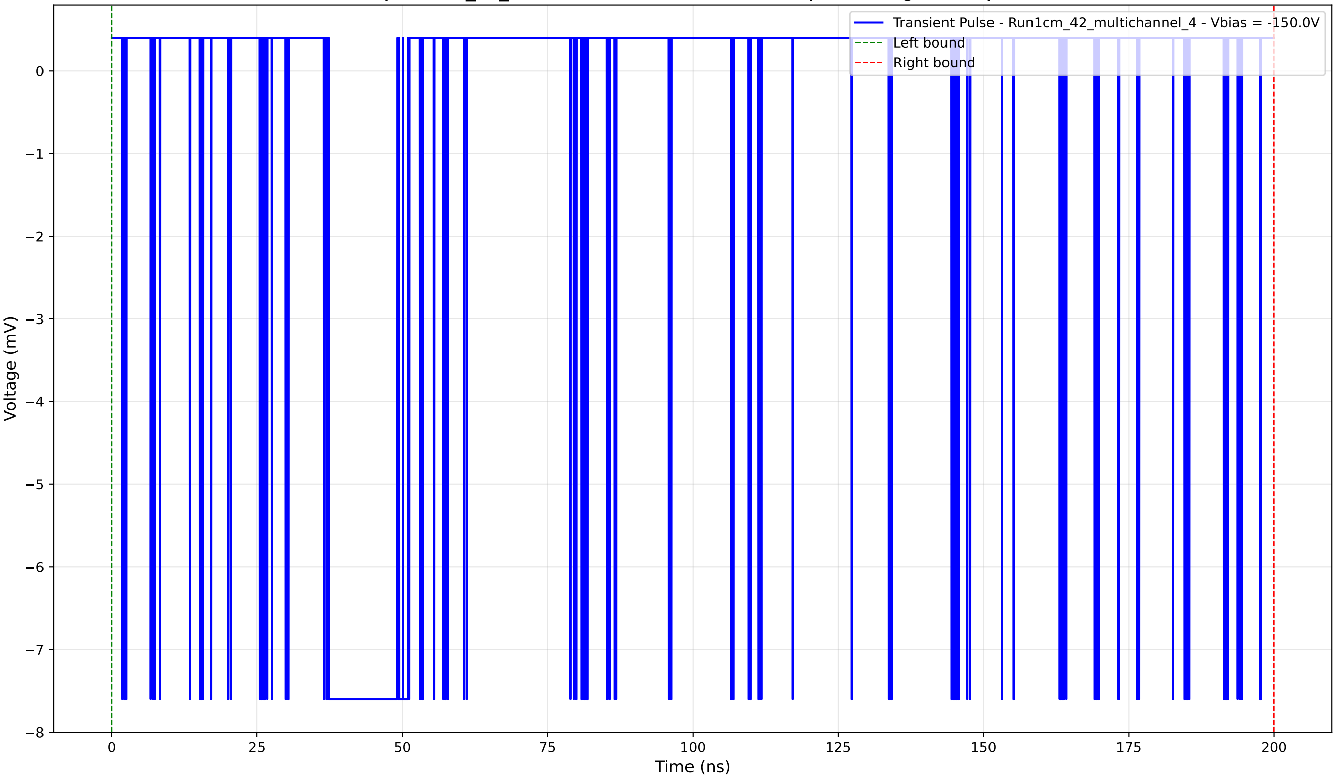
Transient Pulse - Sample: 1cm_42_multichannel - Position: 4445.0 \mu\text{m} - Charge: 2.18 pC - Rise Time: 0.02 ns
