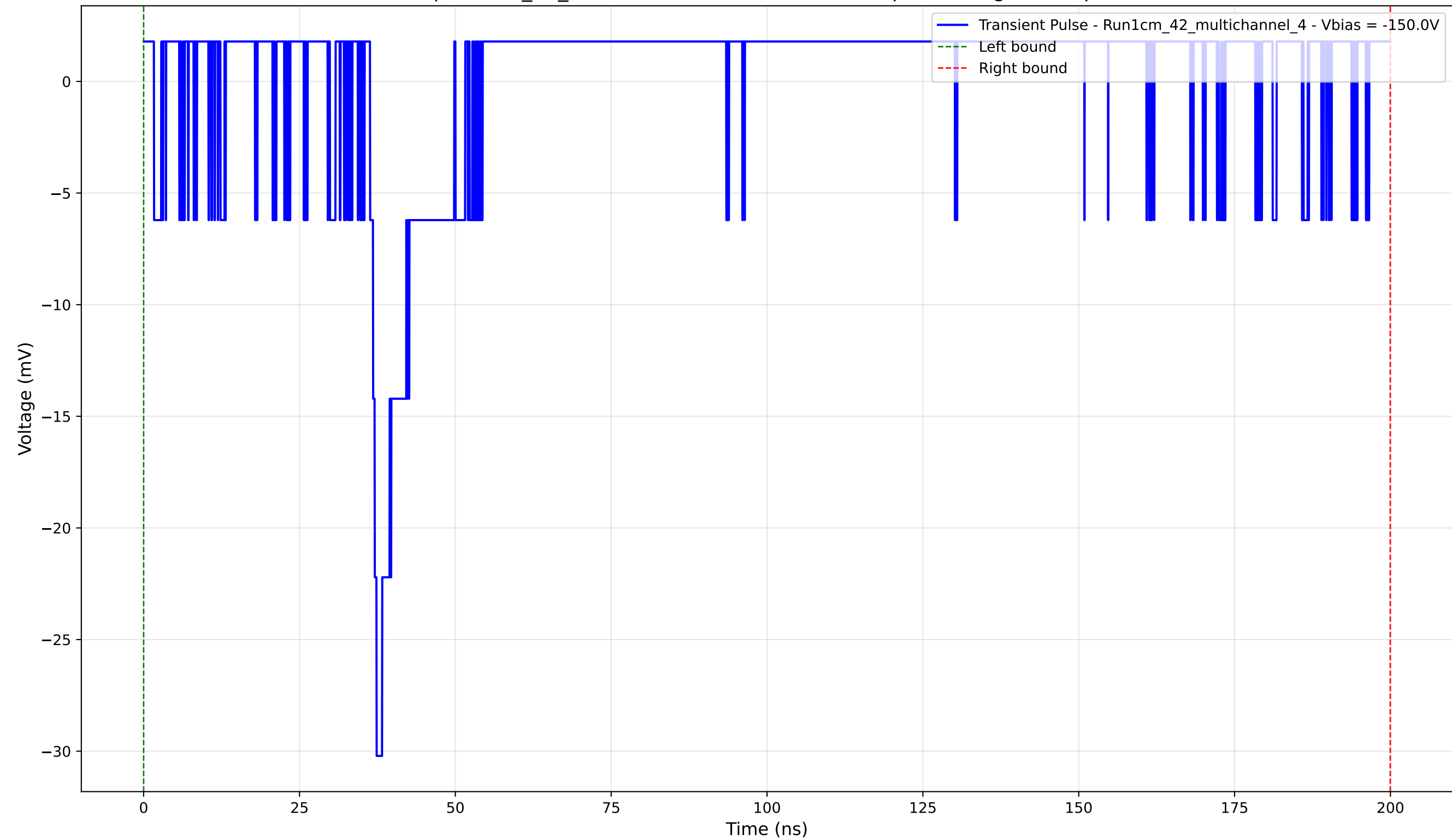
Transient Pulse - Sample: 1cm_42_multichannel - Position: 3090.0 \mu\text{m} - Charge: 0.97 pC - Rise Time: 1.05 ns
