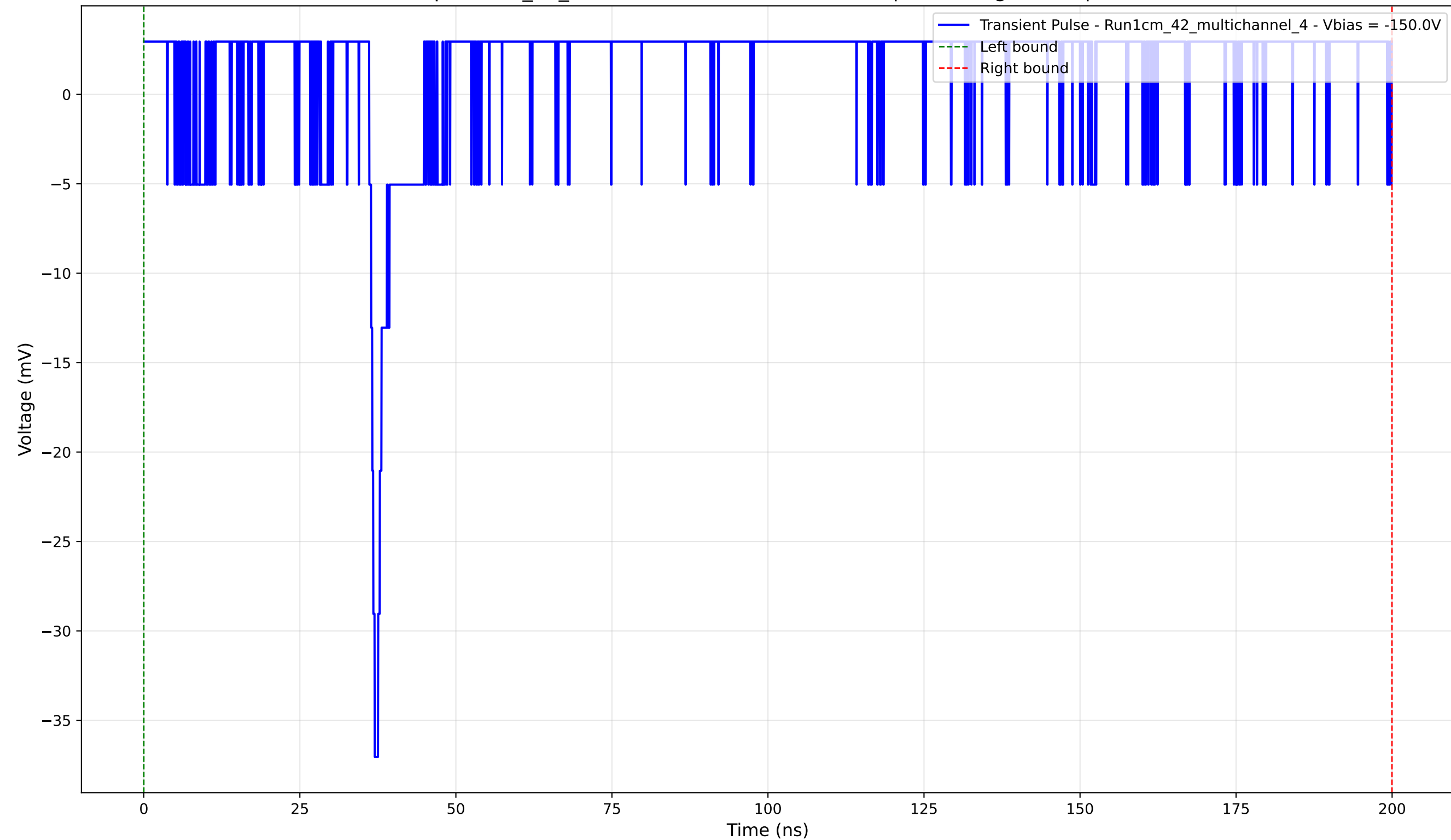
Transient Pulse - Sample: 1cm_42_multichannel - Position: 2435.0 \mu\text{m} - Charge: 6.25 pC - Rise Time: 0.87 ns
