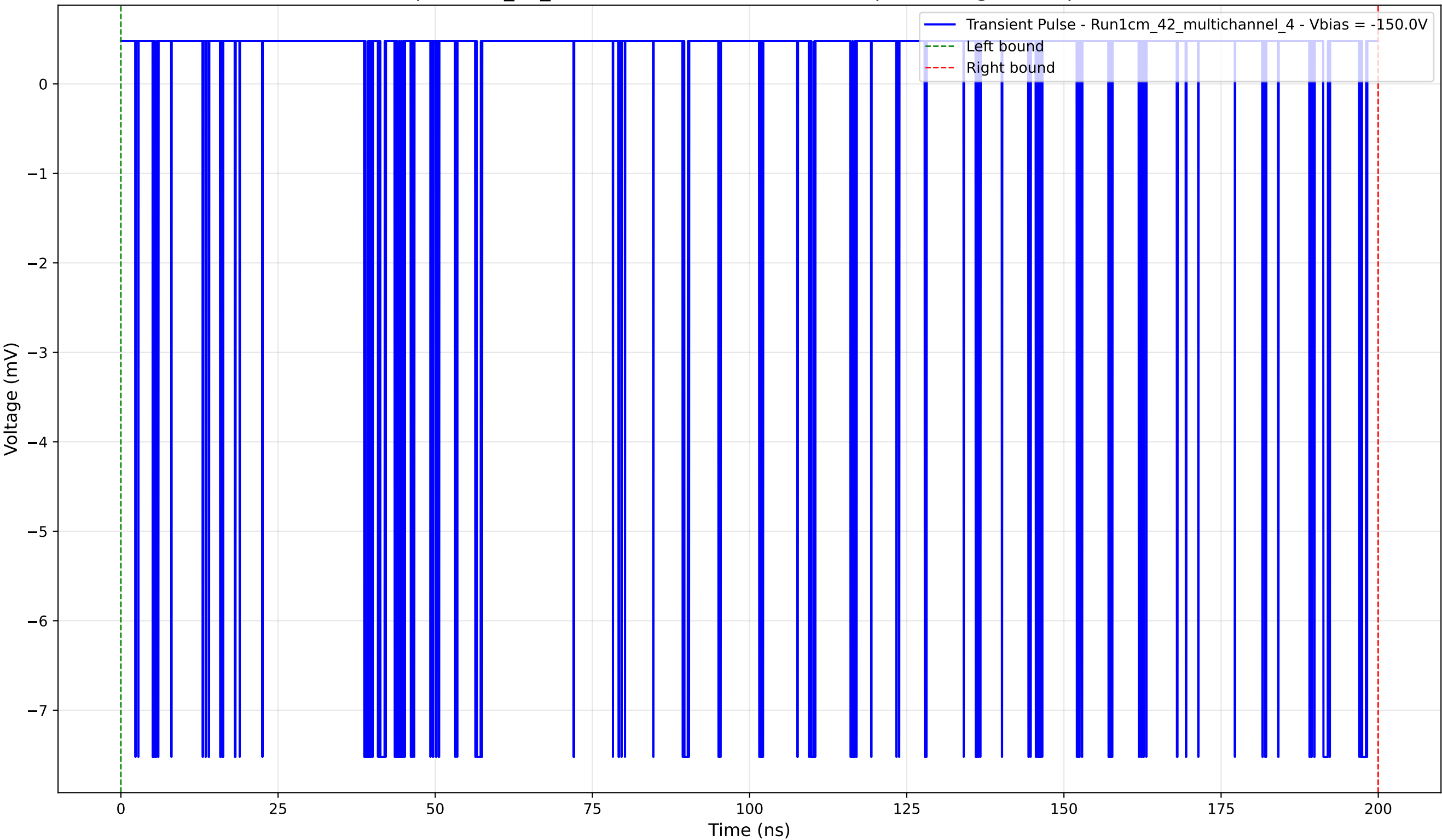
Transient Pulse - Sample: 1cm_42_multichannel - Position: 3880.0 \mu\text{m} - Charge: 0.33 pC - Rise Time: 0.02 ns
