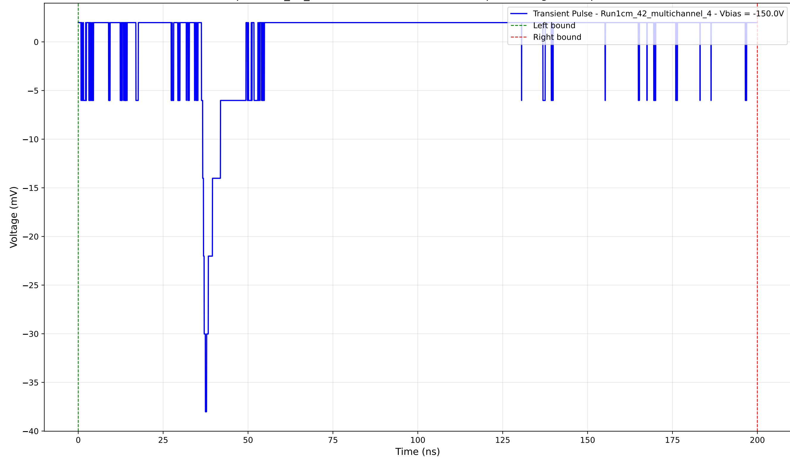
Transient Pulse - Sample: 1cm_42_multichannel - Position: 2960.0 \mu\text{m} - Charge: 2.53 pC - Rise Time: 1.17 ns
