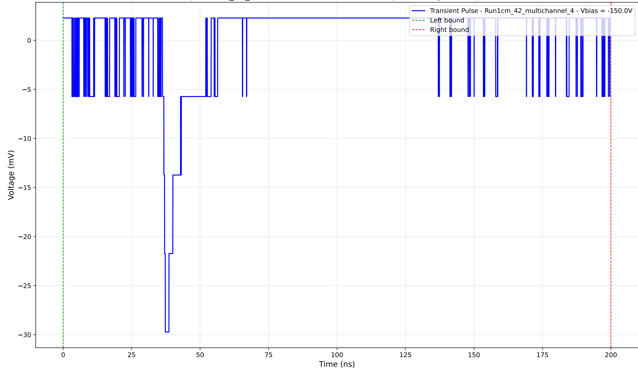
Transient Pulse - Sample: 1cm_42_multichannel - Position: 1635.0 \mu\text{m} - Charge: 1.97 pC - Rise Time: 1.04 ns
