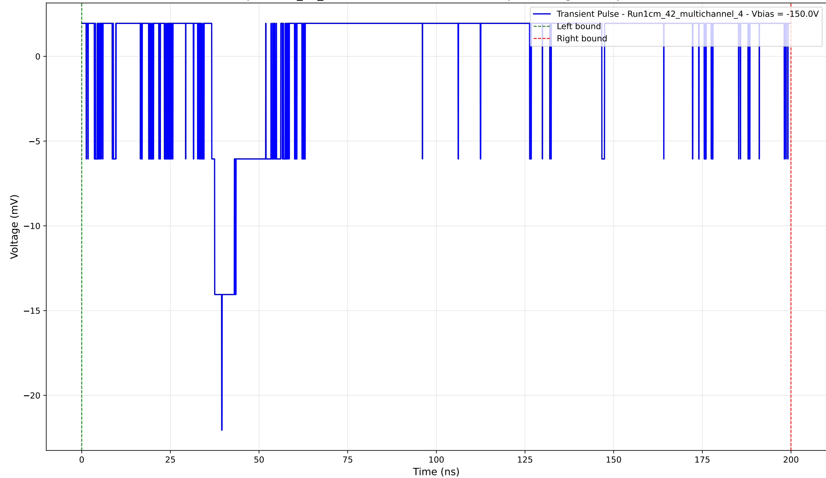
Transient Pulse - Sample: 1cm_42_multichannel - Position: 3690.0 \mu\text{m} - Charge: 2.01 pC - Rise Time: 2.82 ns
