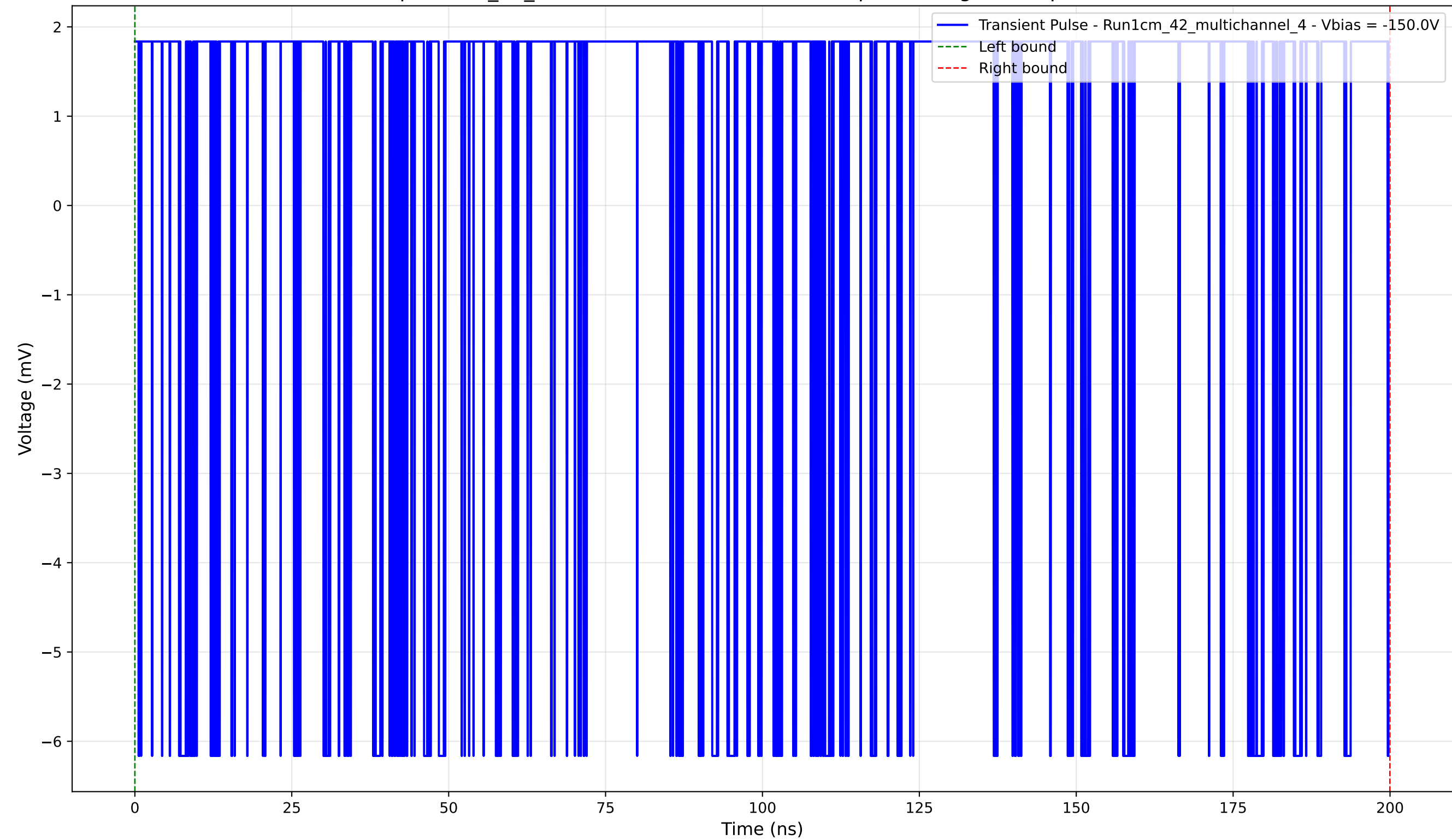
Transient Pulse - Sample: 1cm_42_multichannel - Position: 3415.0 \mu\text{m} - Charge: 2.15 pC - Rise Time: 0.00 ns (N/A)
