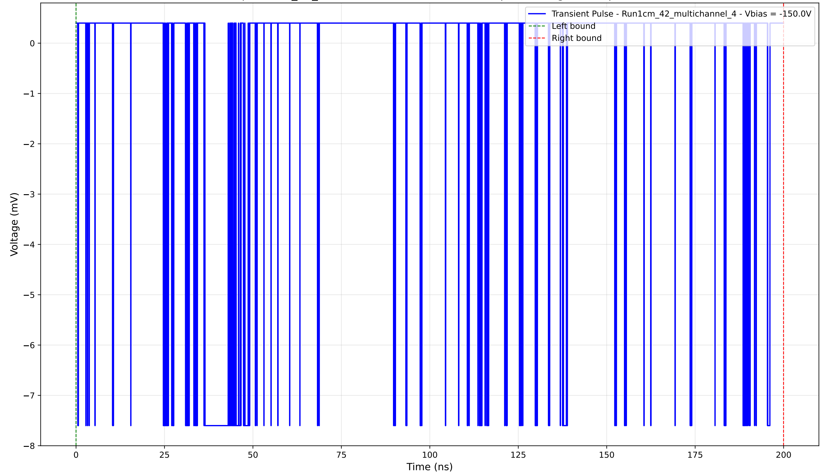
Transient Pulse - Sample: 1cm_42_multichannel - Position: 2930.0 \mu\text{m} - Charge: 1.91 pC - Rise Time: 0.02 ns
