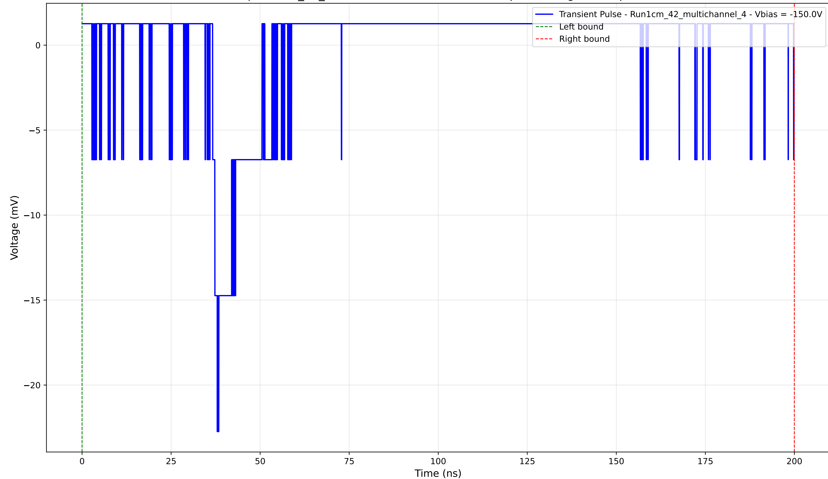
Transient Pulse - Sample: 1cm_42_multichannel - Position: 3465.0 \mu\text{m} - Charge: 0.35 pC - Rise Time: 1.34 ns
