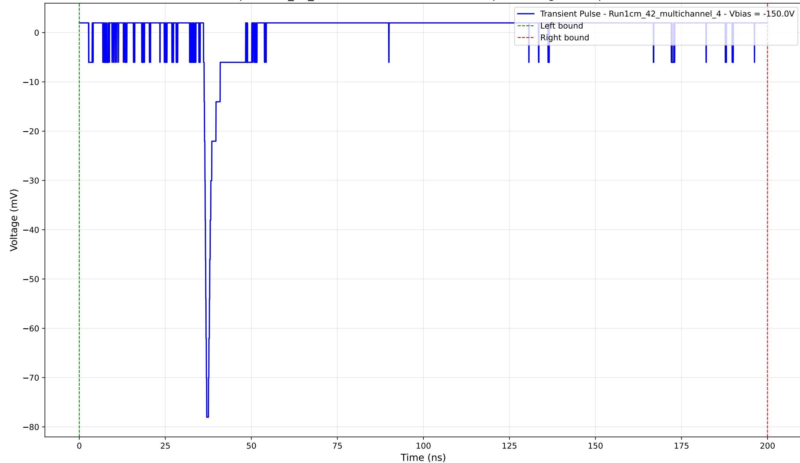
Transient Pulse - Sample: 1cm_42_multichannel - Position: 2265.0 \mu\text{m} - Charge: 1.54 pC - Rise Time: 0.76 ns
