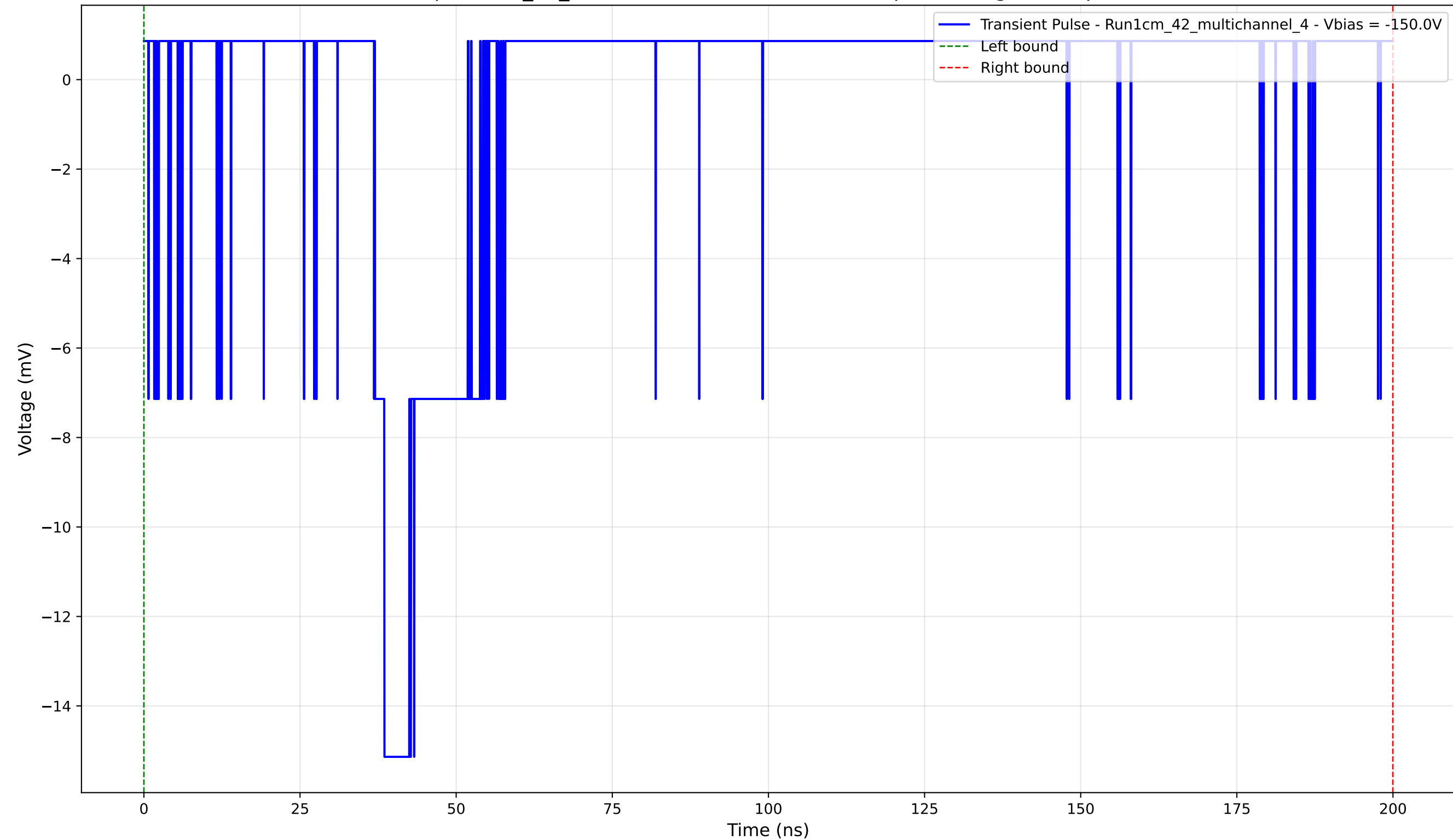
Transient Pulse - Sample: 1cm_42_multichannel - Position: 4685.0 \mu\text{m} - Charge: 0.77 pC - Rise Time: 1.52 ns
