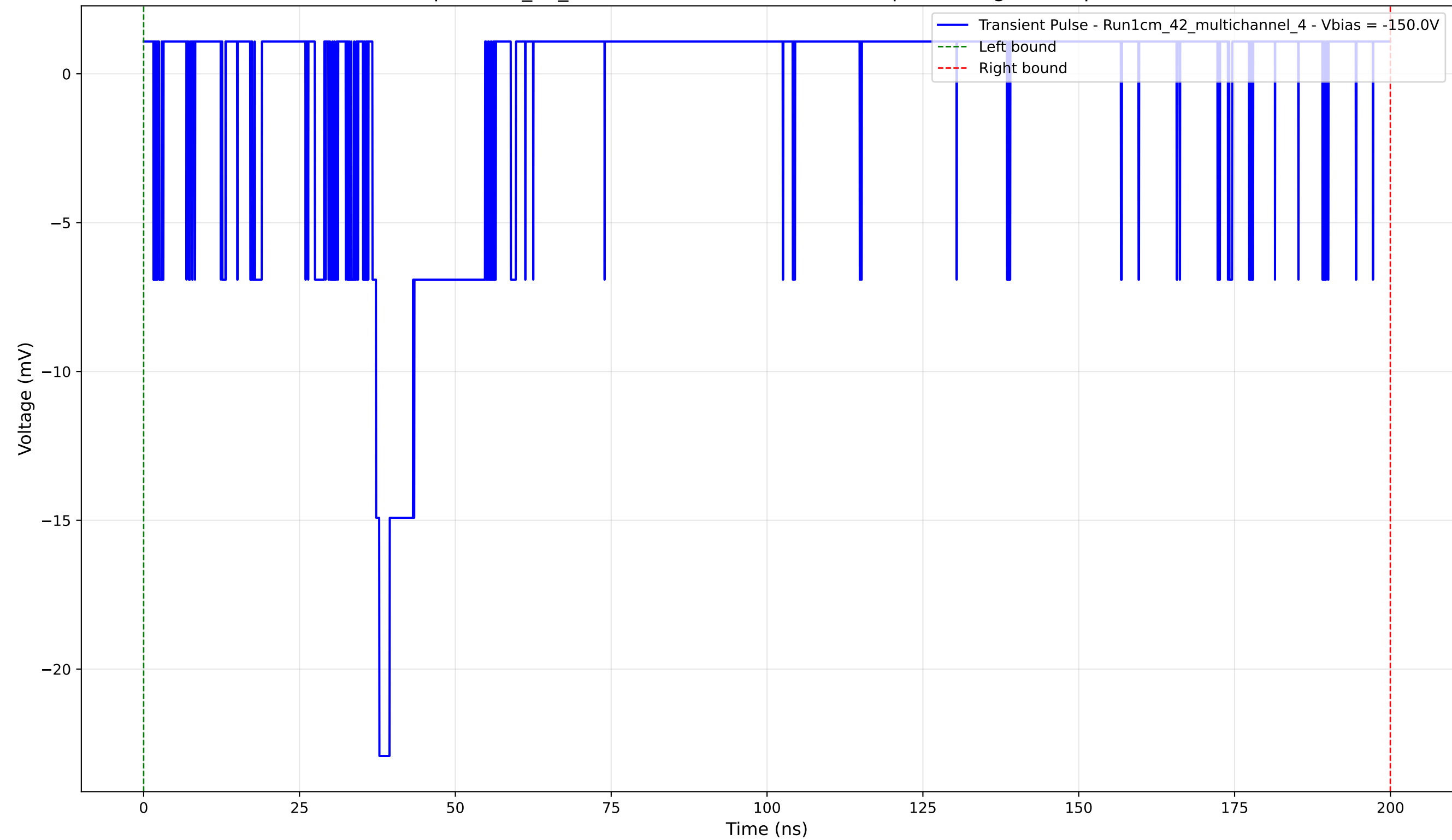
Transient Pulse - Sample: 1cm_42_multichannel - Position: 3515.0 \mu\text{m} - Charge: 1.89 pC - Rise Time: 1.12 ns
