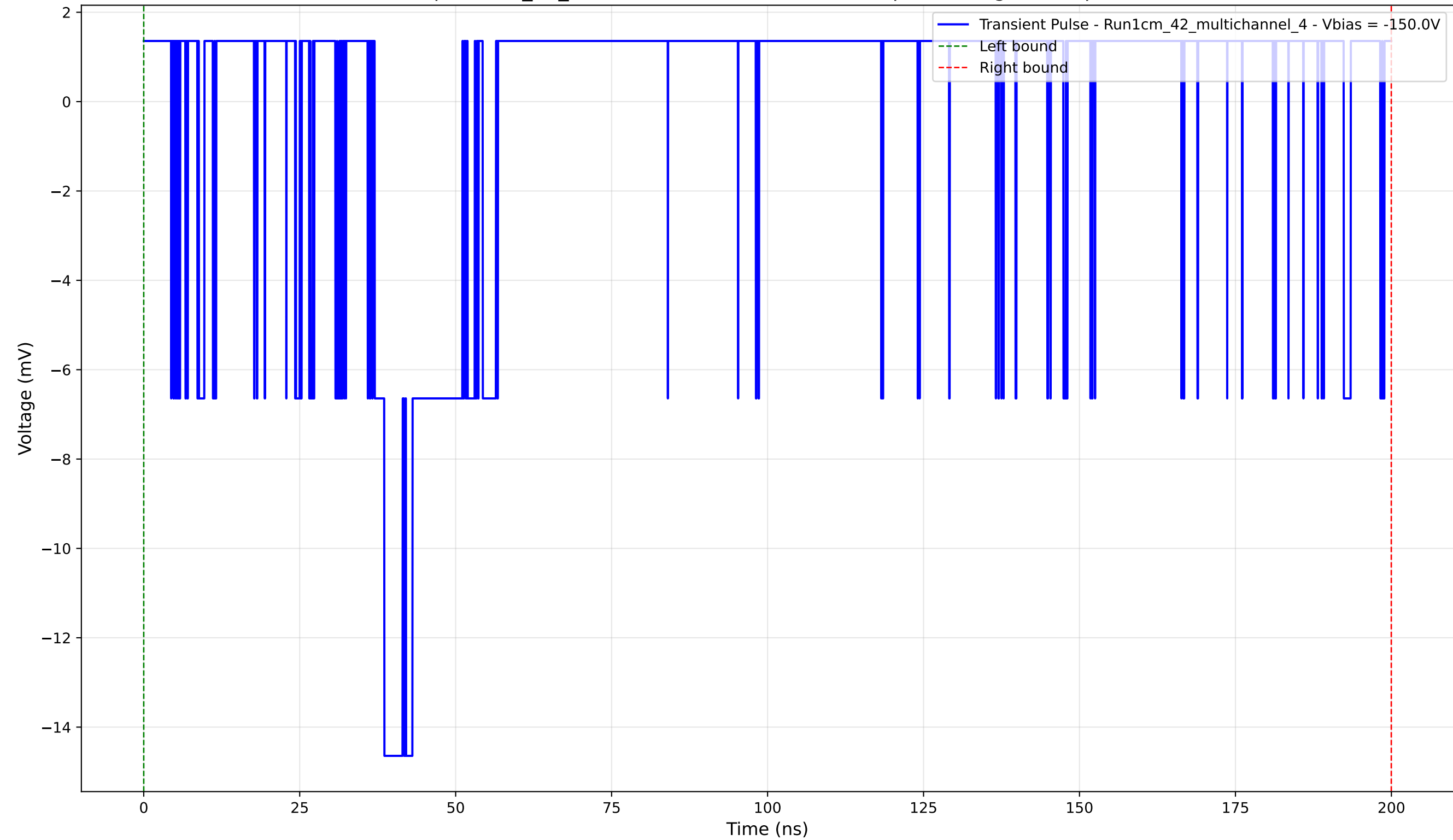
Transient Pulse - Sample: 1cm_42_multichannel - Position: 4485.0 \mu\text{m} - Charge: 0.33 pC - Rise Time: 1.56 ns
