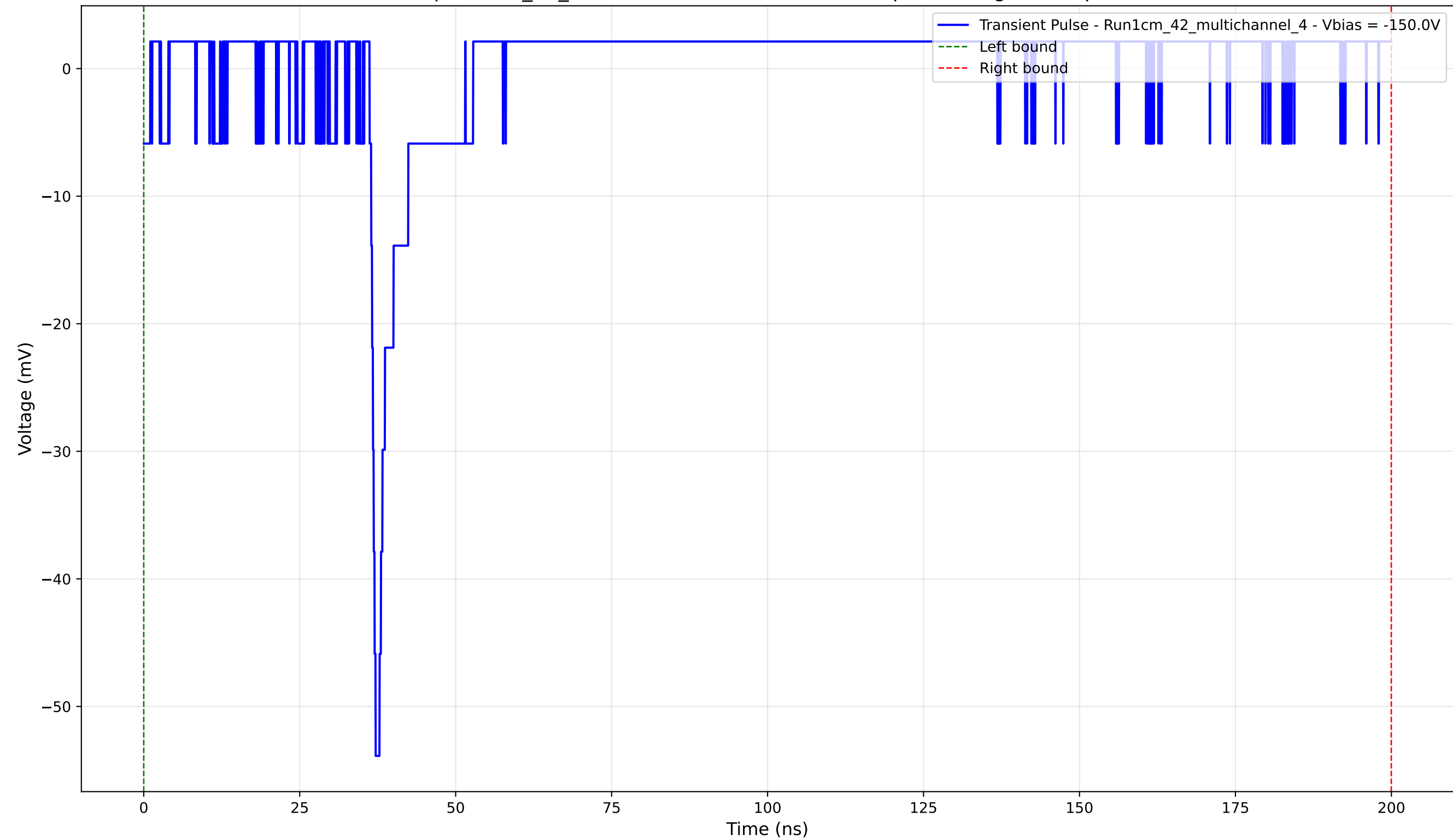
Transient Pulse - Sample: 1cm_42_multichannel - Position: 2030.0 \mu\text{m} - Charge: 1.24 pC - Rise Time: 0.96 ns
