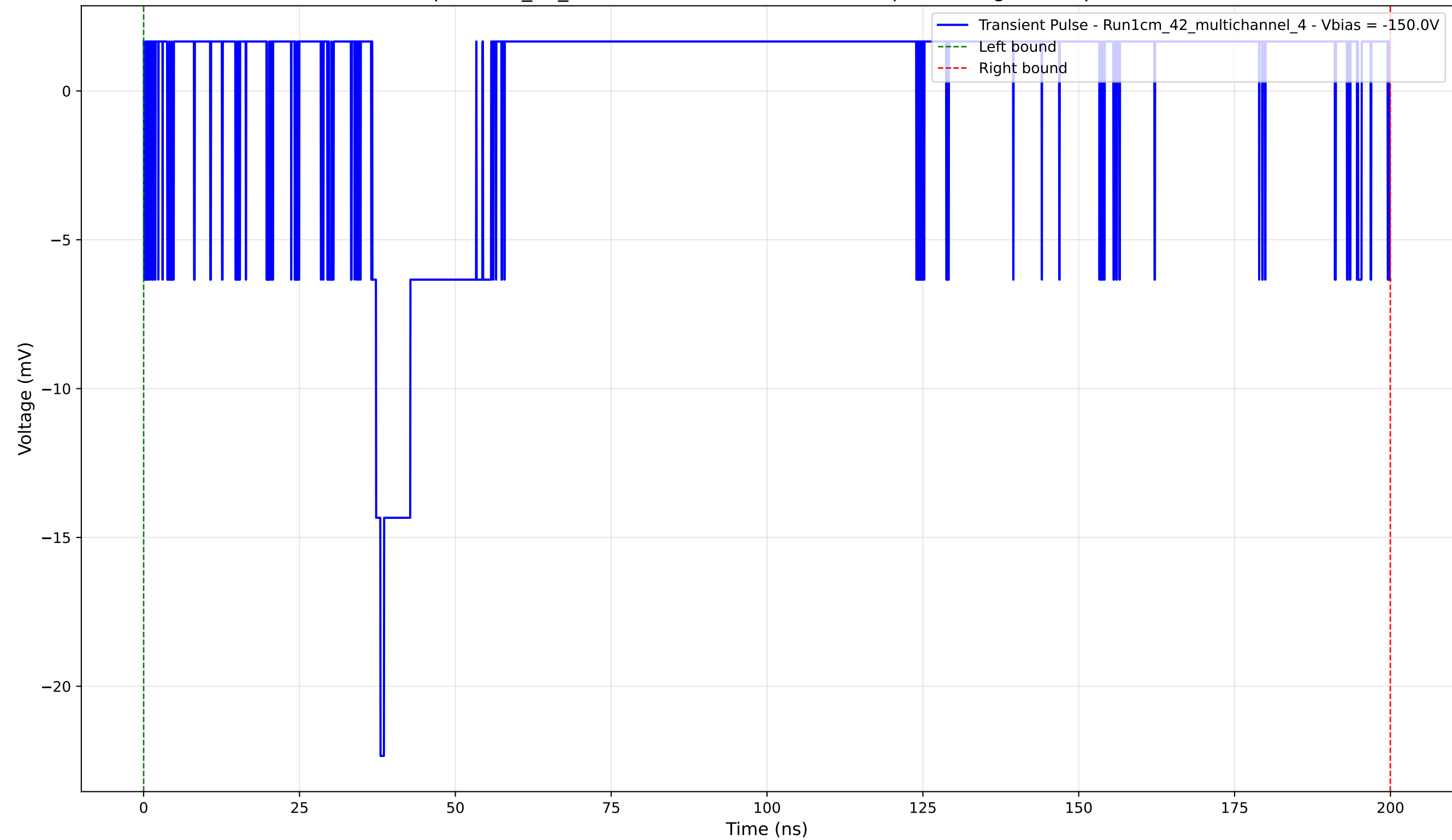
Transient Pulse - Sample: 1cm_42_multichannel - Position: 3570.0 \mu\text{m} - Charge: 1.12 pC - Rise Time: 1.32 ns
