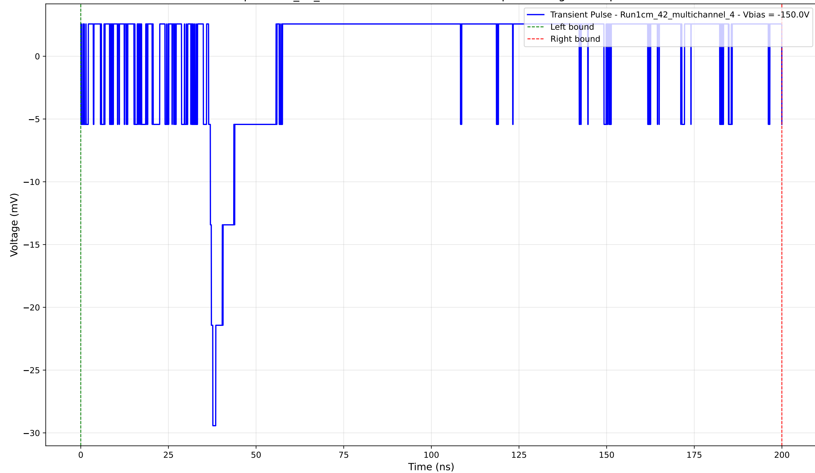
Transient Pulse - Sample: 1cm_42_multichannel - Position: 1460.0 \mu\text{m} - Charge: 2.37 pC - Rise Time: 1.22 ns
