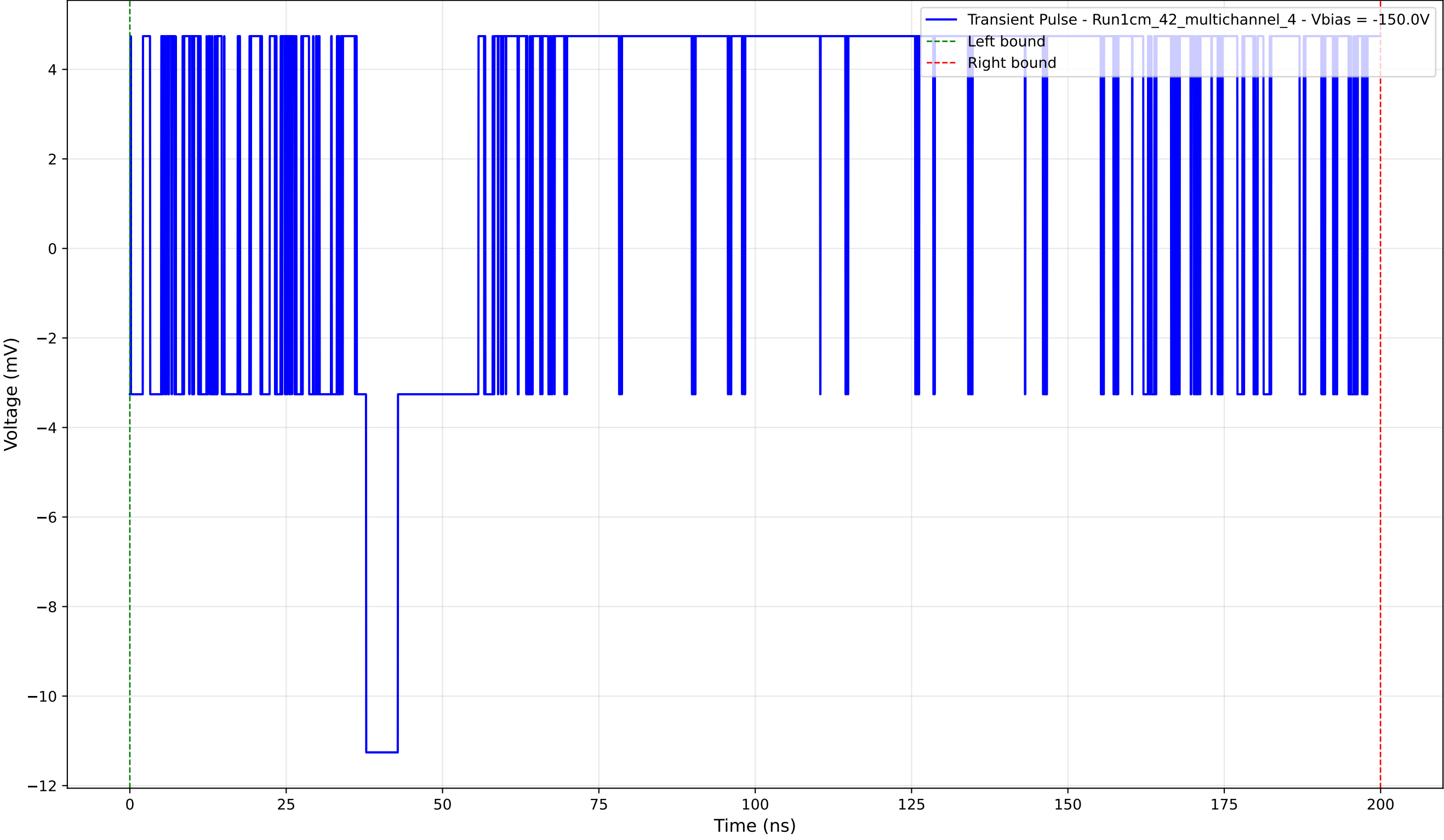
Transient Pulse - Sample: 1cm_42_multichannel - Position: 930.0 \mu\text{m} - Charge: 9.19 pC - Rise Time: 0.00 ns (N/A)
