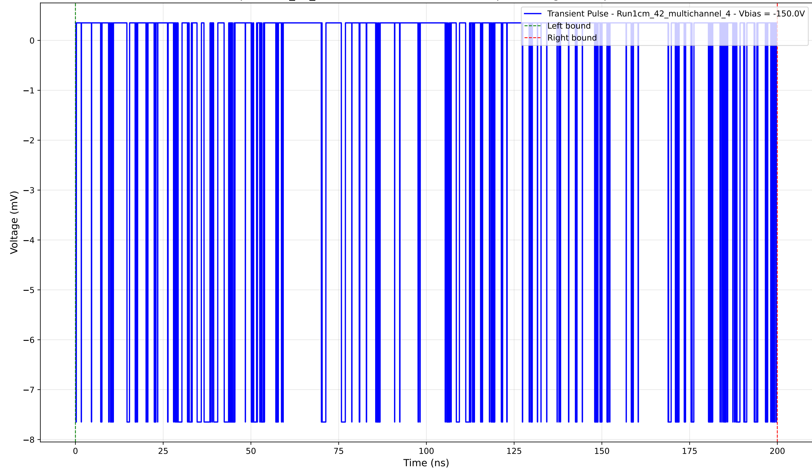
Transient Pulse - Sample: 1cm_42_multichannel - Position: 1885.0 \mu\text{m} - Charge: 3.83 pC - Rise Time: 0.02 ns
