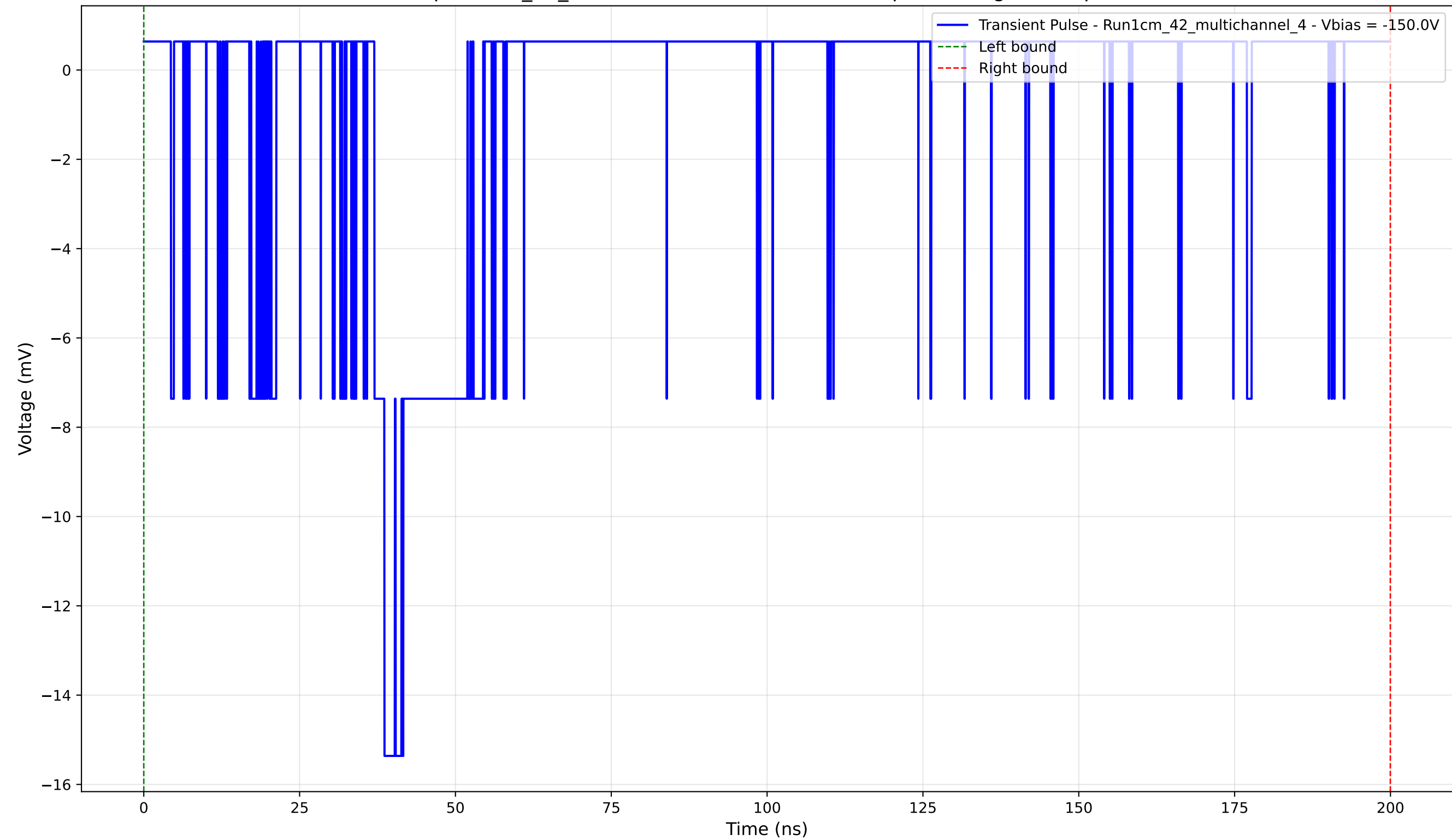
Transient Pulse - Sample: 1cm_42_multichannel - Position: 4780.0 \mu\text{m} - Charge: 2.37 pC - Rise Time: 1.62 ns
