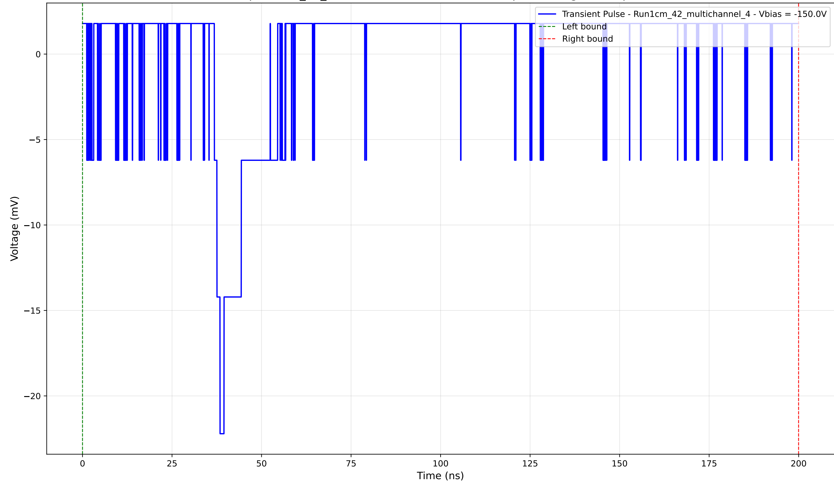
Transient Pulse - Sample: 1cm_42_multichannel - Position: 3680.0 \mu\text{m} - Charge: 1.41 pC - Rise Time: 1.60 ns
