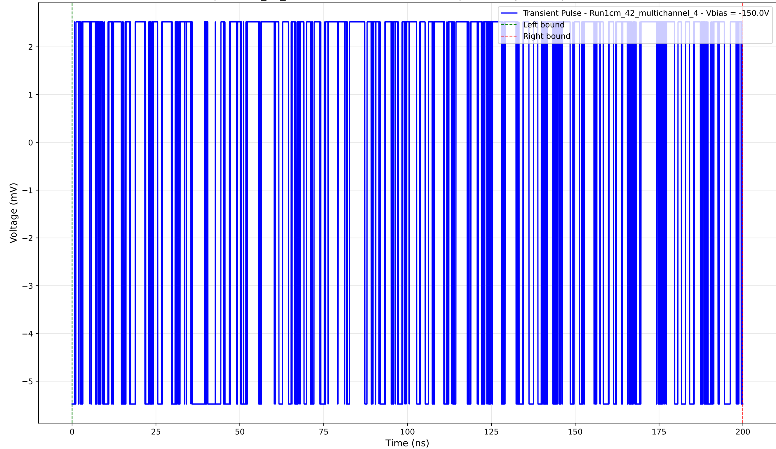
Transient Pulse - Sample: 1cm_42_multichannel - Position: 1890.0 \mu\text{m} - Charge: 0.40 pC - Rise Time: 0.00 ns (N/A)
