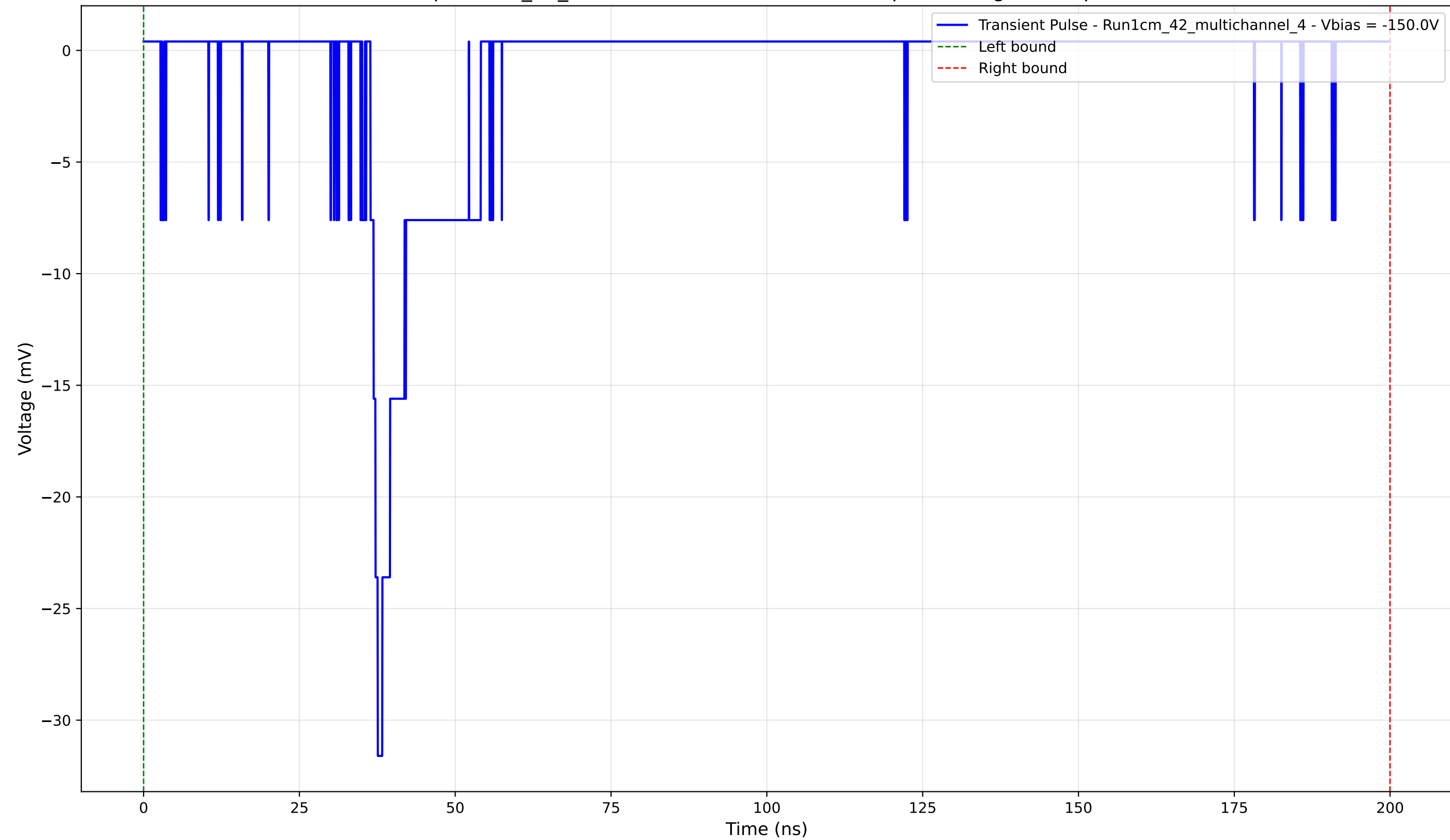
Transient Pulse - Sample: 1cm_42_multichannel - Position: 3190.0 \mu\text{m} - Charge: 3.13 pC - Rise Time: 1.17 ns
