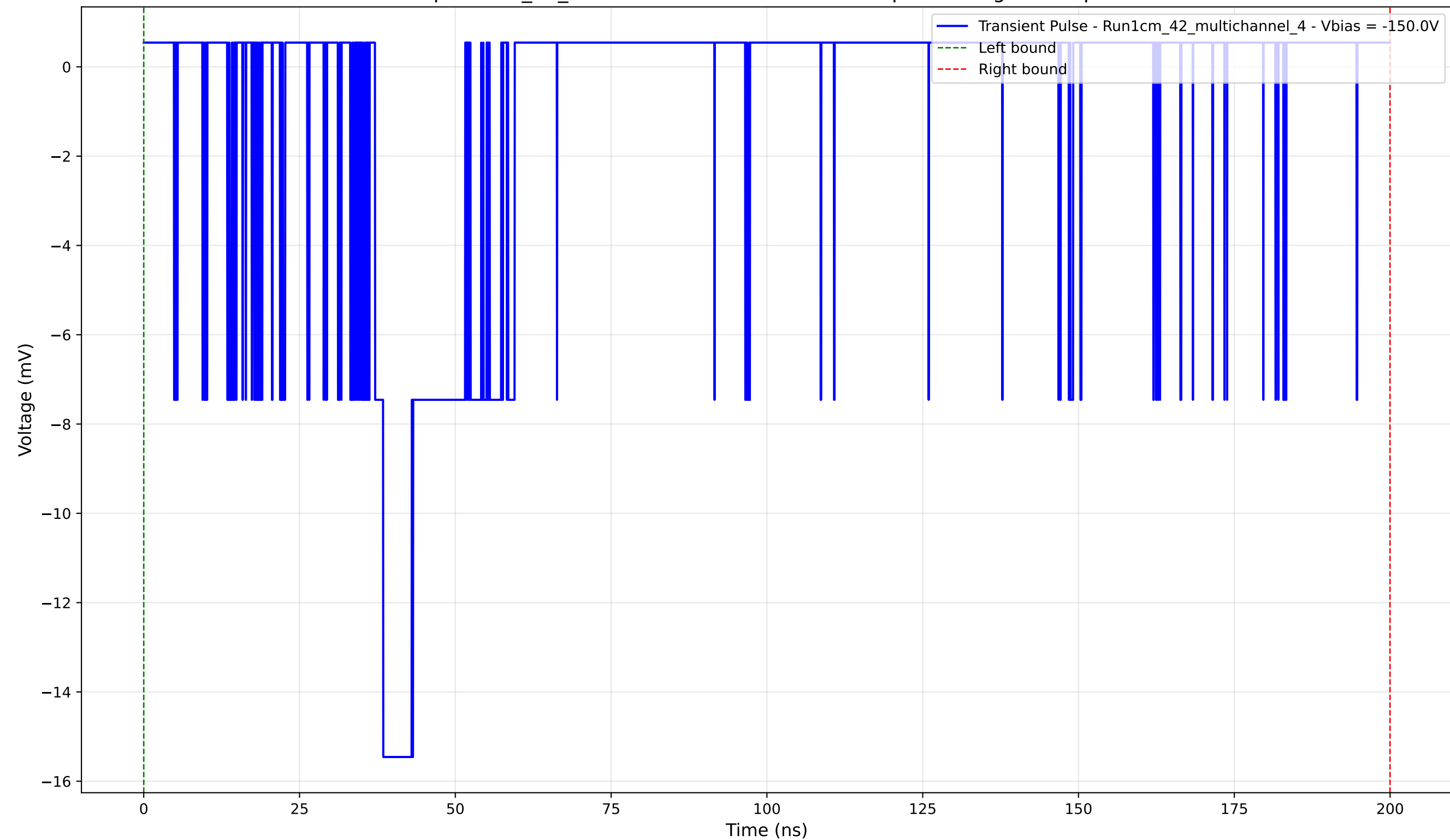
Transient Pulse - Sample: 1cm_42_multichannel - Position: 4325.0 \mu\text{m} - Charge: 3.18 pC - Rise Time: 1.32 ns
