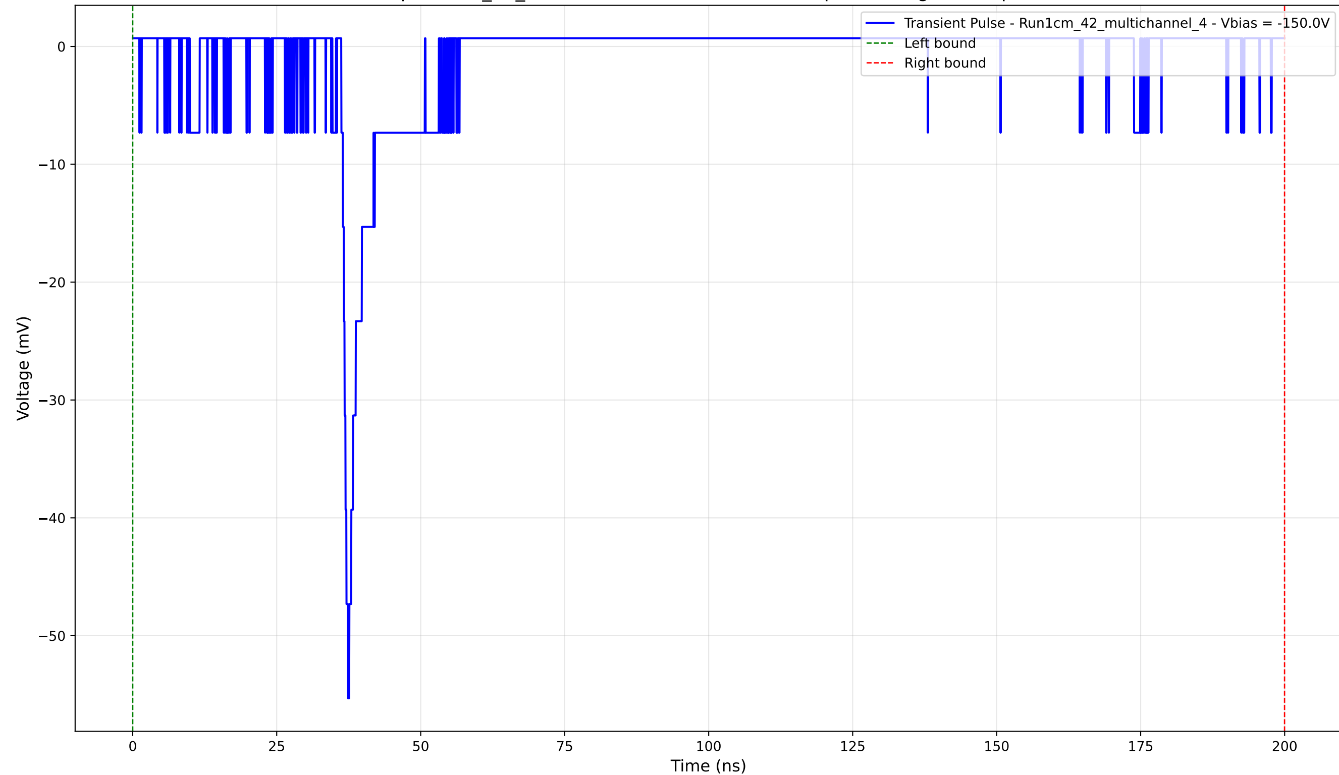
Transient Pulse - Sample: 1cm_42_multichannel - Position: 2785.0 \mu\text{m} - Charge: 3.91 pC - Rise Time: 1.17 ns
