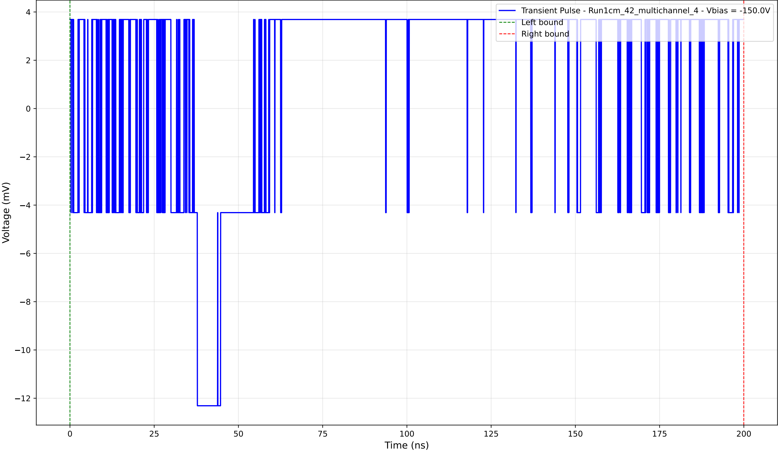
Transient Pulse - Sample: 1cm_42_multichannel - Position: 725.0 \mu\text{m} - Charge: 6.13 pC - Rise Time: 0.00 ns (N/A)
