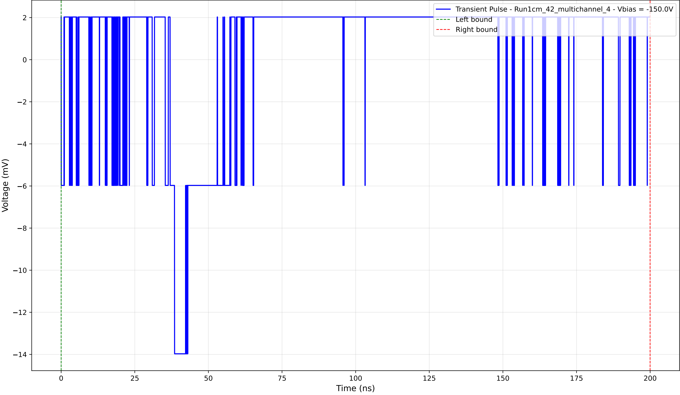
Transient Pulse - Sample: 1cm_42_multichannel - Position: 280.0 \mu\text{m} - Charge: 2.17 pC - Rise Time: 0.00 ns (N/A)
