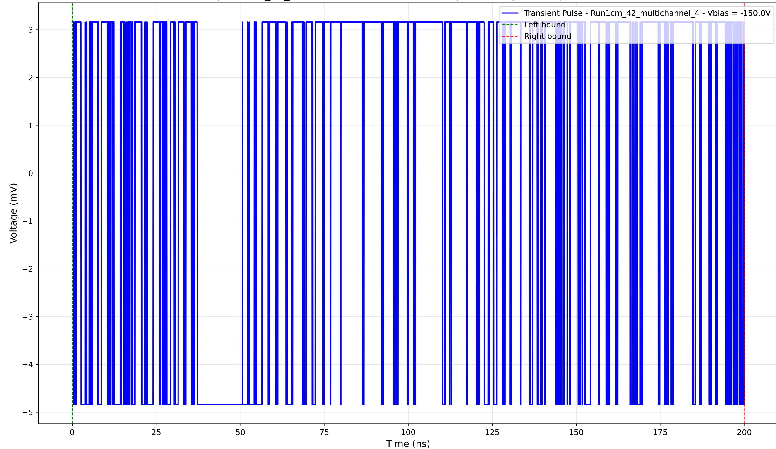
Transient Pulse - Sample: 1cm_42_multichannel - Position: 915.0 \mu\text{m} - Charge: 3.09 pC - Rise Time: 0.00 ns (N/A)
