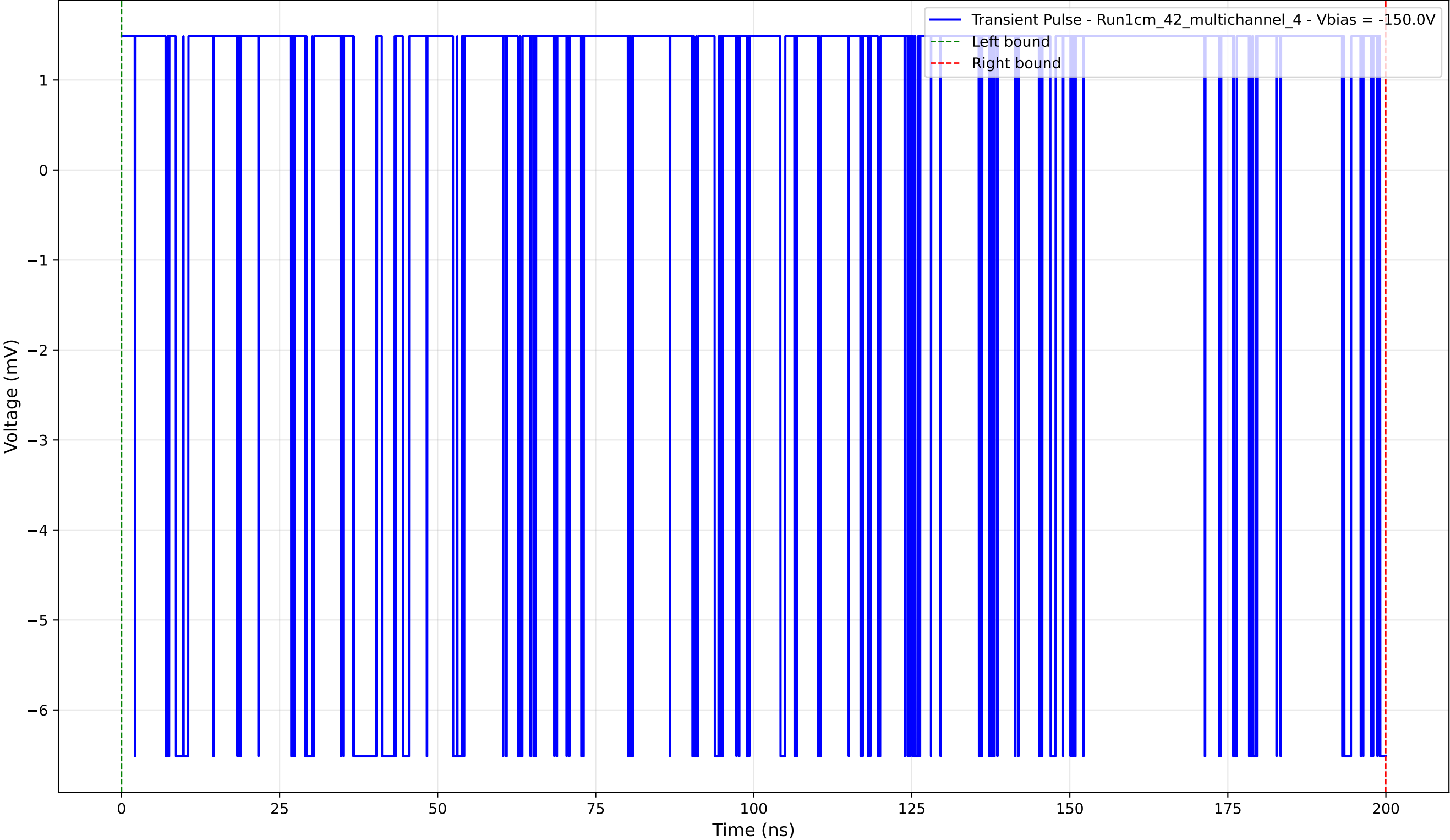
Transient Pulse - Sample: 1cm_42_multichannel - Position: 2920.0 \mu\text{m} - Charge: 1.75 pC - Rise Time: 0.00 ns (N/A)
