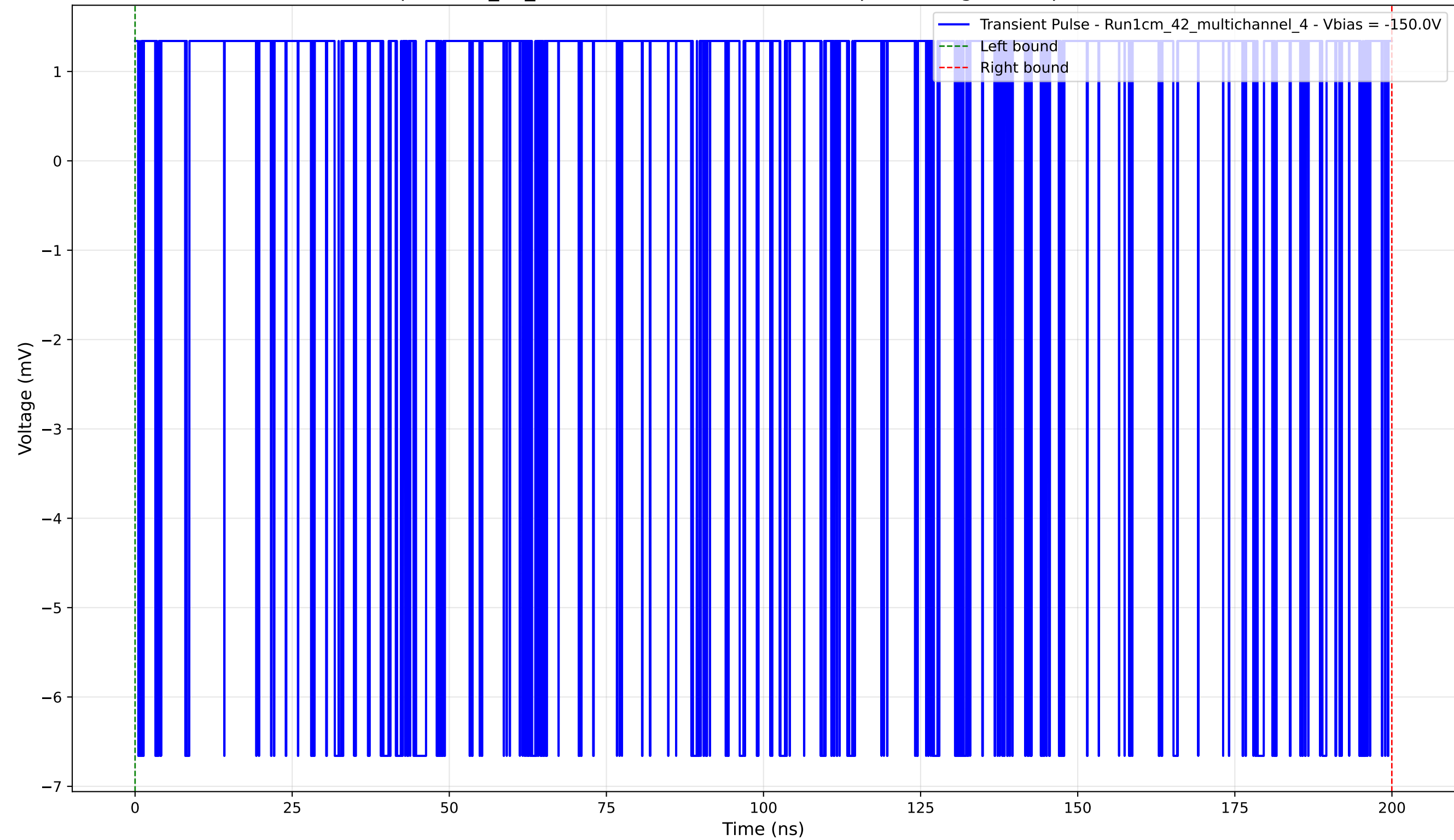
Transient Pulse - Sample: 1cm_42_multichannel - Position: 4390.0 \mu\text{m} - Charge: 0.57 pC - Rise Time: 0.00 ns (N/A)
