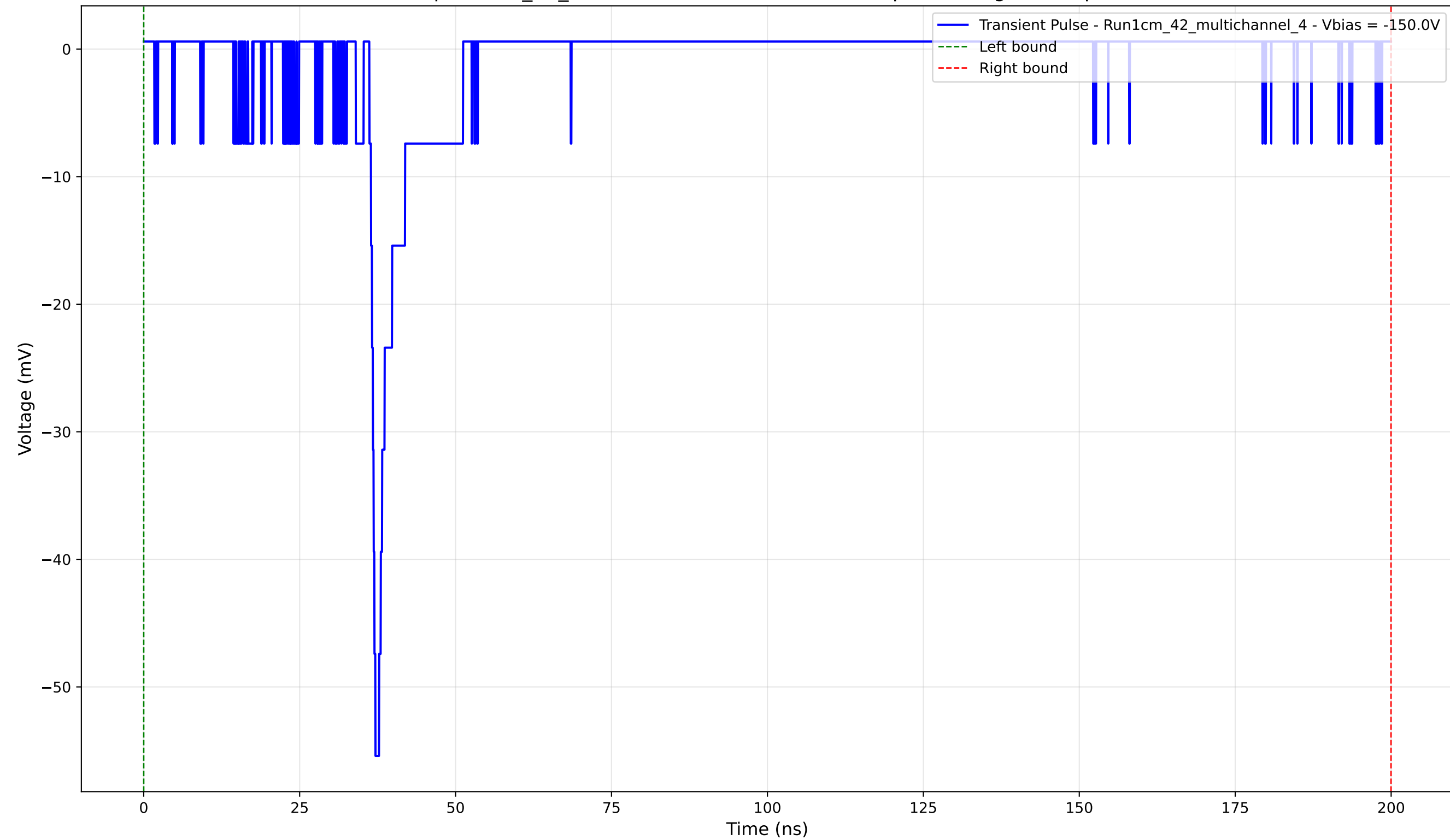
Transient Pulse - Sample: 1cm_42_multichannel - Position: 2050.0 \mu\text{m} - Charge: 3.84 pC - Rise Time: 0.97 ns
