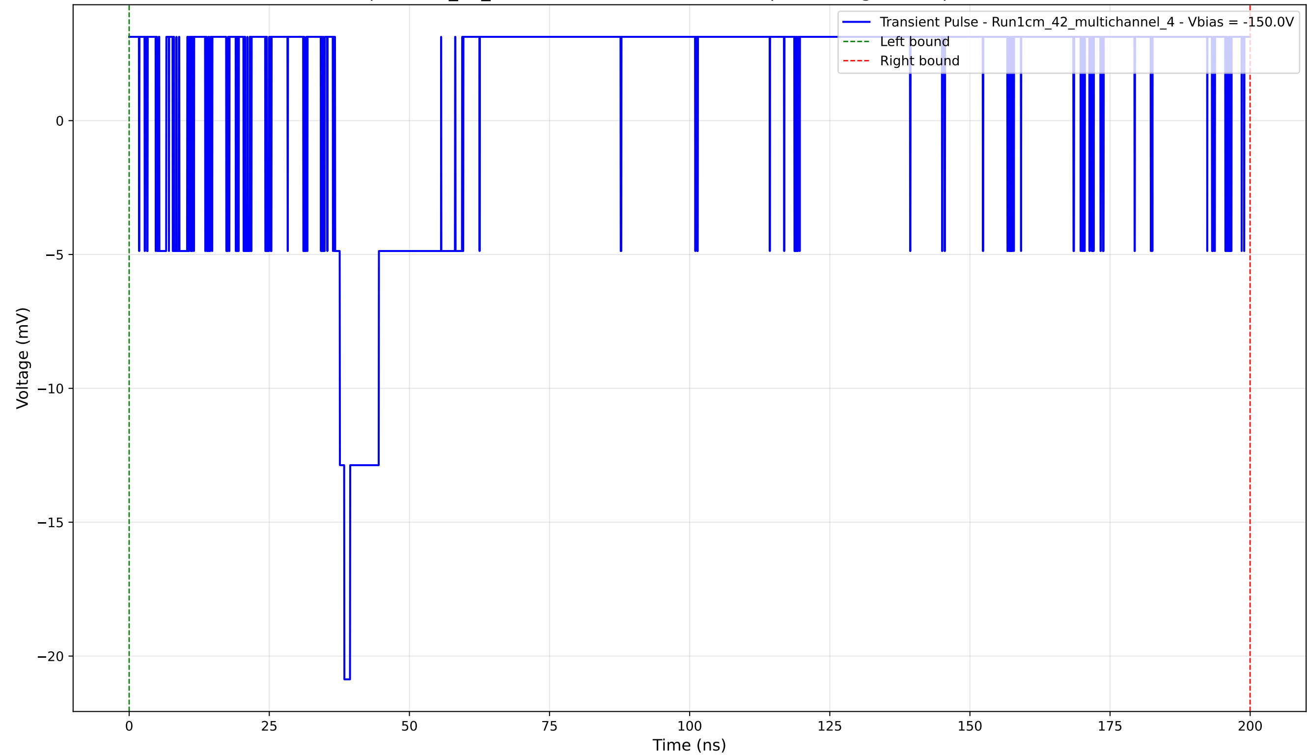
Transient Pulse - Sample: 1cm_42_multichannel - Position: 955.0 \mu\text{m} - Charge: 5.54 pC - Rise Time: 0.00 ns (N/A)
