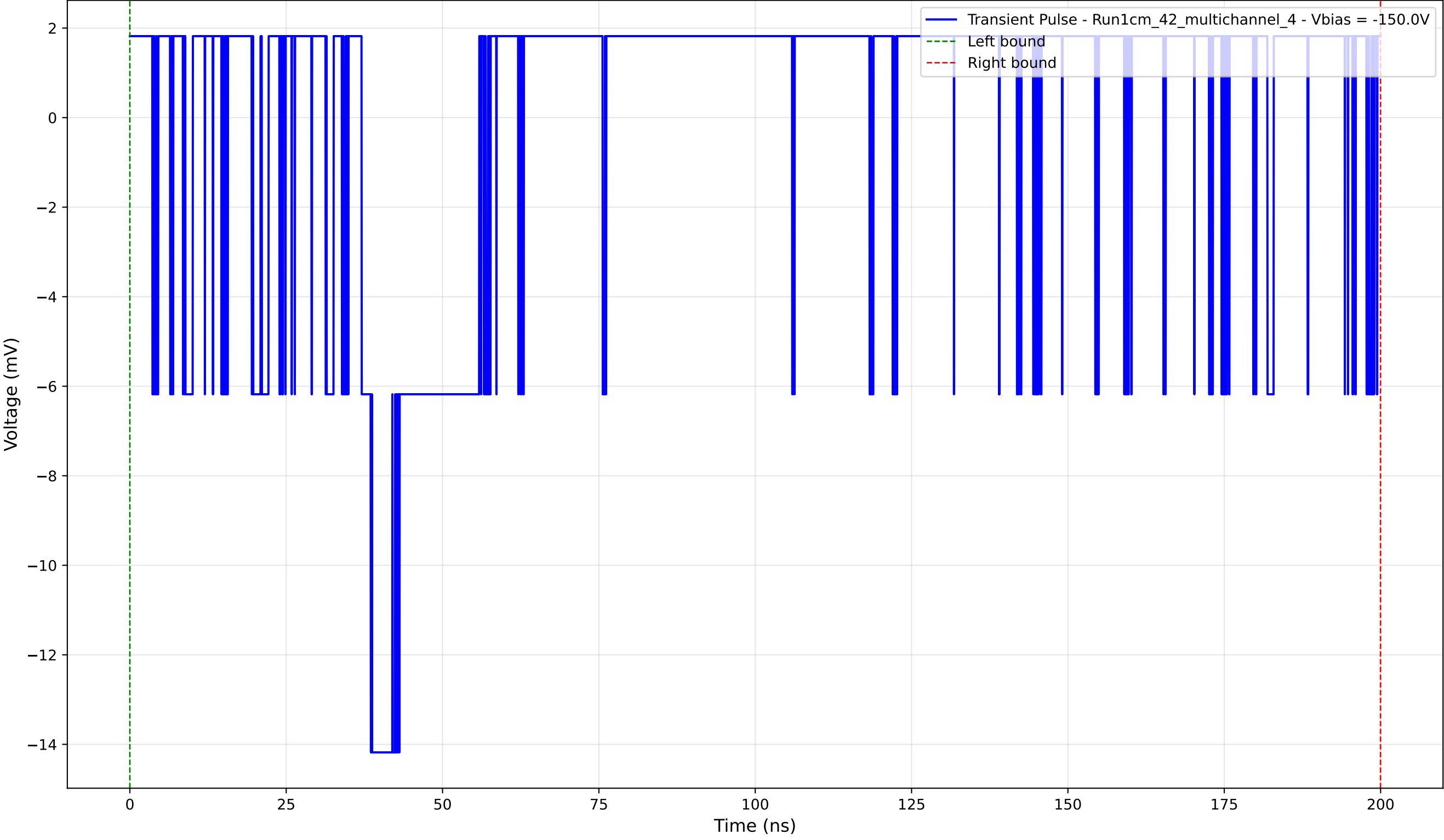
Transient Pulse - Sample: 1cm_42_multichannel - Position: 290.0 \mu\text{m} - Charge: 0.93 pC - Rise Time: 0.00 ns (N/A)
