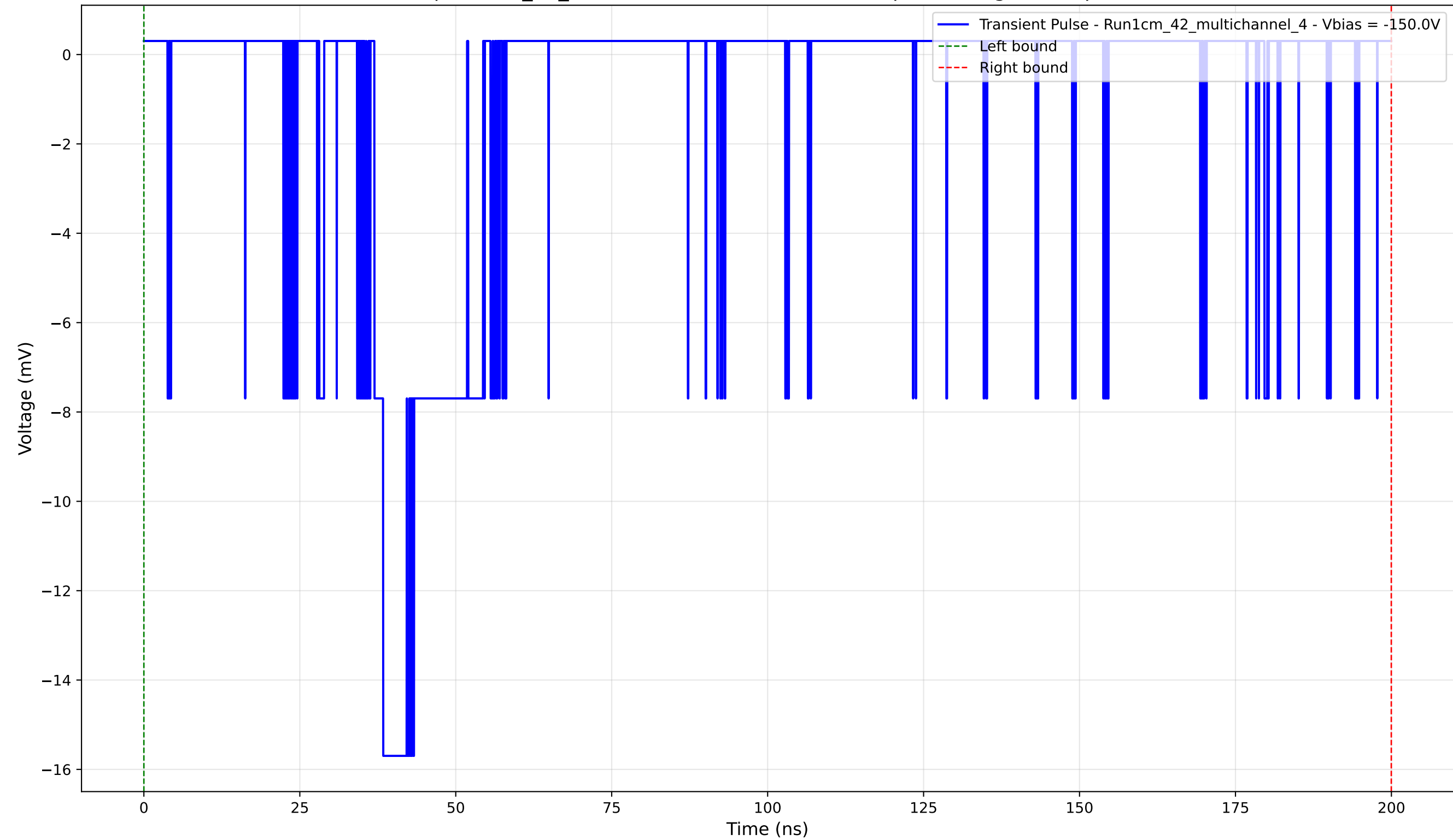
Transient Pulse - Sample: 1cm_42_multichannel - Position: 4755.0 \mu\text{m} - Charge: 3.89 pC - Rise Time: 1.42 ns
