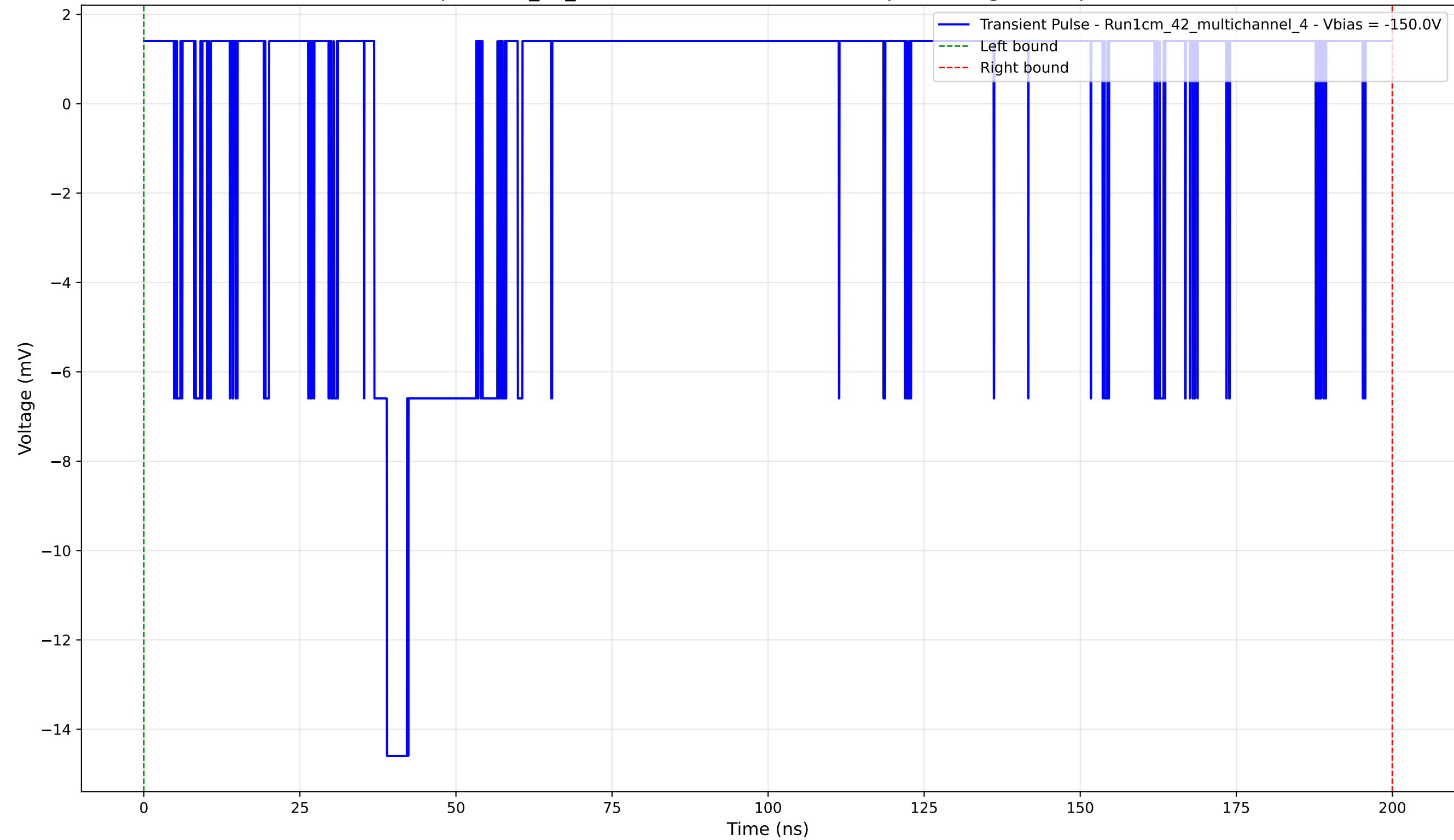
Transient Pulse - Sample: 1cm_42_multichannel - Position: 135.0 \mu\text{m} - Charge: 0.27 pC - Rise Time: 2.02 ns
