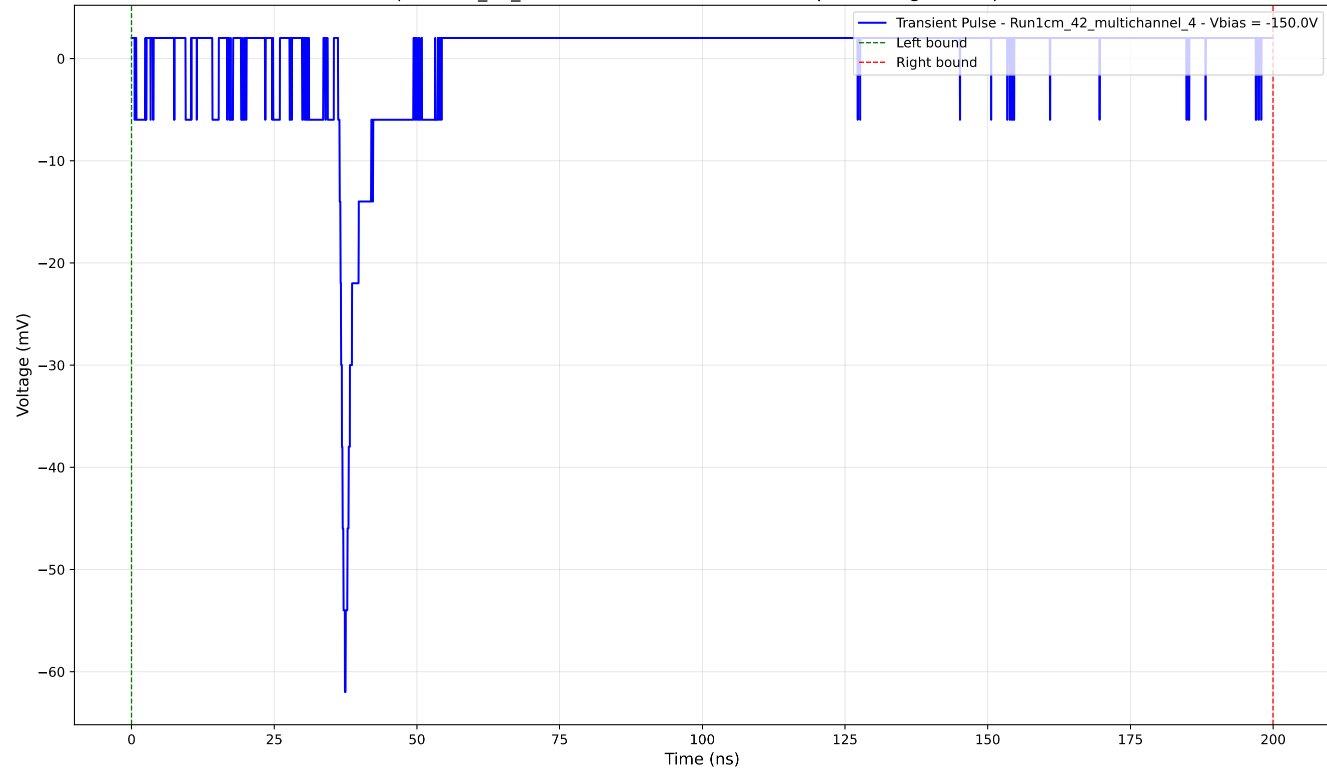
Transient Pulse - Sample: 1cm_42_multichannel - Position: 2040.0 \mu\text{m} - Charge: 1.12 pC - Rise Time: 0.96 ns
