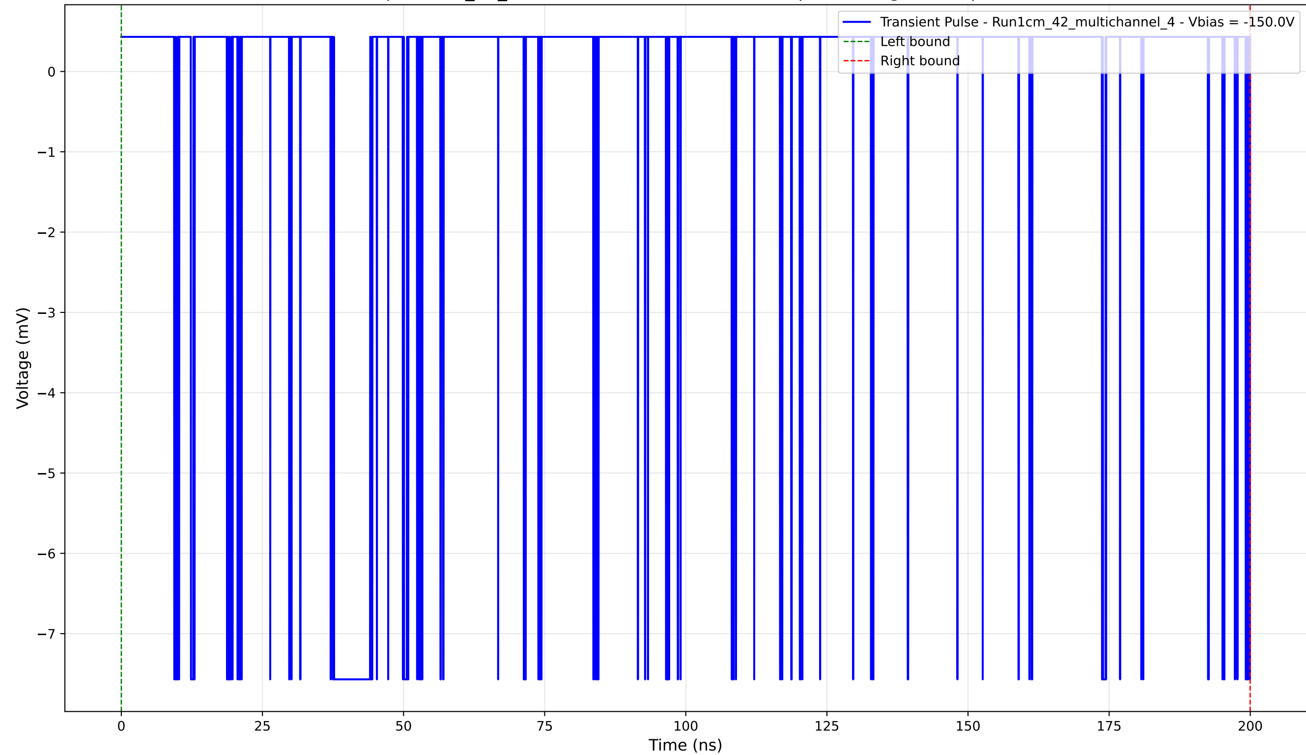
Transient Pulse - Sample: 1cm_42_multichannel - Position: 3940.0 \mu\text{m} - Charge: 0.77 pC - Rise Time: 0.02 ns
