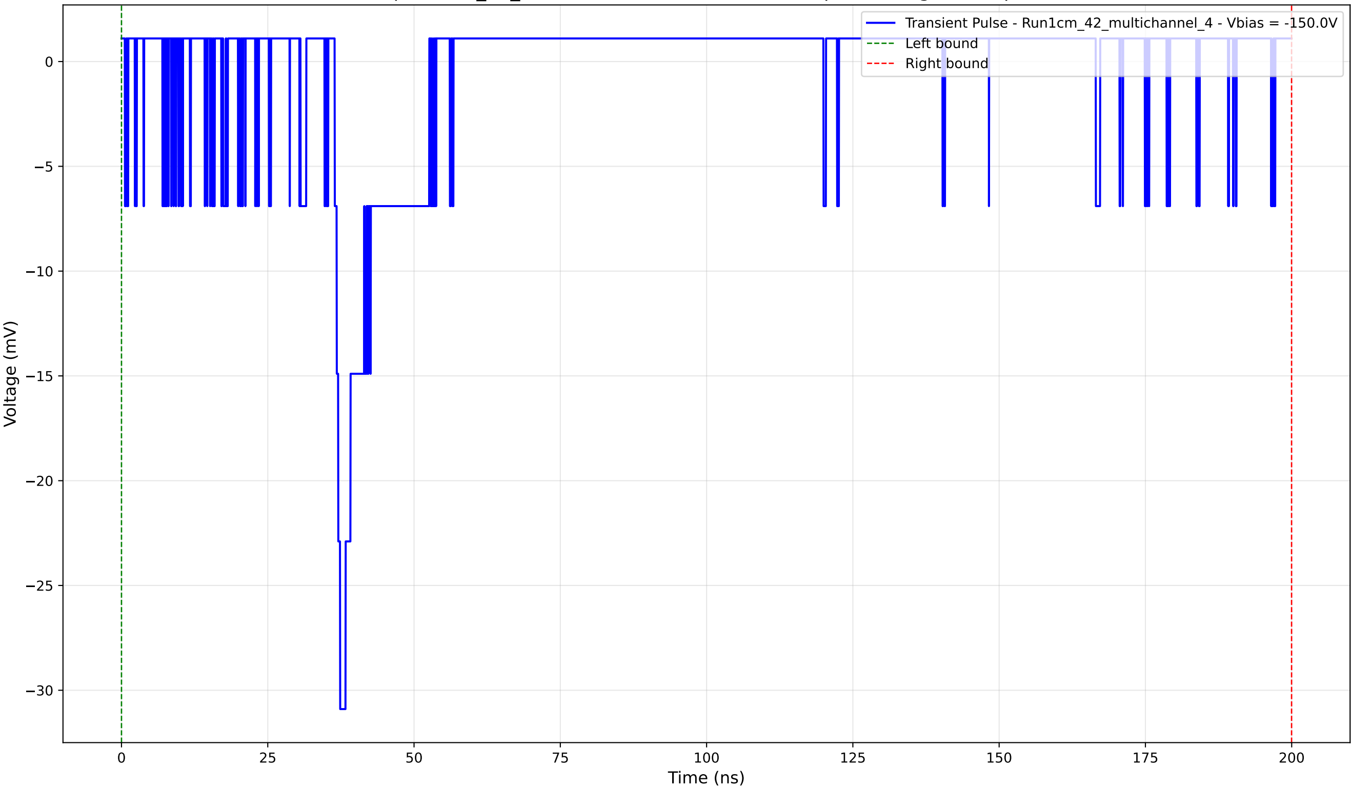
Transient Pulse - Sample: 1cm_42_multichannel - Position: 3105.0 \mu\text{m} - Charge: 1.09 pC - Rise Time: 0.93 ns
