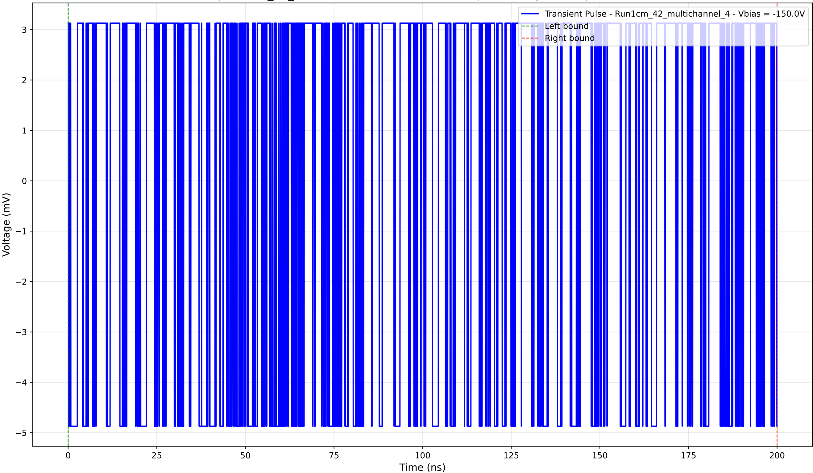
Transient Pulse - Sample: 1cm_42_multichannel - Position: 1360.0 \mu\text{m} - Charge: 2.17 pC - Rise Time: 0.00 ns (N/A)
