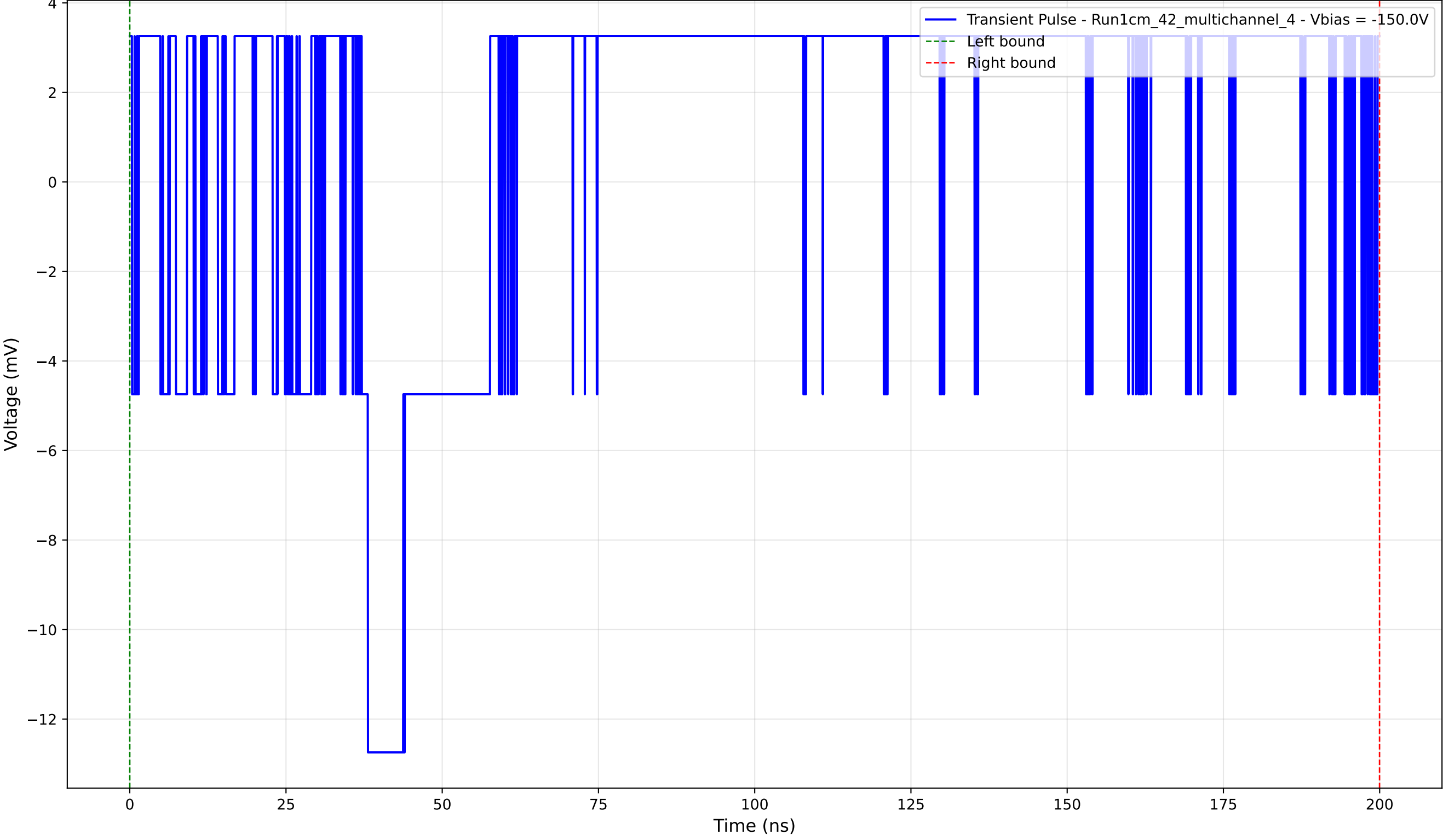
Transient Pulse - Sample: 1cm_42_multichannel - Position: 555.0 \mu\text{m} - Charge: 5.29 pC - Rise Time: 0.00 ns (N/A)
