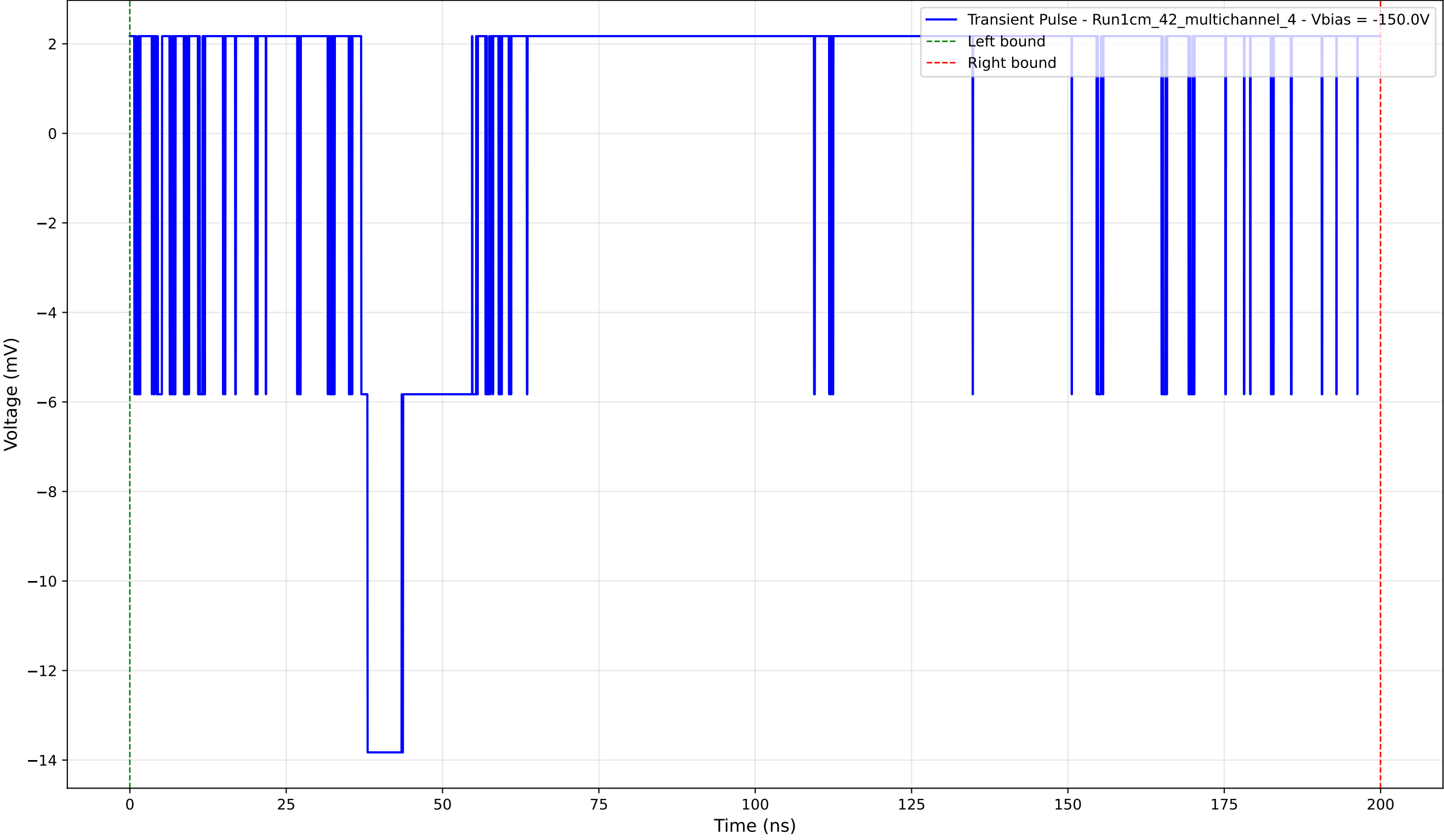
Transient Pulse - Sample: 1cm_42_multichannel - Position: 470.0 \mu\text{m} - Charge: 3.24 pC - Rise Time: 0.00 ns (N/A)
