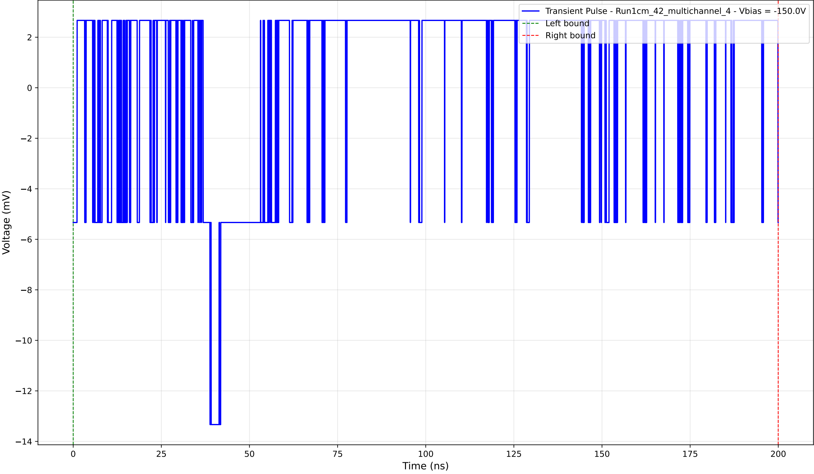
Transient Pulse - Sample: 1cm_42_multichannel - Position: 425.0 \mu\text{m} - Charge: 3.58 pC - Rise Time: 0.00 ns (N/A)
