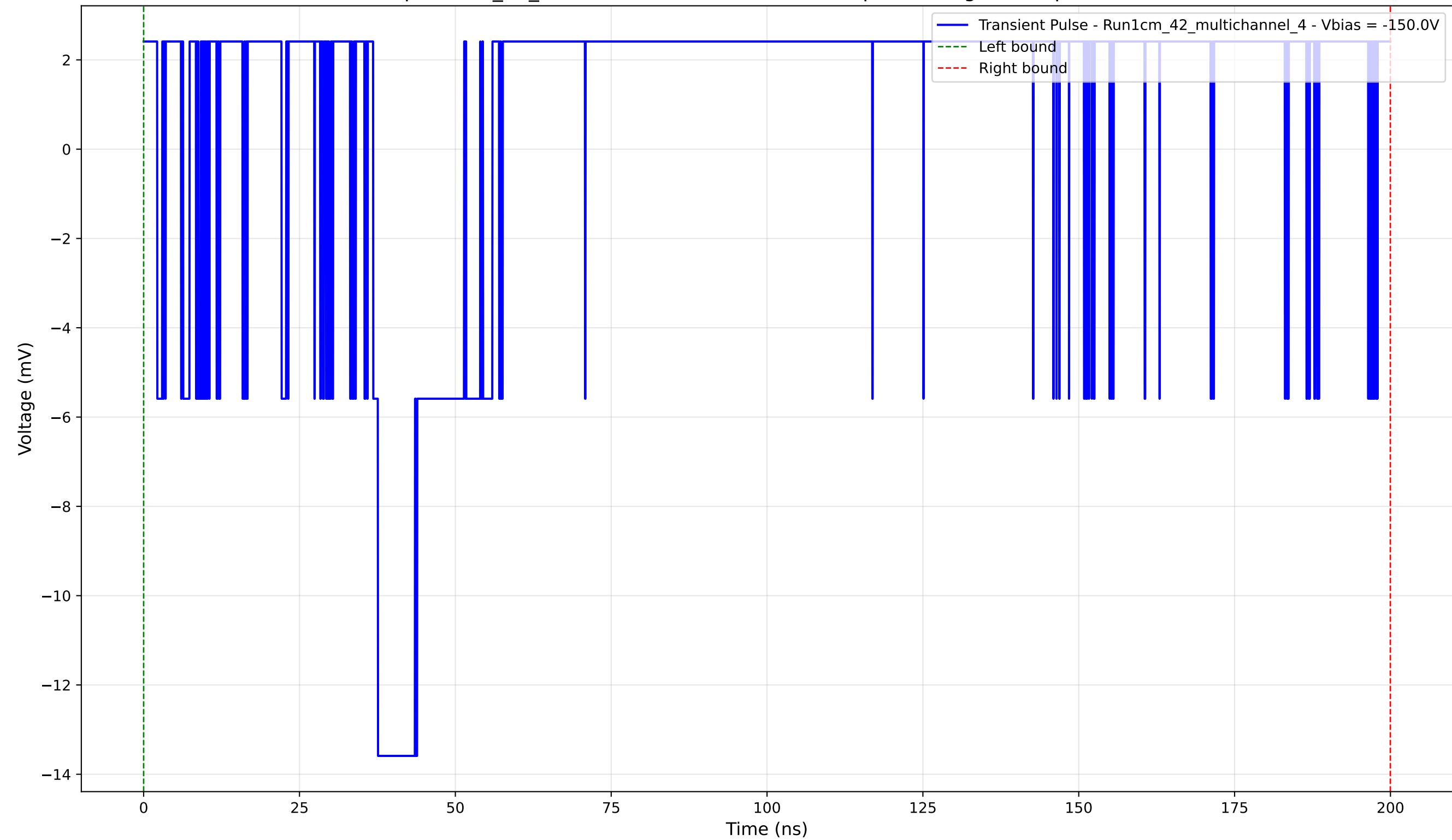
Transient Pulse - Sample: 1cm_42_multichannel - Position: 3770.0 \mu\text{m} - Charge: 3.96 pC - Rise Time: 0.00 ns (N/A)
