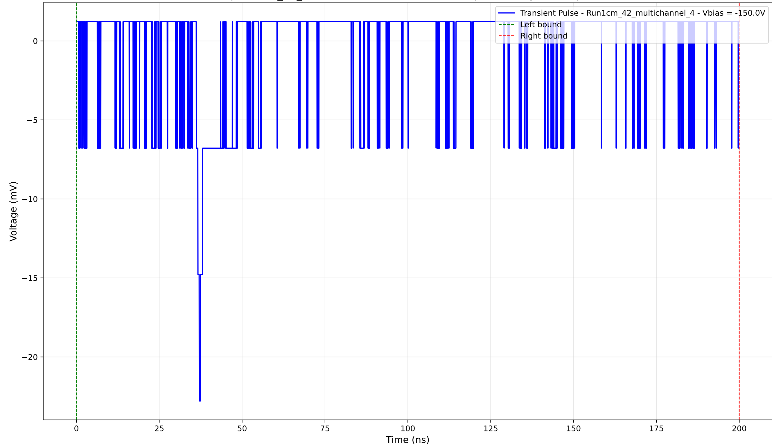
Transient Pulse - Sample: 1cm_42_multichannel - Position: 2425.0 \mu\text{m} - Charge: 0.65 pC - Rise Time: 0.90 ns
