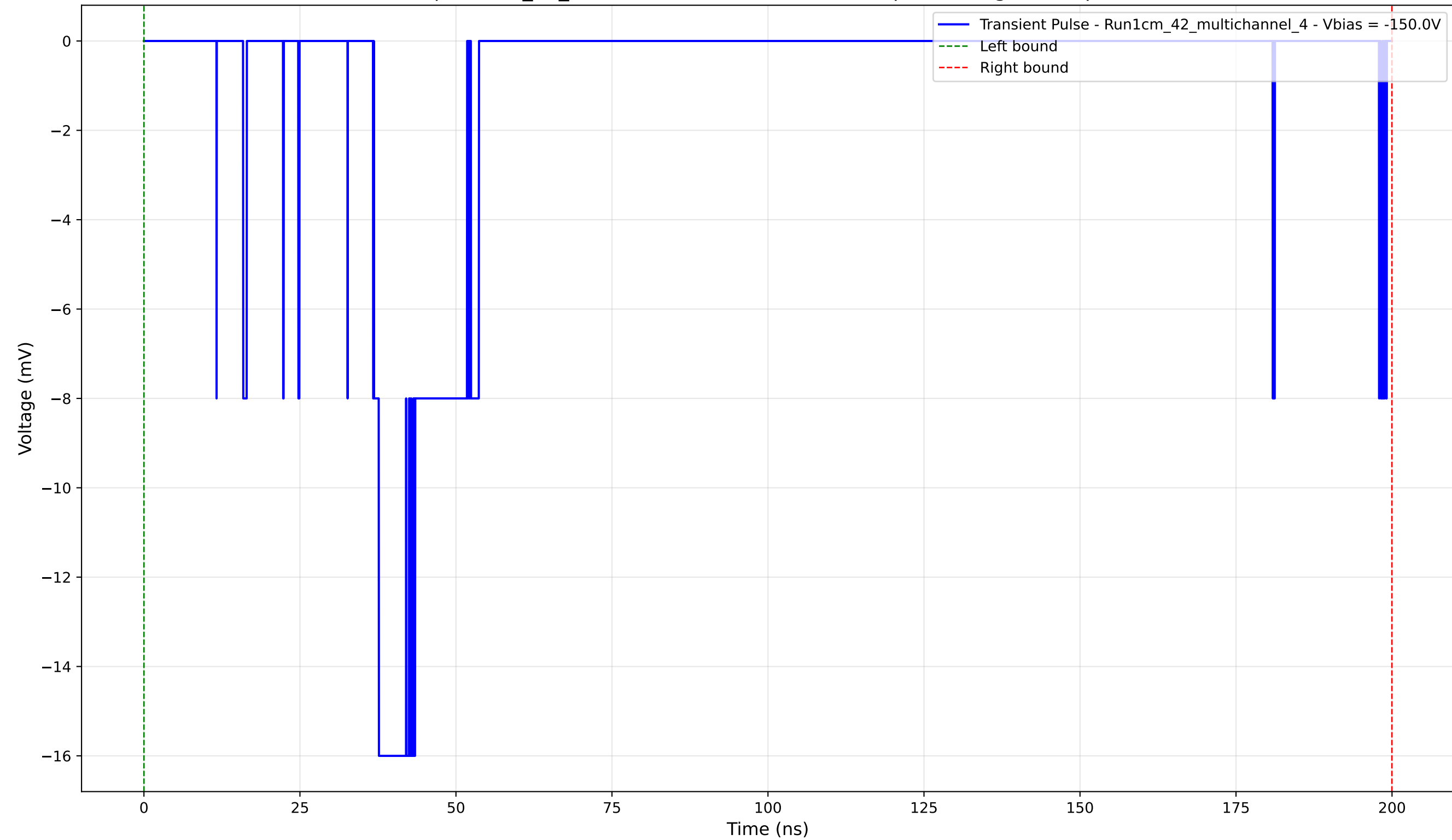
Transient Pulse - Sample: 1cm_42_multichannel - Position: 3795.0 \mu\text{m} - Charge: 3.78 pC - Rise Time: 0.80 ns
