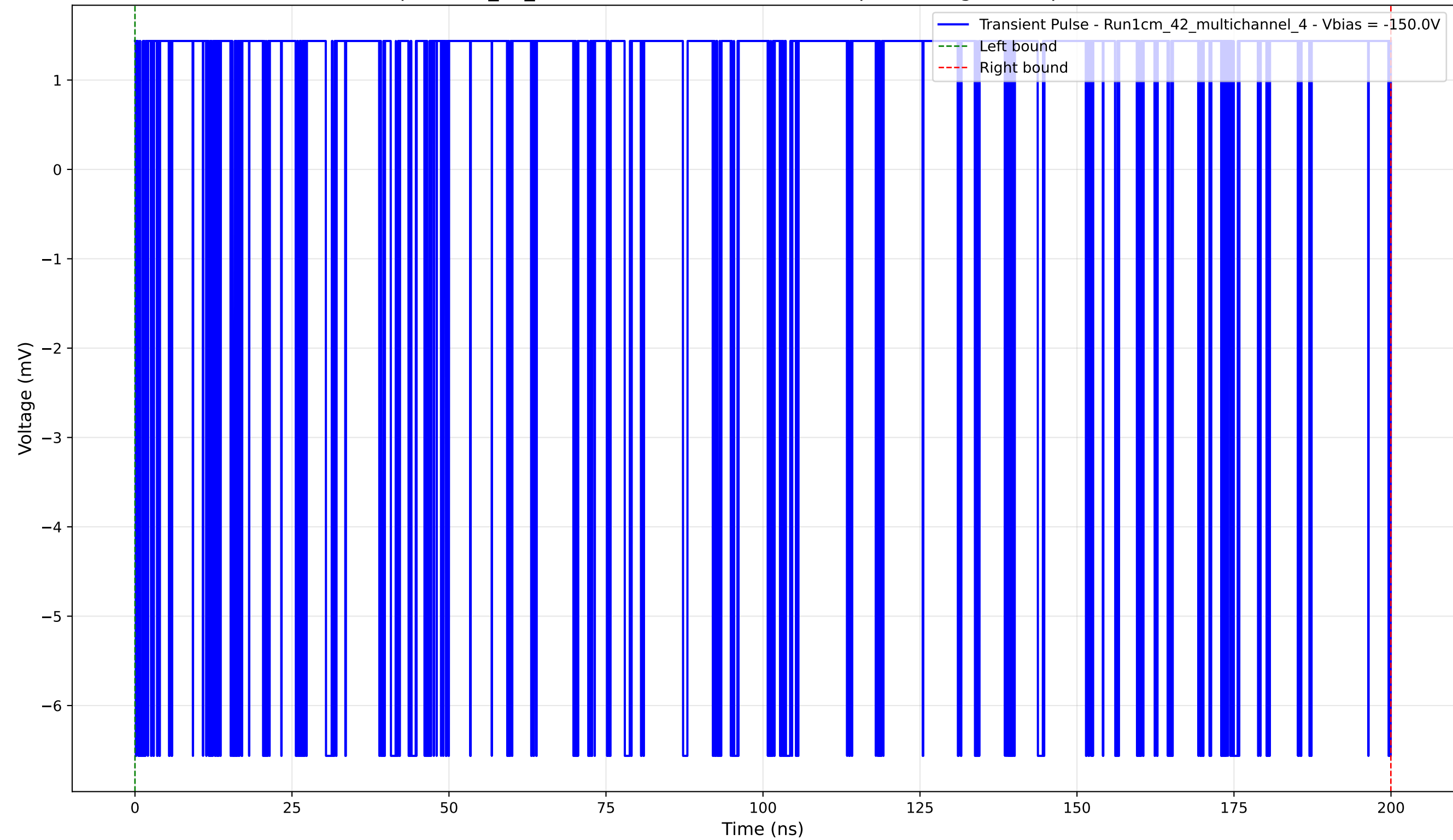
Transient Pulse - Sample: 1cm_42_multichannel - Position: 4400.0 \mu\text{m} - Charge: 1.12 pC - Rise Time: 0.00 ns (N/A)
