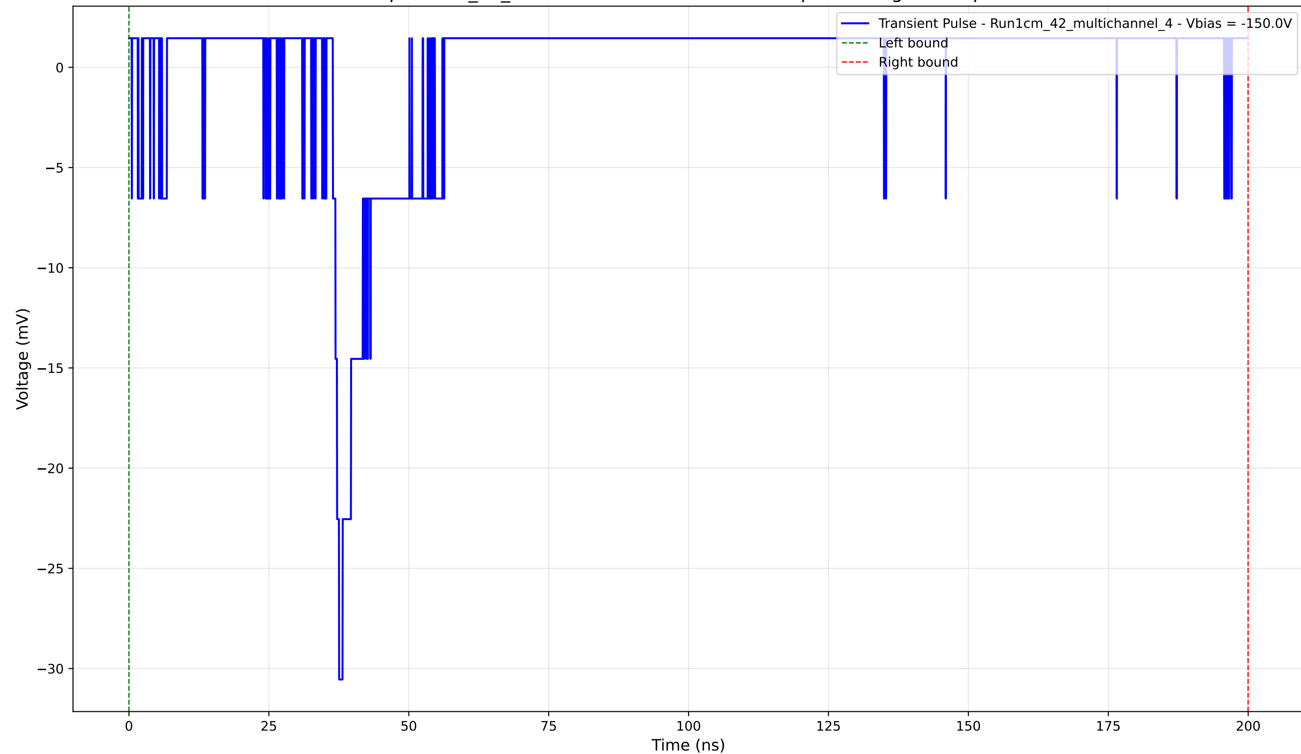
Transient Pulse - Sample: 1cm_42_multichannel - Position: 3195.0 \mu\text{m} - Charge: 0.67 pC - Rise Time: 1.11 ns
