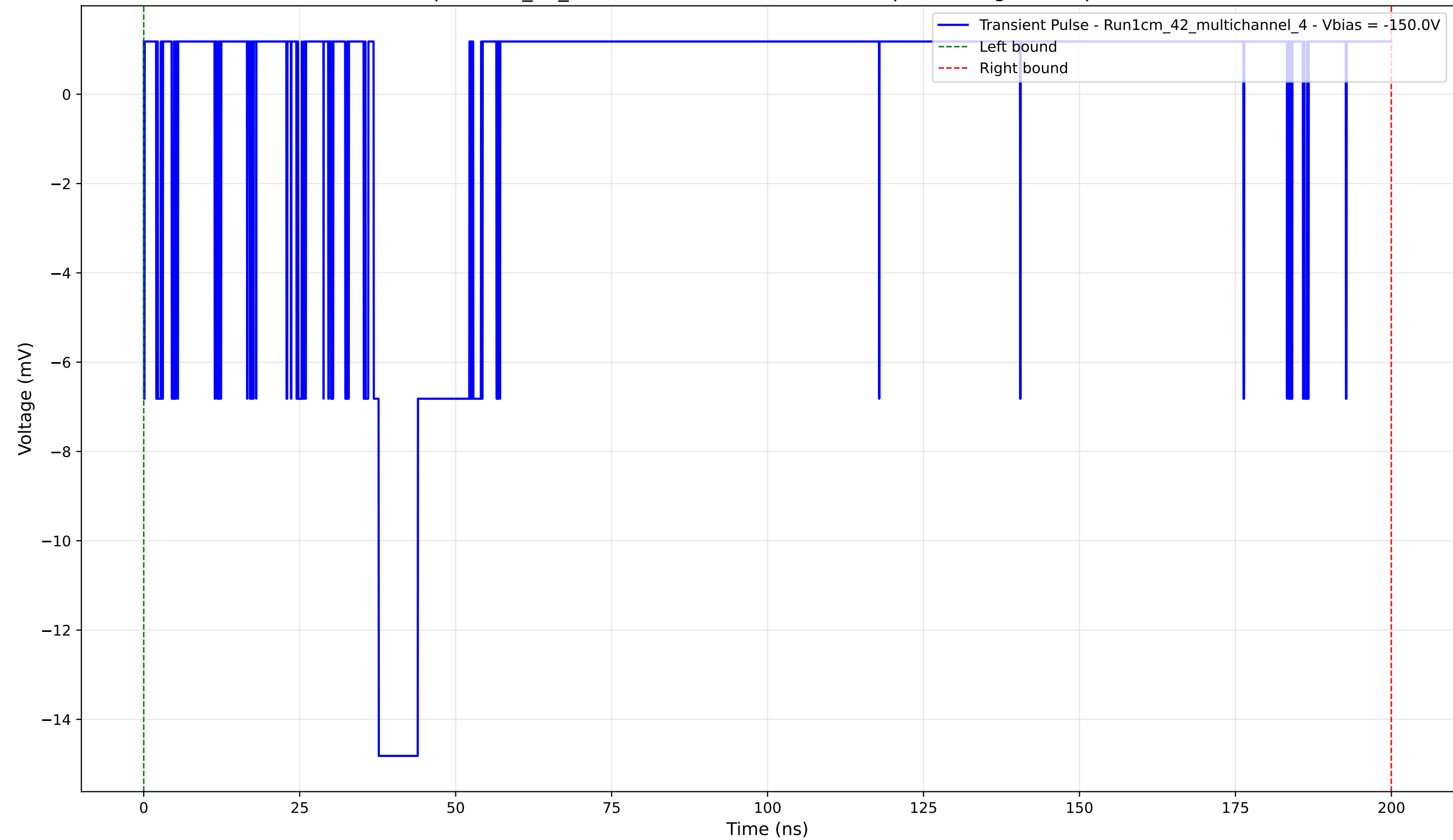
Transient Pulse - Sample: 1cm_42_multichannel - Position: 3800.0 \mu\text{m} - Charge: 0.08 pC - Rise Time: 0.82 ns
