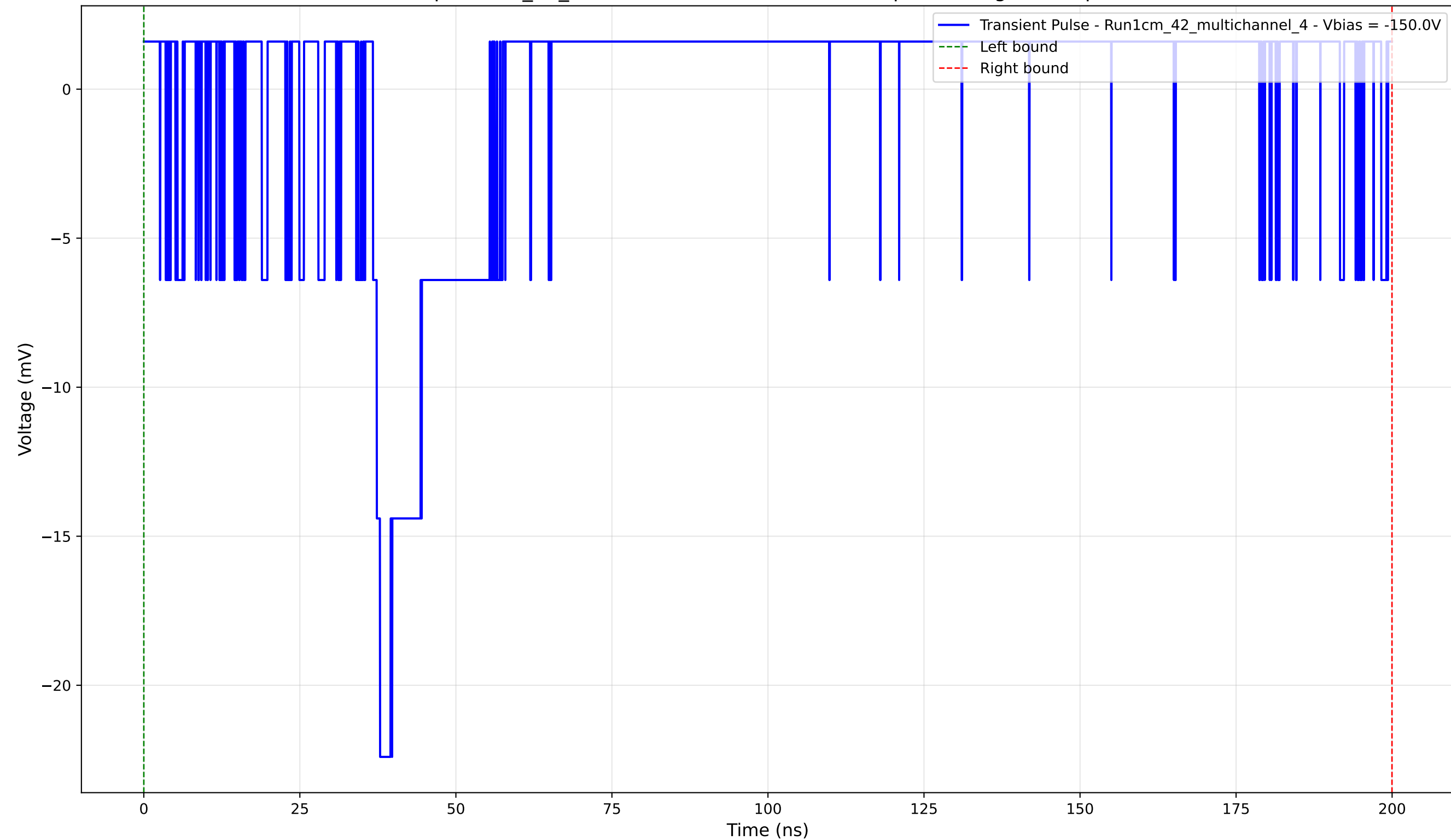
Transient Pulse - Sample: 1cm_42_multichannel - Position: 1135.0 \mu\text{m} - Charge: 0.33 pC - Rise Time: 1.14 ns
