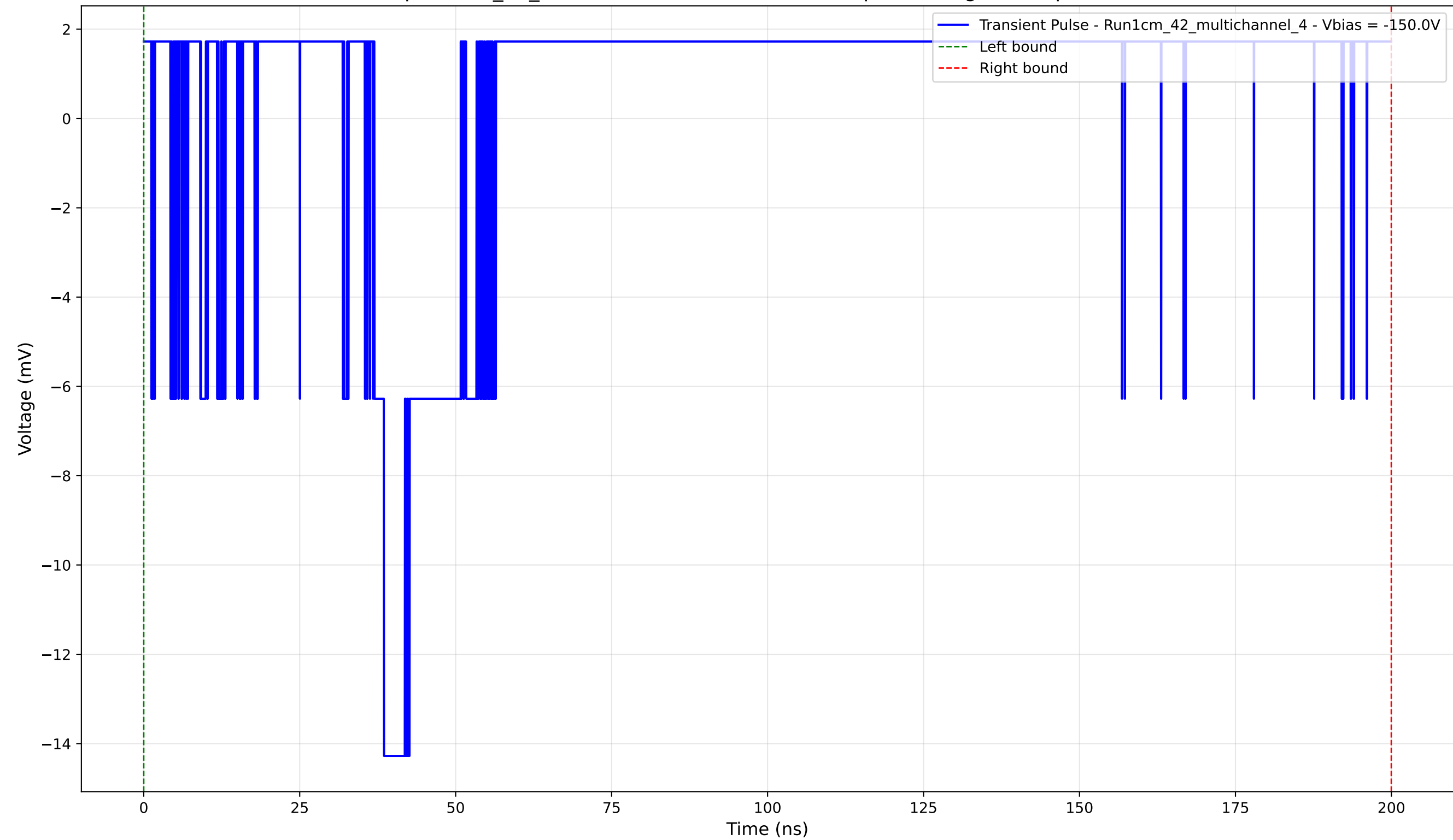
Transient Pulse - Sample: 1cm_42_multichannel - Position: 4175.0 \mu\text{m} - Charge: 2.61 pC - Rise Time: 0.00 ns (N/A)
