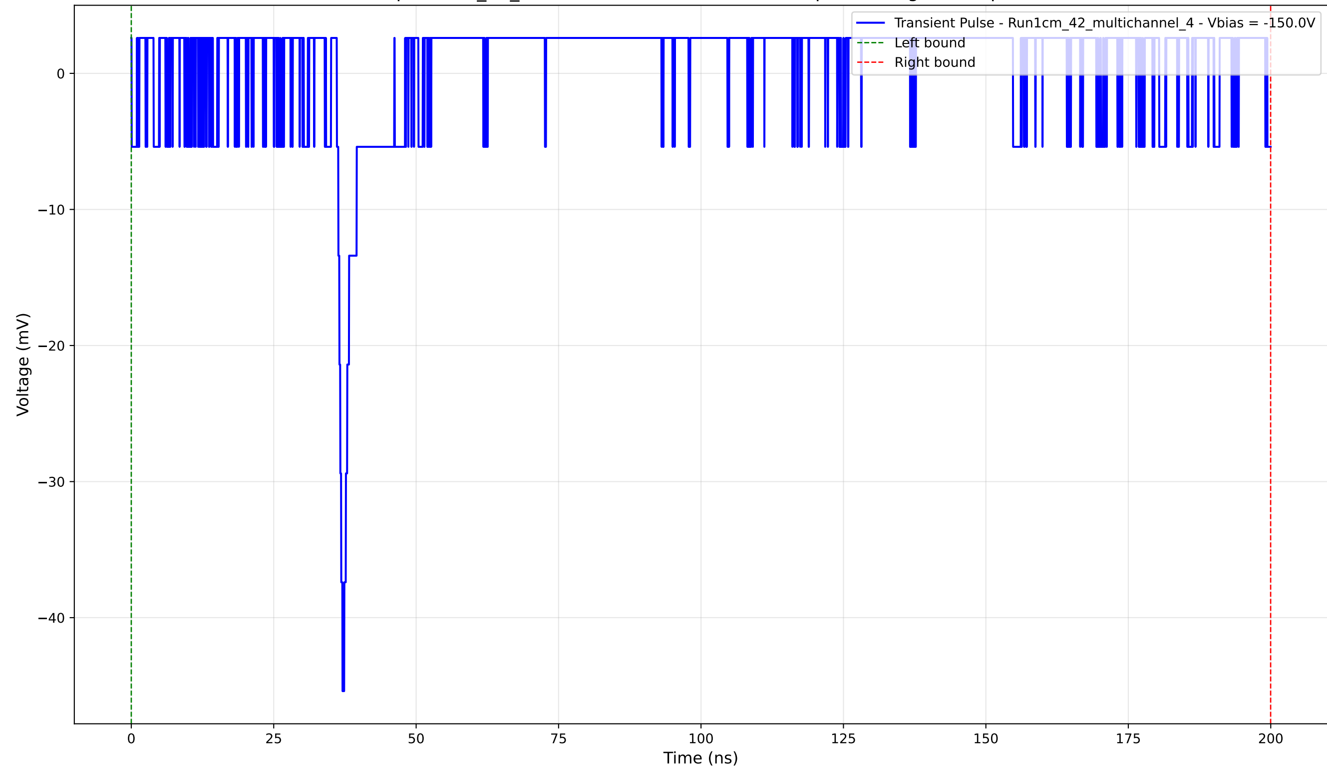
Transient Pulse - Sample: 1cm_42_multichannel - Position: 2335.0 \mu\text{m} - Charge: 3.35 pC - Rise Time: 0.99 ns
