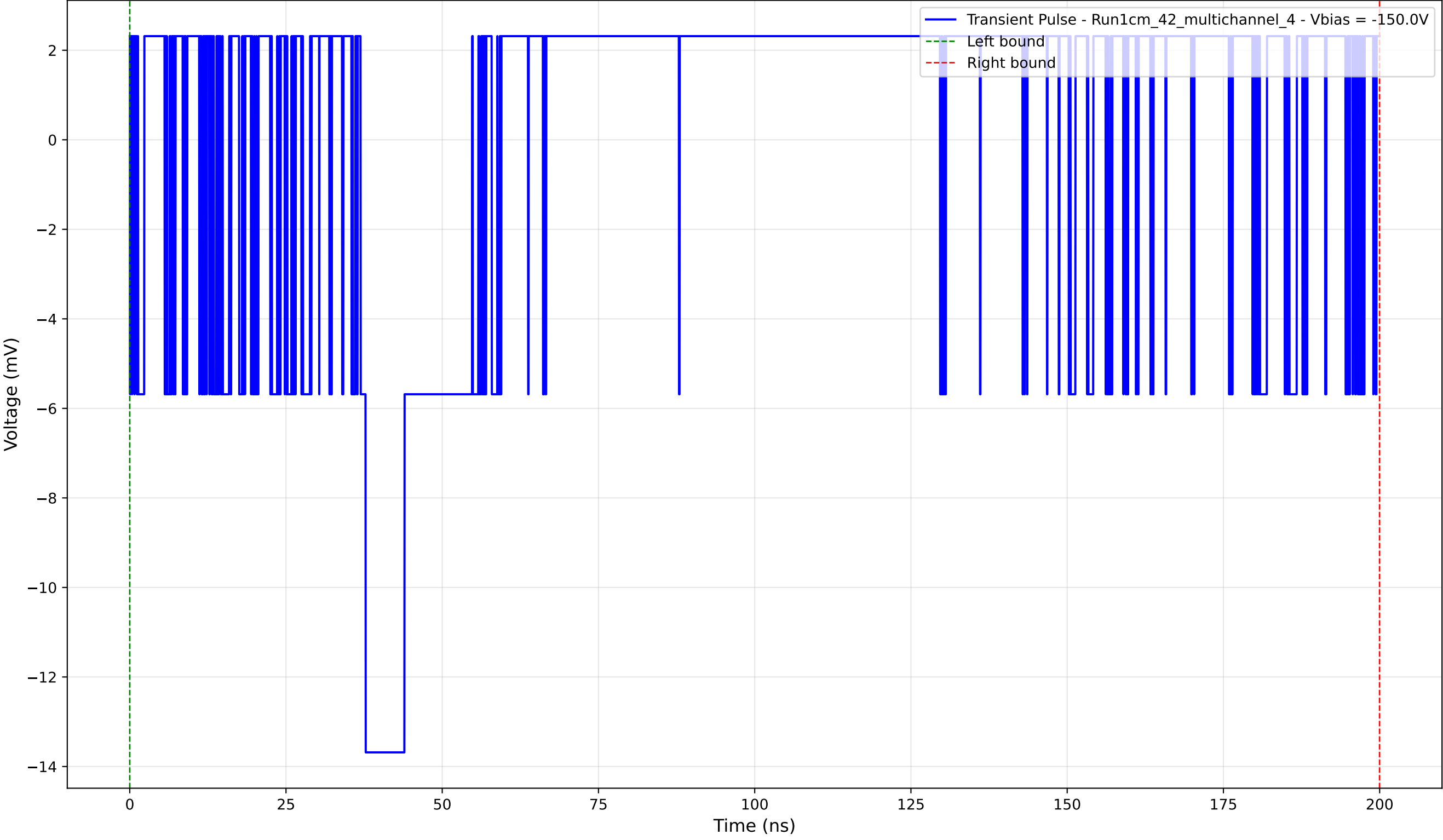
Transient Pulse - Sample: 1cm_42_multichannel - Position: 735.0 \mu\text{m} - Charge: 1.23 pC - Rise Time: 0.00 ns (N/A)
