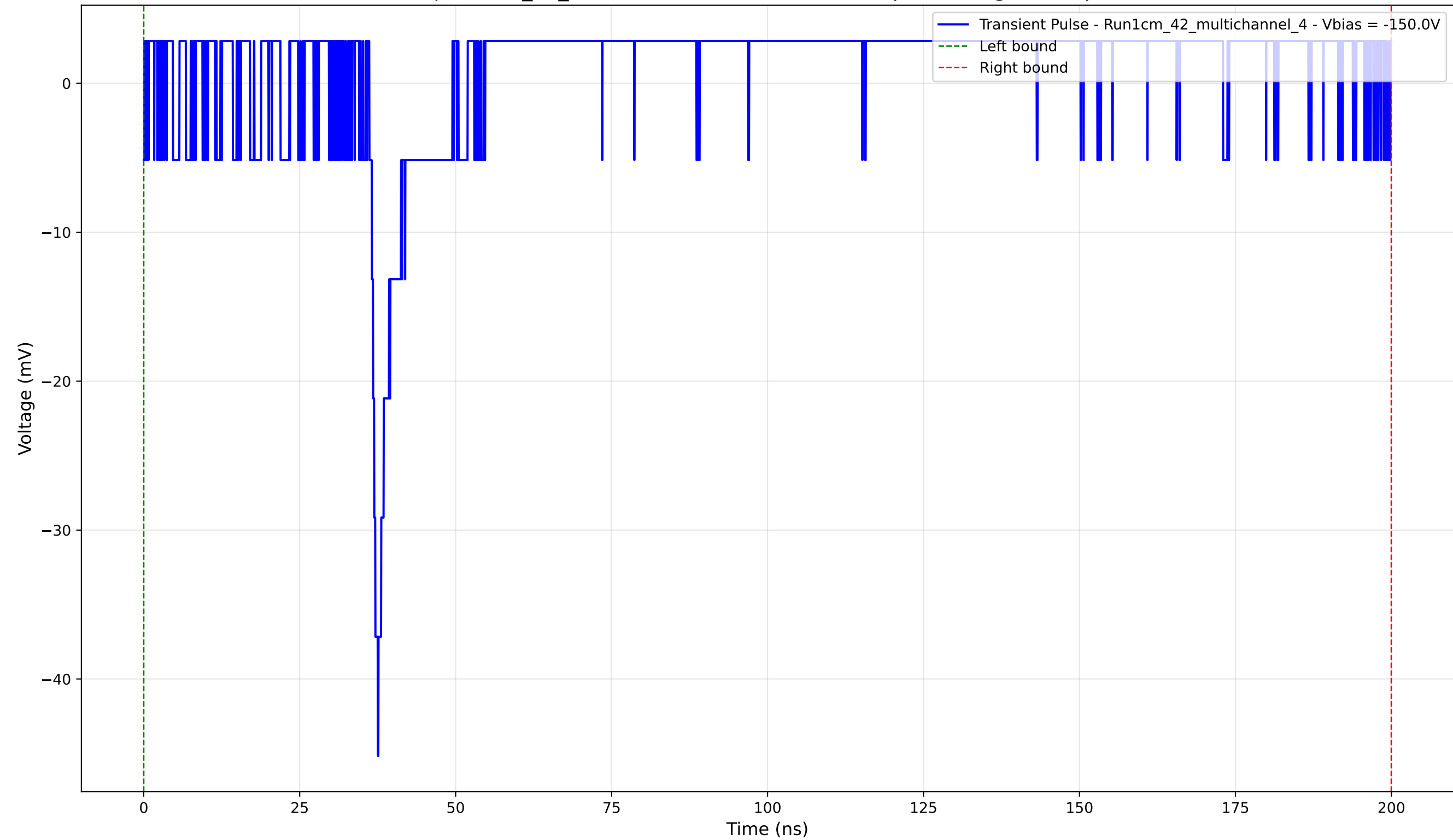
Transient Pulse - Sample: 1cm_42_multichannel - Position: 1945.0 \mu\text{m} - Charge: 4.26 pC - Rise Time: 1.37 ns
