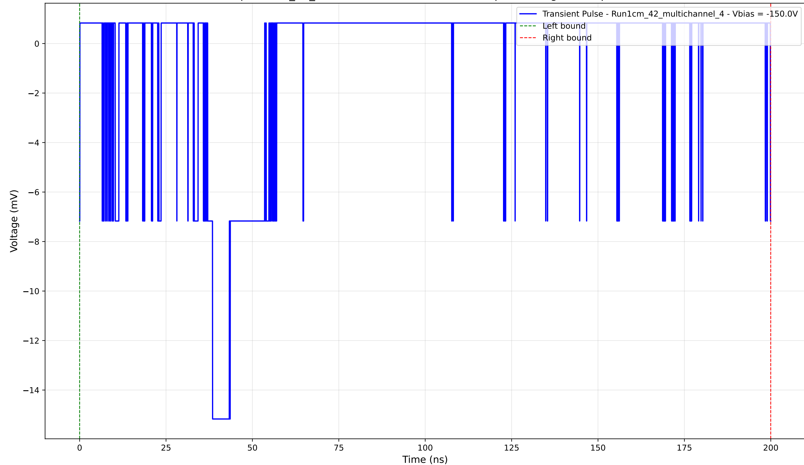
Transient Pulse - Sample: 1cm_42_multichannel - Position: 4500.0 \mu\text{m} - Charge: 1.87 pC - Rise Time: 1.42 ns
