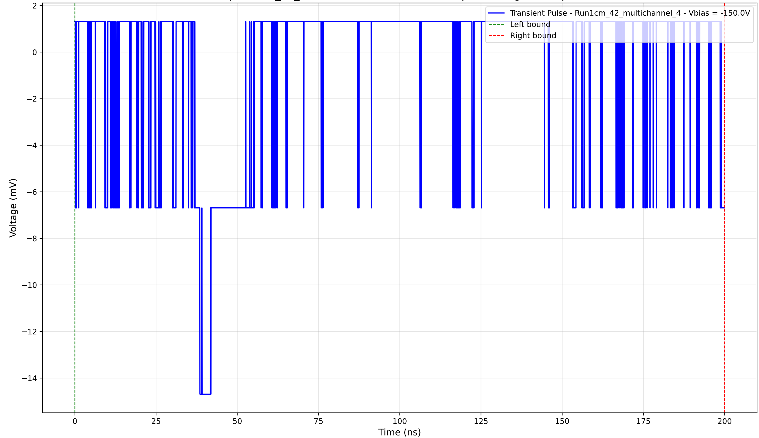
Transient Pulse - Sample: 1cm_42_multichannel - Position: 295.0 \mu\text{m} - Charge: 1.27 pC - Rise Time: 1.54 ns
