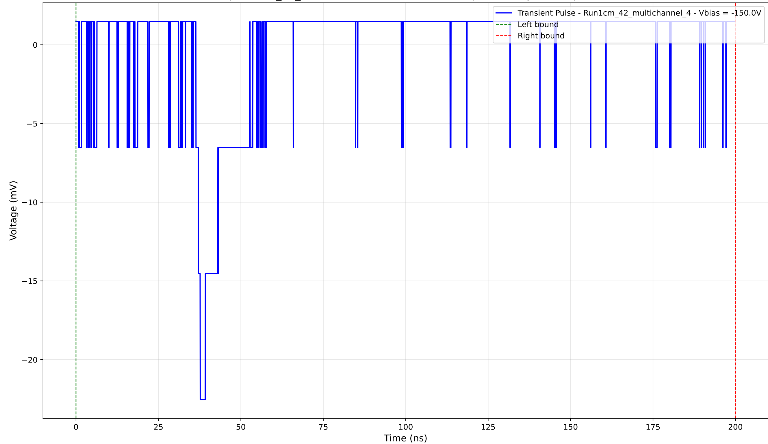
Transient Pulse - Sample: 1cm_42_multichannel - Position: 3480.0 \mu\text{m} - Charge: 0.55 pC - Rise Time: 1.30 ns
