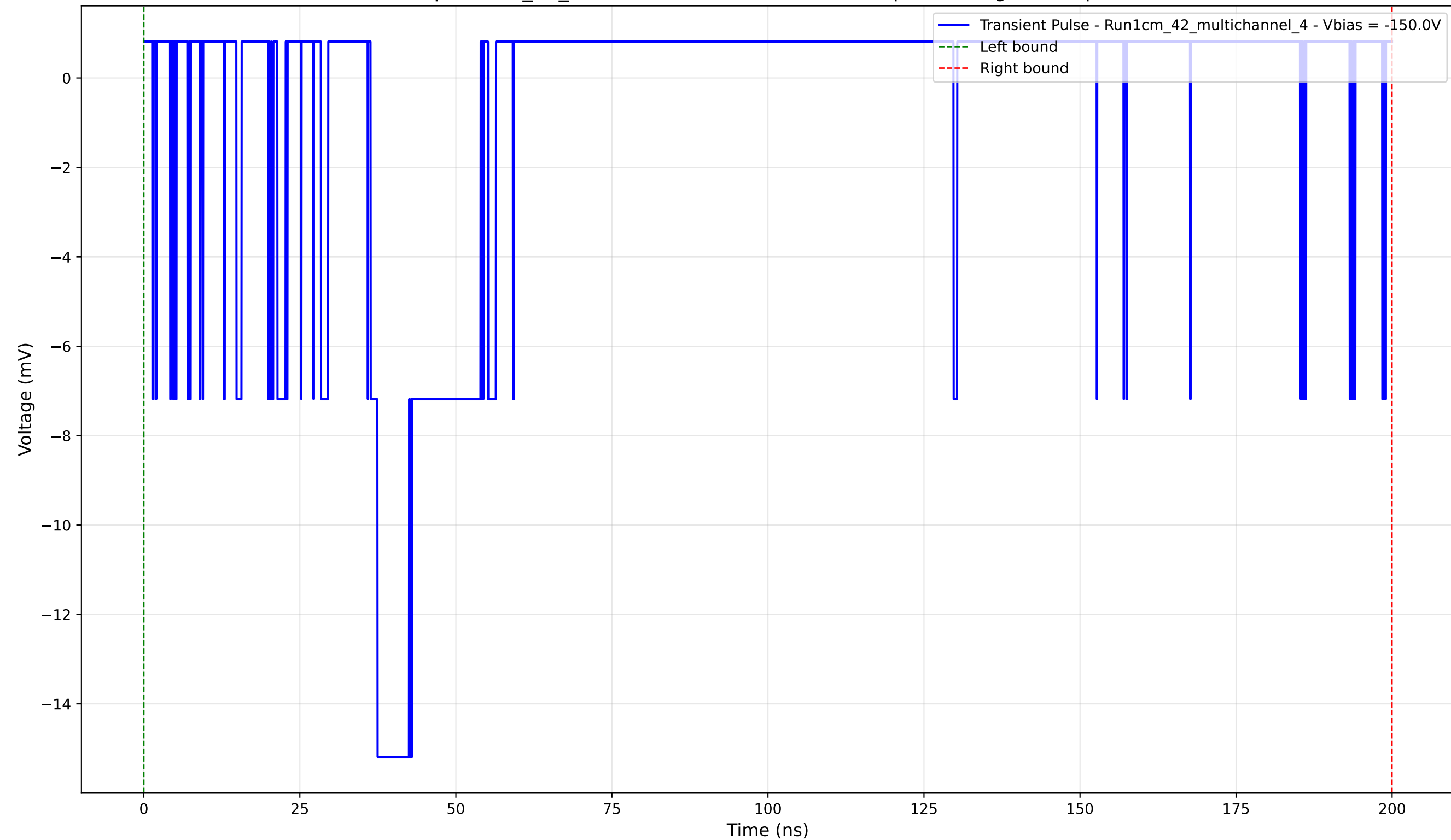
Transient Pulse - Sample: 1cm_42_multichannel - Position: 3650.0 \mu\text{m} - Charge: 1.83 pC - Rise Time: 1.12 ns
