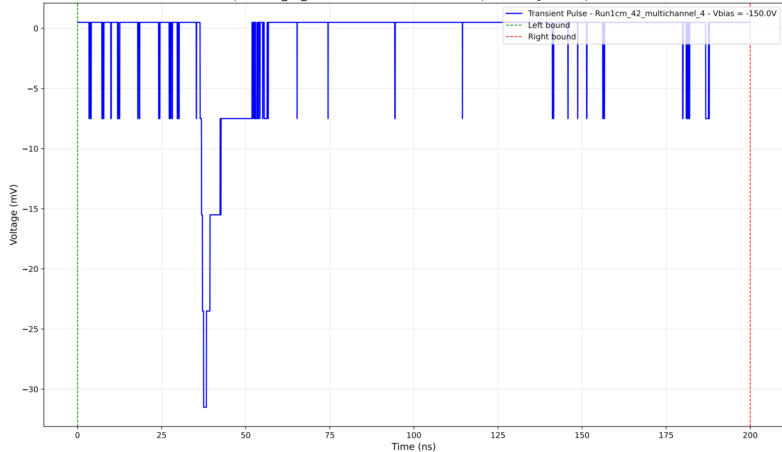
Transient Pulse - Sample: 1cm_42_multichannel - Position: 3155.0 \mu\text{m} - Charge: 3.02 pC - Rise Time: 1.05 ns
