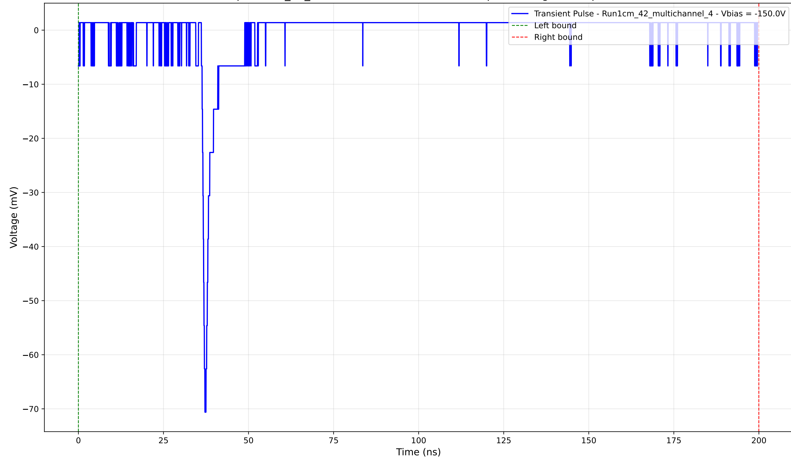
Transient Pulse - Sample: 1cm_42_multichannel - Position: 2175.0 \mu\text{m} - Charge: 0.77 pC - Rise Time: 0.84 ns
