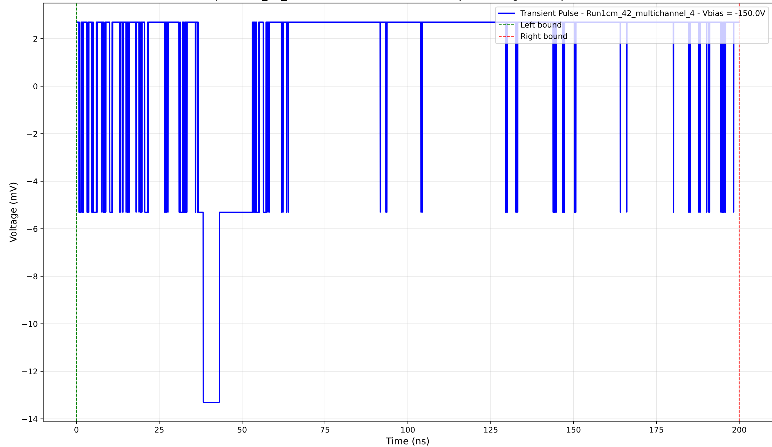
Transient Pulse - Sample: 1cm_42_multichannel - Position: 4190.0 \mu\text{m} - Charge: 4.85 pC - Rise Time: 0.00 ns (N/A)
