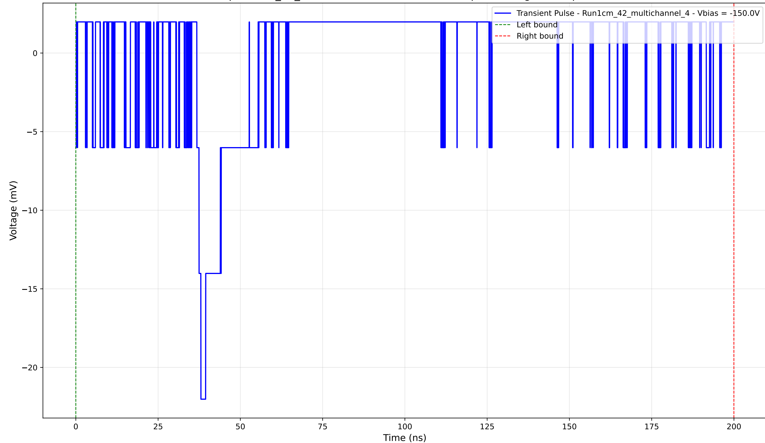
Transient Pulse - Sample: 1cm_42_multichannel - Position: 1100.0 \mu\text{m} - Charge: 0.81 pC - Rise Time: 1.24 ns
