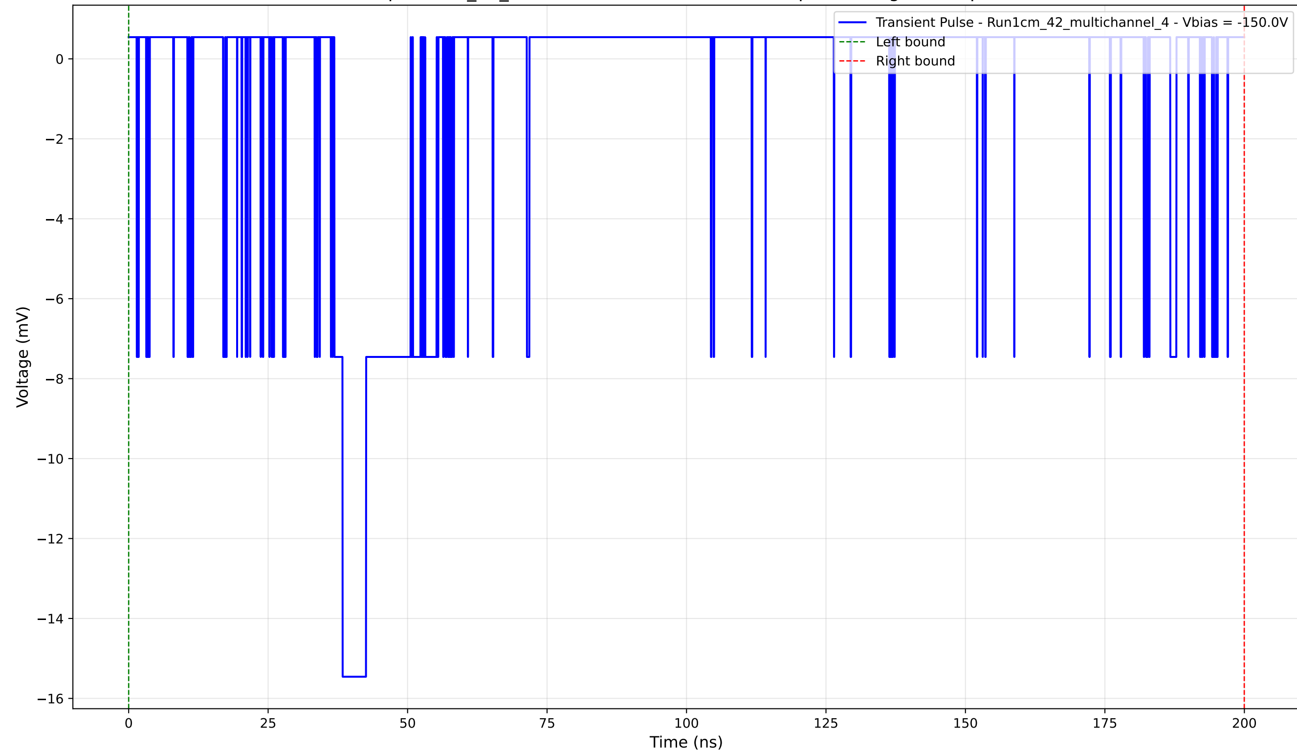
Transient Pulse - Sample: 1cm_42_multichannel - Position: 4695.0 \mu\text{m} - Charge: 2.94 pC - Rise Time: 1.48 ns
