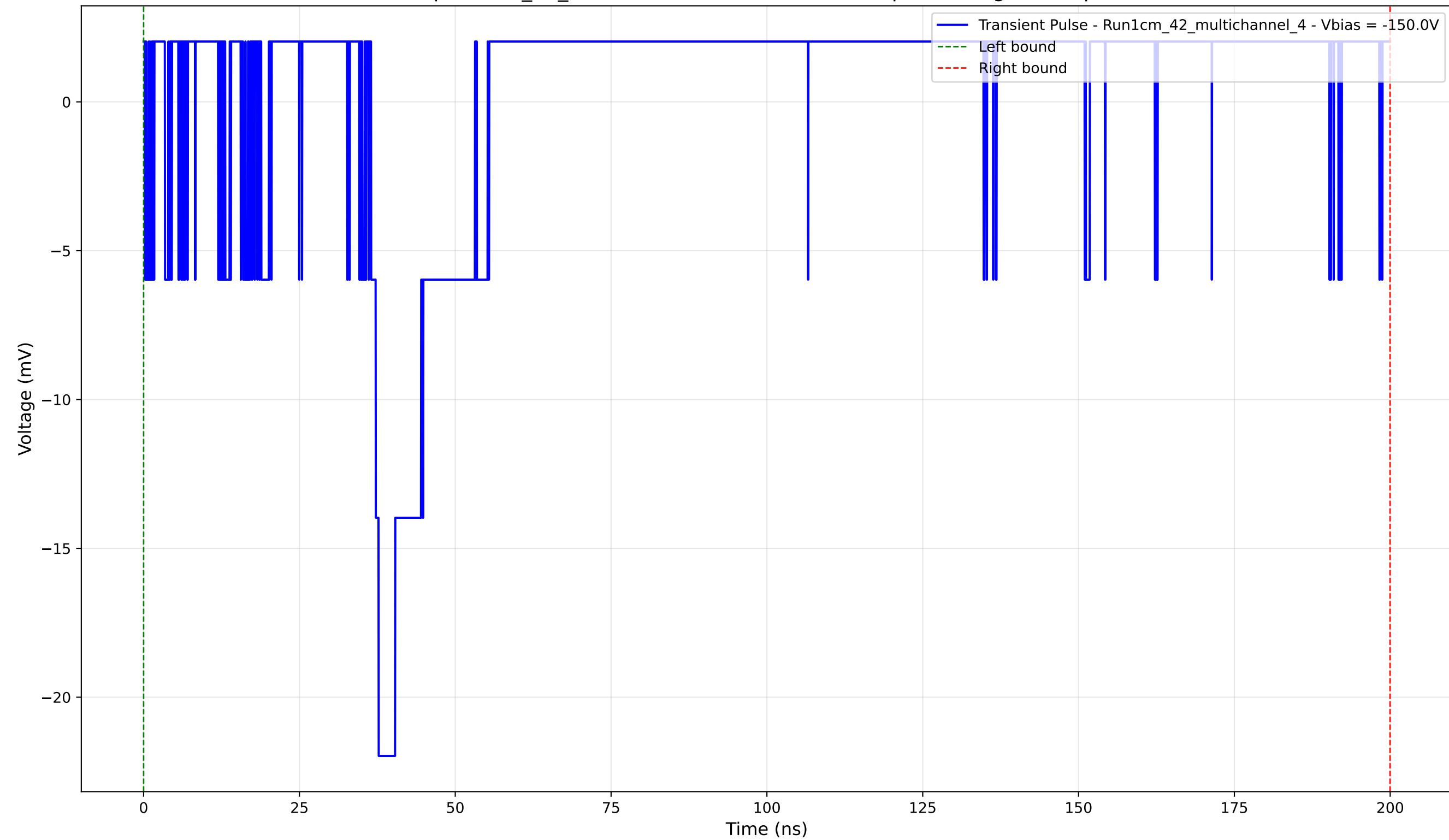
Transient Pulse - Sample: 1cm_42_multichannel - Position: 1225.0 \mu\text{m} - Charge: 1.94 pC - Rise Time: 1.22 ns
