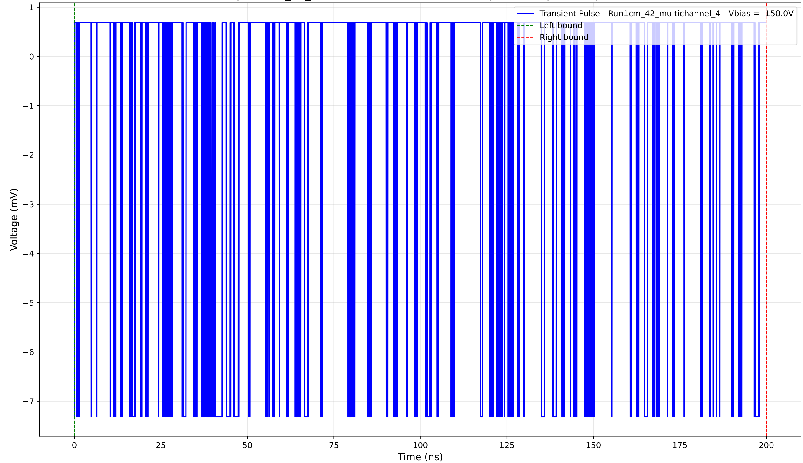
Transient Pulse - Sample: 1cm_42_multichannel - Position: 4375.0 \mu\text{m} - Charge: 2.72 pC - Rise Time: 0.02 ns
