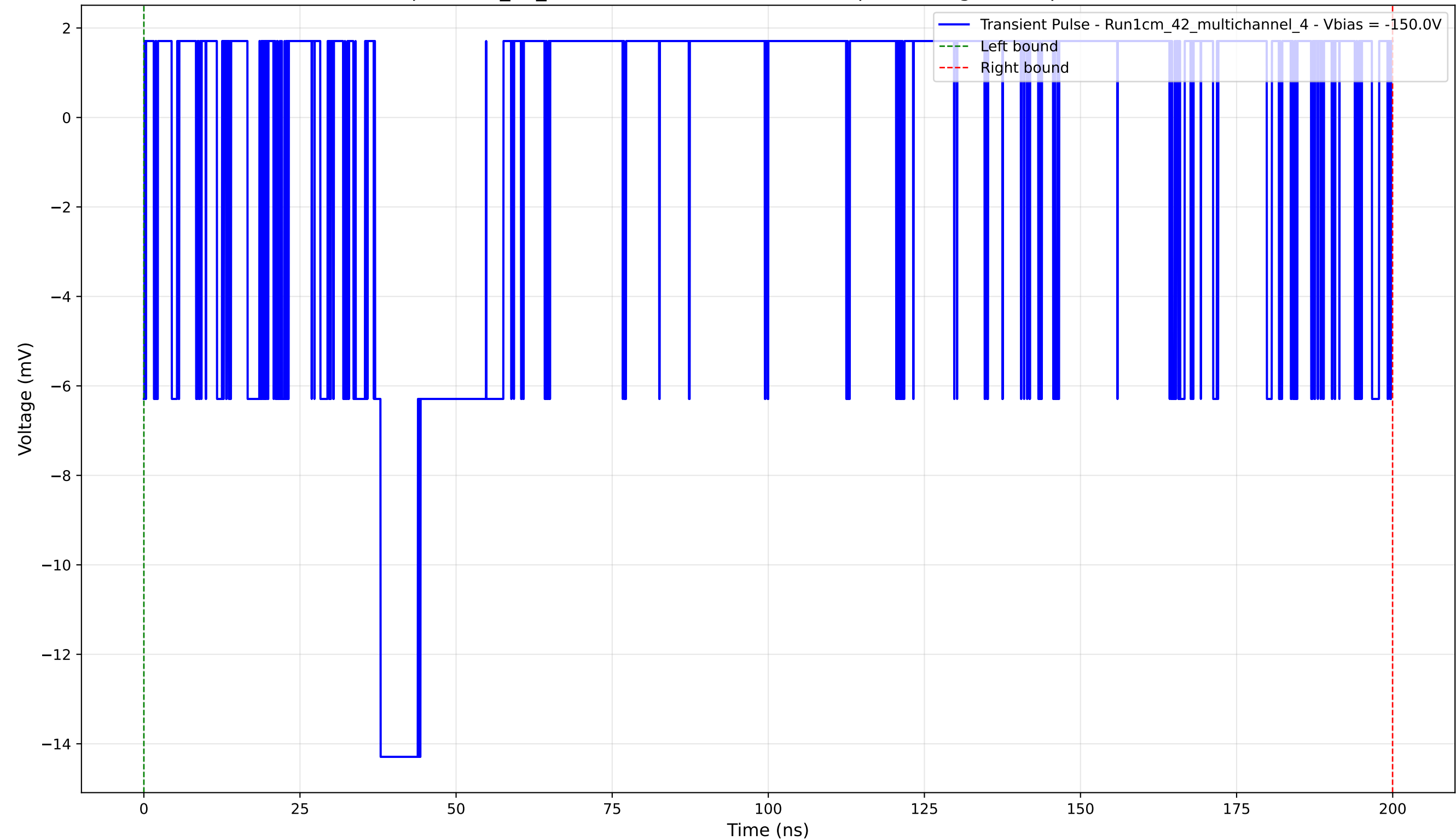
Transient Pulse - Sample: 1cm_42_multichannel - Position: 665.0 \mu\text{m} - Charge: 1.38 pC - Rise Time: 0.00 ns (N/A)
