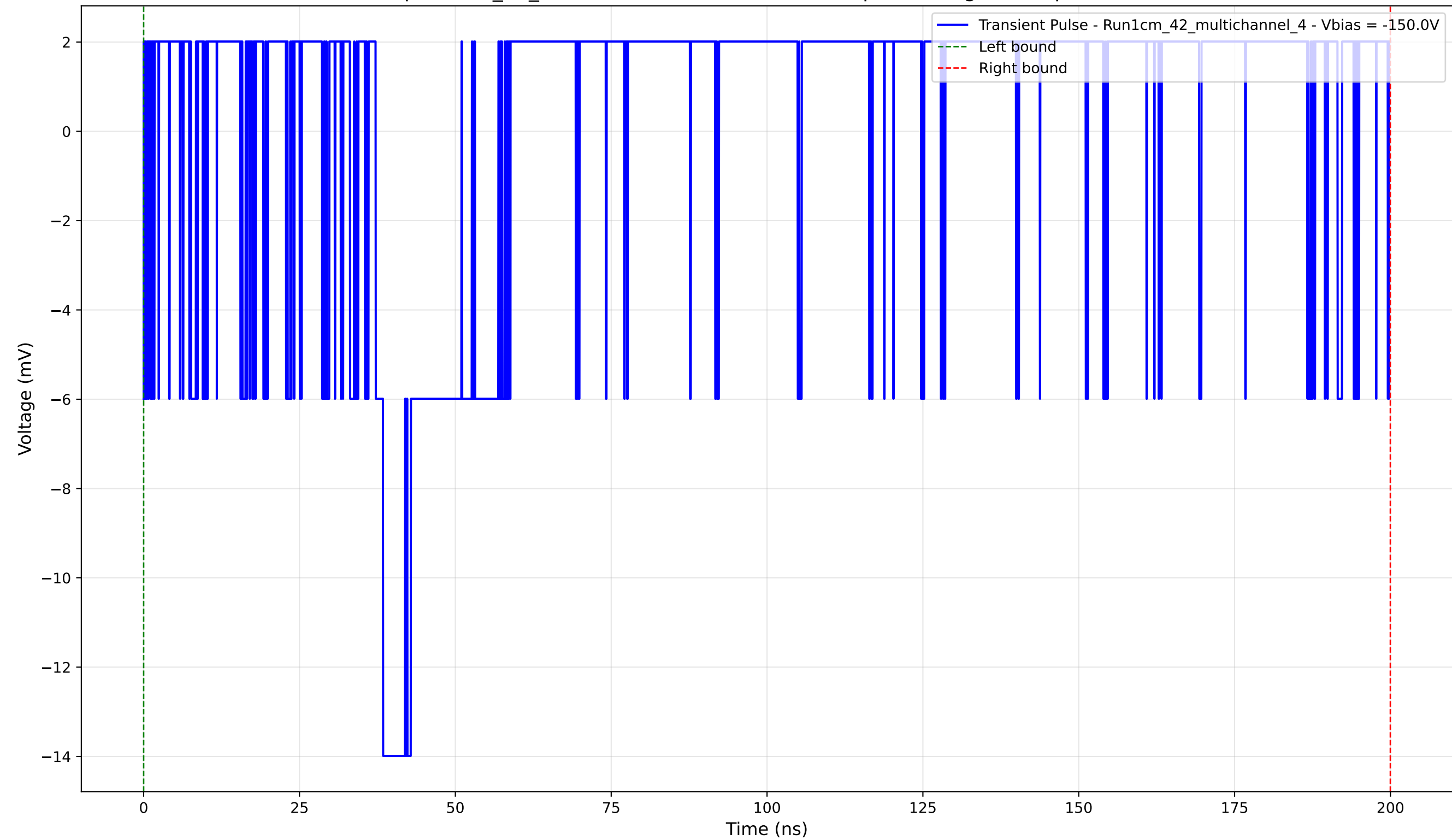
Transient Pulse - Sample: 1cm_42_multichannel - Position: 4335.0 \mu\text{m} - Charge: 1.65 pC - Rise Time: 0.00 ns (N/A)
