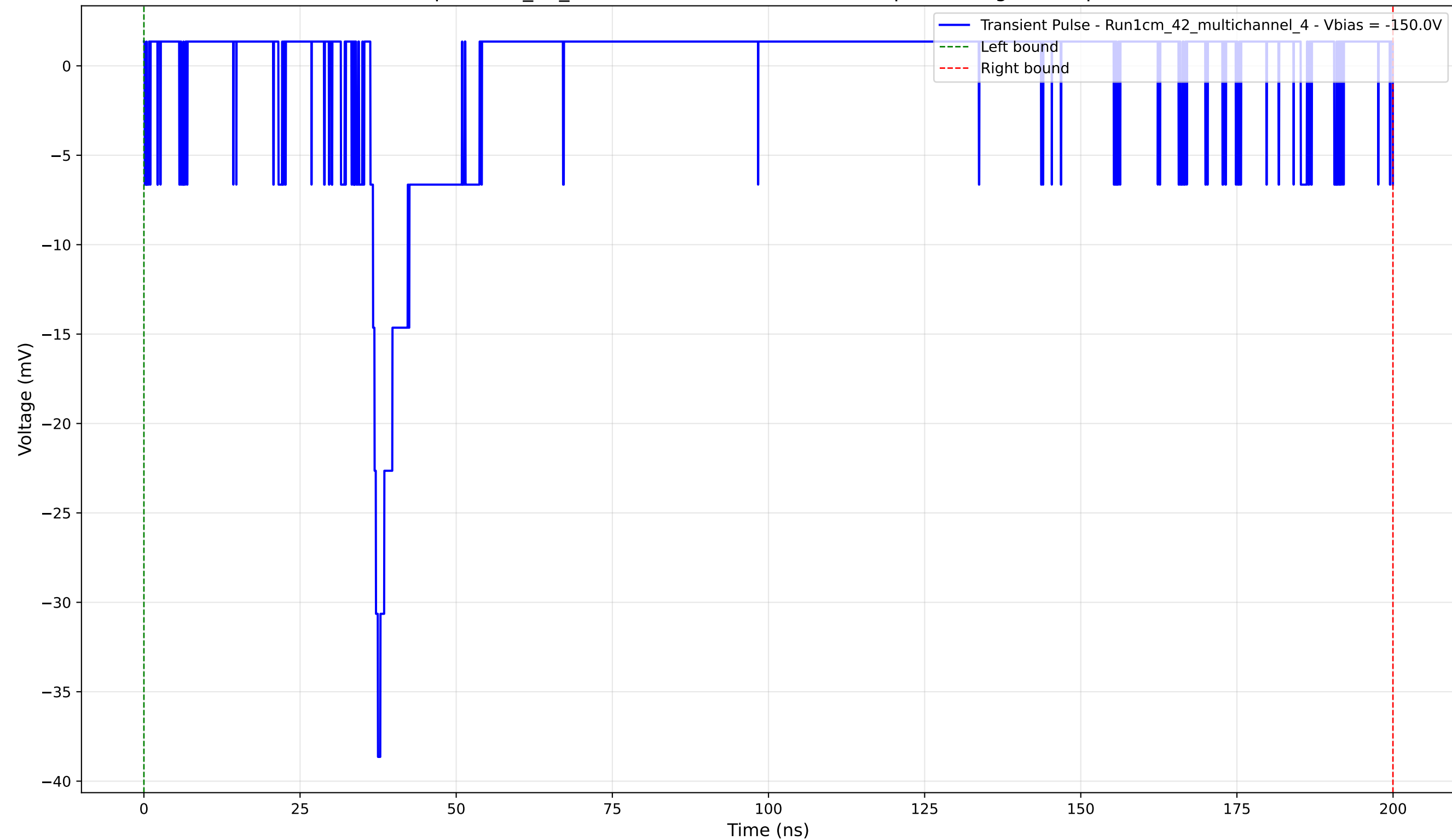
Transient Pulse - Sample: 1cm_42_multichannel - Position: 3030.0 \mu\text{m} - Charge: 0.69 pC - Rise Time: 1.21 ns
