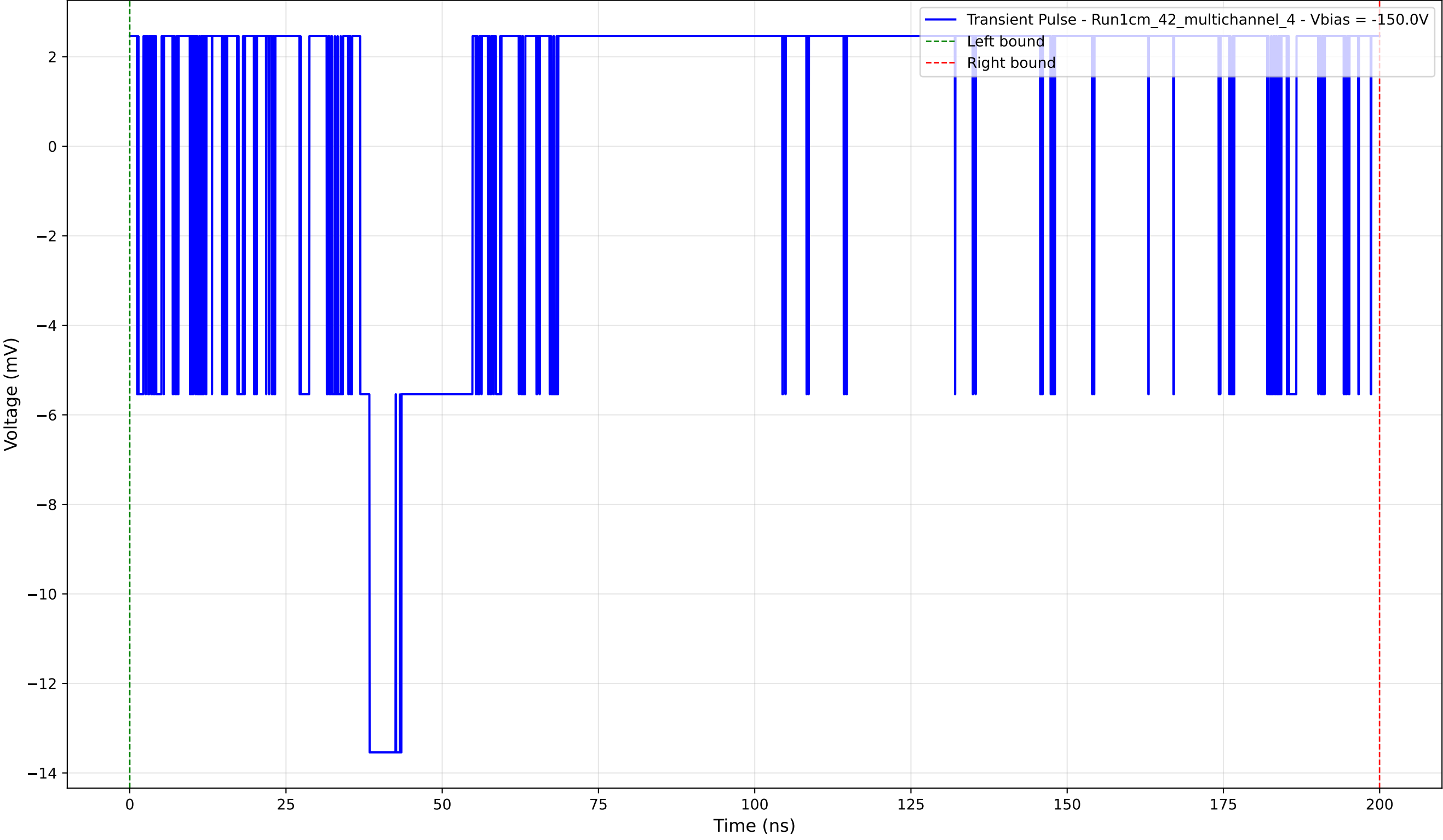
Transient Pulse - Sample: 1cm_42_multichannel - Position: 220.0 \mu\text{m} - Charge: 3.04 pC - Rise Time: 0.00 ns (N/A)
