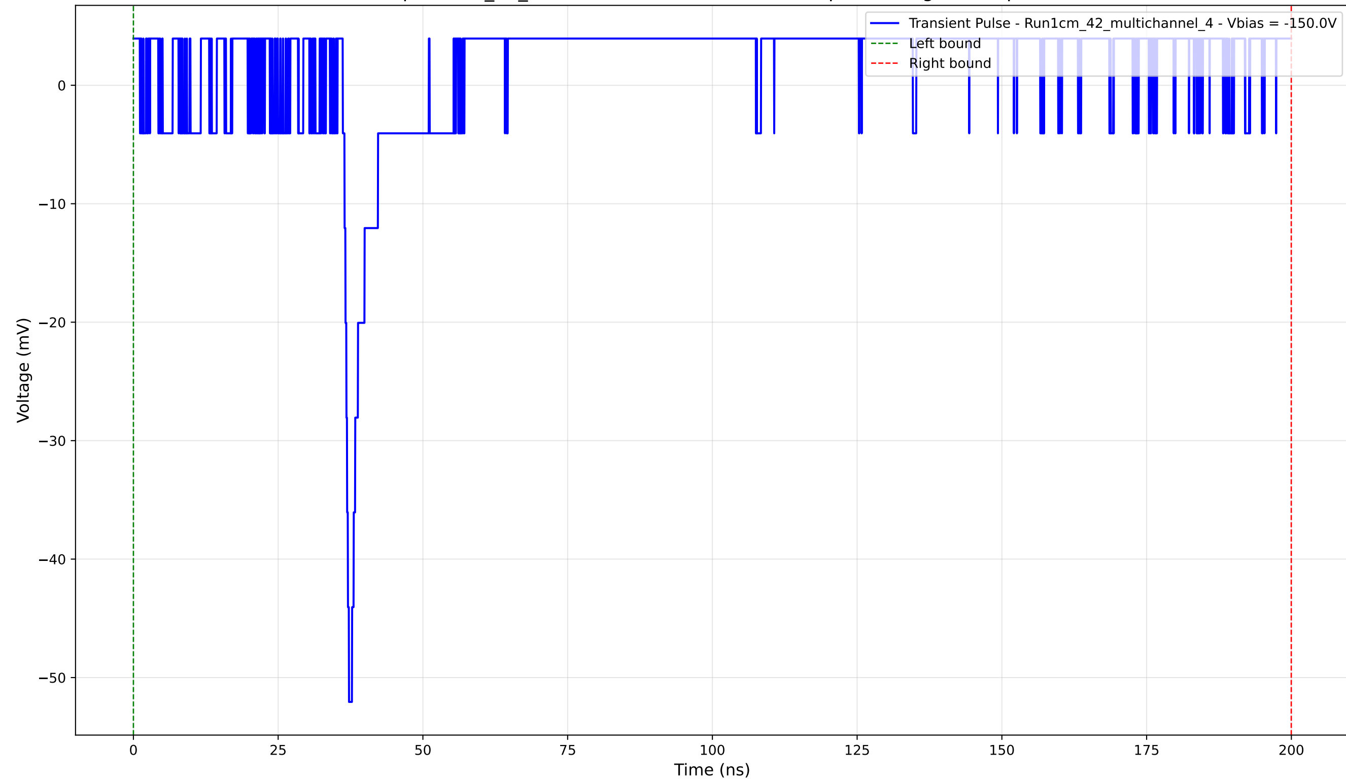
Transient Pulse - Sample: 1cm_42_multichannel - Position: 1990.0 \mu\text{m} - Charge: 6.45 pC - Rise Time: 0.78 ns
