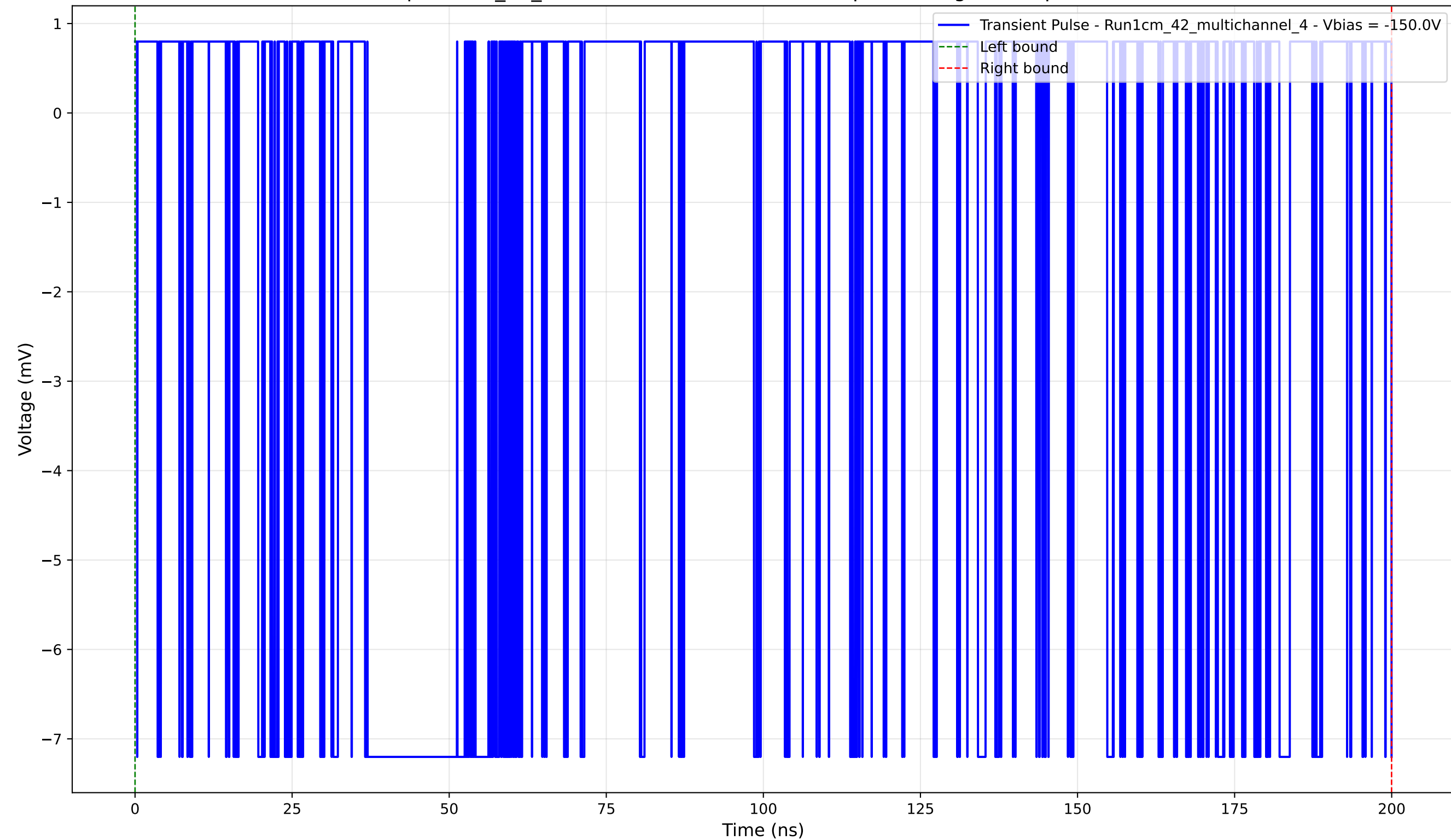
Transient Pulse - Sample: 1cm_42_multichannel - Position: 310.0 \mu\text{m} - Charge: 4.33 pC - Rise Time: 0.00 ns (N/A)
