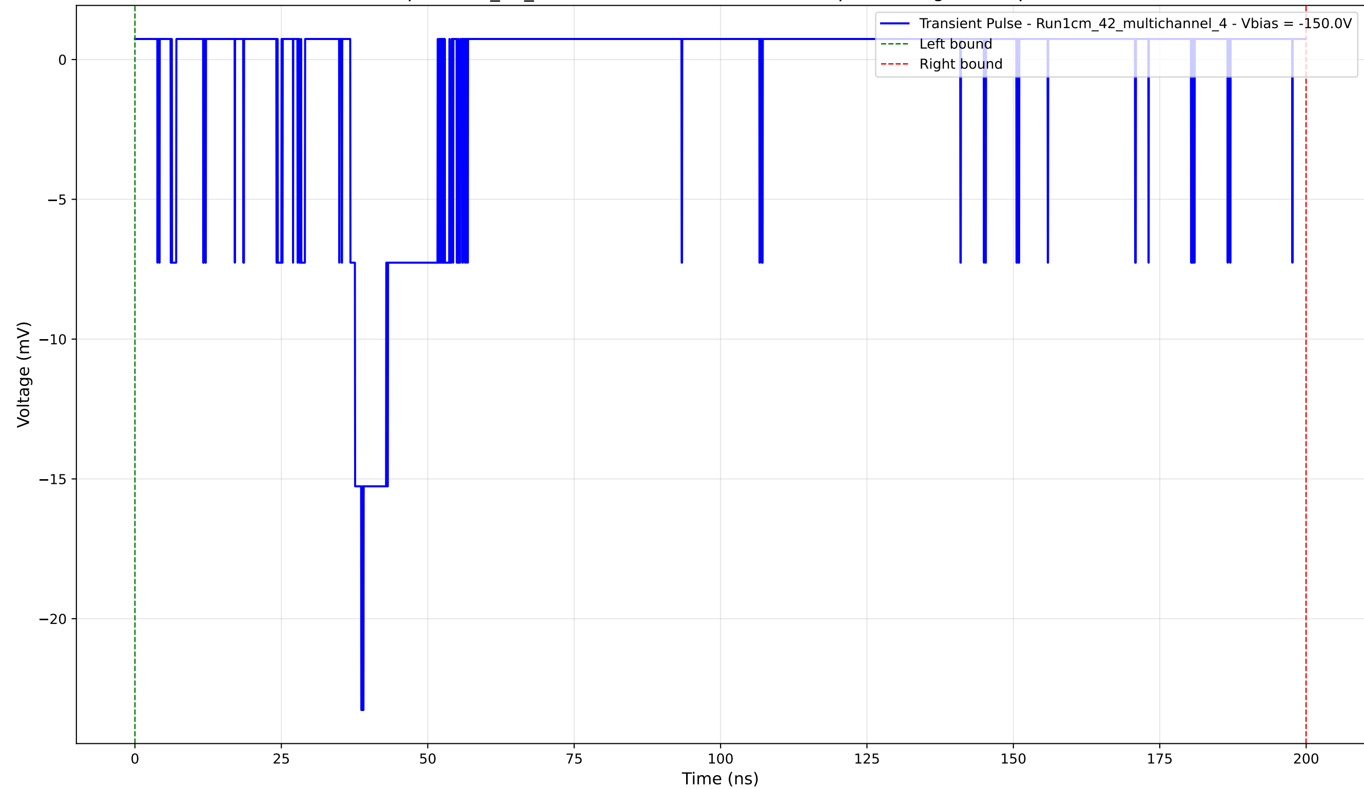
Transient Pulse - Sample: 1cm_42_multichannel - Position: 3735.0 \mu\text{m} - Charge: 1.54 pC - Rise Time: 1.88 ns
