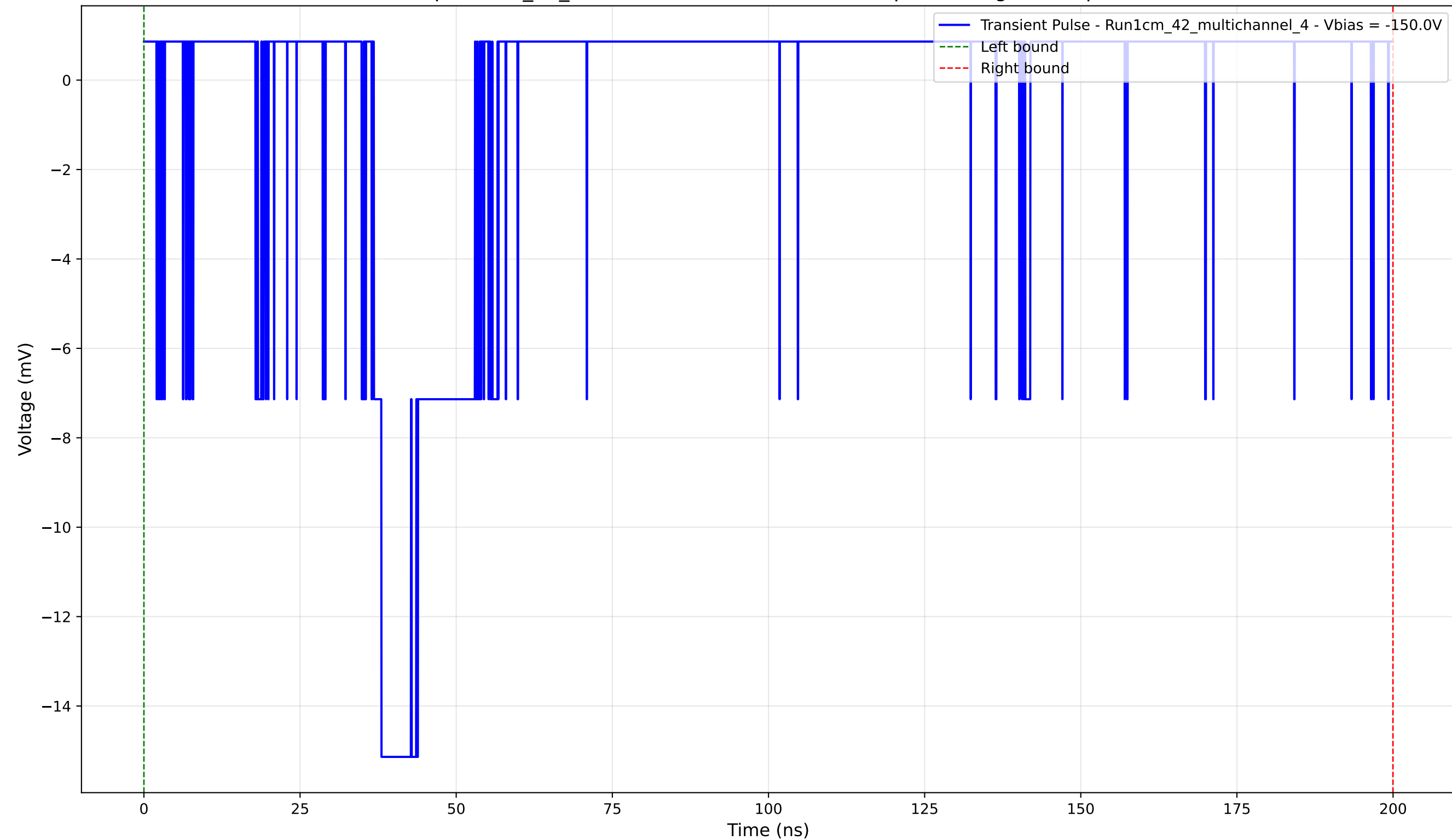
Transient Pulse - Sample: 1cm_42_multichannel - Position: 4020.0 \mu\text{m} - Charge: 1.29 pC - Rise Time: 1.22 ns
