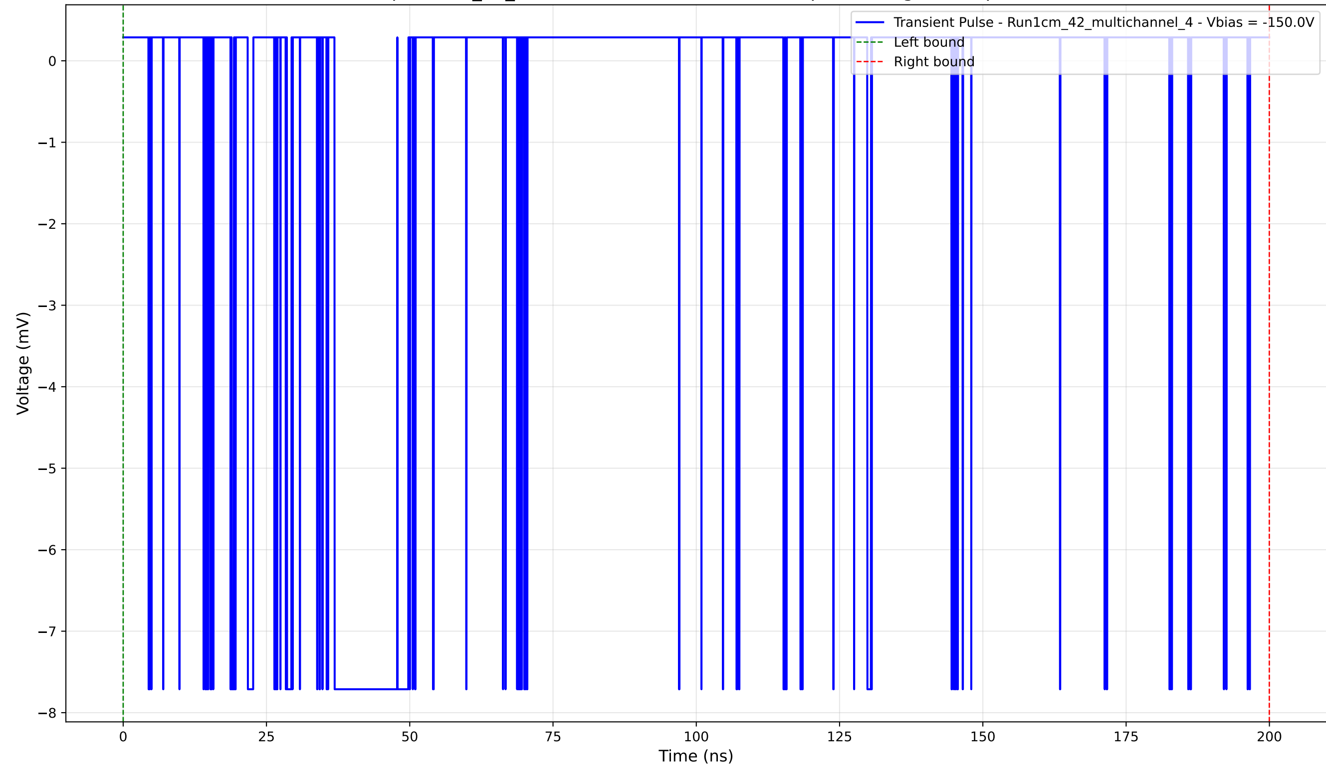
Transient Pulse - Sample: 1cm_42_multichannel - Position: 3445.0 \mu\text{m} - Charge: 2.25 pC - Rise Time: 0.02 ns
