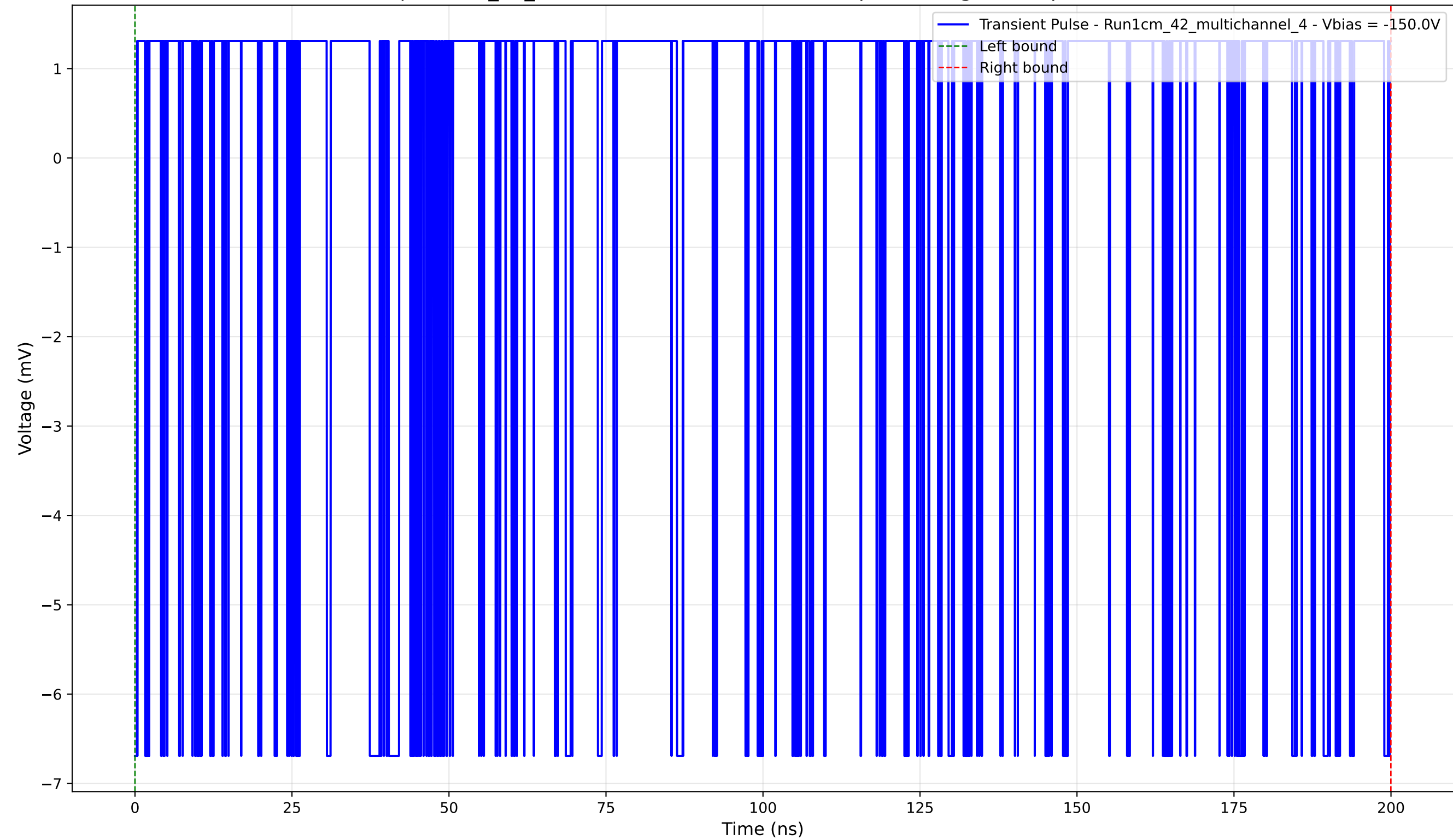
Transient Pulse - Sample: 1cm_42_multichannel - Position: 4425.0 \mu\text{m} - Charge: 0.52 pC - Rise Time: 0.00 ns (N/A)
