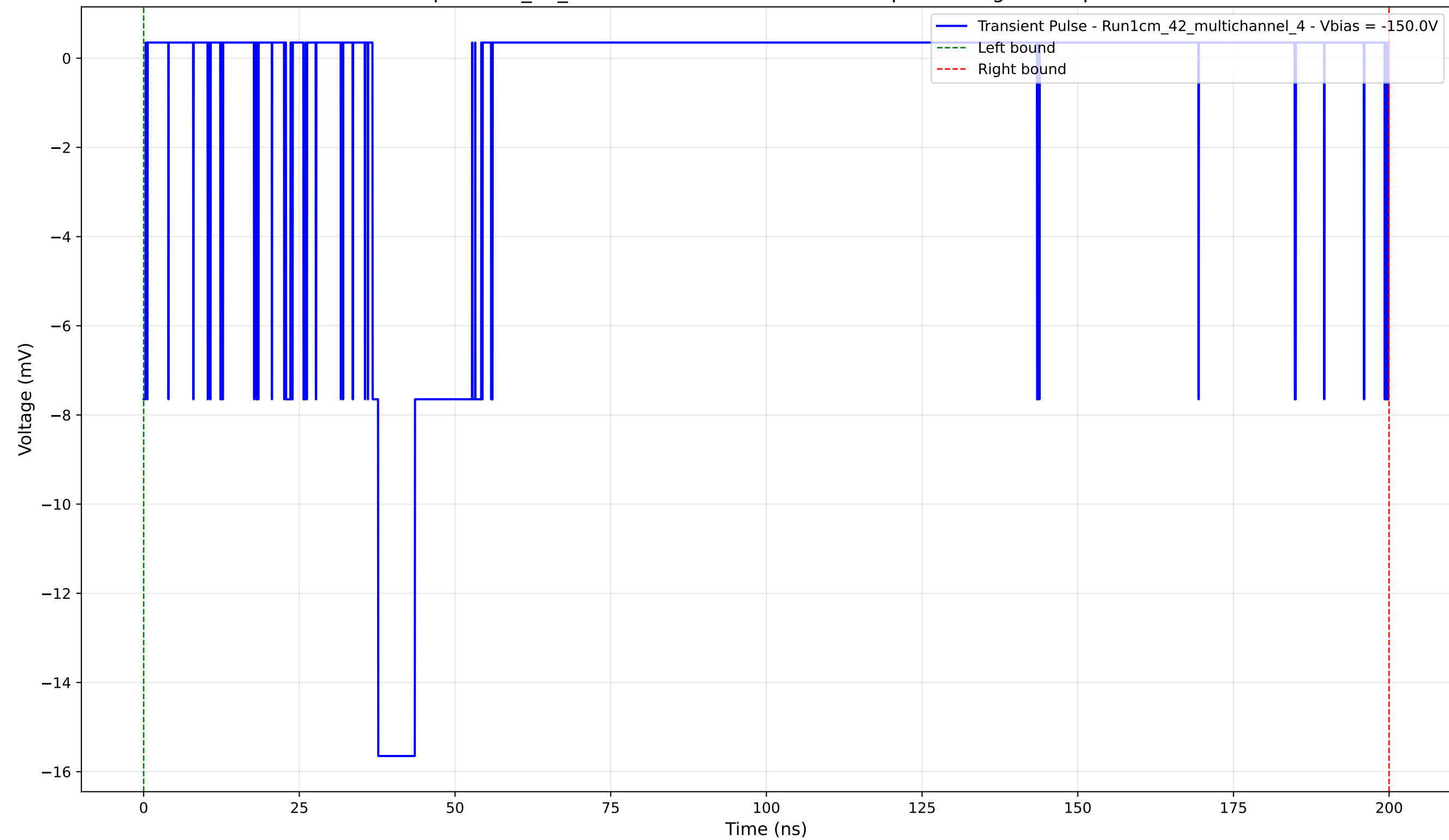
Transient Pulse - Sample: 1cm_42_multichannel - Position: 3760.0 \mu\text{m} - Charge: 2.95 pC - Rise Time: 0.92 ns
