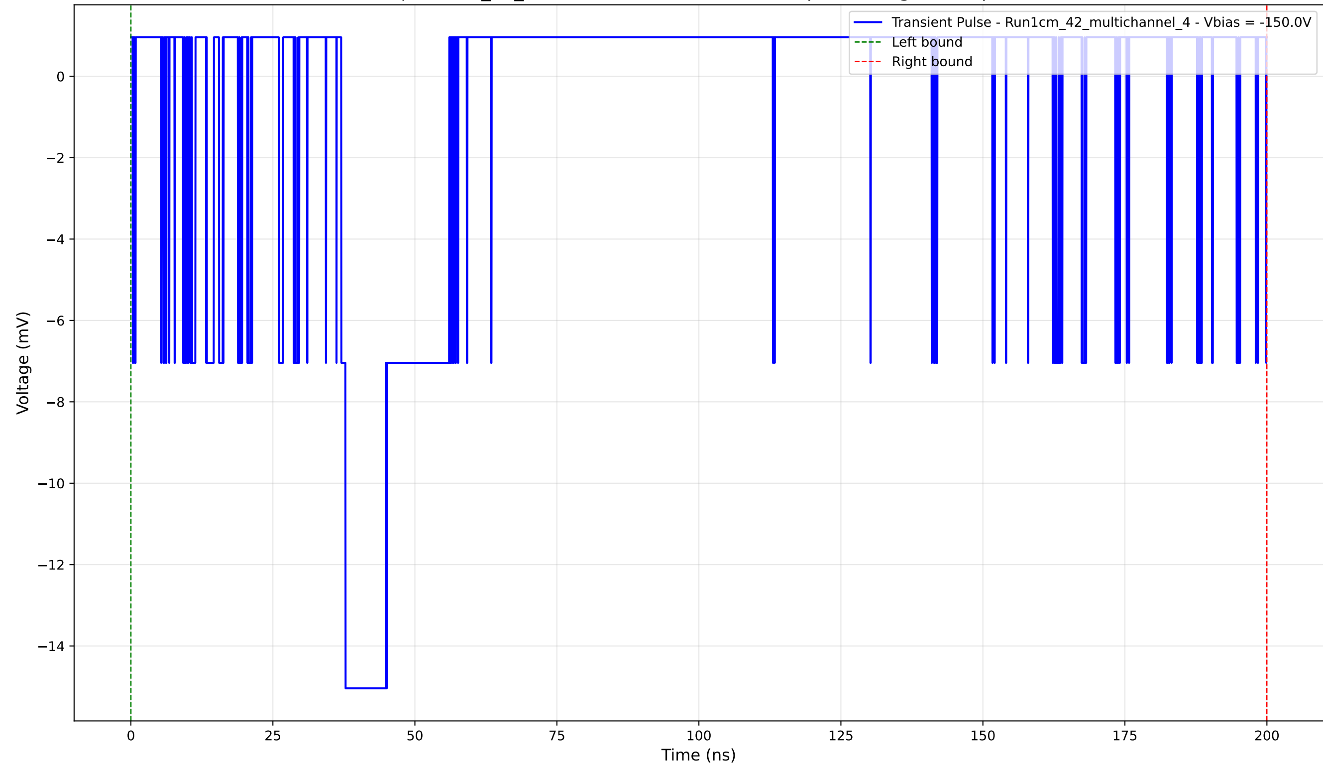
Transient Pulse - Sample: 1cm_42_multichannel - Position: 710.0 \mu\text{m} - Charge: 2.40 pC - Rise Time: 0.76 ns
