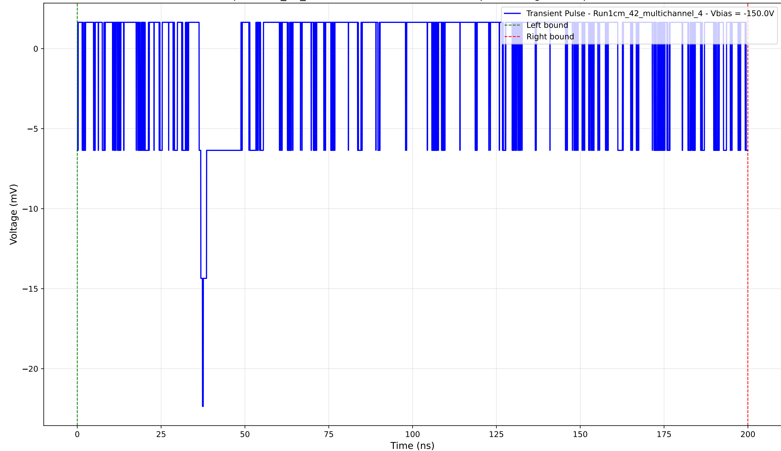
Transient Pulse - Sample: 1cm_42_multichannel - Position: 1925.0 \mu\text{m} - Charge: 0.81 pC - Rise Time: 1.02 ns
