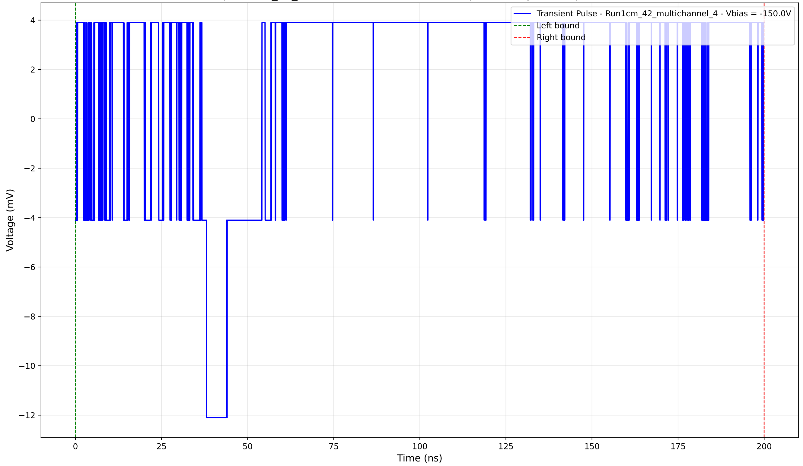
Transient Pulse - Sample: 1cm_42_multichannel - Position: 520.0 \mu\text{m} - Charge: 8.39 pC - Rise Time: 0.00 ns (N/A)
