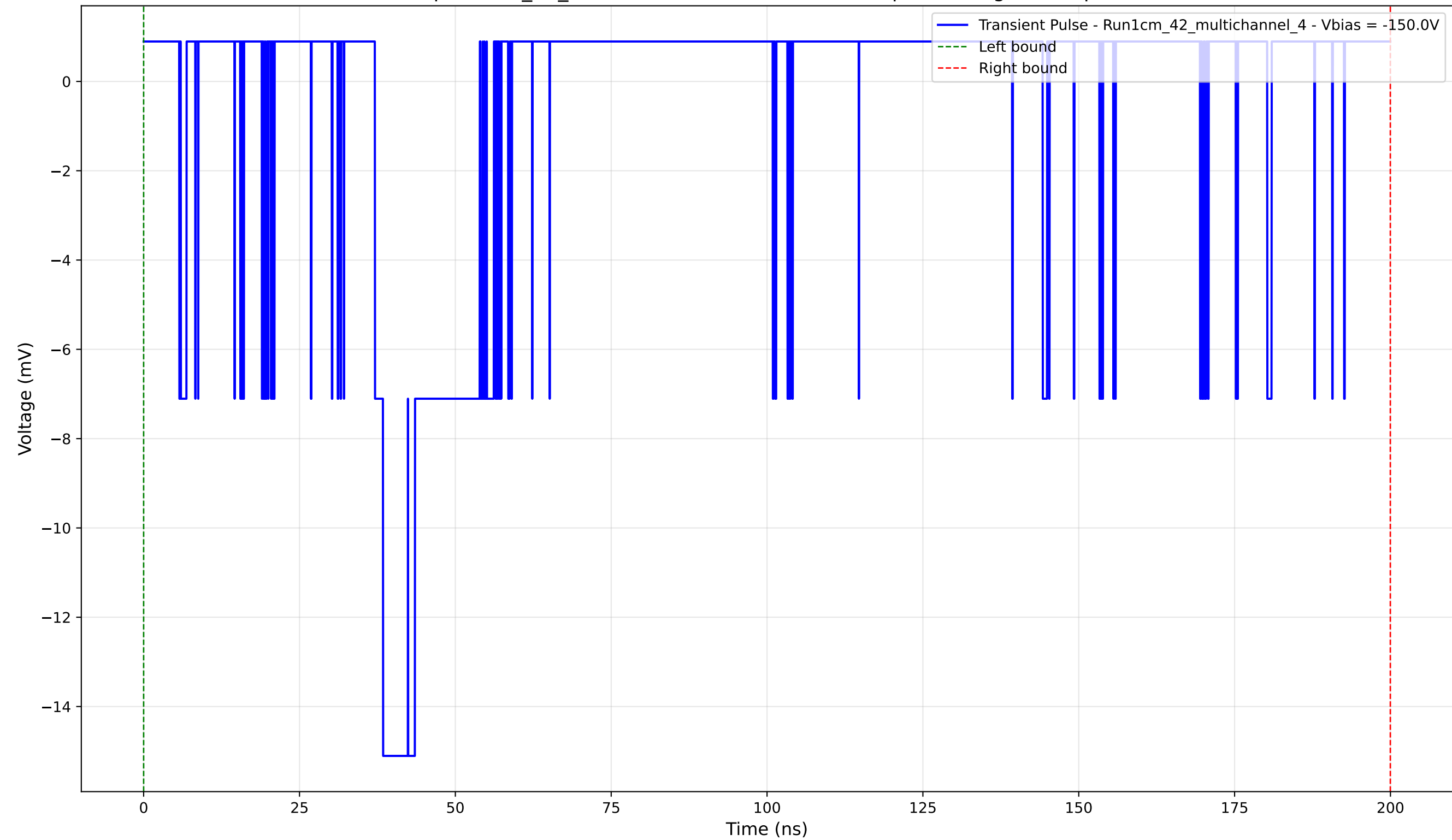
Transient Pulse - Sample: 1cm_42_multichannel - Position: 4255.0 \mu\text{m} - Charge: 1.53 pC - Rise Time: 1.32 ns
