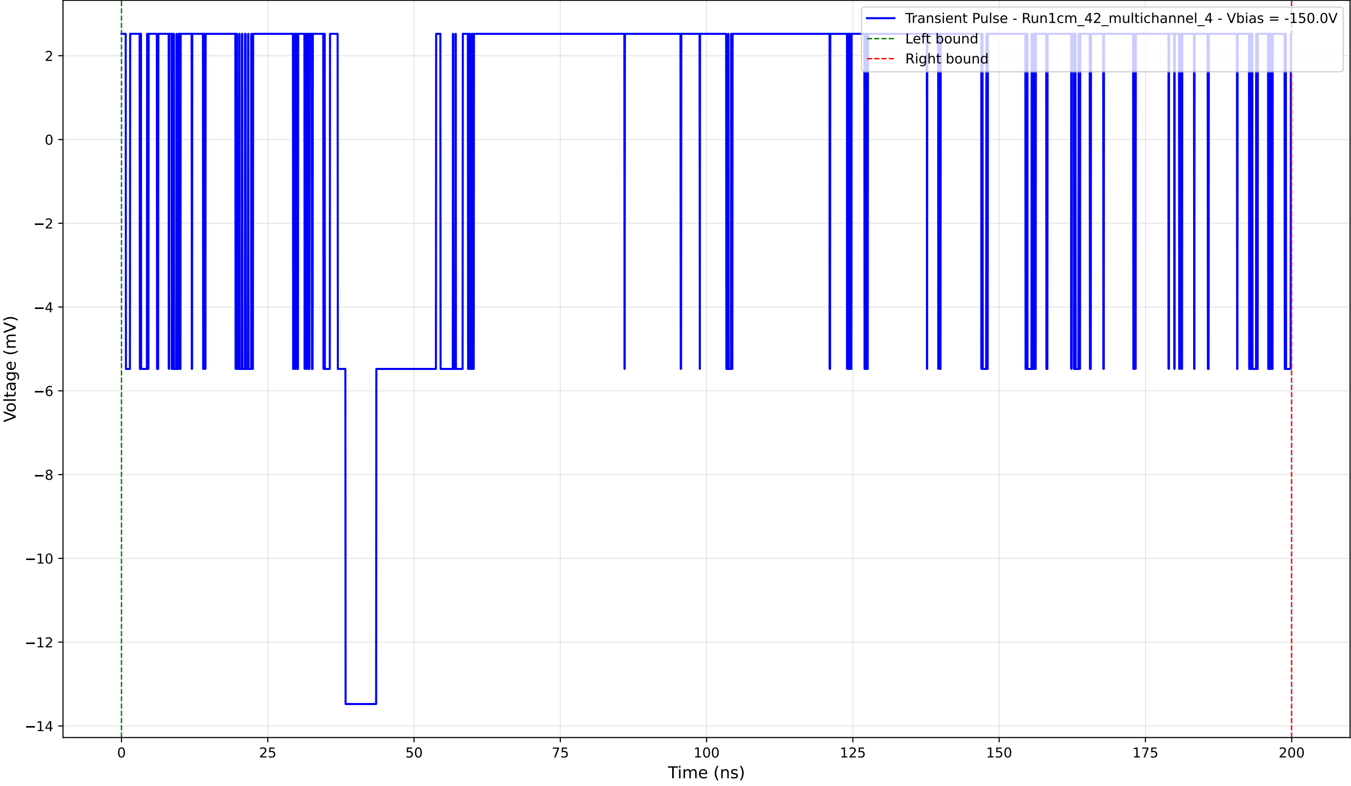
Transient Pulse - Sample: 1cm_42_multichannel - Position: 460.0 \mu\text{m} - Charge: 3.20 pC - Rise Time: 0.00 ns (N/A)
