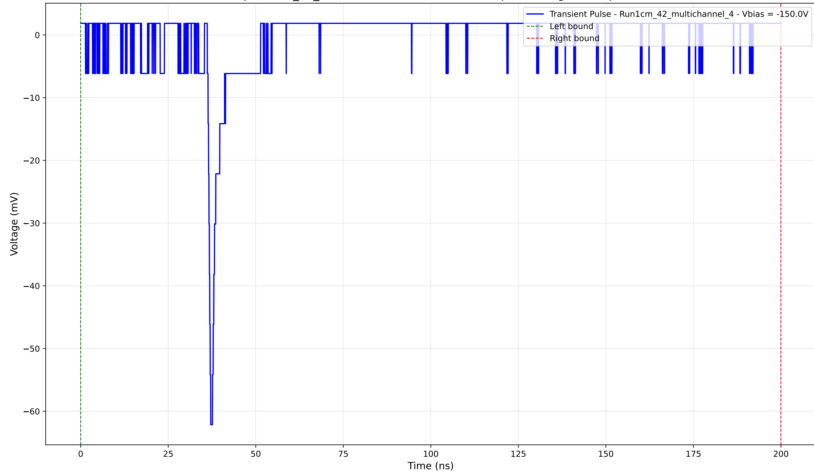
Transient Pulse - Sample: 1cm_42_multichannel - Position: 2140.0 \mu\text{m} - Charge: 0.04 pC - Rise Time: 0.78 ns
