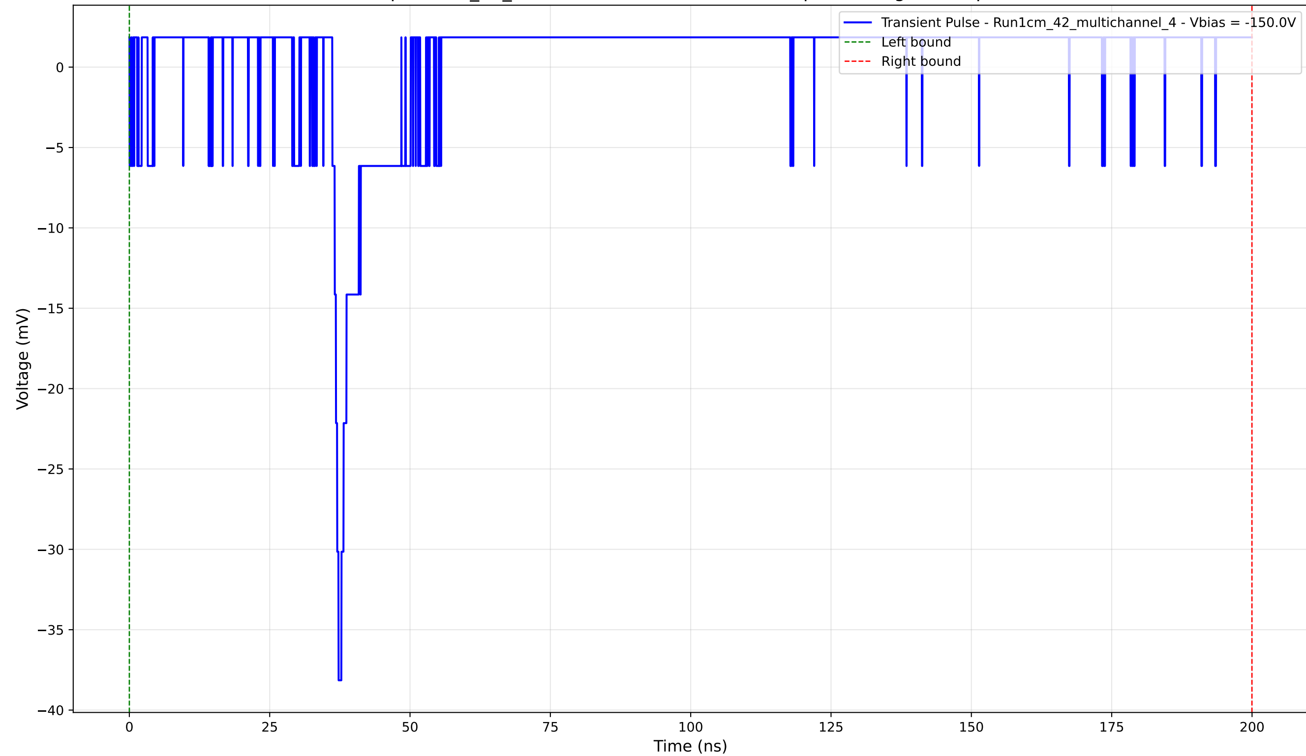
Transient Pulse - Sample: 1cm_42_multichannel - Position: 2830.0 \mu\text{m} - Charge: 2.39 pC - Rise Time: 1.11 ns
