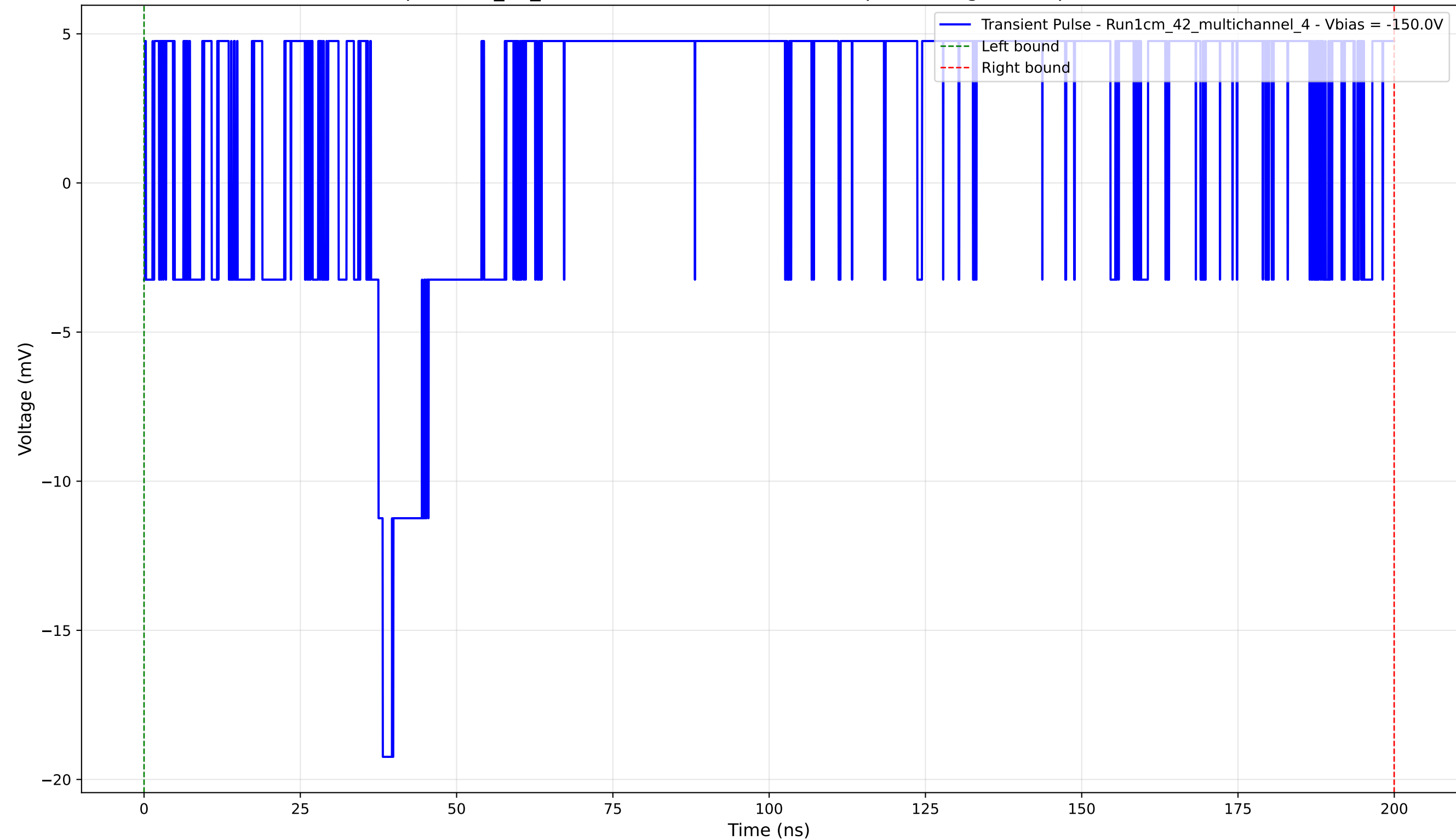
Transient Pulse - Sample: 1cm_42_multichannel - Position: 1010.0 \mu\text{m} - Charge: 9.00 pC - Rise Time: 0.00 ns (N/A)
