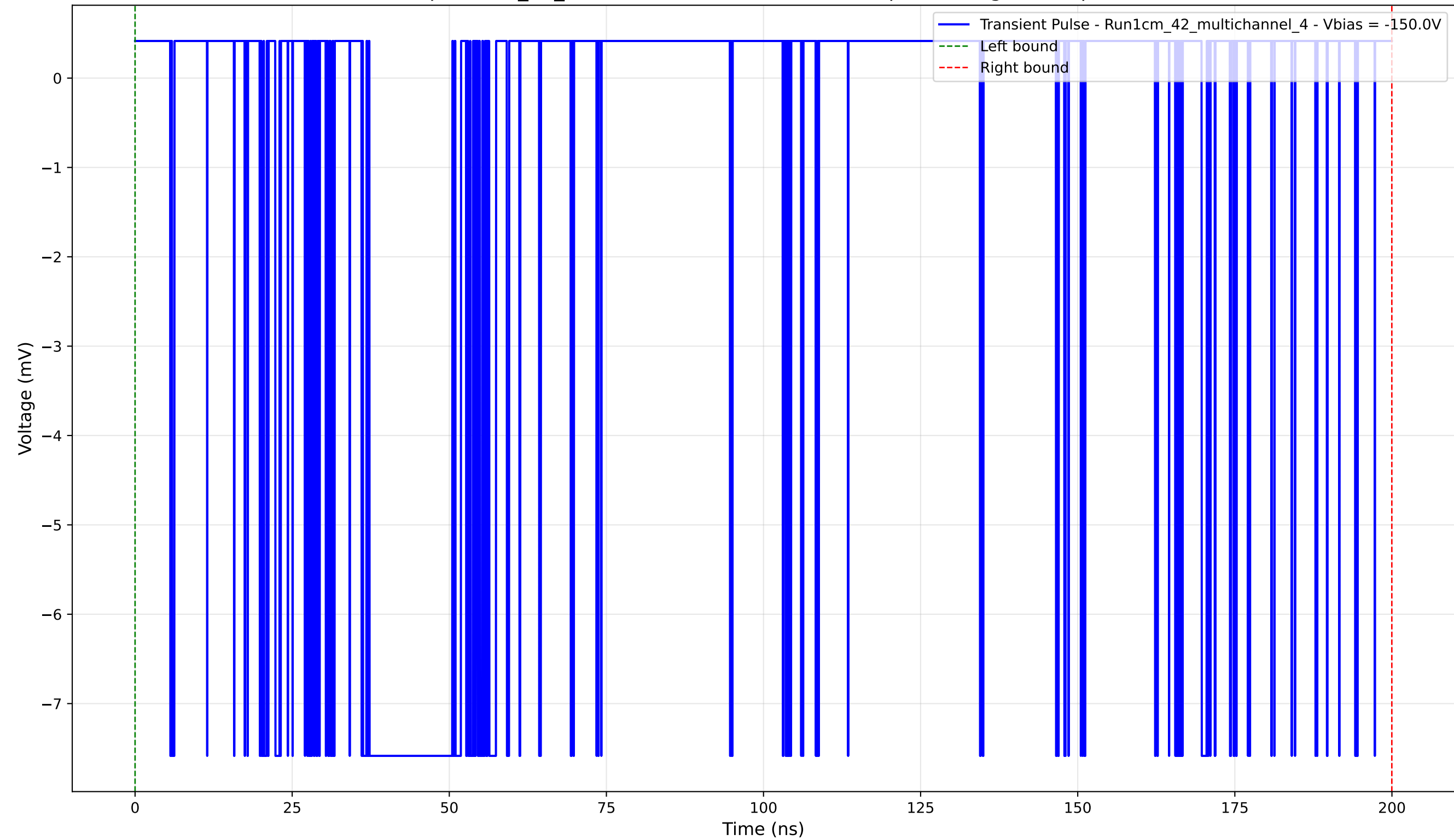
Transient Pulse - Sample: 1cm_42_multichannel - Position: 4850.0 \mu\text{m} - Charge: 3.03 pC - Rise Time: 0.02 ns
