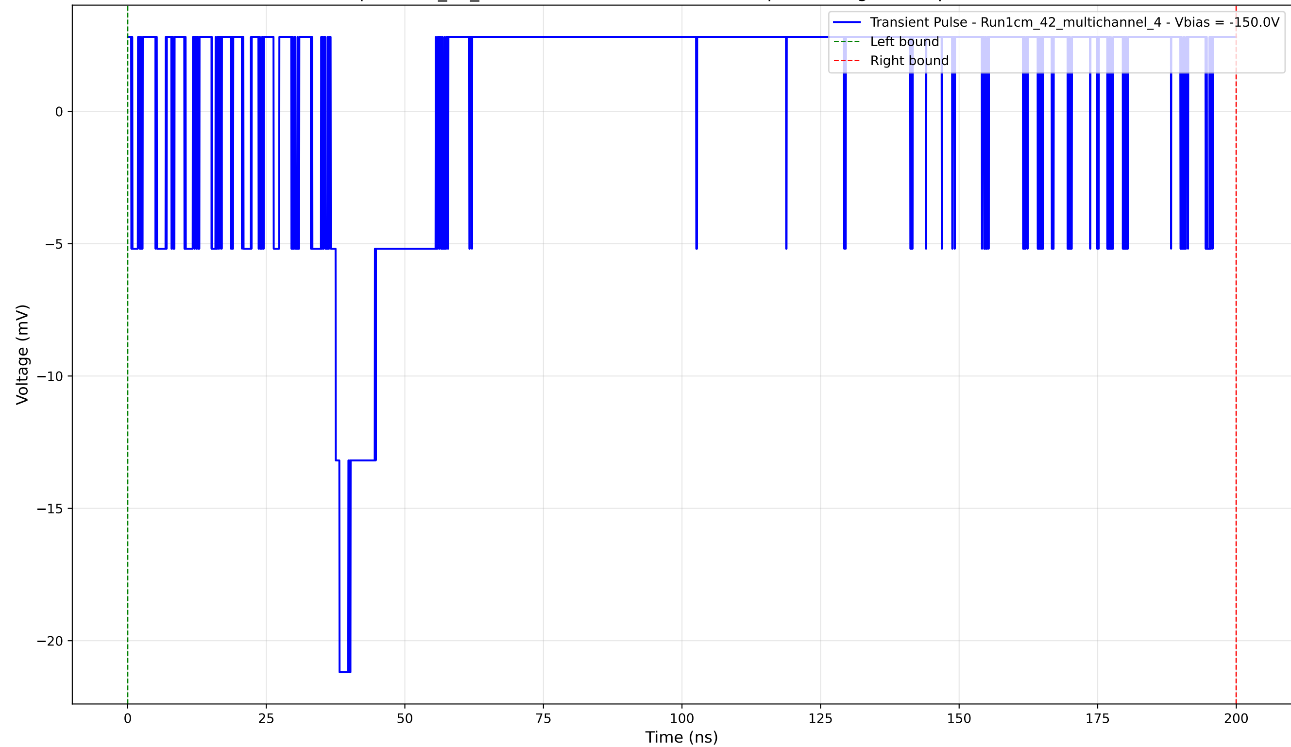
Transient Pulse - Sample: 1cm_42_multichannel - Position: 1020.0 \mu\text{m} - Charge: 3.45 pC - Rise Time: 0.00 ns (N/A)
