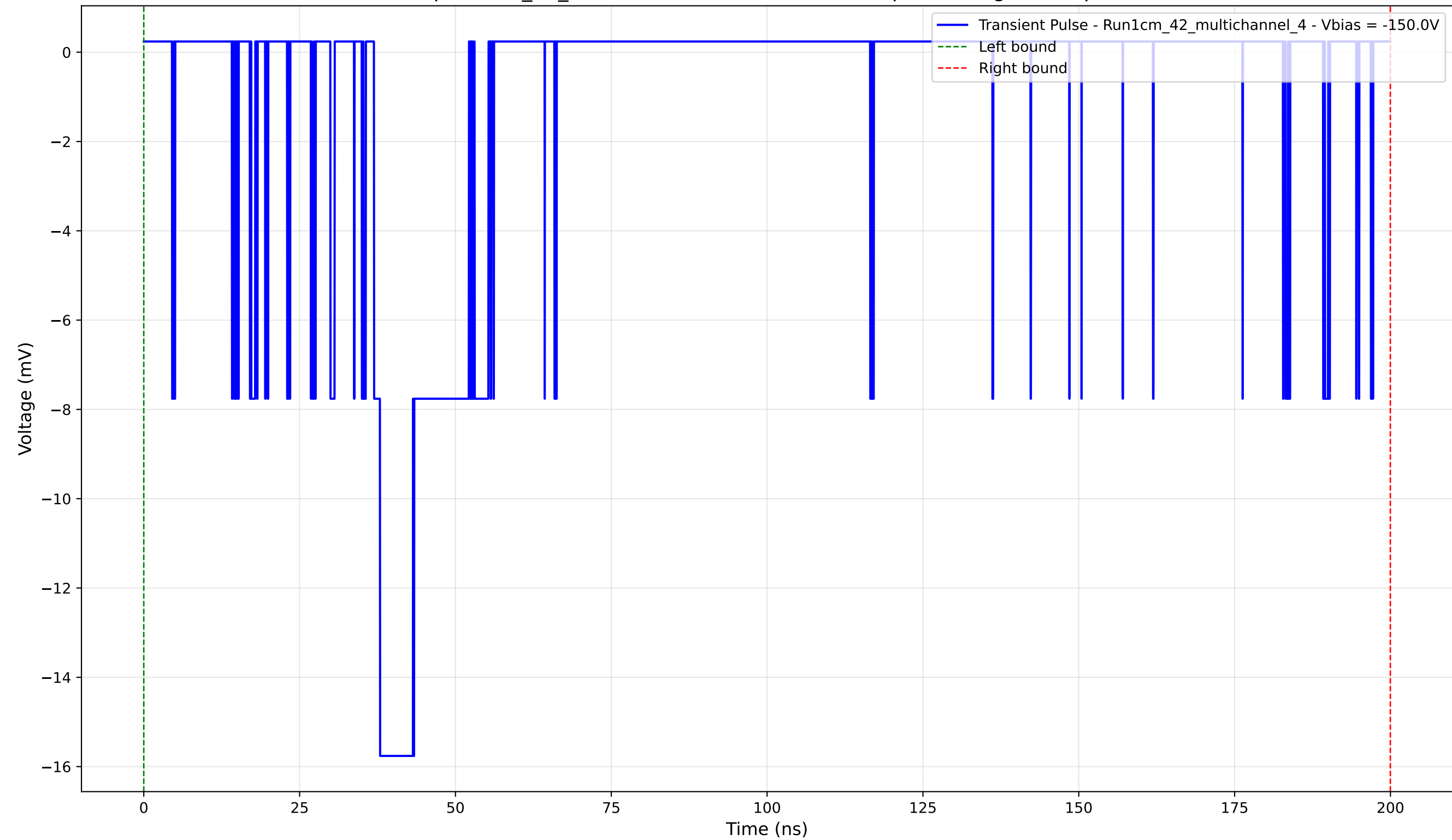
Transient Pulse - Sample: 1cm_42_multichannel - Position: 3990.0 \mu\text{m} - Charge: 3.82 pC - Rise Time: 0.98 ns
