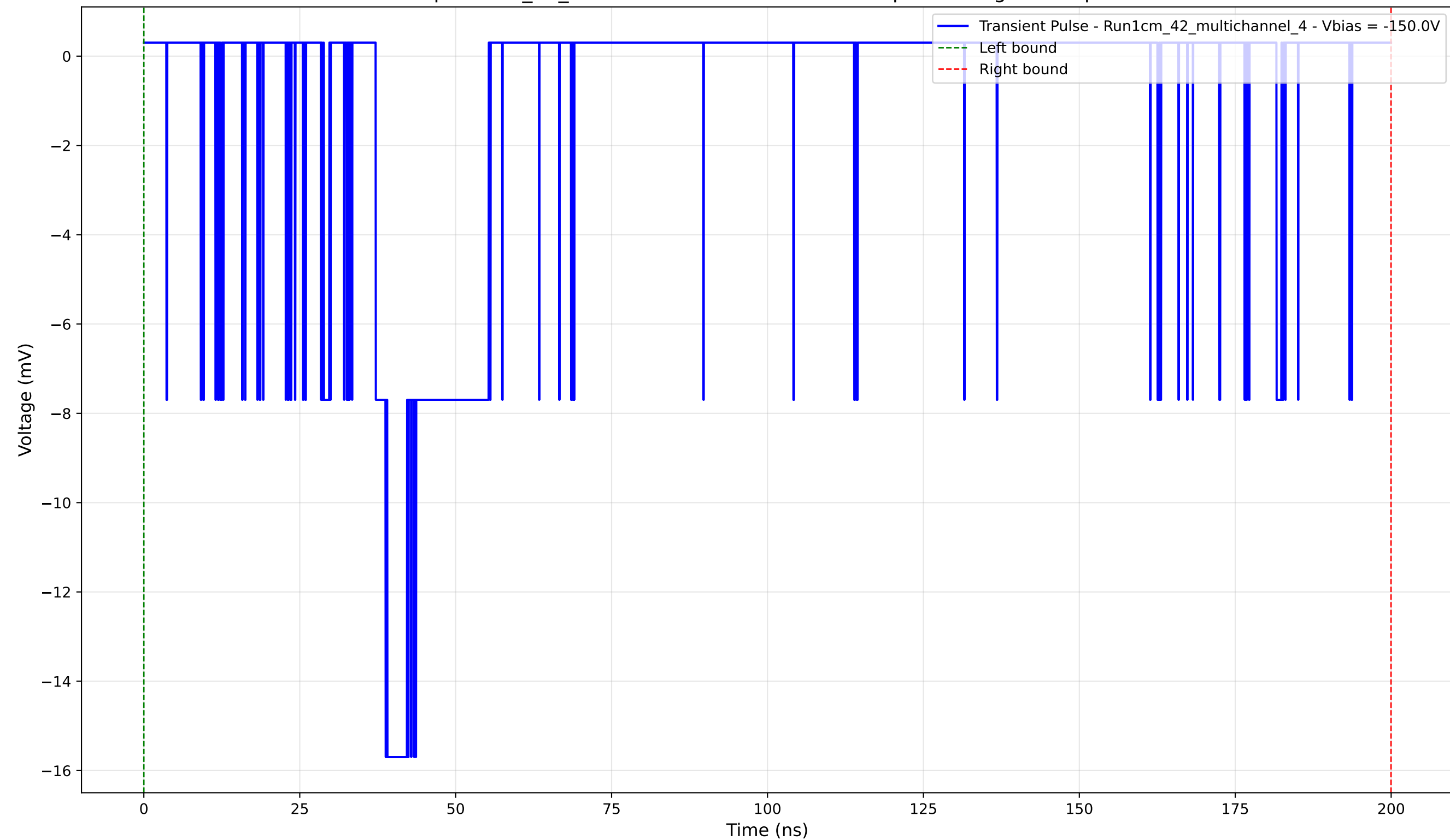
Transient Pulse - Sample: 1cm_42_multichannel - Position: 4620.0 \mu\text{m} - Charge: 3.38 pC - Rise Time: 1.60 ns
