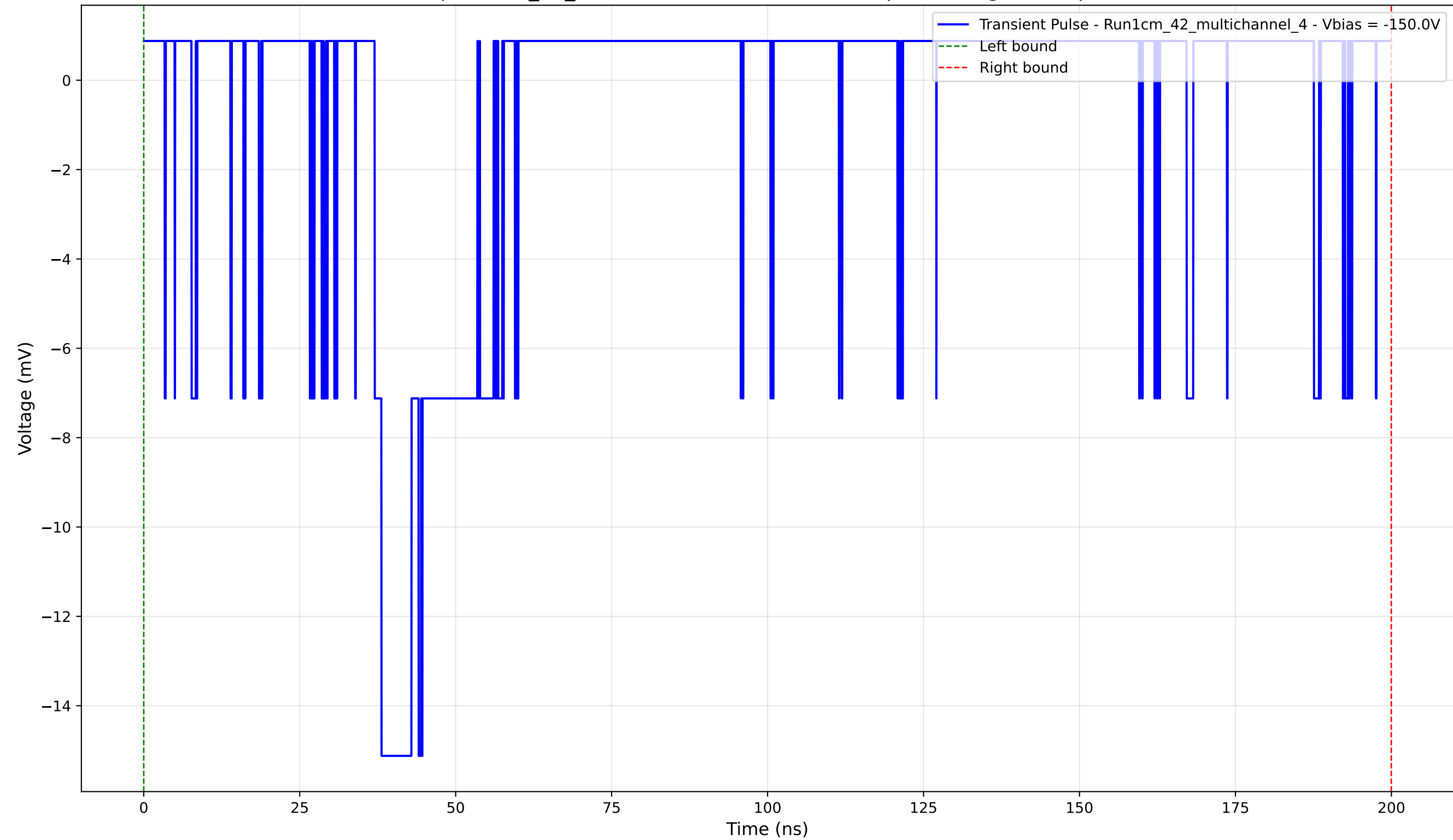
Transient Pulse - Sample: 1cm_42_multichannel - Position: 610.0 \mu\text{m} - Charge: 1.95 pC - Rise Time: 1.10 ns
