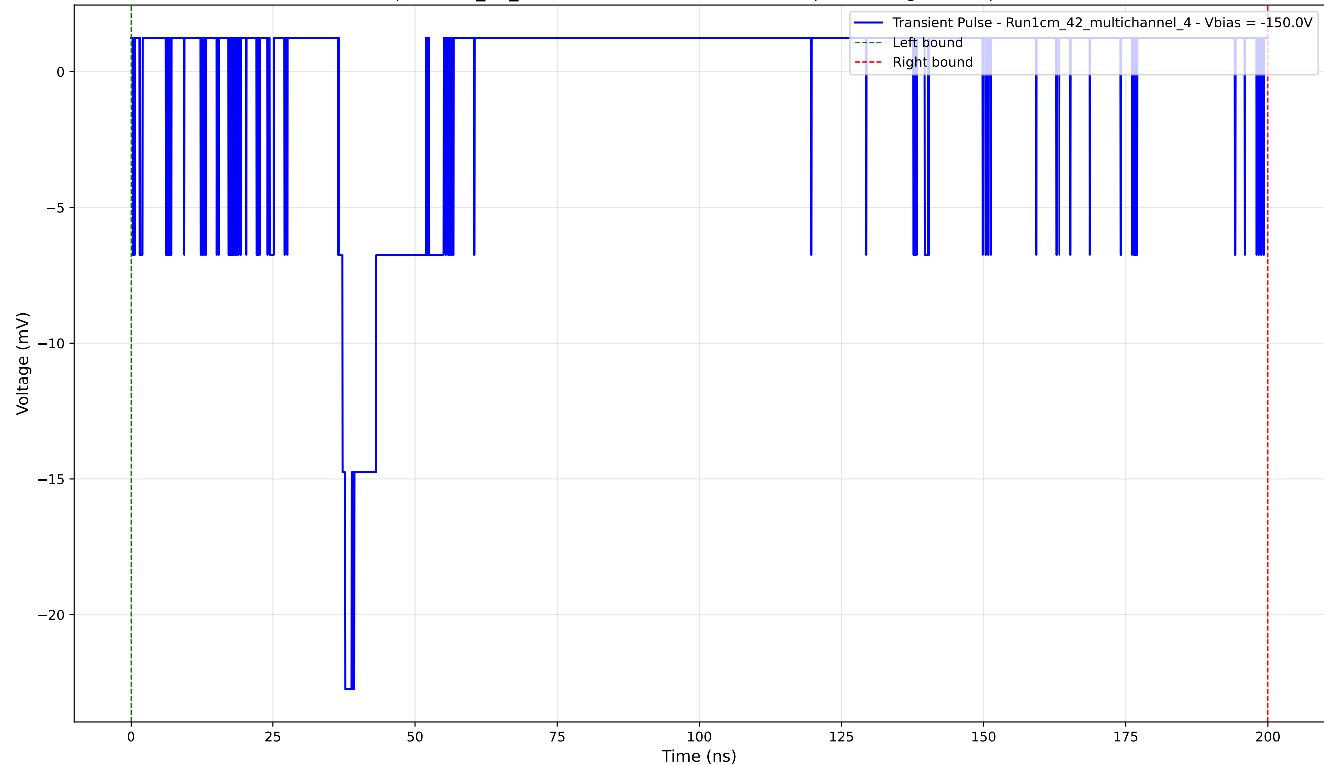
Transient Pulse - Sample: 1cm_42_multichannel - Position: 3500.0 \mu\text{m} - Charge: 0.43 pC - Rise Time: 1.12 ns
