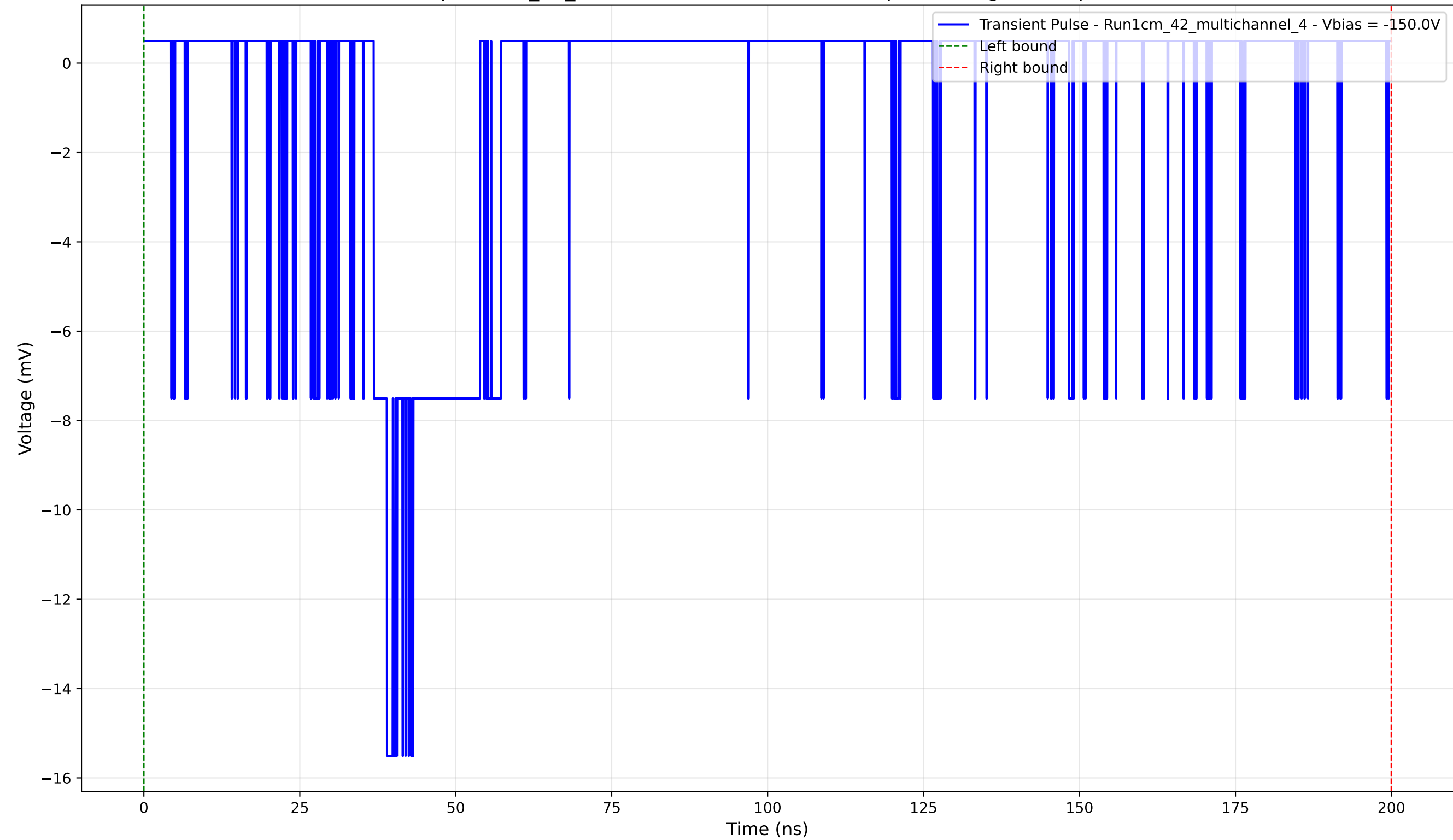
Transient Pulse - Sample: 1cm_42_multichannel - Position: 130.0 \mu\text{m} - Charge: 3.16 pC - Rise Time: 2.12 ns
