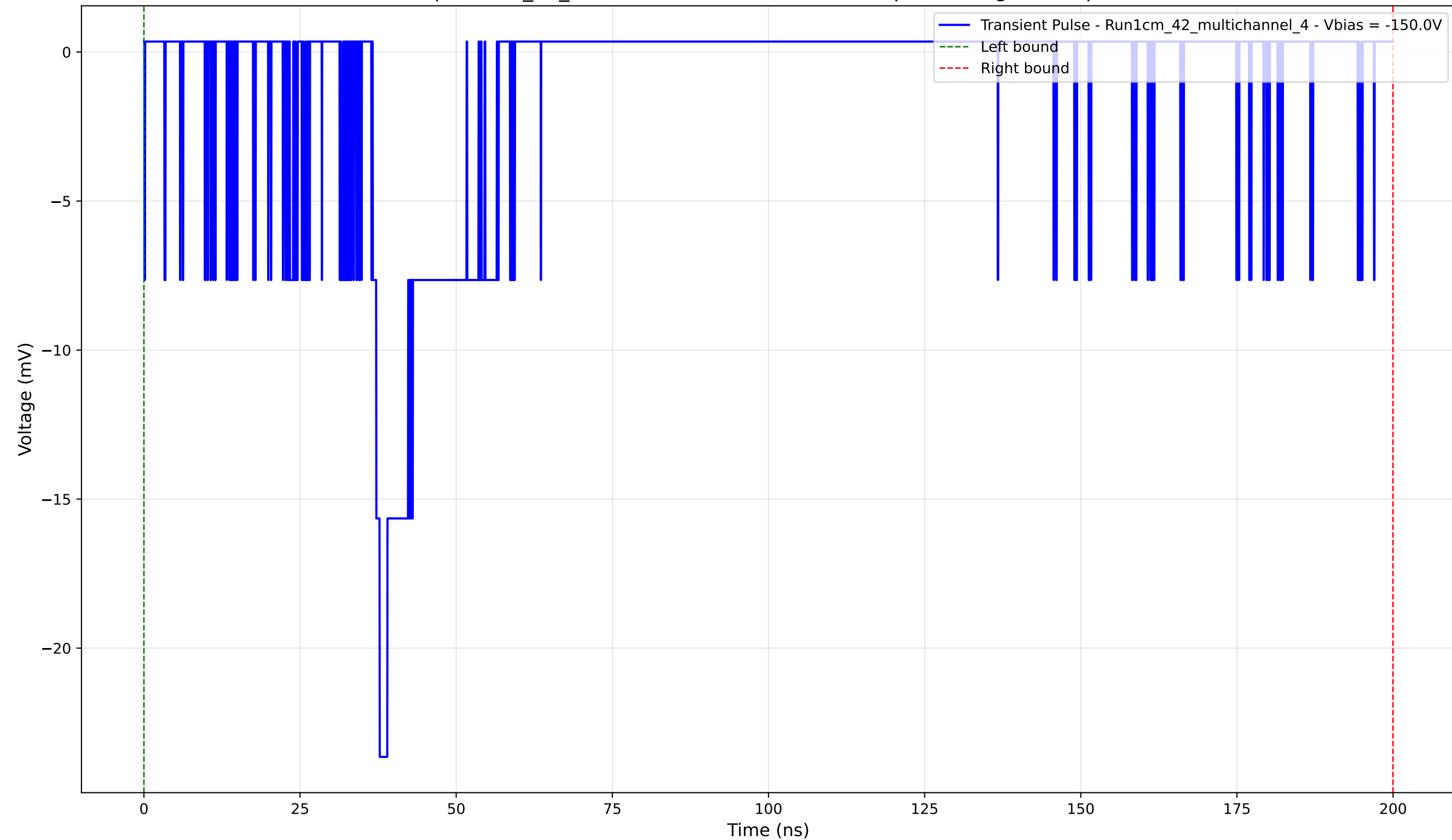
Transient Pulse - Sample: 1cm_42_multichannel - Position: 3475.0 \mu\text{m} - Charge: 4.34 pC - Rise Time: 1.11 ns
