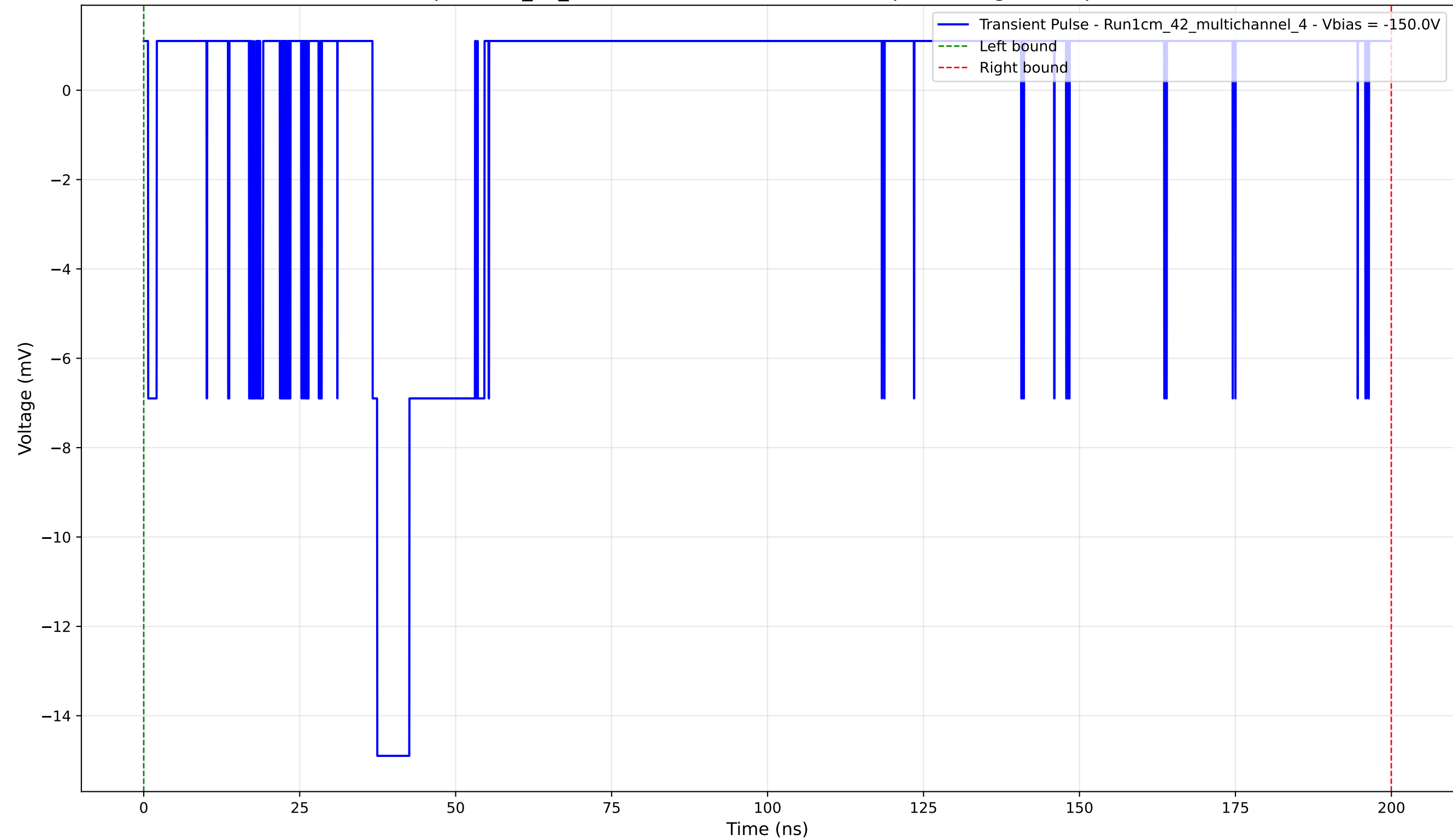
Transient Pulse - Sample: 1cm_42_multichannel - Position: 3630.0 \mu\text{m} - Charge: 0.35 pC - Rise Time: 0.76 ns
