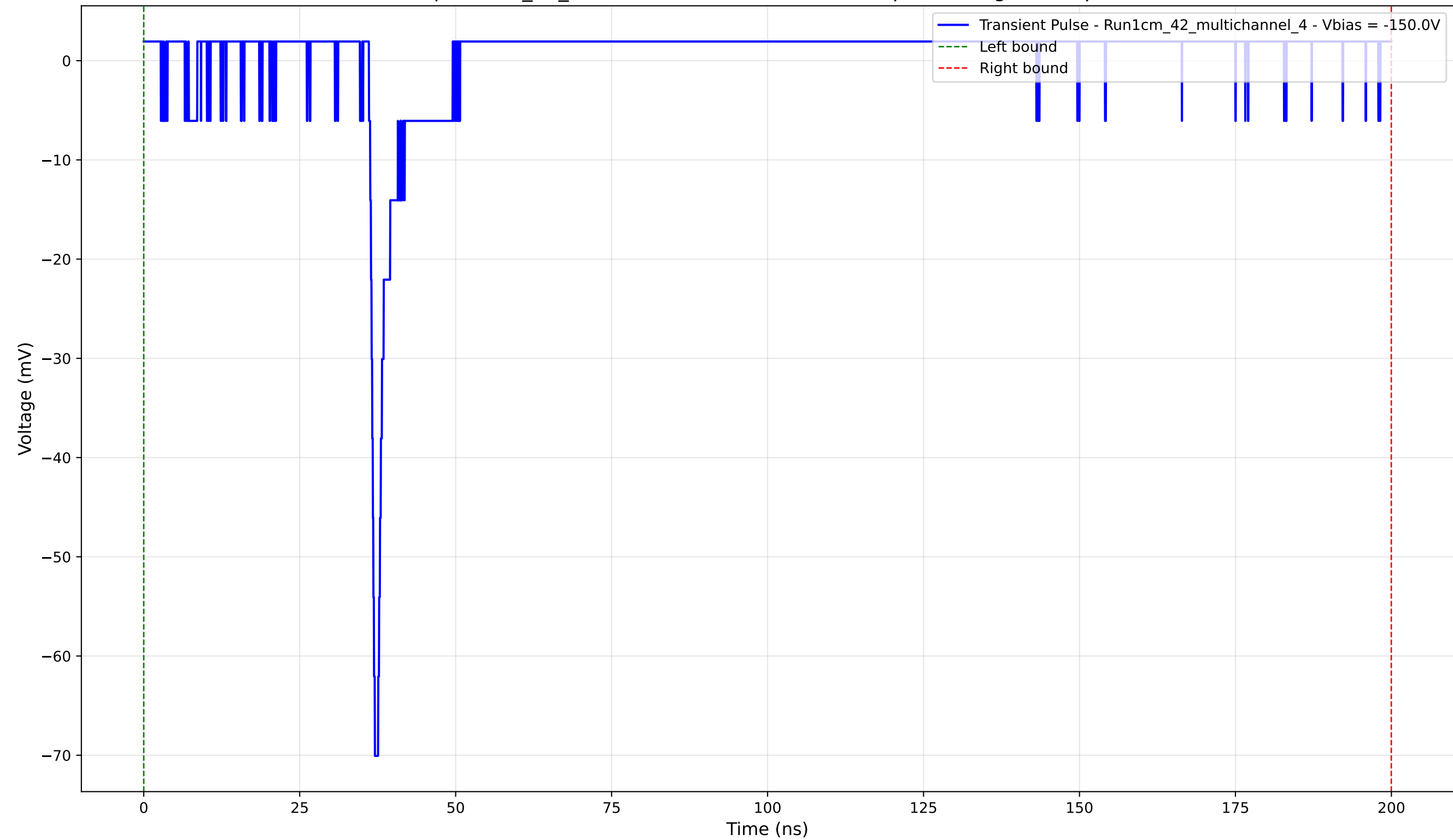
Transient Pulse - Sample: 1cm_42_multichannel - Position: 2540.0 \mu\text{m} - Charge: 1.96 pC - Rise Time: 0.76 ns
