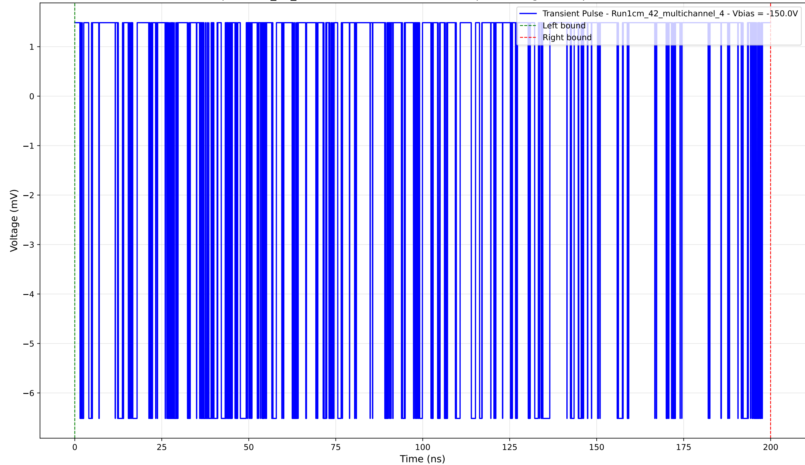
Transient Pulse - Sample: 1cm_42_multichannel - Position: 1380.0 \mu\text{m} - Charge: 1.62 pC - Rise Time: 0.00 ns (N/A)
