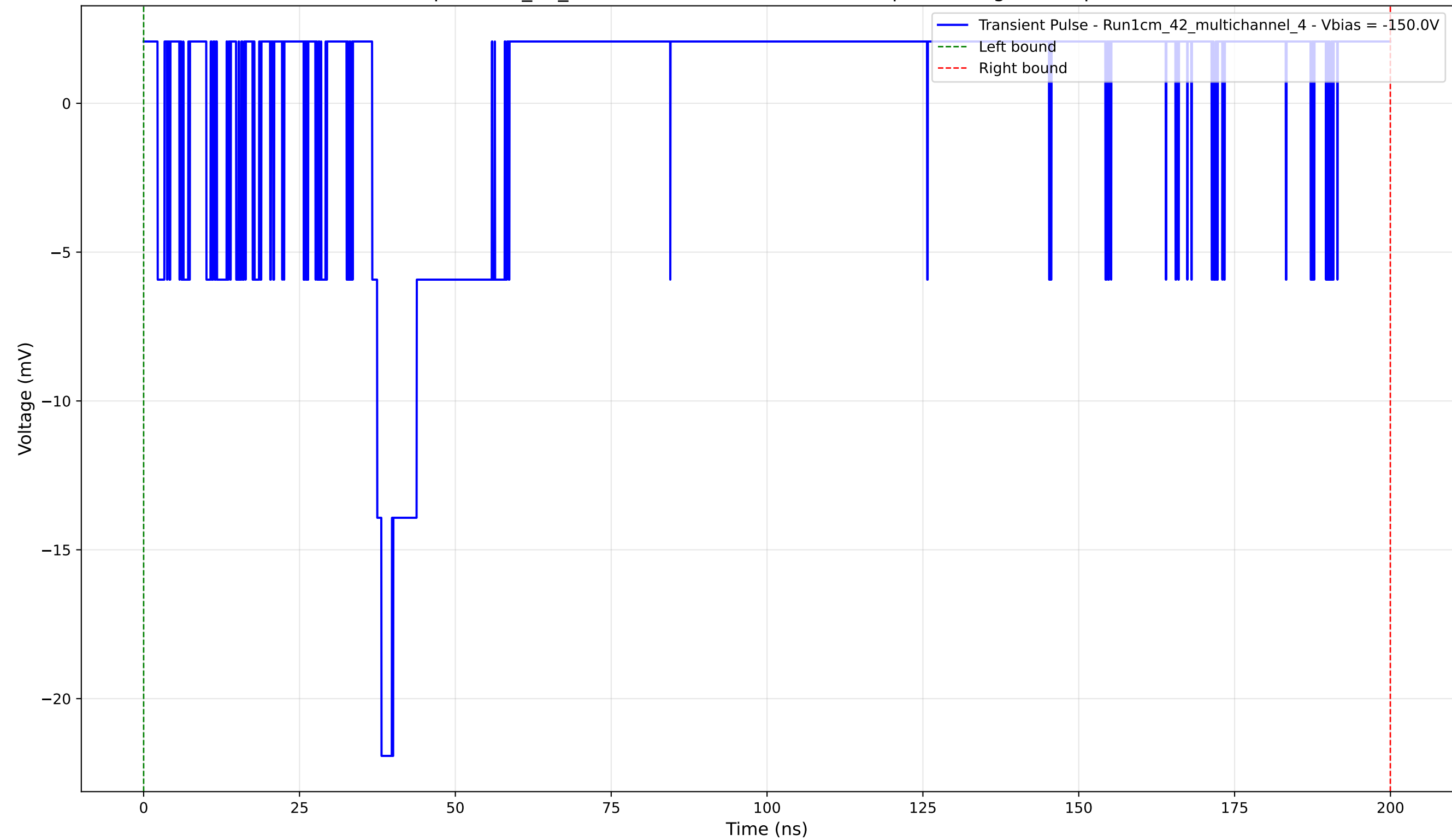
Transient Pulse - Sample: 1cm_42_multichannel - Position: 1105.0 \mu\text{m} - Charge: 1.38 pC - Rise Time: 1.50 ns
