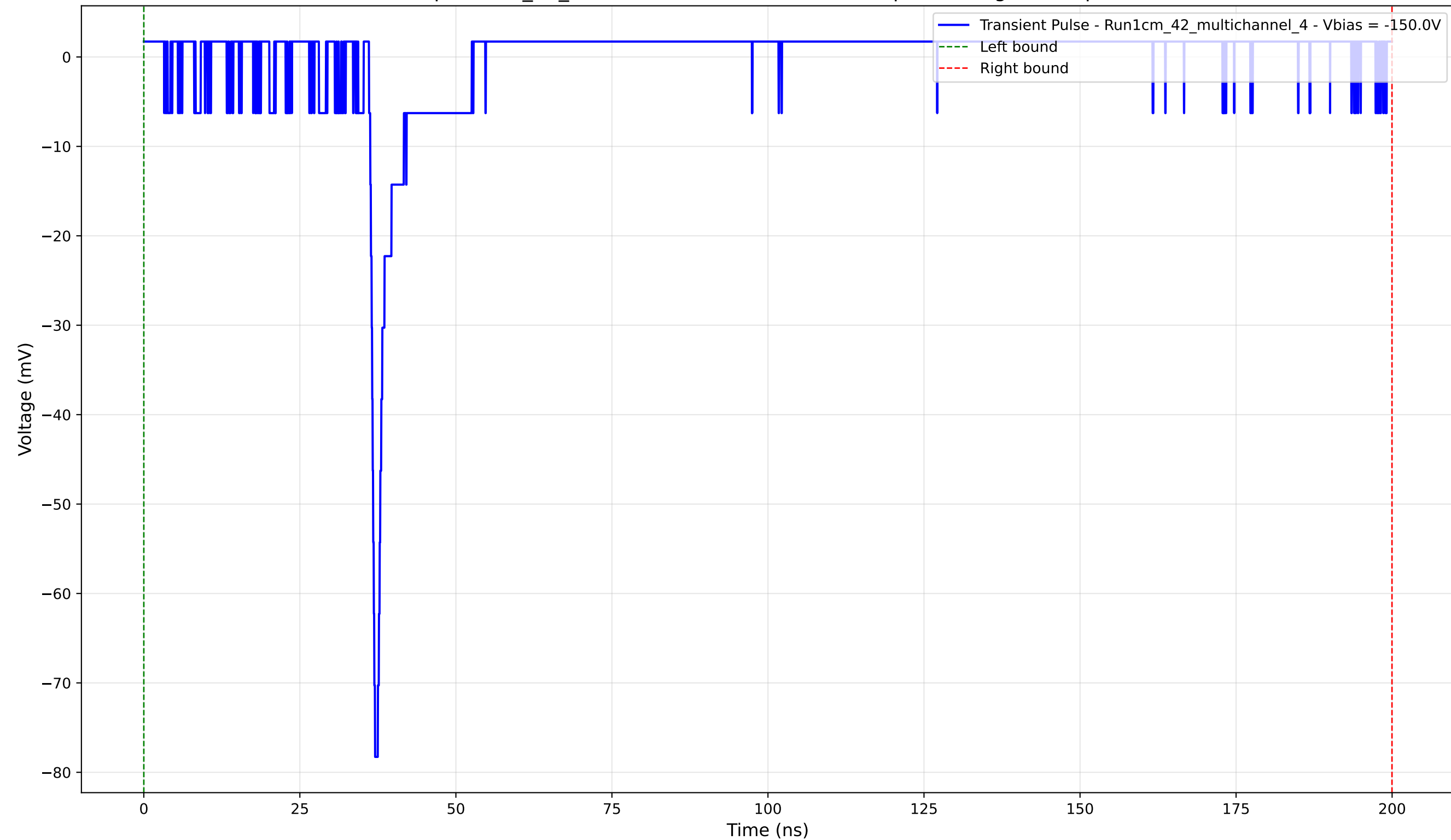
Transient Pulse - Sample: 1cm_42_multichannel - Position: 2260.0 \mu\text{m} - Charge: 0.45 pC - Rise Time: 0.78 ns
