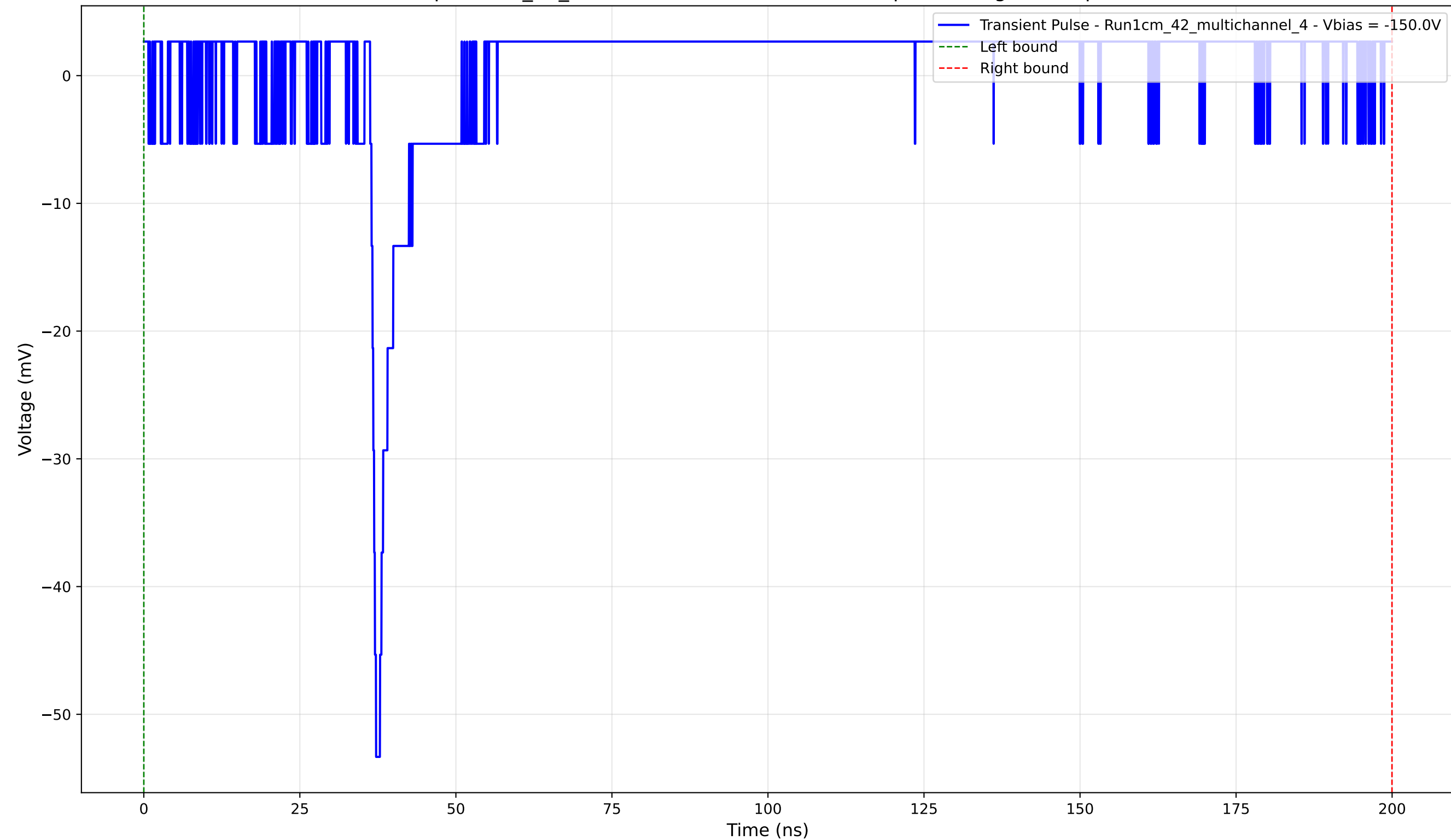
Transient Pulse - Sample: 1cm_42_multichannel - Position: 2000.0 \mu\text{m} - Charge: 2.91 pC - Rise Time: 0.74 ns
