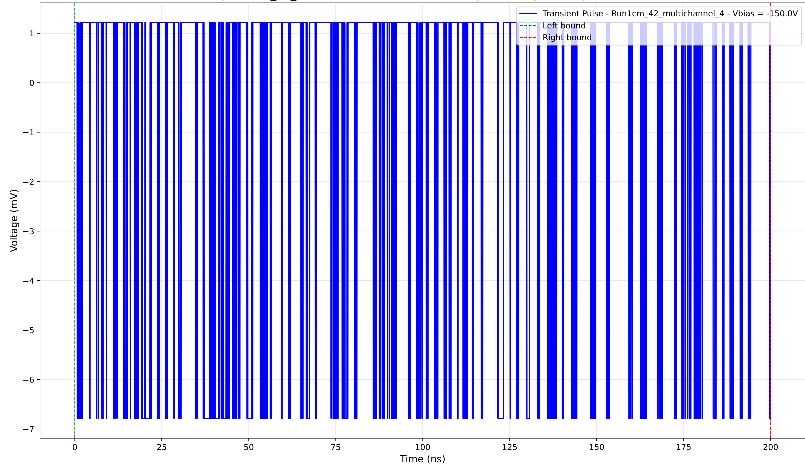
Transient Pulse - Sample: 1cm_42_multichannel - Position: 3400.0 \mu\text{m} - Charge: 1.32 pC - Rise Time: 0.00 ns (N/A)
