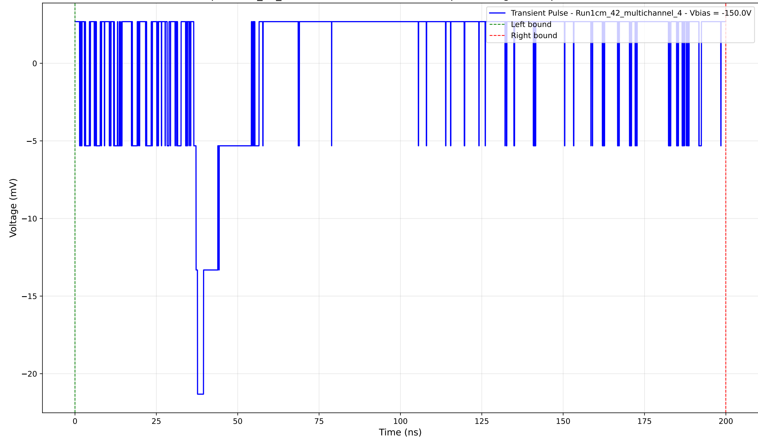
Transient Pulse - Sample: 1cm_42_multichannel - Position: 1300.0 \mu\text{m} - Charge: 3.26 pC - Rise Time: 0.00 ns (N/A)
