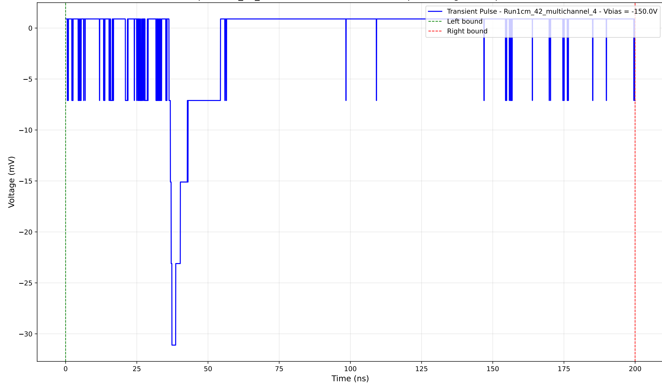
Transient Pulse - Sample: 1cm_42_multichannel - Position: 1620.0 \mu\text{m} - Charge: 2.48 pC - Rise Time: 1.03 ns
