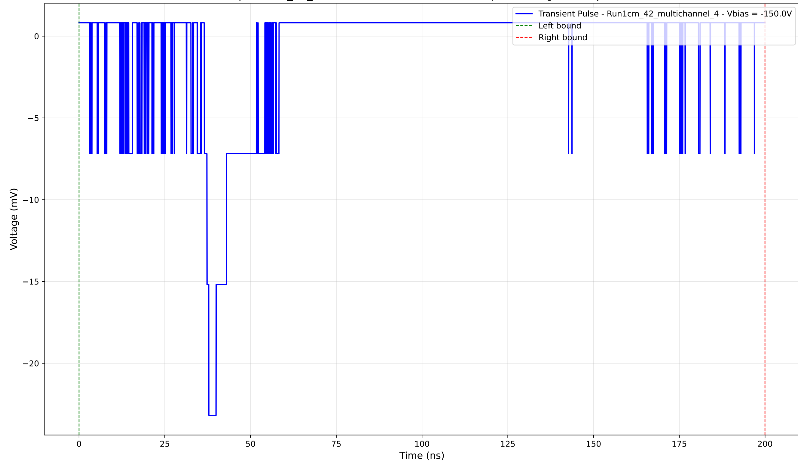
Transient Pulse - Sample: 1cm_42_multichannel - Position: 3565.0 \mu\text{m} - Charge: 2.62 pC - Rise Time: 1.34 ns
