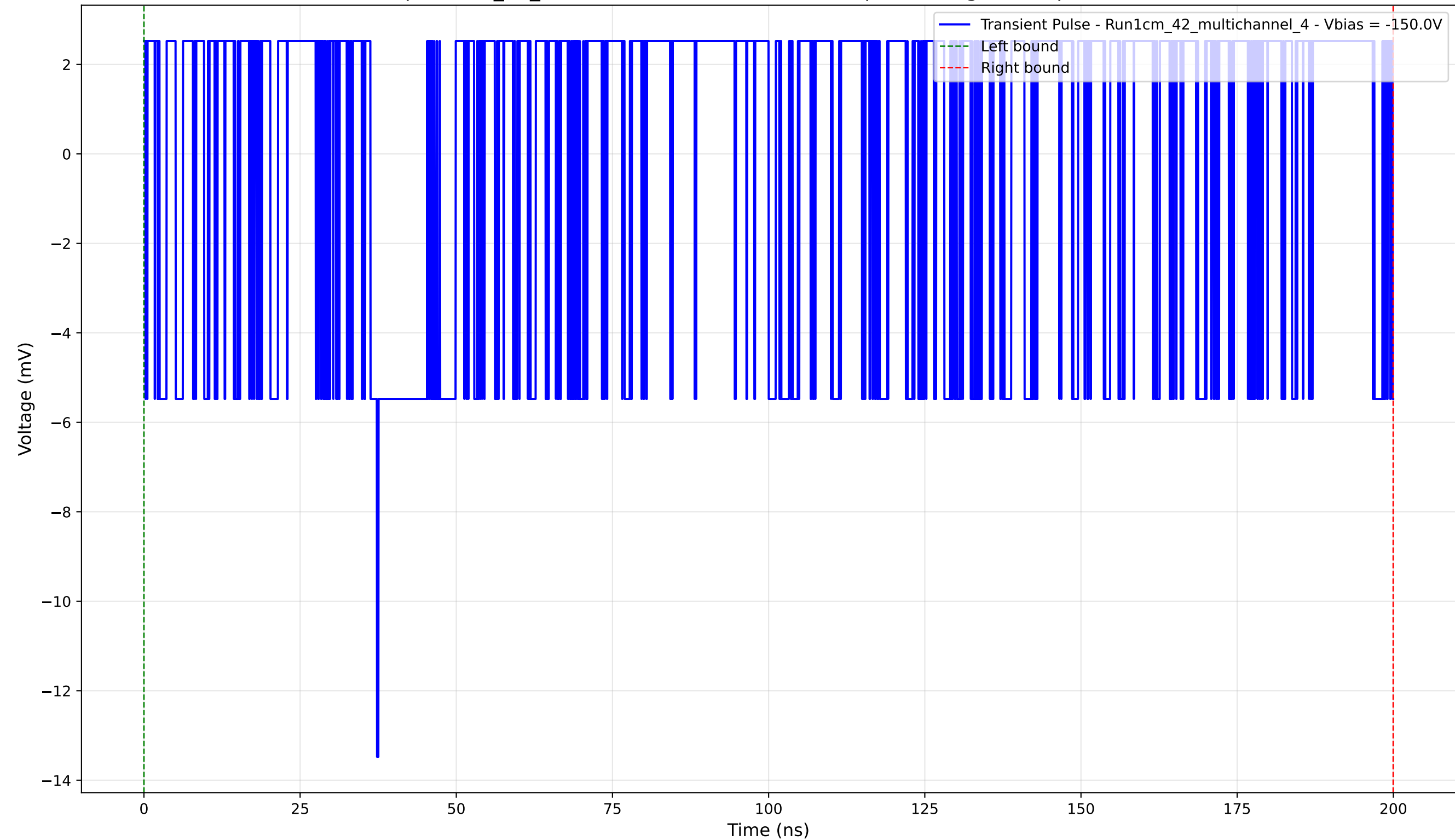
Transient Pulse - Sample: 1cm_42_multichannel - Position: 1915.0 \mu\text{m} - Charge: 0.76 pC - Rise Time: 0.00 ns (N/A)
