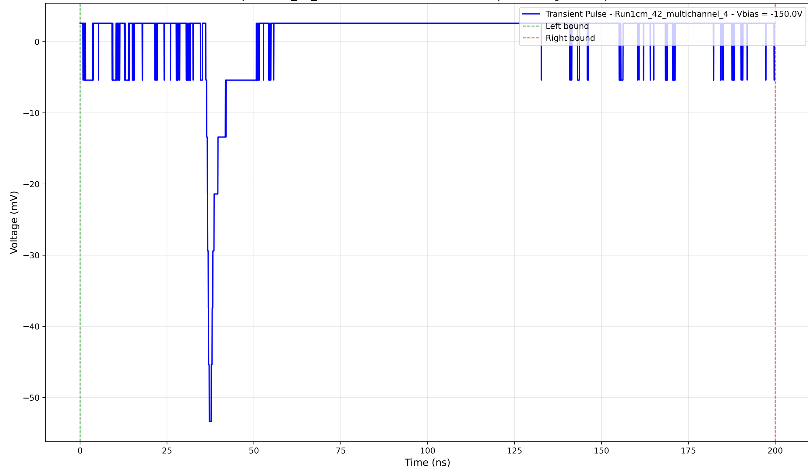
Transient Pulse - Sample: 1cm_42_multichannel - Position: 2715.0 \mu\text{m} - Charge: 3.79 pC - Rise Time: 0.96 ns
