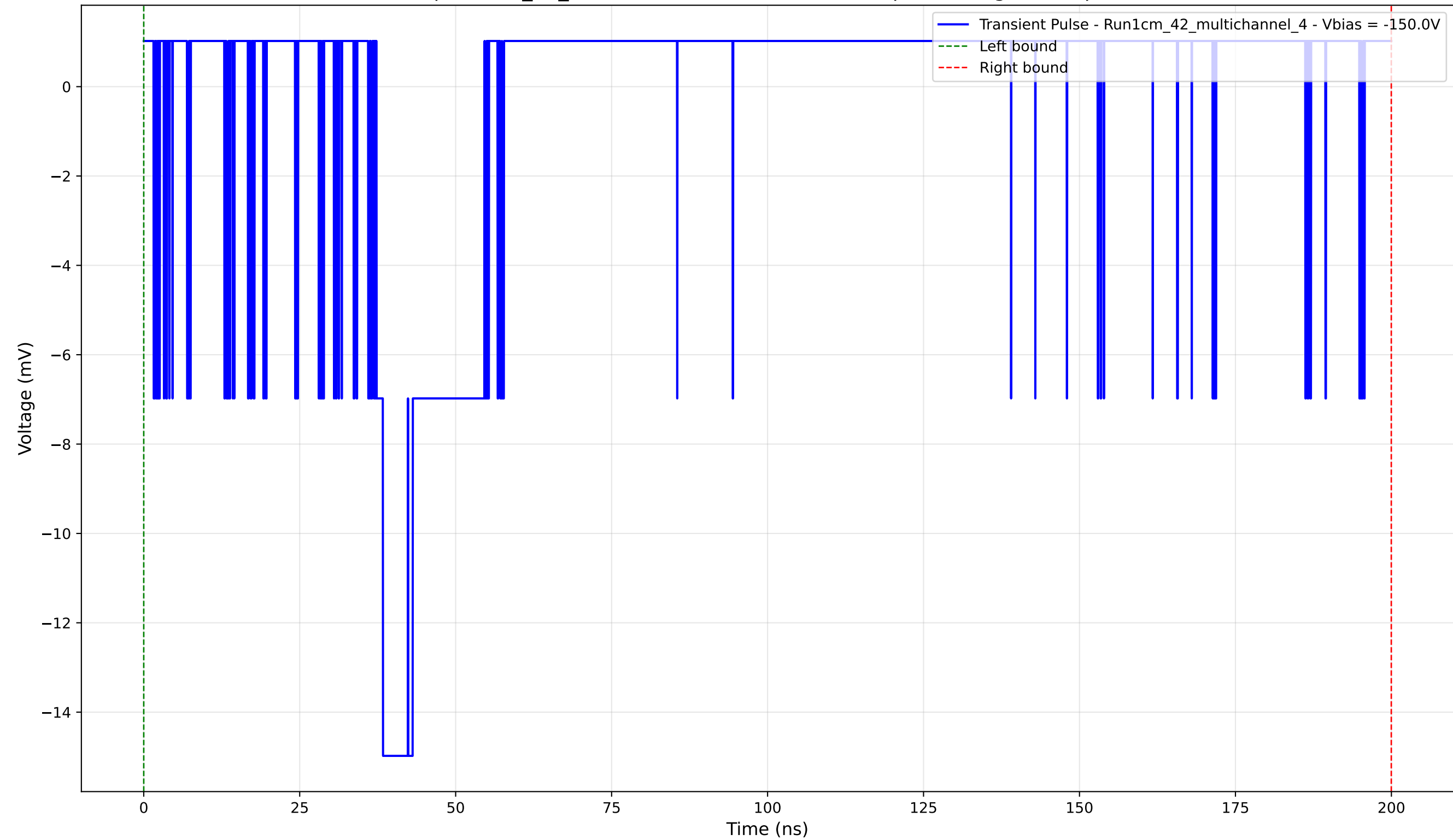
Transient Pulse - Sample: 1cm_42_multichannel - Position: 4520.0 \mu\text{m} - Charge: 0.69 pC - Rise Time: 1.04 ns
