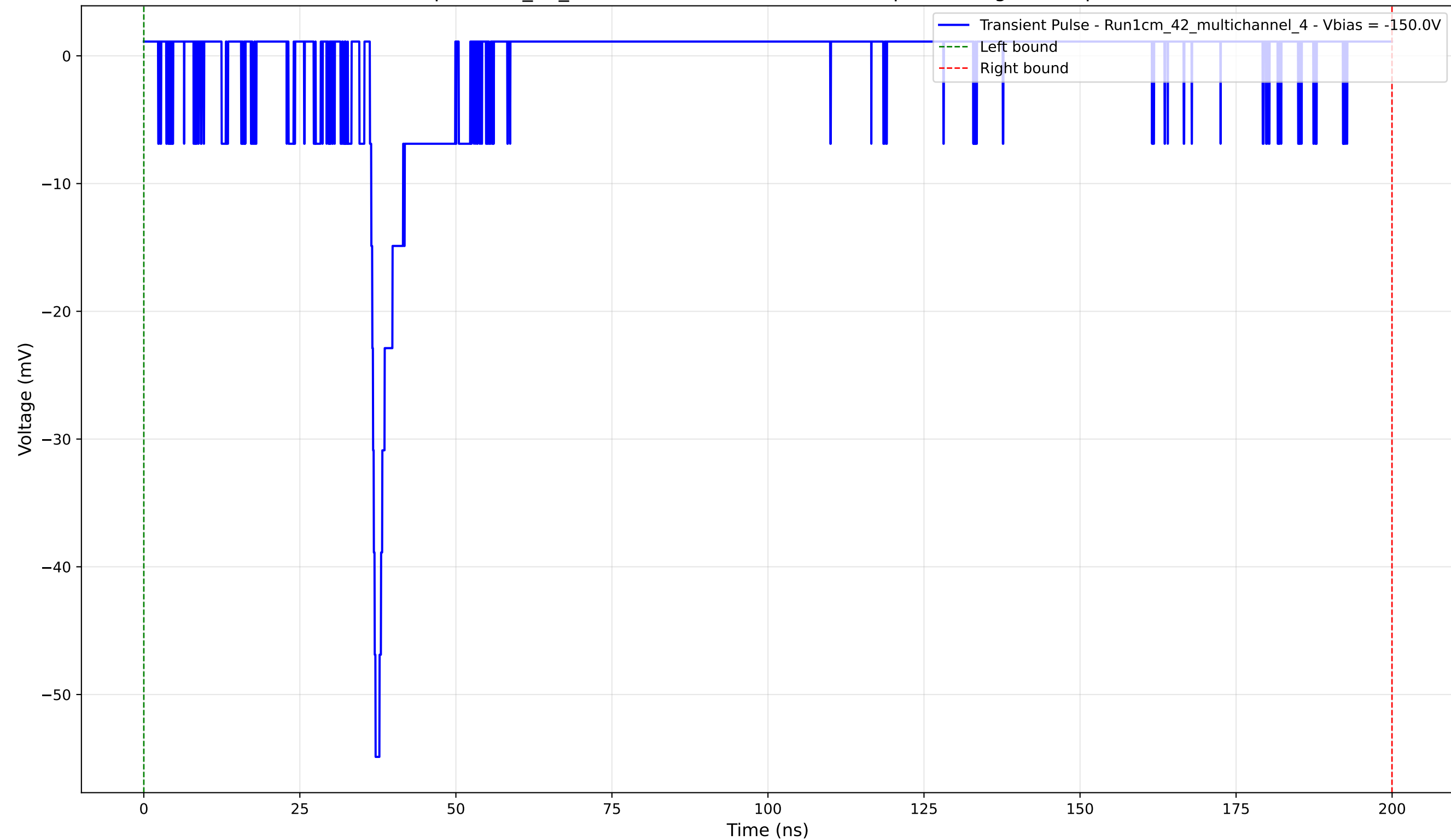
Transient Pulse - Sample: 1cm_42_multichannel - Position: 2700.0 \mu\text{m} - Charge: 2.25 pC - Rise Time: 0.90 ns
