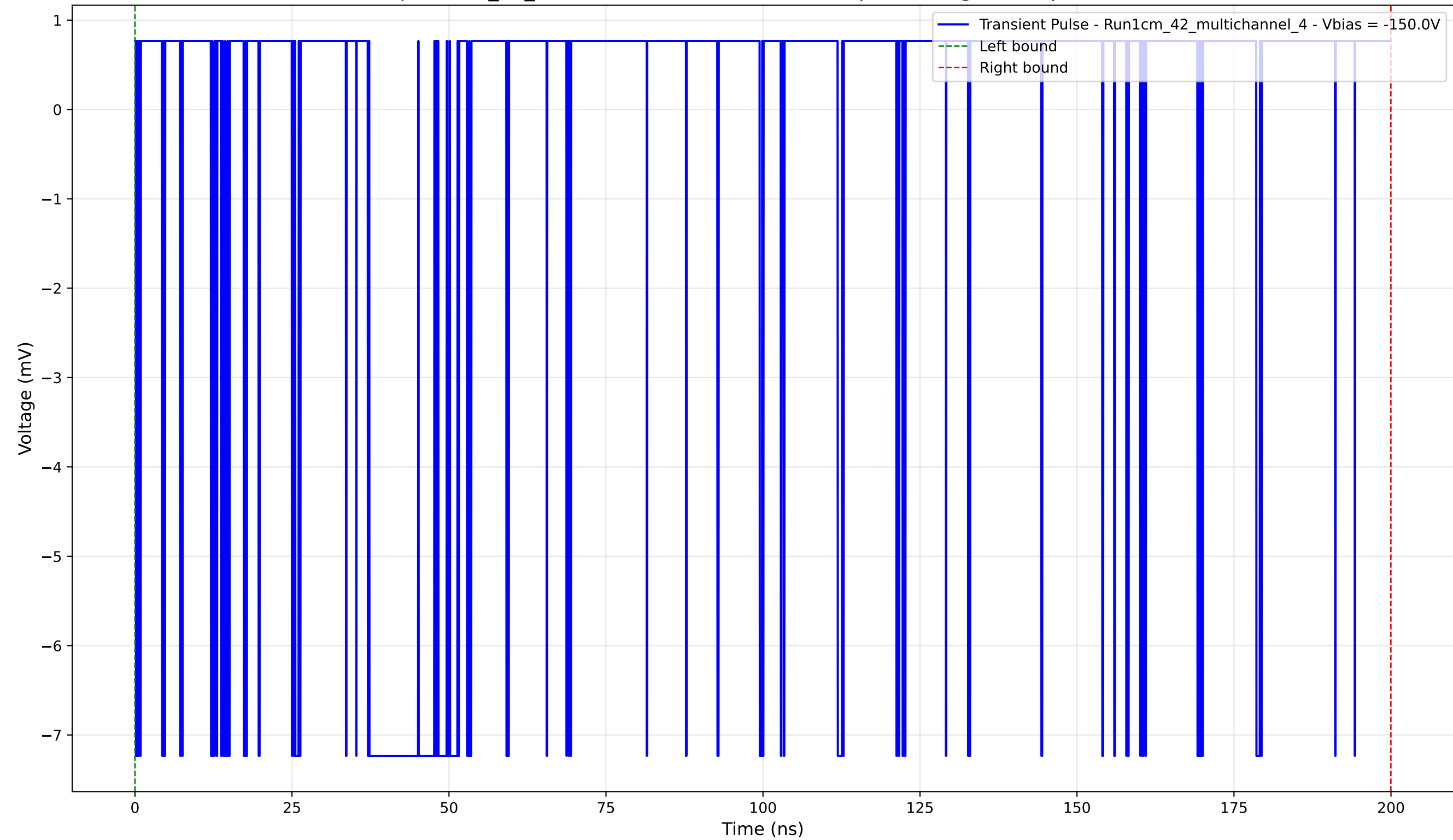
Transient Pulse - Sample: 1cm_42_multichannel - Position: 3860.0 \mu\text{m} - Charge: 0.78 pC - Rise Time: 0.00 ns (N/A)
