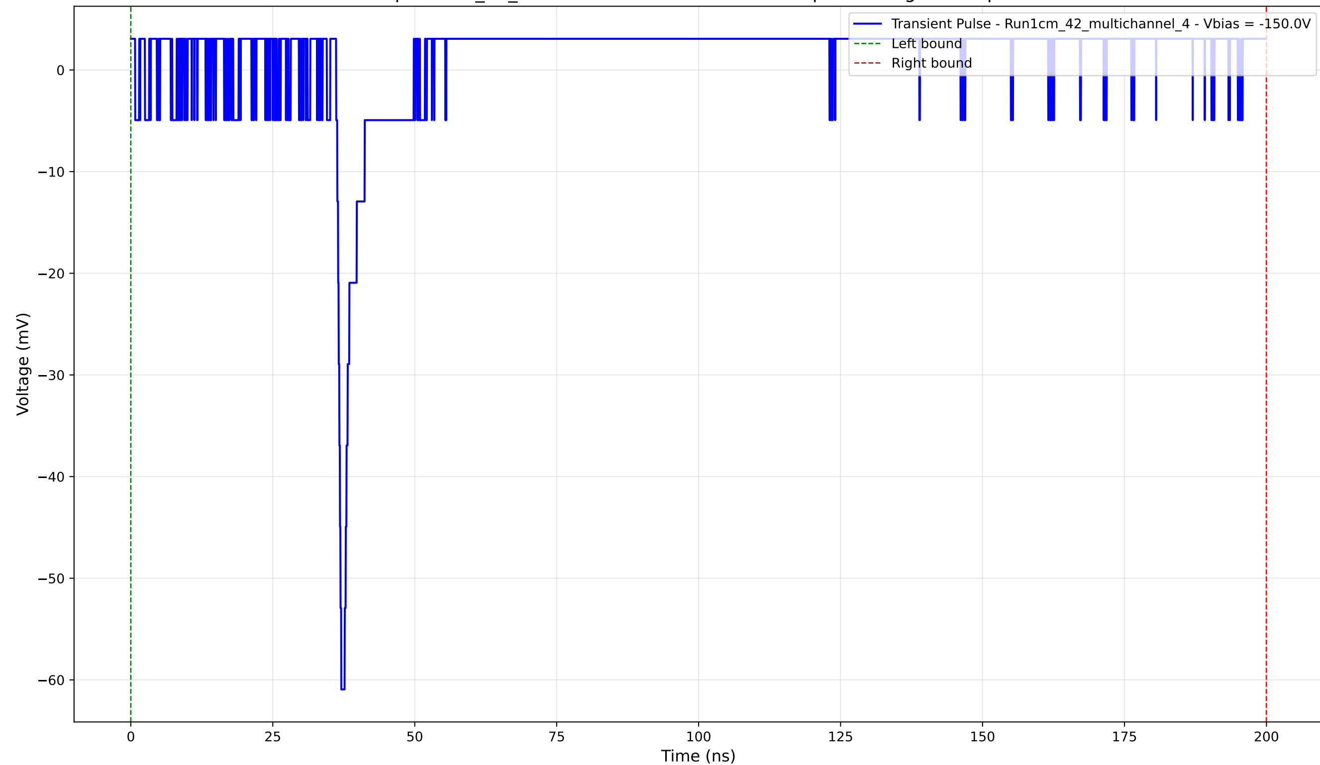
Transient Pulse - Sample: 1cm_42_multichannel - Position: 2605.0 \mu\text{m} - Charge: 5.22 pC - Rise Time: 0.72 ns
