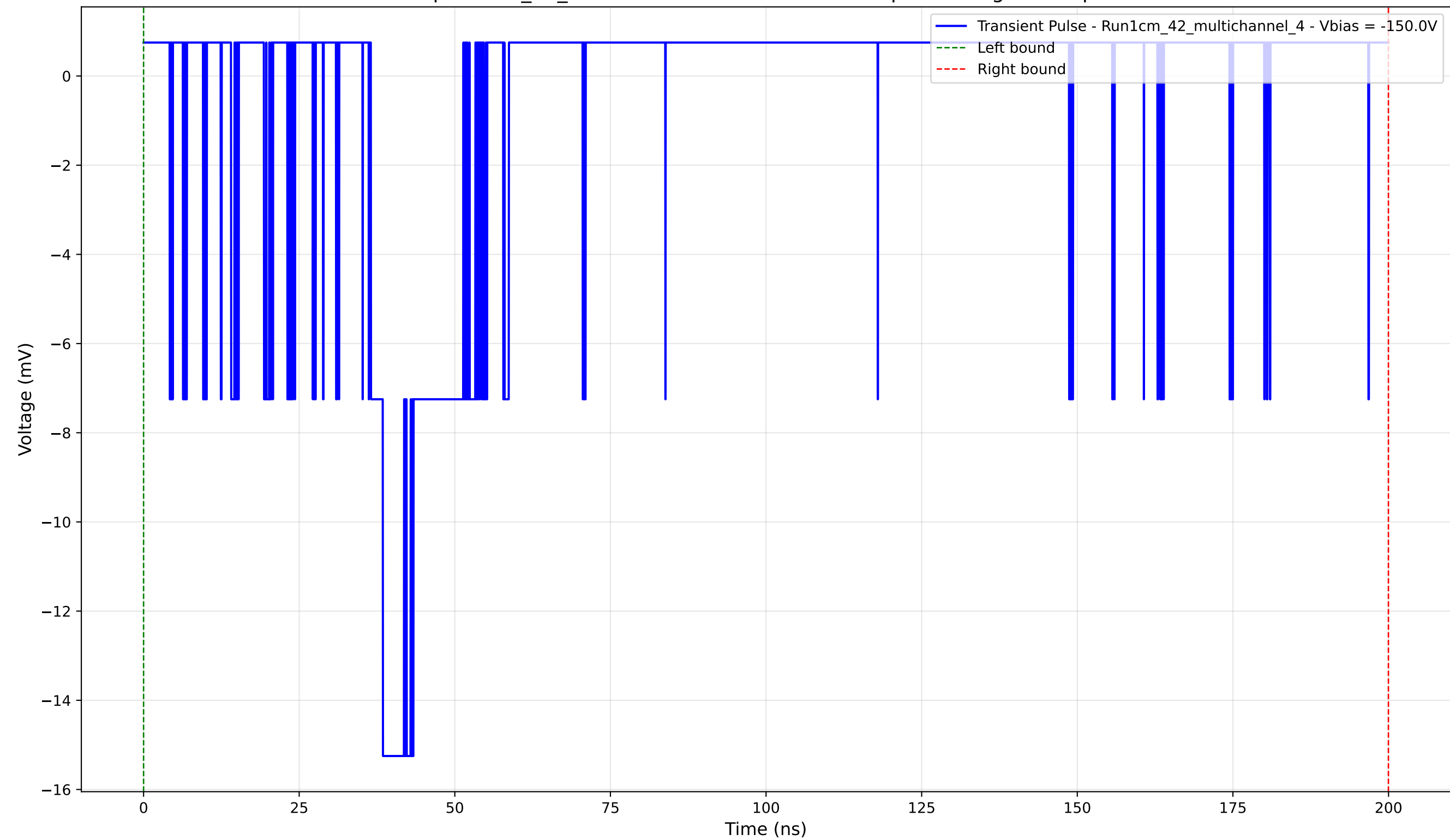
Transient Pulse - Sample: 1cm_42_multichannel - Position: 4680.0 \mu\text{m} - Charge: 1.65 pC - Rise Time: 1.94 ns
