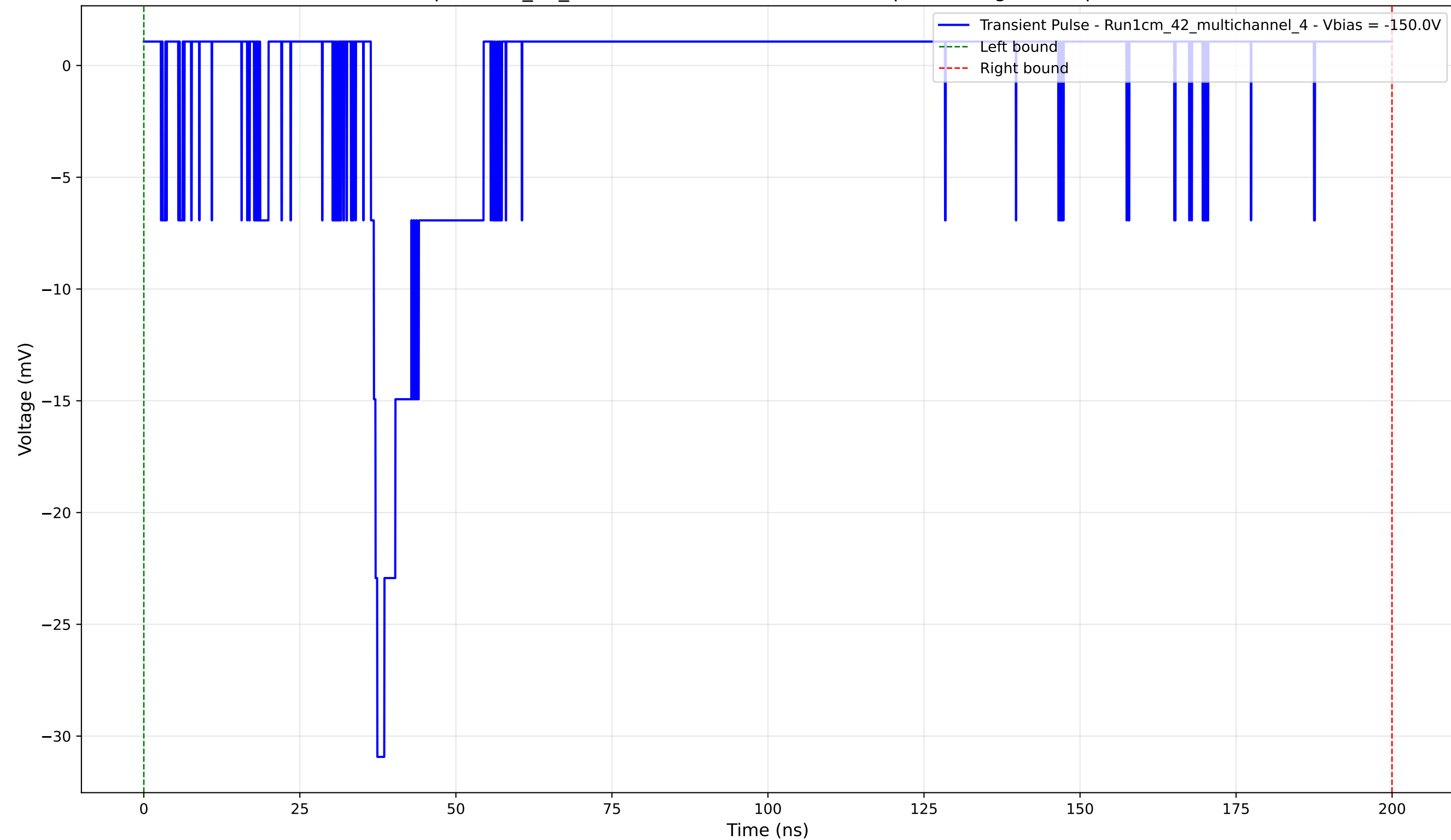
Transient Pulse - Sample: 1cm_42_multichannel - Position: 1565.0 \mu\text{m} - Charge: 1.70 pC - Rise Time: 1.03 ns
