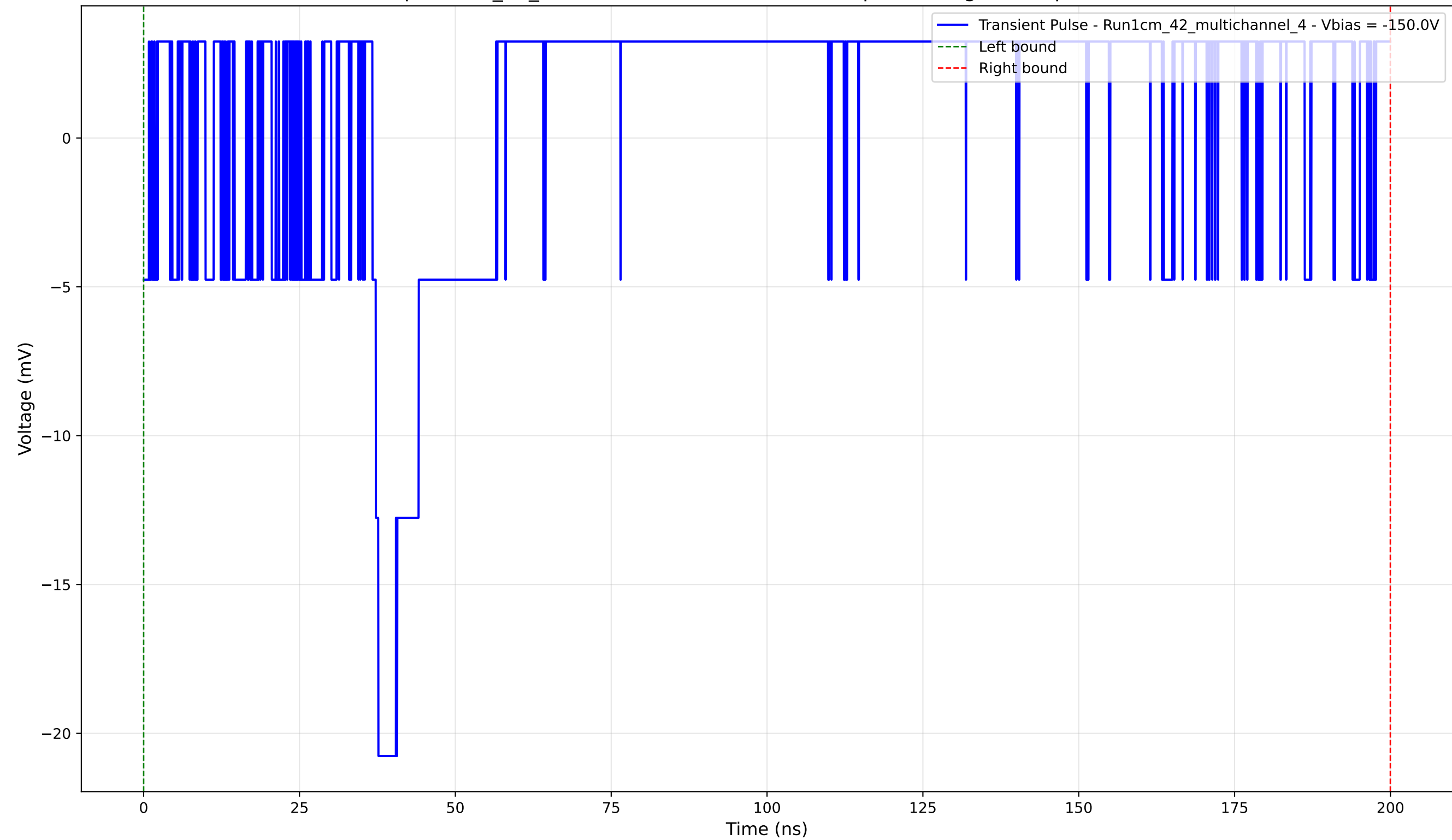
Transient Pulse - Sample: 1cm_42_multichannel - Position: 1215.0 \mu\text{m} - Charge: 4.18 pC - Rise Time: 0.00 ns (N/A)
