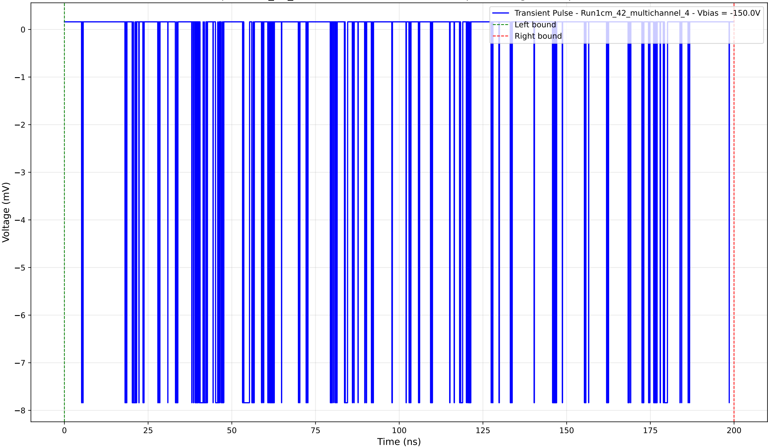
Transient Pulse - Sample: 1cm_42_multichannel - Position: 3925.0 \mu\text{m} - Charge: 2.81 pC - Rise Time: 0.02 ns
