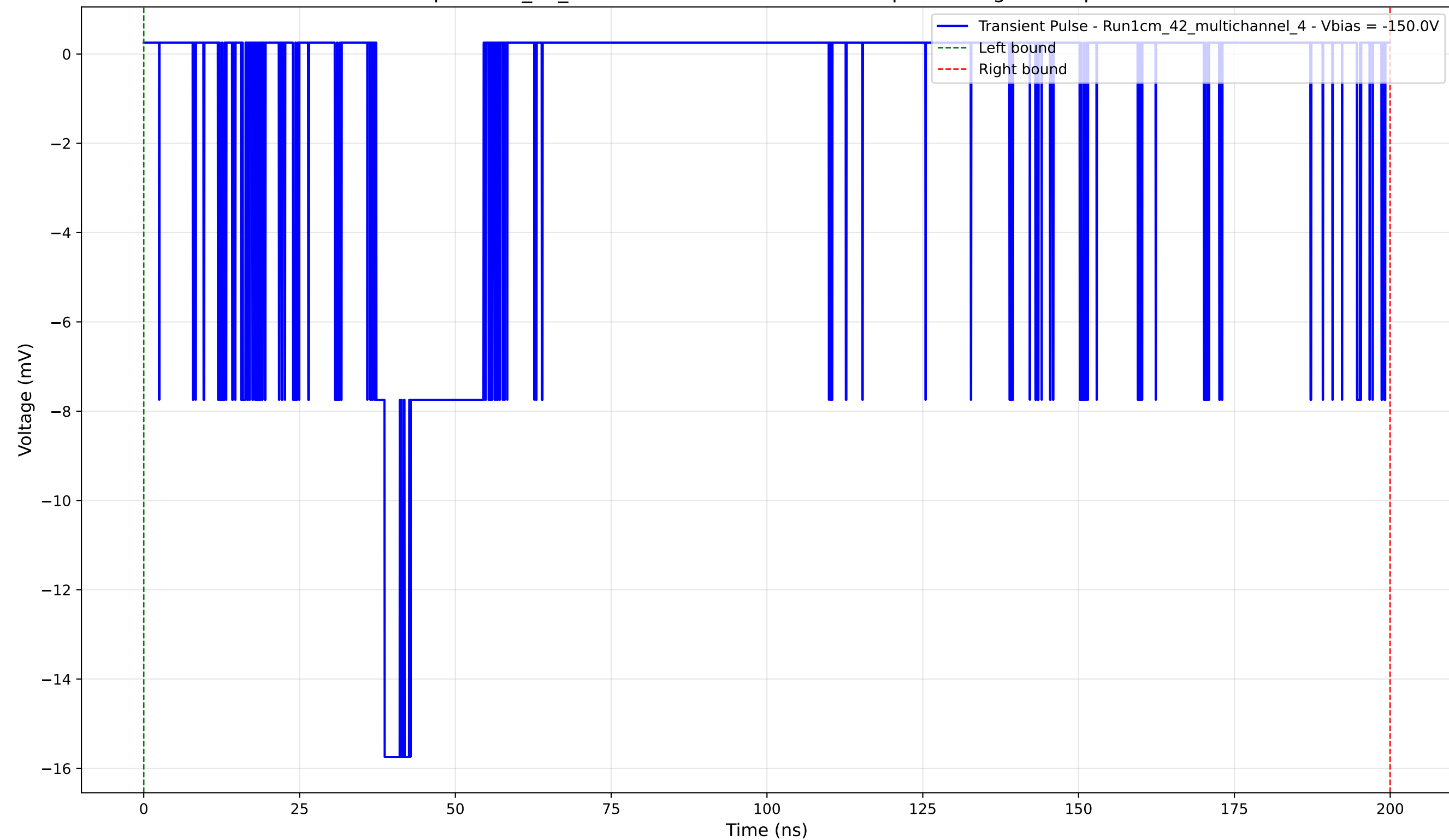
Transient Pulse - Sample: 1cm_42_multichannel - Position: 4475.0 \mu\text{m} - Charge: 4.25 pC - Rise Time: 1.34 ns
