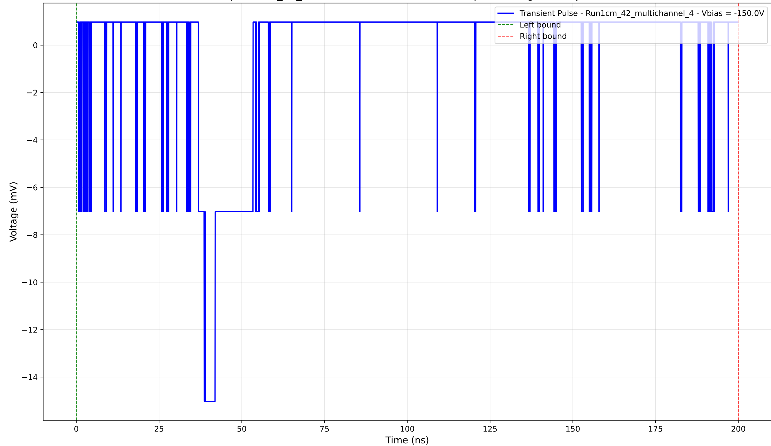
Transient Pulse - Sample: 1cm_42_multichannel - Position: 4765.0 \mu\text{m} - Charge: 0.61 pC - Rise Time: 1.74 ns
