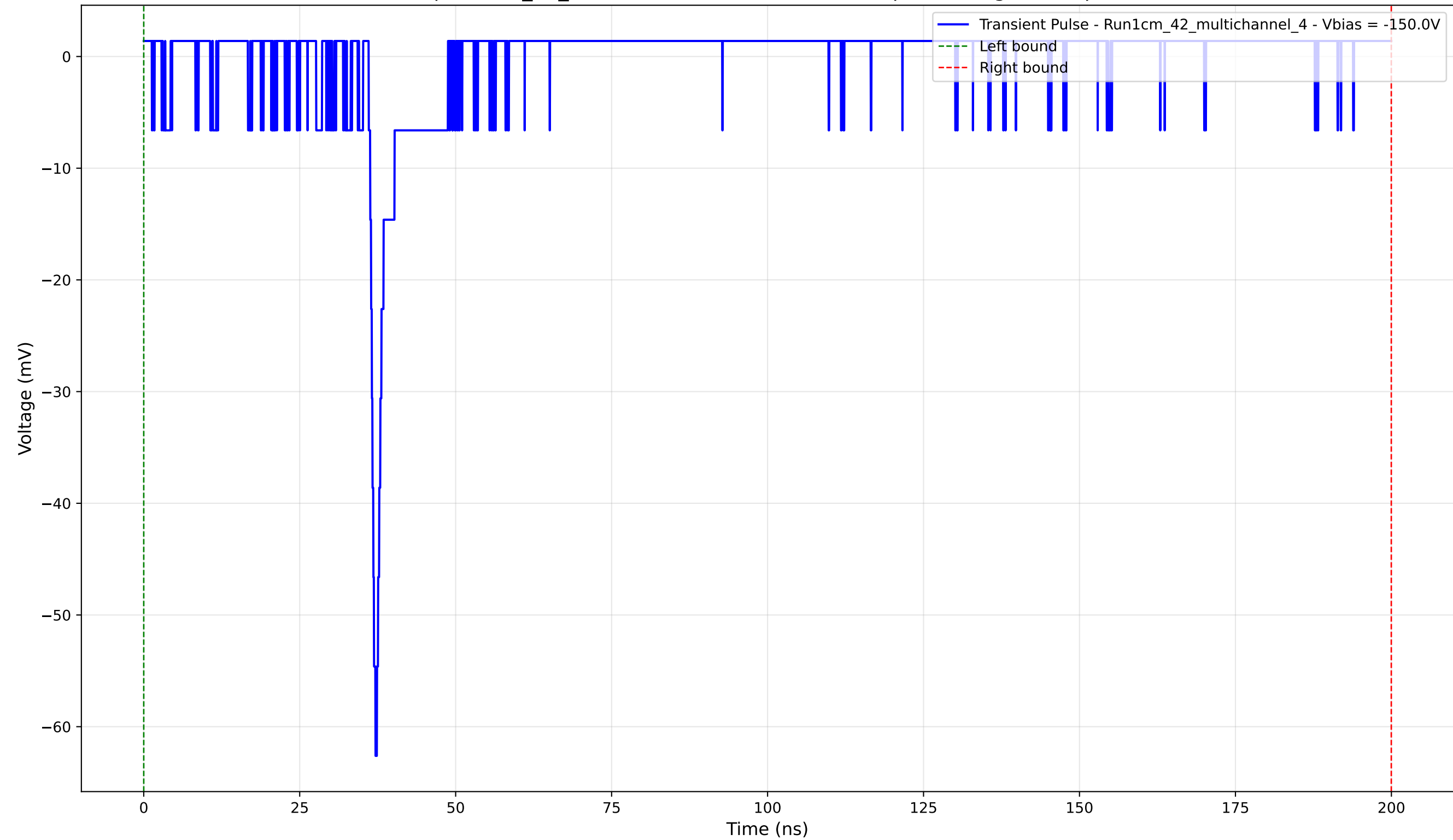
Transient Pulse - Sample: 1cm_42_multichannel - Position: 2445.0 \mu\text{m} - Charge: 0.37 pC - Rise Time: 1.08 ns
