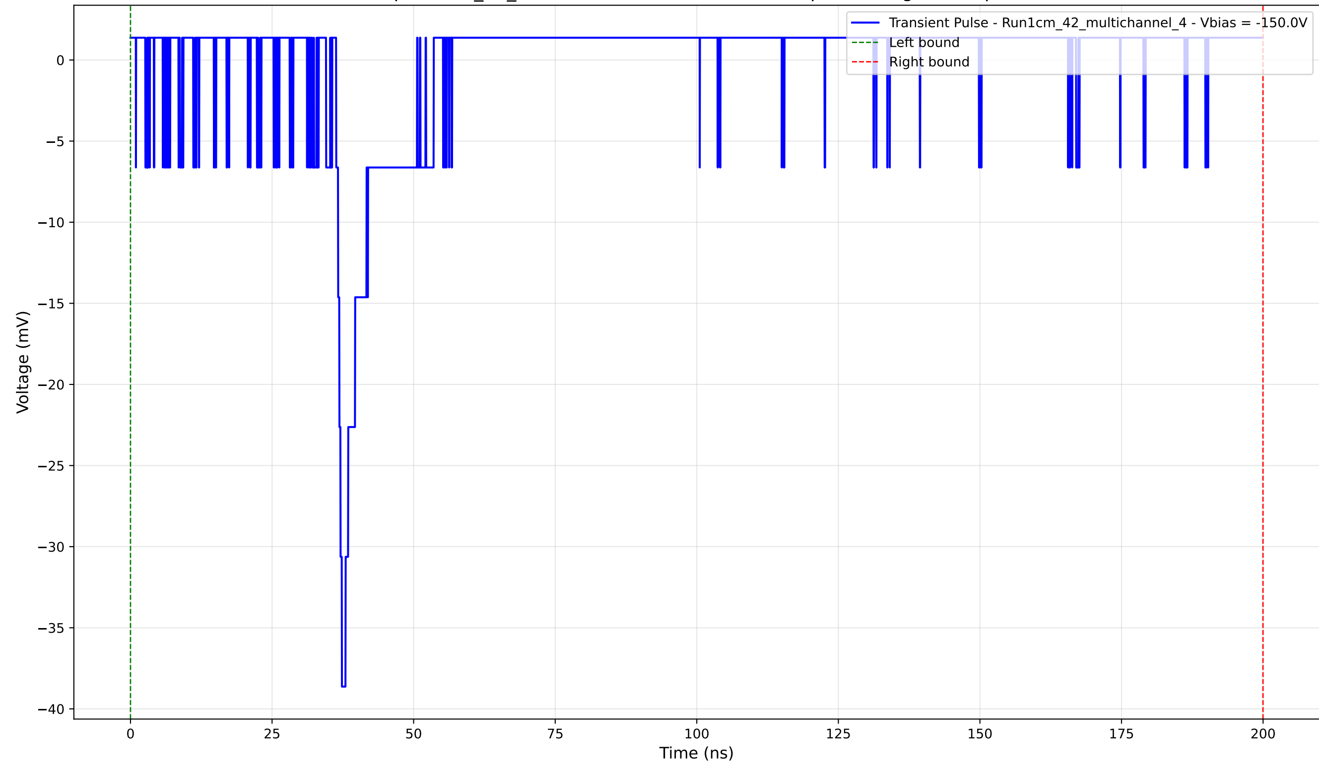
Transient Pulse - Sample: 1cm_42_multichannel - Position: 2970.0 \mu\text{m} - Charge: 0.27 pC - Rise Time: 1.01 ns
