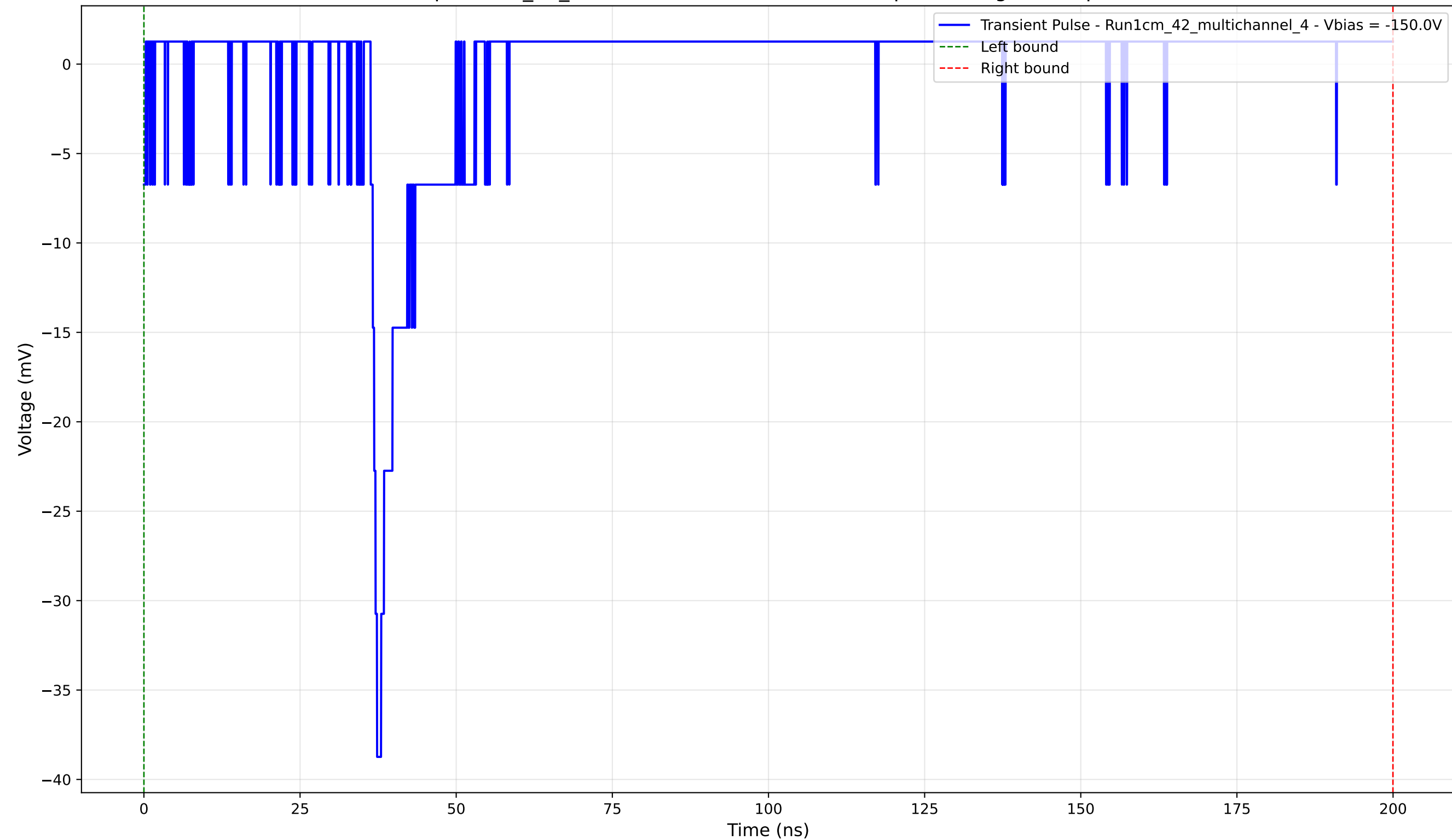
Transient Pulse - Sample: 1cm_42_multichannel - Position: 2995.0 \mu\text{m} - Charge: 0.36 pC - Rise Time: 1.03 ns
