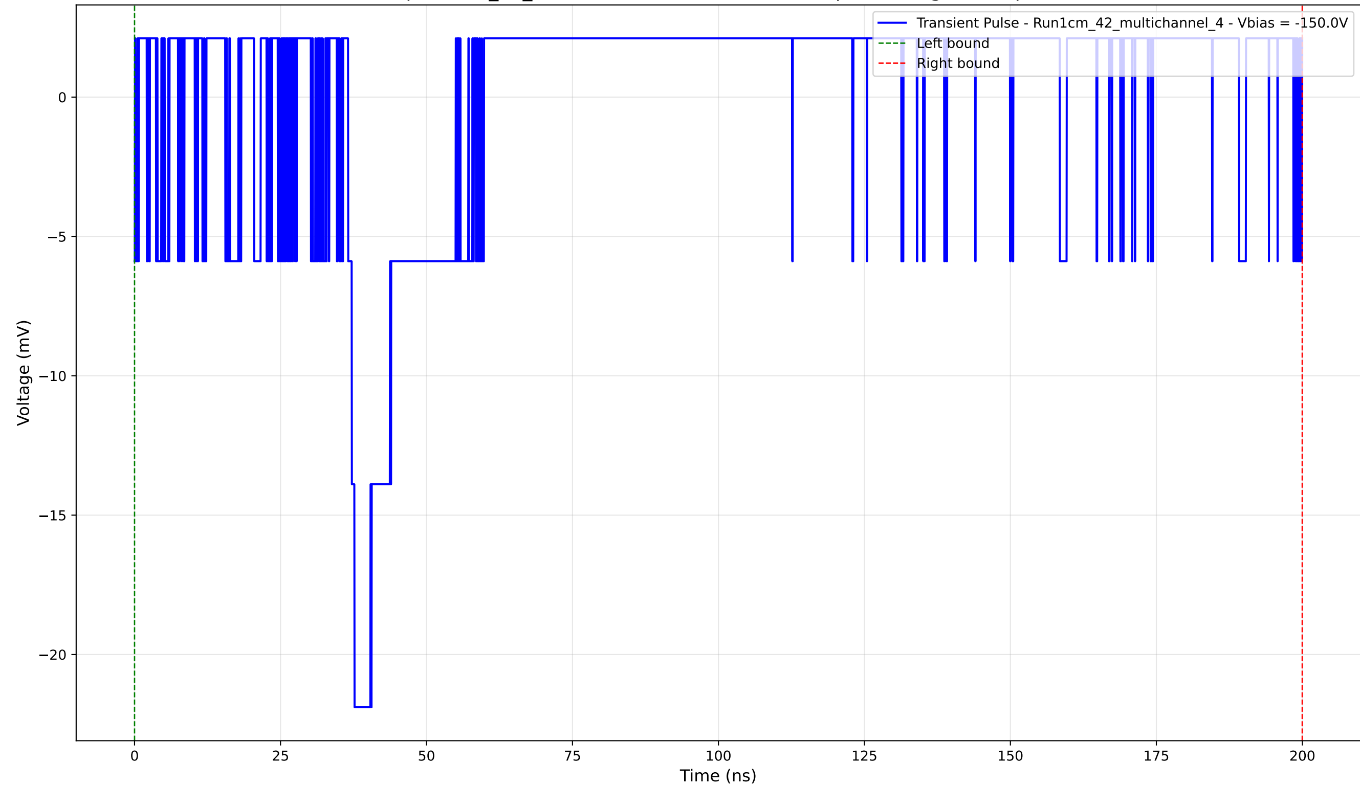
Transient Pulse - Sample: 1cm_42_multichannel - Position: 1205.0 \mu\text{m} - Charge: 0.72 pC - Rise Time: 1.10 ns
