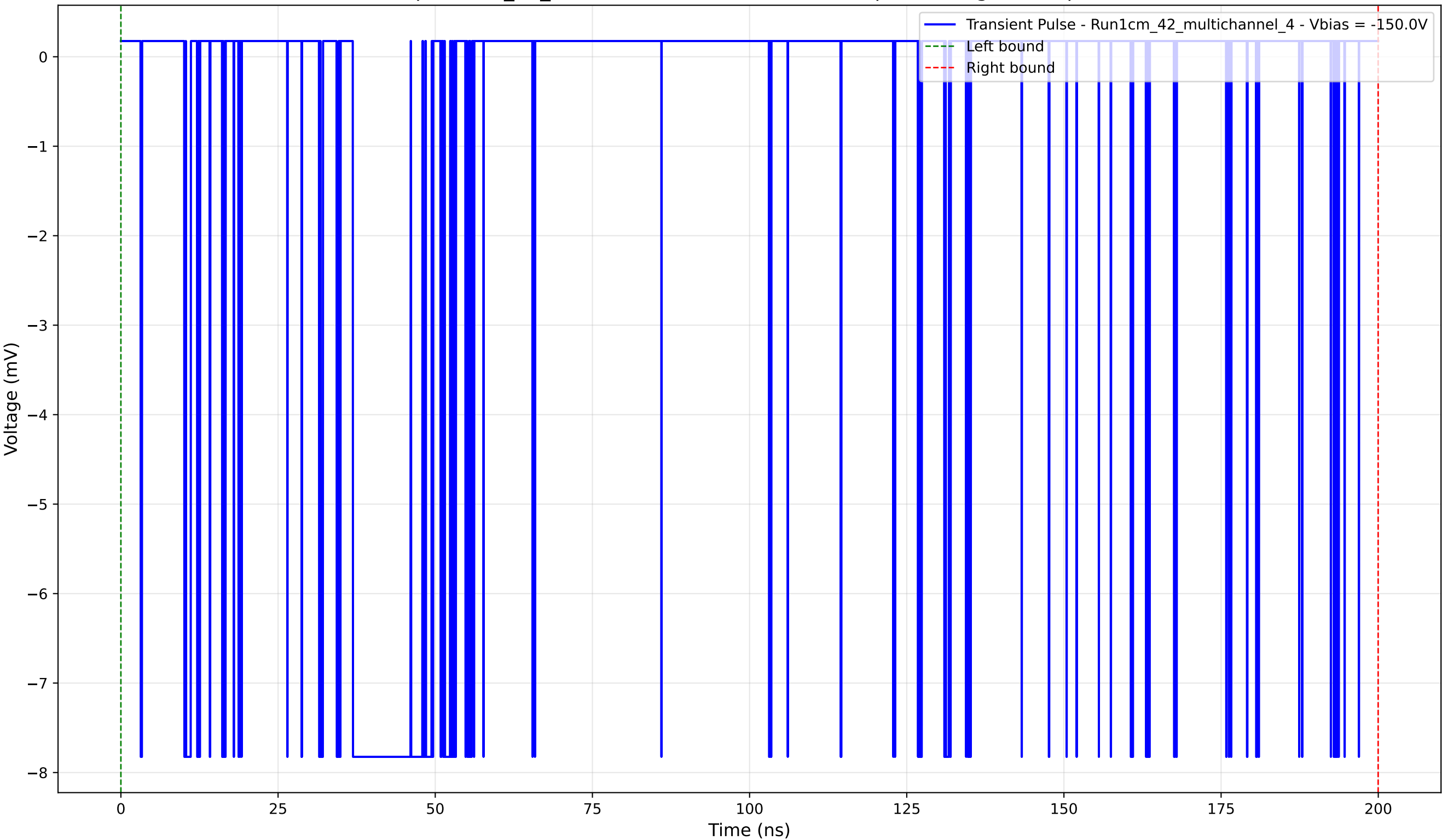
Transient Pulse - Sample: 1cm_42_multichannel - Position: 3950.0 \mu\text{m} - Charge: 2.89 pC - Rise Time: 0.02 ns
