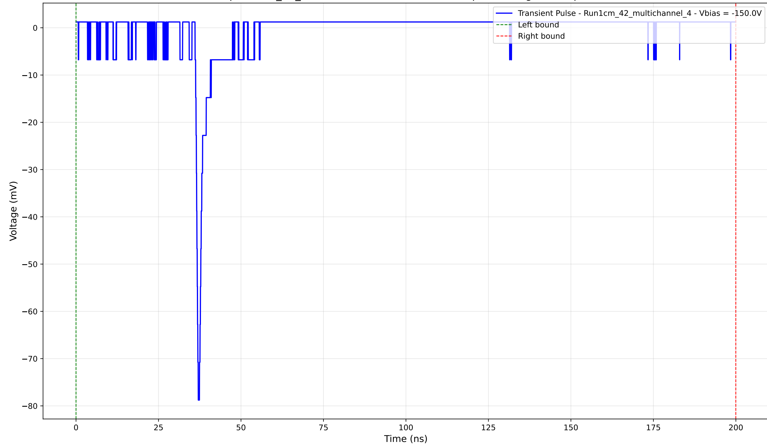
Transient Pulse - Sample: 1cm_42_multichannel - Position: 2460.0 \mu\text{m} - Charge: 1.37 pC - Rise Time: 0.80 ns
