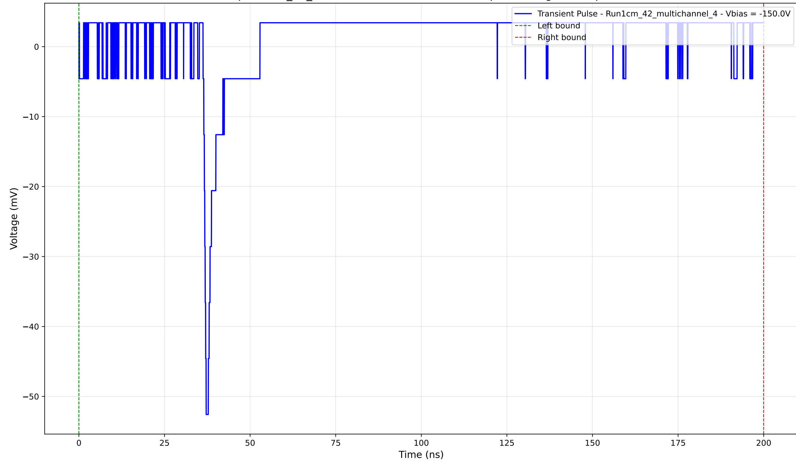
Transient Pulse - Sample: 1cm_42_multichannel - Position: 2015.0 \mu\text{m} - Charge: 6.54 pC - Rise Time: 0.70 ns
