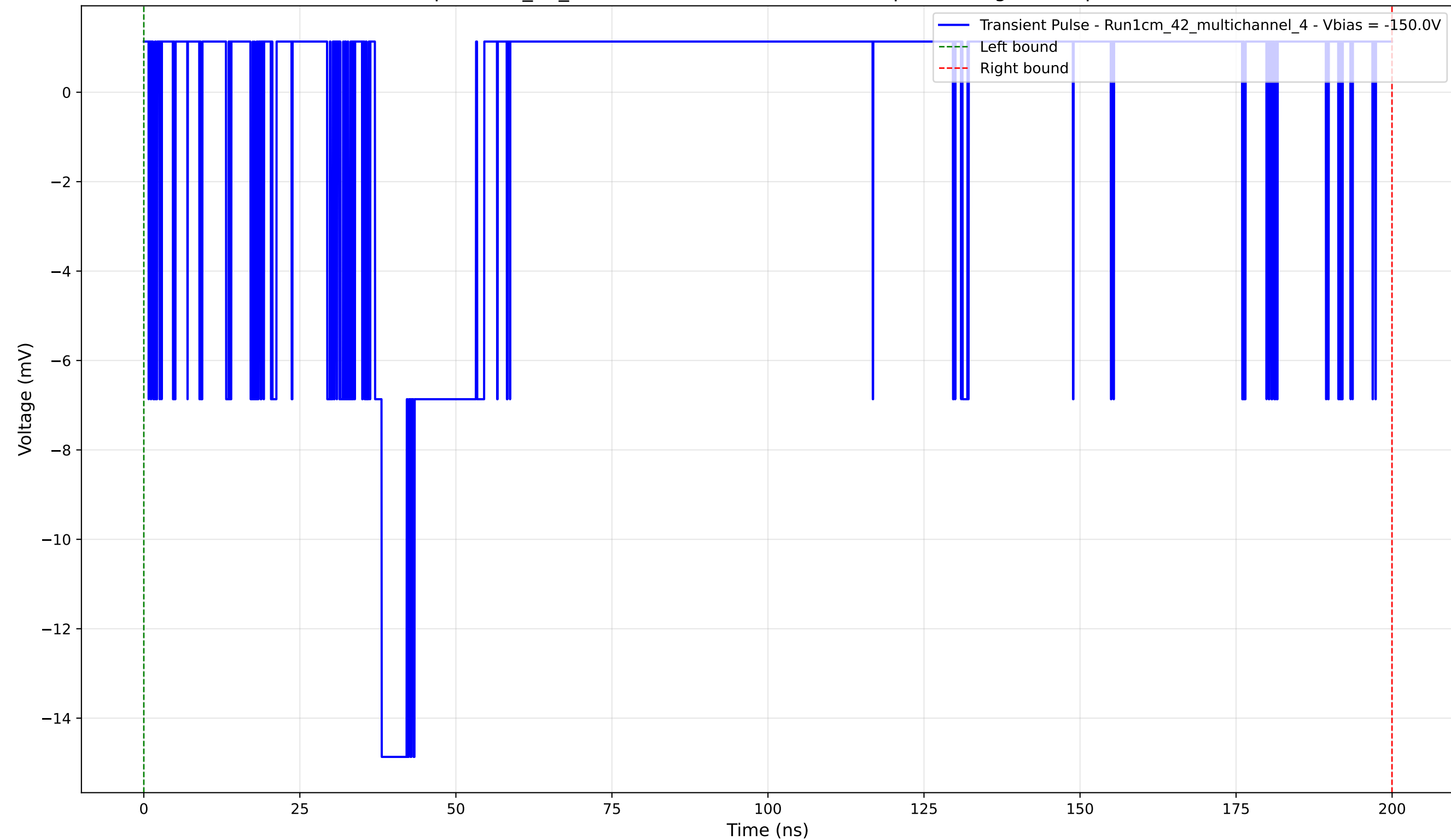
Transient Pulse - Sample: 1cm_42_multichannel - Position: 4070.0 \mu\text{m} - Charge: 0.80 pC - Rise Time: 1.08 ns
