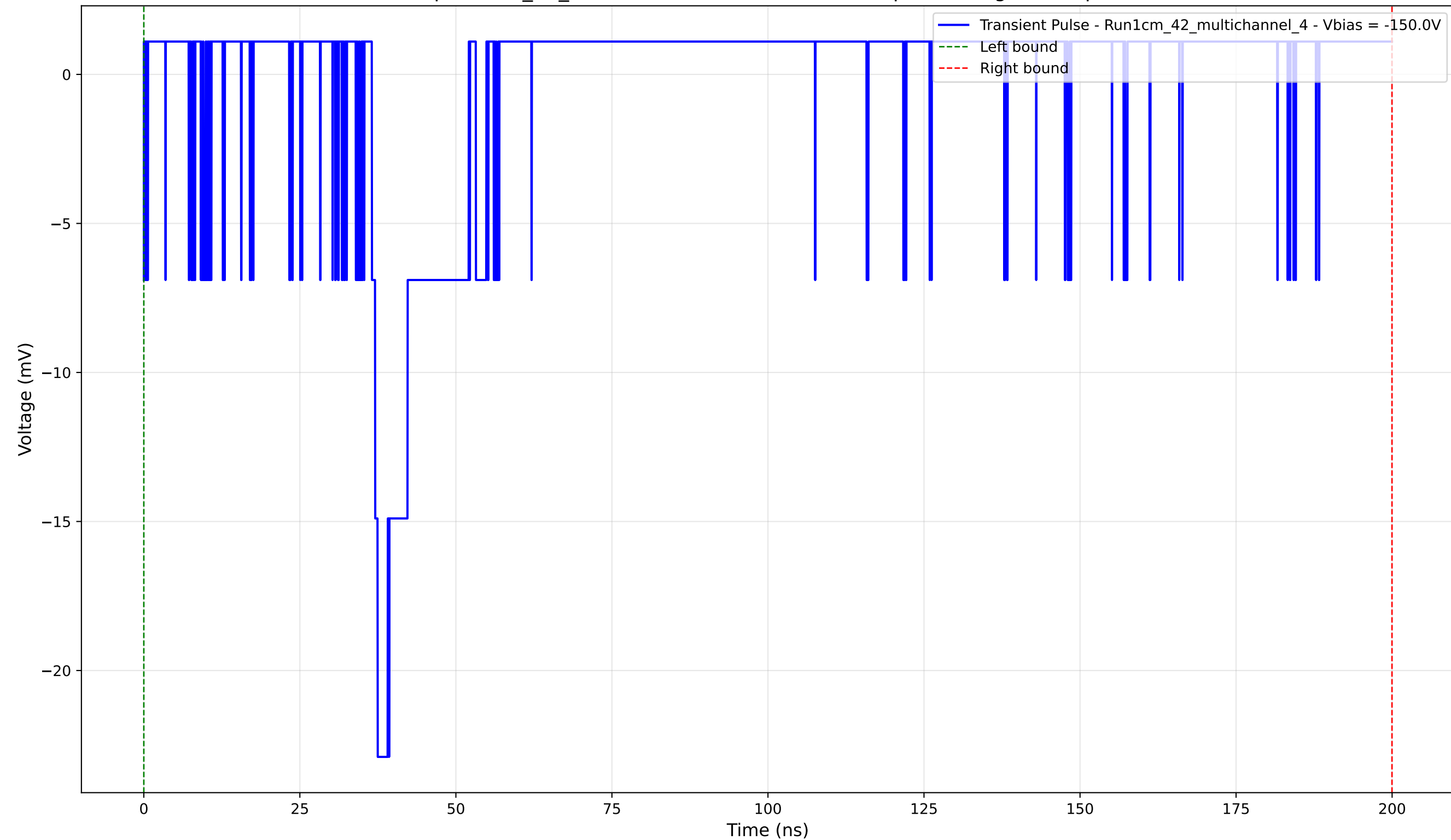
Transient Pulse - Sample: 1cm_42_multichannel - Position: 3325.0 \mu\text{m} - Charge: 0.68 pC - Rise Time: 0.94 ns
