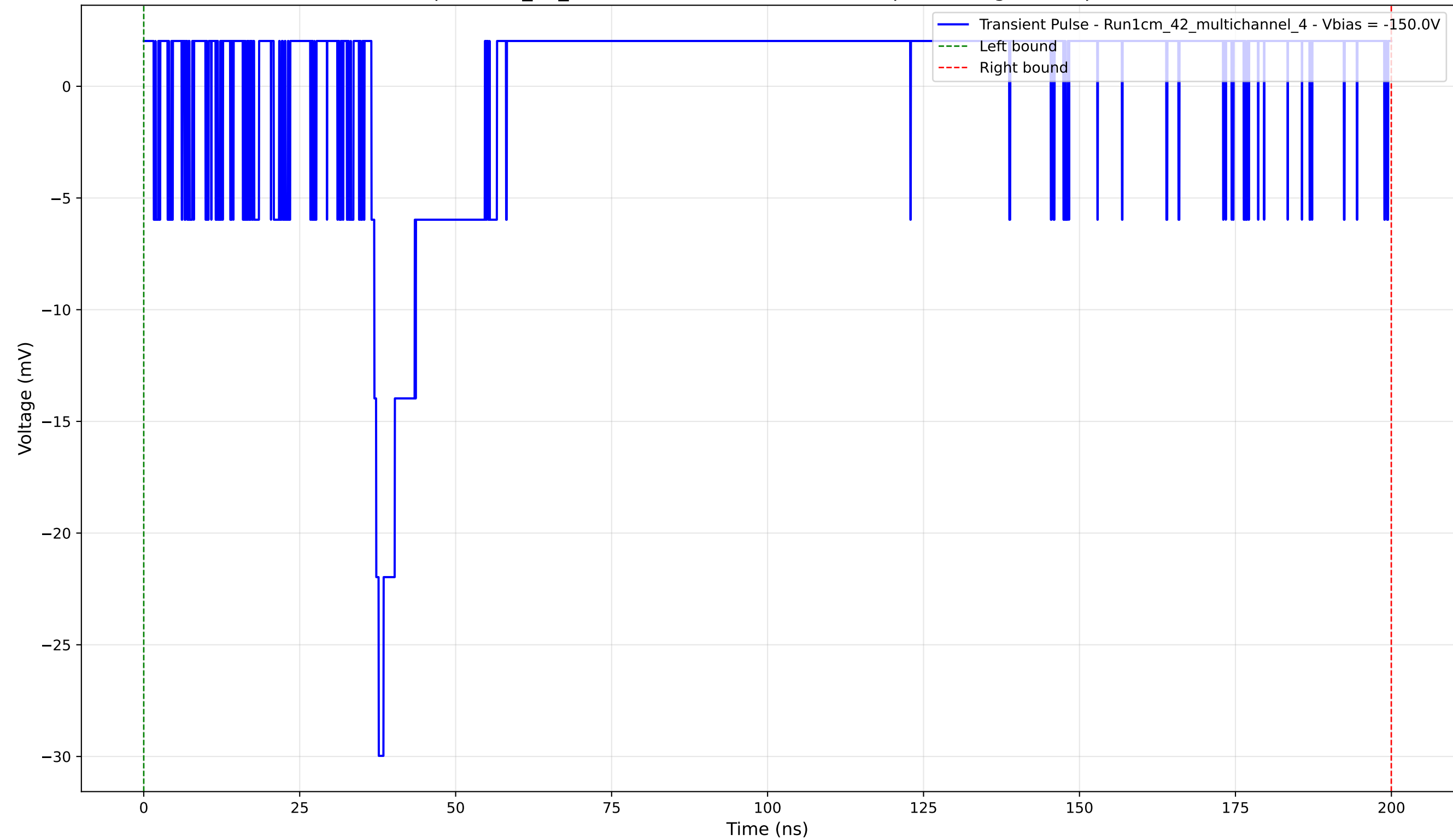
Transient Pulse - Sample: 1cm_42_multichannel - Position: 1475.0 \mu\text{m} - Charge: 1.19 pC - Rise Time: 1.18 ns
