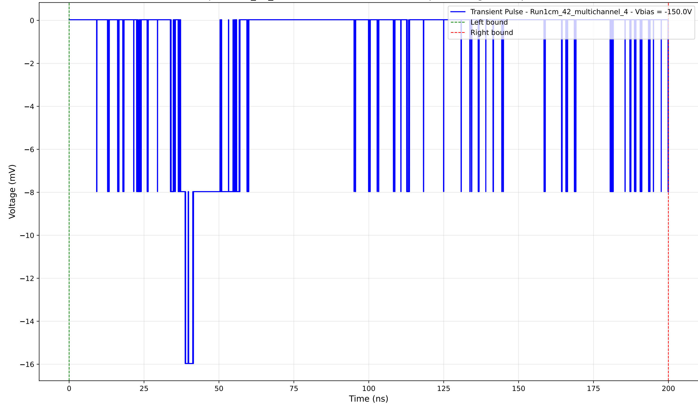
Transient Pulse - Sample: 1cm_42_multichannel - Position: 4470.0 \mu\text{m} - Charge: 4.75 pC - Rise Time: 1.52 ns
