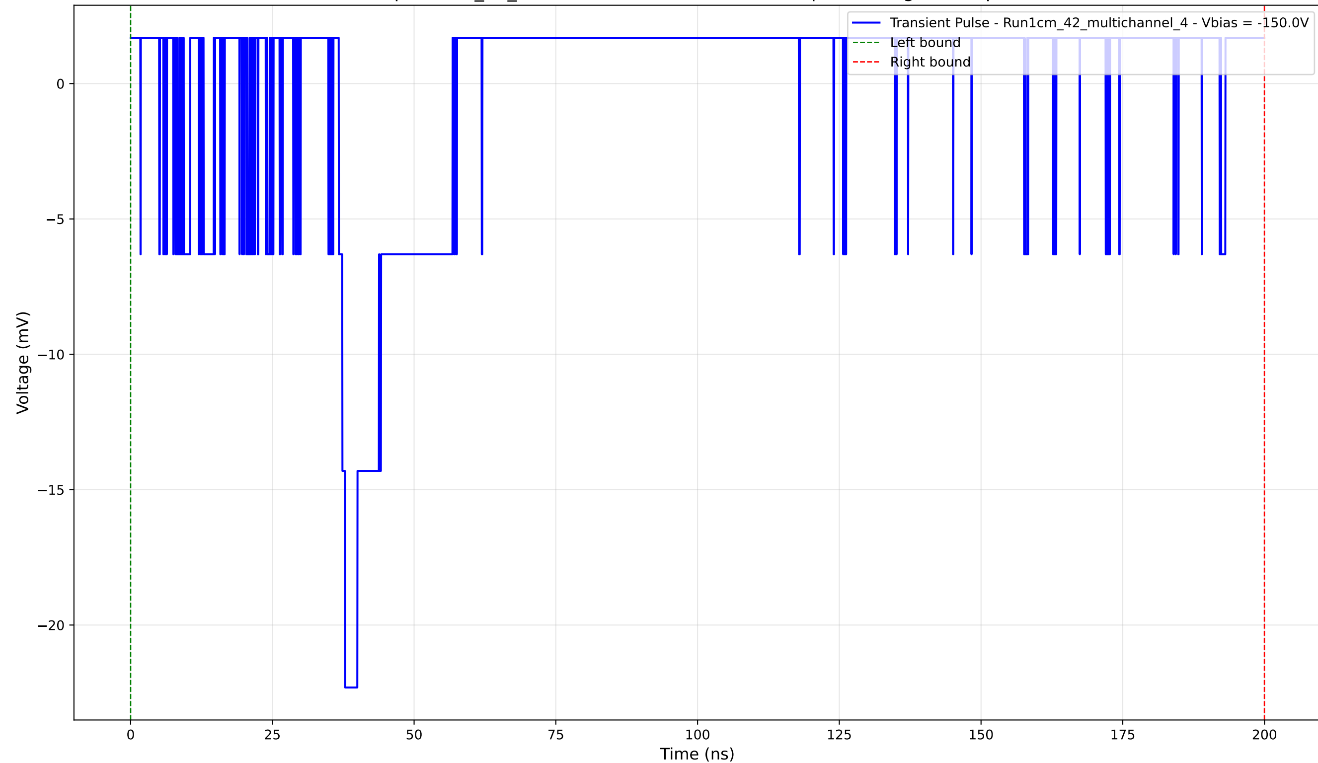
Transient Pulse - Sample: 1cm_42_multichannel - Position: 1155.0 \mu\text{m} - Charge: 0.21 pC - Rise Time: 1.12 ns
