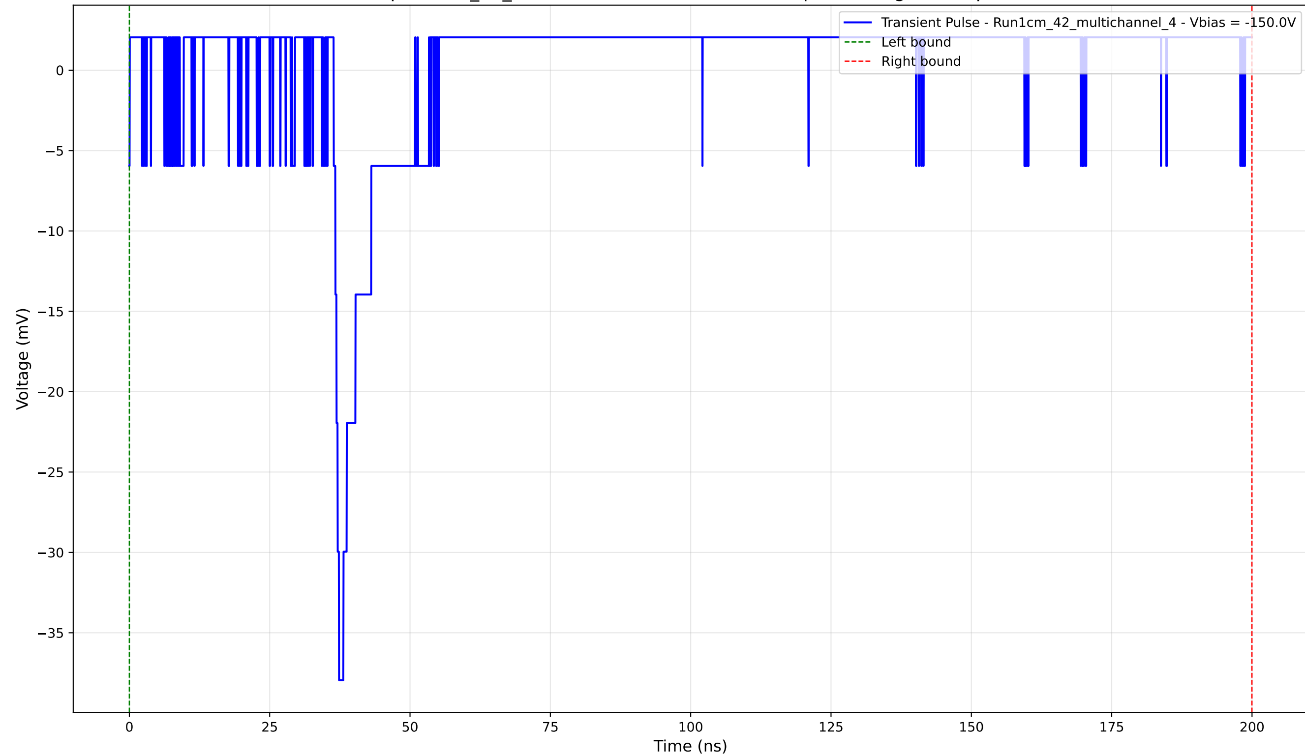
Transient Pulse - Sample: 1cm_42_multichannel - Position: 1735.0 \mu\text{m} - Charge: 2.12 pC - Rise Time: 0.95 ns
