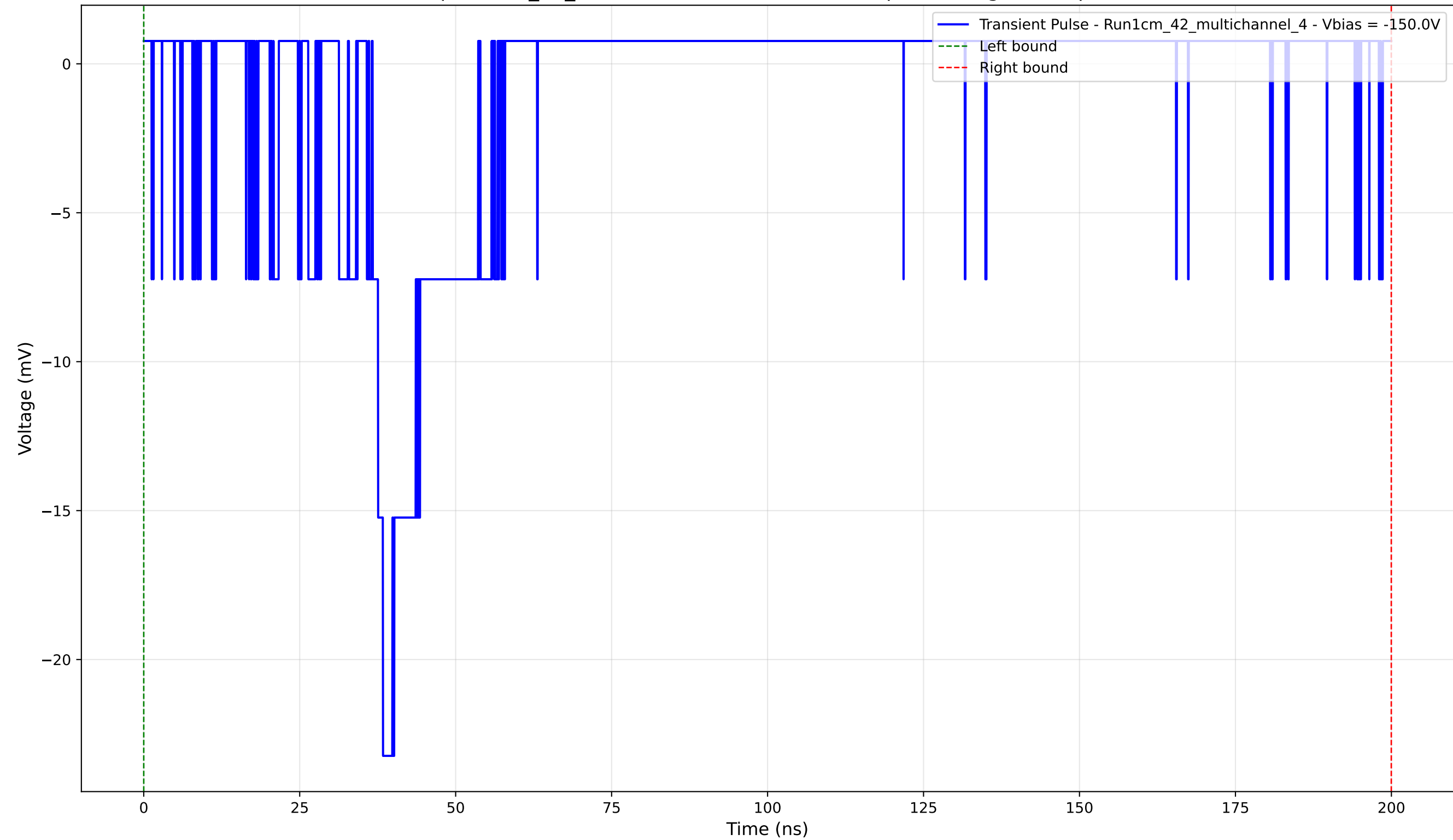
Transient Pulse - Sample: 1cm_42_multichannel - Position: 980.0 \mu\text{m} - Charge: 3.13 pC - Rise Time: 1.66 ns
