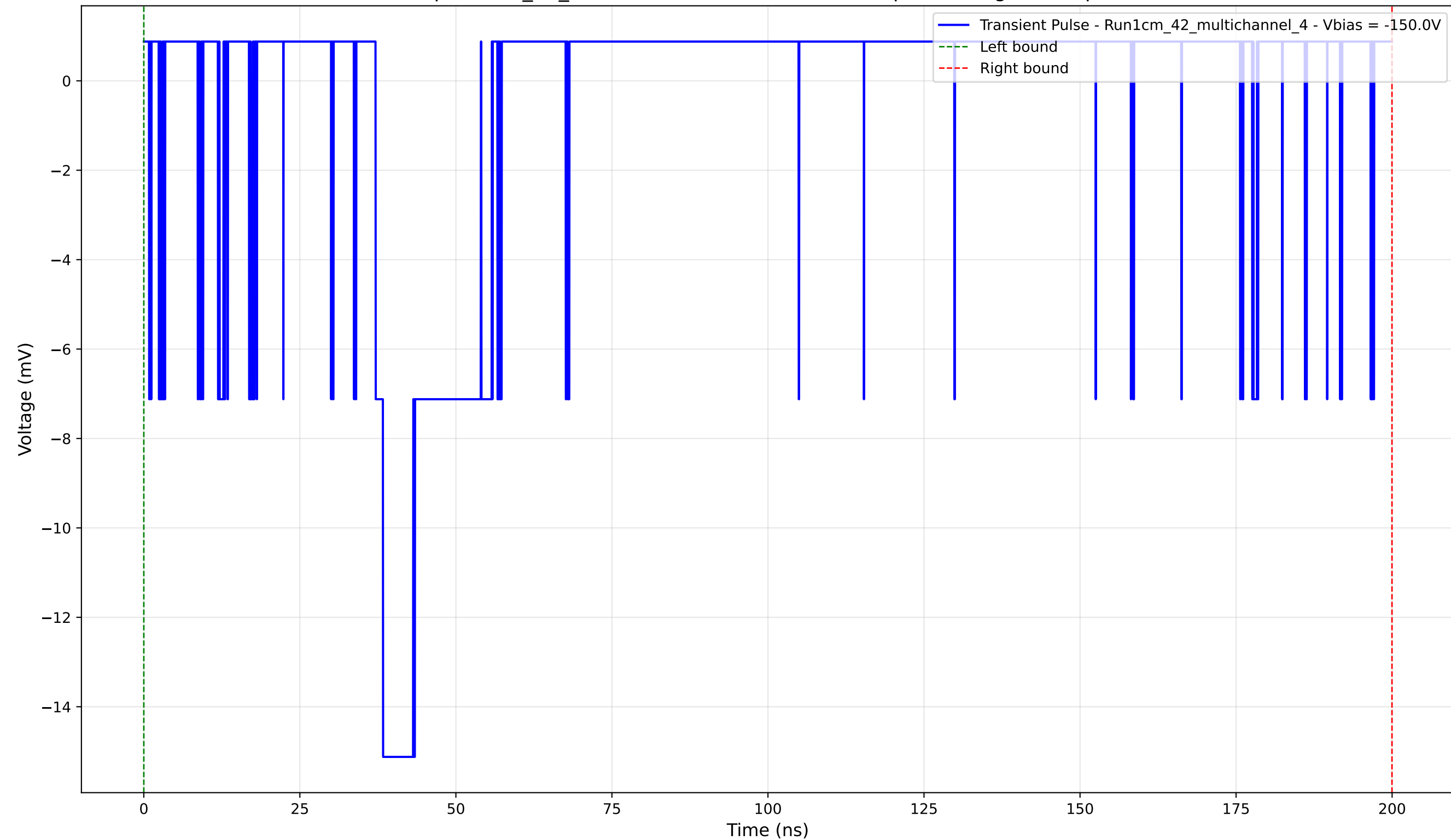
Transient Pulse - Sample: 1cm_42_multichannel - Position: 4145.0 \mu\text{m} - Charge: 1.23 pC - Rise Time: 1.20 ns
