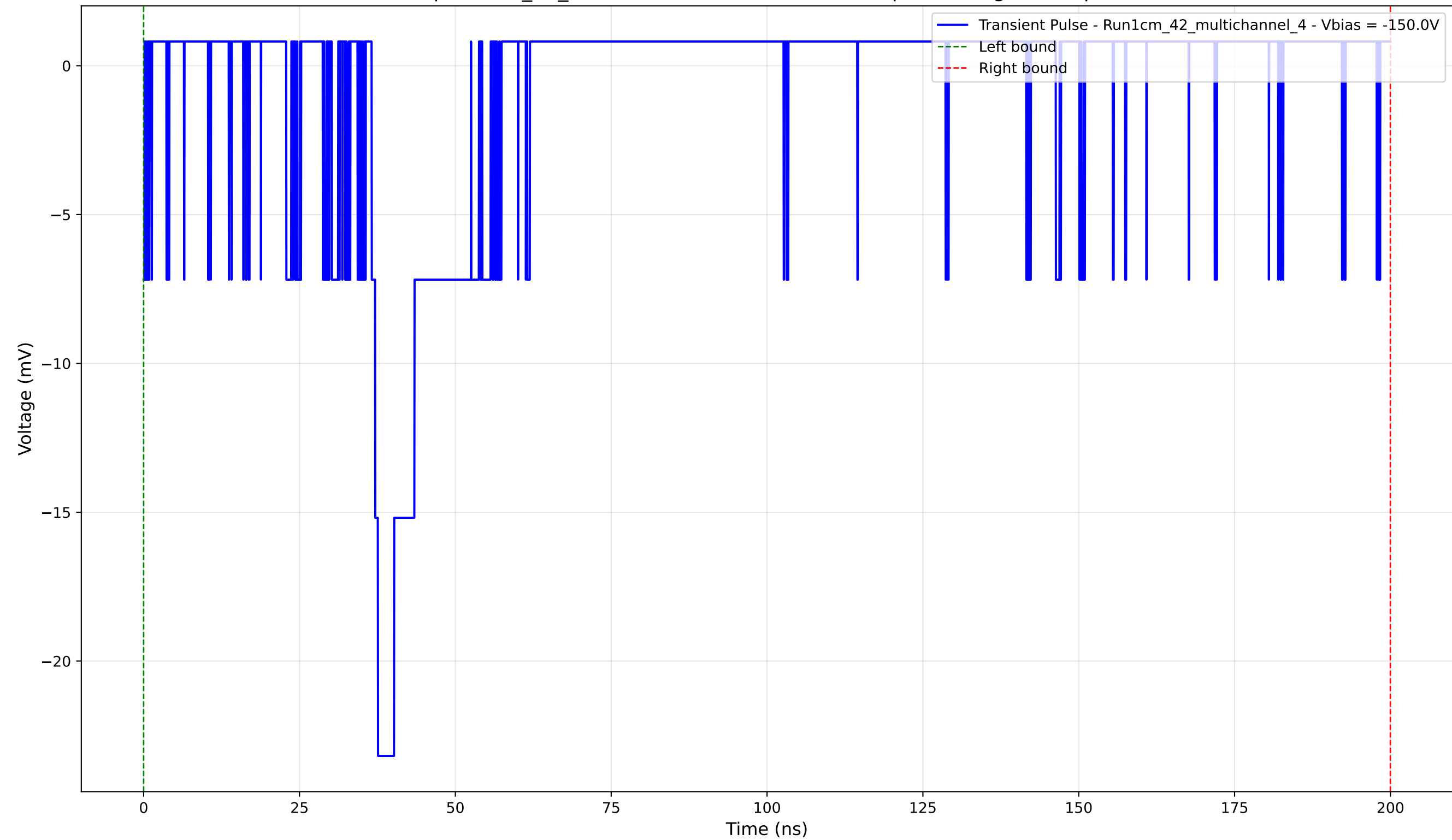
Transient Pulse - Sample: 1cm_42_multichannel - Position: 1290.0 \mu\text{m} - Charge: 3.01 pC - Rise Time: 1.02 ns
