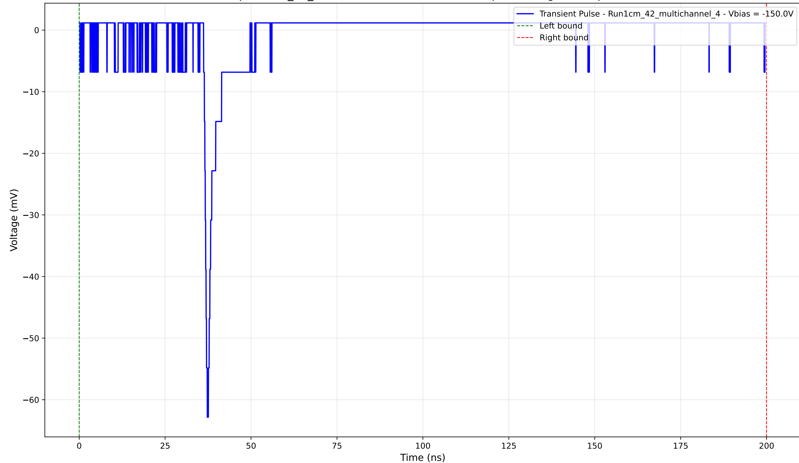
Transient Pulse - Sample: 1cm_42_multichannel - Position: 2090.0 \mu\text{m} - Charge: 1.38 pC - Rise Time: 1.06 ns
