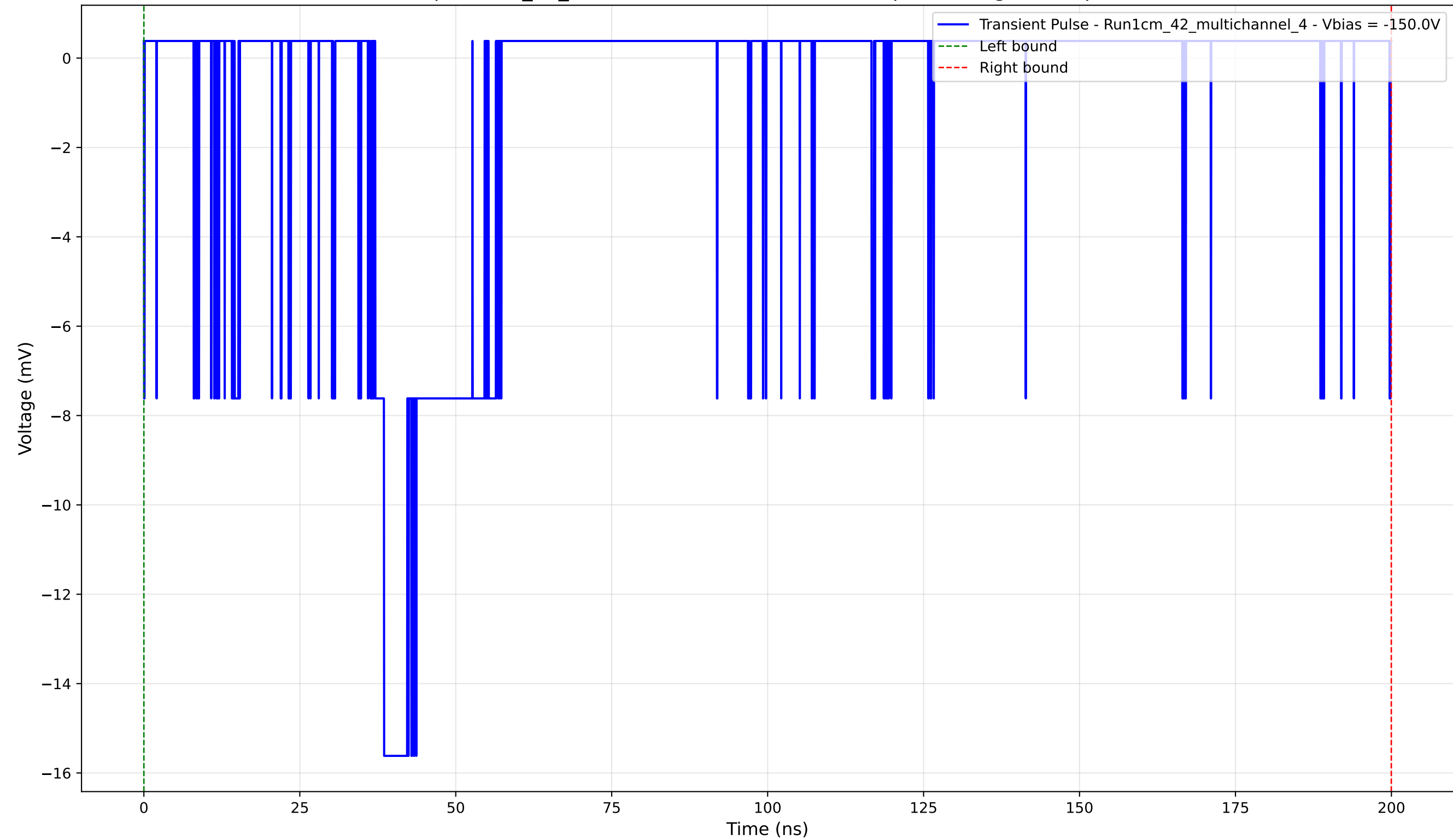
Transient Pulse - Sample: 1cm_42_multichannel - Position: 4590.0 \mu\text{m} - Charge: 3.21 pC - Rise Time: 1.42 ns
