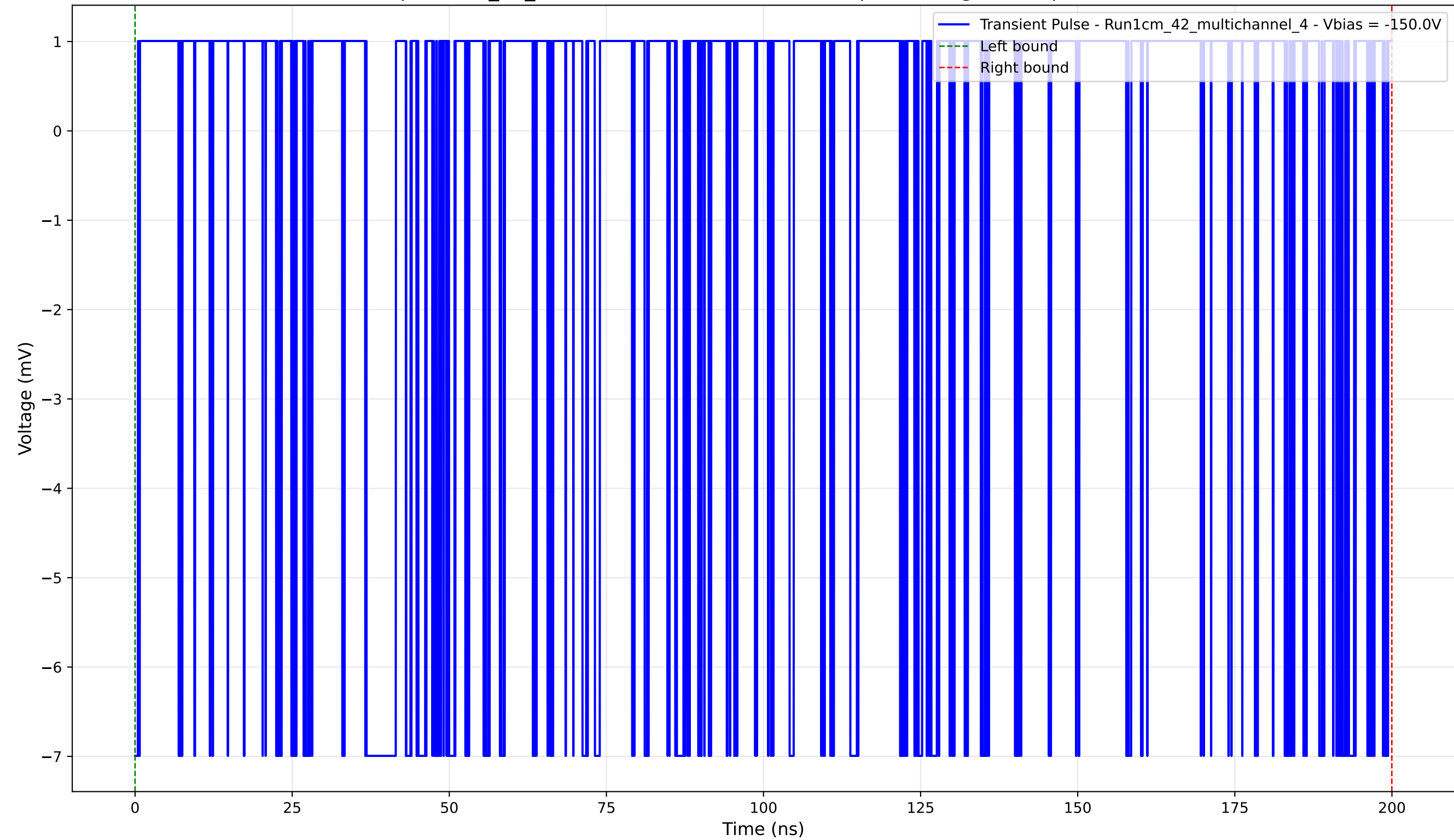
Transient Pulse - Sample: 1cm_42_multichannel - Position: 1400.0 \mu\text{m} - Charge: 1.74 pC - Rise Time: 0.00 ns (N/A)
