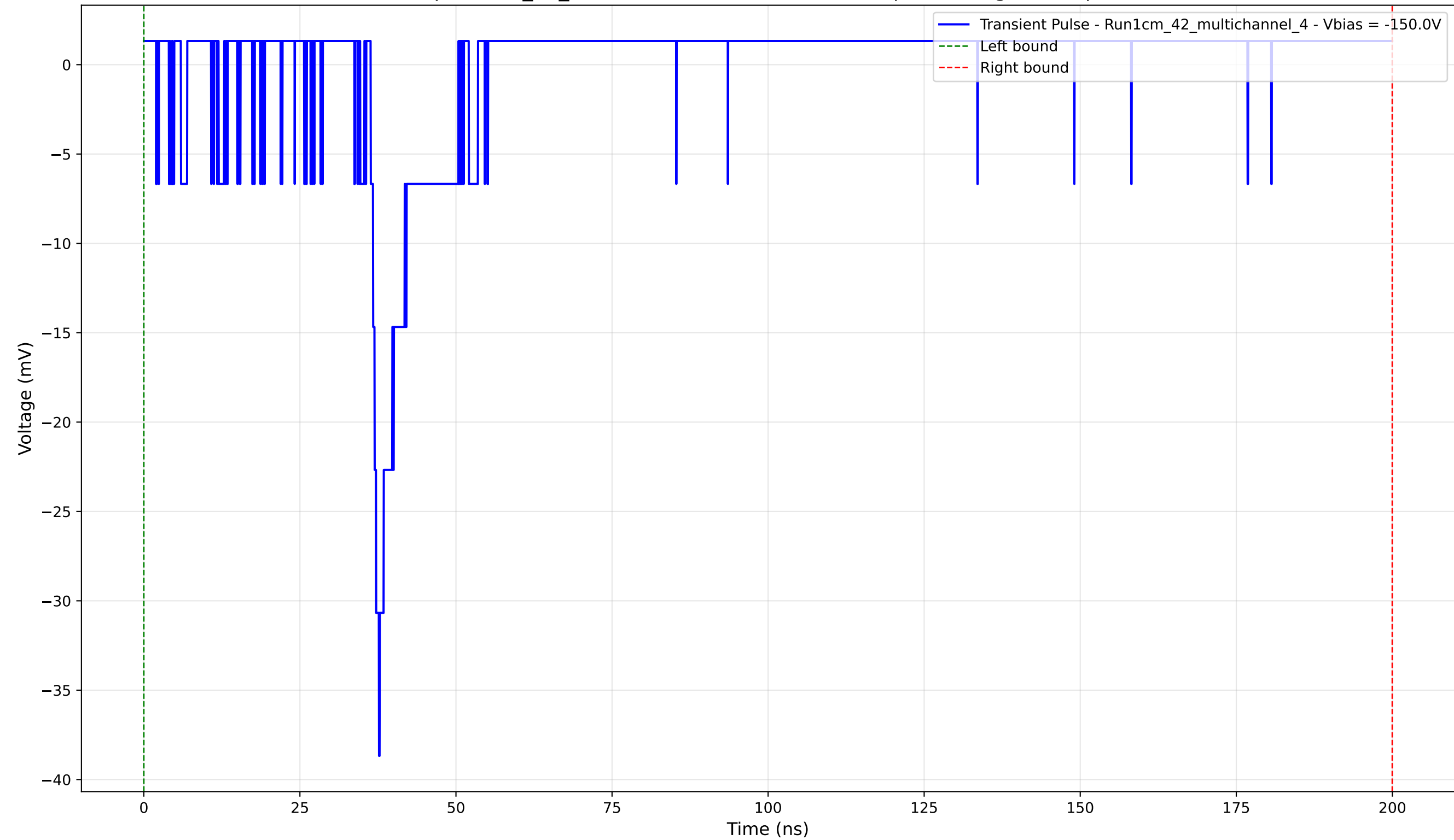
Transient Pulse - Sample: 1cm_42_multichannel - Position: 3055.0 \mu\text{m} - Charge: 0.31 pC - Rise Time: 1.33 ns
