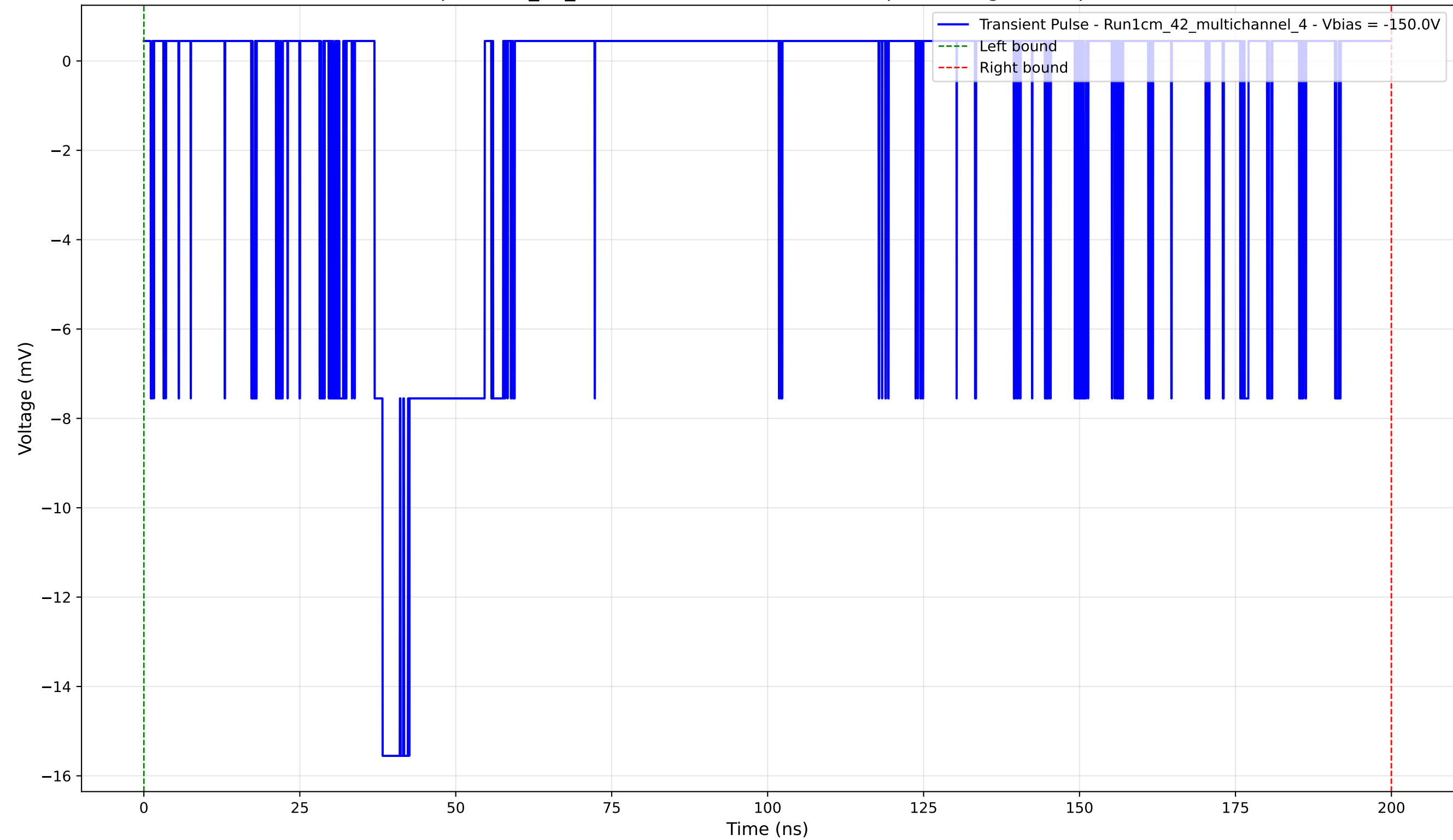
Transient Pulse - Sample: 1cm_42_multichannel - Position: 185.0 \mu\text{m} - Charge: 4.07 pC - Rise Time: 1.30 ns
