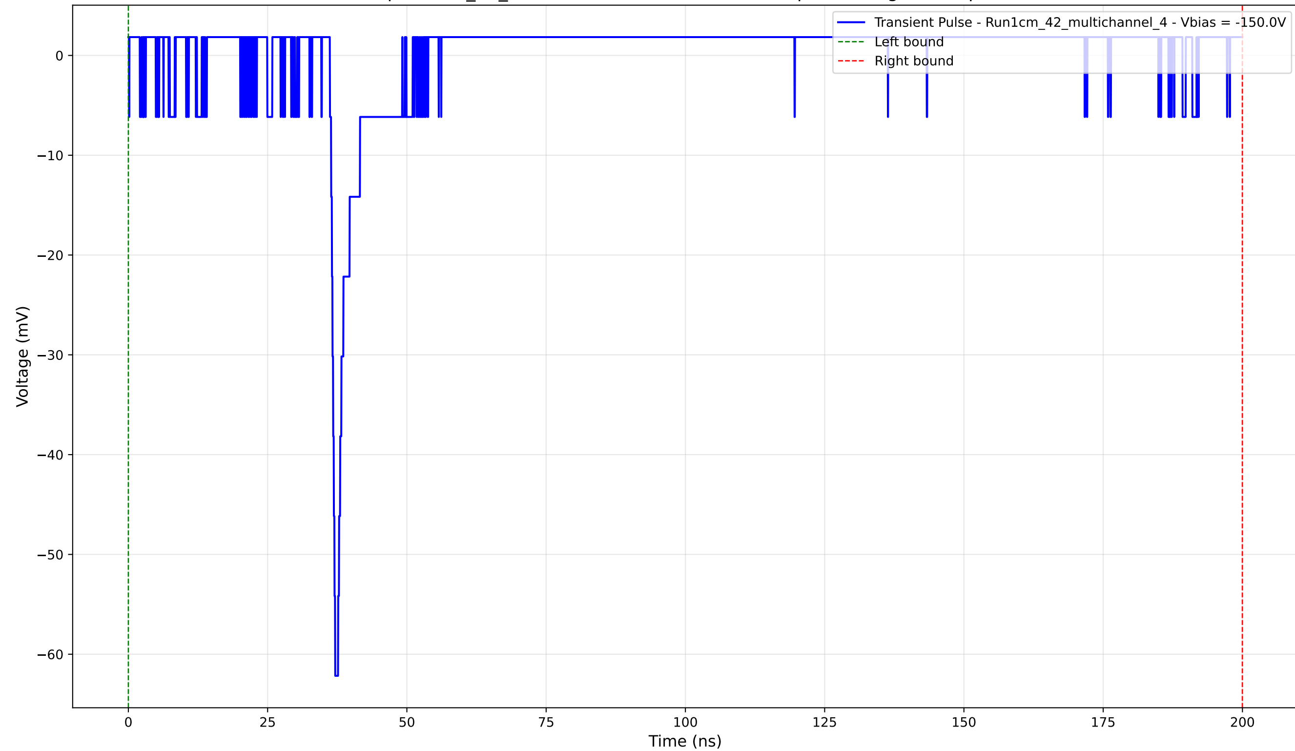
Transient Pulse - Sample: 1cm_42_multichannel - Position: 2130.0 \mu\text{m} - Charge: 0.82 pC - Rise Time: 0.74 ns
