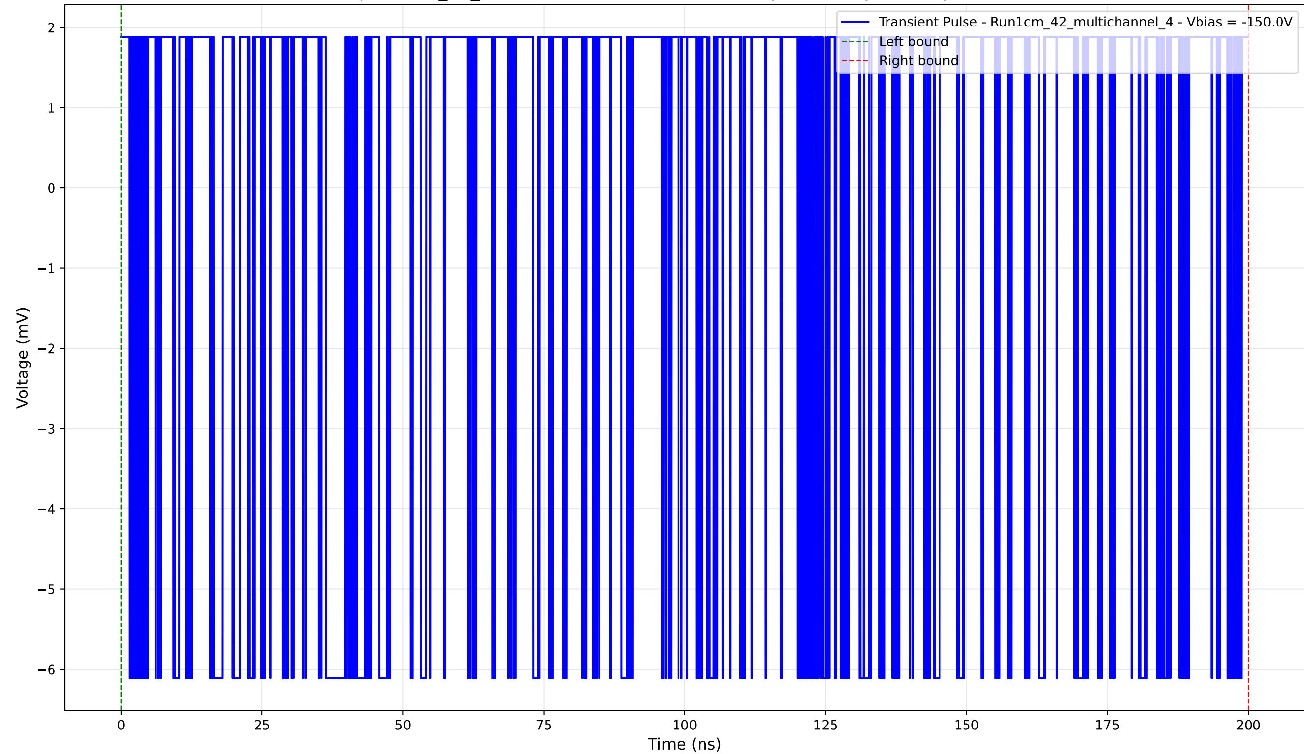
Transient Pulse - Sample: 1cm_42_multichannel - Position: 2405.0 \mu\text{m} - Charge: 0.28 pC - Rise Time: 0.00 ns (N/A)
