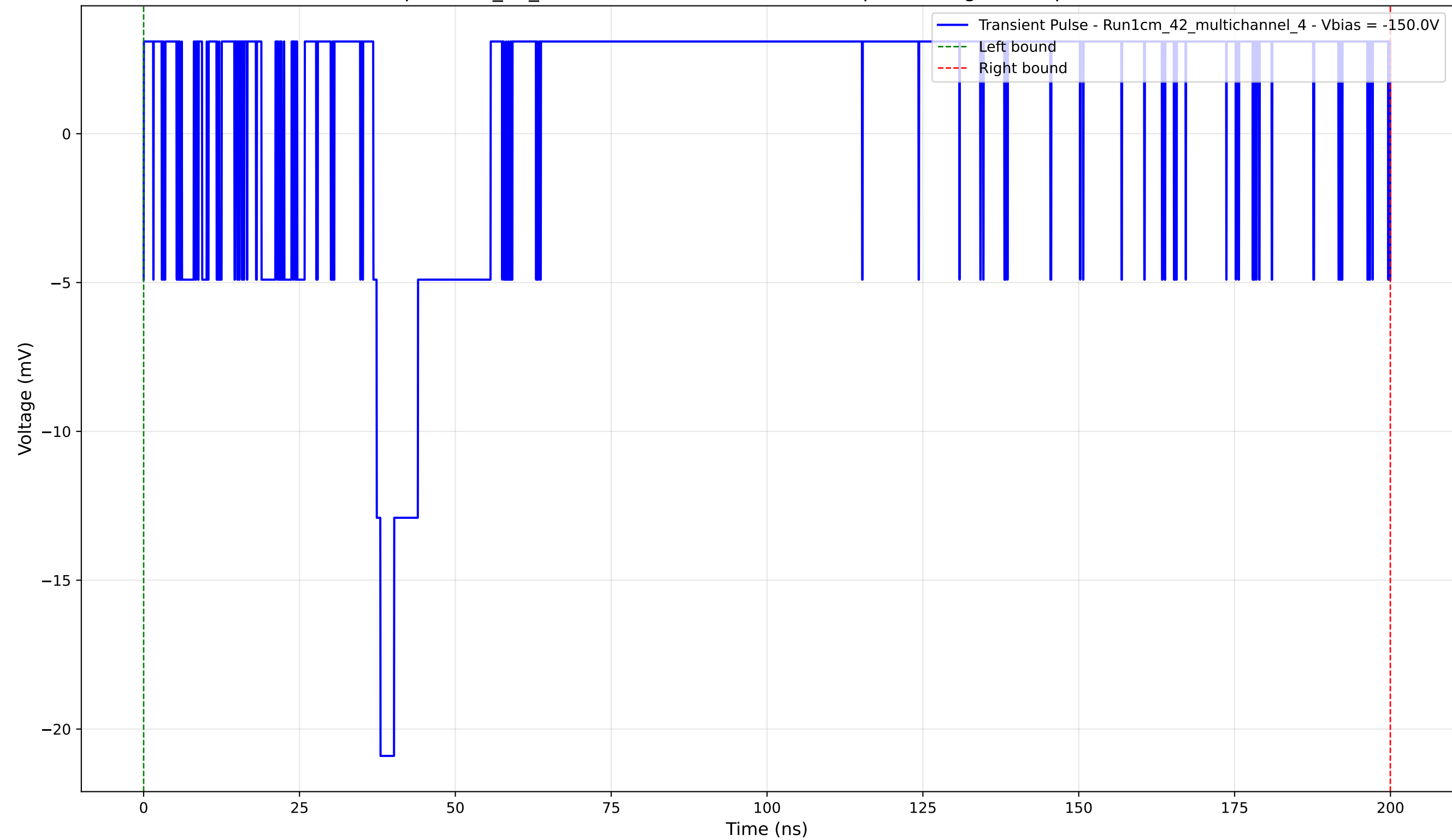
Transient Pulse - Sample: 1cm_42_multichannel - Position: 1090.0 \mu\text{m} - Charge: 5.32 pC - Rise Time: 0.00 ns (N/A)
