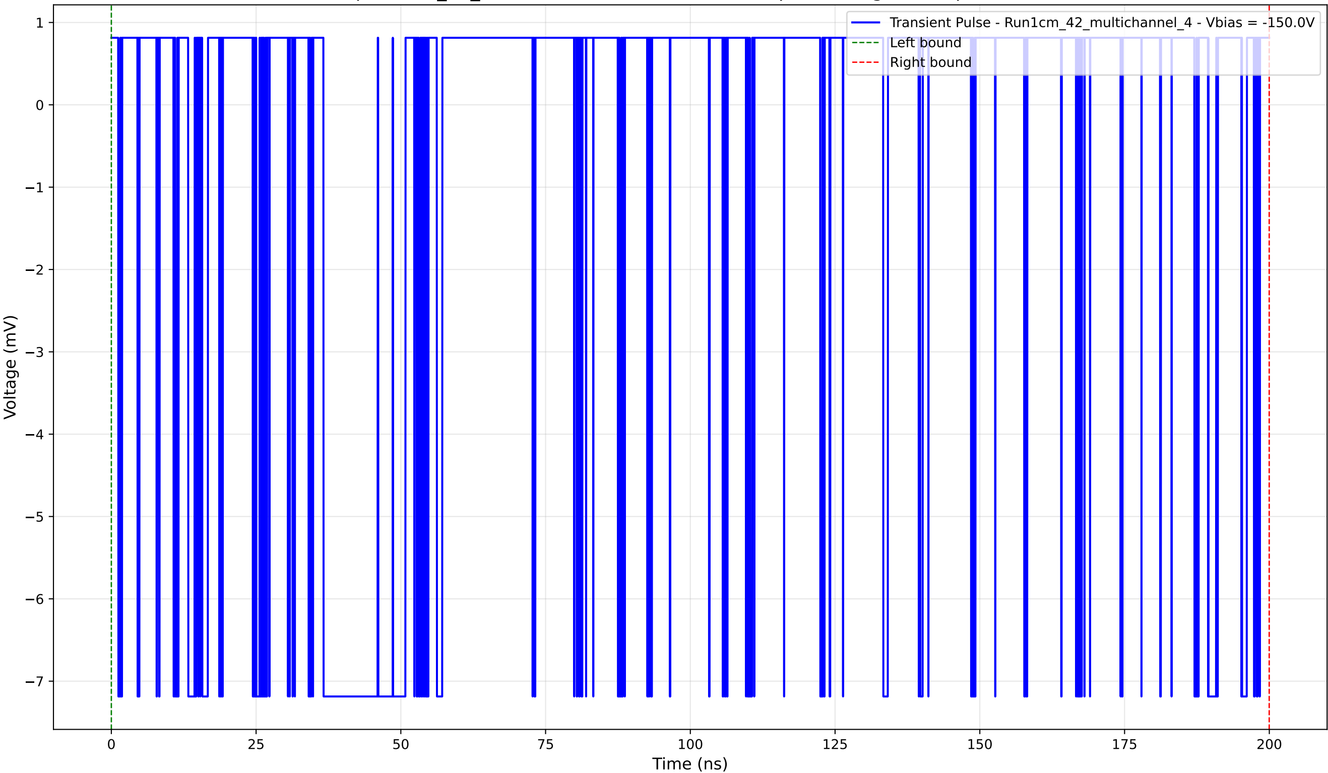
Transient Pulse - Sample: 1cm_42_multichannel - Position: 3355.0 \mu\text{m} - Charge: 2.00 pC - Rise Time: 0.00 ns (N/A)
