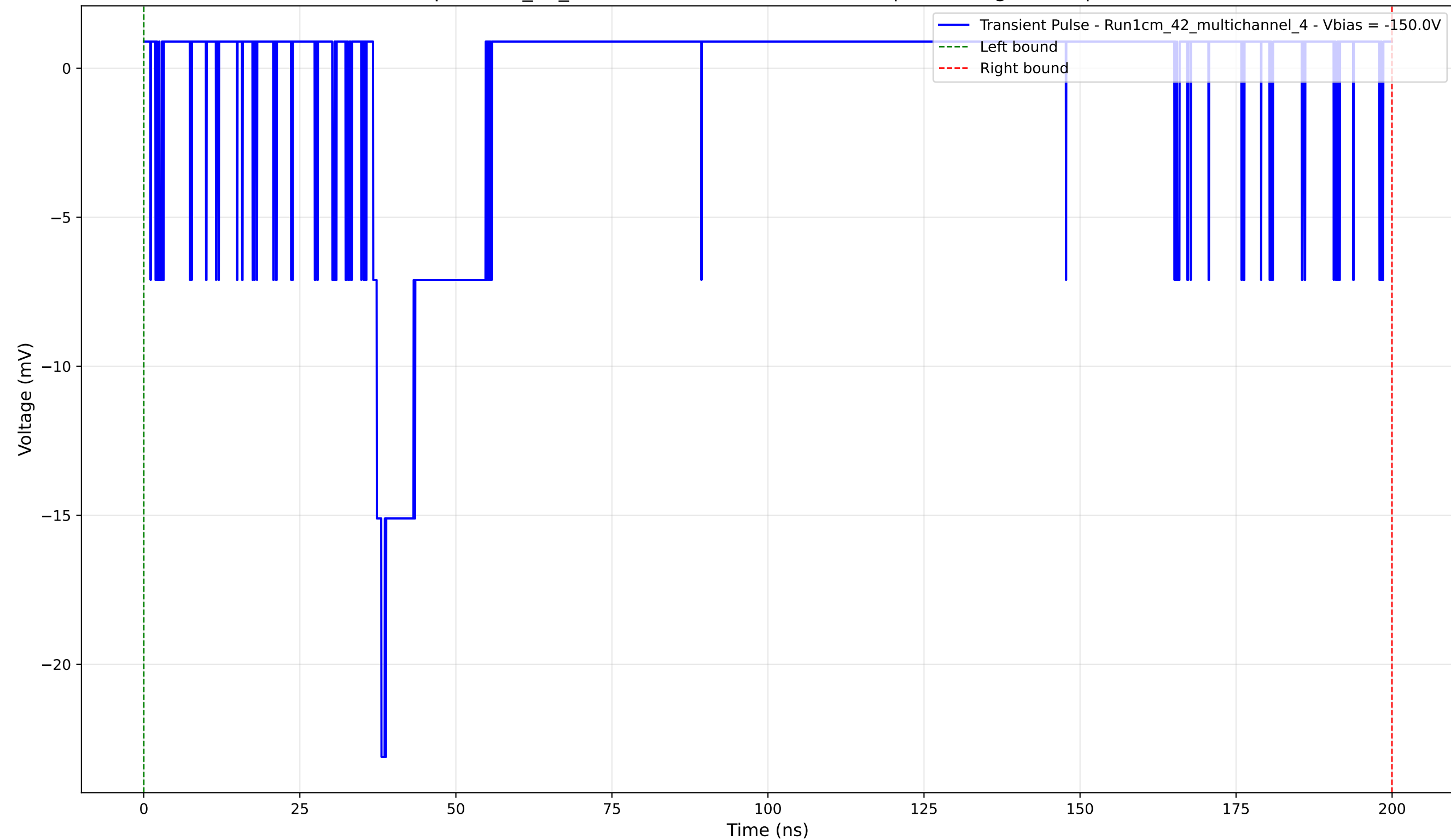
Transient Pulse - Sample: 1cm_42_multichannel - Position: 3635.0 \mu\text{m} - Charge: 1.44 pC - Rise Time: 1.34 ns
