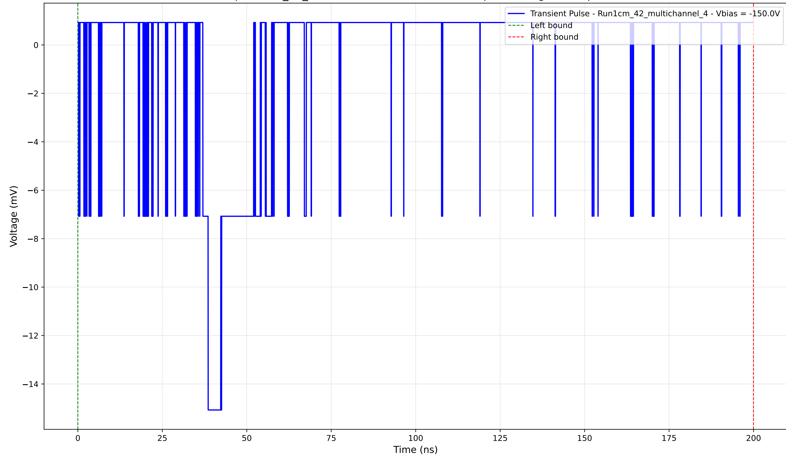
Transient Pulse - Sample: 1cm_42_multichannel - Position: 4610.0 \mu\text{m} - Charge: 1.11 pC - Rise Time: 1.58 ns
