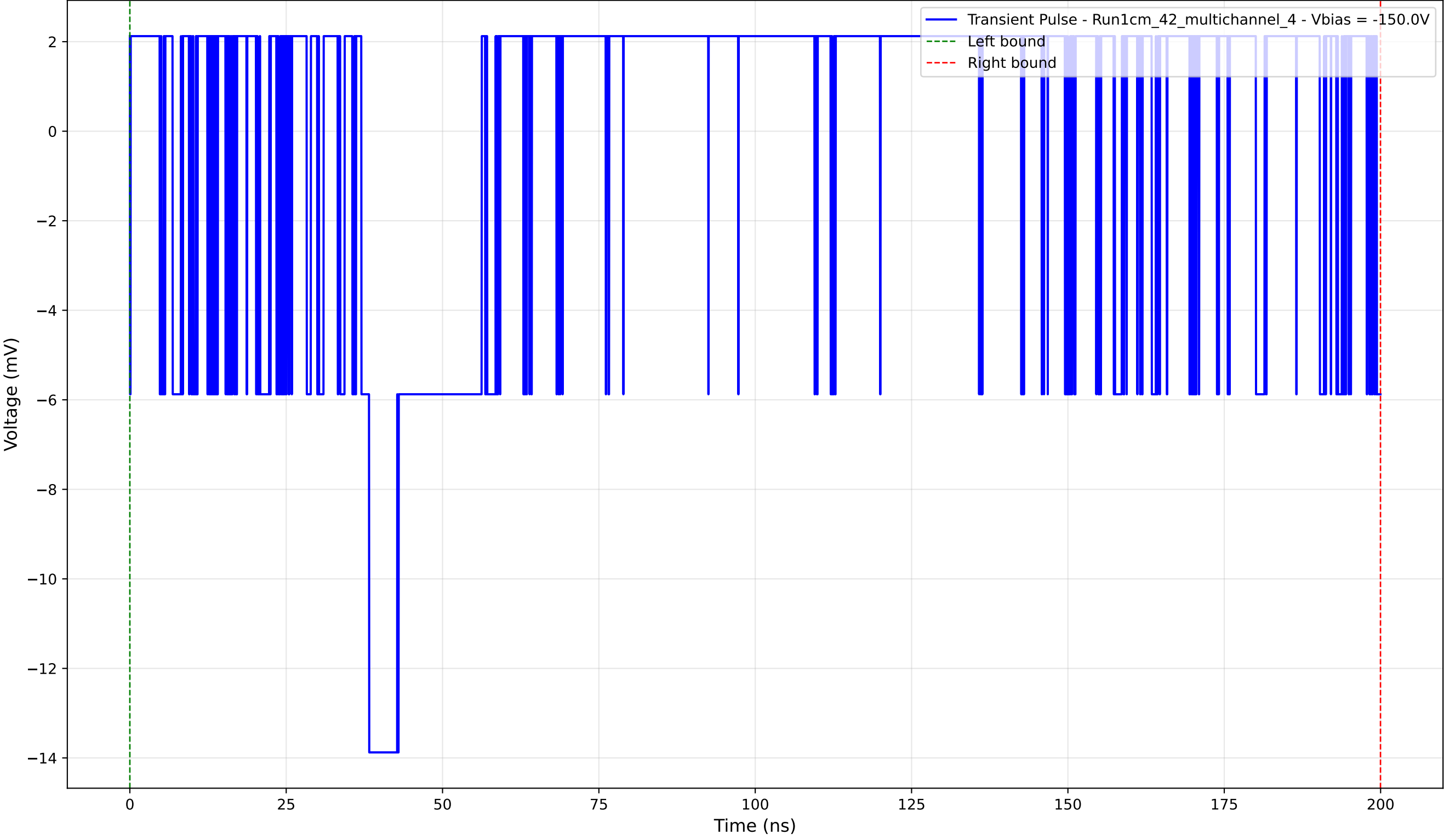
Transient Pulse - Sample: 1cm_42_multichannel - Position: 285.0 \mu\text{m} - Charge: 0.62 pC - Rise Time: 0.00 ns (N/A)
