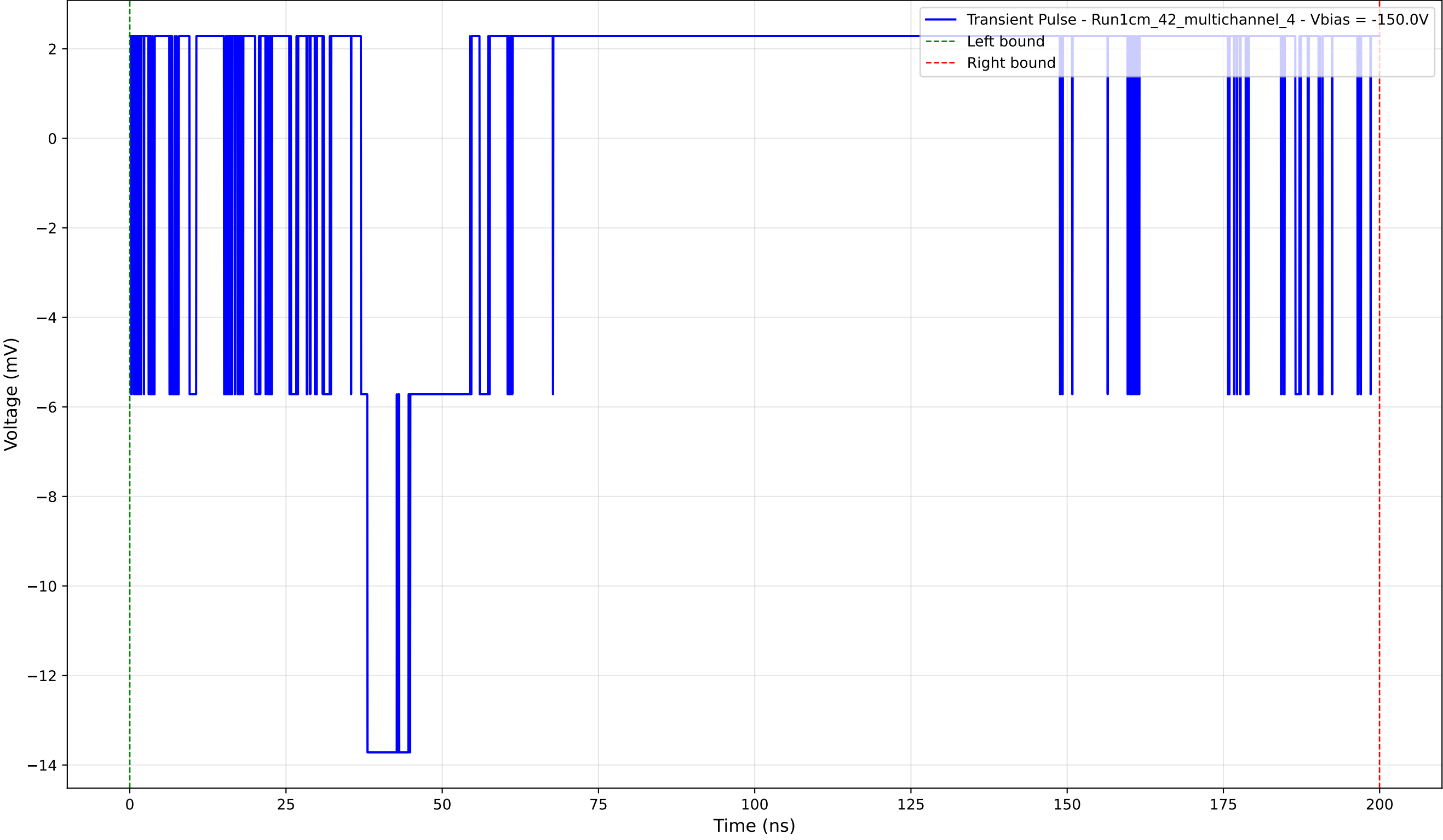
Transient Pulse - Sample: 1cm_42_multichannel - Position: 490.0 \mu\text{m} - Charge: 2.98 pC - Rise Time: 0.00 ns (N/A)
