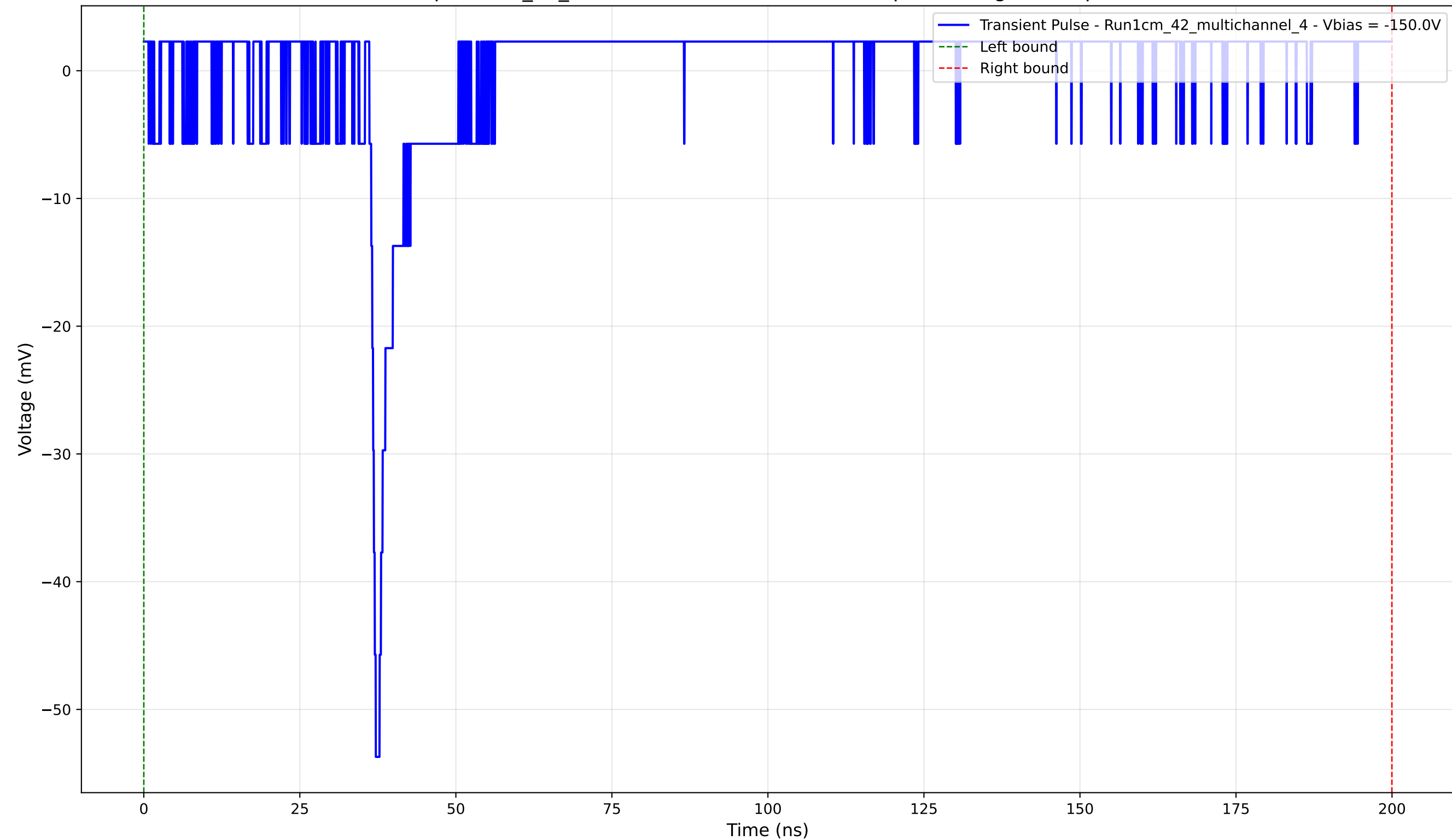
Transient Pulse - Sample: 1cm_42_multichannel - Position: 2730.0 \mu\text{m} - Charge: 1.60 pC - Rise Time: 1.02 ns
