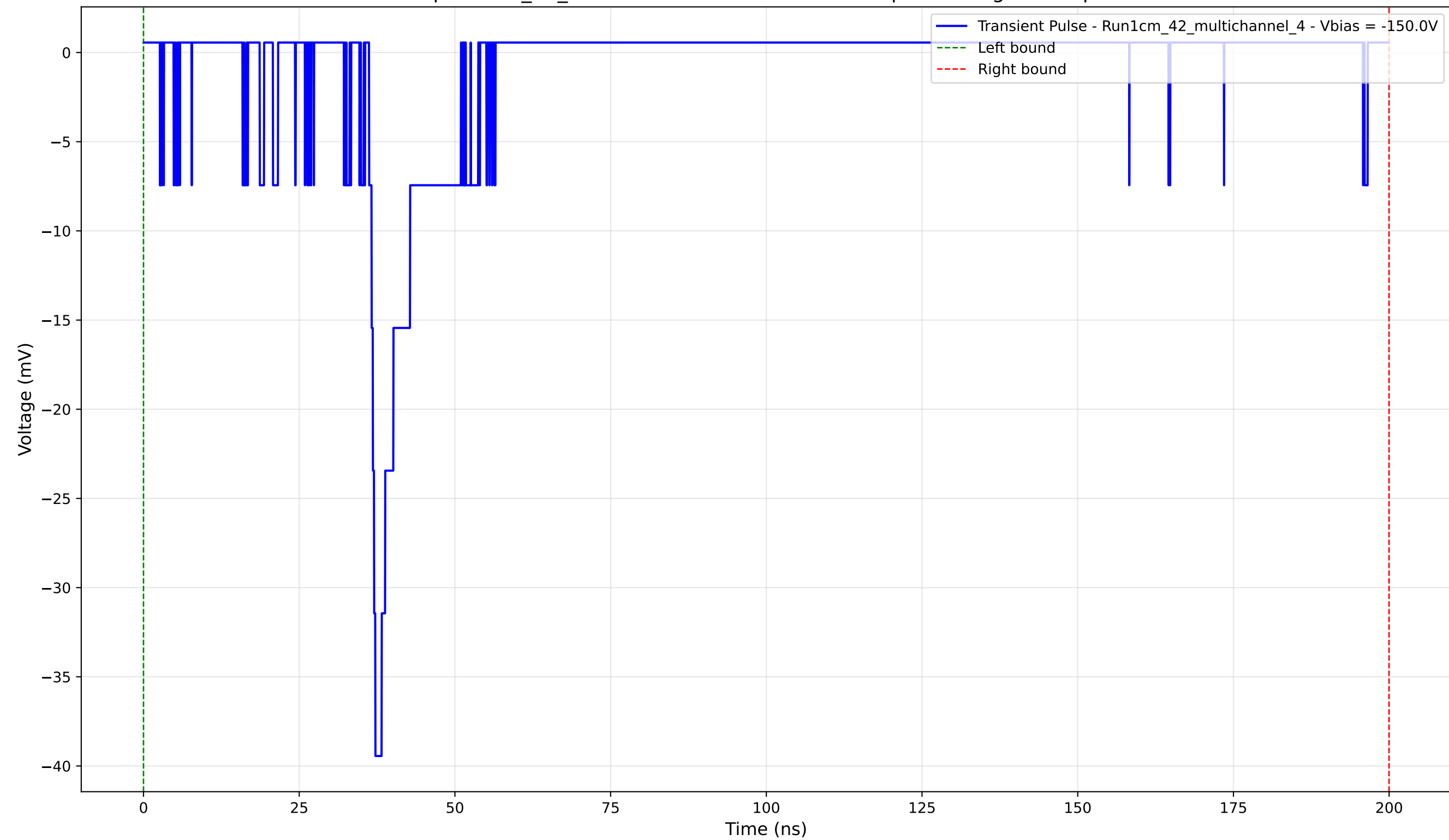
Transient Pulse - Sample: 1cm_42_multichannel - Position: 1775.0 \mu\text{m} - Charge: 3.45 pC - Rise Time: 1.01 ns
