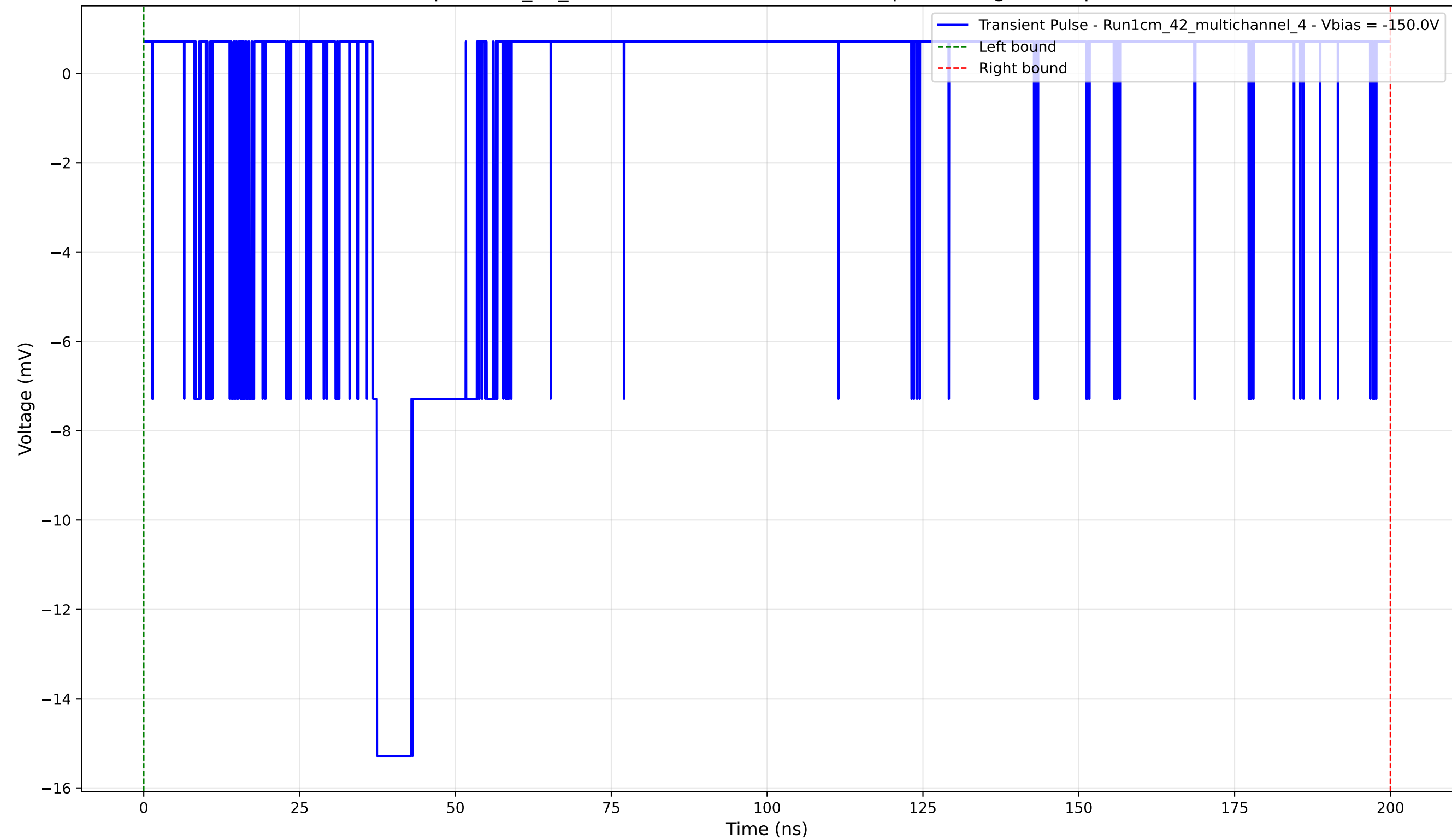
Transient Pulse - Sample: 1cm_42_multichannel - Position: 3610.0 \mu\text{m} - Charge: 2.40 pC - Rise Time: 0.66 ns
