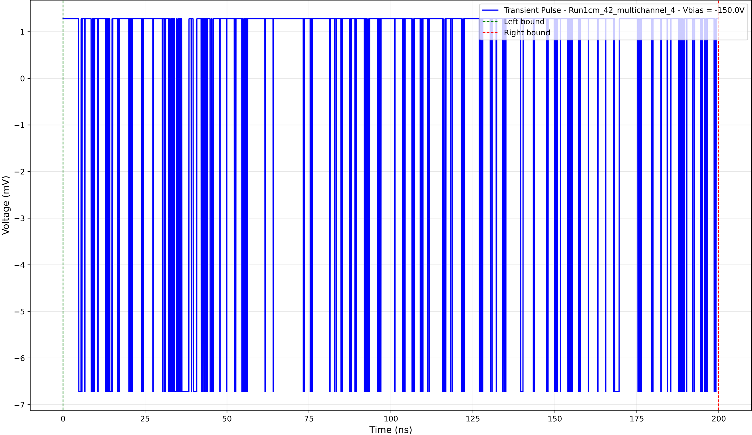
Transient Pulse - Sample: 1cm_42_multichannel - Position: 2400.0 \mu\text{m} - Charge: 0.84 pC - Rise Time: 0.00 ns (N/A)
