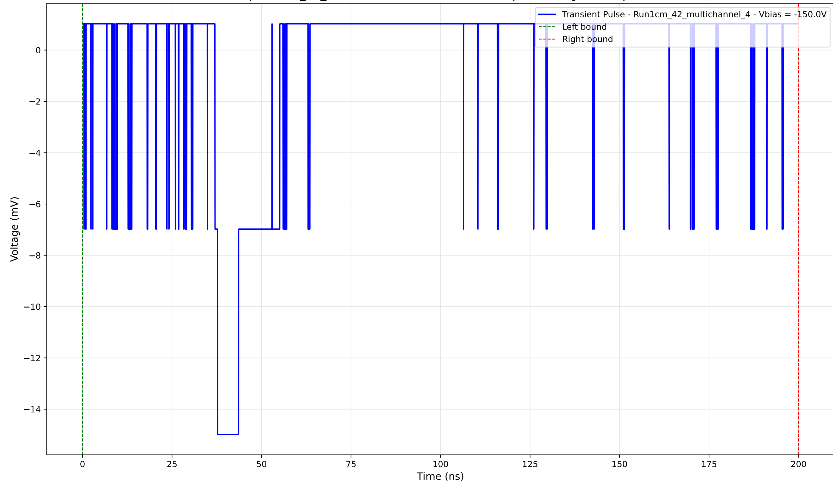
Transient Pulse - Sample: 1cm_42_multichannel - Position: 3810.0 \mu\text{m} - Charge: 0.90 pC - Rise Time: 0.74 ns
