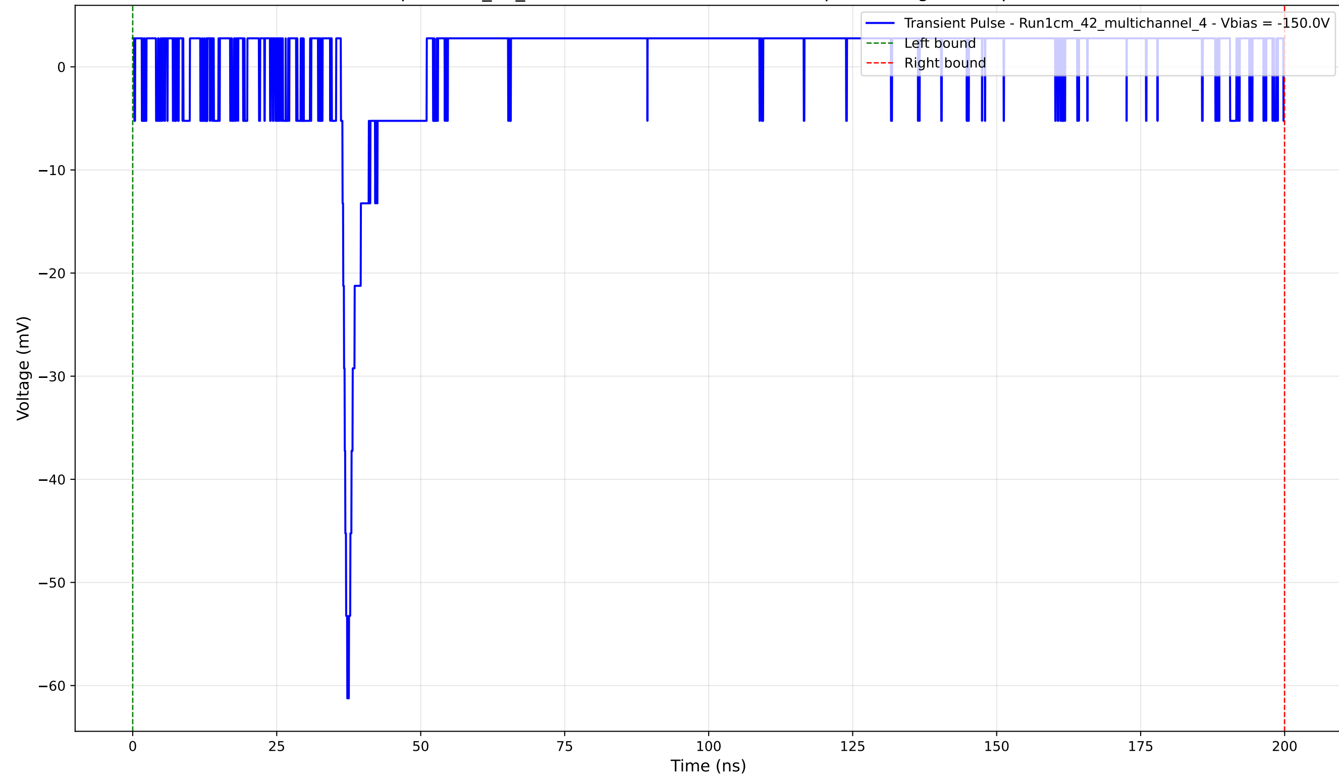
Transient Pulse - Sample: 1cm_42_multichannel - Position: 2655.0 \mu\text{m} - Charge: 3.50 pC - Rise Time: 0.84 ns
