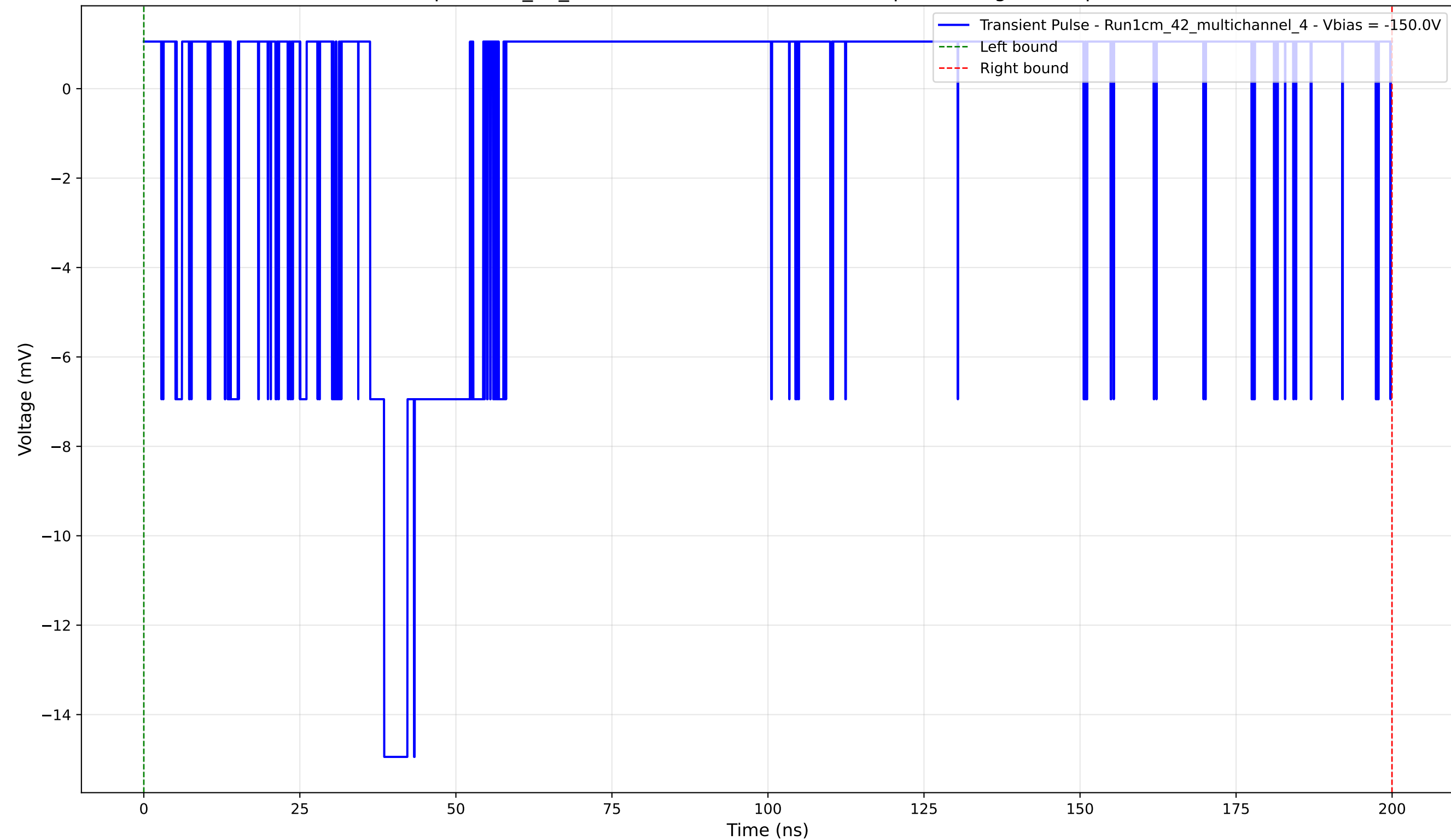
Transient Pulse - Sample: 1cm_42_multichannel - Position: 4650.0 \mu\text{m} - Charge: 1.11 pC - Rise Time: 2.26 ns
