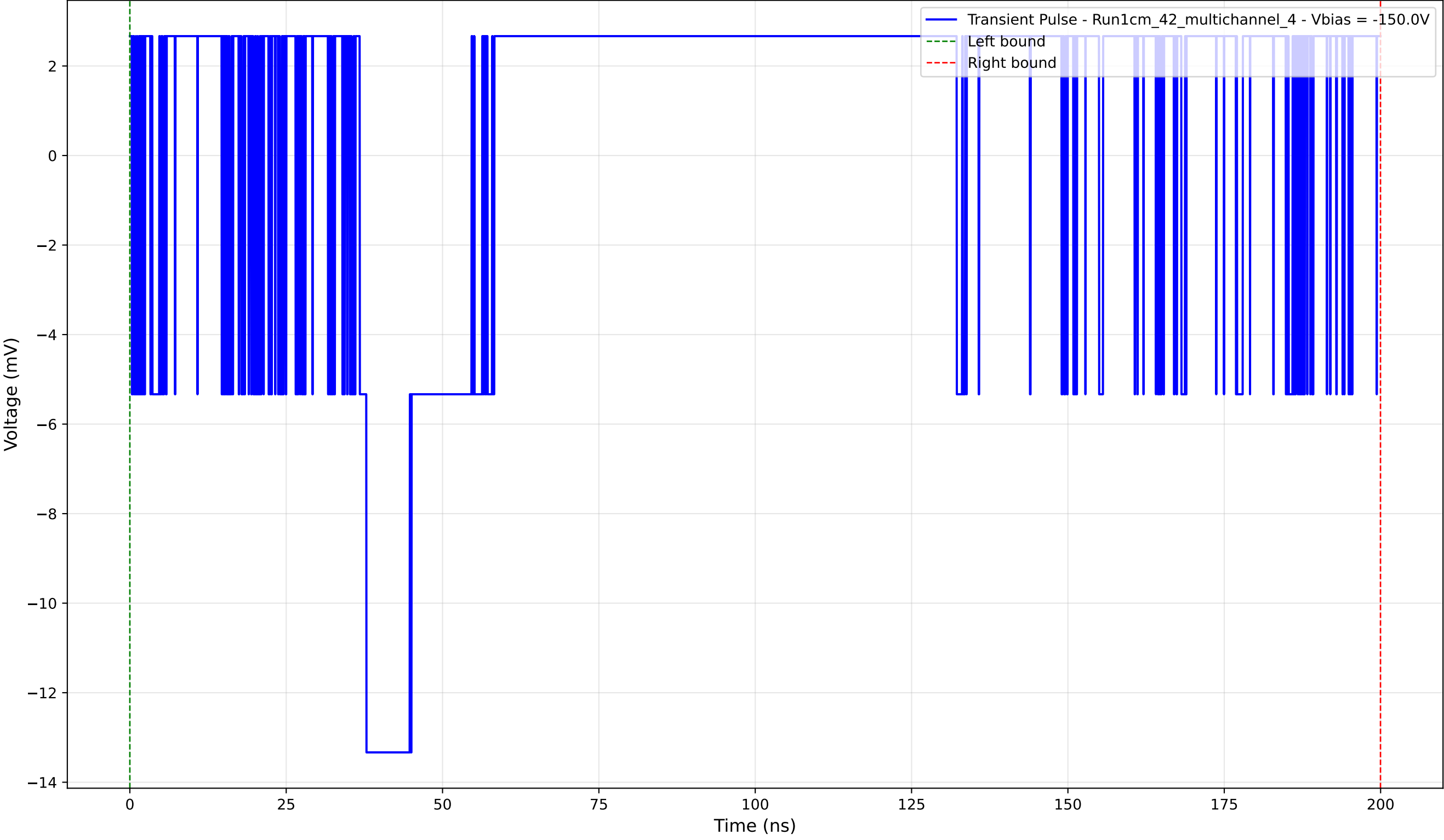
Transient Pulse - Sample: 1cm_42_multichannel - Position: 690.0 \mu\text{m} - Charge: 3.37 pC - Rise Time: 0.00 ns (N/A)
