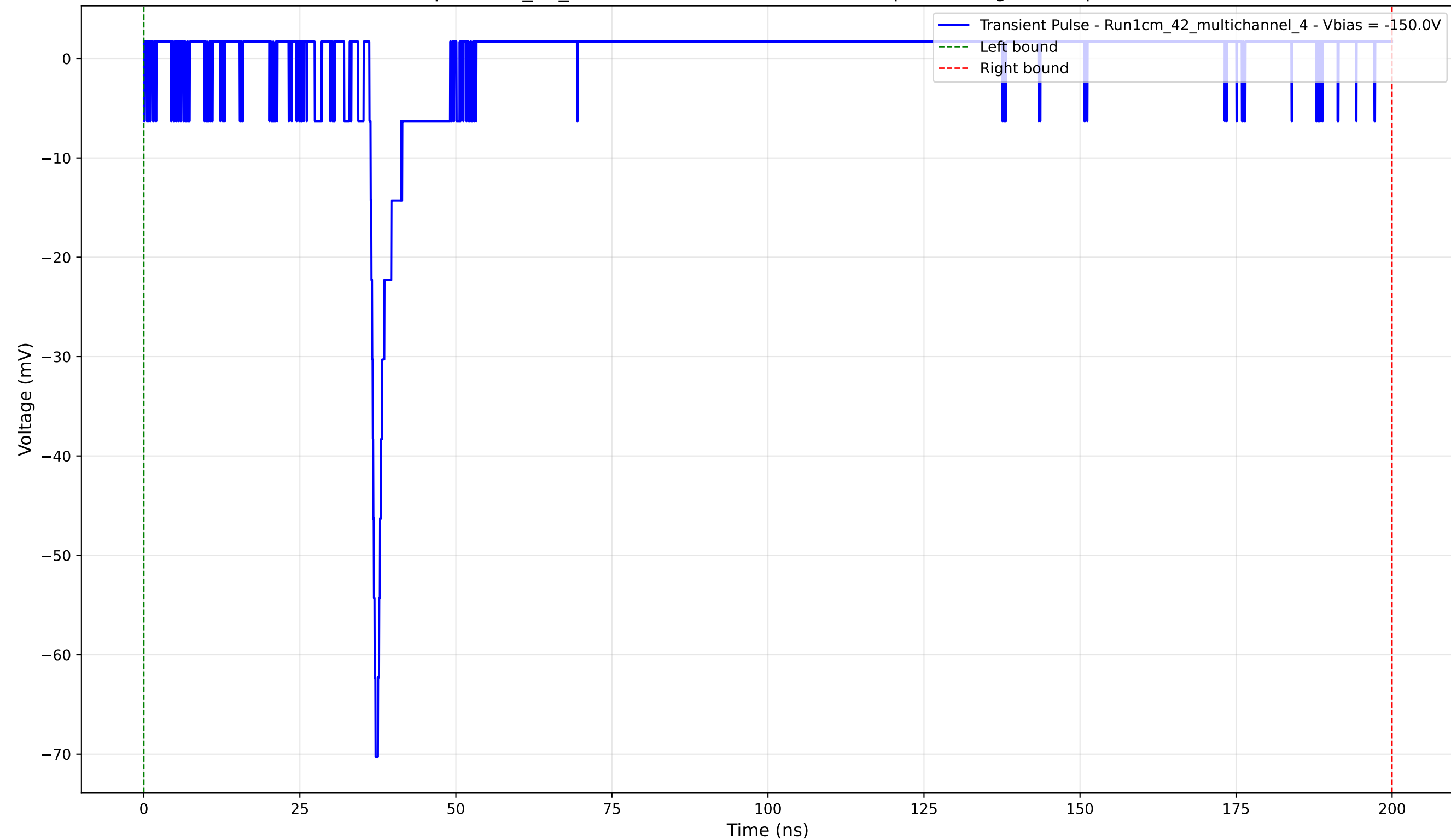
Transient Pulse - Sample: 1cm_42_multichannel - Position: 2205.0 \mu\text{m} - Charge: 0.39 pC - Rise Time: 0.80 ns
