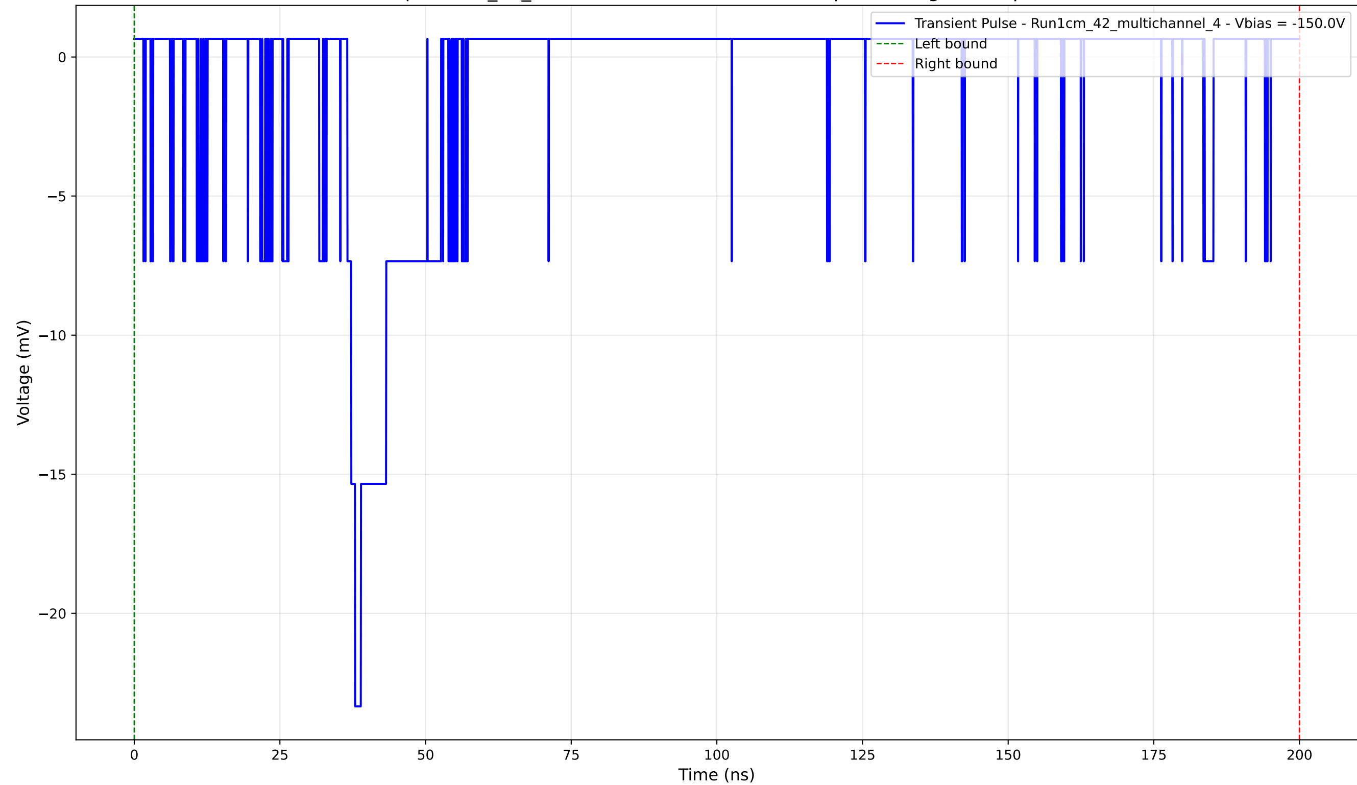
Transient Pulse - Sample: 1cm_42_multichannel - Position: 3550.0 \mu\text{m} - Charge: 2.83 pC - Rise Time: 1.33 ns
