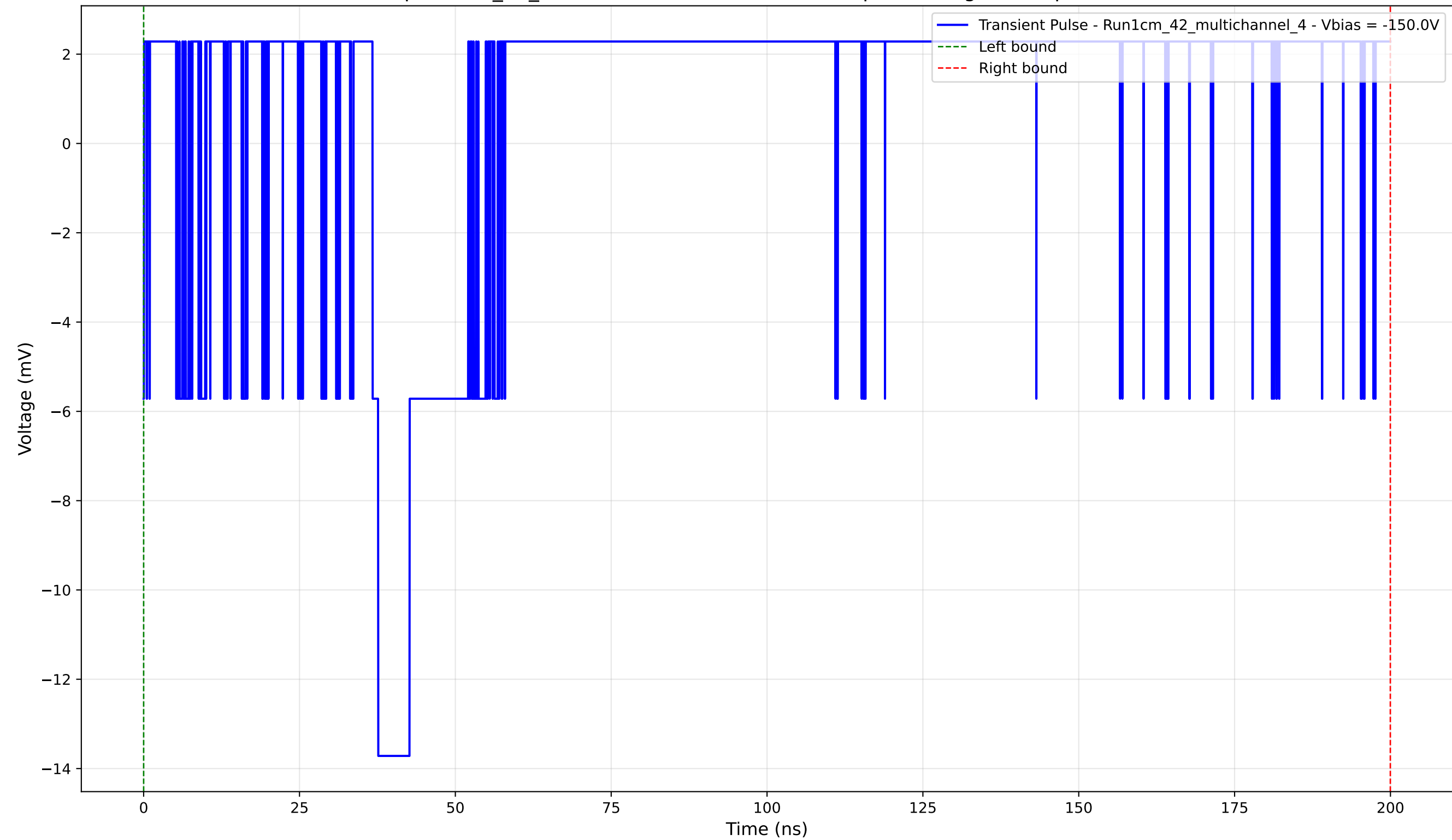
Transient Pulse - Sample: 1cm_42_multichannel - Position: 3720.0 \mu\text{m} - Charge: 3.92 pC - Rise Time: 0.00 ns (N/A)
