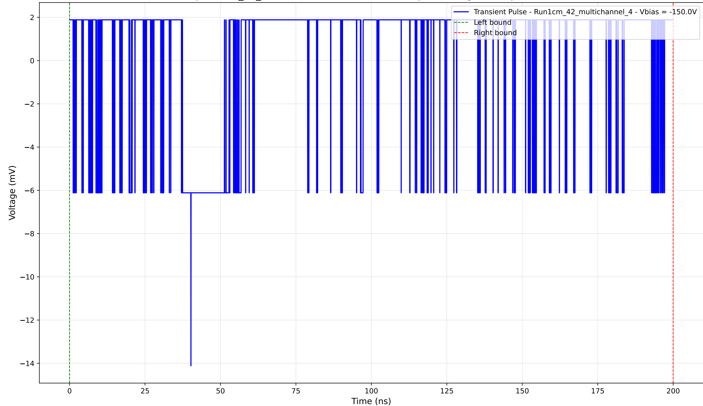
Transient Pulse - Sample: 1cm_42_multichannel - Position: 4350.0 \mu\text{m} - Charge: 2.03 pC - Rise Time: 0.00 ns (N/A)
