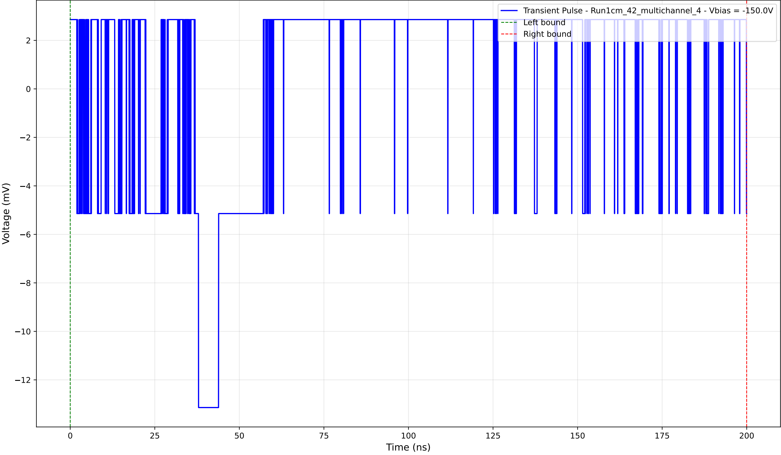
Transient Pulse - Sample: 1cm_42_multichannel - Position: 565.0 \mu\text{m} - Charge: 3.54 pC - Rise Time: 0.00 ns (N/A)
