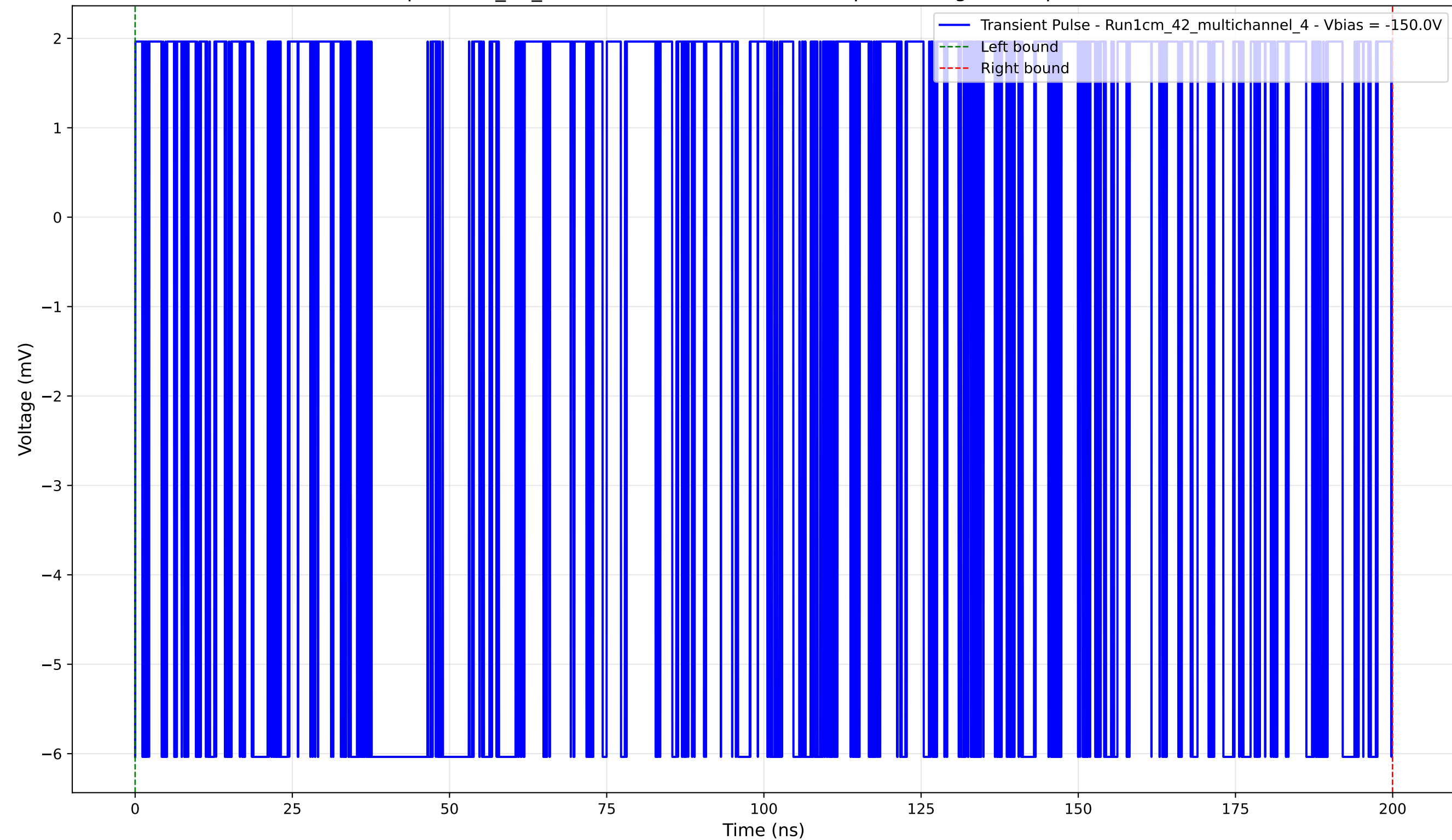
Transient Pulse - Sample: 1cm_42_multichannel - Position: 835.0 \mu\text{m} - Charge: 3.94 pC - Rise Time: 0.00 ns (N/A)
