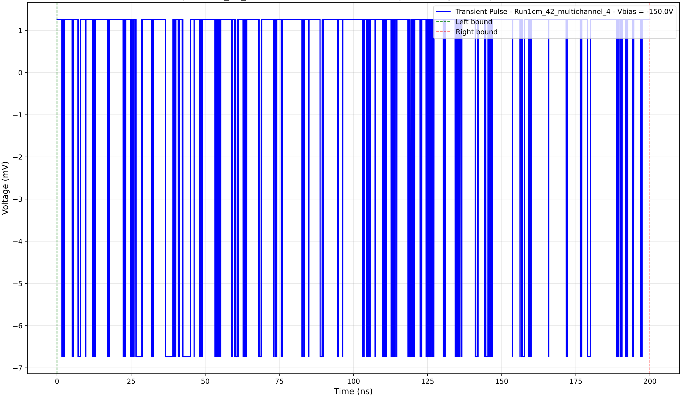
Transient Pulse - Sample: 1cm_42_multichannel - Position: 2390.0 \mu\text{m} - Charge: 0.08 pC - Rise Time: 0.00 ns (N/A)
