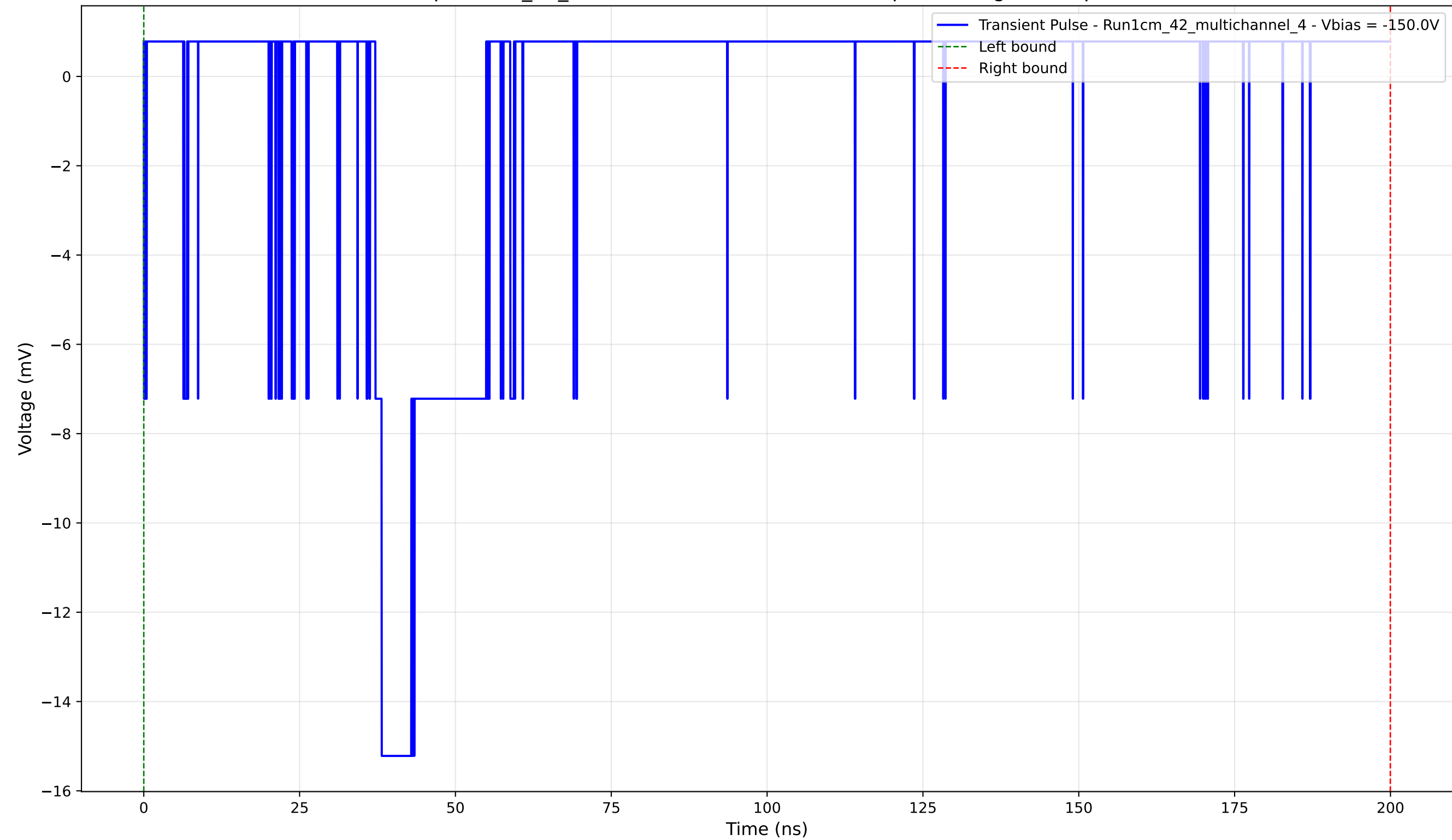
Transient Pulse - Sample: 1cm_42_multichannel - Position: 4130.0 \mu\text{m} - Charge: 1.29 pC - Rise Time: 1.02 ns
