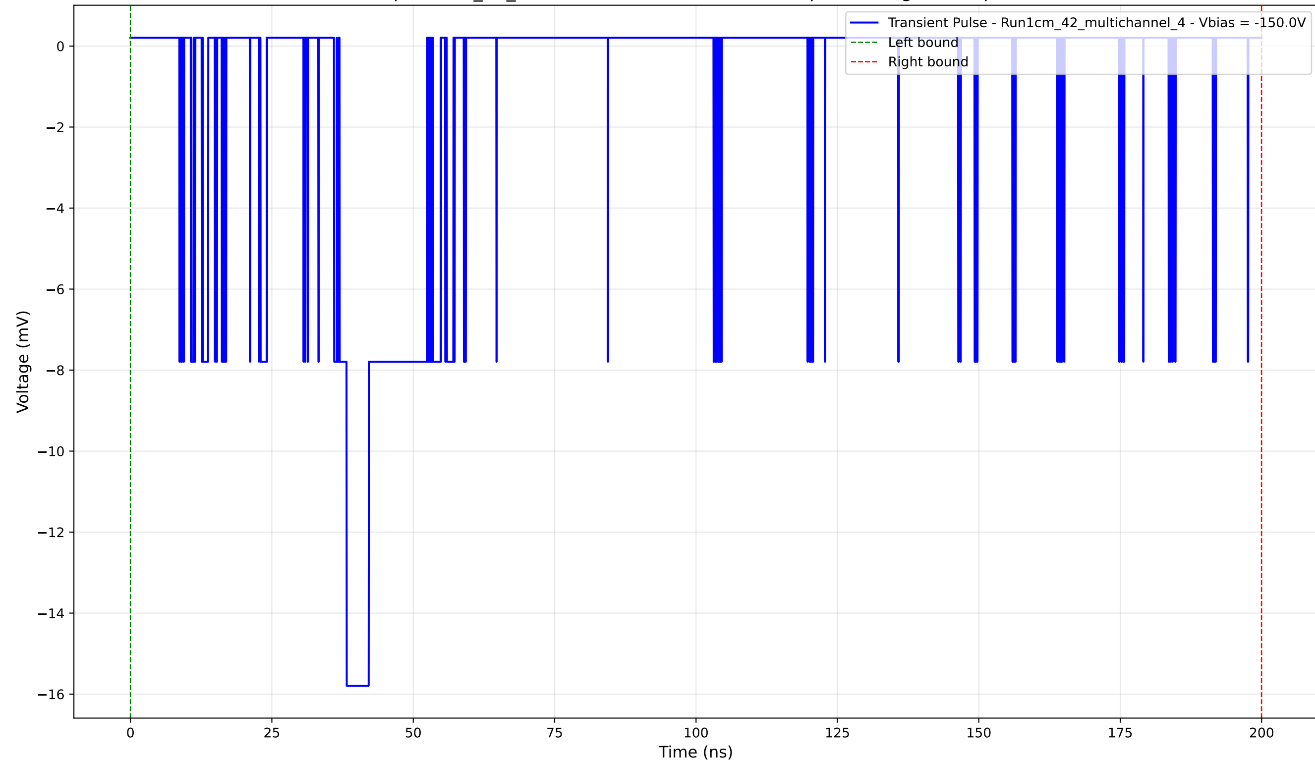
Transient Pulse - Sample: 1cm_42_multichannel - Position: 4745.0 \mu\text{m} - Charge: 4.35 pC - Rise Time: 1.26 ns
