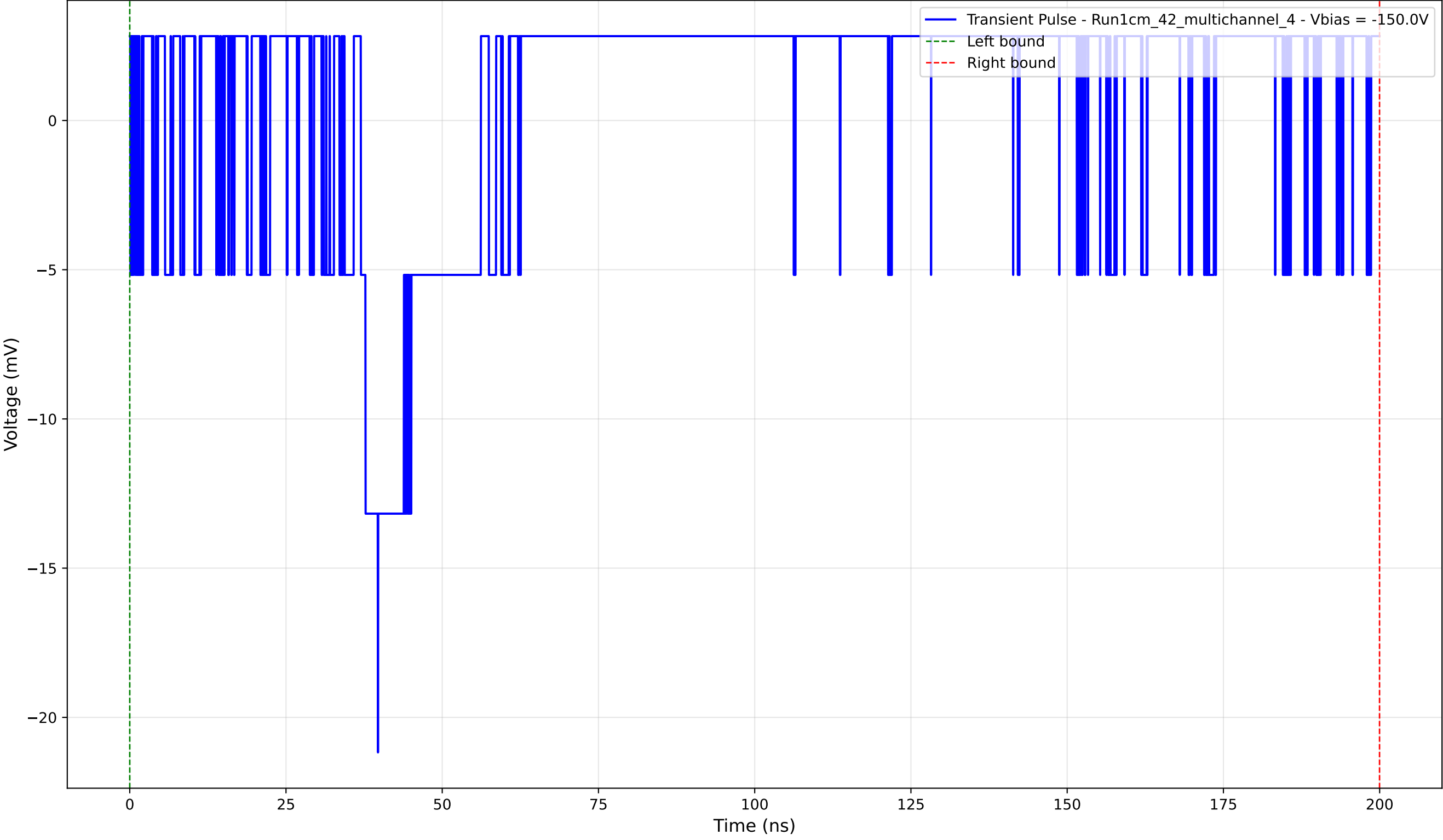
Transient Pulse - Sample: 1cm_42_multichannel - Position: 765.0 \mu\text{m} - Charge: 3.56 pC - Rise Time: 0.00 ns (N/A)
