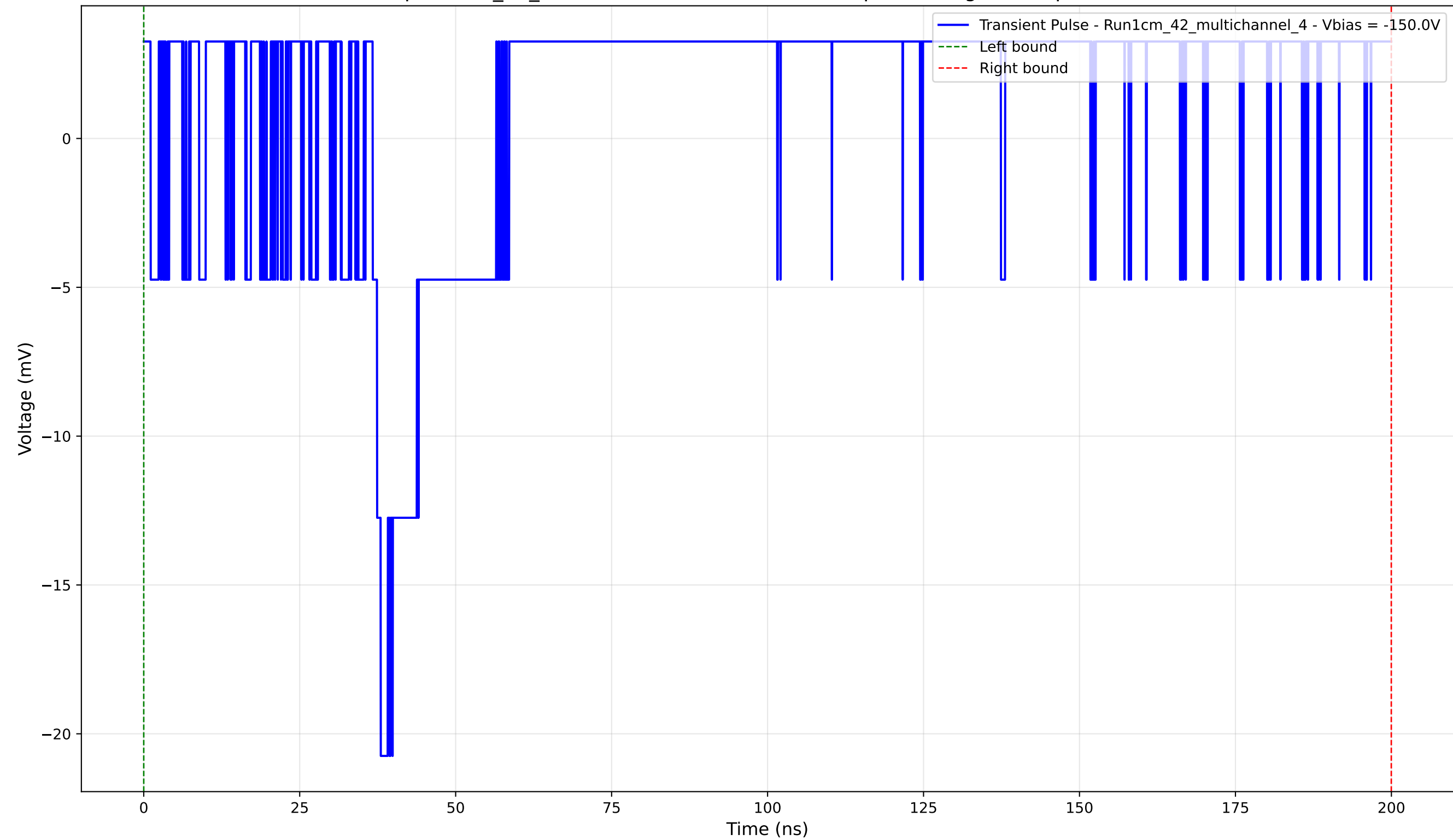
Transient Pulse - Sample: 1cm_42_multichannel - Position: 1080.0 \mu\text{m} - Charge: 5.71 pC - Rise Time: 0.00 ns (N/A)
