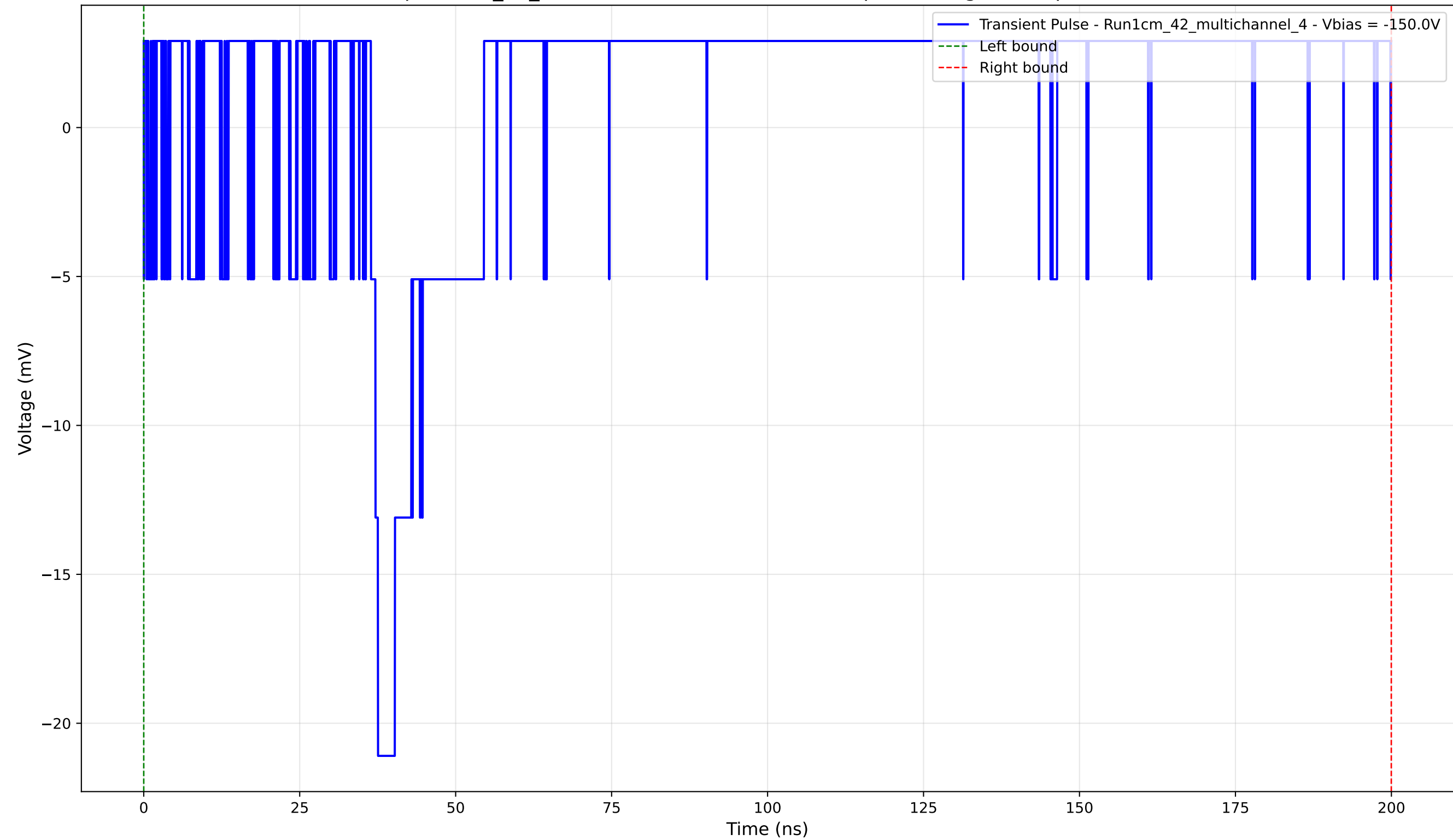
Transient Pulse - Sample: 1cm_42_multichannel - Position: 1280.0 \mu\text{m} - Charge: 5.41 pC - Rise Time: 0.00 ns (N/A)
