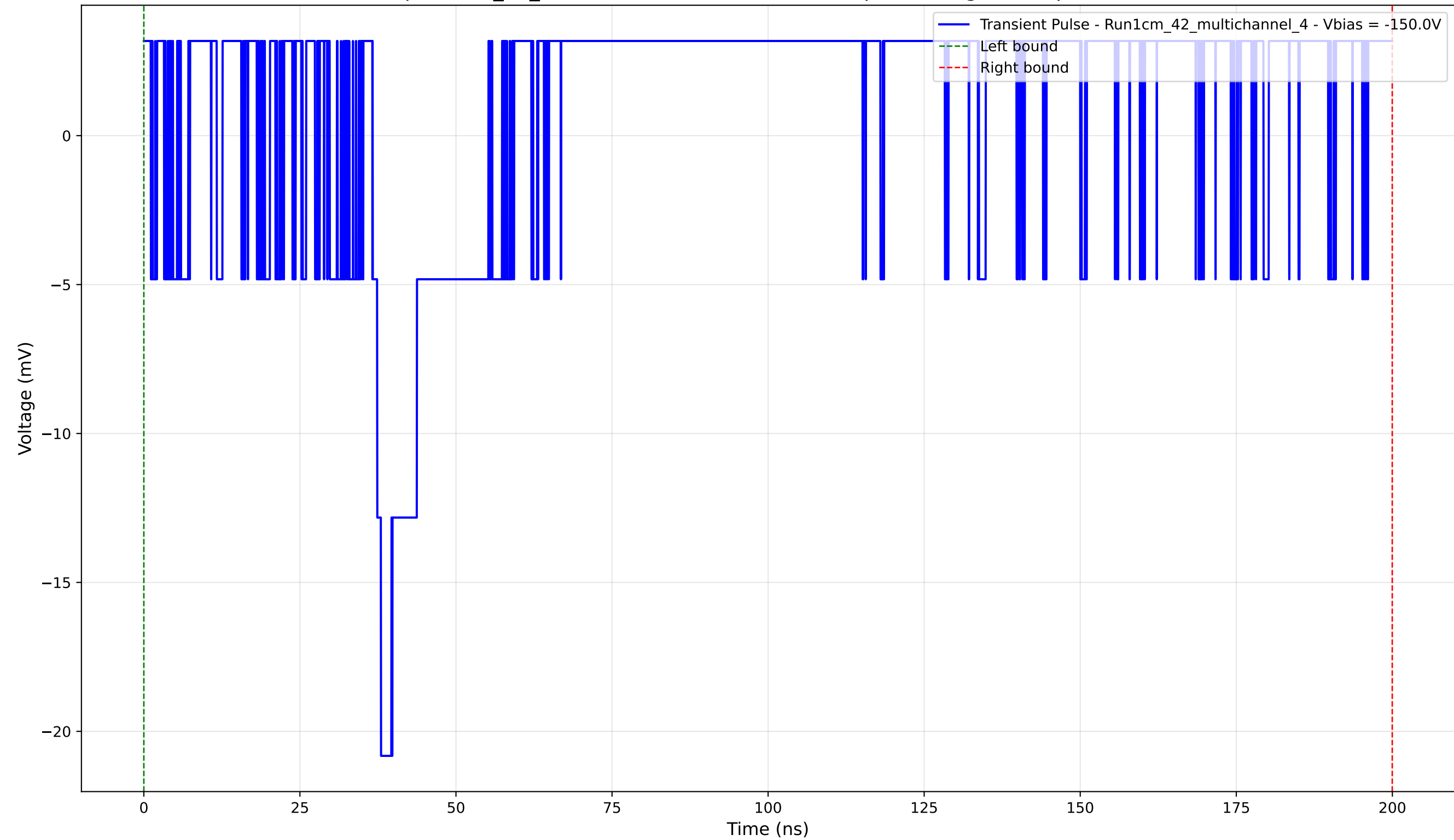
Transient Pulse - Sample: 1cm_42_multichannel - Position: 1075.0 \mu\text{m} - Charge: 4.12 pC - Rise Time: 0.00 ns (N/A)
