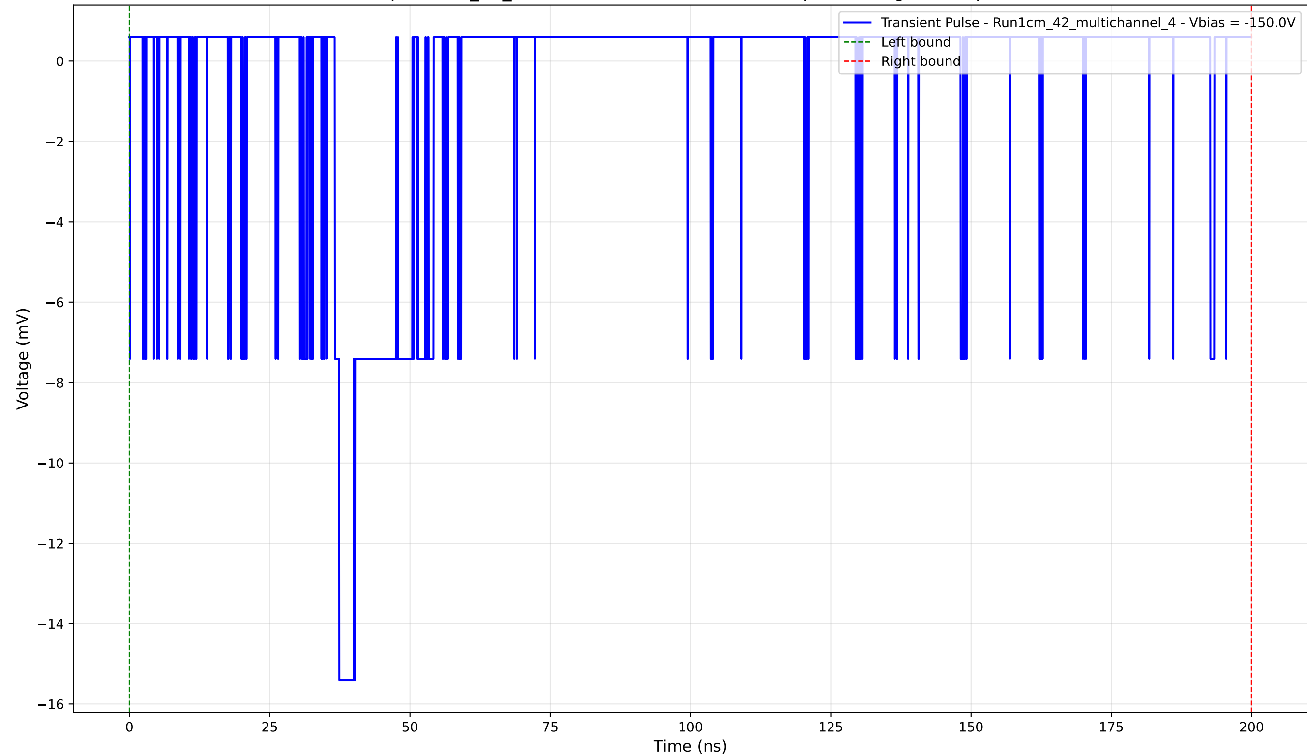
Transient Pulse - Sample: 1cm_42_multichannel - Position: 3345.0 \mu\text{m} - Charge: 2.24 pC - Rise Time: 0.82 ns
