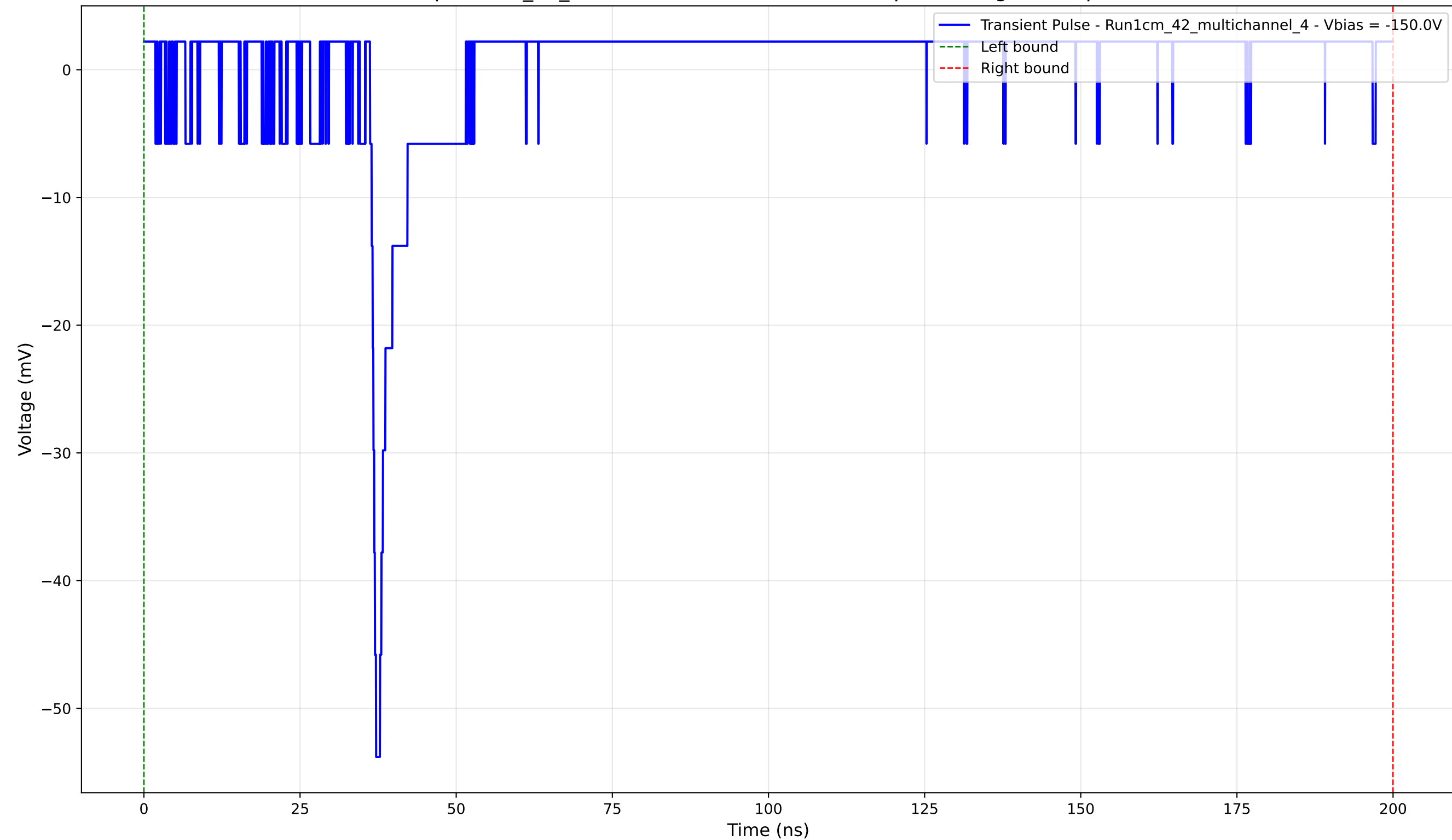
Transient Pulse - Sample: 1cm_42_multichannel - Position: 2035.0 \mu\text{m} - Charge: 2.12 pC - Rise Time: 0.96 ns
