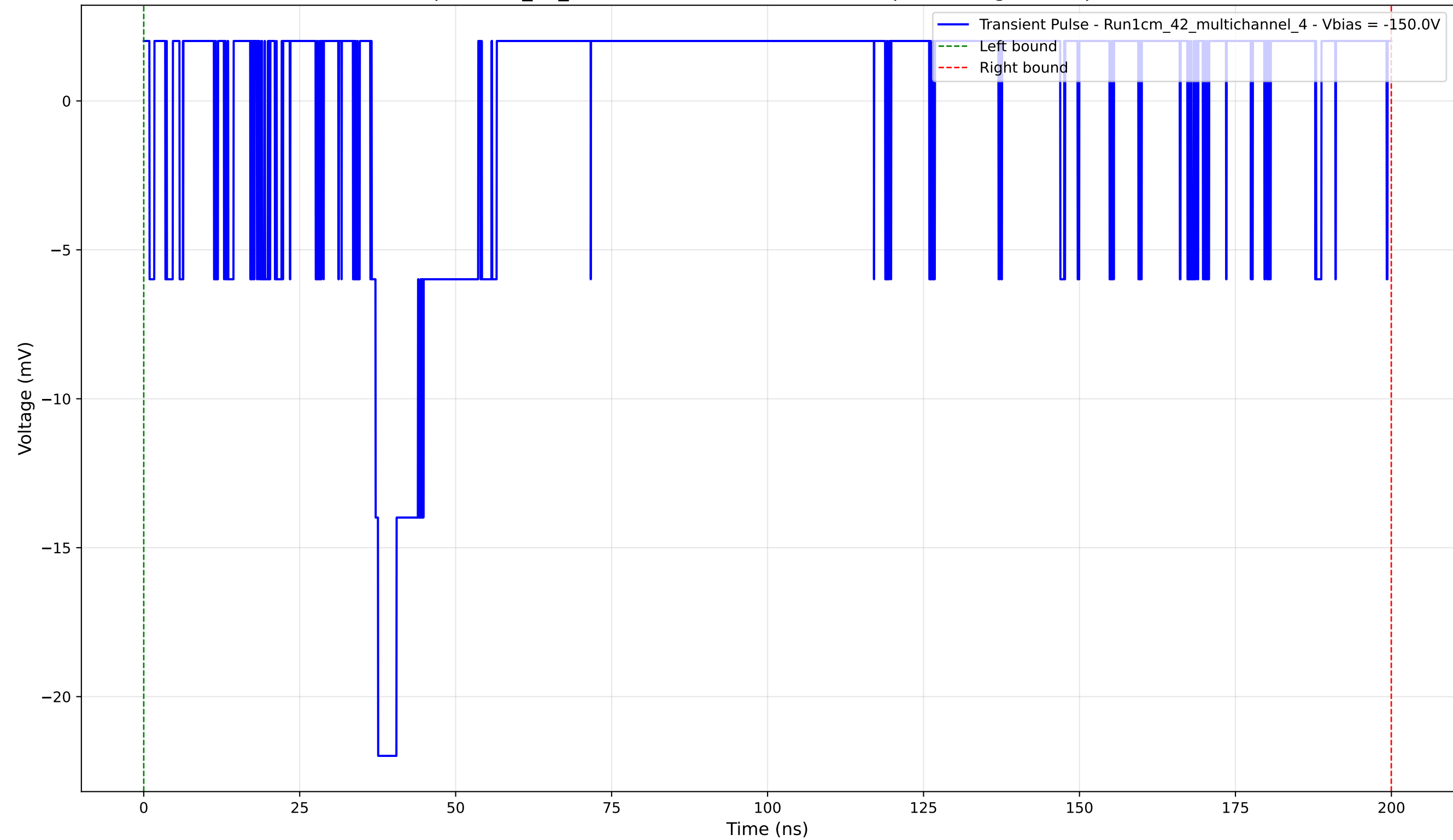
Transient Pulse - Sample: 1cm_42_multichannel - Position: 1260.0 \mu\text{m} - Charge: 0.73 pC - Rise Time: 1.04 ns
