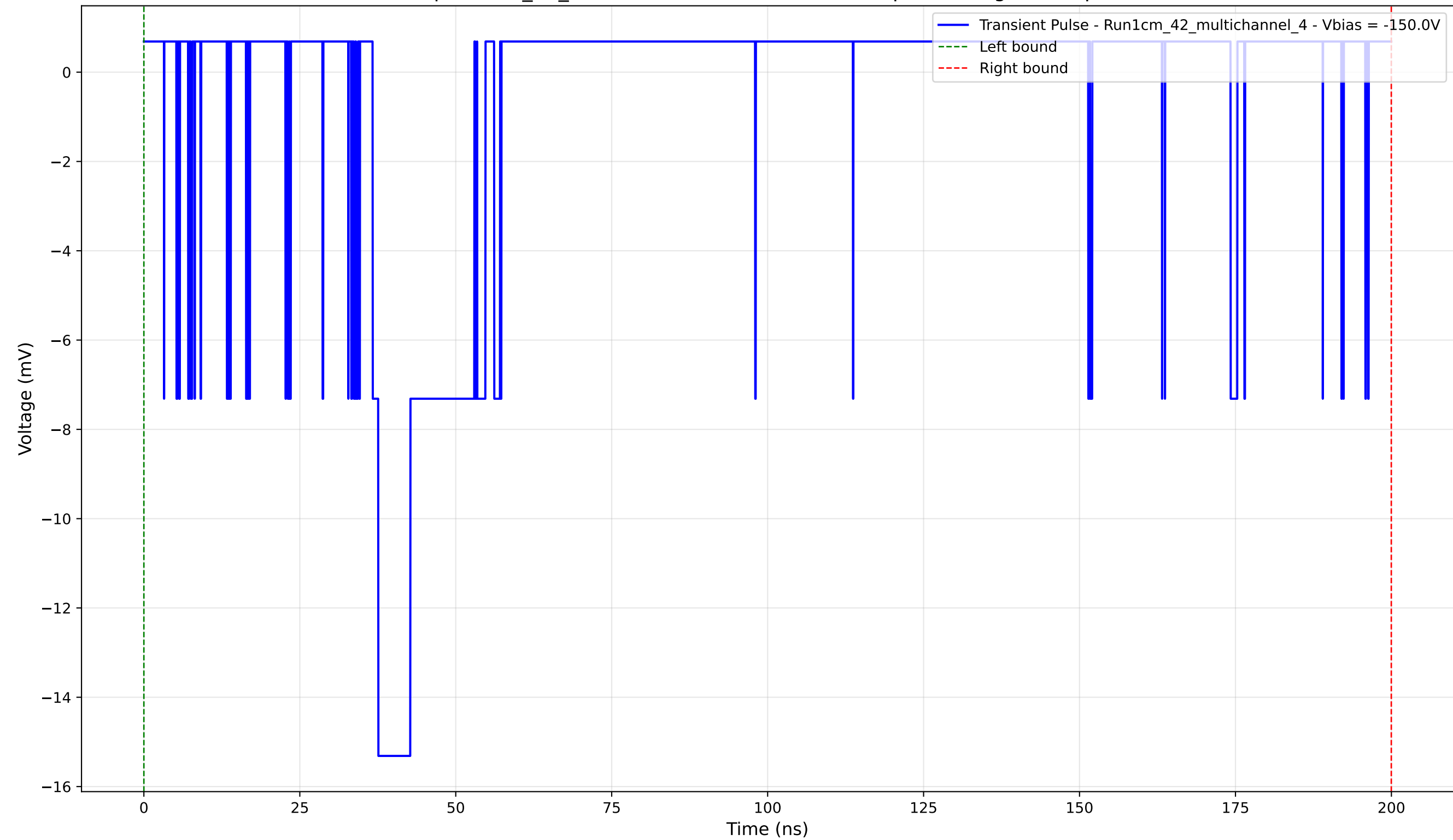
Transient Pulse - Sample: 1cm_42_multichannel - Position: 3705.0 \mu\text{m} - Charge: 1.93 pC - Rise Time: 0.92 ns
