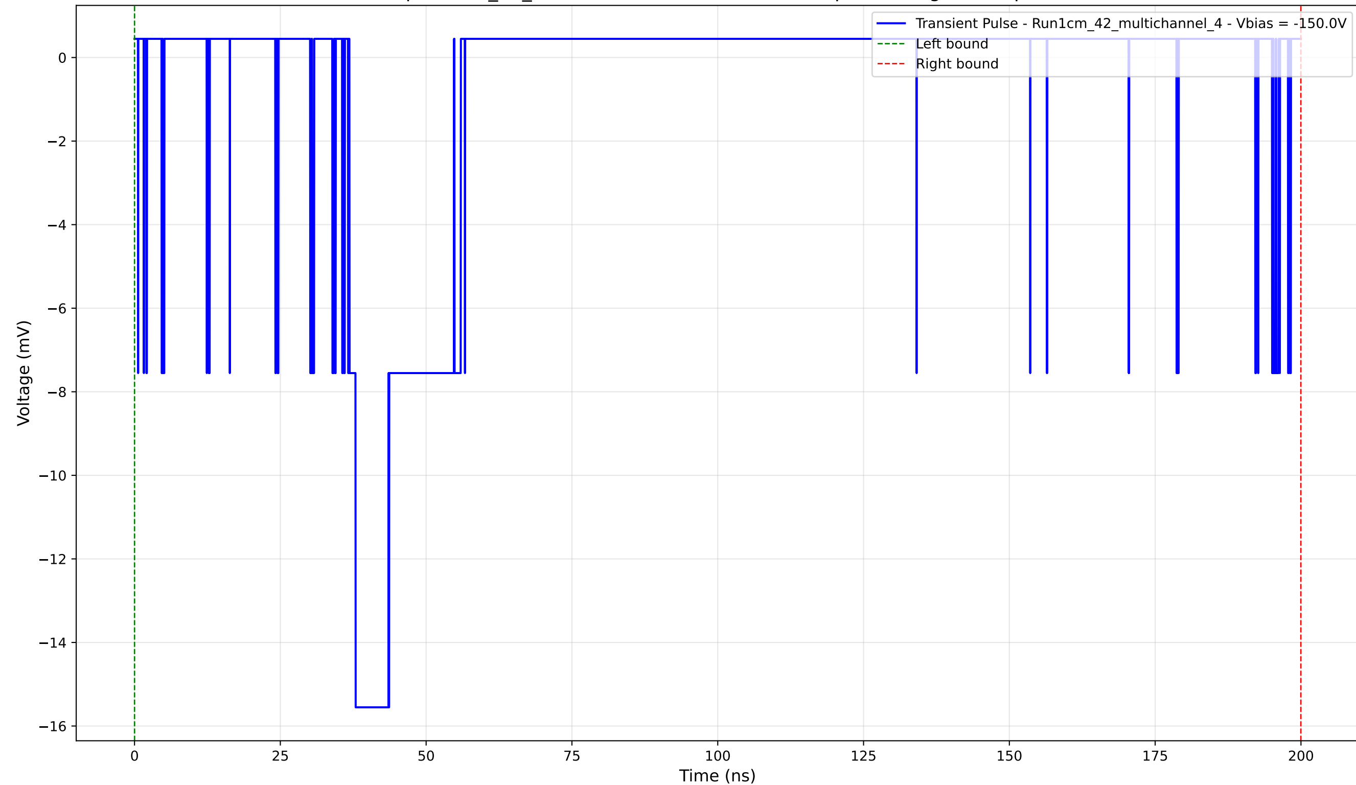
Transient Pulse - Sample: 1cm_42_multichannel - Position: 4000.0 \mu\text{m} - Charge: 2.86 pC - Rise Time: 1.06 ns
