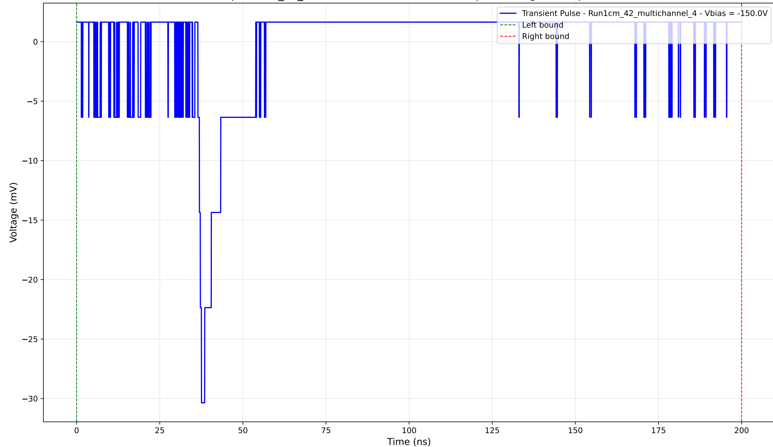
Transient Pulse - Sample: 1cm_42_multichannel - Position: 1490.0 \mu\text{m} - Charge: 0.17 pC - Rise Time: 1.07 ns
