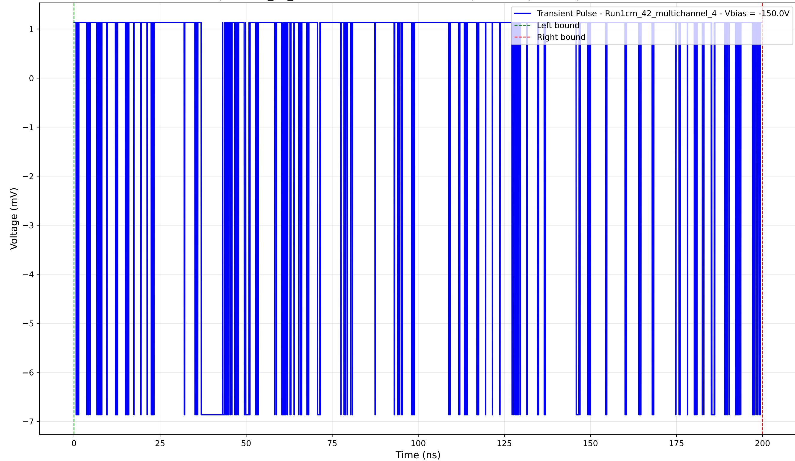
Transient Pulse - Sample: 1cm_42_multichannel - Position: 3430.0 \mu\text{m} - Charge: 0.25 pC - Rise Time: 0.00 ns (N/A)
