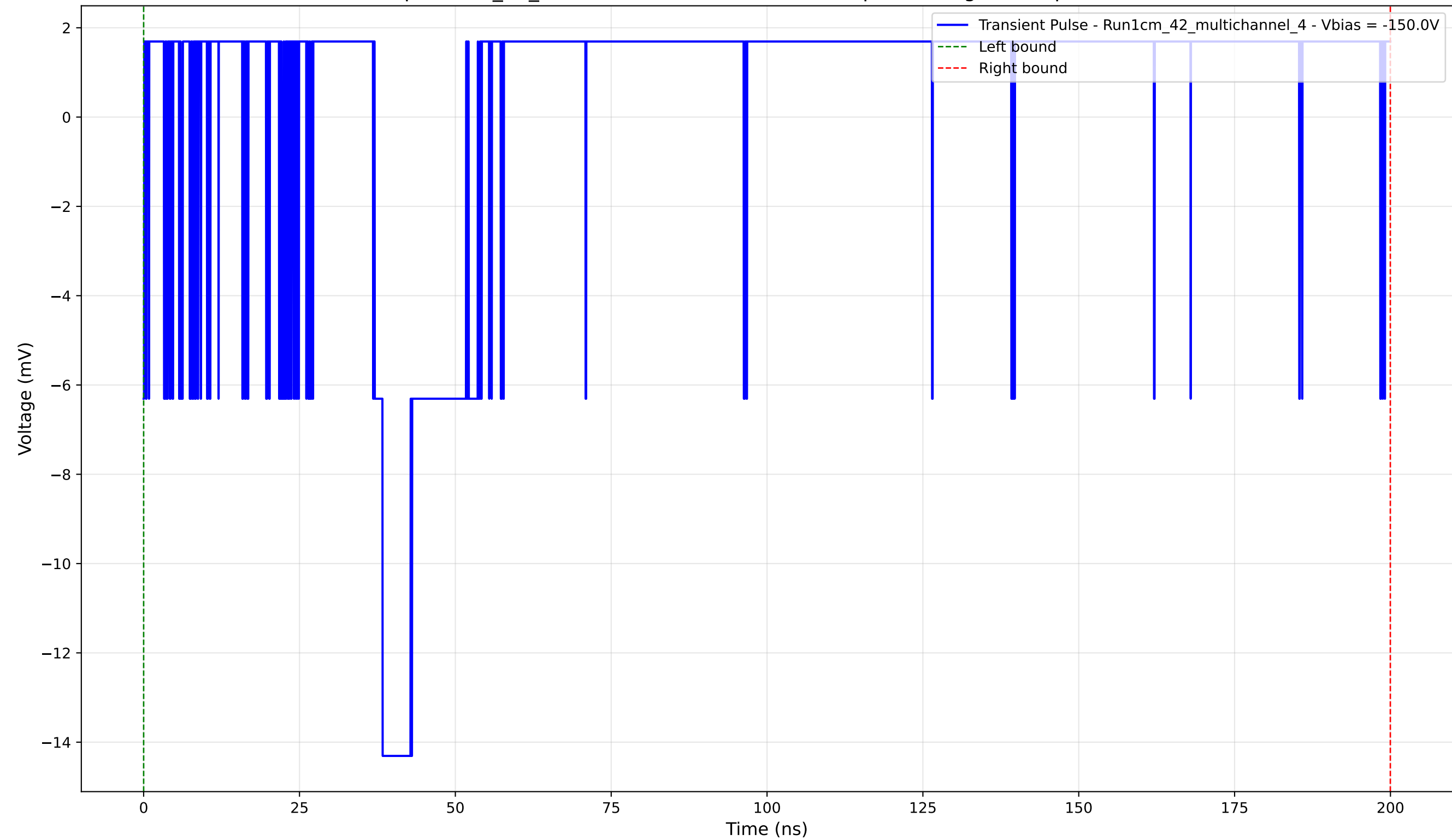
Transient Pulse - Sample: 1cm_42_multichannel - Position: 4170.0 \mu\text{m} - Charge: 2.21 pC - Rise Time: 0.00 ns (N/A)
