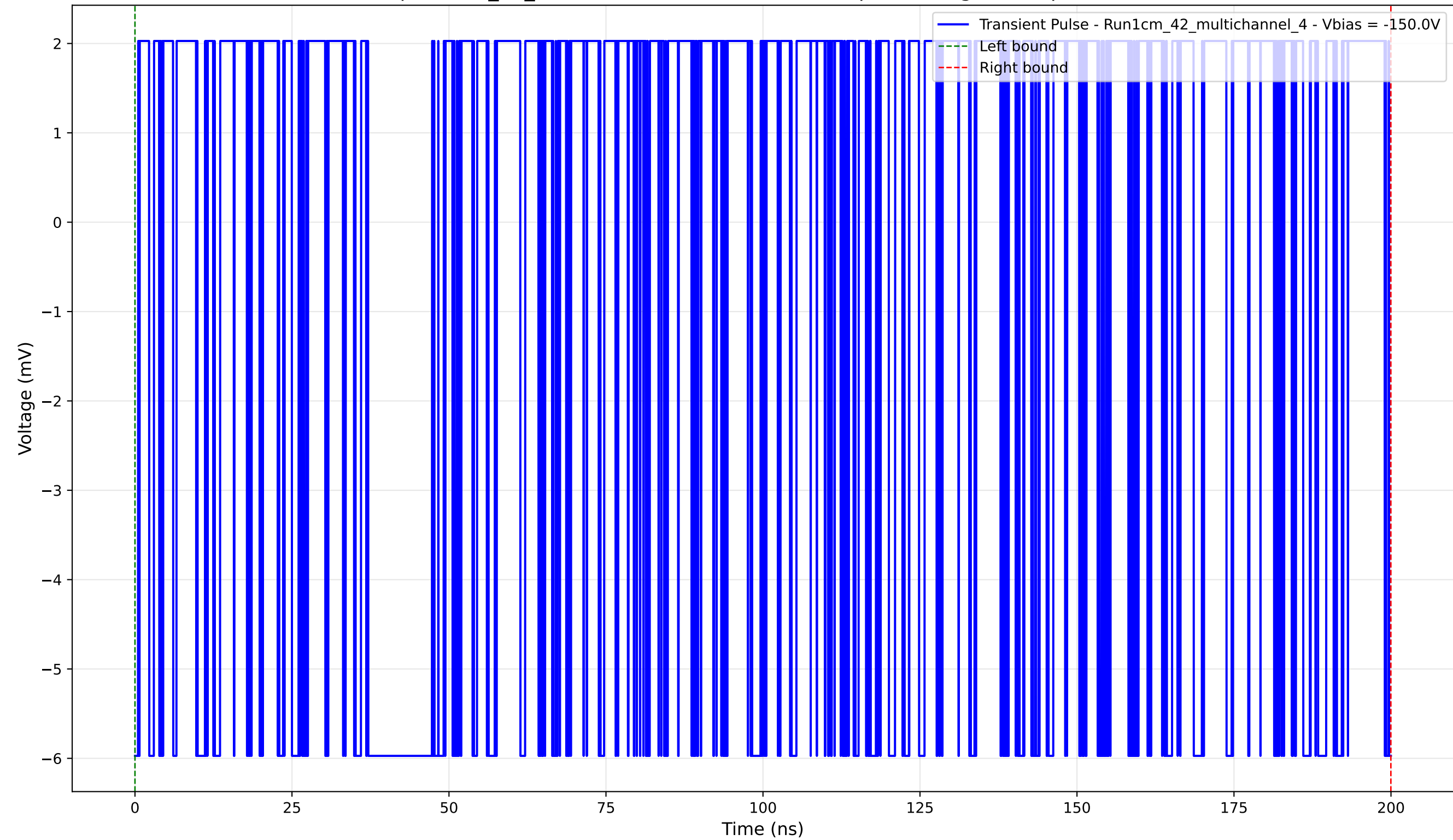
Transient Pulse - Sample: 1cm_42_multichannel - Position: 1340.0 \mu\text{m} - Charge: 1.30 pC - Rise Time: 0.00 ns (N/A)
