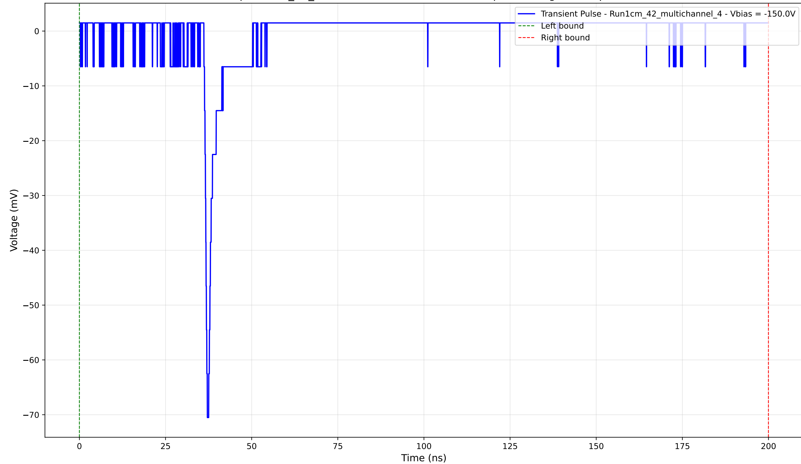
Transient Pulse - Sample: 1cm_42_multichannel - Position: 2180.0 \mu\text{m} - Charge: 0.69 pC - Rise Time: 0.82 ns
