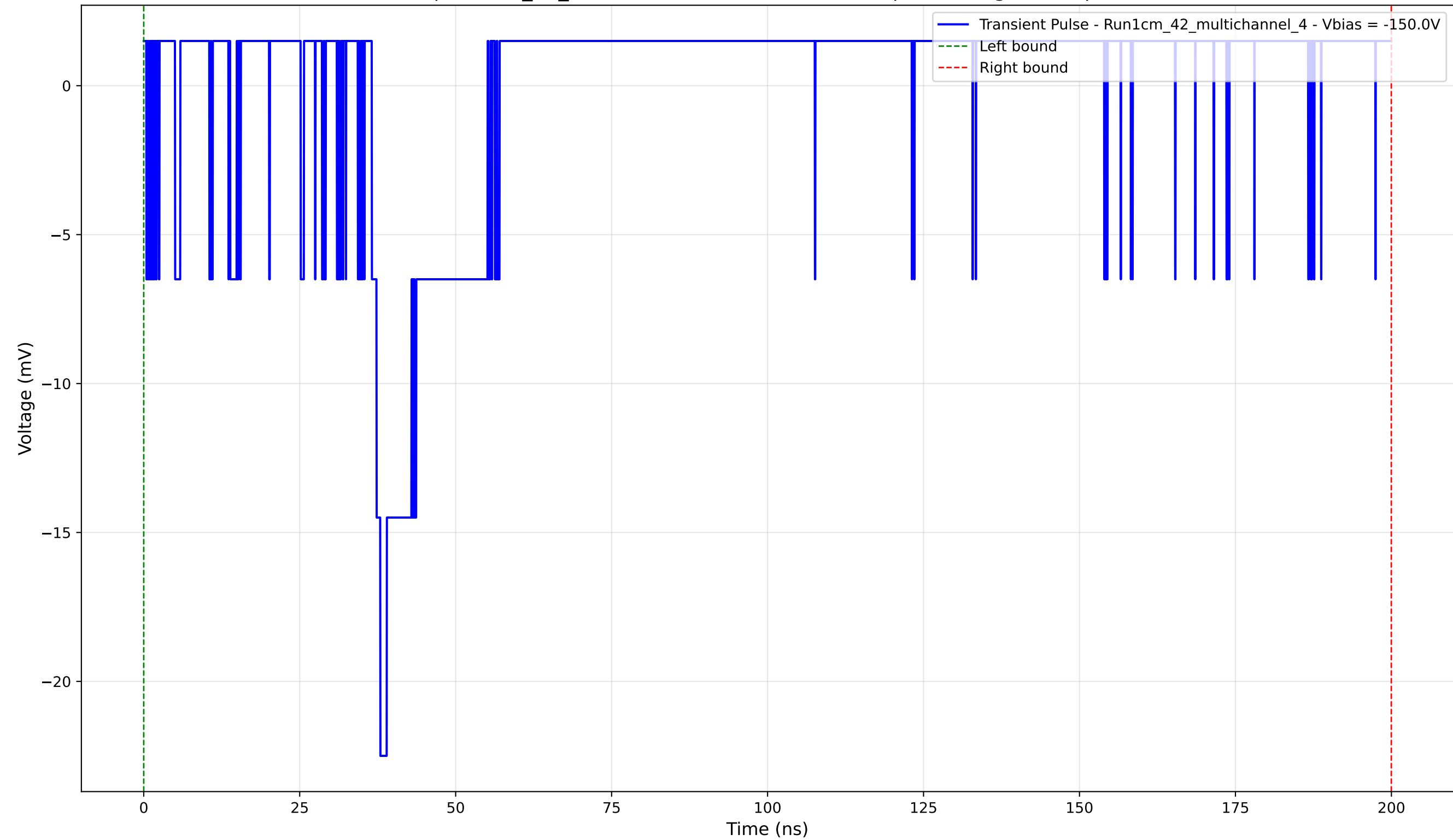
Transient Pulse - Sample: 1cm_42_multichannel - Position: 3540.0 \mu\text{m} - Charge: 0.54 pC - Rise Time: 1.38 ns
