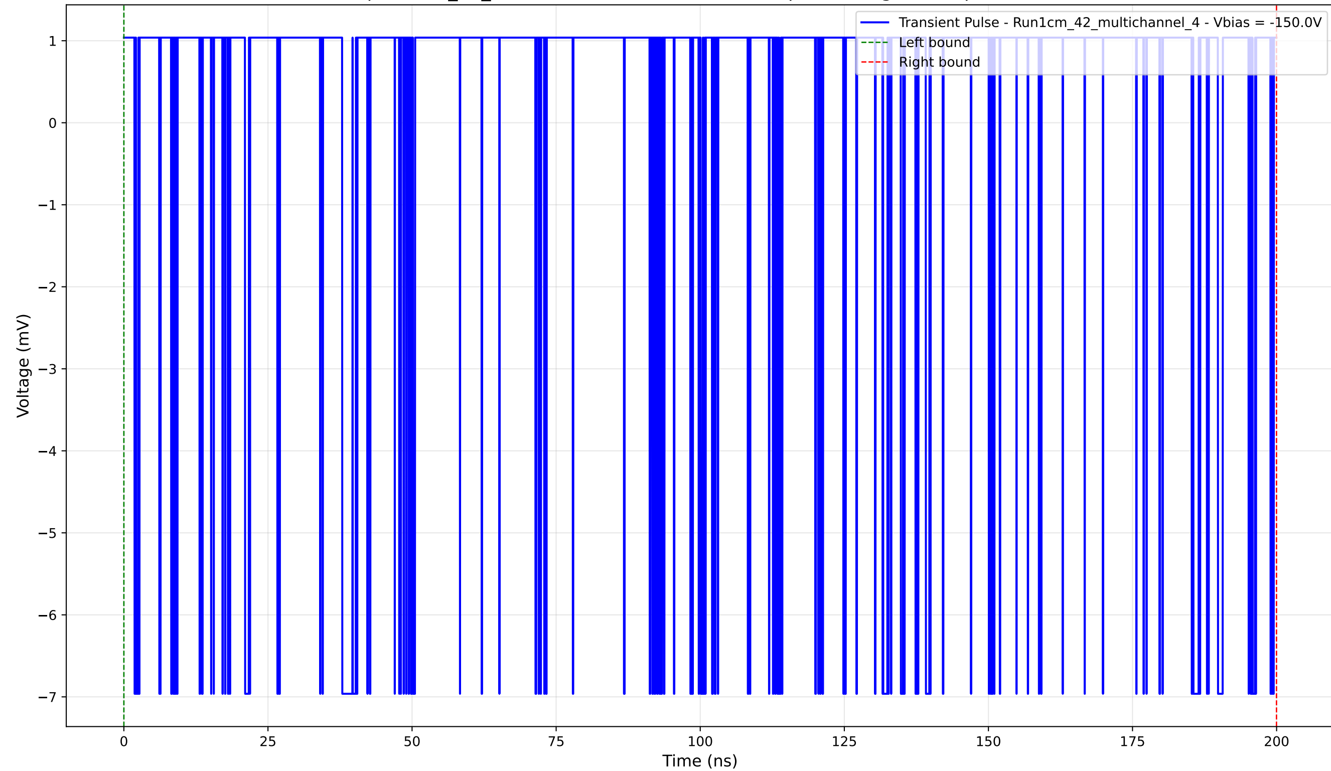
Transient Pulse - Sample: 1cm_42_multichannel - Position: 4420.0 \mu\text{m} - Charge: 1.07 pC - Rise Time: 0.00 ns (N/A)
