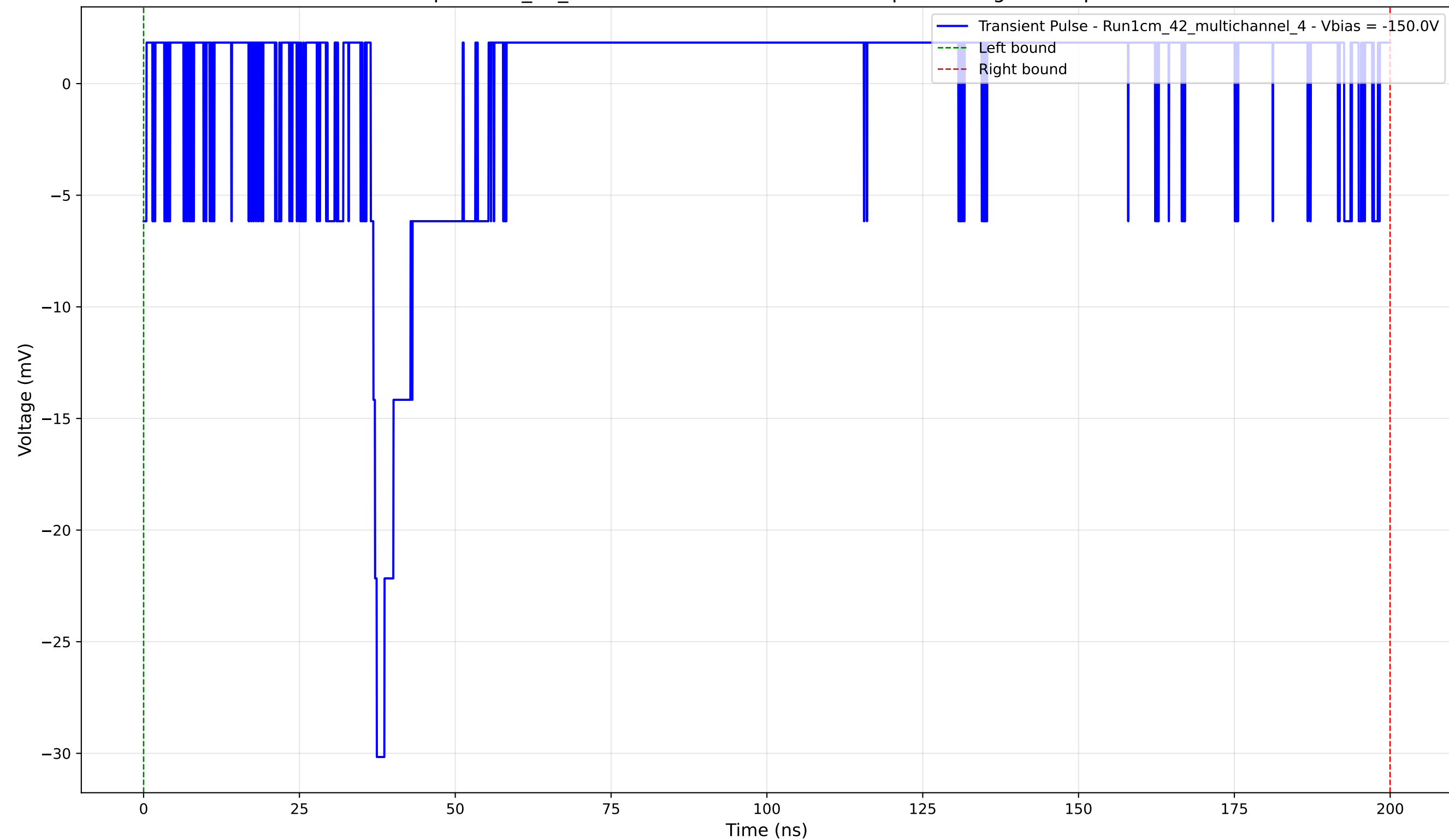
Transient Pulse - Sample: 1cm_42_multichannel - Position: 1580.0 \mu\text{m} - Charge: 0.41 pC - Rise Time: 0.97 ns
