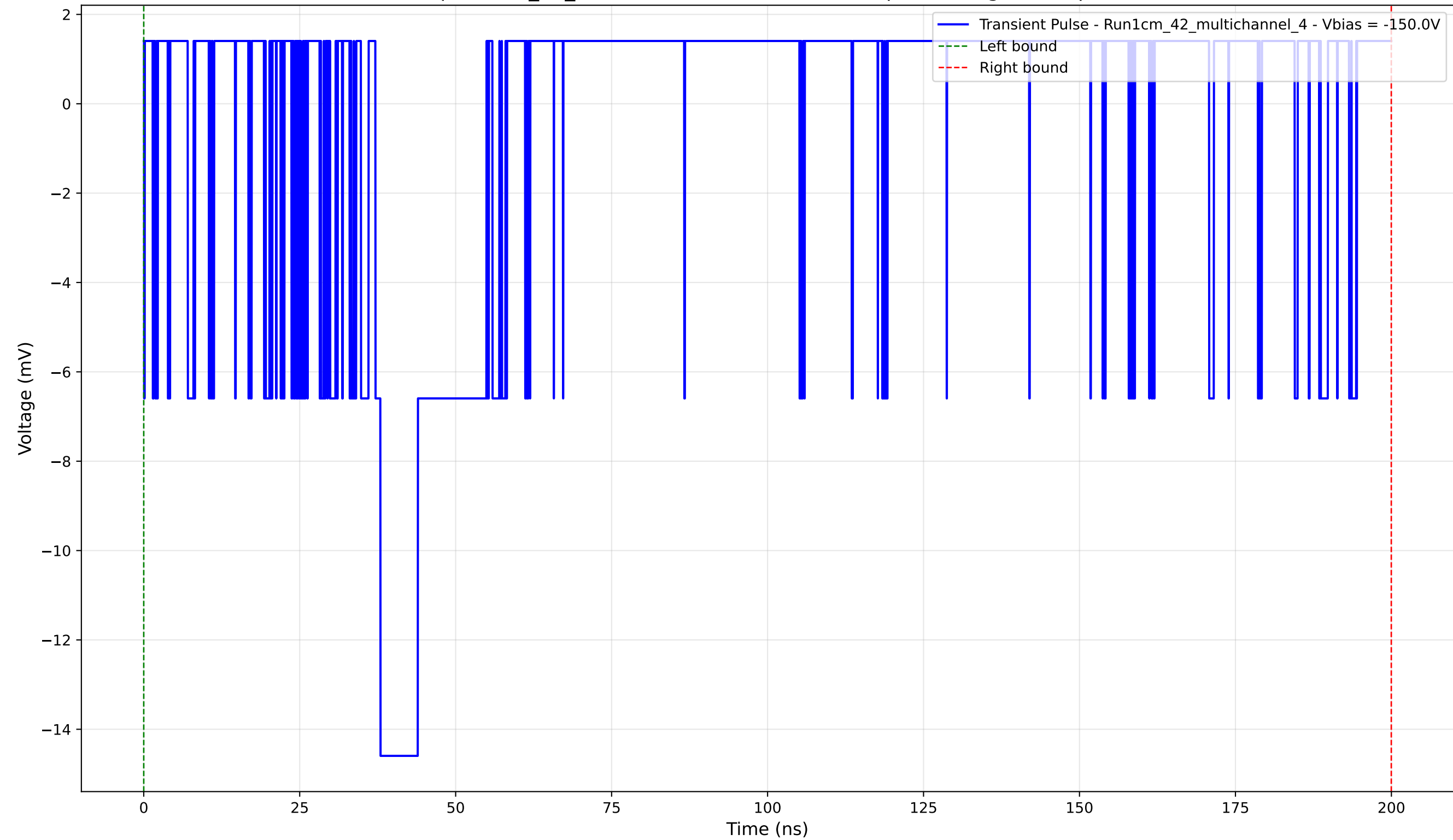
Transient Pulse - Sample: 1cm_42_multichannel - Position: 570.0 \mu\text{m} - Charge: 1.32 pC - Rise Time: 0.82 ns
