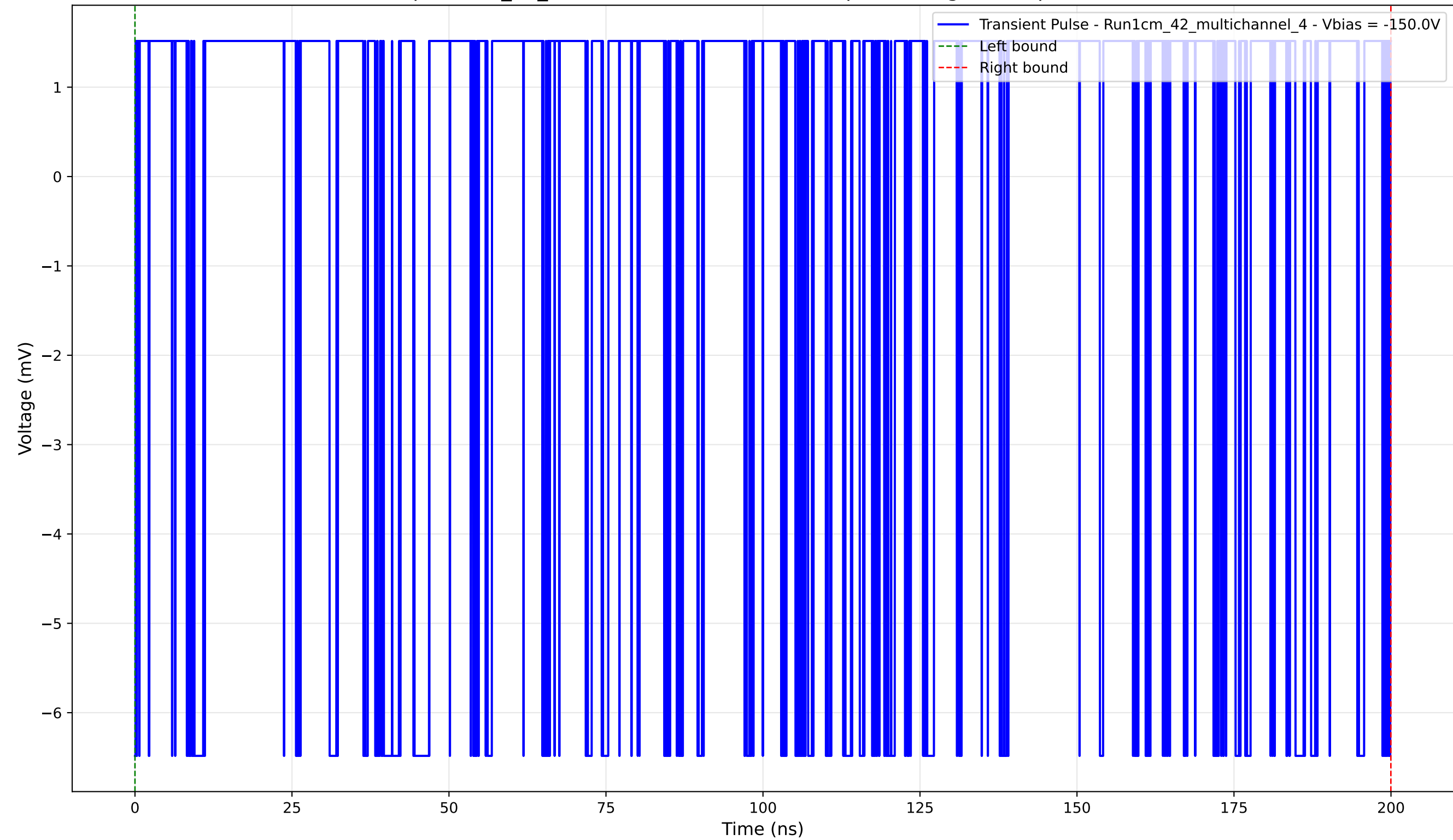
Transient Pulse - Sample: 1cm_42_multichannel - Position: 55.0 \mu\text{m} - Charge: 0.13 pC - Rise Time: 0.00 ns (N/A)
