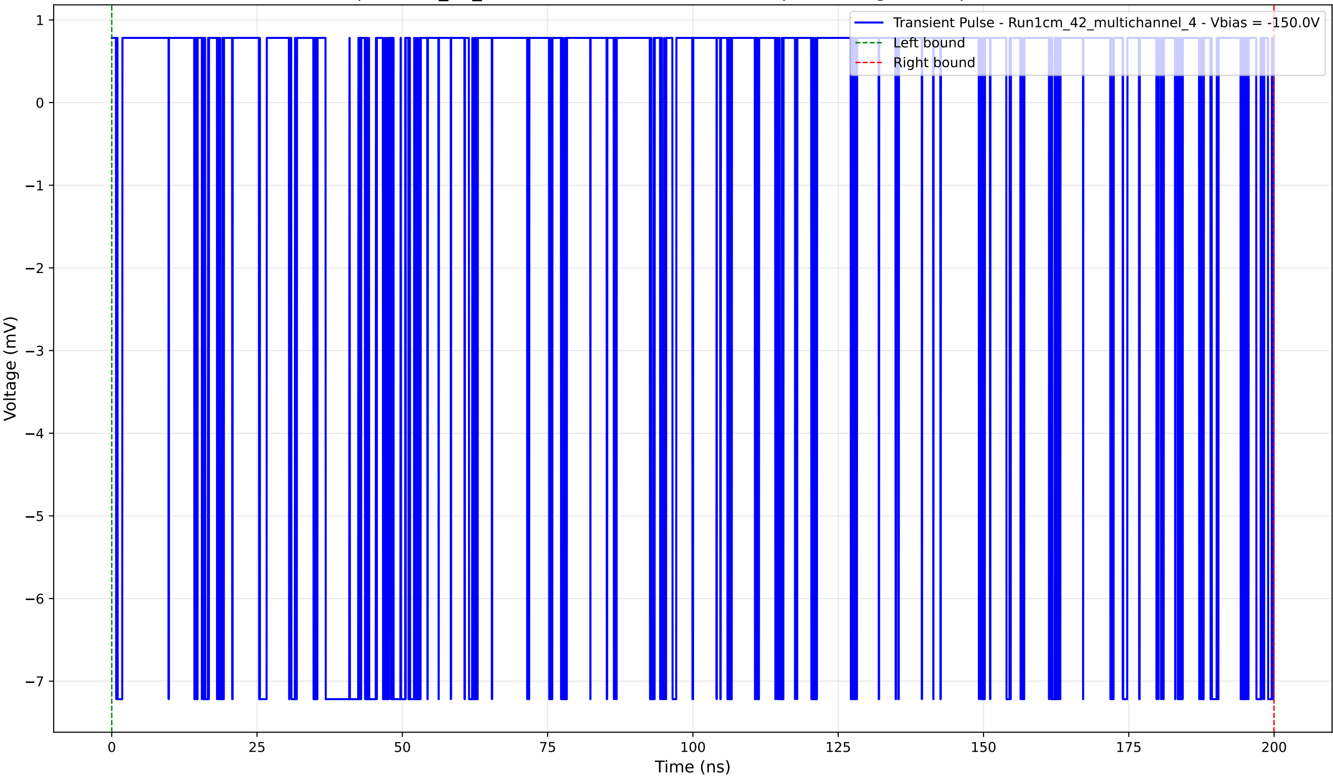
Transient Pulse - Sample: 1cm_42_multichannel - Position: 3365.0 \mu\text{m} - Charge: 2.45 pC - Rise Time: 0.00 ns (N/A)
