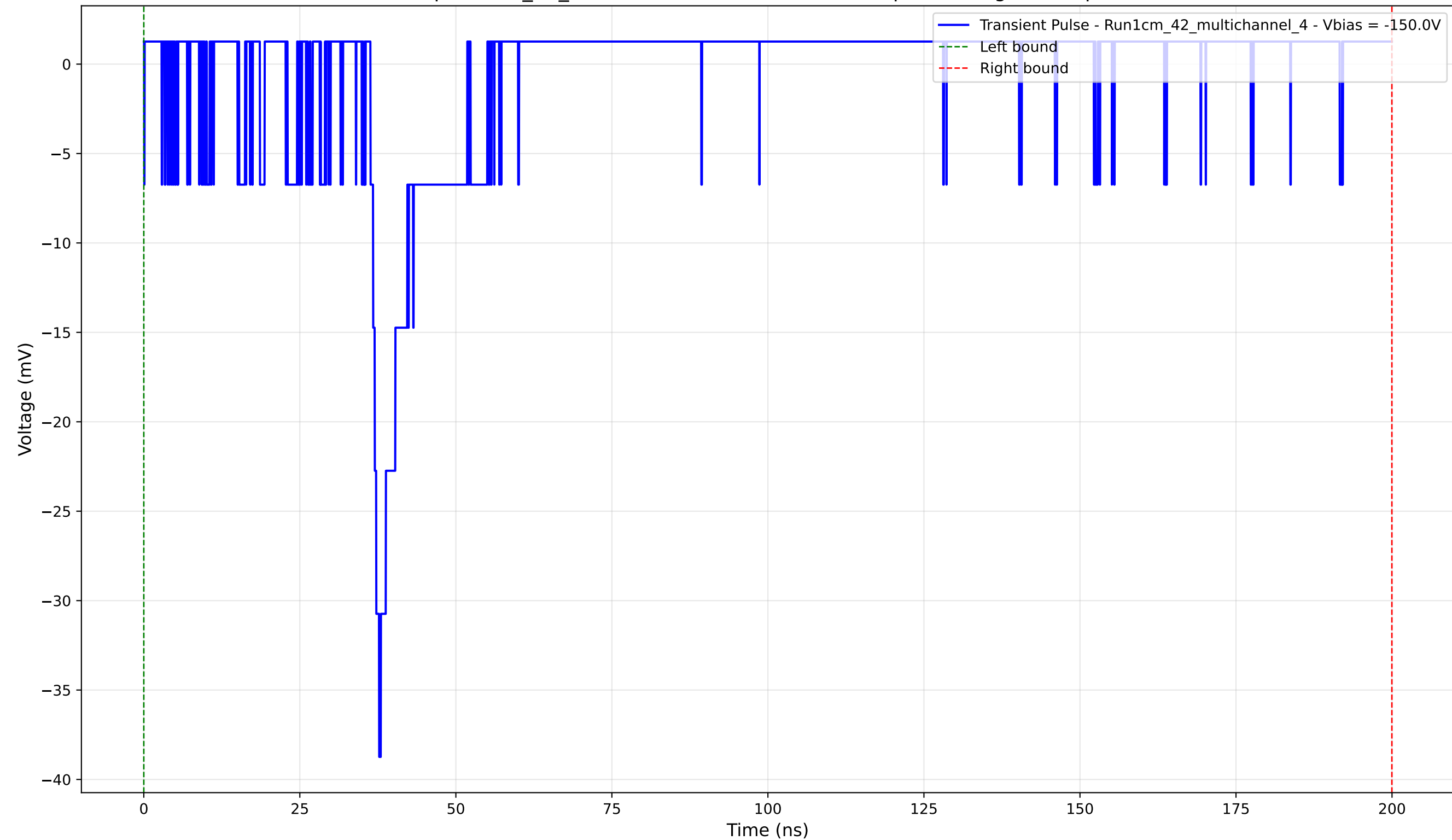
Transient Pulse - Sample: 1cm_42_multichannel - Position: 1645.0 \mu\text{m} - Charge: 1.54 pC - Rise Time: 1.39 ns
