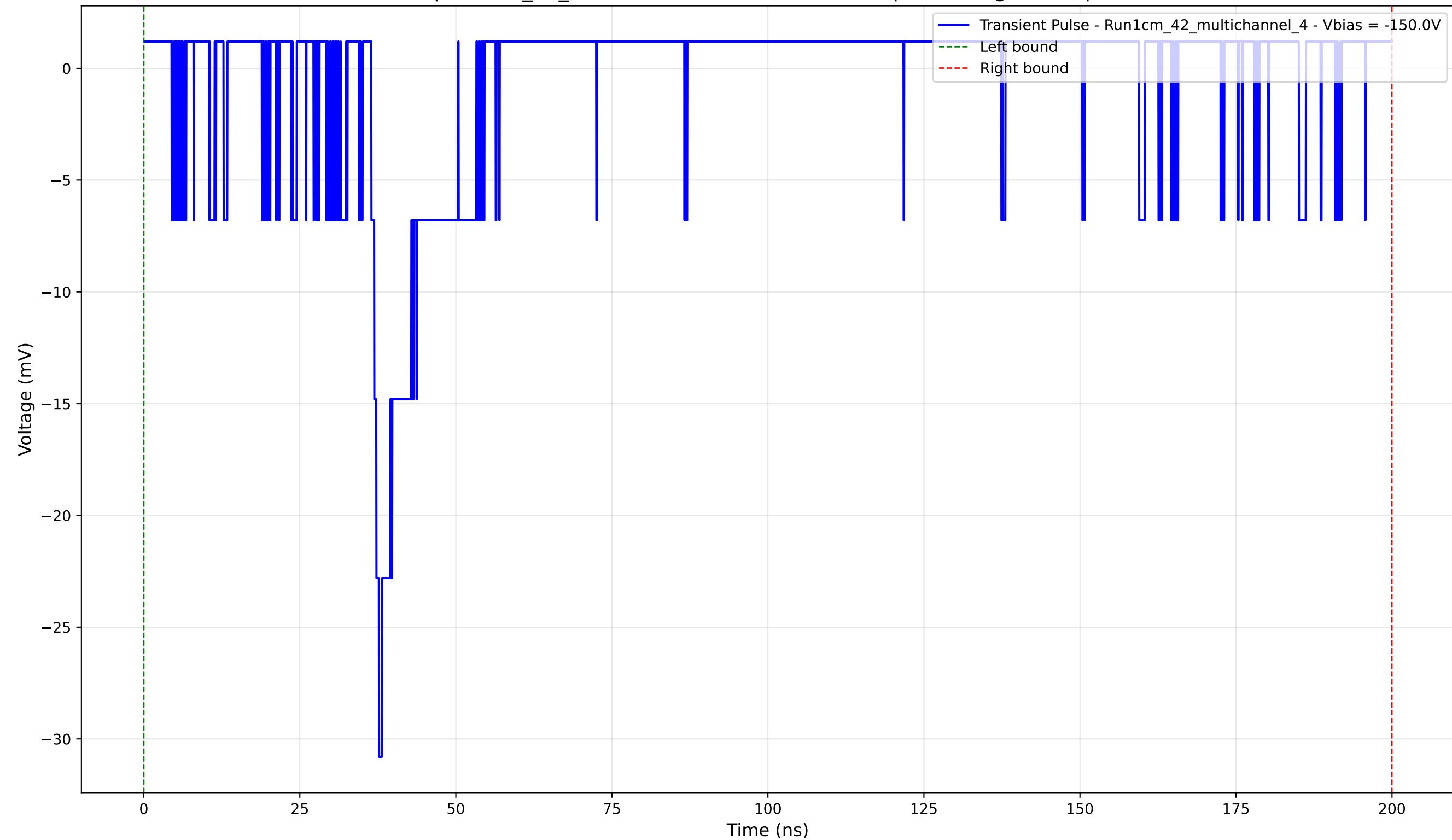
Transient Pulse - Sample: 1cm_42_multichannel - Position: 3265.0 \mu\text{m} - Charge: 1.73 pC - Rise Time: 1.23 ns
