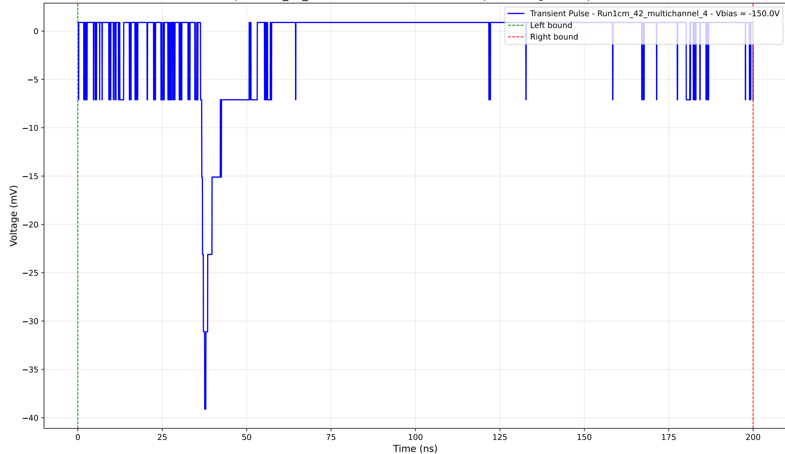
Transient Pulse - Sample: 1cm_42_multichannel - Position: 3045.0 \mu\text{m} - Charge: 2.48 pC - Rise Time: 1.23 ns
