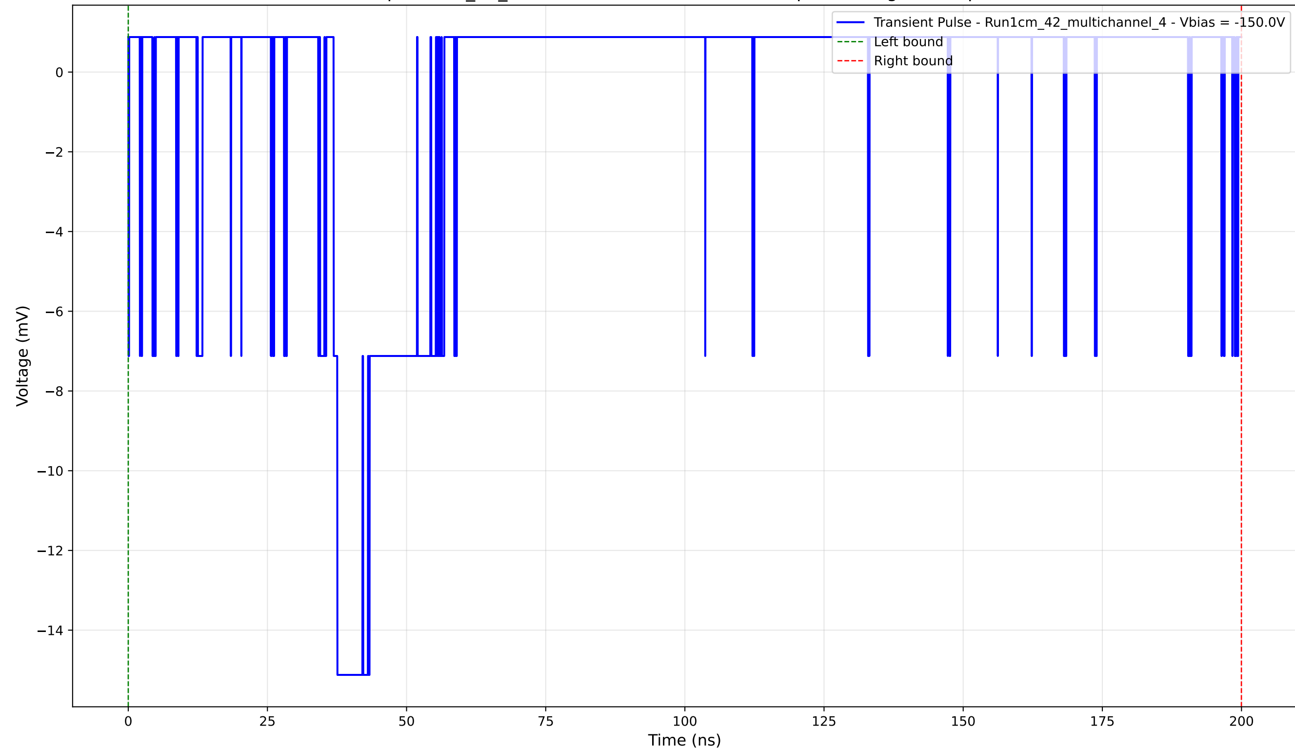
Transient Pulse - Sample: 1cm_42_multichannel - Position: 3725.0 \mu\text{m} - Charge: 1.49 pC - Rise Time: 0.68 ns
