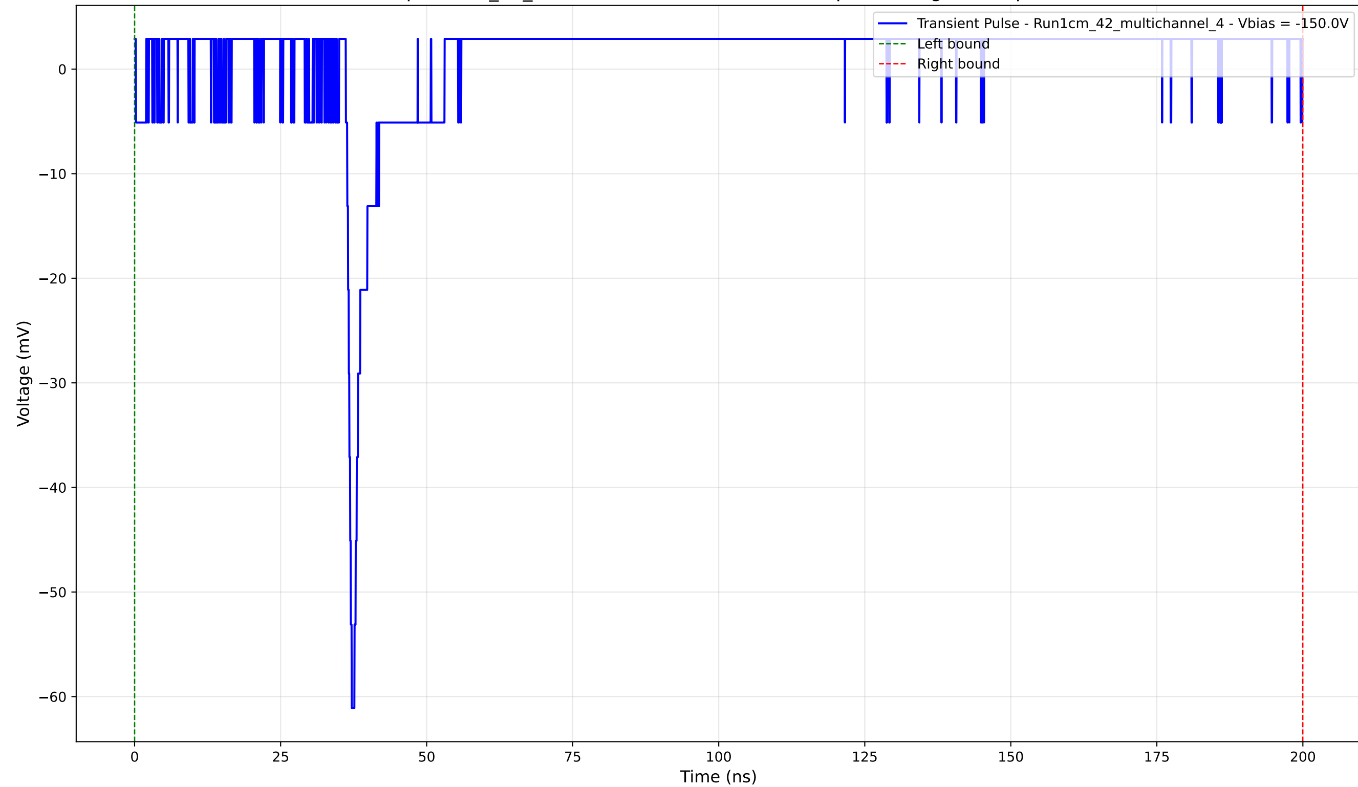
Transient Pulse - Sample: 1cm_42_multichannel - Position: 2110.0 \mu\text{m} - Charge: 4.83 pC - Rise Time: 0.78 ns
