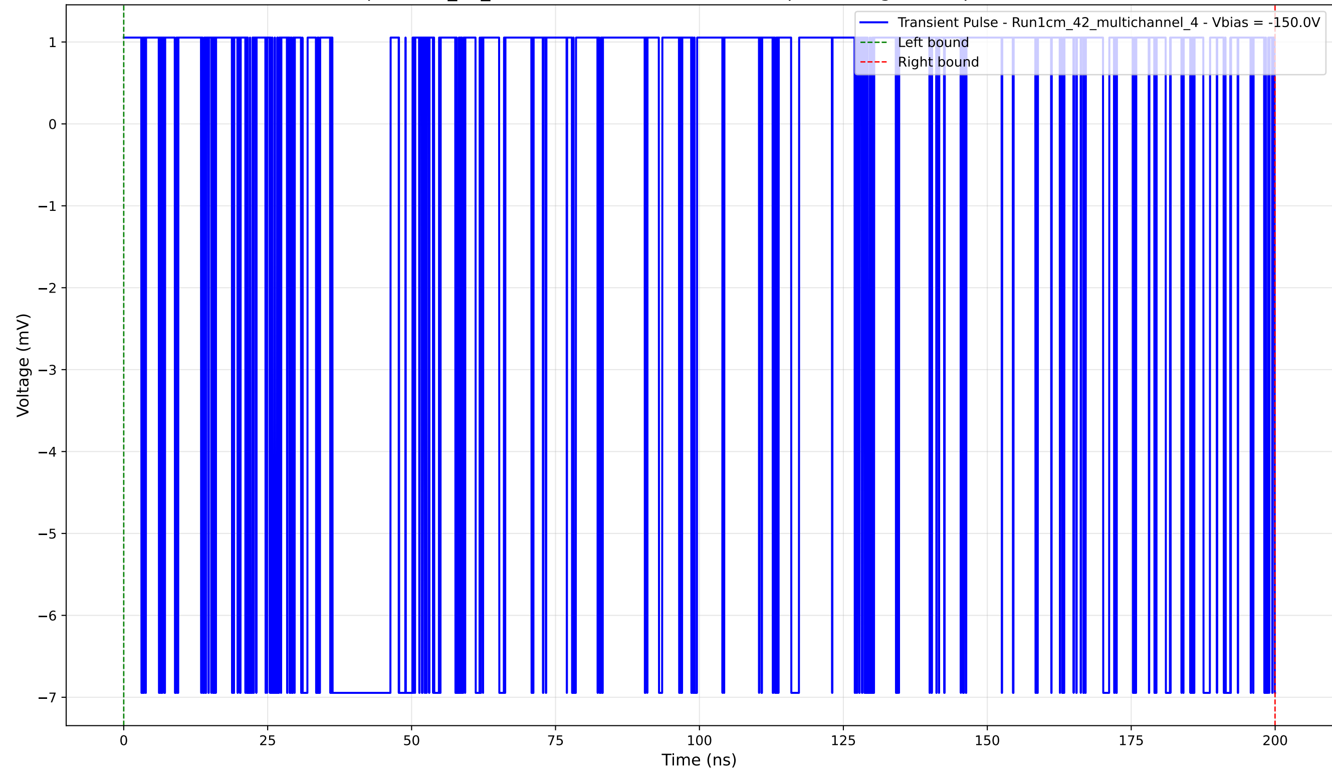
Transient Pulse - Sample: 1cm_42_multichannel - Position: 1410.0 \mu\text{m} - Charge: 2.20 pC - Rise Time: 0.00 ns (N/A)
