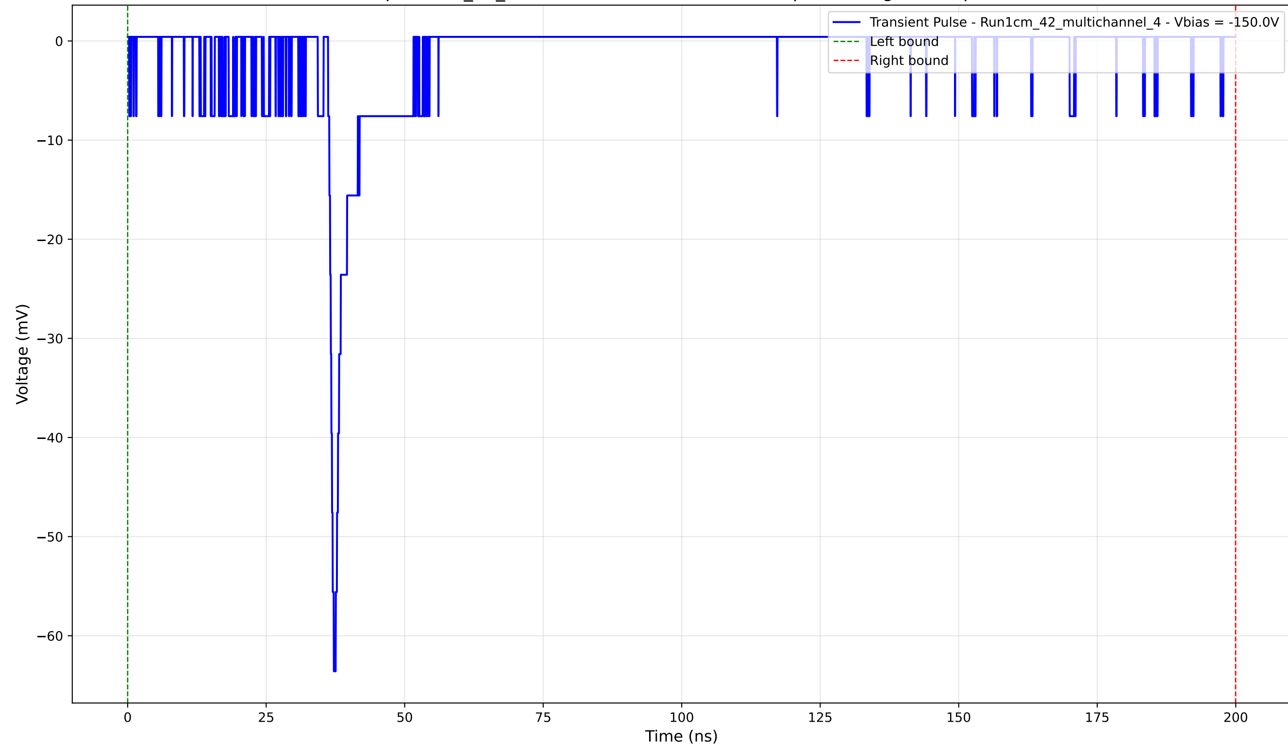
Transient Pulse - Sample: 1cm_42_multichannel - Position: 2645.0 \mu\text{m} - Charge: 5.17 pC - Rise Time: 1.02 ns
