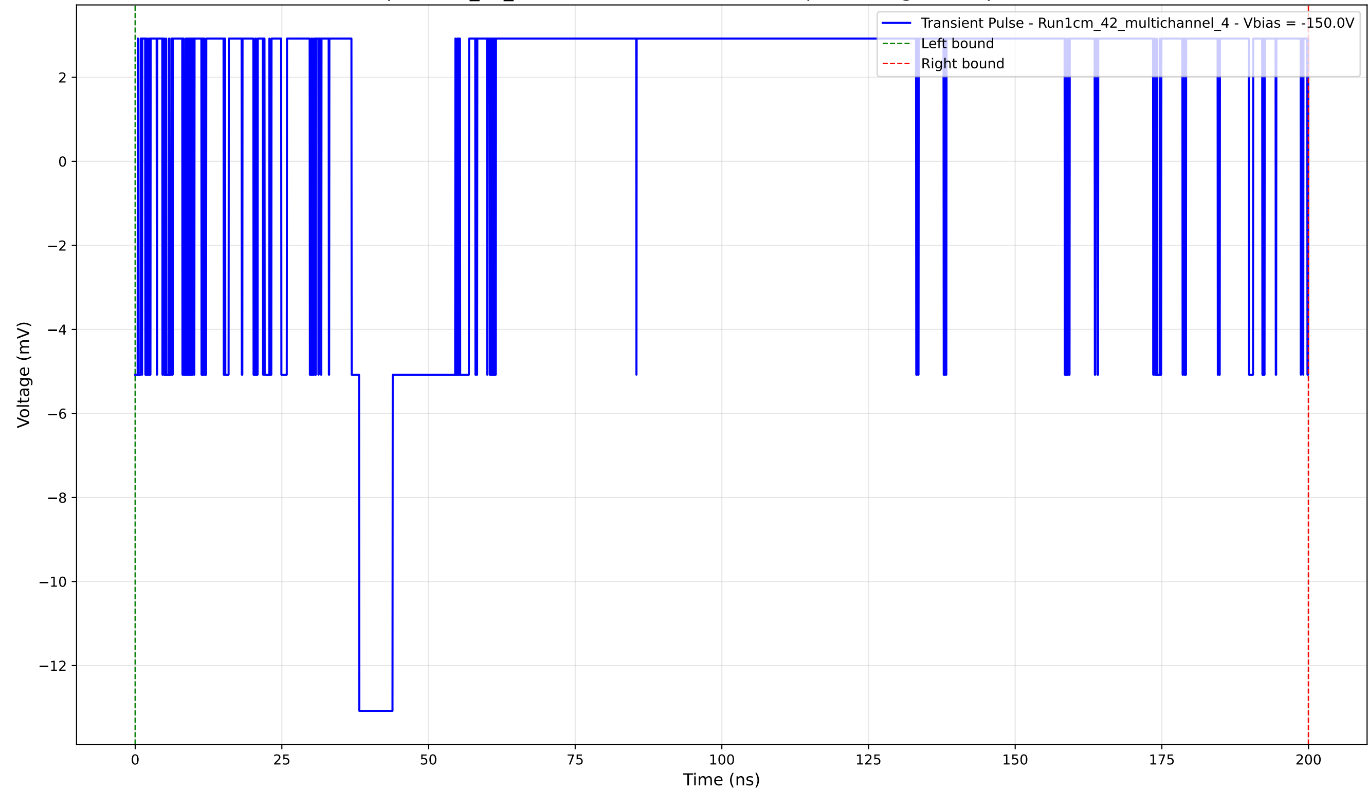
Transient Pulse - Sample: 1cm_42_multichannel - Position: 475.0 \mu\text{m} - Charge: 5.43 pC - Rise Time: 0.00 ns (N/A)
