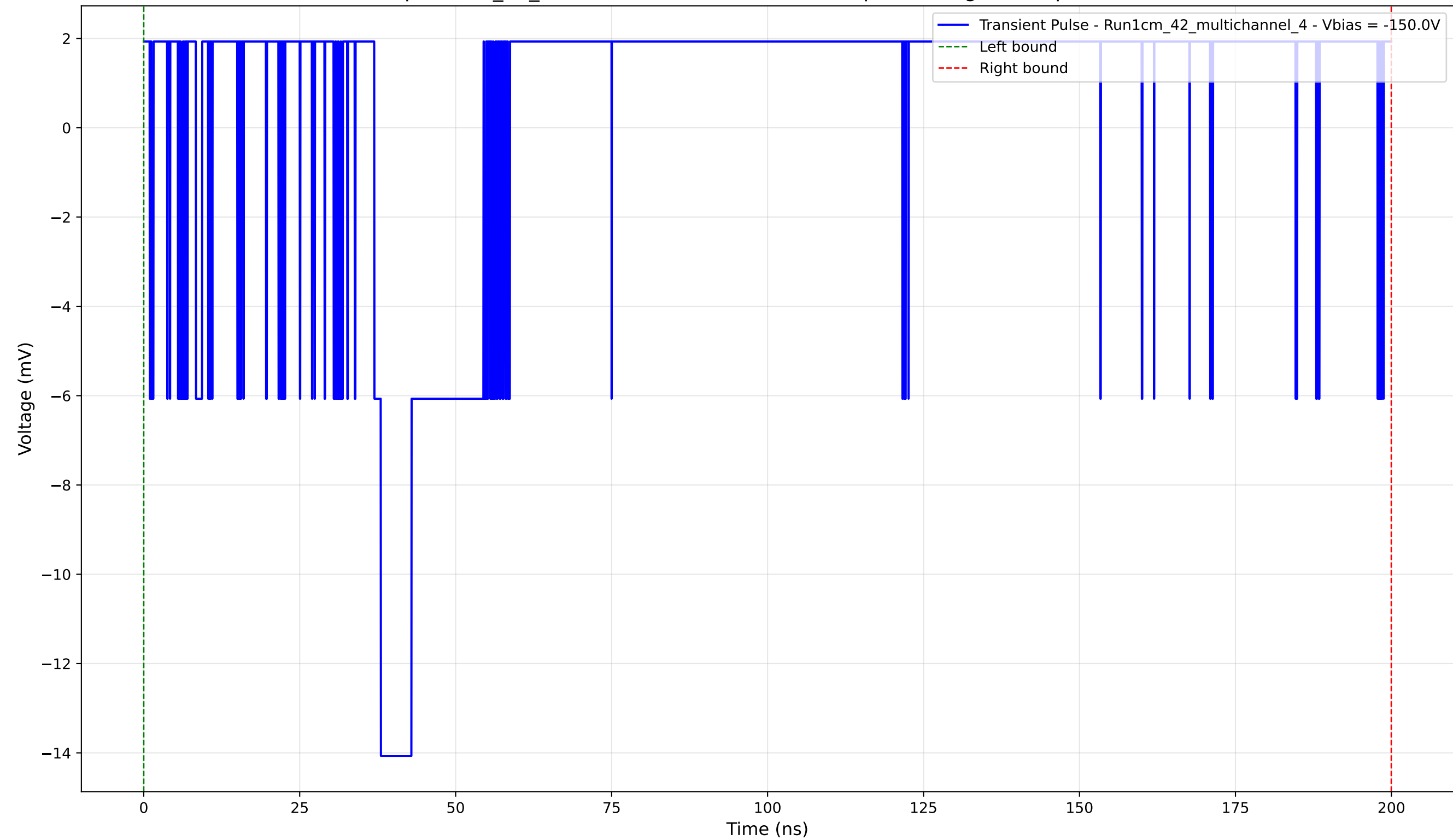
Transient Pulse - Sample: 1cm_42_multichannel - Position: 3975.0 \mu\text{m} - Charge: 2.71 pC - Rise Time: 0.00 ns (N/A)
