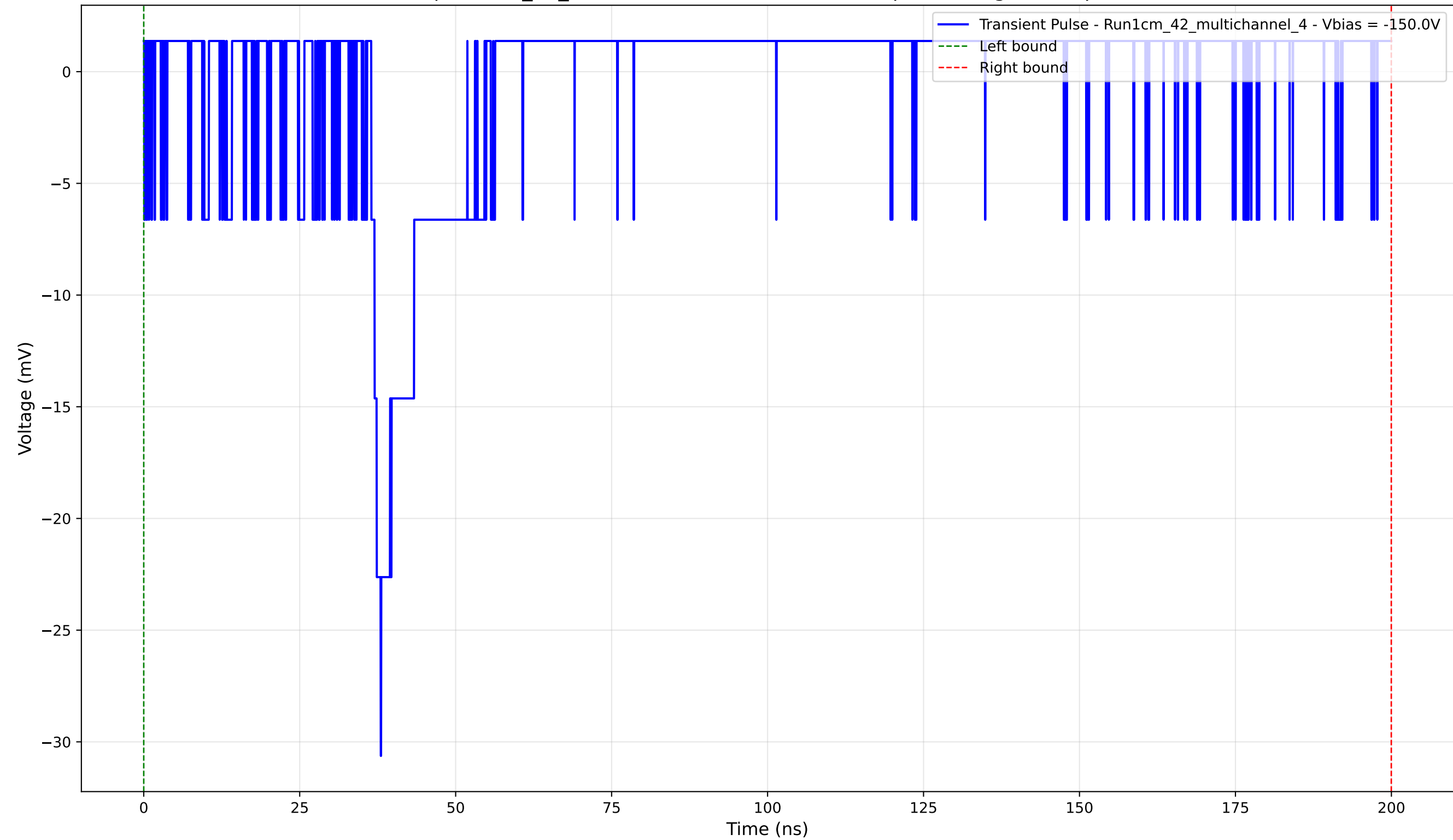
Transient Pulse - Sample: 1cm_42_multichannel - Position: 3300.0 \mu\text{m} - Charge: 0.97 pC - Rise Time: 1.51 ns
