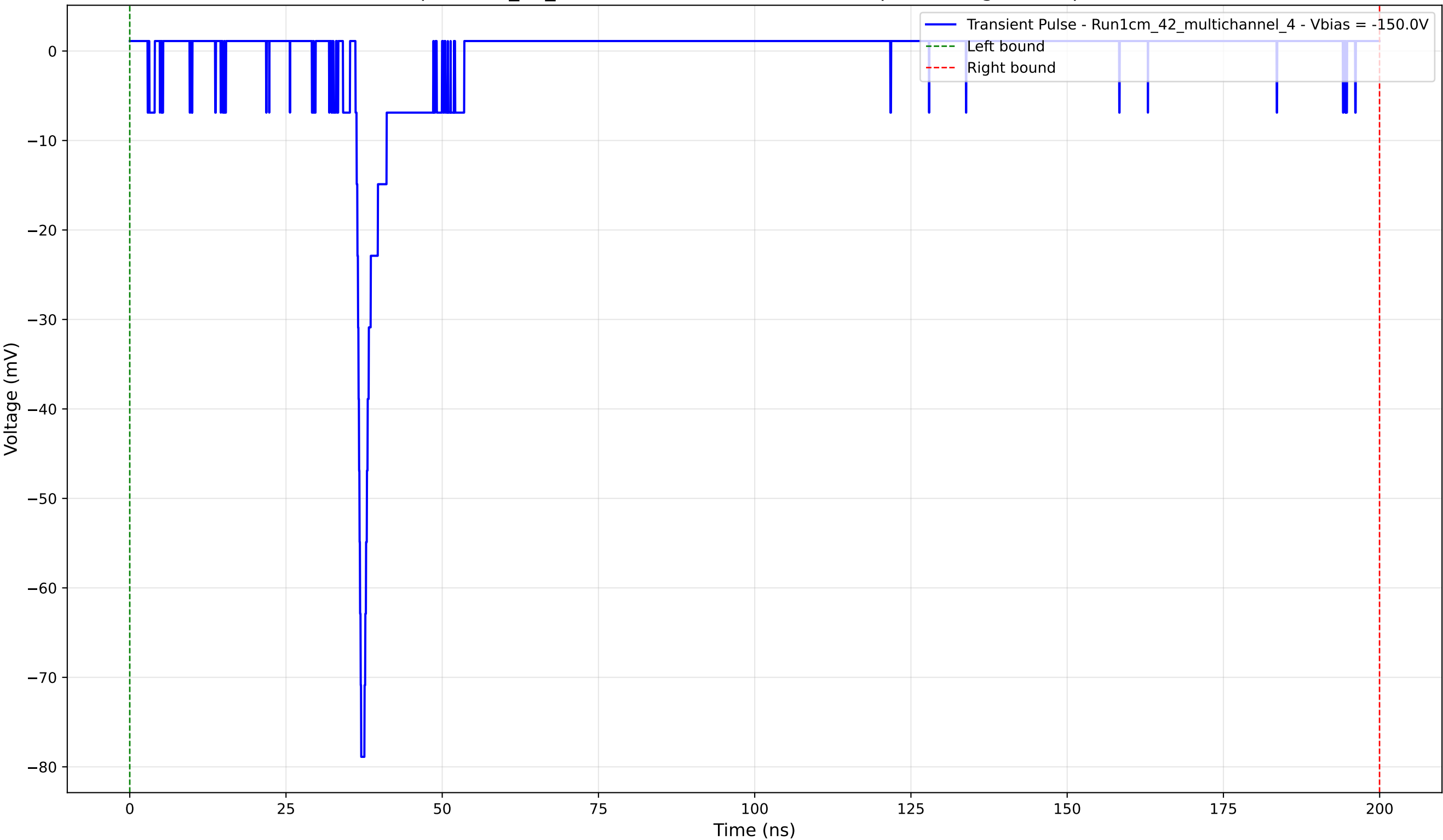
Transient Pulse - Sample: 1cm_42_multichannel - Position: 2250.0 \mu\text{m} - Charge: 1.68 pC - Rise Time: 0.74 ns
