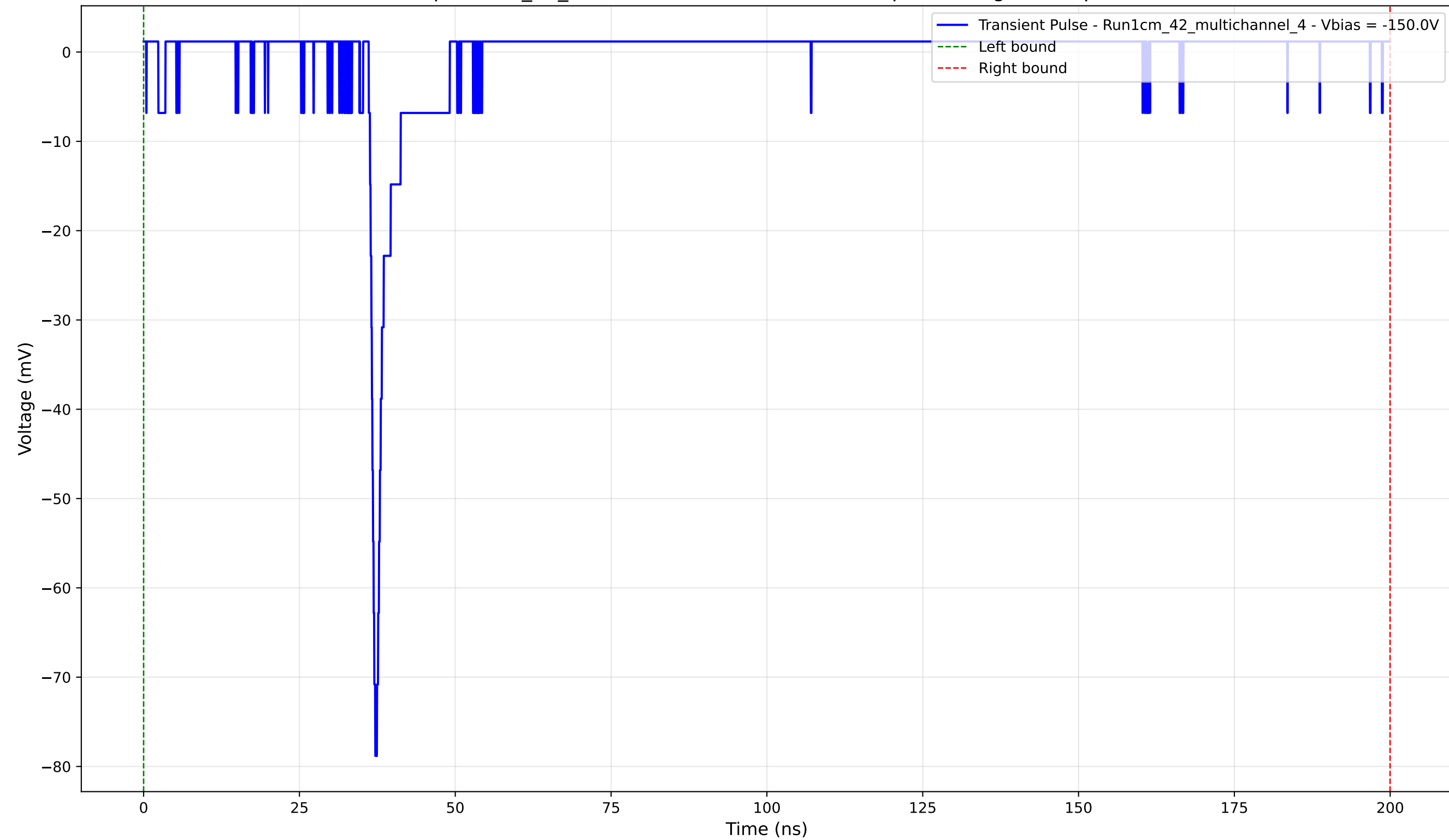
Transient Pulse - Sample: 1cm_42_multichannel - Position: 2225.0 \mu\text{m} - Charge: 1.01 pC - Rise Time: 0.86 ns
