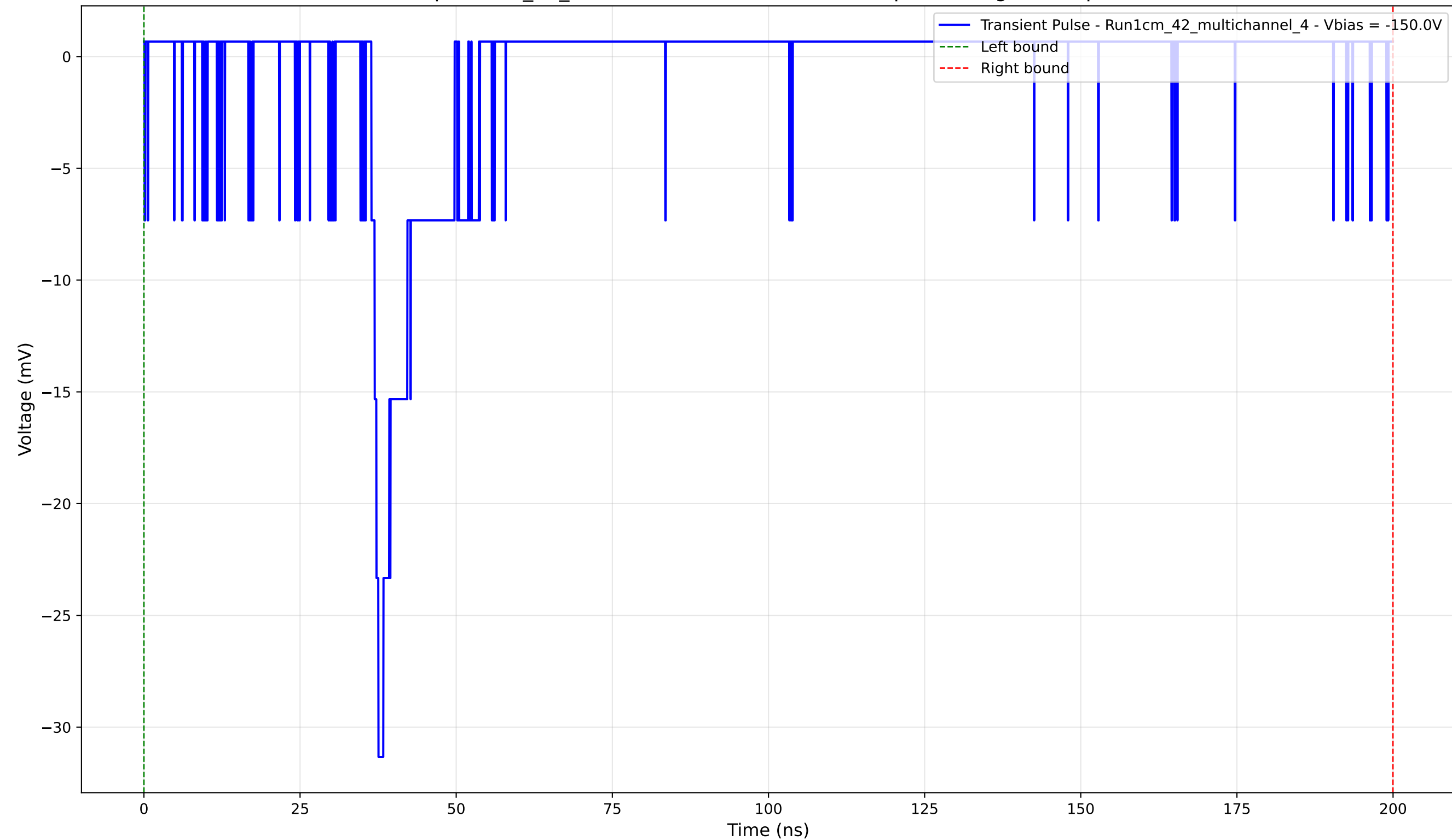
Transient Pulse - Sample: 1cm_42_multichannel - Position: 3215.0 \mu\text{m} - Charge: 2.15 pC - Rise Time: 1.13 ns
