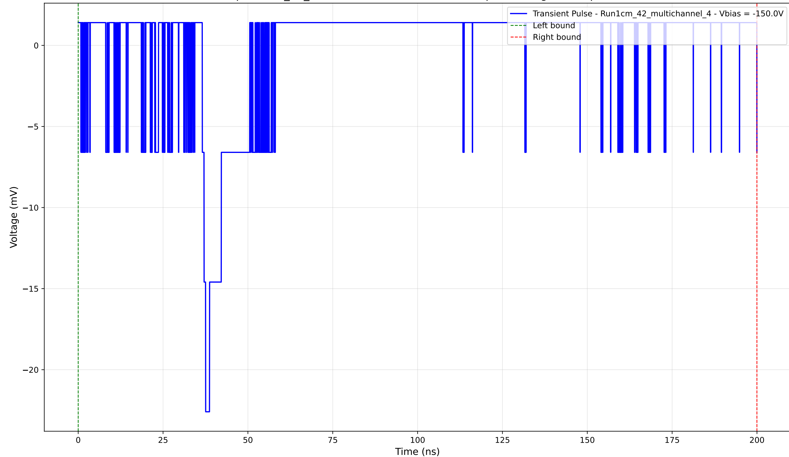
Transient Pulse - Sample: 1cm_42_multichannel - Position: 3330.0 \mu\text{m} - Charge: 0.11 pC - Rise Time: 1.00 ns
