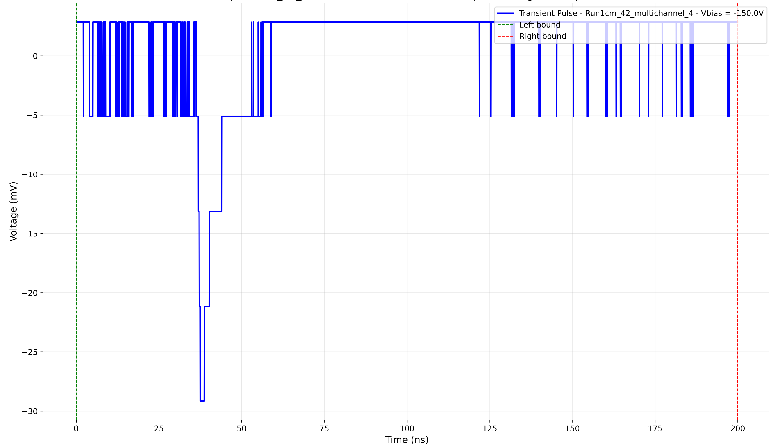
Transient Pulse - Sample: 1cm_42_multichannel - Position: 1525.0 \mu\text{m} - Charge: 4.23 pC - Rise Time: 1.14 ns
