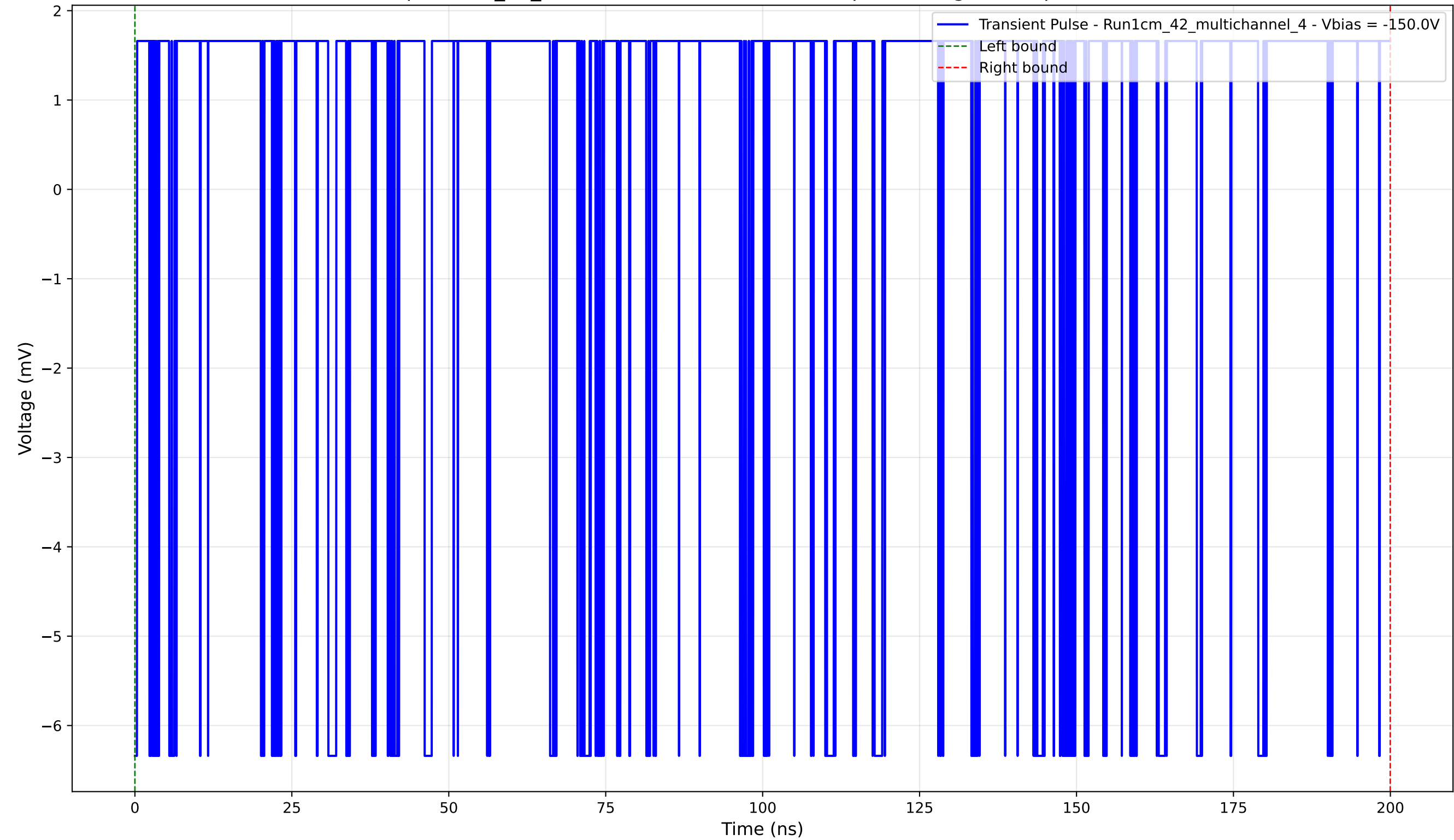
Transient Pulse - Sample: 1cm_42_multichannel - Position: 370.0 \mu\text{m} - Charge: 2.21 pC - Rise Time: 0.00 ns (N/A)
