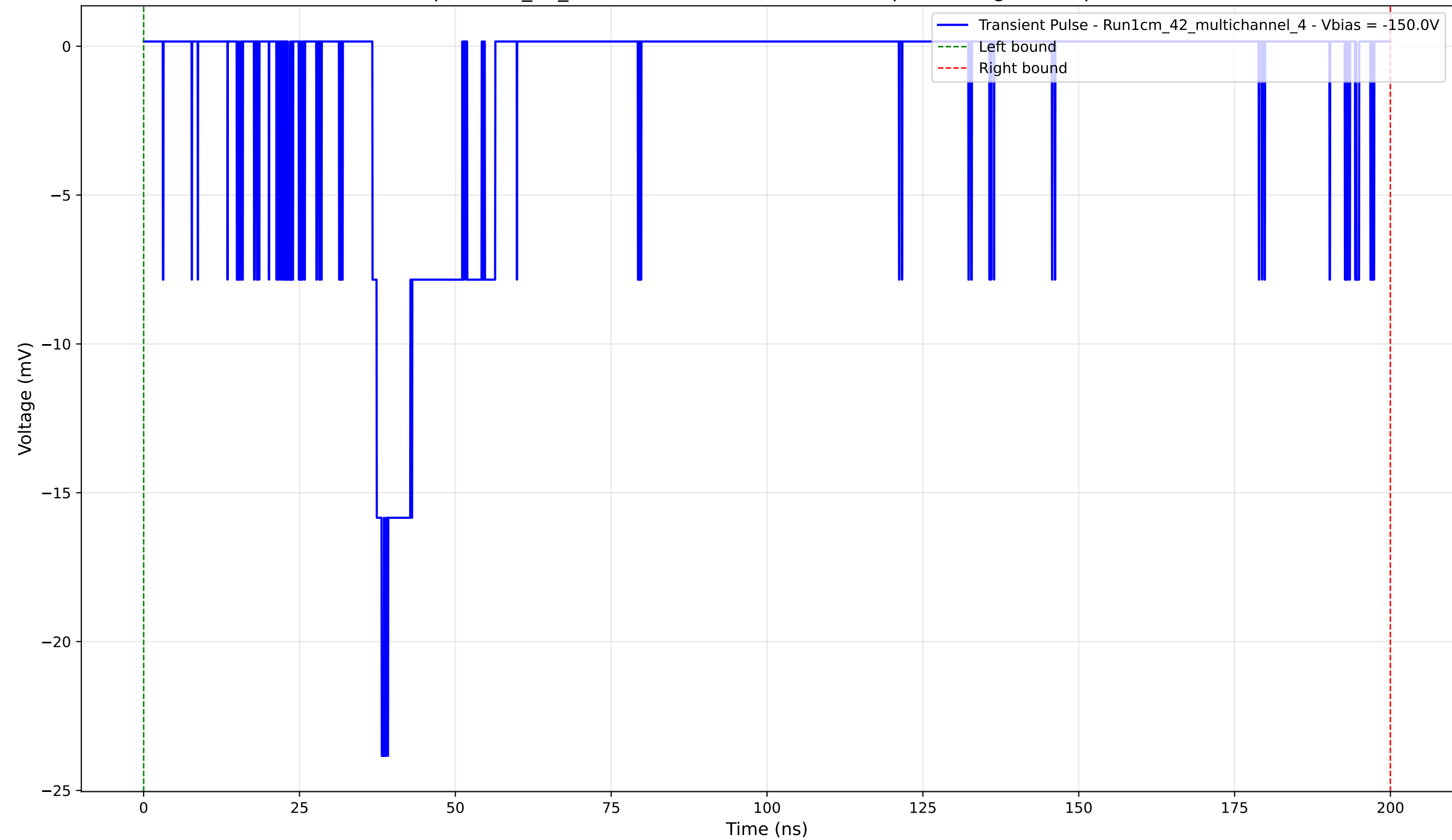
Transient Pulse - Sample: 1cm_42_multichannel - Position: 3590.0 \mu\text{m} - Charge: 4.41 pC - Rise Time: 1.49 ns
