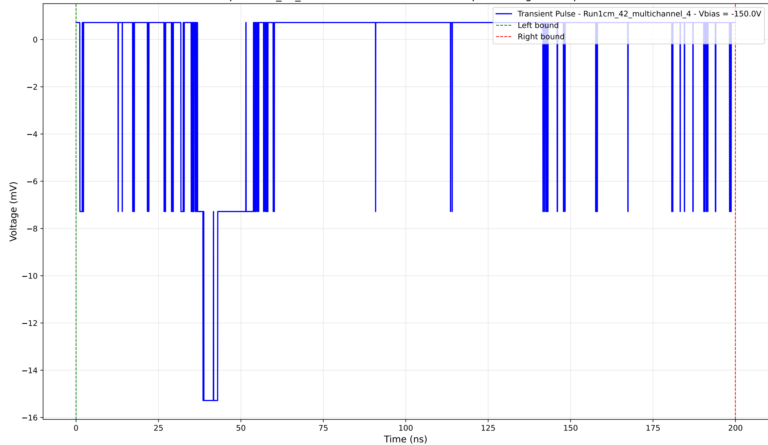
Transient Pulse - Sample: 1cm_42_multichannel - Position: 4690.0 \mu\text{m} - Charge: 1.66 pC - Rise Time: 1.66 ns
