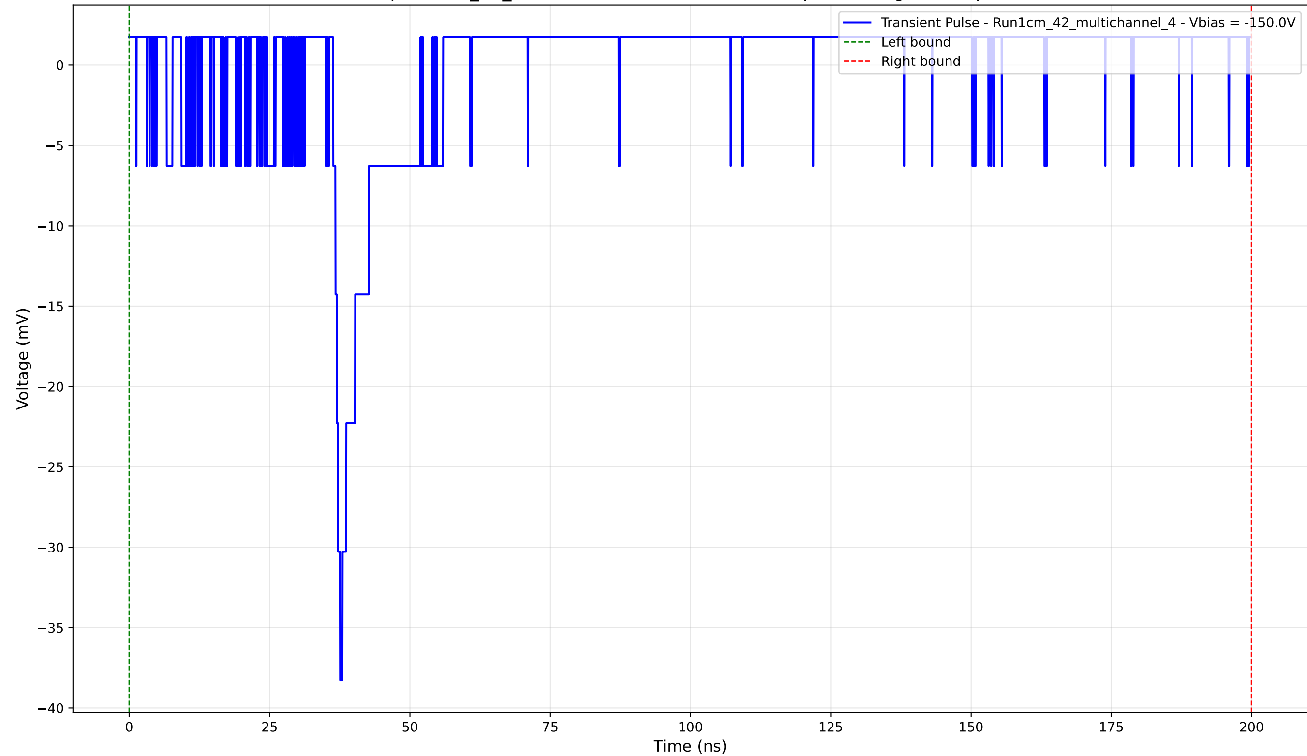
Transient Pulse - Sample: 1cm_42_multichannel - Position: 1665.0 \mu\text{m} - Charge: 0.14 pC - Rise Time: 1.25 ns
