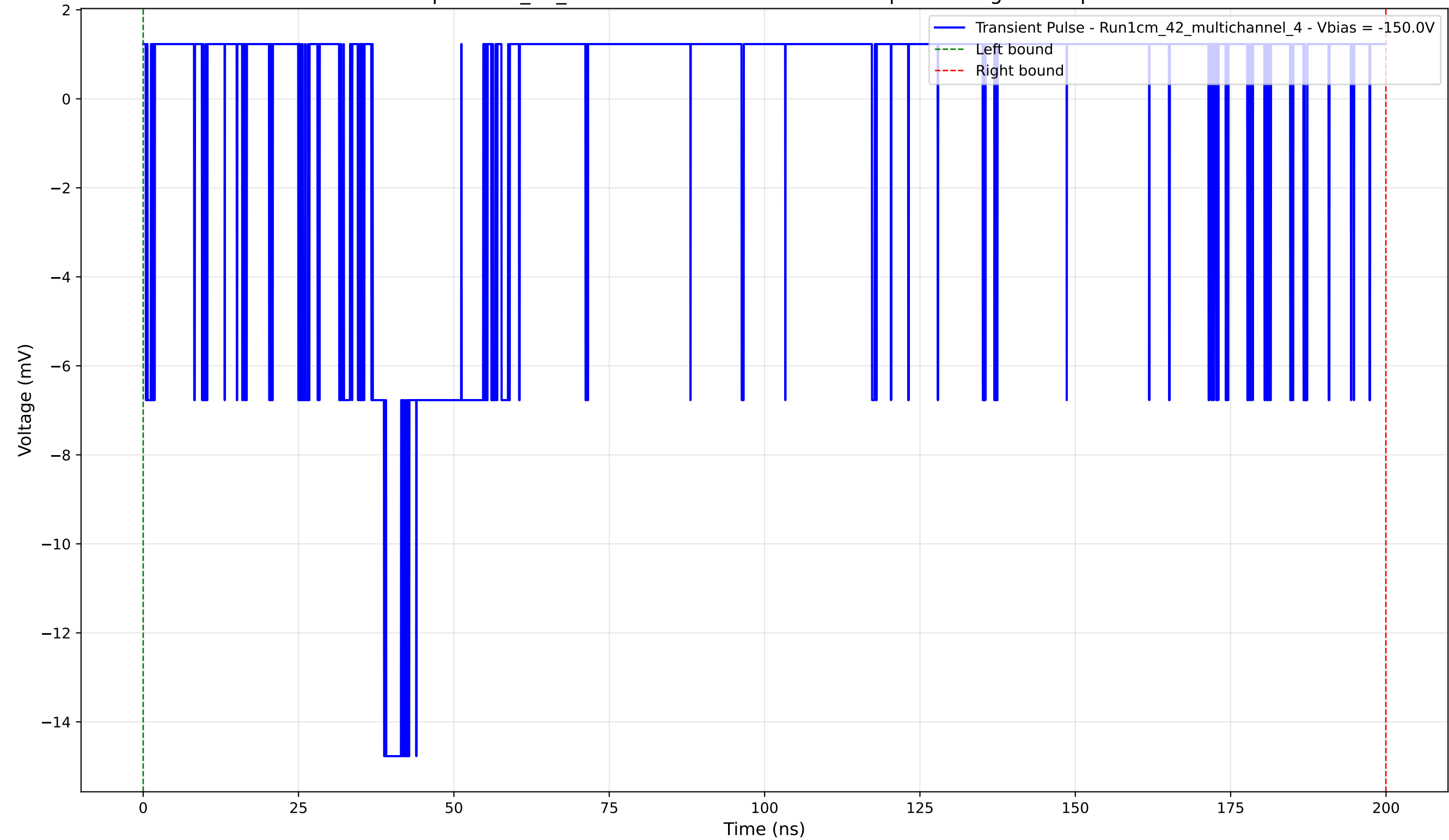
Transient Pulse - Sample: 1cm_42_multichannel - Position: 4480.0 \mu\text{m} - Charge: 0.64 pC - Rise Time: 1.84 ns
