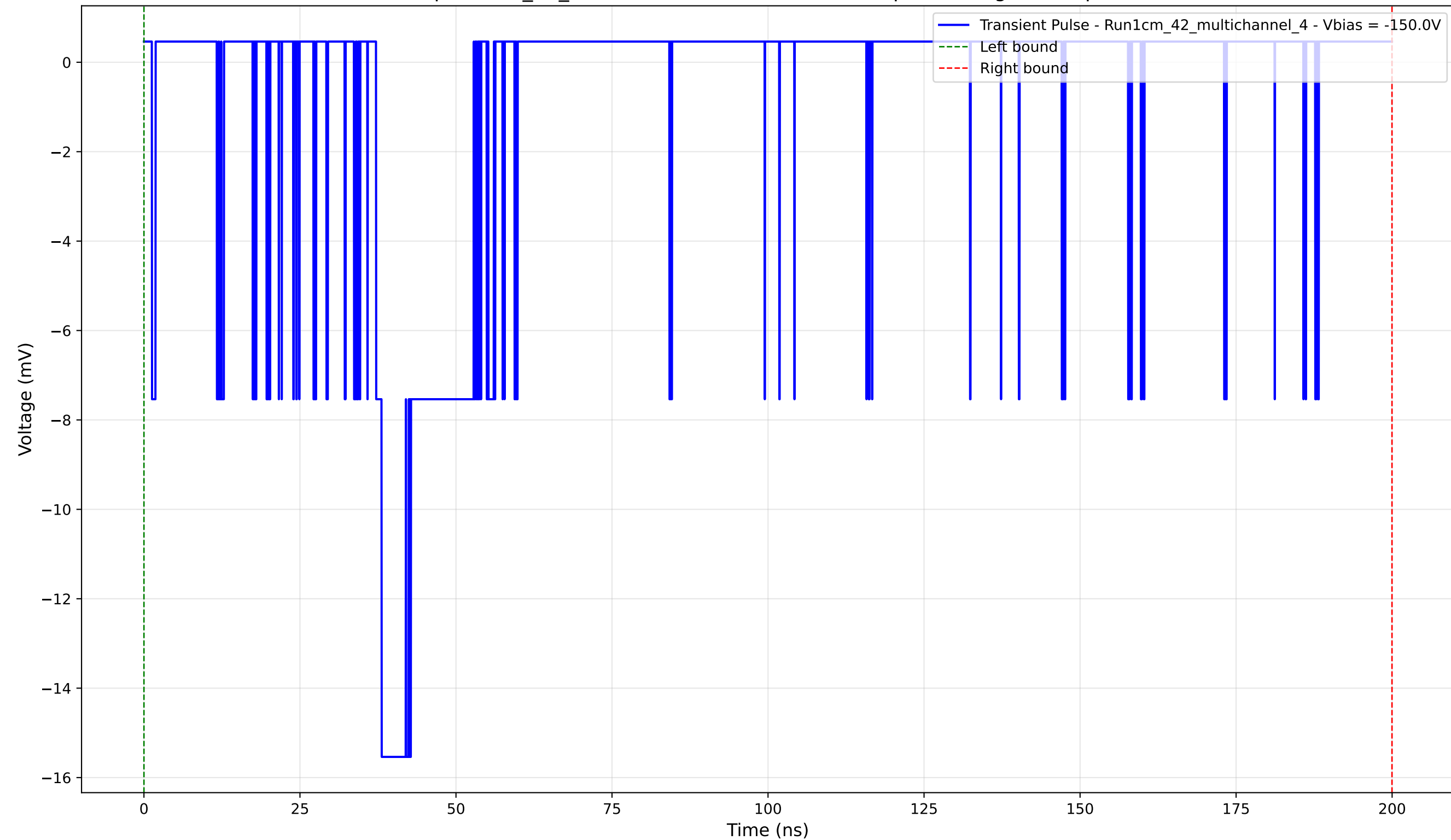
Transient Pulse - Sample: 1cm_42_multichannel - Position: 3970.0 \mu\text{m} - Charge: 2.72 pC - Rise Time: 0.90 ns
