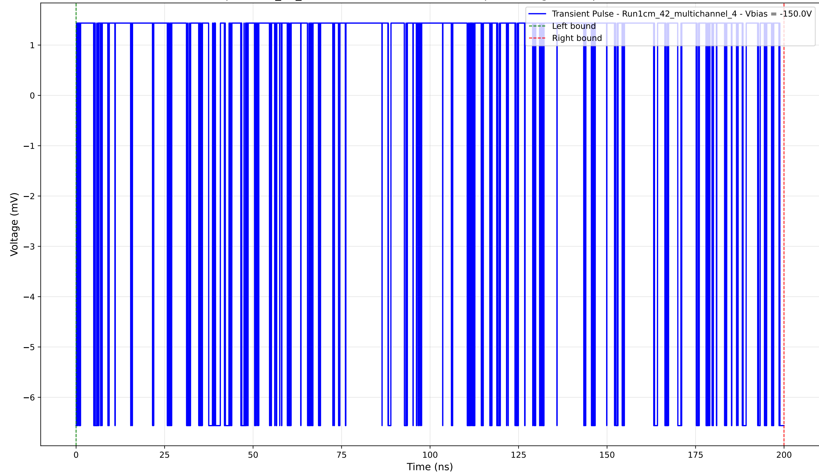
Transient Pulse - Sample: 1cm_42_multichannel - Position: 3385.0 \mu\text{m} - Charge: 0.76 pC - Rise Time: 0.00 ns (N/A)
