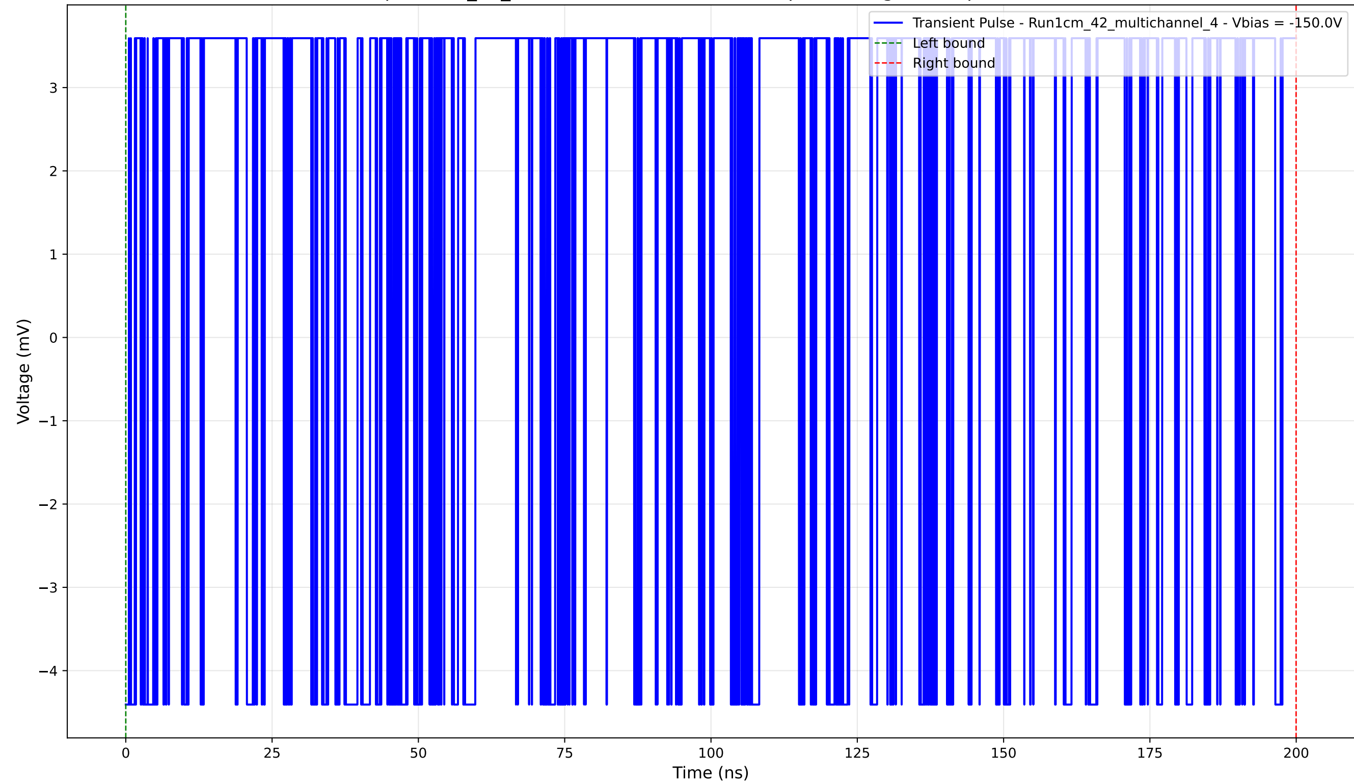
Transient Pulse - Sample: 1cm_42_multichannel - Position: 70.0 \mu\text{m} - Charge: 6.41 pC - Rise Time: 0.00 ns (N/A)
