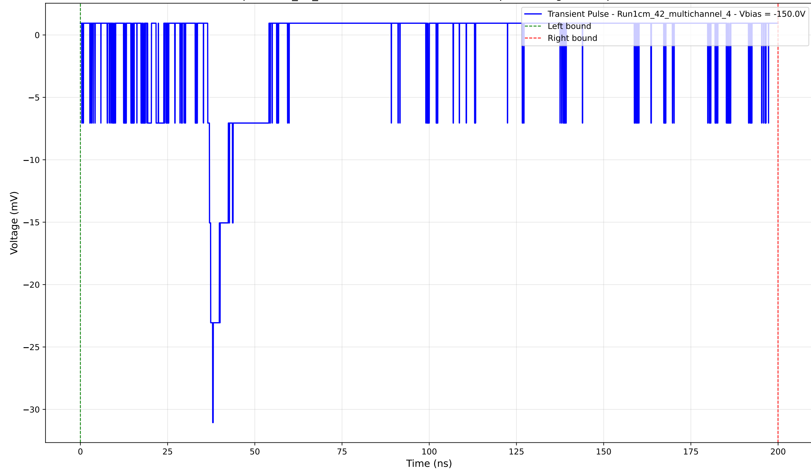
Transient Pulse - Sample: 1cm_42_multichannel - Position: 3280.0 \mu\text{m} - Charge: 2.78 pC - Rise Time: 1.43 ns
