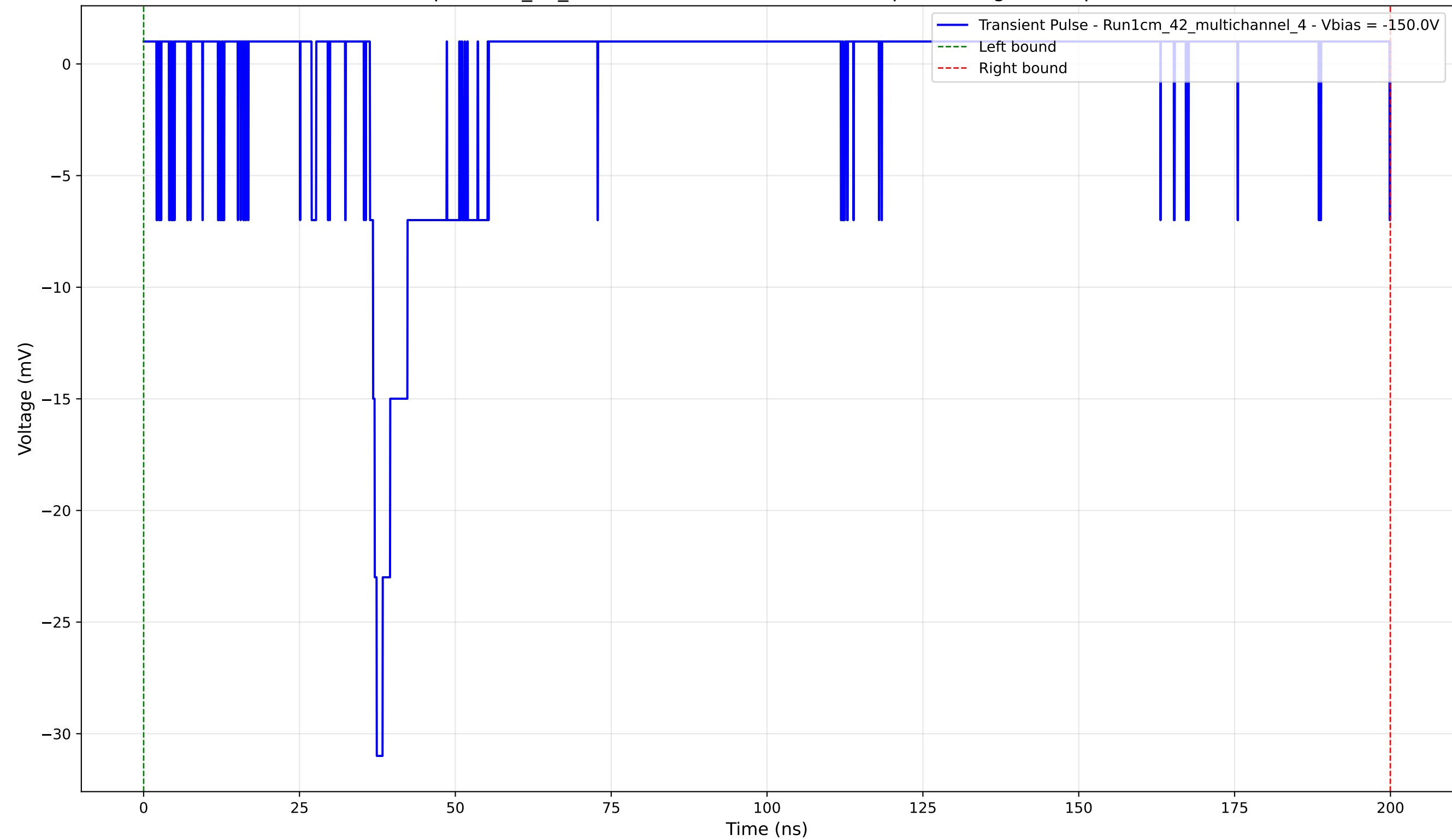
Transient Pulse - Sample: 1cm_42_multichannel - Position: 3135.0 \mu\text{m} - Charge: 1.18 pC - Rise Time: 1.09 ns
