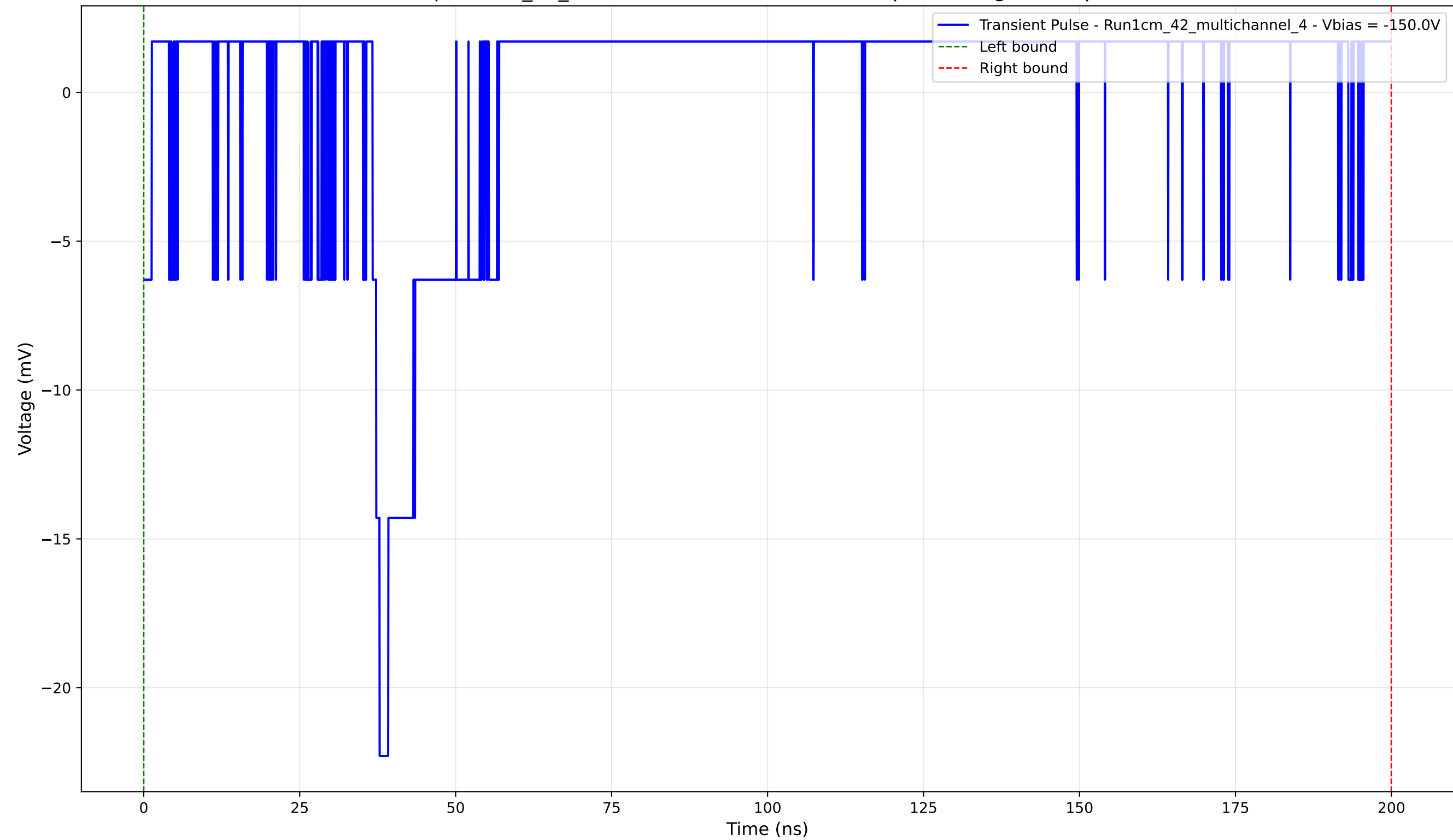
Transient Pulse - Sample: 1cm_42_multichannel - Position: 3520.0 \mu\text{m} - Charge: 1.19 pC - Rise Time: 1.14 ns
