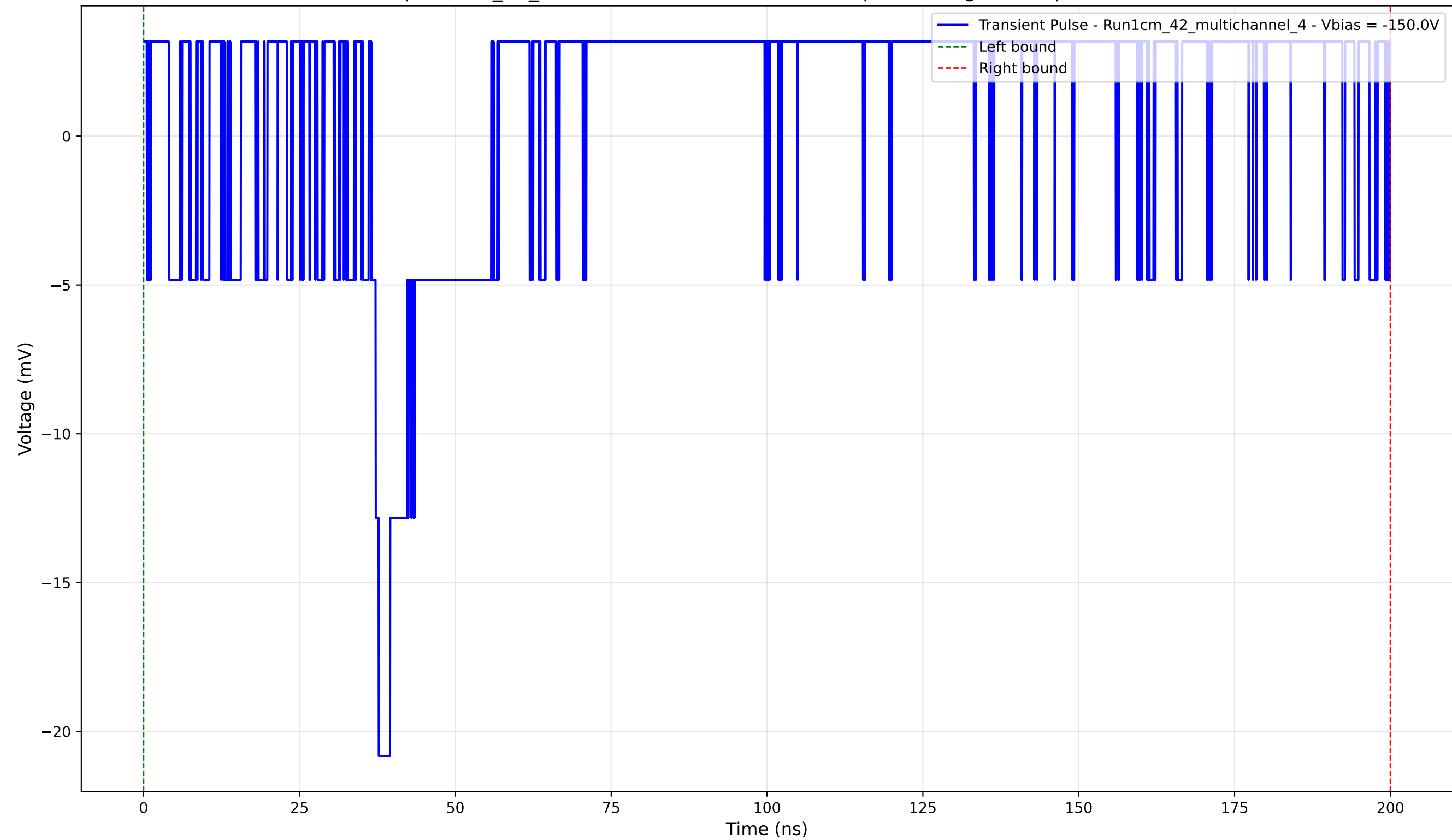
Transient Pulse - Sample: 1cm_42_multichannel - Position: 1305.0 \mu\text{m} - Charge: 4.47 pC - Rise Time: 0.00 ns (N/A)
