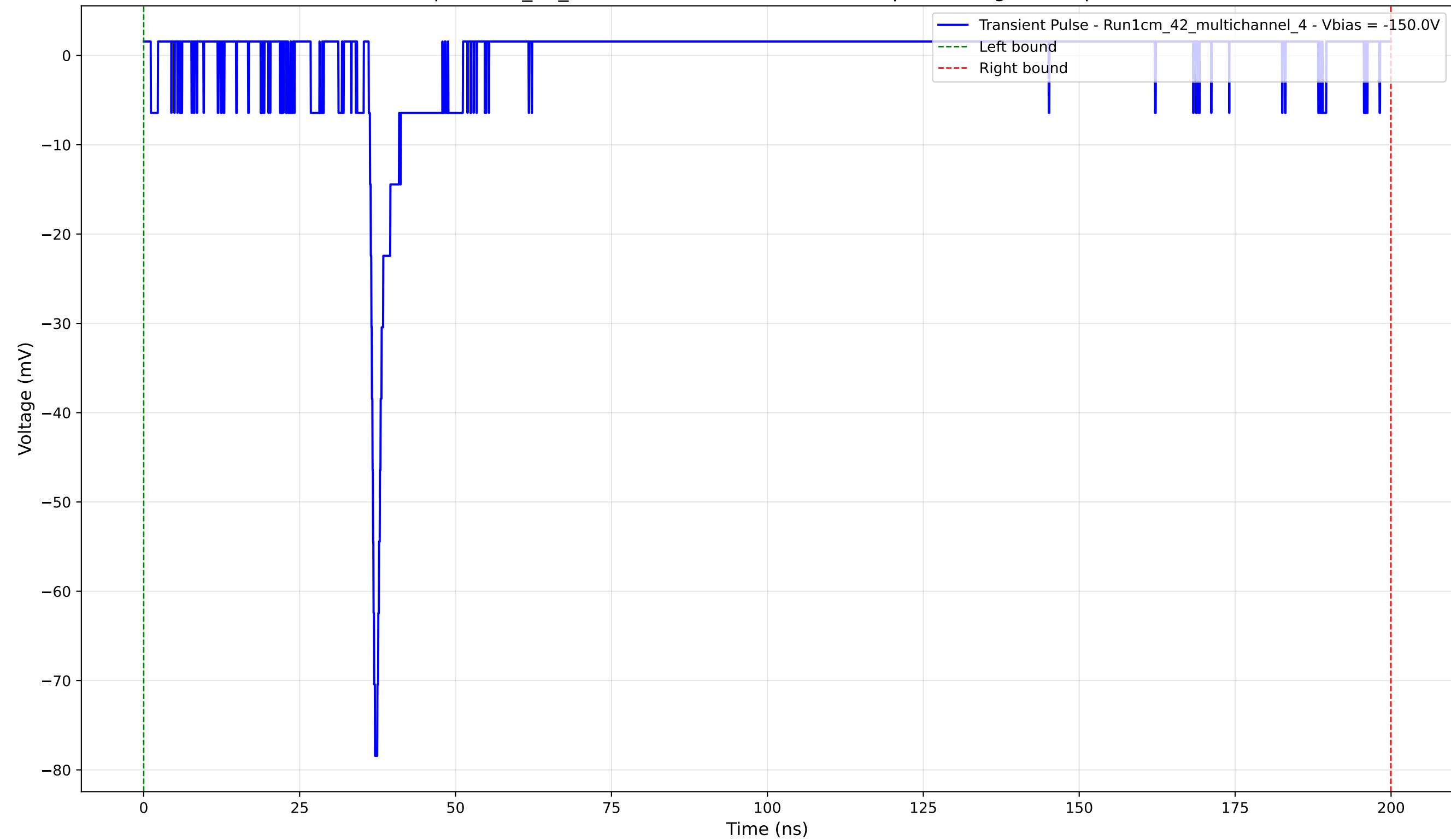
Transient Pulse - Sample: 1cm_42_multichannel - Position: 2275.0 \mu\text{m} - Charge: 0.35 pC - Rise Time: 0.82 ns
