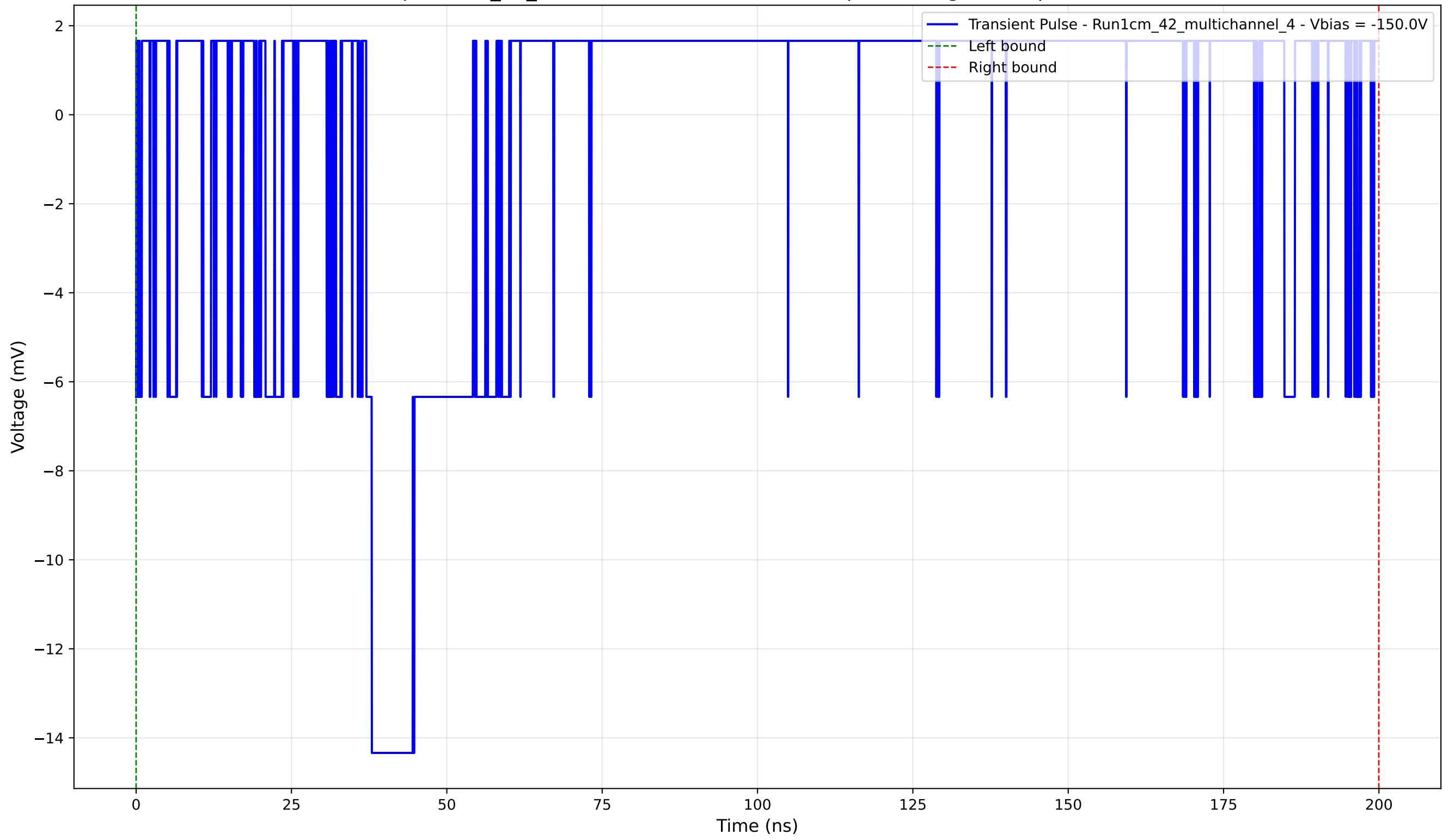
Transient Pulse - Sample: 1cm_42_multichannel - Position: 625.0 \mu\text{m} - Charge: 0.55 pC - Rise Time: 0.00 ns (N/A)
