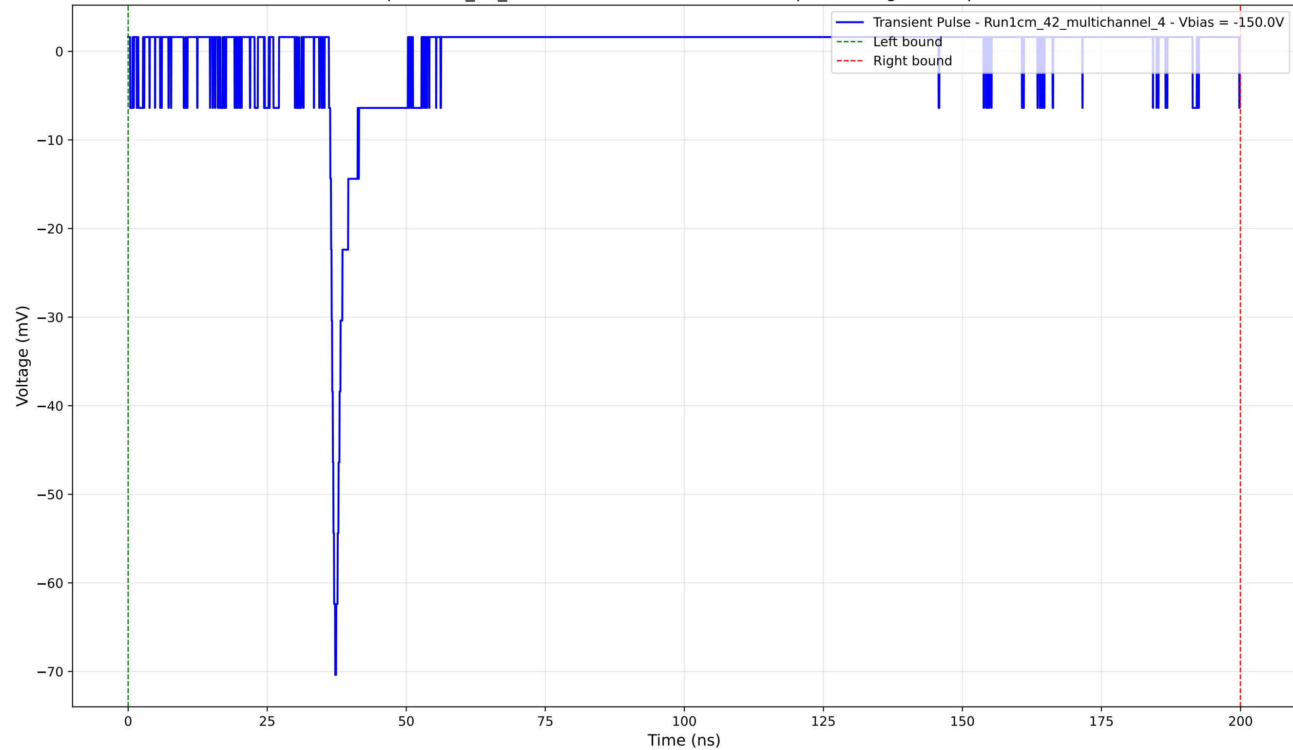
Transient Pulse - Sample: 1cm_42_multichannel - Position: 2575.0 \mu\text{m} - Charge: 0.28 pC - Rise Time: 0.90 ns
