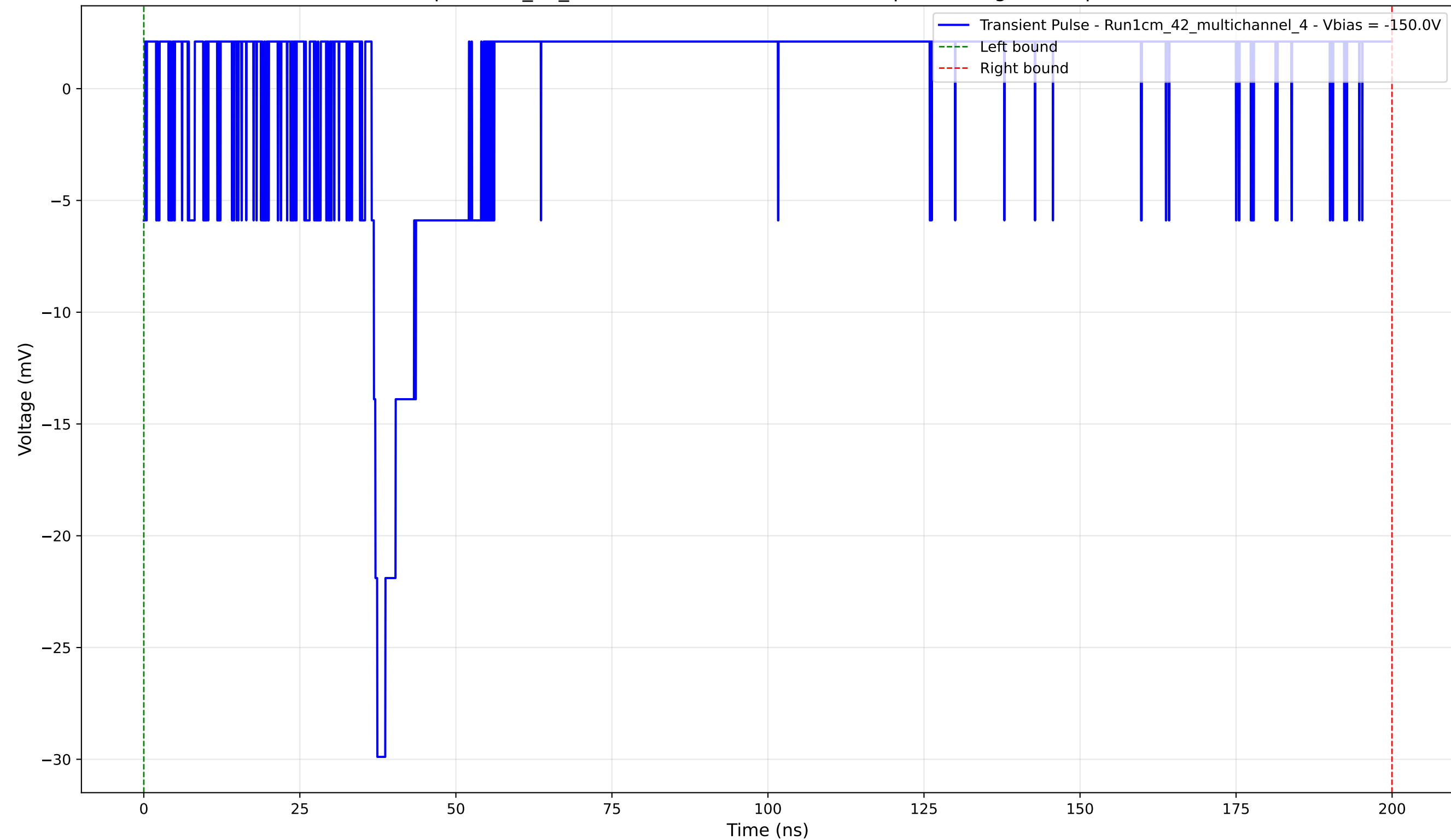
Transient Pulse - Sample: 1cm_42_multichannel - Position: 1570.0 \mu\text{m} - Charge: 2.06 pC - Rise Time: 0.92 ns
