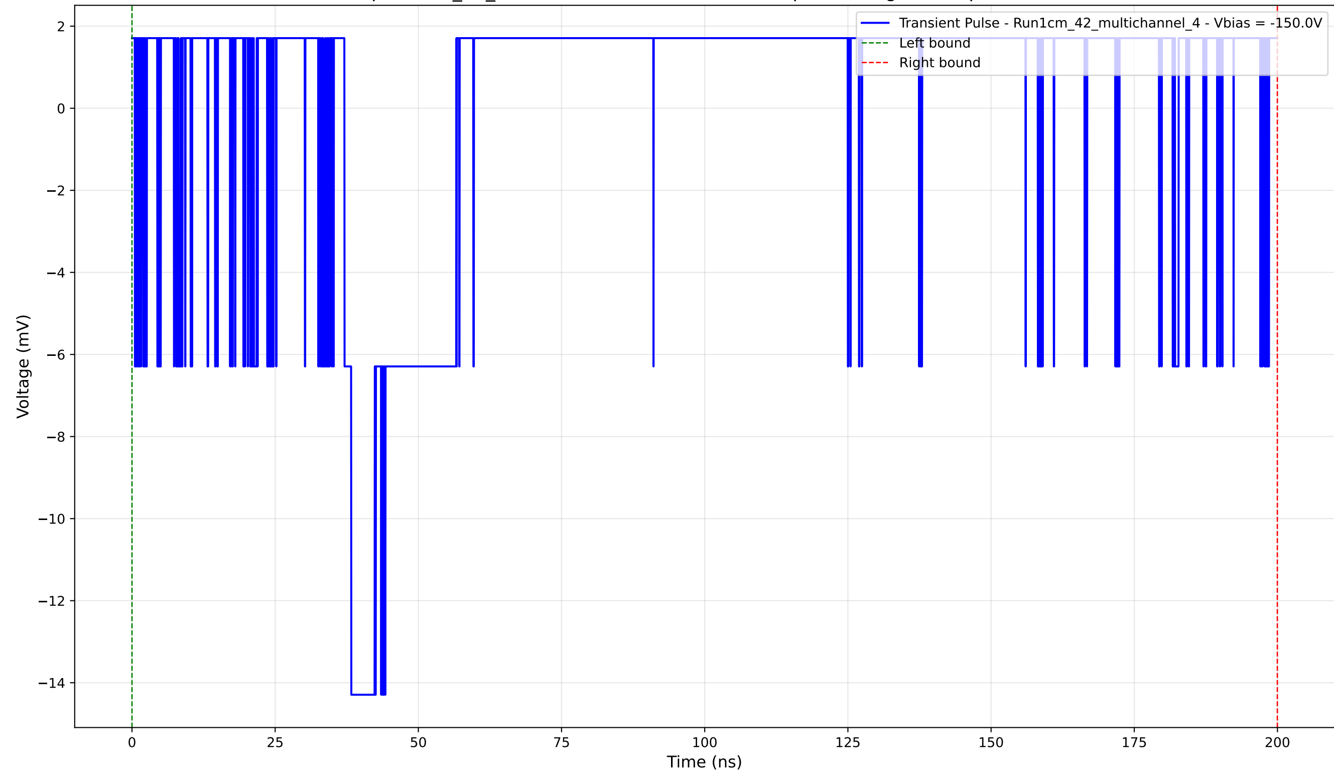
Transient Pulse - Sample: 1cm_42_multichannel - Position: 4515.0 \mu\text{m} - Charge: 1.31 pC - Rise Time: 0.00 ns (N/A)
