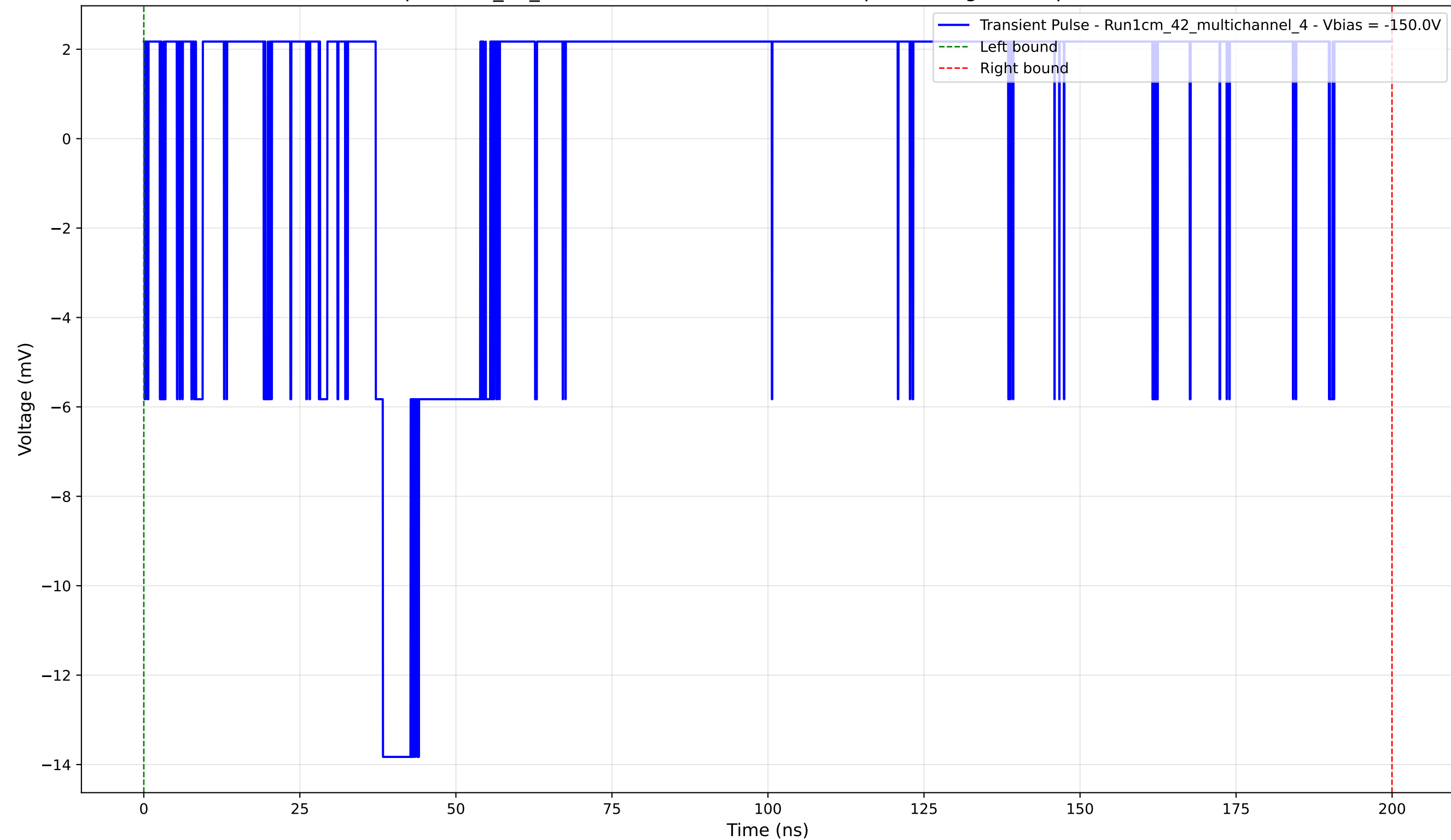
Transient Pulse - Sample: 1cm_42_multichannel - Position: 4295.0 \mu\text{m} - Charge: 3.54 pC - Rise Time: 0.00 ns (N/A)
