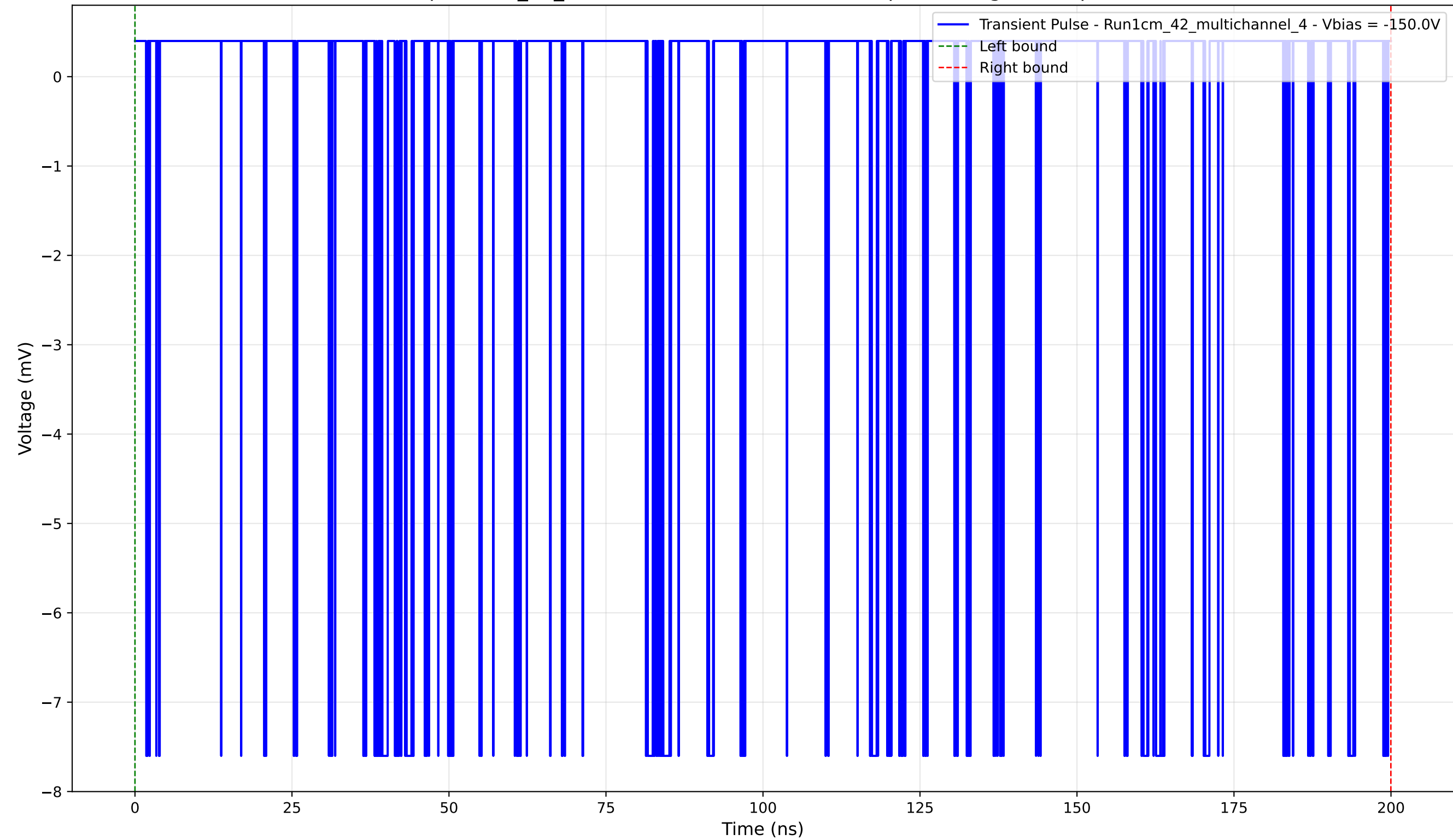
Transient Pulse - Sample: 1cm_42_multichannel - Position: 3410.0 \mu\text{m} - Charge: 1.87 pC - Rise Time: 0.02 ns
