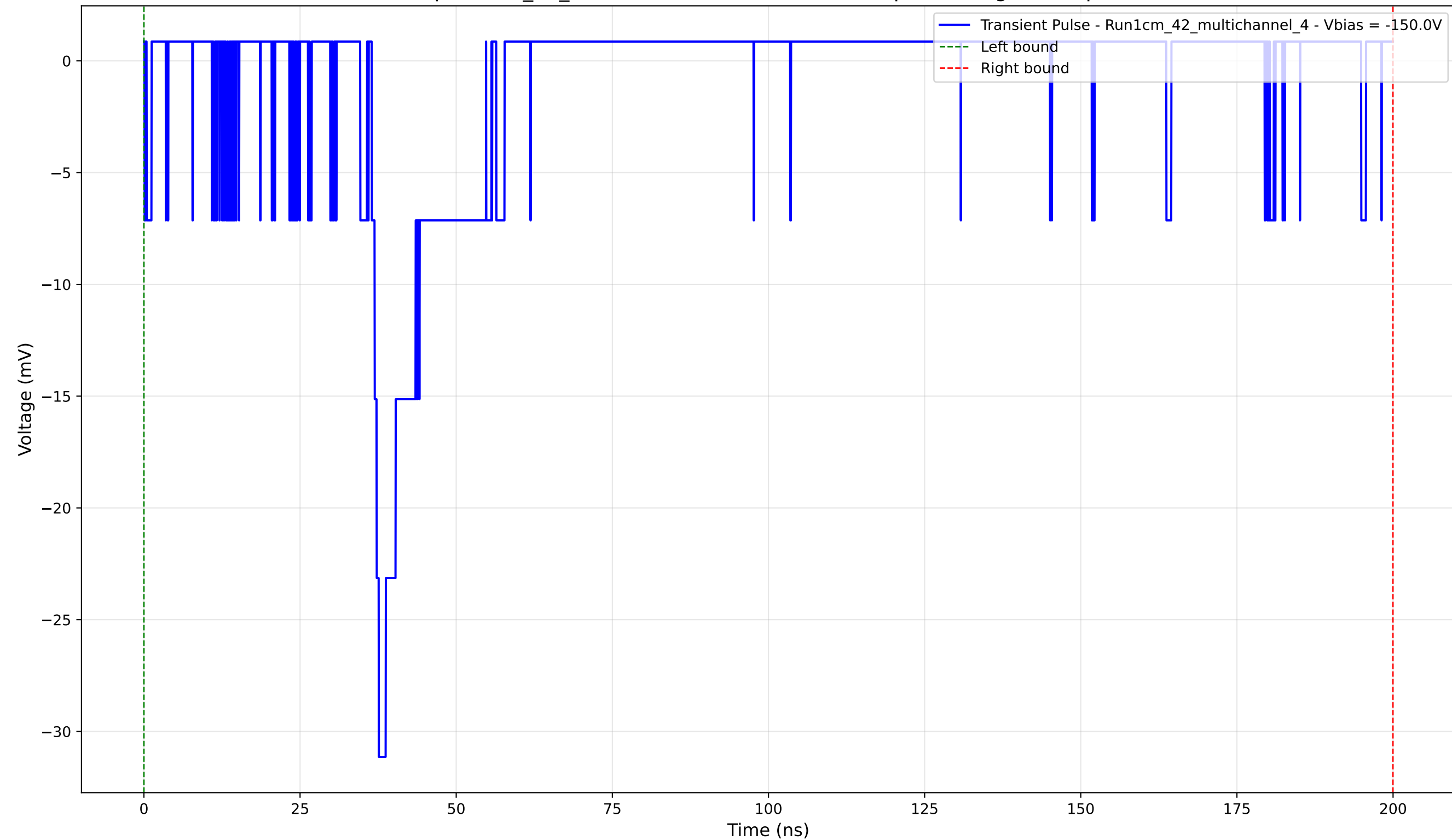
Transient Pulse - Sample: 1cm_42_multichannel - Position: 1480.0 \mu\text{m} - Charge: 3.14 pC - Rise Time: 1.13 ns
