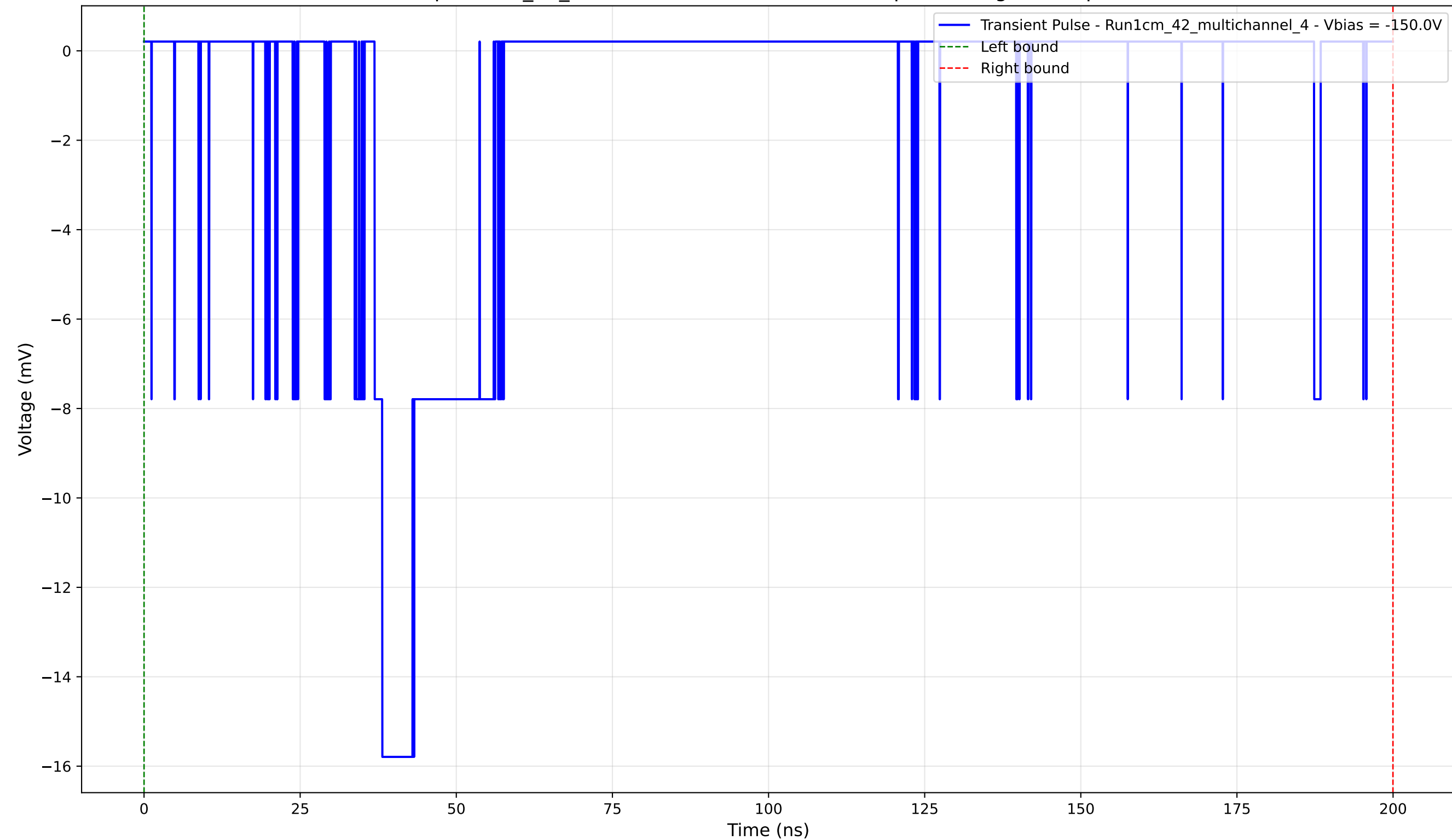
Transient Pulse - Sample: 1cm_42_multichannel - Position: 4035.0 \mu\text{m} - Charge: 4.04 pC - Rise Time: 1.24 ns
