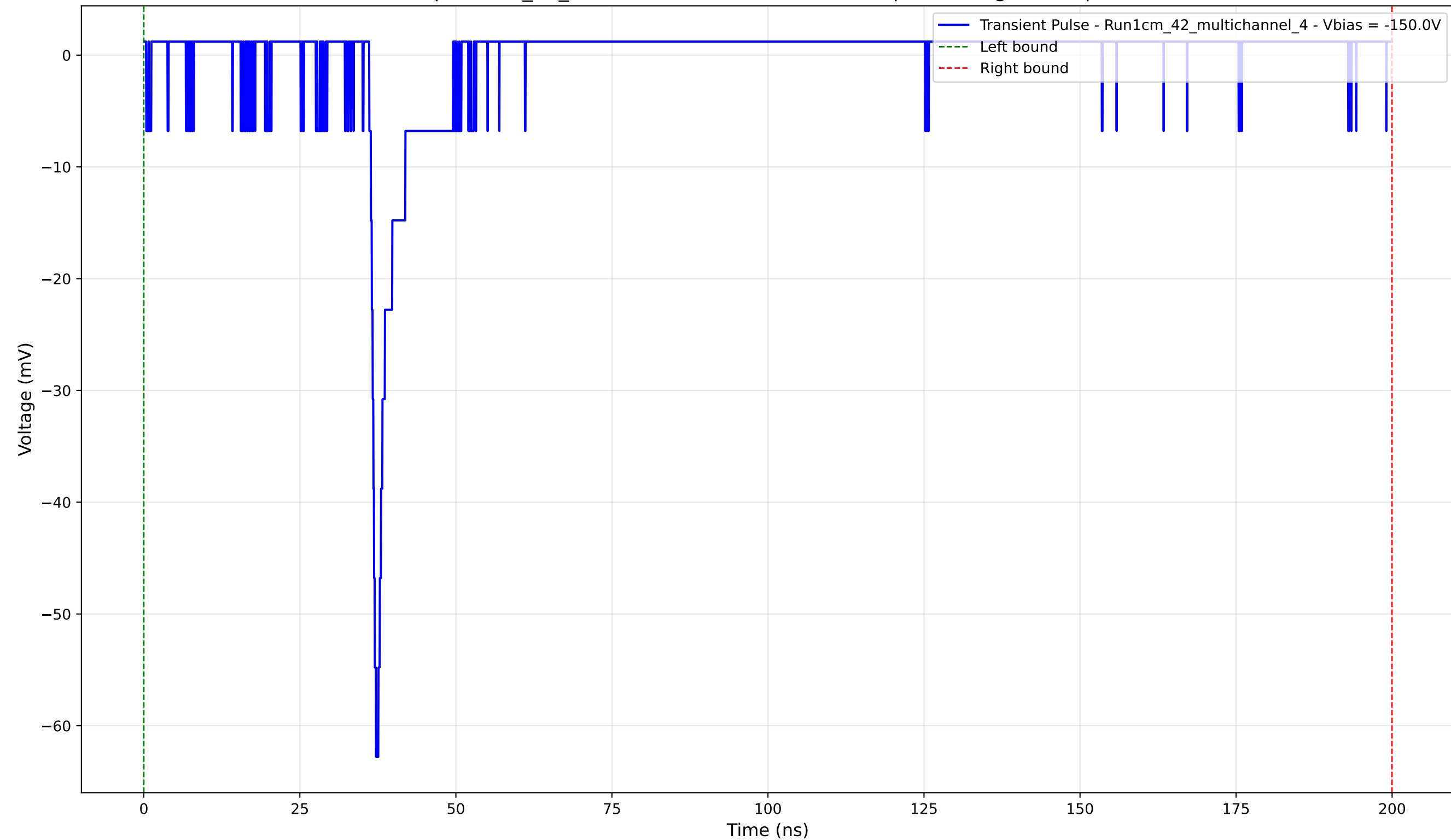
Transient Pulse - Sample: 1cm_42_multichannel - Position: 2115.0 \mu\text{m} - Charge: 1.06 pC - Rise Time: 1.08 ns
