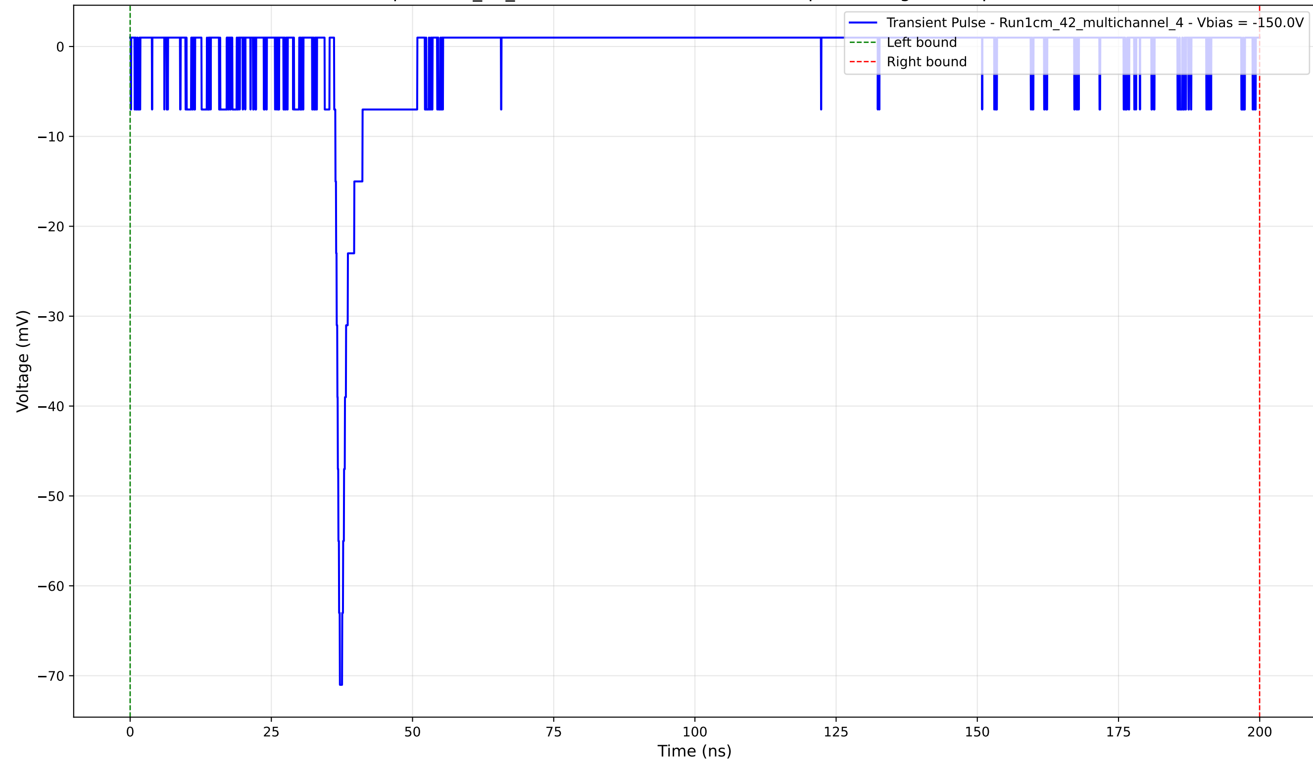
Transient Pulse - Sample: 1cm_42_multichannel - Position: 2190.0 \mu\text{m} - Charge: 3.51 pC - Rise Time: 0.80 ns
