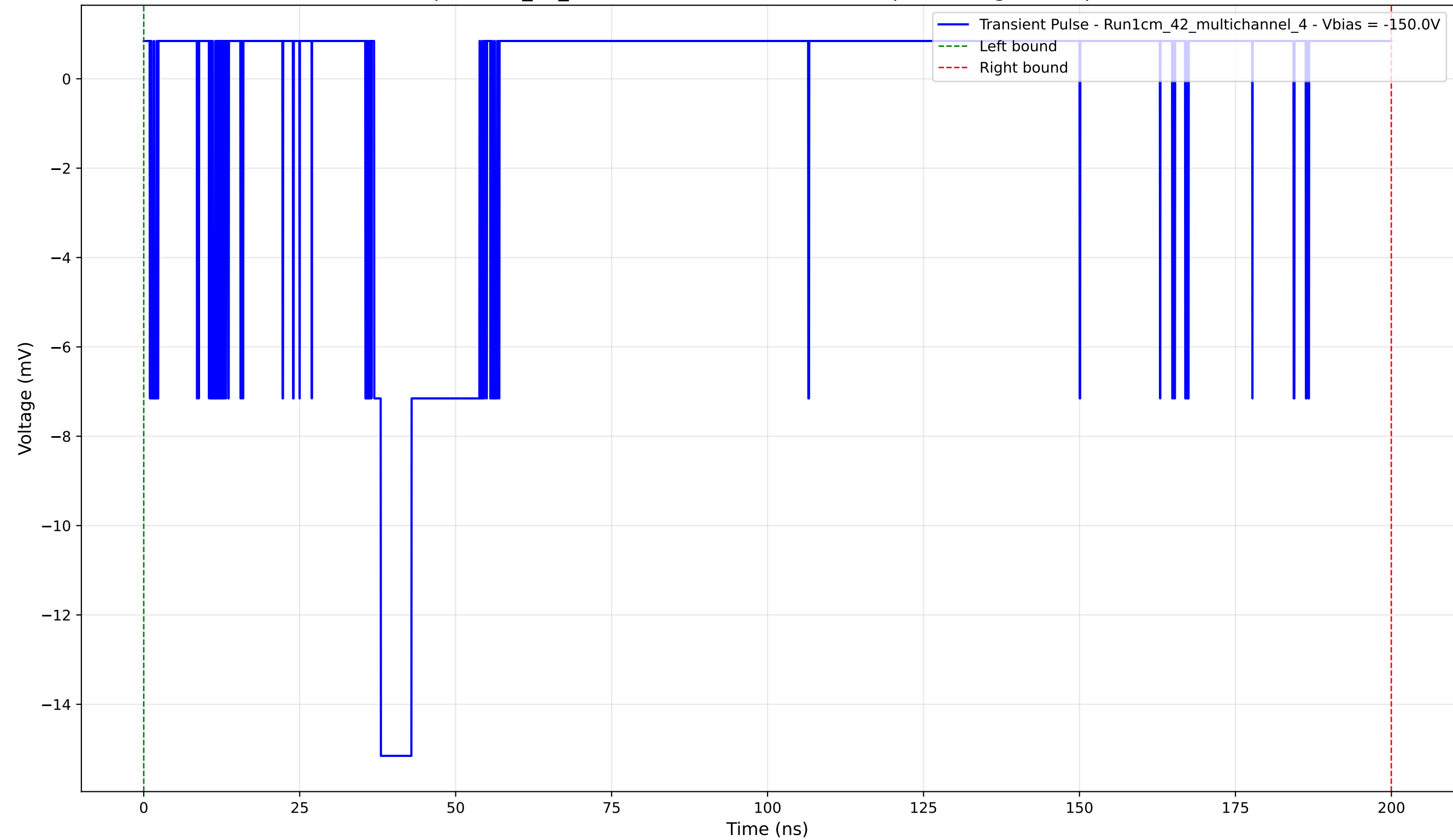
Transient Pulse - Sample: 1cm_42_multichannel - Position: 4065.0 \mu\text{m} - Charge: 1.16 pC - Rise Time: 1.08 ns
