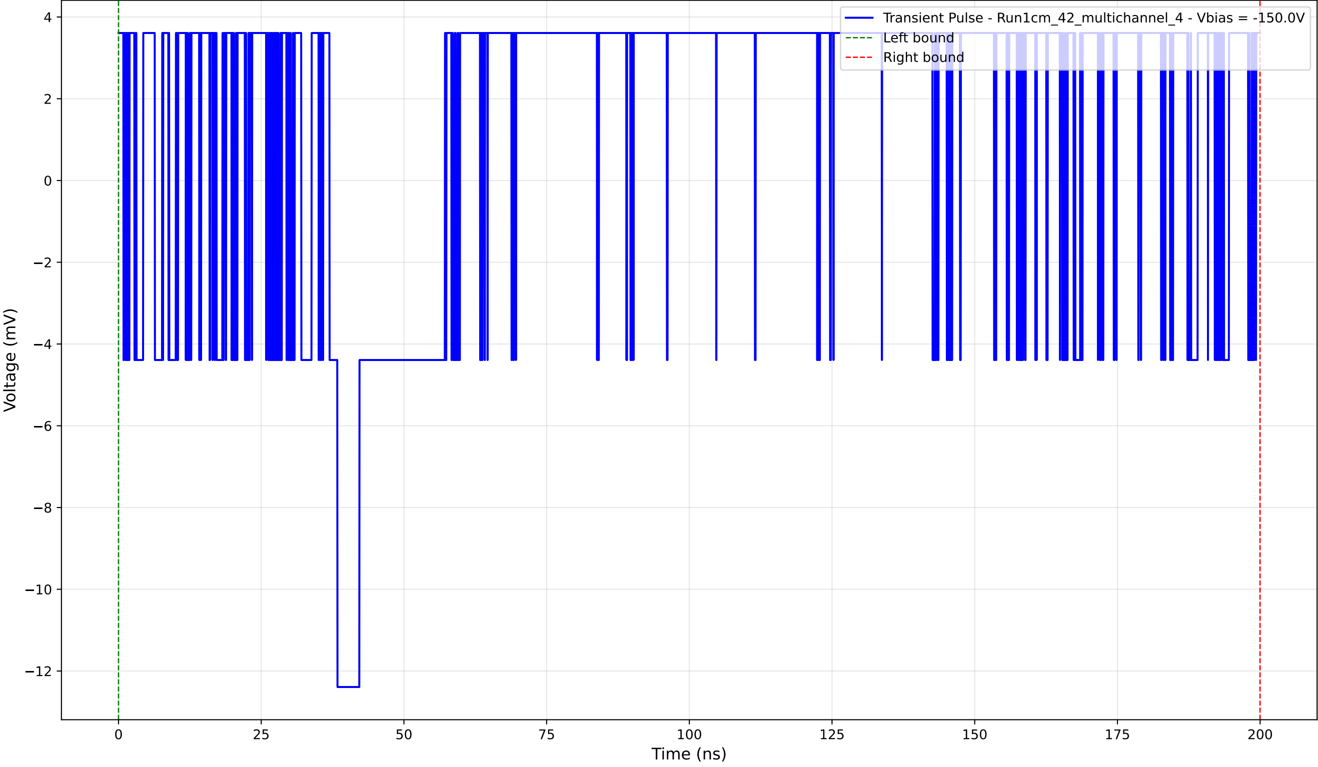
Transient Pulse - Sample: 1cm_42_multichannel - Position: 230.0 \mu\text{m} - Charge: 6.41 pC - Rise Time: 0.00 ns (N/A)
