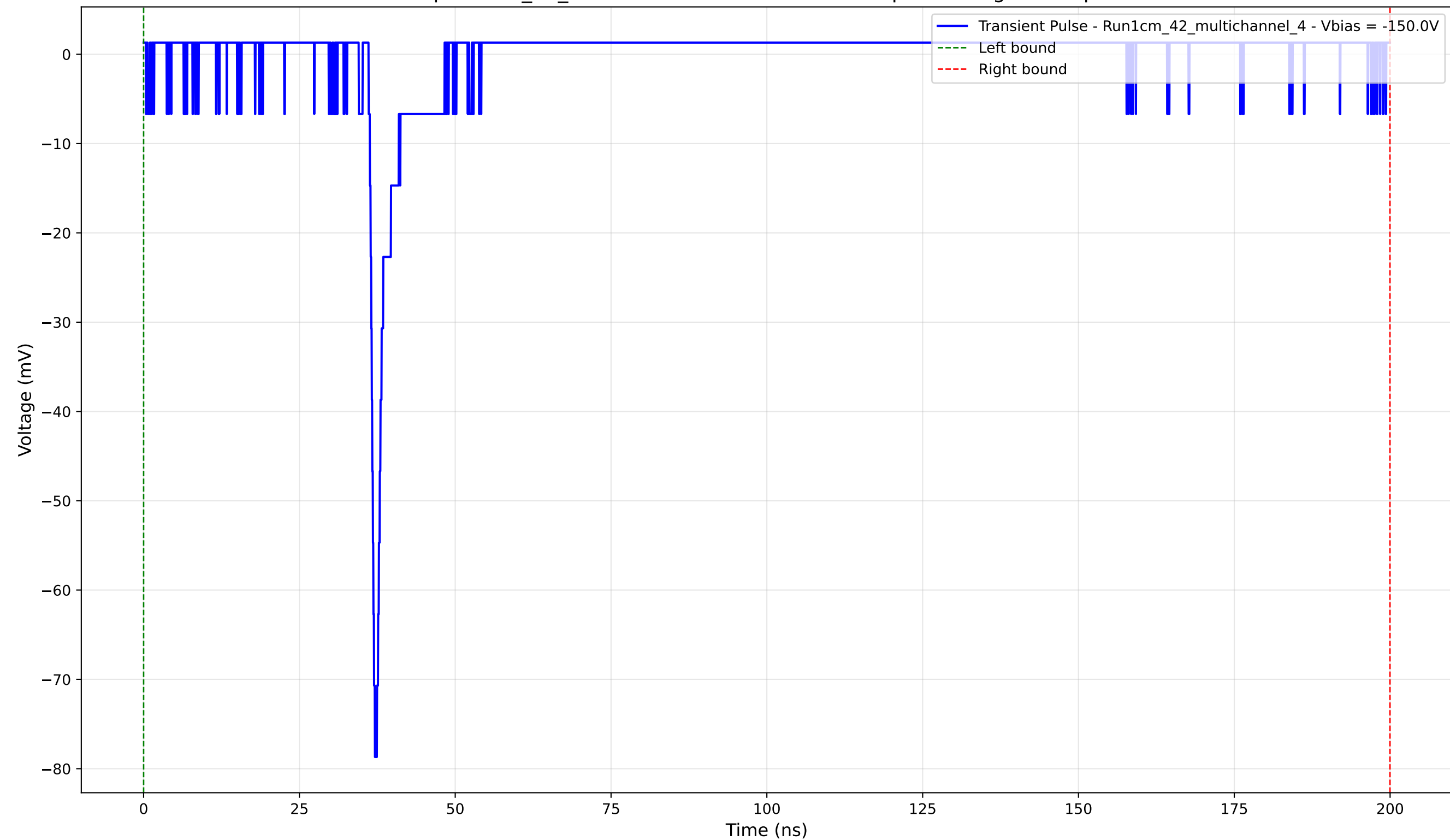
Transient Pulse - Sample: 1cm_42_multichannel - Position: 2520.0 \mu\text{m} - Charge: 0.56 pC - Rise Time: 0.82 ns
