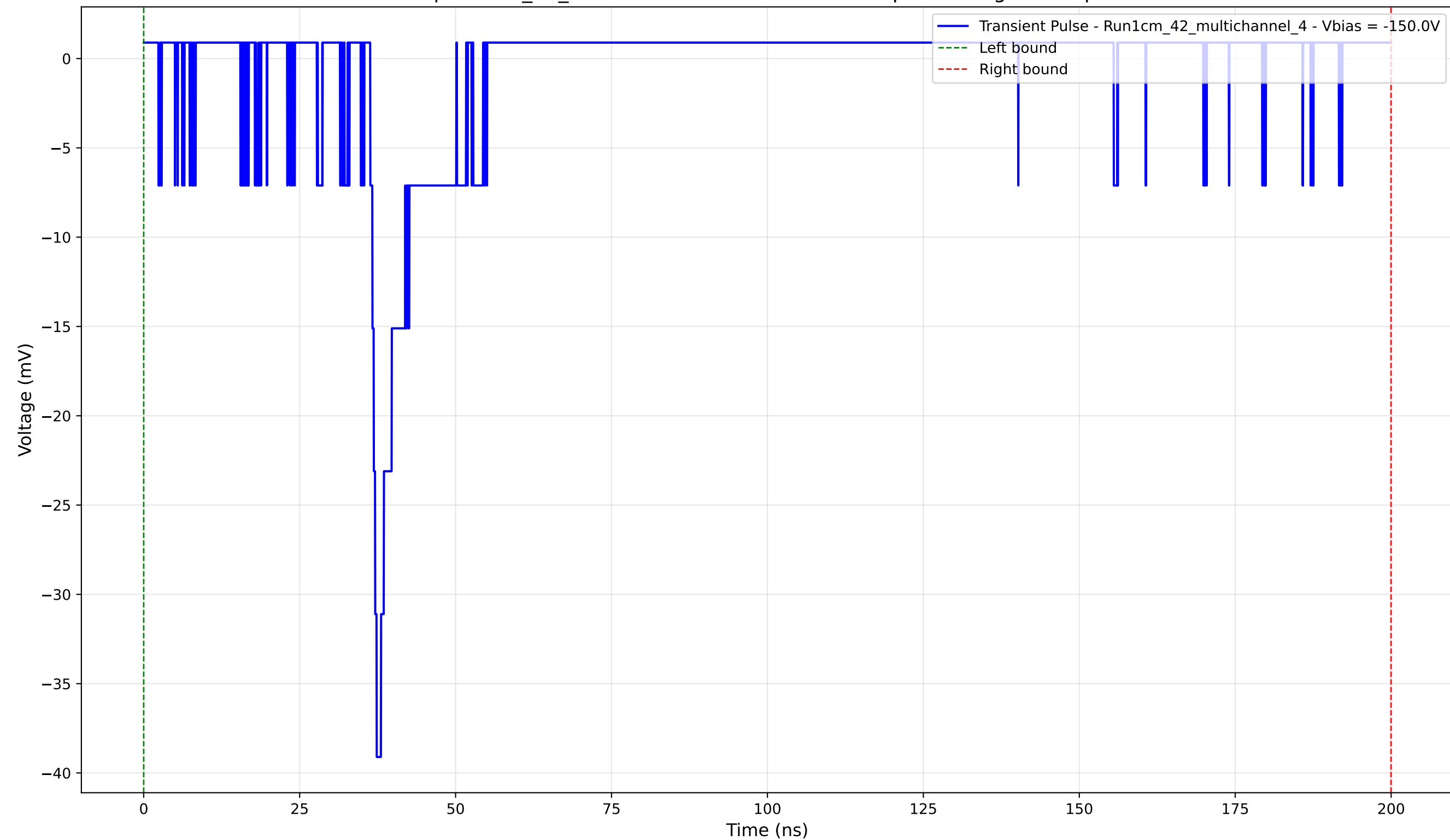
Transient Pulse - Sample: 1cm_42_multichannel - Position: 3010.0 \mu\text{m} - Charge: 2.01 pC - Rise Time: 1.03 ns
