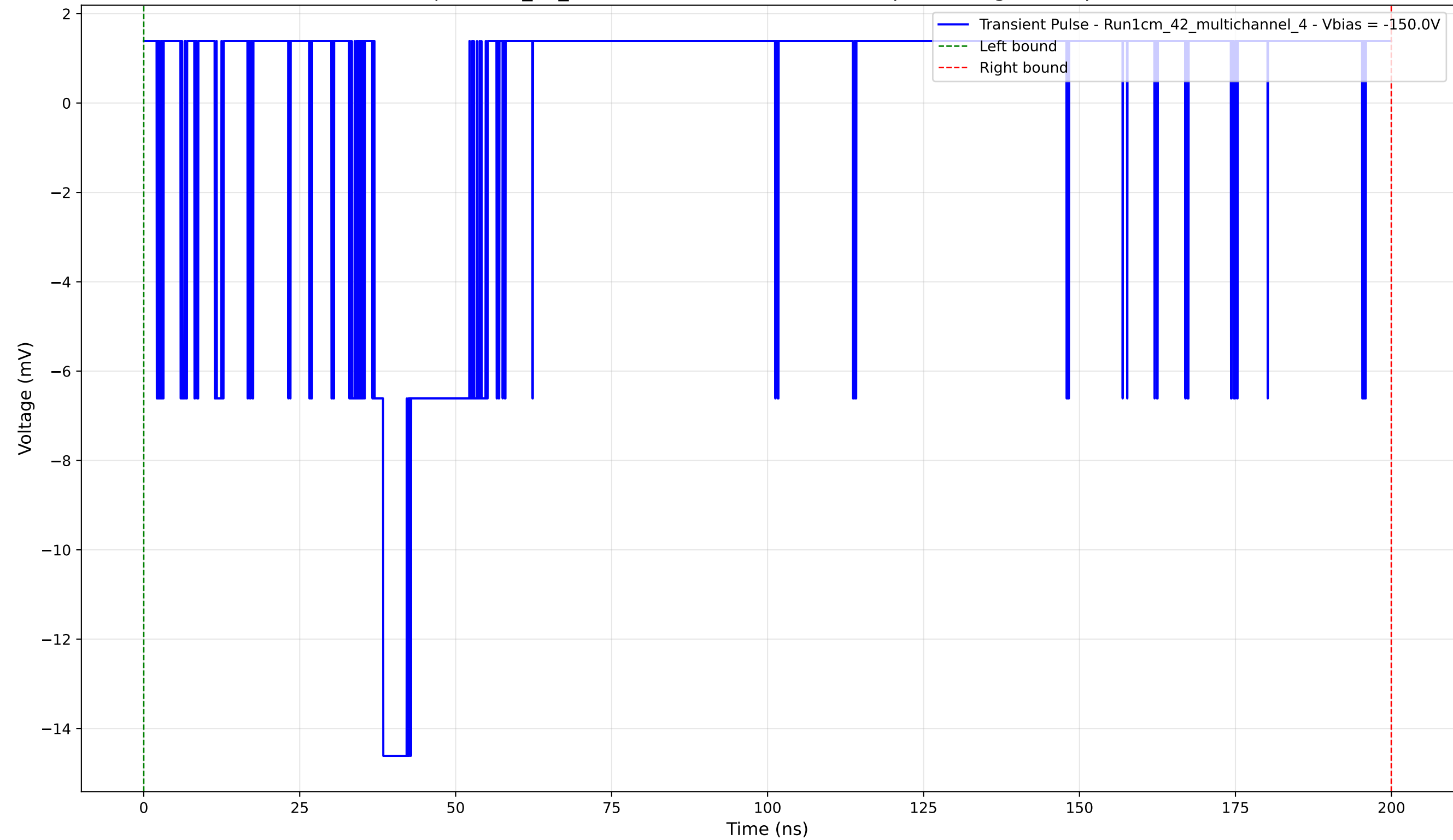
Transient Pulse - Sample: 1cm_42_multichannel - Position: 4670.0 \mu\text{m} - Charge: 0.77 pC - Rise Time: 1.40 ns
