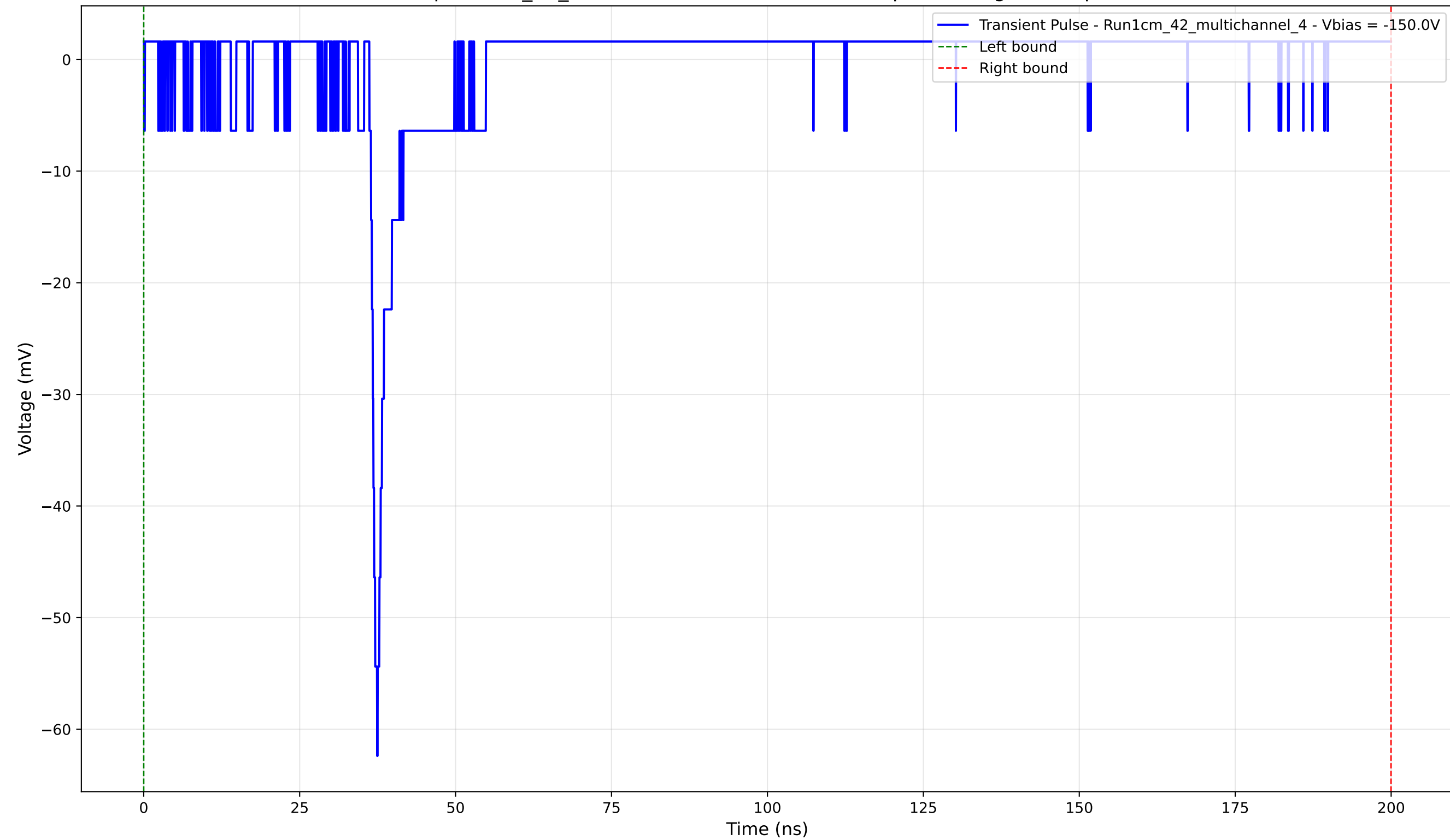
Transient Pulse - Sample: 1cm_42_multichannel - Position: 2075.0 \mu\text{m} - Charge: 0.05 pC - Rise Time: 1.24 ns
