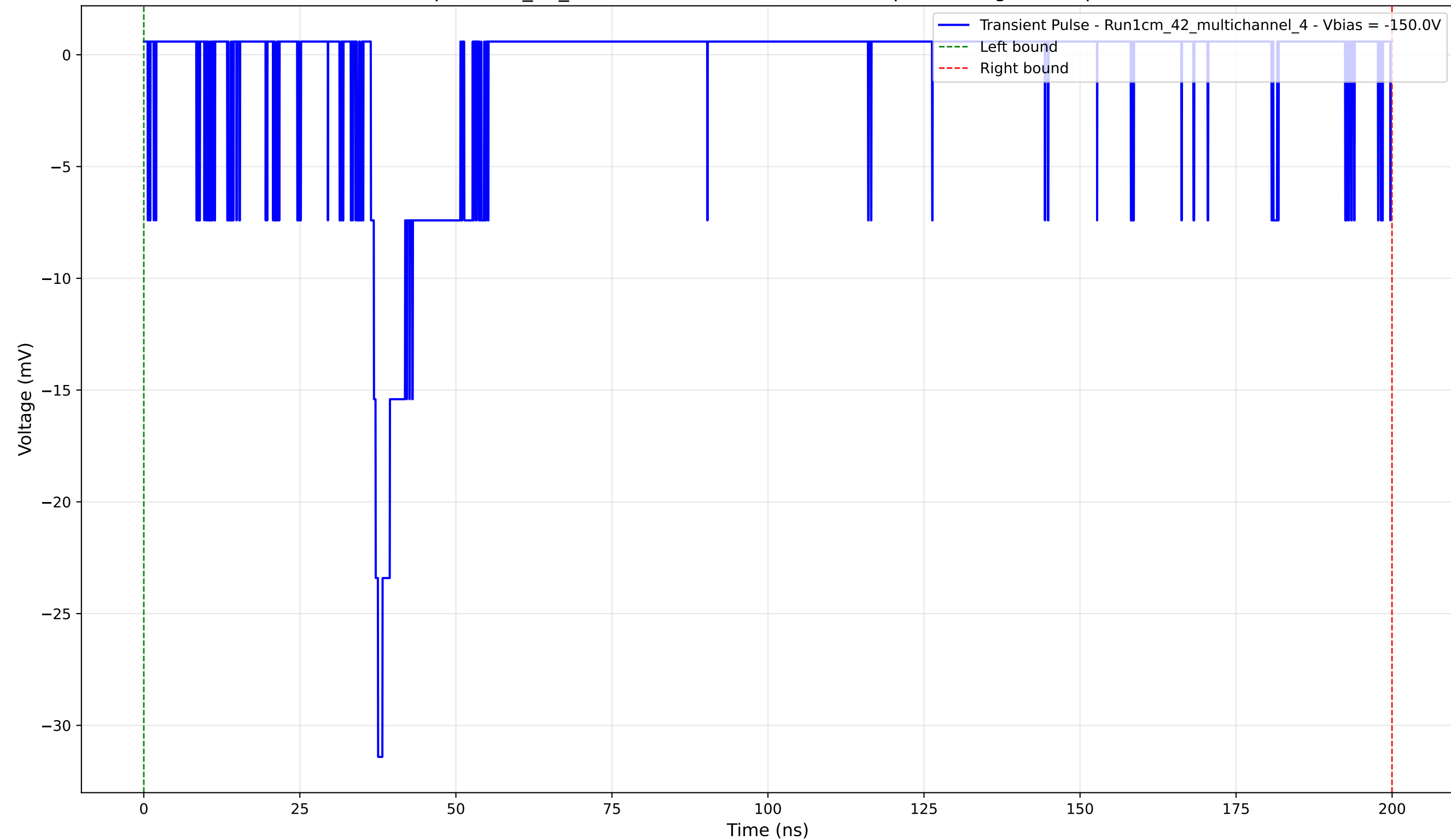
Transient Pulse - Sample: 1cm_42_multichannel - Position: 3165.0 \mu\text{m} - Charge: 2.87 pC - Rise Time: 1.15 ns
