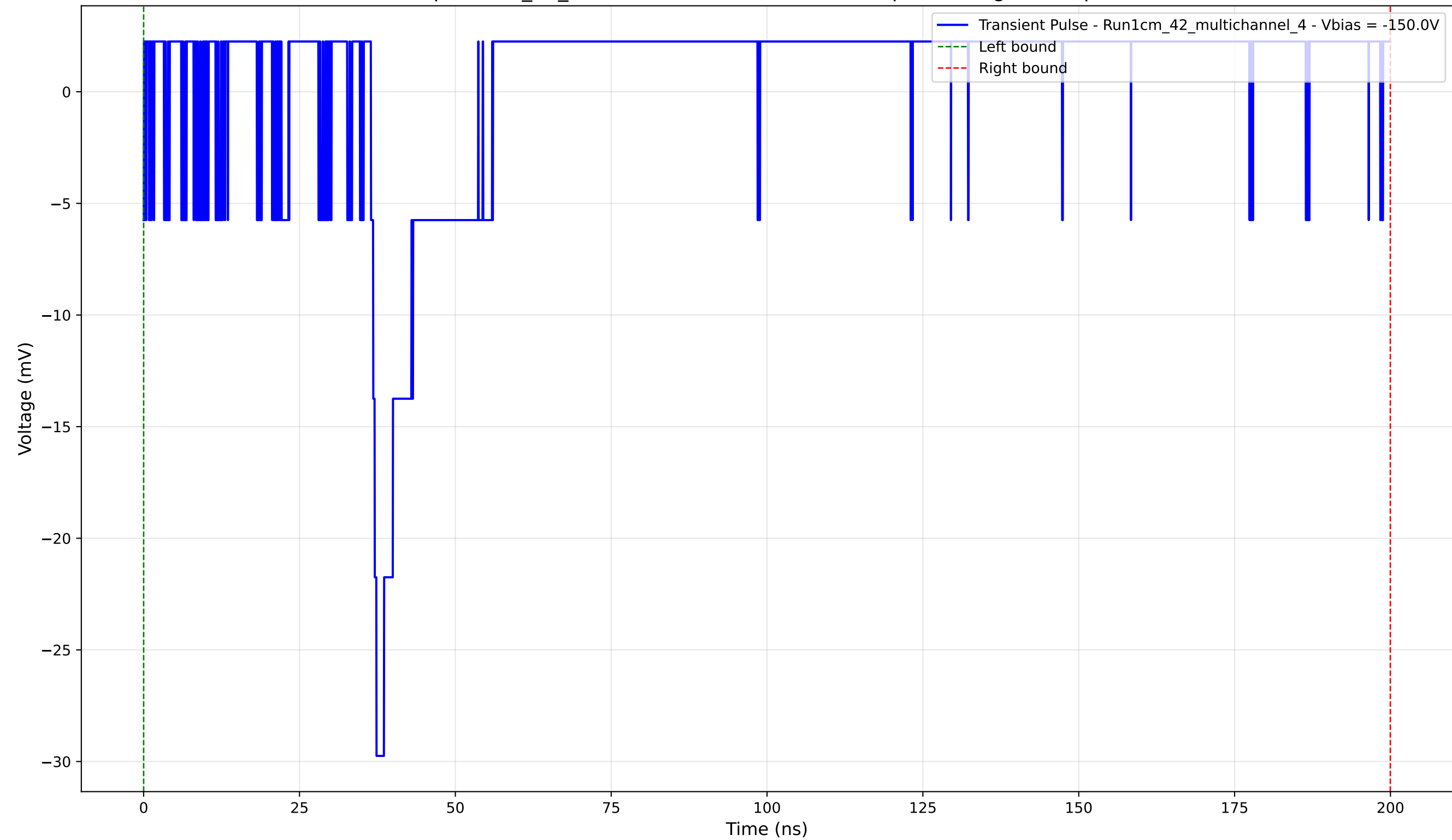
Transient Pulse - Sample: 1cm_42_multichannel - Position: 1630.0 \mu\text{m} - Charge: 2.52 pC - Rise Time: 0.90 ns
