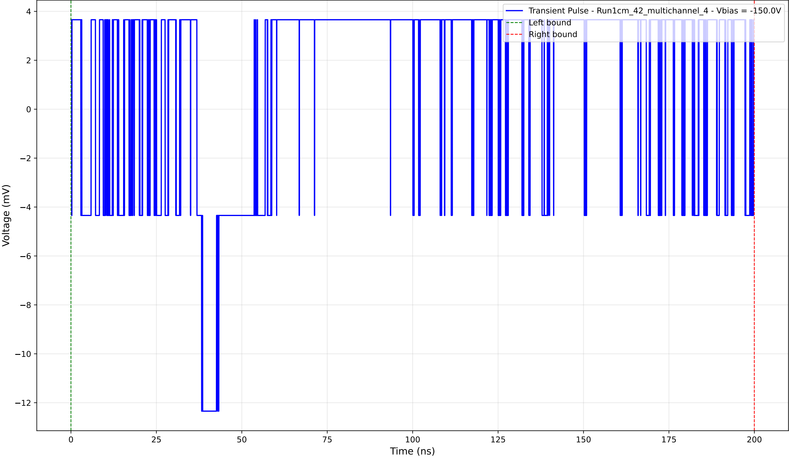
Transient Pulse - Sample: 1cm_42_multichannel - Position: 260.0 \mu\text{m} - Charge: 5.98 pC - Rise Time: 0.00 ns (N/A)
