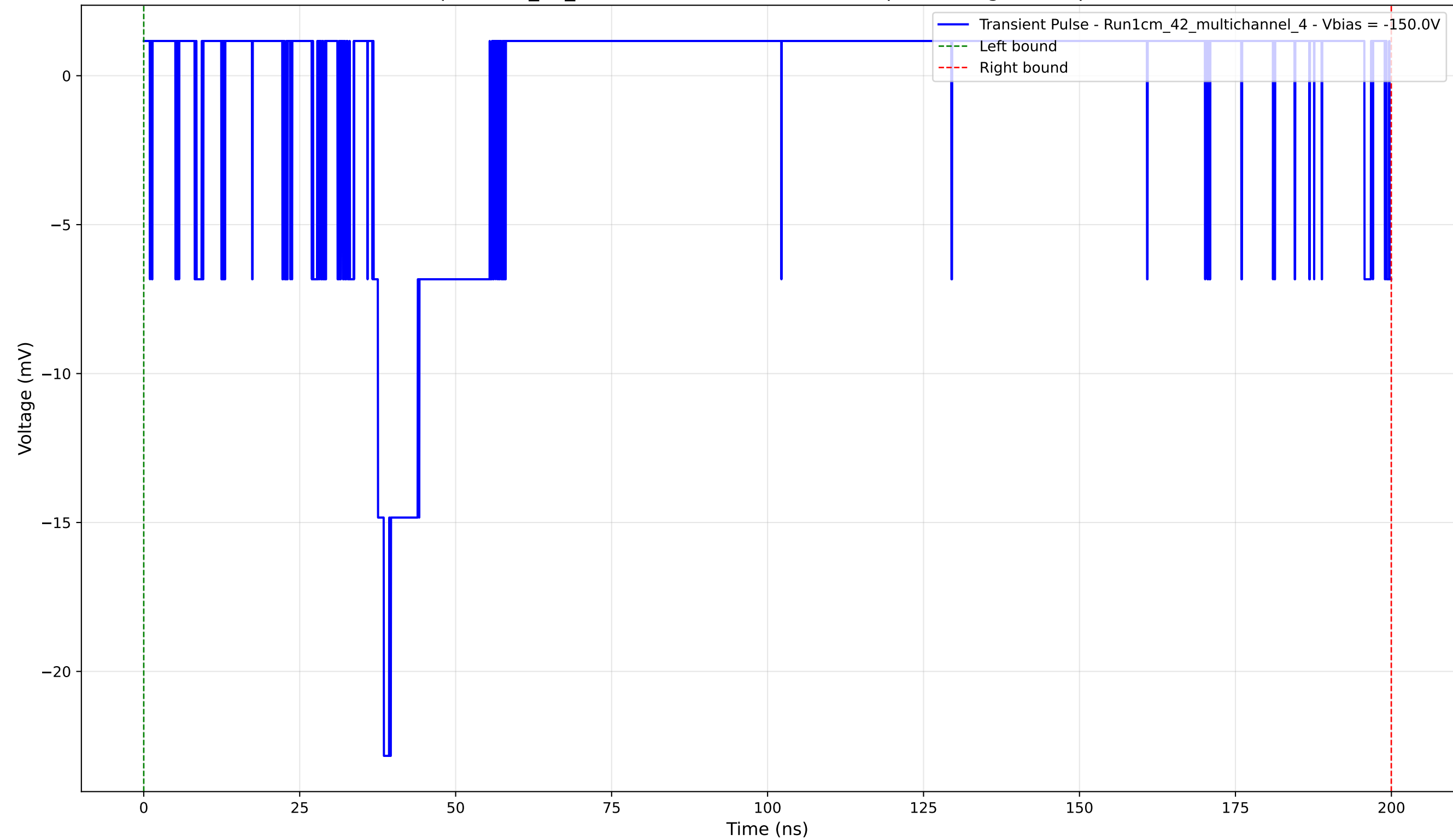
Transient Pulse - Sample: 1cm_42_multichannel - Position: 960.0 \mu\text{m} - Charge: 1.03 pC - Rise Time: 1.66 ns
