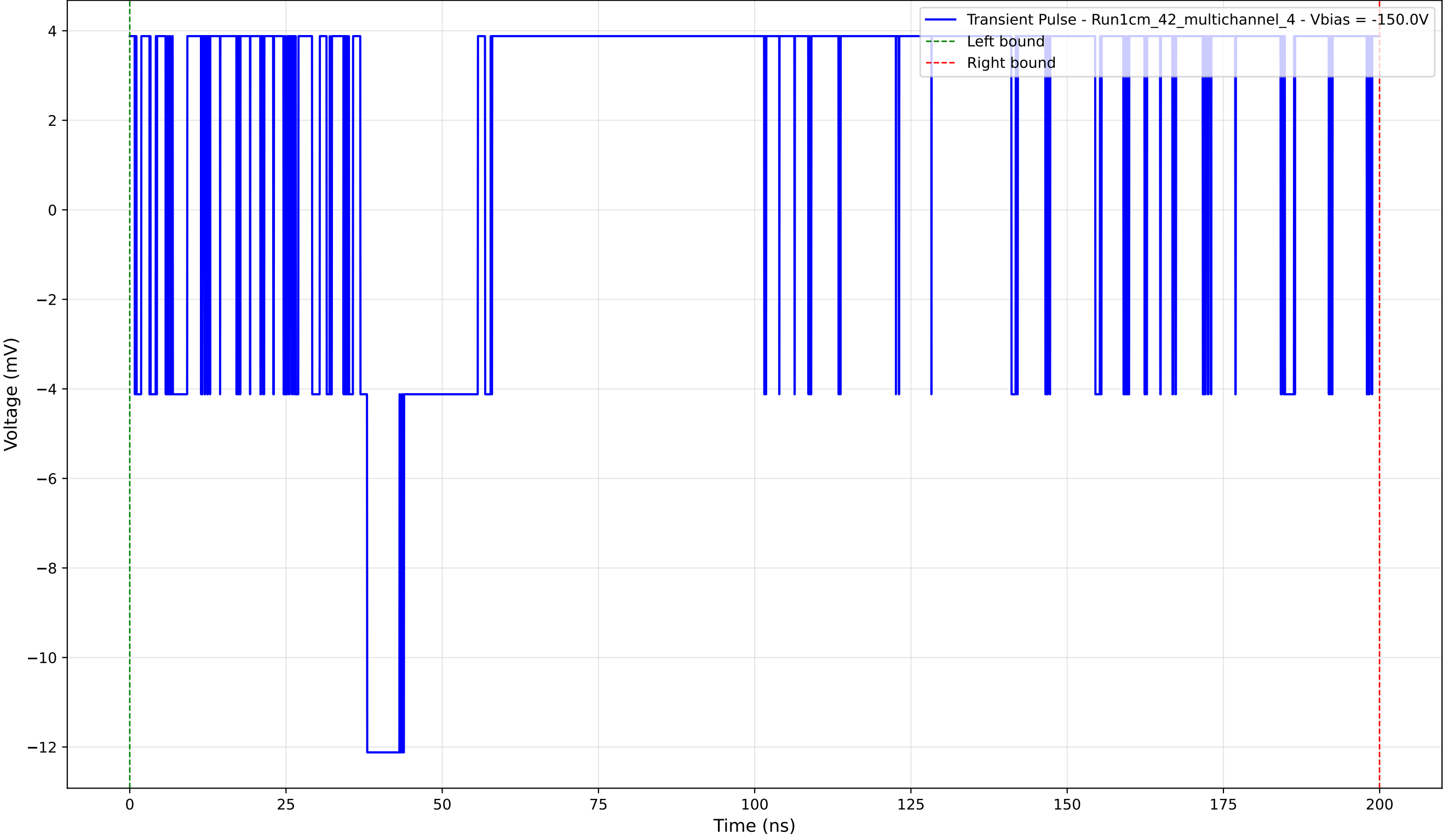
Transient Pulse - Sample: 1cm_42_multichannel - Position: 535.0 \mu\text{m} - Charge: 8.73 pC - Rise Time: 0.00 ns (N/A)
