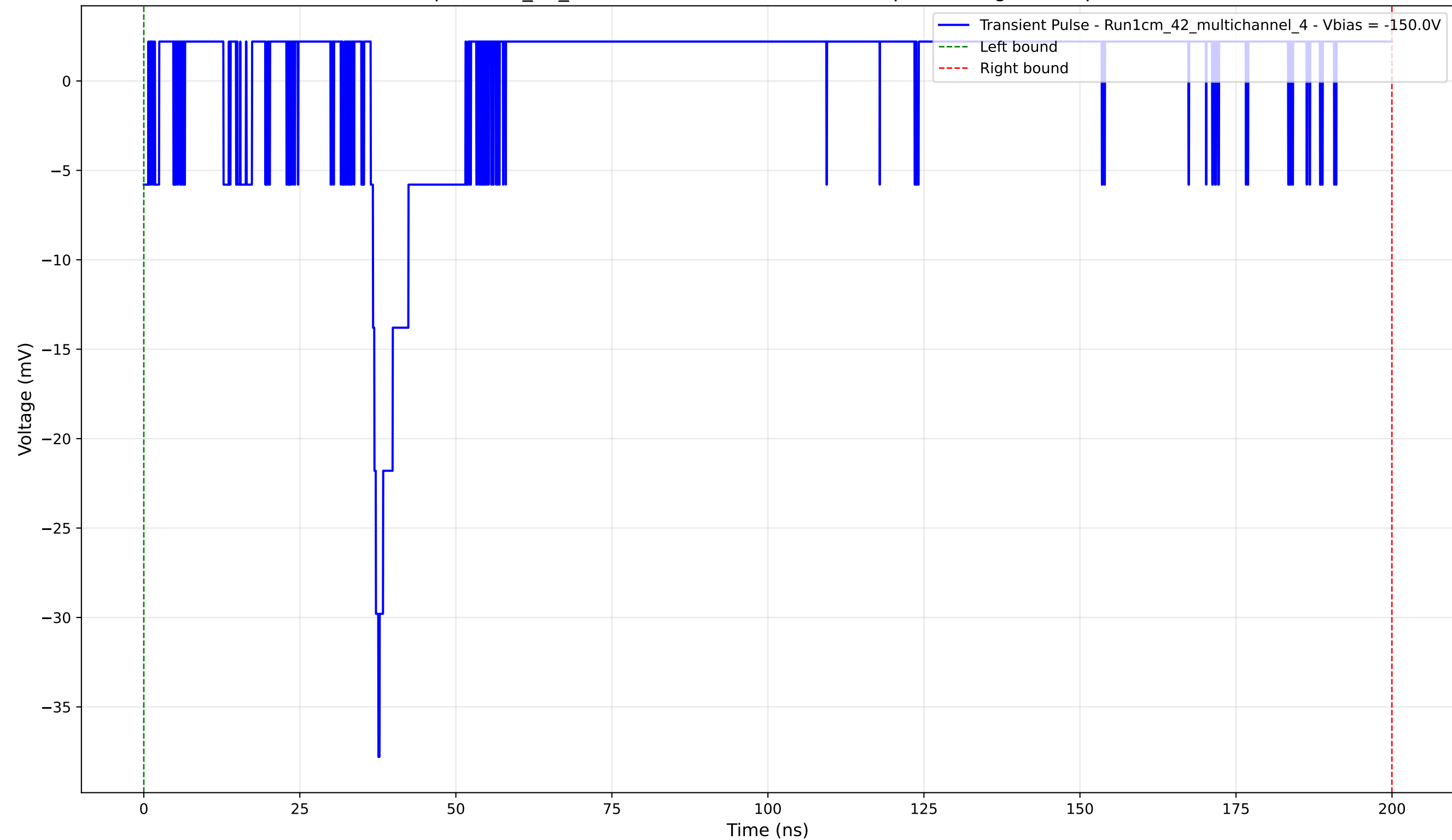
Transient Pulse - Sample: 1cm_42_multichannel - Position: 3040.0 \mu\text{m} - Charge: 2.64 pC - Rise Time: 1.23 ns
