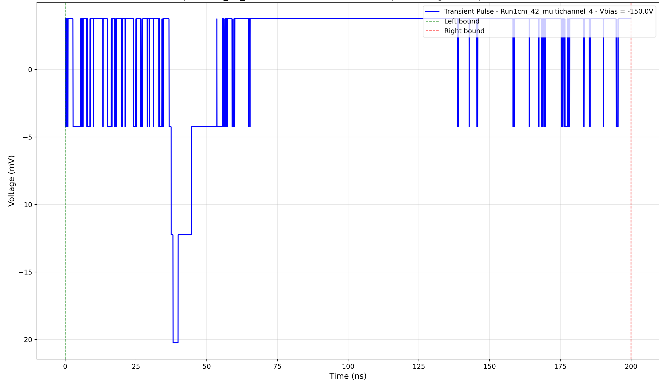
Transient Pulse - Sample: 1cm_42_multichannel - Position: 1030.0 \mu\text{m} - Charge: 8.09 pC - Rise Time: 0.00 ns (N/A)
