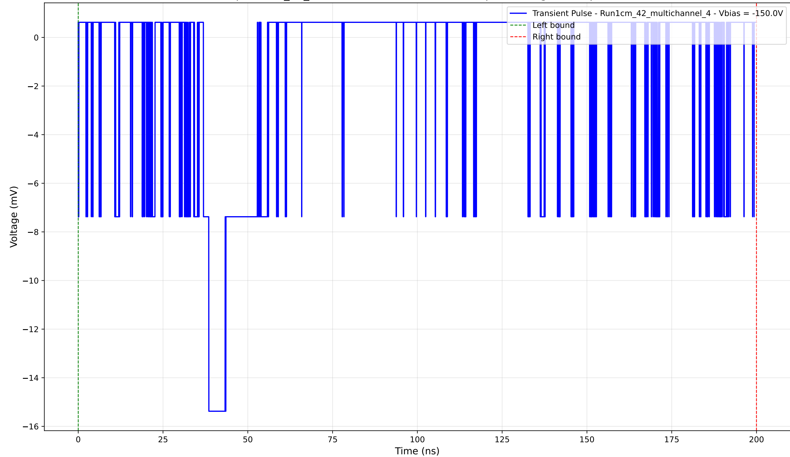
Transient Pulse - Sample: 1cm_42_multichannel - Position: 4555.0 \mu\text{m} - Charge: 4.10 pC - Rise Time: 1.60 ns
