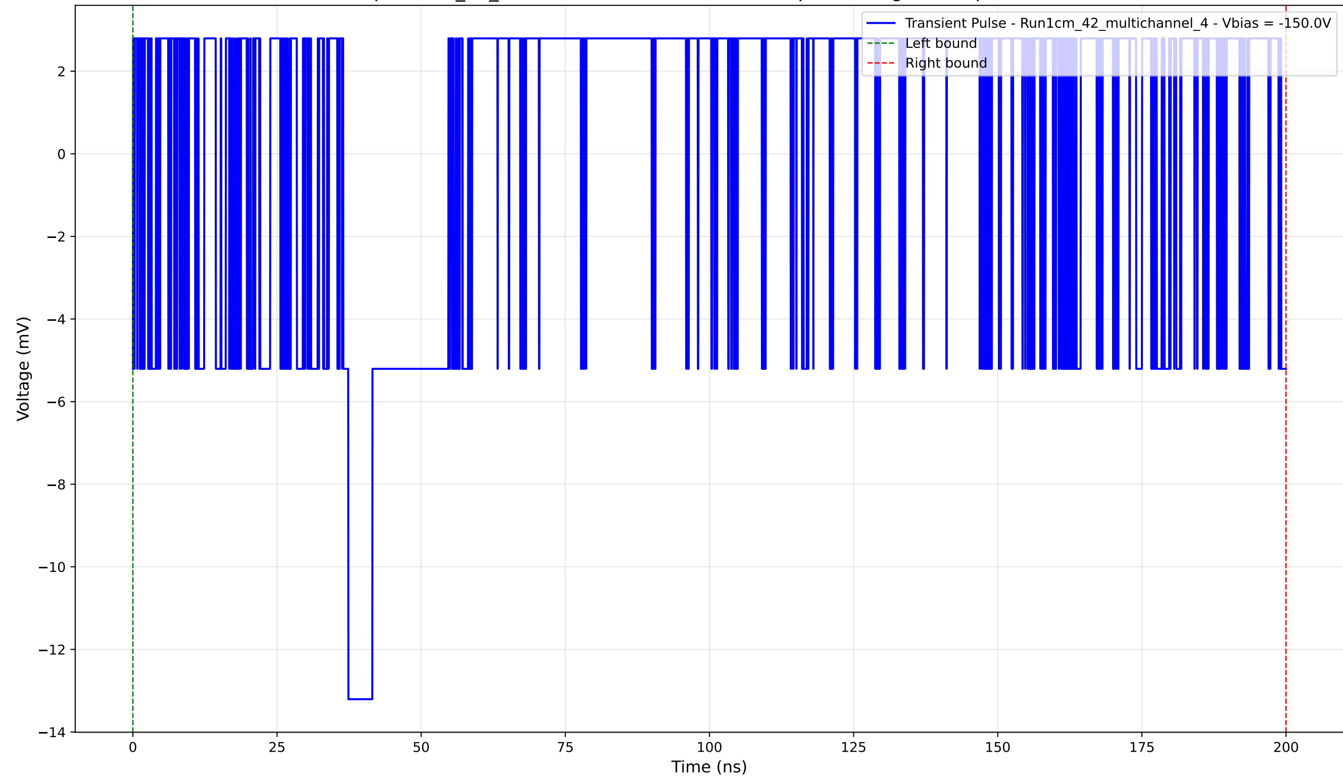
Transient Pulse - Sample: 1cm_42_multichannel - Position: 1320.0 \mu\text{m} - Charge: 1.33 pC - Rise Time: 0.00 ns (N/A)
