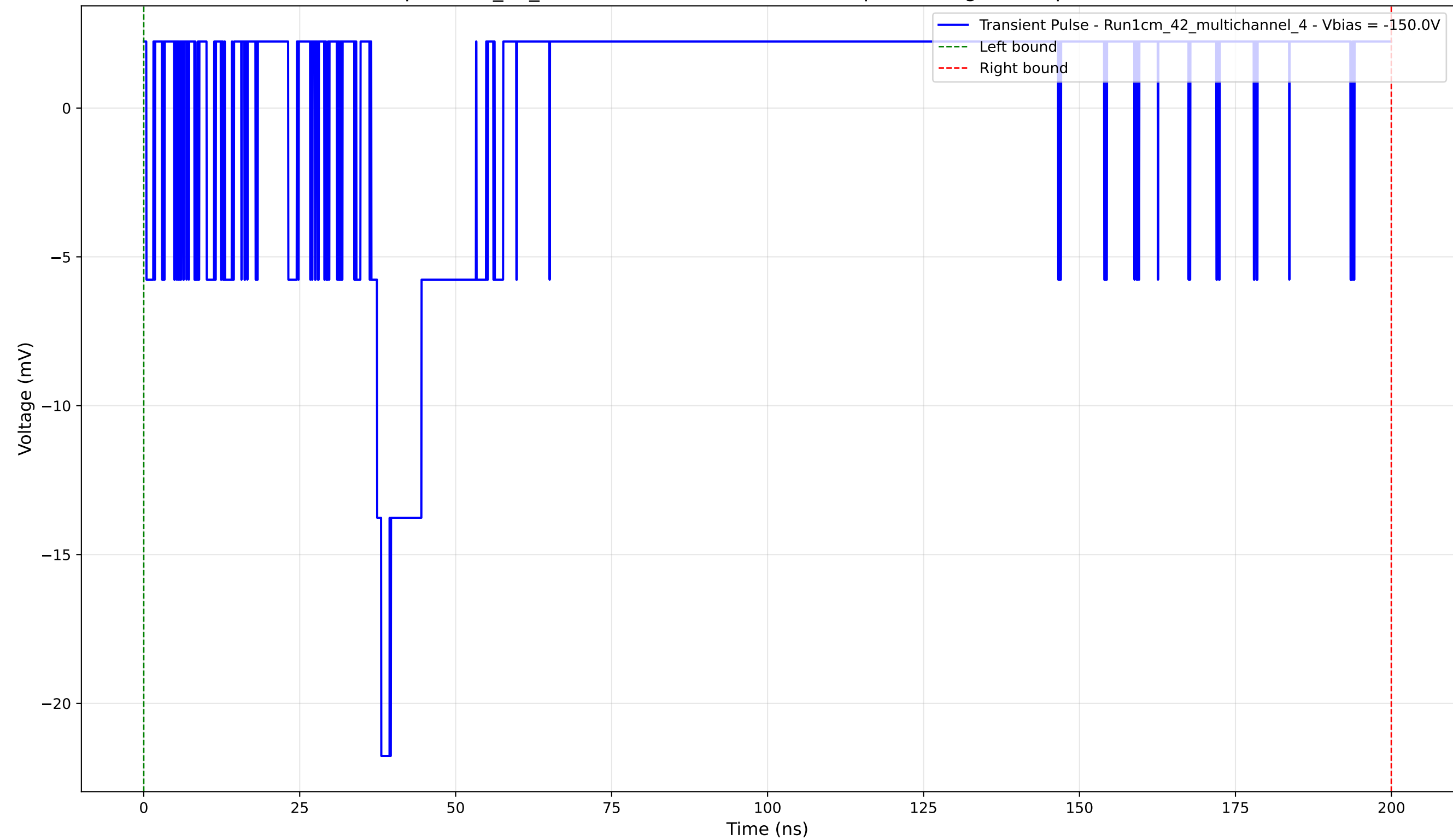
Transient Pulse - Sample: 1cm_42_multichannel - Position: 1125.0 \mu\text{m} - Charge: 2.38 pC - Rise Time: 0.00 ns (N/A)
