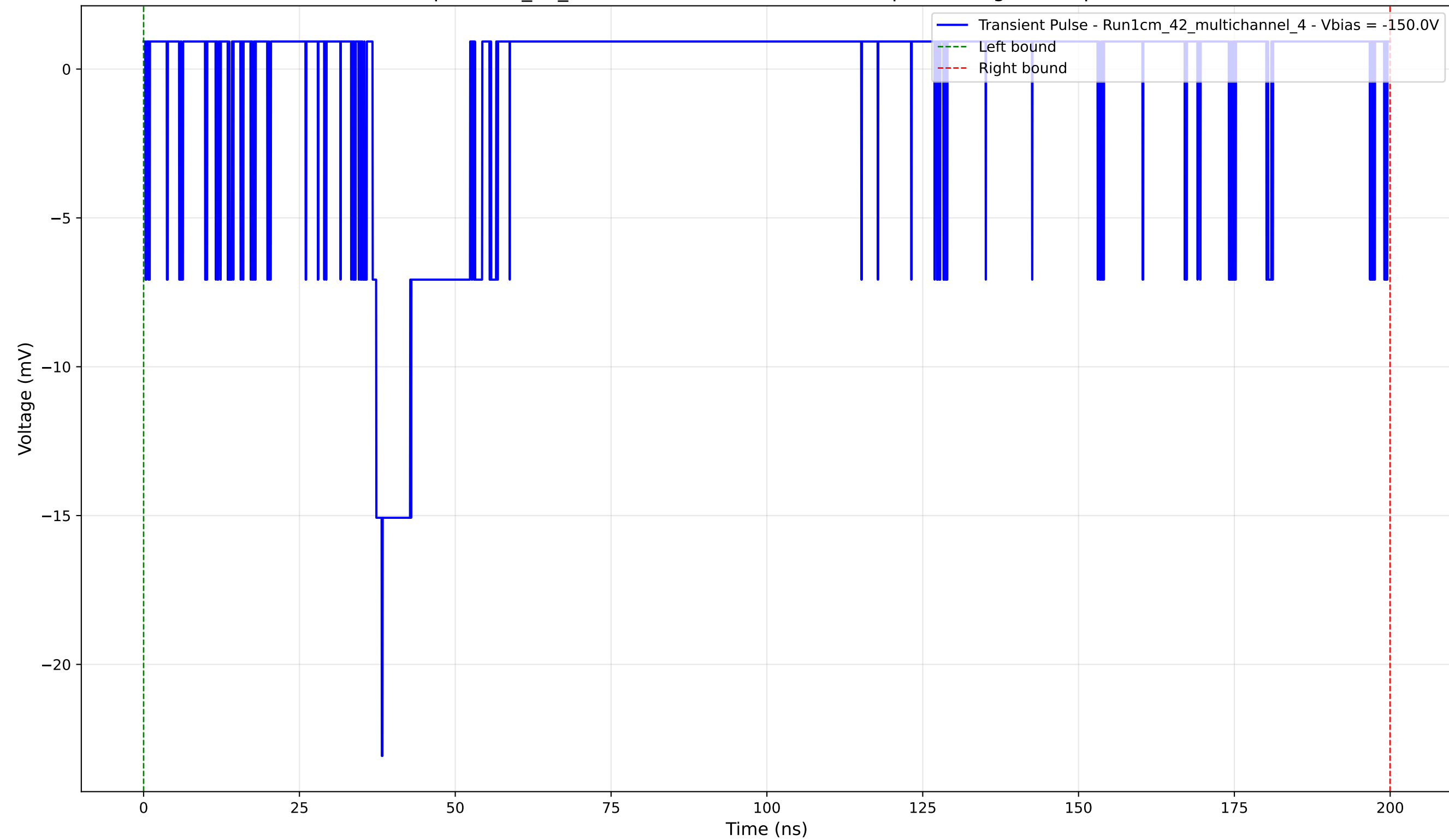
Transient Pulse - Sample: 1cm_42_multichannel - Position: 3580.0 \mu\text{m} - Charge: 1.55 pC - Rise Time: 1.48 ns
