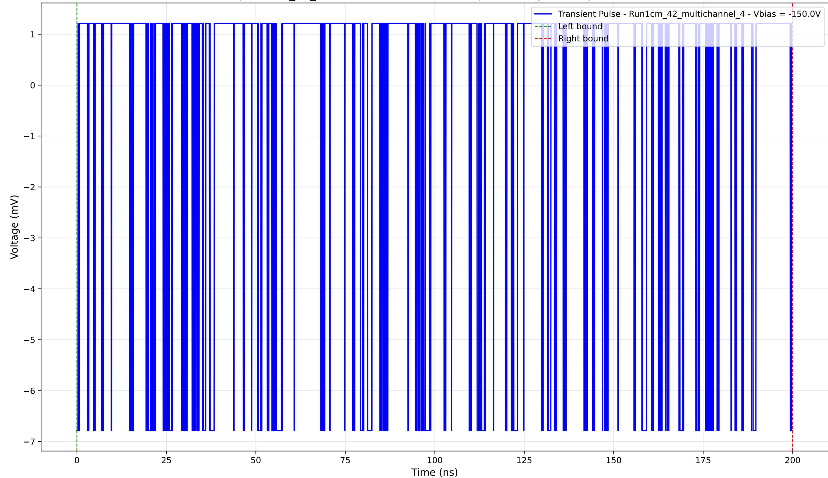
Transient Pulse - Sample: 1cm_42_multichannel - Position: 0.0 \mu\text{m} - Charge: 0.53 pC - Rise Time: 0.00 ns (N/A)
