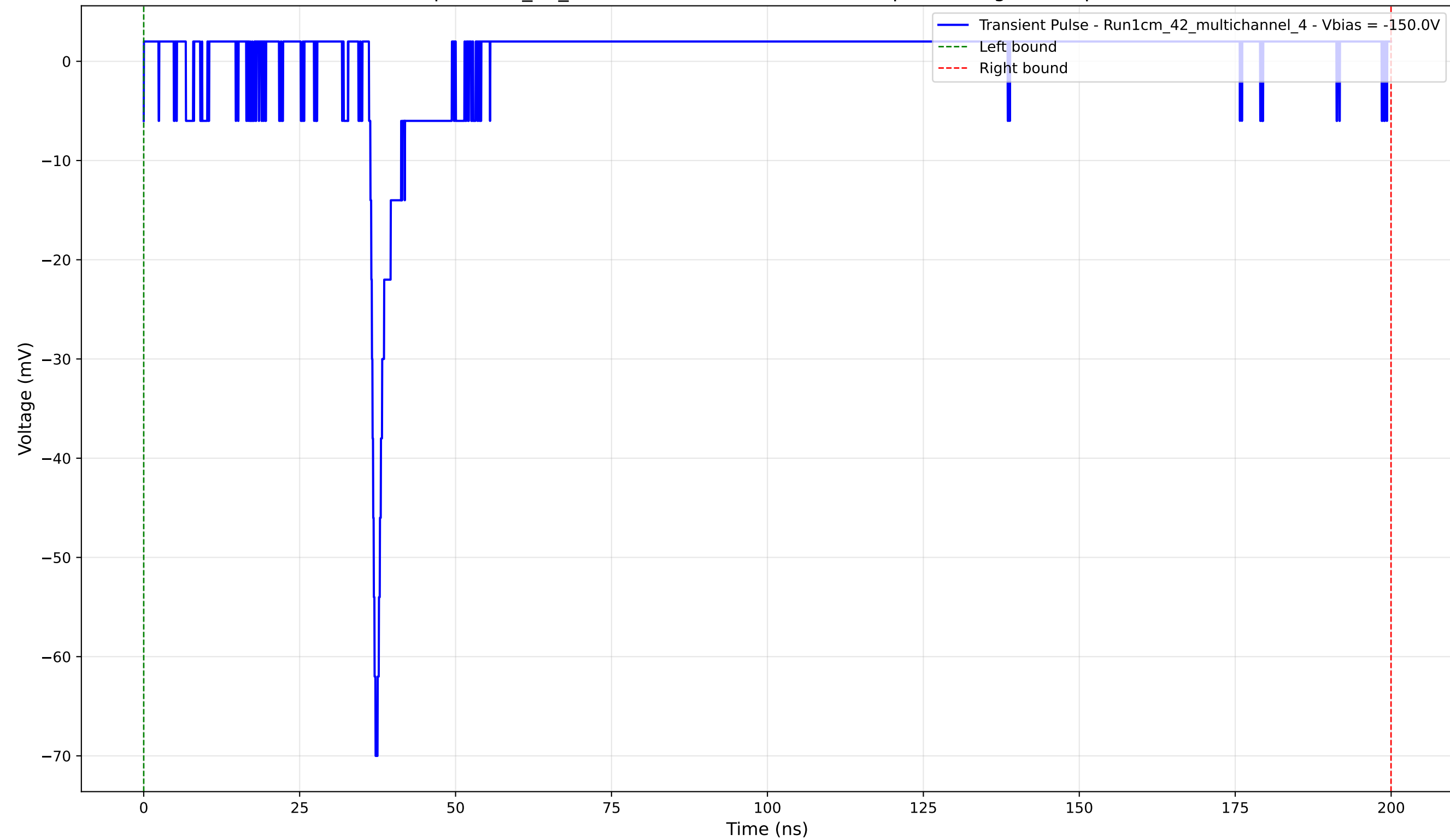
Transient Pulse - Sample: 1cm_42_multichannel - Position: 2185.0 \mu\text{m} - Charge: 1.67 pC - Rise Time: 0.84 ns
