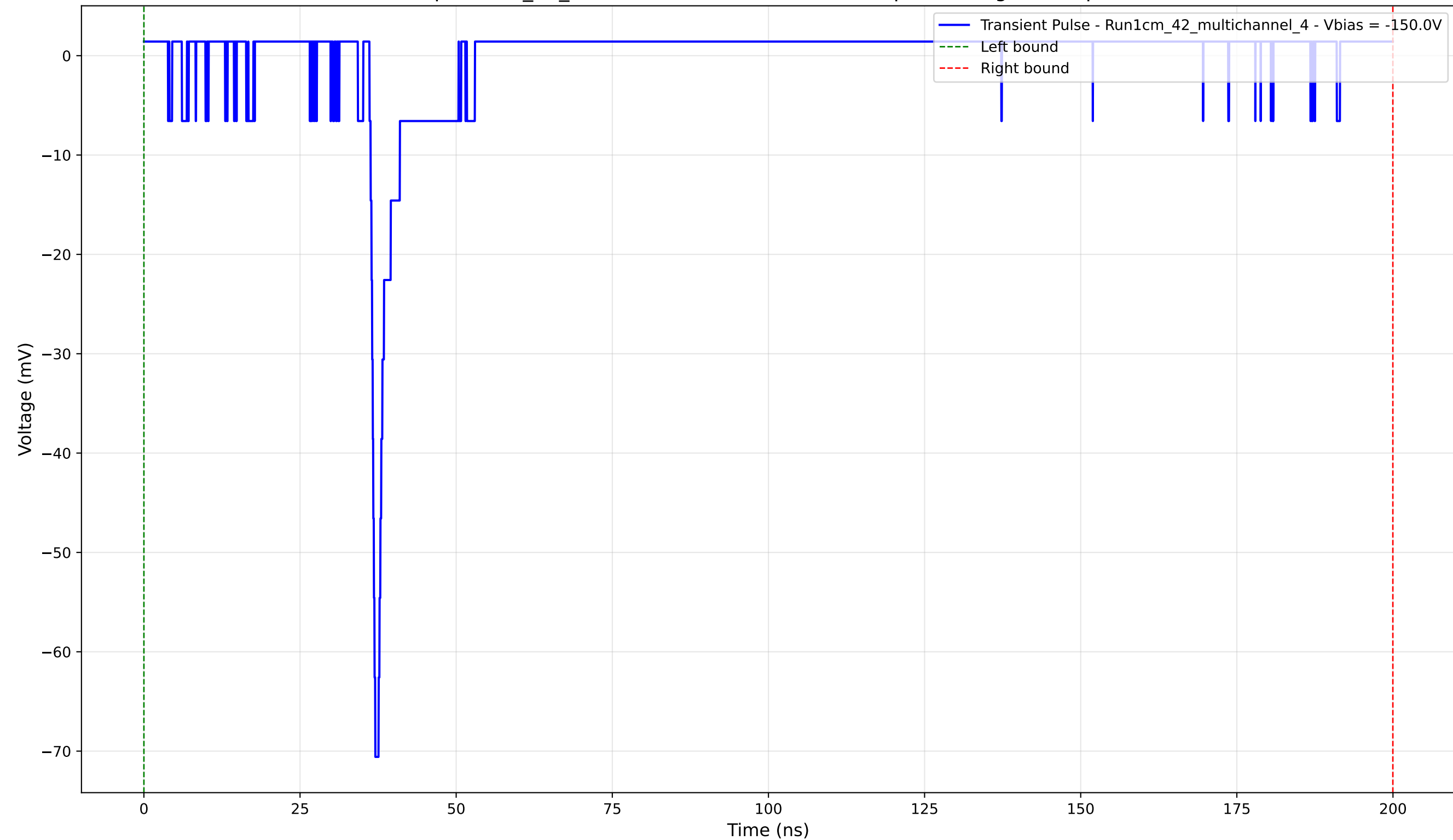
Transient Pulse - Sample: 1cm_42_multichannel - Position: 2545.0 \mu\text{m} - Charge: 0.34 pC - Rise Time: 0.76 ns
