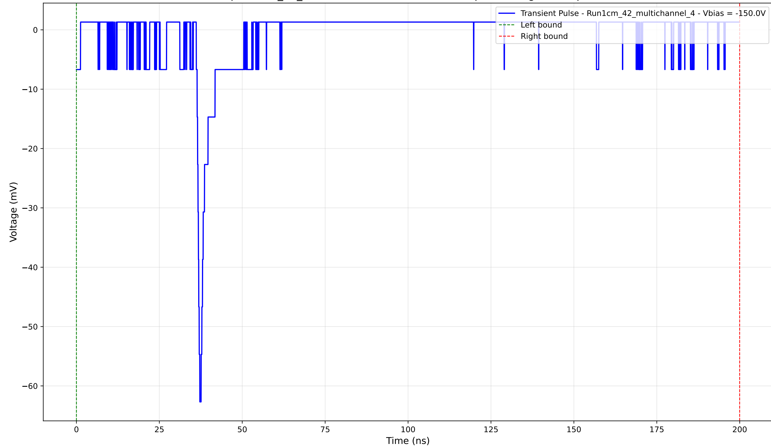
Transient Pulse - Sample: 1cm_42_multichannel - Position: 2100.0 \mu\text{m} - Charge: 2.11 pC - Rise Time: 1.06 ns
