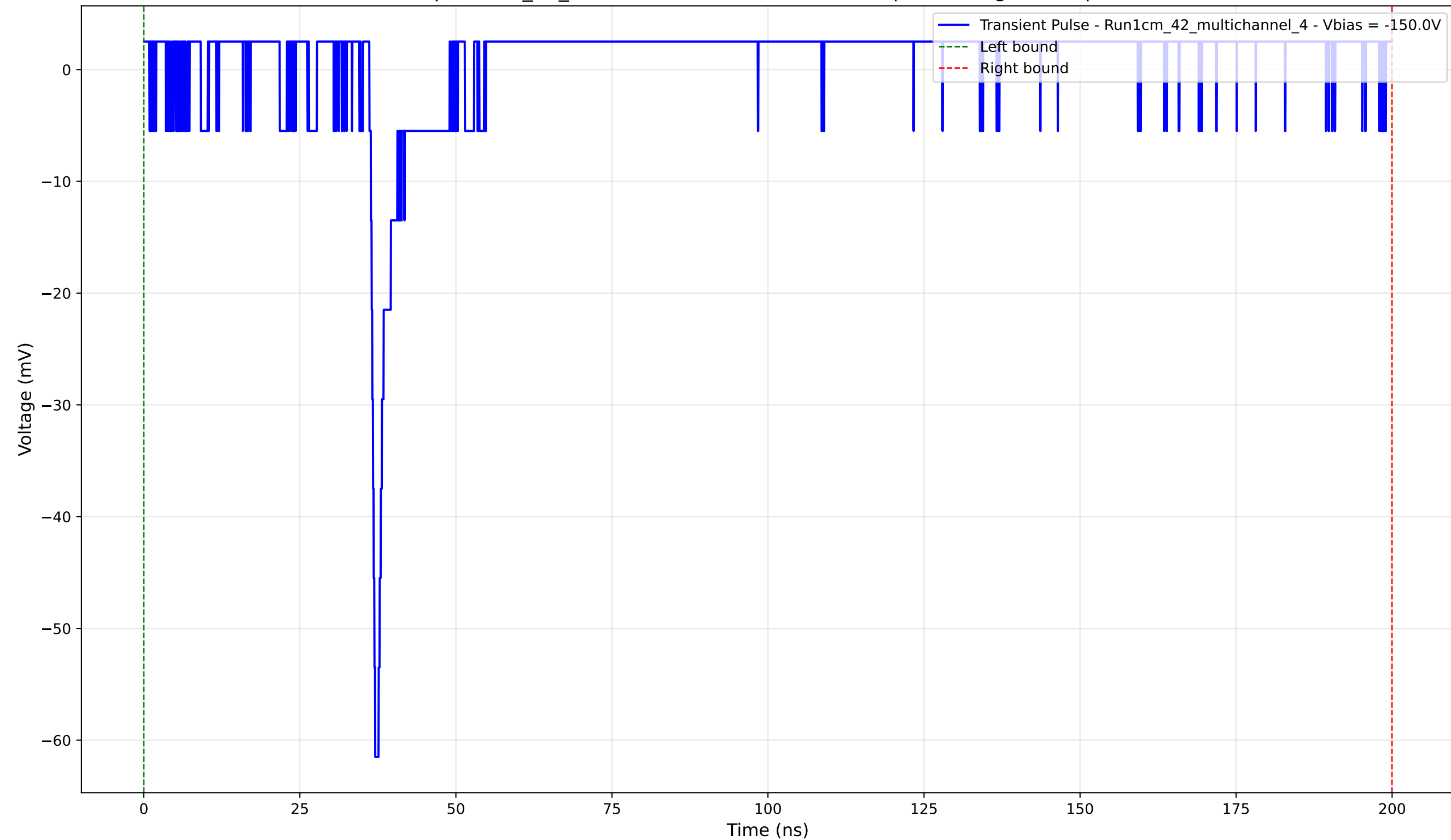
Transient Pulse - Sample: 1cm_42_multichannel - Position: 2595.0 \mu\text{m} - Charge: 3.54 pC - Rise Time: 0.70 ns
