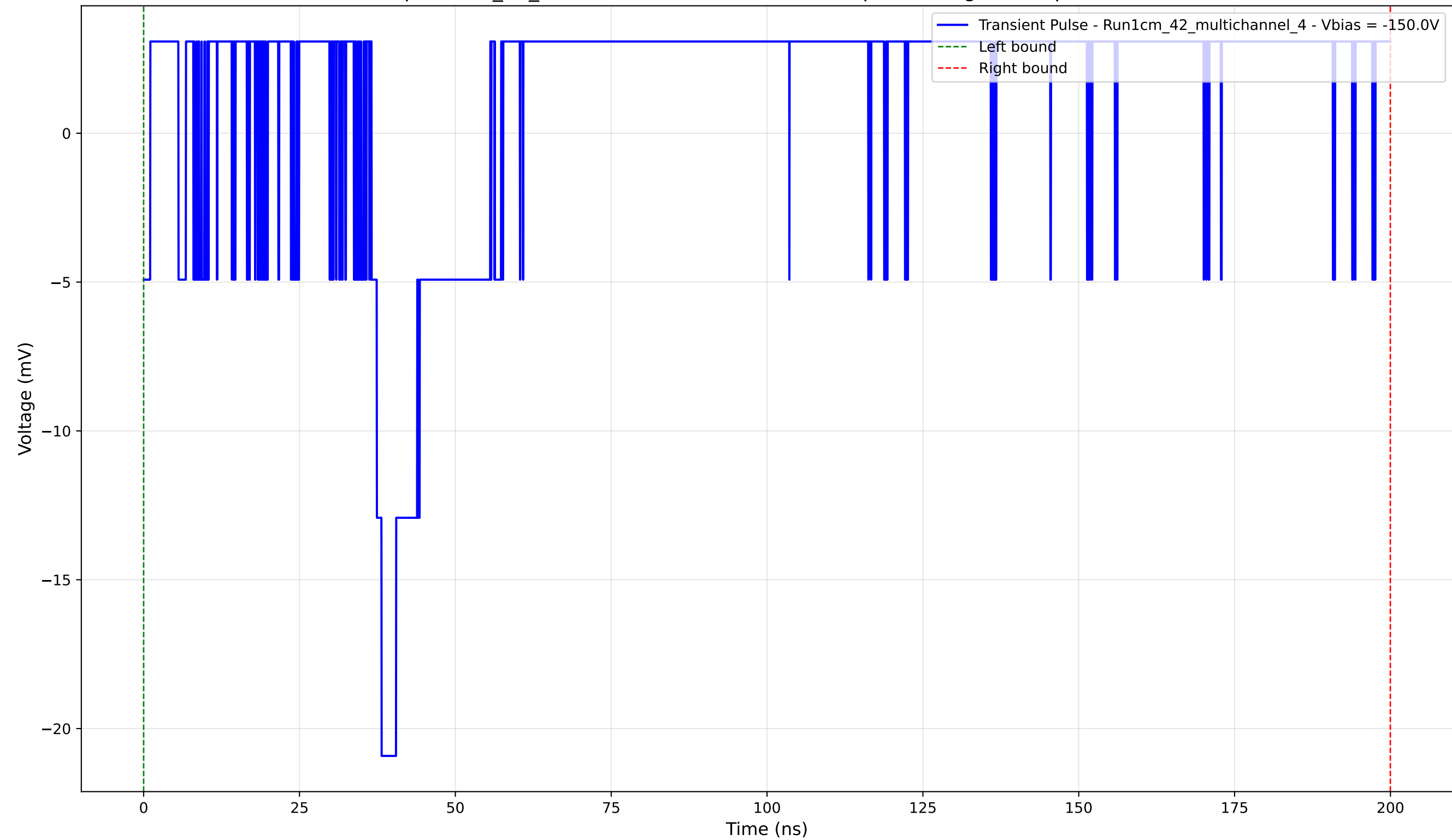
Transient Pulse - Sample: 1cm_42_multichannel - Position: 1035.0 \mu\text{m} - Charge: 5.61 pC - Rise Time: 0.00 ns (N/A)
