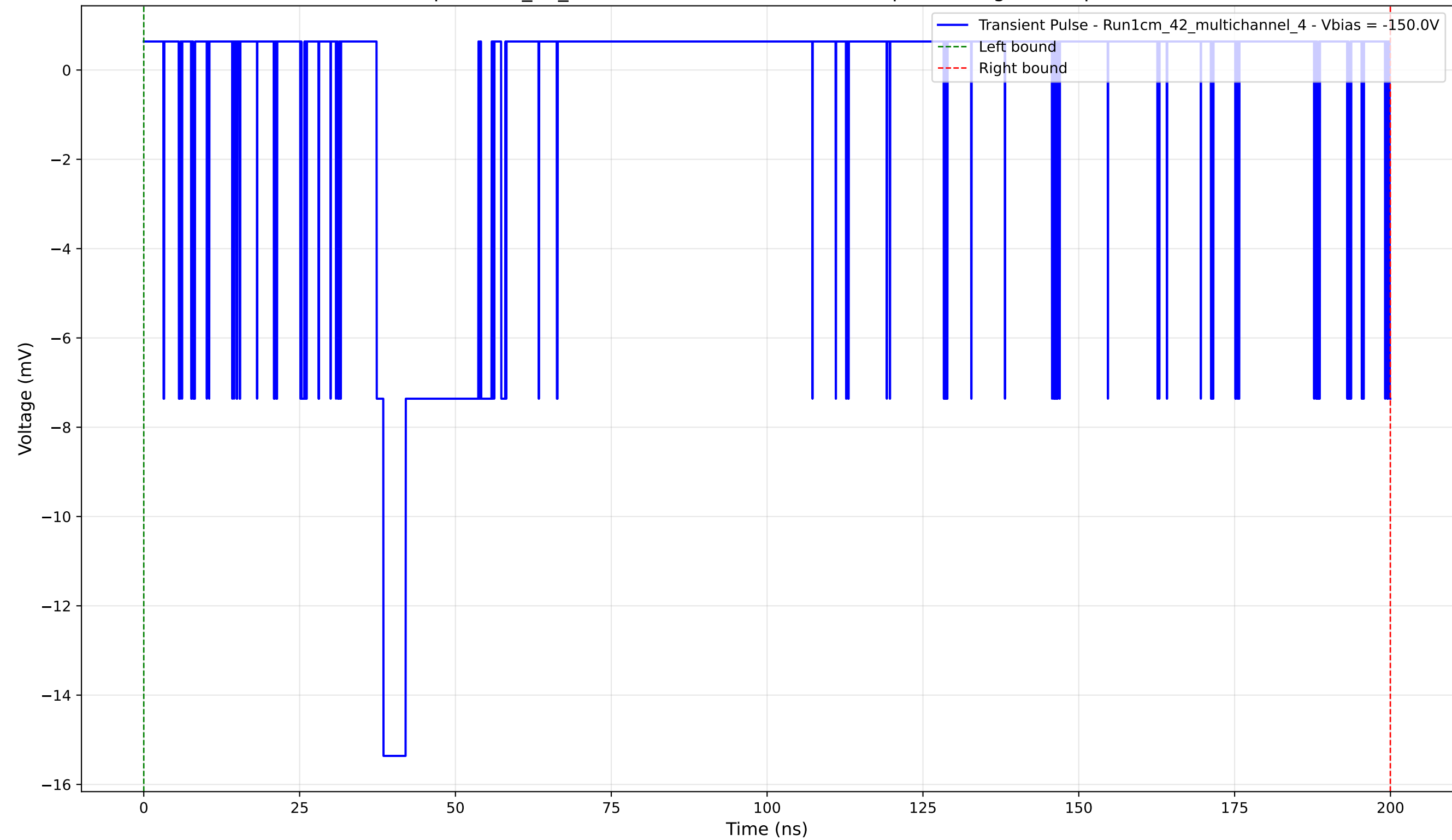
Transient Pulse - Sample: 1cm_42_multichannel - Position: 4330.0 \mu\text{m} - Charge: 2.13 pC - Rise Time: 1.10 ns
