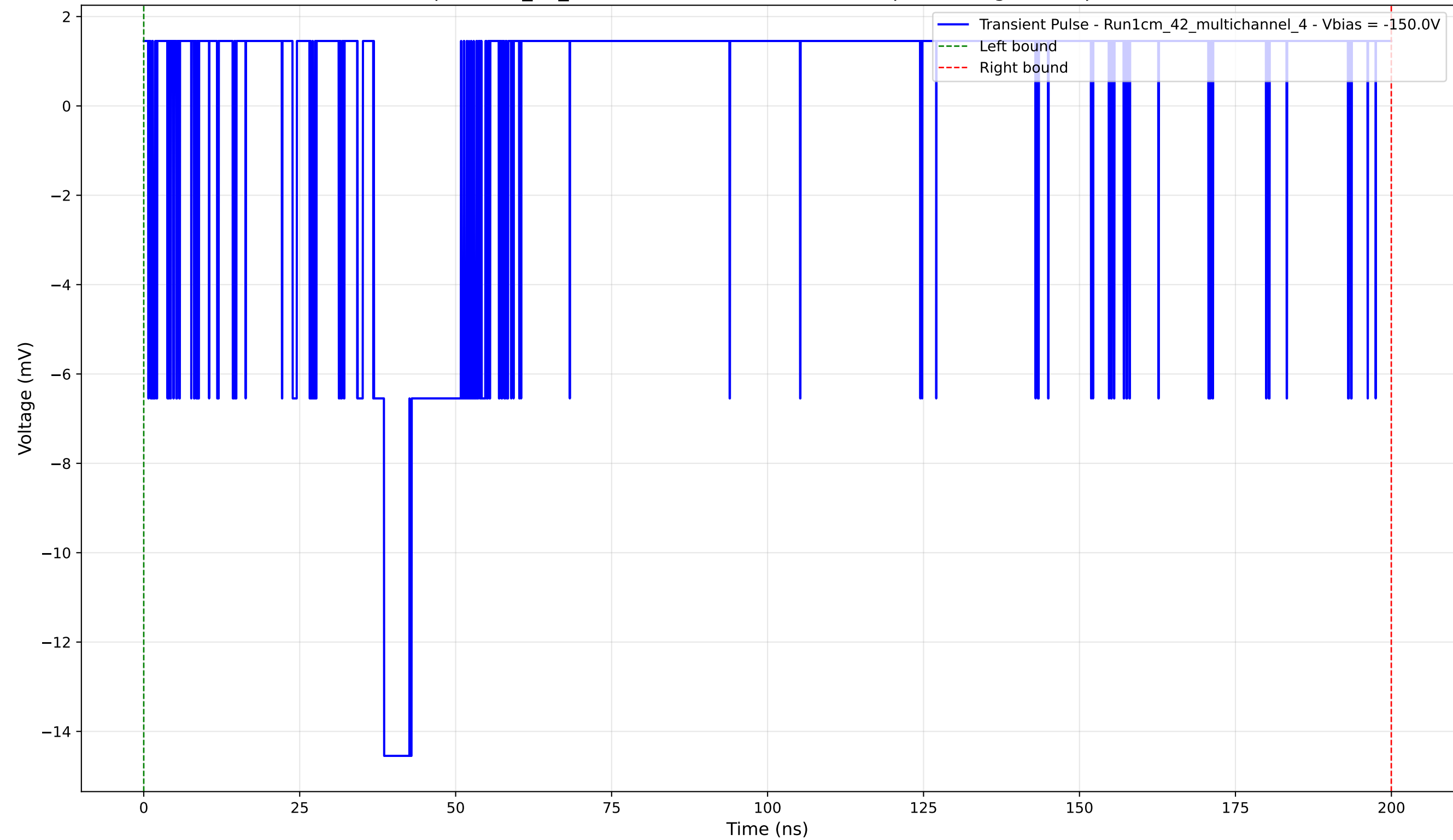
Transient Pulse - Sample: 1cm_42_multichannel - Position: 4655.0 \mu\text{m} - Charge: 0.95 pC - Rise Time: 1.64 ns
