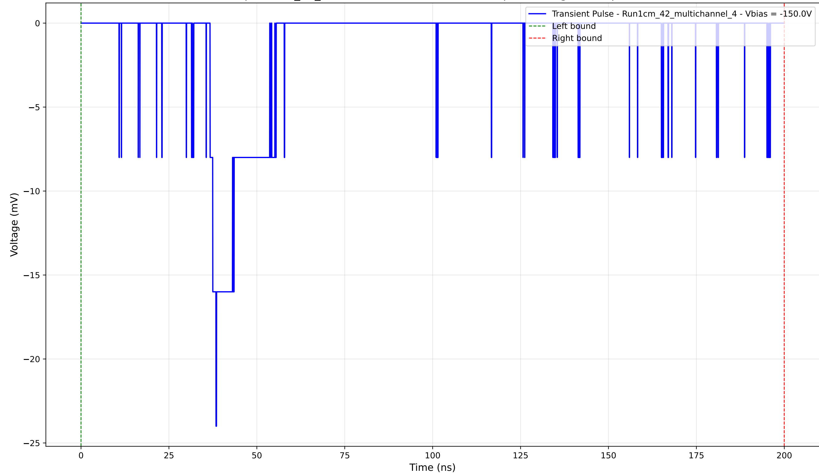
Transient Pulse - Sample: 1cm_42_multichannel - Position: 3660.0 \mu\text{m} - Charge: 4.54 pC - Rise Time: 1.69 ns
