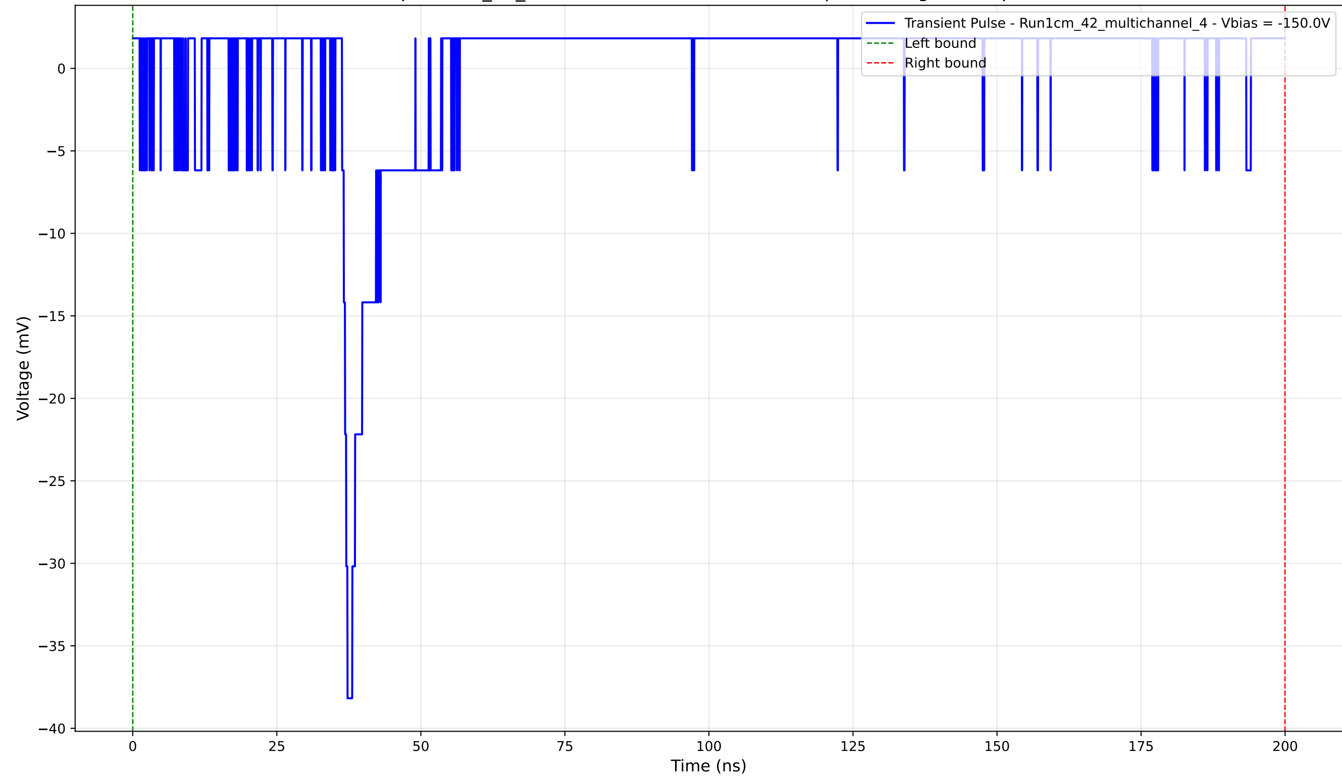
Transient Pulse - Sample: 1cm_42_multichannel - Position: 2985.0 \mu\text{m} - Charge: 1.33 pC - Rise Time: 0.95 ns
