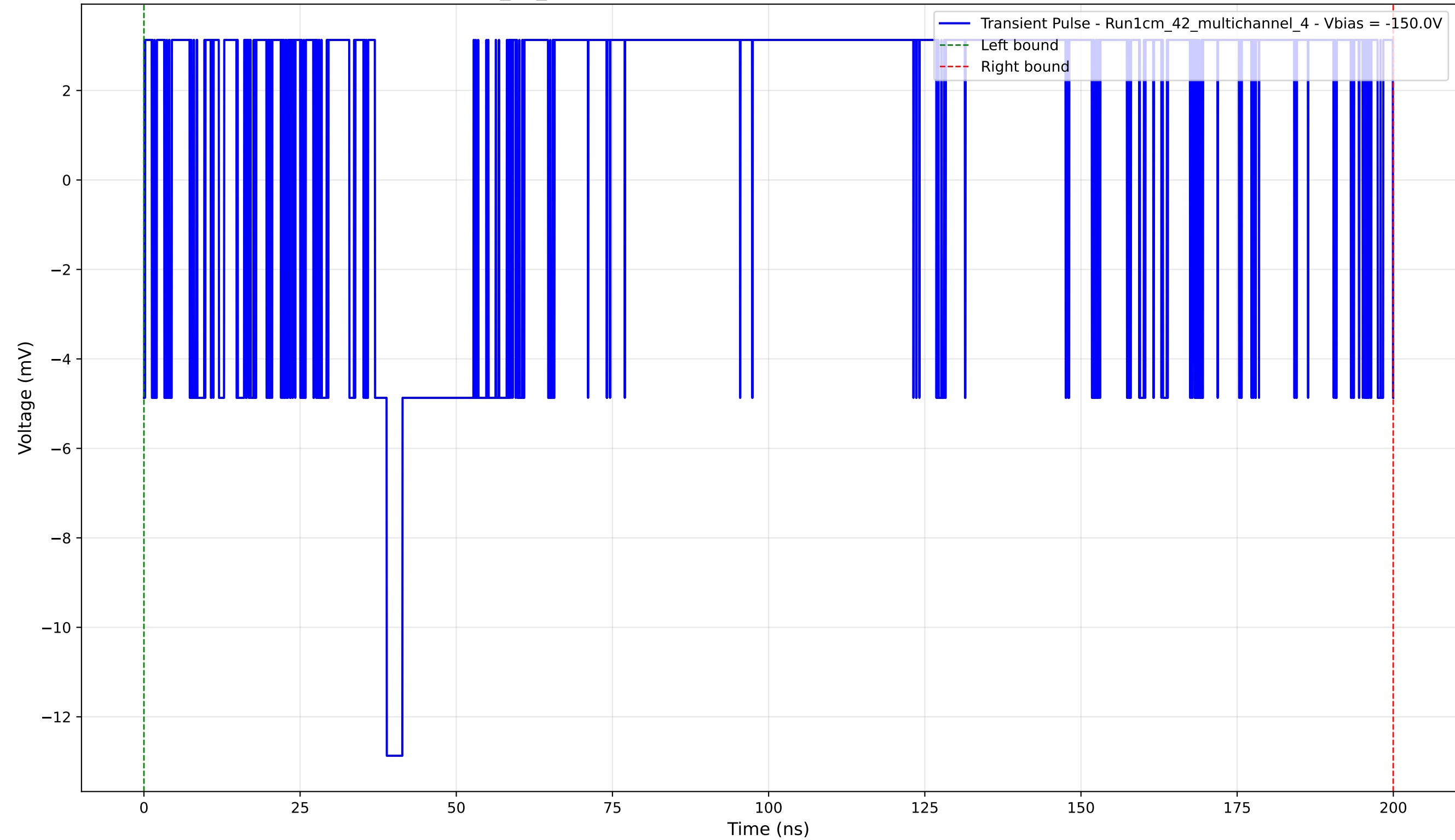
Transient Pulse - Sample: 1cm_42_multichannel - Position: 300.0 \mu\text{m} - Charge: 5.17 pC - Rise Time: 0.00 ns (N/A)
