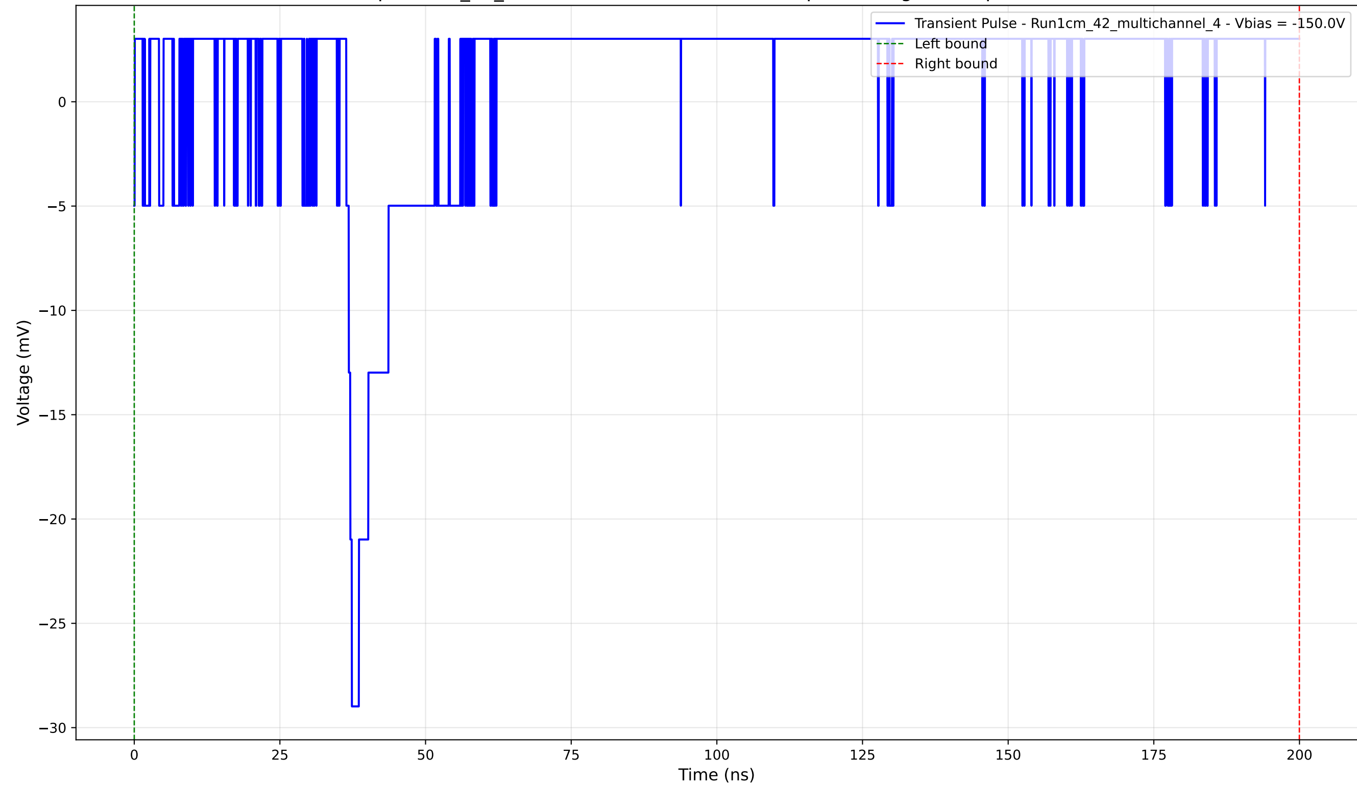
Transient Pulse - Sample: 1cm_42_multichannel - Position: 1605.0 \mu\text{m} - Charge: 5.32 pC - Rise Time: 0.00 ns (N/A)
