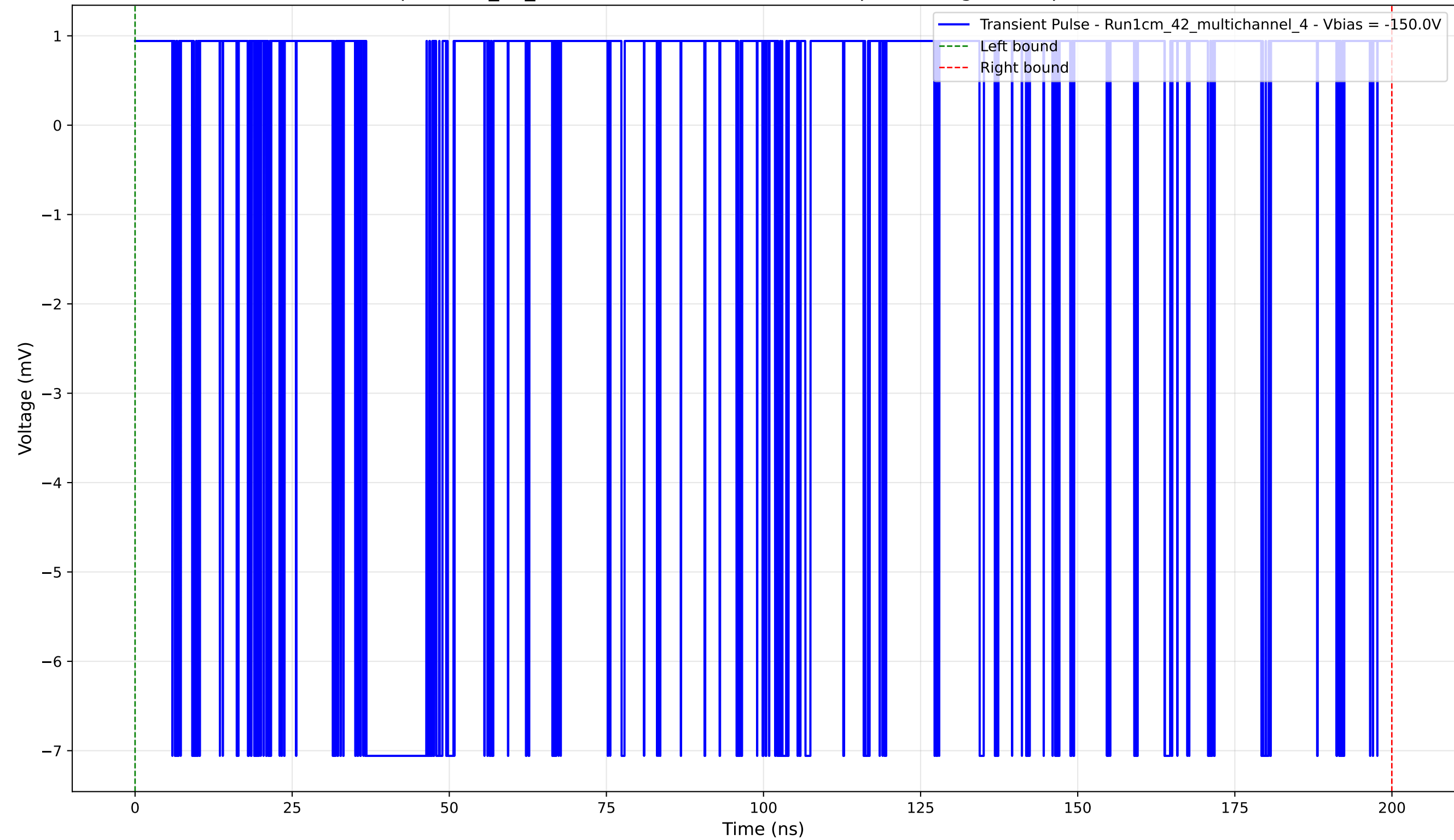
Transient Pulse - Sample: 1cm_42_multichannel - Position: 3435.0 \mu\text{m} - Charge: 1.27 pC - Rise Time: 0.00 ns (N/A)
