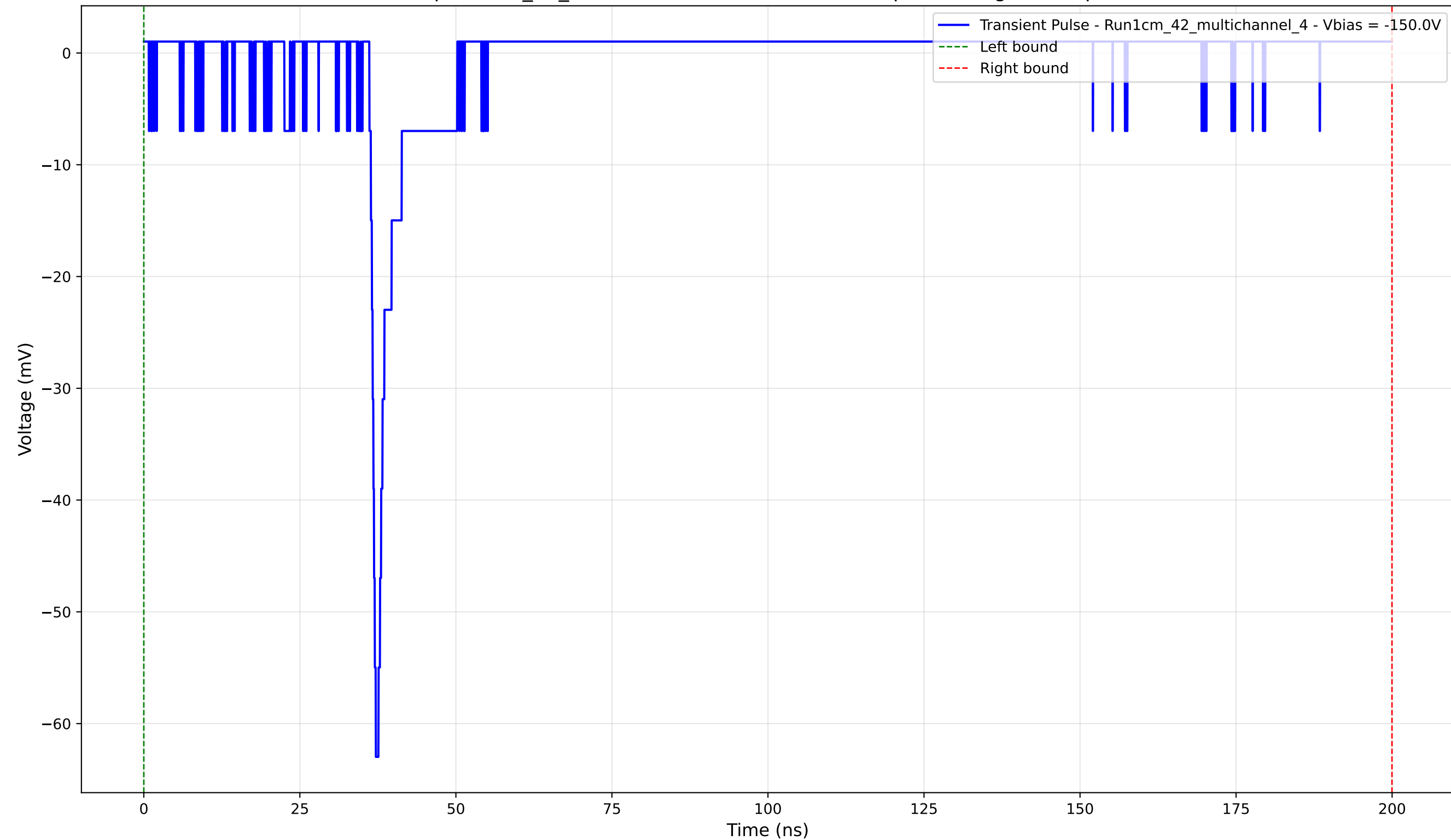
Transient Pulse - Sample: 1cm_42_multichannel - Position: 2120.0 \mu\text{m} - Charge: 1.75 pC - Rise Time: 1.02 ns
