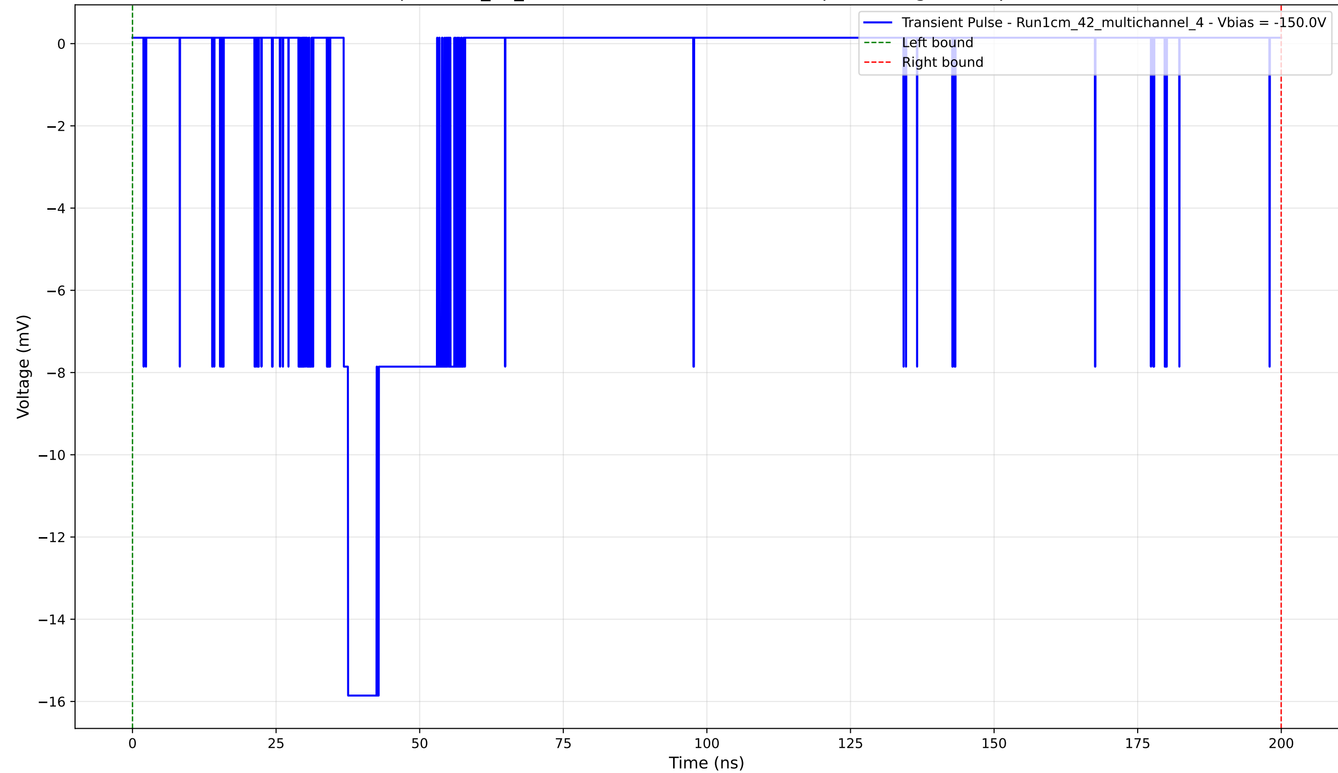
Transient Pulse - Sample: 1cm_42_multichannel - Position: 3625.0 \mu\text{m} - Charge: 4.09 pC - Rise Time: 0.76 ns
