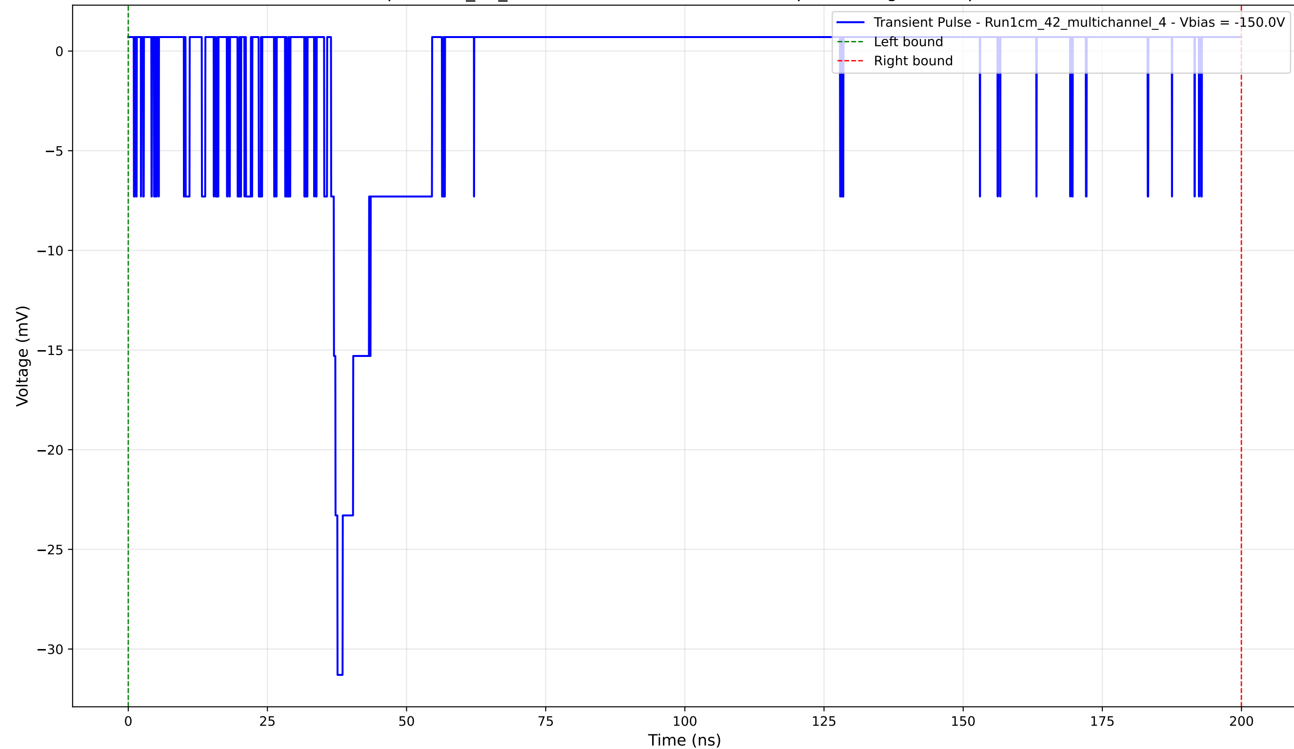
Transient Pulse - Sample: 1cm_42_multichannel - Position: 1495.0 \mu\text{m} - Charge: 3.15 pC - Rise Time: 1.15 ns
