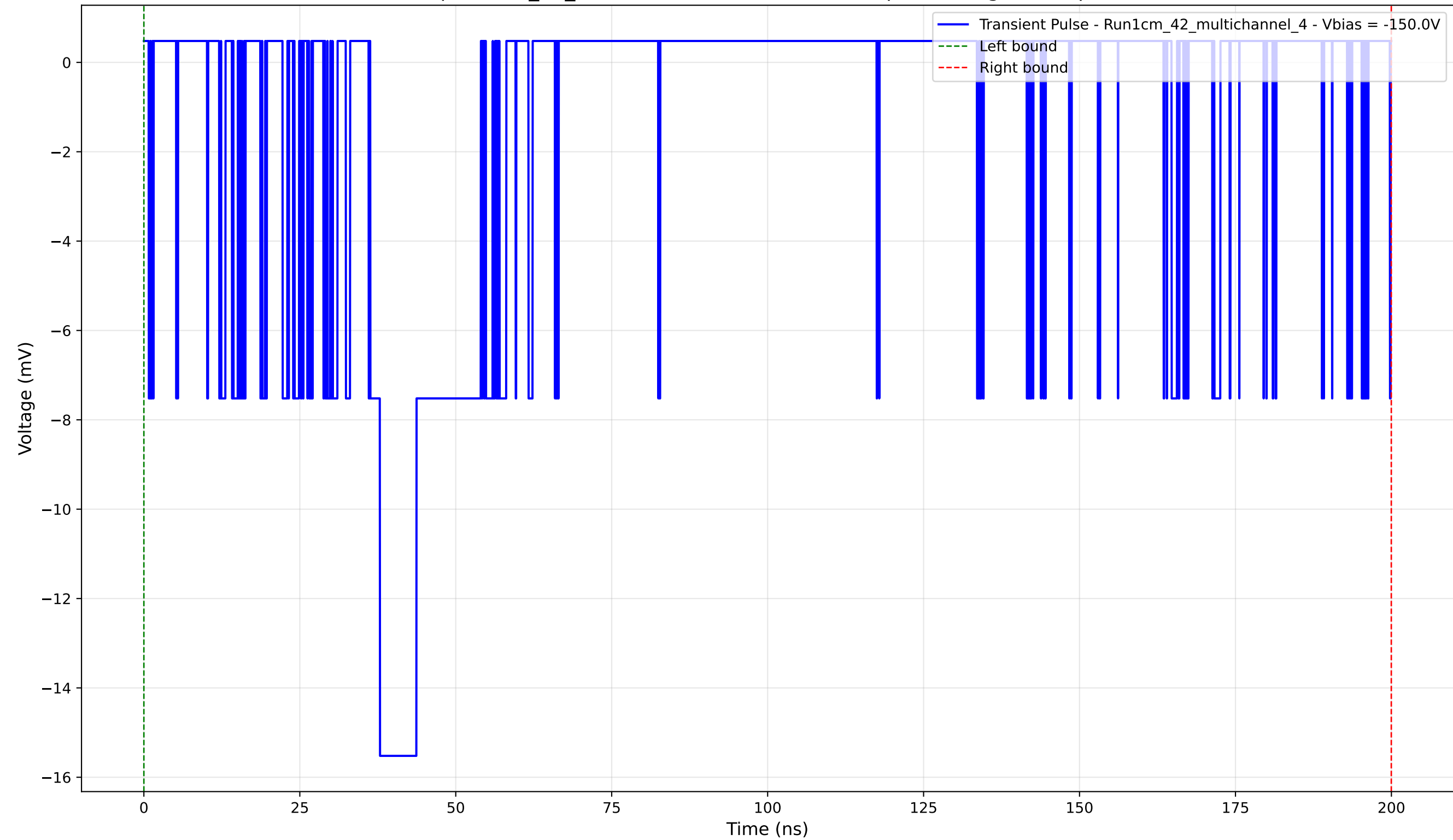
Transient Pulse - Sample: 1cm_42_multichannel - Position: 680.0 \mu\text{m} - Charge: 5.06 pC - Rise Time: 1.56 ns
