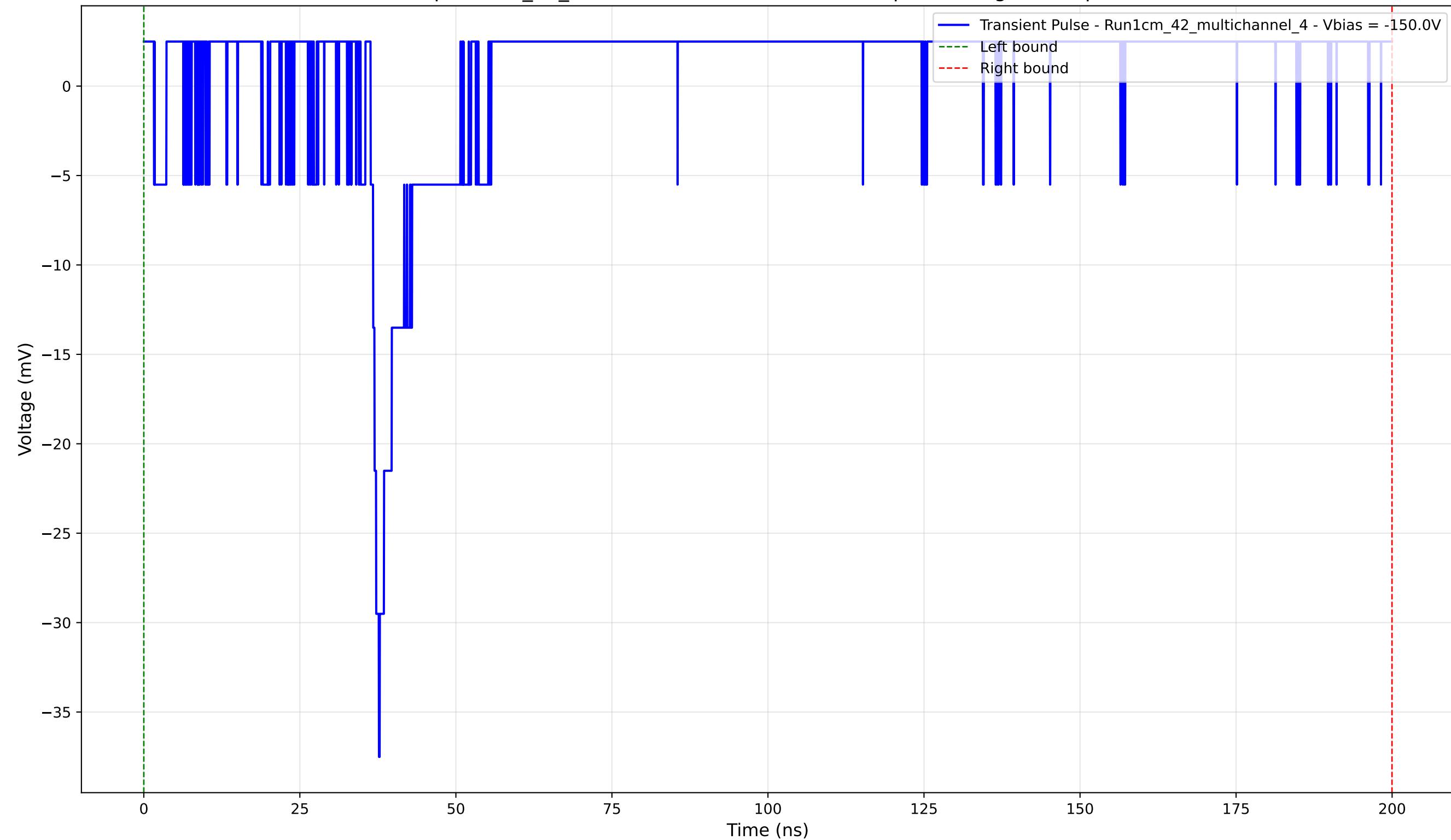
Transient Pulse - Sample: 1cm_42_multichannel - Position: 3065.0 \mu\text{m} - Charge: 3.83 pC - Rise Time: 1.33 ns
