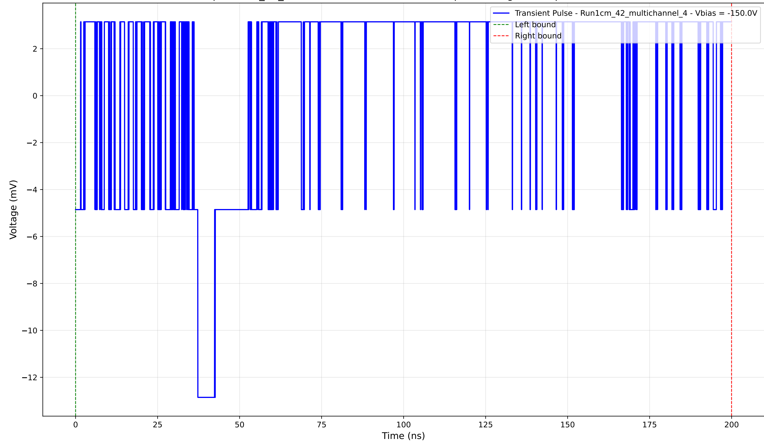
Transient Pulse - Sample: 1cm_42_multichannel - Position: 1315.0 \mu\text{m} - Charge: 4.36 pC - Rise Time: 0.00 ns (N/A)
