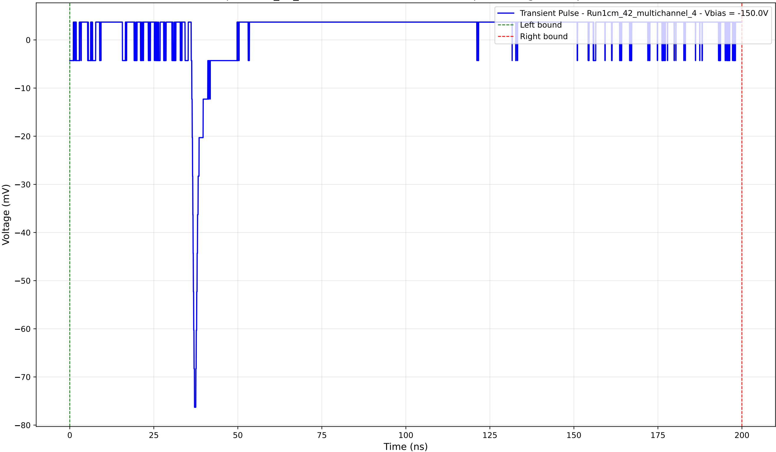
Transient Pulse - Sample: 1cm_42_multichannel - Position: 2255.0 \mu\text{m} - Charge: 7.44 pC - Rise Time: 0.81 ns
