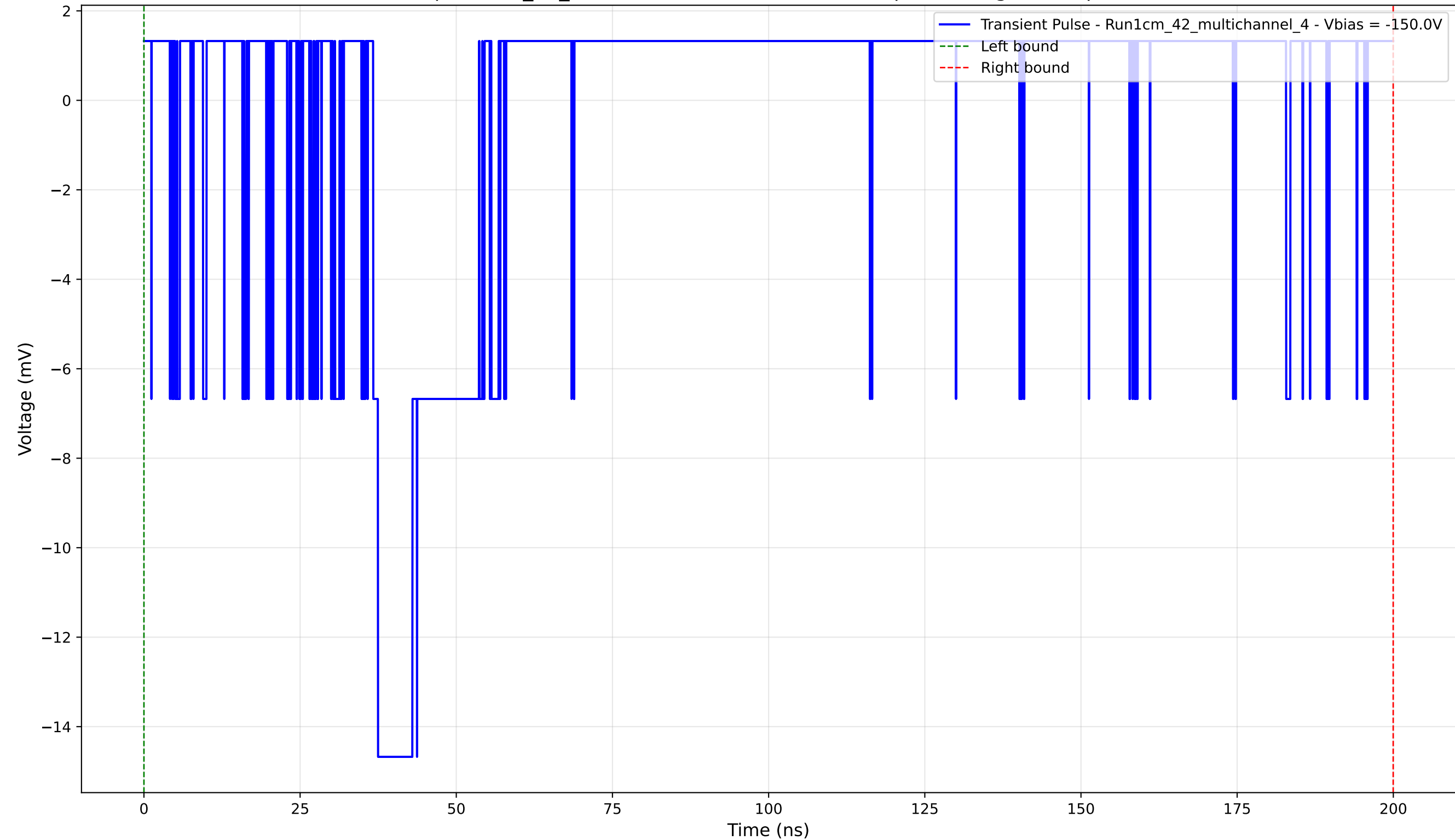
Transient Pulse - Sample: 1cm_42_multichannel - Position: 3665.0 \mu\text{m} - Charge: 0.20 pC - Rise Time: 0.78 ns
