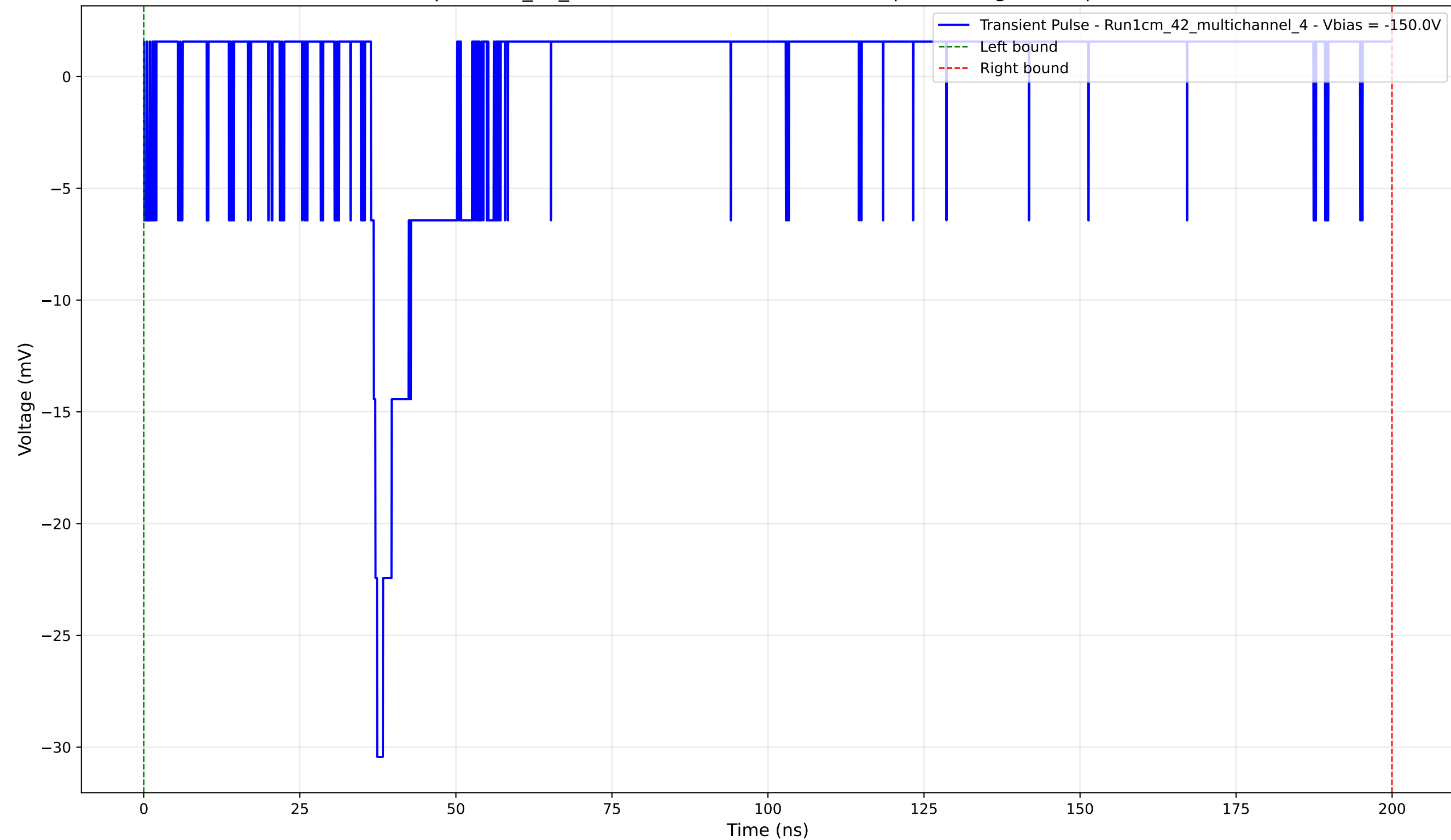
Transient Pulse - Sample: 1cm_42_multichannel - Position: 3130.0 \mu\text{m} - Charge: 0.83 pC - Rise Time: 0.99 ns
