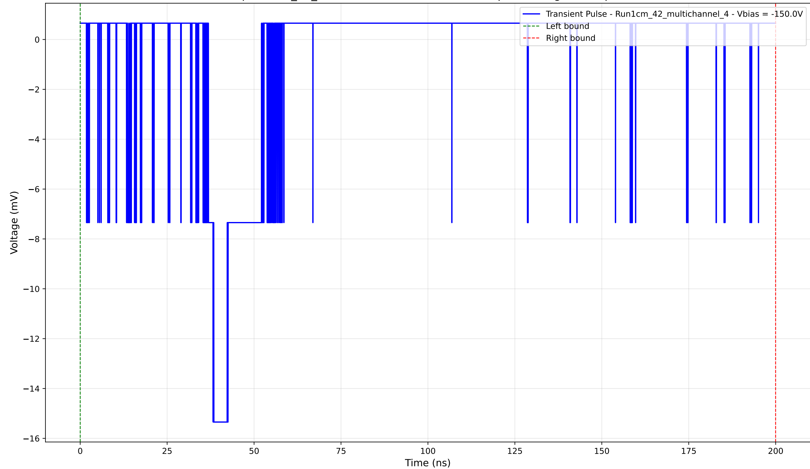
Transient Pulse - Sample: 1cm_42_multichannel - Position: 4160.0 \mu\text{m} - Charge: 1.70 pC - Rise Time: 1.36 ns
