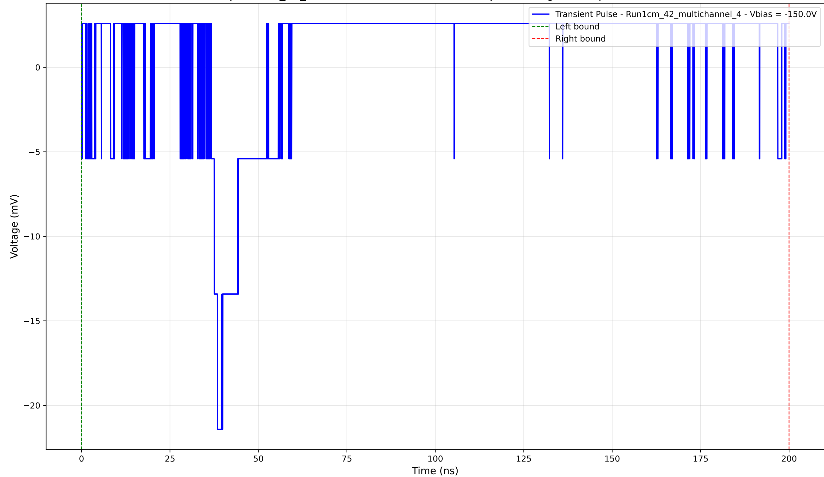
Transient Pulse - Sample: 1cm_42_multichannel - Position: 1060.0 \mu\text{m} - Charge: 3.81 pC - Rise Time: 0.00 ns (N/A)
