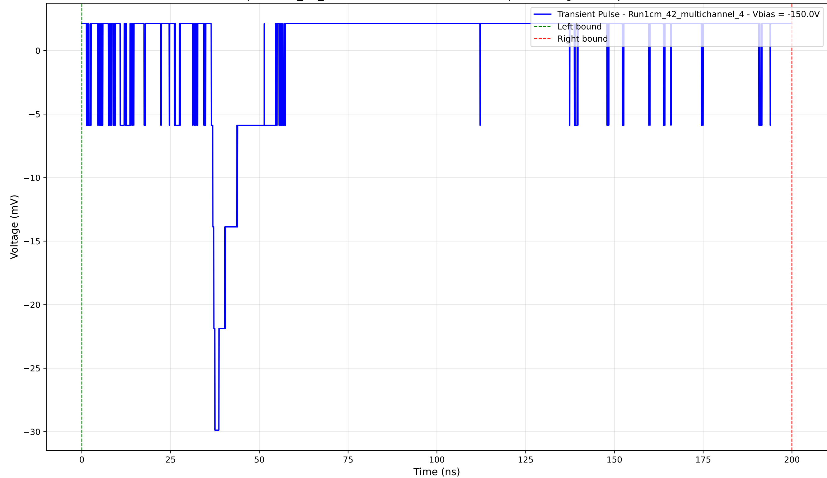
Transient Pulse - Sample: 1cm_42_multichannel - Position: 1510.0 \mu\text{m} - Charge: 1.83 pC - Rise Time: 1.06 ns
