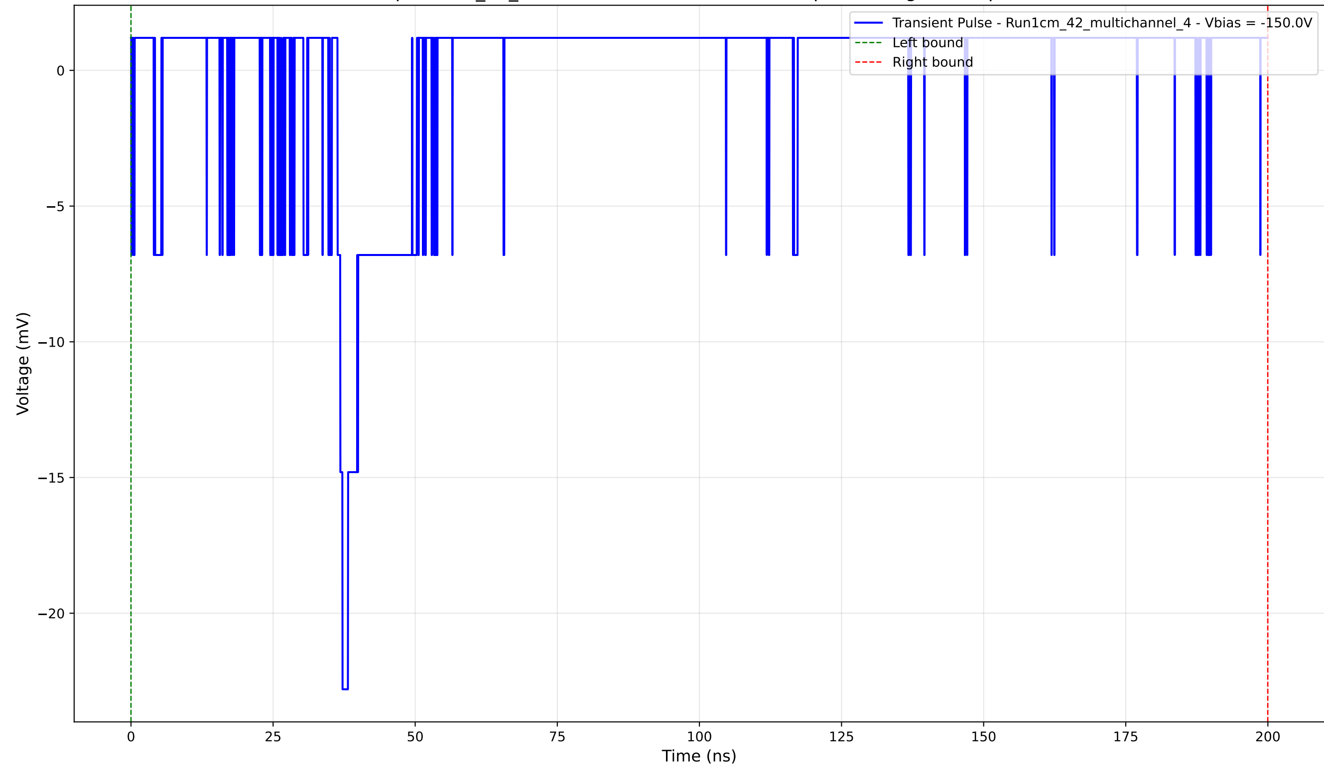
Transient Pulse - Sample: 1cm_42_multichannel - Position: 2945.0 \mu\text{m} - Charge: 0.49 pC - Rise Time: 0.88 ns
