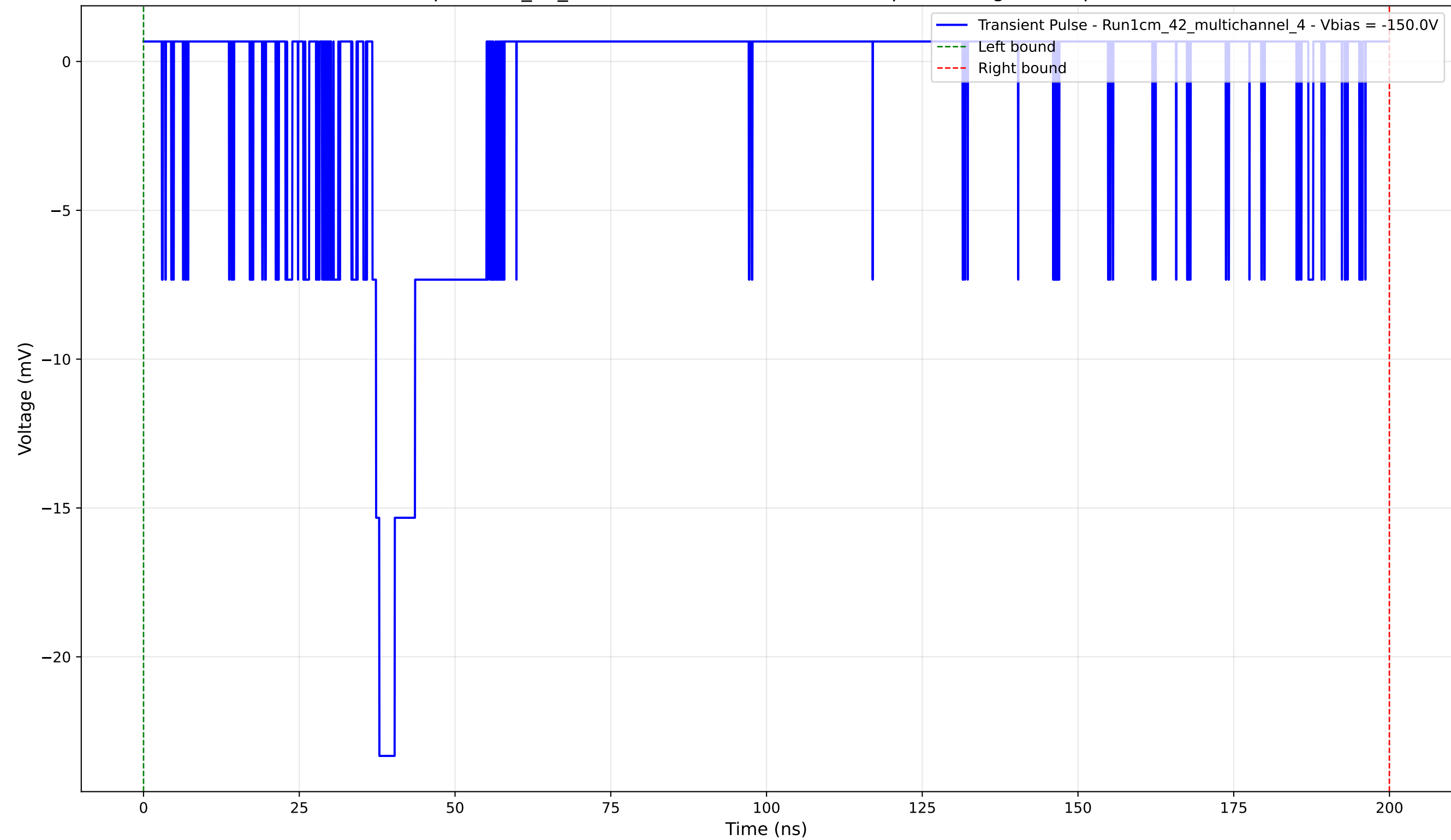
Transient Pulse - Sample: 1cm_42_multichannel - Position: 1170.0 \mu\text{m} - Charge: 3.80 pC - Rise Time: 1.12 ns
