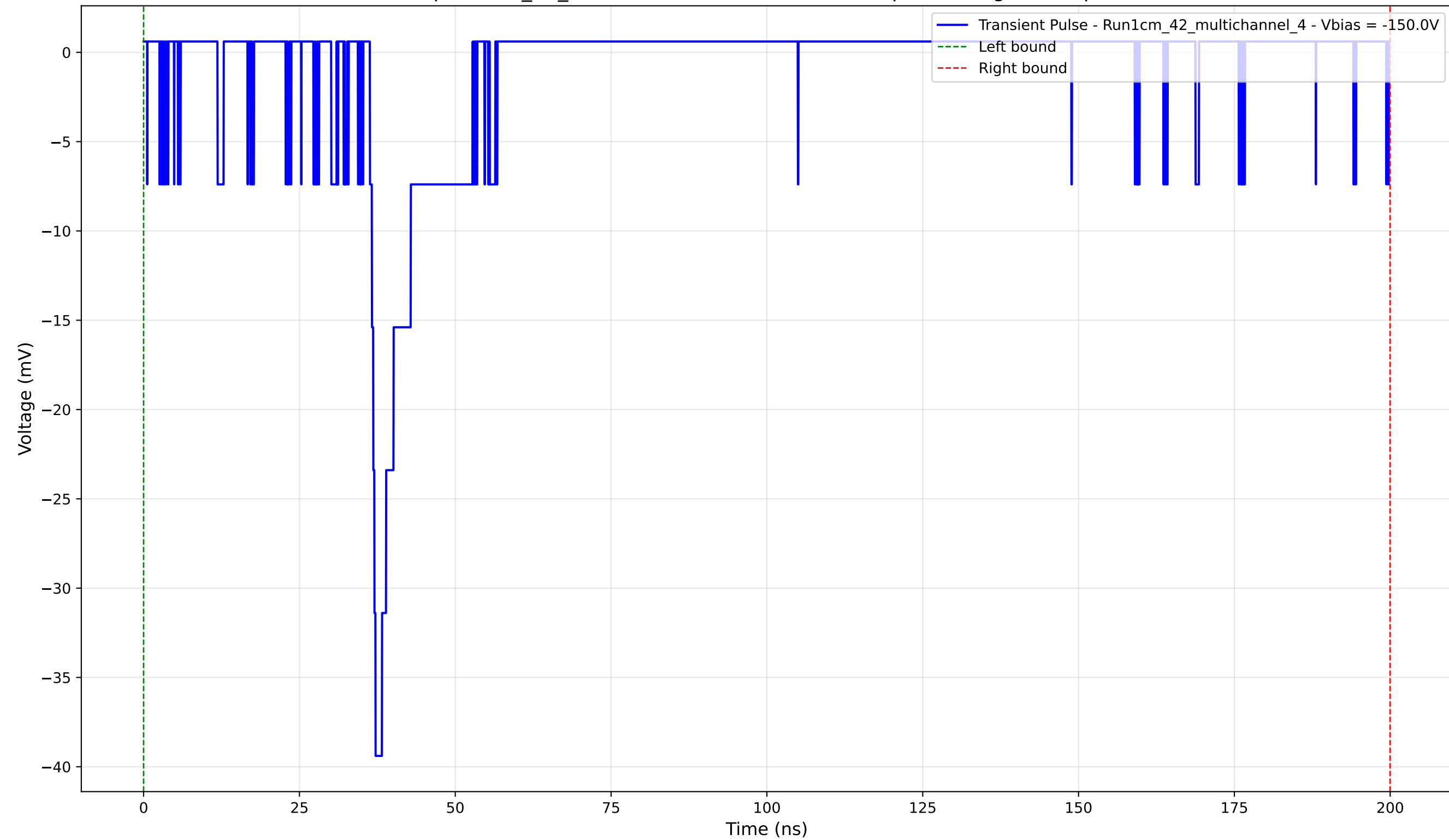
Transient Pulse - Sample: 1cm_42_multichannel - Position: 1770.0 \mu\text{m} - Charge: 3.81 pC - Rise Time: 0.91 ns
