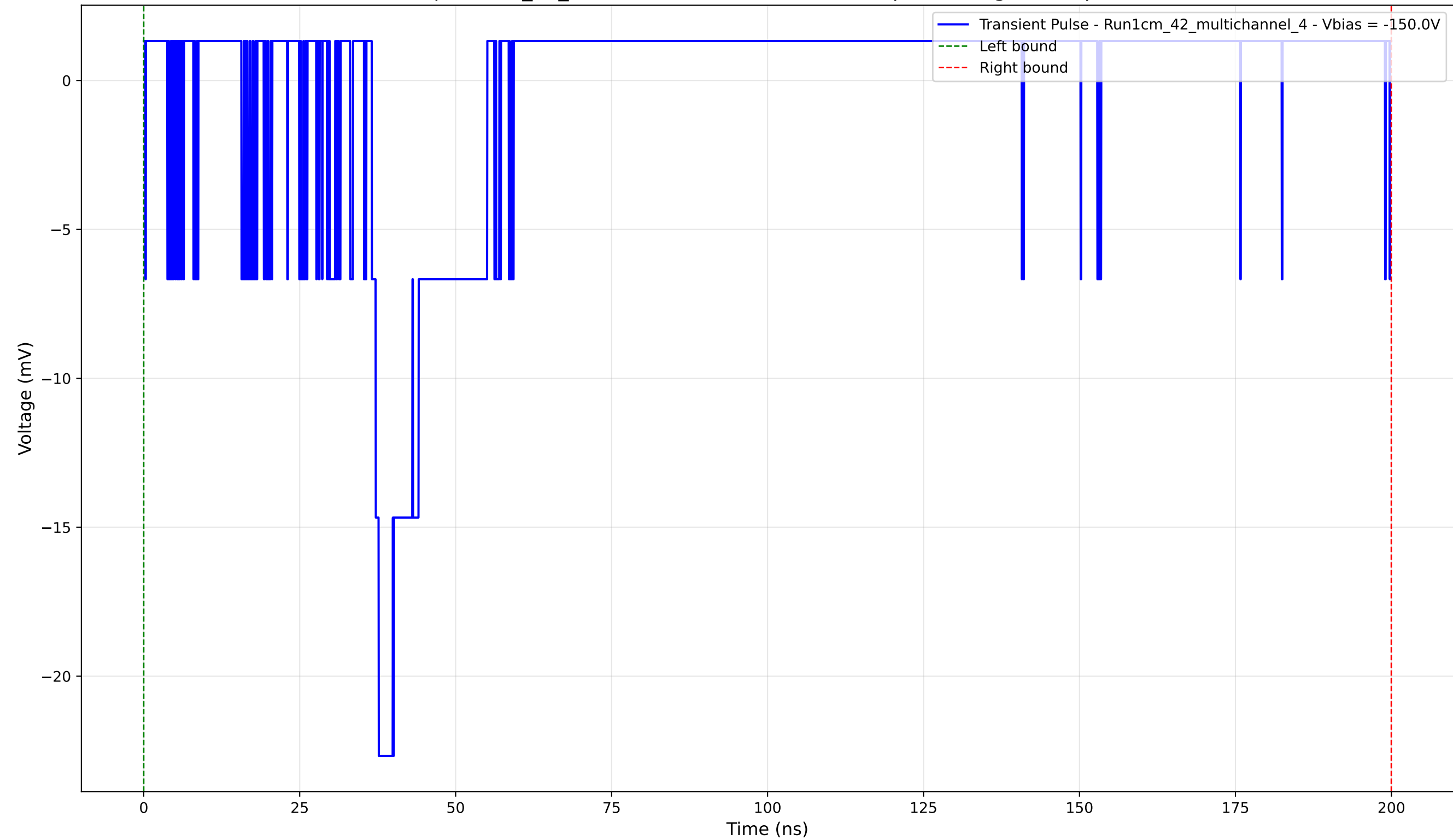
Transient Pulse - Sample: 1cm_42_multichannel - Position: 1295.0 \mu\text{m} - Charge: 0.72 pC - Rise Time: 1.12 ns
