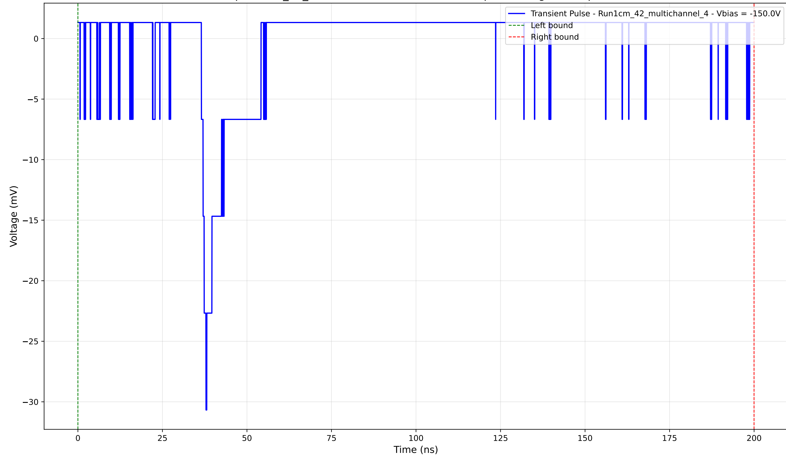
Transient Pulse - Sample: 1cm_42_multichannel - Position: 3305.0 \mu\text{m} - Charge: 0.17 pC - Rise Time: 1.37 ns
