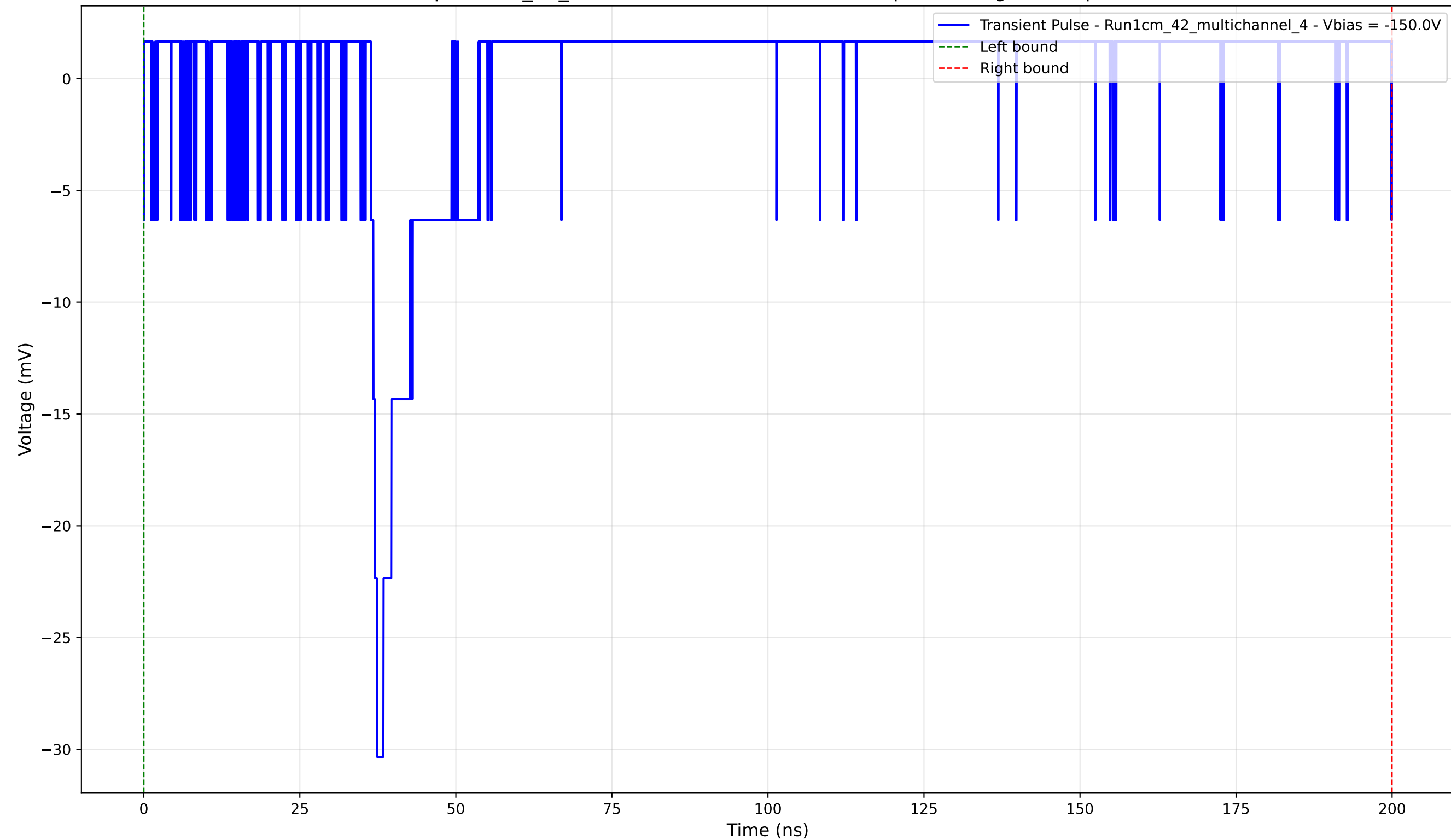
Transient Pulse - Sample: 1cm_42_multichannel - Position: 3140.0 \mu\text{m} - Charge: 1.02 pC - Rise Time: 0.97 ns
