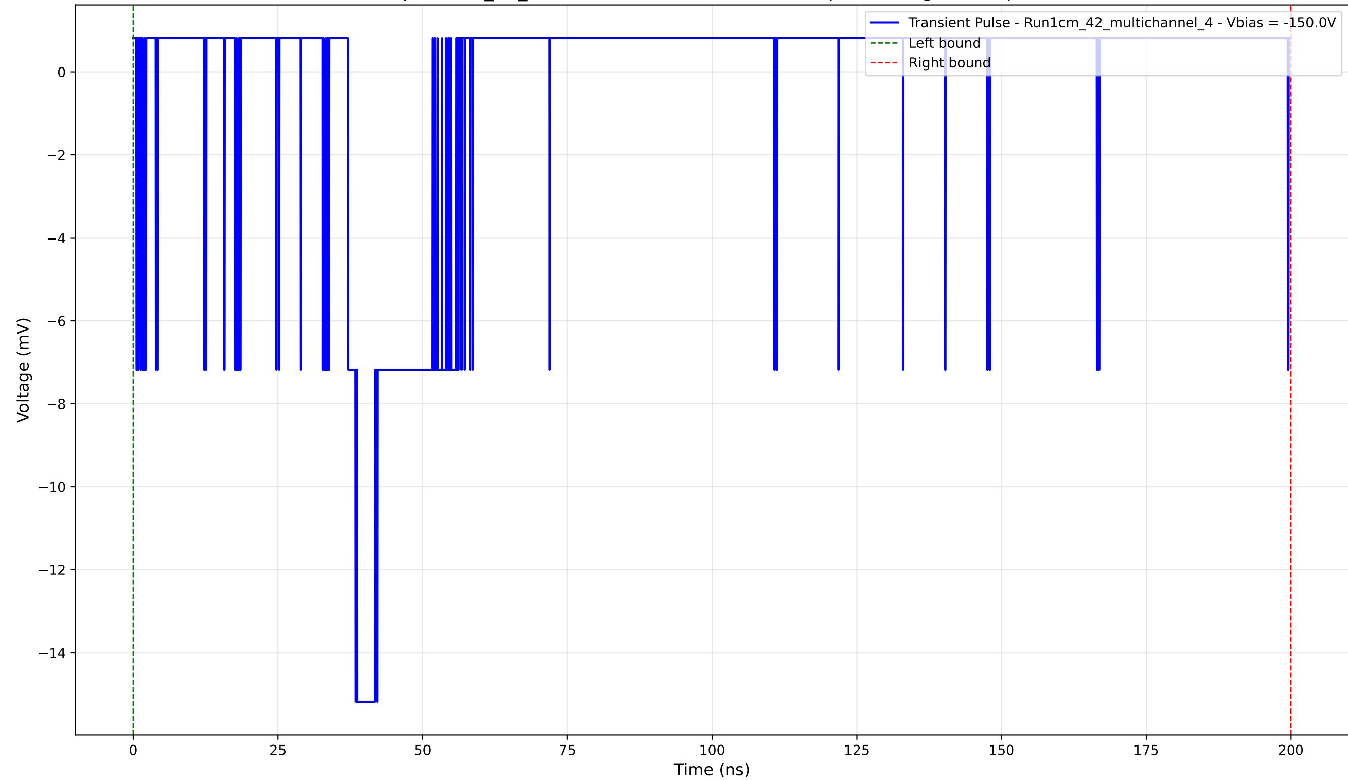
Transient Pulse - Sample: 1cm_42_multichannel - Position: 4660.0 \mu\text{m} - Charge: 0.84 pC - Rise Time: 1.30 ns
