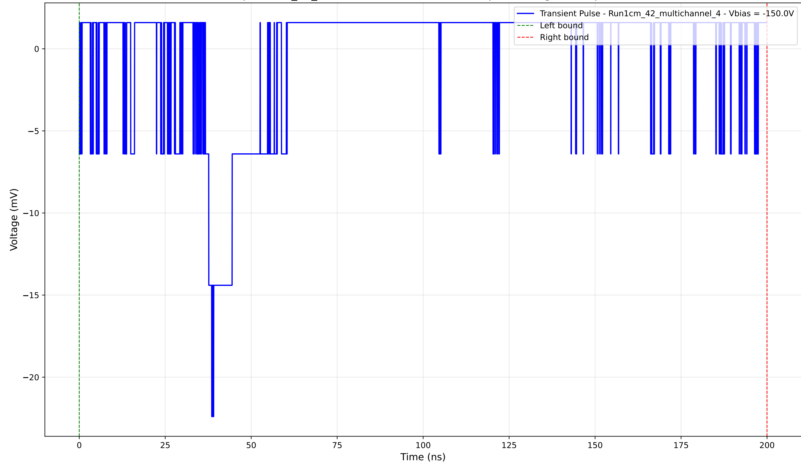
Transient Pulse - Sample: 1cm_42_multichannel - Position: 945.0 \mu\text{m} - Charge: 0.51 pC - Rise Time: 1.84 ns
