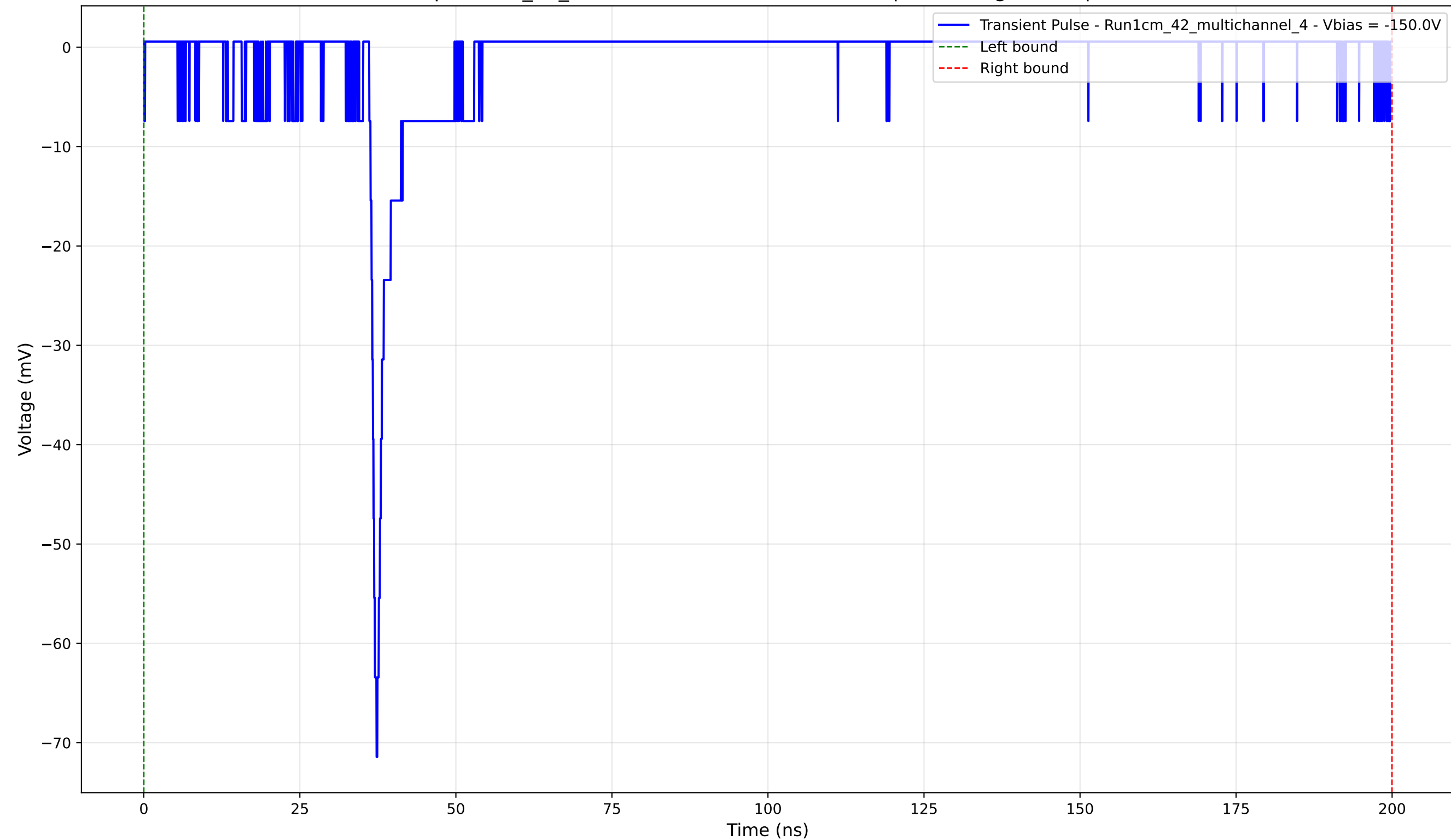
Transient Pulse - Sample: 1cm_42_multichannel - Position: 2585.0 \mu\text{m} - Charge: 4.10 pC - Rise Time: 1.16 ns
