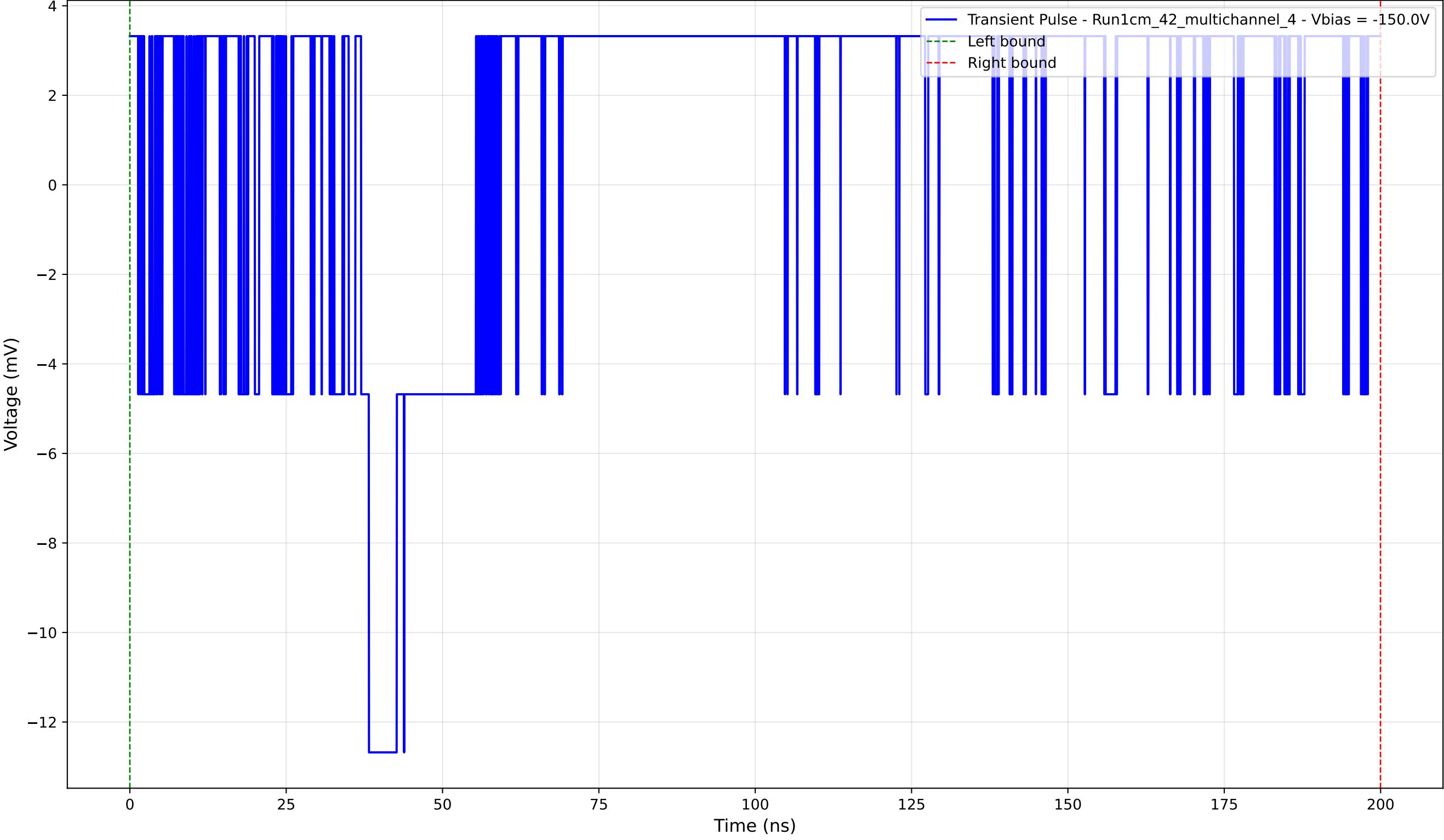
Transient Pulse - Sample: 1cm_42_multichannel - Position: 275.0 \mu\text{m} - Charge: 5.48 pC - Rise Time: 0.00 ns (N/A)
