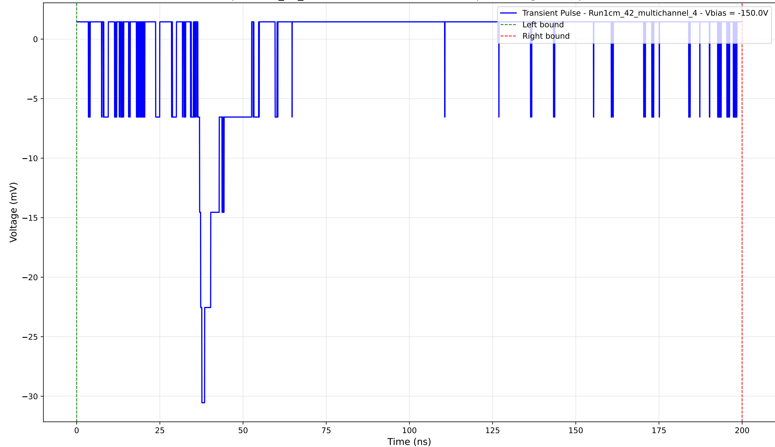
Transient Pulse - Sample: 1cm_42_multichannel - Position: 1470.0 \mu\text{m} - Charge: 0.65 pC - Rise Time: 1.21 ns
