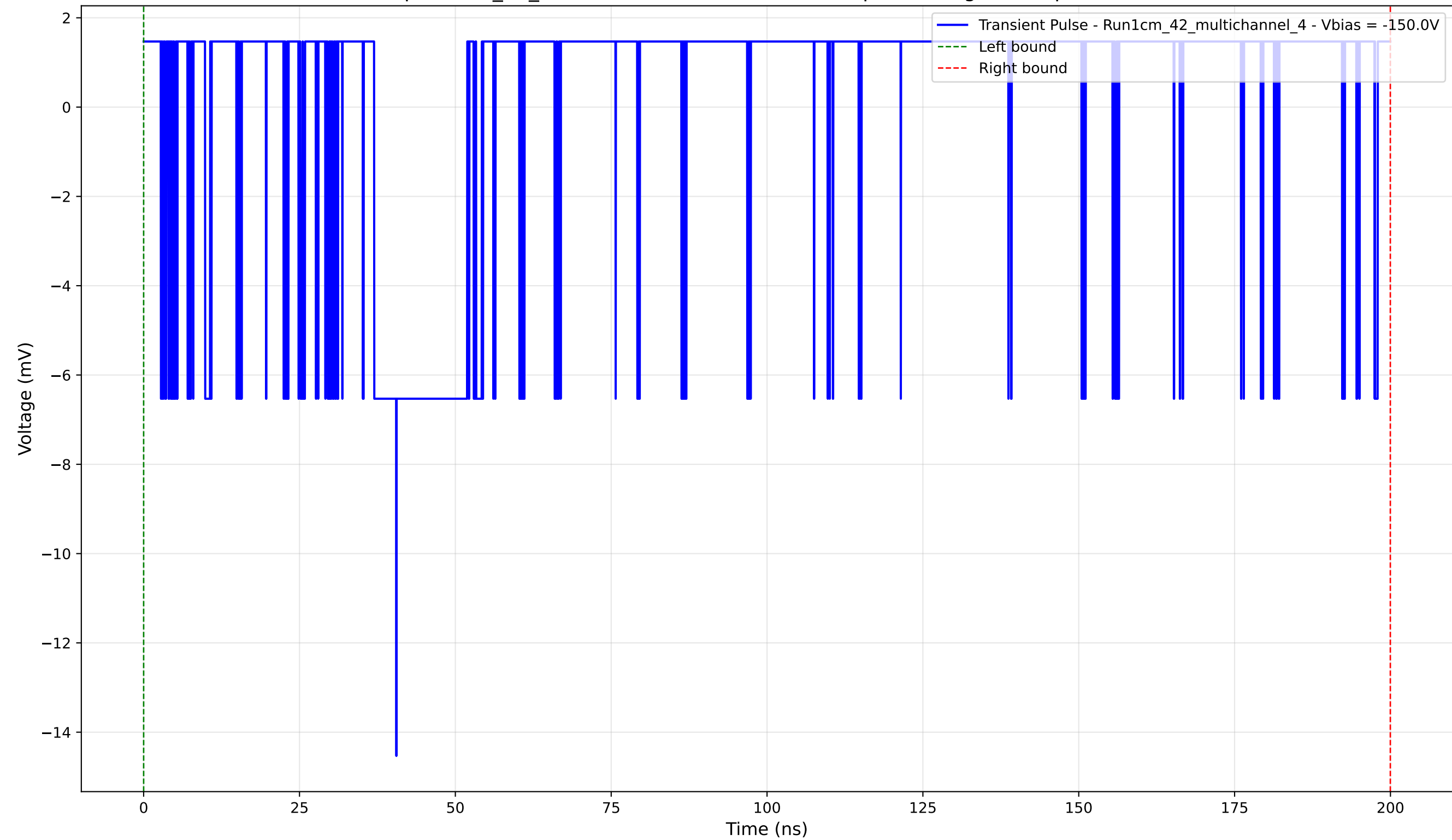
Transient Pulse - Sample: 1cm_42_multichannel - Position: 4840.0 \mu\text{m} - Charge: 1.45 pC - Rise Time: 0.00 ns (N/A)
