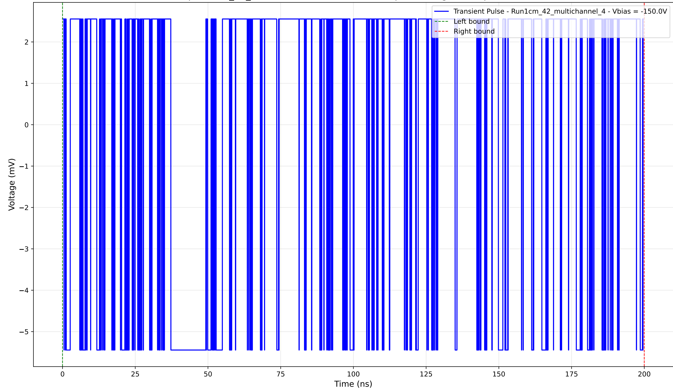
Transient Pulse - Sample: 1cm_42_multichannel - Position: 410.0 \mu\text{m} - Charge: 2.43 pC - Rise Time: 0.00 ns (N/A)
