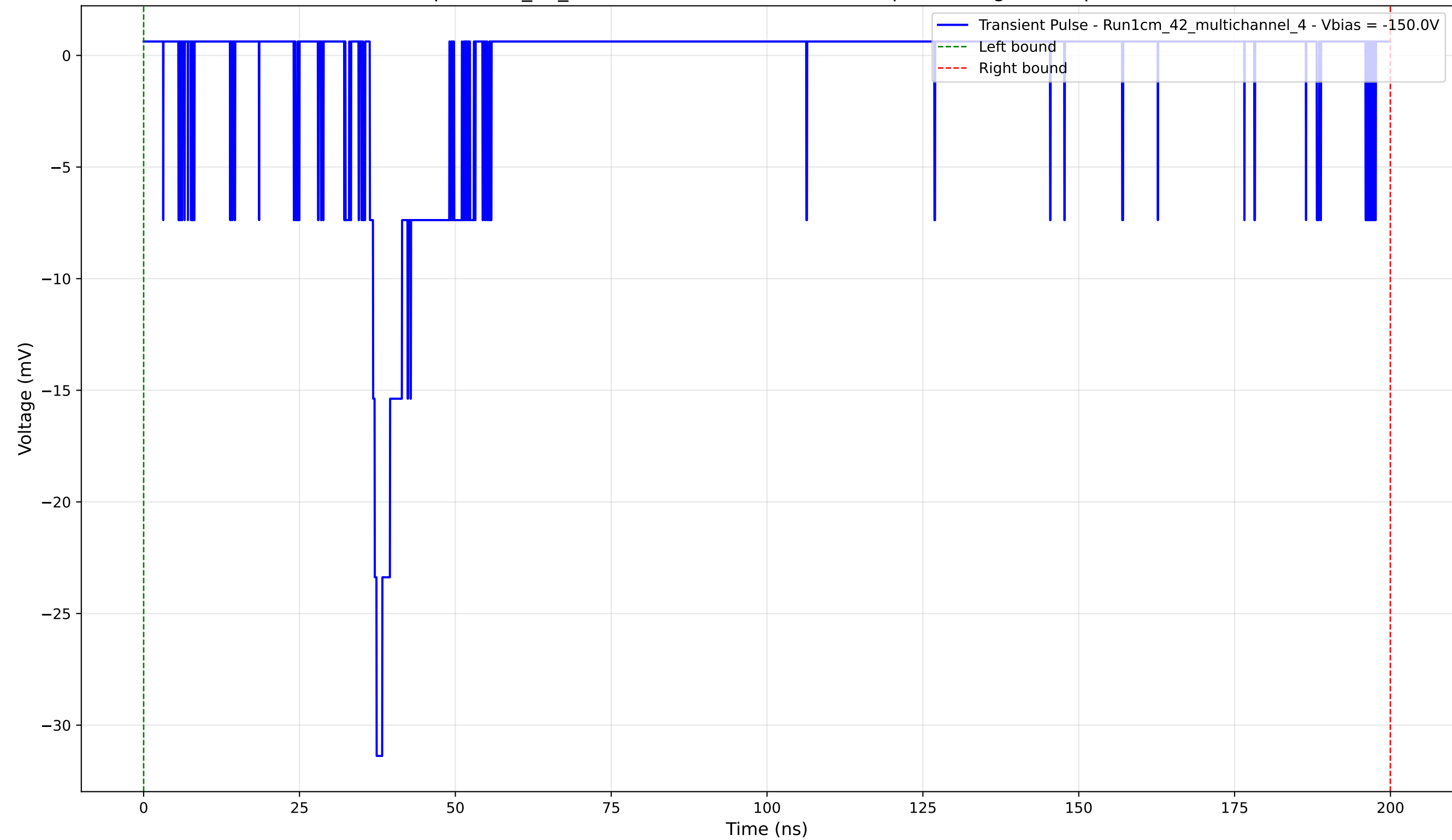
Transient Pulse - Sample: 1cm_42_multichannel - Position: 3095.0 \mu\text{m} - Charge: 2.33 pC - Rise Time: 1.09 ns
