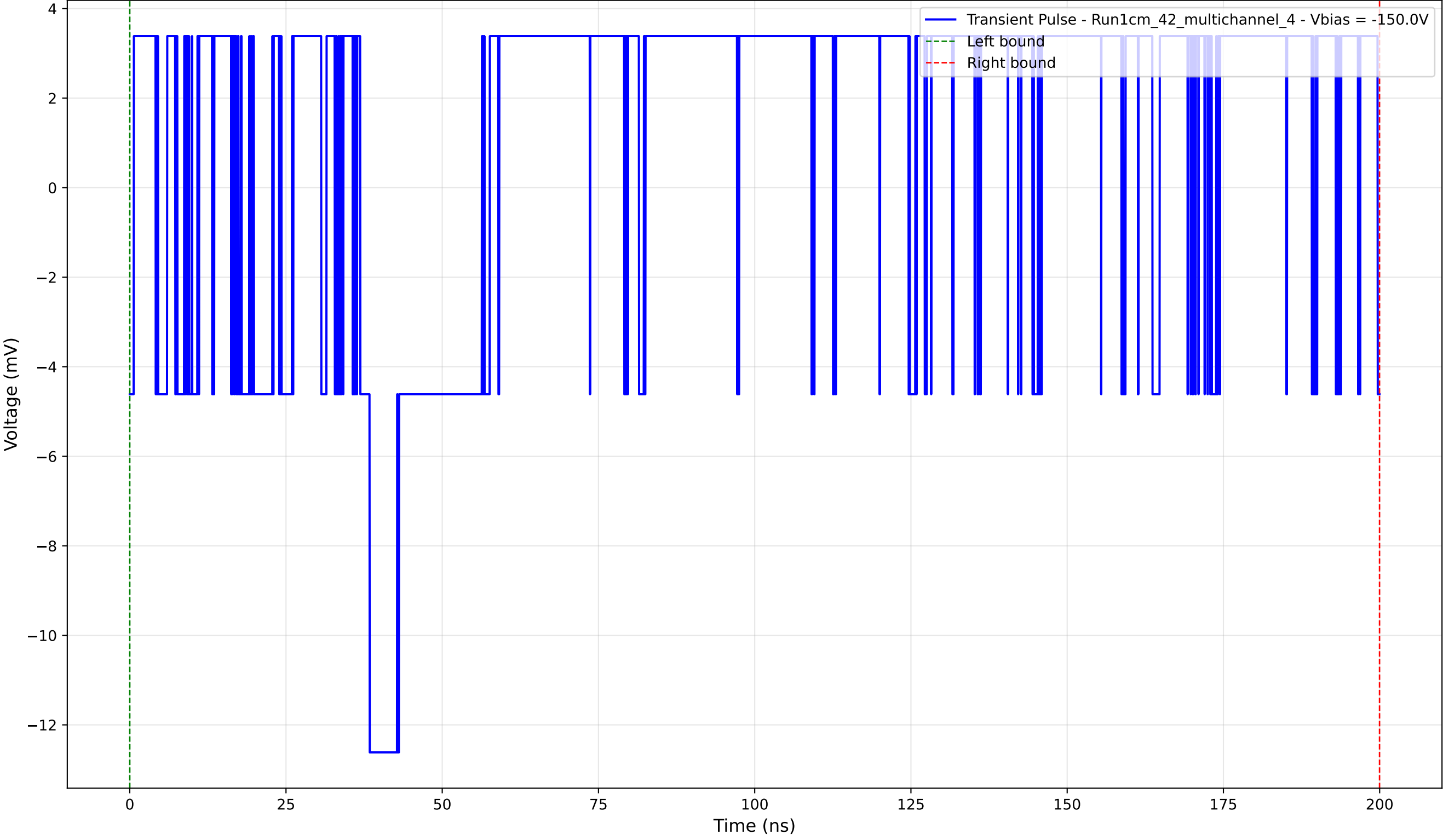
Transient Pulse - Sample: 1cm_42_multichannel - Position: 245.0 \mu\text{m} - Charge: 5.47 pC - Rise Time: 0.00 ns (N/A)
