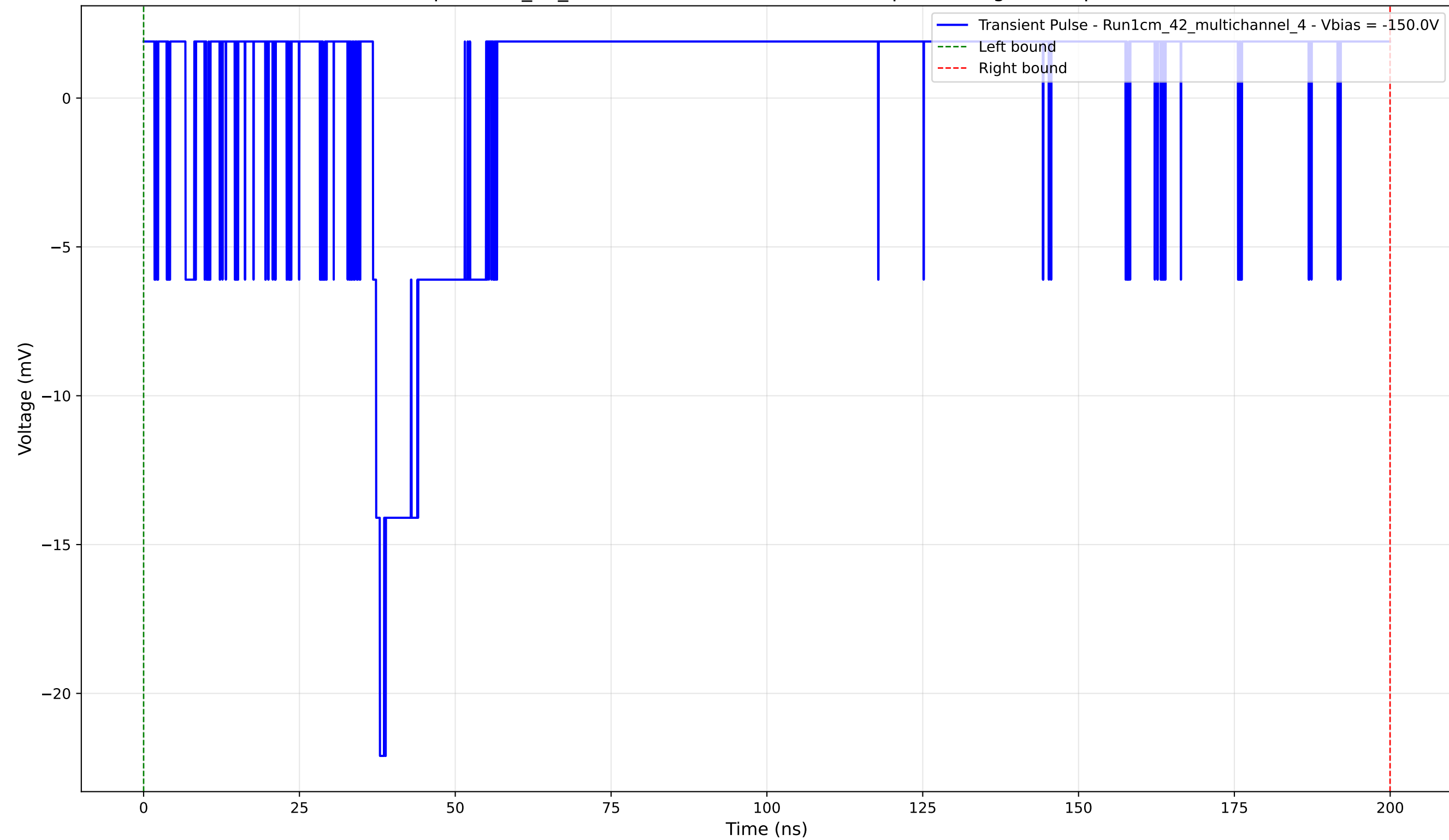
Transient Pulse - Sample: 1cm_42_multichannel - Position: 3575.0 \mu\text{m} - Charge: 2.20 pC - Rise Time: 1.12 ns
