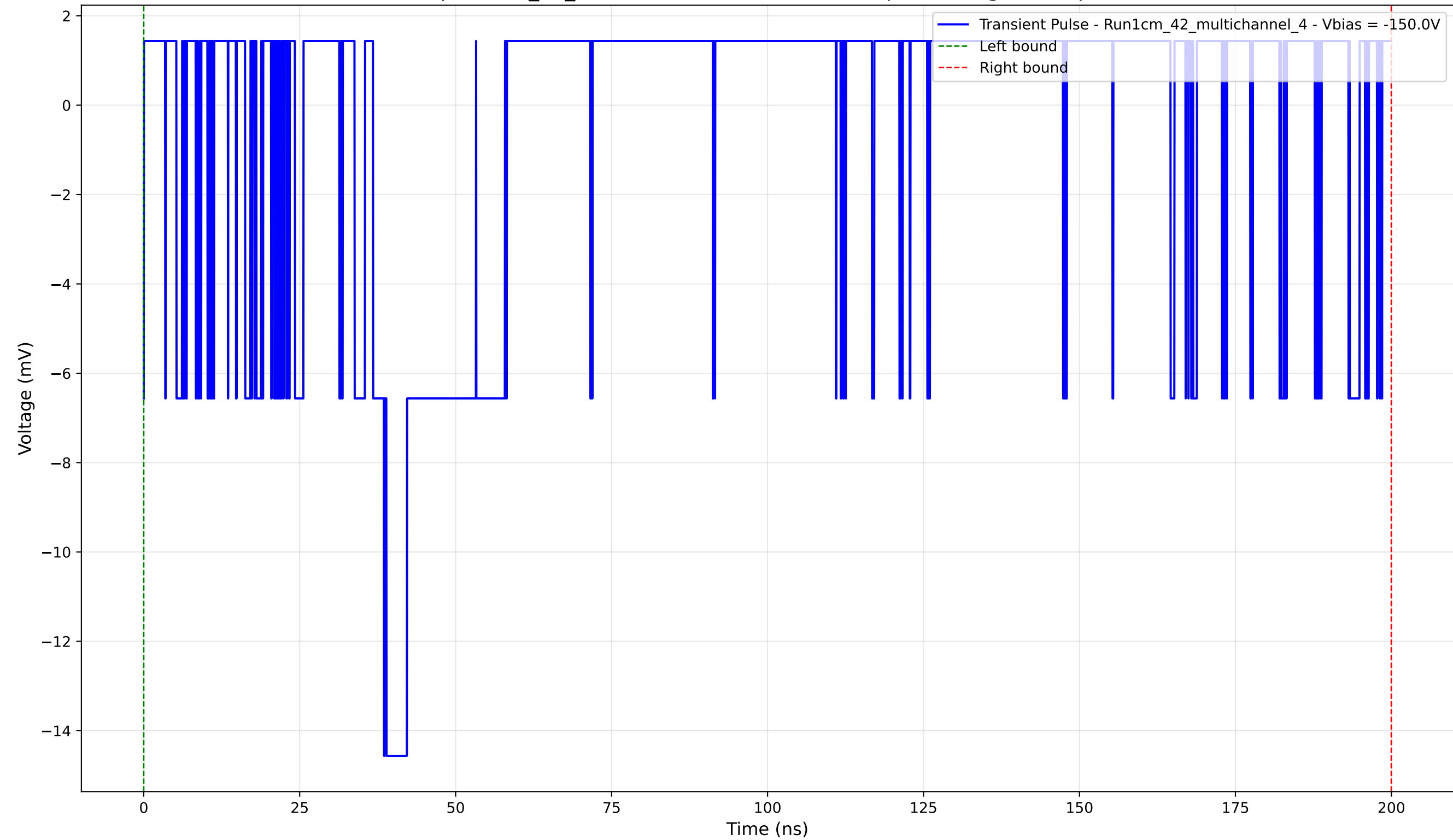
Transient Pulse - Sample: 1cm_42_multichannel - Position: 430.0 \mu\text{m} - Charge: 0.99 pC - Rise Time: 1.76 ns
