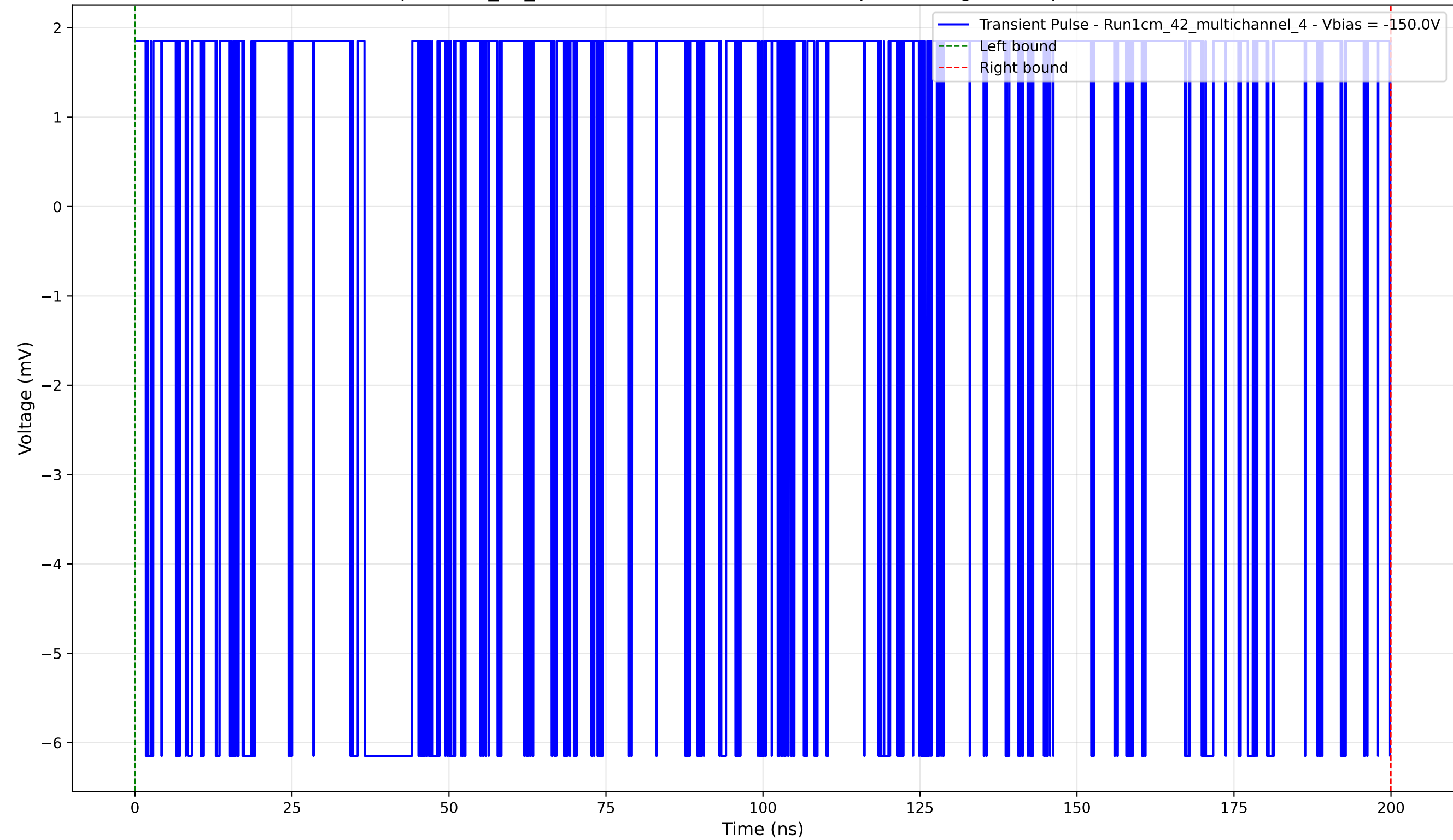
Transient Pulse - Sample: 1cm_42_multichannel - Position: 1850.0 \mu\text{m} - Charge: 0.54 pC - Rise Time: 0.00 ns (N/A)
