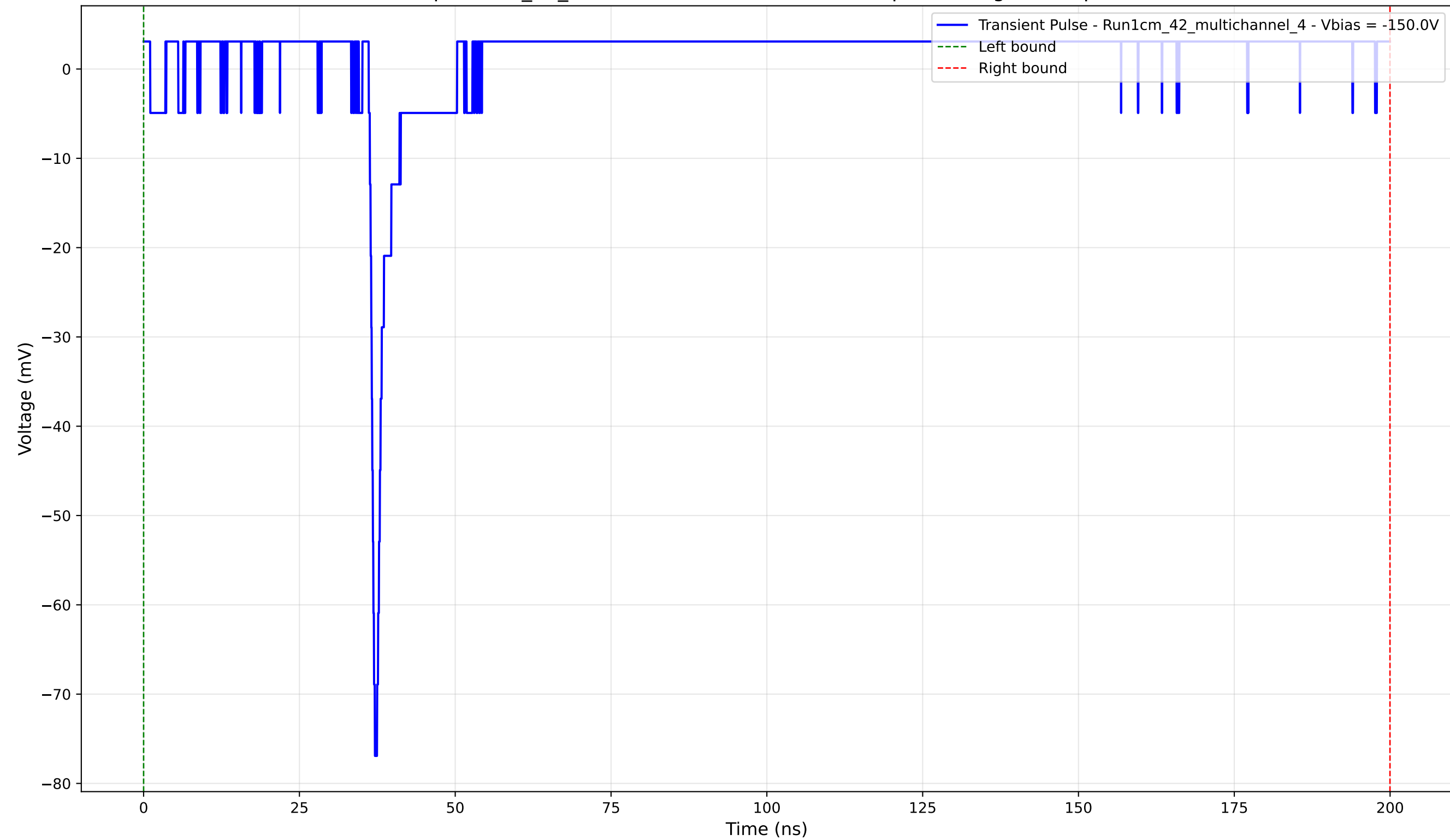
Transient Pulse - Sample: 1cm_42_multichannel - Position: 2235.0 \mu\text{m} - Charge: 5.94 pC - Rise Time: 0.81 ns
