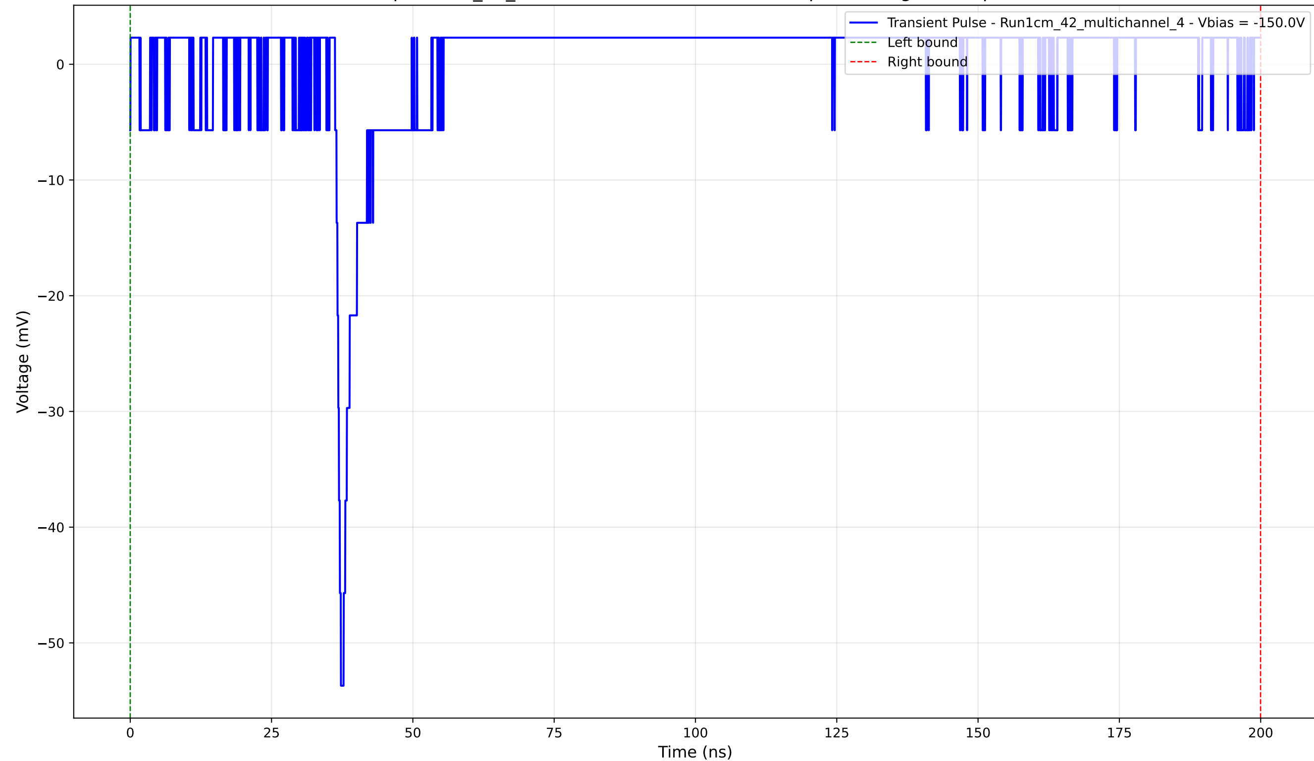
Transient Pulse - Sample: 1cm_42_multichannel - Position: 1975.0 \mu\text{m} - Charge: 1.31 pC - Rise Time: 1.02 ns
