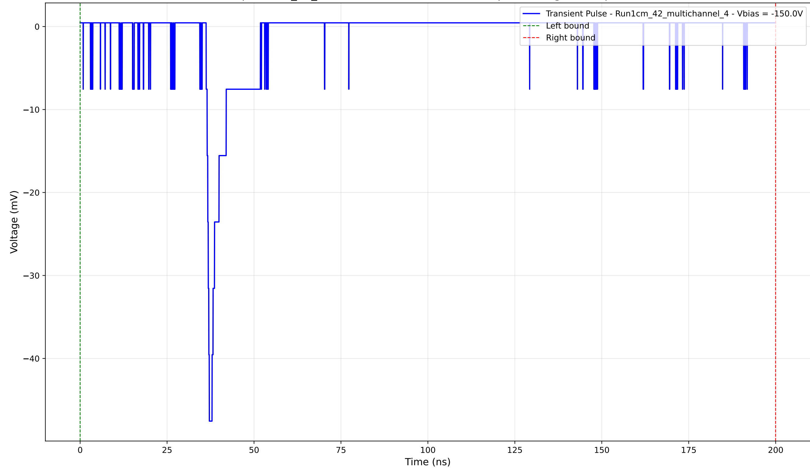
Transient Pulse - Sample: 1cm_42_multichannel - Position: 2810.0 \mu\text{m} - Charge: 3.70 pC - Rise Time: 0.91 ns
