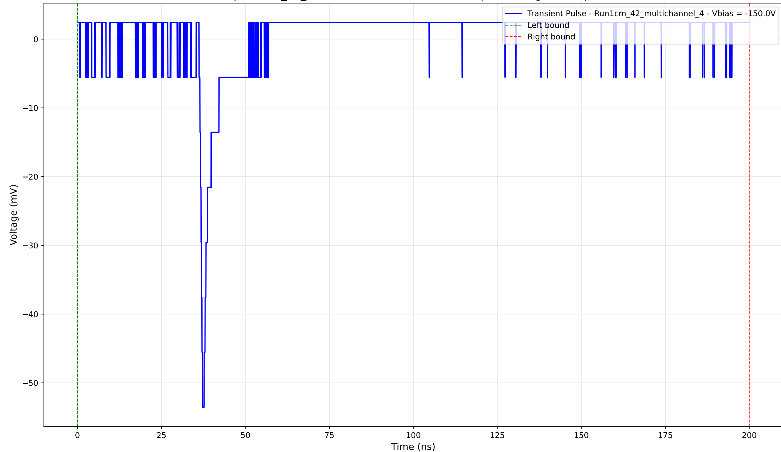
Transient Pulse - Sample: 1cm_42_multichannel - Position: 2775.0 \mu\text{m} - Charge: 2.89 pC - Rise Time: 1.06 ns
