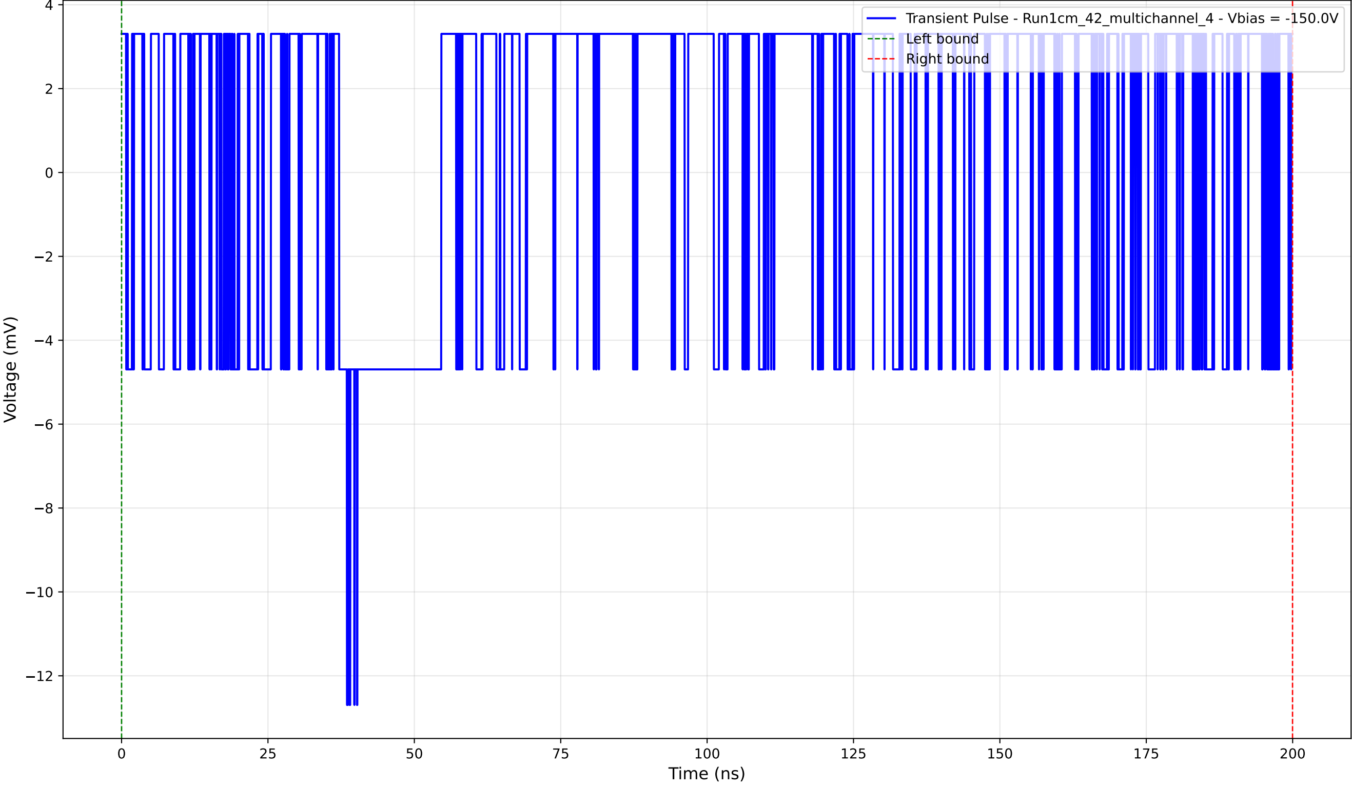
Transient Pulse - Sample: 1cm_42_multichannel - Position: 815.0 \mu\text{m} - Charge: 4.07 pC - Rise Time: 0.00 ns (N/A)
