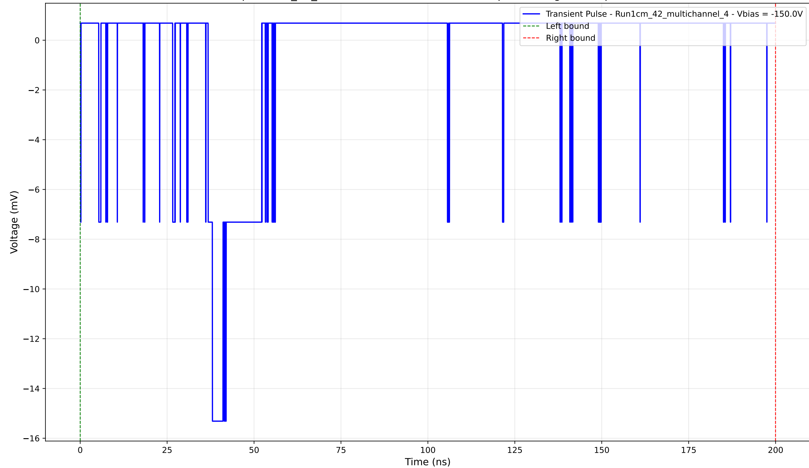
Transient Pulse - Sample: 1cm_42_multichannel - Position: 3840.0 \mu\text{m} - Charge: 1.00 pC - Rise Time: 1.24 ns
