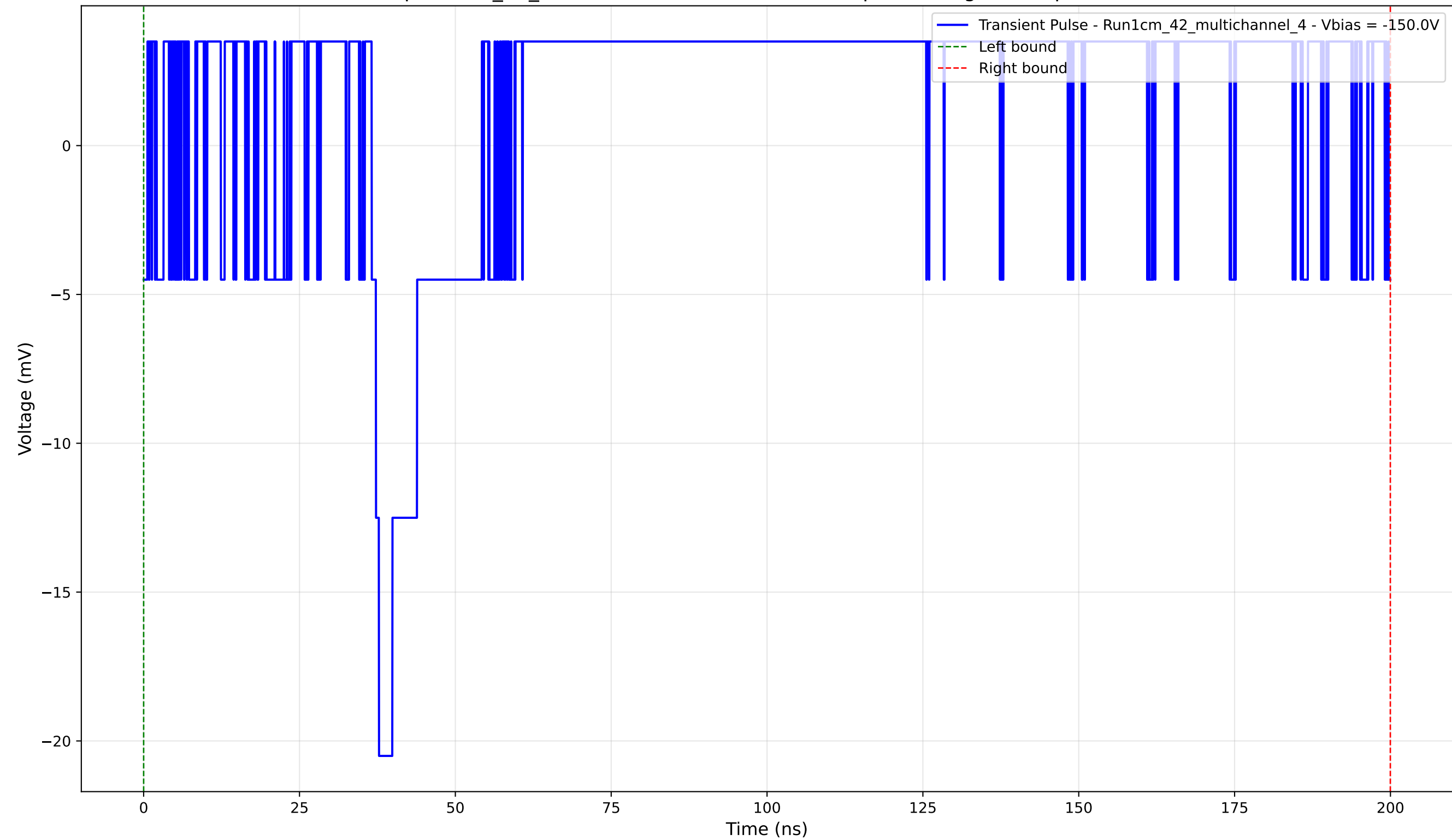
Transient Pulse - Sample: 1cm_42_multichannel - Position: 1195.0 \mu\text{m} - Charge: 5.96 pC - Rise Time: 0.00 ns (N/A)
