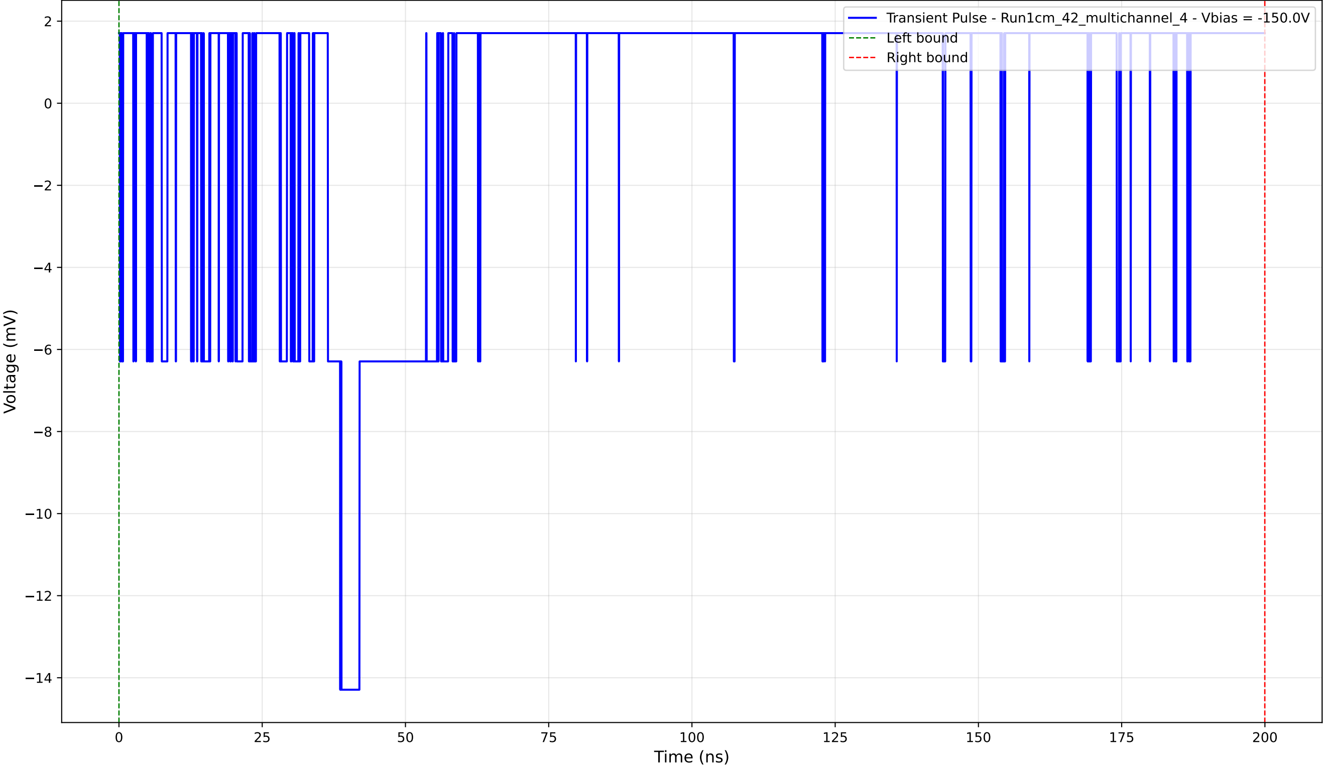
Transient Pulse - Sample: 1cm_42_multichannel - Position: 140.0 \mu\text{m} - Charge: 0.91 pC - Rise Time: 0.00 ns (N/A)
