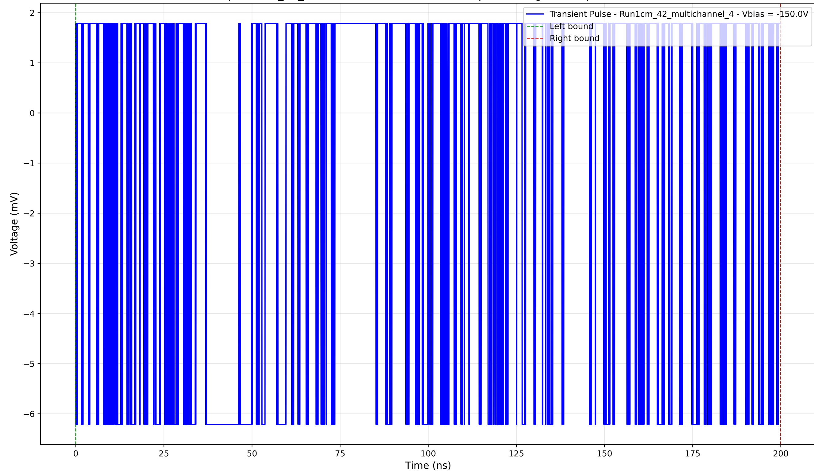
Transient Pulse - Sample: 1cm_42_multichannel - Position: 910.0 \mu\text{m} - Charge: 1.69 pC - Rise Time: 0.00 ns (N/A)
