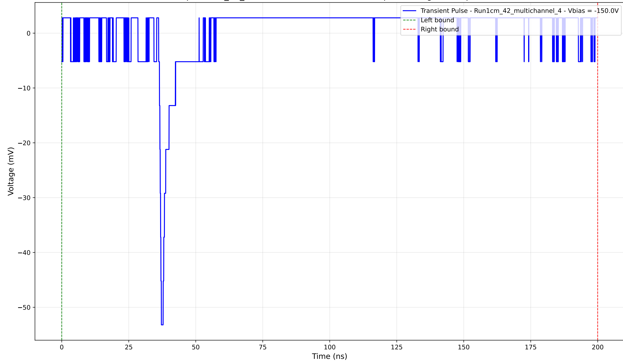
Transient Pulse - Sample: 1cm_42_multichannel - Position: 1995.0 \mu\text{m} - Charge: 2.74 pC - Rise Time: 0.72 ns
