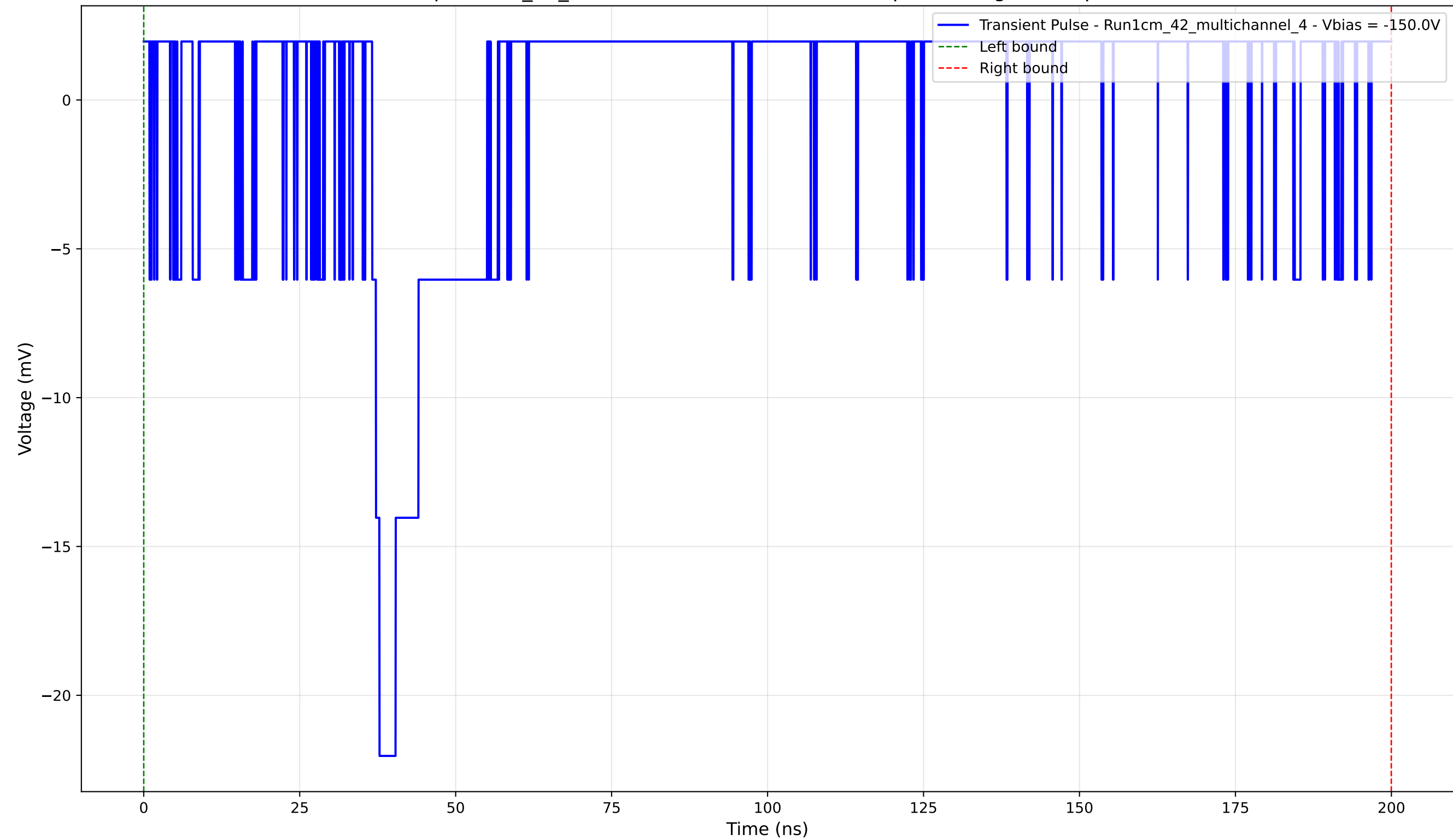
Transient Pulse - Sample: 1cm_42_multichannel - Position: 1190.0 \mu\text{m} - Charge: 0.98 pC - Rise Time: 1.18 ns
