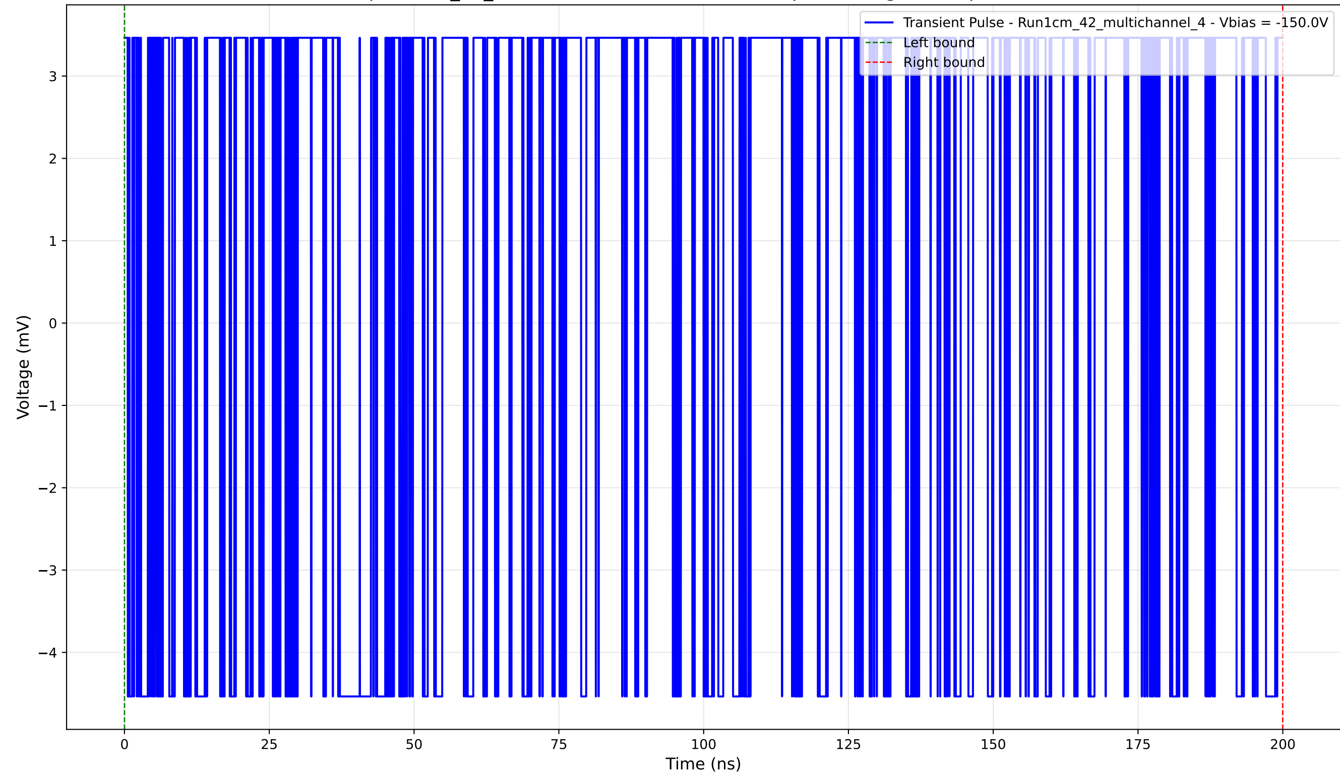
Transient Pulse - Sample: 1cm_42_multichannel - Position: 1345.0 \mu\text{m} - Charge: 5.28 pC - Rise Time: 0.00 ns (N/A)
