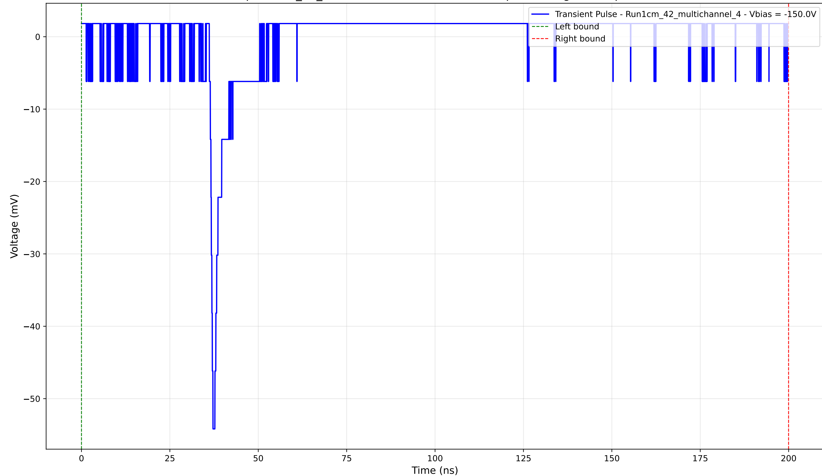
Transient Pulse - Sample: 1cm_42_multichannel - Position: 2750.0 \mu\text{m} - Charge: 0.59 pC - Rise Time: 1.02 ns
