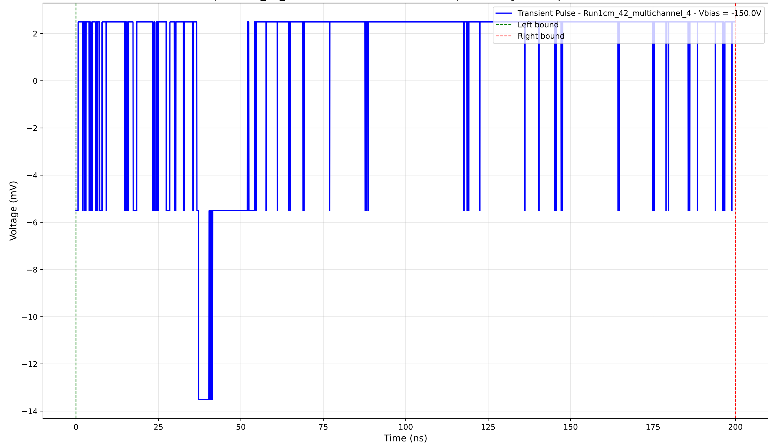
Transient Pulse - Sample: 1cm_42_multichannel - Position: 3340.0 \mu\text{m} - Charge: 4.91 pC - Rise Time: 0.00 ns (N/A)
