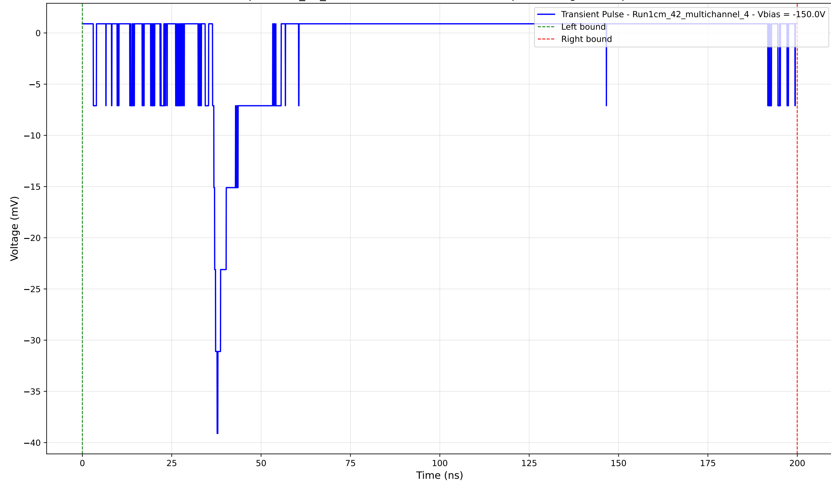
Transient Pulse - Sample: 1cm_42_multichannel - Position: 1640.0 \mu\text{m} - Charge: 2.57 pC - Rise Time: 1.29 ns
