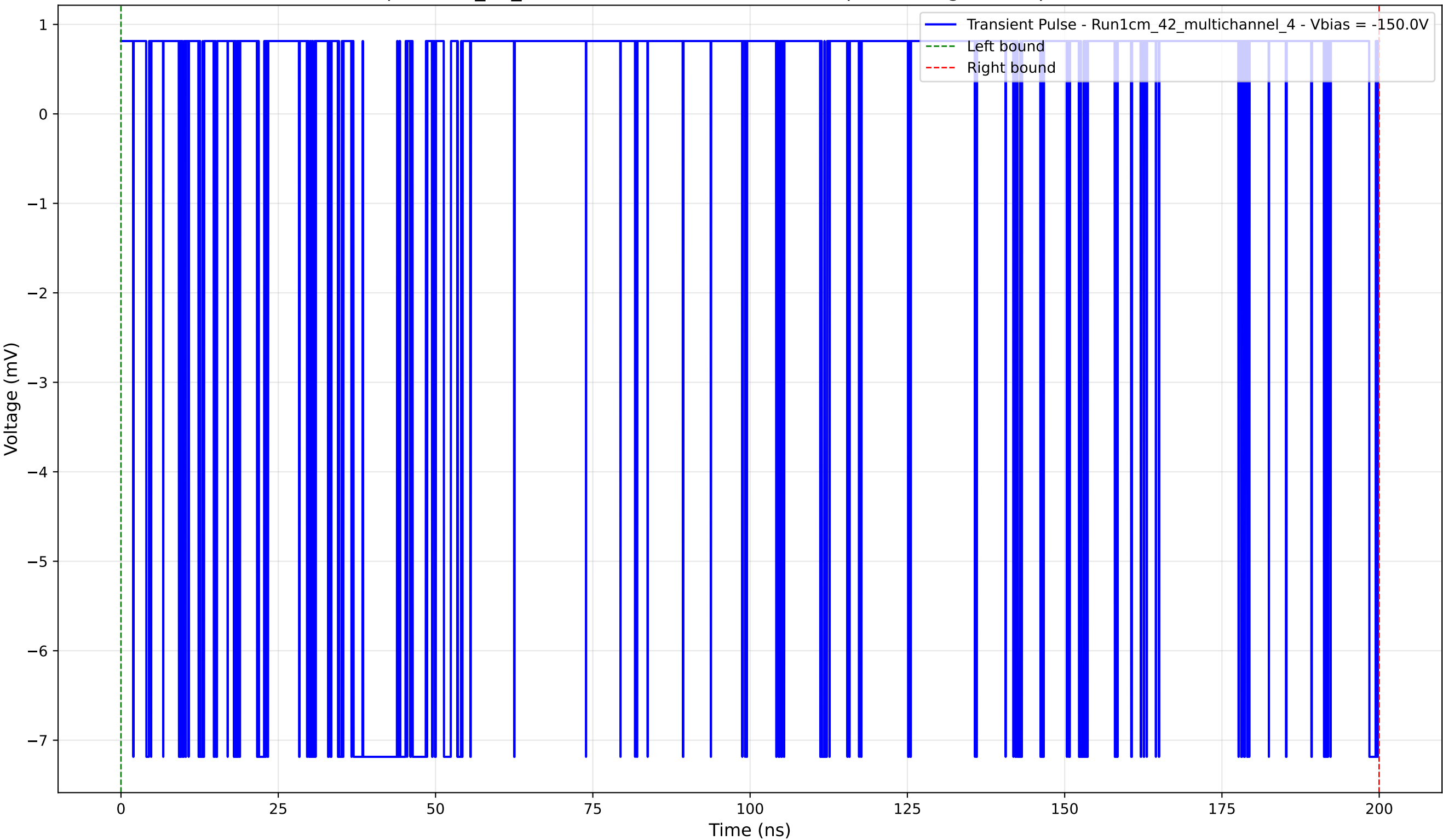
Transient Pulse - Sample: 1cm_42_multichannel - Position: 4365.0 \mu\text{m} - Charge: 0.97 pC - Rise Time: 0.00 ns (N/A)
