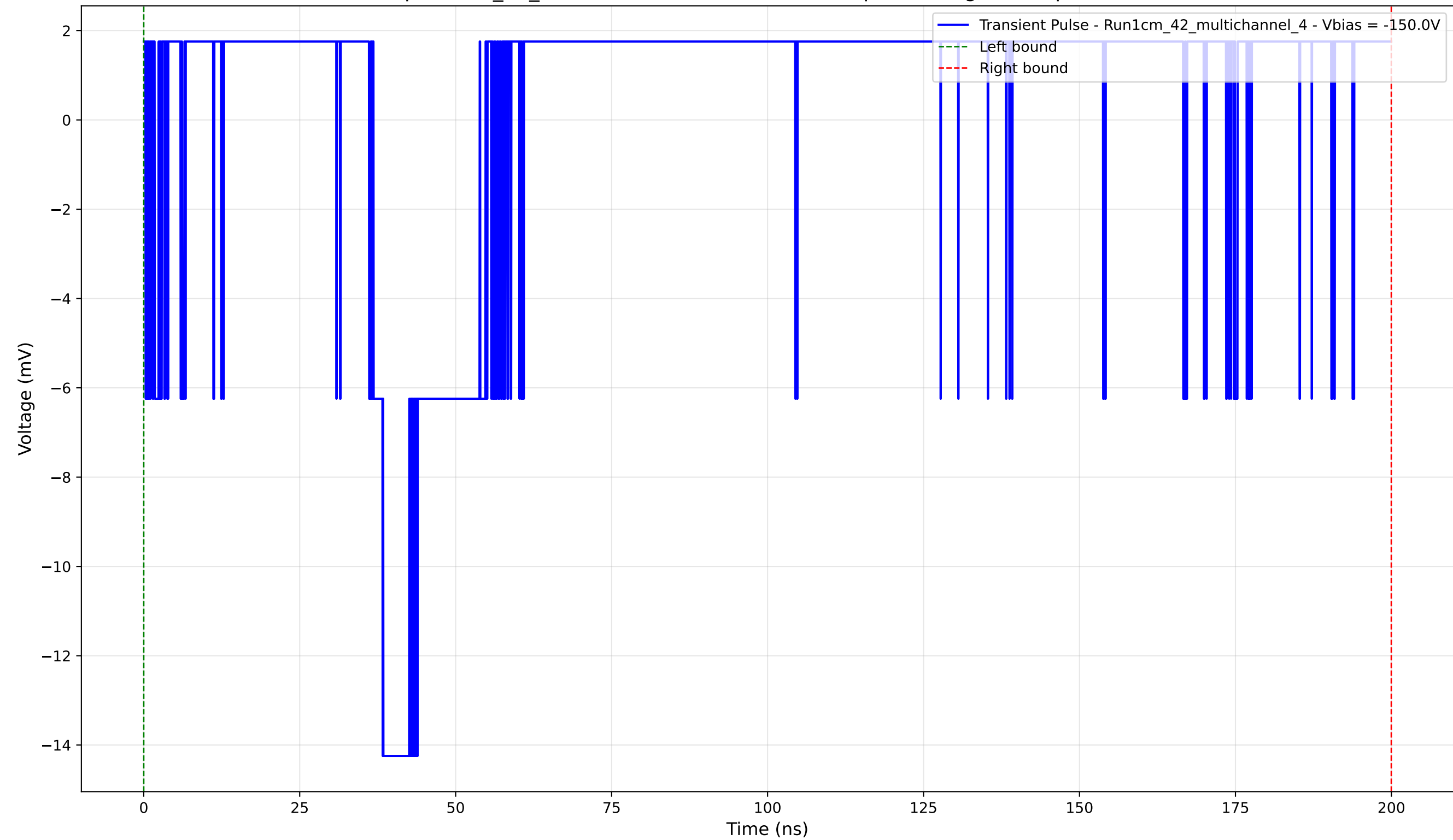
Transient Pulse - Sample: 1cm_42_multichannel - Position: 4540.0 \mu\text{m} - Charge: 2.04 pC - Rise Time: 0.00 ns (N/A)
