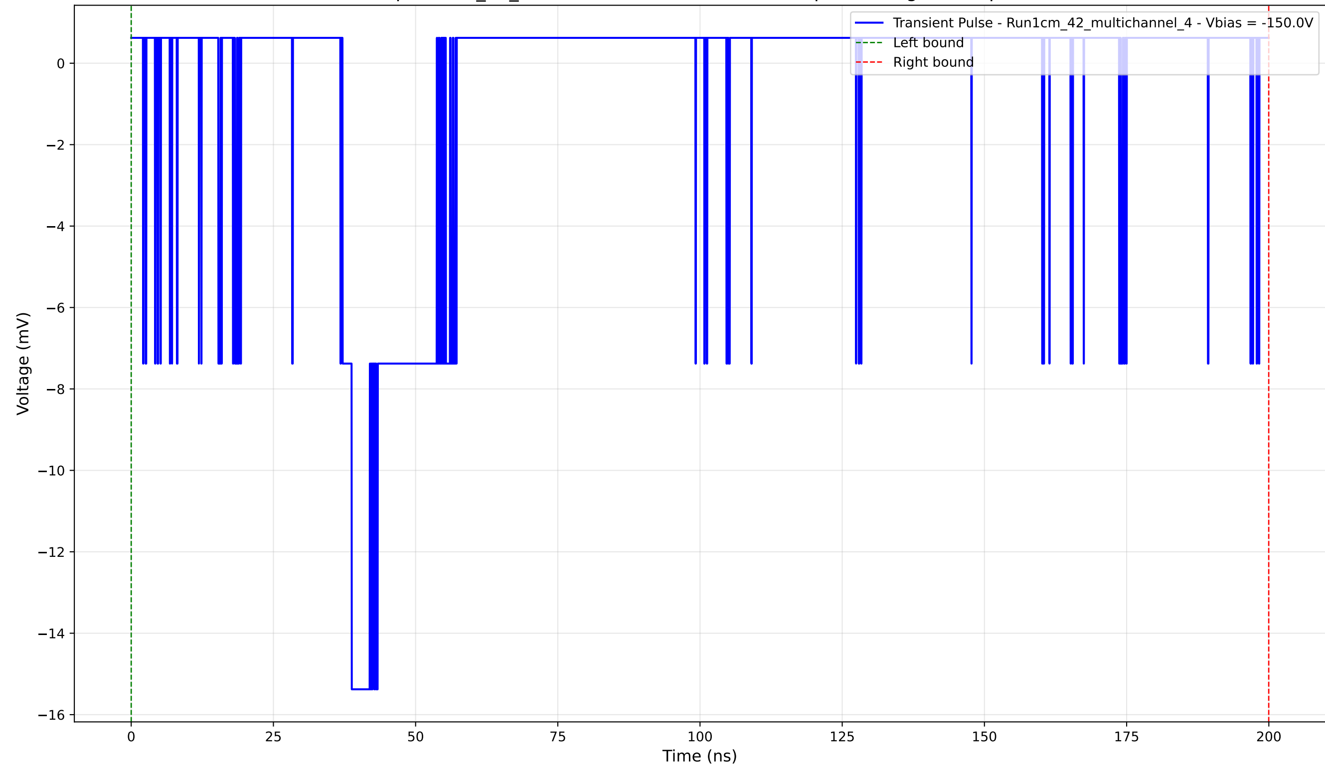
Transient Pulse - Sample: 1cm_42_multichannel - Position: 4645.0 \mu\text{m} - Charge: 1.96 pC - Rise Time: 1.62 ns
