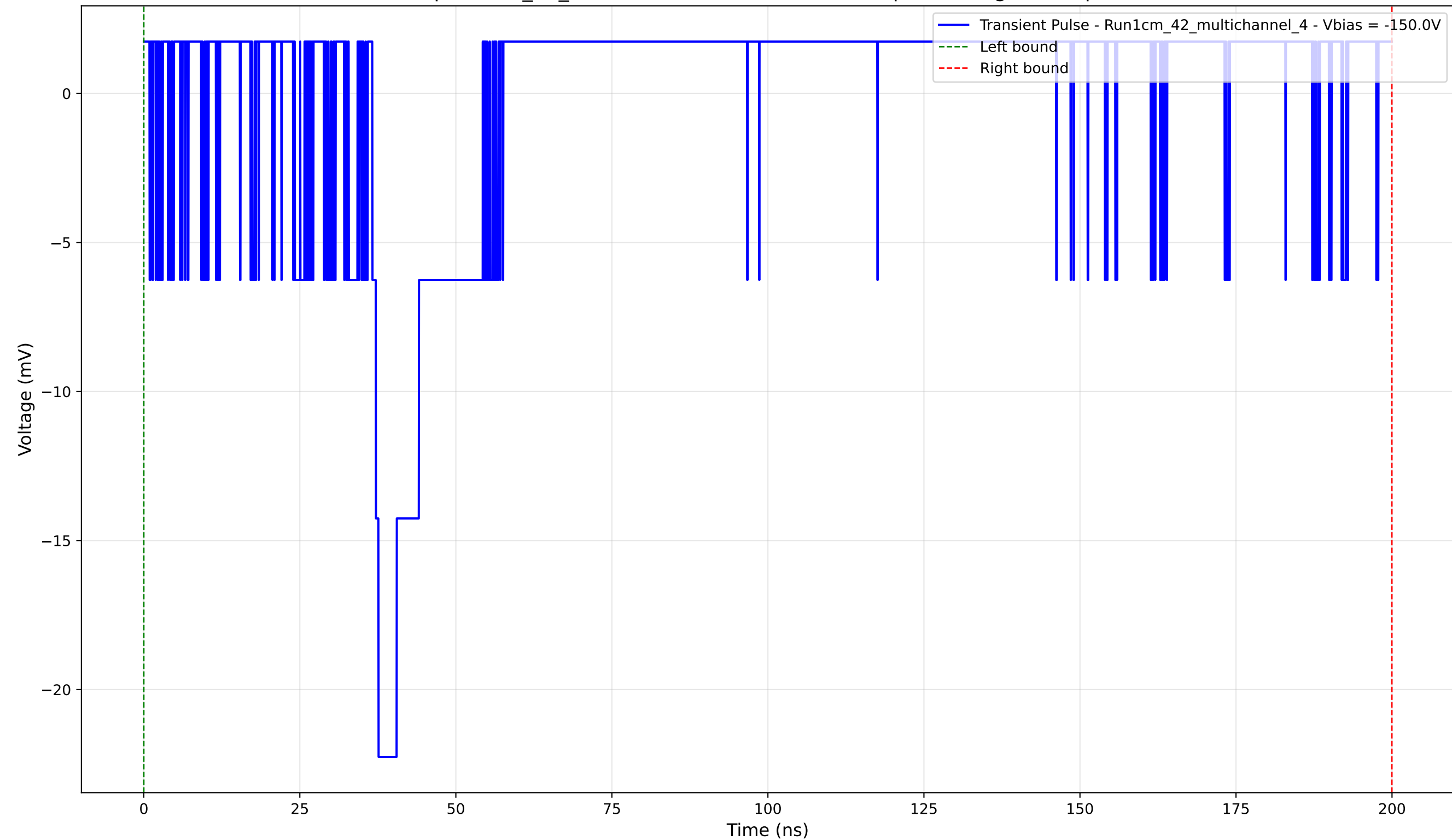
Transient Pulse - Sample: 1cm_42_multichannel - Position: 1270.0 \mu\text{m} - Charge: 0.07 pC - Rise Time: 1.00 ns
