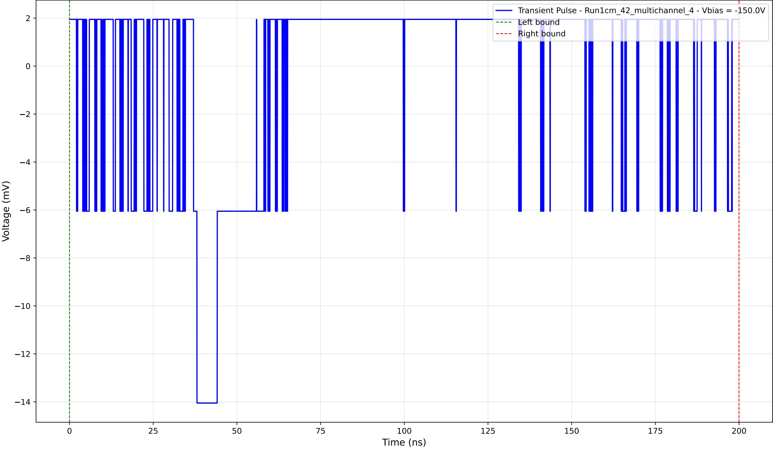
Transient Pulse - Sample: 1cm_42_multichannel - Position: 485.0 \mu\text{m} - Charge: 0.34 pC - Rise Time: 0.00 ns (N/A)
