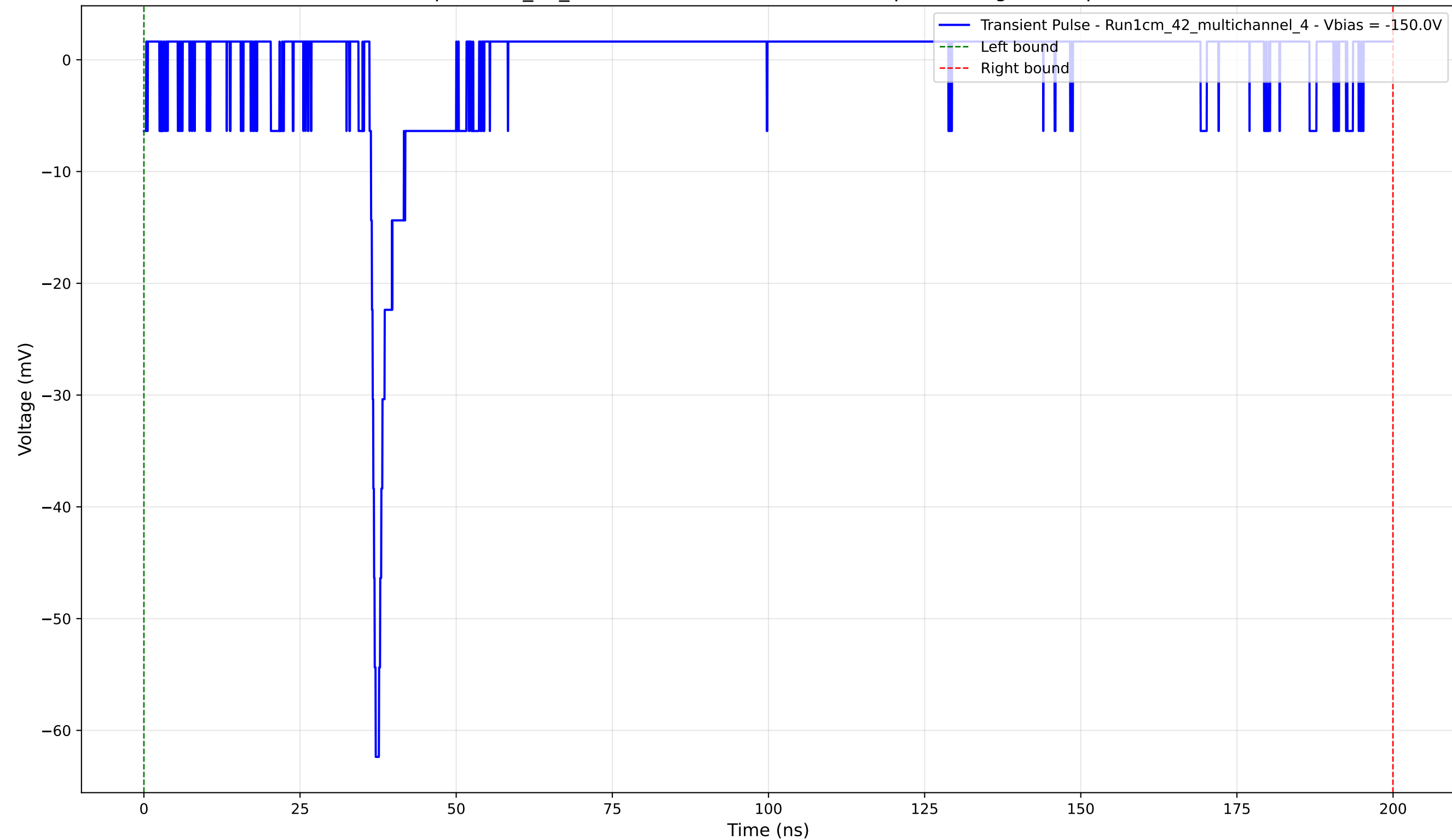
Transient Pulse - Sample: 1cm_42_multichannel - Position: 2150.0 \mu\text{m} - Charge: 0.54 pC - Rise Time: 0.98 ns
