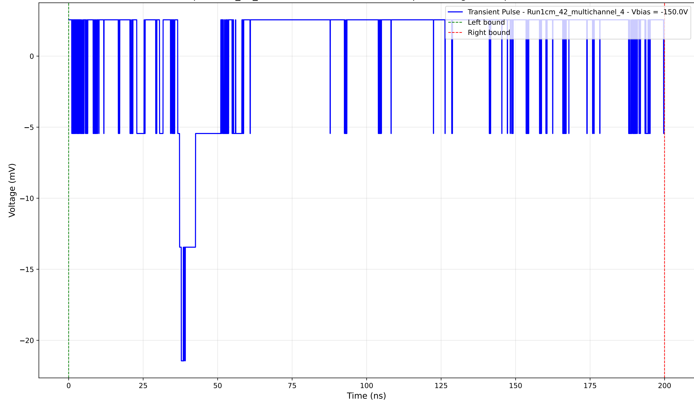
Transient Pulse - Sample: 1cm_42_multichannel - Position: 1310.0 \mu\text{m} - Charge: 3.44 pC - Rise Time: 0.00 ns (N/A)
