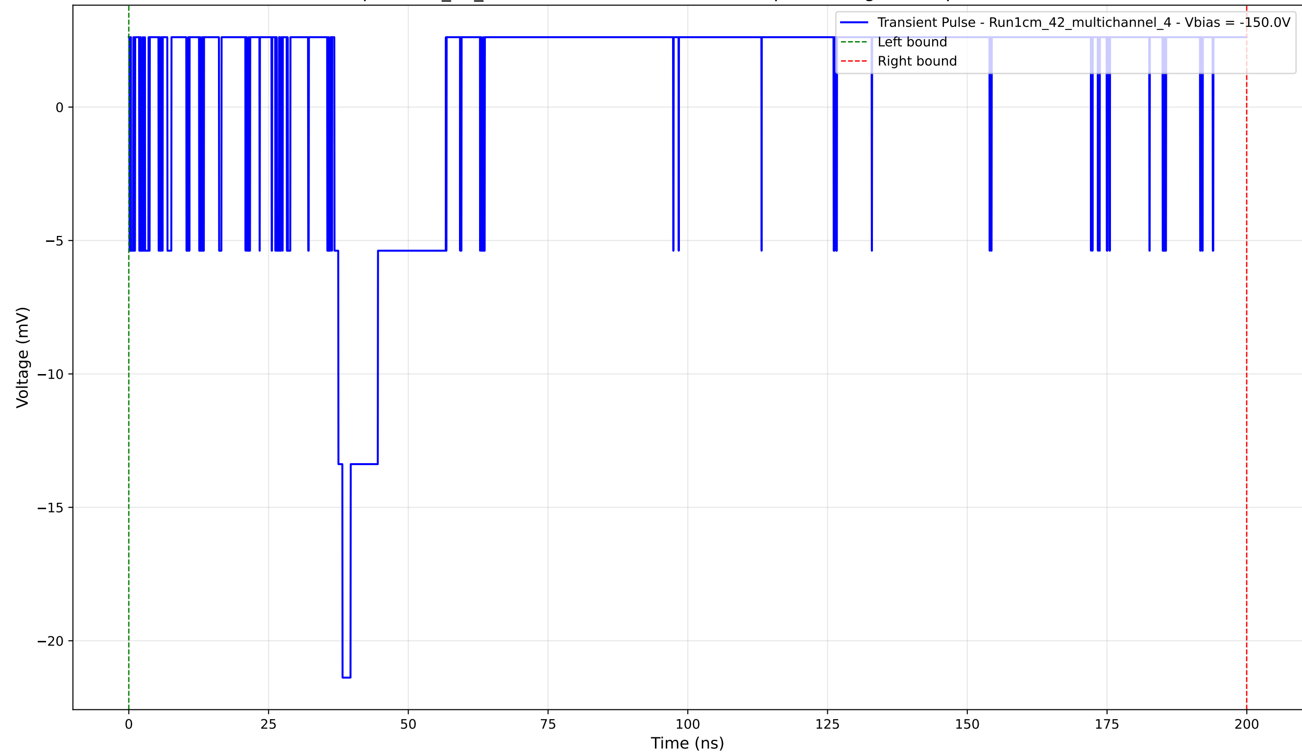
Transient Pulse - Sample: 1cm_42_multichannel - Position: 1015.0 \mu\text{m} - Charge: 4.30 pC - Rise Time: 0.00 ns (N/A)
