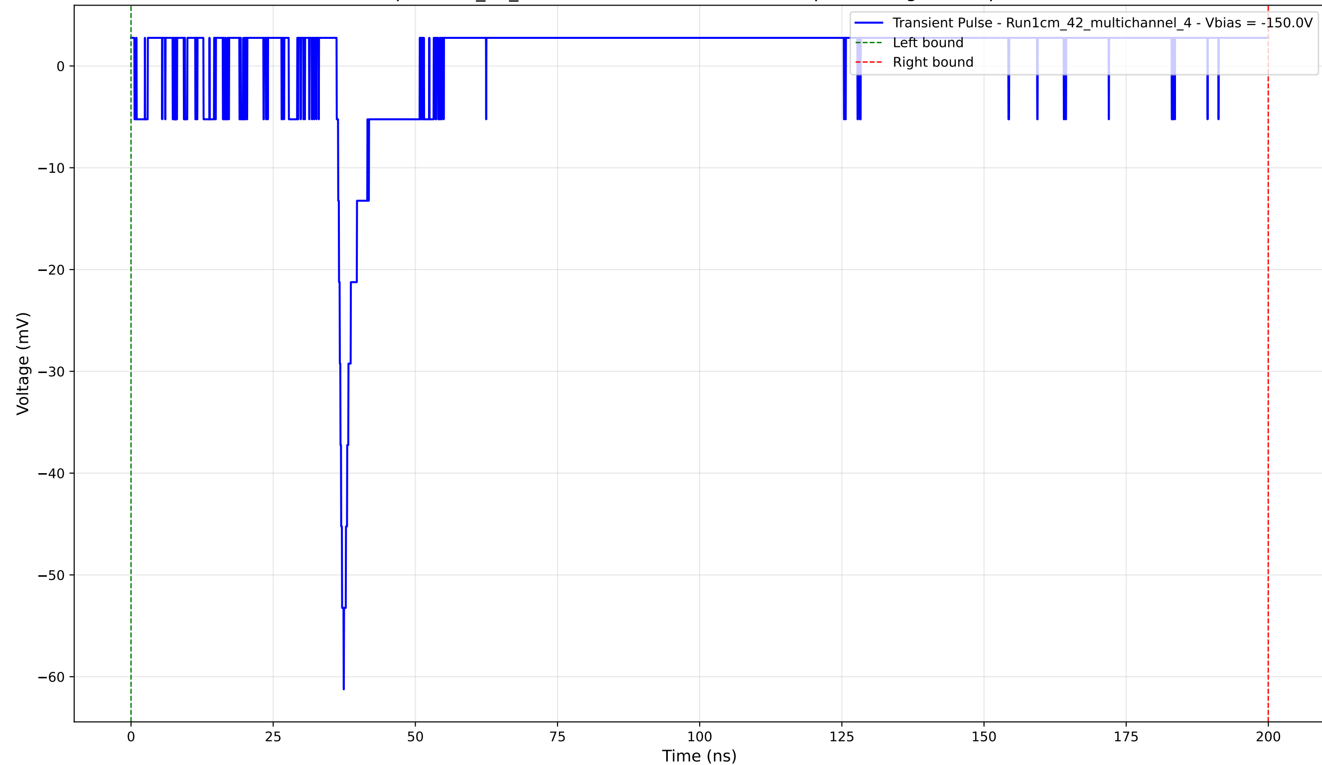
Transient Pulse - Sample: 1cm_42_multichannel - Position: 2065.0 \mu\text{m} - Charge: 4.39 pC - Rise Time: 0.98 ns
