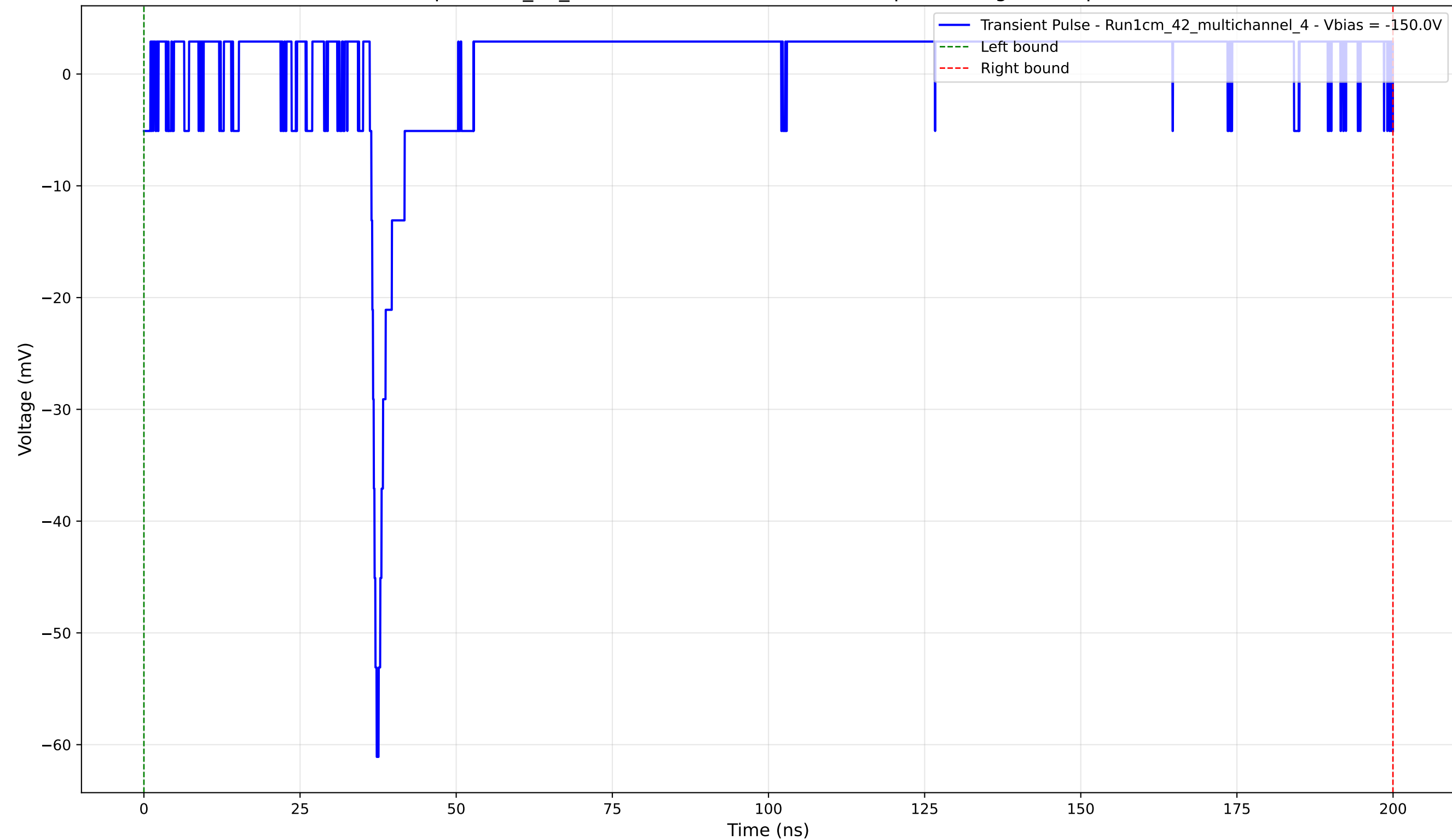
Transient Pulse - Sample: 1cm_42_multichannel - Position: 2085.0 \mu\text{m} - Charge: 4.68 pC - Rise Time: 0.86 ns
