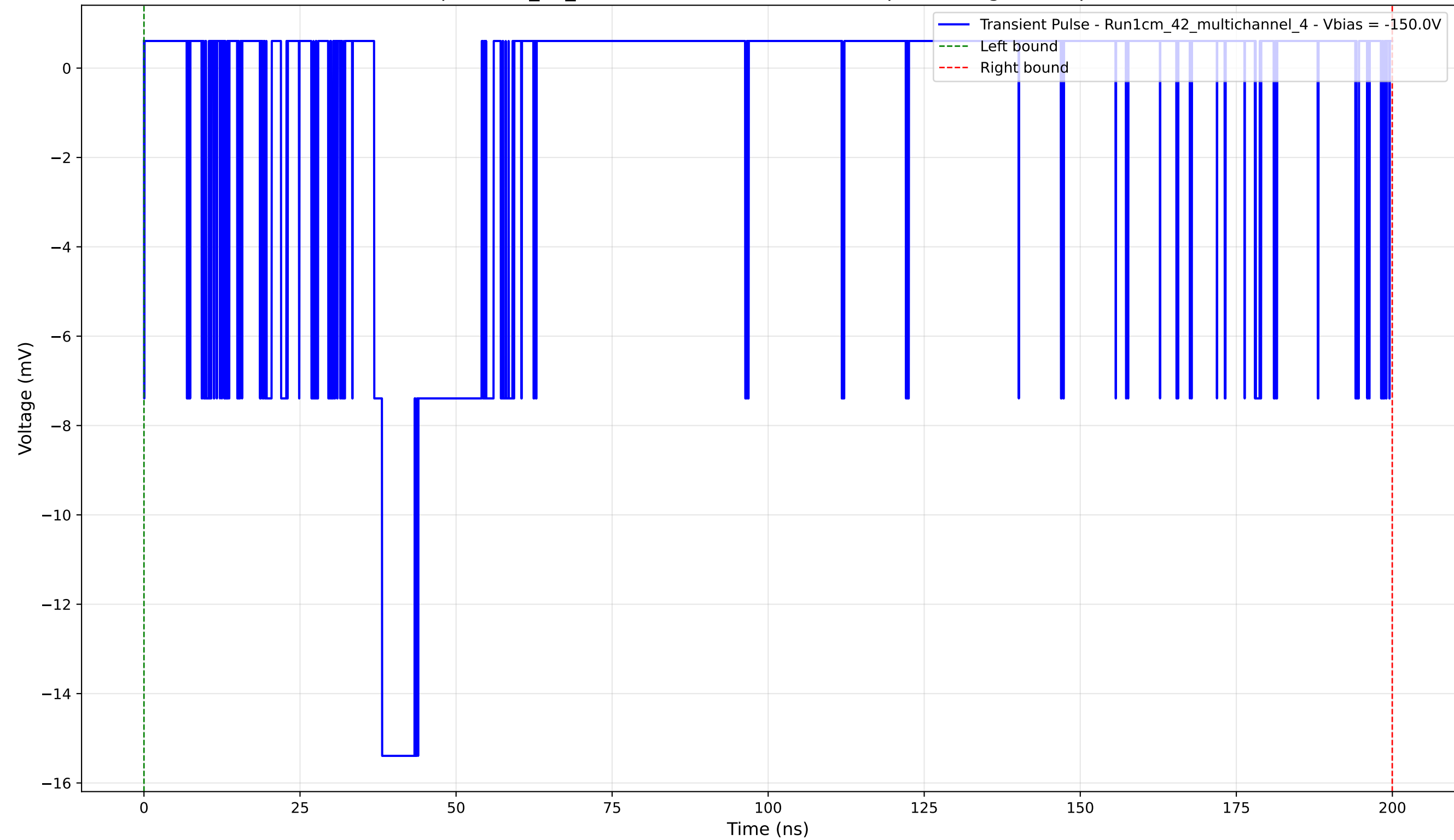
Transient Pulse - Sample: 1cm_42_multichannel - Position: 455.0 \mu\text{m} - Charge: 3.66 pC - Rise Time: 1.28 ns
