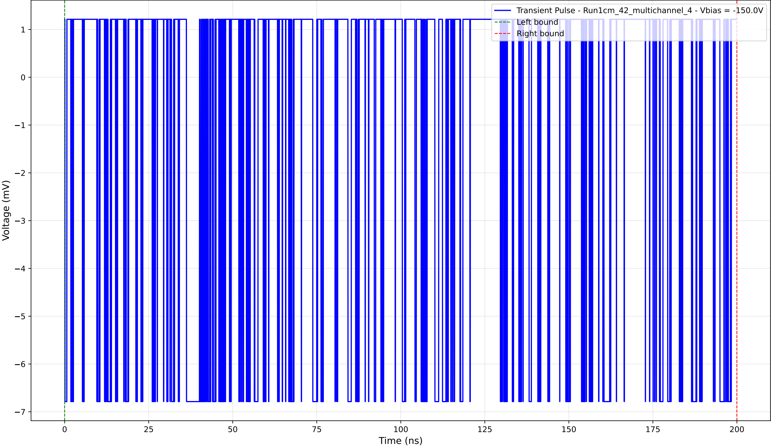
Transient Pulse - Sample: 1cm_42_multichannel - Position: 2360.0 \mu\text{m} - Charge: 2.40 pC - Rise Time: 0.00 ns (N/A)
