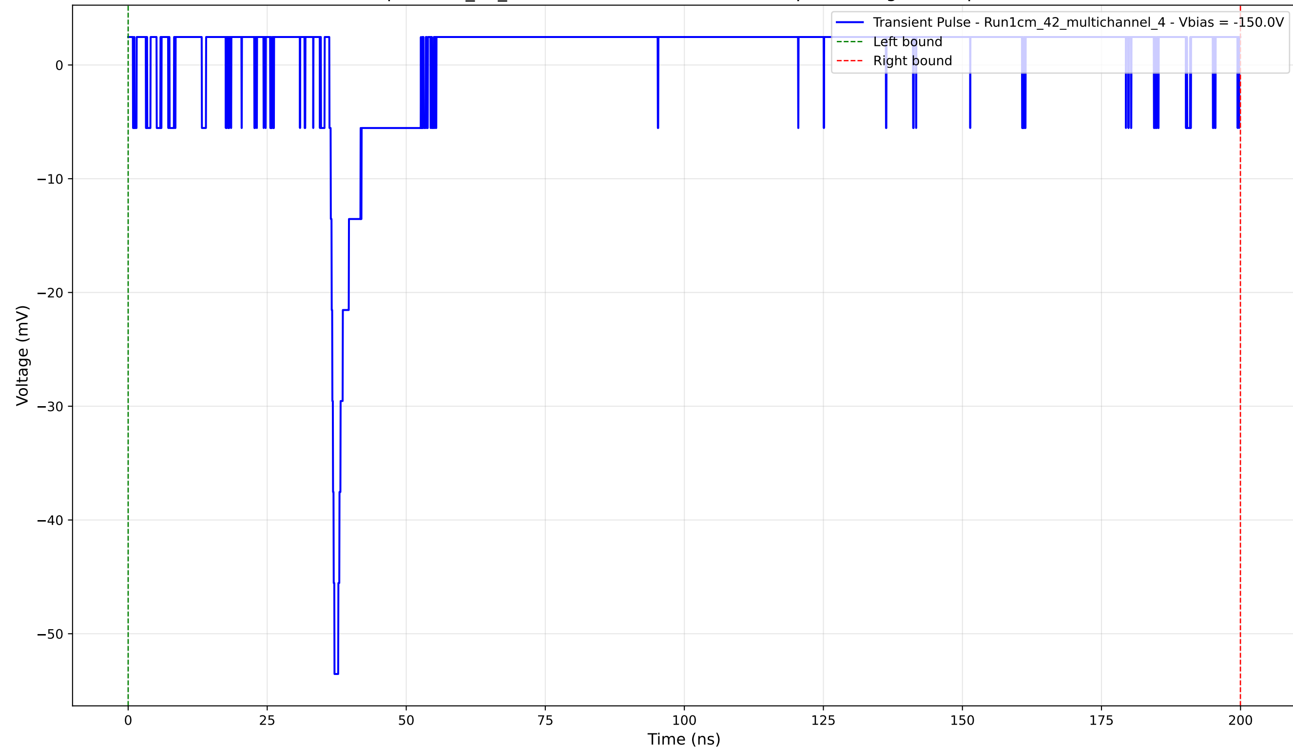
Transient Pulse - Sample: 1cm_42_multichannel - Position: 2685.0 \mu\text{m} - Charge: 3.47 pC - Rise Time: 0.90 ns
