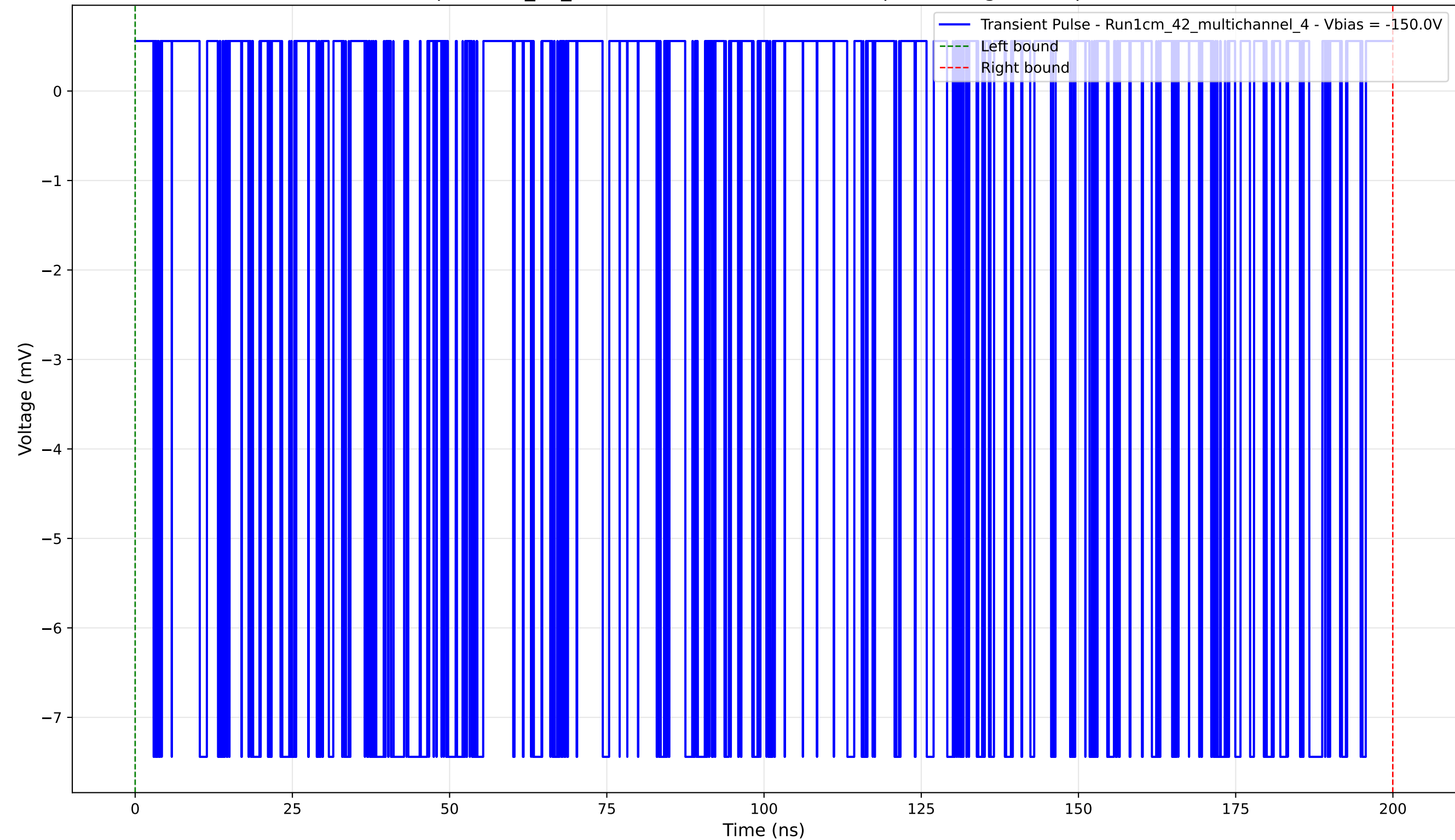
Transient Pulse - Sample: 1cm_42_multichannel - Position: 345.0 \mu\text{m} - Charge: 7.37 pC - Rise Time: 0.02 ns
