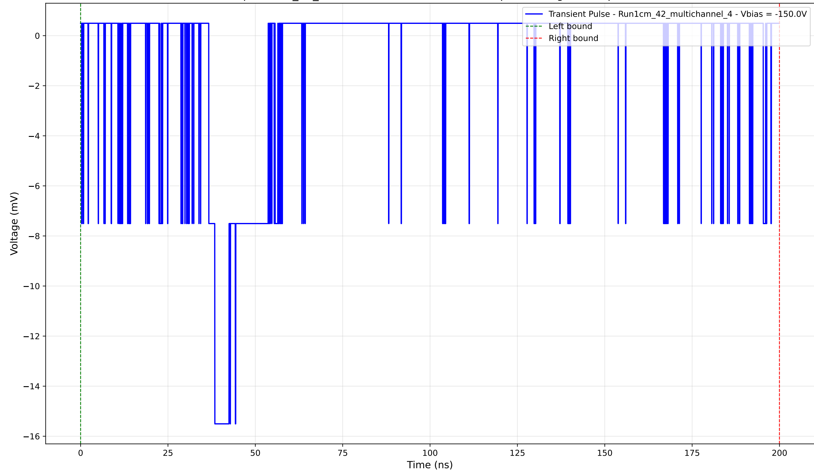
Transient Pulse - Sample: 1cm_42_multichannel - Position: 4570.0 \mu\text{m} - Charge: 3.24 pC - Rise Time: 1.74 ns
