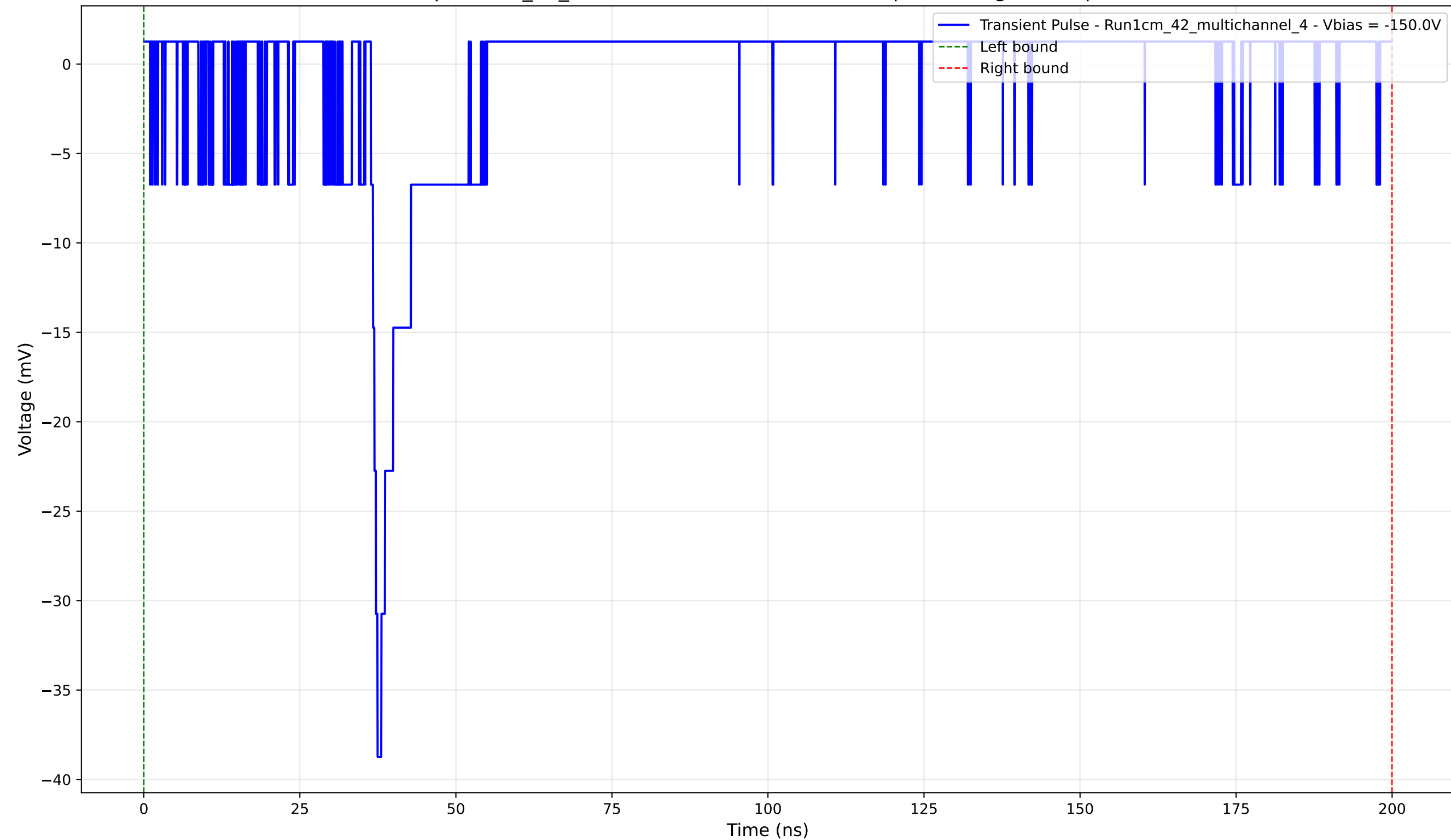
Transient Pulse - Sample: 1cm_42_multichannel - Position: 1695.0 \mu\text{m} - Charge: 2.07 pC - Rise Time: 1.07 ns
