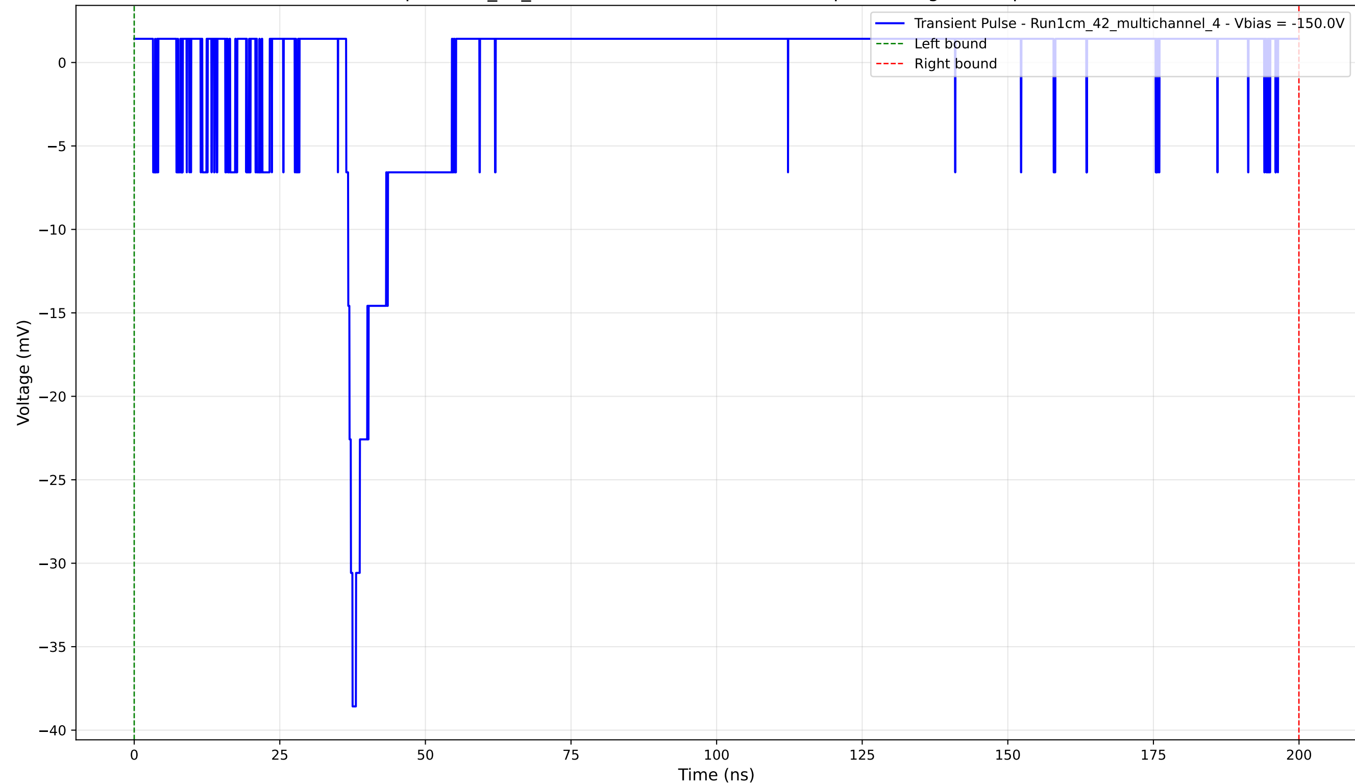
Transient Pulse - Sample: 1cm_42_multichannel - Position: 1690.0 \mu\text{m} - Charge: 0.79 pC - Rise Time: 1.09 ns
