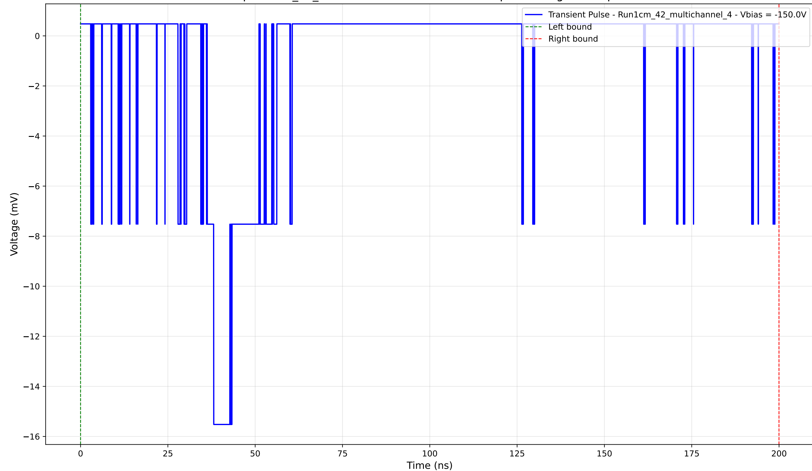
Transient Pulse - Sample: 1cm_42_multichannel - Position: 4080.0 \mu\text{m} - Charge: 2.79 pC - Rise Time: 1.86 ns
