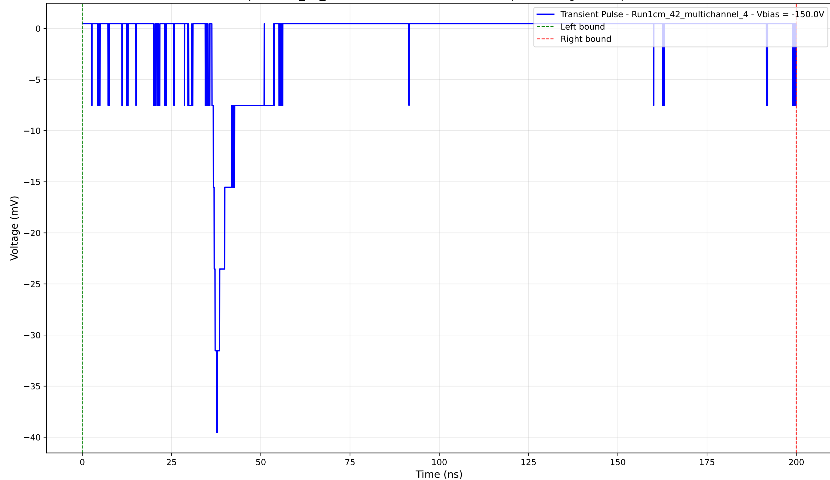
Transient Pulse - Sample: 1cm_42_multichannel - Position: 3060.0 \mu\text{m} - Charge: 3.44 pC - Rise Time: 1.33 ns
