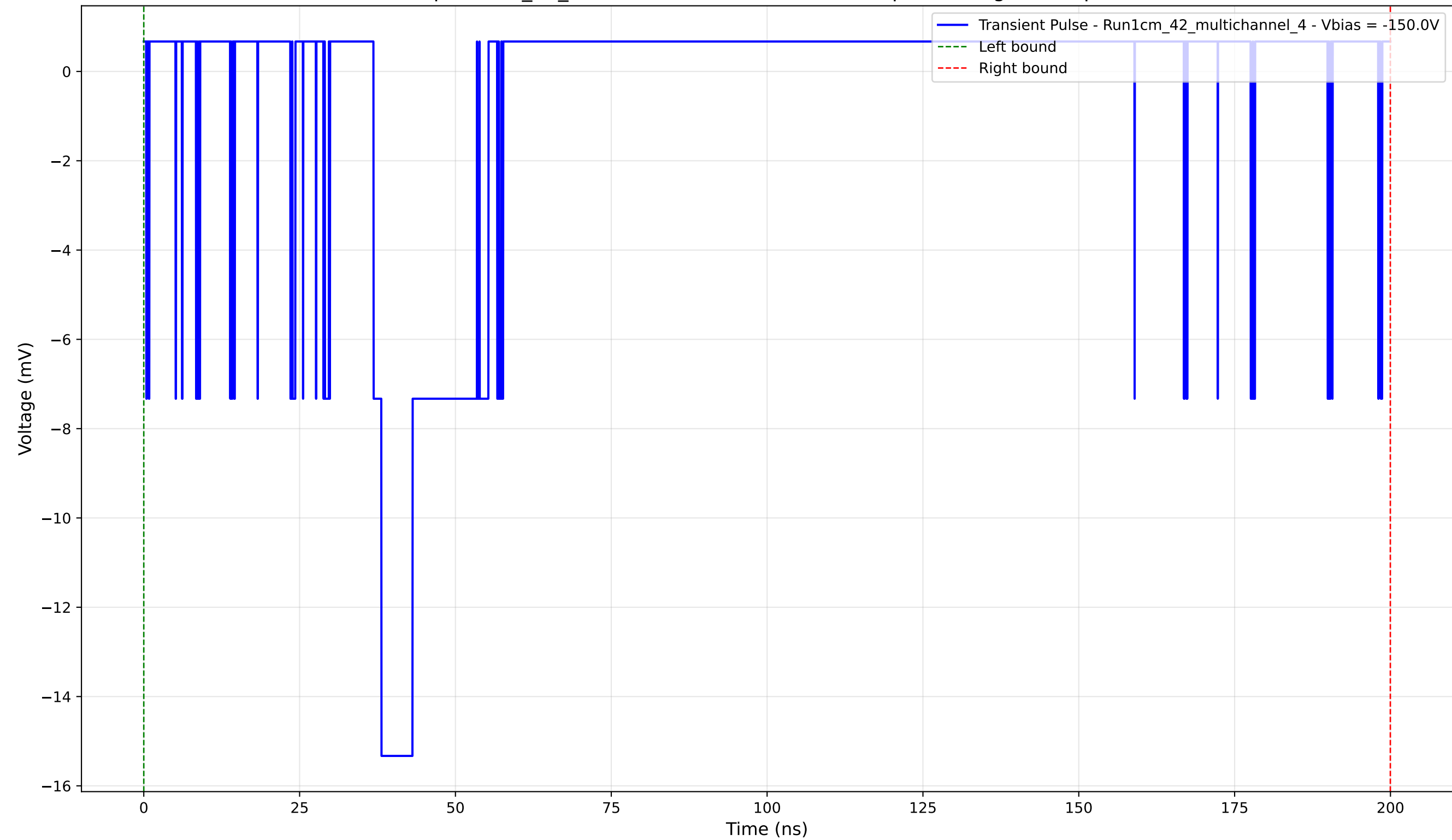
Transient Pulse - Sample: 1cm_42_multichannel - Position: 4025.0 \mu\text{m} - Charge: 1.89 pC - Rise Time: 1.28 ns
