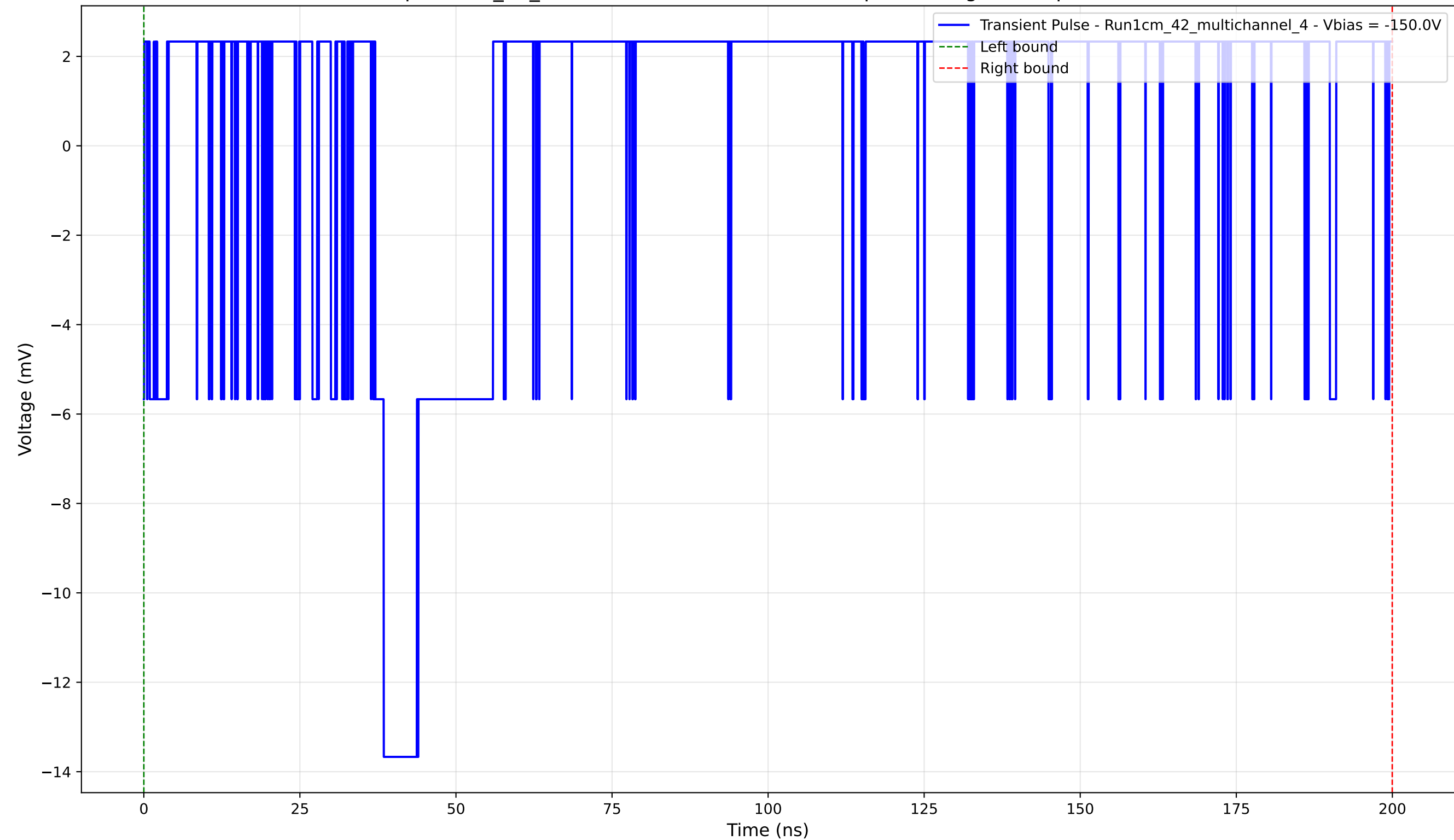
Transient Pulse - Sample: 1cm_42_multichannel - Position: 4495.0 \mu\text{m} - Charge: 3.16 pC - Rise Time: 0.00 ns (N/A)
