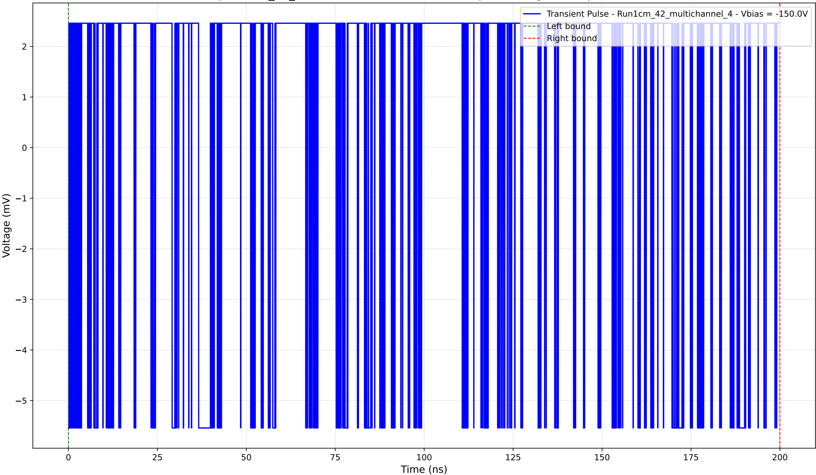
Transient Pulse - Sample: 1cm_42_multichannel - Position: 2880.0 \mu\text{m} - Charge: 3.88 pC - Rise Time: 0.00 ns (N/A)
