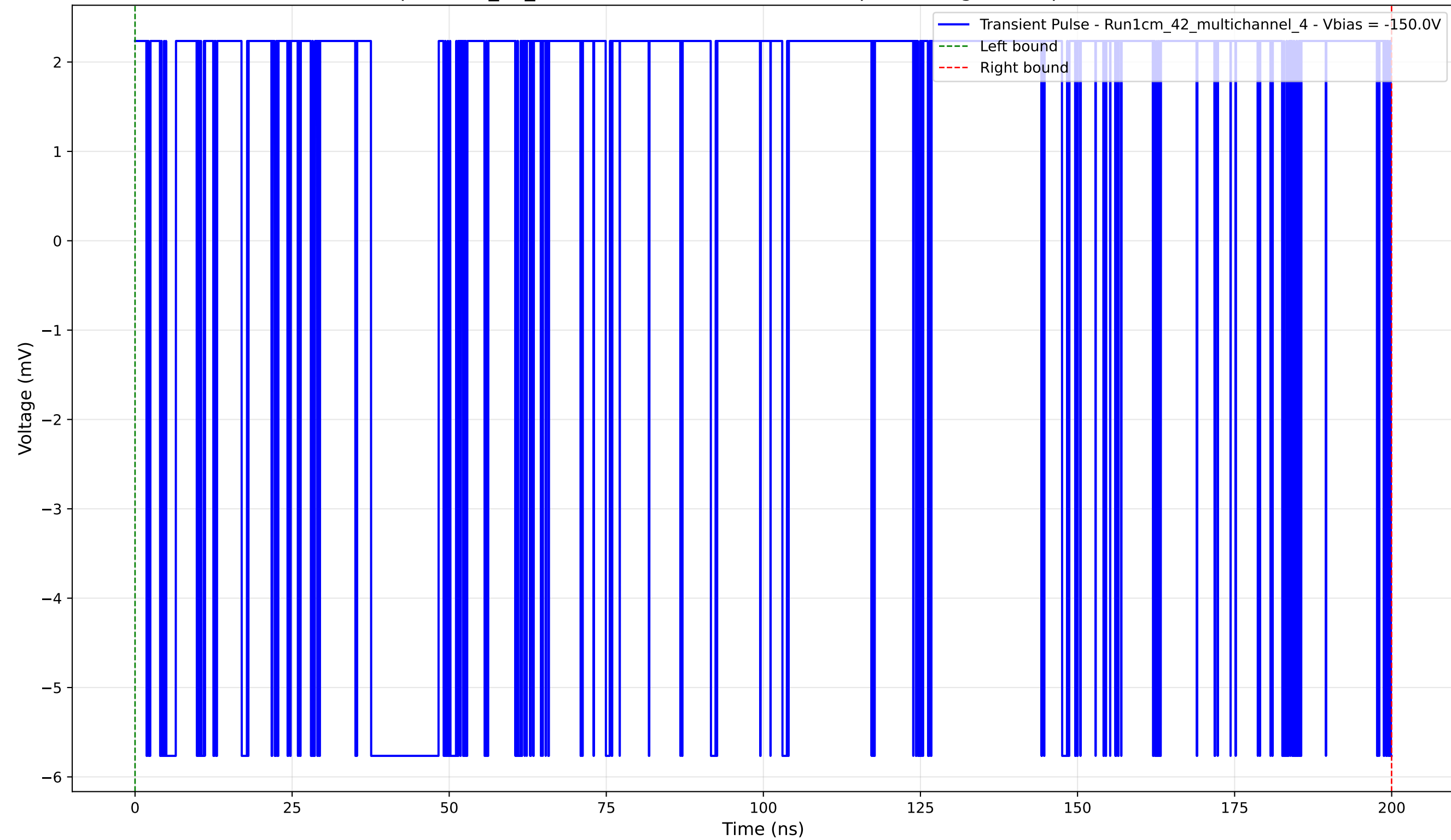
Transient Pulse - Sample: 1cm_42_multichannel - Position: 4440.0 \mu\text{m} - Charge: 3.71 pC - Rise Time: 0.00 ns (N/A)
