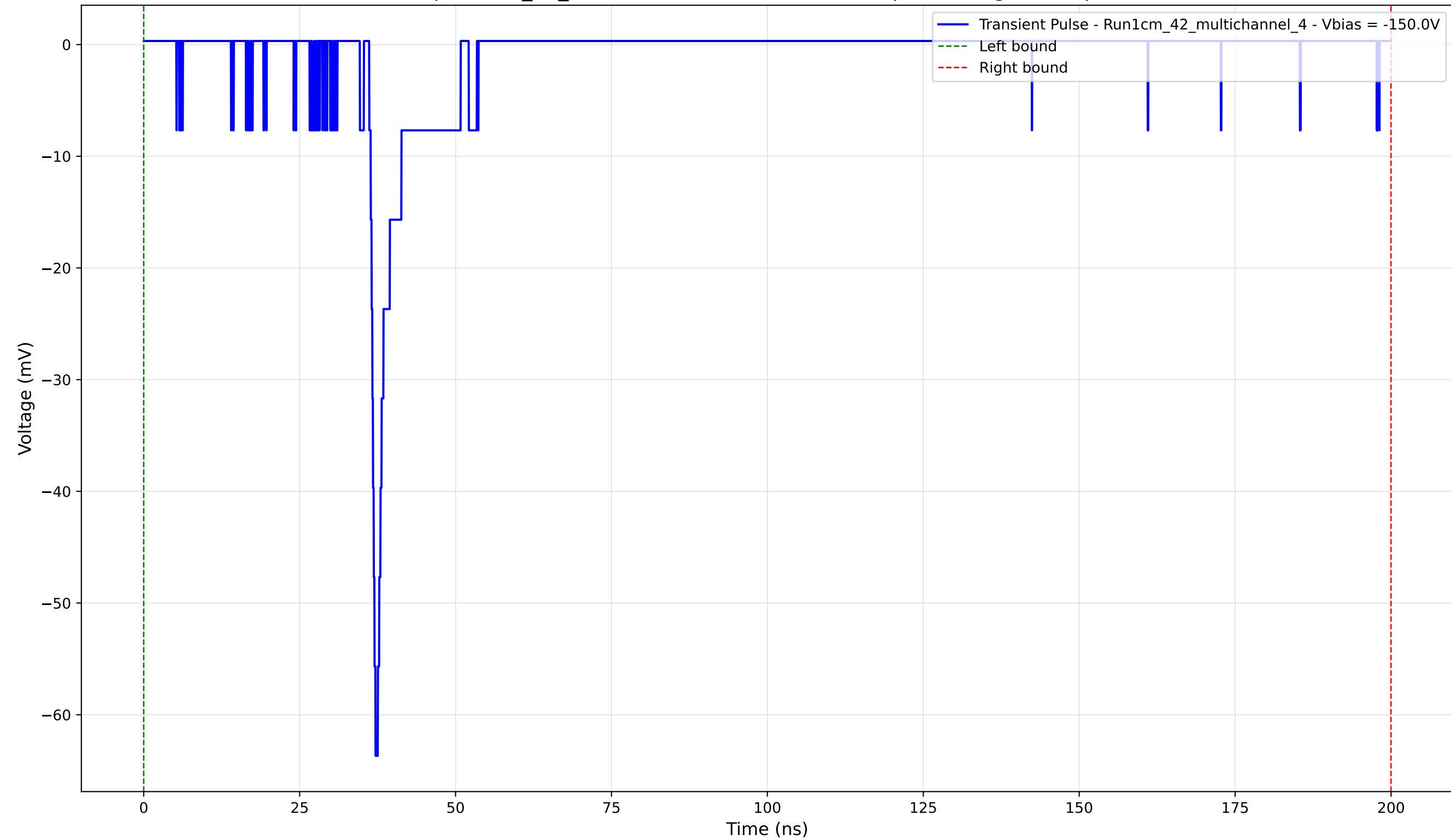
Transient Pulse - Sample: 1cm_42_multichannel - Position: 2630.0 \mu\text{m} - Charge: 4.17 pC - Rise Time: 1.00 ns
