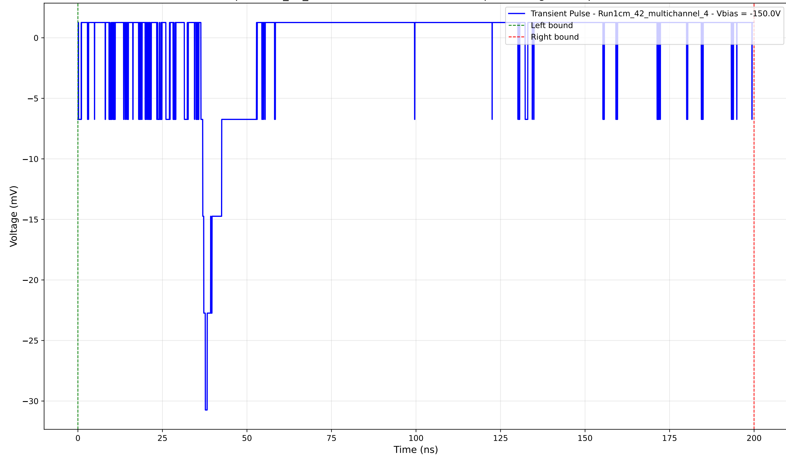
Transient Pulse - Sample: 1cm_42_multichannel - Position: 3230.0 \mu\text{m} - Charge: 0.85 pC - Rise Time: 1.31 ns
