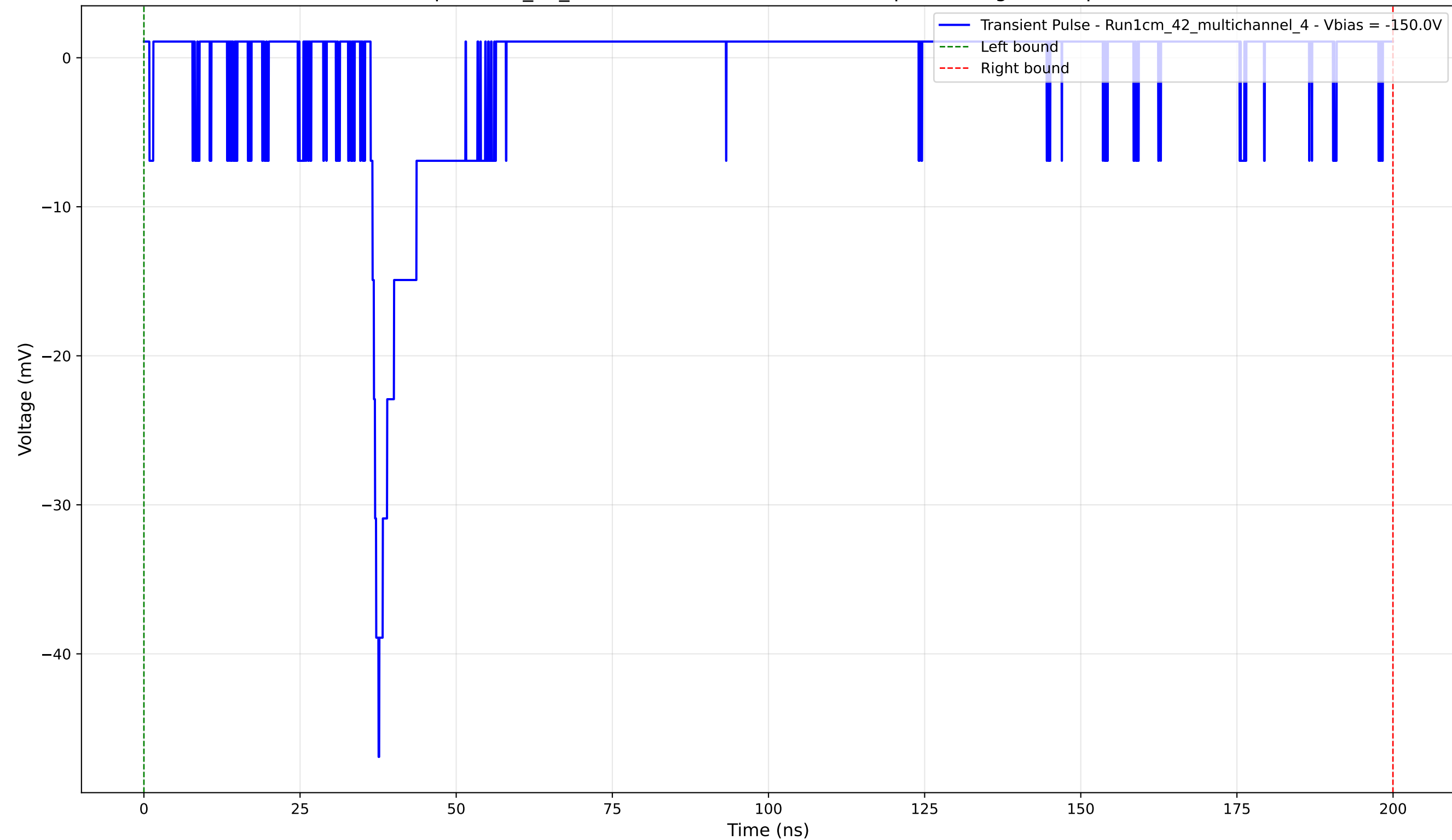
Transient Pulse - Sample: 1cm_42_multichannel - Position: 1785.0 \mu\text{m} - Charge: 2.46 pC - Rise Time: 1.27 ns
