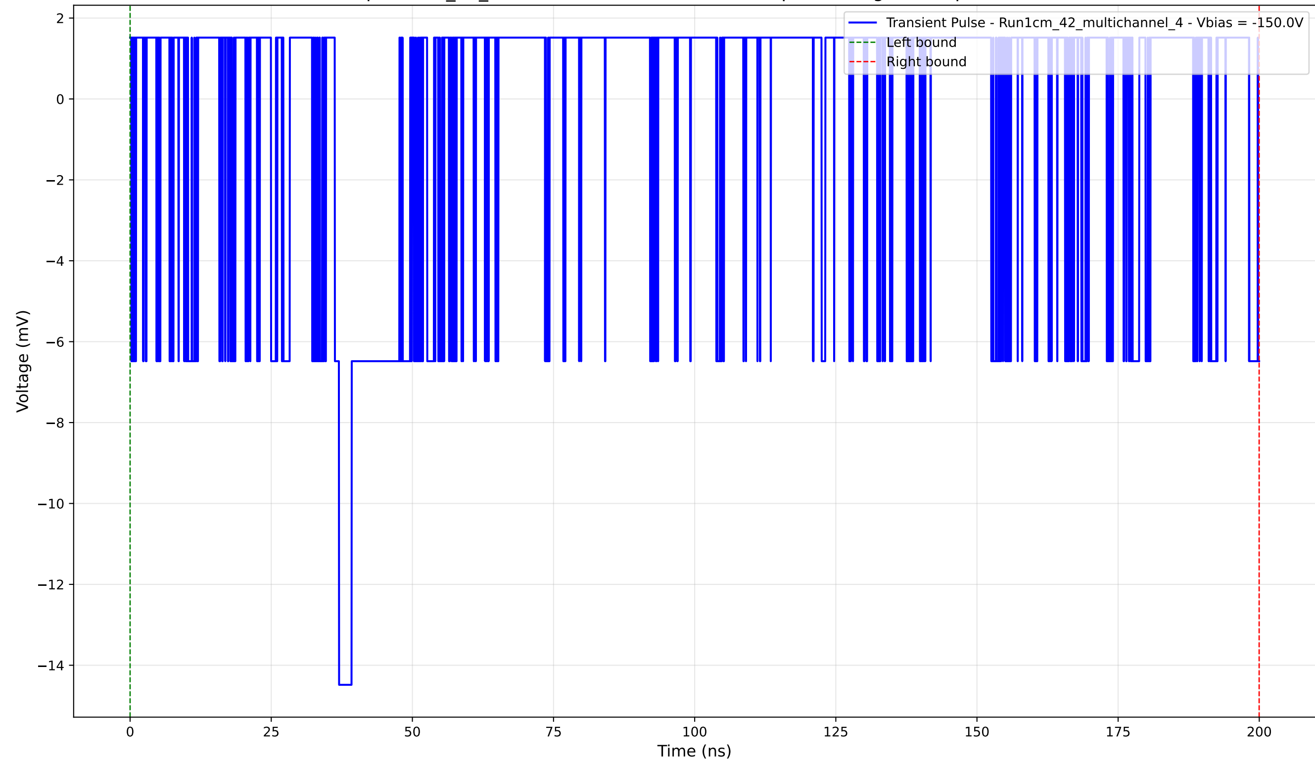
Transient Pulse - Sample: 1cm_42_multichannel - Position: 1835.0 \mu\text{m} - Charge: 1.59 pC - Rise Time: 0.00 ns (N/A)
