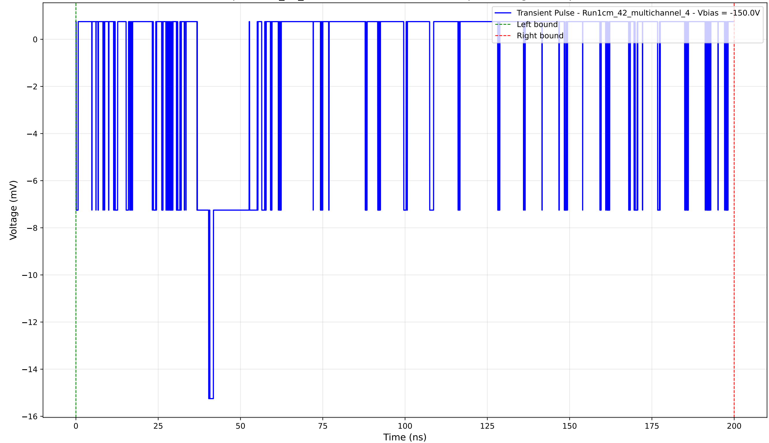
Transient Pulse - Sample: 1cm_42_multichannel - Position: 115.0 \mu\text{m} - Charge: 2.98 pC - Rise Time: 3.48 ns
