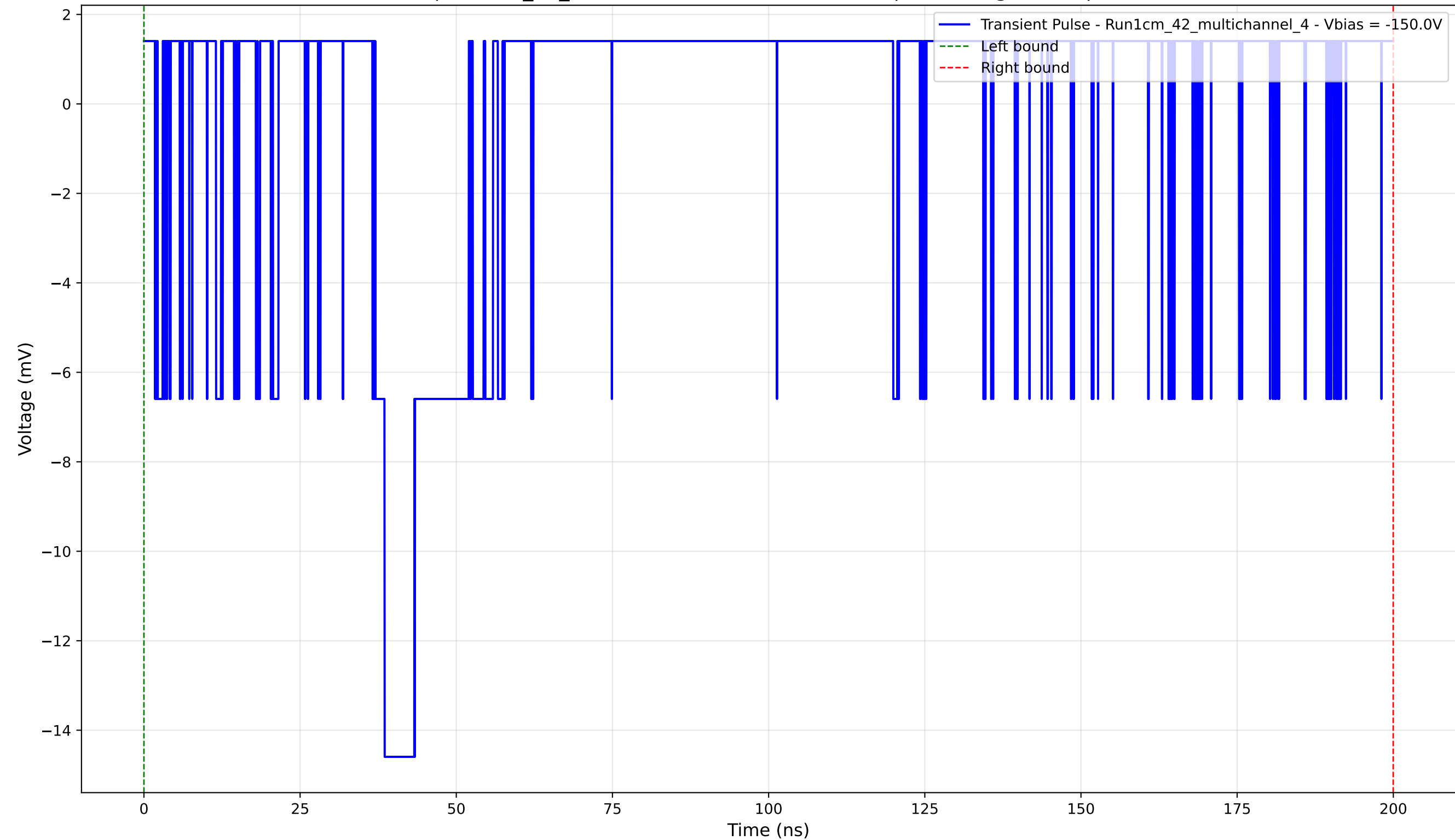
Transient Pulse - Sample: 1cm_42_multichannel - Position: 4625.0 \mu\text{m} - Charge: 0.21 pC - Rise Time: 1.48 ns
