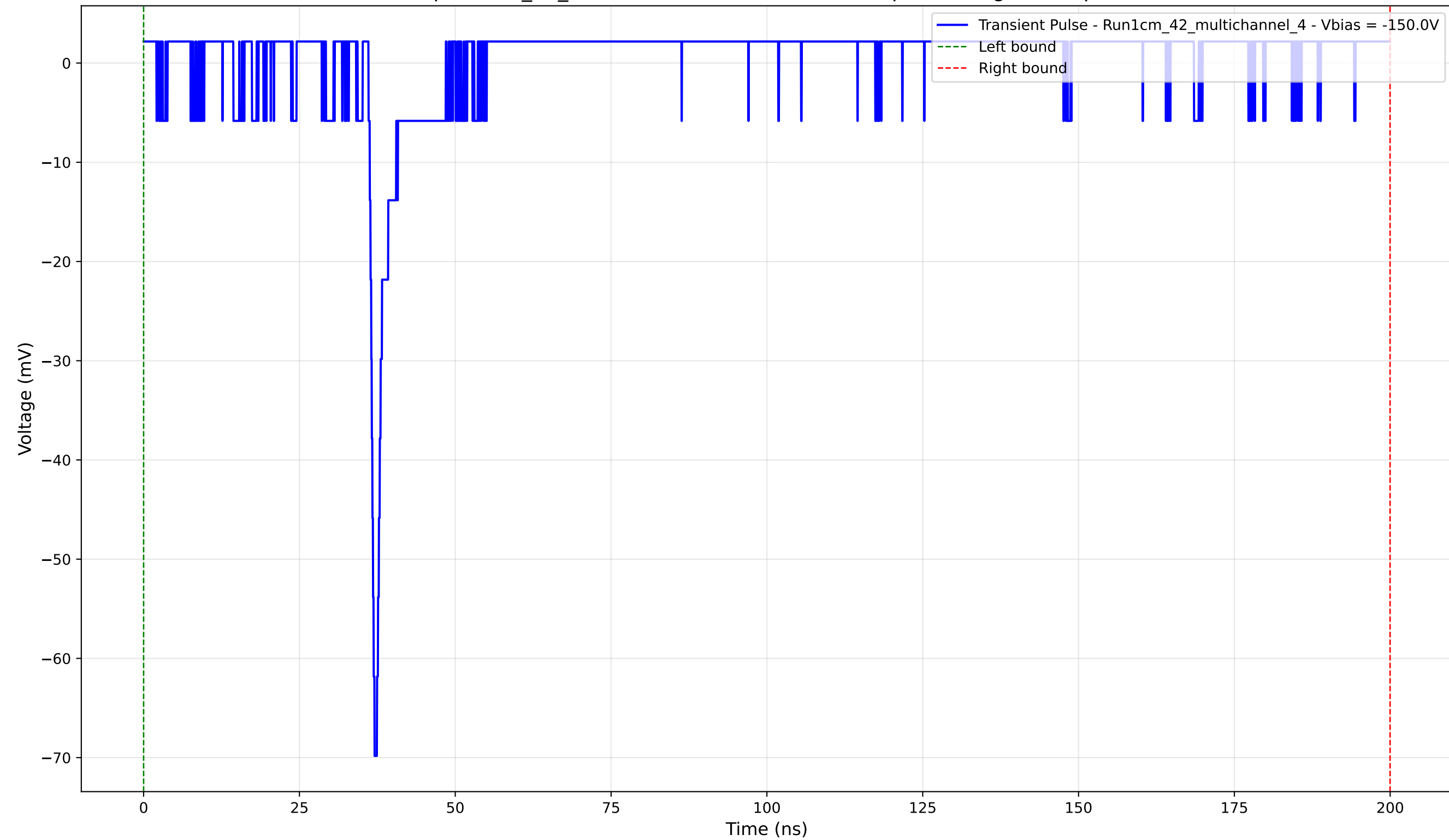
Transient Pulse - Sample: 1cm_42_multichannel - Position: 2315.0 \mu\text{m} - Charge: 1.82 pC - Rise Time: 0.78 ns
