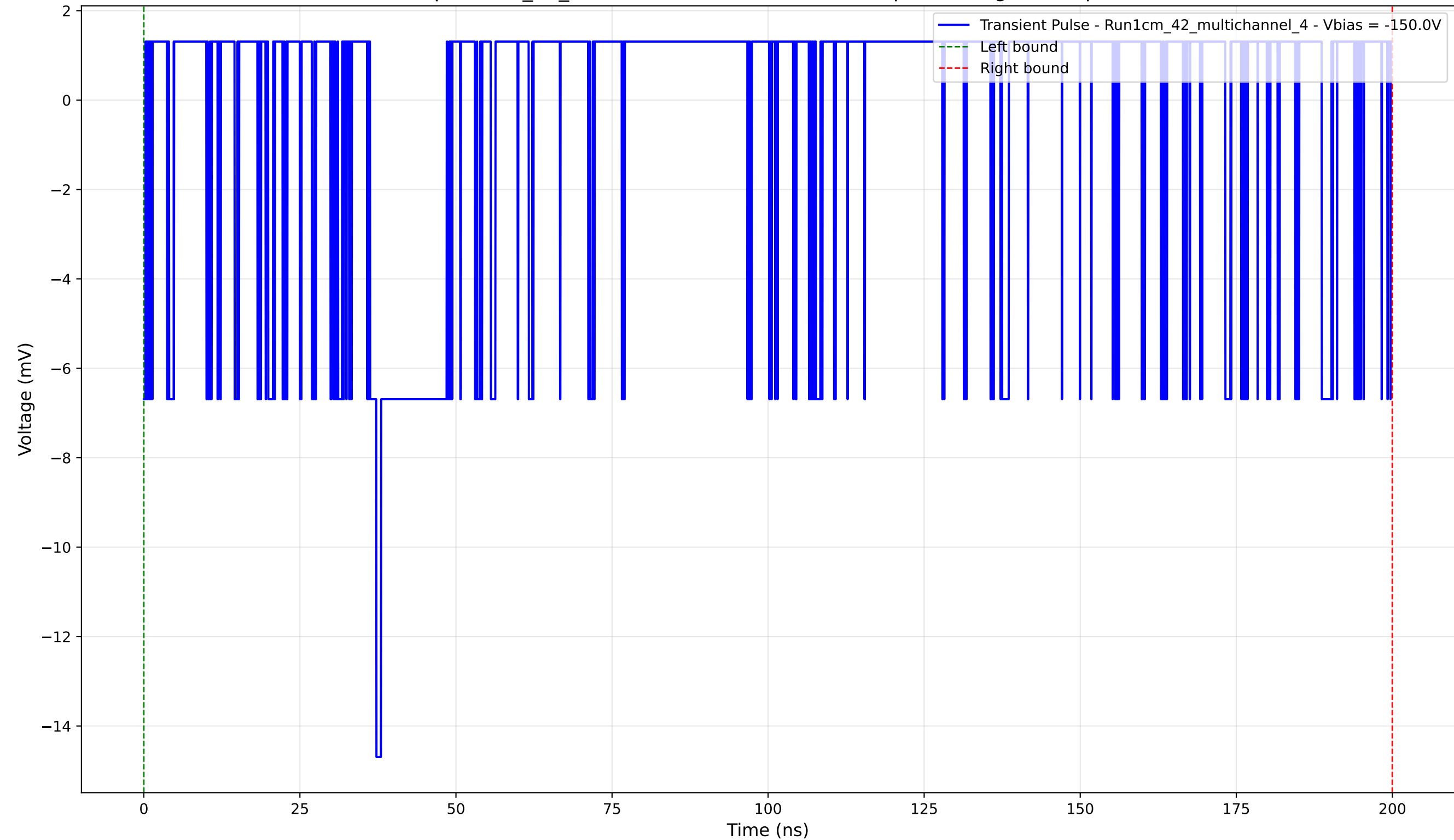
Transient Pulse - Sample: 1cm_42_multichannel - Position: 1840.0 \mu\text{m} - Charge: 0.59 pC - Rise Time: 1.02 ns
