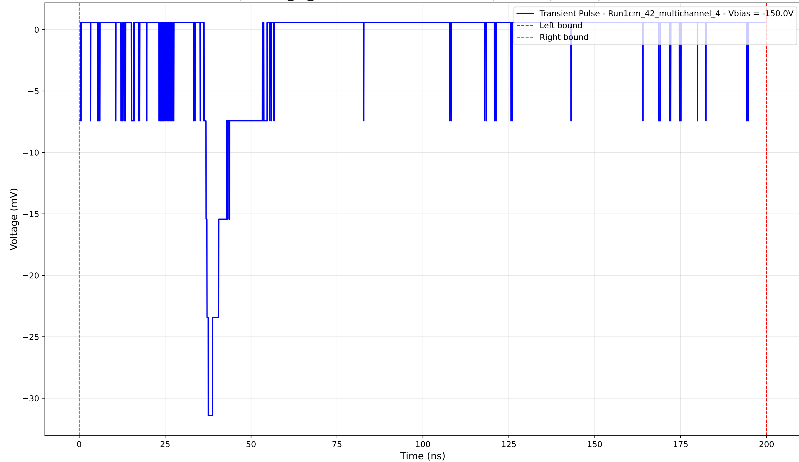
Transient Pulse - Sample: 1cm_42_multichannel - Position: 1515.0 \mu\text{m} - Charge: 3.60 pC - Rise Time: 1.19 ns
