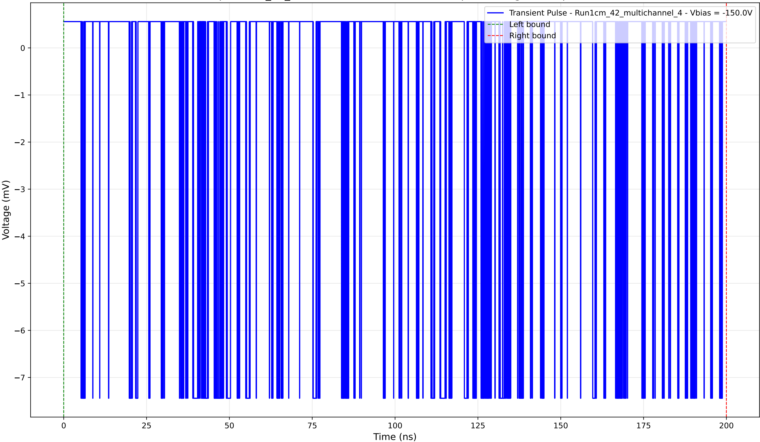
Transient Pulse - Sample: 1cm_42_multichannel - Position: 4415.0 \mu\text{m} - Charge: 2.98 pC - Rise Time: 0.02 ns
