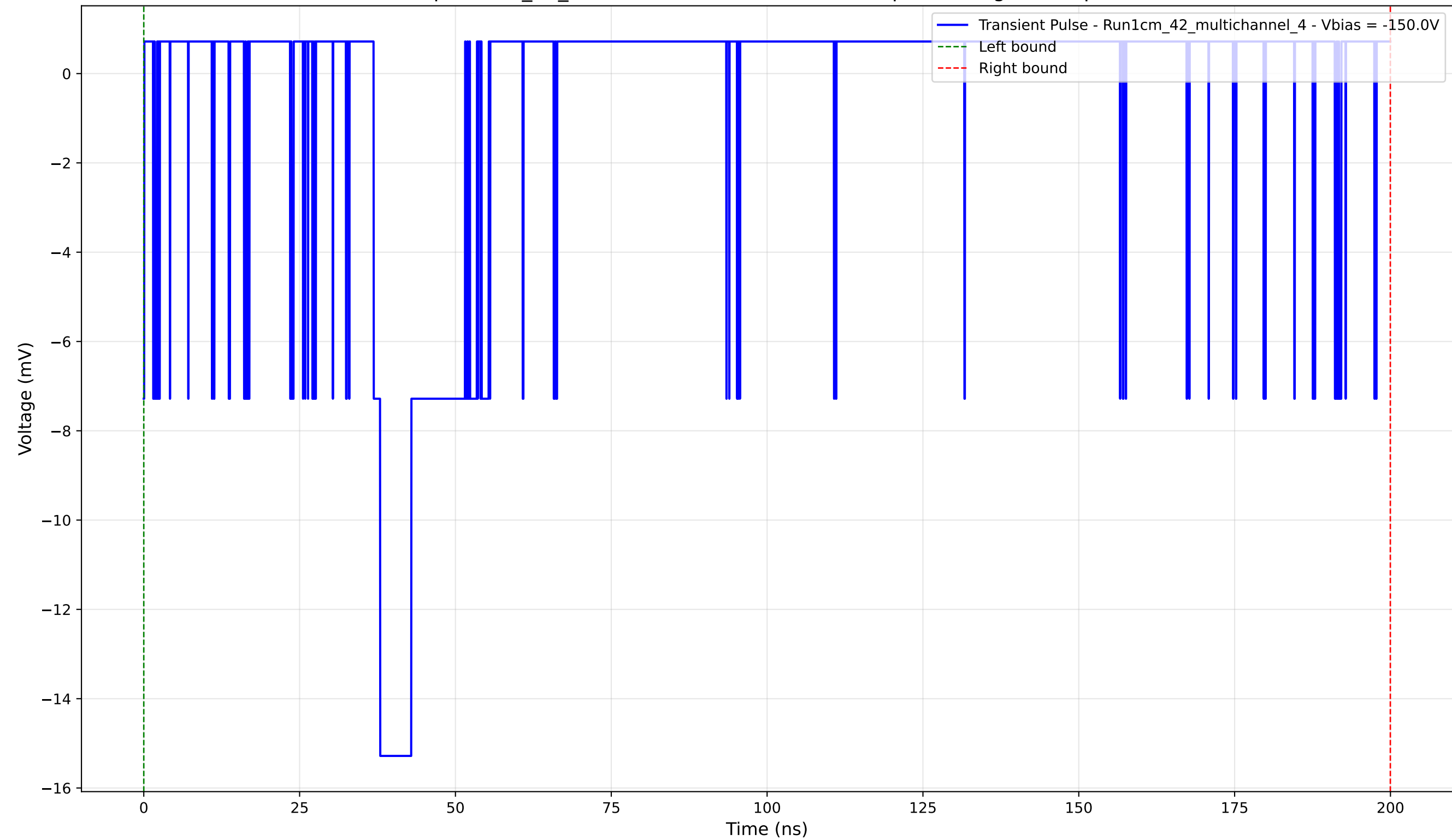
Transient Pulse - Sample: 1cm_42_multichannel - Position: 4050.0 \mu\text{m} - Charge: 1.72 pC - Rise Time: 1.06 ns
