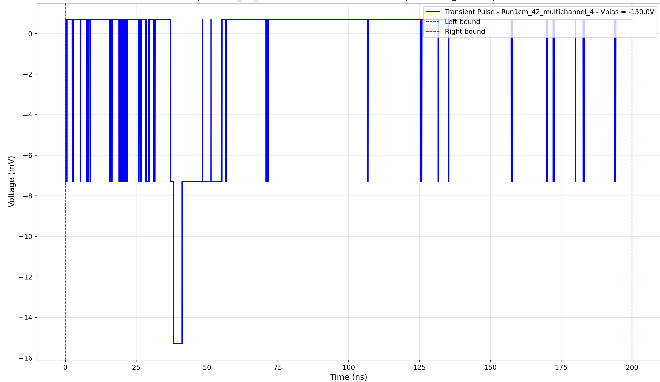
Transient Pulse - Sample: 1cm_42_multichannel - Position: 3965.0 \mu\text{m} - Charge: 1.70 pC - Rise Time: 1.18 ns
