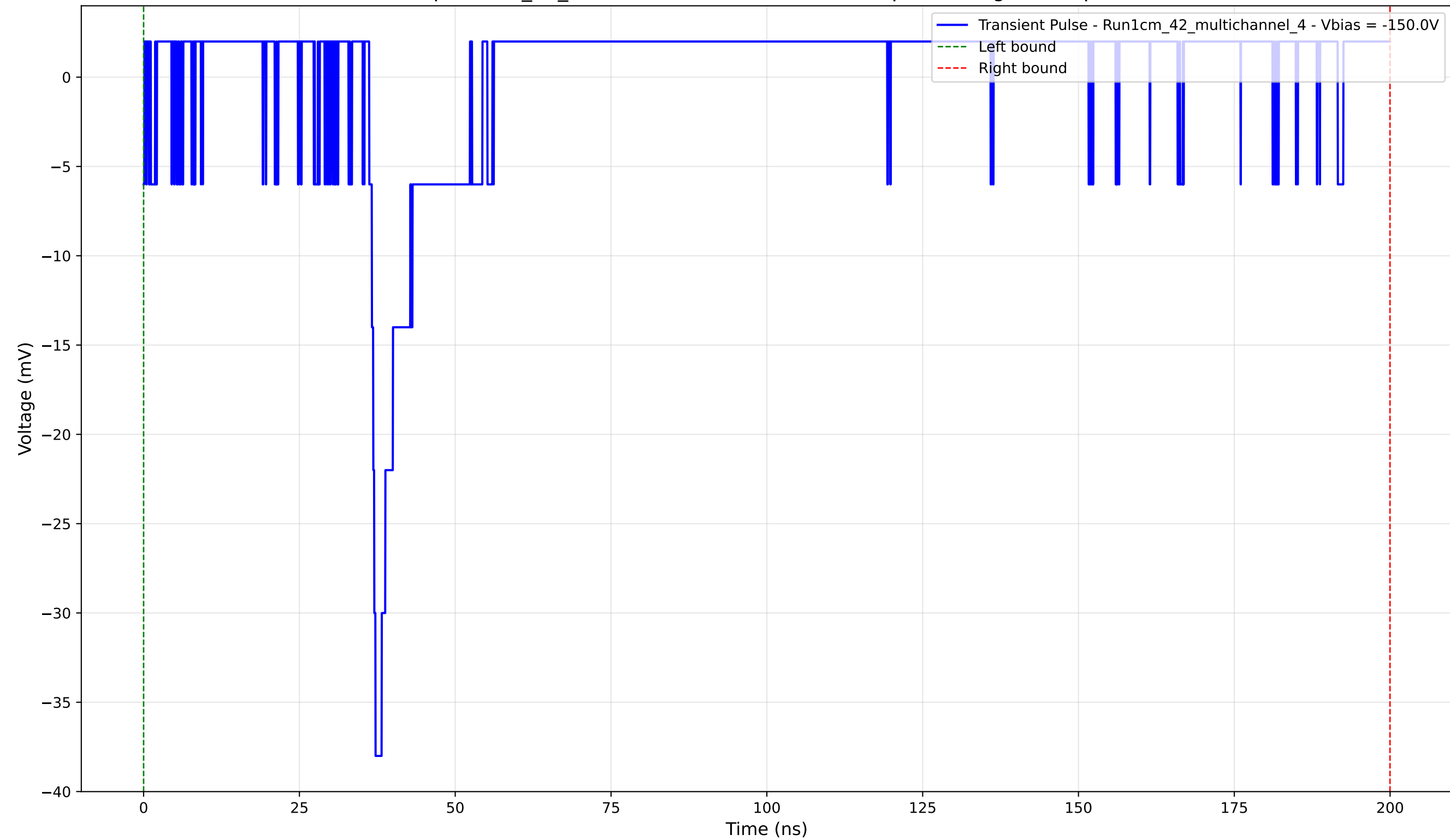
Transient Pulse - Sample: 1cm_42_multichannel - Position: 1800.0 \mu\text{m} - Charge: 1.43 pC - Rise Time: 1.01 ns
