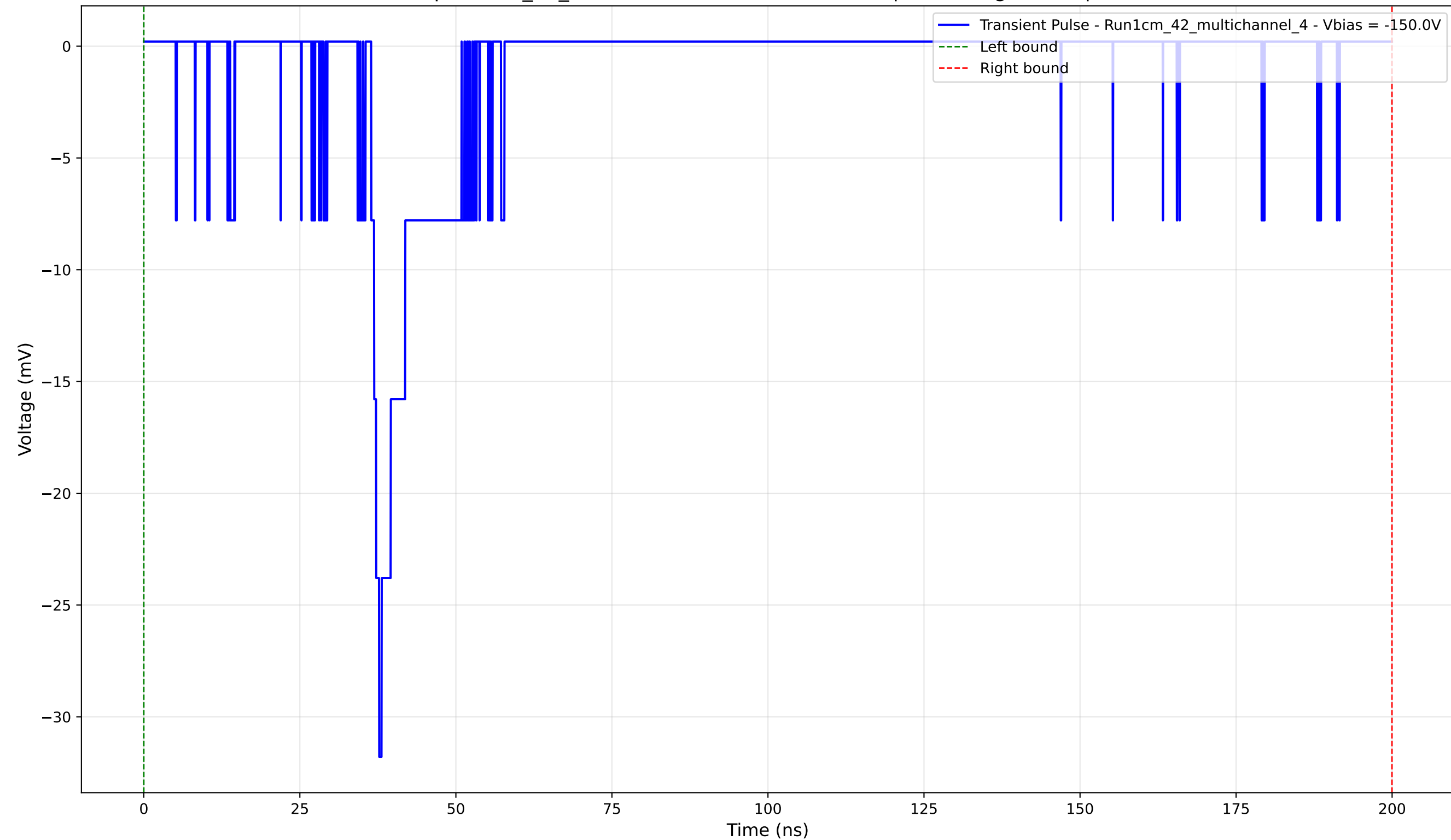
Transient Pulse - Sample: 1cm_42_multichannel - Position: 3175.0 \mu\text{m} - Charge: 3.86 pC - Rise Time: 1.27 ns
