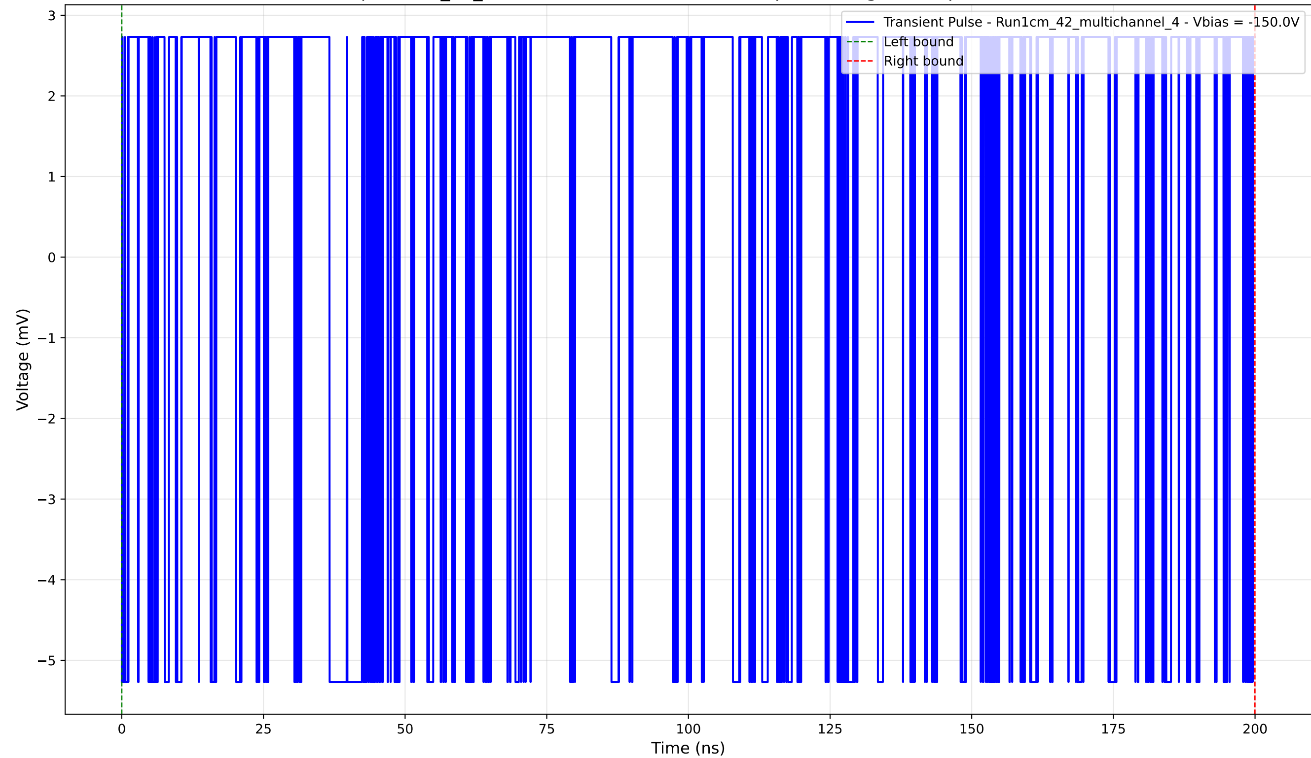
Transient Pulse - Sample: 1cm_42_multichannel - Position: 1855.0 \mu\text{m} - Charge: 4.17 pC - Rise Time: 0.00 ns (N/A)
