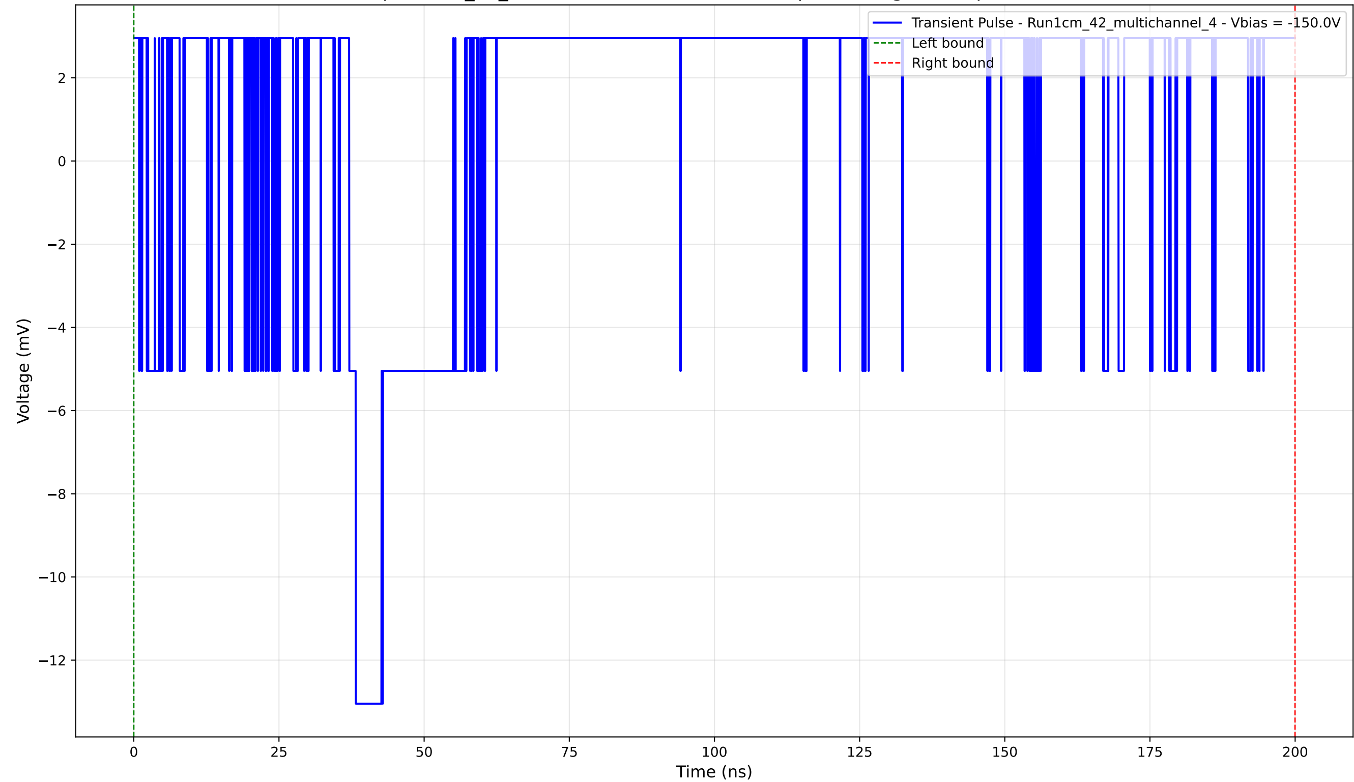
Transient Pulse - Sample: 1cm_42_multichannel - Position: 435.0 \mu\text{m} - Charge: 5.14 pC - Rise Time: 0.00 ns (N/A)
