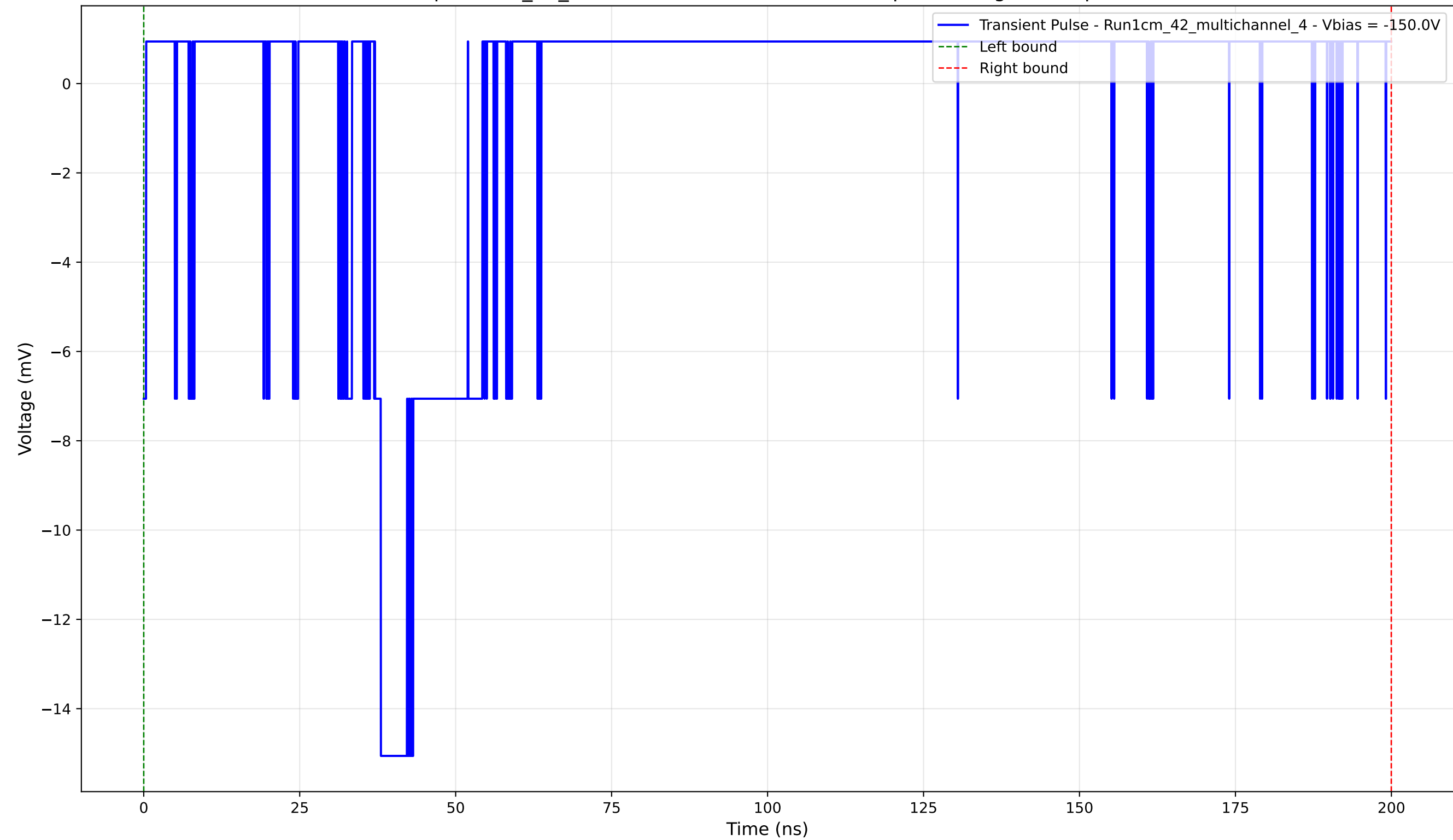
Transient Pulse - Sample: 1cm_42_multichannel - Position: 4085.0 \mu\text{m} - Charge: 0.98 pC - Rise Time: 0.94 ns
