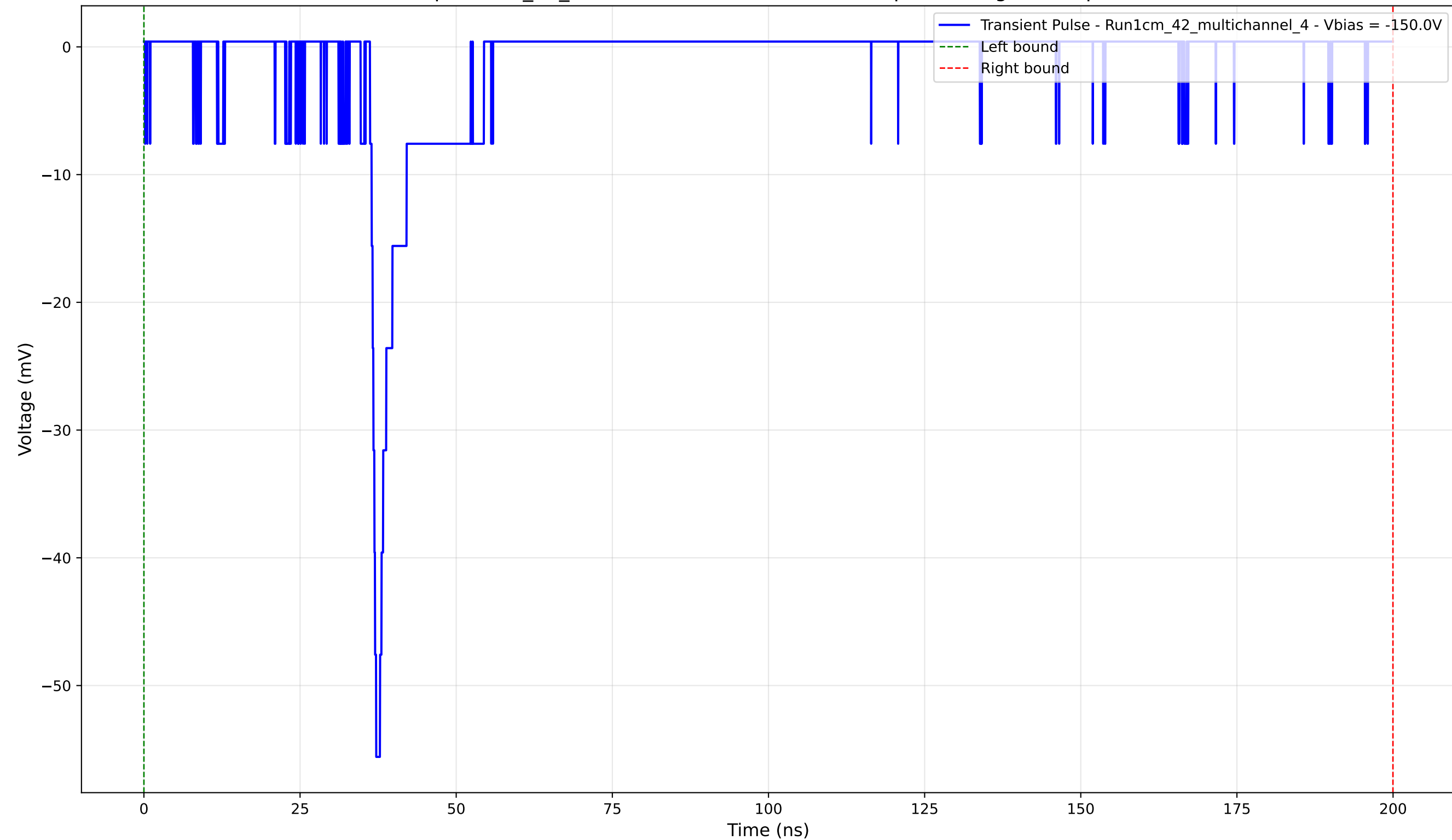
Transient Pulse - Sample: 1cm_42_multichannel - Position: 2025.0 \mu\text{m} - Charge: 4.56 pC - Rise Time: 0.99 ns
