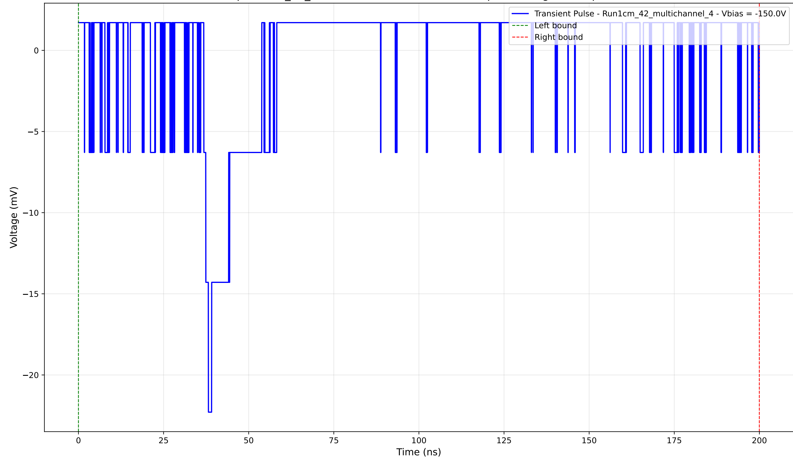
Transient Pulse - Sample: 1cm_42_multichannel - Position: 1085.0 \mu\text{m} - Charge: 0.01 pC - Rise Time: 1.36 ns
