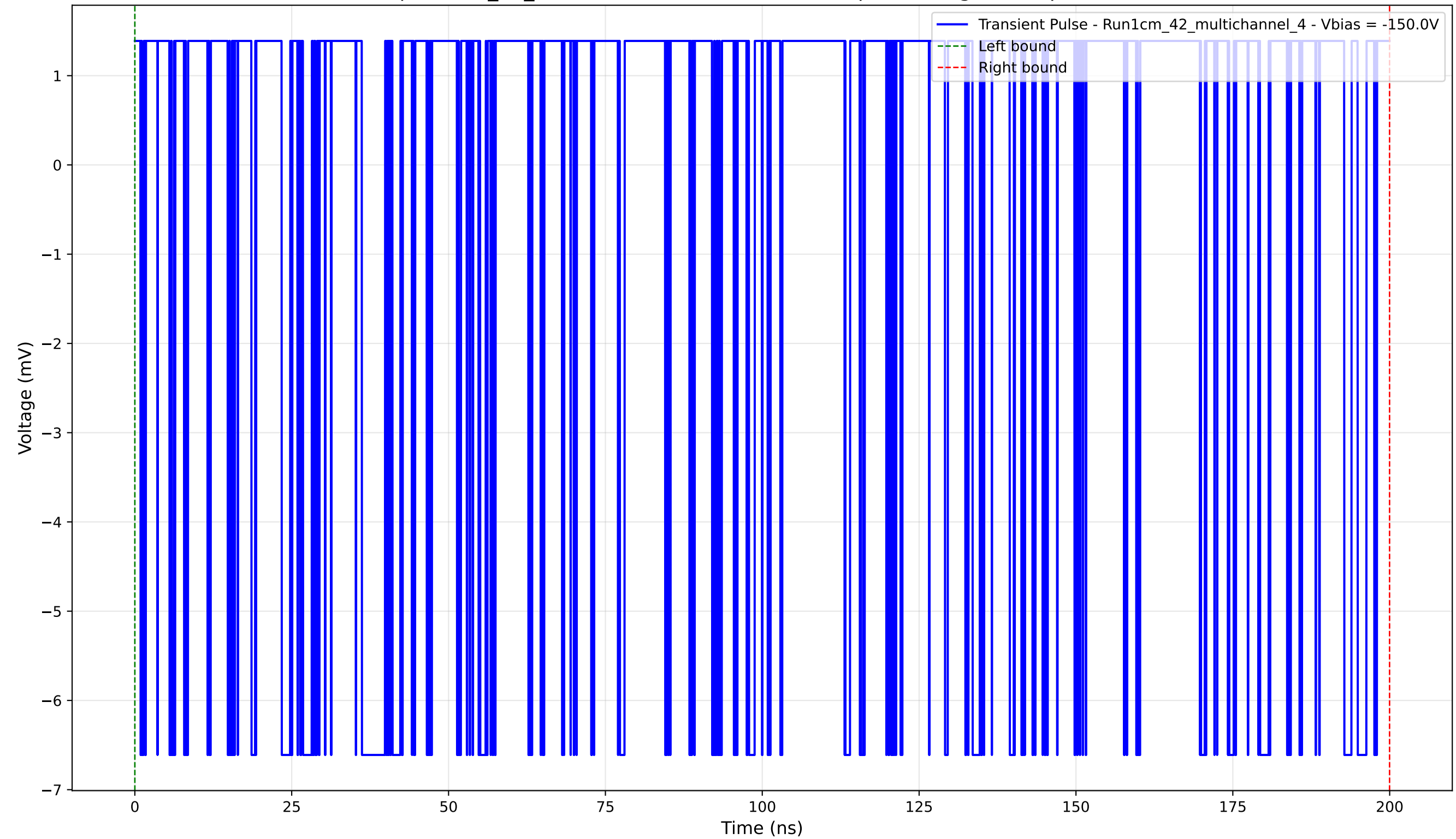
Transient Pulse - Sample: 1cm_42_multichannel - Position: 2370.0 \mu\text{m} - Charge: 0.29 pC - Rise Time: 0.00 ns (N/A)
