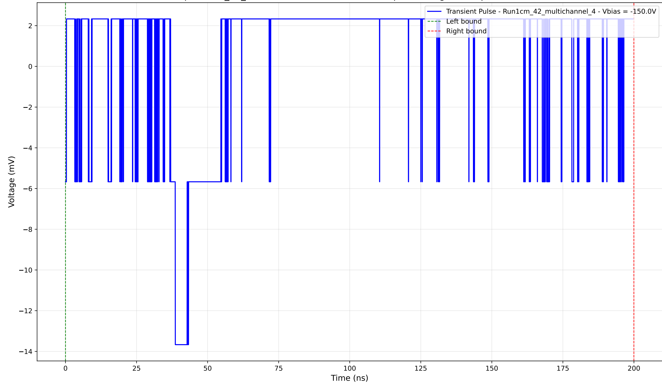
Transient Pulse - Sample: 1cm_42_multichannel - Position: 4510.0 \mu\text{m} - Charge: 3.54 pC - Rise Time: 0.00 ns (N/A)
