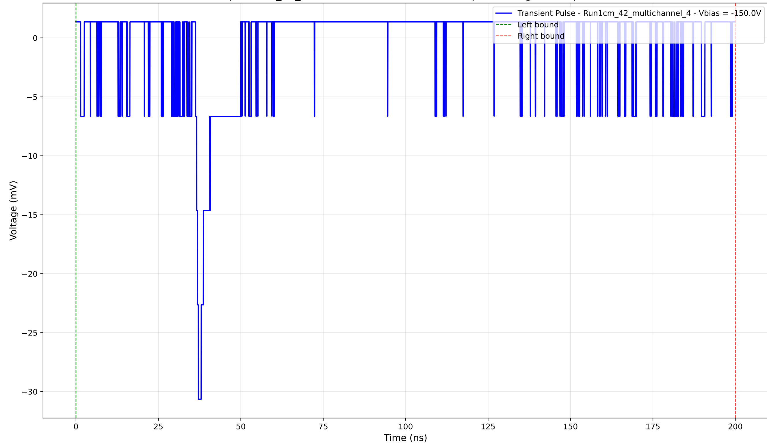
Transient Pulse - Sample: 1cm_42_multichannel - Position: 1935.0 \mu\text{m} - Charge: 0.80 pC - Rise Time: 0.87 ns
