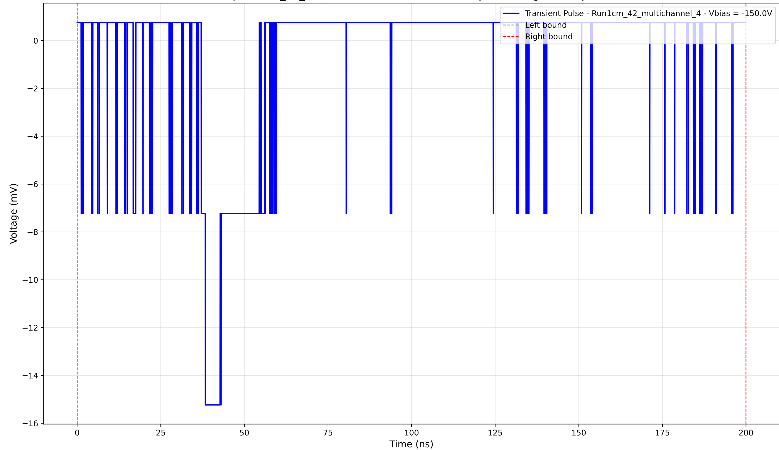
Transient Pulse - Sample: 1cm_42_multichannel - Position: 4630.0 \mu\text{m} - Charge: 1.93 pC - Rise Time: 1.22 ns
