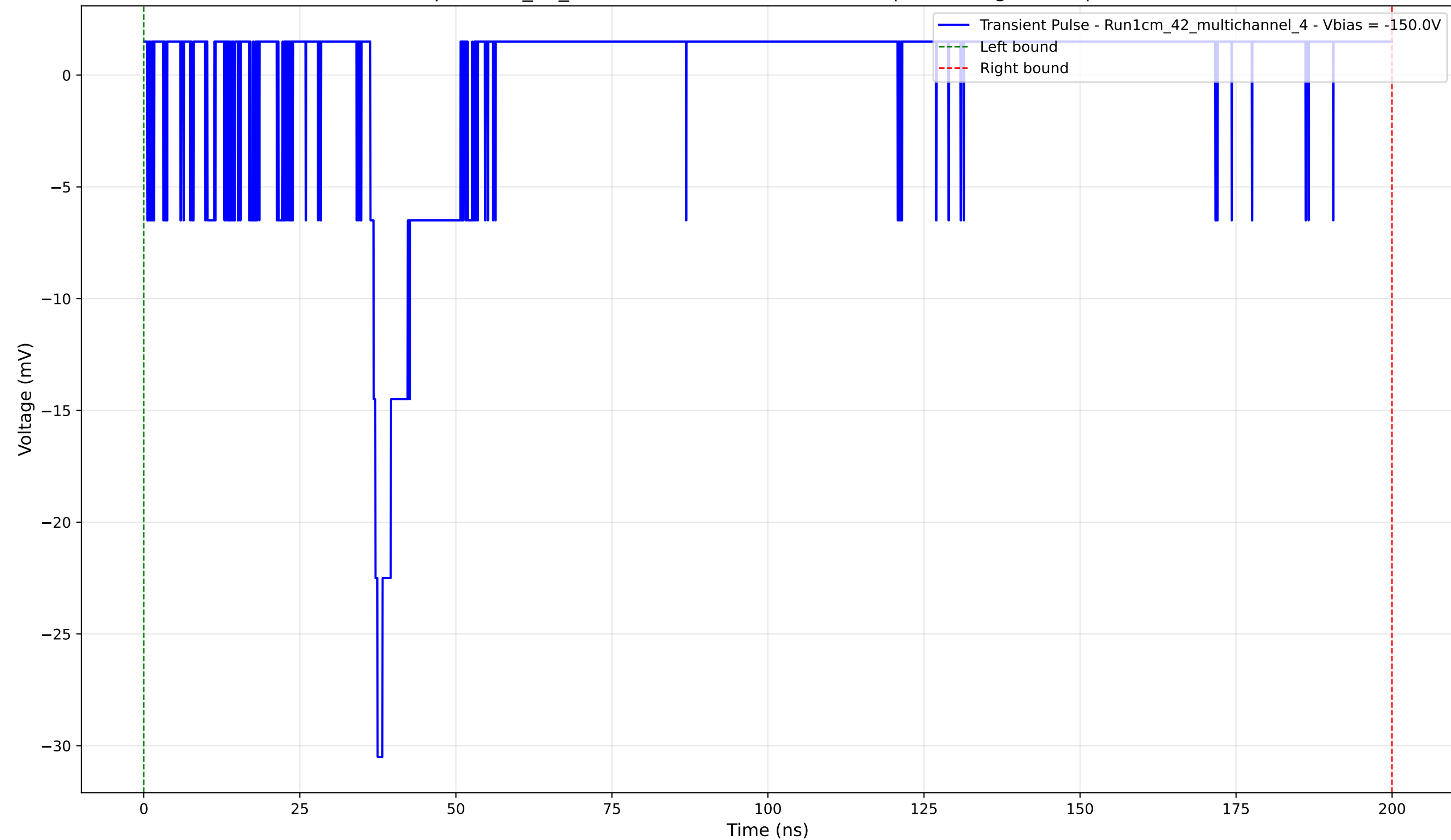
Transient Pulse - Sample: 1cm_42_multichannel - Position: 3145.0 \mu\text{m} - Charge: 0.65 pC - Rise Time: 1.15 ns
