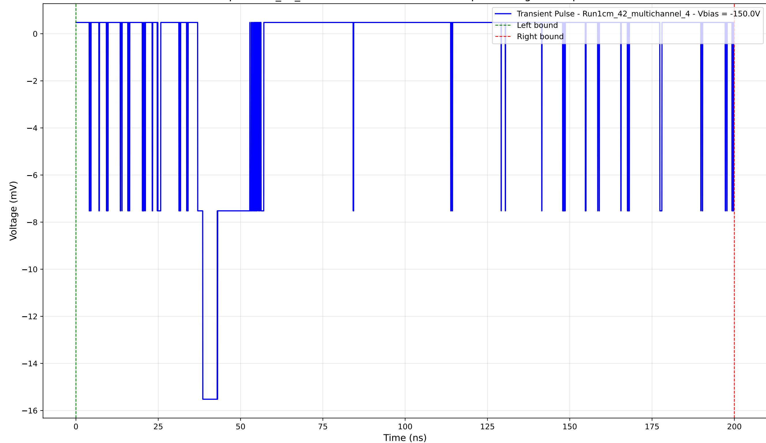
Transient Pulse - Sample: 1cm_42_multichannel - Position: 4260.0 \mu\text{m} - Charge: 2.75 pC - Rise Time: 1.56 ns
