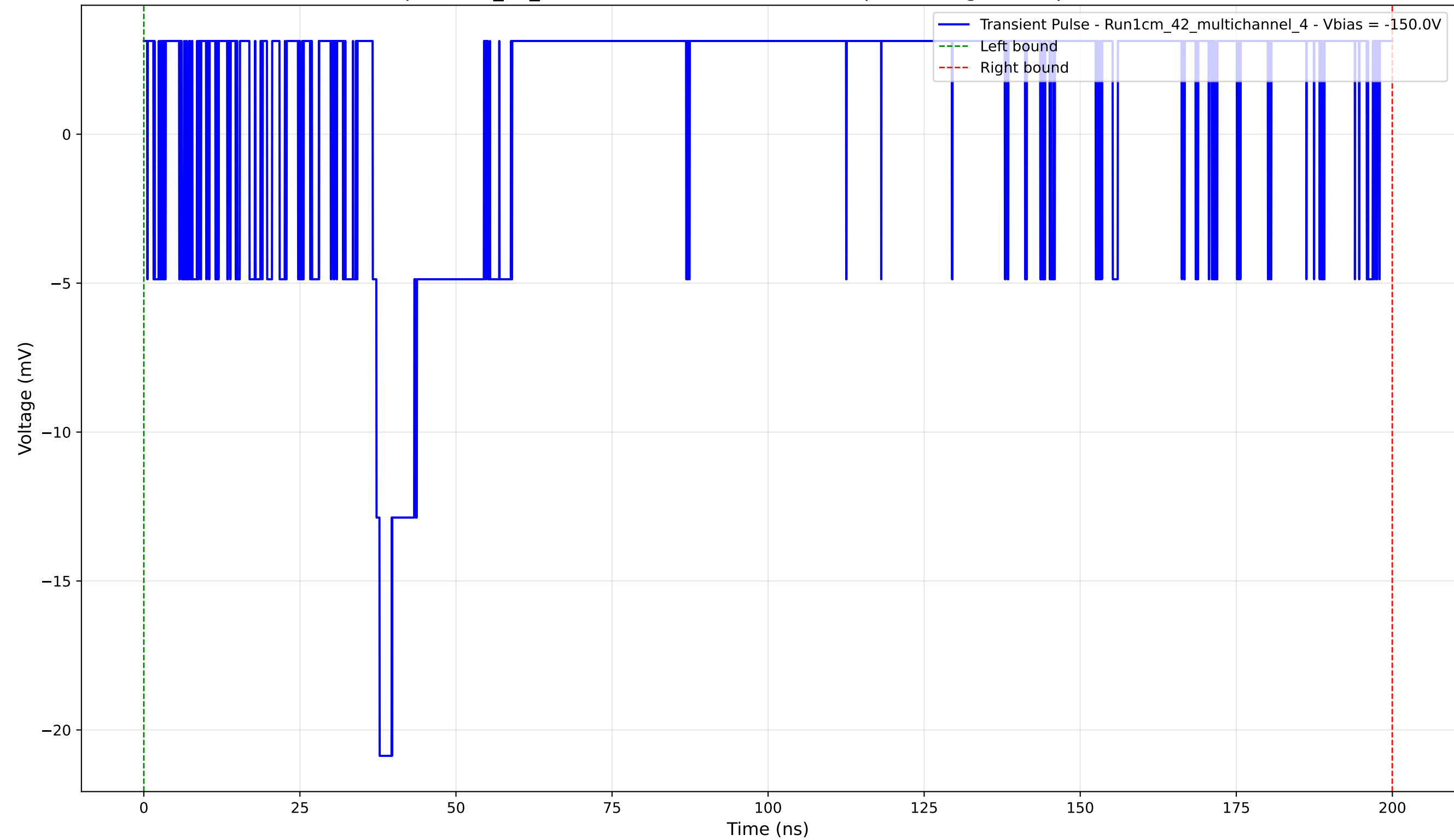
Transient Pulse - Sample: 1cm_42_multichannel - Position: 1180.0 \mu\text{m} - Charge: 4.57 pC - Rise Time: 0.00 ns (N/A)
