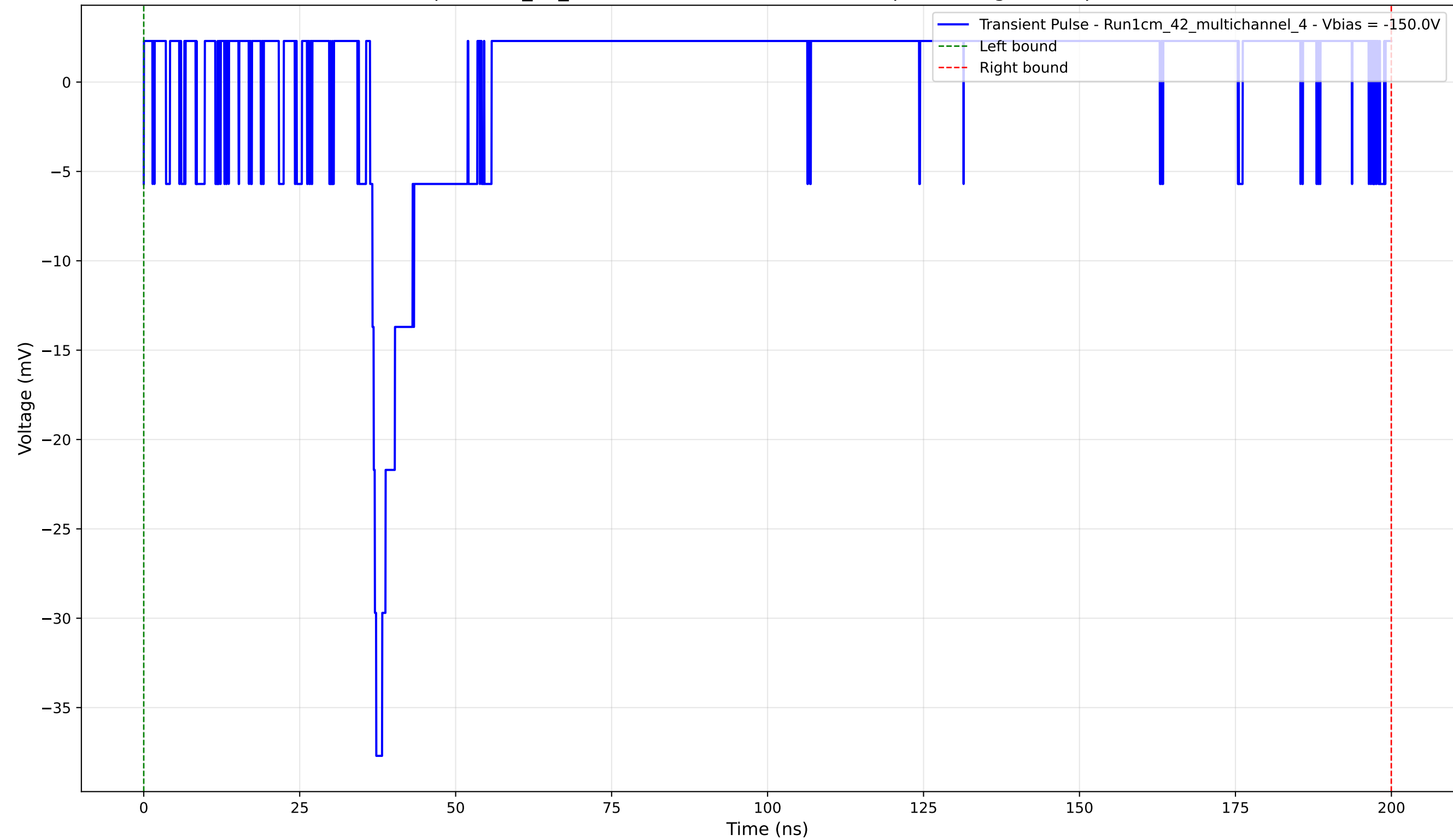
Transient Pulse - Sample: 1cm_42_multichannel - Position: 1750.0 \mu\text{m} - Charge: 2.27 pC - Rise Time: 0.99 ns
