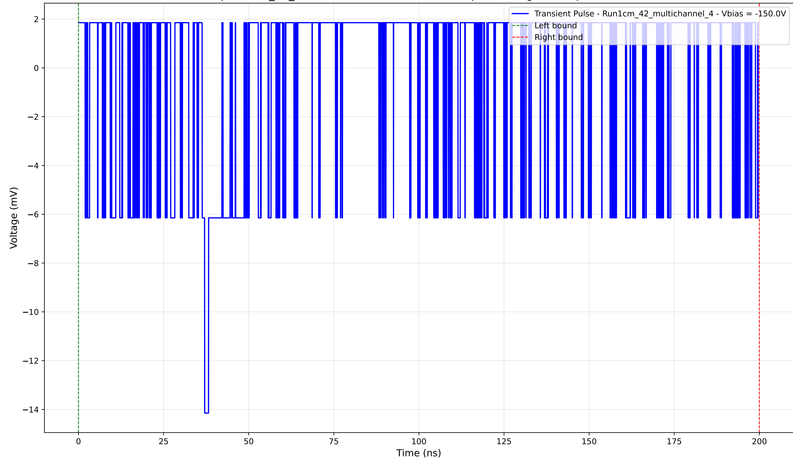
Transient Pulse - Sample: 1cm_42_multichannel - Position: 1920.0 \mu\text{m} - Charge: 0.57 pC - Rise Time: 0.00 ns (N/A)
