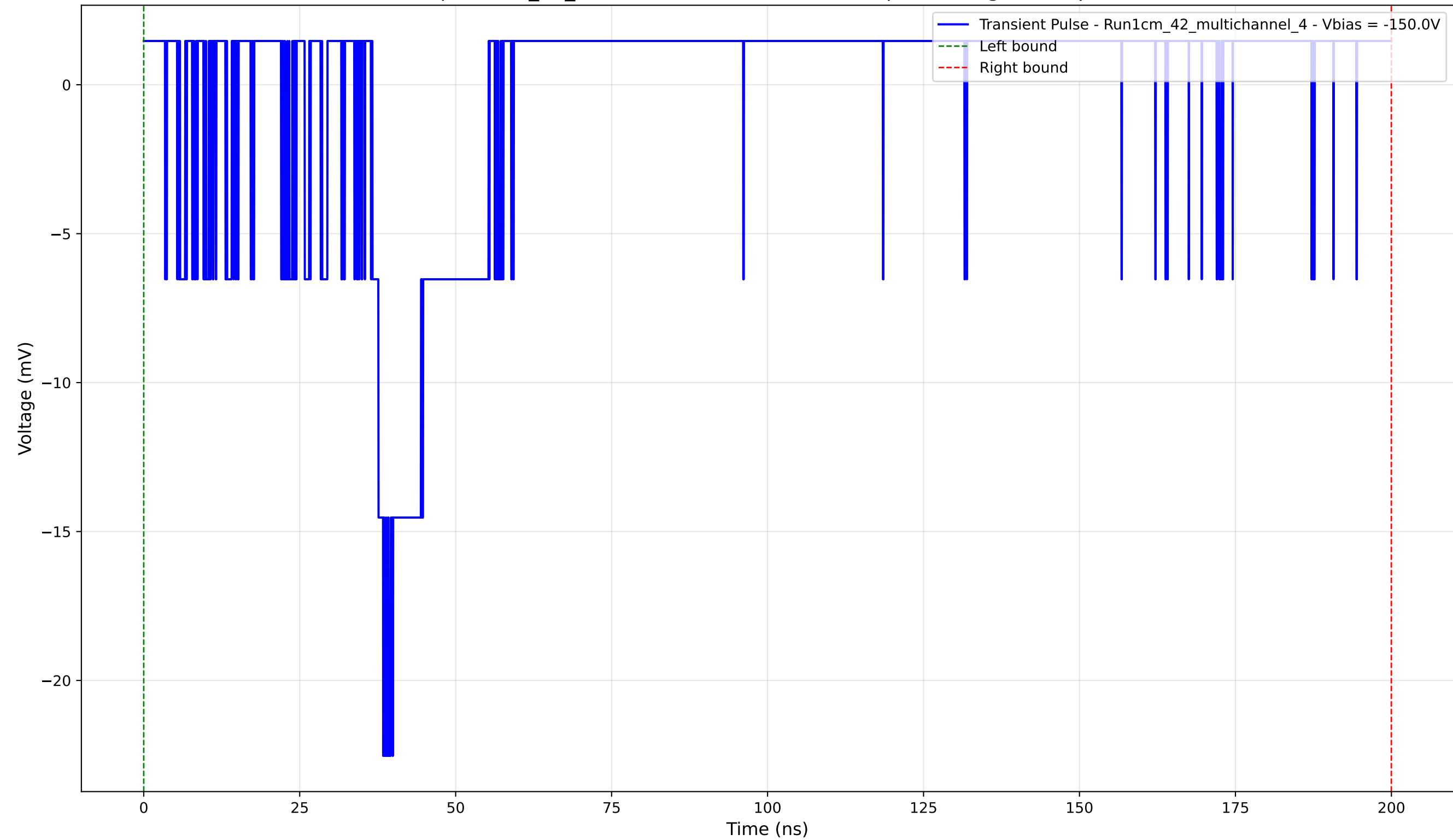
Transient Pulse - Sample: 1cm_42_multichannel - Position: 970.0 \mu\text{m} - Charge: 0.22 pC - Rise Time: 1.74 ns
