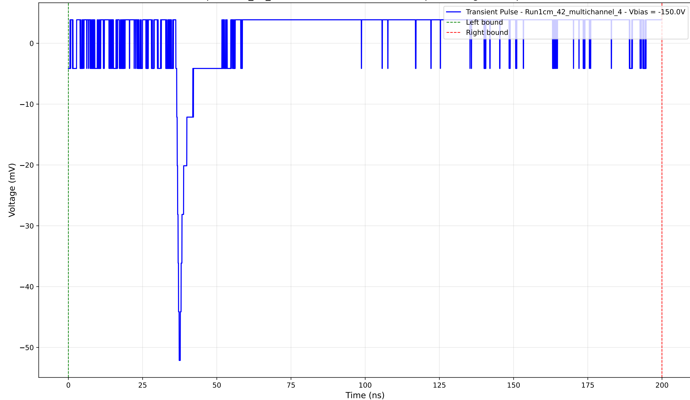
Transient Pulse - Sample: 1cm_42_multichannel - Position: 1965.0 \mu\text{m} - Charge: 7.23 pC - Rise Time: 0.84 ns
