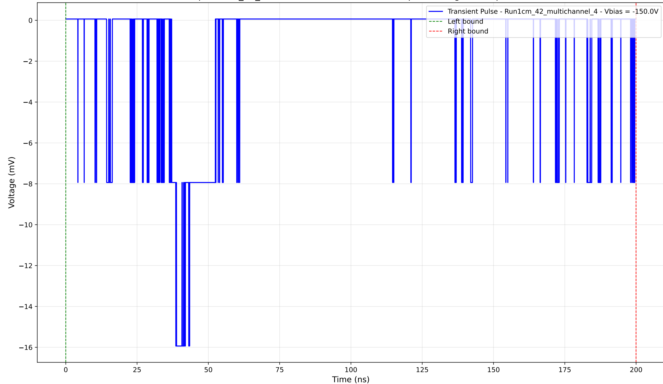
Transient Pulse - Sample: 1cm_42_multichannel - Position: 4800.0 \mu\text{m} - Charge: 4.59 pC - Rise Time: 1.44 ns
