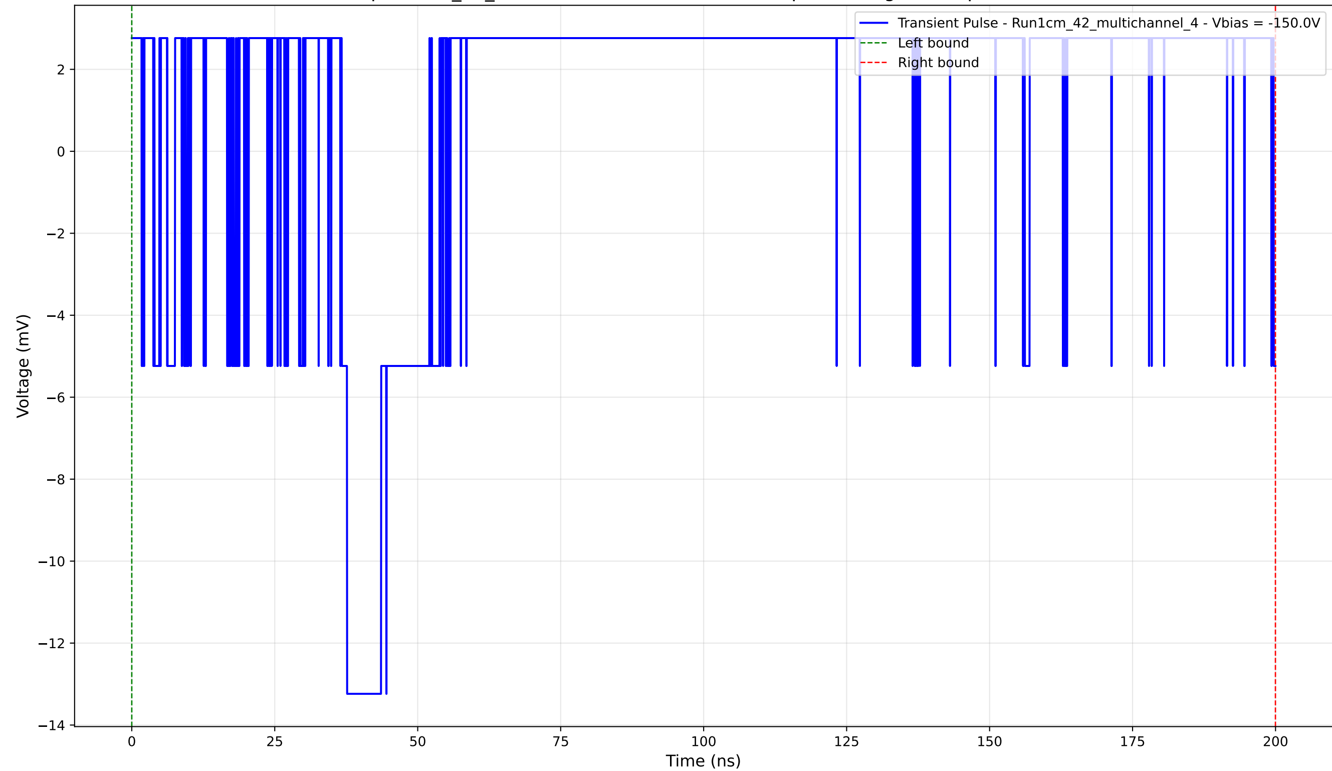
Transient Pulse - Sample: 1cm_42_multichannel - Position: 3780.0 \mu\text{m} - Charge: 5.49 pC - Rise Time: 0.00 ns (N/A)
