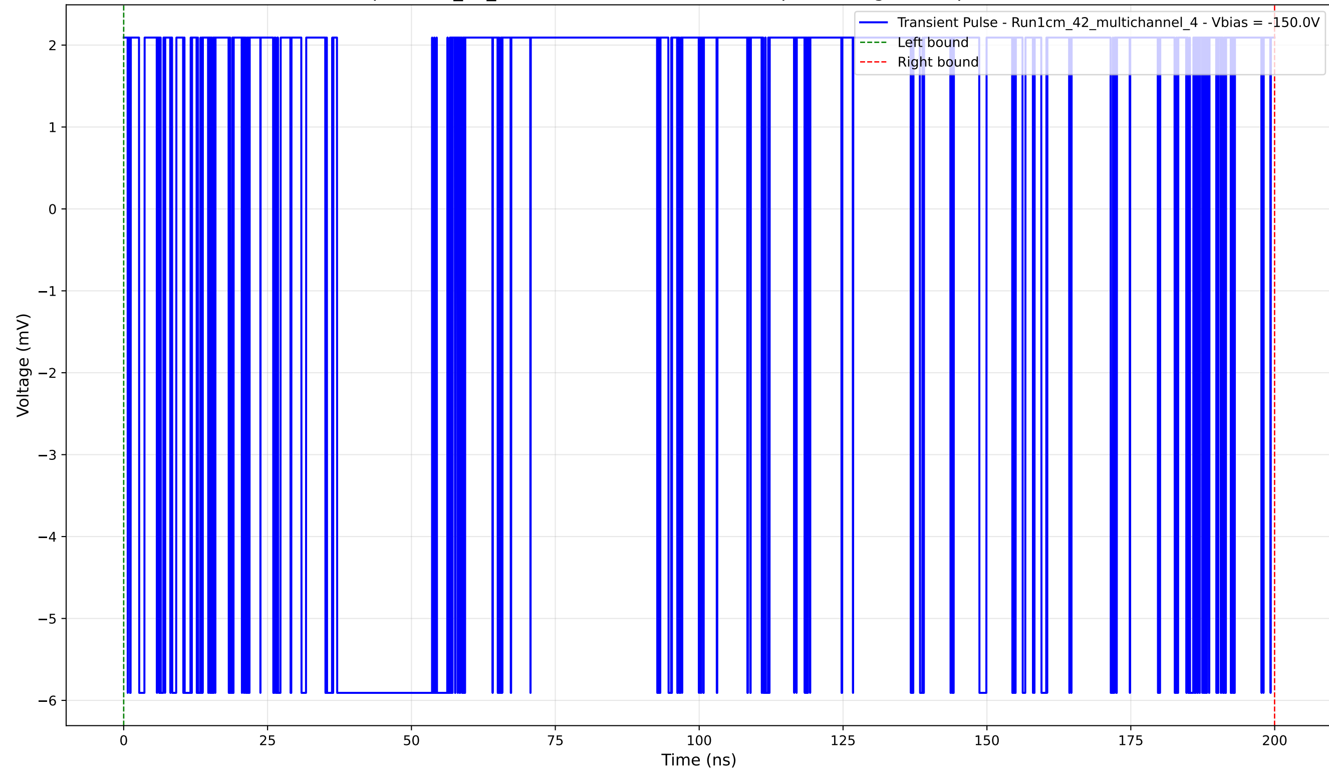
Transient Pulse - Sample: 1cm_42_multichannel - Position: 415.0 \mu\text{m} - Charge: 1.46 pC - Rise Time: 0.00 ns (N/A)
