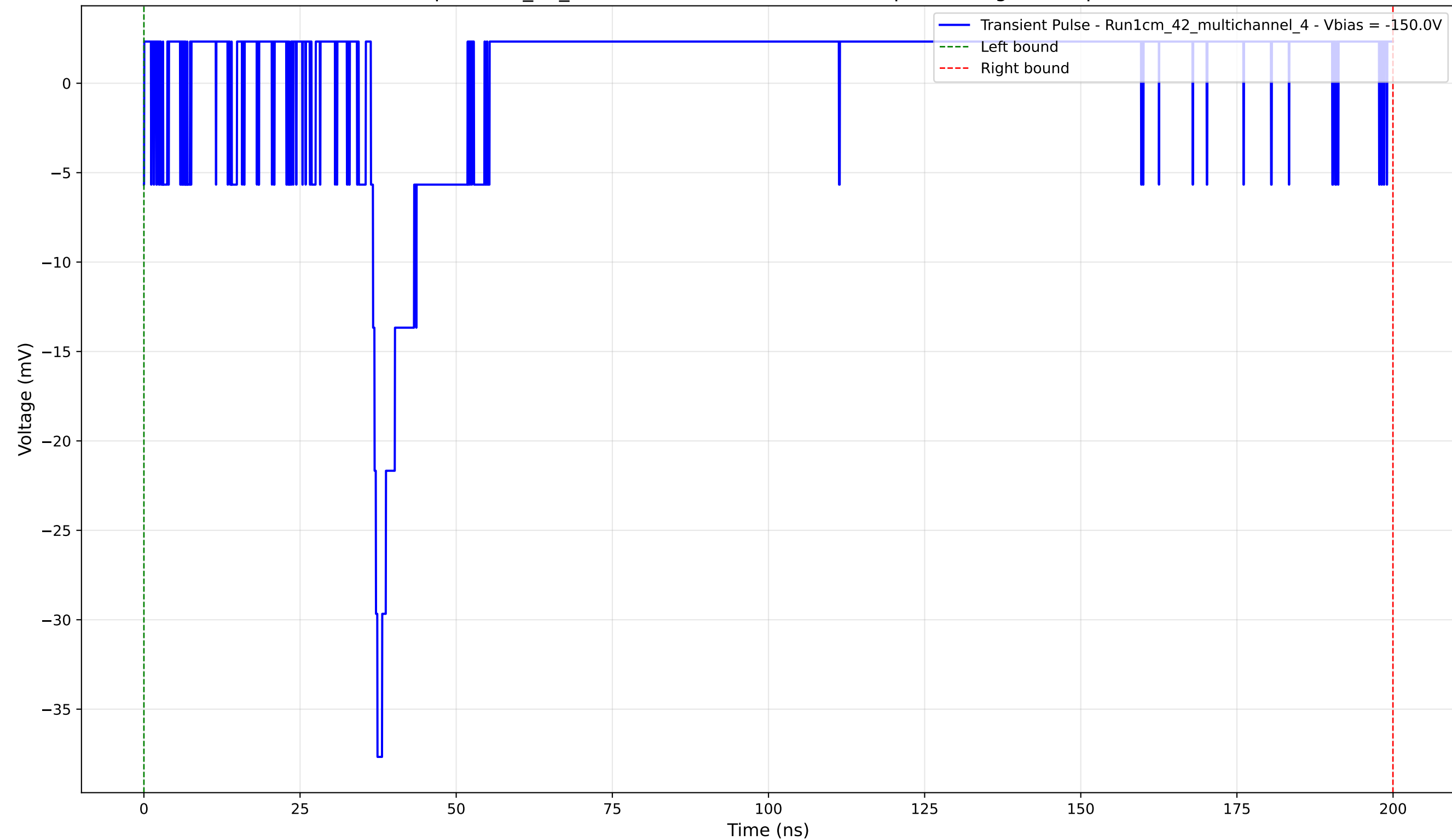
Transient Pulse - Sample: 1cm_42_multichannel - Position: 1715.0 \mu\text{m} - Charge: 2.97 pC - Rise Time: 1.05 ns
