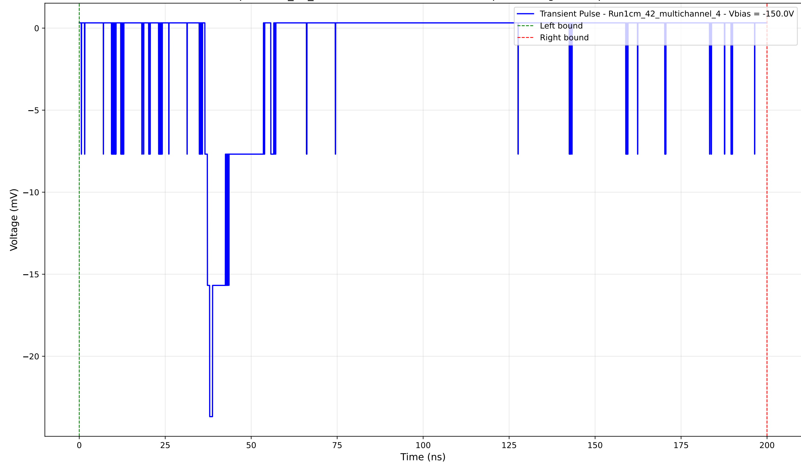
Transient Pulse - Sample: 1cm_42_multichannel - Position: 3560.0 \mu\text{m} - Charge: 3.41 pC - Rise Time: 1.39 ns
