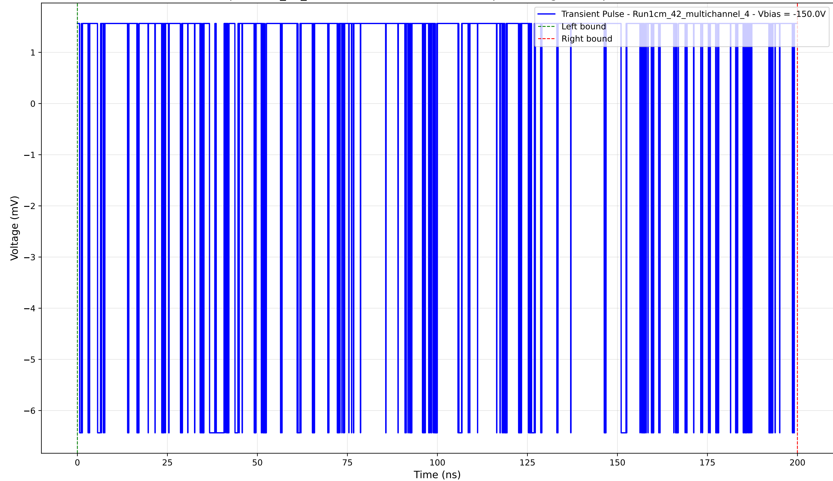
Transient Pulse - Sample: 1cm_42_multichannel - Position: 2395.0 \mu\text{m} - Charge: 1.91 pC - Rise Time: 0.00 ns (N/A)
