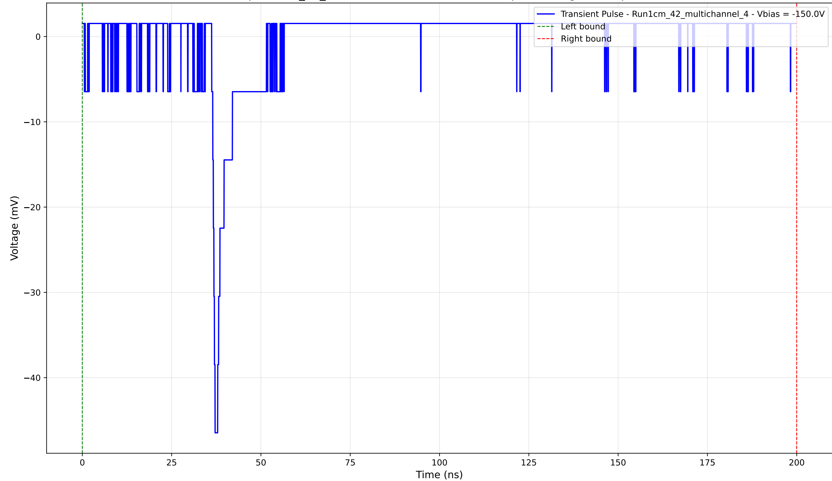
Transient Pulse - Sample: 1cm_42_multichannel - Position: 2800.0 \mu\text{m} - Charge: 0.11 pC - Rise Time: 0.95 ns
