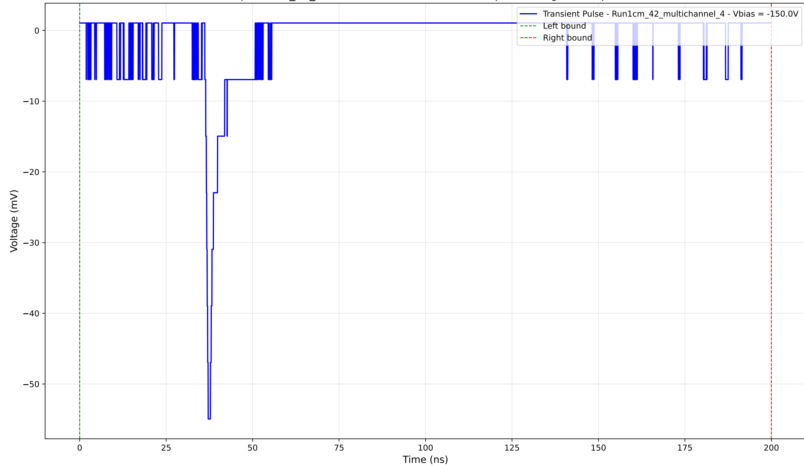
Transient Pulse - Sample: 1cm_42_multichannel - Position: 2045.0 \mu\text{m} - Charge: 2.58 pC - Rise Time: 0.96 ns
