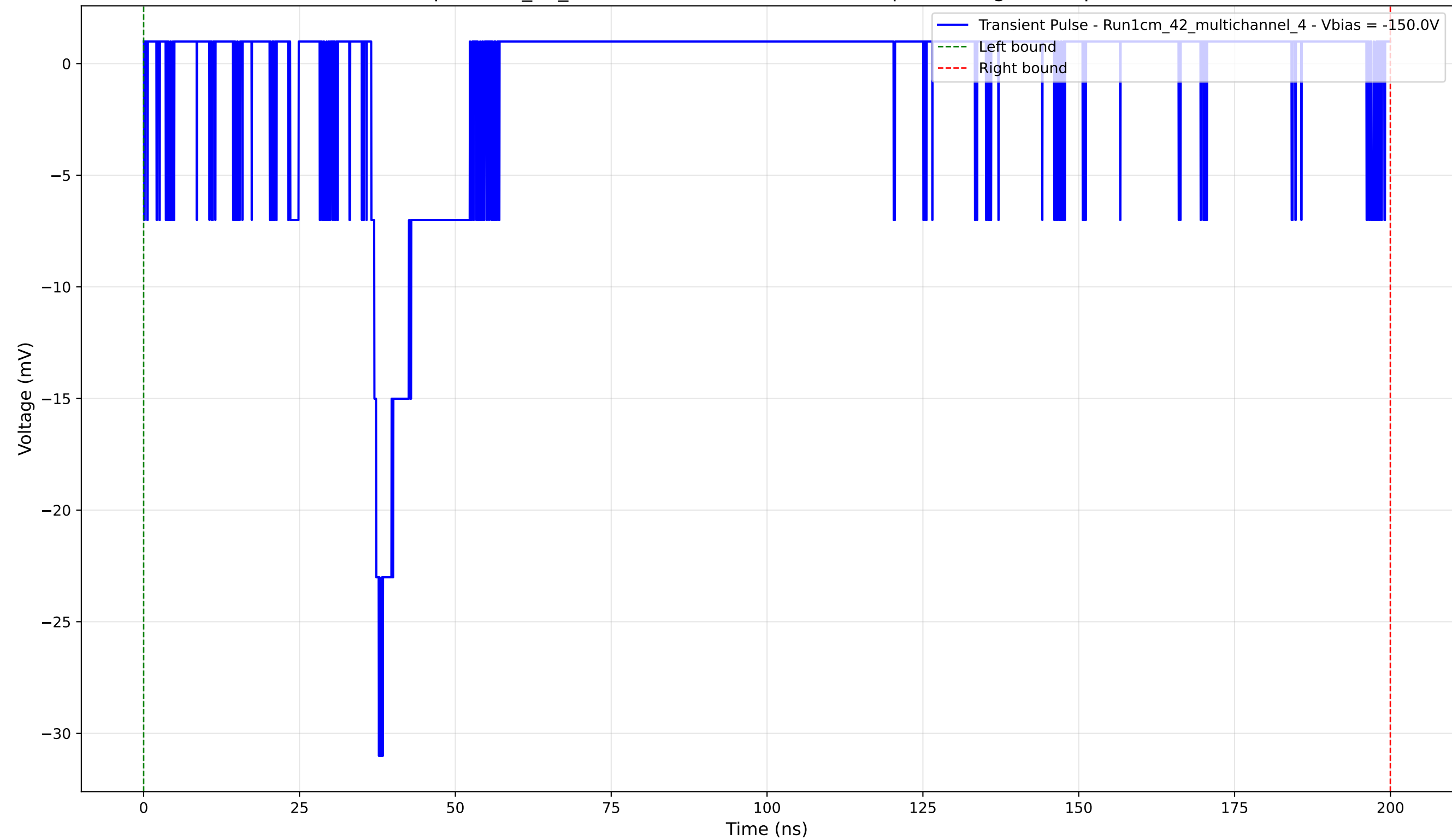
Transient Pulse - Sample: 1cm_42_multichannel - Position: 3295.0 \mu\text{m} - Charge: 2.04 pC - Rise Time: 1.21 ns
