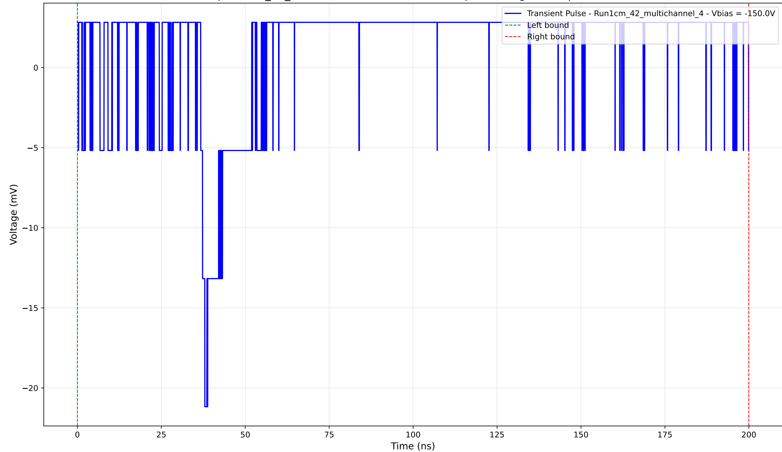
Transient Pulse - Sample: 1cm_42_multichannel - Position: 3555.0 \mu\text{m} - Charge: 5.69 pC - Rise Time: 0.00 ns (N/A)
