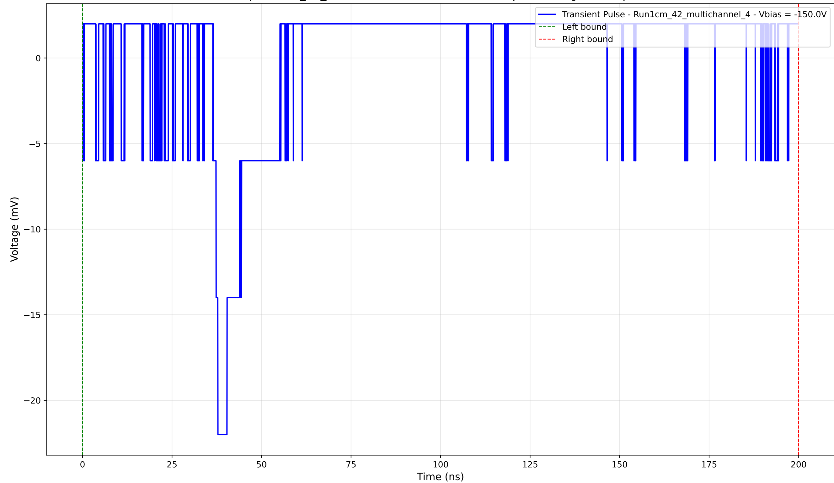
Transient Pulse - Sample: 1cm_42_multichannel - Position: 1175.0 \mu\text{m} - Charge: 1.21 pC - Rise Time: 1.26 ns
