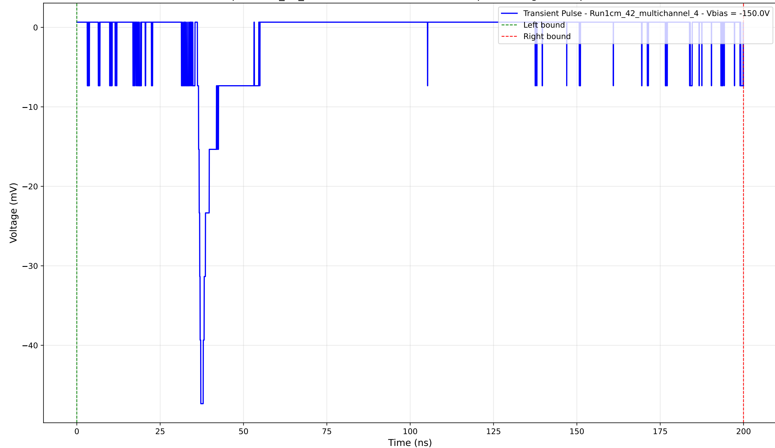
Transient Pulse - Sample: 1cm_42_multichannel - Position: 2795.0 \mu\text{m} - Charge: 3.73 pC - Rise Time: 1.01 ns
