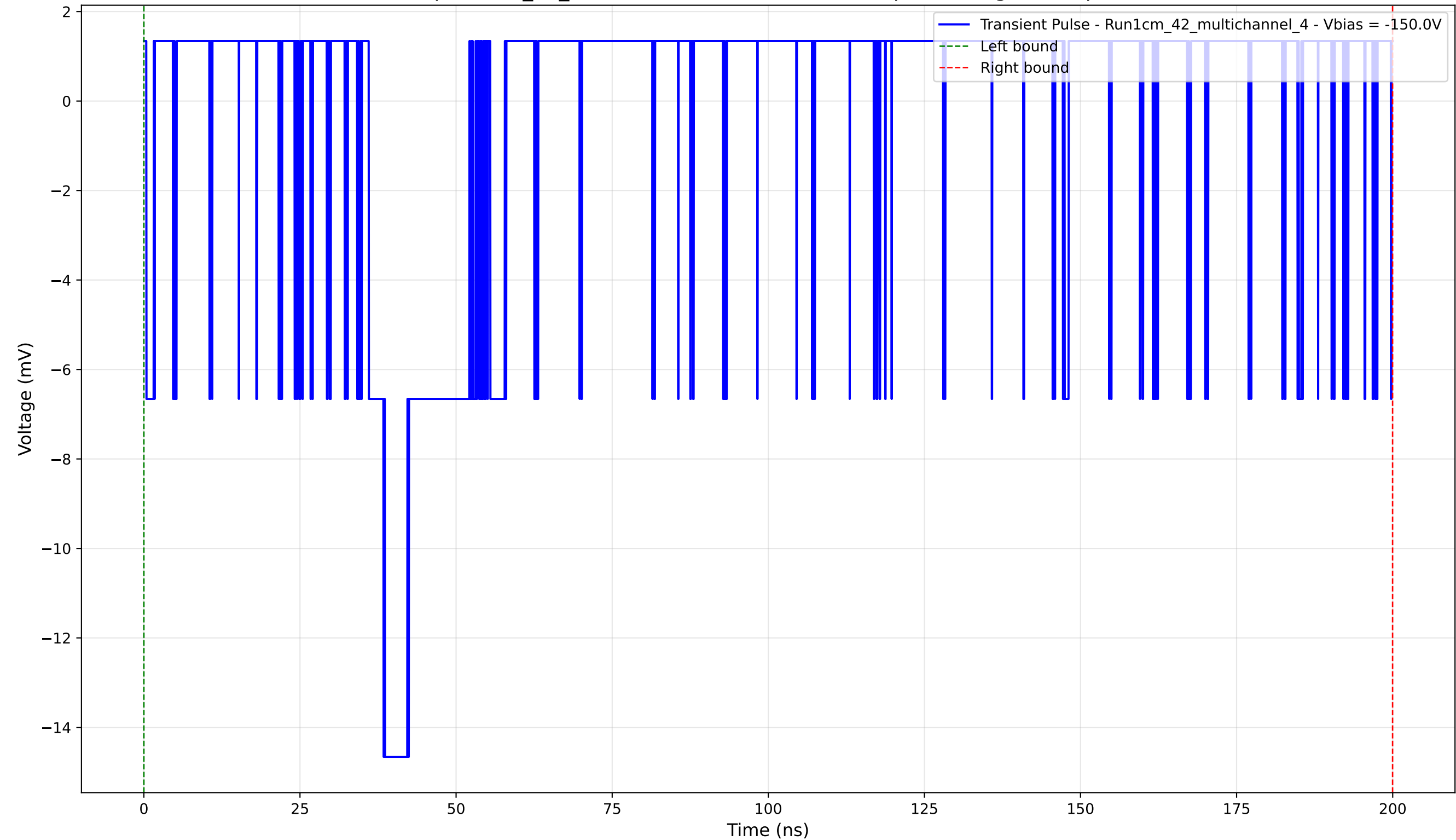
Transient Pulse - Sample: 1cm_42_multichannel - Position: 4795.0 \mu\text{m} - Charge: 0.31 pC - Rise Time: 2.38 ns
