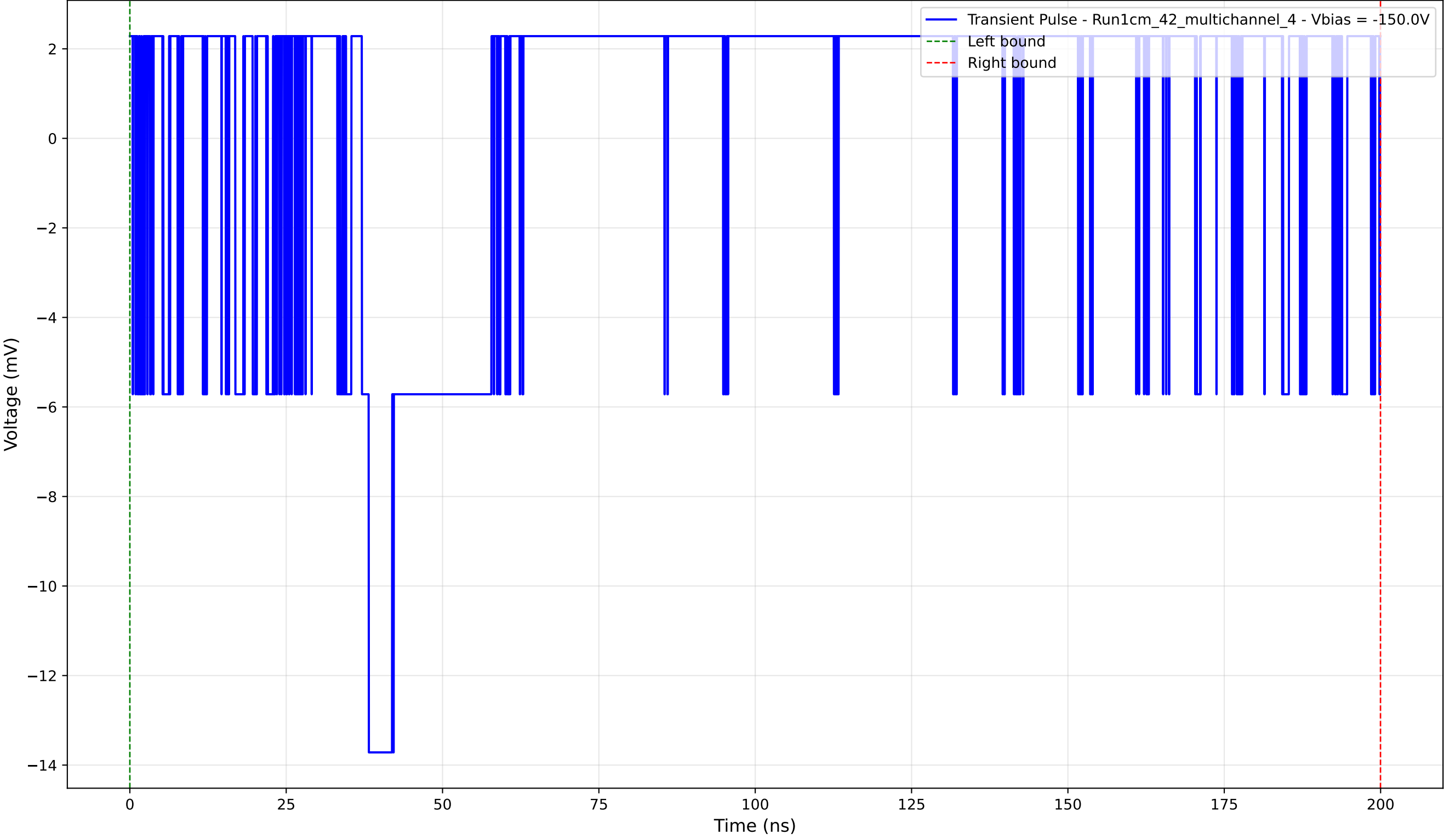
Transient Pulse - Sample: 1cm_42_multichannel - Position: 225.0 \mu\text{m} - Charge: 2.03 pC - Rise Time: 0.00 ns (N/A)
