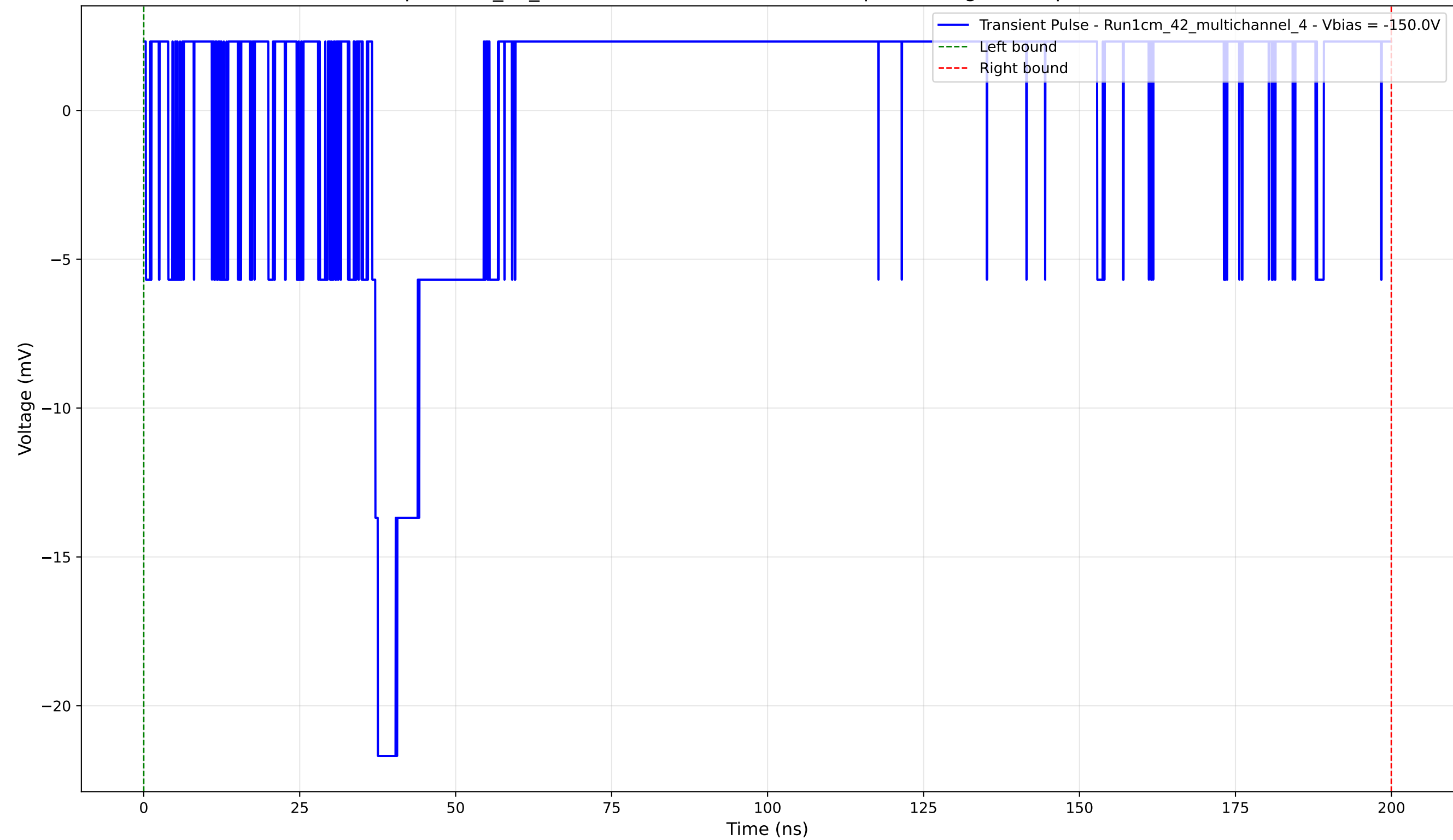
Transient Pulse - Sample: 1cm_42_multichannel - Position: 1275.0 \mu\text{m} - Charge: 2.08 pC - Rise Time: 0.00 ns (N/A)
