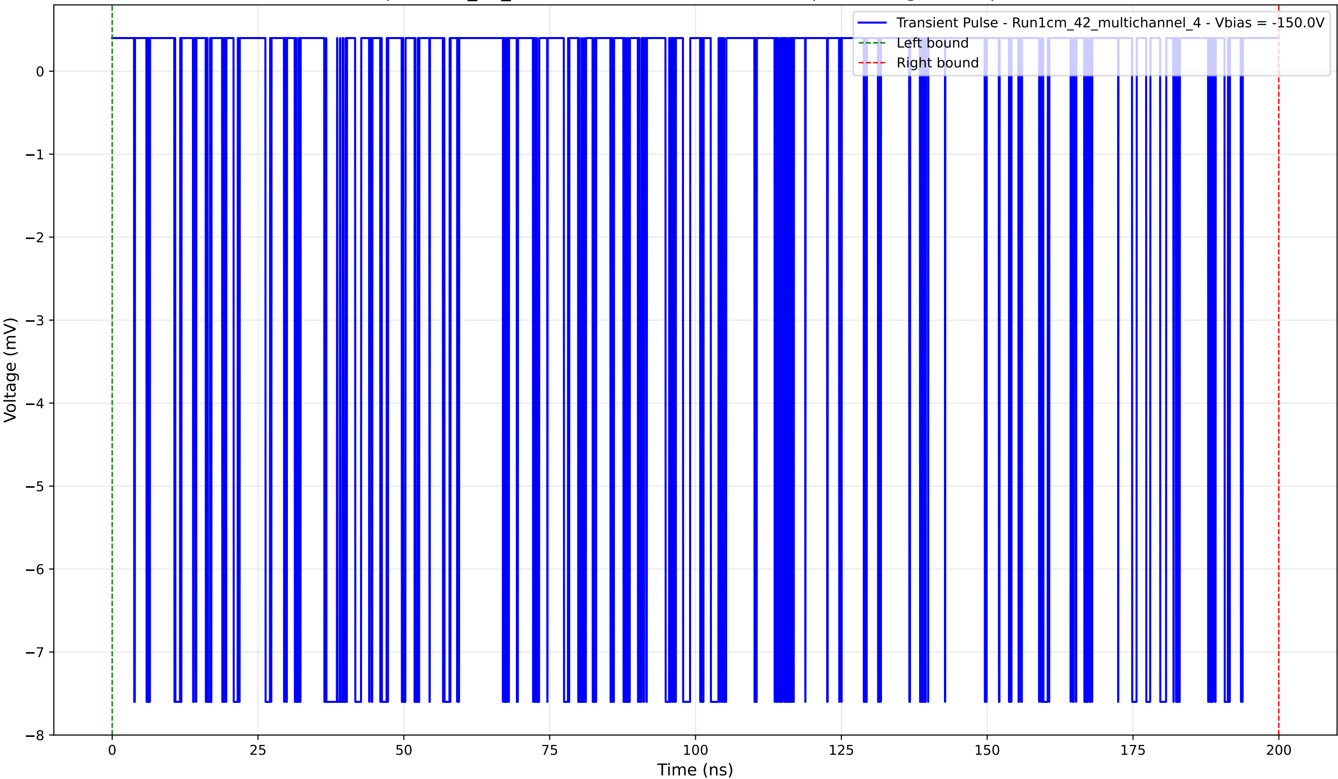
Transient Pulse - Sample: 1cm_42_multichannel - Position: 1895.0 \mu\text{m} - Charge: 3.81 pC - Rise Time: 0.02 ns
