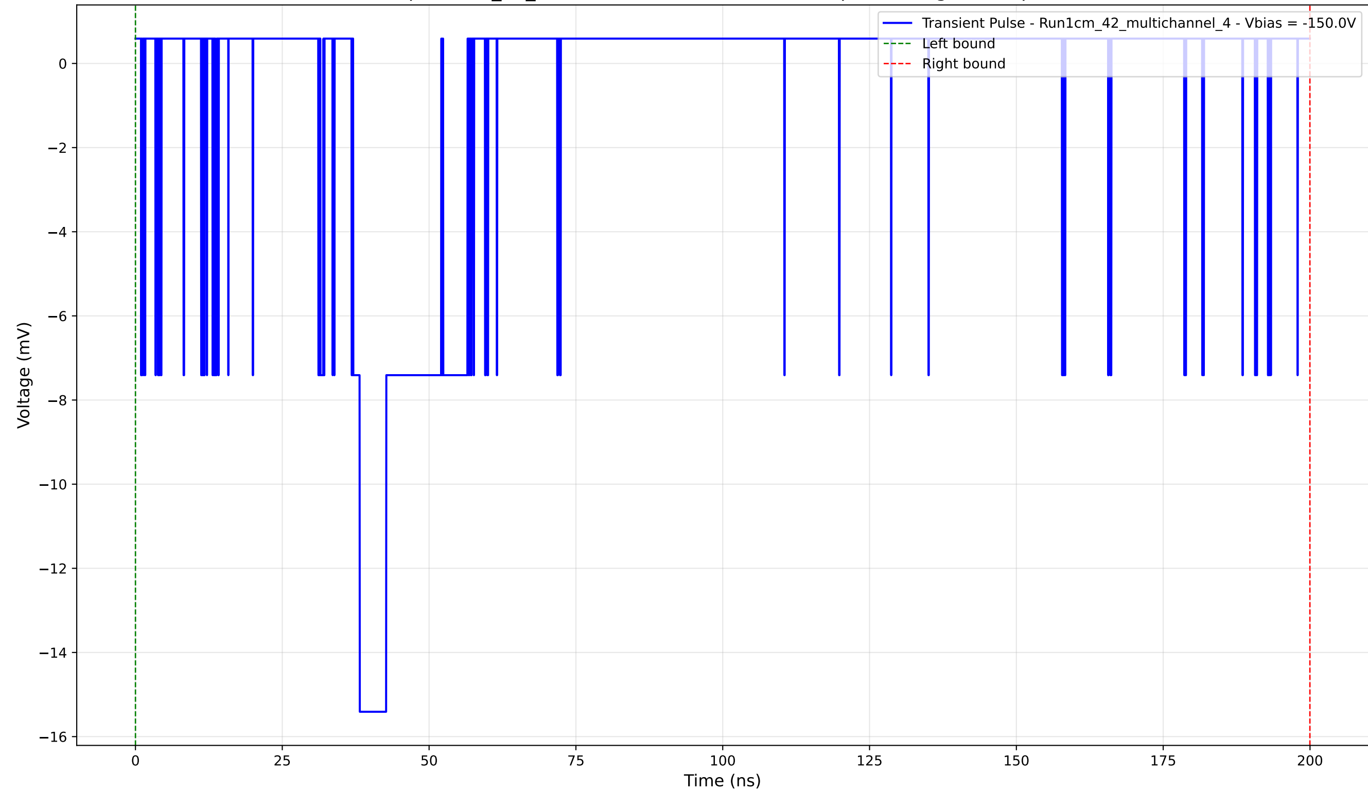
Transient Pulse - Sample: 1cm_42_multichannel - Position: 4135.0 \mu\text{m} - Charge: 2.32 pC - Rise Time: 1.12 ns
