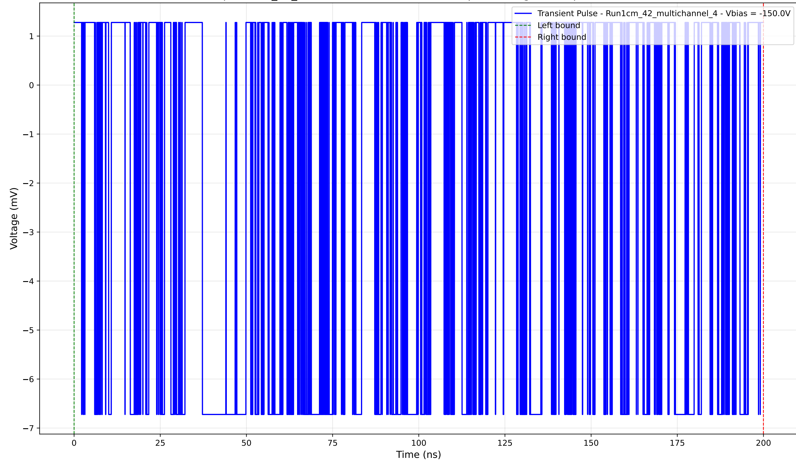
Transient Pulse - Sample: 1cm_42_multichannel - Position: 330.0 \mu\text{m} - Charge: 7.39 pC - Rise Time: 0.00 ns (N/A)
