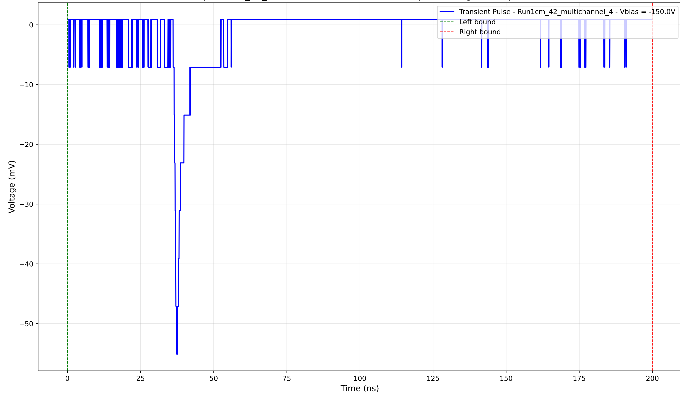
Transient Pulse - Sample: 1cm_42_multichannel - Position: 2780.0 \mu\text{m} - Charge: 3.02 pC - Rise Time: 1.23 ns
