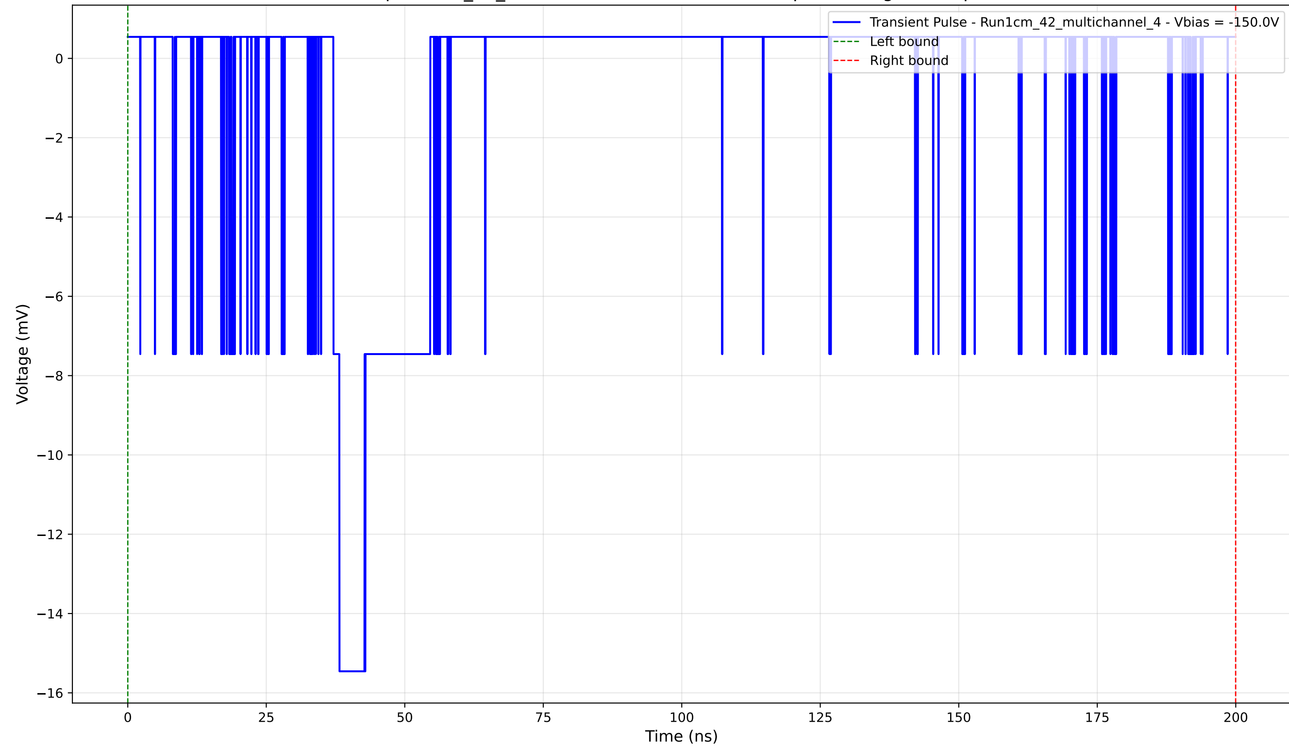
Transient Pulse - Sample: 1cm_42_multichannel - Position: 4545.0 \mu\text{m} - Charge: 2.88 pC - Rise Time: 1.10 ns
