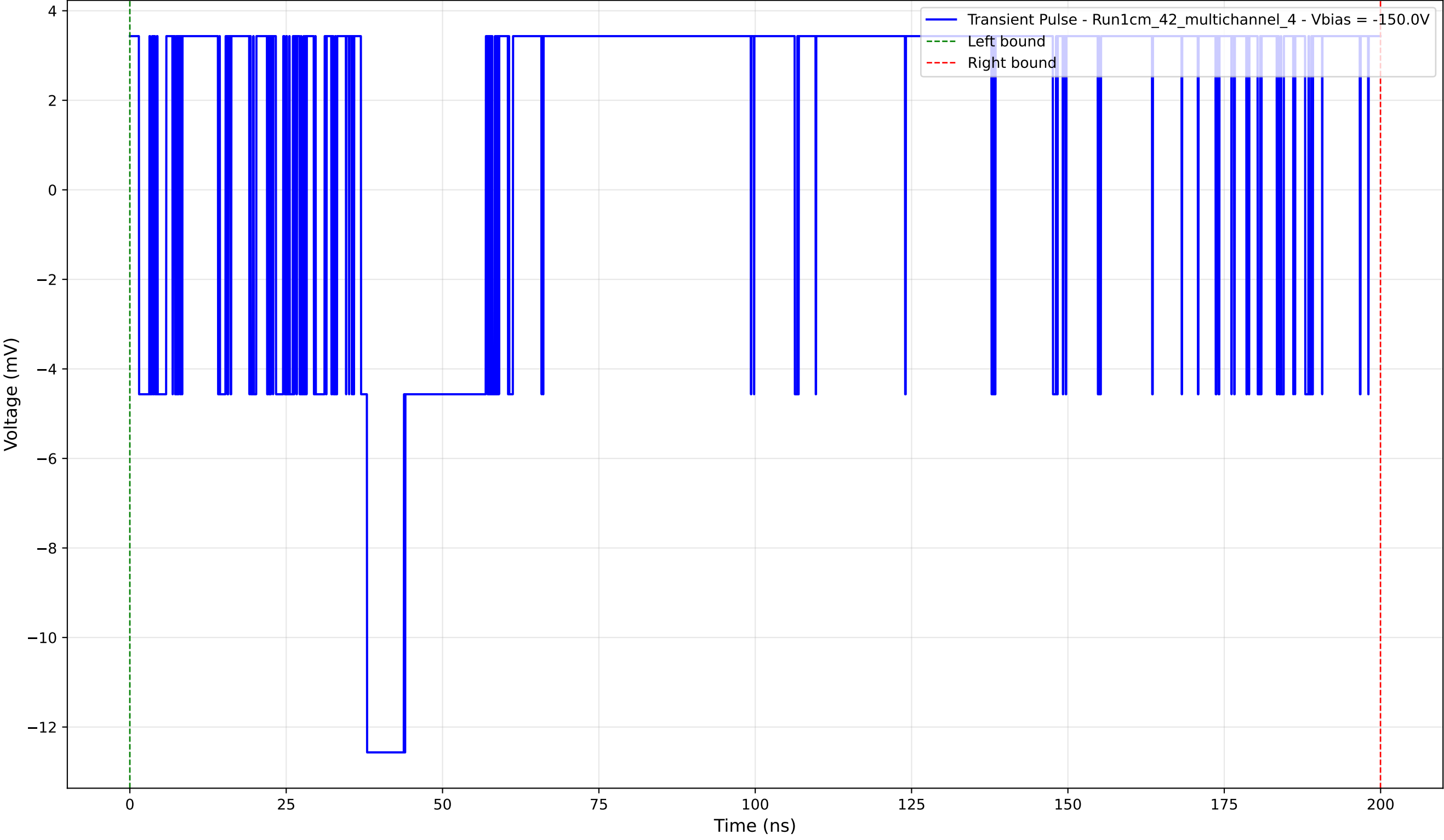
Transient Pulse - Sample: 1cm_42_multichannel - Position: 635.0 \mu\text{m} - Charge: 6.28 pC - Rise Time: 0.00 ns (N/A)
