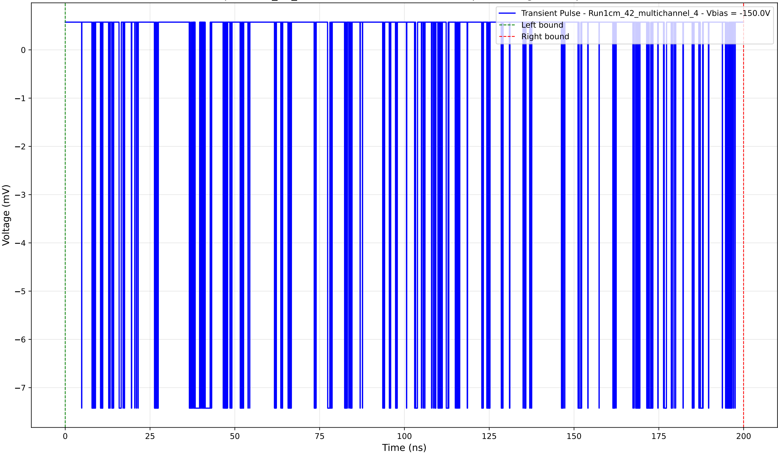
Transient Pulse - Sample: 1cm_42_multichannel - Position: 3390.0 \mu\text{m} - Charge: 2.04 pC - Rise Time: 0.02 ns
