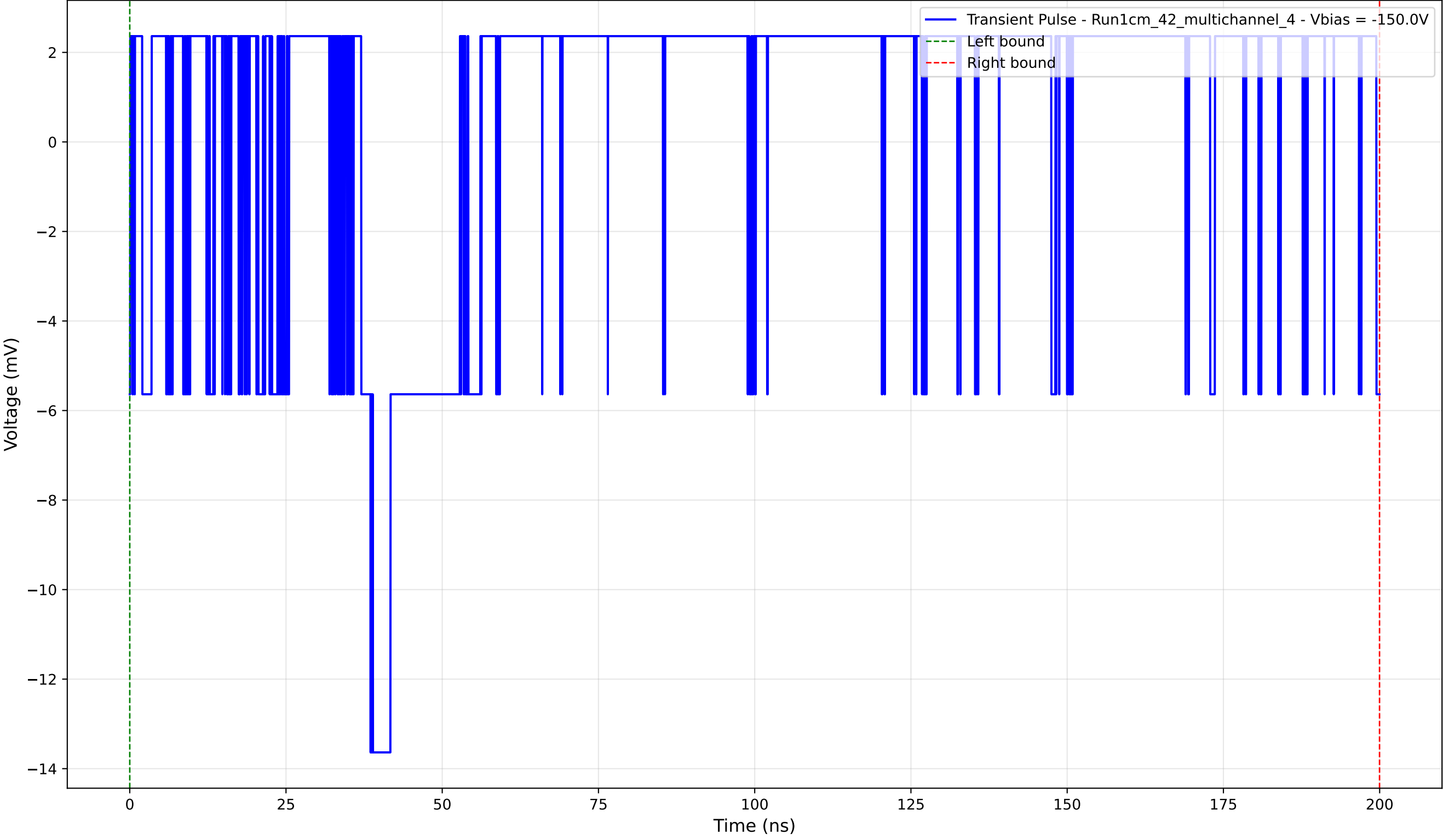
Transient Pulse - Sample: 1cm_42_multichannel - Position: 195.0 \mu\text{m} - Charge: 3.35 pC - Rise Time: 0.00 ns (N/A)
