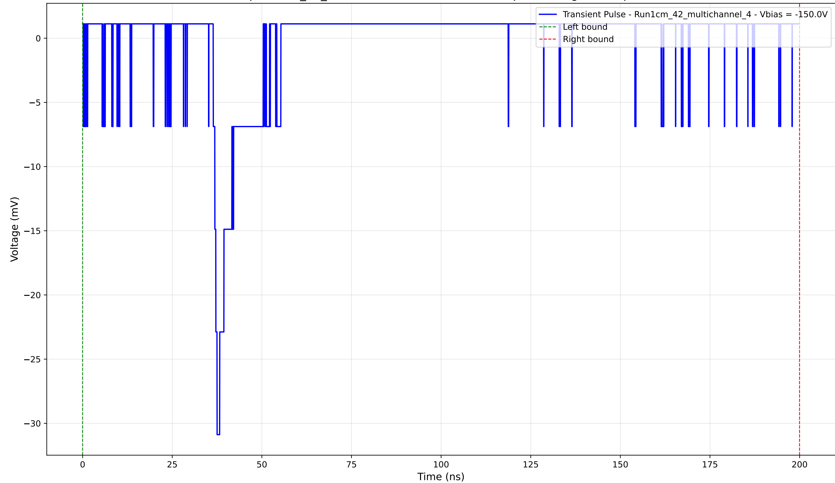
Transient Pulse - Sample: 1cm_42_multichannel - Position: 3150.0 \mu\text{m} - Charge: 0.23 pC - Rise Time: 1.07 ns
