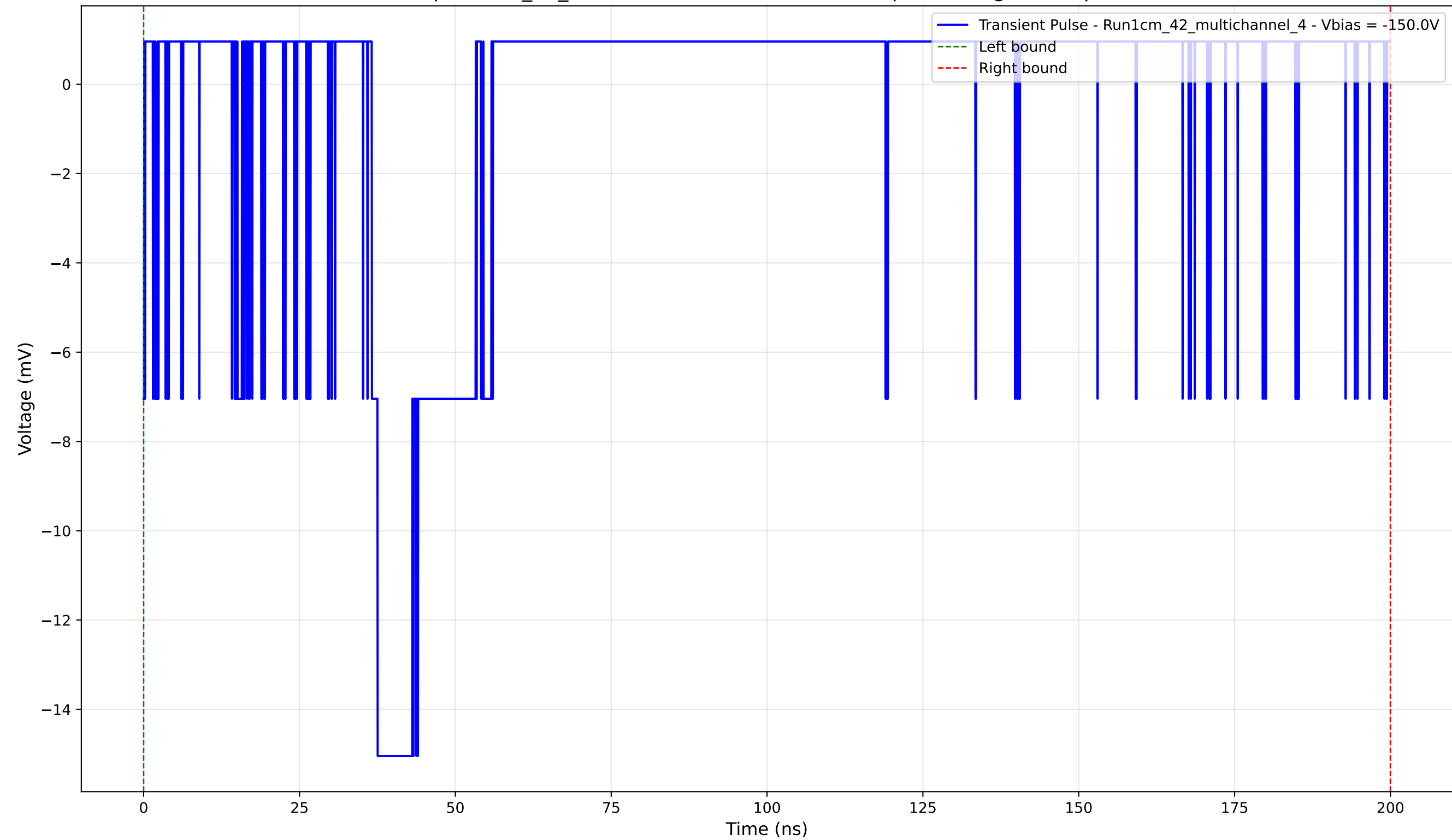
Transient Pulse - Sample: 1cm_42_multichannel - Position: 3750.0 \mu\text{m} - Charge: 1.19 pC - Rise Time: 0.94 ns
