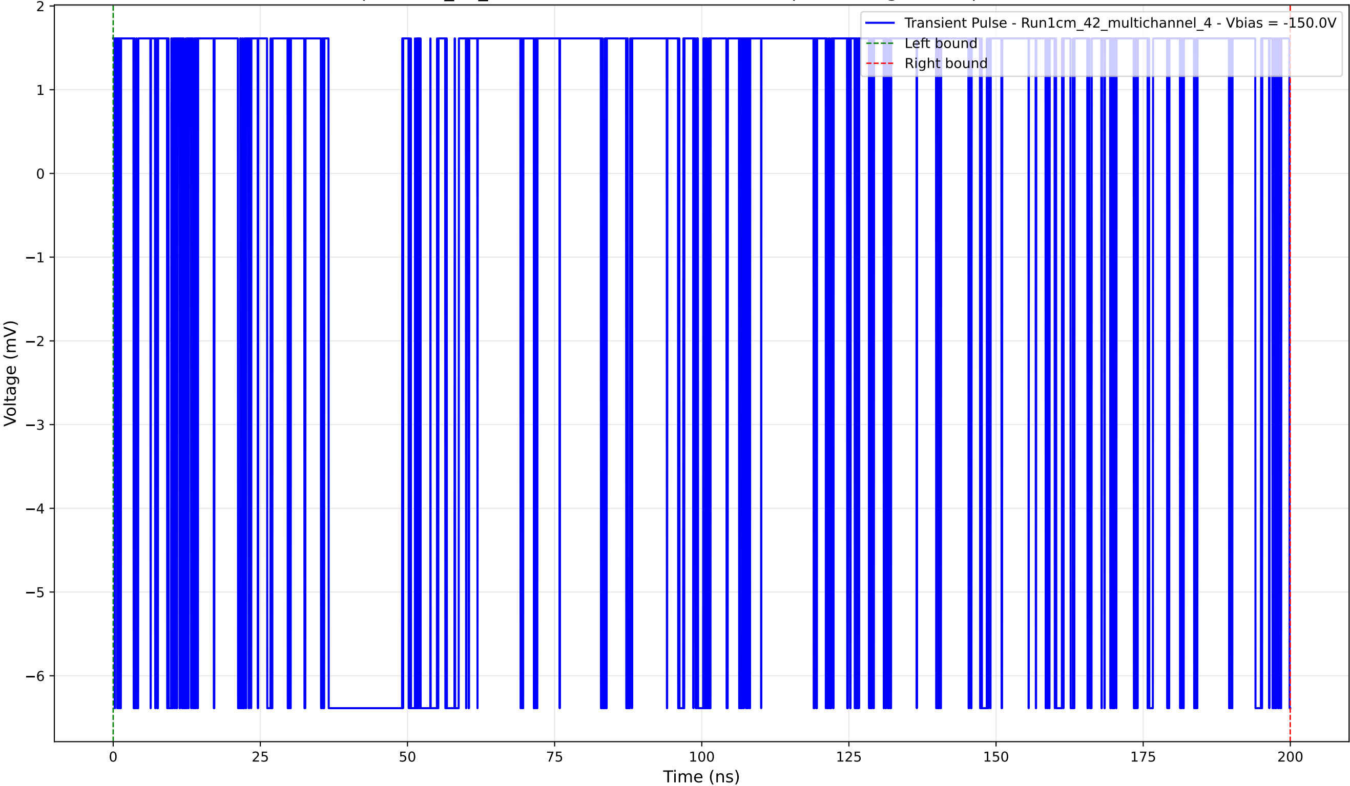
Transient Pulse - Sample: 1cm_42_multichannel - Position: 1335.0 \mu\text{m} - Charge: 0.62 pC - Rise Time: 0.00 ns (N/A)
