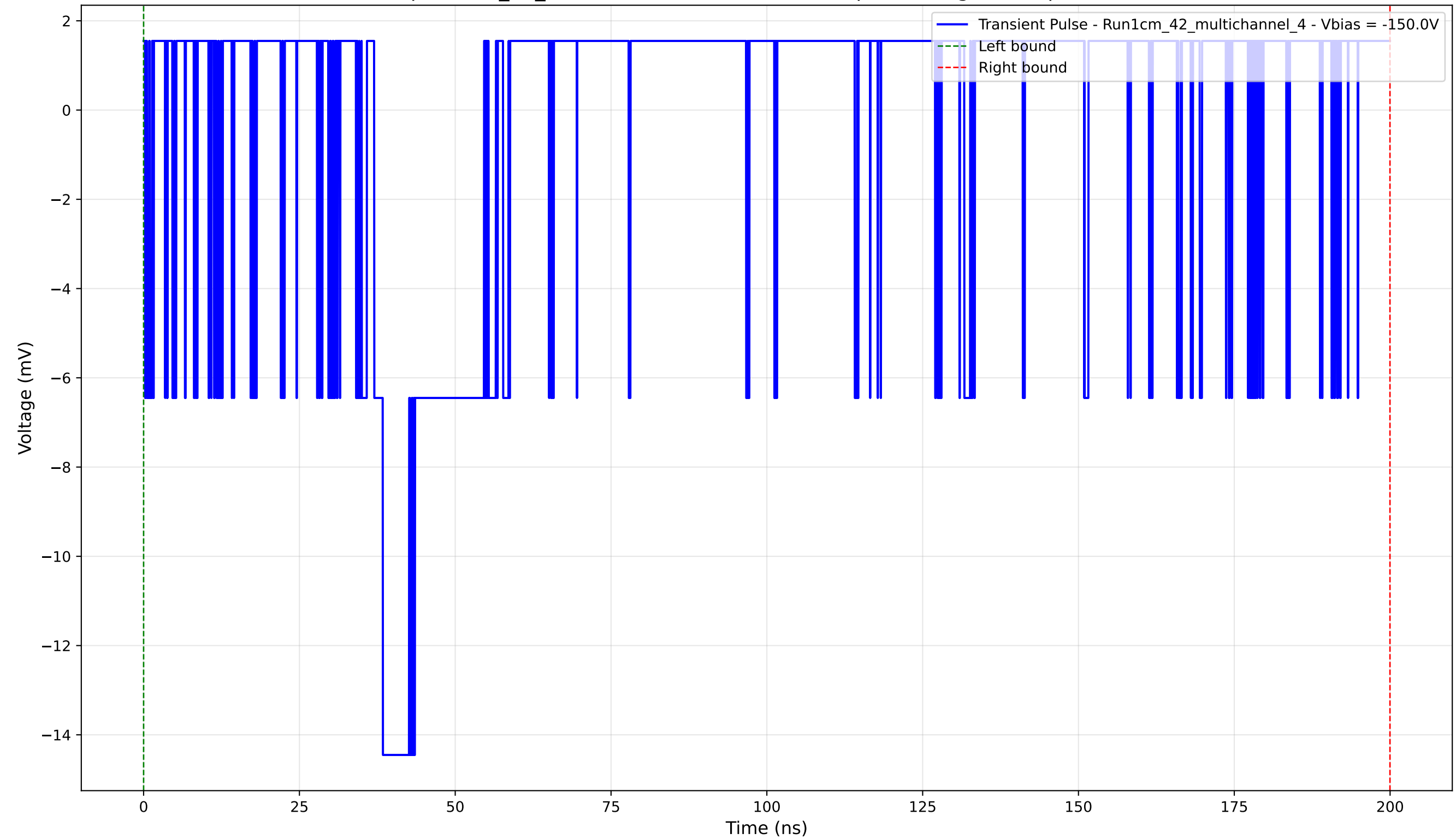
Transient Pulse - Sample: 1cm_42_multichannel - Position: 210.0 \mu\text{m} - Charge: 0.44 pC - Rise Time: 0.00 ns (N/A)
