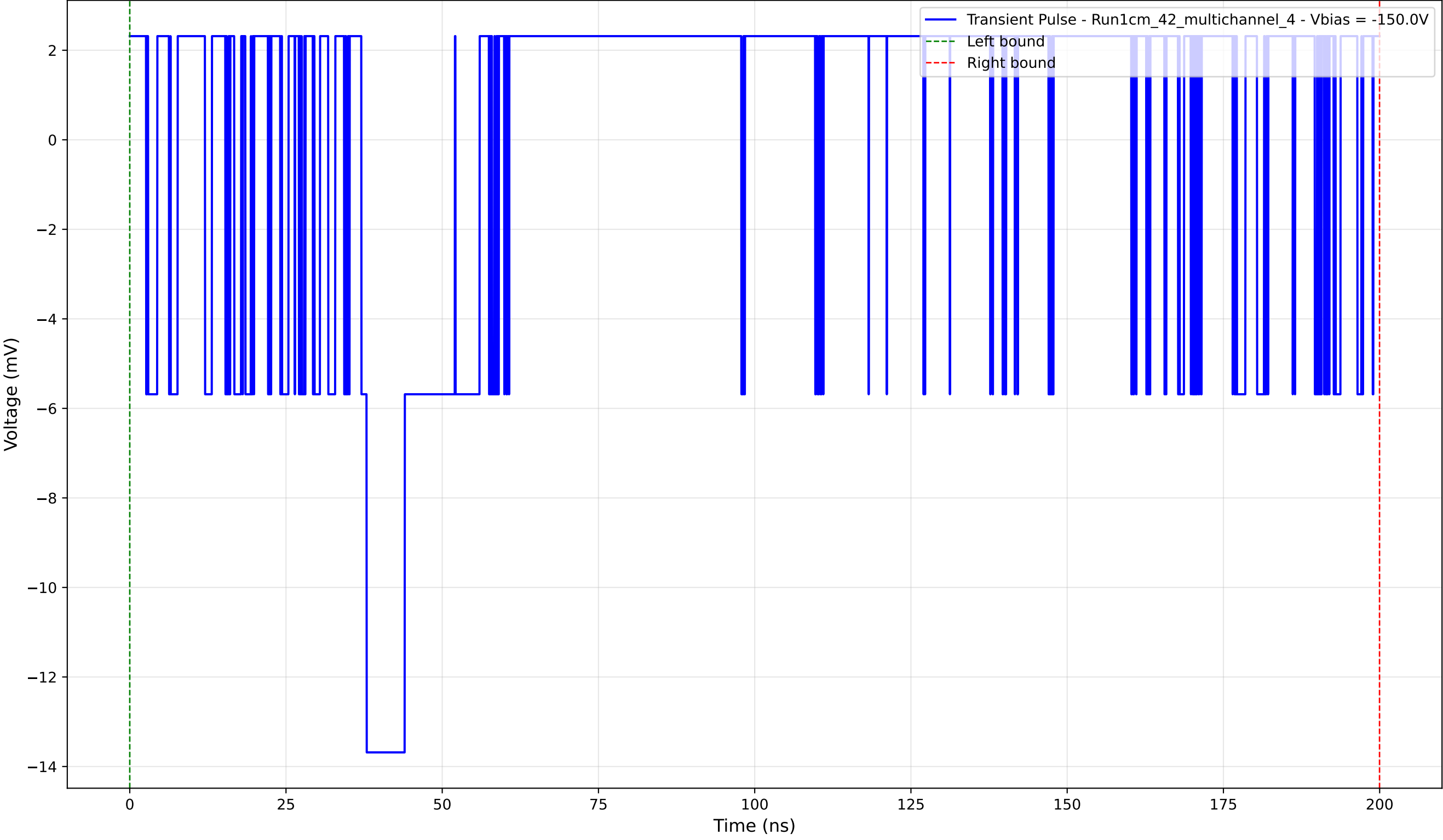
Transient Pulse - Sample: 1cm_42_multichannel - Position: 590.0 \mu\text{m} - Charge: 1.46 pC - Rise Time: 0.00 ns (N/A)
