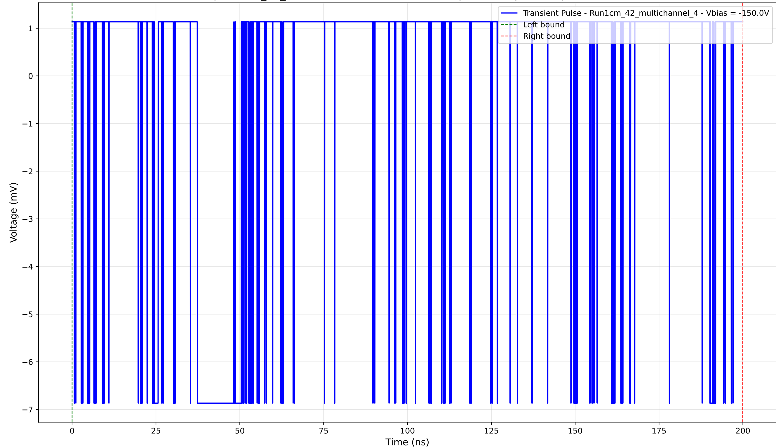
Transient Pulse - Sample: 1cm_42_multichannel - Position: 3945.0 \mu\text{m} - Charge: 0.21 pC - Rise Time: 0.00 ns (N/A)
