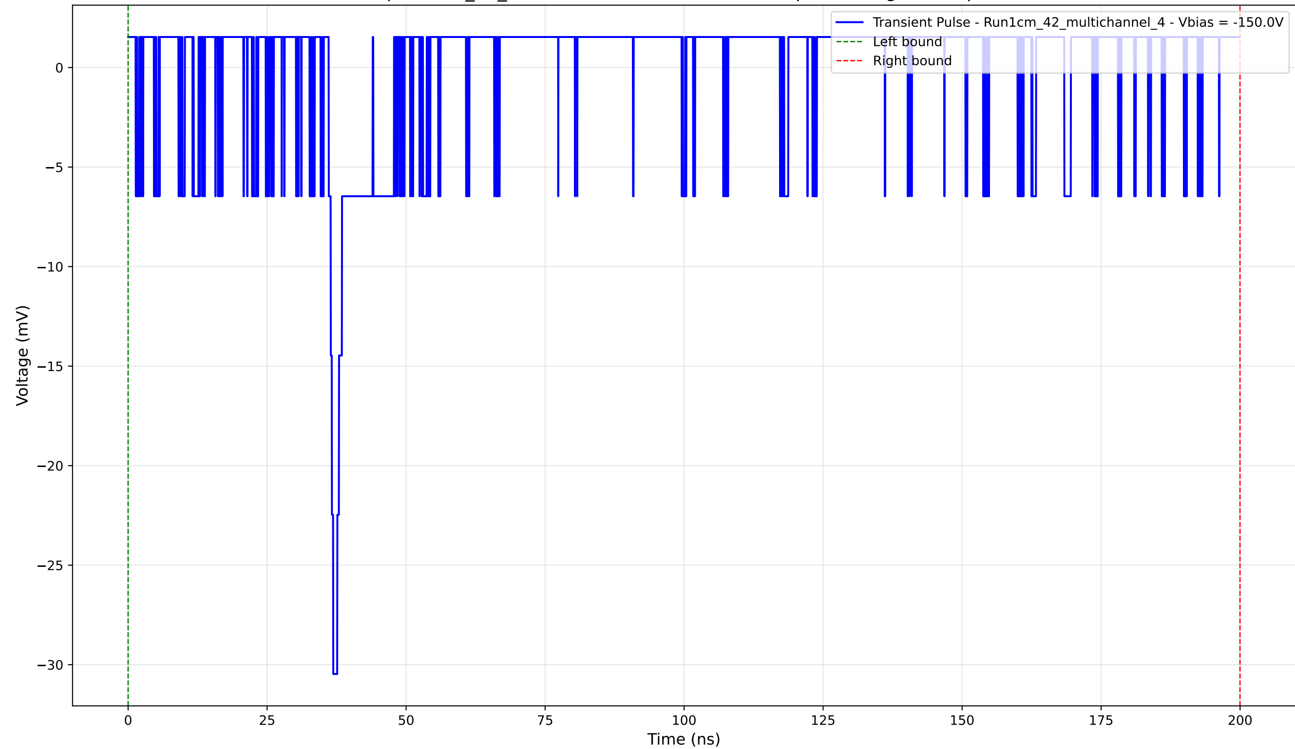
Transient Pulse - Sample: 1cm_42_multichannel - Position: 2340.0 \mu\text{m} - Charge: 0.54 pC - Rise Time: 0.81 ns
