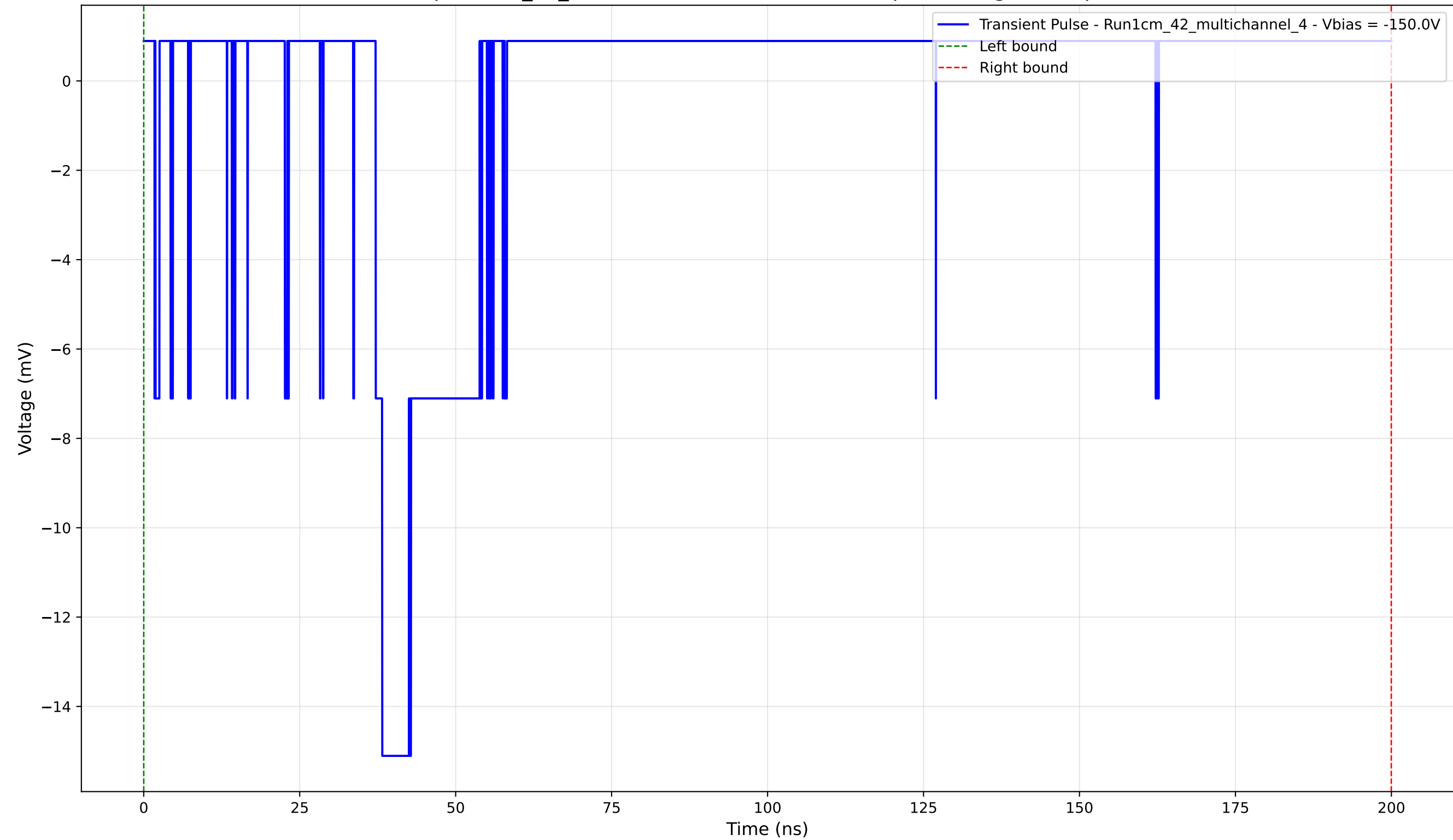
Transient Pulse - Sample: 1cm_42_multichannel - Position: 4180.0 \mu\text{m} - Charge: 0.42 pC - Rise Time: 1.06 ns
