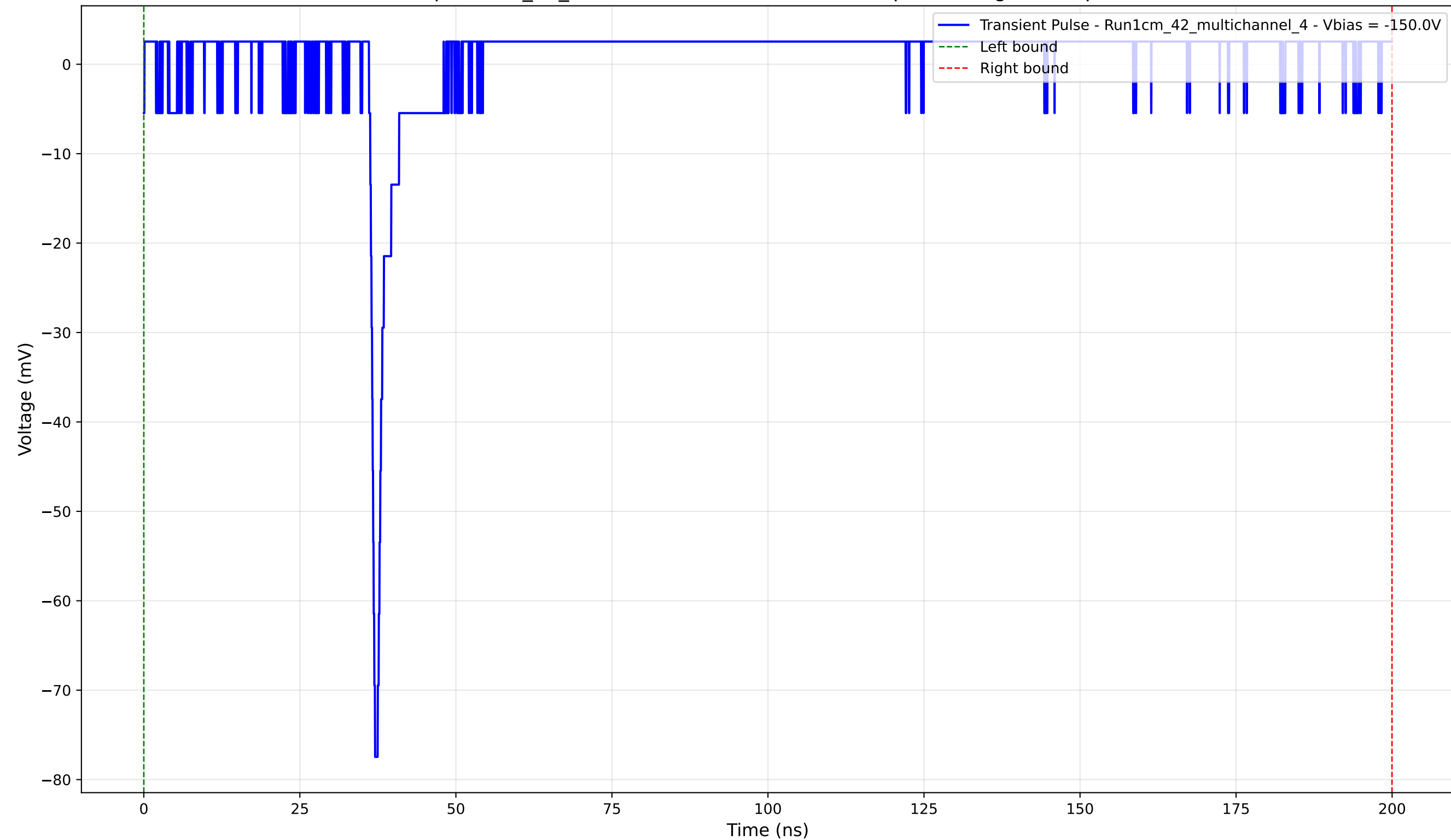
Transient Pulse - Sample: 1cm_42_multichannel - Position: 2500.0 \mu\text{m} - Charge: 3.59 pC - Rise Time: 0.77 ns
