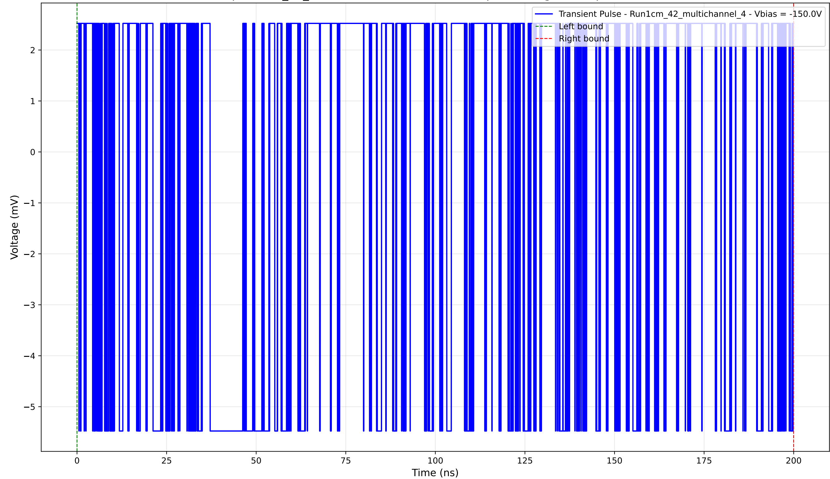
Transient Pulse - Sample: 1cm_42_multichannel - Position: 400.0 \mu\text{m} - Charge: 0.15 pC - Rise Time: 0.00 ns (N/A)
