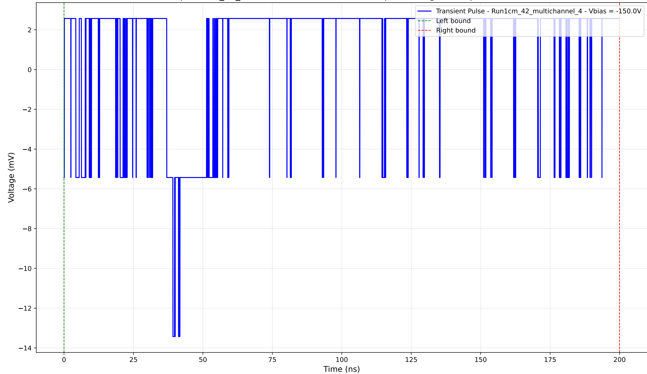
Transient Pulse - Sample: 1cm_42_multichannel - Position: 4835.0 \mu\text{m} - Charge: 5.53 pC - Rise Time: 0.00 ns (N/A)
