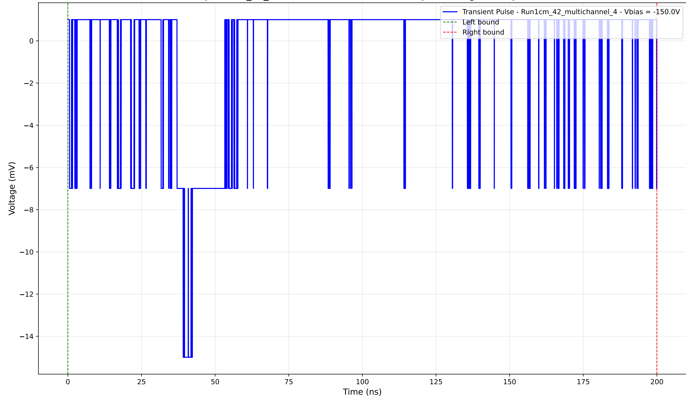
Transient Pulse - Sample: 1cm_42_multichannel - Position: 4340.0 \mu\text{m} - Charge: 1.25 pC - Rise Time: 2.10 ns
