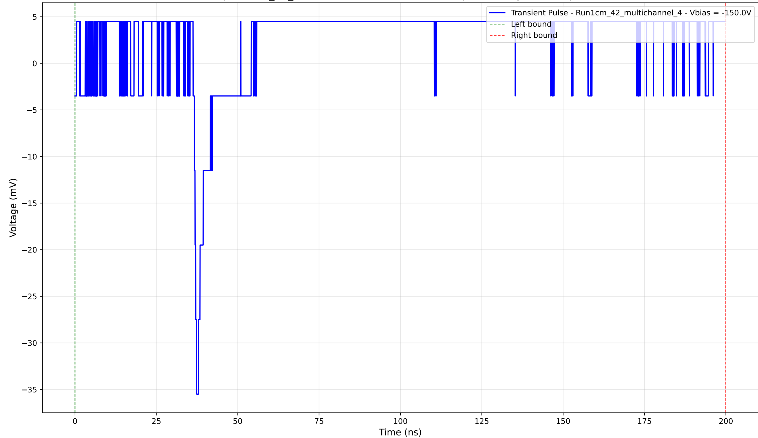
Transient Pulse - Sample: 1cm_42_multichannel - Position: 1810.0 \mu\text{m} - Charge: 10.80 pC - Rise Time: 0.74 ns
