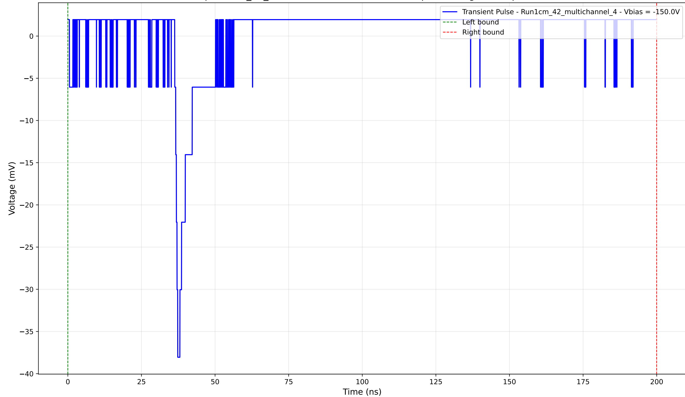
Transient Pulse - Sample: 1cm_42_multichannel - Position: 3005.0 \mu\text{m} - Charge: 1.83 pC - Rise Time: 1.03 ns
