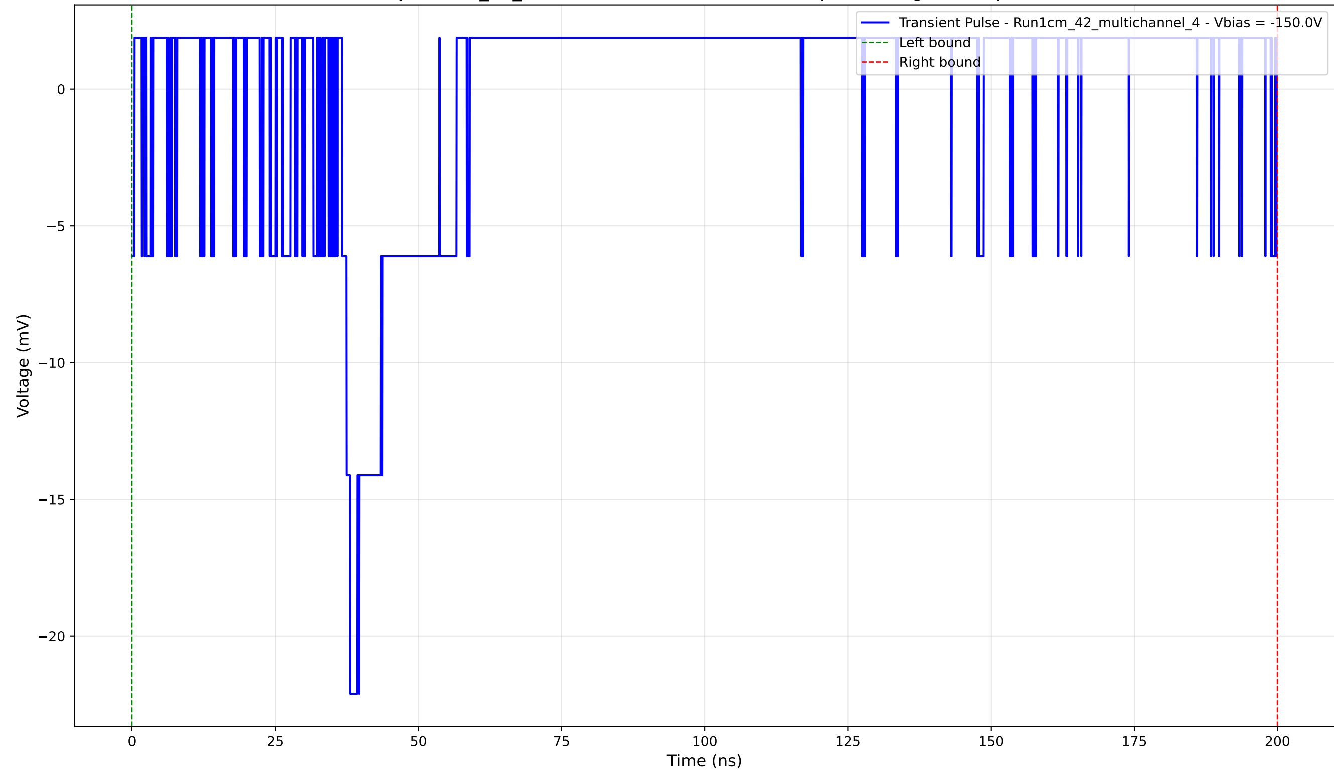
Transient Pulse - Sample: 1cm_42_multichannel - Position: 1115.0 \mu\text{m} - Charge: 1.00 pC - Rise Time: 1.40 ns
