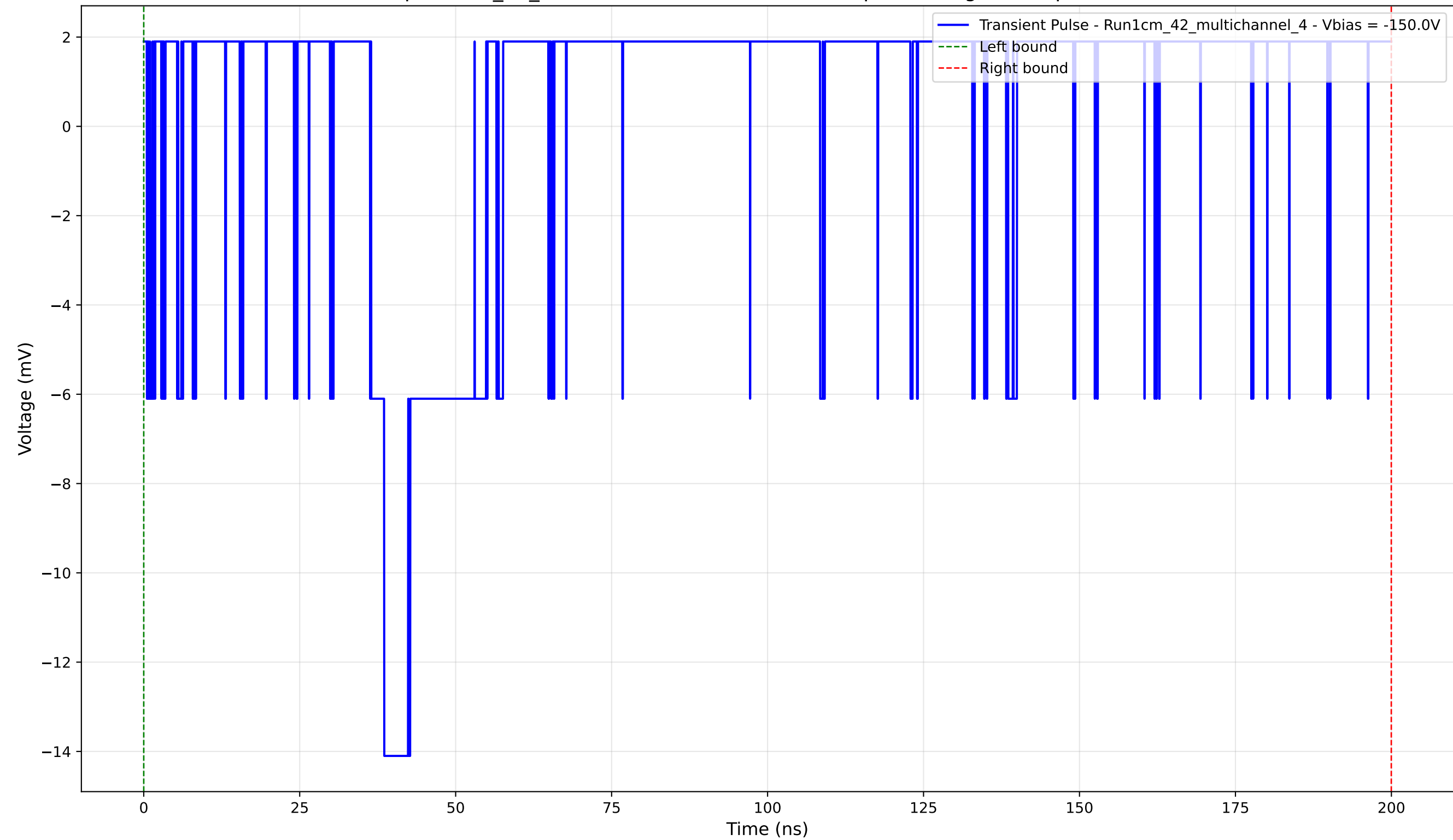
Transient Pulse - Sample: 1cm_42_multichannel - Position: 4740.0 \mu\text{m} - Charge: 2.45 pC - Rise Time: 0.00 ns (N/A)
