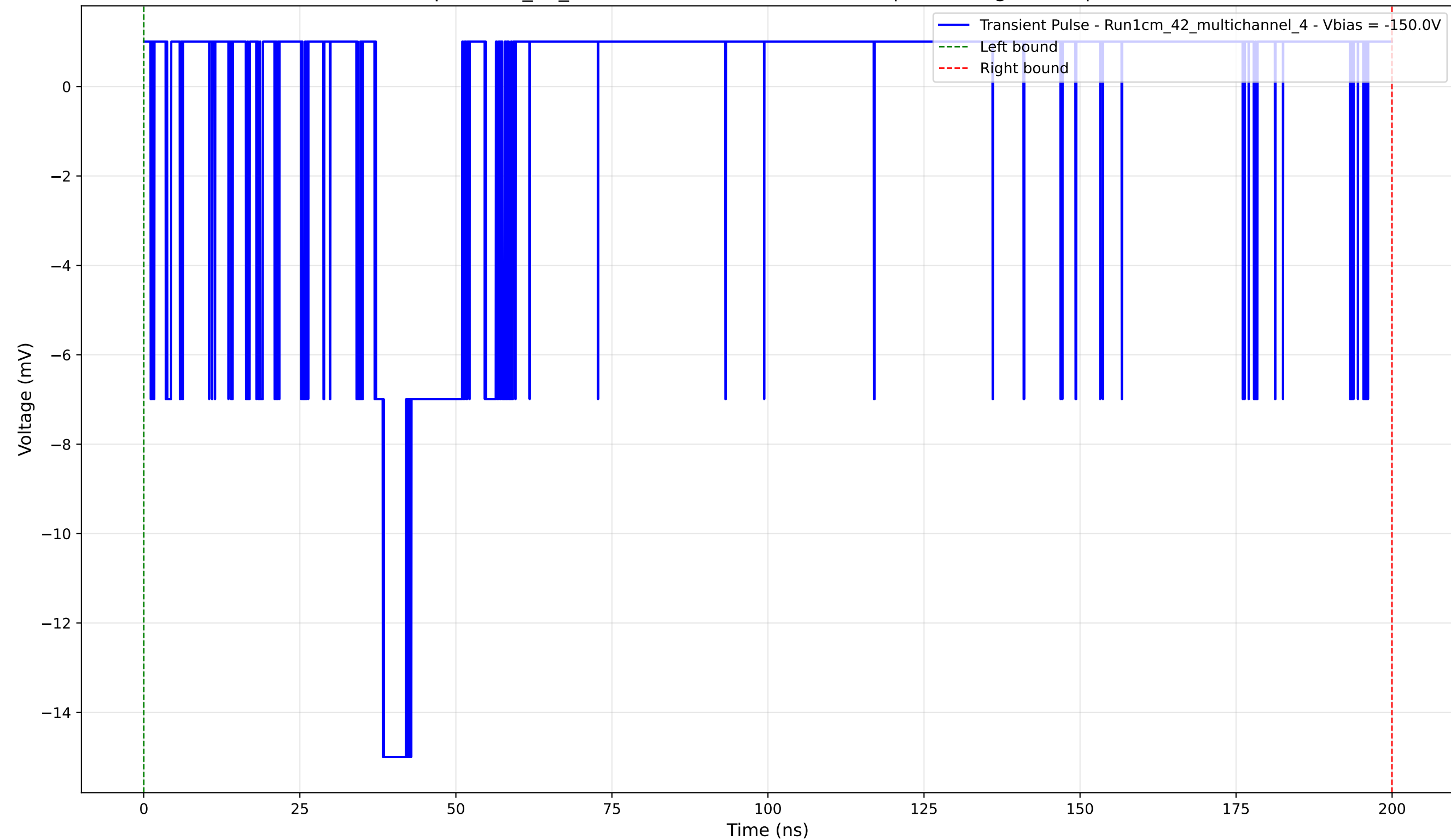
Transient Pulse - Sample: 1cm_42_multichannel - Position: 4635.0 \mu\text{m} - Charge: 0.59 pC - Rise Time: 1.10 ns
