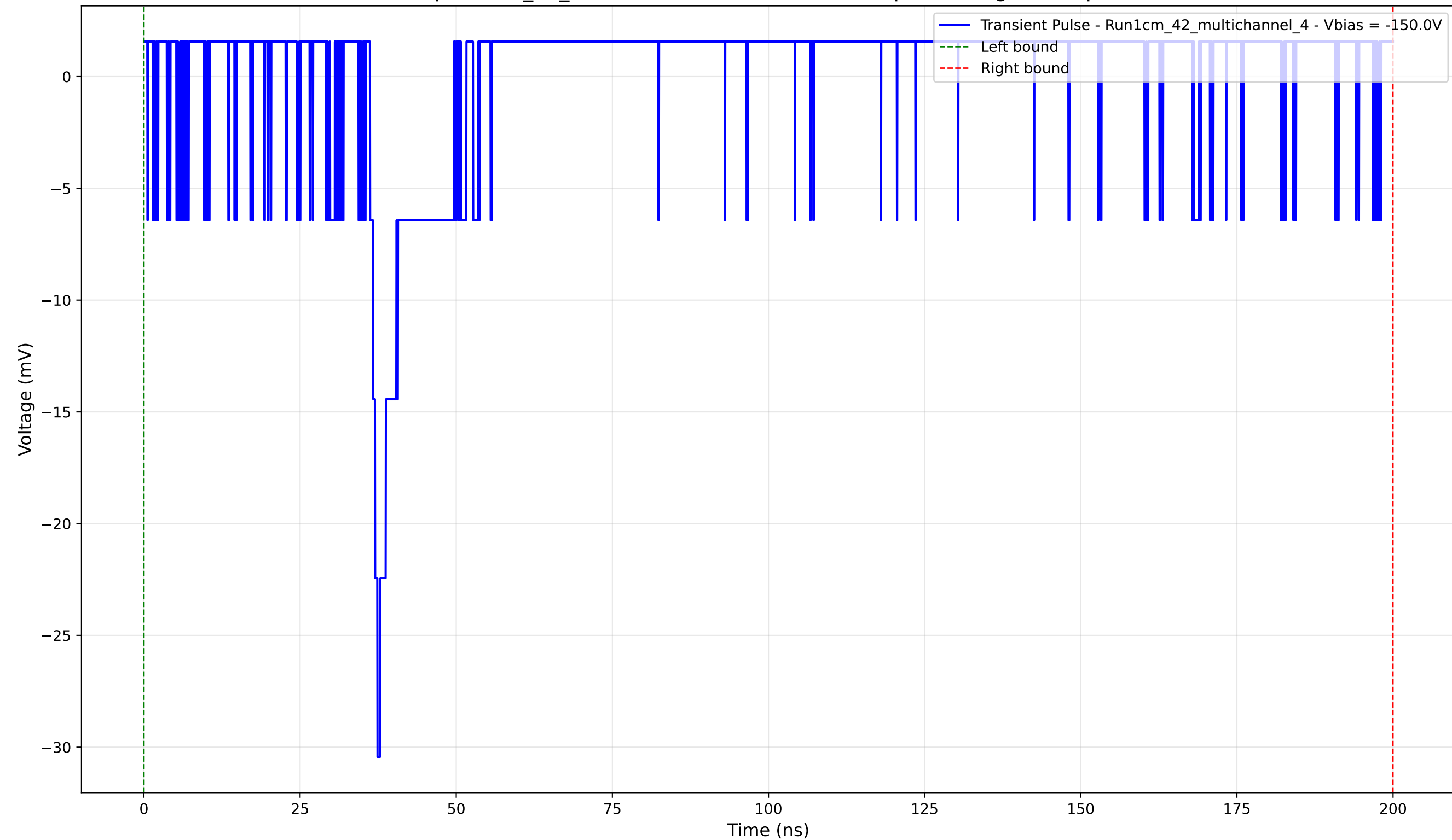
Transient Pulse - Sample: 1cm_42_multichannel - Position: 2950.0 \mu\text{m} - Charge: 1.01 pC - Rise Time: 1.19 ns
