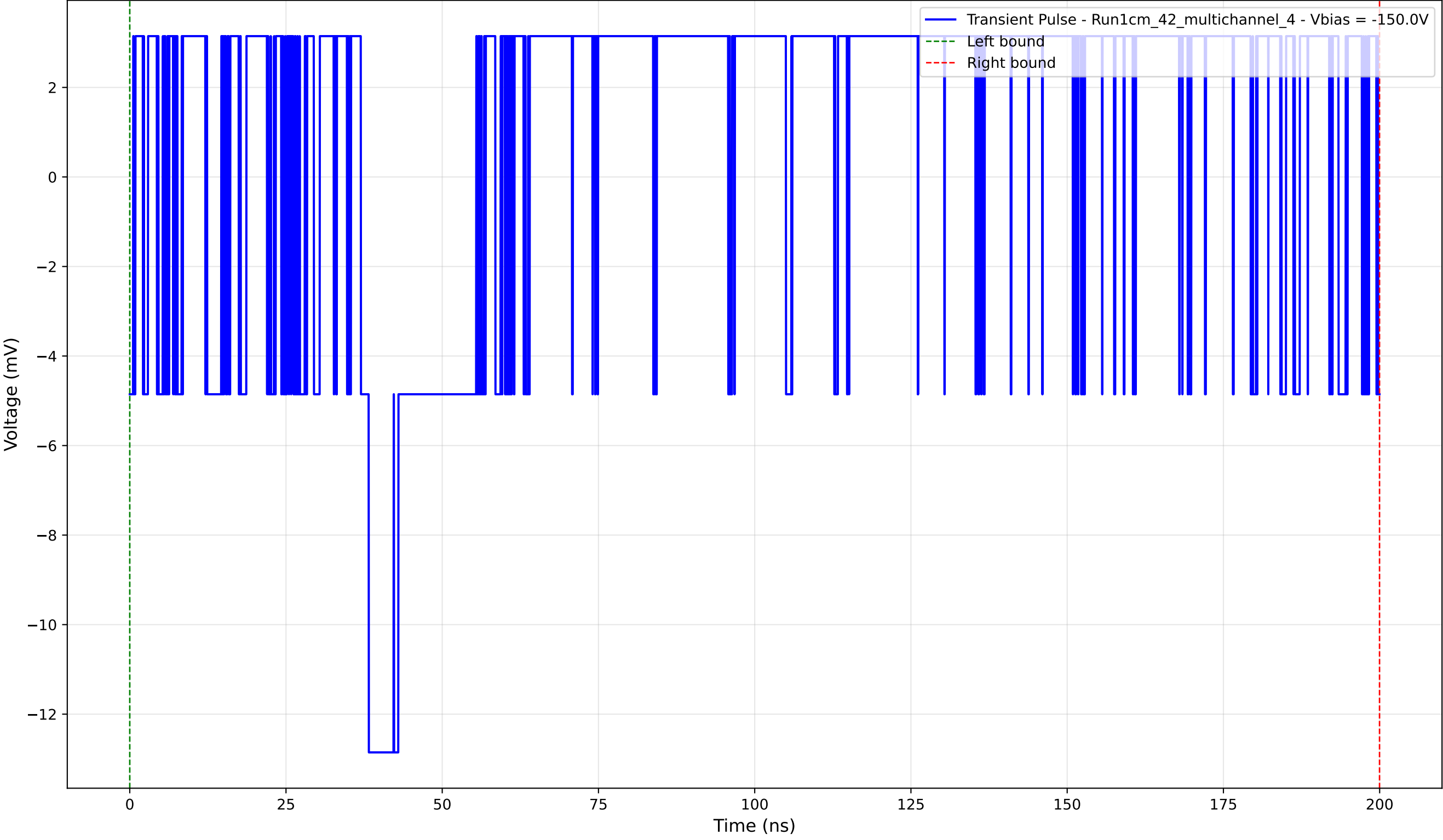
Transient Pulse - Sample: 1cm_42_multichannel - Position: 255.0 \mu\text{m} - Charge: 4.33 pC - Rise Time: 0.00 ns (N/A)
