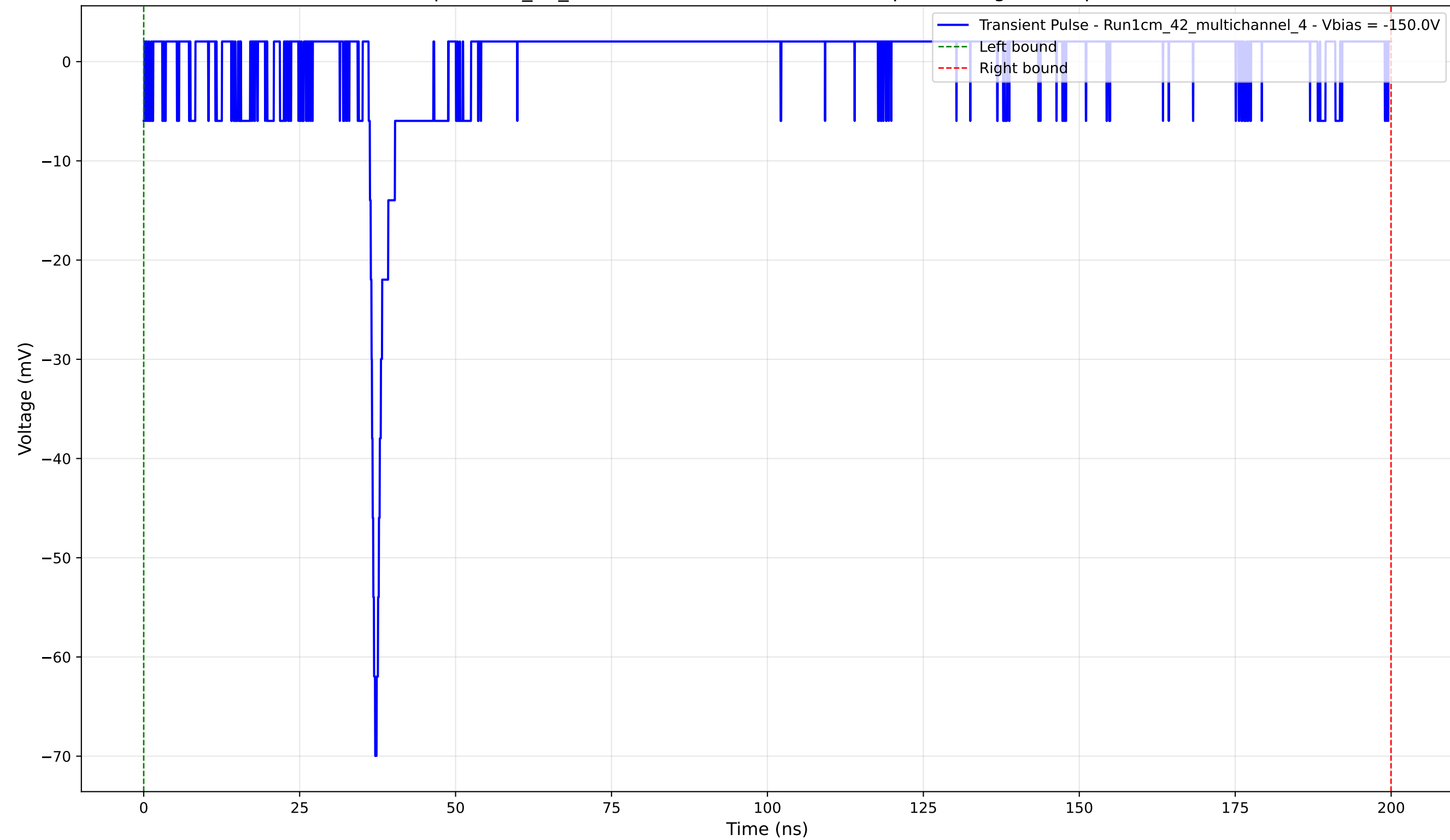
Transient Pulse - Sample: 1cm_42_multichannel - Position: 2450.0 \mu\text{m} - Charge: 1.00 pC - Rise Time: 0.86 ns
