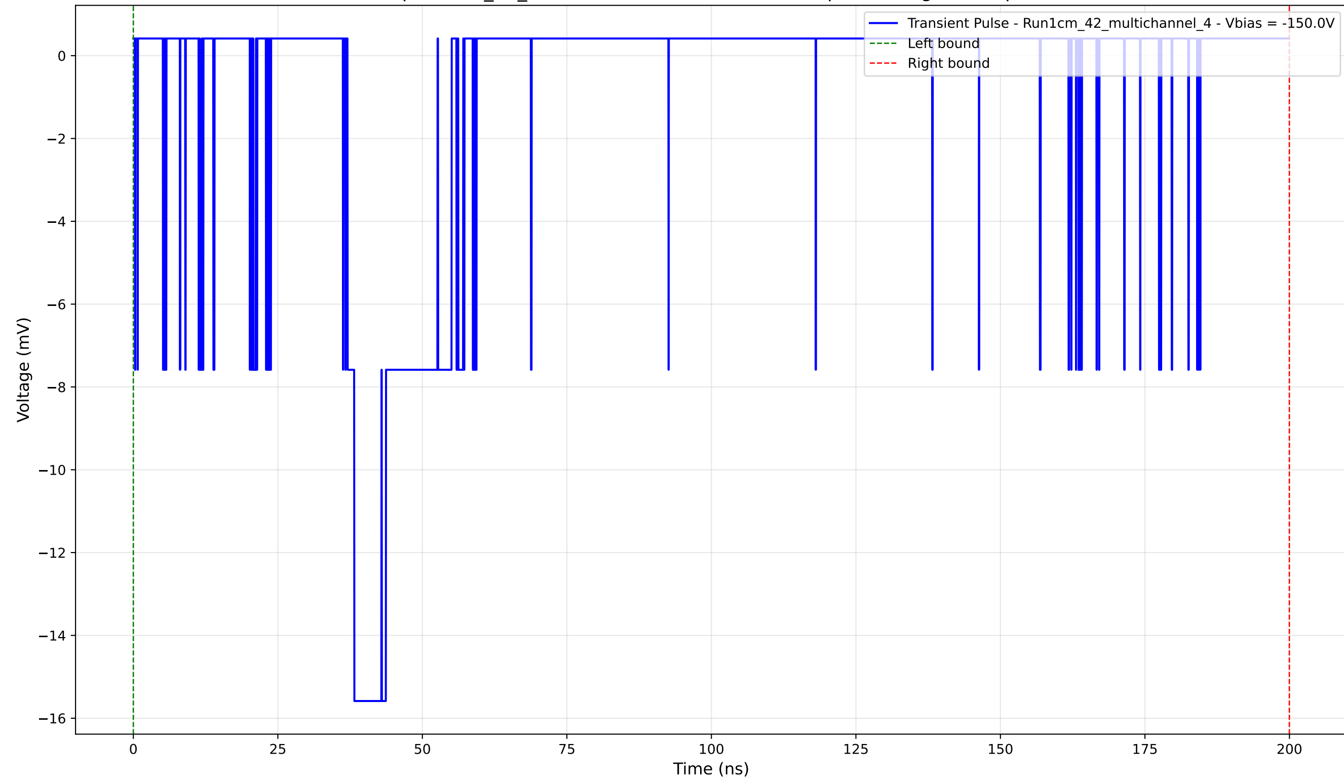
Transient Pulse - Sample: 1cm_42_multichannel - Position: 4095.0 \mu\text{m} - Charge: 3.04 pC - Rise Time: 1.18 ns
