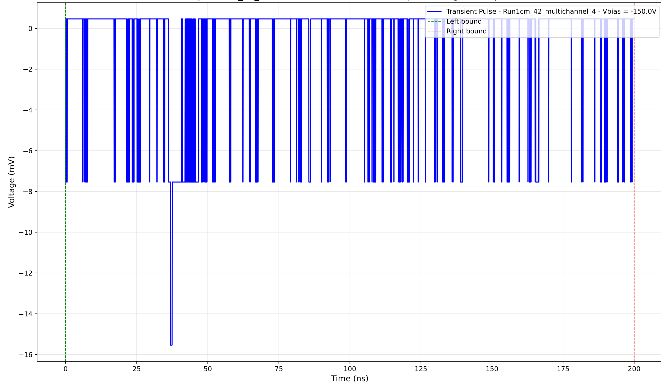
Transient Pulse - Sample: 1cm_42_multichannel - Position: 2355.0 \mu\text{m} - Charge: 2.02 pC - Rise Time: 0.74 ns
