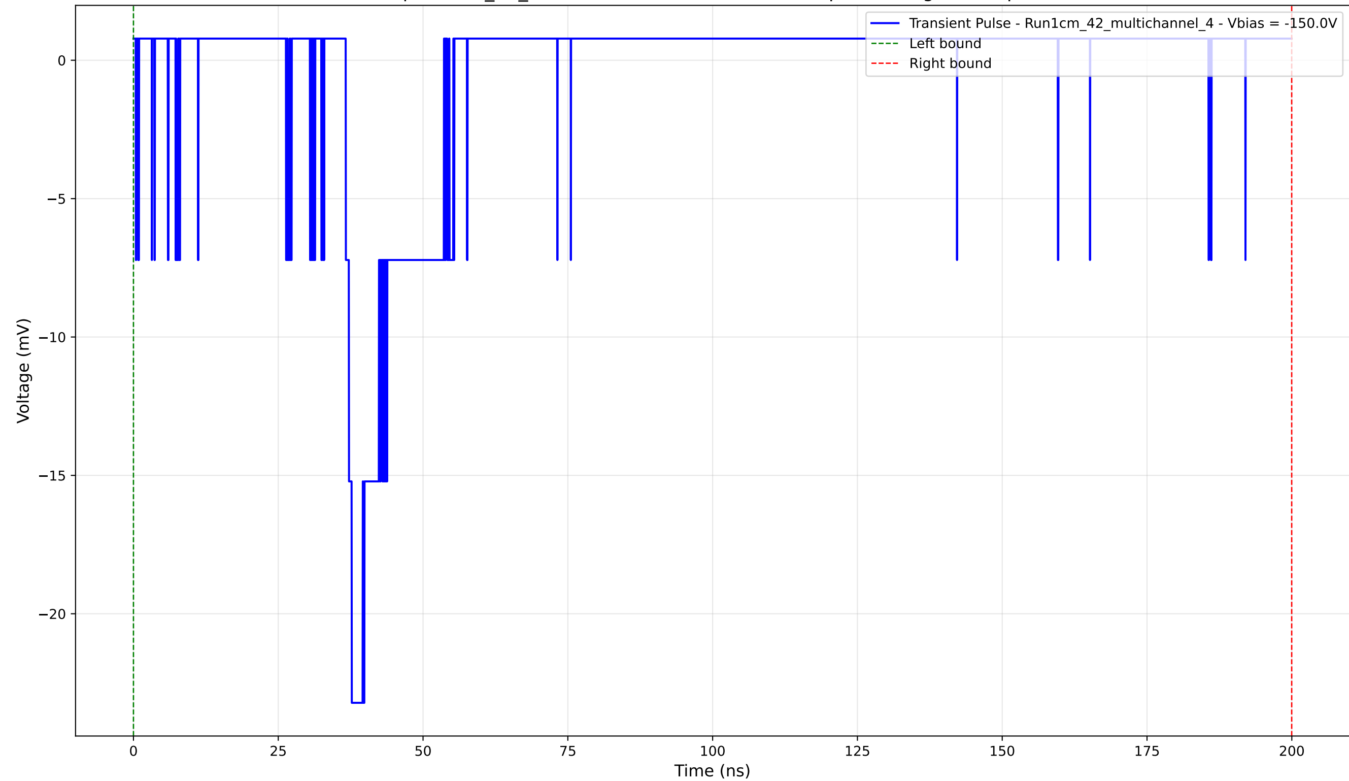
Transient Pulse - Sample: 1cm_42_multichannel - Position: 3505.0 \mu\text{m} - Charge: 1.49 pC - Rise Time: 1.04 ns
