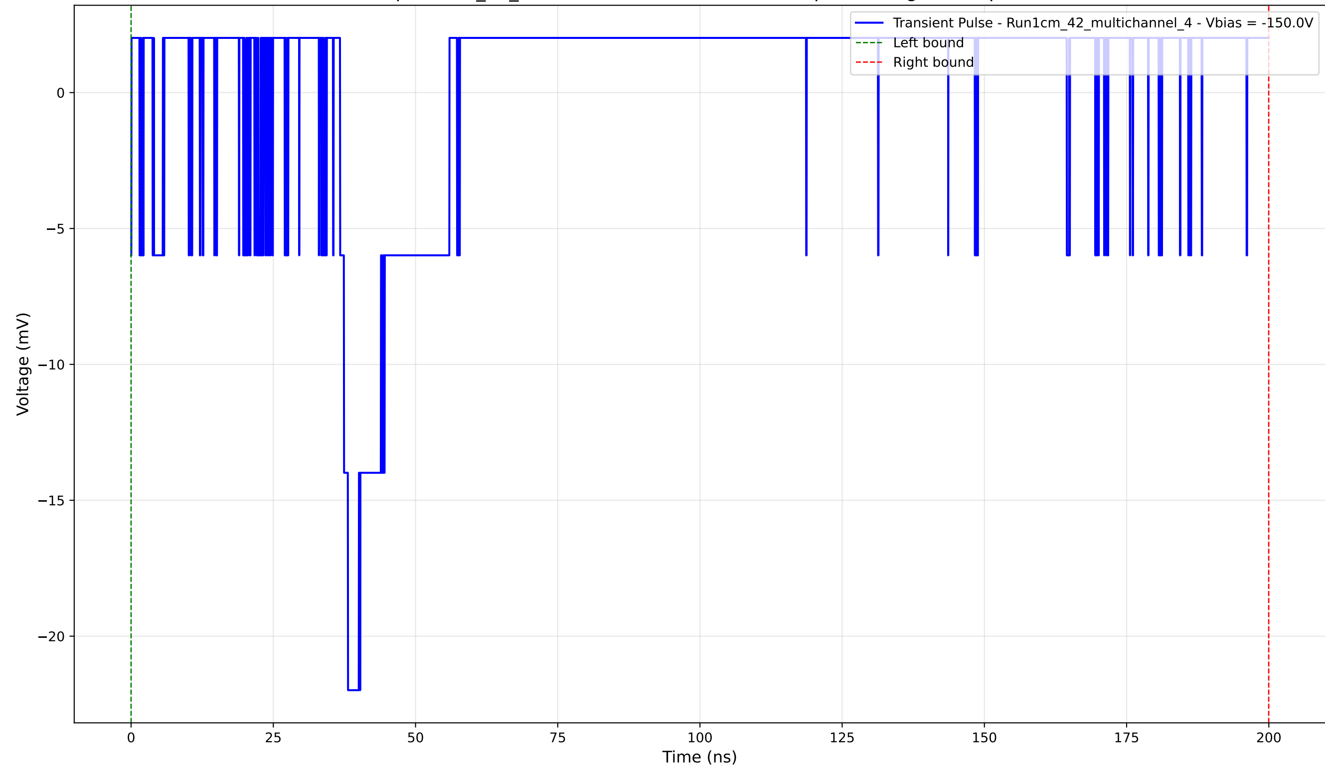
Transient Pulse - Sample: 1cm_42_multichannel - Position: 1005.0 \mu\text{m} - Charge: 1.98 pC - Rise Time: 1.40 ns
