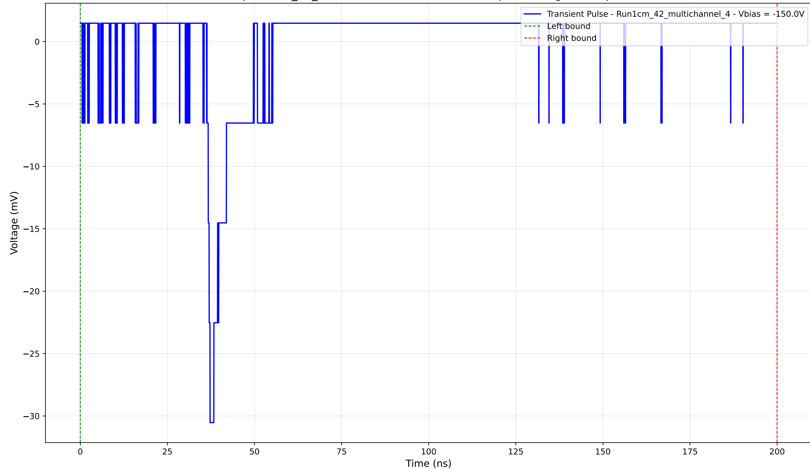
Transient Pulse - Sample: 1cm_42_multichannel - Position: 3070.0 \mu\text{m} - Charge: 0.84 pC - Rise Time: 0.89 ns
