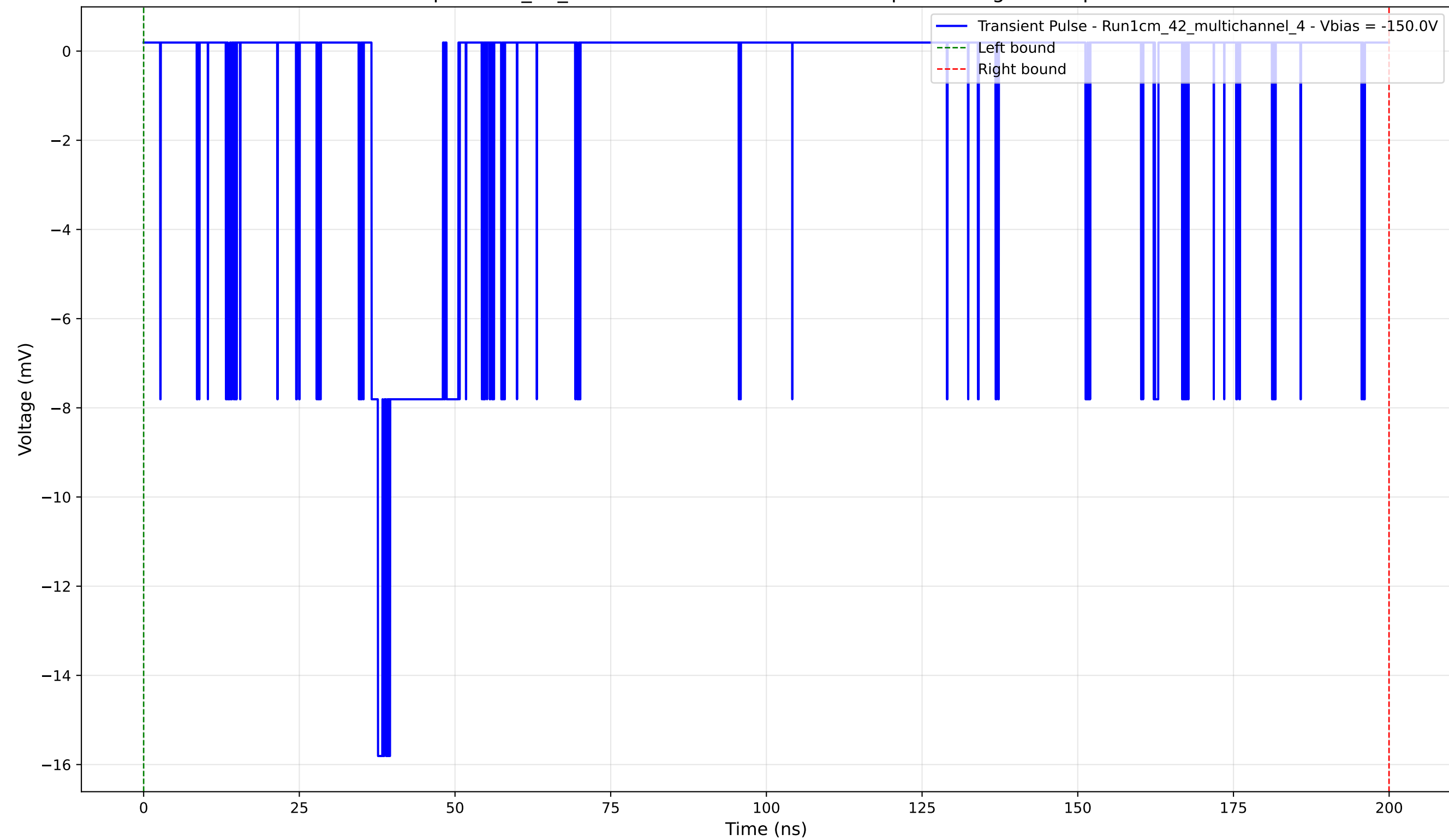
Transient Pulse - Sample: 1cm_42_multichannel - Position: 3350.0 \mu\text{m} - Charge: 2.85 pC - Rise Time: 1.04 ns
