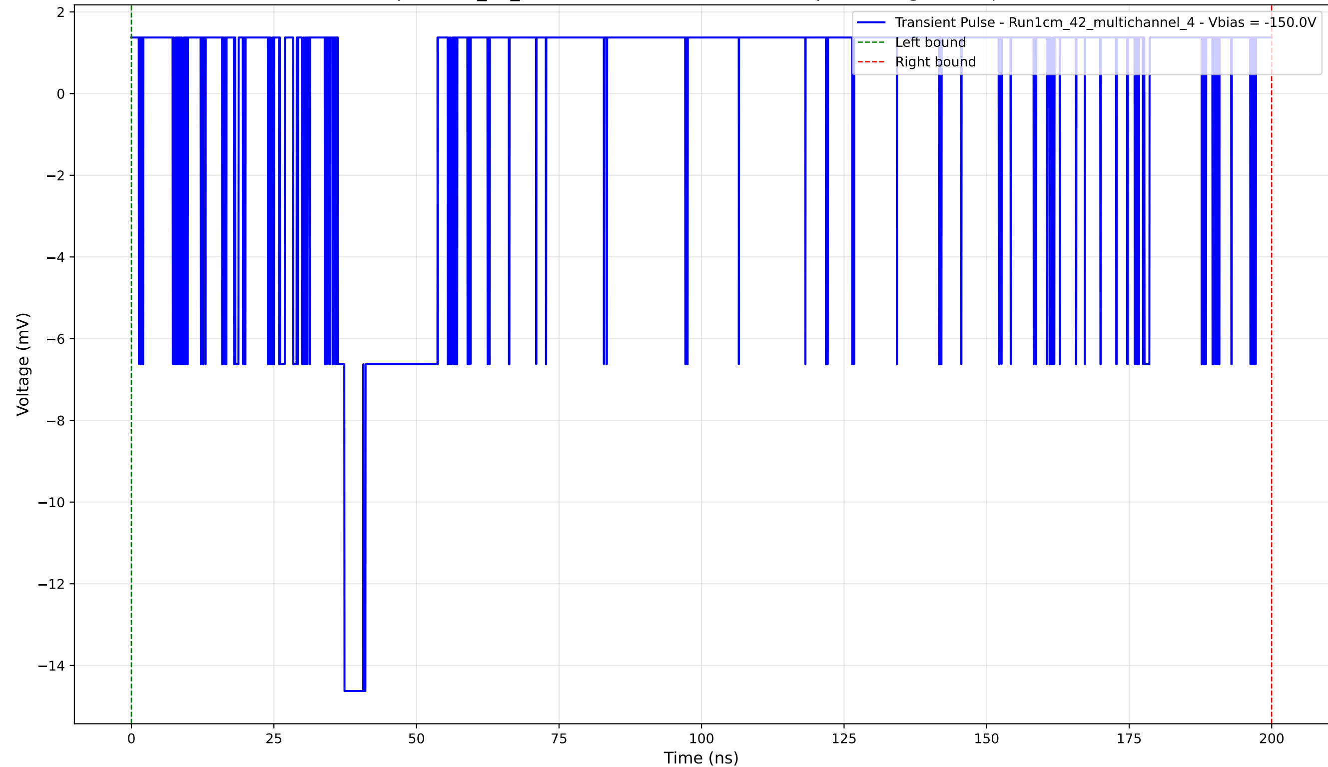
Transient Pulse - Sample: 1cm_42_multichannel - Position: 3455.0 \mu\text{m} - Charge: 0.23 pC - Rise Time: 1.18 ns
