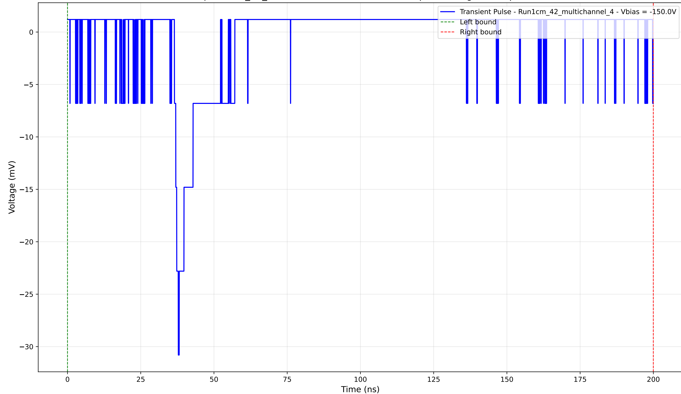
Transient Pulse - Sample: 1cm_42_multichannel - Position: 3285.0 \mu\text{m} - Charge: 1.17 pC - Rise Time: 1.33 ns
