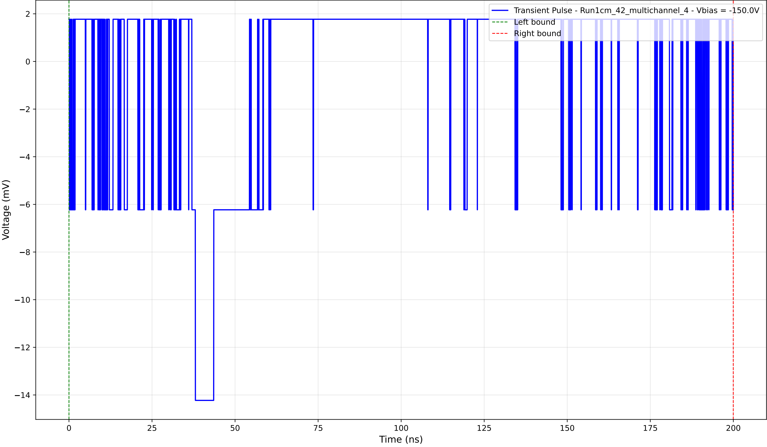
Transient Pulse - Sample: 1cm_42_multichannel - Position: 465.0 \mu\text{m} - Charge: 0.15 pC - Rise Time: 0.00 ns (N/A)
