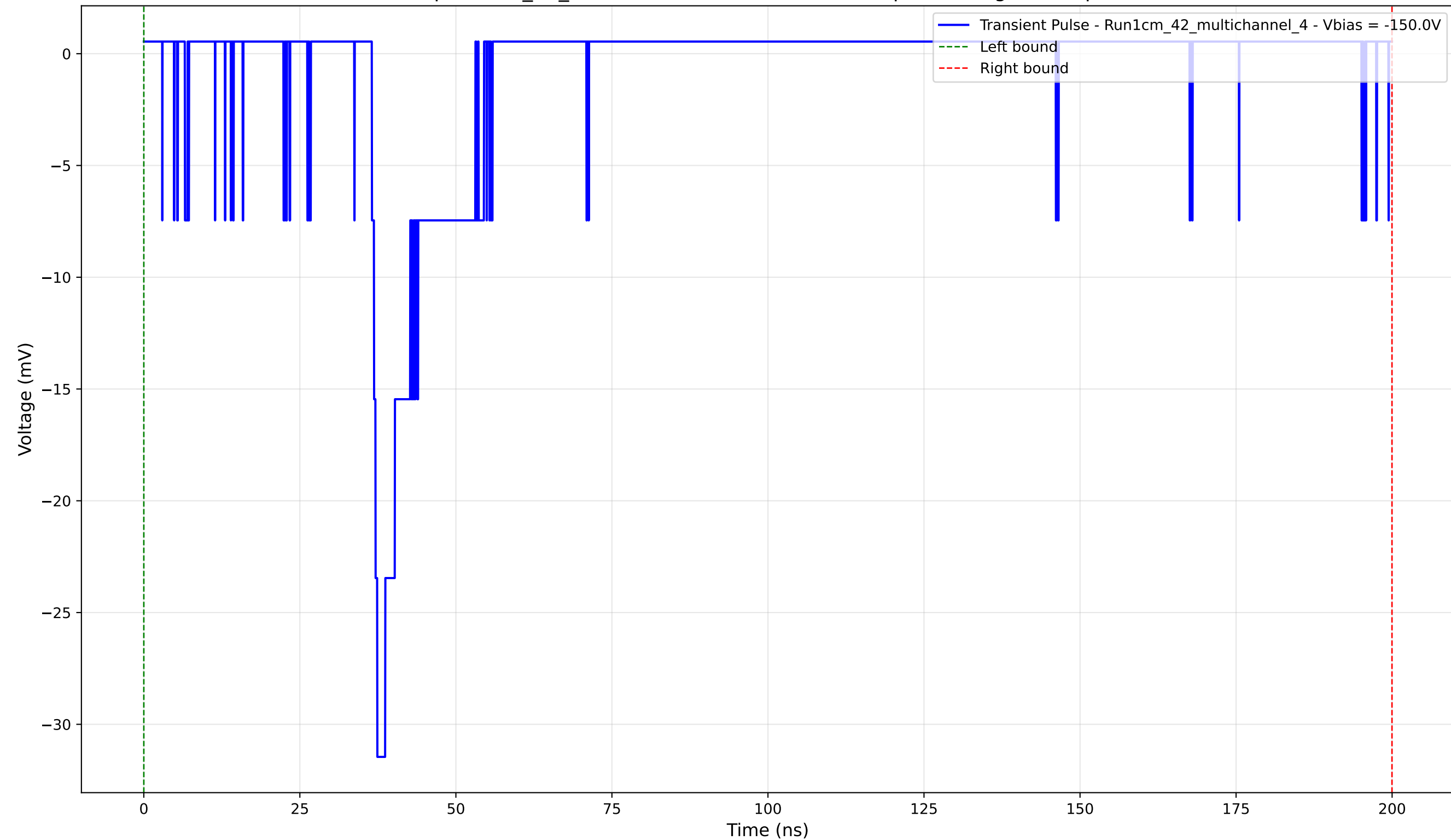
Transient Pulse - Sample: 1cm_42_multichannel - Position: 1550.0 \mu\text{m} - Charge: 2.95 pC - Rise Time: 0.87 ns
