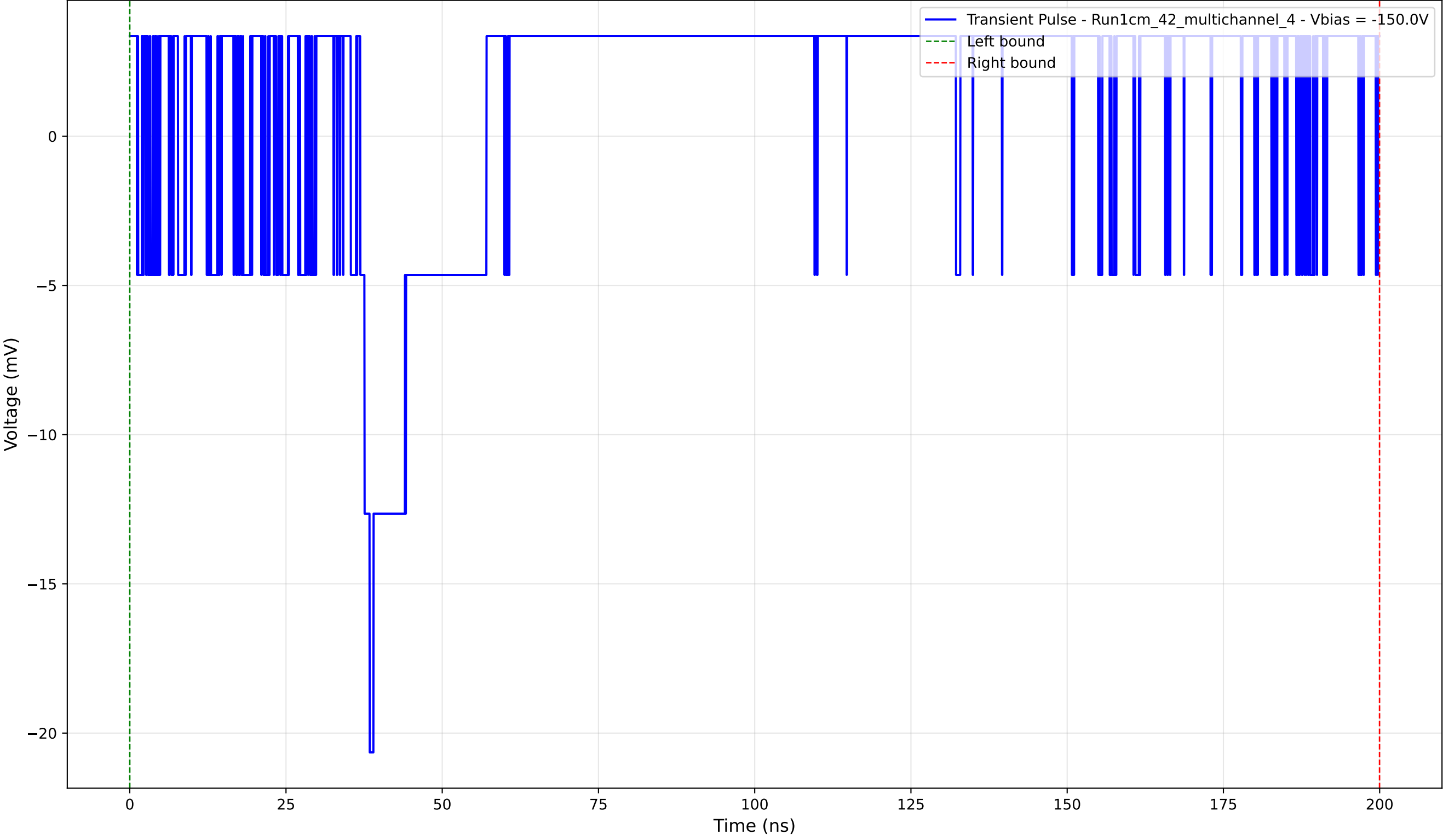
Transient Pulse - Sample: 1cm_42_multichannel - Position: 995.0 \mu\text{m} - Charge: 5.57 pC - Rise Time: 0.00 ns (N/A)
