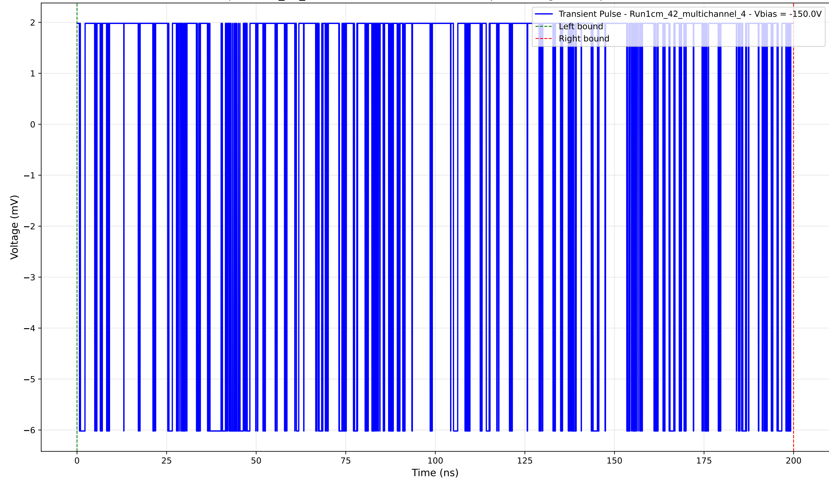
Transient Pulse - Sample: 1cm_42_multichannel - Position: 1390.0 \mu\text{m} - Charge: 0.89 pC - Rise Time: 0.00 ns (N/A)
