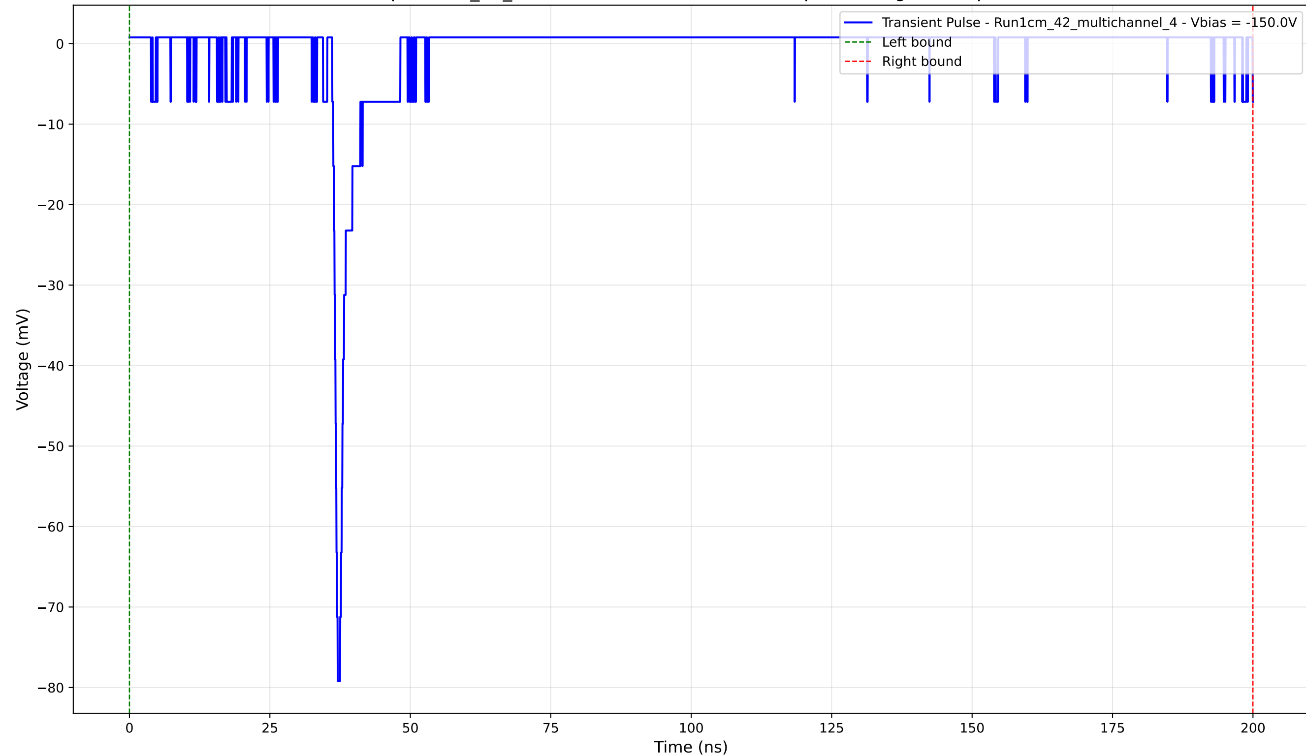
Transient Pulse - Sample: 1cm_42_multichannel - Position: 2515.0 \mu\text{m} - Charge: 2.80 pC - Rise Time: 0.80 ns
