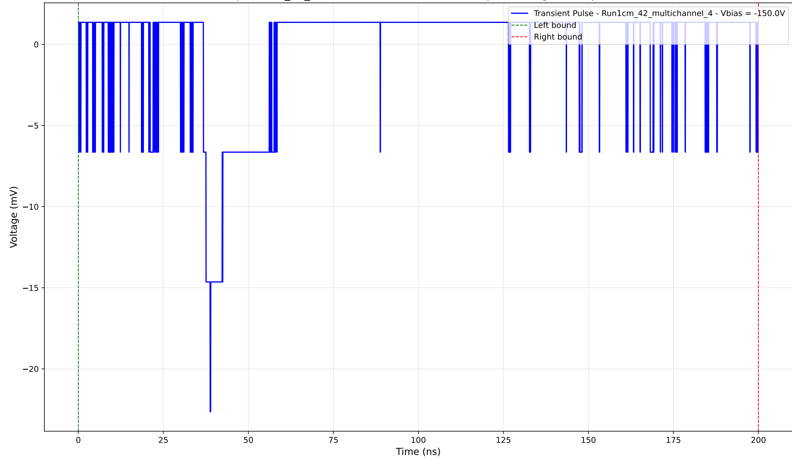
Transient Pulse - Sample: 1cm_42_multichannel - Position: 3685.0 \mu\text{m} - Charge: 0.09 pC - Rise Time: 2.00 ns
