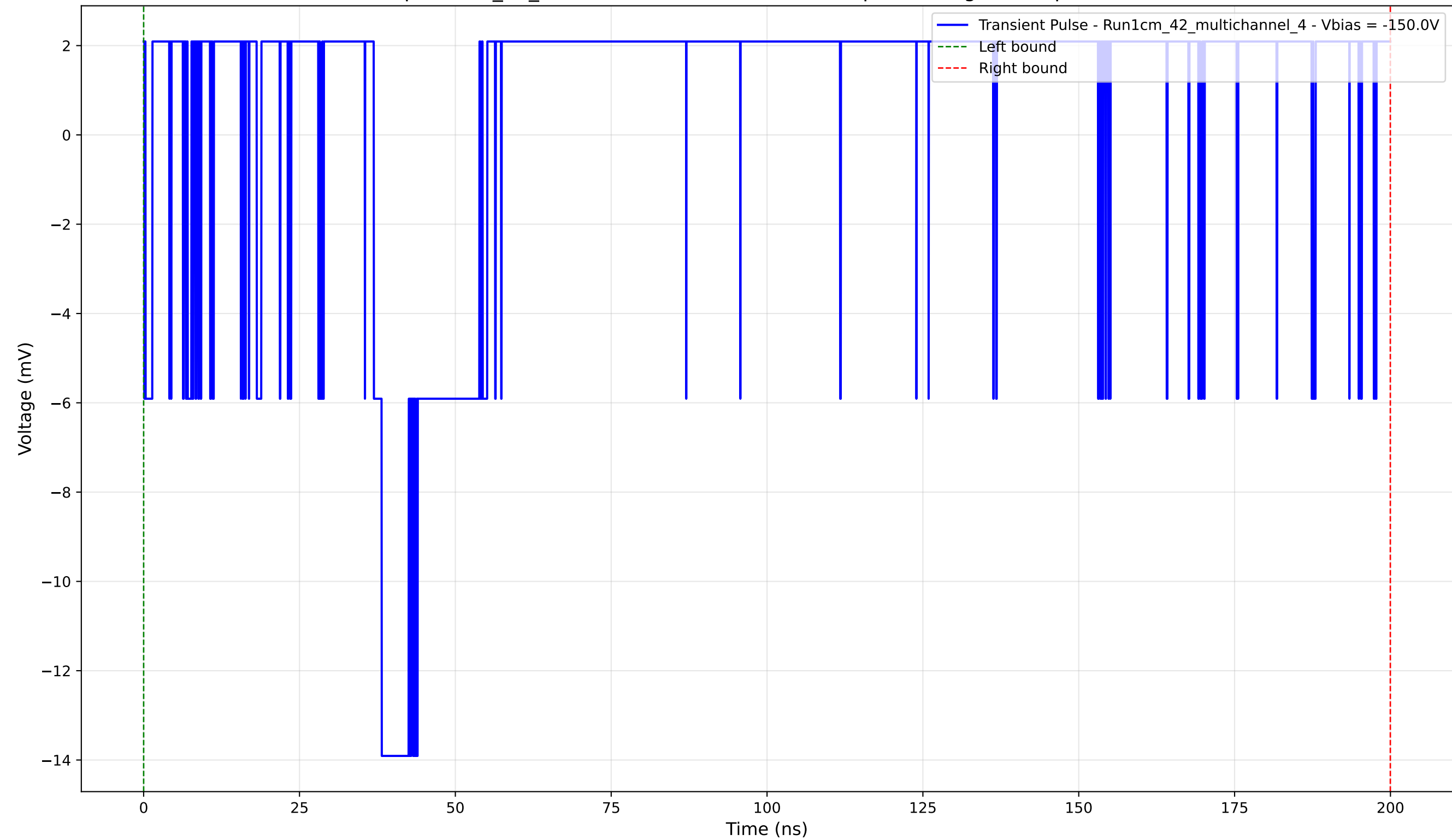
Transient Pulse - Sample: 1cm_42_multichannel - Position: 4090.0 \mu\text{m} - Charge: 3.38 pC - Rise Time: 0.00 ns (N/A)
