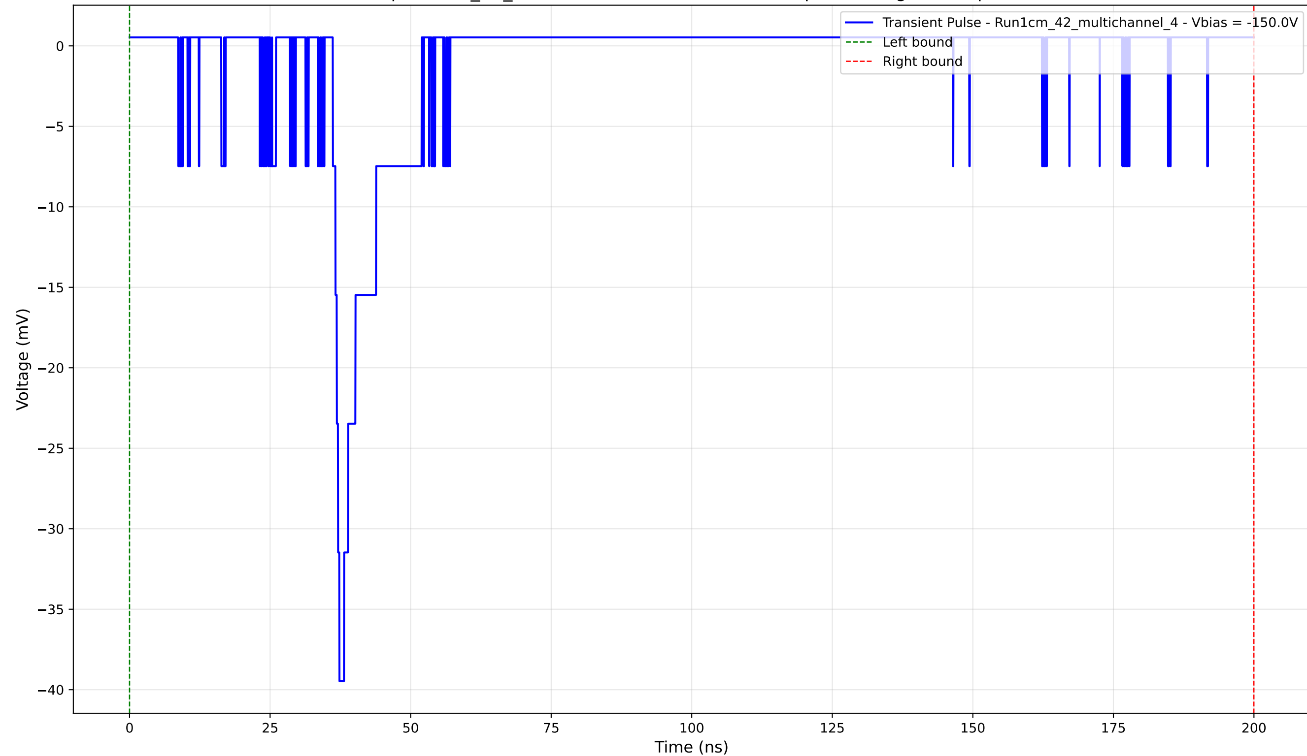
Transient Pulse - Sample: 1cm_42_multichannel - Position: 1730.0 \mu\text{m} - Charge: 3.80 pC - Rise Time: 1.17 ns
