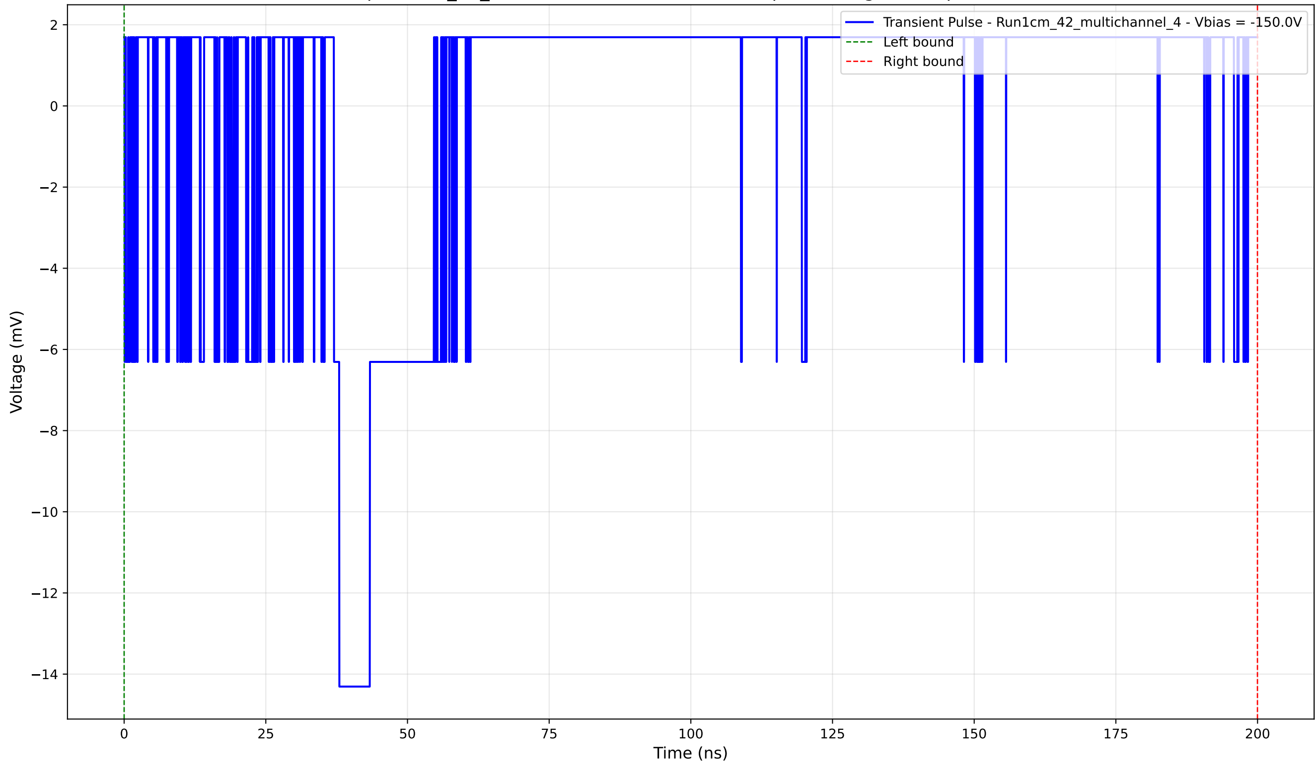
Transient Pulse - Sample: 1cm_42_multichannel - Position: 620.0 \mu\text{m} - Charge: 0.80 pC - Rise Time: 0.00 ns (N/A)
