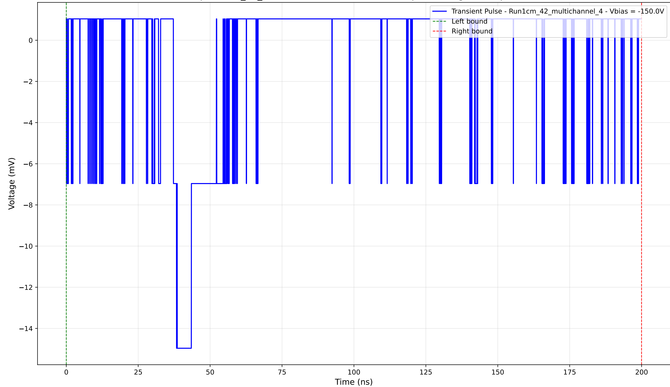
Transient Pulse - Sample: 1cm_42_multichannel - Position: 4580.0 \mu\text{m} - Charge: 1.39 pC - Rise Time: 1.10 ns
