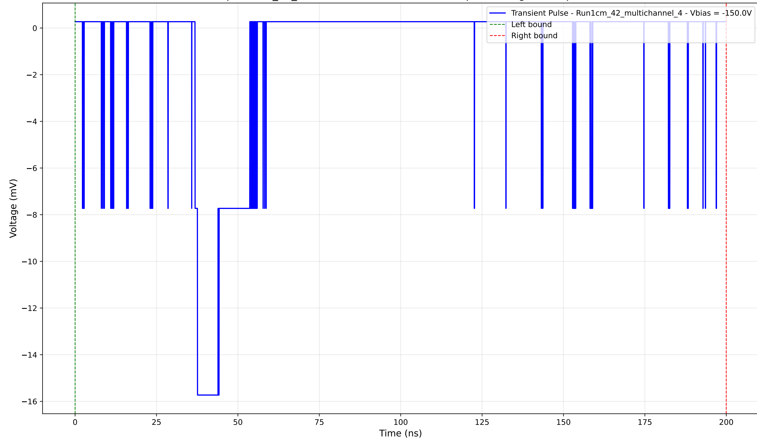
Transient Pulse - Sample: 1cm_42_multichannel - Position: 3745.0 \mu\text{m} - Charge: 3.47 pC - Rise Time: 0.76 ns
