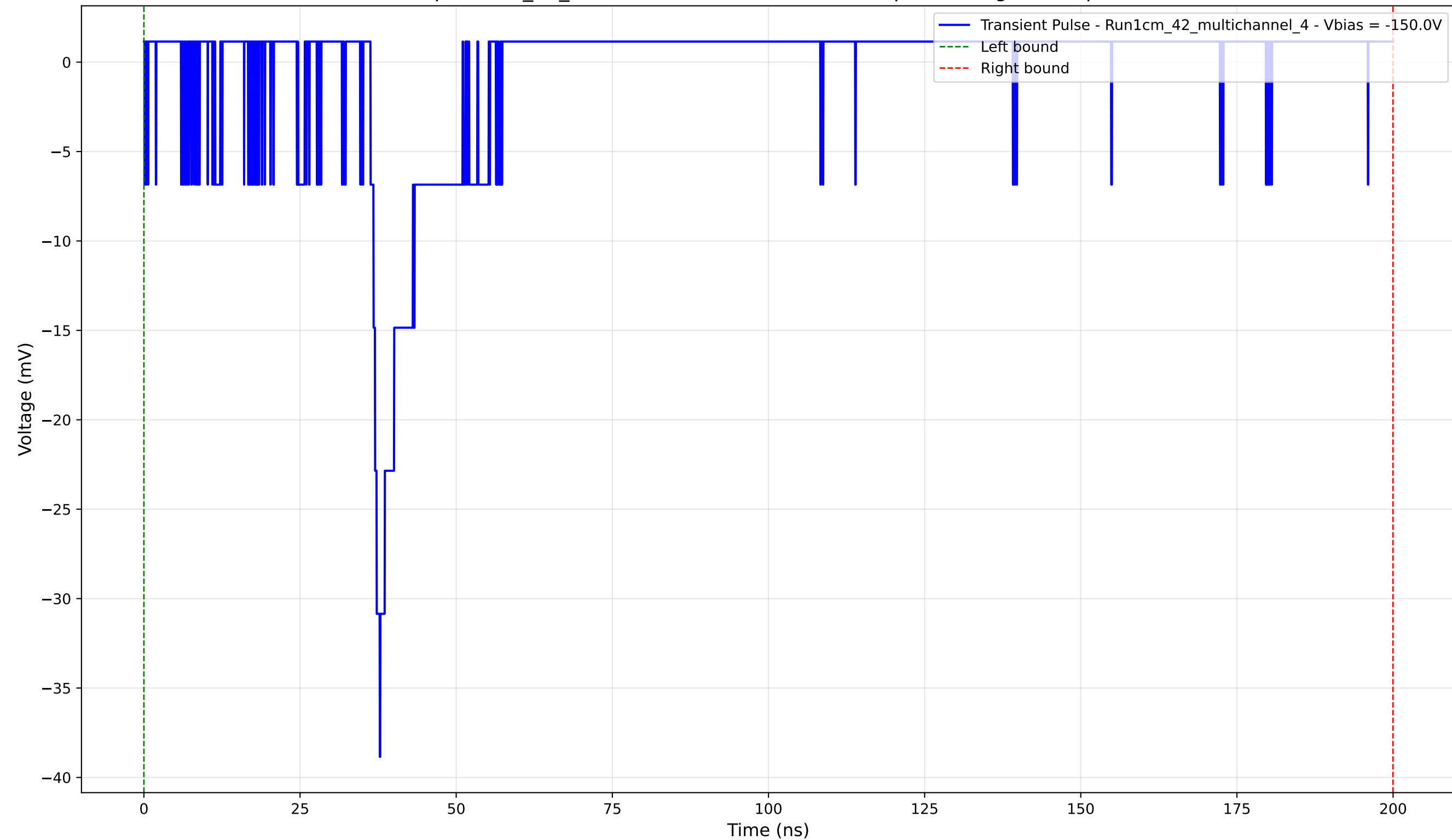
Transient Pulse - Sample: 1cm_42_multichannel - Position: 1650.0 \mu\text{m} - Charge: 1.48 pC - Rise Time: 1.49 ns
