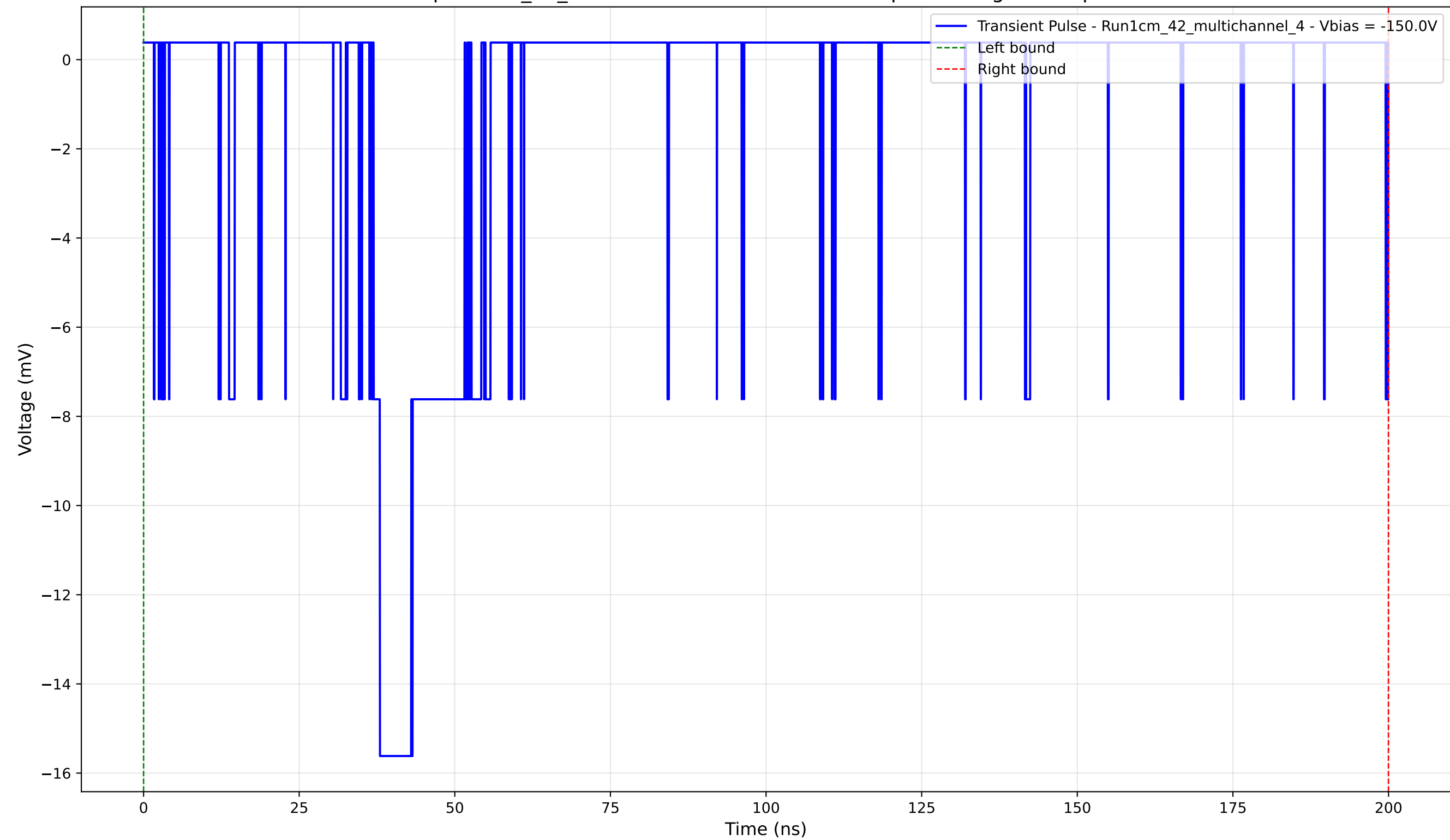
Transient Pulse - Sample: 1cm_42_multichannel - Position: 3980.0 \mu\text{m} - Charge: 3.15 pC - Rise Time: 1.02 ns
