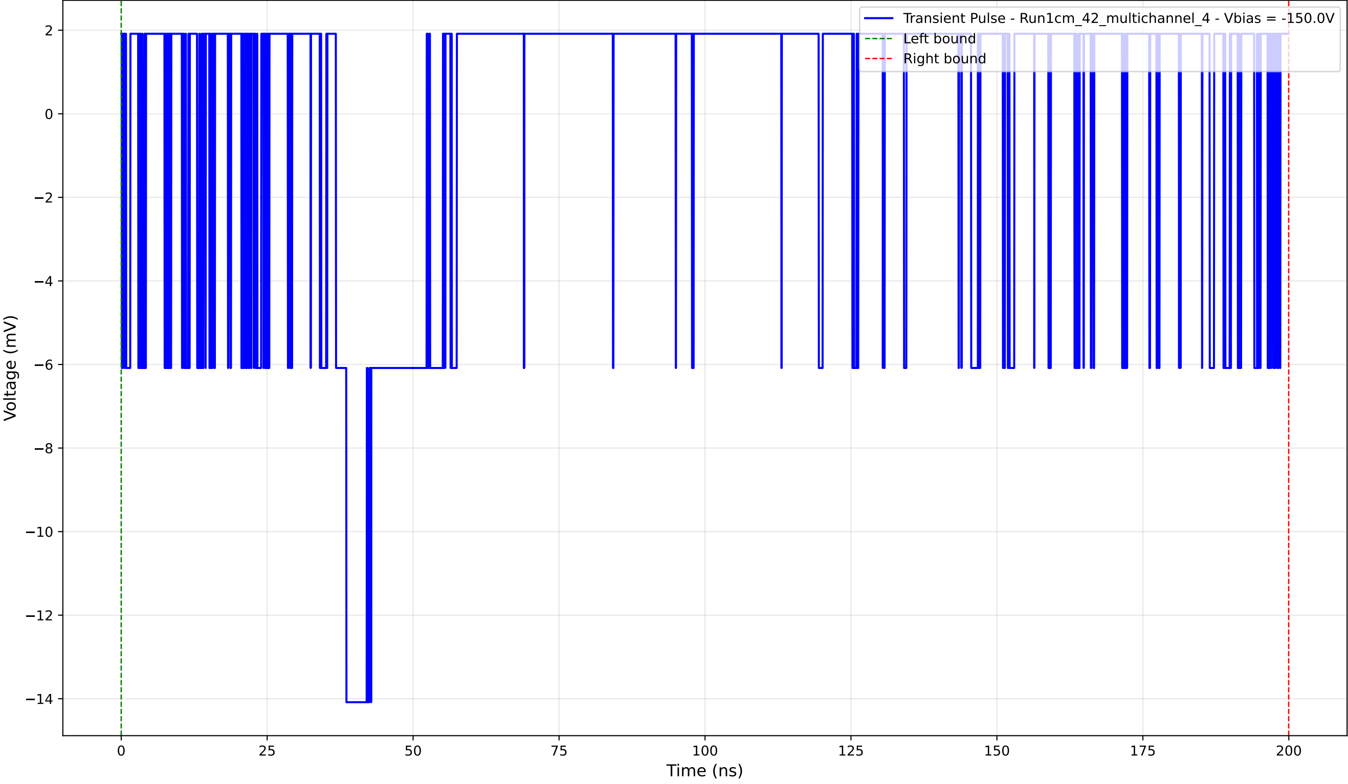
Transient Pulse - Sample: 1cm_42_multichannel - Position: 190.0 \mu\text{m} - Charge: 0.83 pC - Rise Time: 0.00 ns (N/A)
