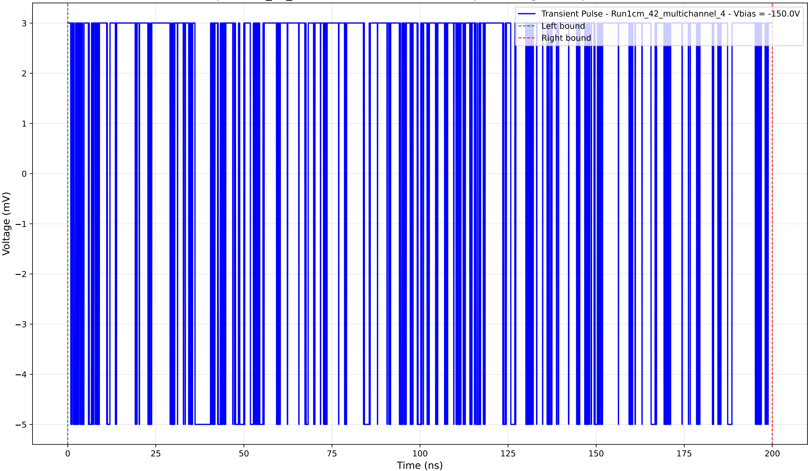
Transient Pulse - Sample: 1cm_42_multichannel - Position: 2410.0 \mu\text{m} - Charge: 5.07 pC - Rise Time: 0.00 ns (N/A)
