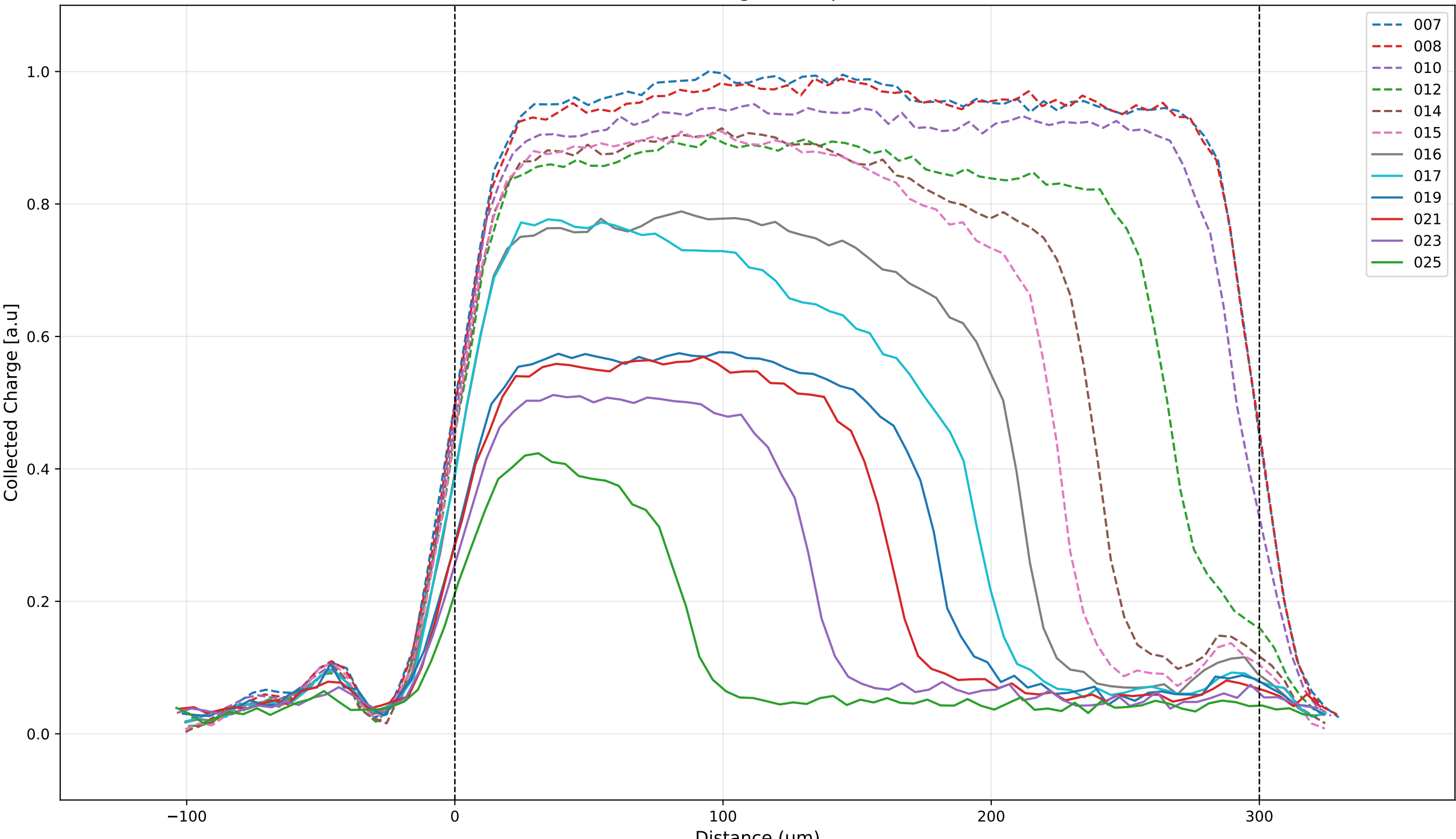
Collected Charge - Sample: 400E
