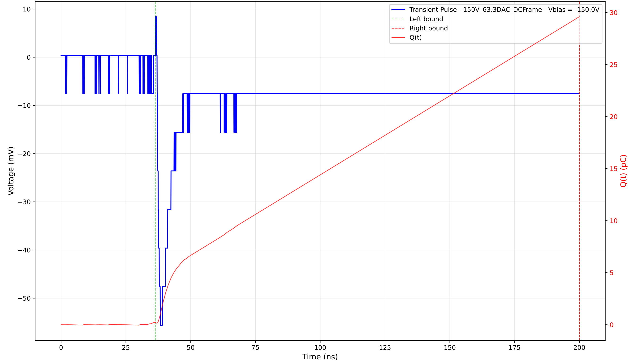
Transient Pulse - Sample: 1cm_42 - Position: 3765.0 \mu\text{m} - Charge: 29.38 pC - Rise Time: 1.21 ns
