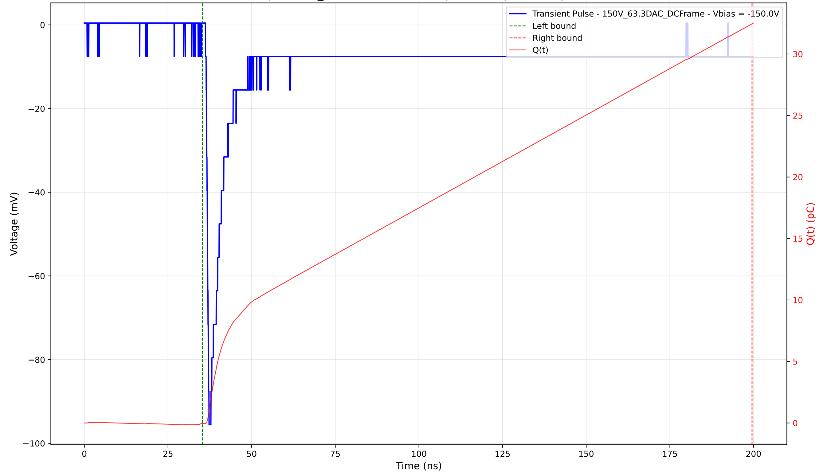
Transient Pulse - Sample: 1cm_42 - Position: 4415.0 \mu\text{m} - Charge: 32.49 pC - Rise Time: 0.75 ns
