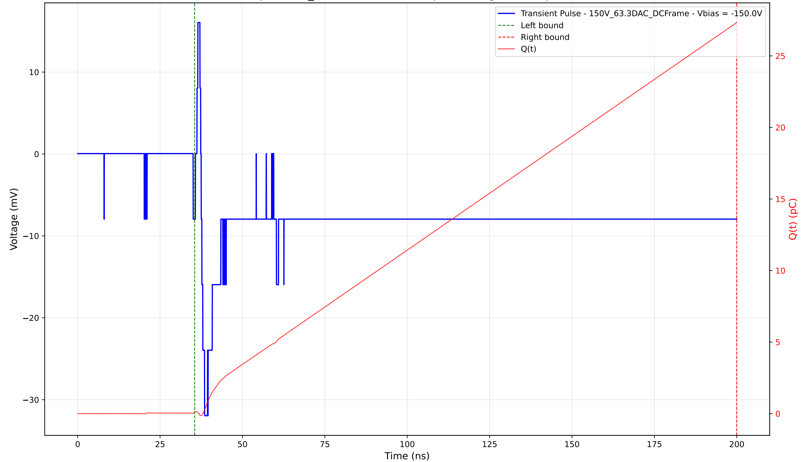
Transient Pulse - Sample: 1cm_42 - Position: 2540.0 \mu\text{m} - Charge: 27.22 pC - Rise Time: 1.03 ns
