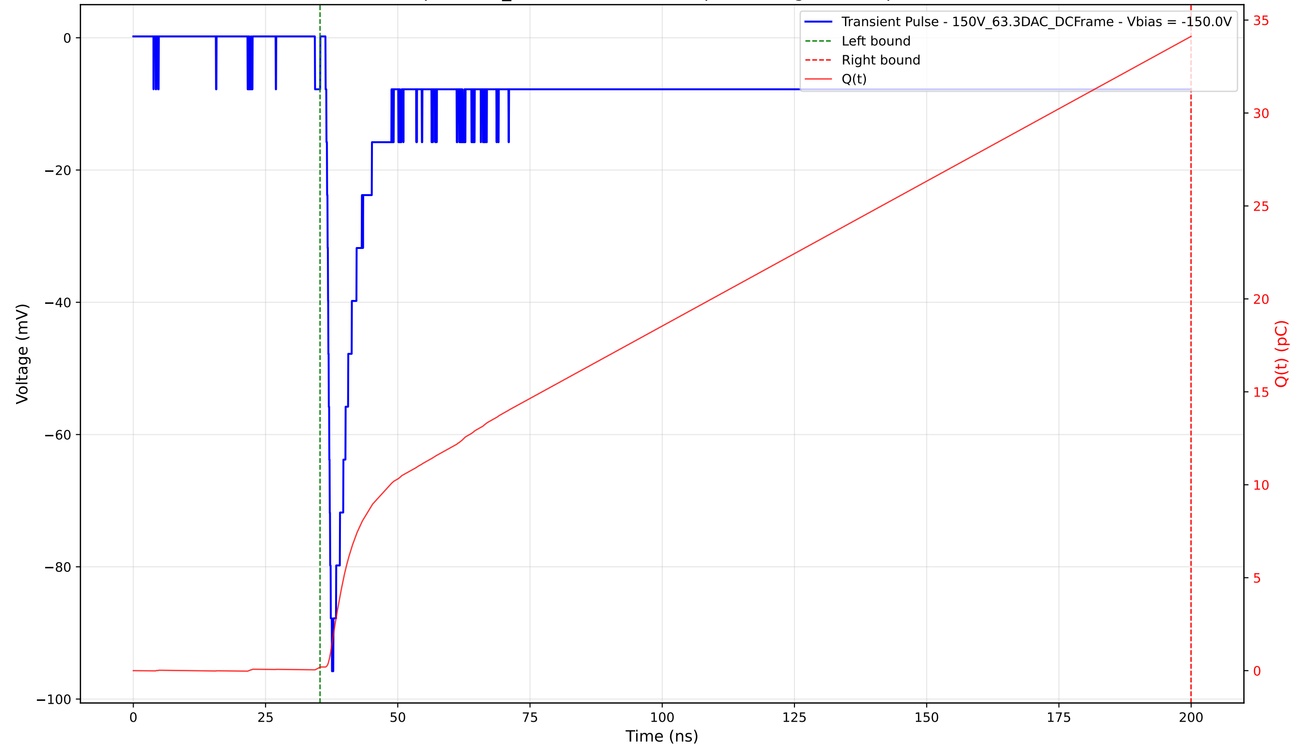
Transient Pulse - Sample: 1cm_42 - Position: 4260.0 \mu\text{m} - Charge: 33.93 pC - Rise Time: 0.84 ns
