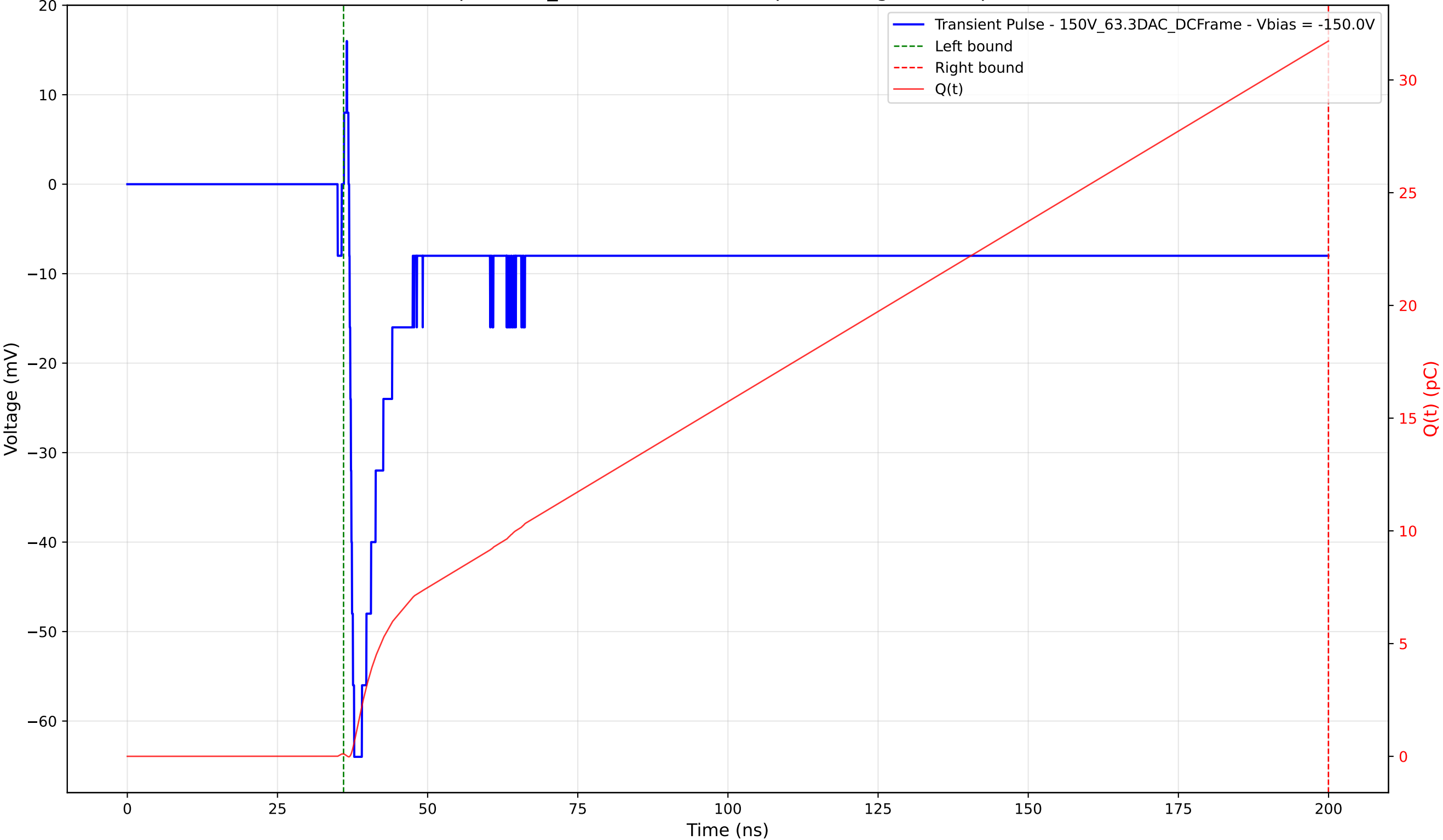
Transient Pulse - Sample: 1cm_42 - Position: 1310.0 \mu\text{m} - Charge: 31.62 pC - Rise Time: 0.82 ns
