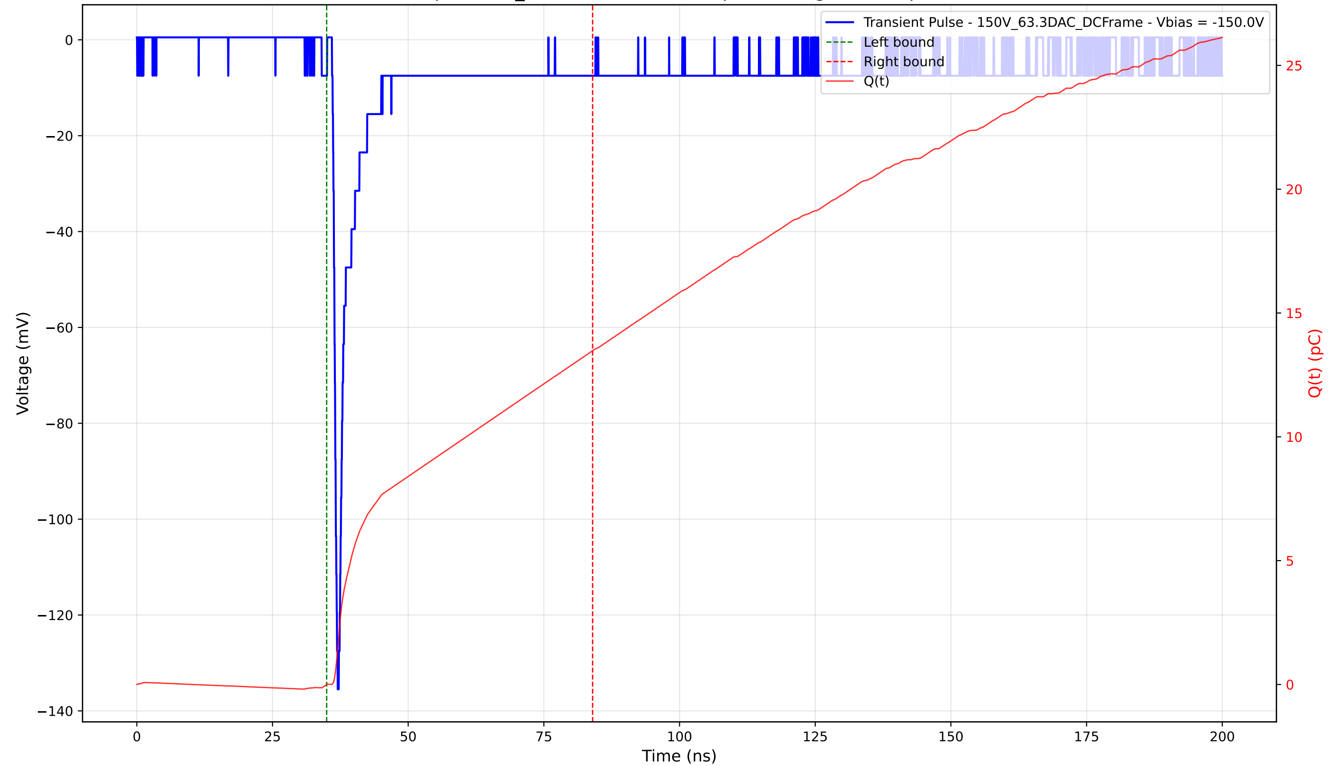
Transient Pulse - Sample: 1cm_42 - Position: 5000.0 \mu\text{m} - Charge: 13.48 pC - Rise Time: 0.80 ns
