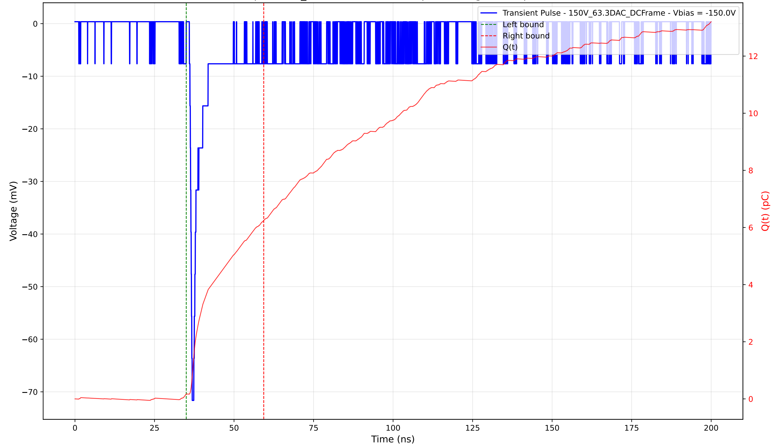
Transient Pulse - Sample: 1cm_42 - Position: 5085.0 \mu\text{m} - Charge: 6.08 pC - Rise Time: 0.88 ns
