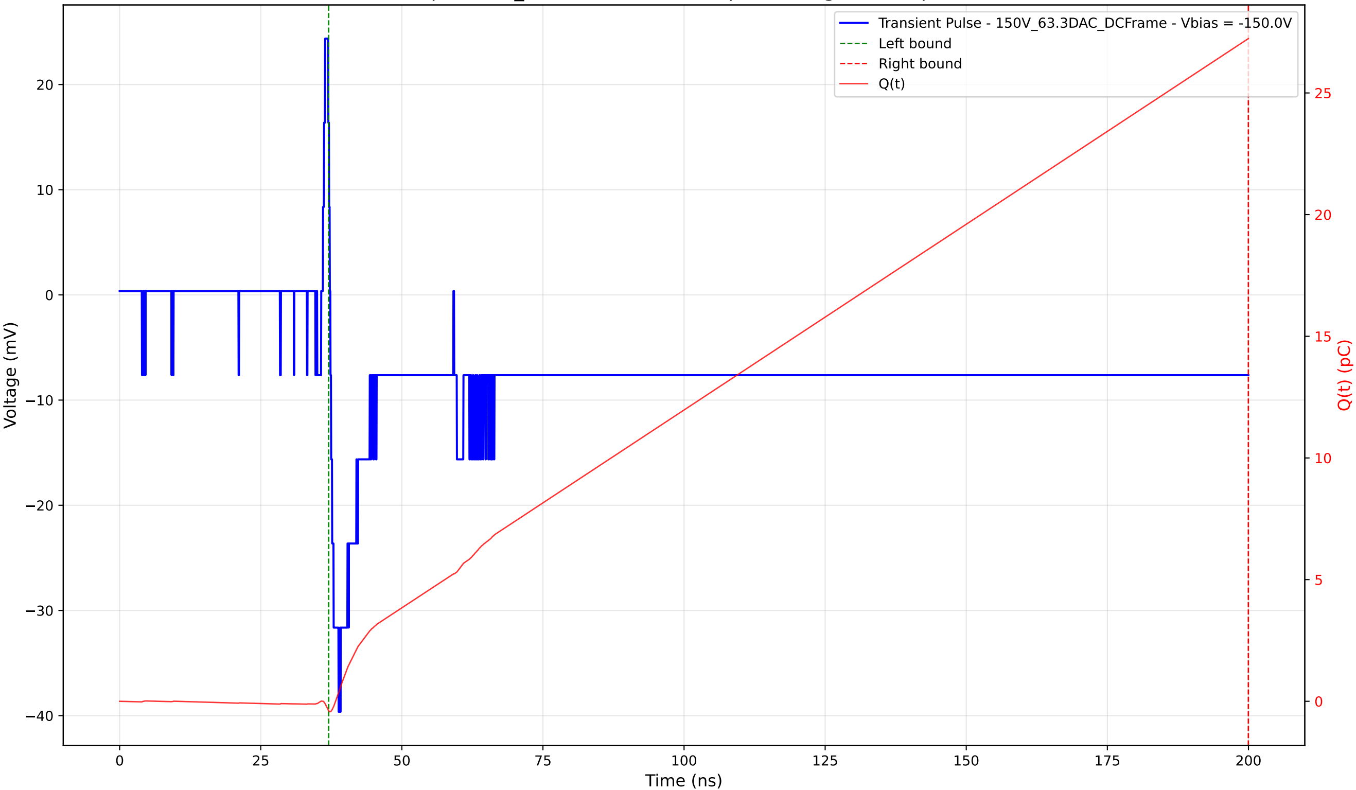
Transient Pulse - Sample: 1cm_42 - Position: 2275.0 \mu\text{m} - Charge: 27.63 pC - Rise Time: 1.45 ns
