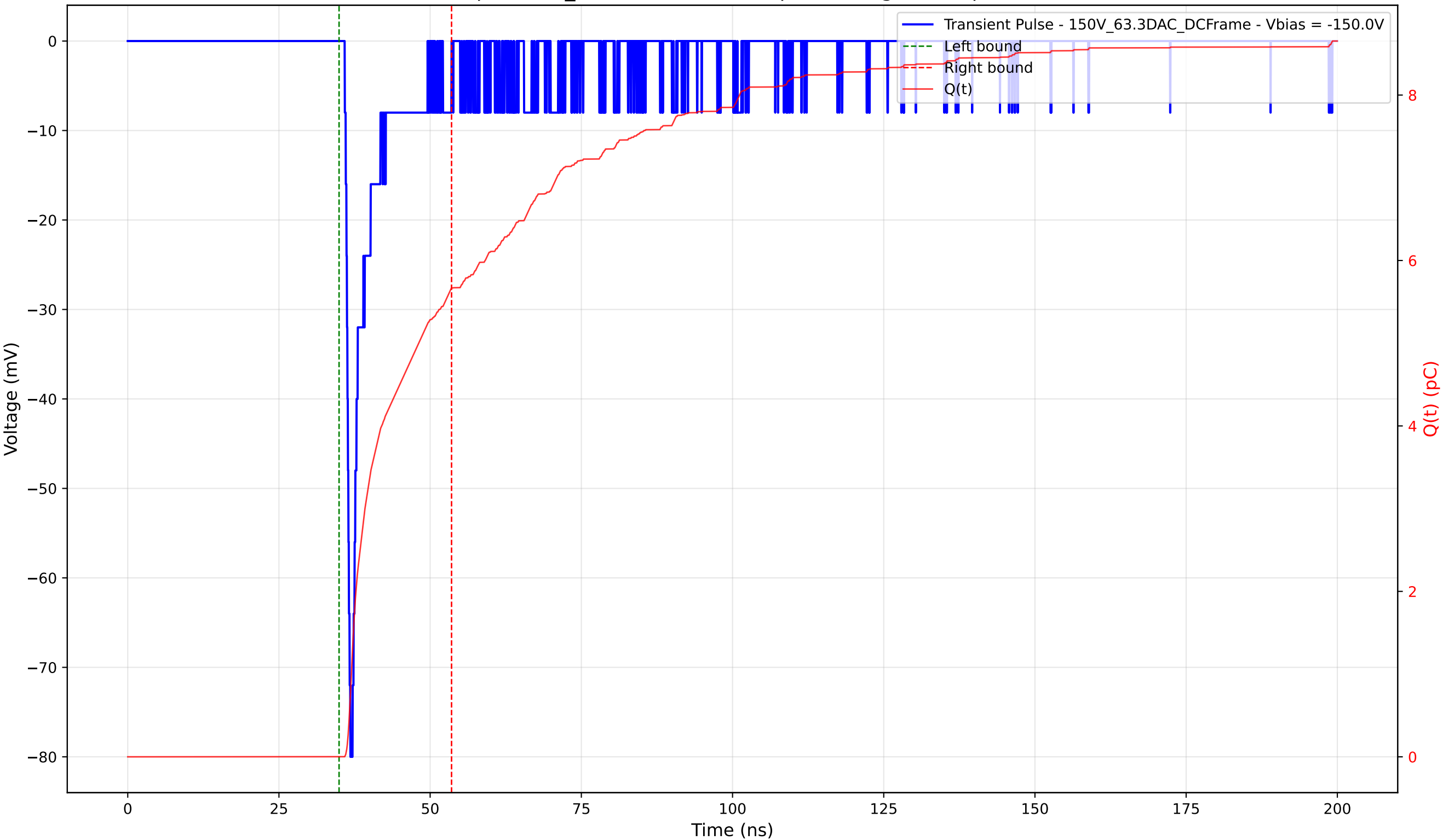
Transient Pulse - Sample: 1cm_42 - Position: 100.0 \mu\text{m} - Charge: 5.67 pC - Rise Time: 0.66 ns
