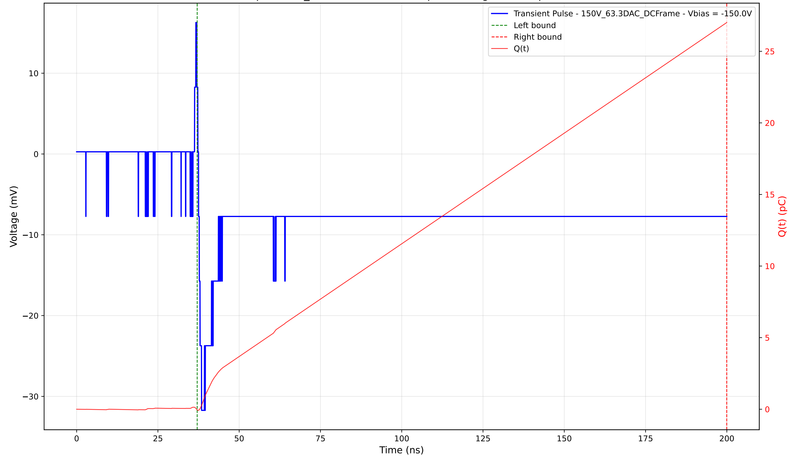
Transient Pulse - Sample: 1cm_42 - Position: 3040.0 \mu\text{m} - Charge: 27.05 pC - Rise Time: 0.93 ns
