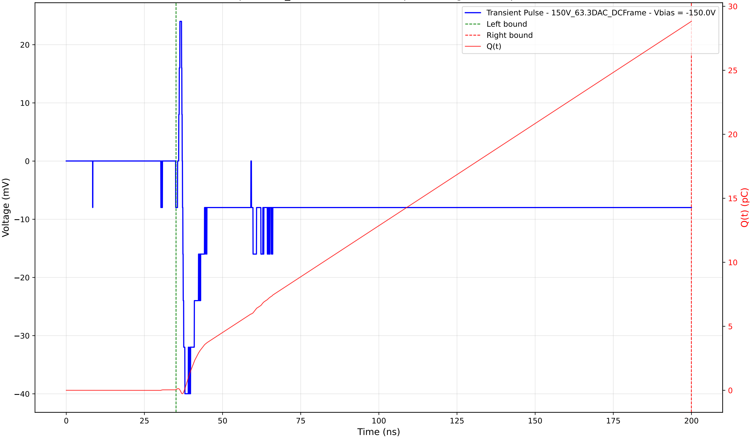
Transient Pulse - Sample: 1cm_42 - Position: 1875.0 \mu\text{m} - Charge: 28.77 pC - Rise Time: 0.77 ns
