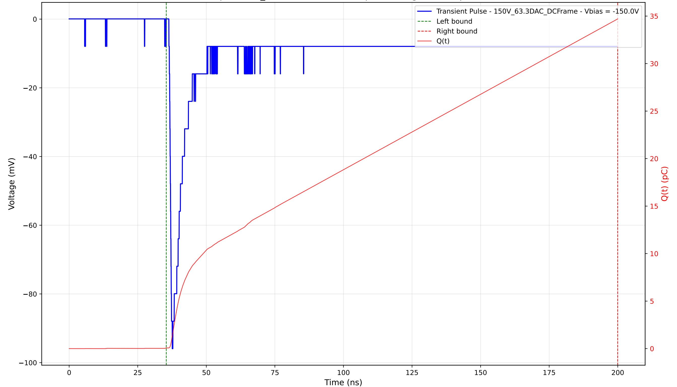
Transient Pulse - Sample: 1cm_42 - Position: 4250.0 \mu\text{m} - Charge: 34.63 pC - Rise Time: 0.80 ns
