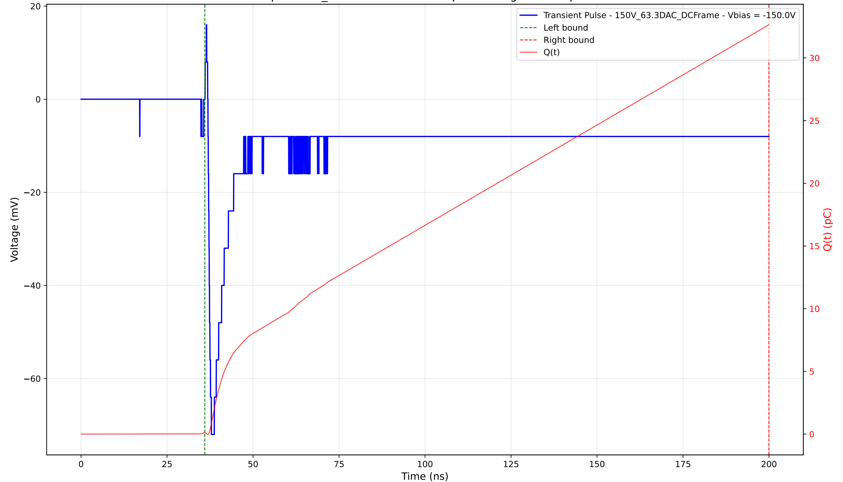
Transient Pulse - Sample: 1cm_42 - Position: 1285.0 \mu\text{m} - Charge: 32.54 pC - Rise Time: 0.98 ns
