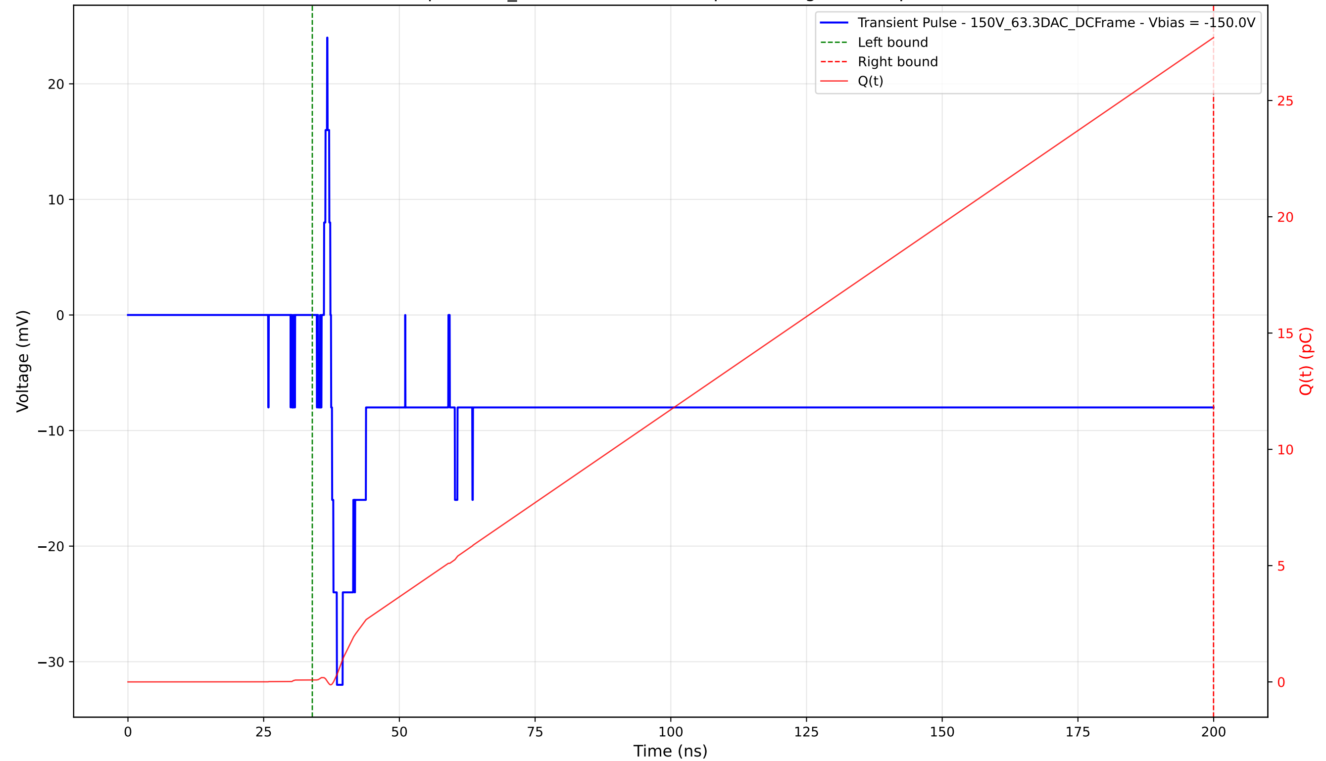
Transient Pulse - Sample: 1cm_42 - Position: 2445.0 \mu\text{m} - Charge: 27.62 pC - Rise Time: 1.07 ns
