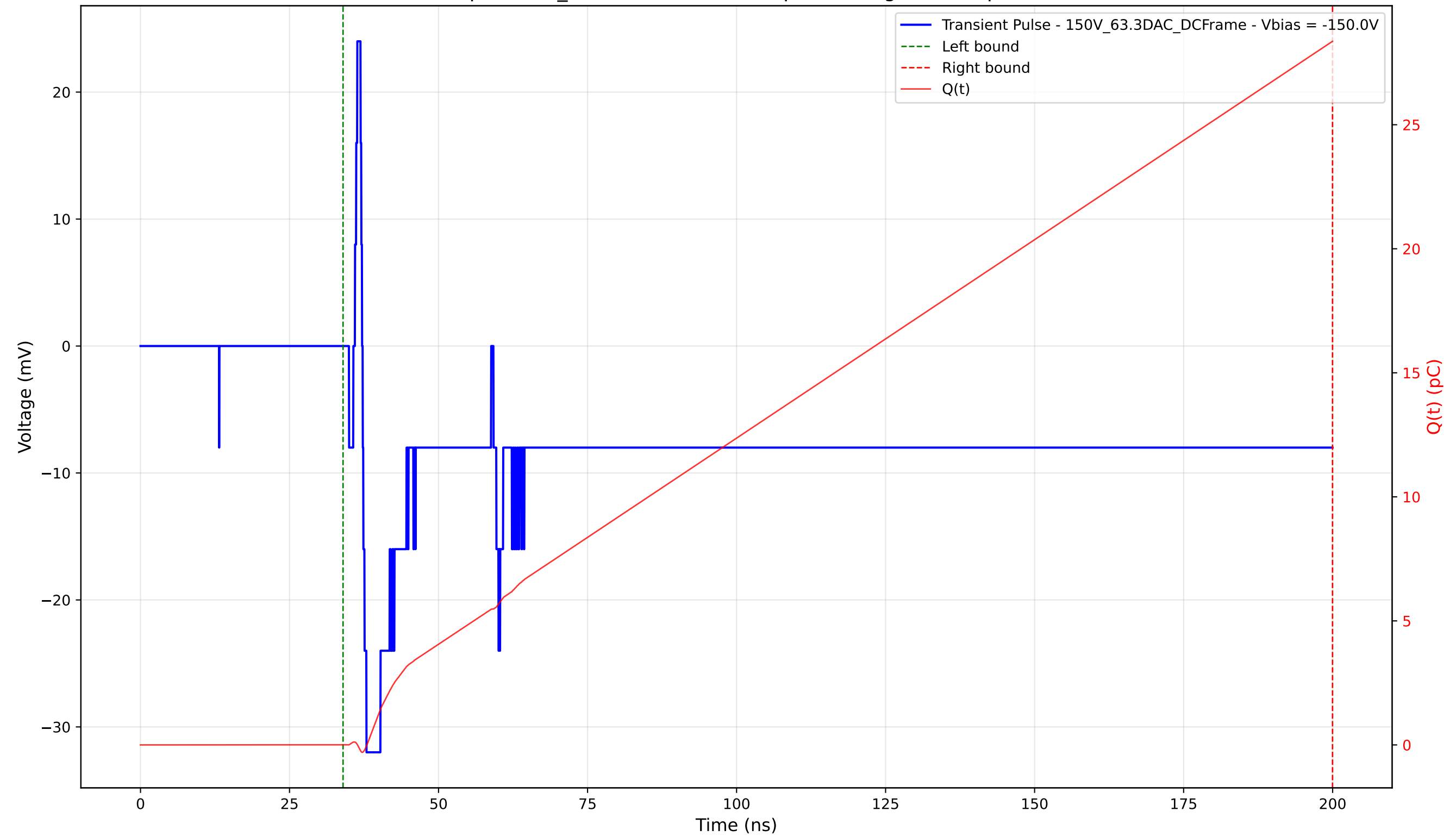
Transient Pulse - Sample: 1cm_42 - Position: 2120.0 \mu\text{m} - Charge: 28.36 pC - Rise Time: 0.63 ns
