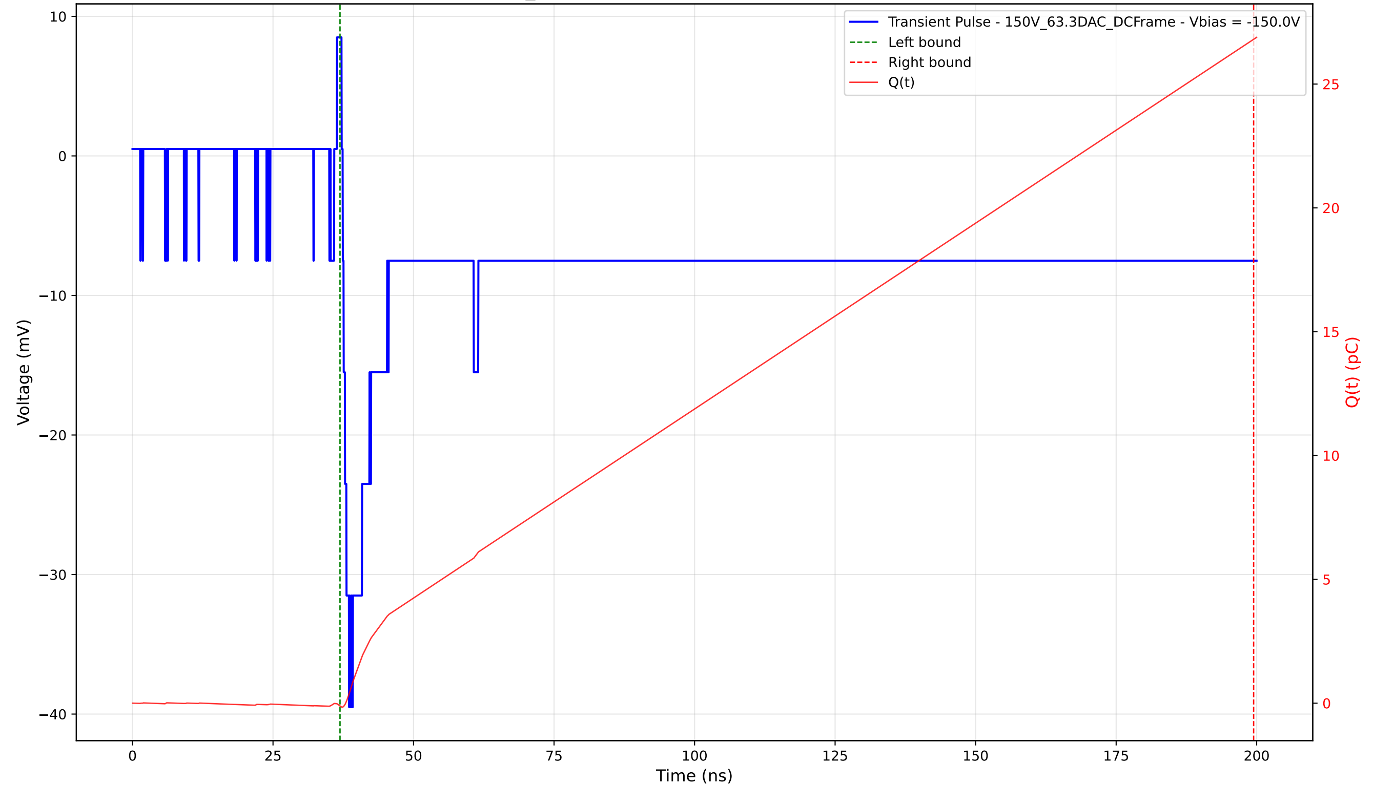
Transient Pulse - Sample: 1cm_42 - Position: 3370.0 \mu\text{m} - Charge: 26.92 pC - Rise Time: 1.13 ns
