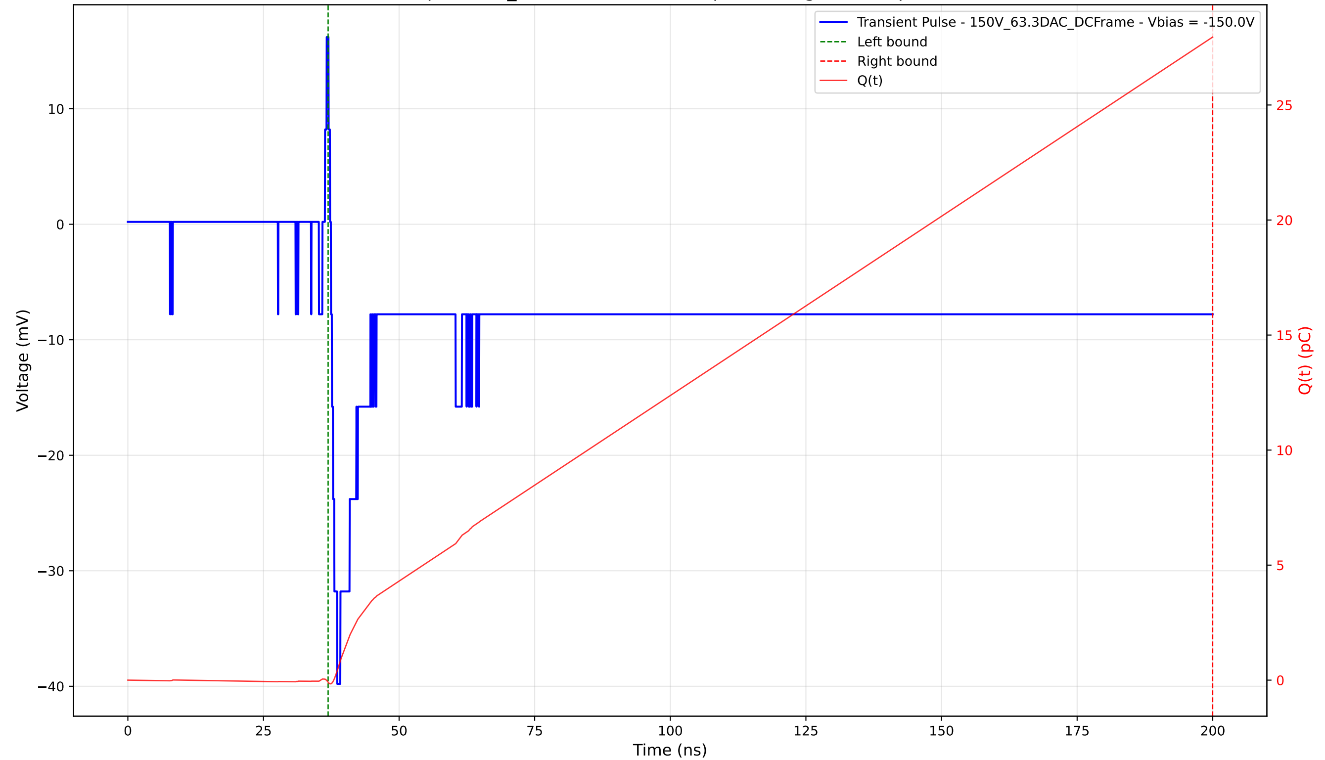
Transient Pulse - Sample: 1cm_42 - Position: 3195.0 \mu\text{m} - Charge: 28.05 pC - Rise Time: 1.15 ns
