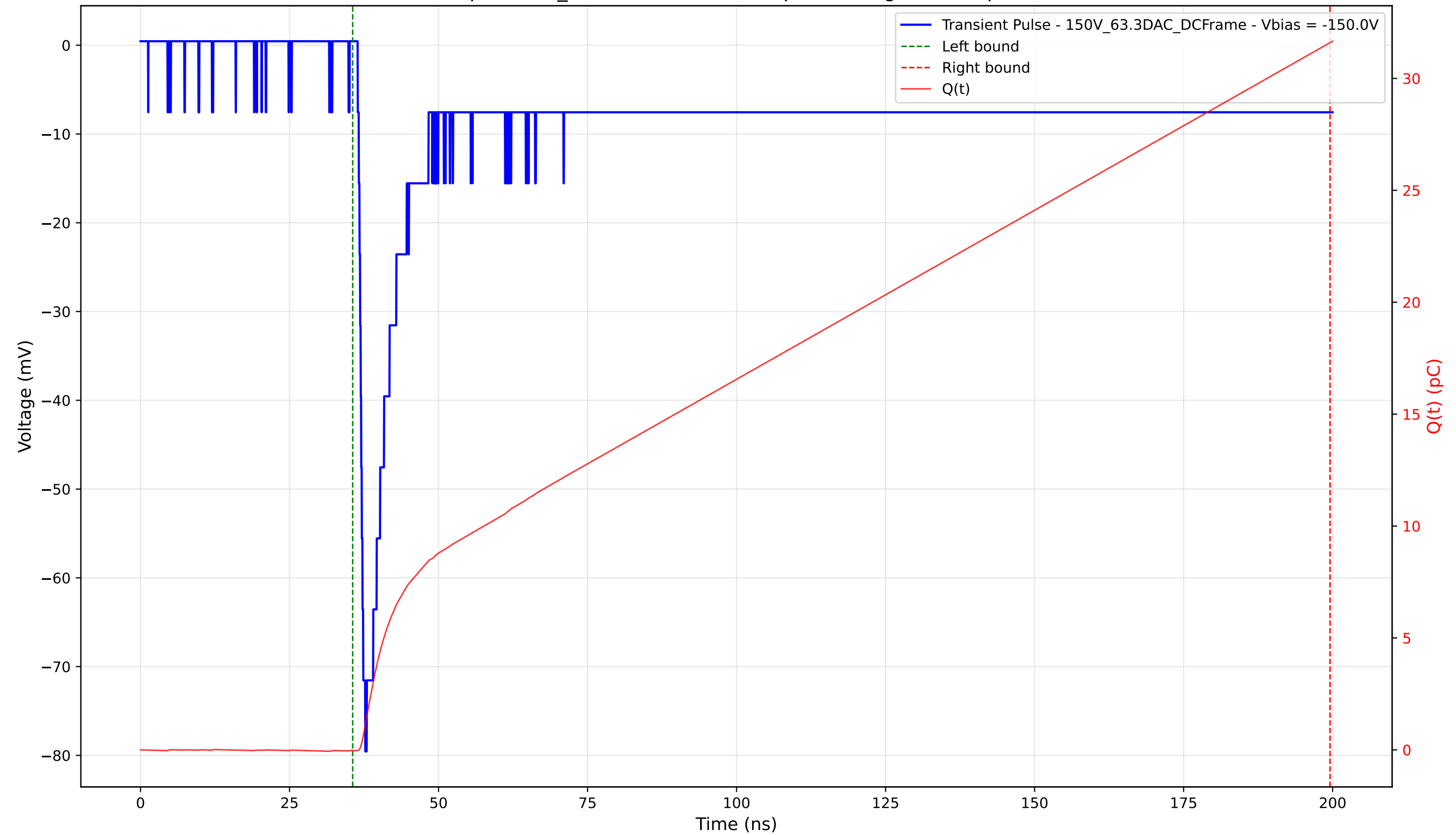
Transient Pulse - Sample: 1cm_42 - Position: 4155.0 \mu\text{m} - Charge: 31.63 pC - Rise Time: 1.10 ns
