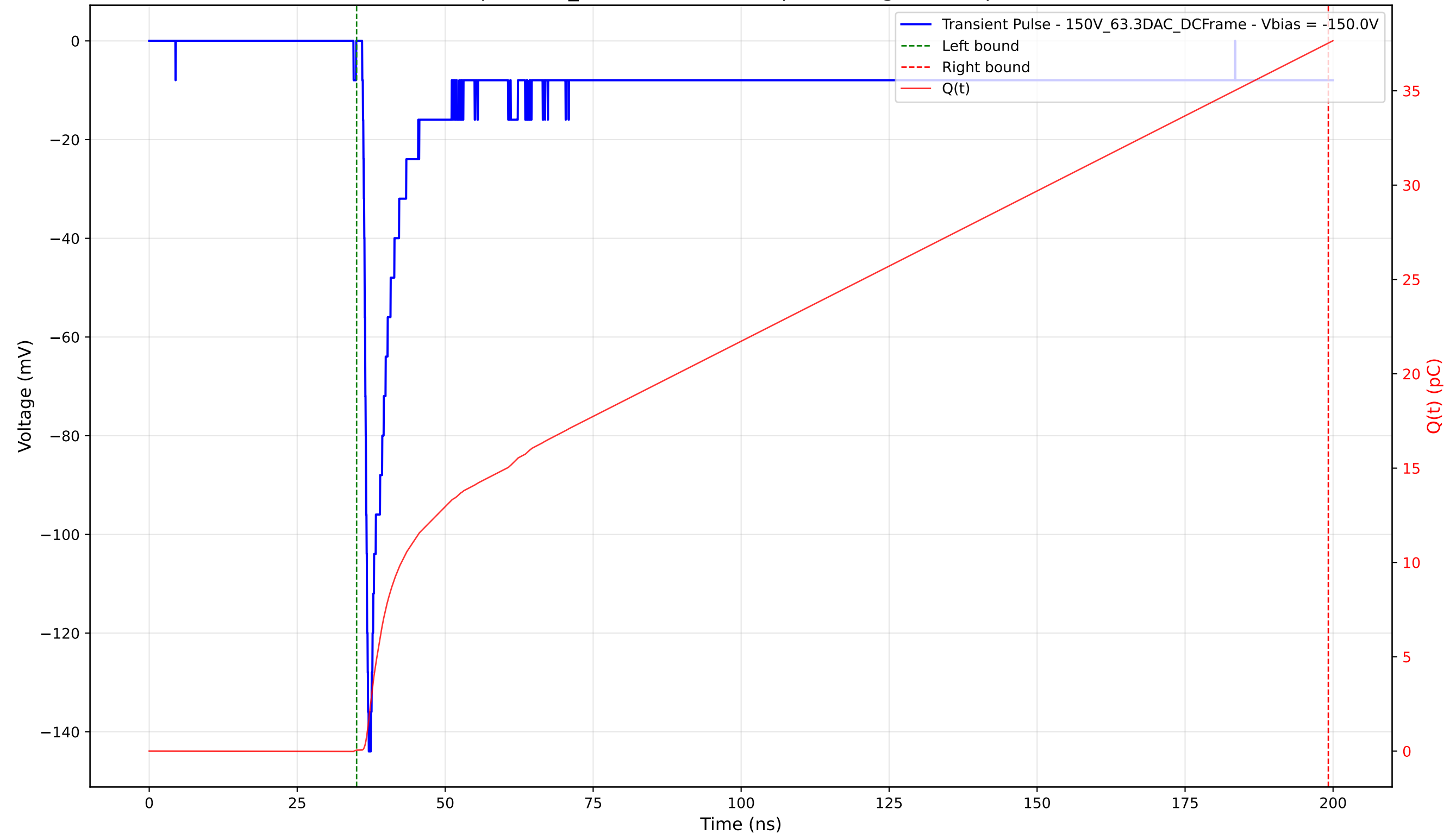
Transient Pulse - Sample: 1cm_42 - Position: 580.0 \mu\text{m} - Charge: 37.47 pC - Rise Time: 0.86 ns
