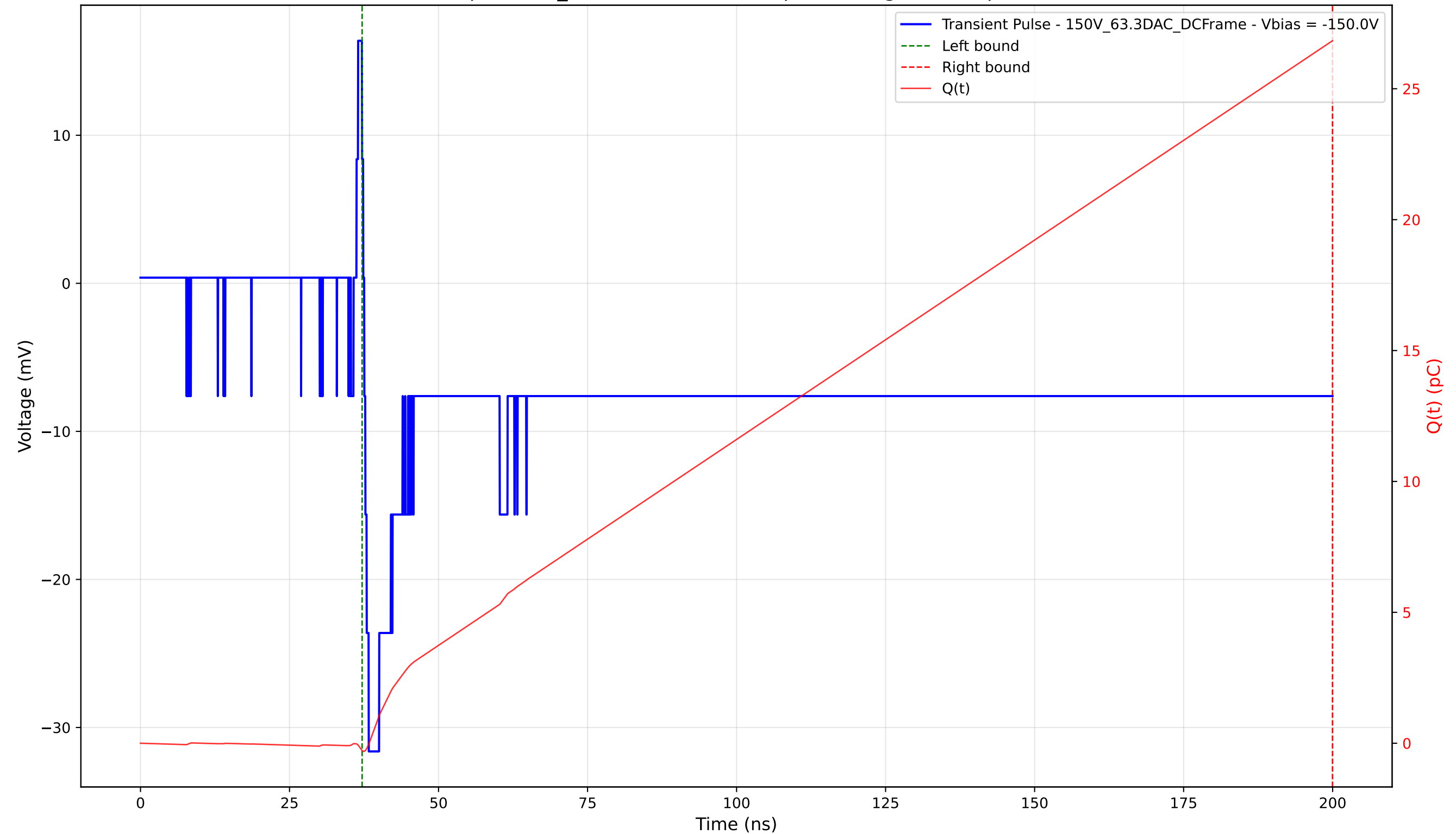
Transient Pulse - Sample: 1cm_42 - Position: 2780.0 \mu\text{m} - Charge: 27.12 pC - Rise Time: 0.75 ns
