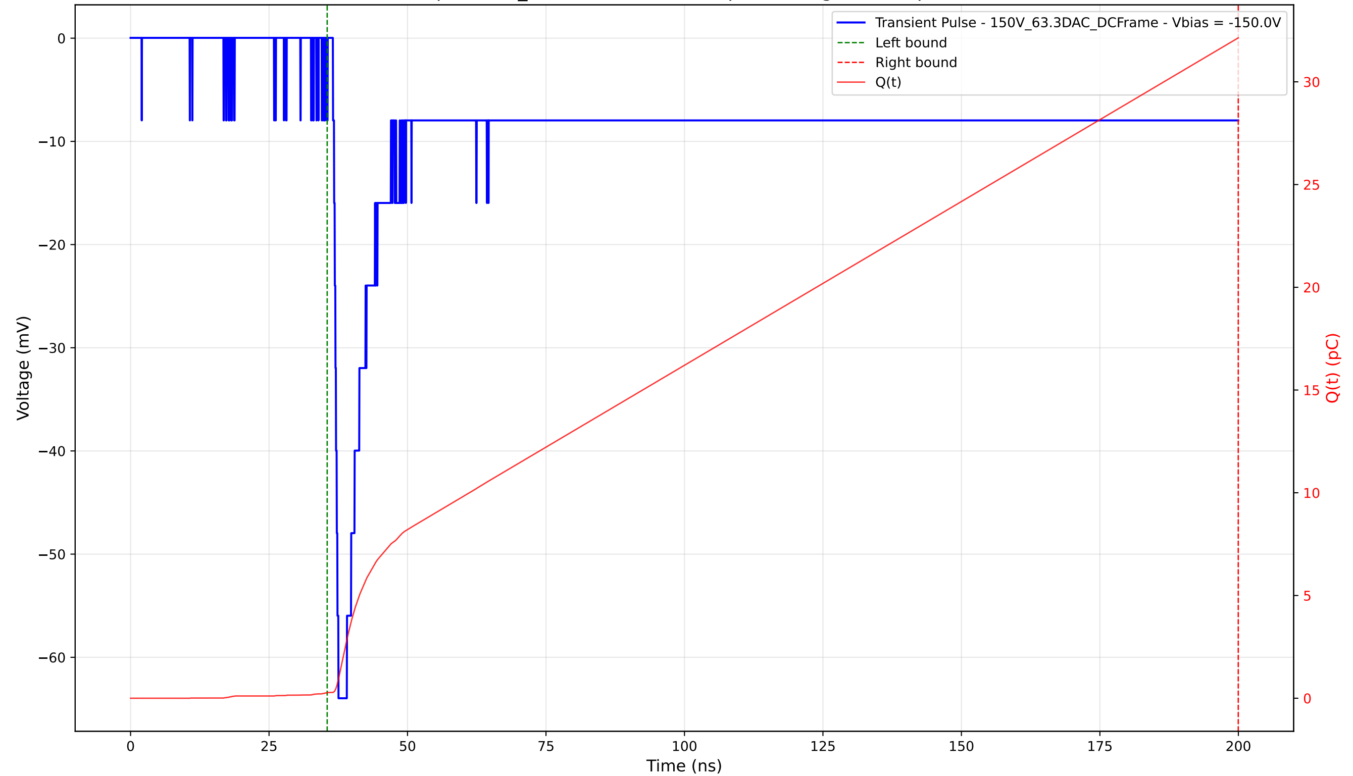
Transient Pulse - Sample: 1cm_42 - Position: 4090.0 \mu\text{m} - Charge: 31.87 pC - Rise Time: 0.98 ns
