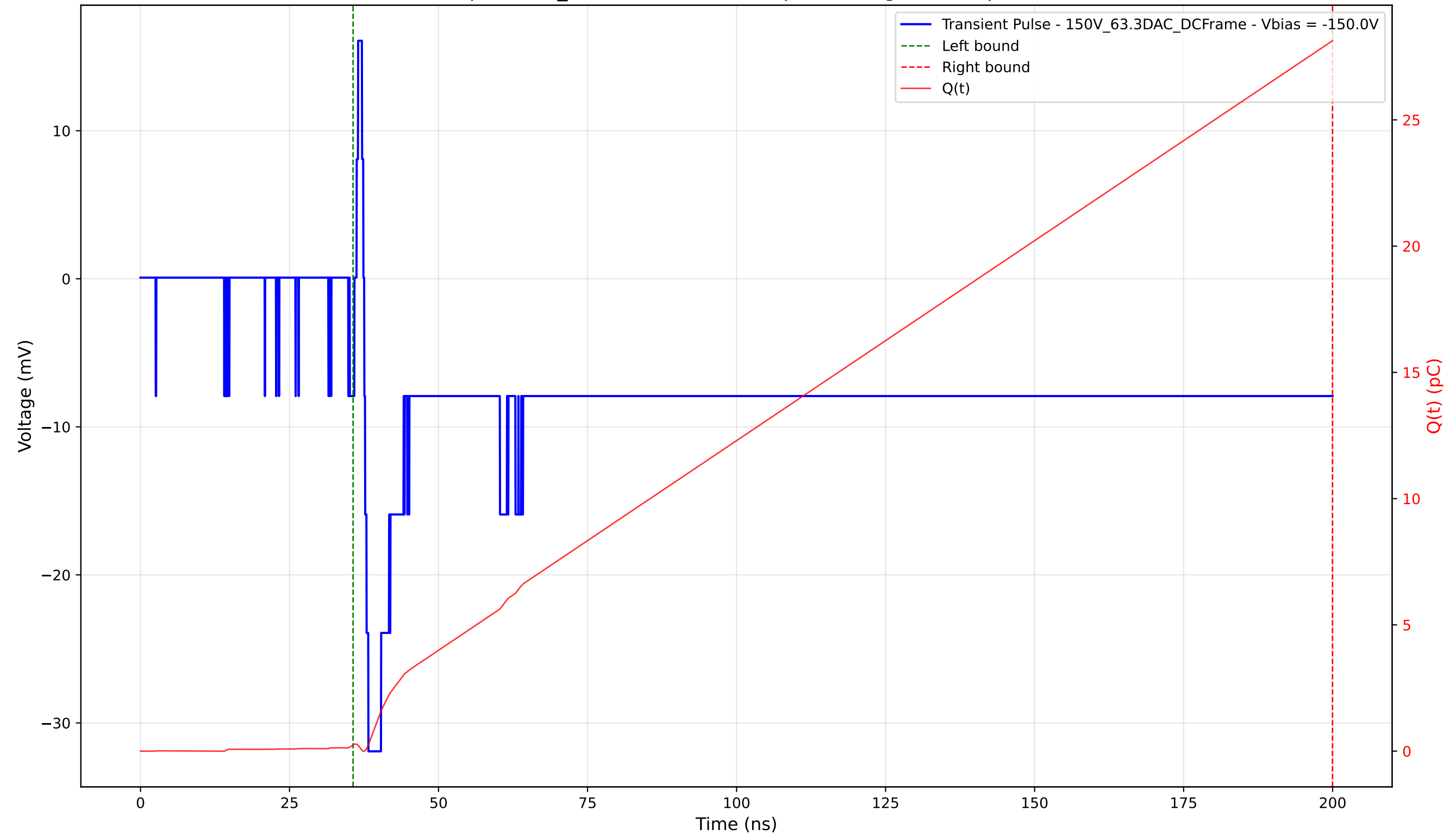
Transient Pulse - Sample: 1cm_42 - Position: 2730.0 \mu\text{m} - Charge: 27.89 pC - Rise Time: 0.69 ns
