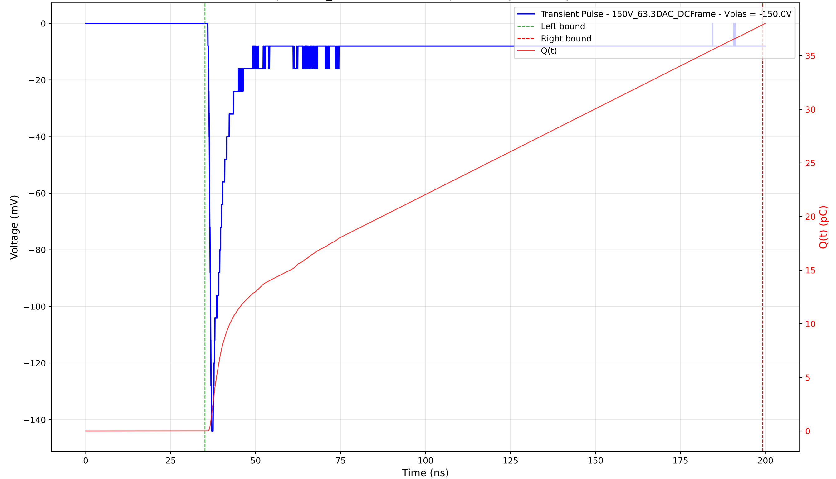
Transient Pulse - Sample: 1cm_42 - Position: 590.0 \mu\text{m} - Charge: 37.90 pC - Rise Time: 0.86 ns
