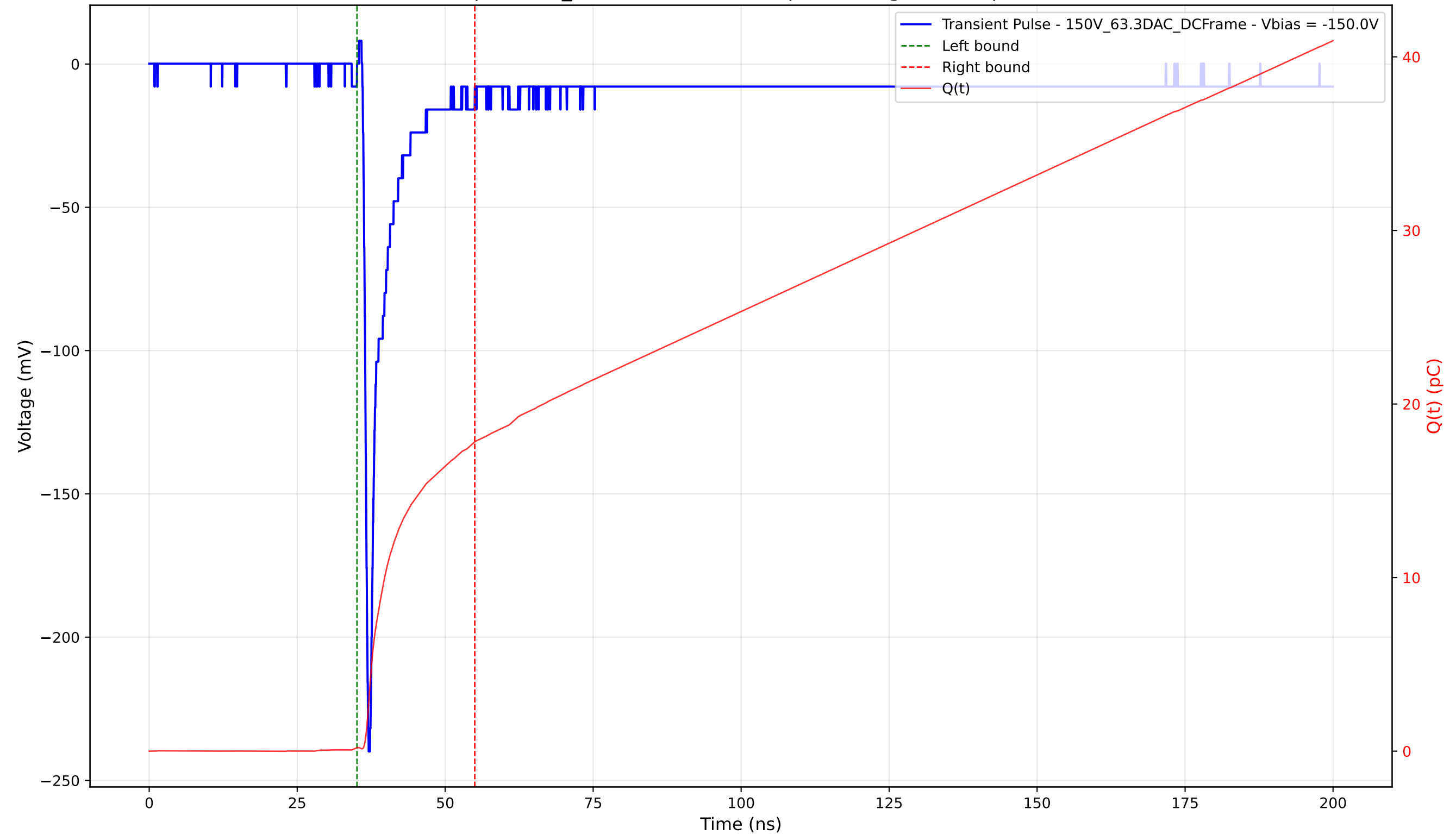
Transient Pulse - Sample: 1cm_42 - Position: 4750.0 \mu\text{m} - Charge: 17.62 pC - Rise Time: 0.78 ns
