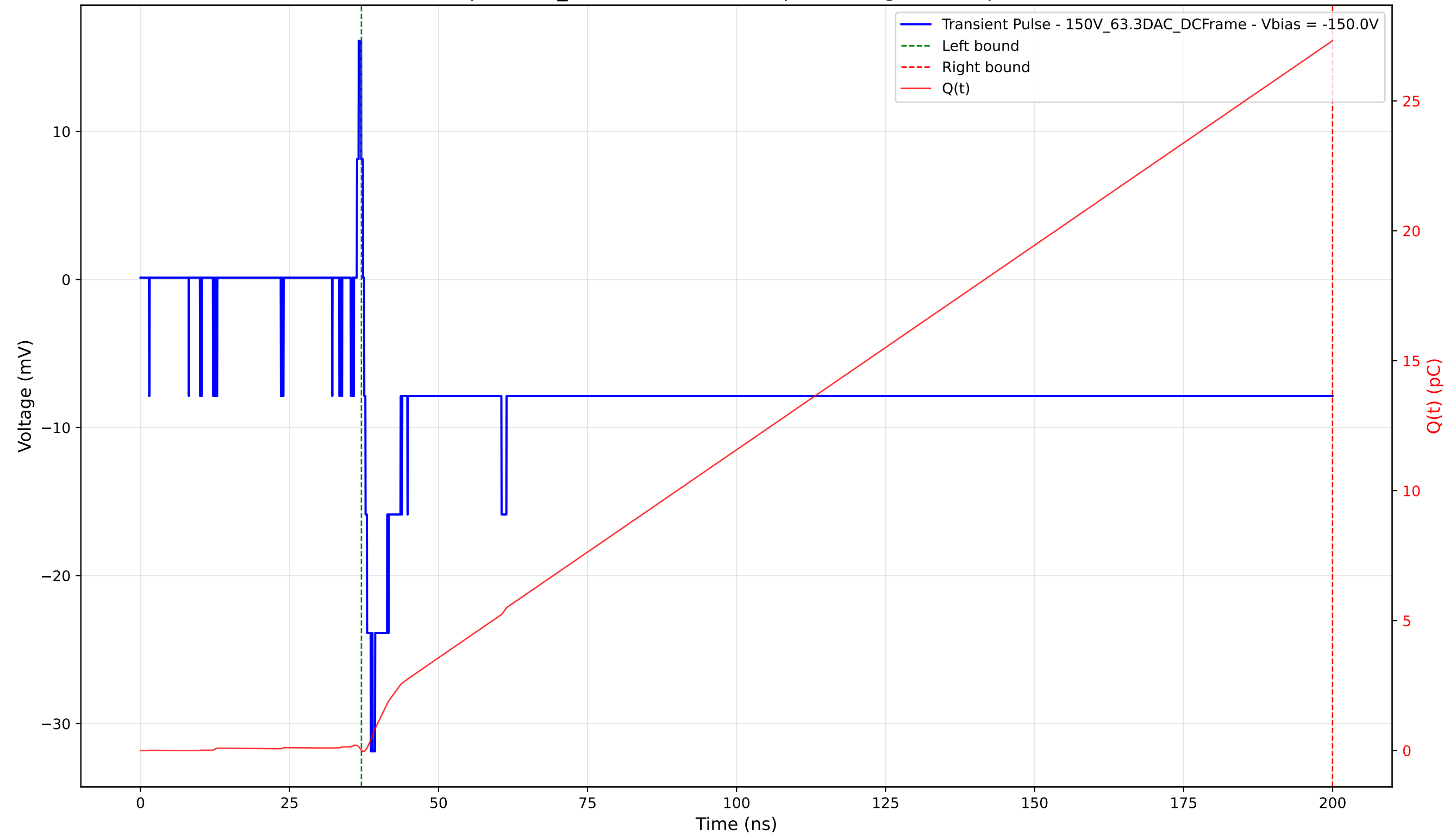
Transient Pulse - Sample: 1cm_42 - Position: 2910.0 \mu\text{m} - Charge: 27.31 pC - Rise Time: 1.13 ns
