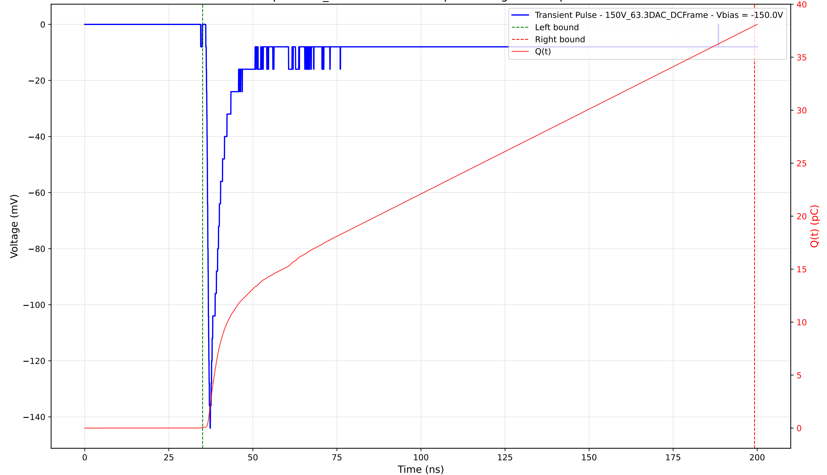
Transient Pulse - Sample: 1cm_42 - Position: 625.0 \mu\text{m} - Charge: 37.90 pC - Rise Time: 0.92 ns
