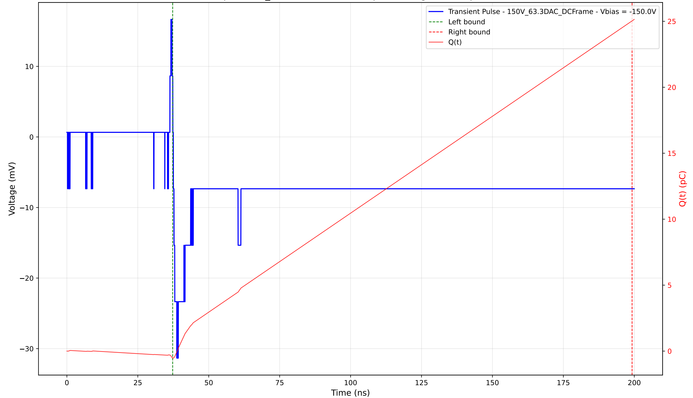
Transient Pulse - Sample: 1cm_42 - Position: 2950.0 \mu\text{m} - Charge: 25.56 pC - Rise Time: 1.25 ns
