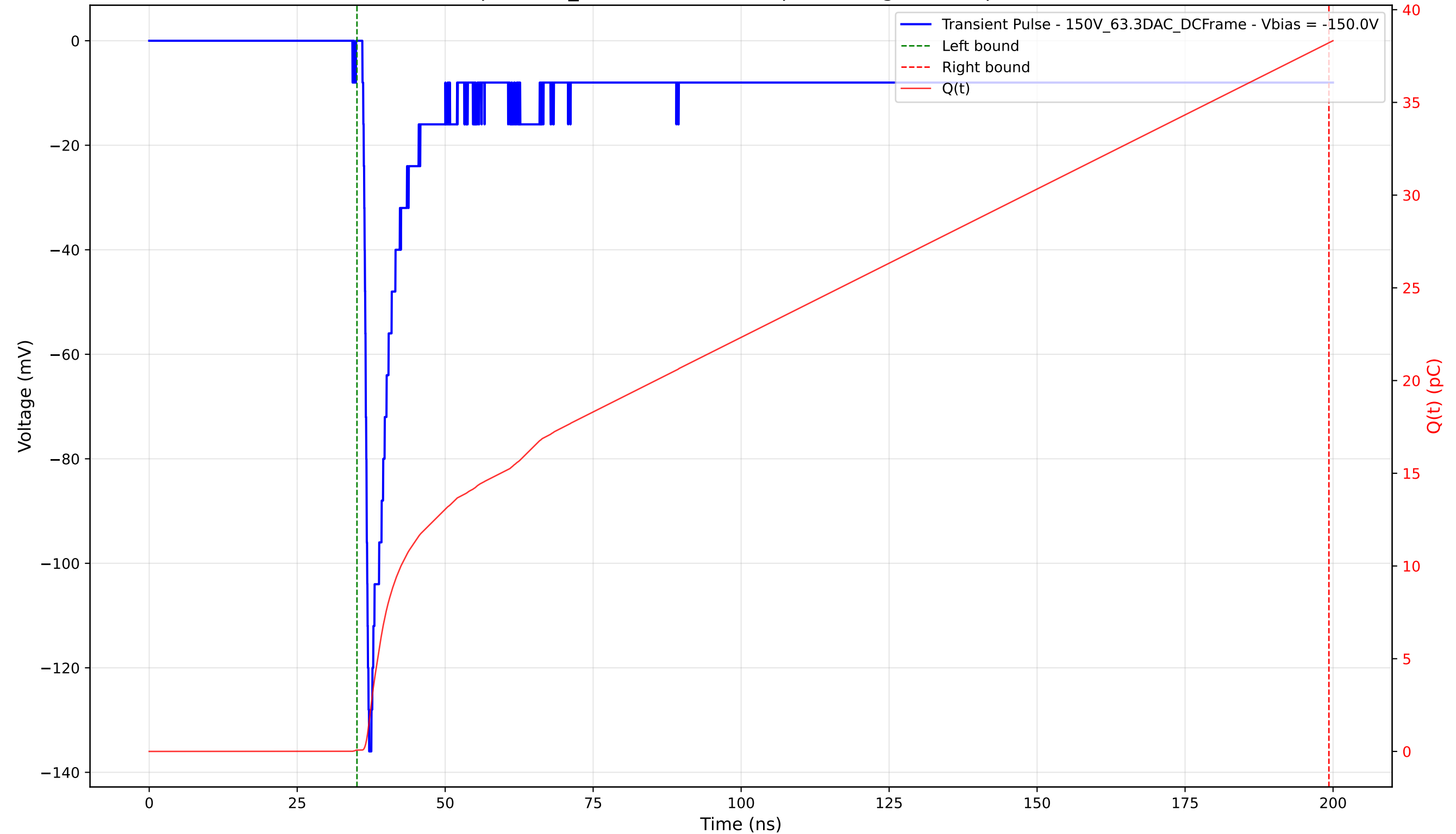
Transient Pulse - Sample: 1cm_42 - Position: 645.0 \mu\text{m} - Charge: 38.15 pC - Rise Time: 0.89 ns
