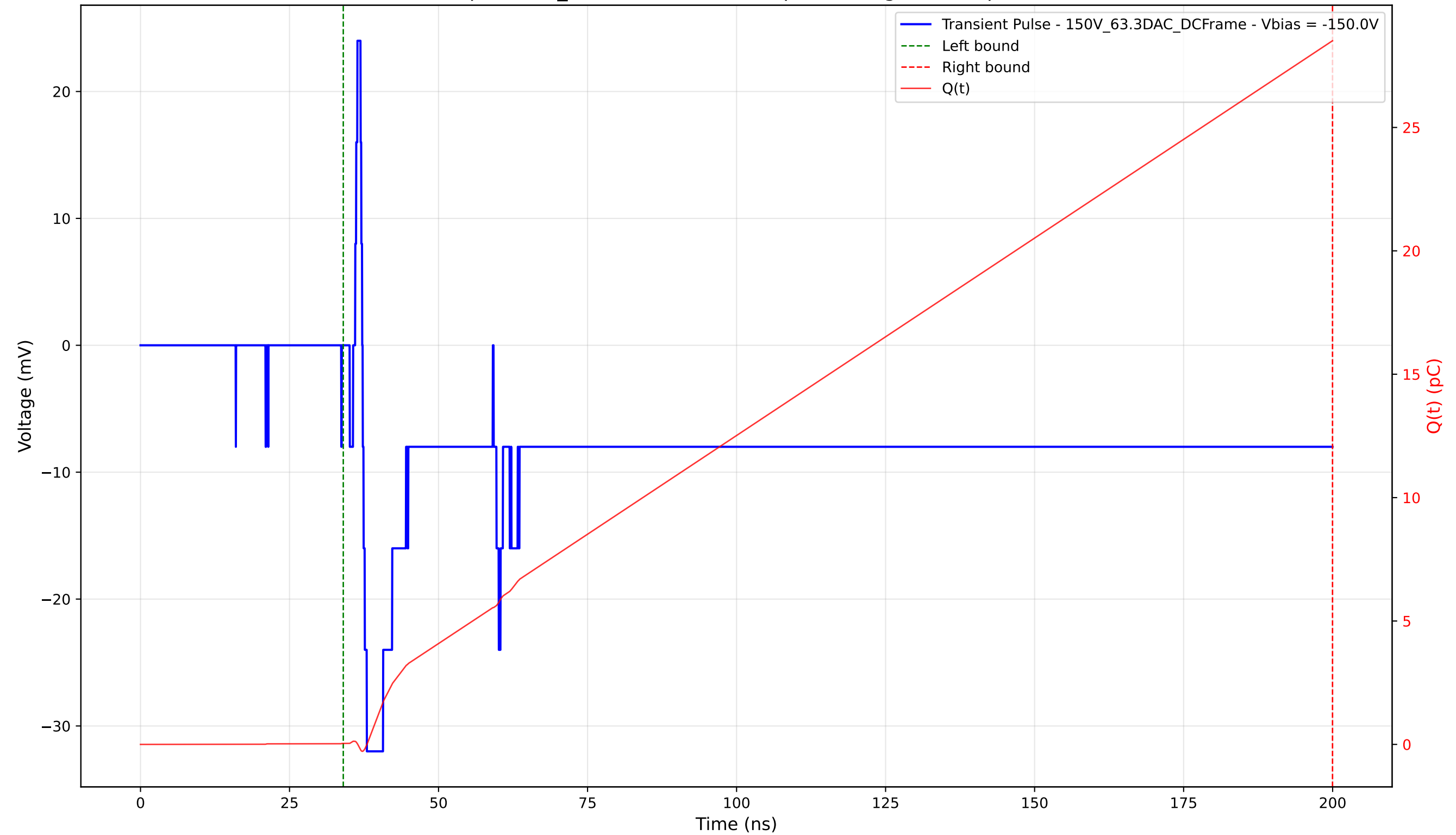
Transient Pulse - Sample: 1cm_42 - Position: 2130.0 \mu\text{m} - Charge: 28.48 pC - Rise Time: 0.69 ns
