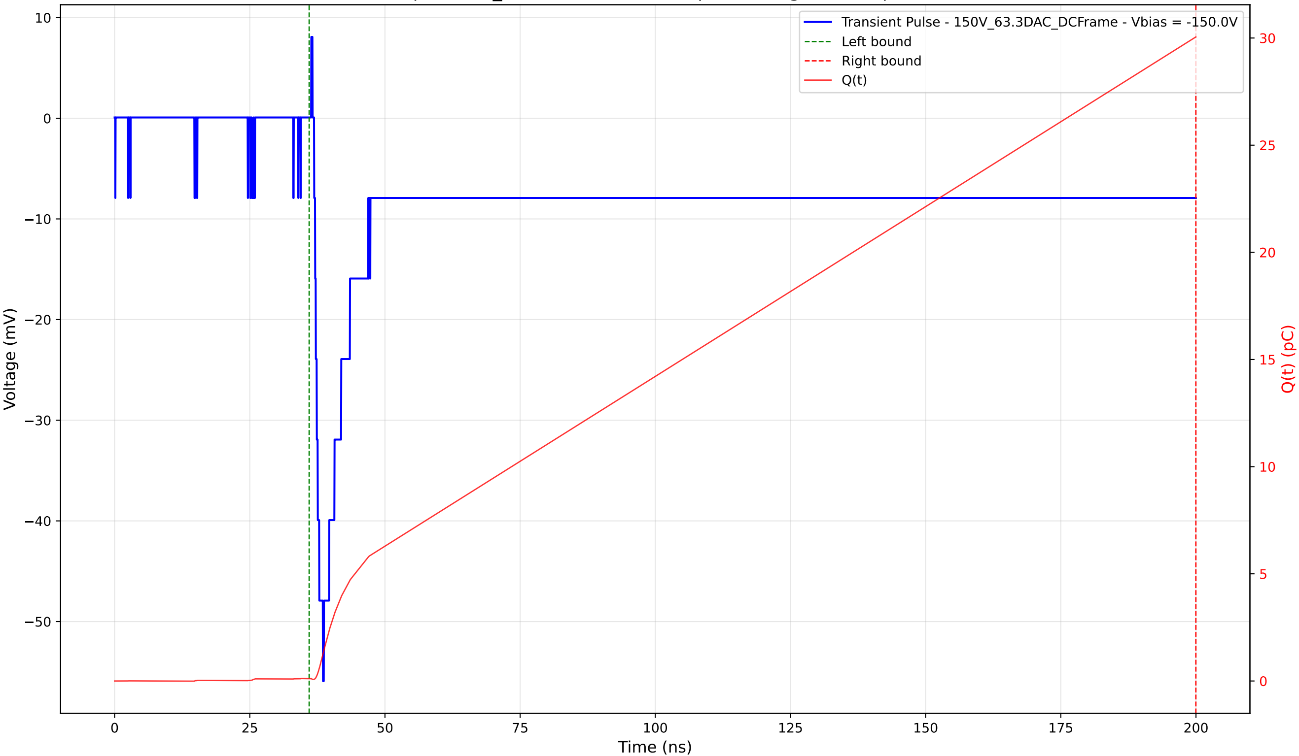
Transient Pulse - Sample: 1cm_42 - Position: 3900.0 \mu\text{m} - Charge: 29.94 pC - Rise Time: 1.63 ns
