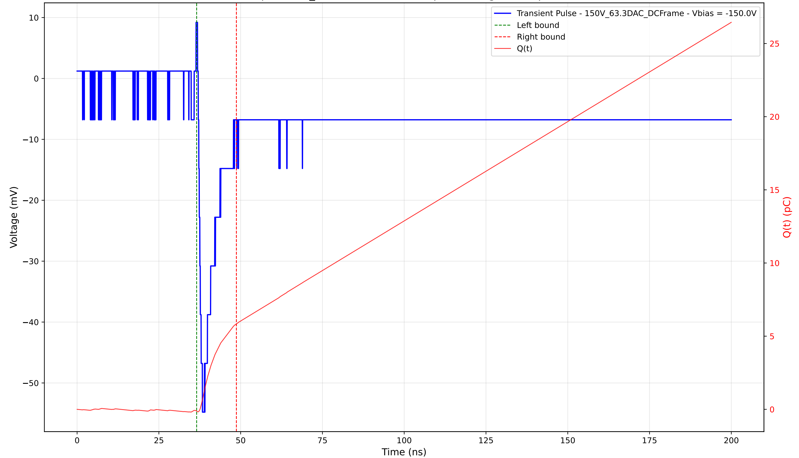
Transient Pulse - Sample: 1cm_42 - Position: 3705.0 \mu\text{m} - Charge: 5.95 pC - Rise Time: 1.26 ns
