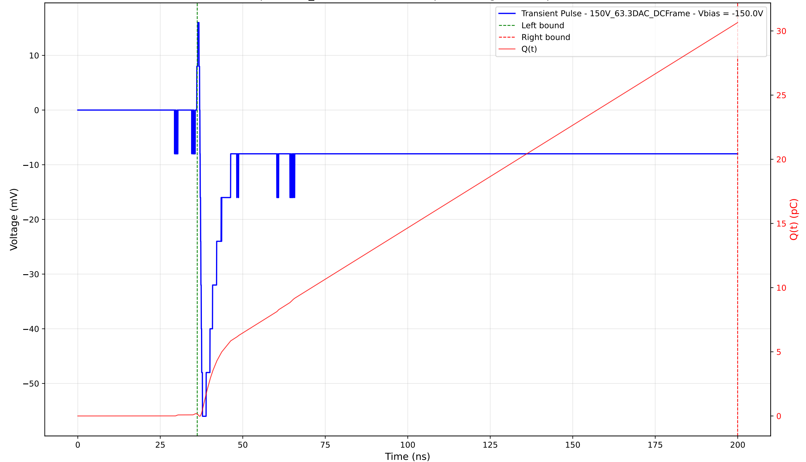
Transient Pulse - Sample: 1cm_42 - Position: 1395.0 \mu\text{m} - Charge: 30.50 pC - Rise Time: 0.77 ns
