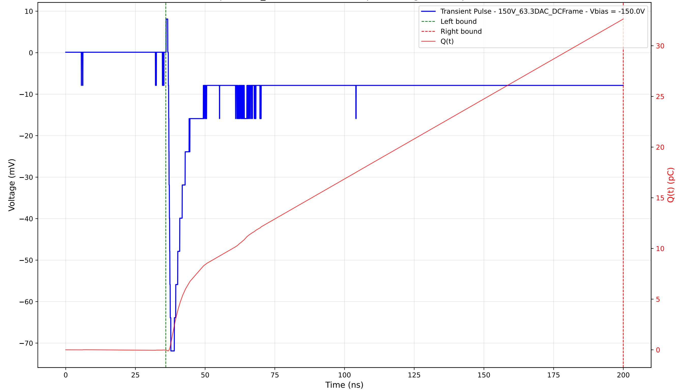
Transient Pulse - Sample: 1cm_42 - Position: 1135.0 \mu\text{m} - Charge: 32.65 pC - Rise Time: 0.90 ns
