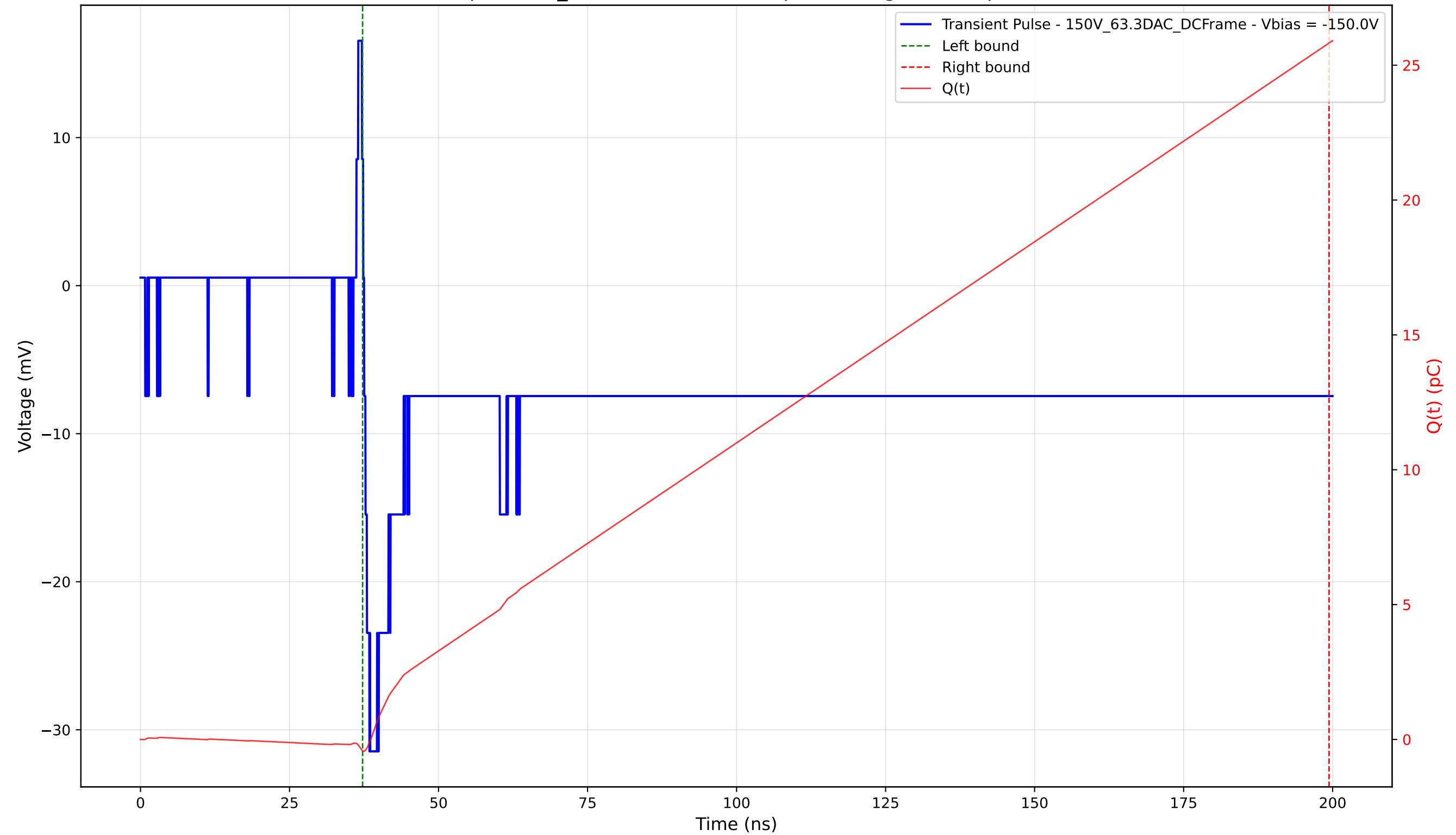
Transient Pulse - Sample: 1cm_42 - Position: 2840.0 \mu\text{m} - Charge: 26.25 pC - Rise Time: 0.89 ns
