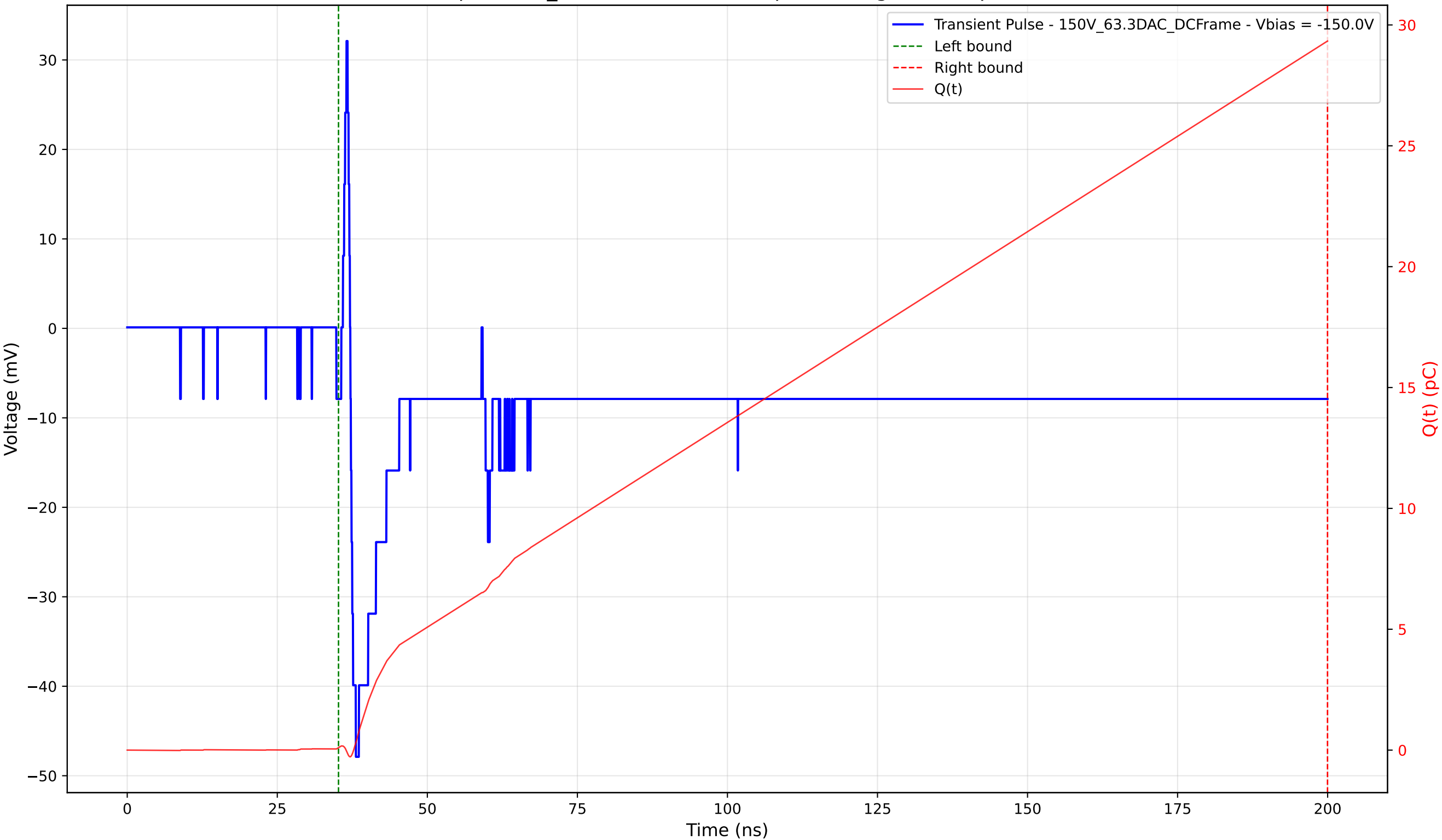
Transient Pulse - Sample: 1cm_42 - Position: 1815.0 \mu\text{m} - Charge: 29.23 pC - Rise Time: 0.91 ns
