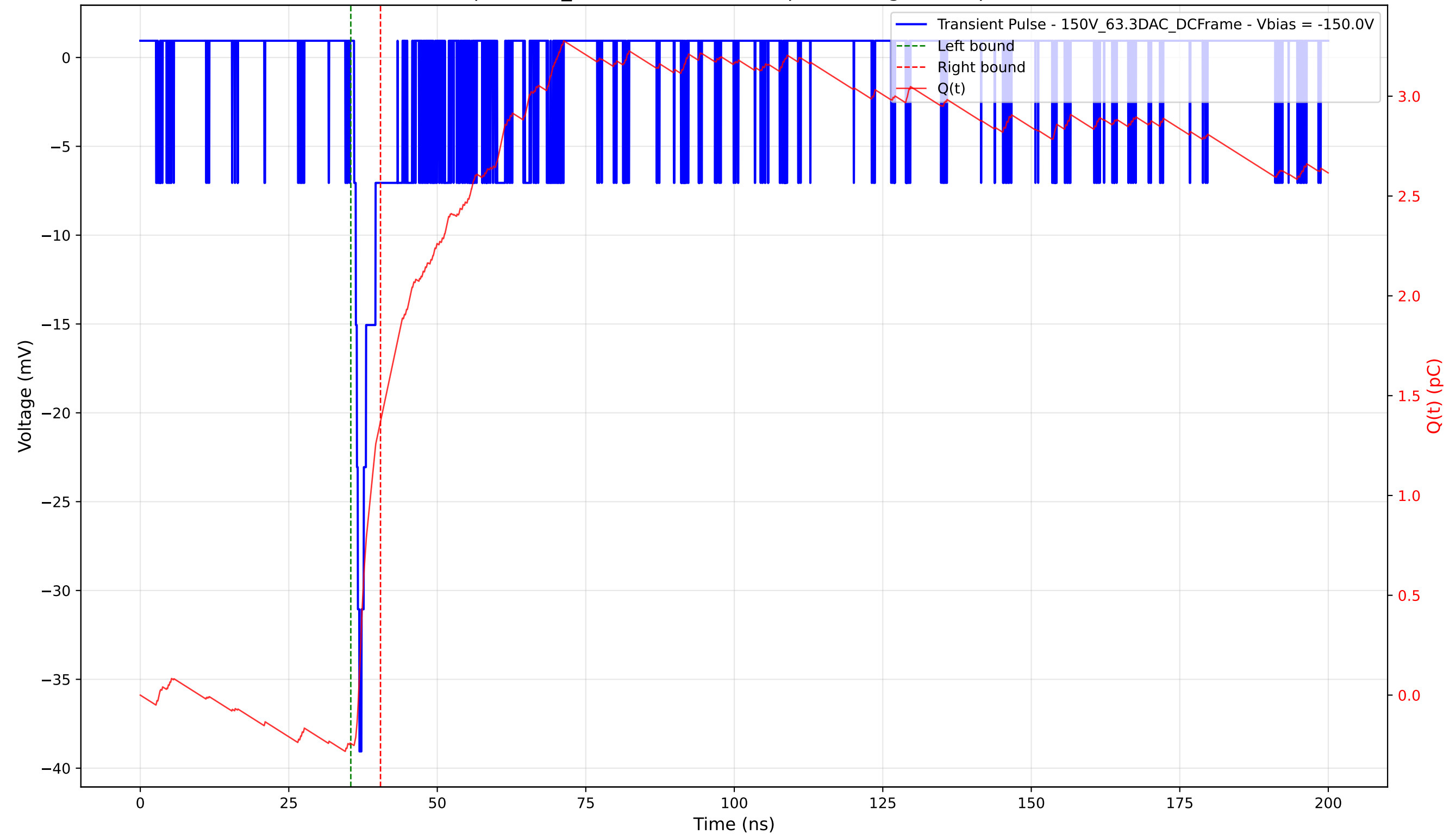
Transient Pulse - Sample: 1cm_42 - Position: 5150.0 \mu\text{m} - Charge: 1.61 pC - Rise Time: 0.89 ns
