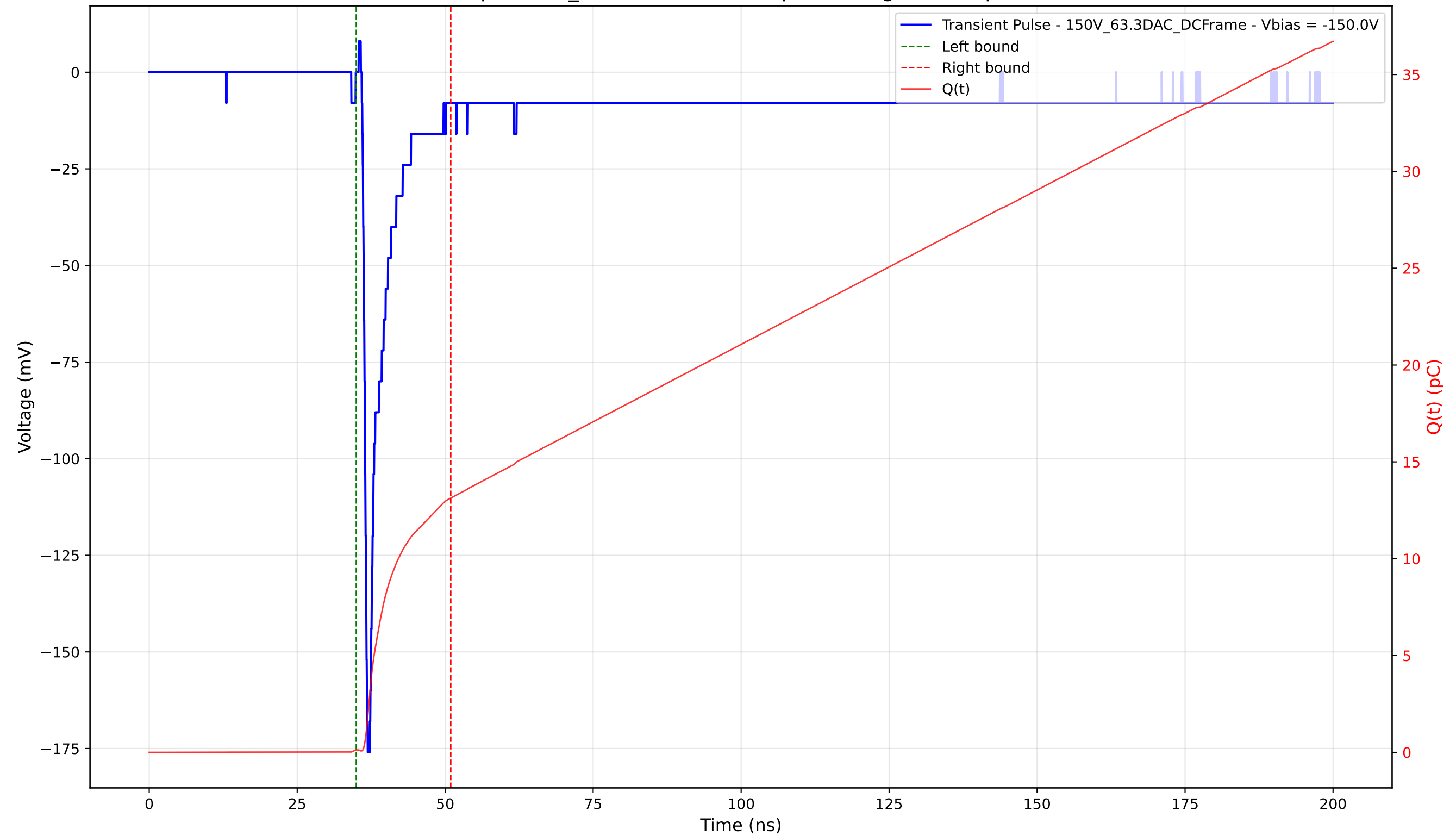
Transient Pulse - Sample: 1cm_42 - Position: 420.0 \mu\text{m} - Charge: 13.00 pC - Rise Time: 0.72 ns
