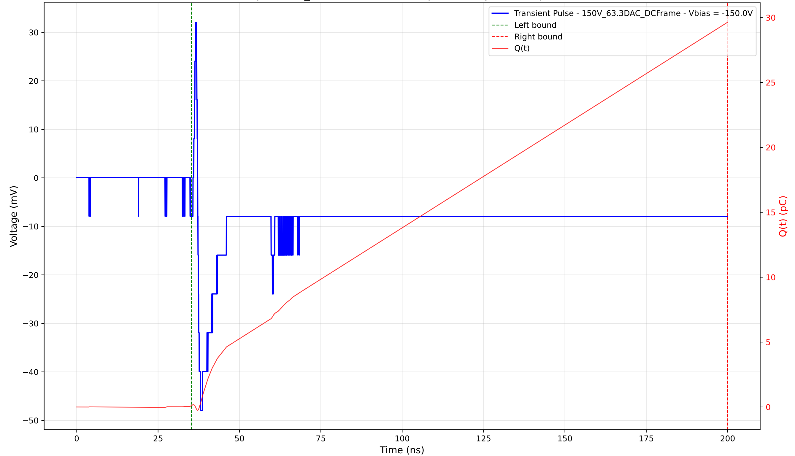
Transient Pulse - Sample: 1cm_42 - Position: 1805.0 \mu\text{m} - Charge: 29.54 pC - Rise Time: 0.89 ns
