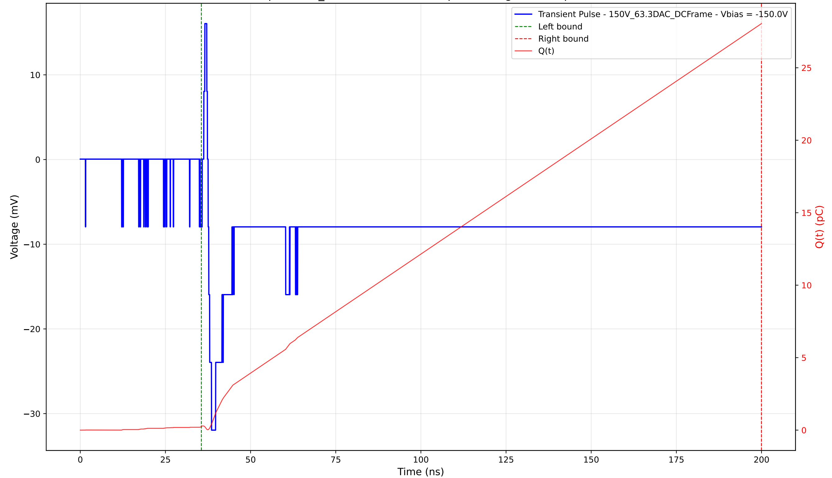
Transient Pulse - Sample: 1cm_42 - Position: 2850.0 \mu\text{m} - Charge: 27.79 pC - Rise Time: 0.99 ns
