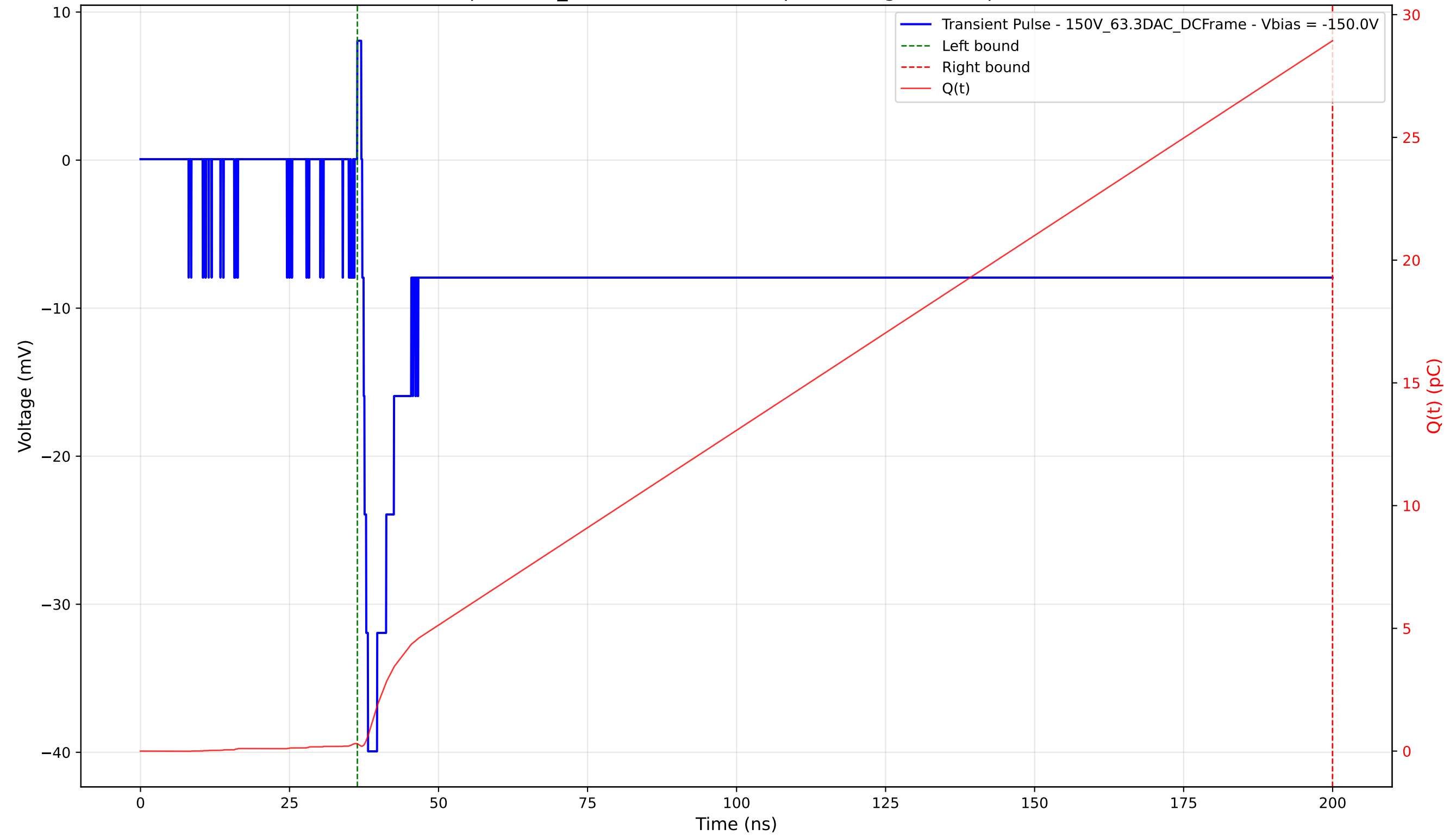
Transient Pulse - Sample: 1cm_42 - Position: 3550.0 \mu\text{m} - Charge: 28.64 pC - Rise Time: 0.97 ns
