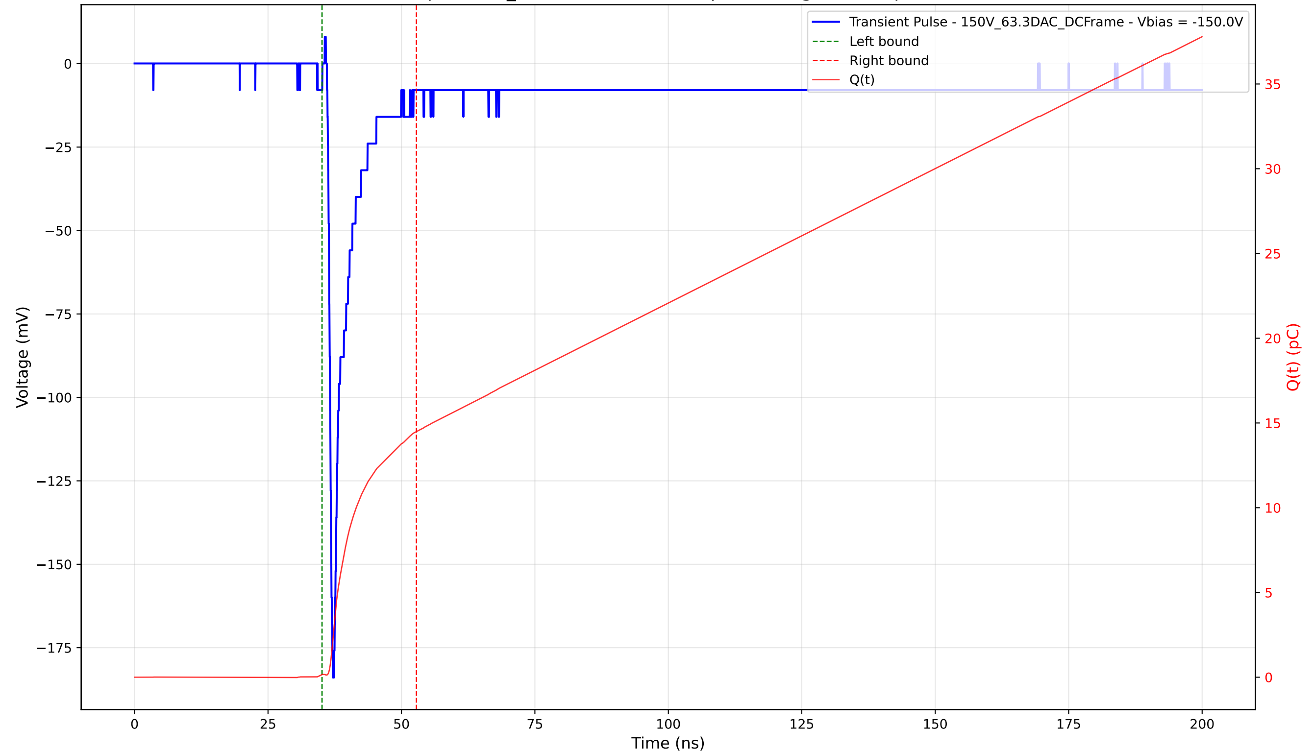
Transient Pulse - Sample: 1cm_42 - Position: 4650.0 \mu\text{m} - Charge: 14.33 pC - Rise Time: 0.77 ns
