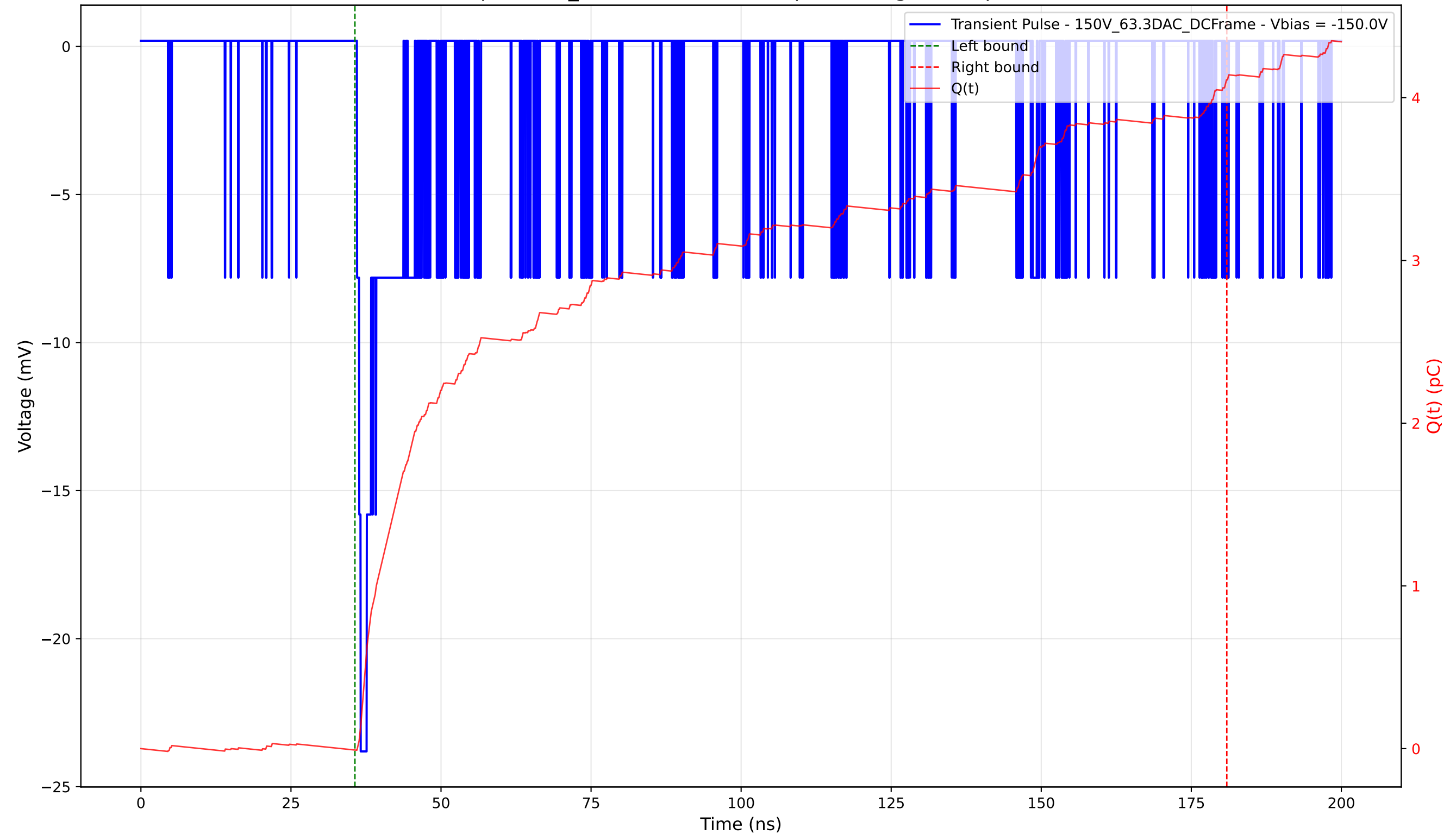
Transient Pulse - Sample: 1cm_42 - Position: 5175.0 \mu\text{m} - Charge: 4.12 pC - Rise Time: 0.61 ns
