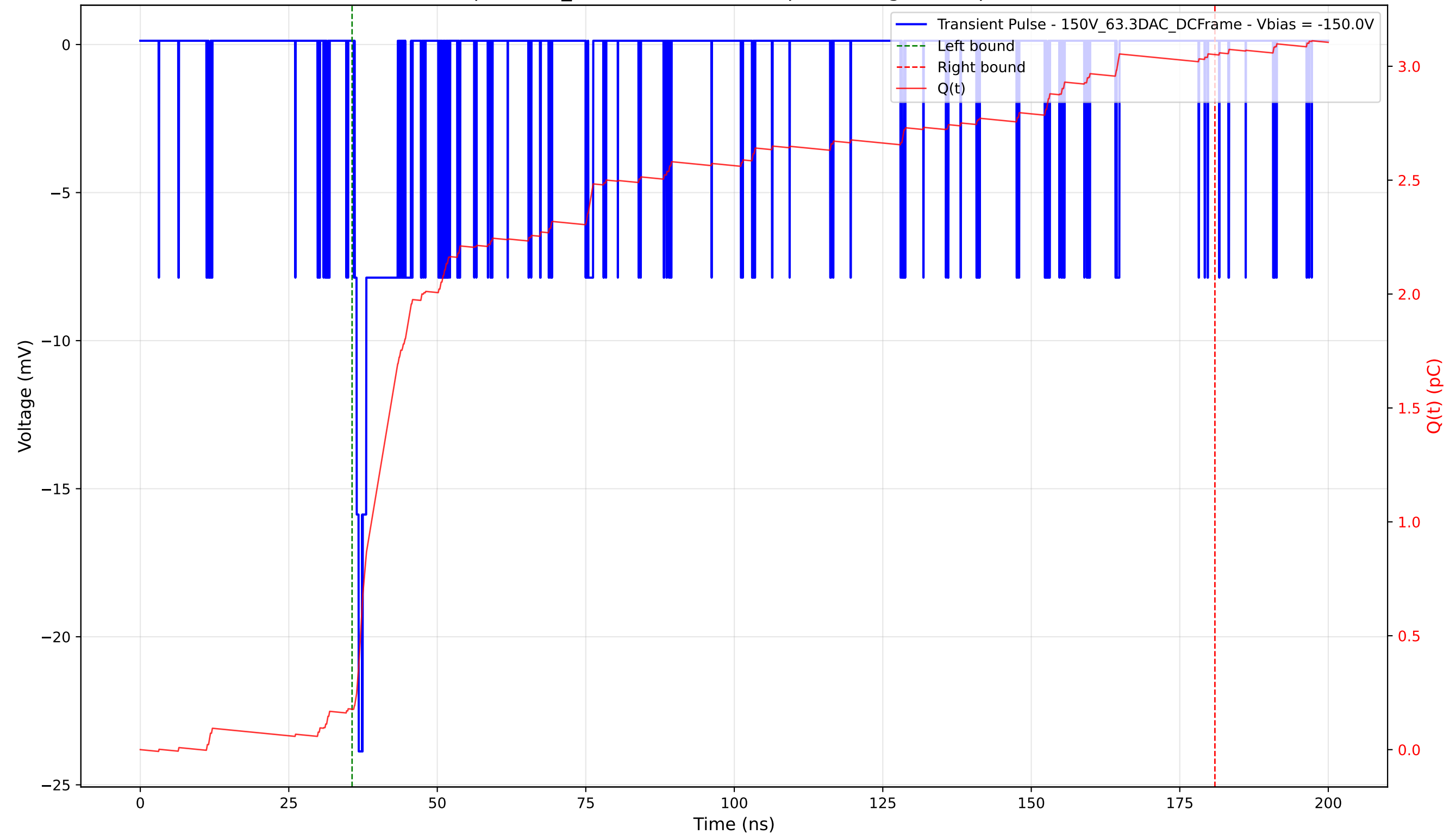
Transient Pulse - Sample: 1cm_42 - Position: 5185.0 \mu\text{m} - Charge: 2.87 pC - Rise Time: 0.67 ns
