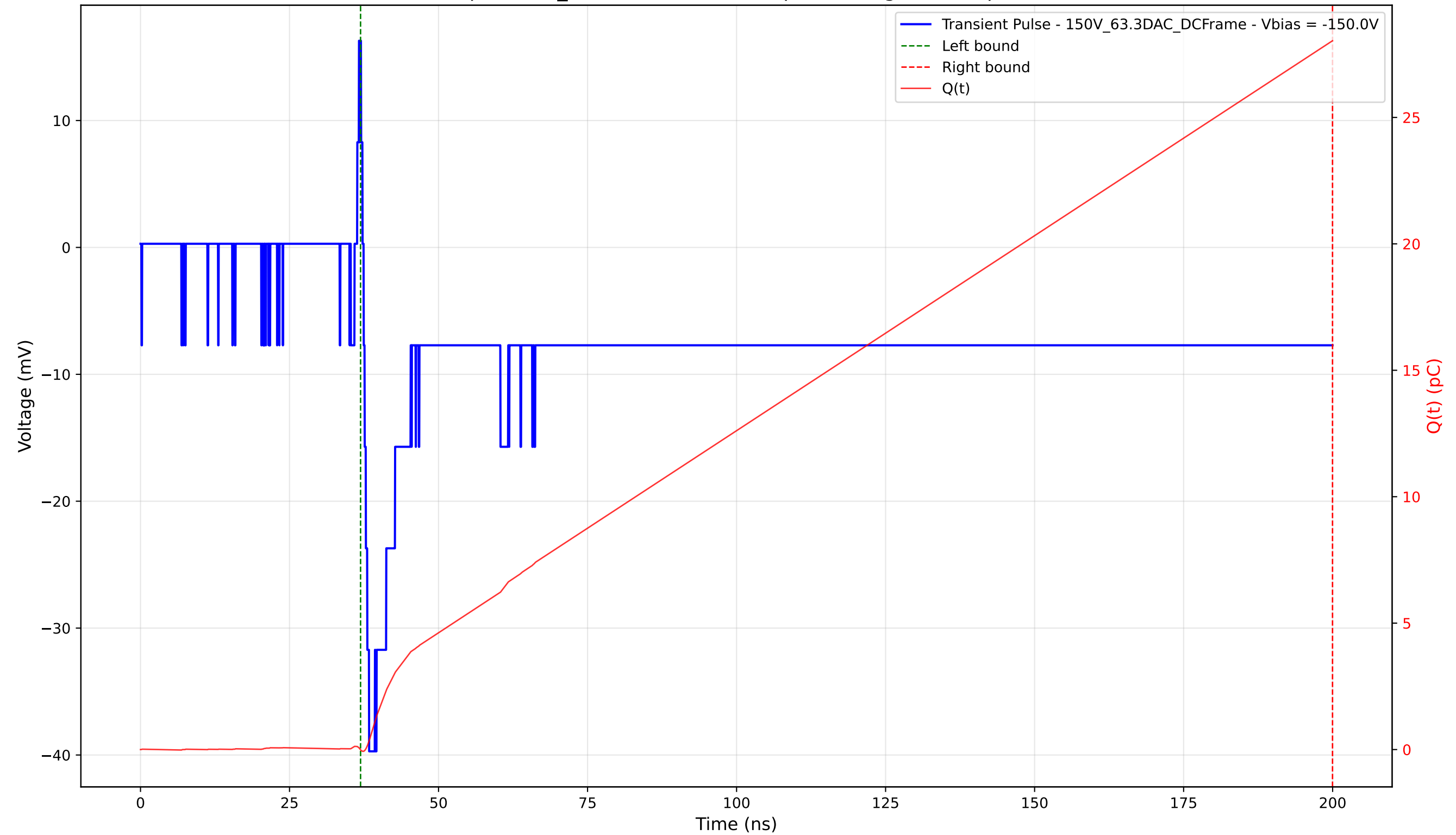
Transient Pulse - Sample: 1cm_42 - Position: 3230.0 \mu\text{m} - Charge: 28.04 pC - Rise Time: 0.91 ns
