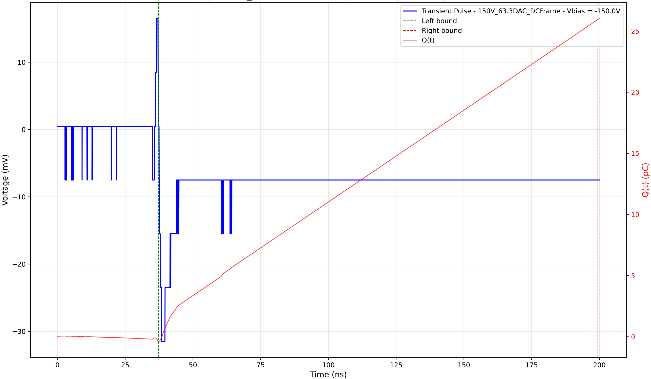
Transient Pulse - Sample: 1cm_42 - Position: 2610.0 \mu\text{m} - Charge: 26.32 pC - Rise Time: 0.99 ns
