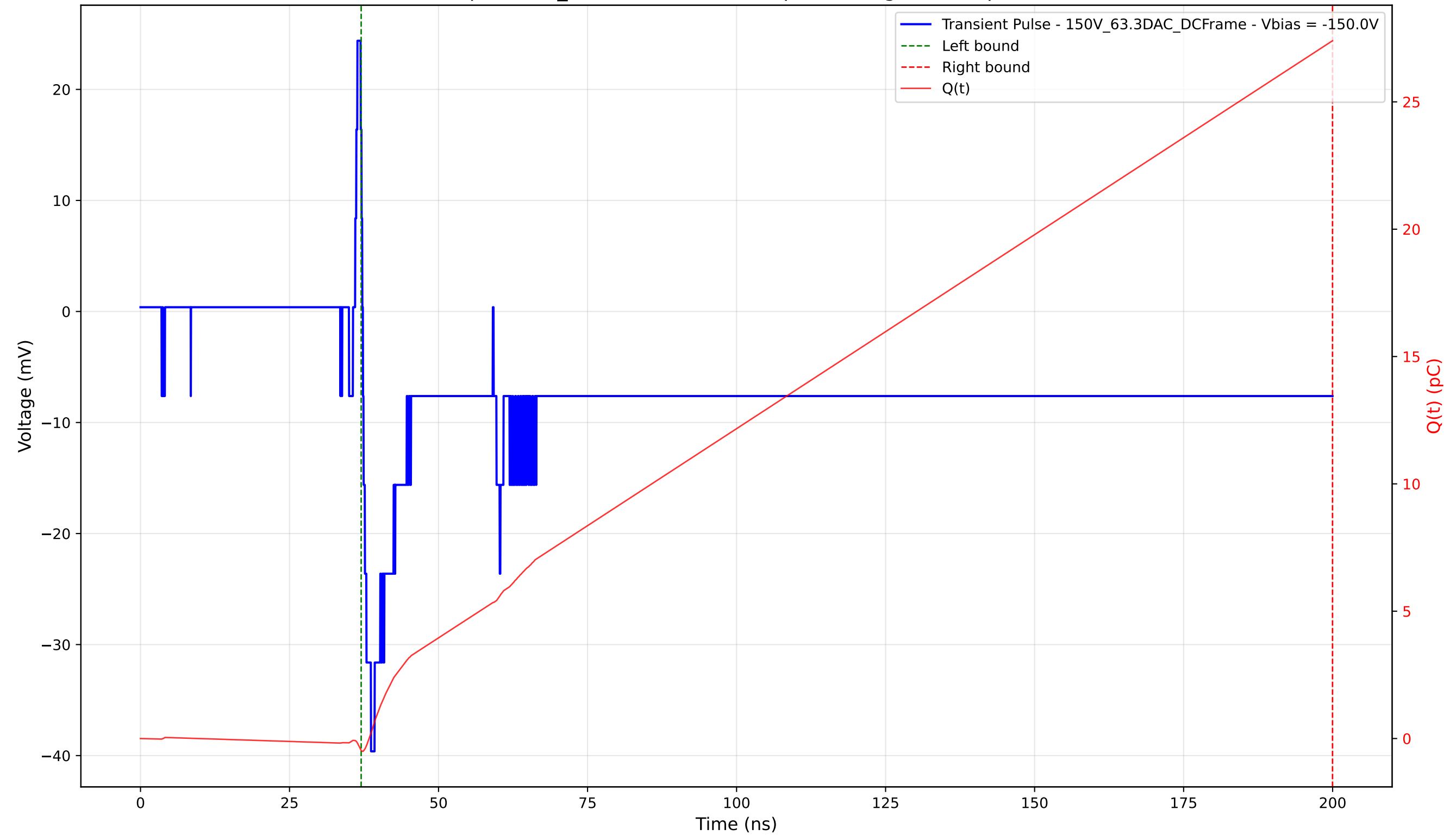
Transient Pulse - Sample: 1cm_42 - Position: 2240.0 \mu\text{m} - Charge: 27.87 pC - Rise Time: 1.35 ns
