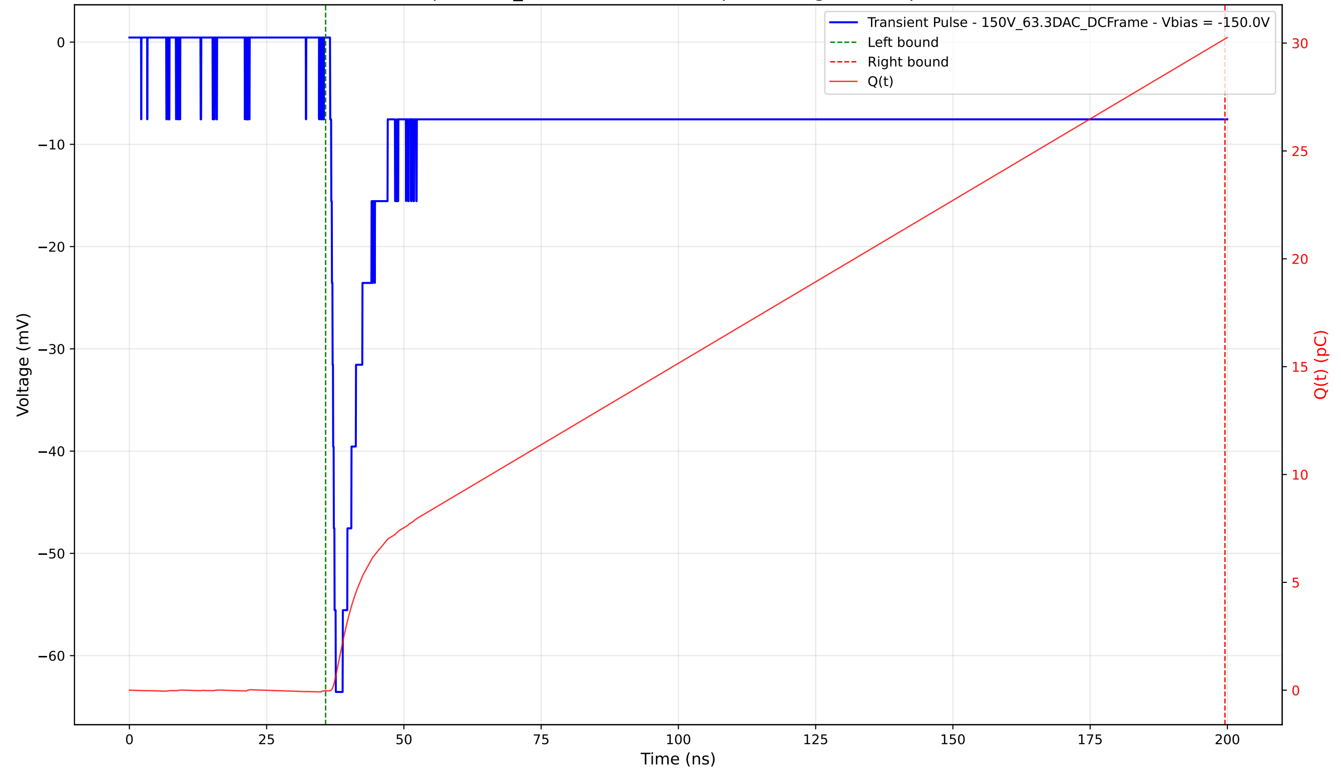
Transient Pulse - Sample: 1cm_42 - Position: 4085.0 \mu\text{m} - Charge: 30.22 pC - Rise Time: 1.02 ns
