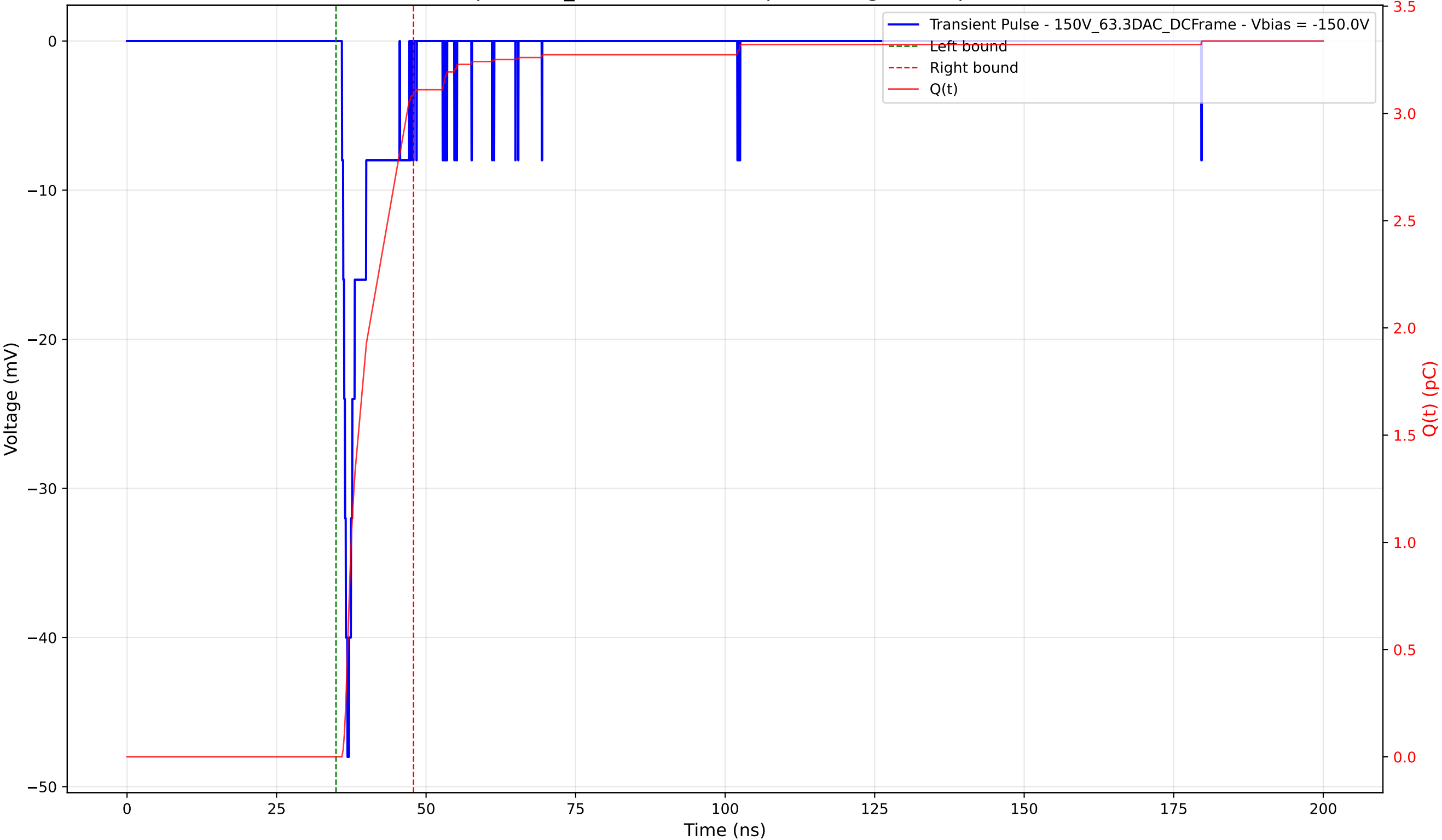
Transient Pulse - Sample: 1cm_42 - Position: 45.0 \mu\text{m} - Charge: 3.10 pC - Rise Time: 0.91 ns
