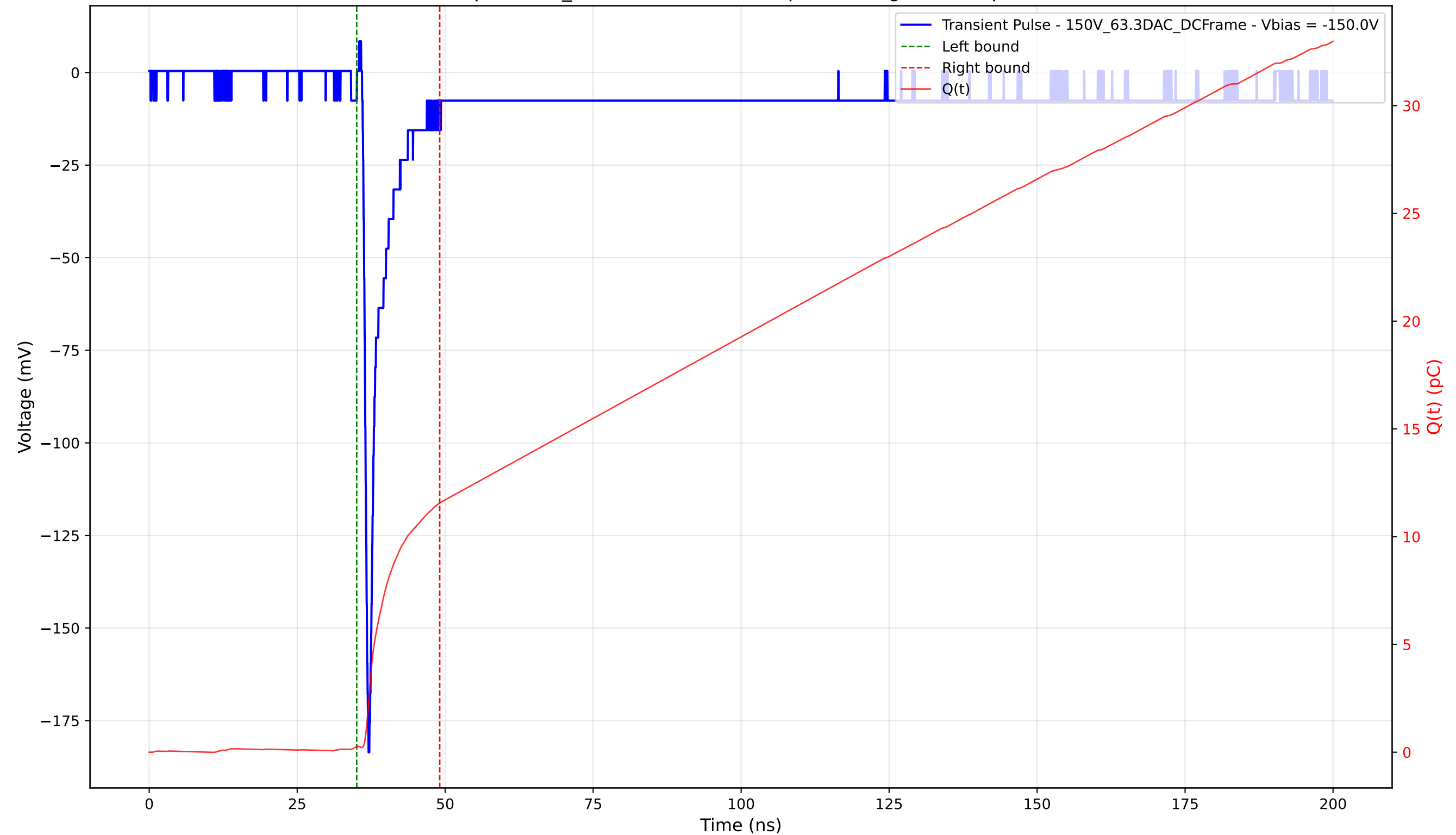
Transient Pulse - Sample: 1cm_42 - Position: 4940.0 \mu\text{m} - Charge: 11.29 pC - Rise Time: 0.77 ns
