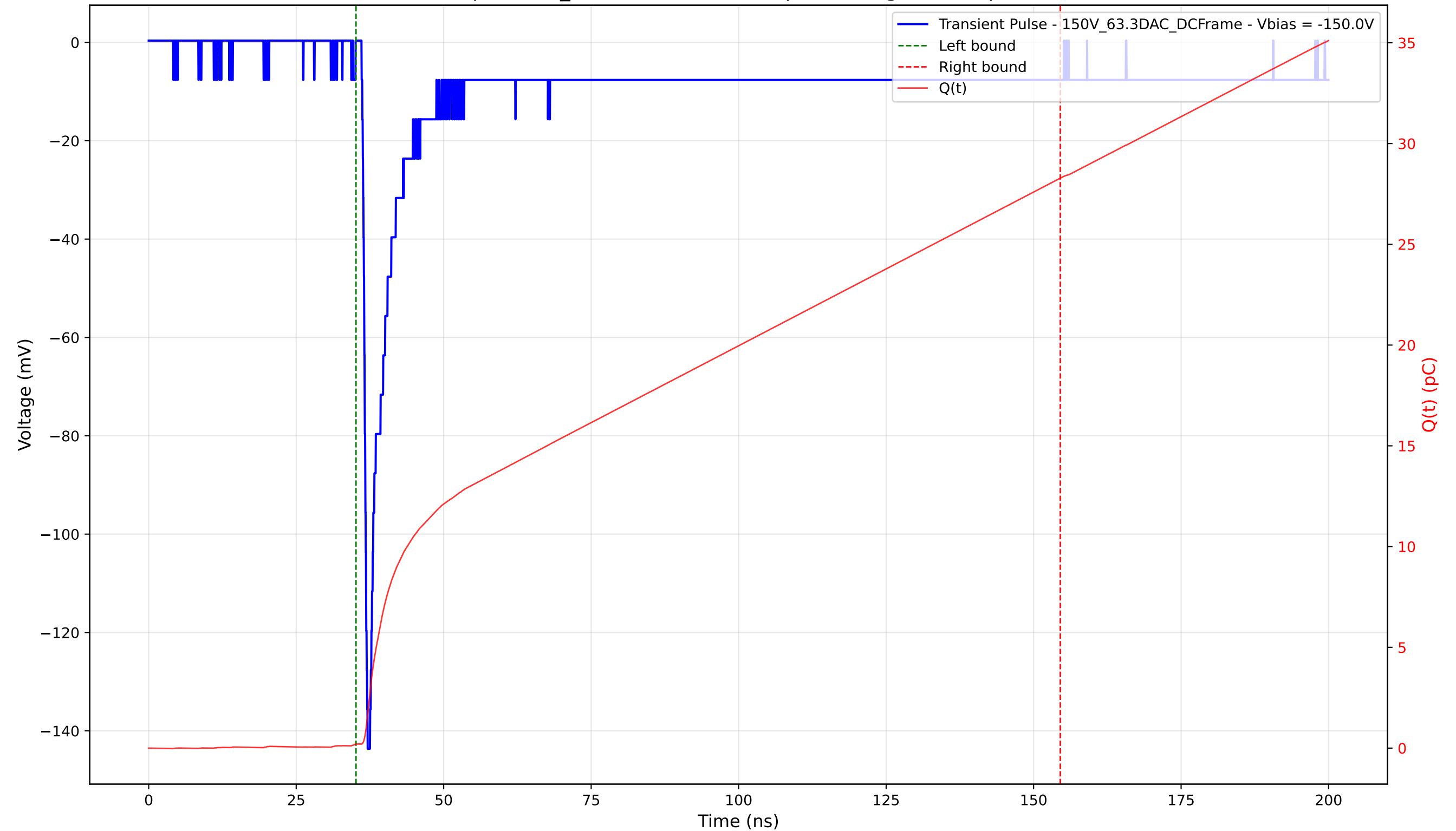
Transient Pulse - Sample: 1cm_42 - Position: 4580.0 \mu\text{m} - Charge: 28.09 pC - Rise Time: 0.82 ns
