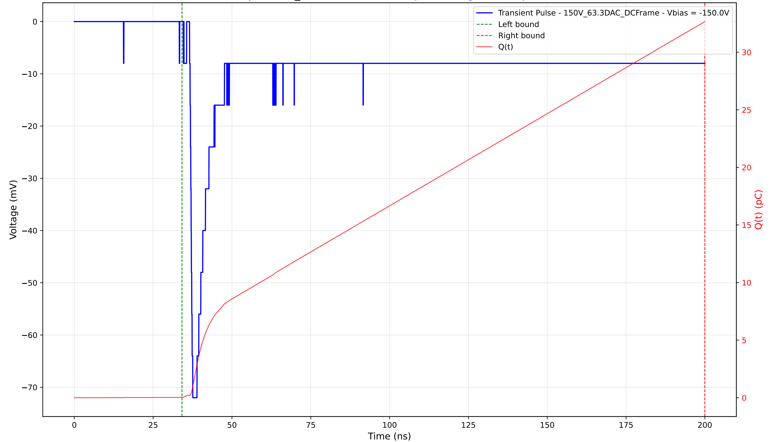
Transient Pulse - Sample: 1cm_42 - Position: 1030.0 \mu\text{m} - Charge: 32.62 pC - Rise Time: 1.00 ns
