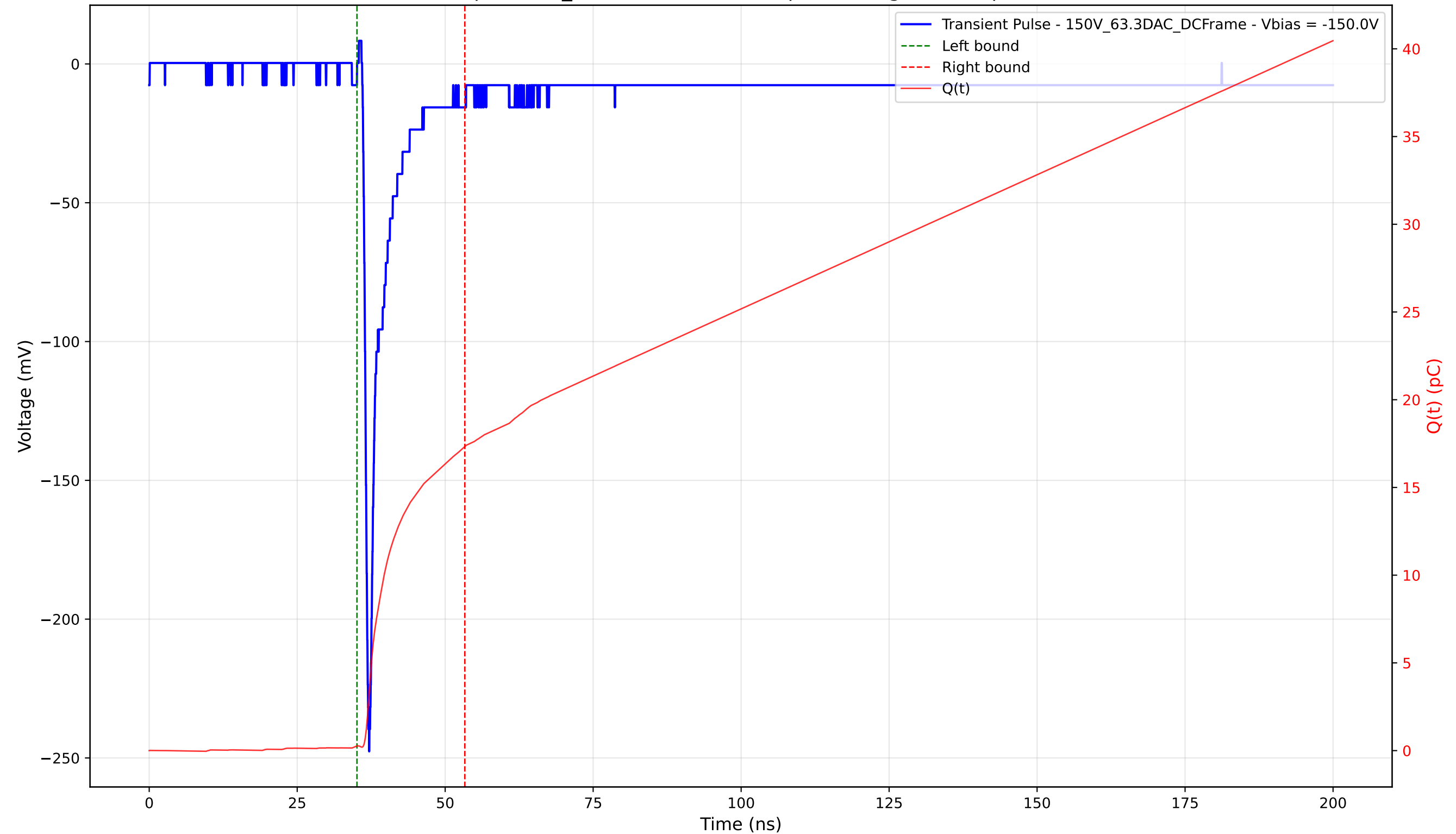
Transient Pulse - Sample: 1cm_42 - Position: 4800.0 \mu\text{m} - Charge: 17.07 pC - Rise Time: 0.78 ns
