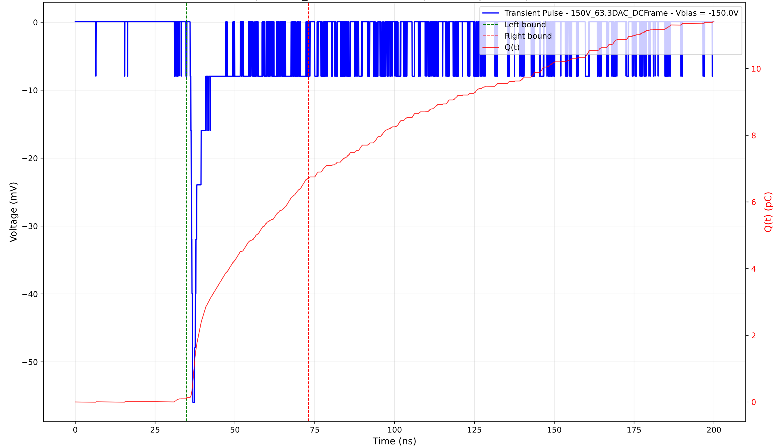
Transient Pulse - Sample: 1cm_42 - Position: 5110.0 \mu\text{m} - Charge: 6.58 pC - Rise Time: 0.85 ns
