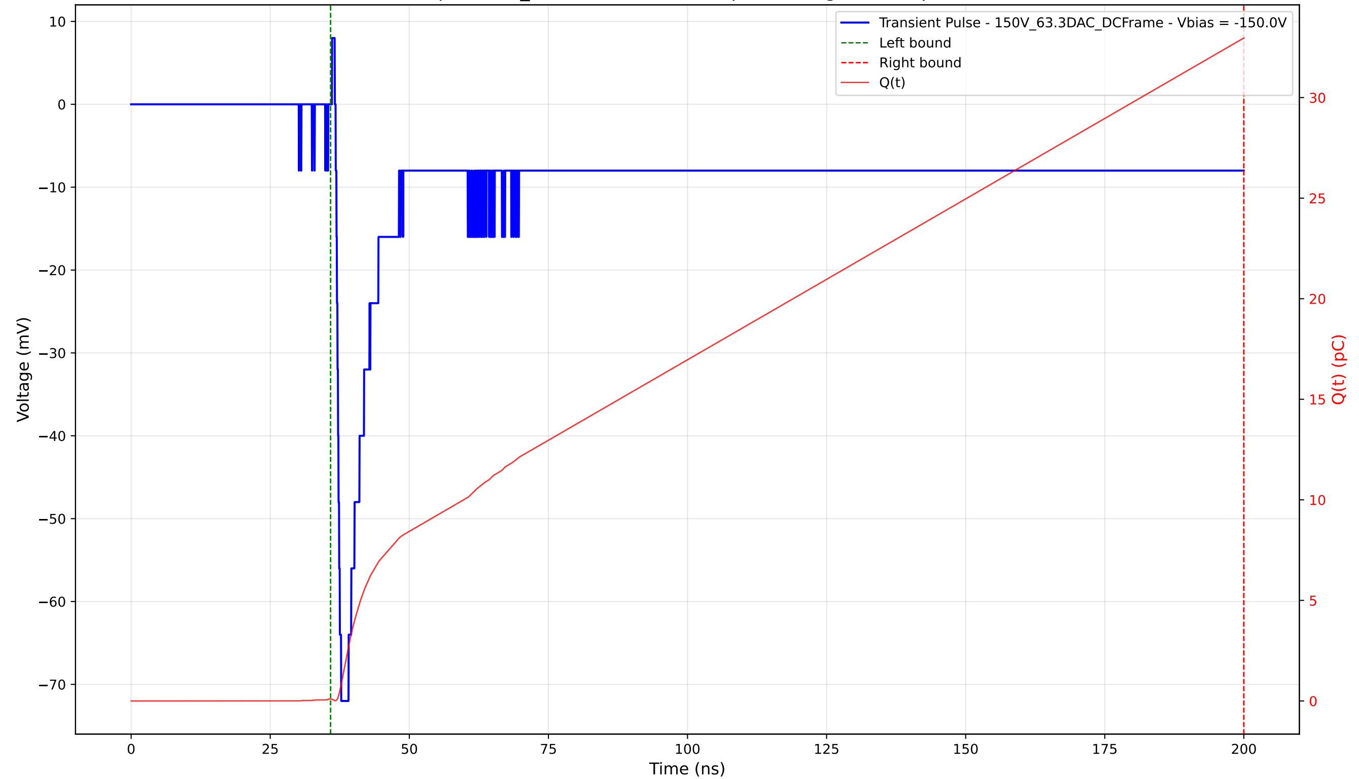
Transient Pulse - Sample: 1cm_42 - Position: 1125.0 \mu\text{m} - Charge: 32.87 pC - Rise Time: 0.98 ns
