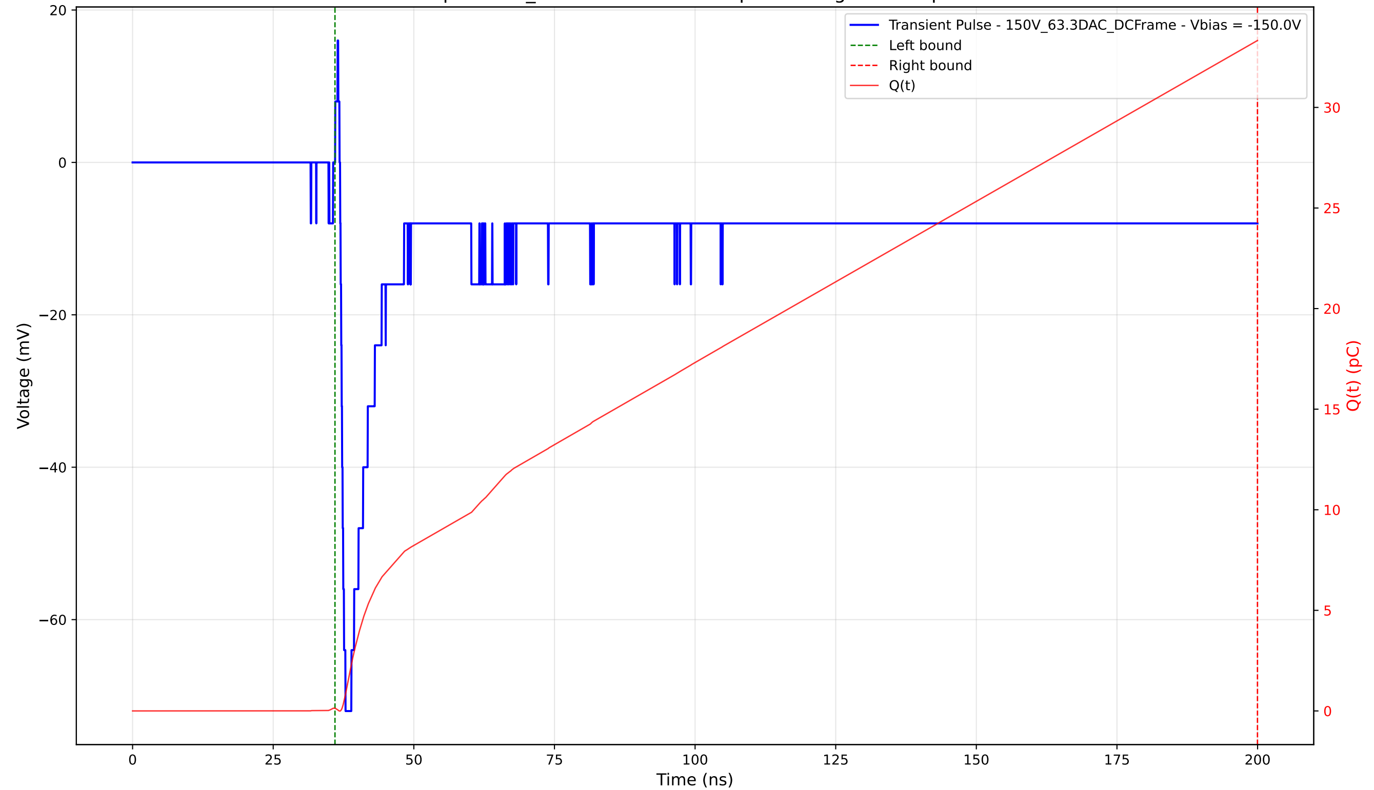
Transient Pulse - Sample: 1cm_42 - Position: 1255.0 \mu\text{m} - Charge: 33.19 pC - Rise Time: 0.94 ns
