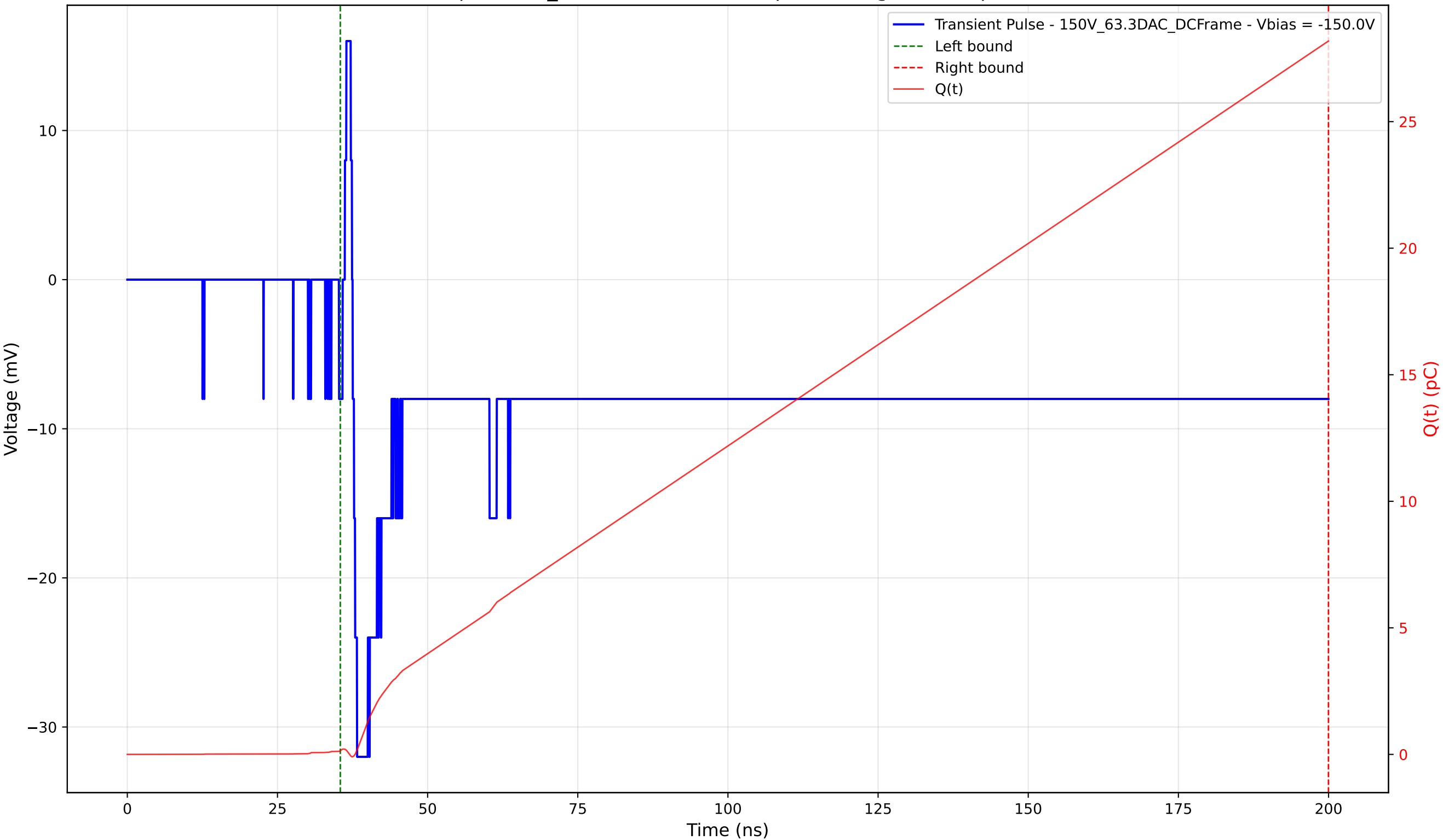
Transient Pulse - Sample: 1cm_42 - Position: 2705.0 \mu\text{m} - Charge: 28.03 pC - Rise Time: 0.73 ns
