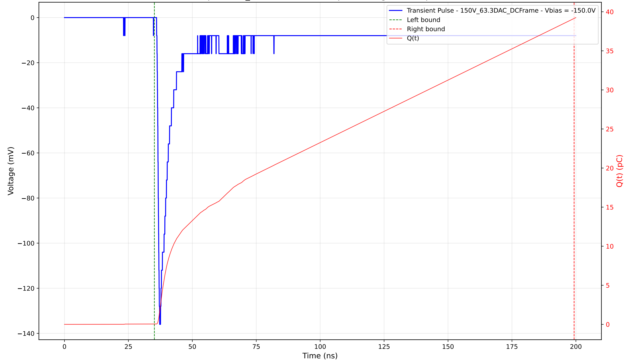
Transient Pulse - Sample: 1cm_42 - Position: 680.0 \mu\text{m} - Charge: 39.10 pC - Rise Time: 0.91 ns
