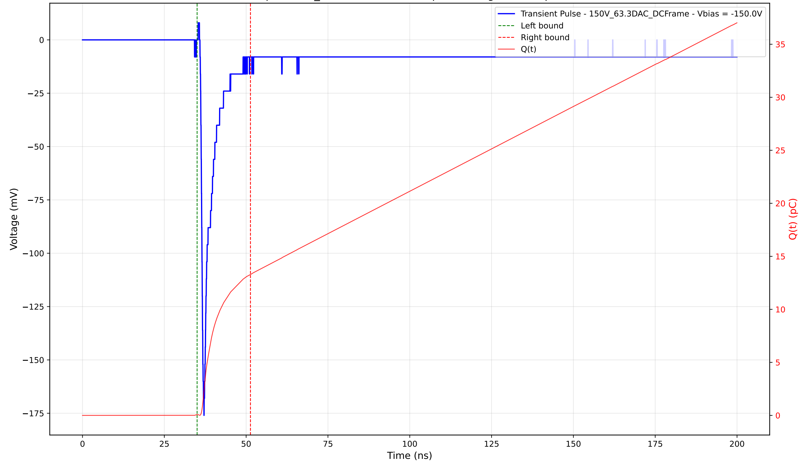
Transient Pulse - Sample: 1cm_42 - Position: 465.0 \mu\text{m} - Charge: 13.21 pC - Rise Time: 0.78 ns
