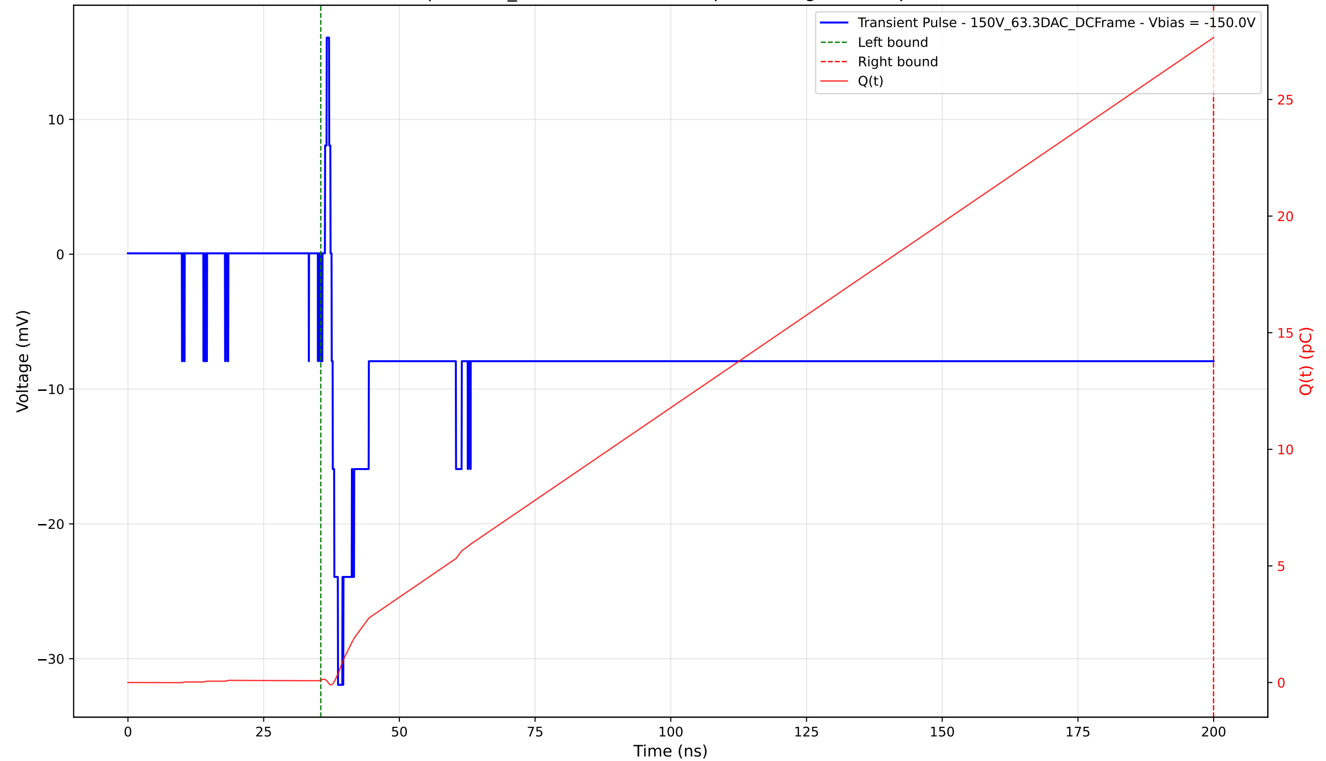
Transient Pulse - Sample: 1cm_42 - Position: 2885.0 \mu\text{m} - Charge: 27.55 pC - Rise Time: 1.17 ns
