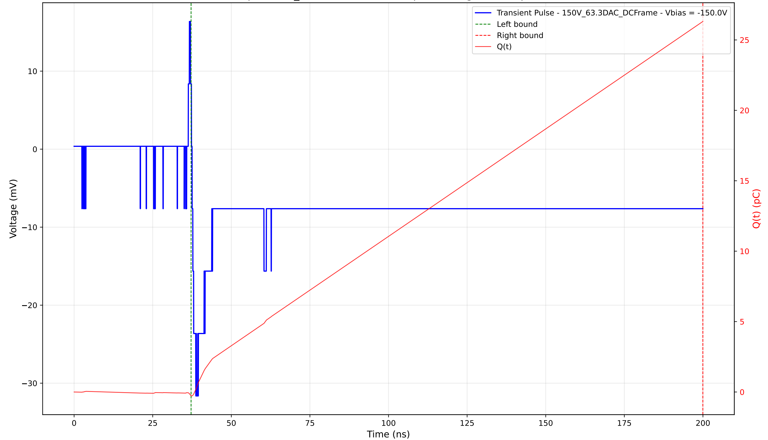
Transient Pulse - Sample: 1cm_42 - Position: 2935.0 \mu\text{m} - Charge: 26.57 pC - Rise Time: 1.19 ns
