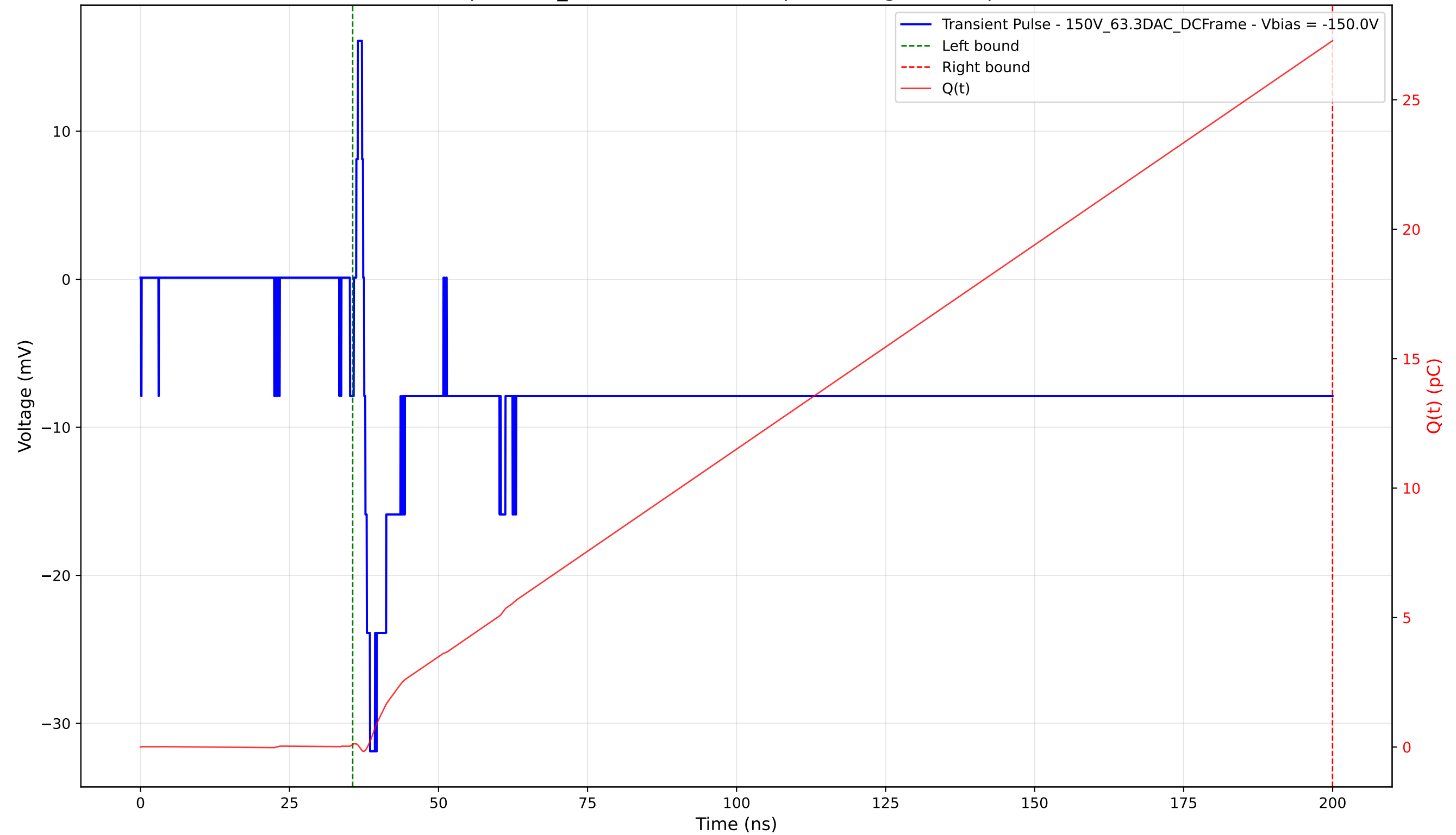
Transient Pulse - Sample: 1cm_42 - Position: 2580.0 \mu\text{m} - Charge: 27.18 pC - Rise Time: 0.99 ns
