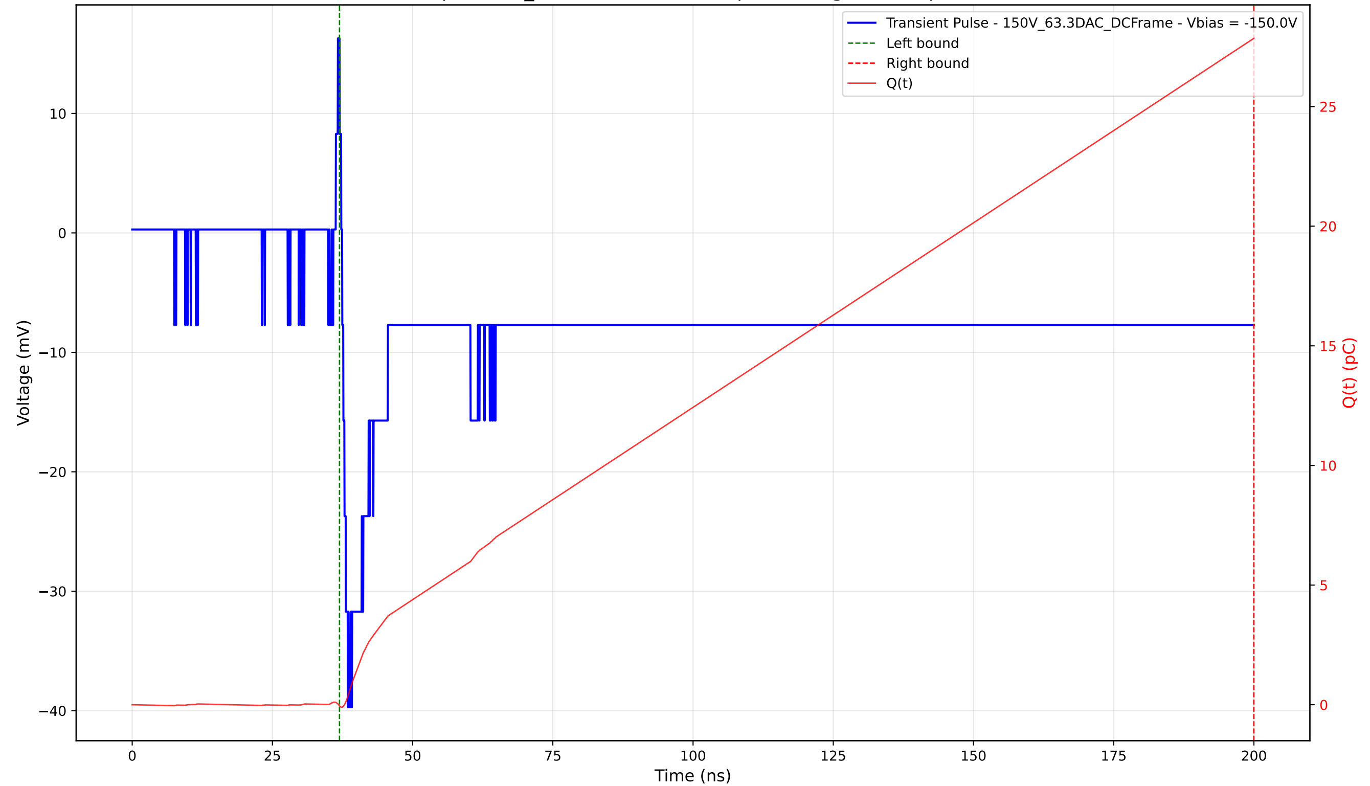
Transient Pulse - Sample: 1cm_42 - Position: 3210.0 \mu\text{m} - Charge: 27.91 pC - Rise Time: 1.01 ns
