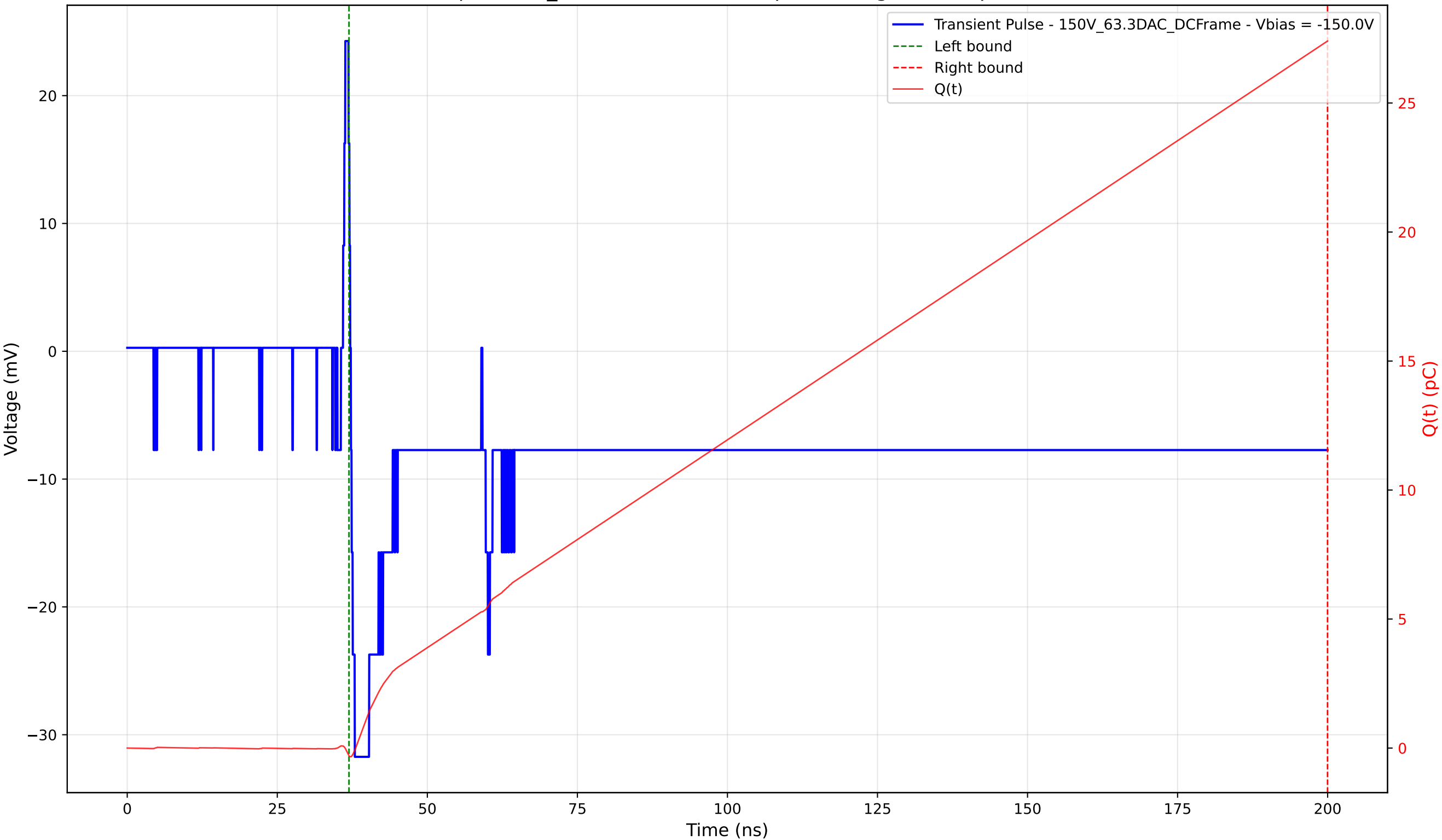
Transient Pulse - Sample: 1cm_42 - Position: 2115.0 \mu\text{m} - Charge: 27.70 pC - Rise Time: 0.65 ns
