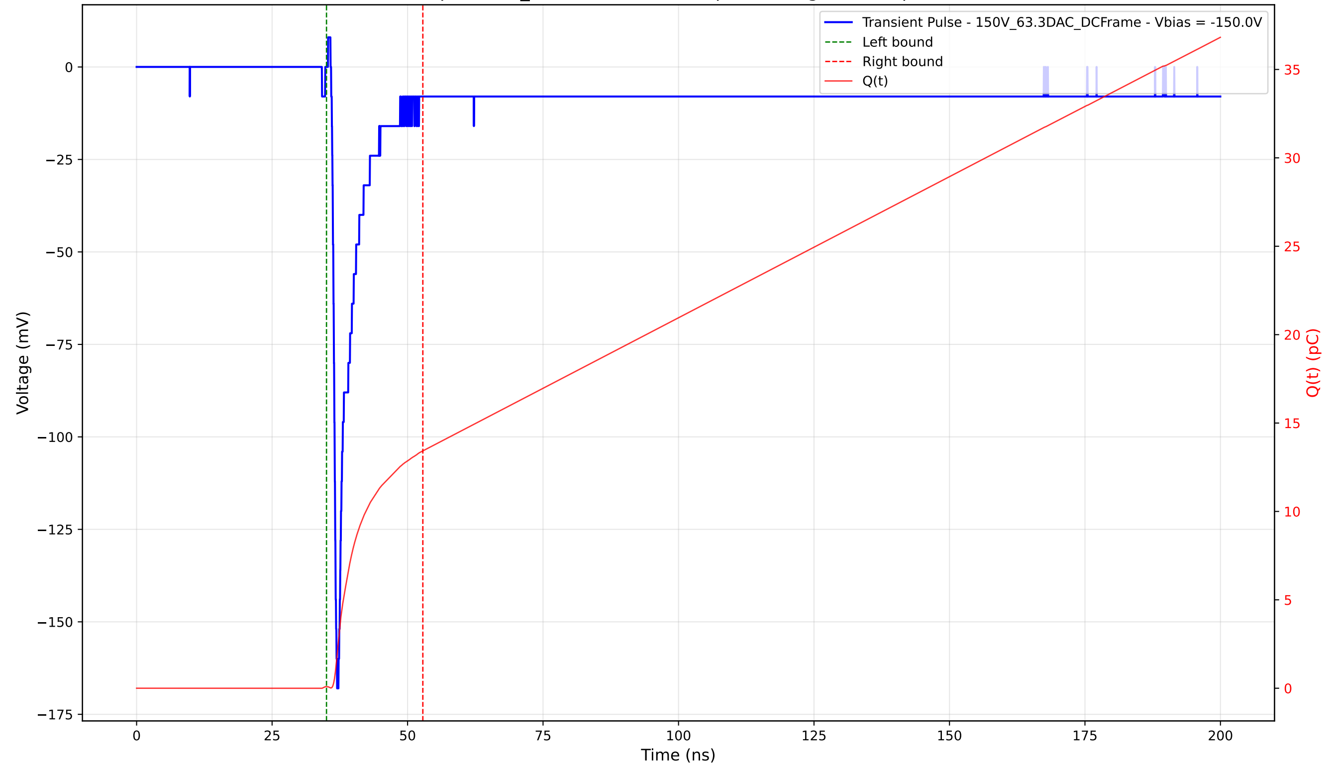
Transient Pulse - Sample: 1cm_42 - Position: 470.0 \mu\text{m} - Charge: 13.34 pC - Rise Time: 0.74 ns
