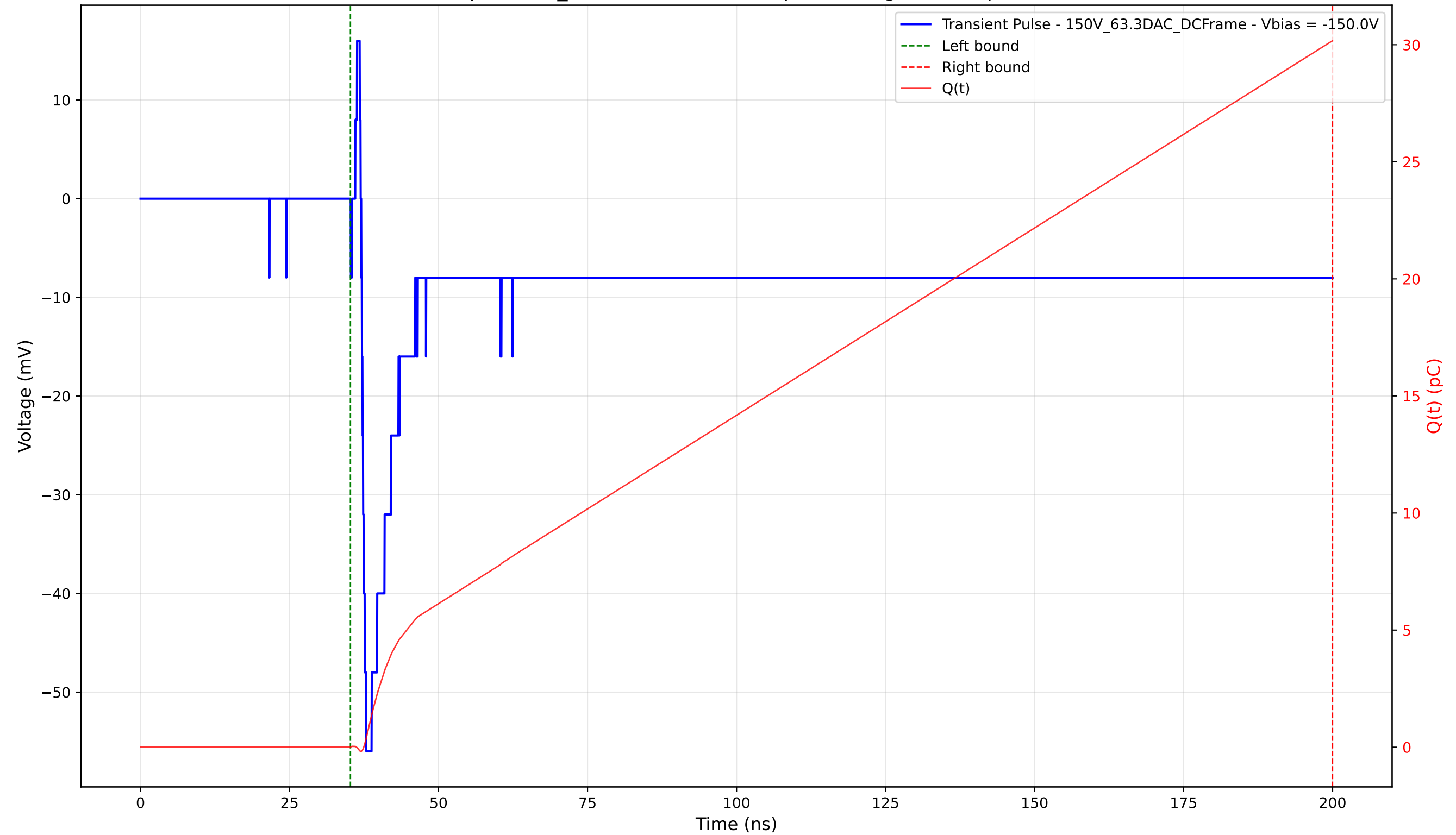
Transient Pulse - Sample: 1cm_42 - Position: 1415.0 \mu\text{m} - Charge: 30.16 pC - Rise Time: 0.83 ns
