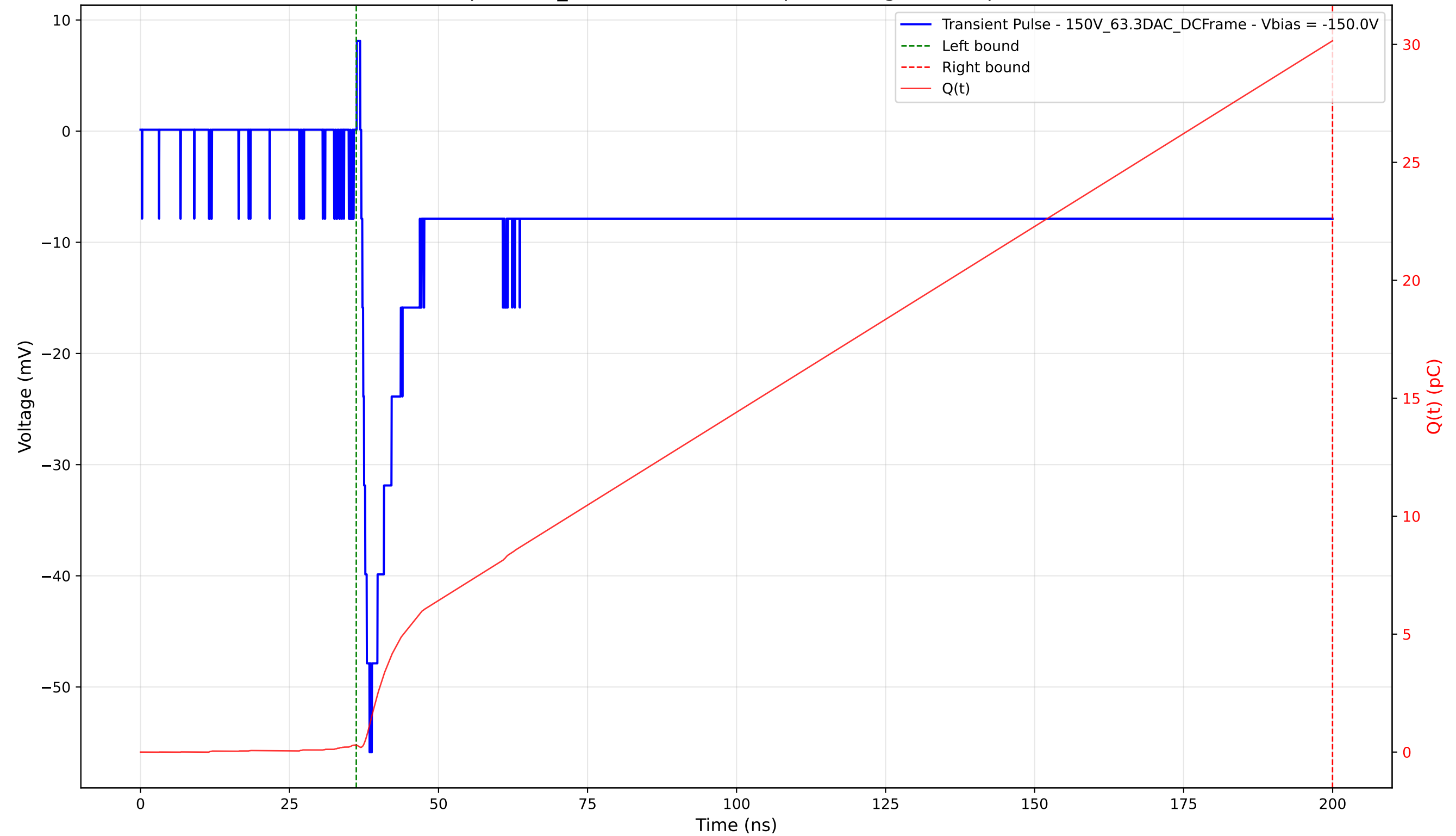
Transient Pulse - Sample: 1cm_42 - Position: 3700.0 \mu\text{m} - Charge: 29.86 pC - Rise Time: 1.39 ns
