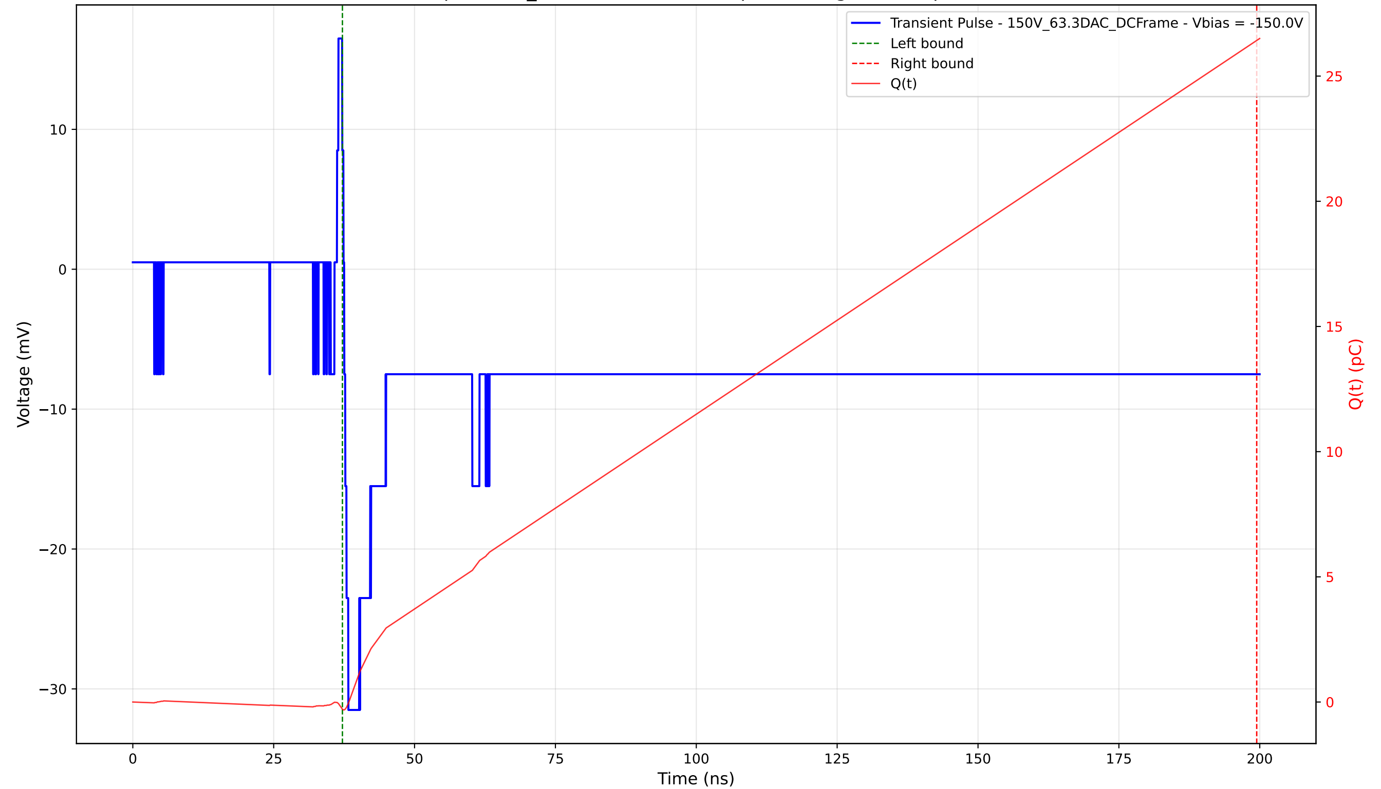
Transient Pulse - Sample: 1cm_42 - Position: 2775.0 \mu\text{m} - Charge: 26.71 pC - Rise Time: 0.73 ns
