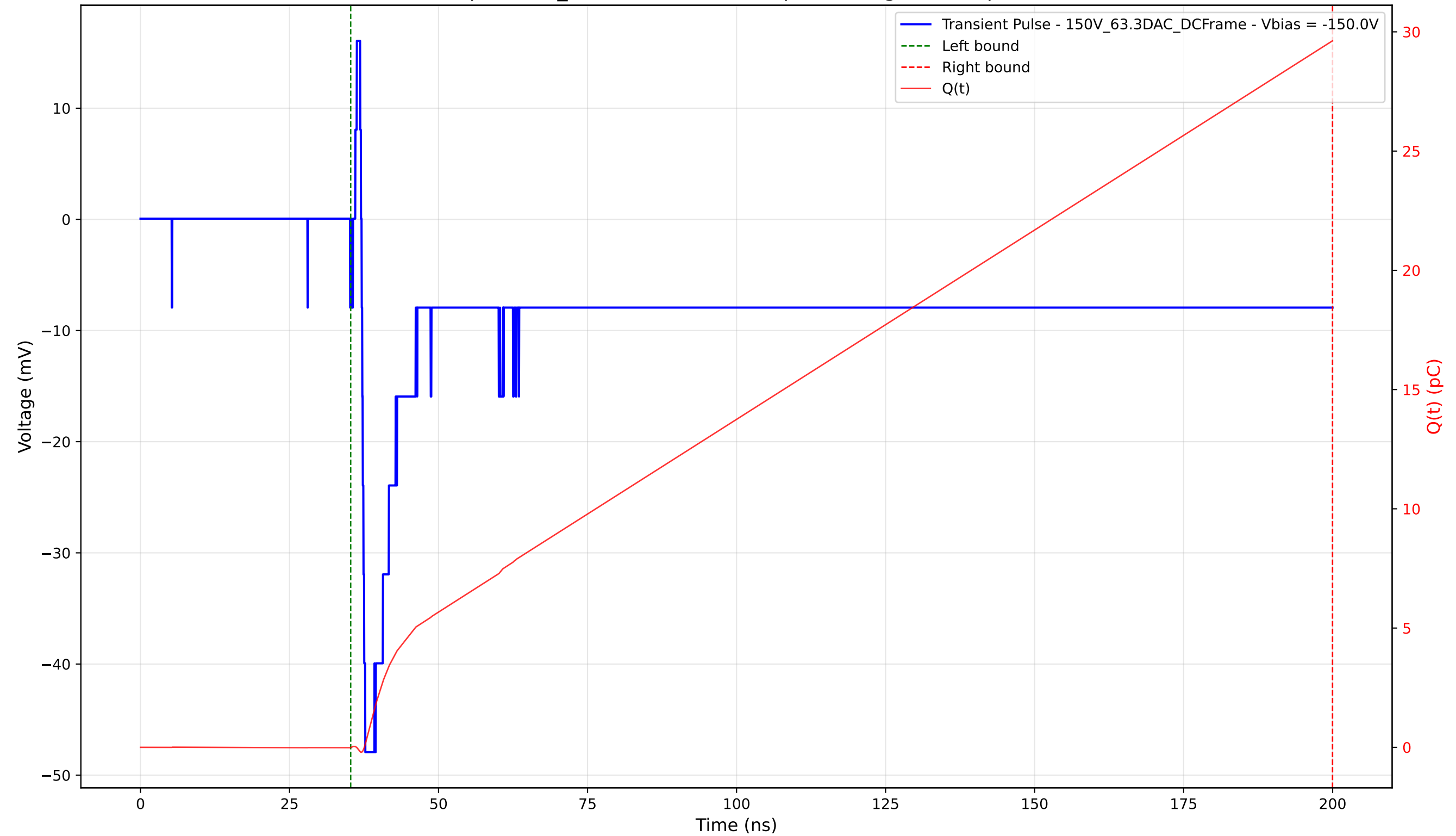
Transient Pulse - Sample: 1cm_42 - Position: 1475.0 \mu\text{m} - Charge: 29.63 pC - Rise Time: 0.61 ns
