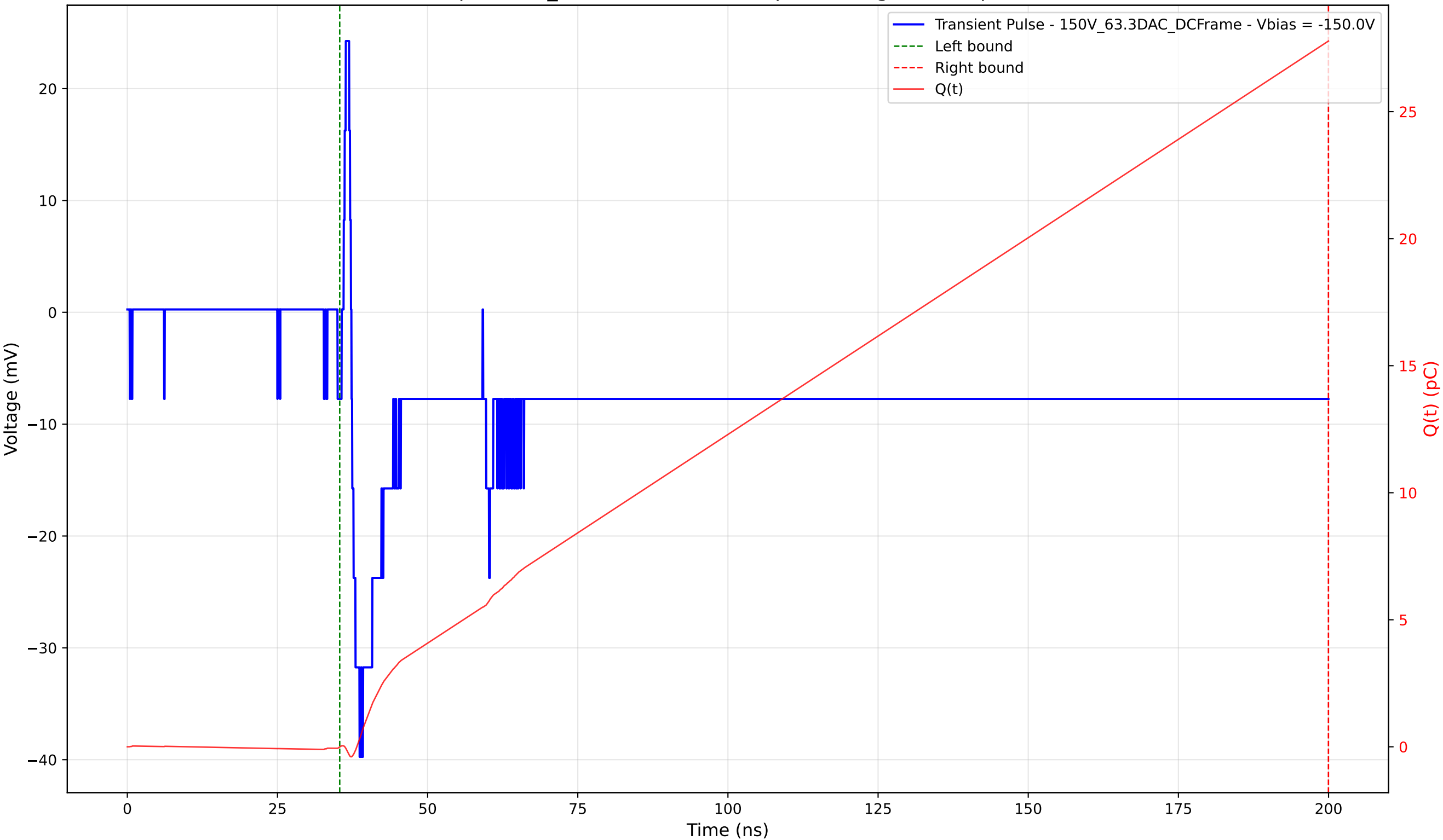
Transient Pulse - Sample: 1cm_42 - Position: 2245.0 \mu\text{m} - Charge: 27.79 pC - Rise Time: 1.35 ns
