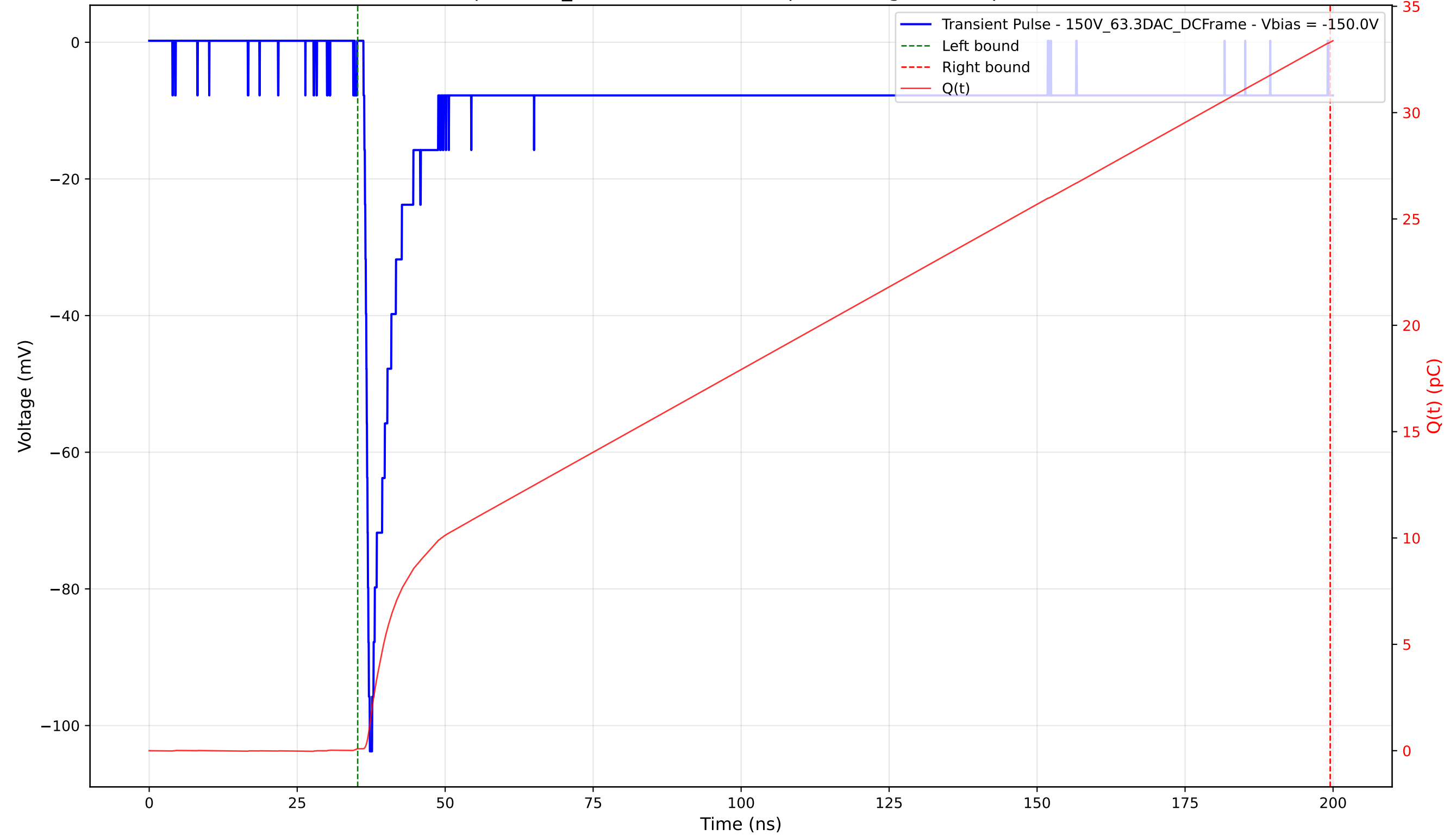
Transient Pulse - Sample: 1cm_42 - Position: 4455.0 \mu\text{m} - Charge: 33.22 pC - Rise Time: 0.77 ns
