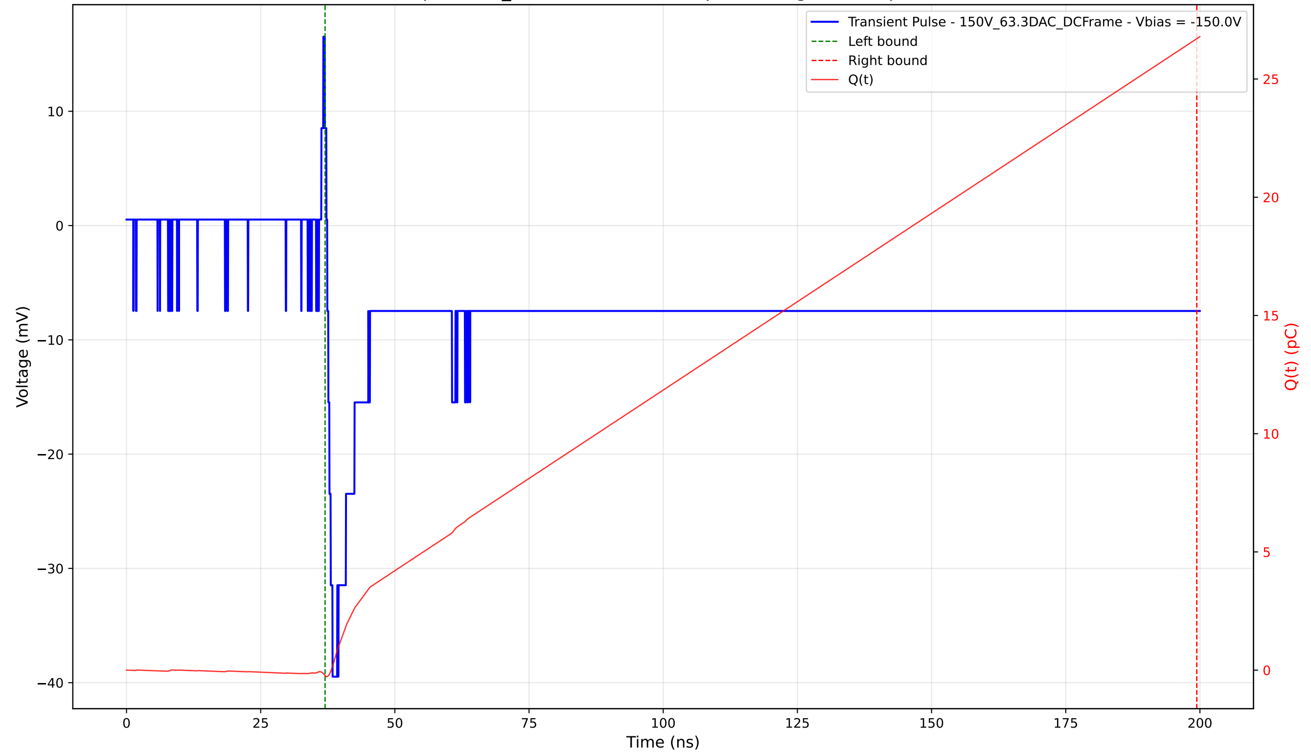
Transient Pulse - Sample: 1cm_42 - Position: 3320.0 \mu\text{m} - Charge: 26.94 pC - Rise Time: 0.99 ns
