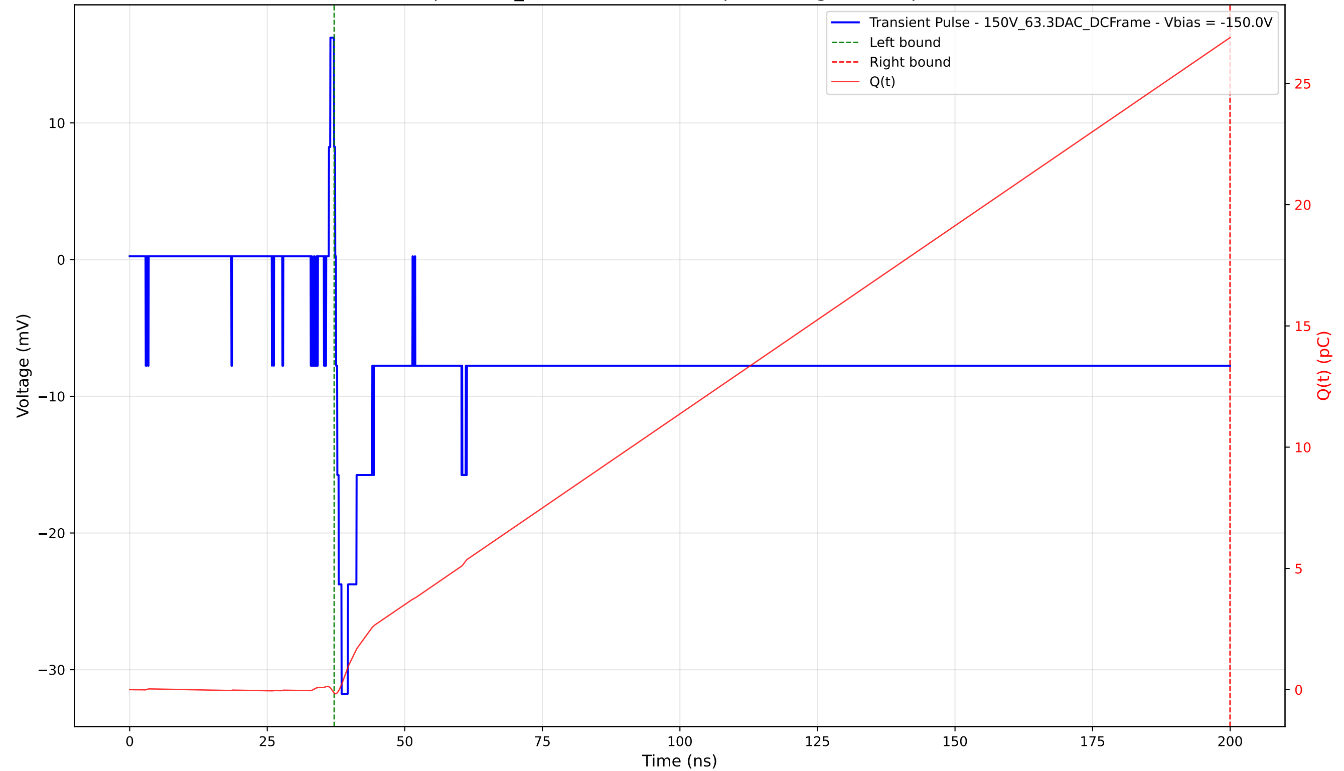
Transient Pulse - Sample: 1cm_42 - Position: 2575.0 \mu\text{m} - Charge: 27.03 pC - Rise Time: 1.01 ns
