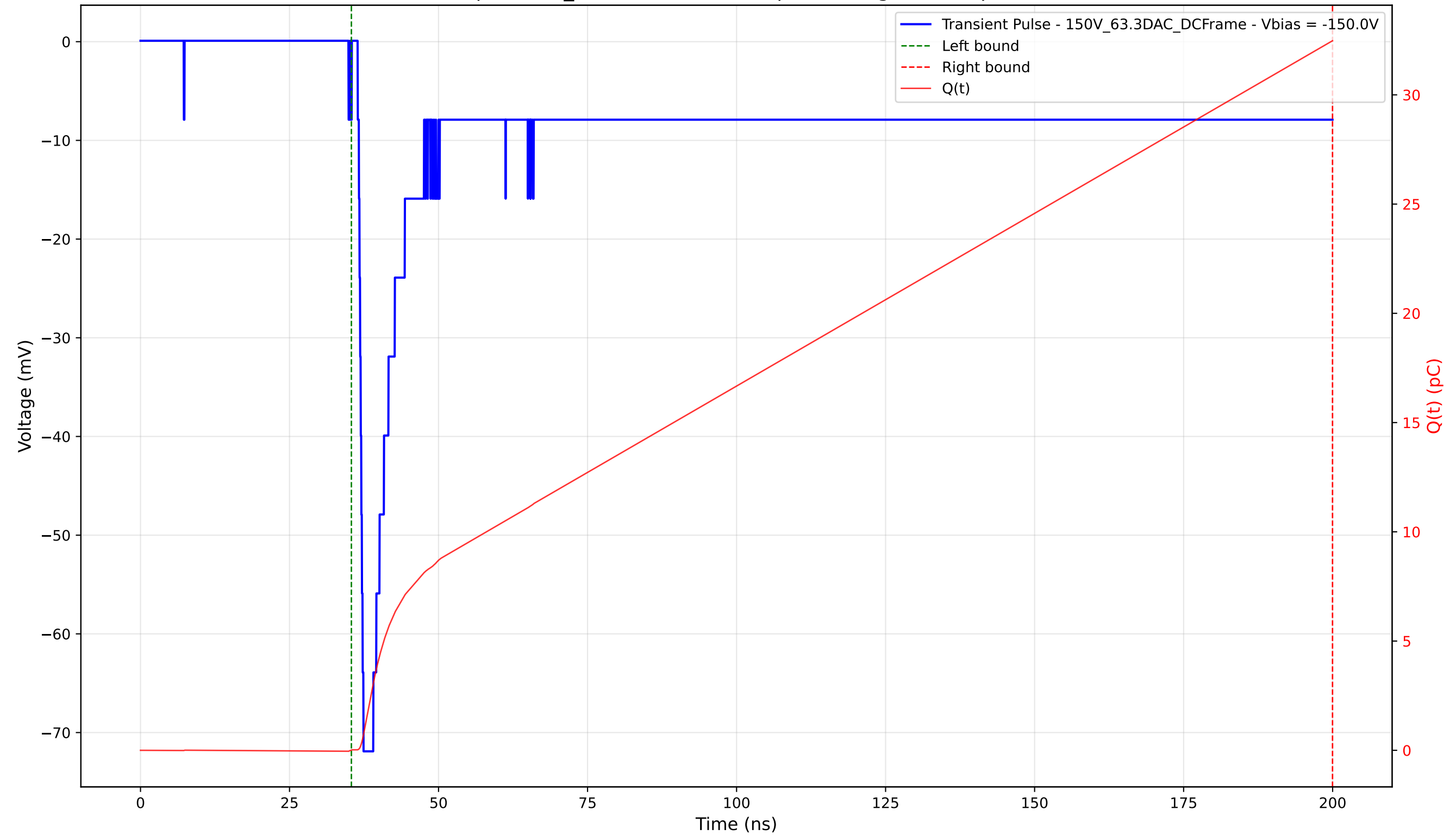
Transient Pulse - Sample: 1cm_42 - Position: 985.0 \mu\text{m} - Charge: 32.46 pC - Rise Time: 0.96 ns
