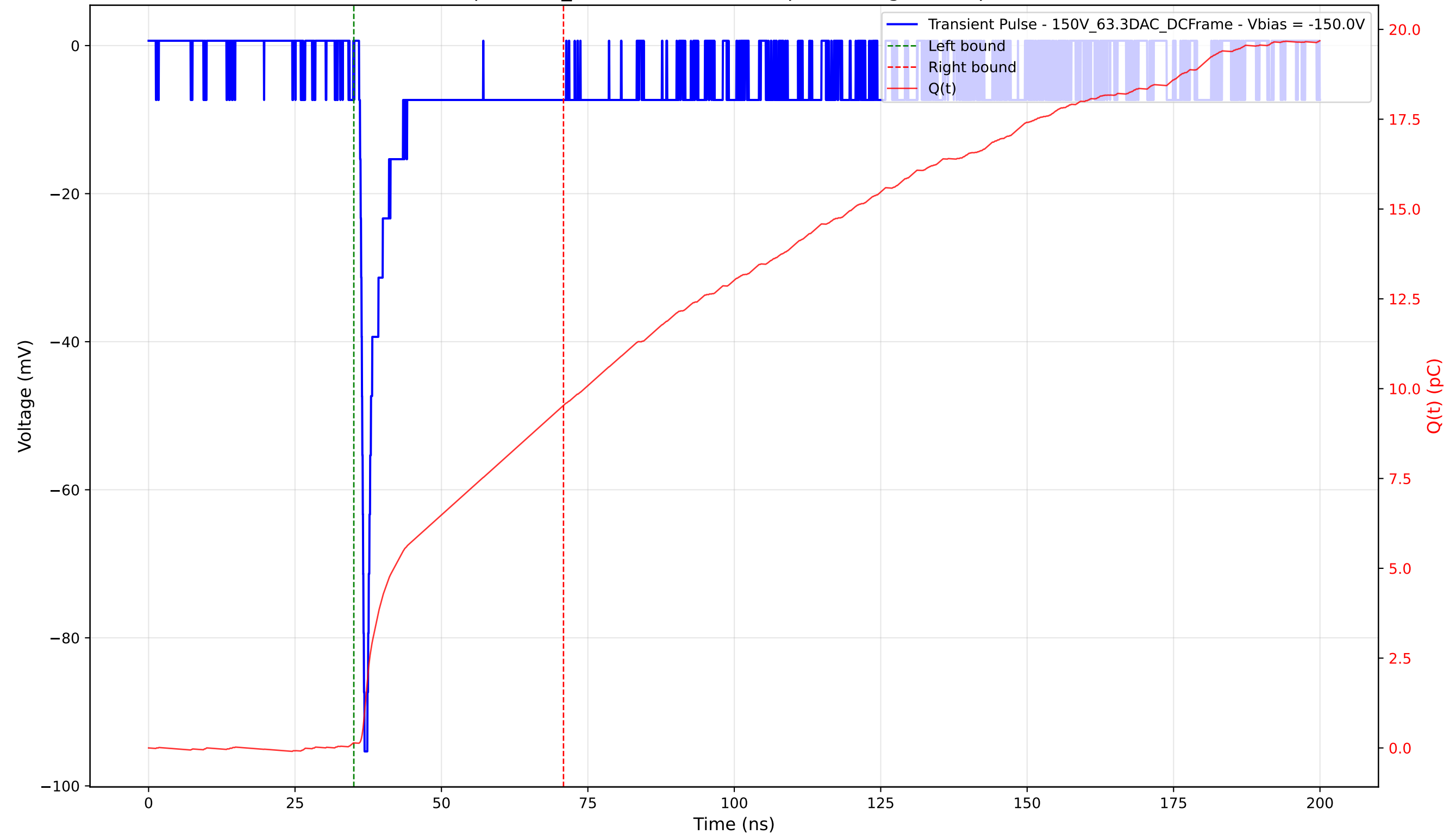
Transient Pulse - Sample: 1cm_42 - Position: 5045.0 \mu\text{m} - Charge: 9.40 pC - Rise Time: 0.67 ns
