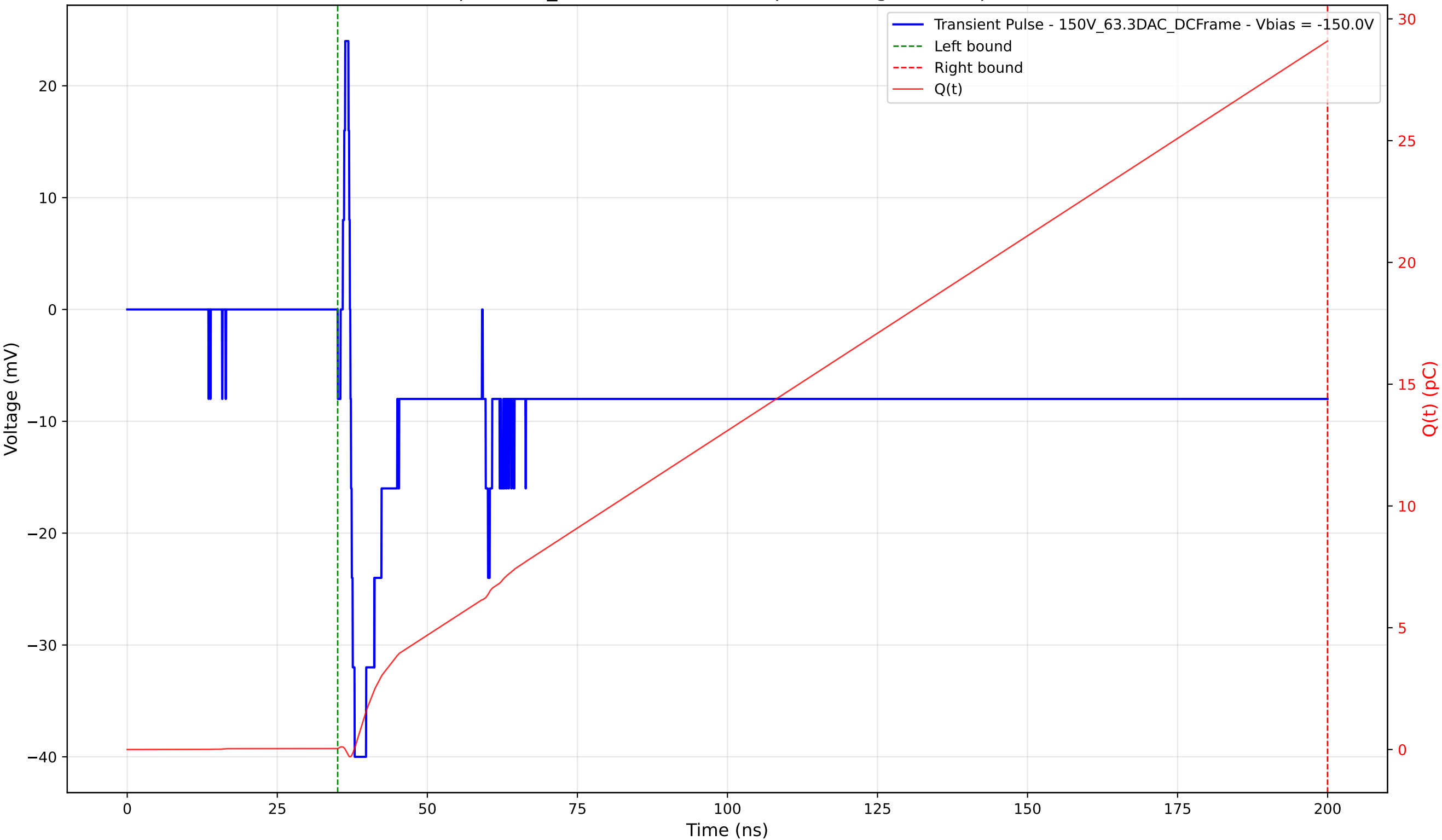
Transient Pulse - Sample: 1cm_42 - Position: 1870.0 \mu\text{m} - Charge: 29.05 pC - Rise Time: 0.71 ns
