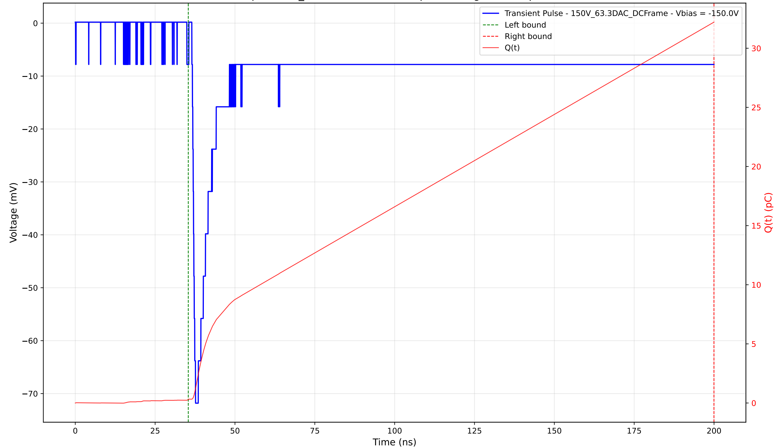
Transient Pulse - Sample: 1cm_42 - Position: 4120.0 \mu\text{m} - Charge: 31.91 pC - Rise Time: 1.14 ns
