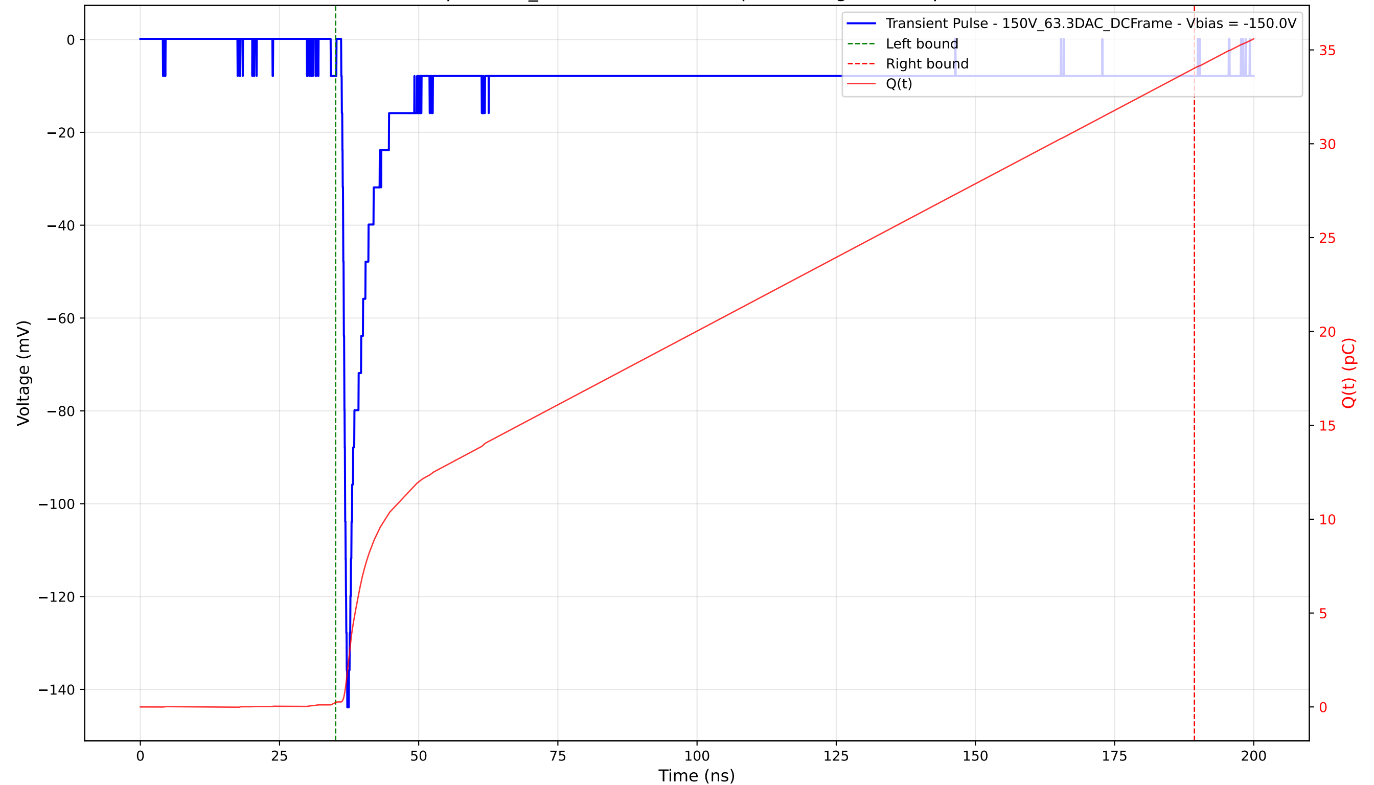
Transient Pulse - Sample: 1cm_42 - Position: 4575.0 \mu\text{m} - Charge: 33.78 pC - Rise Time: 0.88 ns
