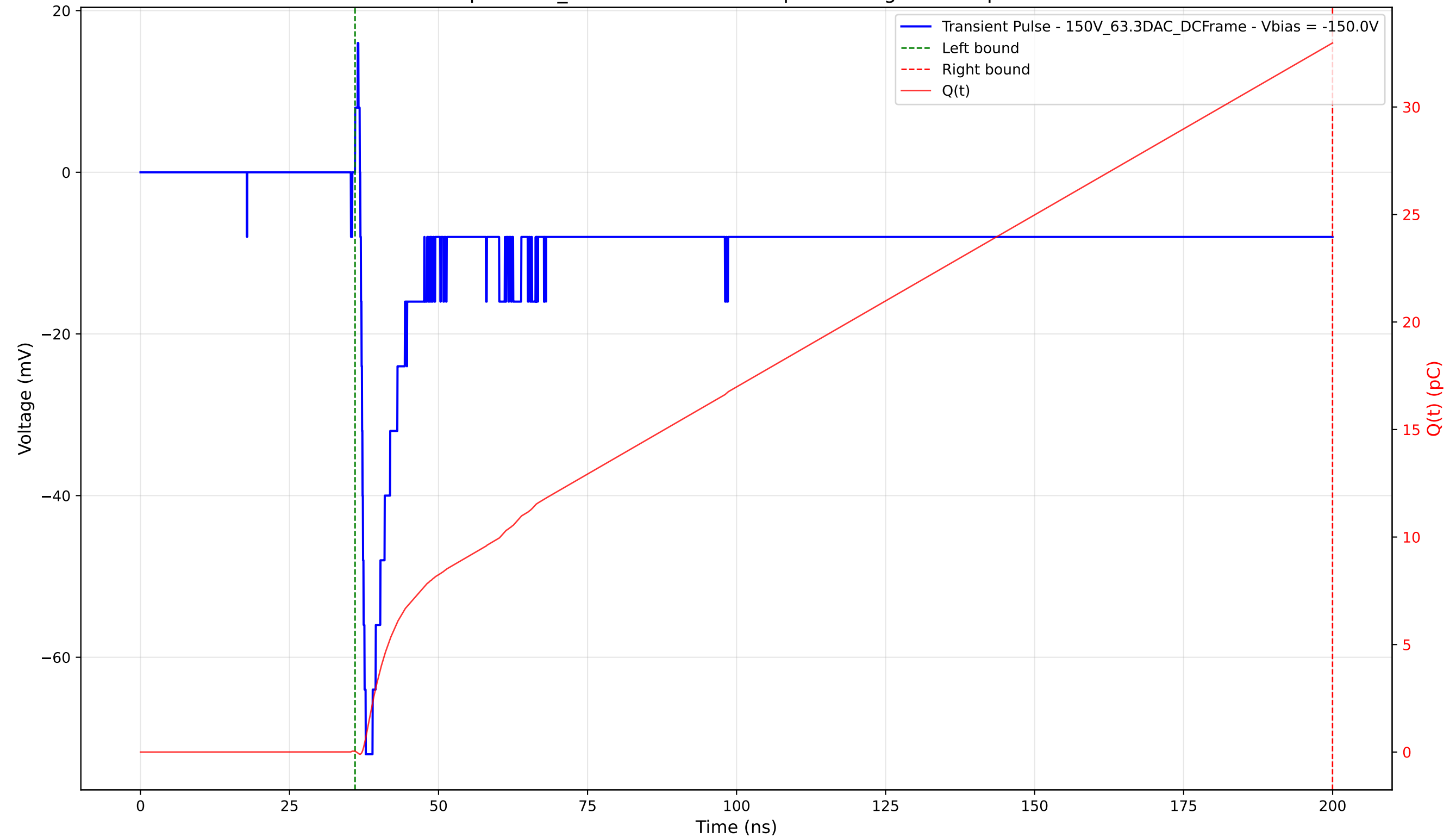
Transient Pulse - Sample: 1cm_42 - Position: 1220.0 \mu\text{m} - Charge: 32.94 pC - Rise Time: 0.90 ns
