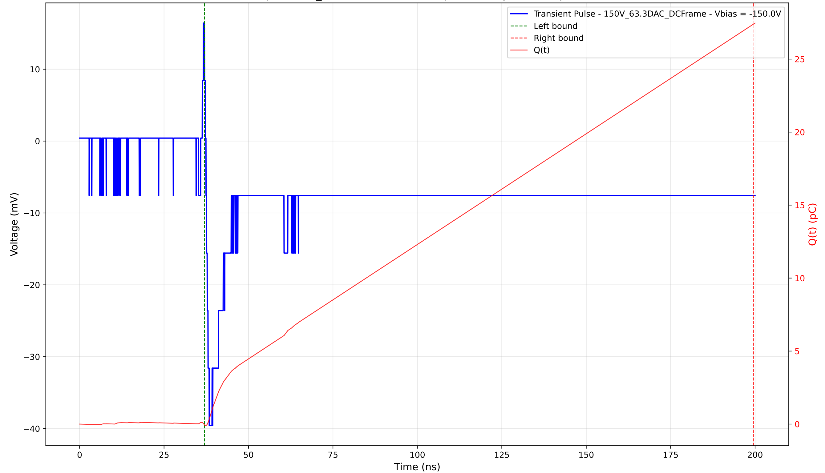
Transient Pulse - Sample: 1cm_42 - Position: 3250.0 \mu\text{m} - Charge: 27.47 pC - Rise Time: 0.95 ns
