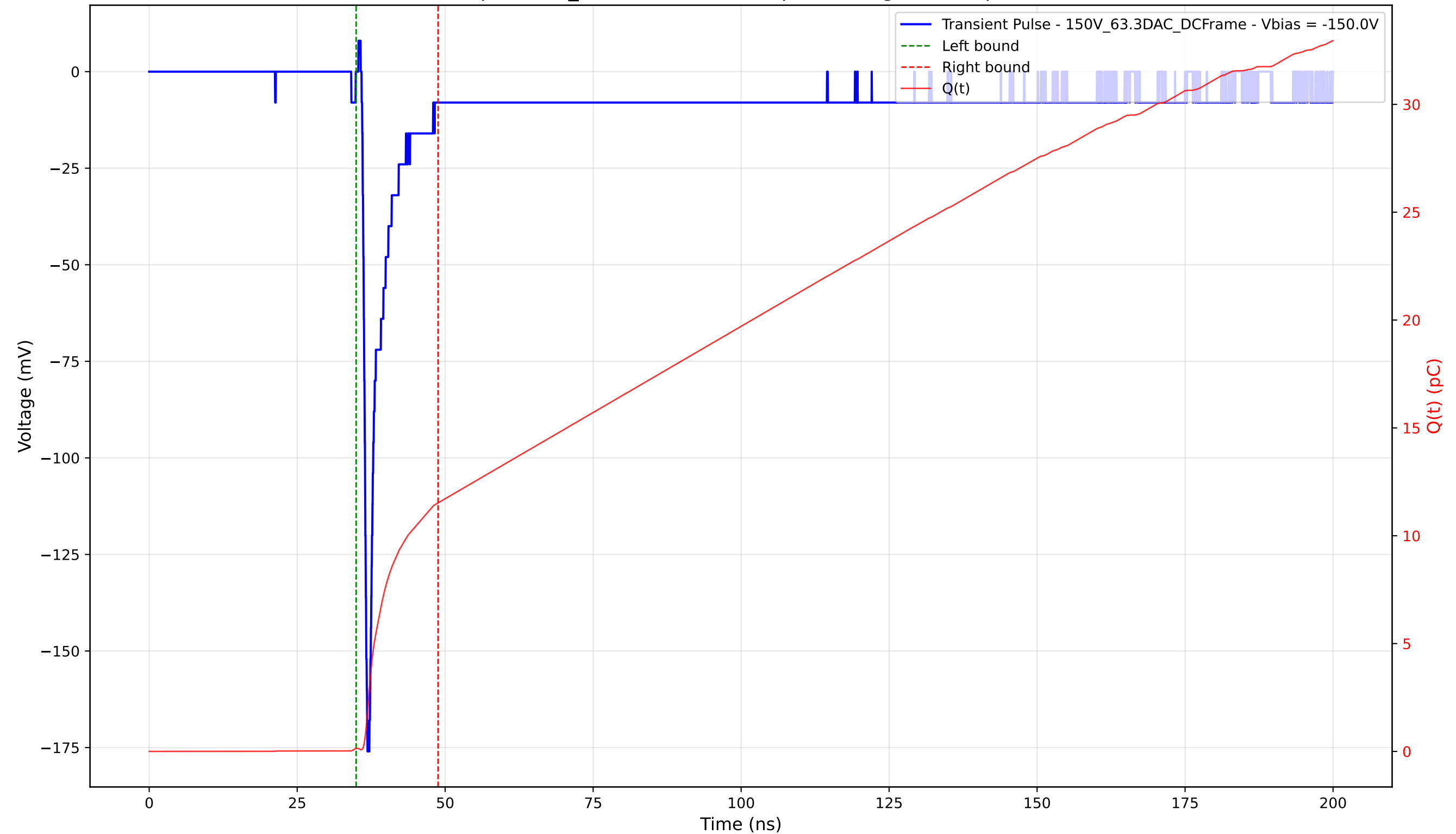
Transient Pulse - Sample: 1cm_42 - Position: 330.0 \mu\text{m} - Charge: 11.39 pC - Rise Time: 0.72 ns
