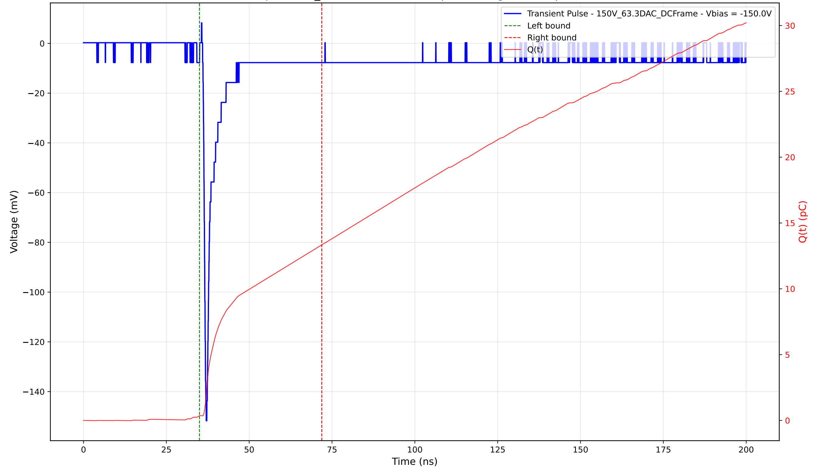
Transient Pulse - Sample: 1cm_42 - Position: 4980.0 \mu\text{m} - Charge: 12.98 pC - Rise Time: 0.84 ns
