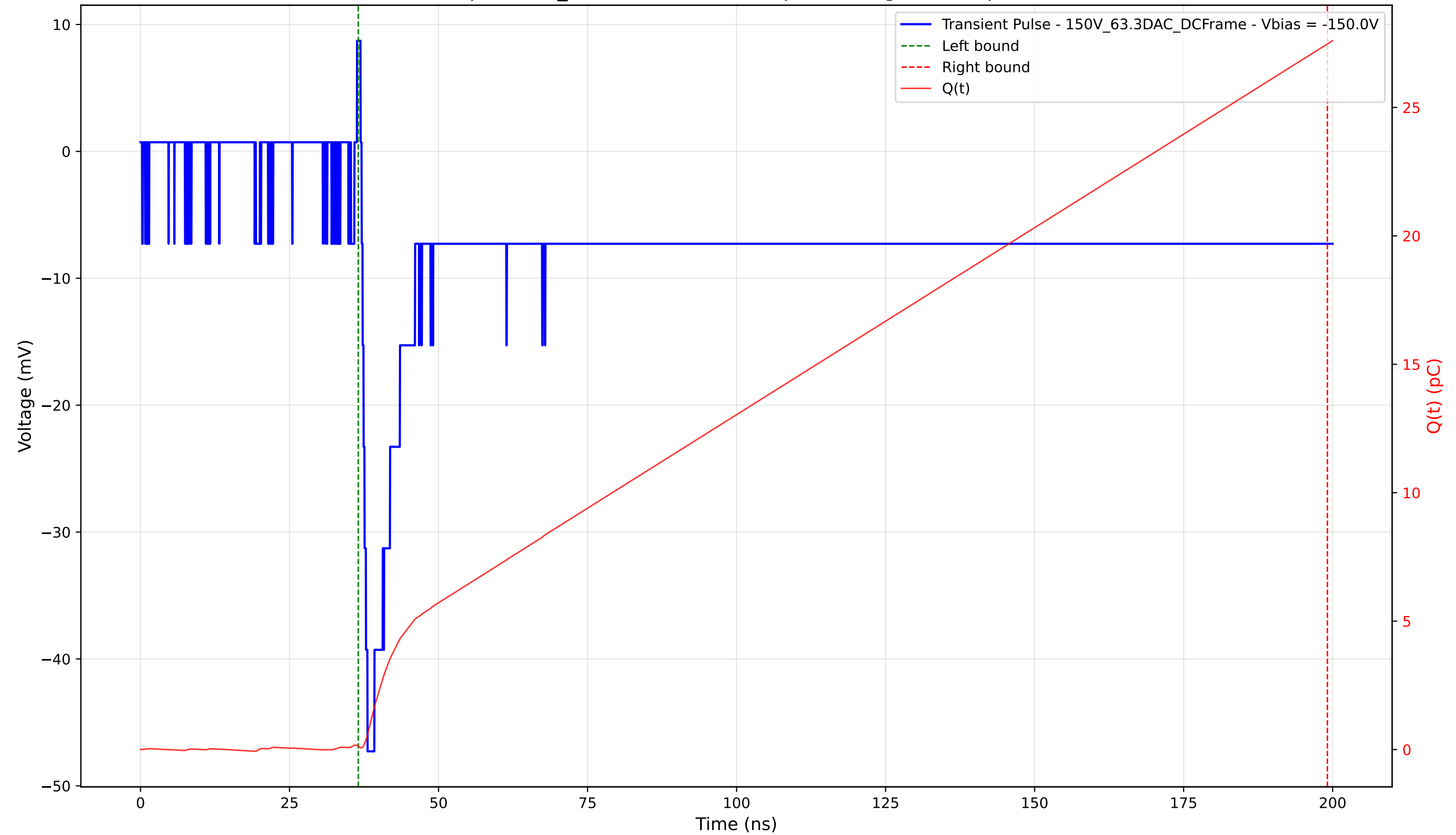
Transient Pulse - Sample: 1cm_42 - Position: 3660.0 \mu\text{m} - Charge: 27.34 pC - Rise Time: 0.99 ns
