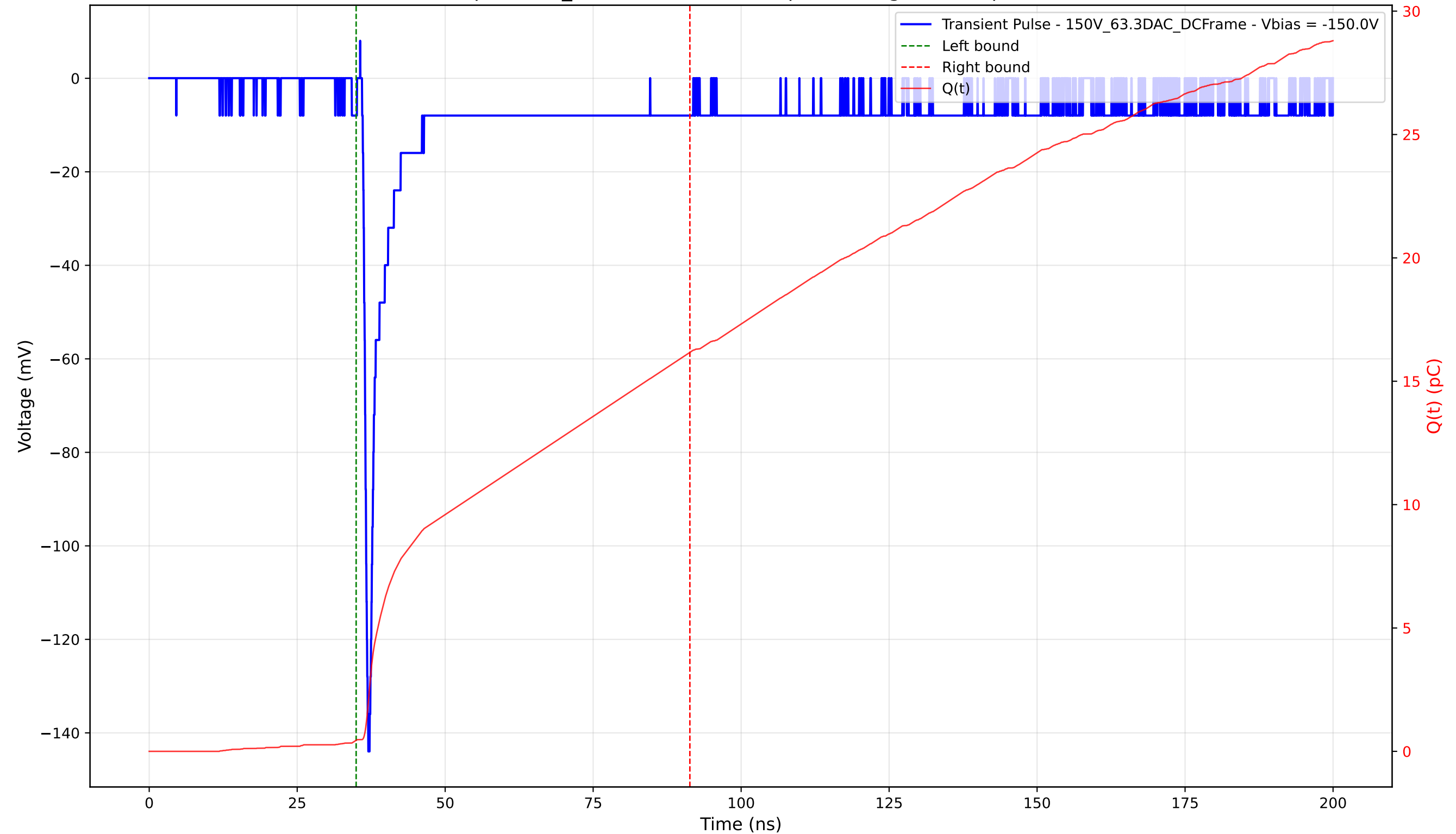
Transient Pulse - Sample: 1cm_42 - Position: 4990.0 \mu\text{m} - Charge: 15.72 pC - Rise Time: 0.82 ns
