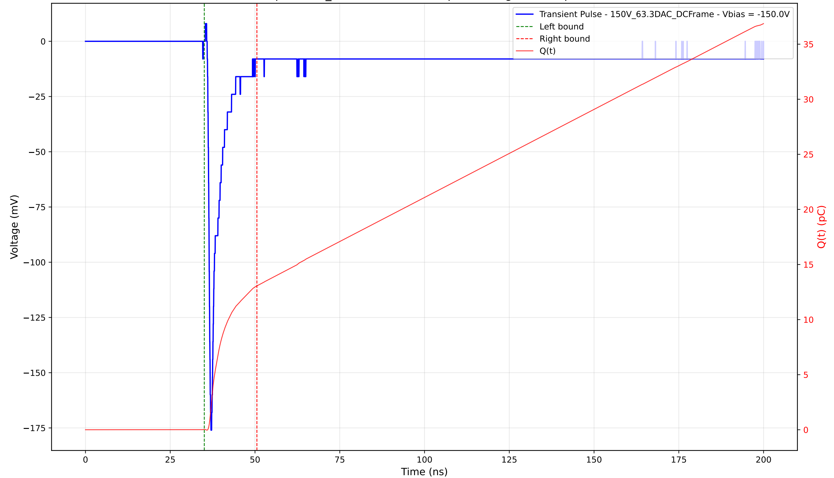
Transient Pulse - Sample: 1cm_42 - Position: 450.0 \mu\text{m} - Charge: 13.03 pC - Rise Time: 0.74 ns
