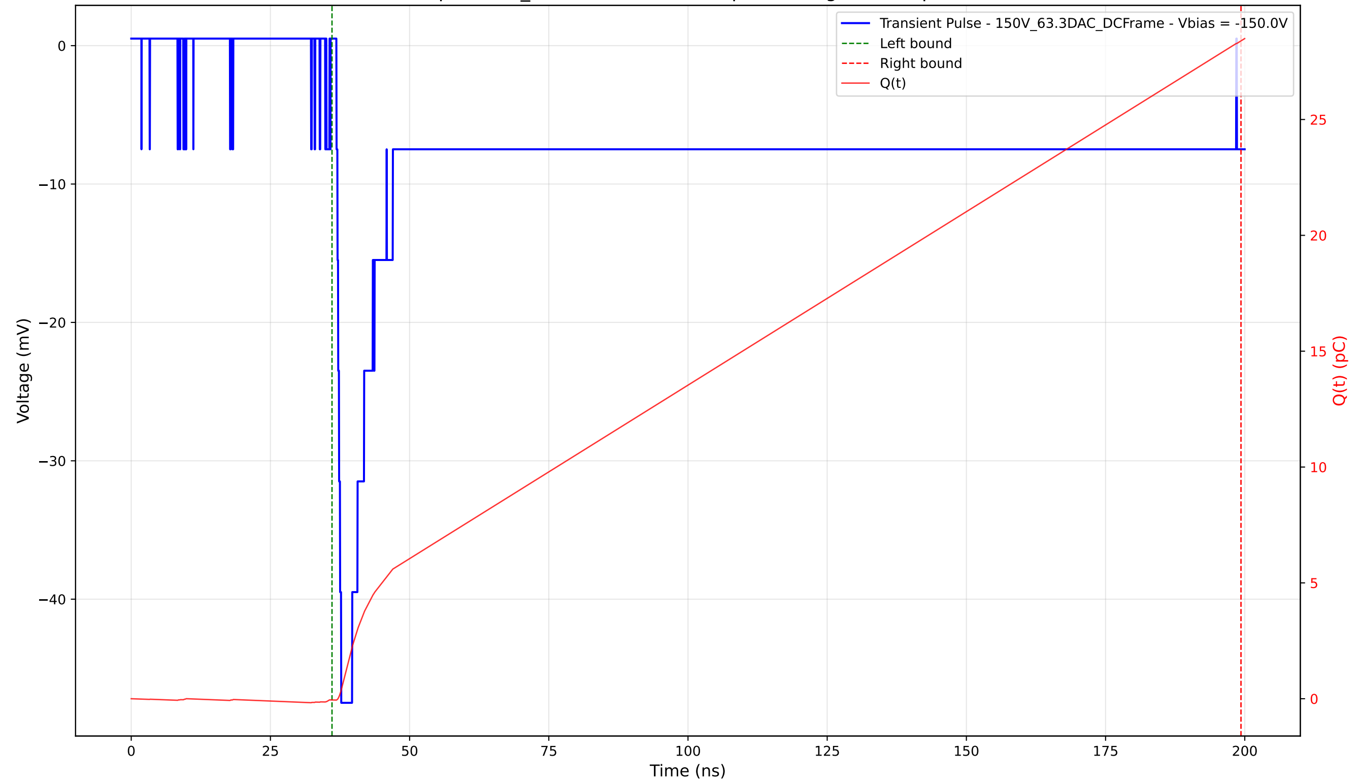
Transient Pulse - Sample: 1cm_42 - Position: 3925.0 \mu\text{m} - Charge: 28.45 pC - Rise Time: 0.85 ns
