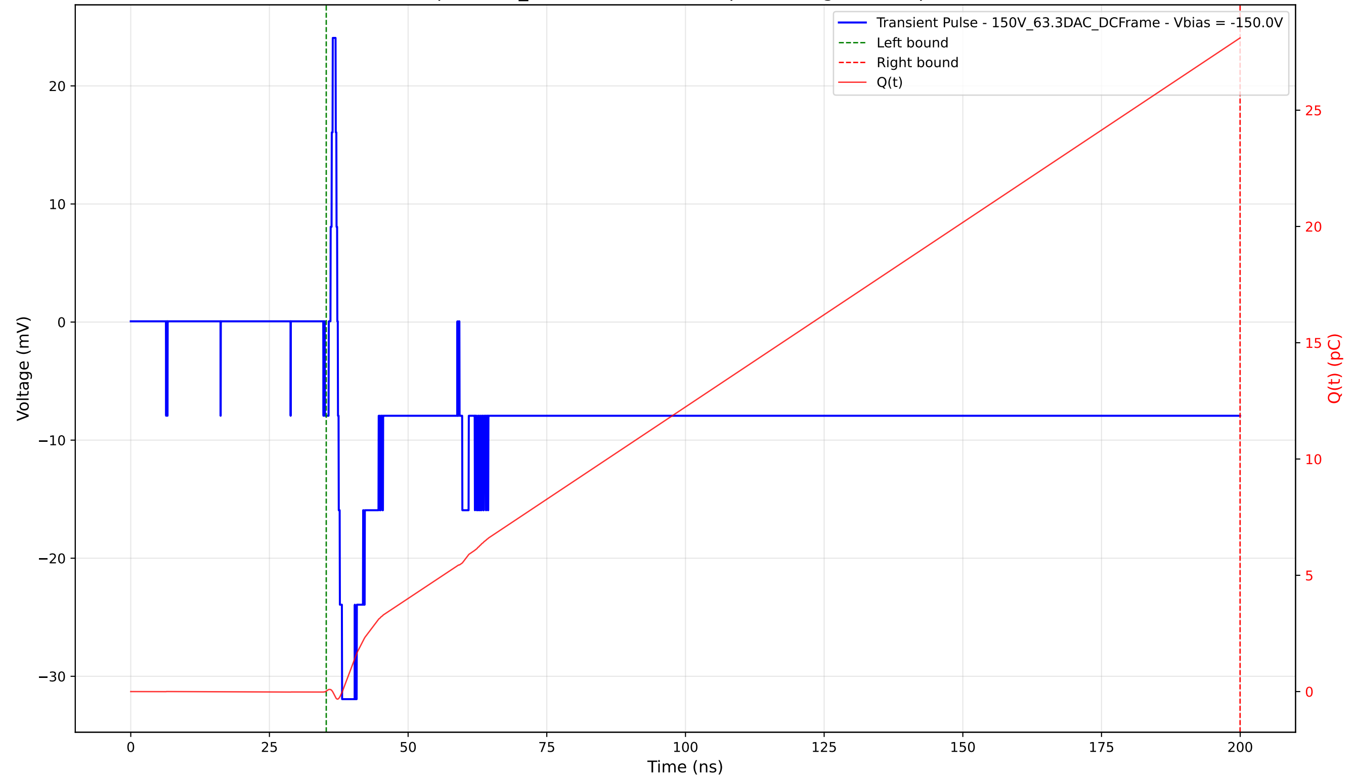
Transient Pulse - Sample: 1cm_42 - Position: 2310.0 \mu\text{m} - Charge: 28.08 pC - Rise Time: 0.75 ns
