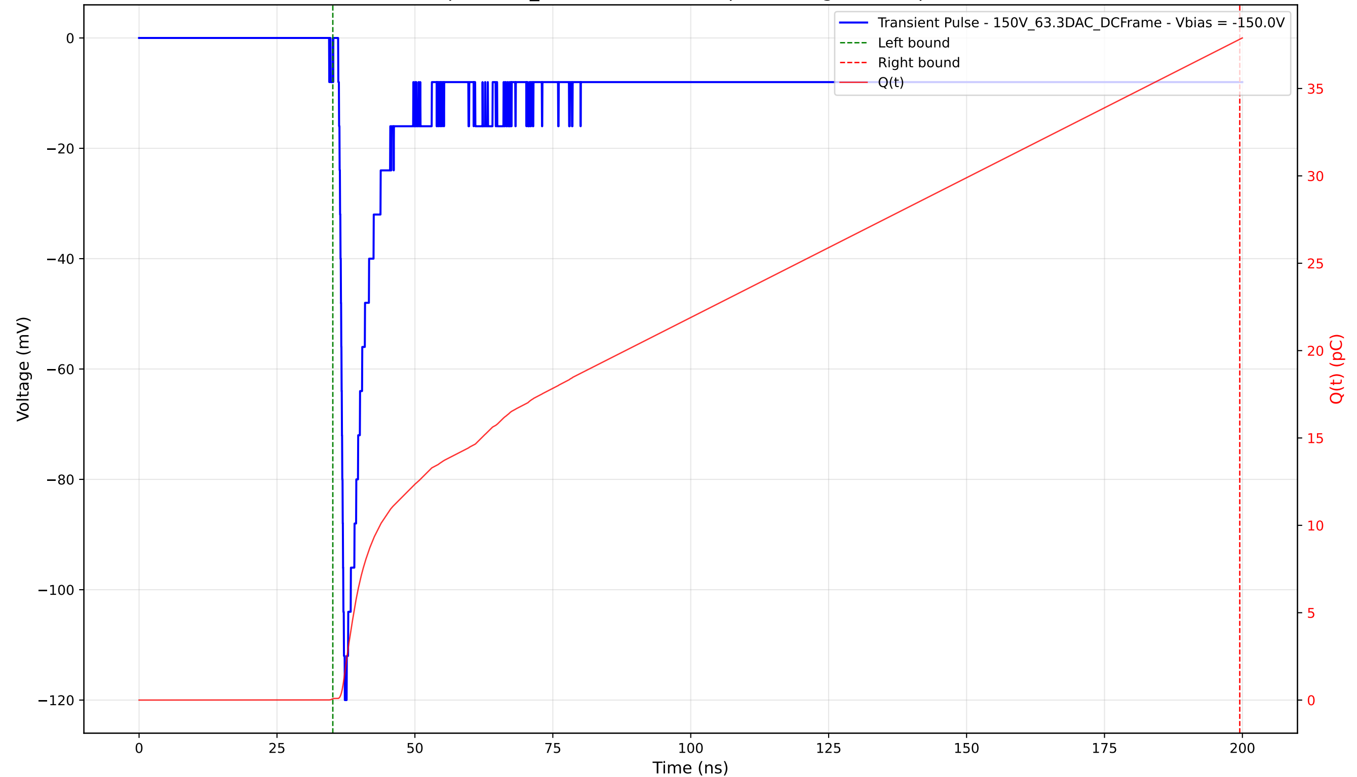
Transient Pulse - Sample: 1cm_42 - Position: 790.0 \mu\text{m} - Charge: 37.74 pC - Rise Time: 0.89 ns
