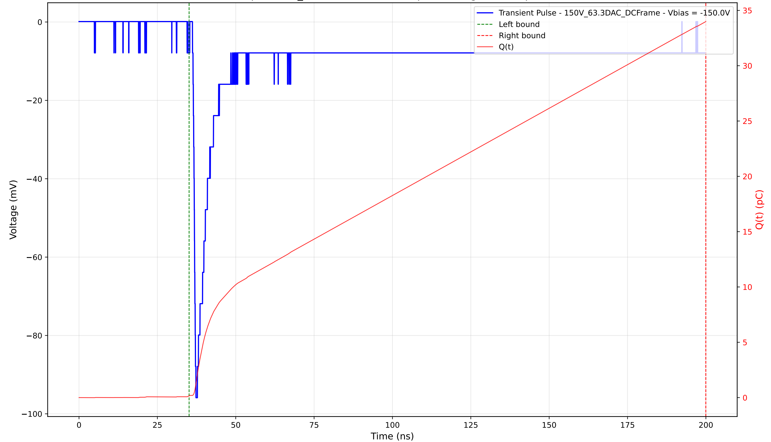
Transient Pulse - Sample: 1cm_42 - Position: 4410.0 \mu\text{m} - Charge: 33.83 pC - Rise Time: 0.78 ns
