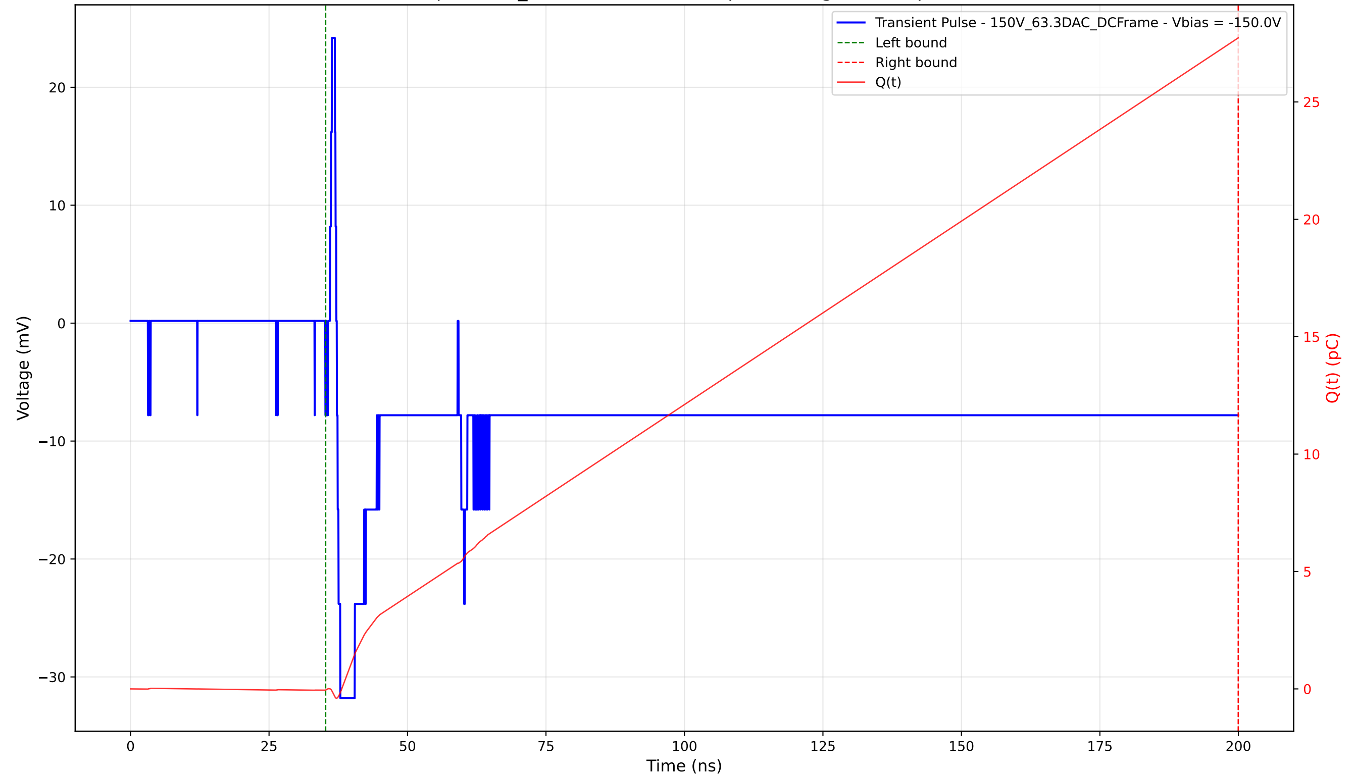
Transient Pulse - Sample: 1cm_42 - Position: 2080.0 \mu\text{m} - Charge: 27.77 pC - Rise Time: 0.63 ns
