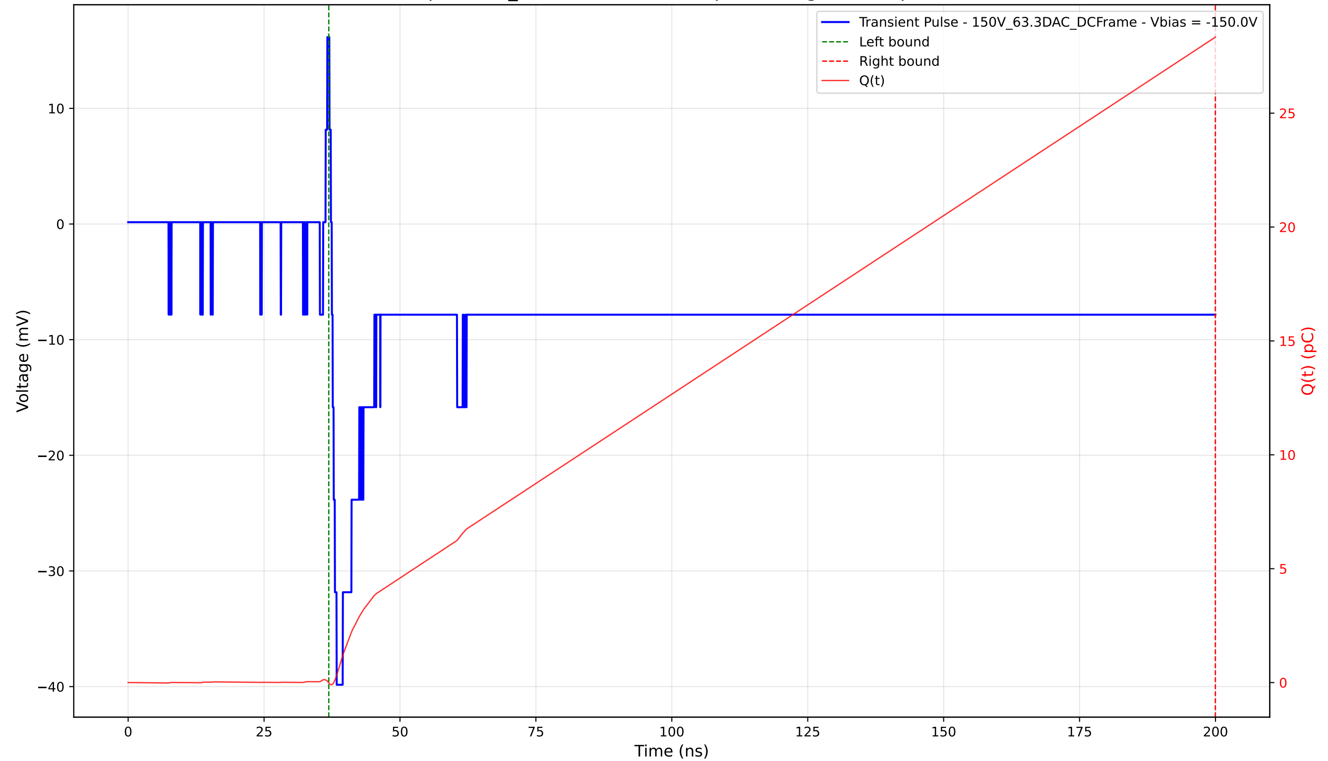
Transient Pulse - Sample: 1cm_42 - Position: 3220.0 \mu\text{m} - Charge: 28.36 pC - Rise Time: 0.89 ns
