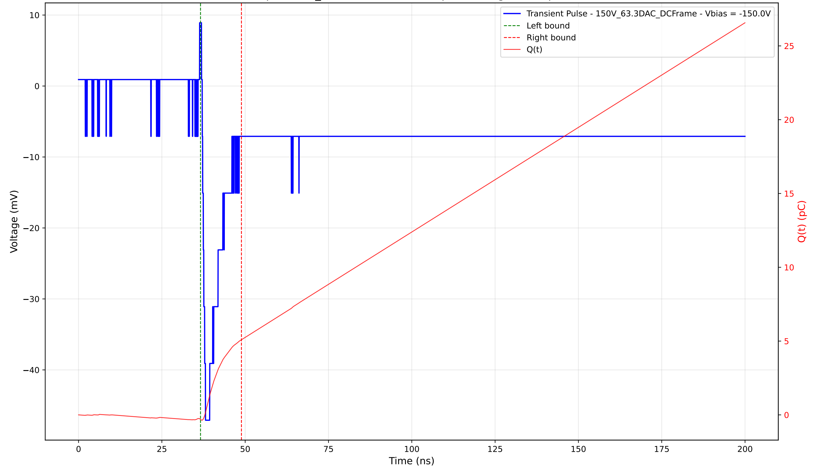
Transient Pulse - Sample: 1cm_42 - Position: 3665.0 \mu\text{m} - Charge: 5.40 pC - Rise Time: 0.97 ns
