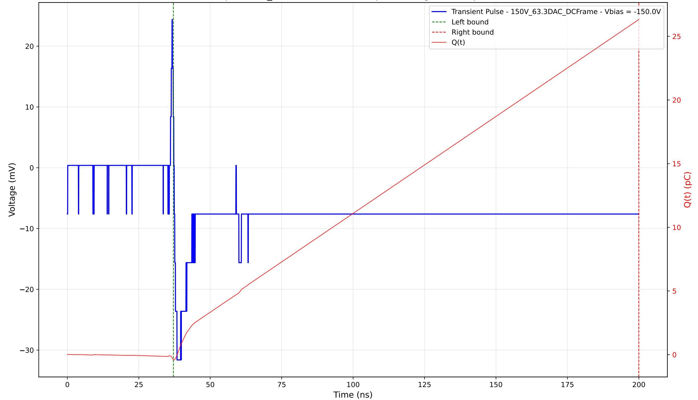
Transient Pulse - Sample: 1cm_42 - Position: 2415.0 \mu\text{m} - Charge: 26.71 pC - Rise Time: 0.97 ns
