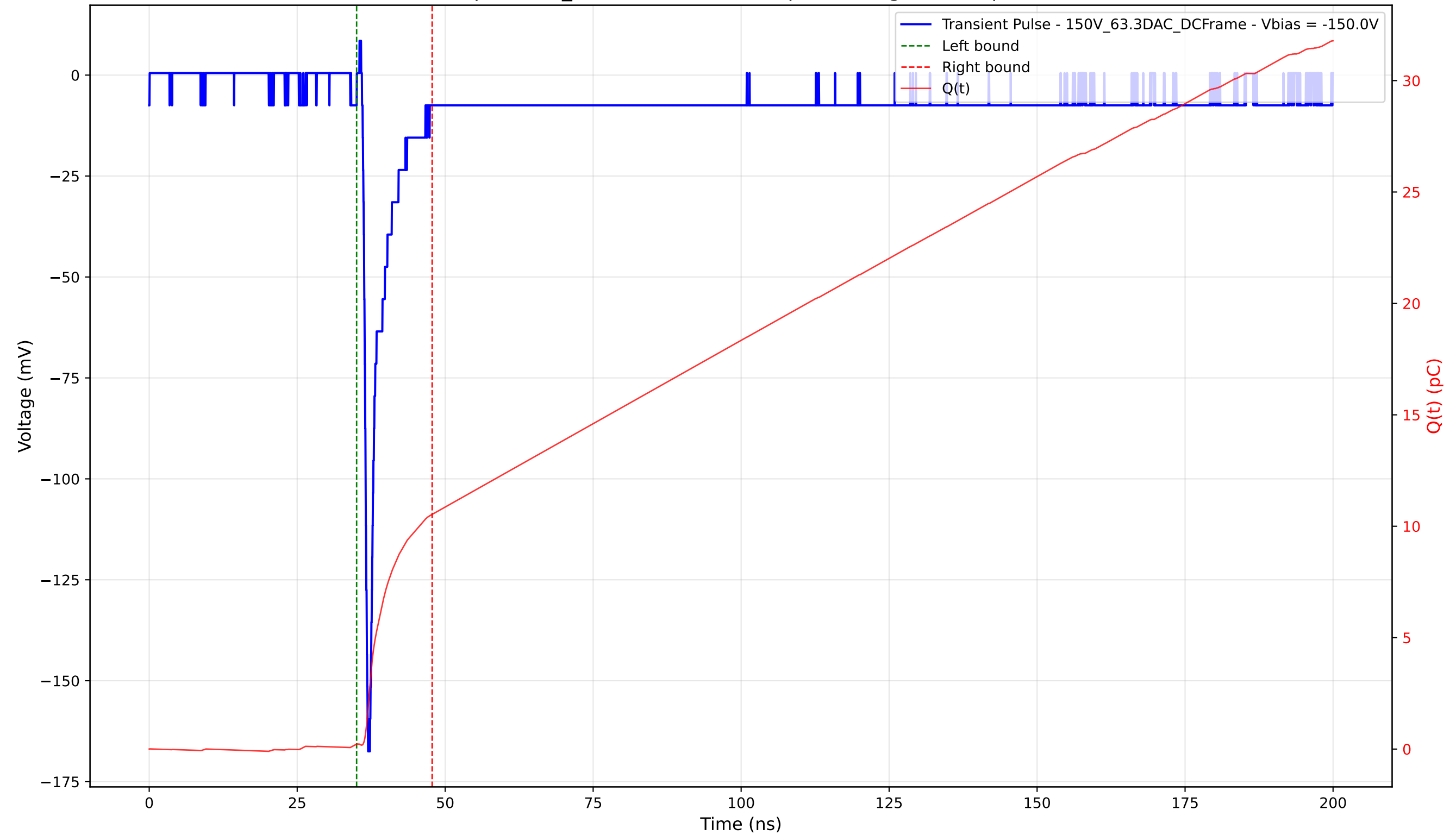
Transient Pulse - Sample: 1cm_42 - Position: 4955.0 \mu\text{m} - Charge: 10.30 pC - Rise Time: 0.72 ns
