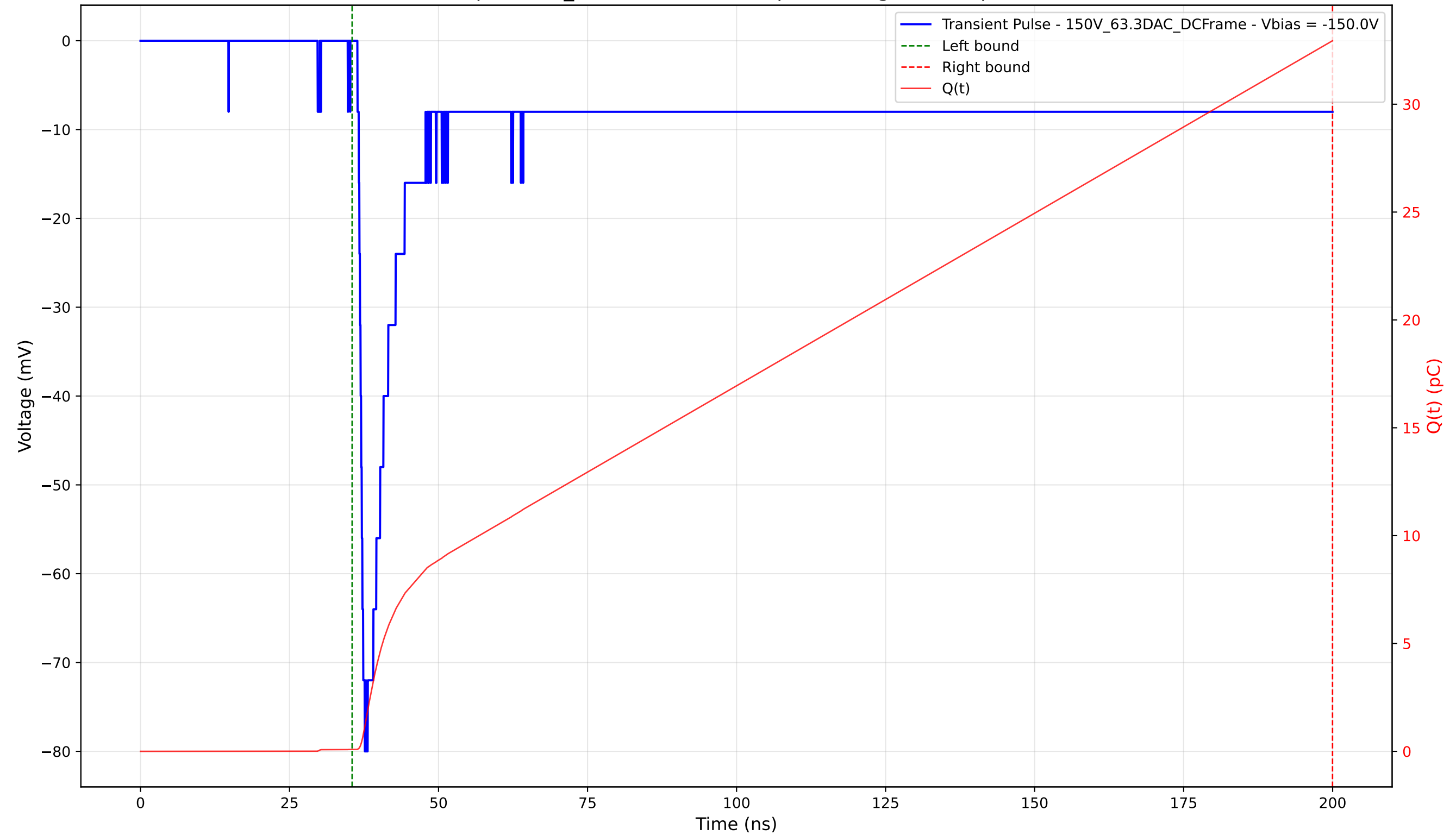
Transient Pulse - Sample: 1cm_42 - Position: 975.0 \mu\text{m} - Charge: 32.85 pC - Rise Time: 0.76 ns
