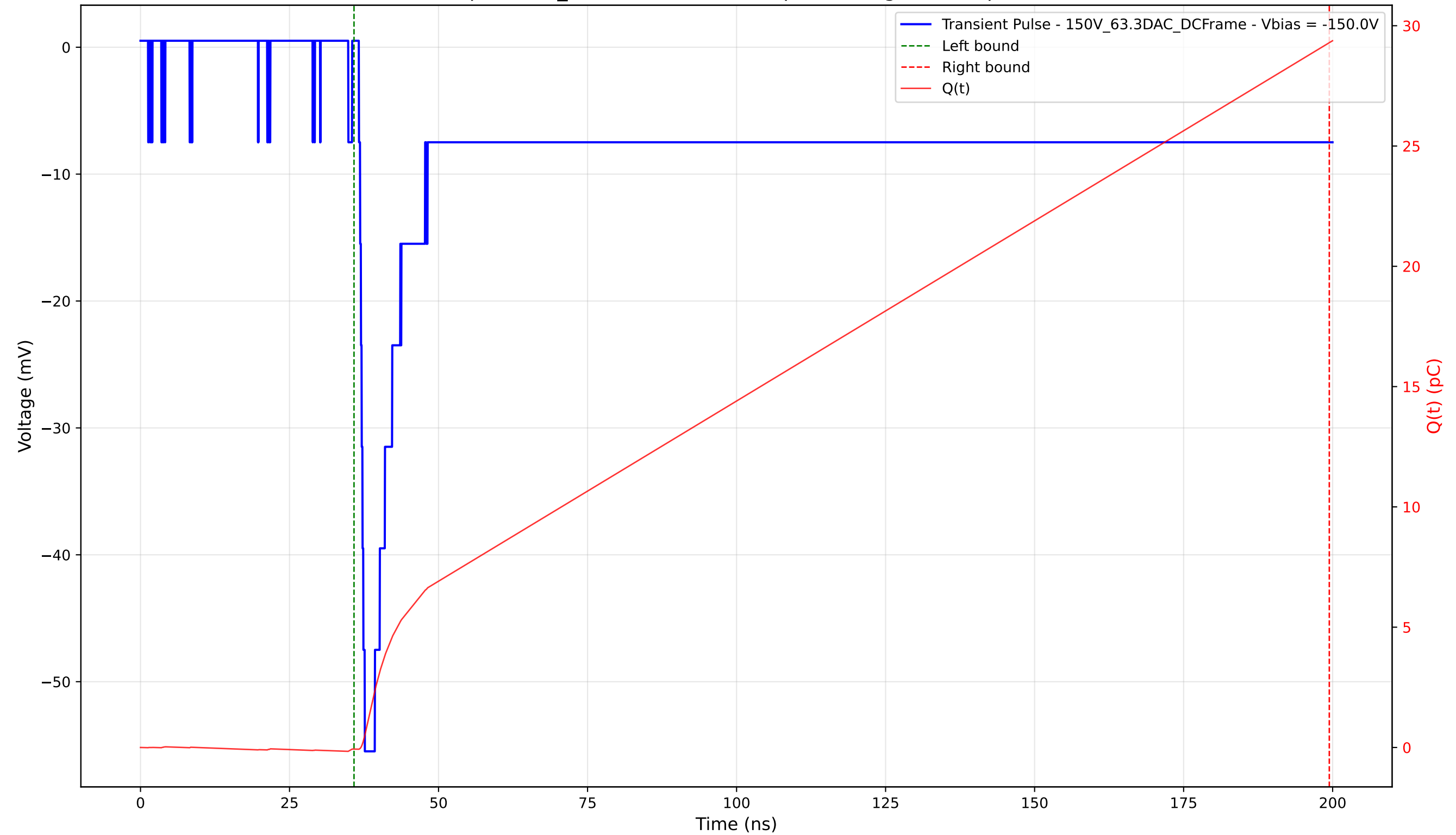
Transient Pulse - Sample: 1cm_42 - Position: 4030.0 \mu\text{m} - Charge: 29.36 pC - Rise Time: 0.99 ns
