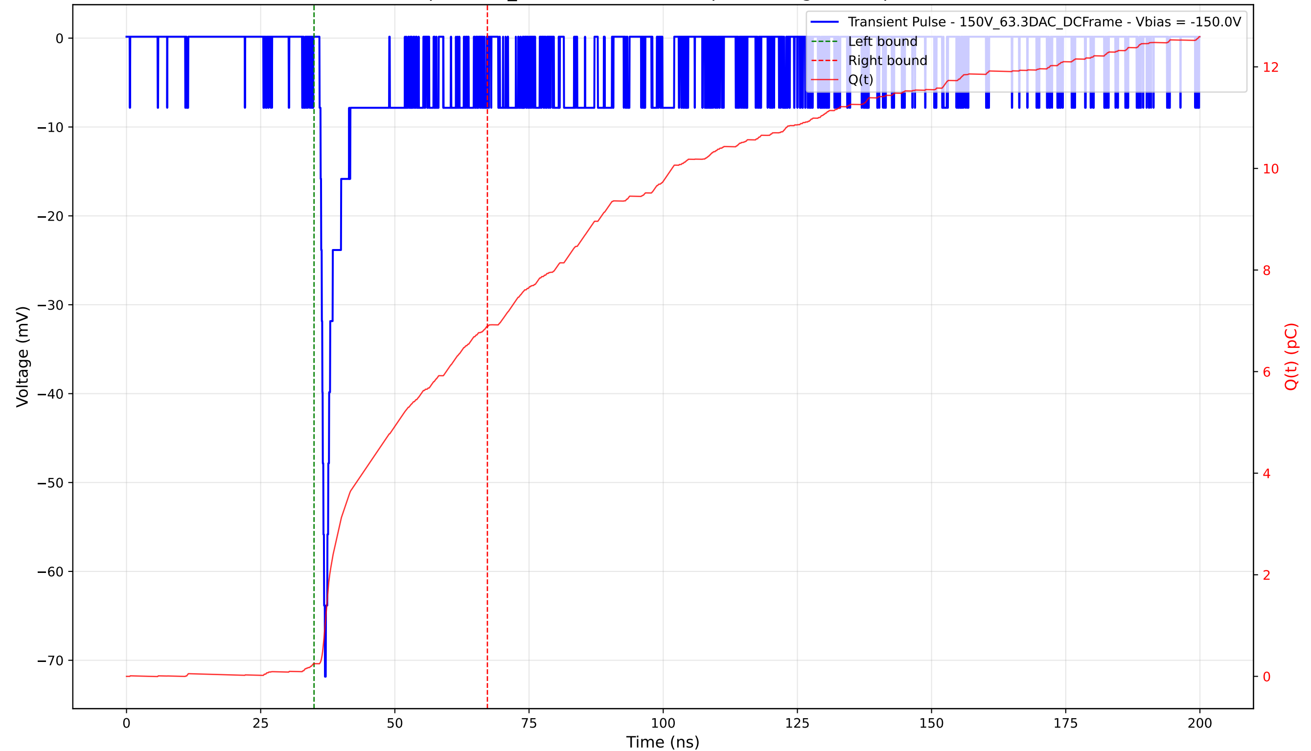
Transient Pulse - Sample: 1cm_42 - Position: 5095.0 \mu\text{m} - Charge: 6.64 pC - Rise Time: 1.00 ns
