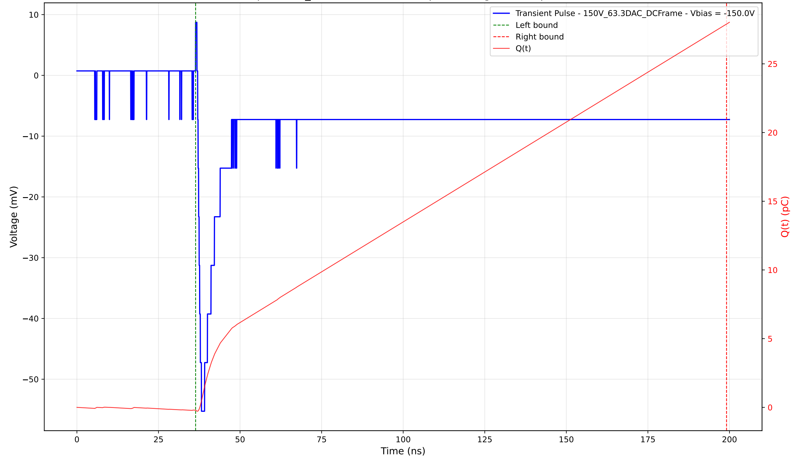
Transient Pulse - Sample: 1cm_42 - Position: 3790.0 \mu\text{m} - Charge: 28.11 pC - Rise Time: 1.15 ns
