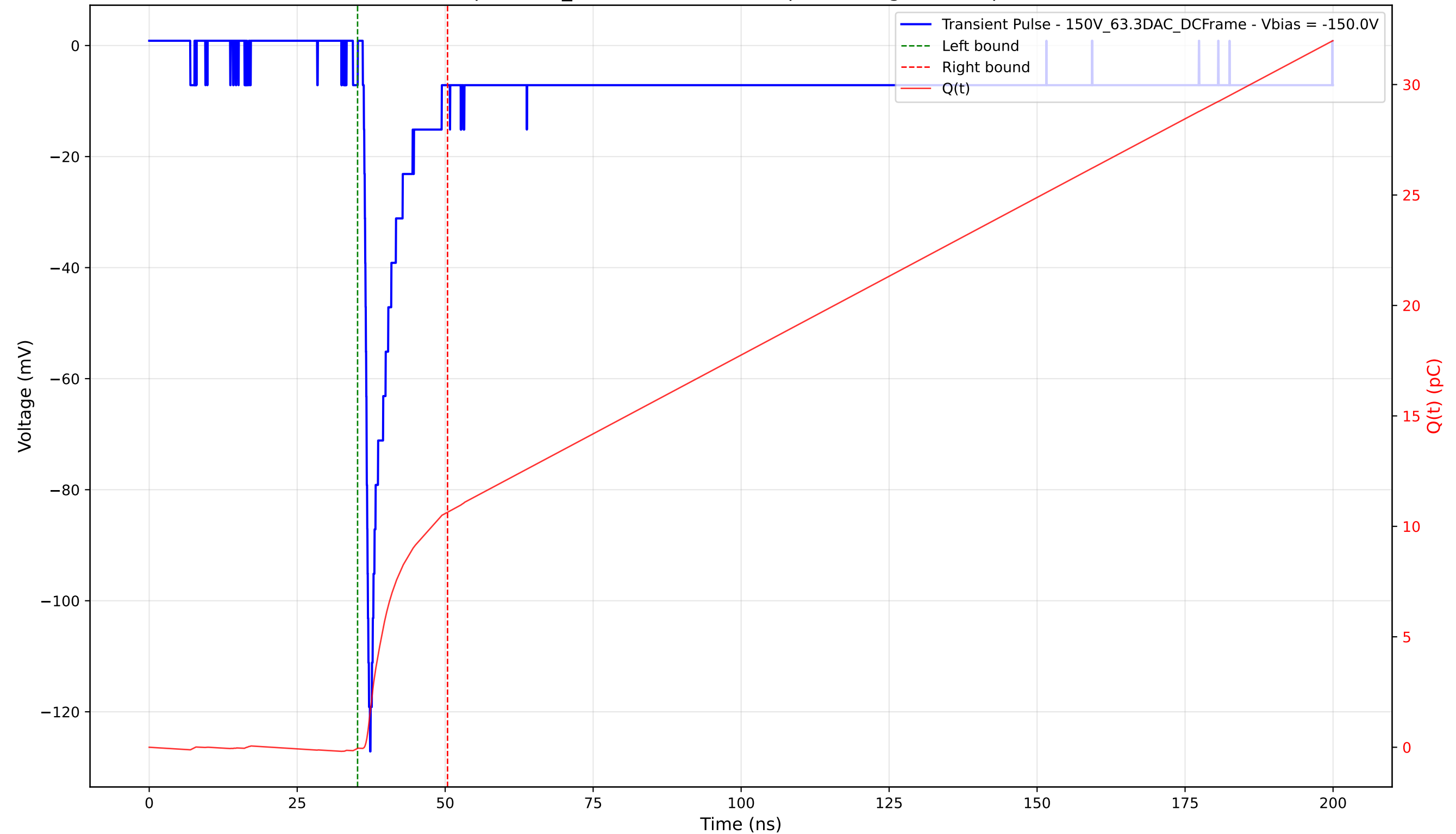
Transient Pulse - Sample: 1cm_42 - Position: 4530.0 \mu\text{m} - Charge: 10.68 pC - Rise Time: 0.87 ns
