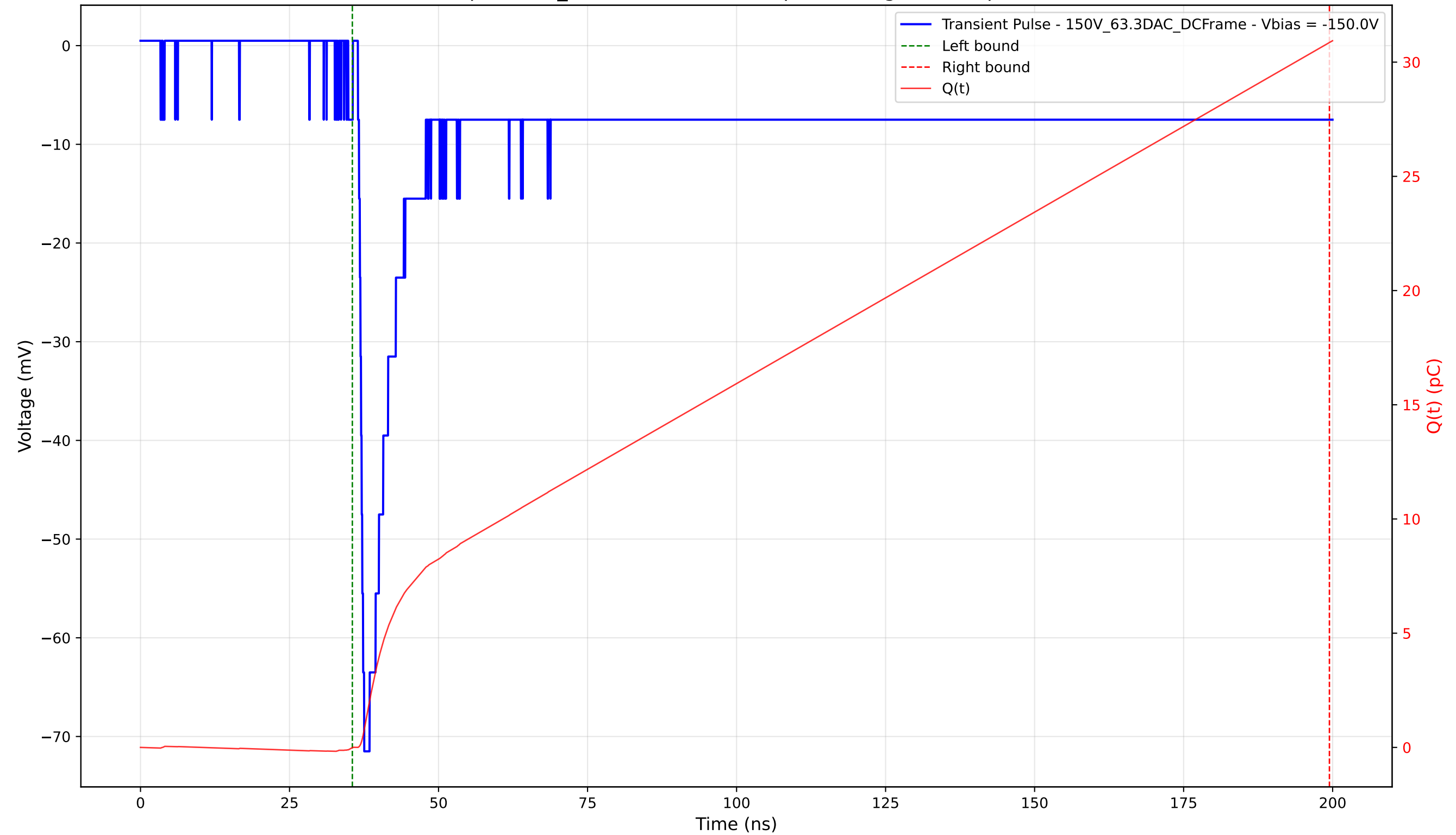
Transient Pulse - Sample: 1cm_42 - Position: 4130.0 \mu\text{m} - Charge: 30.86 pC - Rise Time: 1.04 ns
