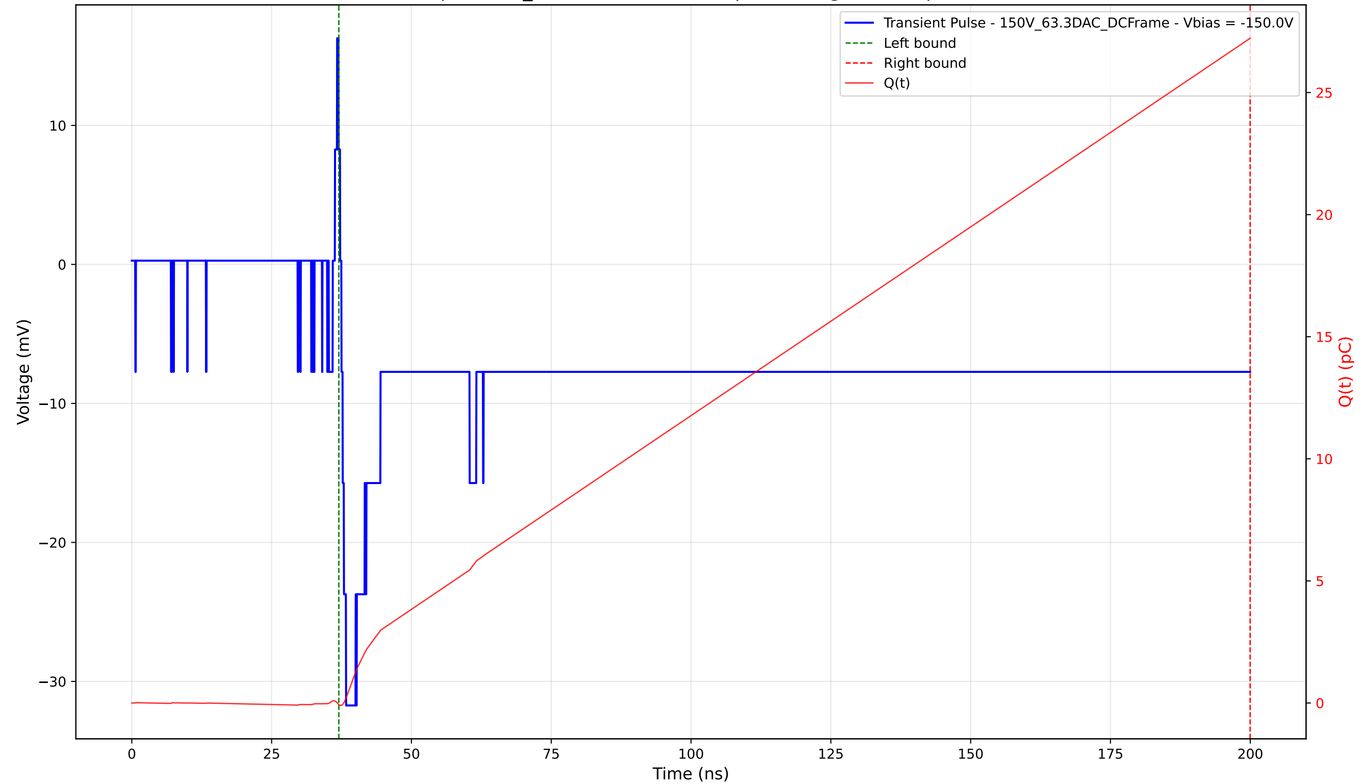
Transient Pulse - Sample: 1cm_42 - Position: 3085.0 \mu\text{m} - Charge: 27.29 pC - Rise Time: 0.83 ns
