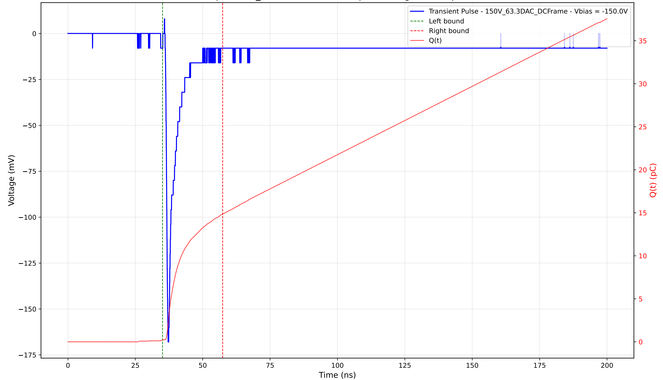
Transient Pulse - Sample: 1cm_42 - Position: 4615.0 \mu\text{m} - Charge: 14.63 pC - Rise Time: 0.76 ns
