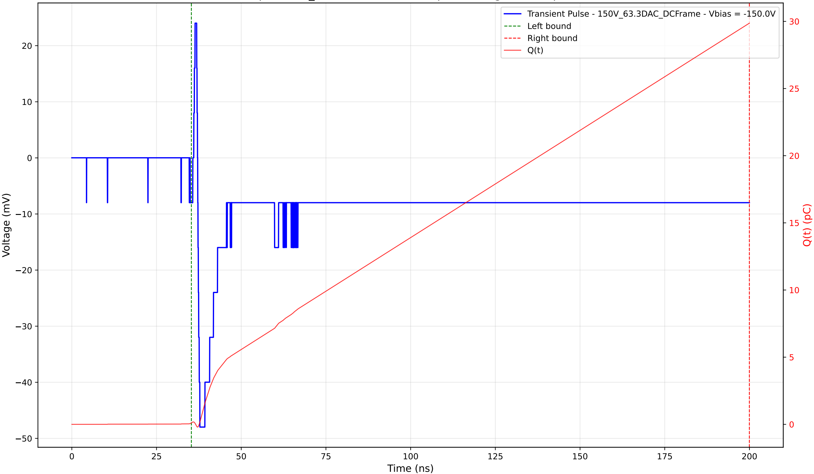
Transient Pulse - Sample: 1cm_42 - Position: 1600.0 \mu\text{m} - Charge: 29.76 pC - Rise Time: 0.63 ns
