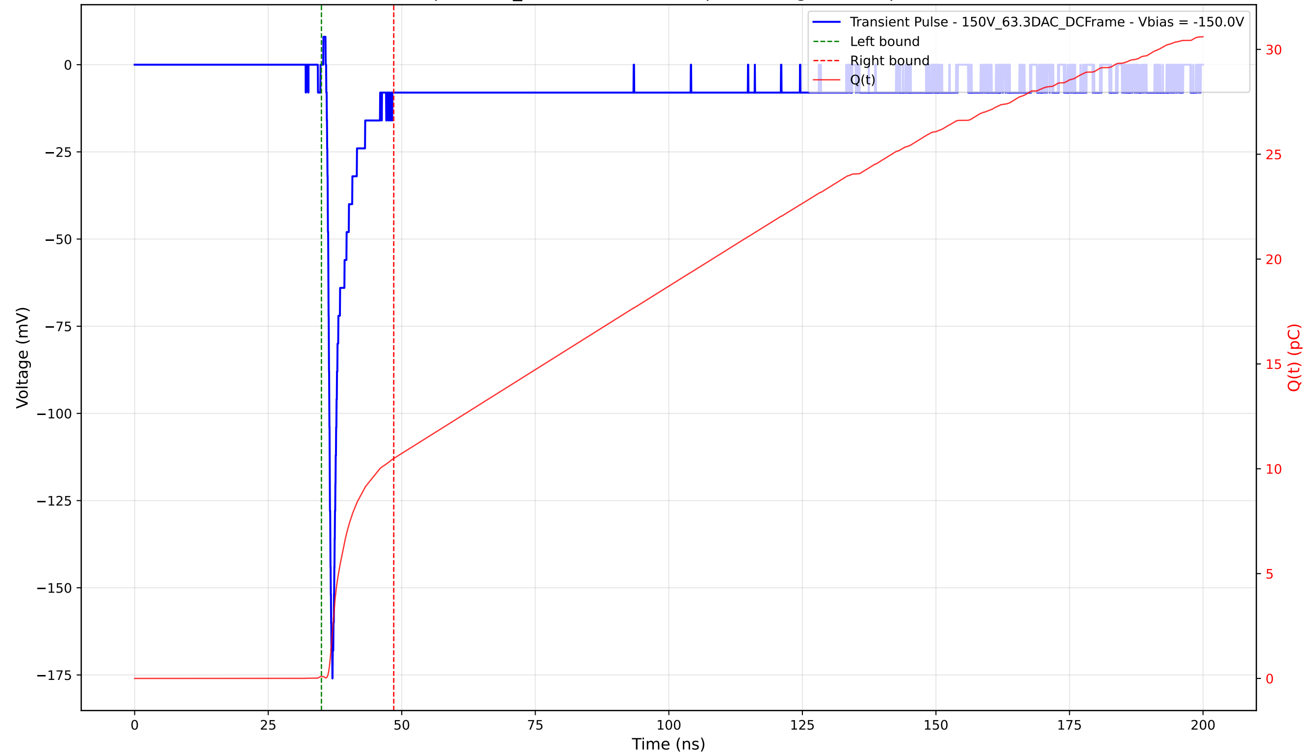
Transient Pulse - Sample: 1cm_42 - Position: 280.0 \mu\text{m} - Charge: 10.40 pC - Rise Time: 0.76 ns
