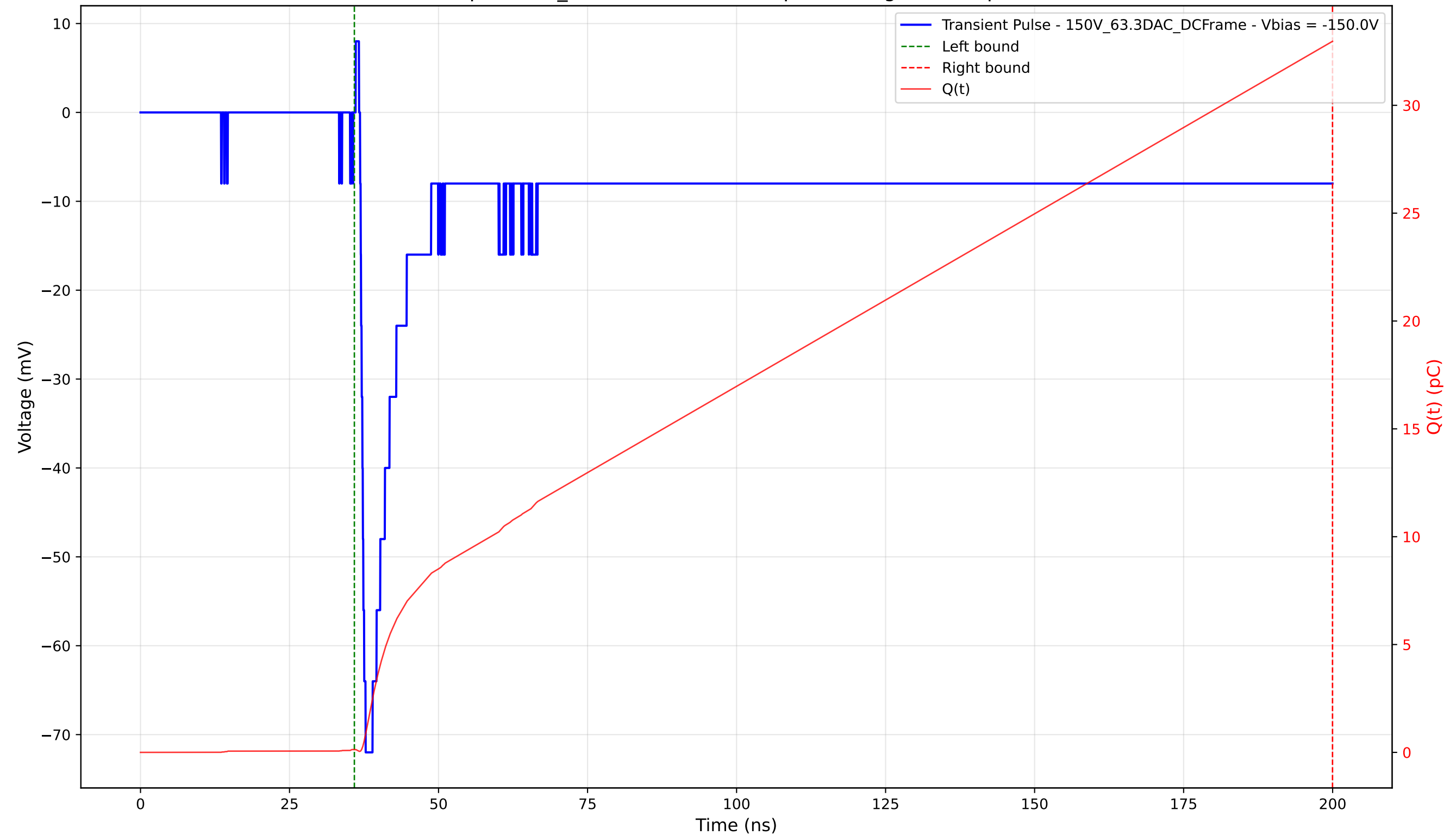
Transient Pulse - Sample: 1cm_42 - Position: 1160.0 \mu\text{m} - Charge: 32.83 pC - Rise Time: 0.92 ns
