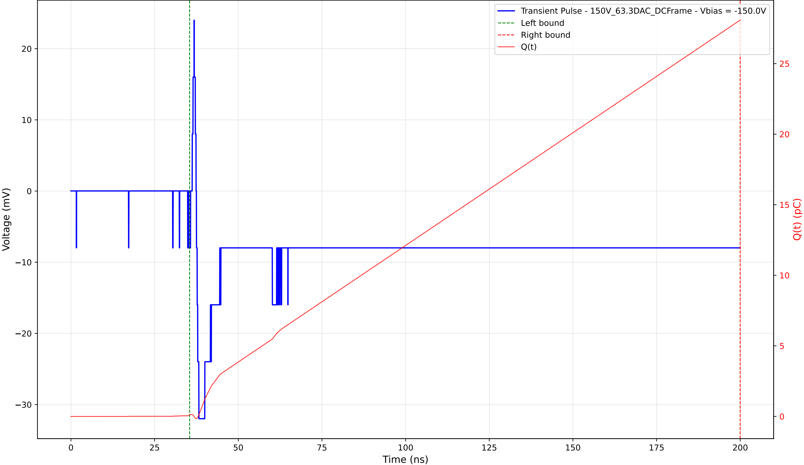
Transient Pulse - Sample: 1cm_42 - Position: 2735.0 \mu\text{m} - Charge: 27.99 pC - Rise Time: 0.73 ns
