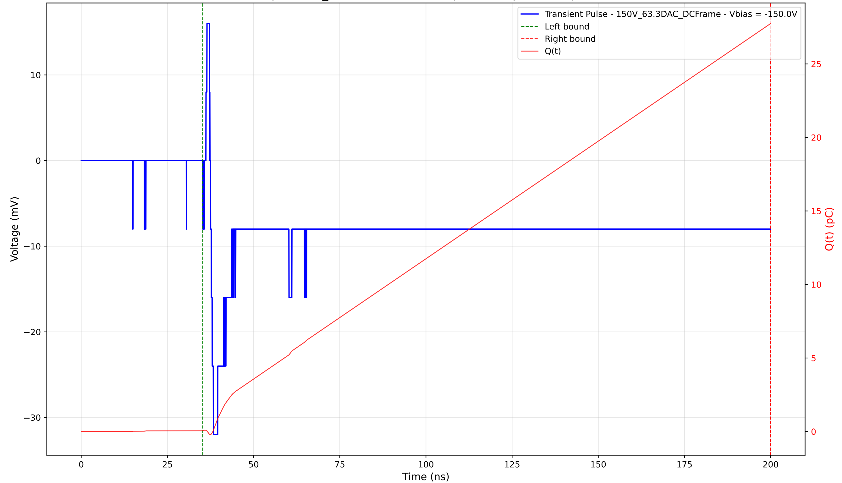
Transient Pulse - Sample: 1cm_42 - Position: 2630.0 \mu\text{m} - Charge: 27.70 pC - Rise Time: 0.81 ns
