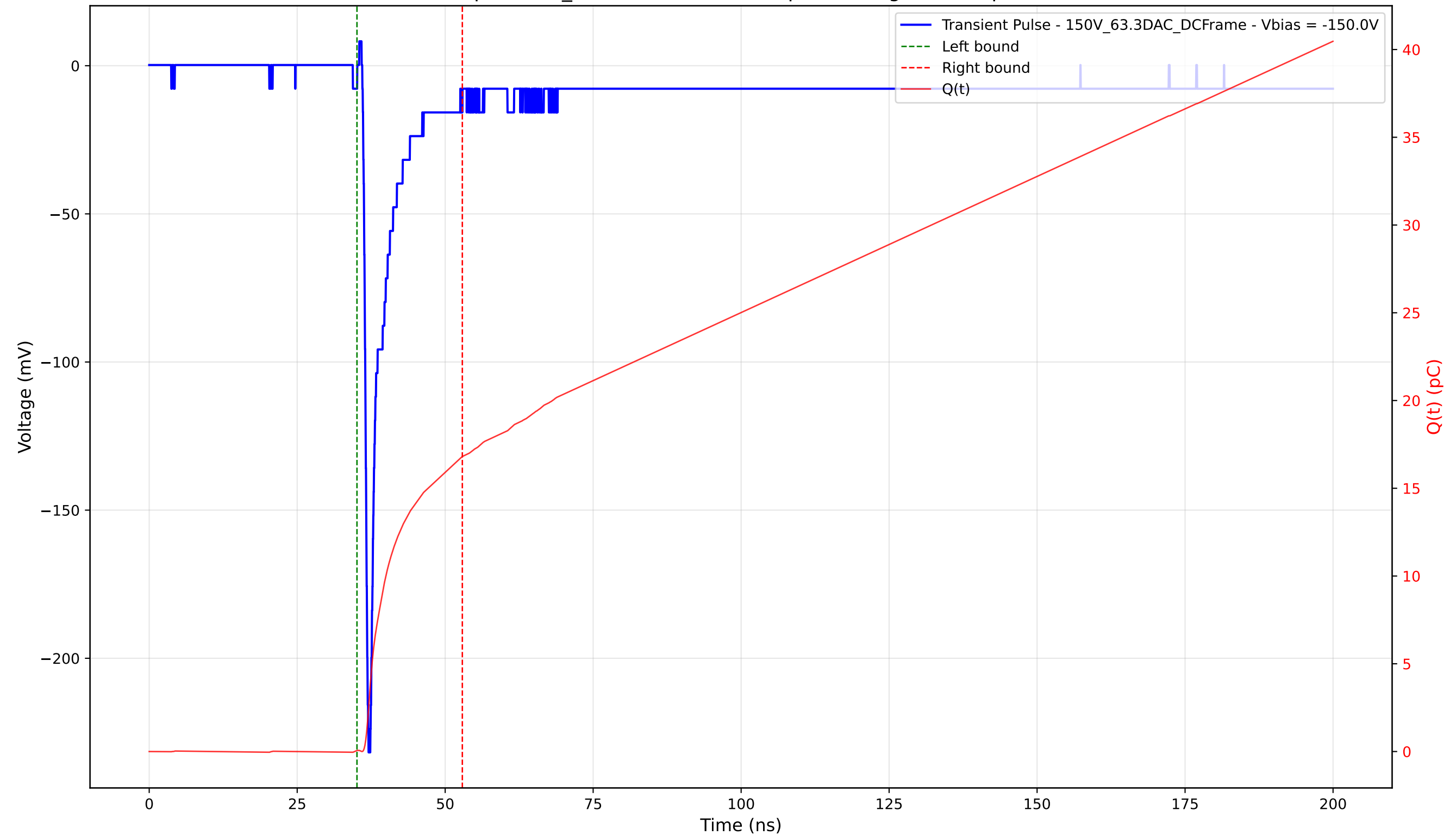
Transient Pulse - Sample: 1cm_42 - Position: 4740.0 \mu\text{m} - Charge: 16.75 pC - Rise Time: 0.78 ns
