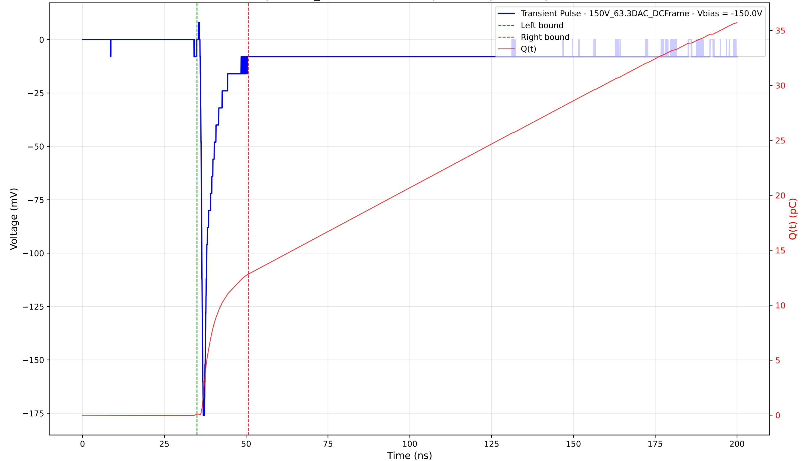
Transient Pulse - Sample: 1cm_42 - Position: 405.0 \mu\text{m} - Charge: 12.73 pC - Rise Time: 0.74 ns
