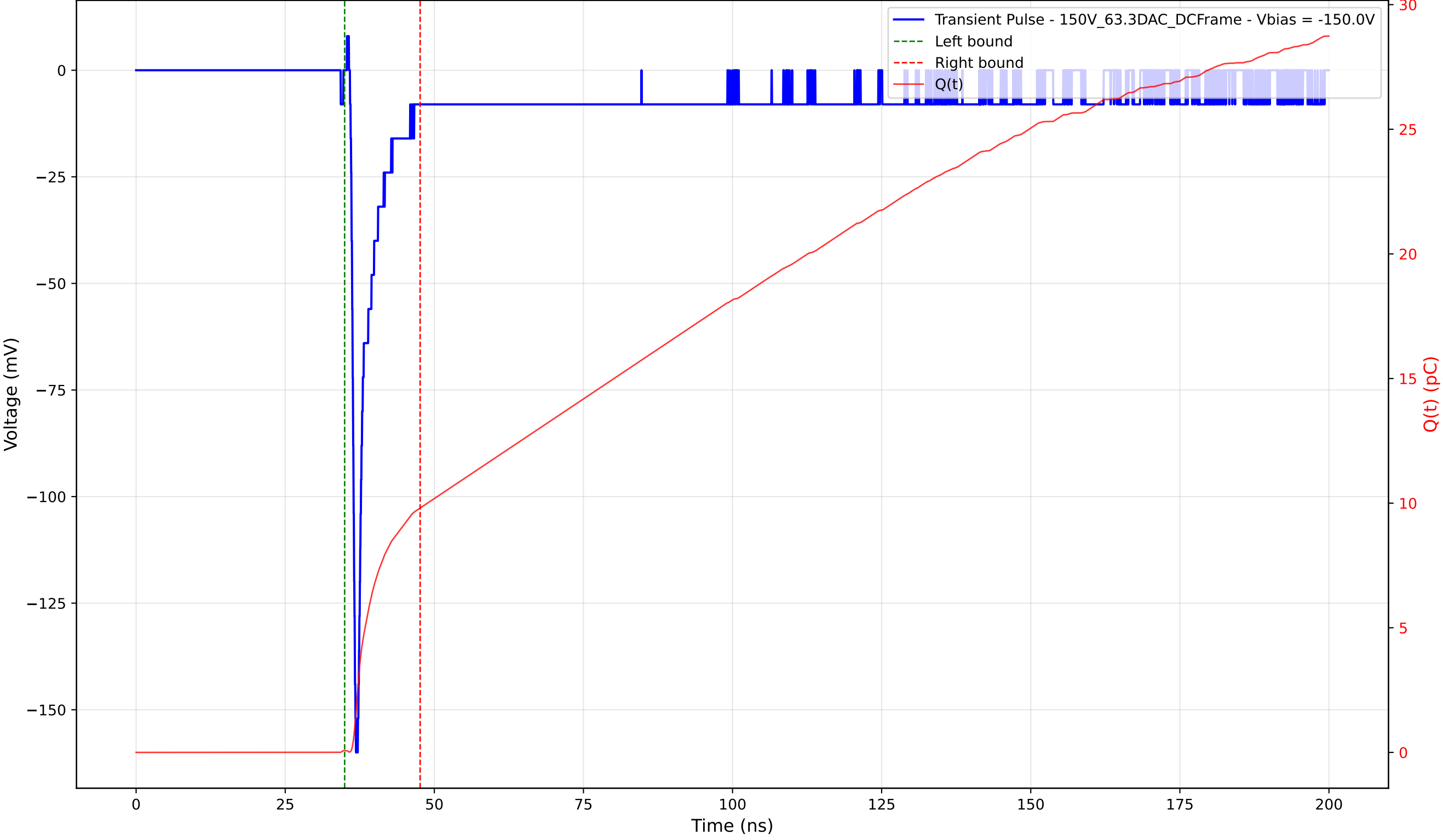
Transient Pulse - Sample: 1cm_42 - Position: 240.0 \mu\text{m} - Charge: 9.73 pC - Rise Time: 0.68 ns
