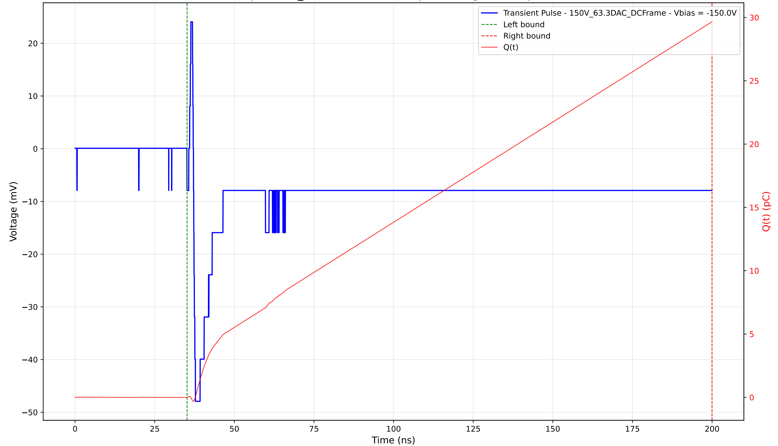
Transient Pulse - Sample: 1cm_42 - Position: 1640.0 \mu\text{m} - Charge: 29.67 pC - Rise Time: 0.61 ns
