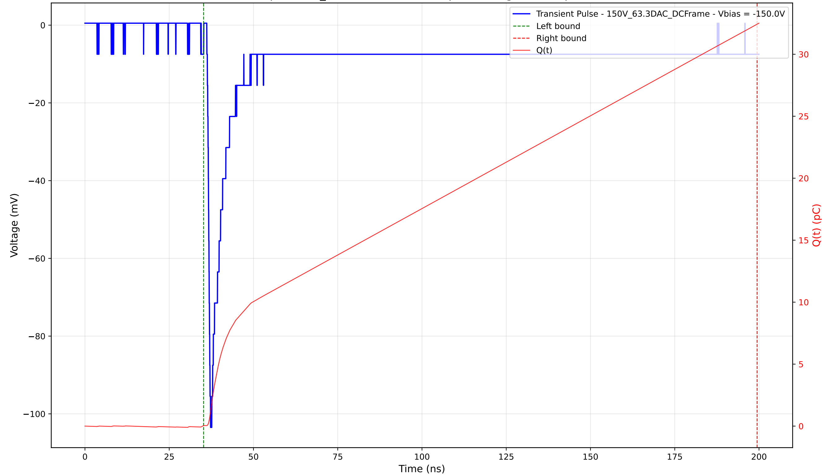
Transient Pulse - Sample: 1cm_42 - Position: 4460.0 \mu\text{m} - Charge: 32.39 pC - Rise Time: 0.79 ns
