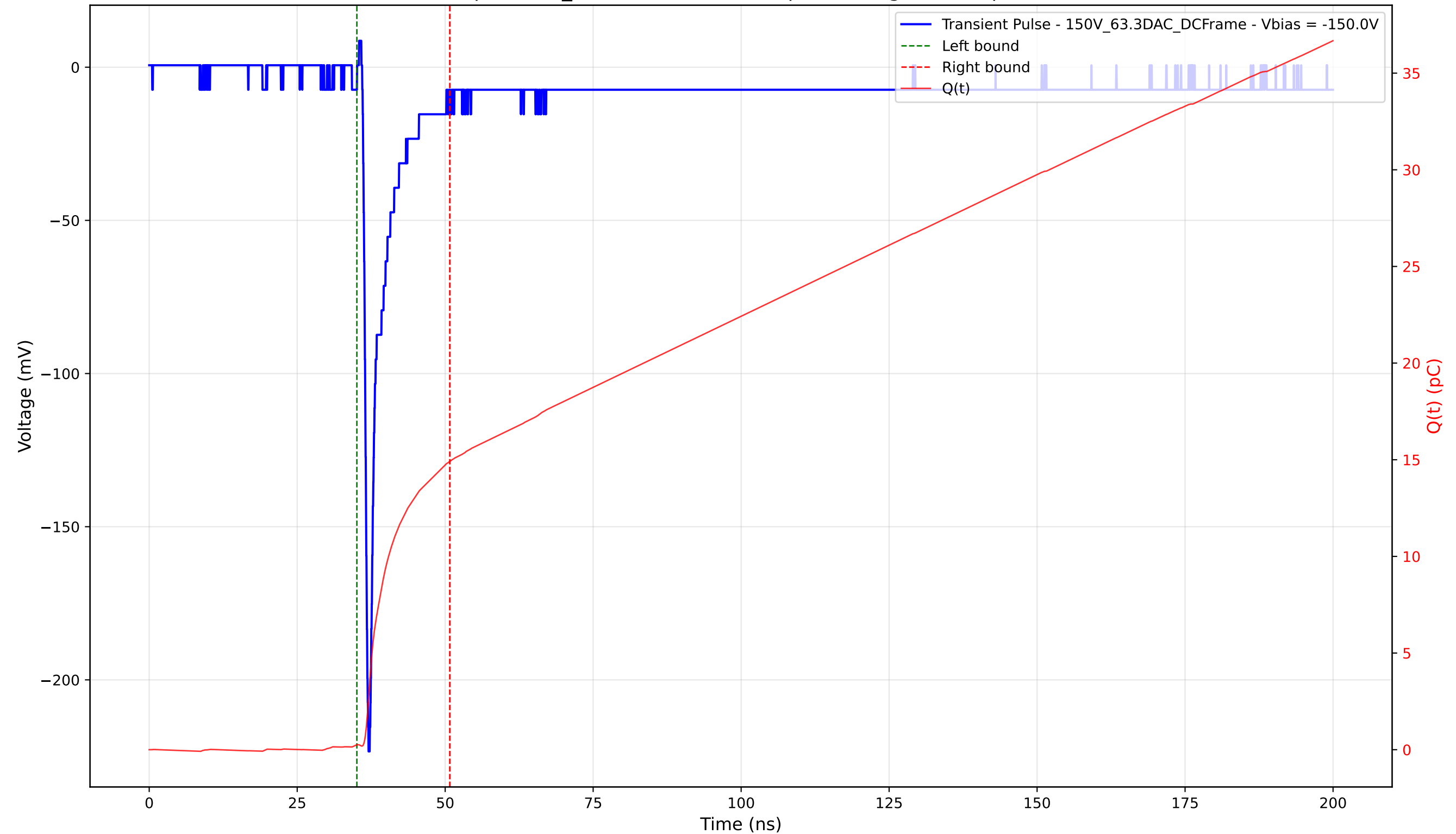
Transient Pulse - Sample: 1cm_42 - Position: 4870.0 \mu\text{m} - Charge: 14.65 pC - Rise Time: 0.78 ns
