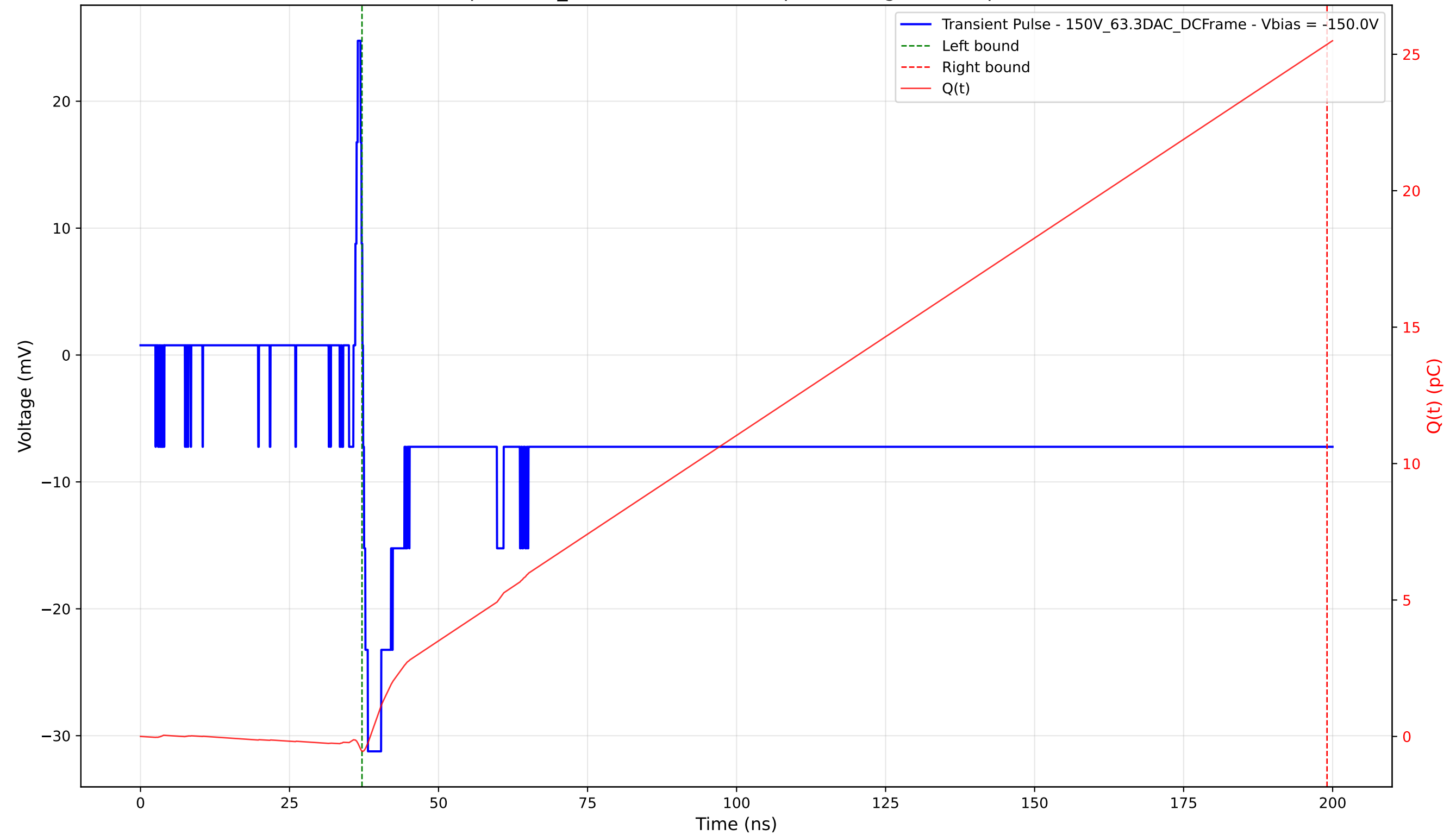
Transient Pulse - Sample: 1cm_42 - Position: 2330.0 \mu\text{m} - Charge: 25.90 pC - Rise Time: 0.81 ns
