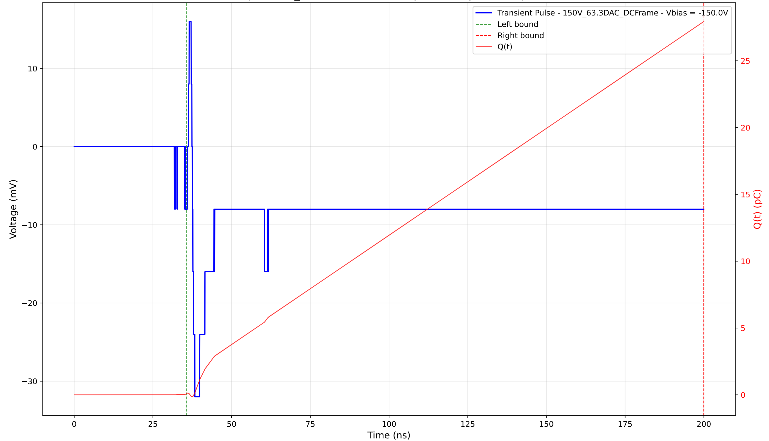
Transient Pulse - Sample: 1cm_42 - Position: 2635.0 \mu\text{m} - Charge: 27.87 pC - Rise Time: 0.81 ns
