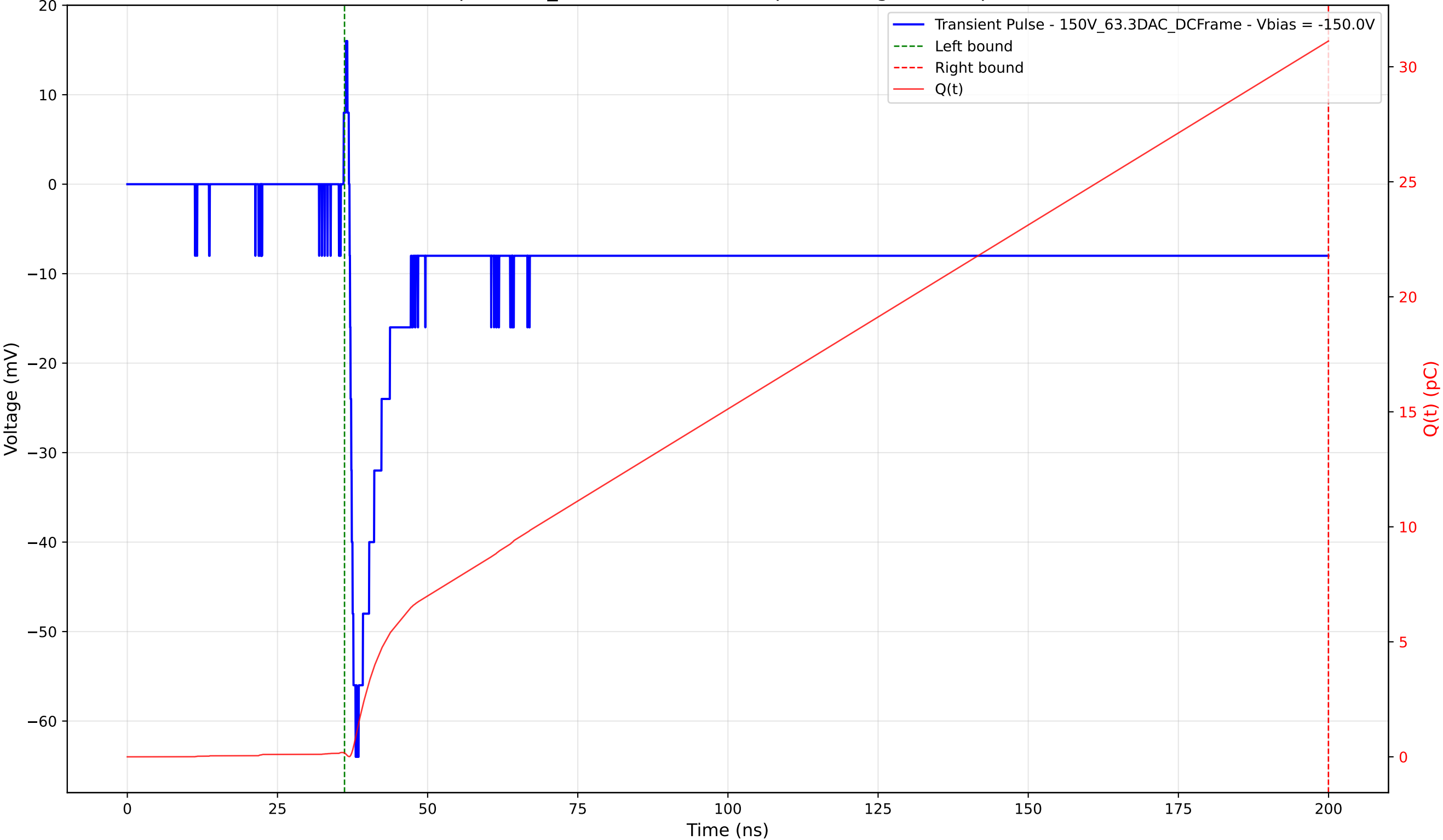
Transient Pulse - Sample: 1cm_42 - Position: 1365.0 \mu\text{m} - Charge: 30.95 pC - Rise Time: 1.00 ns
