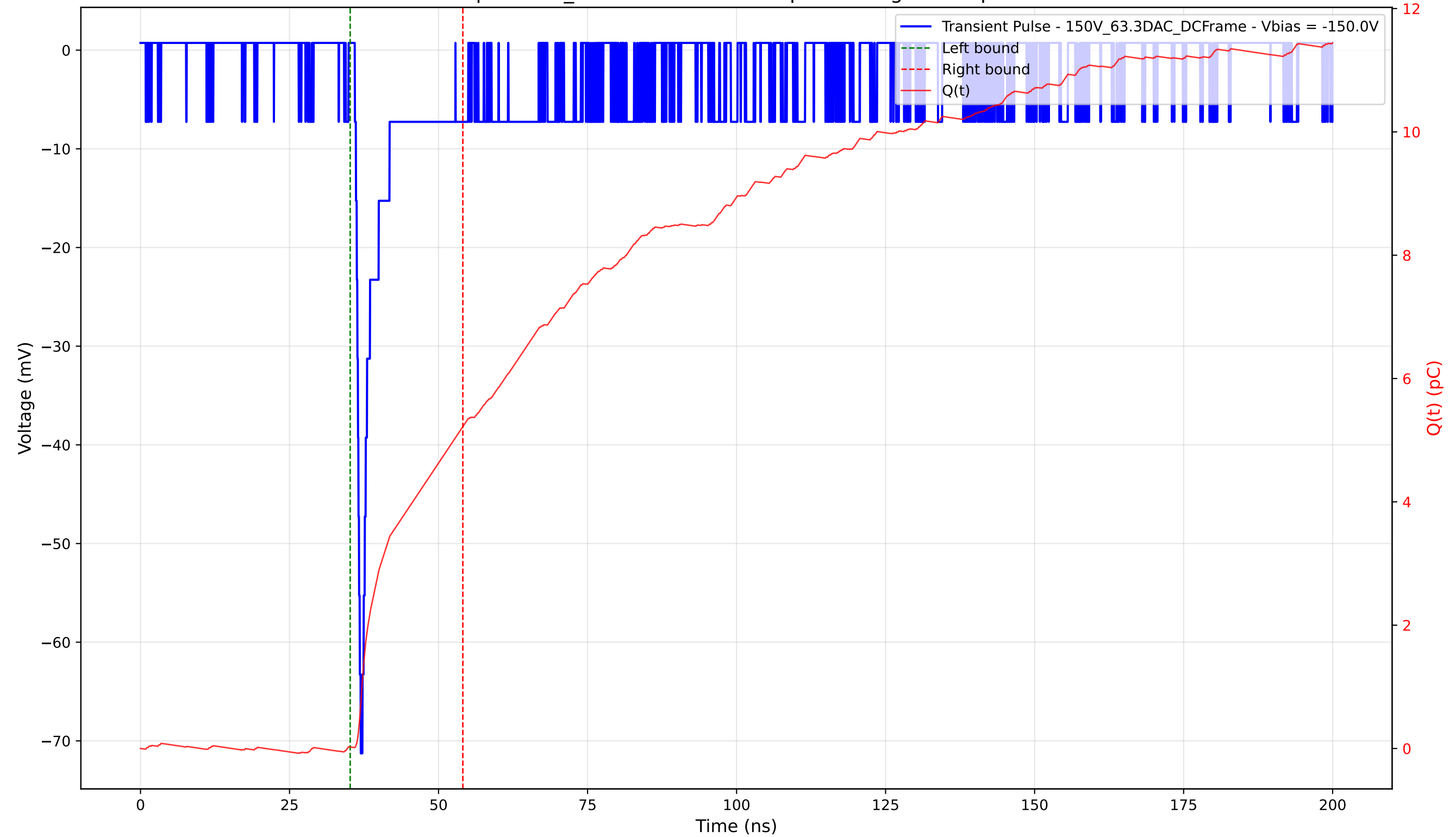
Transient Pulse - Sample: 1cm_42 - Position: 5090.0 \mu\text{m} - Charge: 5.20 pC - Rise Time: 0.98 ns
