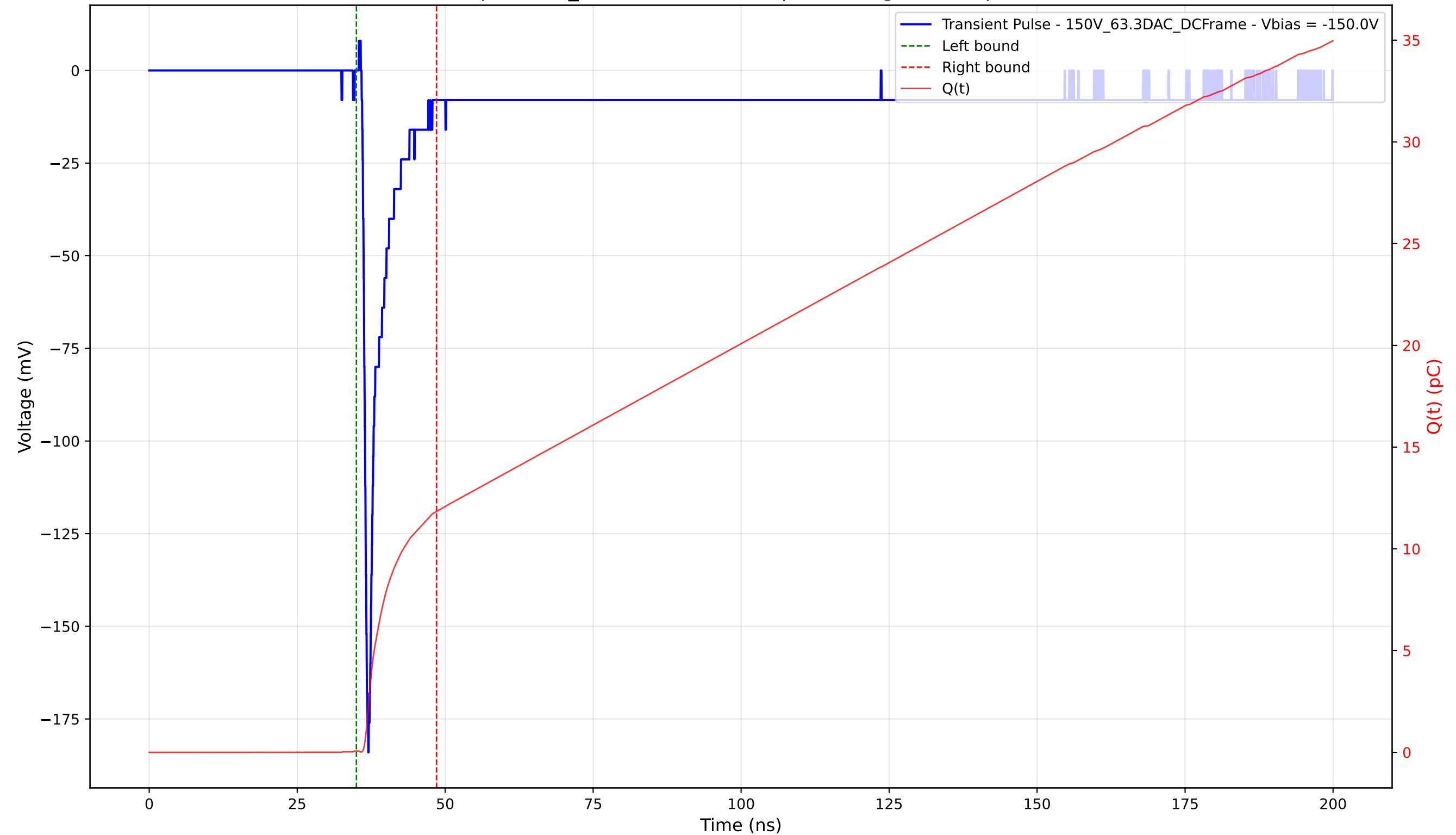
Transient Pulse - Sample: 1cm_42 - Position: 365.0 \mu\text{m} - Charge: 11.77 pC - Rise Time: 0.75 ns
