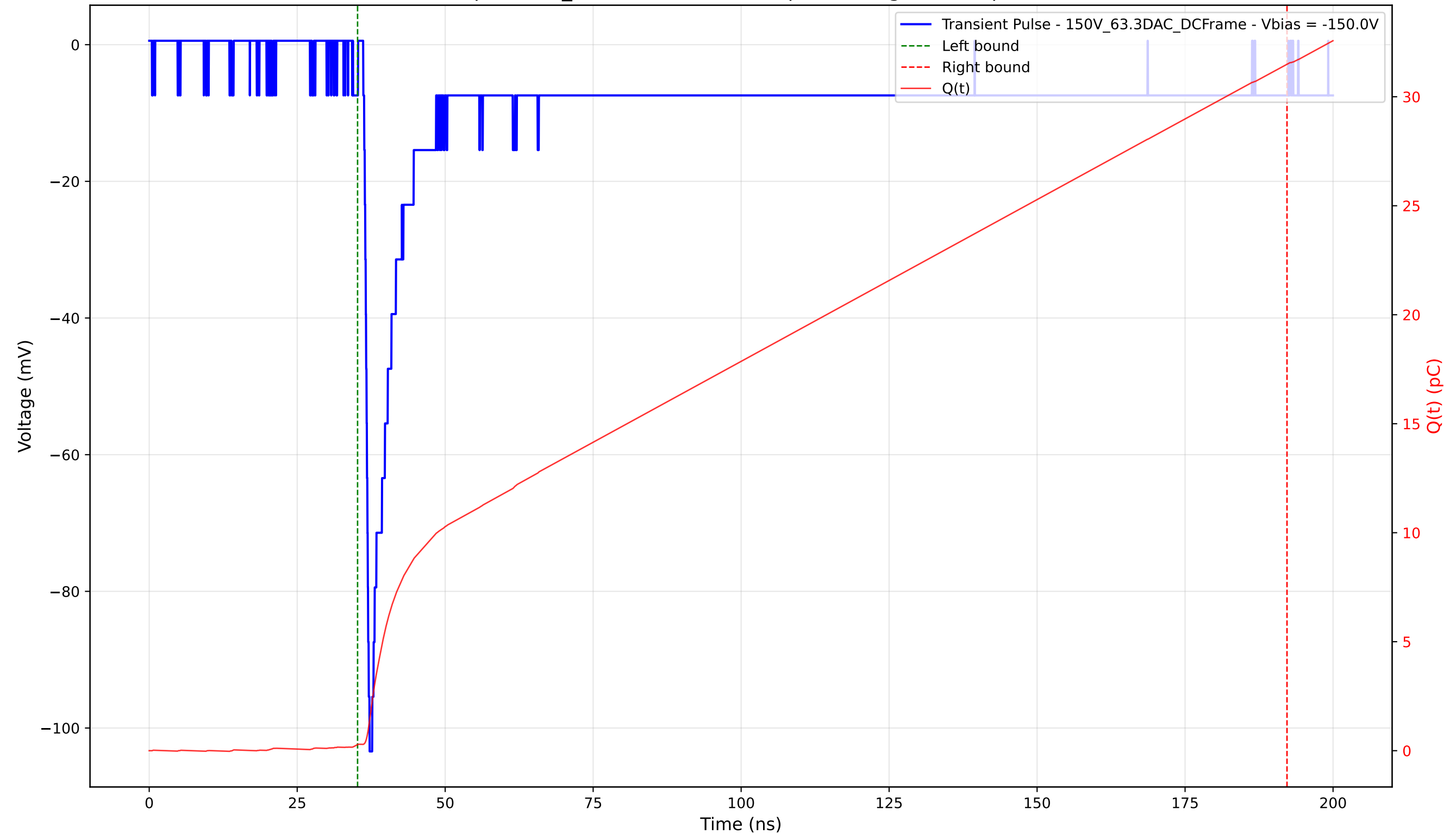
Transient Pulse - Sample: 1cm_42 - Position: 4470.0 \mu\text{m} - Charge: 31.21 pC - Rise Time: 0.77 ns
