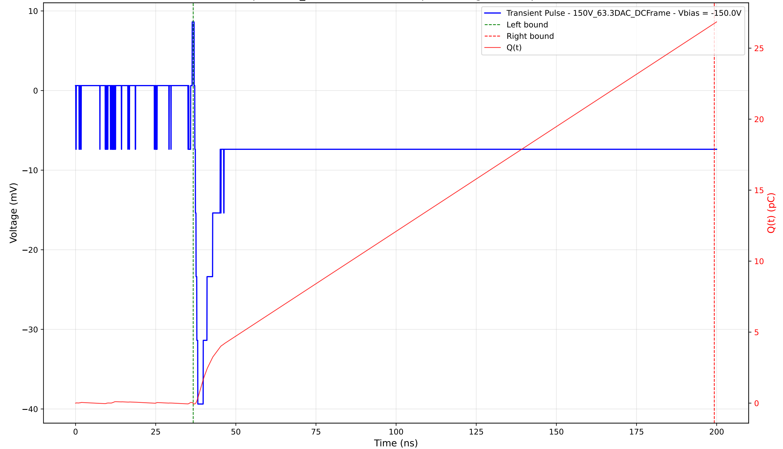
Transient Pulse - Sample: 1cm_42 - Position: 3560.0 \mu\text{m} - Charge: 26.76 pC - Rise Time: 0.93 ns
