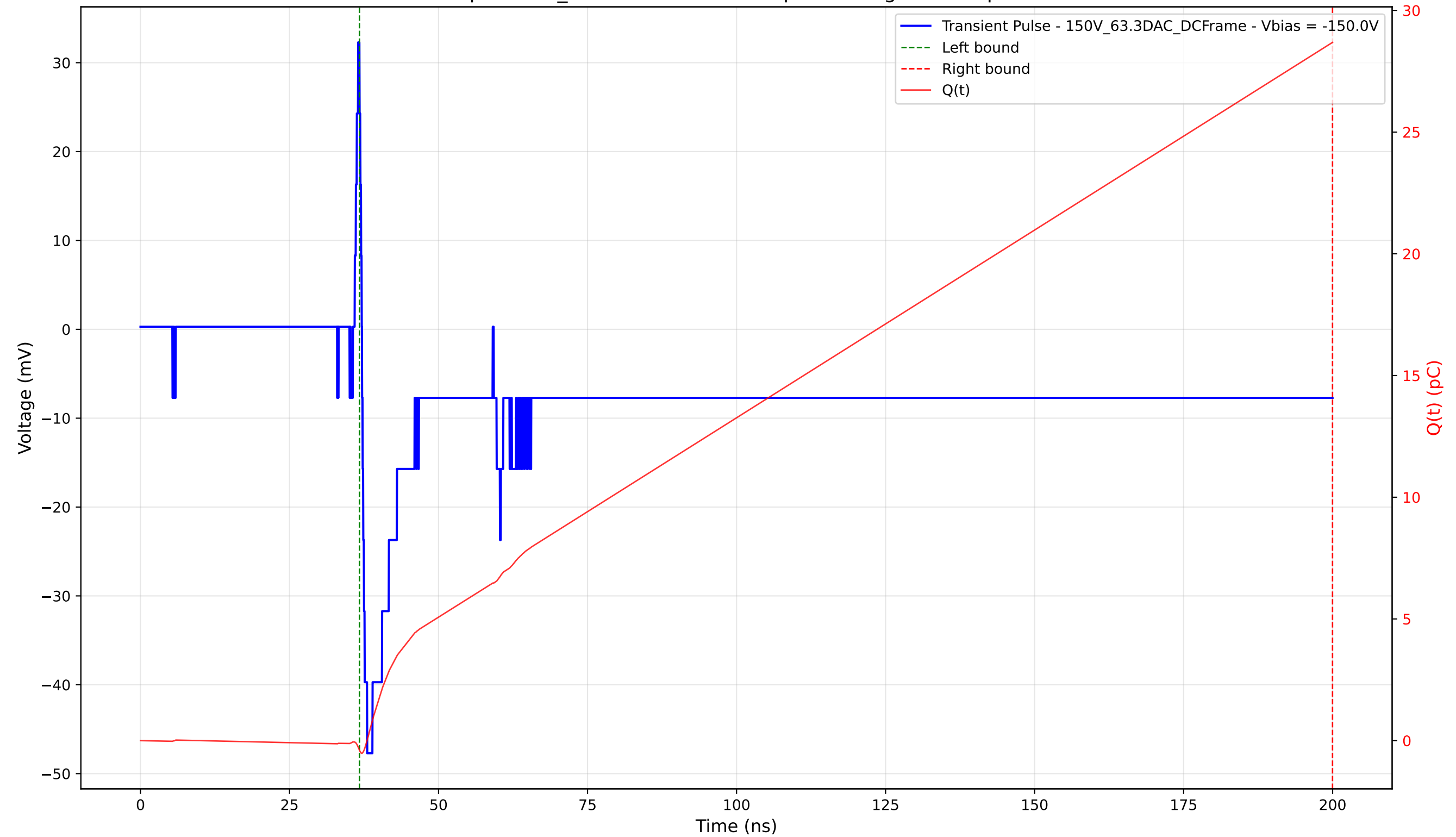
Transient Pulse - Sample: 1cm_42 - Position: 1775.0 \mu\text{m} - Charge: 29.09 pC - Rise Time: 0.87 ns
