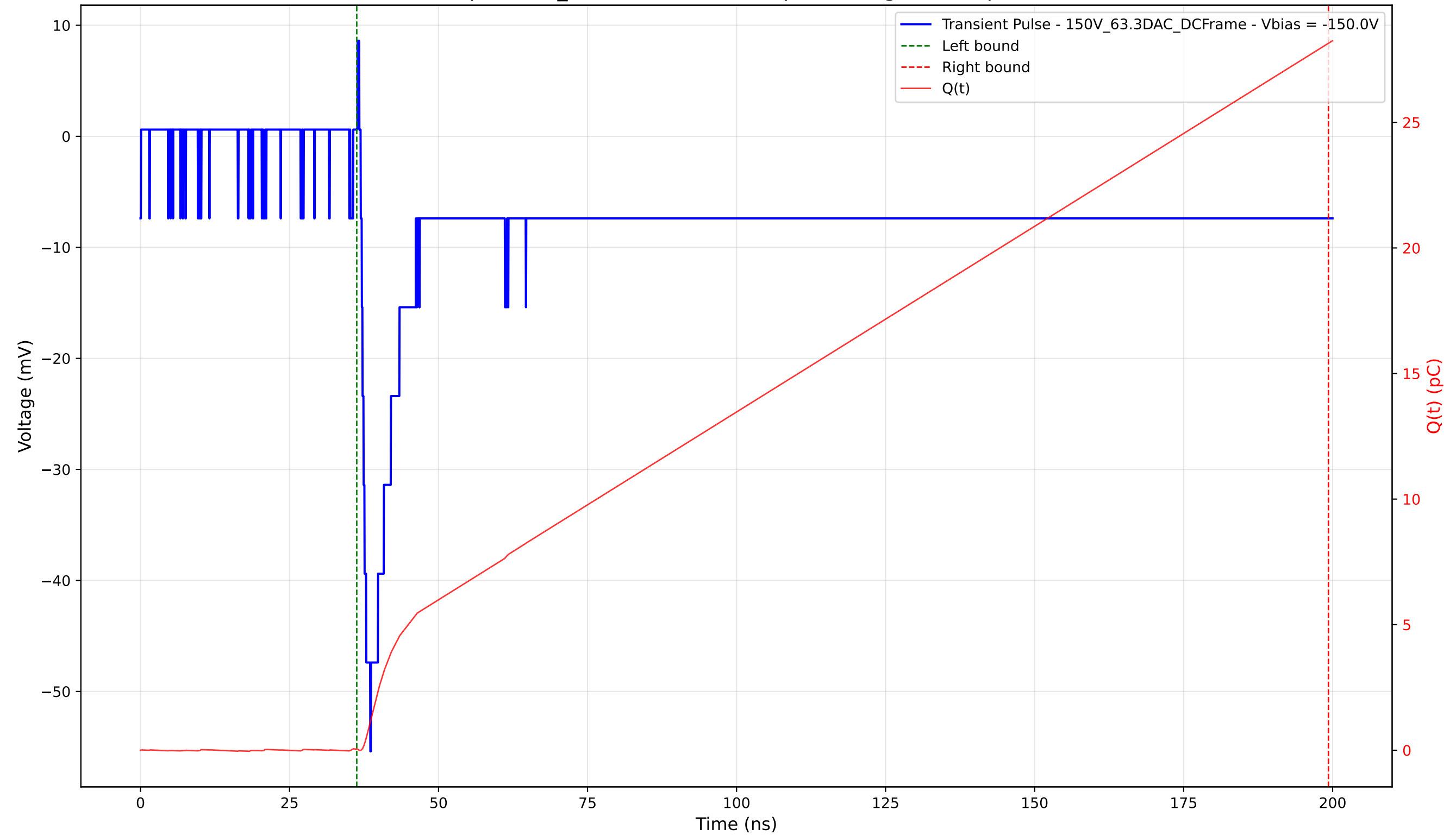
Transient Pulse - Sample: 1cm_42 - Position: 3865.0 \mu\text{m} - Charge: 28.10 pC - Rise Time: 1.61 ns
