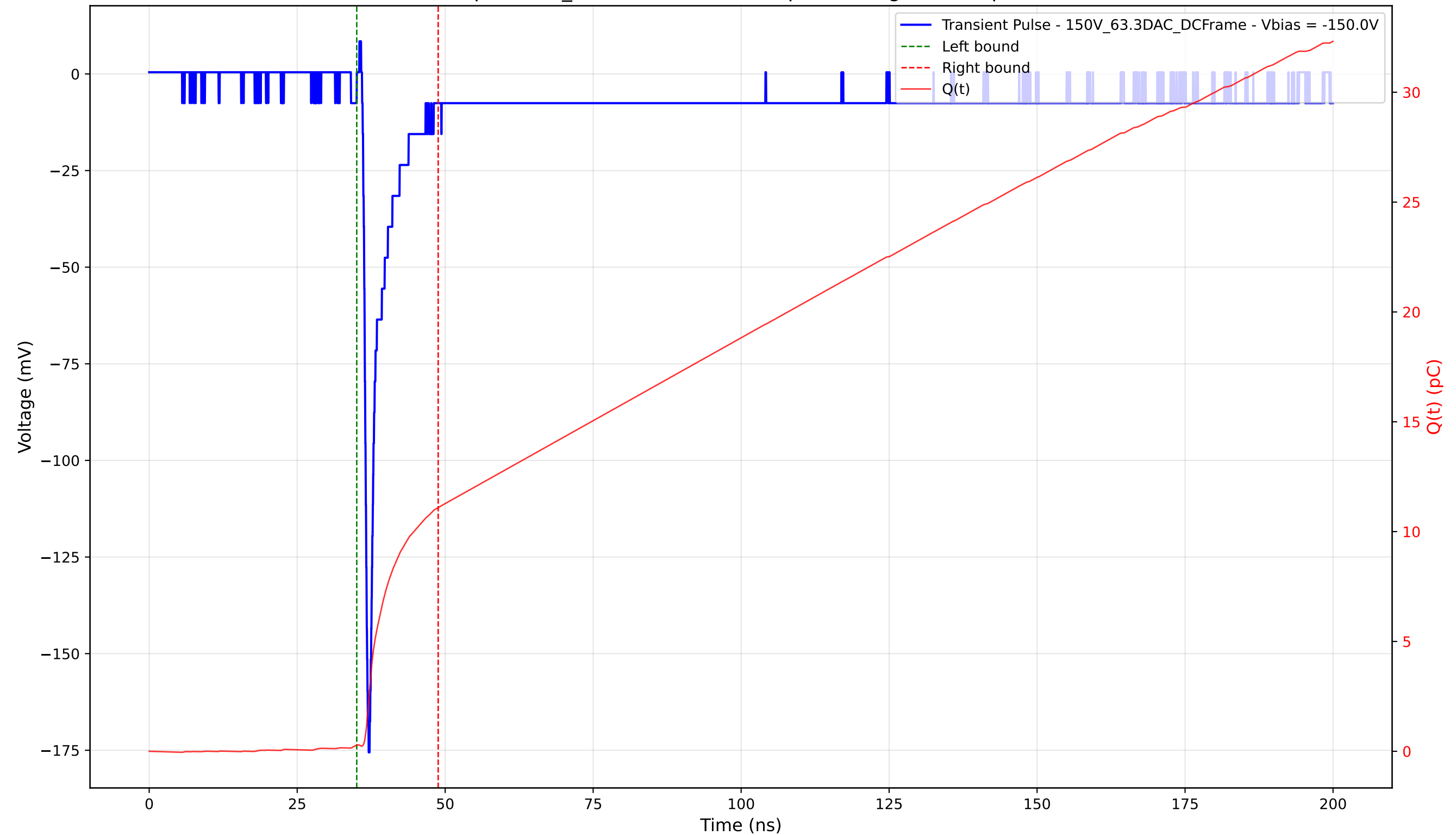
Transient Pulse - Sample: 1cm_42 - Position: 4950.0 \mu\text{m} - Charge: 10.80 pC - Rise Time: 0.73 ns
