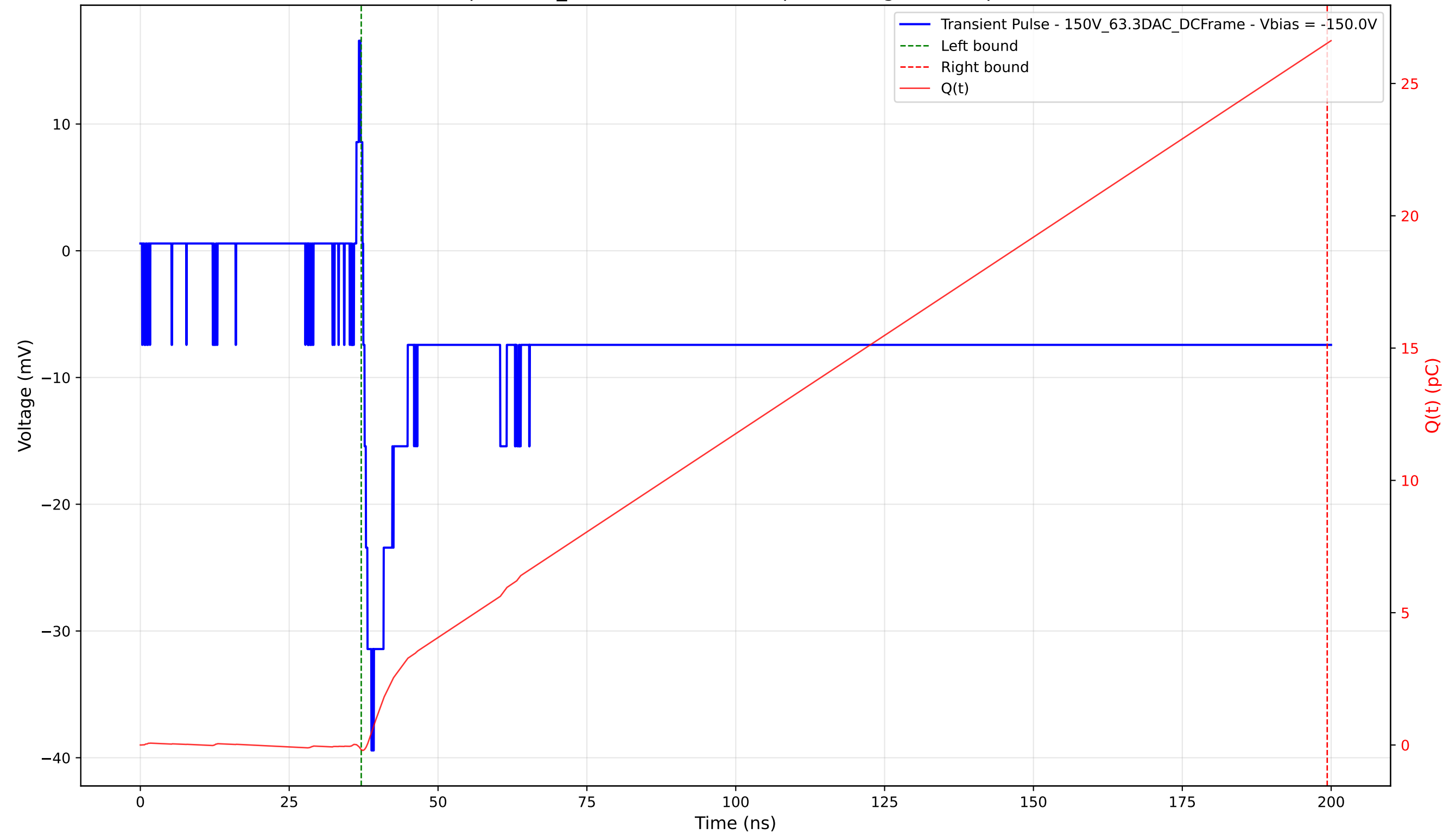
Transient Pulse - Sample: 1cm_42 - Position: 3185.0 \mu\text{m} - Charge: 26.69 pC - Rise Time: 1.37 ns
