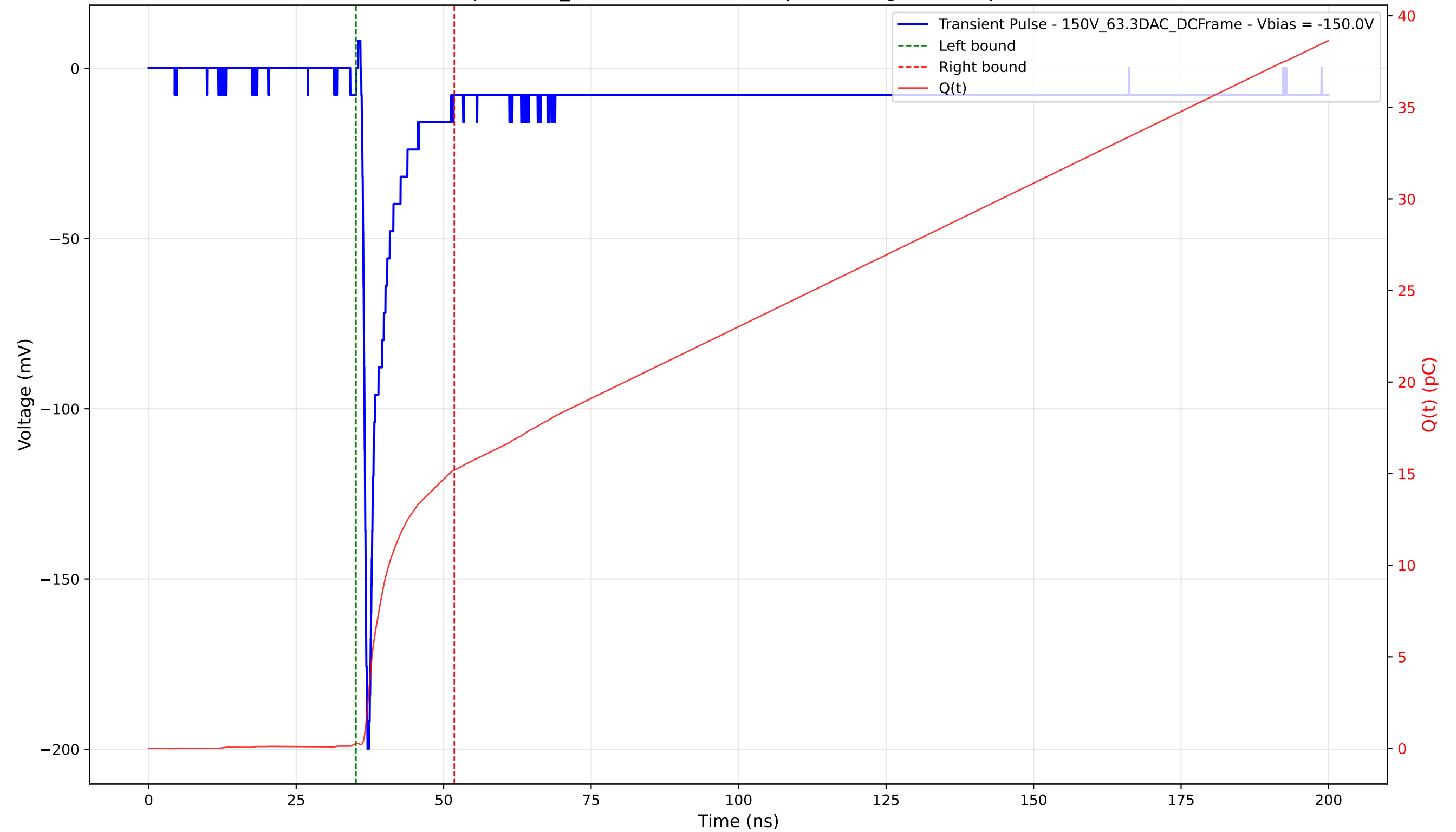
Transient Pulse - Sample: 1cm_42 - Position: 4675.0 \mu\text{m} - Charge: 14.94 pC - Rise Time: 0.79 ns
