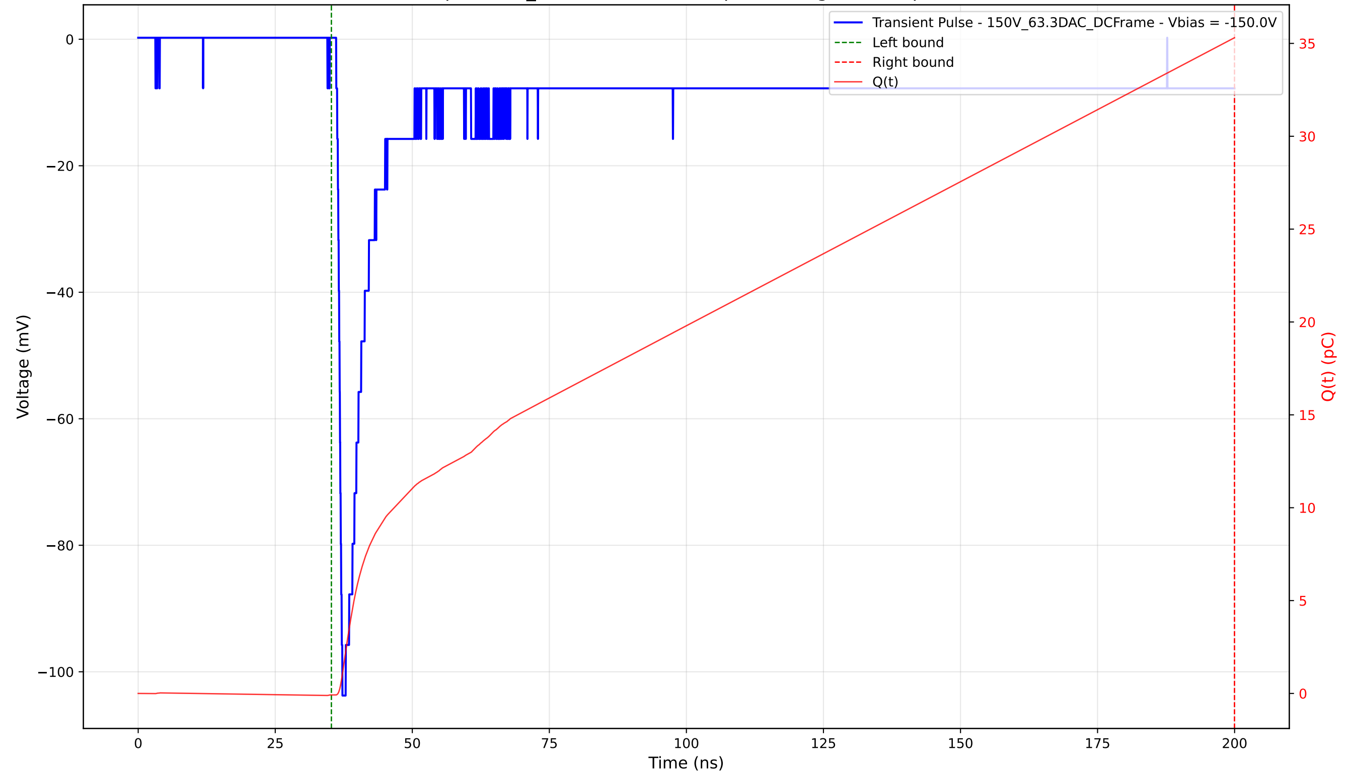
Transient Pulse - Sample: 1cm_42 - Position: 840.0 \mu\text{m} - Charge: 35.39 pC - Rise Time: 0.83 ns
