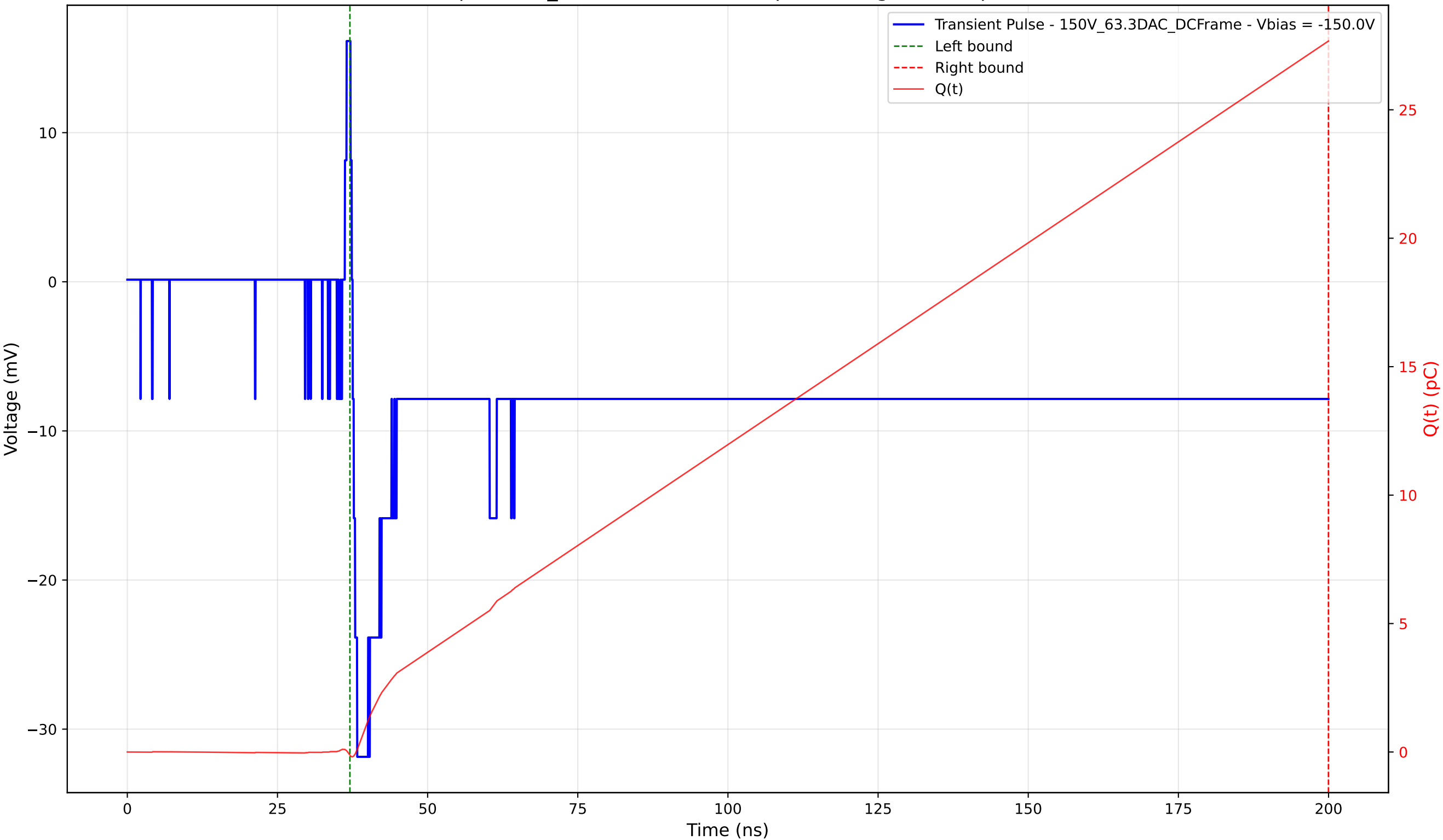
Transient Pulse - Sample: 1cm_42 - Position: 2715.0 \mu\text{m} - Charge: 27.80 pC - Rise Time: 0.75 ns
