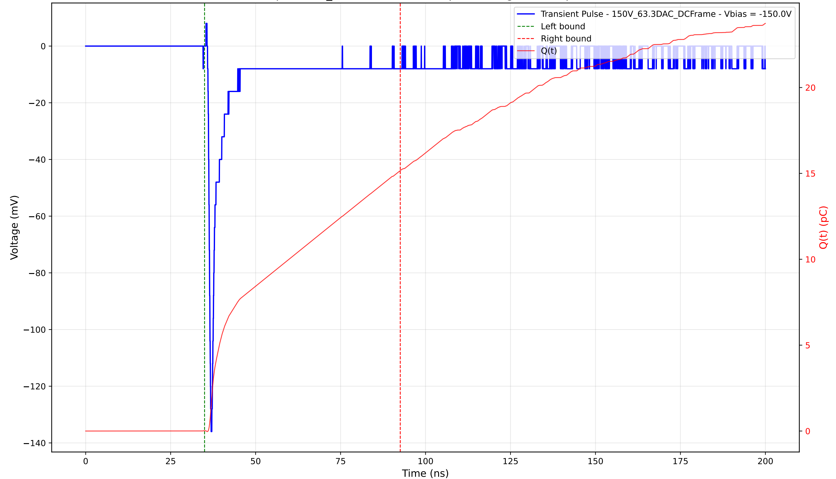
Transient Pulse - Sample: 1cm_42 - Position: 180.0 \mu\text{m} - Charge: 15.15 pC - Rise Time: 0.79 ns
