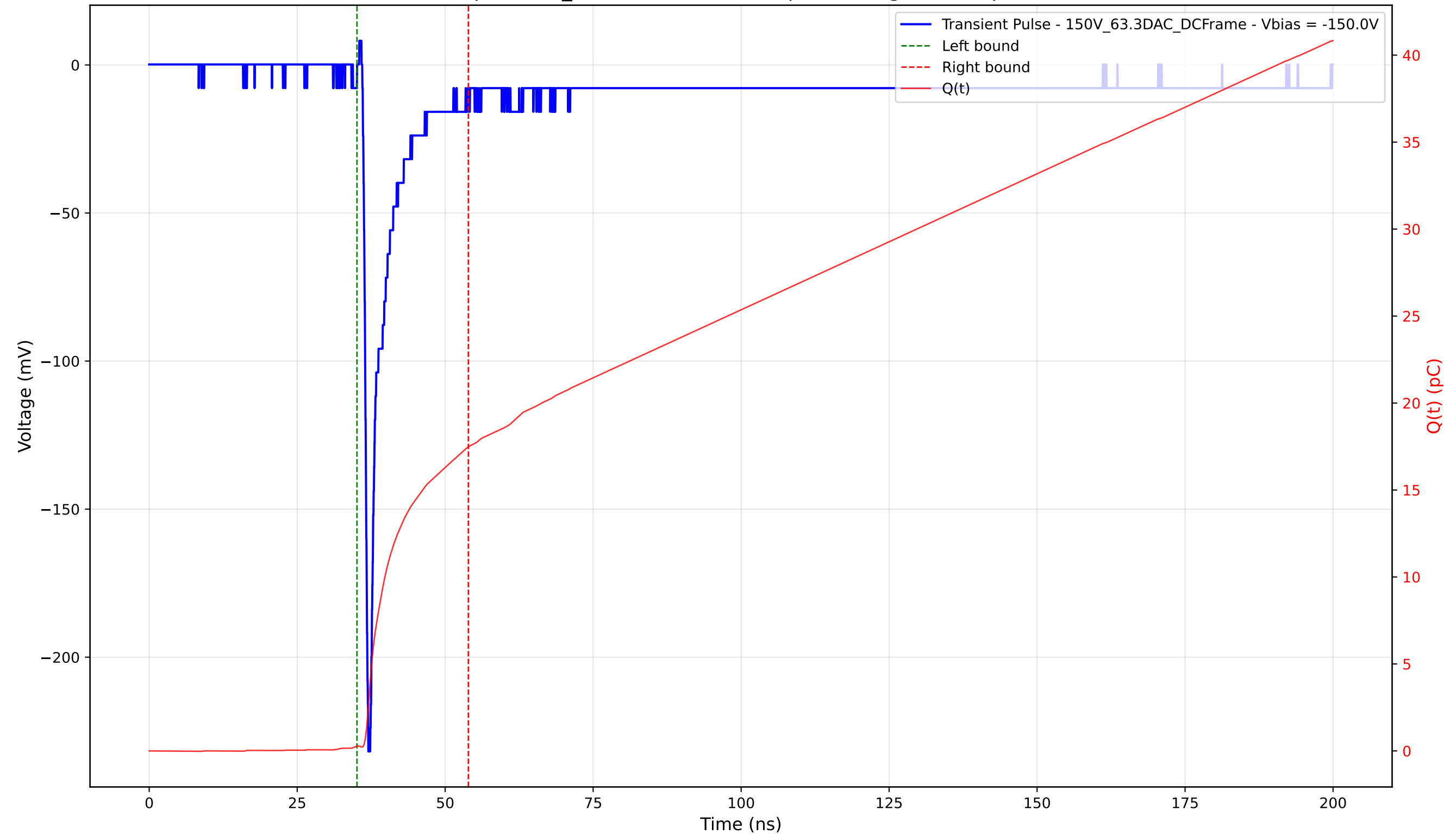
Transient Pulse - Sample: 1cm_42 - Position: 4745.0 \mu\text{m} - Charge: 17.19 pC - Rise Time: 0.80 ns
