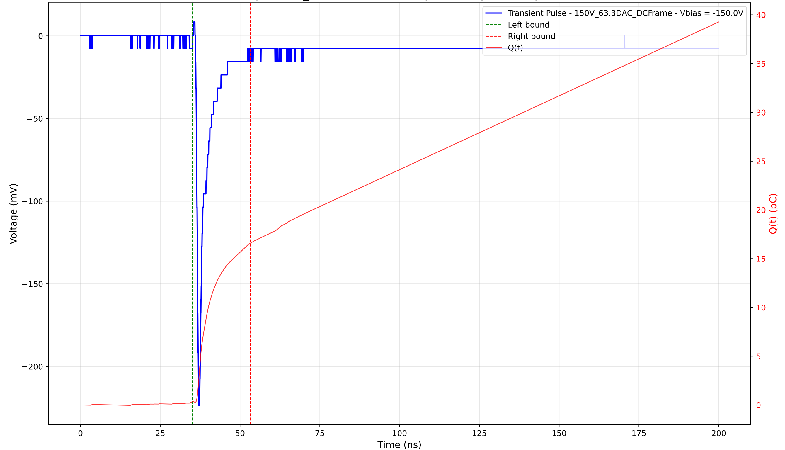
Transient Pulse - Sample: 1cm_42 - Position: 4710.0 \mu\text{m} - Charge: 16.24 pC - Rise Time: 0.80 ns
