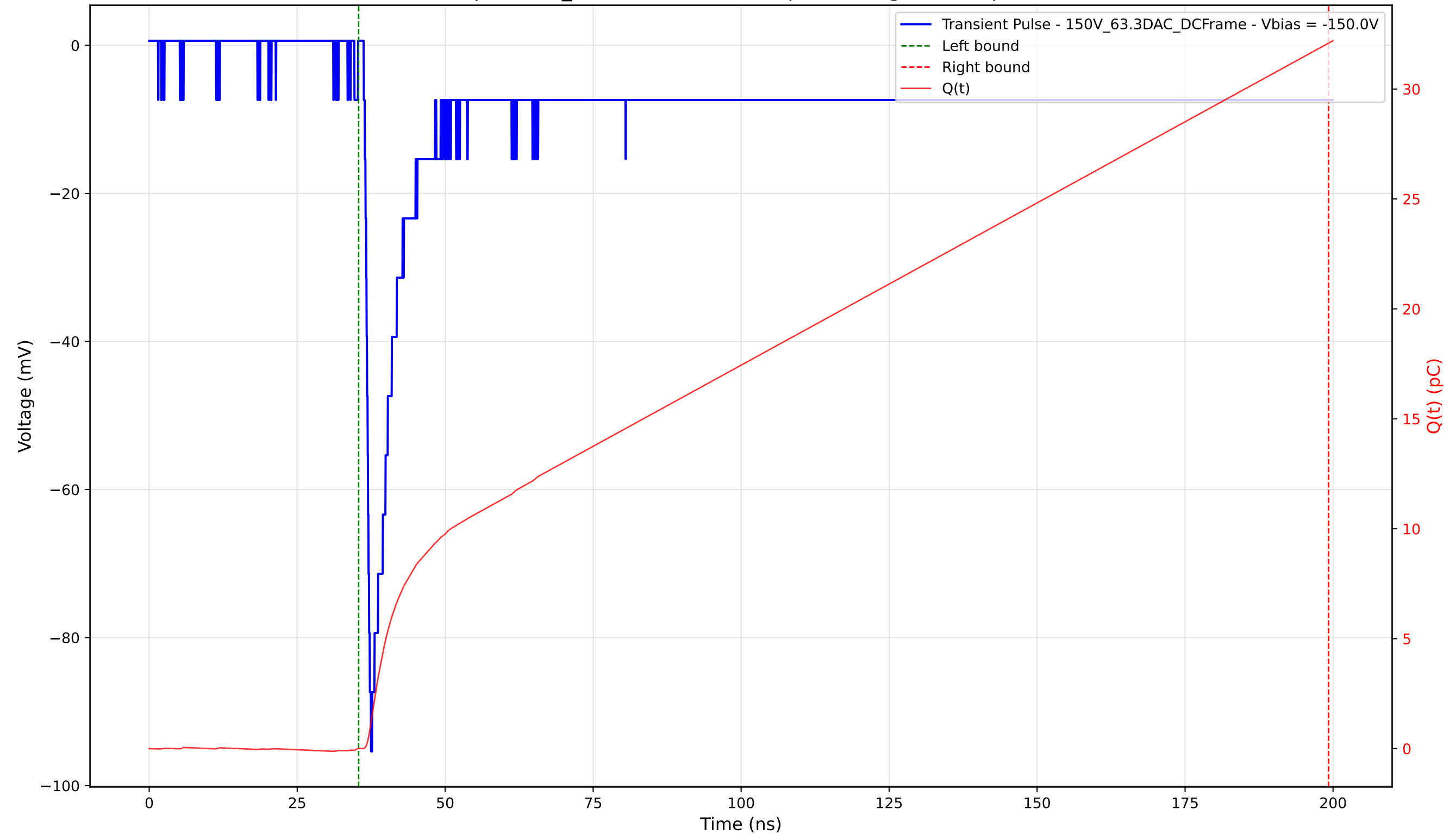
Transient Pulse - Sample: 1cm_42 - Position: 4370.0 \mu\text{m} - Charge: 32.08 pC - Rise Time: 0.85 ns
