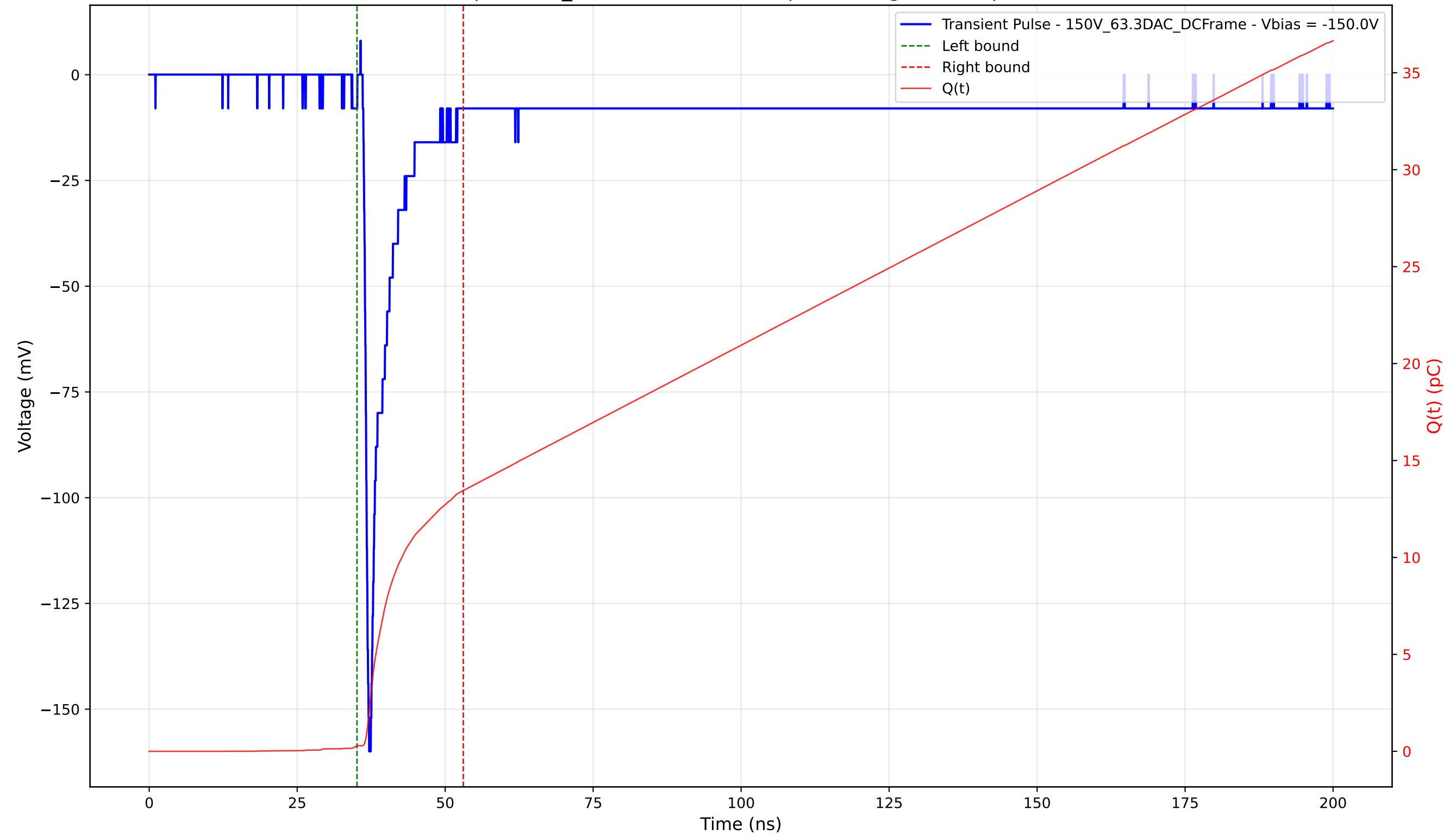
Transient Pulse - Sample: 1cm_42 - Position: 4610.0 \mu\text{m} - Charge: 13.16 pC - Rise Time: 0.82 ns
