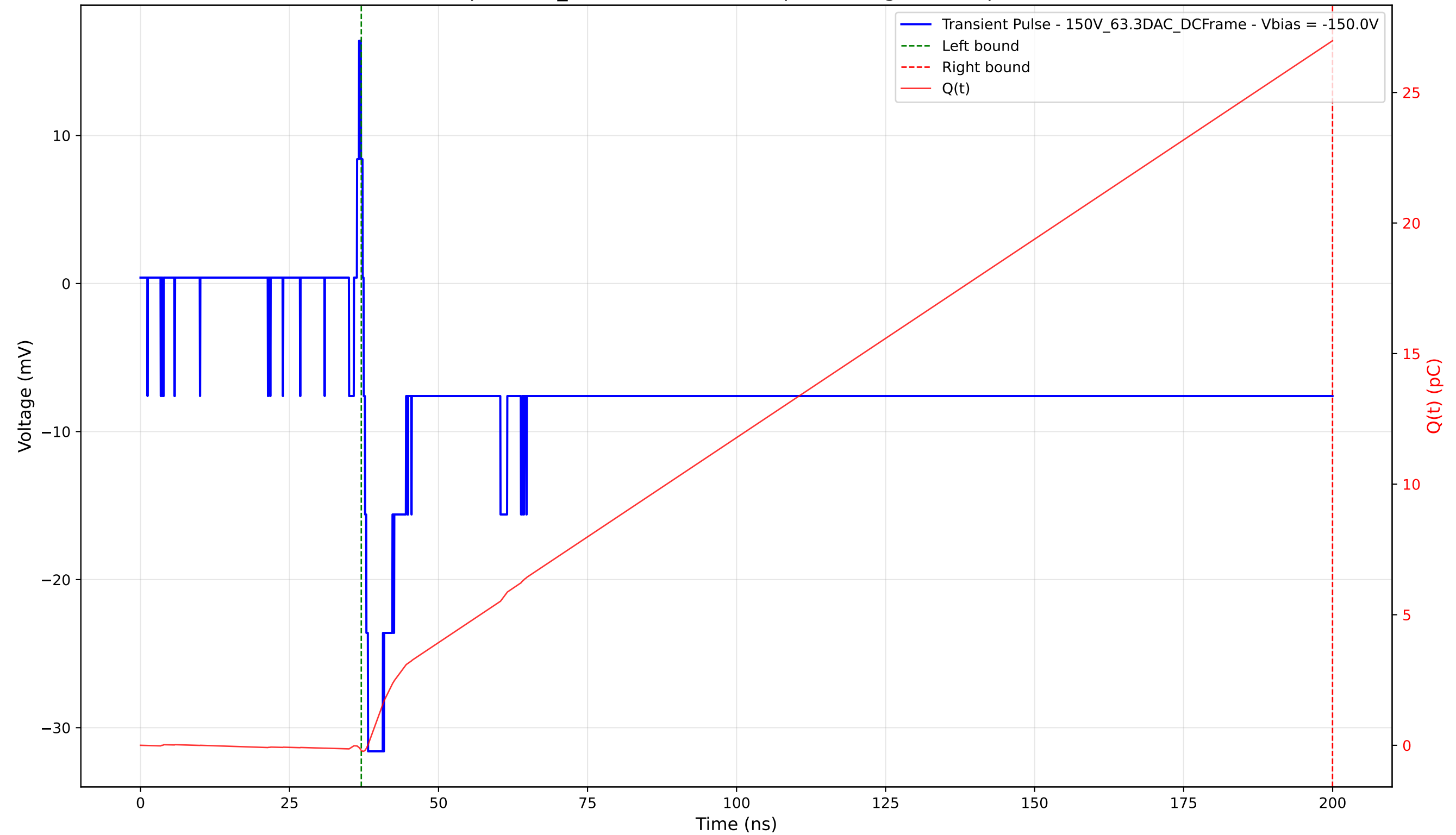
Transient Pulse - Sample: 1cm_42 - Position: 3145.0 \mu\text{m} - Charge: 27.18 pC - Rise Time: 0.73 ns
