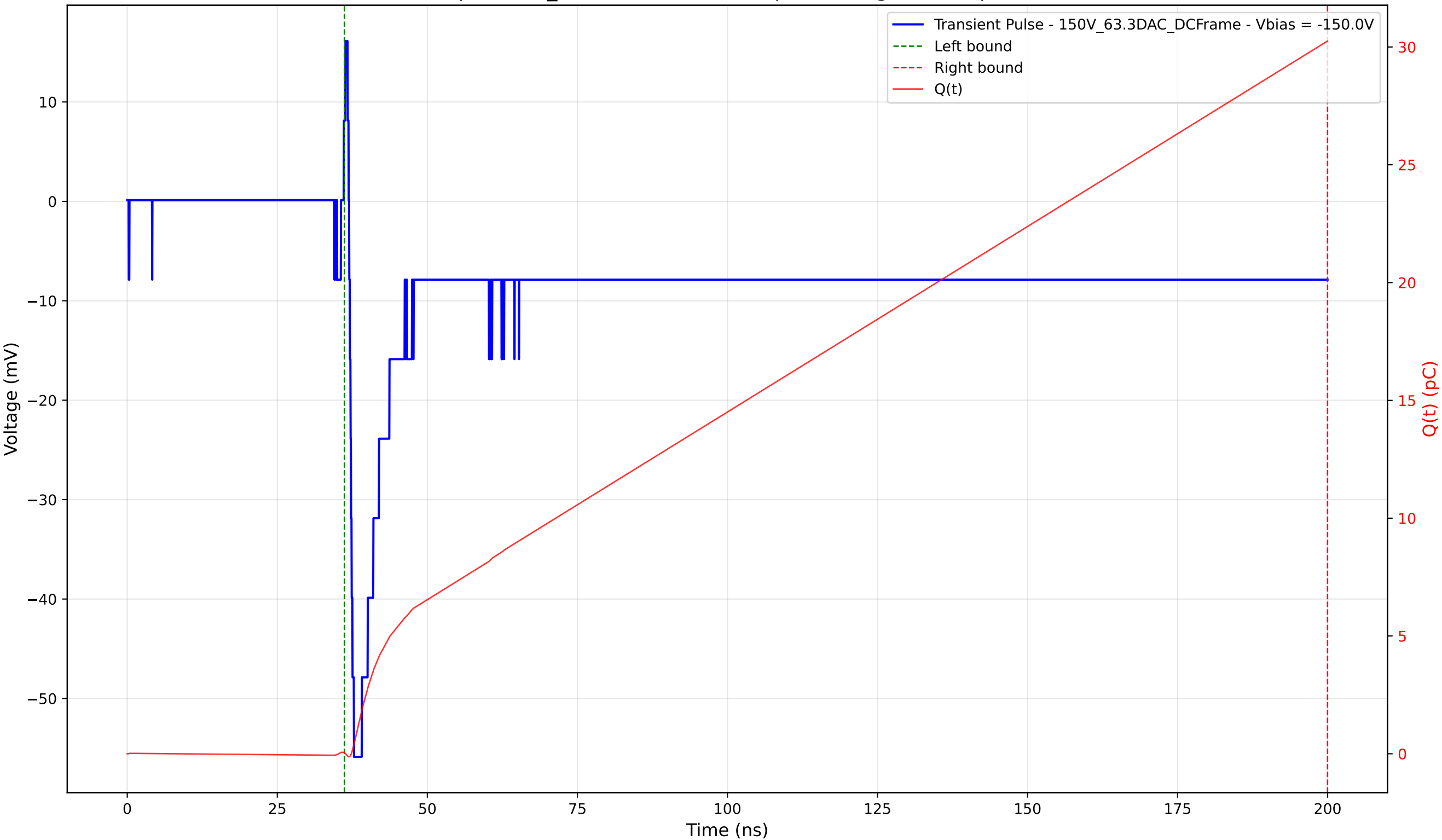
Transient Pulse - Sample: 1cm_42 - Position: 1380.0 \mu\text{m} - Charge: 30.21 pC - Rise Time: 0.79 ns
