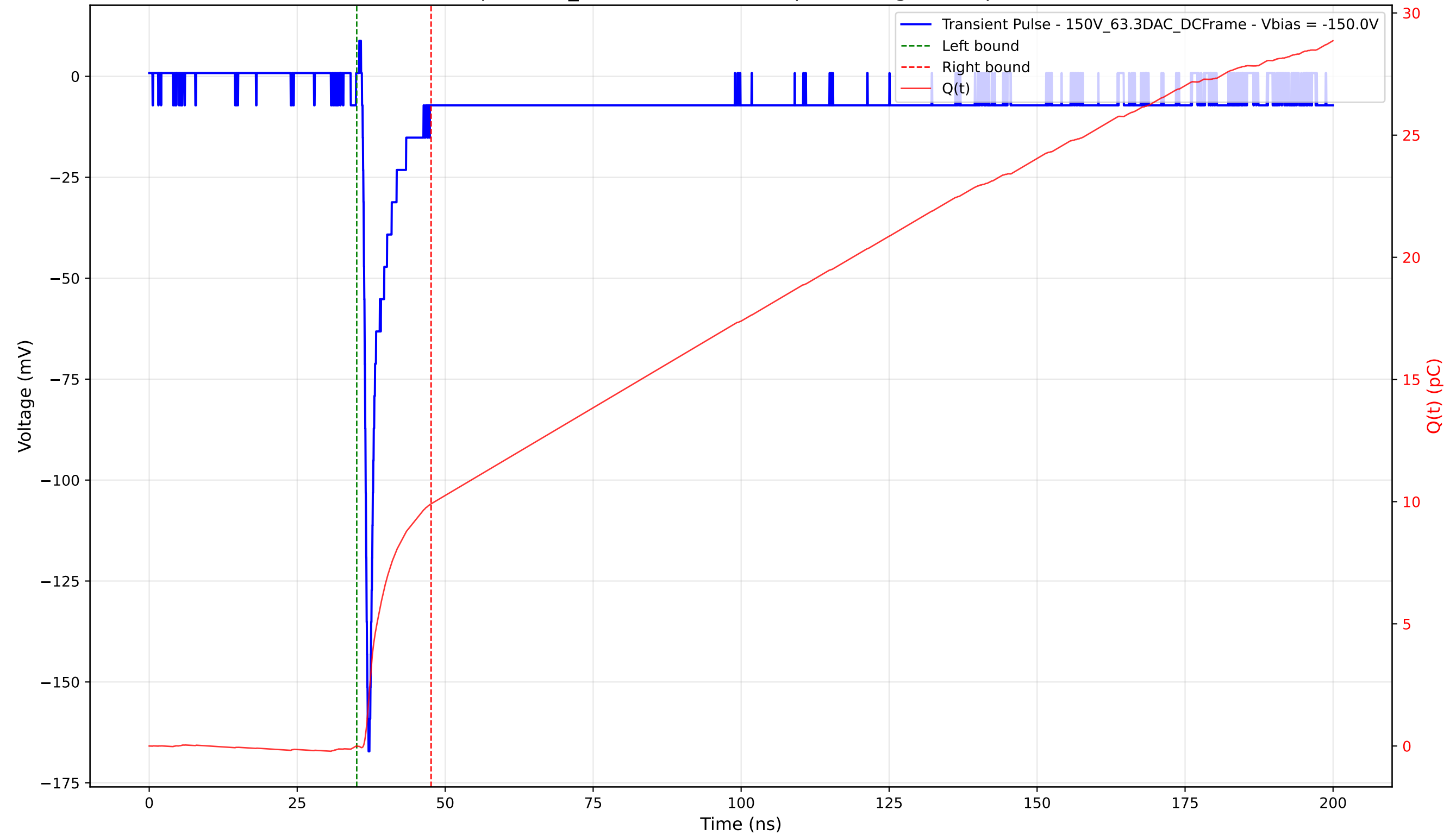
Transient Pulse - Sample: 1cm_42 - Position: 4960.0 \mu\text{m} - Charge: 9.92 pC - Rise Time: 0.74 ns
