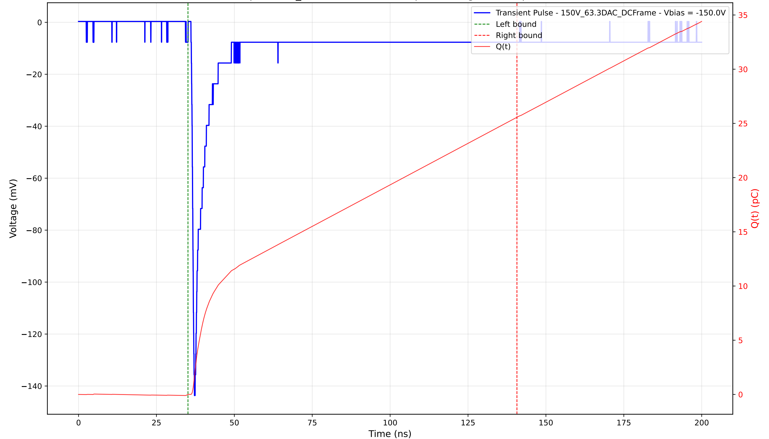
Transient Pulse - Sample: 1cm_42 - Position: 4570.0 \mu\text{m} - Charge: 25.57 pC - Rise Time: 0.86 ns
