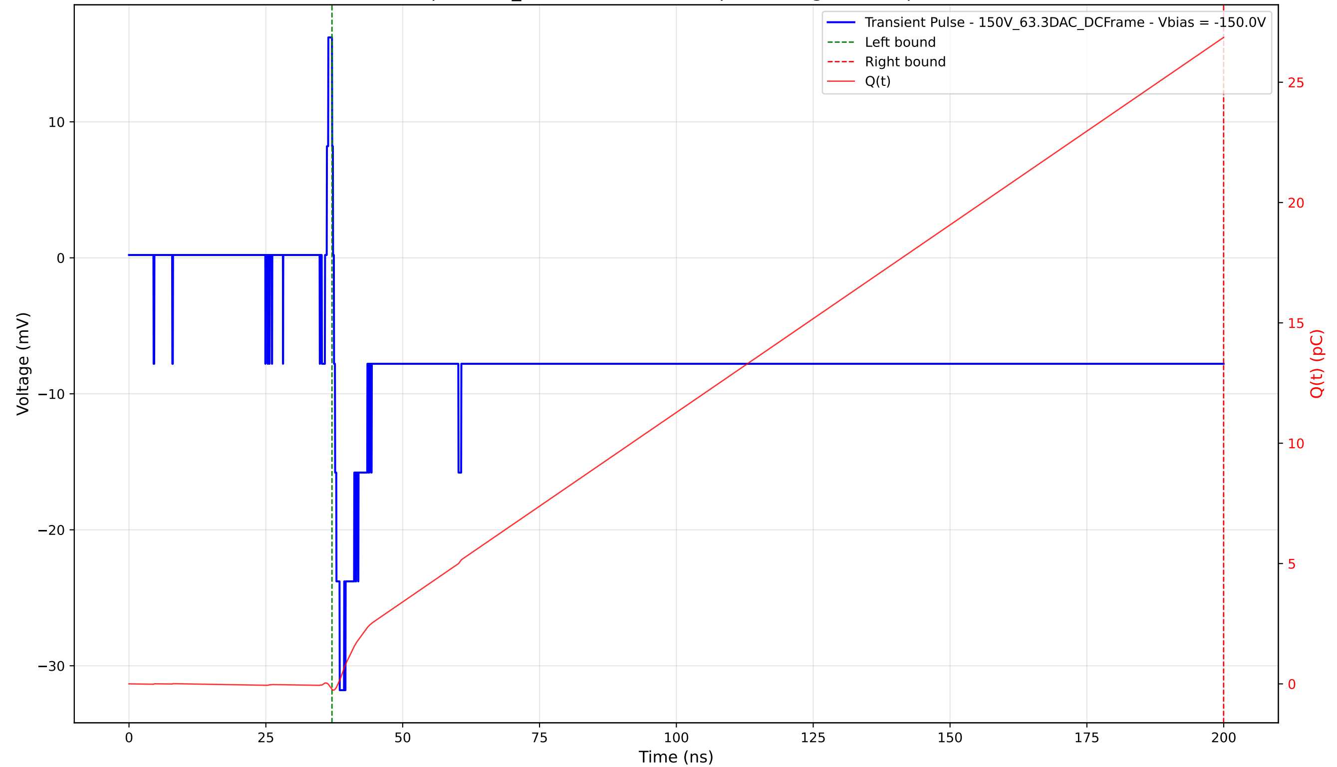
Transient Pulse - Sample: 1cm_42 - Position: 2430.0 \mu\text{m} - Charge: 27.09 pC - Rise Time: 1.05 ns
