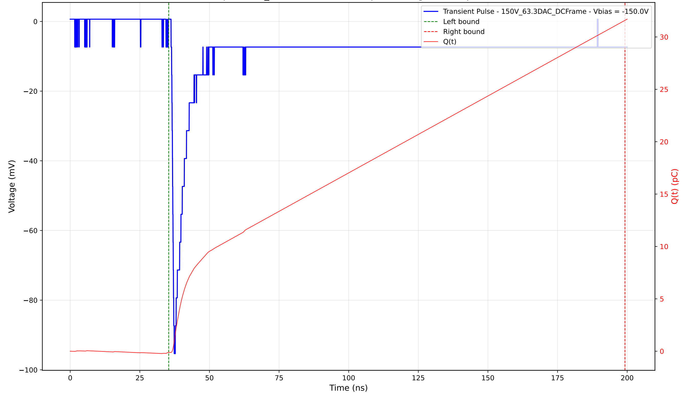
Transient Pulse - Sample: 1cm_42 - Position: 4400.0 \mu\text{m} - Charge: 31.69 pC - Rise Time: 0.77 ns
