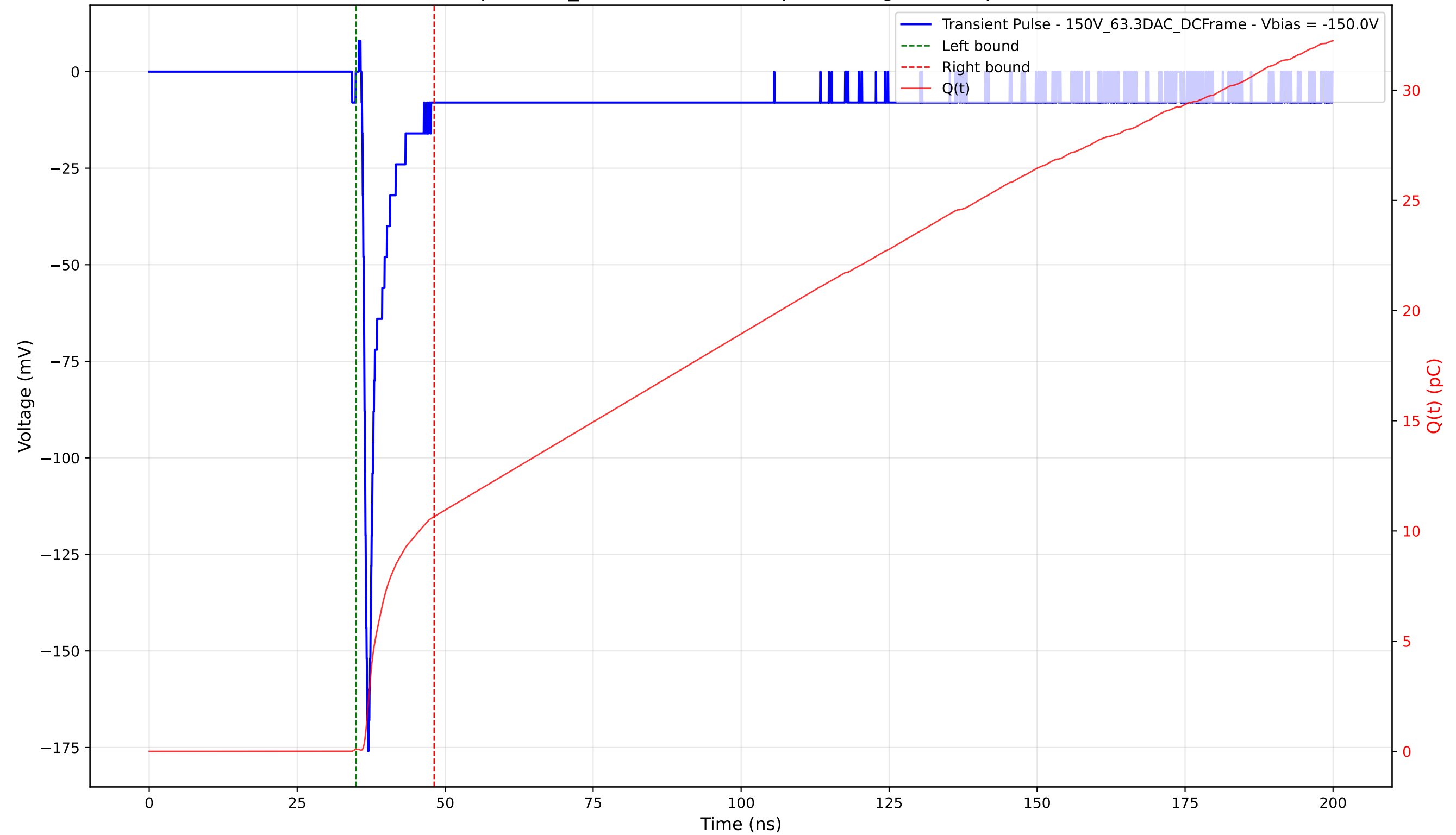
Transient Pulse - Sample: 1cm_42 - Position: 290.0 \mu\text{m} - Charge: 10.56 pC - Rise Time: 0.76 ns
