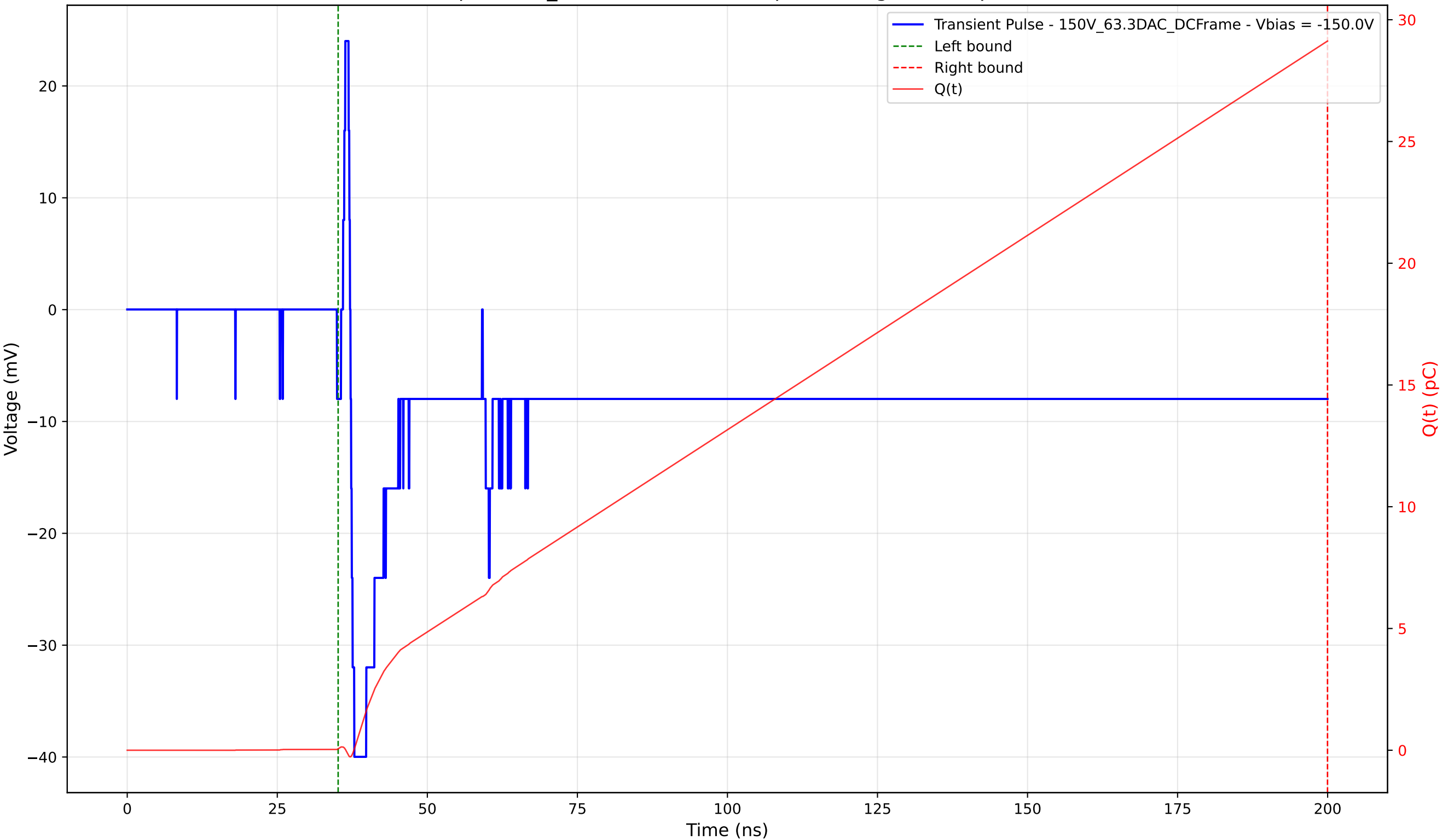
Transient Pulse - Sample: 1cm_42 - Position: 1850.0 \mu\text{m} - Charge: 29.06 pC - Rise Time: 0.63 ns
