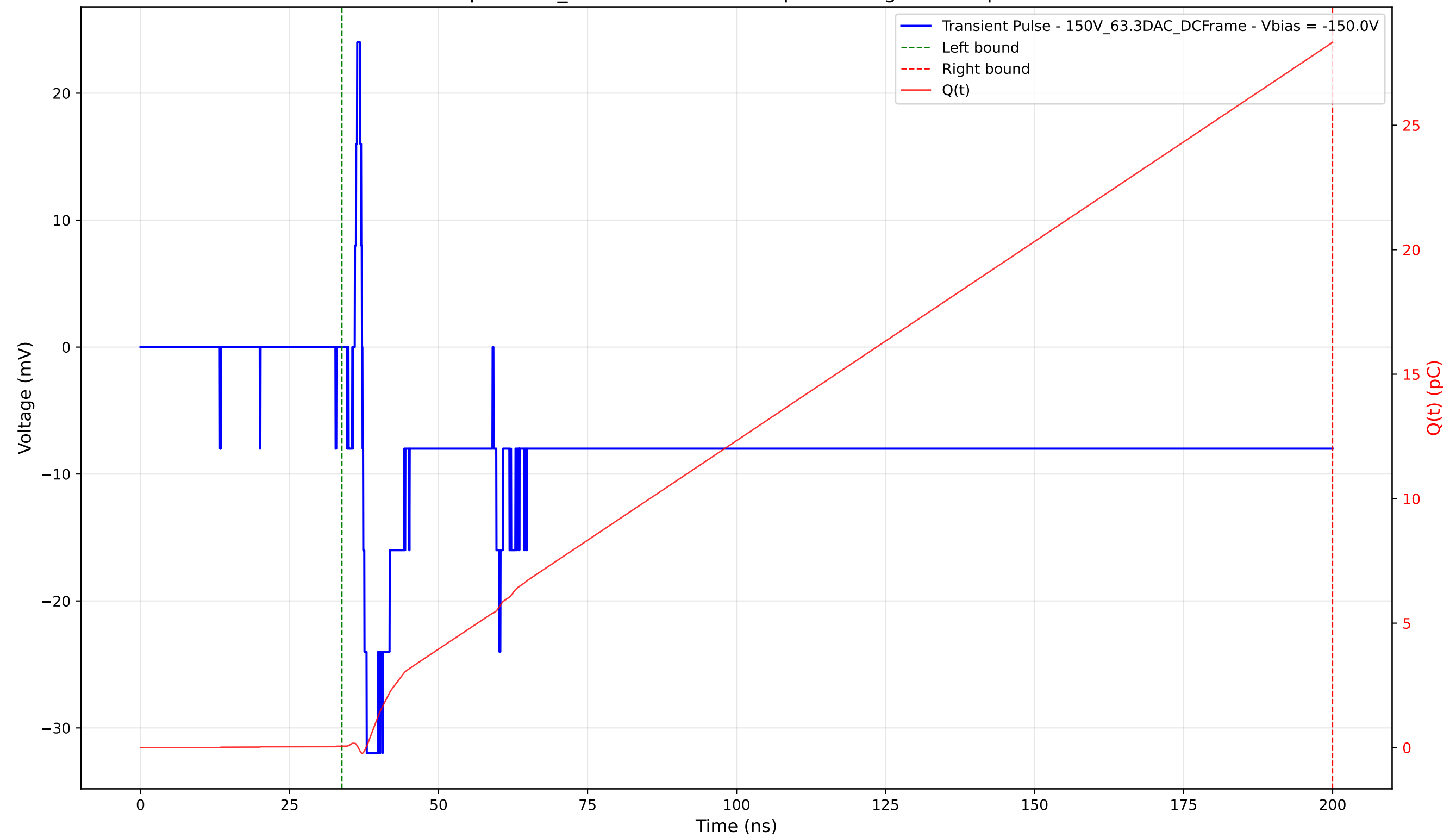
Transient Pulse - Sample: 1cm_42 - Position: 2065.0 \mu\text{m} - Charge: 28.27 pC - Rise Time: 0.71 ns
