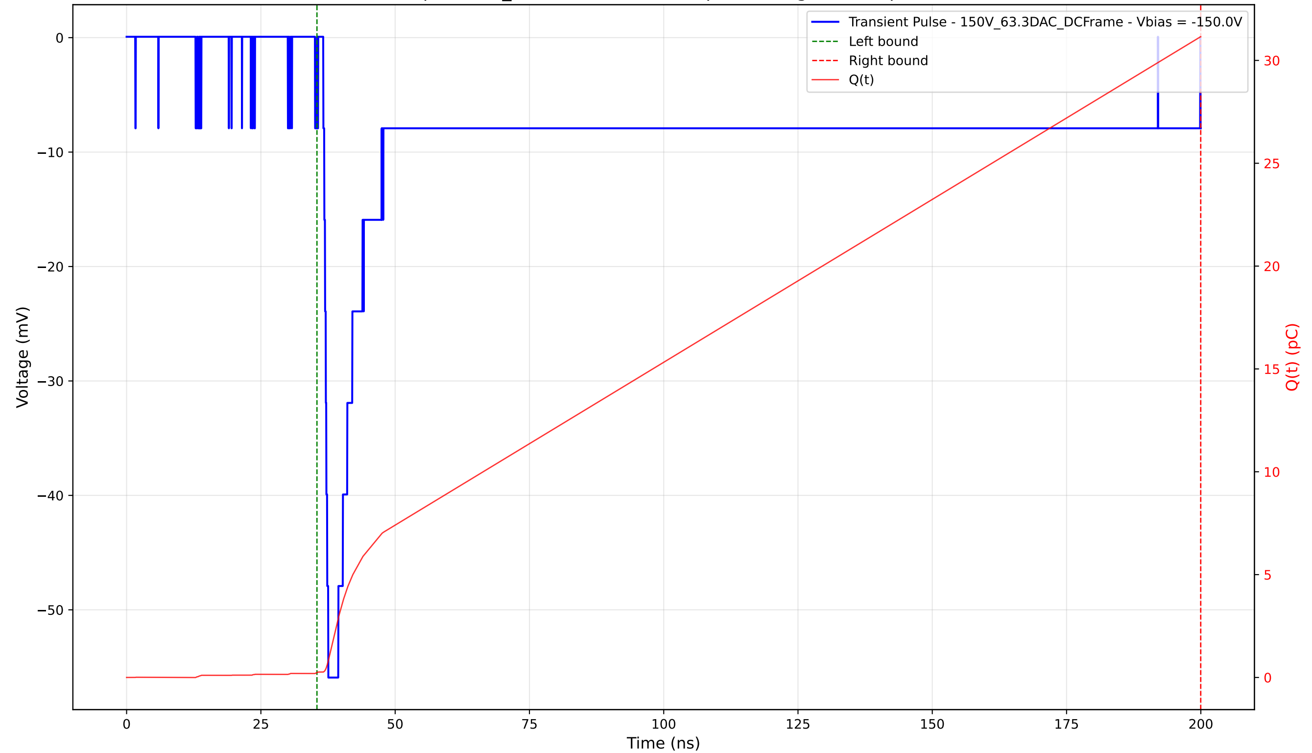
Transient Pulse - Sample: 1cm_42 - Position: 4050.0 \mu\text{m} - Charge: 30.91 pC - Rise Time: 0.93 ns
