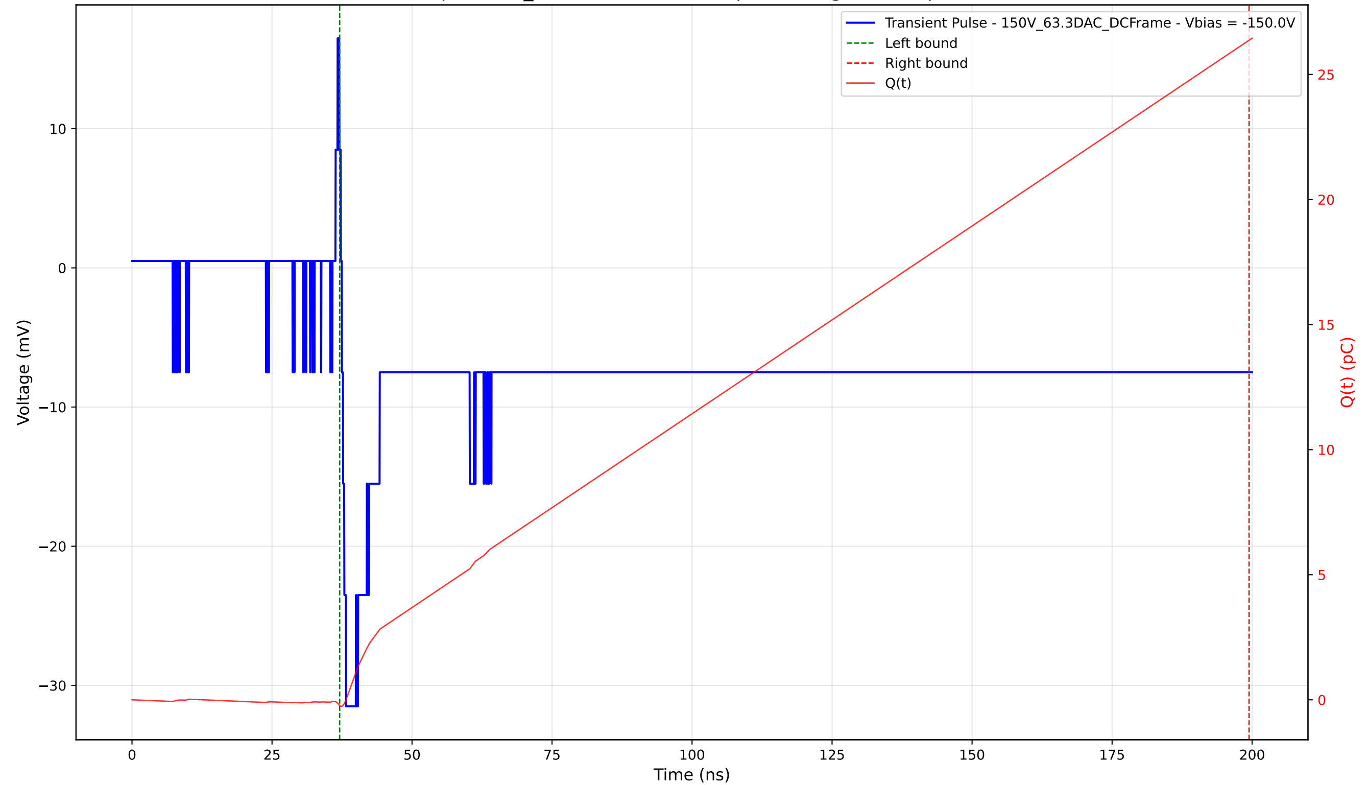
Transient Pulse - Sample: 1cm_42 - Position: 3115.0 \mu\text{m} - Charge: 26.60 pC - Rise Time: 0.75 ns
