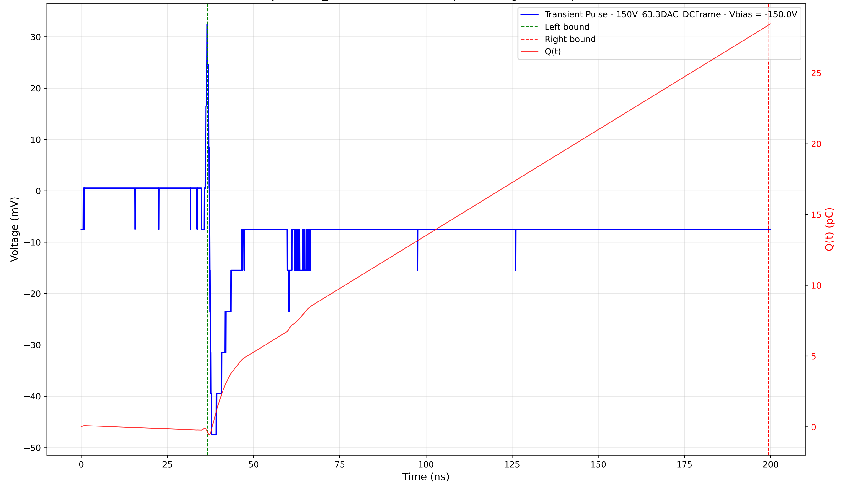
Transient Pulse - Sample: 1cm_42 - Position: 1685.0 \mu\text{m} - Charge: 28.80 pC - Rise Time: 0.67 ns
