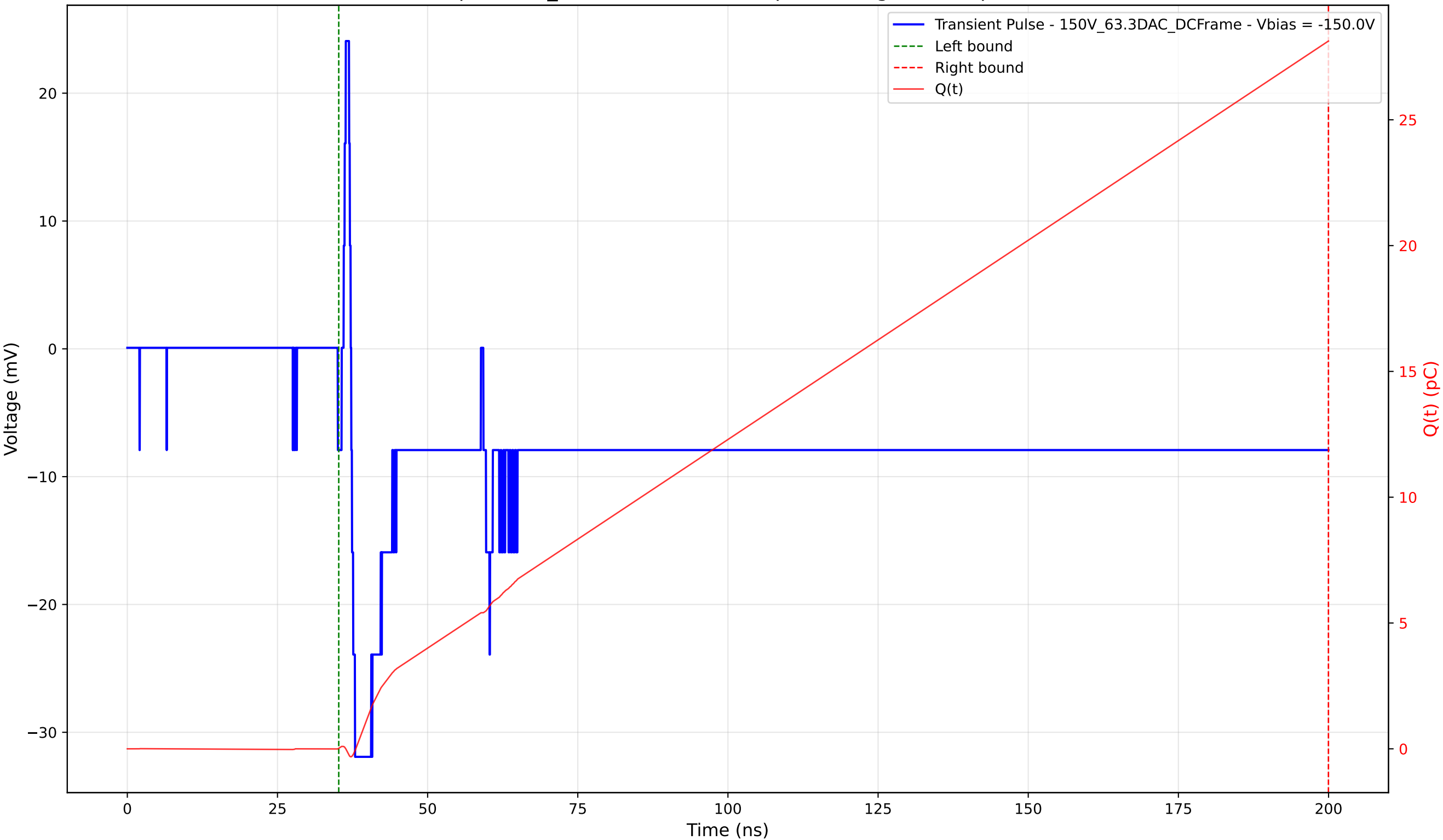
Transient Pulse - Sample: 1cm_42 - Position: 2150.0 \mu\text{m} - Charge: 28.11 pC - Rise Time: 0.63 ns
