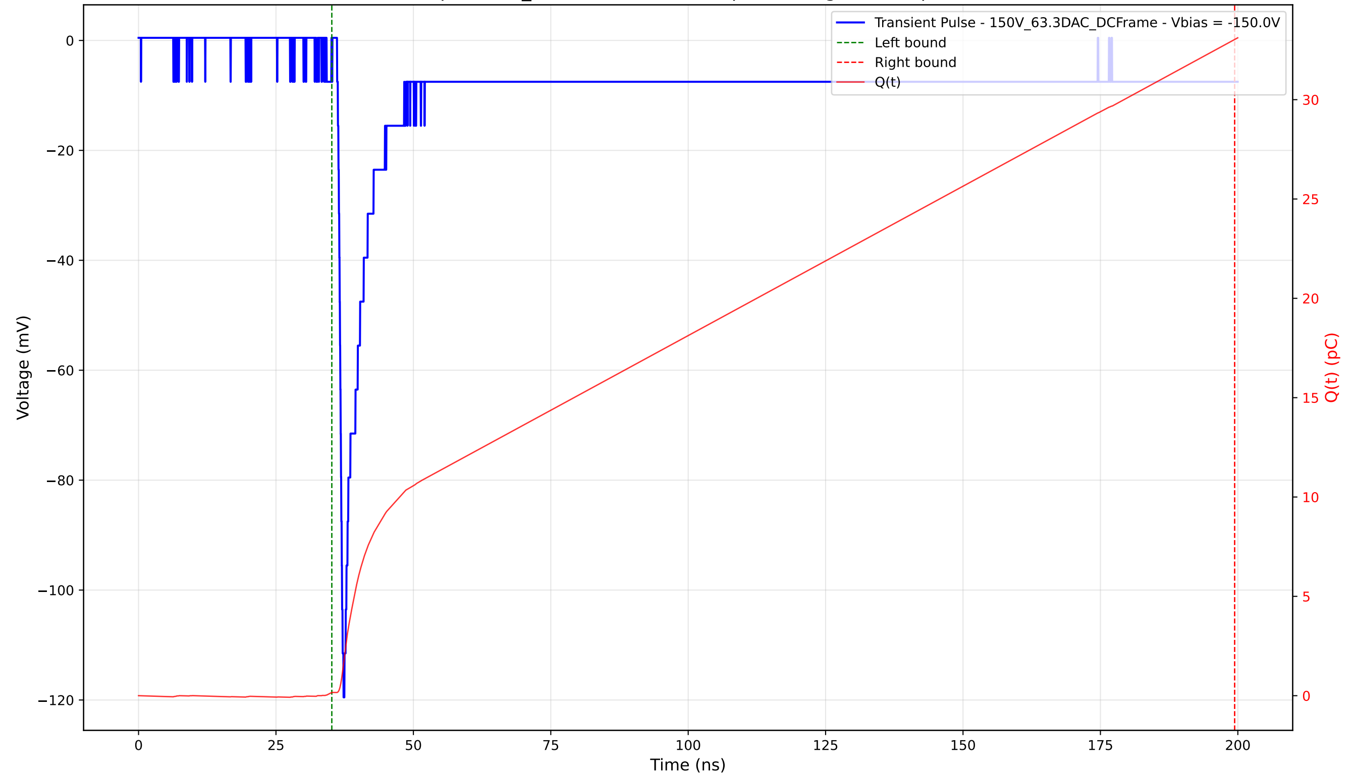
Transient Pulse - Sample: 1cm_42 - Position: 4505.0 \mu\text{m} - Charge: 32.87 pC - Rise Time: 0.87 ns
