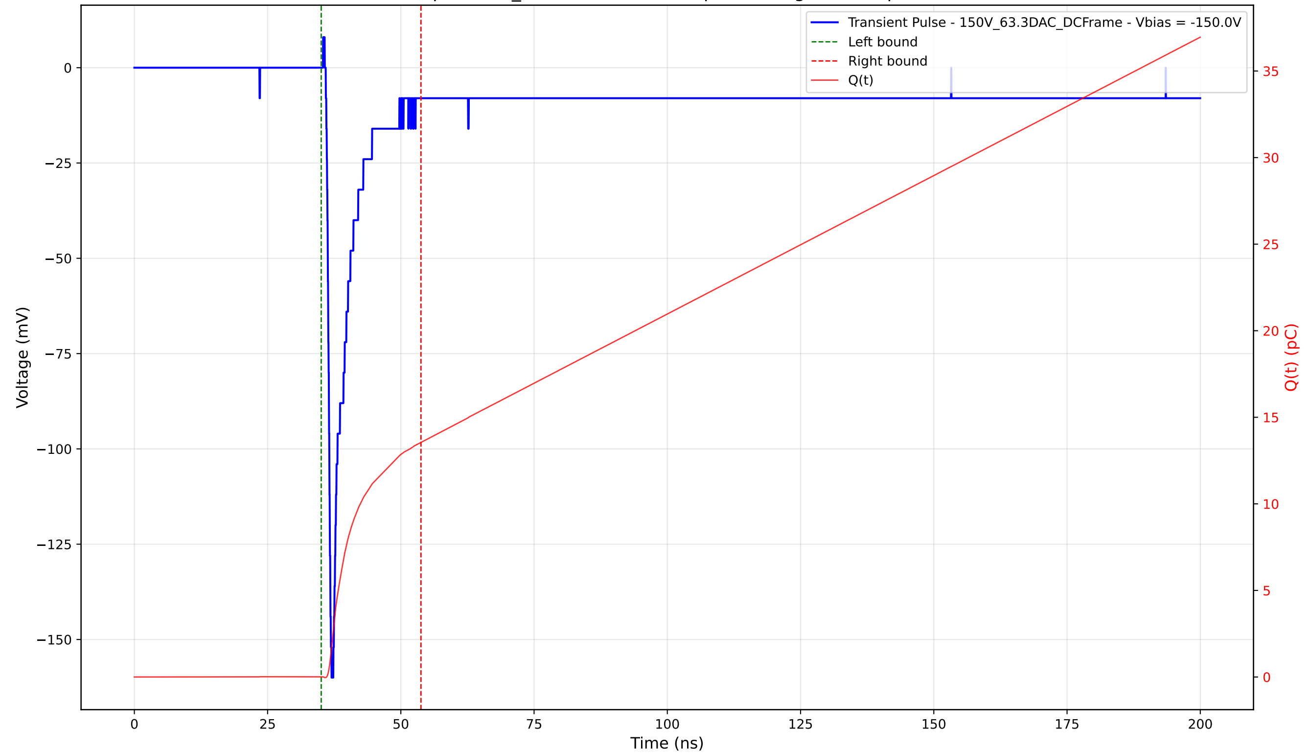
Transient Pulse - Sample: 1cm_42 - Position: 495.0 \mu\text{m} - Charge: 13.54 pC - Rise Time: 0.72 ns
