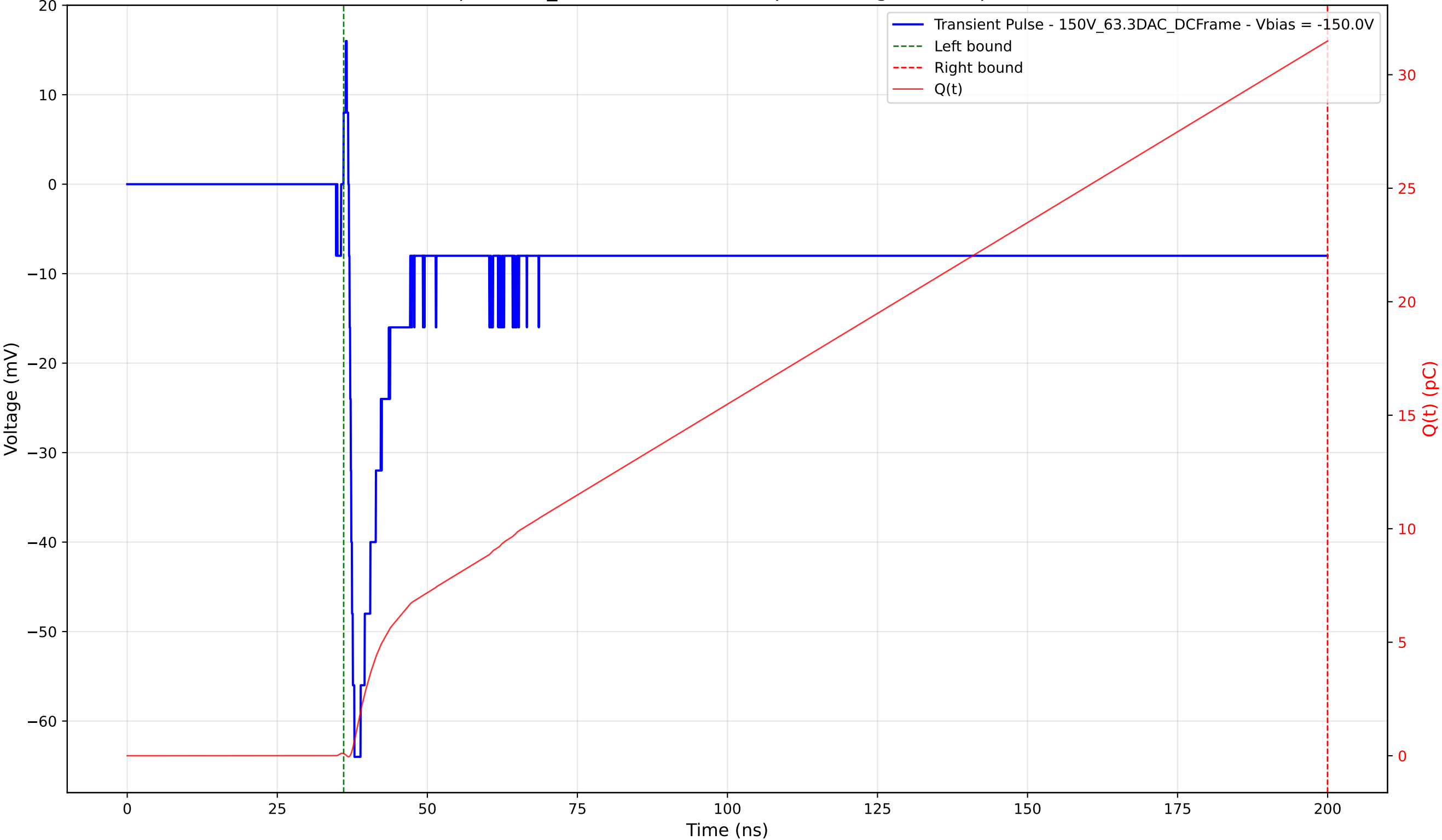
Transient Pulse - Sample: 1cm_42 - Position: 1330.0 \mu\text{m} - Charge: 31.38 pC - Rise Time: 0.90 ns
