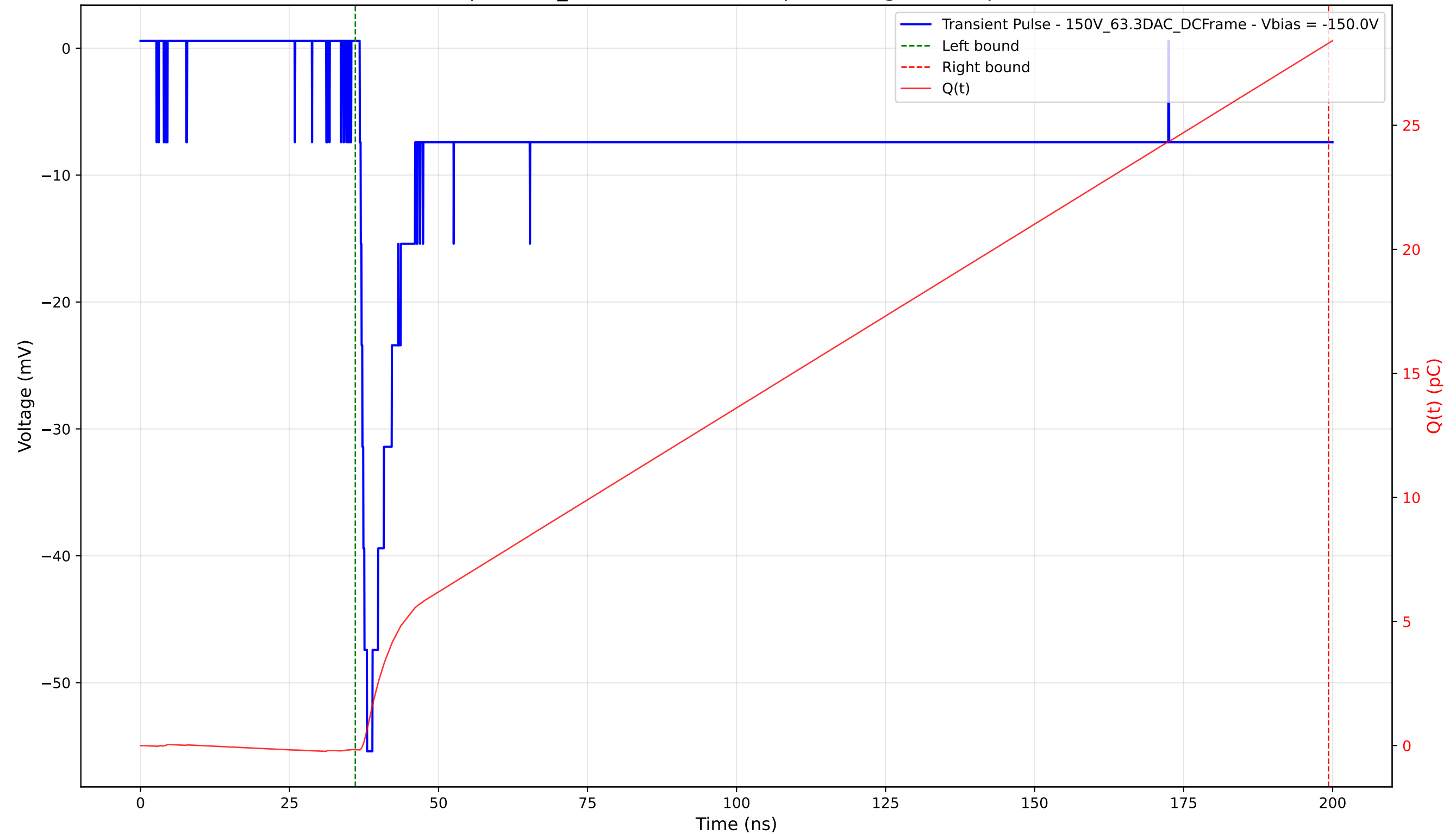
Transient Pulse - Sample: 1cm_42 - Position: 3975.0 \mu\text{m} - Charge: 28.48 pC - Rise Time: 1.23 ns
