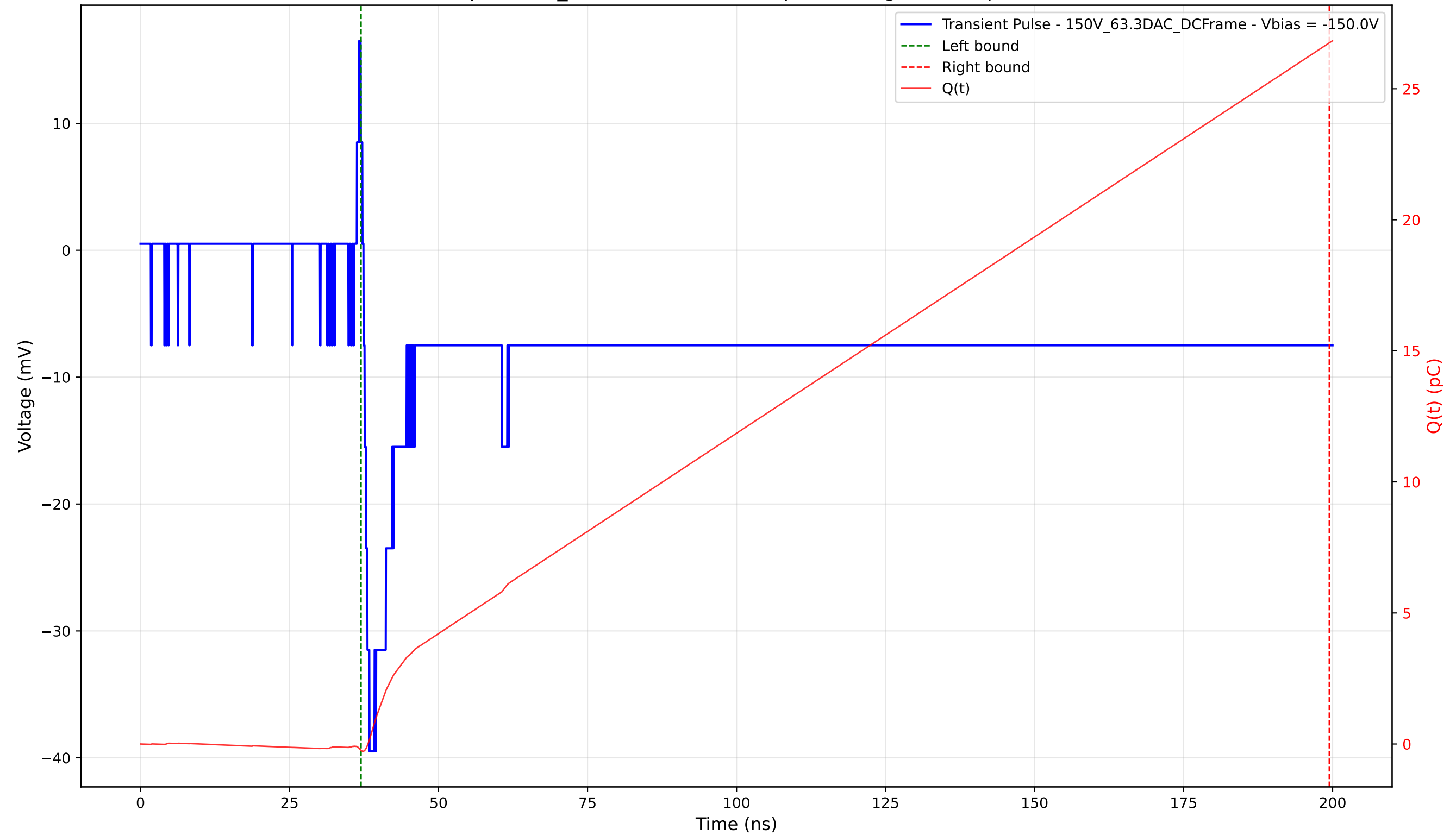
Transient Pulse - Sample: 1cm_42 - Position: 3325.0 \mu\text{m} - Charge: 26.99 pC - Rise Time: 0.99 ns
