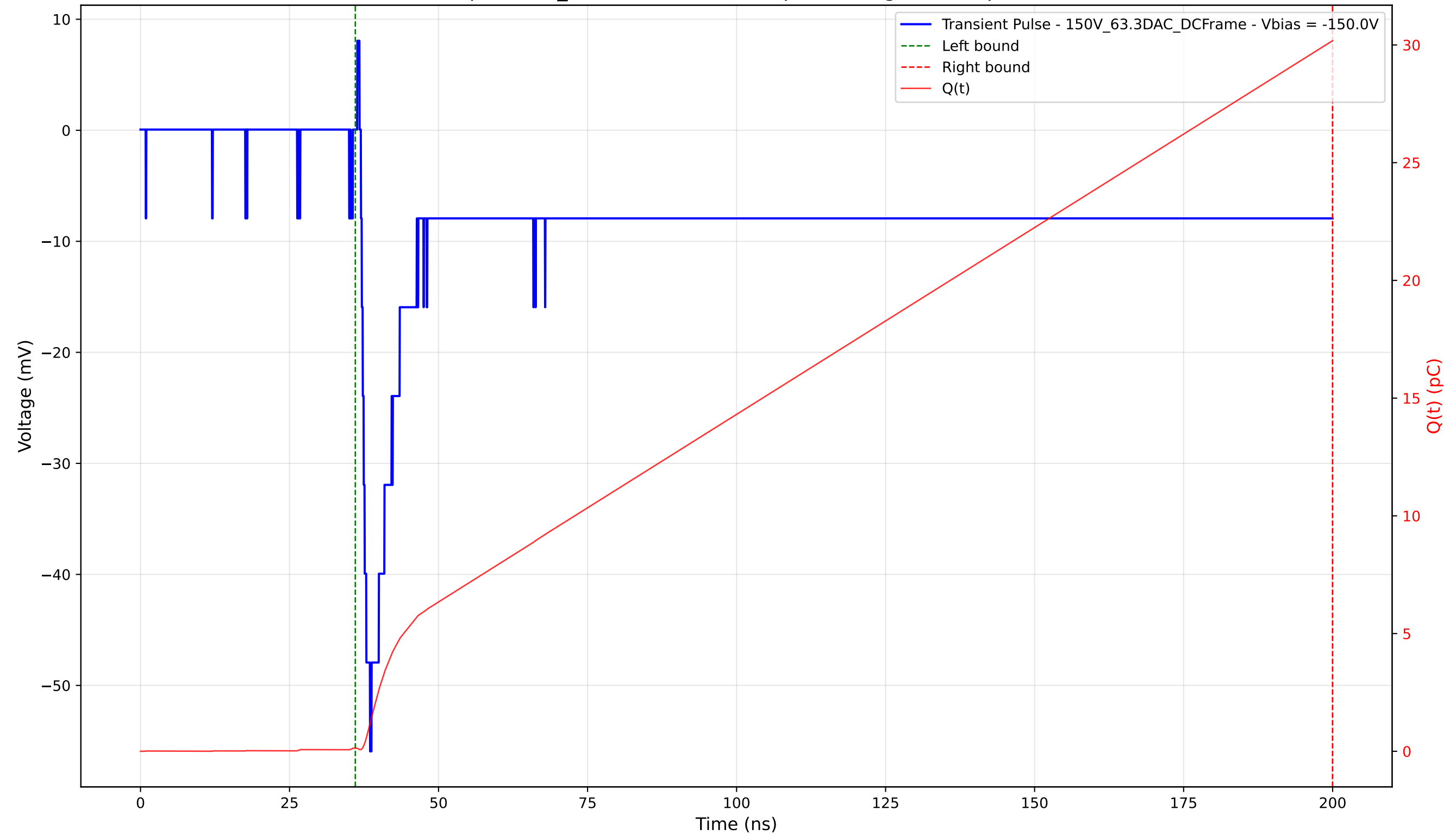
Transient Pulse - Sample: 1cm_42 - Position: 3830.0 \mu\text{m} - Charge: 30.04 pC - Rise Time: 1.53 ns
