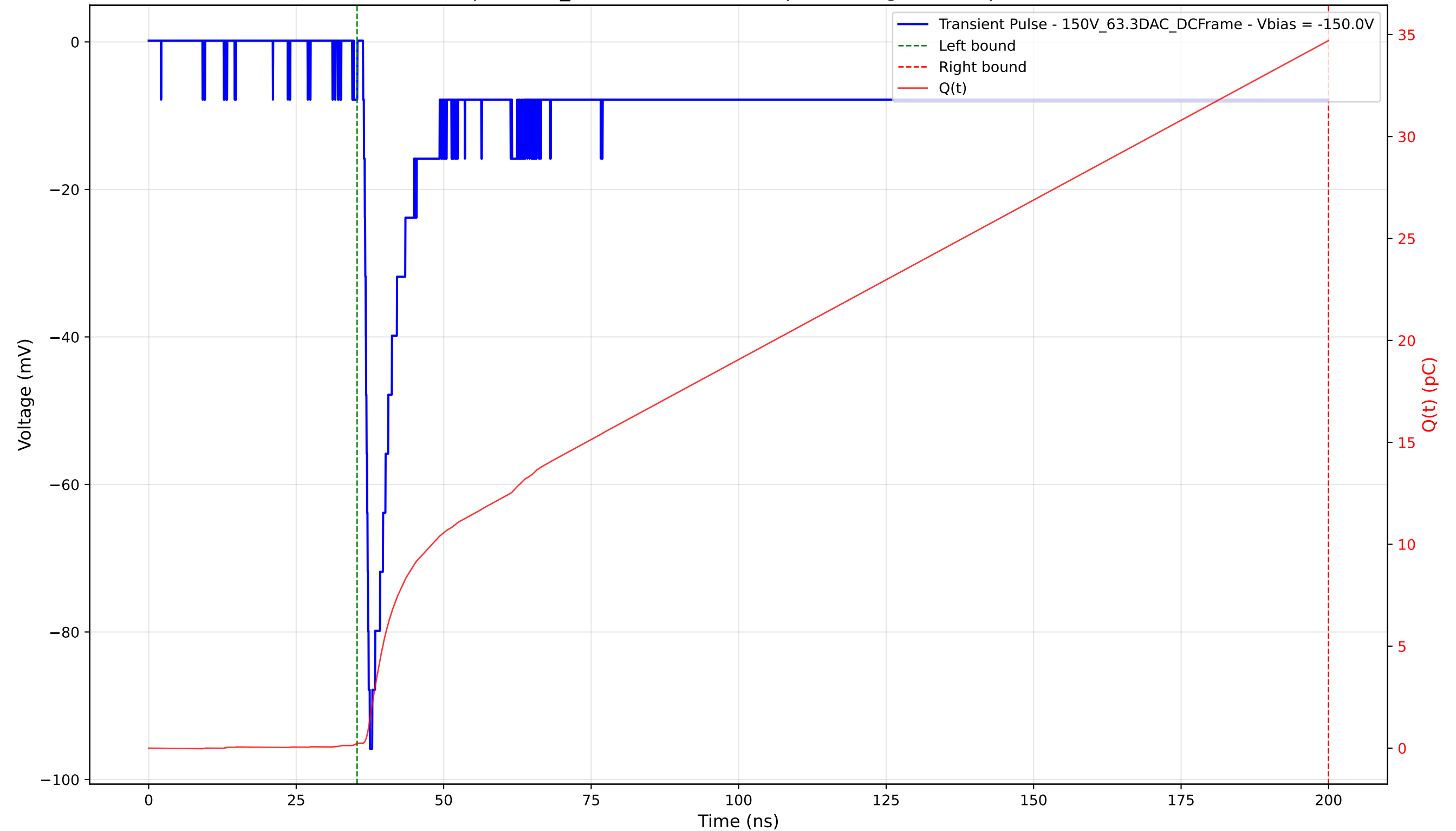
Transient Pulse - Sample: 1cm_42 - Position: 4285.0 \mu\text{m} - Charge: 34.47 pC - Rise Time: 0.82 ns
