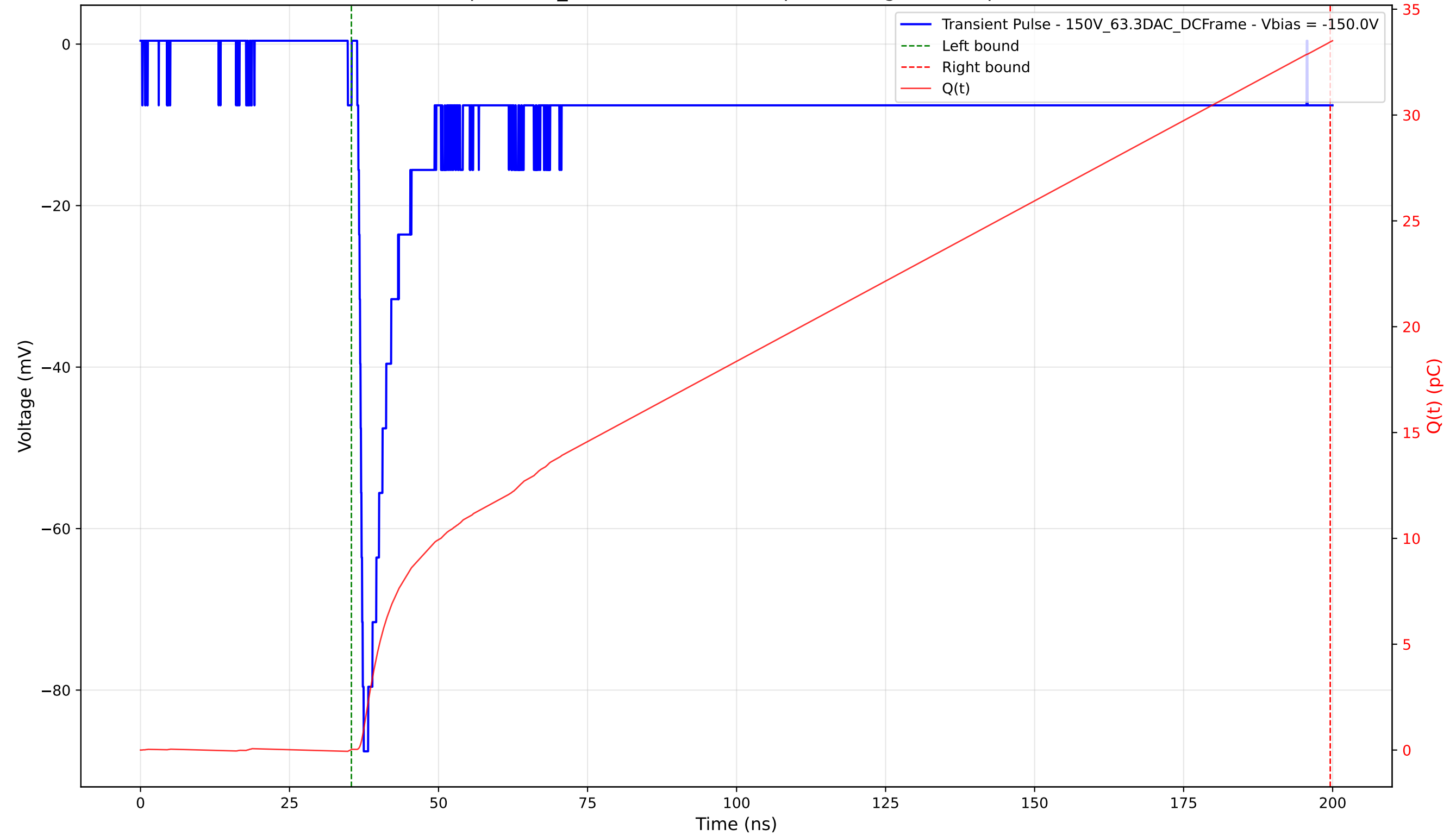
Transient Pulse - Sample: 1cm_42 - Position: 4220.0 \mu\text{m} - Charge: 33.42 pC - Rise Time: 0.76 ns
