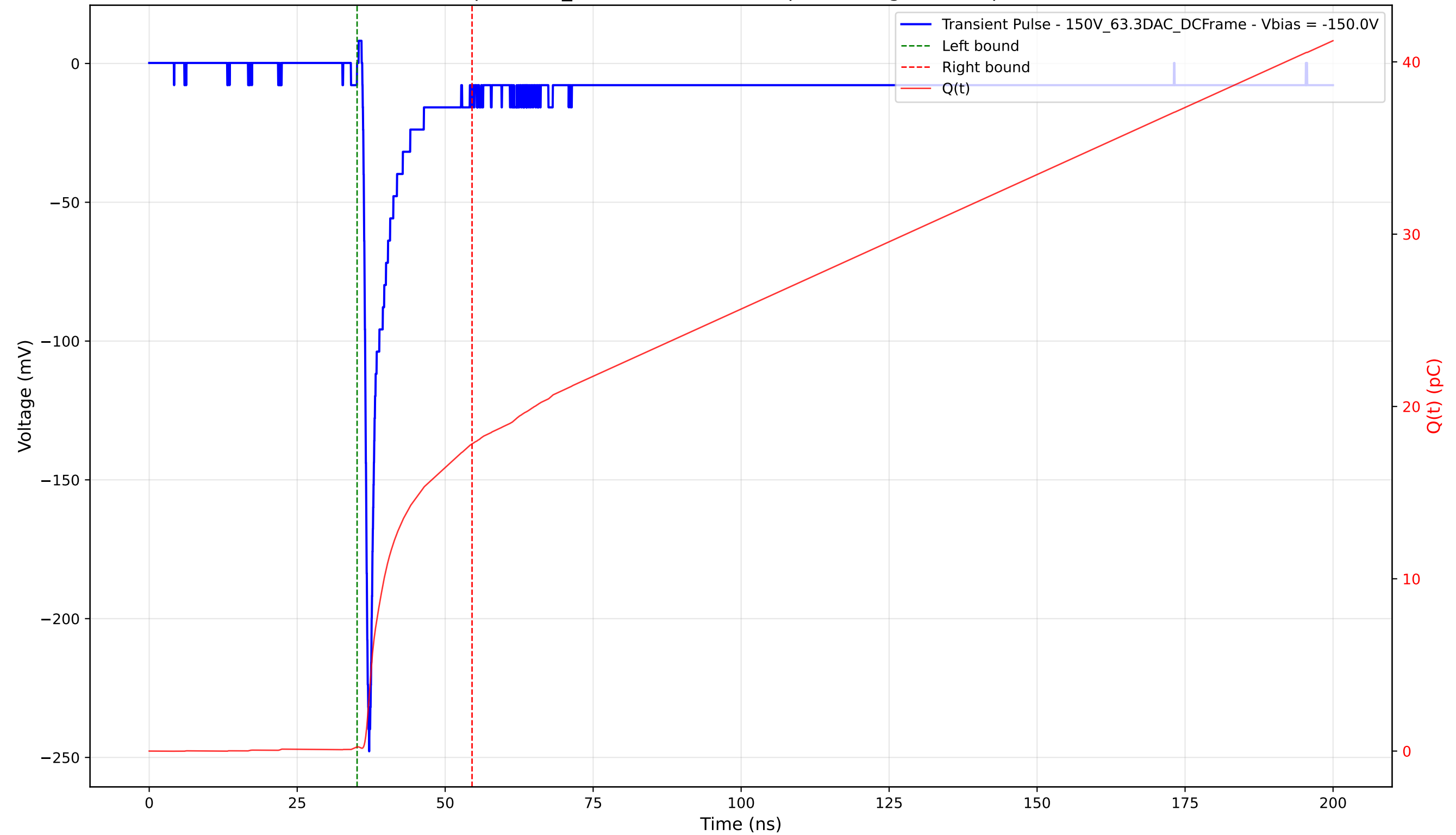
Transient Pulse - Sample: 1cm_42 - Position: 4770.0 \mu\text{m} - Charge: 17.59 pC - Rise Time: 0.76 ns
