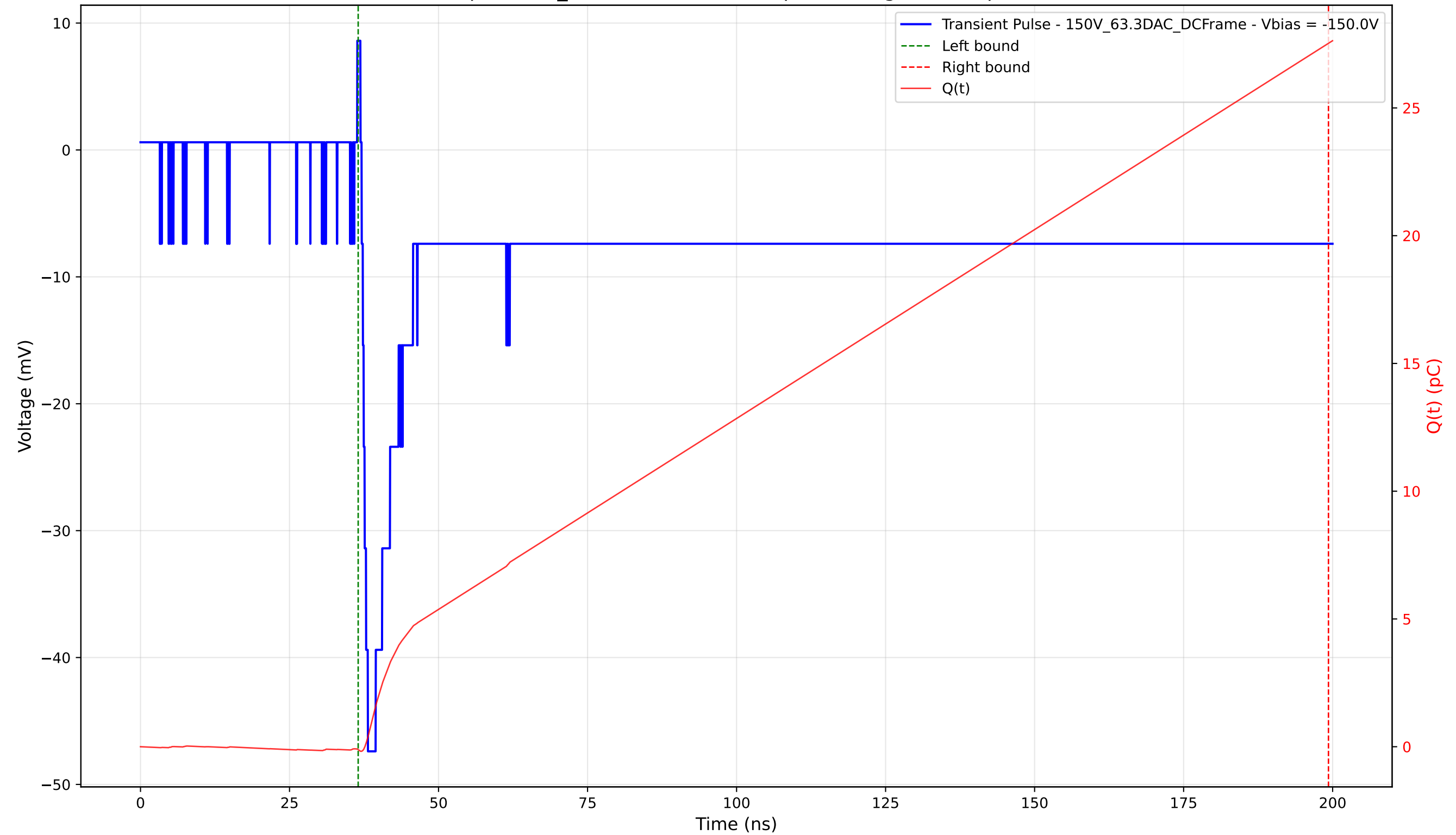
Transient Pulse - Sample: 1cm_42 - Position: 3655.0 \mu\text{m} - Charge: 27.64 pC - Rise Time: 1.05 ns
