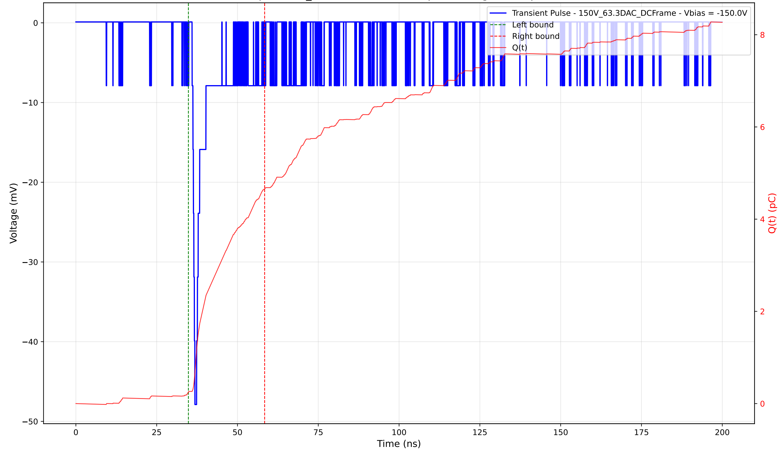
Transient Pulse - Sample: 1cm_42 - Position: 5130.0 \mu\text{m} - Charge: 4.41 pC - Rise Time: 0.87 ns
