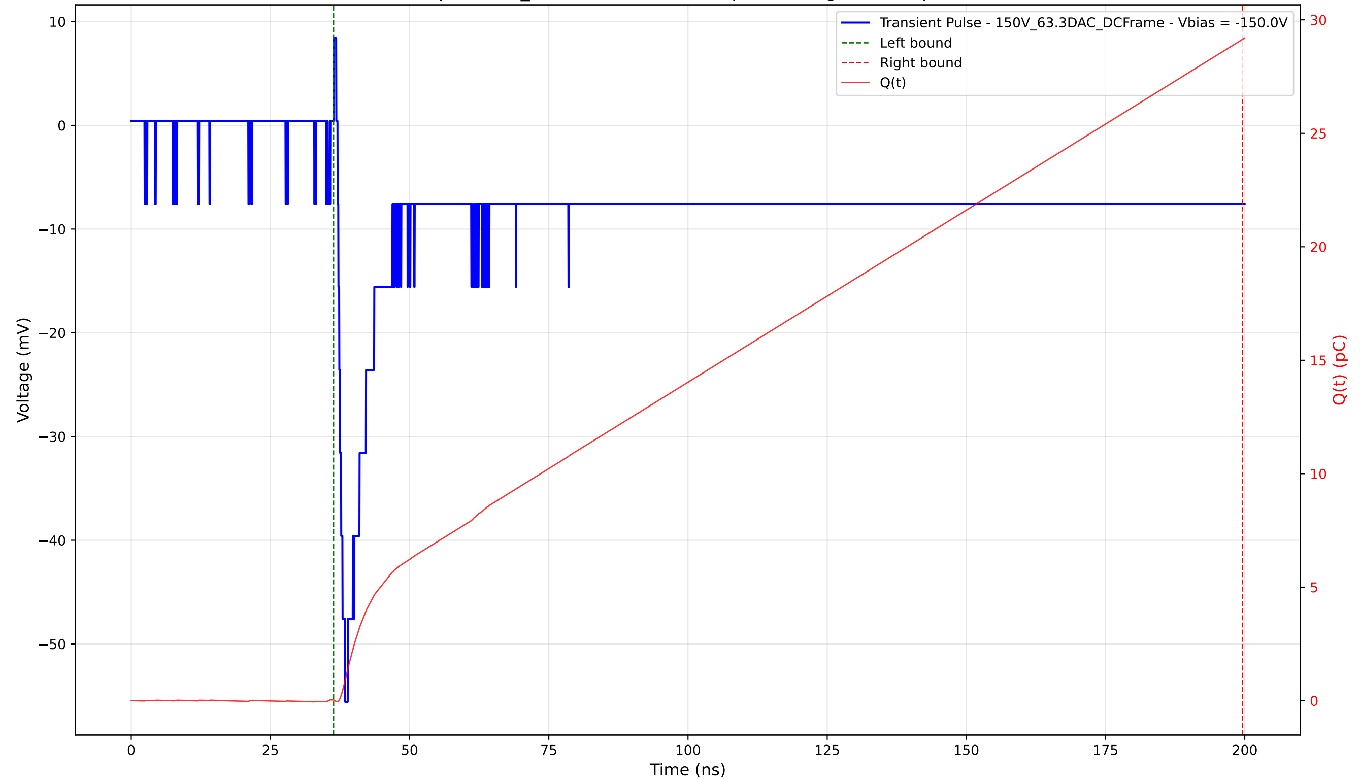
Transient Pulse - Sample: 1cm_42 - Position: 3720.0 \mu\text{m} - Charge: 29.11 pC - Rise Time: 1.35 ns
