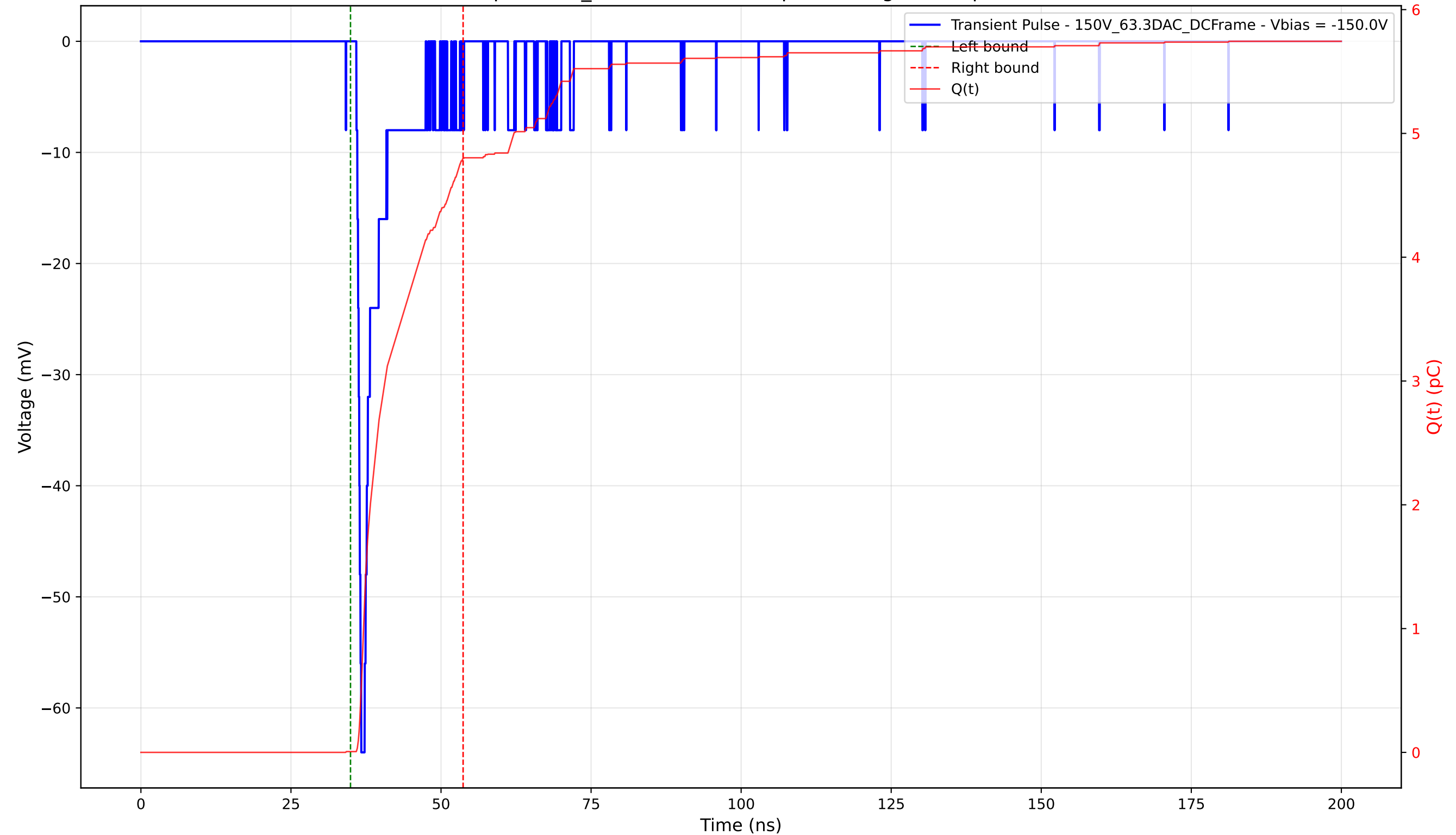
Transient Pulse - Sample: 1cm_42 - Position: 80.0 \mu\text{m} - Charge: 4.79 pC - Rise Time: 0.80 ns
