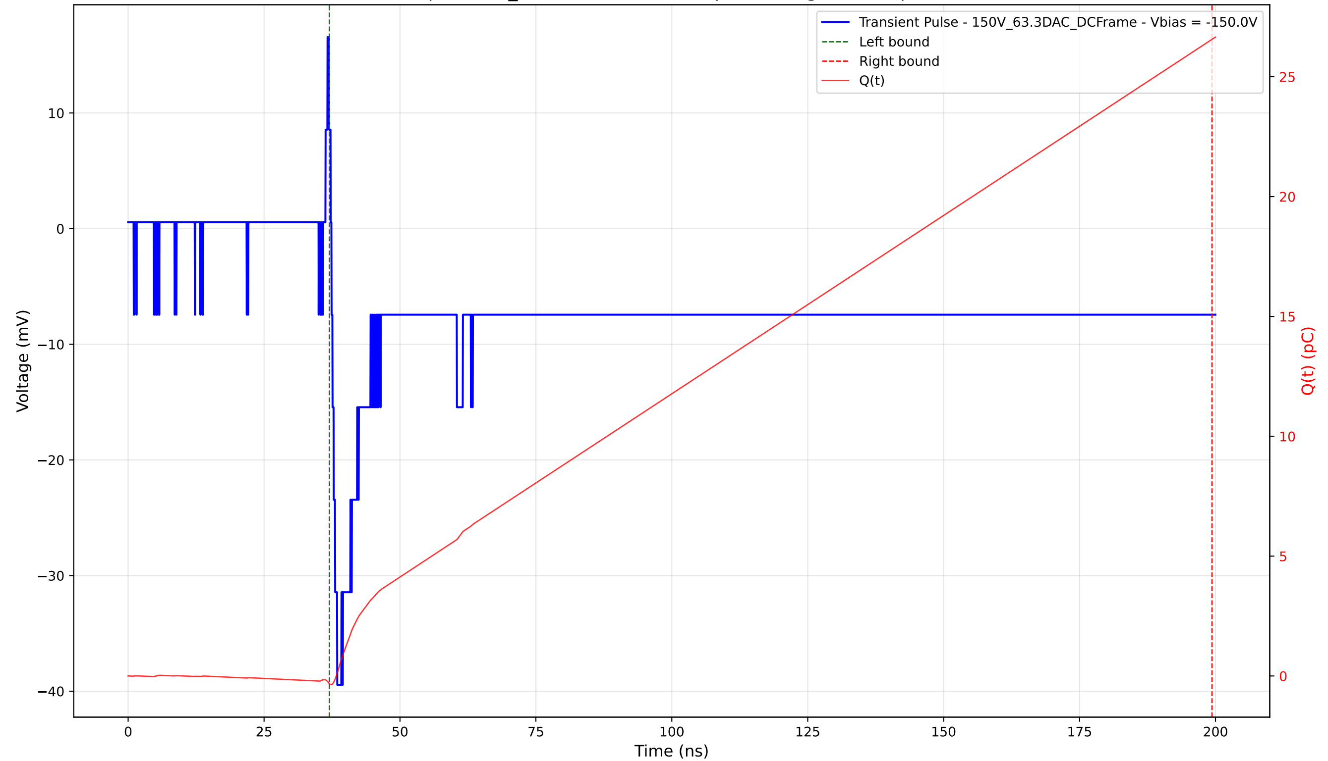
Transient Pulse - Sample: 1cm_42 - Position: 3310.0 \mu\text{m} - Charge: 26.89 pC - Rise Time: 1.05 ns
