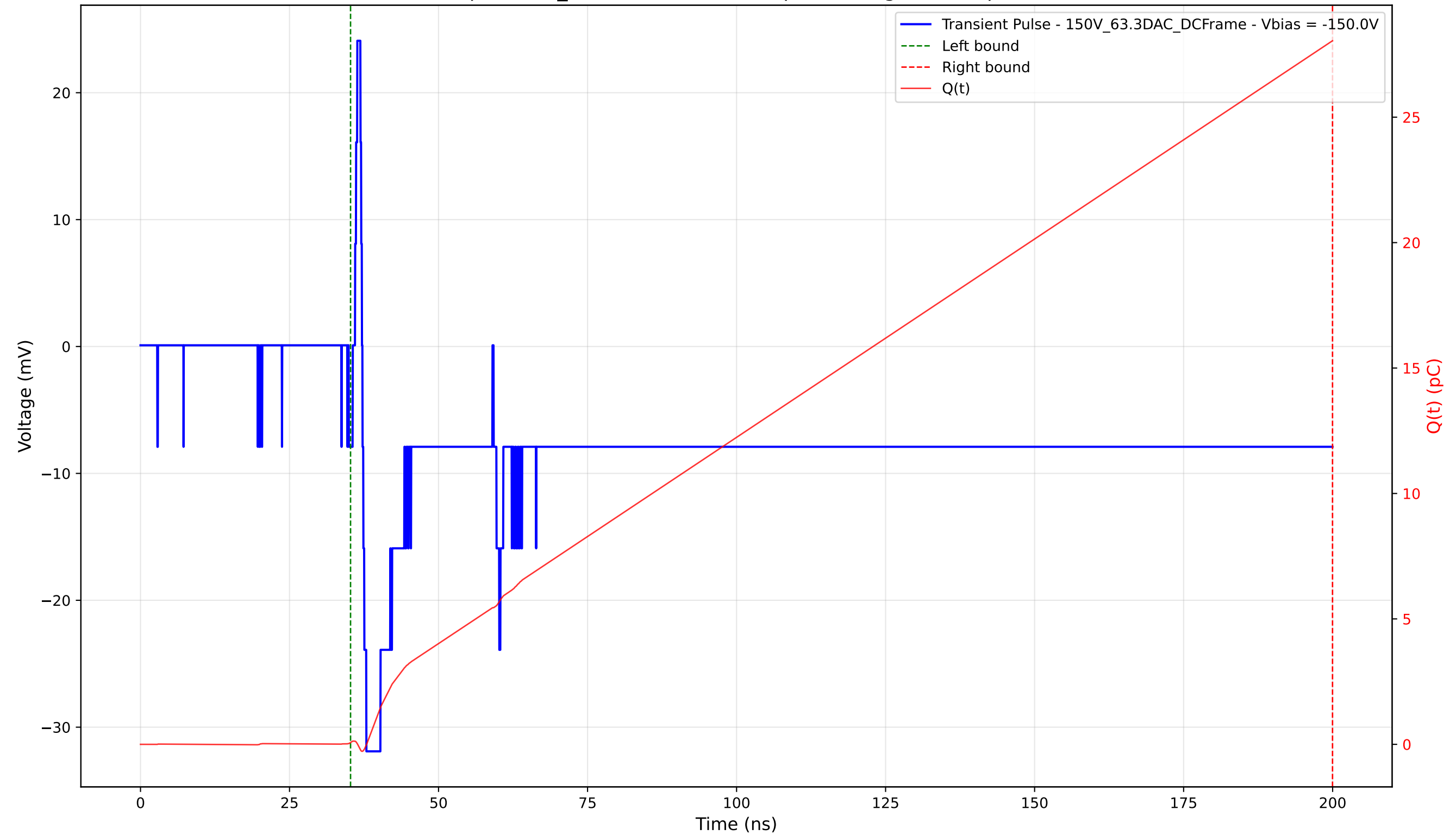
Transient Pulse - Sample: 1cm_42 - Position: 2095.0 \mu\text{m} - Charge: 27.97 pC - Rise Time: 0.65 ns
