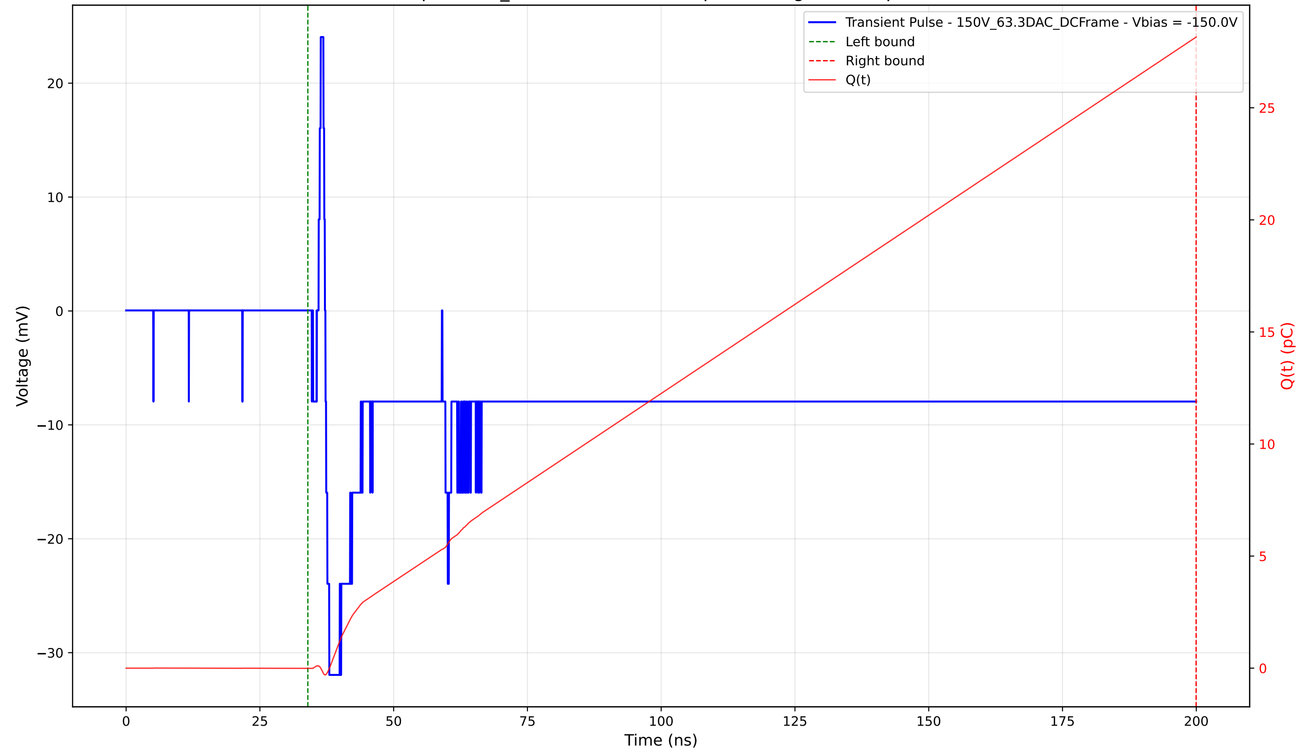
Transient Pulse - Sample: 1cm_42 - Position: 2090.0 \mu\text{m} - Charge: 28.17 pC - Rise Time: 0.71 ns
