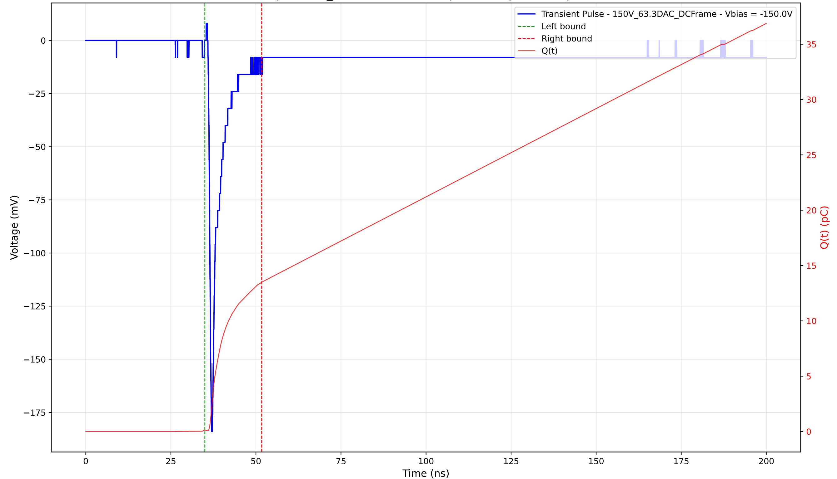
Transient Pulse - Sample: 1cm_42 - Position: 415.0 \mu\text{m} - Charge: 13.37 pC - Rise Time: 0.77 ns
