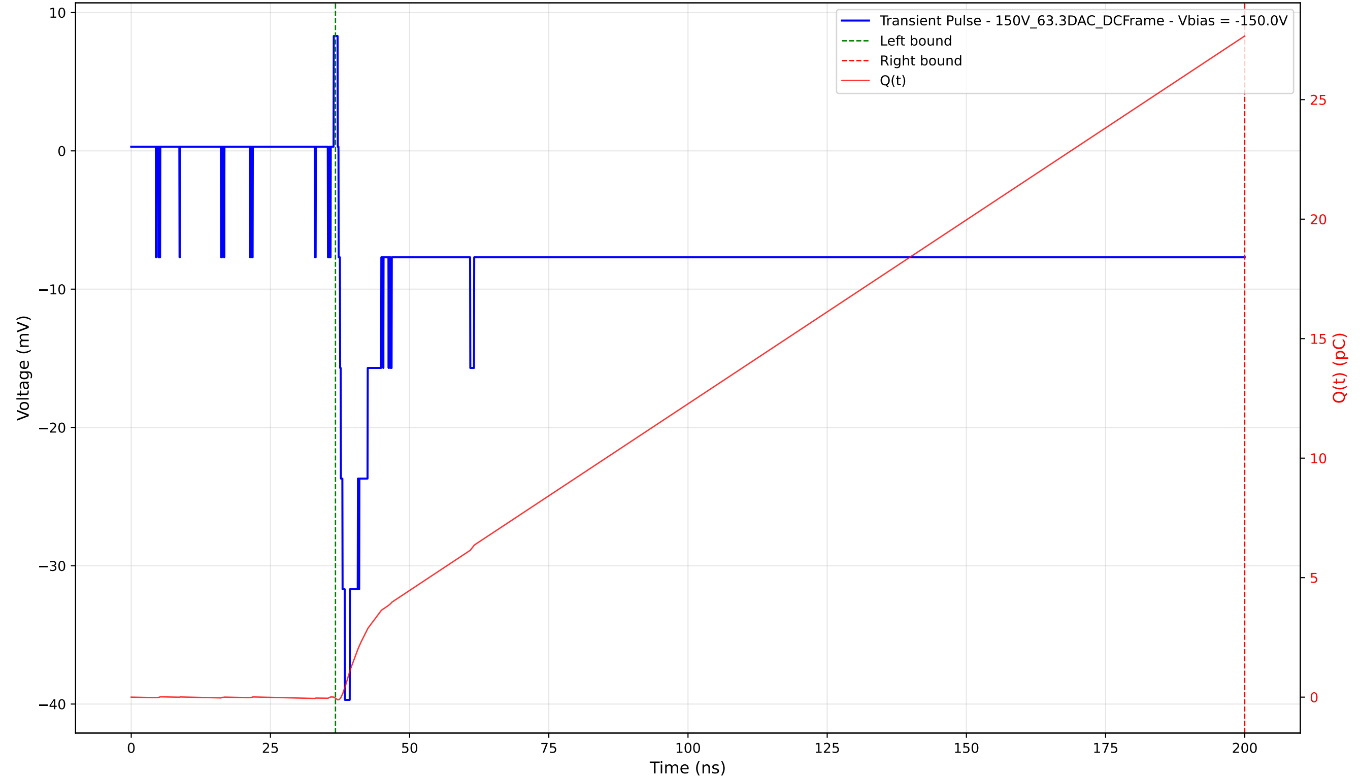
Transient Pulse - Sample: 1cm_42 - Position: 3485.0 \mu\text{m} - Charge: 27.71 pC - Rise Time: 1.13 ns
