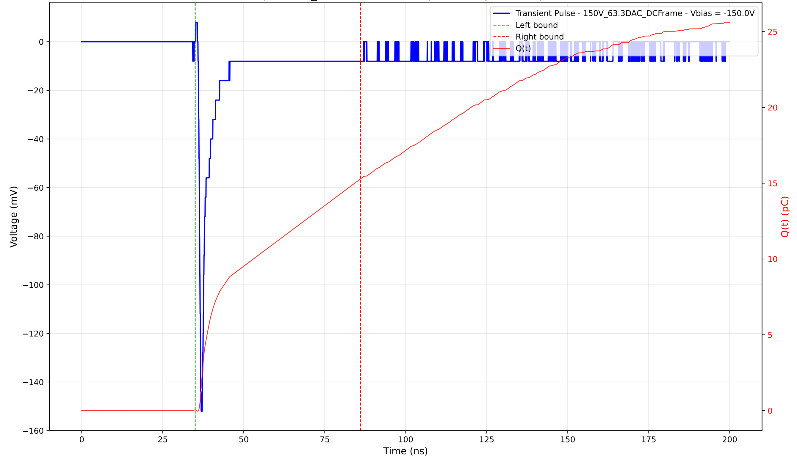
Transient Pulse - Sample: 1cm_42 - Position: 220.0 \mu\text{m} - Charge: 15.26 pC - Rise Time: 0.76 ns
