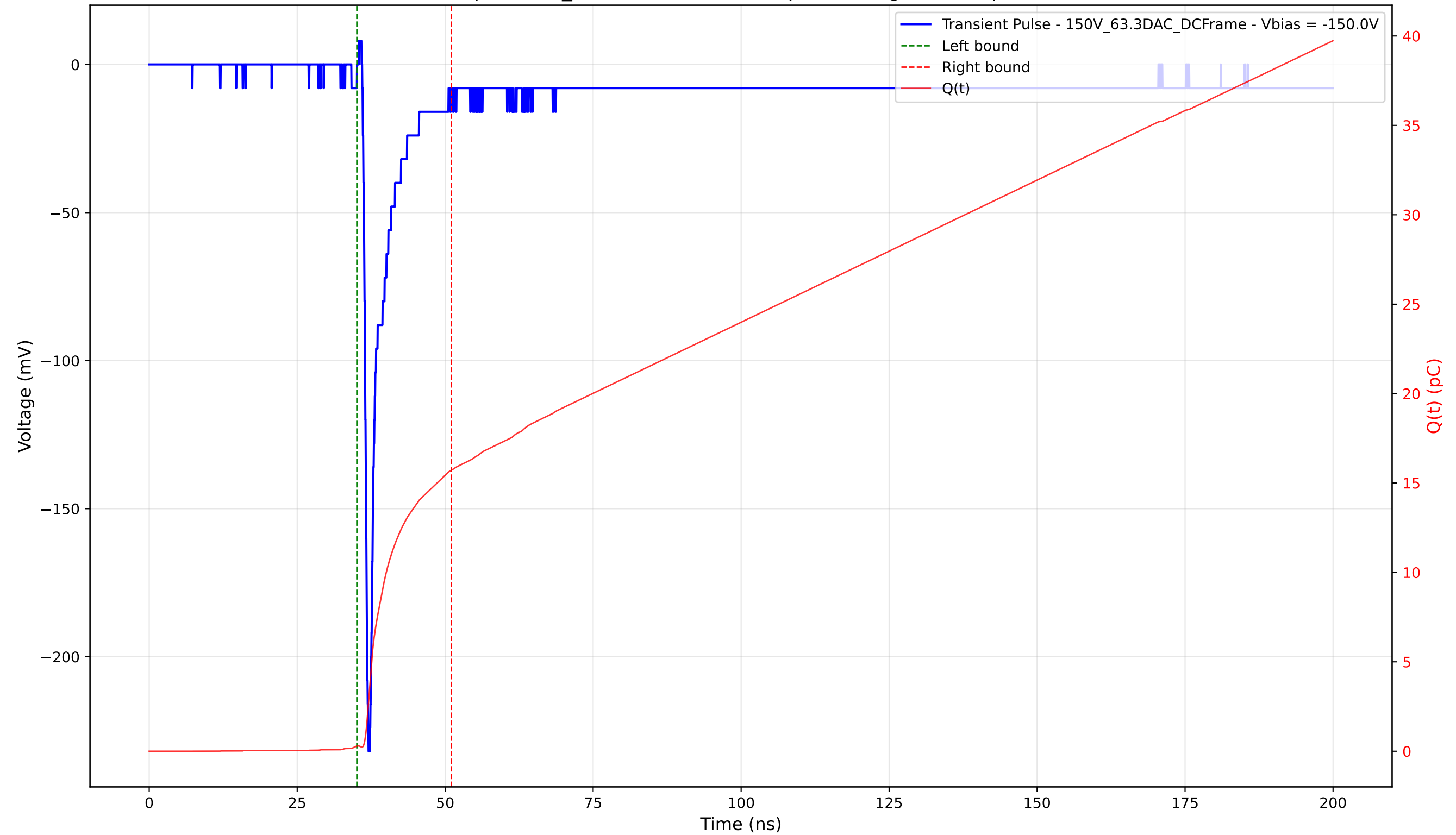
Transient Pulse - Sample: 1cm_42 - Position: 4855.0 \mu\text{m} - Charge: 15.42 pC - Rise Time: 0.80 ns
