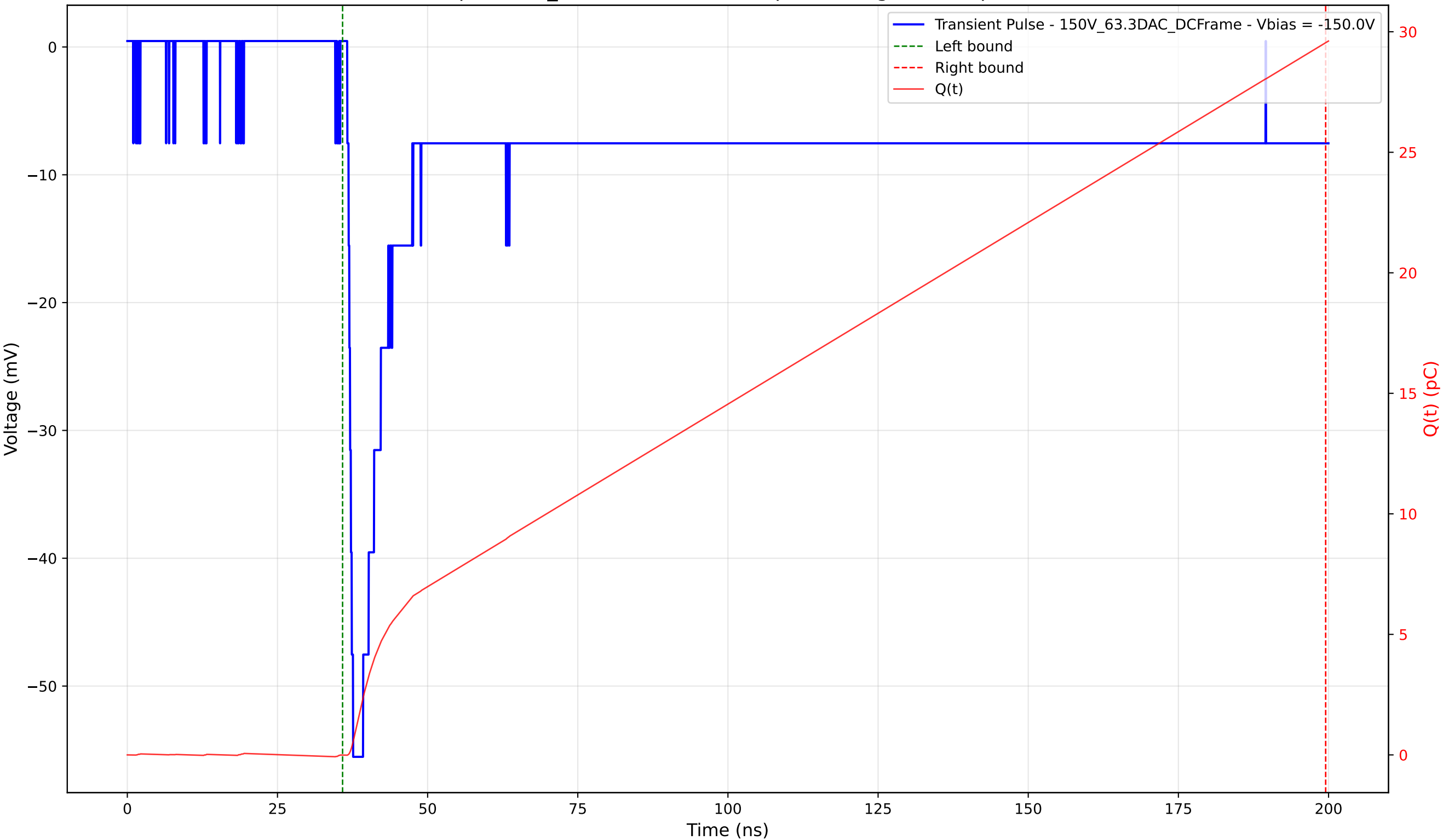
Transient Pulse - Sample: 1cm_42 - Position: 4035.0 \mu\text{m} - Charge: 29.55 pC - Rise Time: 0.97 ns
