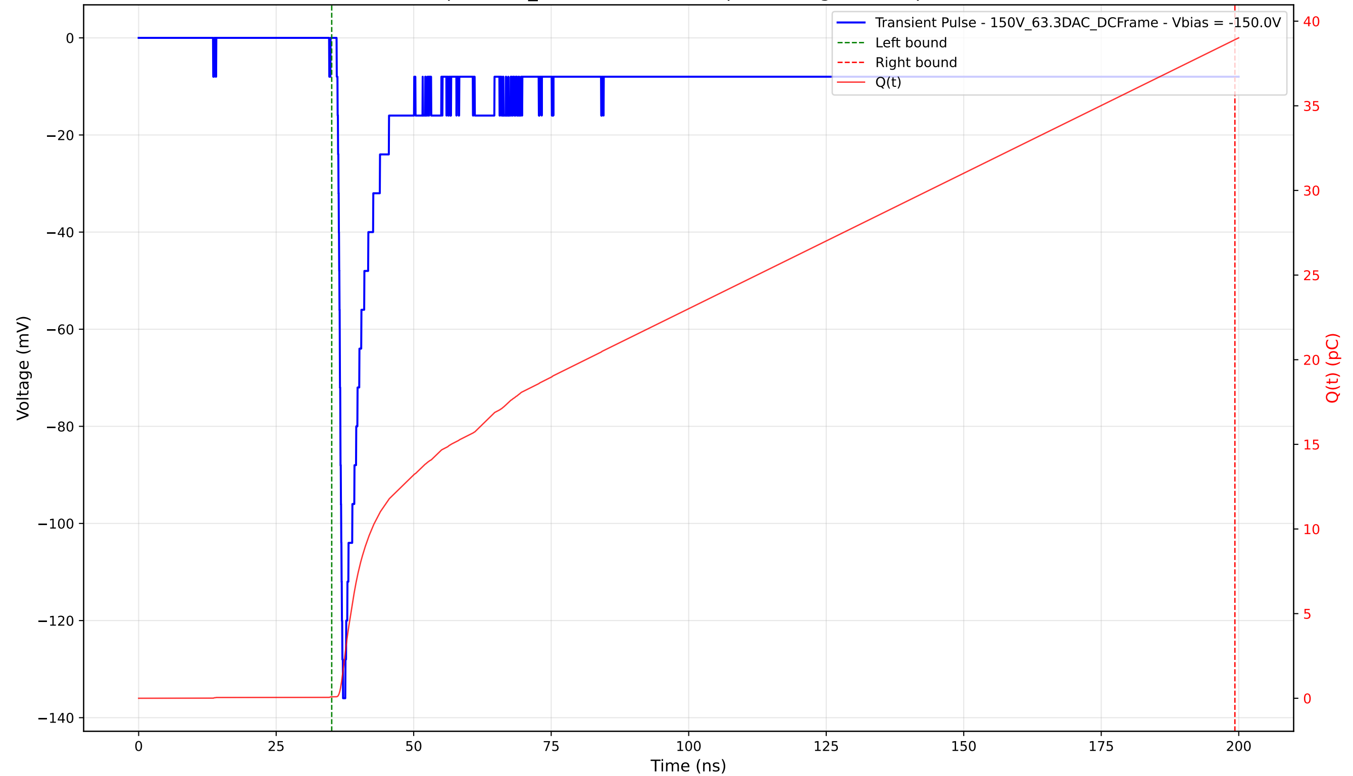
Transient Pulse - Sample: 1cm_42 - Position: 650.0 \mu\text{m} - Charge: 38.82 pC - Rise Time: 0.87 ns
