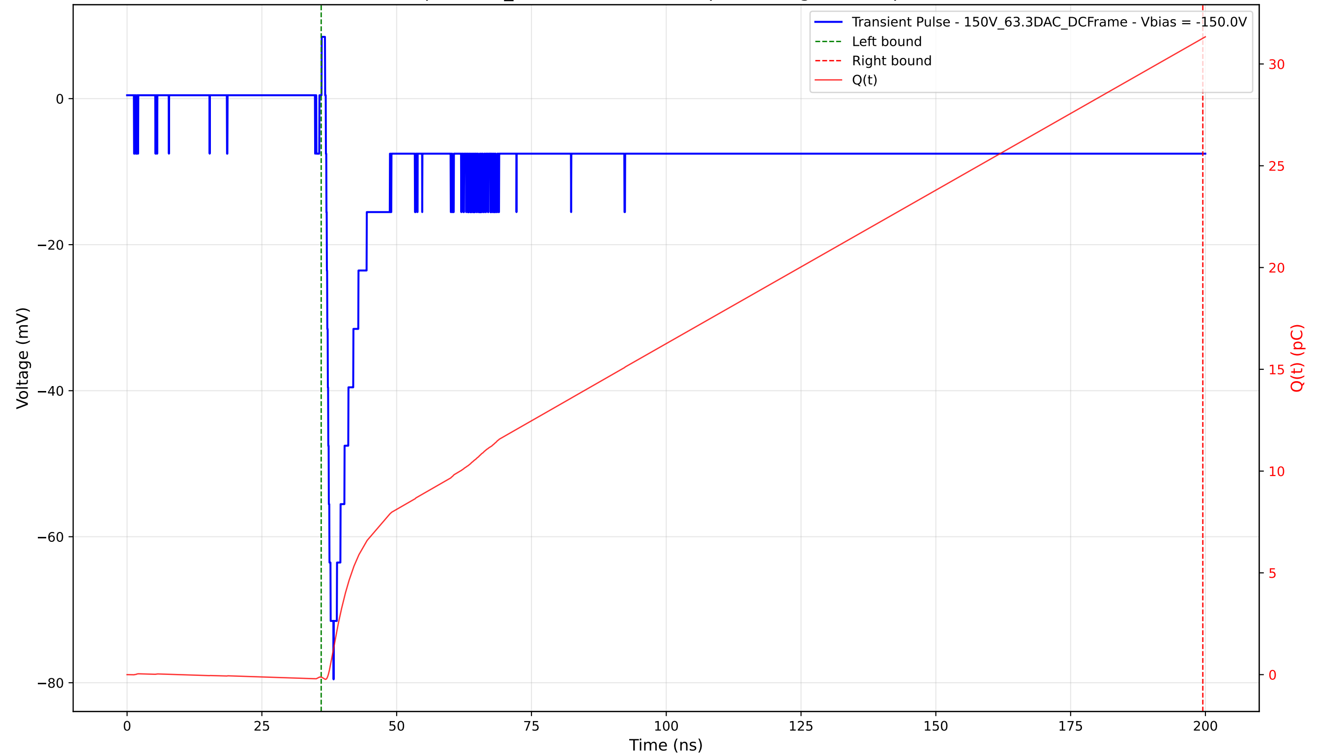
Transient Pulse - Sample: 1cm_42 - Position: 1180.0 \mu\text{m} - Charge: 31.39 pC - Rise Time: 1.34 ns
