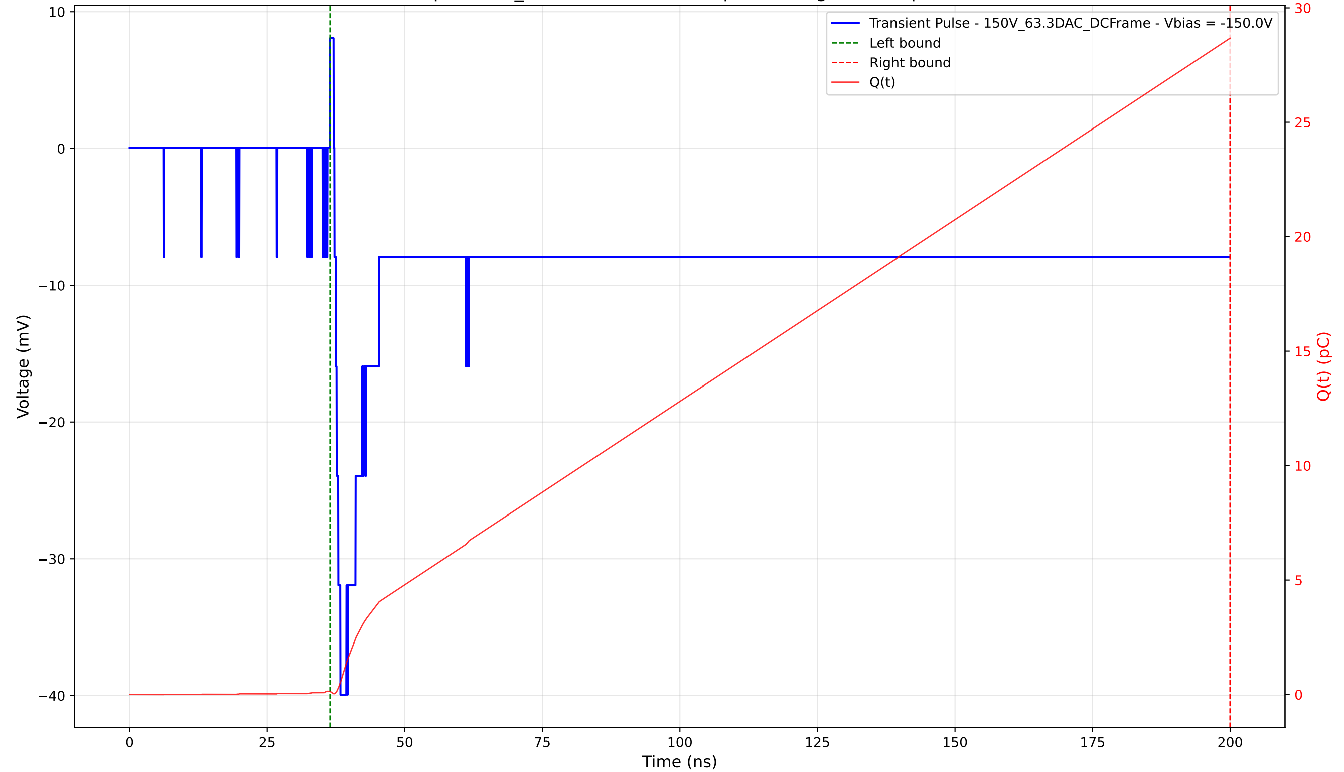
Transient Pulse - Sample: 1cm_42 - Position: 3530.0 \mu\text{m} - Charge: 28.54 pC - Rise Time: 1.09 ns
