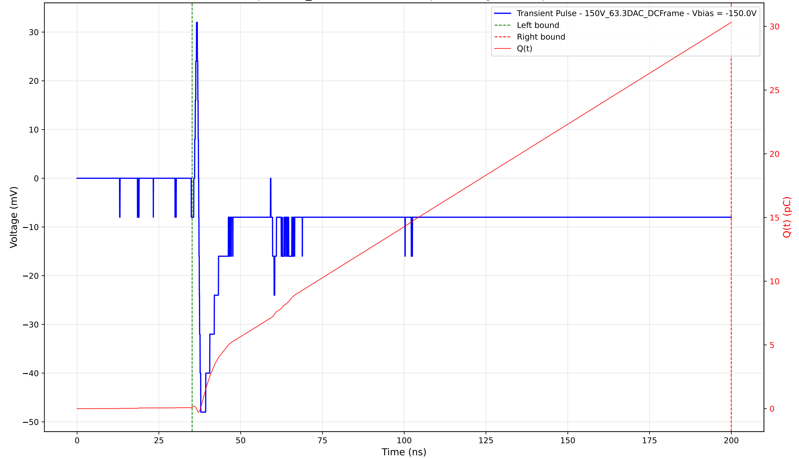
Transient Pulse - Sample: 1cm_42 - Position: 1745.0 \mu\text{m} - Charge: 30.20 pC - Rise Time: 0.63 ns
