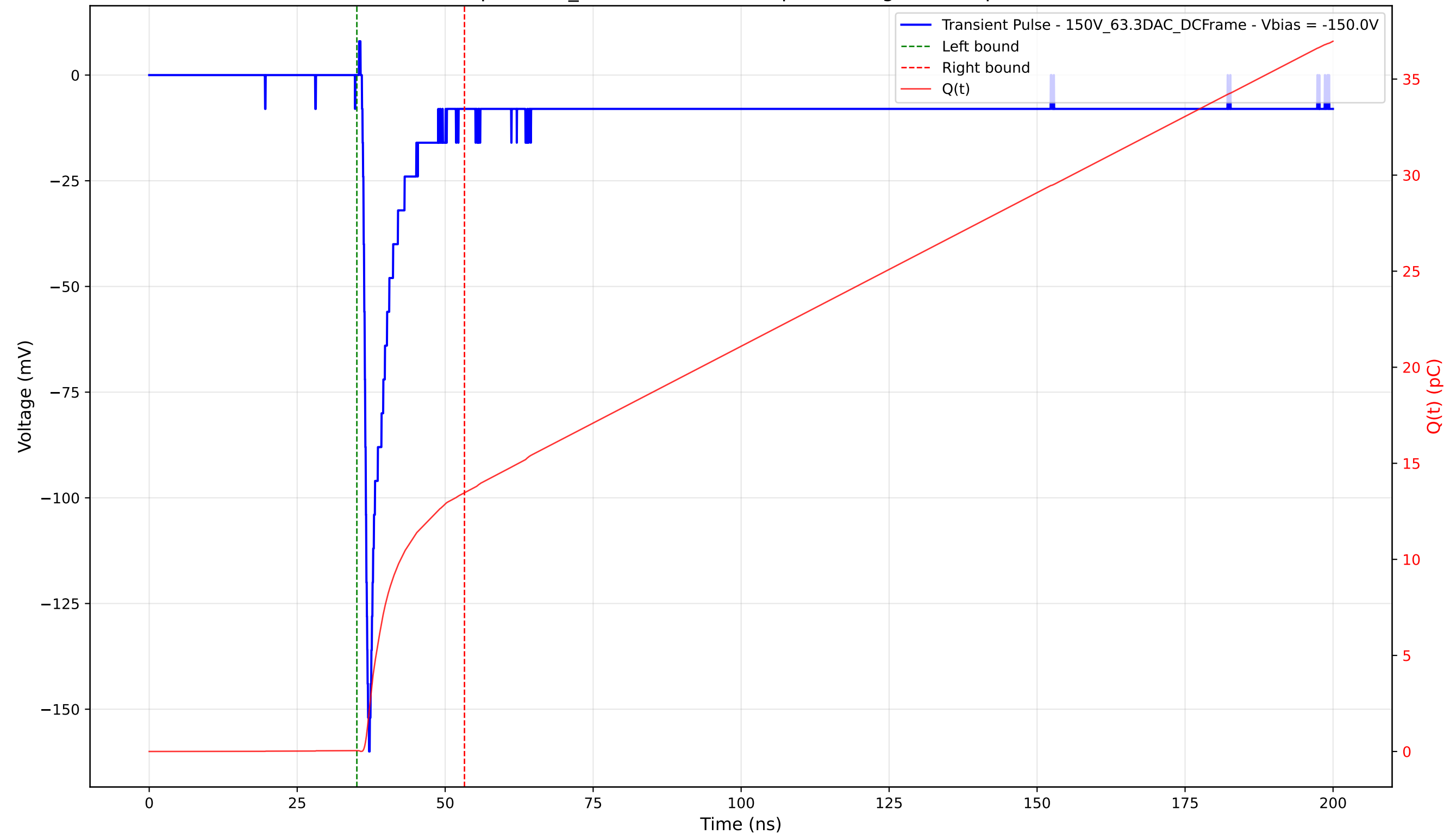
Transient Pulse - Sample: 1cm_42 - Position: 520.0 \mu\text{m} - Charge: 13.42 pC - Rise Time: 0.78 ns
