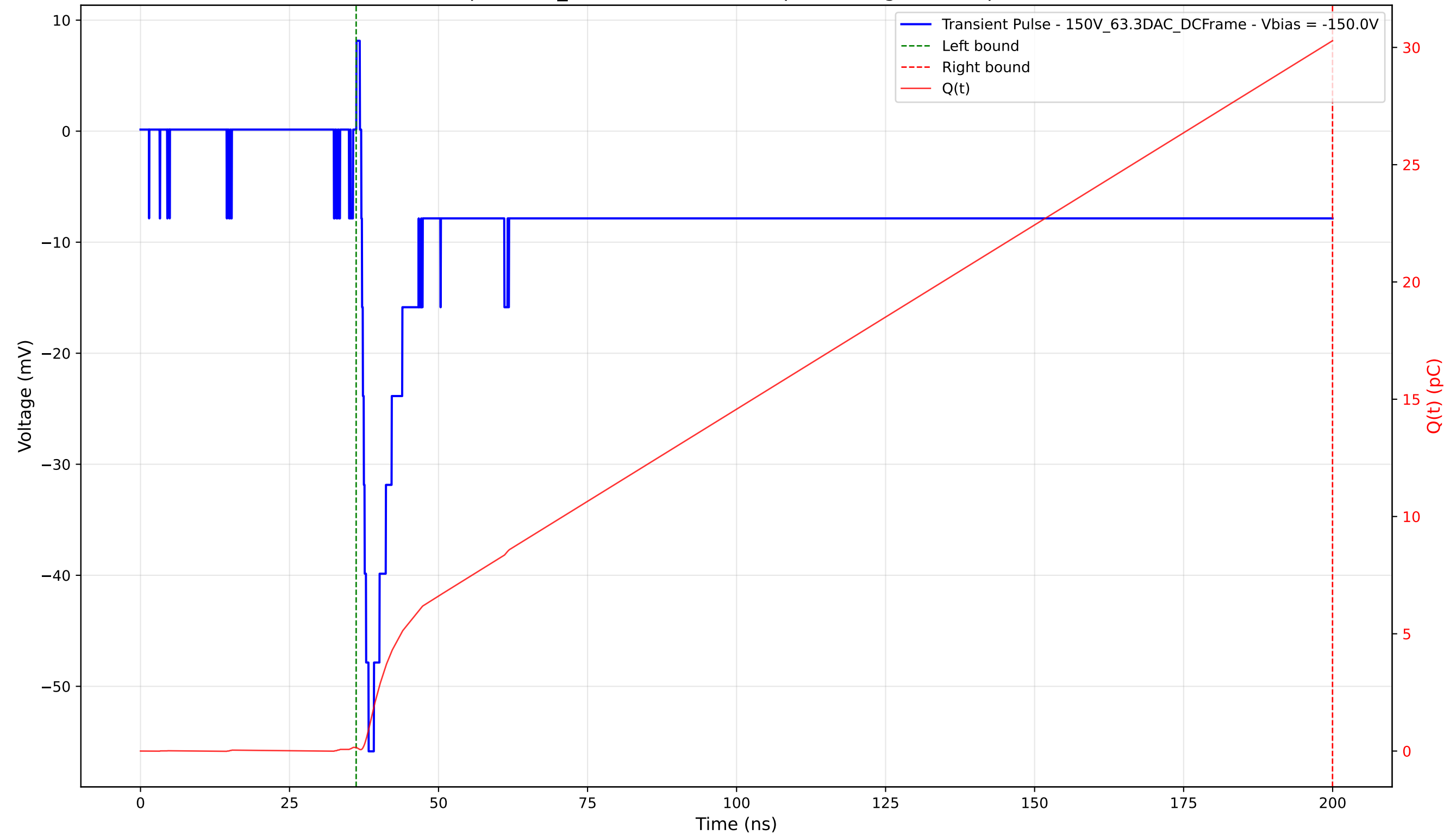
Transient Pulse - Sample: 1cm_42 - Position: 3785.0 \mu\text{m} - Charge: 30.13 pC - Rise Time: 1.23 ns
