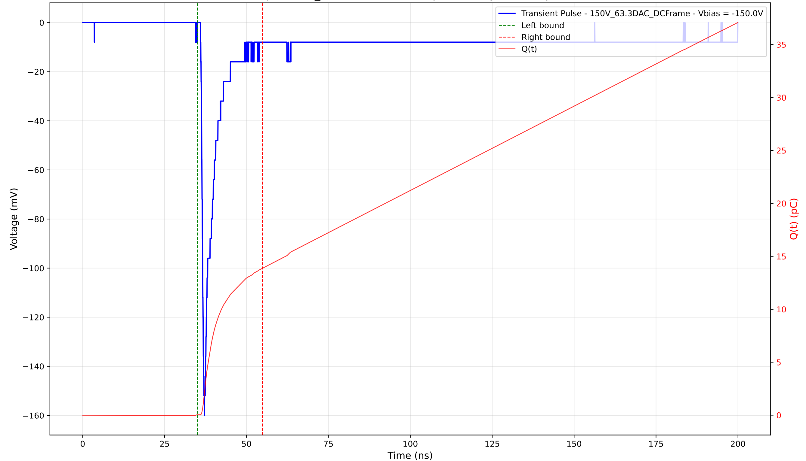
Transient Pulse - Sample: 1cm_42 - Position: 530.0 \mu\text{m} - Charge: 13.83 pC - Rise Time: 0.88 ns
