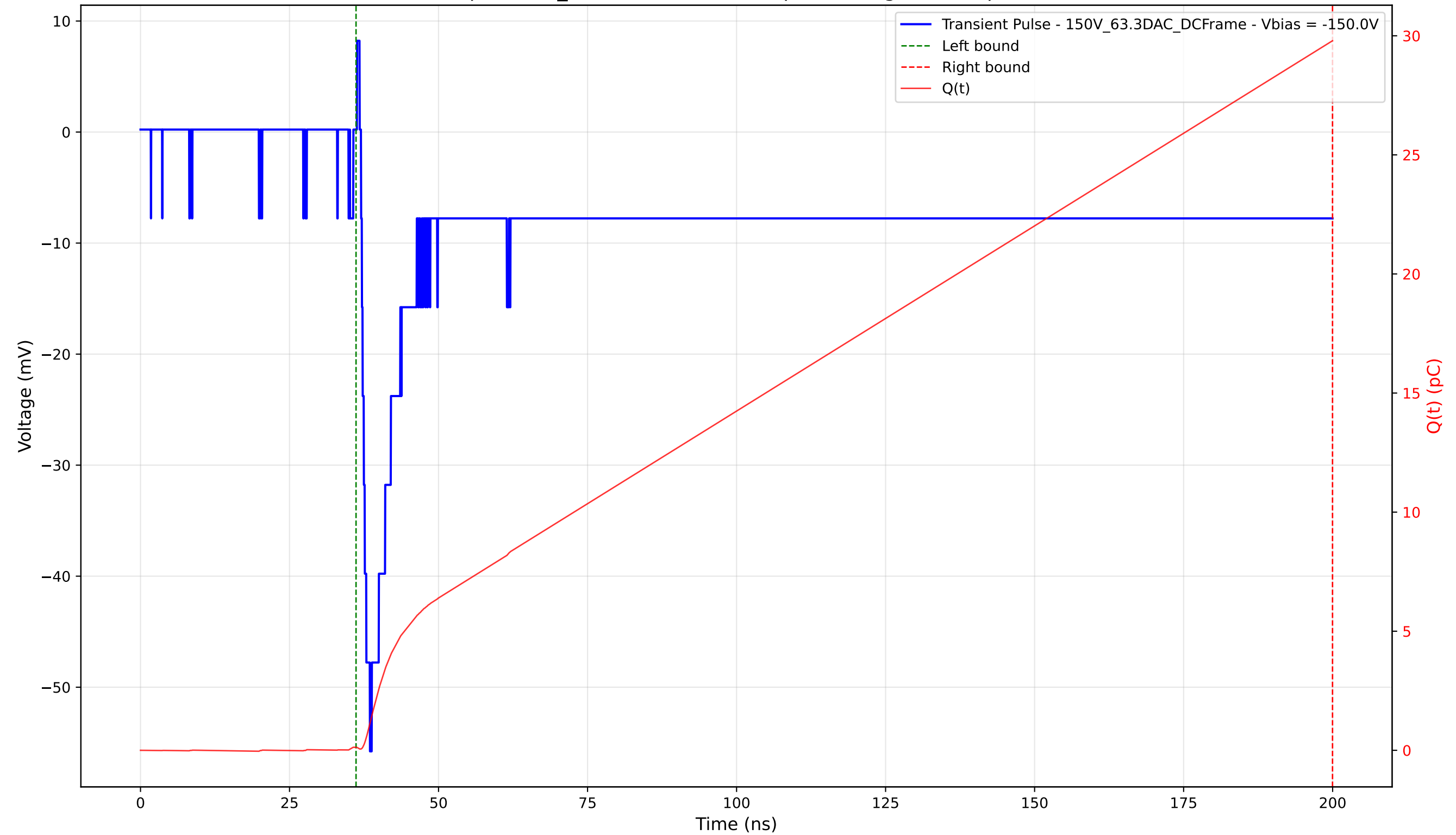
Transient Pulse - Sample: 1cm_42 - Position: 3825.0 \mu\text{m} - Charge: 29.67 pC - Rise Time: 1.49 ns
