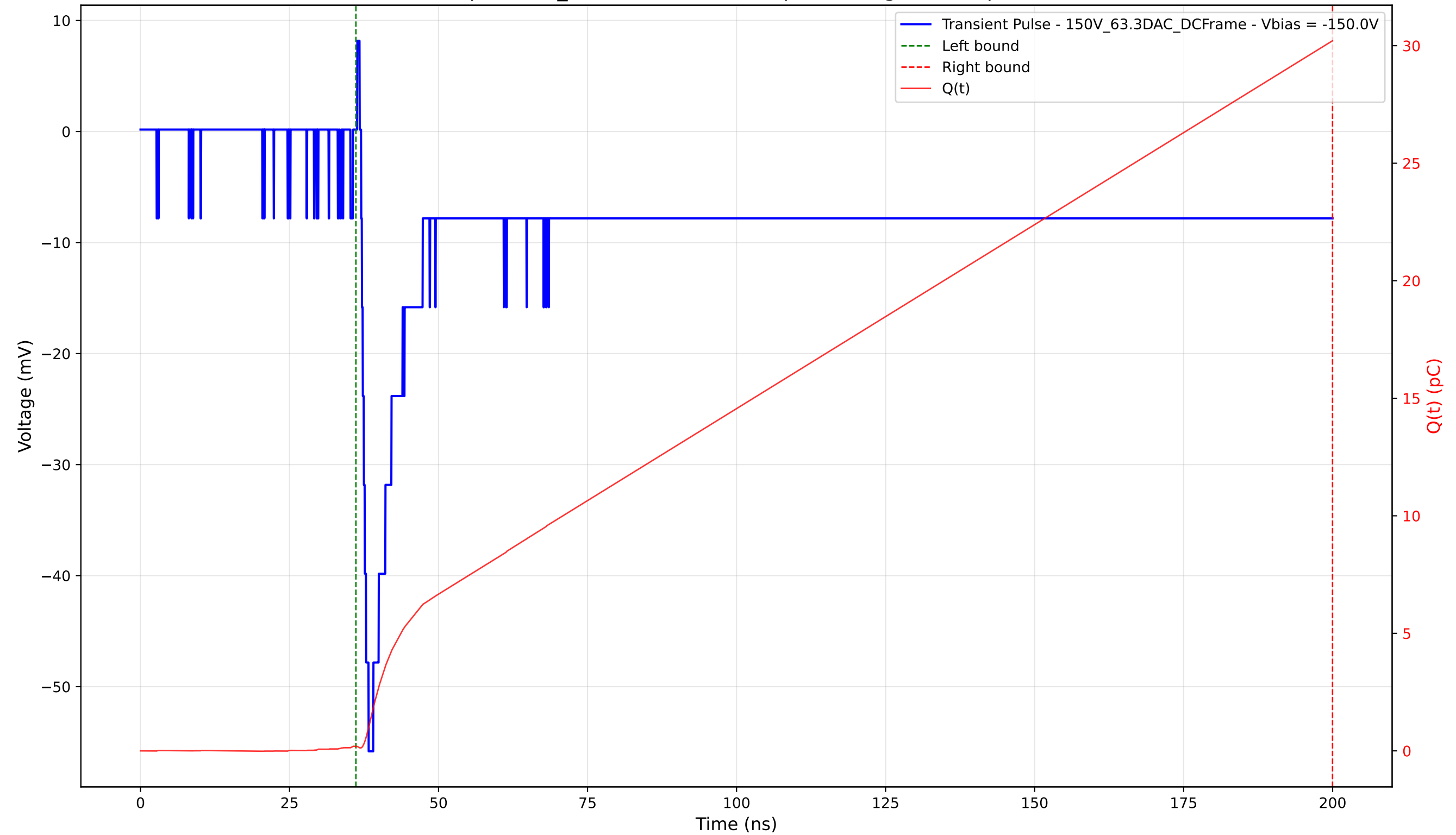
Transient Pulse - Sample: 1cm_42 - Position: 3805.0 \mu\text{m} - Charge: 30.02 pC - Rise Time: 1.25 ns
