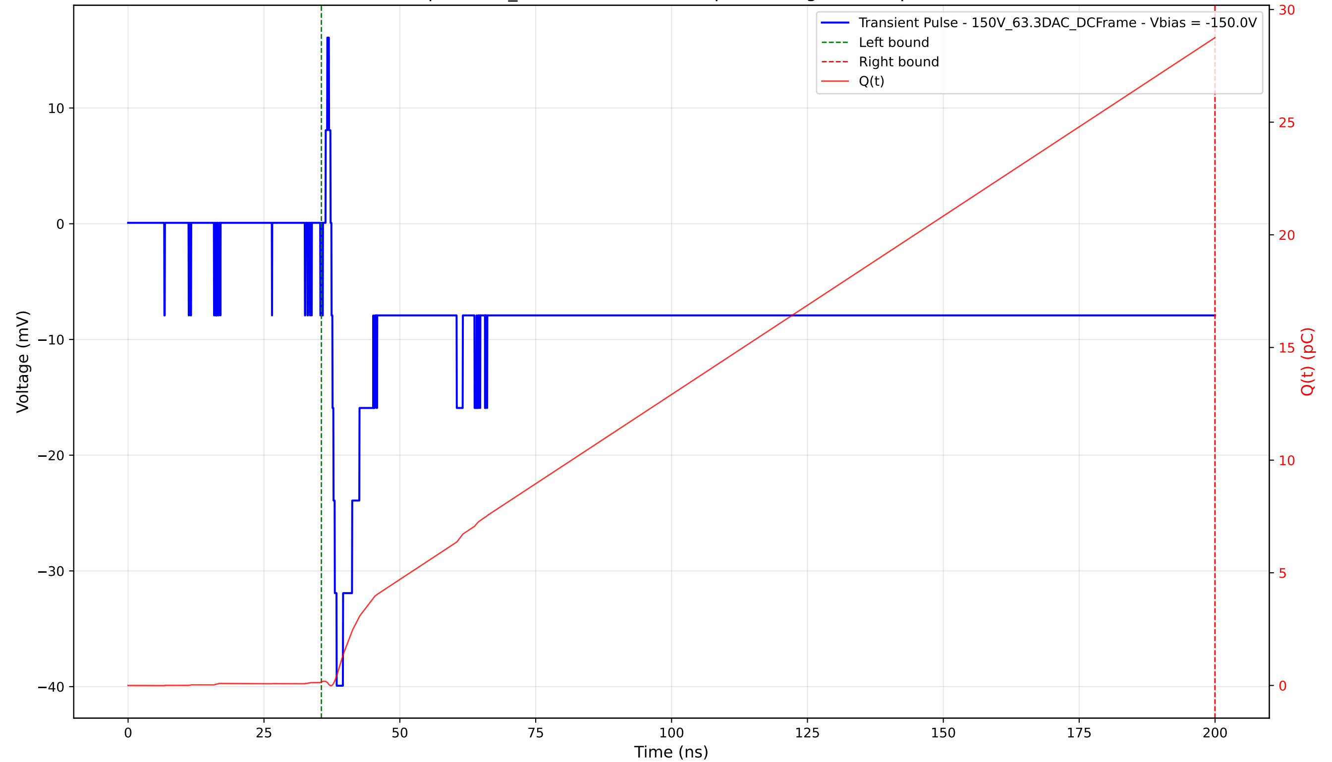
Transient Pulse - Sample: 1cm_42 - Position: 3255.0 \mu\text{m} - Charge: 28.59 pC - Rise Time: 0.95 ns
