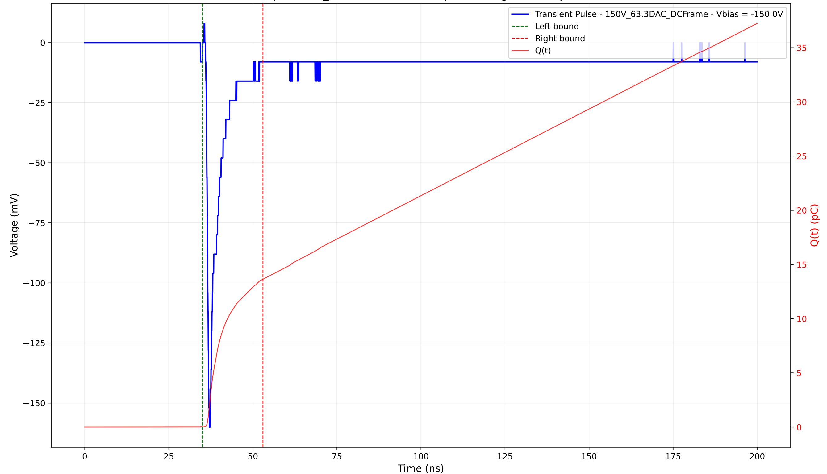
Transient Pulse - Sample: 1cm_42 - Position: 505.0 \mu\text{m} - Charge: 13.55 pC - Rise Time: 0.74 ns
