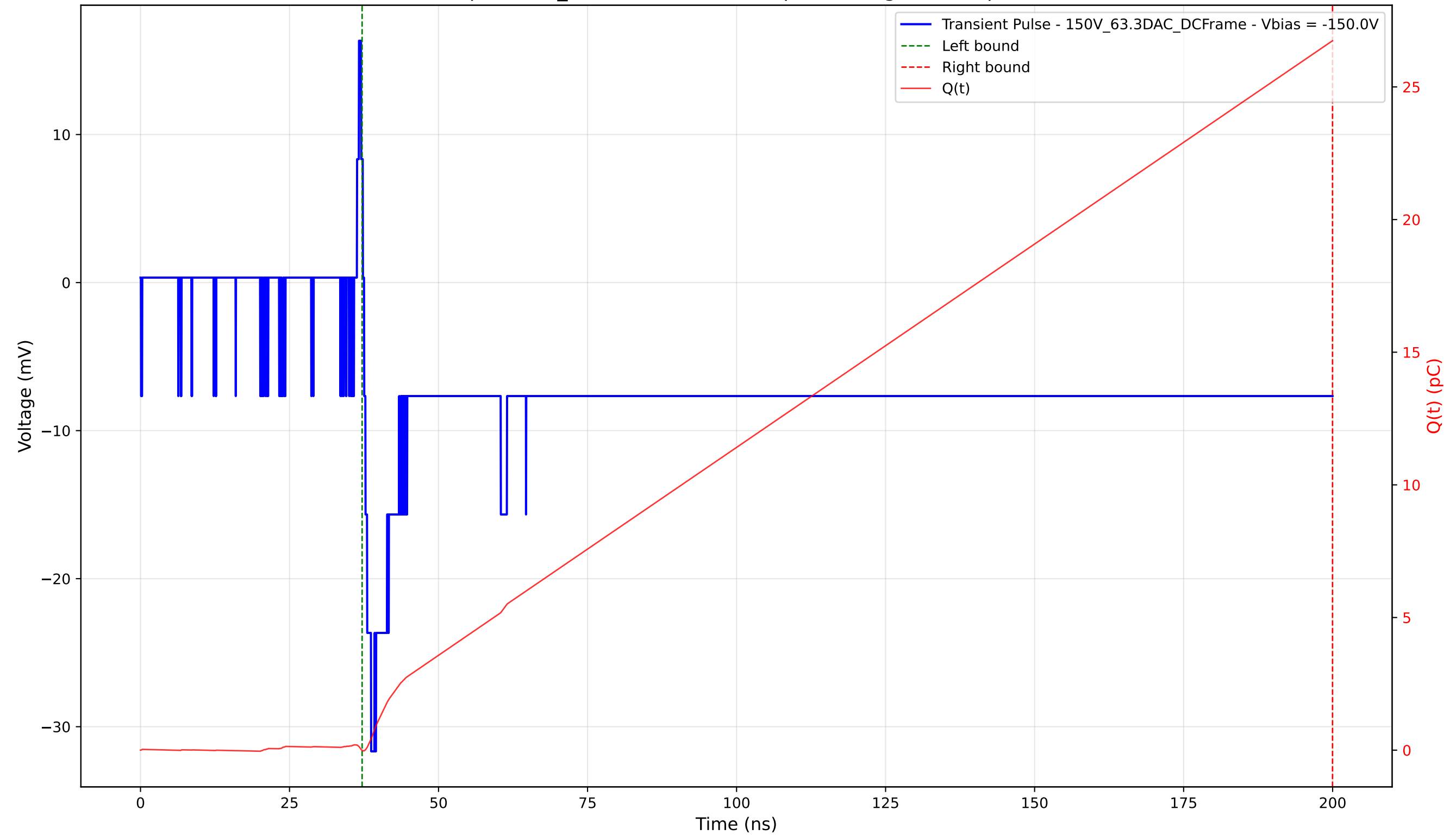
Transient Pulse - Sample: 1cm_42 - Position: 2940.0 \mu\text{m} - Charge: 26.75 pC - Rise Time: 1.17 ns
