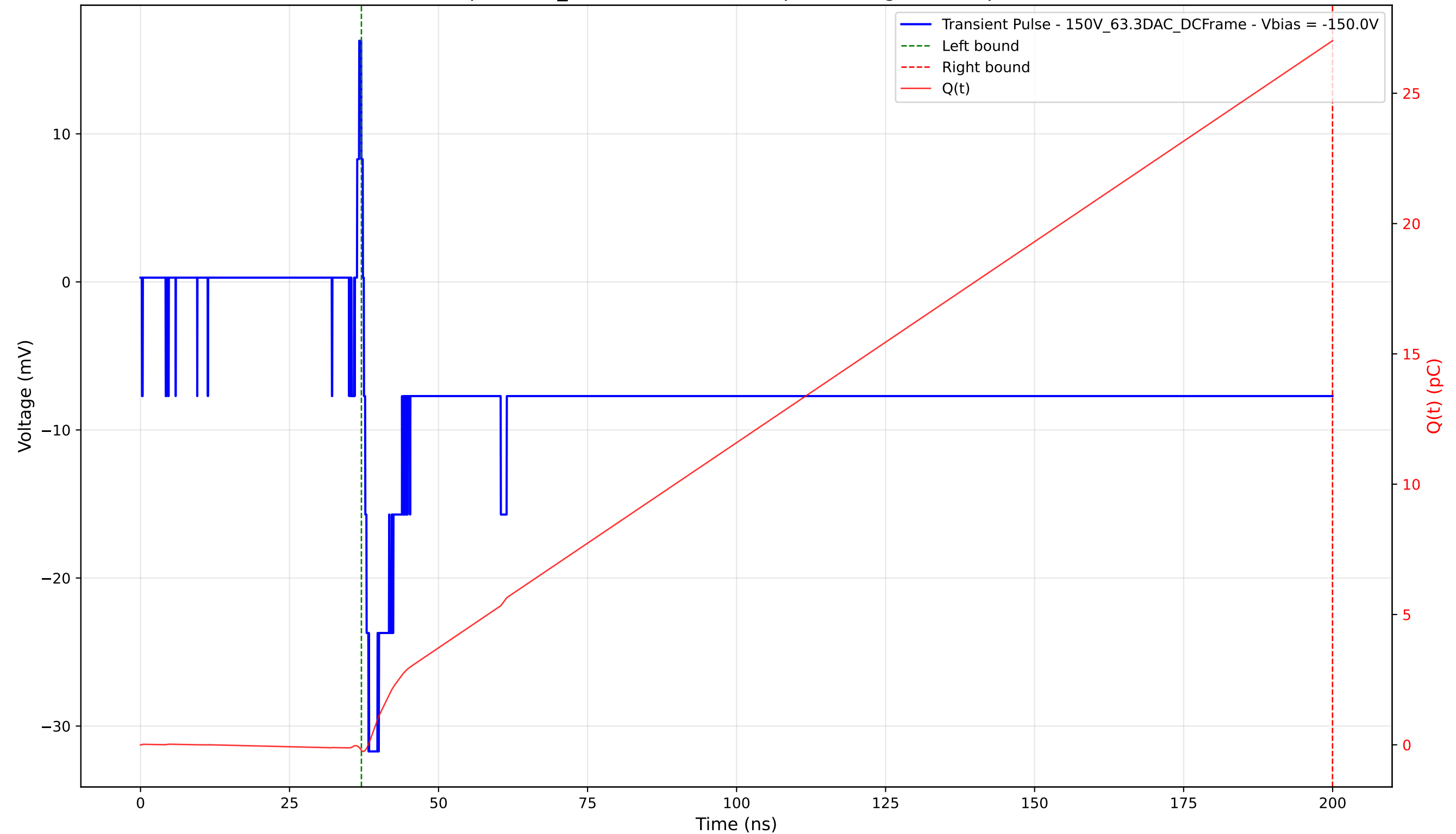
Transient Pulse - Sample: 1cm_42 - Position: 3095.0 \mu\text{m} - Charge: 27.23 pC - Rise Time: 0.77 ns
