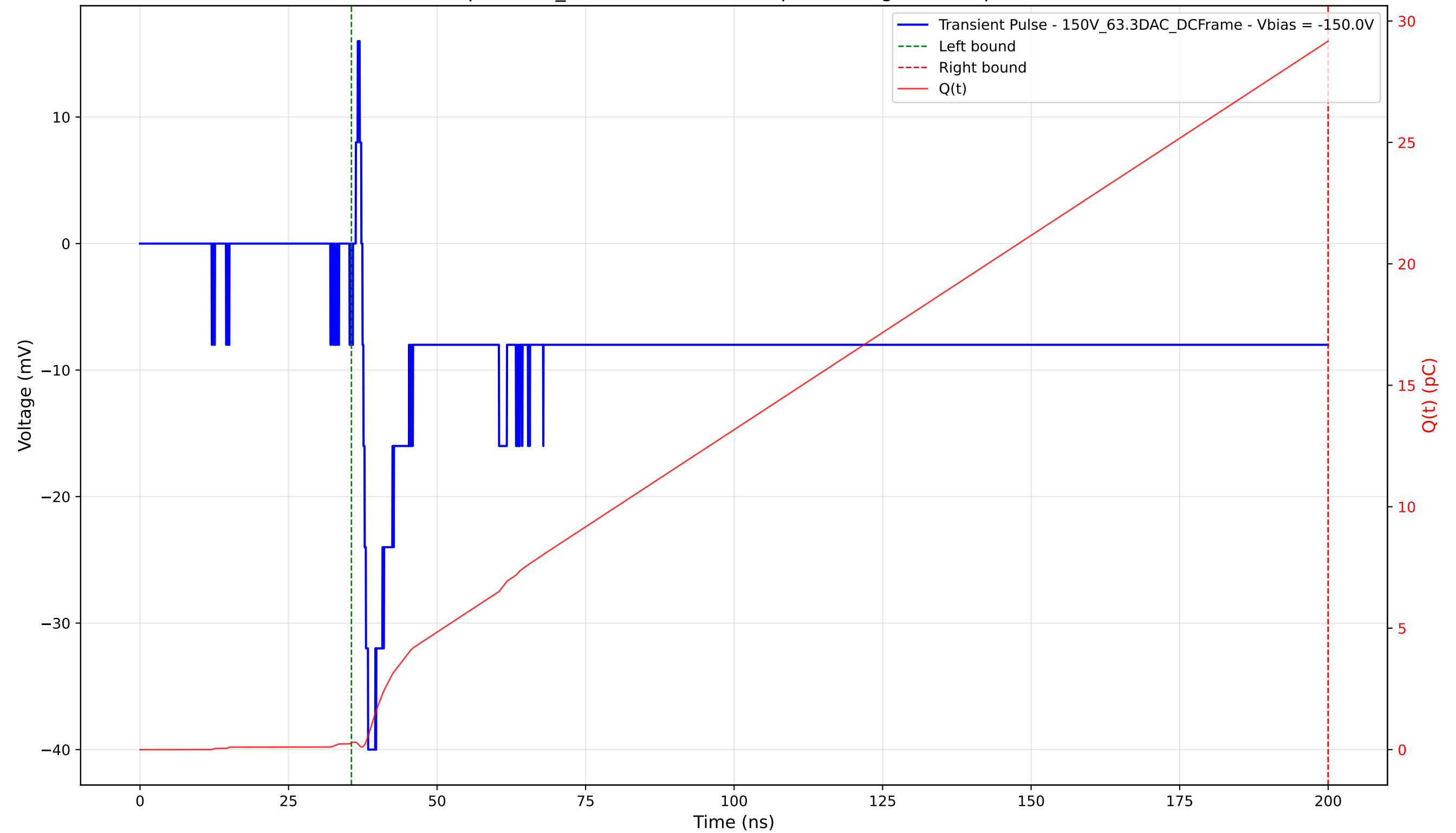
Transient Pulse - Sample: 1cm_42 - Position: 3240.0 \mu\text{m} - Charge: 28.89 pC - Rise Time: 0.95 ns
