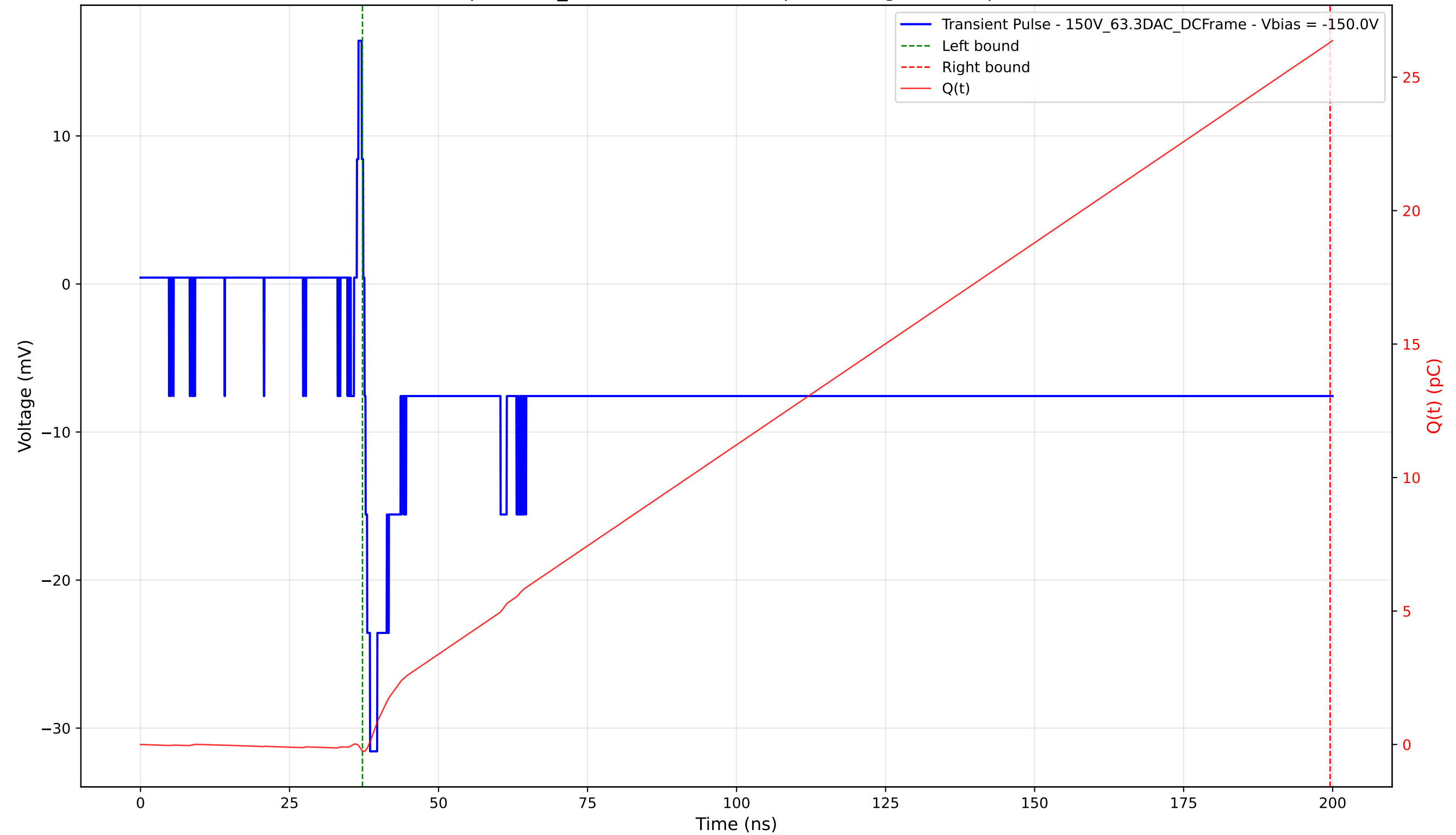
Transient Pulse - Sample: 1cm_42 - Position: 2860.0 \mu\text{m} - Charge: 26.54 pC - Rise Time: 0.93 ns
