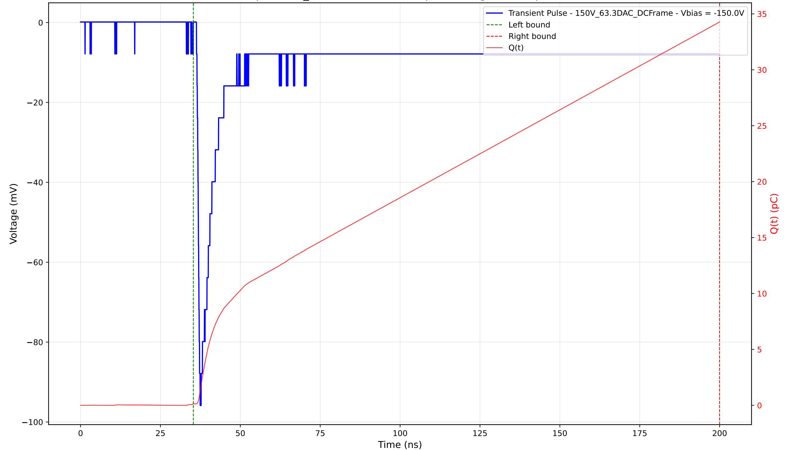
Transient Pulse - Sample: 1cm_42 - Position: 4355.0 \mu\text{m} - Charge: 34.14 pC - Rise Time: 0.82 ns
