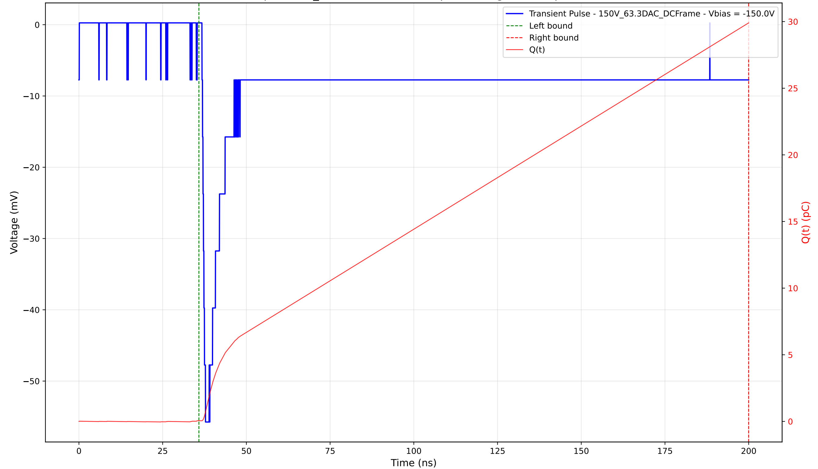
Transient Pulse - Sample: 1cm_42 - Position: 4010.0 \mu\text{m} - Charge: 29.85 pC - Rise Time: 1.05 ns
