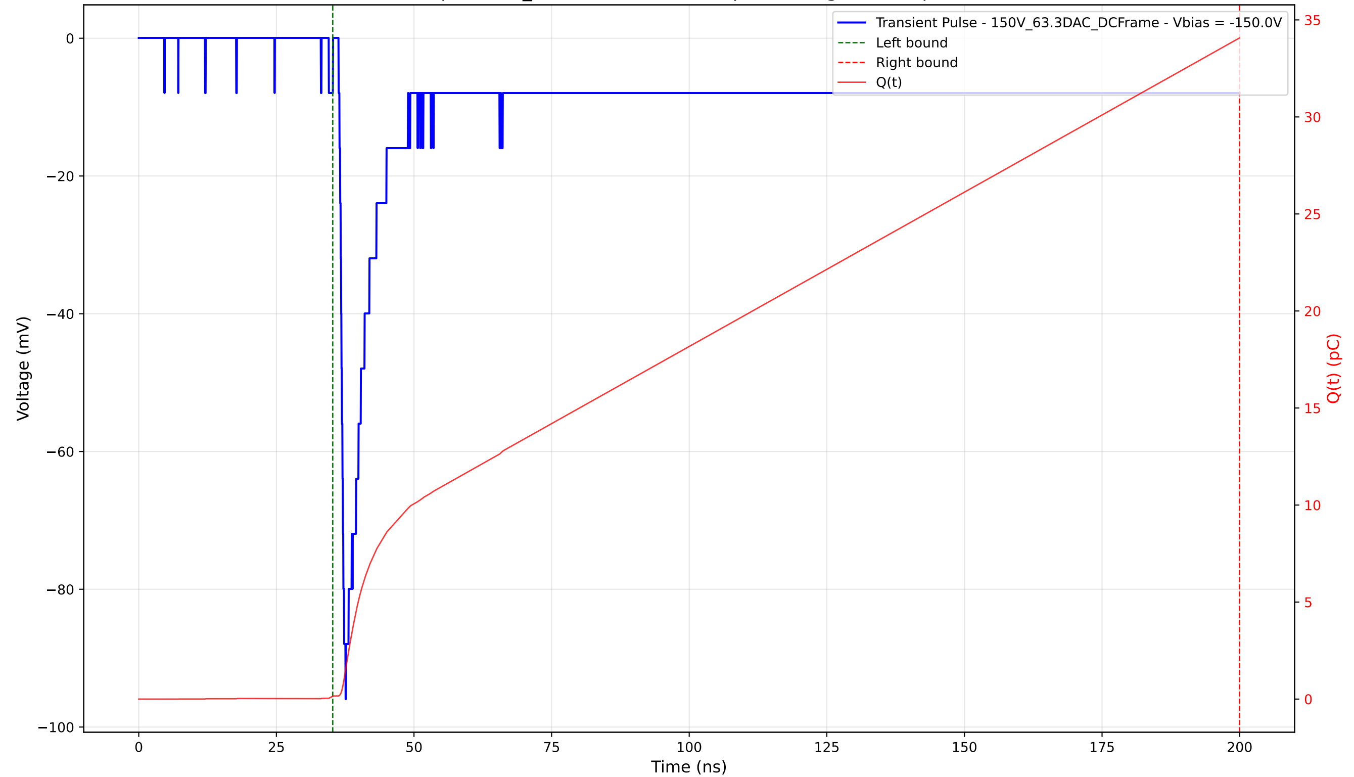
Transient Pulse - Sample: 1cm_42 - Position: 4345.0 \mu\text{m} - Charge: 33.92 pC - Rise Time: 0.86 ns
