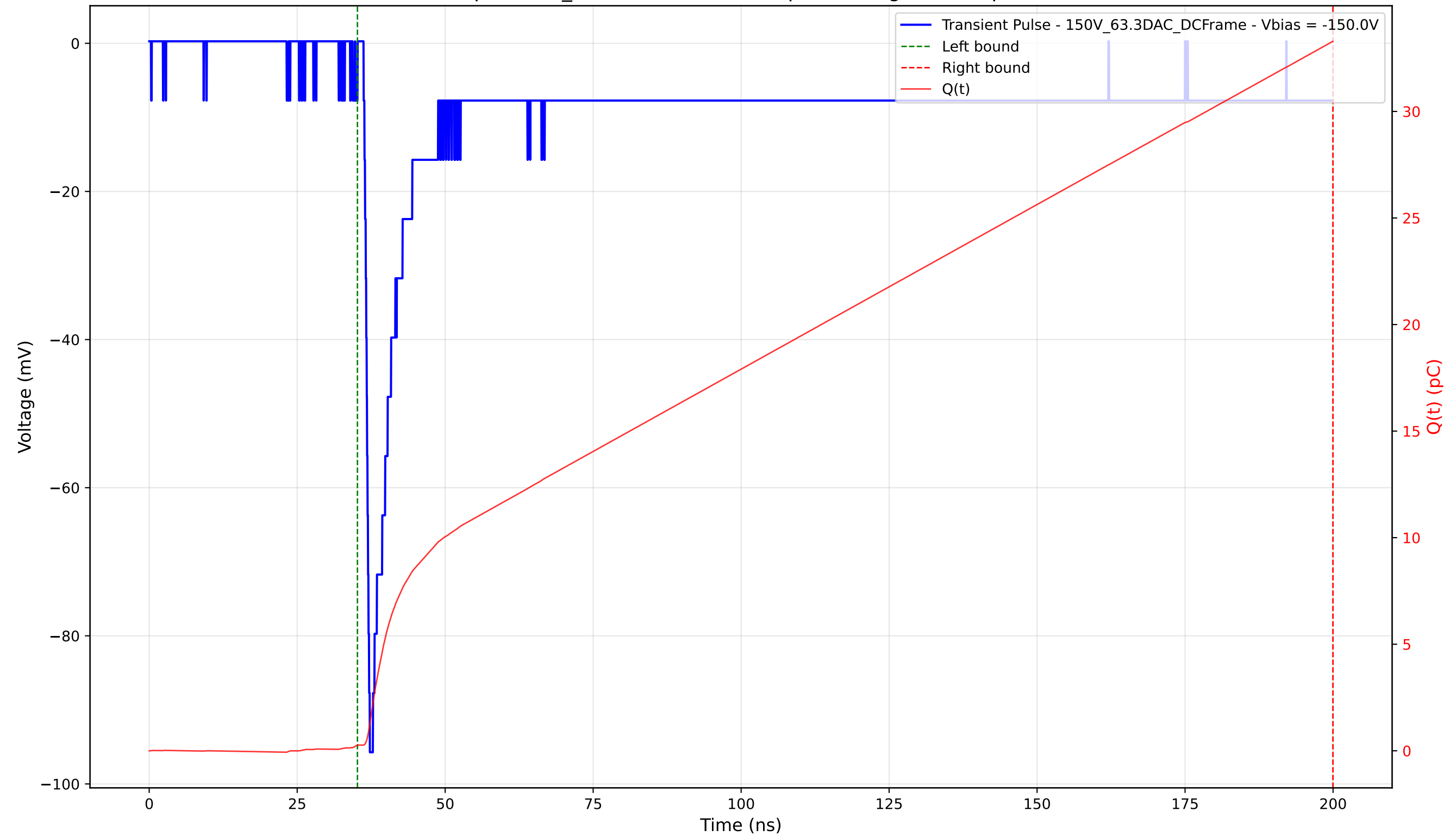
Transient Pulse - Sample: 1cm_42 - Position: 4420.0 \mu\text{m} - Charge: 33.03 pC - Rise Time: 0.80 ns
