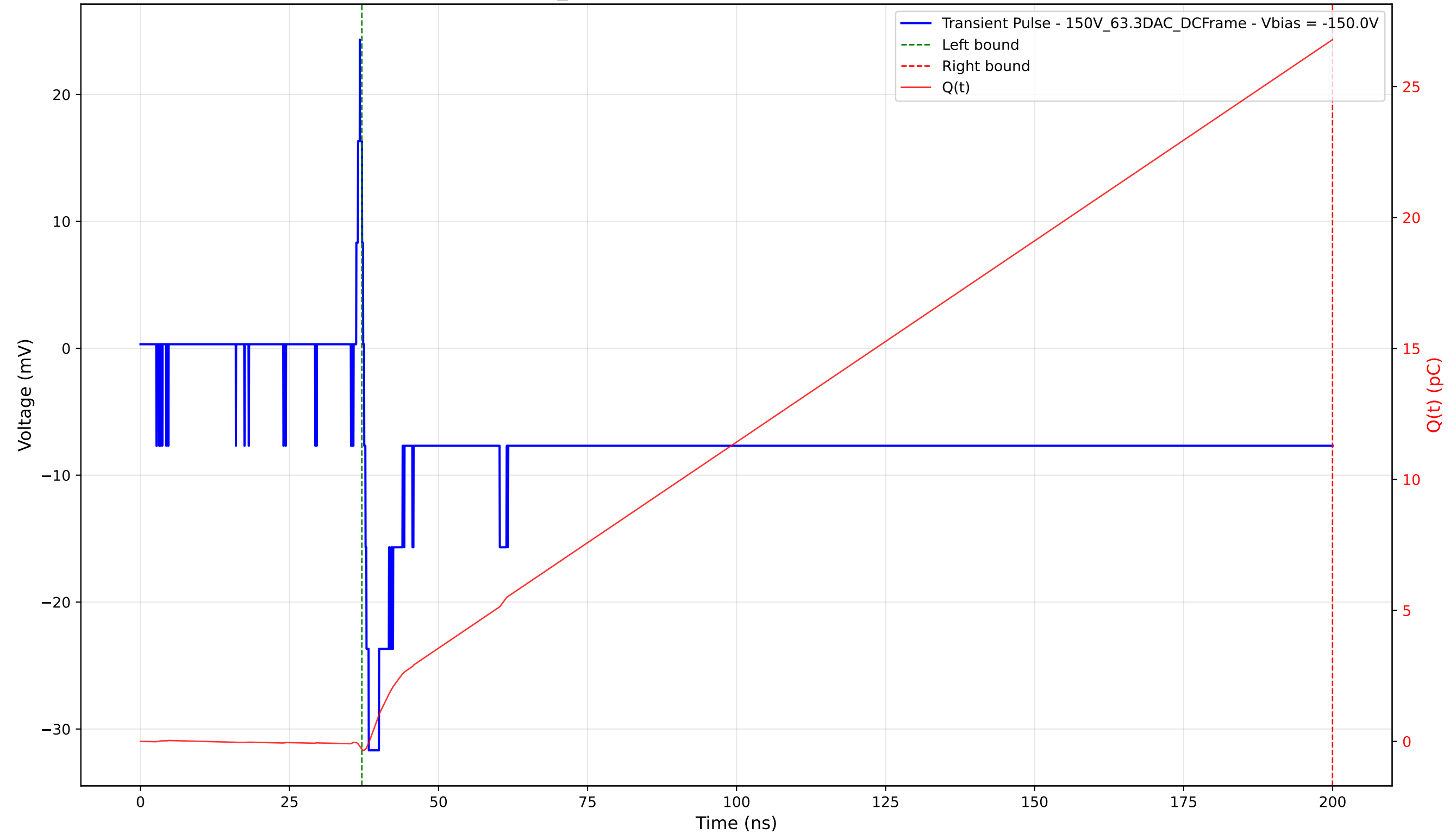
Transient Pulse - Sample: 1cm_42 - Position: 2680.0 \mu\text{m} - Charge: 27.10 pC - Rise Time: 0.77 ns
