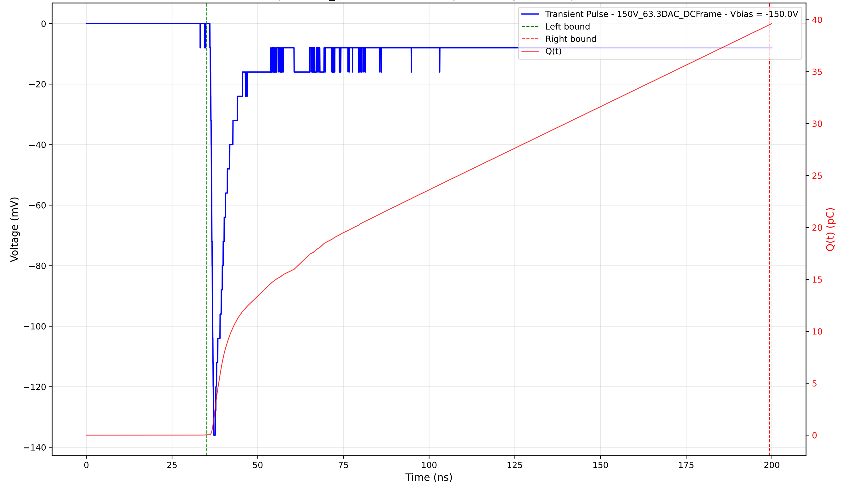
Transient Pulse - Sample: 1cm_42 - Position: 675.0 \mu\text{m} - Charge: 39.48 pC - Rise Time: 0.89 ns
