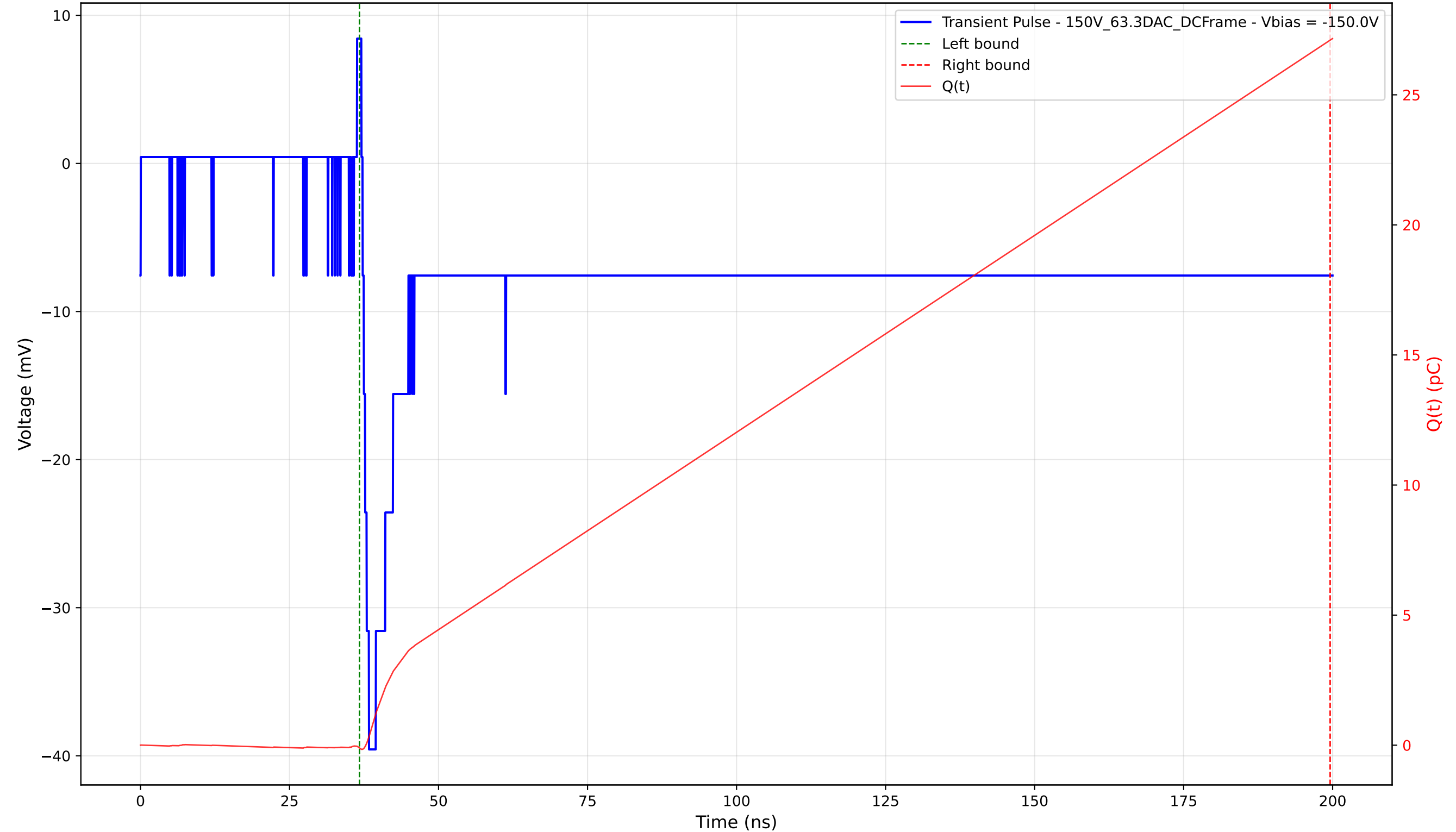
Transient Pulse - Sample: 1cm_42 - Position: 3510.0 \mu\text{m} - Charge: 27.21 pC - Rise Time: 1.07 ns
