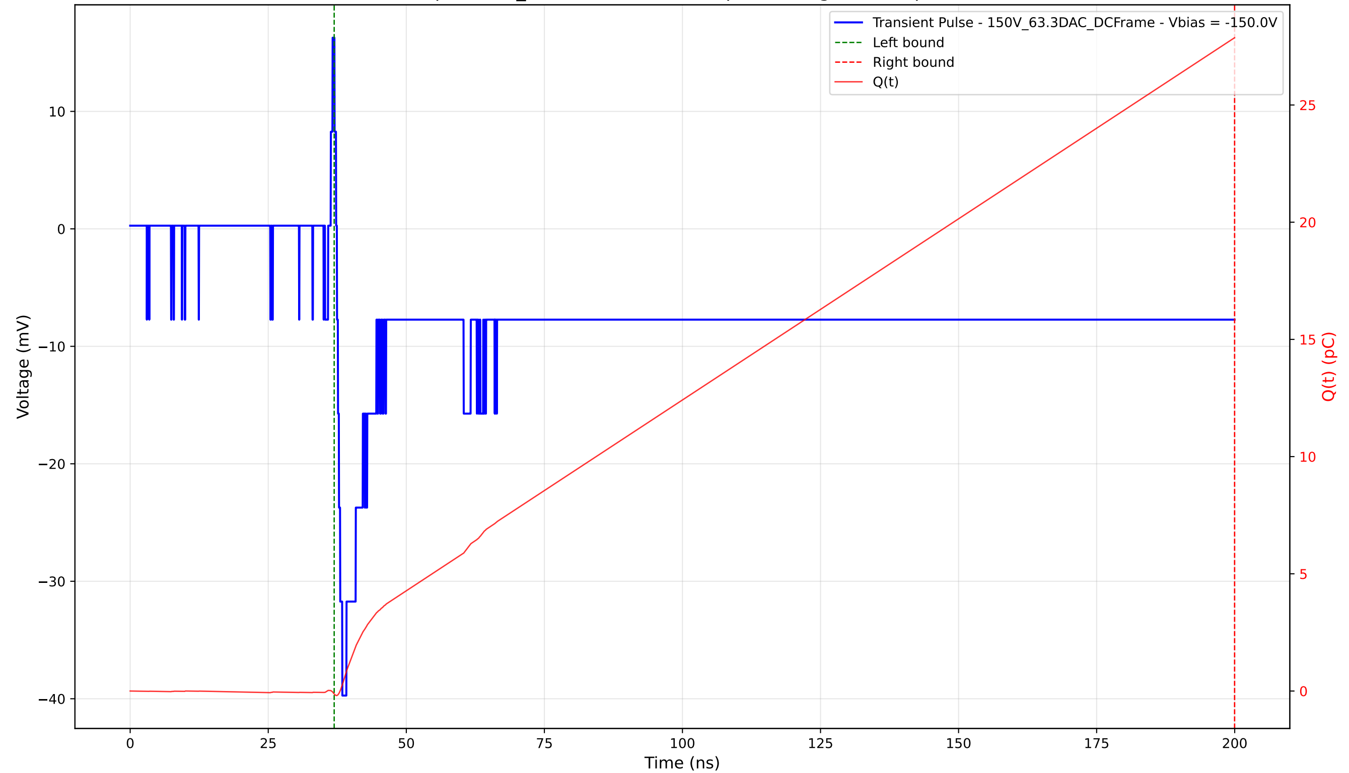
Transient Pulse - Sample: 1cm_42 - Position: 3205.0 \mu\text{m} - Charge: 28.00 pC - Rise Time: 0.97 ns
