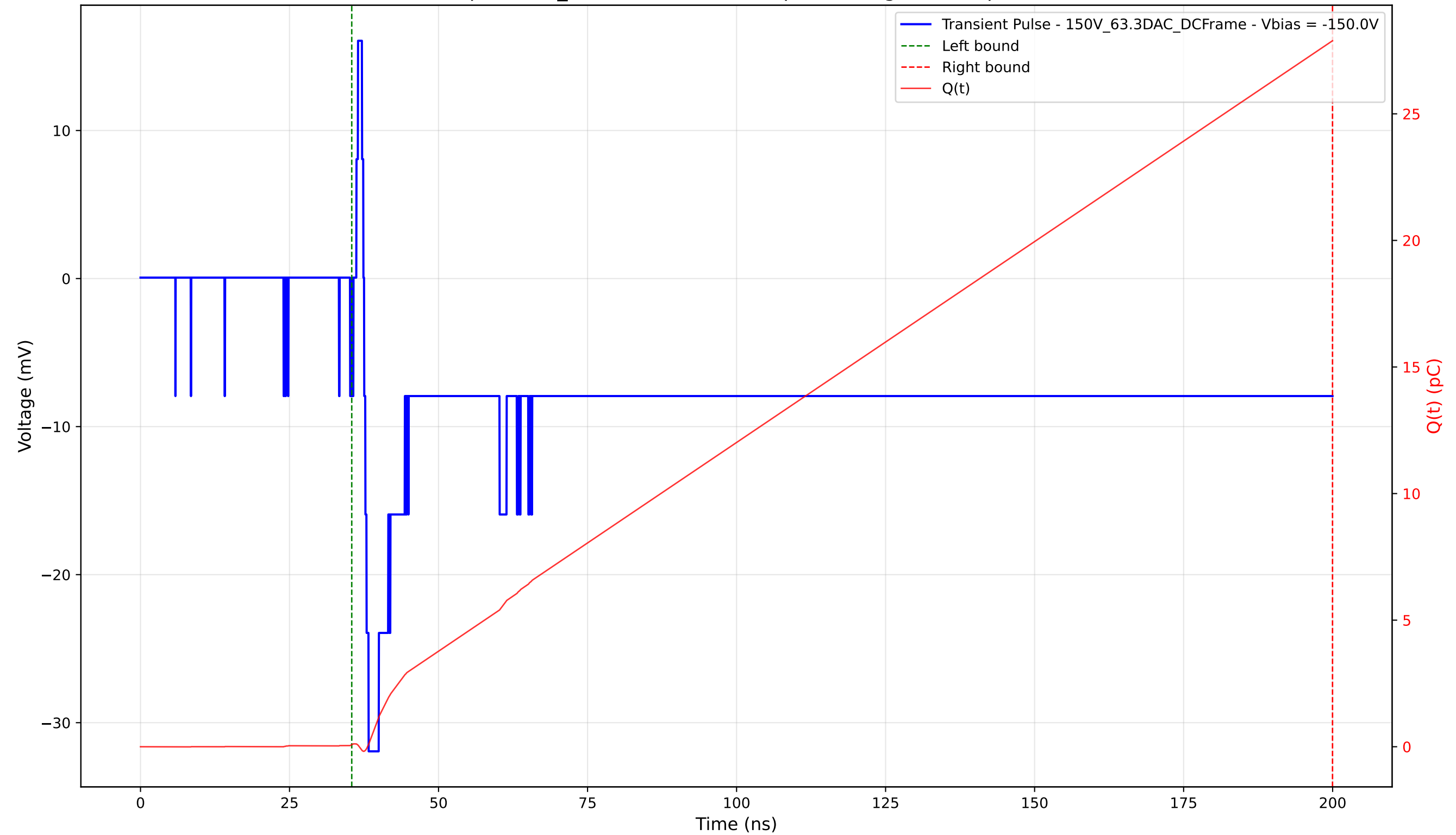
Transient Pulse - Sample: 1cm_42 - Position: 2665.0 \mu\text{m} - Charge: 27.80 pC - Rise Time: 0.75 ns
