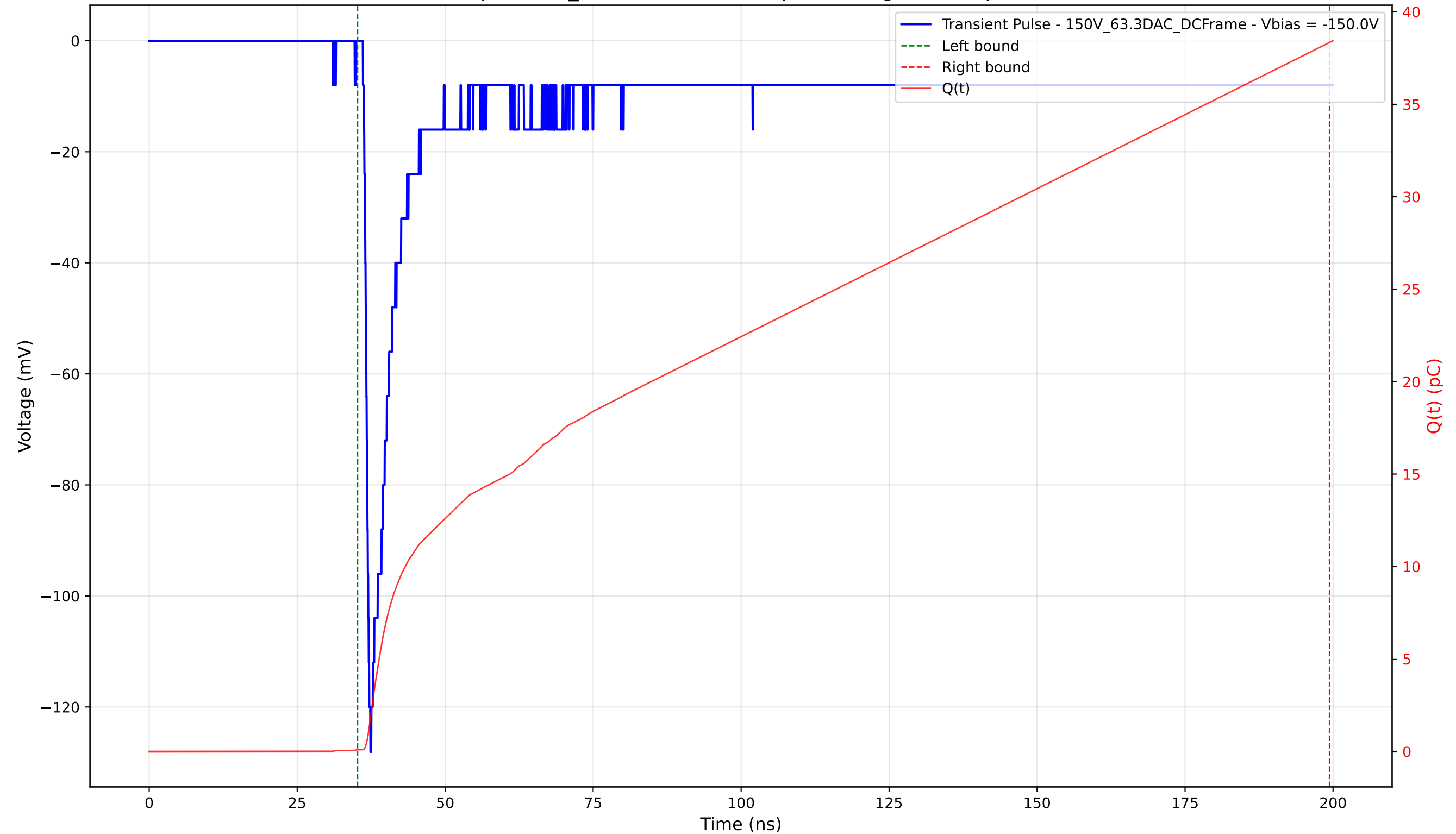
Transient Pulse - Sample: 1cm_42 - Position: 775.0 \mu\text{m} - Charge: 38.26 pC - Rise Time: 0.93 ns
