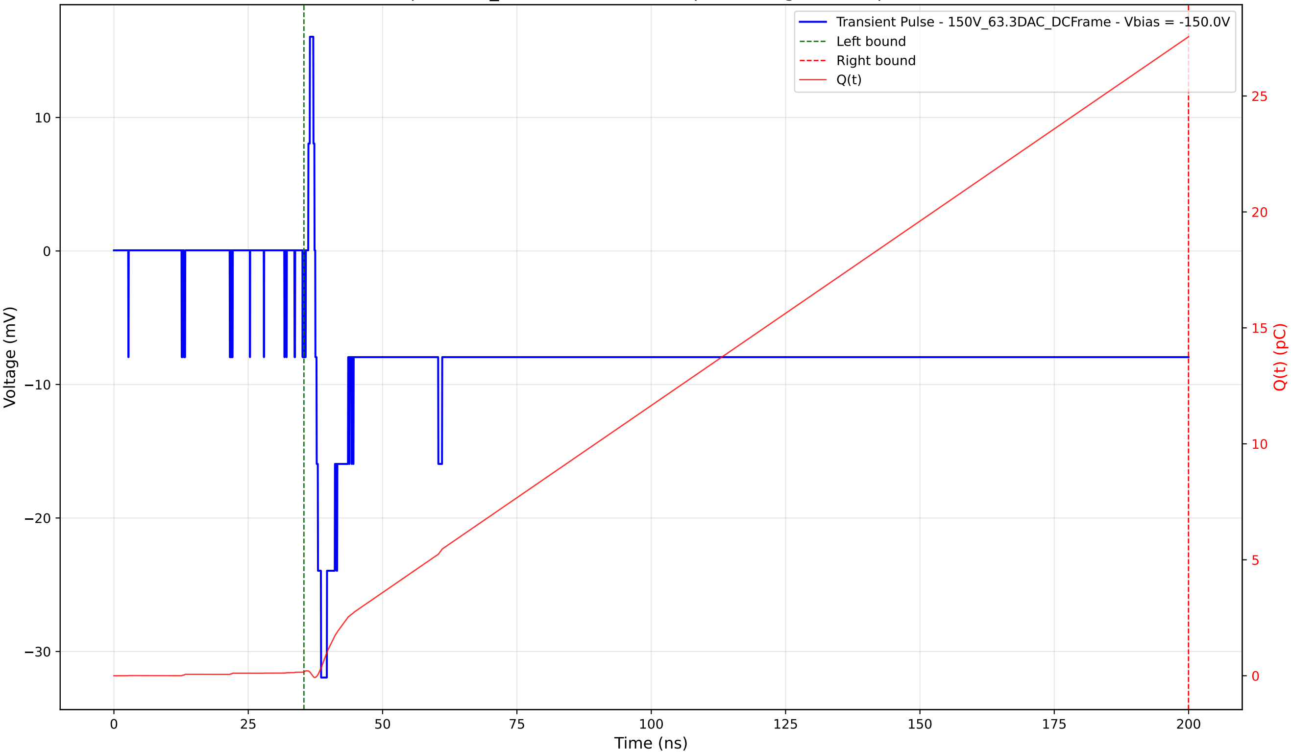
Transient Pulse - Sample: 1cm_42 - Position: 2590.0 \mu\text{m} - Charge: 27.38 pC - Rise Time: 1.07 ns
