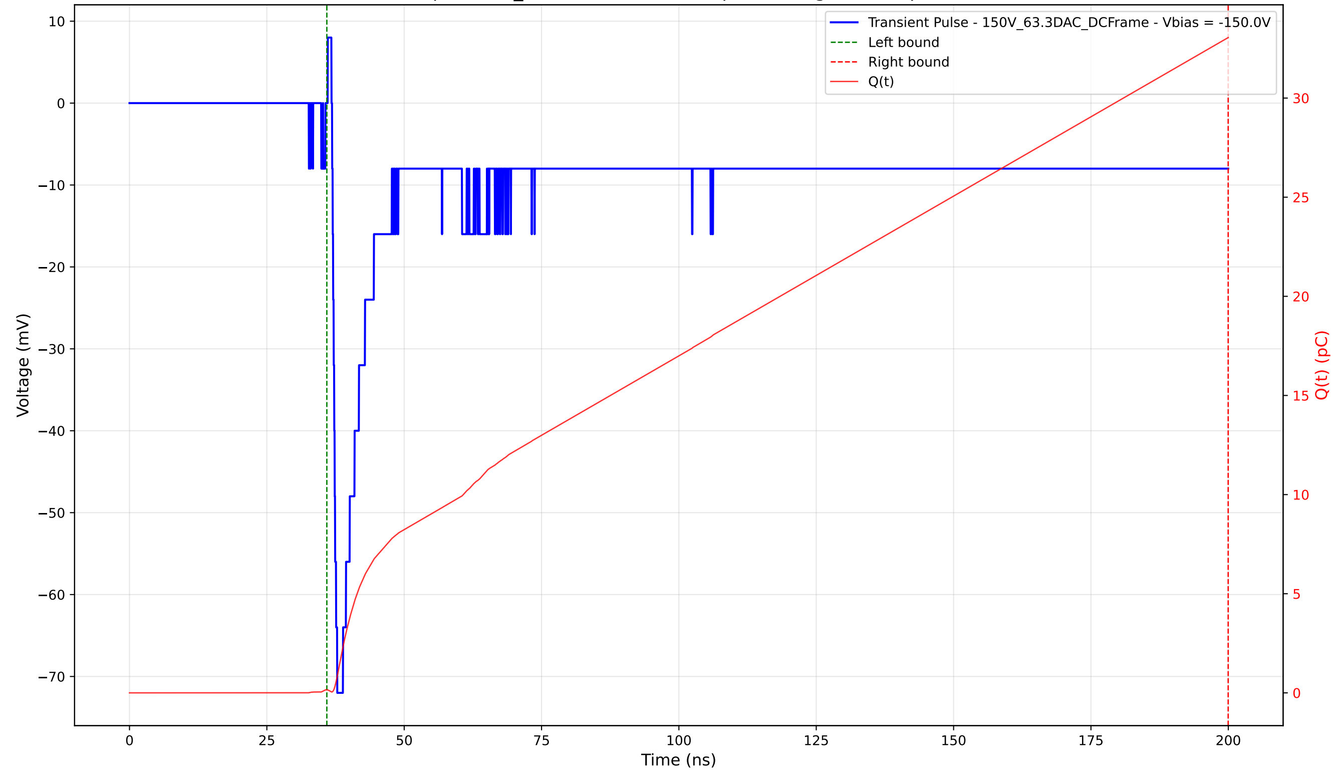
Transient Pulse - Sample: 1cm_42 - Position: 1245.0 \mu\text{m} - Charge: 32.90 pC - Rise Time: 0.92 ns
