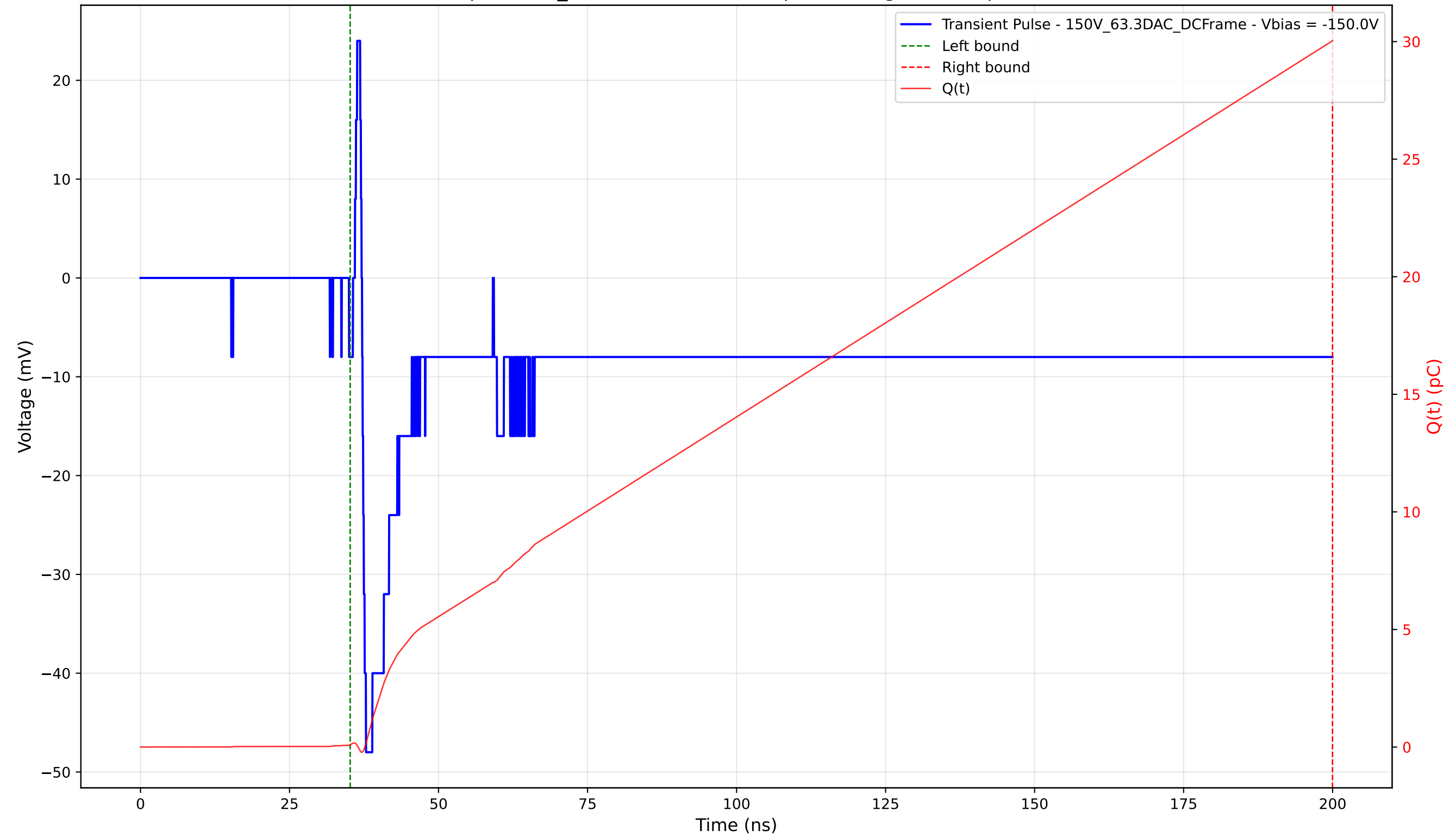
Transient Pulse - Sample: 1cm_42 - Position: 1645.0 \mu\text{m} - Charge: 29.93 pC - Rise Time: 0.65 ns
