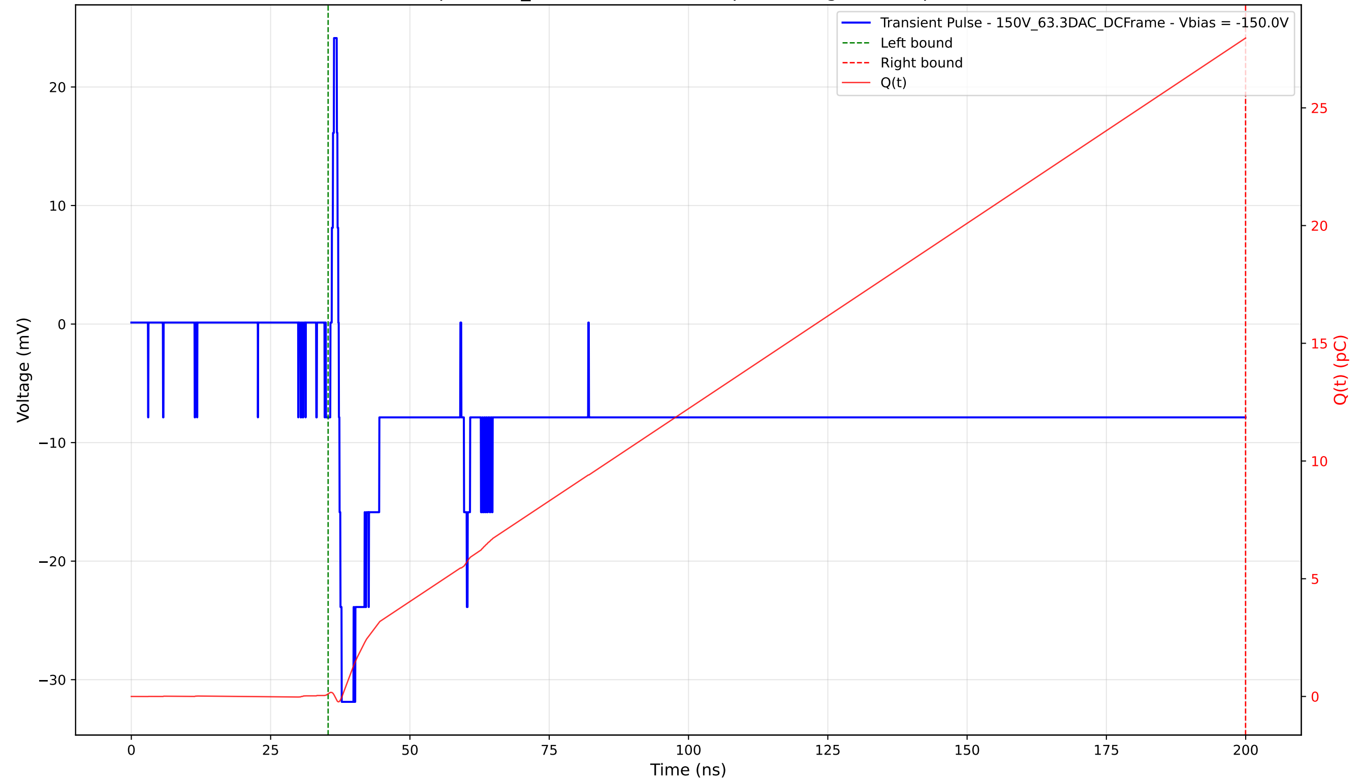
Transient Pulse - Sample: 1cm_42 - Position: 2045.0 \mu\text{m} - Charge: 27.85 pC - Rise Time: 0.51 ns
