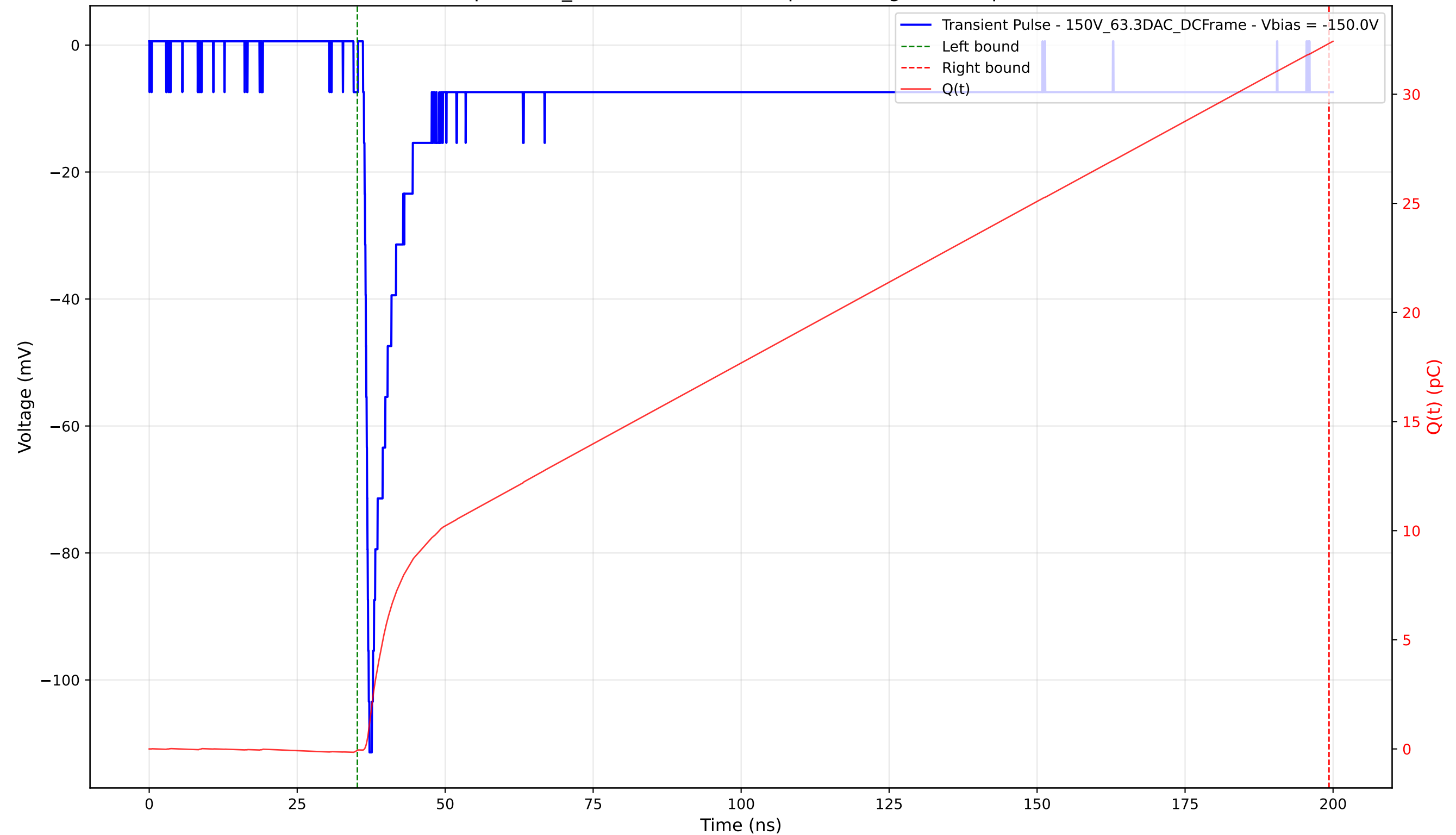
Transient Pulse - Sample: 1cm_42 - Position: 4495.0 \mu\text{m} - Charge: 32.39 pC - Rise Time: 0.81 ns
