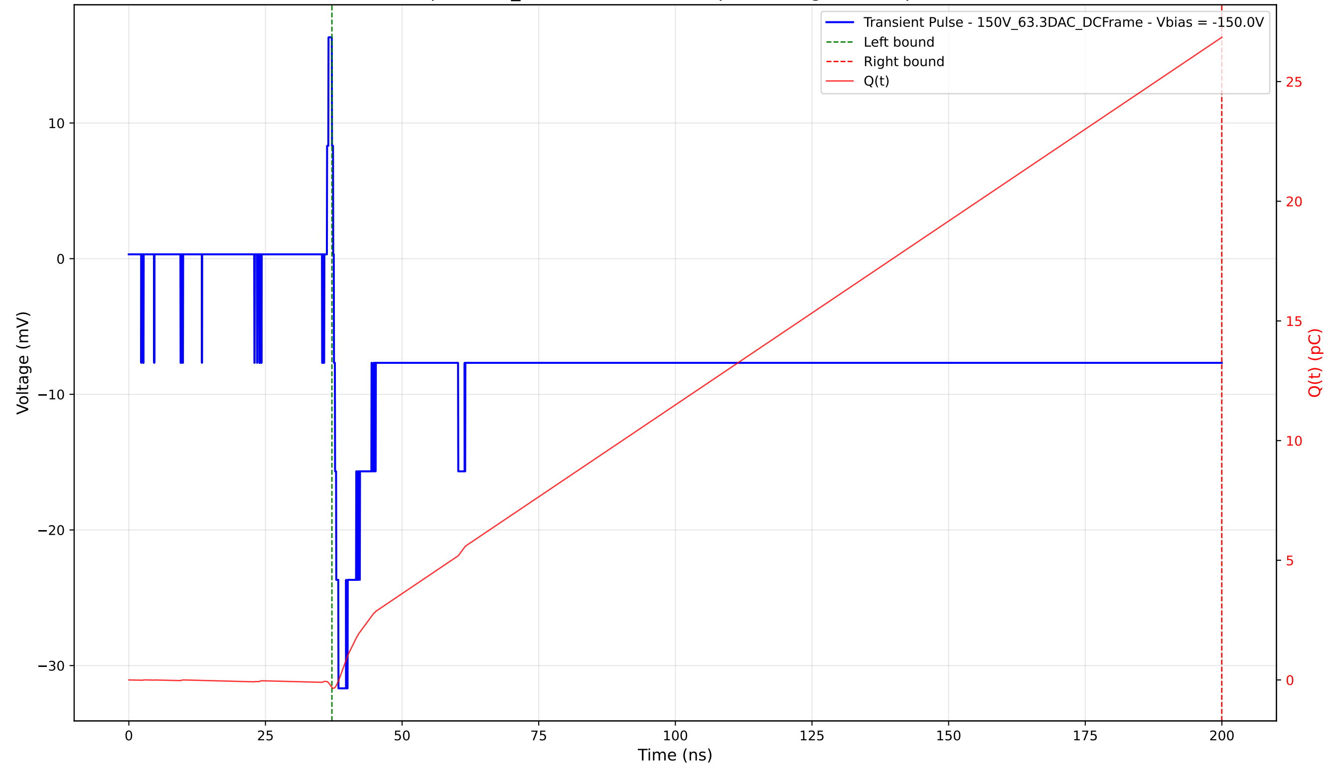
Transient Pulse - Sample: 1cm_42 - Position: 2810.0 \mu\text{m} - Charge: 27.16 pC - Rise Time: 0.83 ns
