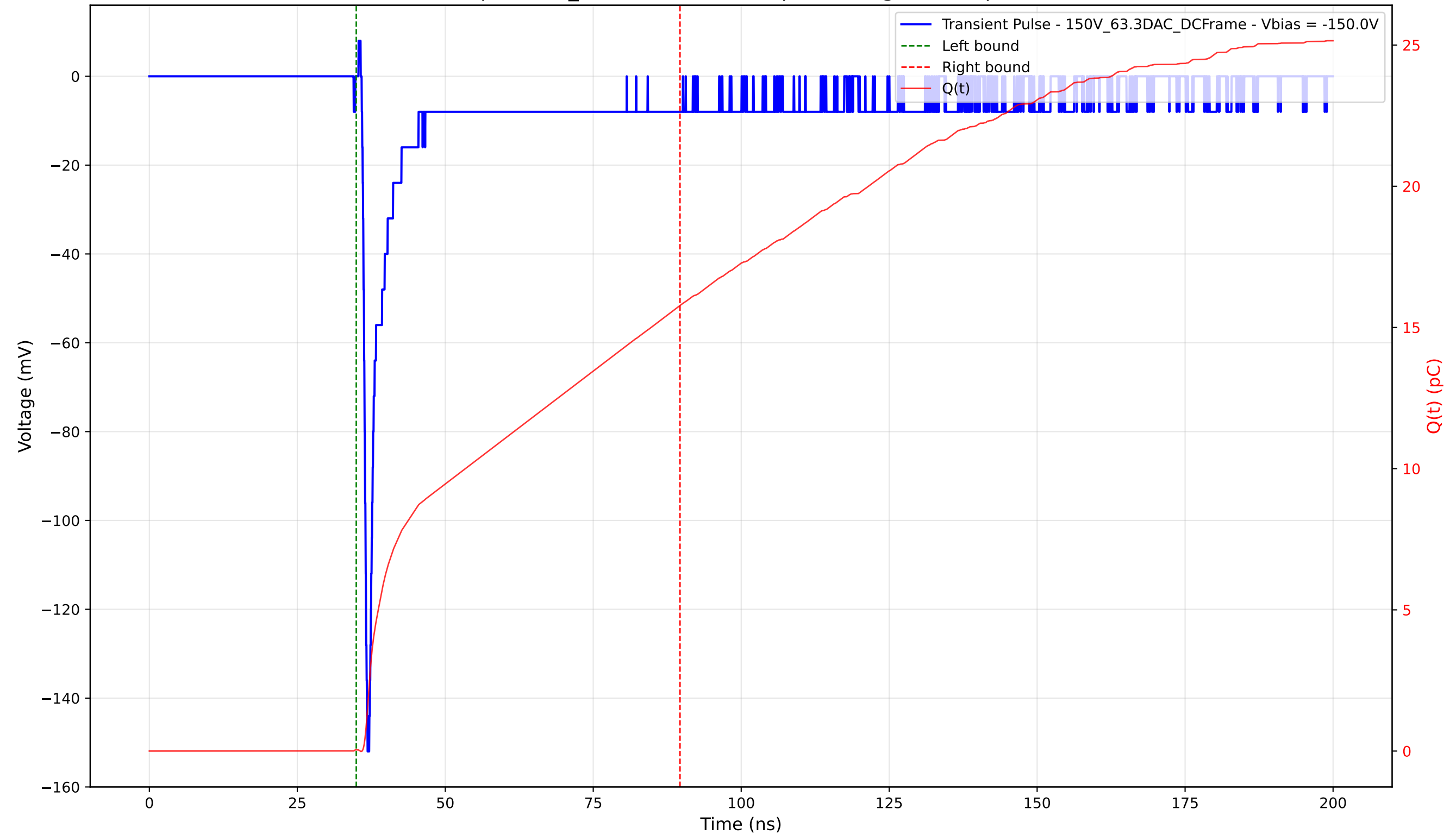
Transient Pulse - Sample: 1cm_42 - Position: 210.0 \mu\text{m} - Charge: 15.74 pC - Rise Time: 0.80 ns
