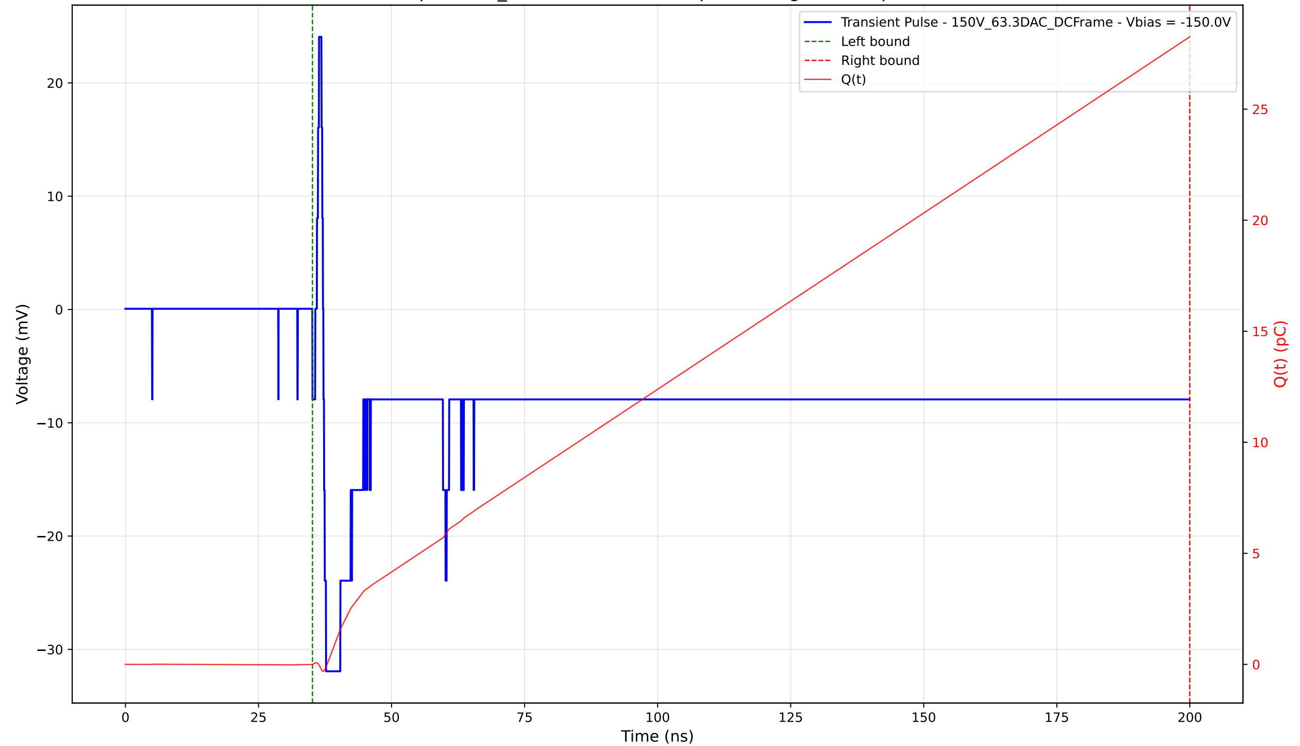
Transient Pulse - Sample: 1cm_42 - Position: 1985.0 \mu\text{m} - Charge: 28.26 pC - Rise Time: 0.49 ns
