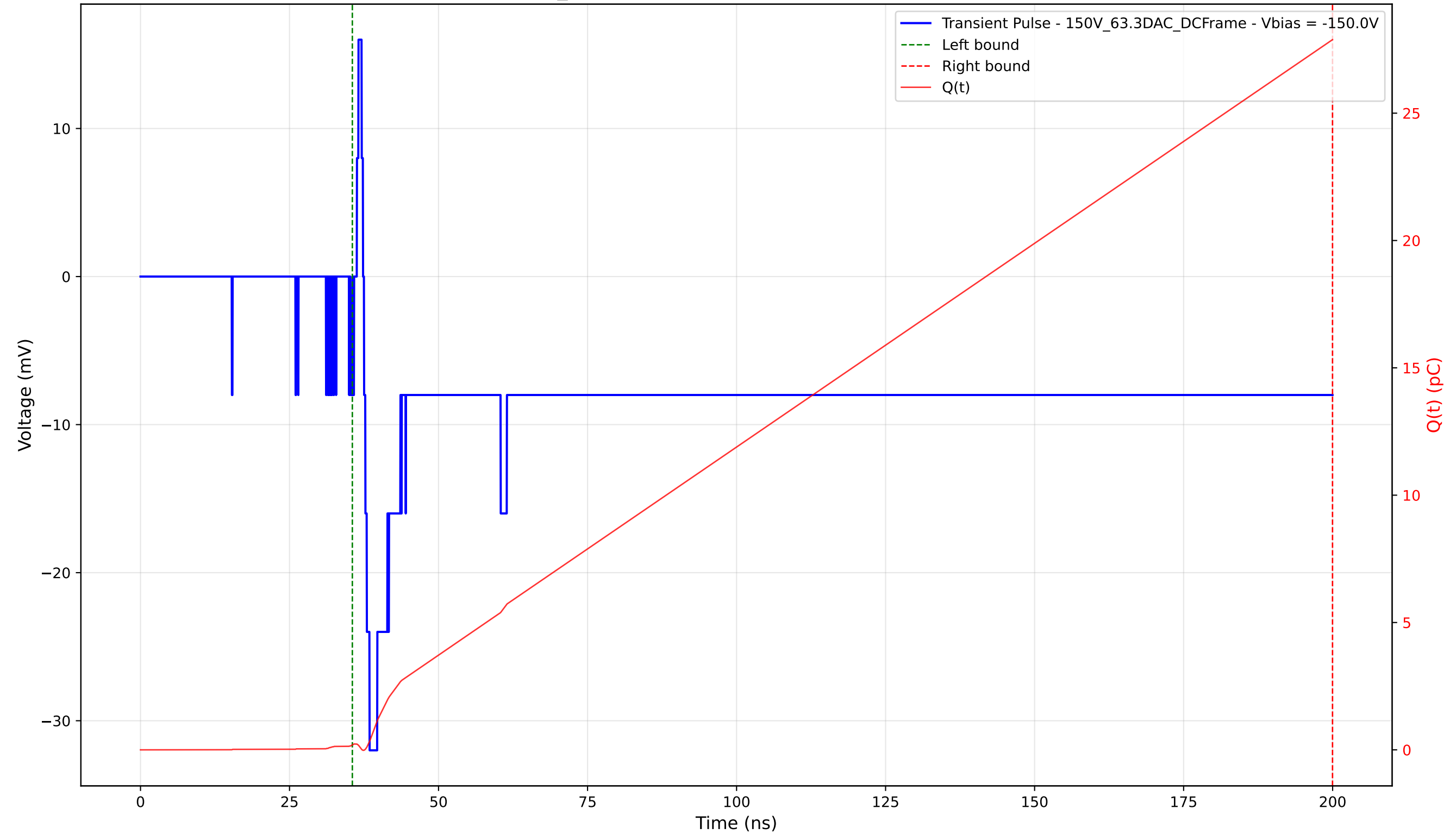
Transient Pulse - Sample: 1cm_42 - Position: 2865.0 \mu\text{m} - Charge: 27.69 pC - Rise Time: 0.93 ns
