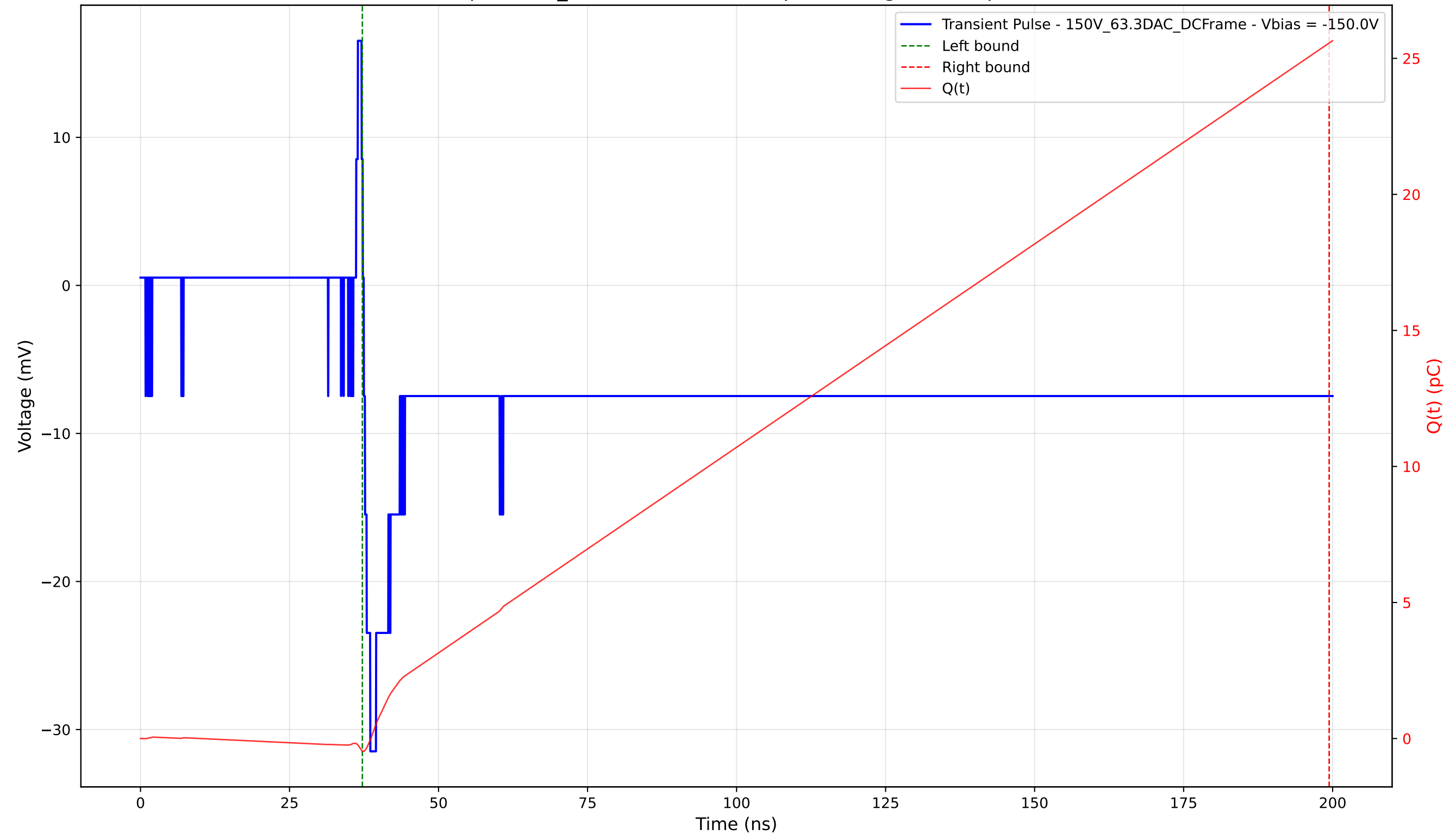
Transient Pulse - Sample: 1cm_42 - Position: 2535.0 \mu\text{m} - Charge: 26.02 pC - Rise Time: 1.09 ns
