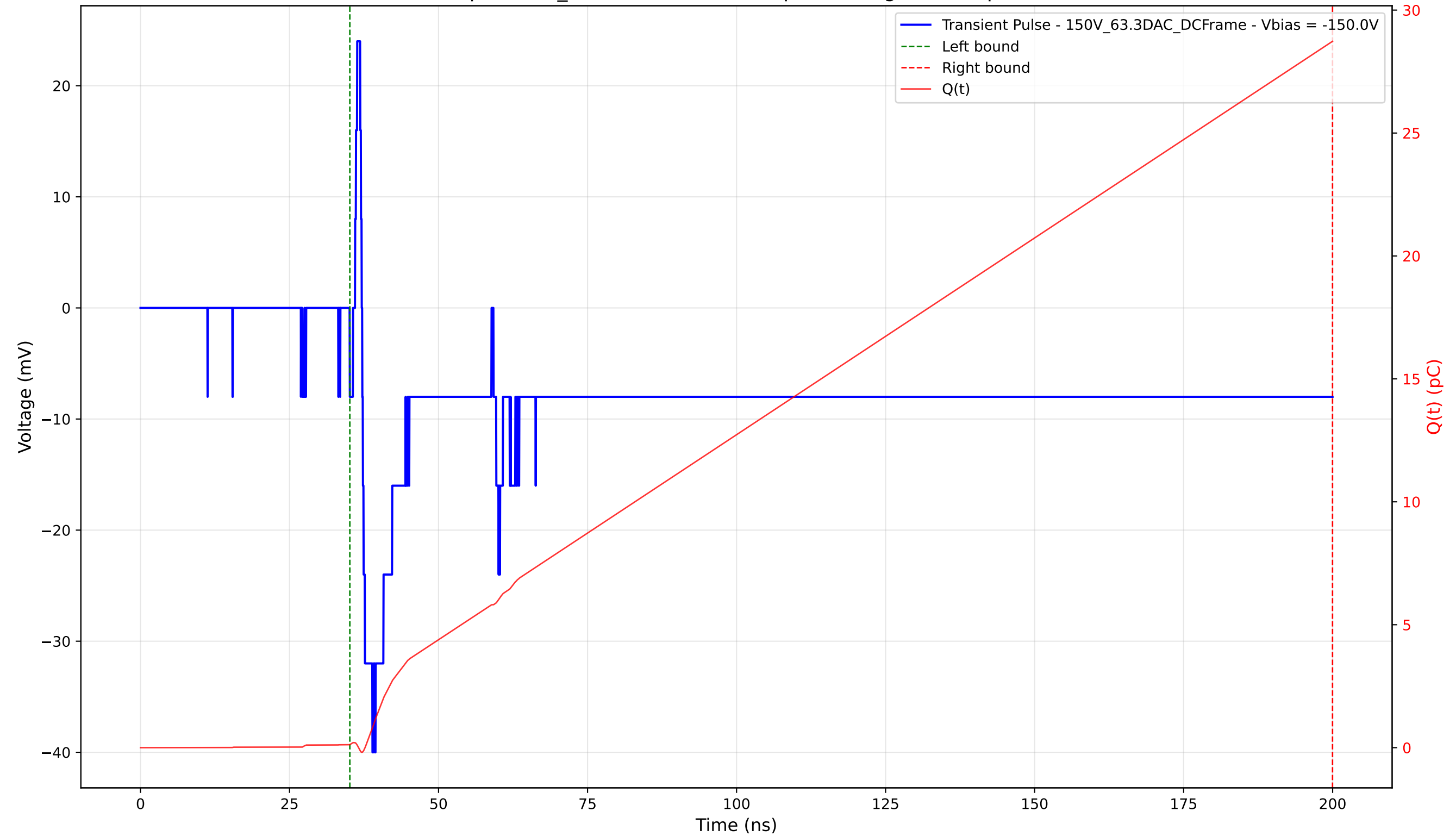
Transient Pulse - Sample: 1cm_42 - Position: 1920.0 \mu\text{m} - Charge: 28.61 pC - Rise Time: 1.71 ns
