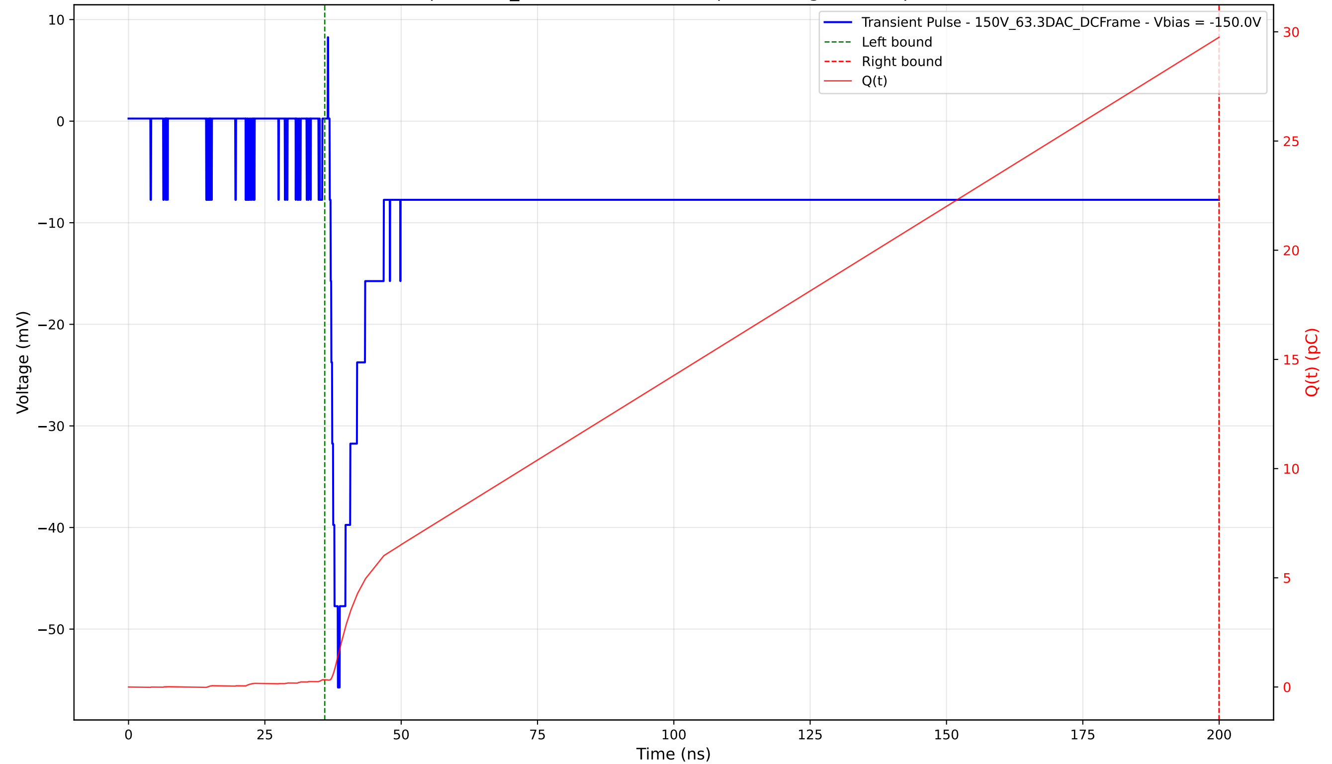
Transient Pulse - Sample: 1cm_42 - Position: 3905.0 \mu\text{m} - Charge: 29.42 pC - Rise Time: 1.51 ns
