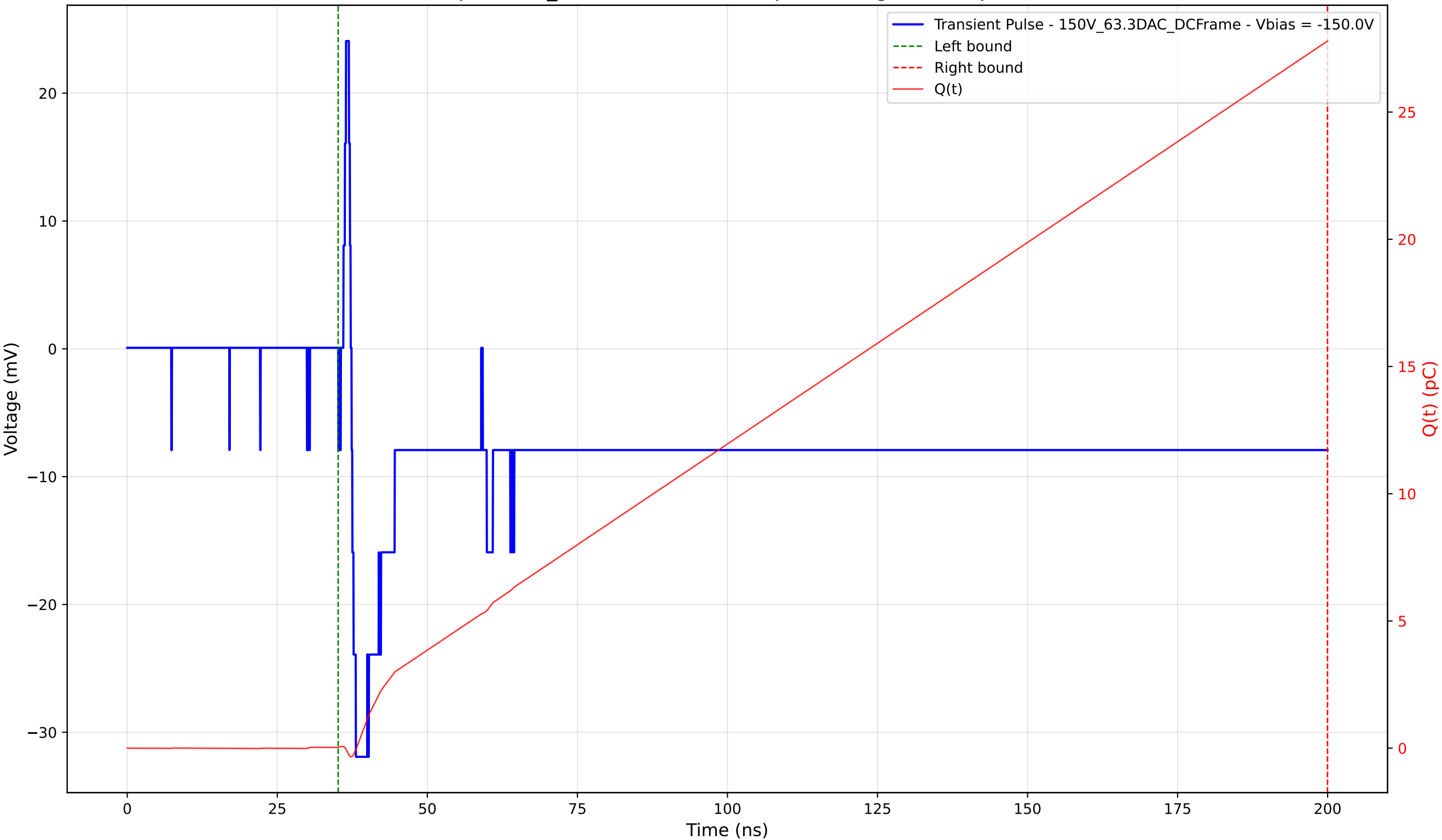
Transient Pulse - Sample: 1cm_42 - Position: 2340.0 \mu\text{m} - Charge: 27.77 pC - Rise Time: 0.71 ns
