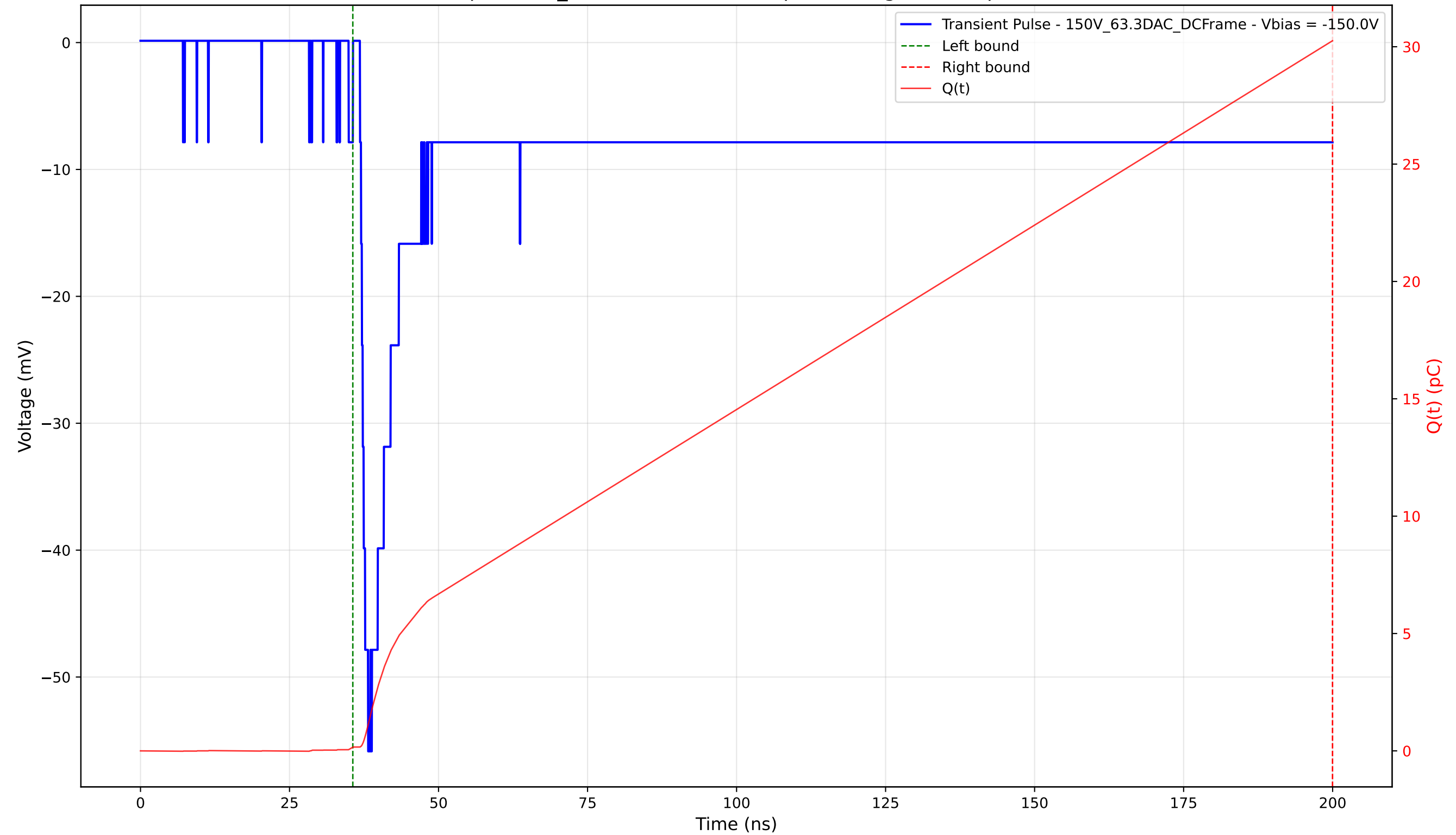
Transient Pulse - Sample: 1cm_42 - Position: 3940.0 \mu\text{m} - Charge: 30.09 pC - Rise Time: 1.37 ns
