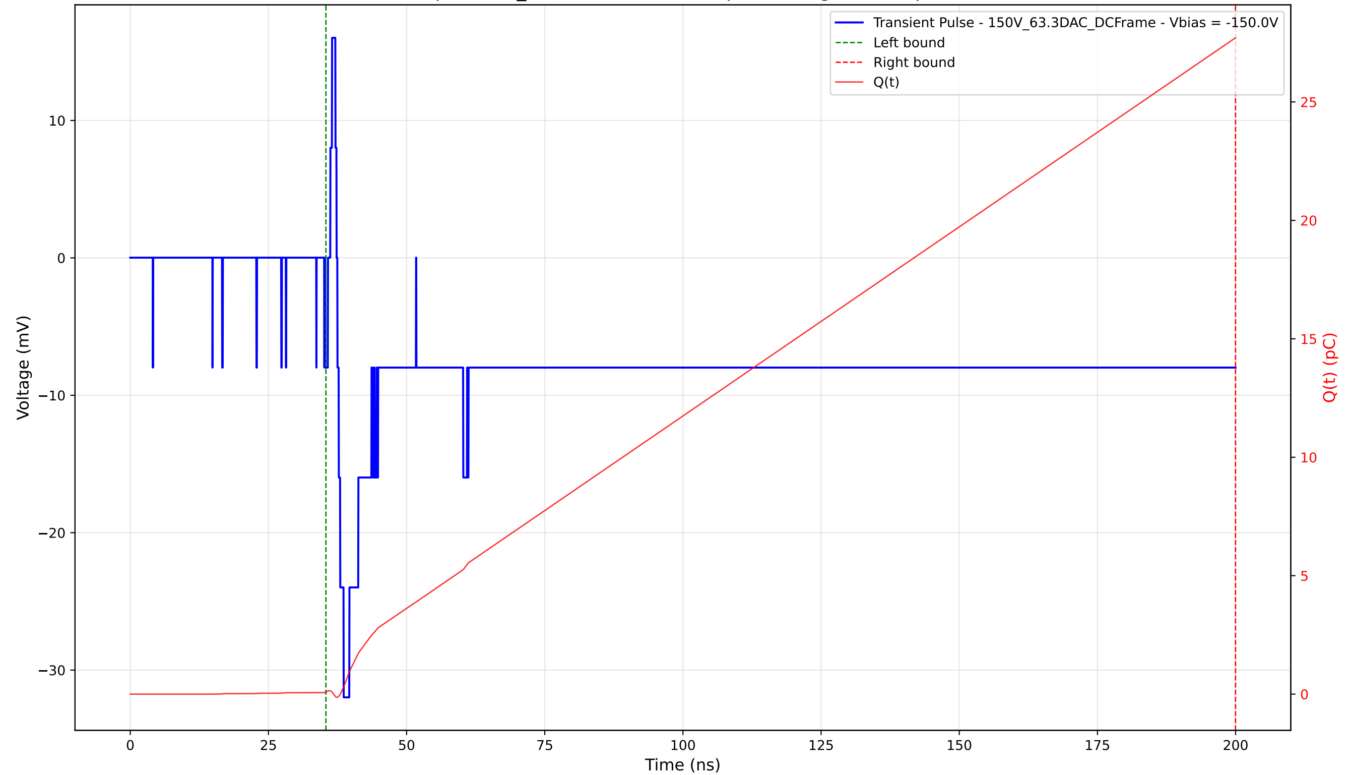
Transient Pulse - Sample: 1cm_42 - Position: 2550.0 \mu\text{m} - Charge: 27.62 pC - Rise Time: 1.13 ns
