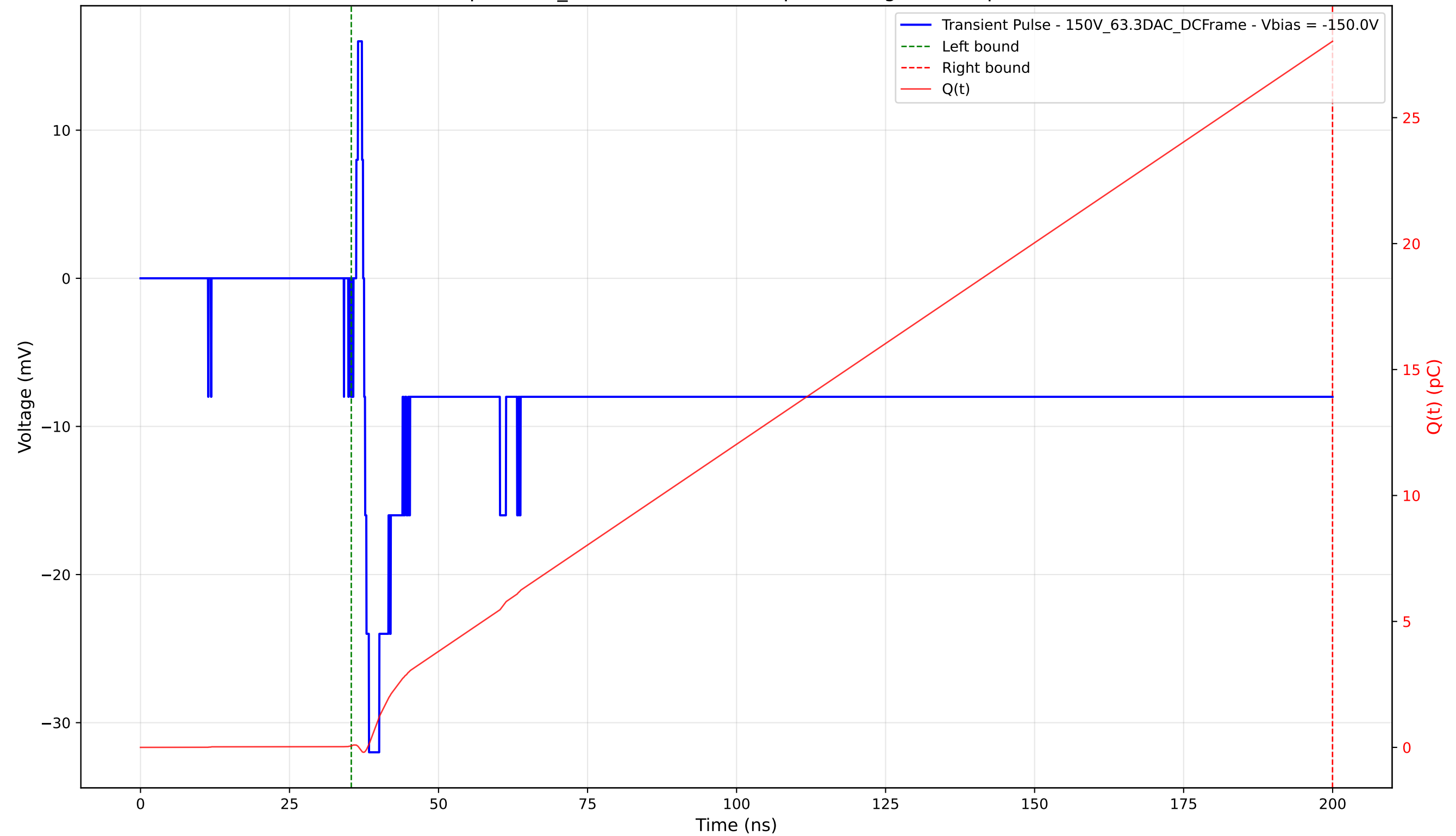
Transient Pulse - Sample: 1cm_42 - Position: 2645.0 \mu\text{m} - Charge: 27.97 pC - Rise Time: 0.81 ns
