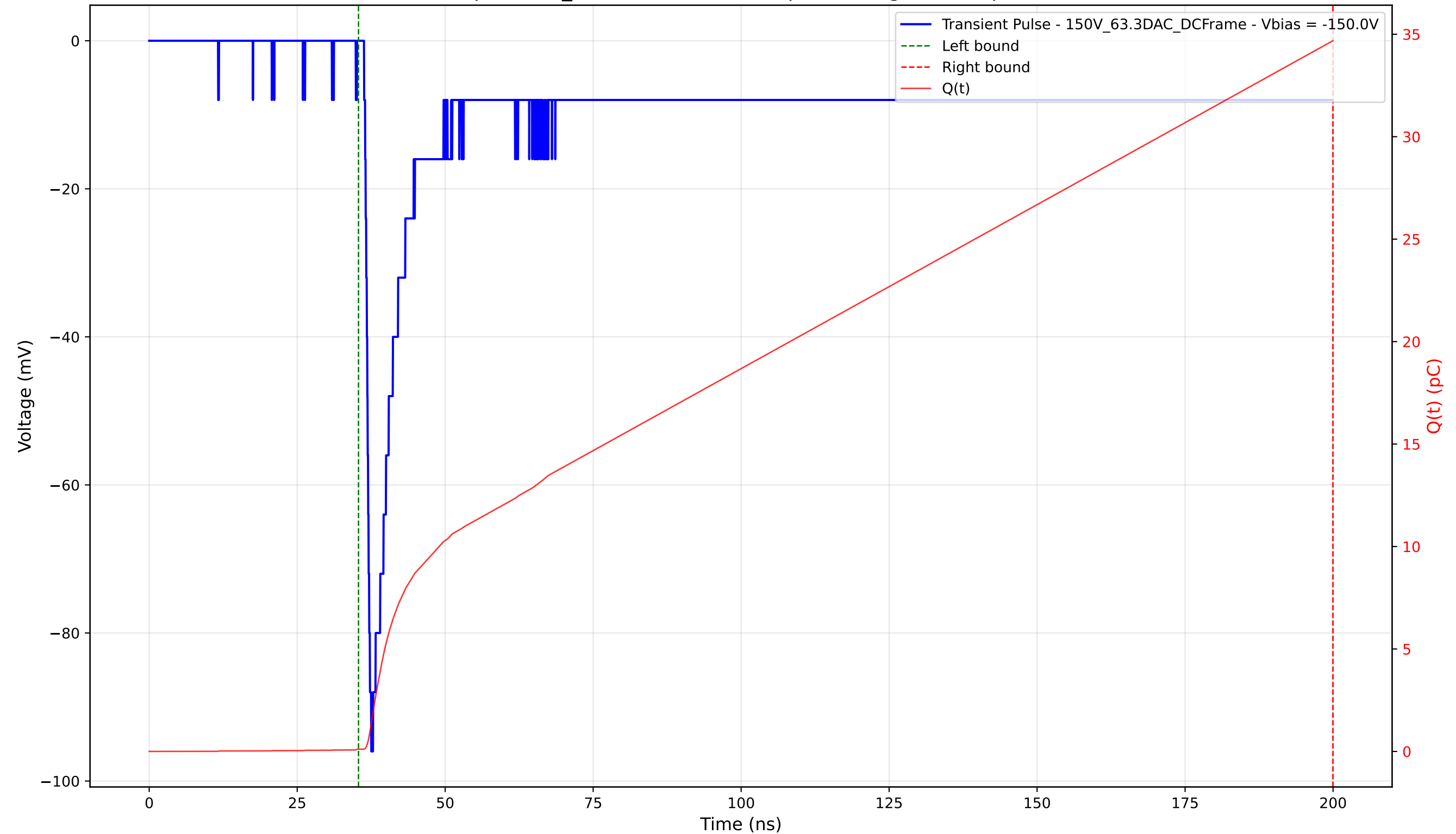
Transient Pulse - Sample: 1cm_42 - Position: 4335.0 \mu\text{m} - Charge: 34.58 pC - Rise Time: 0.82 ns
