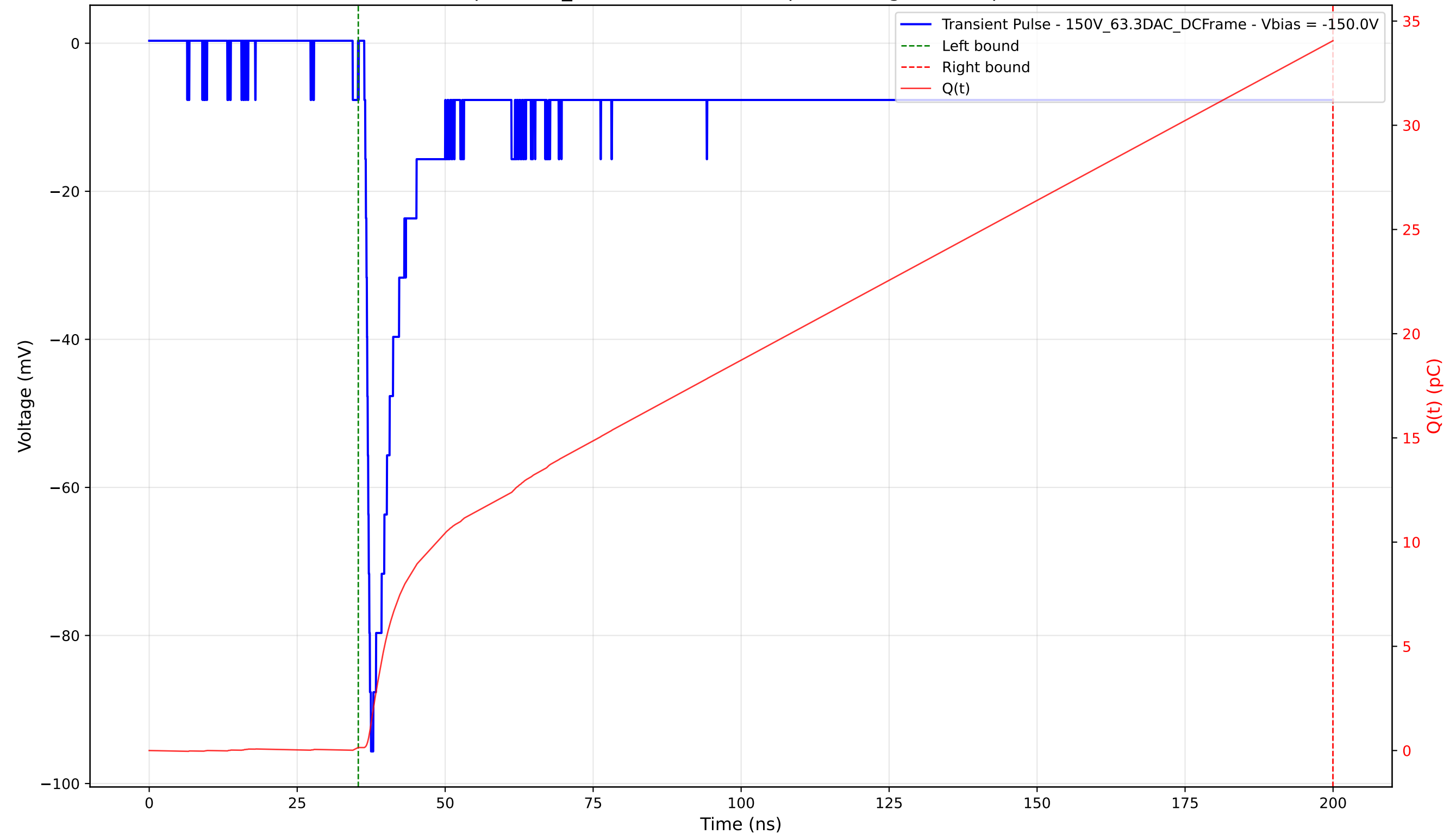
Transient Pulse - Sample: 1cm_42 - Position: 4295.0 \mu\text{m} - Charge: 33.91 pC - Rise Time: 0.80 ns
