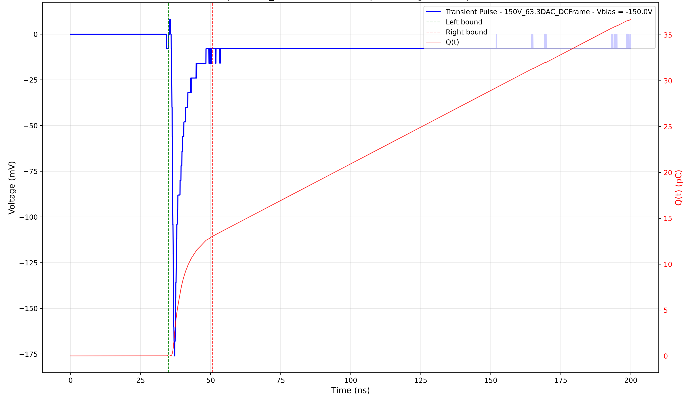
Transient Pulse - Sample: 1cm_42 - Position: 460.0 \mu\text{m} - Charge: 12.95 pC - Rise Time: 0.76 ns
