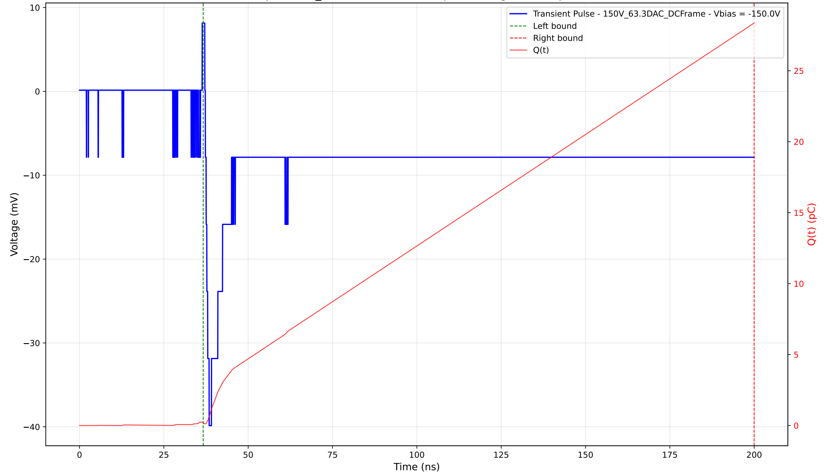
Transient Pulse - Sample: 1cm_42 - Position: 3465.0 \mu\text{m} - Charge: 28.17 pC - Rise Time: 1.13 ns
