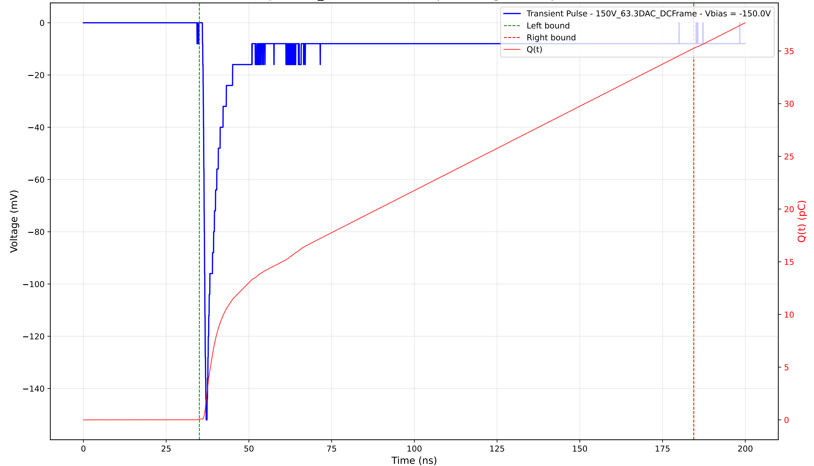
Transient Pulse - Sample: 1cm_42 - Position: 555.0 \mu\text{m} - Charge: 35.19 pC - Rise Time: 0.92 ns
