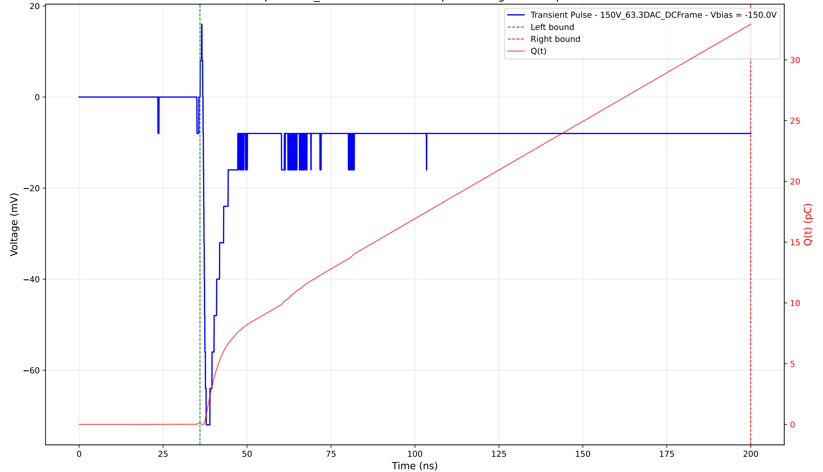
Transient Pulse - Sample: 1cm_42 - Position: 1240.0 \mu\text{m} - Charge: 32.83 pC - Rise Time: 0.92 ns
