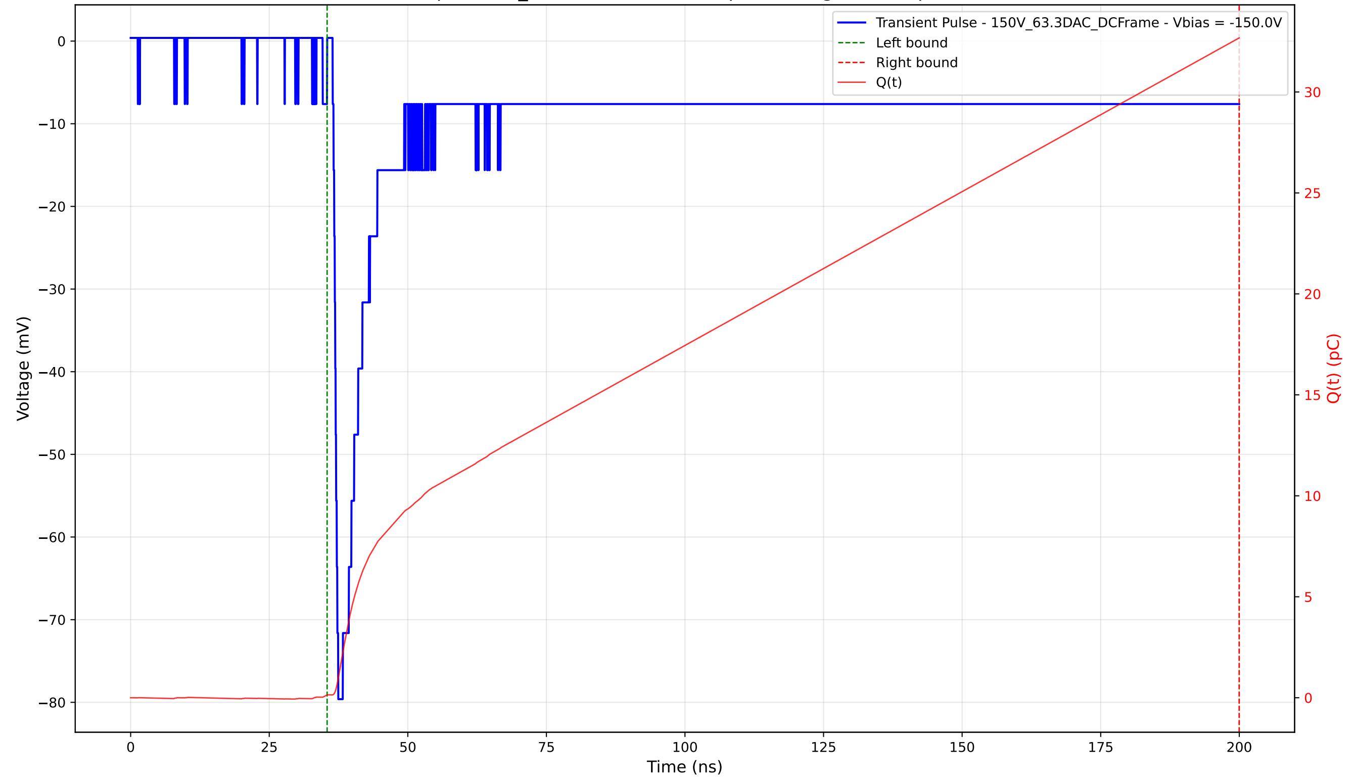
Transient Pulse - Sample: 1cm_42 - Position: 4175.0 \mu\text{m} - Charge: 32.53 pC - Rise Time: 0.86 ns
