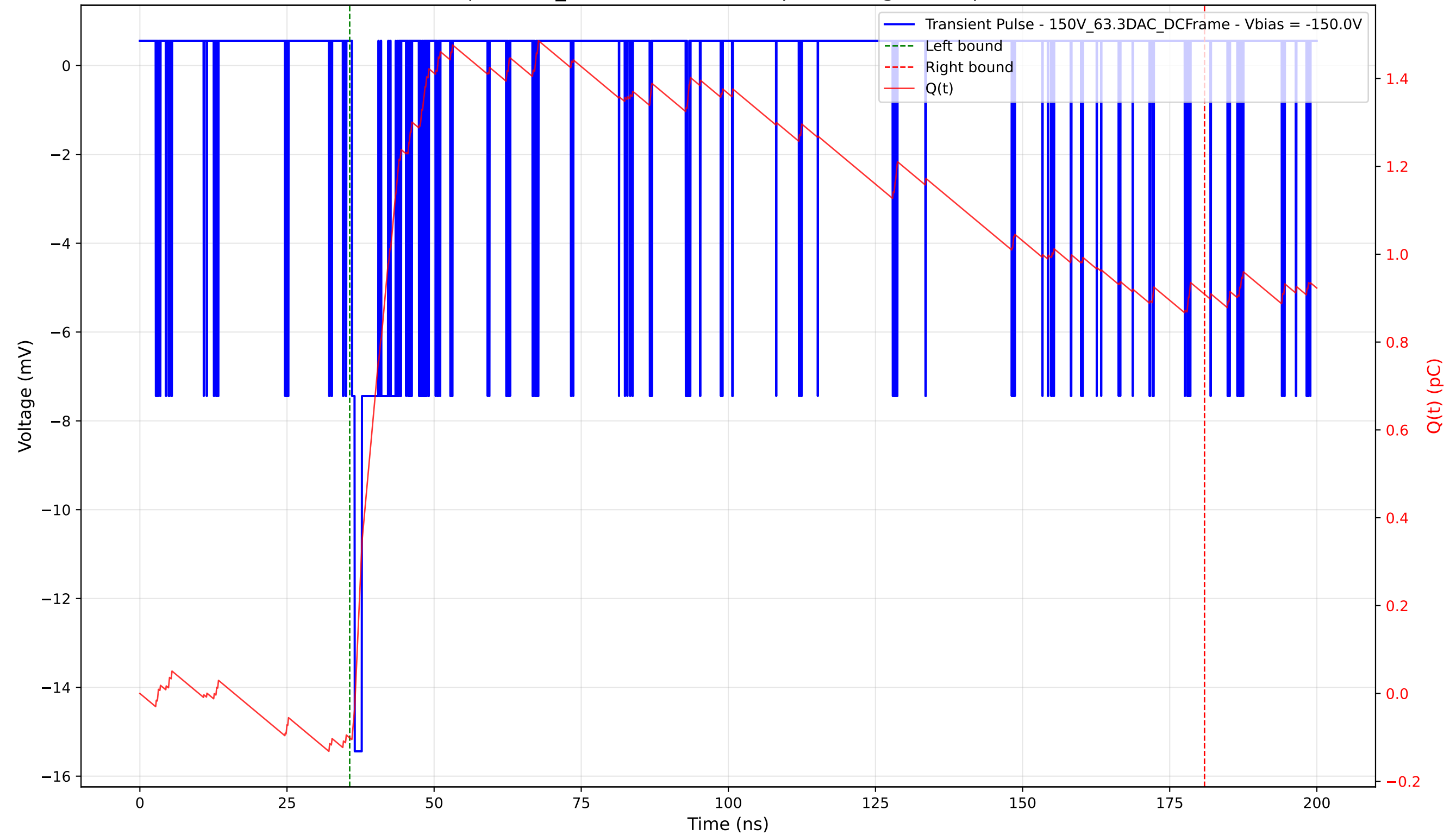
Transient Pulse - Sample: 1cm_42 - Position: 5195.0 \mu\text{m} - Charge: 1.01 pC - Rise Time: 0.48 ns
