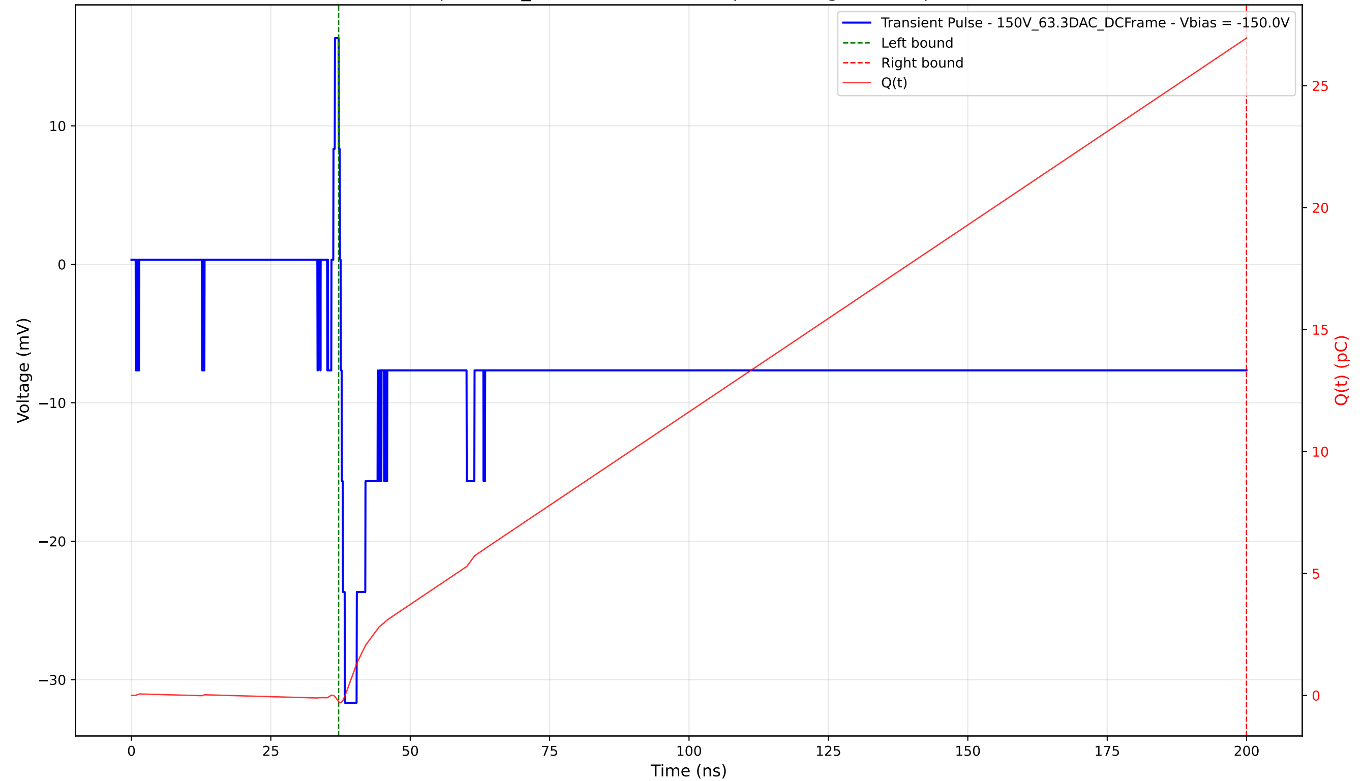
Transient Pulse - Sample: 1cm_42 - Position: 2710.0 \mu\text{m} - Charge: 27.22 pC - Rise Time: 0.73 ns
