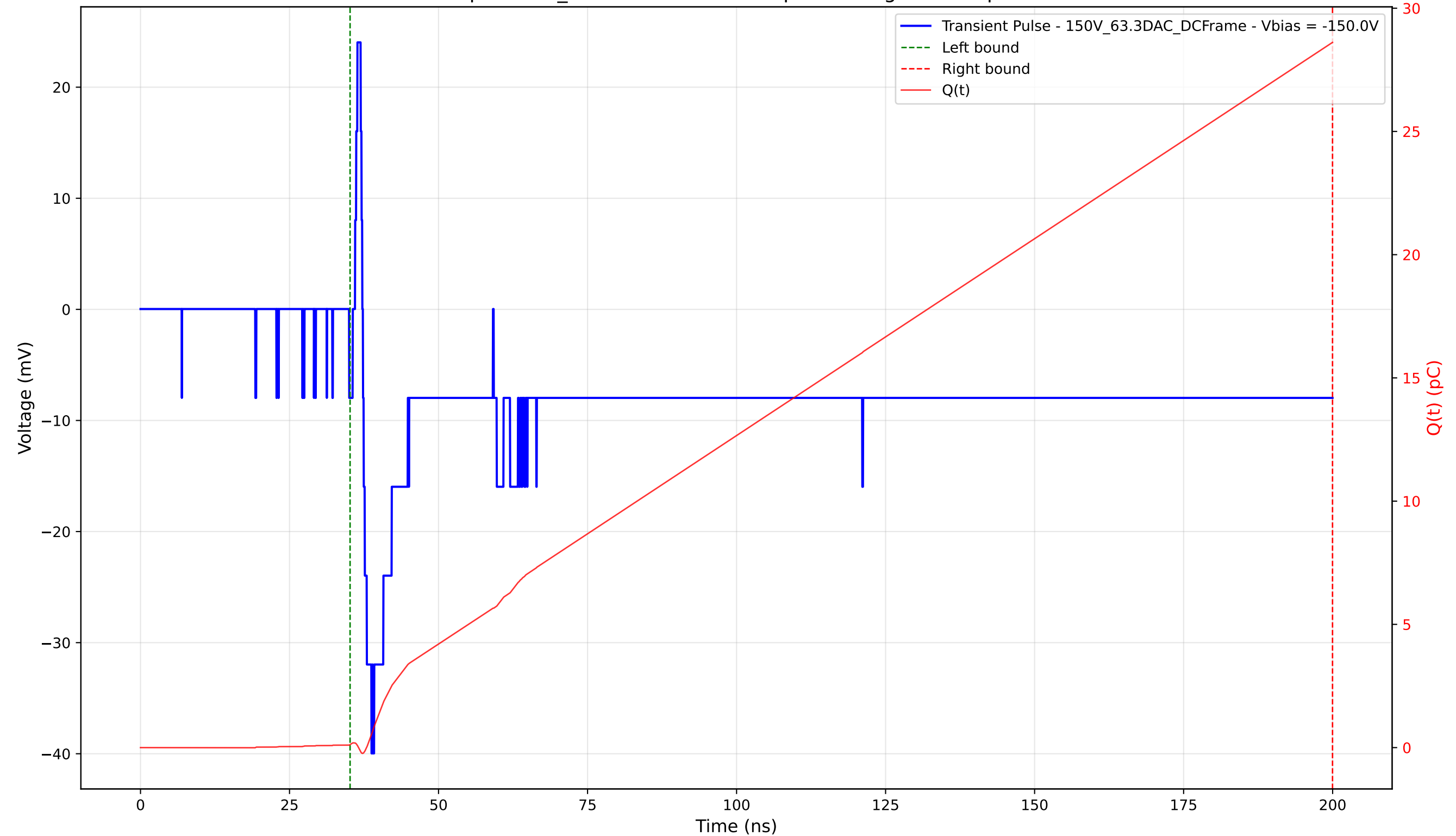
Transient Pulse - Sample: 1cm_42 - Position: 2250.0 \mu\text{m} - Charge: 28.49 pC - Rise Time: 1.43 ns
