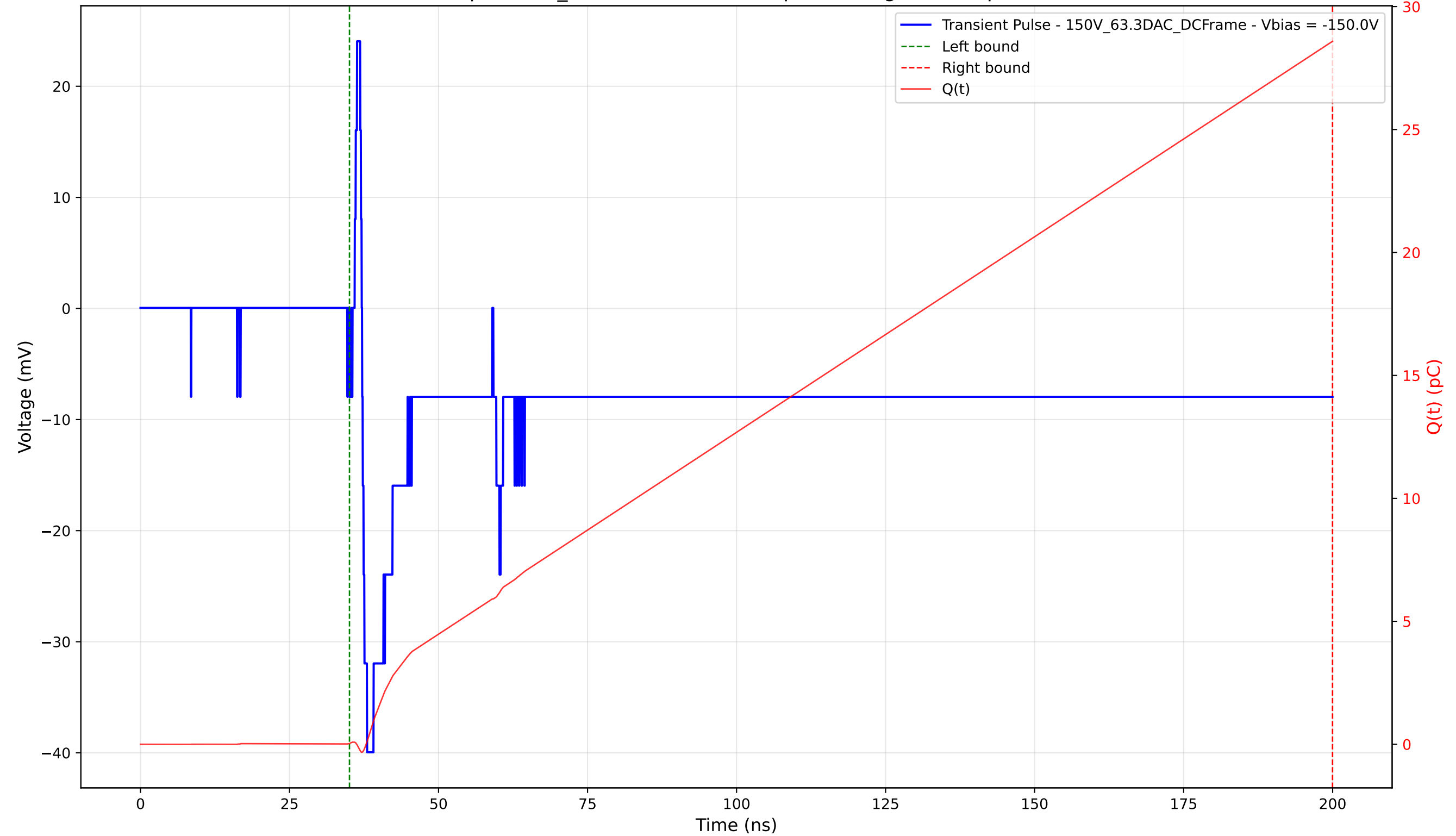
Transient Pulse - Sample: 1cm_42 - Position: 1895.0 \mu\text{m} - Charge: 28.56 pC - Rise Time: 0.83 ns
