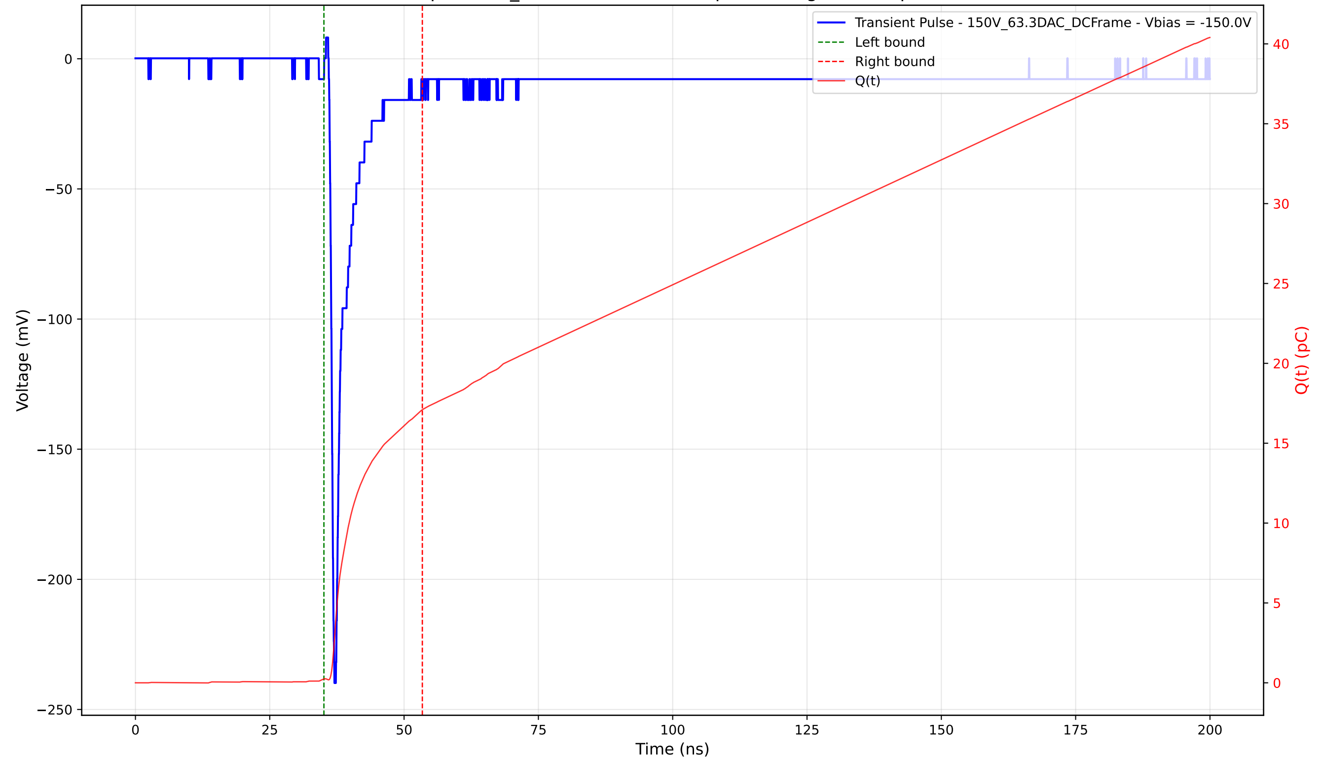
Transient Pulse - Sample: 1cm_42 - Position: 4820.0 \mu\text{m} - Charge: 16.84 pC - Rise Time: 0.76 ns
