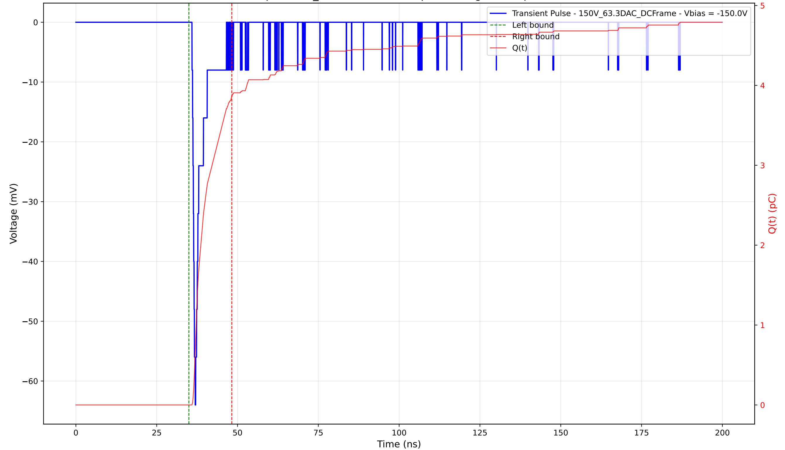
Transient Pulse - Sample: 1cm_42 - Position: 70.0 \mu\text{m} - Charge: 3.86 pC - Rise Time: 0.98 ns
