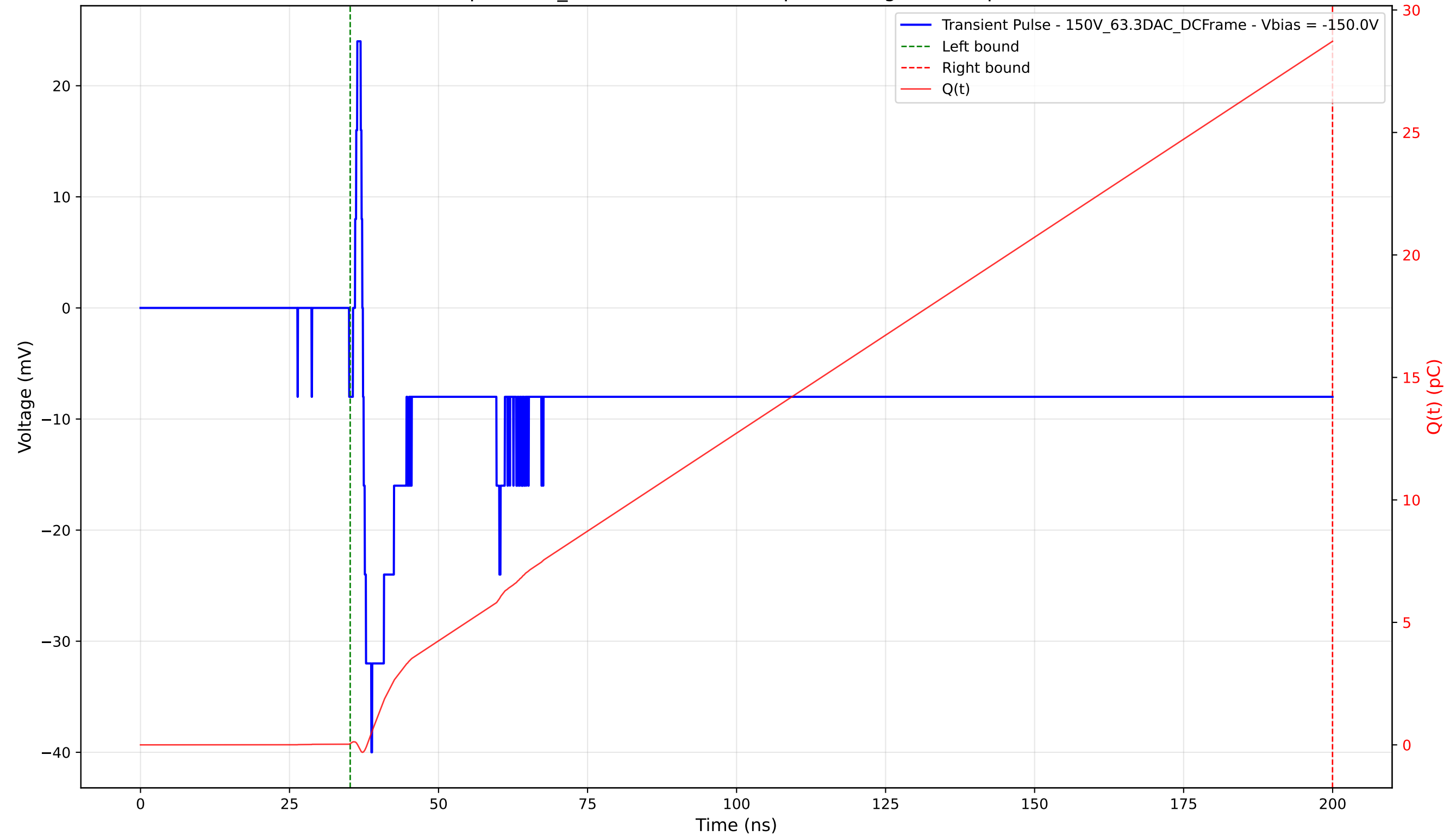
Transient Pulse - Sample: 1cm_42 - Position: 2200.0 \mu\text{m} - Charge: 28.67 pC - Rise Time: 1.41 ns
