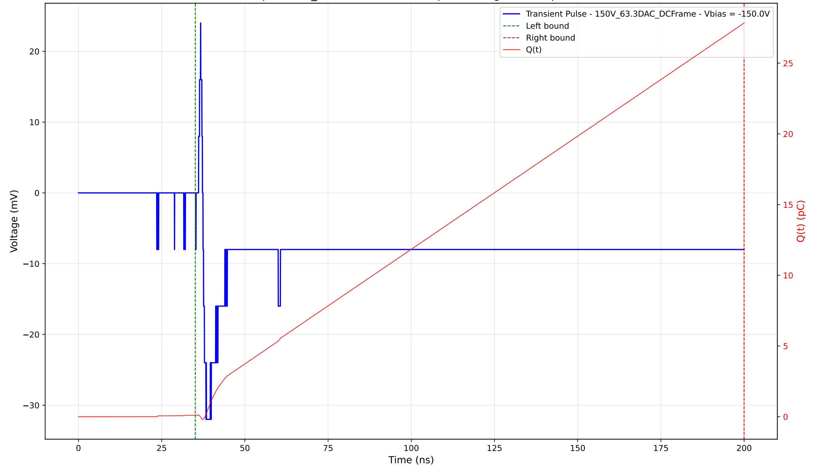
Transient Pulse - Sample: 1cm_42 - Position: 2420.0 \mu\text{m} - Charge: 27.74 pC - Rise Time: 0.89 ns
