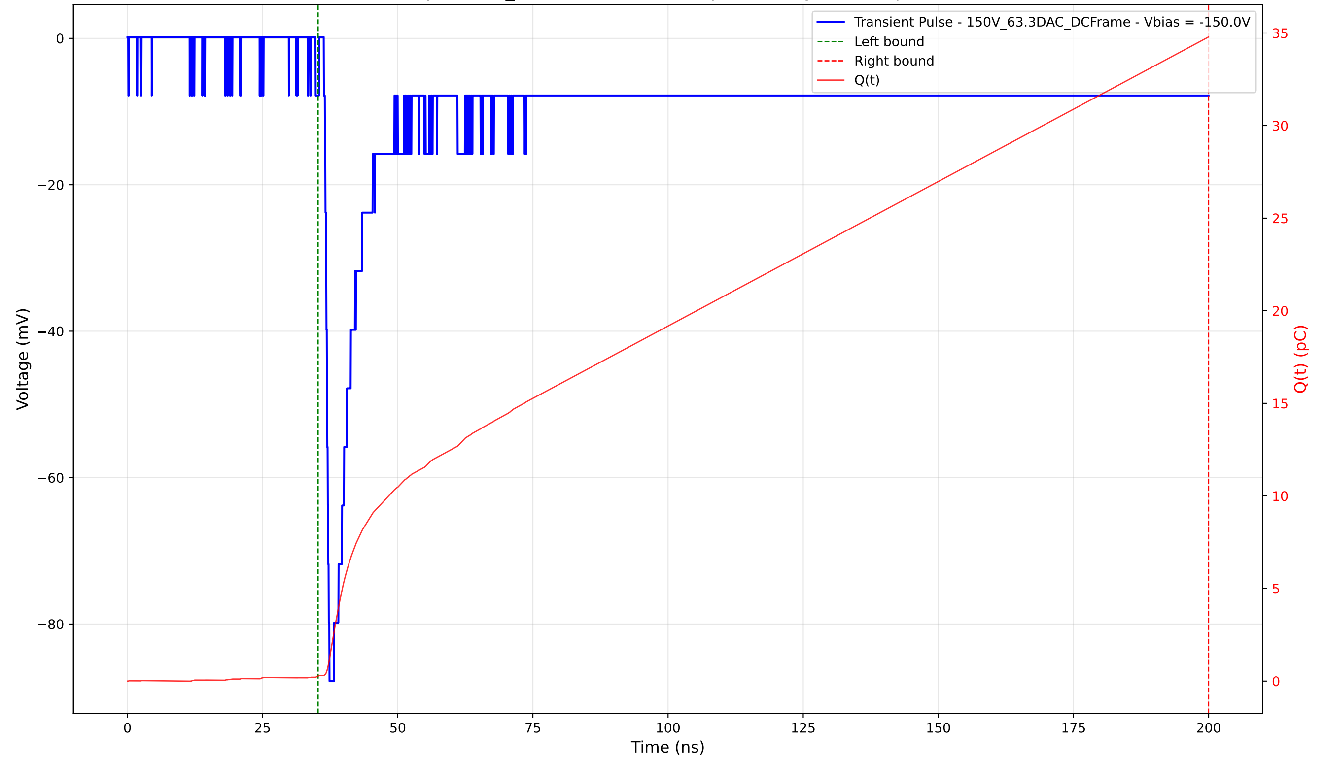
Transient Pulse - Sample: 1cm_42 - Position: 4245.0 \mu\text{m} - Charge: 34.51 pC - Rise Time: 0.72 ns
