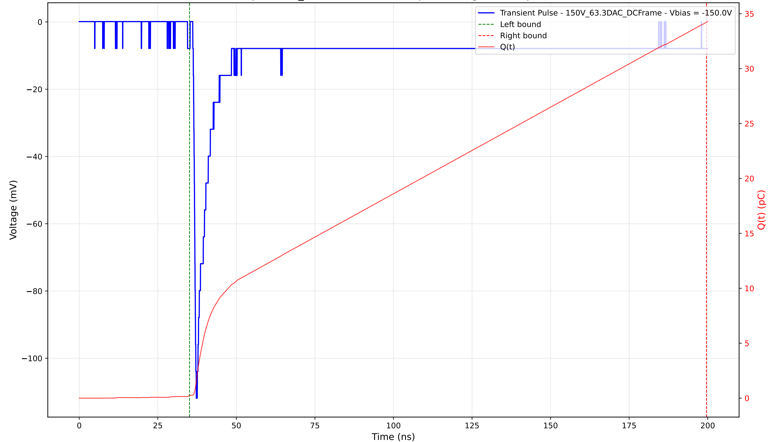
Transient Pulse - Sample: 1cm_42 - Position: 4490.0 \mu\text{m} - Charge: 33.98 pC - Rise Time: 0.81 ns
