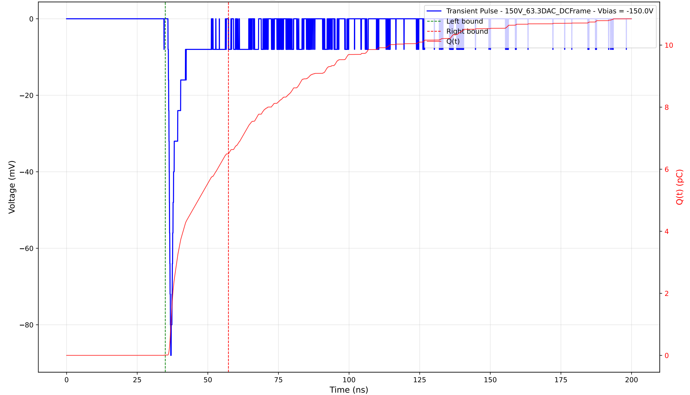
Transient Pulse - Sample: 1cm_42 - Position: 105.0 \mu\text{m} - Charge: 6.48 pC - Rise Time: 0.72 ns
