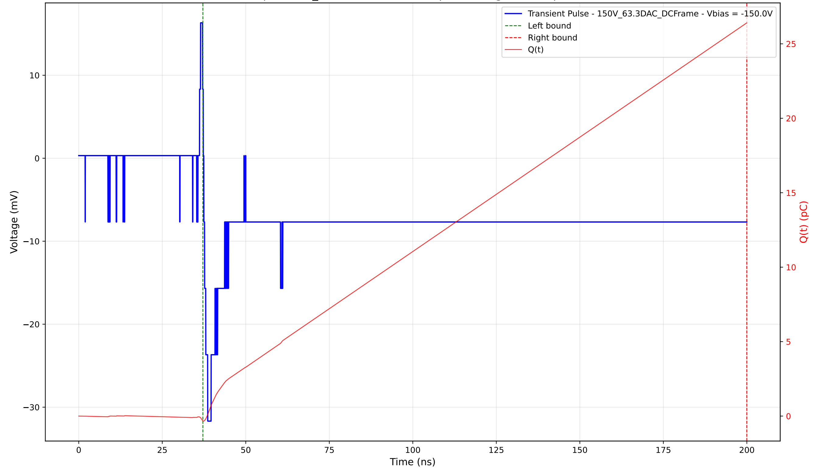
Transient Pulse - Sample: 1cm_42 - Position: 2500.0 \mu\text{m} - Charge: 26.73 pC - Rise Time: 1.17 ns
