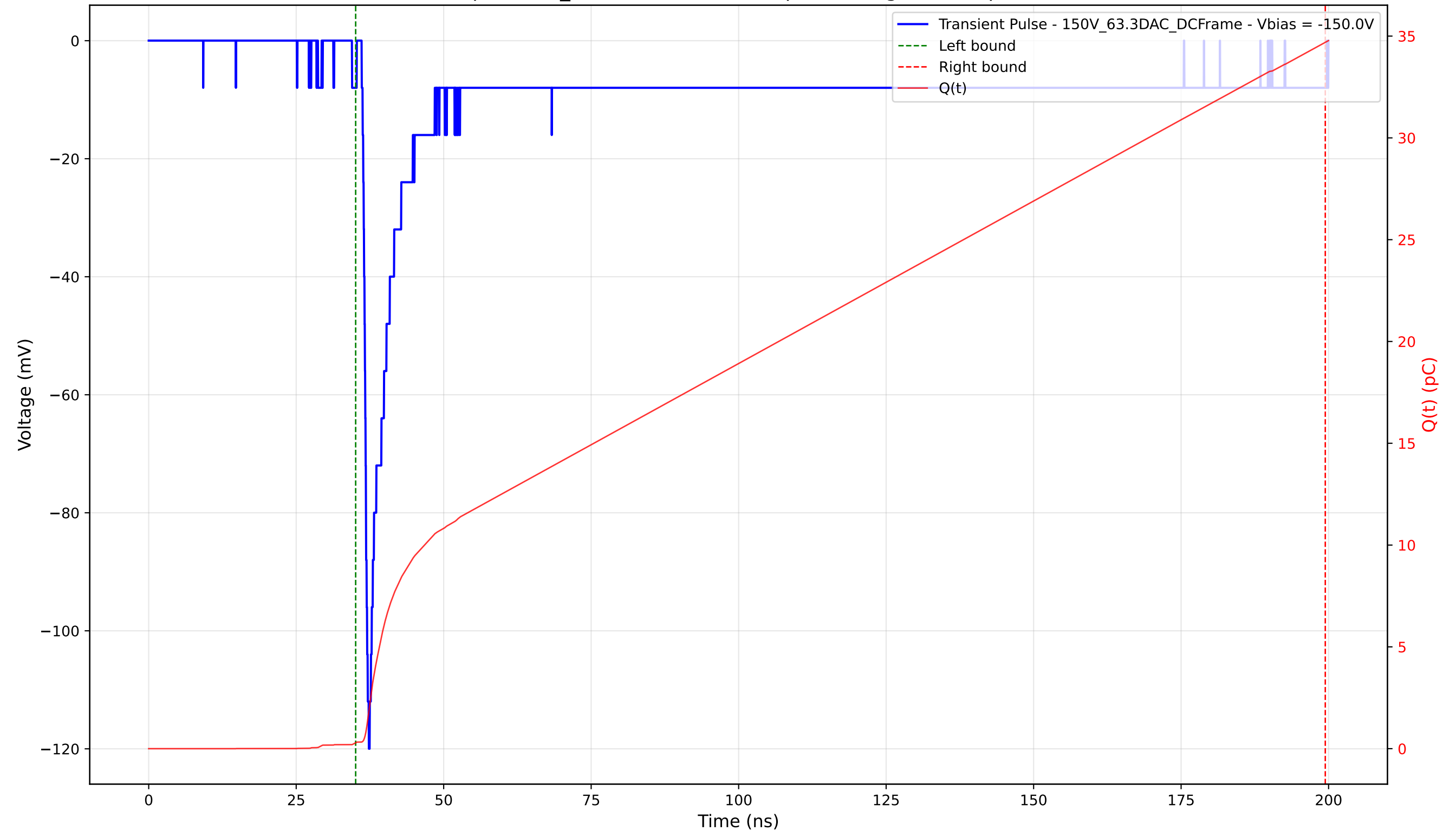
Transient Pulse - Sample: 1cm_42 - Position: 4510.0 \mu\text{m} - Charge: 34.41 pC - Rise Time: 0.87 ns
