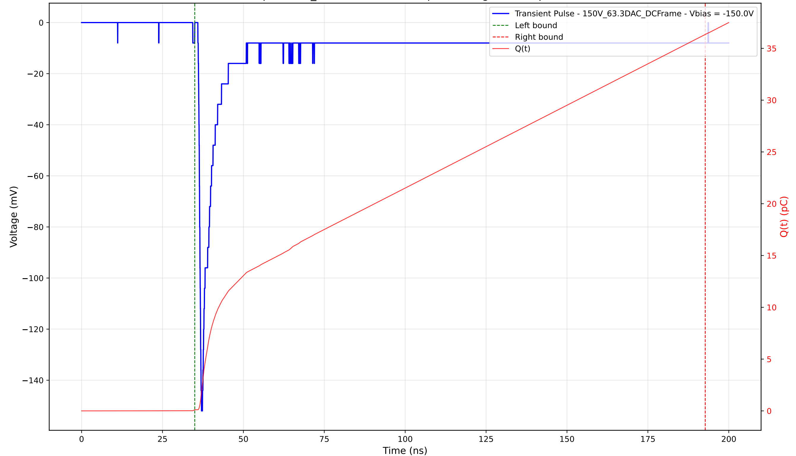
Transient Pulse - Sample: 1cm_42 - Position: 535.0 \mu\text{m} - Charge: 36.24 pC - Rise Time: 0.86 ns
