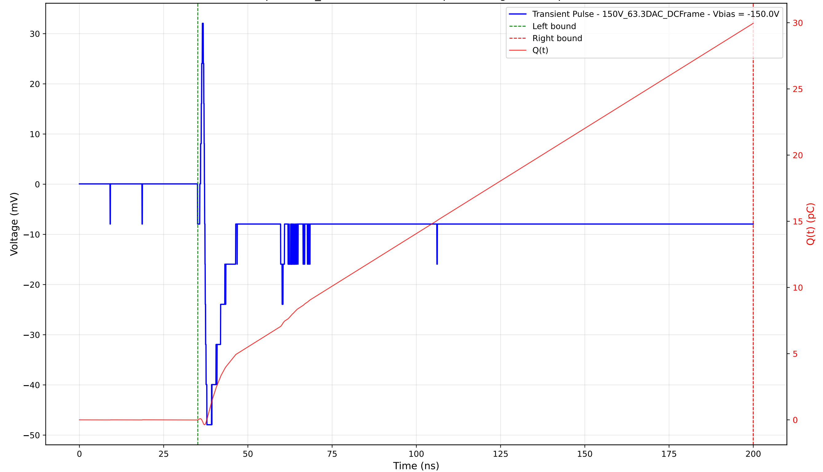
Transient Pulse - Sample: 1cm_42 - Position: 1730.0 \mu\text{m} - Charge: 29.96 pC - Rise Time: 0.67 ns
