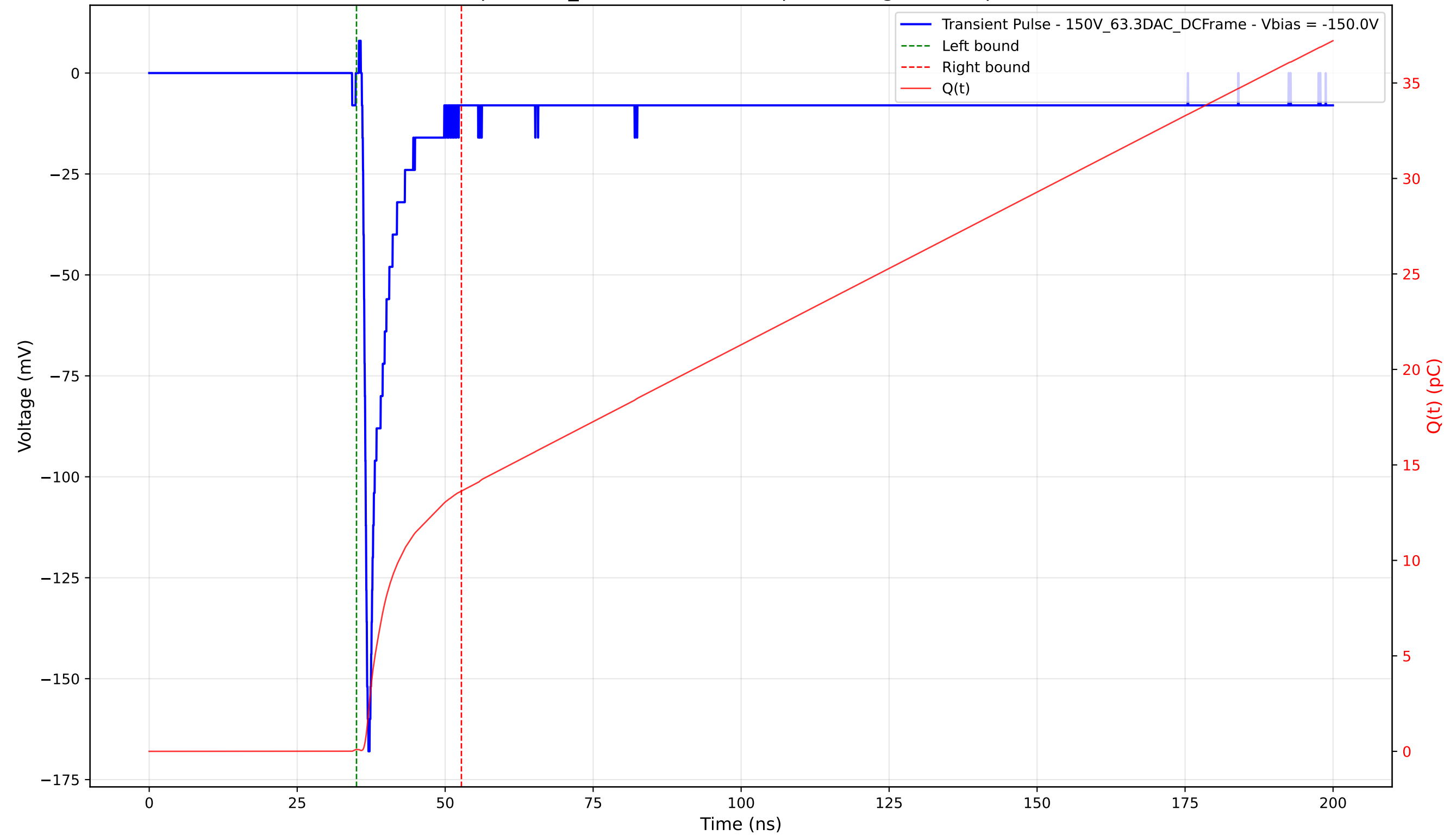
Transient Pulse - Sample: 1cm_42 - Position: 480.0 \mu\text{m} - Charge: 13.53 pC - Rise Time: 0.74 ns
