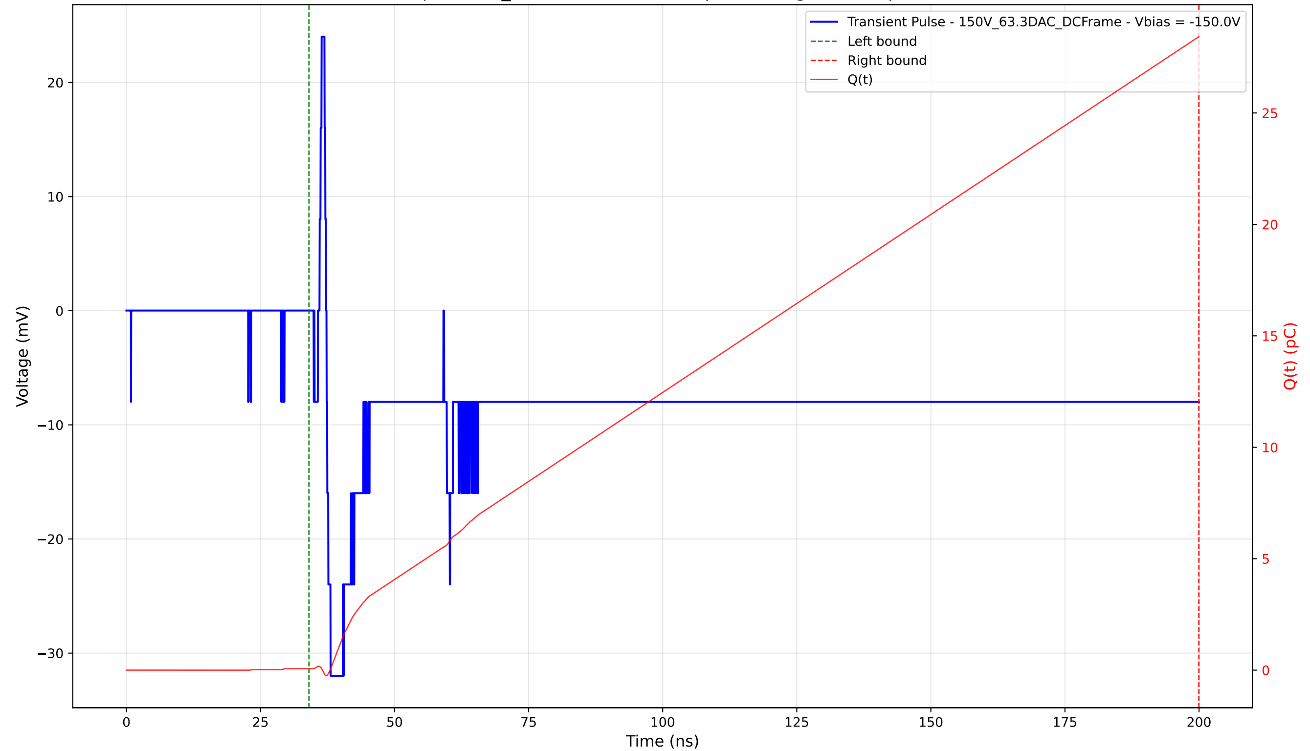
Transient Pulse - Sample: 1cm_42 - Position: 2190.0 \mu\text{m} - Charge: 28.36 pC - Rise Time: 0.75 ns
