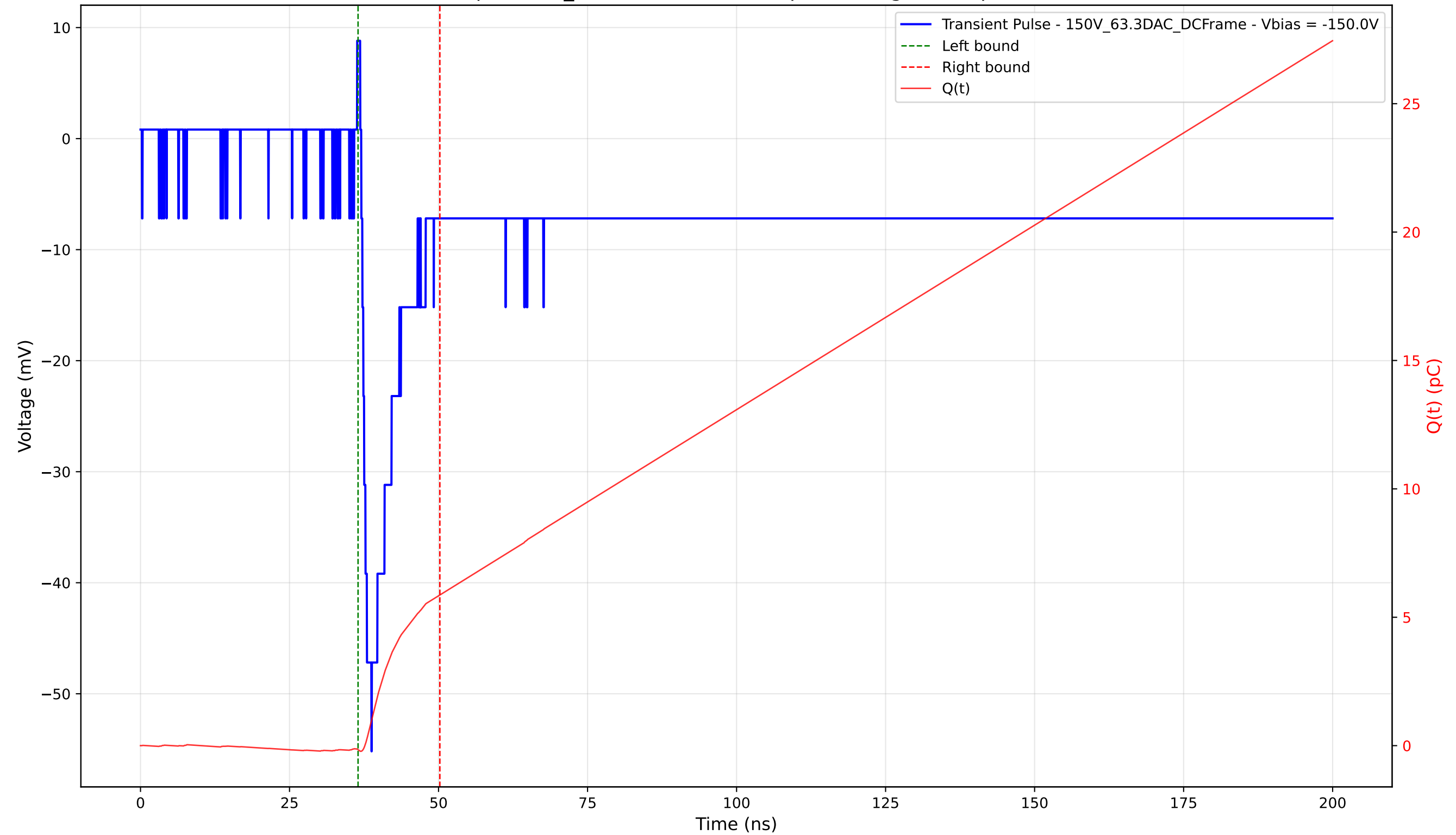
Transient Pulse - Sample: 1cm_42 - Position: 3690.0 \mu\text{m} - Charge: 6.03 pC - Rise Time: 1.71 ns
