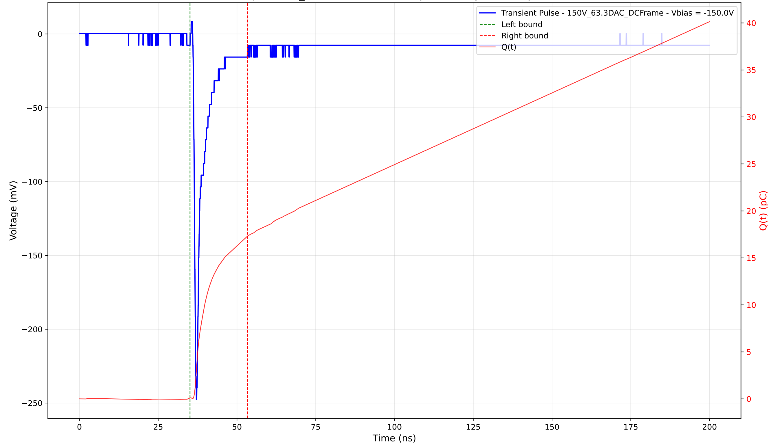
Transient Pulse - Sample: 1cm_42 - Position: 4795.0 \mu\text{m} - Charge: 17.22 pC - Rise Time: 0.76 ns
