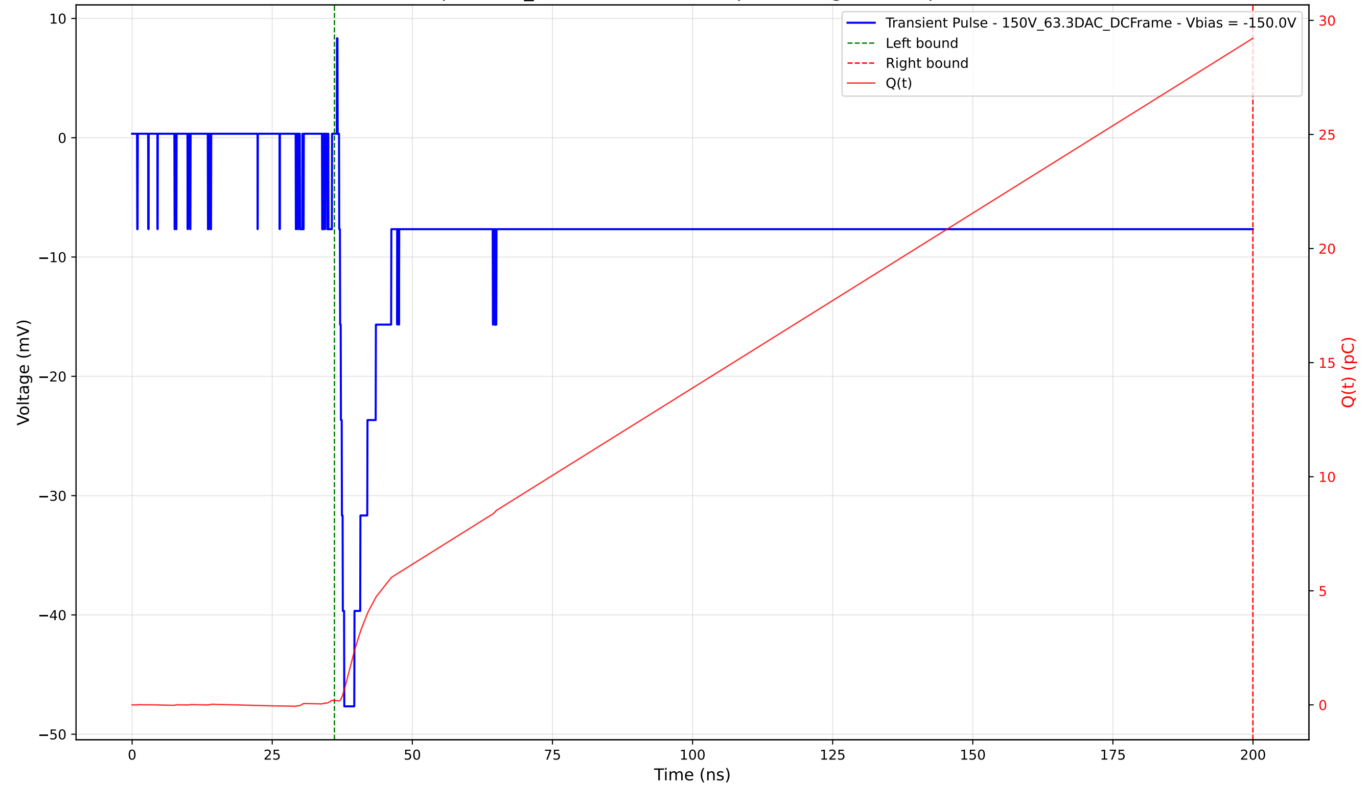
Transient Pulse - Sample: 1cm_42 - Position: 3875.0 \mu\text{m} - Charge: 29.02 pC - Rise Time: 0.91 ns
