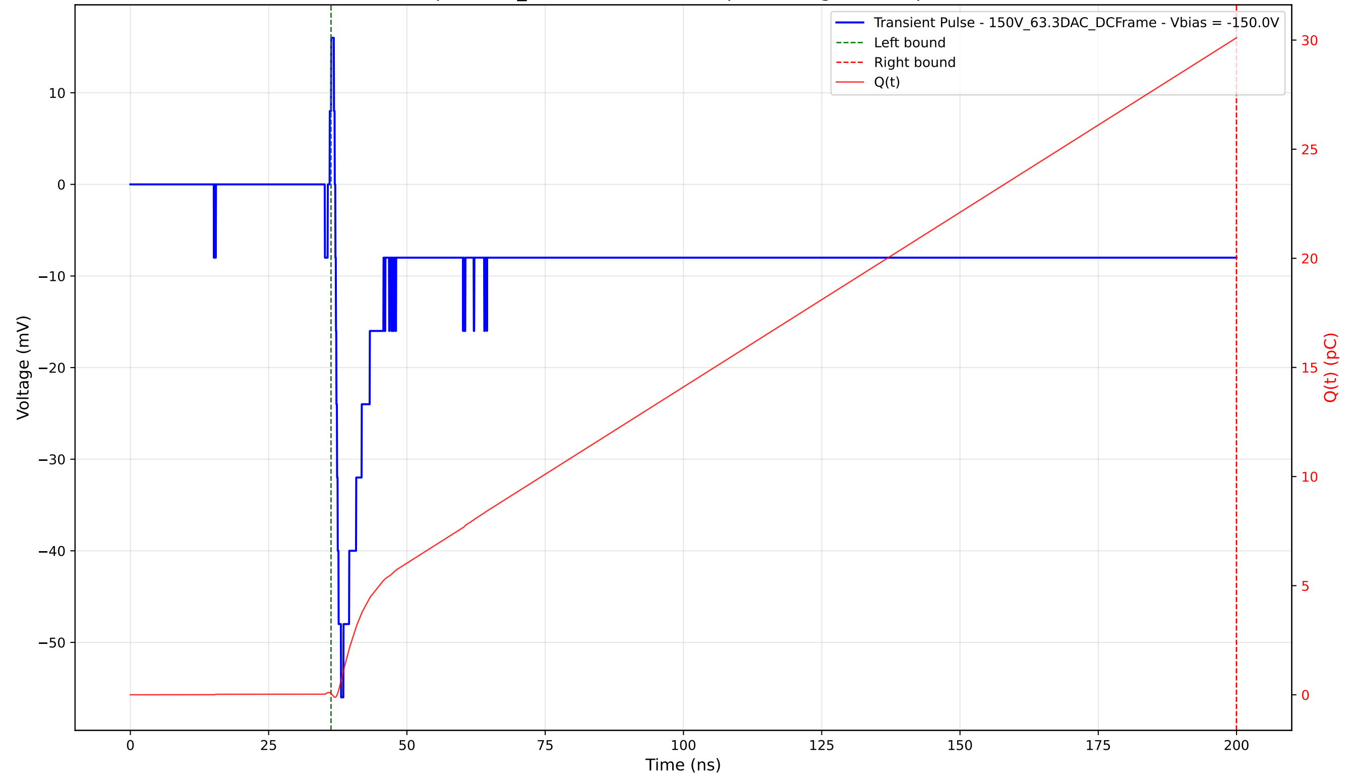
Transient Pulse - Sample: 1cm_42 - Position: 1440.0 \mu\text{m} - Charge: 30.04 pC - Rise Time: 1.03 ns
