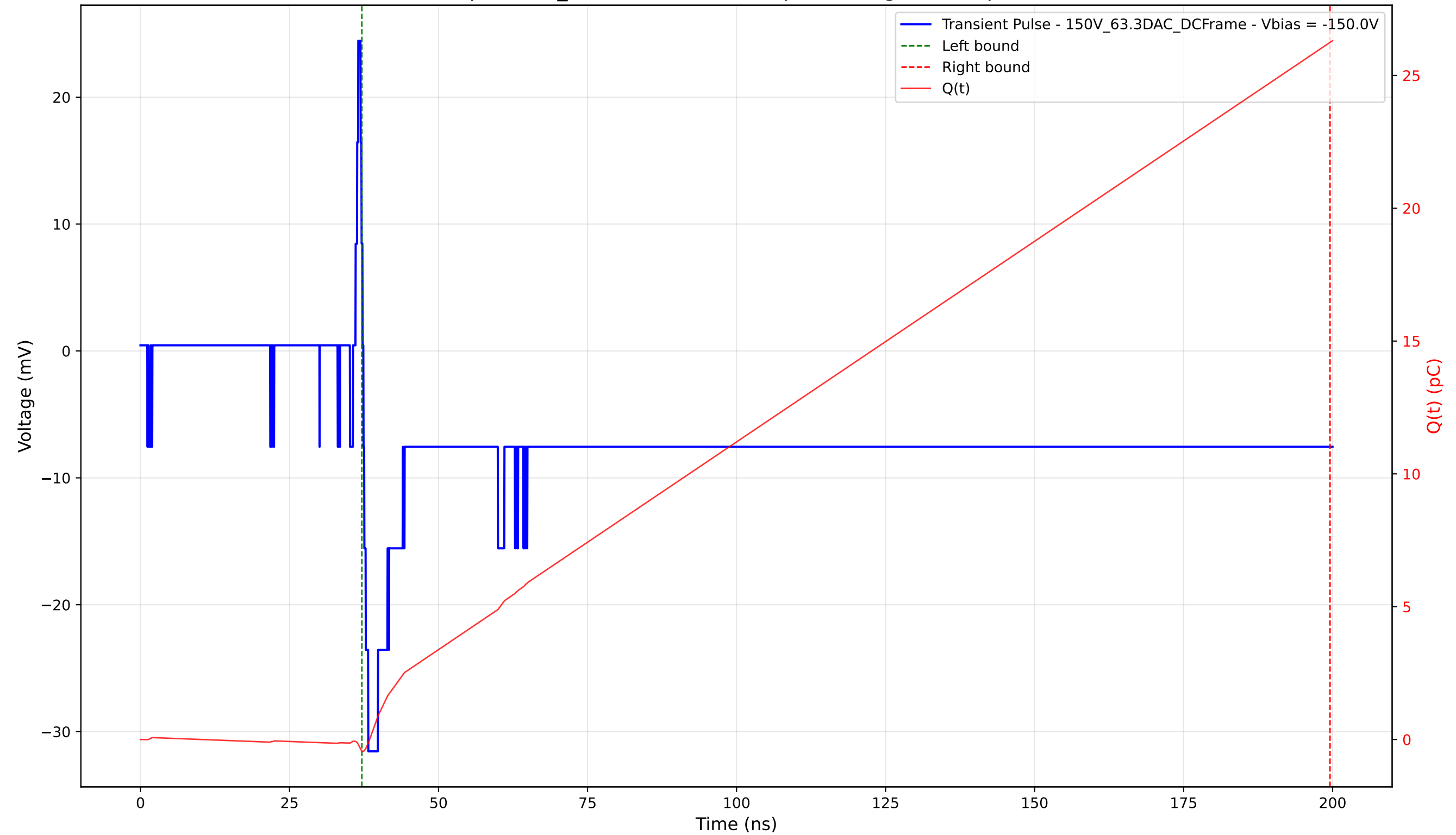
Transient Pulse - Sample: 1cm_42 - Position: 2375.0 \mu\text{m} - Charge: 26.67 pC - Rise Time: 0.81 ns
