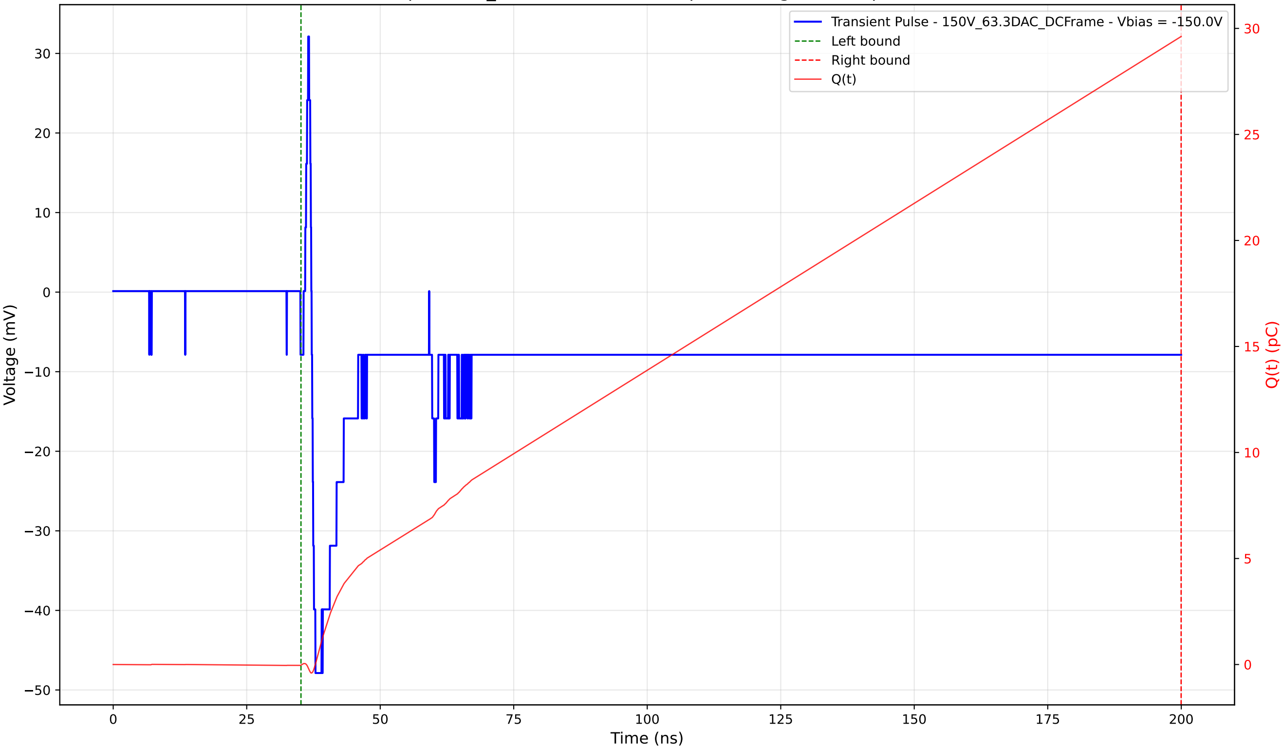
Transient Pulse - Sample: 1cm_42 - Position: 1760.0 \mu\text{m} - Charge: 29.65 pC - Rise Time: 0.71 ns
