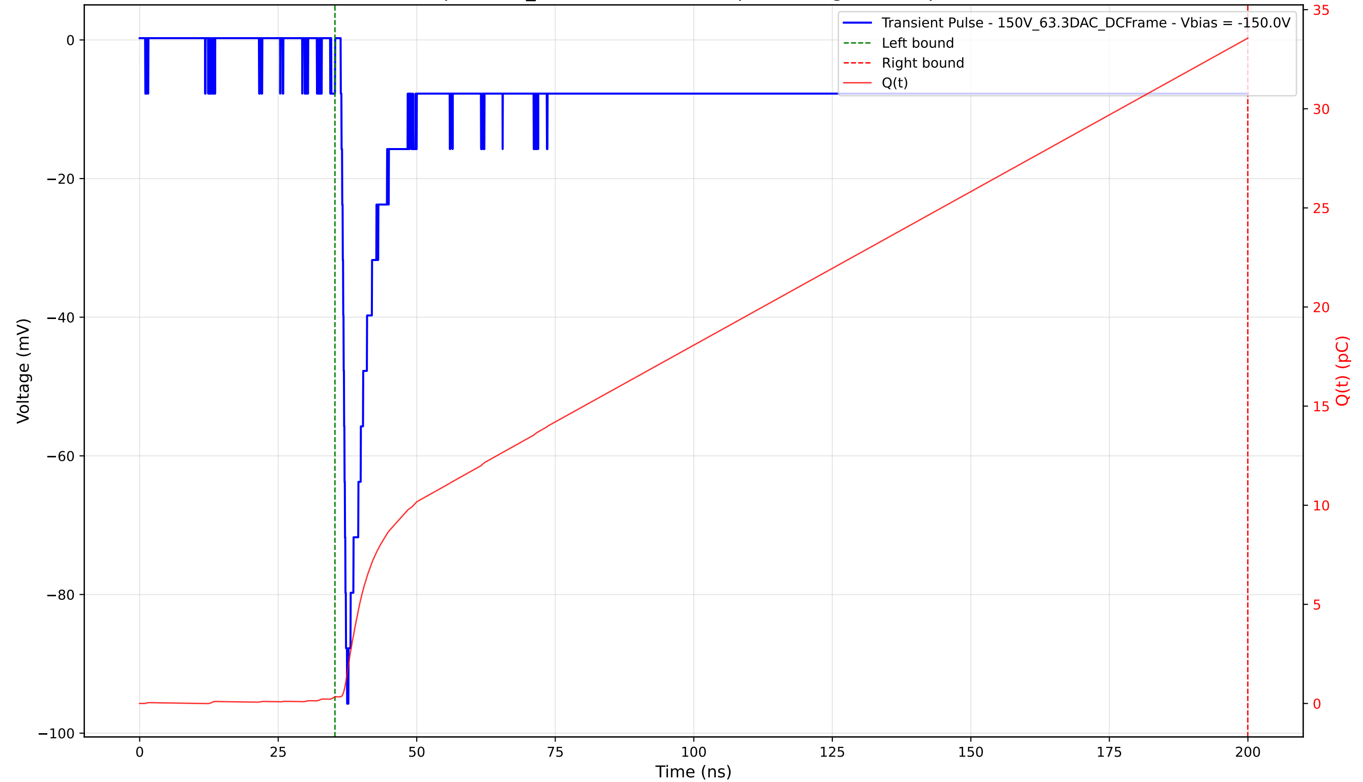
Transient Pulse - Sample: 1cm_42 - Position: 4375.0 \mu\text{m} - Charge: 33.23 pC - Rise Time: 0.82 ns
