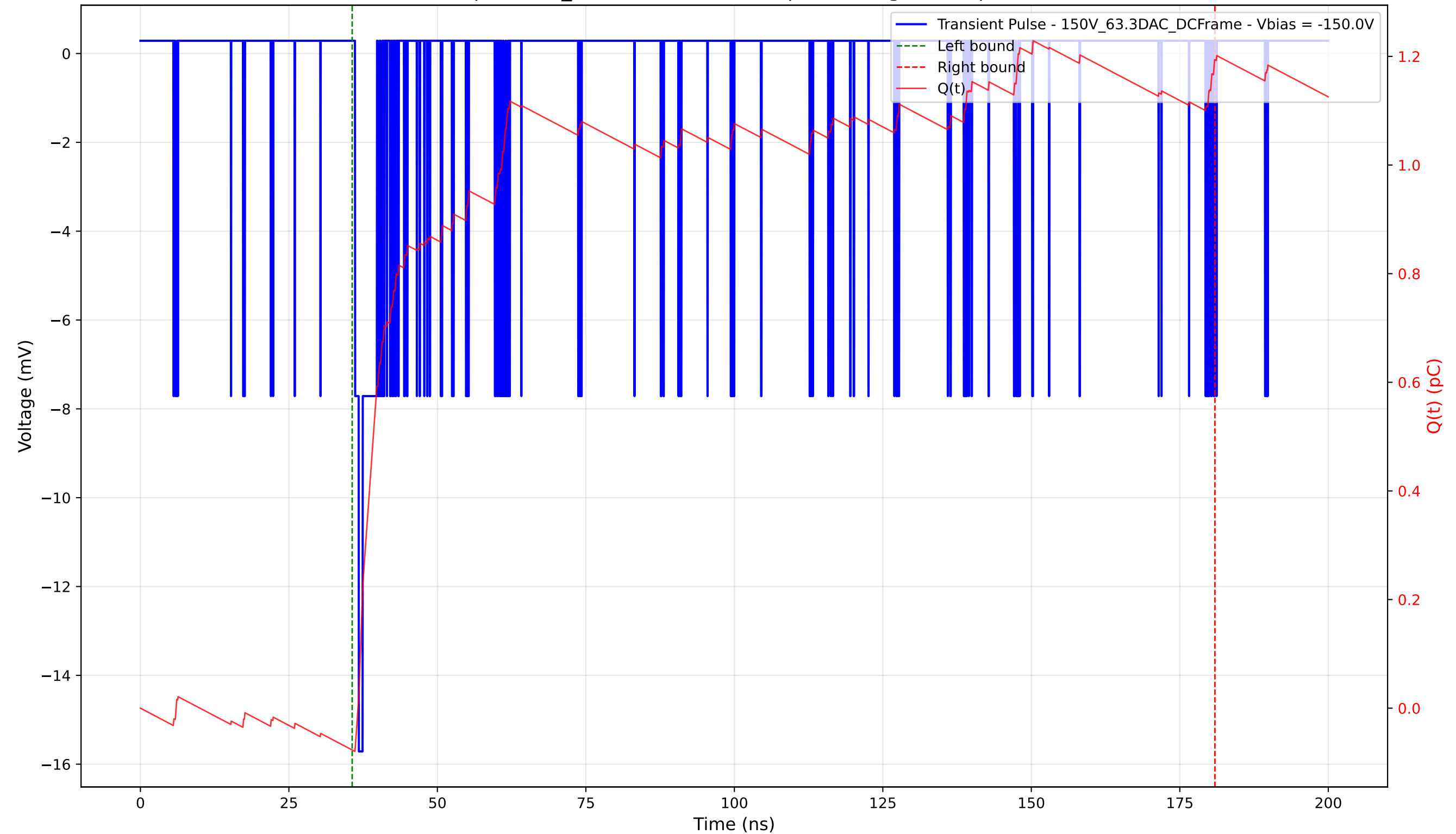
Transient Pulse - Sample: 1cm_42 - Position: 5210.0 \mu\text{m} - Charge: 1.27 pC - Rise Time: 0.64 ns
