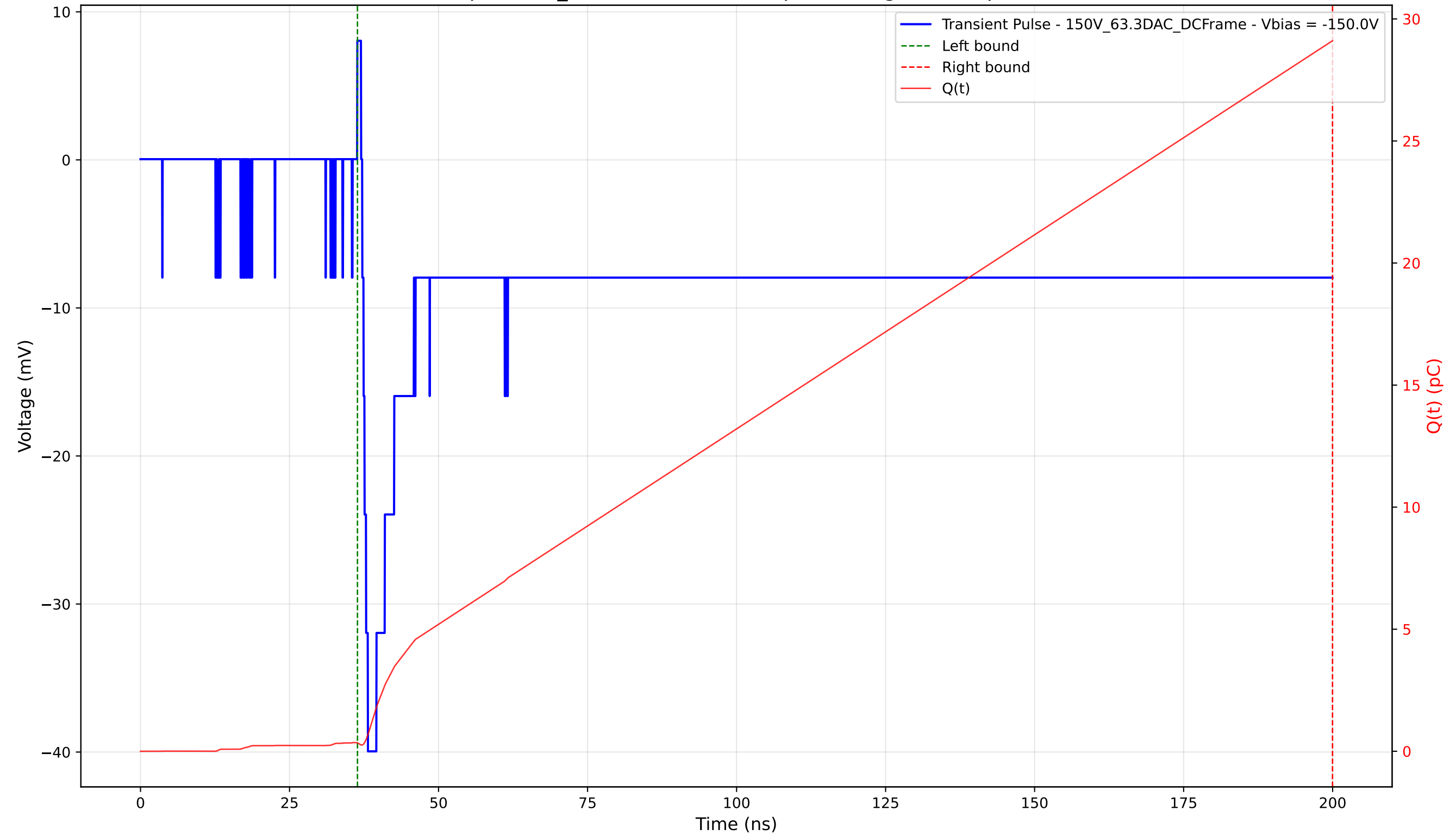
Transient Pulse - Sample: 1cm_42 - Position: 3545.0 \mu\text{m} - Charge: 28.76 pC - Rise Time: 0.95 ns
