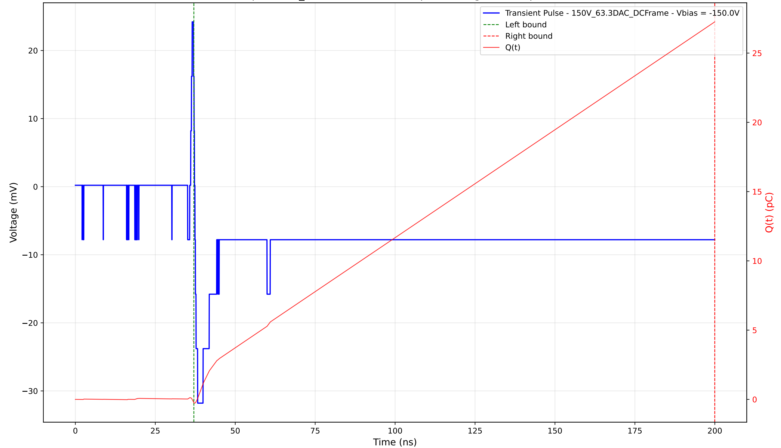
Transient Pulse - Sample: 1cm_42 - Position: 2360.0 \mu\text{m} - Charge: 27.49 pC - Rise Time: 0.85 ns
