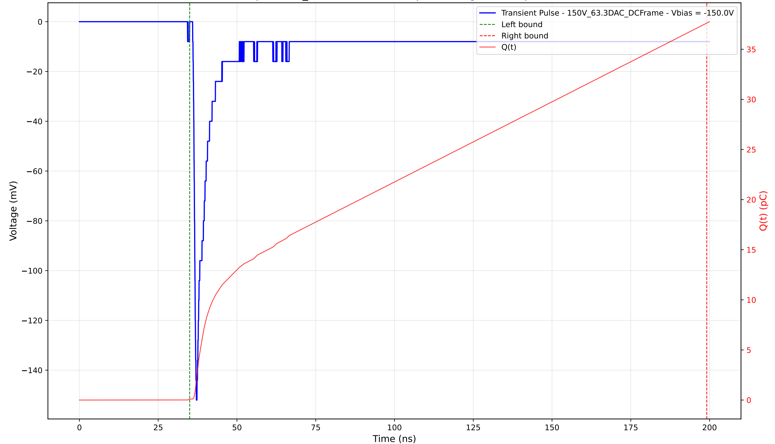
Transient Pulse - Sample: 1cm_42 - Position: 550.0 \mu\text{m} - Charge: 37.52 pC - Rise Time: 0.92 ns
