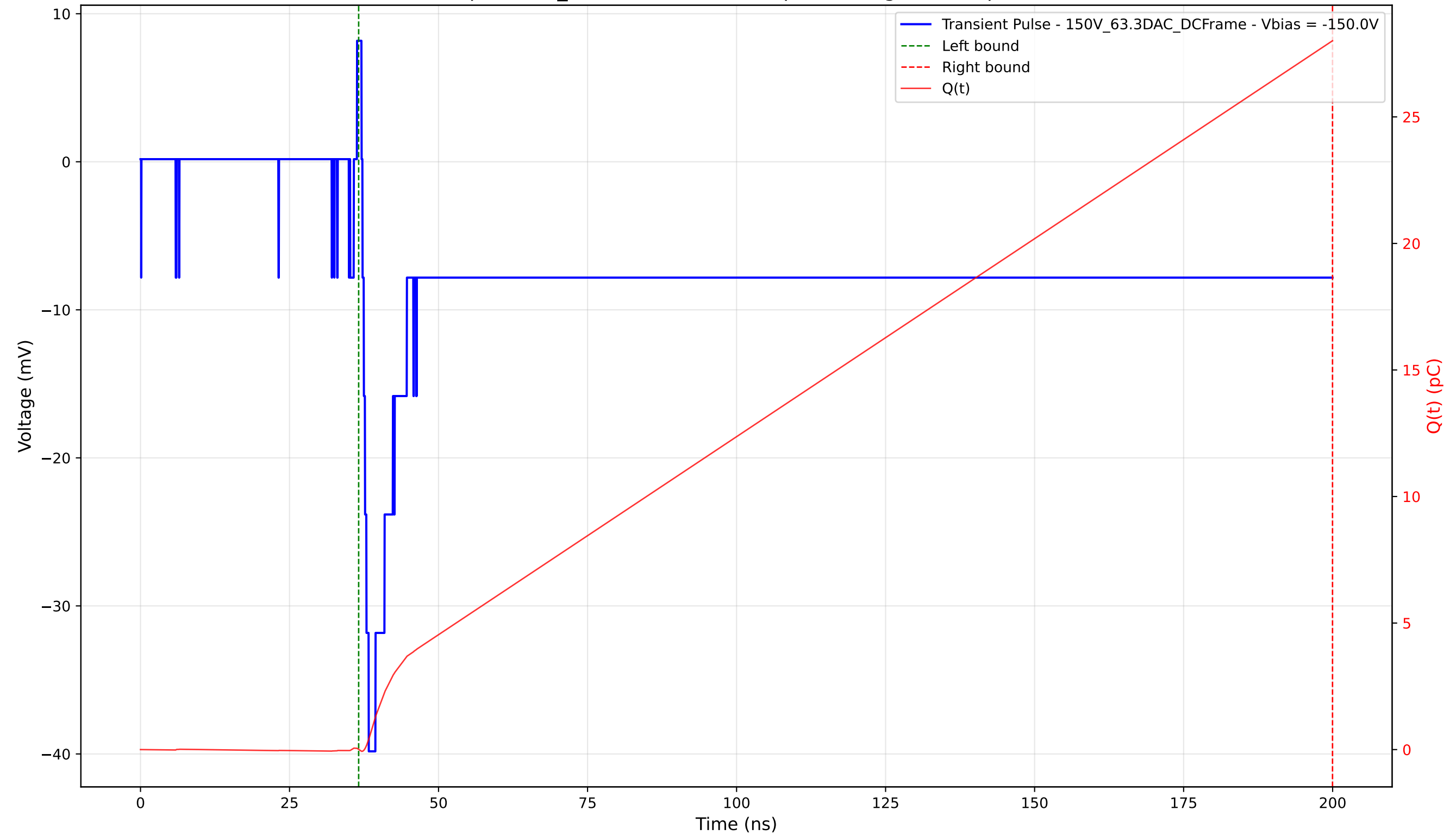
Transient Pulse - Sample: 1cm_42 - Position: 3495.0 \mu\text{m} - Charge: 28.00 pC - Rise Time: 1.05 ns
