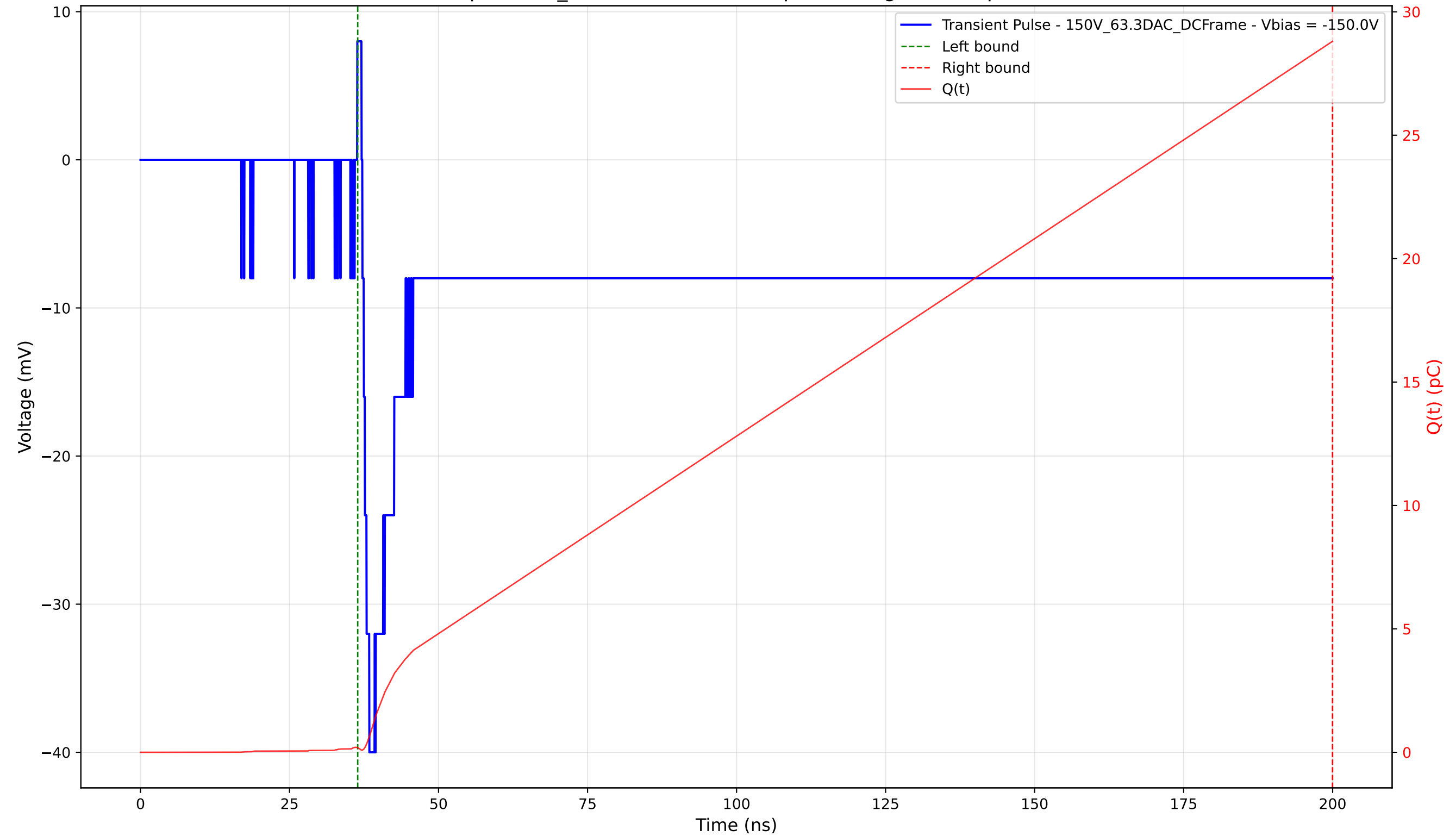
Transient Pulse - Sample: 1cm_42 - Position: 3520.0 \mu\text{m} - Charge: 28.62 pC - Rise Time: 1.17 ns
