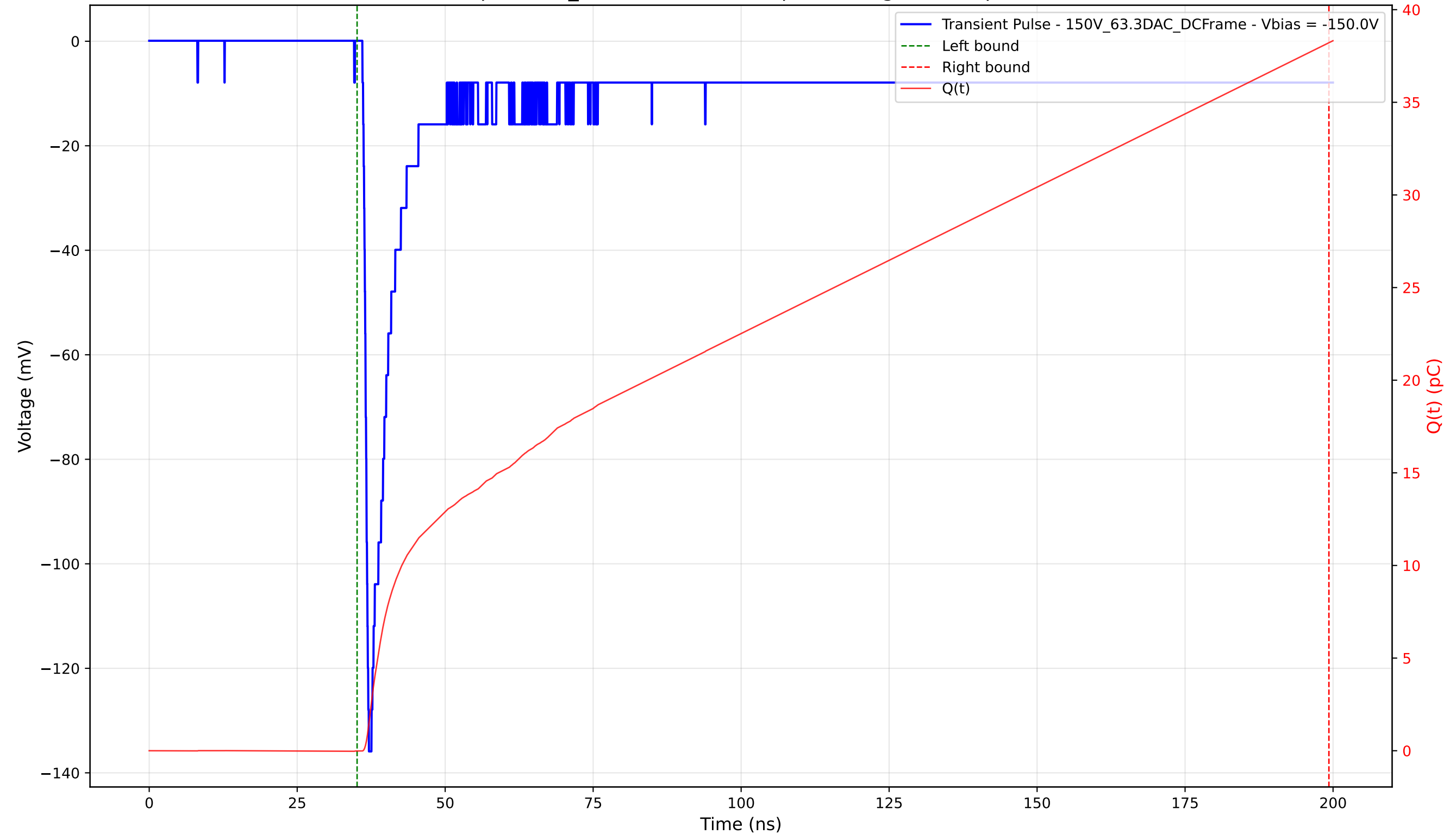
Transient Pulse - Sample: 1cm_42 - Position: 630.0 \mu\text{m} - Charge: 38.23 pC - Rise Time: 0.87 ns
