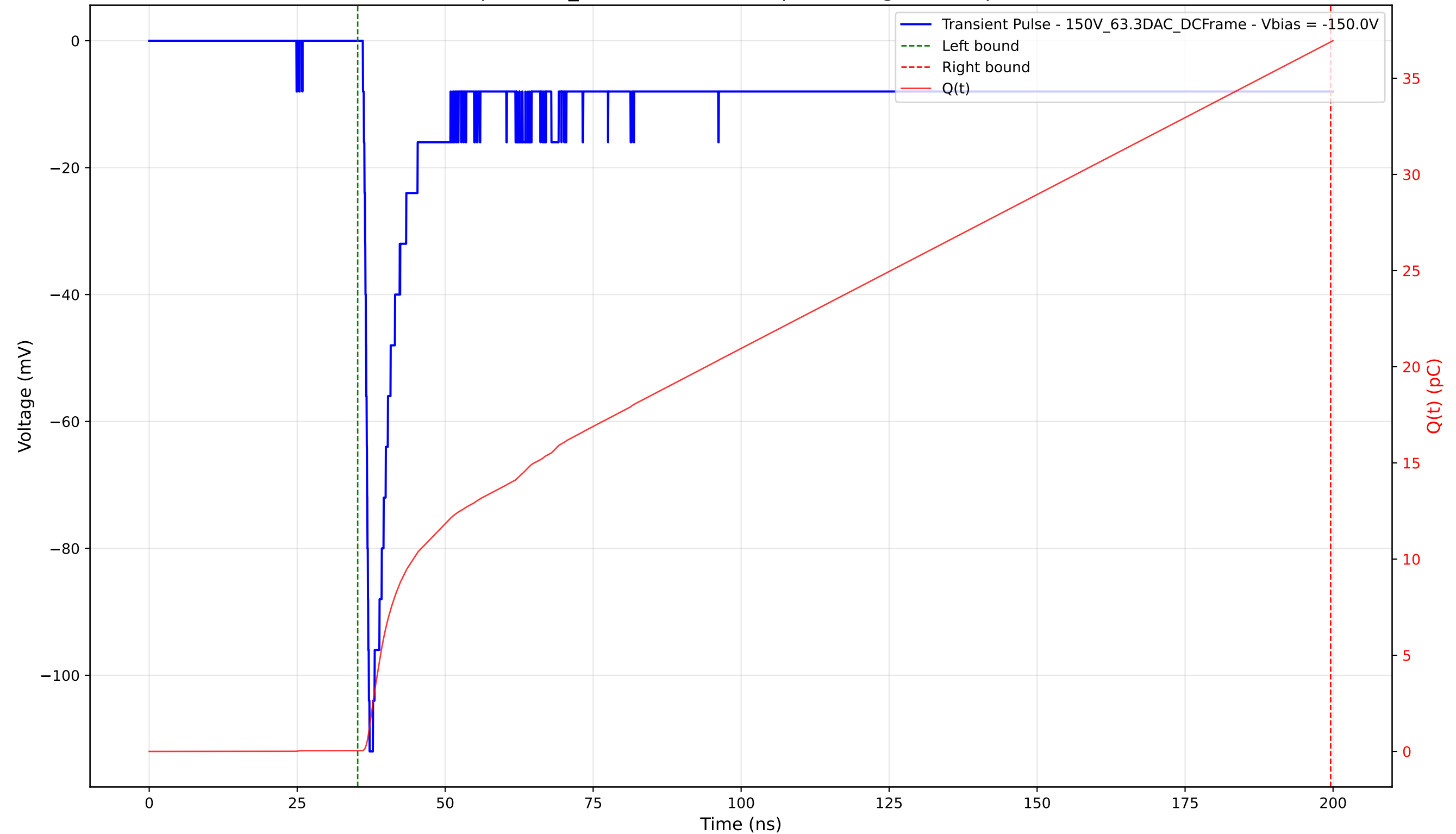
Transient Pulse - Sample: 1cm_42 - Position: 810.0 \mu\text{m} - Charge: 36.84 pC - Rise Time: 0.85 ns
