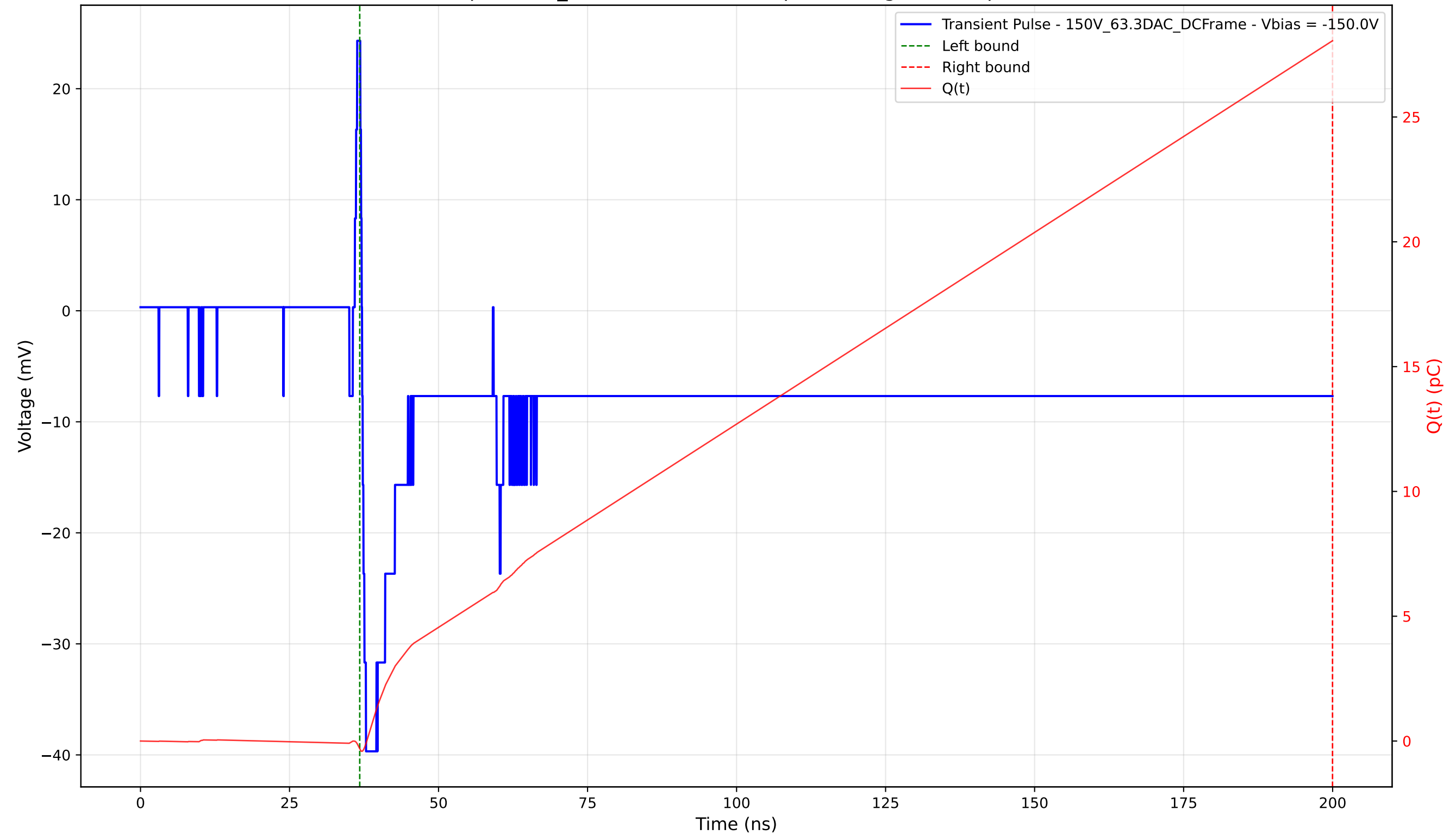
Transient Pulse - Sample: 1cm_42 - Position: 1860.0 \mu\text{m} - Charge: 28.37 pC - Rise Time: 0.65 ns
