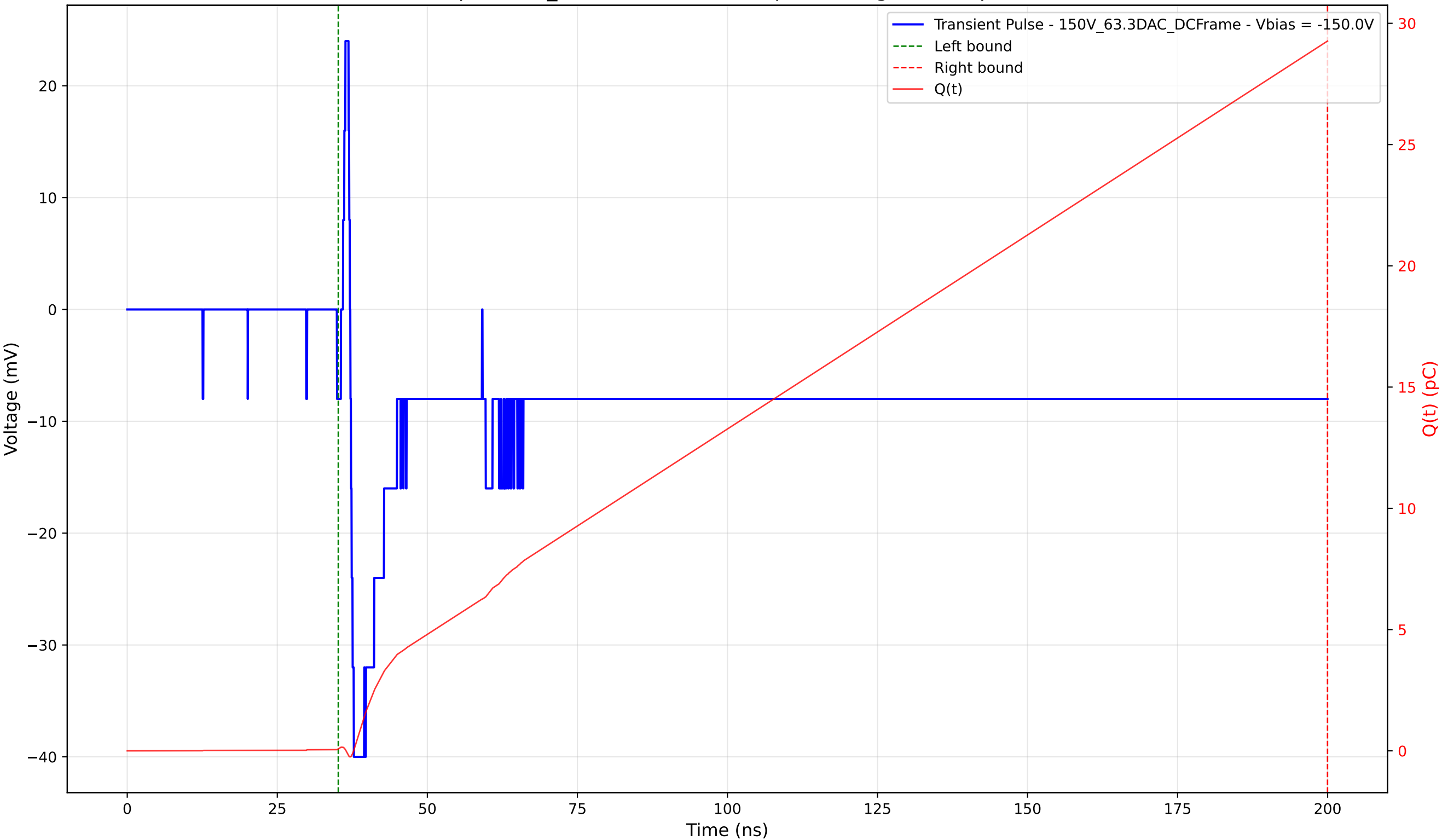
Transient Pulse - Sample: 1cm_42 - Position: 1855.0 \mu\text{m} - Charge: 29.19 pC - Rise Time: 0.57 ns
