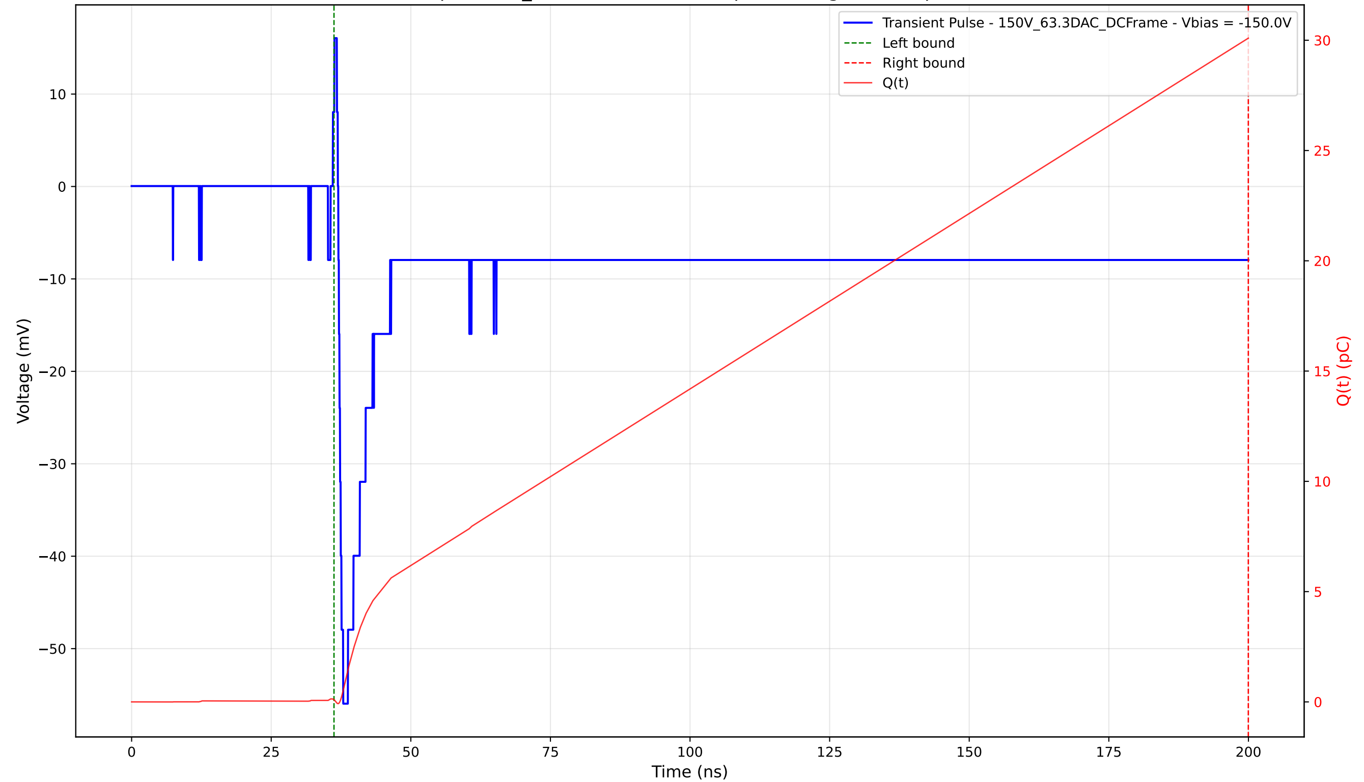
Transient Pulse - Sample: 1cm_42 - Position: 1425.0 \mu\text{m} - Charge: 29.99 pC - Rise Time: 0.87 ns
