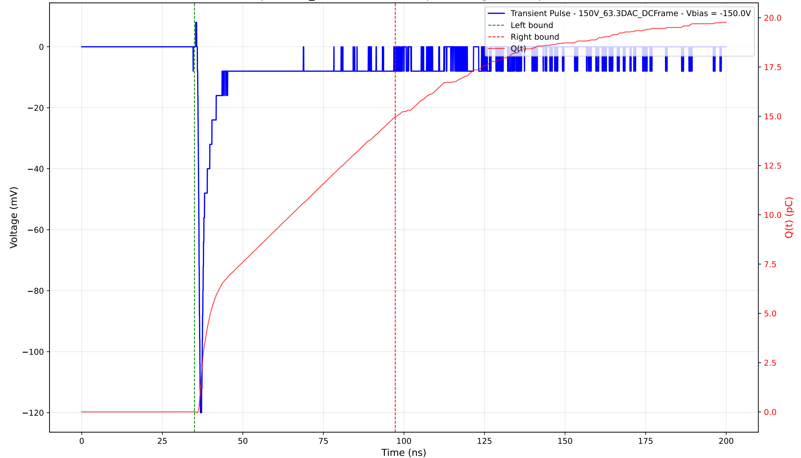
Transient Pulse - Sample: 1cm_42 - Position: 160.0 \mu\text{m} - Charge: 14.96 pC - Rise Time: 0.73 ns
