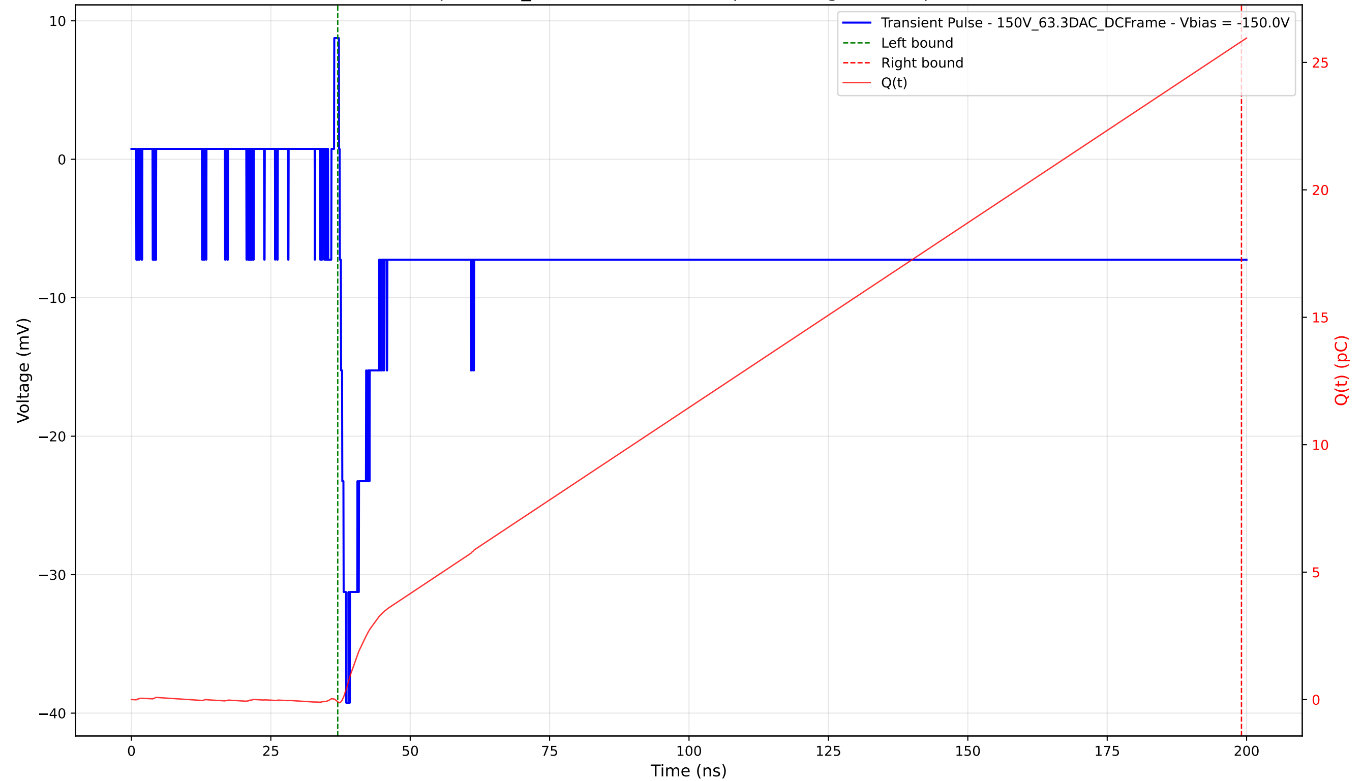
Transient Pulse - Sample: 1cm_42 - Position: 3385.0 \mu\text{m} - Charge: 25.91 pC - Rise Time: 1.15 ns
