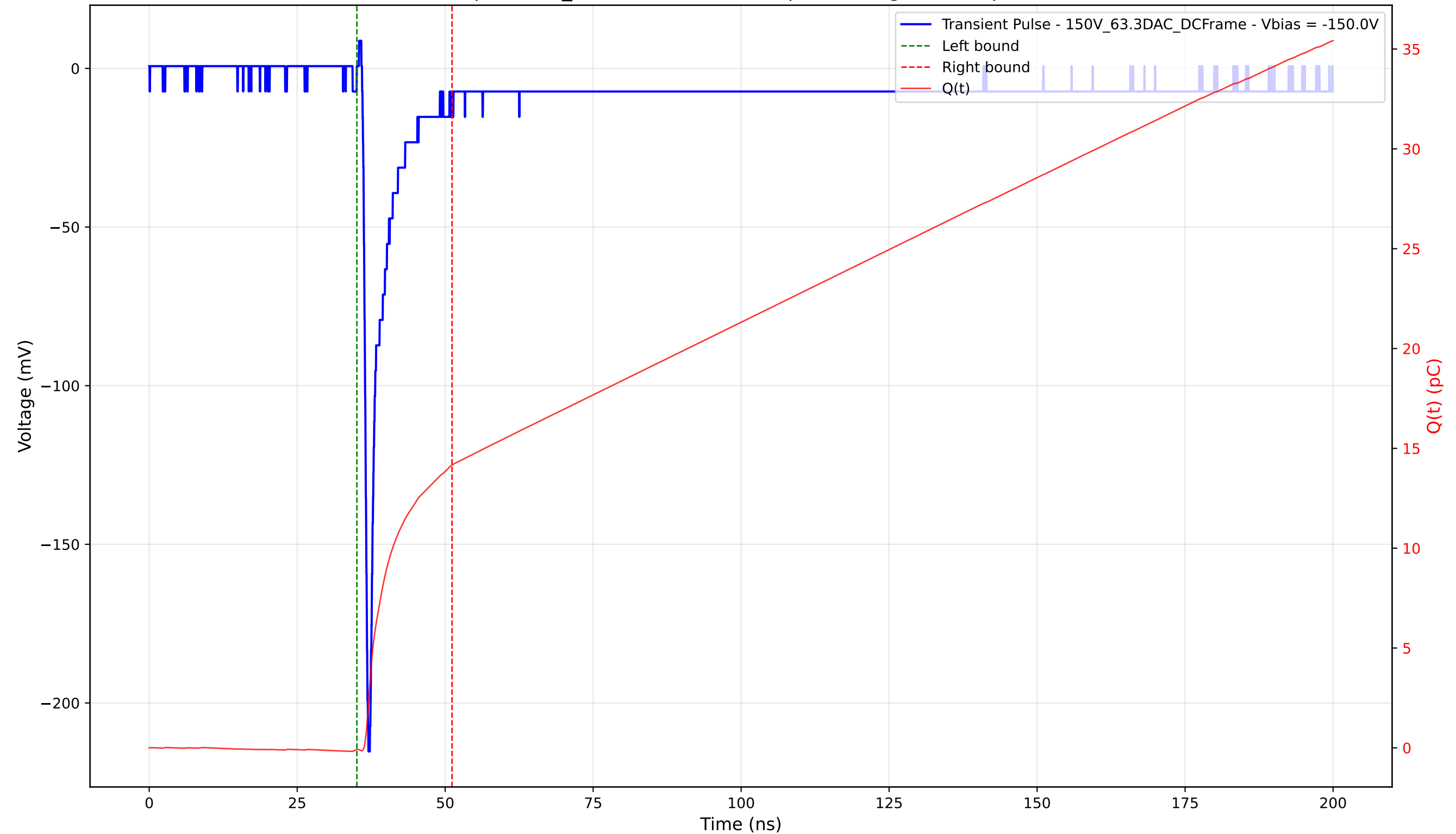
Transient Pulse - Sample: 1cm_42 - Position: 4885.0 \mu\text{m} - Charge: 14.24 pC - Rise Time: 0.78 ns
