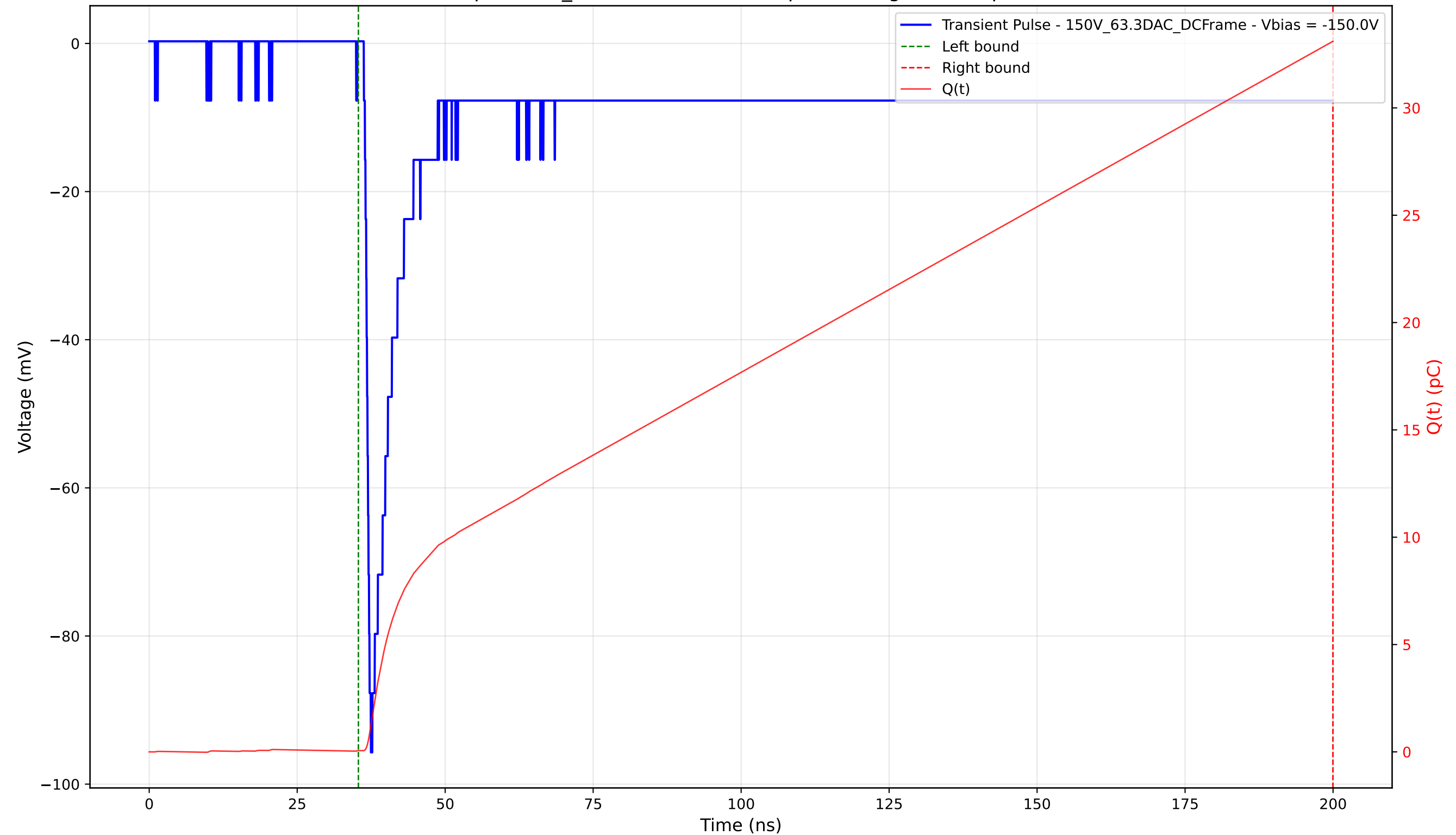
Transient Pulse - Sample: 1cm_42 - Position: 4365.0 \mu\text{m} - Charge: 33.04 pC - Rise Time: 0.80 ns
