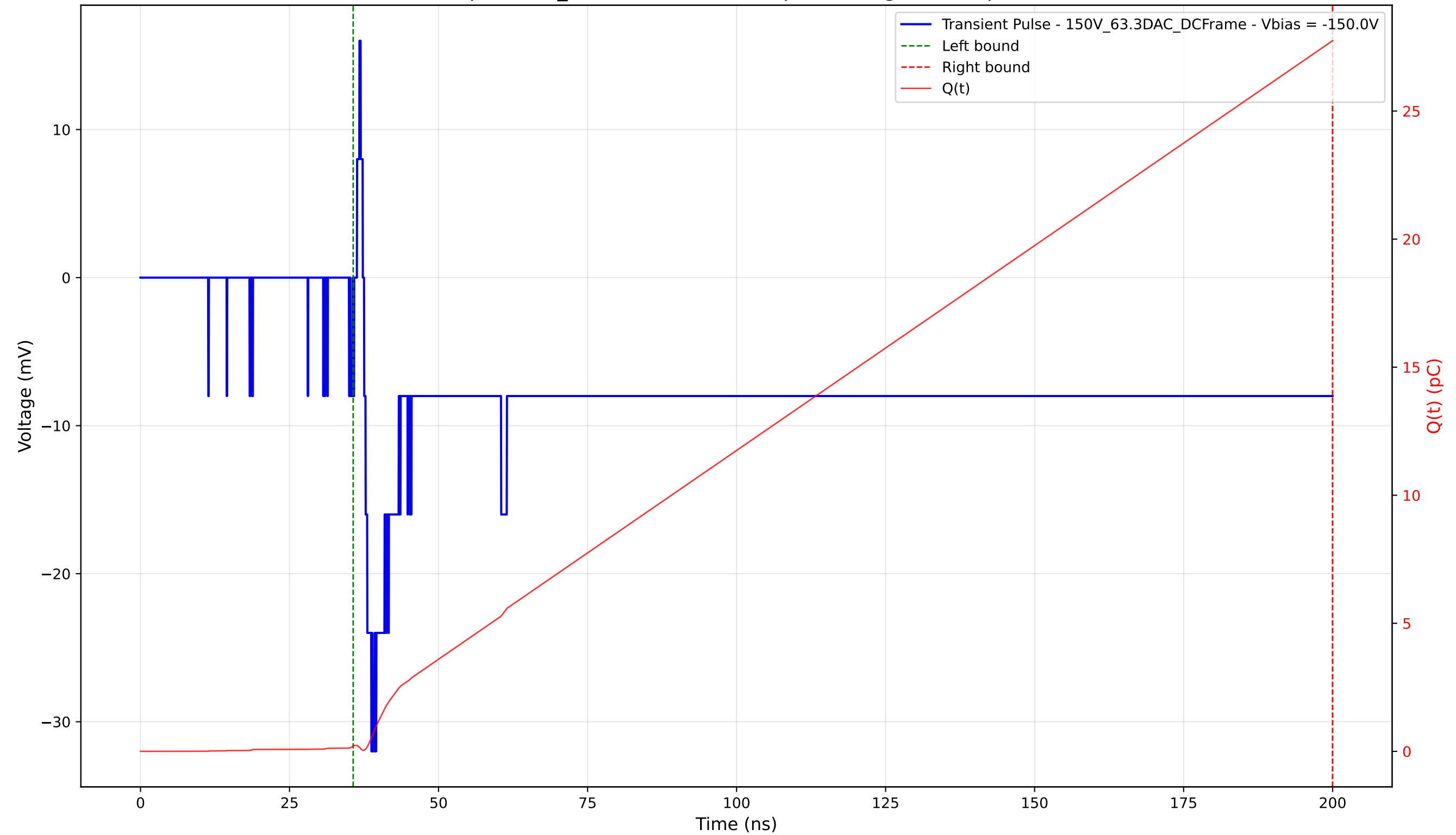
Transient Pulse - Sample: 1cm_42 - Position: 2990.0 \mu\text{m} - Charge: 27.54 pC - Rise Time: 1.21 ns
