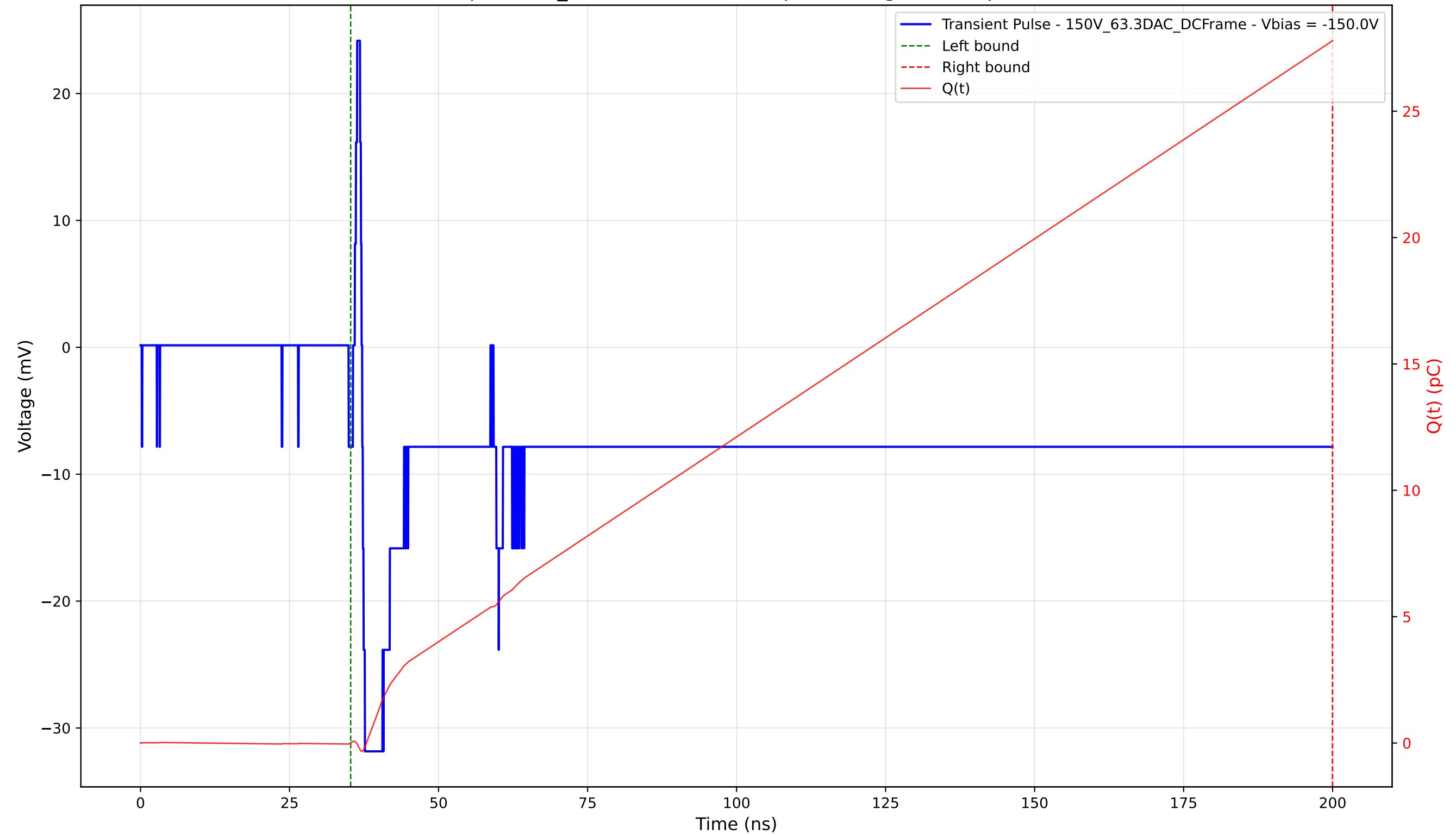
Transient Pulse - Sample: 1cm_42 - Position: 1965.0 \mu\text{m} - Charge: 27.78 pC - Rise Time: 0.45 ns
