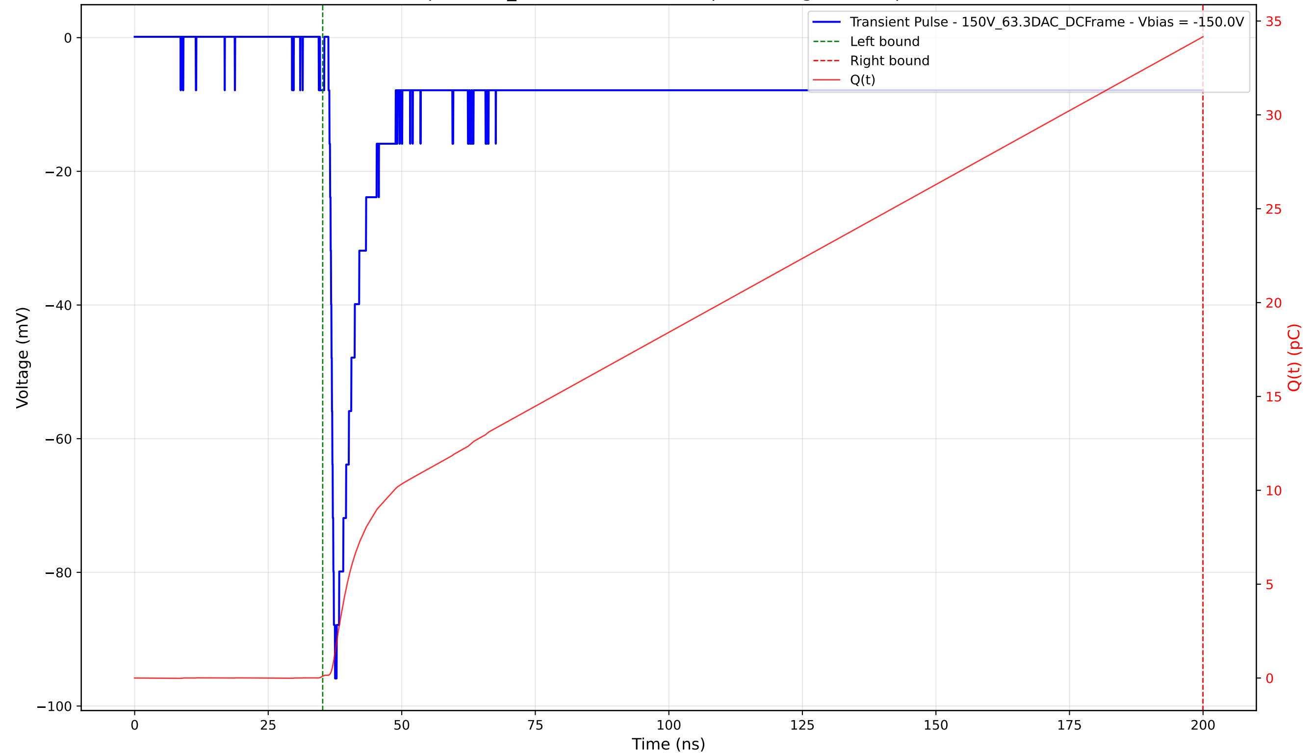
Transient Pulse - Sample: 1cm_42 - Position: 4325.0 \mu\text{m} - Charge: 34.06 pC - Rise Time: 0.84 ns
