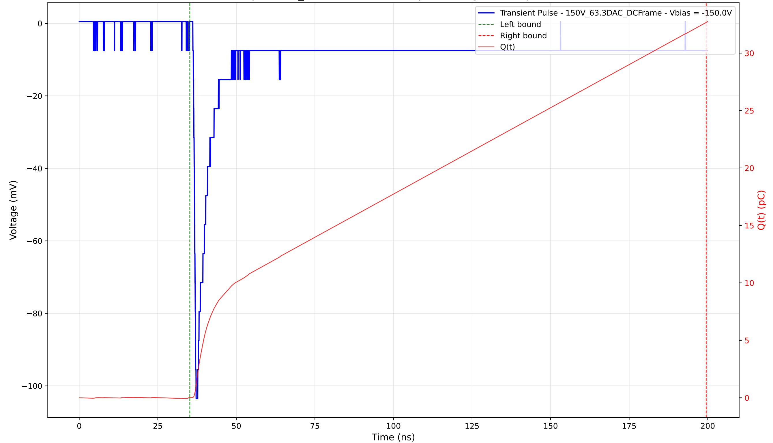
Transient Pulse - Sample: 1cm_42 - Position: 4475.0 \mu\text{m} - Charge: 32.63 pC - Rise Time: 0.75 ns
