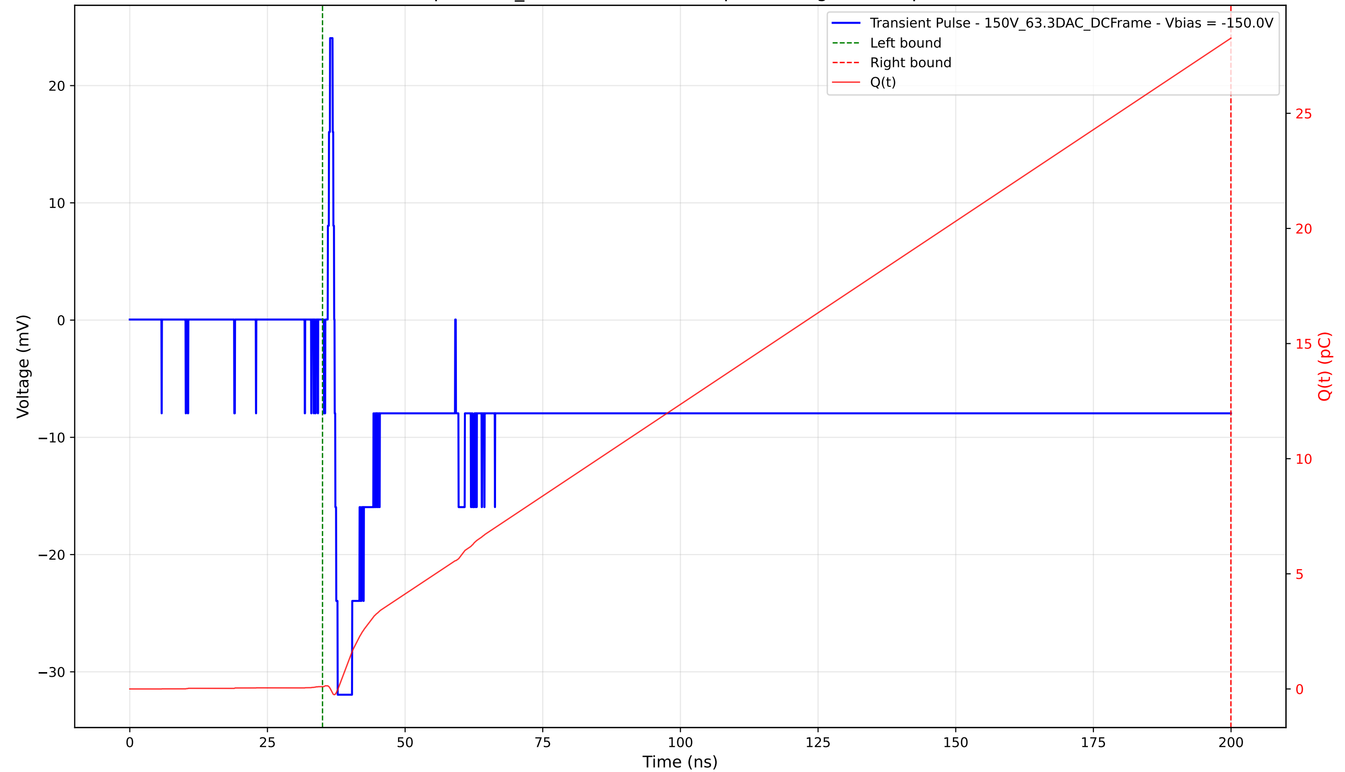
Transient Pulse - Sample: 1cm_42 - Position: 2015.0 \mu\text{m} - Charge: 28.17 pC - Rise Time: 0.55 ns
