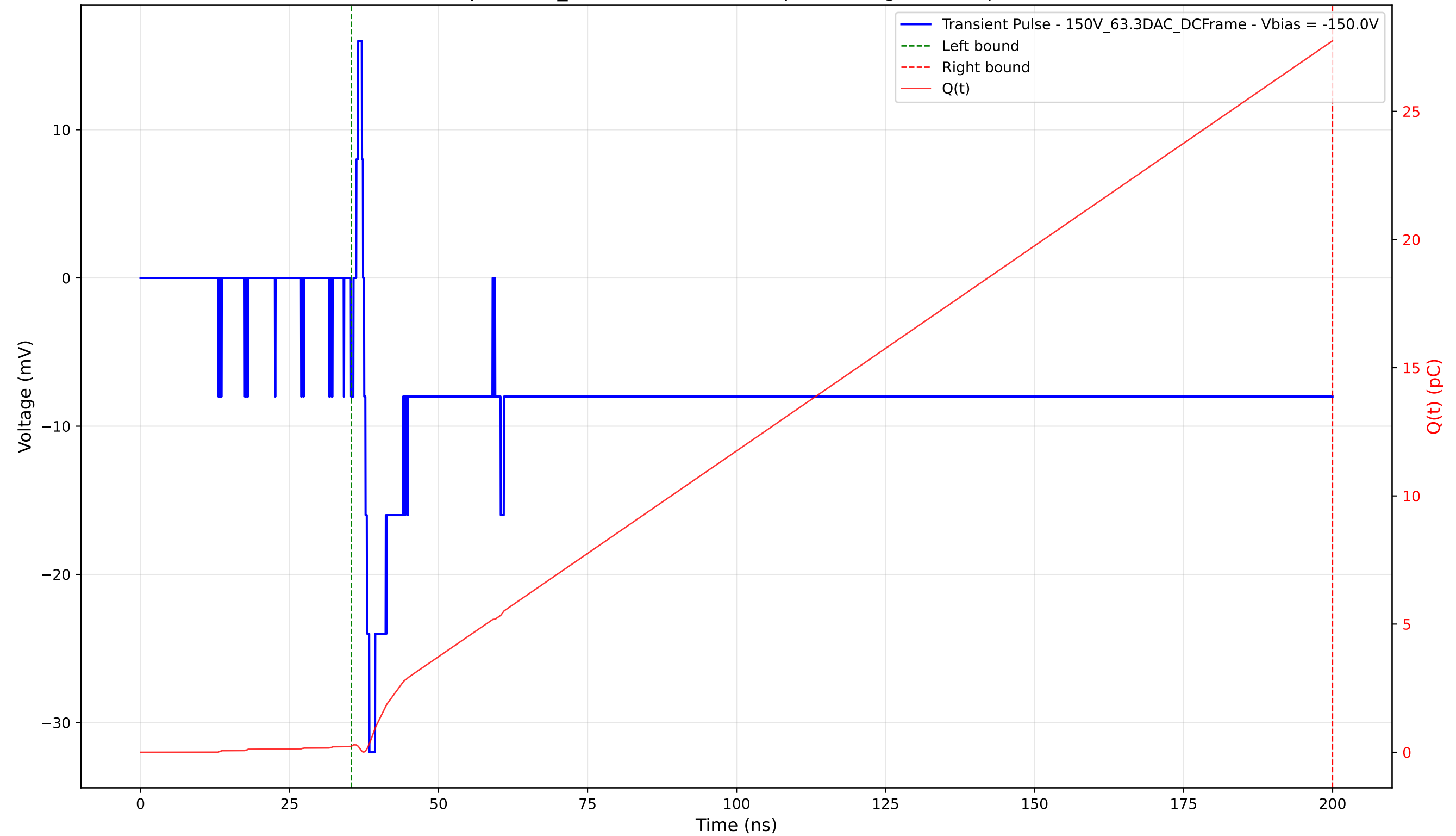
Transient Pulse - Sample: 1cm_42 - Position: 2555.0 \mu\text{m} - Charge: 27.51 pC - Rise Time: 0.87 ns
