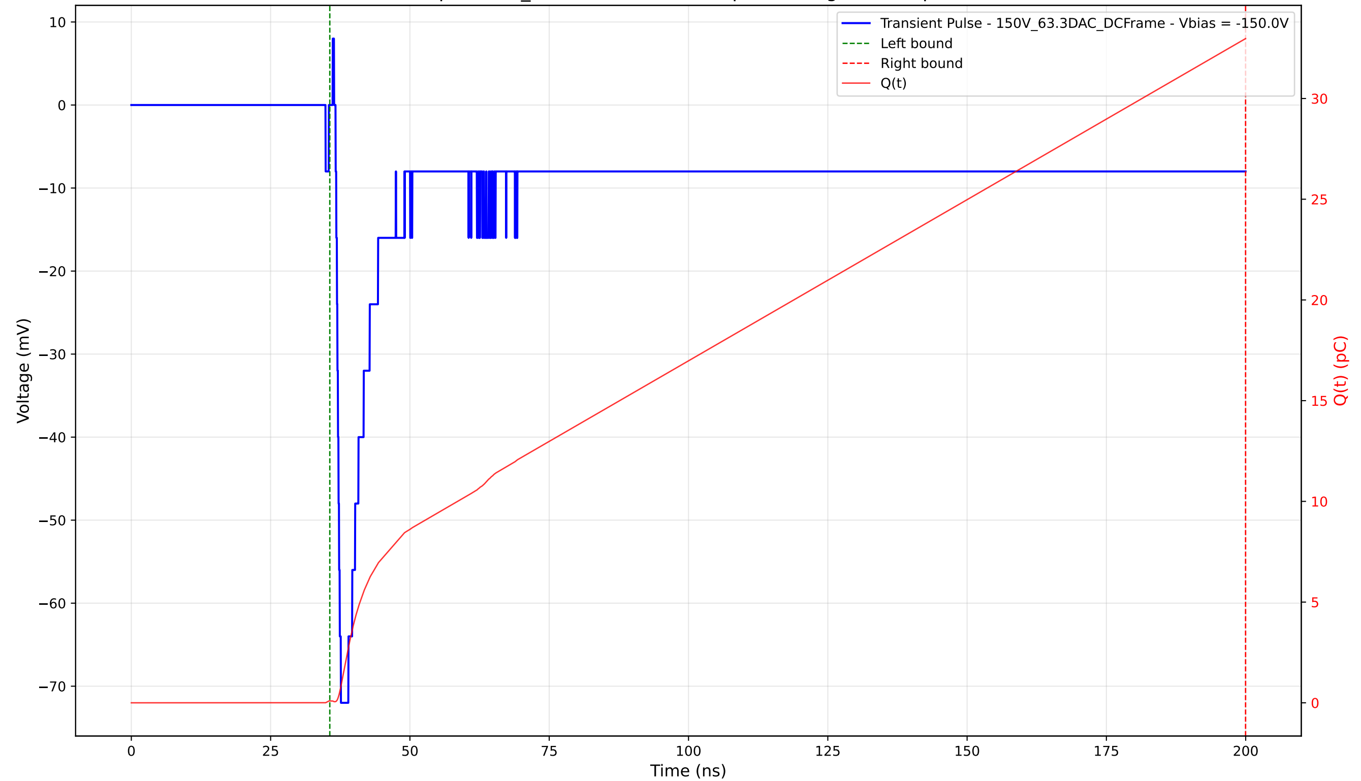
Transient Pulse - Sample: 1cm_42 - Position: 1060.0 \mu\text{m} - Charge: 32.88 pC - Rise Time: 0.94 ns
