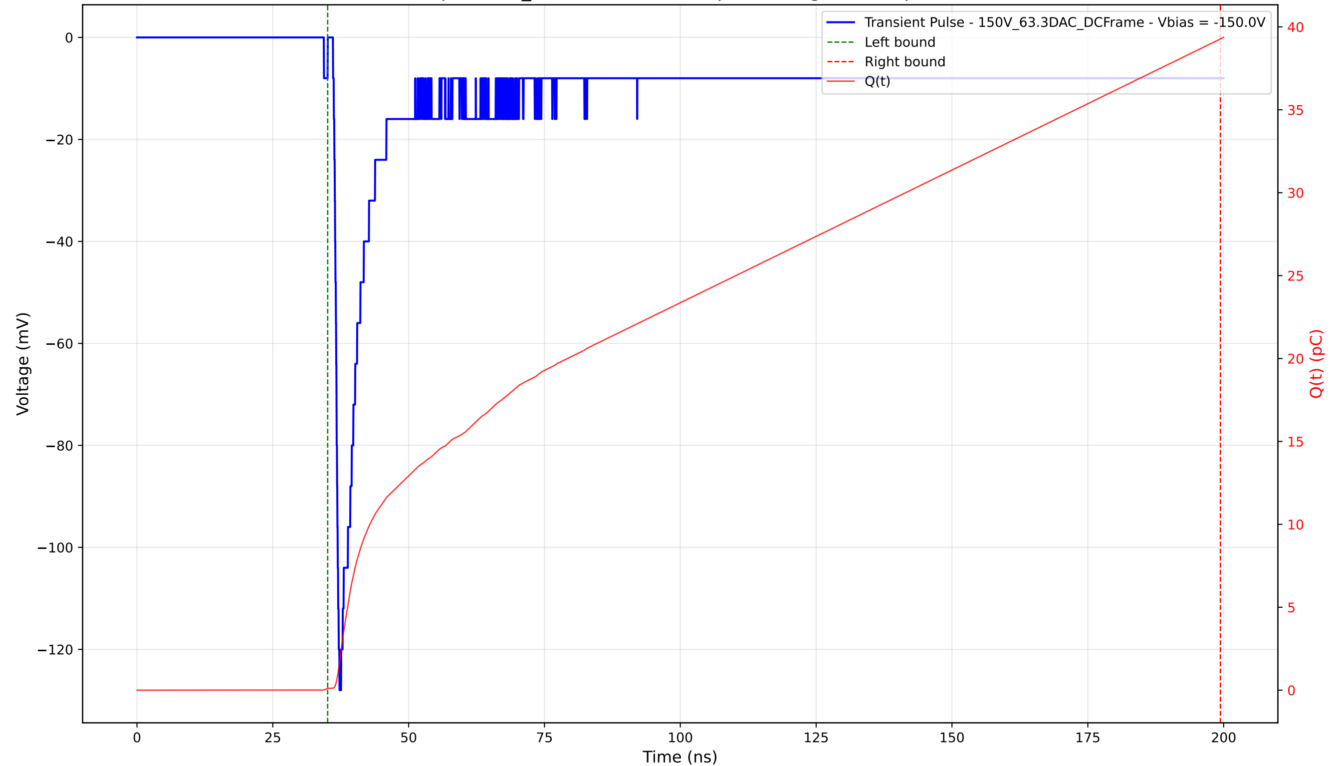
Transient Pulse - Sample: 1cm_42 - Position: 760.0 \mu\text{m} - Charge: 39.16 pC - Rise Time: 0.91 ns
