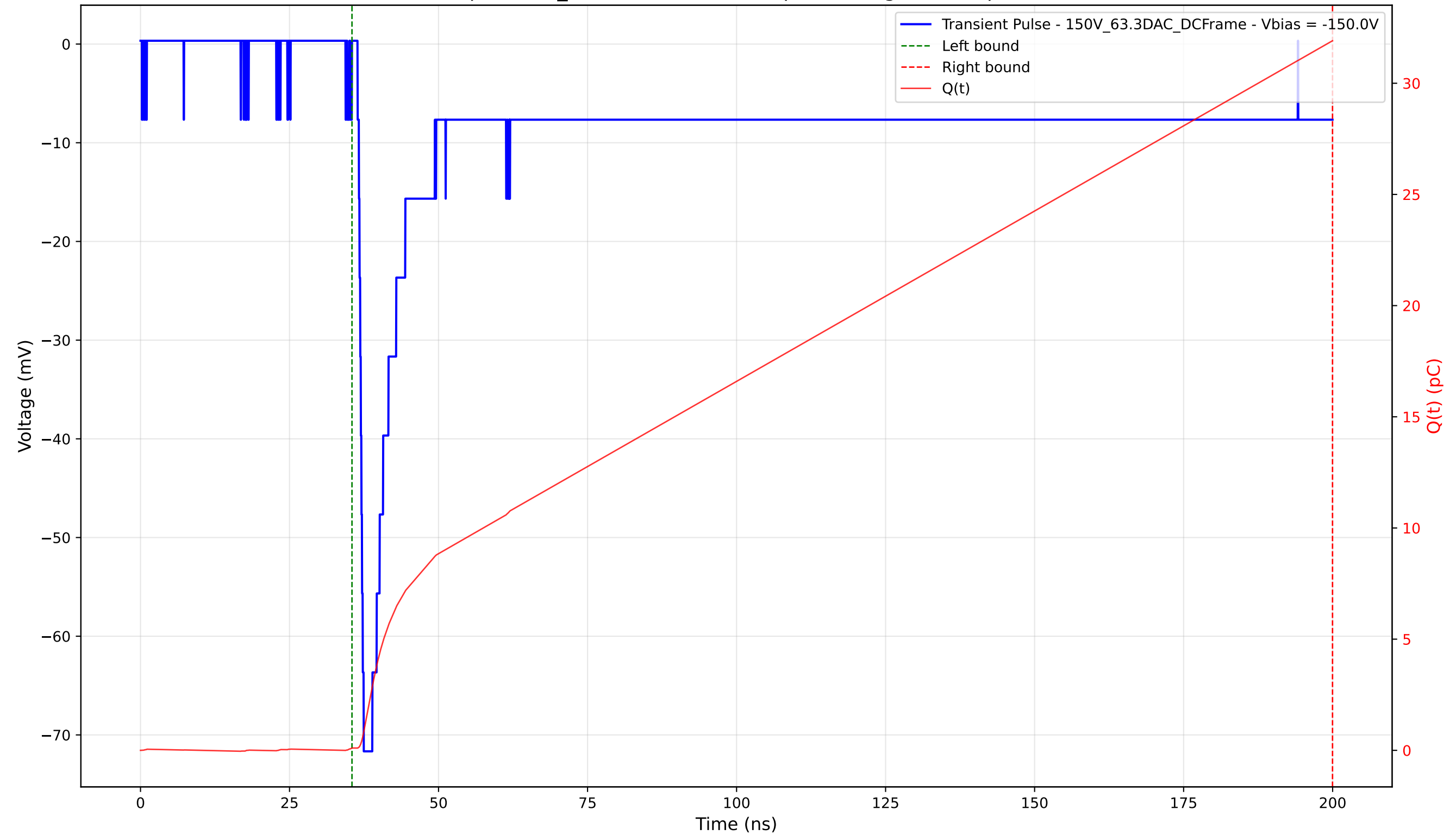
Transient Pulse - Sample: 1cm_42 - Position: 4145.0 \mu\text{m} - Charge: 31.81 pC - Rise Time: 1.02 ns
