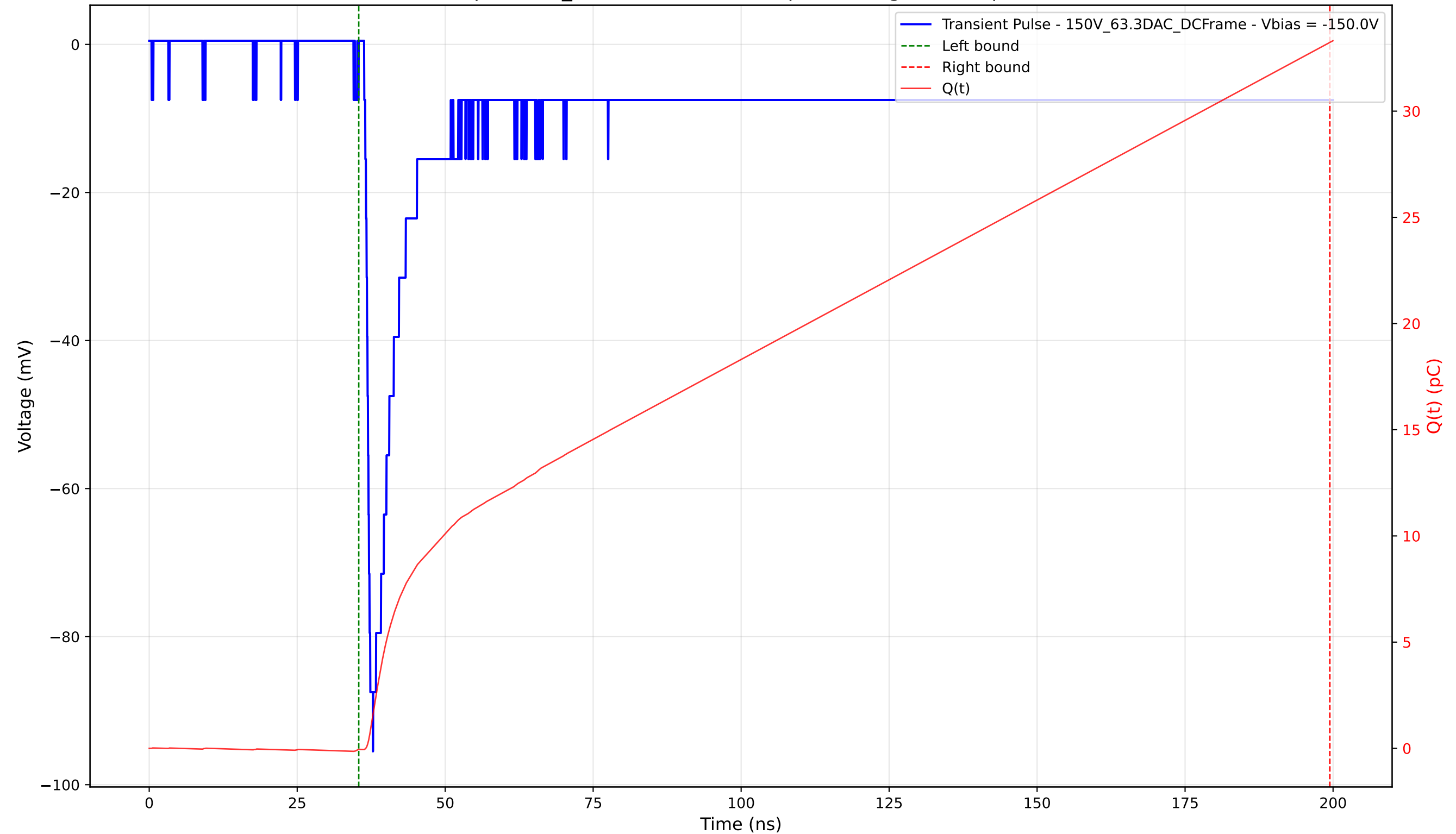
Transient Pulse - Sample: 1cm_42 - Position: 4255.0 \mu\text{m} - Charge: 33.29 pC - Rise Time: 0.85 ns
