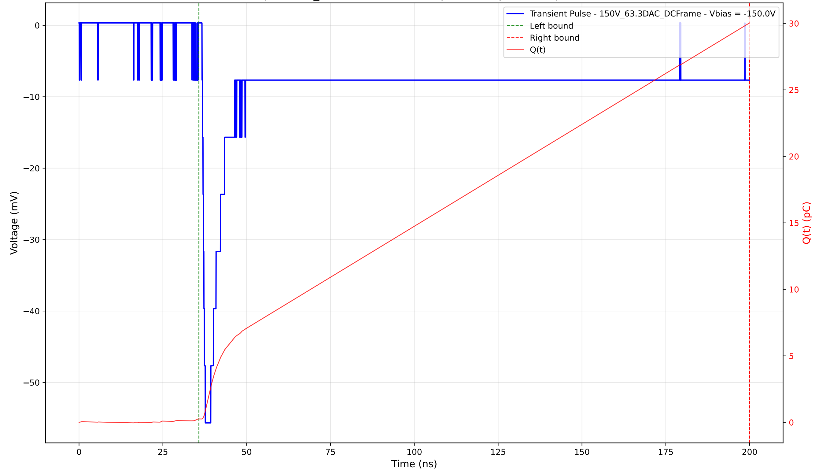
Transient Pulse - Sample: 1cm_42 - Position: 4025.0 \mu\text{m} - Charge: 29.78 pC - Rise Time: 0.97 ns
