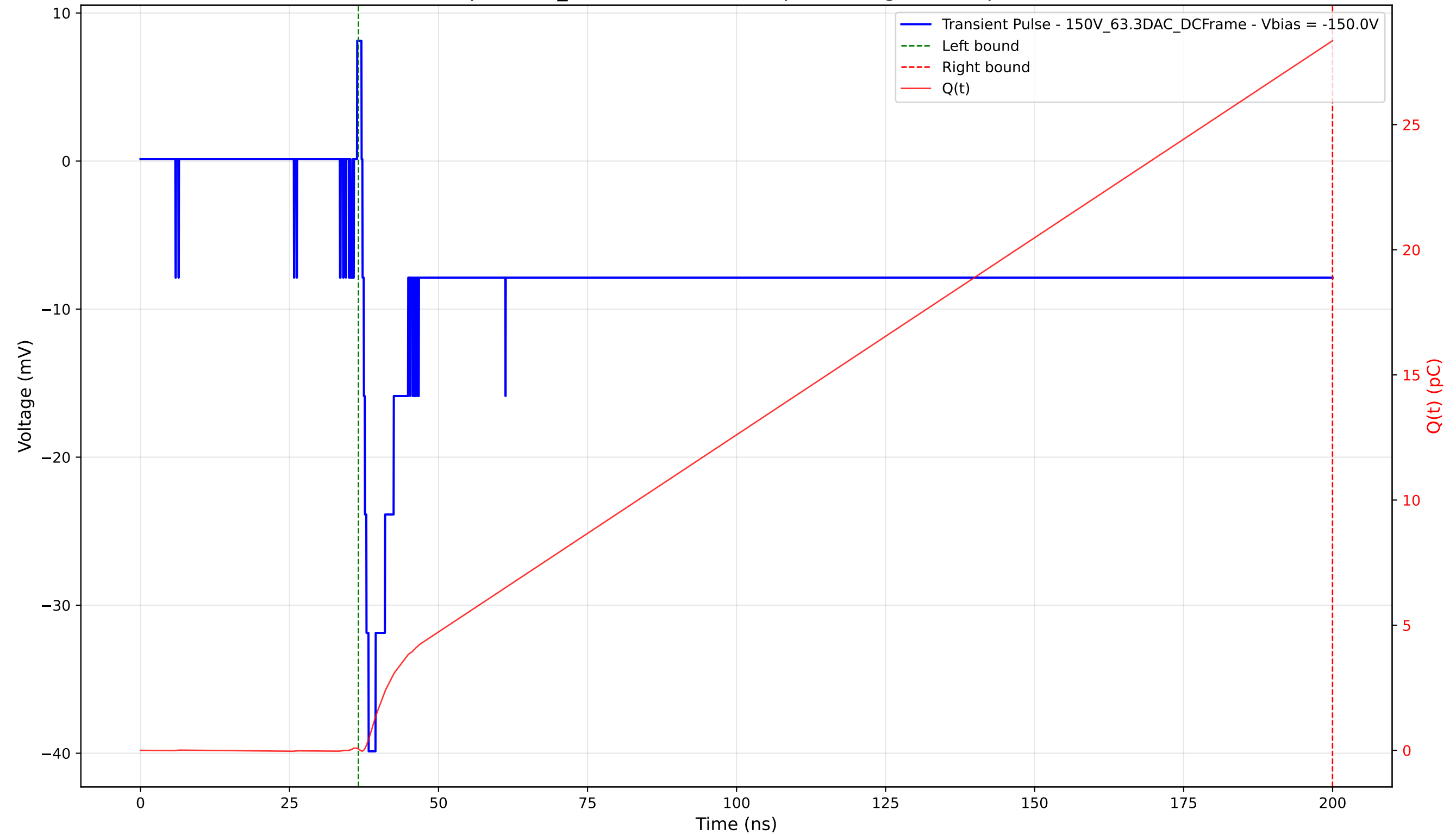
Transient Pulse - Sample: 1cm_42 - Position: 3515.0 \mu\text{m} - Charge: 28.30 pC - Rise Time: 1.03 ns
