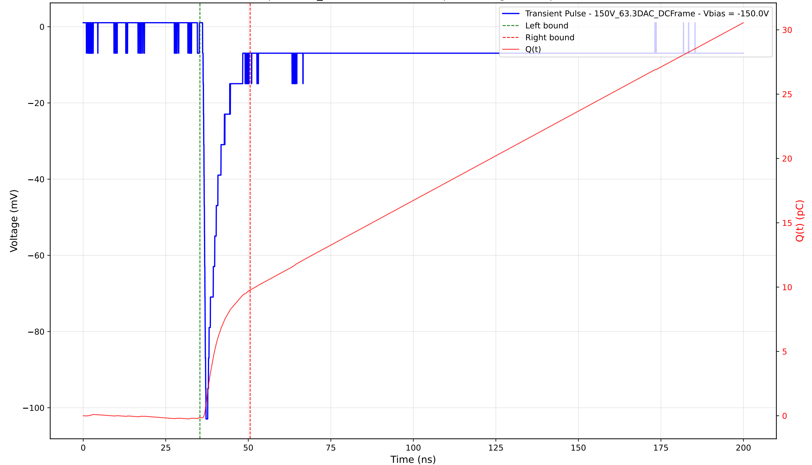
Transient Pulse - Sample: 1cm_42 - Position: 4465.0 \mu\text{m} - Charge: 9.92 pC - Rise Time: 0.77 ns
