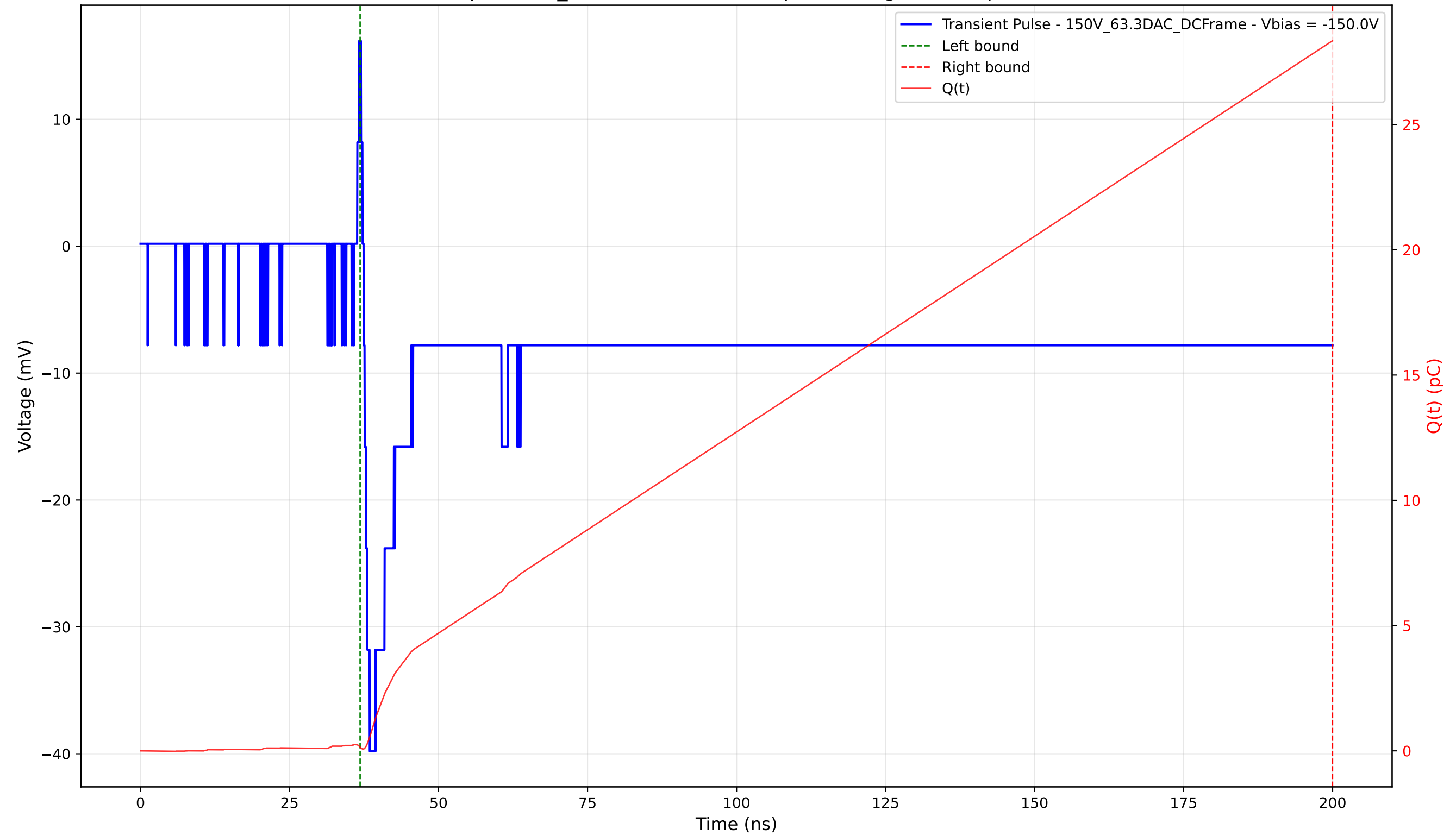
Transient Pulse - Sample: 1cm_42 - Position: 3300.0 \mu\text{m} - Charge: 28.19 pC - Rise Time: 1.01 ns
