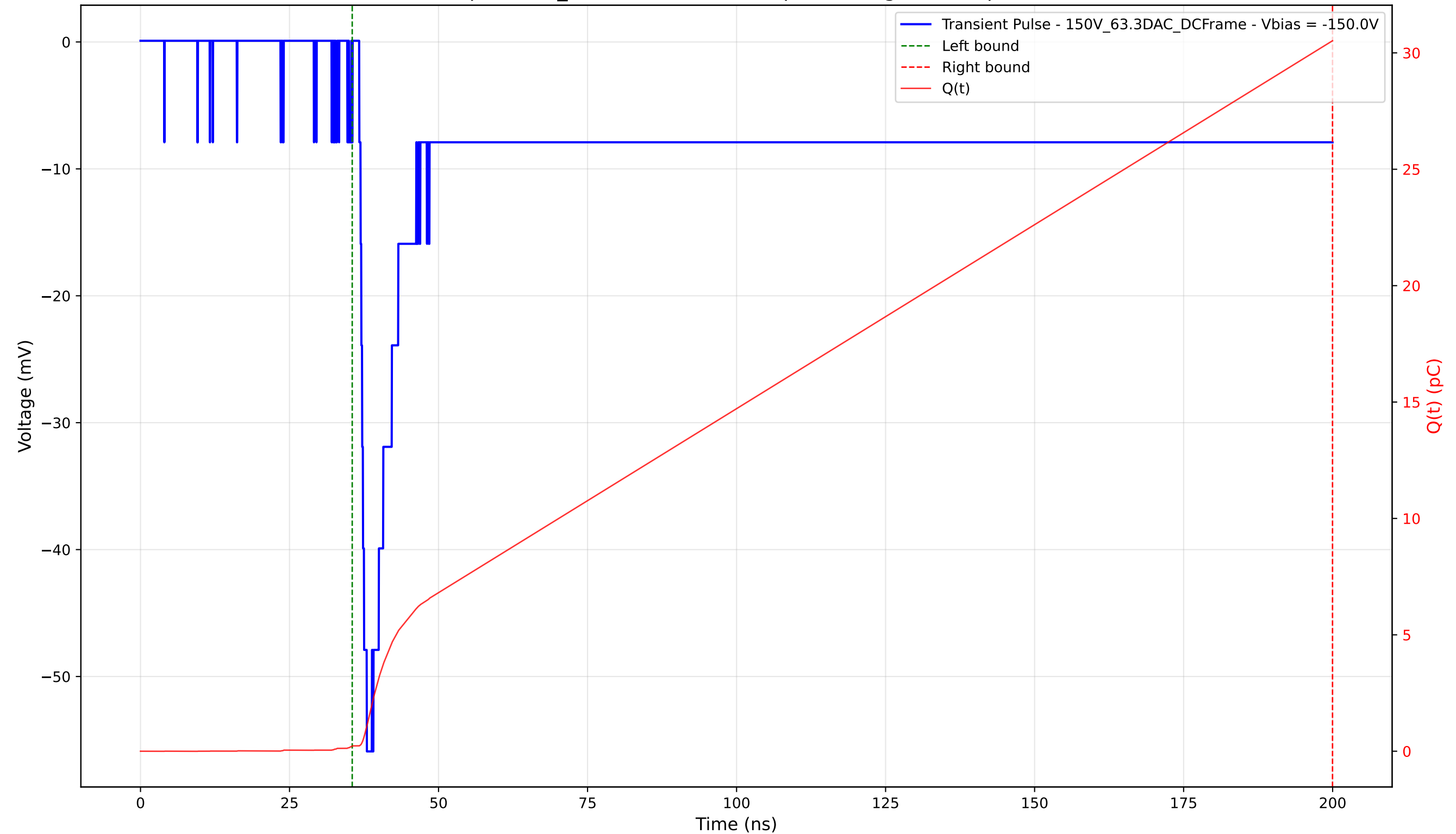
Transient Pulse - Sample: 1cm_42 - Position: 4000.0 \mu\text{m} - Charge: 30.30 pC - Rise Time: 1.27 ns
