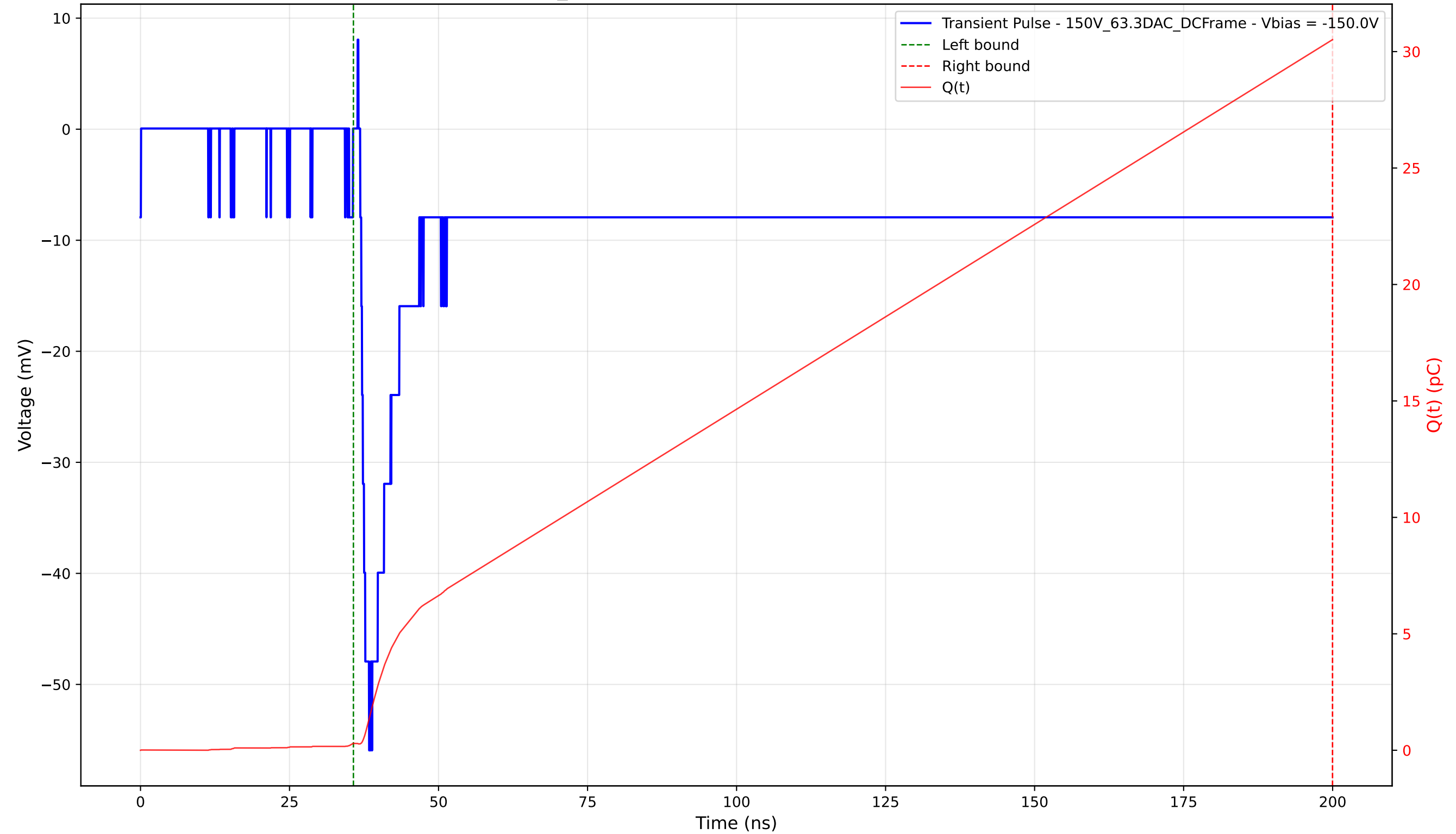
Transient Pulse - Sample: 1cm_42 - Position: 3920.0 \mu\text{m} - Charge: 30.22 pC - Rise Time: 1.49 ns
