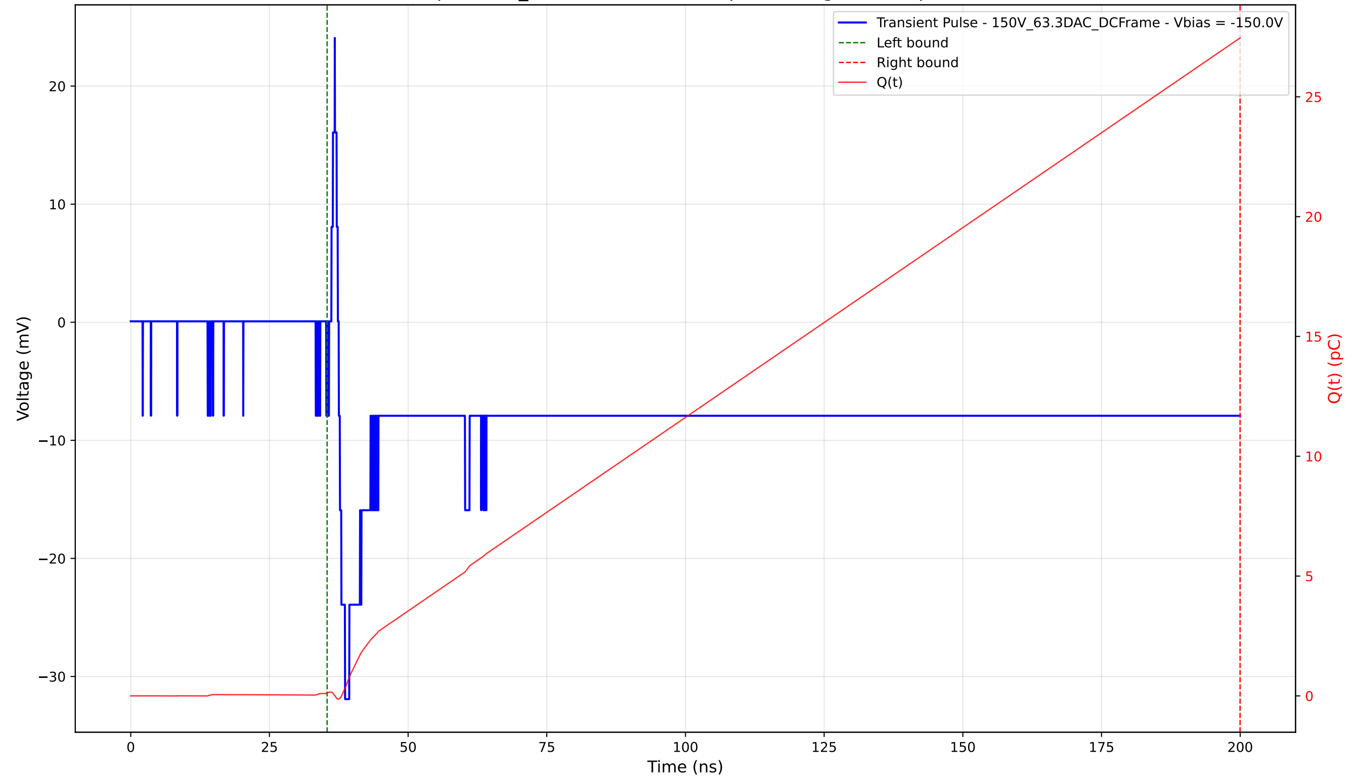
Transient Pulse - Sample: 1cm_42 - Position: 2530.0 \mu\text{m} - Charge: 27.34 pC - Rise Time: 1.13 ns
