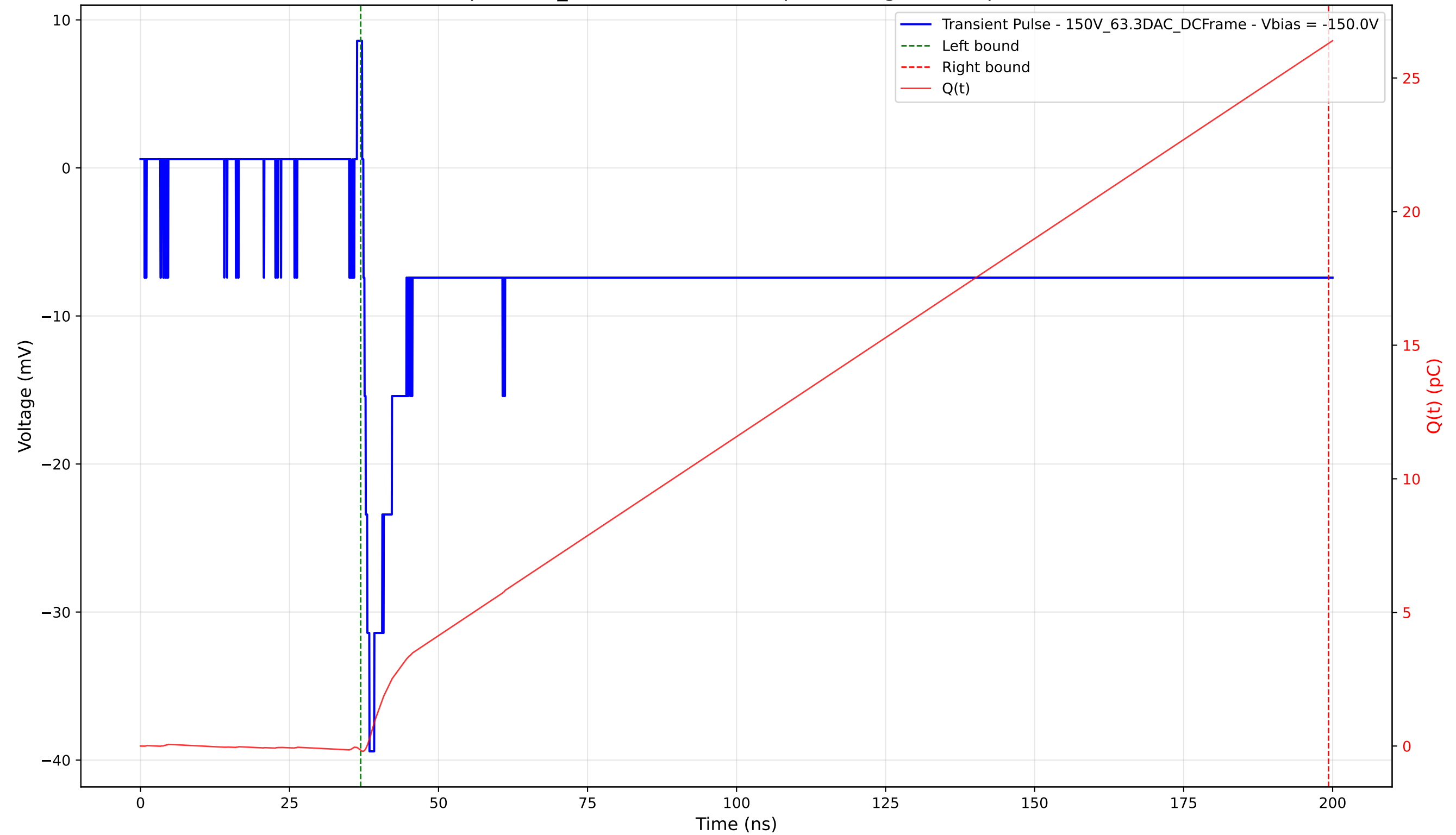
Transient Pulse - Sample: 1cm_42 - Position: 3380.0 \mu\text{m} - Charge: 26.45 pC - Rise Time: 1.01 ns
