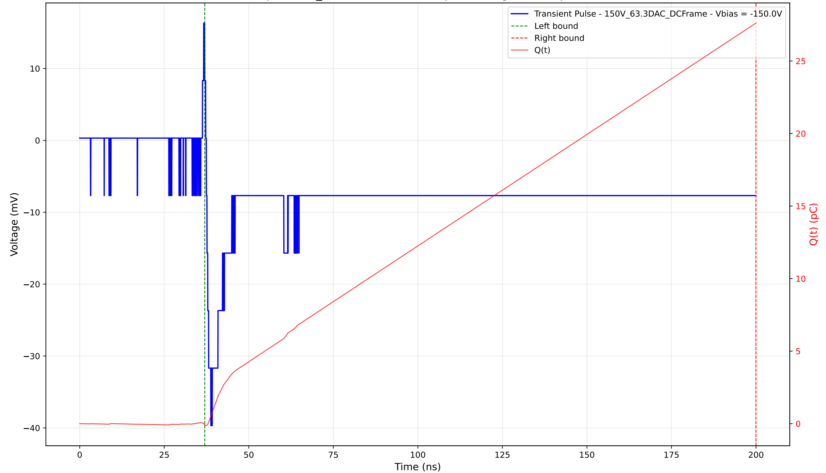
Transient Pulse - Sample: 1cm_42 - Position: 3180.0 \mu\text{m} - Charge: 27.70 pC - Rise Time: 1.35 ns
