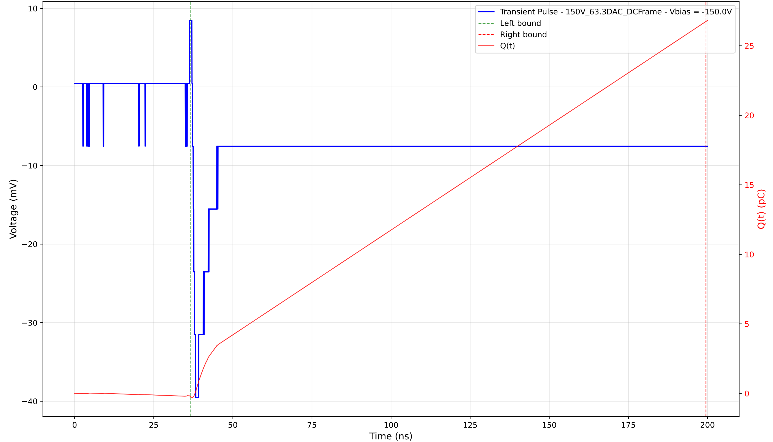
Transient Pulse - Sample: 1cm_42 - Position: 3505.0 \mu\text{m} - Charge: 27.00 pC - Rise Time: 1.01 ns
