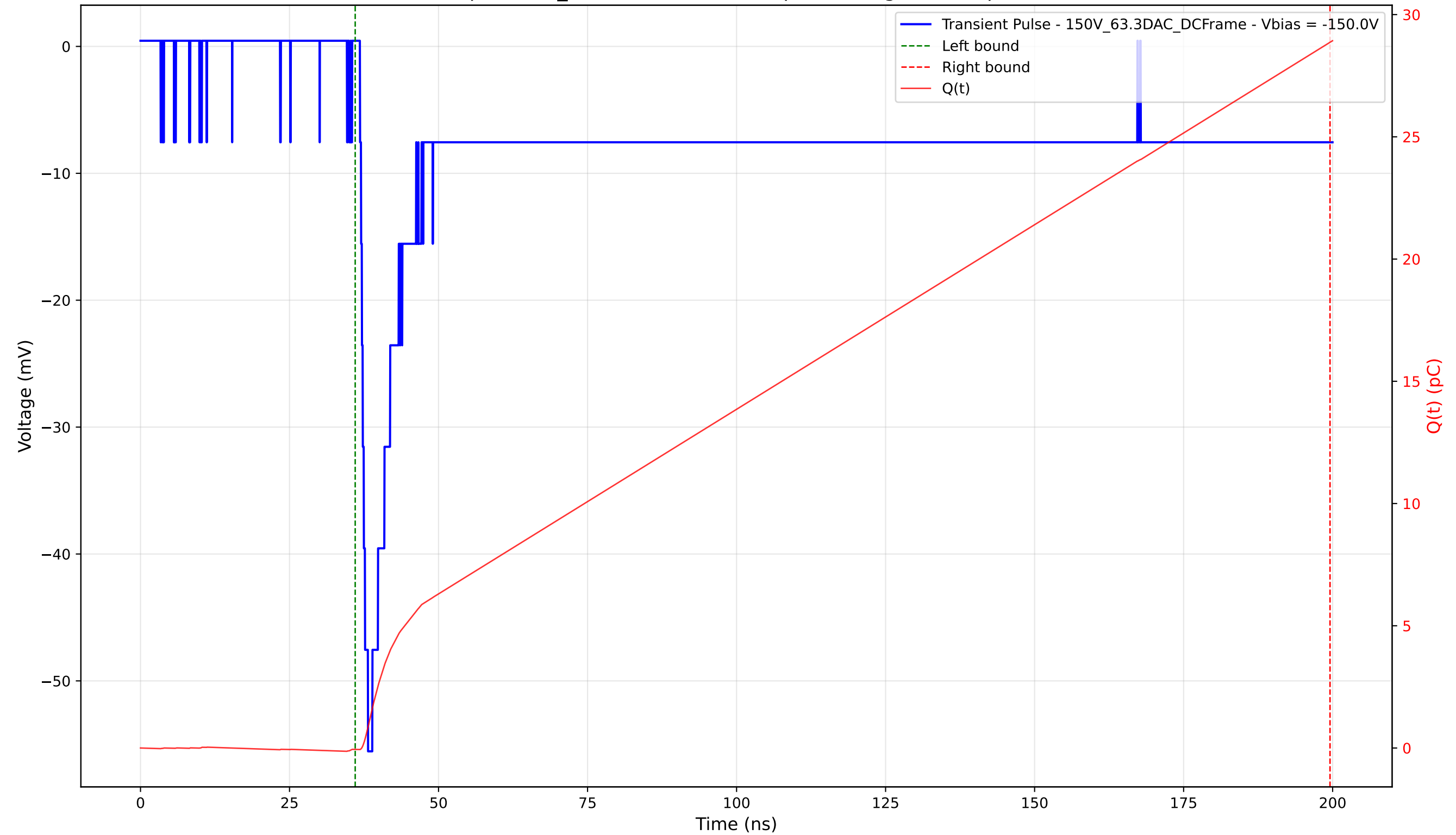
Transient Pulse - Sample: 1cm_42 - Position: 3950.0 \mu\text{m} - Charge: 28.93 pC - Rise Time: 1.35 ns
