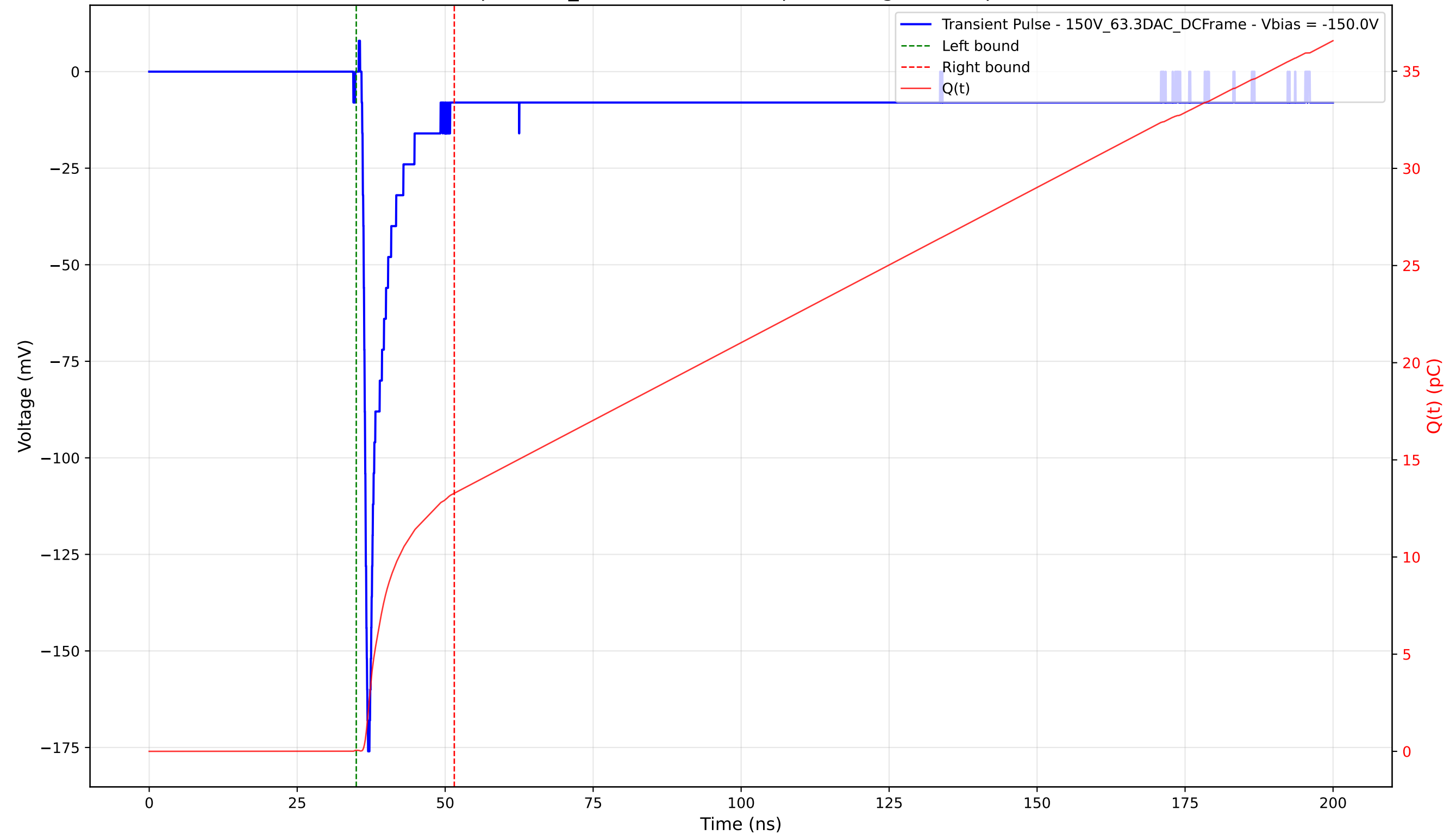
Transient Pulse - Sample: 1cm_42 - Position: 440.0 \mu\text{m} - Charge: 13.23 pC - Rise Time: 0.76 ns
