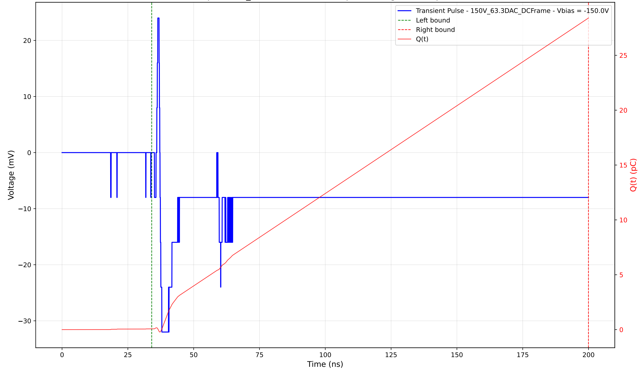
Transient Pulse - Sample: 1cm_42 - Position: 2050.0 \mu\text{m} - Charge: 28.33 pC - Rise Time: 0.69 ns
