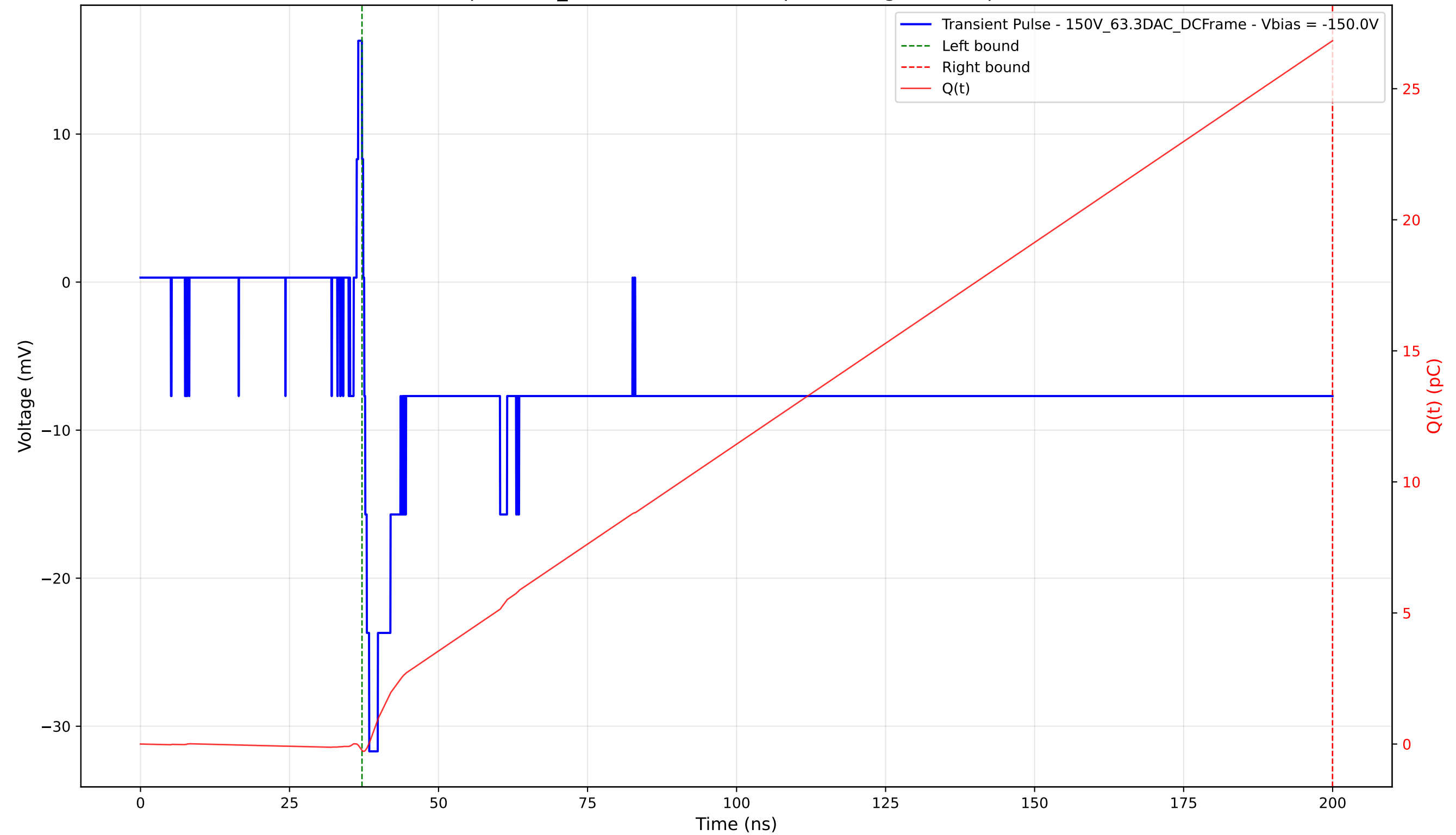
Transient Pulse - Sample: 1cm_42 - Position: 2835.0 \mu\text{m} - Charge: 27.08 pC - Rise Time: 0.83 ns
