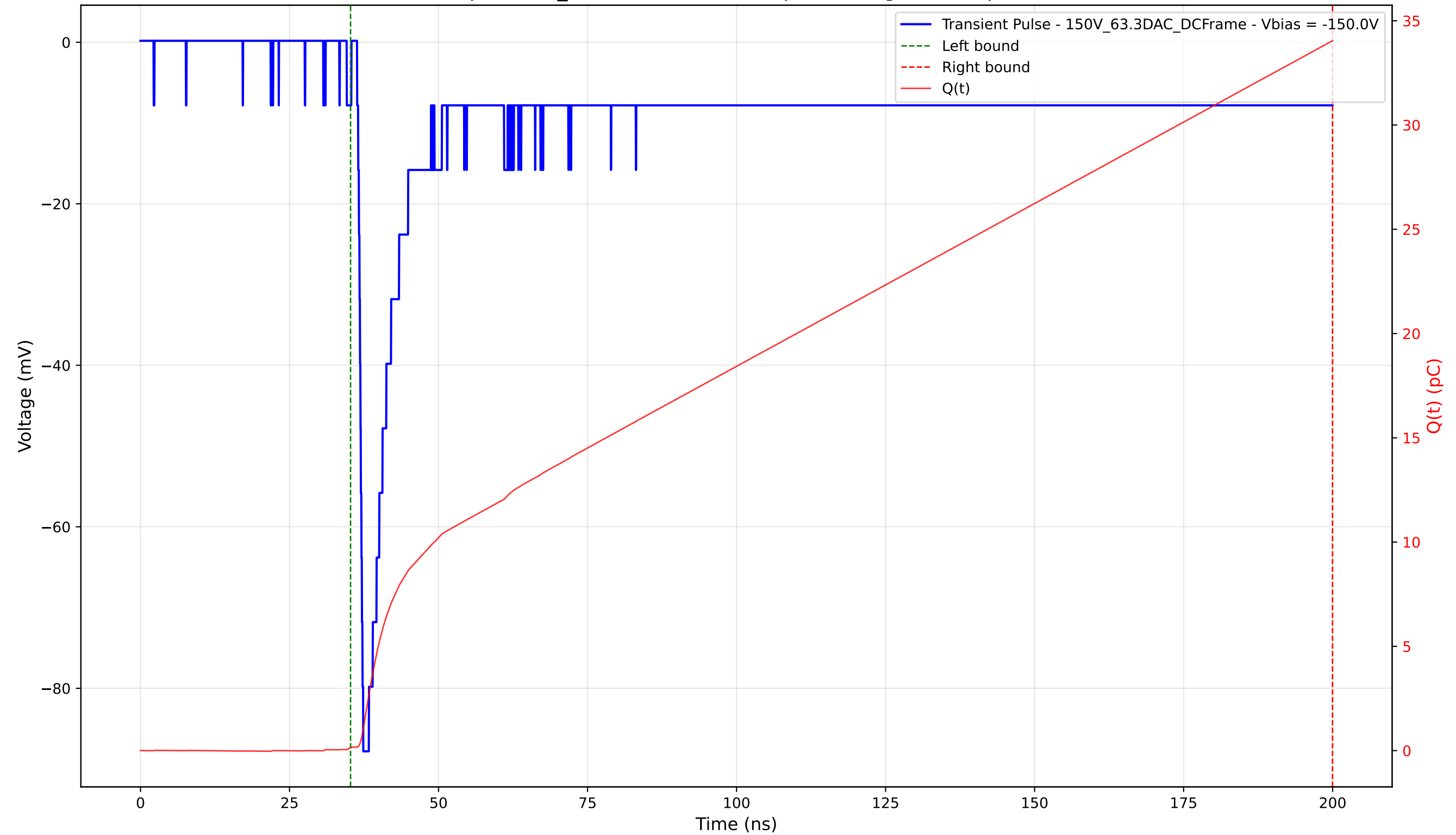
Transient Pulse - Sample: 1cm_42 - Position: 4240.0 \mu\text{m} - Charge: 33.90 pC - Rise Time: 0.74 ns
