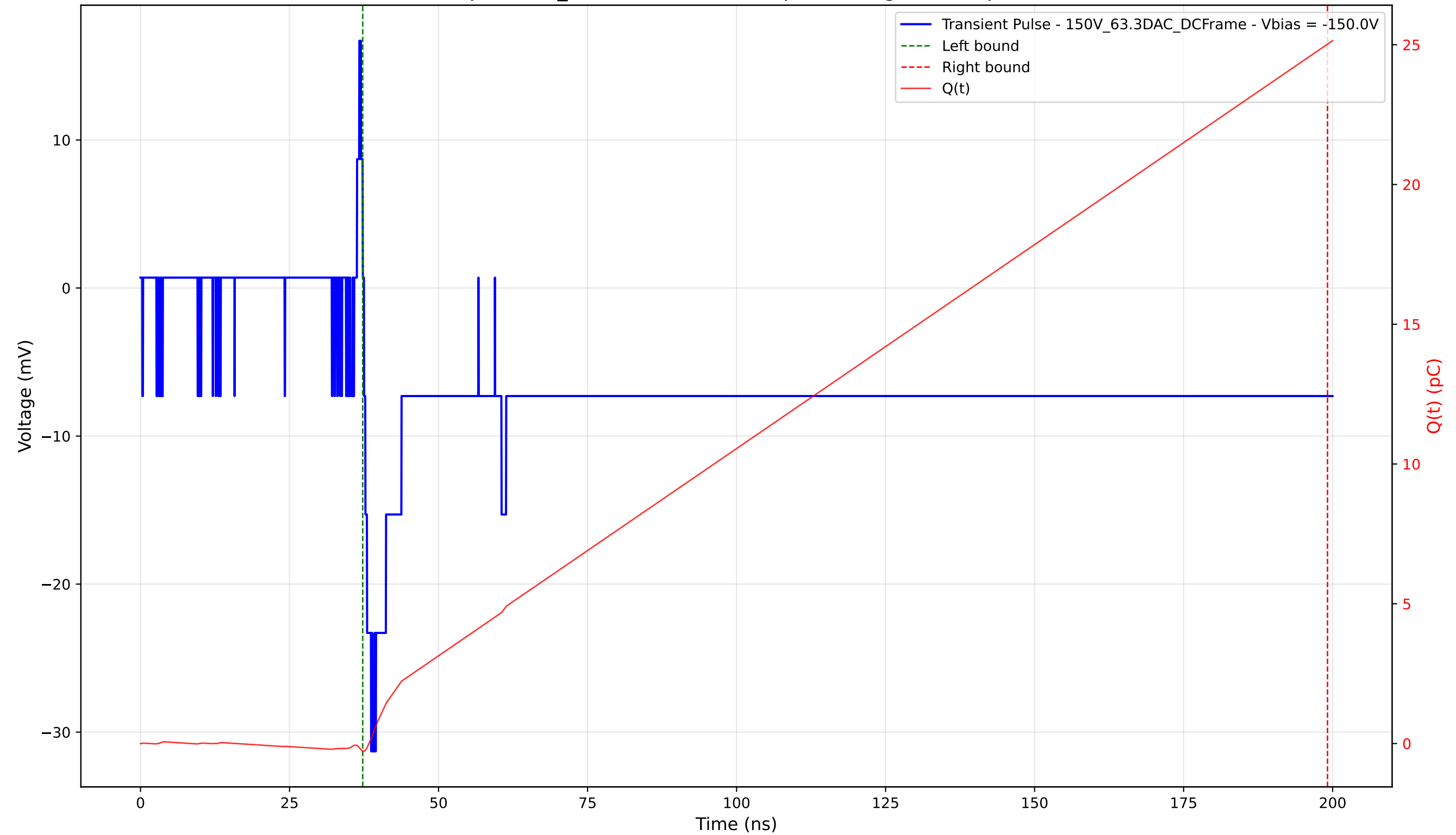
Transient Pulse - Sample: 1cm_42 - Position: 2975.0 \mu\text{m} - Charge: 25.30 pC - Rise Time: 1.19 ns
