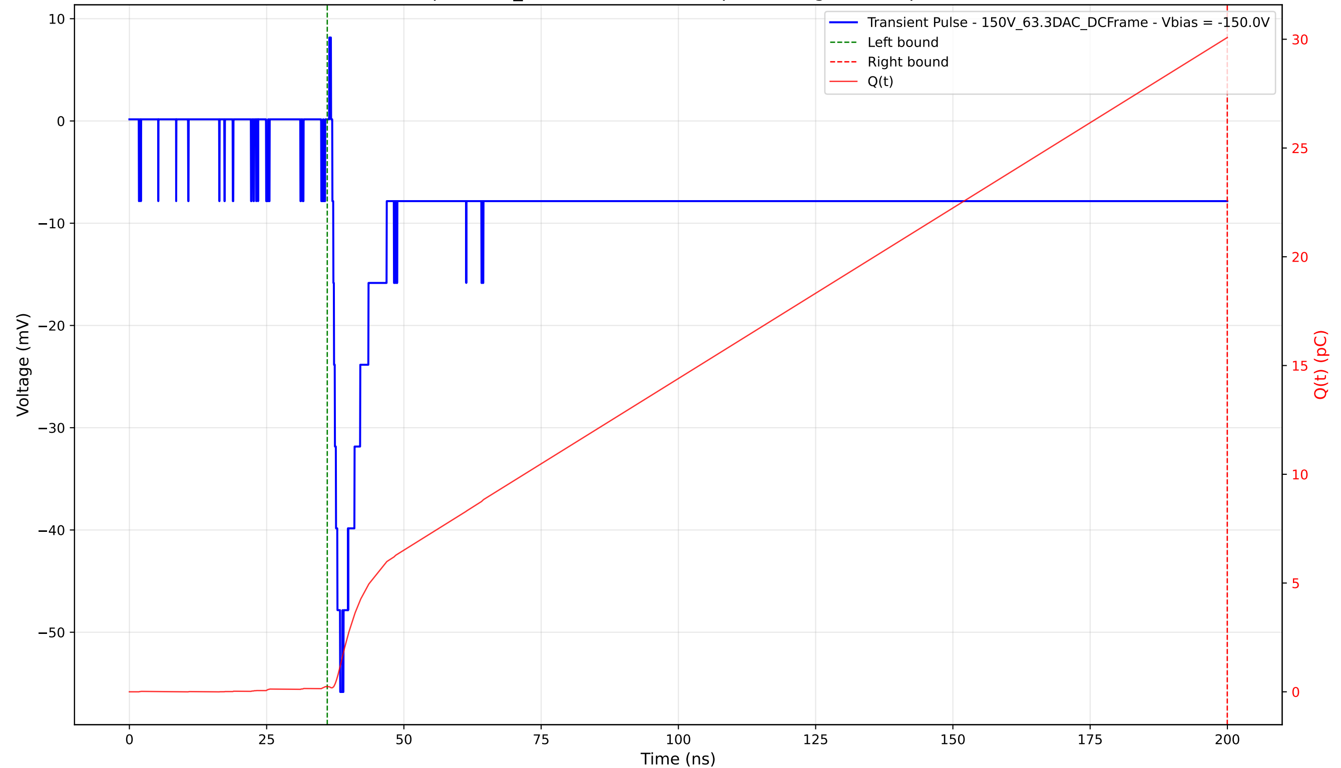
Transient Pulse - Sample: 1cm_42 - Position: 3840.0 \mu\text{m} - Charge: 29.84 pC - Rise Time: 1.43 ns
