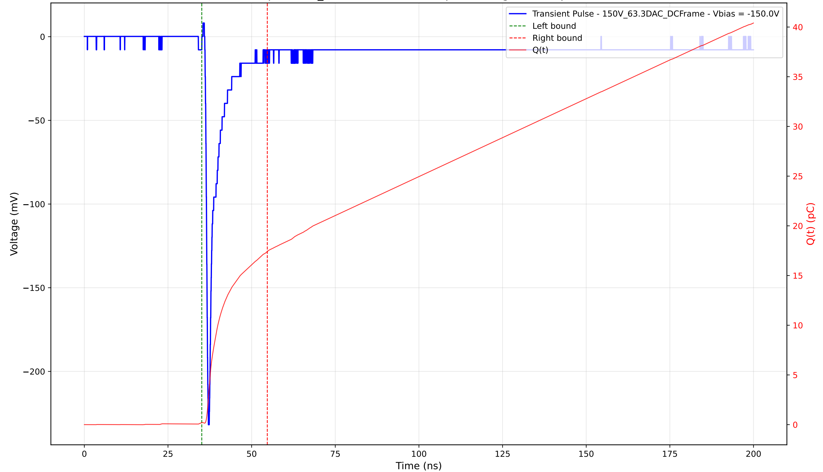
Transient Pulse - Sample: 1cm_42 - Position: 4735.0 \mu\text{m} - Charge: 17.21 pC - Rise Time: 0.82 ns
