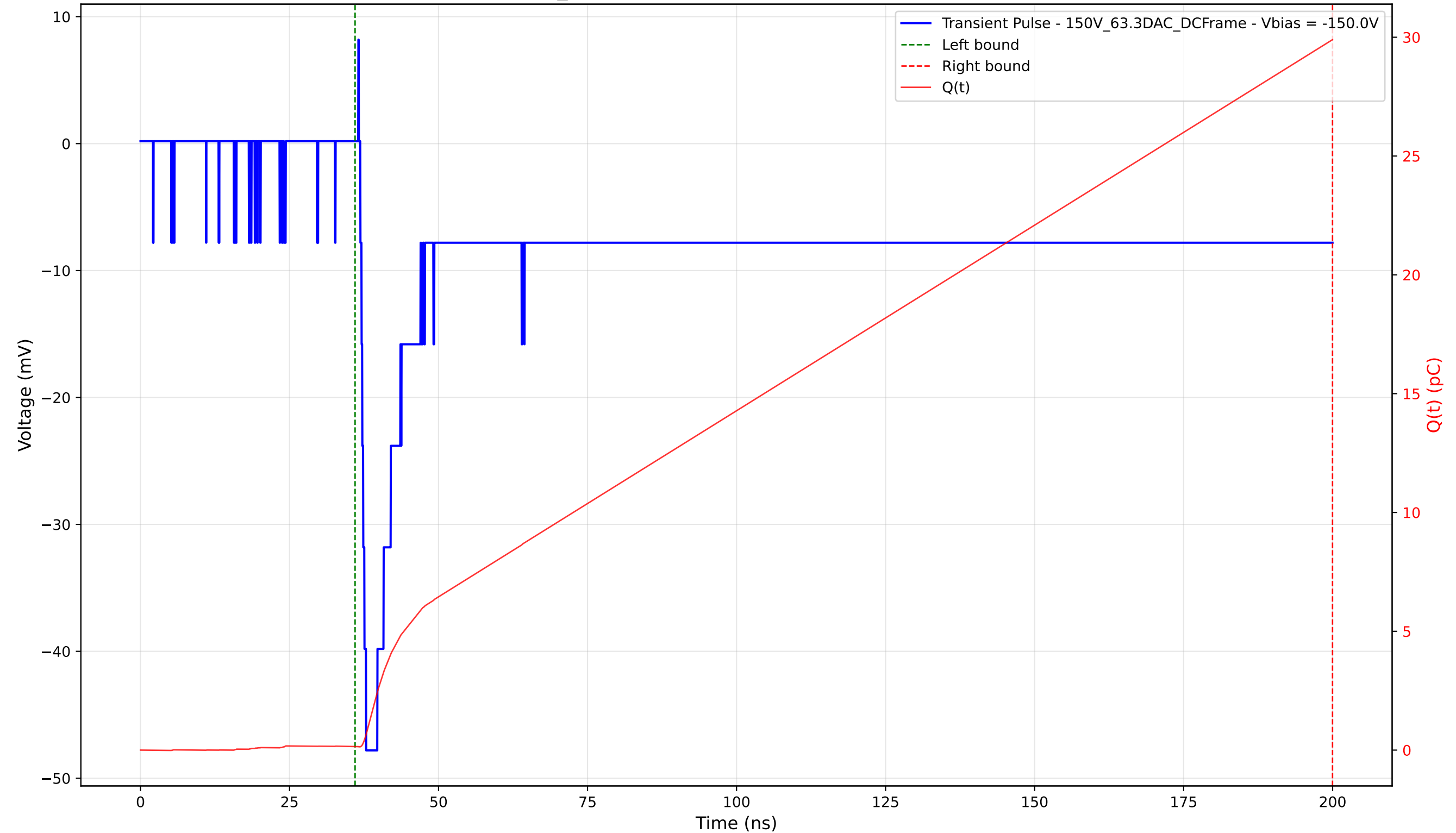
Transient Pulse - Sample: 1cm_42 - Position: 3910.0 \mu\text{m} - Charge: 29.74 pC - Rise Time: 0.97 ns
