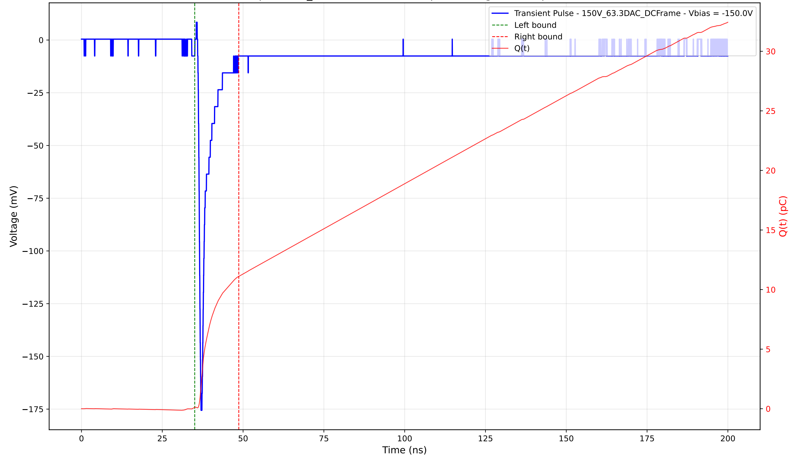
Transient Pulse - Sample: 1cm_42 - Position: 4945.0 \mu\text{m} - Charge: 10.99 pC - Rise Time: 0.74 ns
