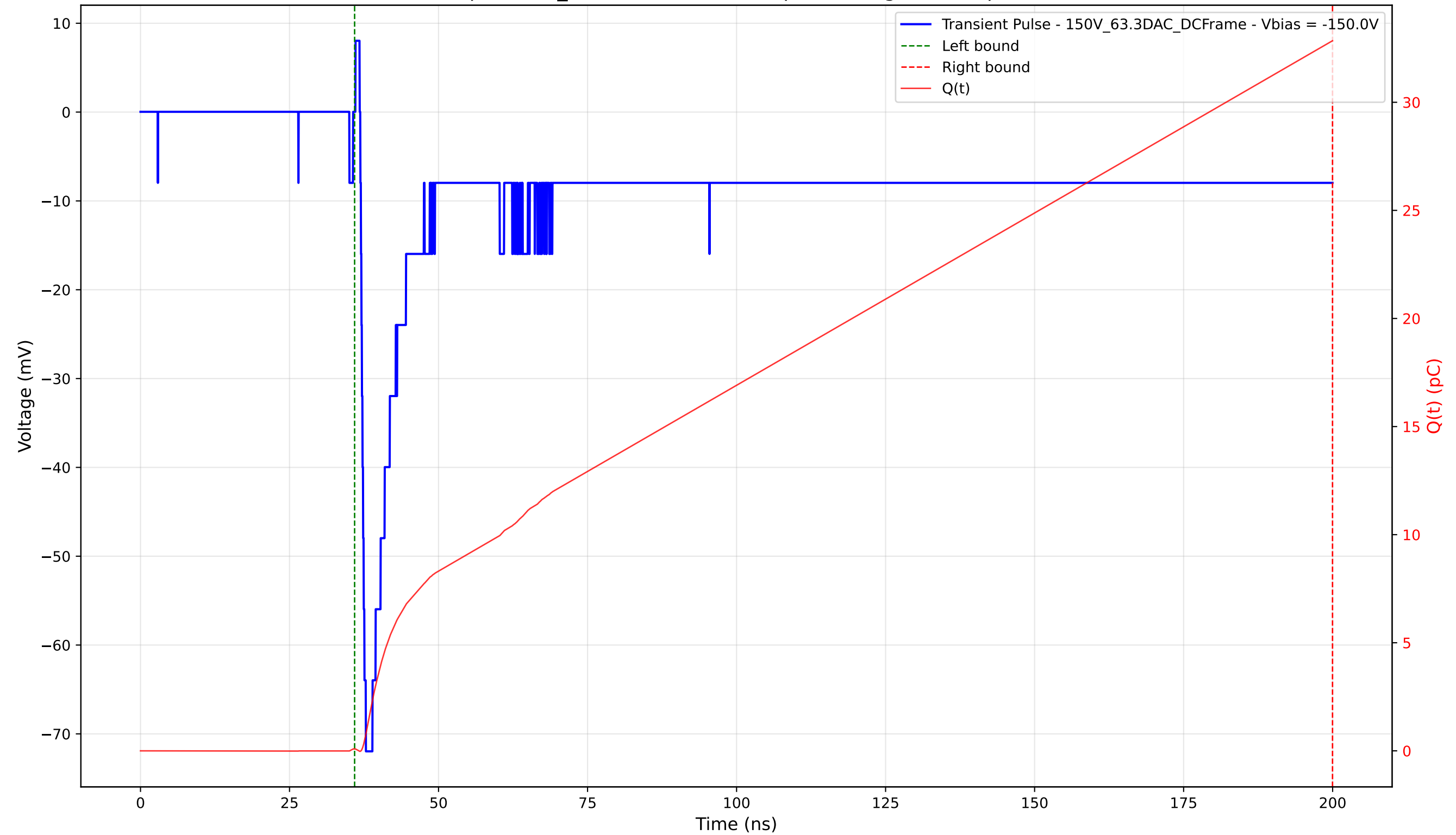
Transient Pulse - Sample: 1cm_42 - Position: 1235.0 \mu\text{m} - Charge: 32.76 pC - Rise Time: 0.92 ns
