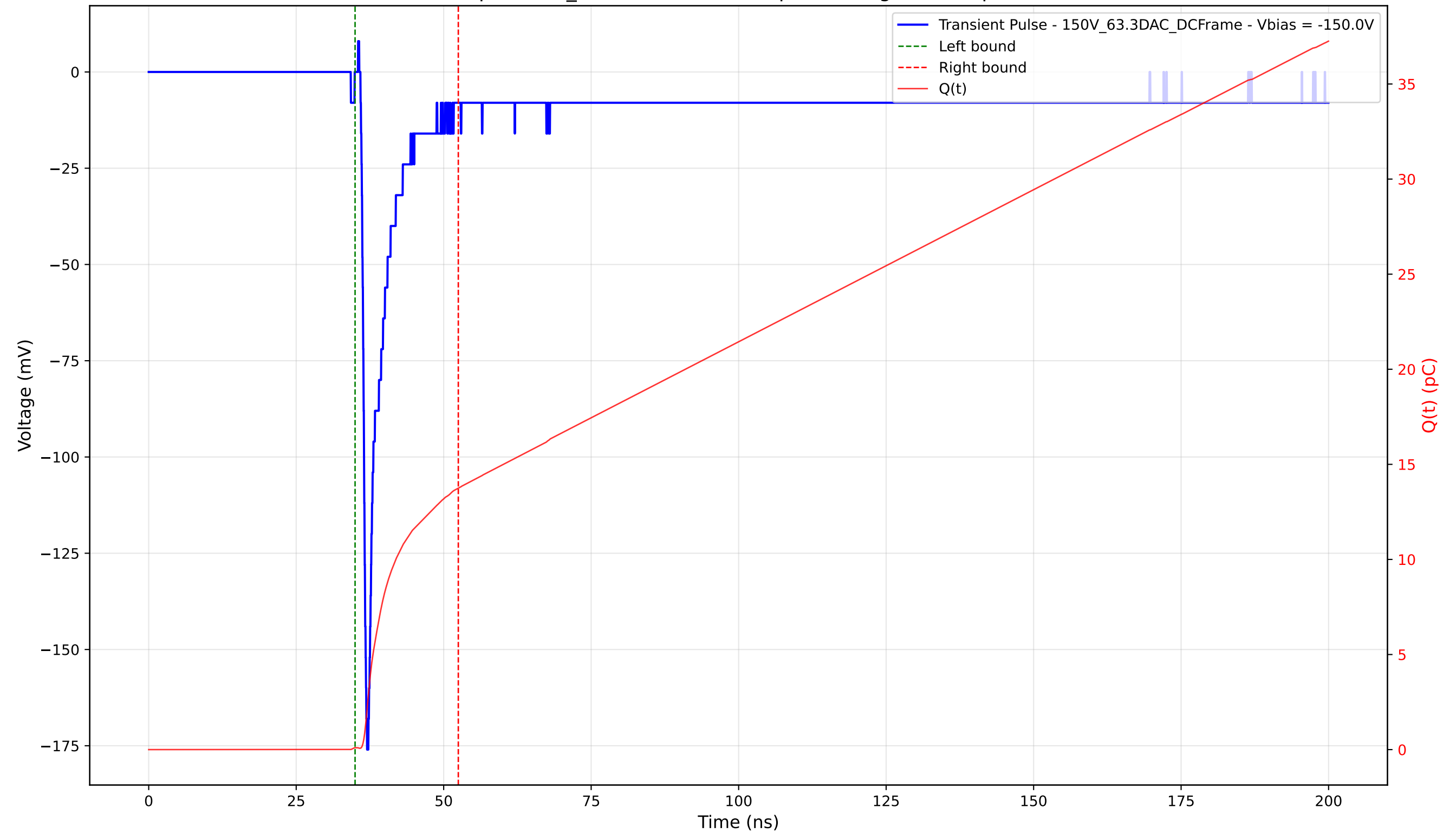
Transient Pulse - Sample: 1cm_42 - Position: 455.0 \mu\text{m} - Charge: 13.64 pC - Rise Time: 0.78 ns
