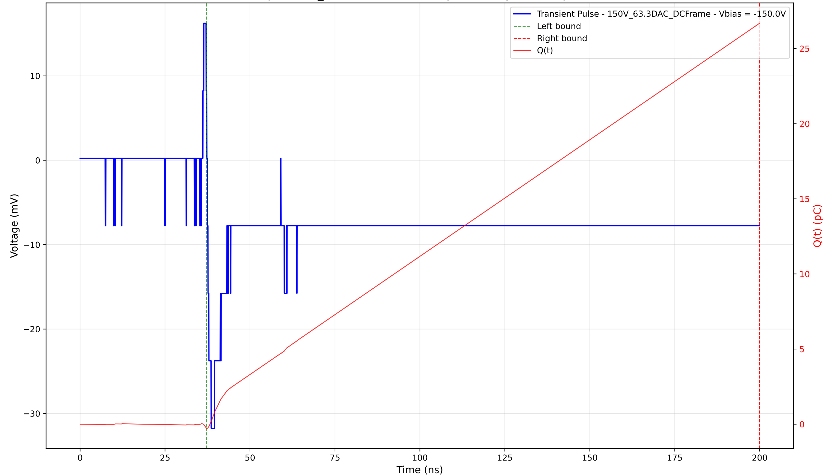
Transient Pulse - Sample: 1cm_42 - Position: 2470.0 \mu\text{m} - Charge: 26.93 pC - Rise Time: 1.13 ns
