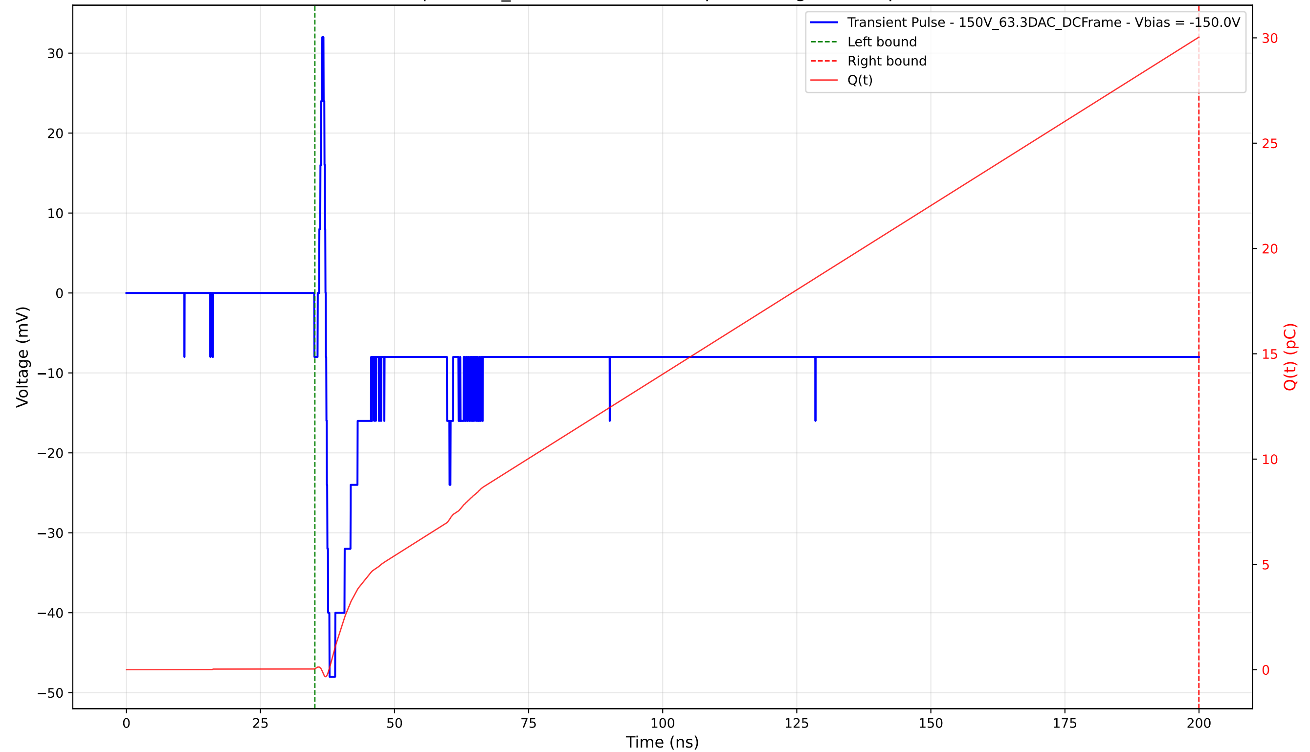
Transient Pulse - Sample: 1cm_42 - Position: 1750.0 \mu\text{m} - Charge: 29.99 pC - Rise Time: 0.69 ns
