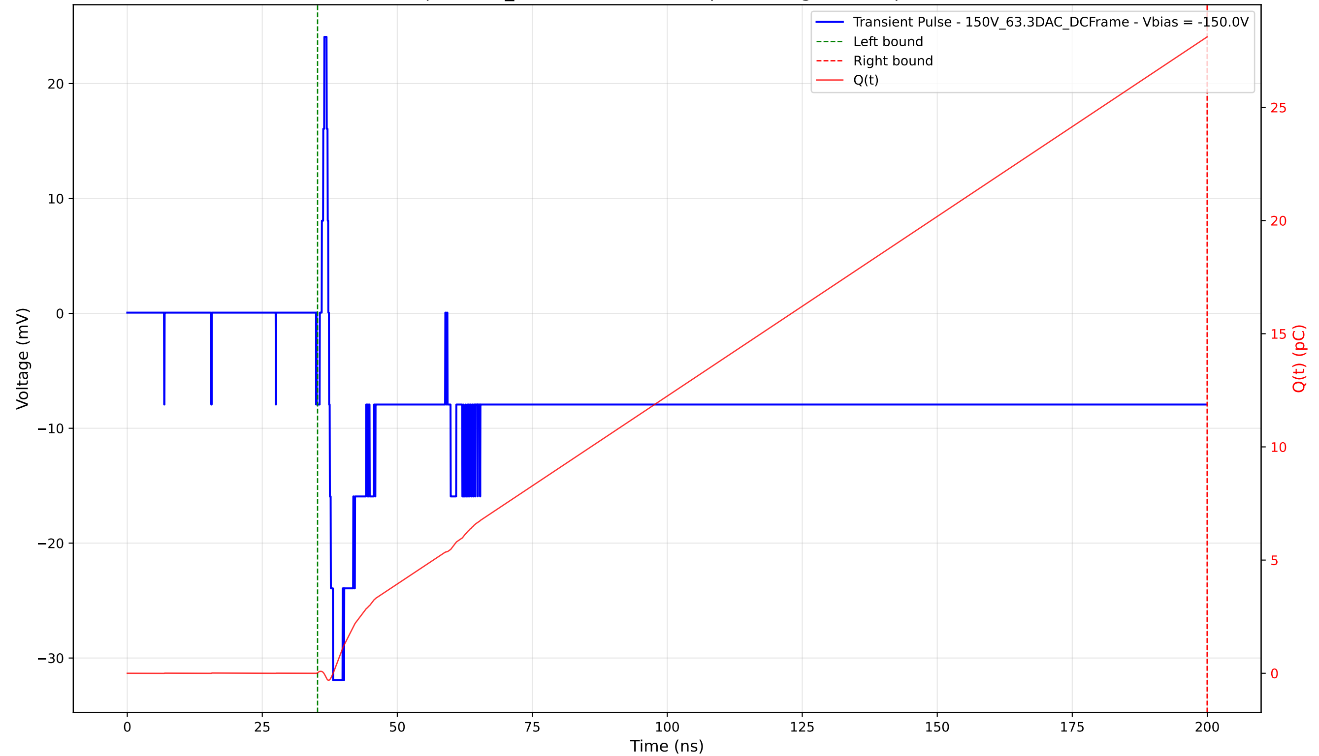
Transient Pulse - Sample: 1cm_42 - Position: 2345.0 \mu\text{m} - Charge: 28.09 pC - Rise Time: 0.75 ns
