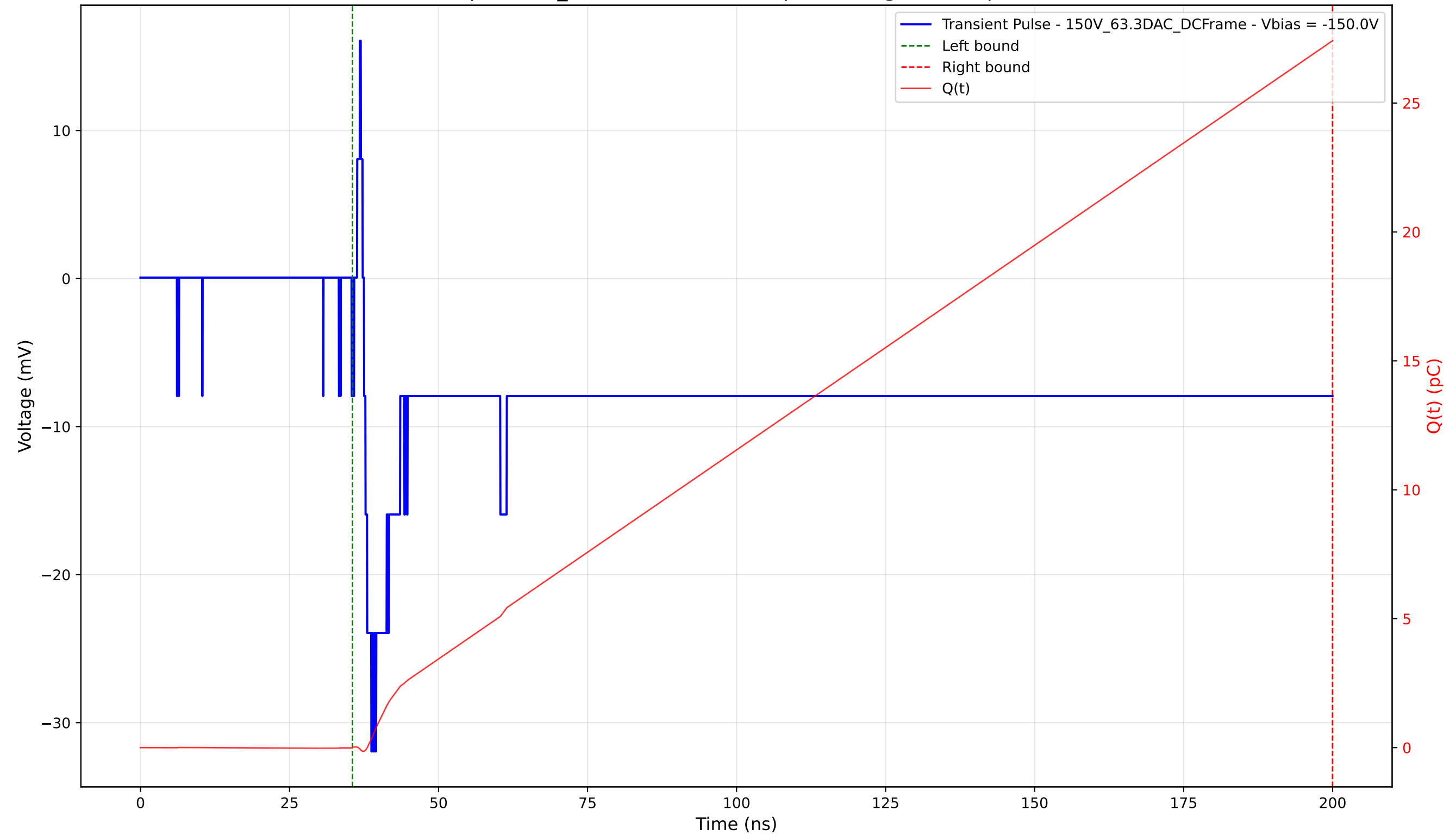
Transient Pulse - Sample: 1cm_42 - Position: 2970.0 \mu\text{m} - Charge: 27.41 pC - Rise Time: 1.23 ns
