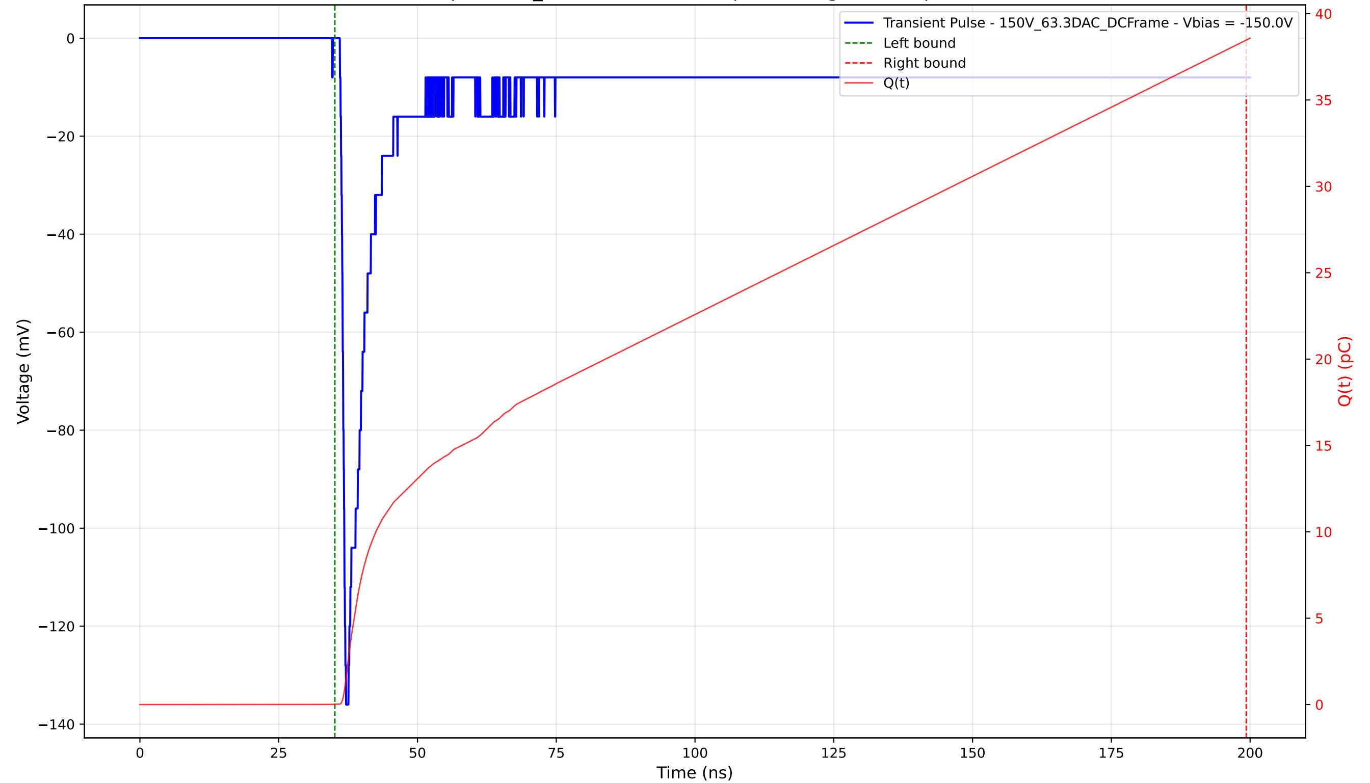
Transient Pulse - Sample: 1cm_42 - Position: 640.0 \mu\text{m} - Charge: 38.45 pC - Rise Time: 0.87 ns
