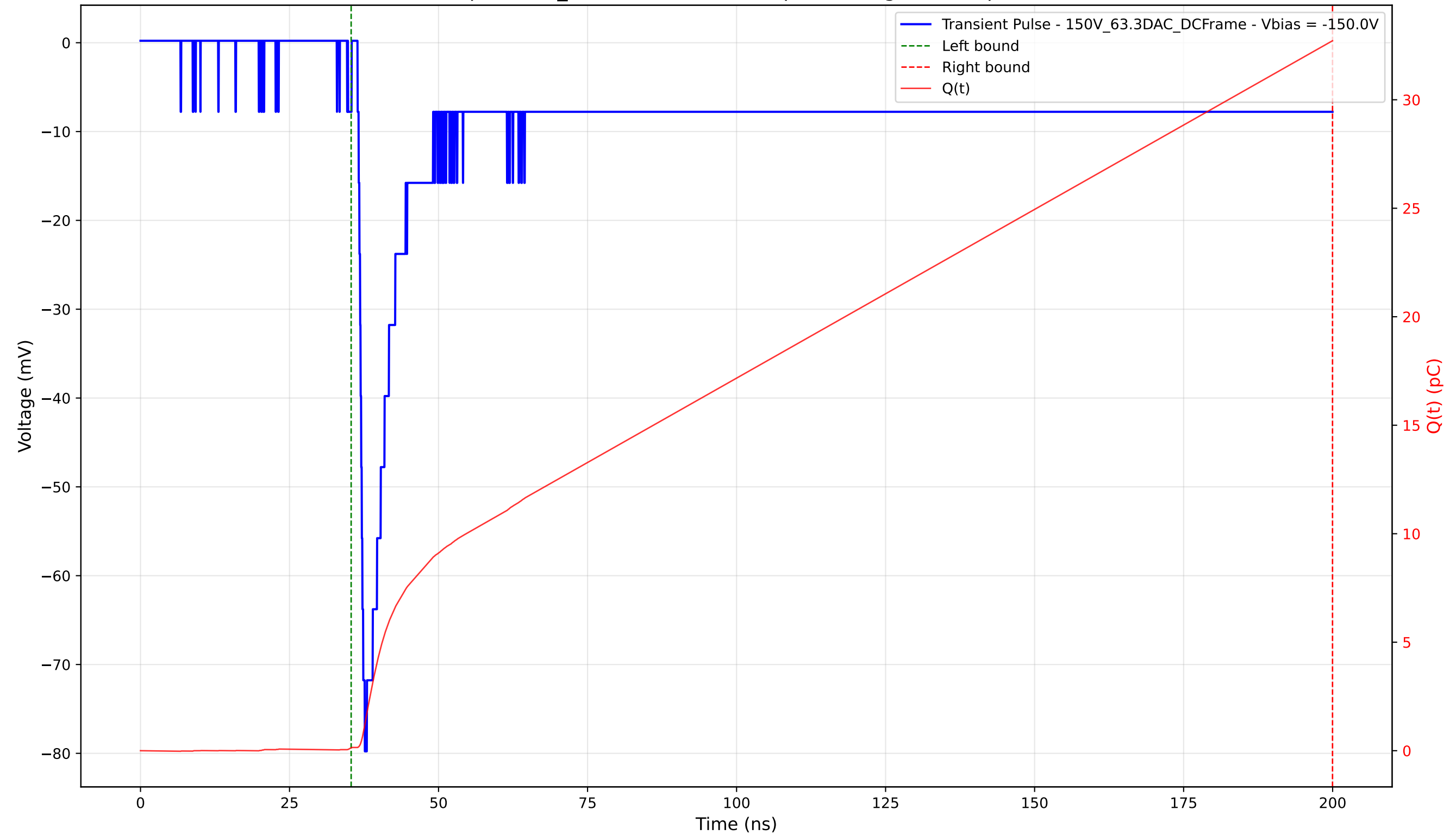
Transient Pulse - Sample: 1cm_42 - Position: 4160.0 \mu\text{m} - Charge: 32.58 pC - Rise Time: 1.04 ns
