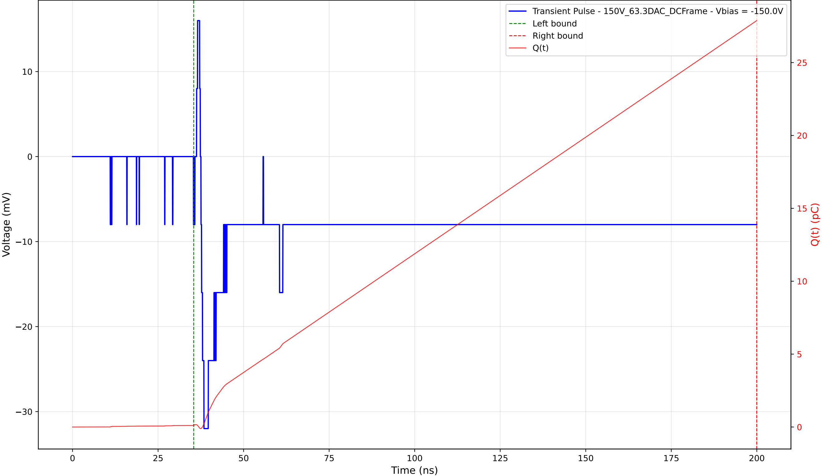
Transient Pulse - Sample: 1cm_42 - Position: 2845.0 \mu\text{m} - Charge: 27.77 pC - Rise Time: 0.87 ns
