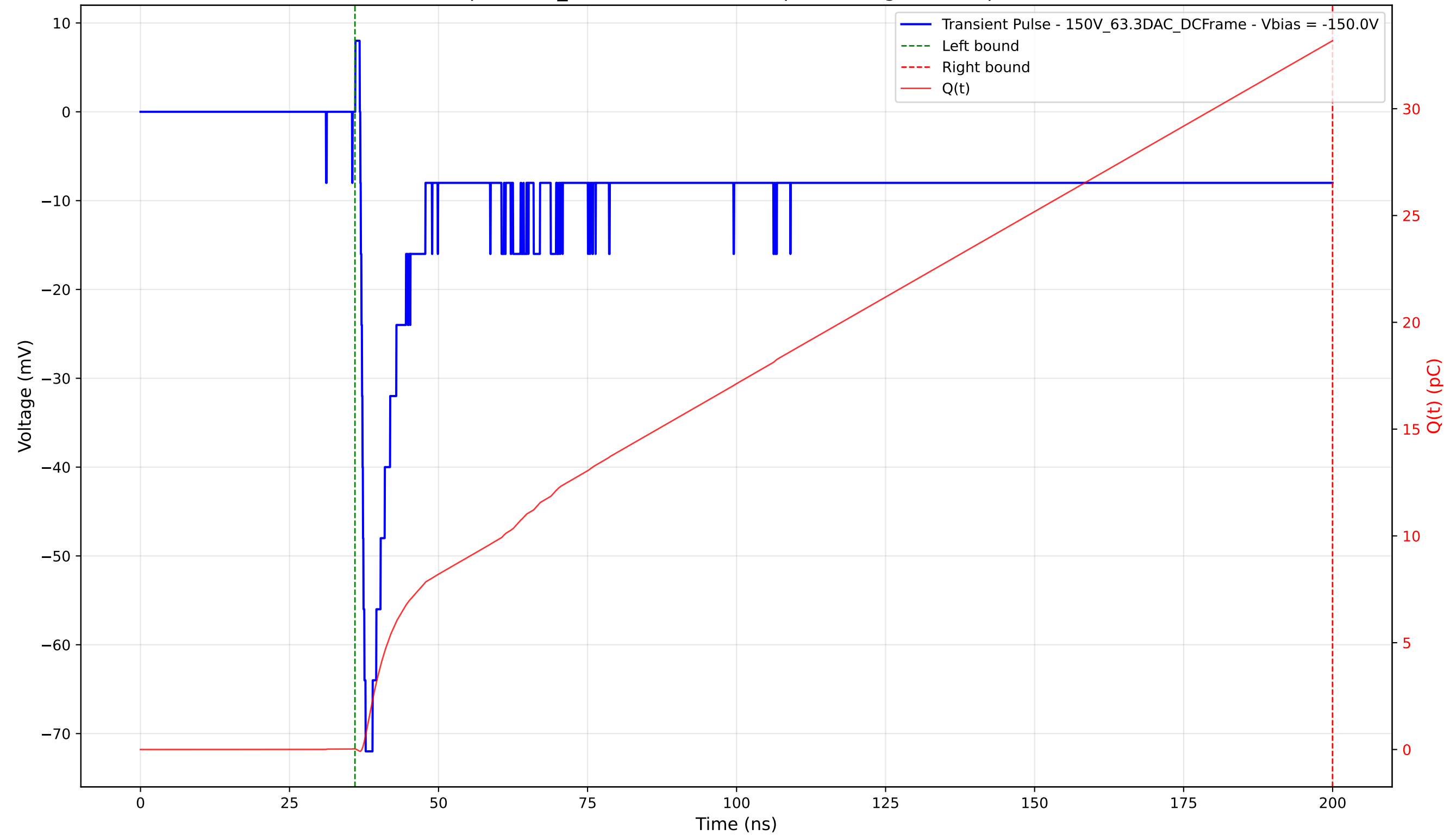
Transient Pulse - Sample: 1cm_42 - Position: 1225.0 \mu\text{m} - Charge: 33.15 pC - Rise Time: 0.88 ns
