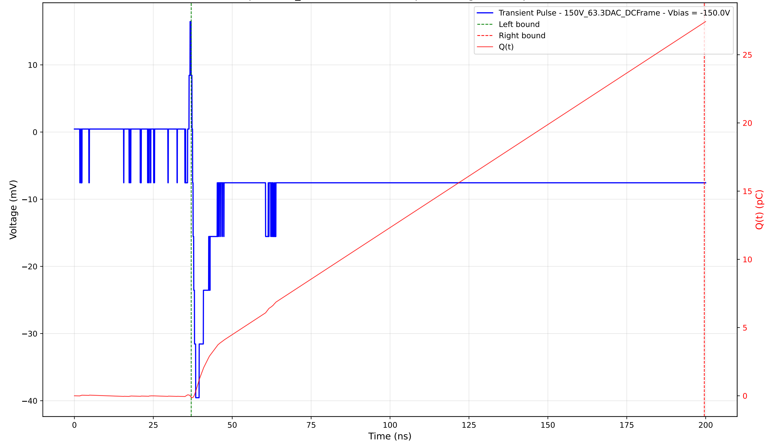
Transient Pulse - Sample: 1cm_42 - Position: 3285.0 \mu\text{m} - Charge: 27.47 pC - Rise Time: 0.99 ns
