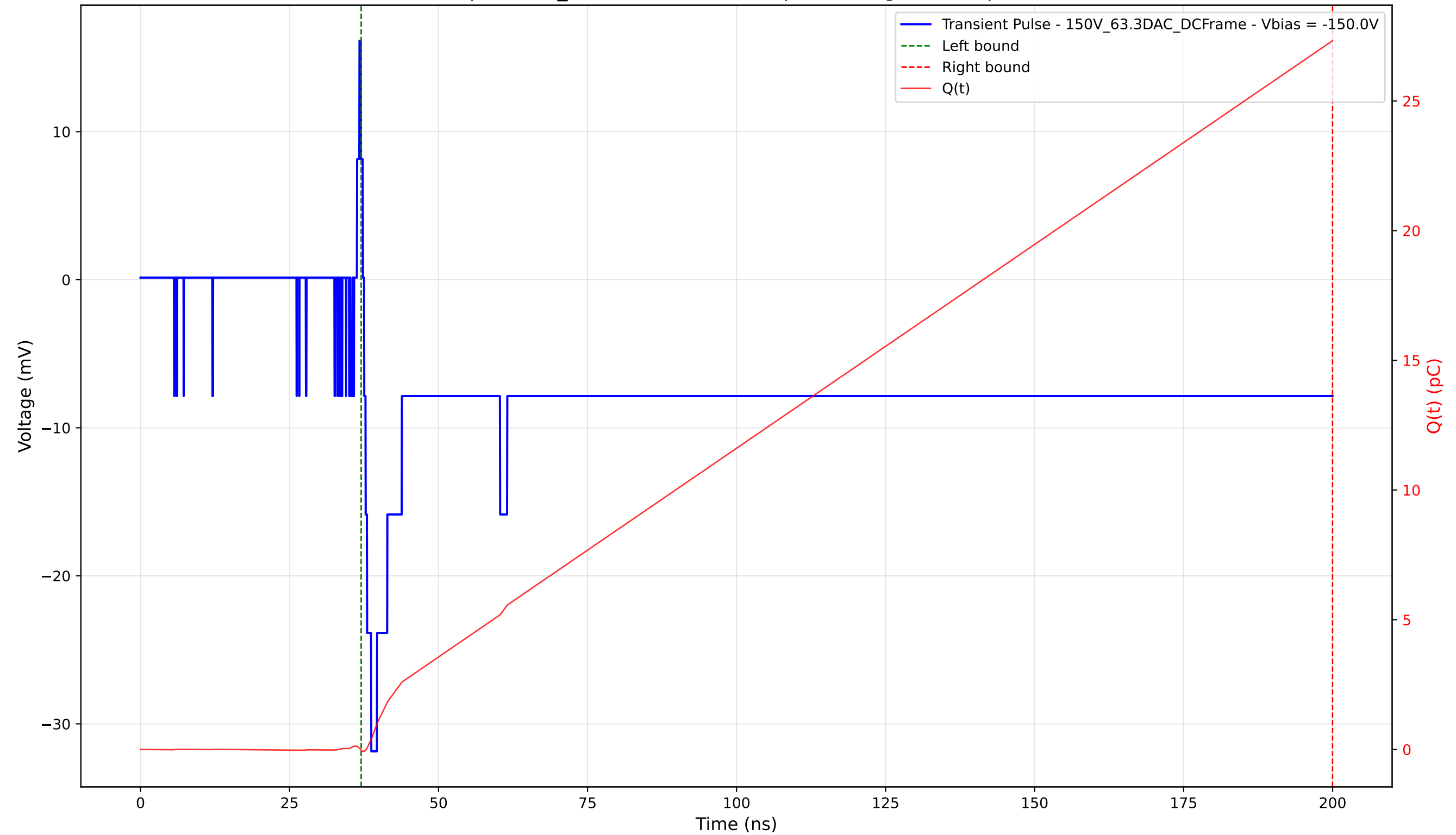
Transient Pulse - Sample: 1cm_42 - Position: 3015.0 \mu\text{m} - Charge: 27.35 pC - Rise Time: 1.19 ns
