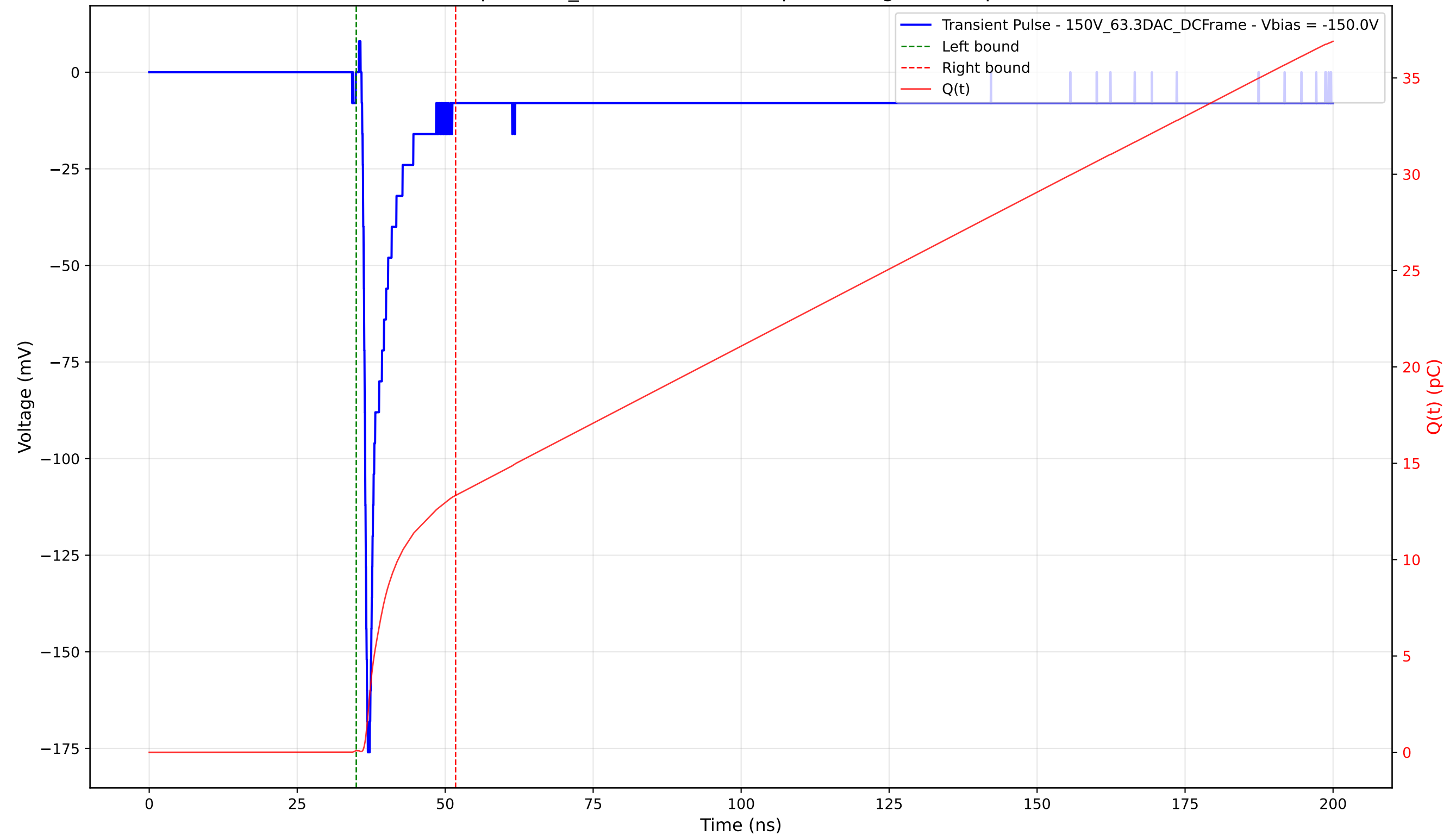
Transient Pulse - Sample: 1cm_42 - Position: 430.0 \mu\text{m} - Charge: 13.24 pC - Rise Time: 0.74 ns
