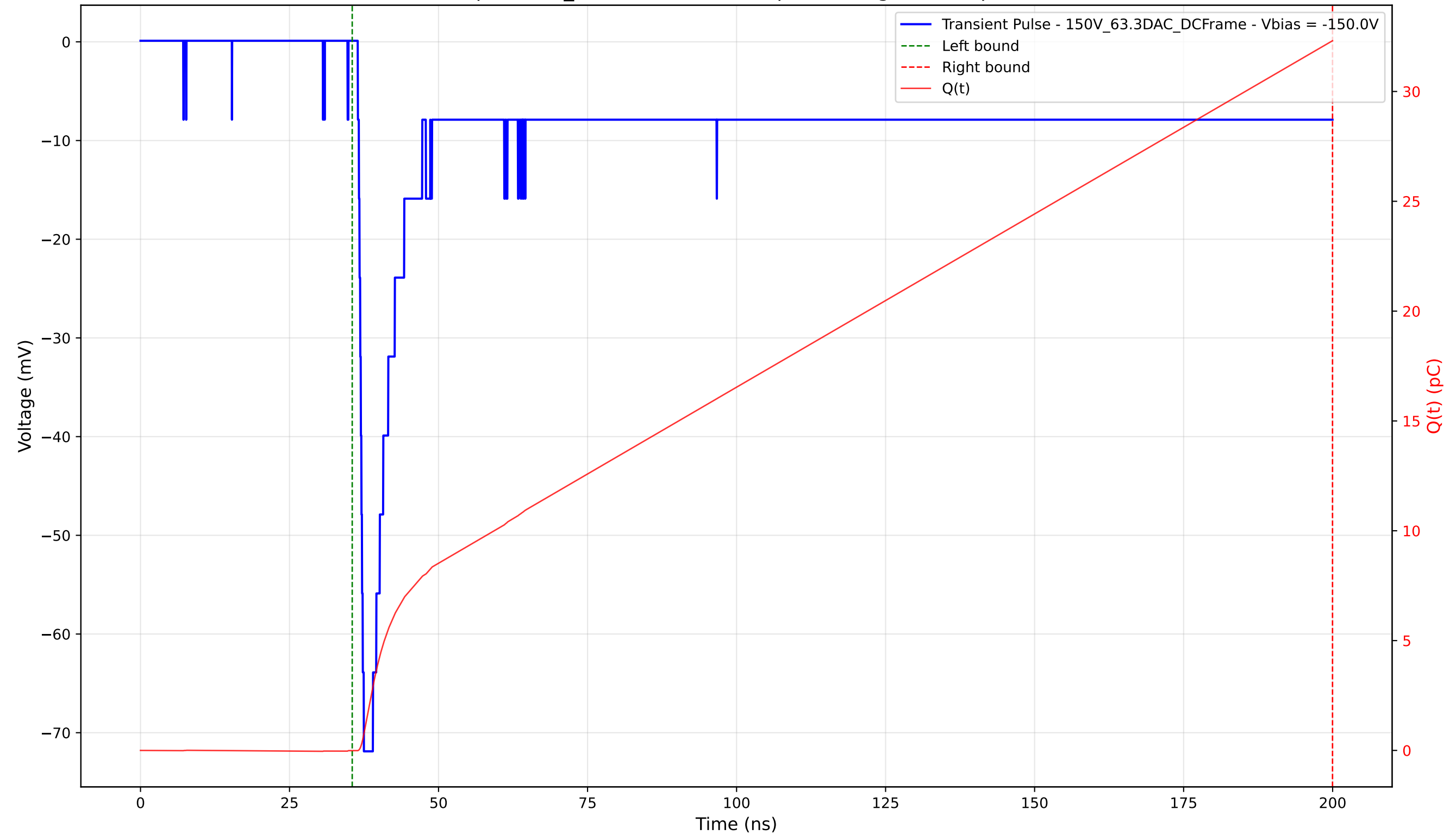
Transient Pulse - Sample: 1cm_42 - Position: 990.0 \mu\text{m} - Charge: 32.32 pC - Rise Time: 1.00 ns
