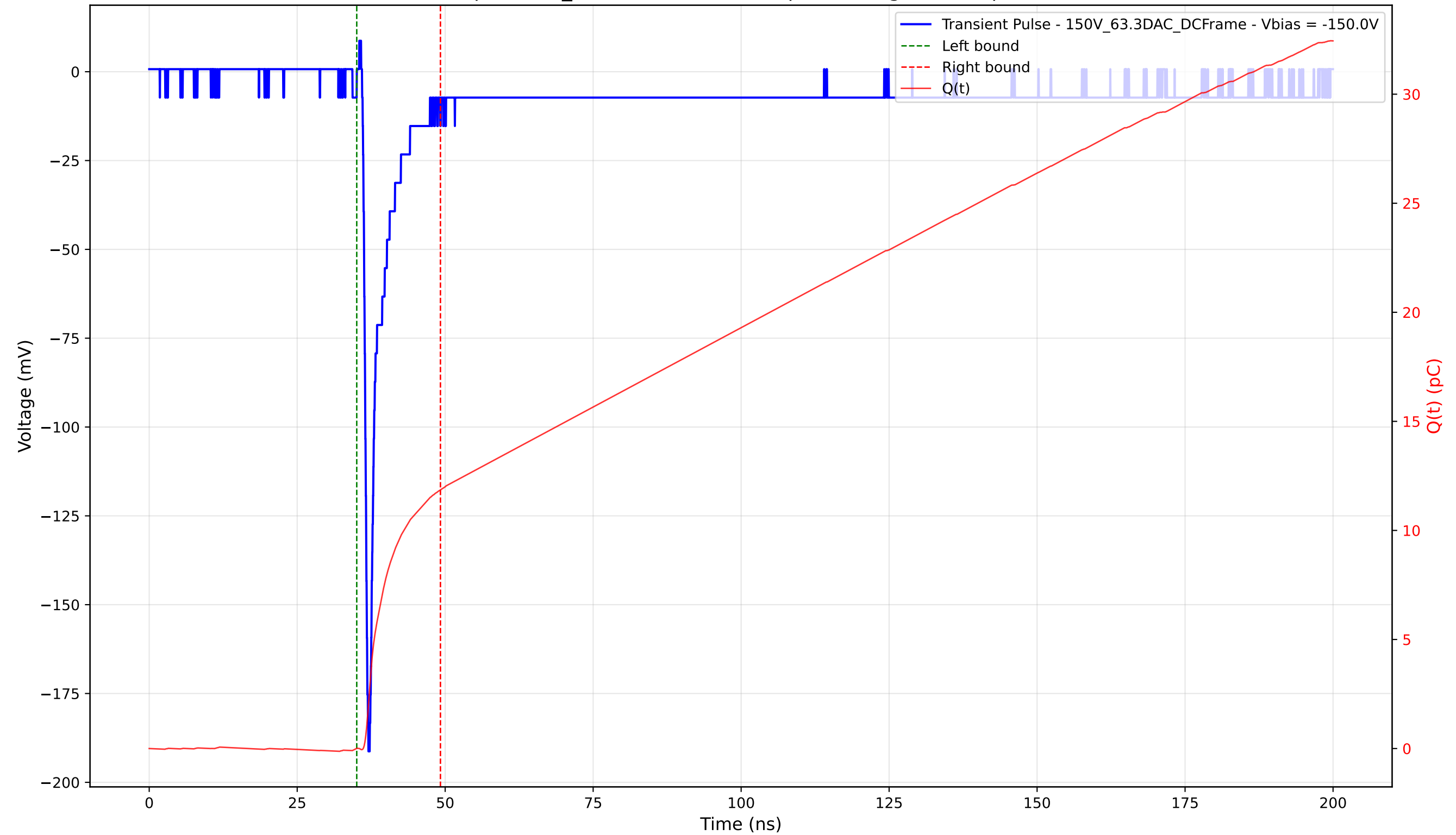
Transient Pulse - Sample: 1cm_42 - Position: 4925.0 \mu\text{m} - Charge: 11.84 pC - Rise Time: 0.75 ns
