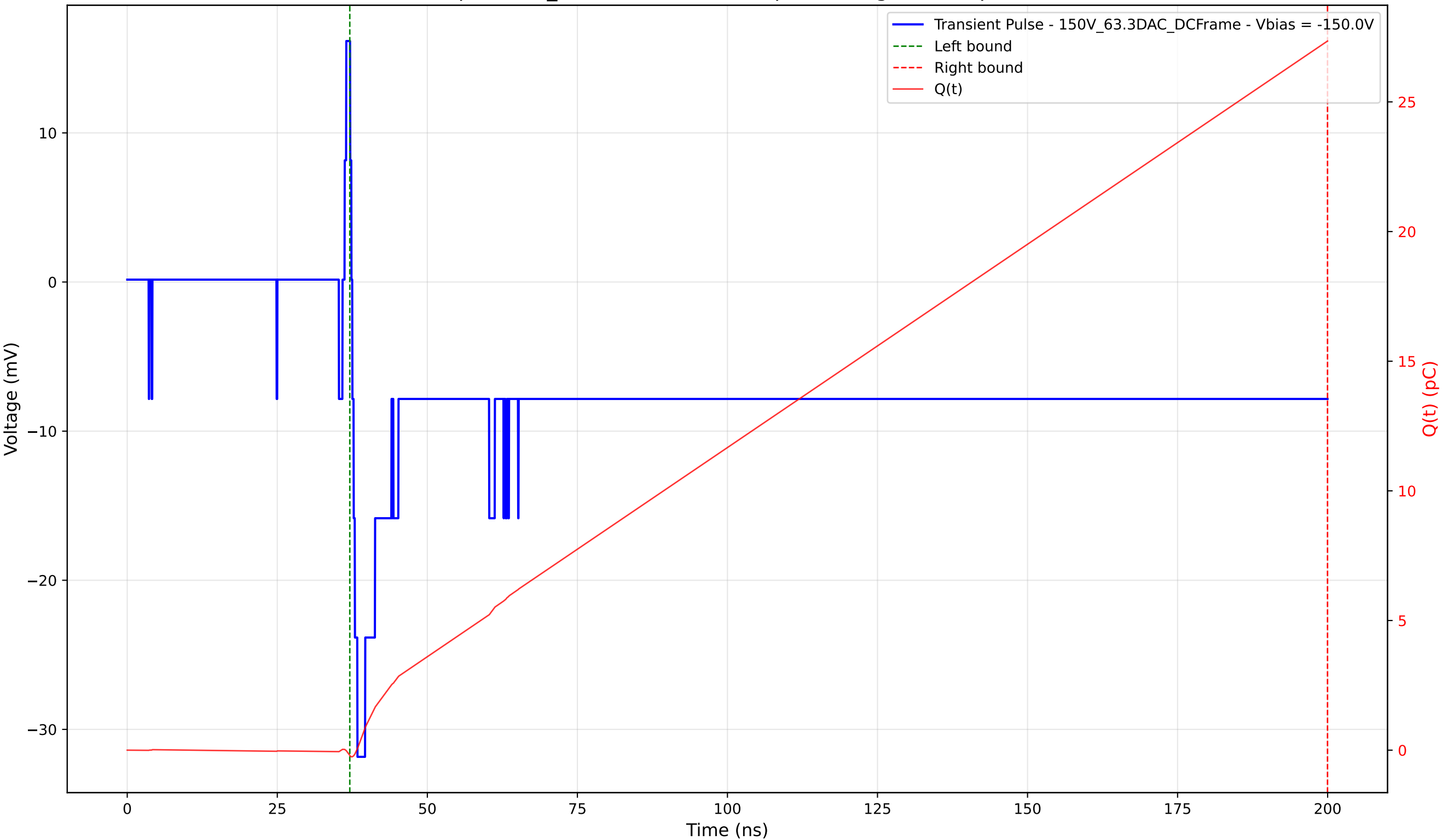
Transient Pulse - Sample: 1cm_42 - Position: 2620.0 \mu\text{m} - Charge: 27.55 pC - Rise Time: 0.85 ns
