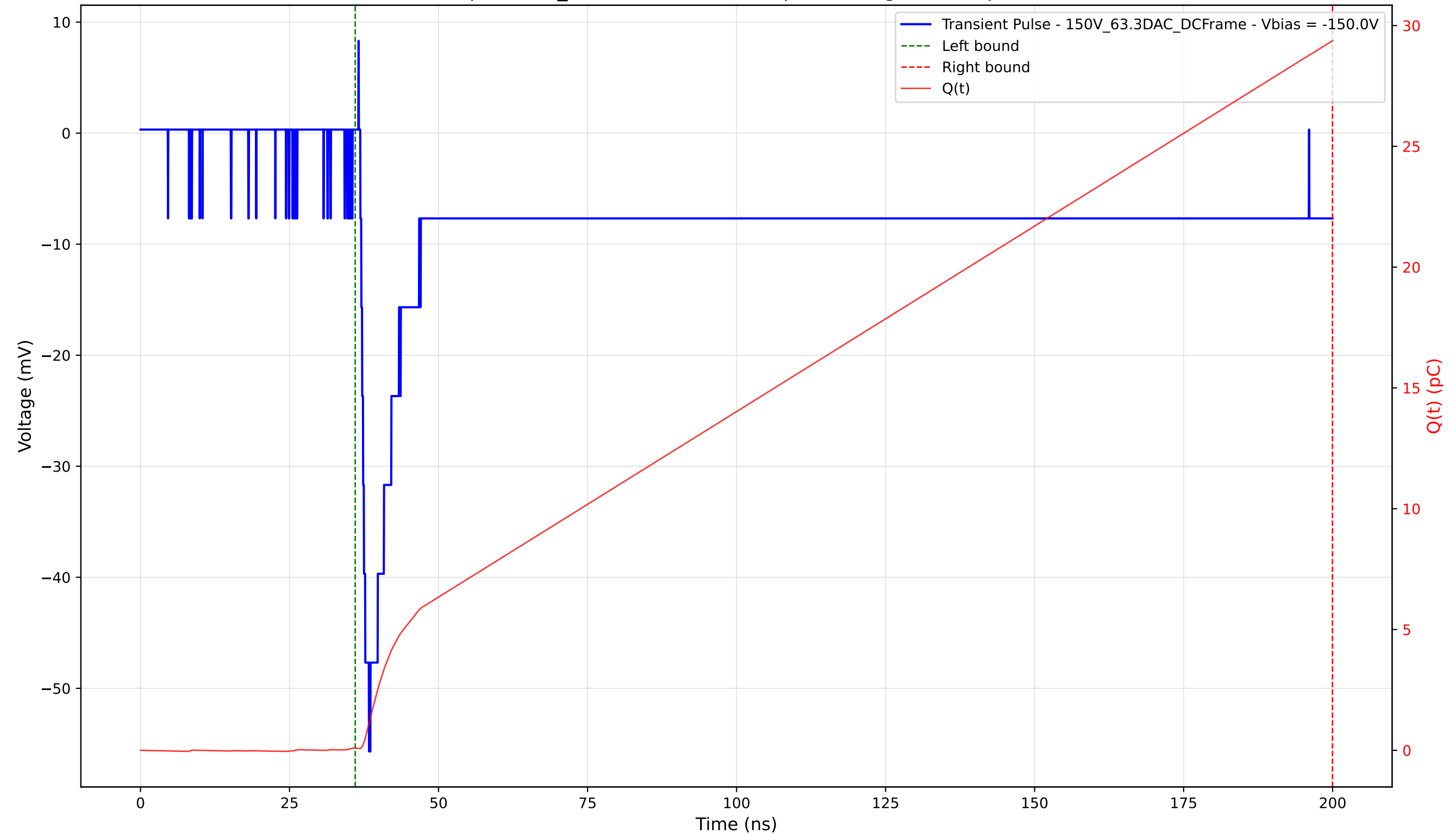
Transient Pulse - Sample: 1cm_42 - Position: 3930.0 \mu\text{m} - Charge: 29.28 pC - Rise Time: 1.45 ns
