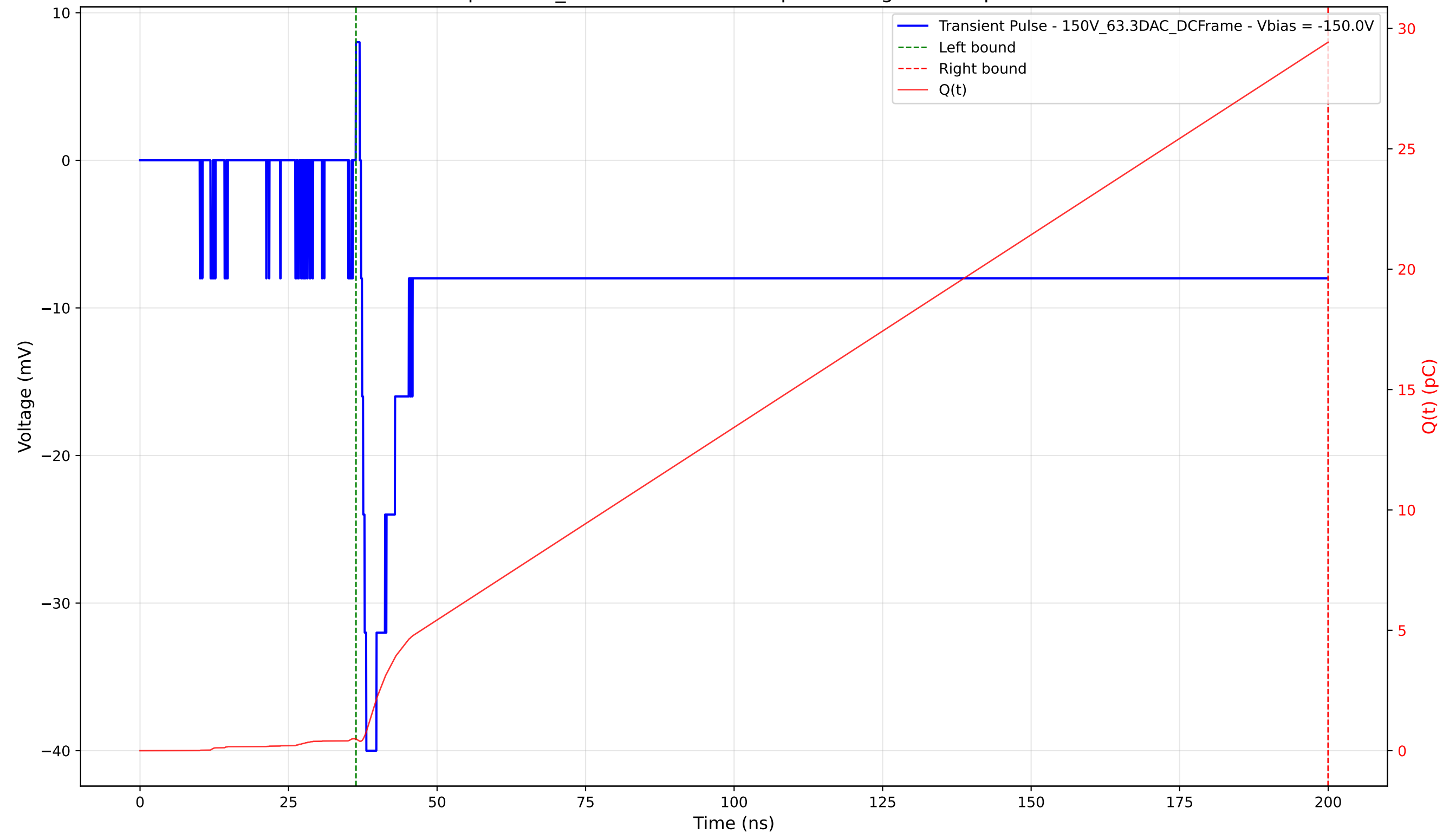
Transient Pulse - Sample: 1cm_42 - Position: 3570.0 \mu\text{m} - Charge: 28.94 pC - Rise Time: 0.89 ns
