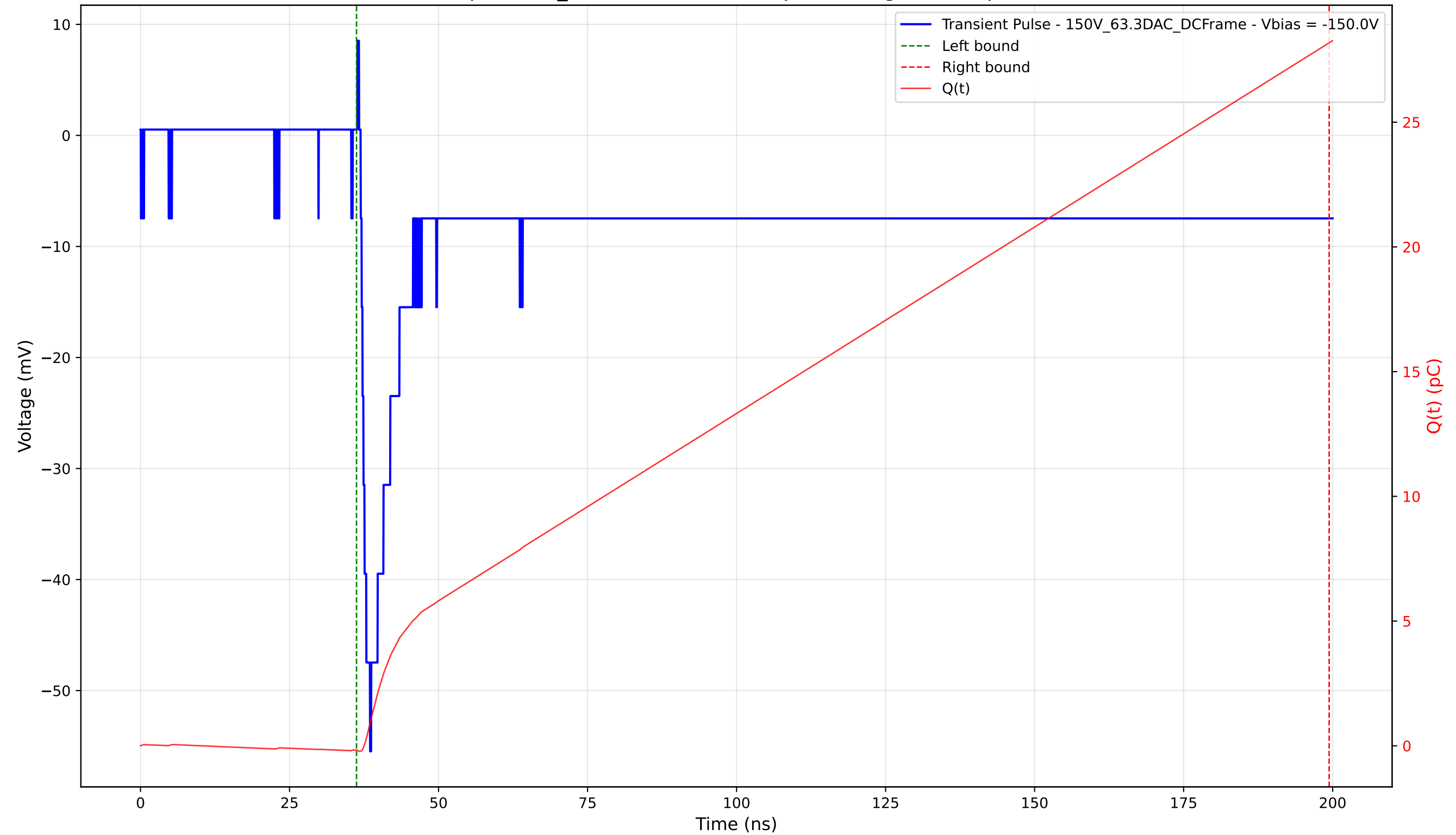
Transient Pulse - Sample: 1cm_42 - Position: 3880.0 \mu\text{m} - Charge: 28.35 pC - Rise Time: 1.57 ns
