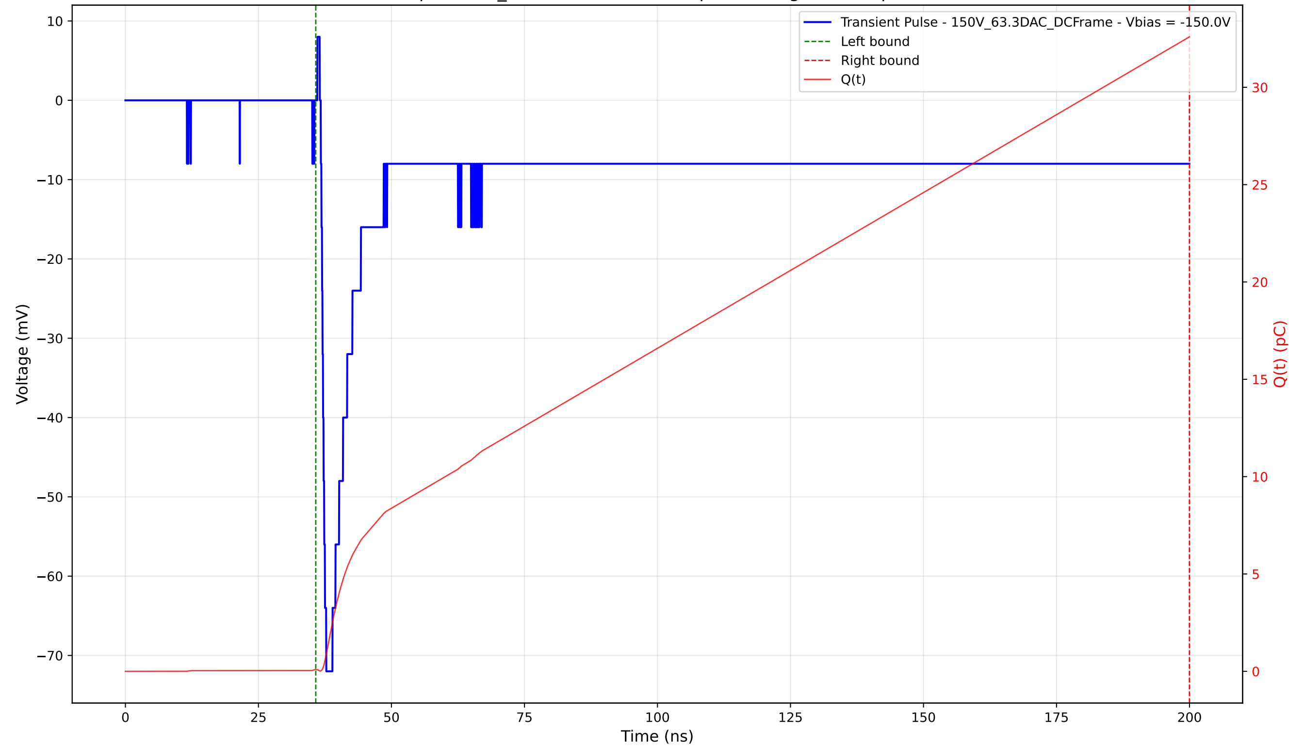
Transient Pulse - Sample: 1cm_42 - Position: 1095.0 \mu\text{m} - Charge: 32.50 pC - Rise Time: 1.02 ns
