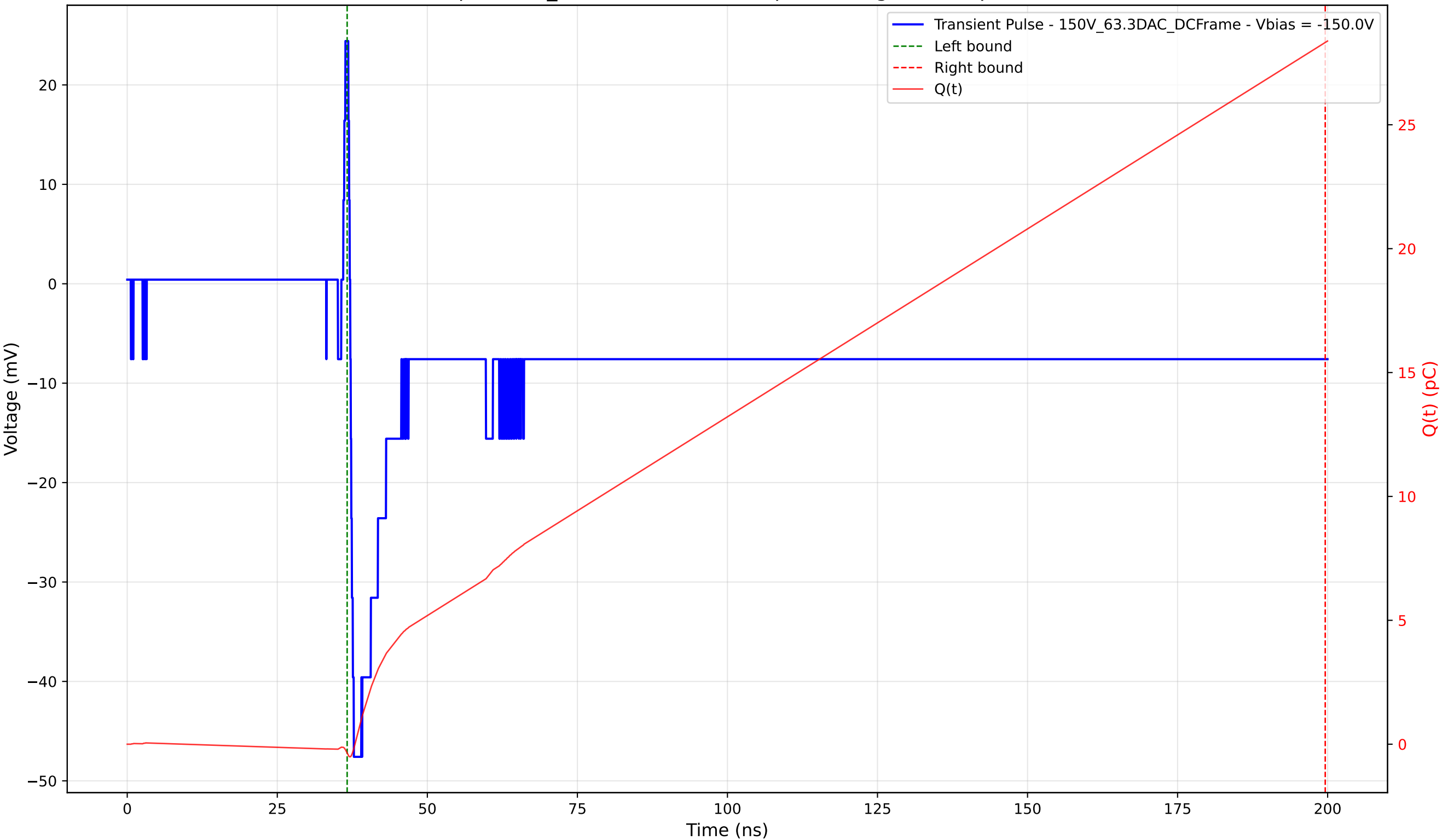
Transient Pulse - Sample: 1cm_42 - Position: 1625.0 \mu\text{m} - Charge: 28.68 pC - Rise Time: 0.59 ns
