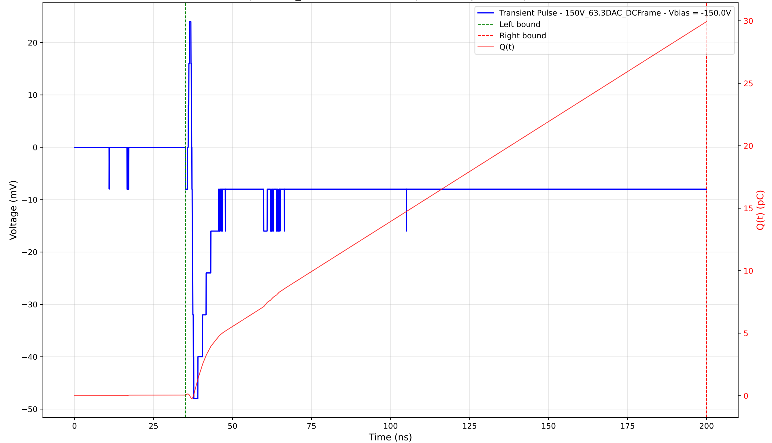
Transient Pulse - Sample: 1cm_42 - Position: 1615.0 \mu\text{m} - Charge: 29.88 pC - Rise Time: 0.59 ns
