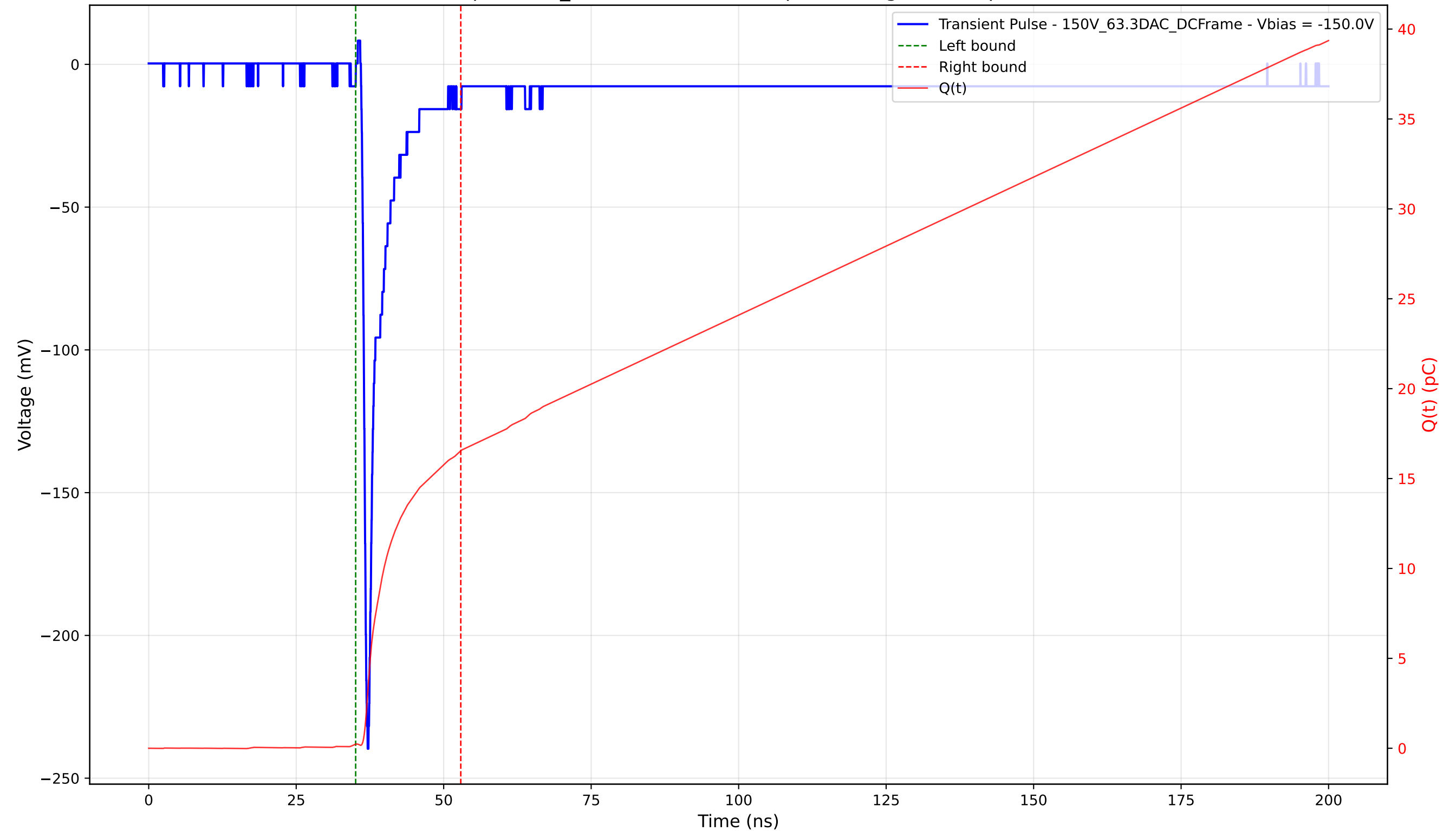
Transient Pulse - Sample: 1cm_42 - Position: 4830.0 \mu\text{m} - Charge: 16.31 pC - Rise Time: 0.78 ns
