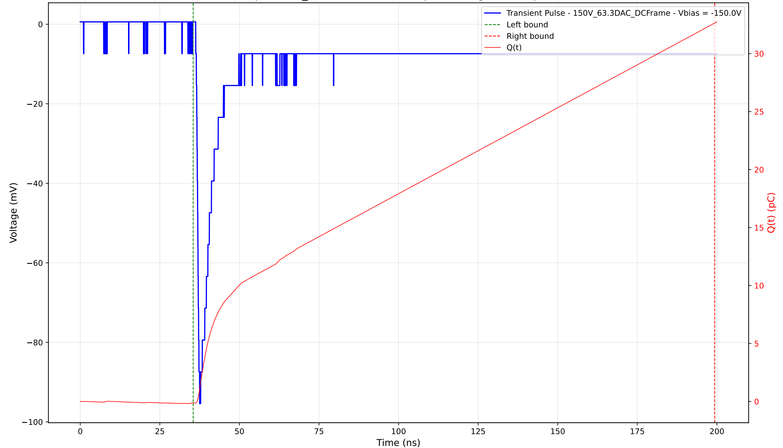
Transient Pulse - Sample: 1cm_42 - Position: 4300.0 \mu\text{m} - Charge: 32.76 pC - Rise Time: 0.81 ns
