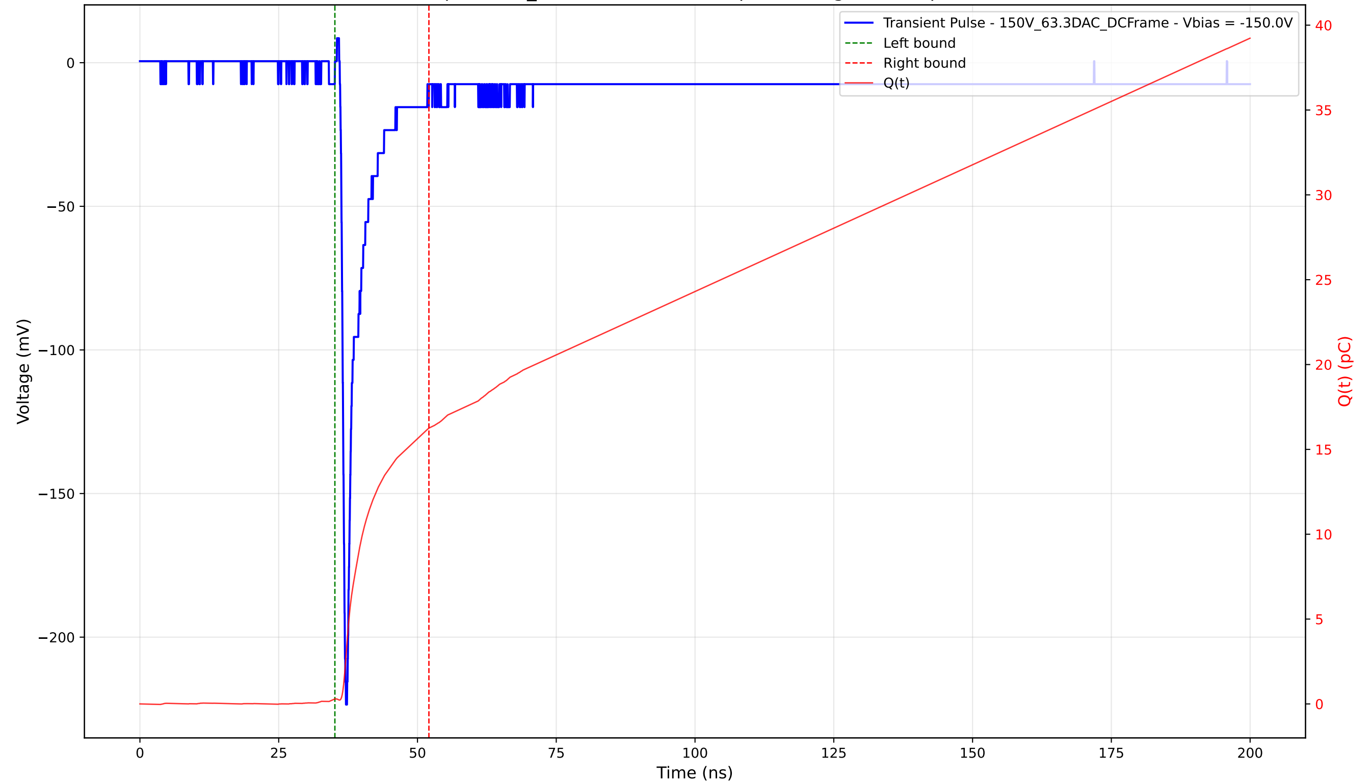
Transient Pulse - Sample: 1cm_42 - Position: 4715.0 \mu\text{m} - Charge: 15.96 pC - Rise Time: 0.80 ns
