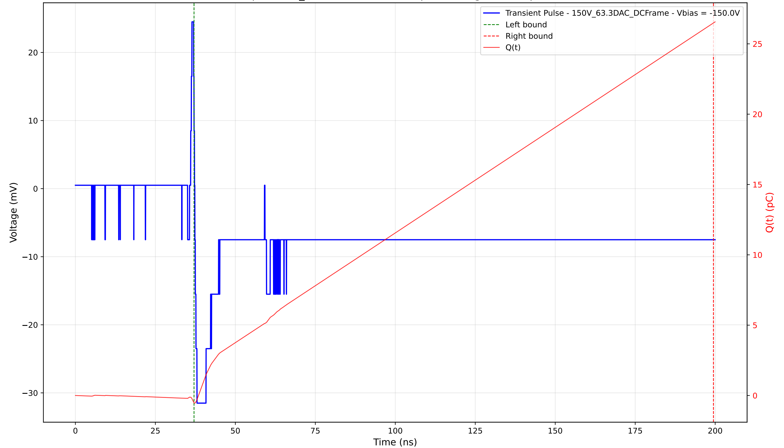
Transient Pulse - Sample: 1cm_42 - Position: 2300.0 \mu\text{m} - Charge: 27.00 pC - Rise Time: 0.67 ns
