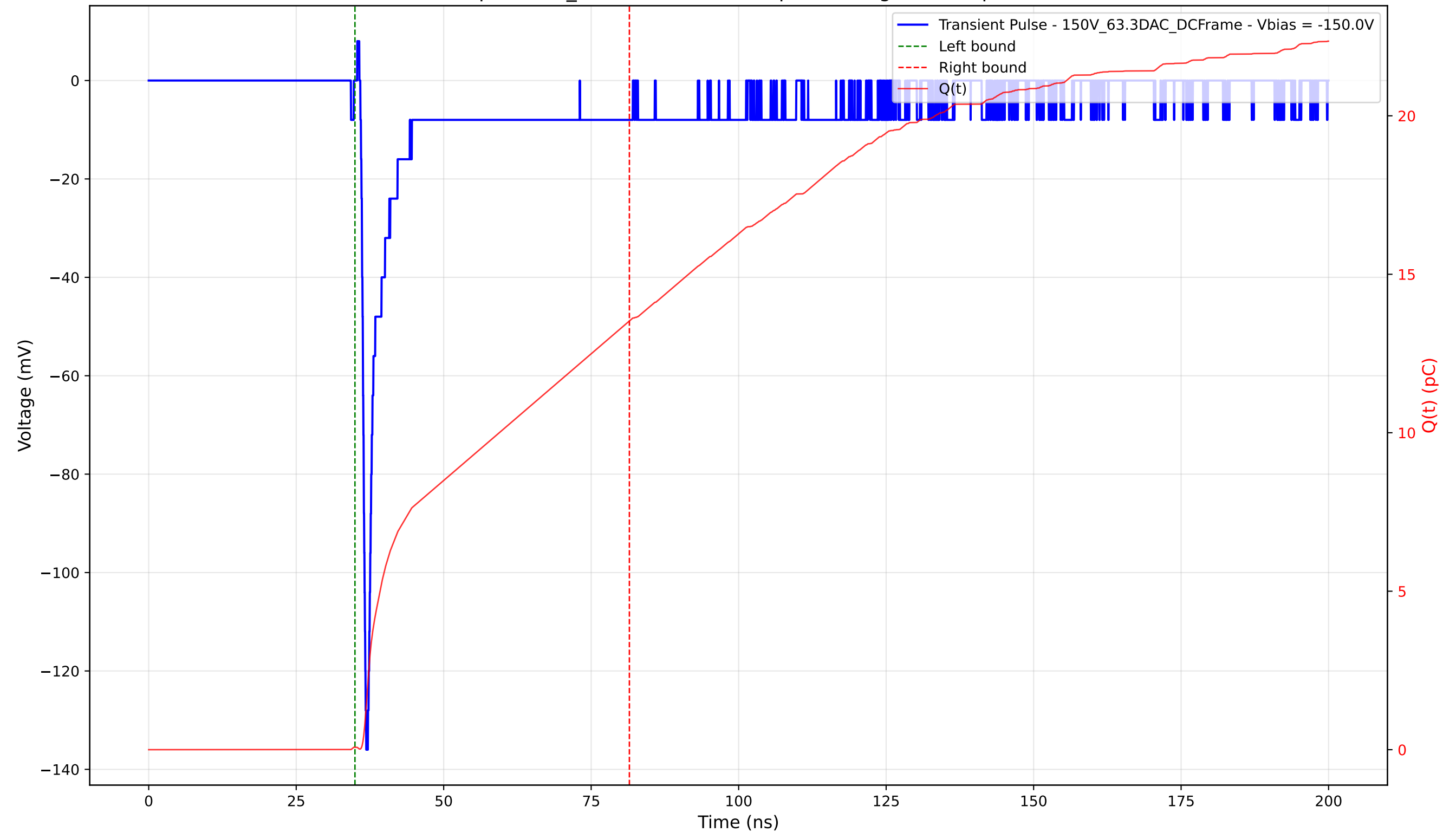
Transient Pulse - Sample: 1cm_42 - Position: 185.0 \mu\text{m} - Charge: 13.45 pC - Rise Time: 0.79 ns
