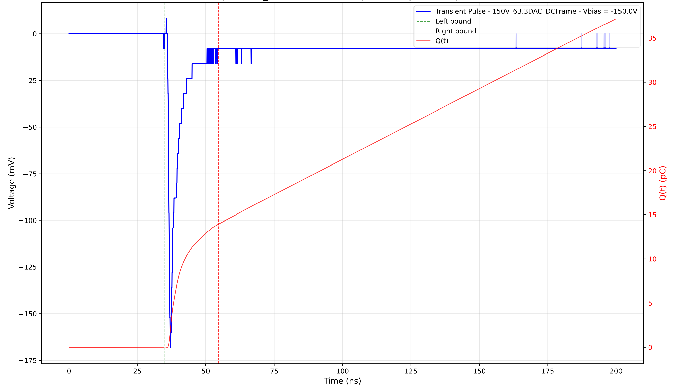
Transient Pulse - Sample: 1cm_42 - Position: 490.0 \mu\text{m} - Charge: 13.92 pC - Rise Time: 0.78 ns
