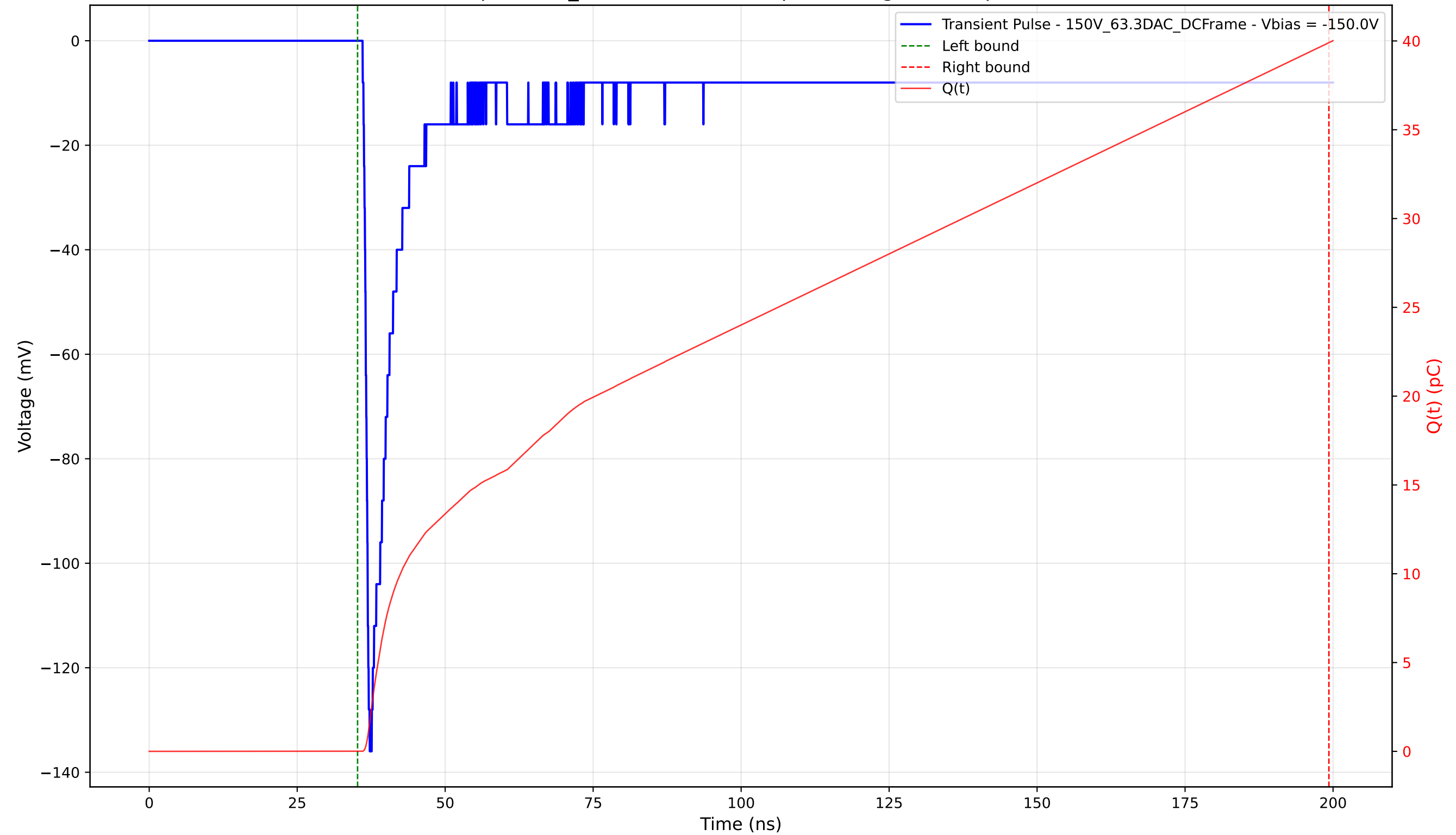
Transient Pulse - Sample: 1cm_42 - Position: 705.0 \mu\text{m} - Charge: 39.90 pC - Rise Time: 0.89 ns
