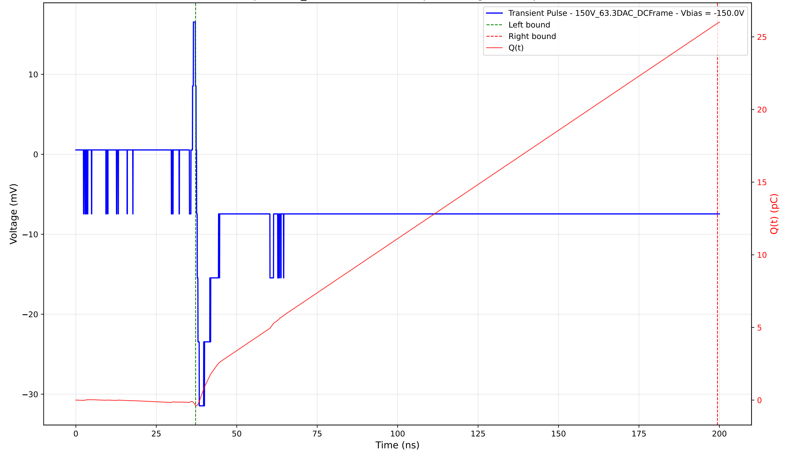
Transient Pulse - Sample: 1cm_42 - Position: 2815.0 \mu\text{m} - Charge: 26.31 pC - Rise Time: 0.83 ns
