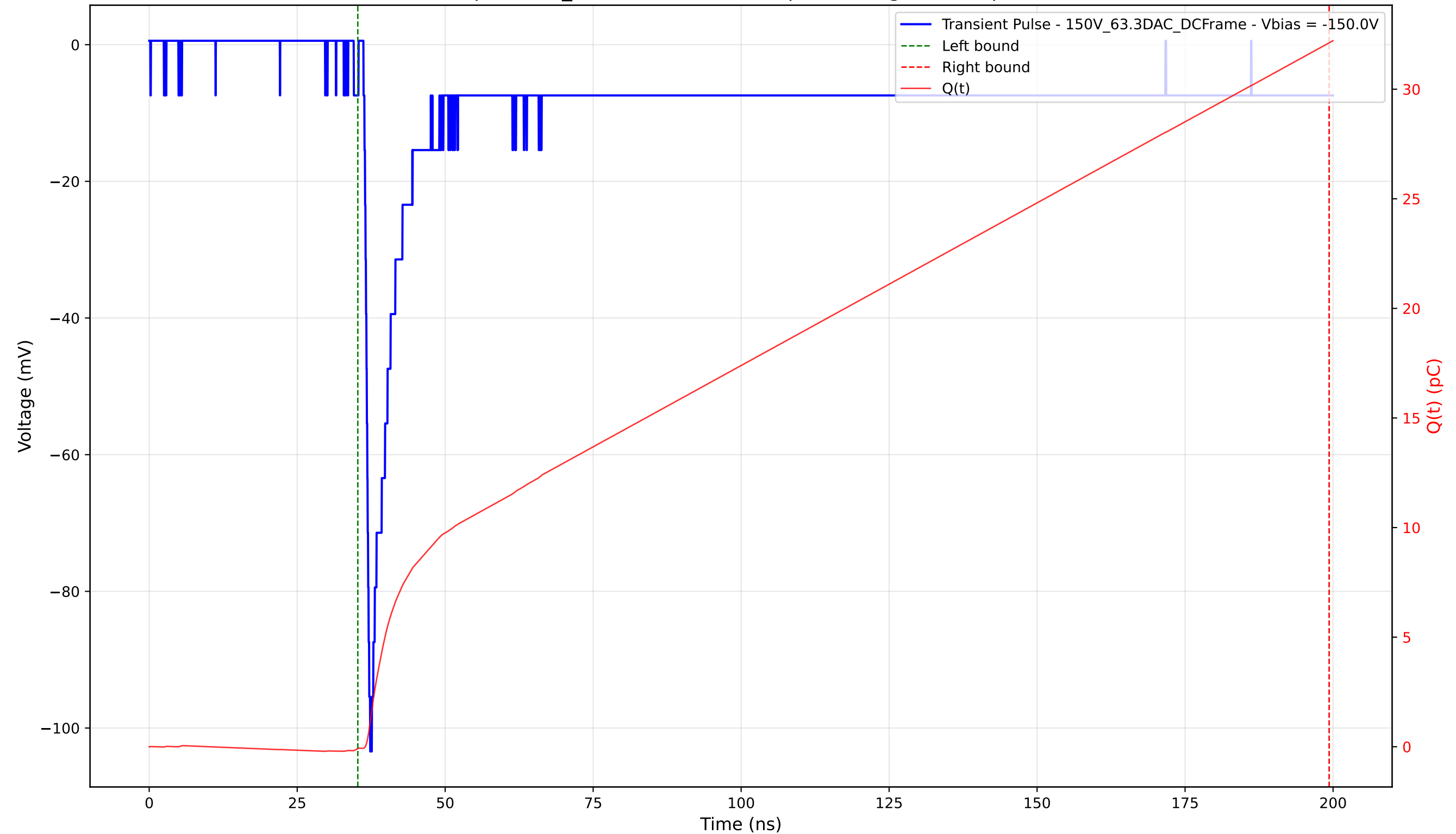
Transient Pulse - Sample: 1cm_42 - Position: 4445.0 \mu\text{m} - Charge: 32.20 pC - Rise Time: 0.81 ns
