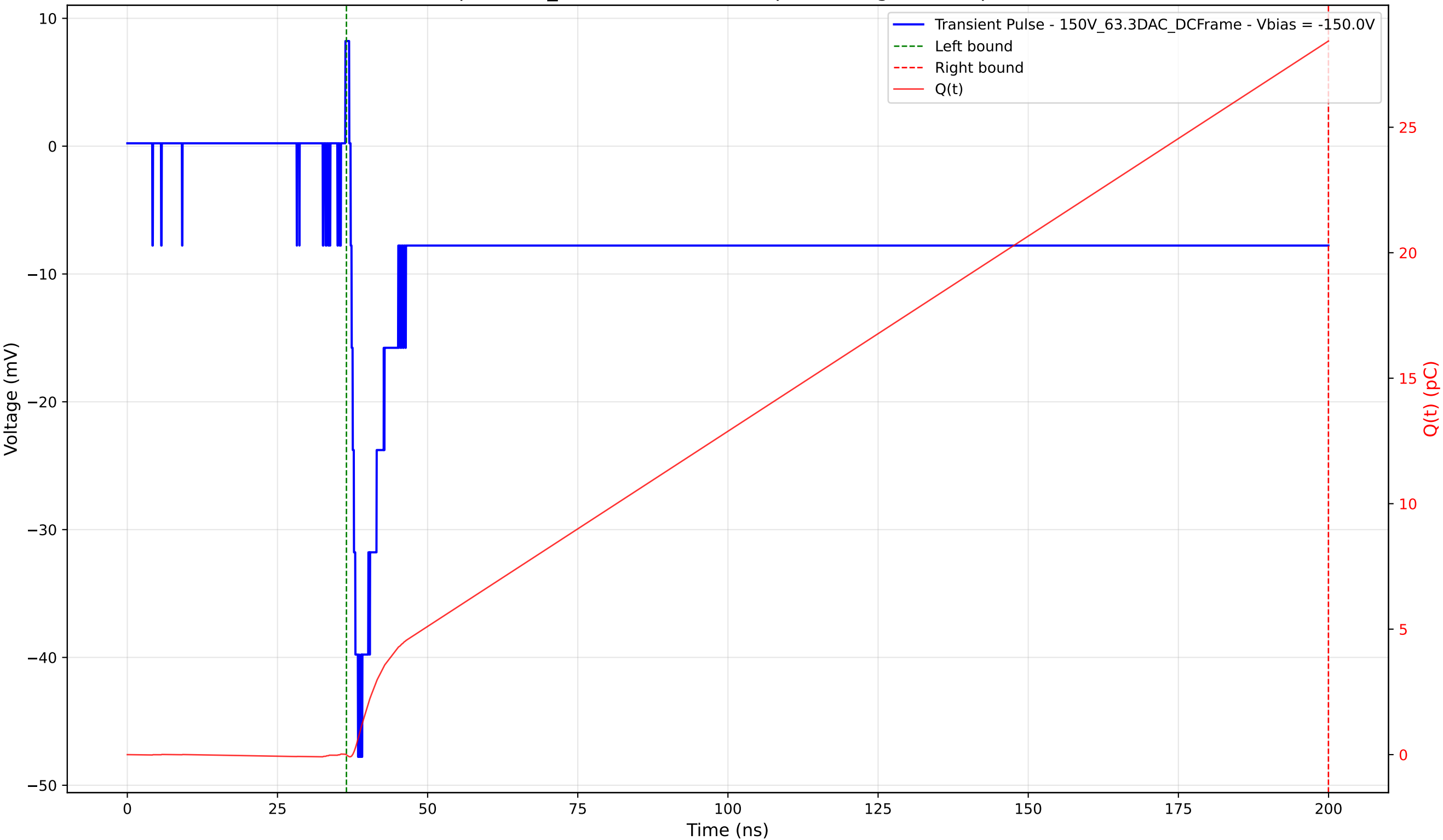
Transient Pulse - Sample: 1cm_42 - Position: 3610.0 \mu\text{m} - Charge: 28.45 pC - Rise Time: 1.23 ns
