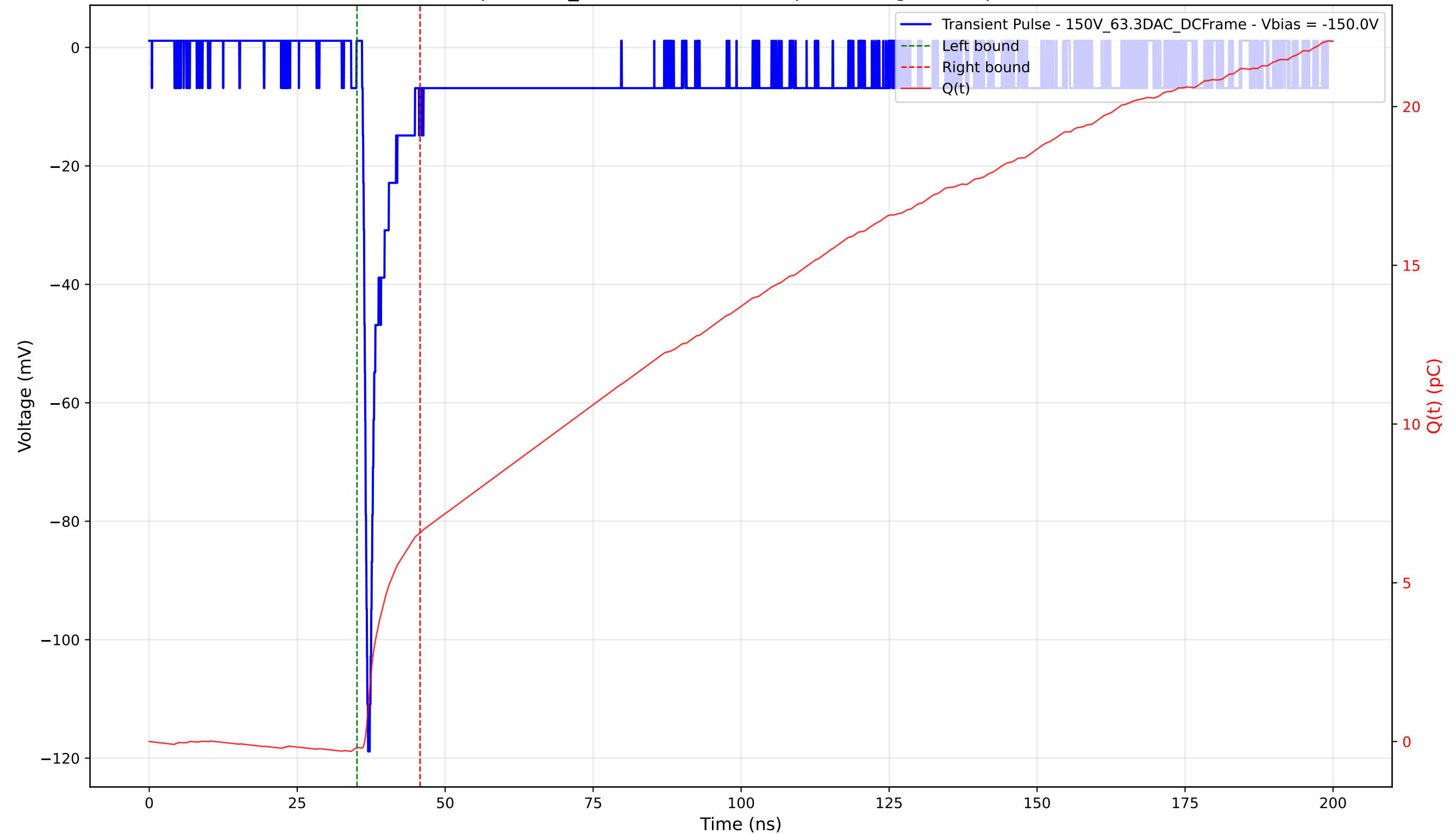
Transient Pulse - Sample: 1cm_42 - Position: 5020.0 \mu\text{m} - Charge: 6.76 pC - Rise Time: 0.77 ns
