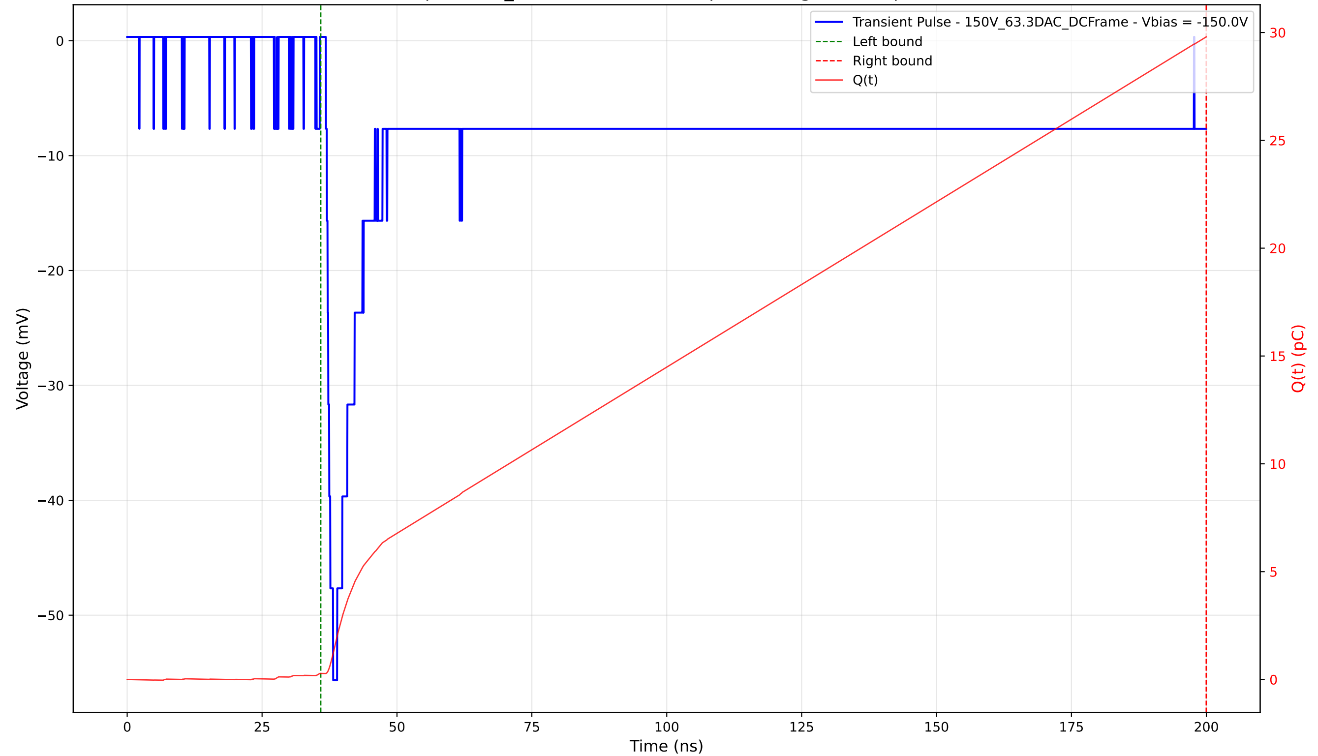
Transient Pulse - Sample: 1cm_42 - Position: 3945.0 \mu\text{m} - Charge: 29.52 pC - Rise Time: 1.35 ns
