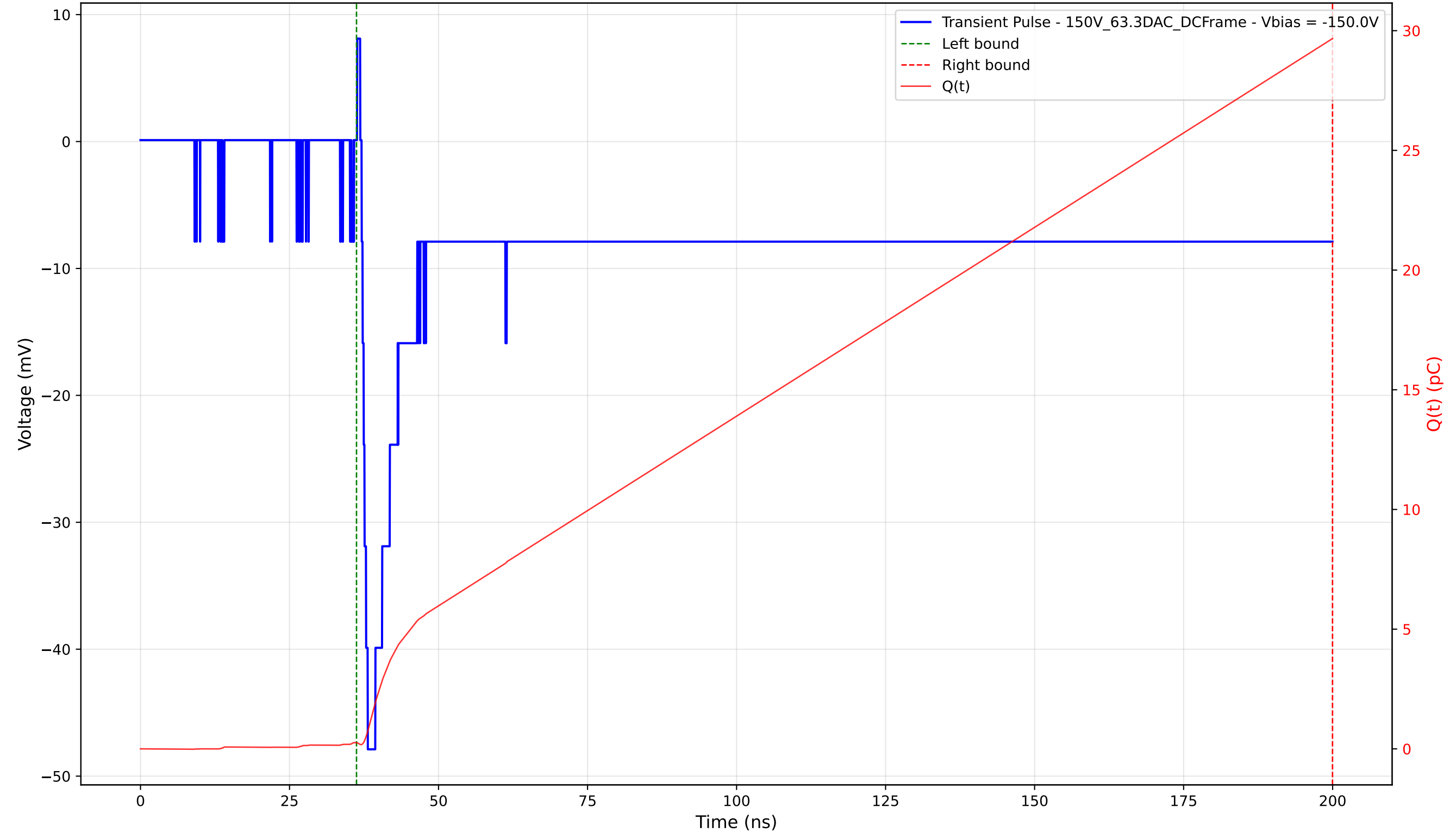
Transient Pulse - Sample: 1cm_42 - Position: 3650.0 \mu\text{m} - Charge: 29.41 pC - Rise Time: 1.03 ns
