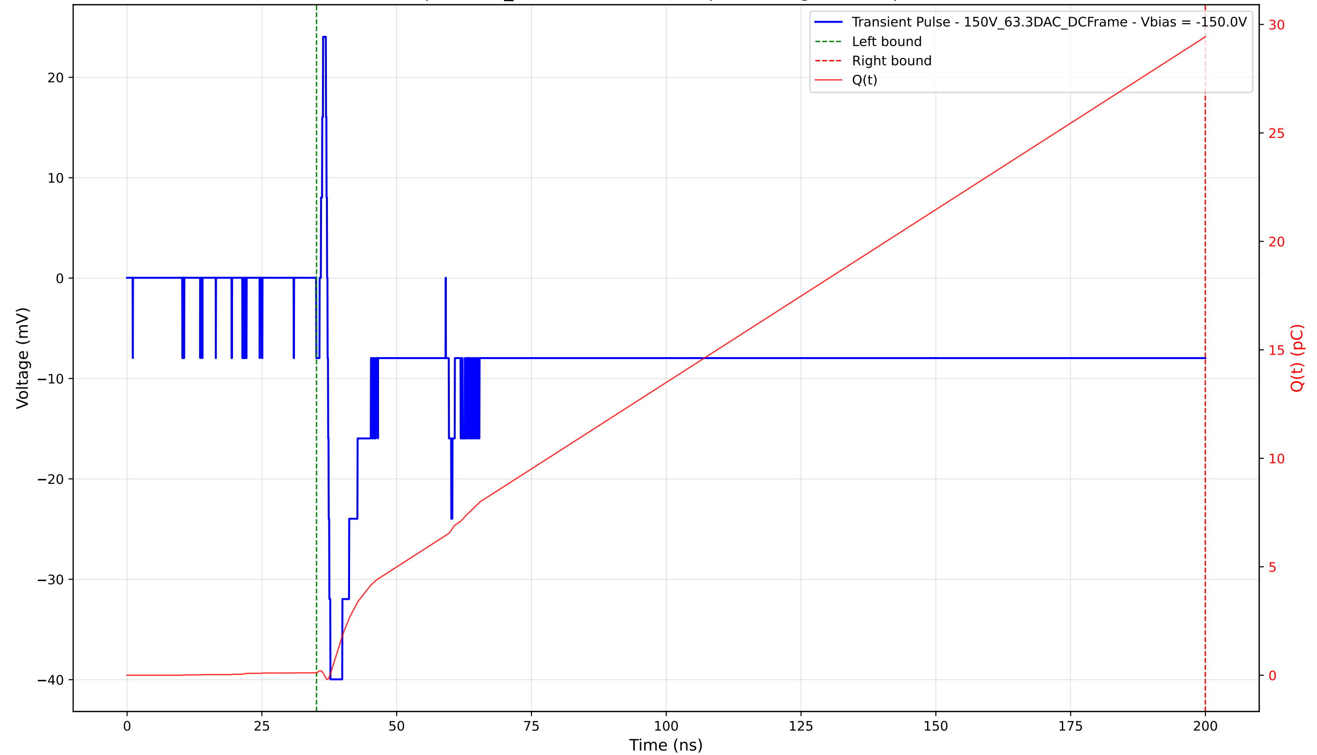
Transient Pulse - Sample: 1cm_42 - Position: 1840.0 \mu\text{m} - Charge: 29.31 pC - Rise Time: 0.53 ns
