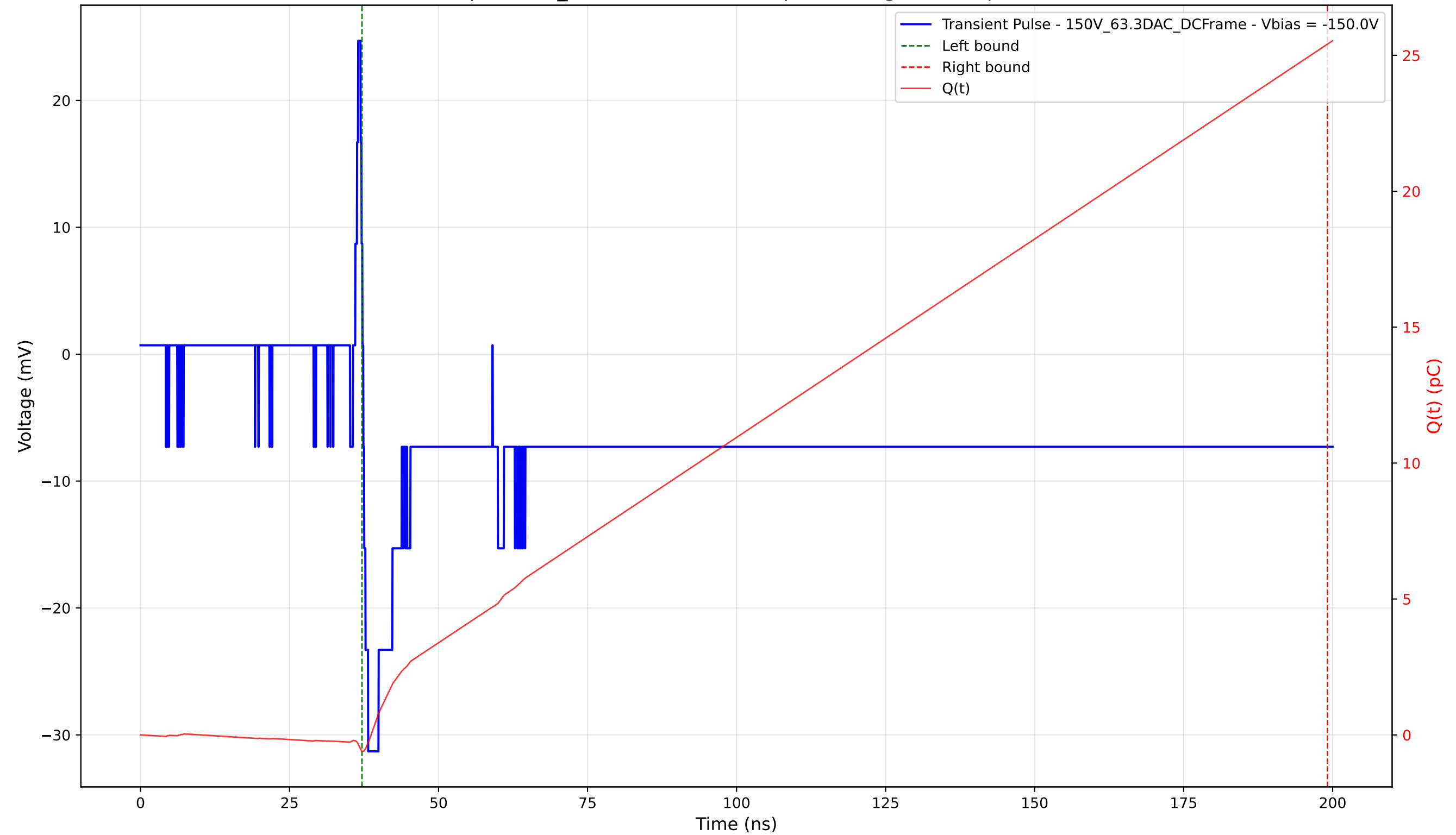
Transient Pulse - Sample: 1cm_42 - Position: 2370.0 \mu\text{m} - Charge: 26.01 pC - Rise Time: 0.81 ns
