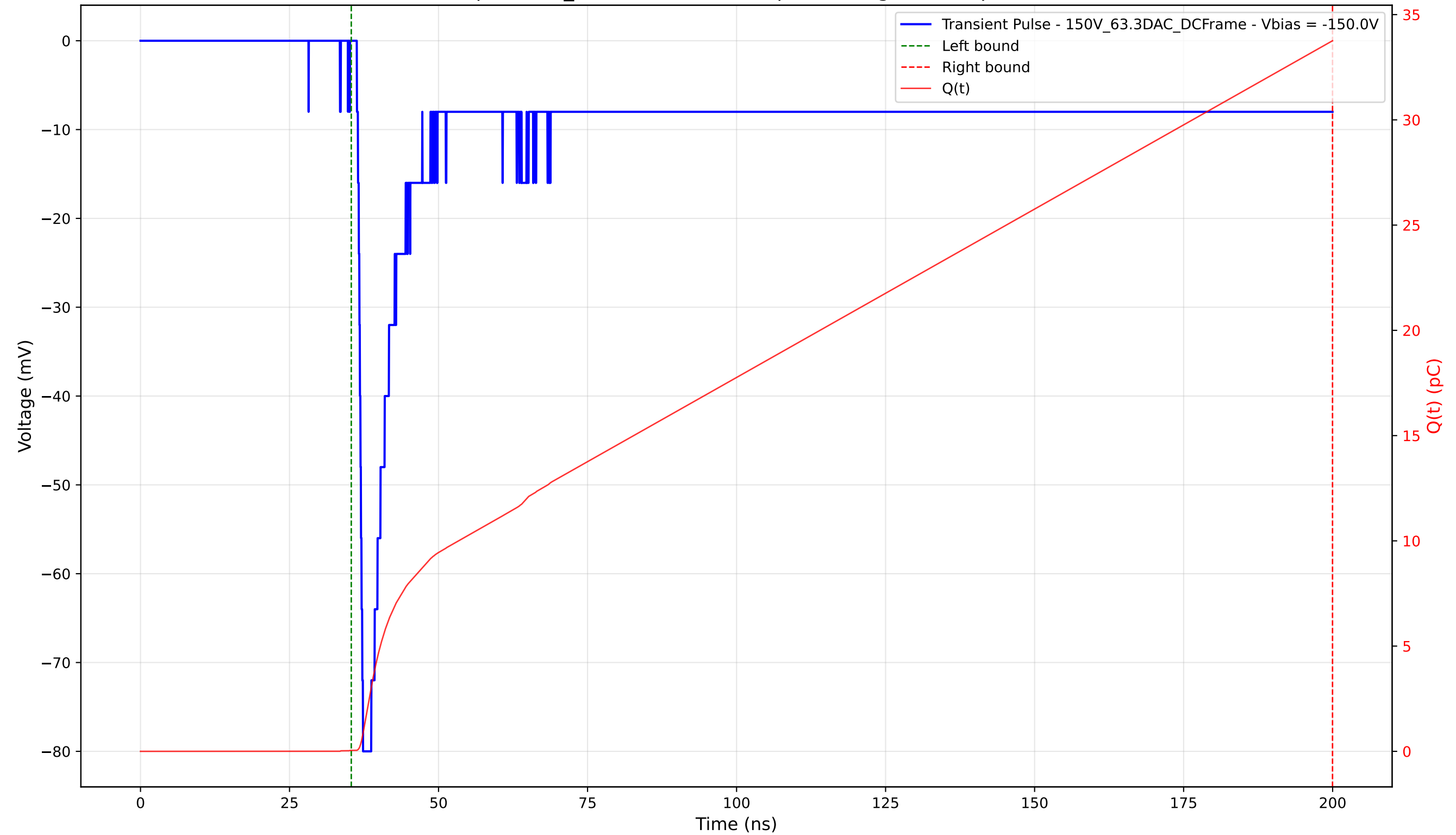
Transient Pulse - Sample: 1cm_42 - Position: 935.0 \mu\text{m} - Charge: 33.71 pC - Rise Time: 0.74 ns
