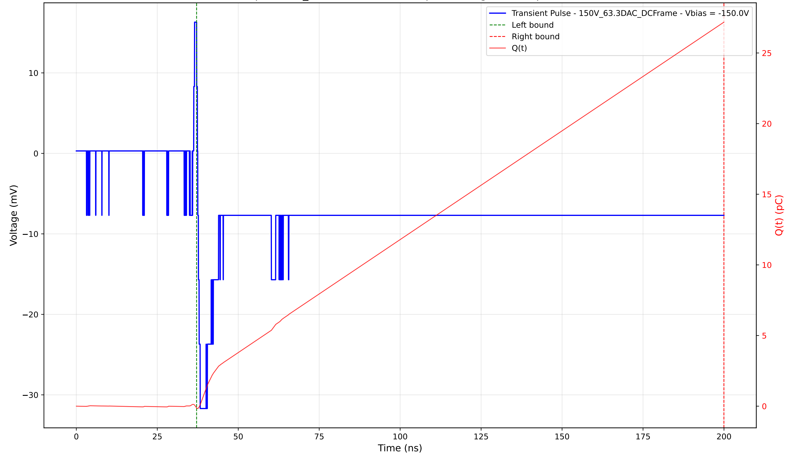
Transient Pulse - Sample: 1cm_42 - Position: 2765.0 \mu\text{m} - Charge: 27.31 pC - Rise Time: 0.75 ns
