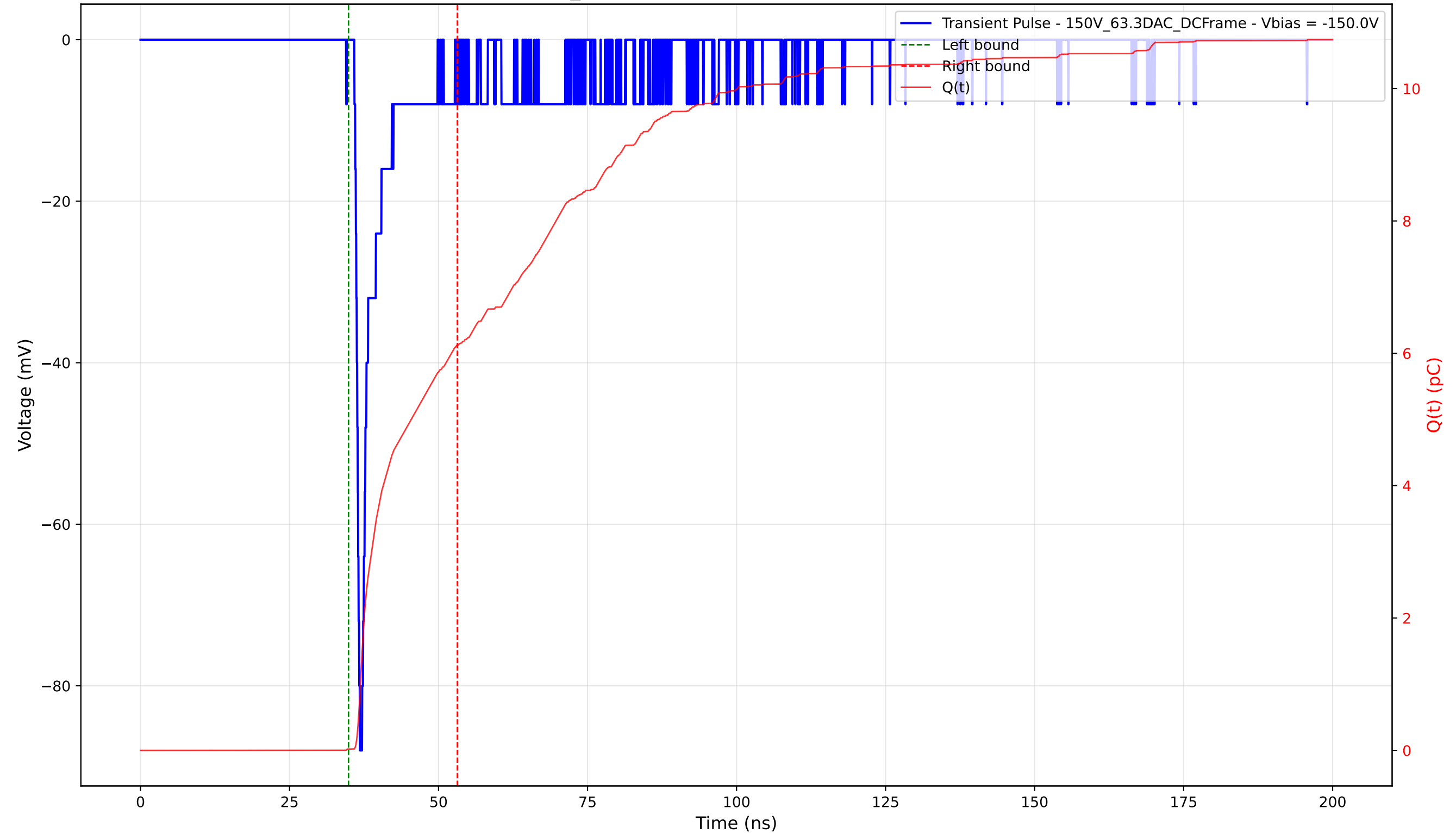
Transient Pulse - Sample: 1cm_42 - Position: 110.0 \mu\text{m} - Charge: 6.10 pC - Rise Time: 0.68 ns
