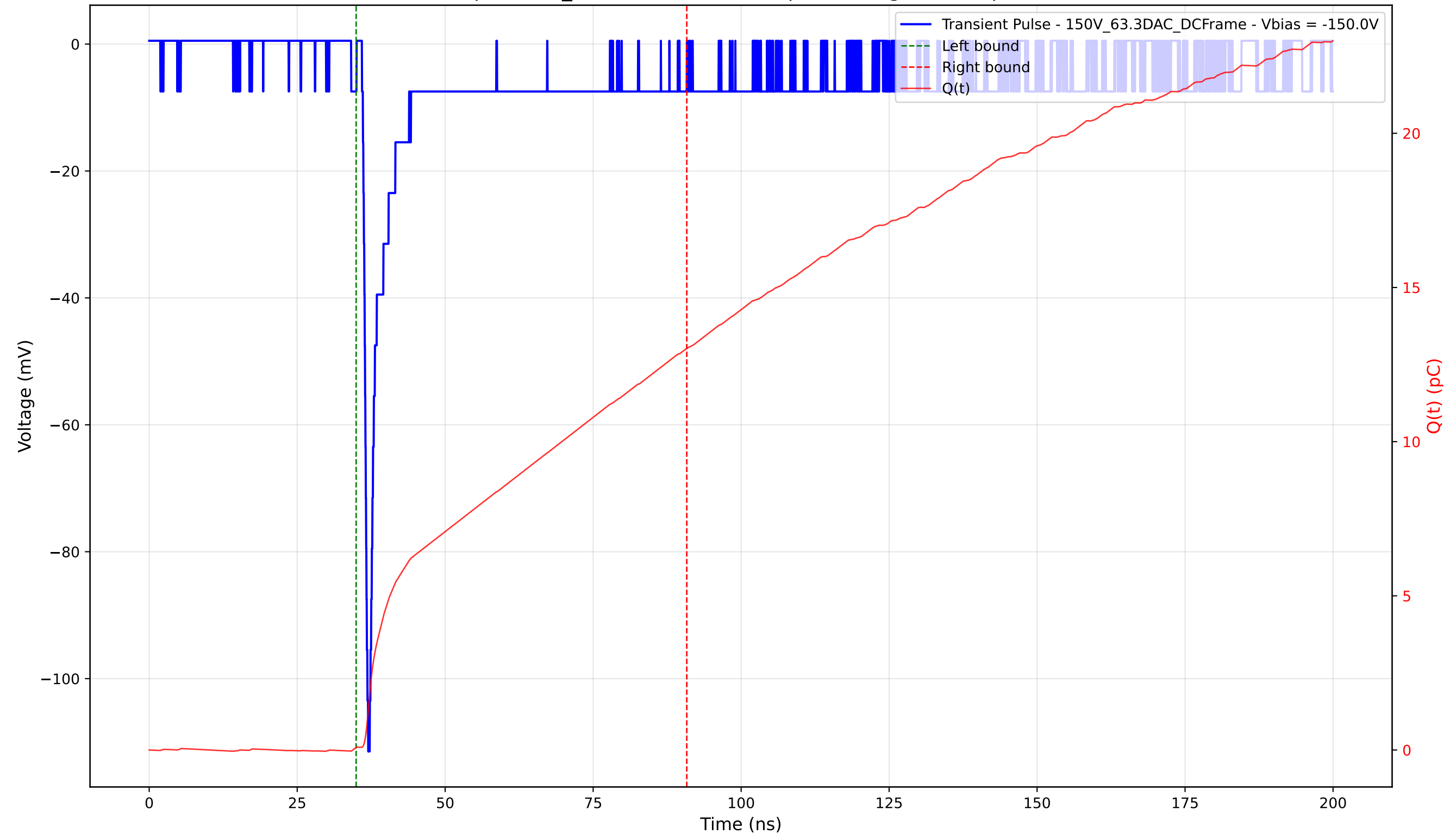
Transient Pulse - Sample: 1cm_42 - Position: 5030.0 \mu\text{m} - Charge: 12.94 pC - Rise Time: 0.77 ns
