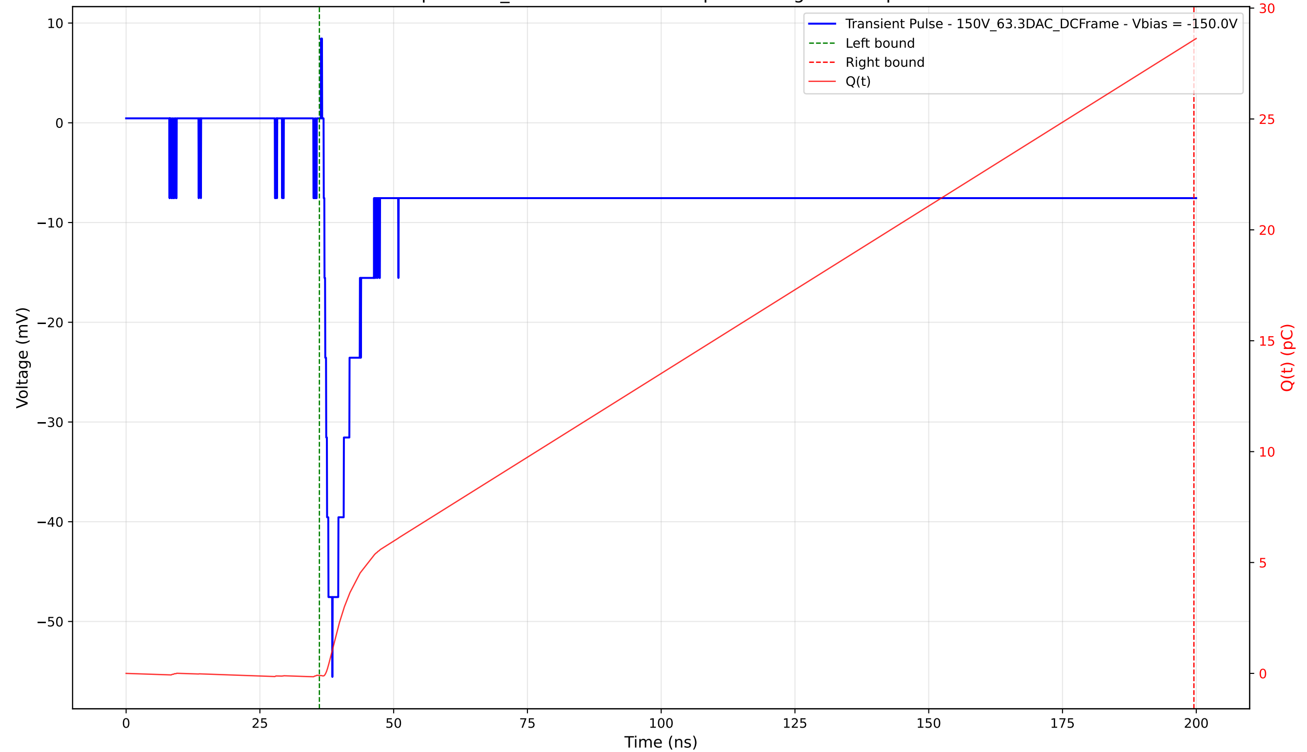
Transient Pulse - Sample: 1cm_42 - Position: 3895.0 \mu\text{m} - Charge: 28.65 pC - Rise Time: 1.61 ns
