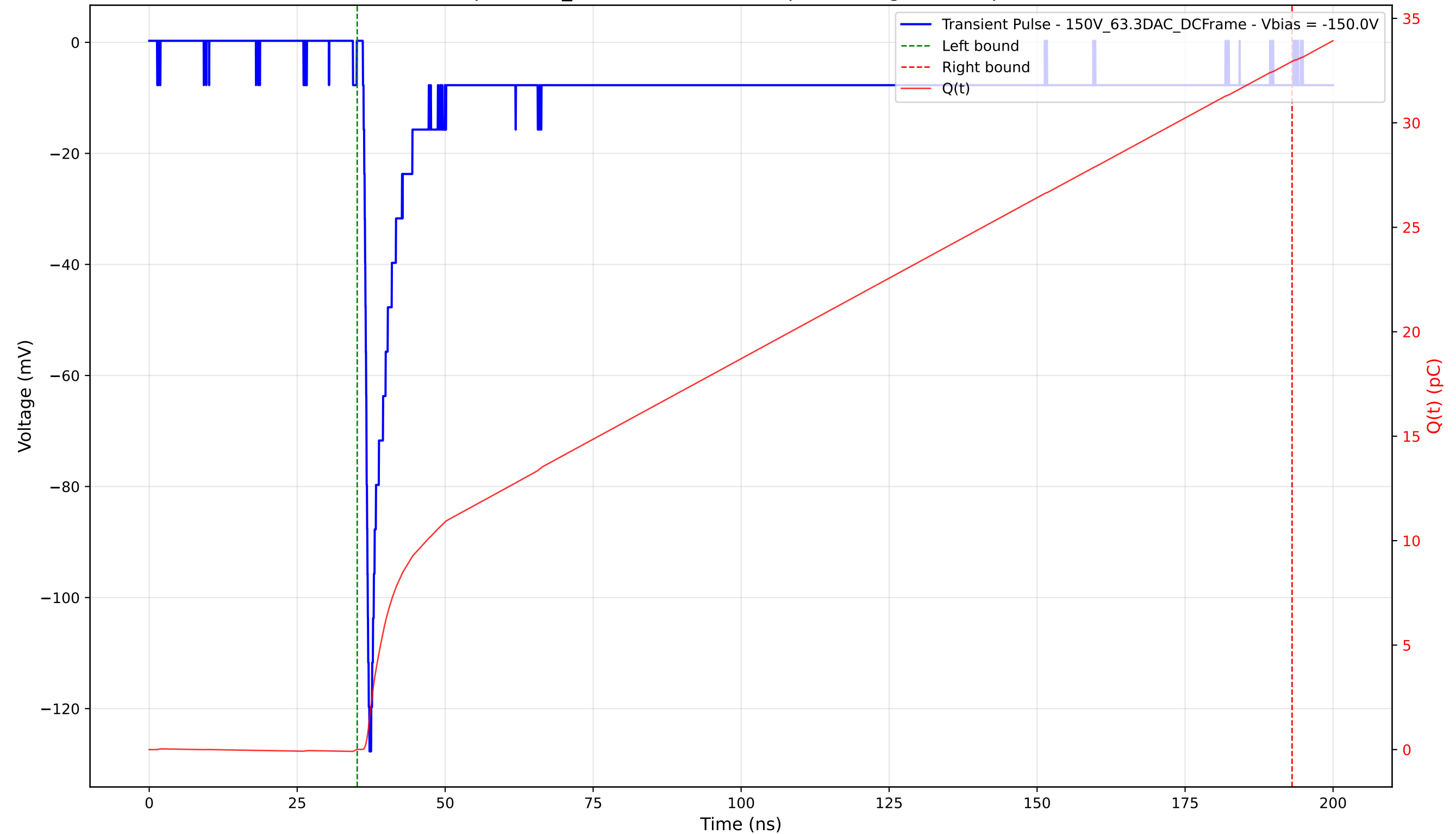
Transient Pulse - Sample: 1cm_42 - Position: 4540.0 \mu\text{m} - Charge: 32.94 pC - Rise Time: 0.87 ns
