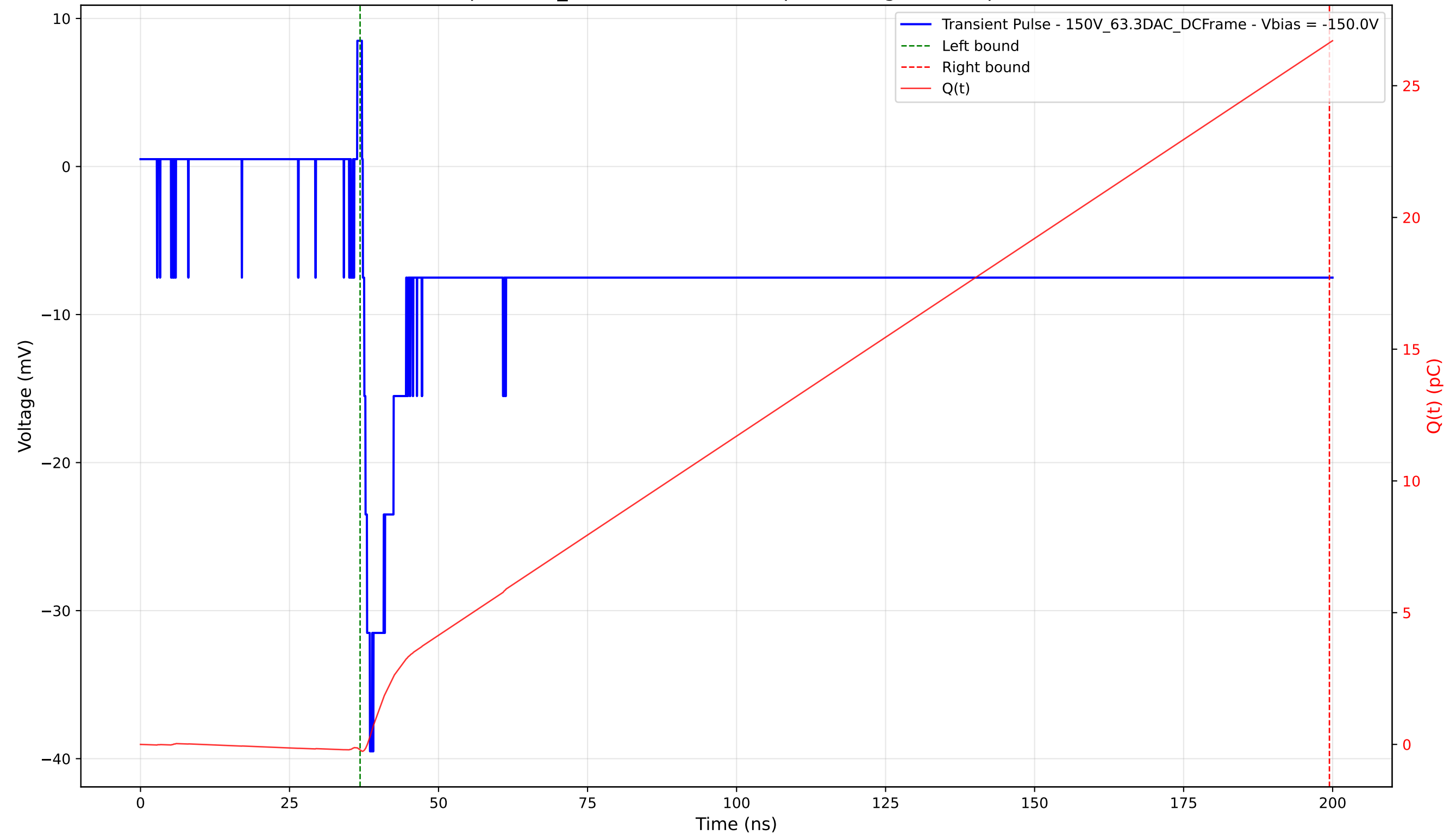
Transient Pulse - Sample: 1cm_42 - Position: 3435.0 \mu\text{m} - Charge: 26.84 pC - Rise Time: 1.19 ns
