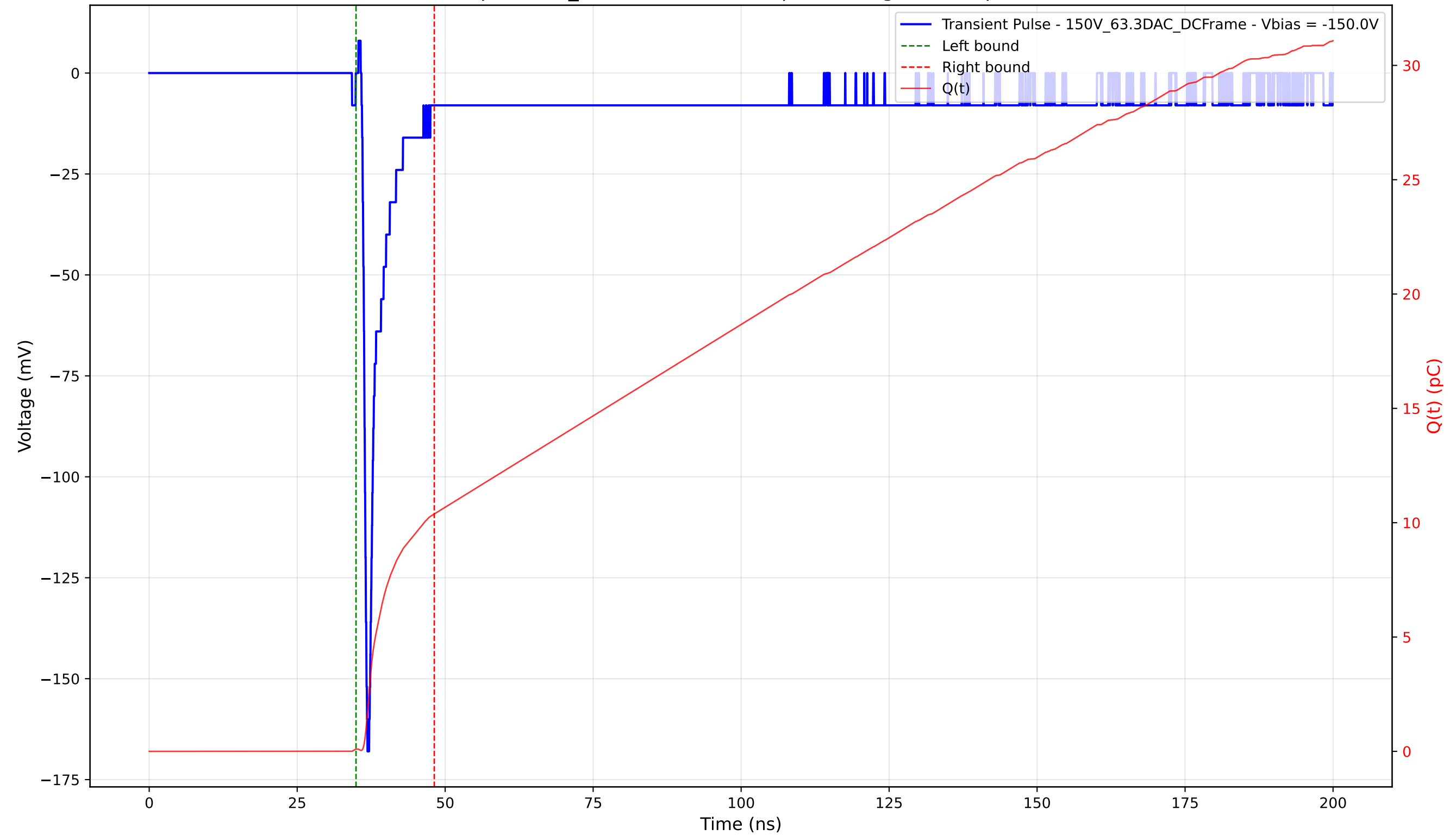
Transient Pulse - Sample: 1cm_42 - Position: 270.0 \mu\text{m} - Charge: 10.28 pC - Rise Time: 0.70 ns
