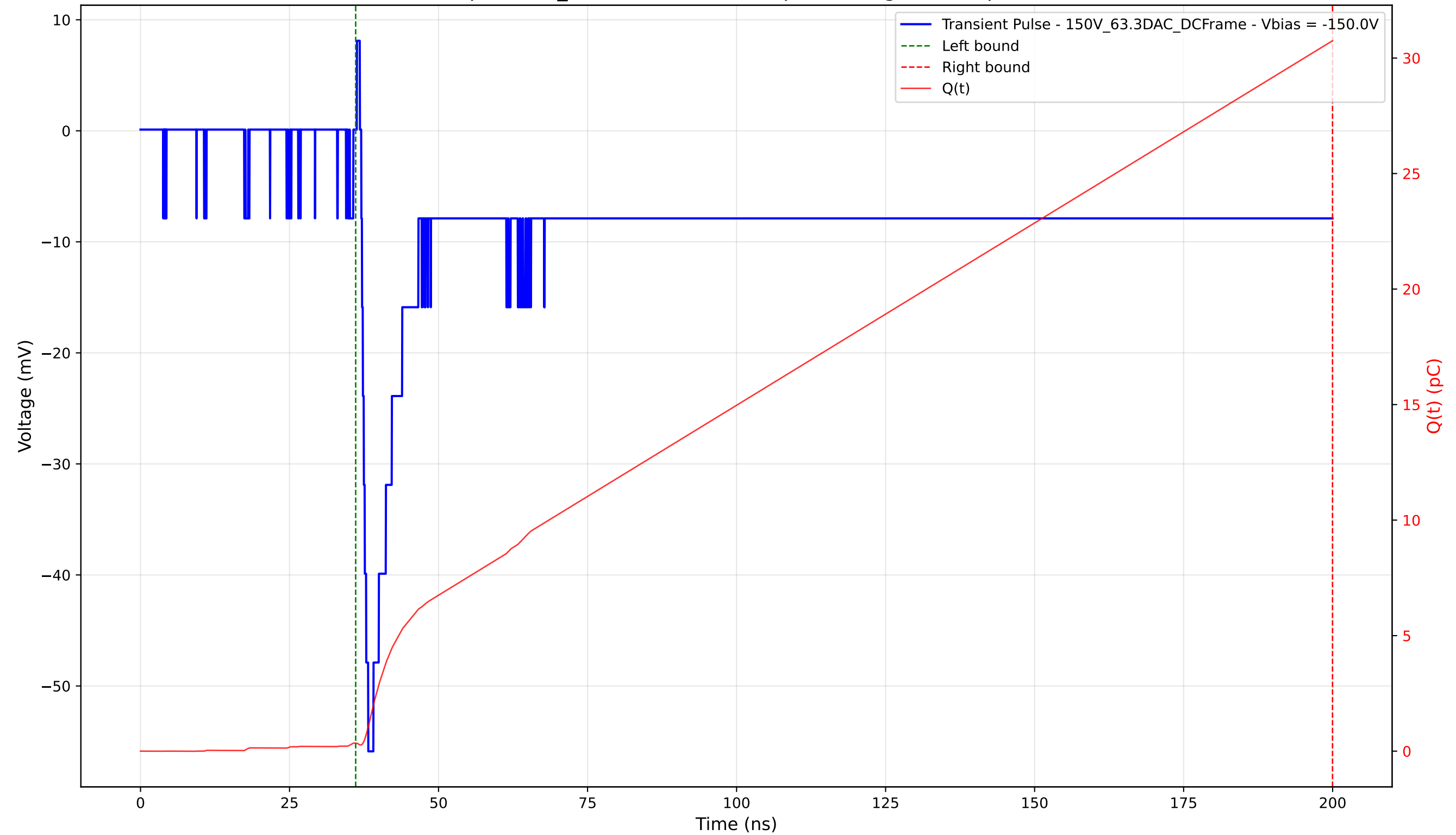
Transient Pulse - Sample: 1cm_42 - Position: 3775.0 \mu\text{m} - Charge: 30.40 pC - Rise Time: 1.17 ns
