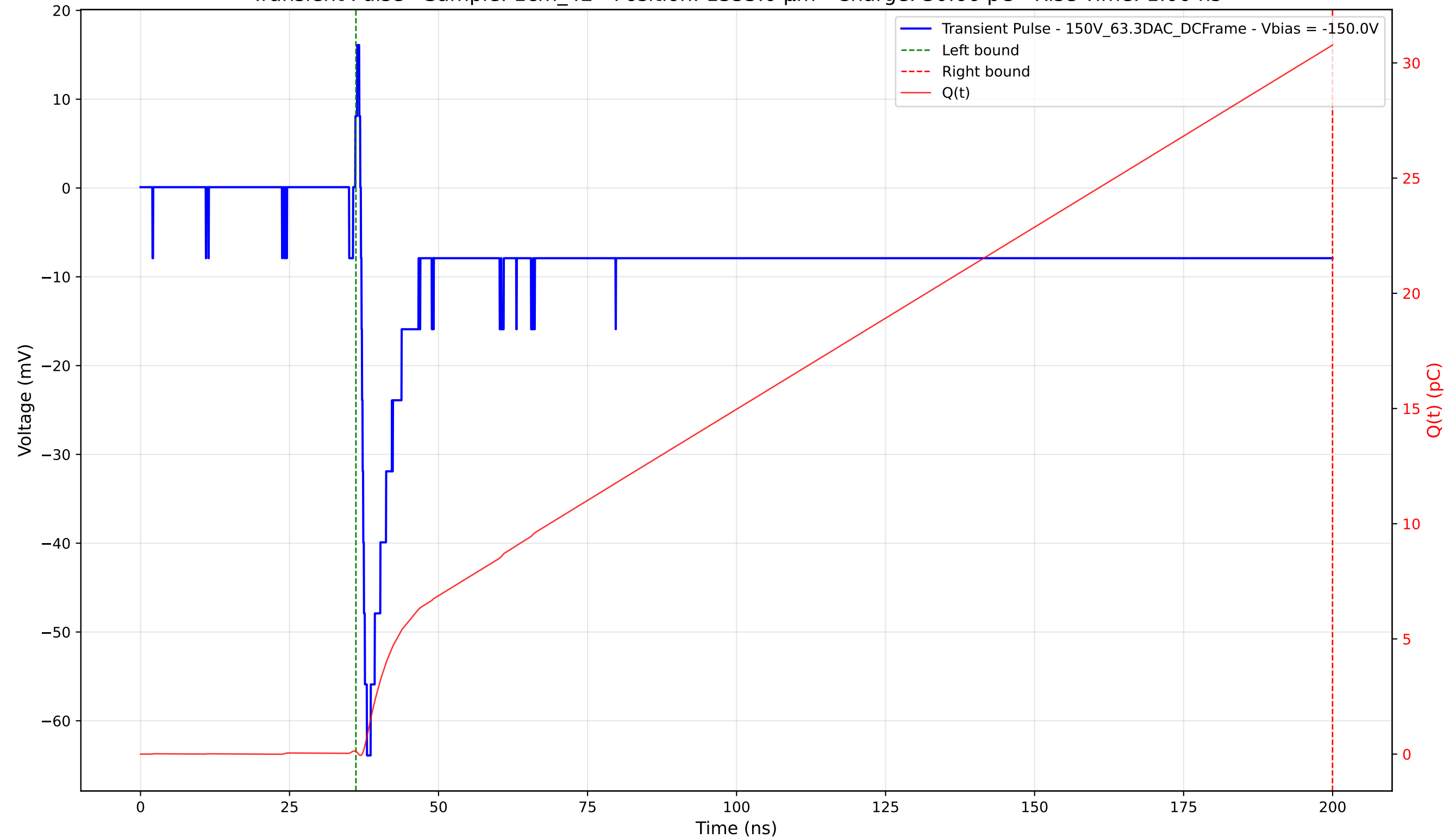
Transient Pulse - Sample: 1cm_42 - Position: 1355.0 \mu\text{m} - Charge: 30.66 pC - Rise Time: 1.00 ns
