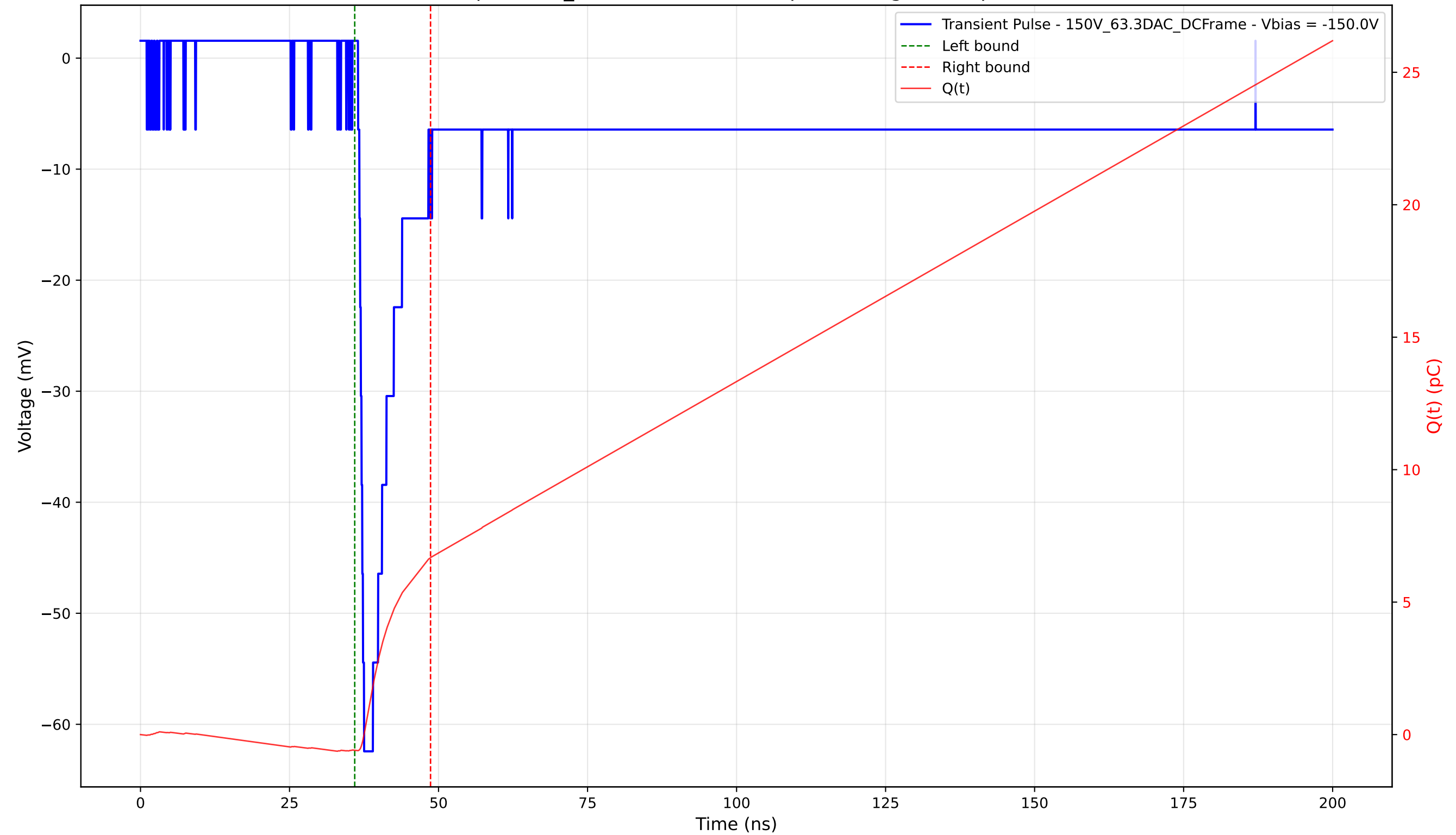
Transient Pulse - Sample: 1cm_42 - Position: 4095.0 \mu\text{m} - Charge: 7.28 pC - Rise Time: 1.00 ns
