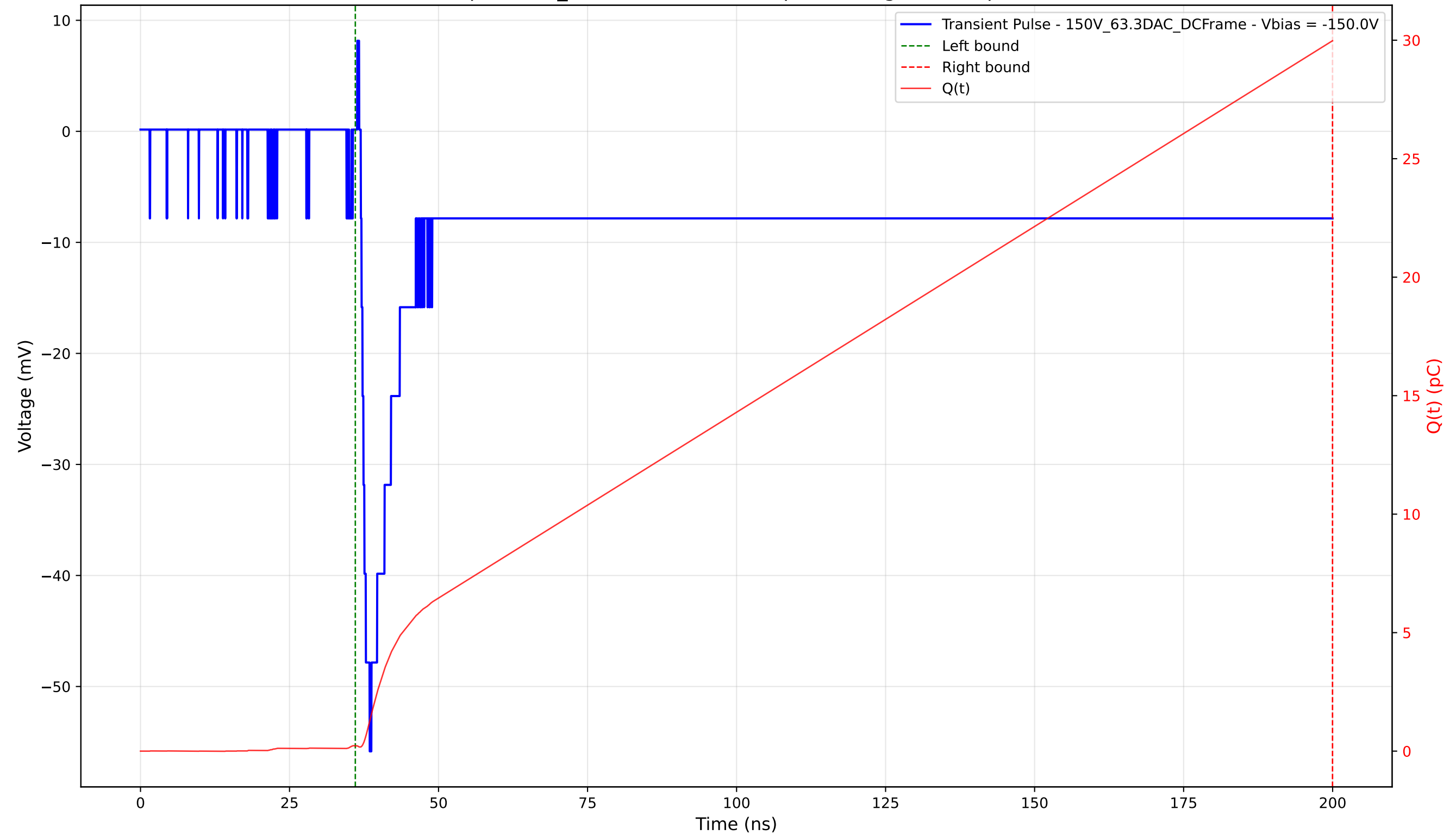
Transient Pulse - Sample: 1cm_42 - Position: 3870.0 \mu\text{m} - Charge: 29.75 pC - Rise Time: 1.49 ns
