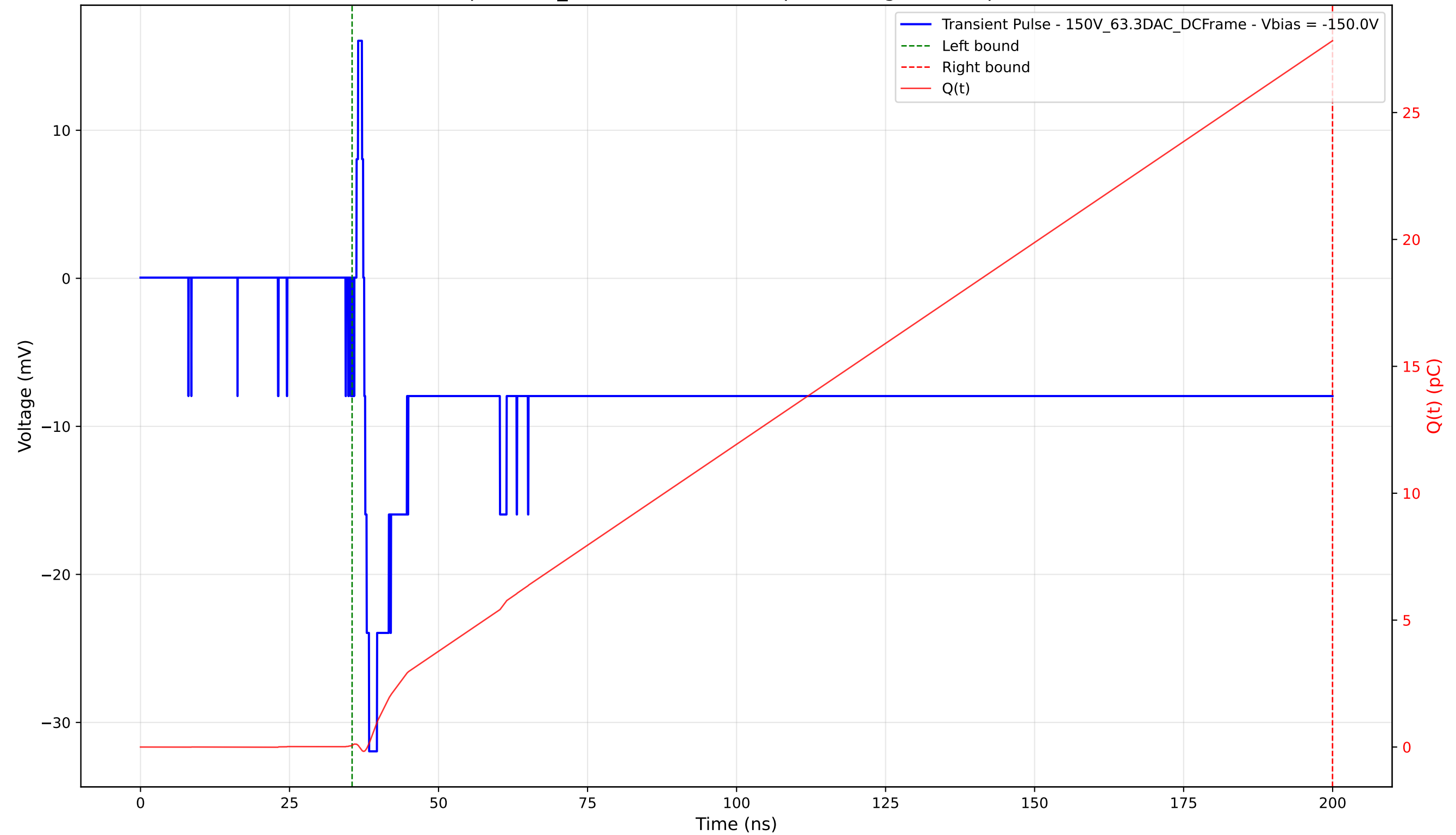
Transient Pulse - Sample: 1cm_42 - Position: 2660.0 \mu\text{m} - Charge: 27.75 pC - Rise Time: 0.81 ns
