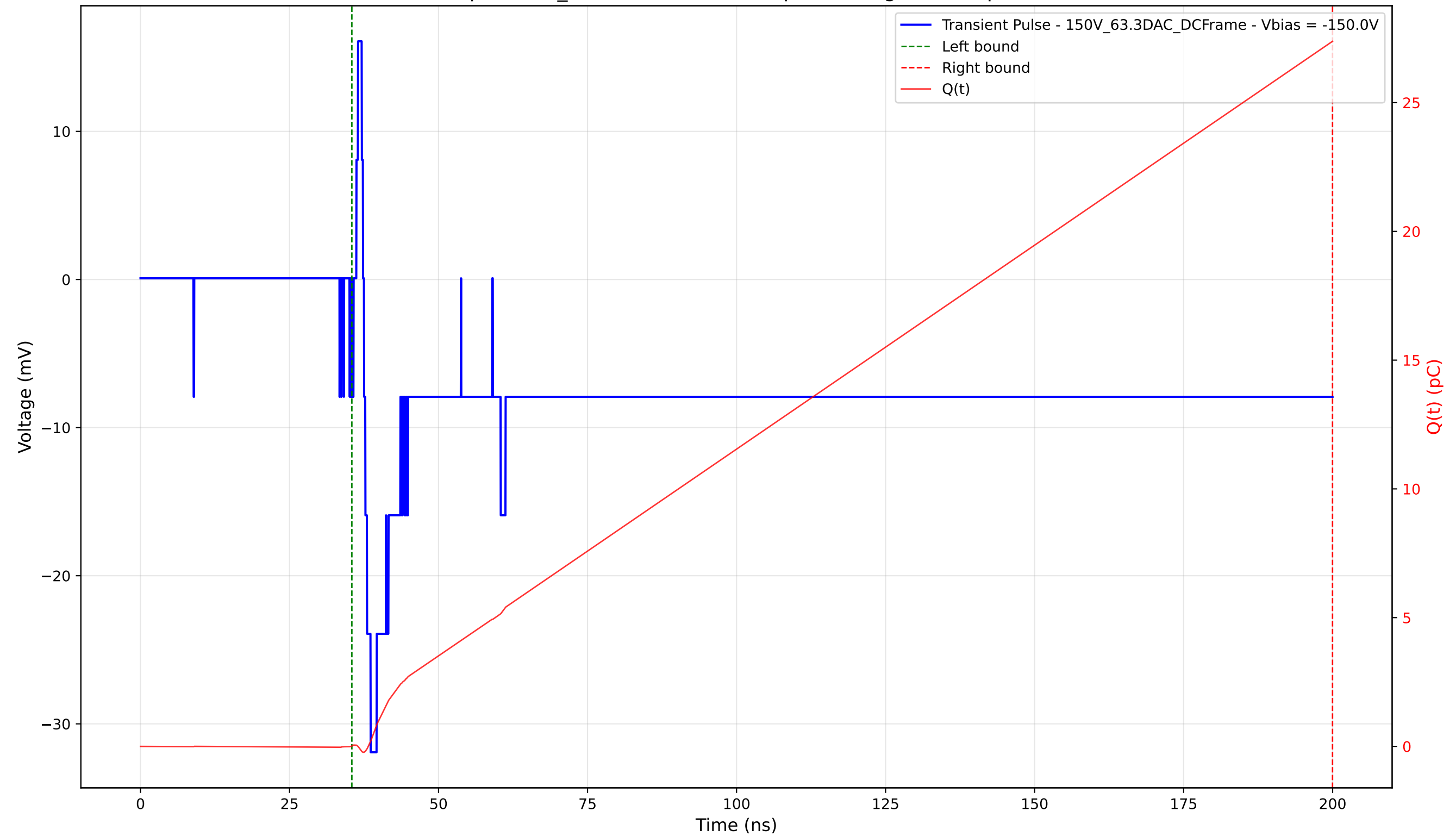
Transient Pulse - Sample: 1cm_42 - Position: 2570.0 \mu\text{m} - Charge: 27.36 pC - Rise Time: 1.11 ns
