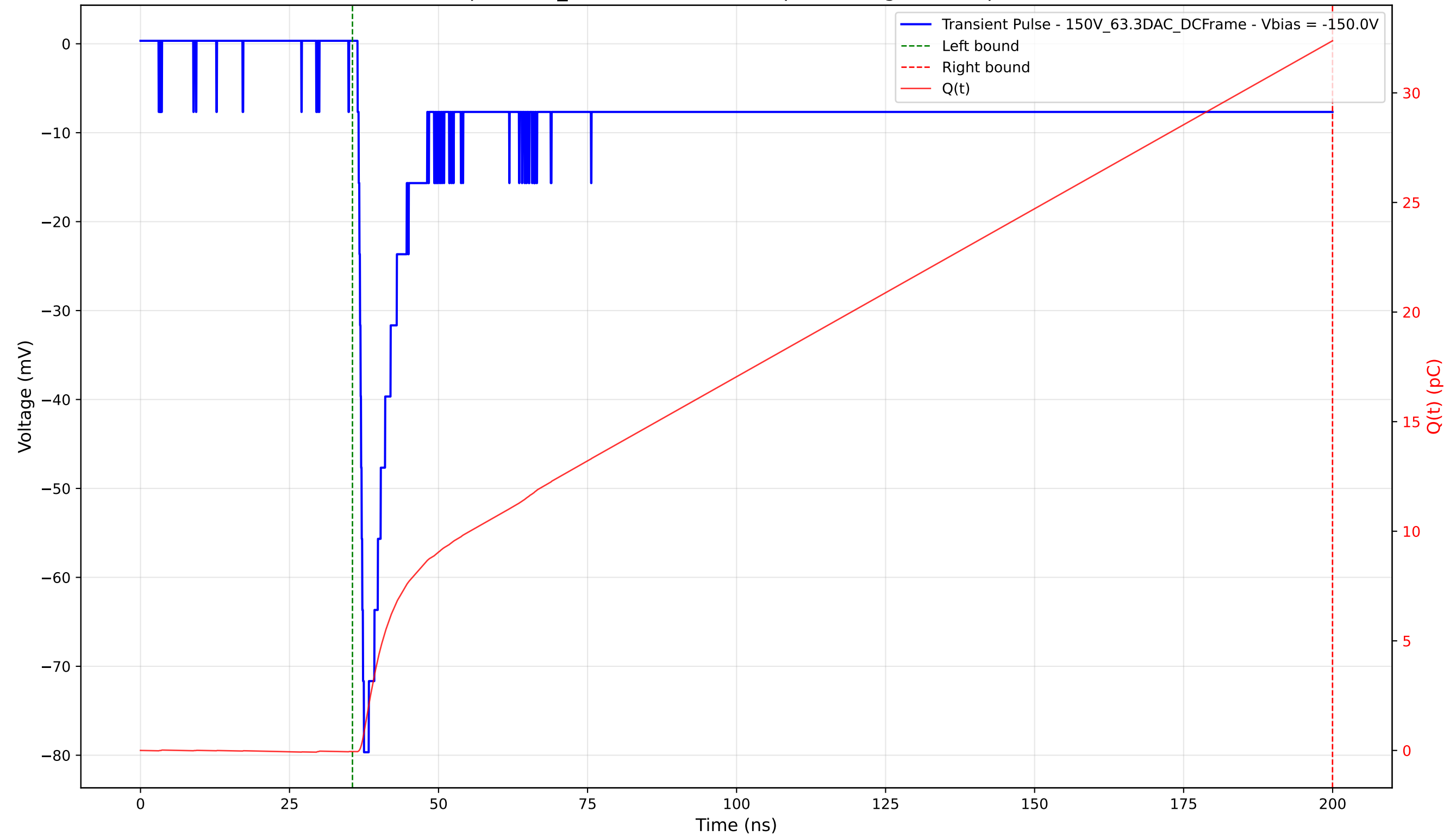
Transient Pulse - Sample: 1cm_42 - Position: 4170.0 \mu\text{m} - Charge: 32.43 pC - Rise Time: 0.90 ns
