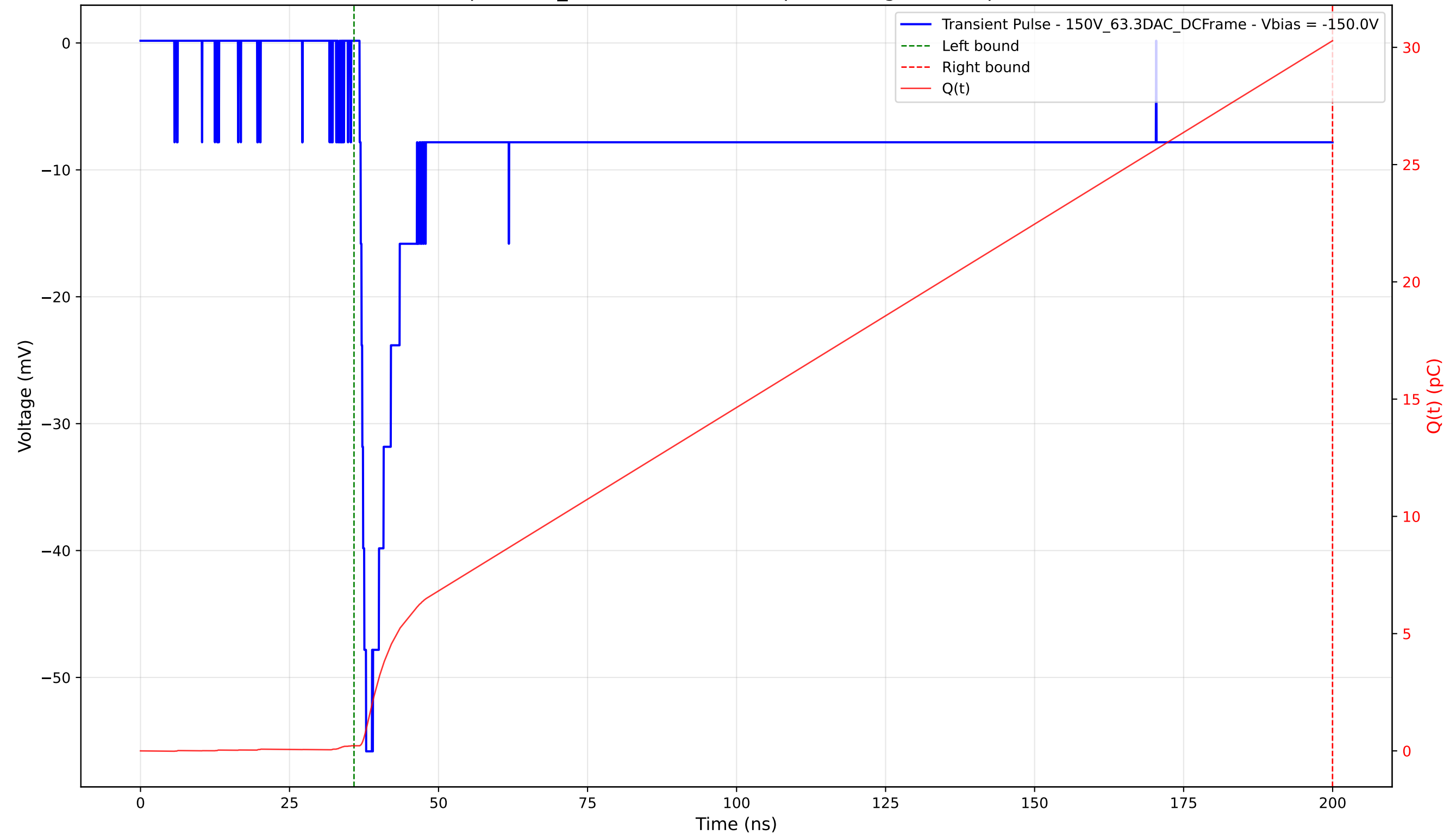
Transient Pulse - Sample: 1cm_42 - Position: 3985.0 \mu\text{m} - Charge: 30.06 pC - Rise Time: 1.09 ns
