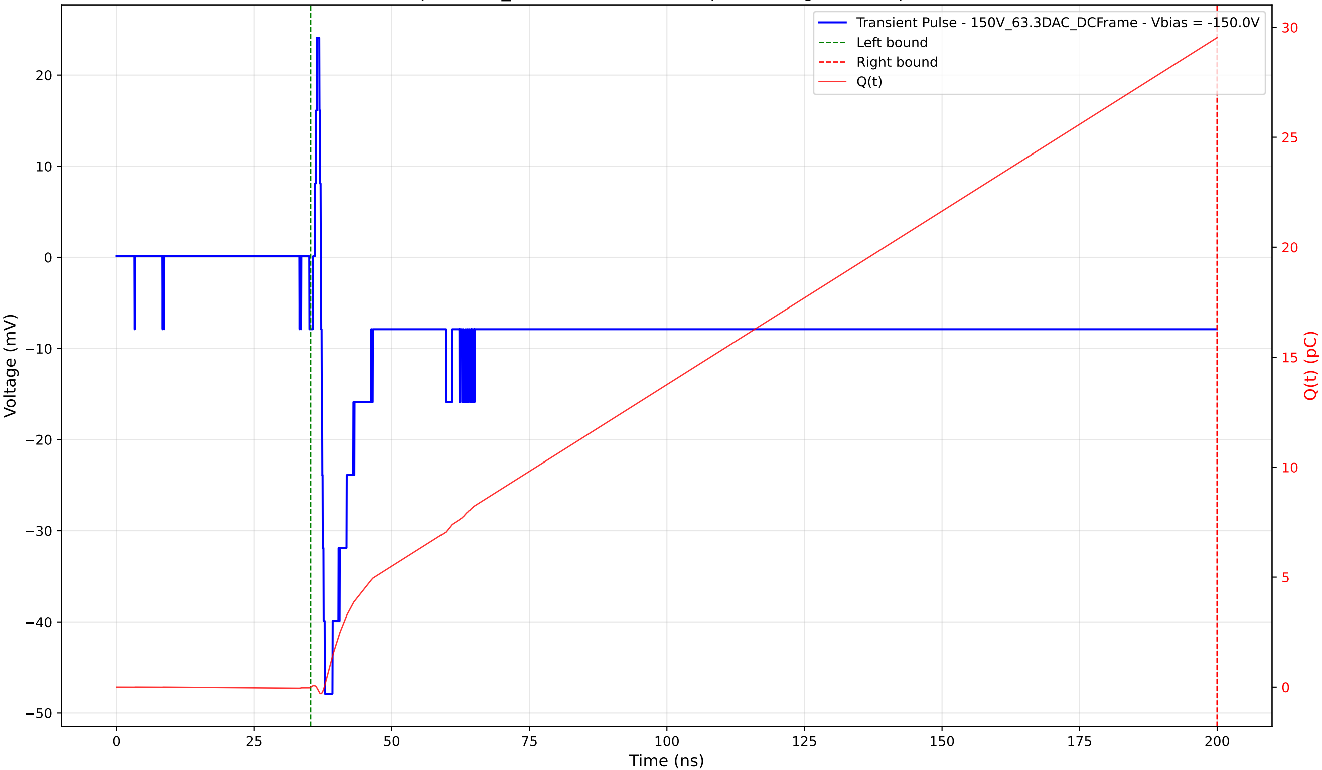
Transient Pulse - Sample: 1cm_42 - Position: 1595.0 \mu\text{m} - Charge: 29.53 pC - Rise Time: 0.67 ns
