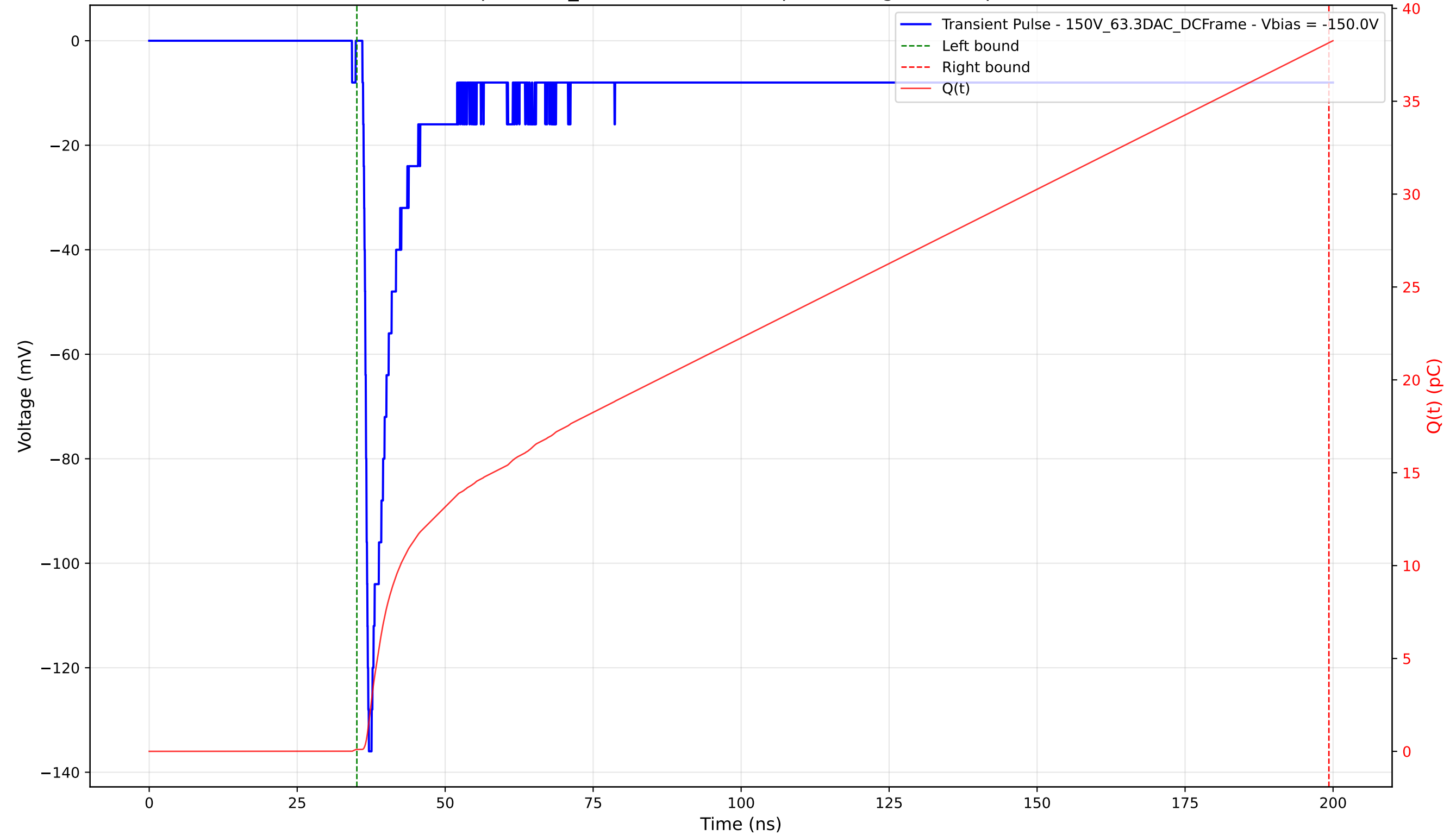
Transient Pulse - Sample: 1cm_42 - Position: 635.0 \mu\text{m} - Charge: 38.05 pC - Rise Time: 0.87 ns
