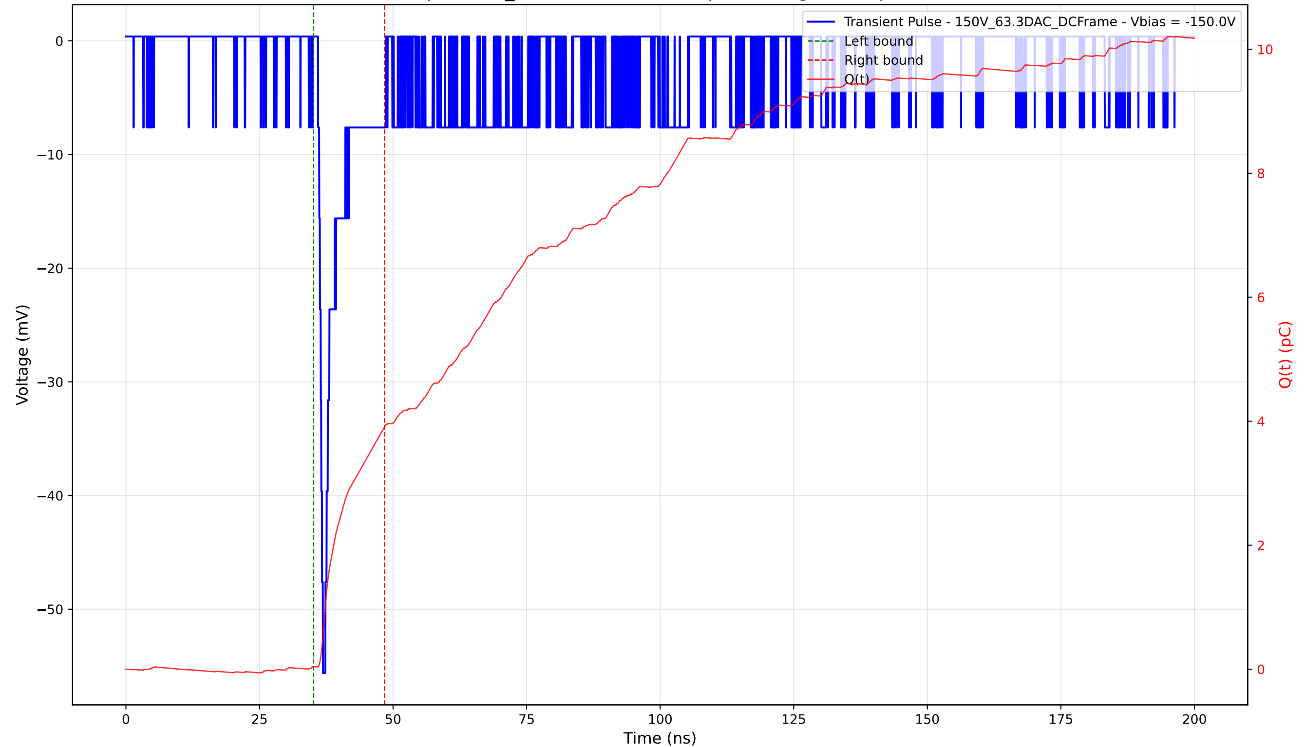
Transient Pulse - Sample: 1cm_42 - Position: 5115.0 \mu\text{m} - Charge: 3.87 pC - Rise Time: 0.91 ns
