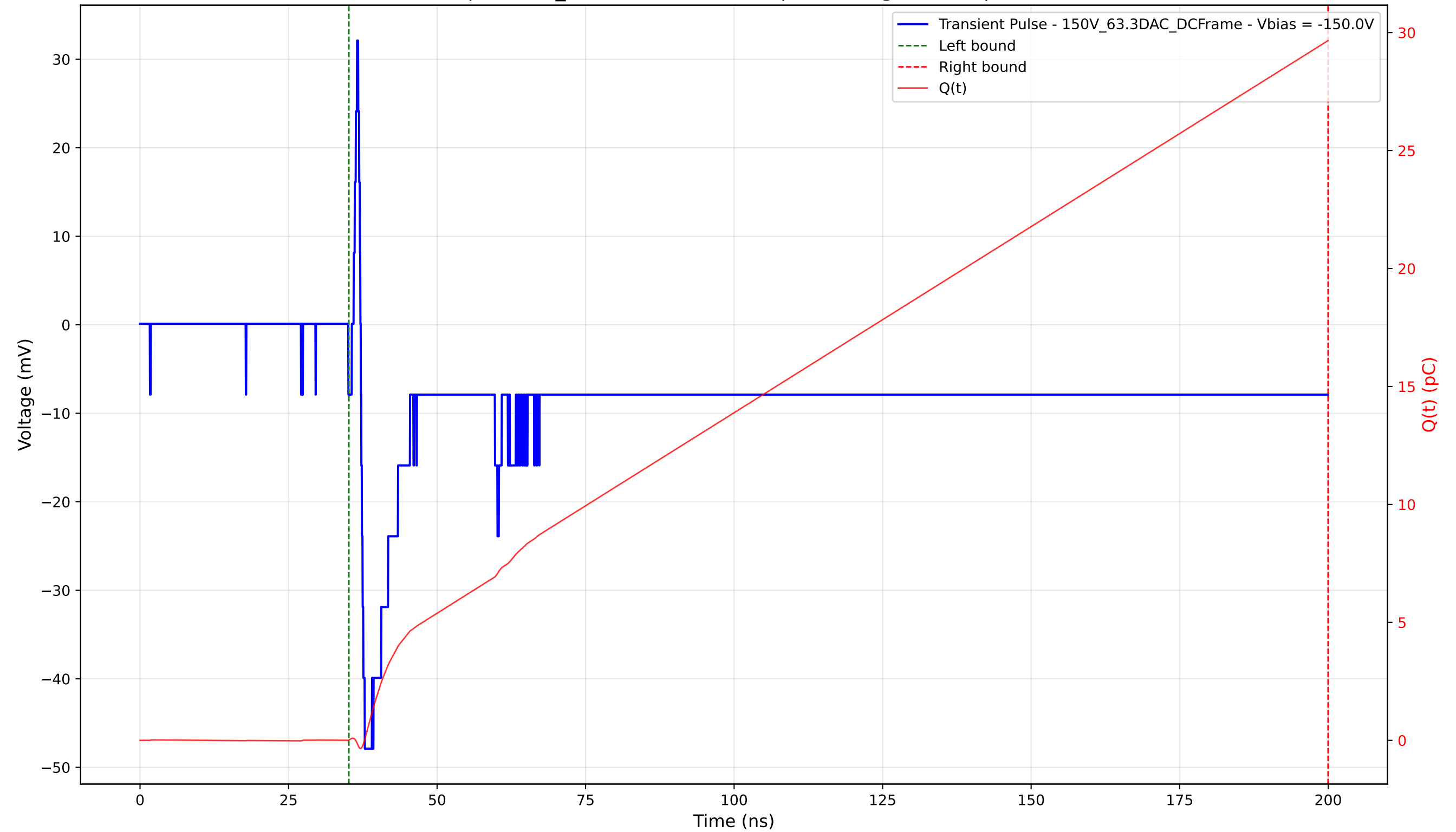
Transient Pulse - Sample: 1cm_42 - Position: 1720.0 \mu\text{m} - Charge: 29.64 pC - Rise Time: 0.67 ns
