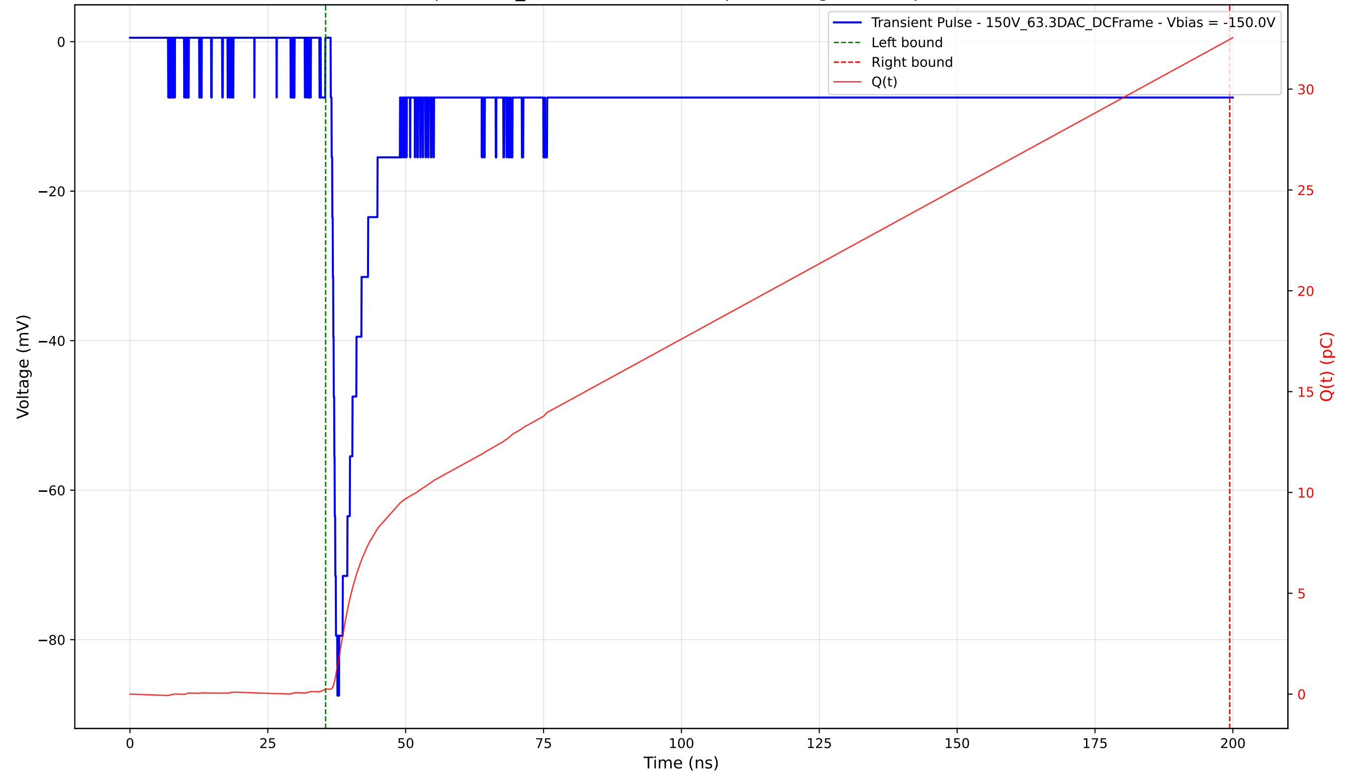
Transient Pulse - Sample: 1cm_42 - Position: 4200.0 \mu\text{m} - Charge: 32.22 pC - Rise Time: 0.80 ns
