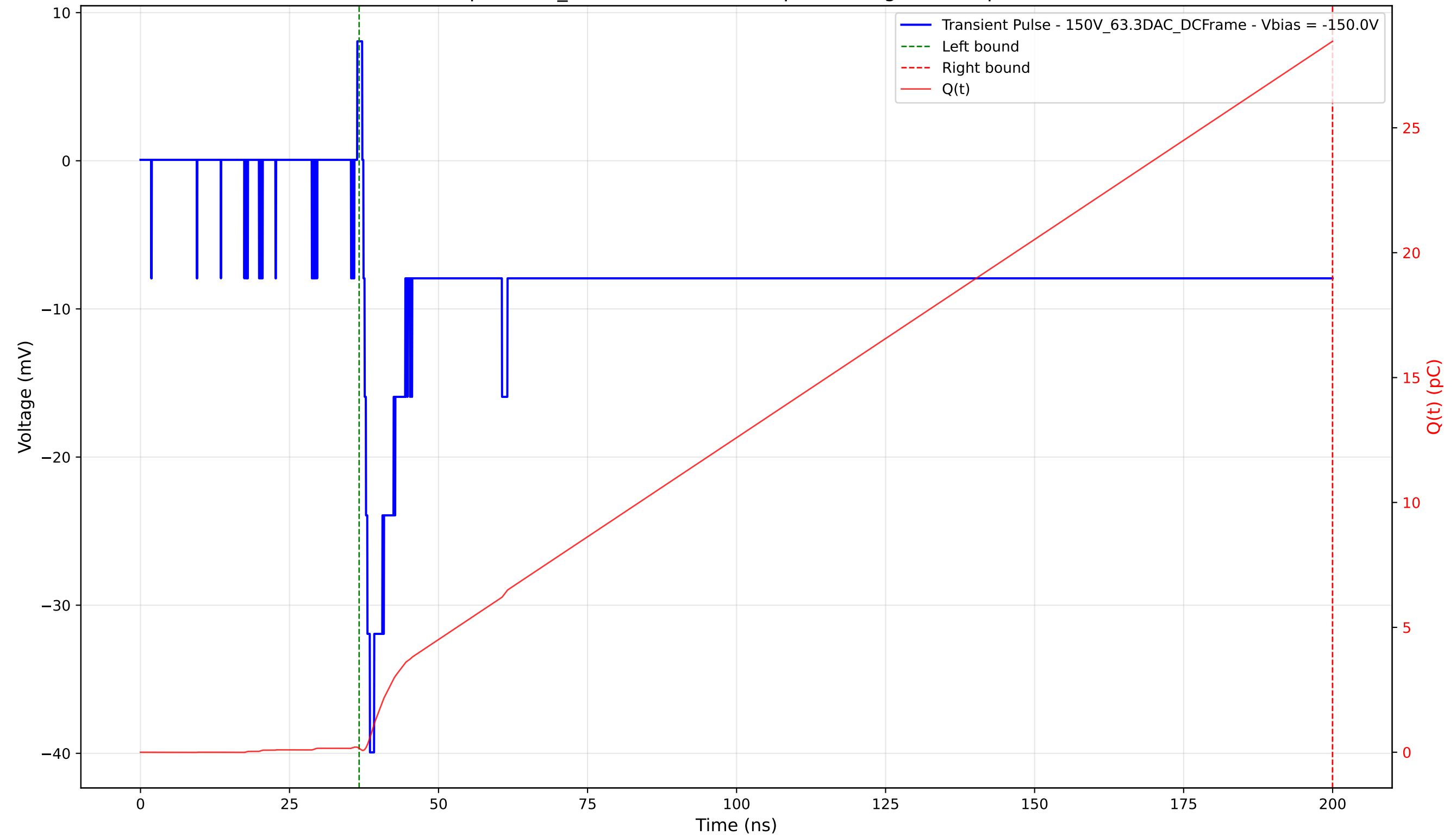
Transient Pulse - Sample: 1cm_42 - Position: 3350.0 \mu\text{m} - Charge: 28.31 pC - Rise Time: 1.09 ns
