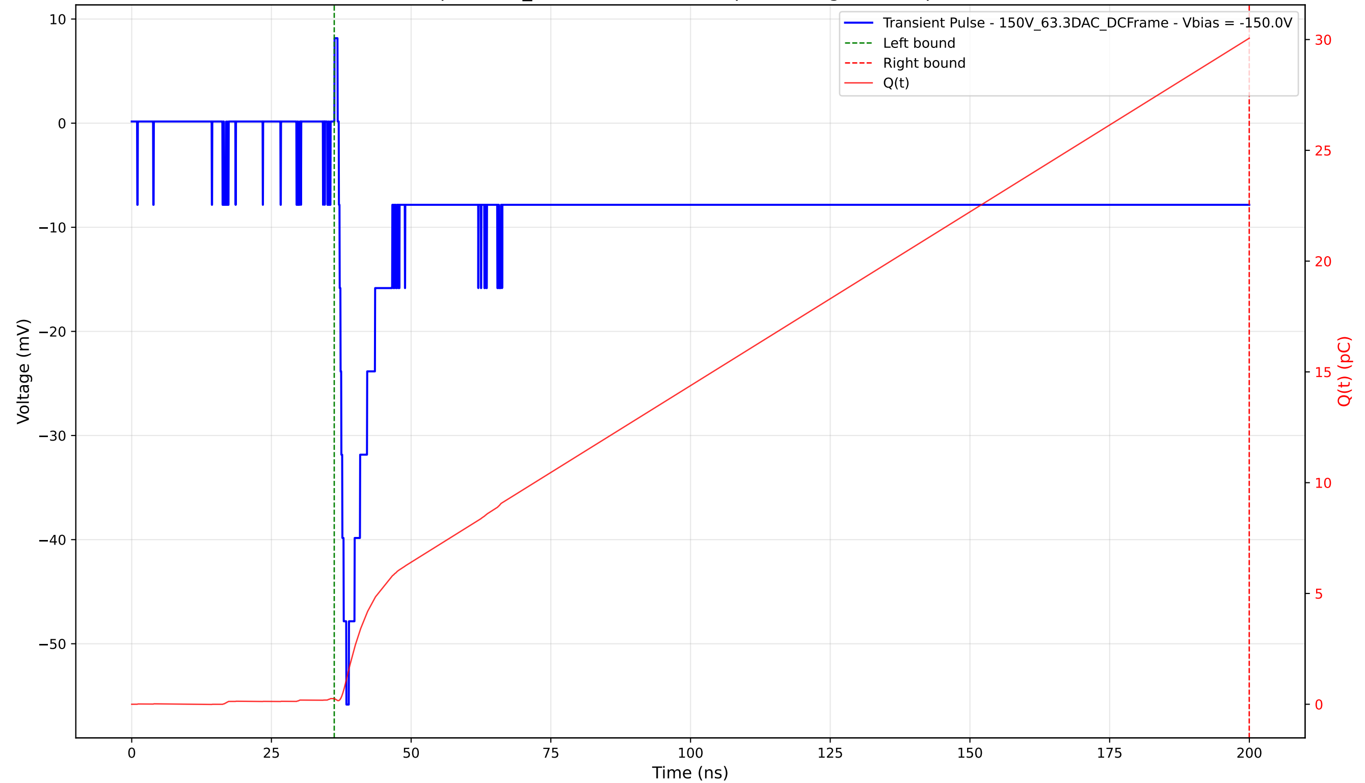
Transient Pulse - Sample: 1cm_42 - Position: 3715.0 \mu\text{m} - Charge: 29.81 pC - Rise Time: 1.35 ns
