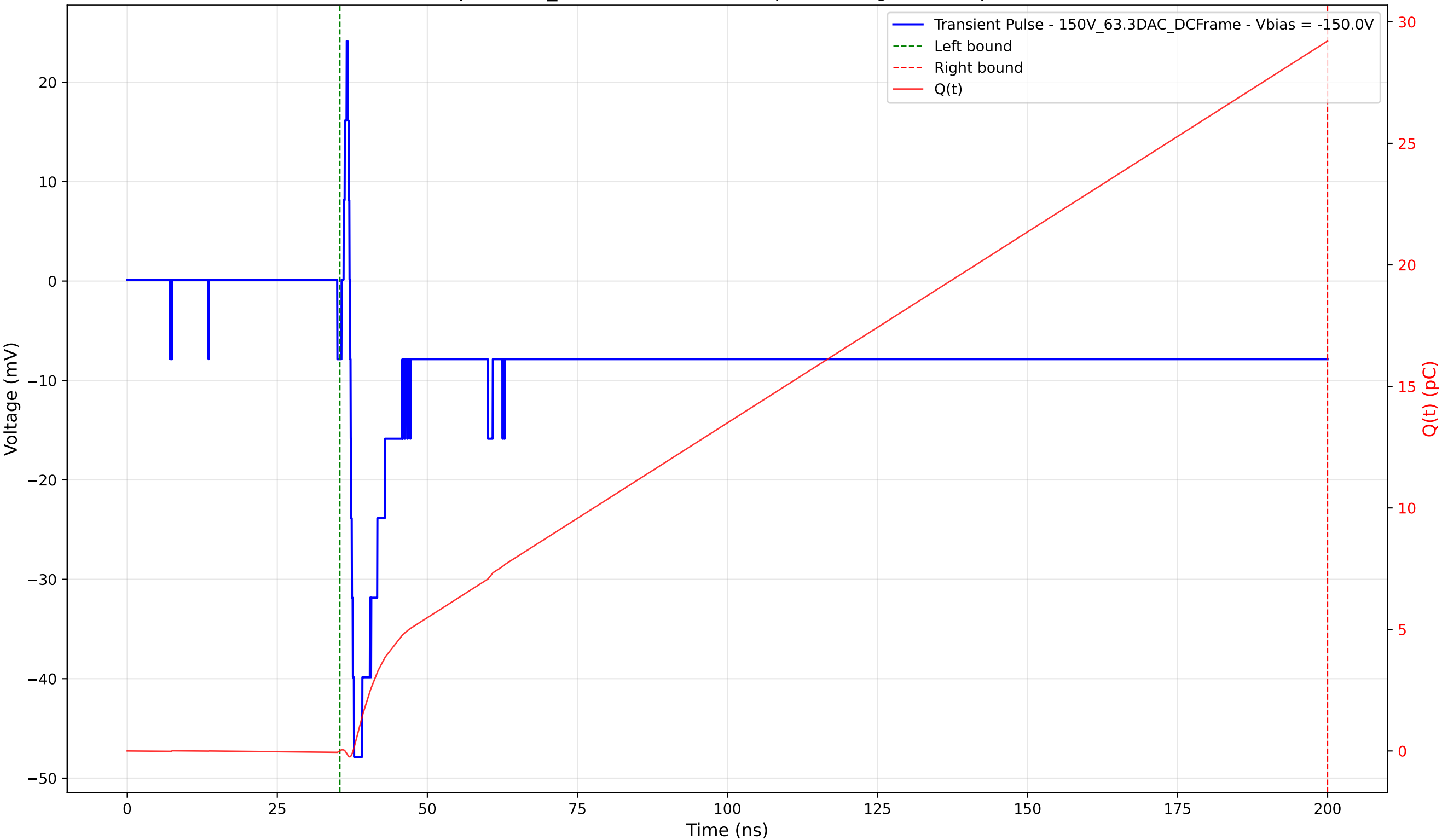
Transient Pulse - Sample: 1cm_42 - Position: 1535.0 \mu\text{m} - Charge: 29.20 pC - Rise Time: 0.65 ns
