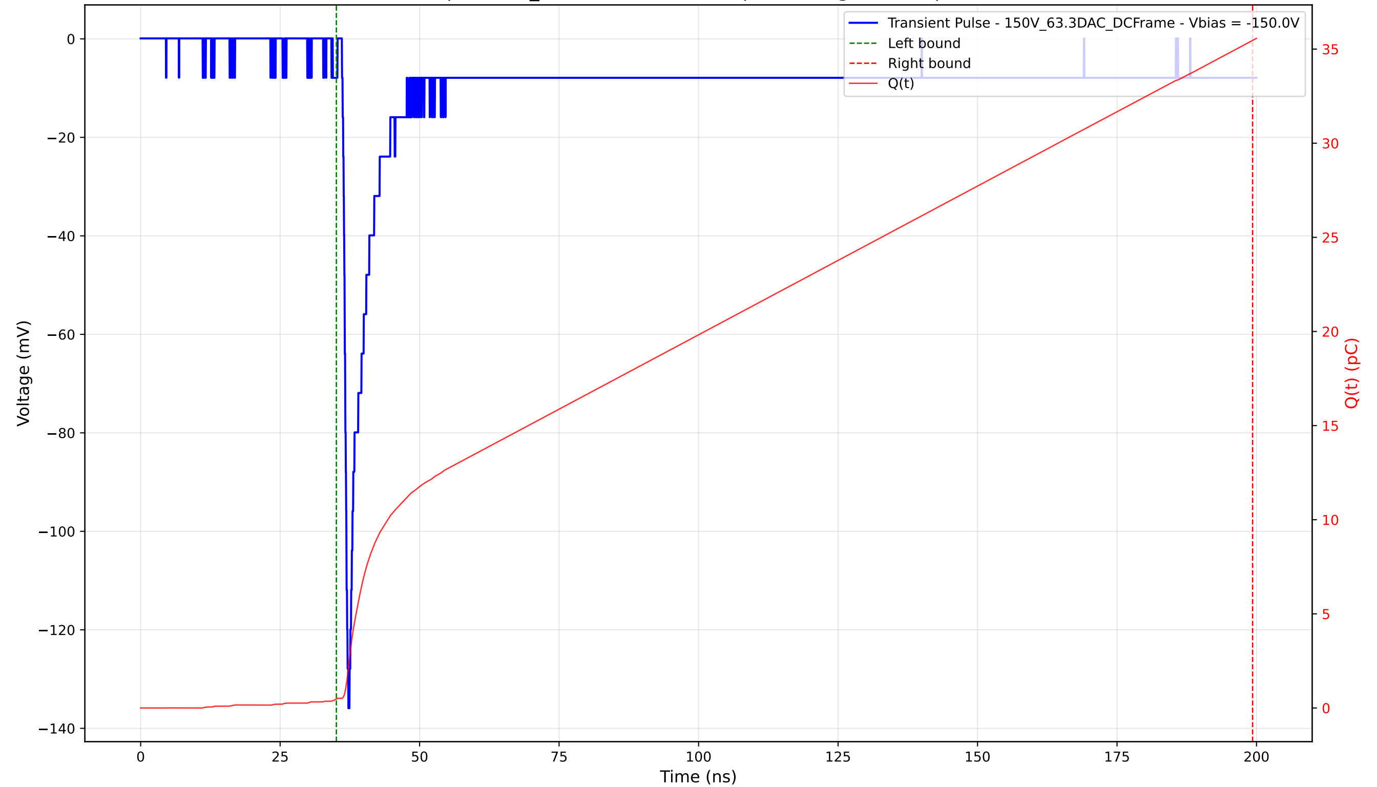
Transient Pulse - Sample: 1cm_42 - Position: 4550.0 \mu\text{m} - Charge: 34.98 pC - Rise Time: 0.89 ns
