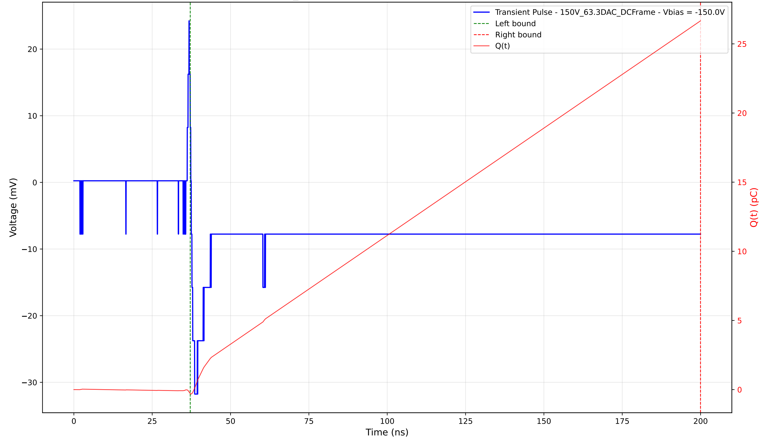
Transient Pulse - Sample: 1cm_42 - Position: 2505.0 \mu\text{m} - Charge: 26.96 pC - Rise Time: 1.09 ns
