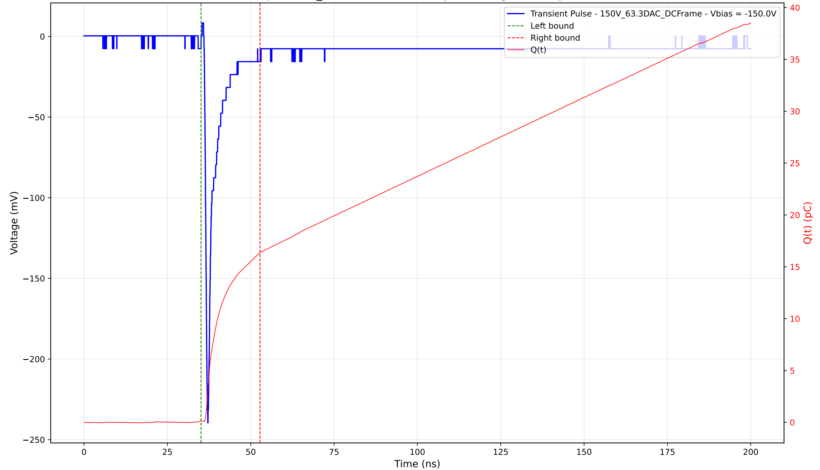
Transient Pulse - Sample: 1cm_42 - Position: 4840.0 \mu\text{m} - Charge: 16.22 pC - Rise Time: 0.80 ns
