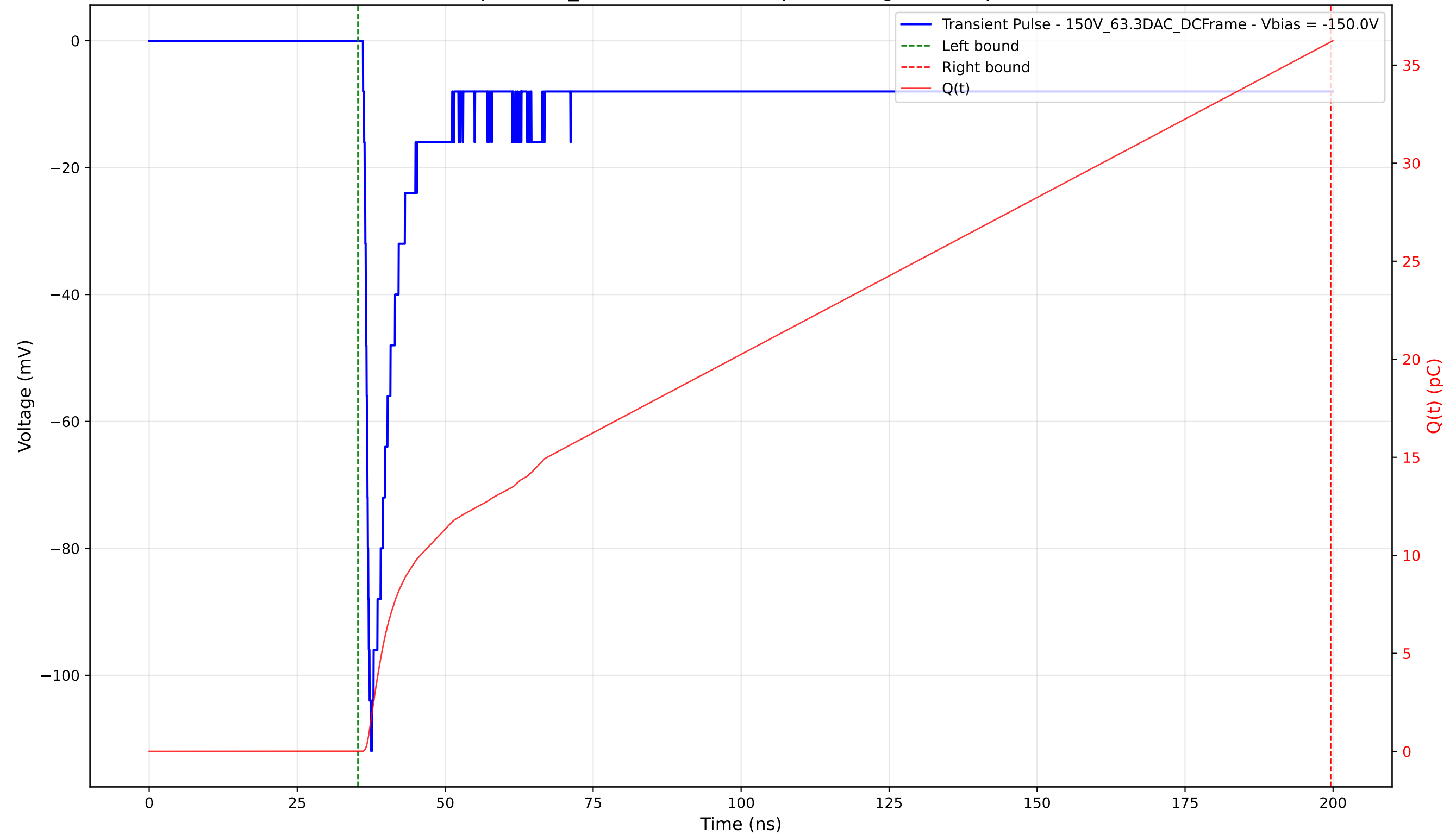
Transient Pulse - Sample: 1cm_42 - Position: 830.0 \mu\text{m} - Charge: 36.18 pC - Rise Time: 0.93 ns
