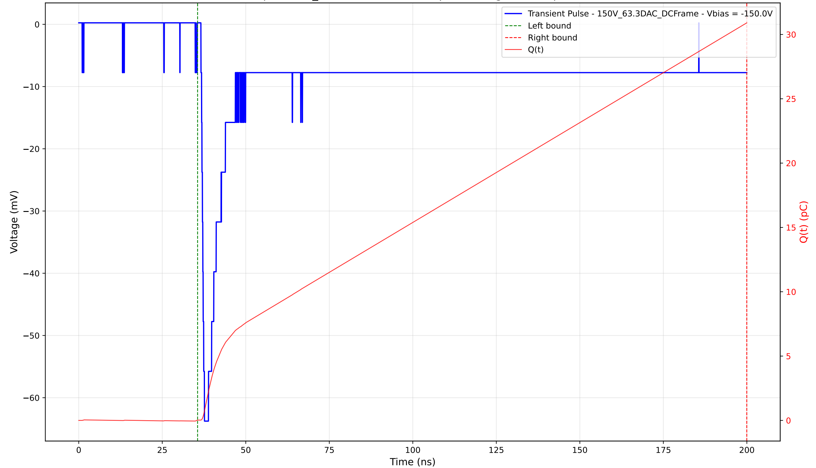
Transient Pulse - Sample: 1cm_42 - Position: 4080.0 \mu\text{m} - Charge: 30.88 pC - Rise Time: 1.04 ns
