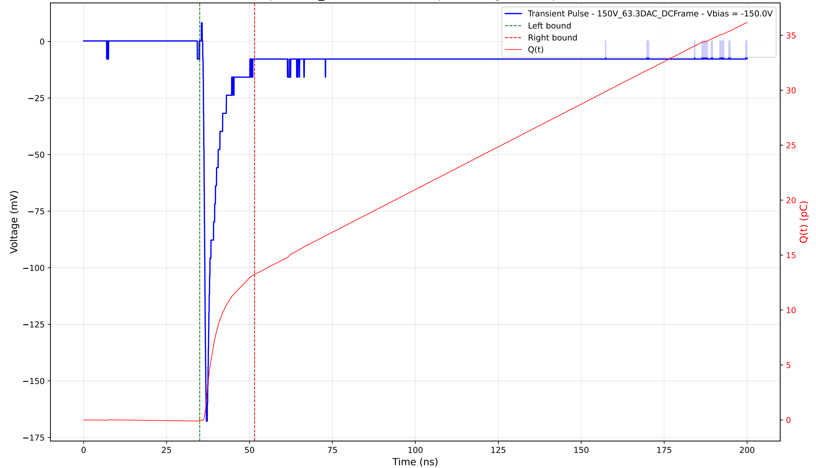
Transient Pulse - Sample: 1cm_42 - Position: 475.0 \mu\text{m} - Charge: 13.26 pC - Rise Time: 0.74 ns
