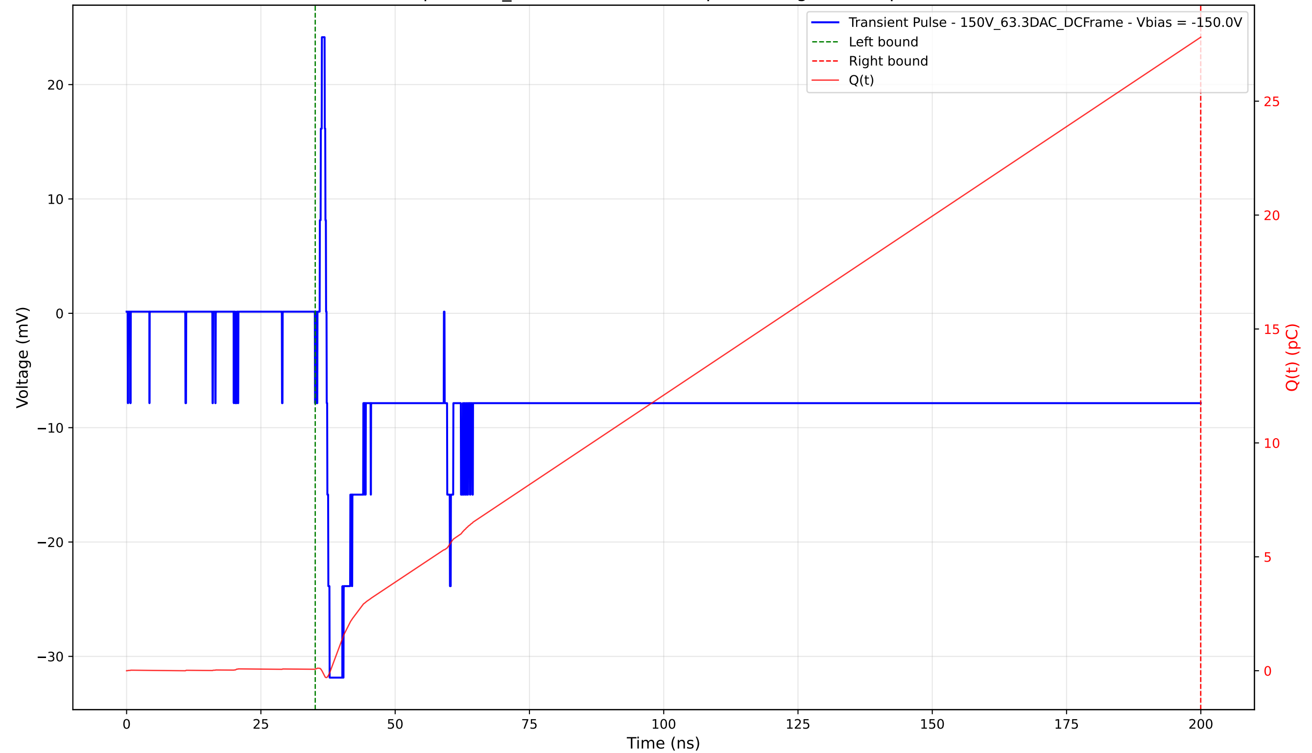
Transient Pulse - Sample: 1cm_42 - Position: 2075.0 \mu\text{m} - Charge: 27.74 pC - Rise Time: 0.55 ns
