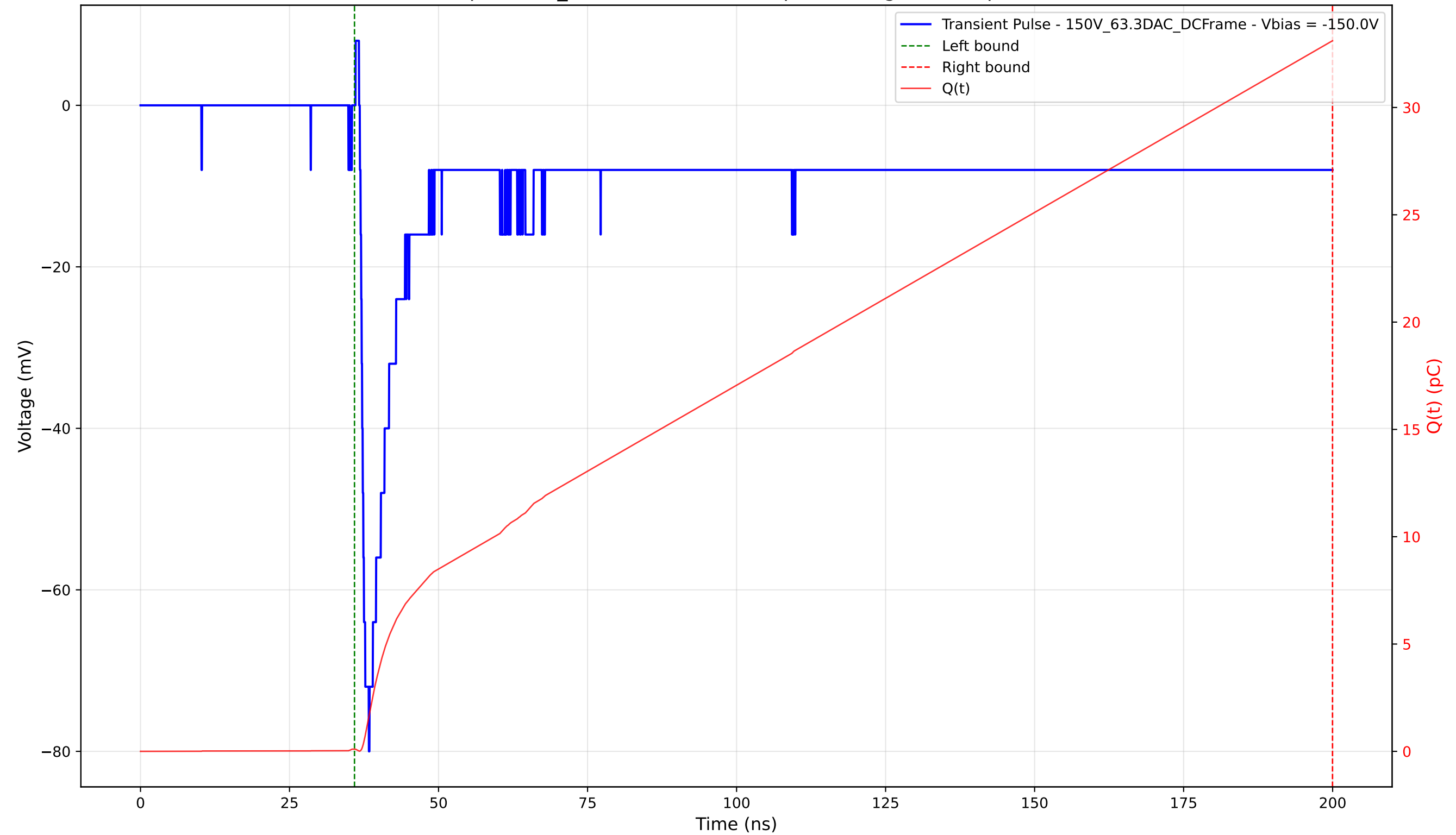
Transient Pulse - Sample: 1cm_42 - Position: 1145.0 \mu\text{m} - Charge: 33.01 pC - Rise Time: 0.80 ns
