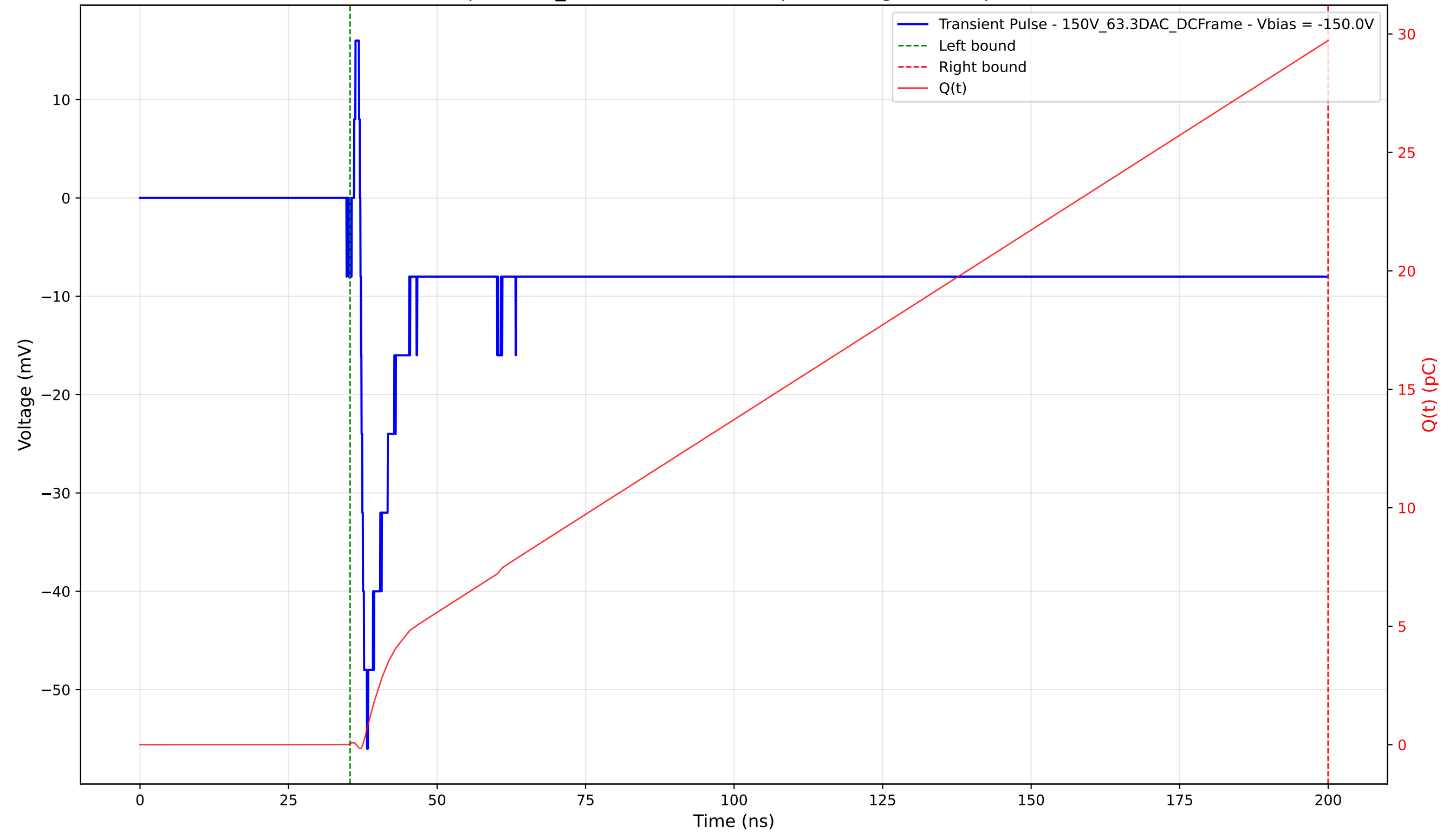
Transient Pulse - Sample: 1cm_42 - Position: 1490.0 \mu\text{m} - Charge: 29.67 pC - Rise Time: 1.11 ns
