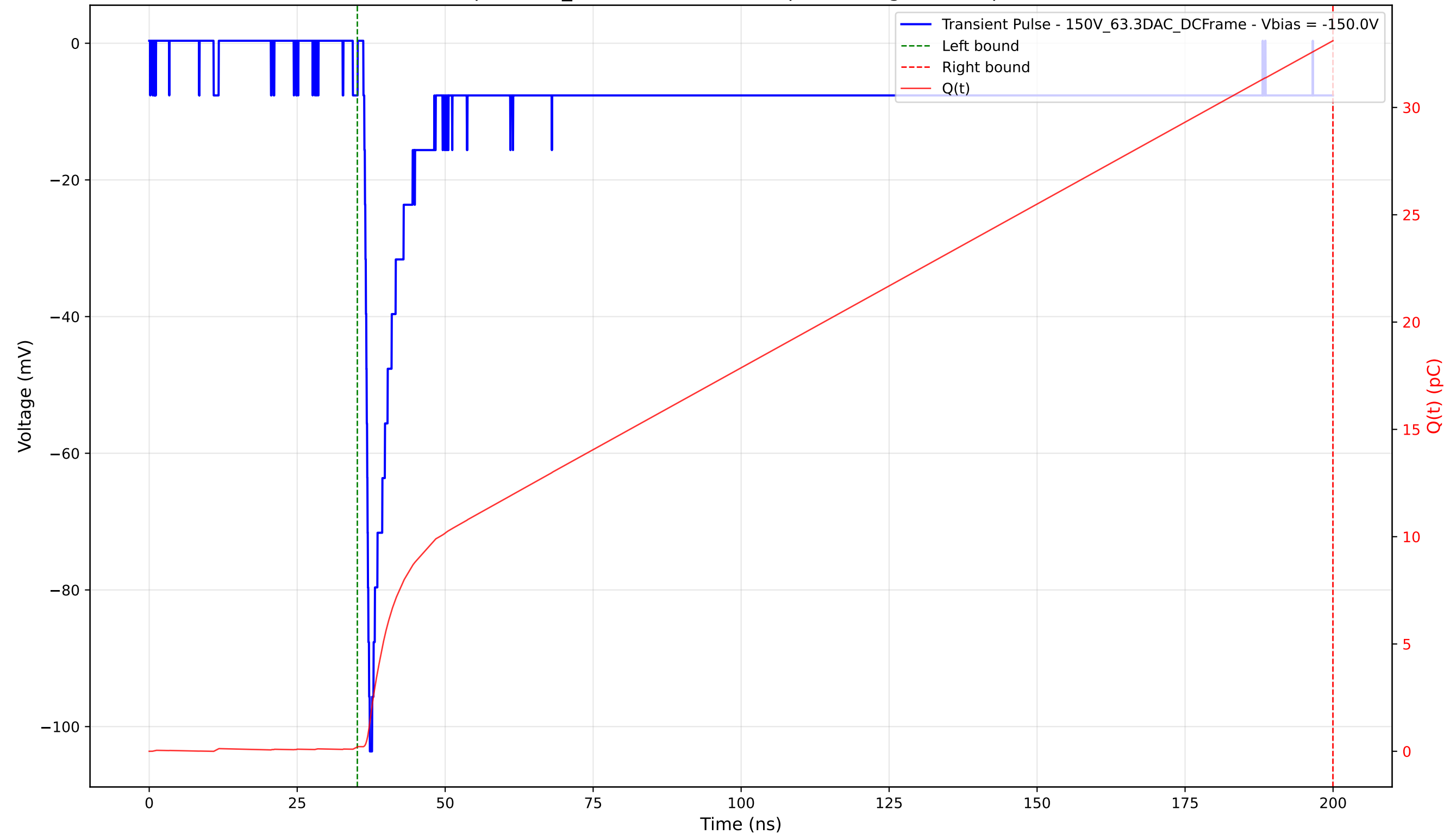
Transient Pulse - Sample: 1cm_42 - Position: 4450.0 \mu\text{m} - Charge: 32.90 pC - Rise Time: 0.81 ns
