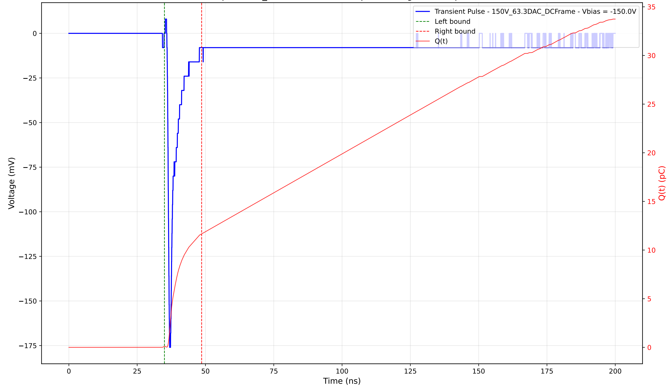
Transient Pulse - Sample: 1cm_42 - Position: 360.0 \mu\text{m} - Charge: 11.57 pC - Rise Time: 0.72 ns
