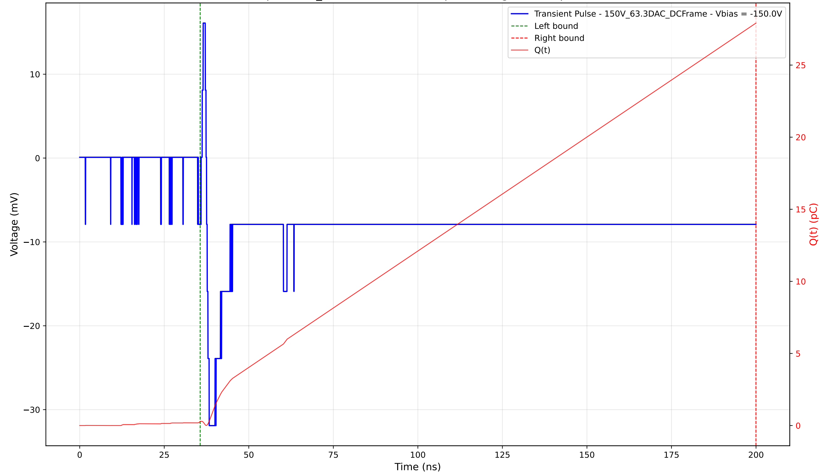
Transient Pulse - Sample: 1cm_42 - Position: 2675.0 \mu\text{m} - Charge: 27.64 pC - Rise Time: 0.77 ns
