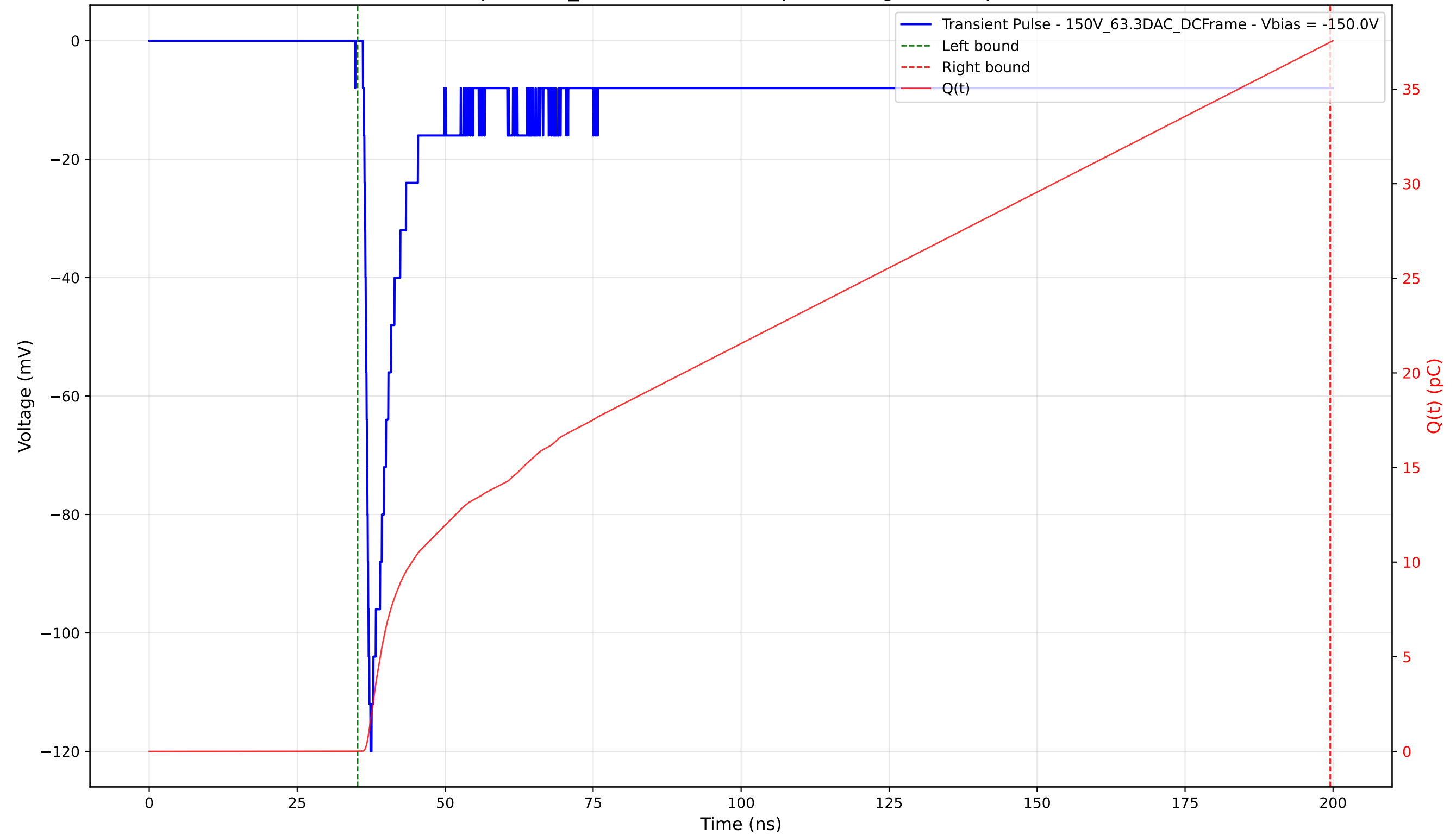
Transient Pulse - Sample: 1cm_42 - Position: 805.0 \mu\text{m} - Charge: 37.47 pC - Rise Time: 0.93 ns
