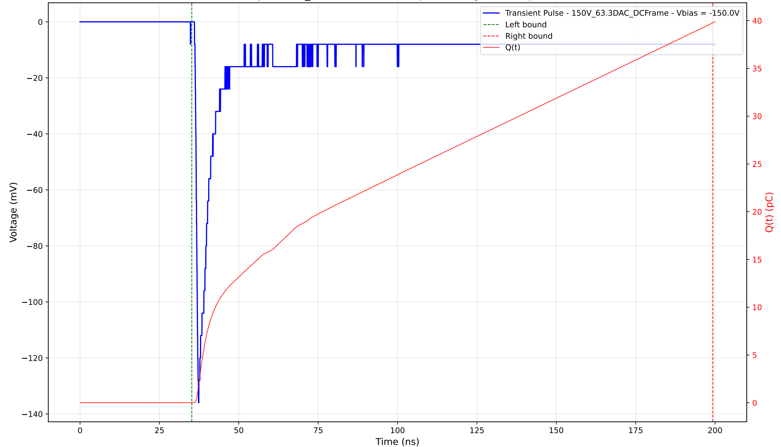
Transient Pulse - Sample: 1cm_42 - Position: 730.0 \mu\text{m} - Charge: 39.75 pC - Rise Time: 0.95 ns
