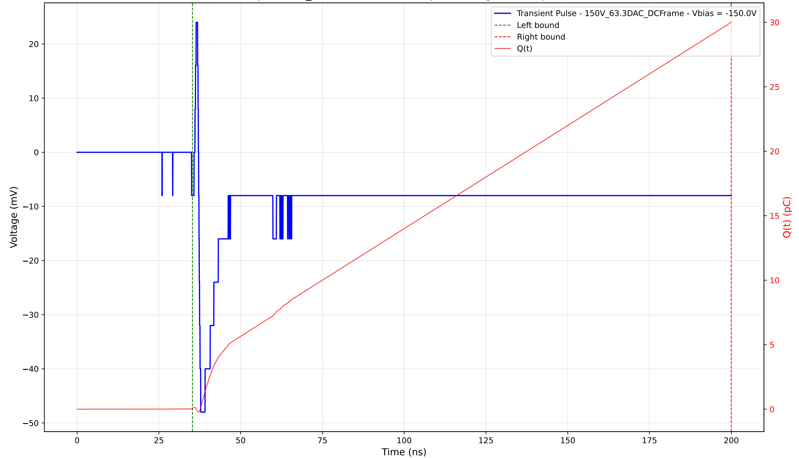
Transient Pulse - Sample: 1cm_42 - Position: 1620.0 \mu\text{m} - Charge: 29.94 pC - Rise Time: 0.63 ns
