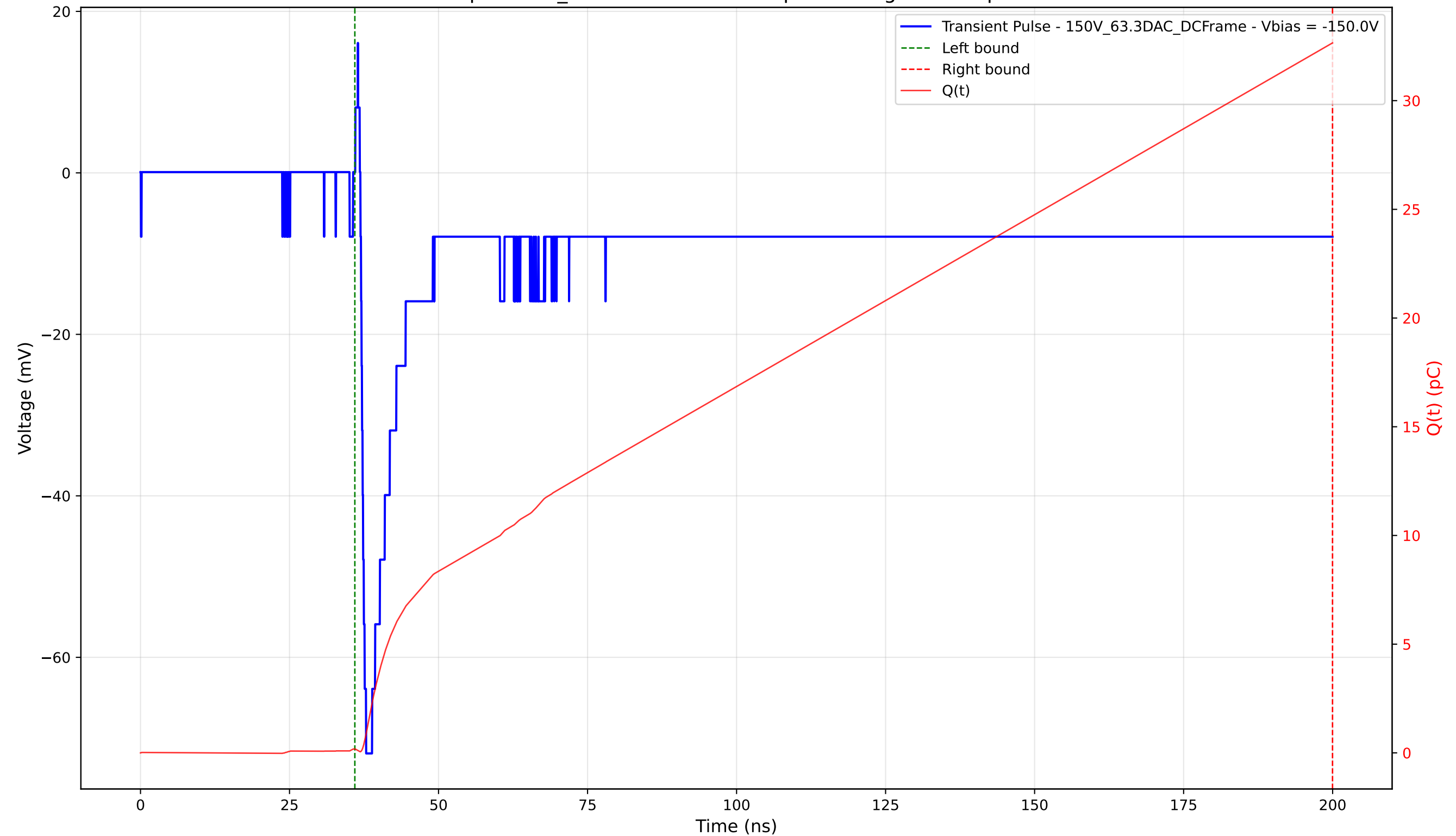
Transient Pulse - Sample: 1cm_42 - Position: 1260.0 \mu\text{m} - Charge: 32.48 pC - Rise Time: 0.94 ns
