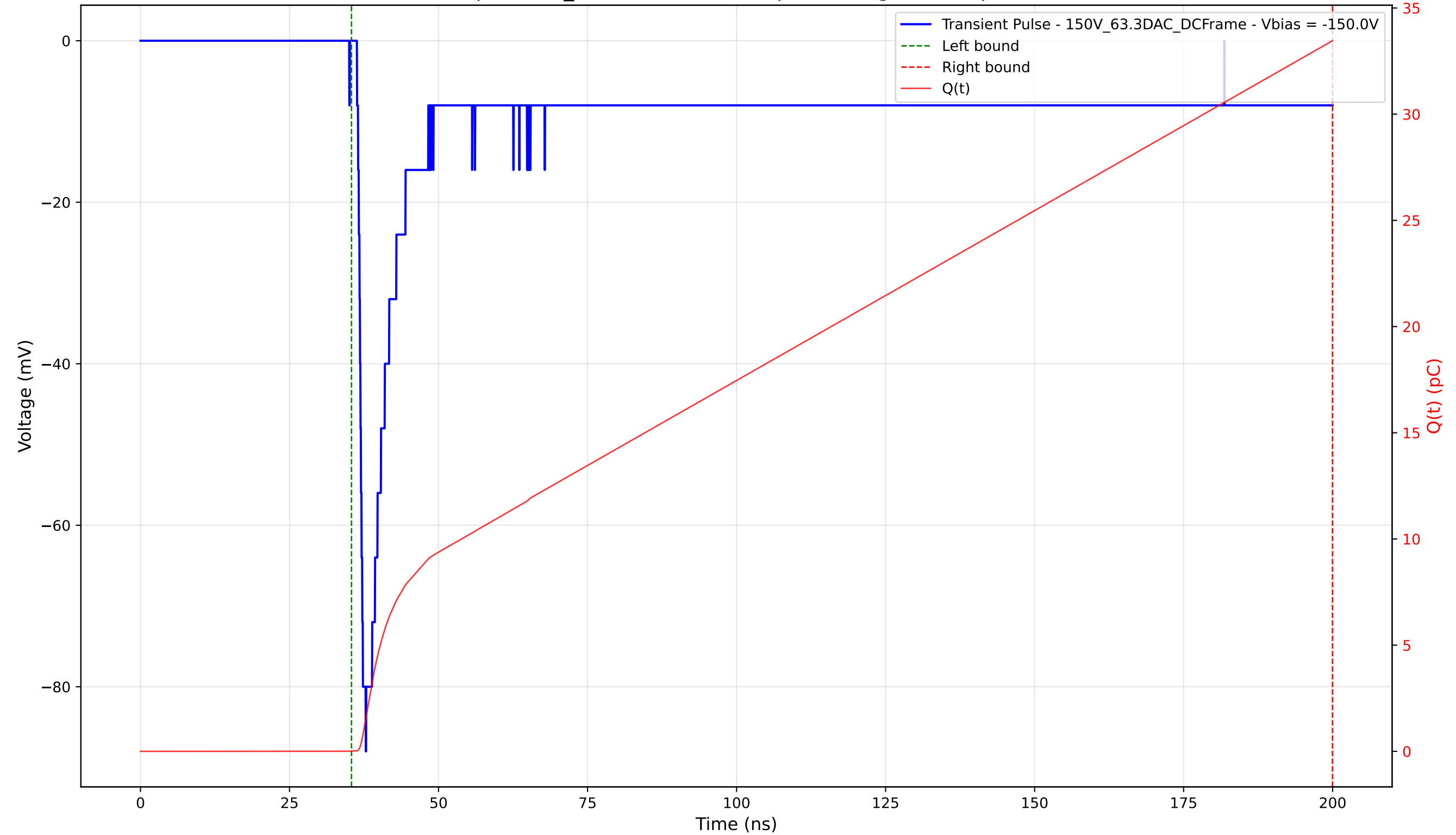
Transient Pulse - Sample: 1cm_42 - Position: 930.0 \mu\text{m} - Charge: 33.44 pC - Rise Time: 0.82 ns
