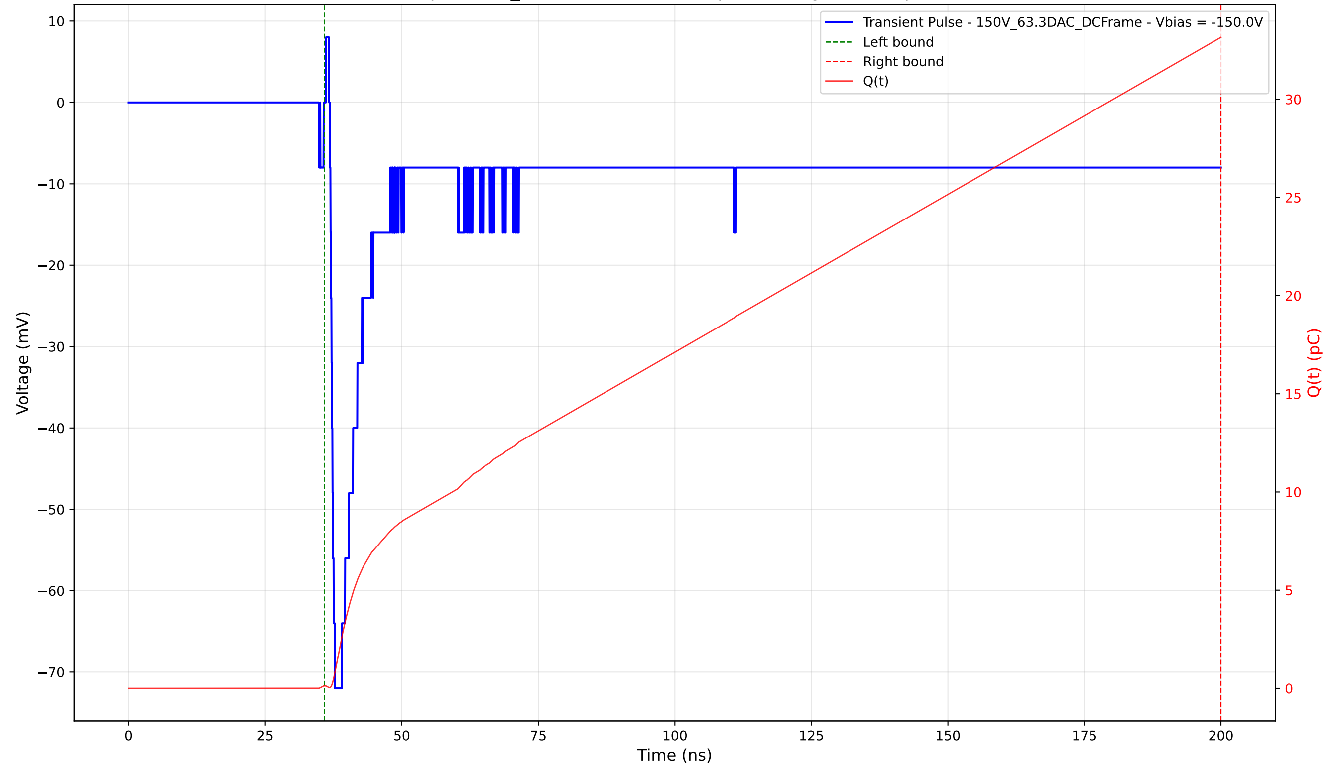
Transient Pulse - Sample: 1cm_42 - Position: 1170.0 \mu\text{m} - Charge: 33.03 pC - Rise Time: 0.90 ns
