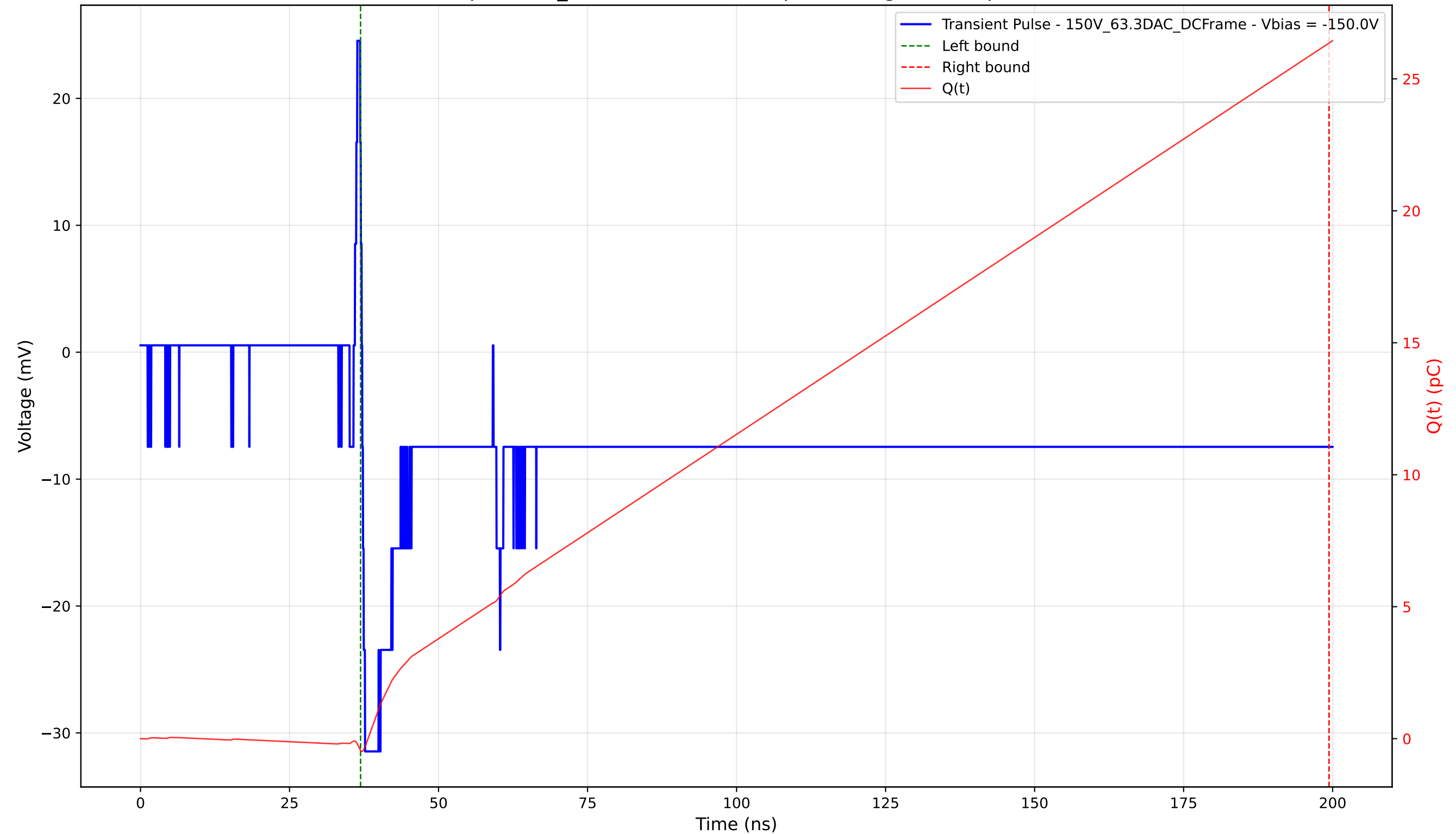
Transient Pulse - Sample: 1cm_42 - Position: 1995.0 \mu\text{m} - Charge: 26.81 pC - Rise Time: 0.47 ns
