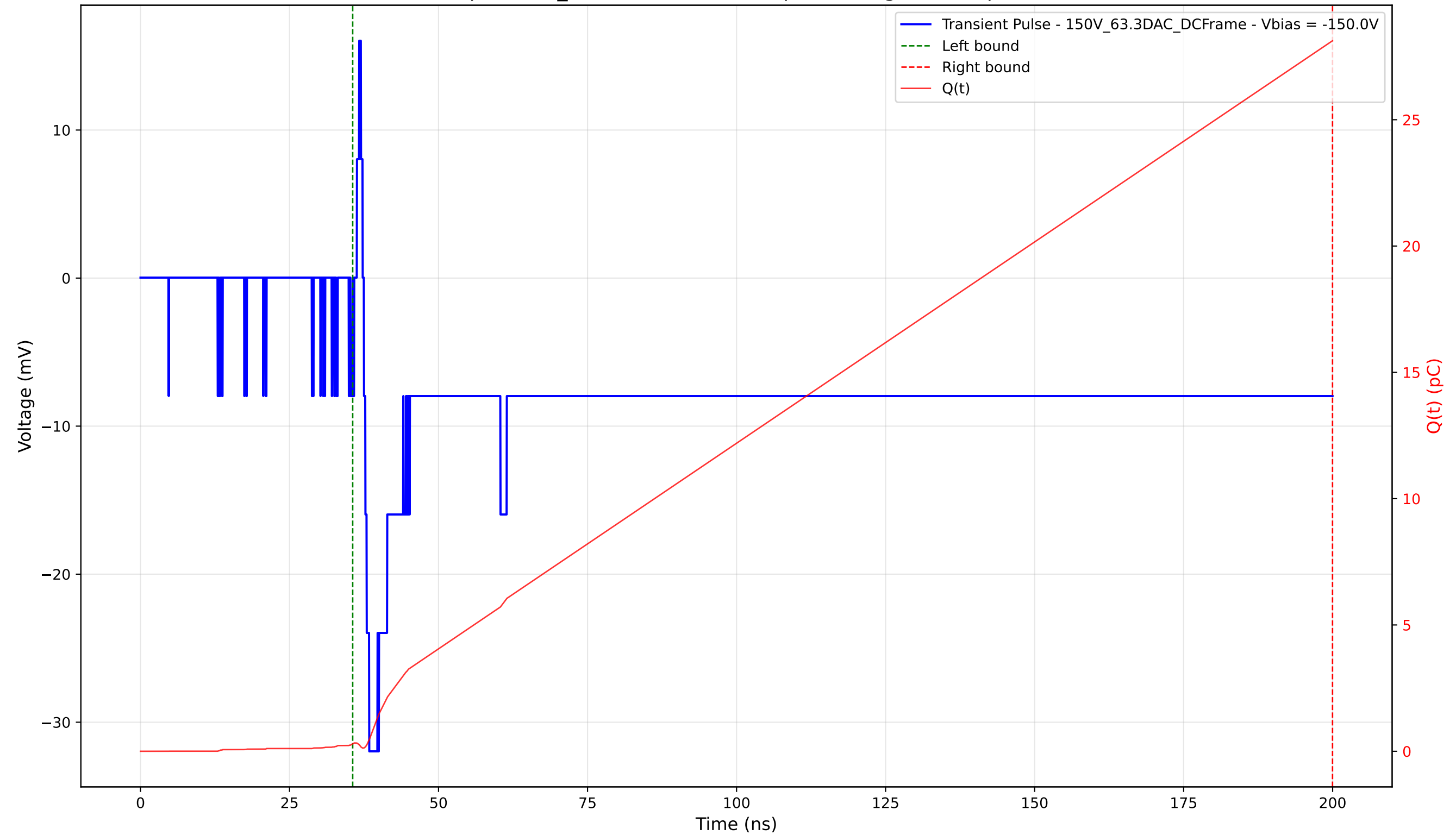
Transient Pulse - Sample: 1cm_42 - Position: 3070.0 \mu\text{m} - Charge: 27.83 pC - Rise Time: 0.89 ns
