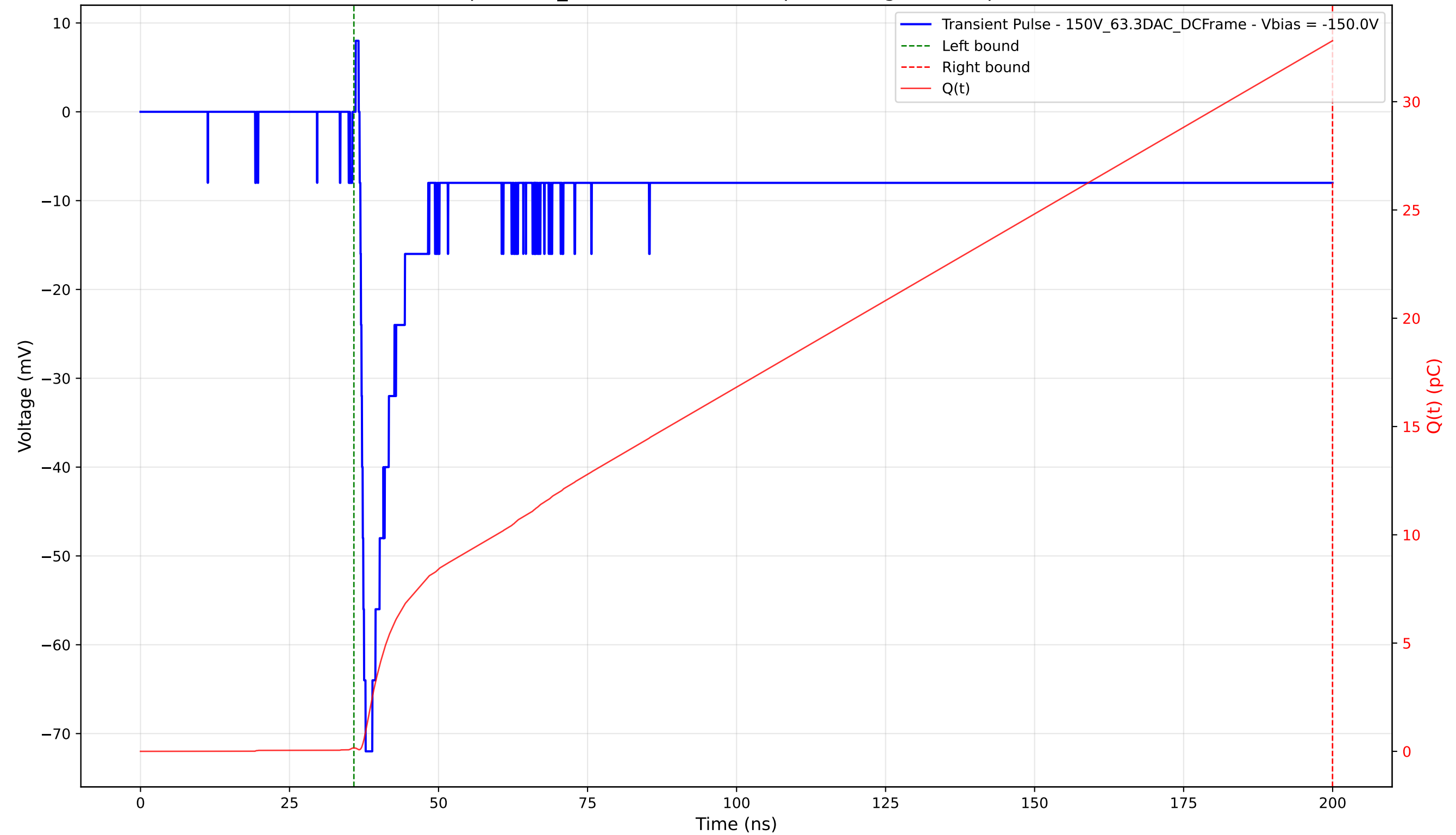
Transient Pulse - Sample: 1cm_42 - Position: 1120.0 \mu\text{m} - Charge: 32.66 pC - Rise Time: 1.00 ns
