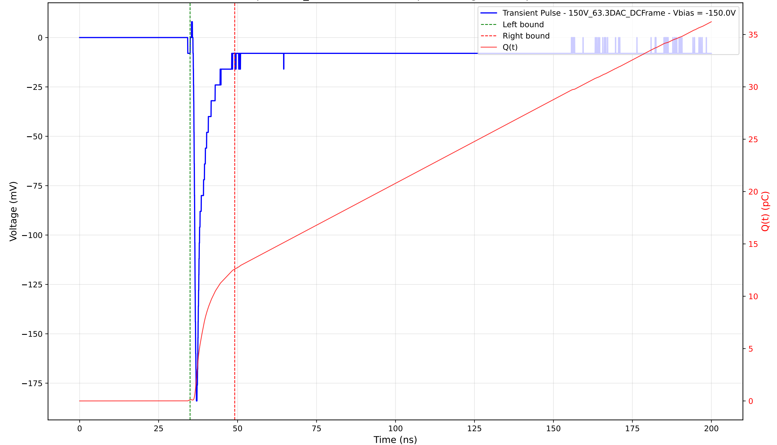
Transient Pulse - Sample: 1cm_42 - Position: 400.0 \mu\text{m} - Charge: 12.46 pC - Rise Time: 0.77 ns
