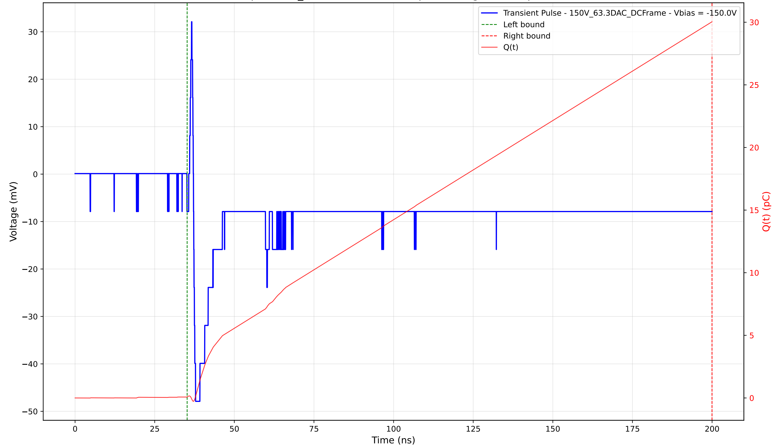
Transient Pulse - Sample: 1cm_42 - Position: 1695.0 \mu\text{m} - Charge: 29.95 pC - Rise Time: 0.65 ns
