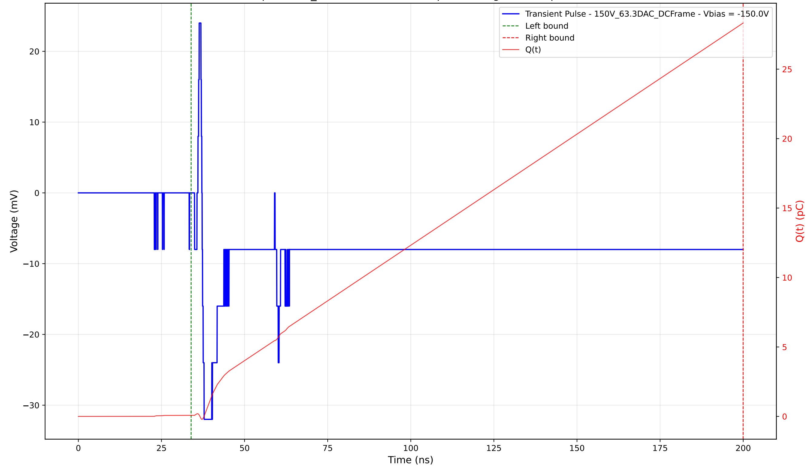
Transient Pulse - Sample: 1cm_42 - Position: 2055.0 \mu\text{m} - Charge: 28.24 pC - Rise Time: 0.59 ns
