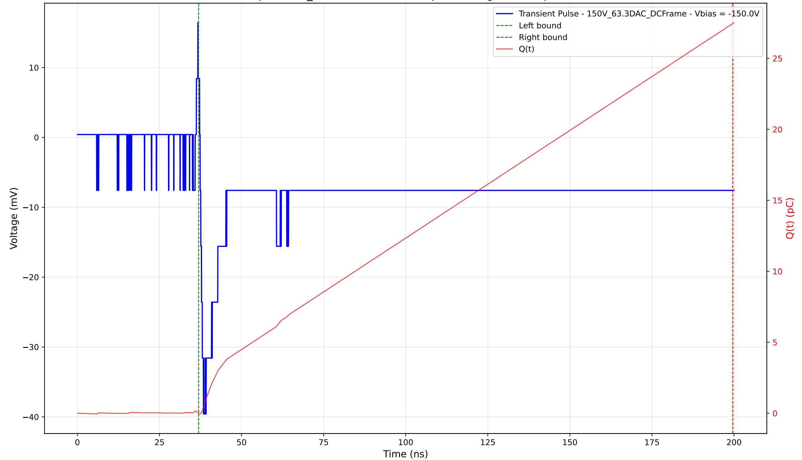
Transient Pulse - Sample: 1cm_42 - Position: 3330.0 \mu\text{m} - Charge: 27.44 pC - Rise Time: 1.01 ns
