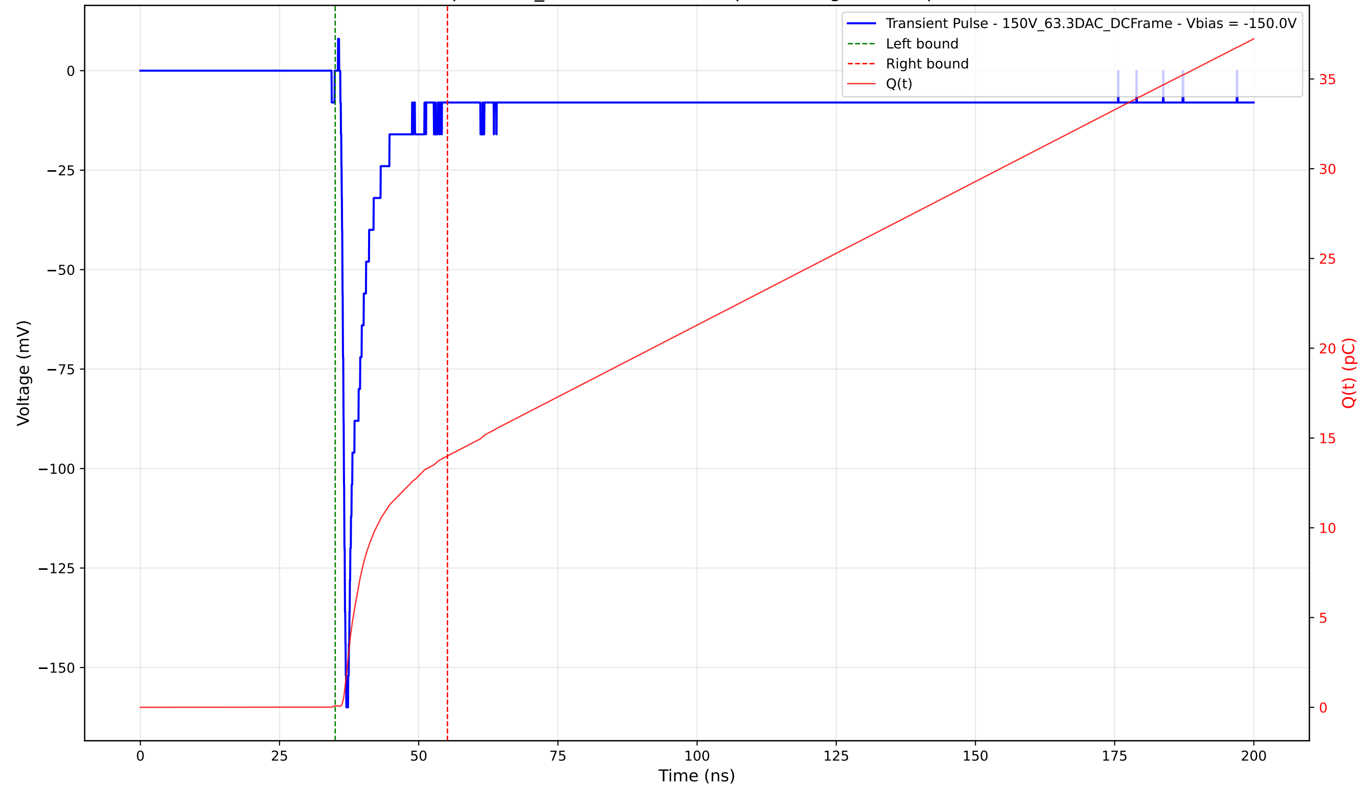
Transient Pulse - Sample: 1cm_42 - Position: 500.0 \mu\text{m} - Charge: 13.92 pC - Rise Time: 0.74 ns
