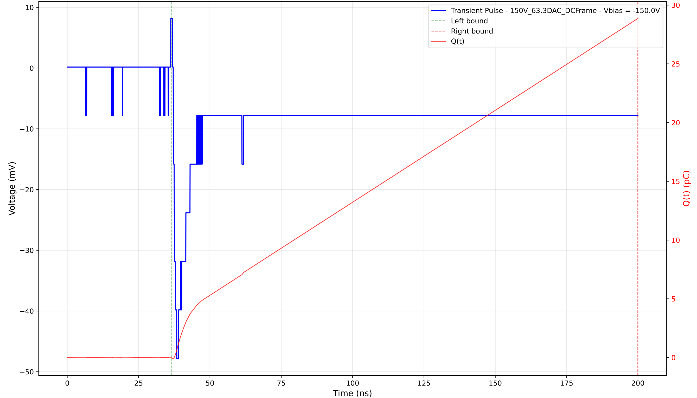
Transient Pulse - Sample: 1cm_42 - Position: 3615.0 \mu\text{m} - Charge: 28.86 pC - Rise Time: 1.25 ns
