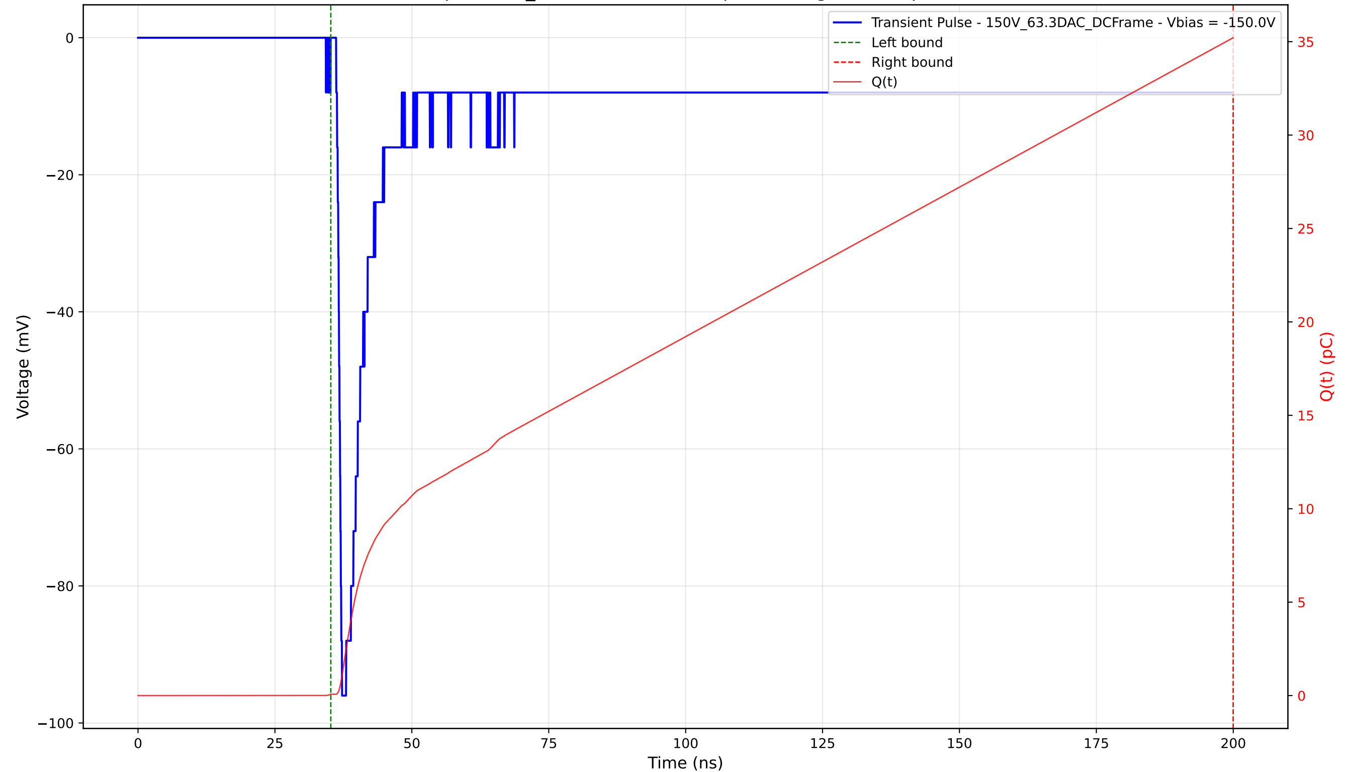
Transient Pulse - Sample: 1cm_42 - Position: 860.0 \mu\text{m} - Charge: 35.14 pC - Rise Time: 0.78 ns
