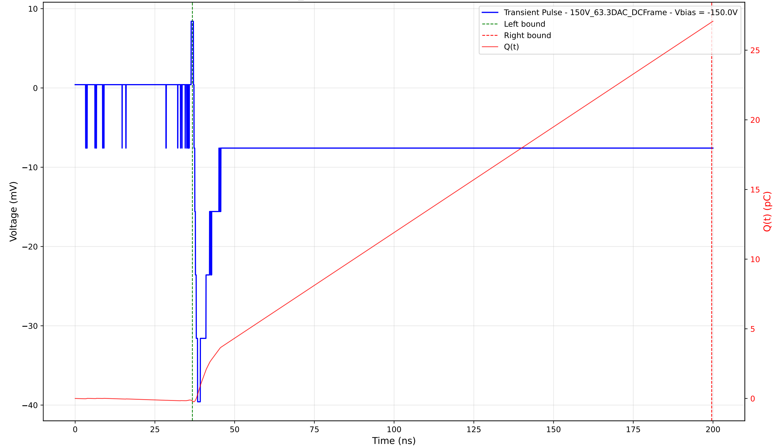
Transient Pulse - Sample: 1cm_42 - Position: 3475.0 \mu\text{m} - Charge: 27.20 pC - Rise Time: 1.13 ns
