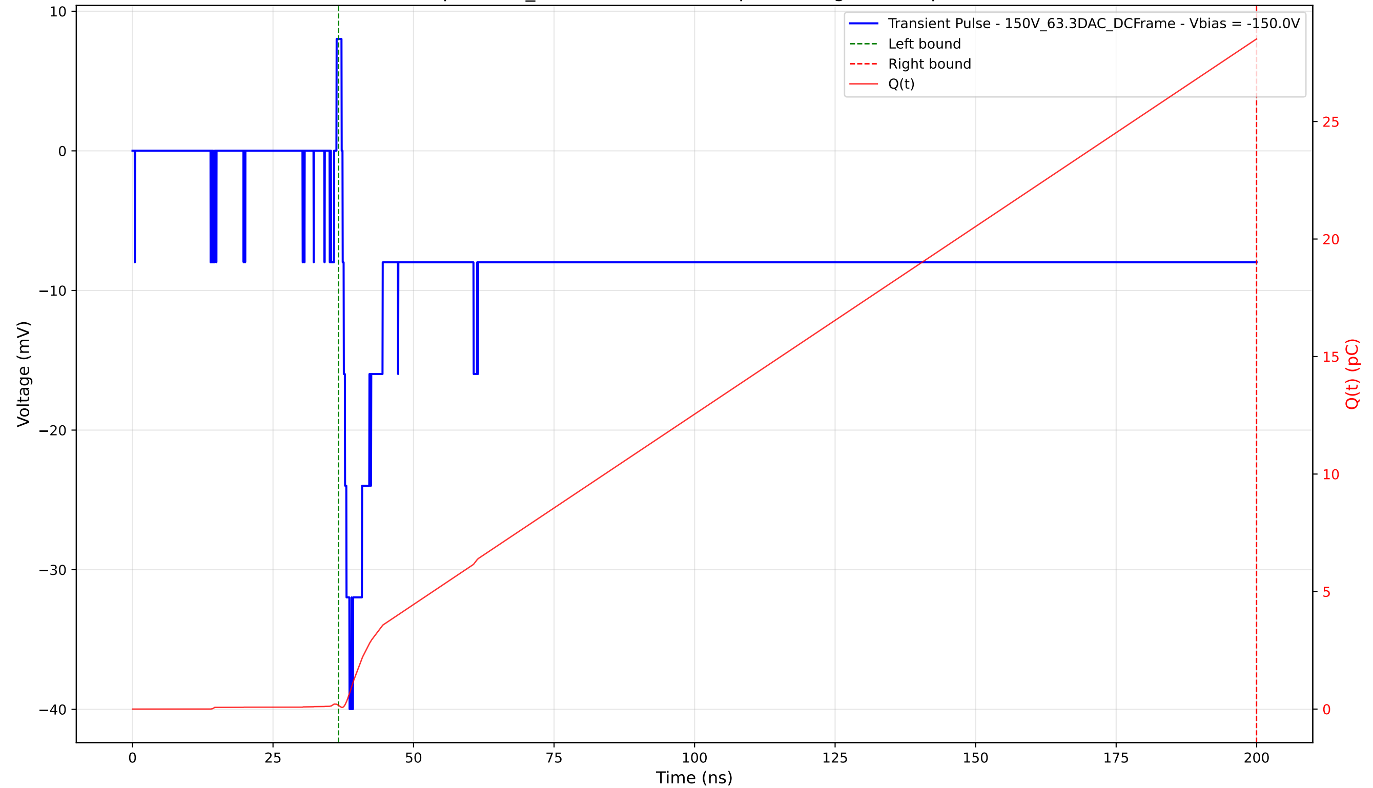
Transient Pulse - Sample: 1cm_42 - Position: 3375.0 \mu\text{m} - Charge: 28.36 pC - Rise Time: 1.23 ns
