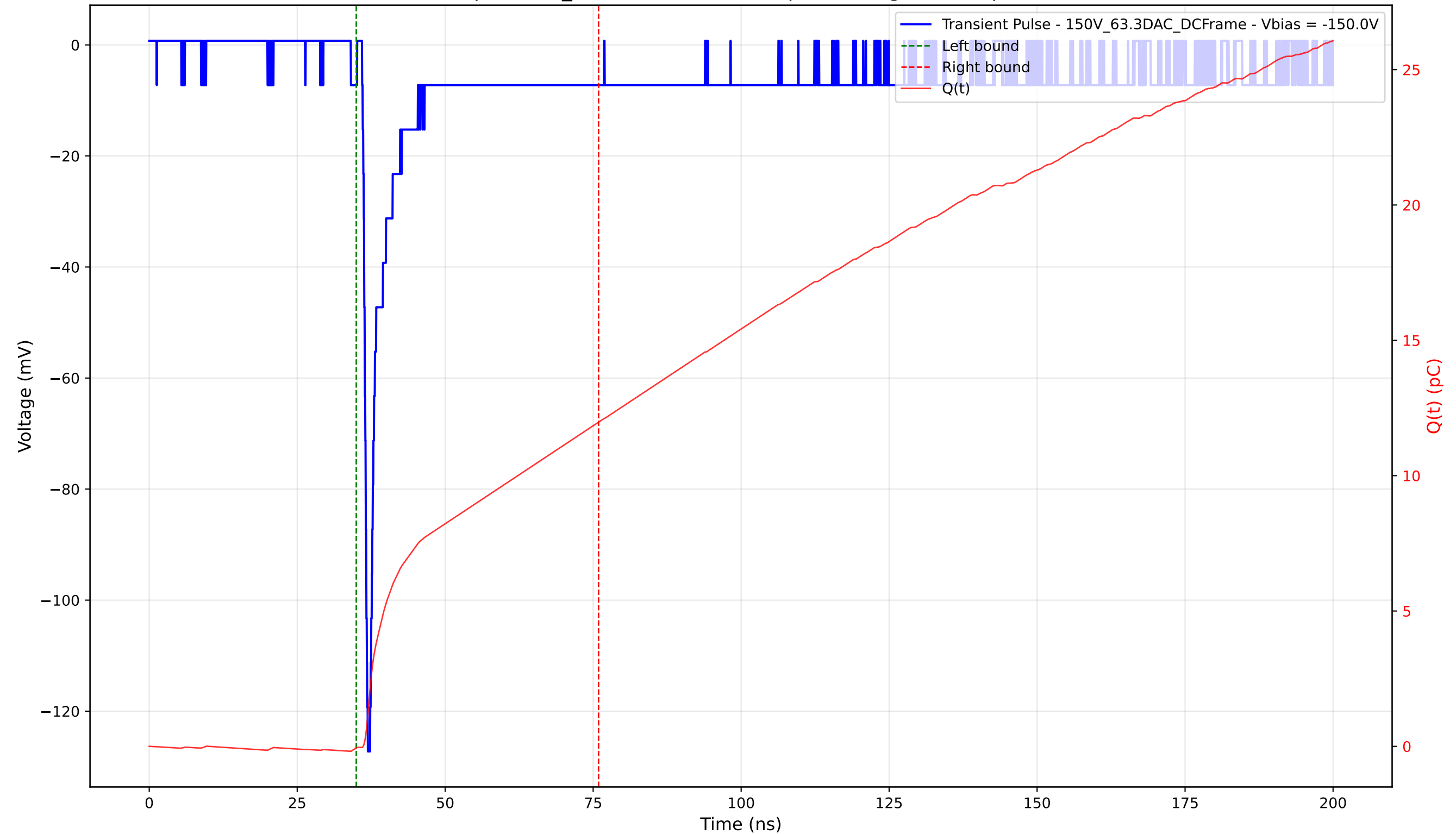
Transient Pulse - Sample: 1cm_42 - Position: 5005.0 \mu\text{m} - Charge: 12.04 pC - Rise Time: 0.77 ns
