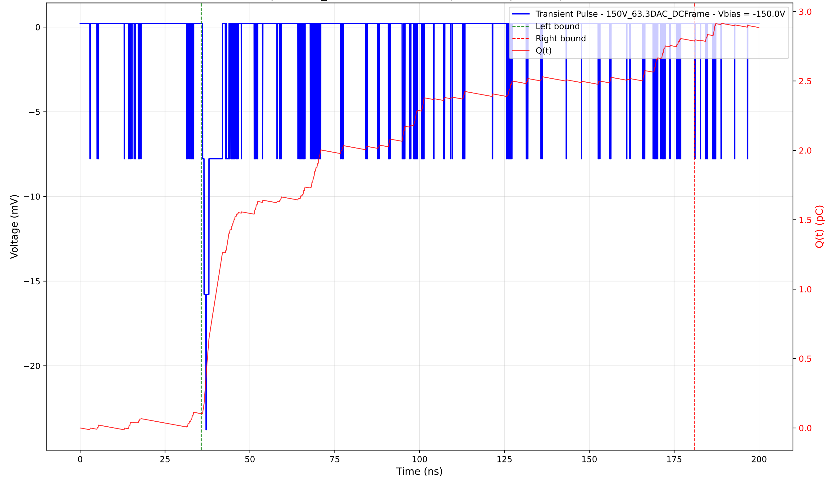
Transient Pulse - Sample: 1cm_42 - Position: 5190.0 \mu\text{m} - Charge: 2.69 pC - Rise Time: 1.01 ns
