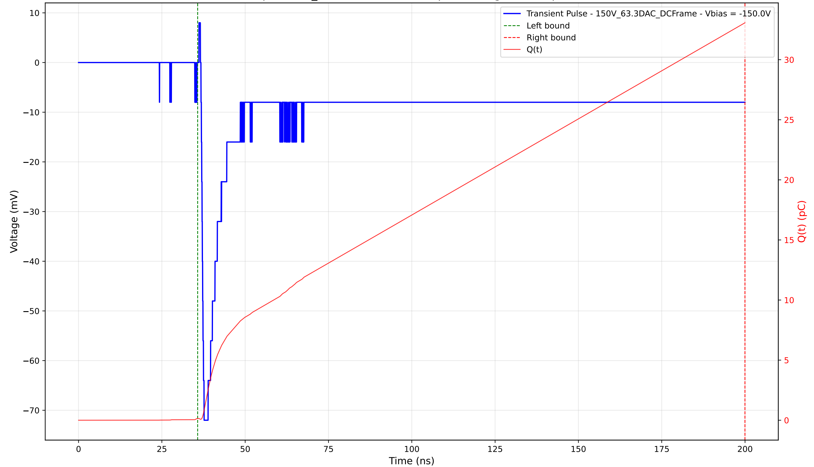
Transient Pulse - Sample: 1cm_42 - Position: 1110.0 \mu\text{m} - Charge: 32.93 pC - Rise Time: 0.92 ns
