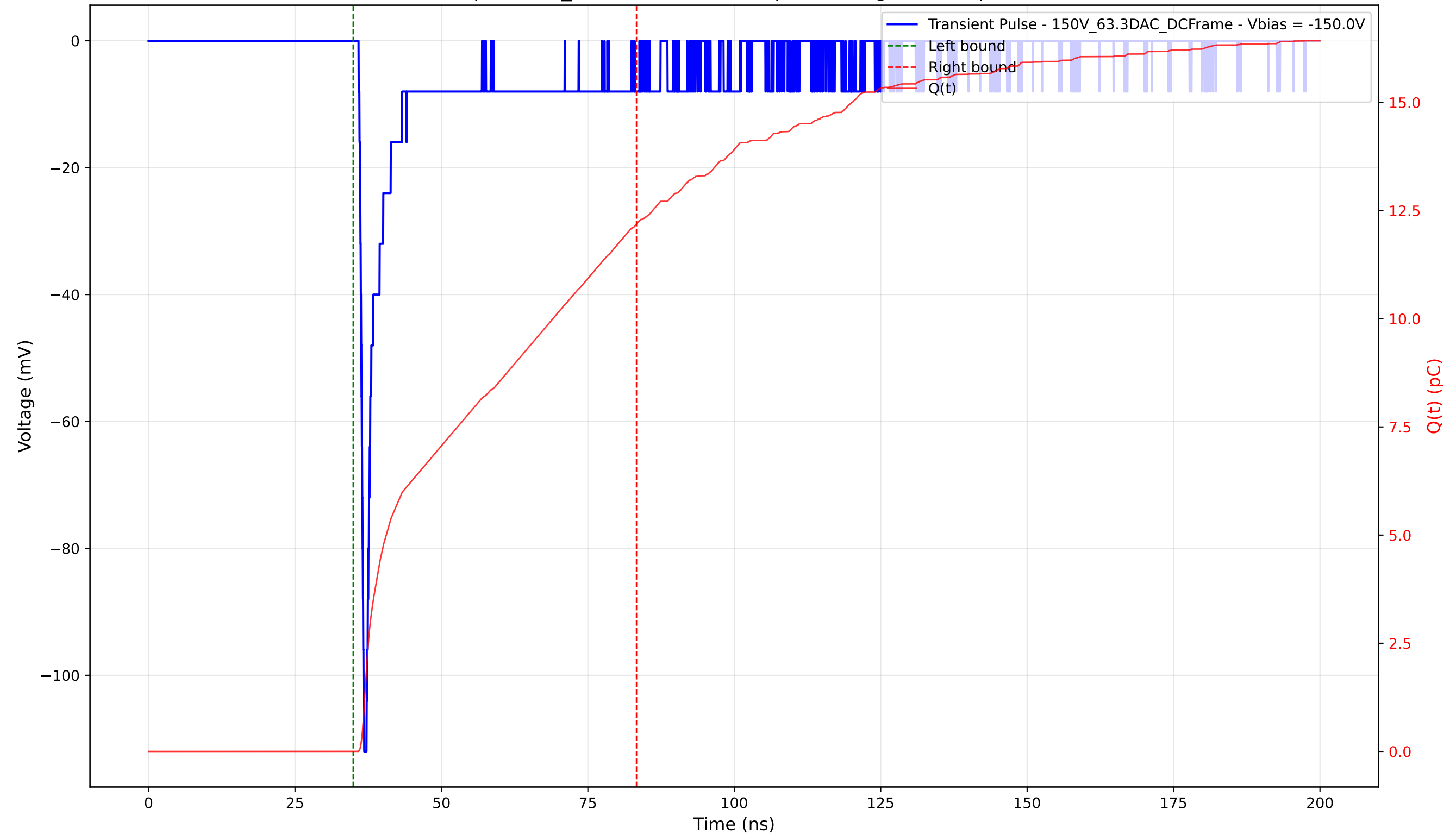
Transient Pulse - Sample: 1cm_42 - Position: 150.0 \mu\text{m} - Charge: 12.19 pC - Rise Time: 0.71 ns
