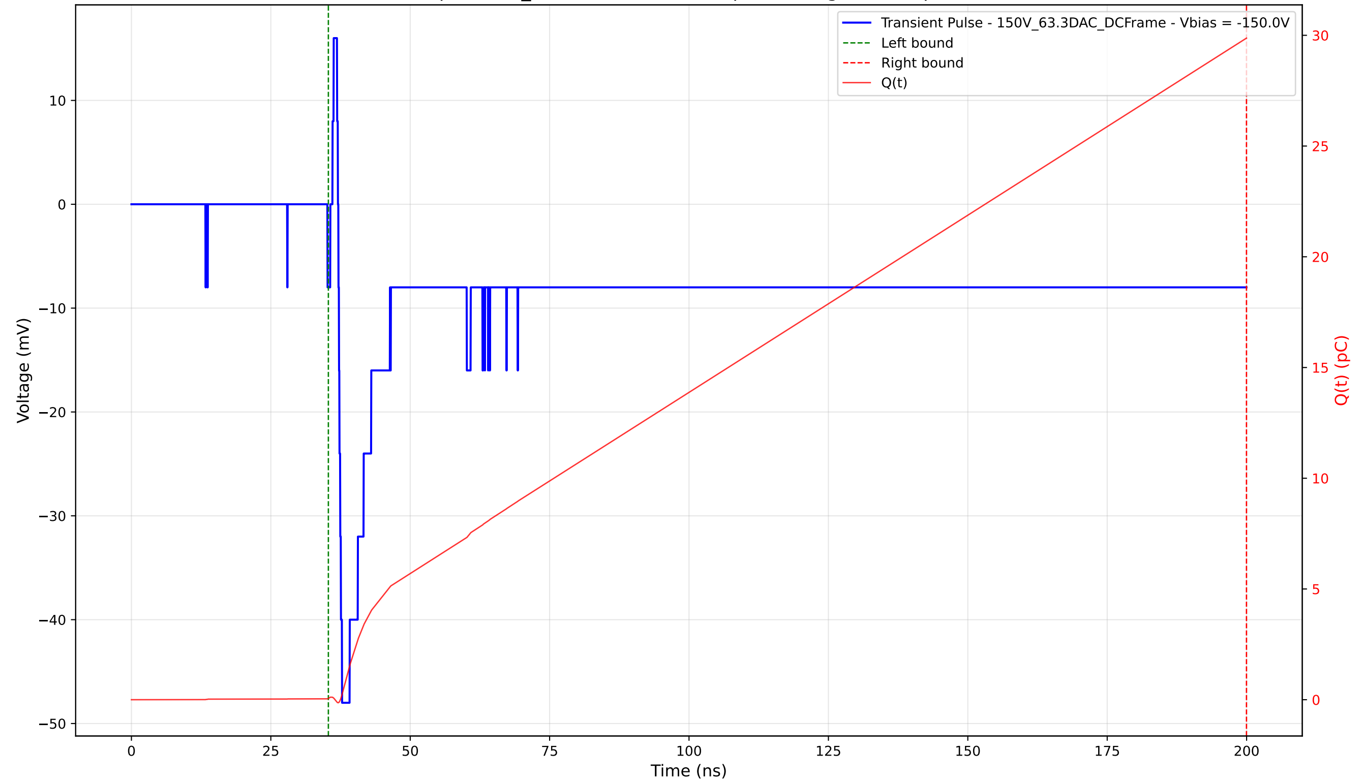
Transient Pulse - Sample: 1cm_42 - Position: 1510.0 \mu\text{m} - Charge: 29.81 pC - Rise Time: 0.65 ns
