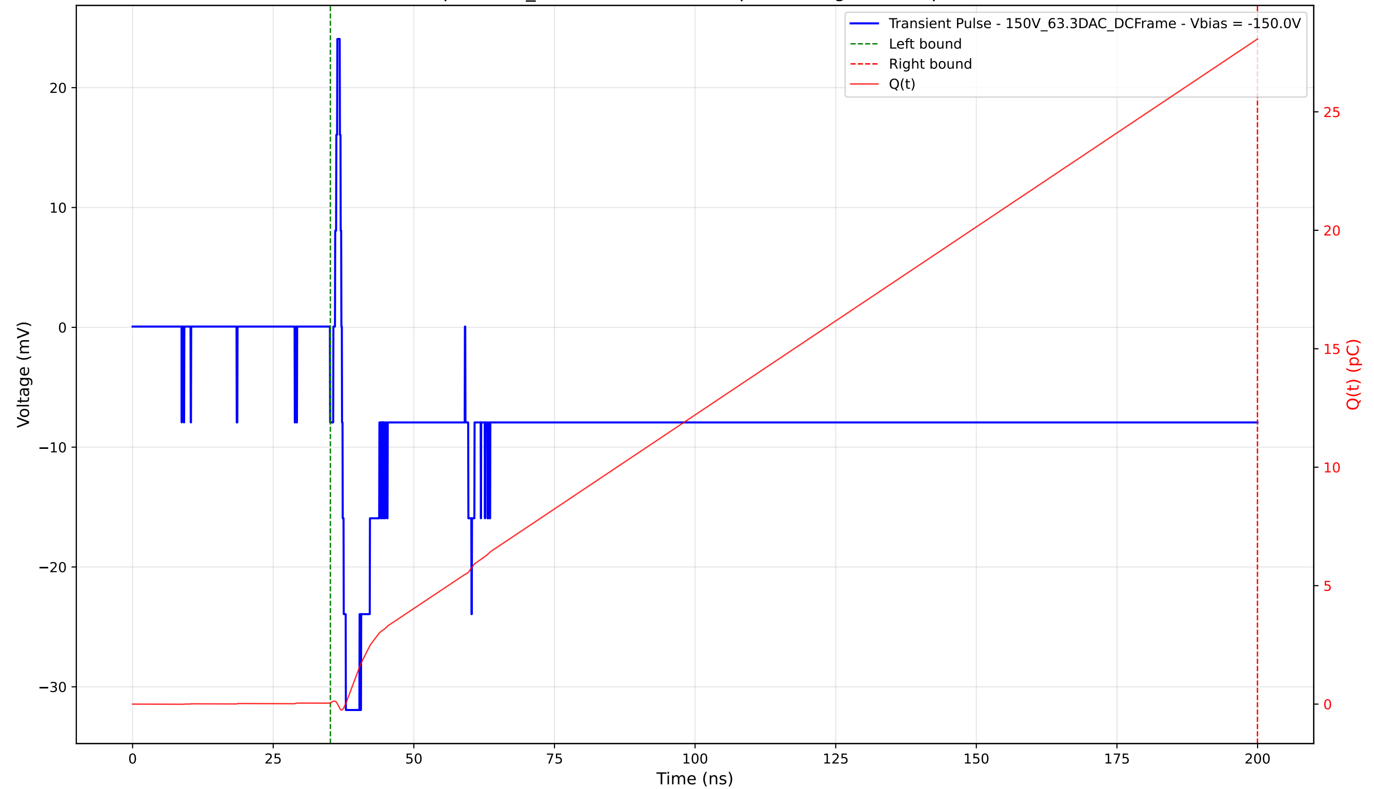
Transient Pulse - Sample: 1cm_42 - Position: 2005.0 \mu\text{m} - Charge: 28.03 pC - Rise Time: 0.69 ns
