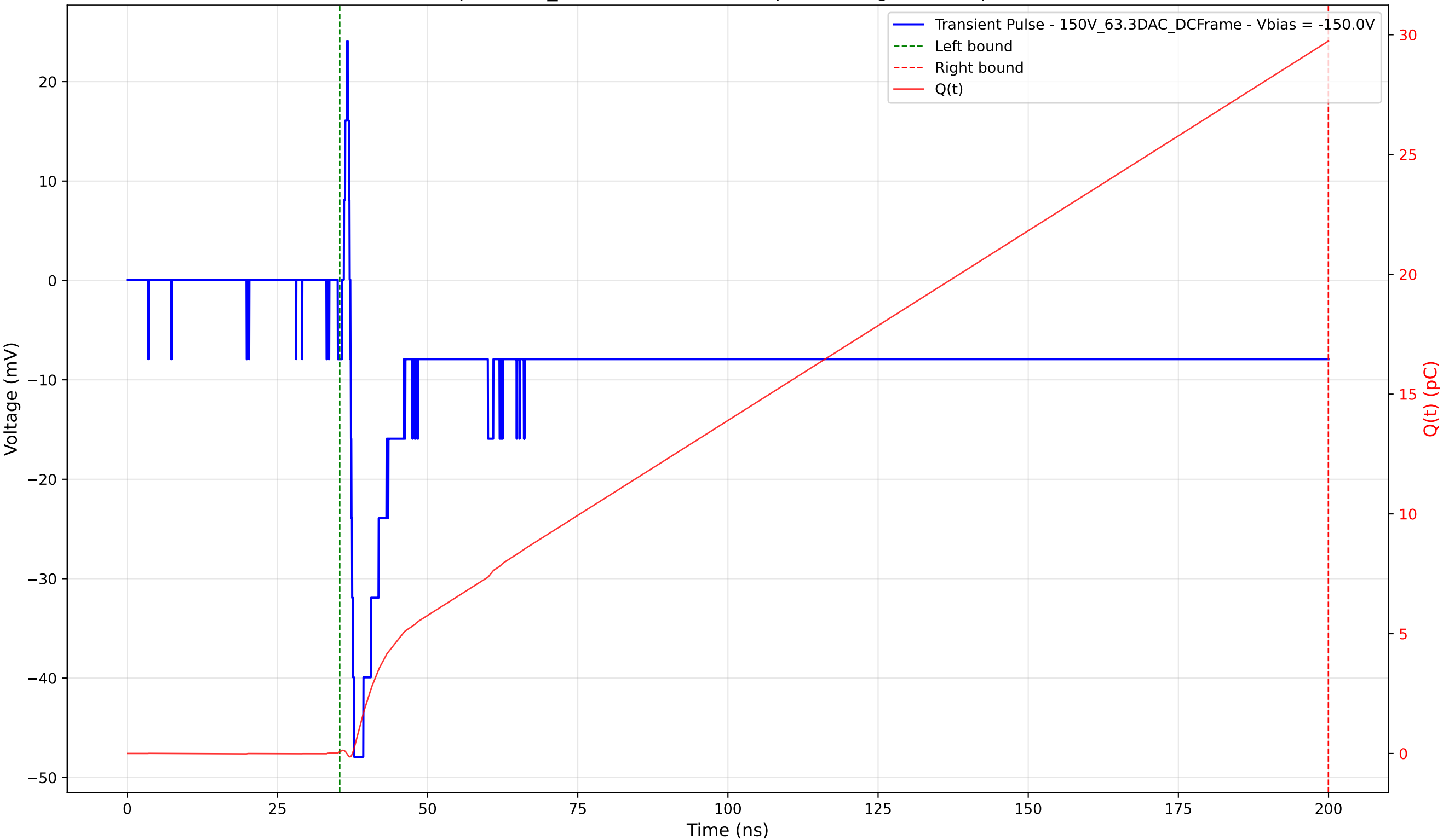
Transient Pulse - Sample: 1cm_42 - Position: 1520.0 \mu\text{m} - Charge: 29.66 pC - Rise Time: 0.61 ns
