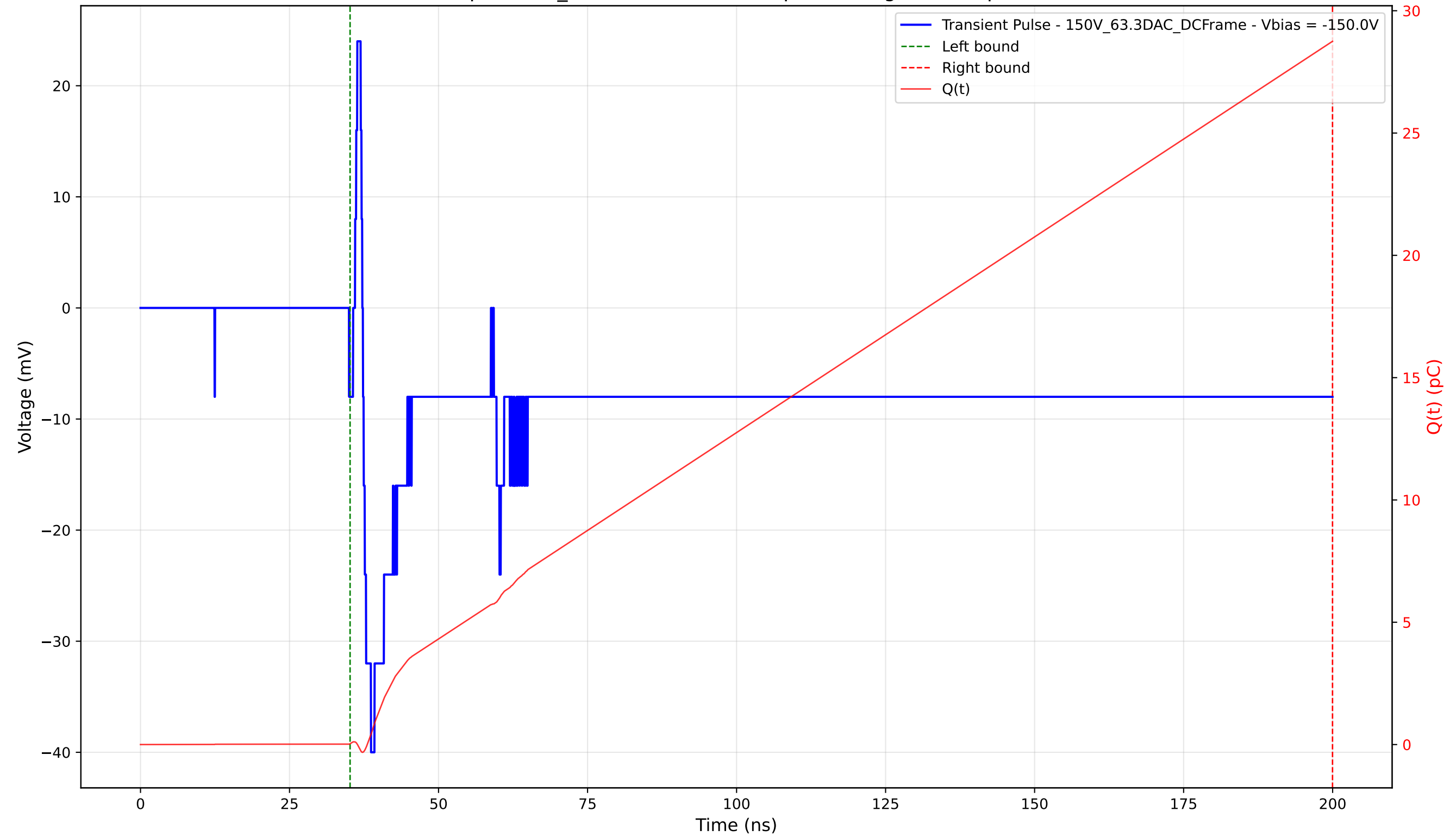
Transient Pulse - Sample: 1cm_42 - Position: 2220.0 \mu\text{m} - Charge: 28.72 pC - Rise Time: 1.35 ns
