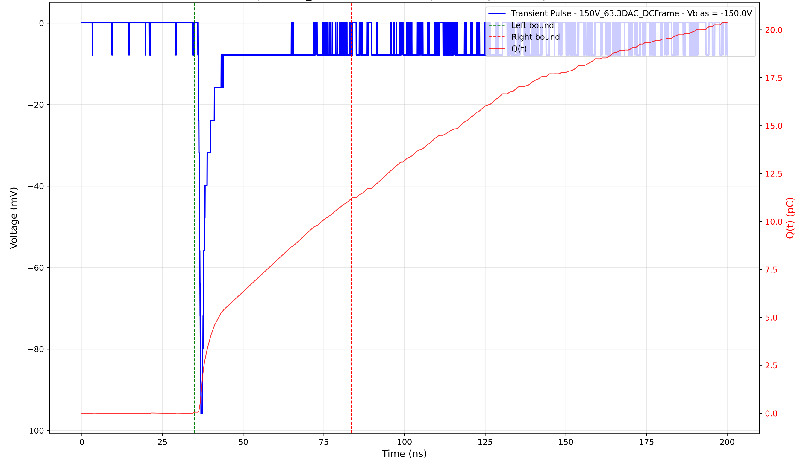
Transient Pulse - Sample: 1cm_42 - Position: 5050.0 \mu\text{m} - Charge: 11.14 pC - Rise Time: 0.70 ns
