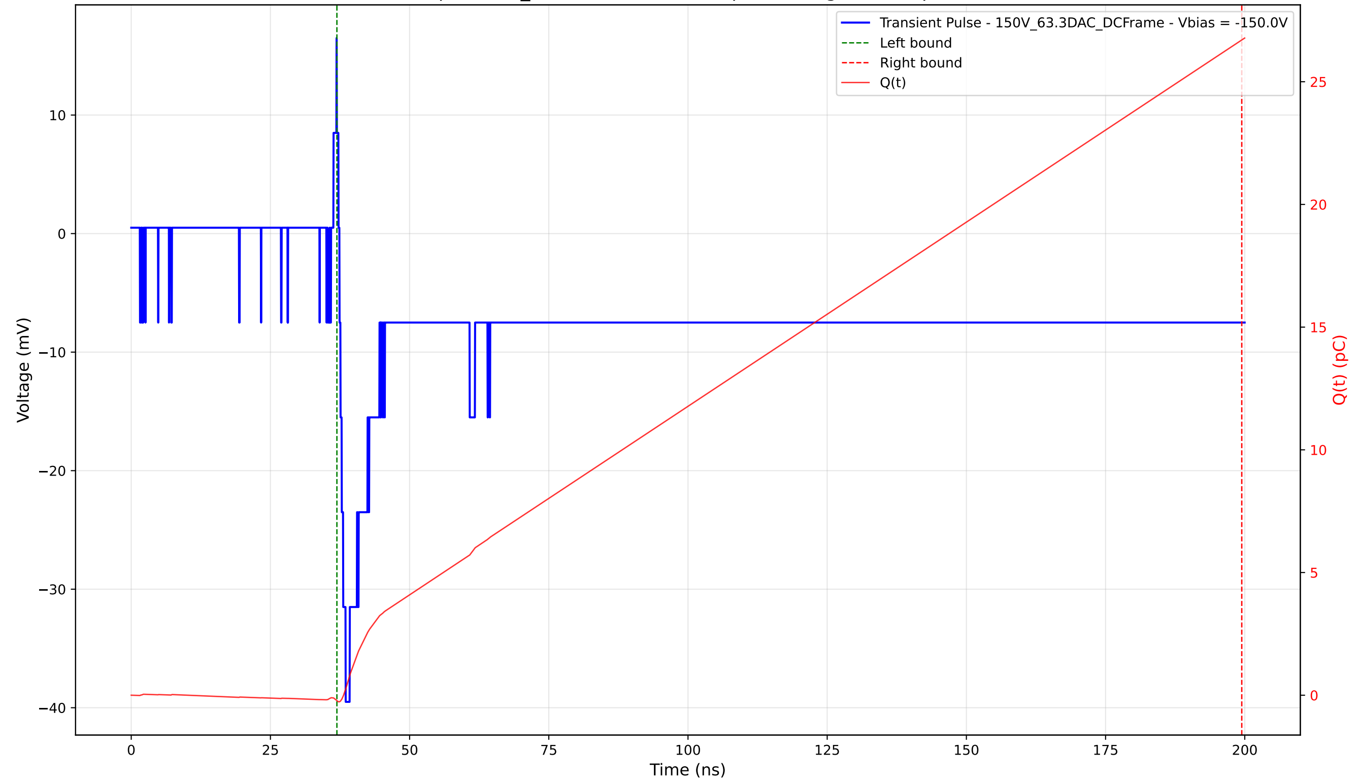
Transient Pulse - Sample: 1cm_42 - Position: 3335.0 \mu\text{m} - Charge: 26.93 pC - Rise Time: 1.11 ns
