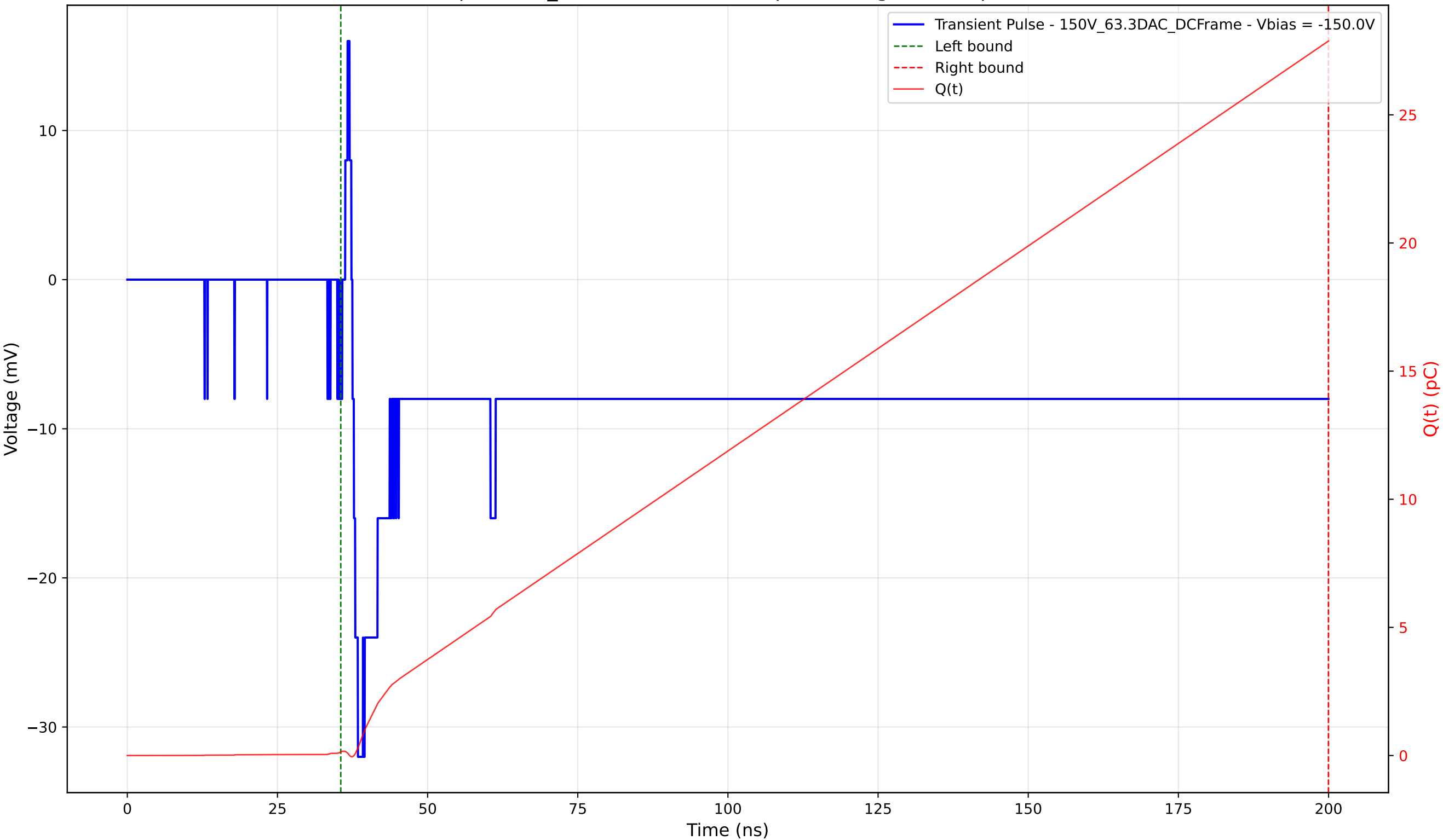
Transient Pulse - Sample: 1cm_42 - Position: 3065.0 \mu\text{m} - Charge: 27.74 pC - Rise Time: 0.91 ns
