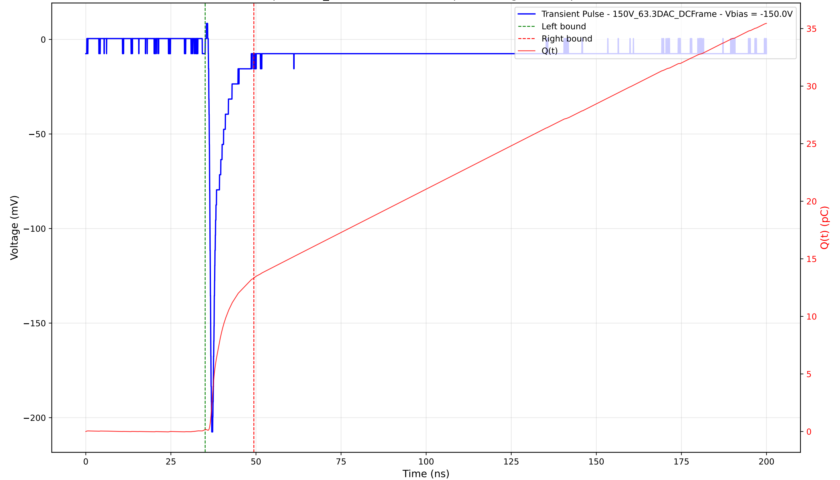
Transient Pulse - Sample: 1cm_42 - Position: 4900.0 \mu\text{m} - Charge: 13.16 pC - Rise Time: 0.77 ns
