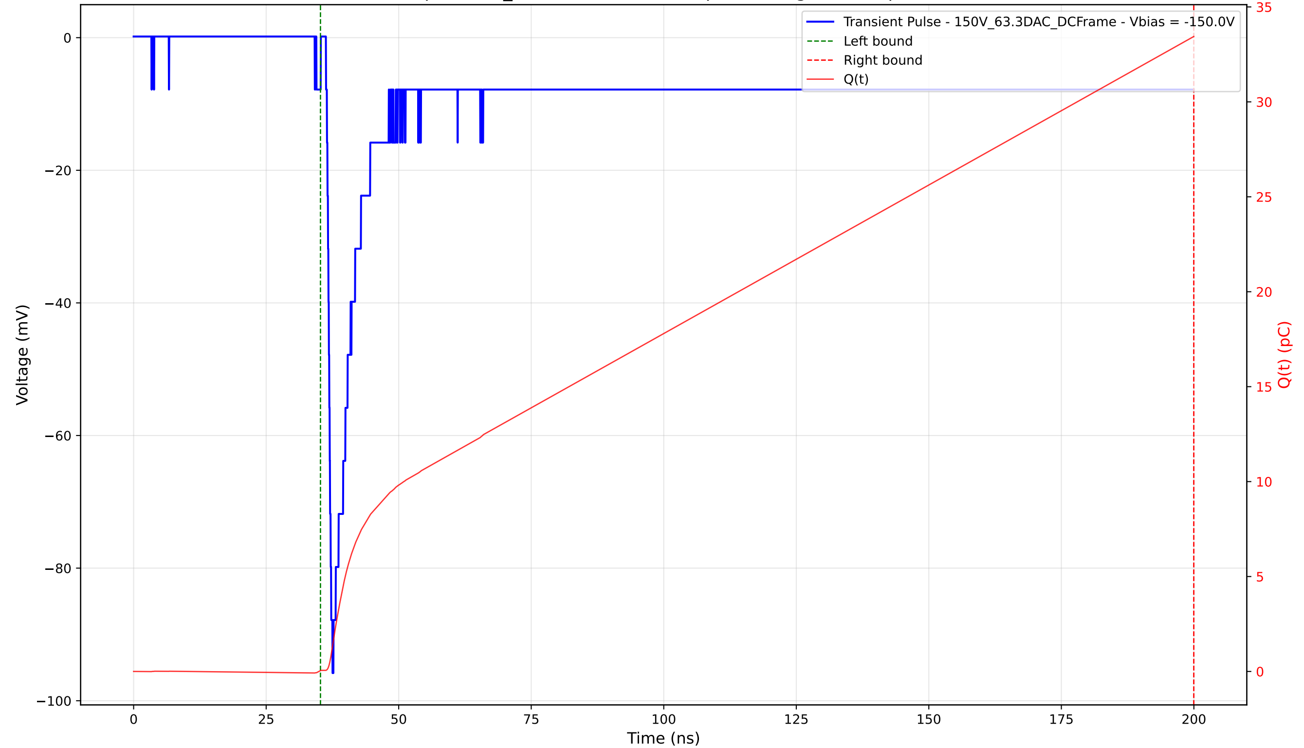
Transient Pulse - Sample: 1cm_42 - Position: 4360.0 \mu\text{m} - Charge: 33.39 pC - Rise Time: 0.82 ns
