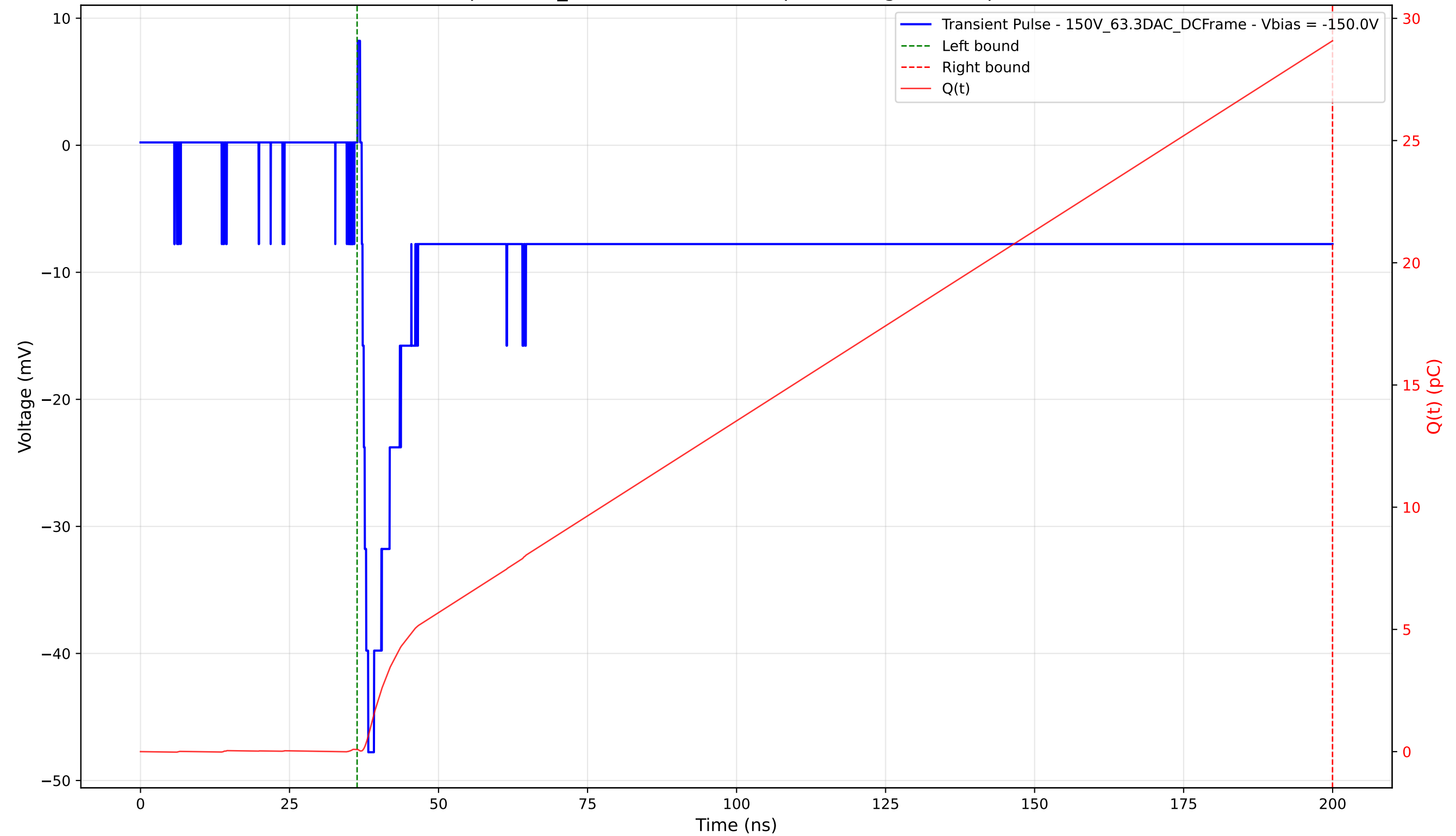
Transient Pulse - Sample: 1cm_42 - Position: 3640.0 \mu\text{m} - Charge: 28.99 pC - Rise Time: 1.09 ns
