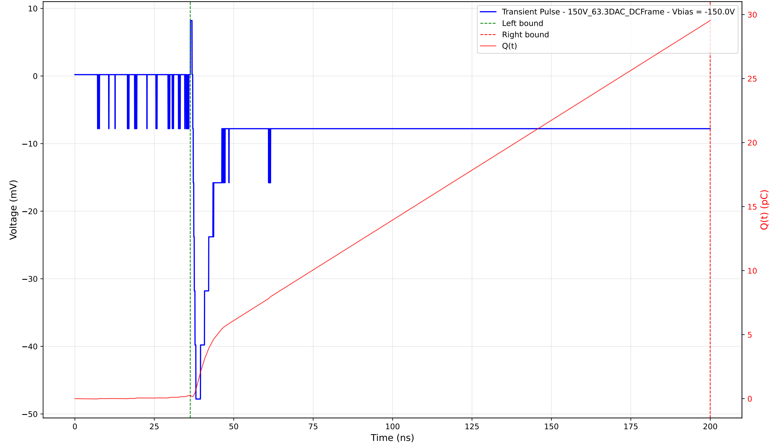
Transient Pulse - Sample: 1cm_42 - Position: 3675.0 \mu\text{m} - Charge: 29.28 pC - Rise Time: 0.99 ns
