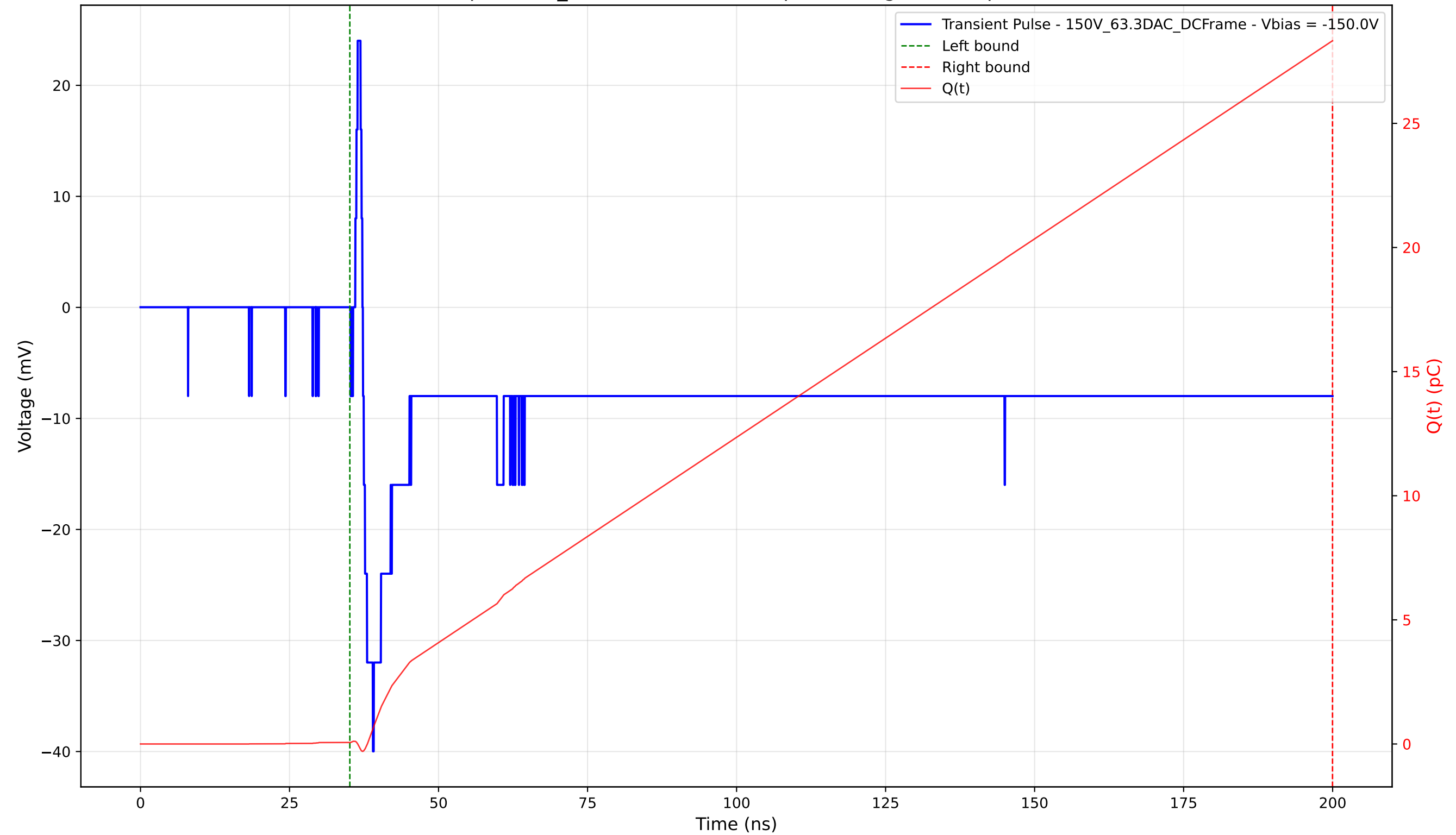
Transient Pulse - Sample: 1cm_42 - Position: 2305.0 \mu\text{m} - Charge: 28.27 pC - Rise Time: 1.67 ns
