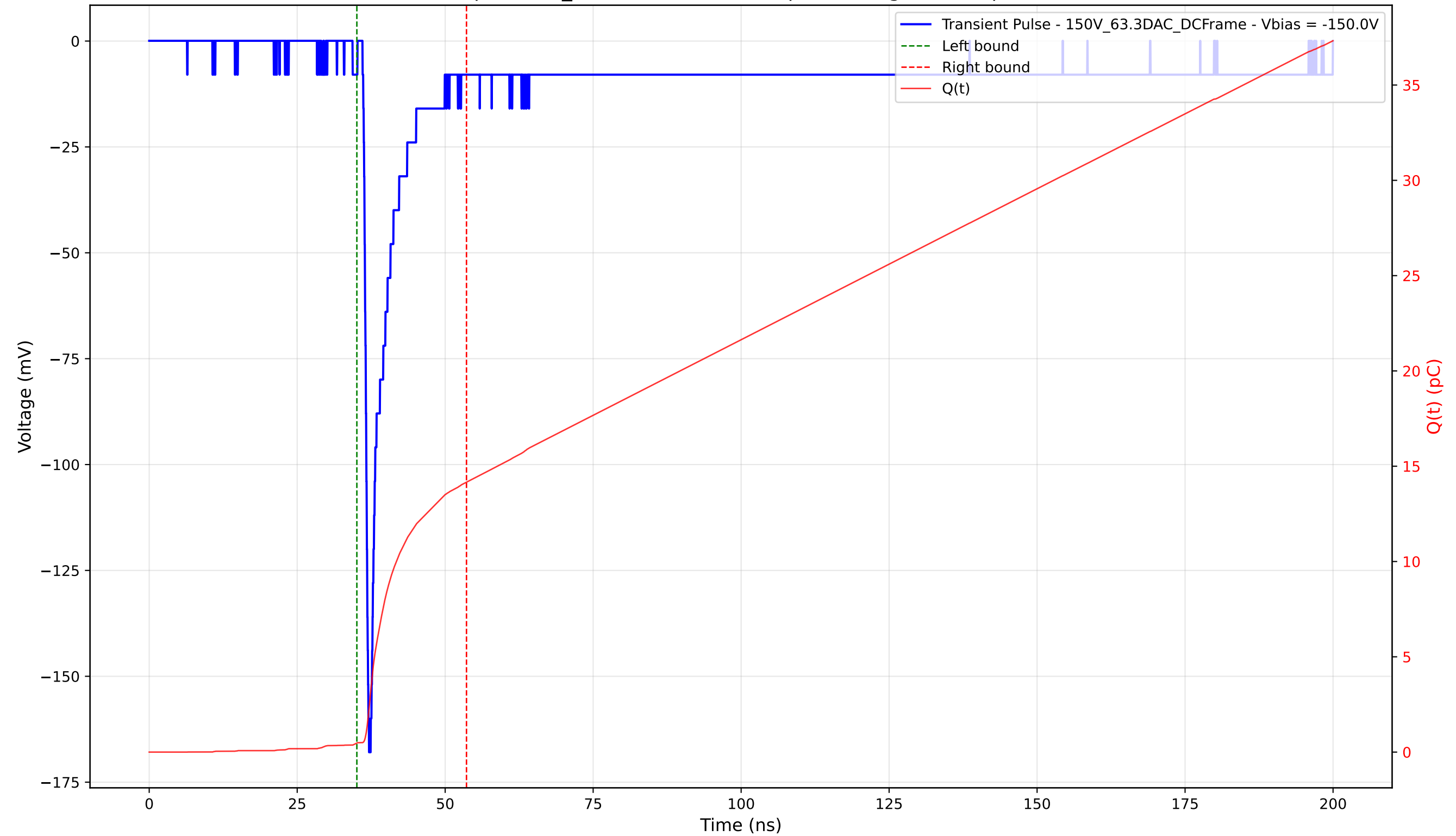
Transient Pulse - Sample: 1cm_42 - Position: 4620.0 \mu\text{m} - Charge: 13.68 pC - Rise Time: 0.74 ns
