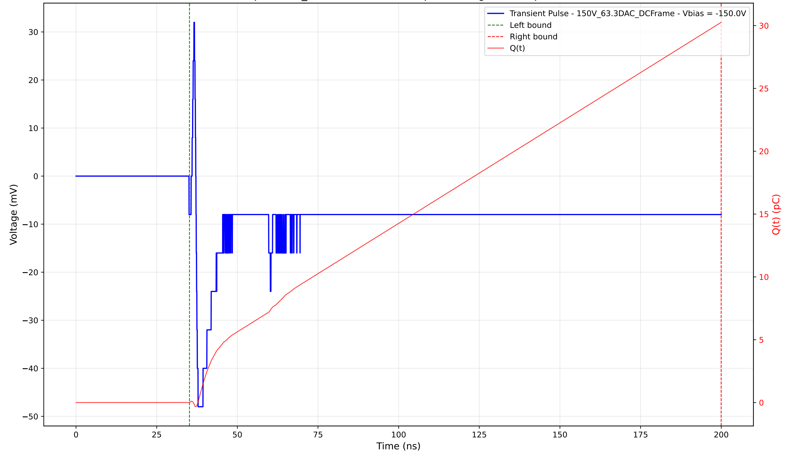
Transient Pulse - Sample: 1cm_42 - Position: 1710.0 \mu\text{m} - Charge: 30.23 pC - Rise Time: 0.65 ns
