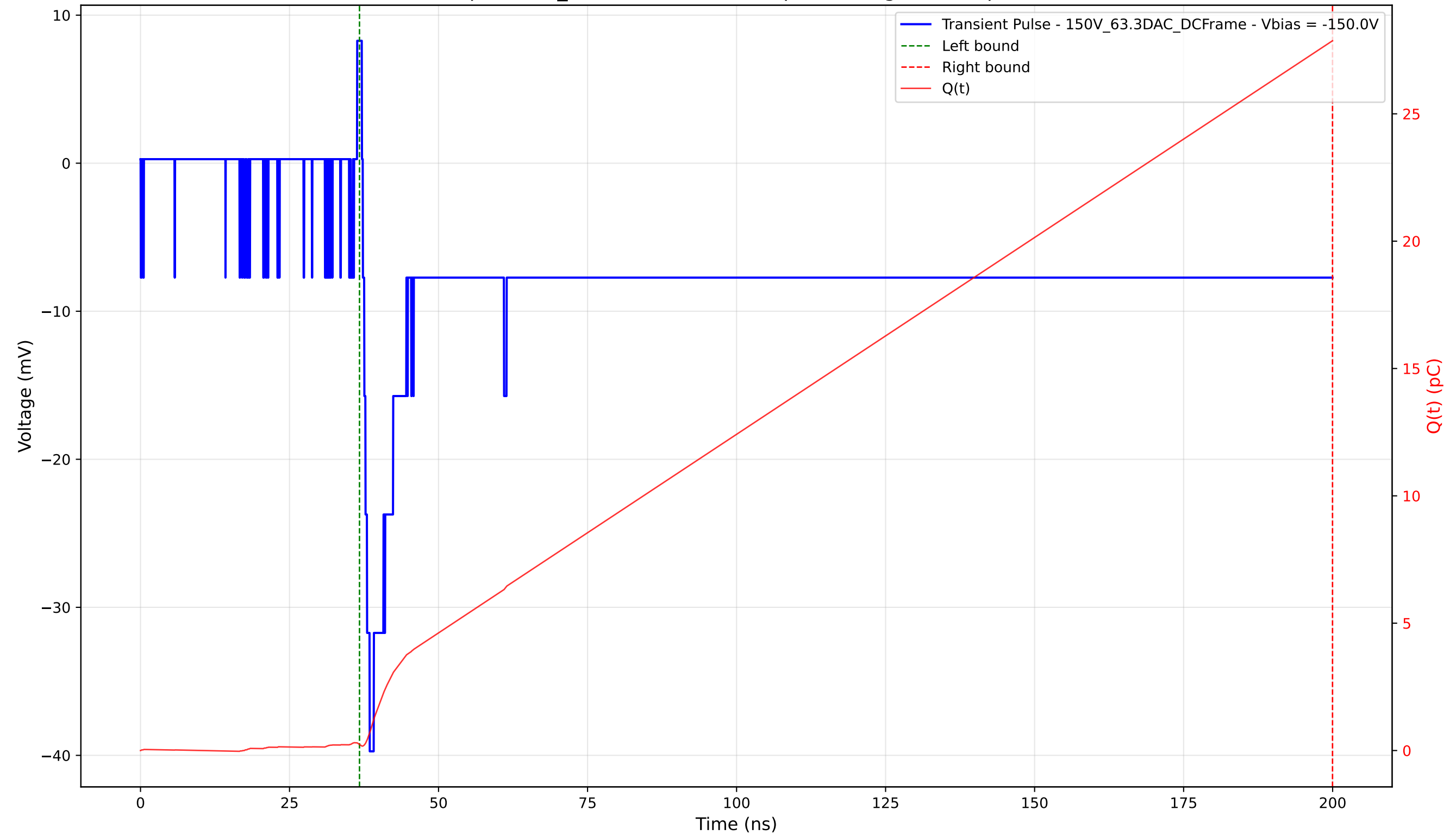
Transient Pulse - Sample: 1cm_42 - Position: 3440.0 \mu\text{m} - Charge: 27.63 pC - Rise Time: 1.15 ns
