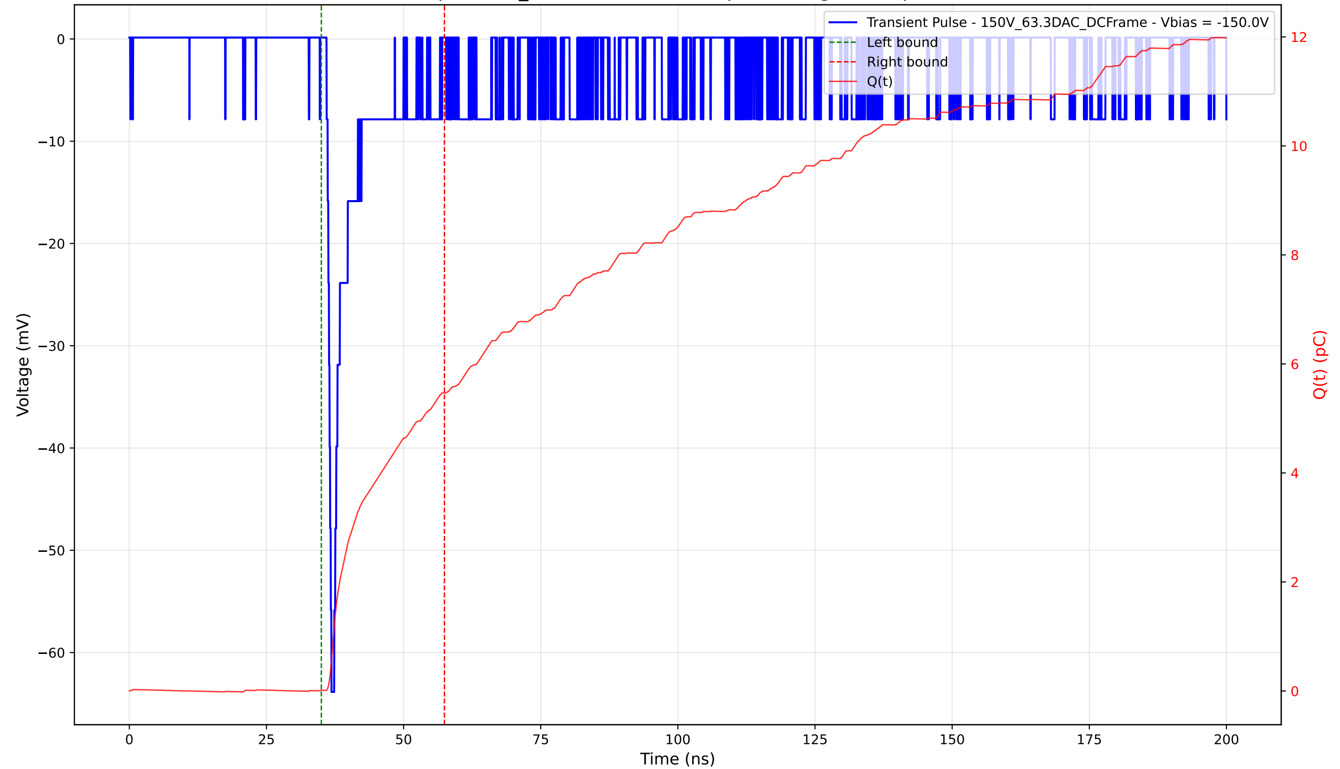
Transient Pulse - Sample: 1cm_42 - Position: 5100.0 \mu\text{m} - Charge: 5.46 pC - Rise Time: 0.88 ns
