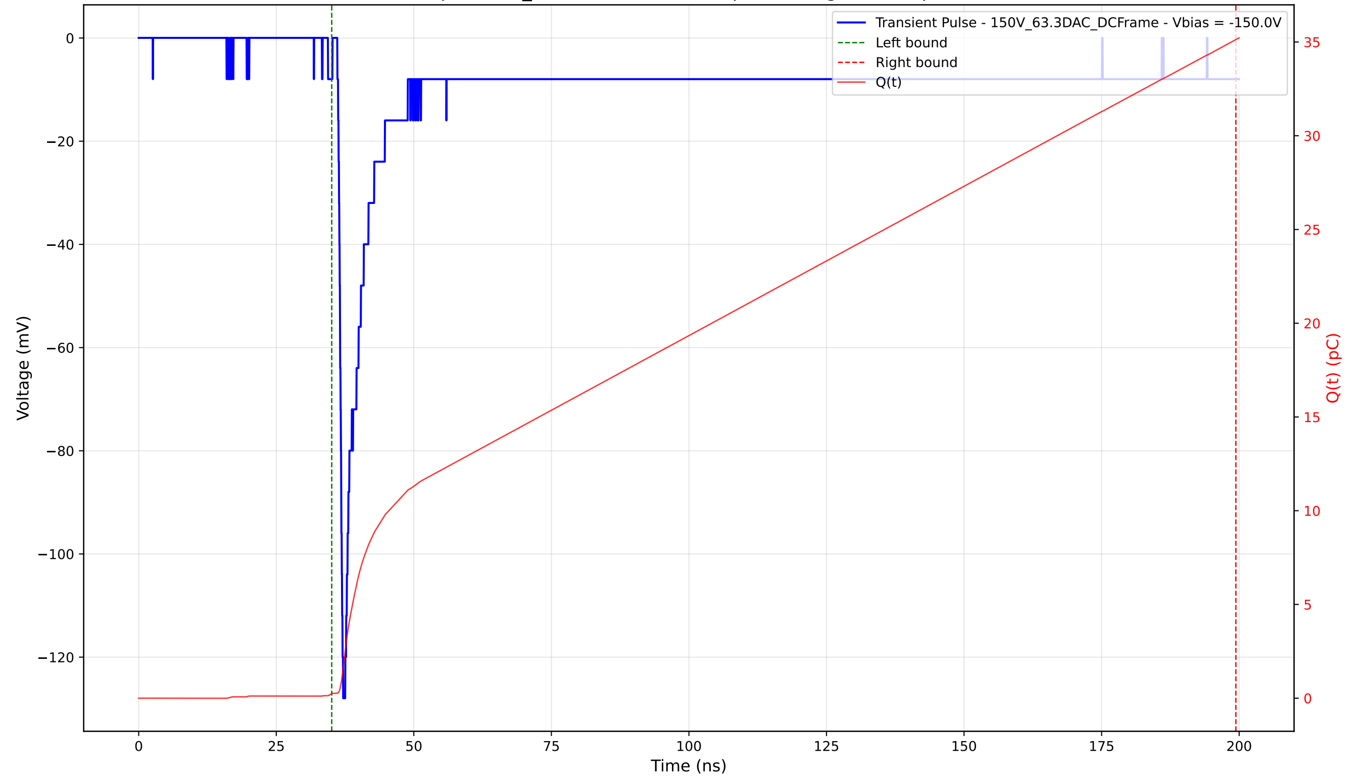
Transient Pulse - Sample: 1cm_42 - Position: 4545.0 \mu\text{m} - Charge: 34.89 pC - Rise Time: 0.81 ns
