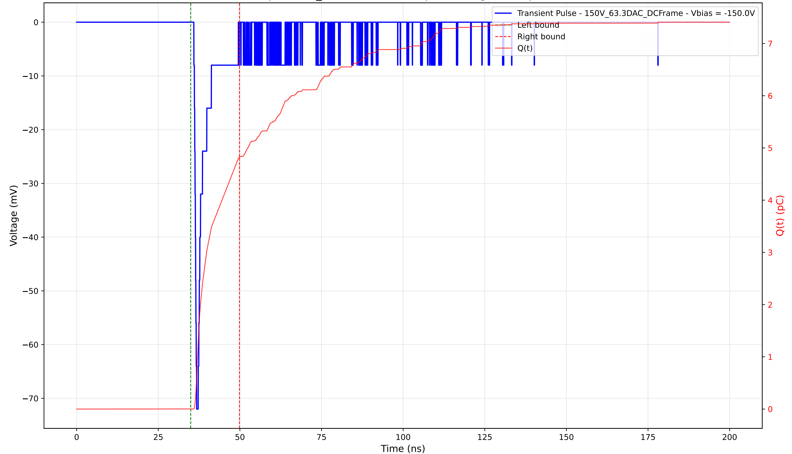
Transient Pulse - Sample: 1cm_42 - Position: 90.0 \mu\text{m} - Charge: 4.83 pC - Rise Time: 0.84 ns
