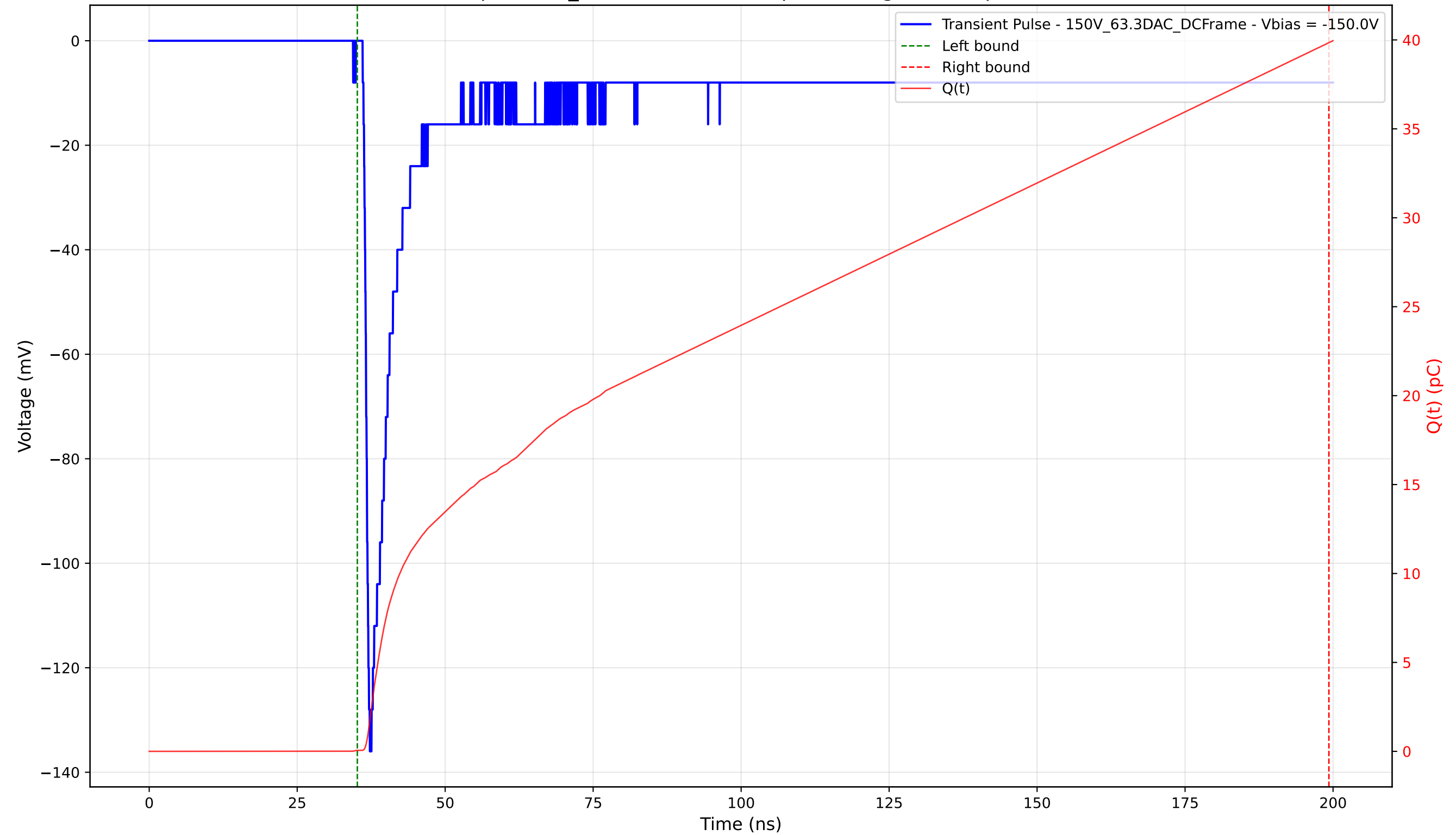
Transient Pulse - Sample: 1cm_42 - Position: 710.0 \mu\text{m} - Charge: 39.79 pC - Rise Time: 0.93 ns
