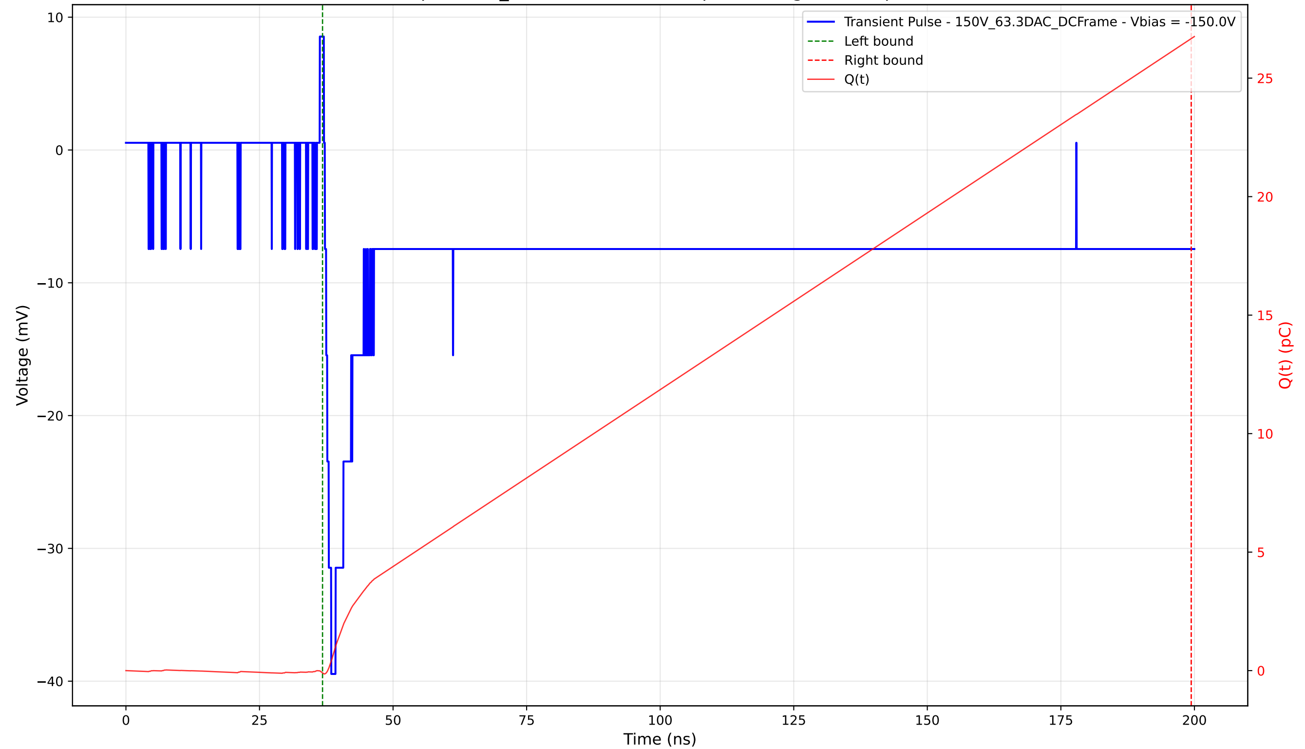
Transient Pulse - Sample: 1cm_42 - Position: 3490.0 \mu\text{m} - Charge: 26.77 pC - Rise Time: 1.19 ns
