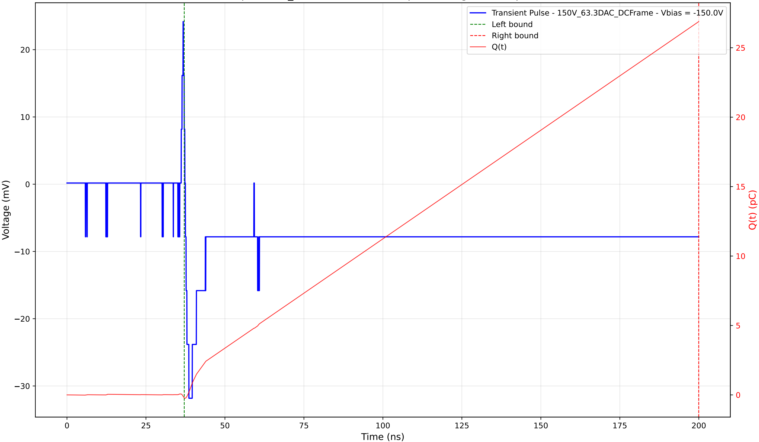
Transient Pulse - Sample: 1cm_42 - Position: 2515.0 \mu\text{m} - Charge: 27.10 pC - Rise Time: 1.11 ns
