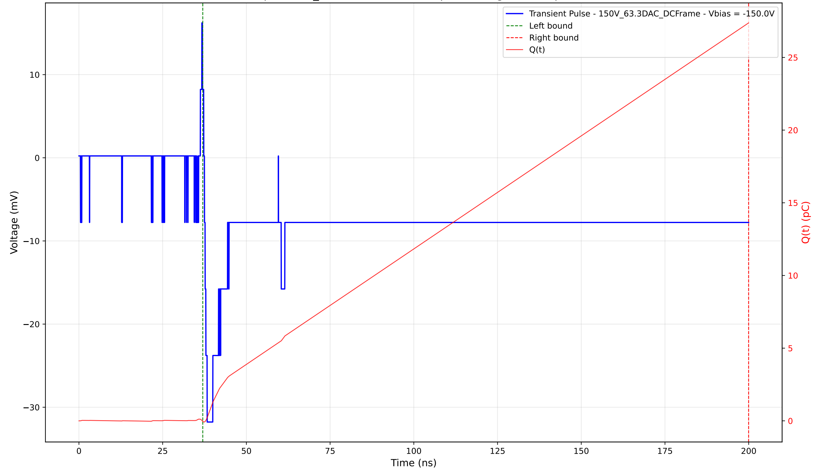
Transient Pulse - Sample: 1cm_42 - Position: 3080.0 \mu\text{m} - Charge: 27.41 pC - Rise Time: 0.81 ns
