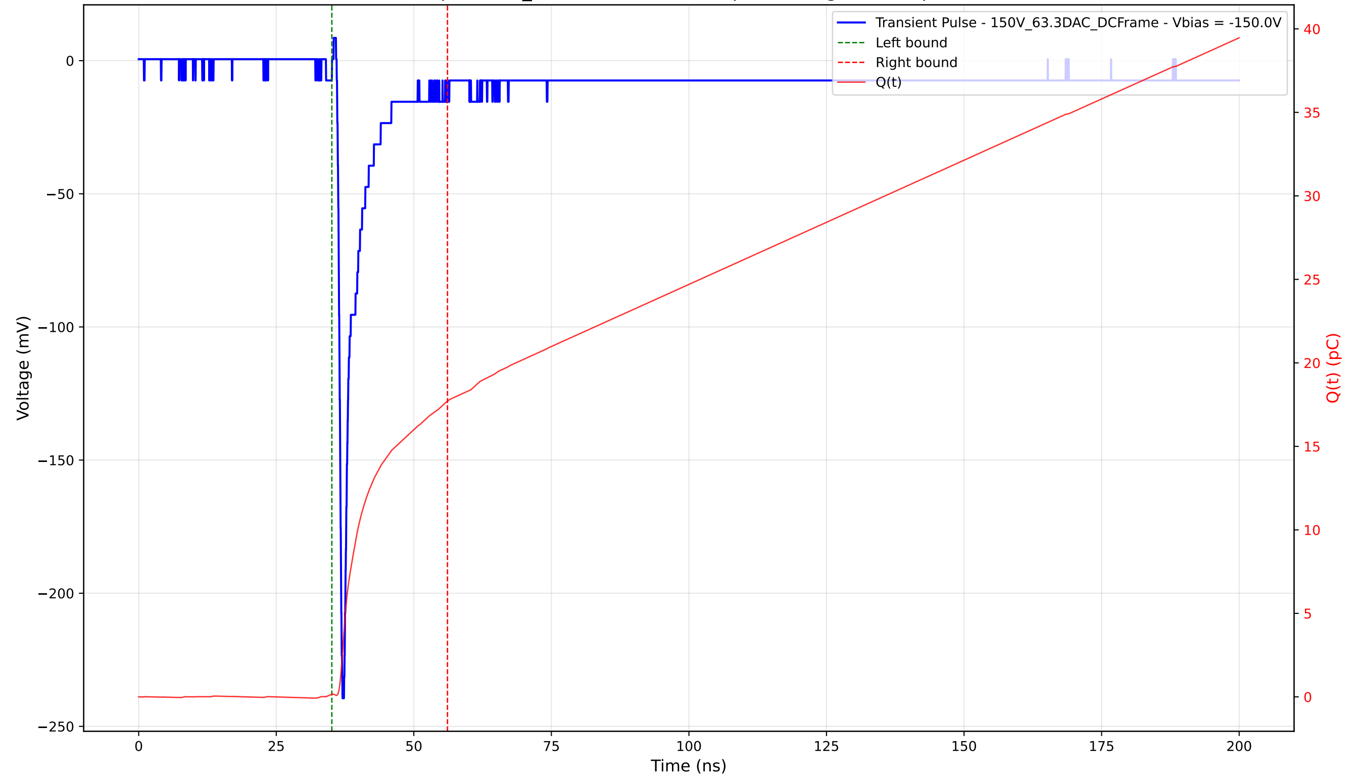
Transient Pulse - Sample: 1cm_42 - Position: 4815.0 \mu\text{m} - Charge: 17.55 pC - Rise Time: 0.76 ns
