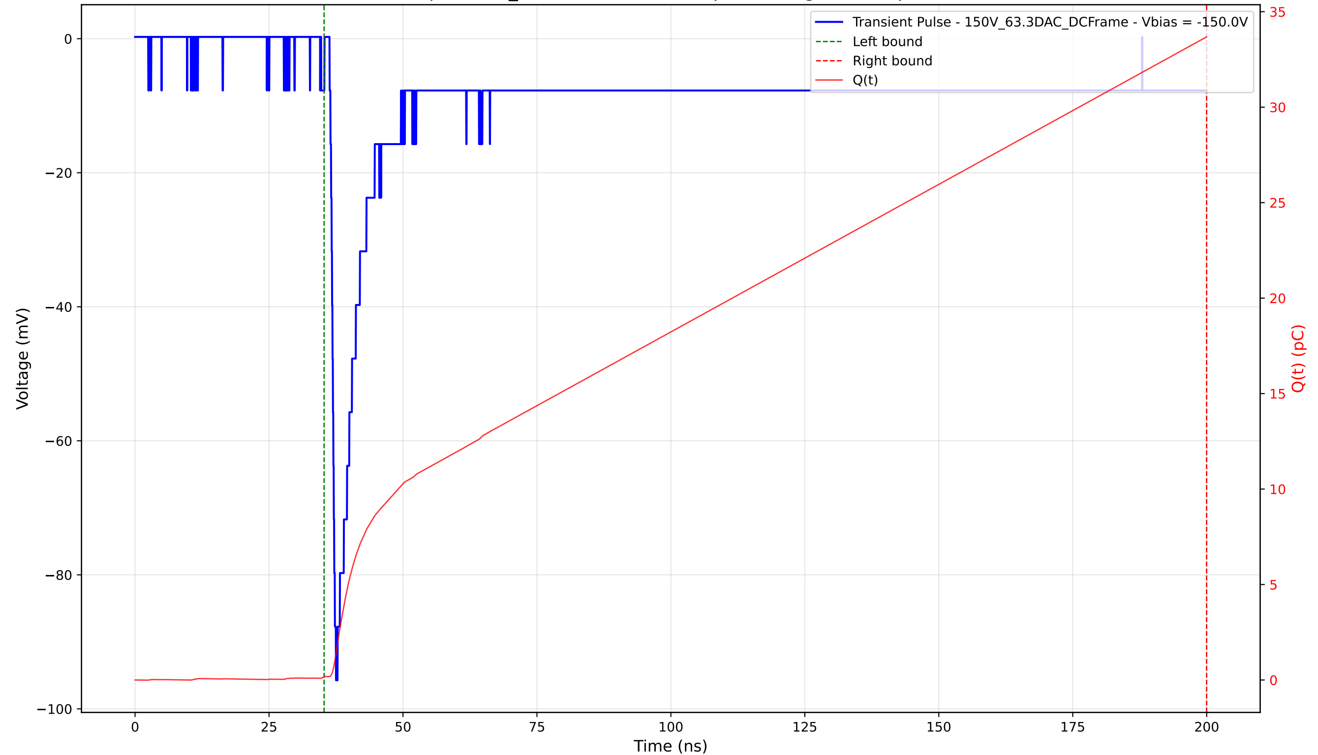
Transient Pulse - Sample: 1cm_42 - Position: 4330.0 \mu\text{m} - Charge: 33.51 pC - Rise Time: 0.84 ns
