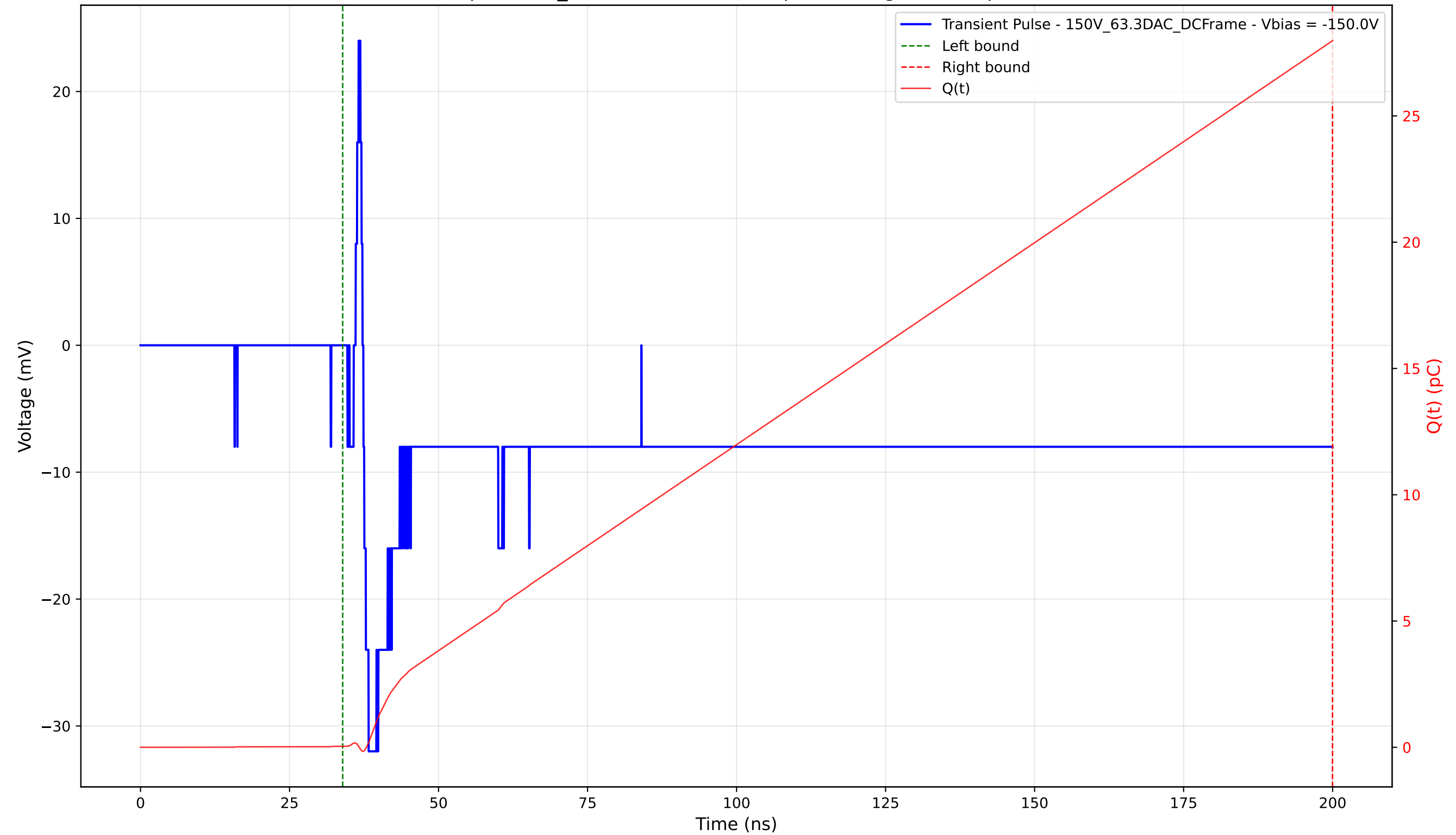
Transient Pulse - Sample: 1cm_42 - Position: 2395.0 \mu\text{m} - Charge: 27.94 pC - Rise Time: 0.87 ns
