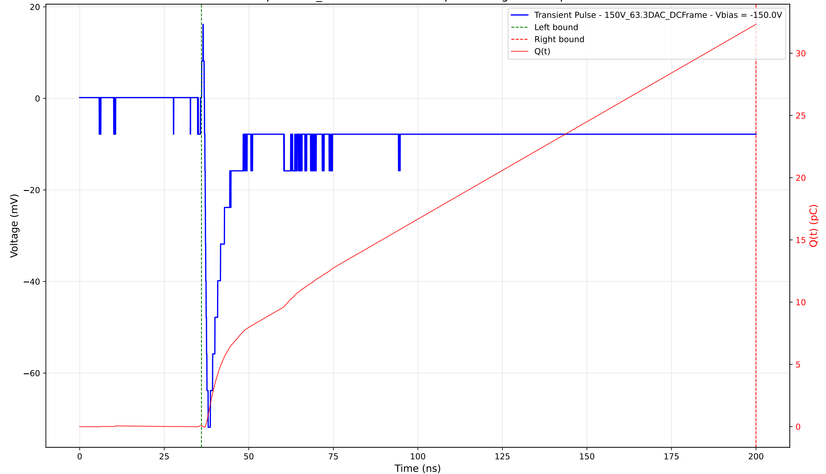
Transient Pulse - Sample: 1cm_42 - Position: 1290.0 \mu\text{m} - Charge: 32.23 pC - Rise Time: 1.08 ns
