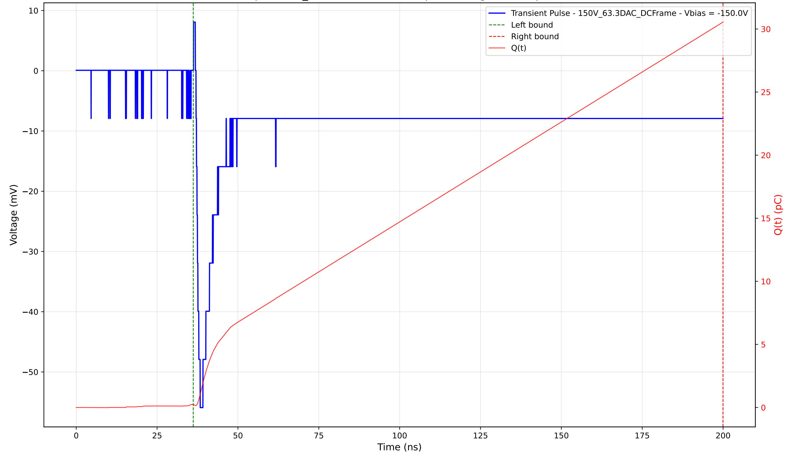
Transient Pulse - Sample: 1cm_42 - Position: 3750.0 \mu\text{m} - Charge: 30.31 pC - Rise Time: 1.29 ns
