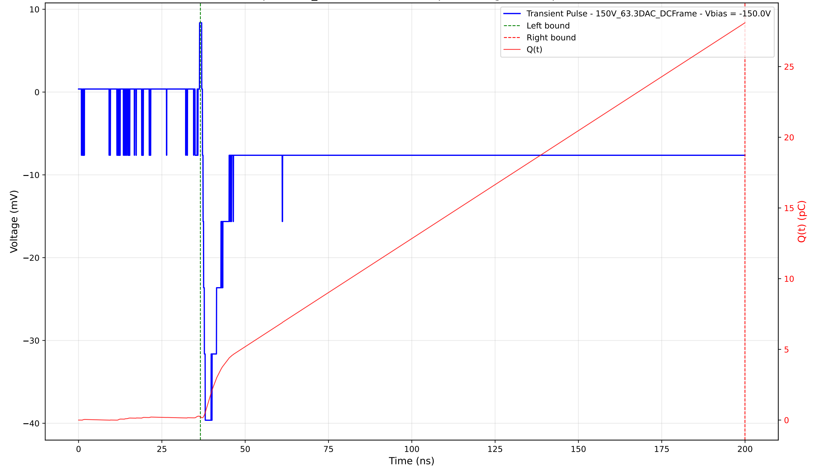
Transient Pulse - Sample: 1cm_42 - Position: 3585.0 \mu\text{m} - Charge: 27.87 pC - Rise Time: 0.83 ns
