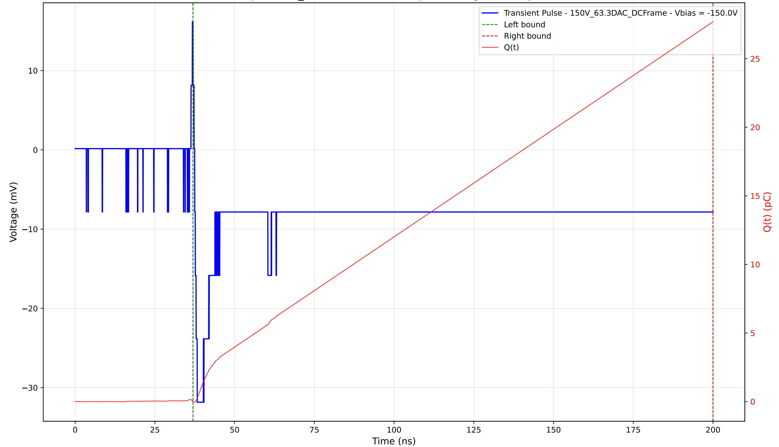
Transient Pulse - Sample: 1cm_42 - Position: 3090.0 \mu\text{m} - Charge: 27.68 pC - Rise Time: 0.79 ns
