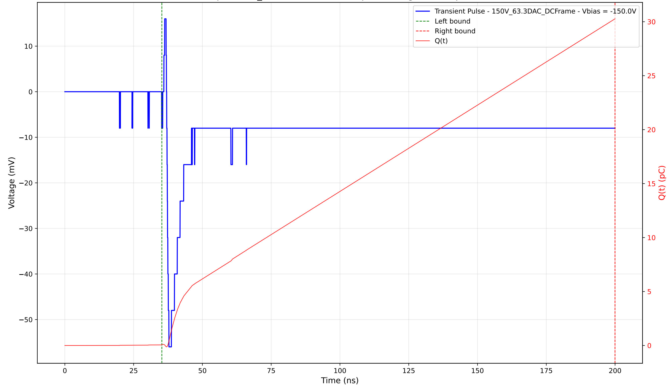
Transient Pulse - Sample: 1cm_42 - Position: 1420.0 \mu\text{m} - Charge: 30.21 pC - Rise Time: 0.81 ns
