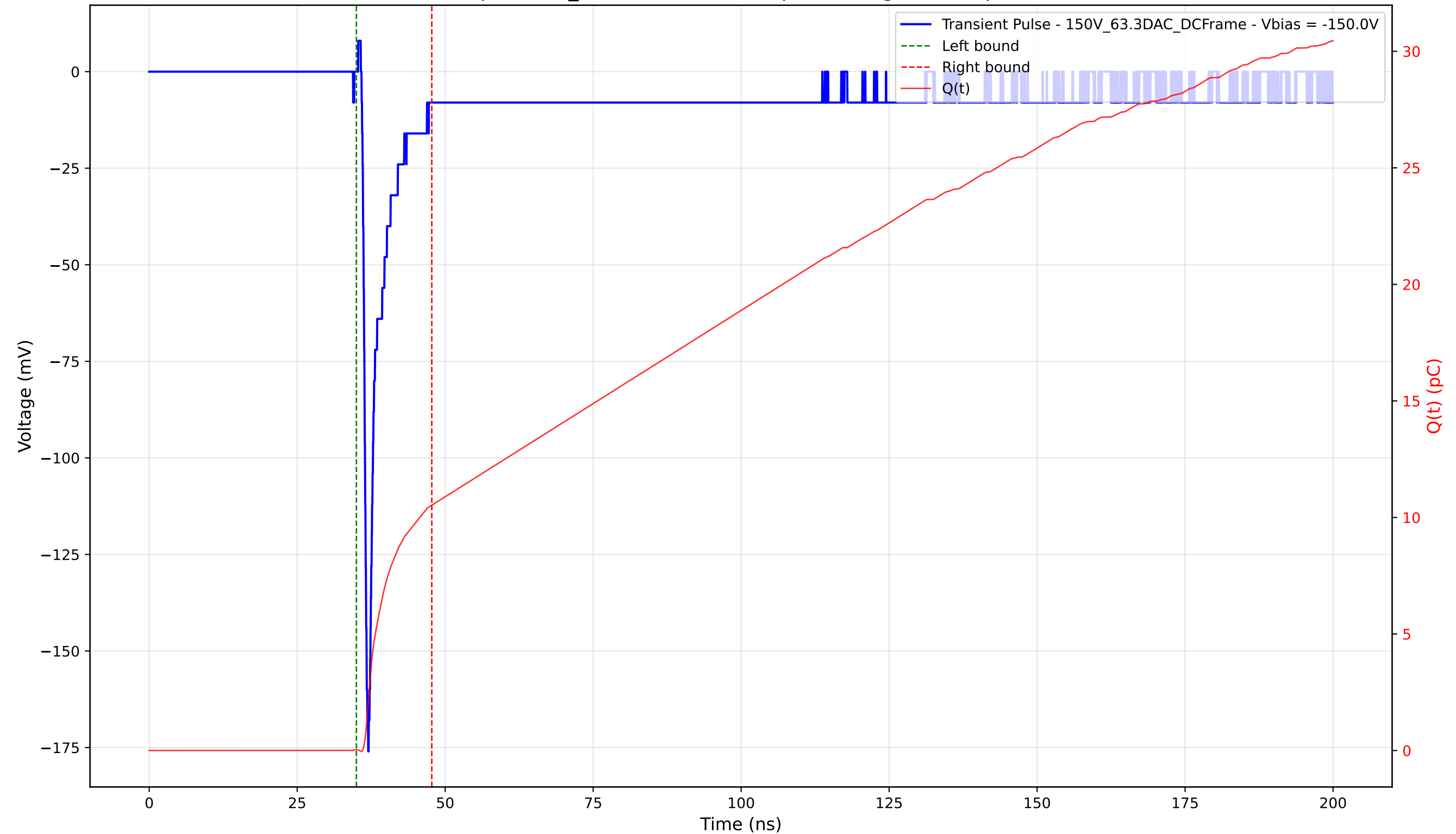
Transient Pulse - Sample: 1cm_42 - Position: 300.0 \mu\text{m} - Charge: 10.50 pC - Rise Time: 0.74 ns
