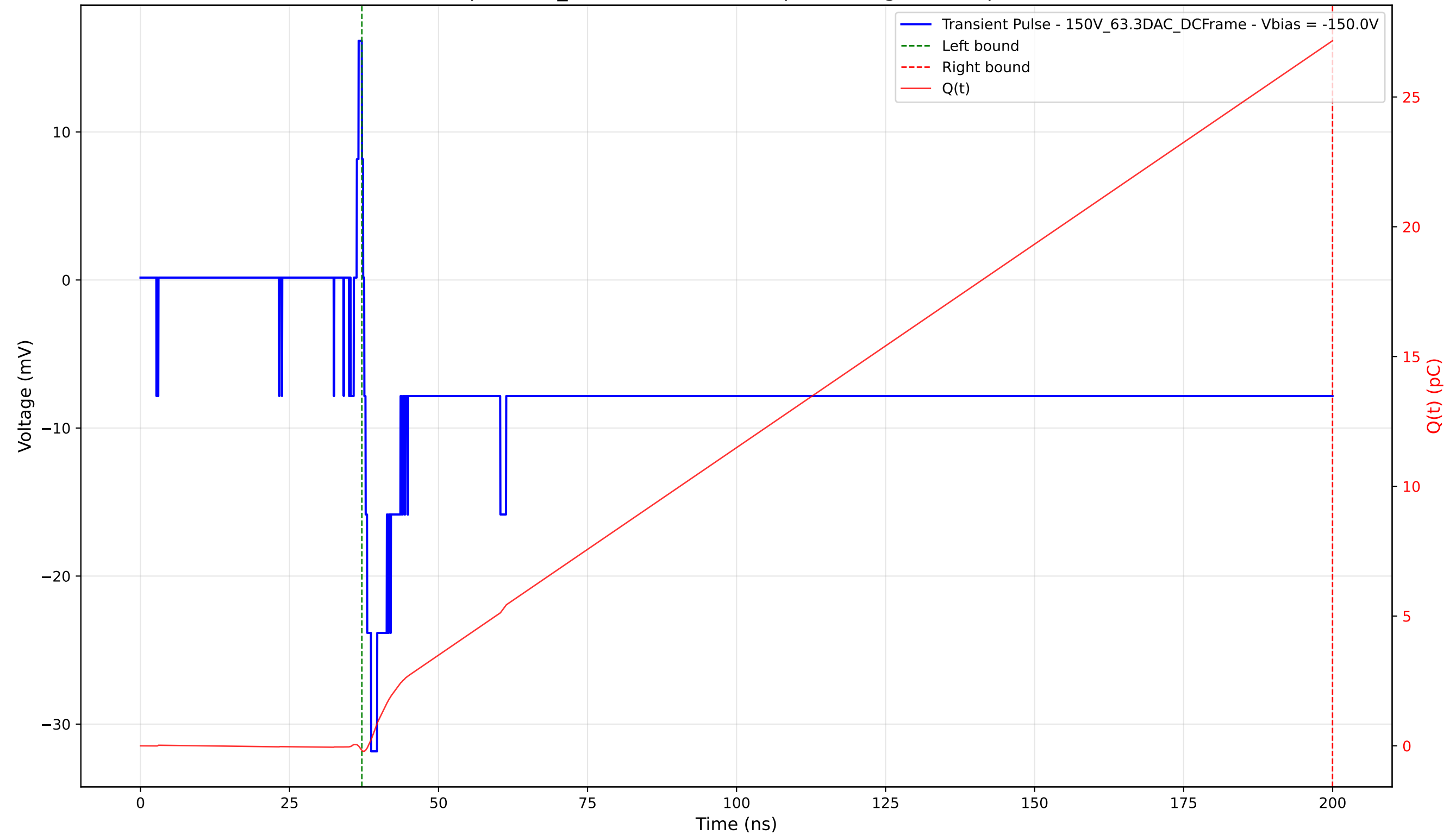
Transient Pulse - Sample: 1cm_42 - Position: 2880.0 \mu\text{m} - Charge: 27.35 pC - Rise Time: 1.15 ns
