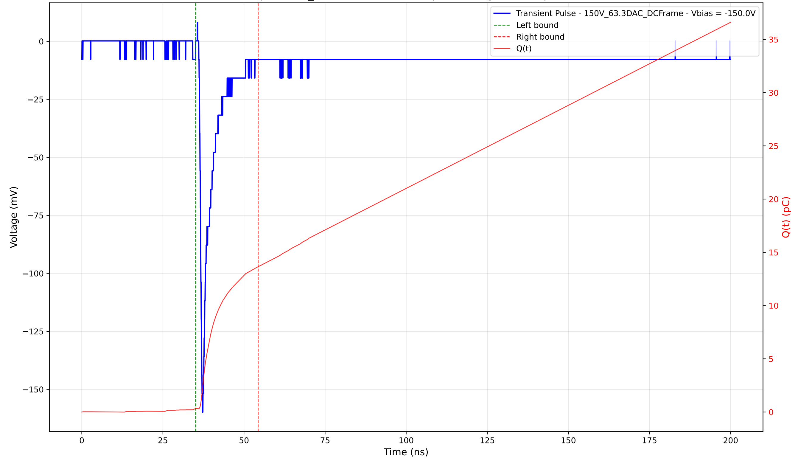
Transient Pulse - Sample: 1cm_42 - Position: 4600.0 \mu\text{m} - Charge: 13.31 pC - Rise Time: 0.84 ns
