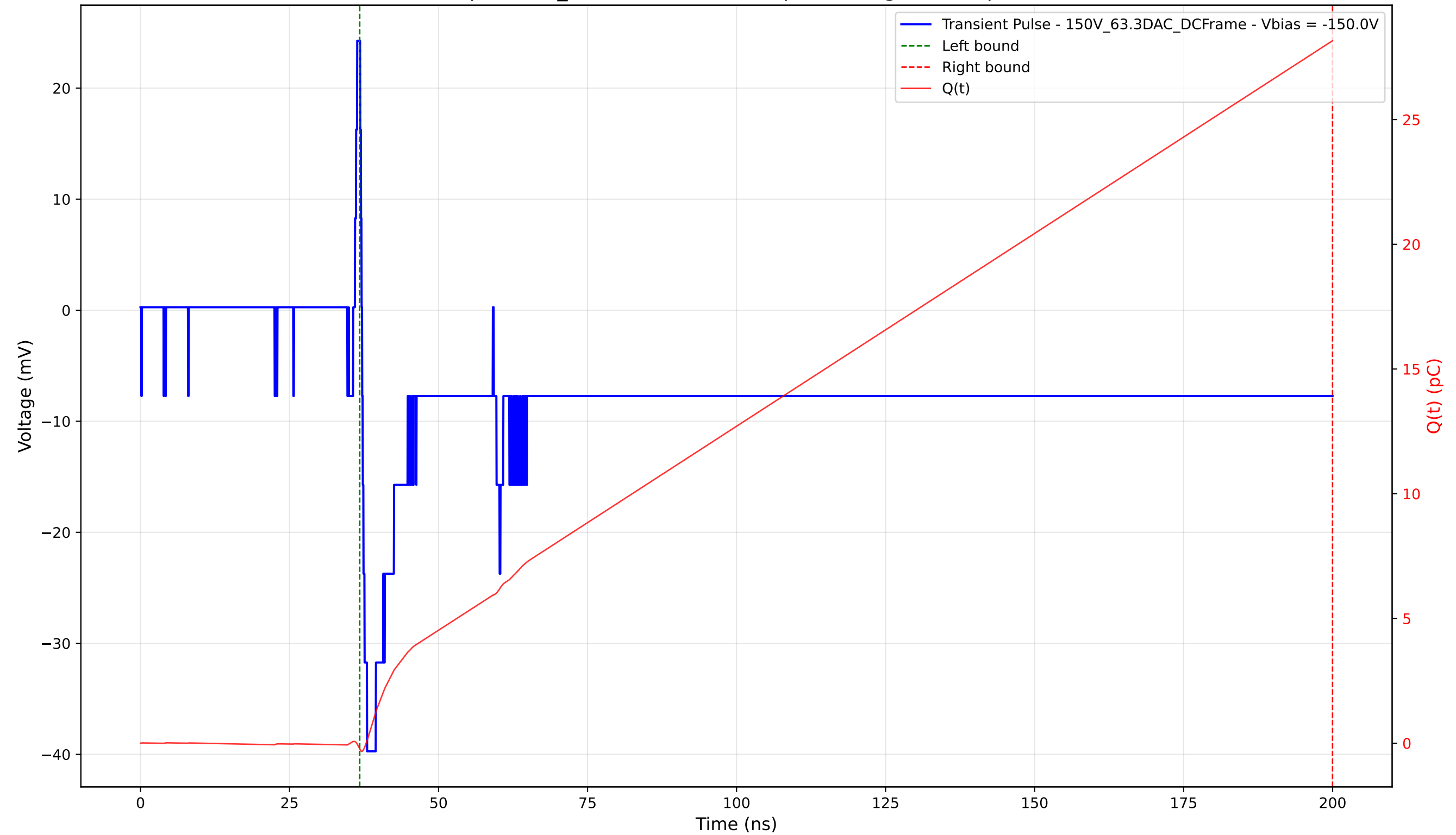
Transient Pulse - Sample: 1cm_42 - Position: 1890.0 \mu\text{m} - Charge: 28.40 pC - Rise Time: 0.83 ns
