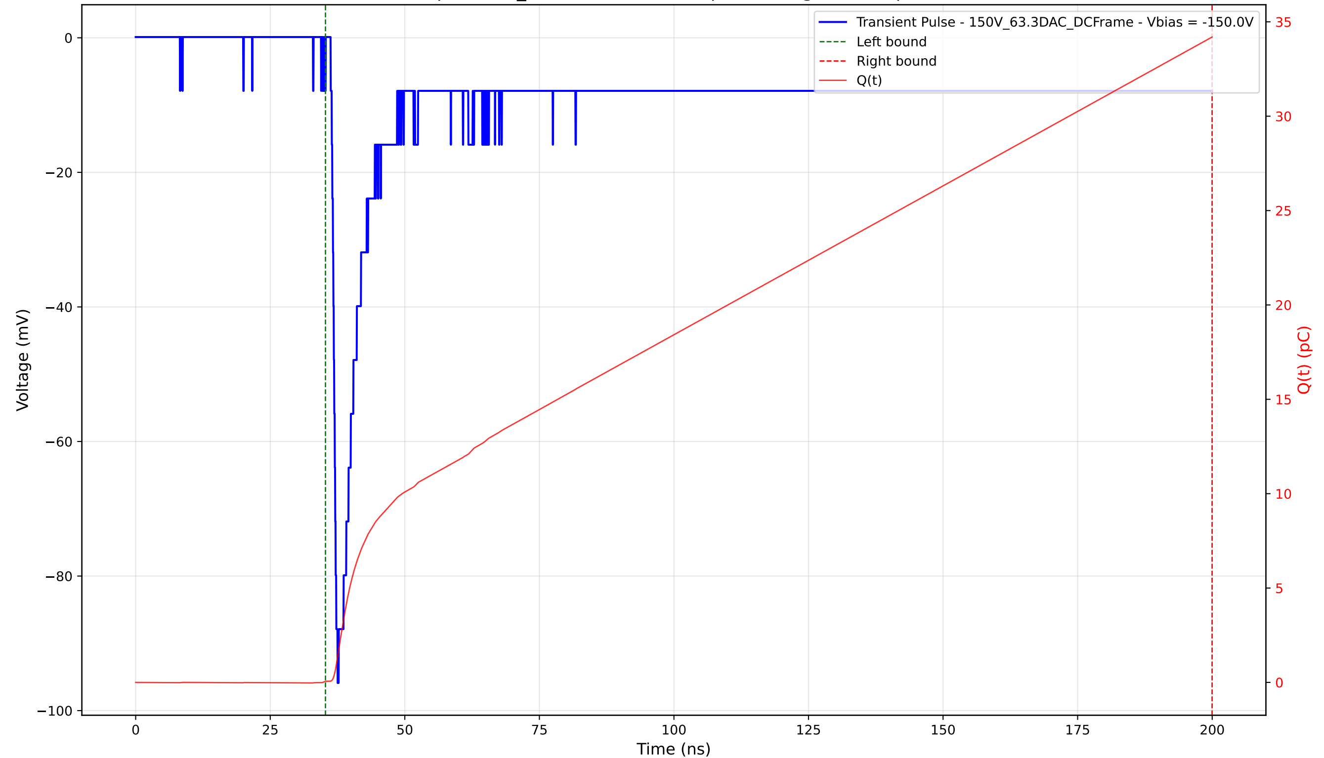
Transient Pulse - Sample: 1cm_42 - Position: 890.0 \mu\text{m} - Charge: 34.14 pC - Rise Time: 0.86 ns
