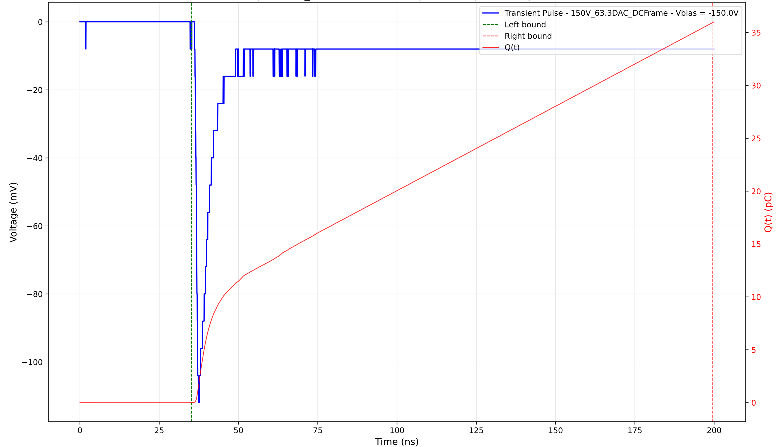
Transient Pulse - Sample: 1cm_42 - Position: 820.0 \mu\text{m} - Charge: 35.93 pC - Rise Time: 0.87 ns
