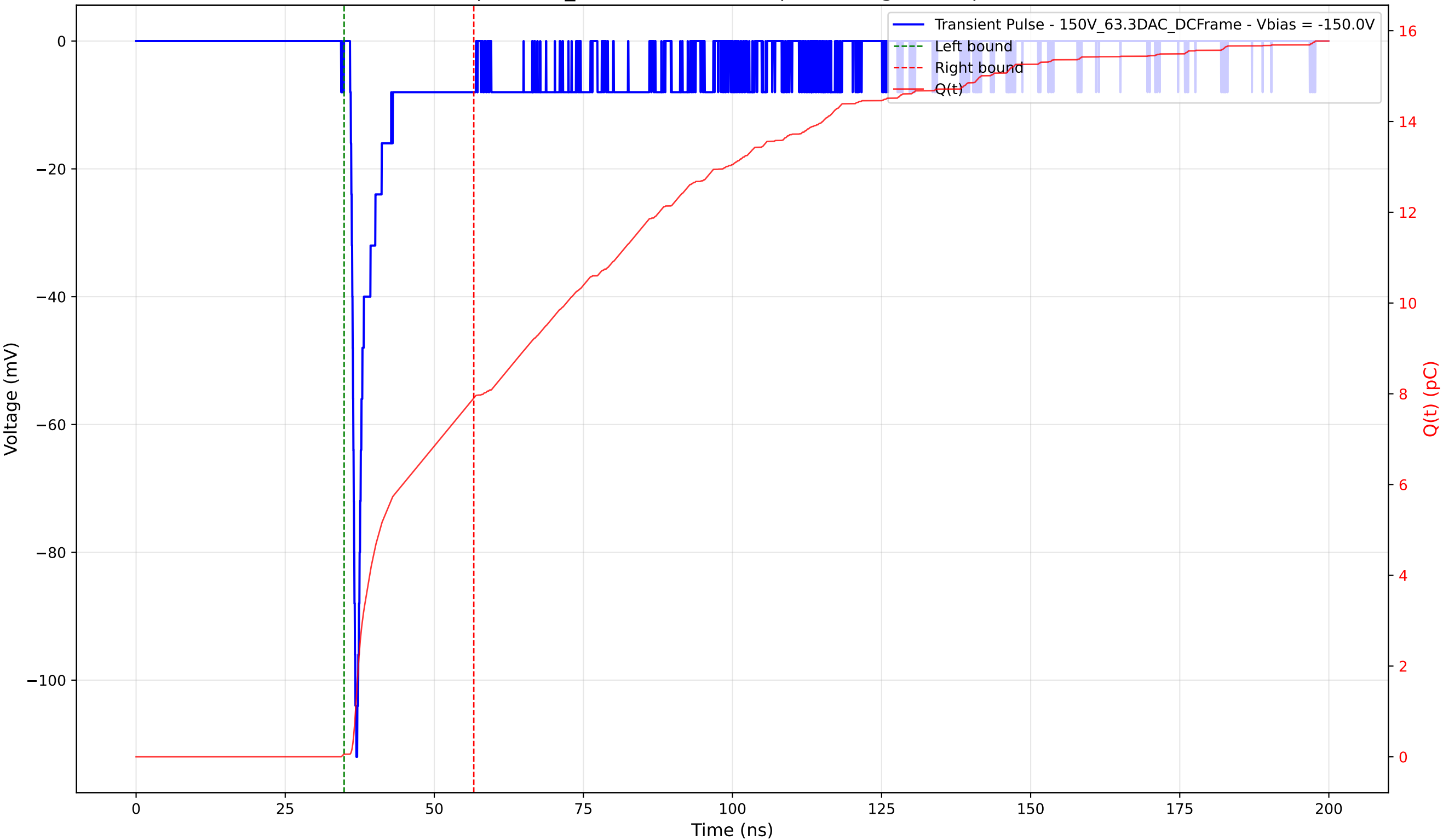
Transient Pulse - Sample: 1cm_42 - Position: 140.0 \mu\text{m} - Charge: 7.85 pC - Rise Time: 0.77 ns
