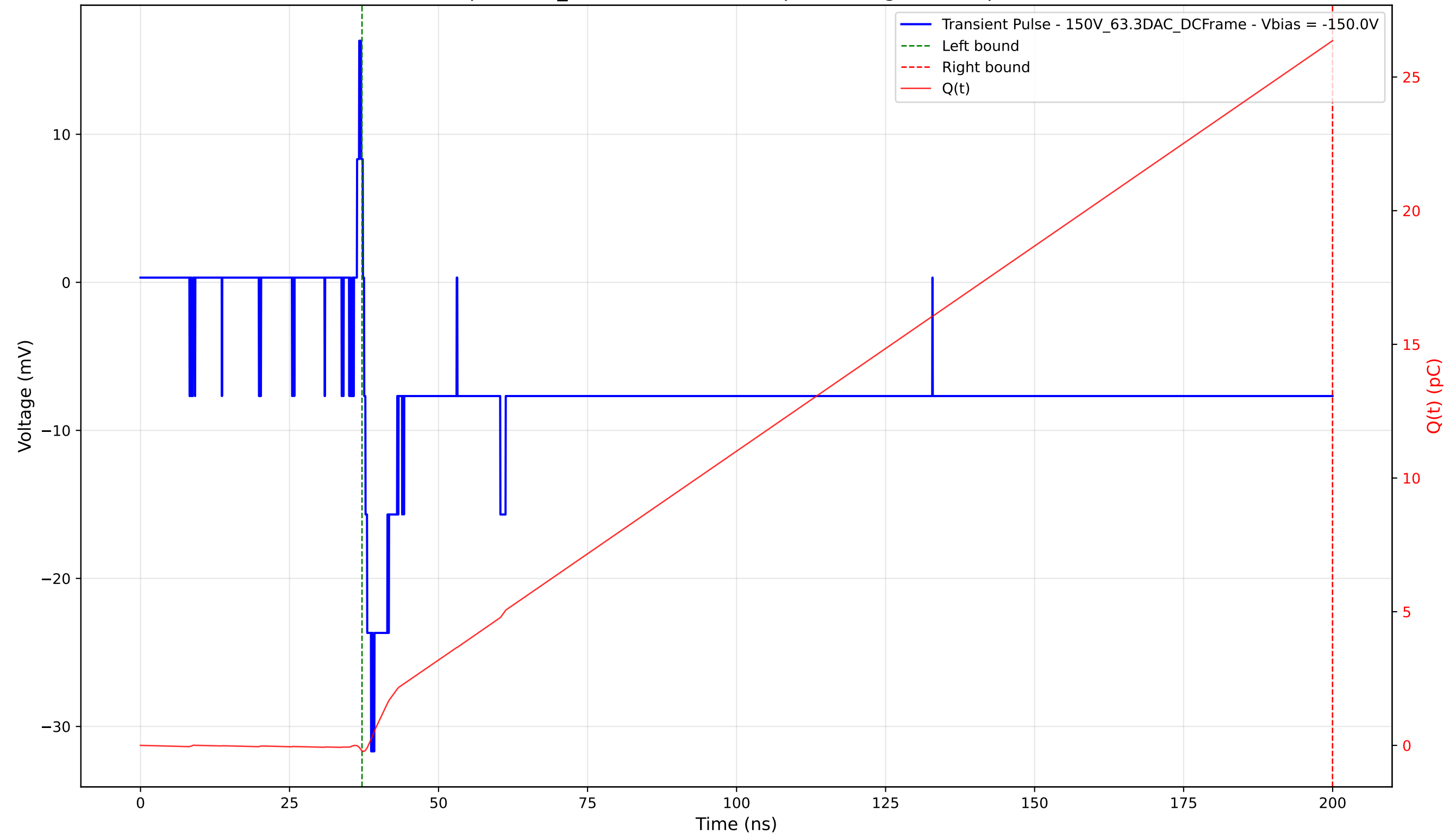
Transient Pulse - Sample: 1cm_42 - Position: 2960.0 \mu\text{m} - Charge: 26.56 pC - Rise Time: 1.17 ns
