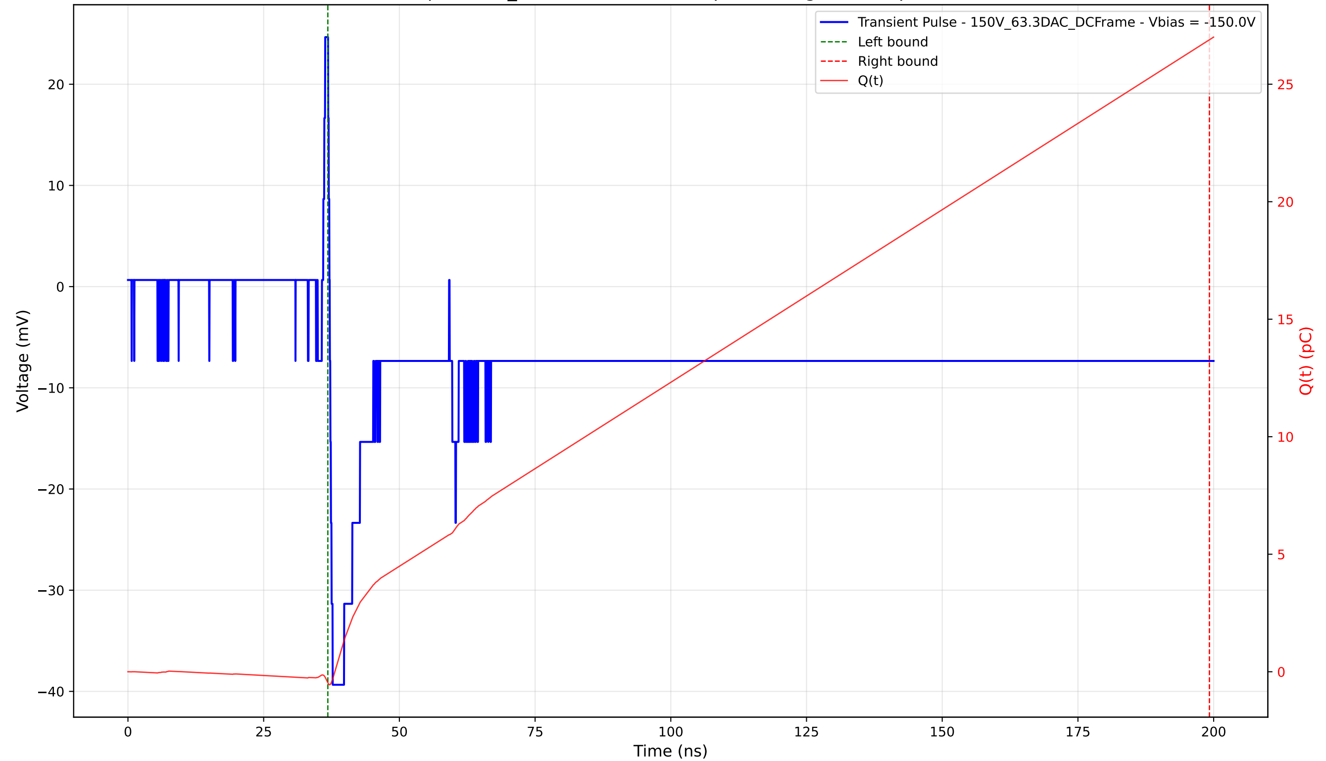
Transient Pulse - Sample: 1cm_42 - Position: 1845.0 \mu\text{m} - Charge: 27.36 pC - Rise Time: 0.53 ns
