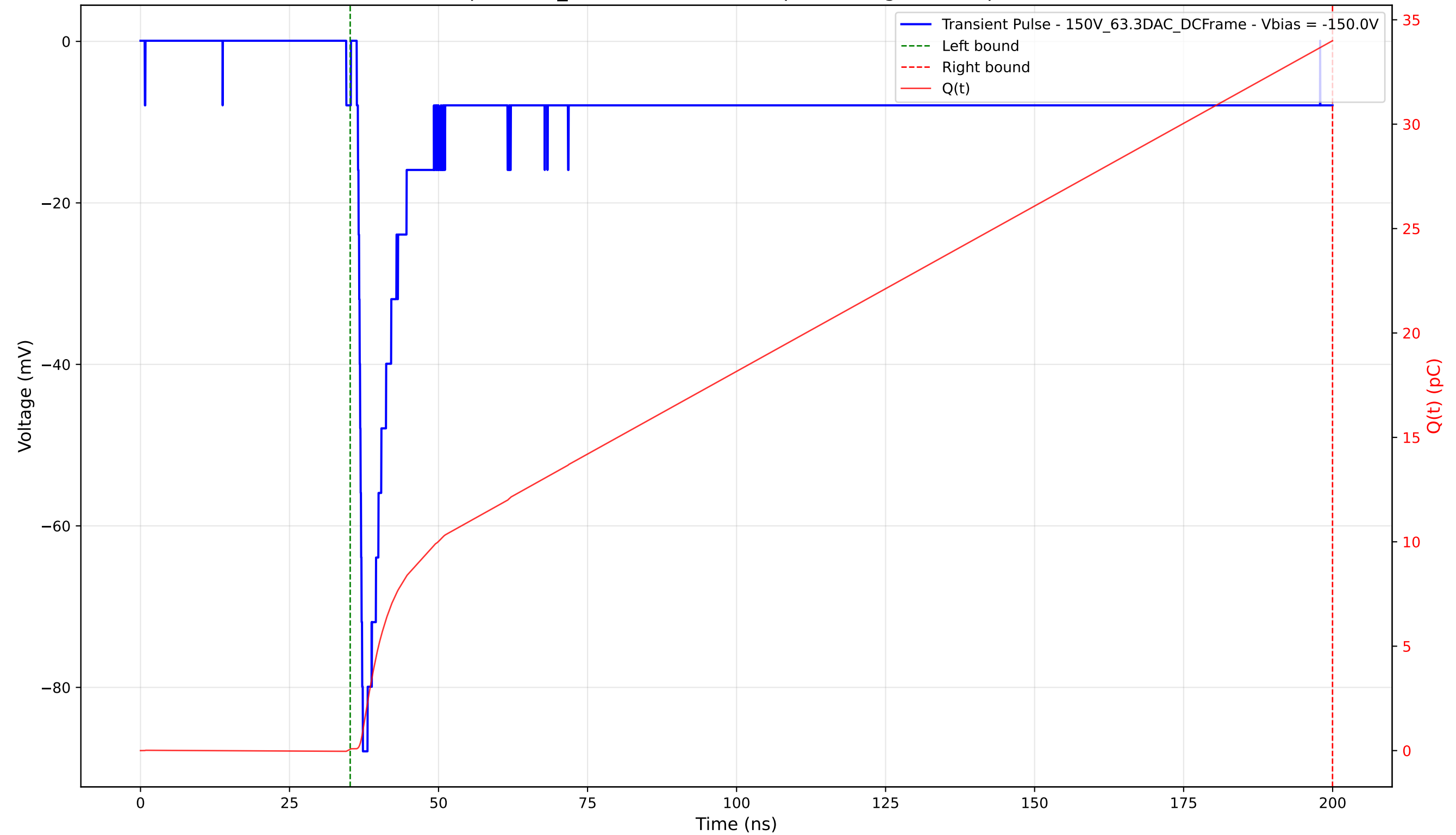
Transient Pulse - Sample: 1cm_42 - Position: 4340.0 \mu\text{m} - Charge: 33.93 pC - Rise Time: 0.72 ns
