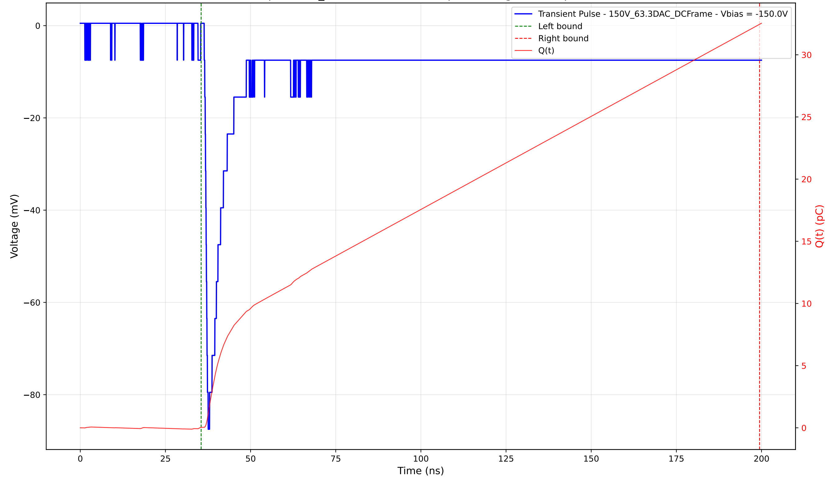
Transient Pulse - Sample: 1cm_42 - Position: 4205.0 \mu\text{m} - Charge: 32.41 pC - Rise Time: 0.80 ns
