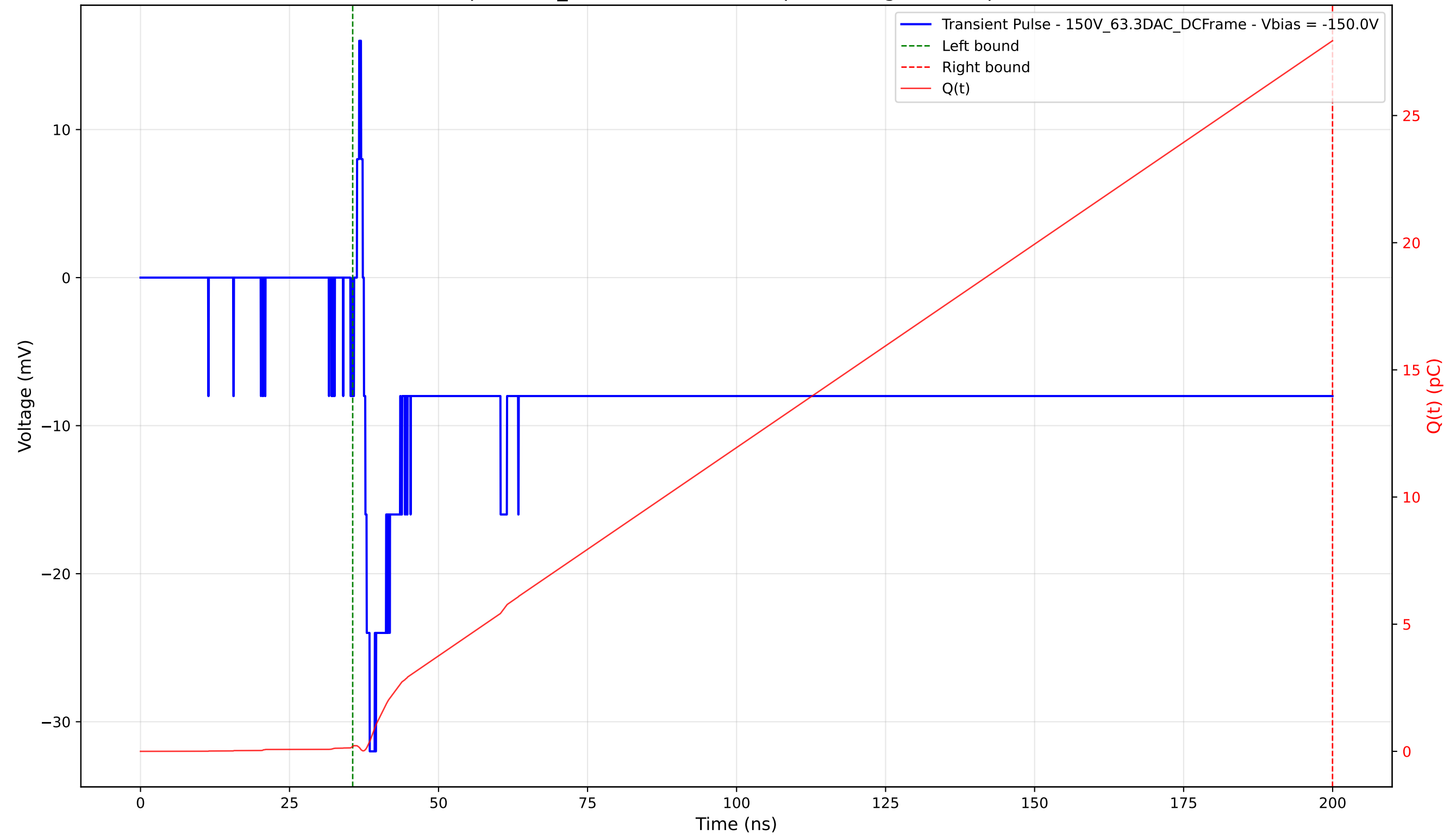
Transient Pulse - Sample: 1cm_42 - Position: 3035.0 \mu\text{m} - Charge: 27.75 pC - Rise Time: 0.97 ns
