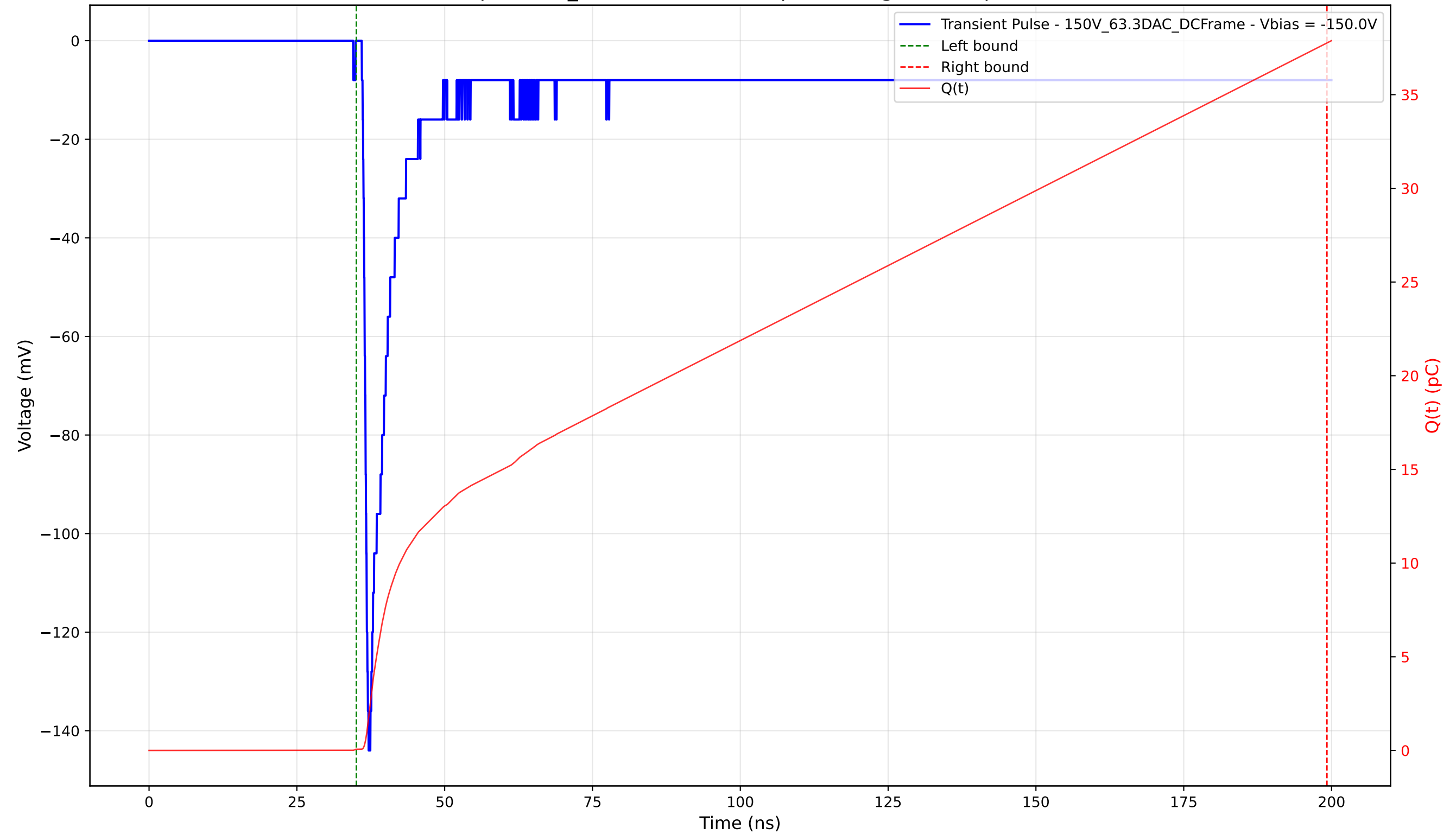
Transient Pulse - Sample: 1cm_42 - Position: 595.0 \mu\text{m} - Charge: 37.70 pC - Rise Time: 0.88 ns
