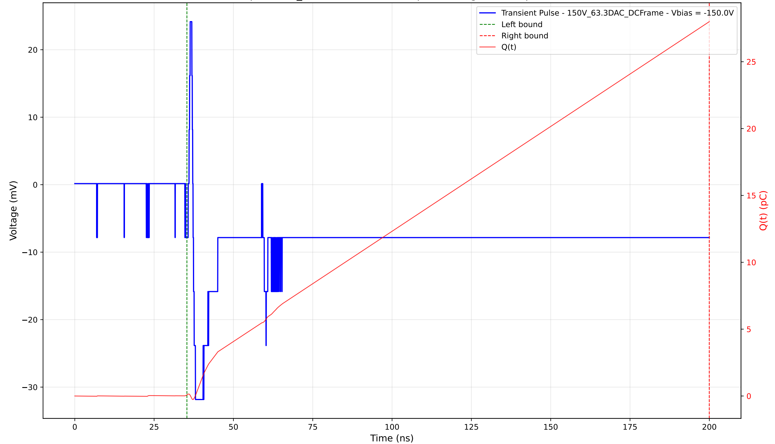
Transient Pulse - Sample: 1cm_42 - Position: 2145.0 \mu\text{m} - Charge: 27.91 pC - Rise Time: 0.75 ns
