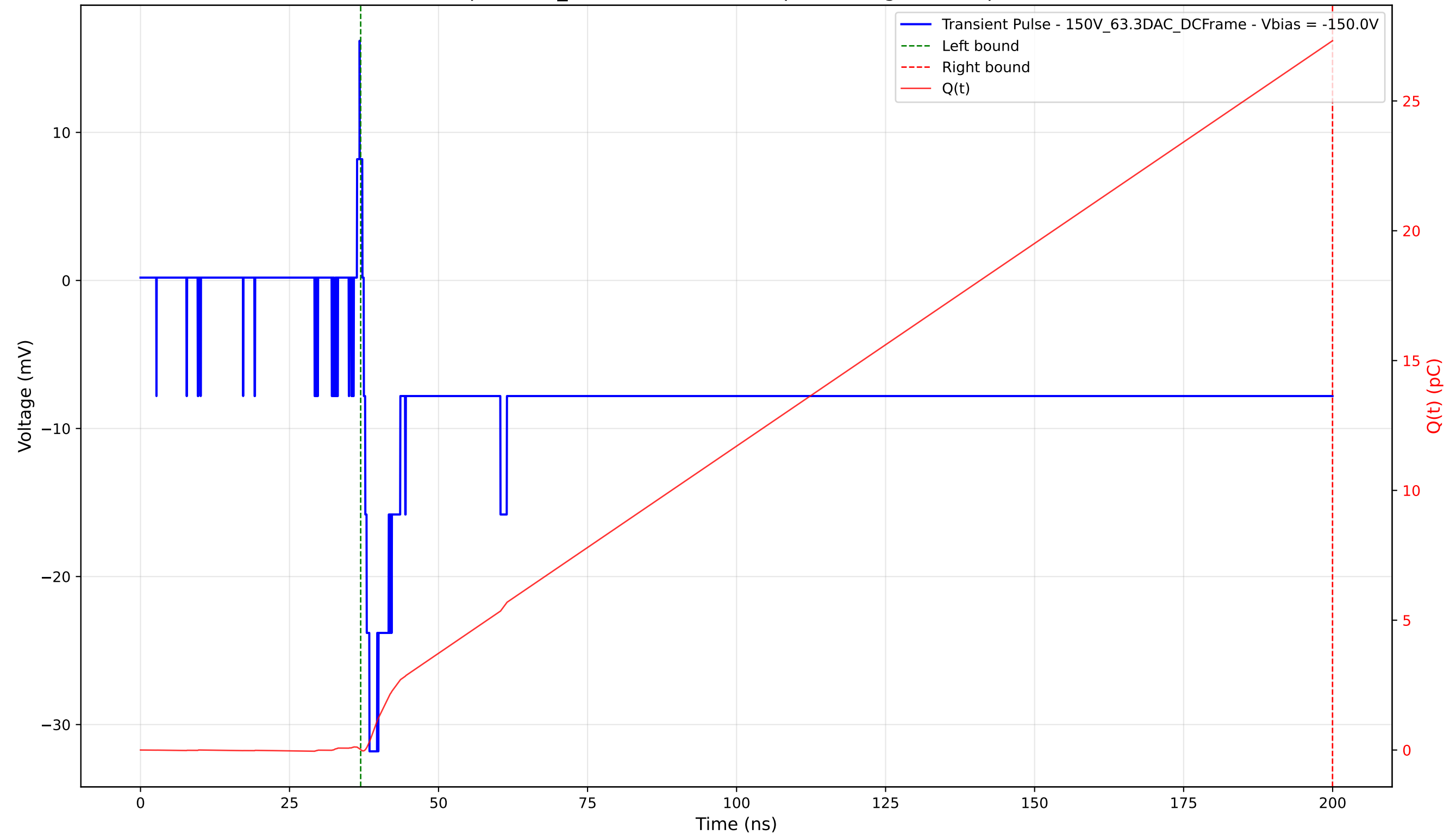
Transient Pulse - Sample: 1cm_42 - Position: 3075.0 \mu\text{m} - Charge: 27.31 pC - Rise Time: 0.95 ns
