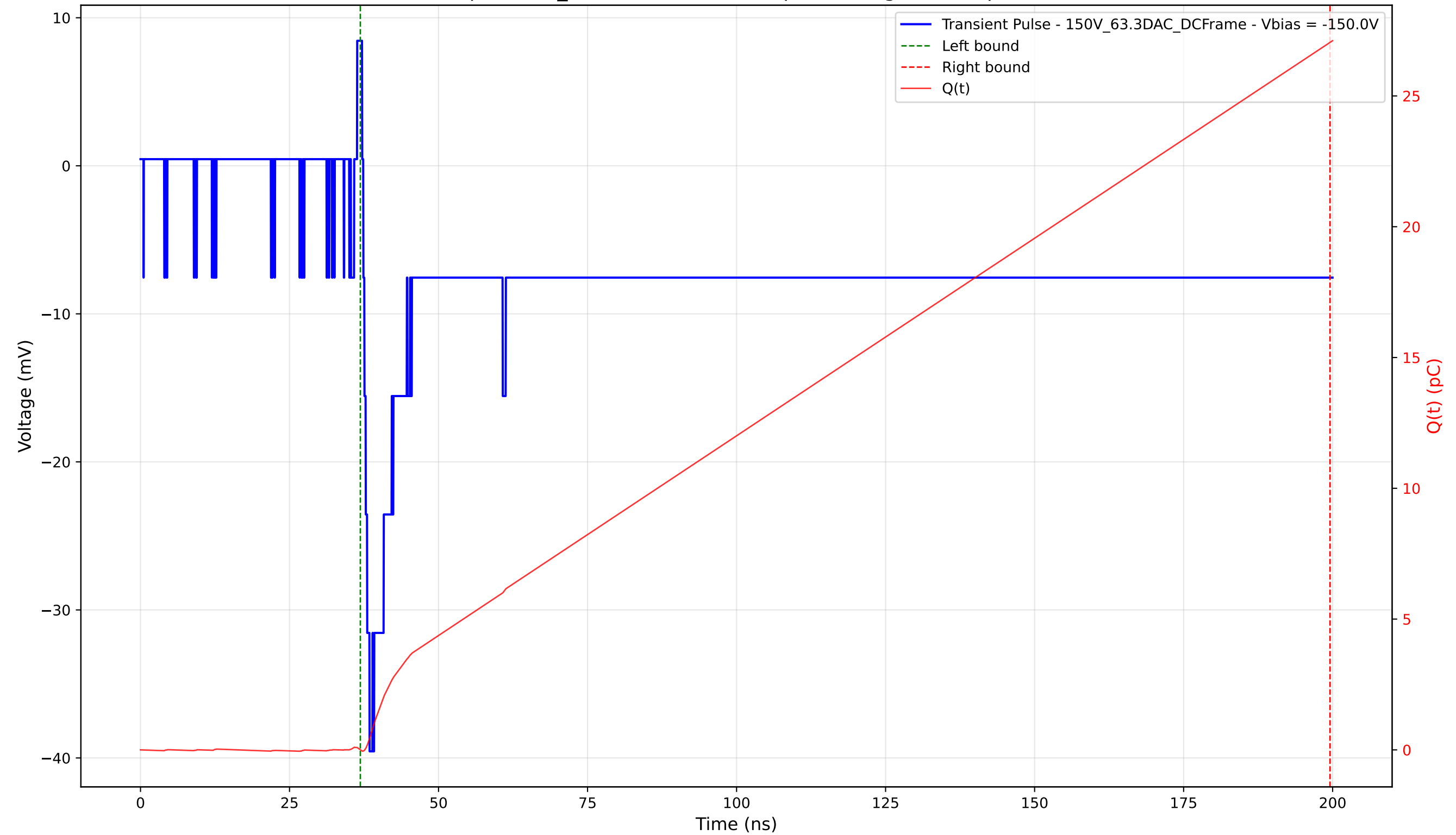
Transient Pulse - Sample: 1cm_42 - Position: 3390.0 \mu\text{m} - Charge: 27.04 pC - Rise Time: 1.05 ns
