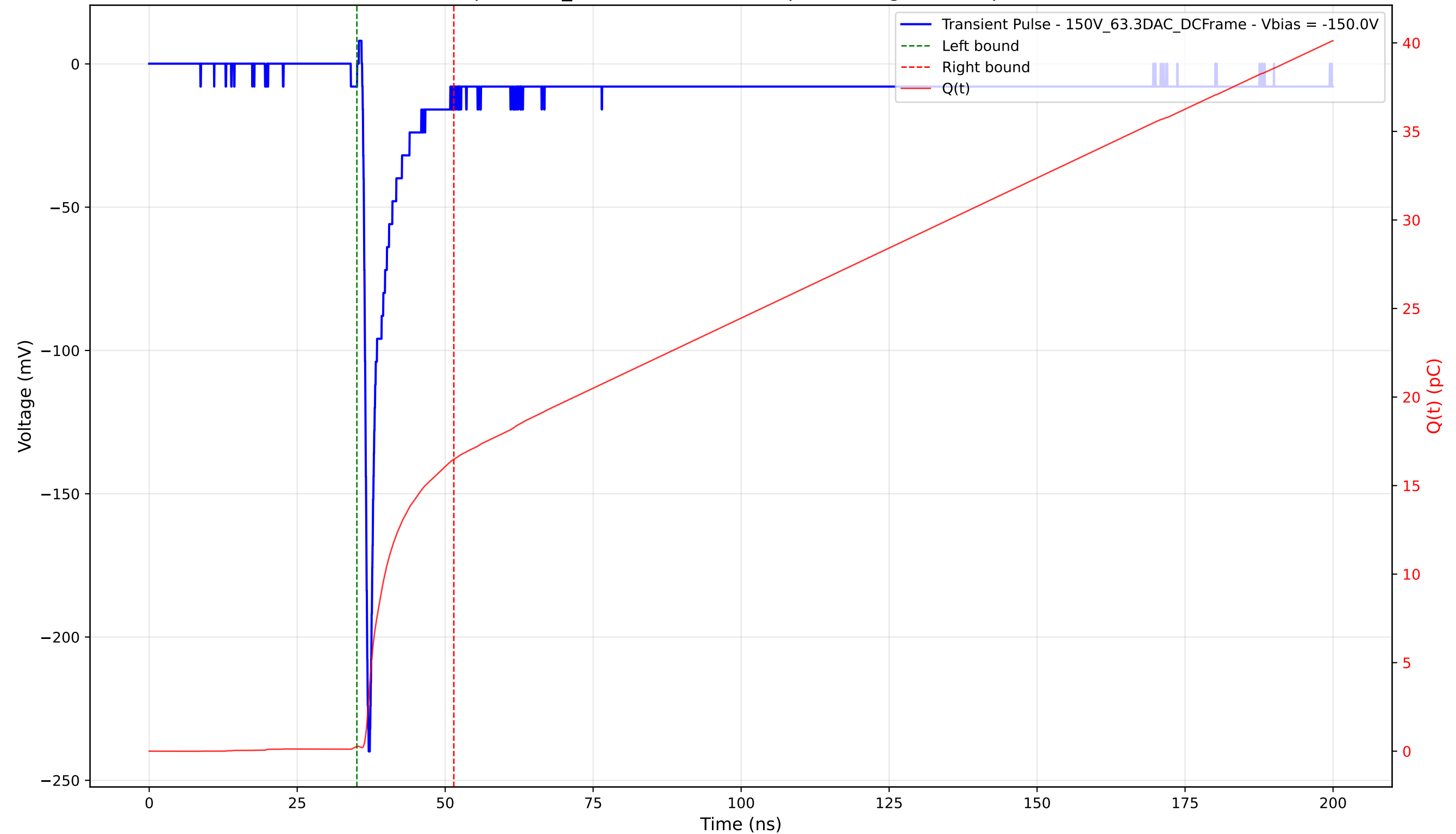
Transient Pulse - Sample: 1cm_42 - Position: 4825.0 \mu\text{m} - Charge: 16.22 pC - Rise Time: 0.78 ns
