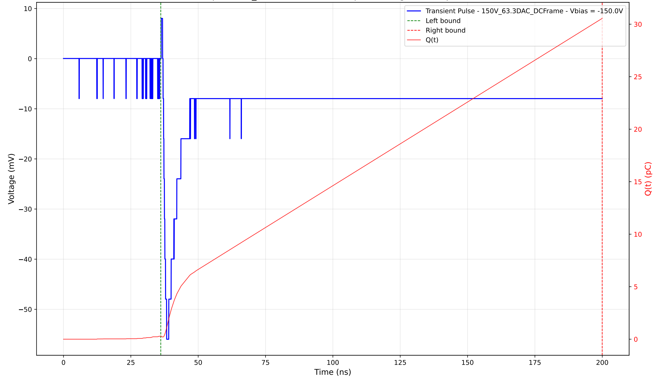
Transient Pulse - Sample: 1cm_42 - Position: 3835.0 \mu\text{m} - Charge: 30.26 pC - Rise Time: 1.33 ns
