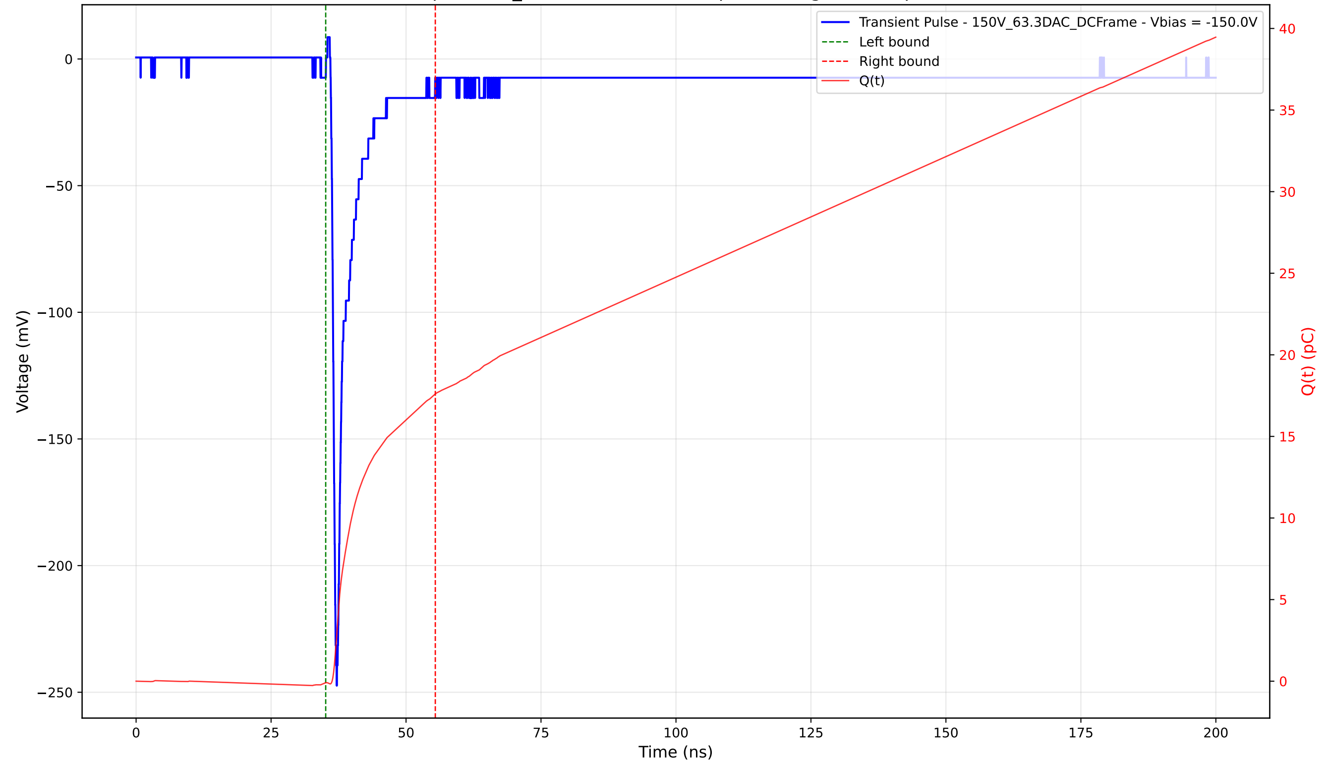
Transient Pulse - Sample: 1cm_42 - Position: 4765.0 \mu\text{m} - Charge: 17.70 pC - Rise Time: 0.78 ns
