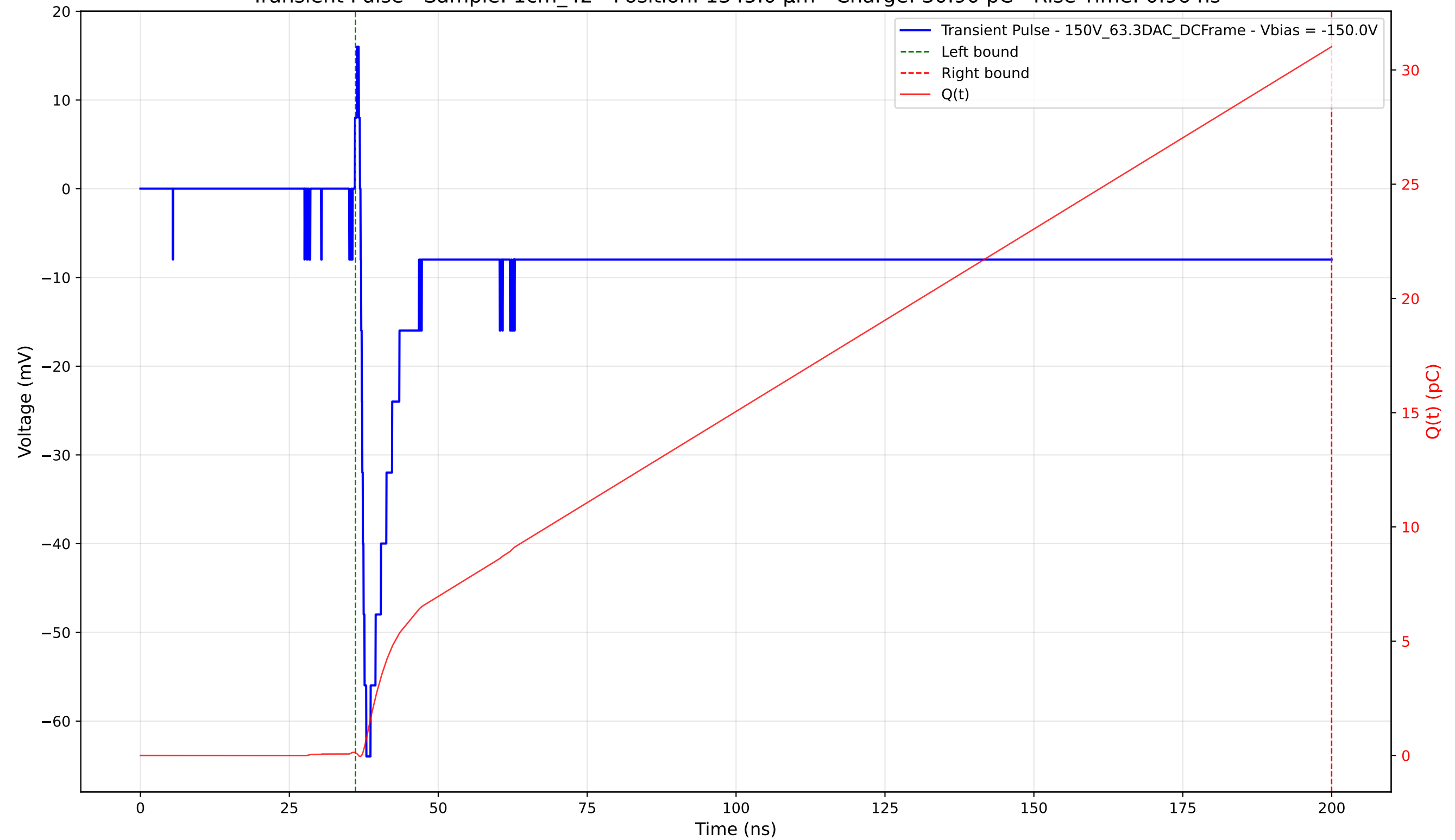
Transient Pulse - Sample: 1cm_42 - Position: 1345.0 \mu\text{m} - Charge: 30.90 pC - Rise Time: 0.96 ns
