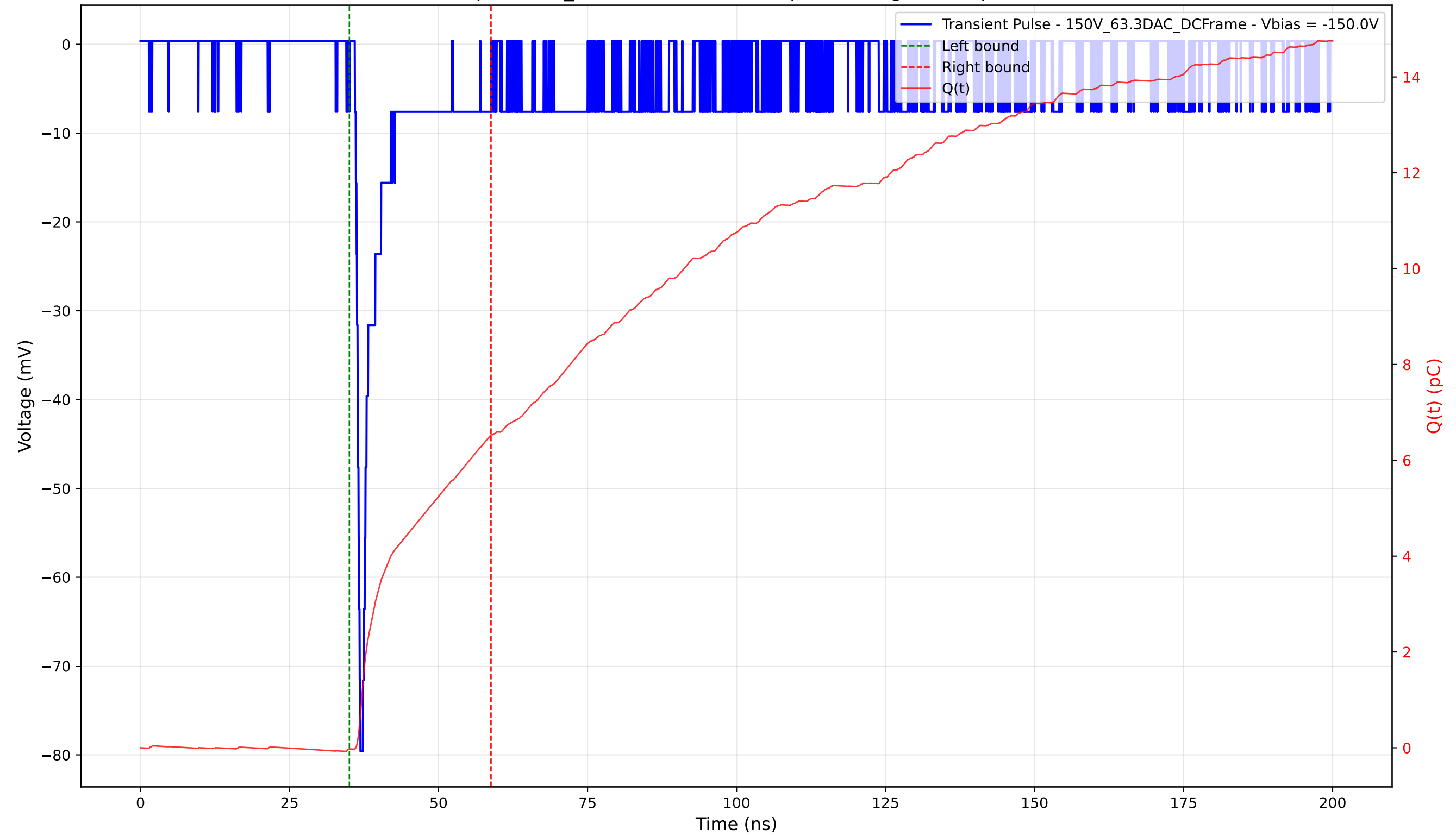
Transient Pulse - Sample: 1cm_42 - Position: 5075.0 \mu\text{m} - Charge: 6.56 pC - Rise Time: 0.78 ns
