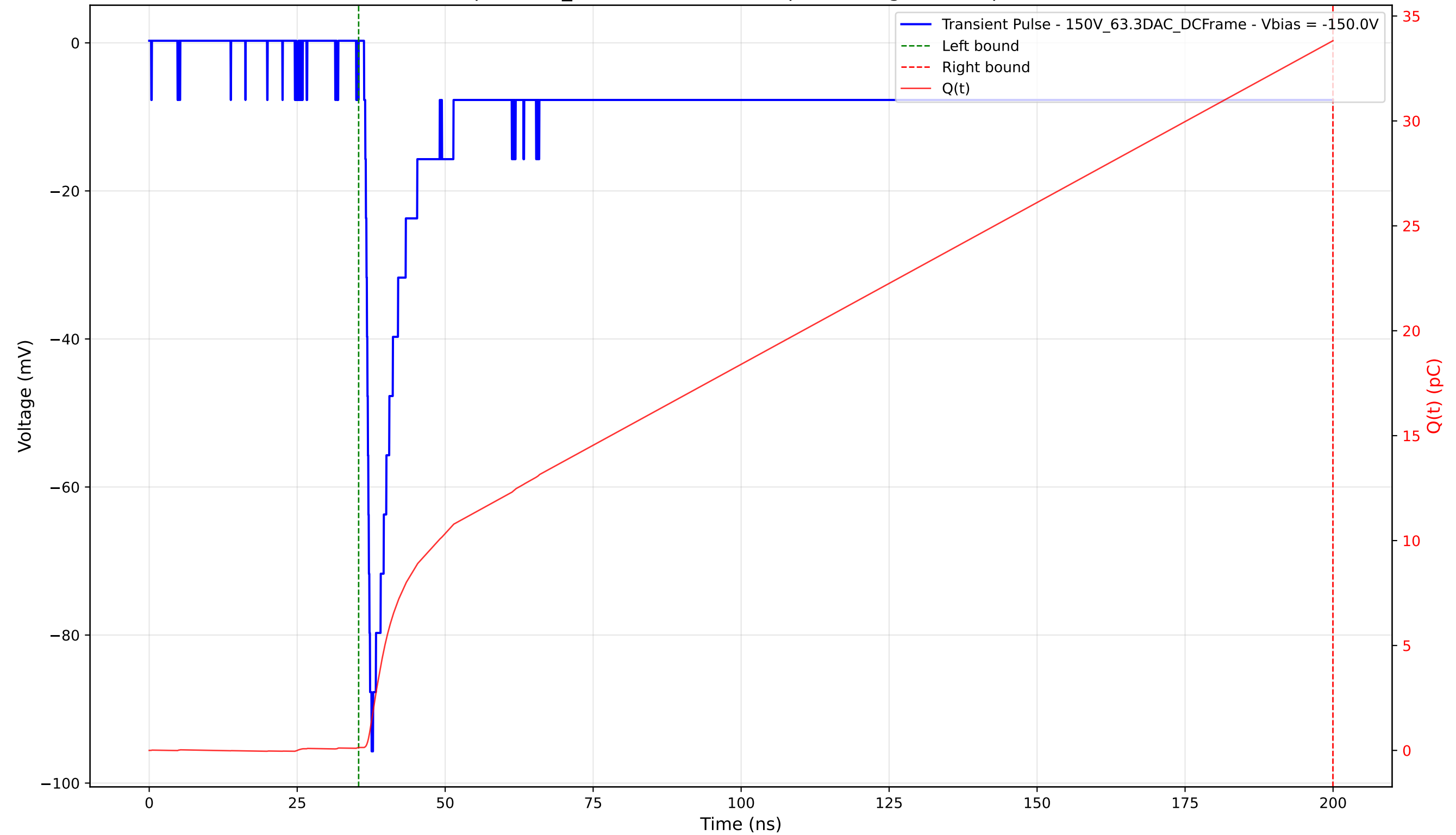
Transient Pulse - Sample: 1cm_42 - Position: 4305.0 \mu\text{m} - Charge: 33.68 pC - Rise Time: 0.82 ns
