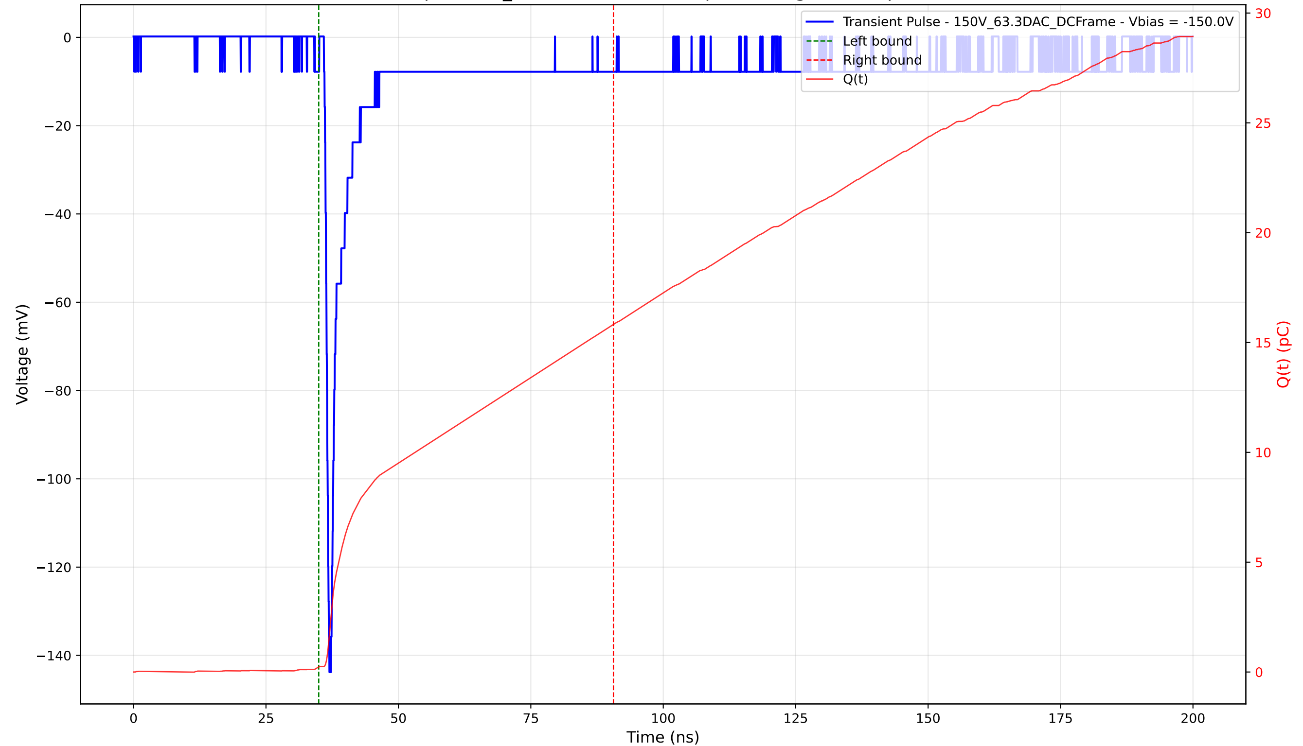
Transient Pulse - Sample: 1cm_42 - Position: 4985.0 \mu\text{m} - Charge: 15.59 pC - Rise Time: 0.80 ns
