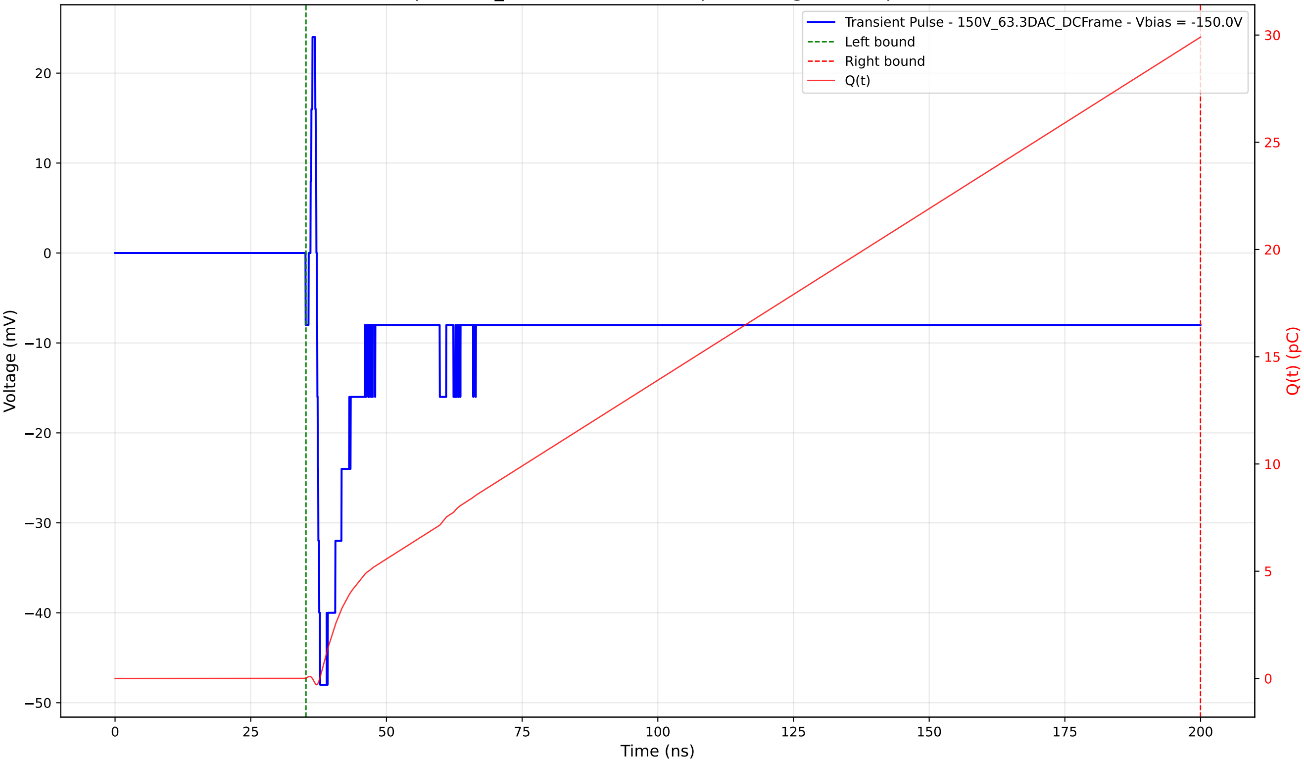
Transient Pulse - Sample: 1cm_42 - Position: 1630.0 \mu\text{m} - Charge: 29.89 pC - Rise Time: 0.59 ns
