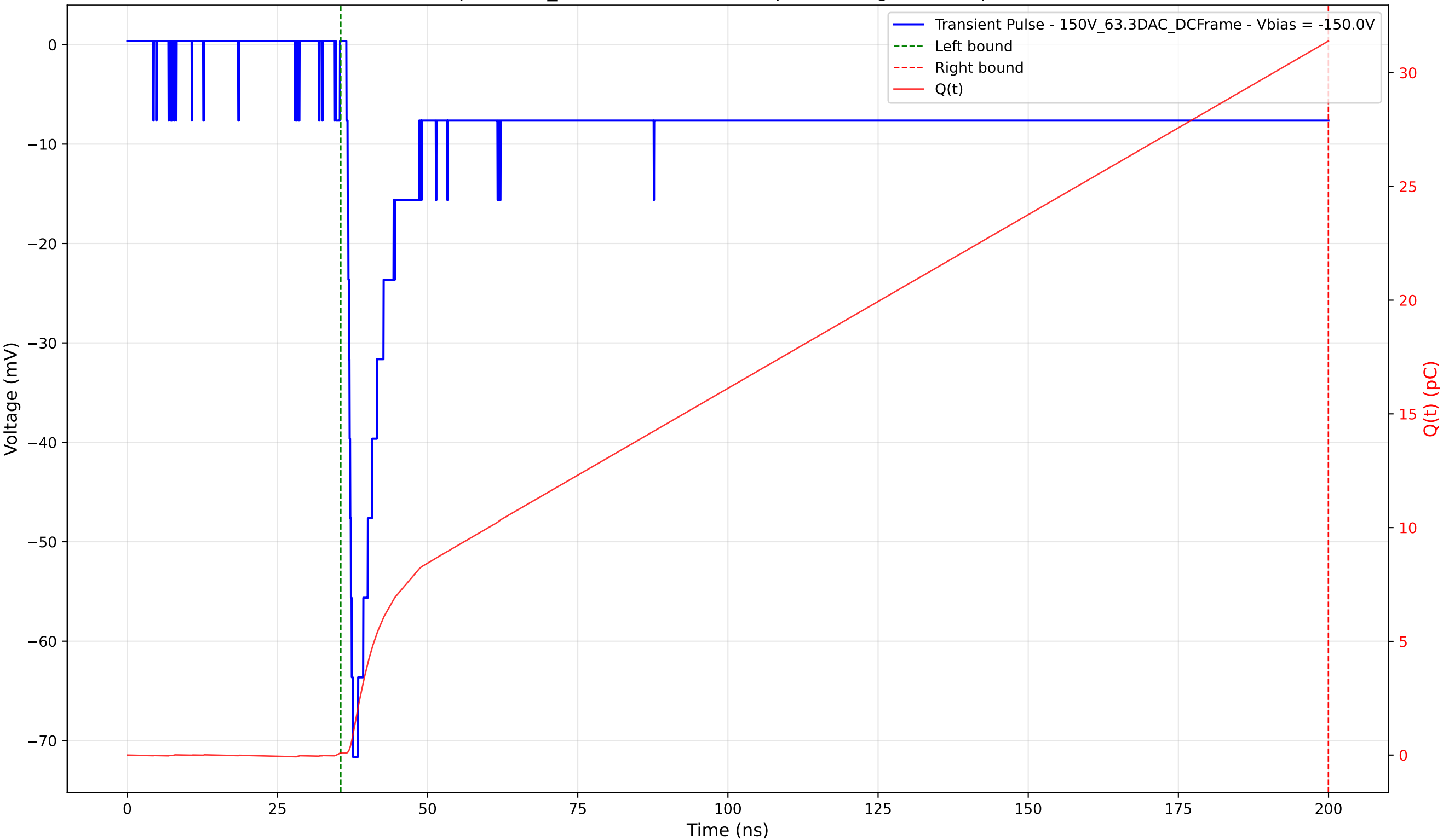
Transient Pulse - Sample: 1cm_42 - Position: 4125.0 \mu\text{m} - Charge: 31.30 pC - Rise Time: 1.06 ns
