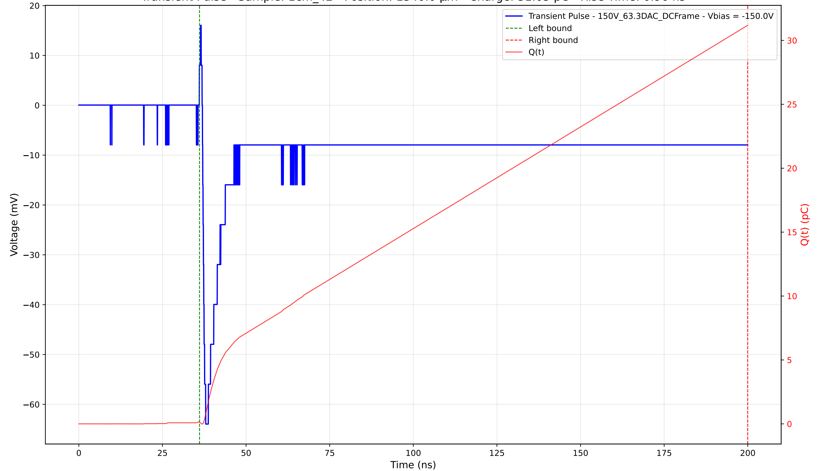
Transient Pulse - Sample: 1cm_42 - Position: 1340.0 \mu\text{m} - Charge: 31.05 pC - Rise Time: 0.96 ns
