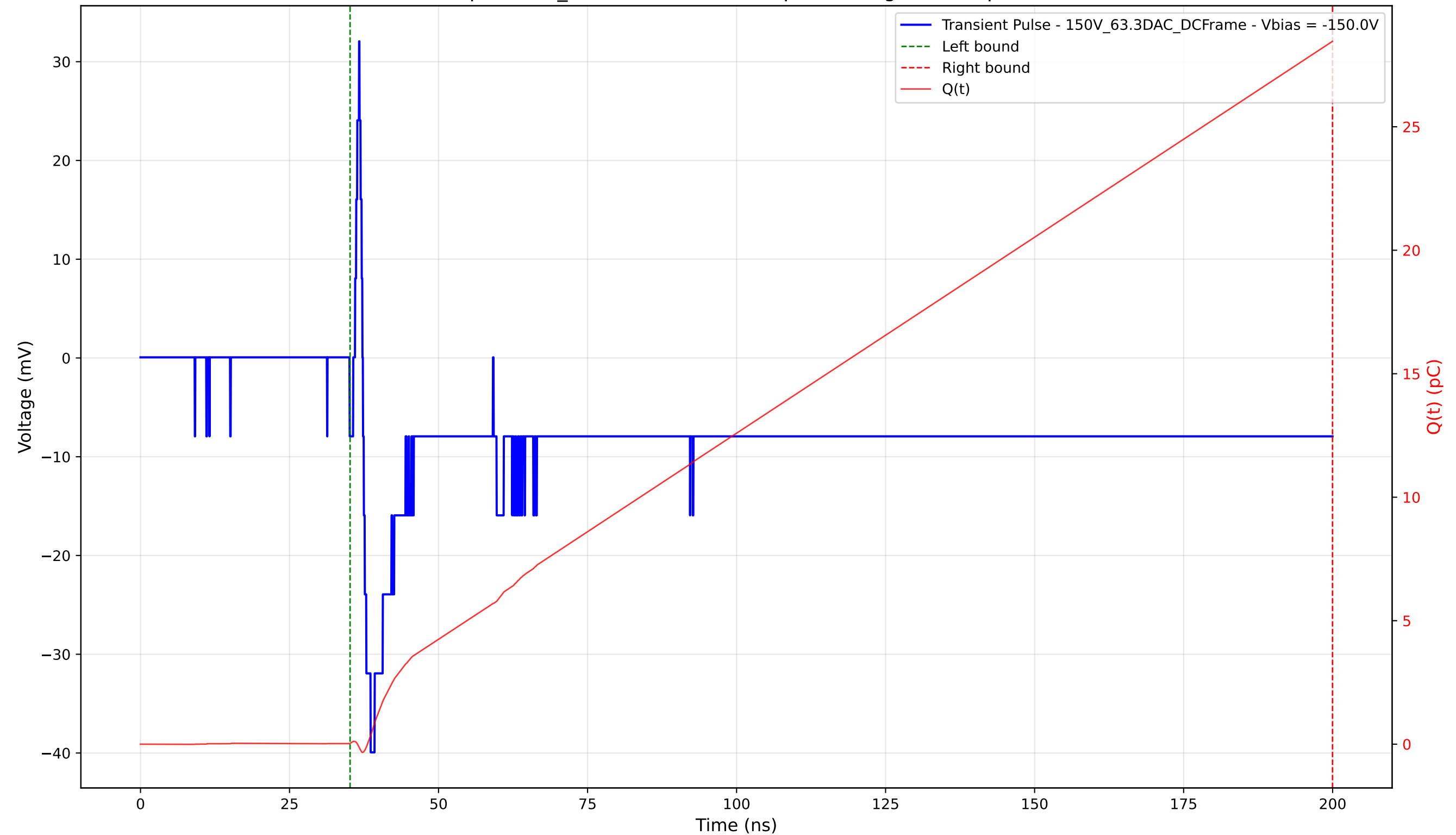
Transient Pulse - Sample: 1cm_42 - Position: 2265.0 \mu\text{m} - Charge: 28.43 pC - Rise Time: 1.29 ns
