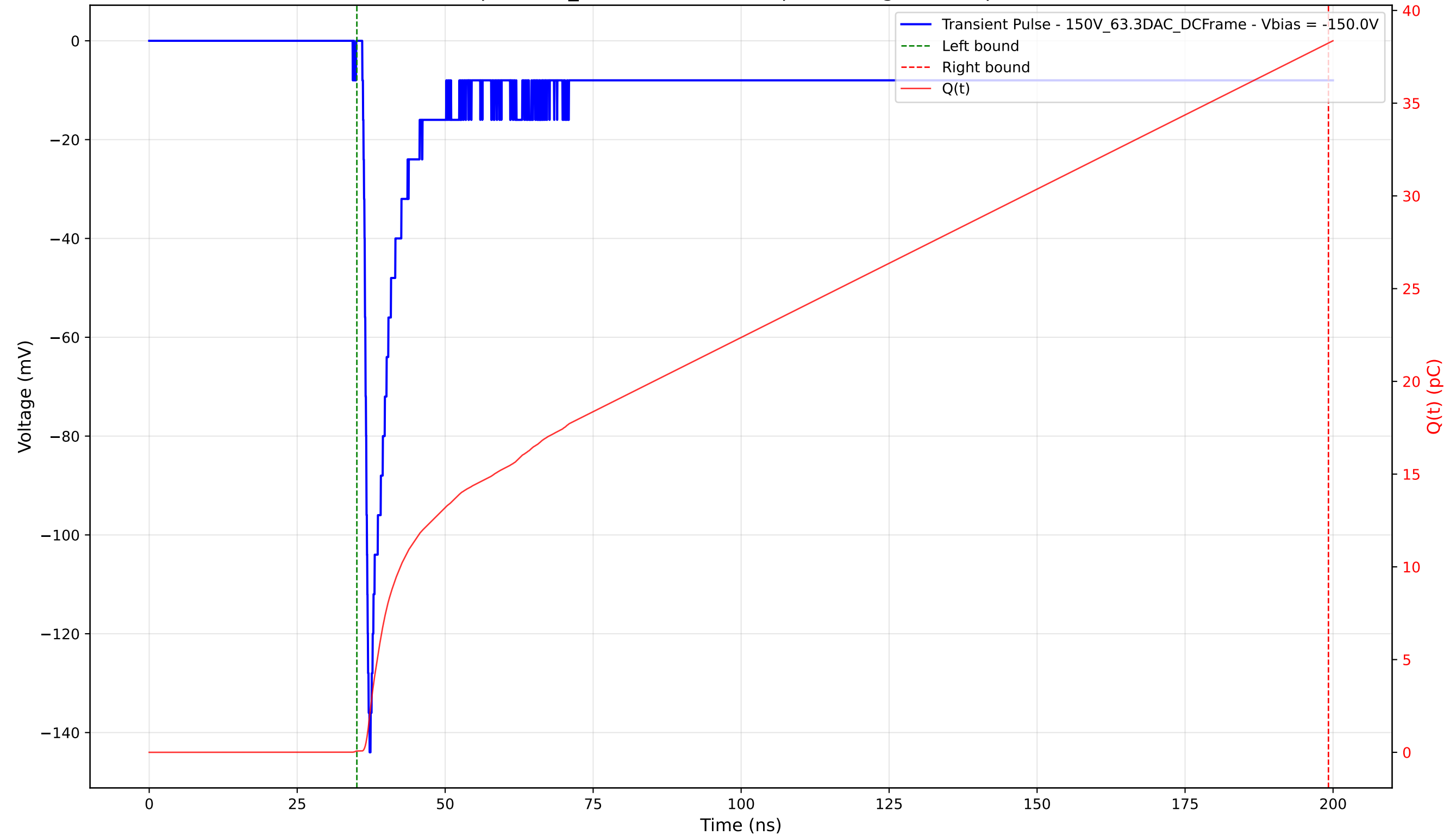
Transient Pulse - Sample: 1cm_42 - Position: 620.0 \mu\text{m} - Charge: 38.17 pC - Rise Time: 0.94 ns
