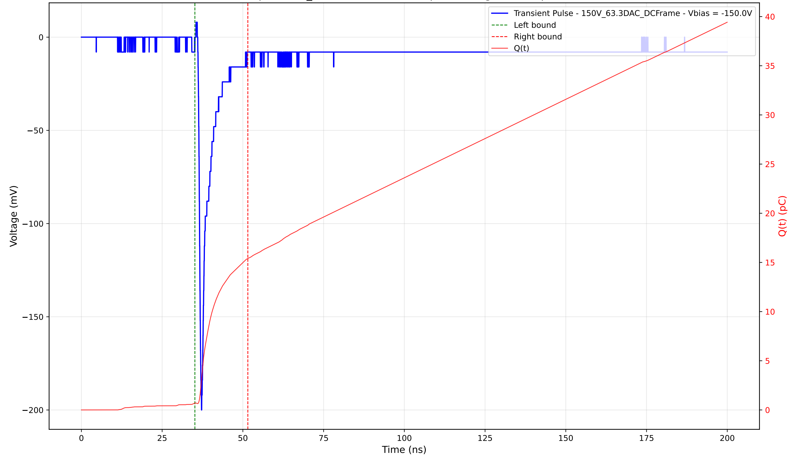
Transient Pulse - Sample: 1cm_42 - Position: 4670.0 \mu\text{m} - Charge: 14.70 pC - Rise Time: 0.81 ns
