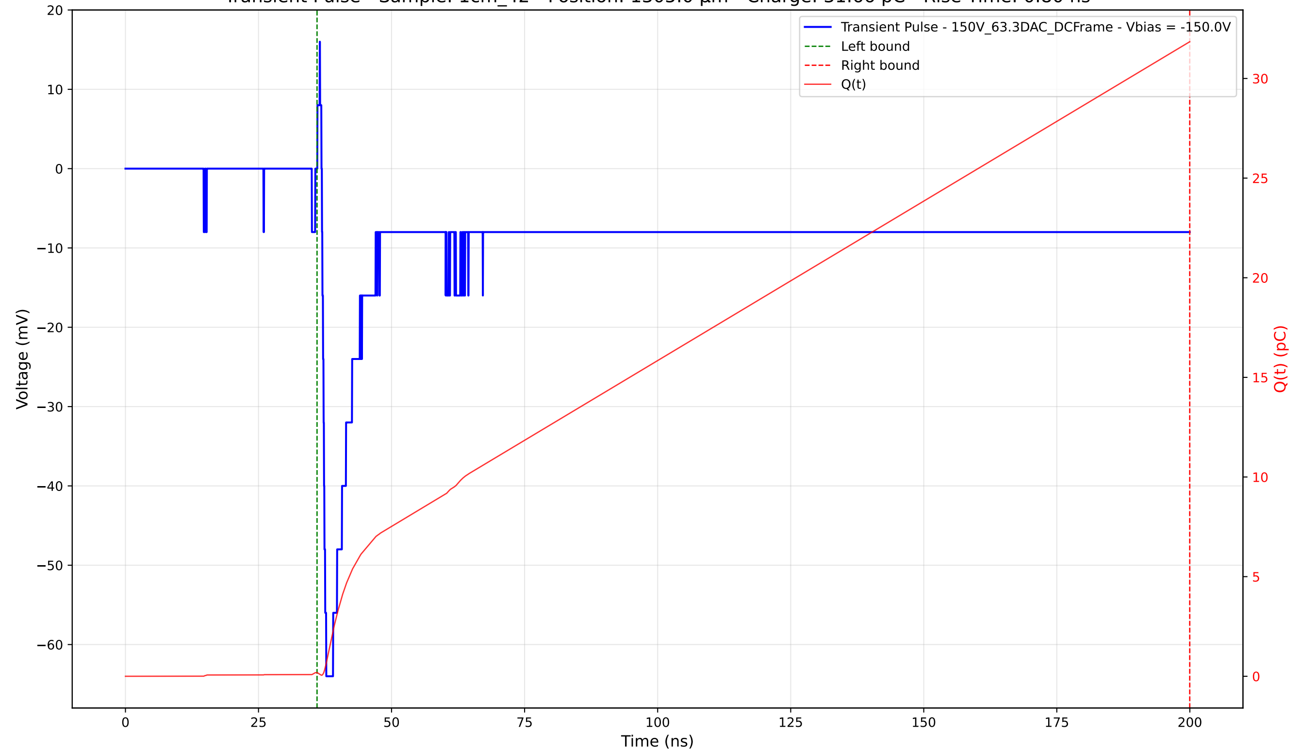
Transient Pulse - Sample: 1cm_42 - Position: 1305.0 \mu\text{m} - Charge: 31.66 pC - Rise Time: 0.80 ns
