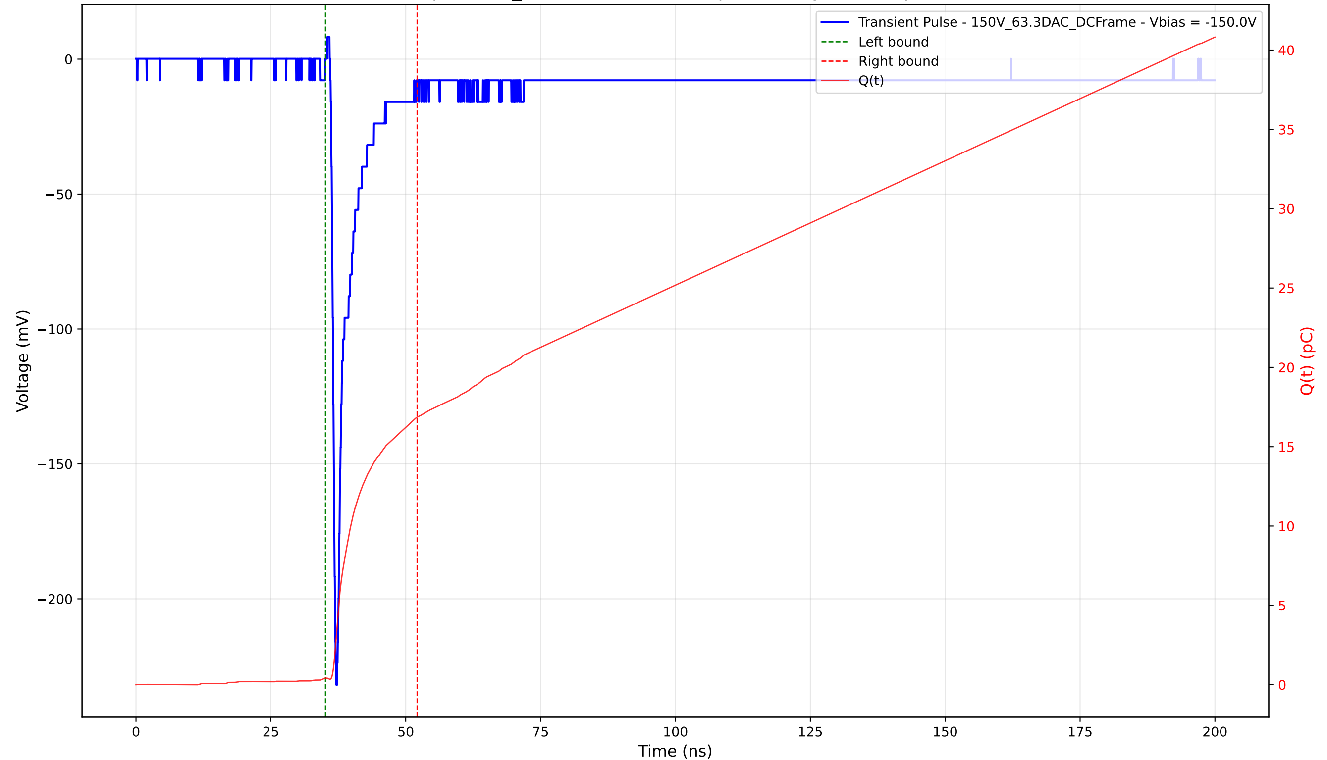
Transient Pulse - Sample: 1cm_42 - Position: 4730.0 \mu\text{m} - Charge: 16.44 pC - Rise Time: 0.80 ns
