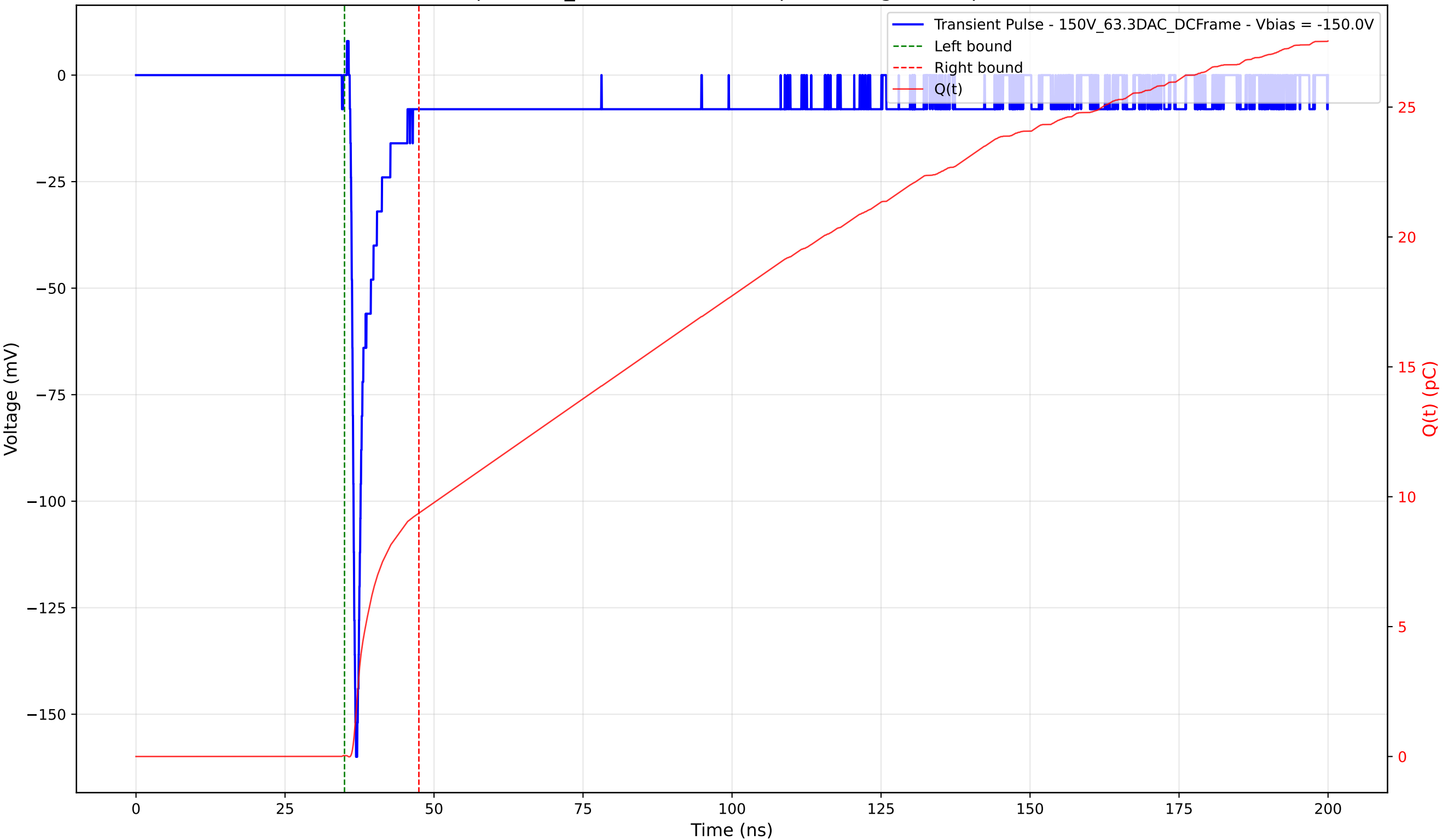
Transient Pulse - Sample: 1cm_42 - Position: 230.0 \mu\text{m} - Charge: 9.33 pC - Rise Time: 0.72 ns
