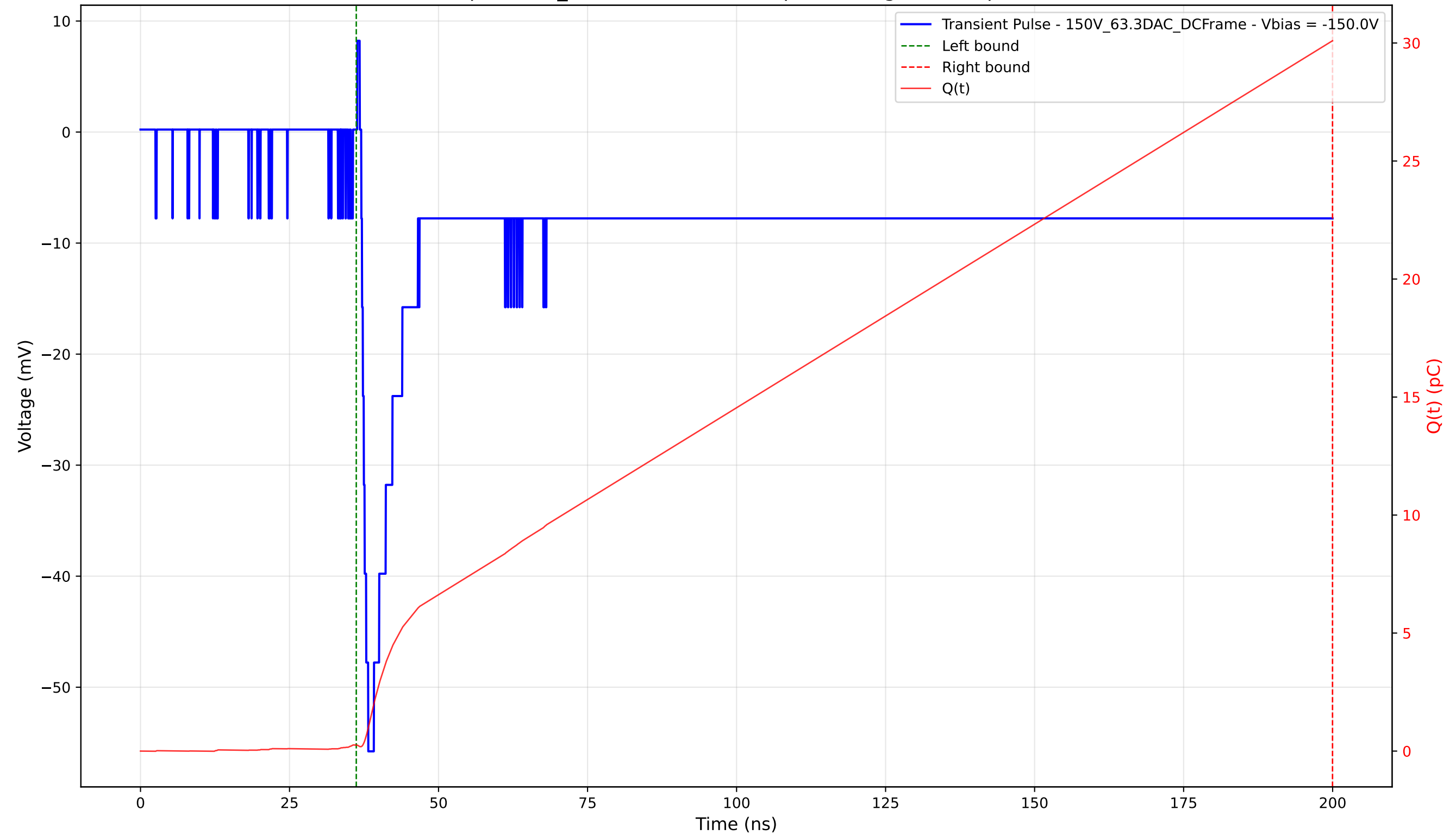
Transient Pulse - Sample: 1cm_42 - Position: 3780.0 \mu\text{m} - Charge: 29.84 pC - Rise Time: 1.17 ns
