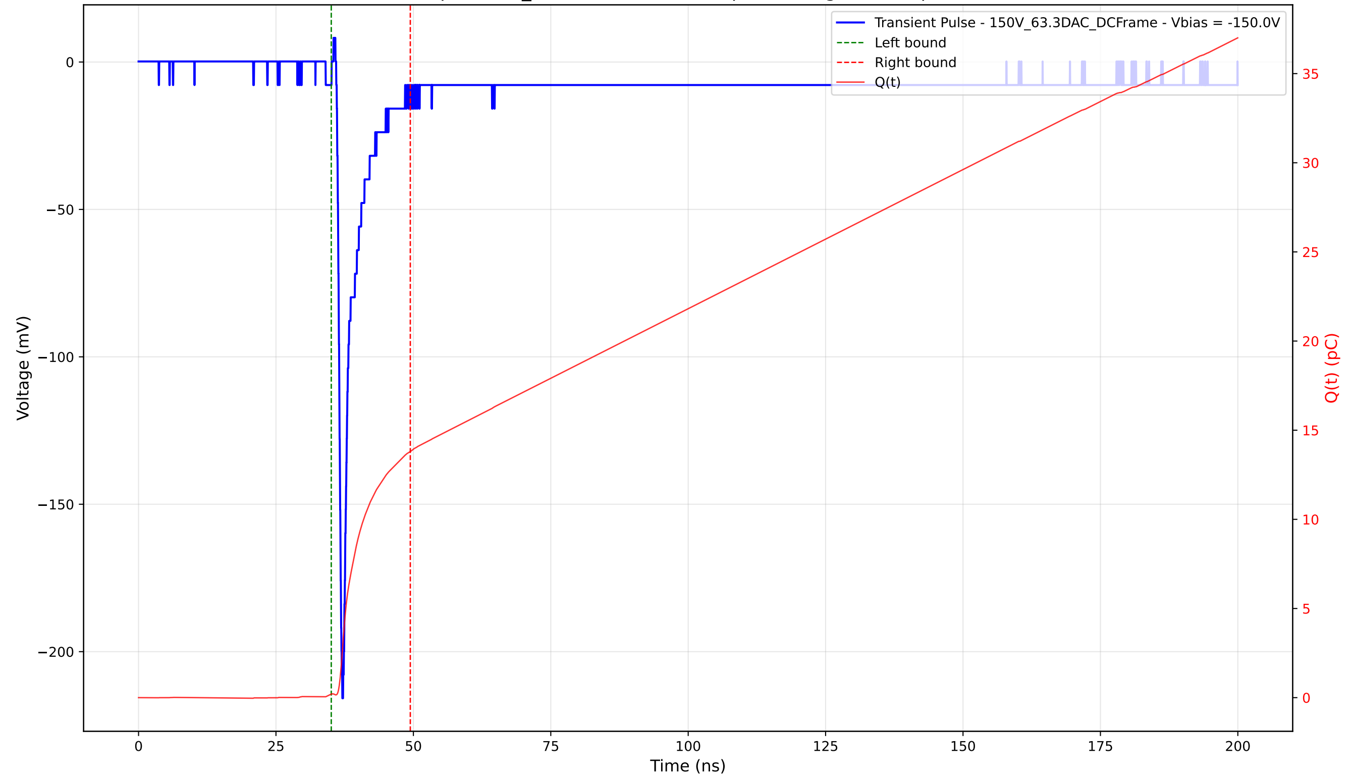
Transient Pulse - Sample: 1cm_42 - Position: 4890.0 \mu\text{m} - Charge: 13.59 pC - Rise Time: 0.79 ns
