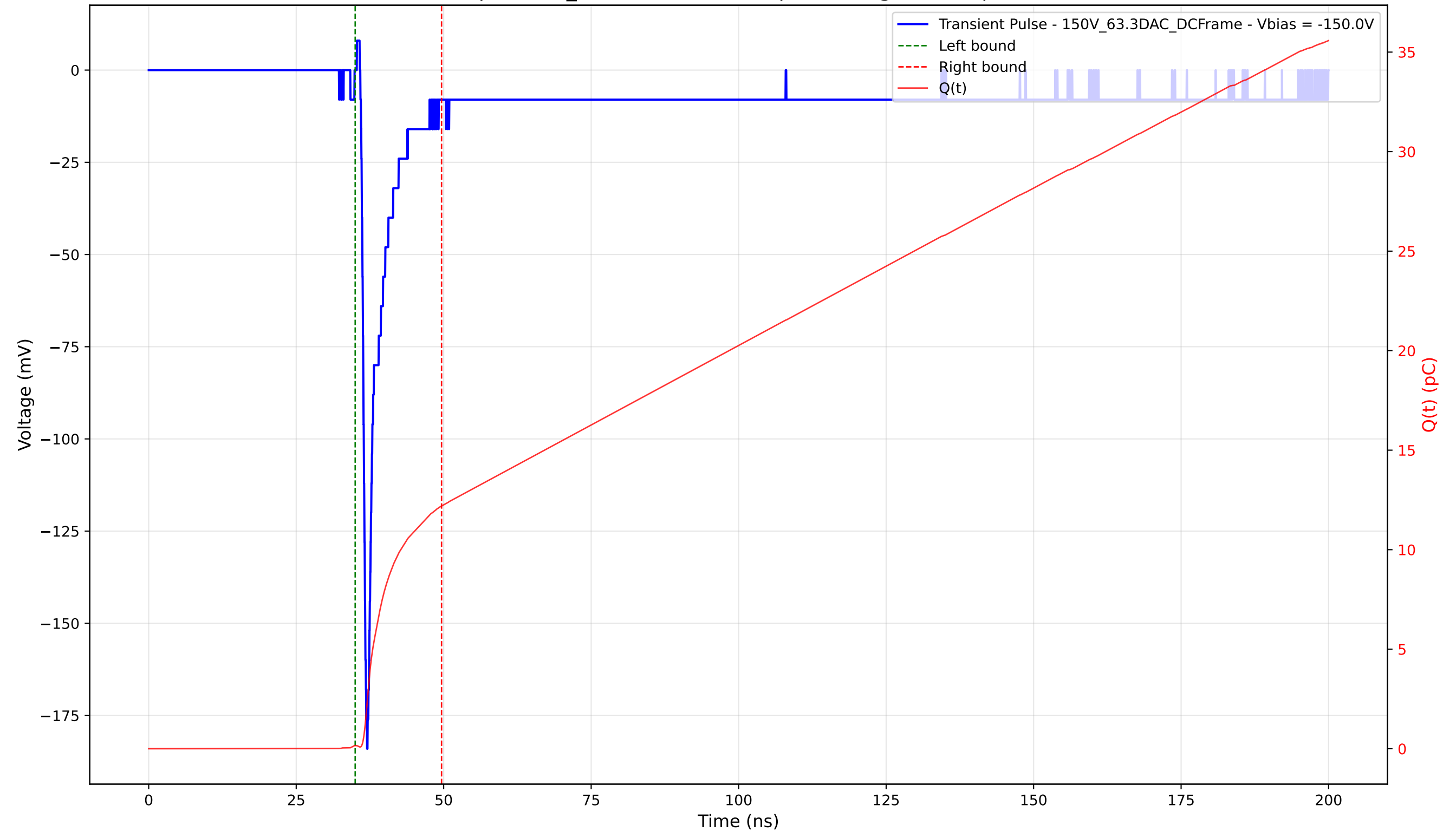
Transient Pulse - Sample: 1cm_42 - Position: 370.0 \mu\text{m} - Charge: 12.03 pC - Rise Time: 0.77 ns
