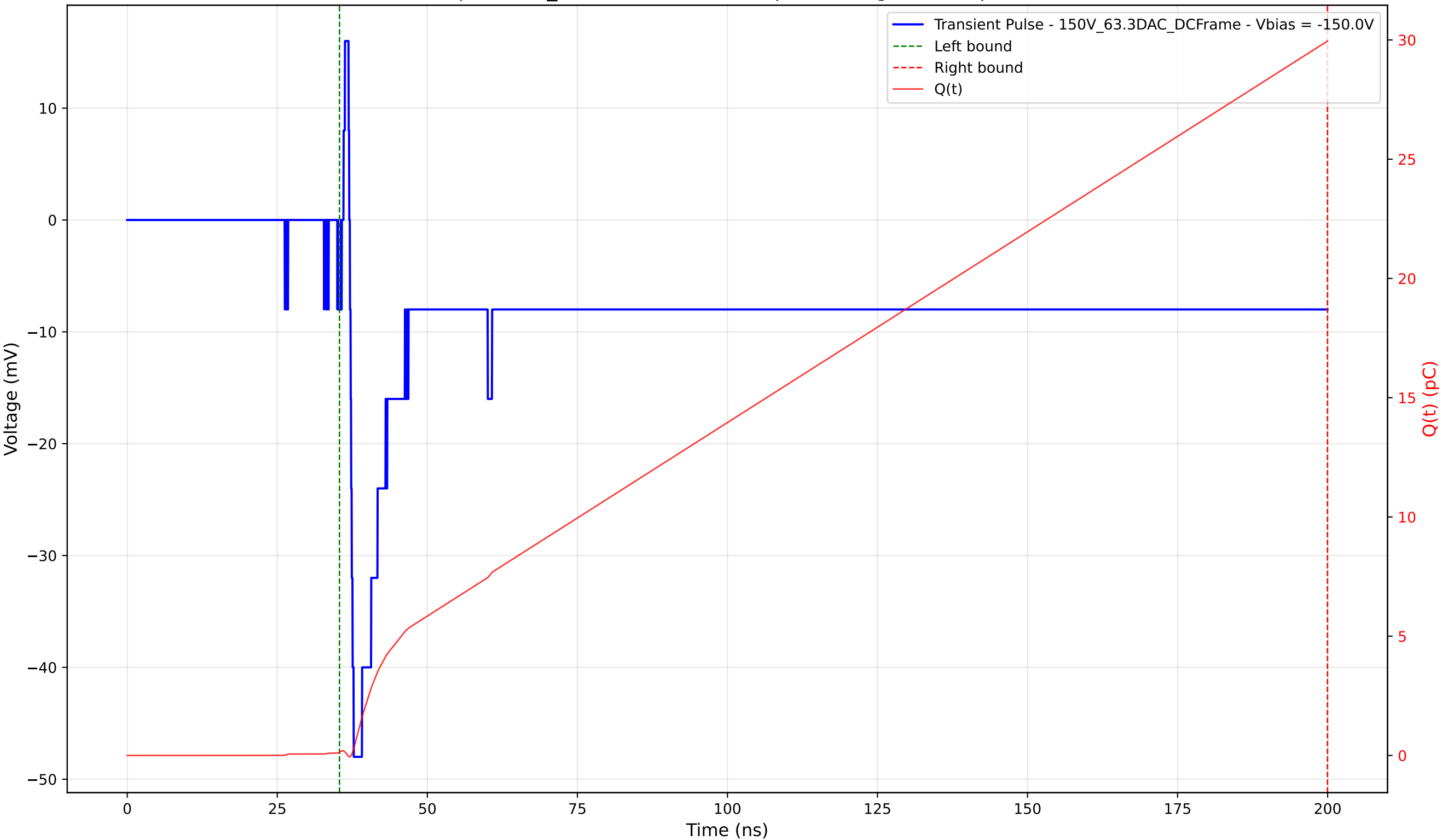
Transient Pulse - Sample: 1cm_42 - Position: 1485.0 \mu\text{m} - Charge: 29.82 pC - Rise Time: 0.63 ns
