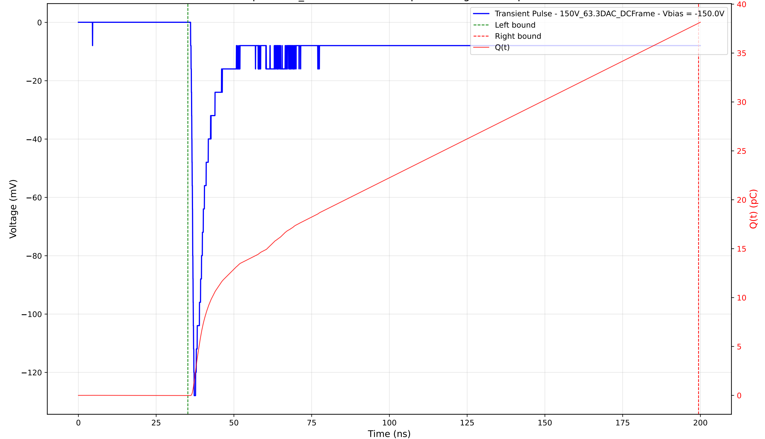
Transient Pulse - Sample: 1cm_42 - Position: 755.0 \mu\text{m} - Charge: 38.08 pC - Rise Time: 0.91 ns
