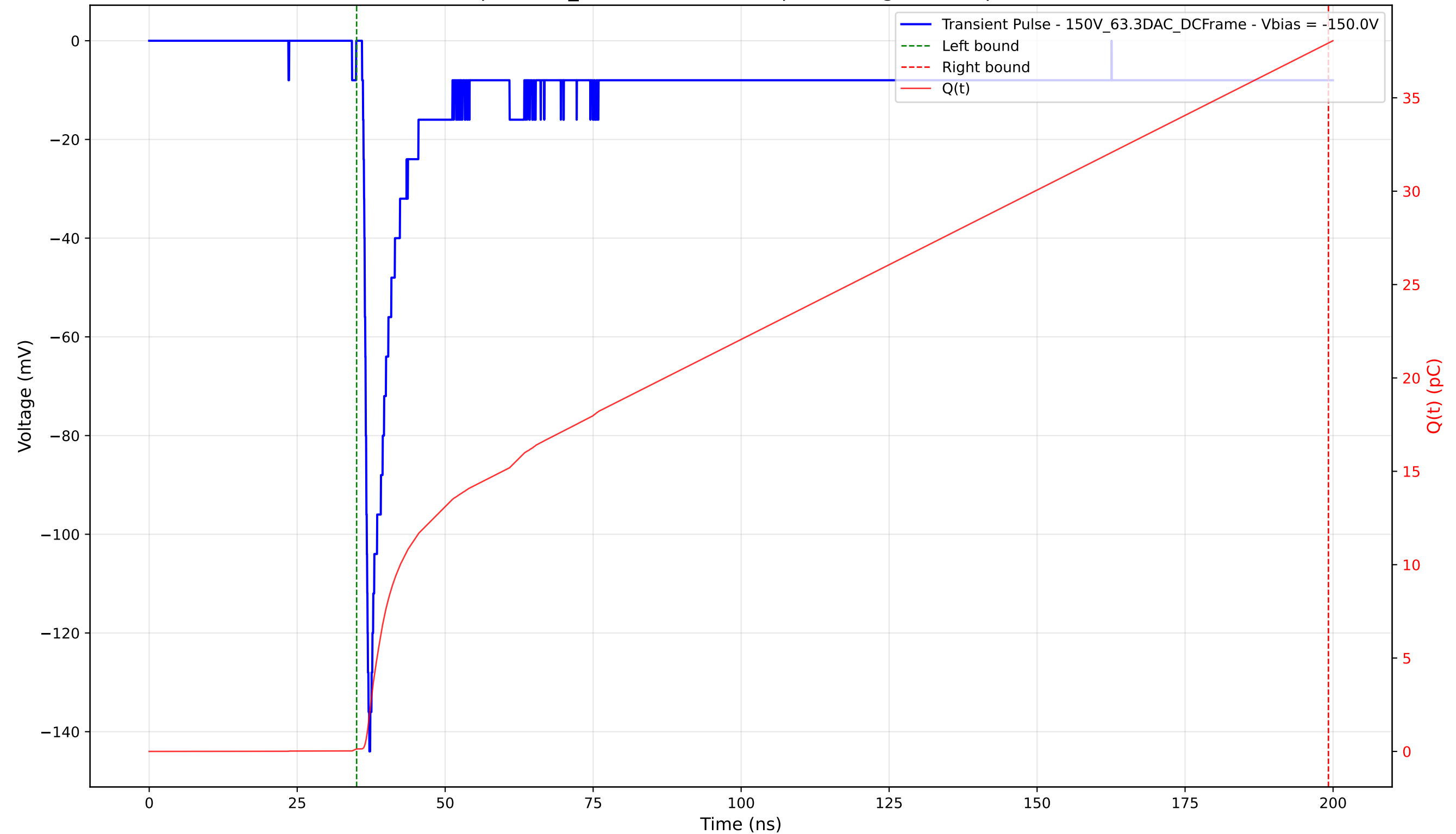
Transient Pulse - Sample: 1cm_42 - Position: 605.0 \mu\text{m} - Charge: 37.80 pC - Rise Time: 0.92 ns
