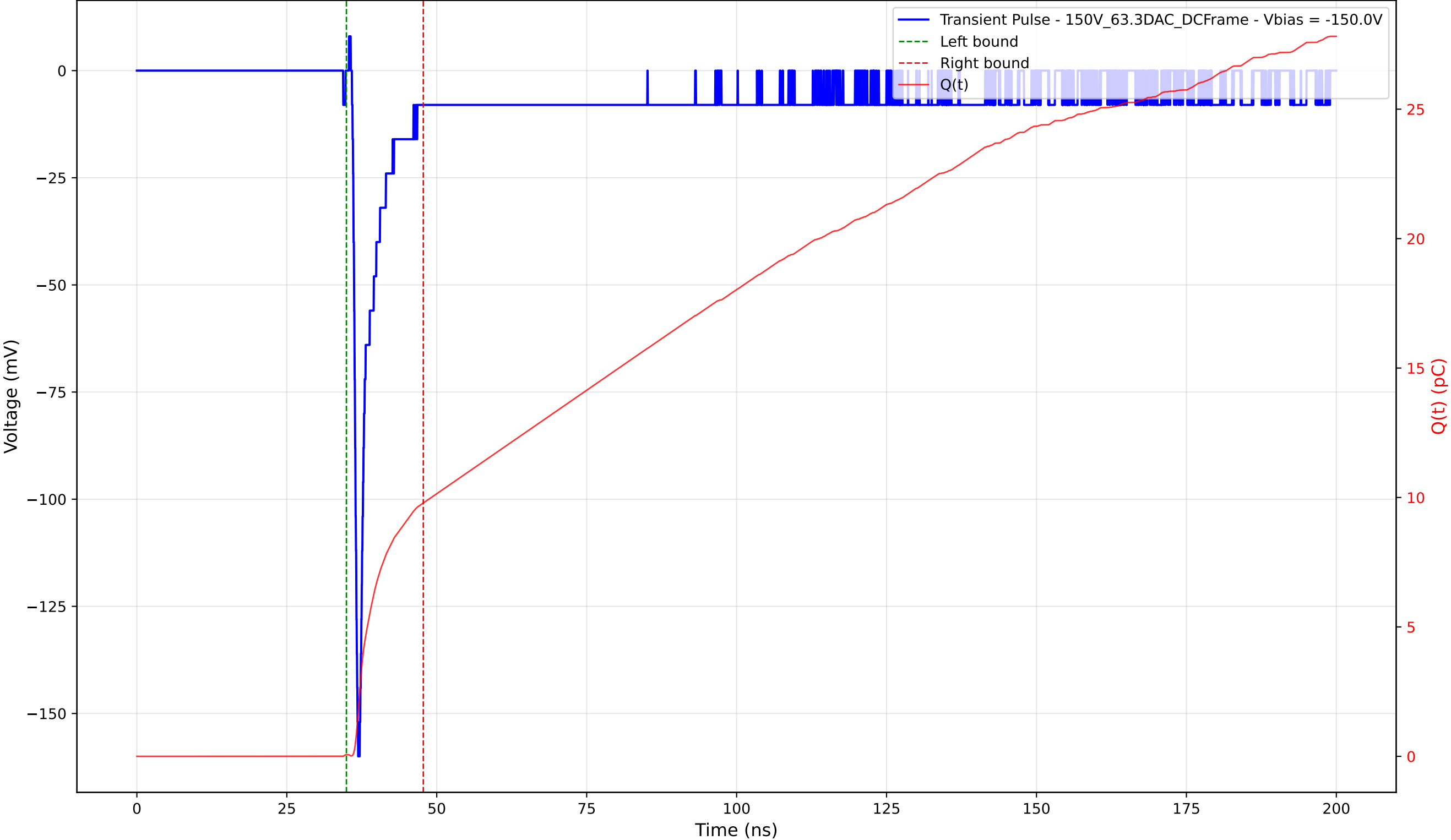
Transient Pulse - Sample: 1cm_42 - Position: 235.0 \mu\text{m} - Charge: 9.72 pC - Rise Time: 0.70 ns
