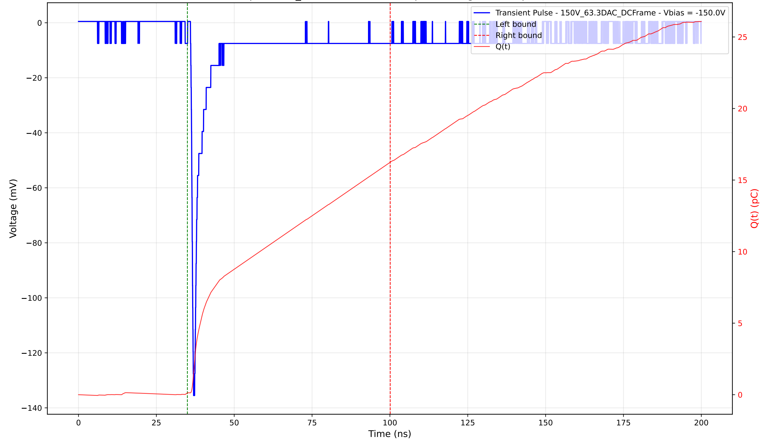
Transient Pulse - Sample: 1cm_42 - Position: 4995.0 \mu\text{m} - Charge: 16.12 pC - Rise Time: 0.78 ns
