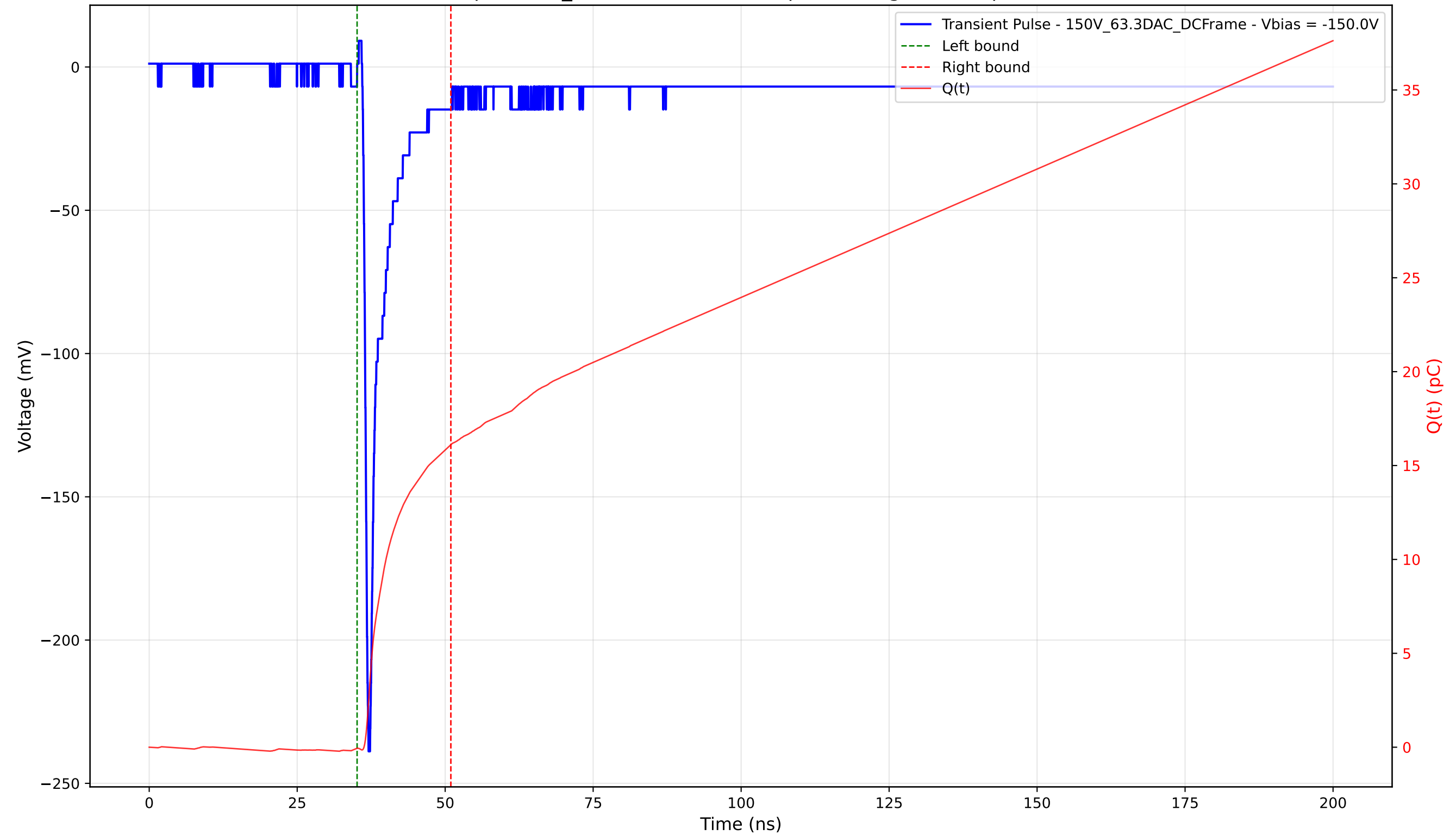
Transient Pulse - Sample: 1cm_42 - Position: 4785.0 \mu\text{m} - Charge: 16.17 pC - Rise Time: 0.78 ns
