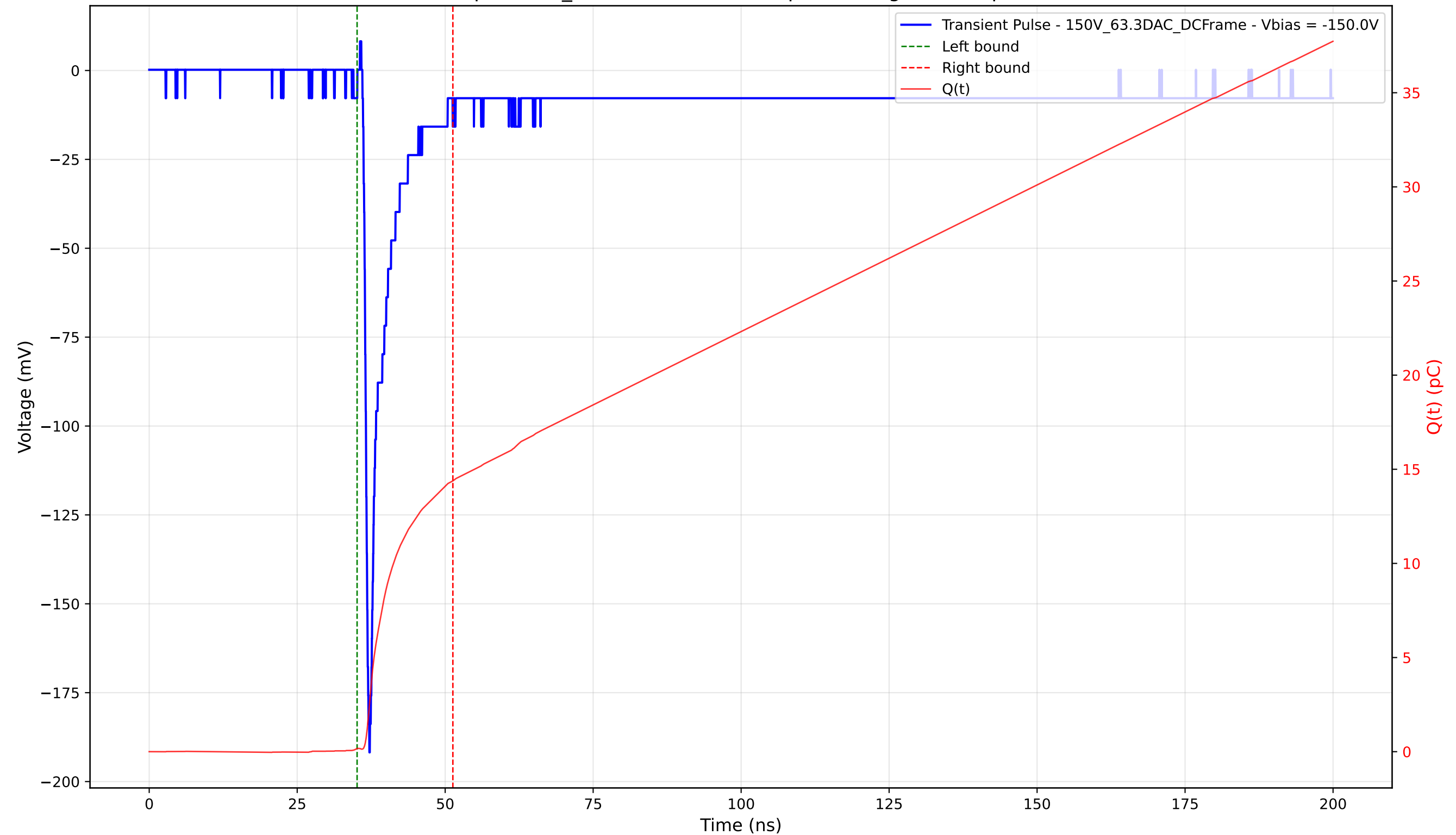
Transient Pulse - Sample: 1cm_42 - Position: 4655.0 \mu\text{m} - Charge: 14.21 pC - Rise Time: 0.79 ns
