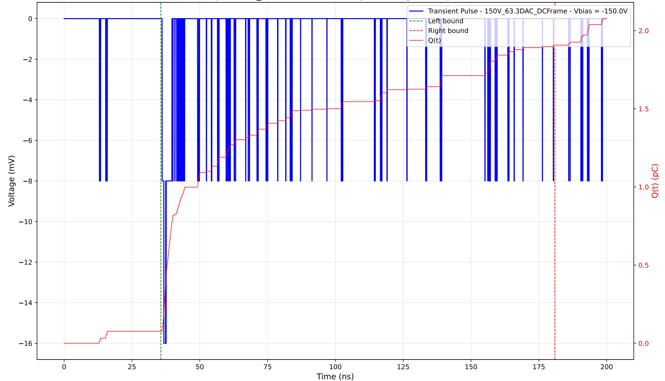
Transient Pulse - Sample: 1cm_42 - Position: 5205.0 \mu\text{m} - Charge: 1.83 pC - Rise Time: 0.66 ns
