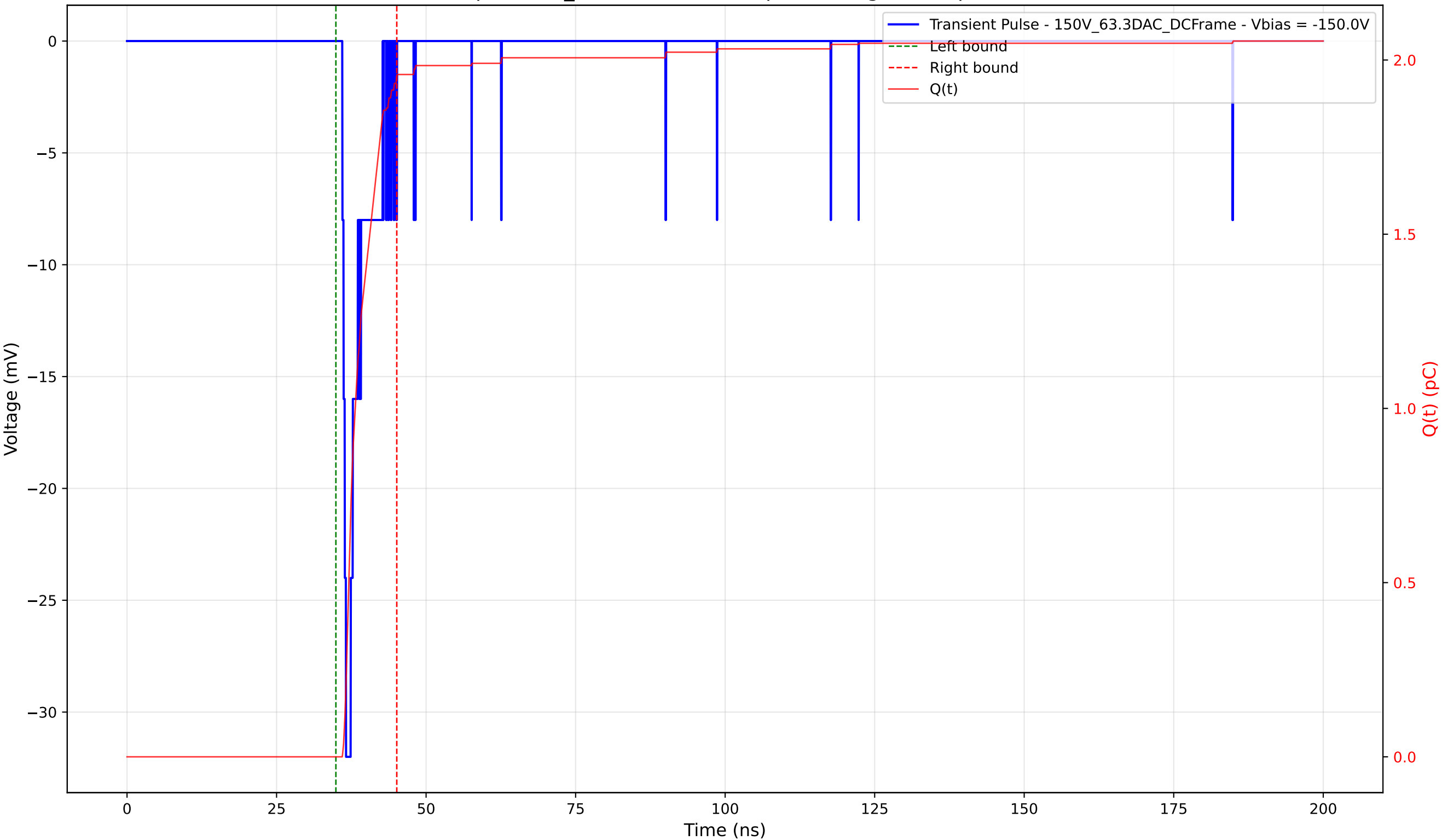
Transient Pulse - Sample: 1cm_42 - Position: 25.0 \mu\text{m} - Charge: 1.95 pC - Rise Time: 0.61 ns
