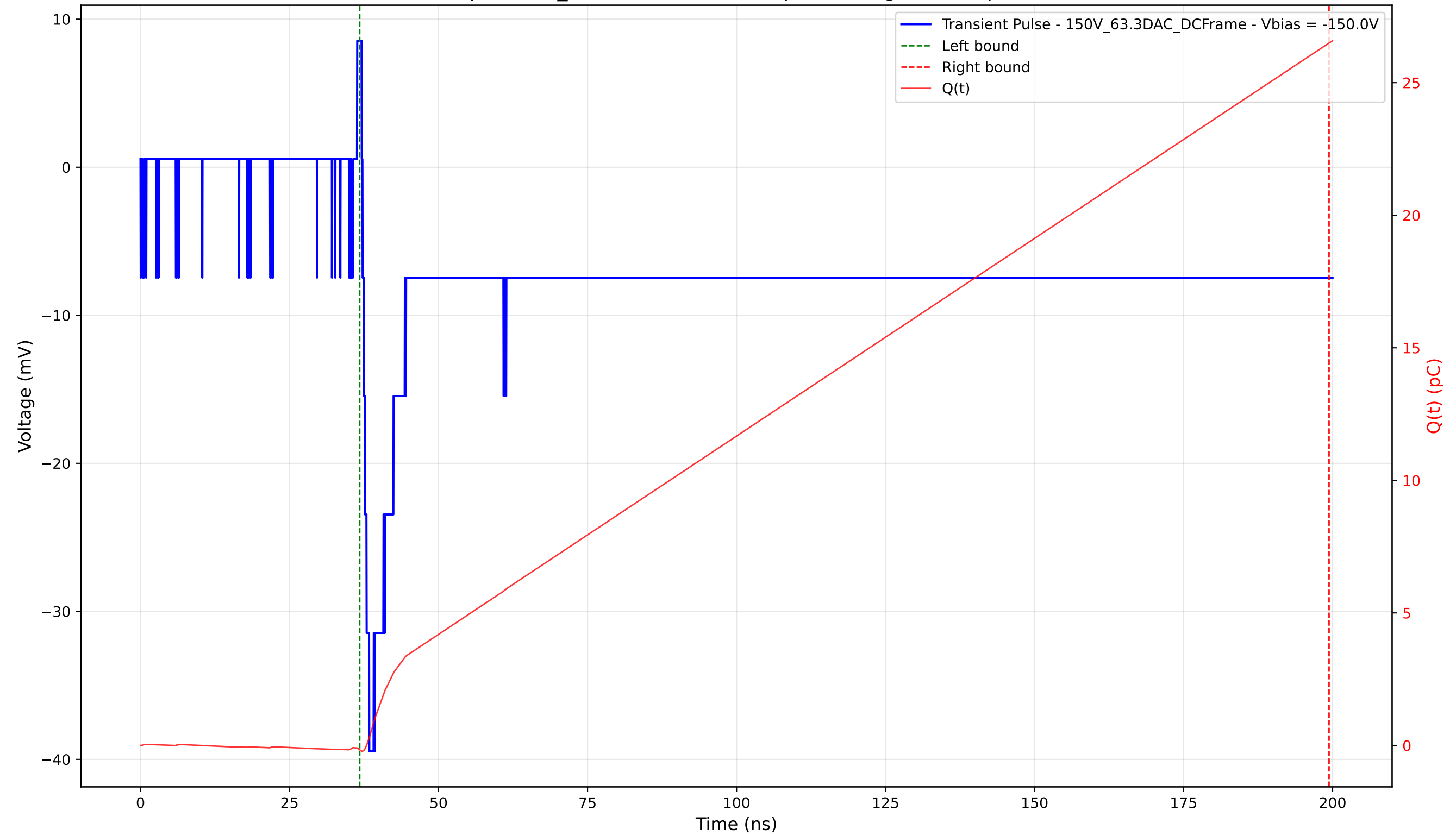
Transient Pulse - Sample: 1cm_42 - Position: 3500.0 \mu\text{m} - Charge: 26.66 pC - Rise Time: 1.13 ns
