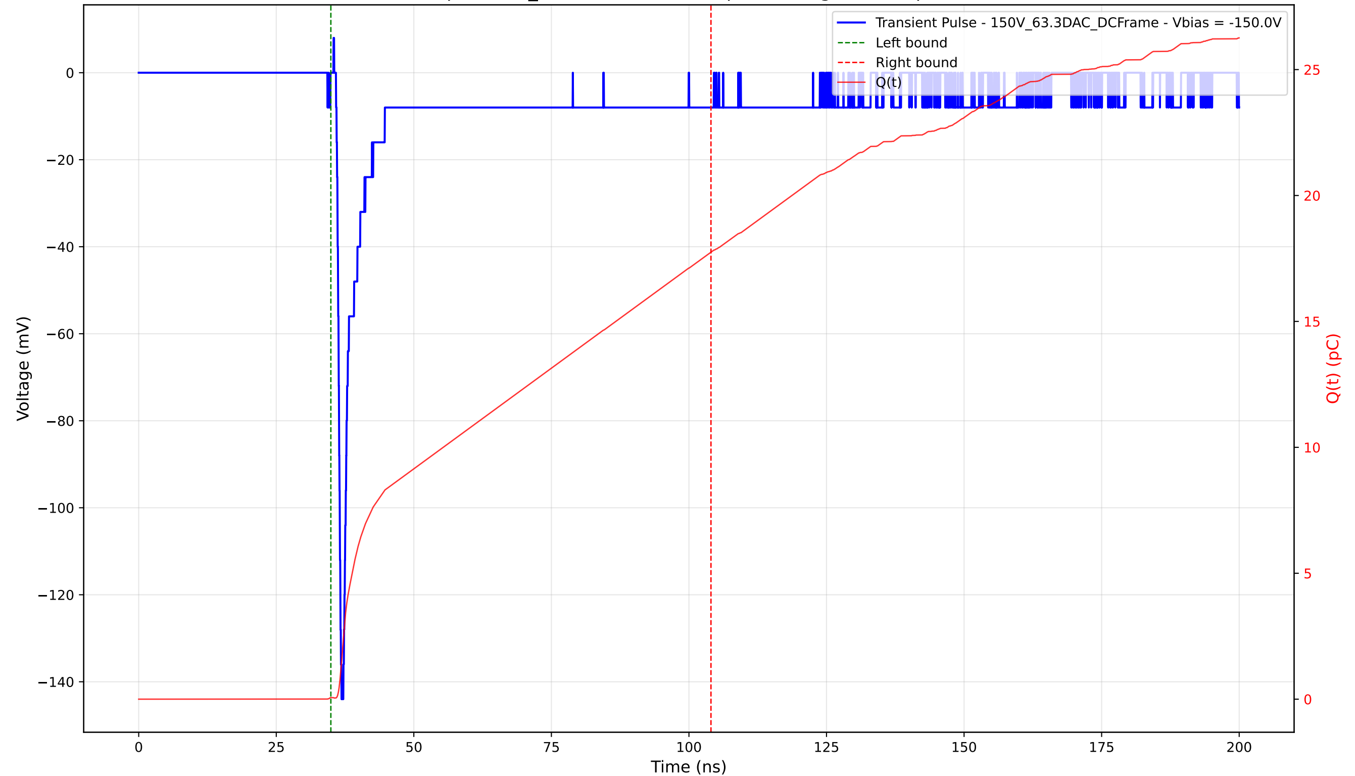
Transient Pulse - Sample: 1cm_42 - Position: 200.0 \mu\text{m} - Charge: 17.69 pC - Rise Time: 0.78 ns
