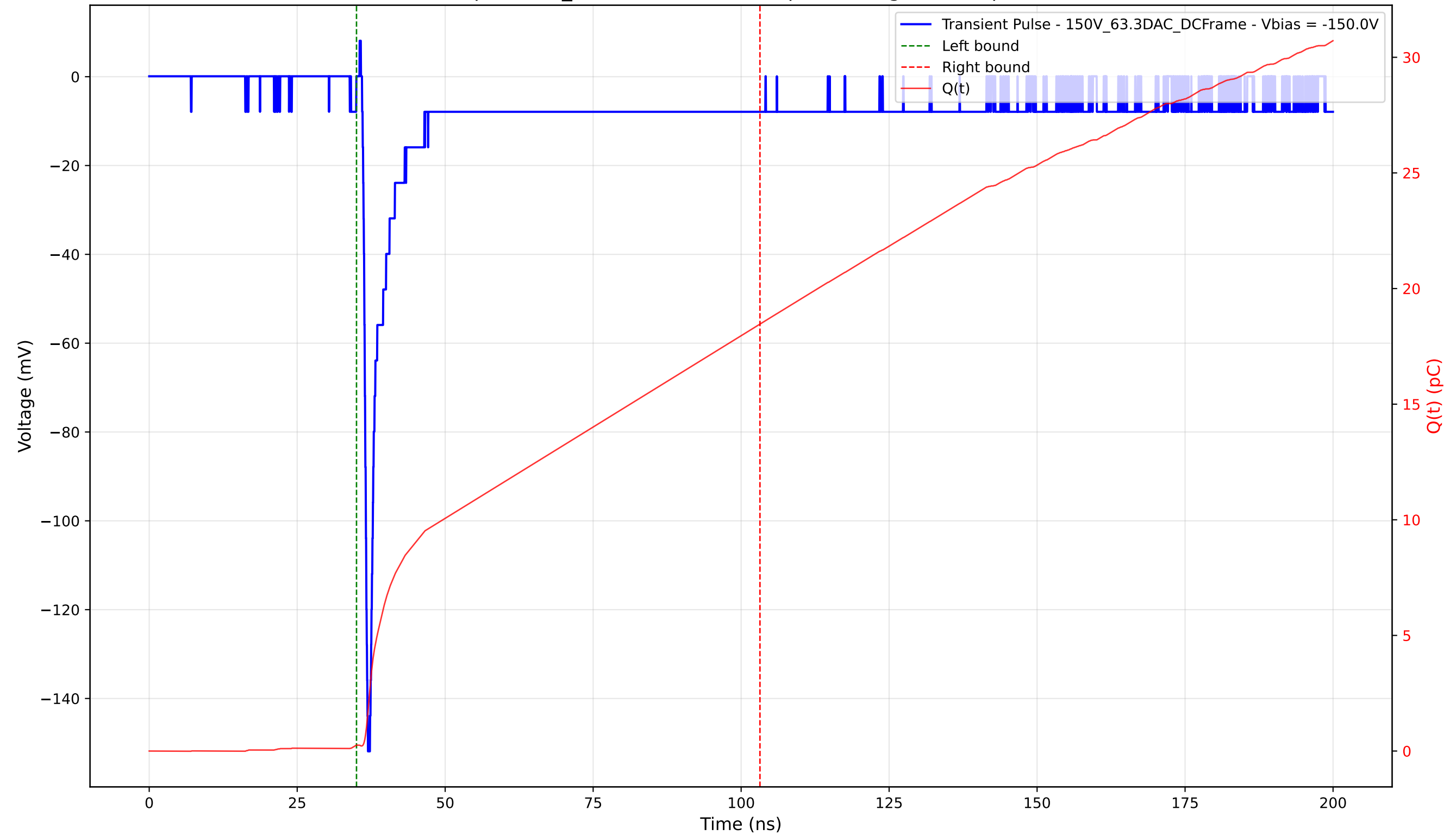
Transient Pulse - Sample: 1cm_42 - Position: 4975.0 \mu\text{m} - Charge: 18.22 pC - Rise Time: 0.80 ns
