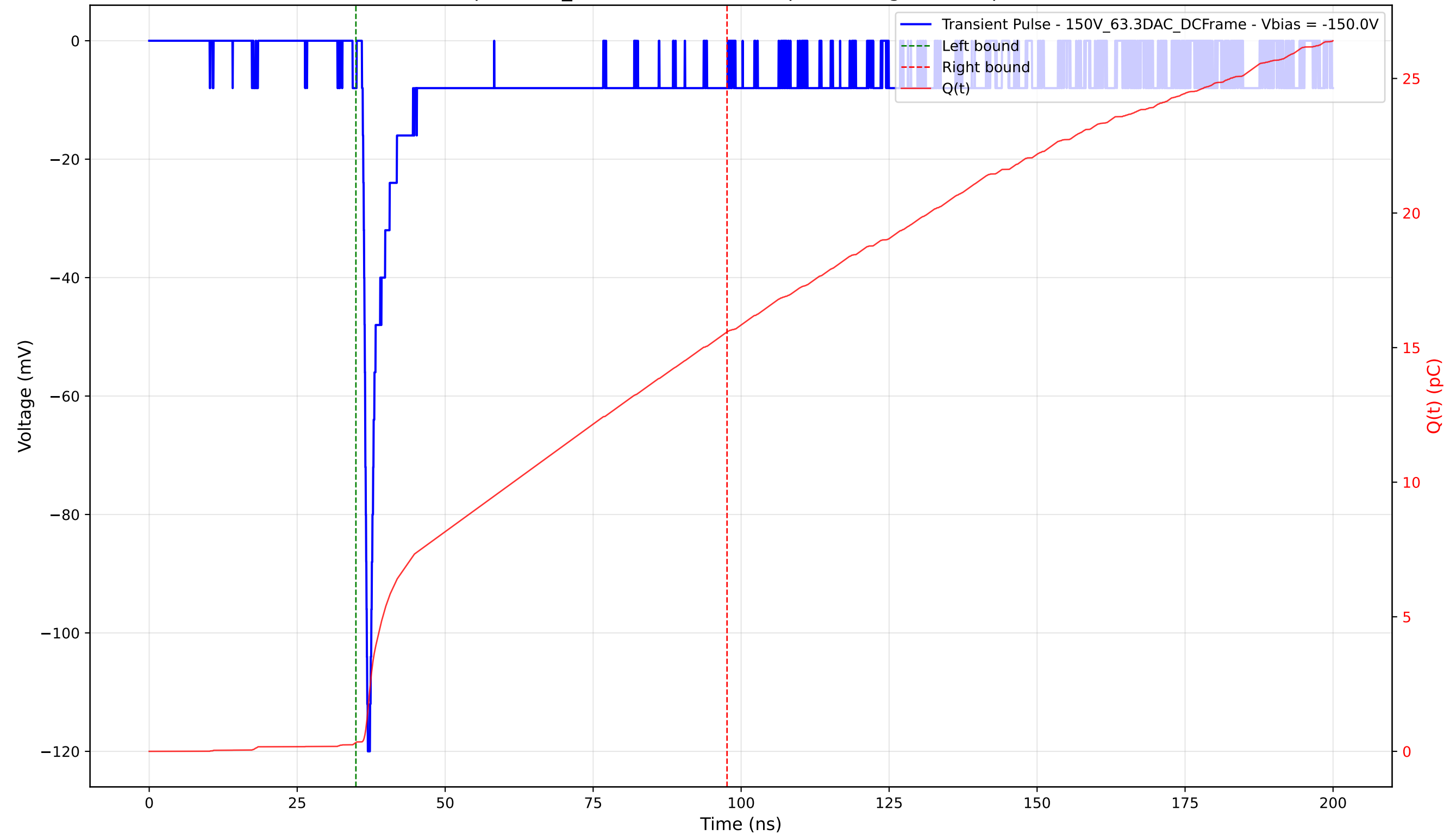
Transient Pulse - Sample: 1cm_42 - Position: 5015.0 \mu\text{m} - Charge: 15.26 pC - Rise Time: 0.75 ns
