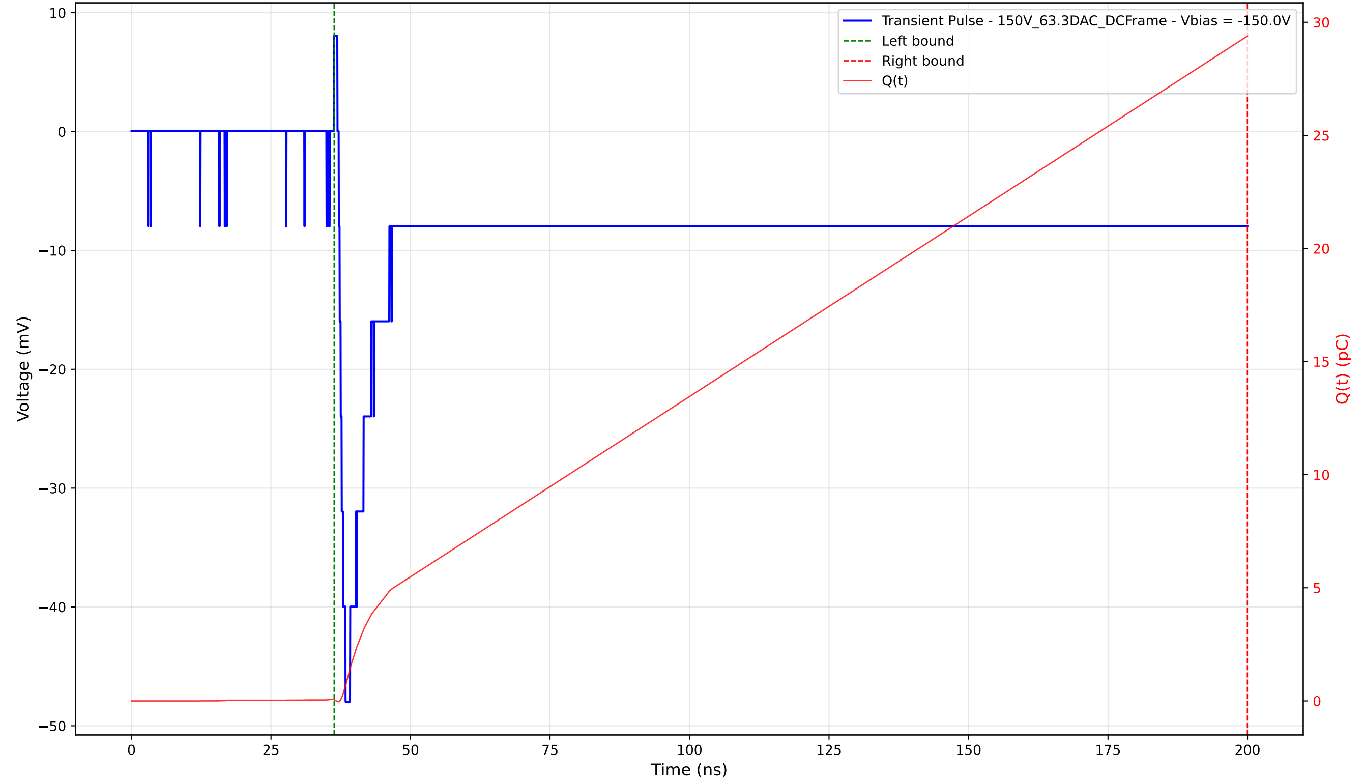
Transient Pulse - Sample: 1cm_42 - Position: 3625.0 \mu\text{m} - Charge: 29.33 pC - Rise Time: 1.21 ns
