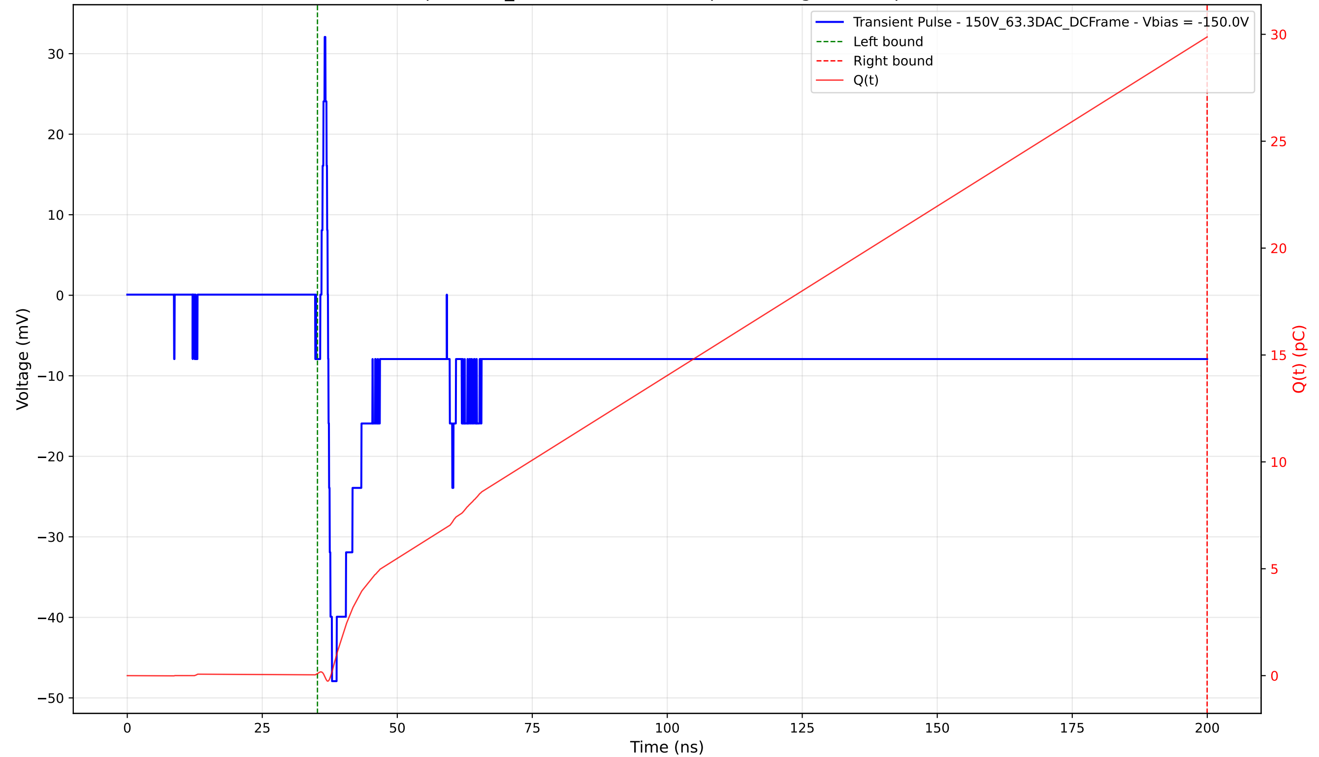
Transient Pulse - Sample: 1cm_42 - Position: 1790.0 \mu\text{m} - Charge: 29.78 pC - Rise Time: 0.73 ns
