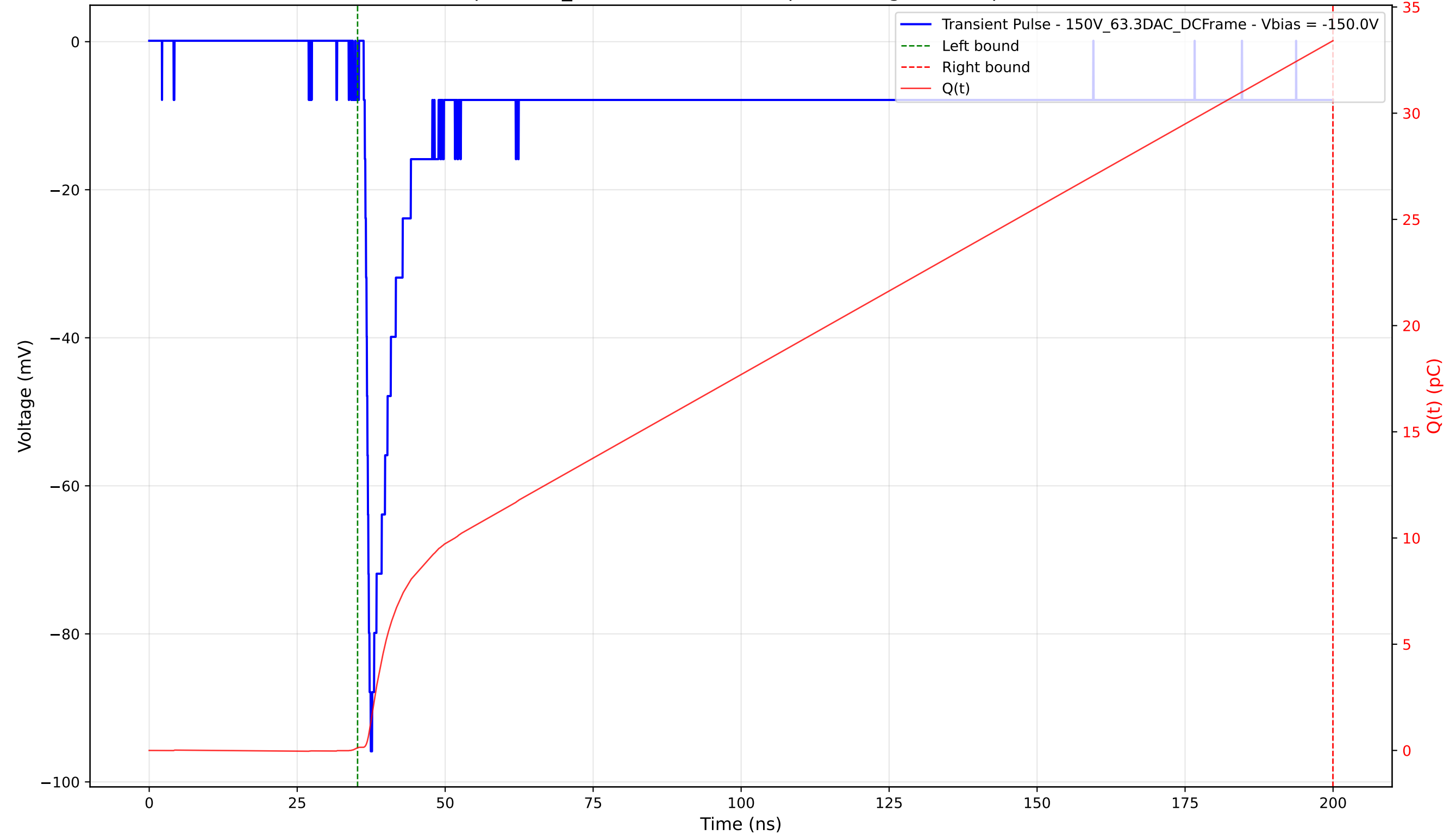
Transient Pulse - Sample: 1cm_42 - Position: 4395.0 \mu\text{m} - Charge: 33.28 pC - Rise Time: 0.82 ns
