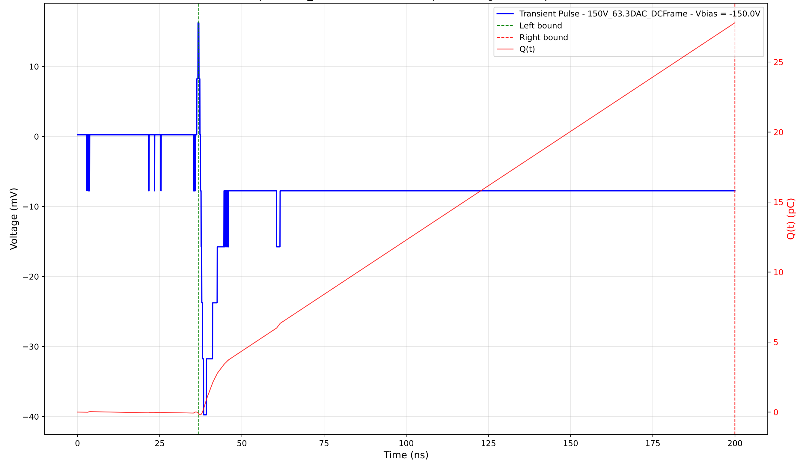
Transient Pulse - Sample: 1cm_42 - Position: 3305.0 \mu\text{m} - Charge: 27.94 pC - Rise Time: 0.95 ns
