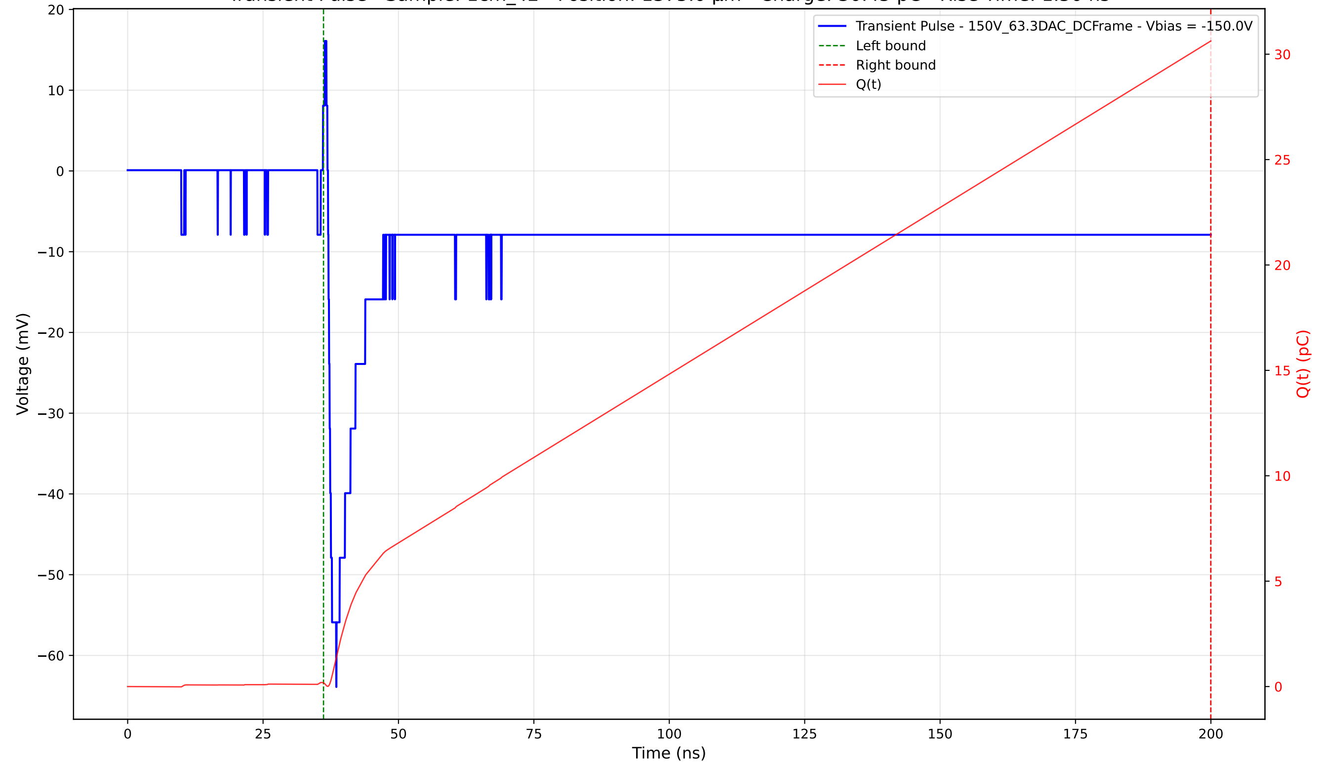
Transient Pulse - Sample: 1cm_42 - Position: 1375.0 \mu\text{m} - Charge: 30.45 pC - Rise Time: 1.50 ns
