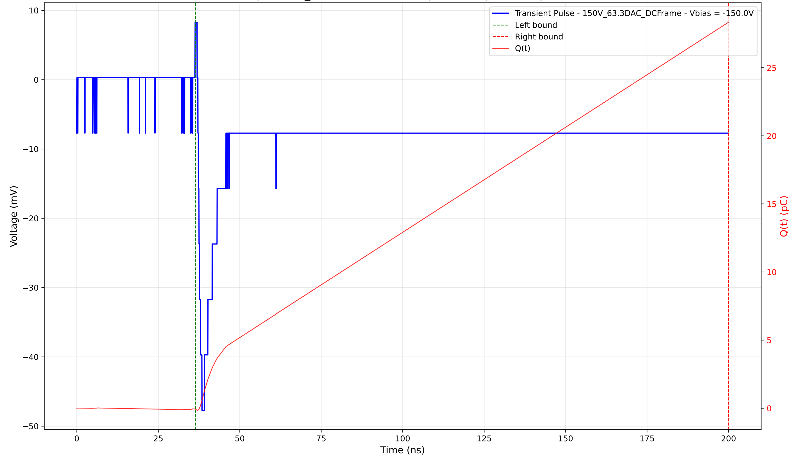
Transient Pulse - Sample: 1cm_42 - Position: 3620.0 \mu\text{m} - Charge: 28.42 pC - Rise Time: 1.25 ns
