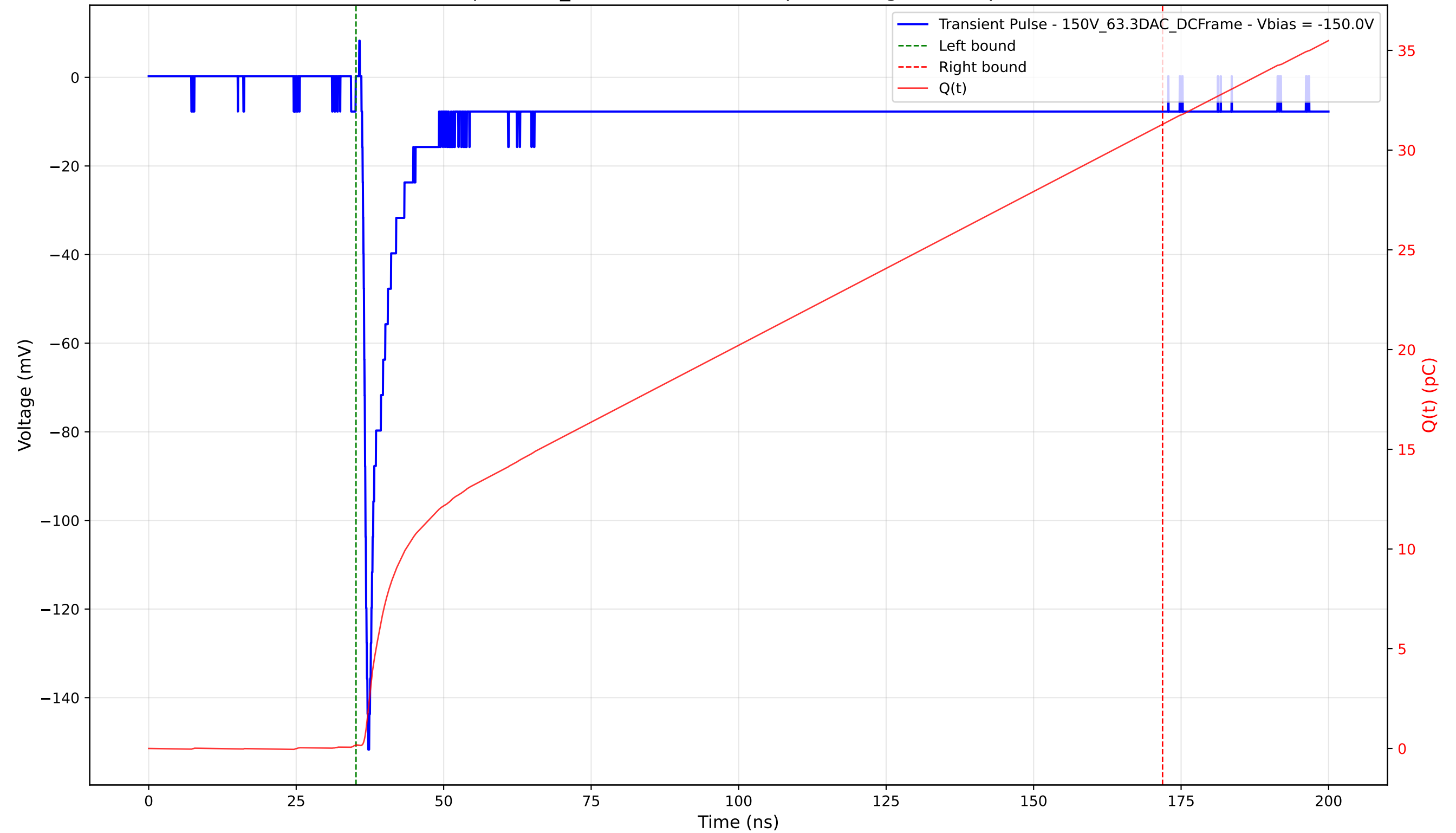
Transient Pulse - Sample: 1cm_42 - Position: 4585.0 \mu\text{m} - Charge: 31.13 pC - Rise Time: 0.90 ns
