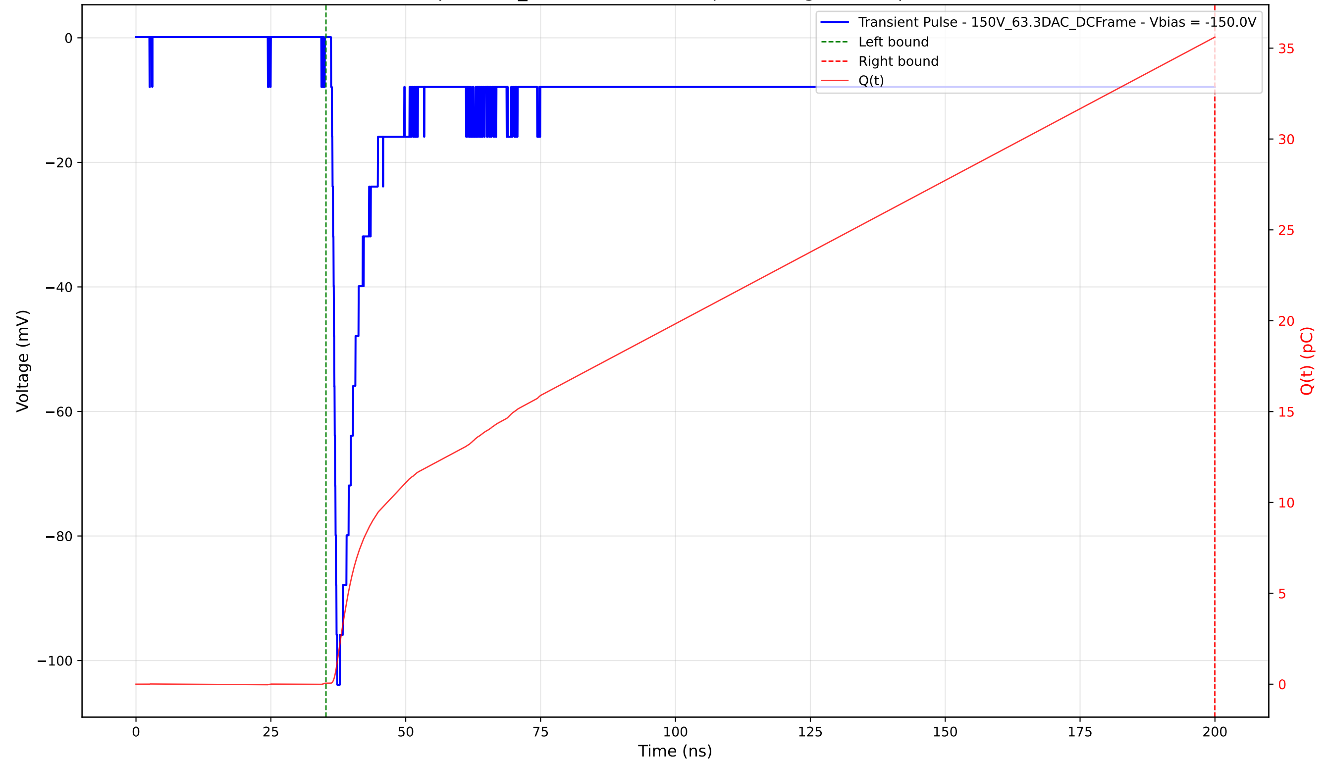
Transient Pulse - Sample: 1cm_42 - Position: 845.0 \mu\text{m} - Charge: 35.55 pC - Rise Time: 0.85 ns
