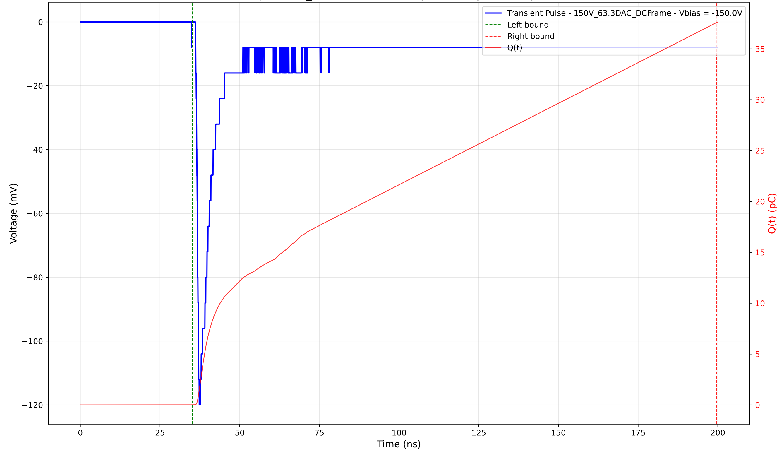
Transient Pulse - Sample: 1cm_42 - Position: 795.0 \mu\text{m} - Charge: 37.56 pC - Rise Time: 0.91 ns
