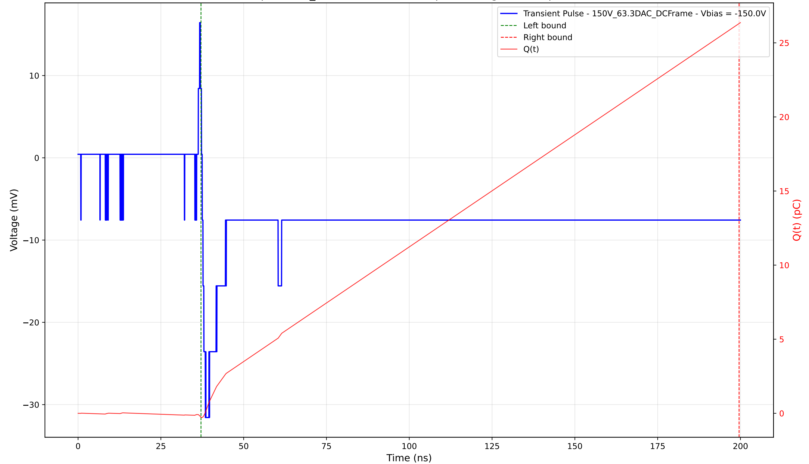
Transient Pulse - Sample: 1cm_42 - Position: 3055.0 \mu\text{m} - Charge: 26.56 pC - Rise Time: 0.95 ns
