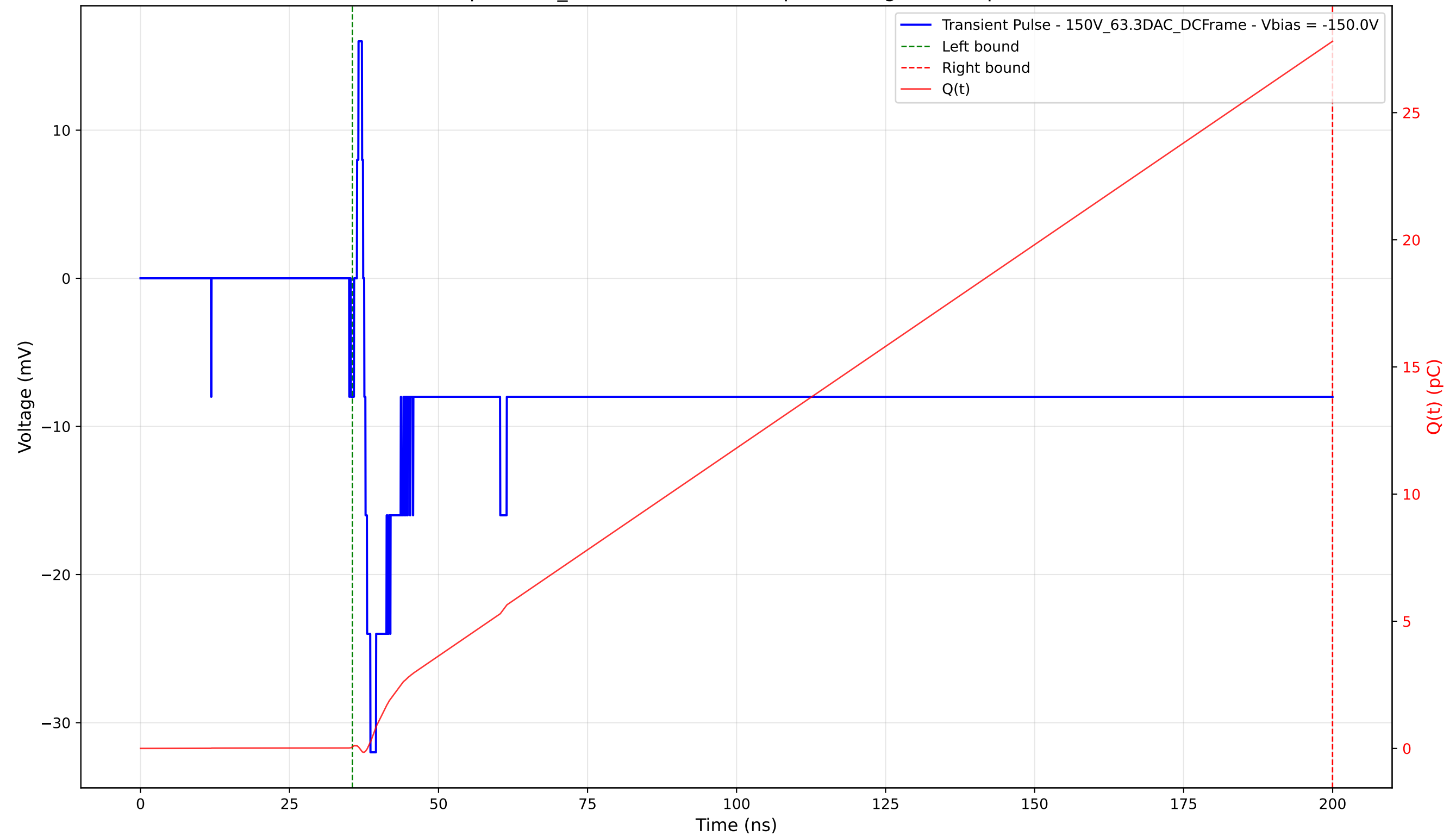
Transient Pulse - Sample: 1cm_42 - Position: 2875.0 \mu\text{m} - Charge: 27.74 pC - Rise Time: 1.03 ns
