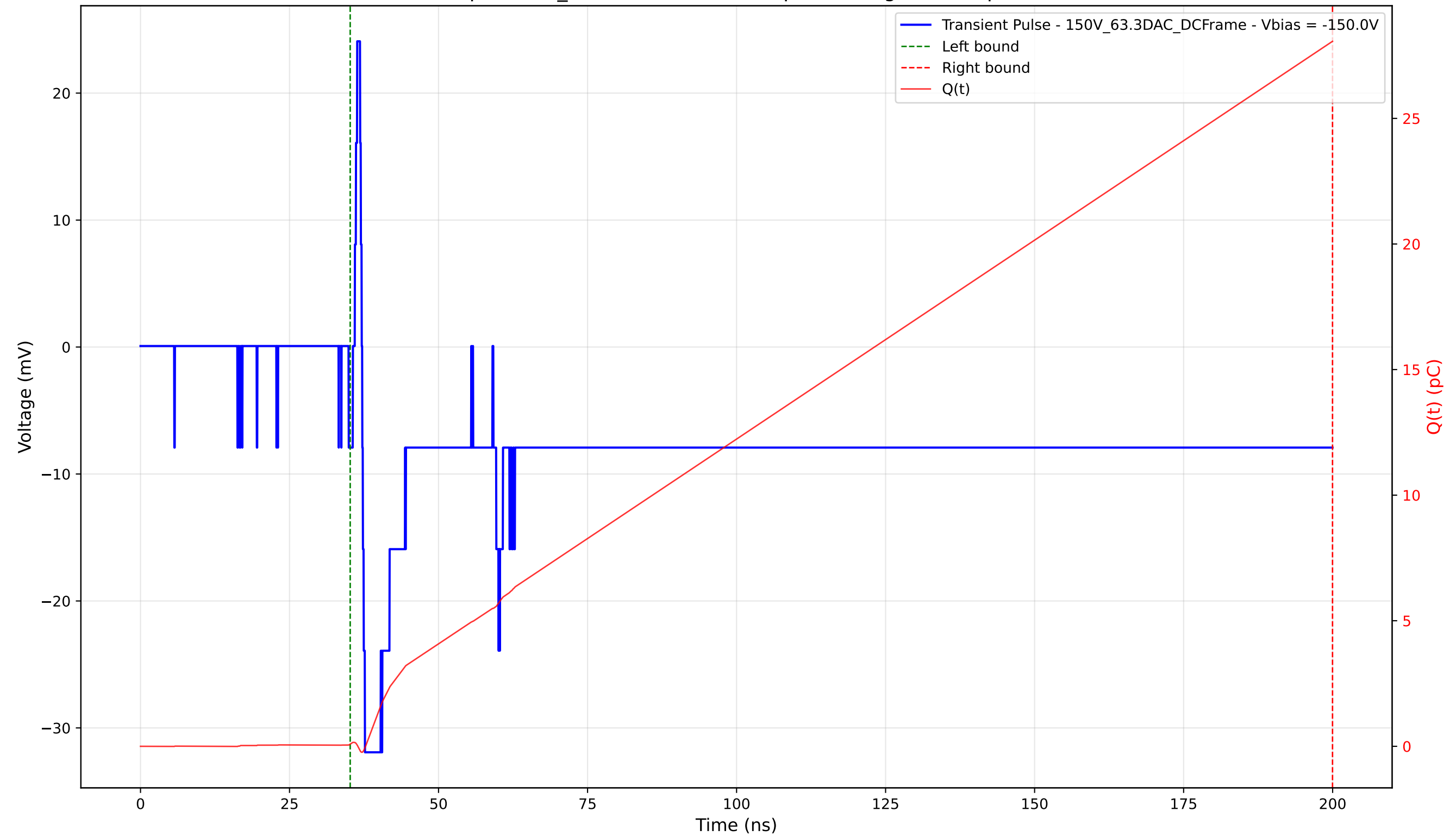
Transient Pulse - Sample: 1cm_42 - Position: 1960.0 \mu\text{m} - Charge: 27.98 pC - Rise Time: 0.45 ns
