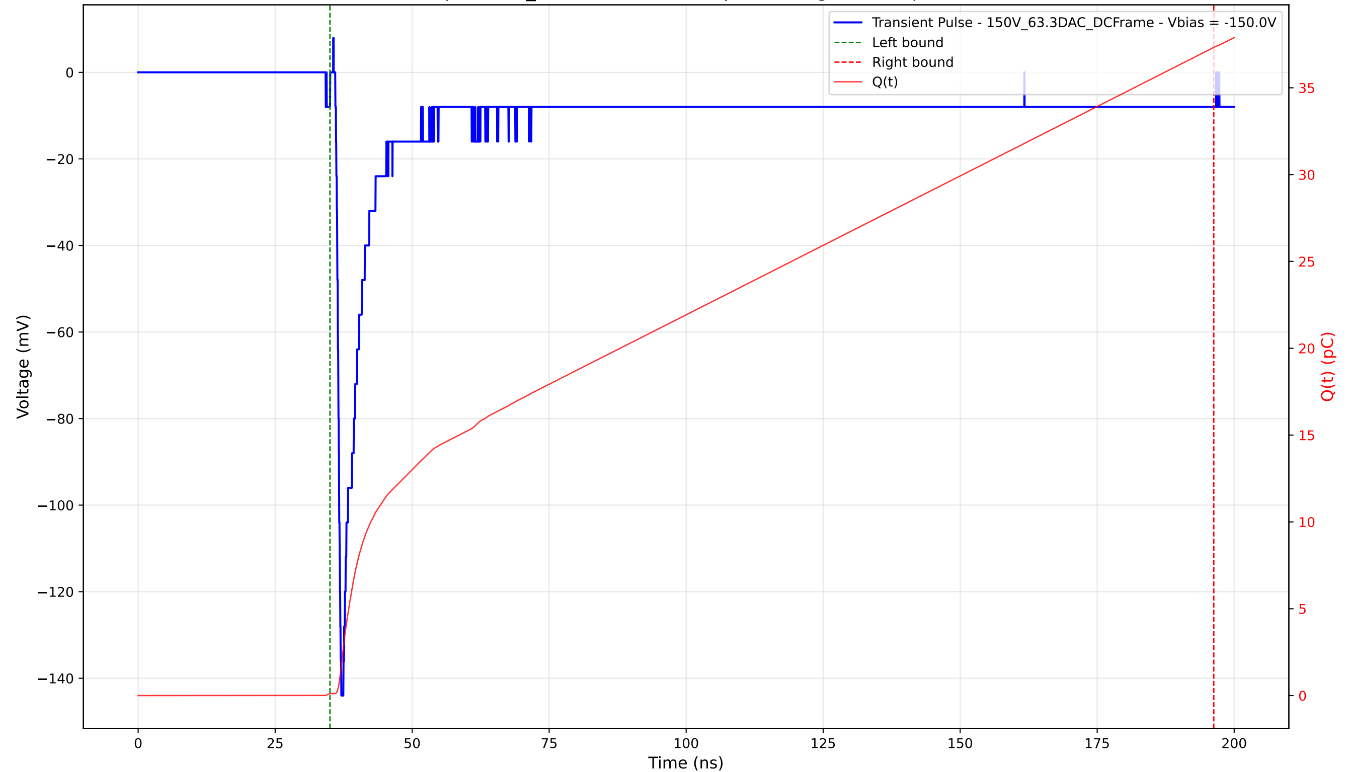
Transient Pulse - Sample: 1cm_42 - Position: 575.0 \mu\text{m} - Charge: 37.21 pC - Rise Time: 0.84 ns
