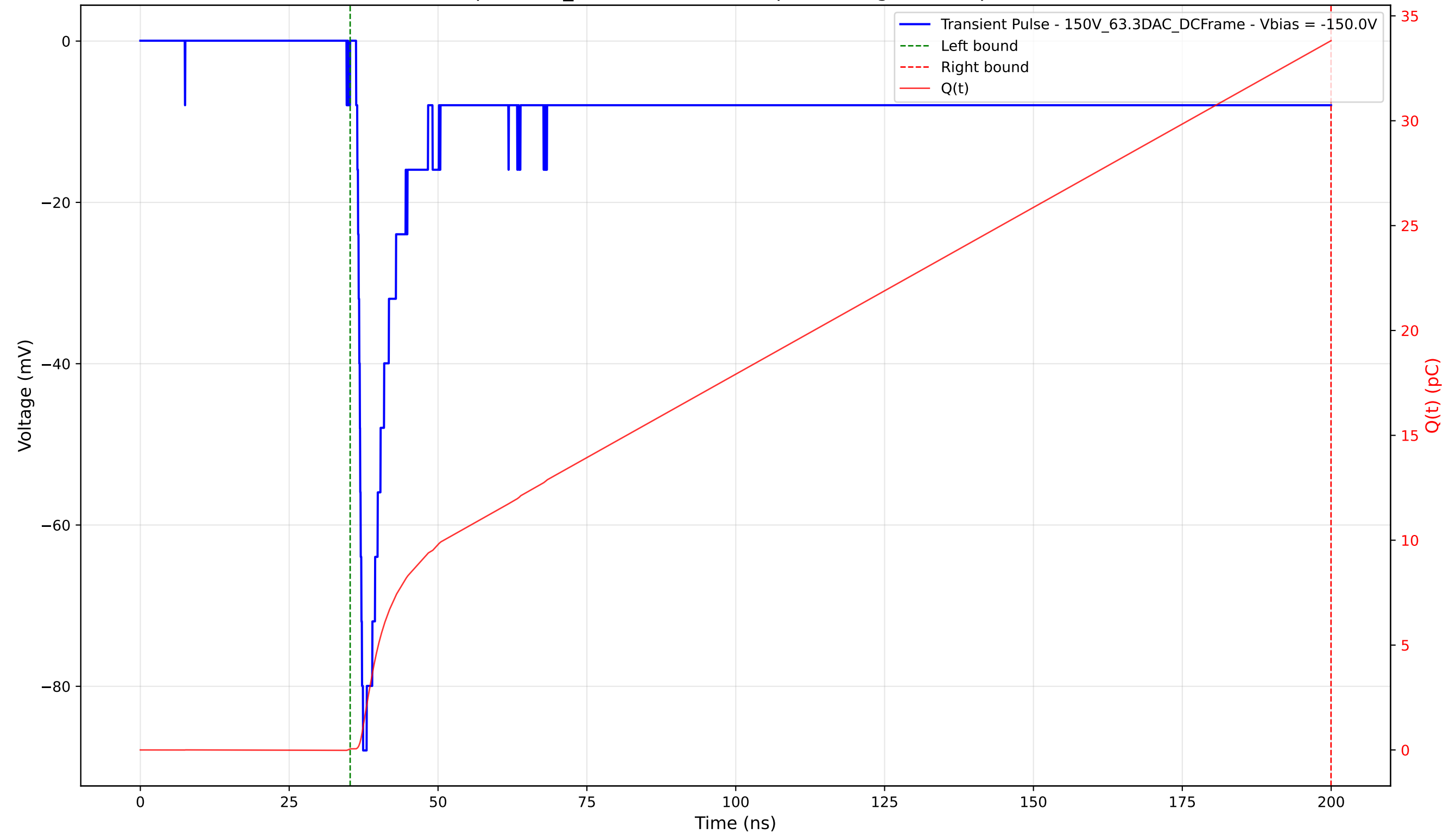
Transient Pulse - Sample: 1cm_42 - Position: 910.0 \mu\text{m} - Charge: 33.76 pC - Rise Time: 0.80 ns
