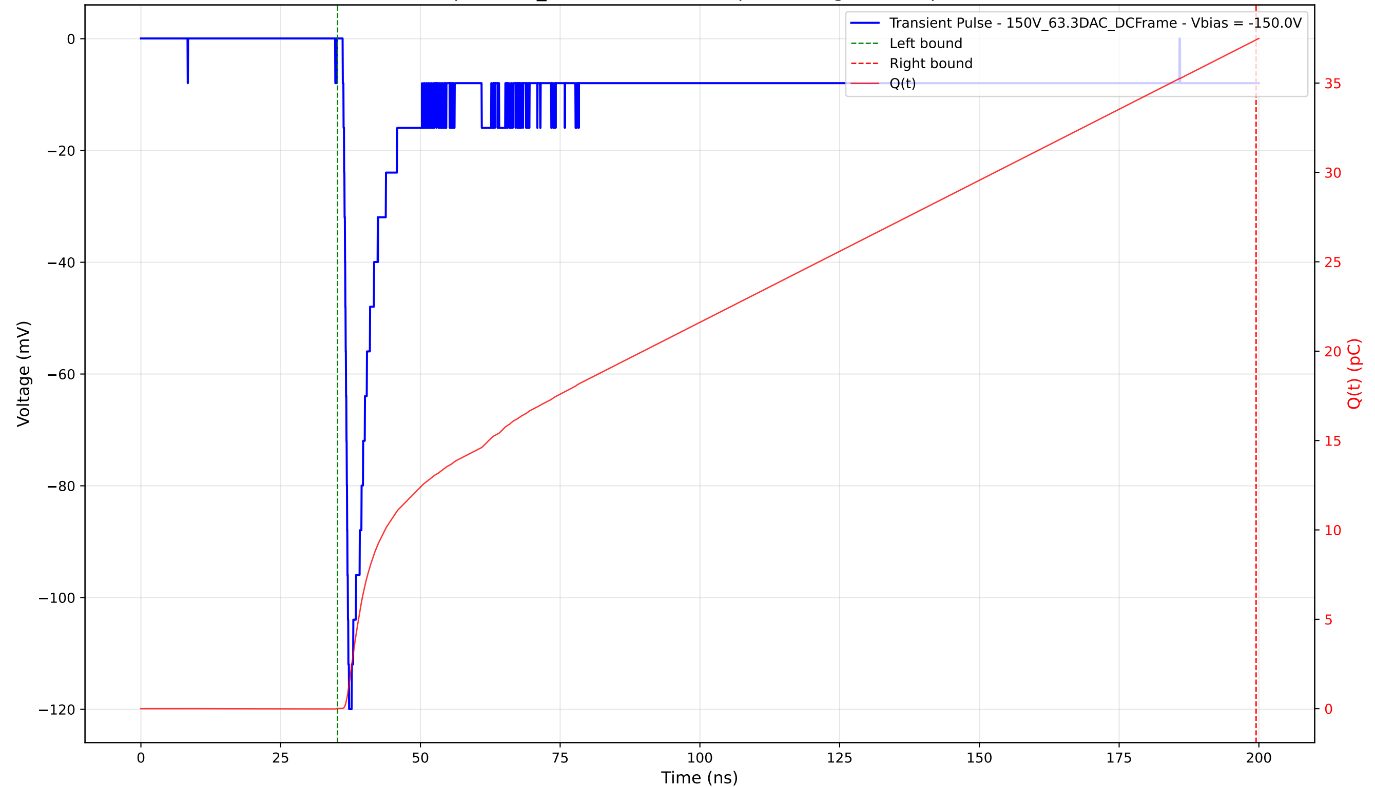
Transient Pulse - Sample: 1cm_42 - Position: 785.0 \mu\text{m} - Charge: 37.41 pC - Rise Time: 0.87 ns
