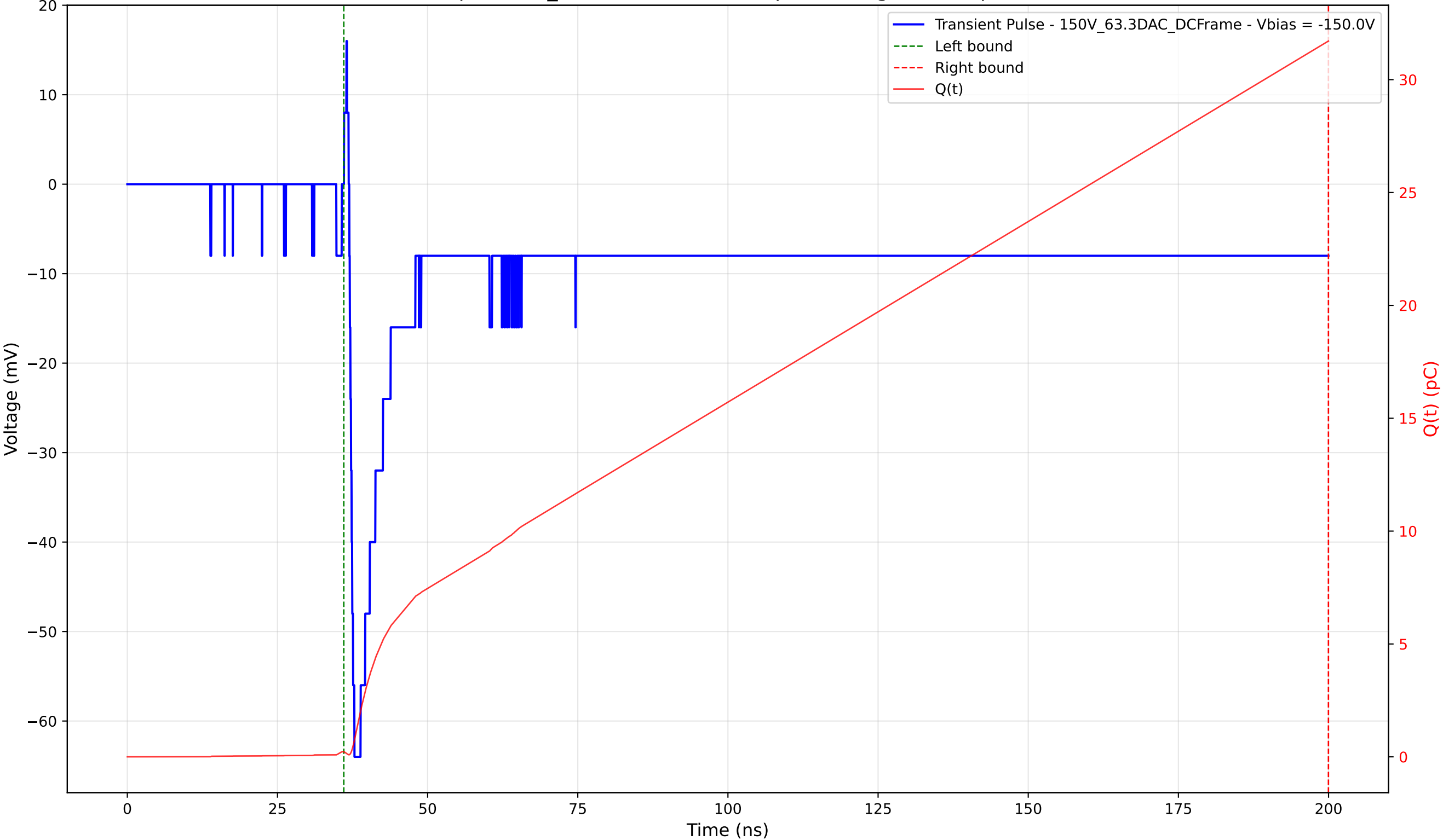
Transient Pulse - Sample: 1cm_42 - Position: 1325.0 \mu\text{m} - Charge: 31.48 pC - Rise Time: 0.84 ns
