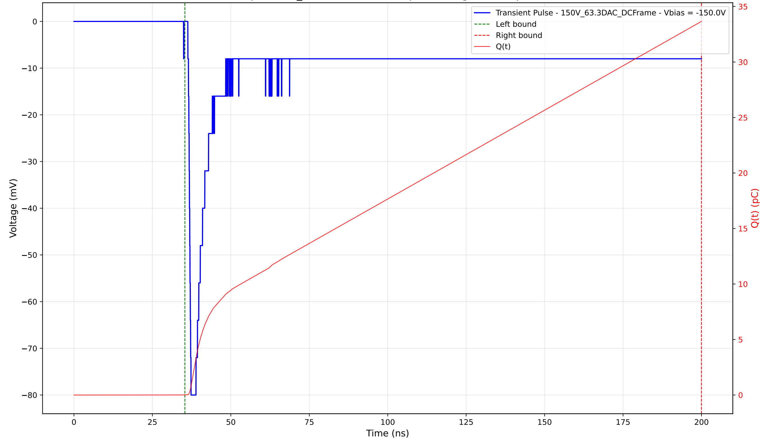
Transient Pulse - Sample: 1cm_42 - Position: 925.0 \mu\text{m} - Charge: 33.64 pC - Rise Time: 0.70 ns
