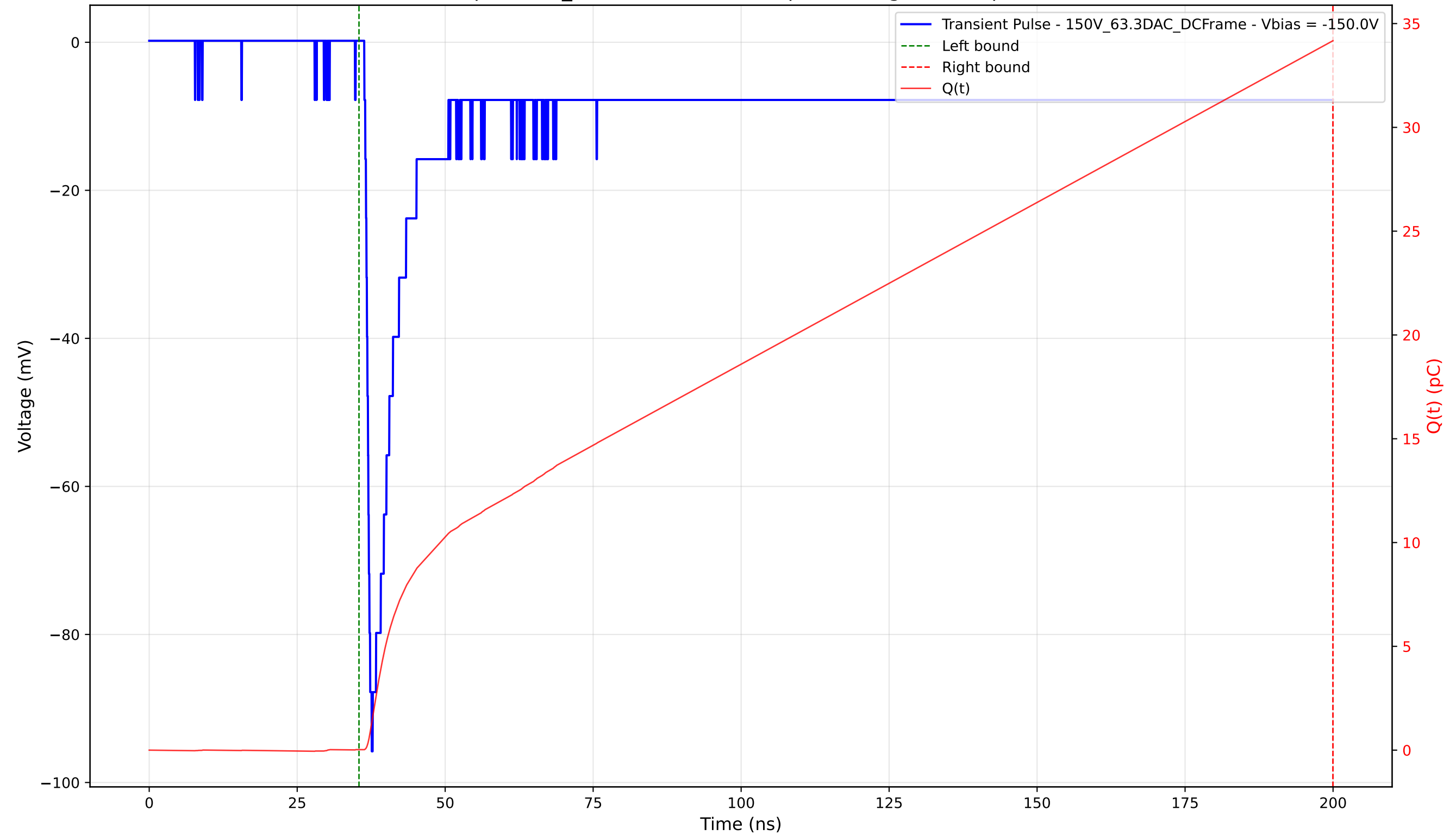
Transient Pulse - Sample: 1cm_42 - Position: 4270.0 \mu\text{m} - Charge: 34.15 pC - Rise Time: 0.84 ns
