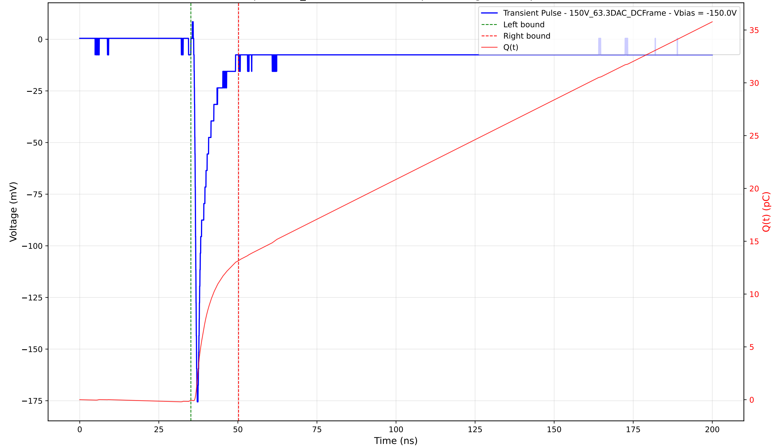
Transient Pulse - Sample: 1cm_42 - Position: 4630.0 \mu\text{m} - Charge: 13.21 pC - Rise Time: 0.75 ns
