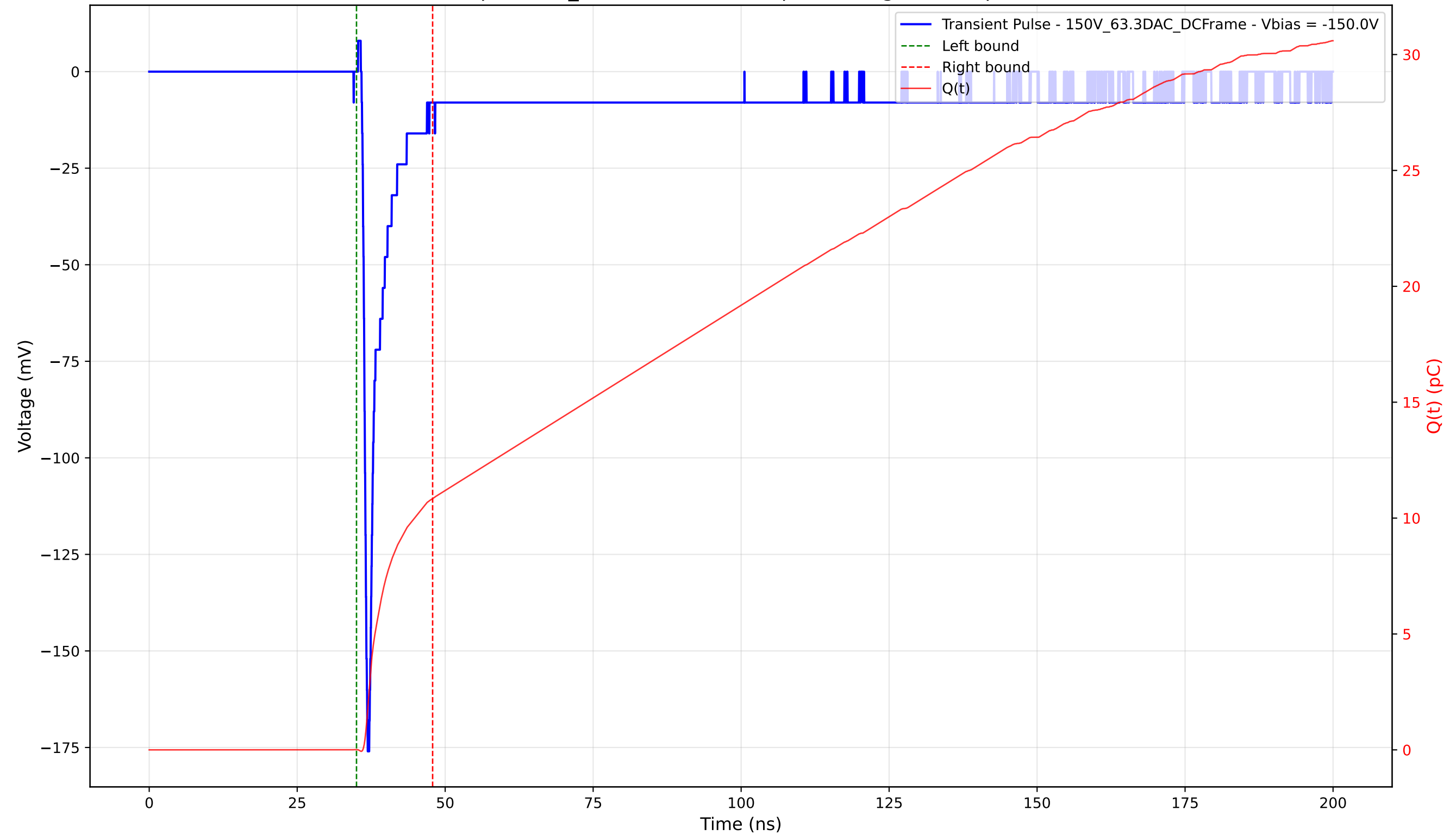
Transient Pulse - Sample: 1cm_42 - Position: 320.0 \mu\text{m} - Charge: 10.83 pC - Rise Time: 0.74 ns
