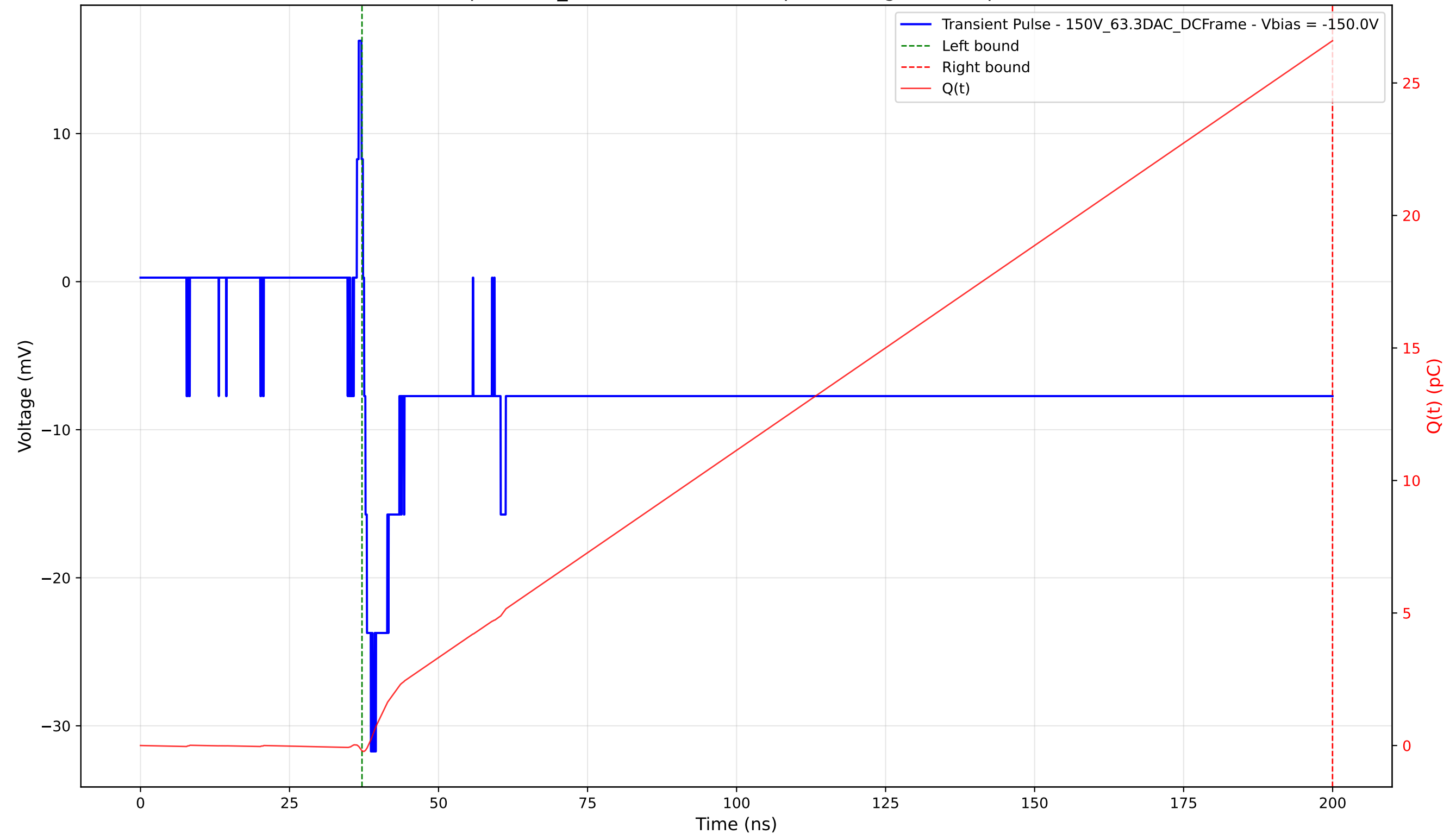
Transient Pulse - Sample: 1cm_42 - Position: 2925.0 \mu\text{m} - Charge: 26.79 pC - Rise Time: 1.13 ns
