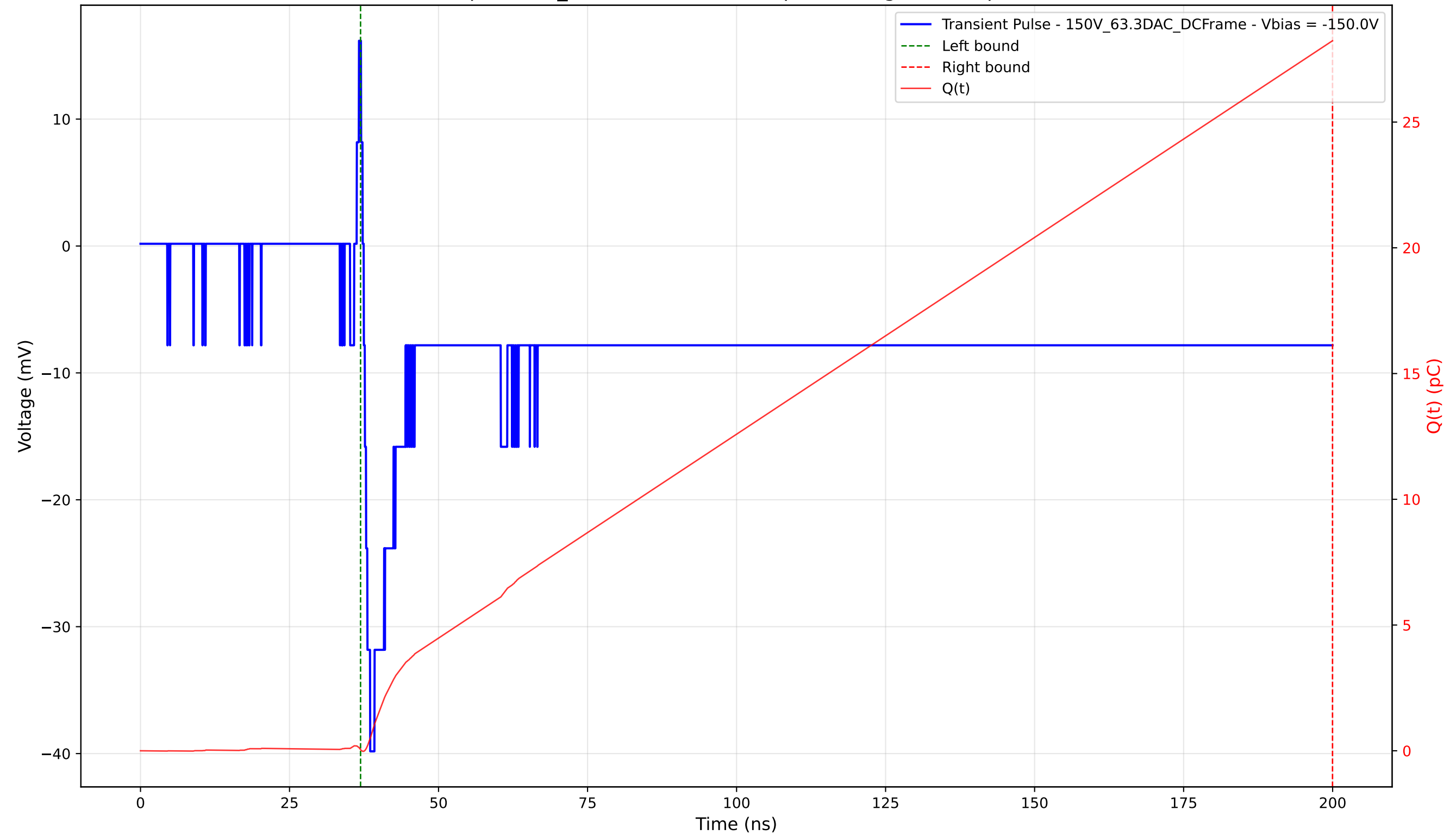
Transient Pulse - Sample: 1cm_42 - Position: 3190.0 \mu\text{m} - Charge: 28.19 pC - Rise Time: 1.07 ns
