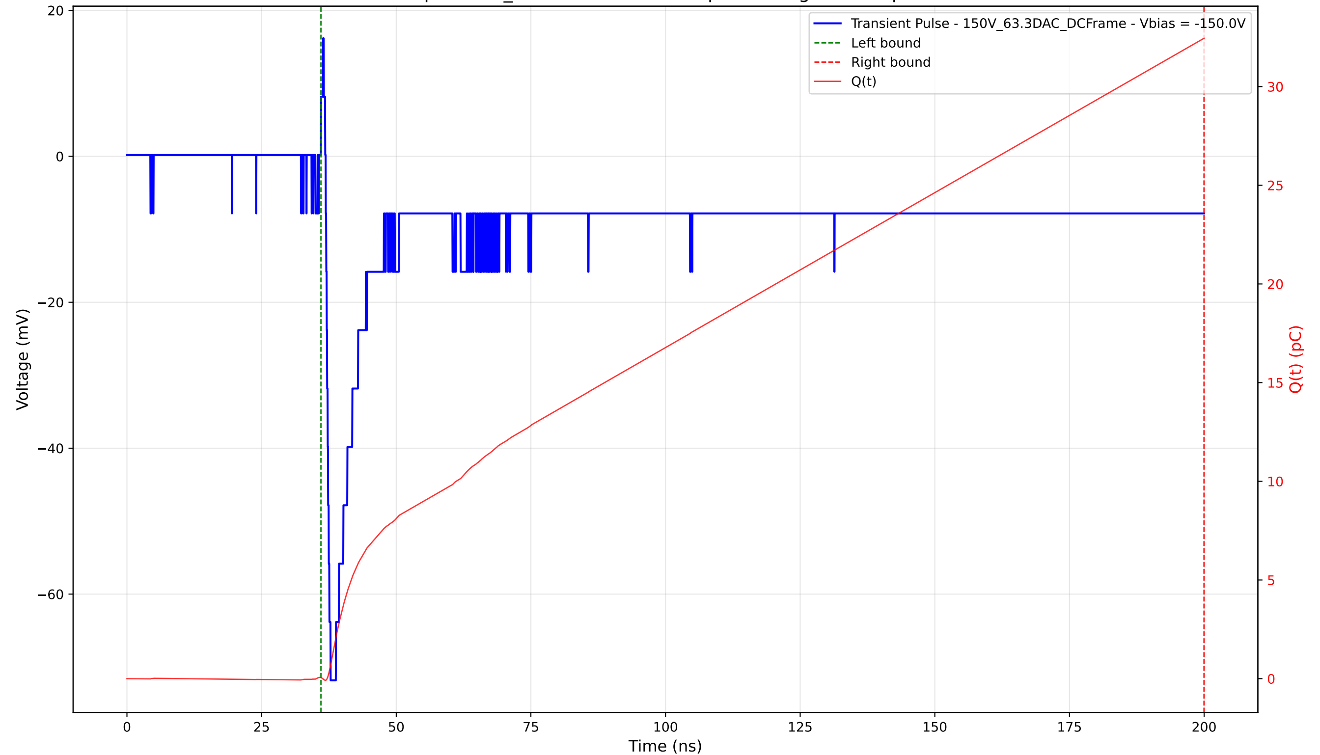
Transient Pulse - Sample: 1cm_42 - Position: 1270.0 \mu\text{m} - Charge: 32.39 pC - Rise Time: 0.90 ns
