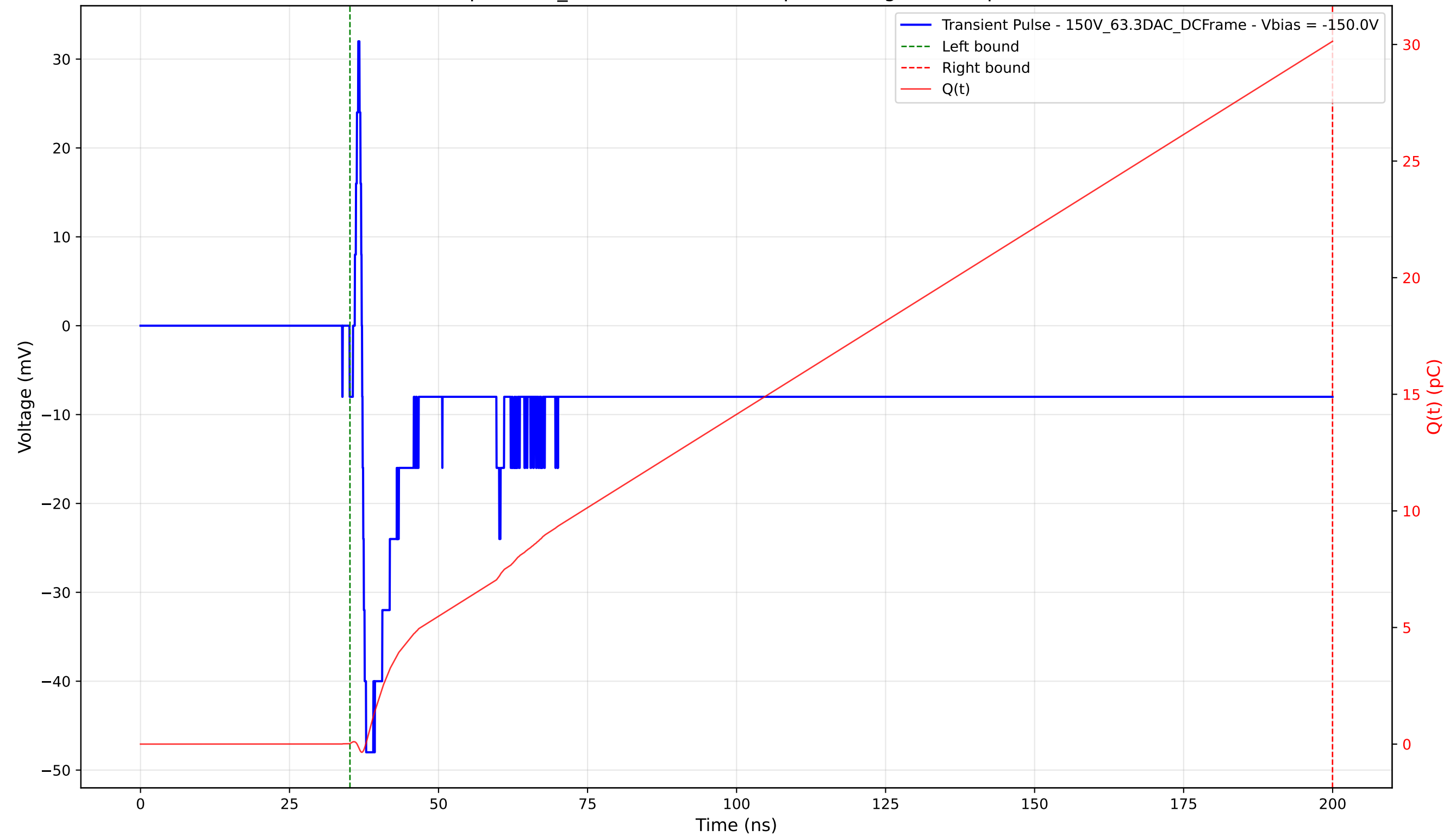
Transient Pulse - Sample: 1cm_42 - Position: 1755.0 \mu\text{m} - Charge: 30.11 pC - Rise Time: 0.67 ns
