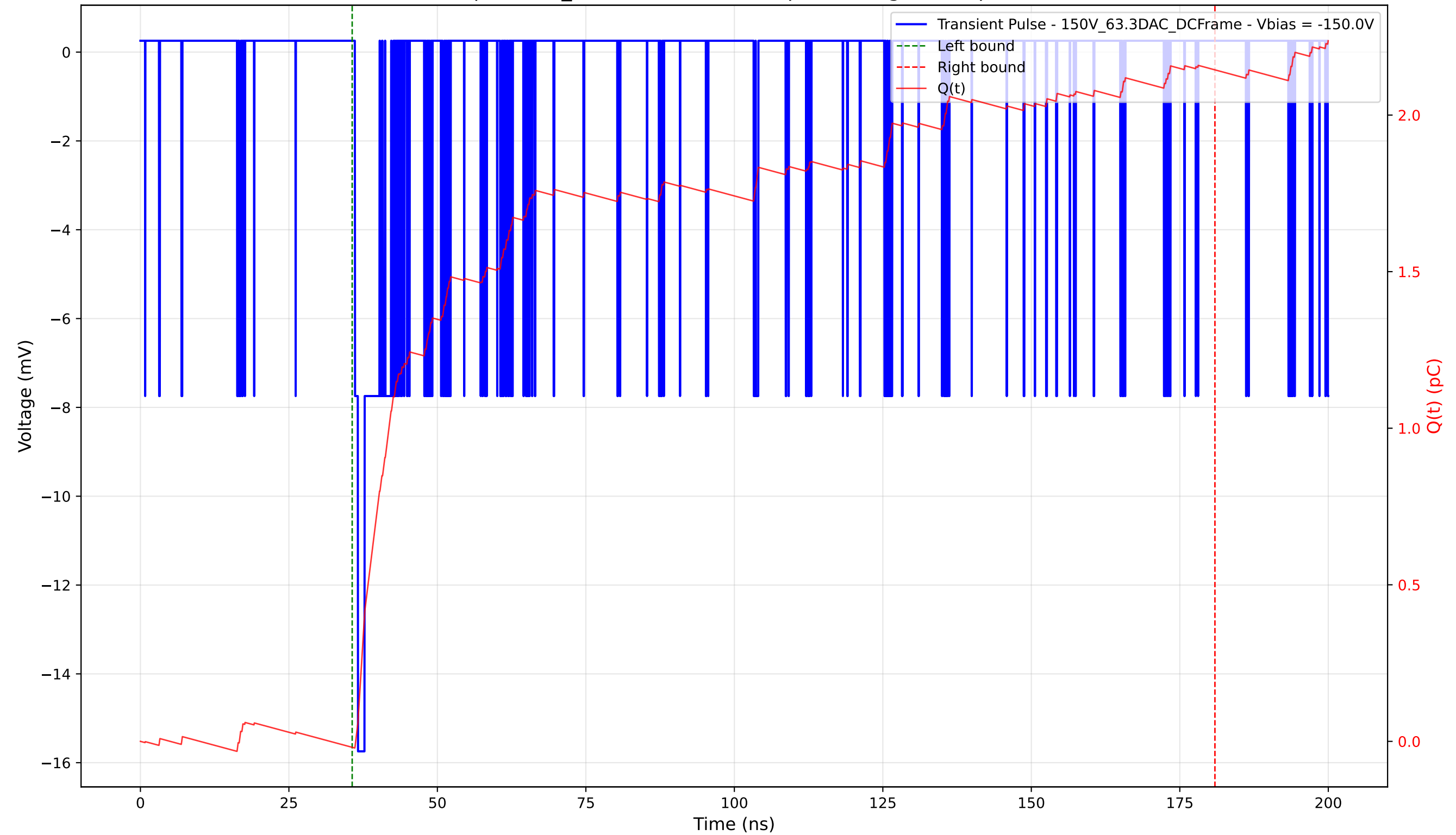
Transient Pulse - Sample: 1cm_42 - Position: 5200.0 \mu\text{m} - Charge: 2.16 pC - Rise Time: 0.52 ns
