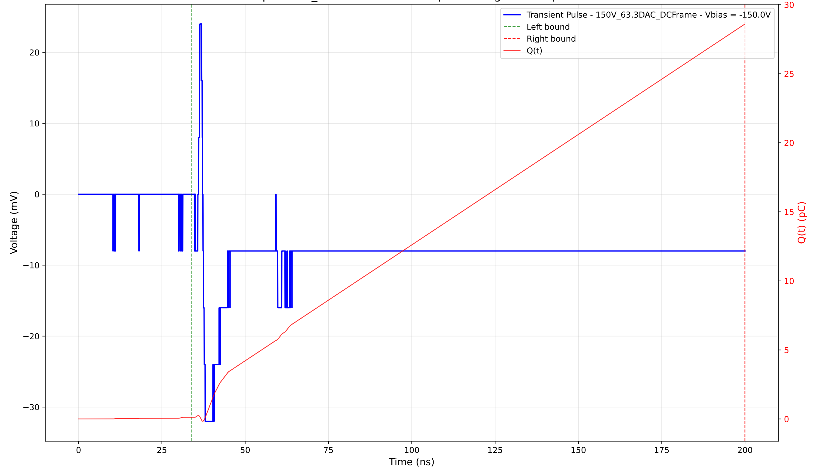
Transient Pulse - Sample: 1cm_42 - Position: 2285.0 \mu\text{m} - Charge: 28.48 pC - Rise Time: 0.65 ns
