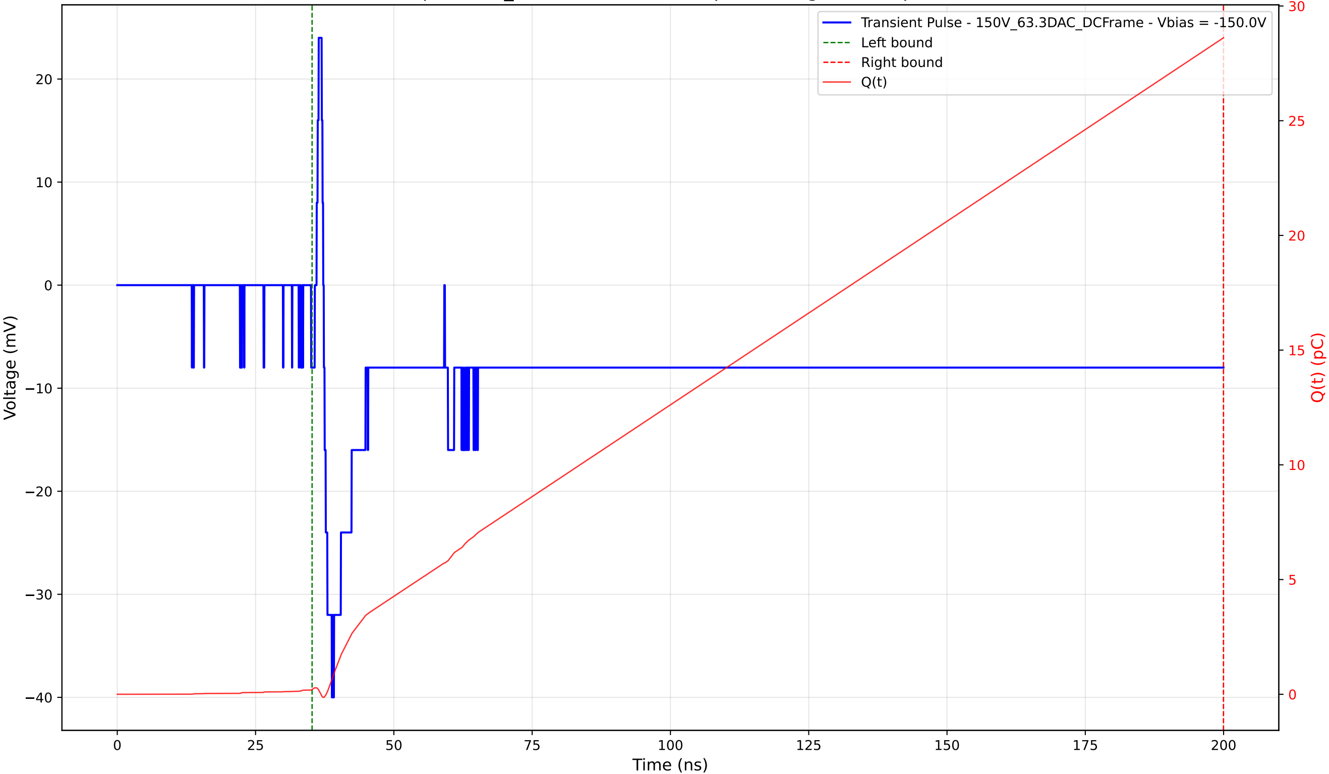
Transient Pulse - Sample: 1cm_42 - Position: 2295.0 \mu\text{m} - Charge: 28.40 pC - Rise Time: 1.45 ns
