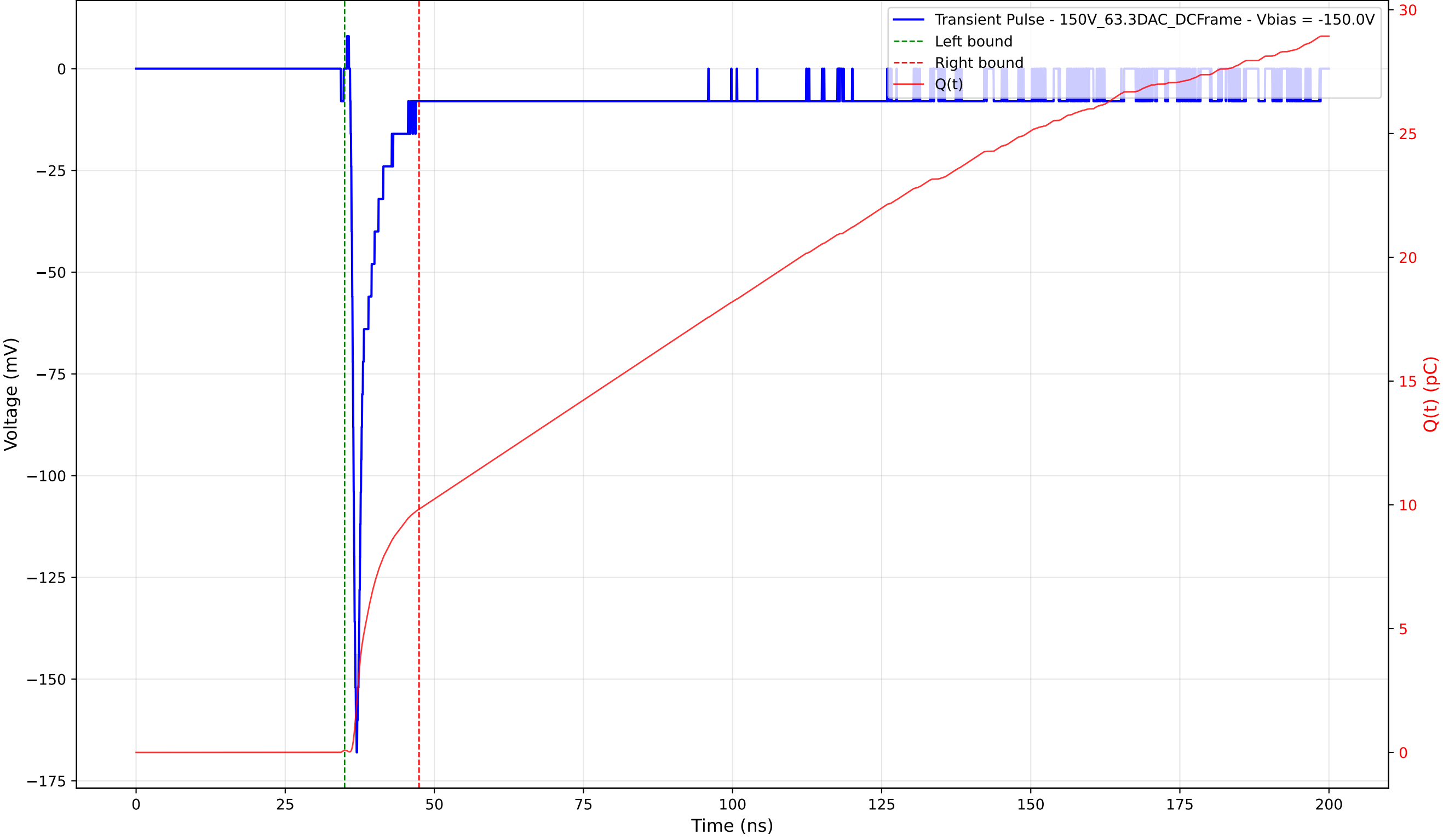
Transient Pulse - Sample: 1cm_42 - Position: 250.0 \mu\text{m} - Charge: 9.75 pC - Rise Time: 0.74 ns
