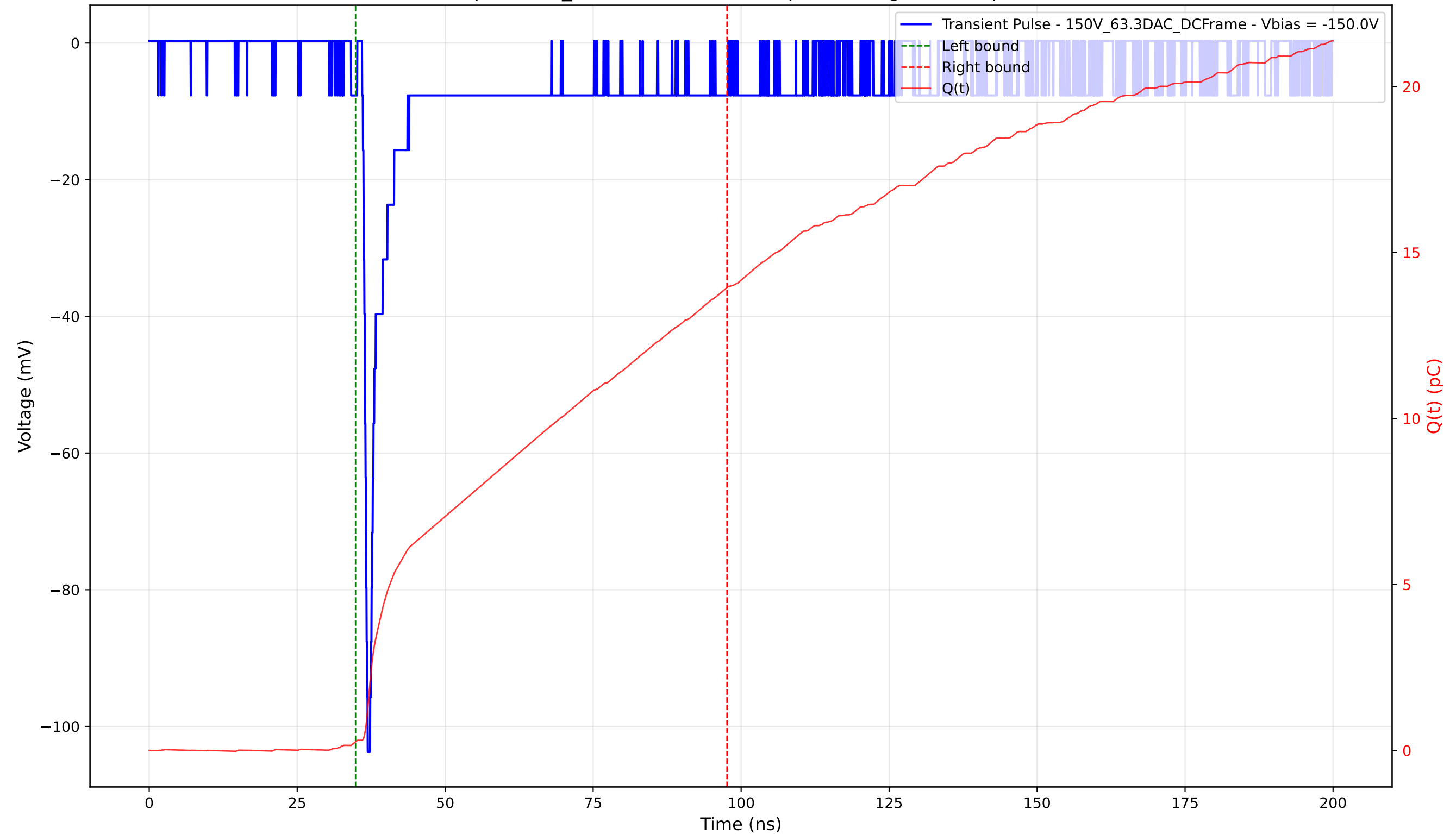
Transient Pulse - Sample: 1cm_42 - Position: 5035.0 \mu\text{m} - Charge: 13.68 pC - Rise Time: 0.71 ns
