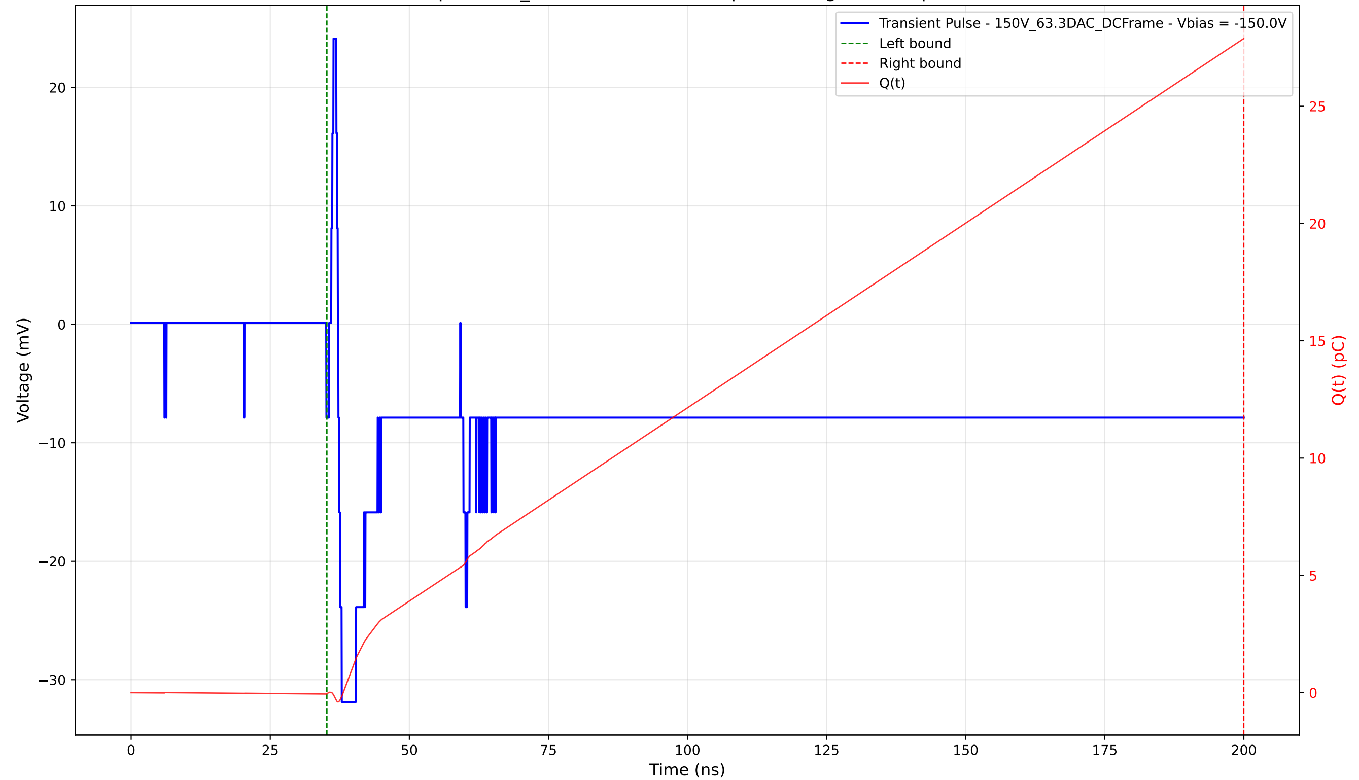
Transient Pulse - Sample: 1cm_42 - Position: 2085.0 \mu\text{m} - Charge: 27.93 pC - Rise Time: 0.61 ns
