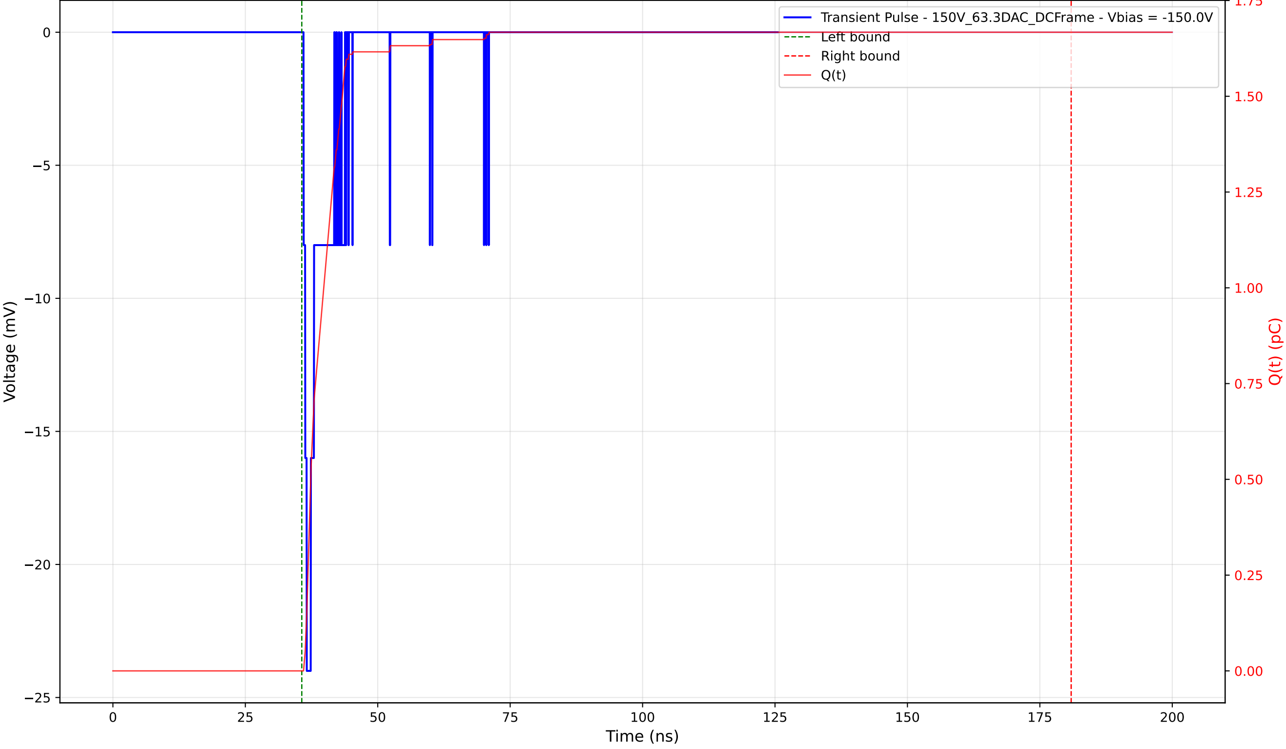
Transient Pulse - Sample: 1cm_42 - Position: 5.0 \mu\text{m} - Charge: 1.67 pC - Rise Time: 0.59 ns
