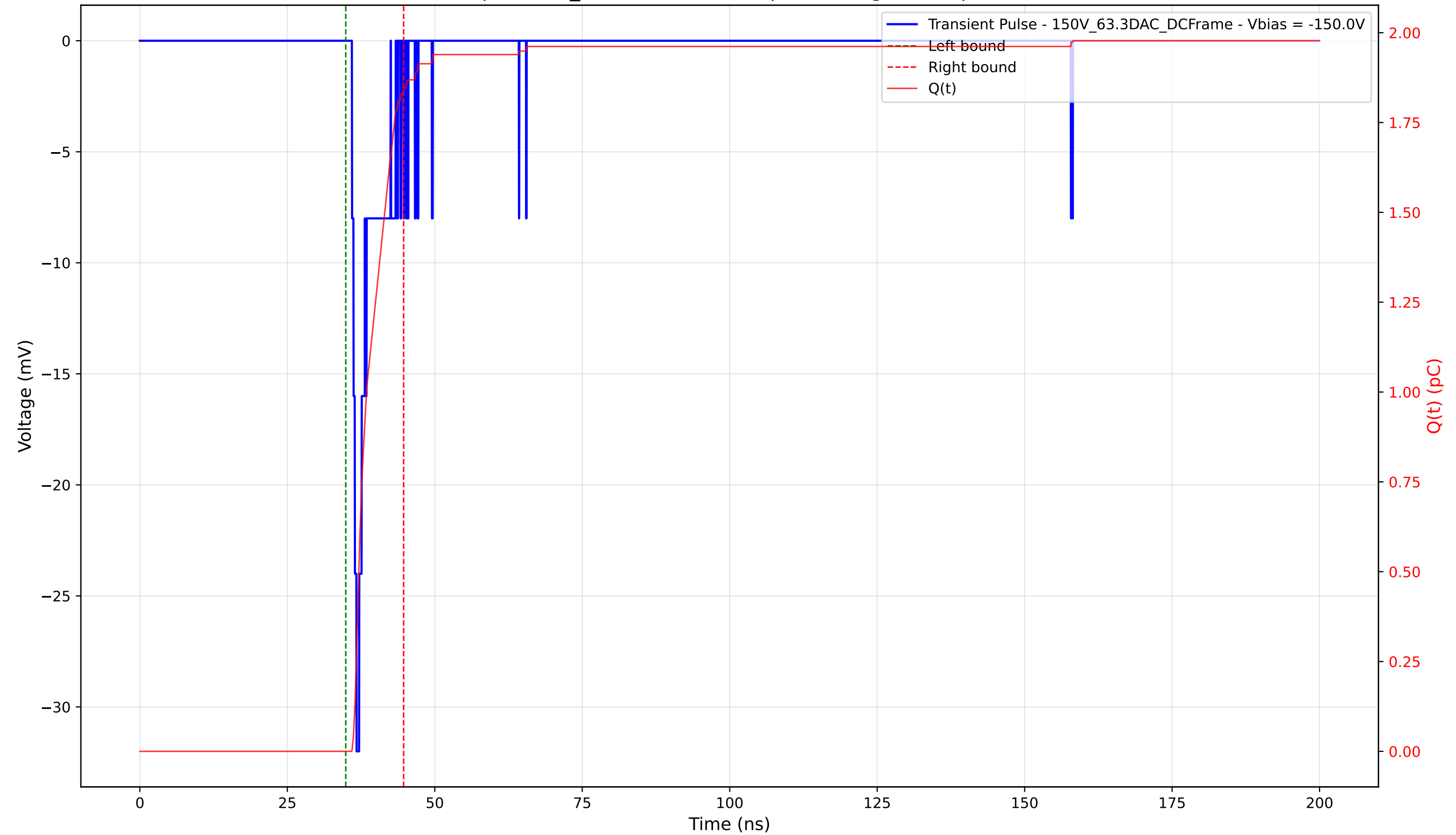
Transient Pulse - Sample: 1cm_42 - Position: 15.0 \mu\text{m} - Charge: 1.84 pC - Rise Time: 0.77 ns
