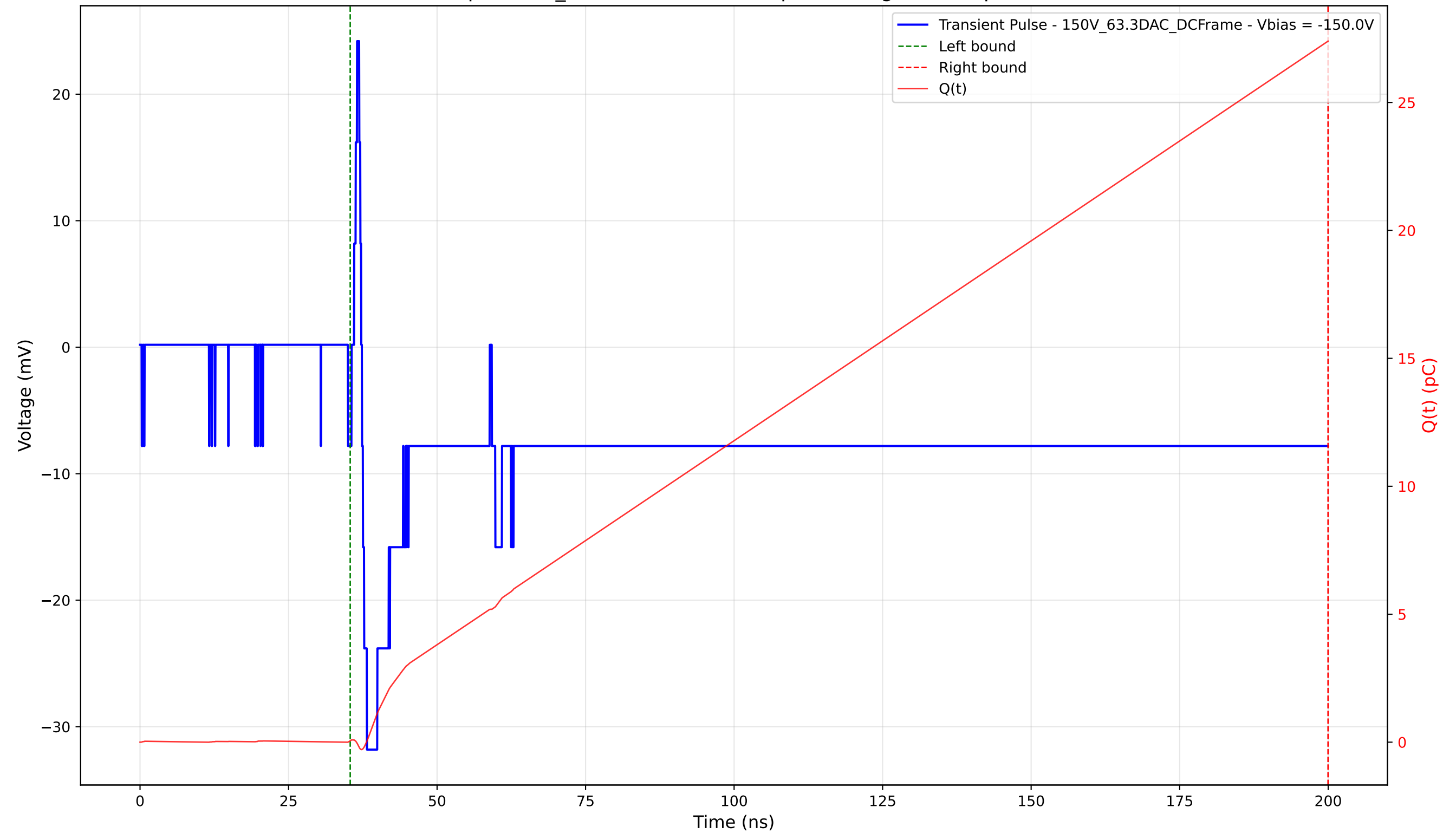
Transient Pulse - Sample: 1cm_42 - Position: 2355.0 \mu\text{m} - Charge: 27.34 pC - Rise Time: 0.83 ns
