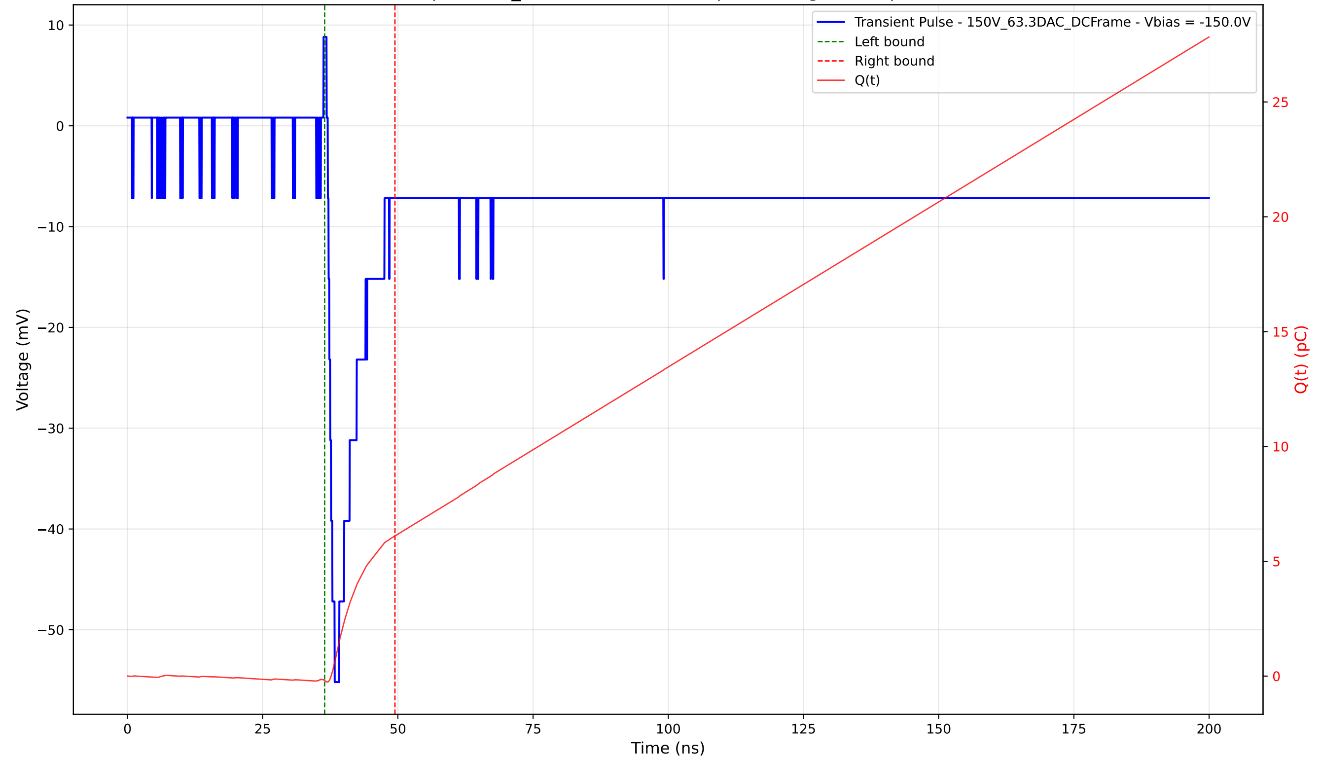
Transient Pulse - Sample: 1cm_42 - Position: 3740.0 \mu\text{m} - Charge: 6.30 pC - Rise Time: 1.27 ns
