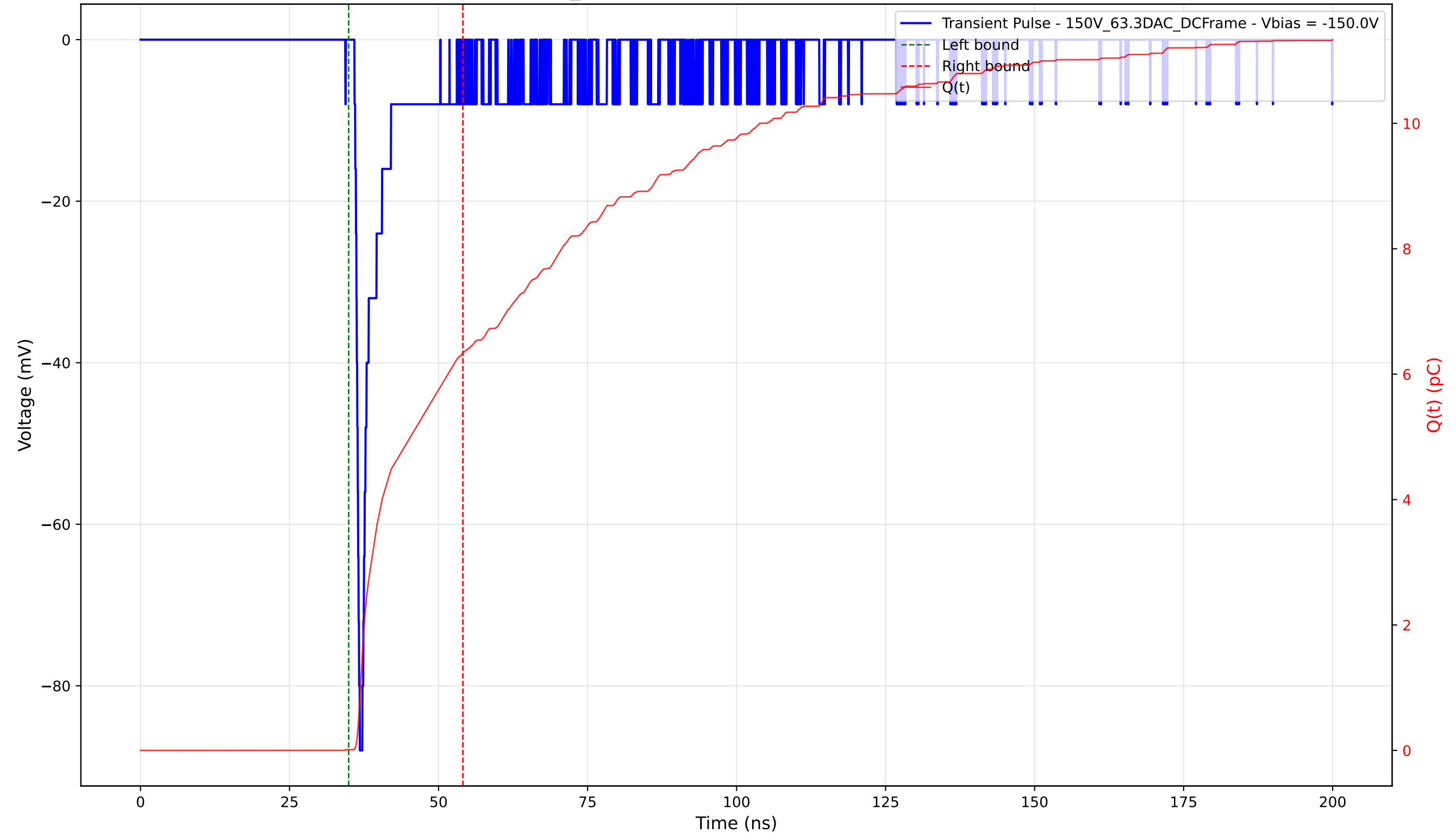
Transient Pulse - Sample: 1cm_42 - Position: 115.0 \mu\text{m} - Charge: 6.33 pC - Rise Time: 0.66 ns
