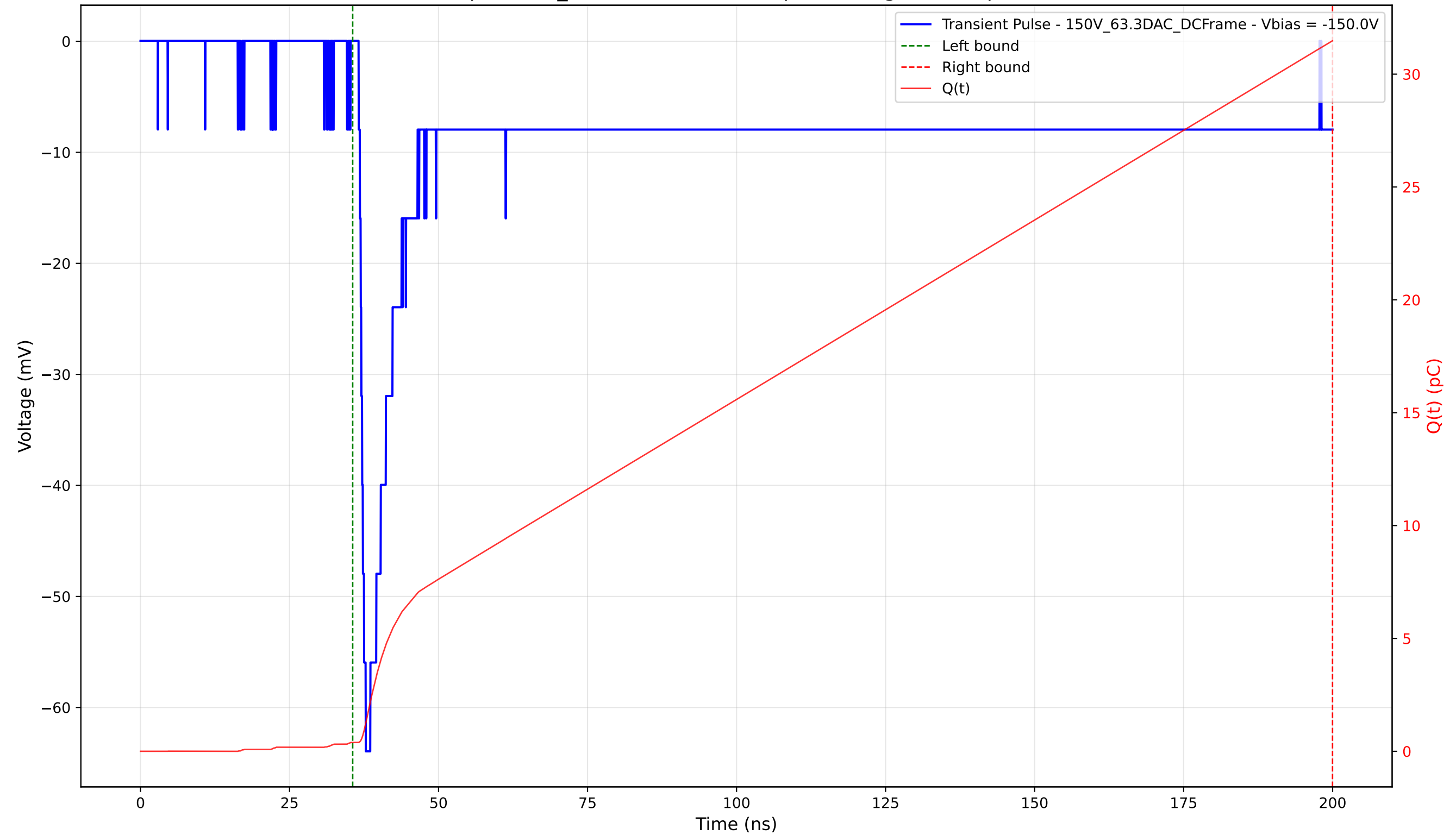
Transient Pulse - Sample: 1cm_42 - Position: 4060.0 \mu\text{m} - Charge: 31.09 pC - Rise Time: 1.18 ns
