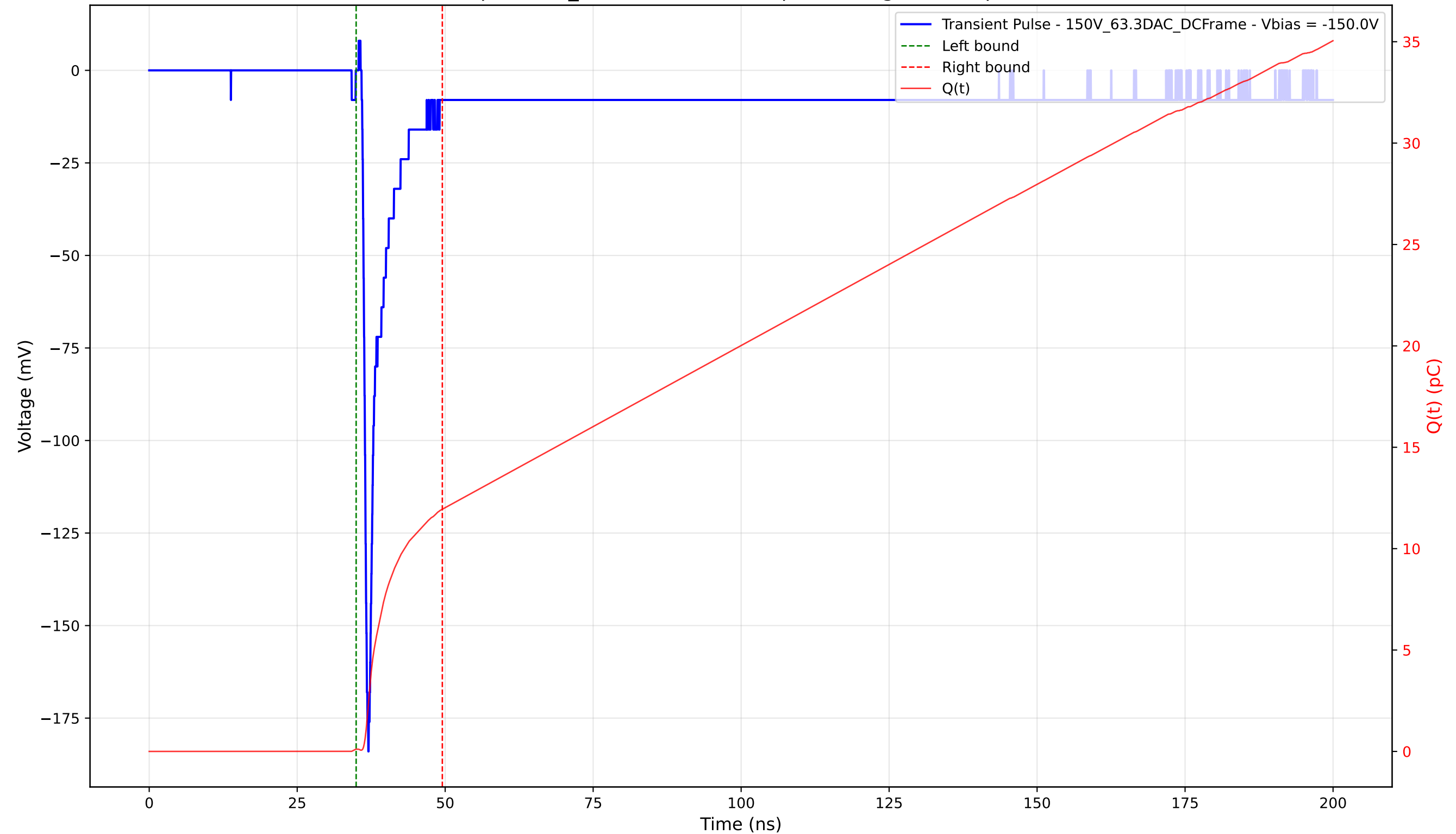
Transient Pulse - Sample: 1cm_42 - Position: 345.0 \mu\text{m} - Charge: 11.83 pC - Rise Time: 0.75 ns
