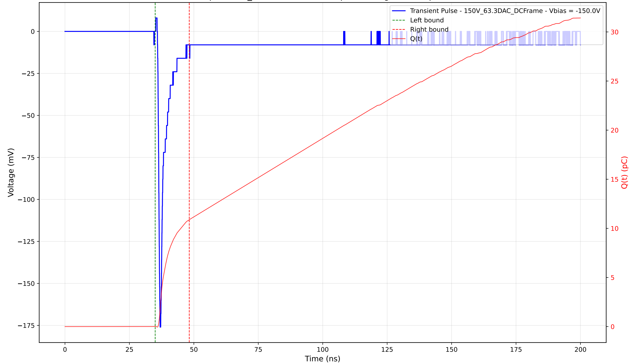
Transient Pulse - Sample: 1cm_42 - Position: 310.0 \mu\text{m} - Charge: 10.84 pC - Rise Time: 0.74 ns
