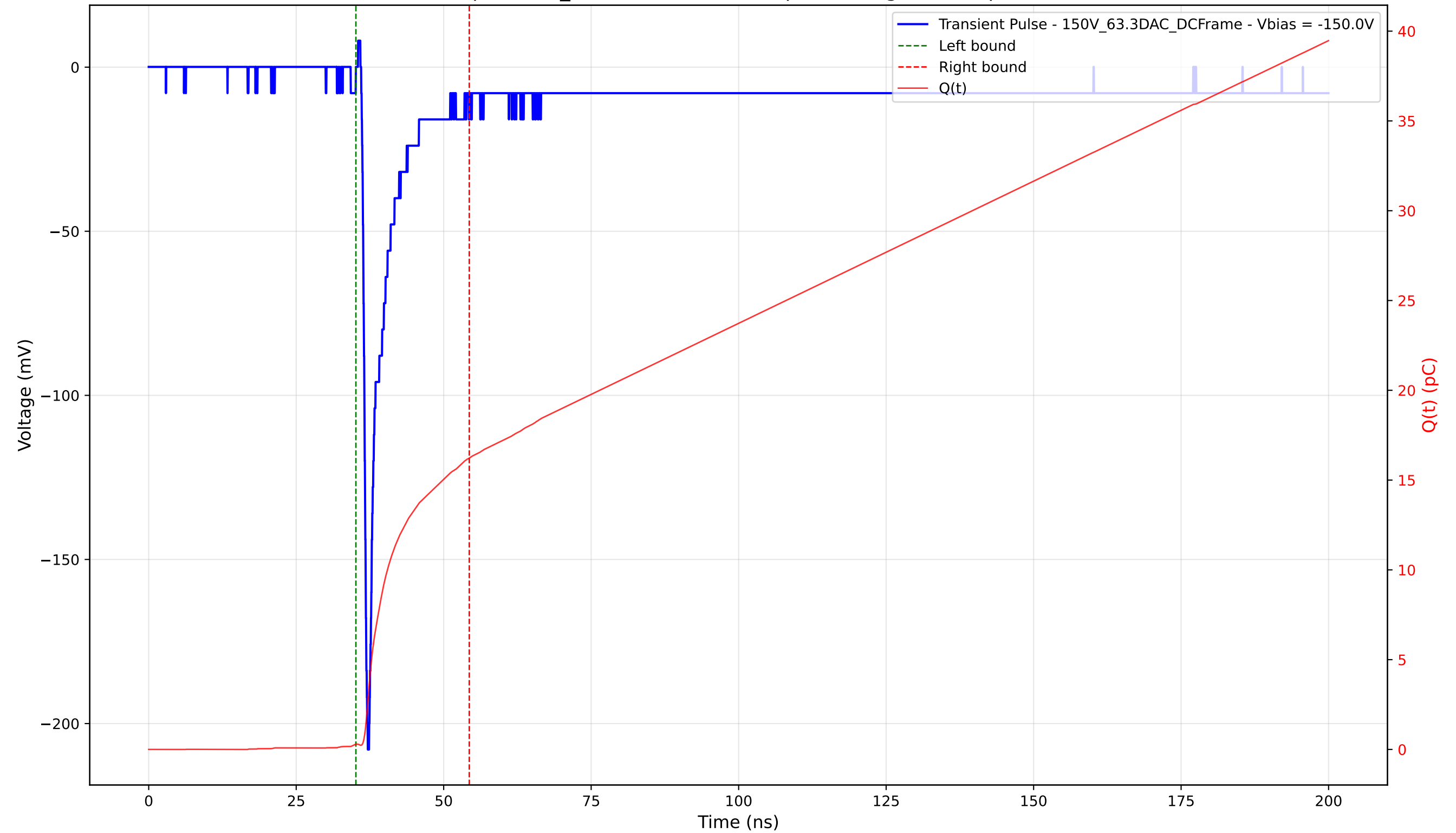
Transient Pulse - Sample: 1cm_42 - Position: 4685.0 \mu\text{m} - Charge: 15.93 pC - Rise Time: 0.81 ns
