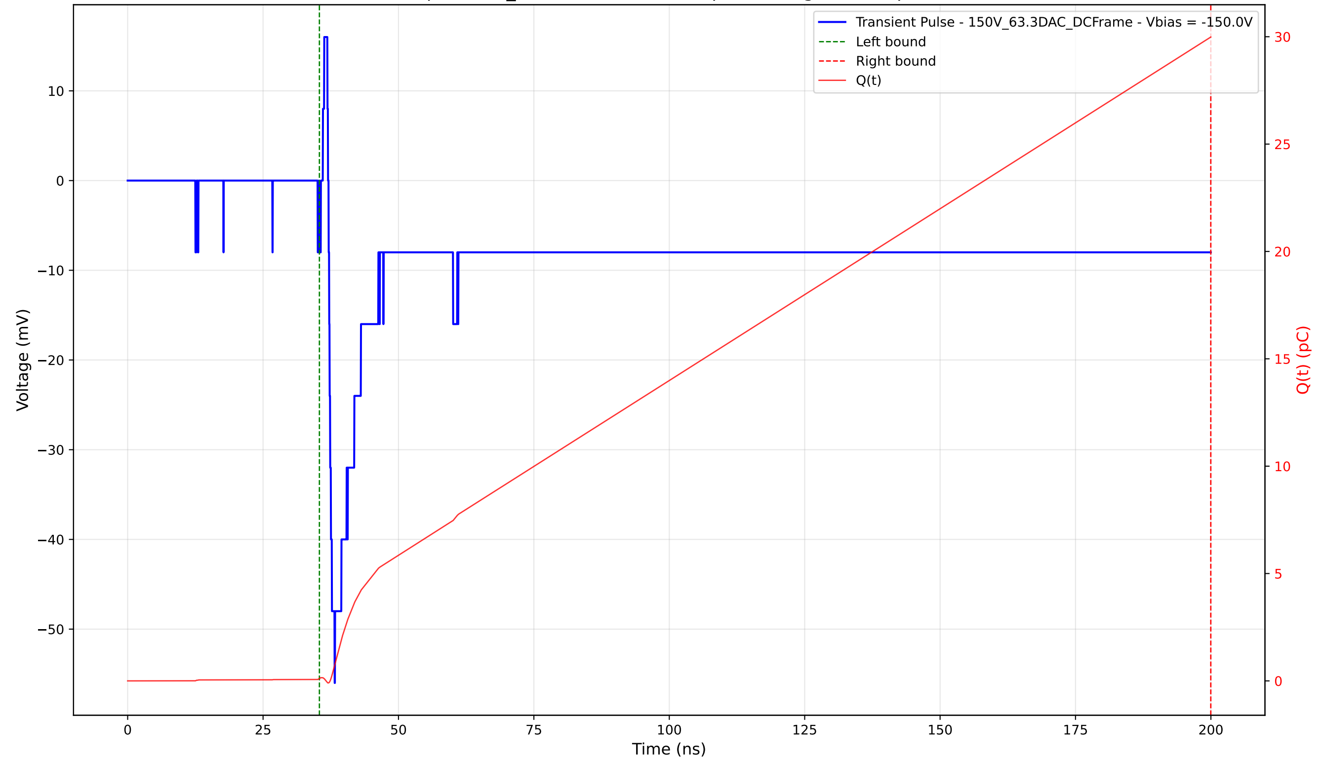
Transient Pulse - Sample: 1cm_42 - Position: 1495.0 \mu\text{m} - Charge: 29.88 pC - Rise Time: 1.11 ns
