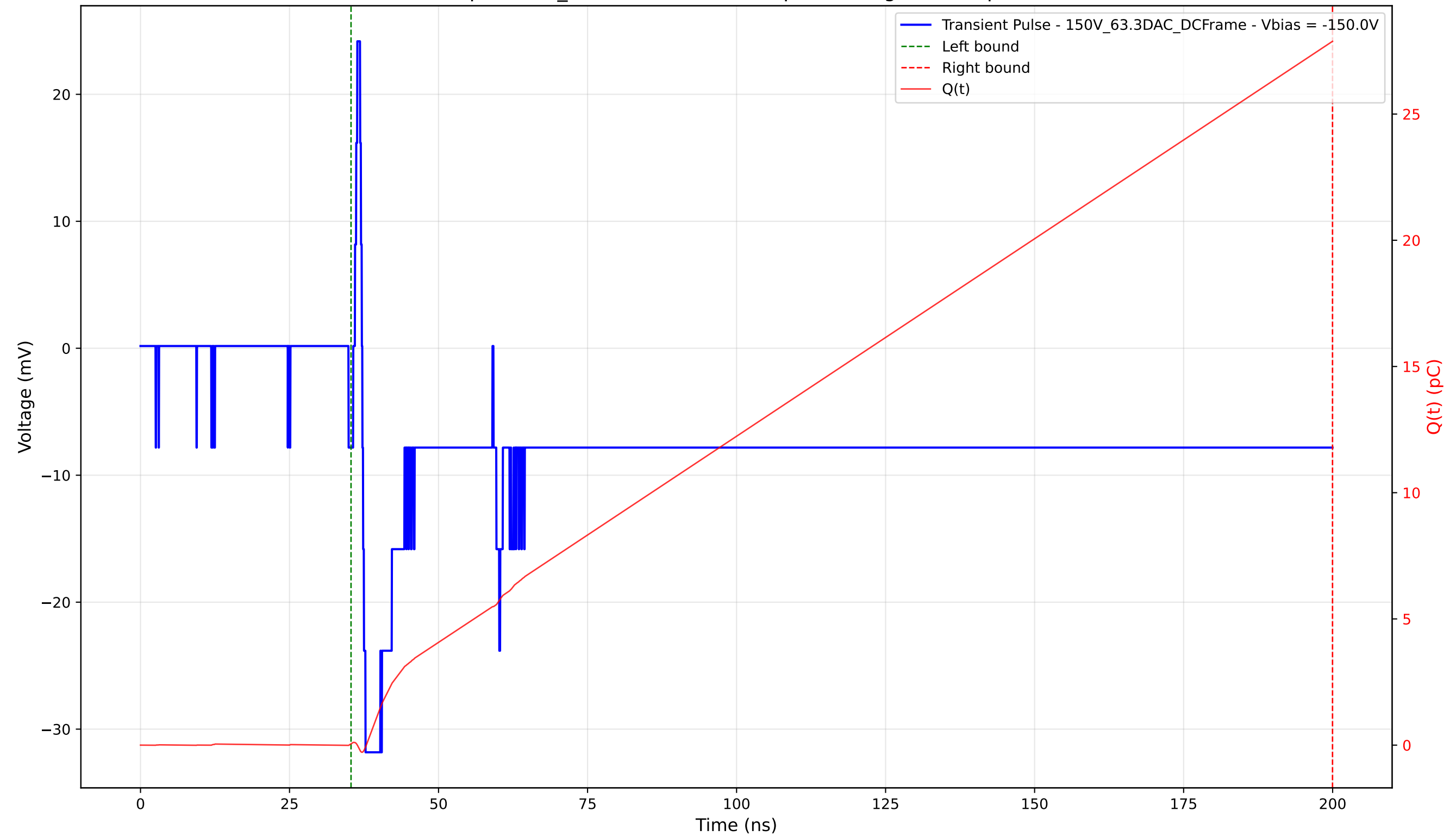
Transient Pulse - Sample: 1cm_42 - Position: 2035.0 \mu\text{m} - Charge: 27.83 pC - Rise Time: 0.53 ns
