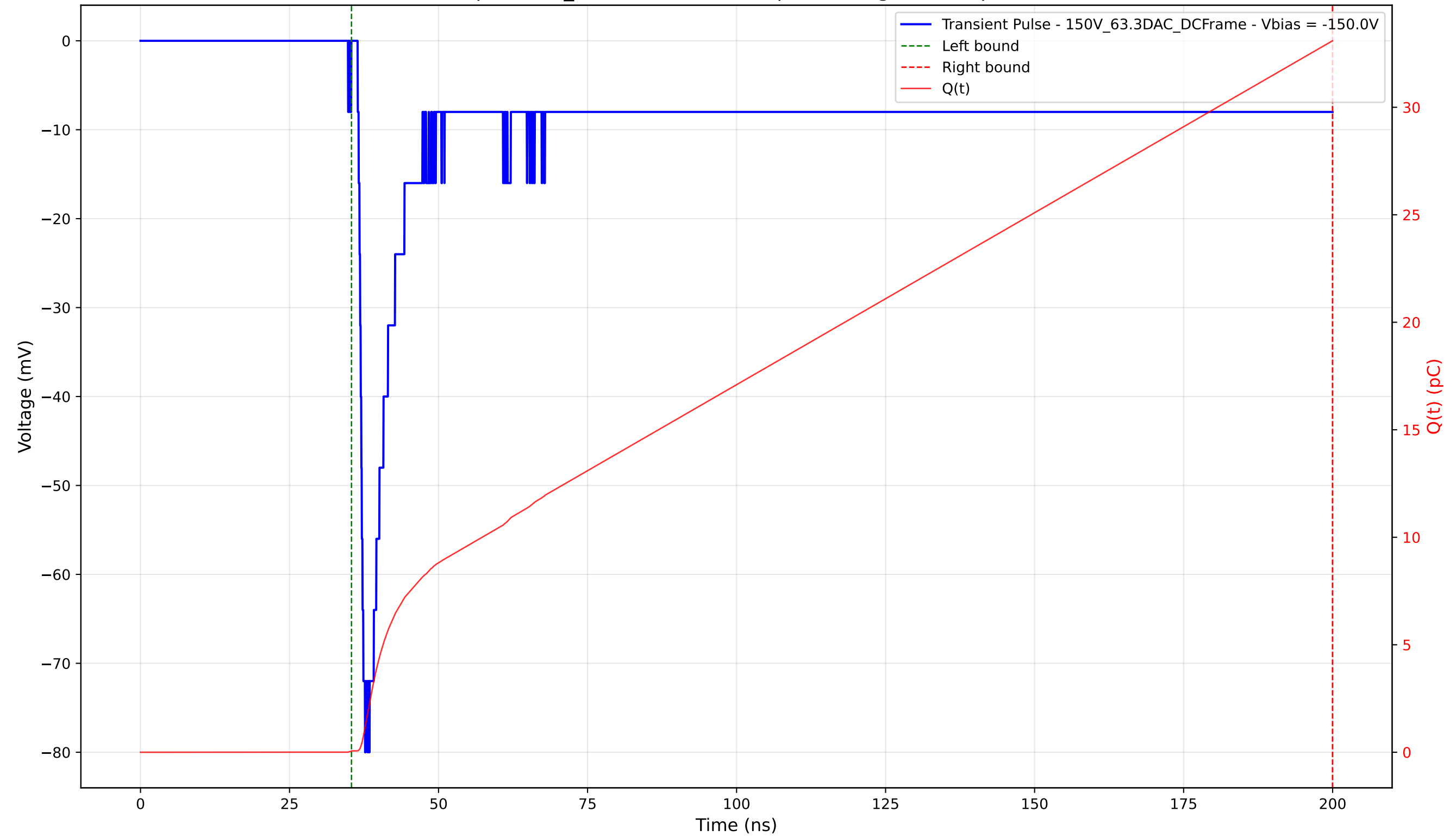
Transient Pulse - Sample: 1cm_42 - Position: 980.0 \mu\text{m} - Charge: 33.03 pC - Rise Time: 0.80 ns
