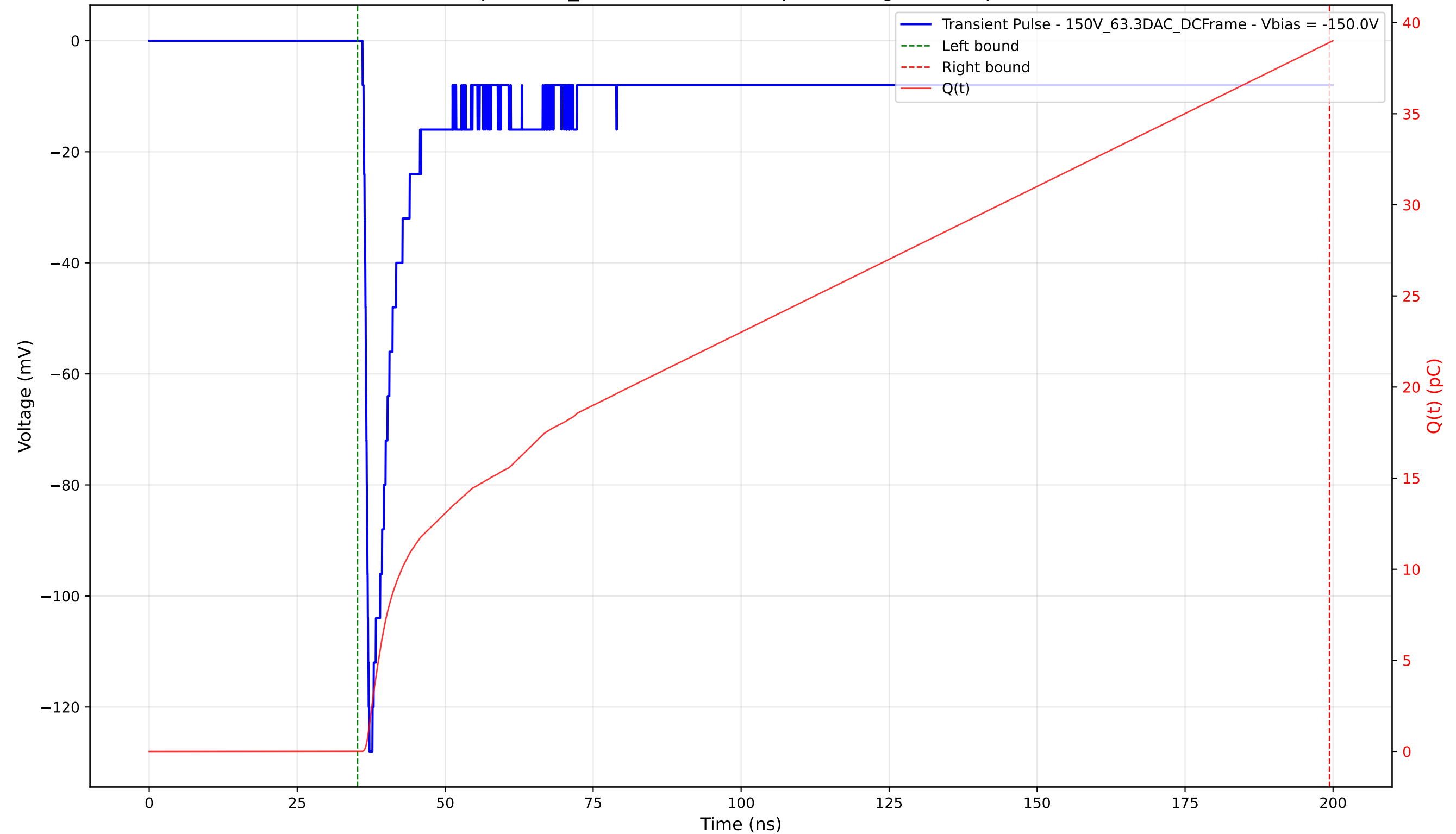
Transient Pulse - Sample: 1cm_42 - Position: 740.0 \mu\text{m} - Charge: 38.91 pC - Rise Time: 0.85 ns
