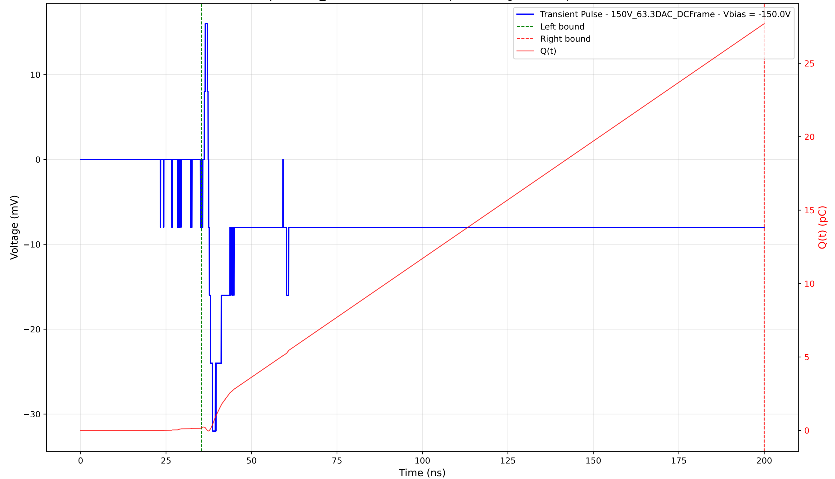
Transient Pulse - Sample: 1cm_42 - Position: 2525.0 \mu\text{m} - Charge: 27.52 pC - Rise Time: 1.13 ns
