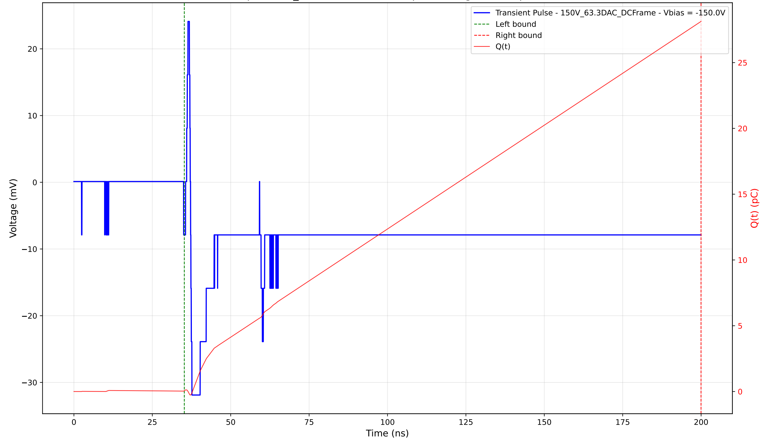
Transient Pulse - Sample: 1cm_42 - Position: 1945.0 \mu\text{m} - Charge: 28.07 pC - Rise Time: 0.43 ns
