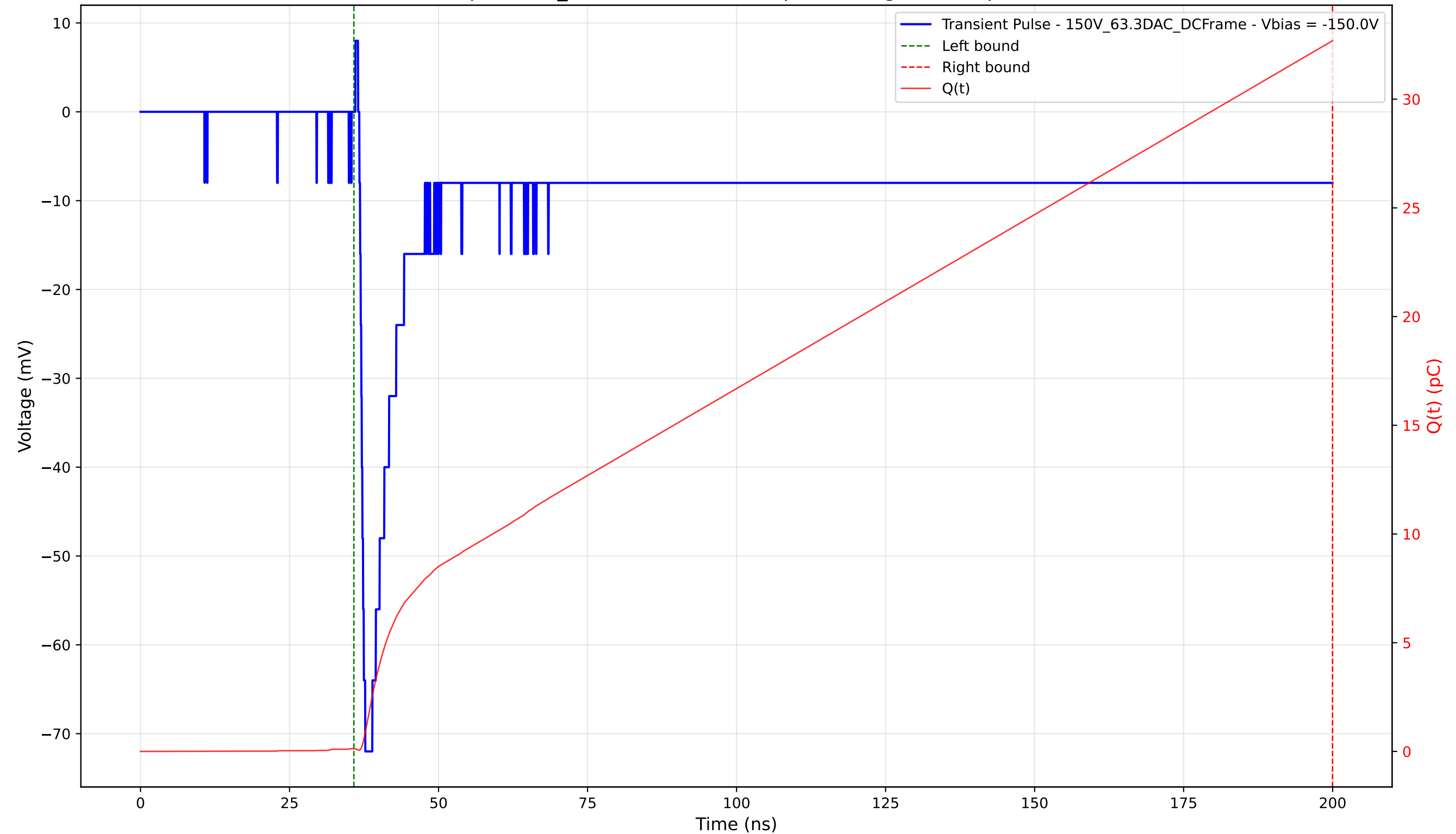
Transient Pulse - Sample: 1cm_42 - Position: 1090.0 \mu\text{m} - Charge: 32.56 pC - Rise Time: 0.98 ns
