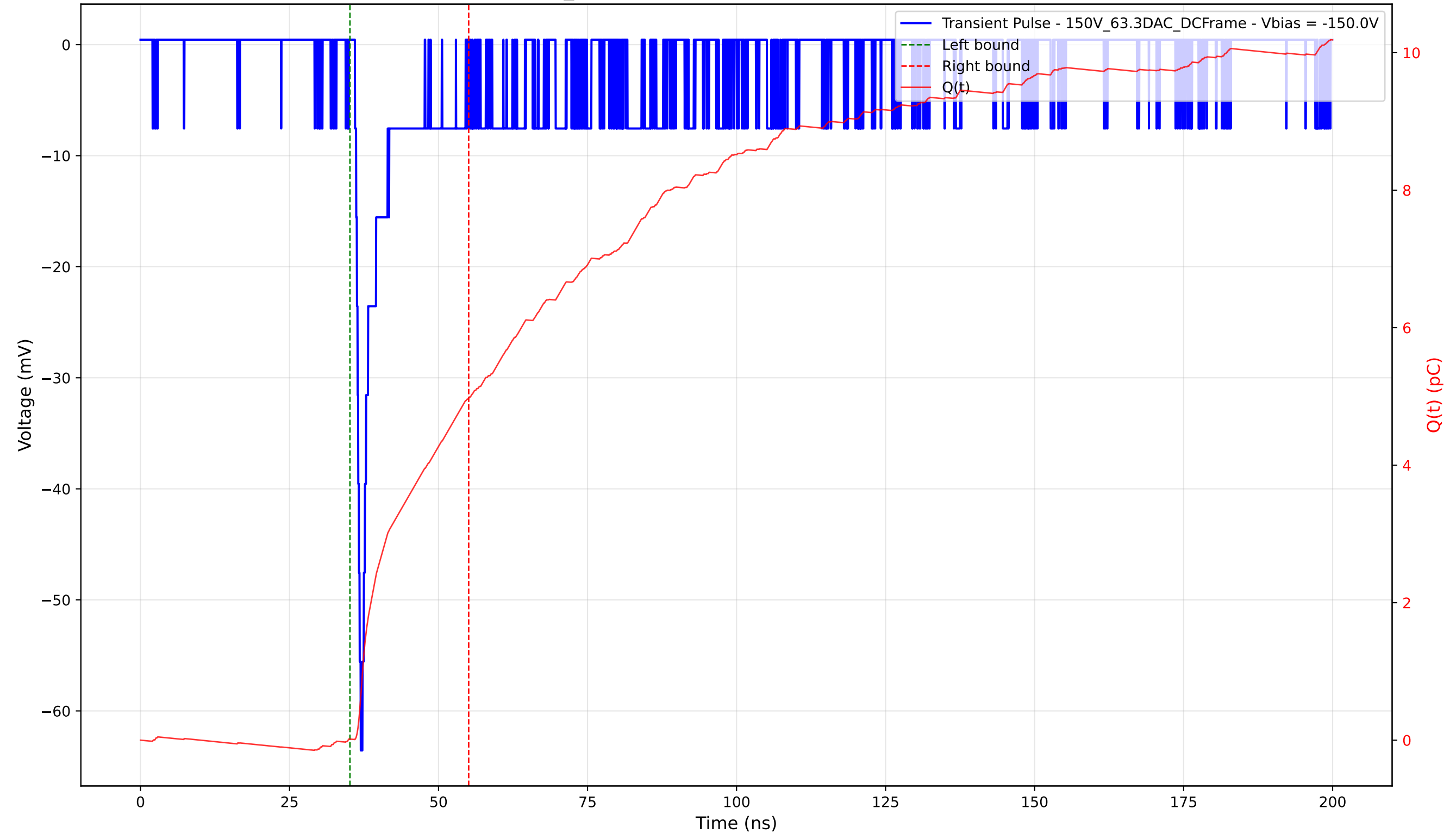
Transient Pulse - Sample: 1cm_42 - Position: 5105.0 \mu\text{m} - Charge: 4.96 pC - Rise Time: 0.96 ns
