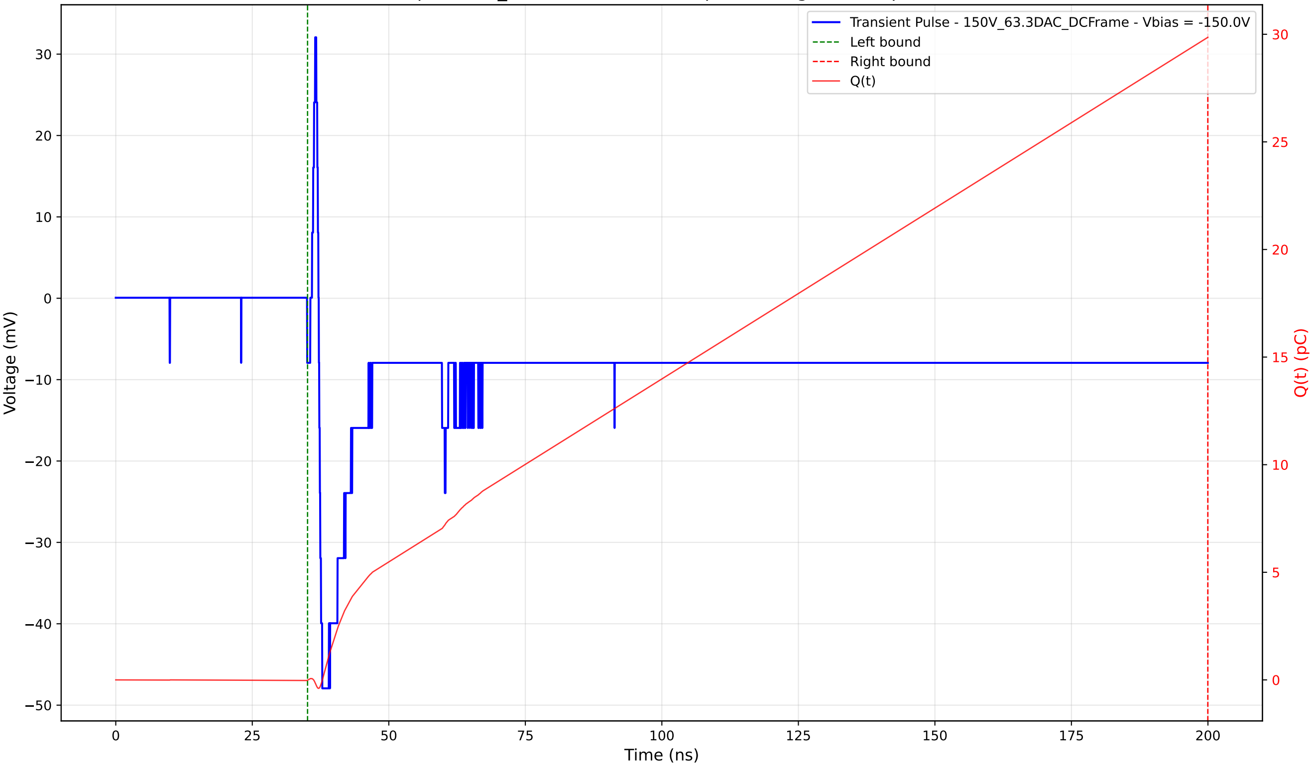
Transient Pulse - Sample: 1cm_42 - Position: 1715.0 \mu\text{m} - Charge: 29.87 pC - Rise Time: 0.63 ns
