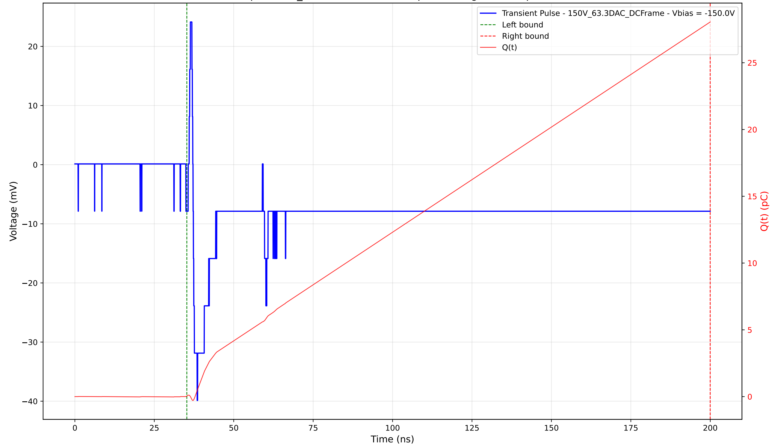
Transient Pulse - Sample: 1cm_42 - Position: 1915.0 \mu\text{m} - Charge: 28.00 pC - Rise Time: 1.29 ns
