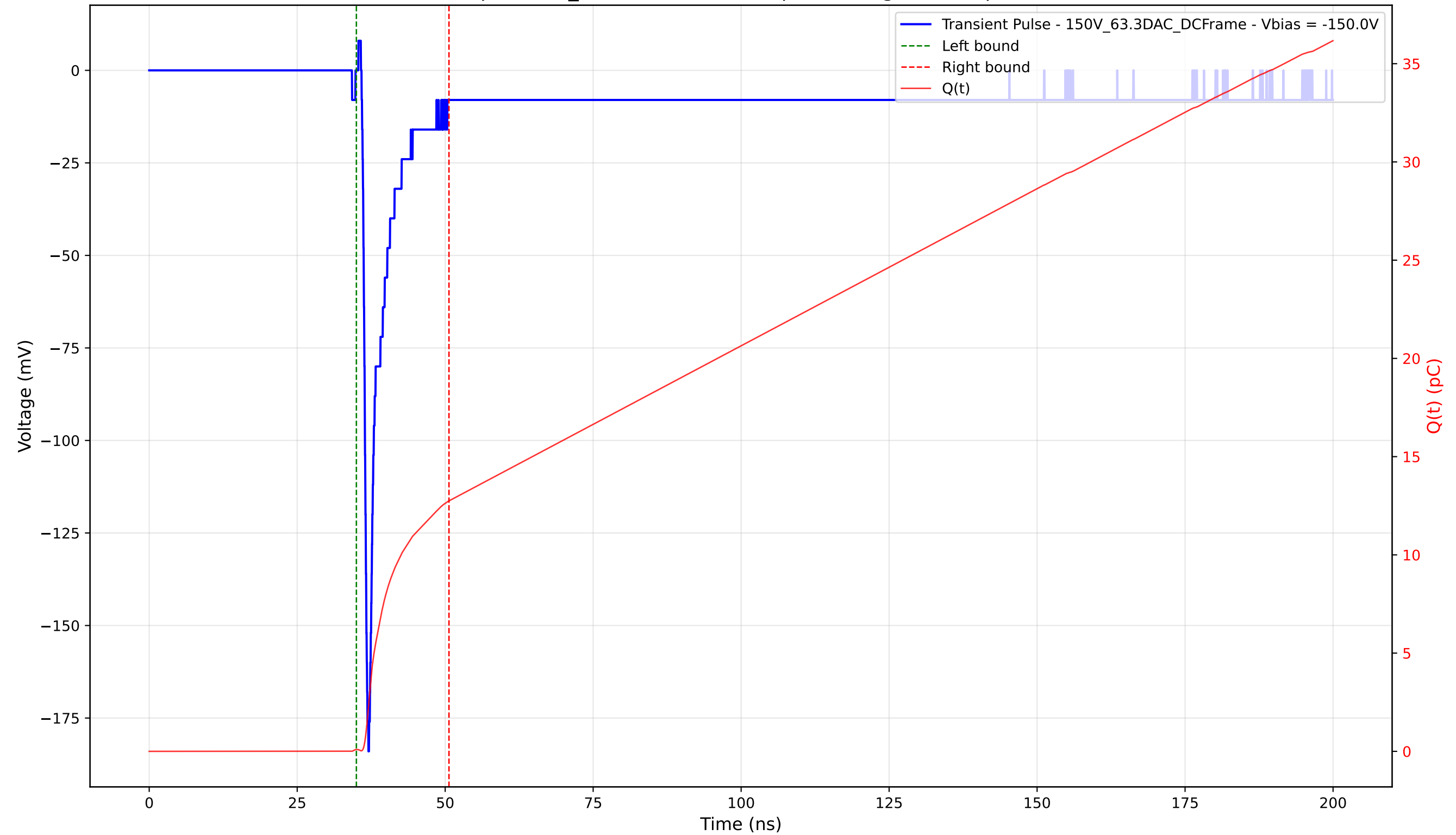
Transient Pulse - Sample: 1cm_42 - Position: 385.0 \mu\text{m} - Charge: 12.65 pC - Rise Time: 0.77 ns
