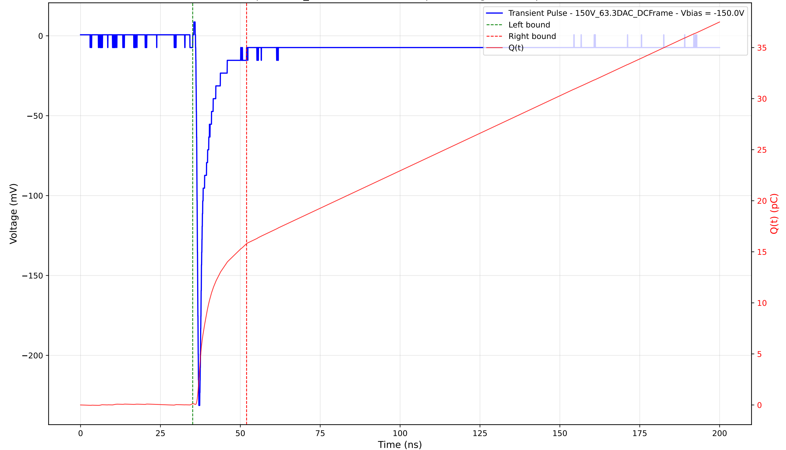
Transient Pulse - Sample: 1cm_42 - Position: 4850.0 \mu\text{m} - Charge: 15.68 pC - Rise Time: 0.78 ns
