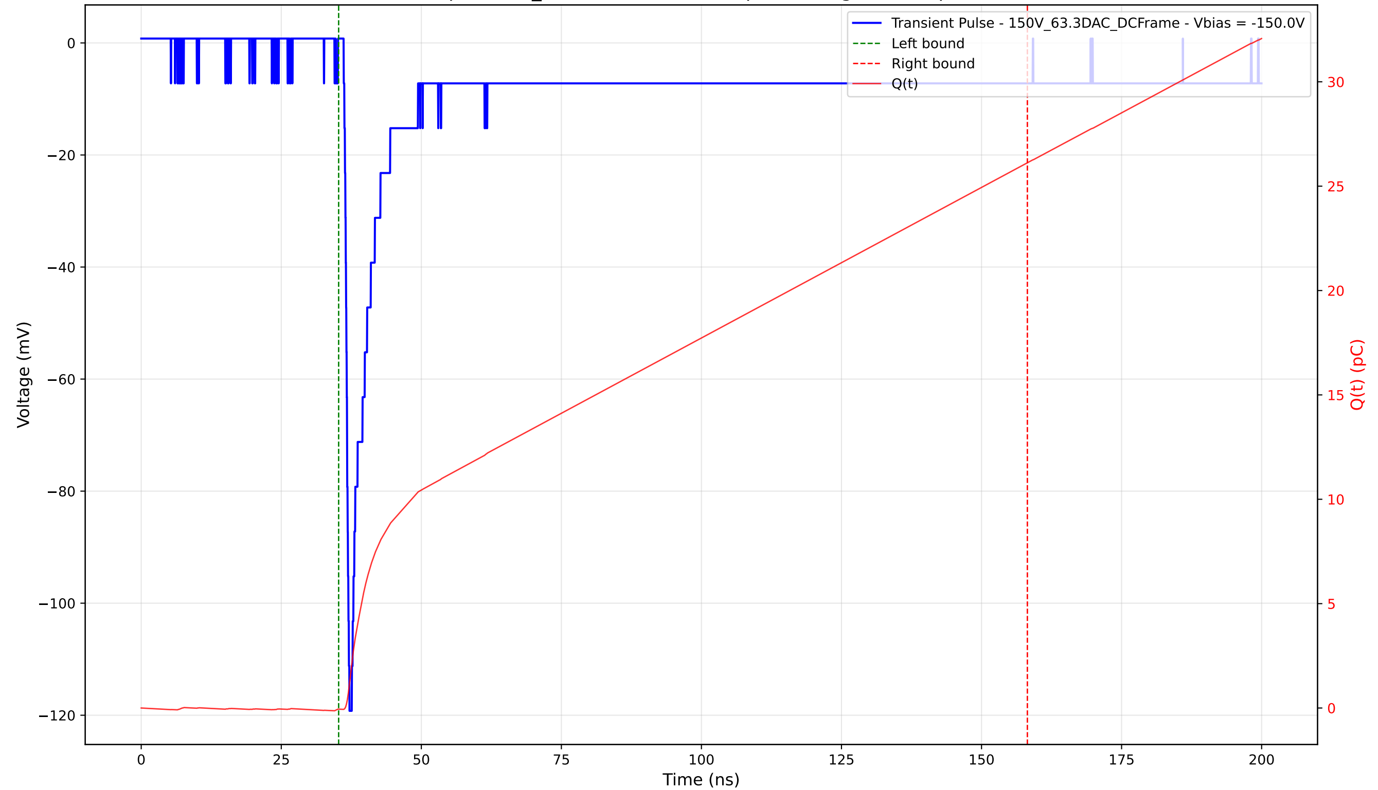
Transient Pulse - Sample: 1cm_42 - Position: 4525.0 \mu\text{m} - Charge: 26.18 pC - Rise Time: 0.81 ns
