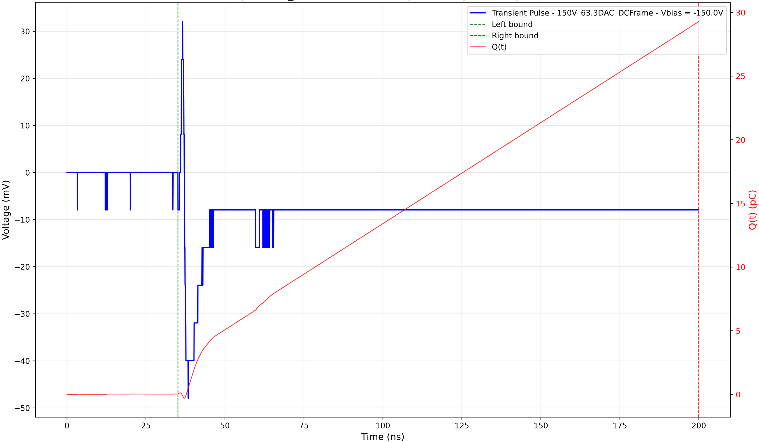
Transient Pulse - Sample: 1cm_42 - Position: 1810.0 \mu\text{m} - Charge: 29.25 pC - Rise Time: 1.17 ns
