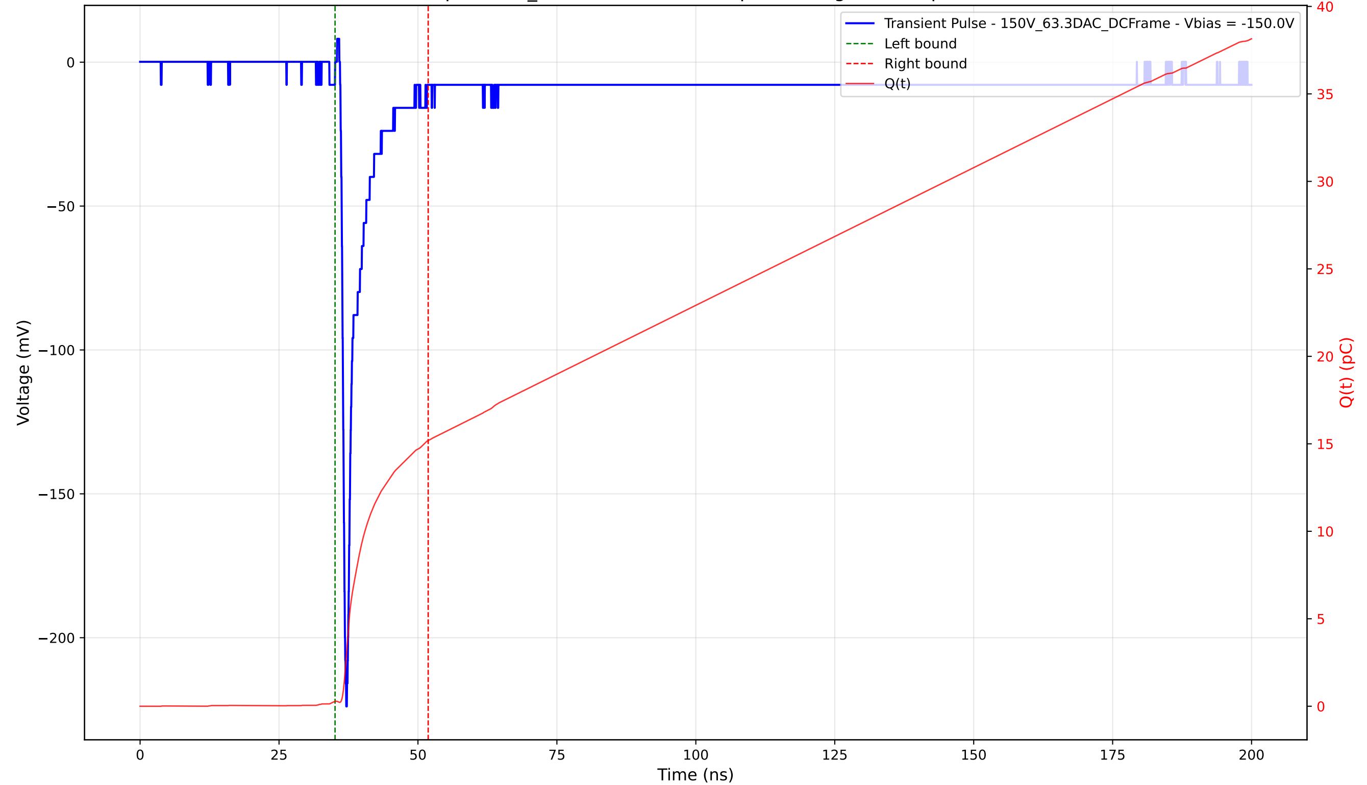
Transient Pulse - Sample: 1cm_42 - Position: 4875.0 \mu\text{m} - Charge: 14.90 pC - Rise Time: 0.80 ns
