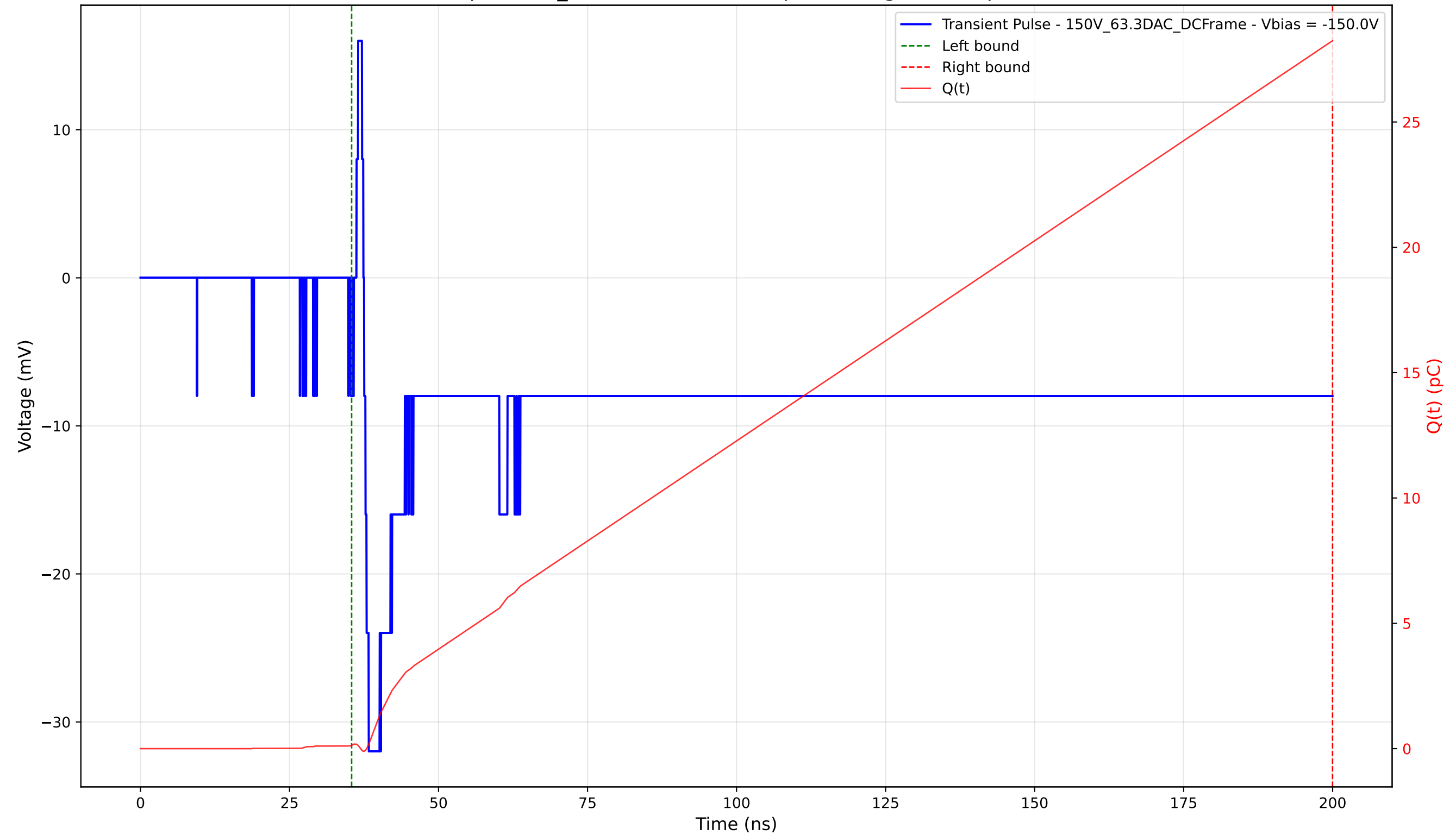
Transient Pulse - Sample: 1cm_42 - Position: 2790.0 \mu\text{m} - Charge: 28.11 pC - Rise Time: 0.77 ns
