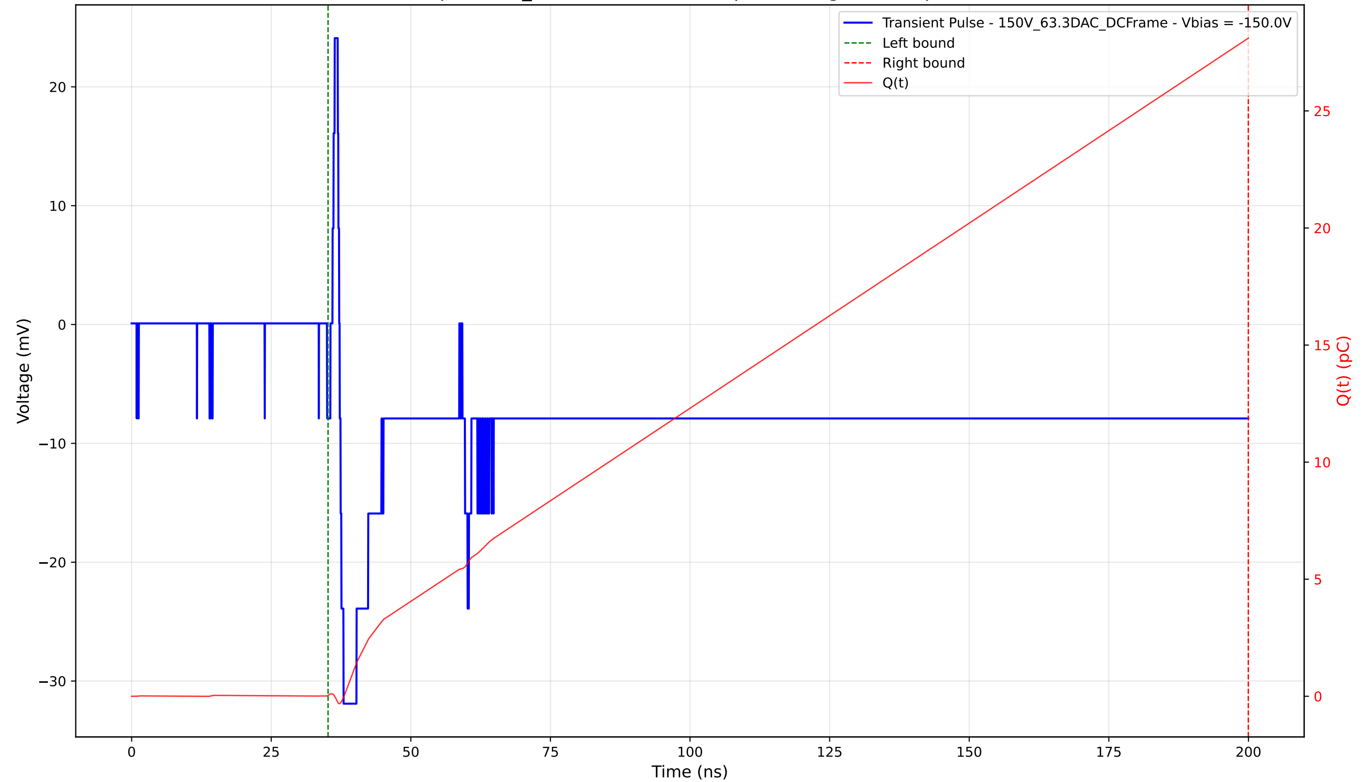
Transient Pulse - Sample: 1cm_42 - Position: 2135.0 \mu\text{m} - Charge: 28.07 pC - Rise Time: 0.69 ns
