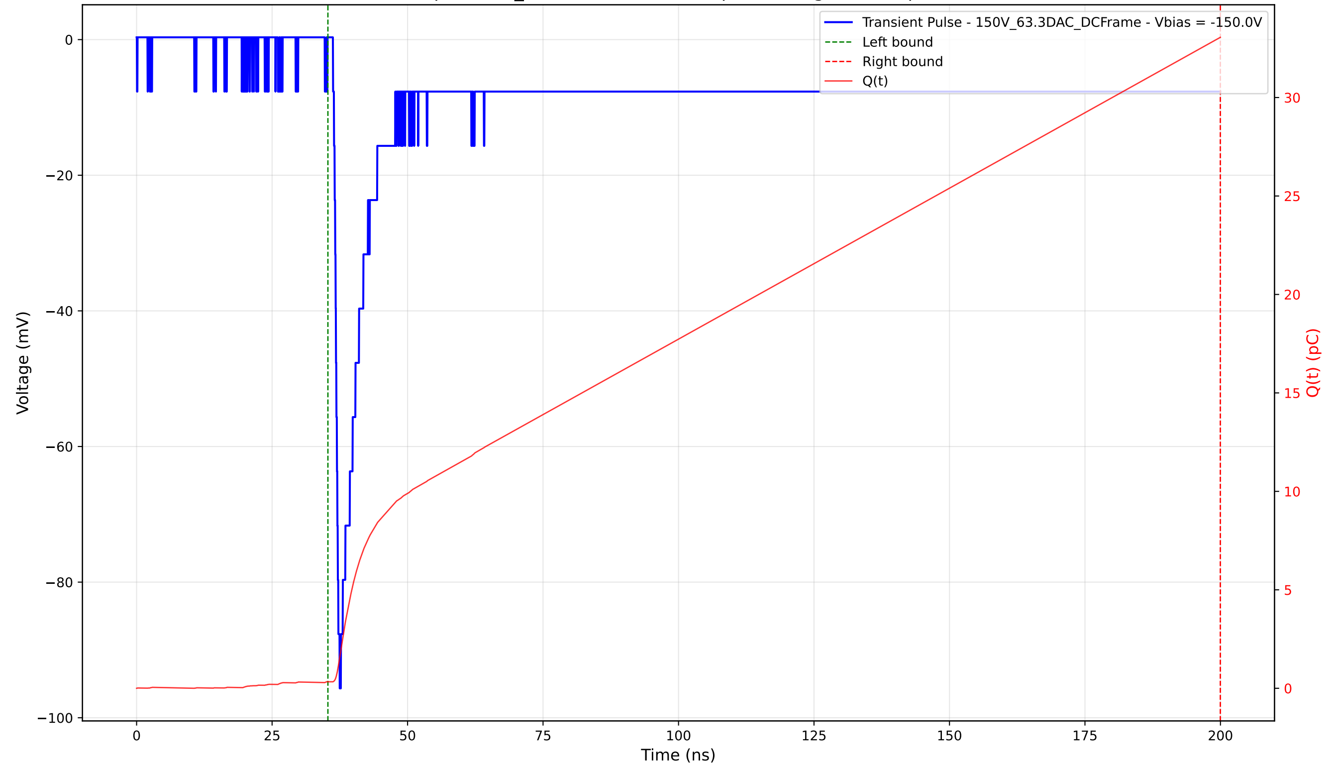
Transient Pulse - Sample: 1cm_42 - Position: 4385.0 \mu\text{m} - Charge: 32.72 pC - Rise Time: 0.82 ns
