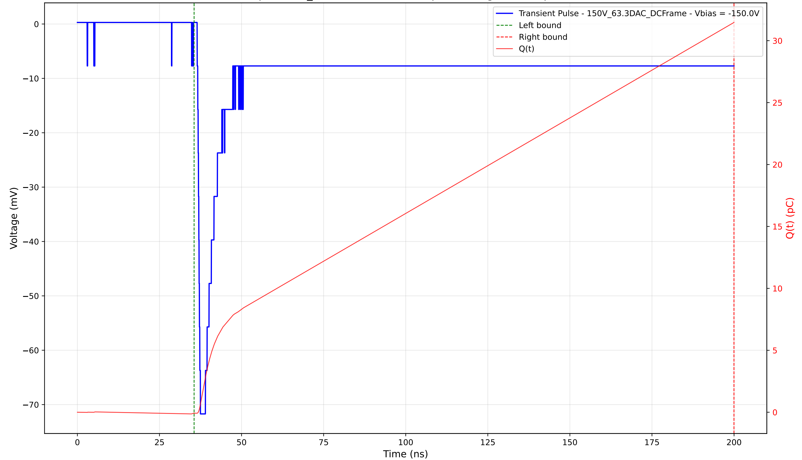
Transient Pulse - Sample: 1cm_42 - Position: 1000.0 \mu\text{m} - Charge: 31.55 pC - Rise Time: 0.98 ns
