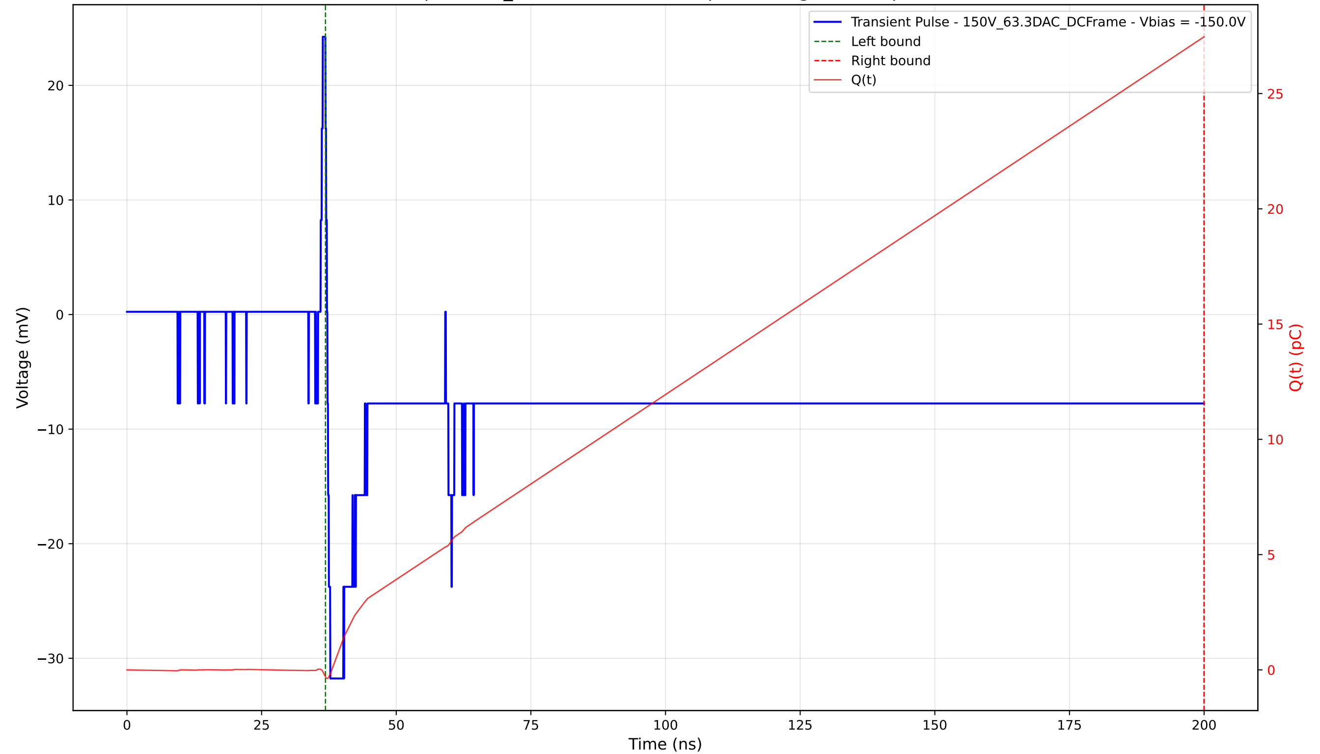
Transient Pulse - Sample: 1cm_42 - Position: 2025.0 \mu\text{m} - Charge: 27.78 pC - Rise Time: 0.53 ns
