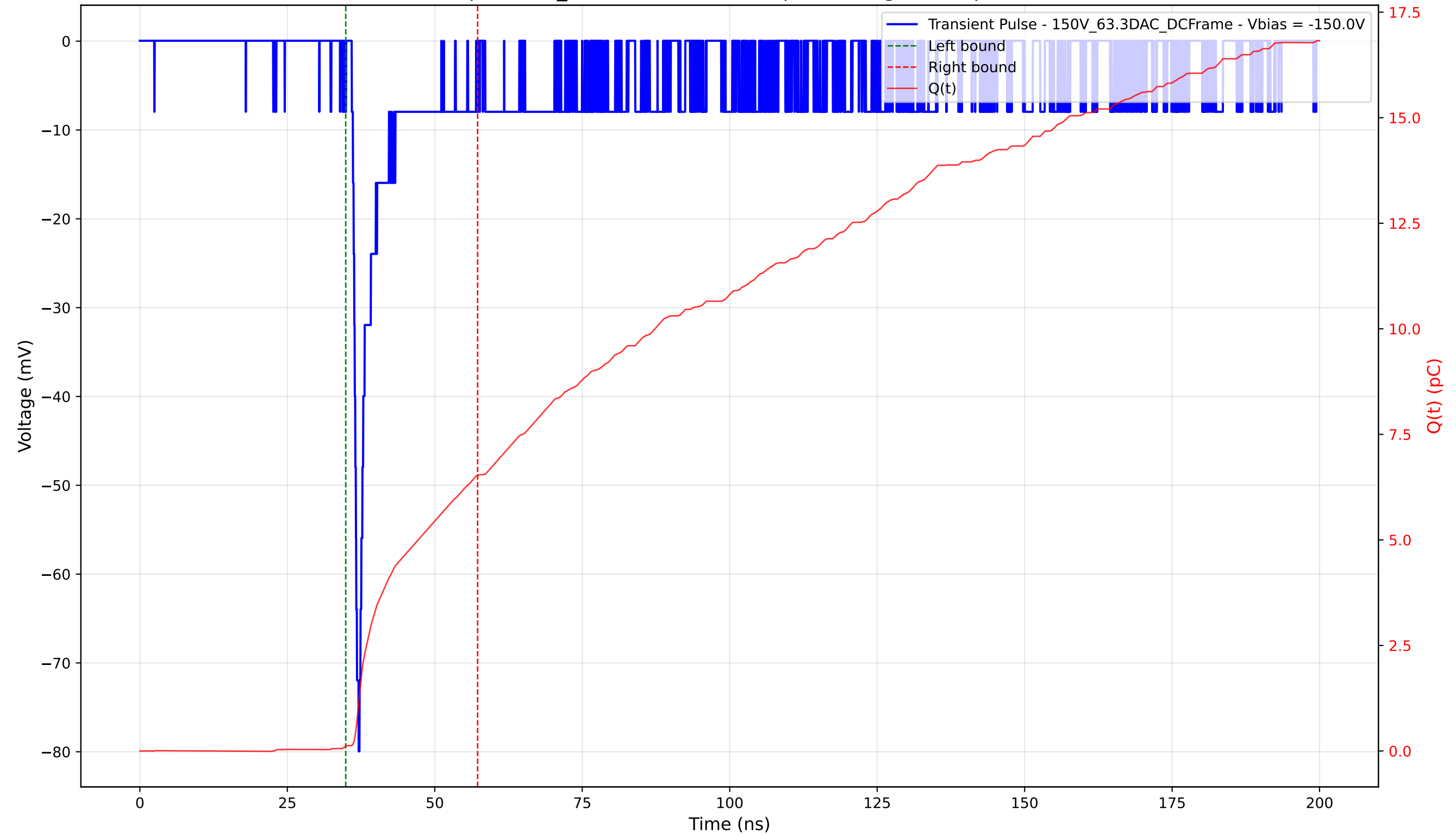
Transient Pulse - Sample: 1cm_42 - Position: 5080.0 \mu\text{m} - Charge: 6.42 pC - Rise Time: 0.98 ns
