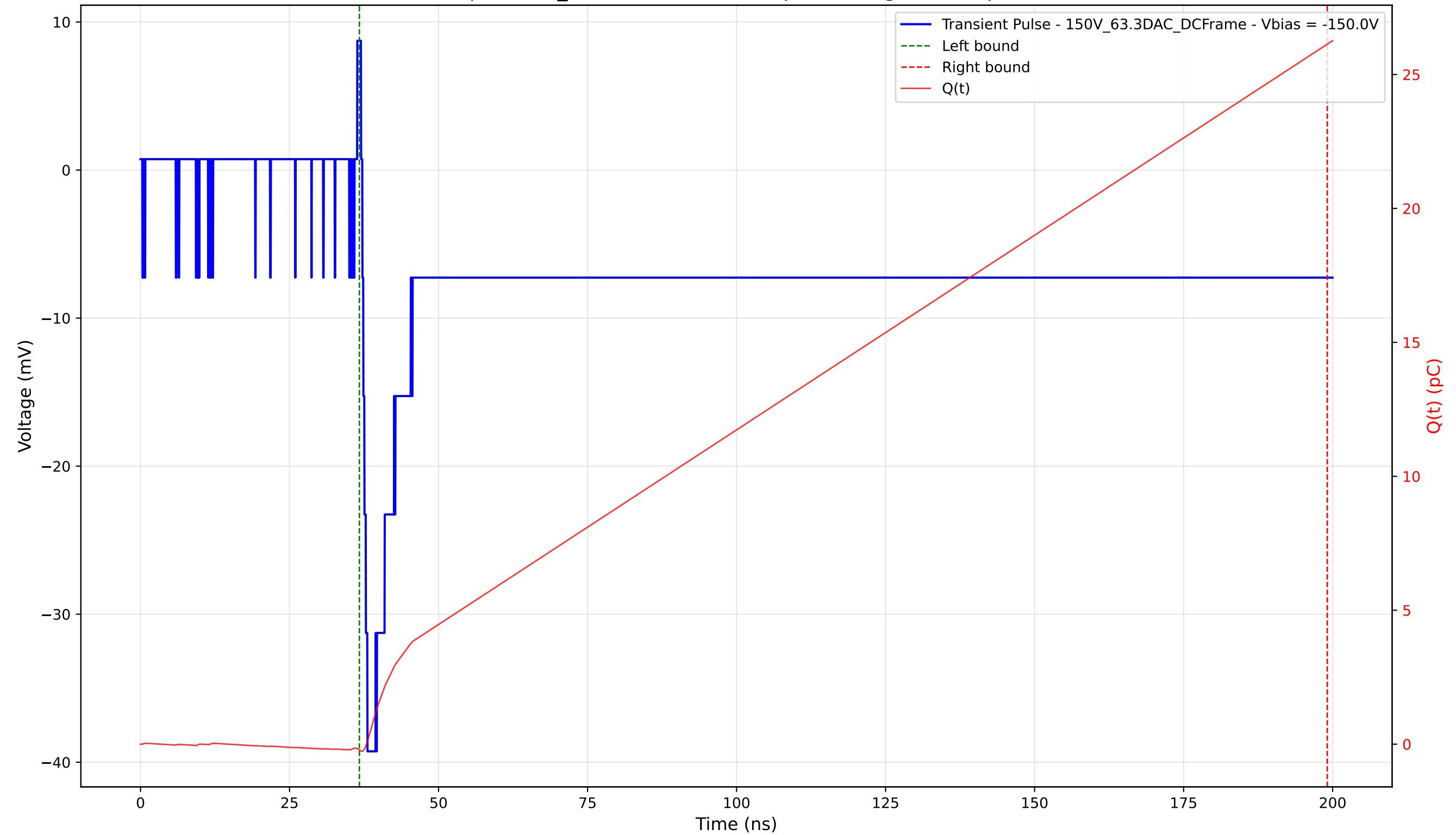
Transient Pulse - Sample: 1cm_42 - Position: 3555.0 \mu\text{m} - Charge: 26.35 pC - Rise Time: 0.85 ns
