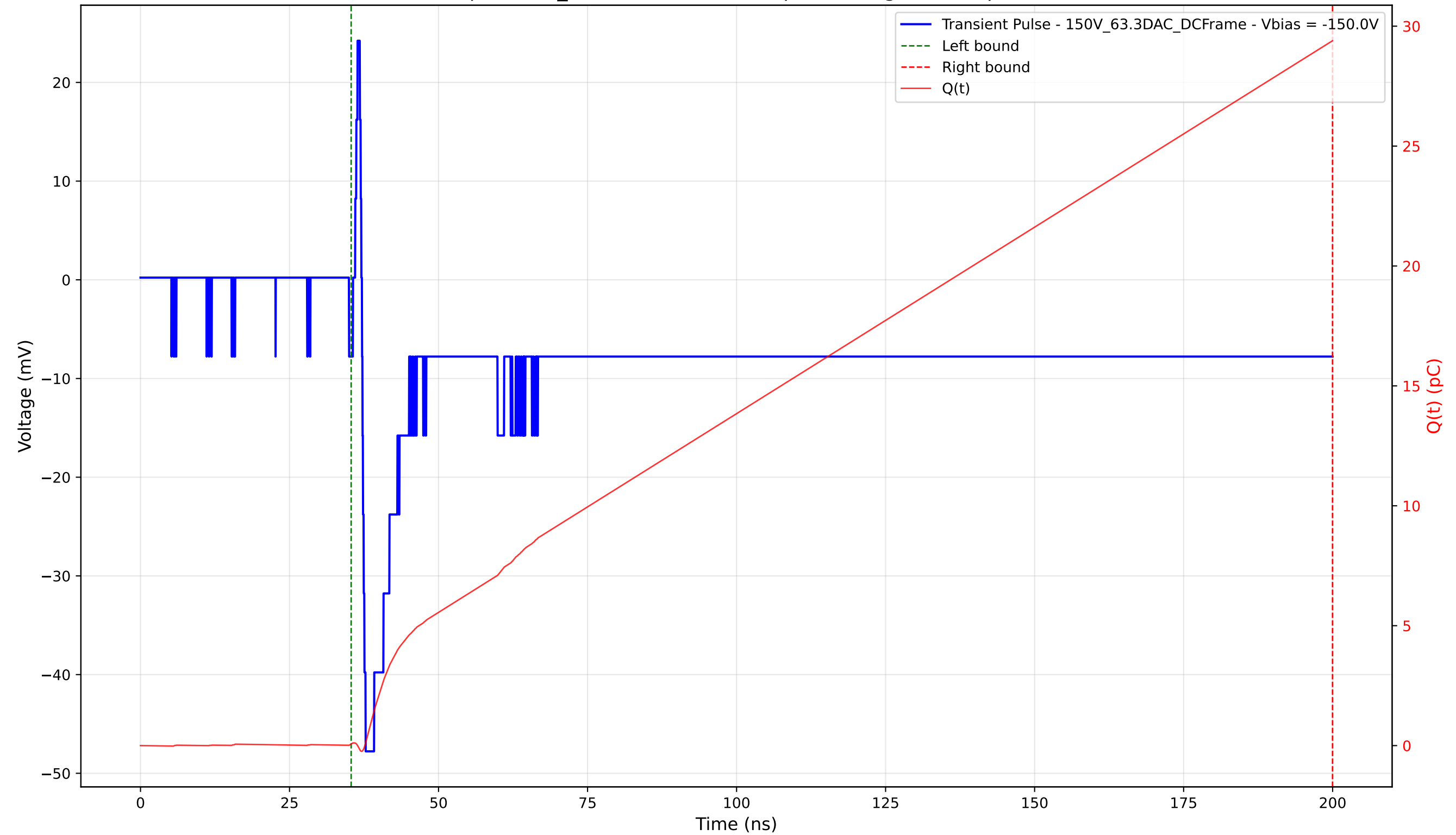
Transient Pulse - Sample: 1cm_42 - Position: 1585.0 \mu\text{m} - Charge: 29.32 pC - Rise Time: 0.61 ns
