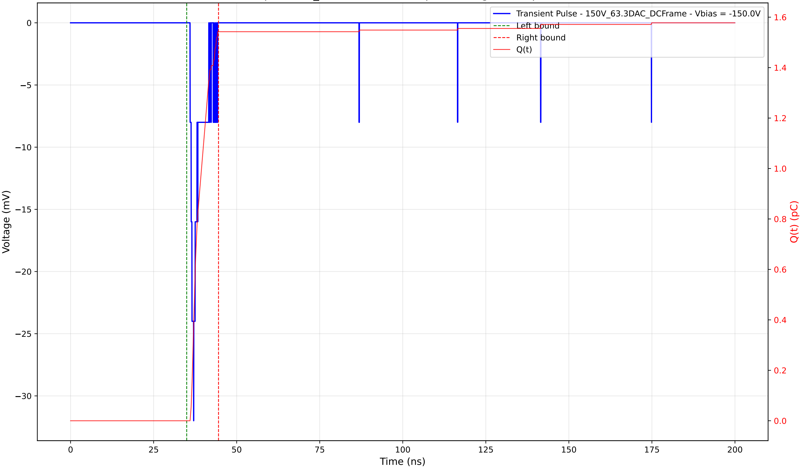
Transient Pulse - Sample: 1cm_42 - Position: 10.0 \mu\text{m} - Charge: 1.54 pC - Rise Time: 1.07 ns
