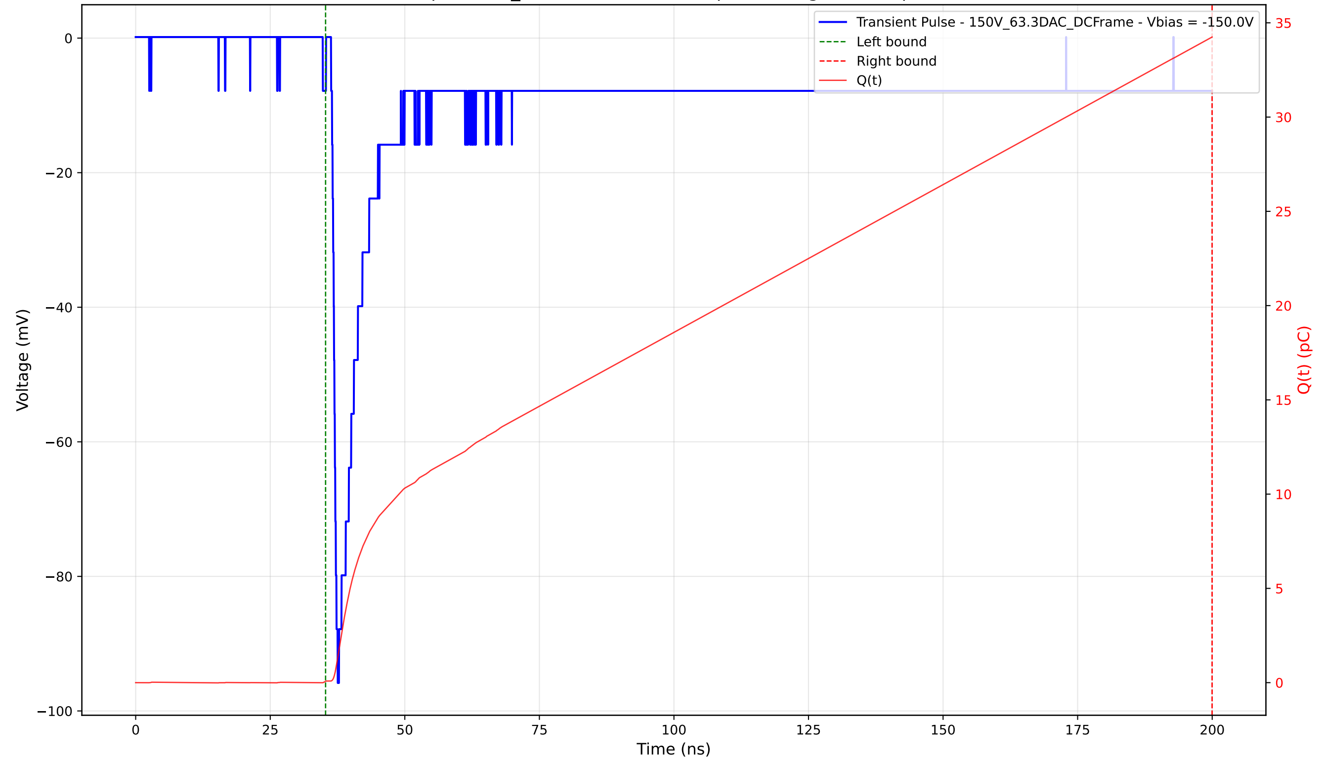
Transient Pulse - Sample: 1cm_42 - Position: 4315.0 \mu\text{m} - Charge: 34.17 pC - Rise Time: 0.84 ns
