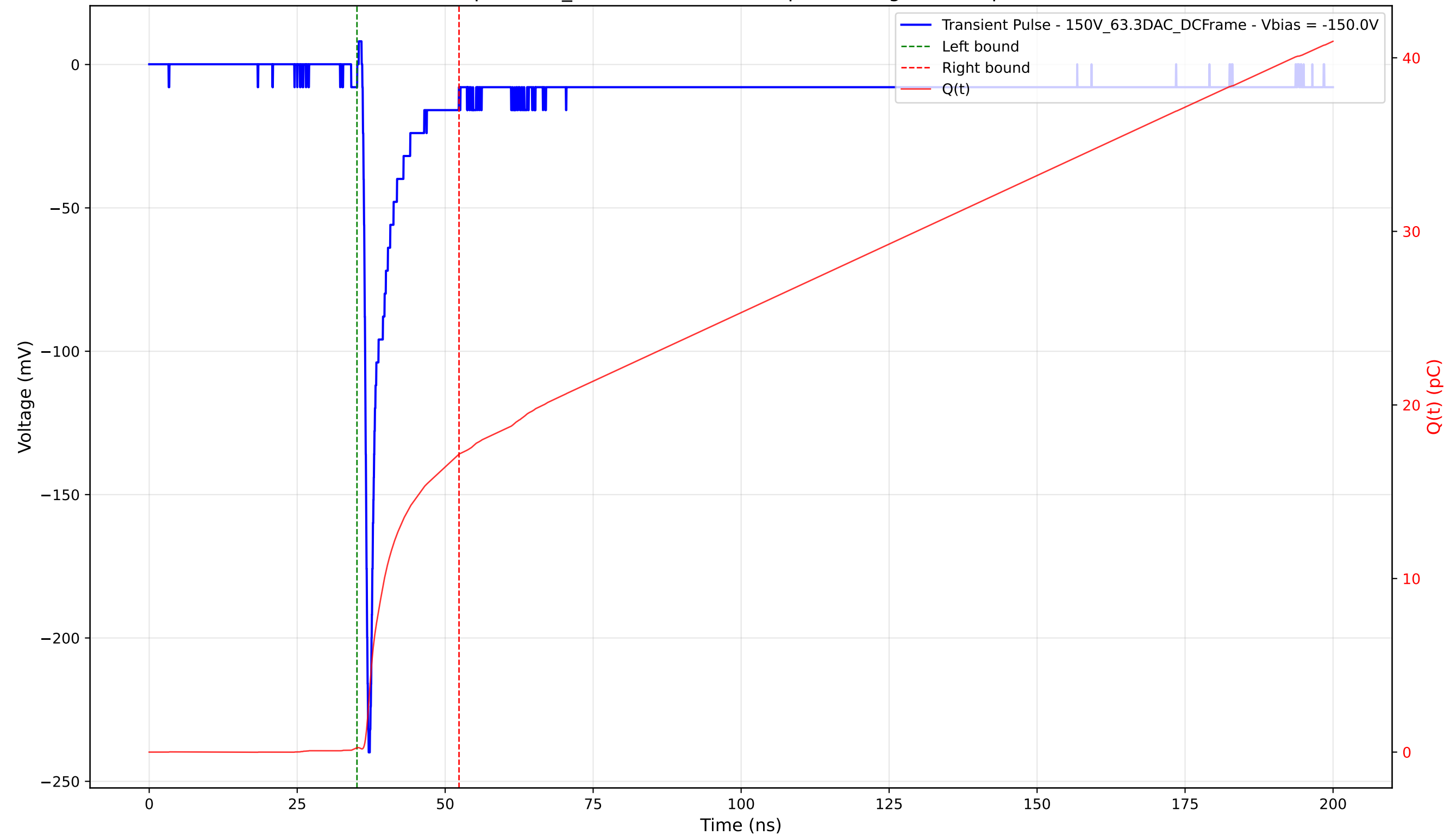
Transient Pulse - Sample: 1cm_42 - Position: 4755.0 \mu\text{m} - Charge: 16.91 pC - Rise Time: 0.78 ns
