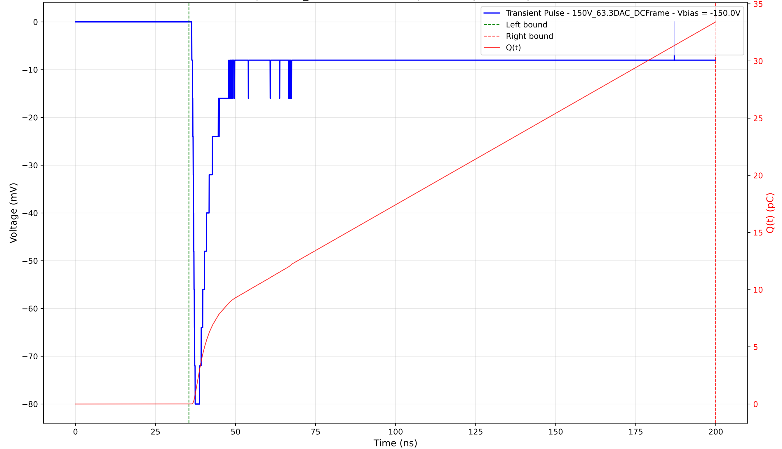
Transient Pulse - Sample: 1cm_42 - Position: 950.0 \mu\text{m} - Charge: 33.42 pC - Rise Time: 0.72 ns
