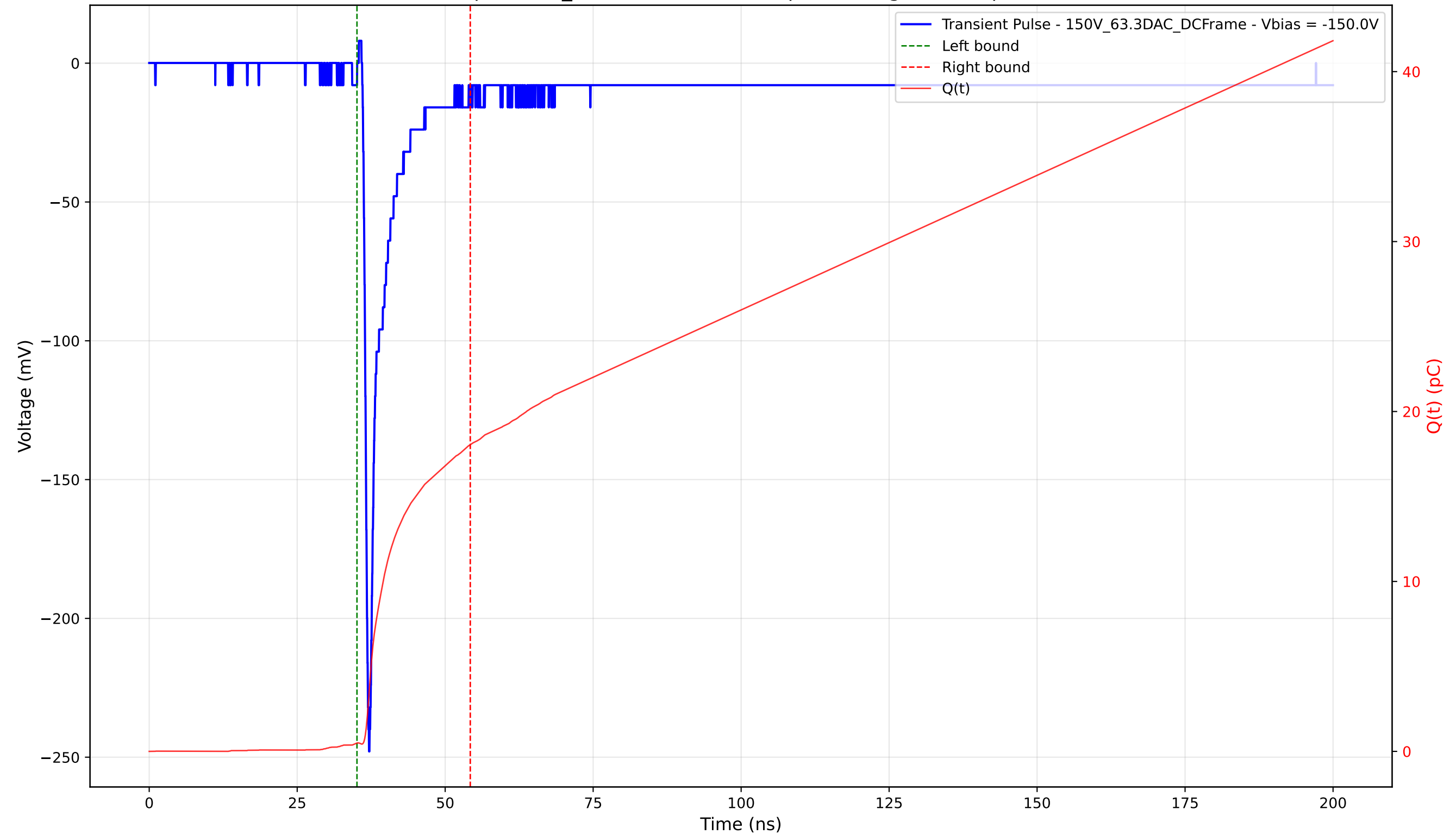
Transient Pulse - Sample: 1cm_42 - Position: 4780.0 \mu\text{m} - Charge: 17.56 pC - Rise Time: 0.78 ns
