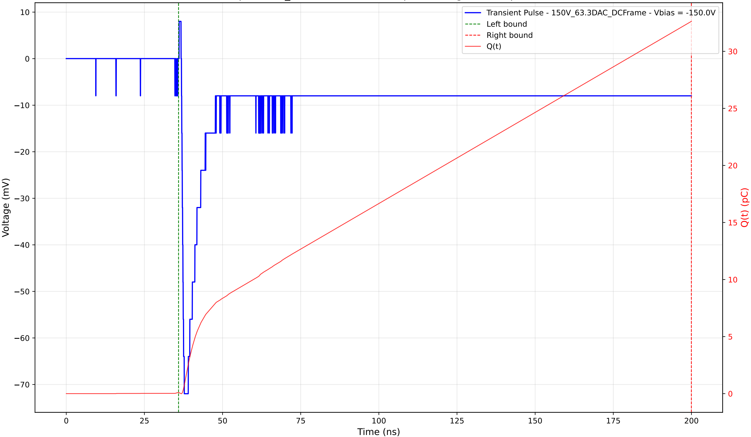
Transient Pulse - Sample: 1cm_42 - Position: 1185.0 \mu\text{m} - Charge: 32.54 pC - Rise Time: 0.88 ns
