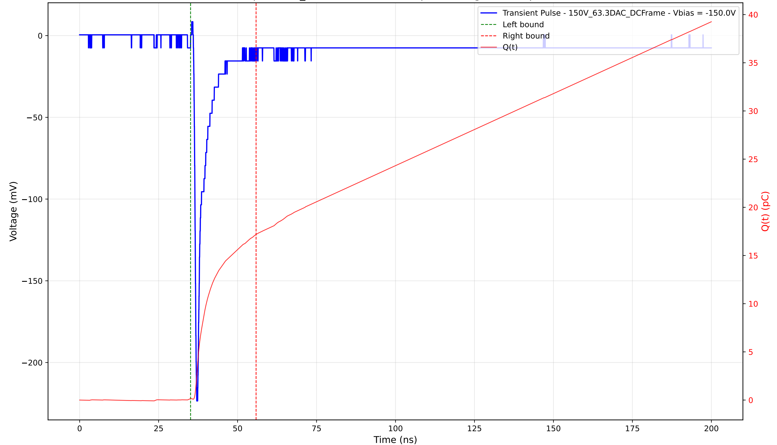
Transient Pulse - Sample: 1cm_42 - Position: 4720.0 \mu\text{m} - Charge: 17.02 pC - Rise Time: 0.78 ns
