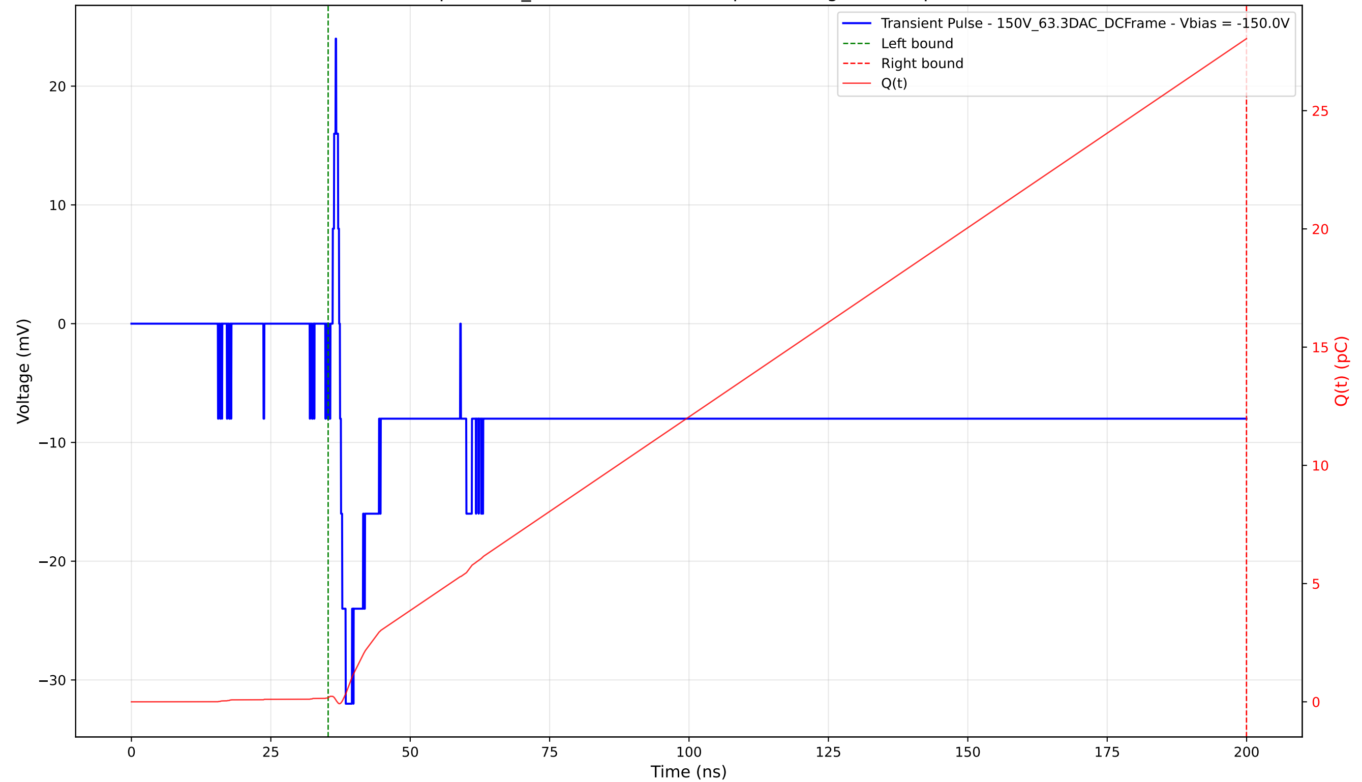
Transient Pulse - Sample: 1cm_42 - Position: 2410.0 \mu\text{m} - Charge: 27.87 pC - Rise Time: 1.03 ns
