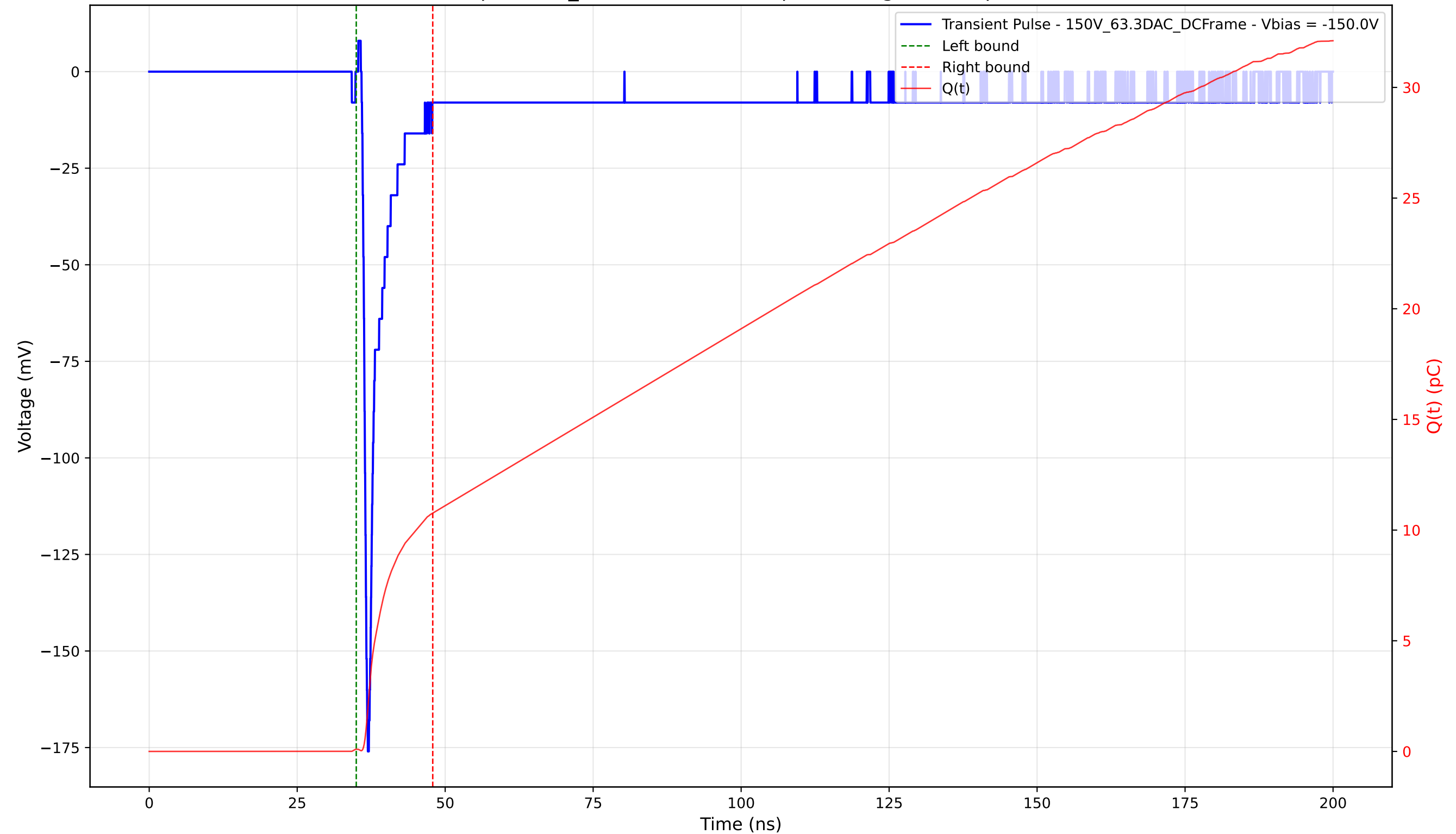
Transient Pulse - Sample: 1cm_42 - Position: 305.0 \mu\text{m} - Charge: 10.67 pC - Rise Time: 0.74 ns
