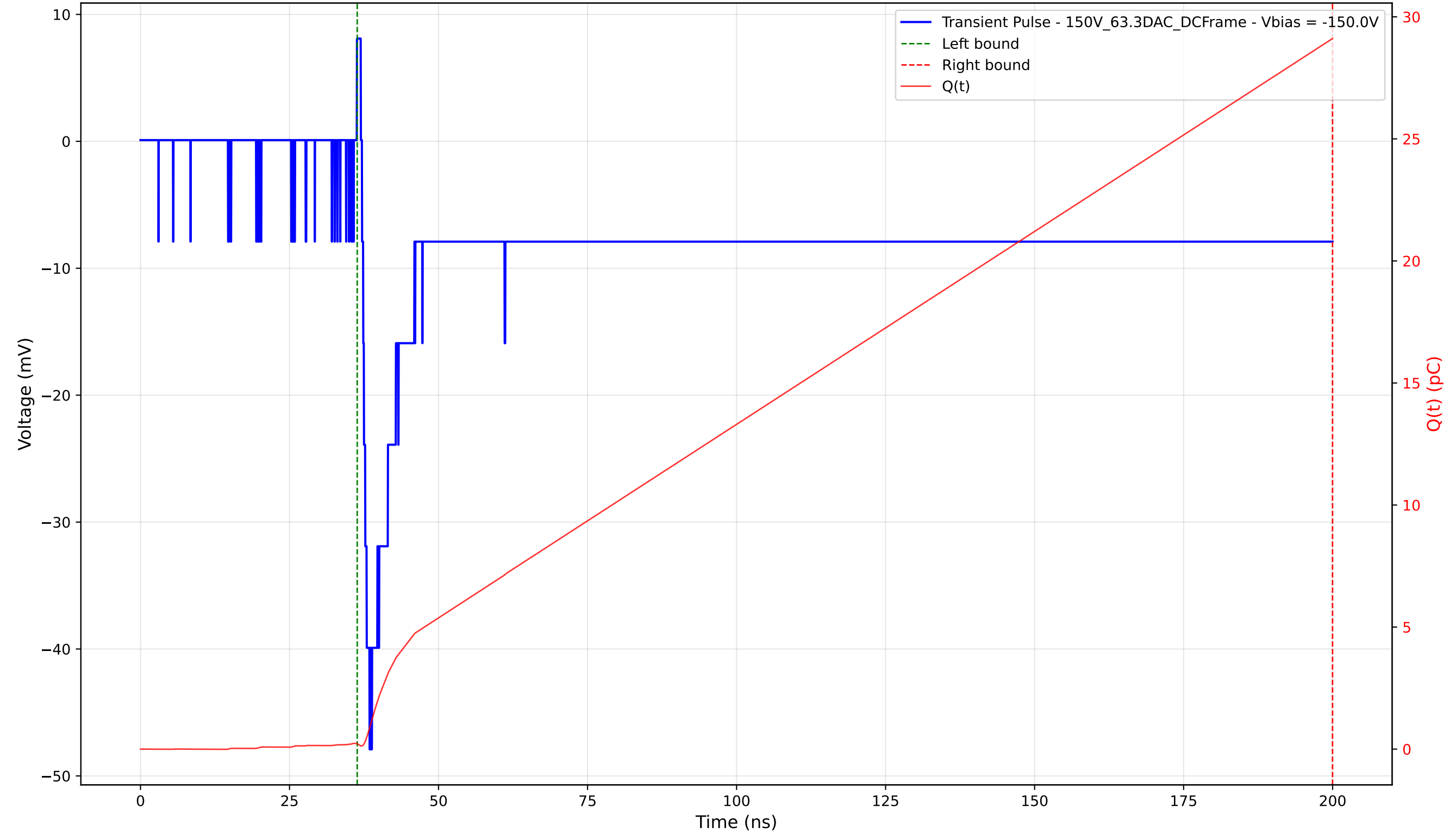
Transient Pulse - Sample: 1cm_42 - Position: 3605.0 \mu\text{m} - Charge: 28.89 pC - Rise Time: 1.27 ns
