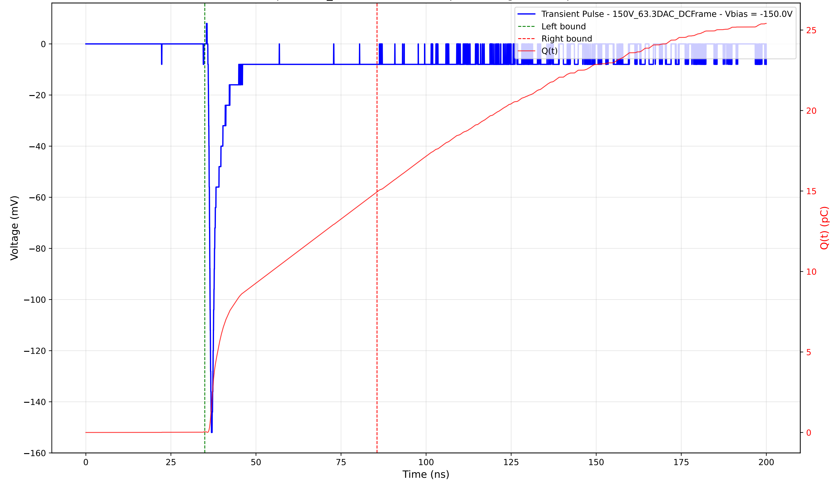
Transient Pulse - Sample: 1cm_42 - Position: 205.0 \mu\text{m} - Charge: 14.90 pC - Rise Time: 0.82 ns
