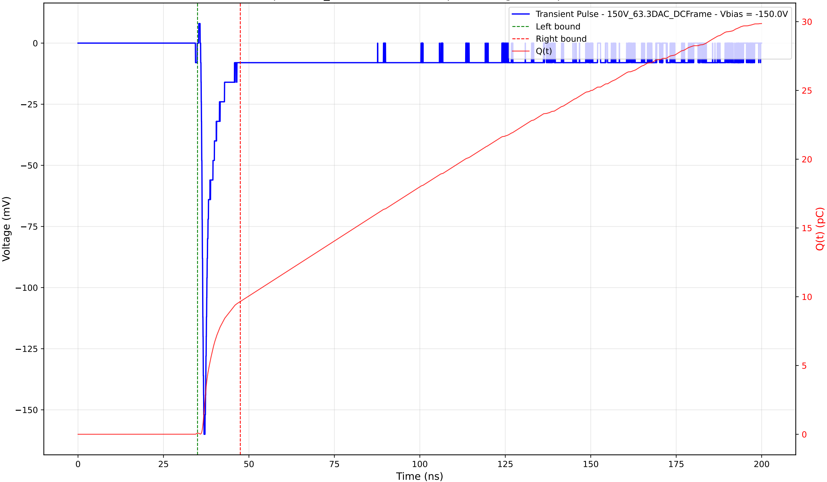
Transient Pulse - Sample: 1cm_42 - Position: 245.0 \mu\text{m} - Charge: 9.57 pC - Rise Time: 0.70 ns
