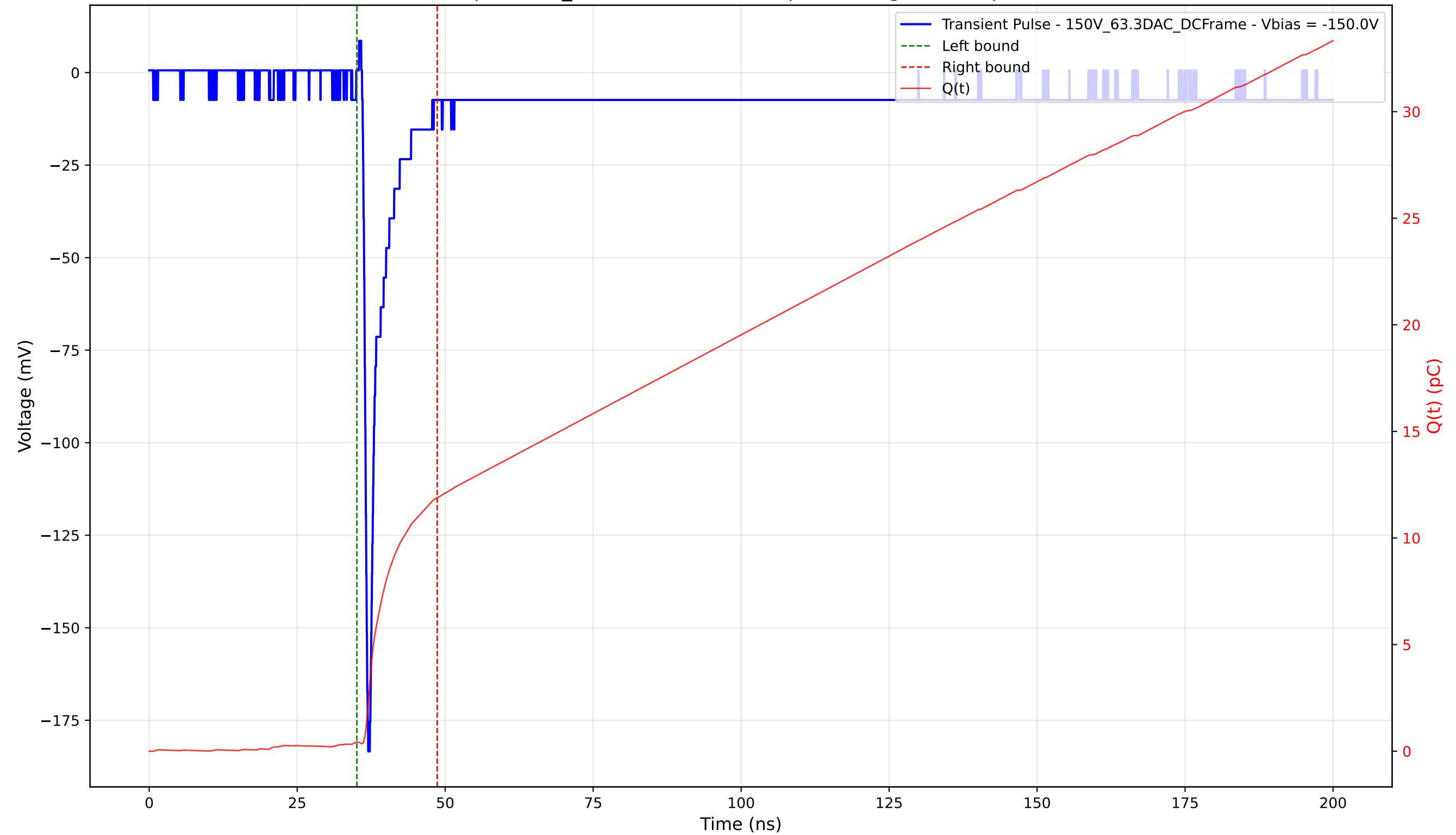
Transient Pulse - Sample: 1cm_42 - Position: 4935.0 \mu\text{m} - Charge: 11.46 pC - Rise Time: 0.73 ns
