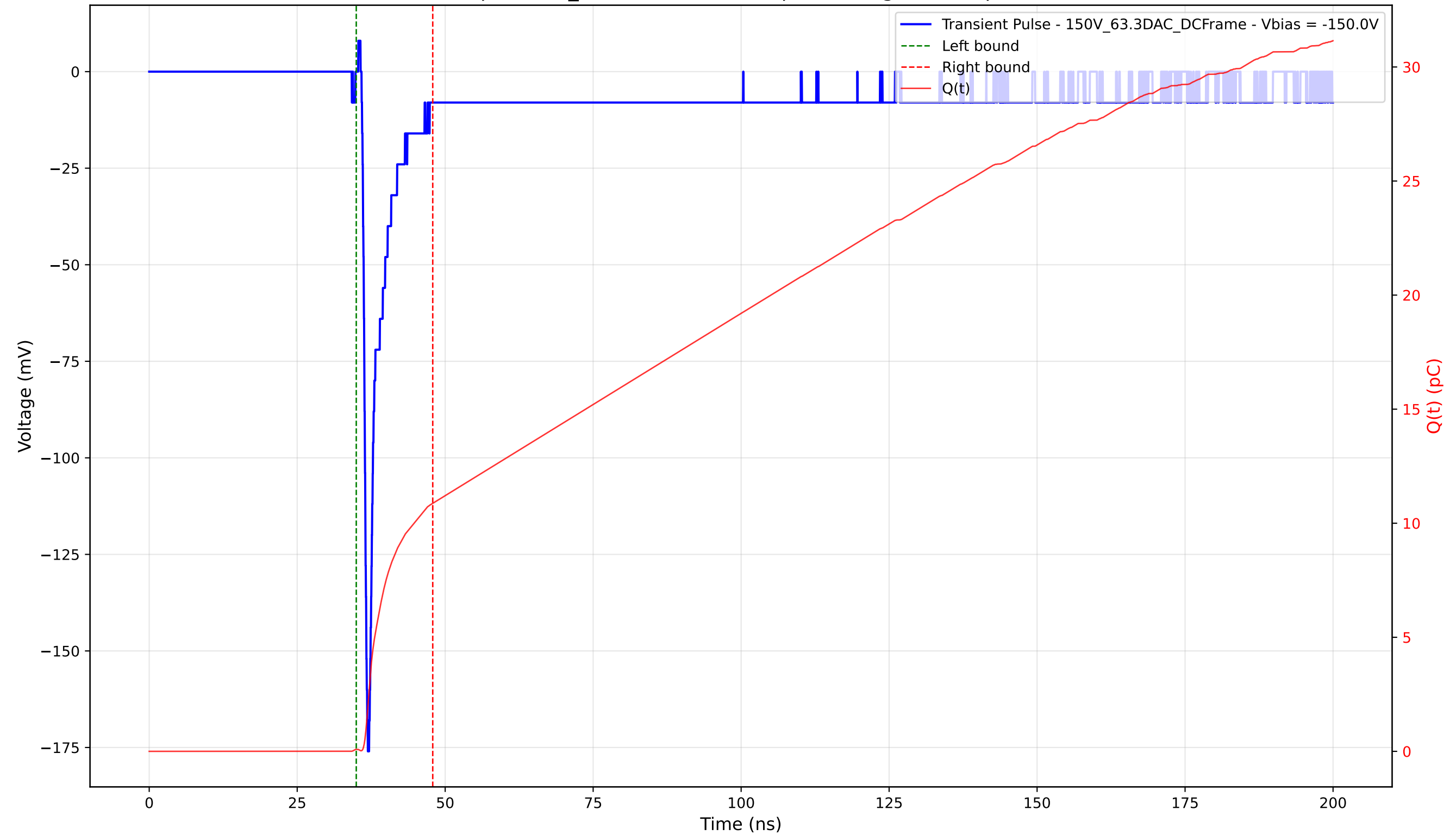
Transient Pulse - Sample: 1cm_42 - Position: 315.0 \mu\text{m} - Charge: 10.79 pC - Rise Time: 0.72 ns
