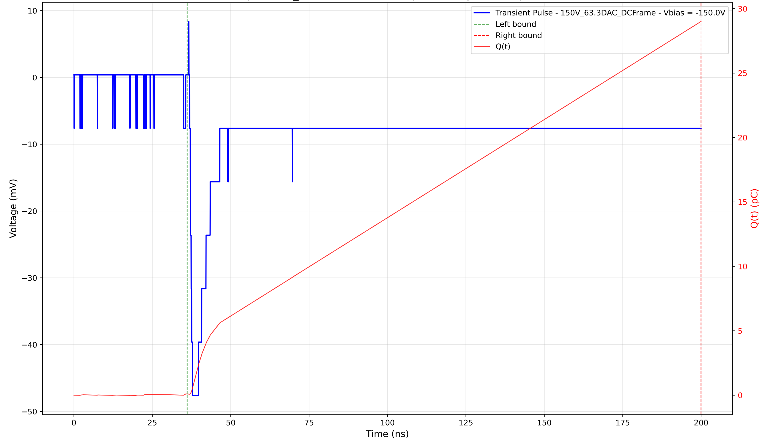
Transient Pulse - Sample: 1cm_42 - Position: 3885.0 \mu\text{m} - Charge: 28.91 pC - Rise Time: 0.93 ns
