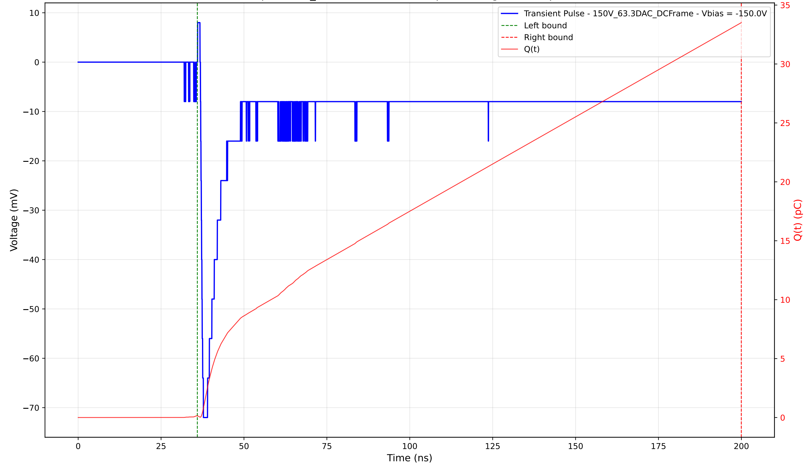
Transient Pulse - Sample: 1cm_42 - Position: 1210.0 \mu\text{m} - Charge: 33.36 pC - Rise Time: 0.88 ns
