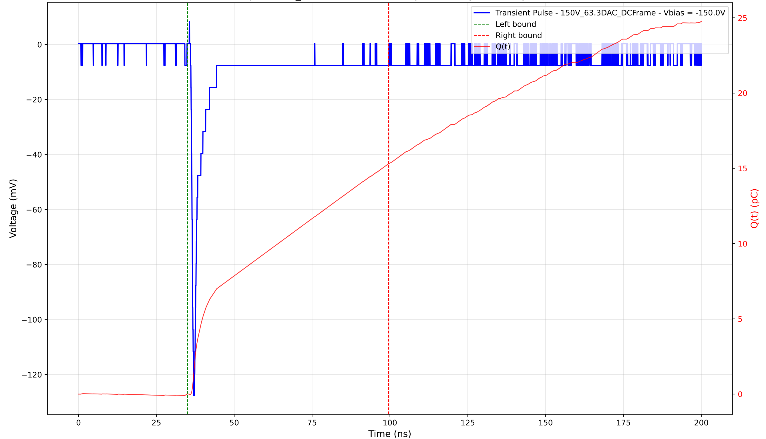
Transient Pulse - Sample: 1cm_42 - Position: 5010.0 \mu\text{m} - Charge: 15.30 pC - Rise Time: 0.79 ns
