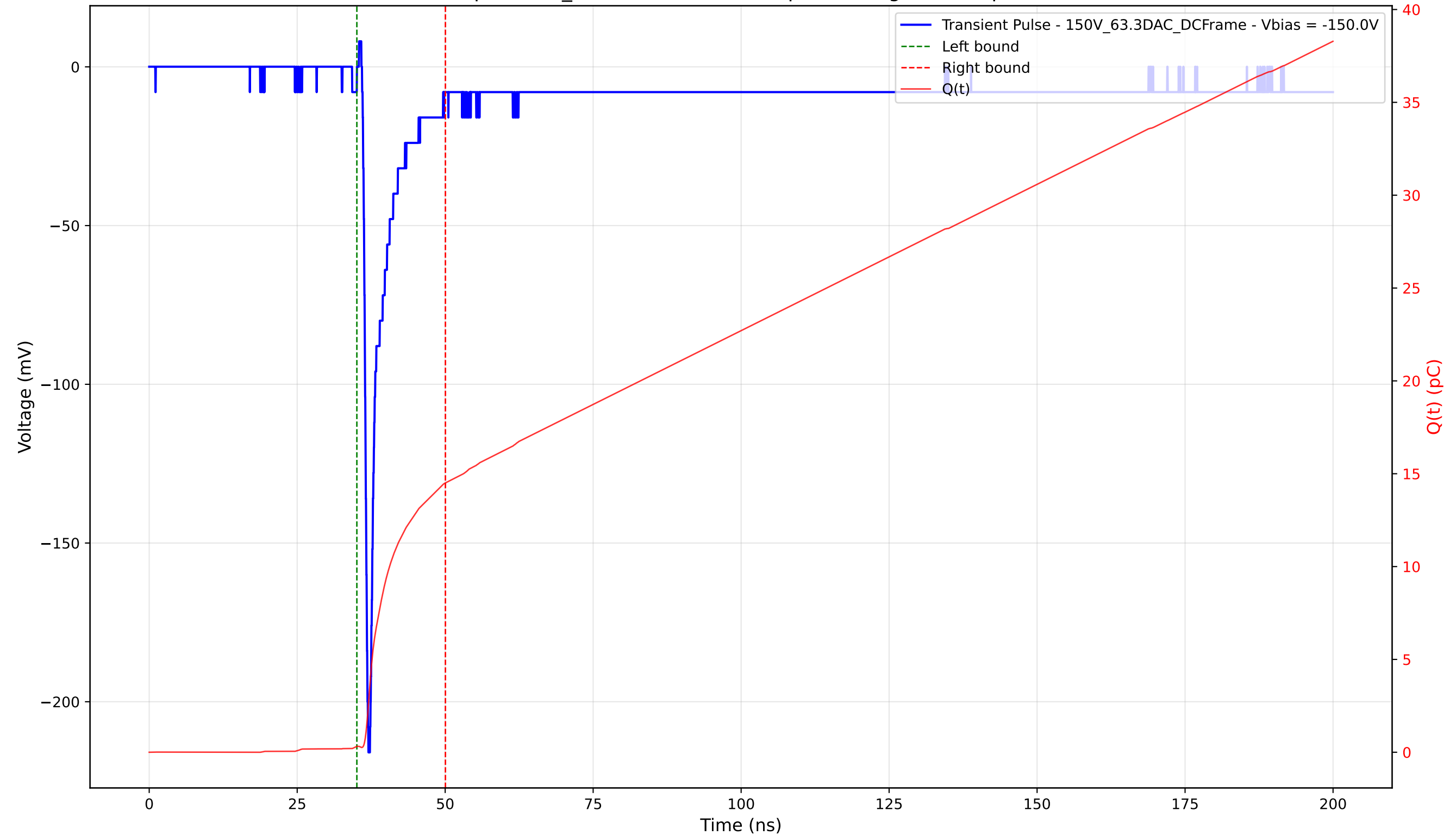
Transient Pulse - Sample: 1cm_42 - Position: 4880.0 \mu\text{m} - Charge: 14.18 pC - Rise Time: 0.77 ns
