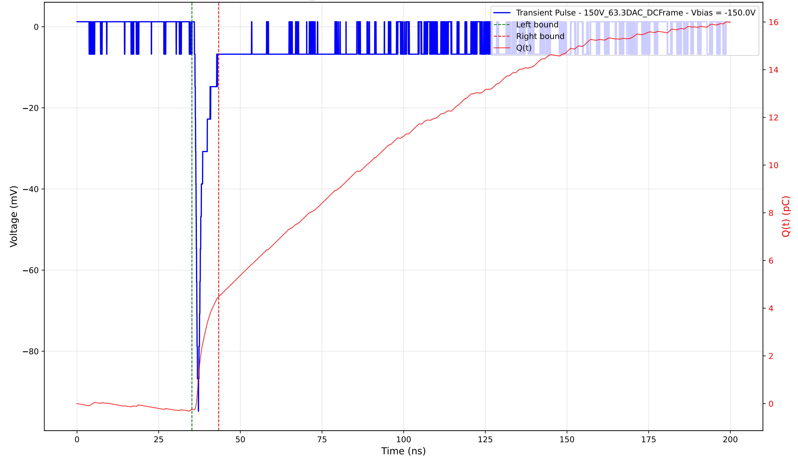
Transient Pulse - Sample: 1cm_42 - Position: 5055.0 \mu\text{m} - Charge: 4.72 pC - Rise Time: 0.75 ns
