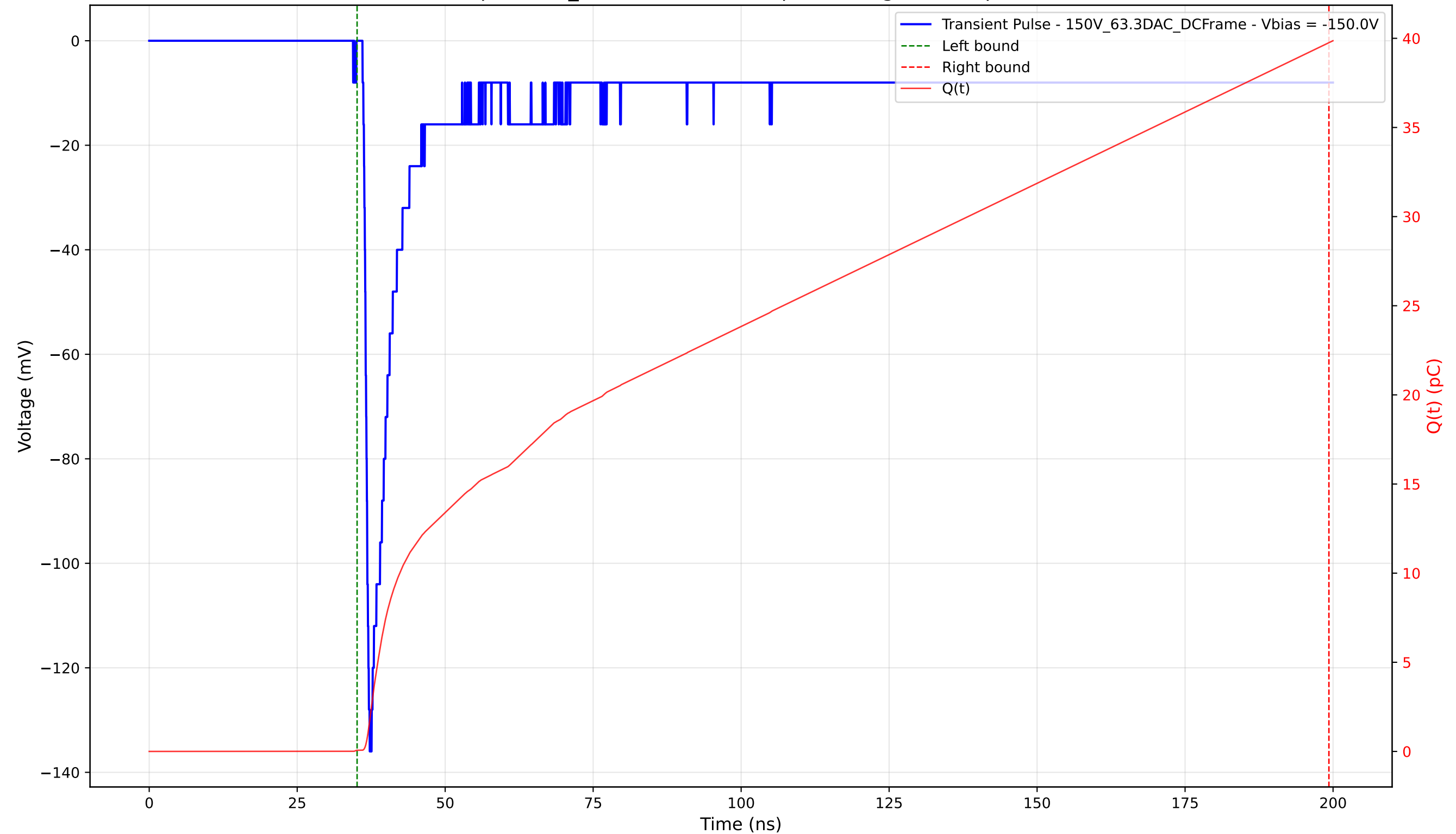
Transient Pulse - Sample: 1cm_42 - Position: 700.0 \mu\text{m} - Charge: 39.69 pC - Rise Time: 0.93 ns
