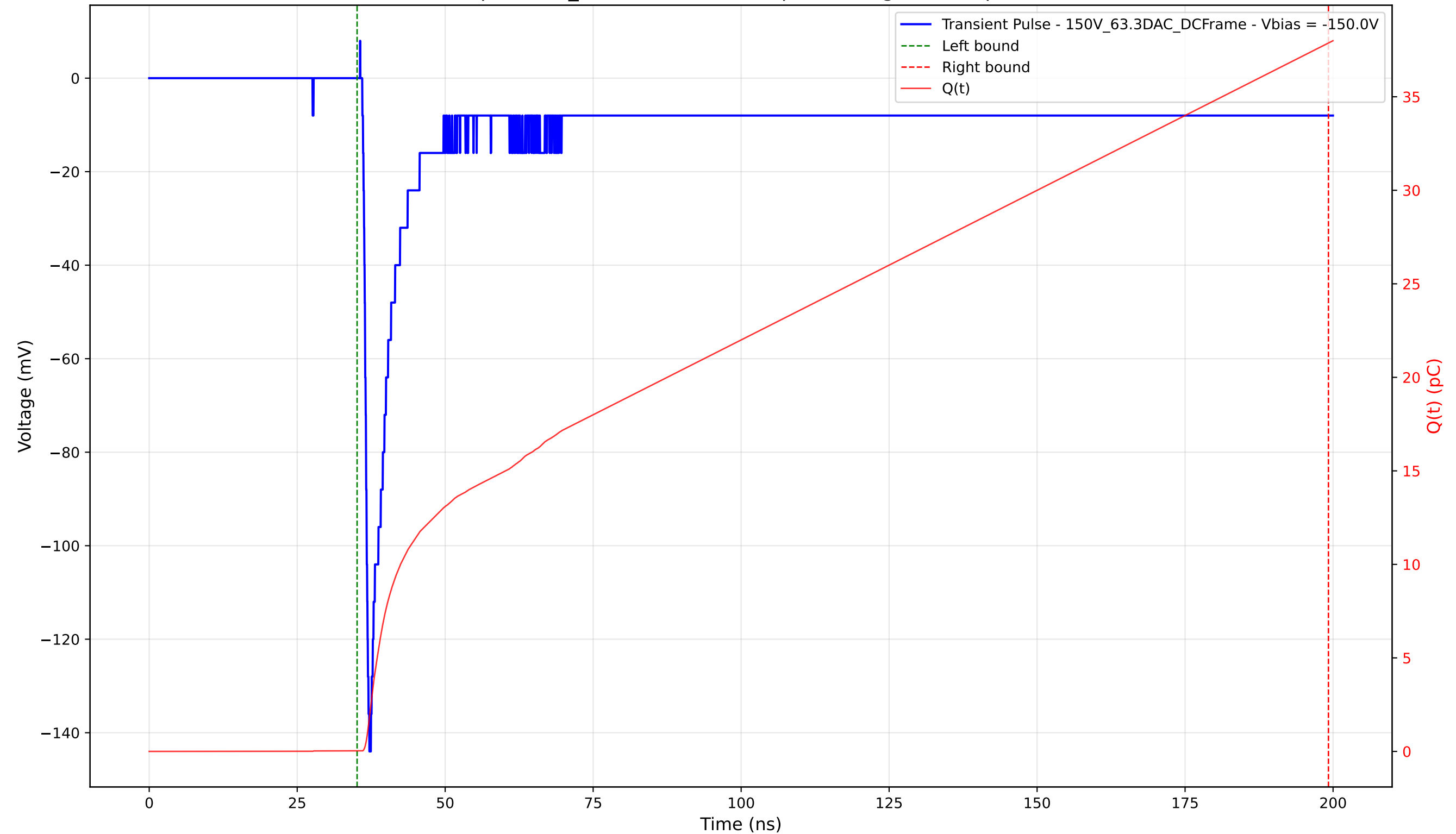
Transient Pulse - Sample: 1cm_42 - Position: 610.0 \mu\text{m} - Charge: 37.85 pC - Rise Time: 0.92 ns
