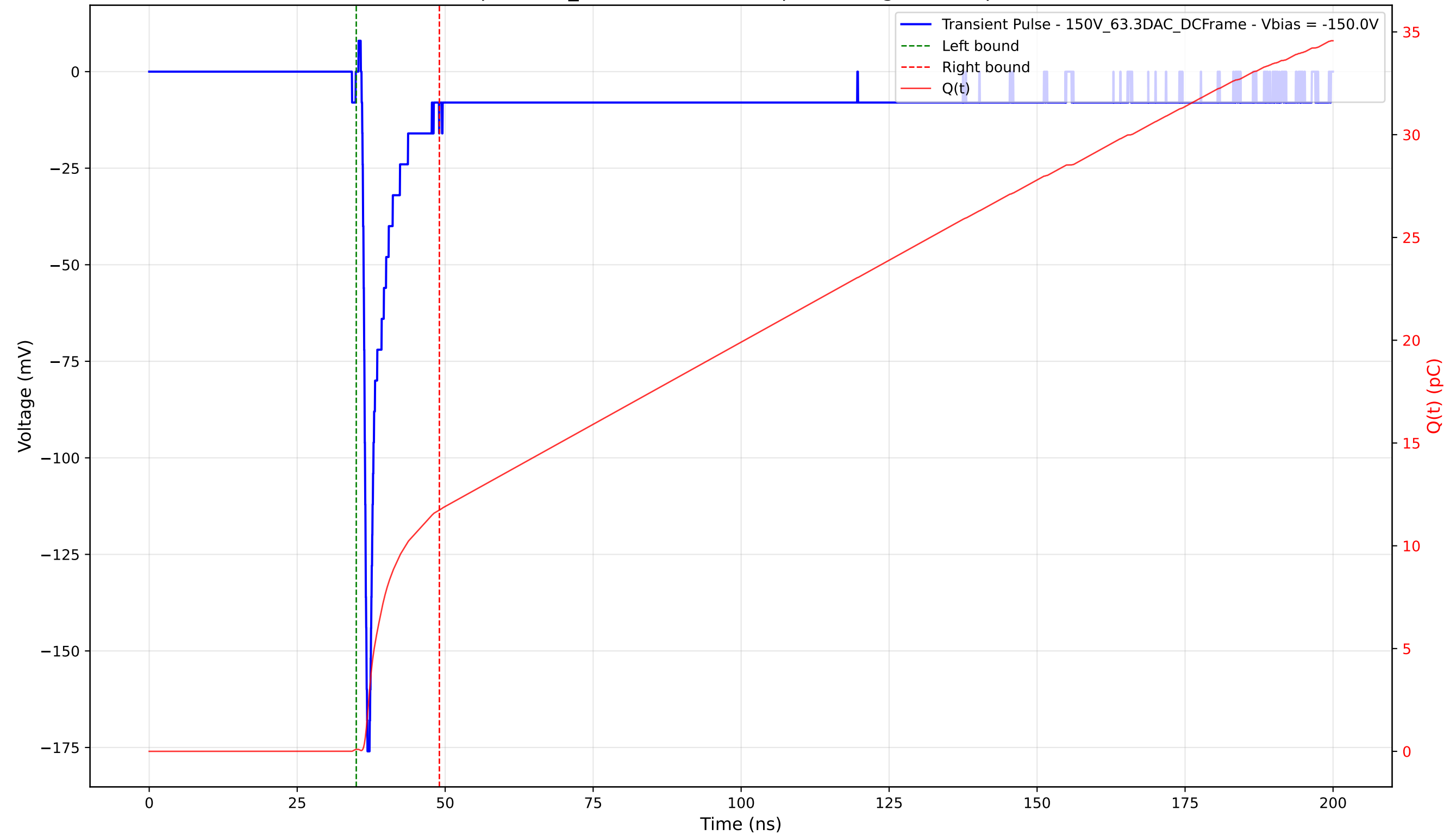
Transient Pulse - Sample: 1cm_42 - Position: 350.0 \mu\text{m} - Charge: 11.64 pC - Rise Time: 0.72 ns
