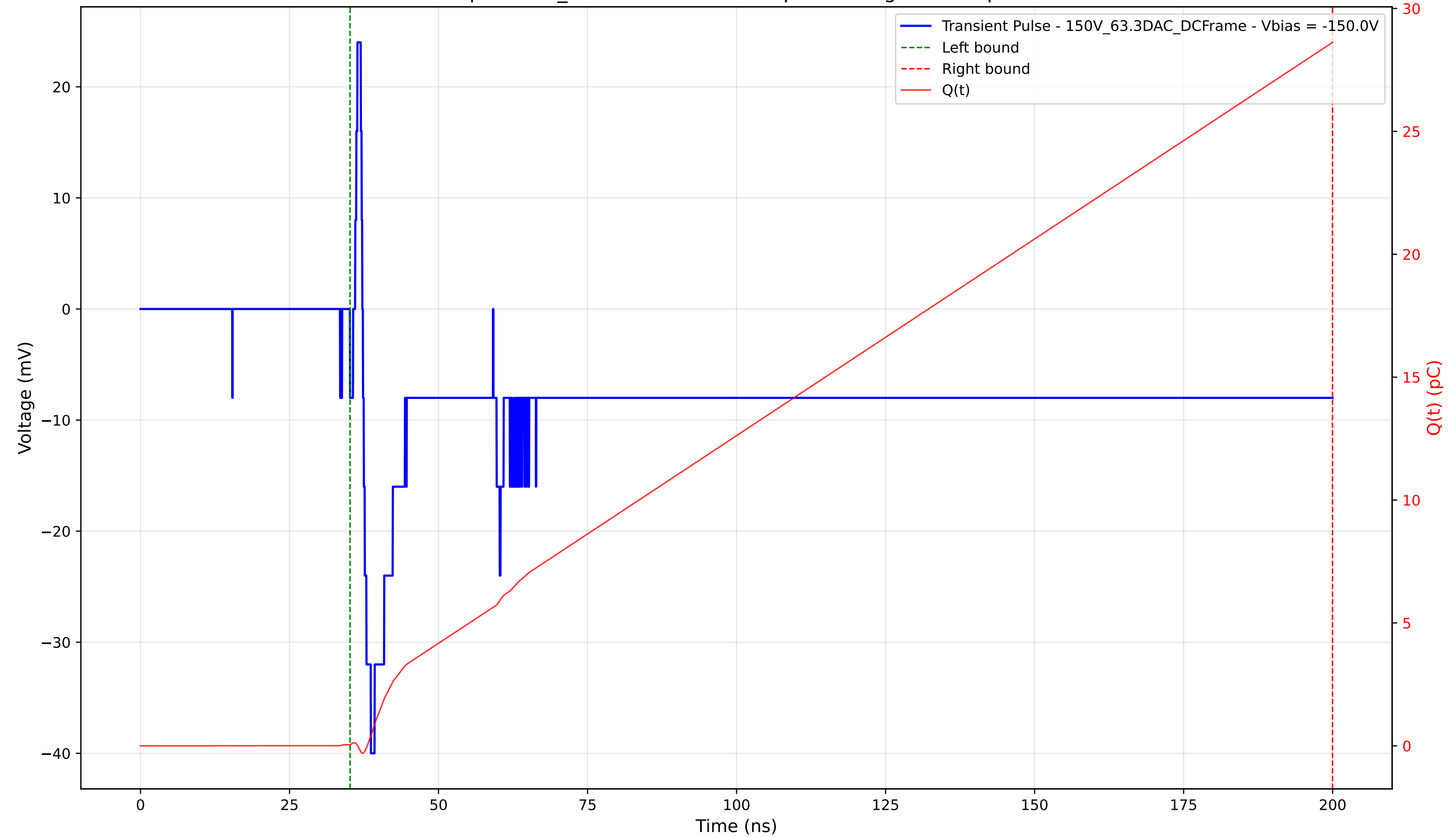
Transient Pulse - Sample: 1cm_42 - Position: 2235.0 \mu\text{m} - Charge: 28.58 pC - Rise Time: 1.33 ns
