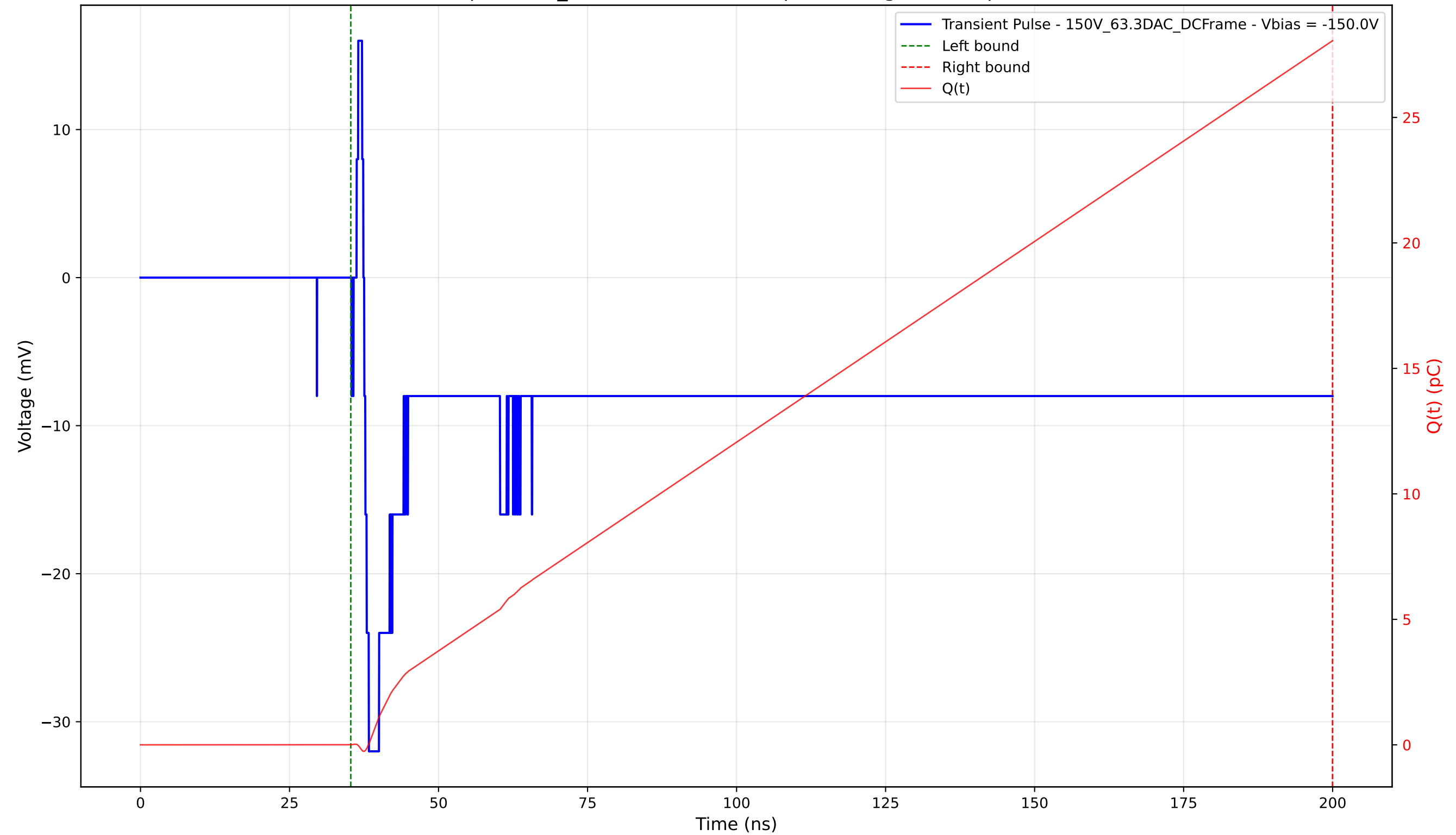
Transient Pulse - Sample: 1cm_42 - Position: 2800.0 \mu\text{m} - Charge: 28.05 pC - Rise Time: 0.77 ns
