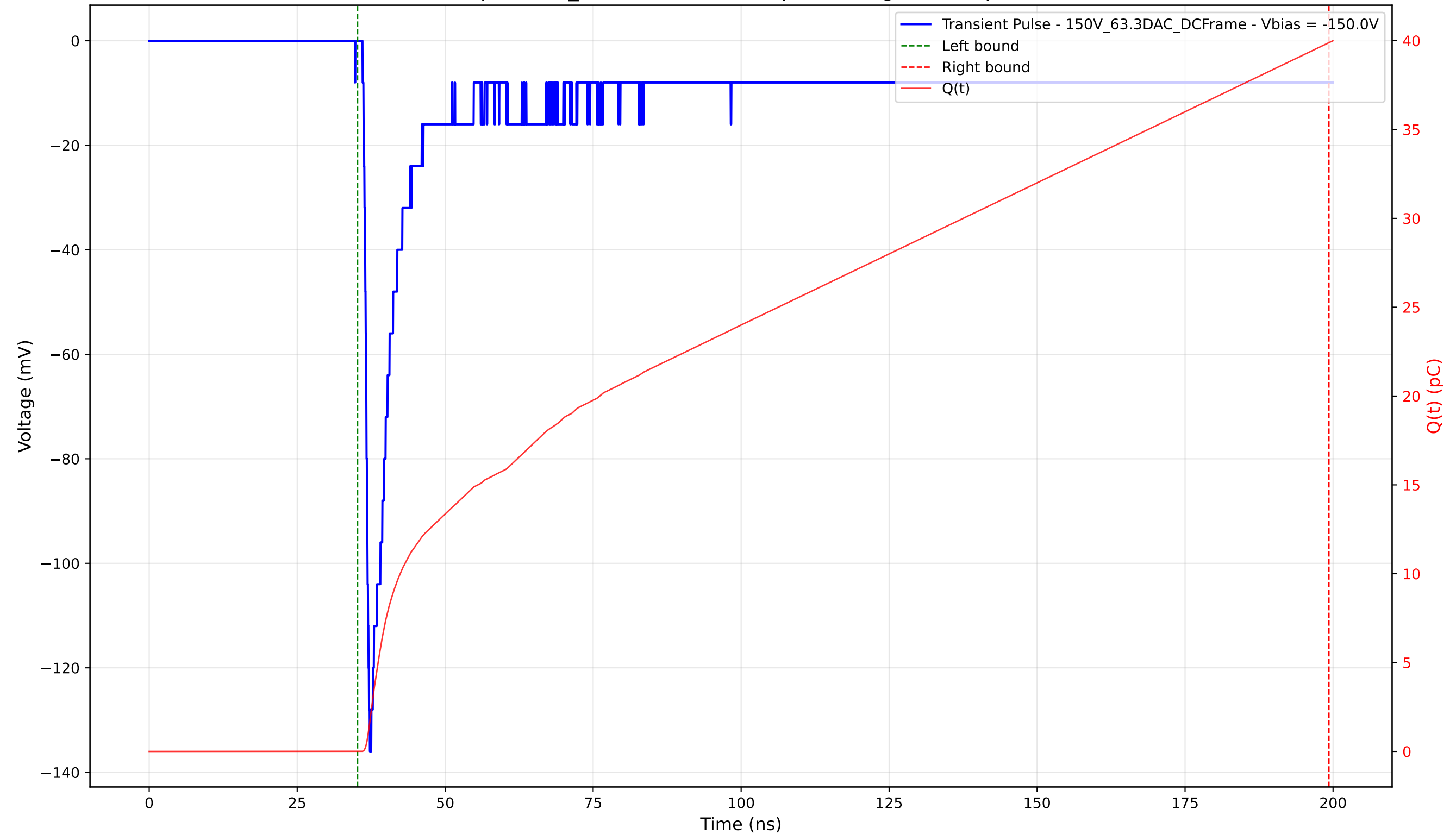
Transient Pulse - Sample: 1cm_42 - Position: 715.0 \mu\text{m} - Charge: 39.88 pC - Rise Time: 0.93 ns
