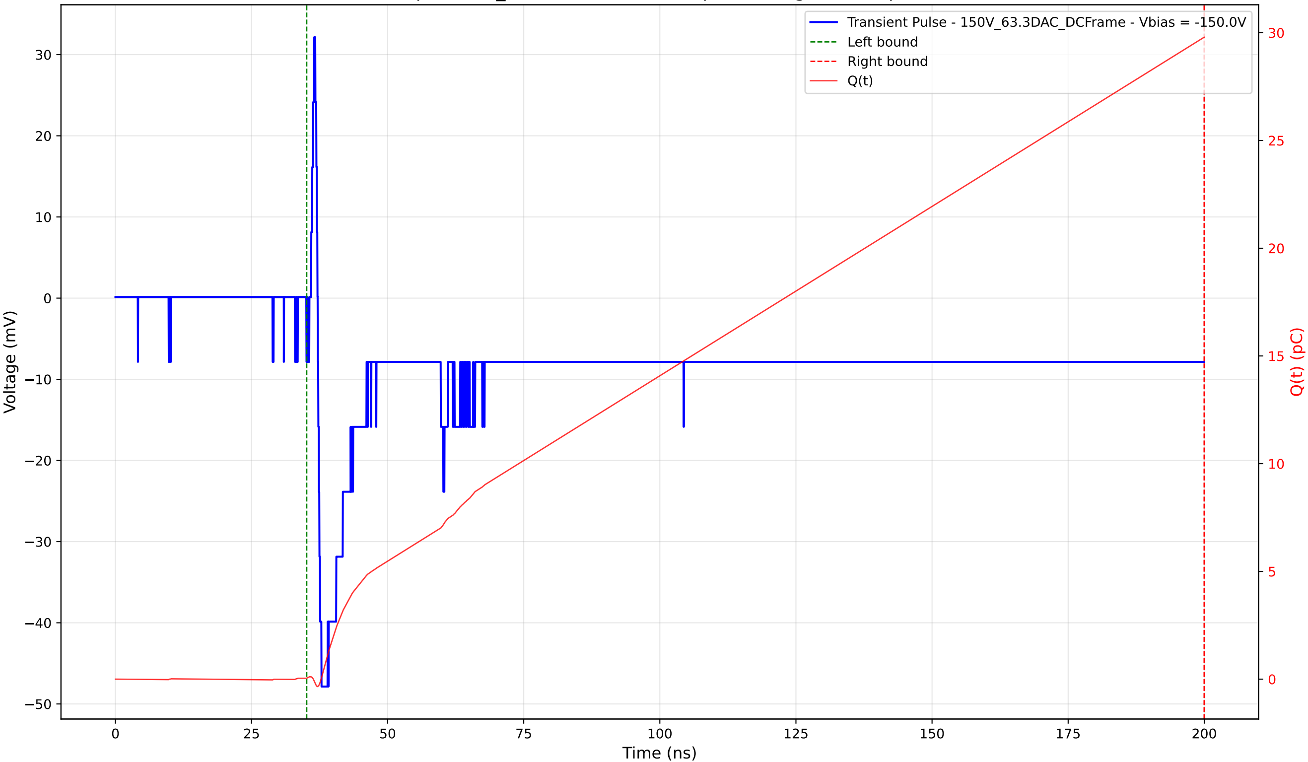
Transient Pulse - Sample: 1cm_42 - Position: 1735.0 \mu\text{m} - Charge: 29.74 pC - Rise Time: 0.69 ns
