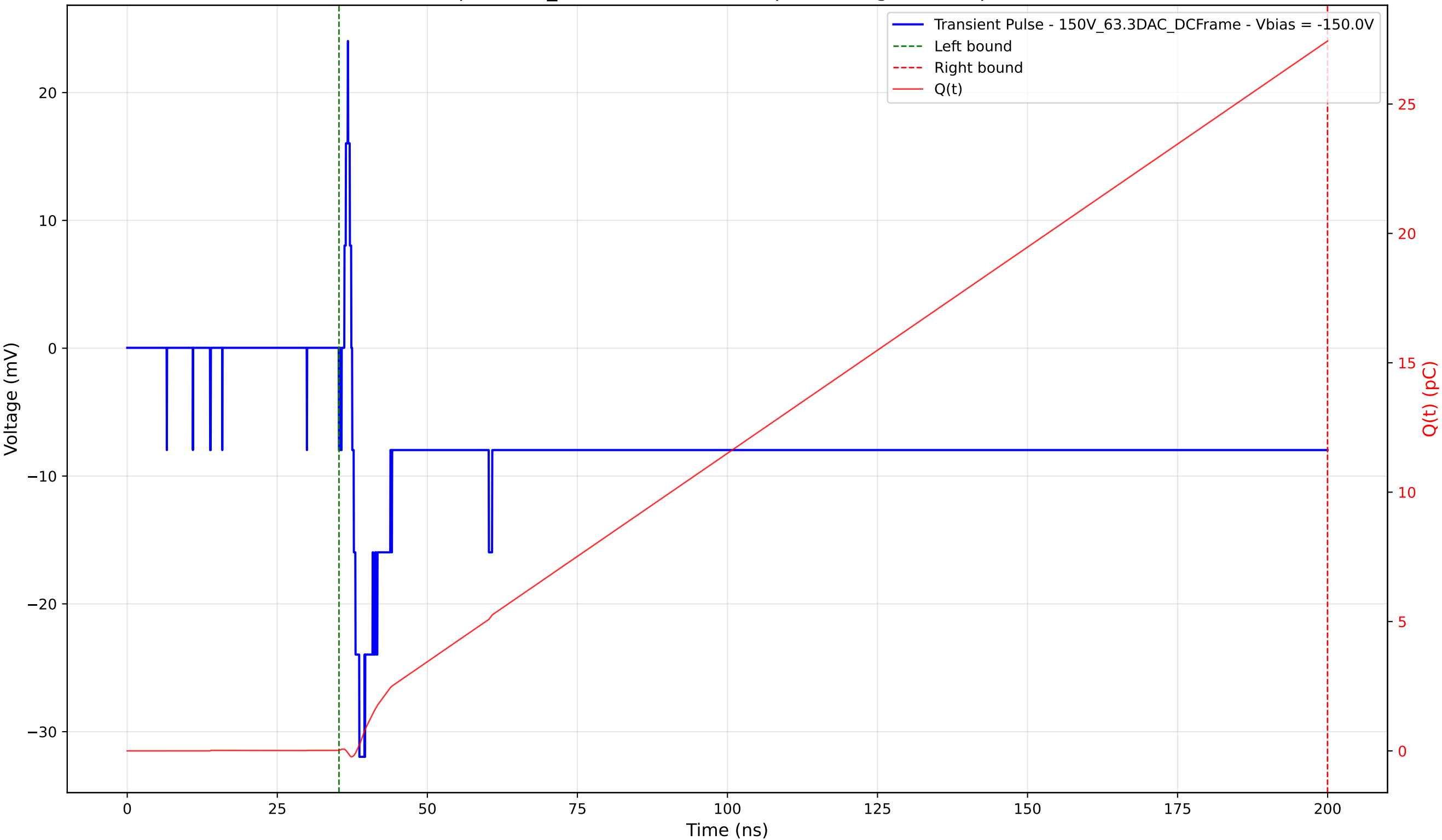
Transient Pulse - Sample: 1cm_42 - Position: 2485.0 \mu\text{m} - Charge: 27.41 pC - Rise Time: 1.19 ns
