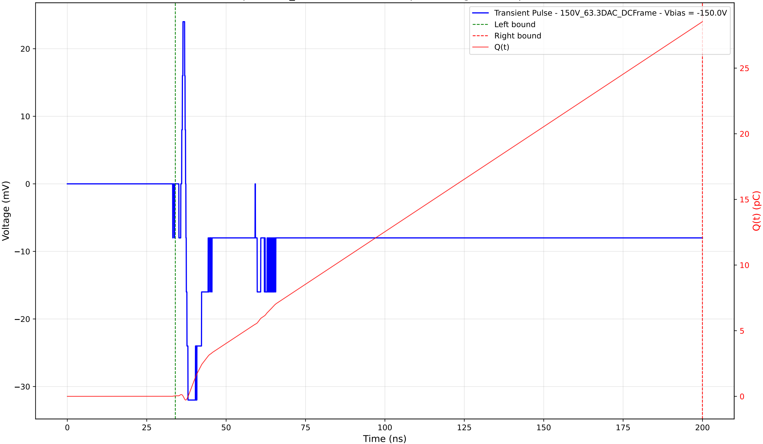
Transient Pulse - Sample: 1cm_42 - Position: 2290.0 \mu\text{m} - Charge: 28.50 pC - Rise Time: 0.65 ns
