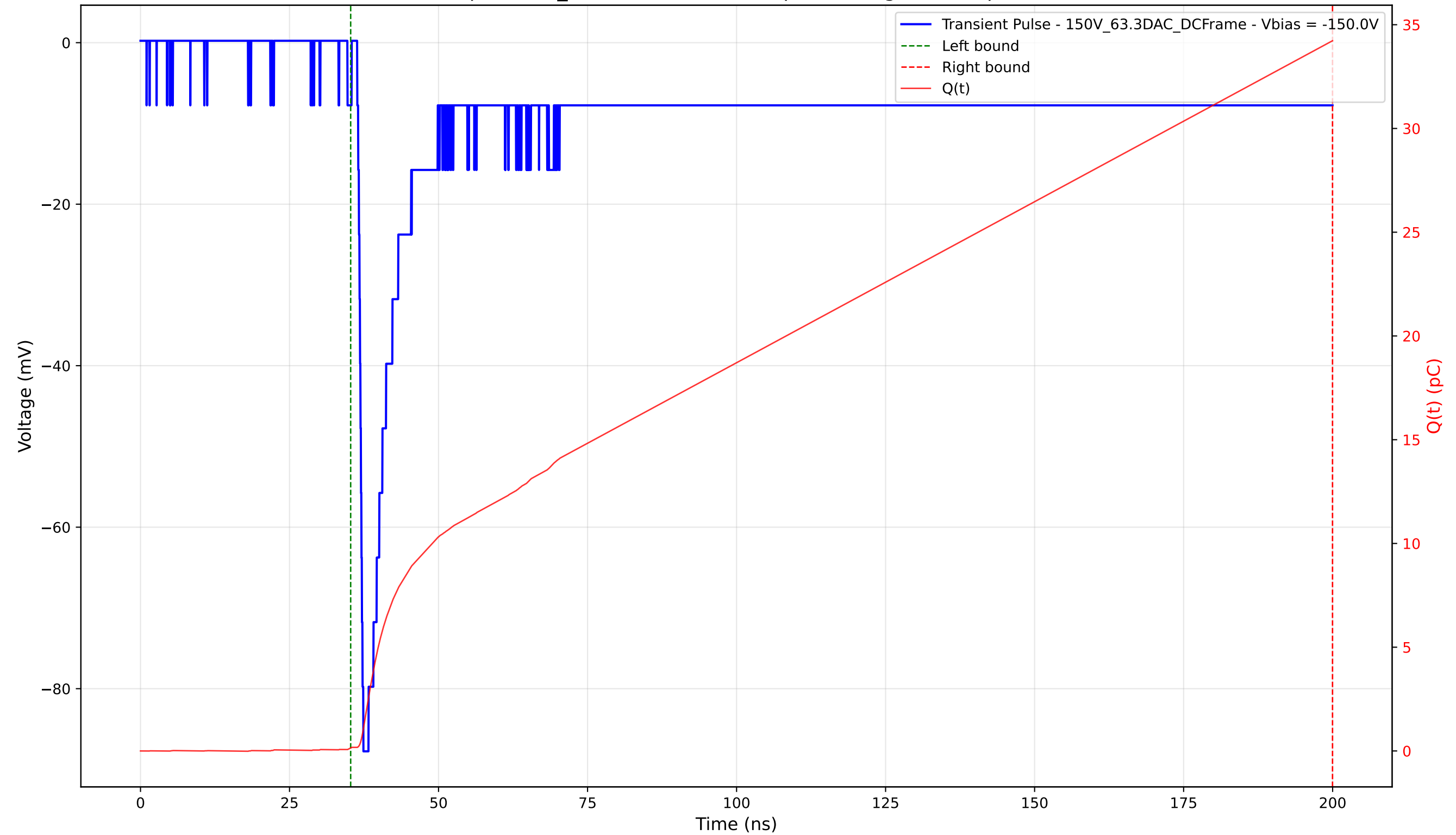
Transient Pulse - Sample: 1cm_42 - Position: 4230.0 \mu\text{m} - Charge: 34.08 pC - Rise Time: 0.74 ns
