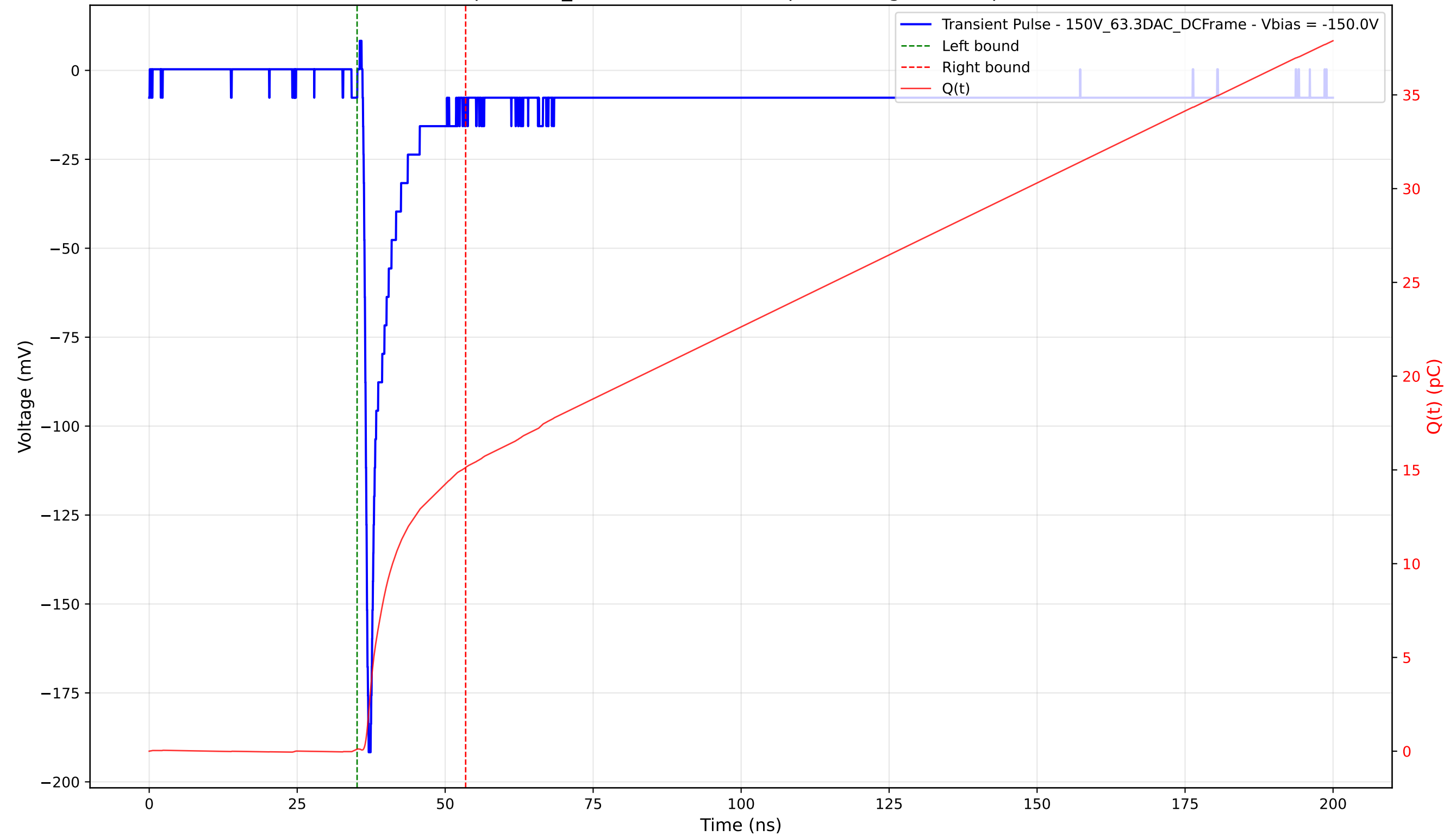
Transient Pulse - Sample: 1cm_42 - Position: 4665.0 \mu\text{m} - Charge: 15.02 pC - Rise Time: 0.77 ns
