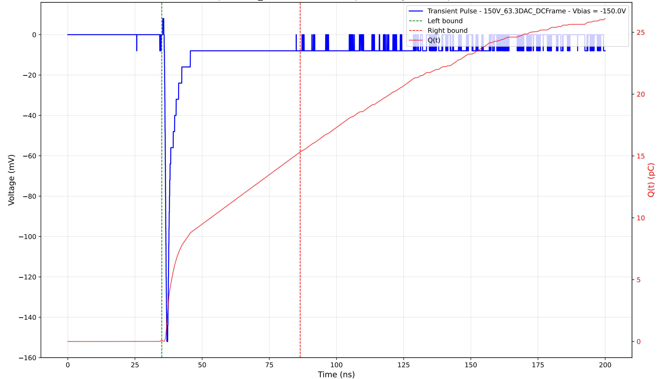
Transient Pulse - Sample: 1cm_42 - Position: 215.0 \mu\text{m} - Charge: 15.25 pC - Rise Time: 0.78 ns
