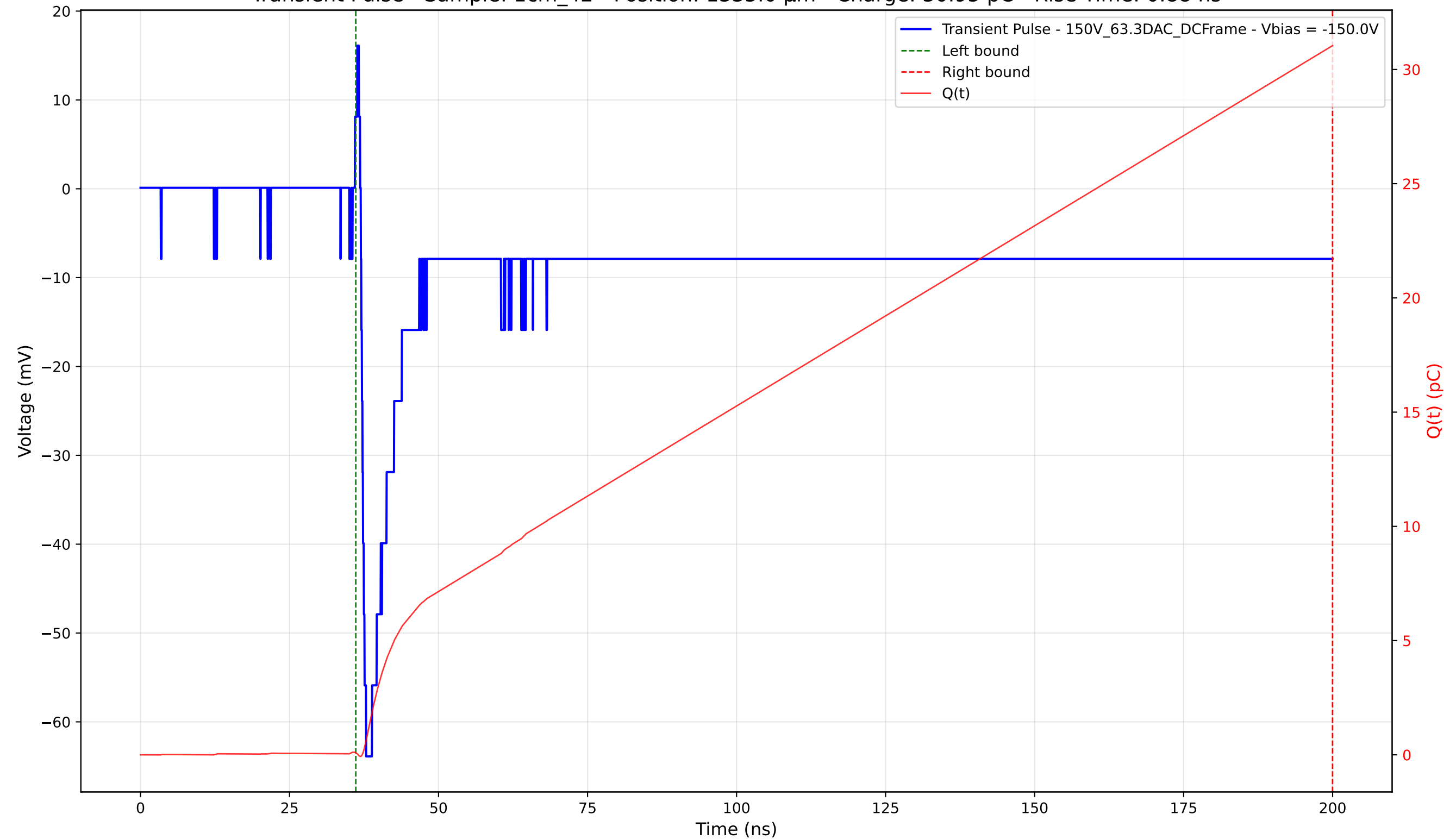
Transient Pulse - Sample: 1cm_42 - Position: 1335.0 \mu\text{m} - Charge: 30.95 pC - Rise Time: 0.88 ns
