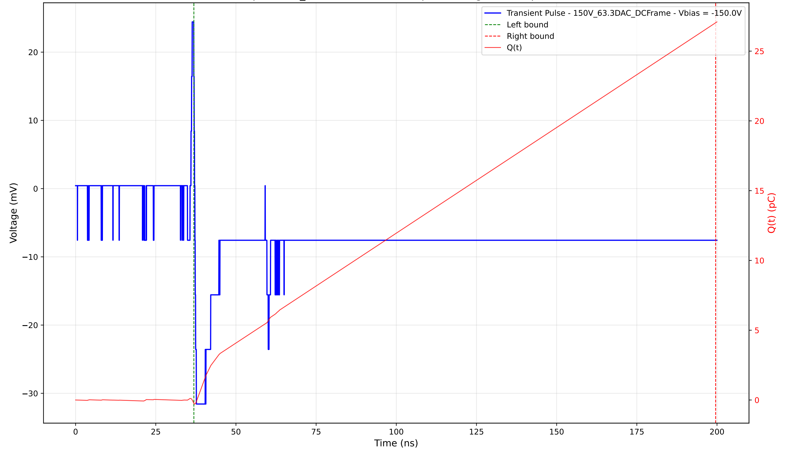
Transient Pulse - Sample: 1cm_42 - Position: 1950.0 \mu\text{m} - Charge: 27.28 pC - Rise Time: 0.45 ns
