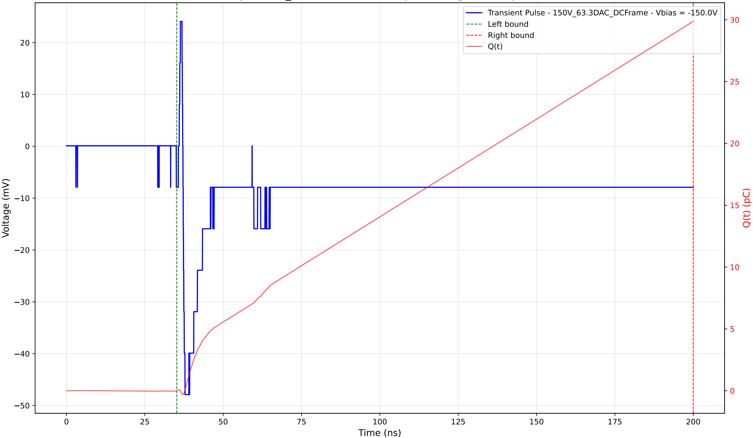
Transient Pulse - Sample: 1cm_42 - Position: 1675.0 \mu\text{m} - Charge: 29.87 pC - Rise Time: 0.65 ns
