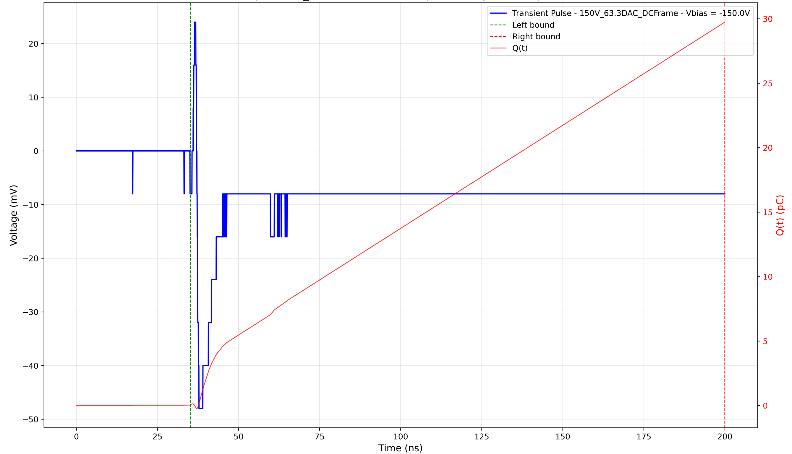
Transient Pulse - Sample: 1cm_42 - Position: 1605.0 \mu\text{m} - Charge: 29.68 pC - Rise Time: 0.63 ns
