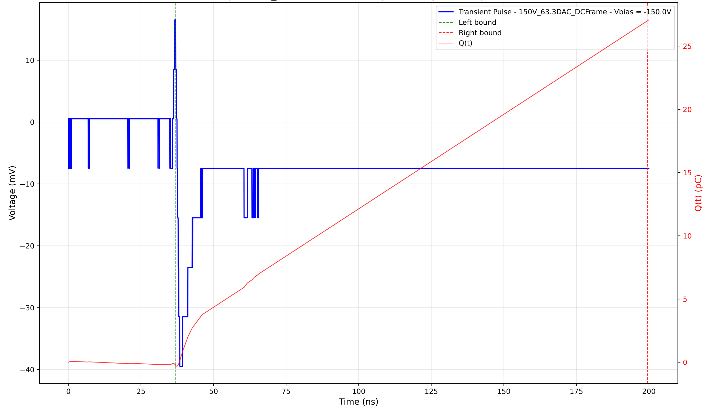
Transient Pulse - Sample: 1cm_42 - Position: 3265.0 \mu\text{m} - Charge: 27.26 pC - Rise Time: 0.95 ns
