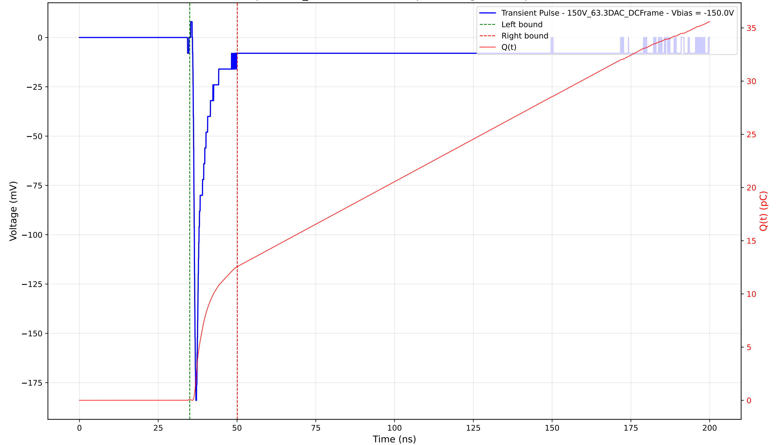
Transient Pulse - Sample: 1cm_42 - Position: 375.0 \mu\text{m} - Charge: 12.50 pC - Rise Time: 0.75 ns
