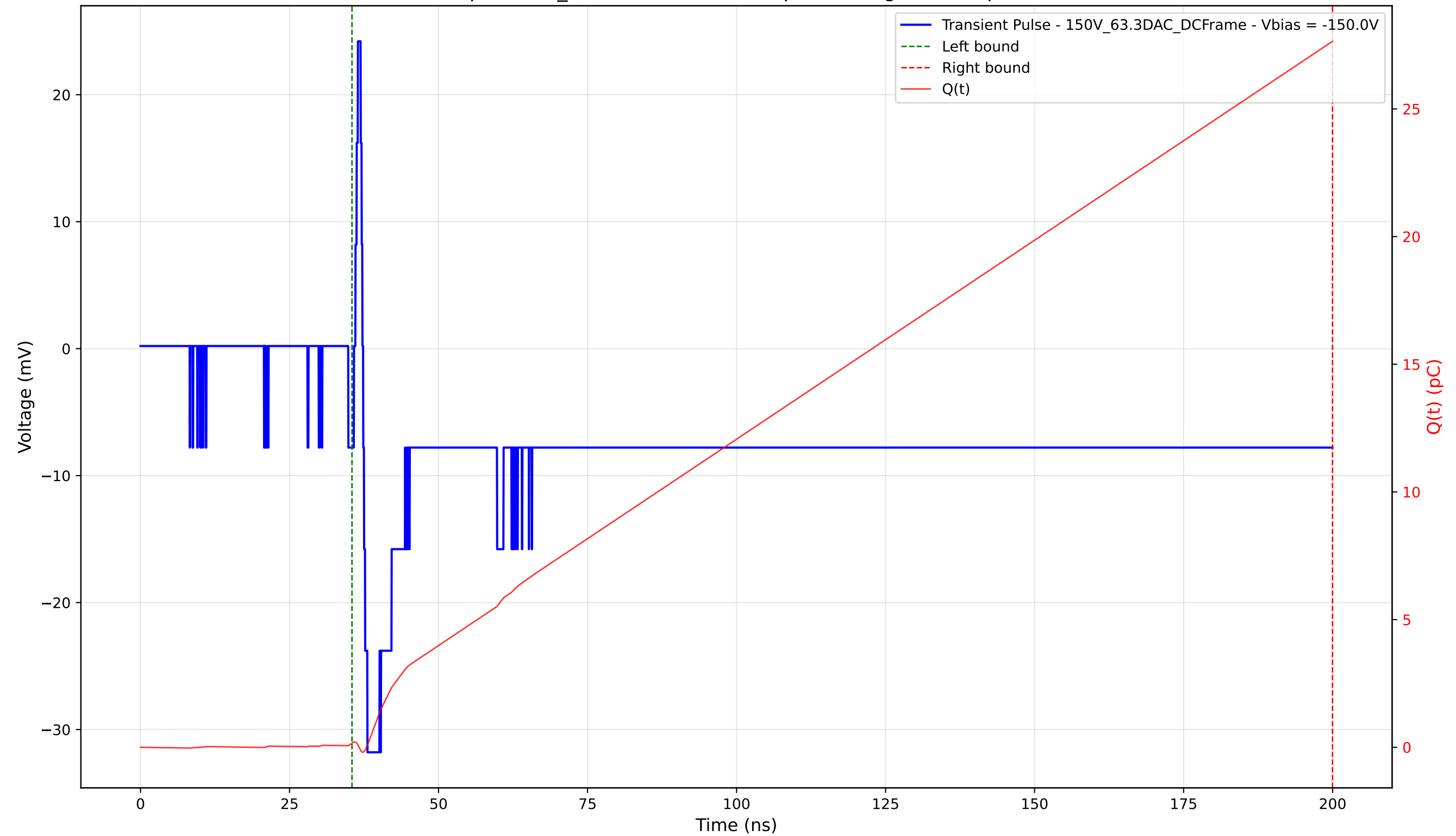
Transient Pulse - Sample: 1cm_42 - Position: 2320.0 \mu\text{m} - Charge: 27.49 pC - Rise Time: 0.71 ns
