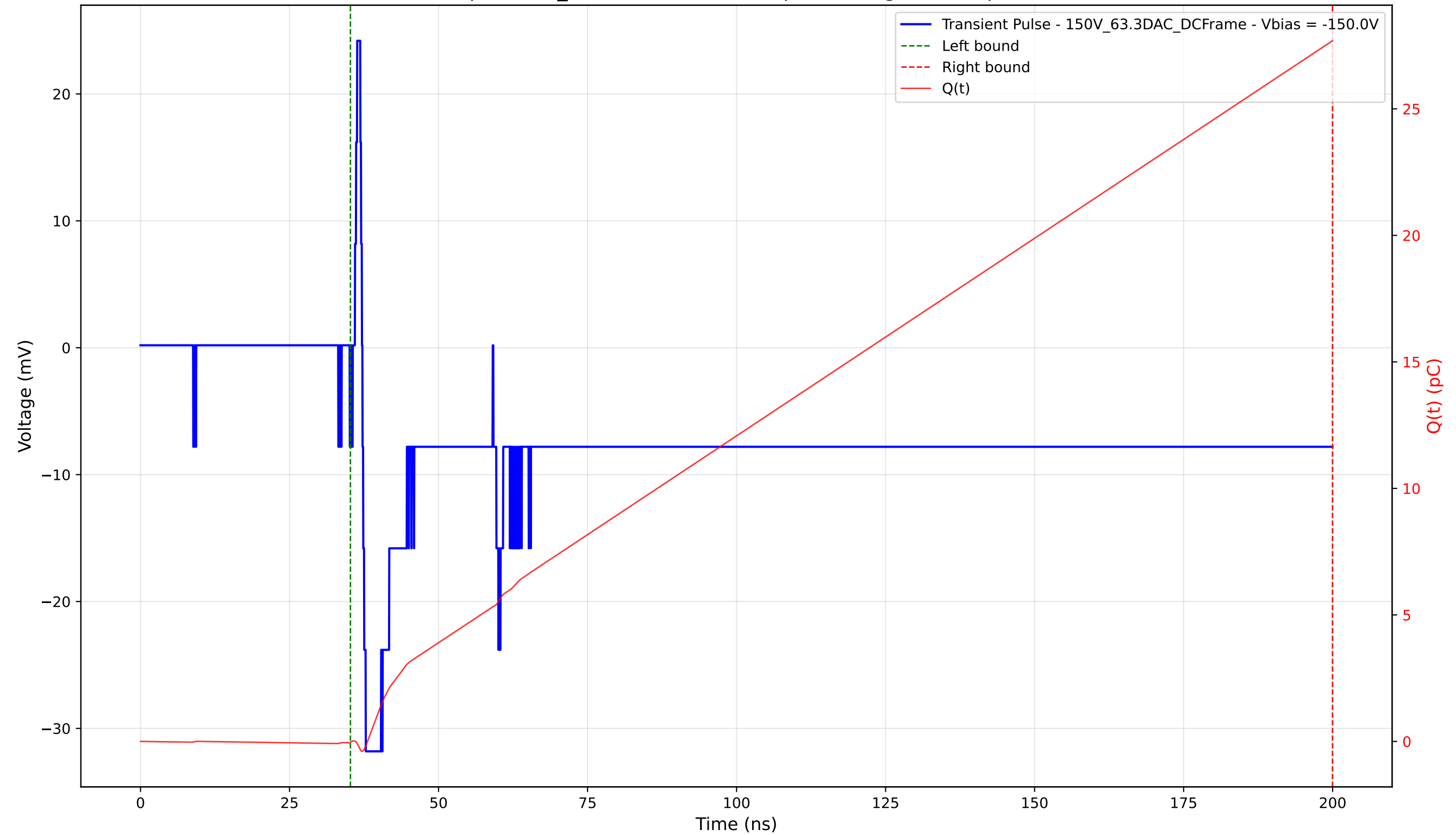
Transient Pulse - Sample: 1cm_42 - Position: 2100.0 \mu\text{m} - Charge: 27.73 pC - Rise Time: 0.55 ns
