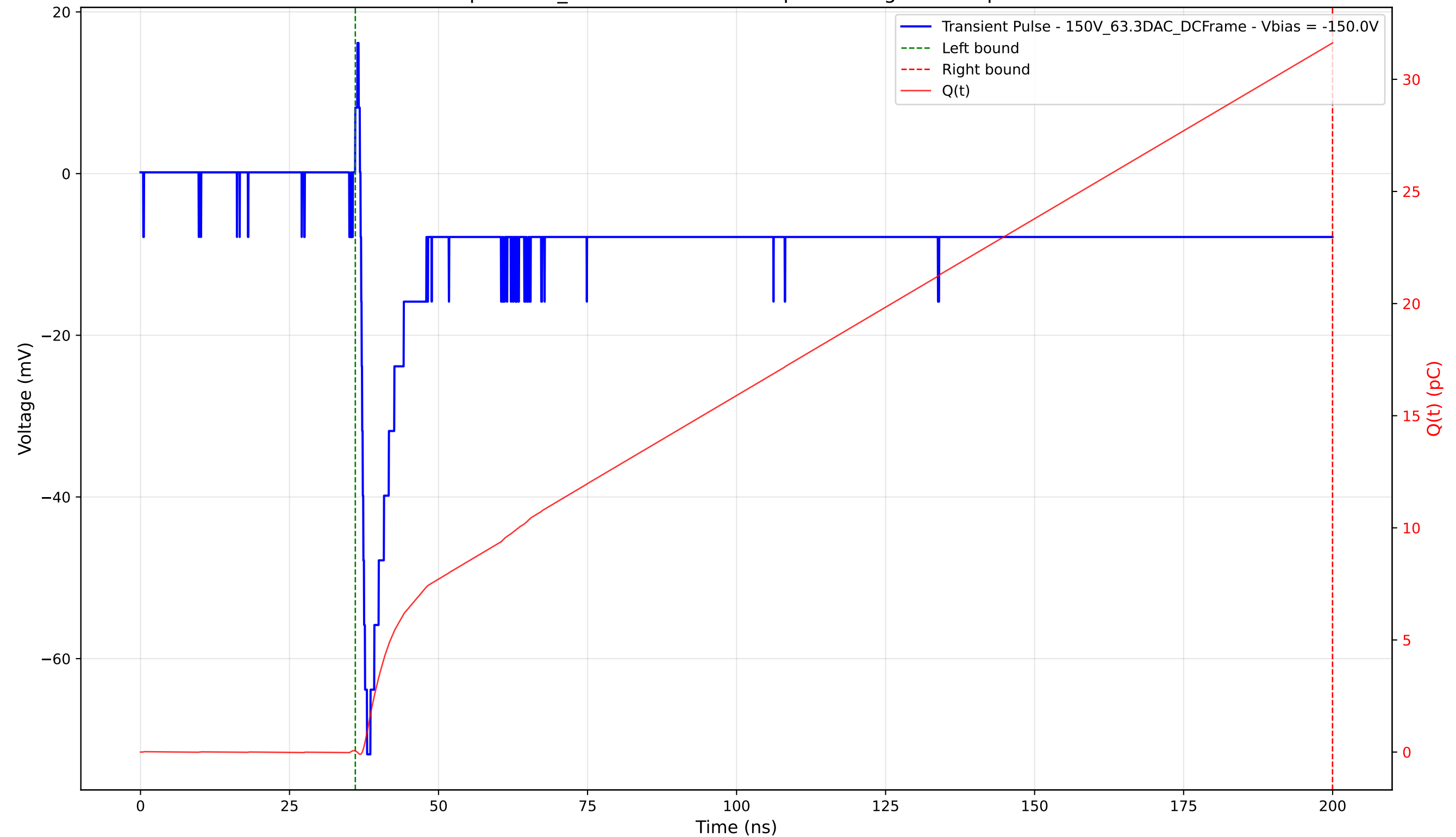
Transient Pulse - Sample: 1cm_42 - Position: 1295.0 \mu\text{m} - Charge: 31.57 pC - Rise Time: 1.08 ns
