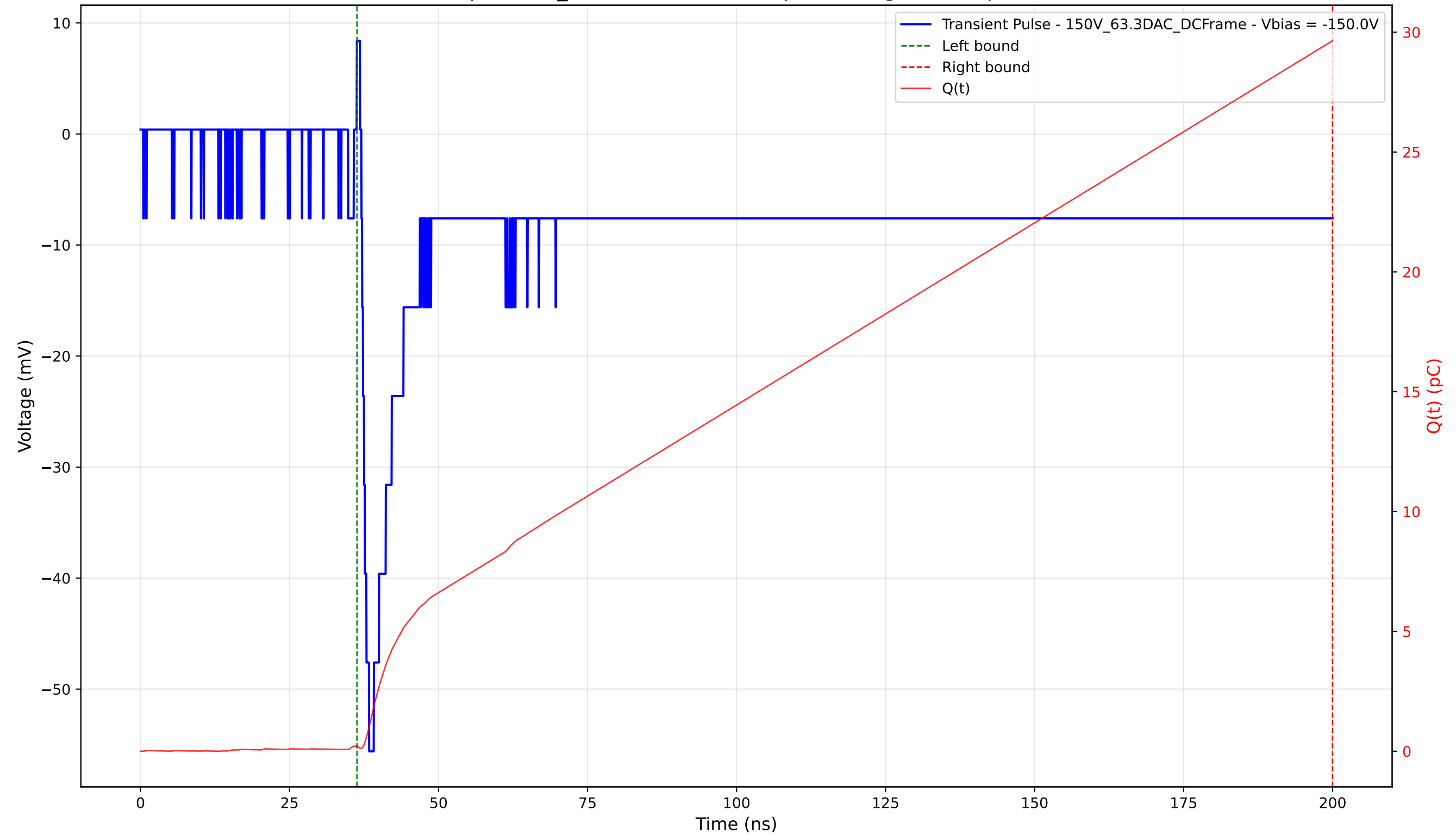
Transient Pulse - Sample: 1cm_42 - Position: 3730.0 \mu\text{m} - Charge: 29.44 pC - Rise Time: 1.29 ns
