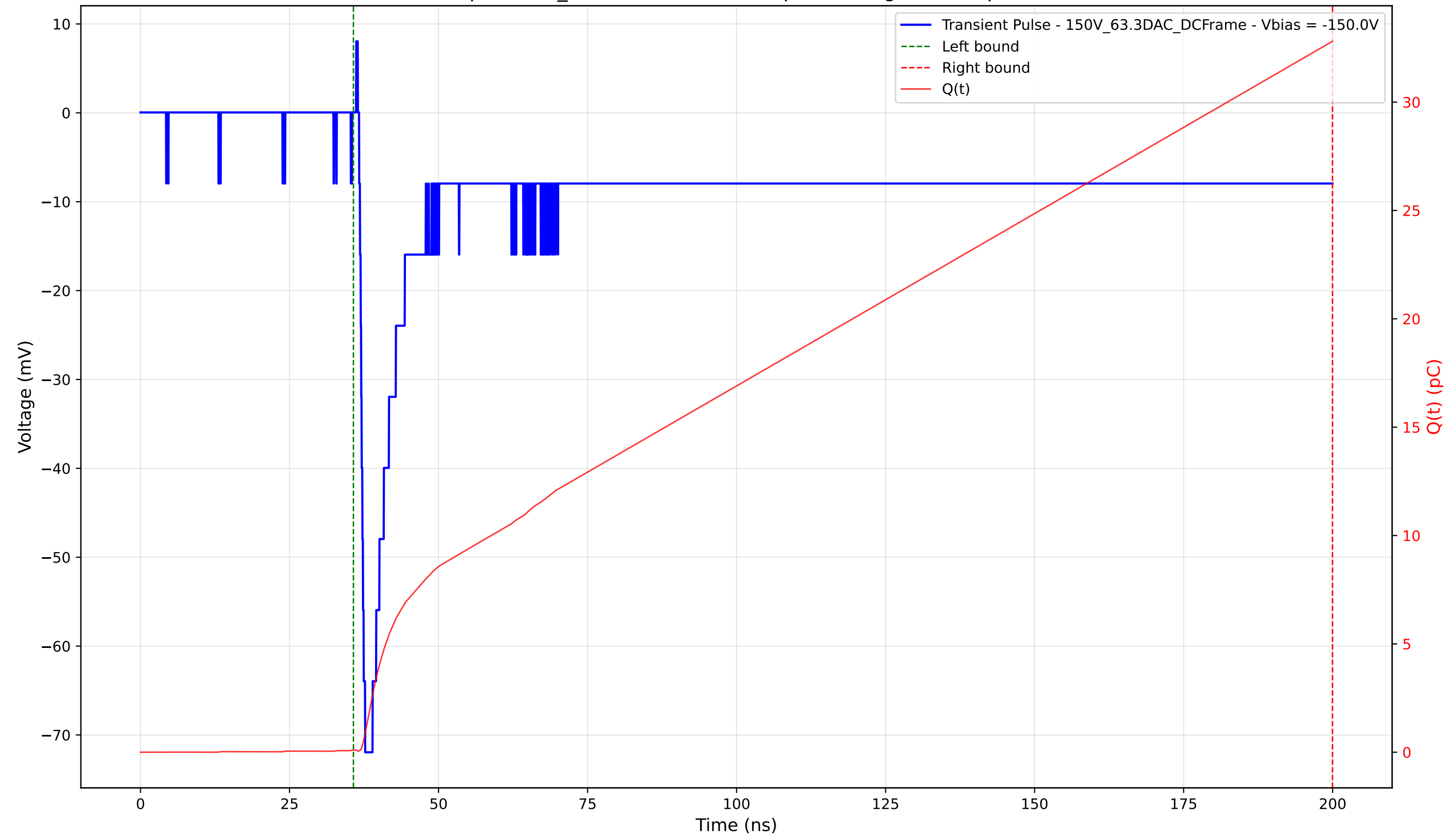
Transient Pulse - Sample: 1cm_42 - Position: 1075.0 \mu\text{m} - Charge: 32.71 pC - Rise Time: 1.00 ns
