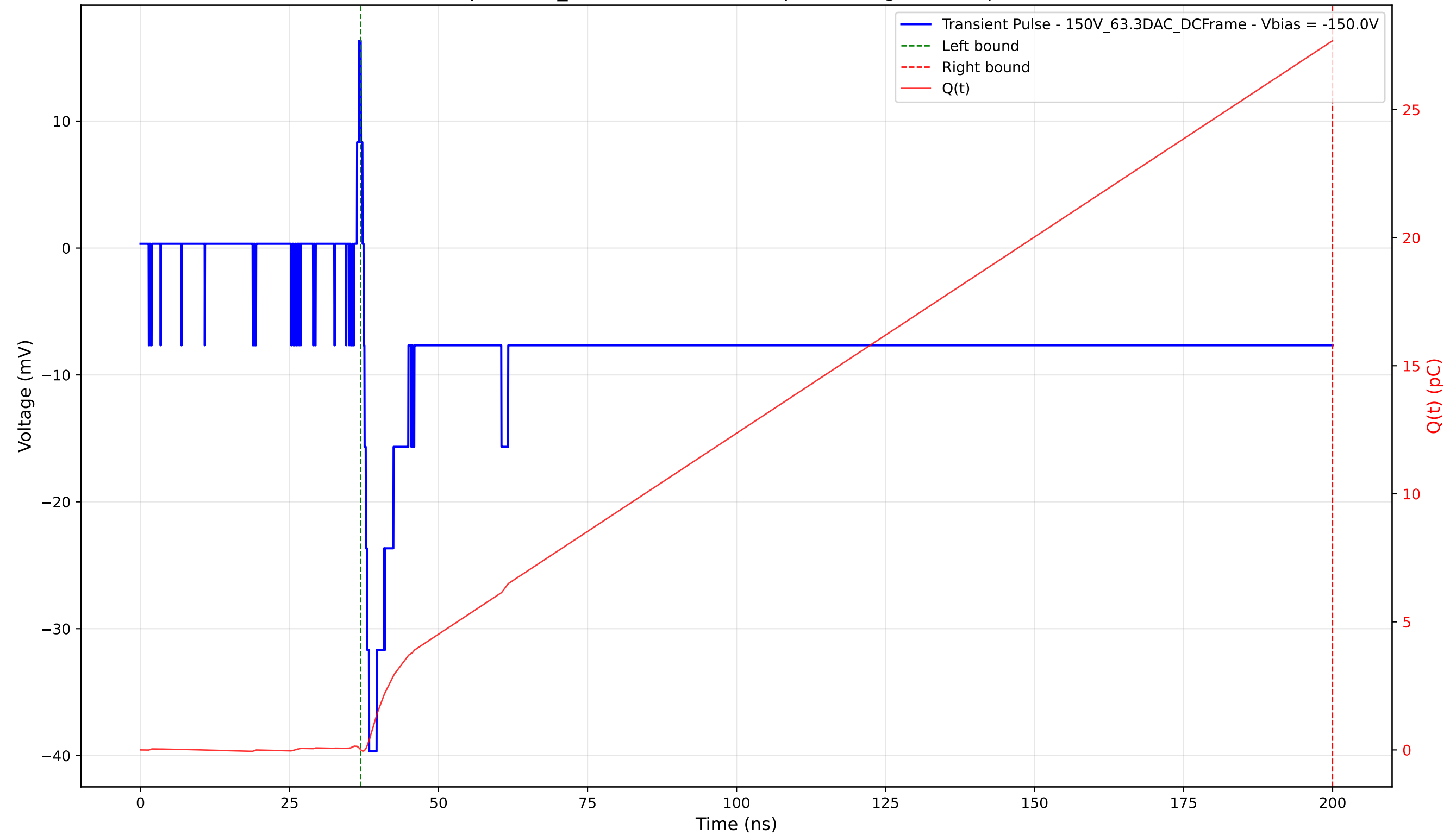
Transient Pulse - Sample: 1cm_42 - Position: 3235.0 \mu\text{m} - Charge: 27.68 pC - Rise Time: 0.91 ns
