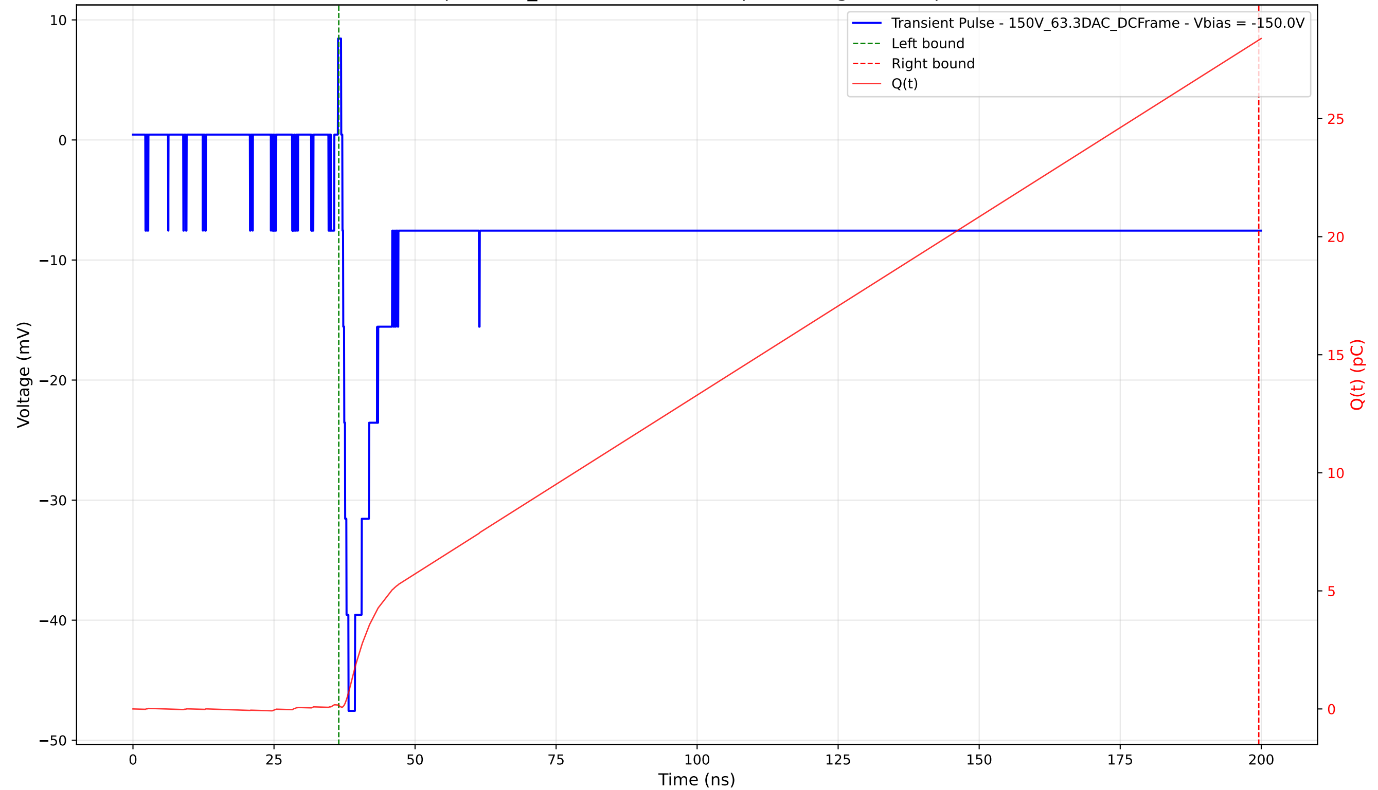
Transient Pulse - Sample: 1cm_42 - Position: 3645.0 \mu\text{m} - Charge: 28.18 pC - Rise Time: 1.09 ns
