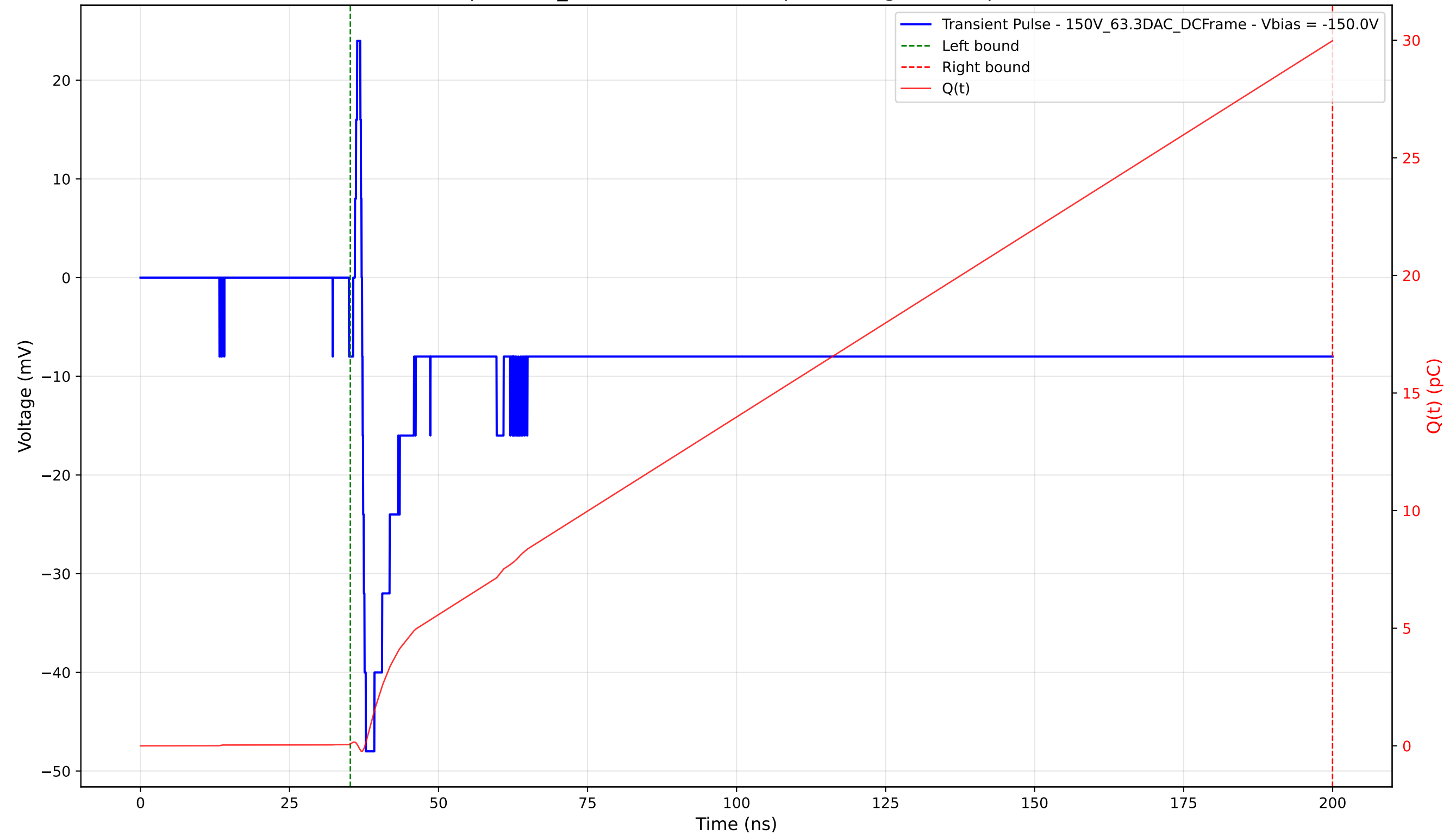
Transient Pulse - Sample: 1cm_42 - Position: 1670.0 \mu\text{m} - Charge: 29.89 pC - Rise Time: 0.63 ns
