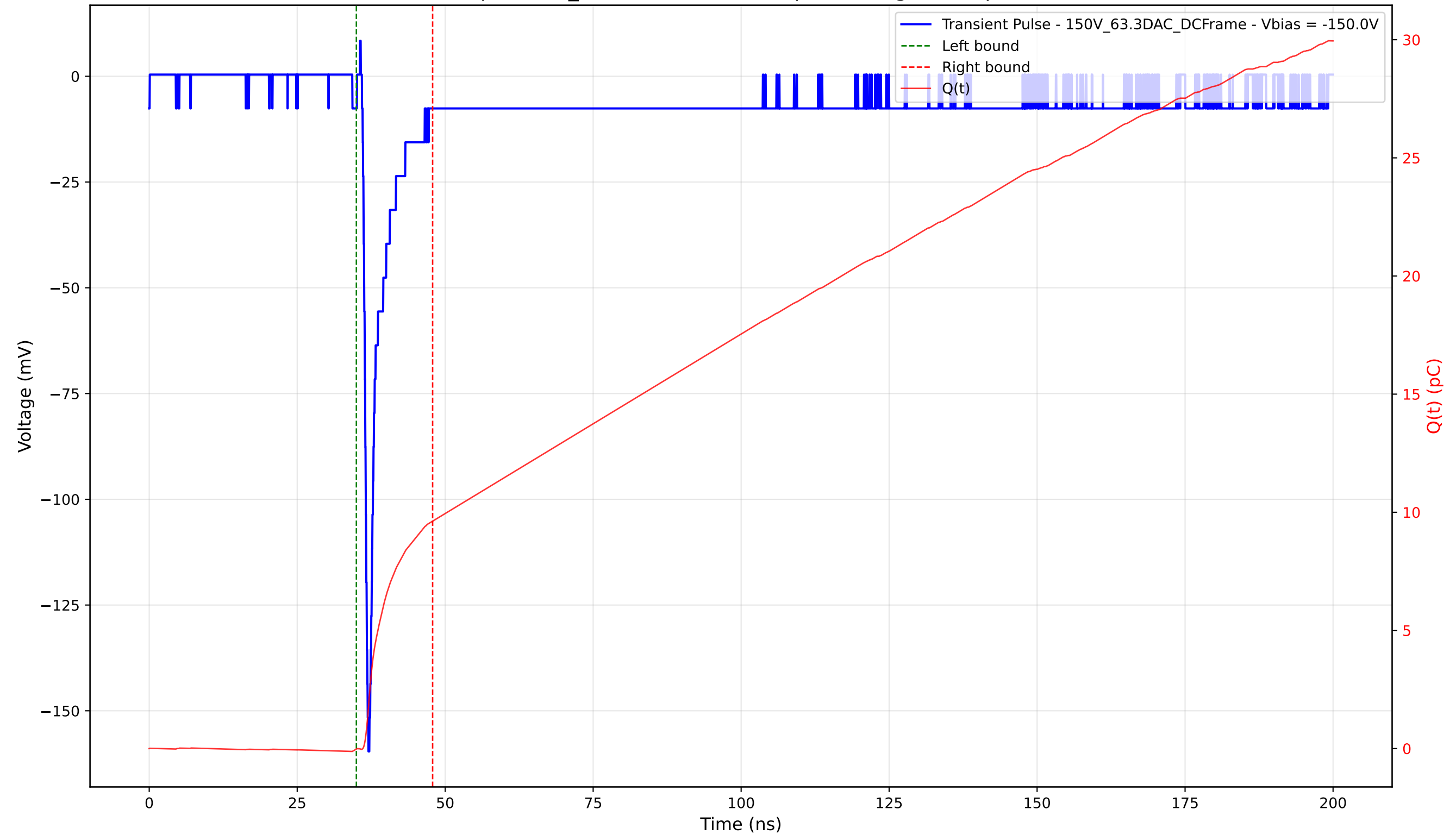
Transient Pulse - Sample: 1cm_42 - Position: 4970.0 \mu\text{m} - Charge: 9.64 pC - Rise Time: 0.80 ns
