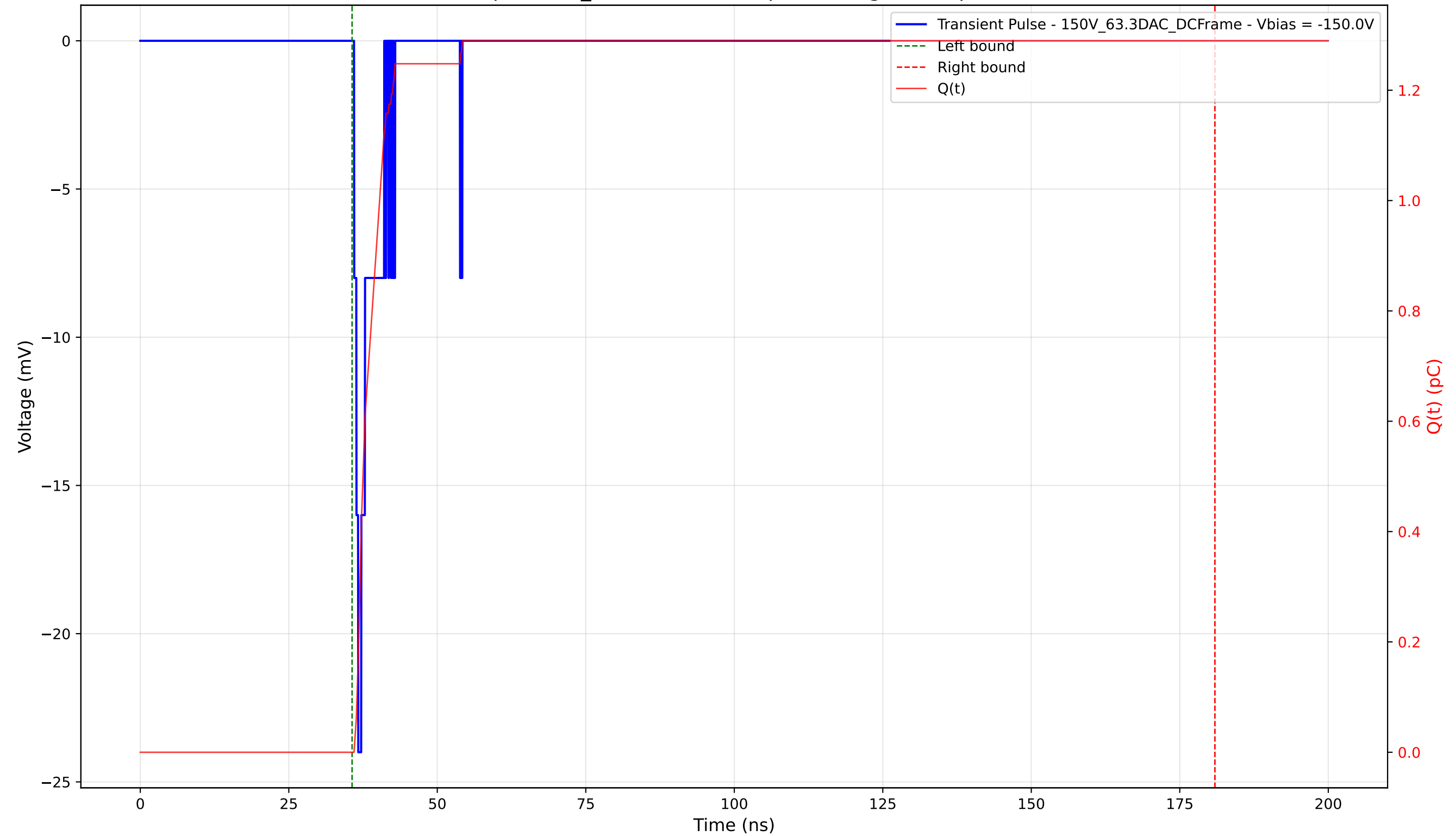
Transient Pulse - Sample: 1cm_42 - Position: 0.0 \mu\text{m} - Charge: 1.29 pC - Rise Time: 0.69 ns
