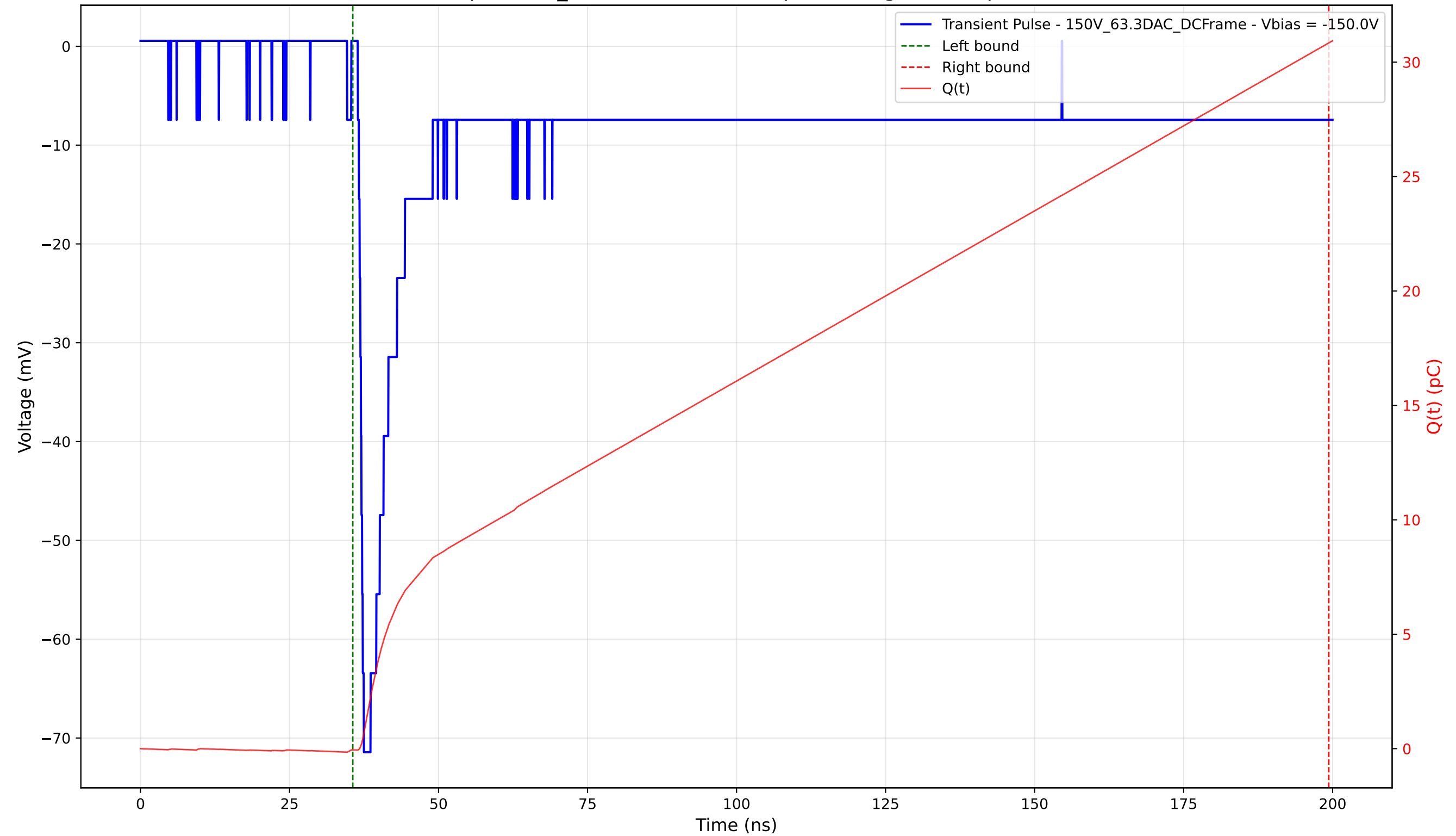
Transient Pulse - Sample: 1cm_42 - Position: 4140.0 \mu\text{m} - Charge: 30.90 pC - Rise Time: 1.00 ns
