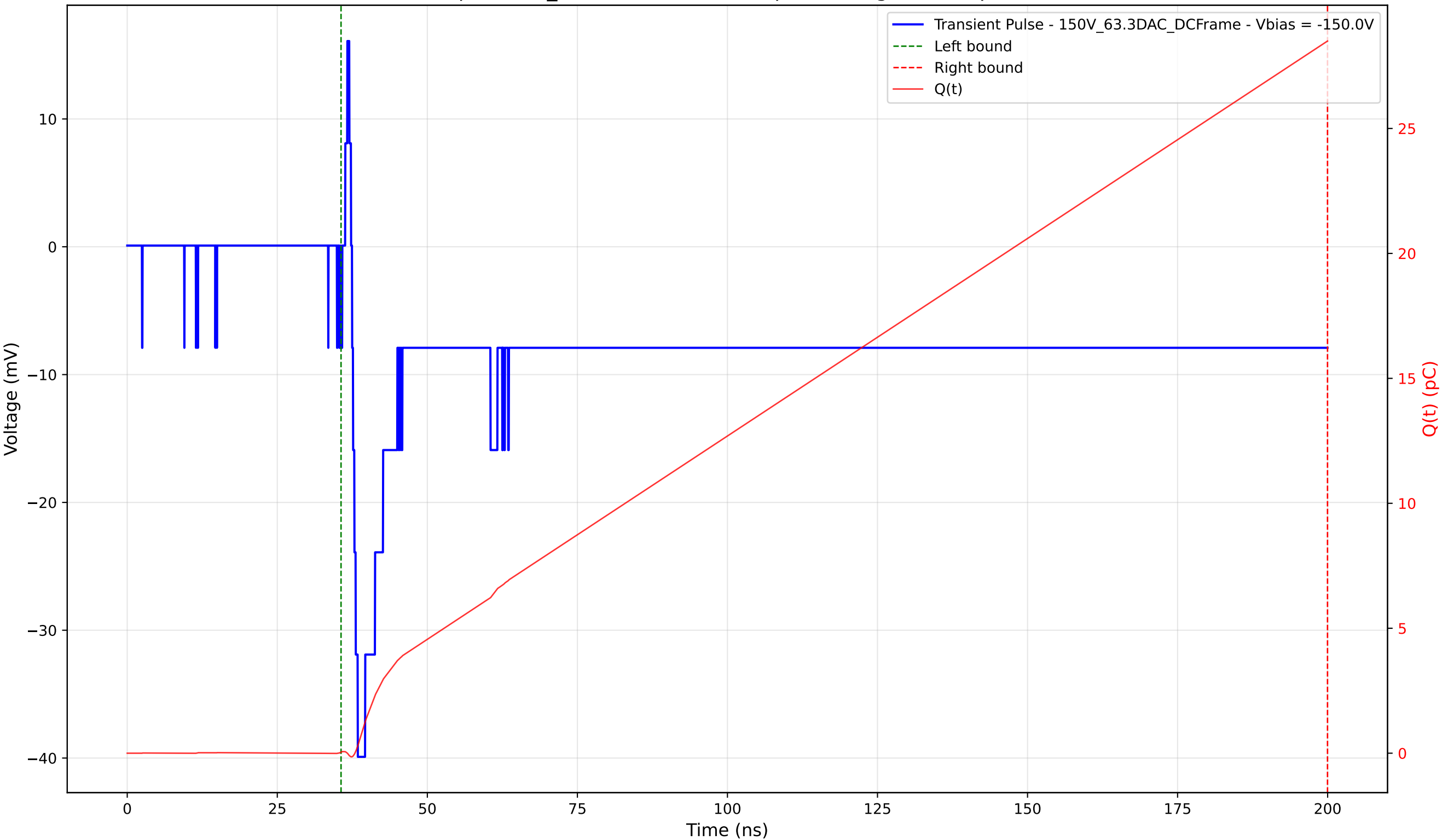
Transient Pulse - Sample: 1cm_42 - Position: 3270.0 \mu\text{m} - Charge: 28.46 pC - Rise Time: 0.95 ns
