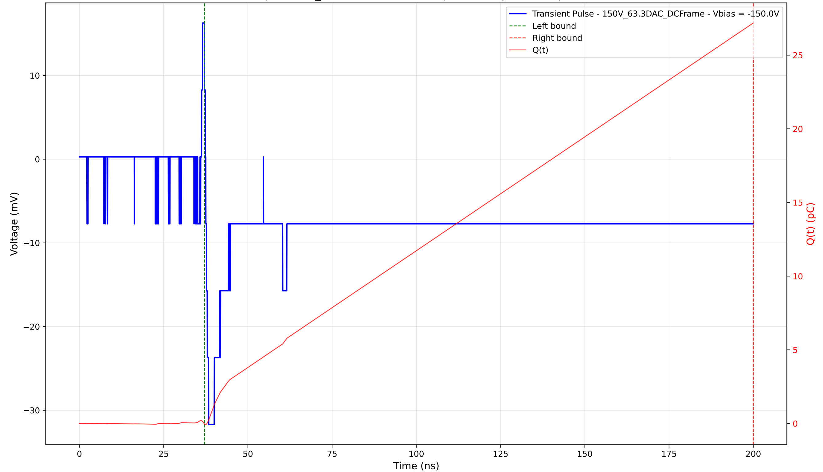
Transient Pulse - Sample: 1cm_42 - Position: 2830.0 \mu\text{m} - Charge: 27.22 pC - Rise Time: 0.85 ns
