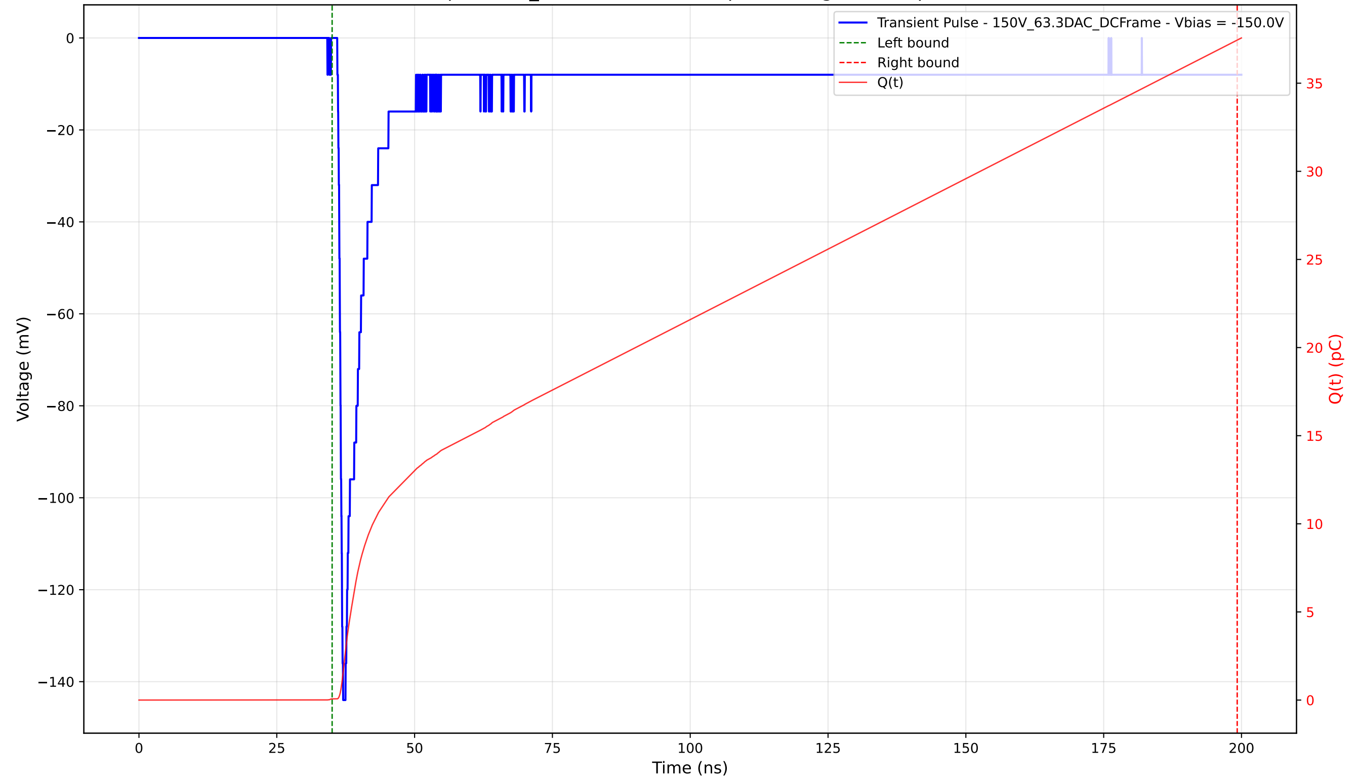
Transient Pulse - Sample: 1cm_42 - Position: 570.0 \mu\text{m} - Charge: 37.38 pC - Rise Time: 0.82 ns
