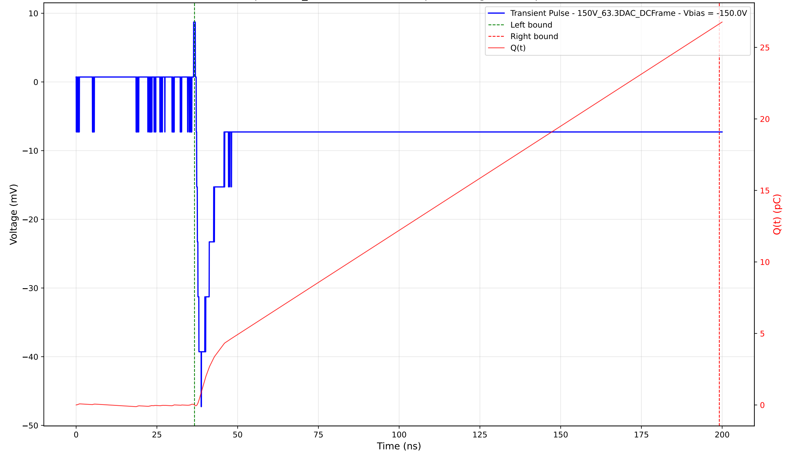
Transient Pulse - Sample: 1cm_42 - Position: 3580.0 \mu\text{m} - Charge: 26.65 pC - Rise Time: 1.57 ns
