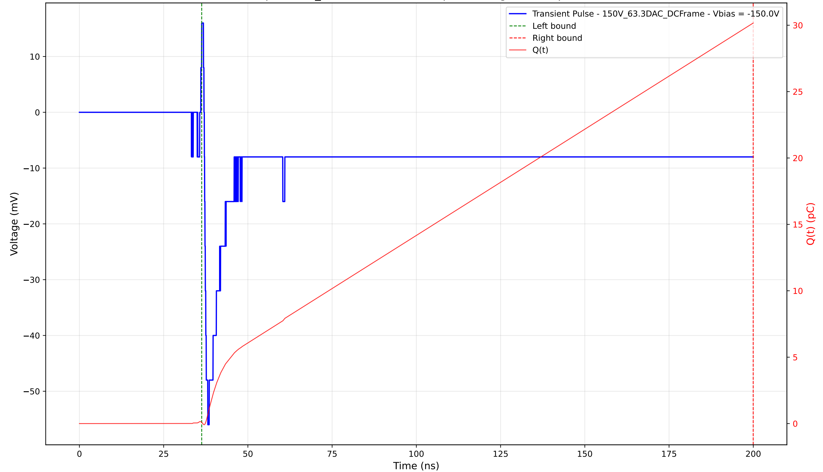
Transient Pulse - Sample: 1cm_42 - Position: 1450.0 \mu\text{m} - Charge: 30.07 pC - Rise Time: 1.03 ns
