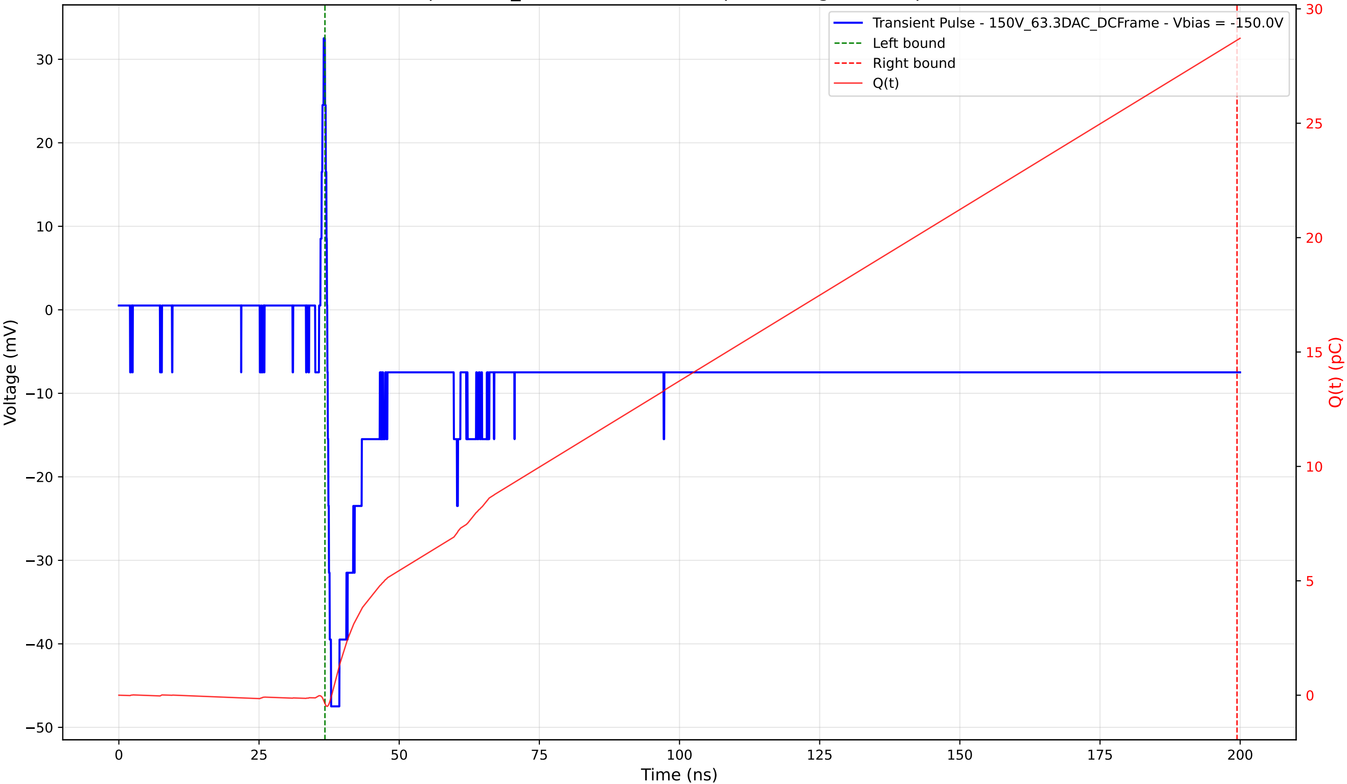
Transient Pulse - Sample: 1cm_42 - Position: 1700.0 \mu\text{m} - Charge: 29.00 pC - Rise Time: 0.67 ns
