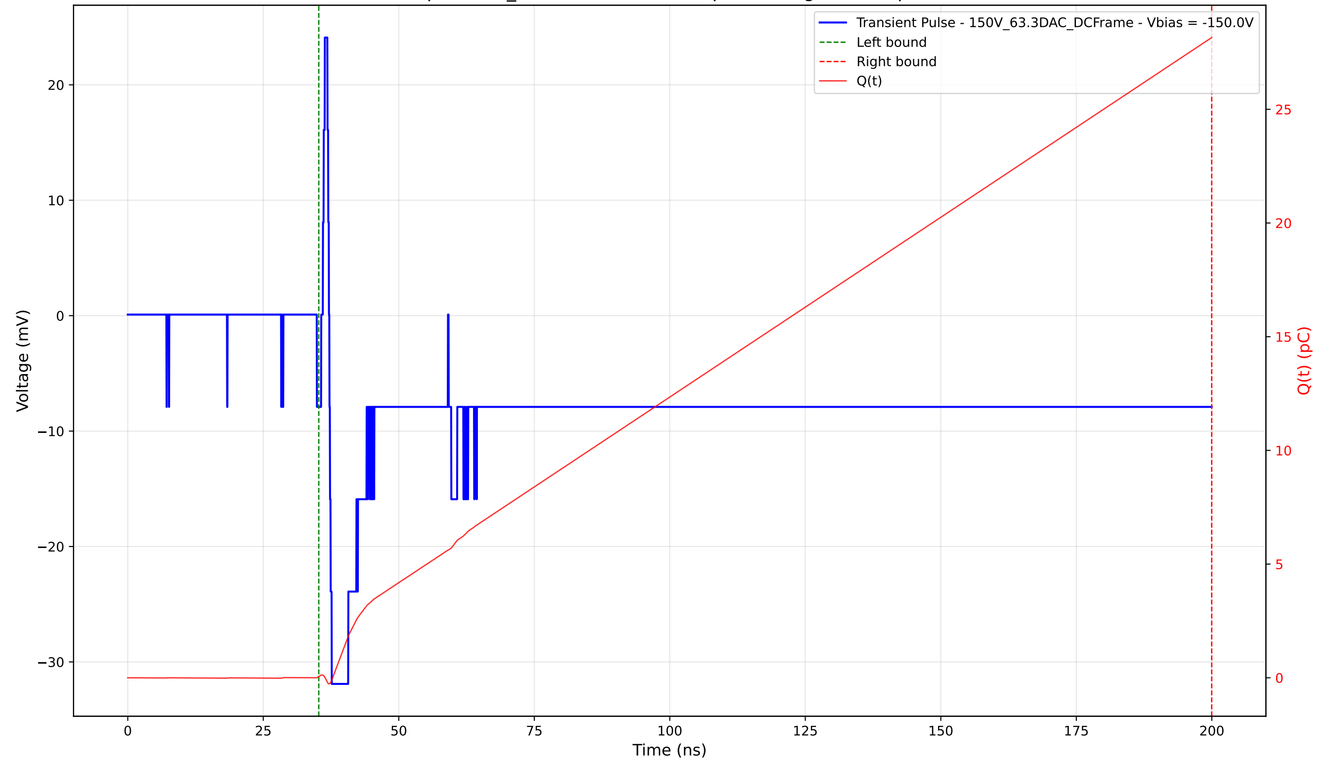
Transient Pulse - Sample: 1cm_42 - Position: 1955.0 \mu\text{m} - Charge: 28.10 pC - Rise Time: 0.43 ns
