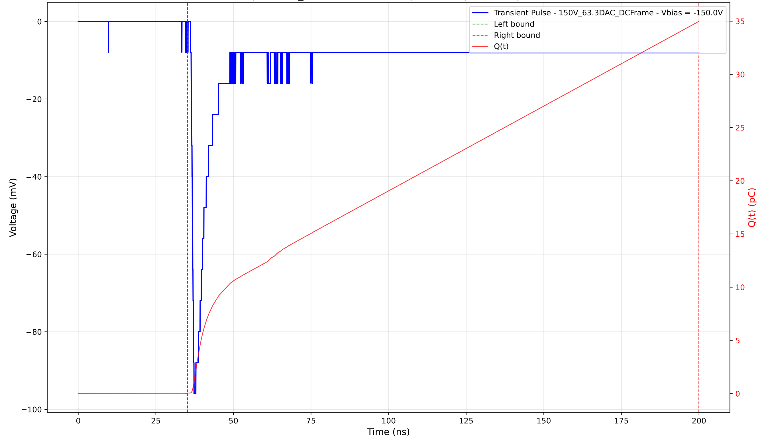
Transient Pulse - Sample: 1cm_42 - Position: 870.0 \mu\text{m} - Charge: 34.94 pC - Rise Time: 0.78 ns
