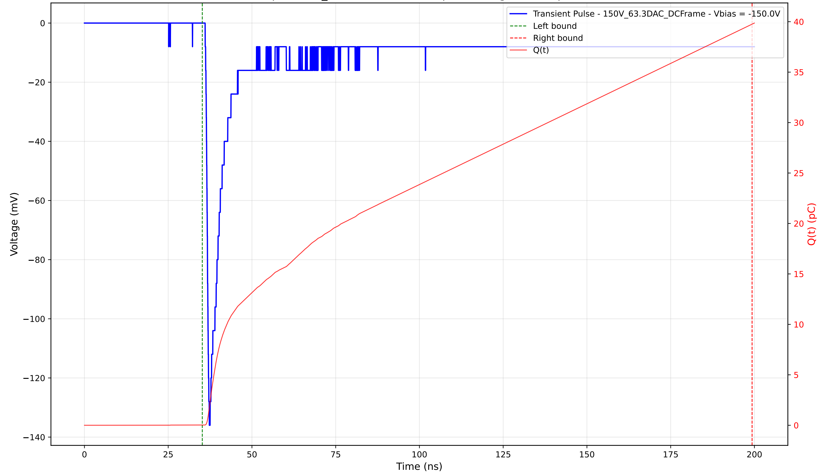
Transient Pulse - Sample: 1cm_42 - Position: 695.0 \mu\text{m} - Charge: 39.73 pC - Rise Time: 0.95 ns
