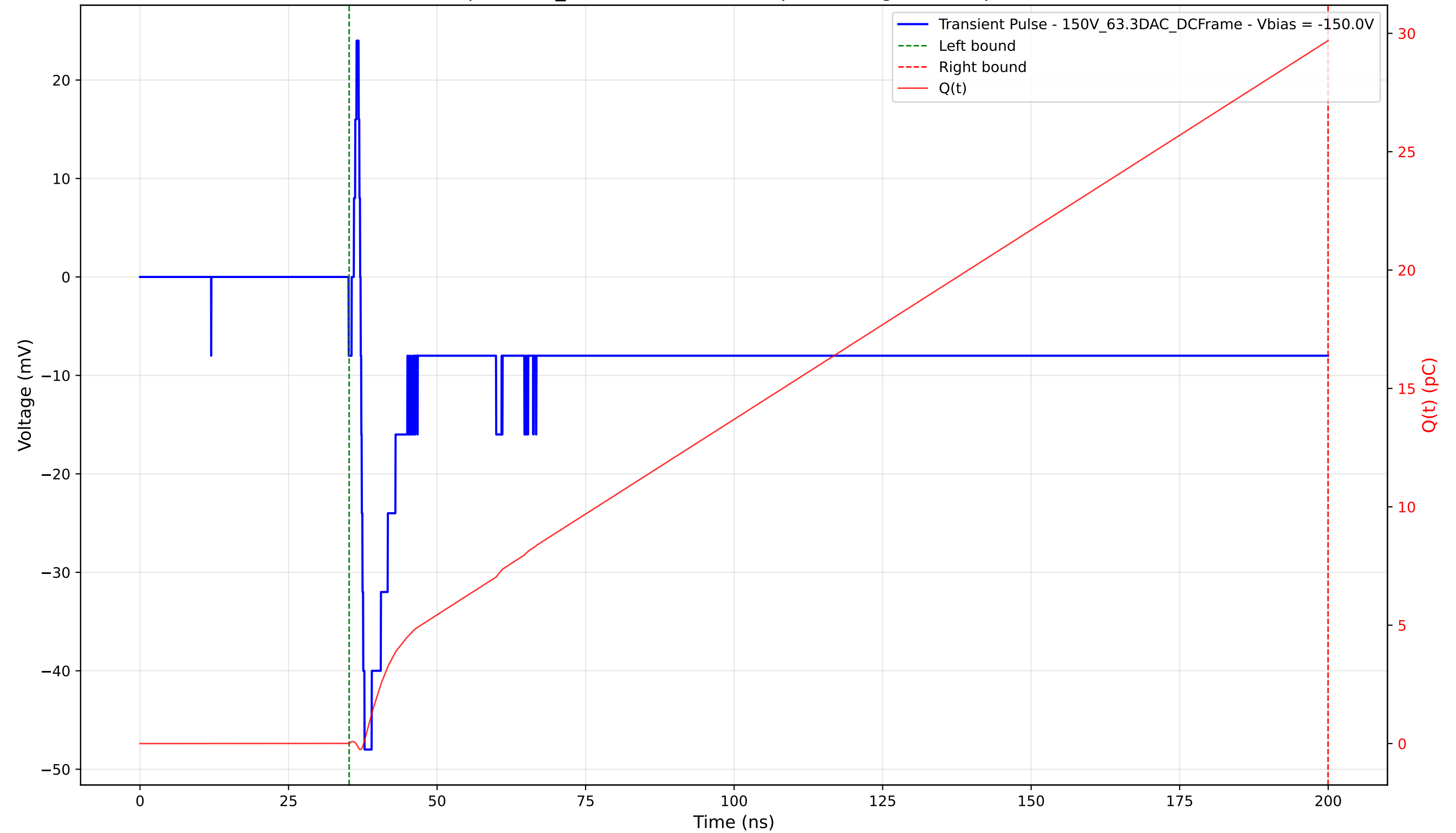
Transient Pulse - Sample: 1cm_42 - Position: 1560.0 \mu\text{m} - Charge: 29.67 pC - Rise Time: 0.65 ns
