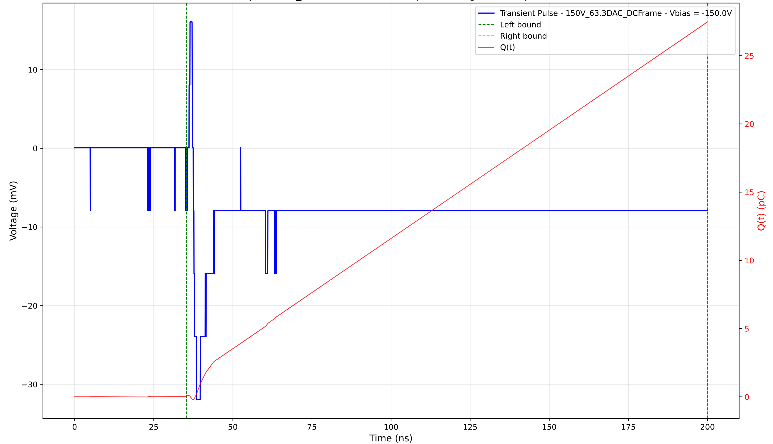
Transient Pulse - Sample: 1cm_42 - Position: 2615.0 \mu\text{m} - Charge: 27.42 pC - Rise Time: 0.97 ns
