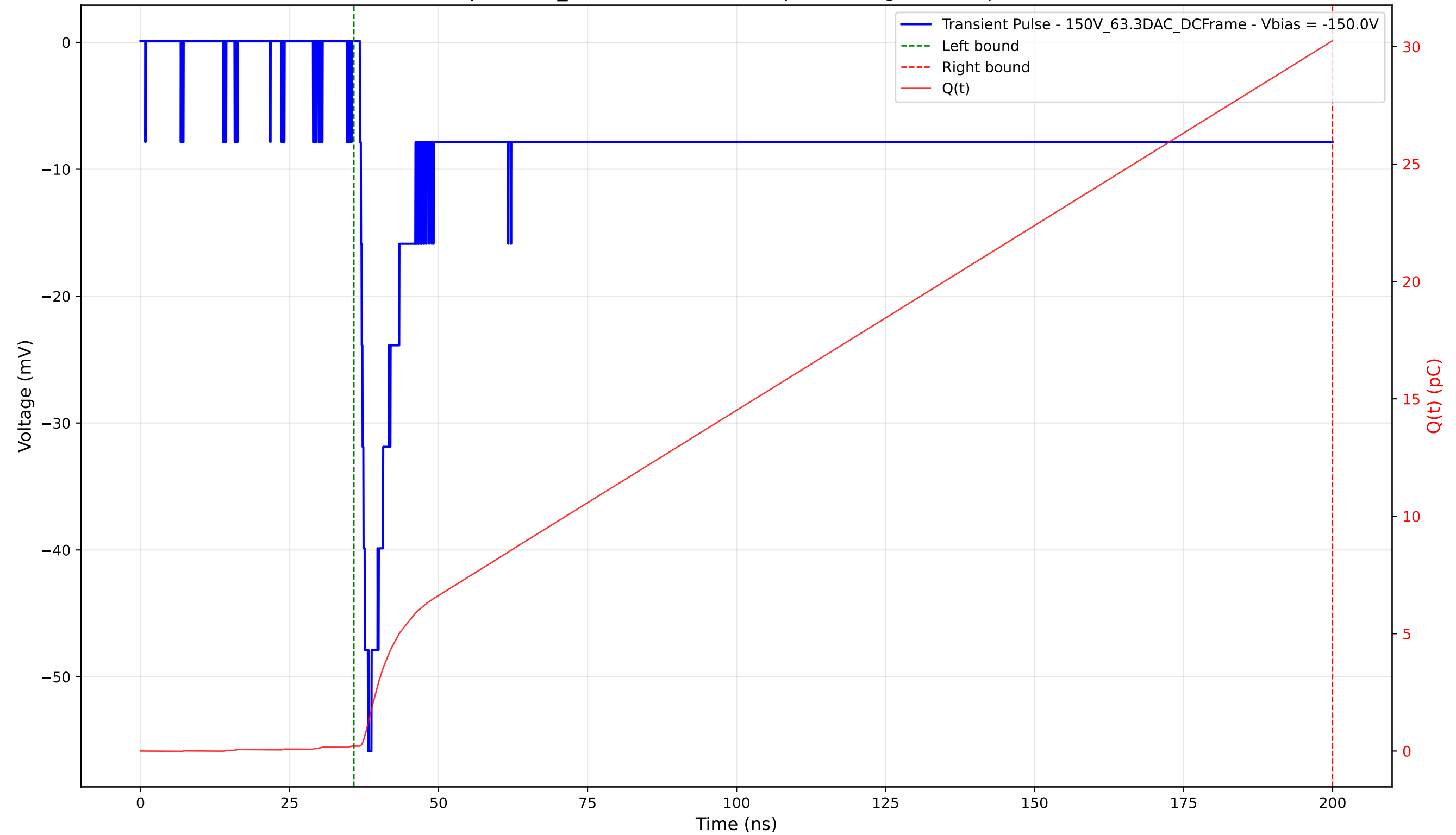
Transient Pulse - Sample: 1cm_42 - Position: 3960.0 \mu\text{m} - Charge: 30.05 pC - Rise Time: 1.37 ns
