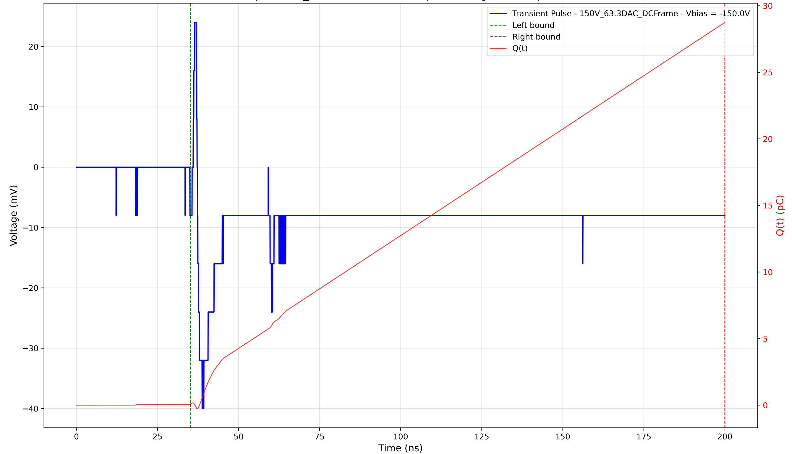
Transient Pulse - Sample: 1cm_42 - Position: 2225.0 \mu\text{m} - Charge: 28.65 pC - Rise Time: 1.45 ns
