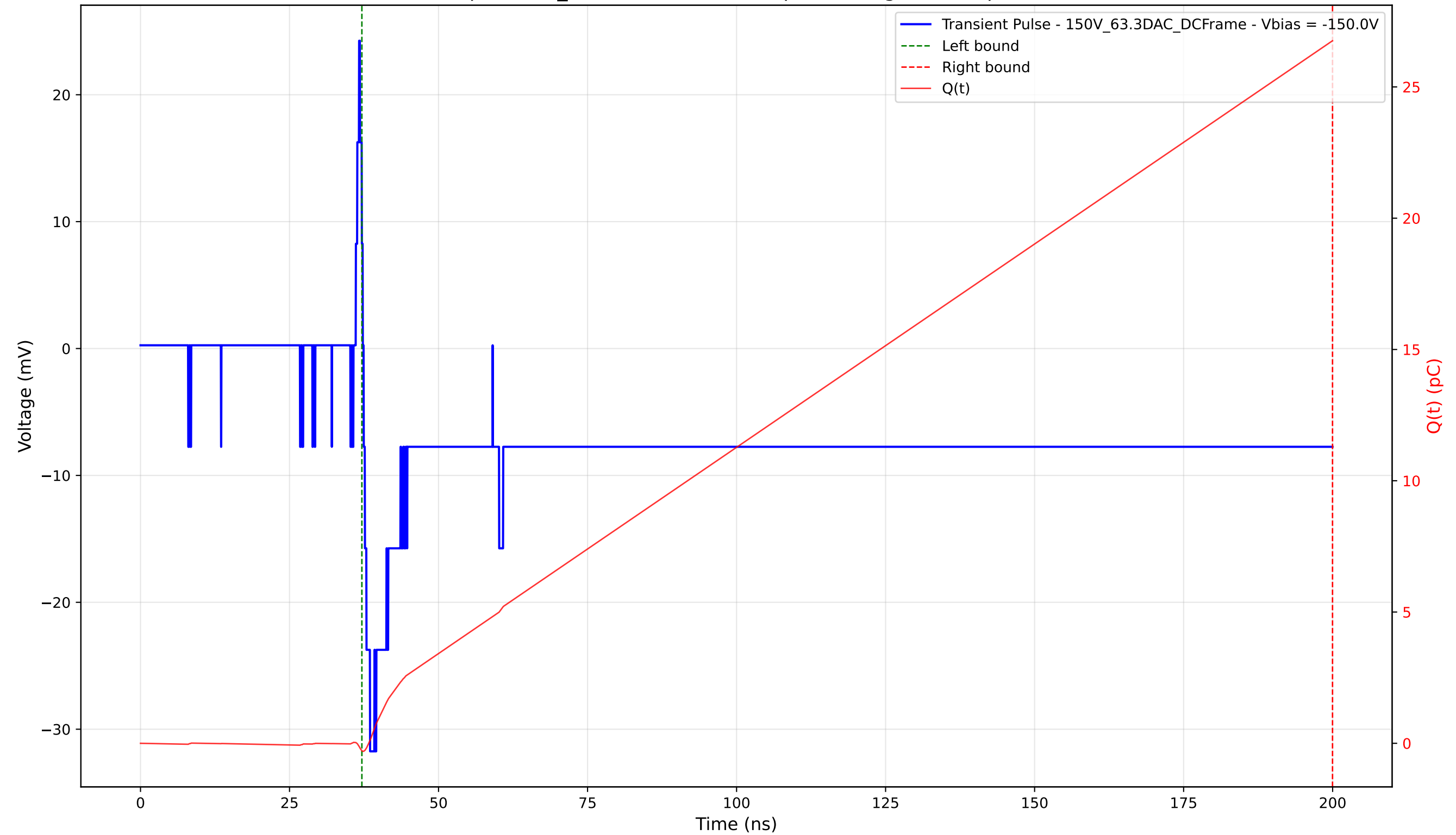
Transient Pulse - Sample: 1cm_42 - Position: 2435.0 \mu\text{m} - Charge: 27.04 pC - Rise Time: 1.07 ns
