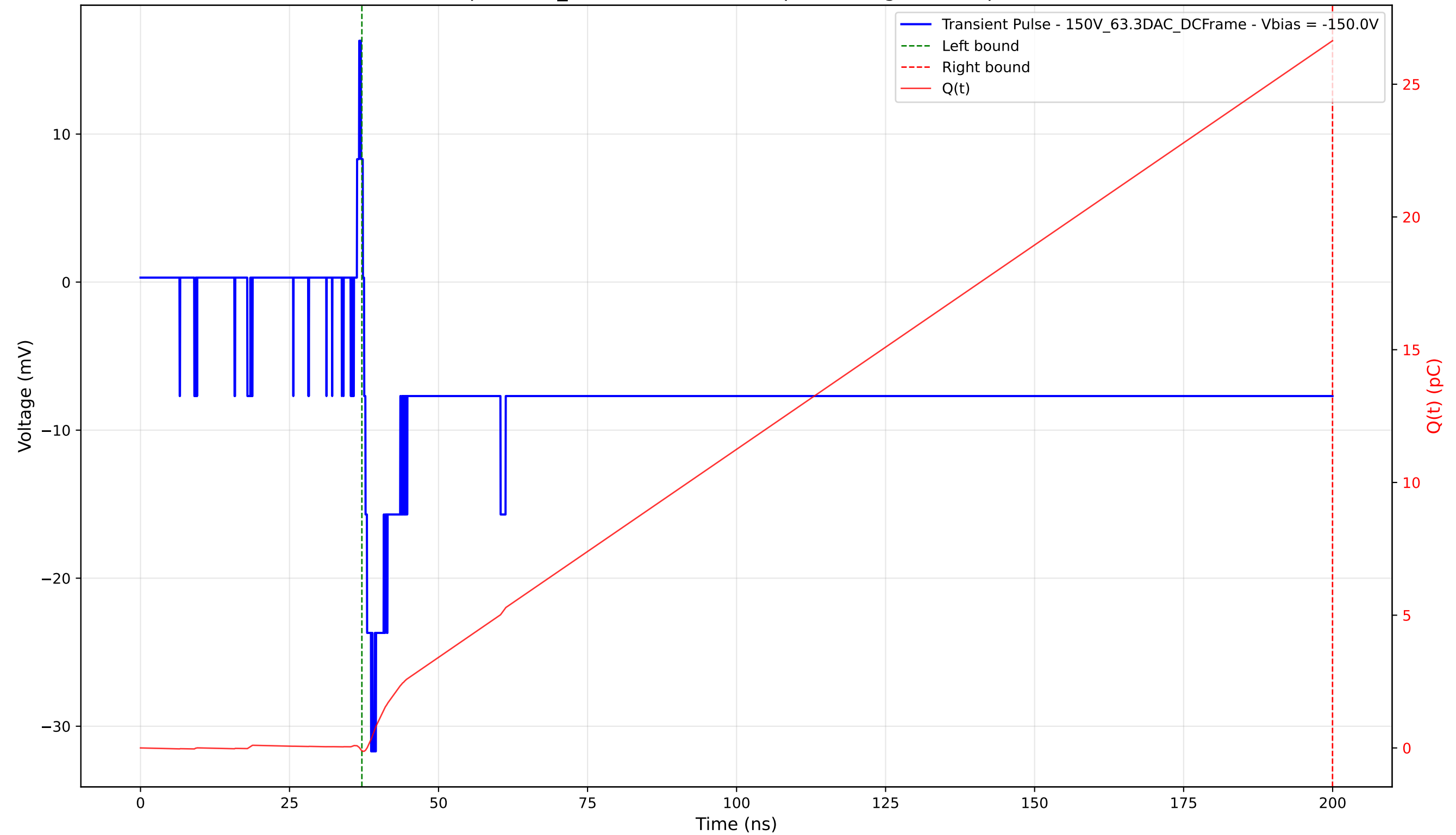
Transient Pulse - Sample: 1cm_42 - Position: 2980.0 \mu\text{m} - Charge: 26.74 pC - Rise Time: 1.17 ns
