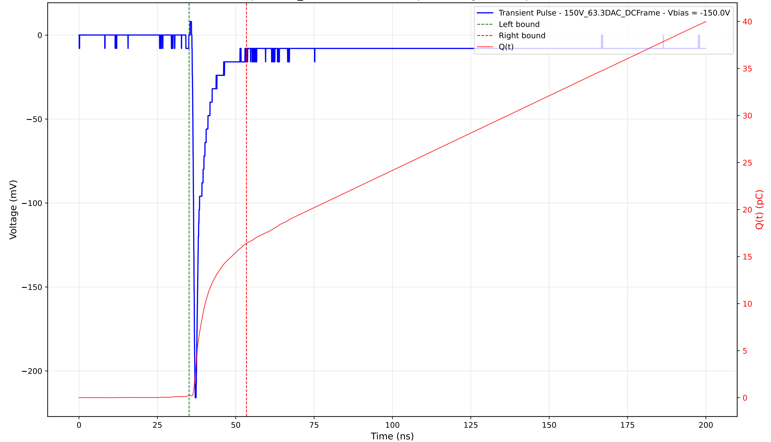
Transient Pulse - Sample: 1cm_42 - Position: 4705.0 \mu\text{m} - Charge: 16.16 pC - Rise Time: 0.81 ns
