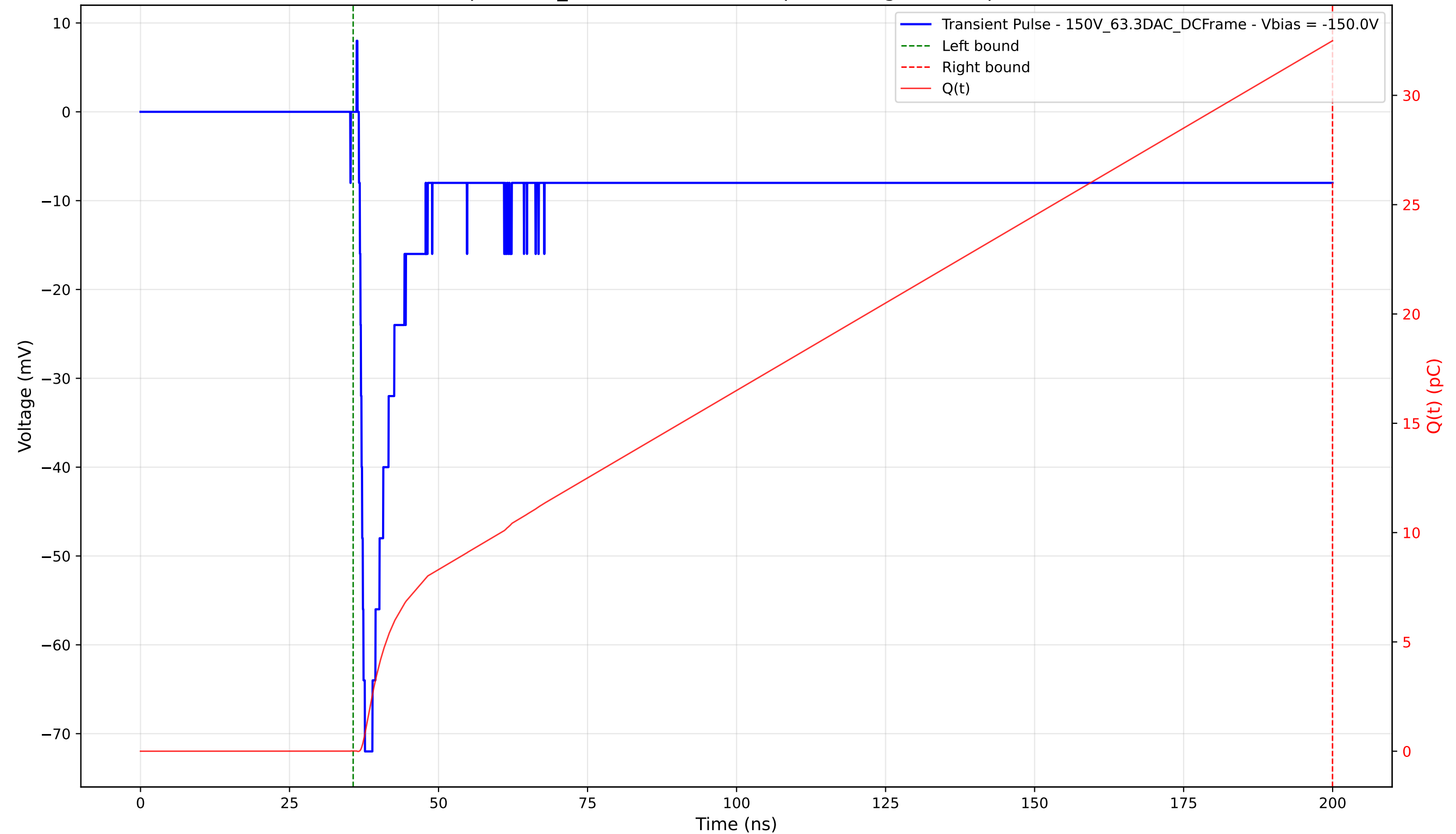
Transient Pulse - Sample: 1cm_42 - Position: 1055.0 \mu\text{m} - Charge: 32.48 pC - Rise Time: 1.00 ns
