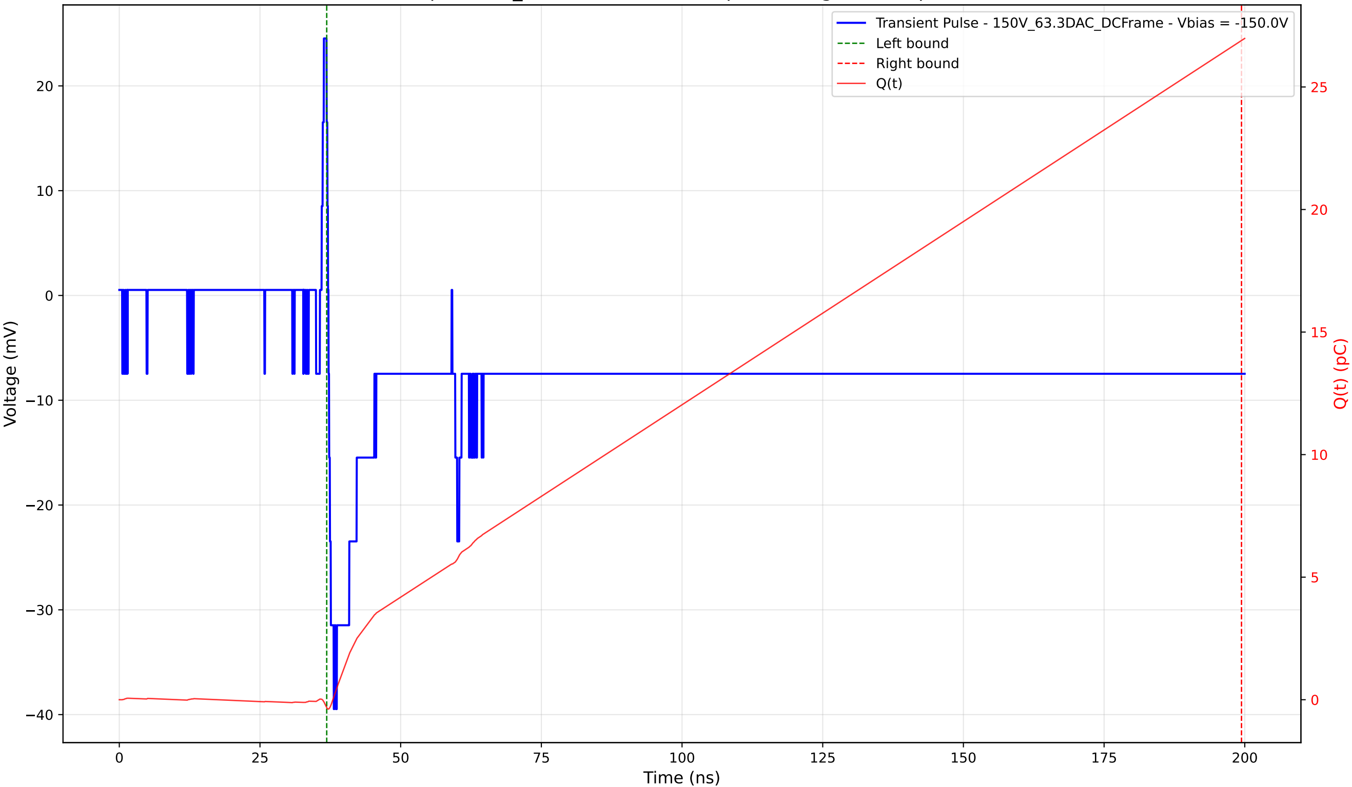
Transient Pulse - Sample: 1cm_42 - Position: 1930.0 \mu\text{m} - Charge: 27.22 pC - Rise Time: 0.93 ns
