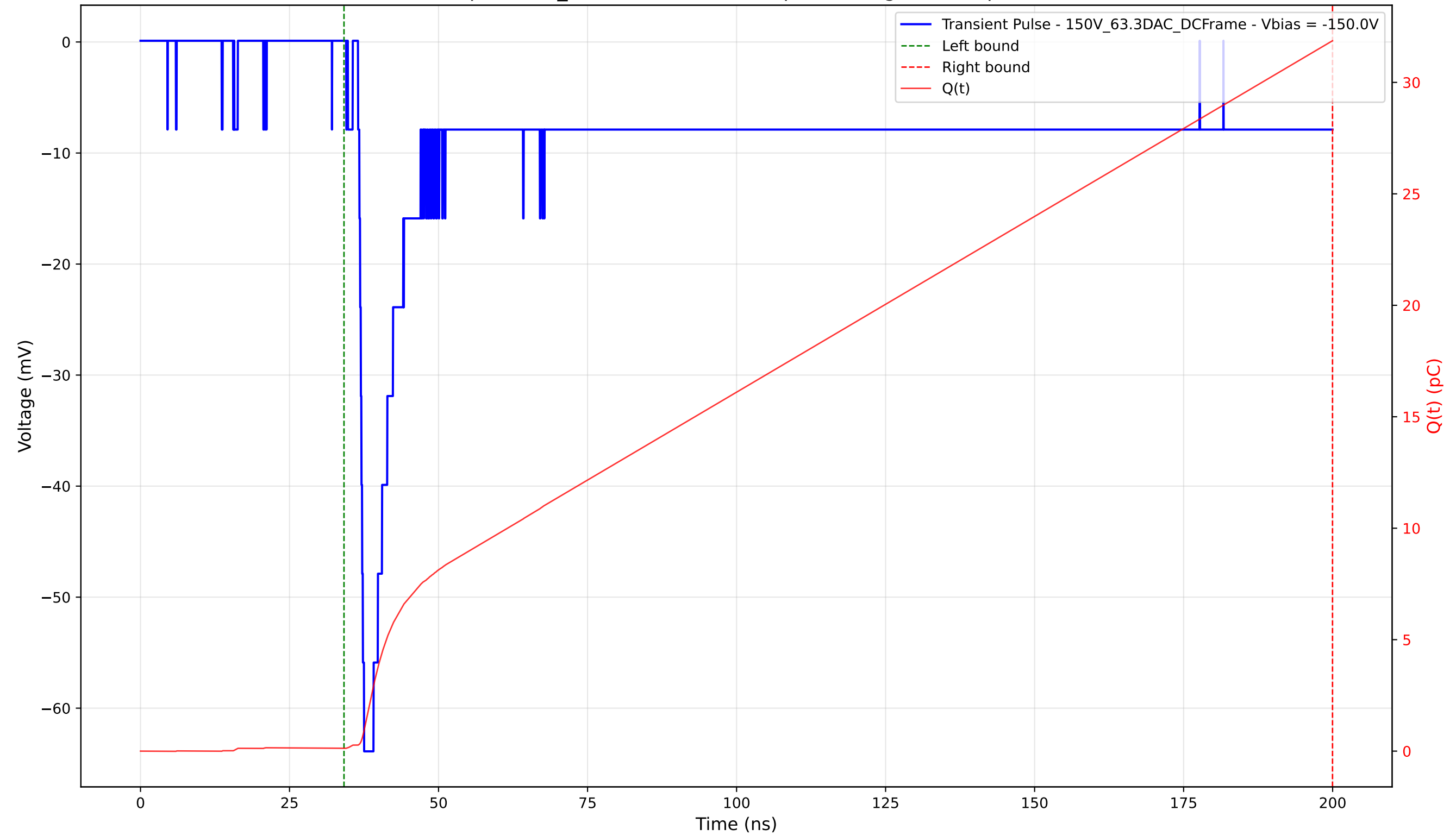
Transient Pulse - Sample: 1cm_42 - Position: 4100.0 \mu\text{m} - Charge: 31.74 pC - Rise Time: 1.00 ns
