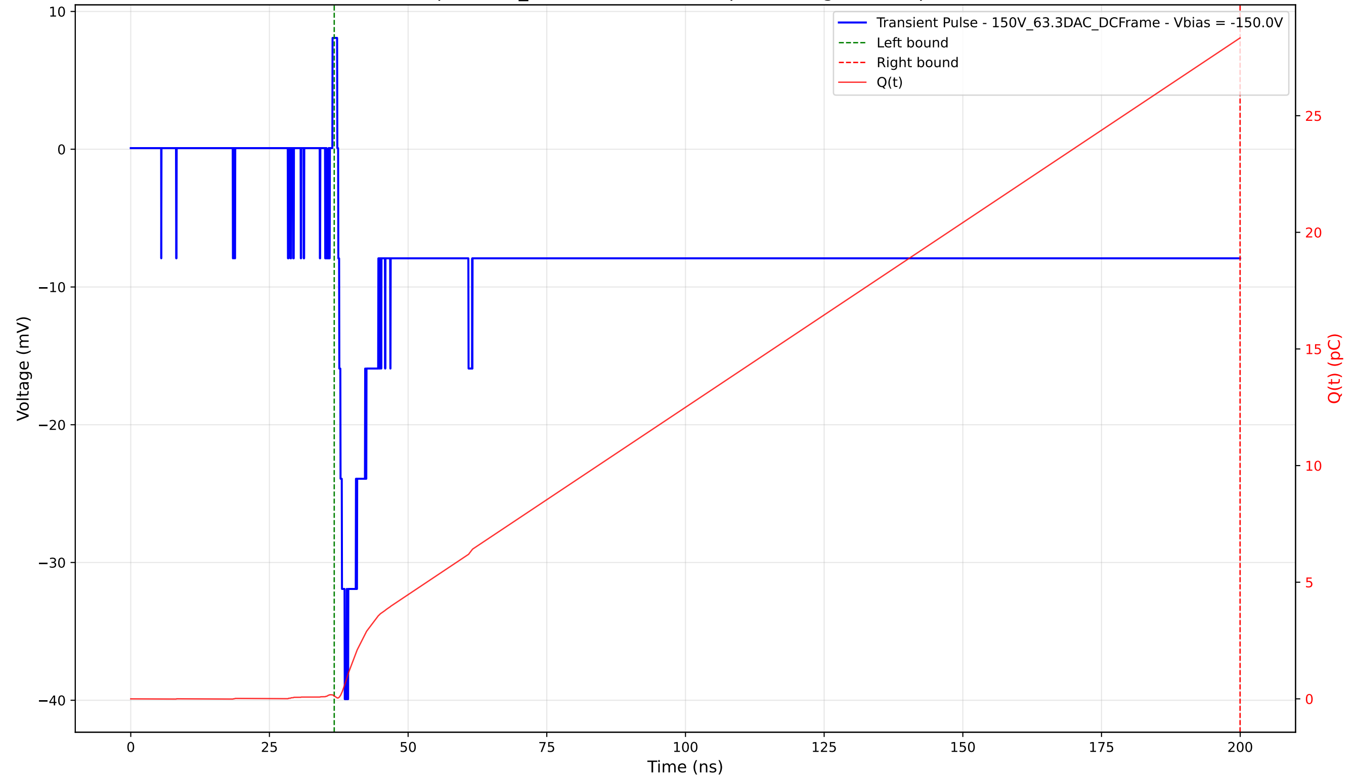
Transient Pulse - Sample: 1cm_42 - Position: 3365.0 \mu\text{m} - Charge: 28.21 pC - Rise Time: 1.17 ns
