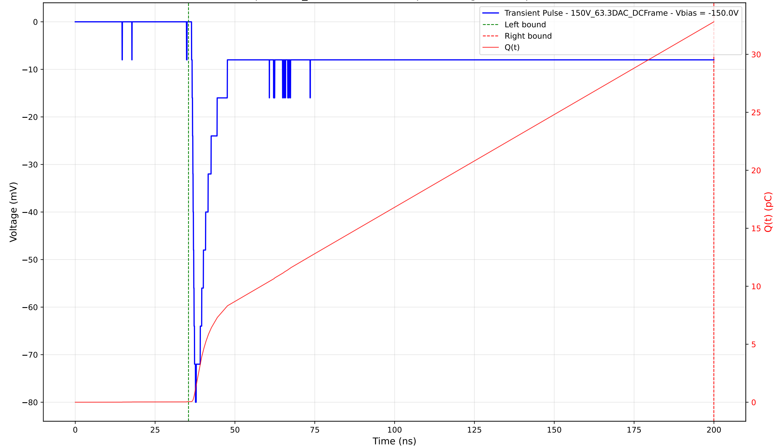
Transient Pulse - Sample: 1cm_42 - Position: 970.0 \mu\text{m} - Charge: 32.76 pC - Rise Time: 0.76 ns
