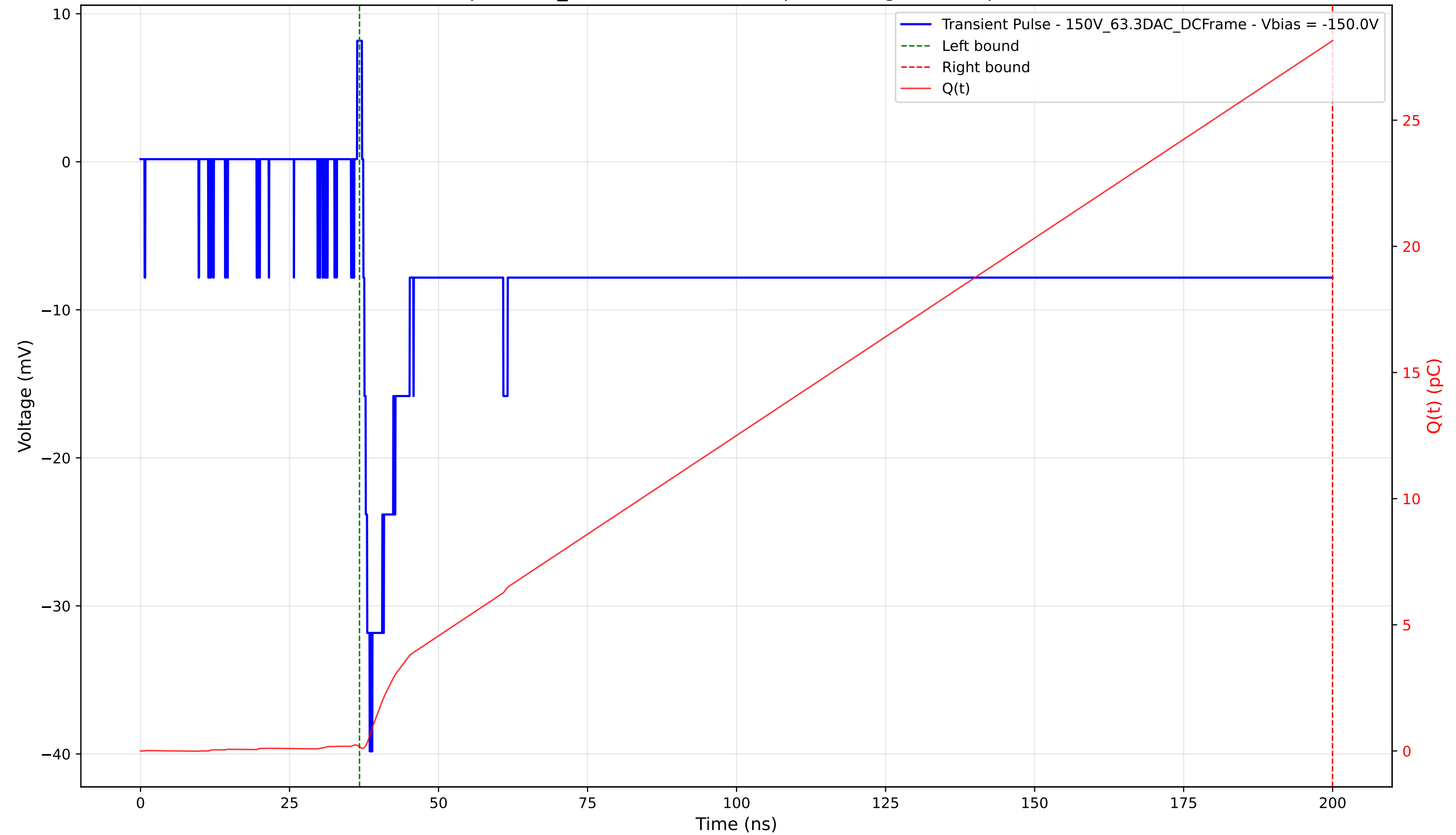
Transient Pulse - Sample: 1cm_42 - Position: 3405.0 \mu\text{m} - Charge: 27.98 pC - Rise Time: 1.07 ns
