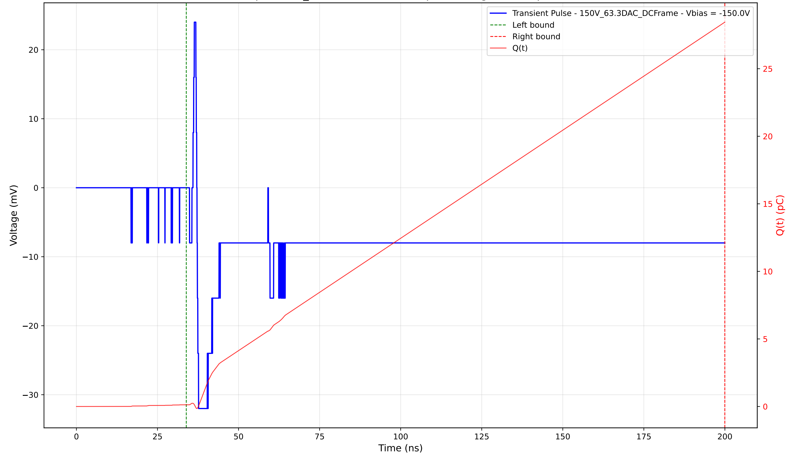
Transient Pulse - Sample: 1cm_42 - Position: 1975.0 \mu\text{m} - Charge: 28.32 pC - Rise Time: 0.47 ns
