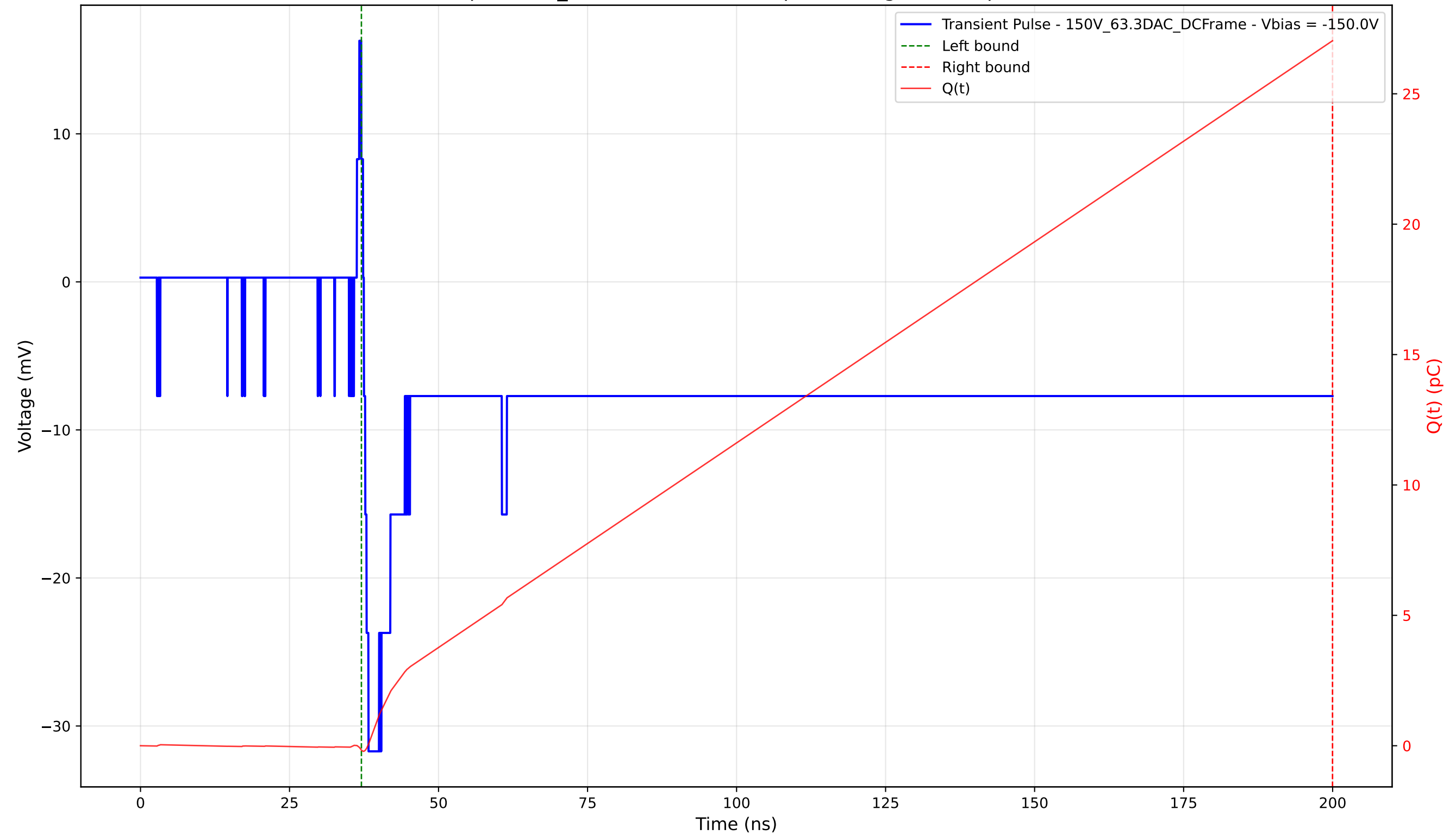
Transient Pulse - Sample: 1cm_42 - Position: 3110.0 \mu\text{m} - Charge: 27.20 pC - Rise Time: 0.77 ns
