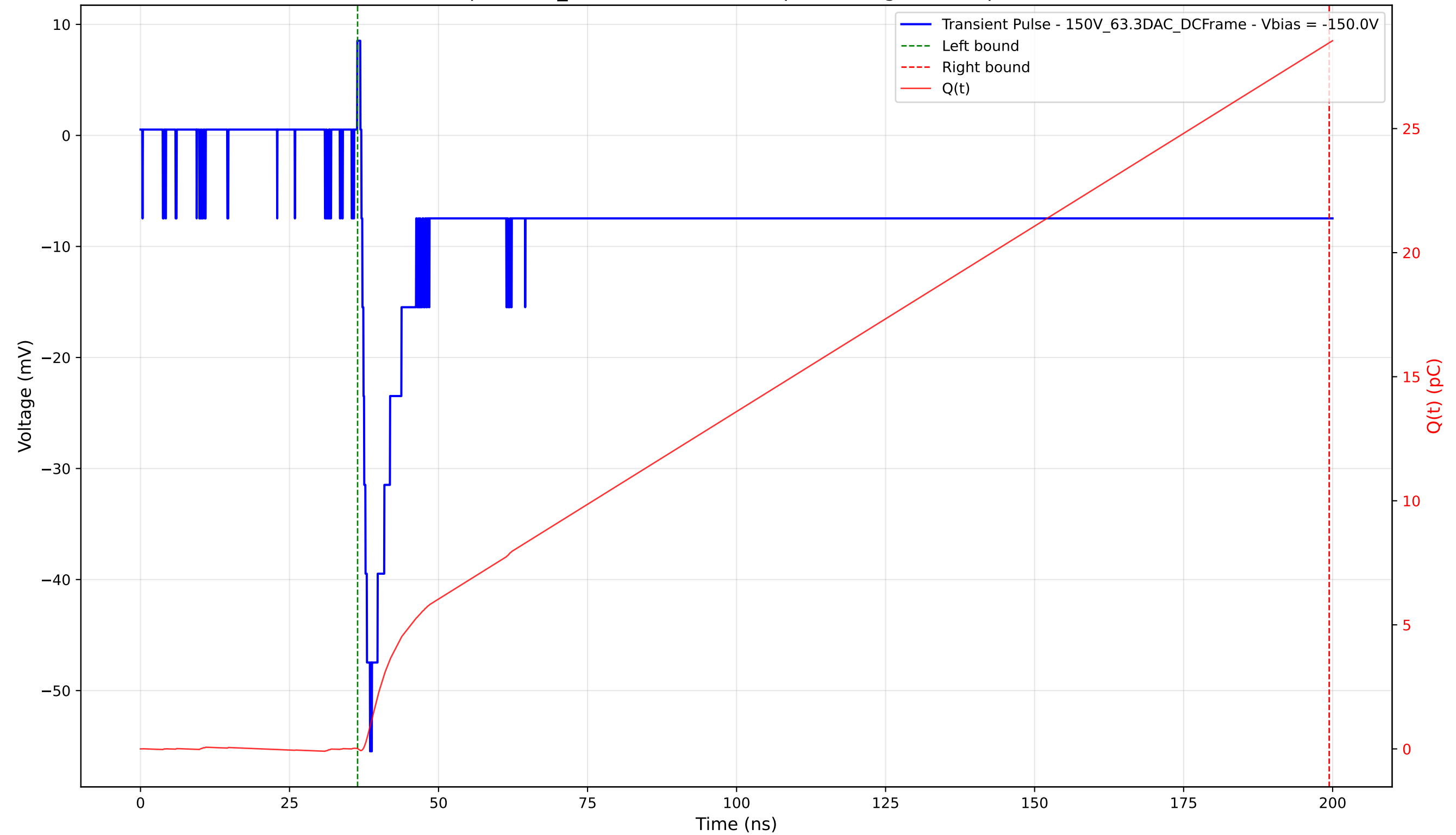
Transient Pulse - Sample: 1cm_42 - Position: 3695.0 \mu\text{m} - Charge: 28.45 pC - Rise Time: 1.45 ns
