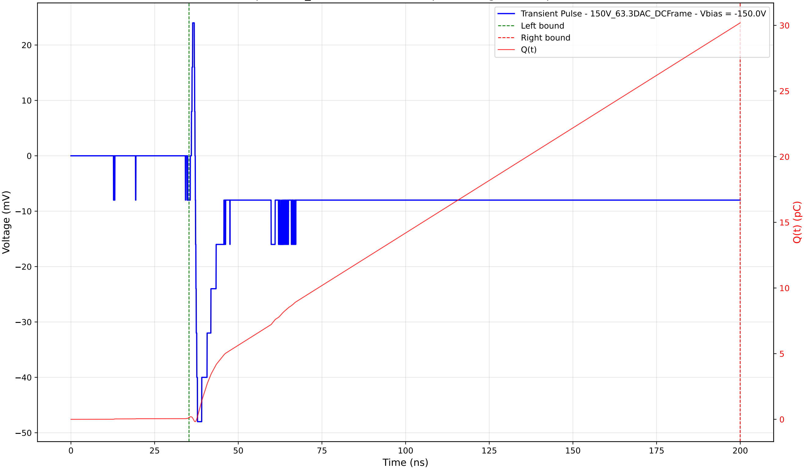
Transient Pulse - Sample: 1cm_42 - Position: 1635.0 \mu\text{m} - Charge: 30.05 pC - Rise Time: 0.65 ns
