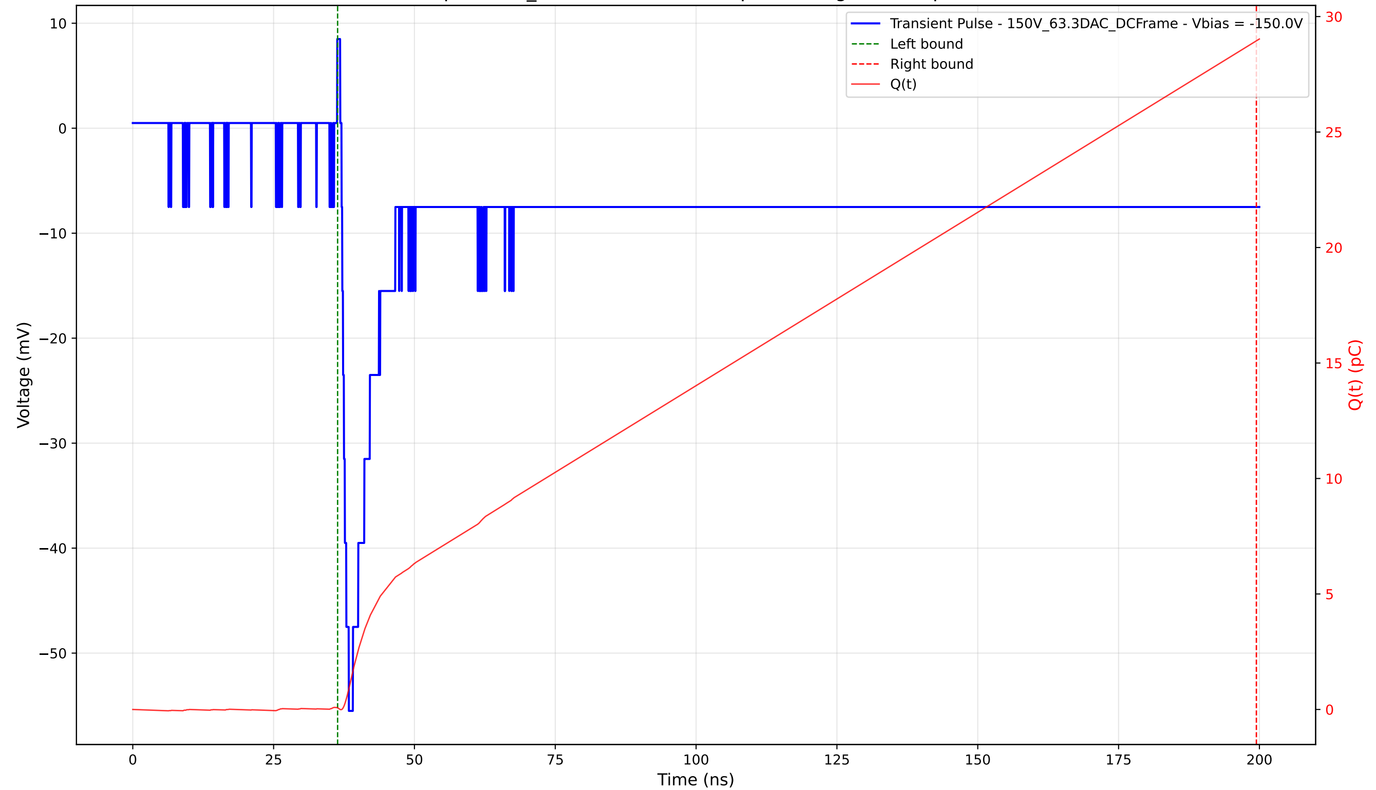
Transient Pulse - Sample: 1cm_42 - Position: 3735.0 \mu\text{m} - Charge: 28.88 pC - Rise Time: 1.29 ns
