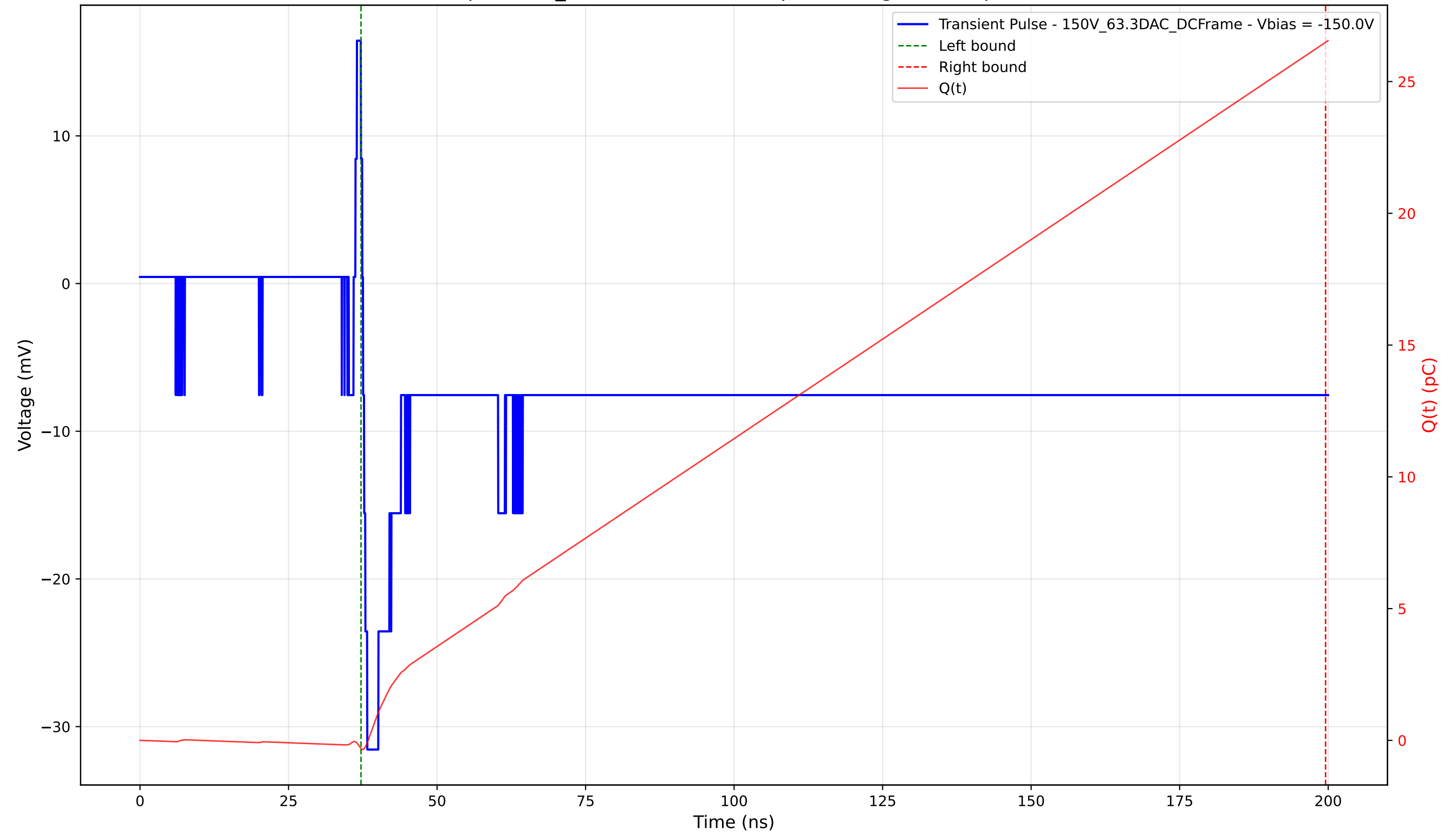
Transient Pulse - Sample: 1cm_42 - Position: 2745.0 \mu\text{m} - Charge: 26.80 pC - Rise Time: 0.71 ns
