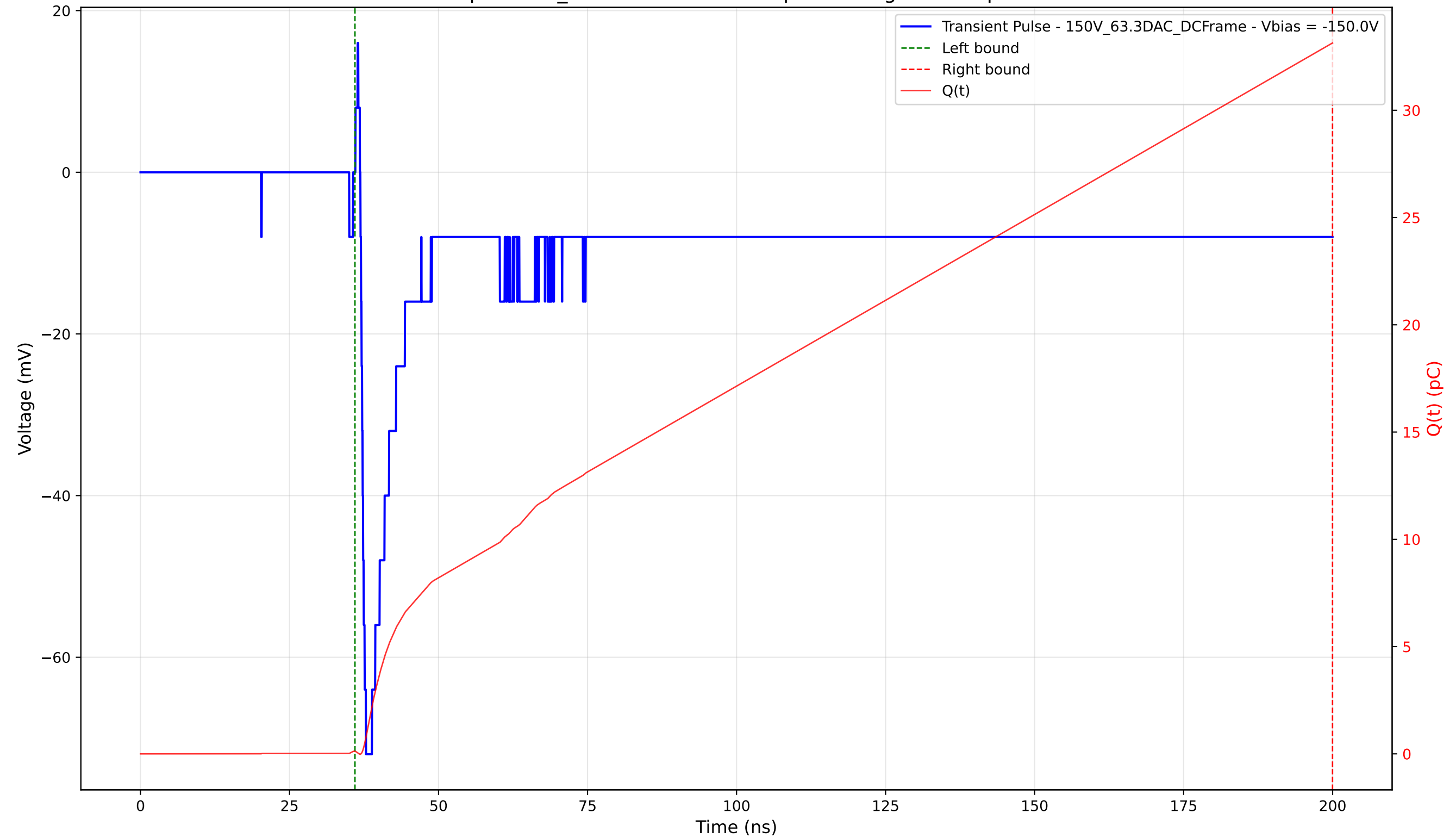
Transient Pulse - Sample: 1cm_42 - Position: 1265.0 \mu\text{m} - Charge: 33.02 pC - Rise Time: 0.92 ns
