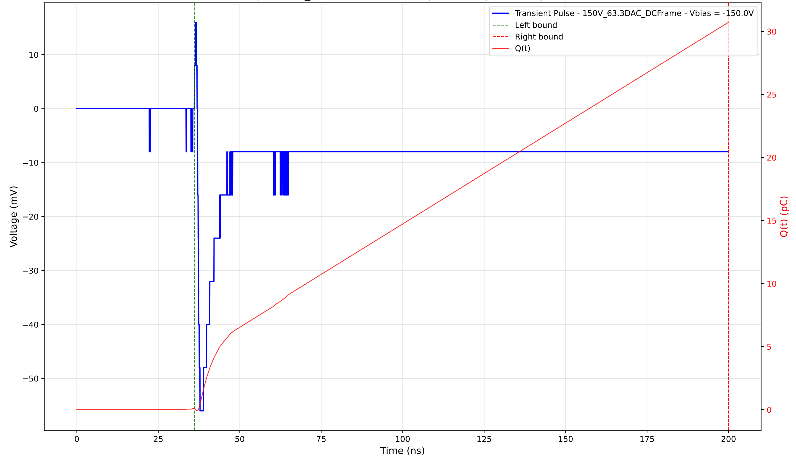
Transient Pulse - Sample: 1cm_42 - Position: 1400.0 \mu\text{m} - Charge: 30.65 pC - Rise Time: 0.79 ns
