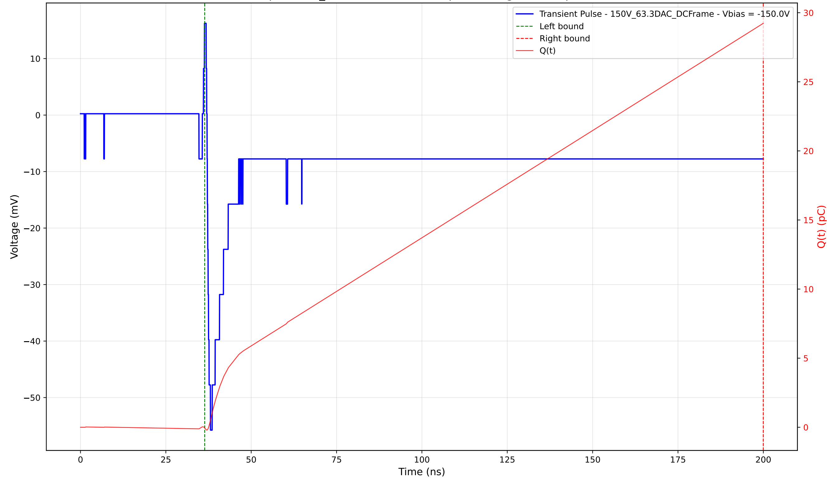
Transient Pulse - Sample: 1cm_42 - Position: 1455.0 \mu\text{m} - Charge: 29.28 pC - Rise Time: 0.99 ns
