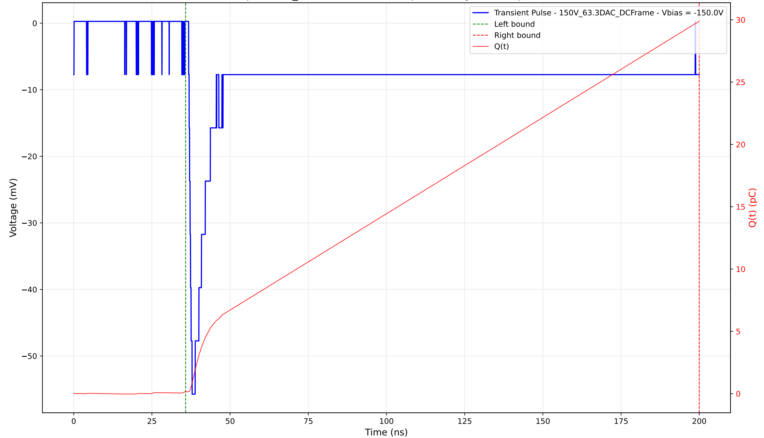
Transient Pulse - Sample: 1cm_42 - Position: 3990.0 \mu\text{m} - Charge: 29.72 pC - Rise Time: 1.11 ns
