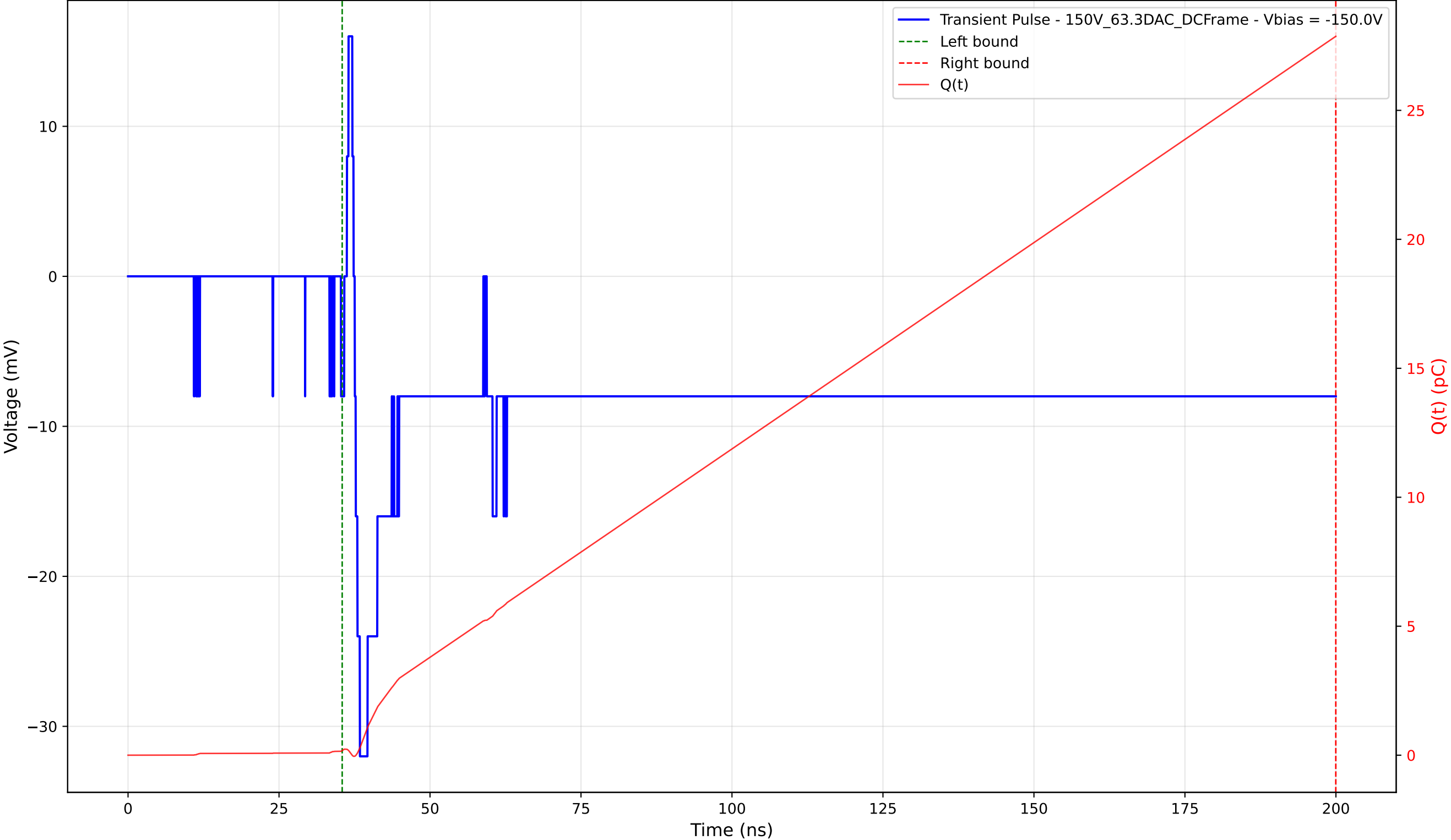
Transient Pulse - Sample: 1cm_42 - Position: 2595.0 \mu\text{m} - Charge: 27.69 pC - Rise Time: 0.85 ns
