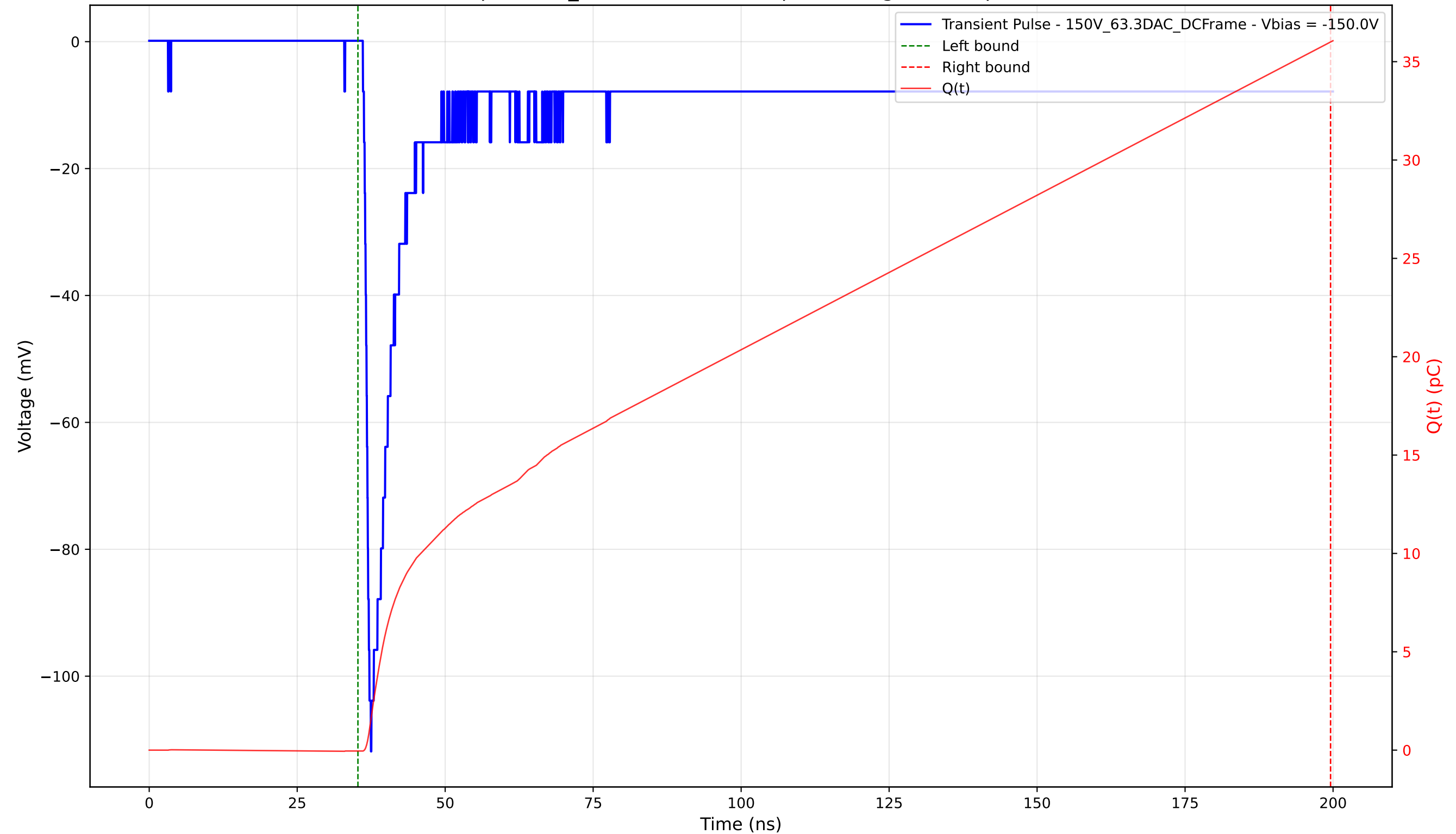
Transient Pulse - Sample: 1cm_42 - Position: 825.0 \mu\text{m} - Charge: 36.05 pC - Rise Time: 0.93 ns
