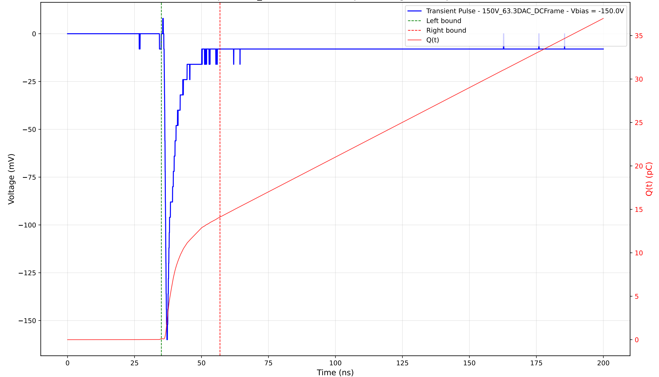
Transient Pulse - Sample: 1cm_42 - Position: 515.0 \mu\text{m} - Charge: 13.99 pC - Rise Time: 0.76 ns
