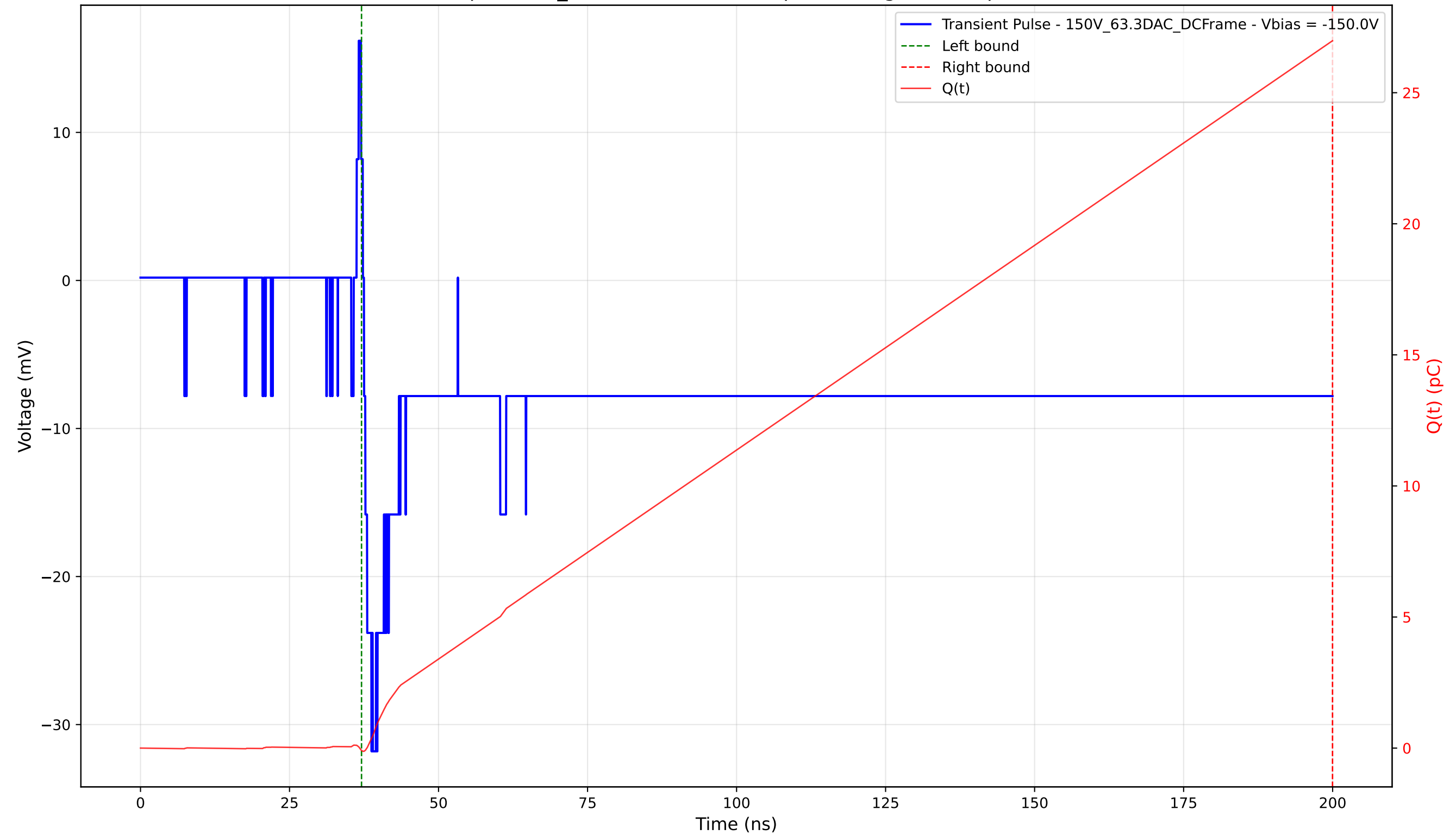
Transient Pulse - Sample: 1cm_42 - Position: 2915.0 \mu\text{m} - Charge: 27.07 pC - Rise Time: 1.25 ns
