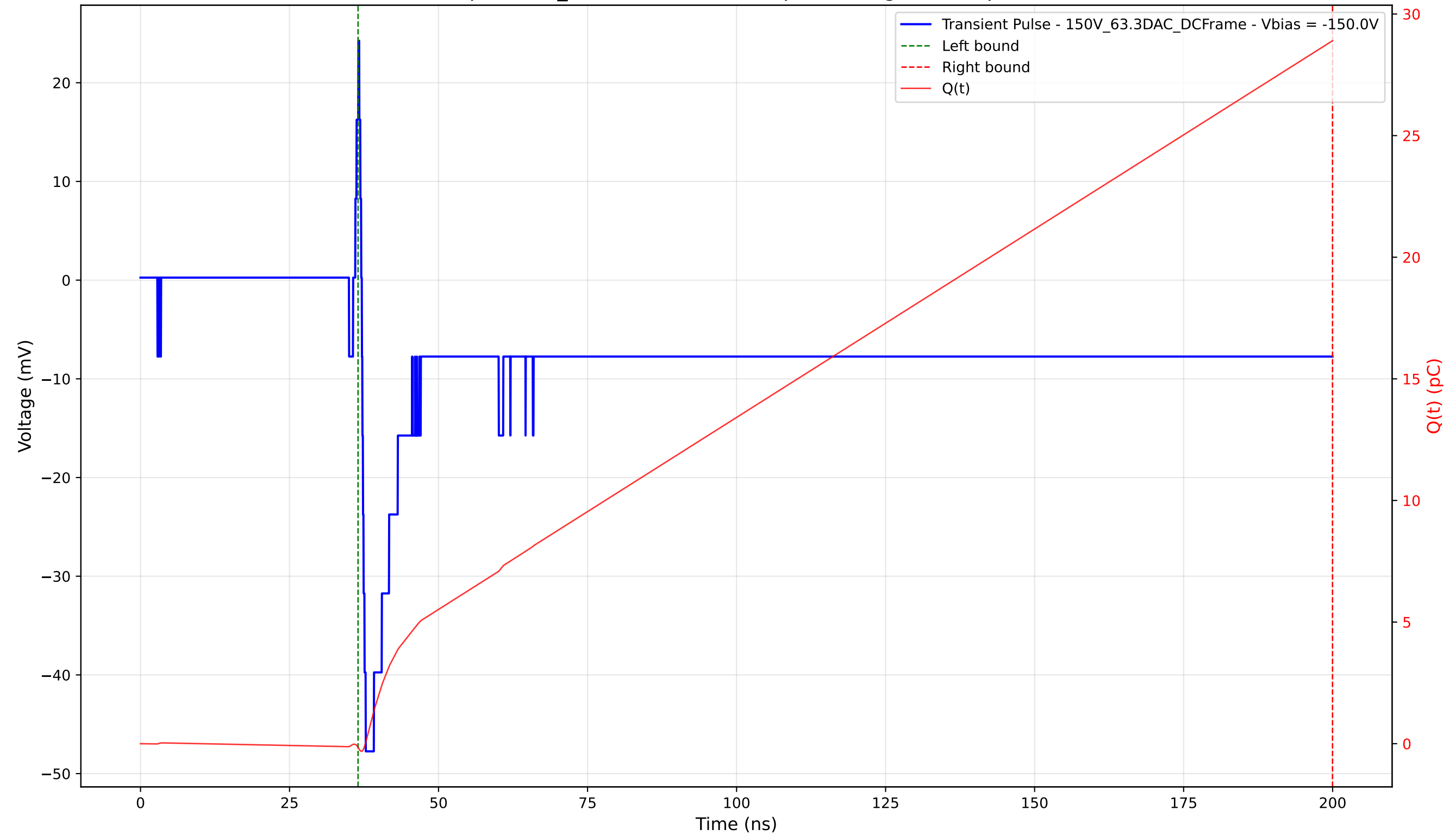
Transient Pulse - Sample: 1cm_42 - Position: 1515.0 \mu\text{m} - Charge: 29.04 pC - Rise Time: 0.65 ns
