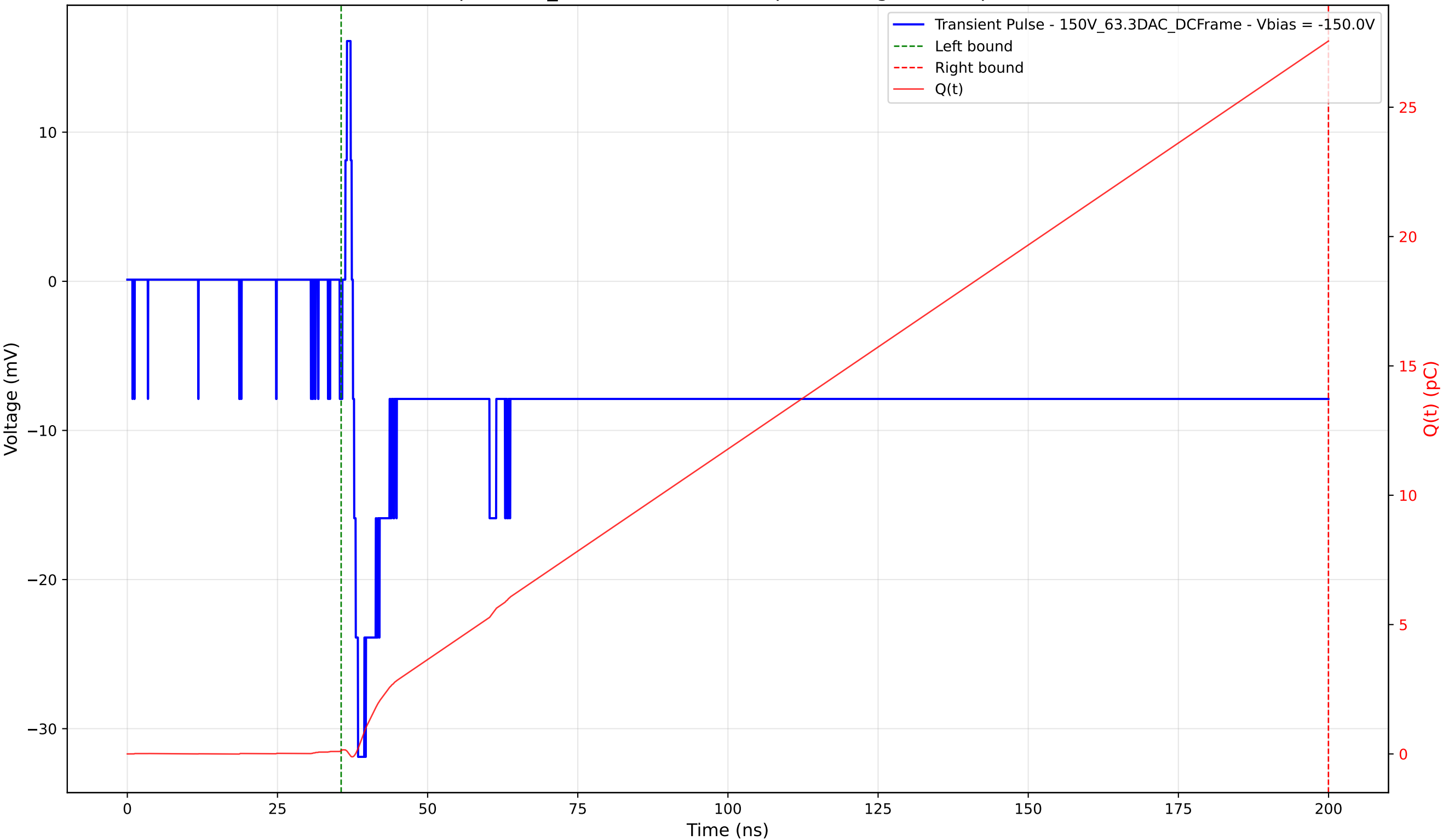
Transient Pulse - Sample: 1cm_42 - Position: 2855.0 \mu\text{m} - Charge: 27.43 pC - Rise Time: 0.85 ns
