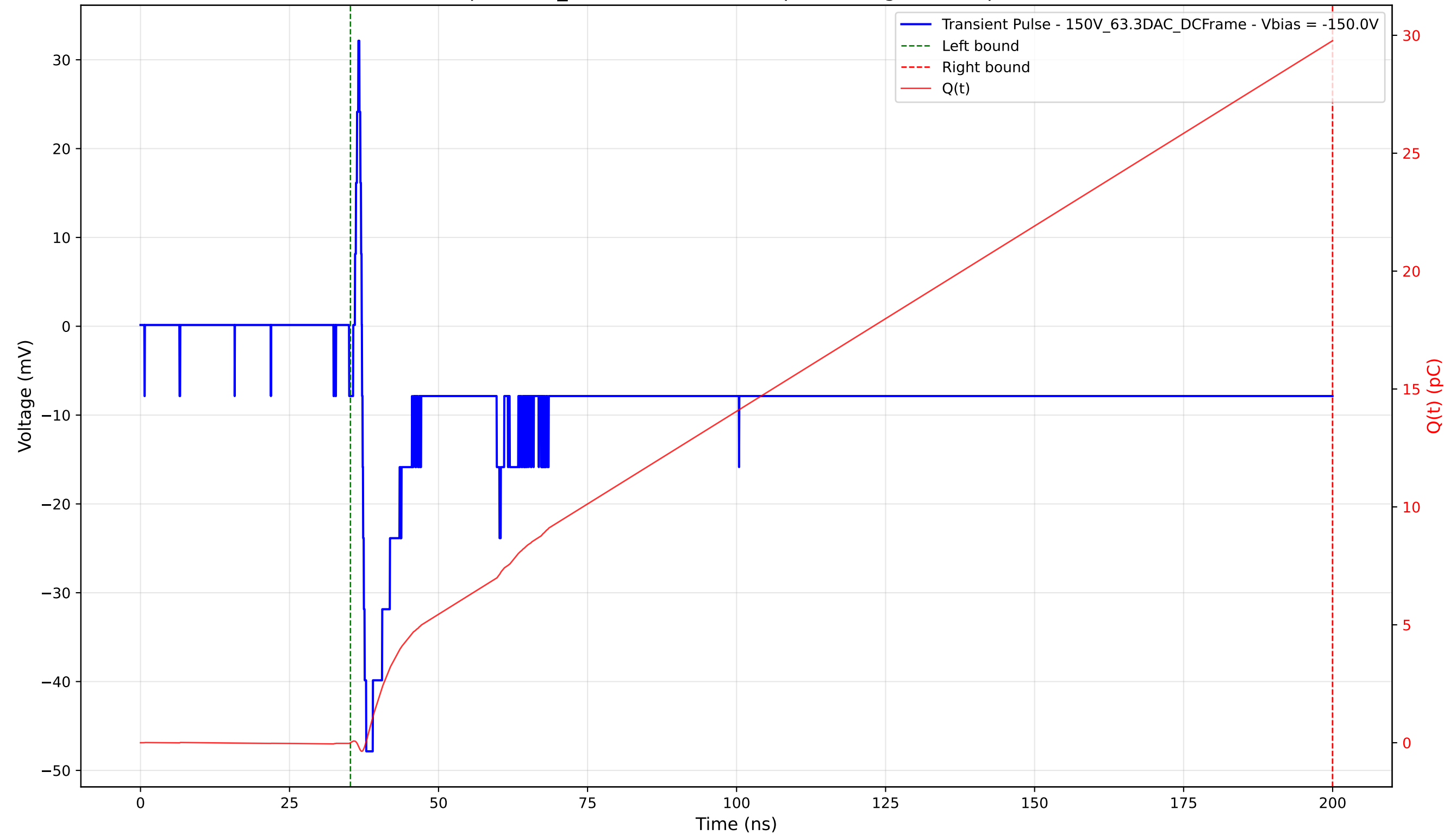
Transient Pulse - Sample: 1cm_42 - Position: 1765.0 \mu\text{m} - Charge: 29.77 pC - Rise Time: 0.71 ns
