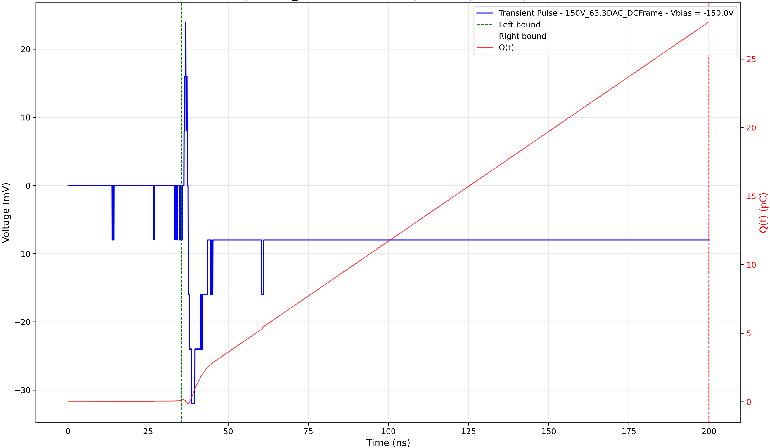
Transient Pulse - Sample: 1cm_42 - Position: 2565.0 \mu\text{m} - Charge: 27.59 pC - Rise Time: 1.03 ns
