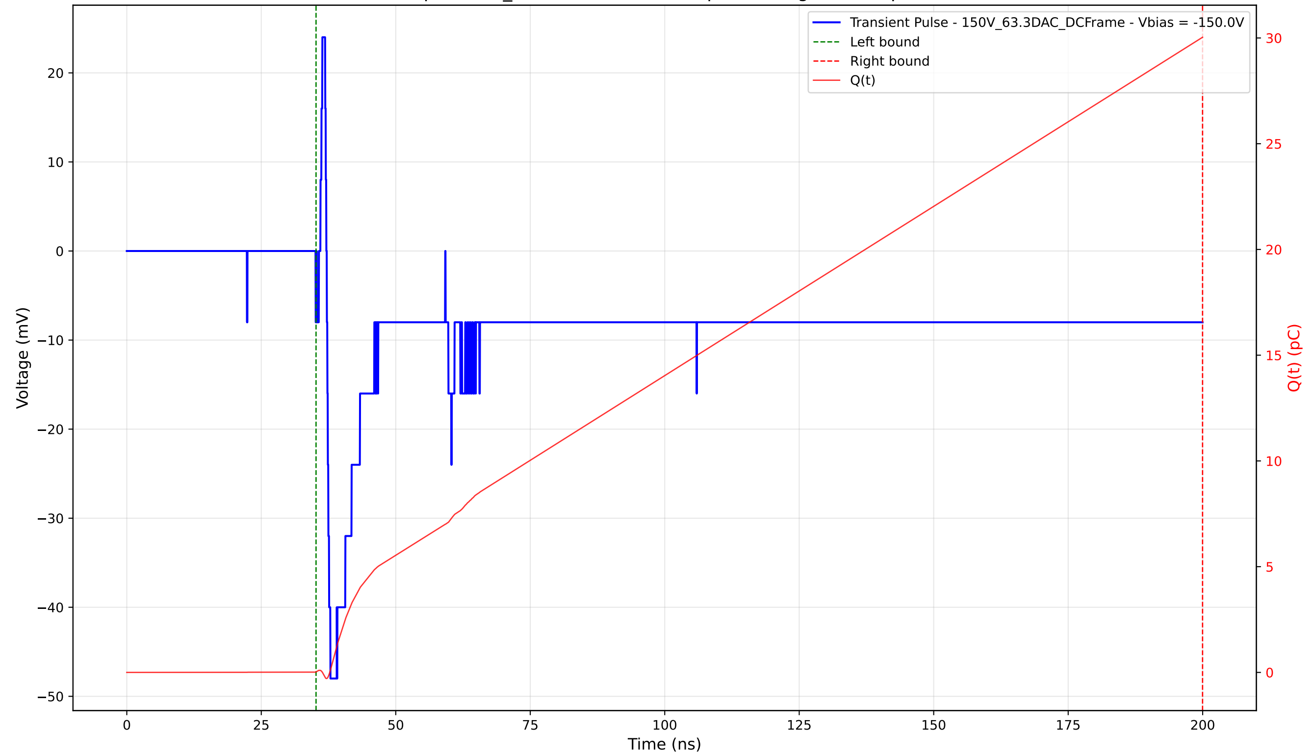
Transient Pulse - Sample: 1cm_42 - Position: 1660.0 \mu\text{m} - Charge: 30.01 pC - Rise Time: 0.67 ns
