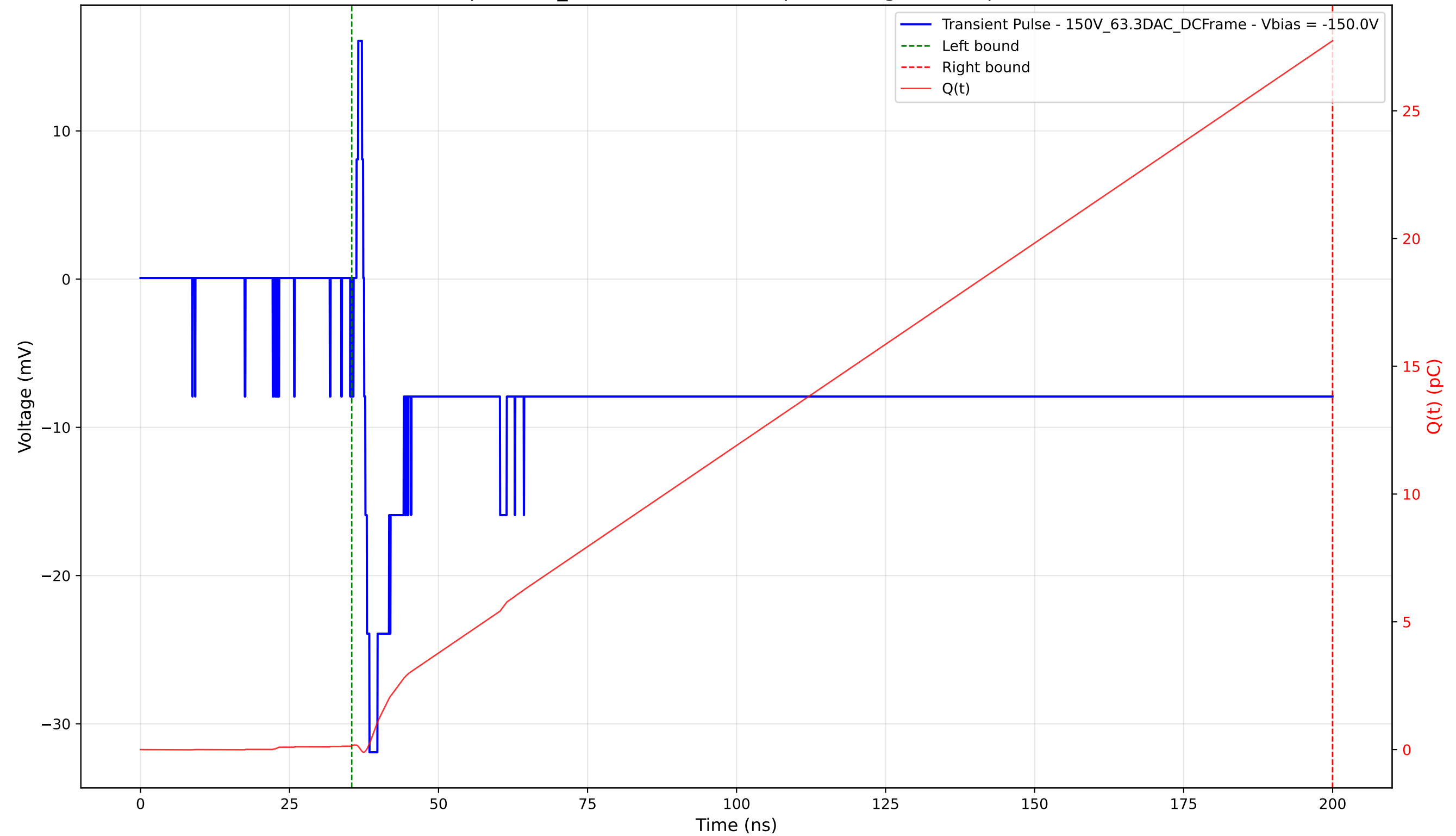
Transient Pulse - Sample: 1cm_42 - Position: 2825.0 \mu\text{m} - Charge: 27.59 pC - Rise Time: 0.89 ns
