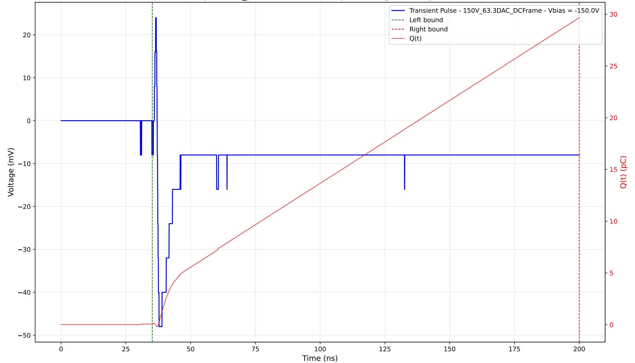
Transient Pulse - Sample: 1cm_42 - Position: 1540.0 \mu\text{m} - Charge: 29.59 pC - Rise Time: 0.69 ns
