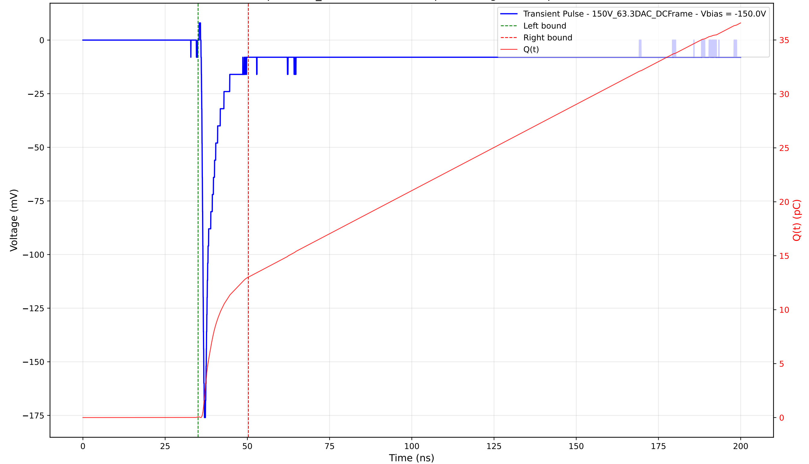
Transient Pulse - Sample: 1cm_42 - Position: 435.0 \mu\text{m} - Charge: 12.95 pC - Rise Time: 0.74 ns
