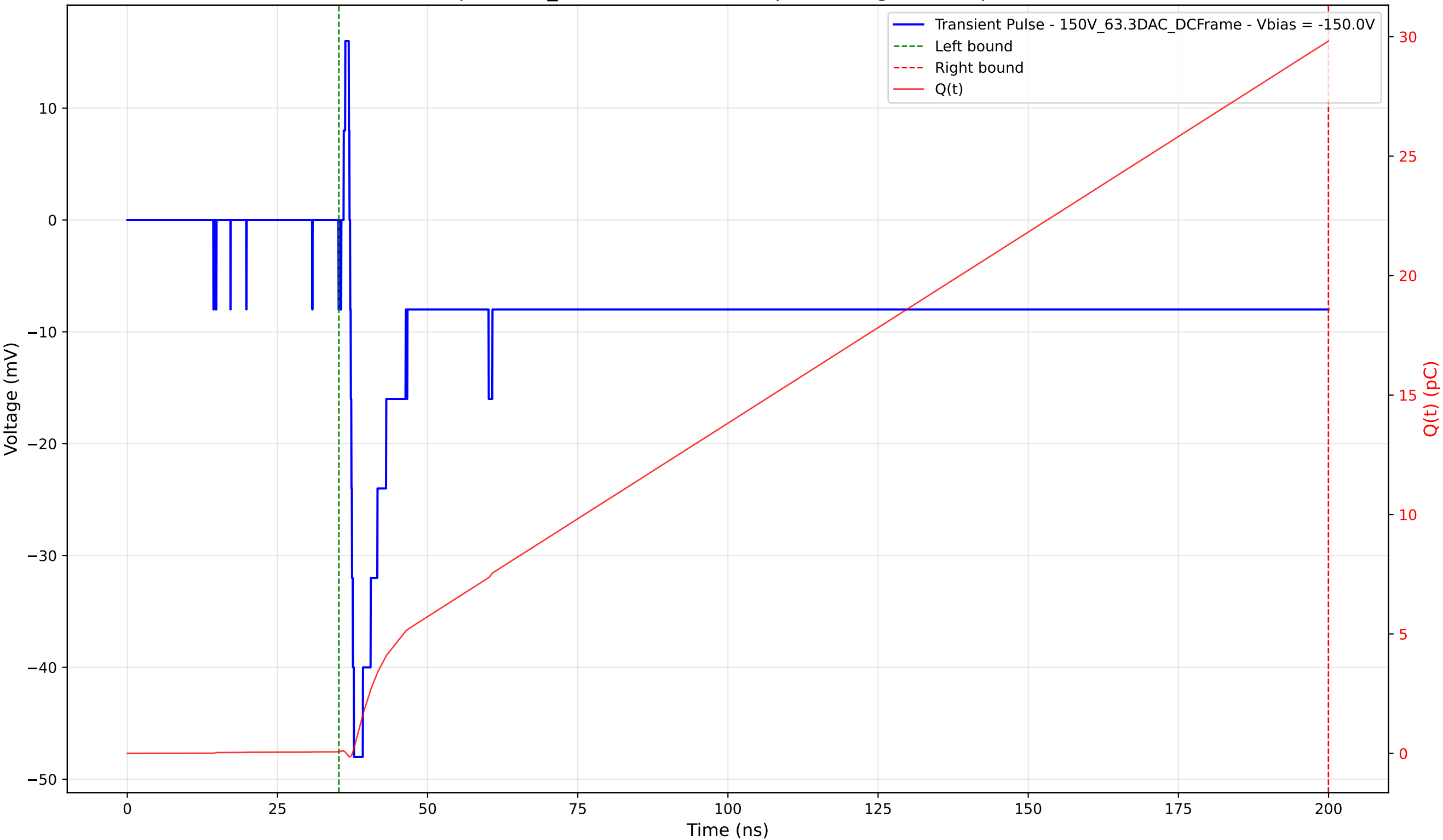
Transient Pulse - Sample: 1cm_42 - Position: 1500.0 \mu\text{m} - Charge: 29.75 pC - Rise Time: 0.63 ns
