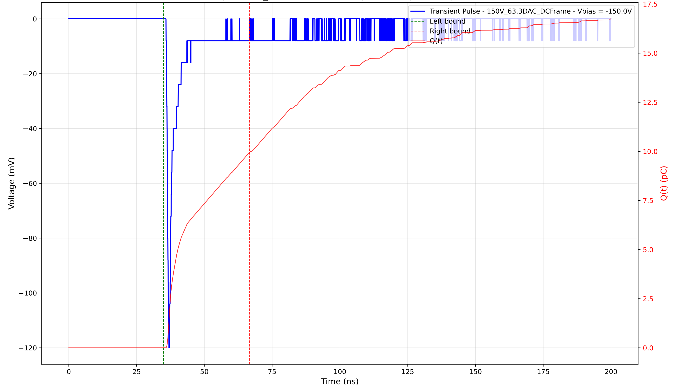
Transient Pulse - Sample: 1cm_42 - Position: 155.0 \mu\text{m} - Charge: 9.94 pC - Rise Time: 0.77 ns
