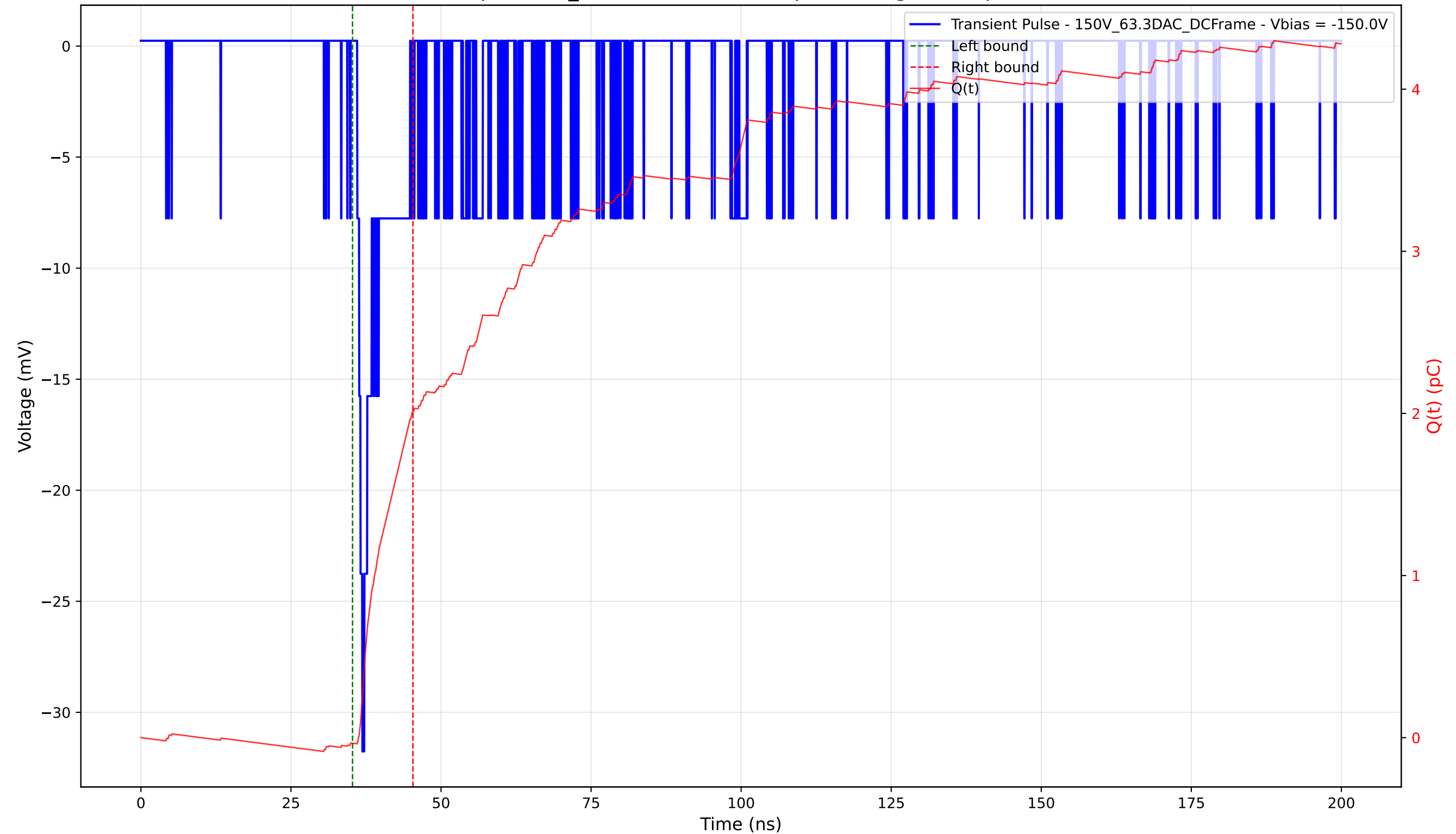
Transient Pulse - Sample: 1cm_42 - Position: 5170.0 \mu\text{m} - Charge: 2.04 pC - Rise Time: 0.85 ns
