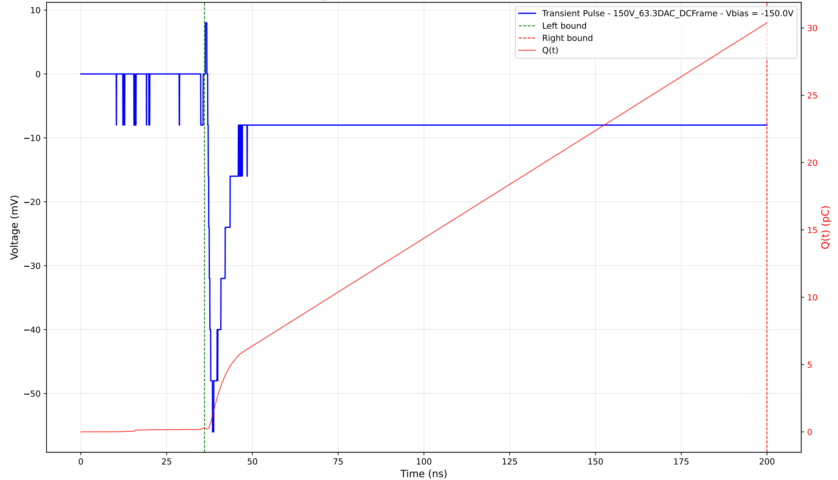
Transient Pulse - Sample: 1cm_42 - Position: 3860.0 \mu\text{m} - Charge: 30.09 pC - Rise Time: 1.39 ns
