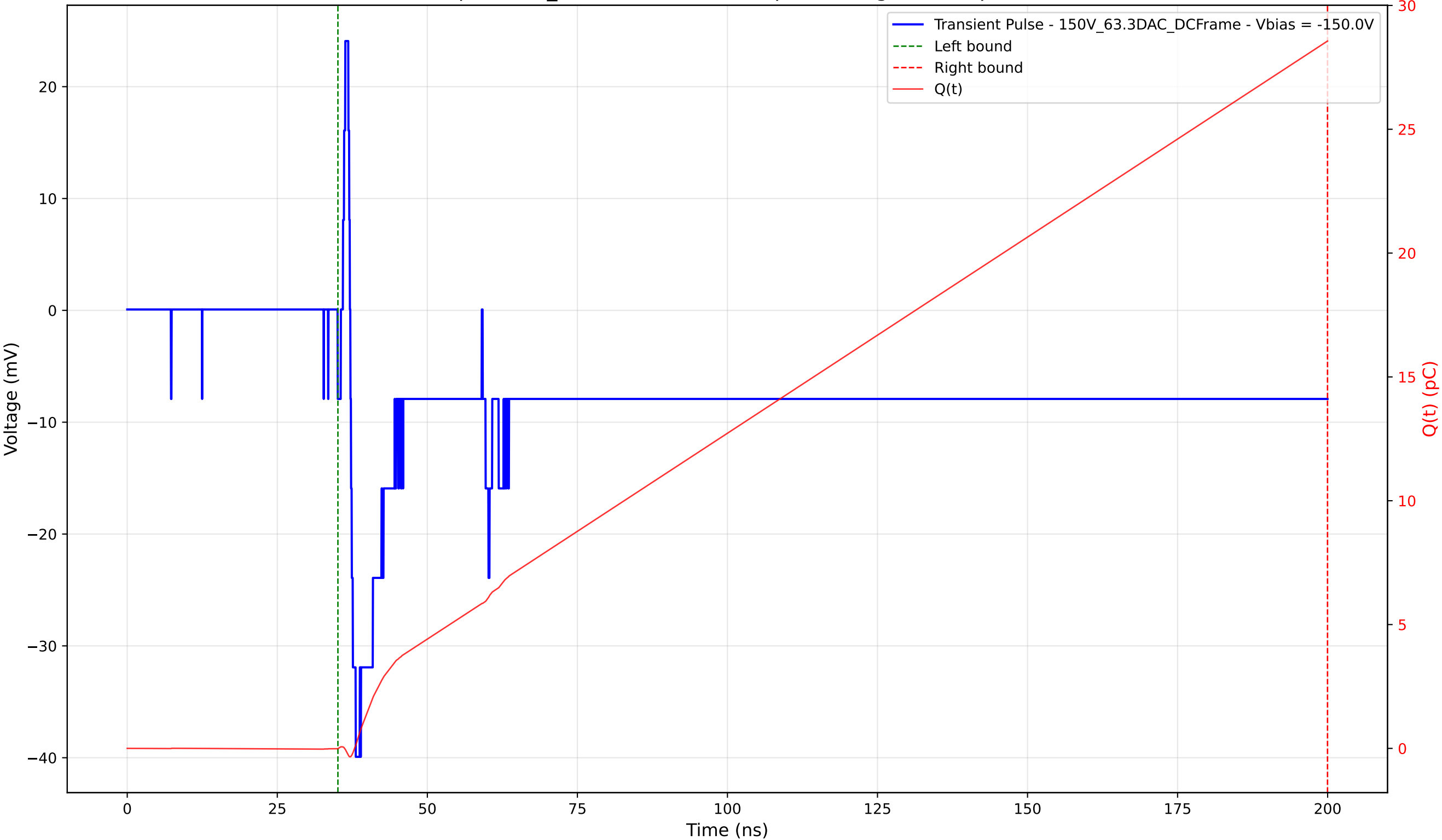
Transient Pulse - Sample: 1cm_42 - Position: 1900.0 \mu\text{m} - Charge: 28.57 pC - Rise Time: 0.89 ns
