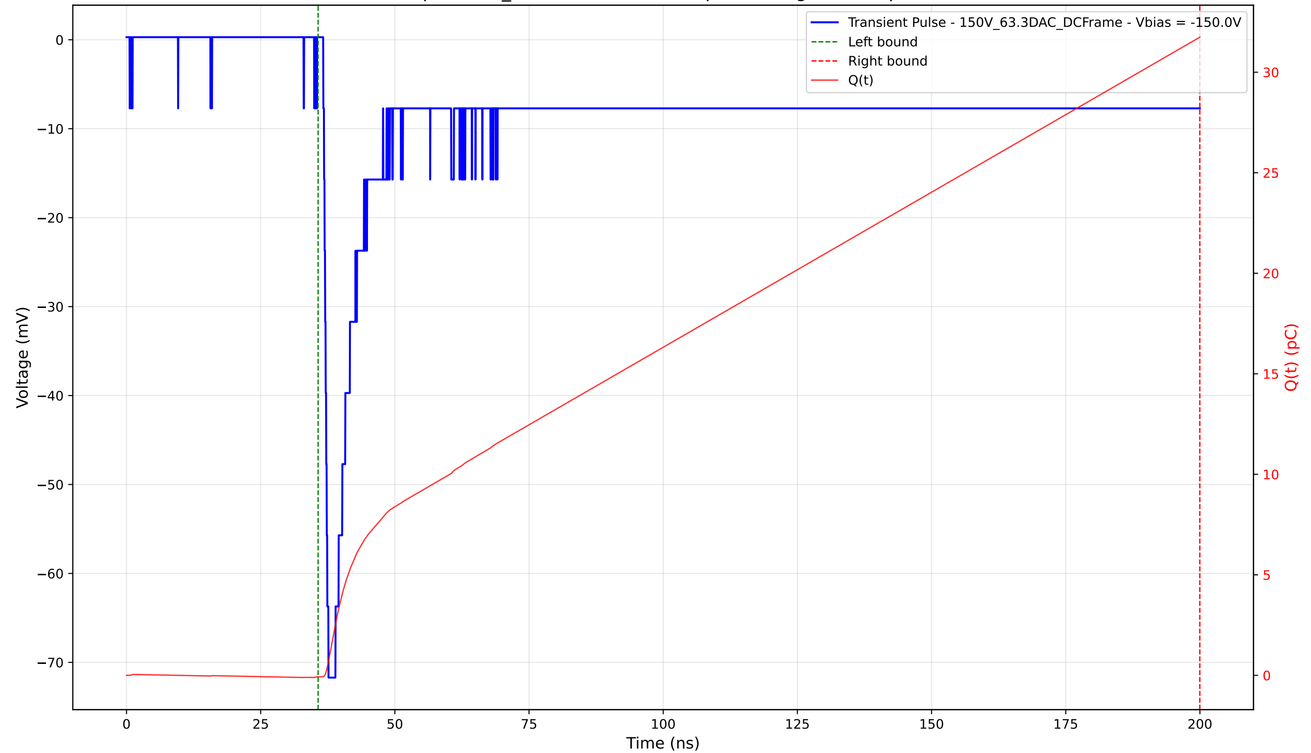
Transient Pulse - Sample: 1cm_42 - Position: 1065.0 \mu\text{m} - Charge: 31.81 pC - Rise Time: 0.96 ns
