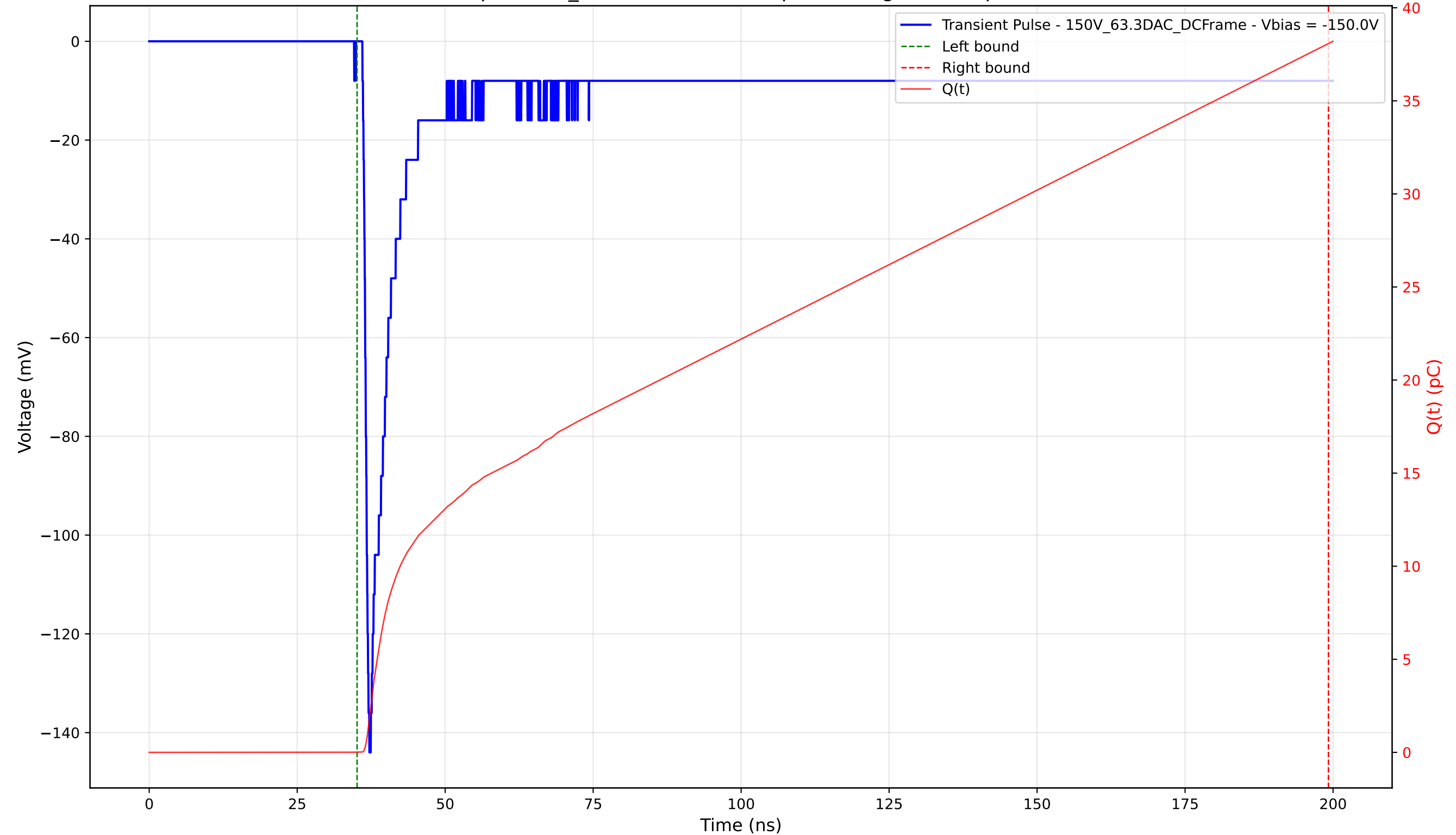
Transient Pulse - Sample: 1cm_42 - Position: 615.0 \mu\text{m} - Charge: 38.06 pC - Rise Time: 0.92 ns
