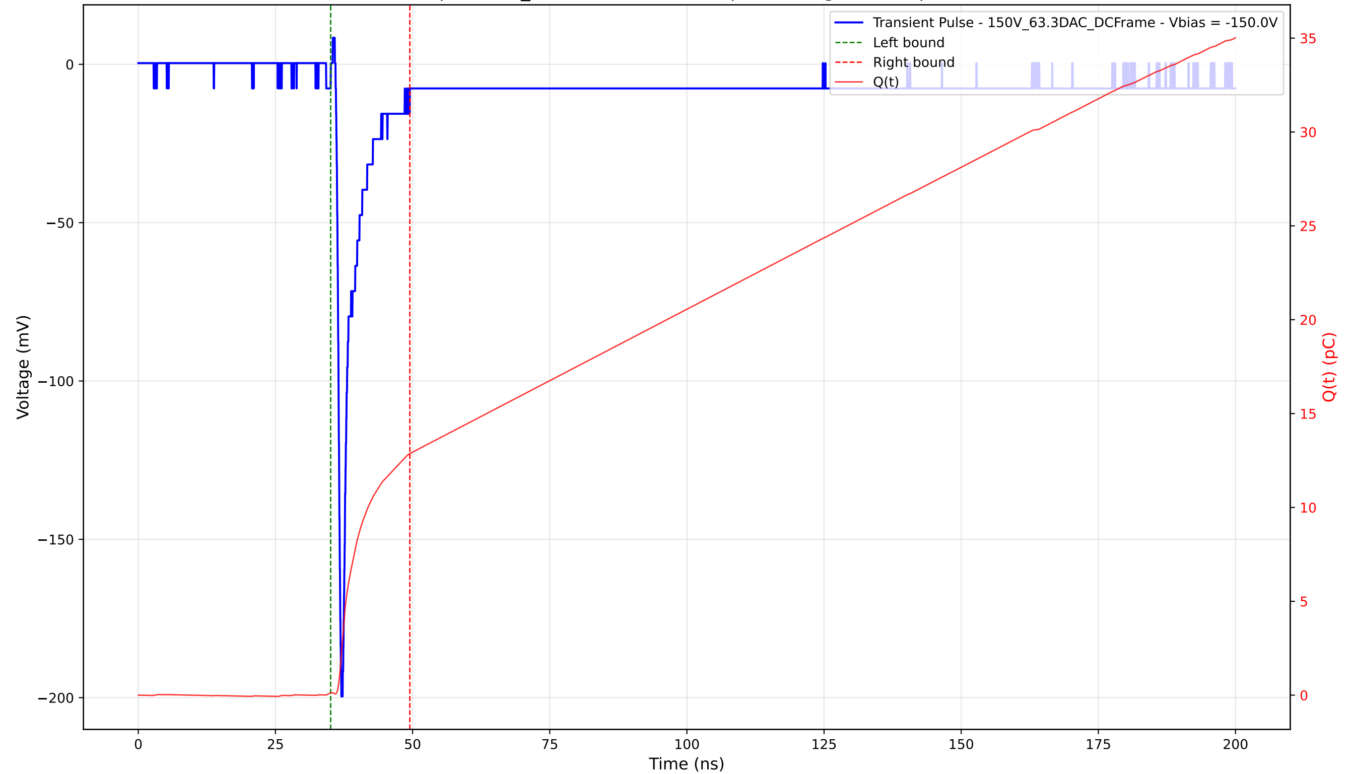
Transient Pulse - Sample: 1cm_42 - Position: 4915.0 \mu\text{m} - Charge: 12.74 pC - Rise Time: 0.77 ns
