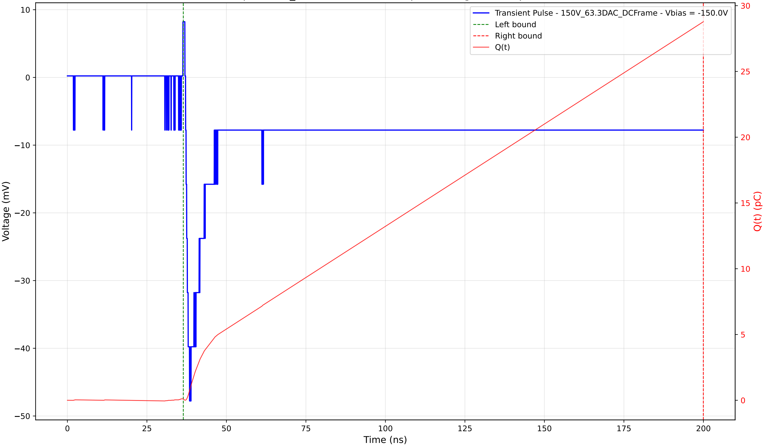
Transient Pulse - Sample: 1cm_42 - Position: 3600.0 \mu\text{m} - Charge: 28.69 pC - Rise Time: 1.25 ns
