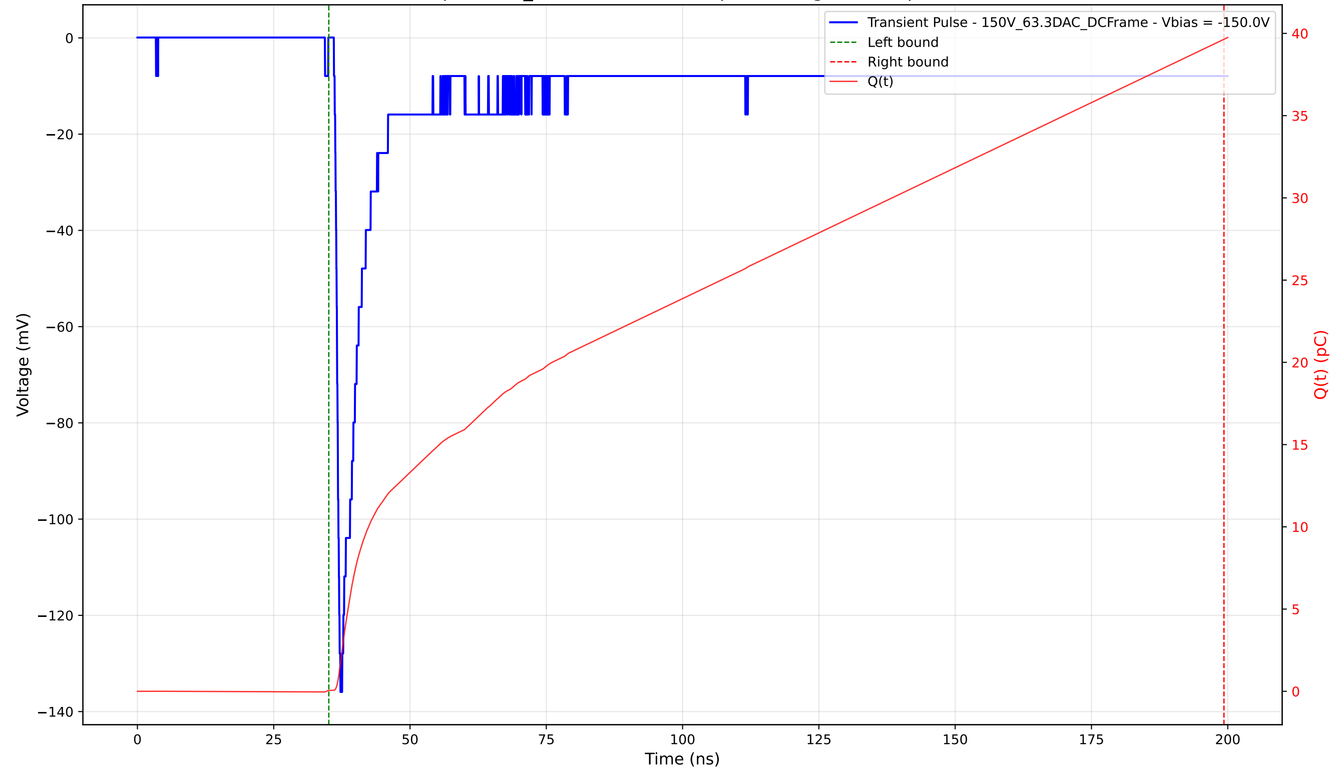
Transient Pulse - Sample: 1cm_42 - Position: 690.0 \mu\text{m} - Charge: 39.59 pC - Rise Time: 0.91 ns
