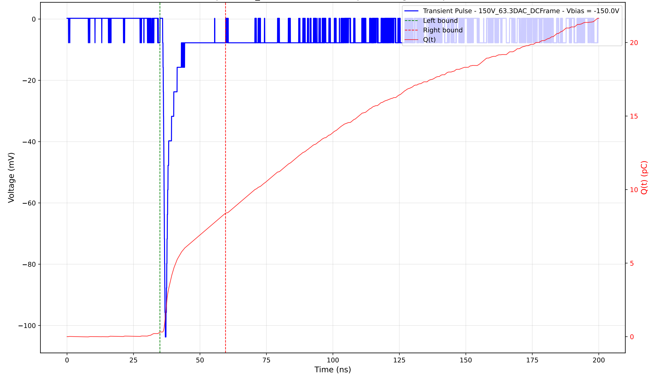
Transient Pulse - Sample: 1cm_42 - Position: 5040.0 \mu\text{m} - Charge: 8.09 pC - Rise Time: 0.73 ns
