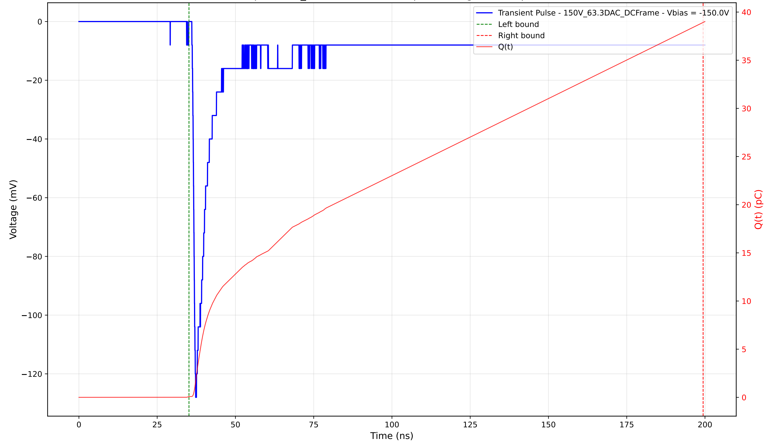
Transient Pulse - Sample: 1cm_42 - Position: 770.0 \mu\text{m} - Charge: 38.84 pC - Rise Time: 0.95 ns
