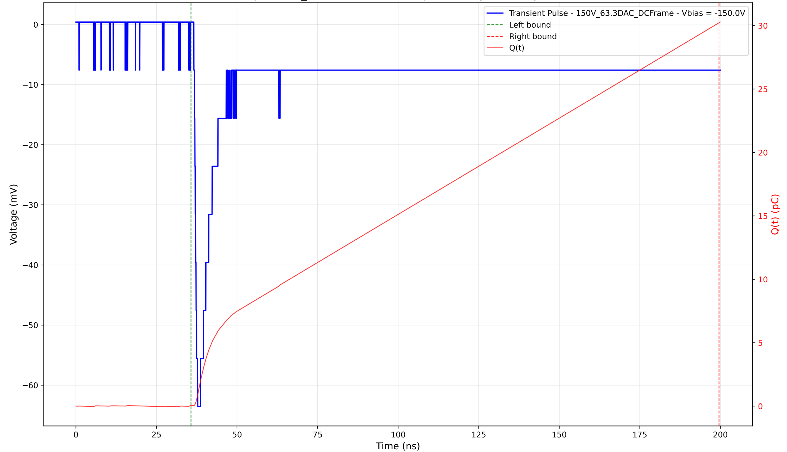
Transient Pulse - Sample: 1cm_42 - Position: 4065.0 \mu\text{m} - Charge: 30.18 pC - Rise Time: 1.20 ns
