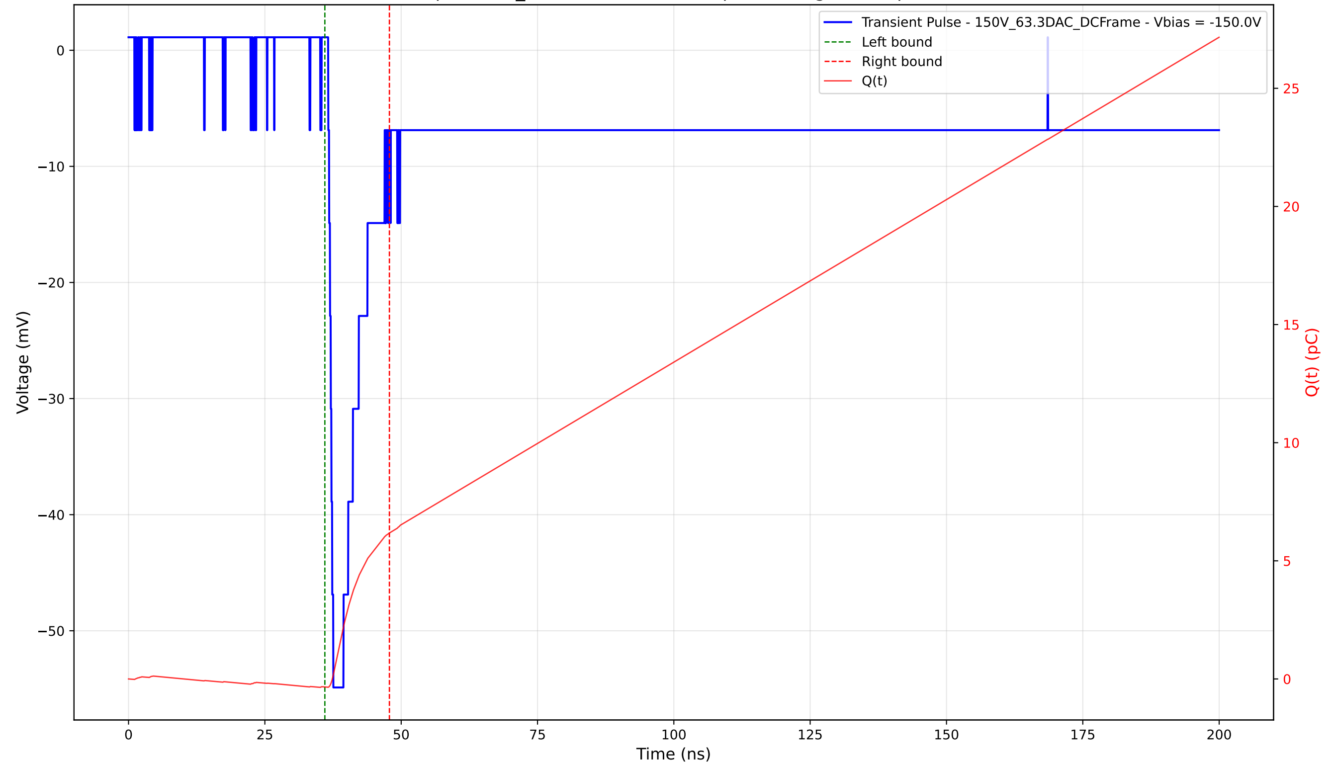
Transient Pulse - Sample: 1cm_42 - Position: 4045.0 \mu\text{m} - Charge: 6.52 pC - Rise Time: 0.92 ns
