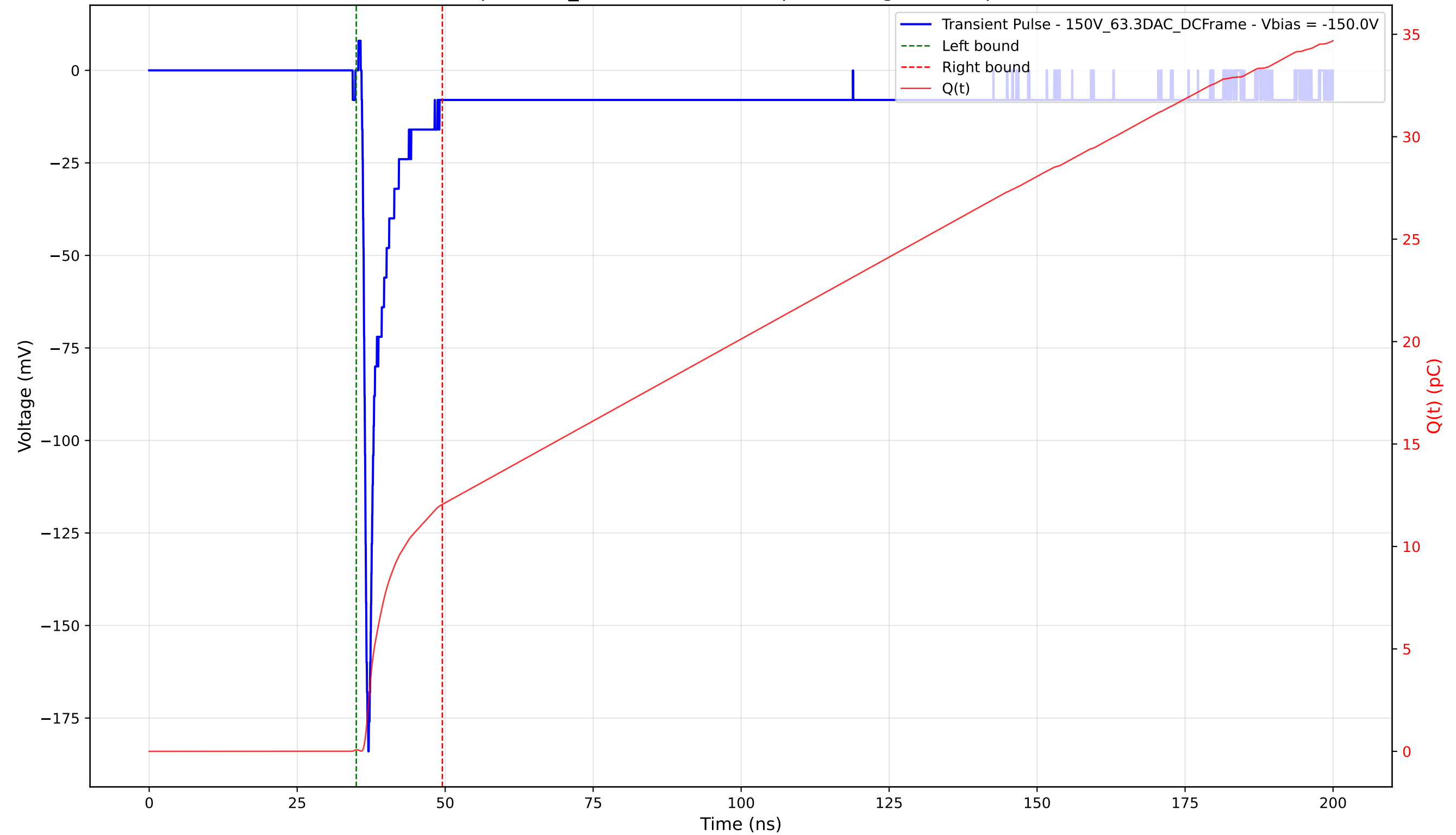
Transient Pulse - Sample: 1cm_42 - Position: 355.0 \mu\text{m} - Charge: 11.98 pC - Rise Time: 0.75 ns
