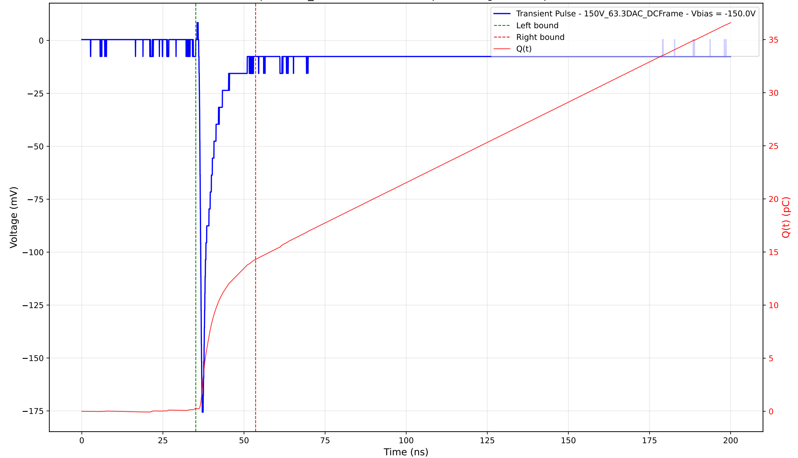
Transient Pulse - Sample: 1cm_42 - Position: 4635.0 \mu\text{m} - Charge: 14.03 pC - Rise Time: 0.76 ns
