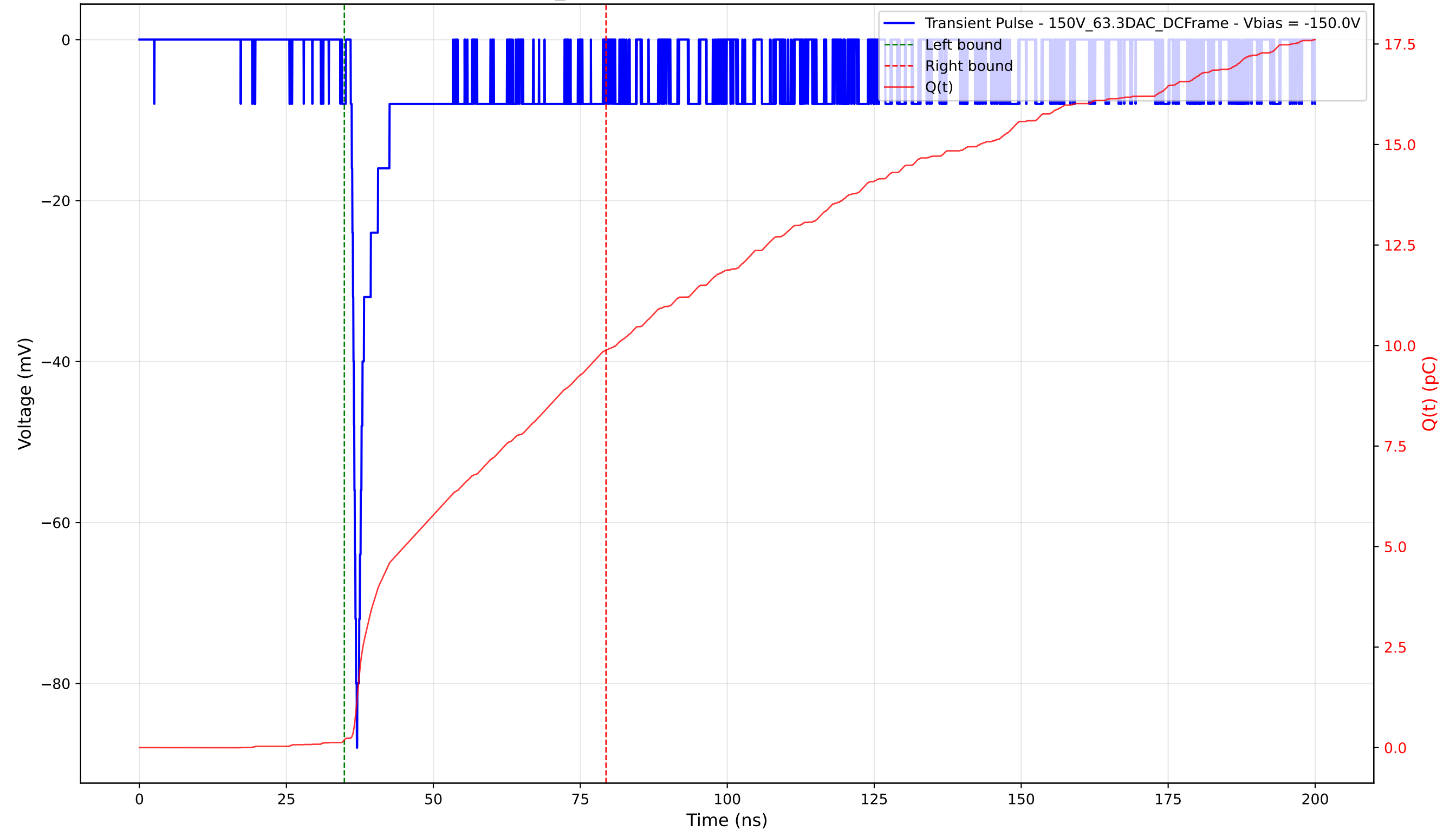
Transient Pulse - Sample: 1cm_42 - Position: 5070.0 \mu\text{m} - Charge: 9.69 pC - Rise Time: 0.74 ns
