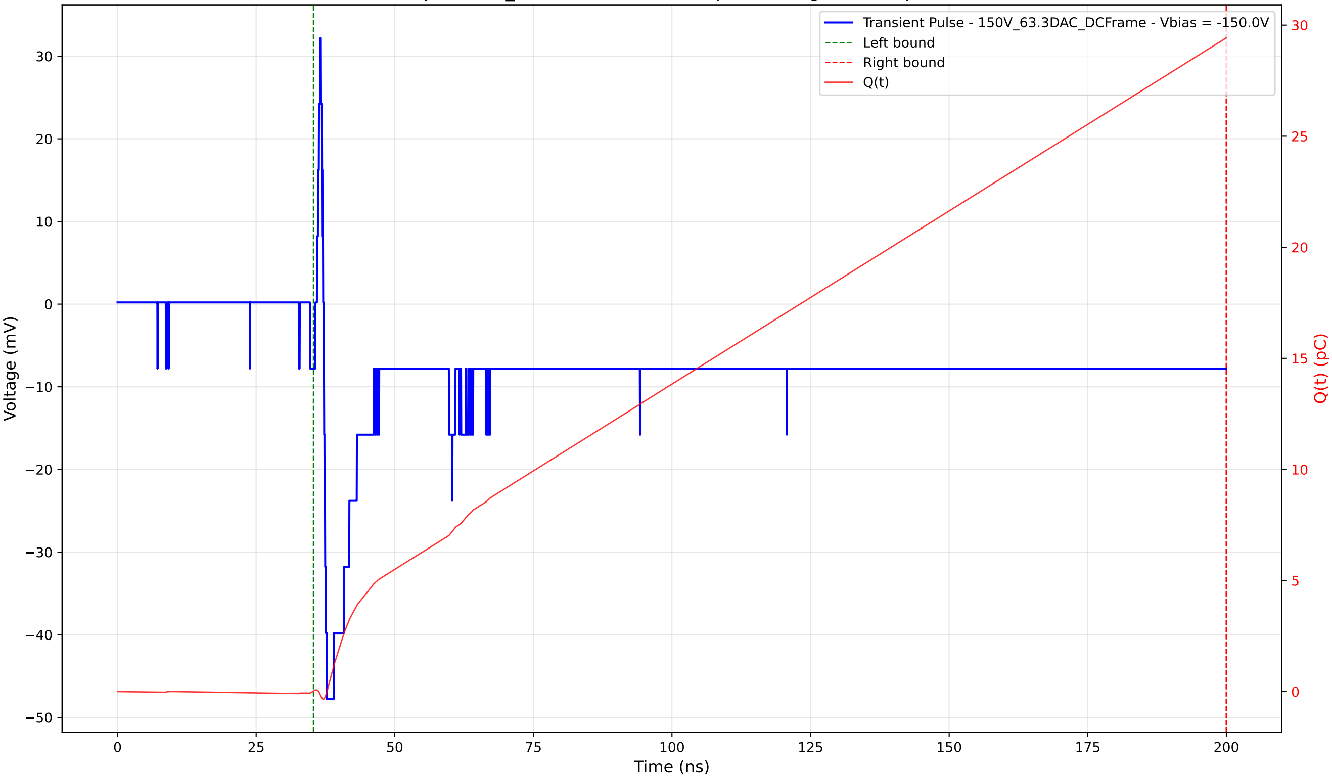
Transient Pulse - Sample: 1cm_42 - Position: 1680.0 \mu\text{m} - Charge: 29.40 pC - Rise Time: 0.59 ns
