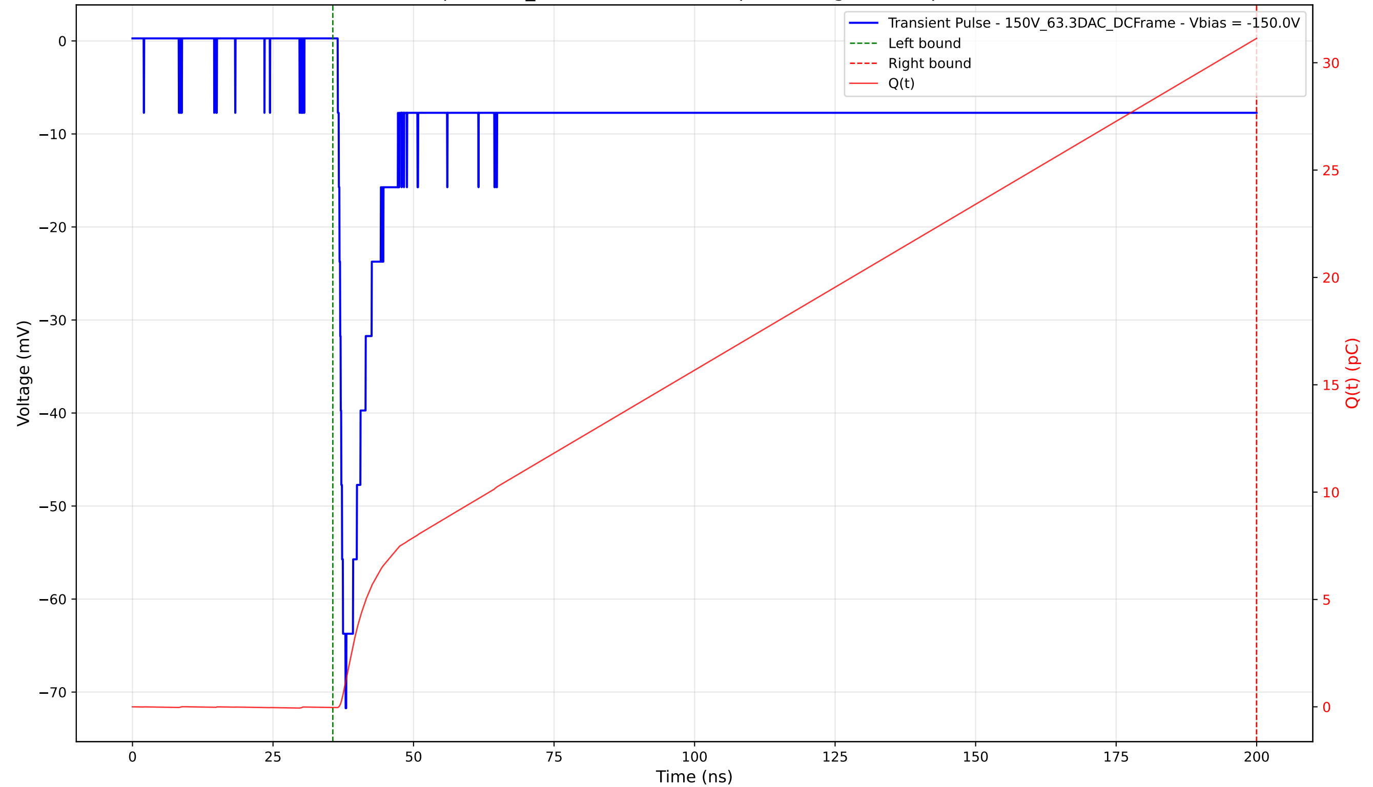
Transient Pulse - Sample: 1cm_42 - Position: 4115.0 \mu\text{m} - Charge: 31.16 pC - Rise Time: 1.38 ns
