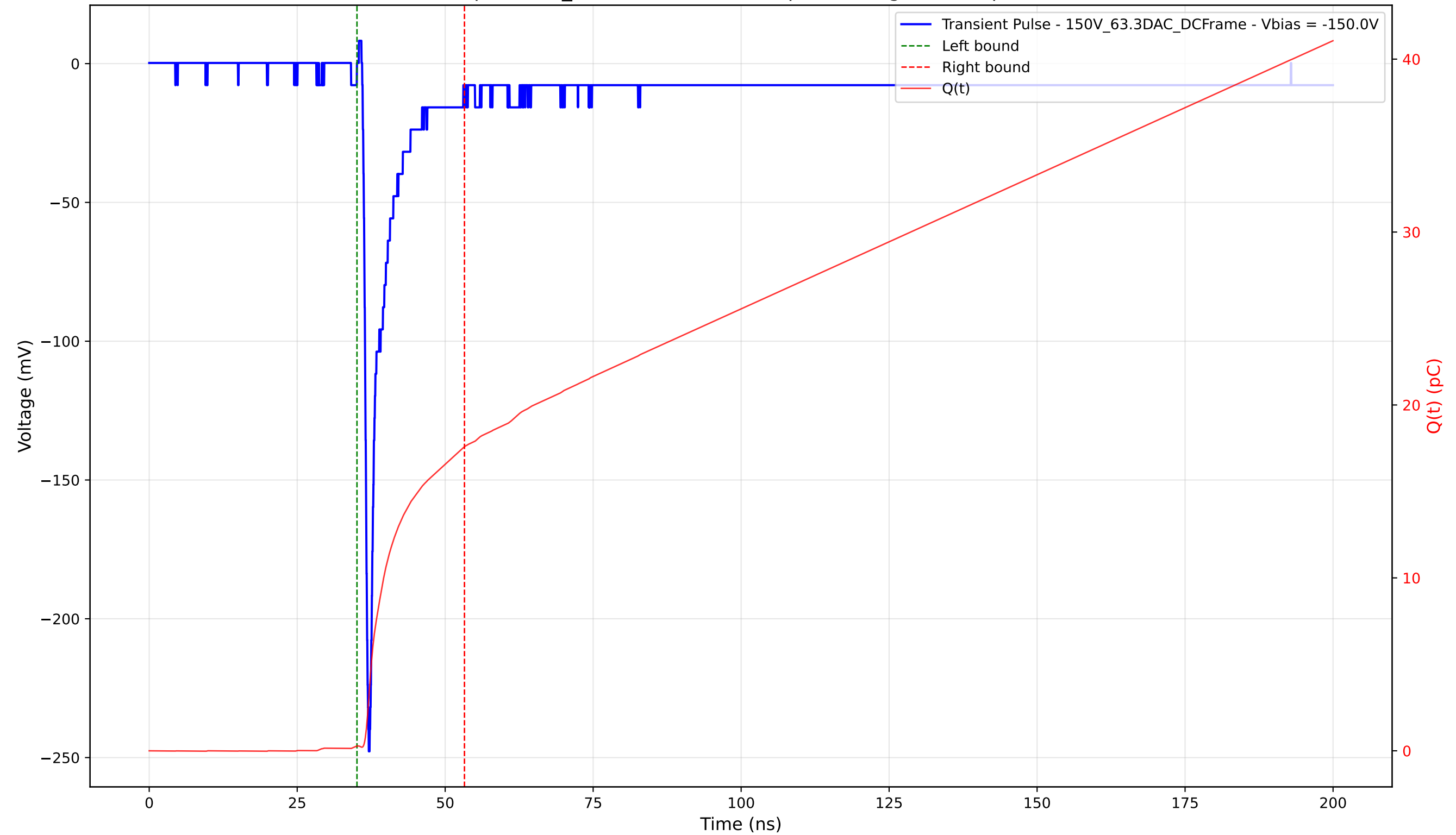
Transient Pulse - Sample: 1cm_42 - Position: 4790.0 \mu\text{m} - Charge: 17.30 pC - Rise Time: 0.76 ns
