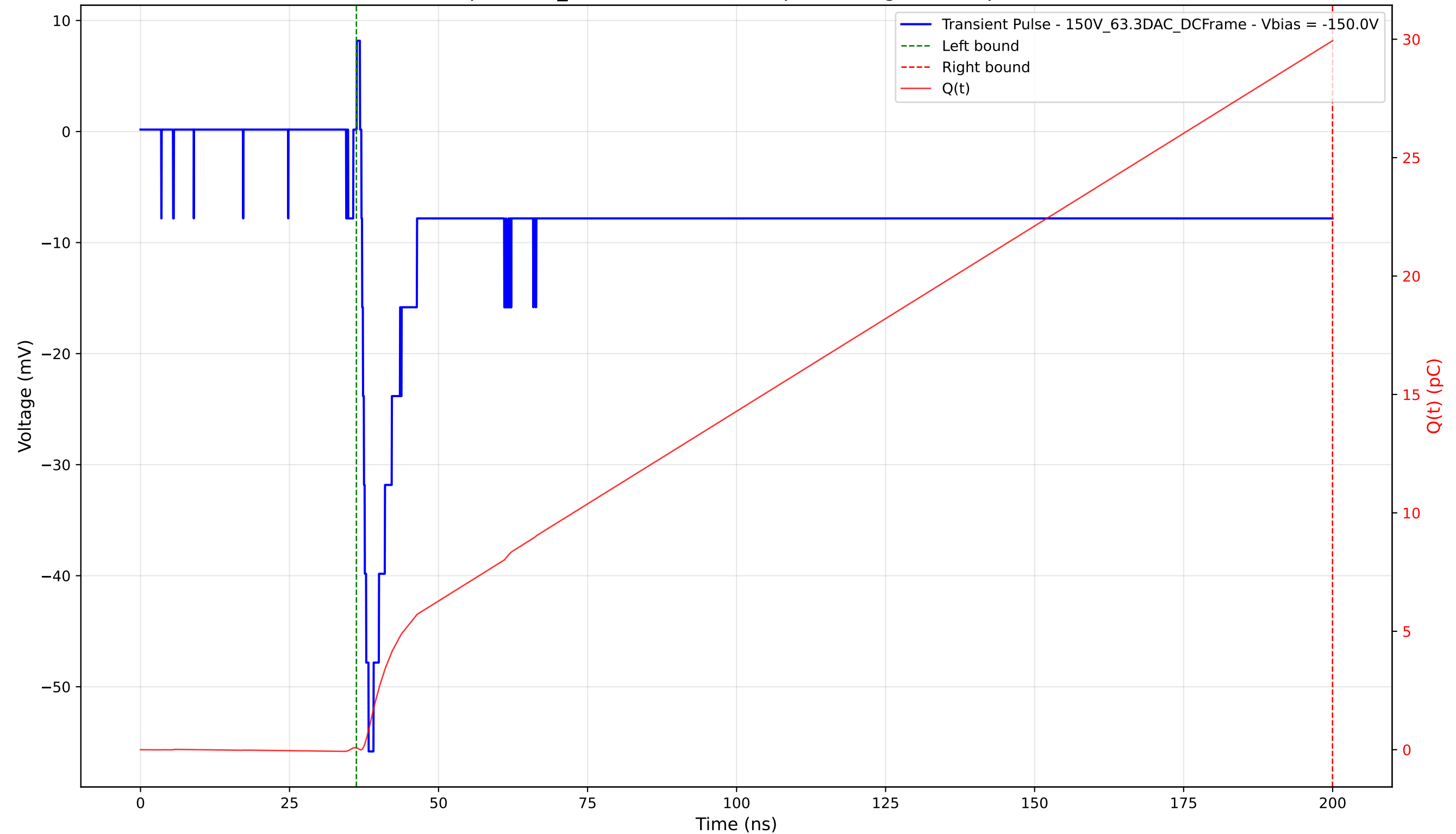
Transient Pulse - Sample: 1cm_42 - Position: 3745.0 \mu\text{m} - Charge: 29.85 pC - Rise Time: 1.21 ns
