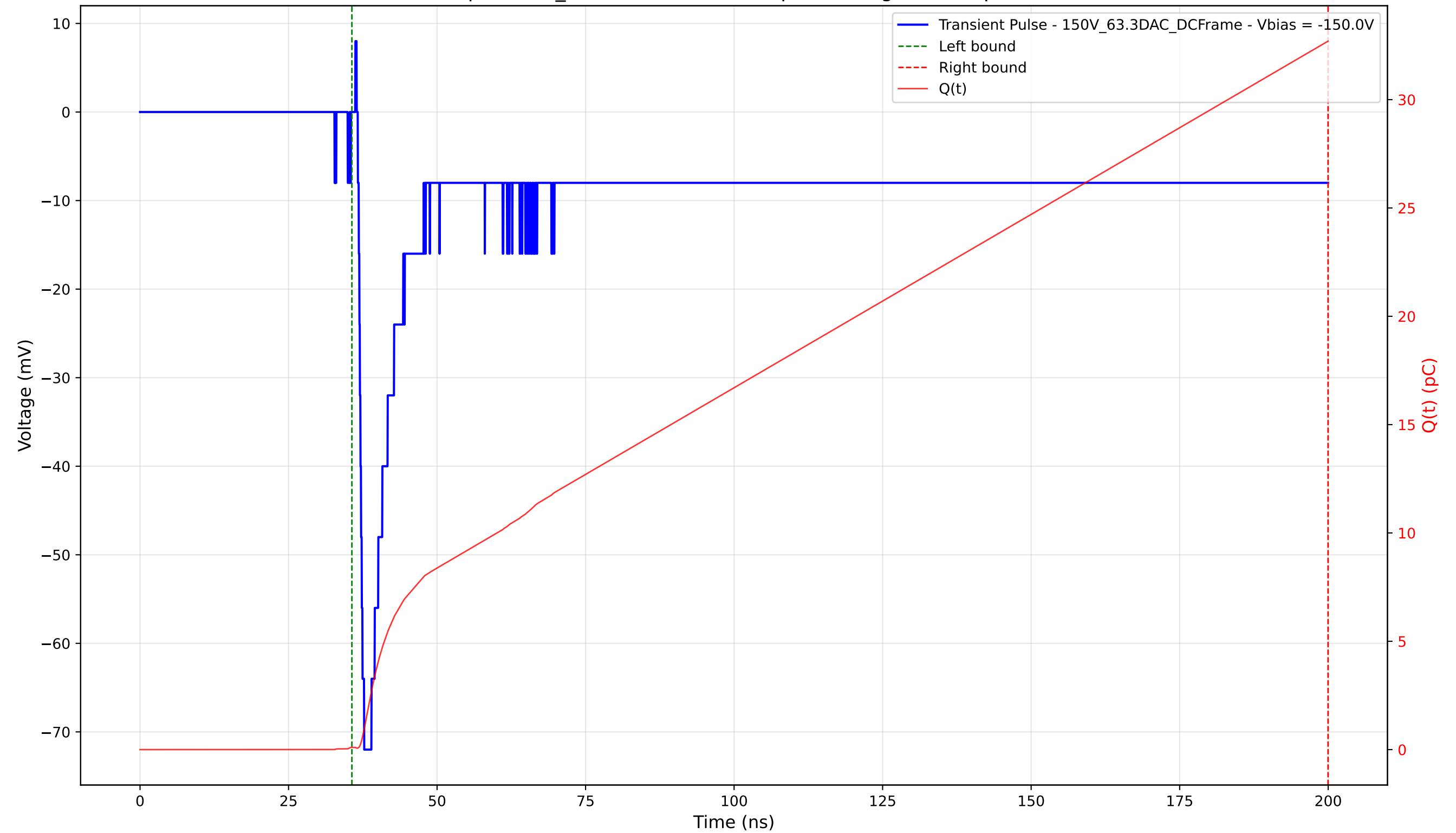
Transient Pulse - Sample: 1cm_42 - Position: 1070.0 \mu\text{m} - Charge: 32.60 pC - Rise Time: 1.06 ns
