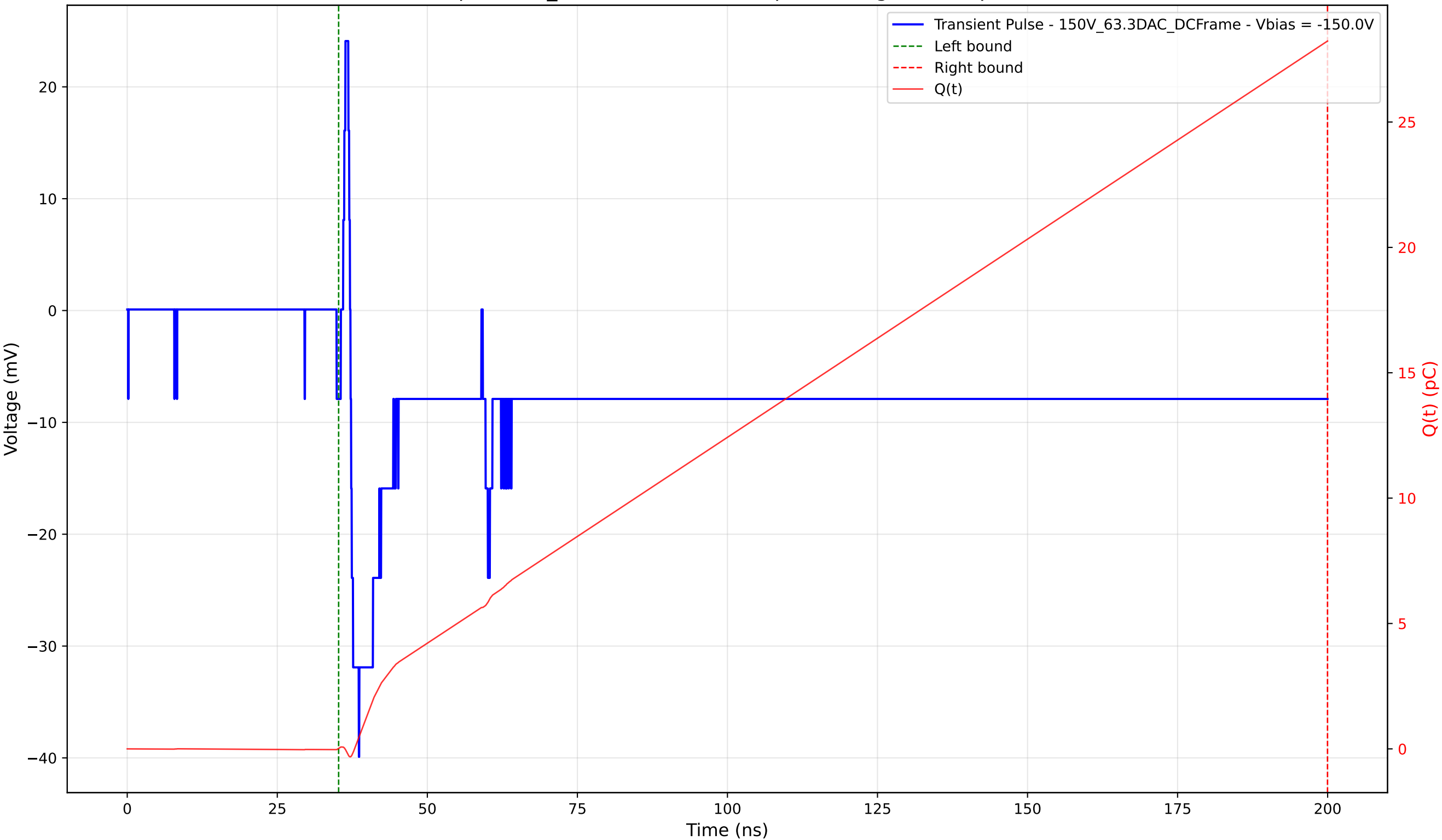
Transient Pulse - Sample: 1cm_42 - Position: 1925.0 \mu\text{m} - Charge: 28.21 pC - Rise Time: 1.39 ns
