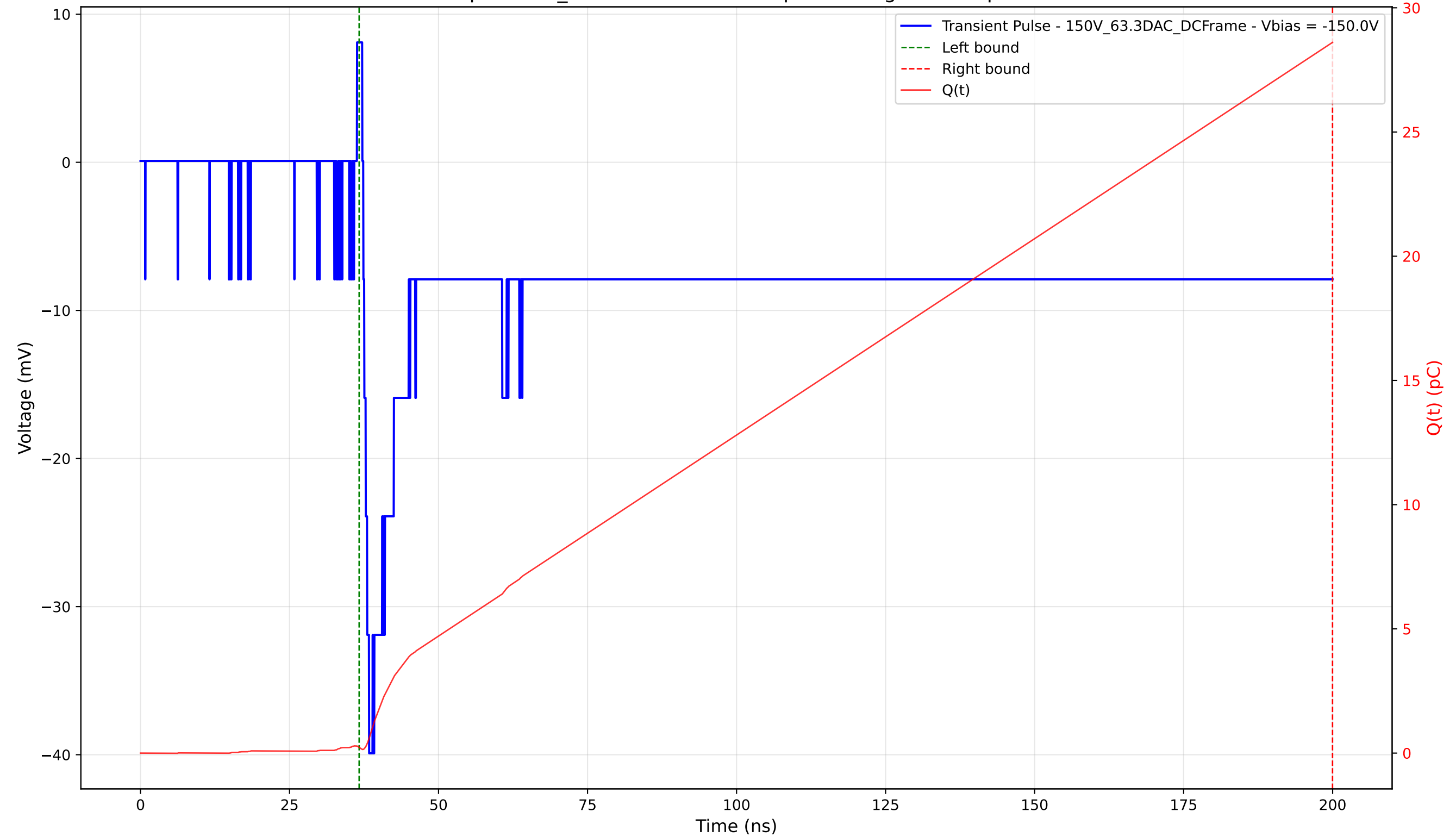
Transient Pulse - Sample: 1cm_42 - Position: 3355.0 \mu\text{m} - Charge: 28.38 pC - Rise Time: 0.97 ns
