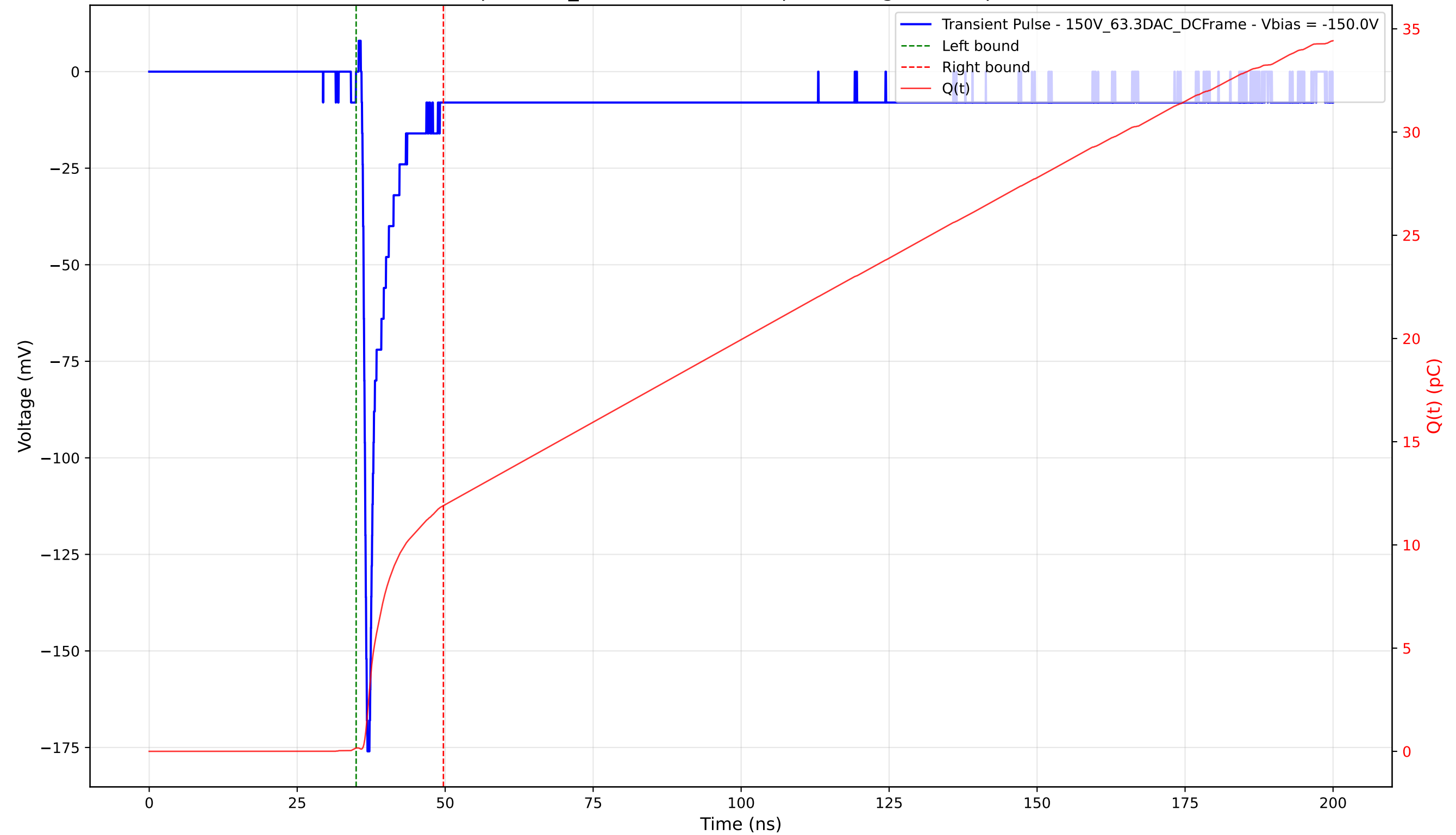
Transient Pulse - Sample: 1cm_42 - Position: 340.0 \mu\text{m} - Charge: 11.74 pC - Rise Time: 0.72 ns
