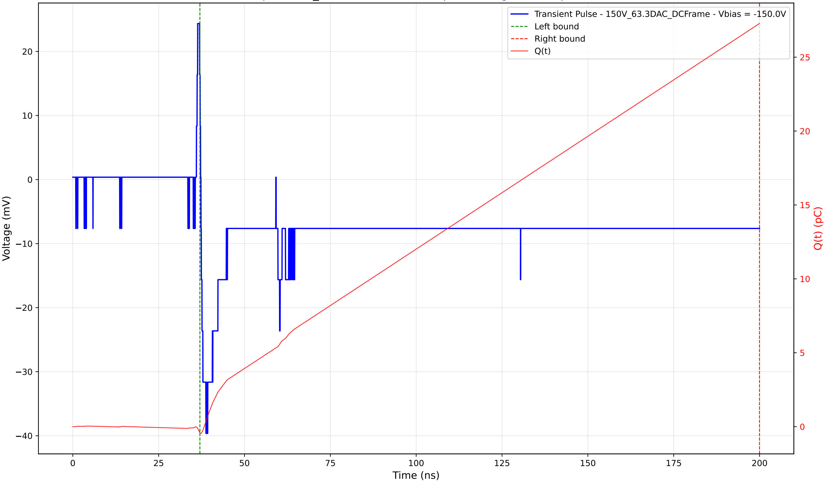
Transient Pulse - Sample: 1cm_42 - Position: 2210.0 \mu\text{m} - Charge: 27.70 pC - Rise Time: 1.45 ns
