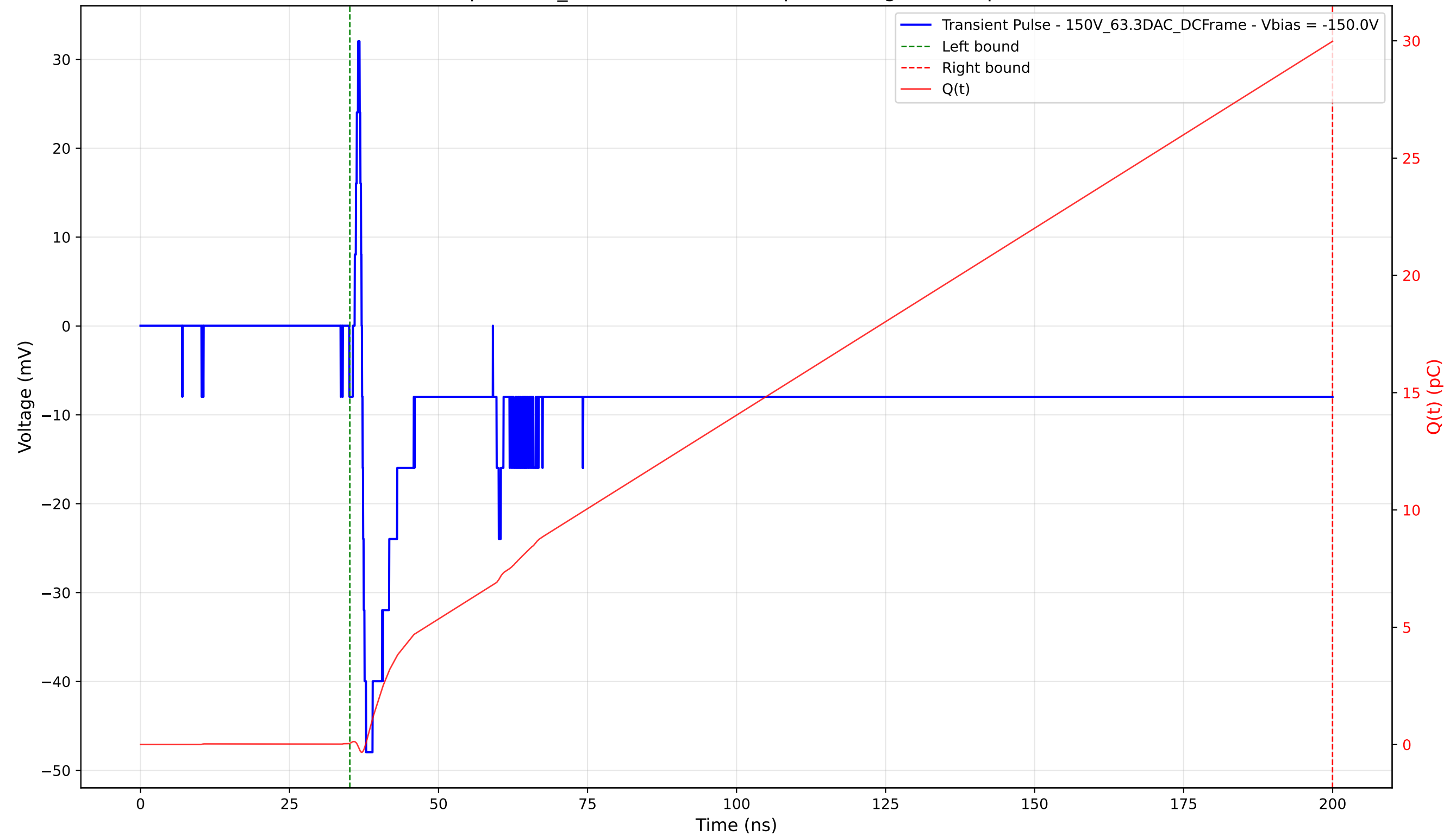
Transient Pulse - Sample: 1cm_42 - Position: 1770.0 \mu\text{m} - Charge: 29.93 pC - Rise Time: 0.69 ns
