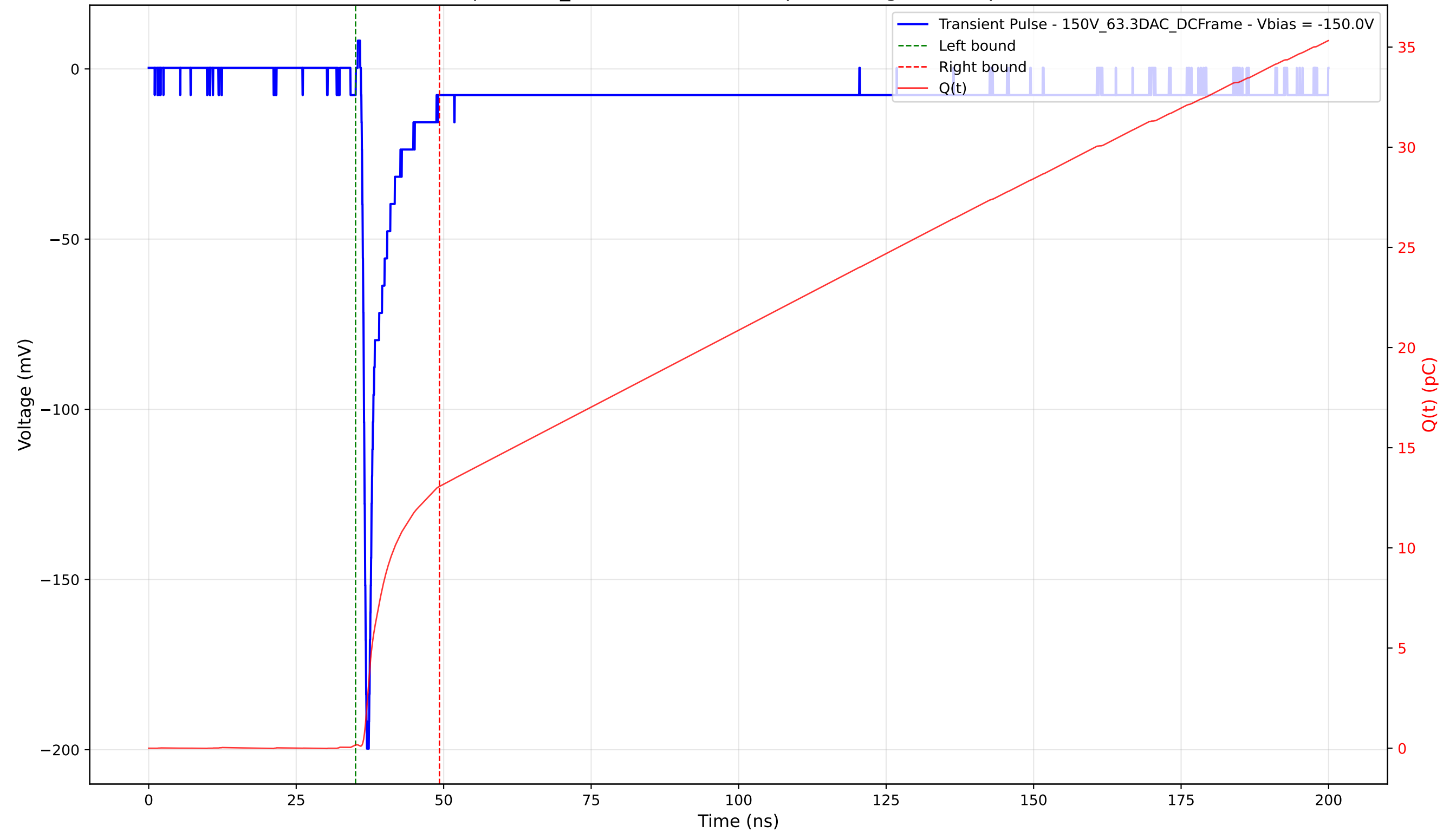
Transient Pulse - Sample: 1cm_42 - Position: 4910.0 \mu\text{m} - Charge: 12.89 pC - Rise Time: 0.75 ns
