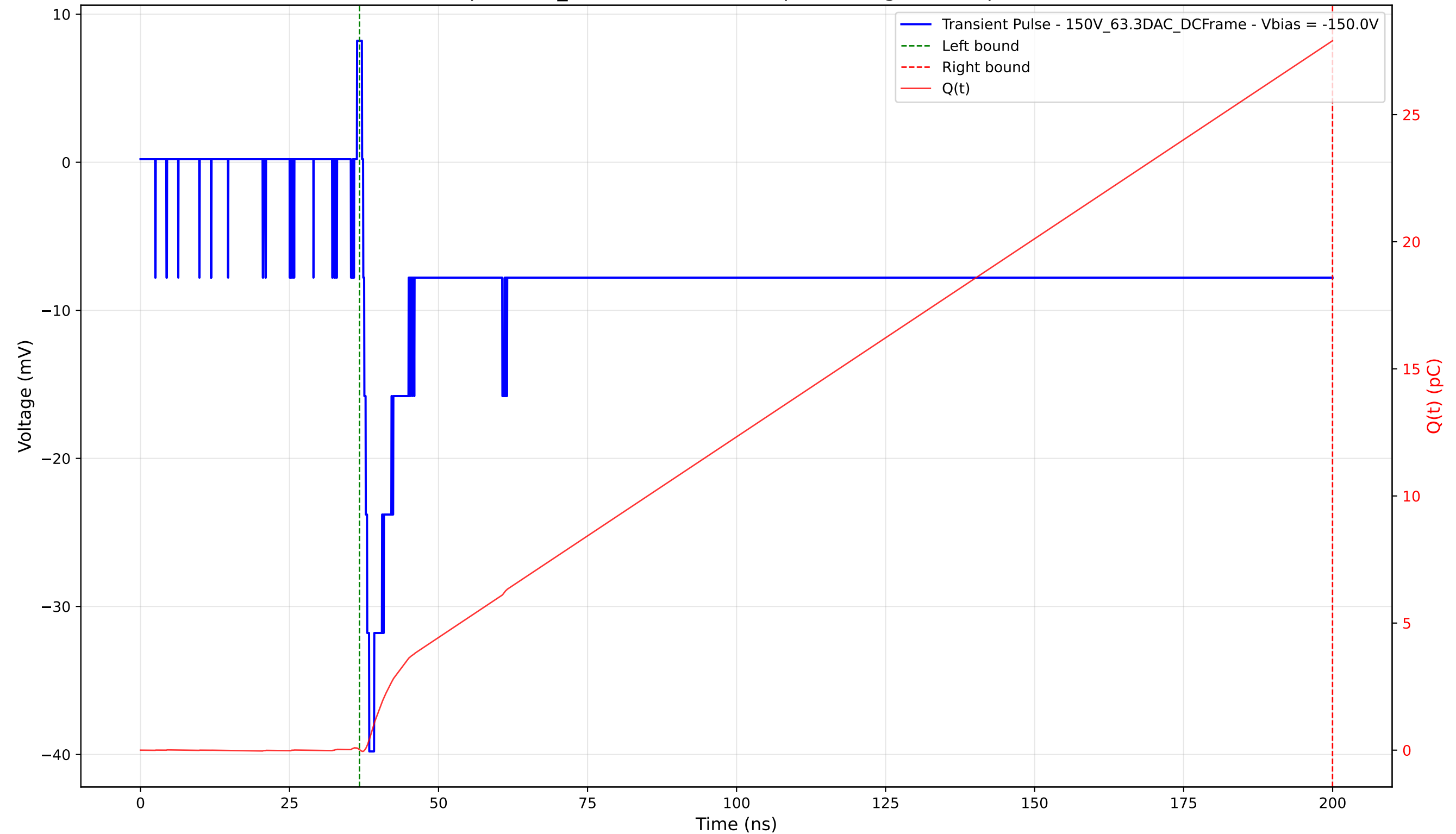
Transient Pulse - Sample: 1cm_42 - Position: 3400.0 \mu\text{m} - Charge: 27.89 pC - Rise Time: 1.01 ns
