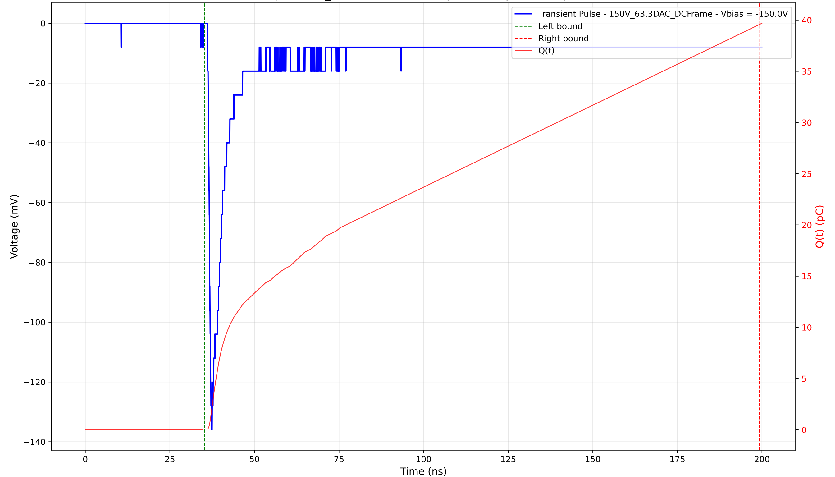
Transient Pulse - Sample: 1cm_42 - Position: 735.0 \mu\text{m} - Charge: 39.51 pC - Rise Time: 0.95 ns
