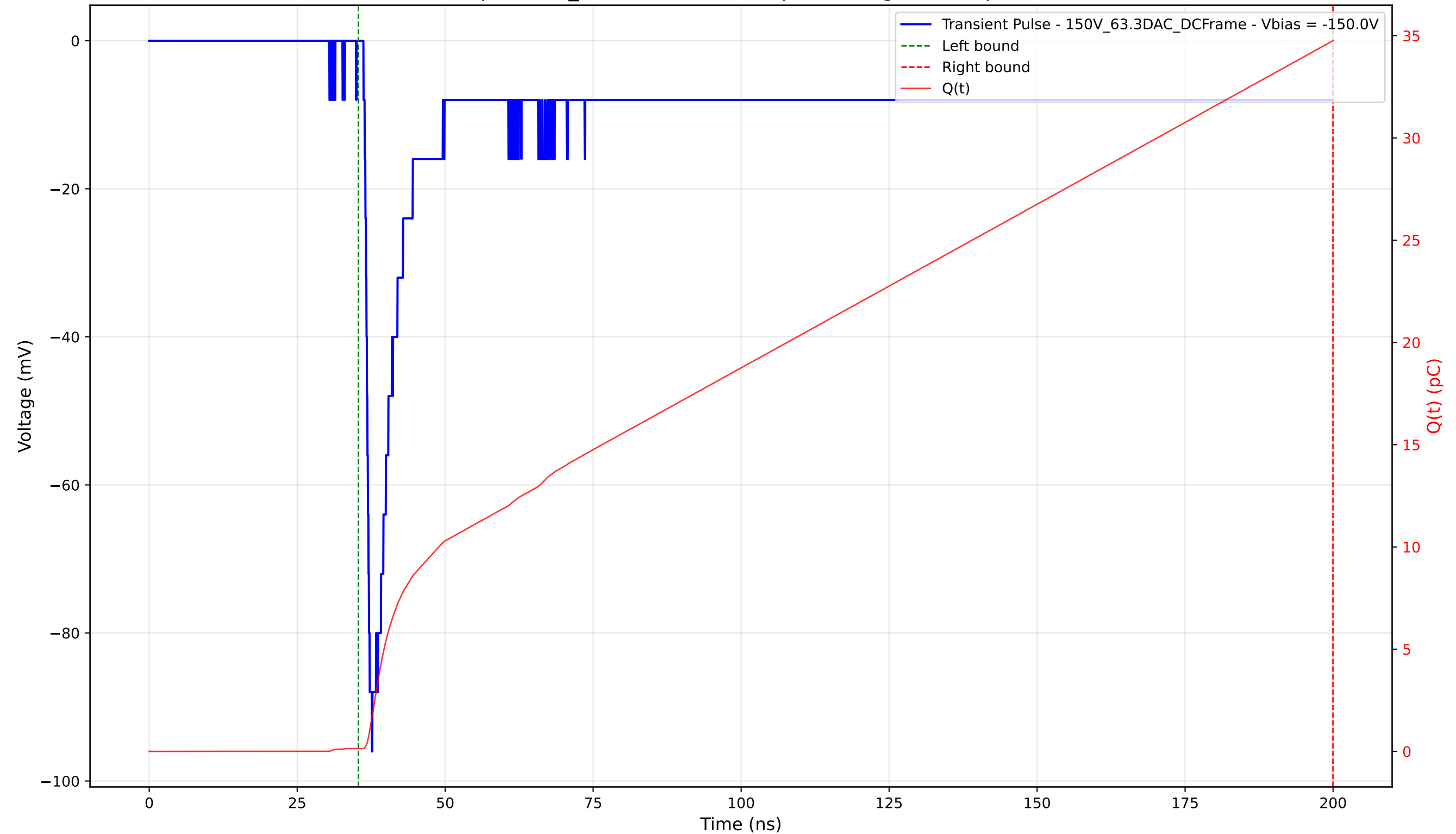
Transient Pulse - Sample: 1cm_42 - Position: 885.0 \mu\text{m} - Charge: 34.61 pC - Rise Time: 0.86 ns
