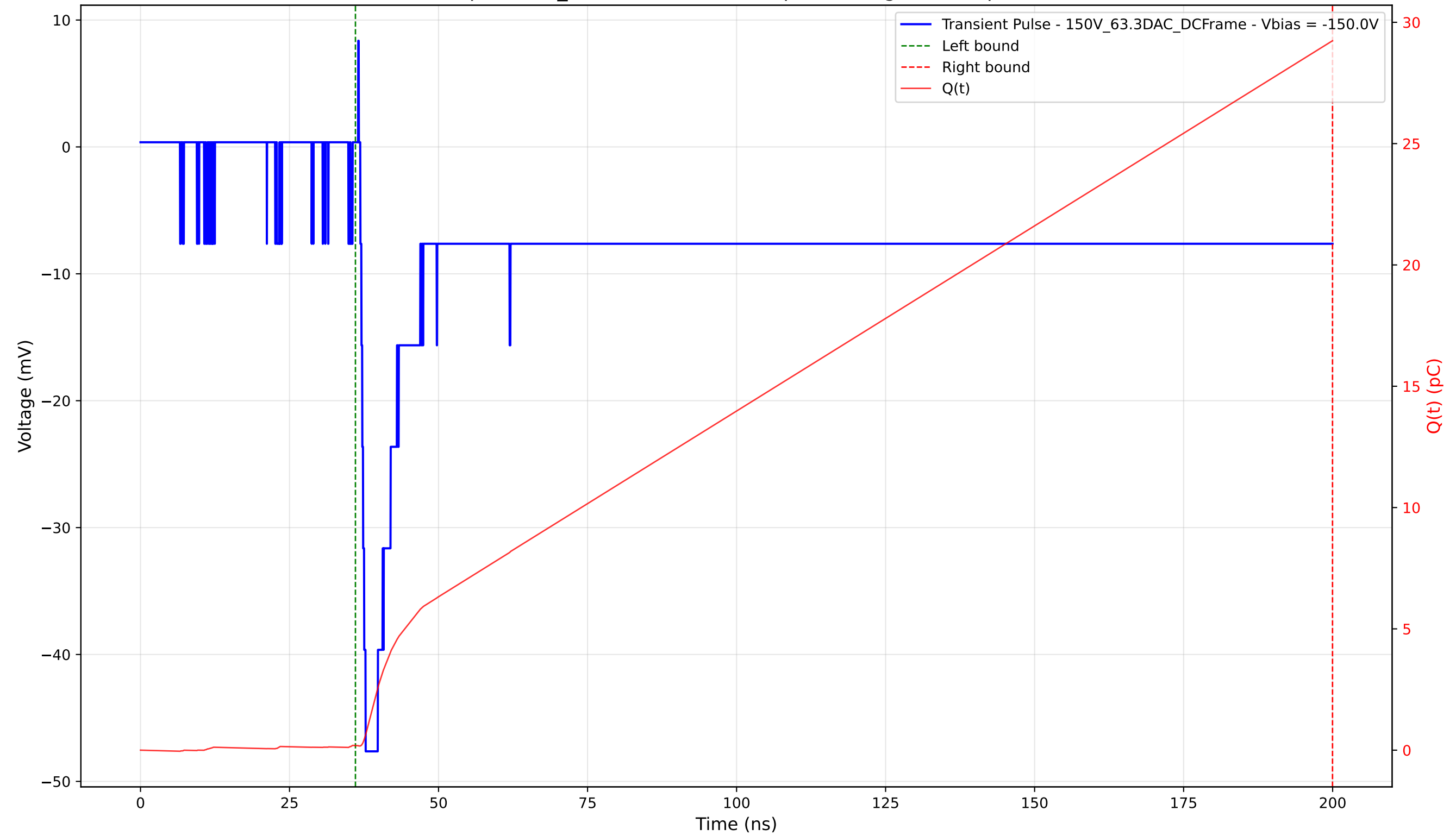
Transient Pulse - Sample: 1cm_42 - Position: 3915.0 \mu\text{m} - Charge: 29.05 pC - Rise Time: 0.89 ns
