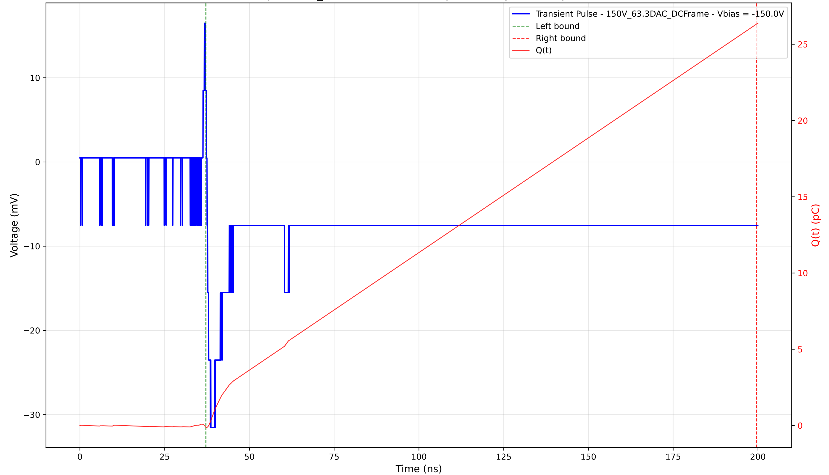
Transient Pulse - Sample: 1cm_42 - Position: 3025.0 \mu\text{m} - Charge: 26.42 pC - Rise Time: 0.97 ns
