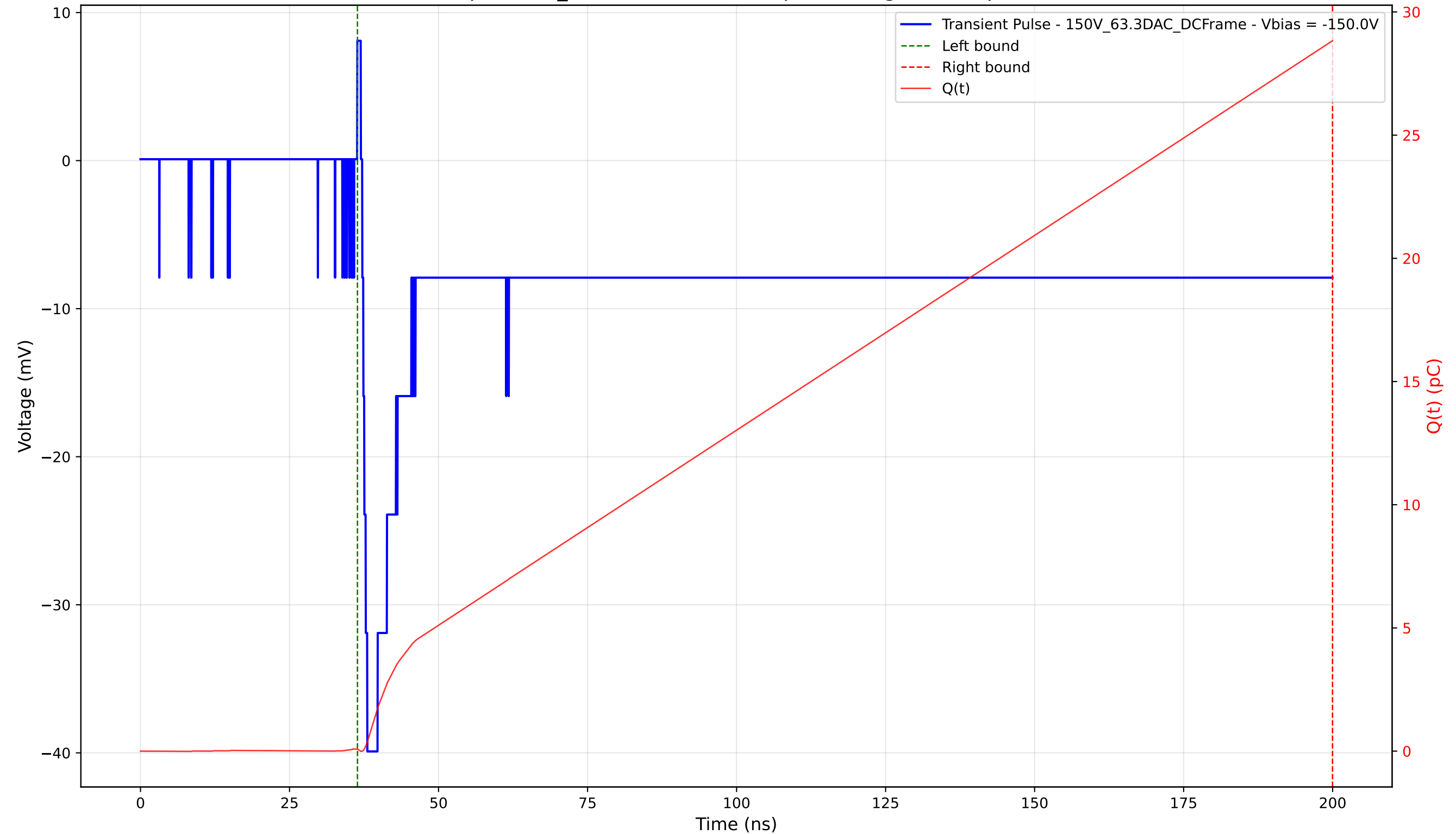
Transient Pulse - Sample: 1cm_42 - Position: 3575.0 \mu\text{m} - Charge: 28.75 pC - Rise Time: 0.85 ns
