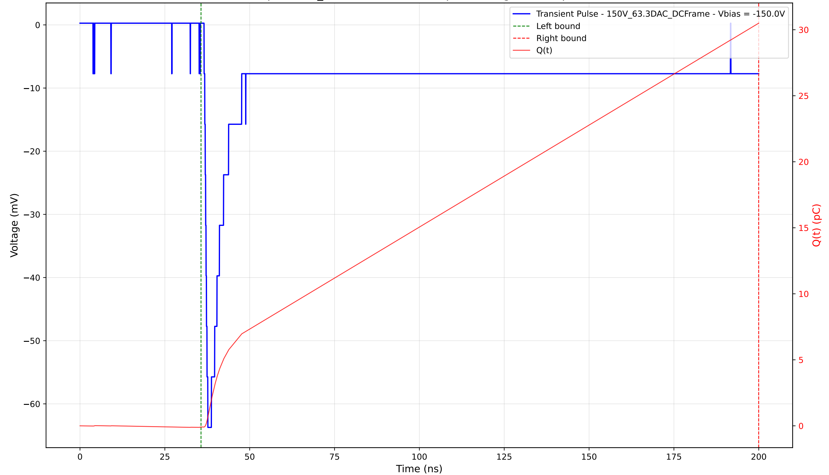
Transient Pulse - Sample: 1cm_42 - Position: 4075.0 \mu\text{m} - Charge: 30.59 pC - Rise Time: 1.10 ns
