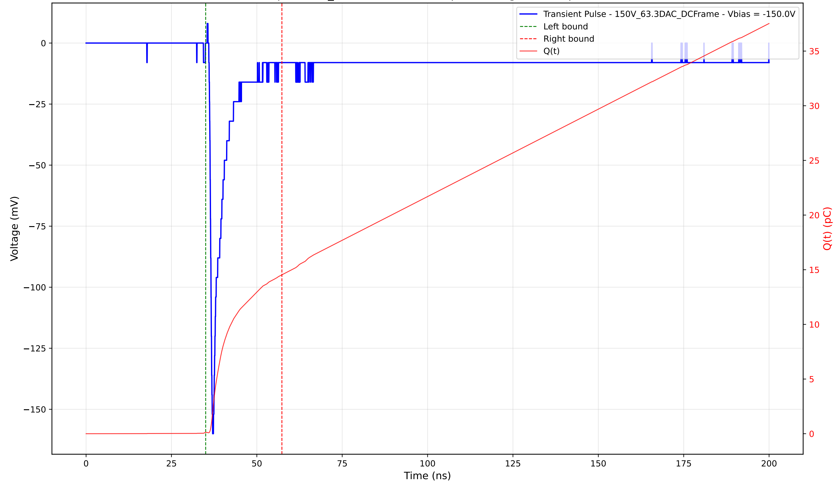
Transient Pulse - Sample: 1cm_42 - Position: 510.0 \mu\text{m} - Charge: 14.41 pC - Rise Time: 0.74 ns
