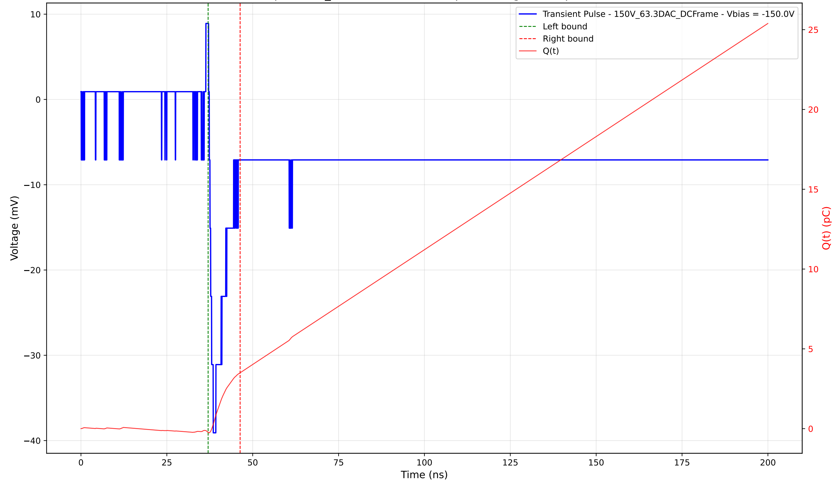
Transient Pulse - Sample: 1cm_42 - Position: 3395.0 \mu\text{m} - Charge: 3.74 pC - Rise Time: 1.15 ns
