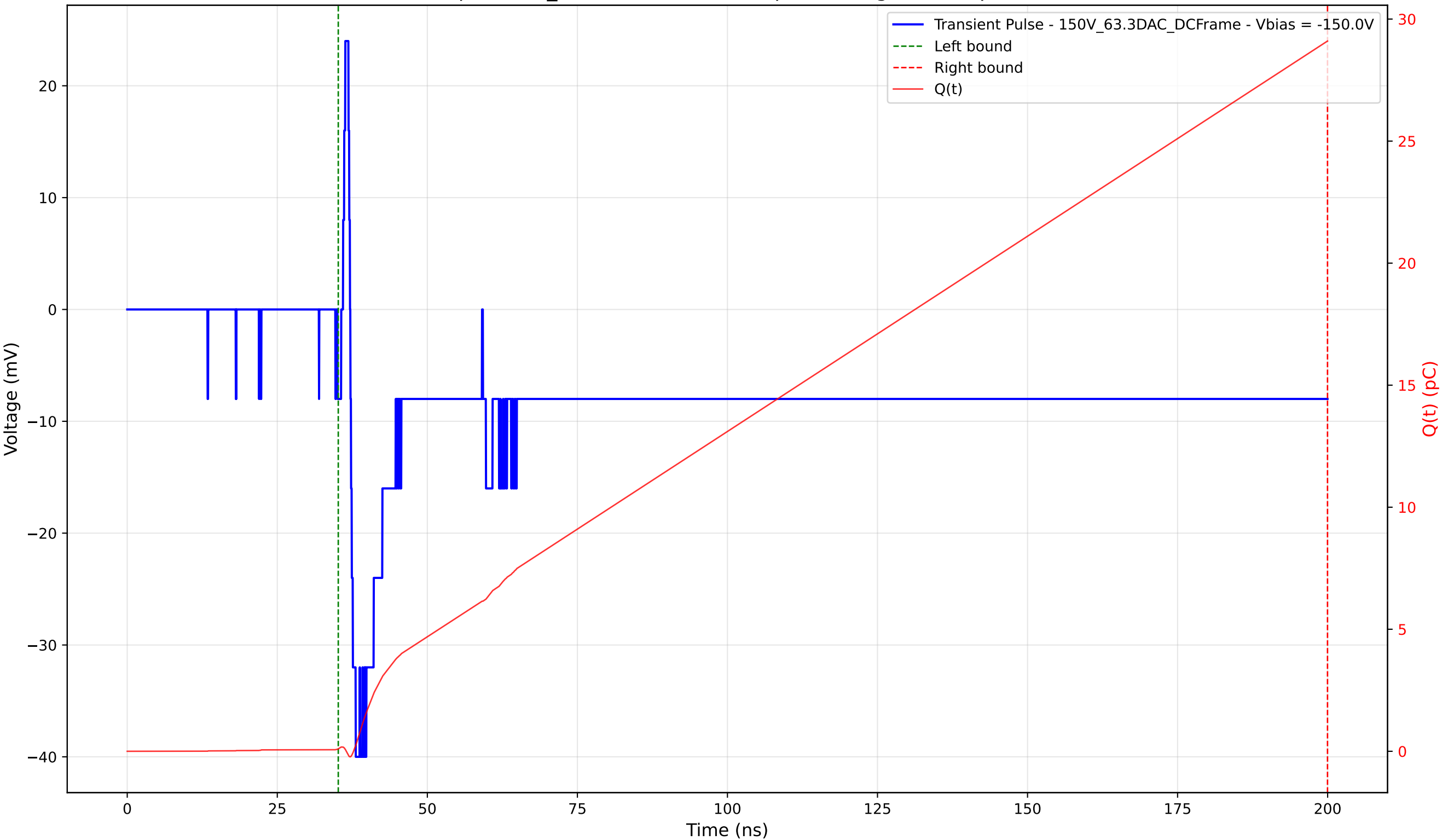
Transient Pulse - Sample: 1cm_42 - Position: 1865.0 \mu\text{m} - Charge: 29.00 pC - Rise Time: 0.89 ns
