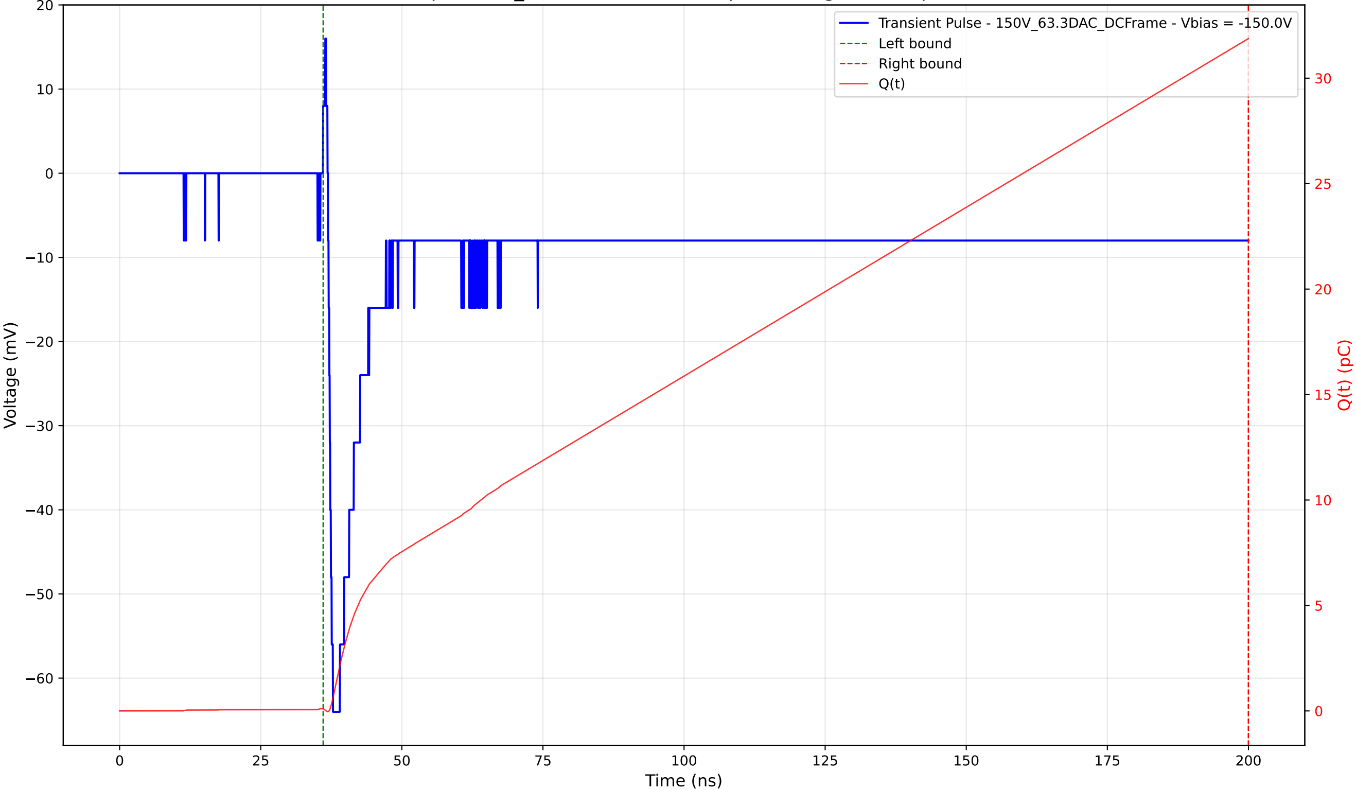
Transient Pulse - Sample: 1cm_42 - Position: 1315.0 \mu\text{m} - Charge: 31.77 pC - Rise Time: 0.86 ns
