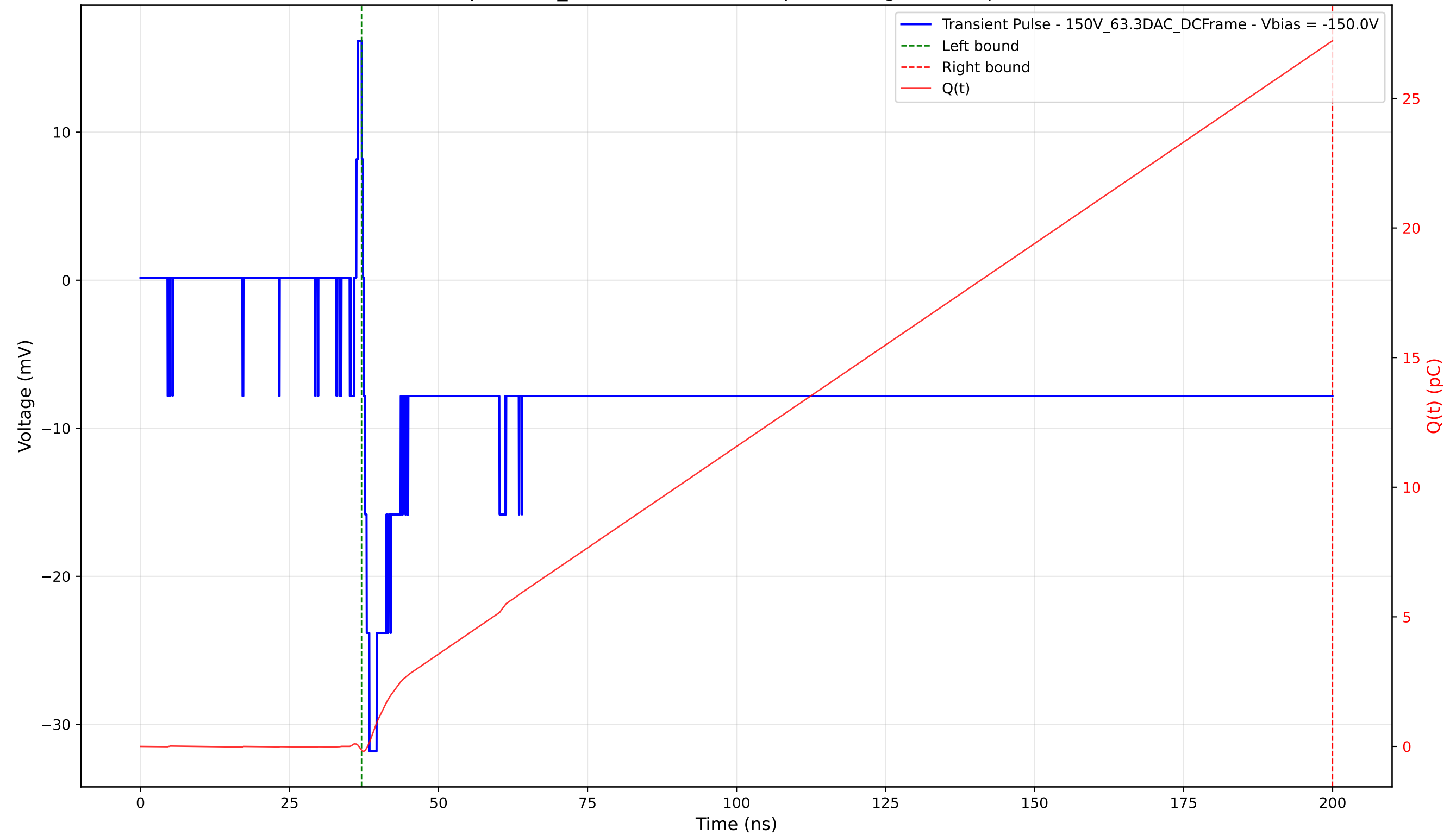
Transient Pulse - Sample: 1cm_42 - Position: 2560.0 \mu\text{m} - Charge: 27.37 pC - Rise Time: 0.93 ns
