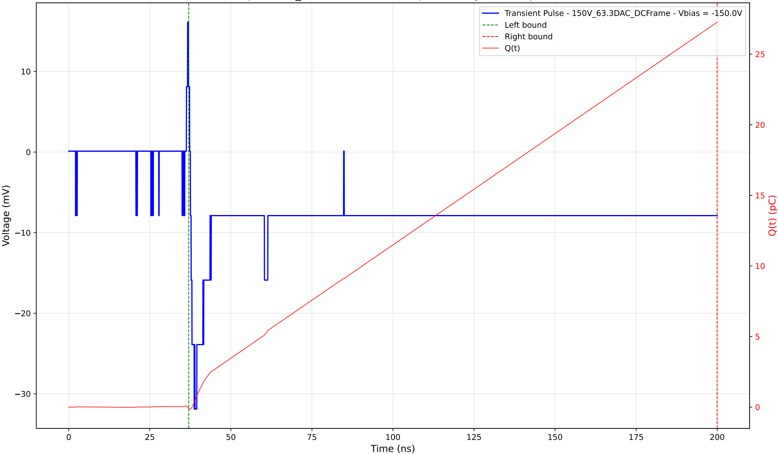
Transient Pulse - Sample: 1cm_42 - Position: 2920.0 \mu\text{m} - Charge: 27.36 pC - Rise Time: 1.17 ns
