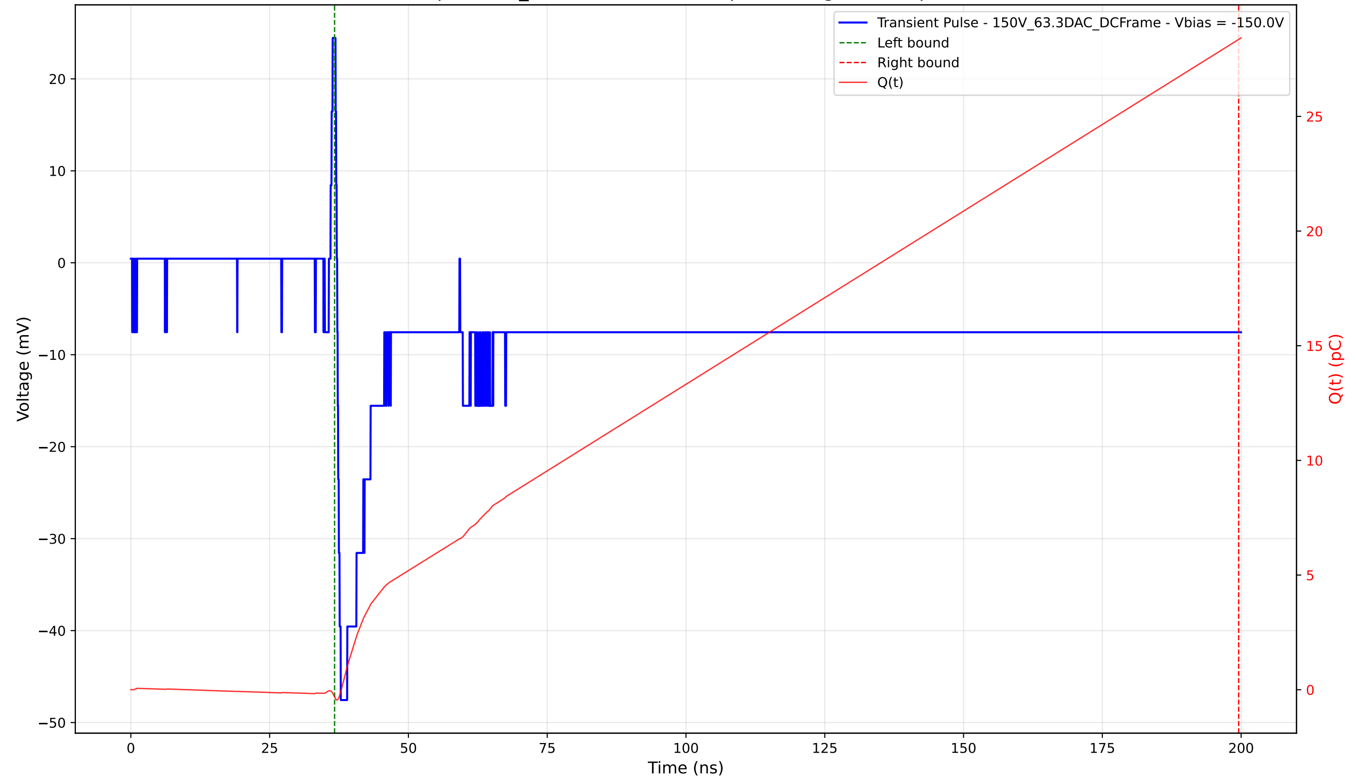
Transient Pulse - Sample: 1cm_42 - Position: 1665.0 \mu\text{m} - Charge: 28.67 pC - Rise Time: 0.63 ns
