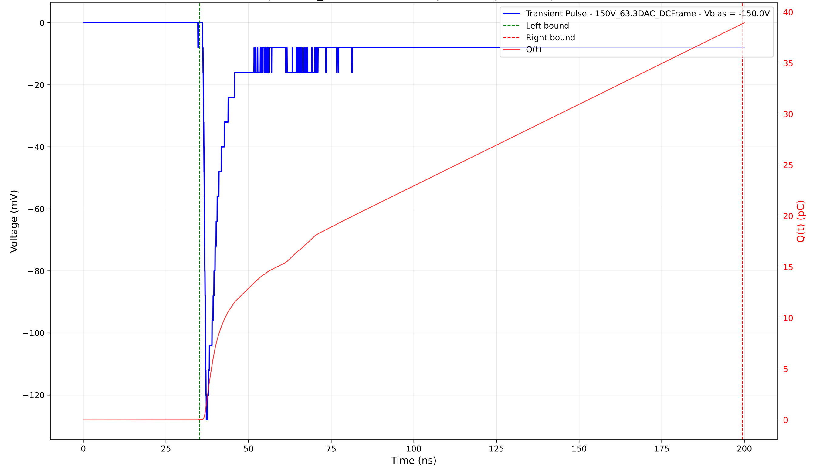
Transient Pulse - Sample: 1cm_42 - Position: 745.0 \mu\text{m} - Charge: 38.82 pC - Rise Time: 0.89 ns
