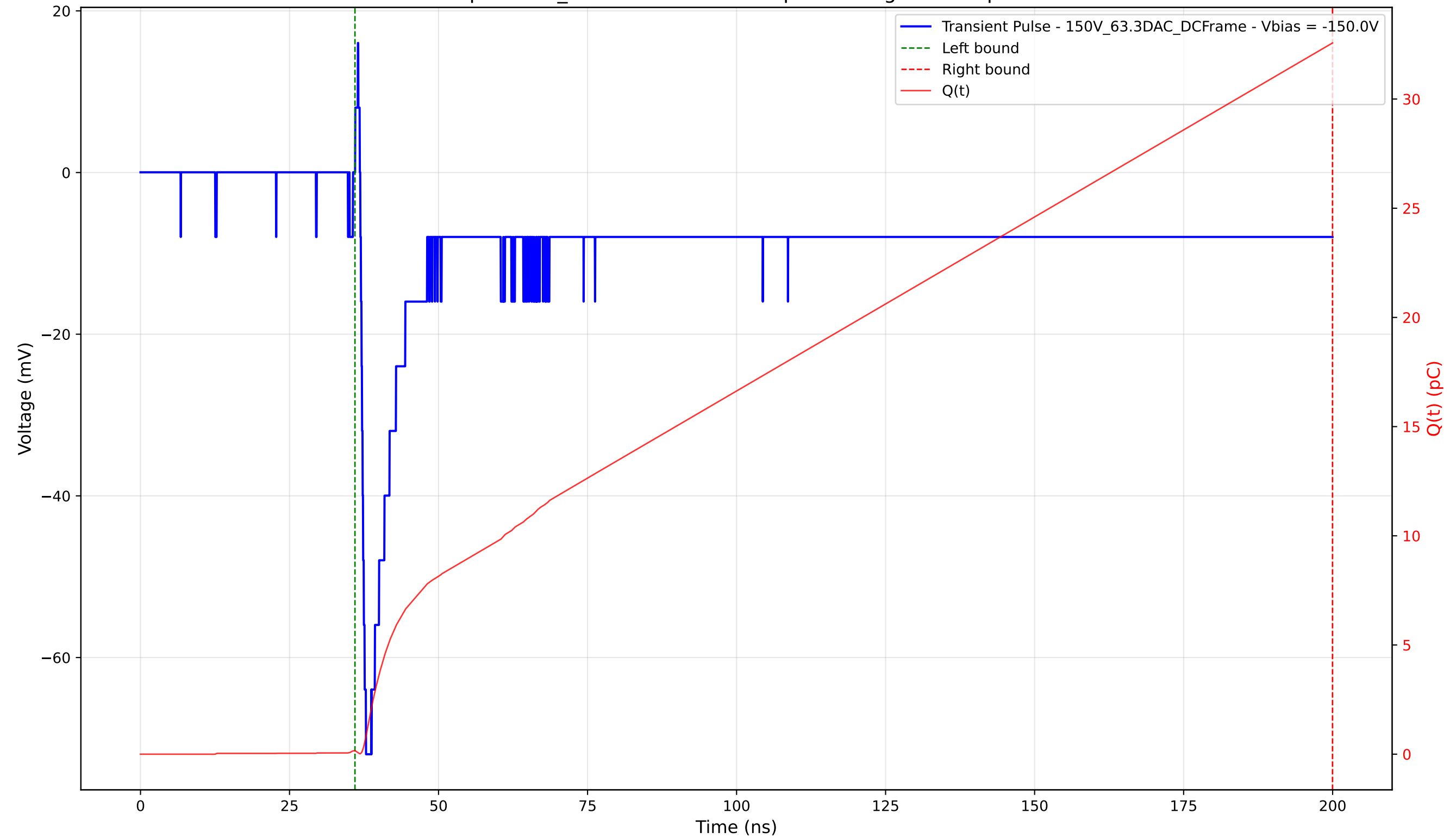
Transient Pulse - Sample: 1cm_42 - Position: 1275.0 \mu\text{m} - Charge: 32.41 pC - Rise Time: 0.94 ns
