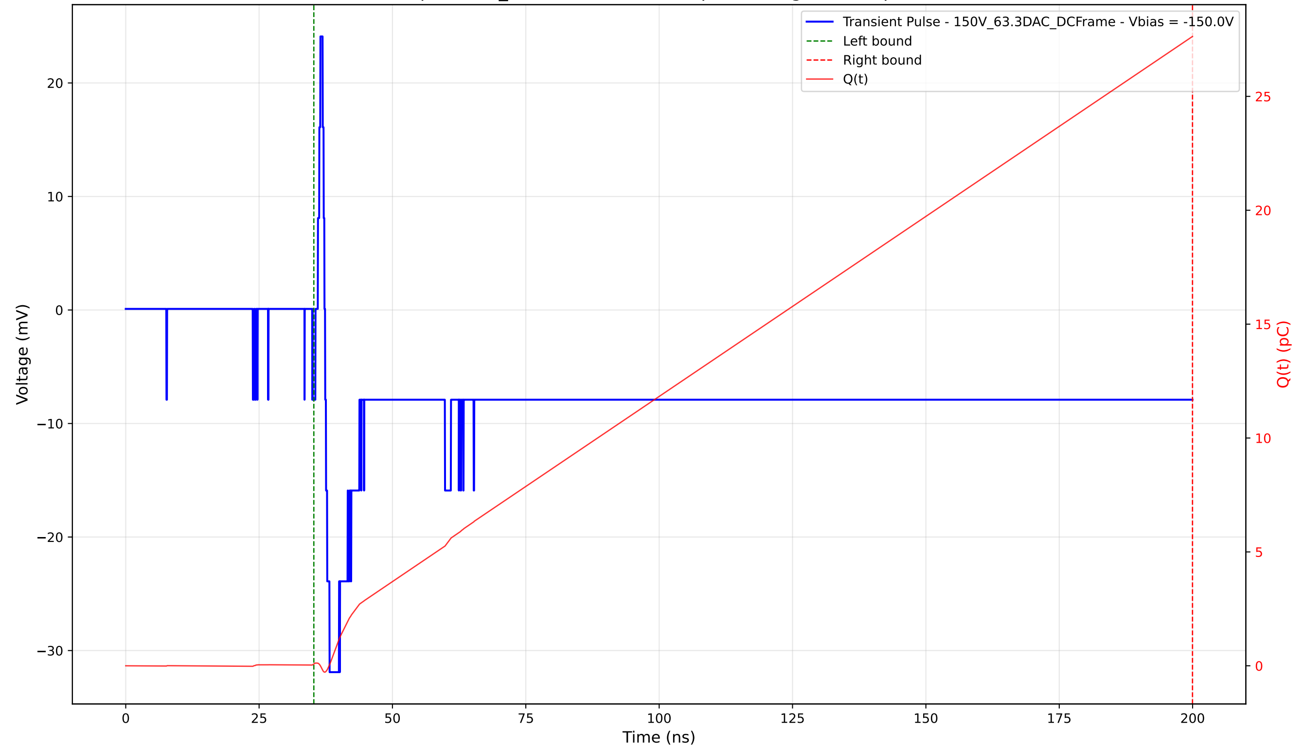
Transient Pulse - Sample: 1cm_42 - Position: 2350.0 \mu\text{m} - Charge: 27.56 pC - Rise Time: 0.83 ns
