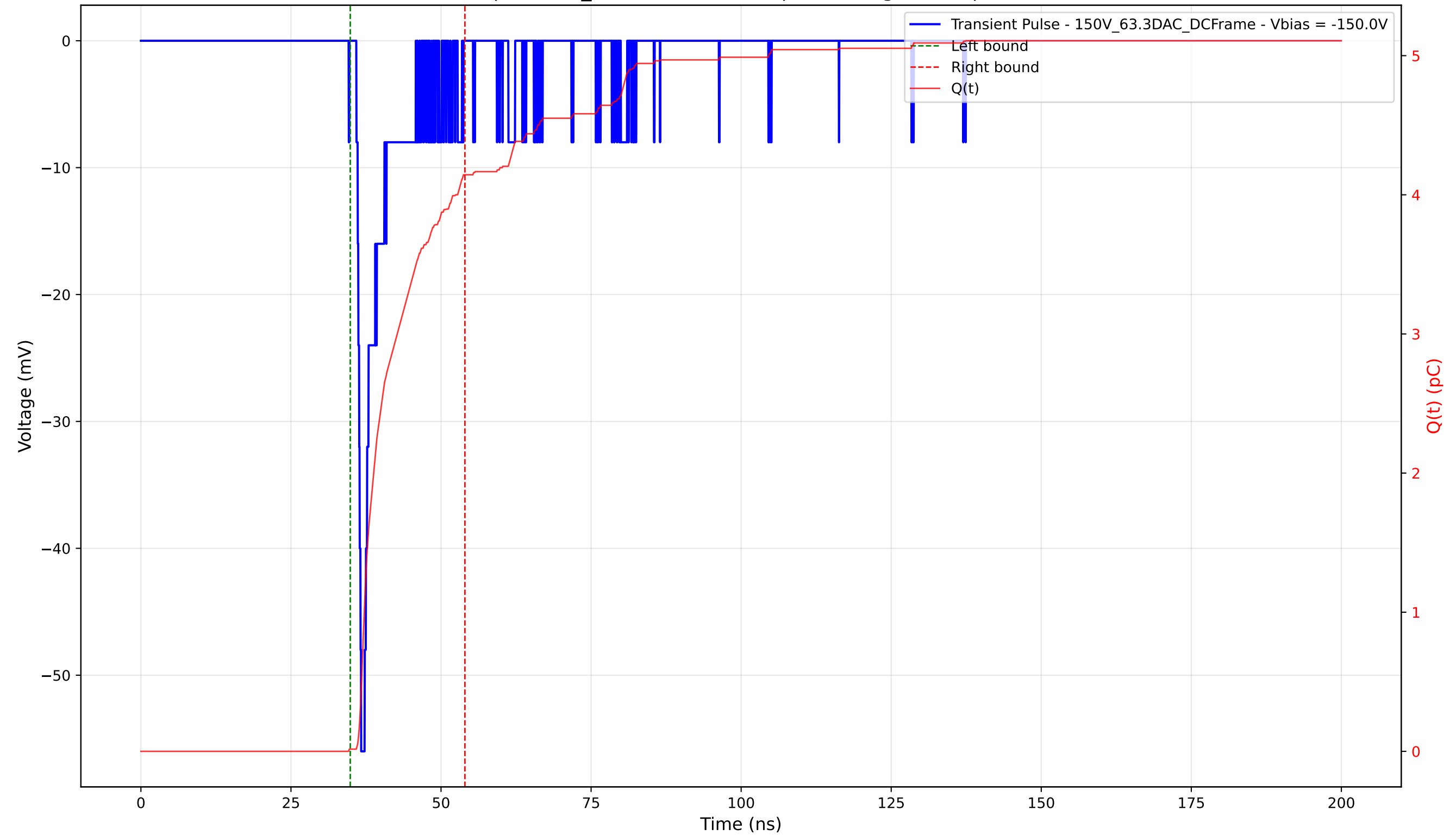
Transient Pulse - Sample: 1cm_42 - Position: 65.0 \mu\text{m} - Charge: 4.13 pC - Rise Time: 0.79 ns
