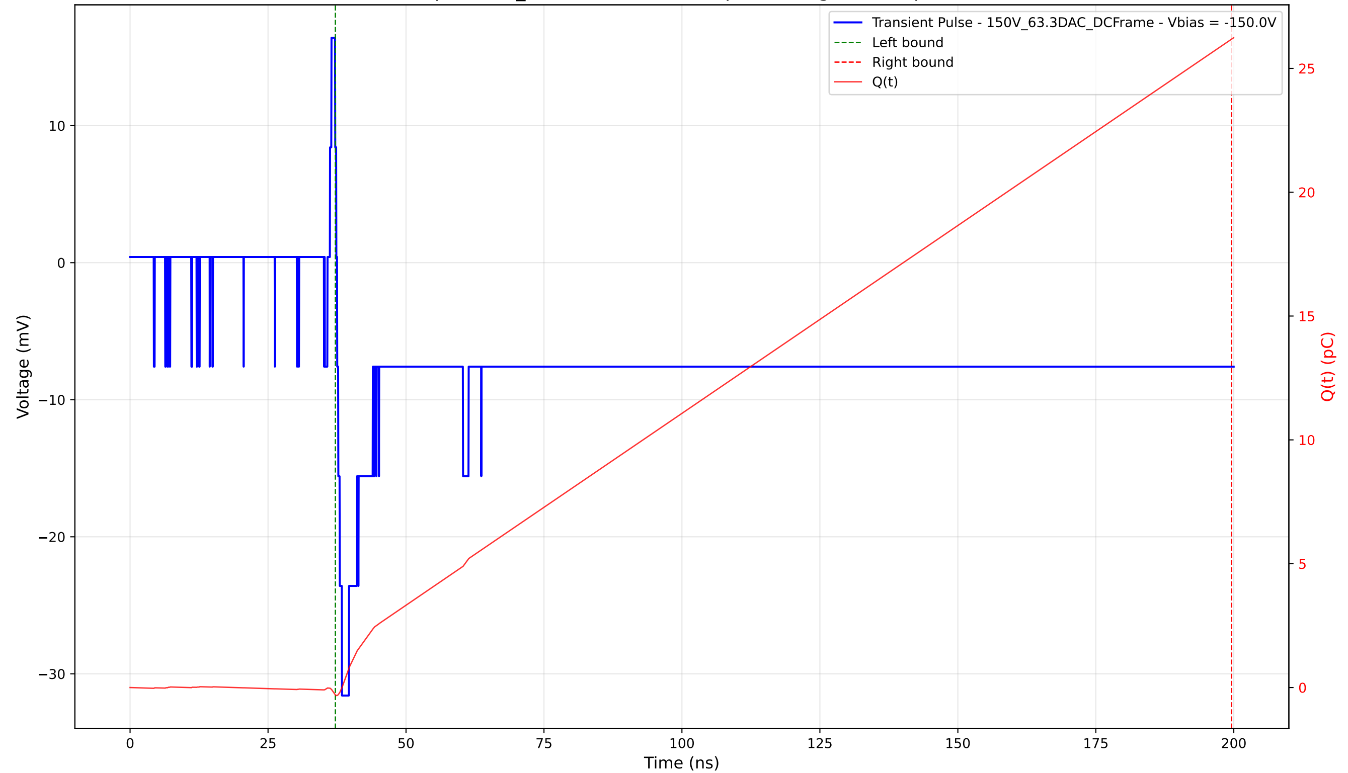
Transient Pulse - Sample: 1cm_42 - Position: 2585.0 \mu\text{m} - Charge: 26.48 pC - Rise Time: 0.87 ns
