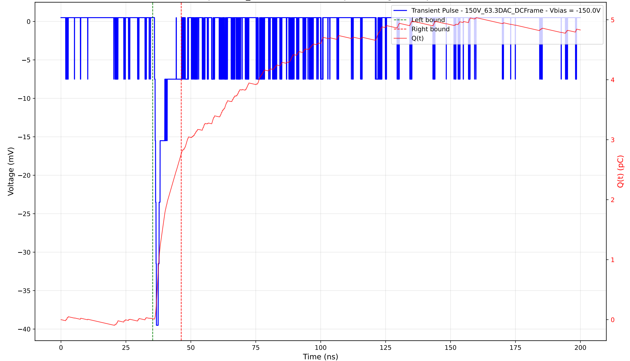
Transient Pulse - Sample: 1cm_42 - Position: 5140.0 \mu\text{m} - Charge: 2.75 pC - Rise Time: 0.73 ns
