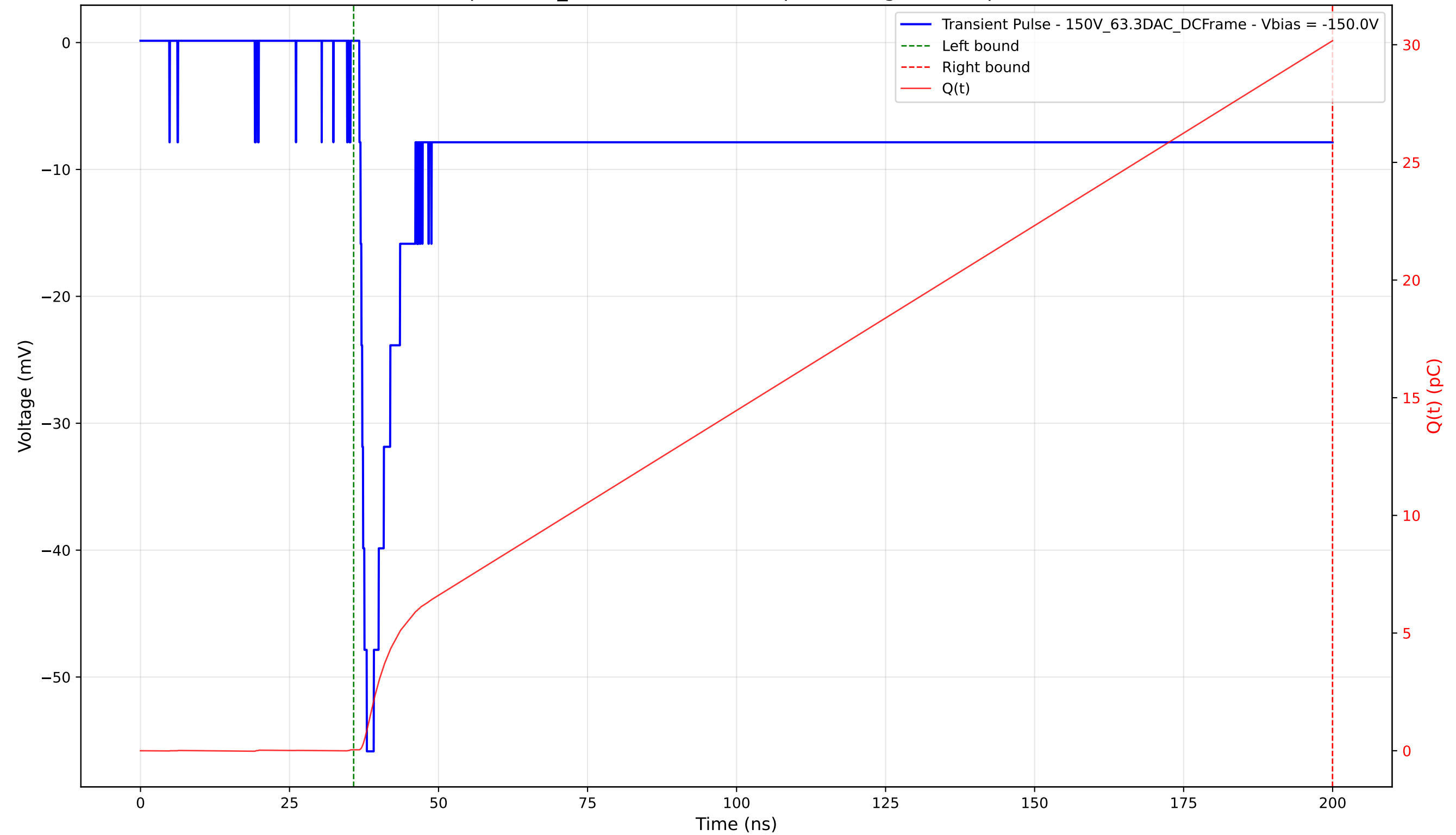
Transient Pulse - Sample: 1cm_42 - Position: 3995.0 \mu\text{m} - Charge: 30.13 pC - Rise Time: 1.25 ns
