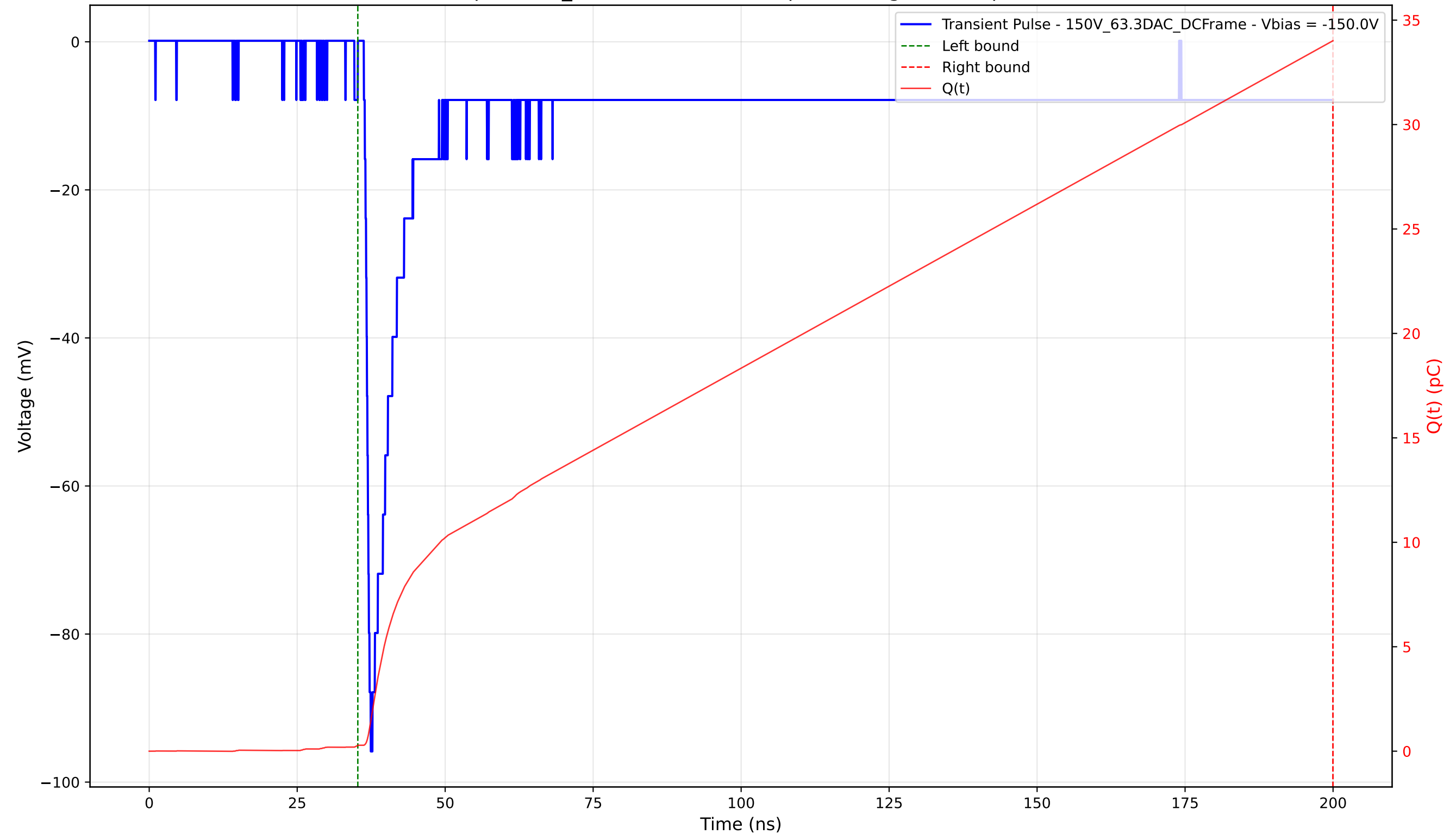
Transient Pulse - Sample: 1cm_42 - Position: 4380.0 \mu\text{m} - Charge: 33.73 pC - Rise Time: 0.82 ns
