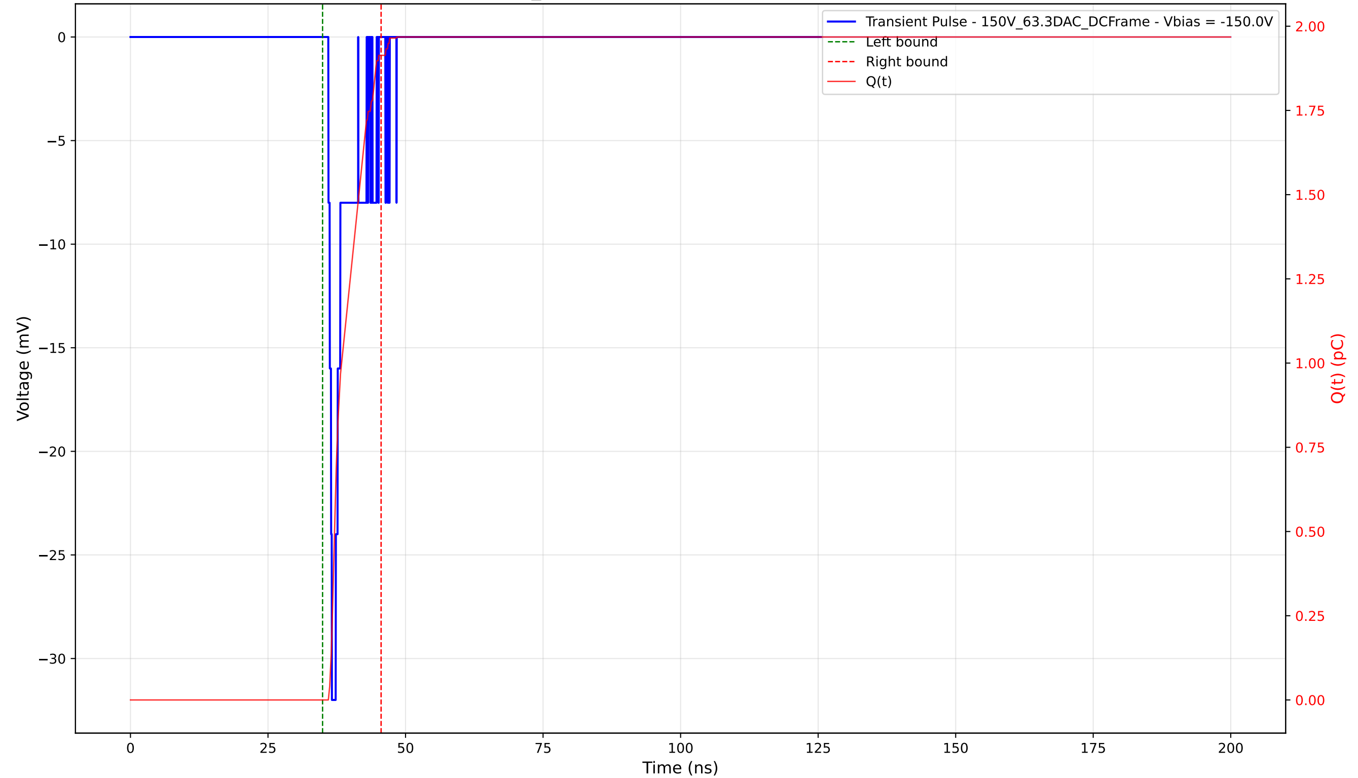
Transient Pulse - Sample: 1cm_42 - Position: 20.0 \mu\text{m} - Charge: 1.91 pC - Rise Time: 0.63 ns
