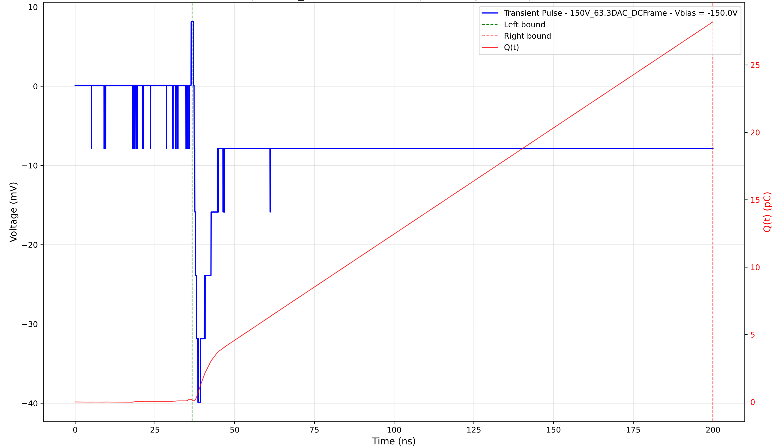
Transient Pulse - Sample: 1cm_42 - Position: 3450.0 \mu\text{m} - Charge: 28.05 pC - Rise Time: 1.17 ns
