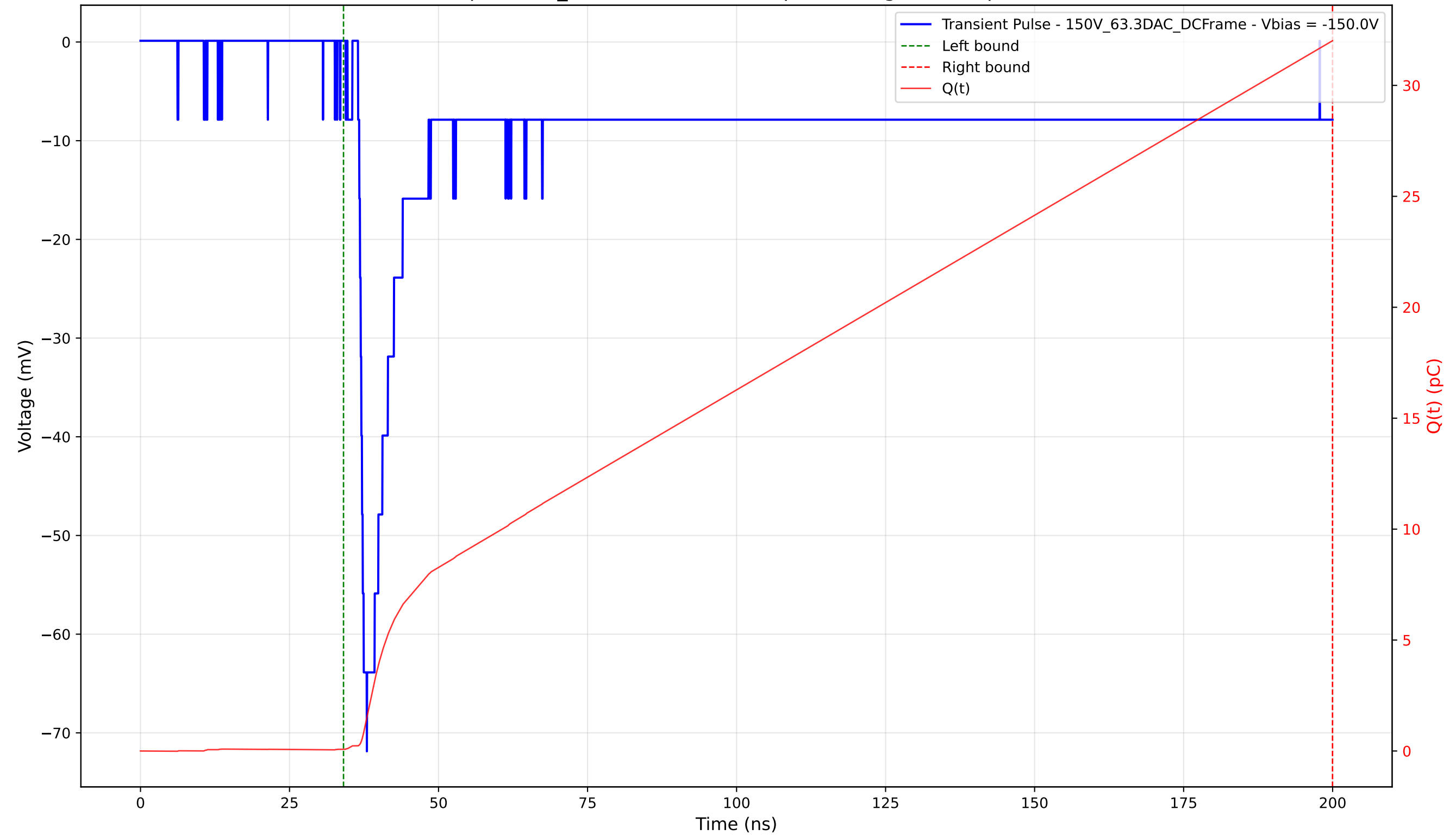
Transient Pulse - Sample: 1cm_42 - Position: 4110.0 \mu\text{m} - Charge: 31.93 pC - Rise Time: 1.46 ns
