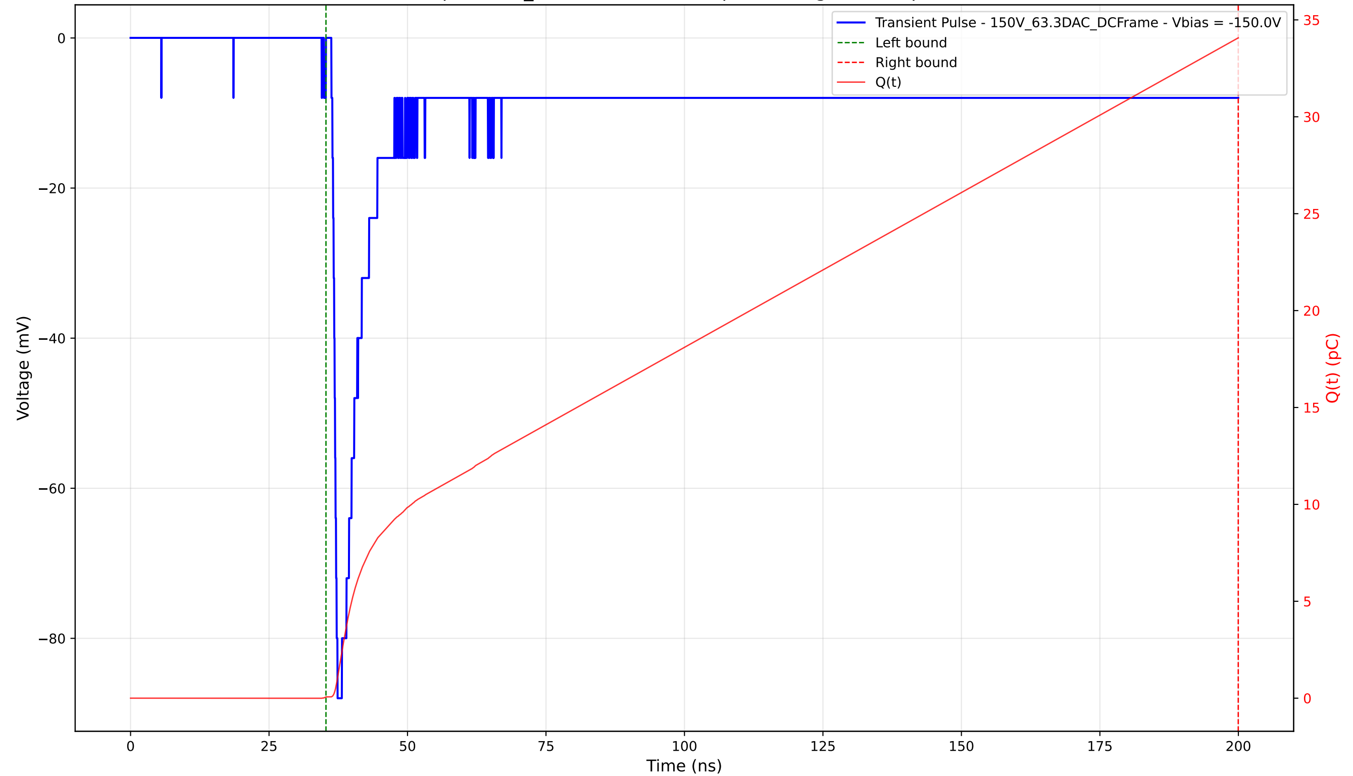
Transient Pulse - Sample: 1cm_42 - Position: 905.0 \mu\text{m} - Charge: 34.01 pC - Rise Time: 0.78 ns
