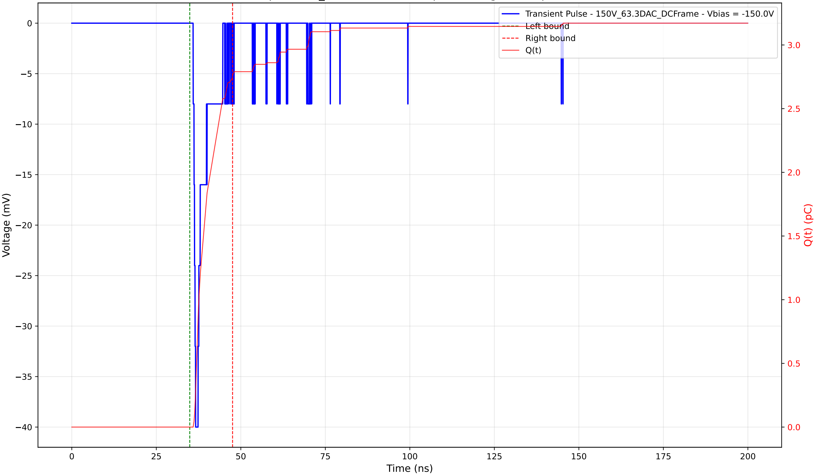
Transient Pulse - Sample: 1cm_42 - Position: 40.0 \mu\text{m} - Charge: 2.76 pC - Rise Time: 0.73 ns
