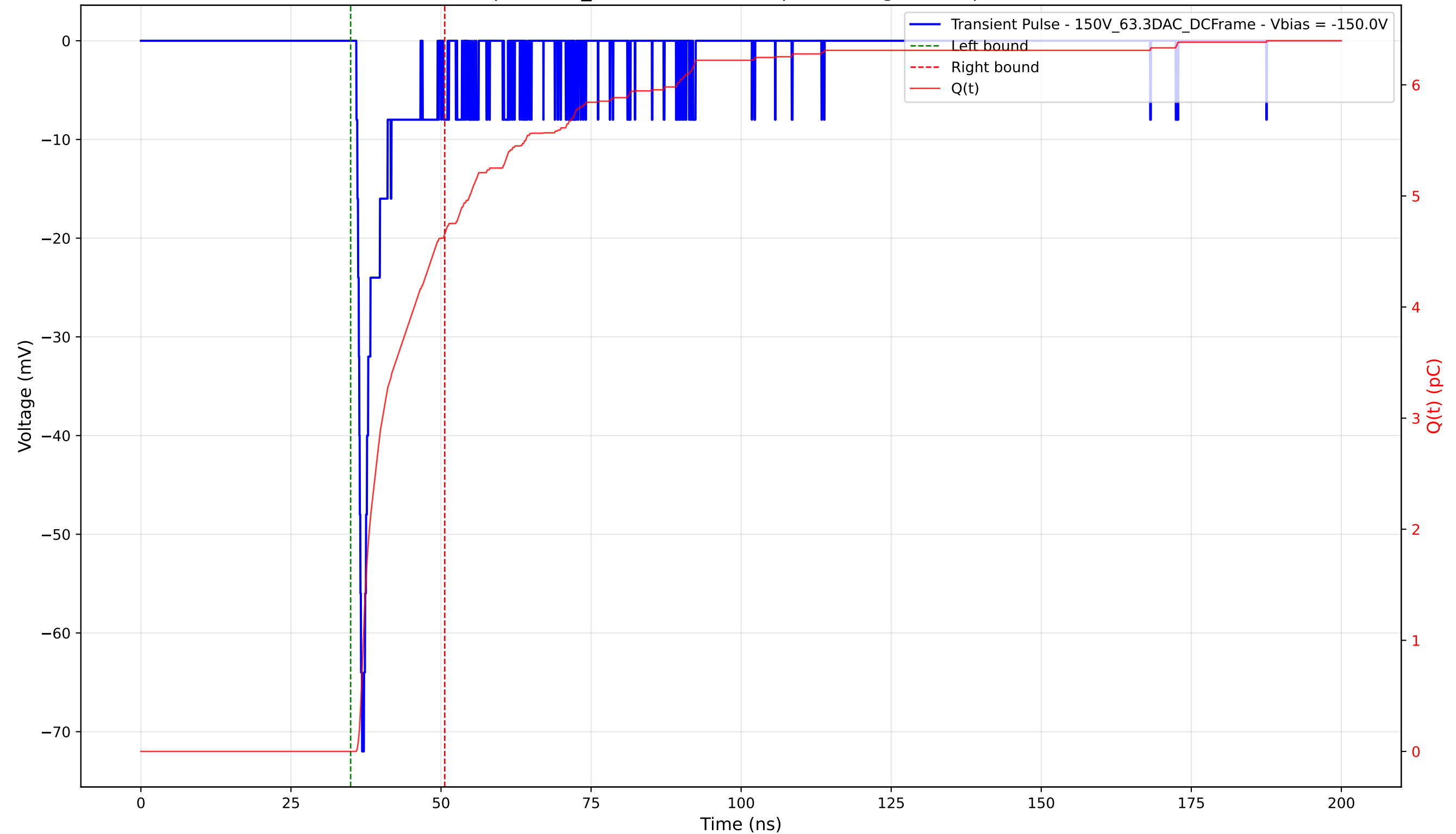
Transient Pulse - Sample: 1cm_42 - Position: 85.0 \mu\text{m} - Charge: 4.66 pC - Rise Time: 0.94 ns
