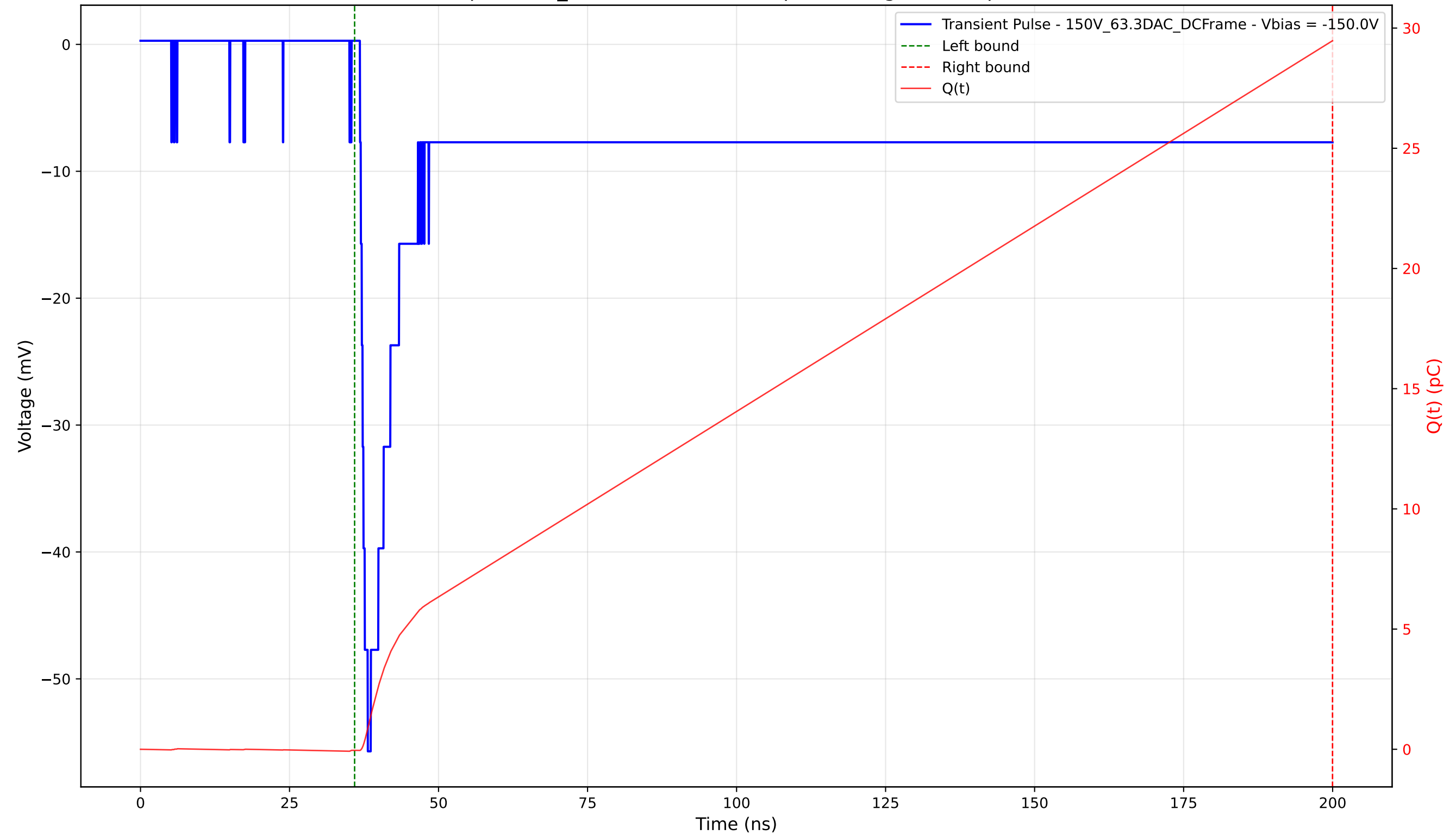
Transient Pulse - Sample: 1cm_42 - Position: 3955.0 \mu\text{m} - Charge: 29.52 pC - Rise Time: 1.31 ns
