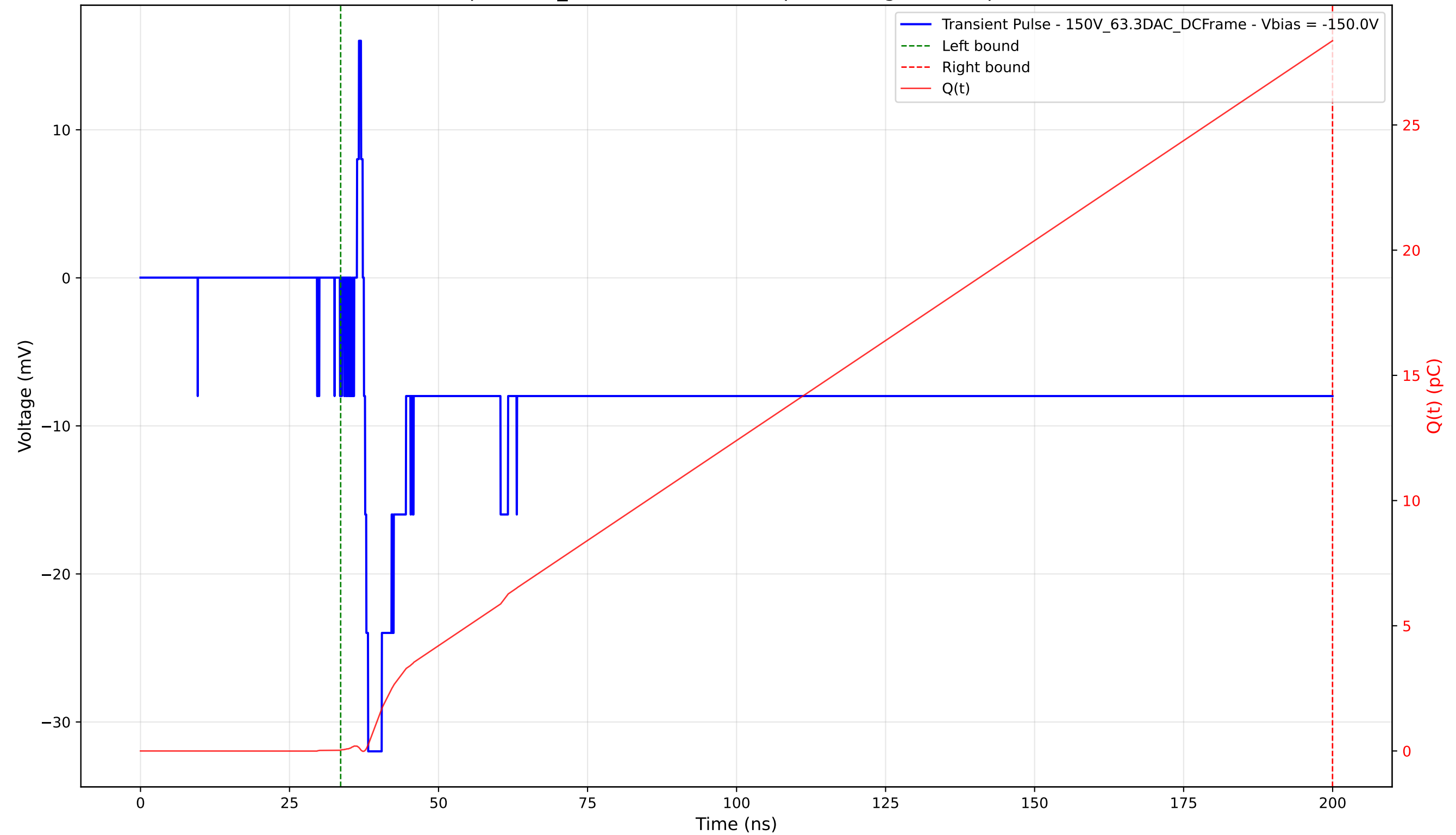
Transient Pulse - Sample: 1cm_42 - Position: 3150.0 \mu\text{m} - Charge: 28.32 pC - Rise Time: 0.71 ns
