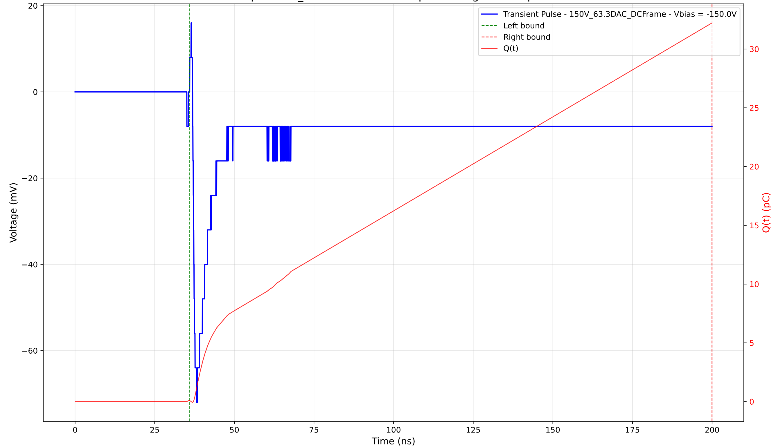
Transient Pulse - Sample: 1cm_42 - Position: 1300.0 \mu\text{m} - Charge: 32.14 pC - Rise Time: 1.16 ns
