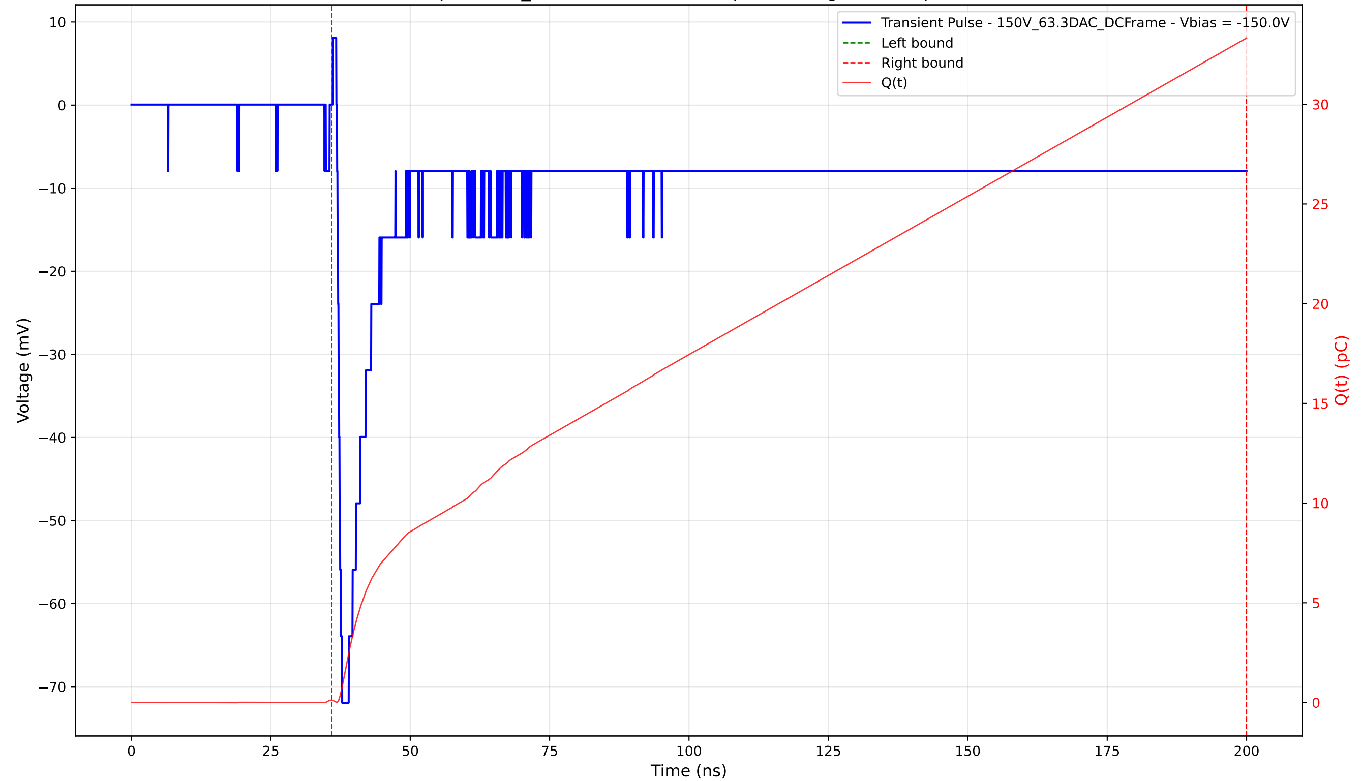
Transient Pulse - Sample: 1cm_42 - Position: 1195.0 \mu\text{m} - Charge: 33.20 pC - Rise Time: 0.90 ns
