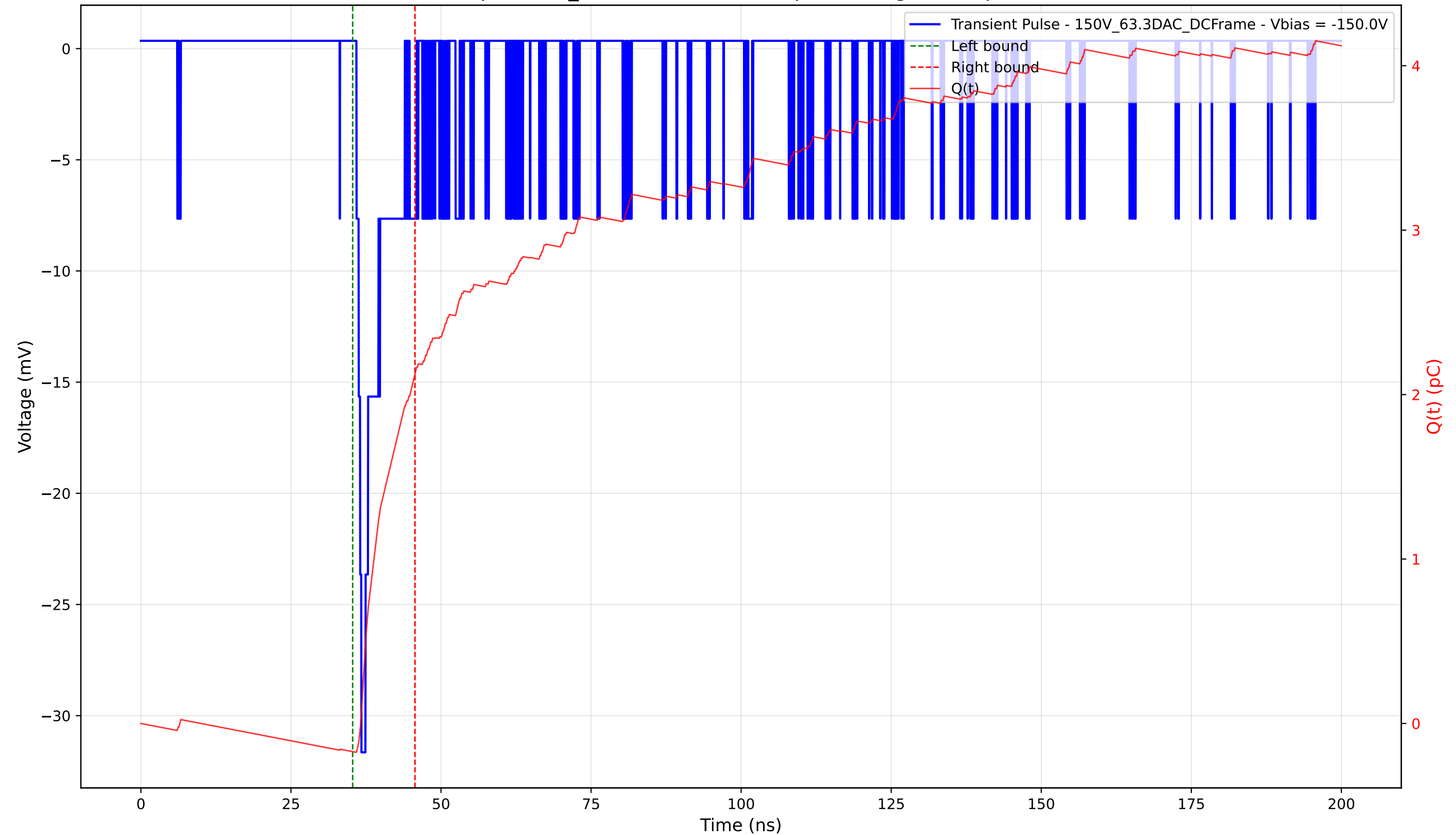
Transient Pulse - Sample: 1cm_42 - Position: 5160.0 \mu\text{m} - Charge: 2.30 pC - Rise Time: 0.81 ns
