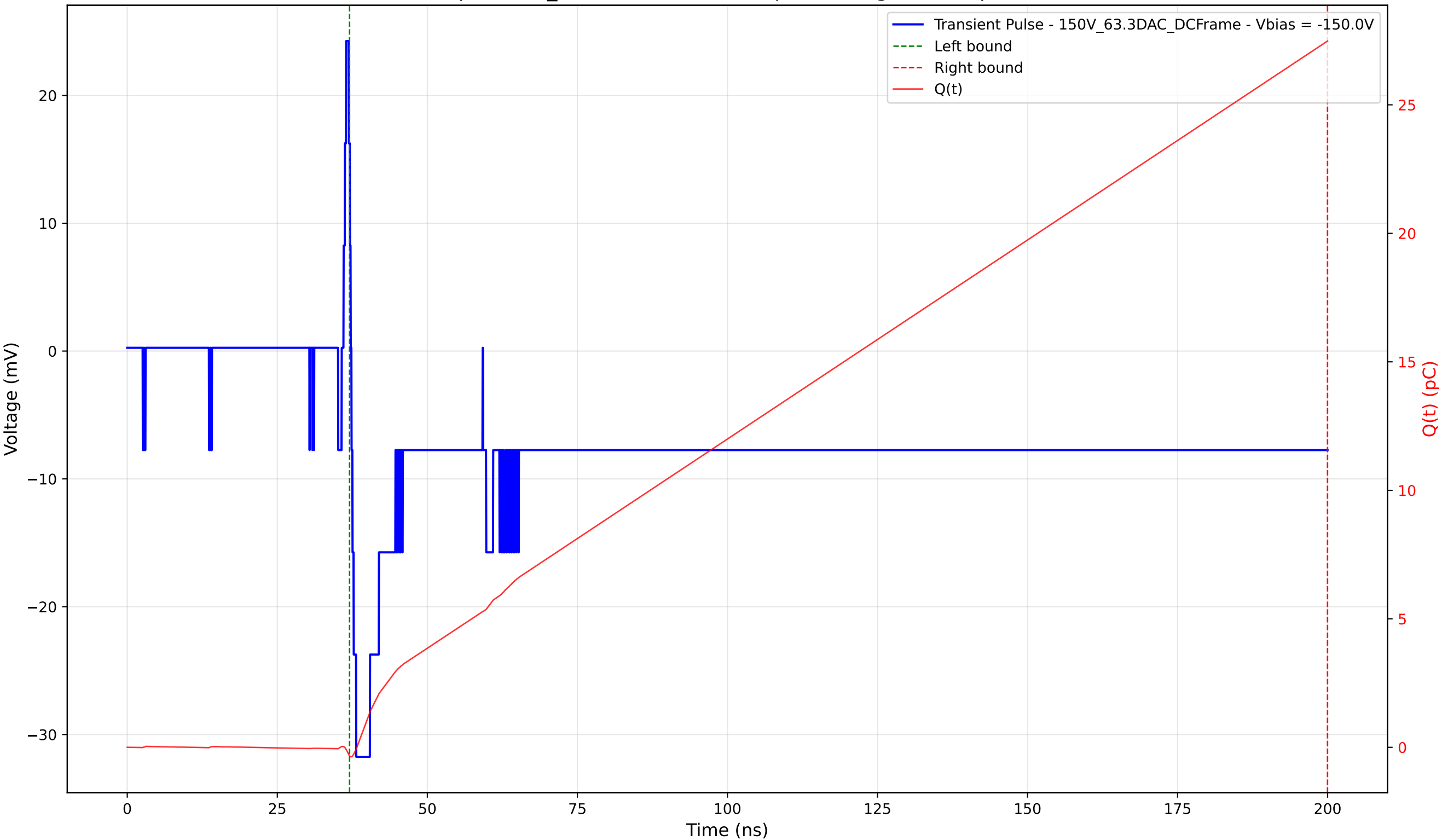
Transient Pulse - Sample: 1cm_42 - Position: 2325.0 \mu\text{m} - Charge: 27.82 pC - Rise Time: 0.79 ns
