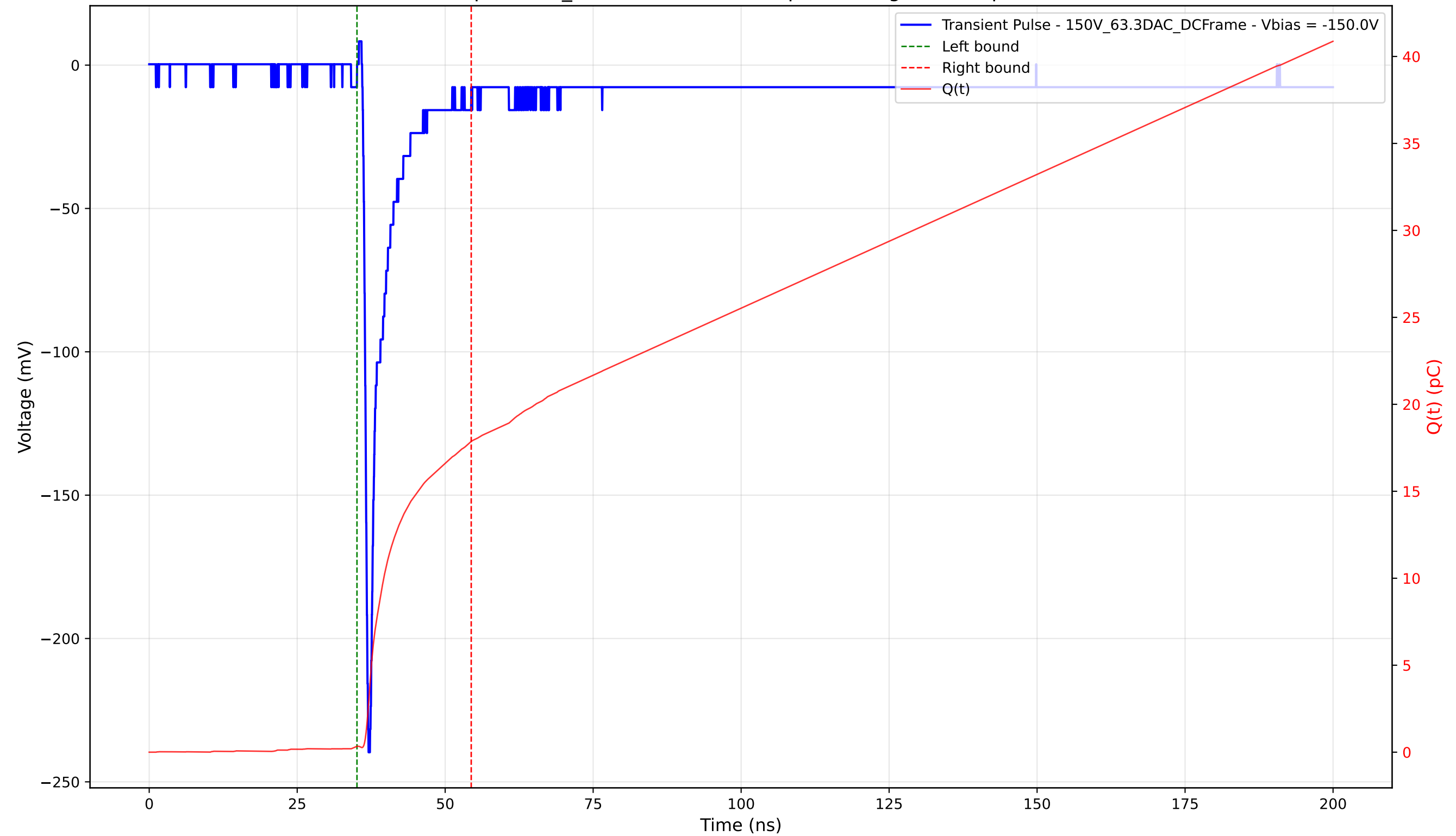
Transient Pulse - Sample: 1cm_42 - Position: 4760.0 \mu\text{m} - Charge: 17.53 pC - Rise Time: 0.80 ns
