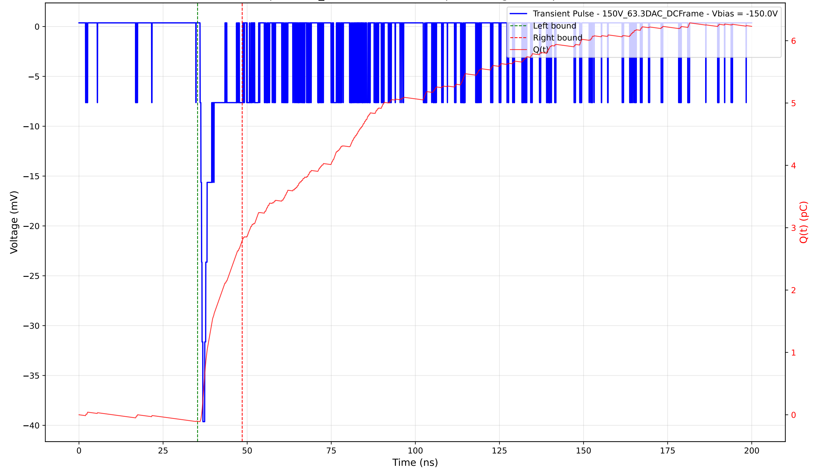
Transient Pulse - Sample: 1cm_42 - Position: 5145.0 \mu\text{m} - Charge: 2.90 pC - Rise Time: 0.83 ns
