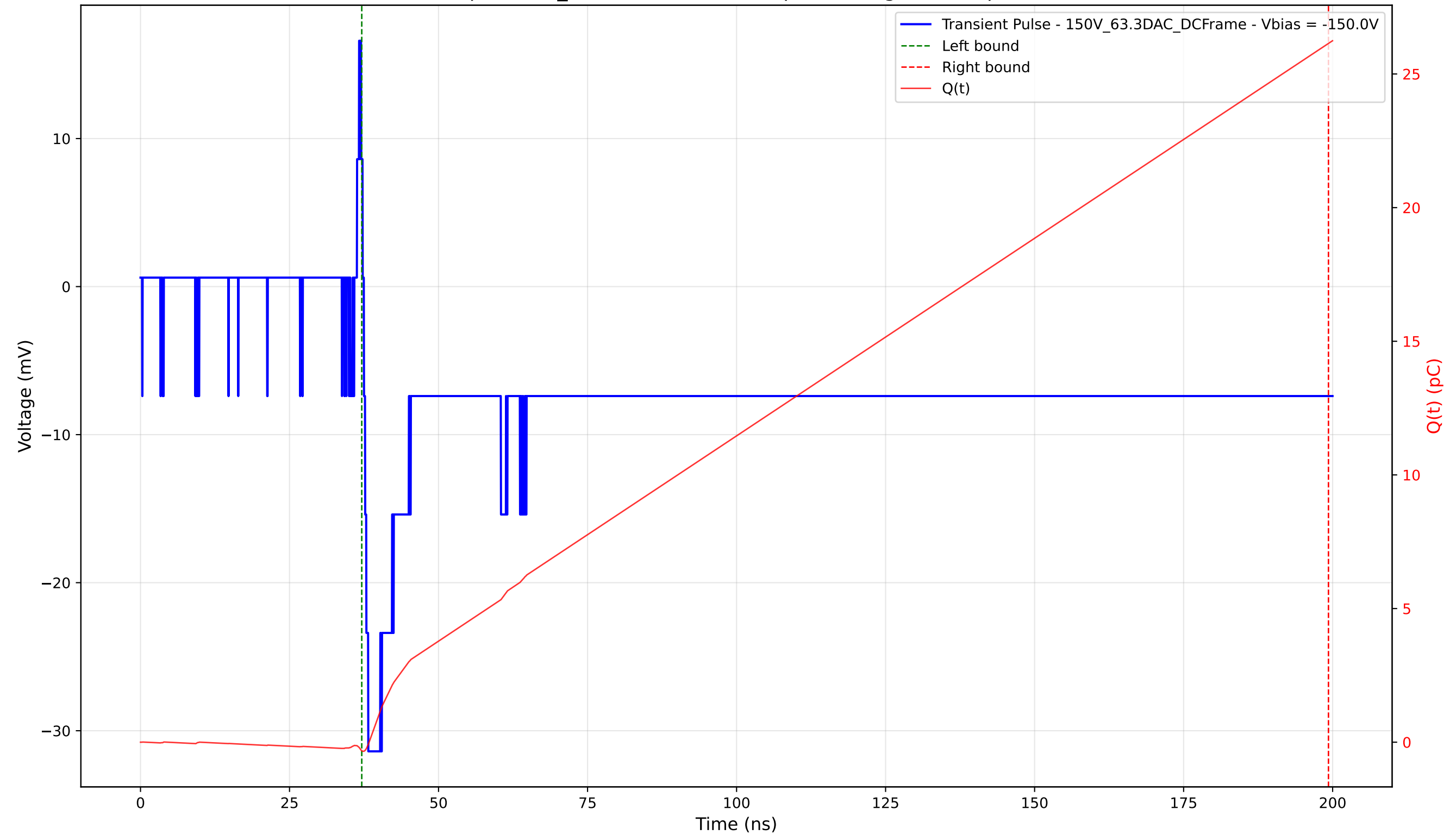
Transient Pulse - Sample: 1cm_42 - Position: 3130.0 \mu\text{m} - Charge: 26.46 pC - Rise Time: 0.73 ns
