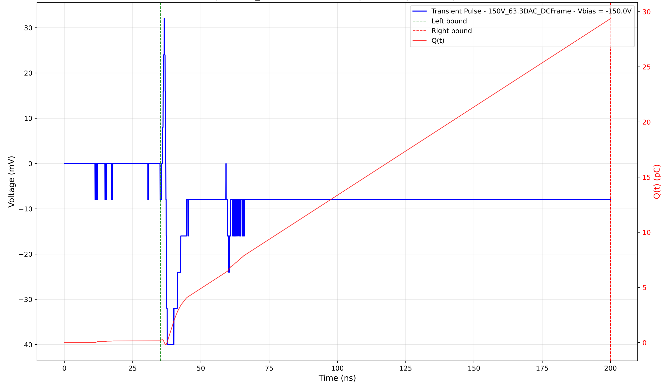
Transient Pulse - Sample: 1cm_42 - Position: 1825.0 \mu\text{m} - Charge: 29.19 pC - Rise Time: 0.49 ns
