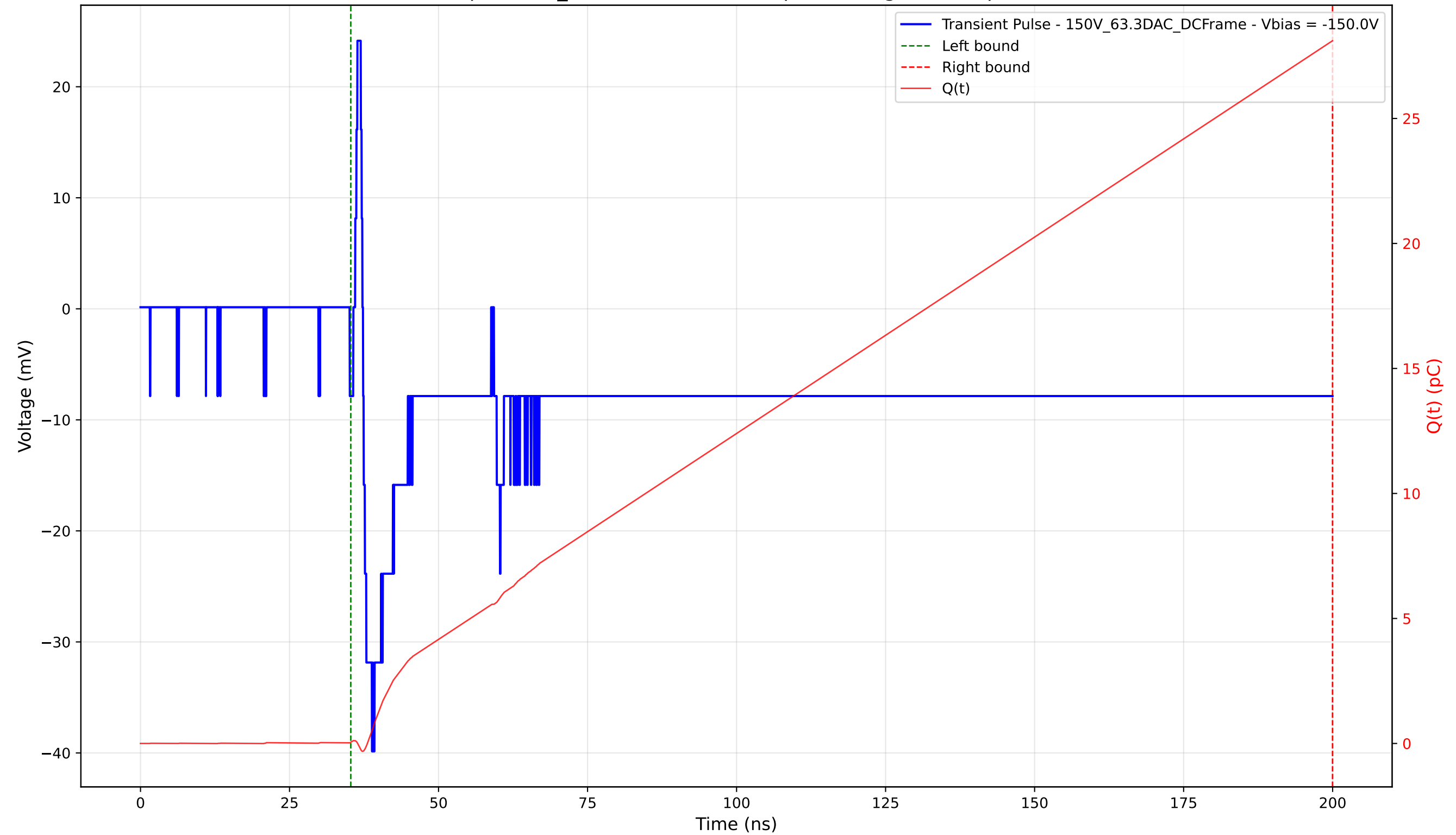
Transient Pulse - Sample: 1cm_42 - Position: 2270.0 \mu\text{m} - Charge: 28.06 pC - Rise Time: 1.49 ns
