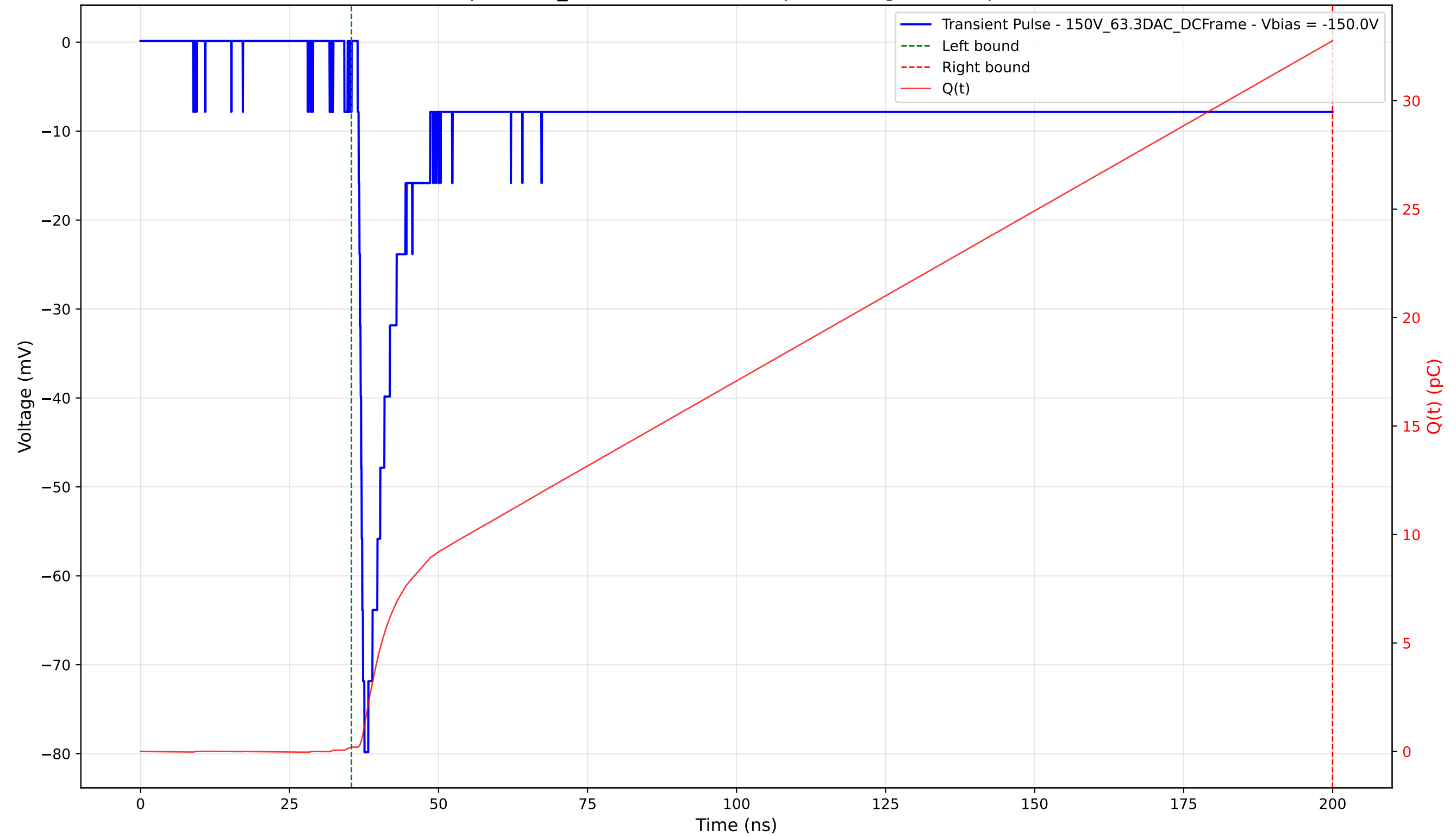
Transient Pulse - Sample: 1cm_42 - Position: 4165.0 \mu\text{m} - Charge: 32.56 pC - Rise Time: 0.98 ns
