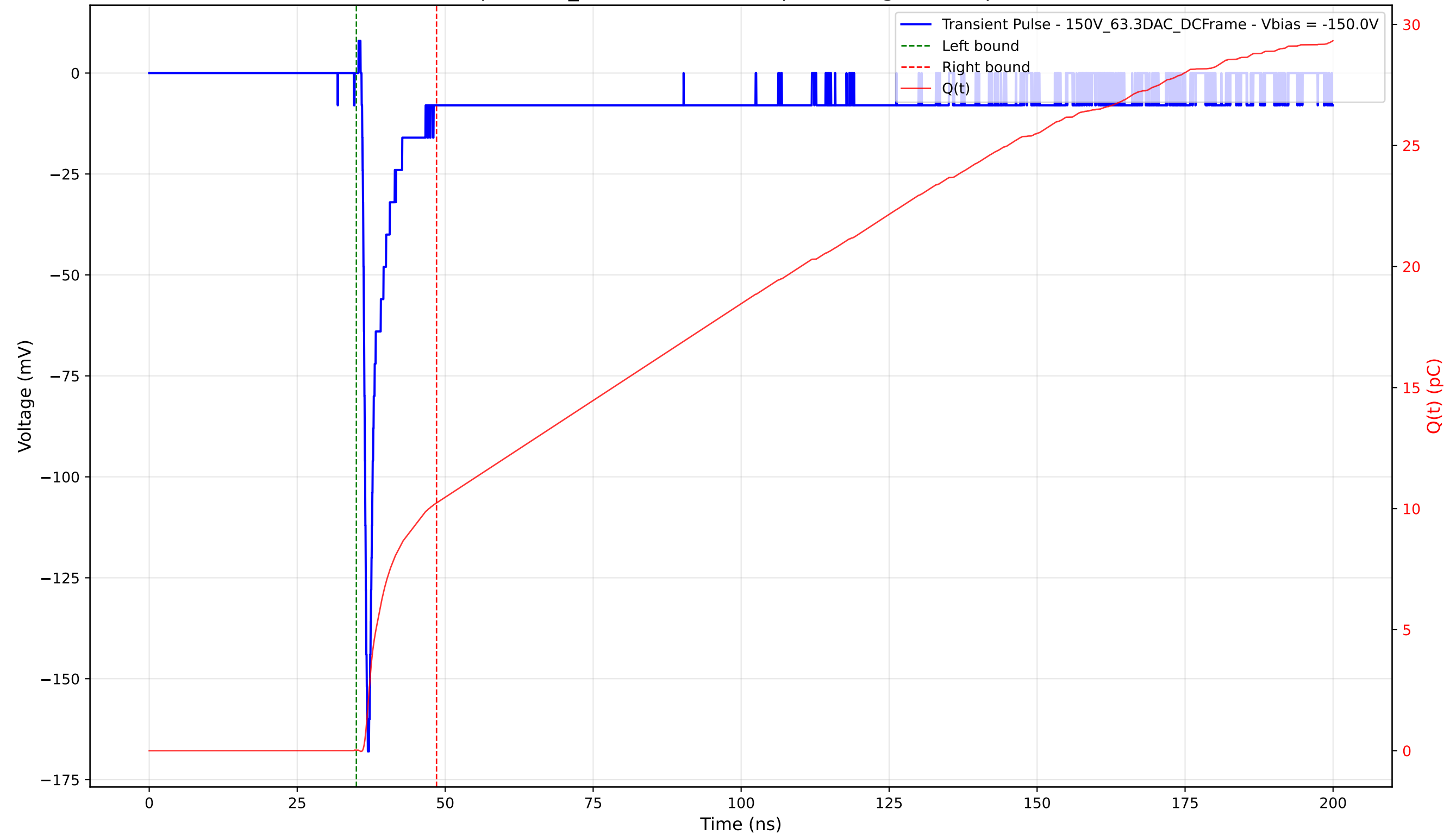
Transient Pulse - Sample: 1cm_42 - Position: 255.0 \mu\text{m} - Charge: 10.21 pC - Rise Time: 0.72 ns
