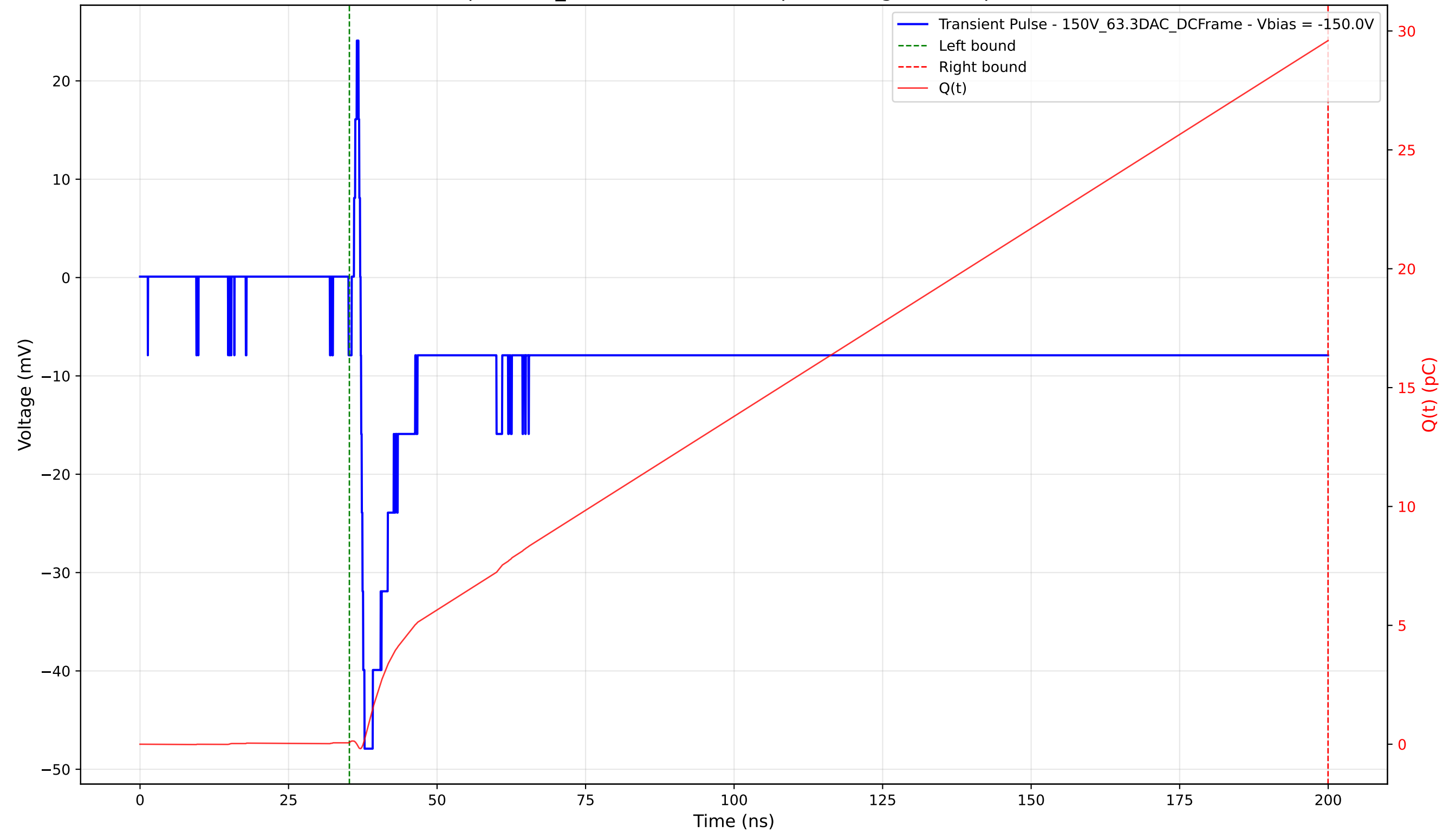
Transient Pulse - Sample: 1cm_42 - Position: 1550.0 \mu\text{m} - Charge: 29.52 pC - Rise Time: 0.65 ns
