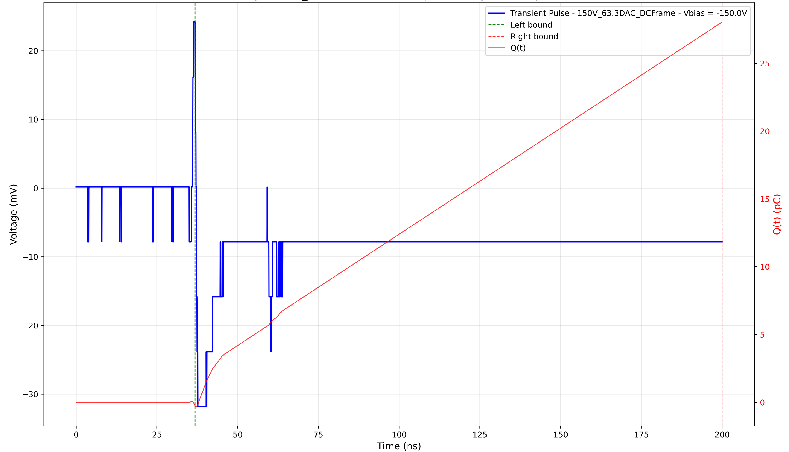
Transient Pulse - Sample: 1cm_42 - Position: 1970.0 \mu\text{m} - Charge: 28.29 pC - Rise Time: 0.45 ns
