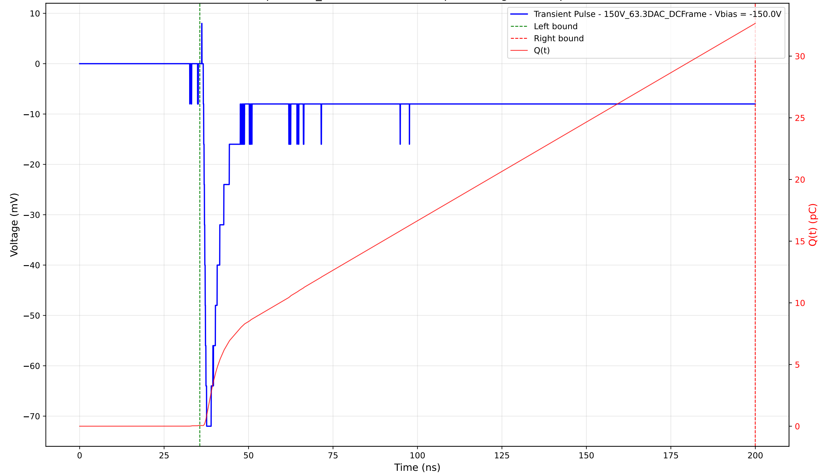
Transient Pulse - Sample: 1cm_42 - Position: 1040.0 \mu\text{m} - Charge: 32.59 pC - Rise Time: 0.98 ns
