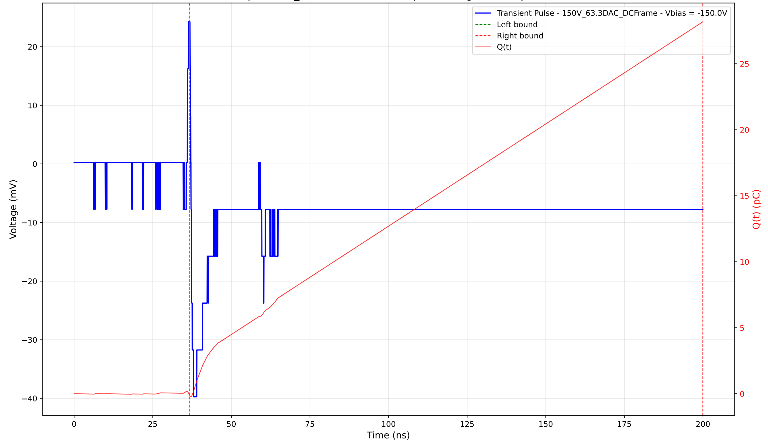
Transient Pulse - Sample: 1cm_42 - Position: 1885.0 \mu\text{m} - Charge: 28.32 pC - Rise Time: 0.85 ns
