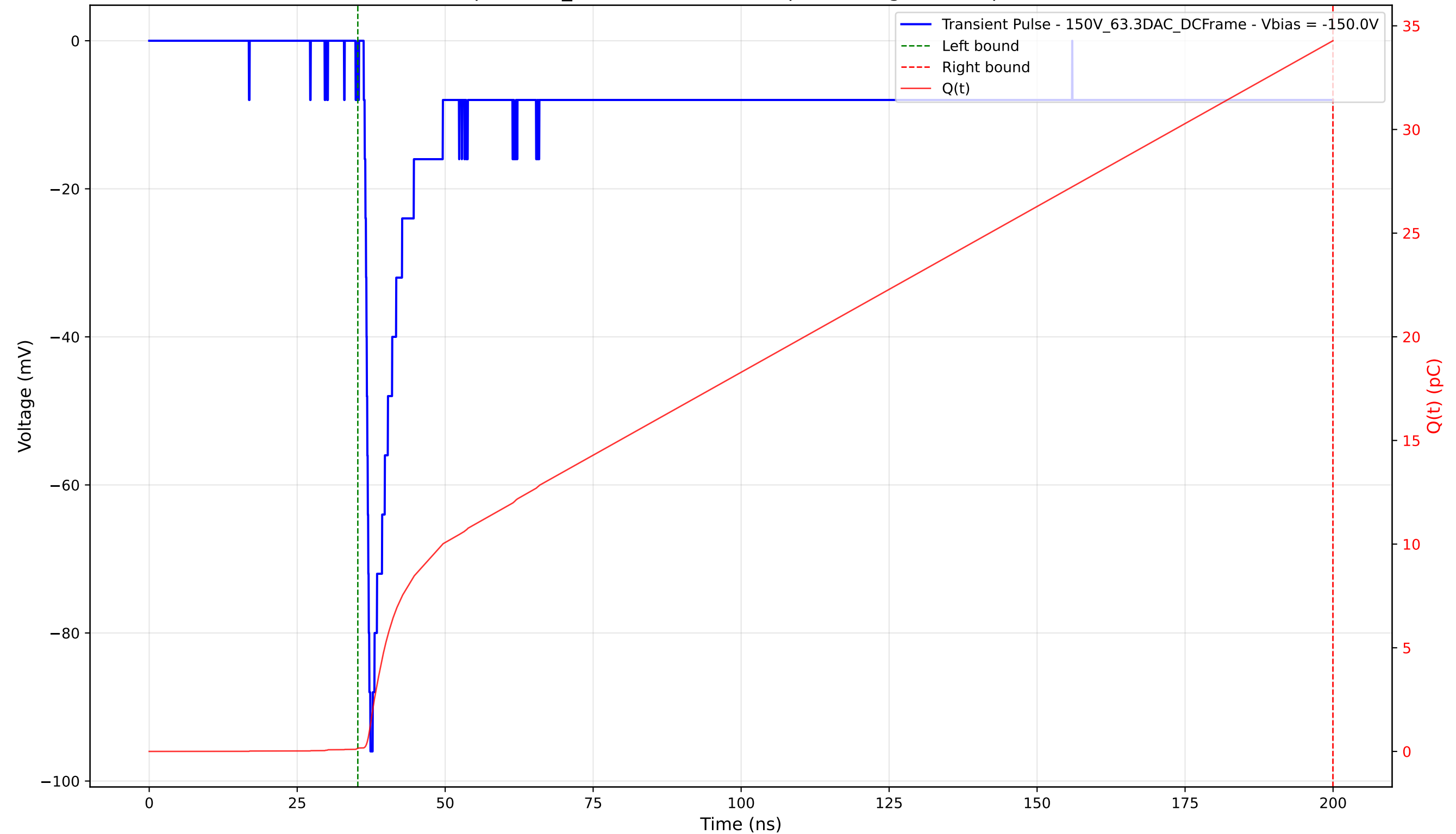
Transient Pulse - Sample: 1cm_42 - Position: 4405.0 \mu\text{m} - Charge: 34.13 pC - Rise Time: 0.80 ns
