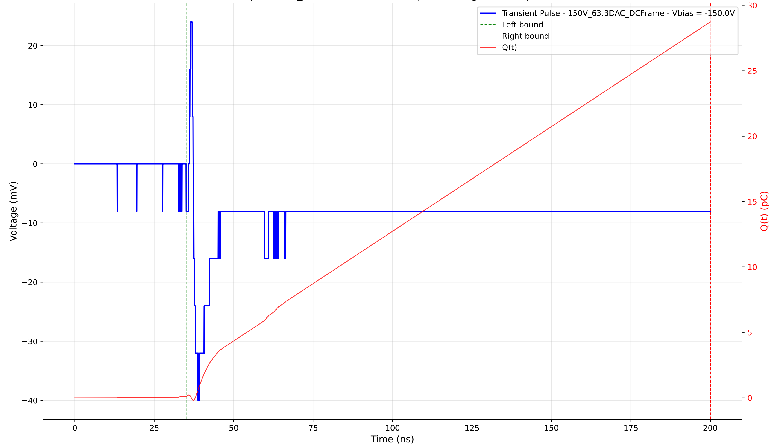
Transient Pulse - Sample: 1cm_42 - Position: 2260.0 \mu\text{m} - Charge: 28.59 pC - Rise Time: 1.35 ns
