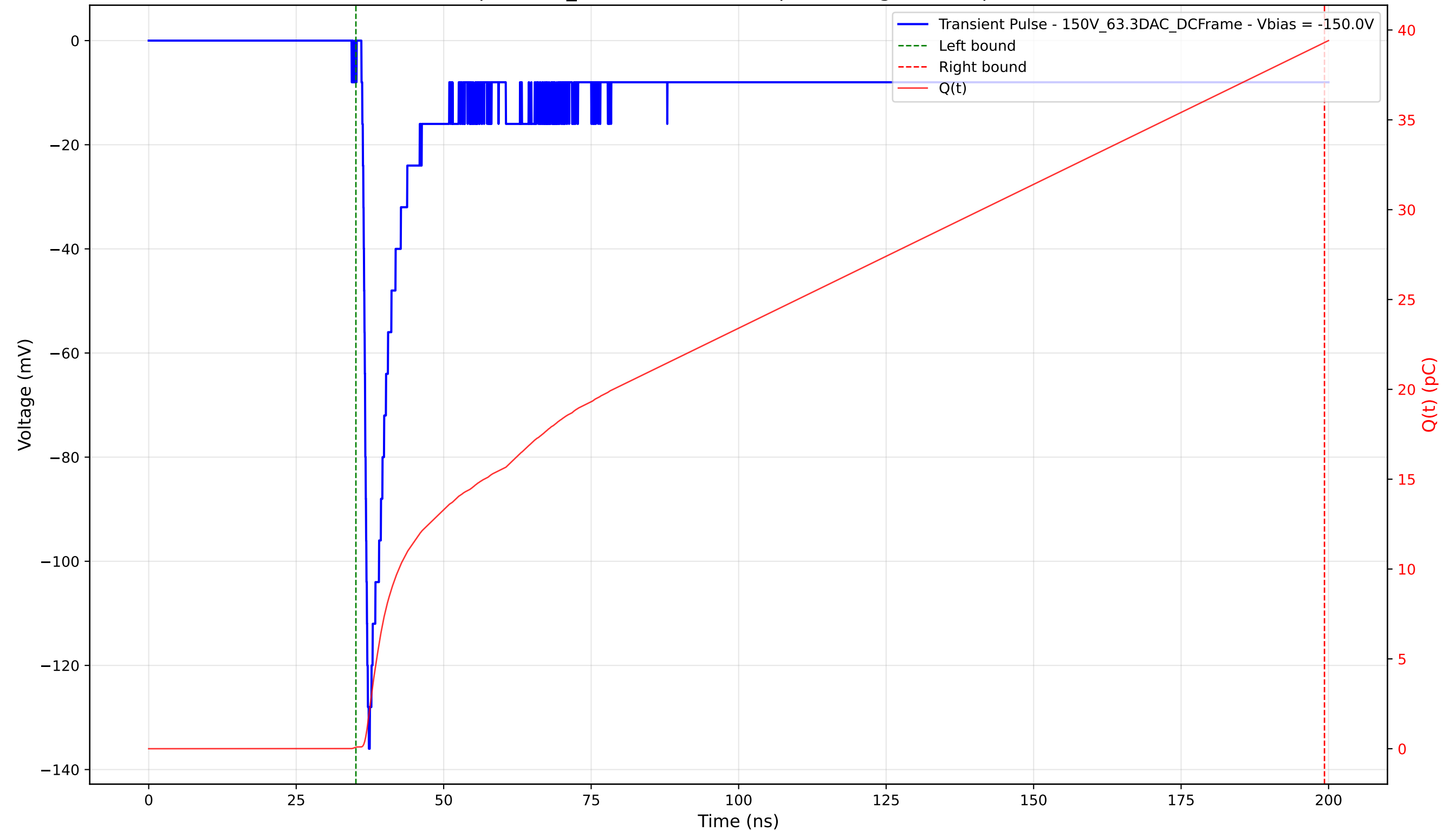
Transient Pulse - Sample: 1cm_42 - Position: 725.0 \mu\text{m} - Charge: 39.22 pC - Rise Time: 0.95 ns
