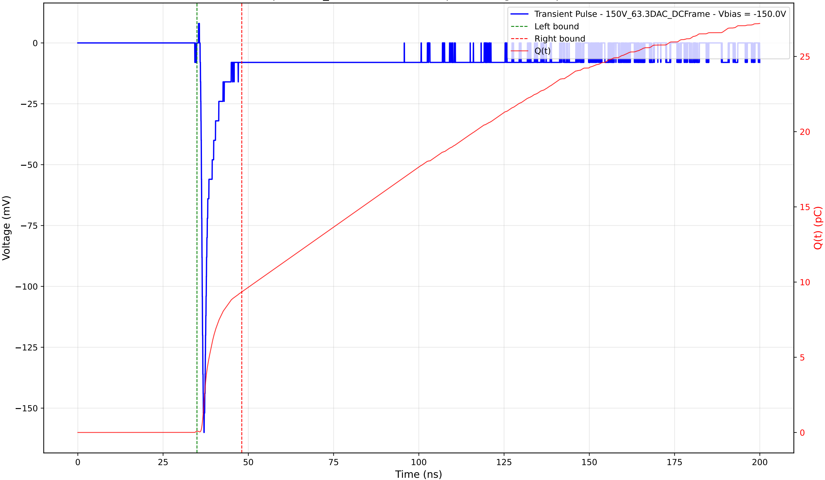
Transient Pulse - Sample: 1cm_42 - Position: 225.0 \mu\text{m} - Charge: 9.27 pC - Rise Time: 0.72 ns
