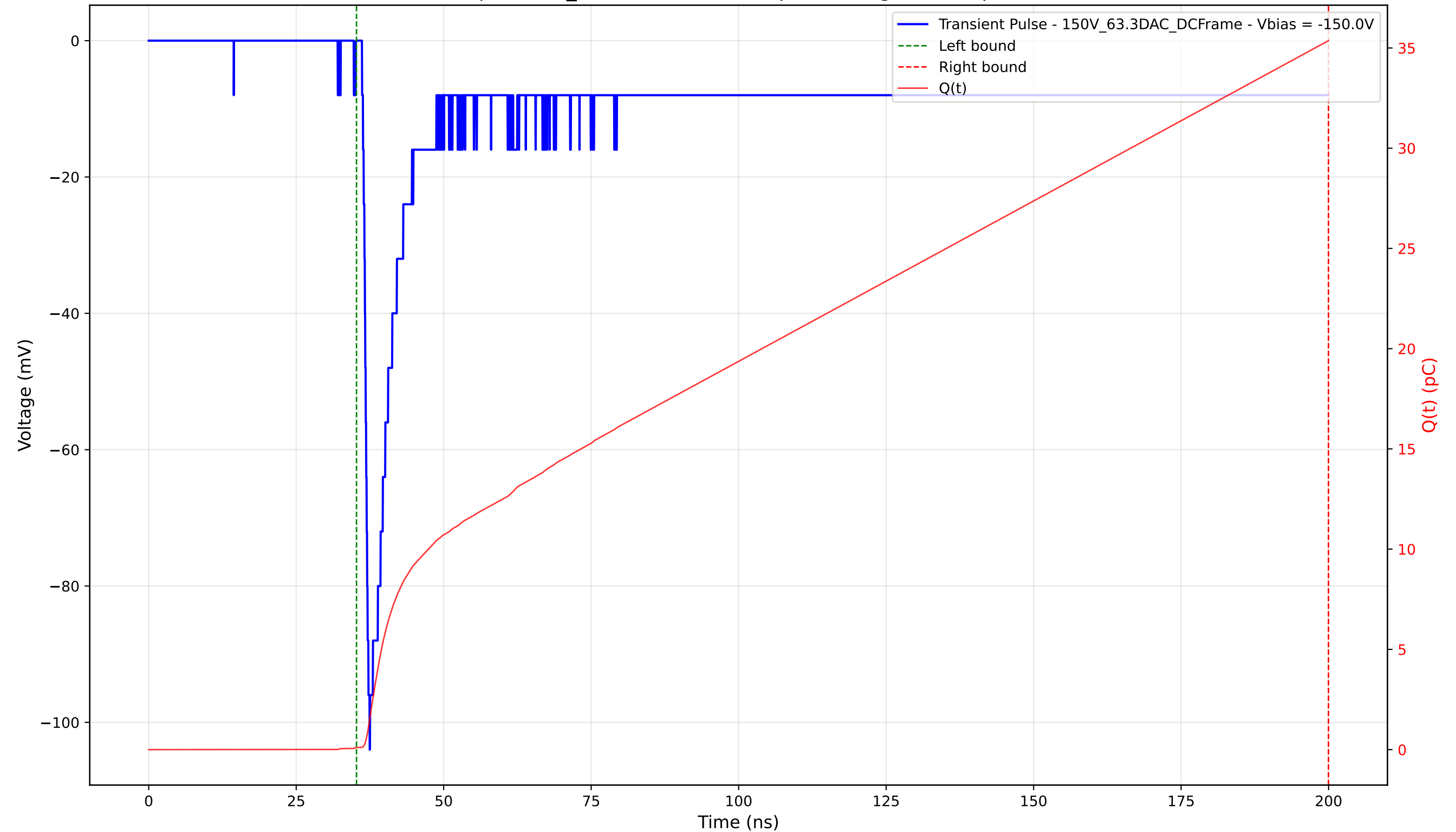
Transient Pulse - Sample: 1cm_42 - Position: 855.0 \mu\text{m} - Charge: 35.26 pC - Rise Time: 0.93 ns
