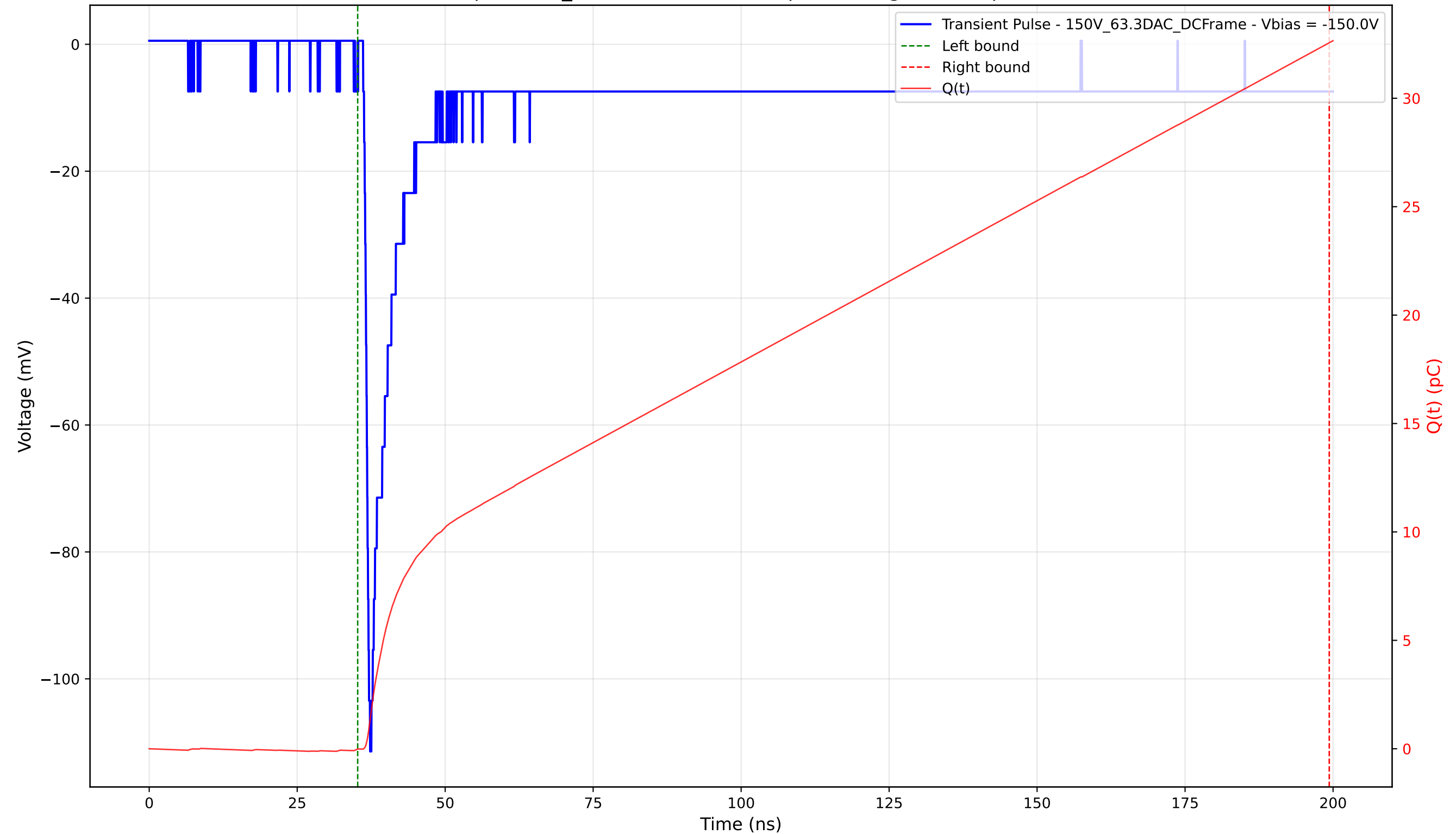
Transient Pulse - Sample: 1cm_42 - Position: 4480.0 \mu\text{m} - Charge: 32.57 pC - Rise Time: 0.83 ns
