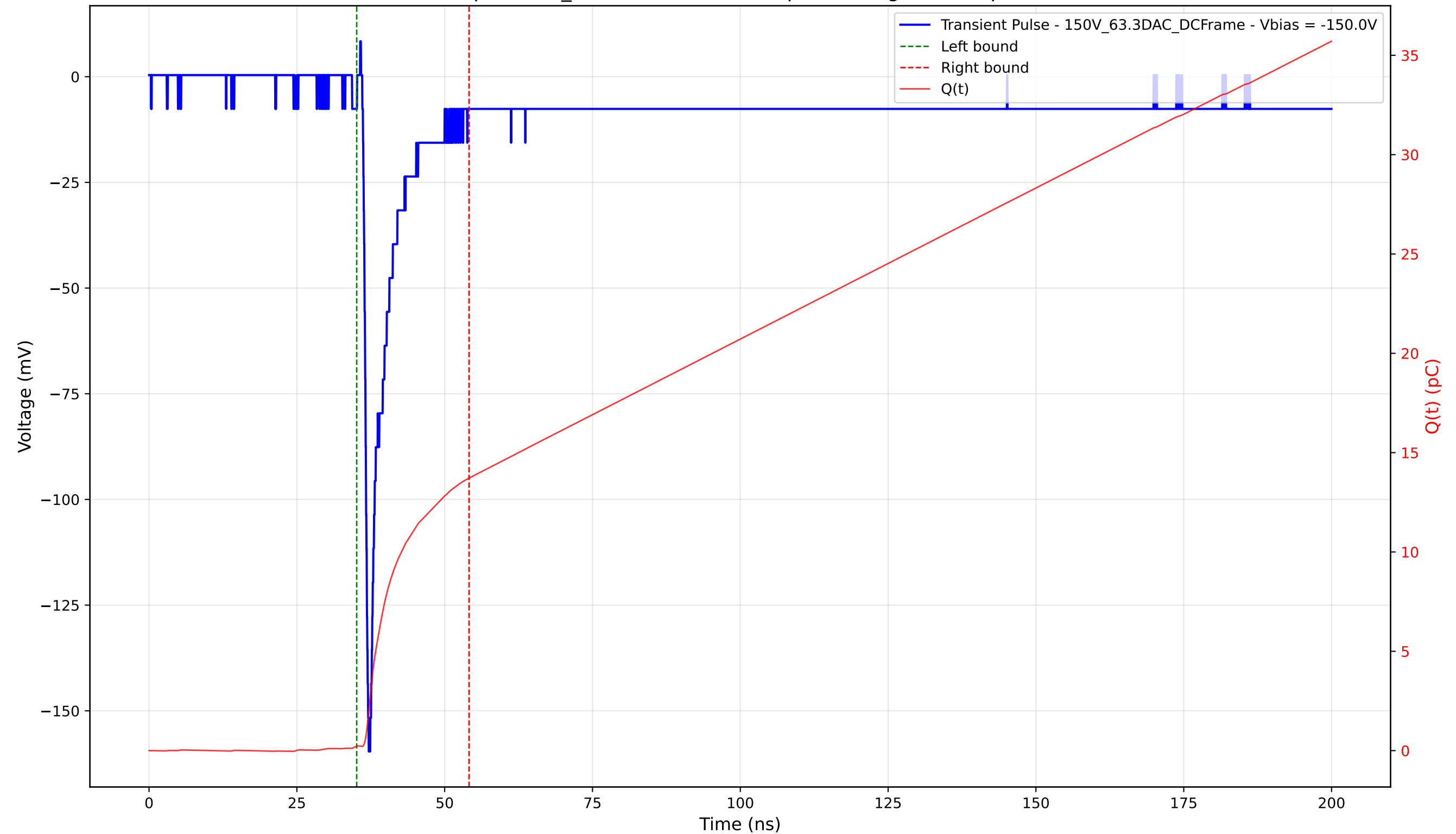
Transient Pulse - Sample: 1cm_42 - Position: 4605.0 \mu\text{m} - Charge: 13.49 pC - Rise Time: 0.82 ns
