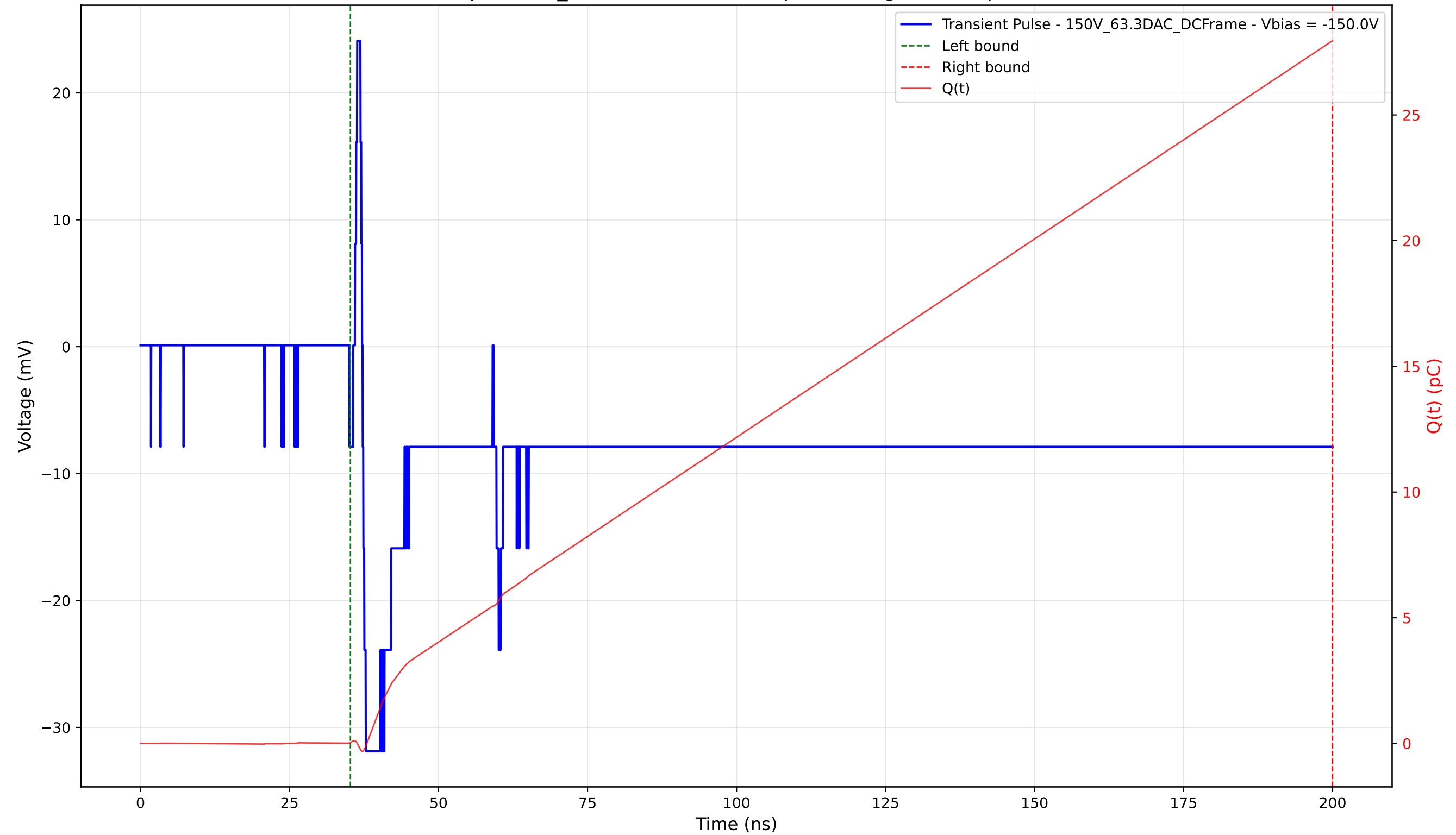
Transient Pulse - Sample: 1cm_42 - Position: 2125.0 \mu\text{m} - Charge: 27.92 pC - Rise Time: 0.53 ns
