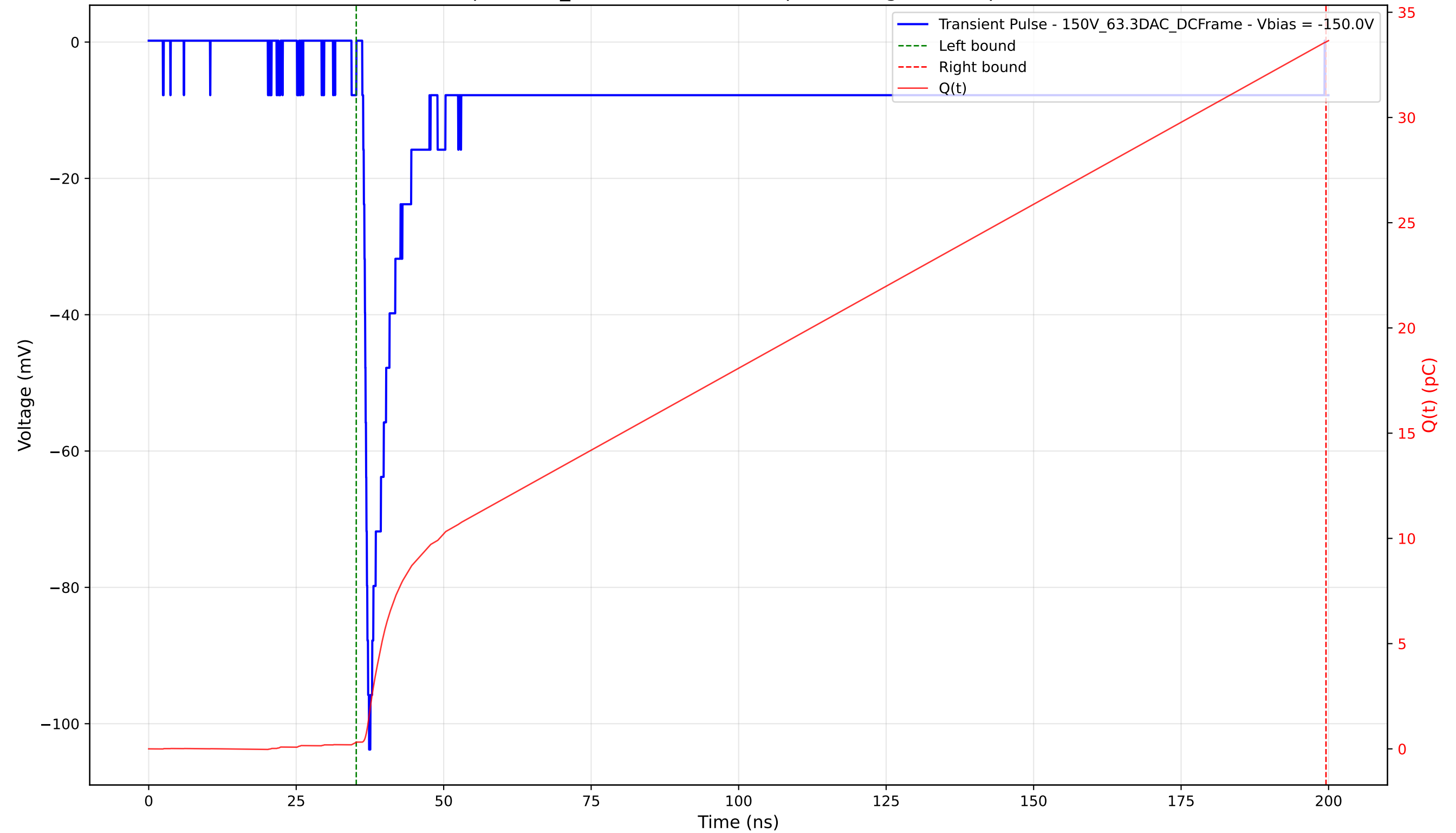
Transient Pulse - Sample: 1cm_42 - Position: 4440.0 \mu\text{m} - Charge: 33.27 pC - Rise Time: 0.83 ns
