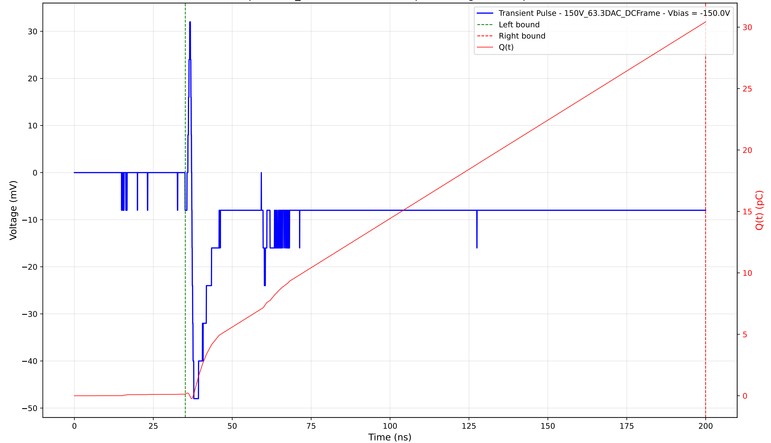
Transient Pulse - Sample: 1cm_42 - Position: 1740.0 \mu\text{m} - Charge: 30.29 pC - Rise Time: 0.65 ns
