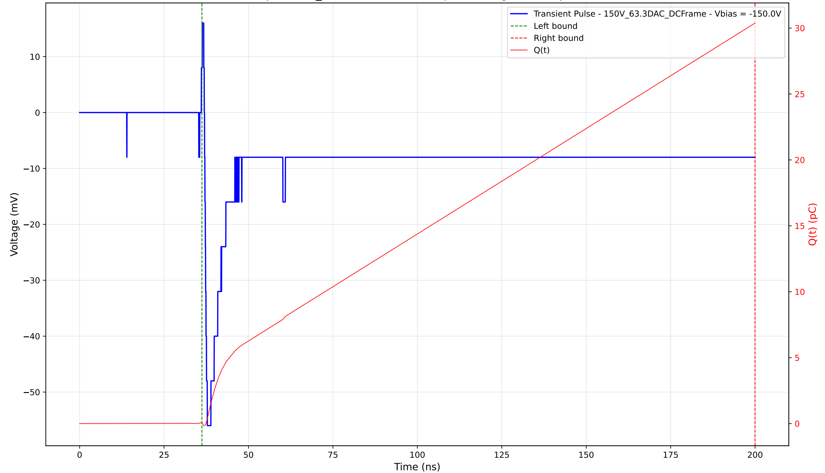
Transient Pulse - Sample: 1cm_42 - Position: 1405.0 \mu\text{m} - Charge: 30.36 pC - Rise Time: 0.81 ns
