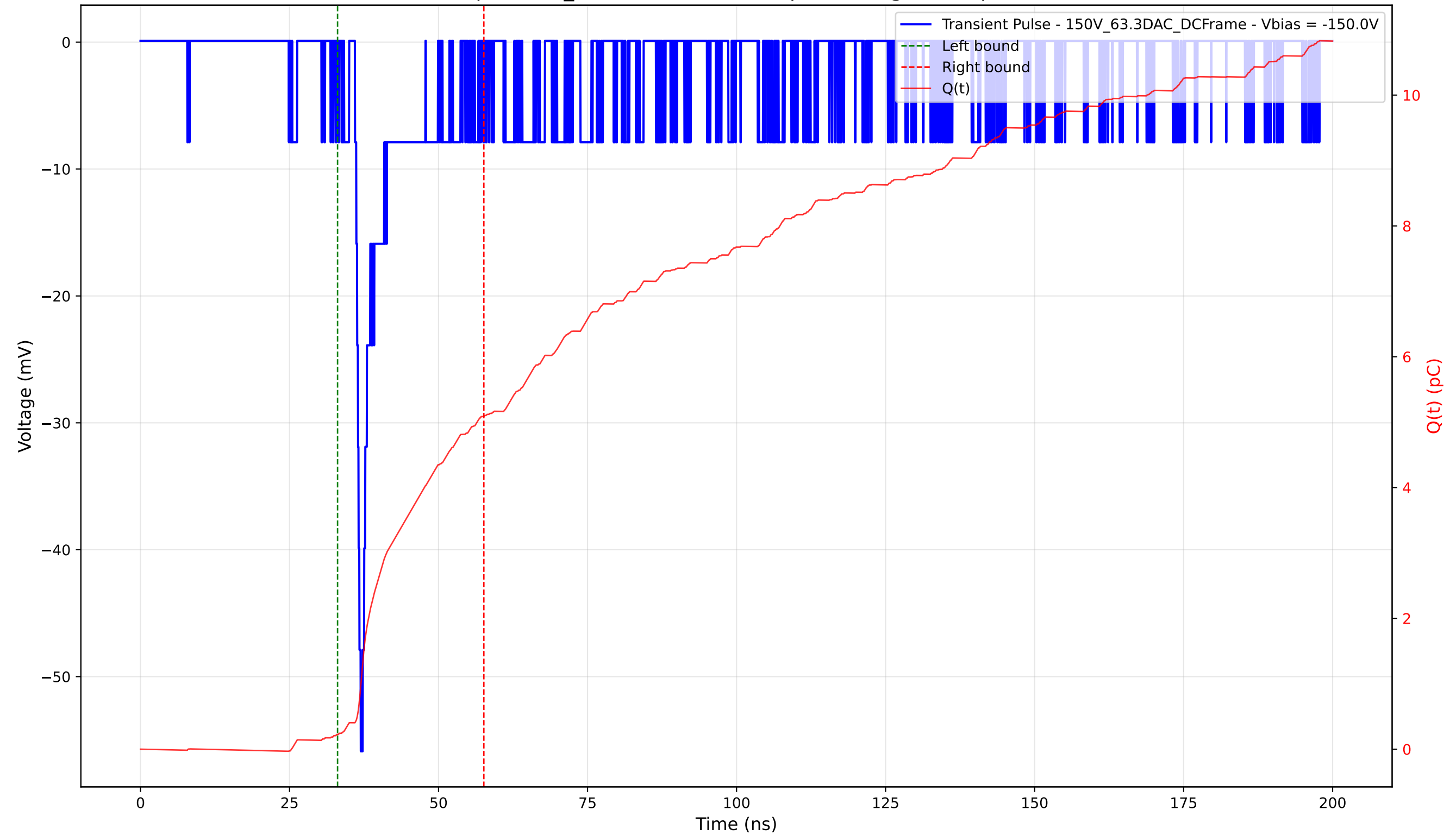
Transient Pulse - Sample: 1cm_42 - Position: 5120.0 \mu\text{m} - Charge: 4.87 pC - Rise Time: 0.97 ns
