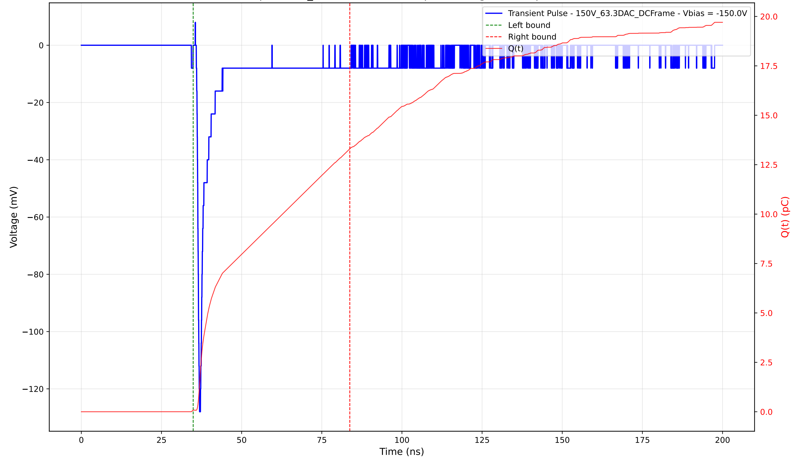
Transient Pulse - Sample: 1cm_42 - Position: 170.0 \mu\text{m} - Charge: 13.22 pC - Rise Time: 0.79 ns
