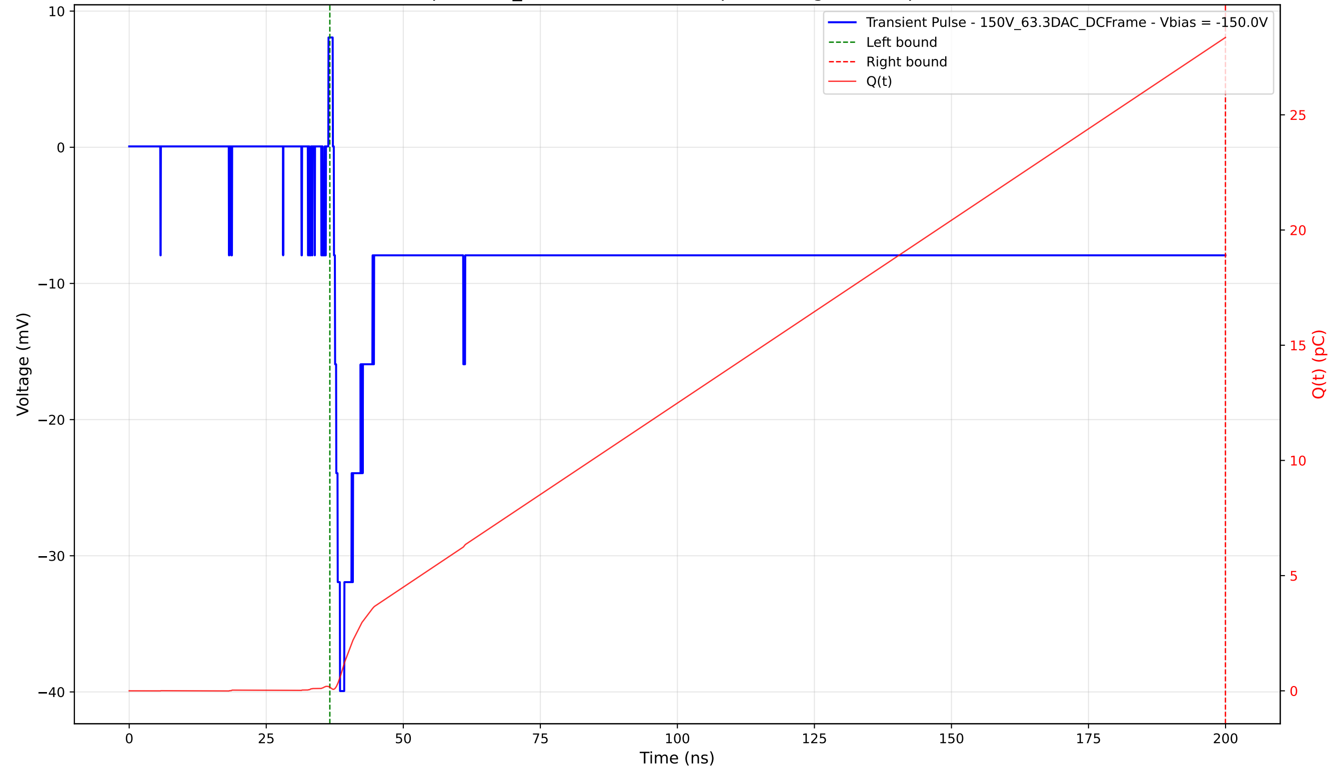
Transient Pulse - Sample: 1cm_42 - Position: 3420.0 \mu\text{m} - Charge: 28.21 pC - Rise Time: 1.11 ns
