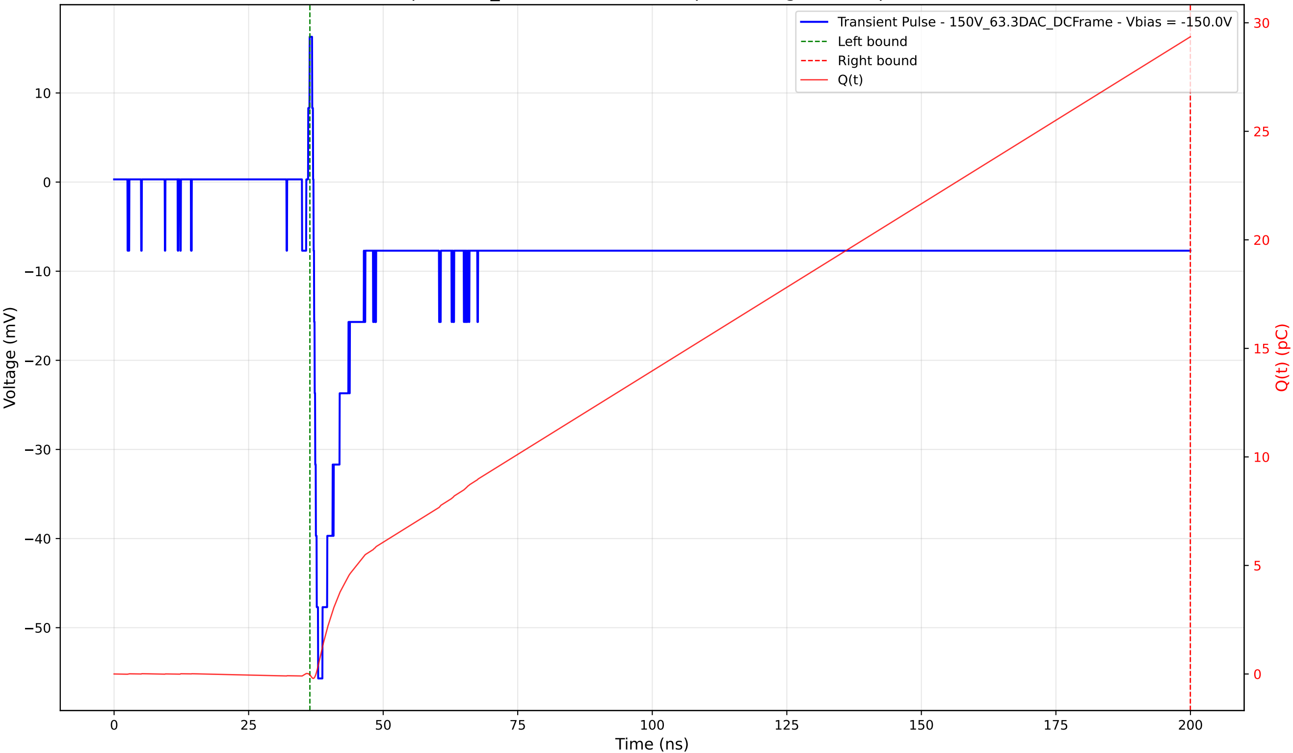
Transient Pulse - Sample: 1cm_42 - Position: 1435.0 \mu\text{m} - Charge: 29.40 pC - Rise Time: 0.85 ns
