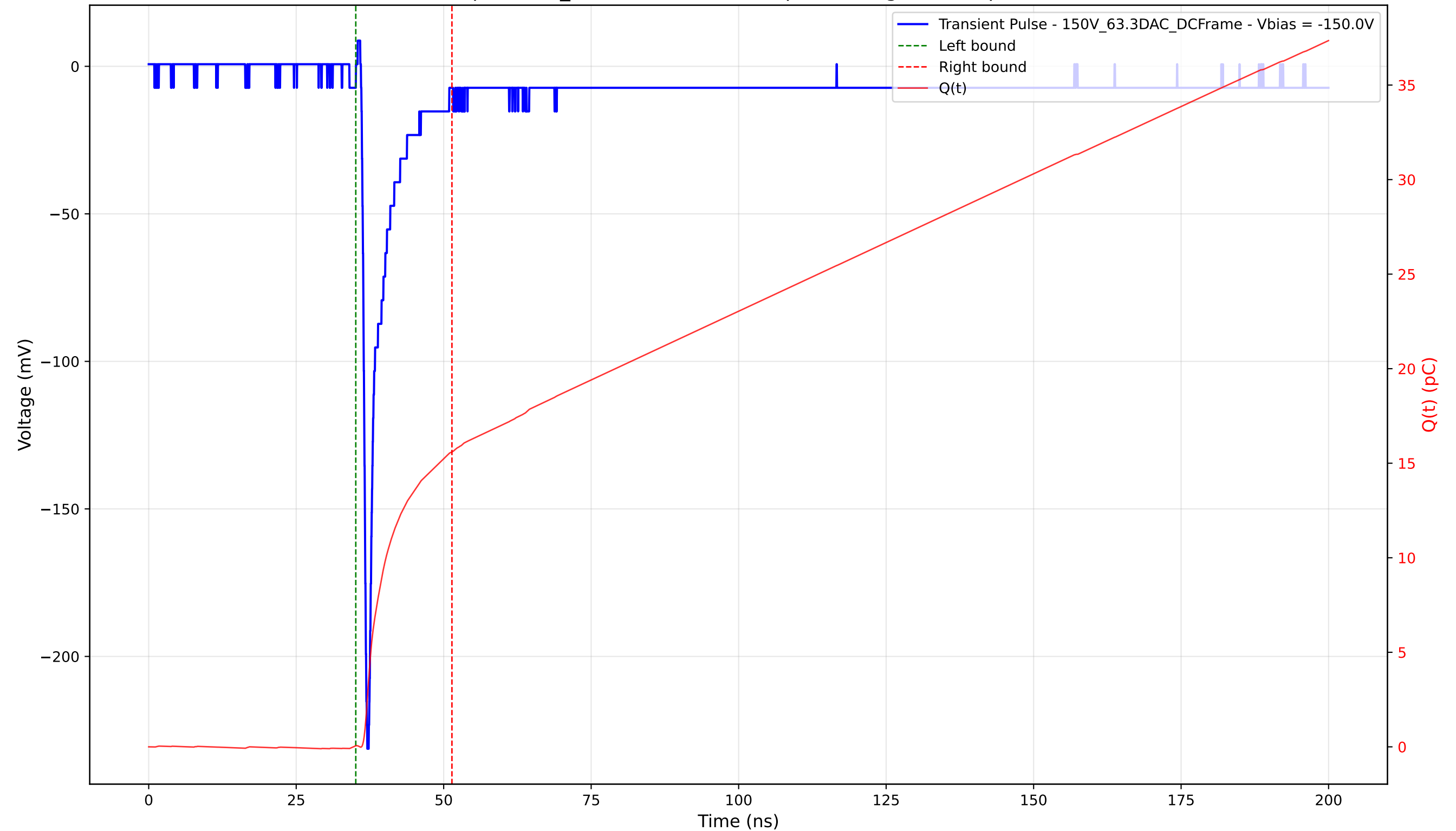
Transient Pulse - Sample: 1cm_42 - Position: 4845.0 \mu\text{m} - Charge: 15.53 pC - Rise Time: 0.78 ns
