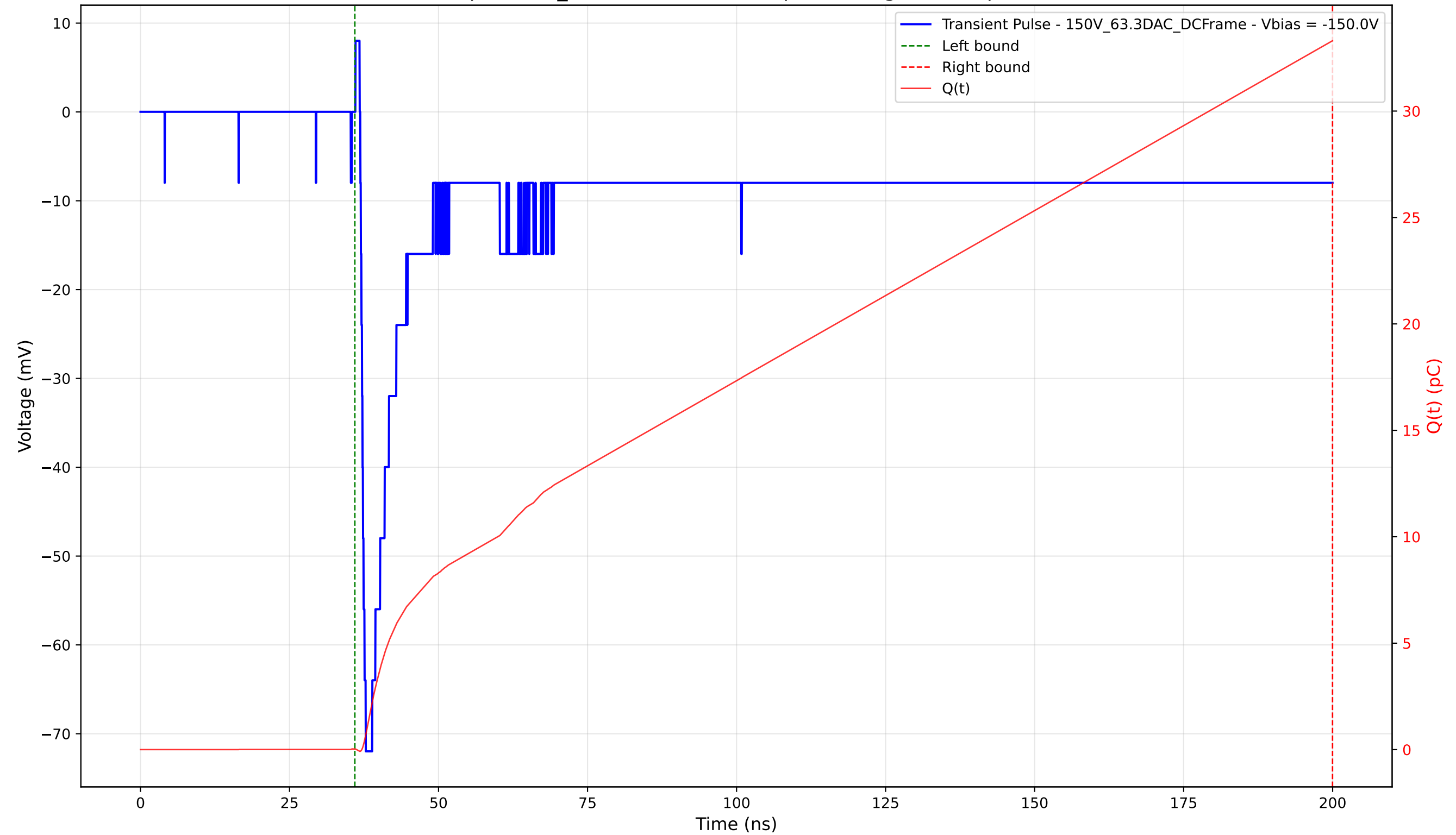
Transient Pulse - Sample: 1cm_42 - Position: 1250.0 \mu\text{m} - Charge: 33.27 pC - Rise Time: 0.90 ns
