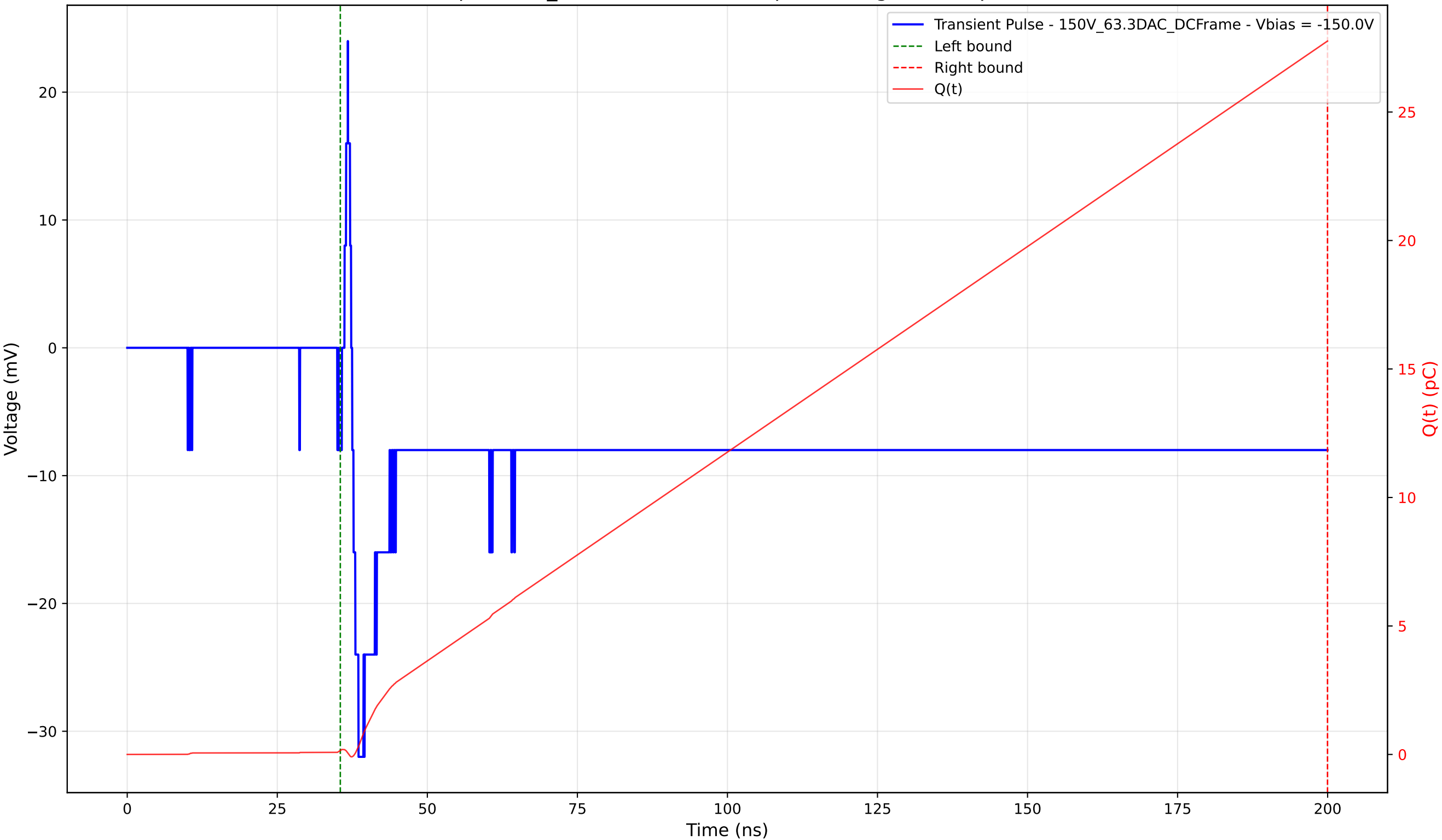
Transient Pulse - Sample: 1cm_42 - Position: 2510.0 \mu\text{m} - Charge: 27.61 pC - Rise Time: 1.05 ns
