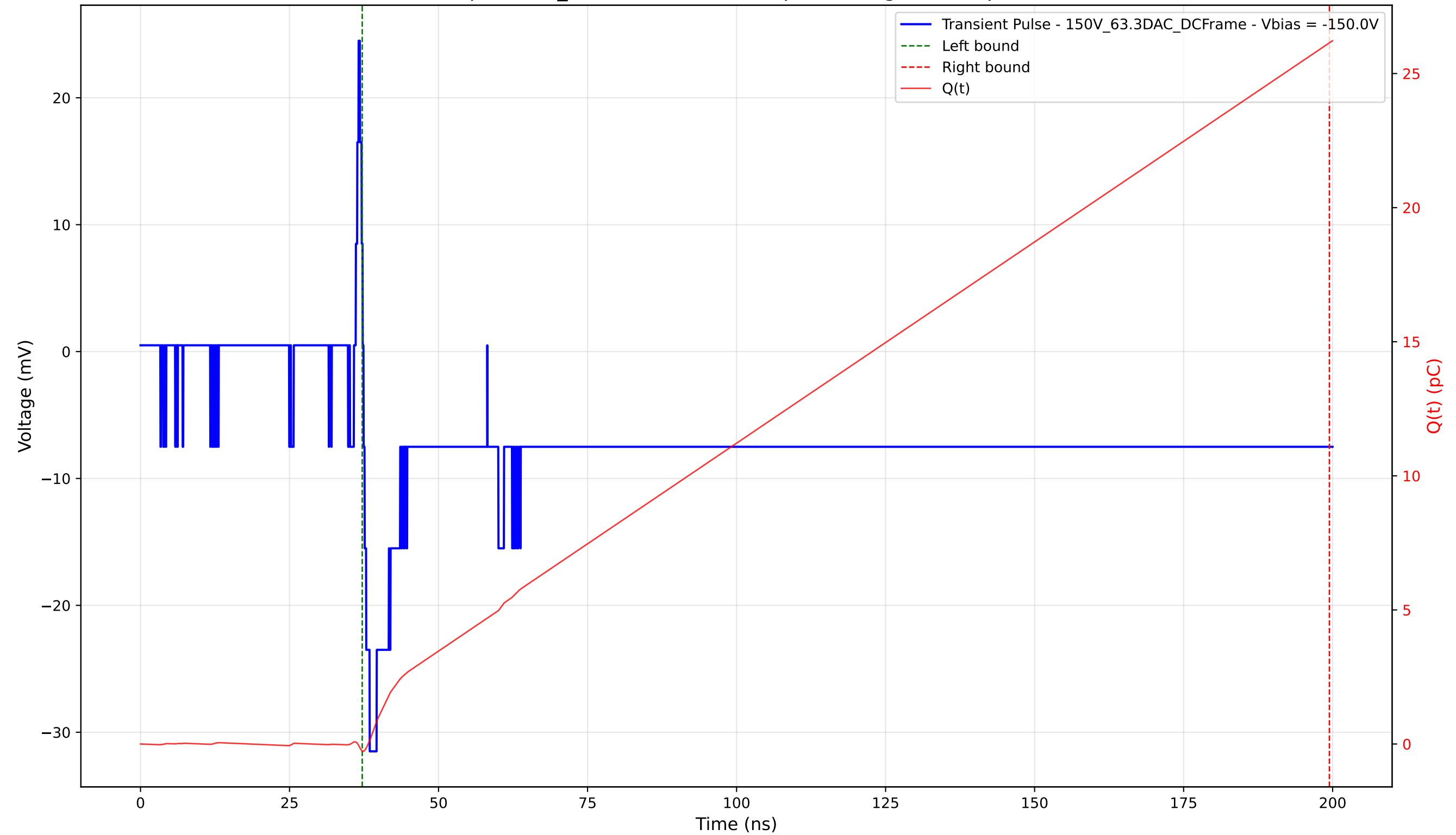
Transient Pulse - Sample: 1cm_42 - Position: 2400.0 \mu\text{m} - Charge: 26.41 pC - Rise Time: 1.03 ns
