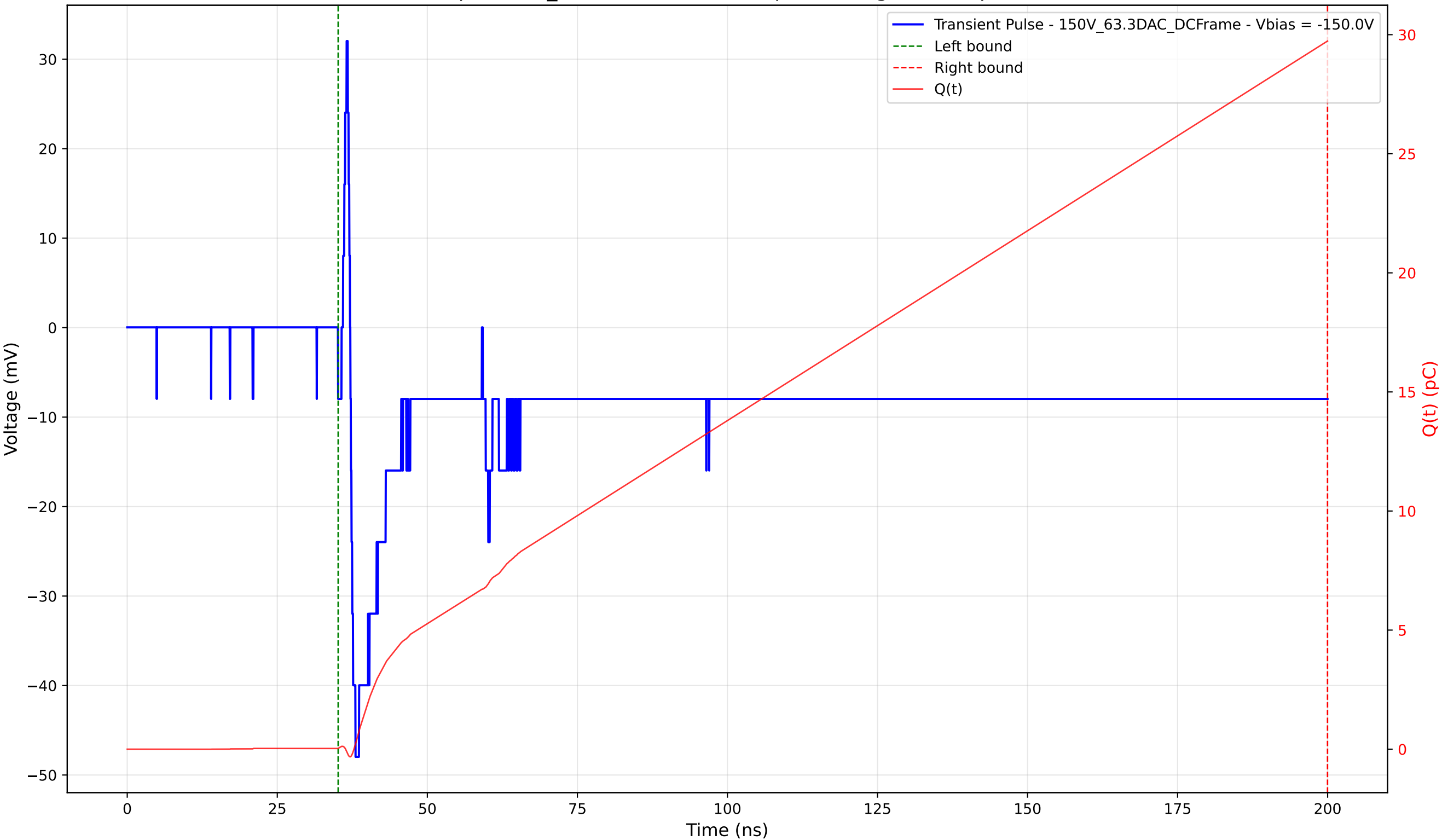
Transient Pulse - Sample: 1cm_42 - Position: 1795.0 \mu\text{m} - Charge: 29.70 pC - Rise Time: 0.85 ns
