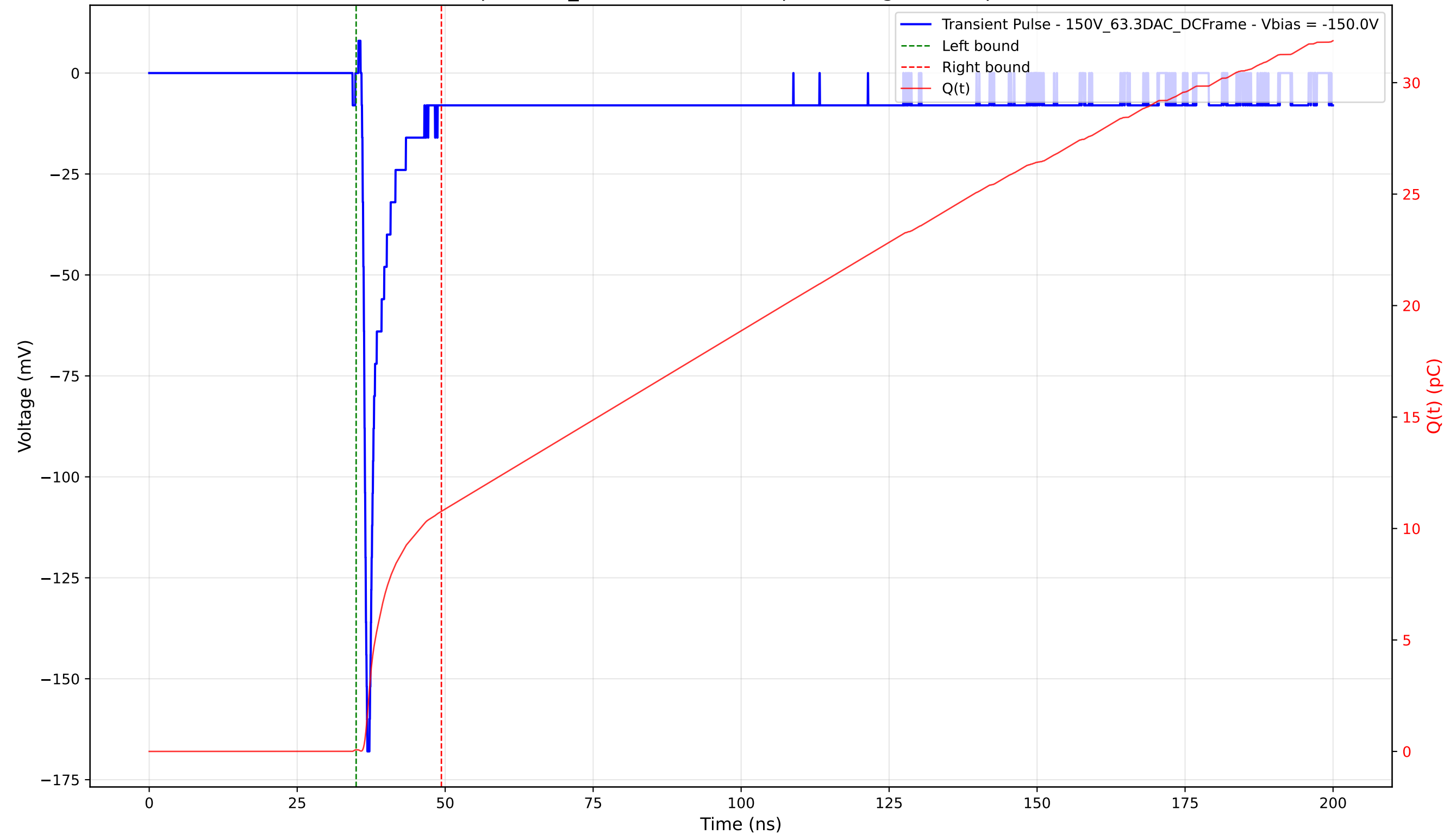
Transient Pulse - Sample: 1cm_42 - Position: 295.0 \mu\text{m} - Charge: 10.70 pC - Rise Time: 0.70 ns
