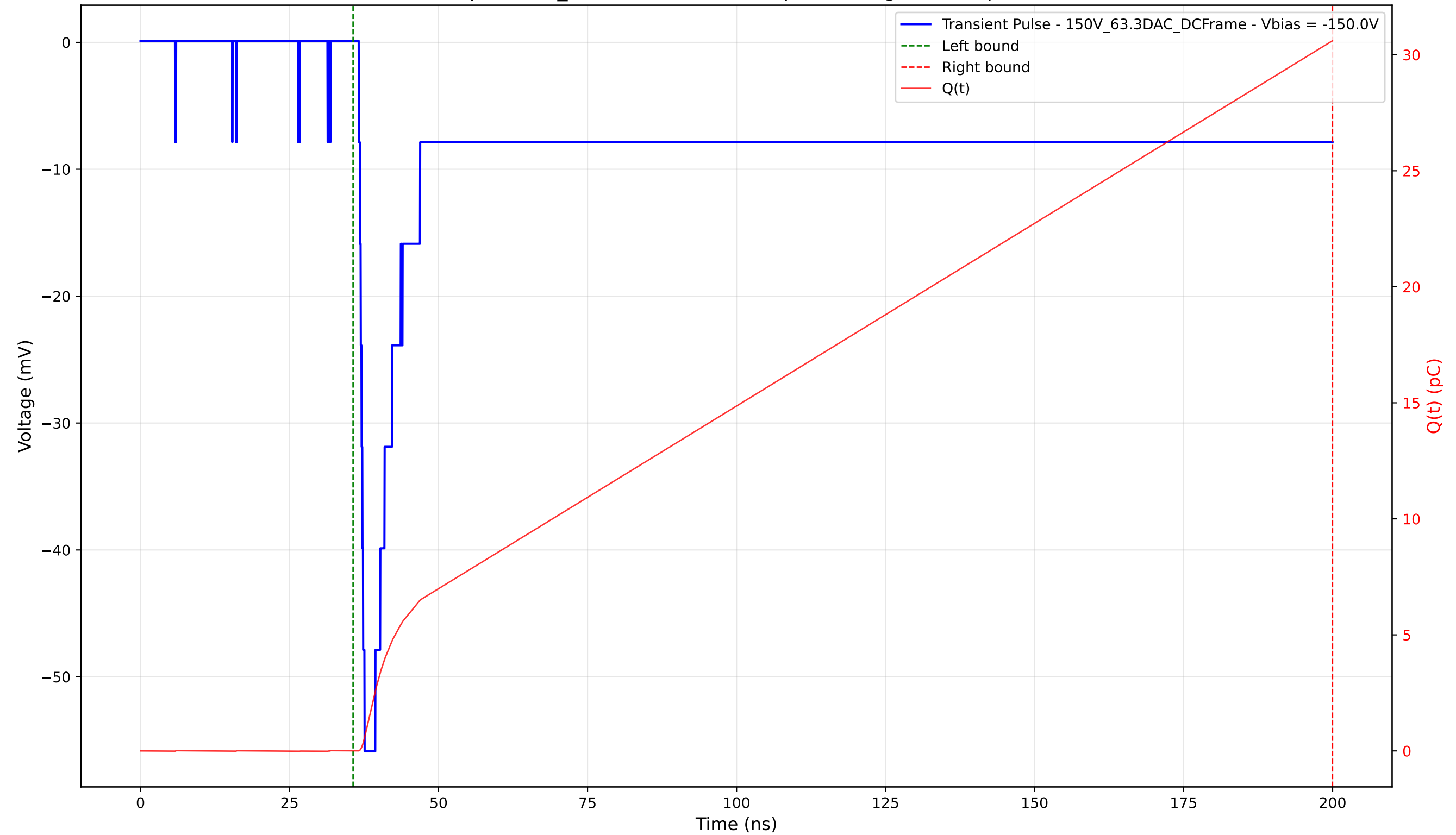
Transient Pulse - Sample: 1cm_42 - Position: 4040.0 \mu\text{m} - Charge: 30.60 pC - Rise Time: 0.97 ns
