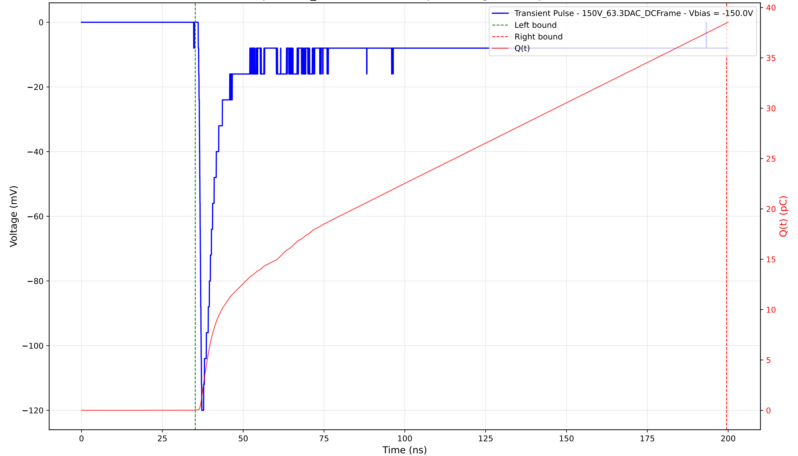
Transient Pulse - Sample: 1cm_42 - Position: 780.0 \mu\text{m} - Charge: 38.42 pC - Rise Time: 0.85 ns
