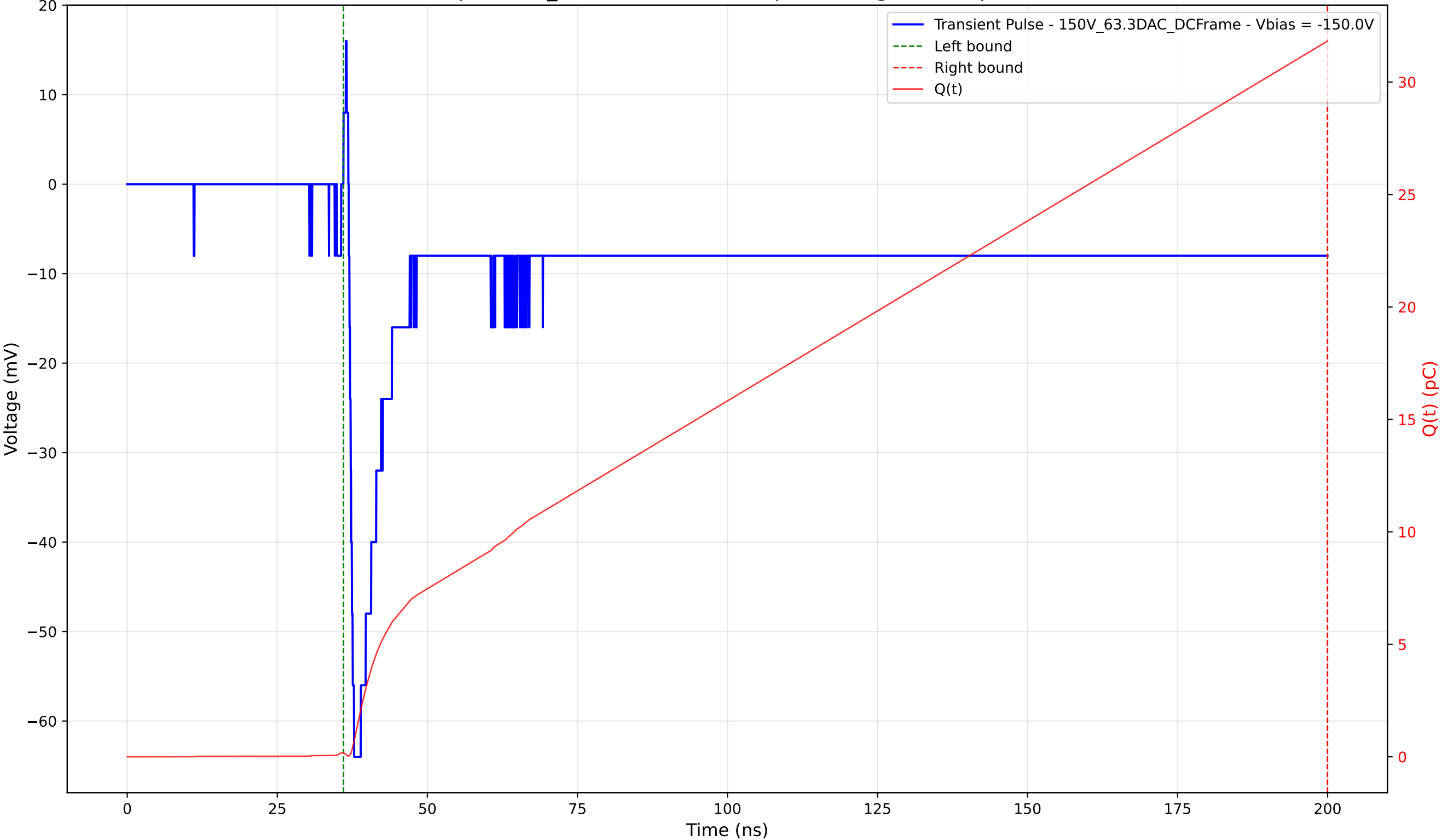
Transient Pulse - Sample: 1cm_42 - Position: 1320.0 \mu\text{m} - Charge: 31.64 pC - Rise Time: 0.86 ns
