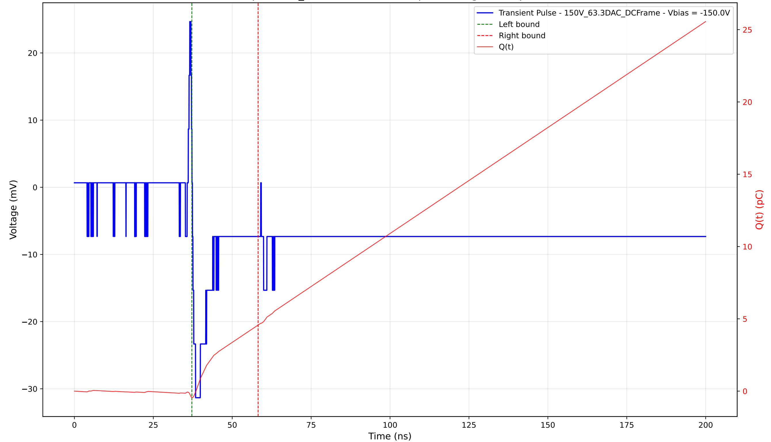
Transient Pulse - Sample: 1cm_42 - Position: 2380.0 \mu\text{m} - Charge: 5.03 pC - Rise Time: 0.99 ns
