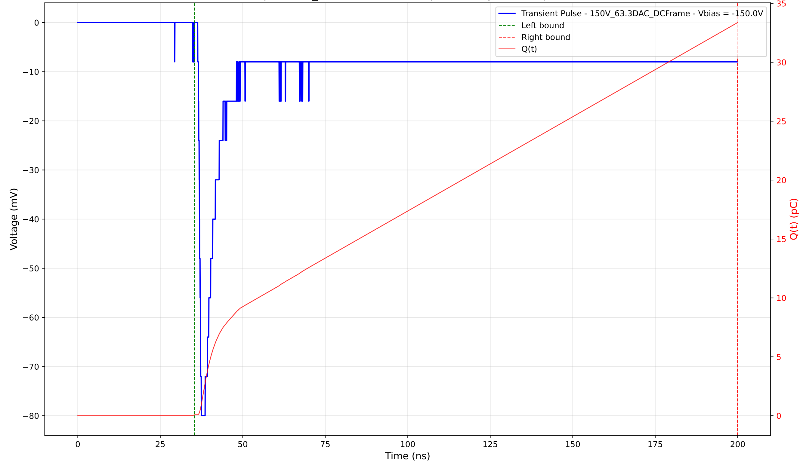
Transient Pulse - Sample: 1cm_42 - Position: 955.0 \mu\text{m} - Charge: 33.30 pC - Rise Time: 0.72 ns
