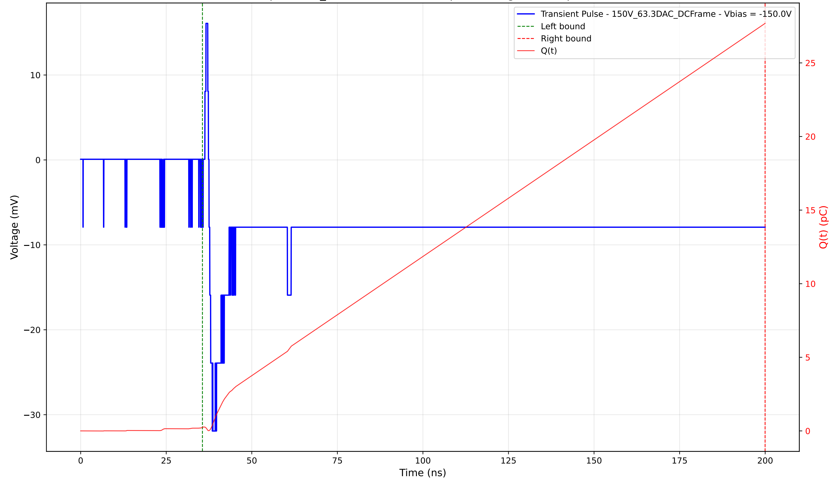
Transient Pulse - Sample: 1cm_42 - Position: 2890.0 \mu\text{m} - Charge: 27.44 pC - Rise Time: 0.95 ns
