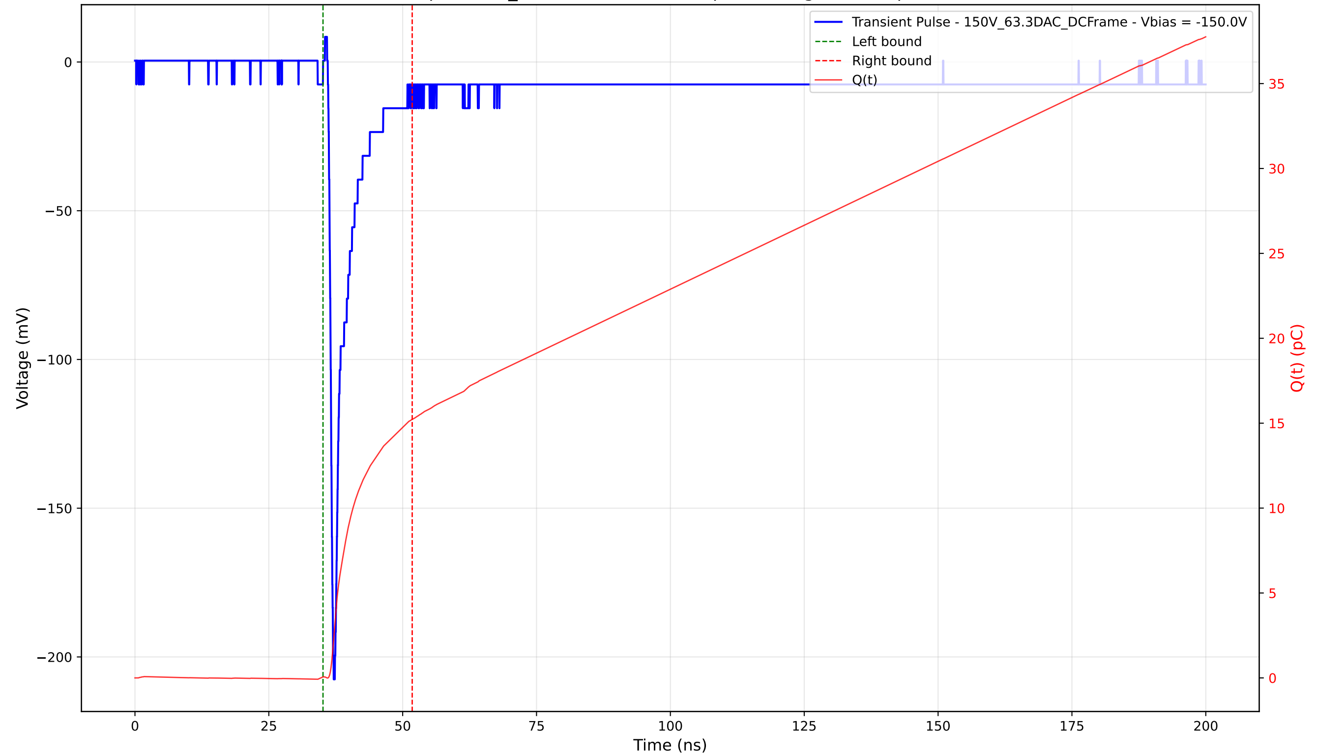
Transient Pulse - Sample: 1cm_42 - Position: 4690.0 \mu\text{m} - Charge: 15.16 pC - Rise Time: 0.81 ns
