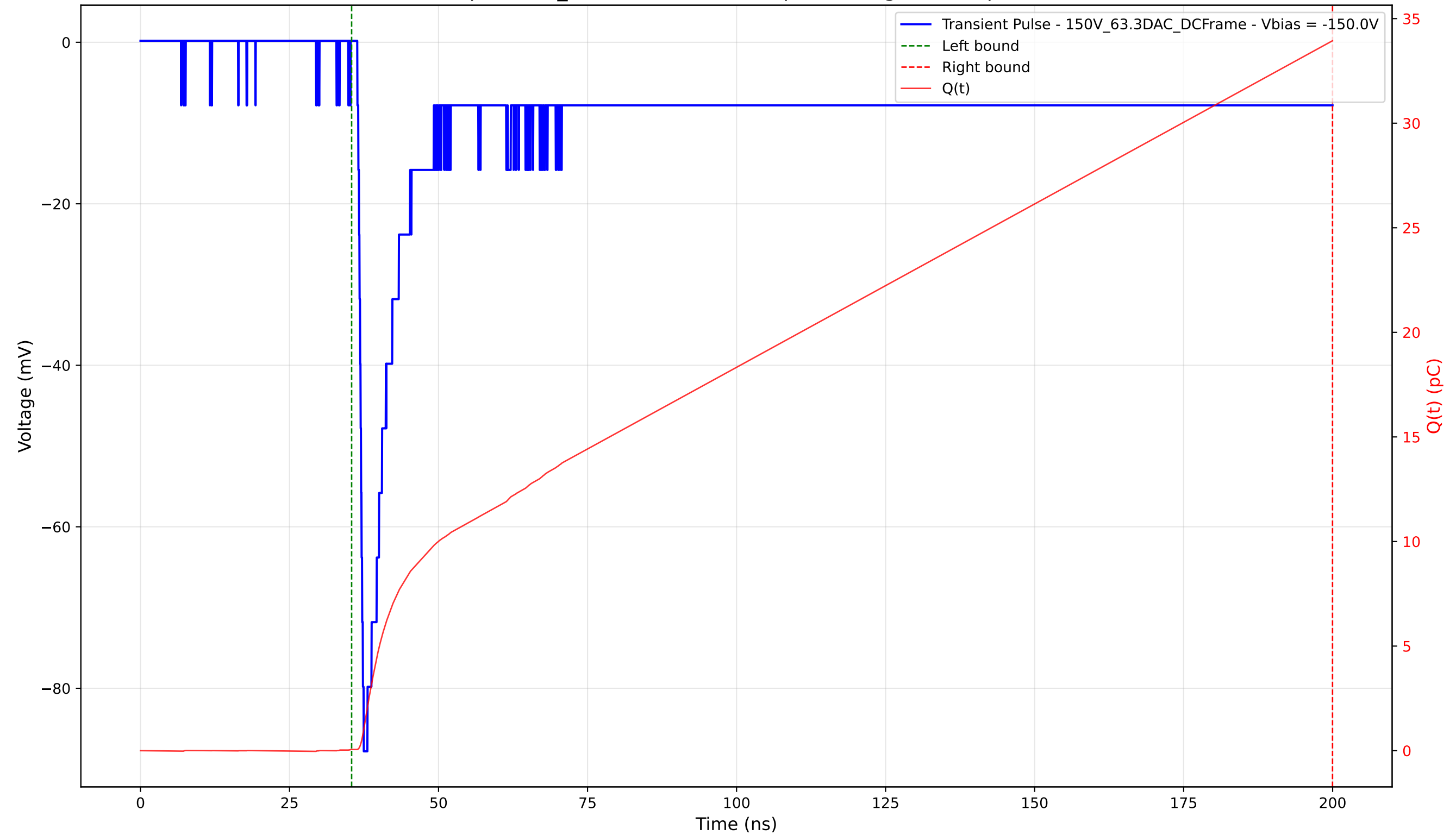
Transient Pulse - Sample: 1cm_42 - Position: 4215.0 \mu\text{m} - Charge: 33.89 pC - Rise Time: 0.78 ns
