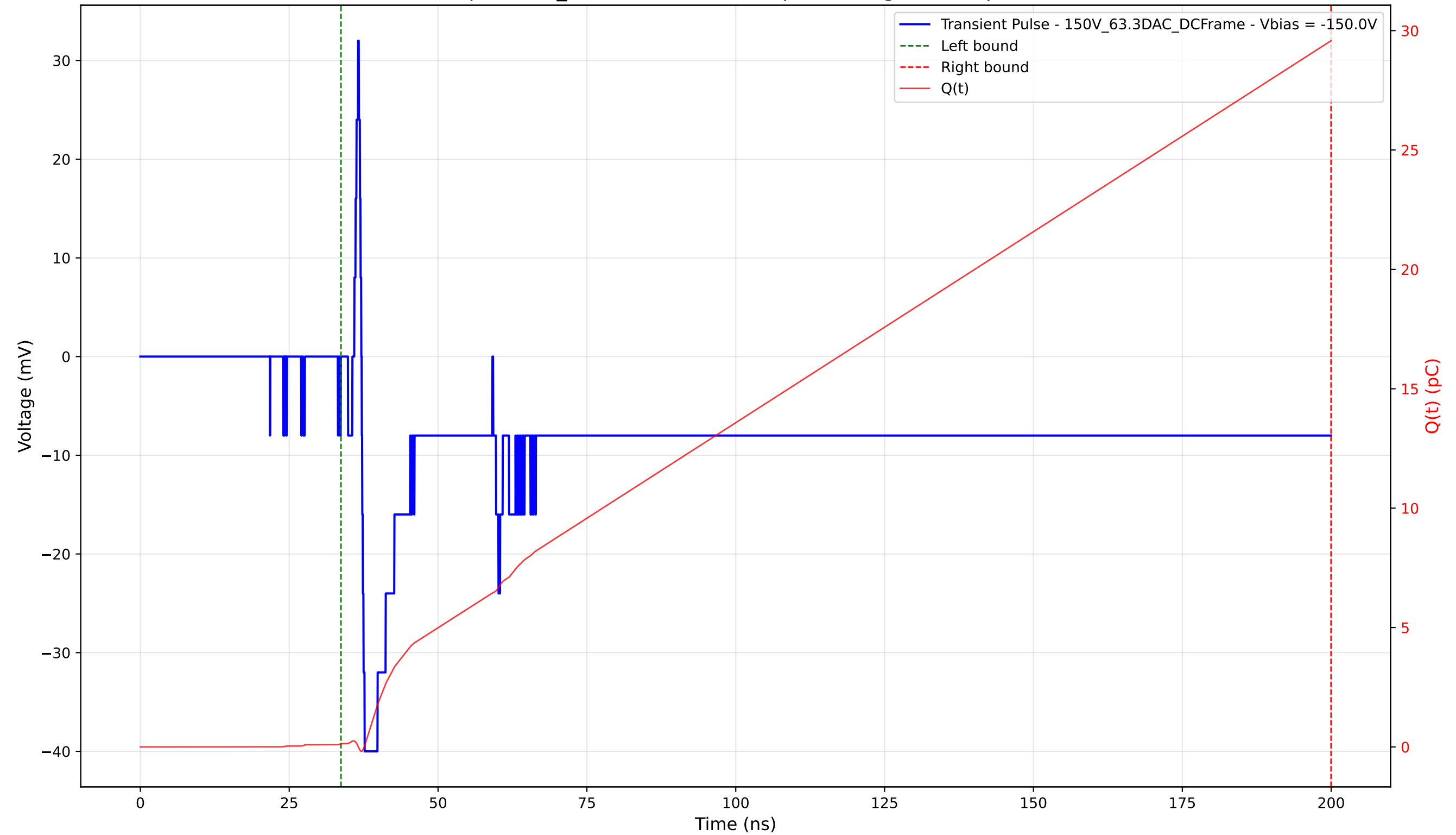
Transient Pulse - Sample: 1cm_42 - Position: 1835.0 \mu\text{m} - Charge: 29.44 pC - Rise Time: 0.49 ns
