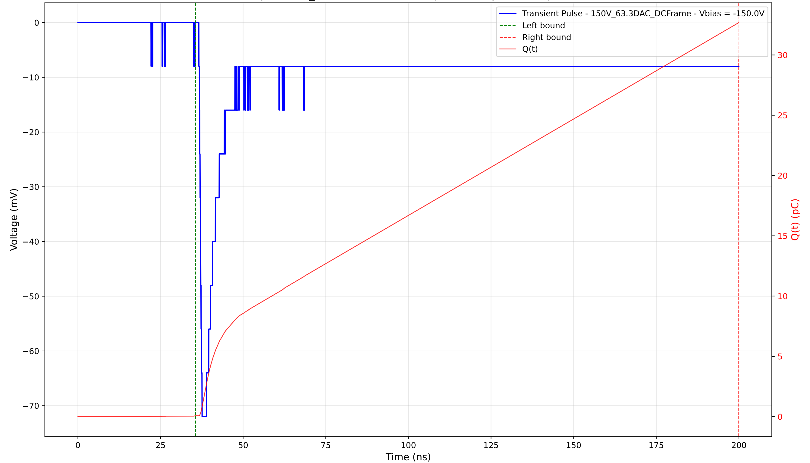
Transient Pulse - Sample: 1cm_42 - Position: 1045.0 \mu\text{m} - Charge: 32.62 pC - Rise Time: 0.96 ns
