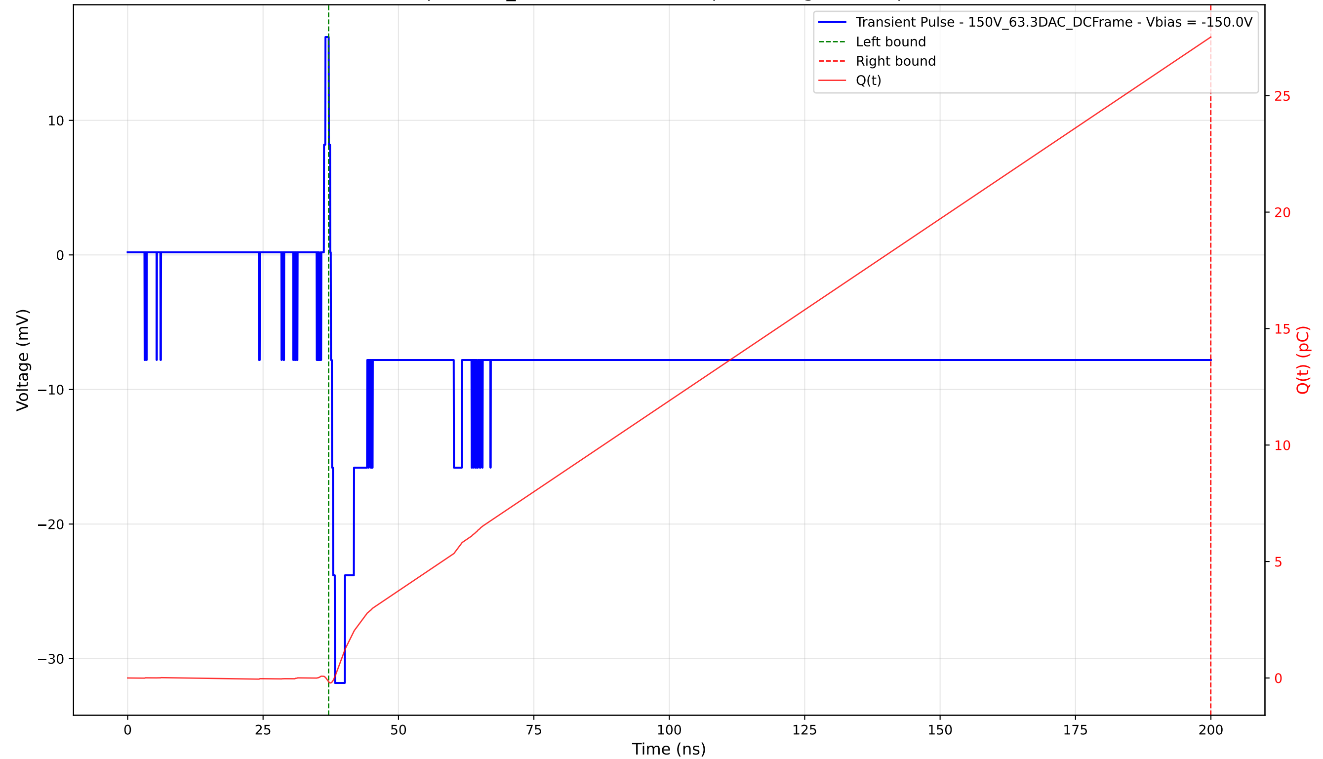
Transient Pulse - Sample: 1cm_42 - Position: 2785.0 \mu\text{m} - Charge: 27.68 pC - Rise Time: 0.75 ns
