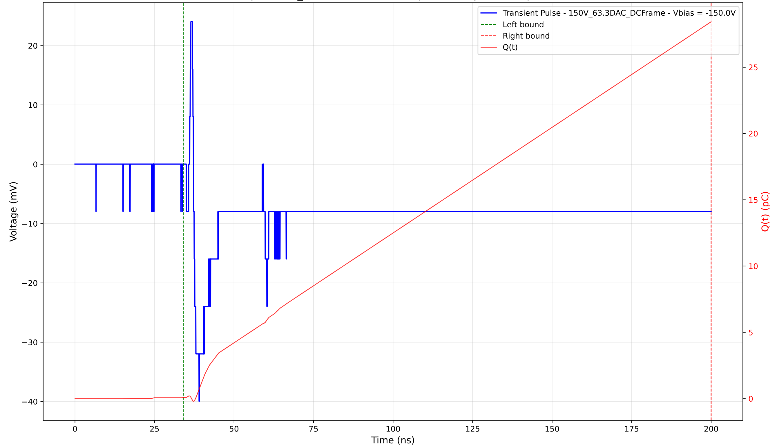
Transient Pulse - Sample: 1cm_42 - Position: 2280.0 \mu\text{m} - Charge: 28.35 pC - Rise Time: 1.69 ns
