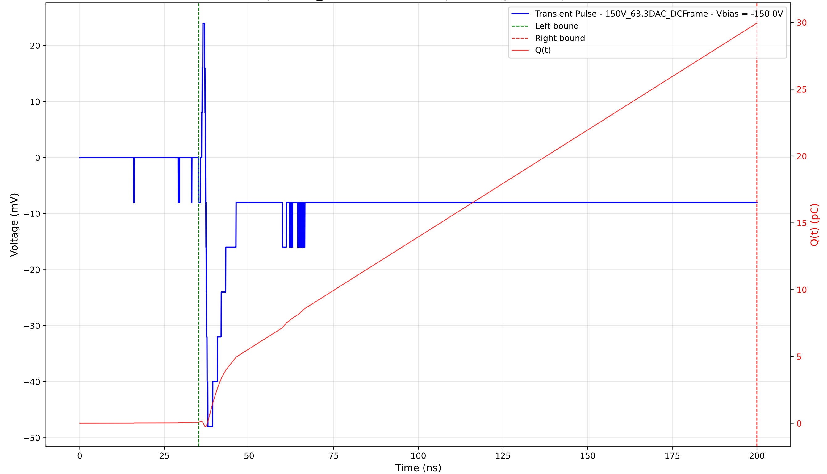
Transient Pulse - Sample: 1cm_42 - Position: 1610.0 \mu\text{m} - Charge: 29.87 pC - Rise Time: 0.67 ns
