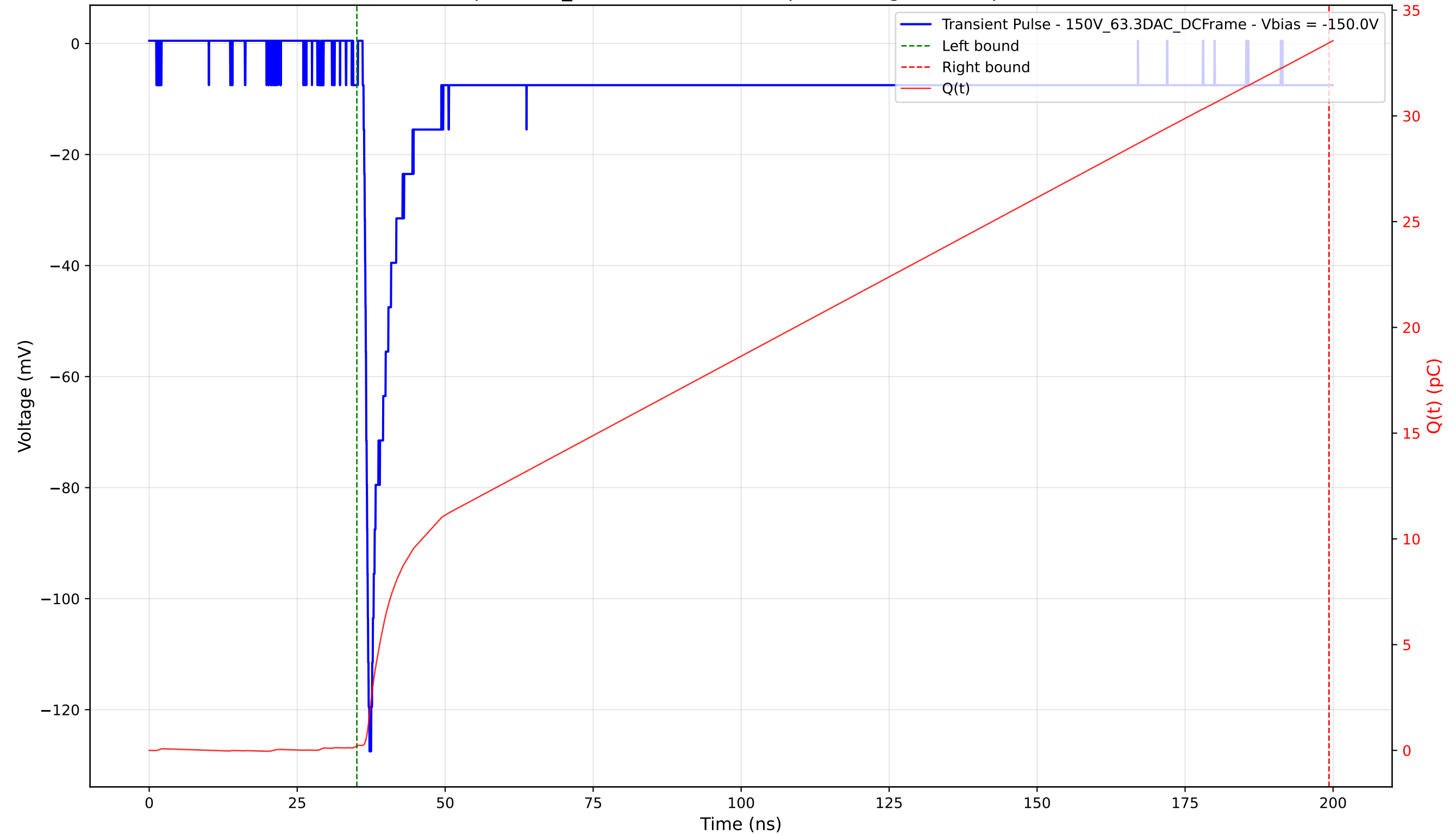
Transient Pulse - Sample: 1cm_42 - Position: 4535.0 \mu\text{m} - Charge: 33.24 pC - Rise Time: 0.85 ns
