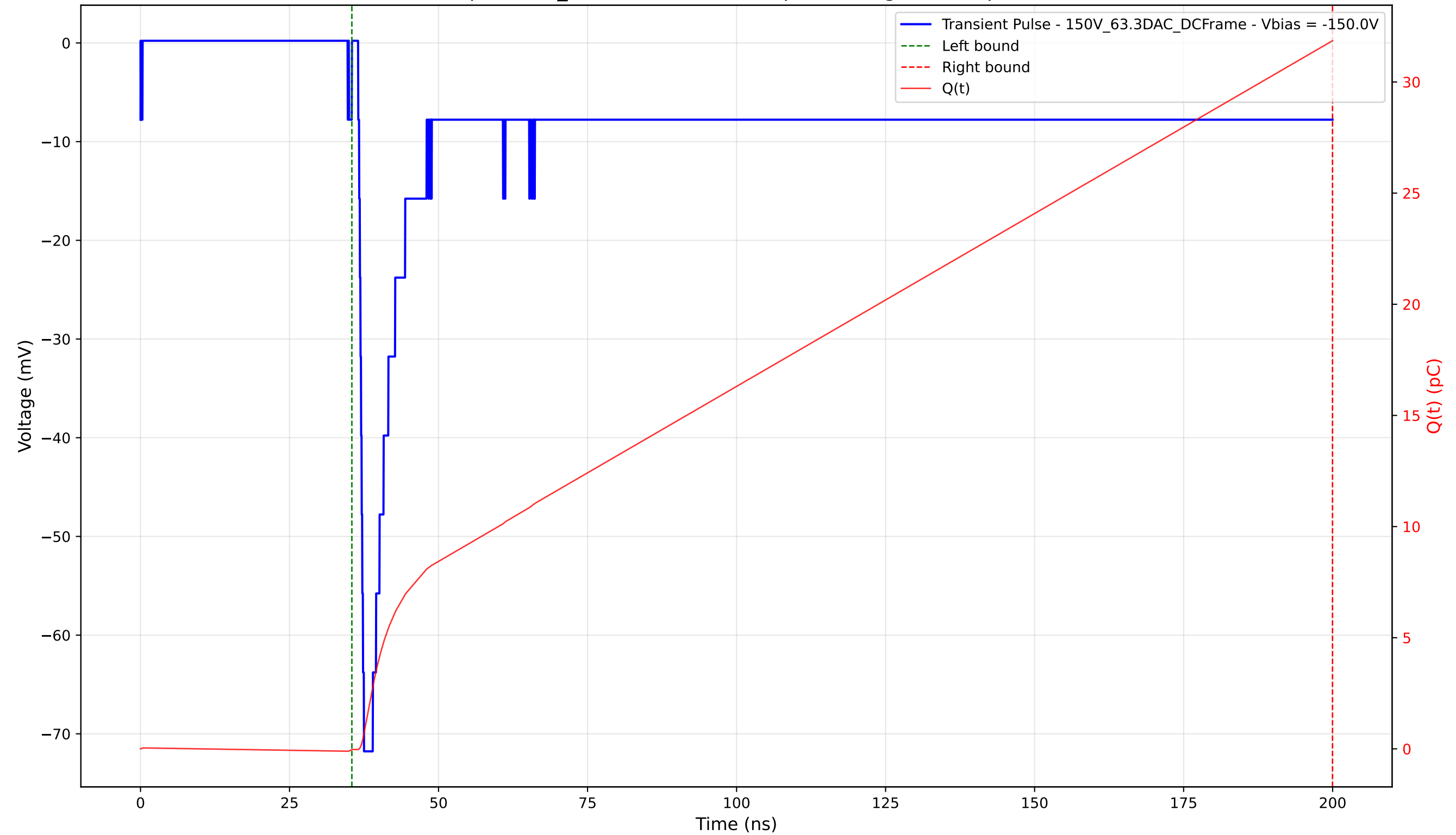
Transient Pulse - Sample: 1cm_42 - Position: 1010.0 \mu\text{m} - Charge: 31.88 pC - Rise Time: 0.96 ns
