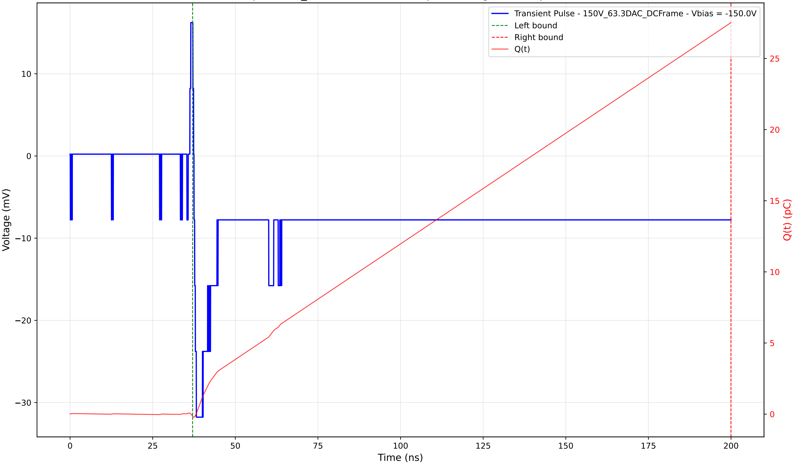
Transient Pulse - Sample: 1cm_42 - Position: 2720.0 \mu\text{m} - Charge: 27.67 pC - Rise Time: 0.71 ns
