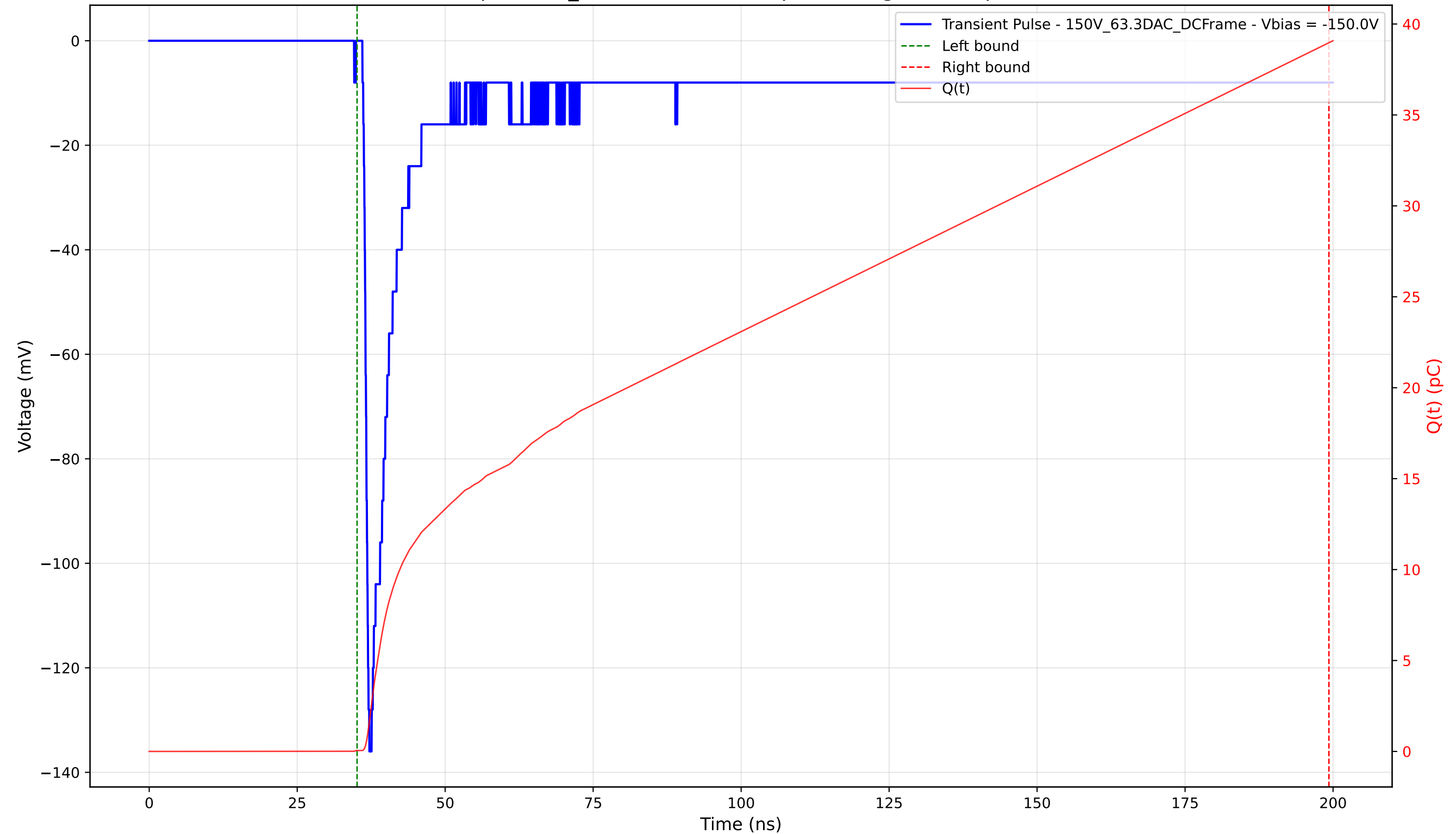
Transient Pulse - Sample: 1cm_42 - Position: 670.0 \mu\text{m} - Charge: 38.92 pC - Rise Time: 0.89 ns
