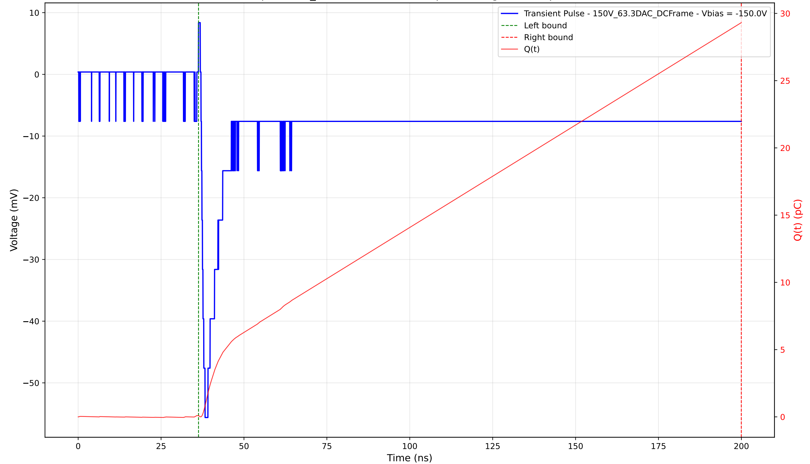
Transient Pulse - Sample: 1cm_42 - Position: 3725.0 \mu\text{m} - Charge: 29.23 pC - Rise Time: 1.23 ns
