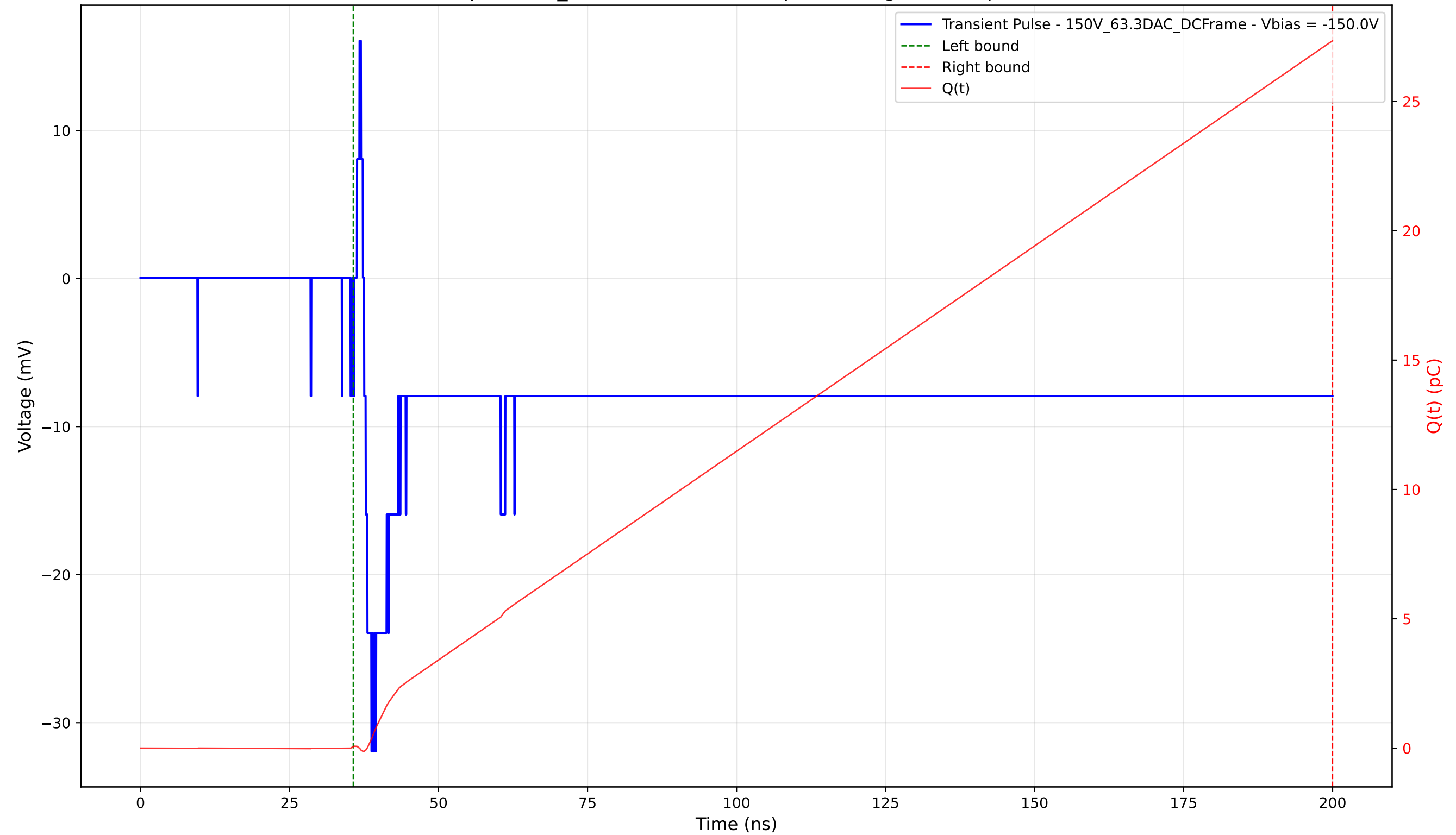
Transient Pulse - Sample: 1cm_42 - Position: 2985.0 \mu\text{m} - Charge: 27.29 pC - Rise Time: 1.23 ns
