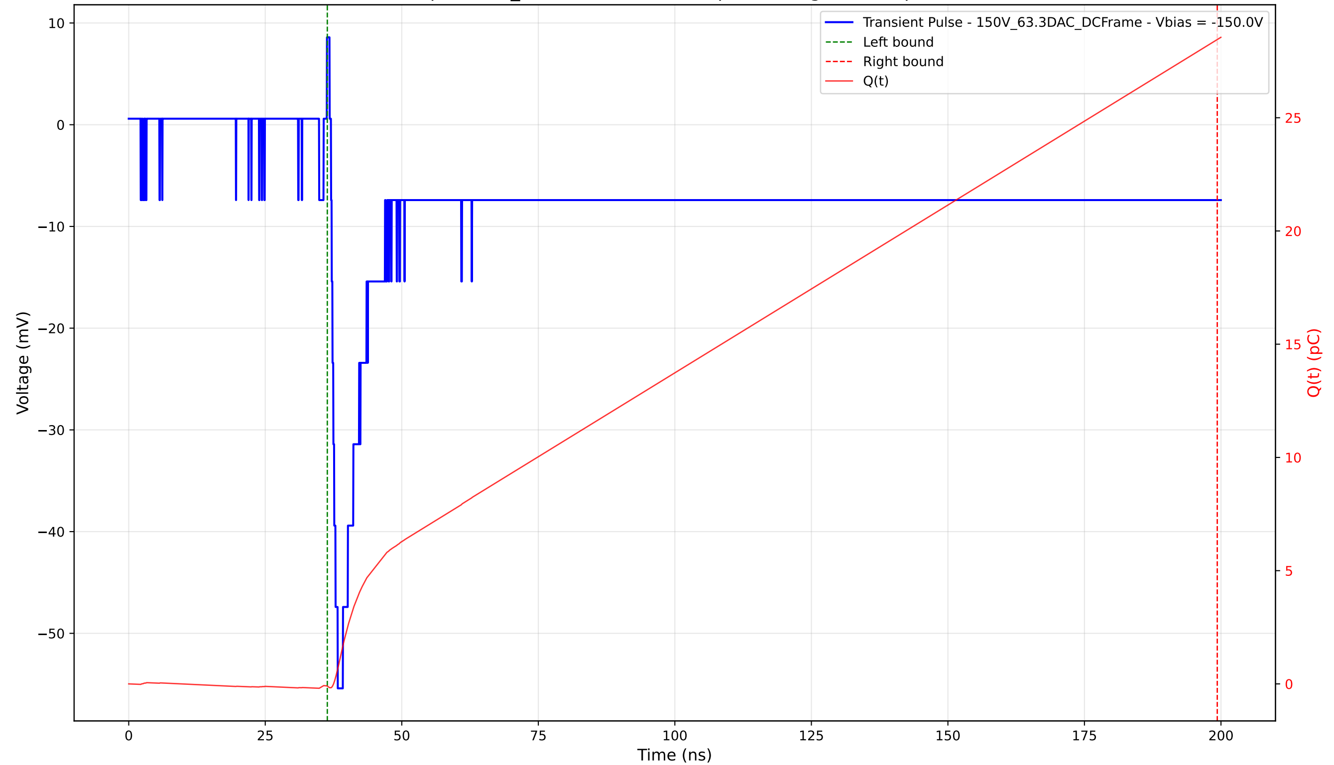
Transient Pulse - Sample: 1cm_42 - Position: 3795.0 \mu\text{m} - Charge: 28.55 pC - Rise Time: 1.23 ns
