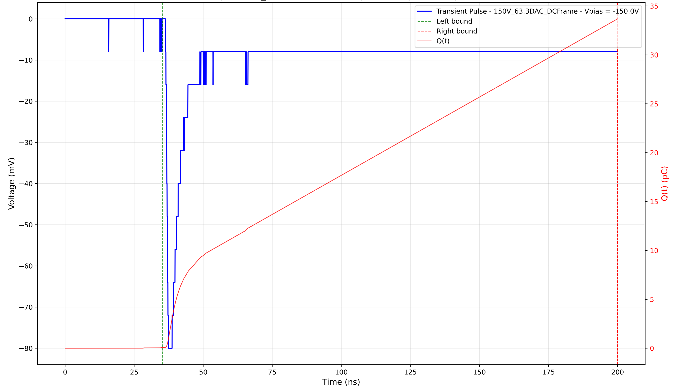
Transient Pulse - Sample: 1cm_42 - Position: 945.0 \mu\text{m} - Charge: 33.60 pC - Rise Time: 0.74 ns
