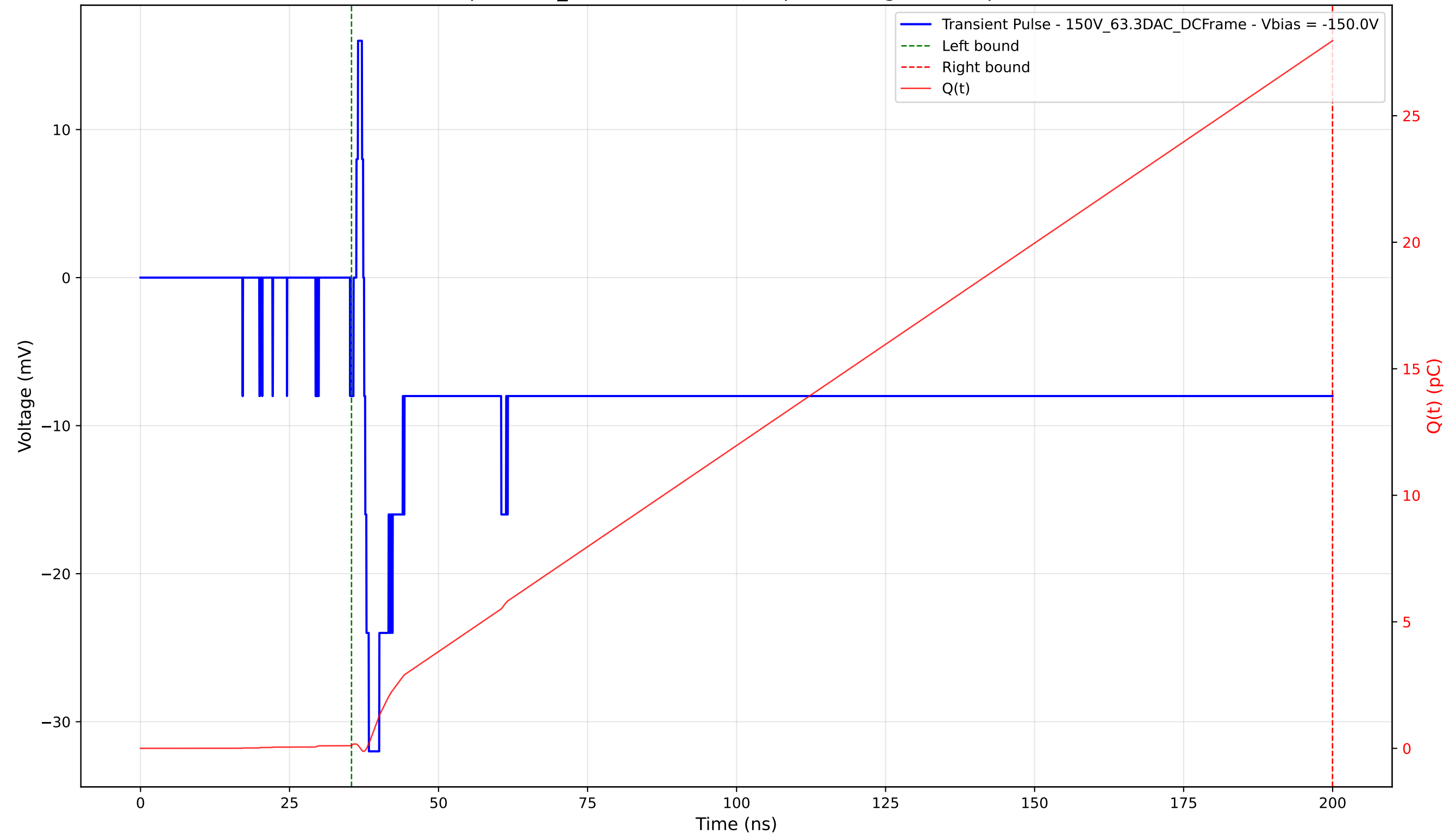
Transient Pulse - Sample: 1cm_42 - Position: 2685.0 \mu\text{m} - Charge: 27.84 pC - Rise Time: 0.79 ns
