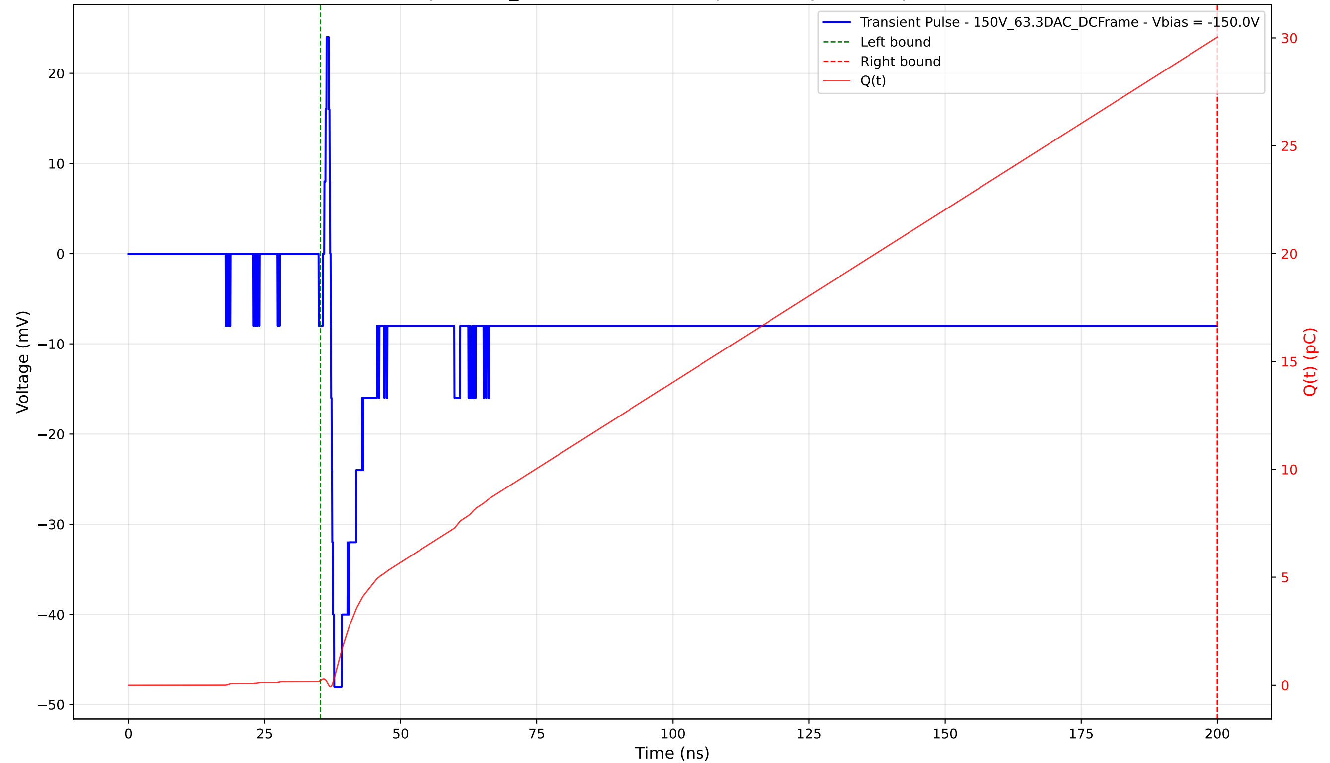
Transient Pulse - Sample: 1cm_42 - Position: 1590.0 \mu\text{m} - Charge: 29.82 pC - Rise Time: 0.65 ns
