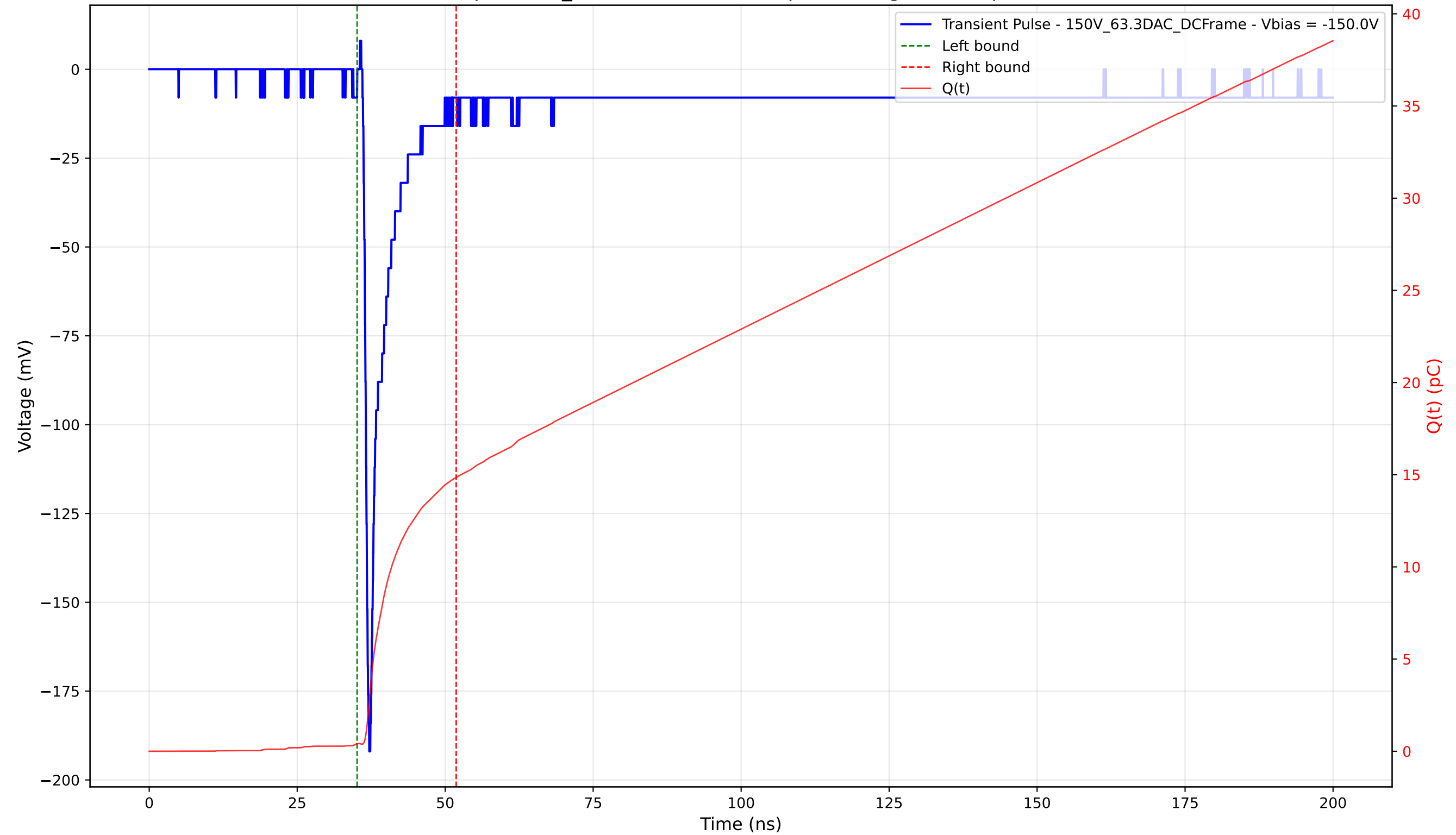
Transient Pulse - Sample: 1cm_42 - Position: 4660.0 \mu\text{m} - Charge: 14.43 pC - Rise Time: 0.77 ns
