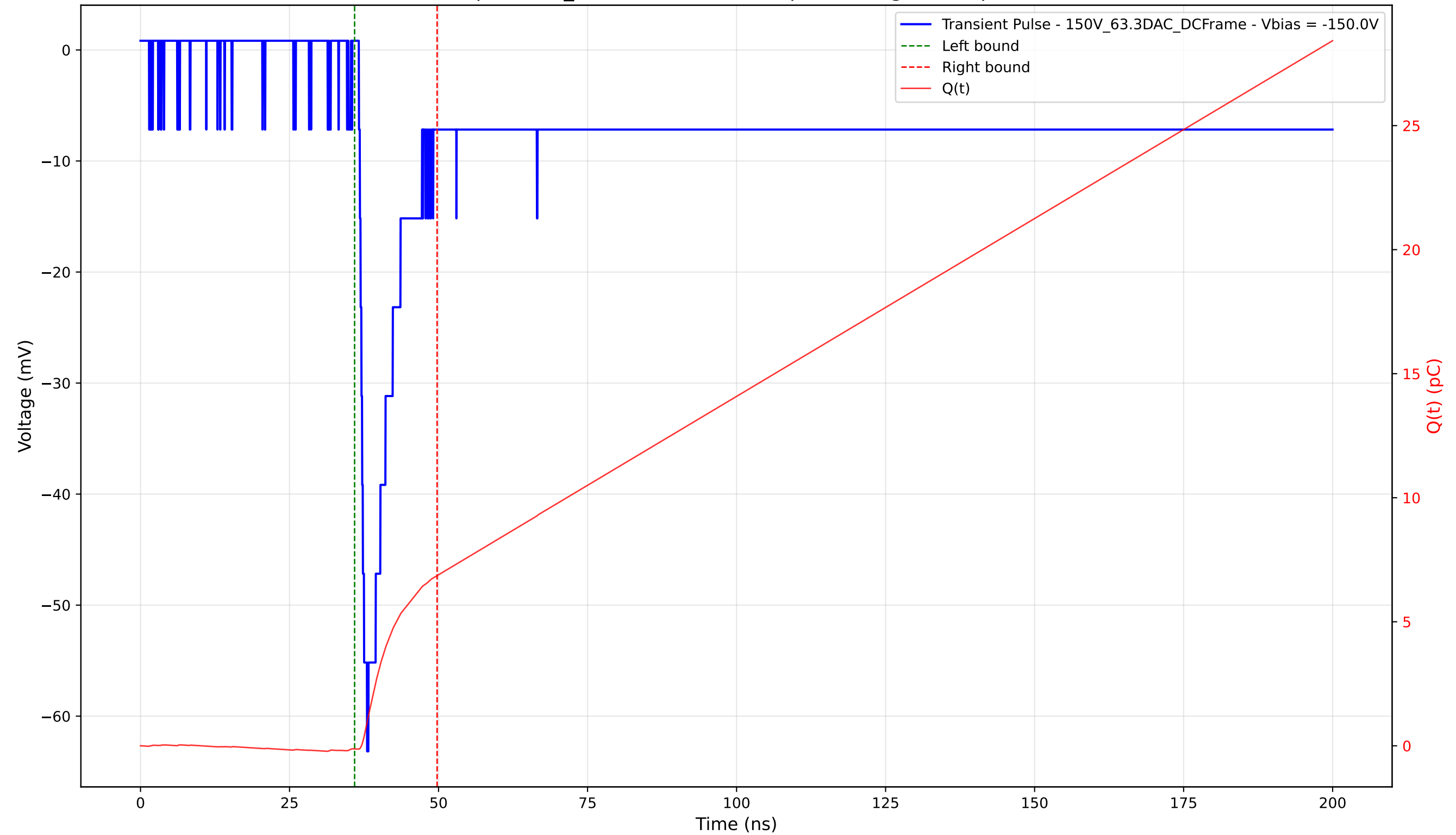
Transient Pulse - Sample: 1cm_42 - Position: 4055.0 \mu\text{m} - Charge: 6.99 pC - Rise Time: 1.36 ns
