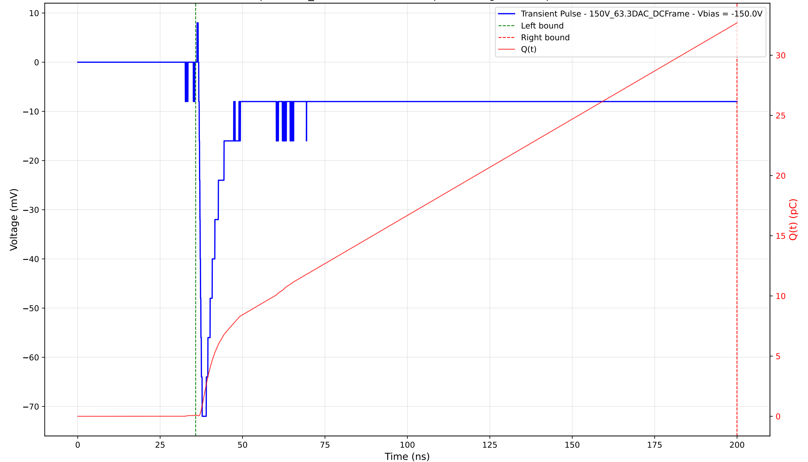
Transient Pulse - Sample: 1cm_42 - Position: 1100.0 \mu\text{m} - Charge: 32.60 pC - Rise Time: 1.02 ns
