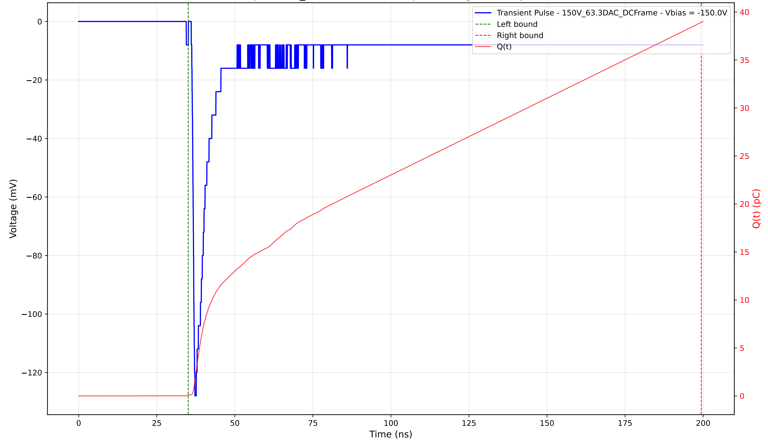
Transient Pulse - Sample: 1cm_42 - Position: 750.0 \mu\text{m} - Charge: 38.82 pC - Rise Time: 0.87 ns
