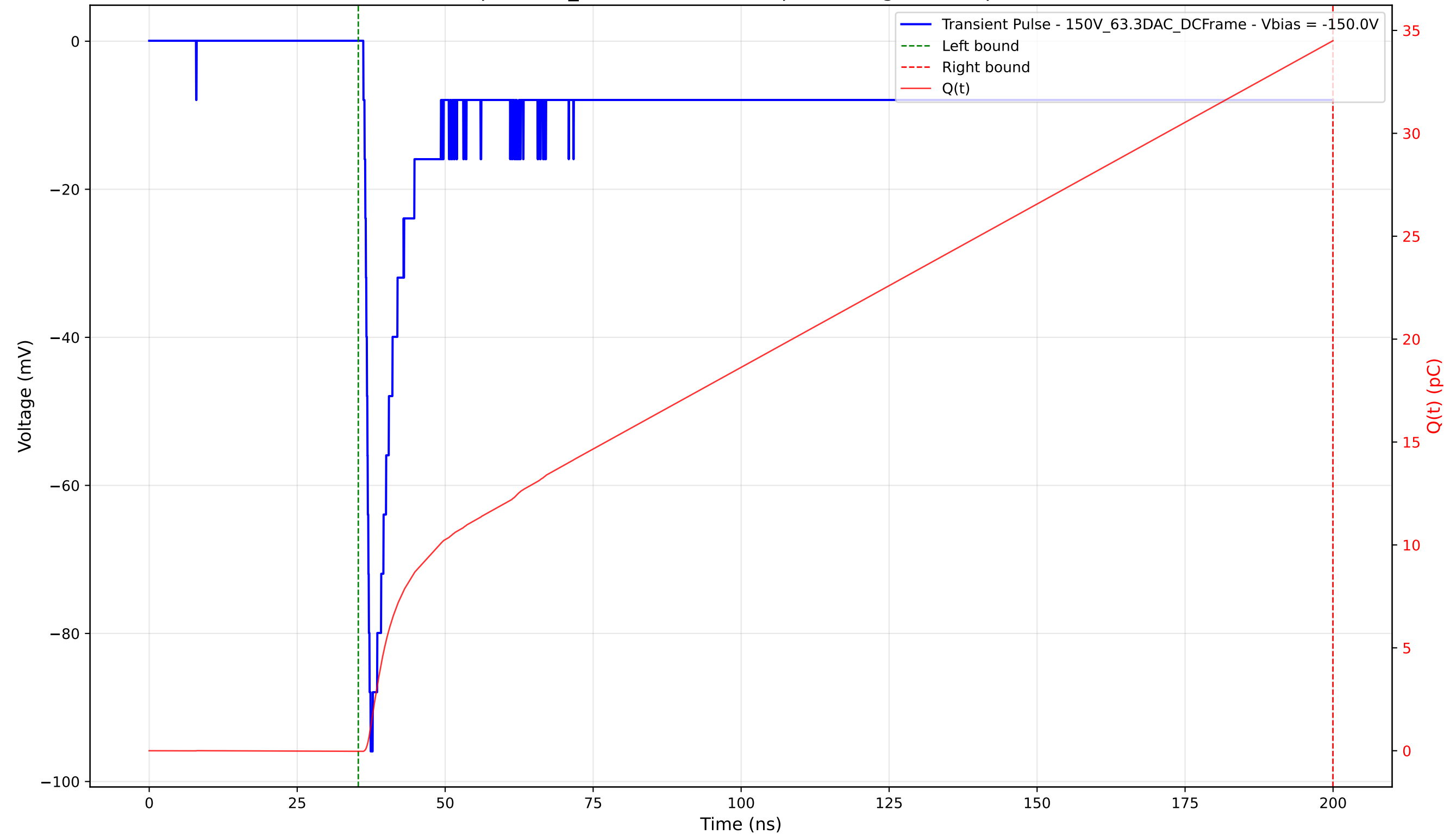
Transient Pulse - Sample: 1cm_42 - Position: 880.0 \mu\text{m} - Charge: 34.53 pC - Rise Time: 0.86 ns
