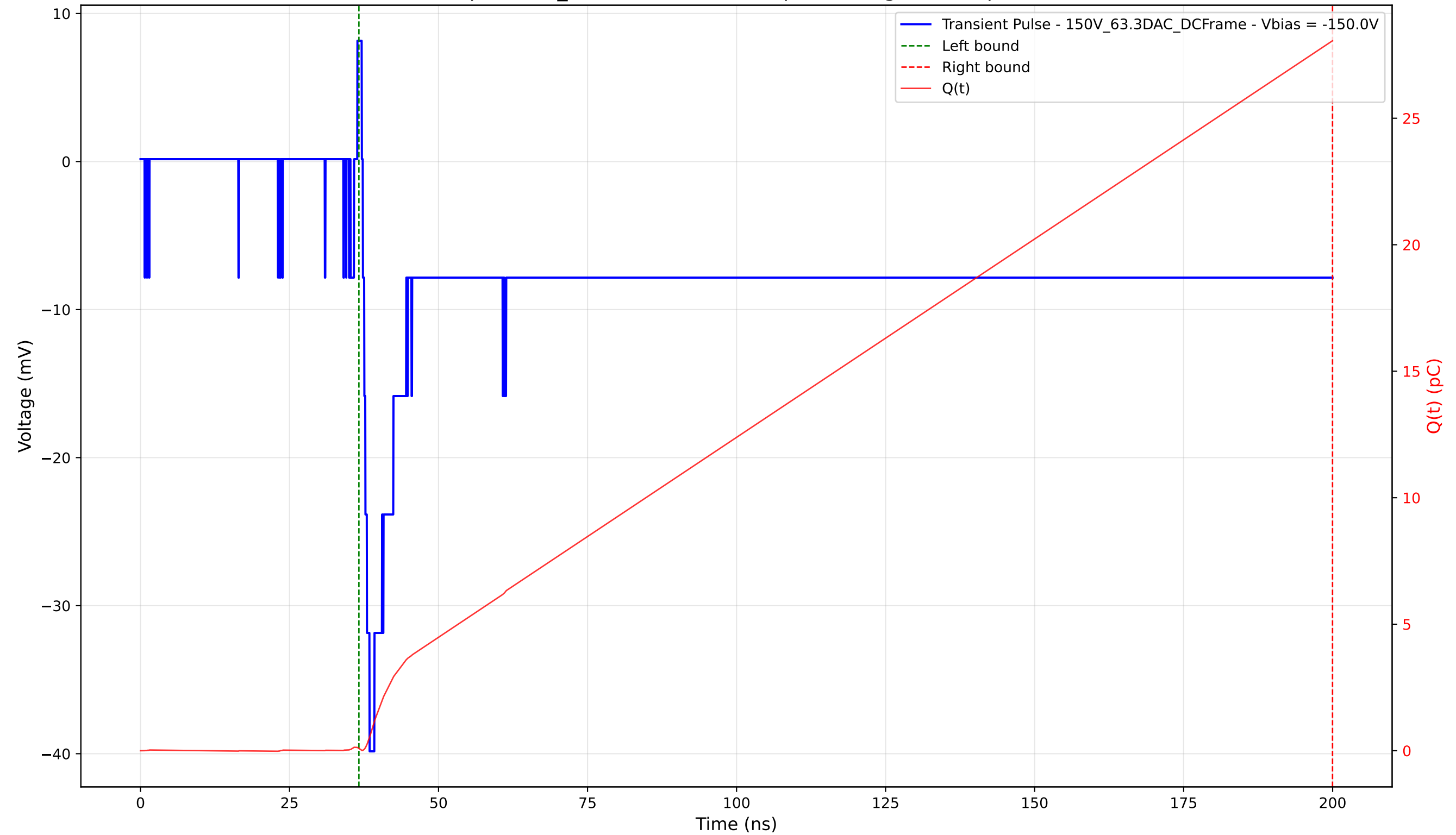
Transient Pulse - Sample: 1cm_42 - Position: 3445.0 \mu\text{m} - Charge: 27.97 pC - Rise Time: 1.13 ns
