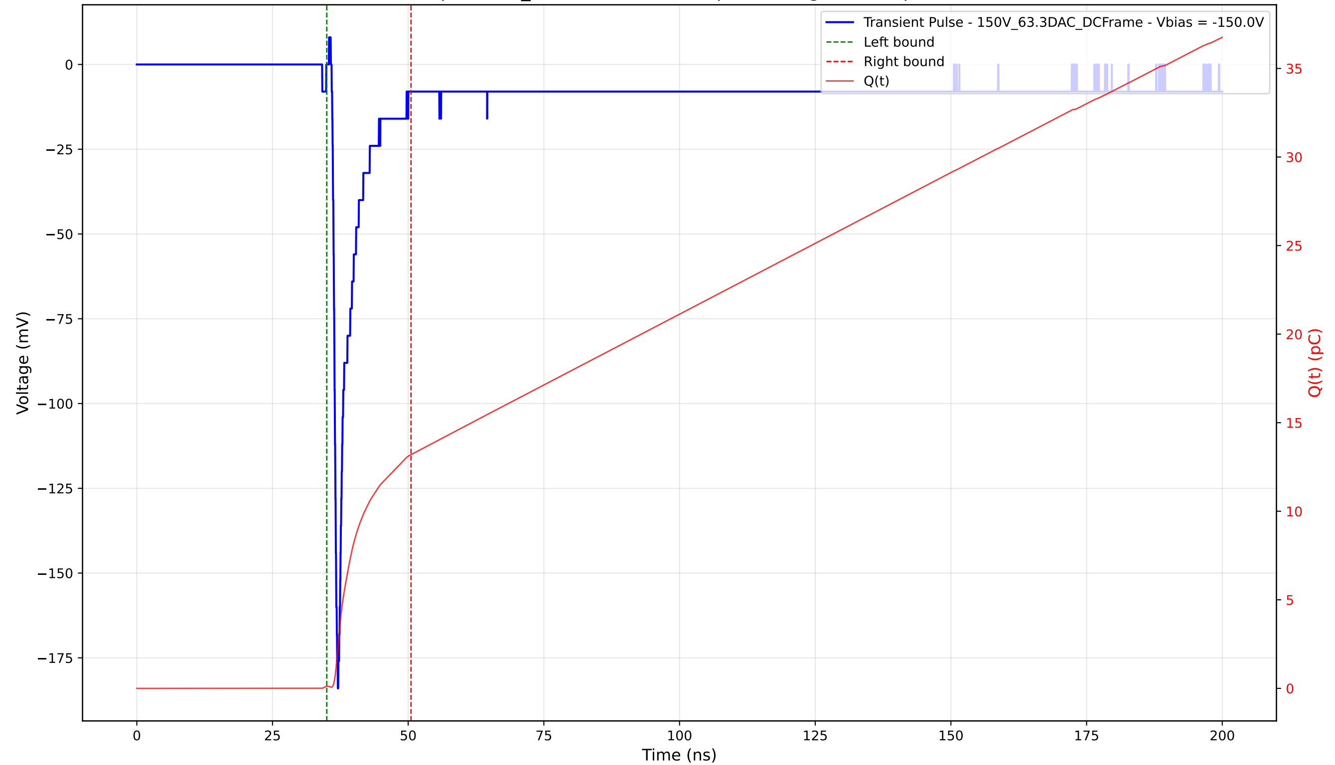
Transient Pulse - Sample: 1cm_42 - Position: 425.0 \mu\text{m} - Charge: 13.08 pC - Rise Time: 0.79 ns
