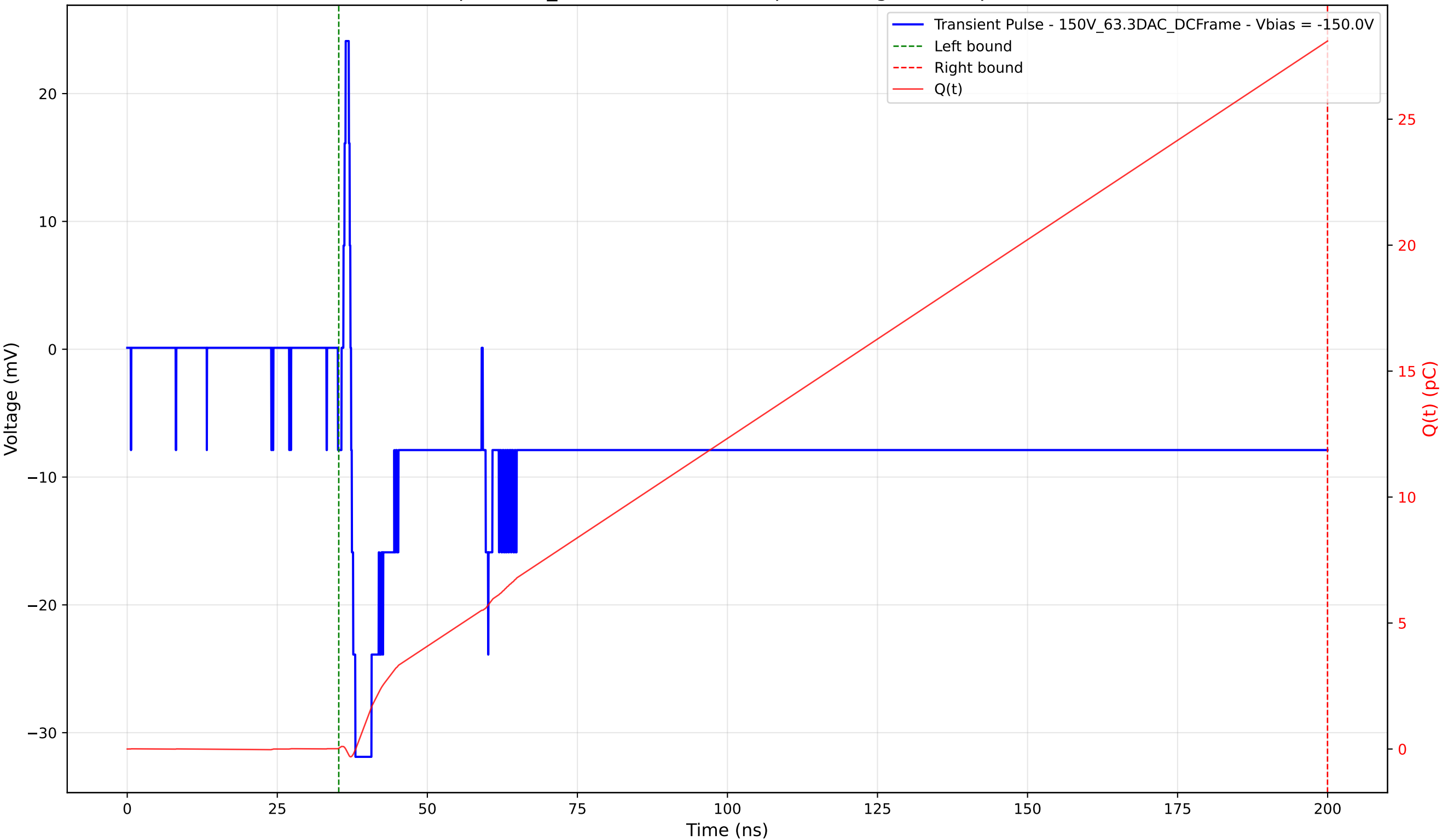
Transient Pulse - Sample: 1cm_42 - Position: 2170.0 \mu\text{m} - Charge: 28.07 pC - Rise Time: 0.71 ns
