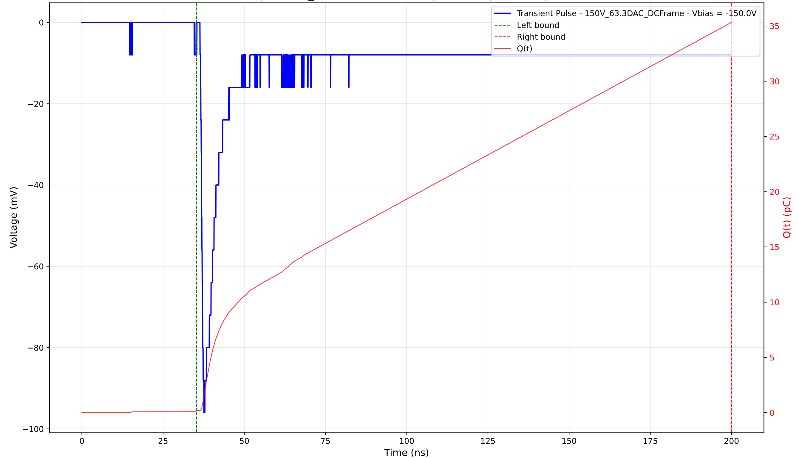
Transient Pulse - Sample: 1cm_42 - Position: 4265.0 \mu\text{m} - Charge: 35.15 pC - Rise Time: 0.82 ns
