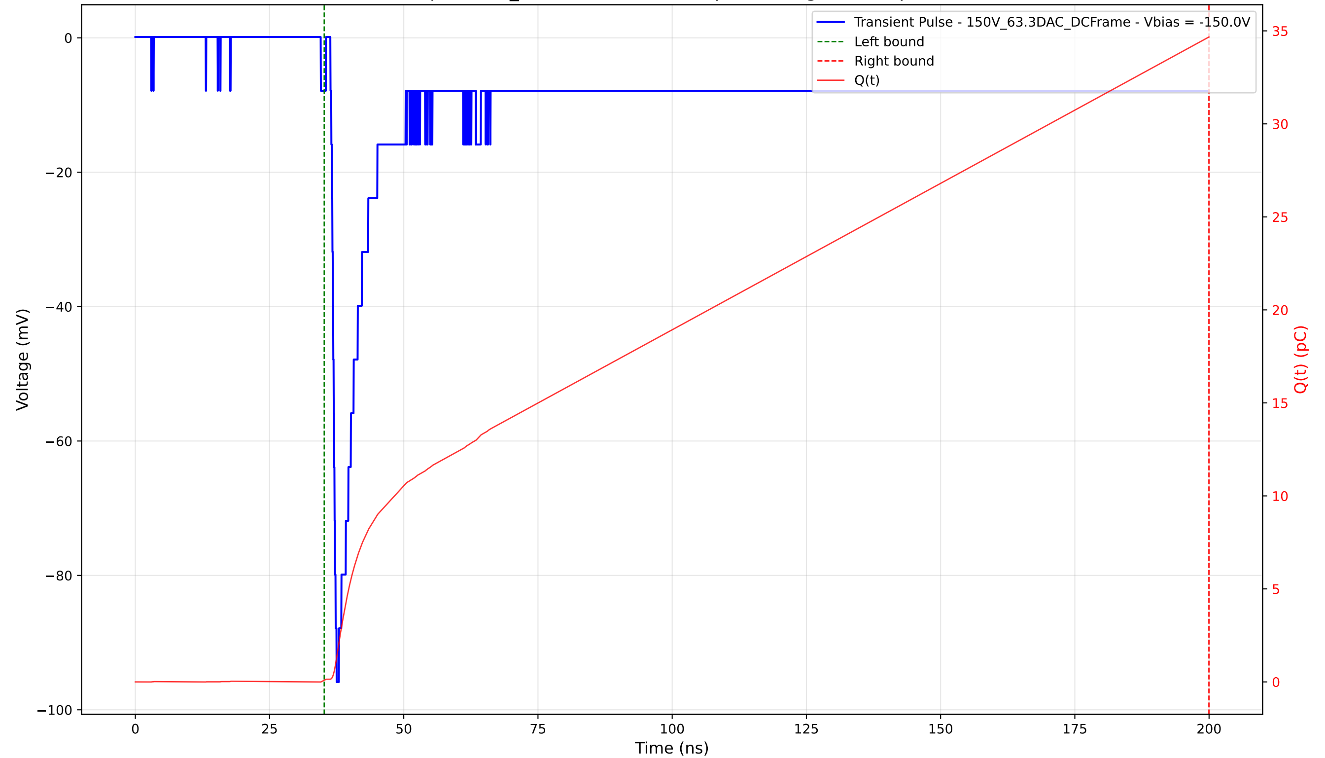
Transient Pulse - Sample: 1cm_42 - Position: 4275.0 \mu\text{m} - Charge: 34.58 pC - Rise Time: 0.82 ns
