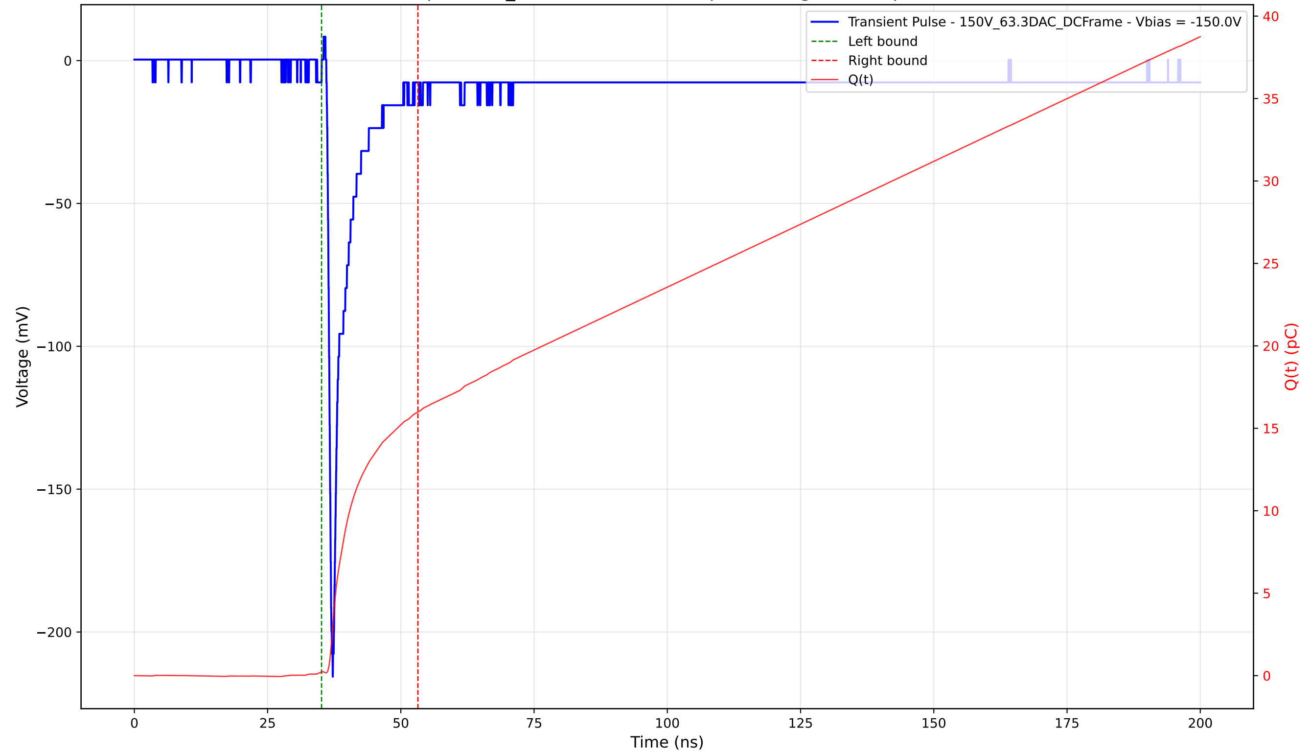
Transient Pulse - Sample: 1cm_42 - Position: 4695.0 \mu\text{m} - Charge: 15.74 pC - Rise Time: 0.81 ns
