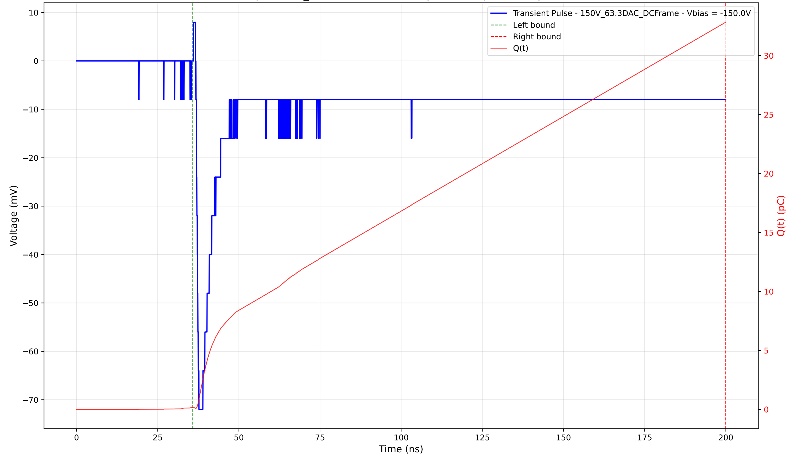
Transient Pulse - Sample: 1cm_42 - Position: 1130.0 \mu\text{m} - Charge: 32.66 pC - Rise Time: 0.92 ns
