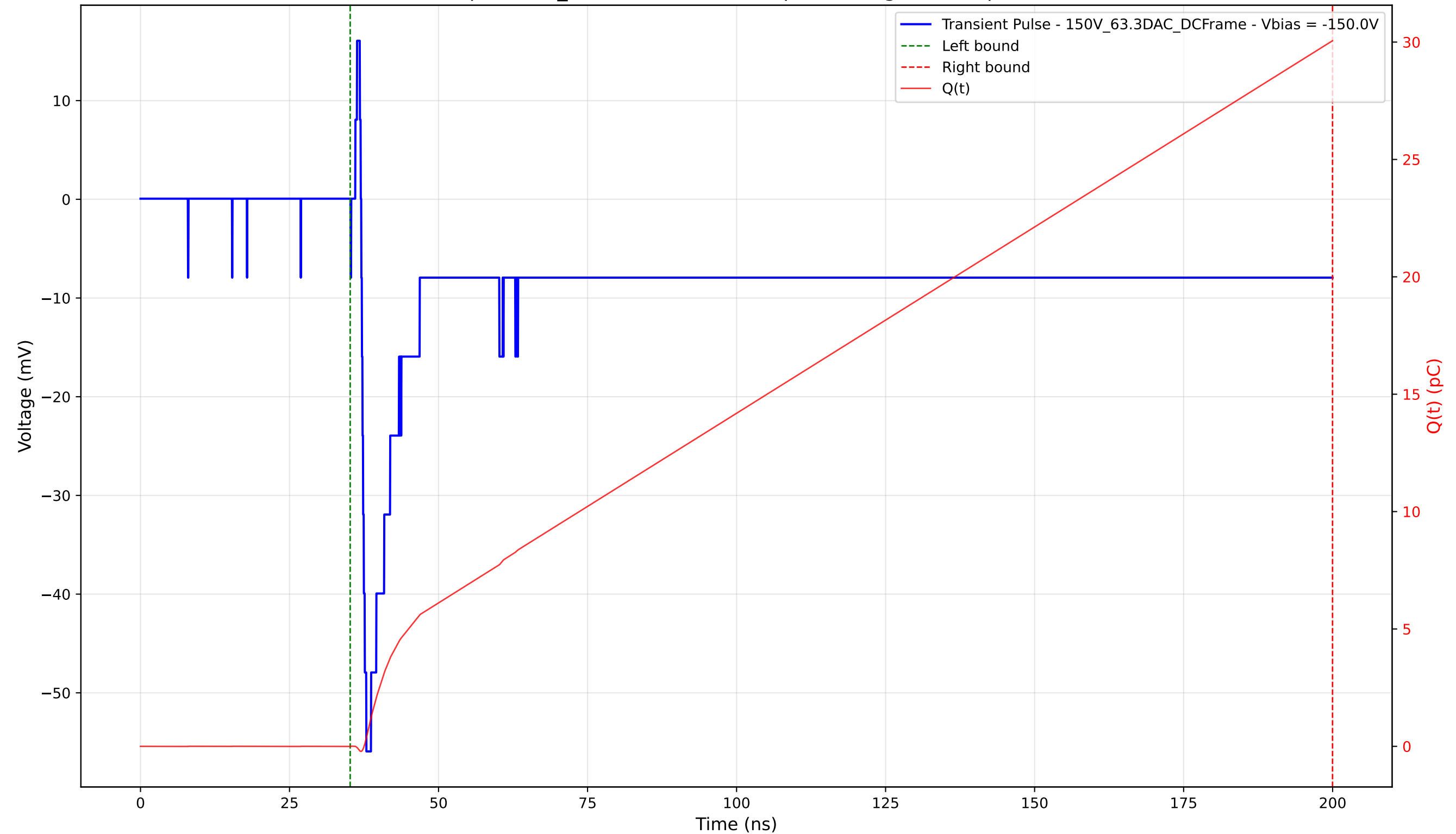
Transient Pulse - Sample: 1cm_42 - Position: 1430.0 \mu\text{m} - Charge: 30.07 pC - Rise Time: 0.85 ns
