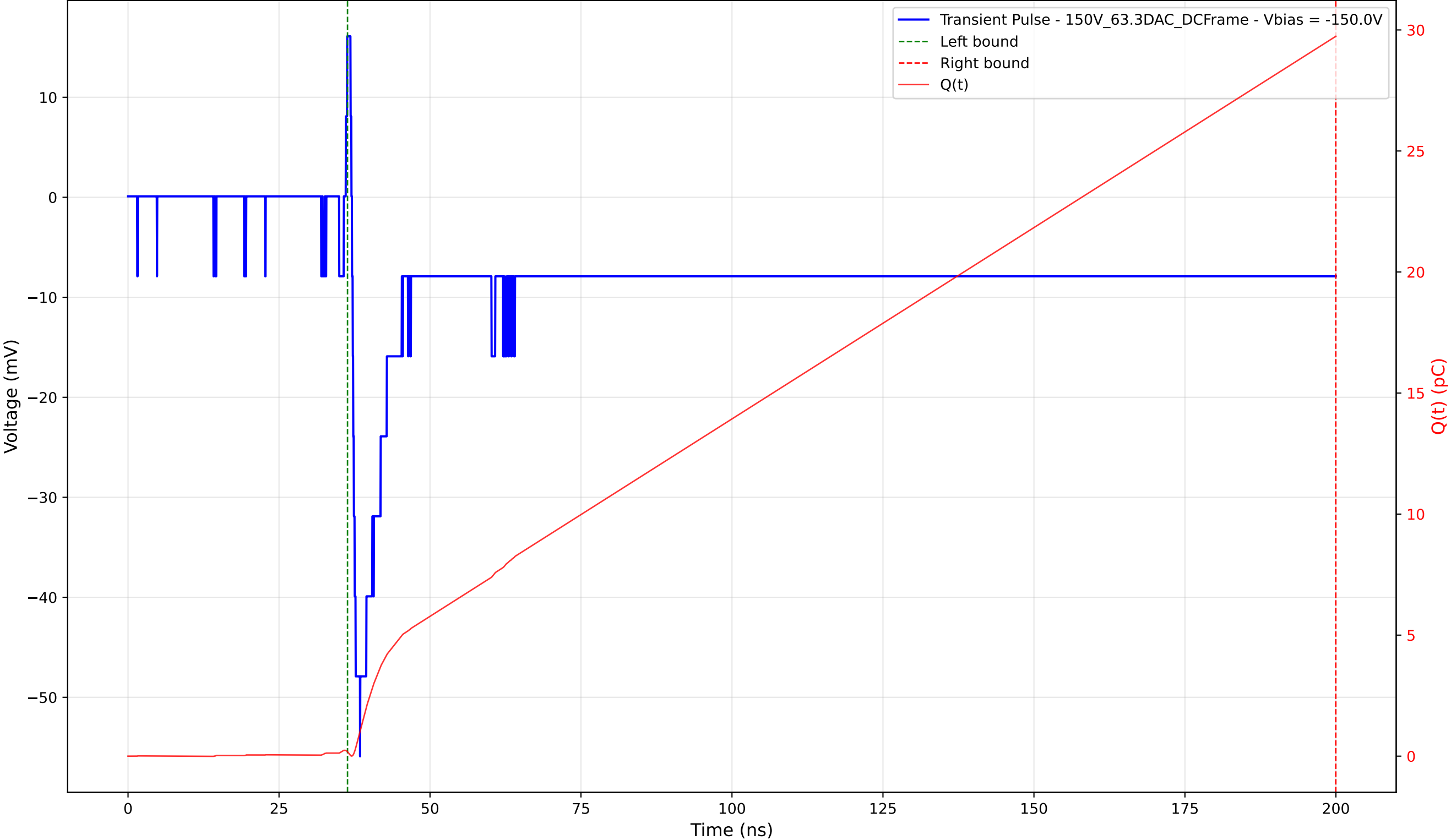
Transient Pulse - Sample: 1cm_42 - Position: 1480.0 \mu\text{m} - Charge: 29.55 pC - Rise Time: 1.35 ns
