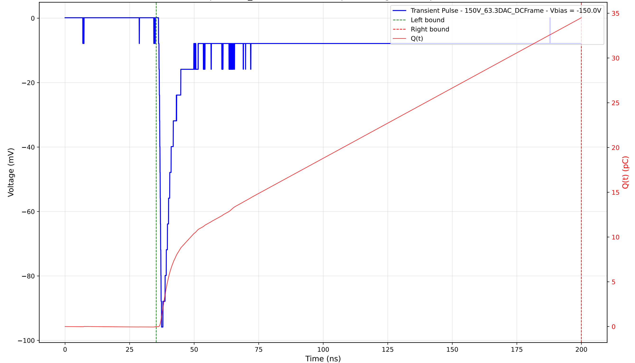
Transient Pulse - Sample: 1cm_42 - Position: 875.0 \mu\text{m} - Charge: 34.51 pC - Rise Time: 0.82 ns
