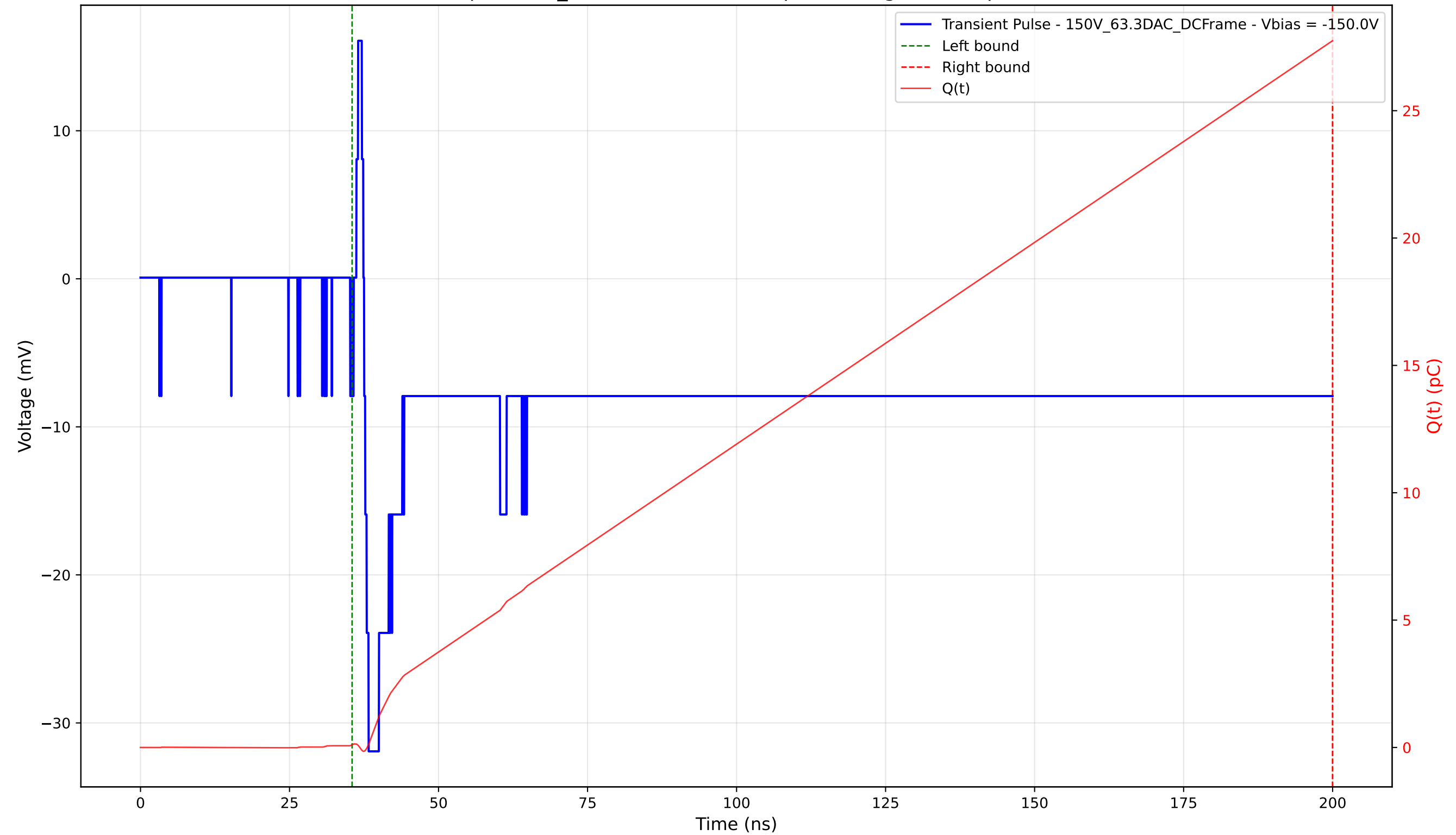
Transient Pulse - Sample: 1cm_42 - Position: 2795.0 \mu\text{m} - Charge: 27.64 pC - Rise Time: 0.75 ns
