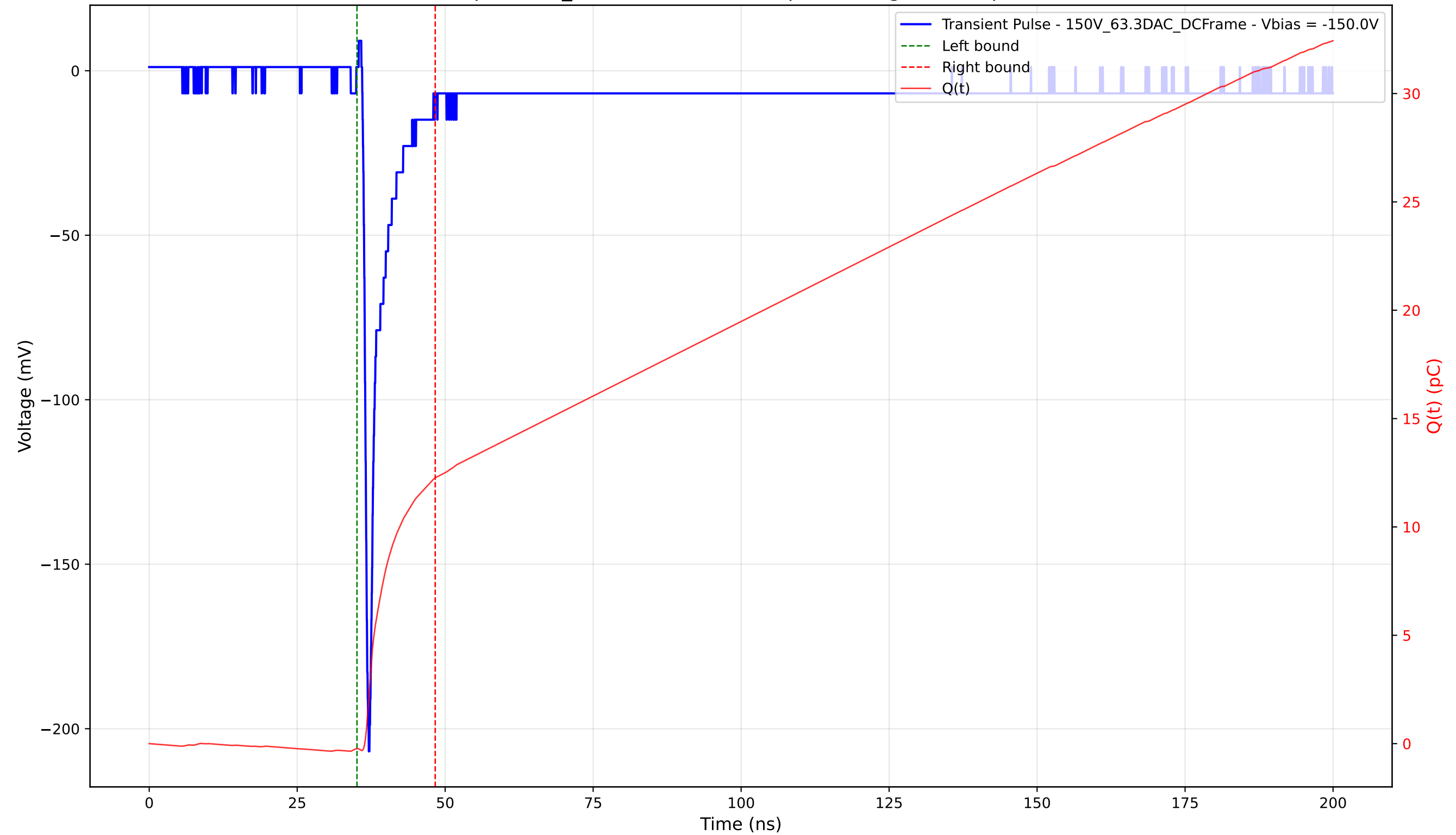
Transient Pulse - Sample: 1cm_42 - Position: 4905.0 \mu\text{m} - Charge: 12.50 pC - Rise Time: 0.81 ns
