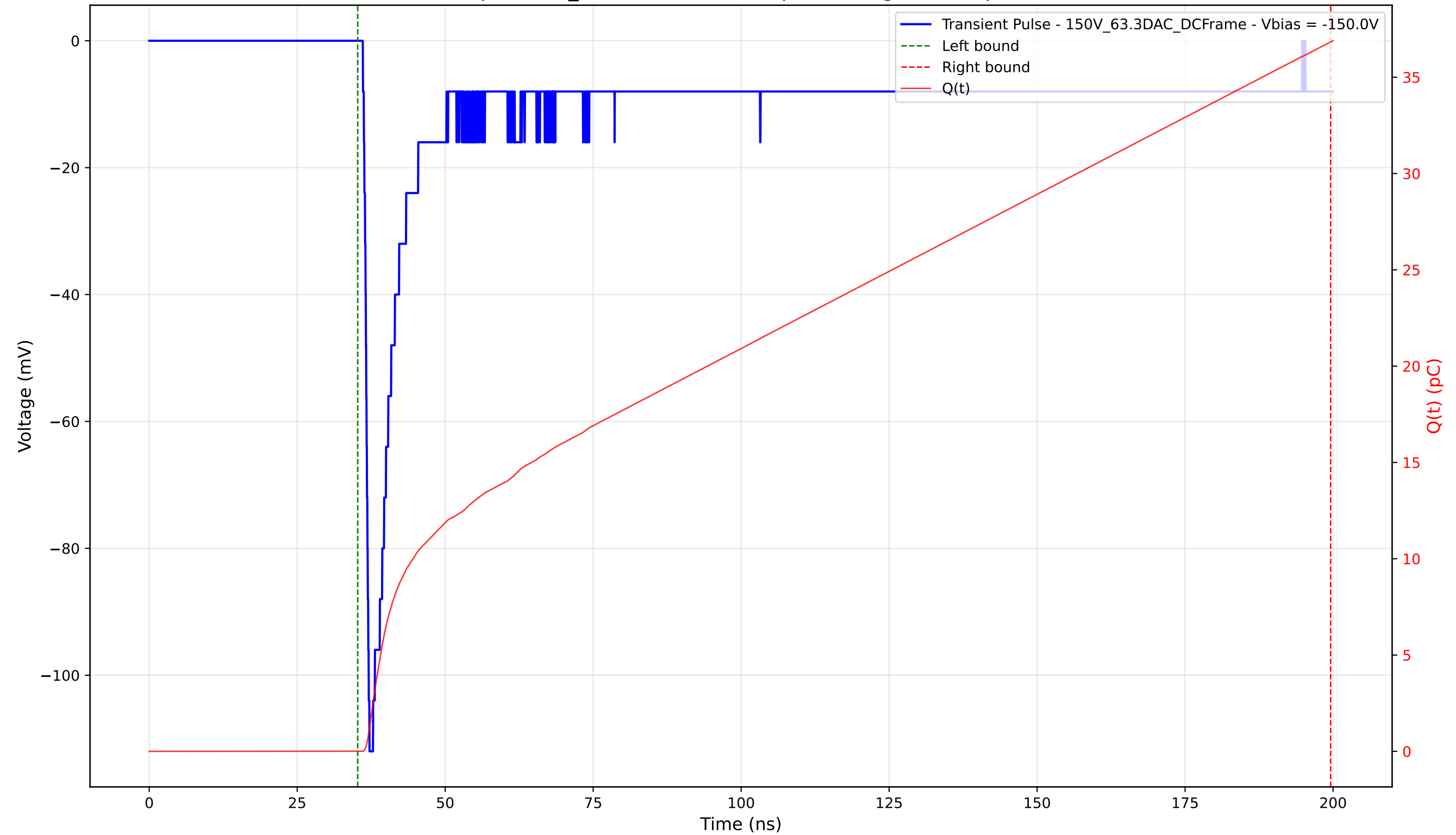
Transient Pulse - Sample: 1cm_42 - Position: 800.0 \mu\text{m} - Charge: 36.83 pC - Rise Time: 0.83 ns
