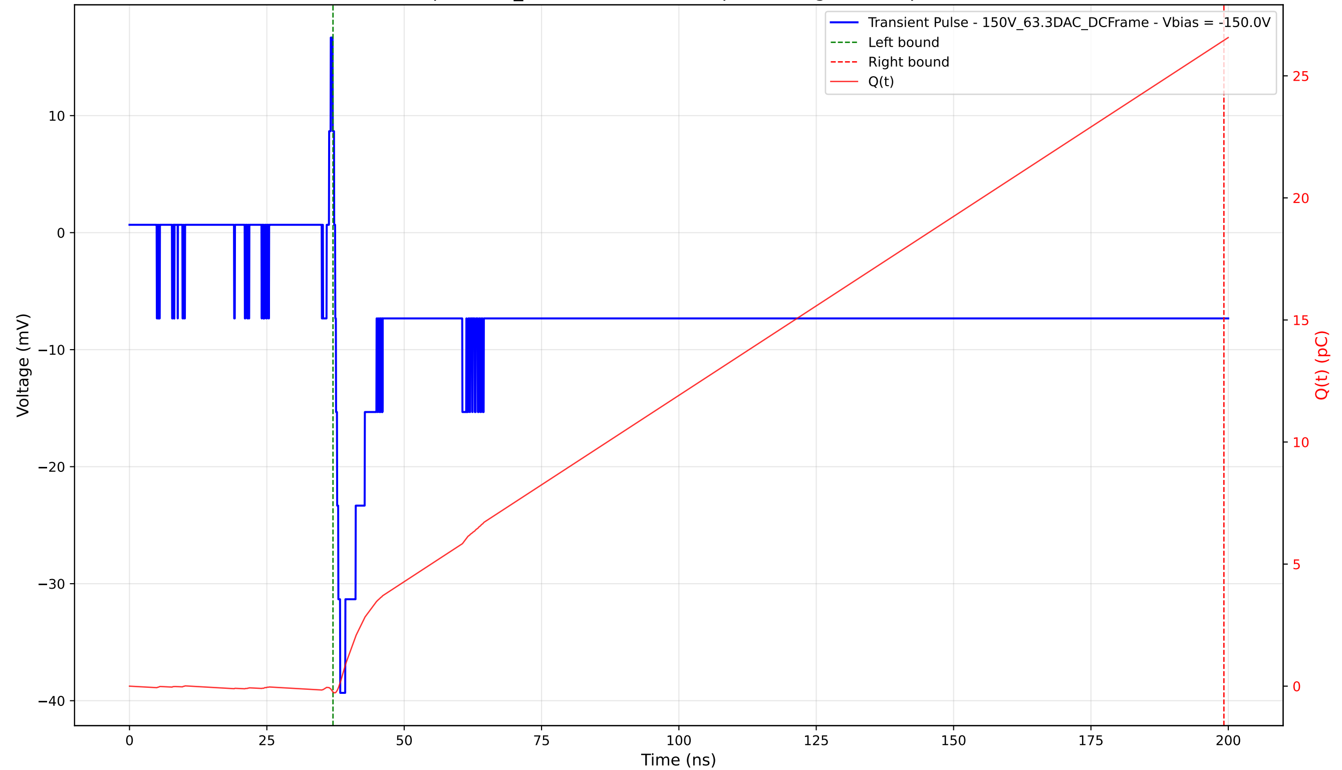
Transient Pulse - Sample: 1cm_42 - Position: 3245.0 \mu\text{m} - Charge: 26.69 pC - Rise Time: 0.91 ns
