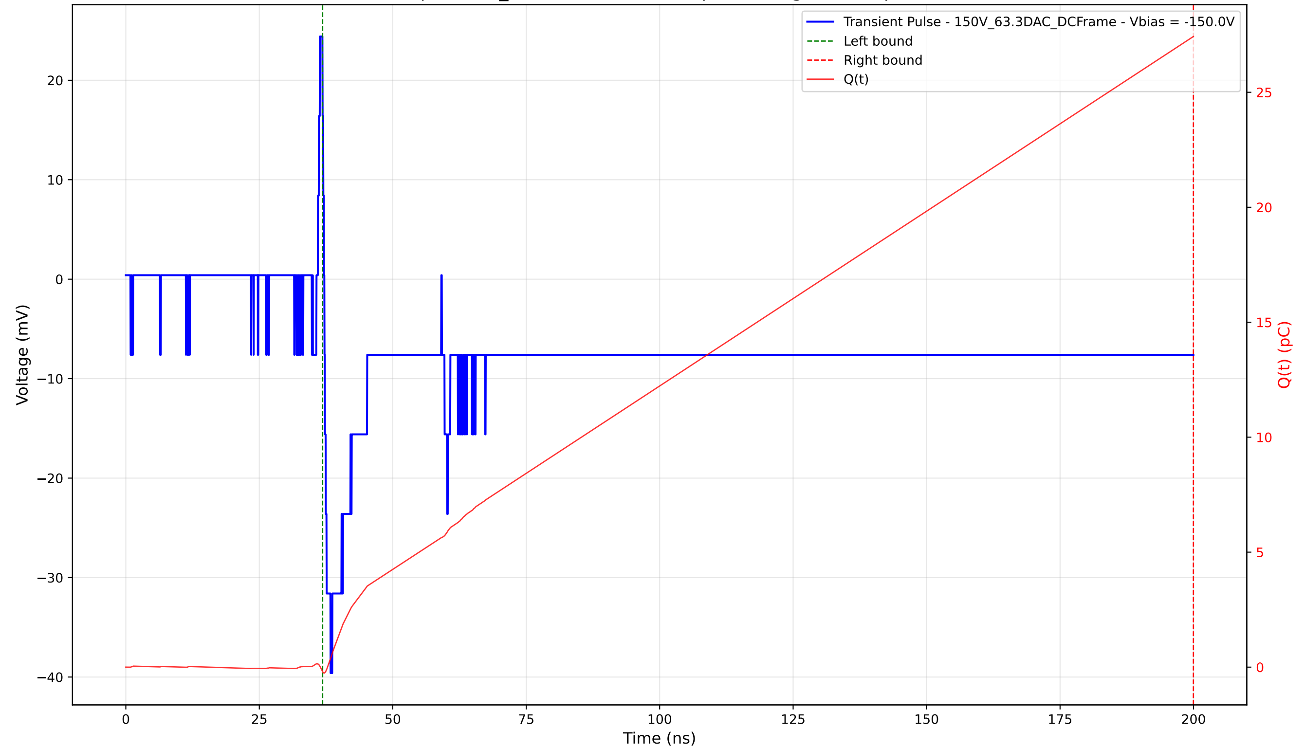
Transient Pulse - Sample: 1cm_42 - Position: 1935.0 \mu\text{m} - Charge: 27.63 pC - Rise Time: 1.15 ns
