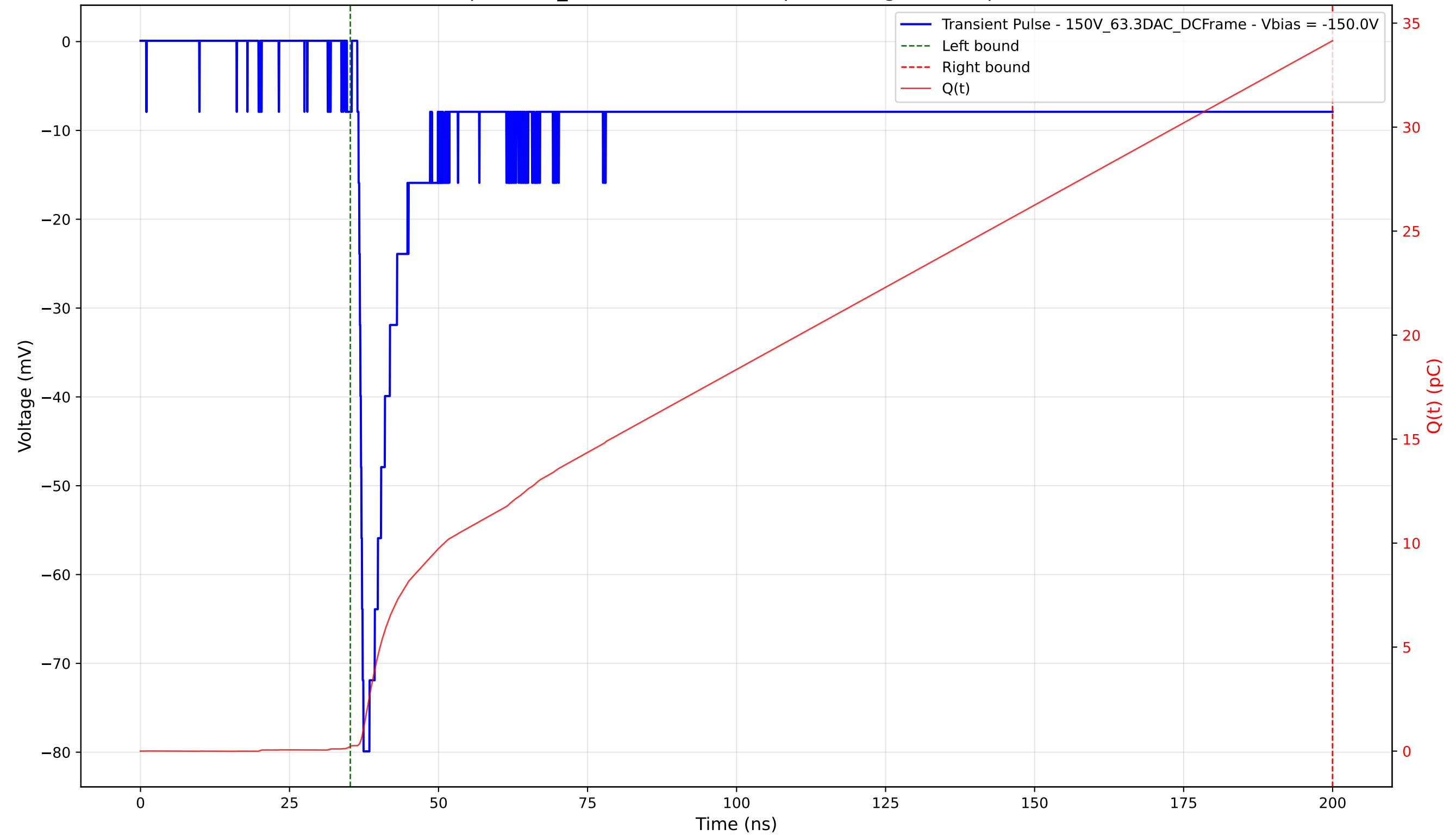
Transient Pulse - Sample: 1cm_42 - Position: 4185.0 \mu\text{m} - Charge: 33.93 pC - Rise Time: 0.84 ns
