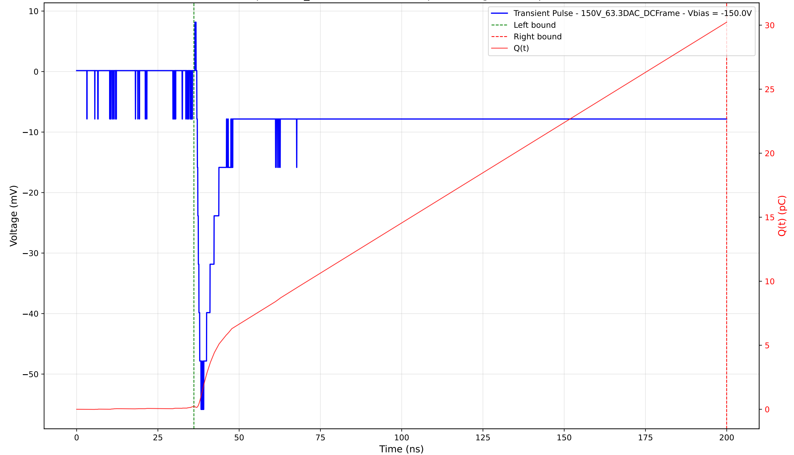
Transient Pulse - Sample: 1cm_42 - Position: 3820.0 \mu\text{m} - Charge: 30.03 pC - Rise Time: 1.29 ns
