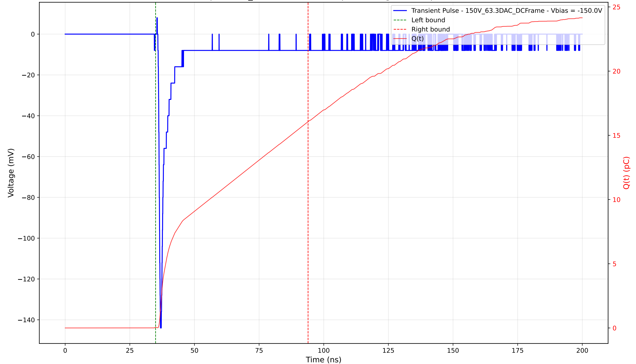
Transient Pulse - Sample: 1cm_42 - Position: 195.0 \mu\text{m} - Charge: 16.02 pC - Rise Time: 0.78 ns
