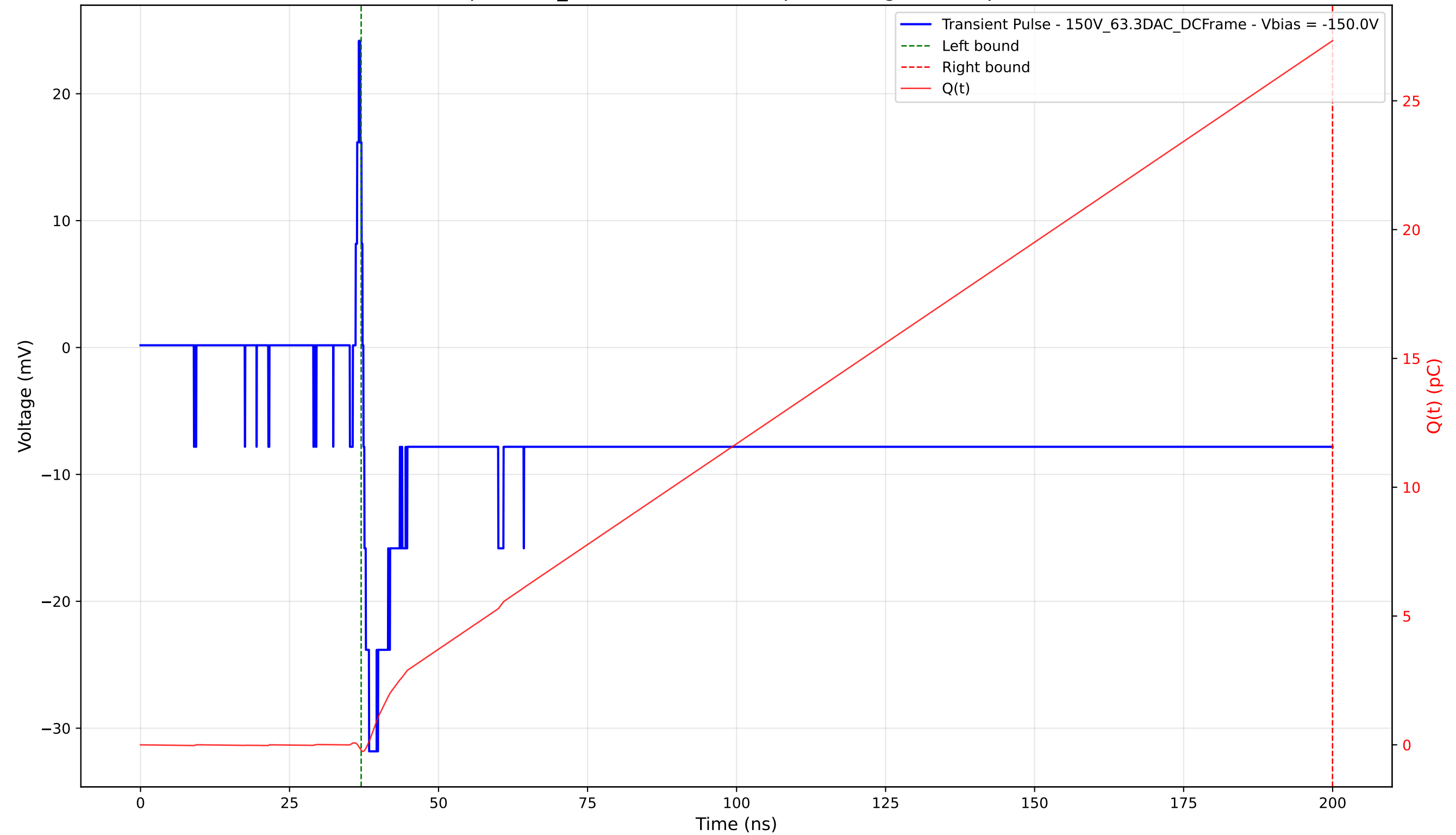
Transient Pulse - Sample: 1cm_42 - Position: 2405.0 \mu\text{m} - Charge: 27.54 pC - Rise Time: 0.95 ns
