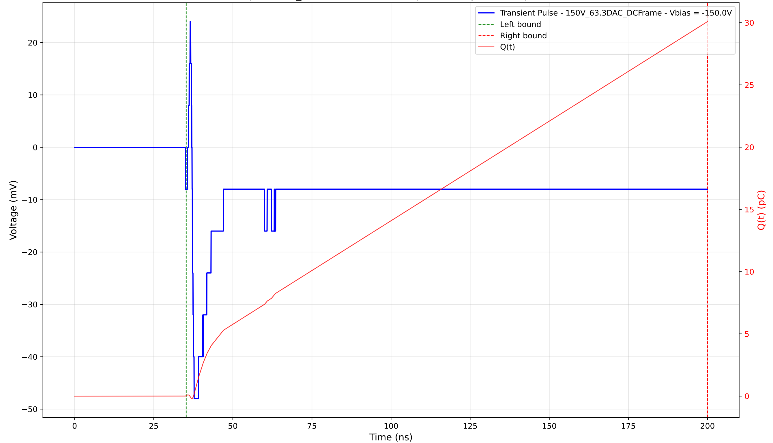
Transient Pulse - Sample: 1cm_42 - Position: 1530.0 \mu\text{m} - Charge: 30.05 pC - Rise Time: 0.65 ns
