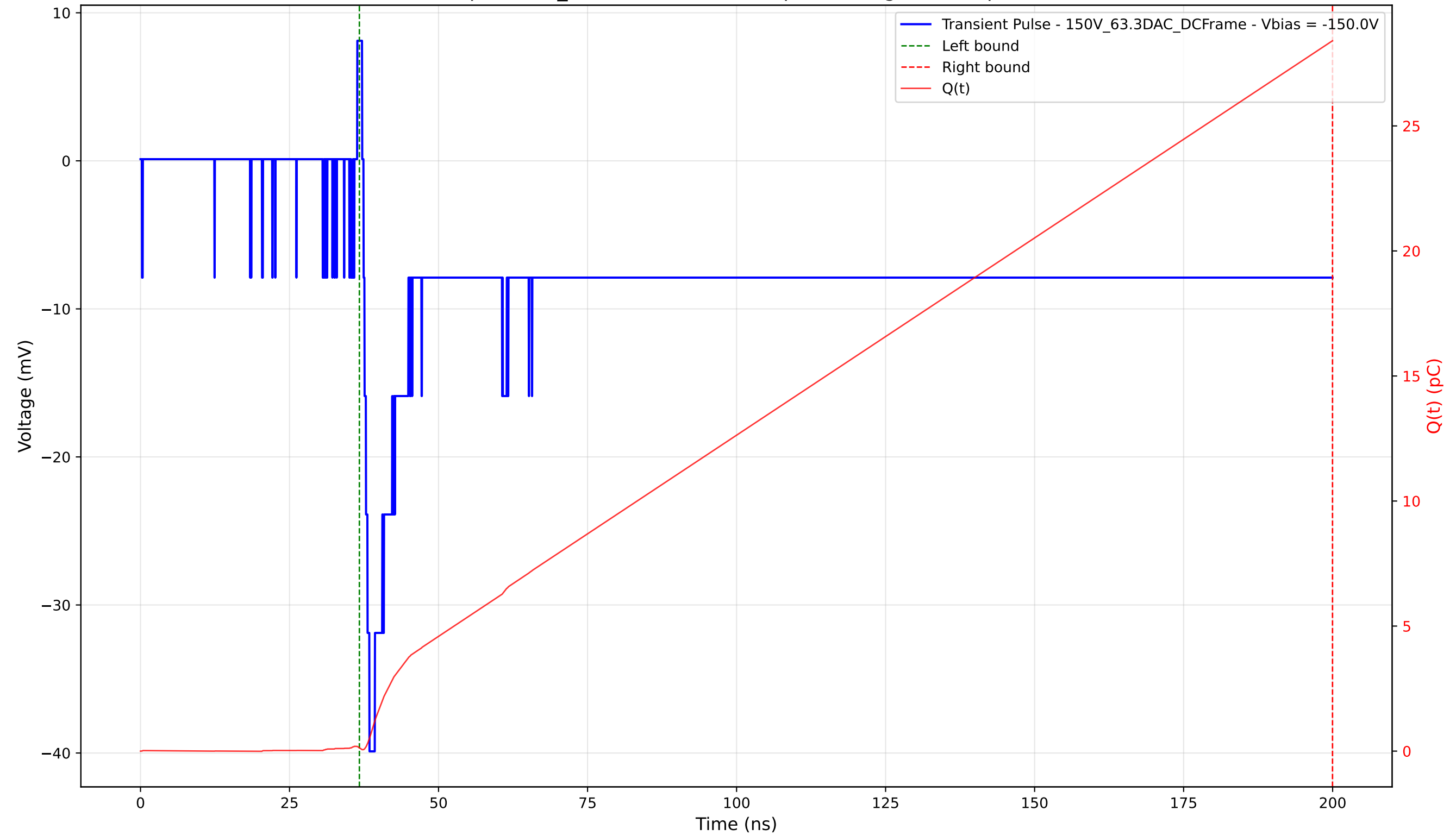
Transient Pulse - Sample: 1cm_42 - Position: 3360.0 \mu\text{m} - Charge: 28.28 pC - Rise Time: 0.99 ns
