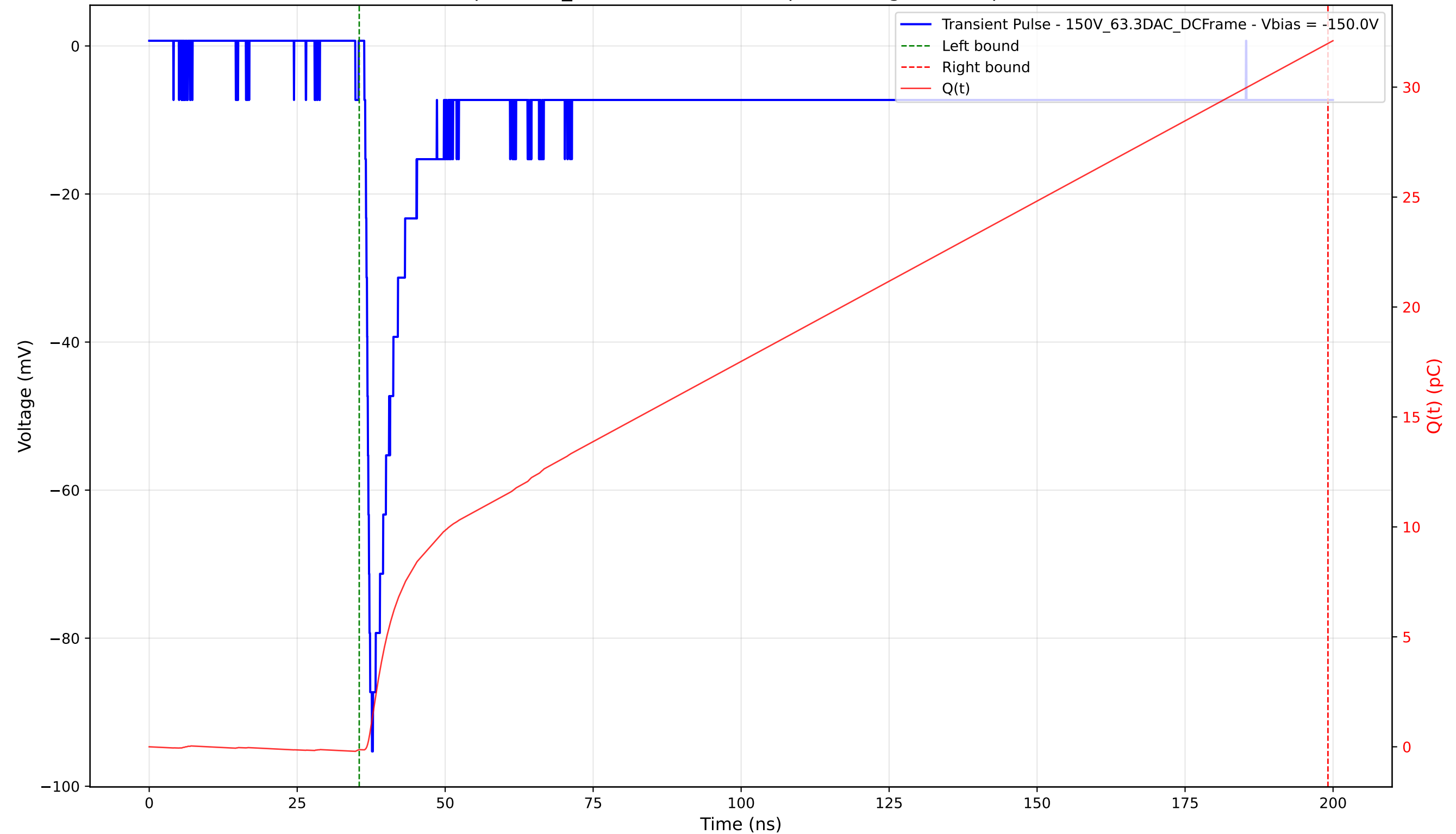
Transient Pulse - Sample: 1cm_42 - Position: 4310.0 \mu\text{m} - Charge: 32.12 pC - Rise Time: 0.83 ns
