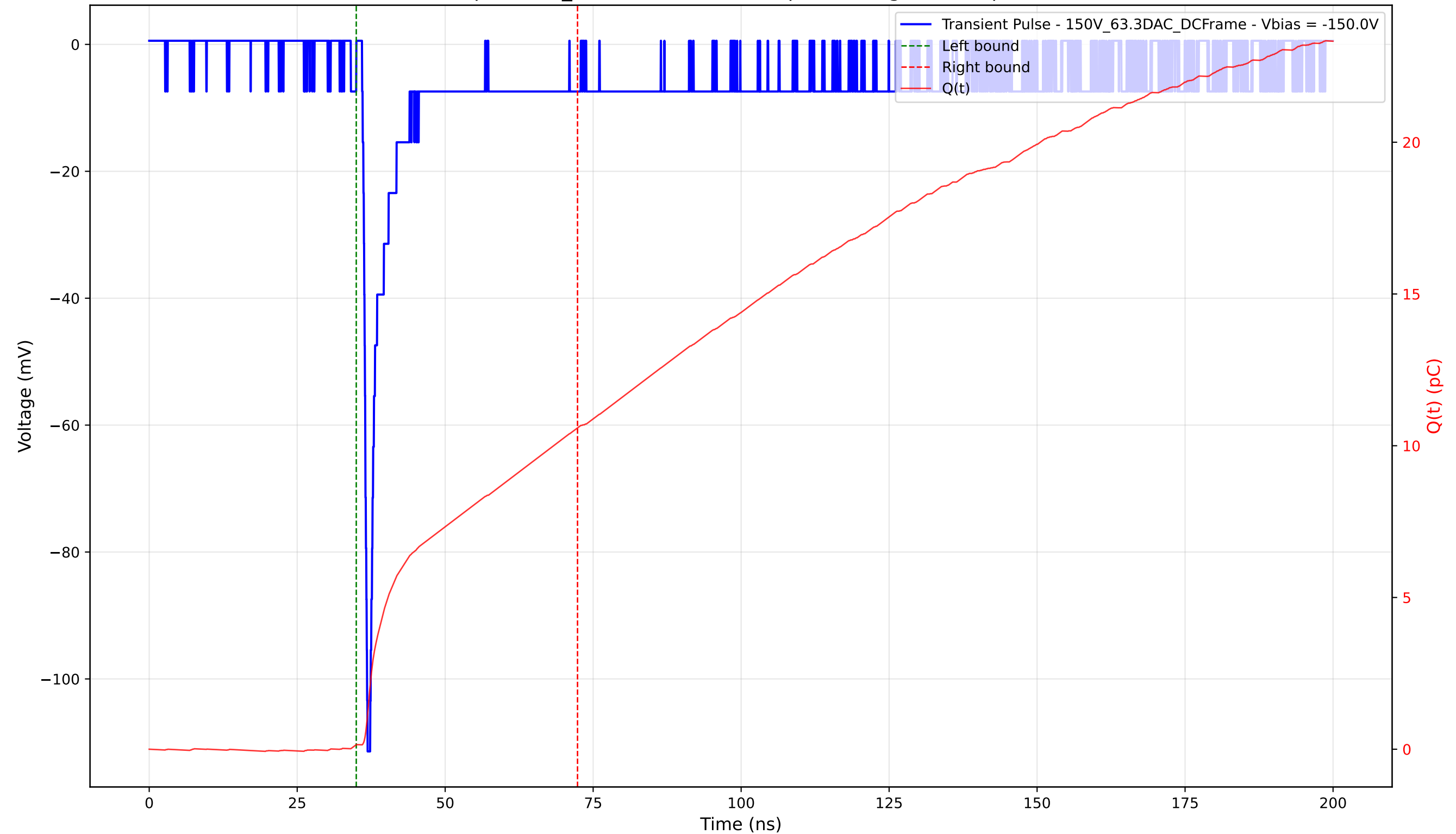
Transient Pulse - Sample: 1cm_42 - Position: 5025.0 \mu\text{m} - Charge: 10.44 pC - Rise Time: 0.75 ns
