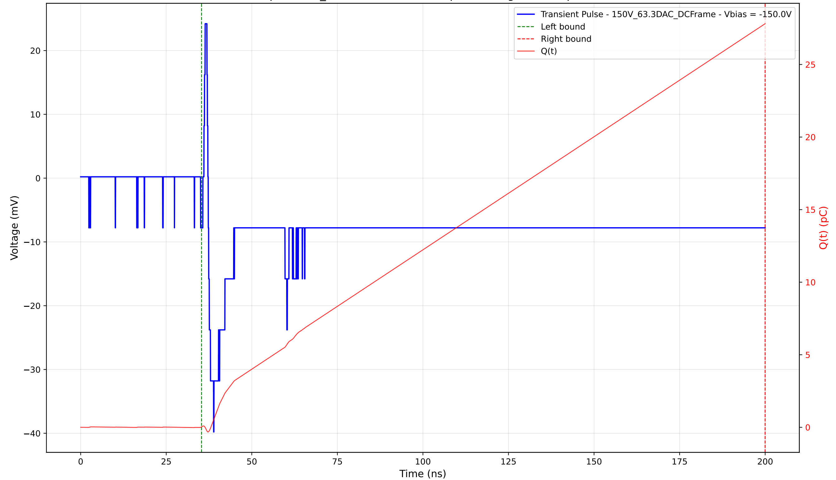
Transient Pulse - Sample: 1cm_42 - Position: 2140.0 \mu\text{m} - Charge: 27.78 pC - Rise Time: 1.57 ns
