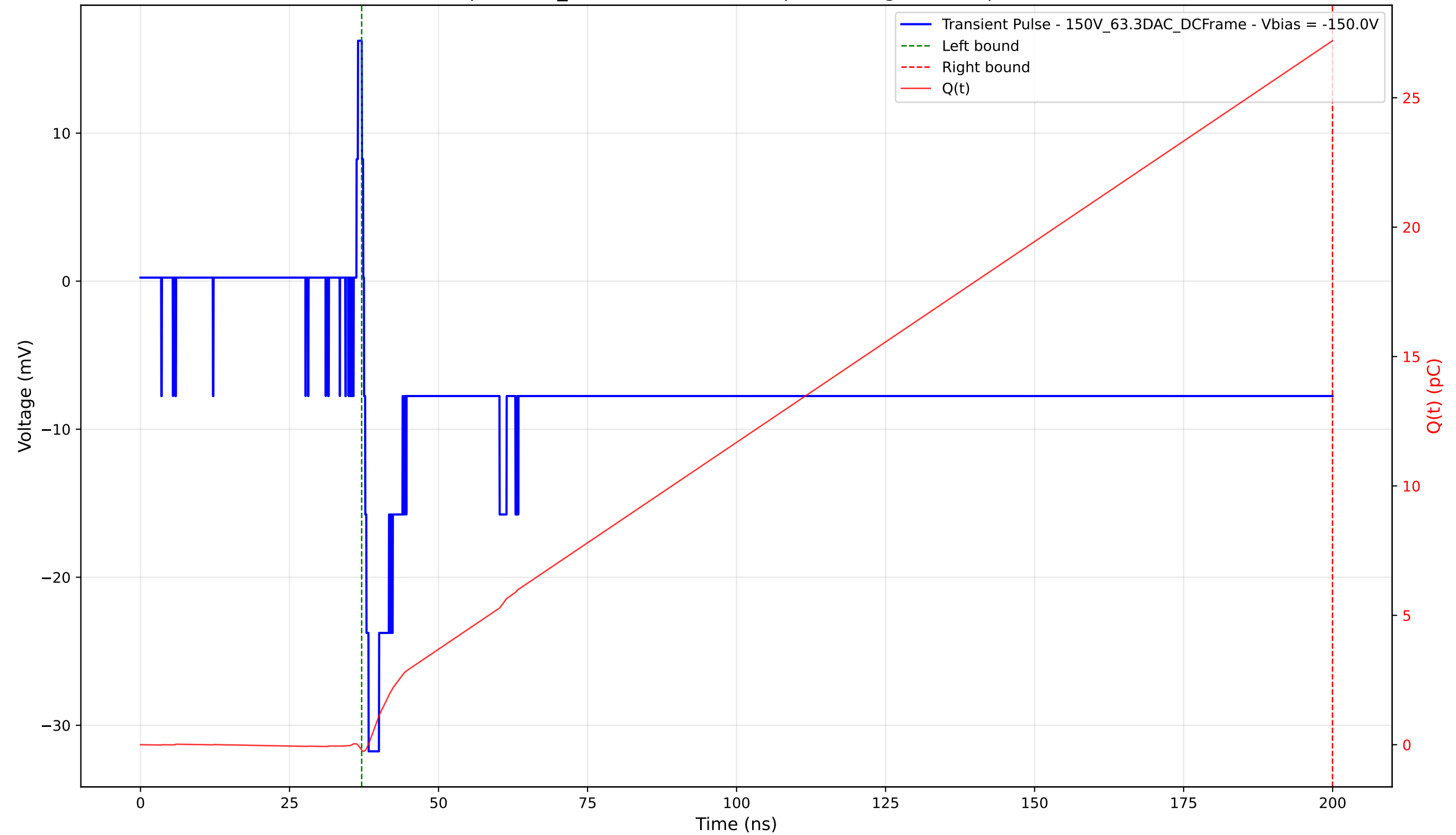
Transient Pulse - Sample: 1cm_42 - Position: 2690.0 \mu\text{m} - Charge: 27.41 pC - Rise Time: 0.77 ns
