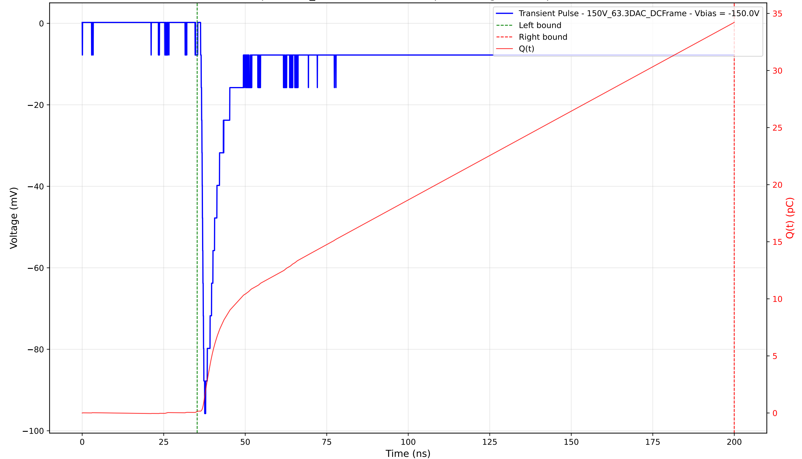
Transient Pulse - Sample: 1cm_42 - Position: 4280.0 \mu\text{m} - Charge: 34.08 pC - Rise Time: 0.82 ns
