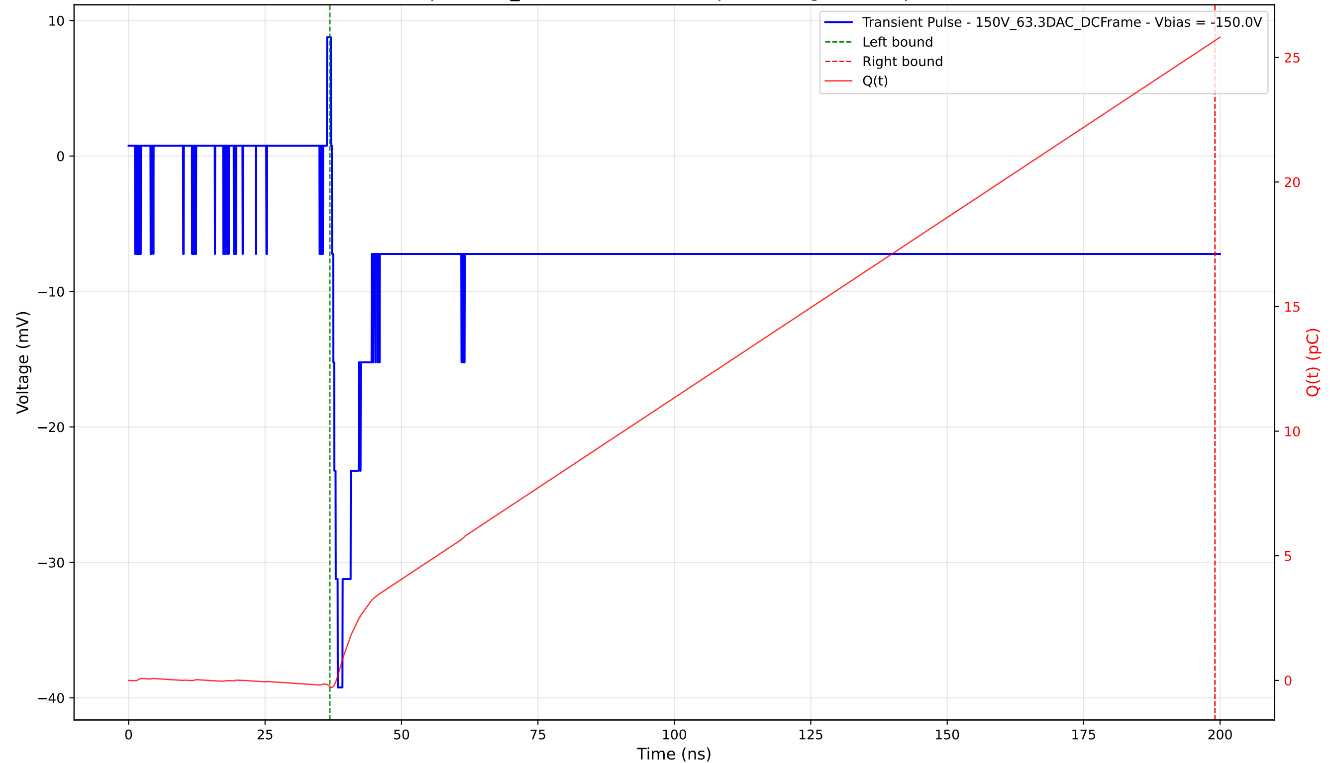
Transient Pulse - Sample: 1cm_42 - Position: 3480.0 \mu\text{m} - Charge: 25.92 pC - Rise Time: 1.07 ns
