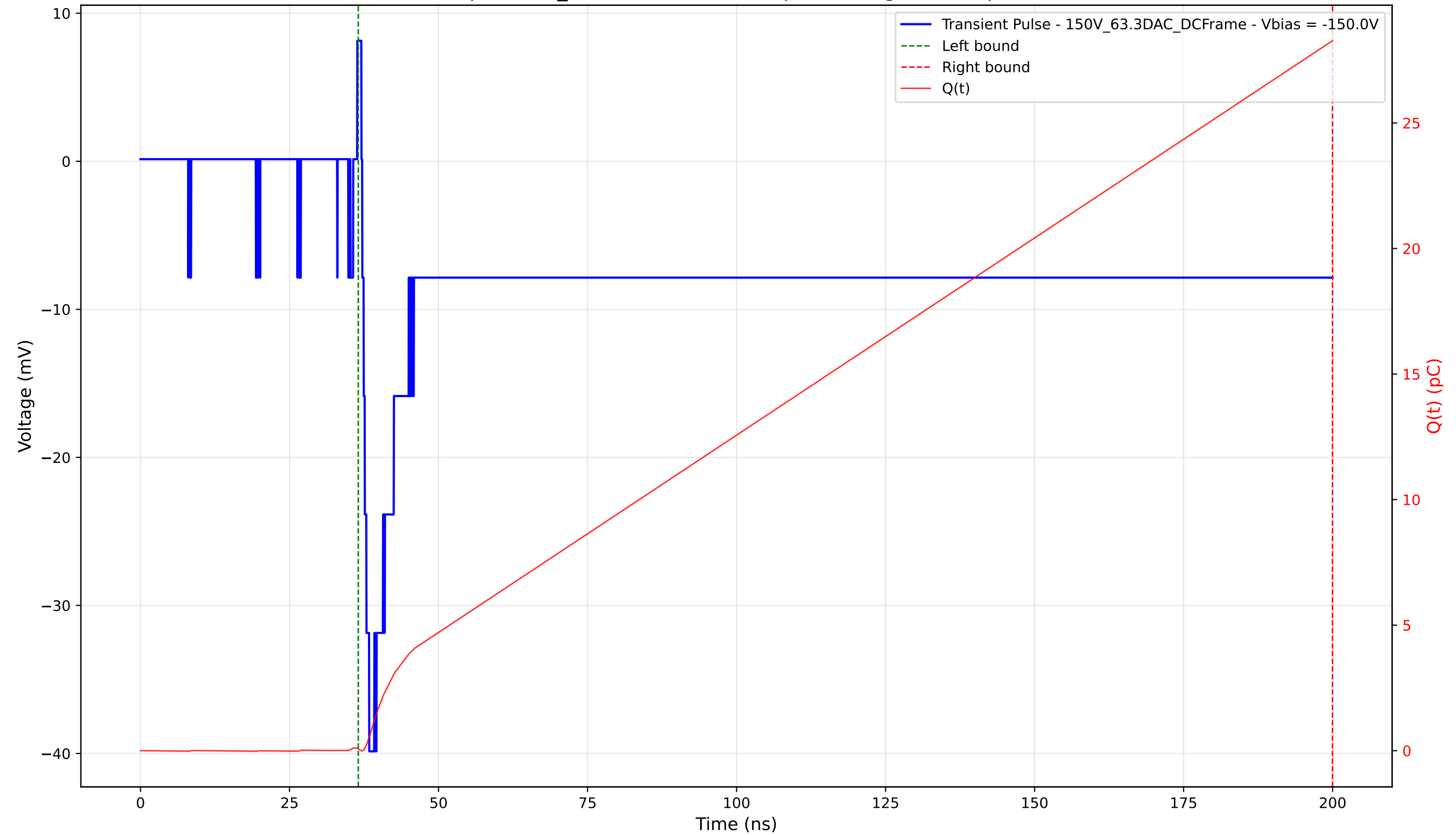
Transient Pulse - Sample: 1cm_42 - Position: 3525.0 \mu\text{m} - Charge: 28.20 pC - Rise Time: 1.17 ns
