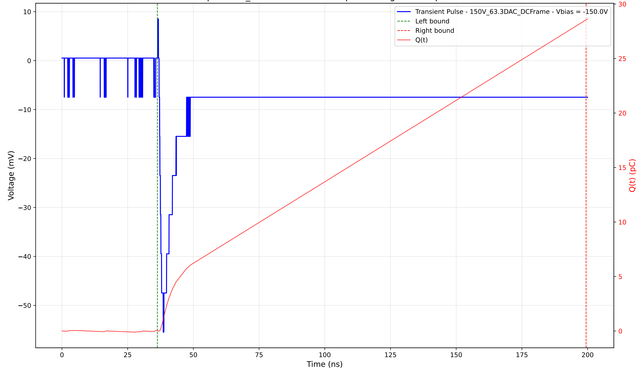
Transient Pulse - Sample: 1cm_42 - Position: 3850.0 \mu\text{m} - Charge: 28.51 pC - Rise Time: 1.57 ns
