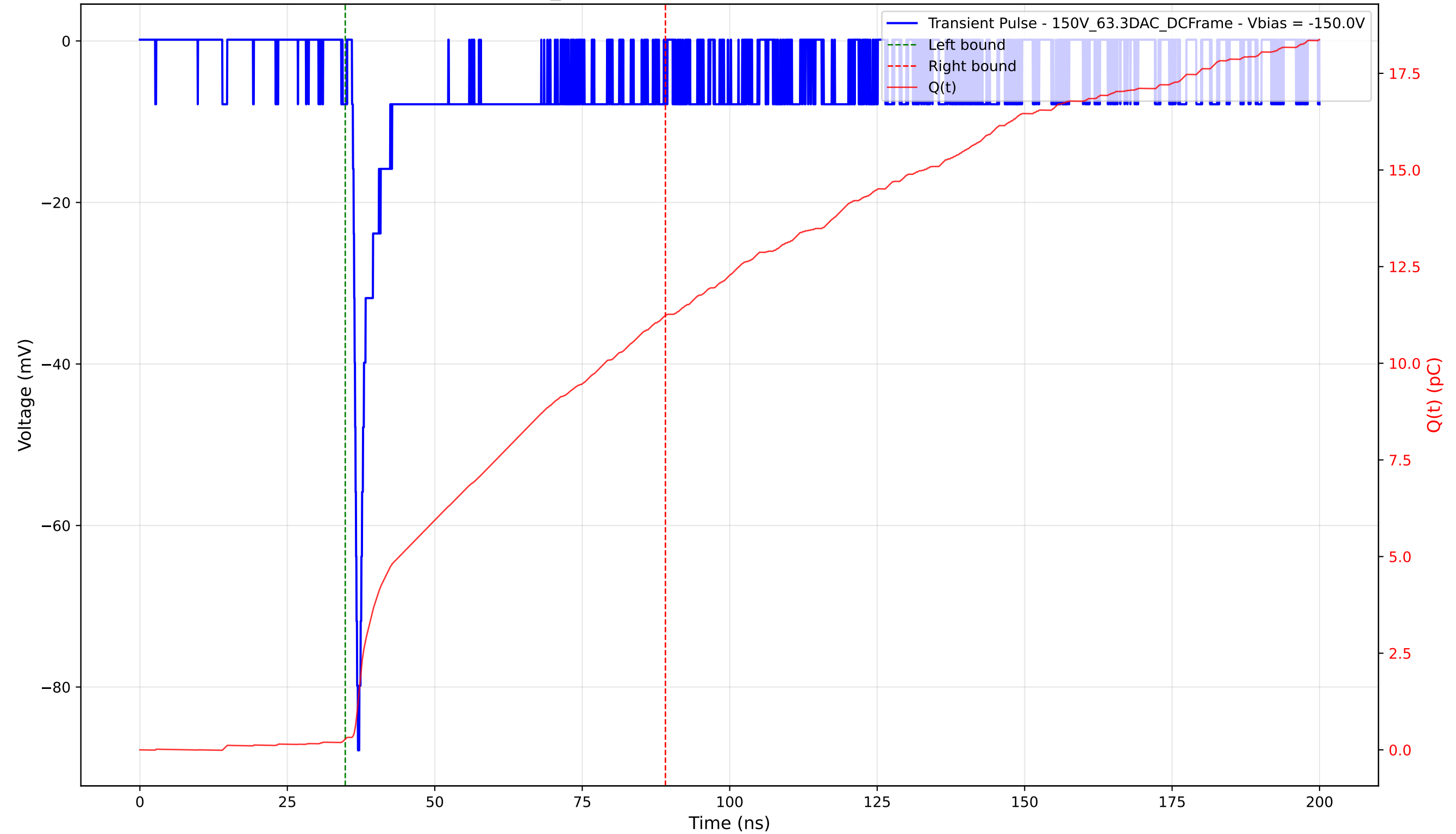
Transient Pulse - Sample: 1cm_42 - Position: 5065.0 \mu\text{m} - Charge: 10.96 pC - Rise Time: 0.72 ns
