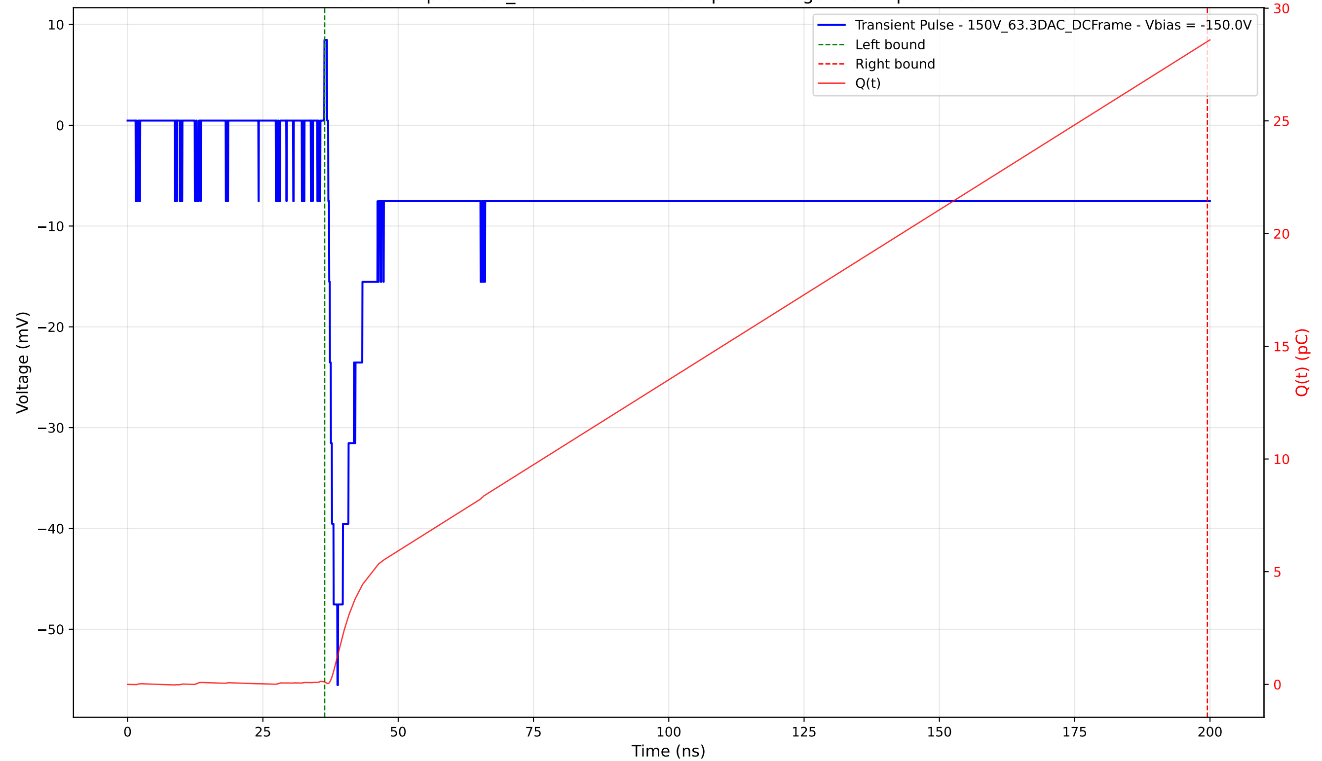
Transient Pulse - Sample: 1cm_42 - Position: 3685.0 \mu\text{m} - Charge: 28.41 pC - Rise Time: 1.69 ns
