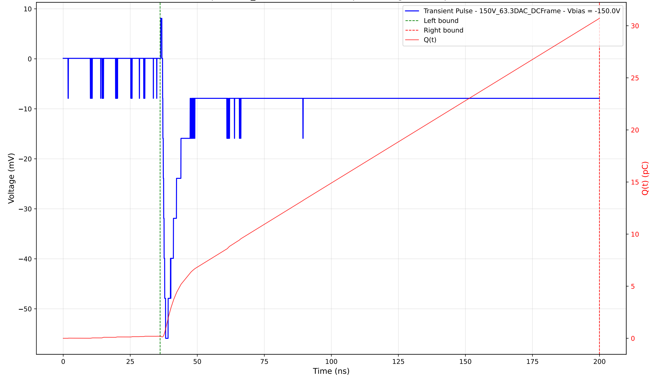
Transient Pulse - Sample: 1cm_42 - Position: 3755.0 \mu\text{m} - Charge: 30.51 pC - Rise Time: 1.13 ns
