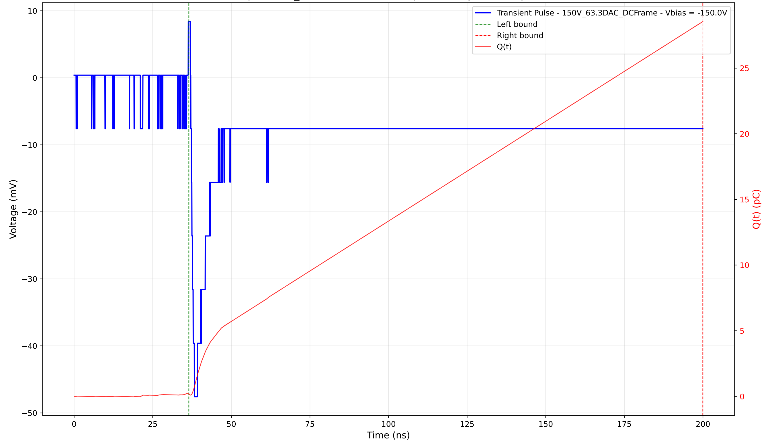
Transient Pulse - Sample: 1cm_42 - Position: 3635.0 \mu\text{m} - Charge: 28.38 pC - Rise Time: 1.13 ns
