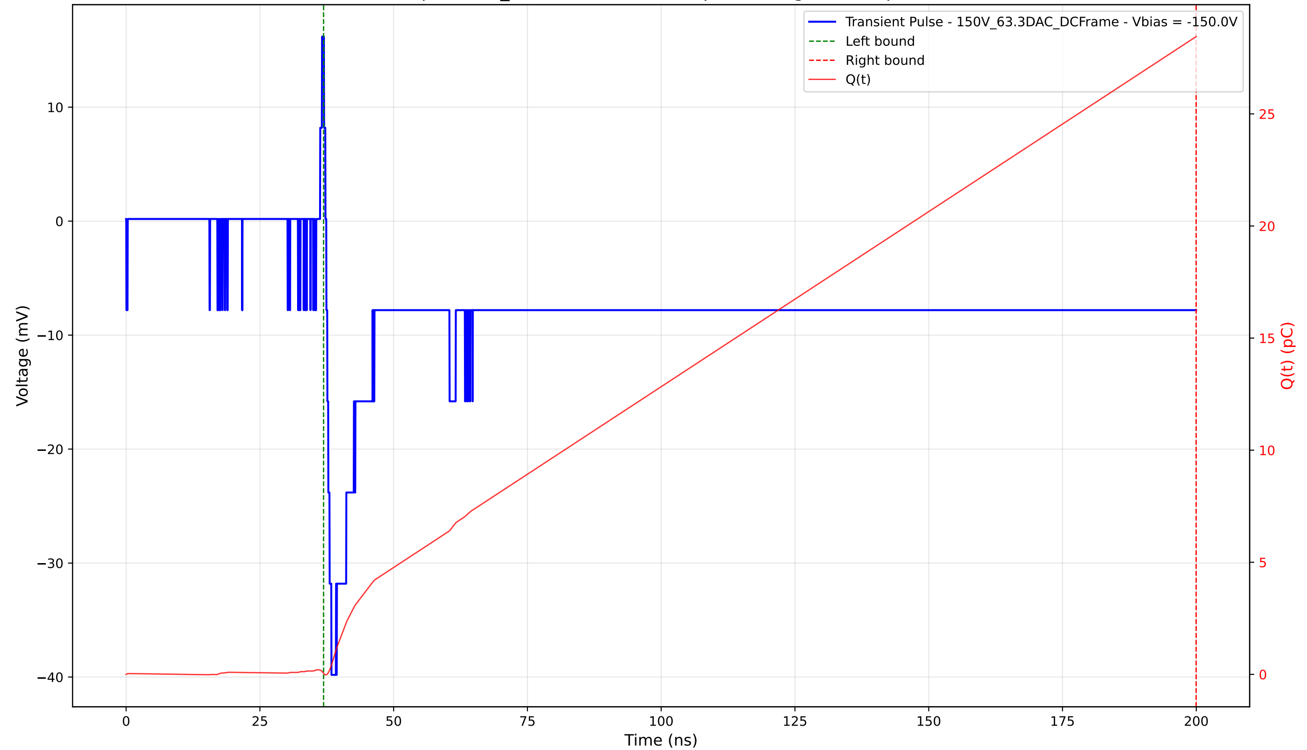
Transient Pulse - Sample: 1cm_42 - Position: 3275.0 \mu\text{m} - Charge: 28.40 pC - Rise Time: 0.95 ns
