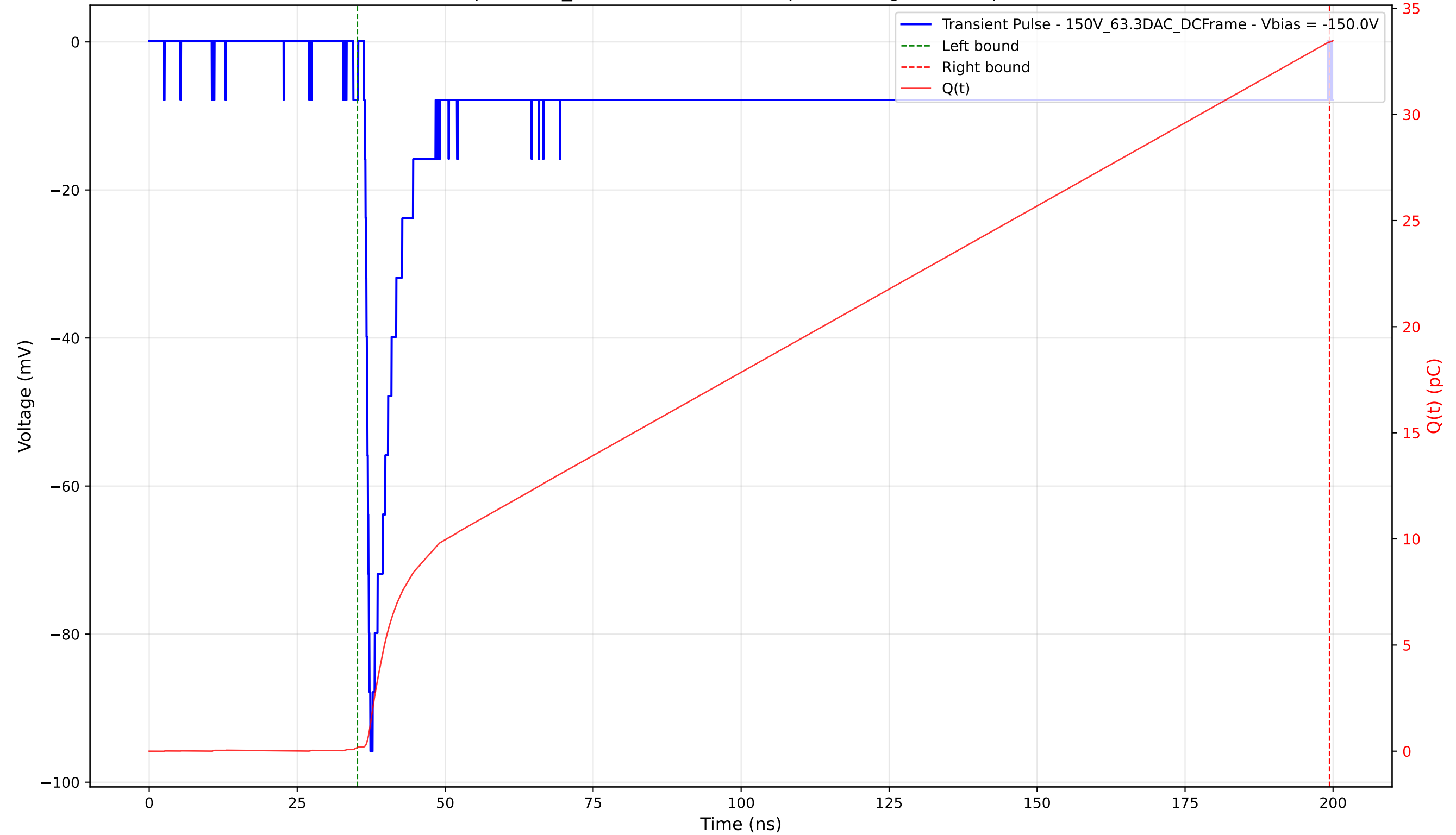
Transient Pulse - Sample: 1cm_42 - Position: 4390.0 \mu\text{m} - Charge: 33.22 pC - Rise Time: 0.80 ns
