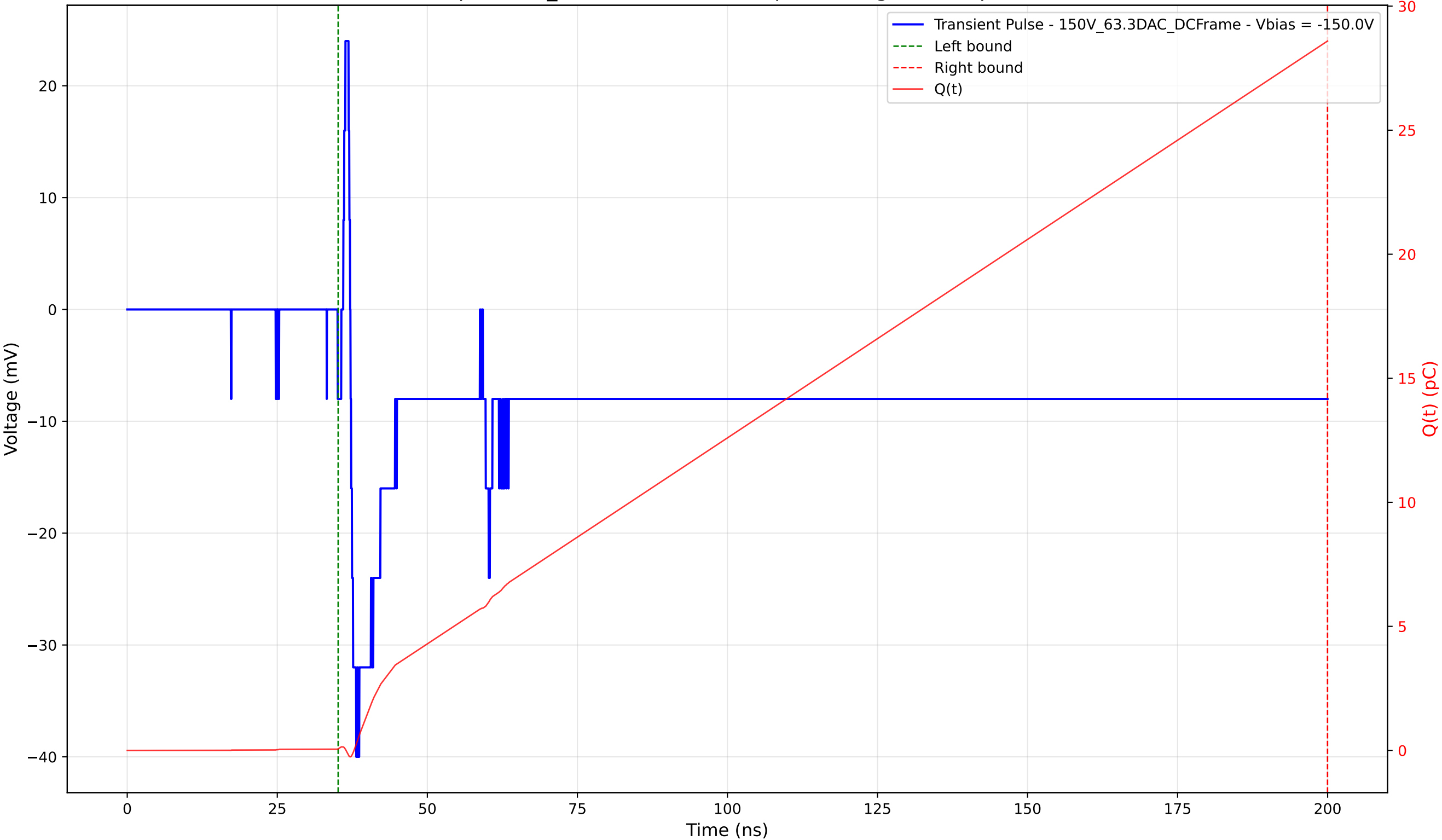
Transient Pulse - Sample: 1cm_42 - Position: 1910.0 \mu\text{m} - Charge: 28.53 pC - Rise Time: 0.95 ns
