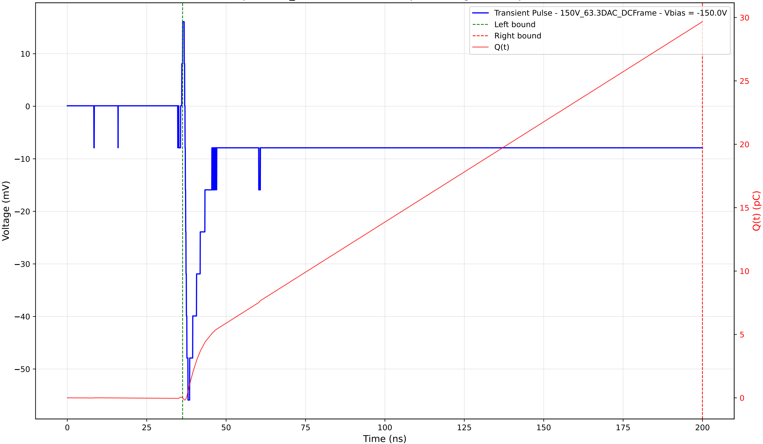
Transient Pulse - Sample: 1cm_42 - Position: 1445.0 \mu\text{m} - Charge: 29.66 pC - Rise Time: 0.93 ns
