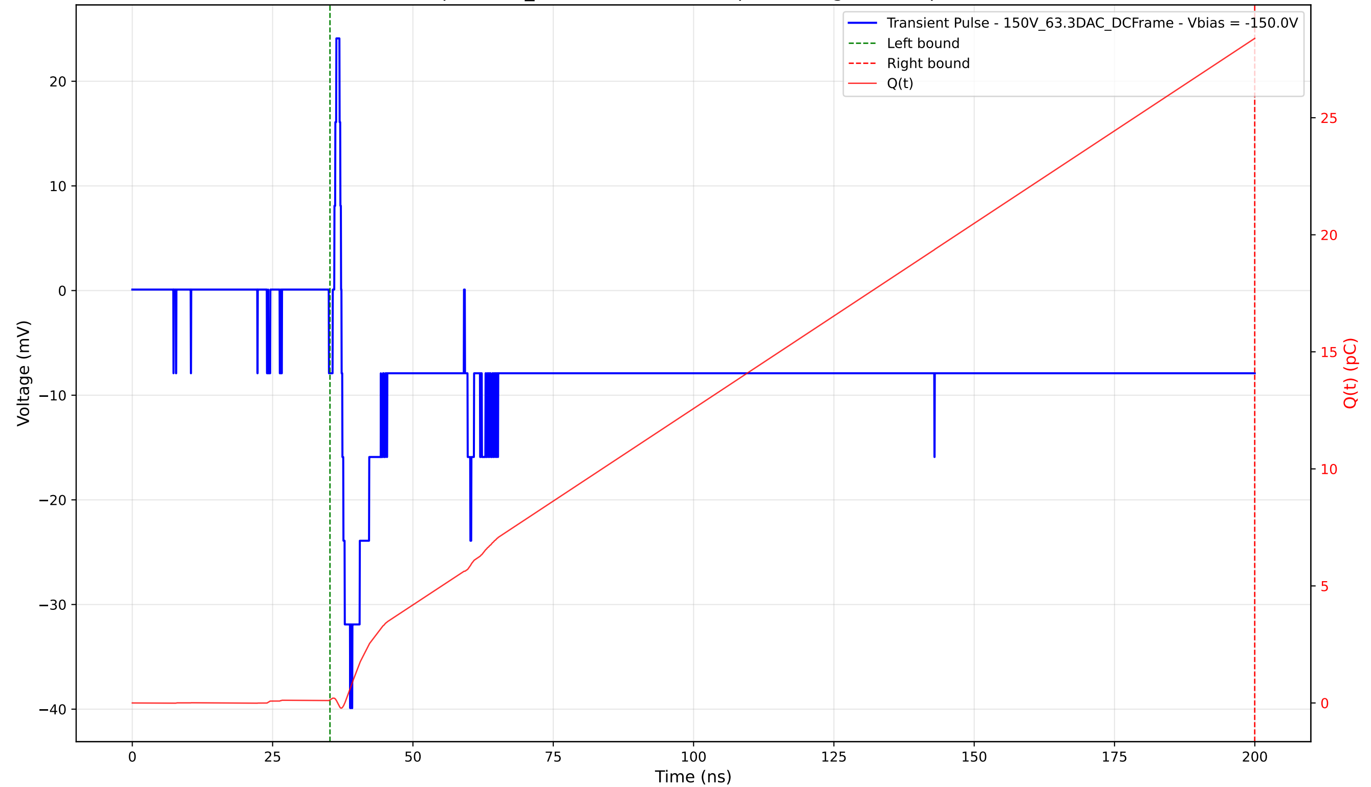
Transient Pulse - Sample: 1cm_42 - Position: 2165.0 \mu\text{m} - Charge: 28.26 pC - Rise Time: 1.53 ns
