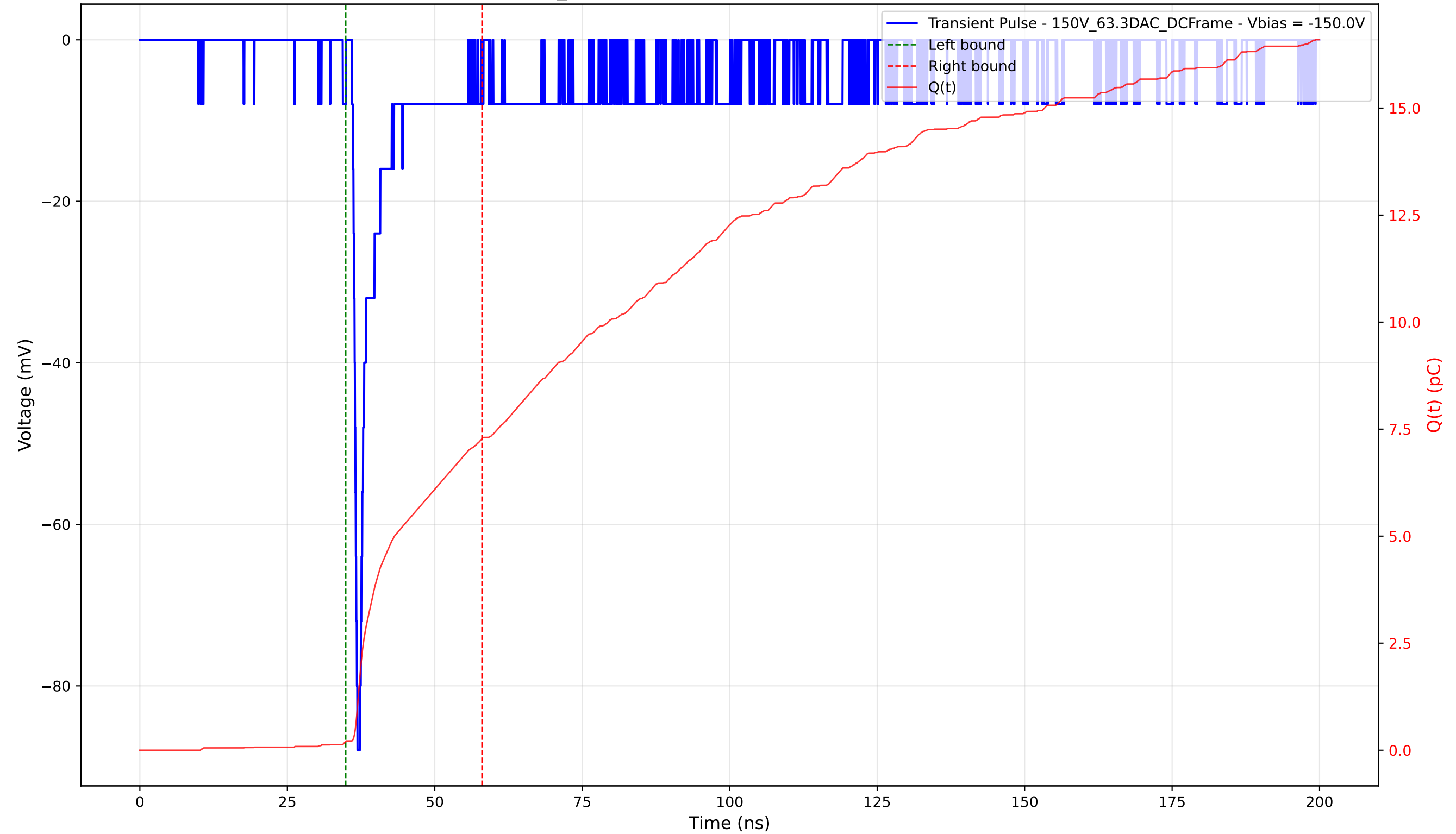
Transient Pulse - Sample: 1cm_42 - Position: 5060.0 \mu\text{m} - Charge: 7.06 pC - Rise Time: 0.68 ns
