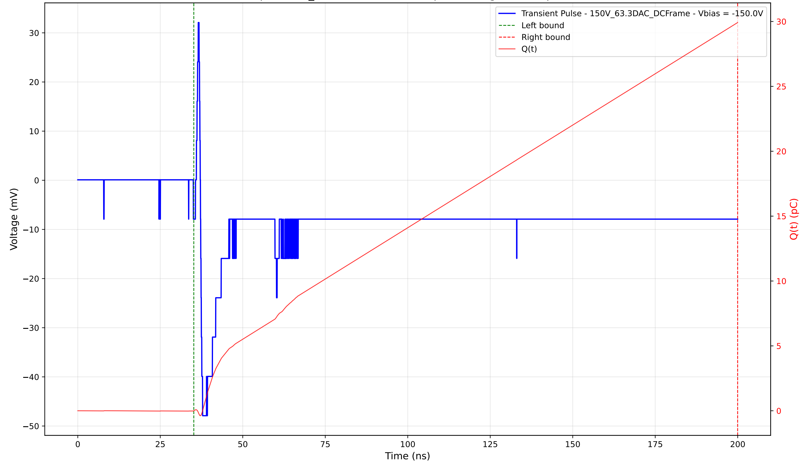
Transient Pulse - Sample: 1cm_42 - Position: 1725.0 \mu\text{m} - Charge: 29.92 pC - Rise Time: 0.65 ns
