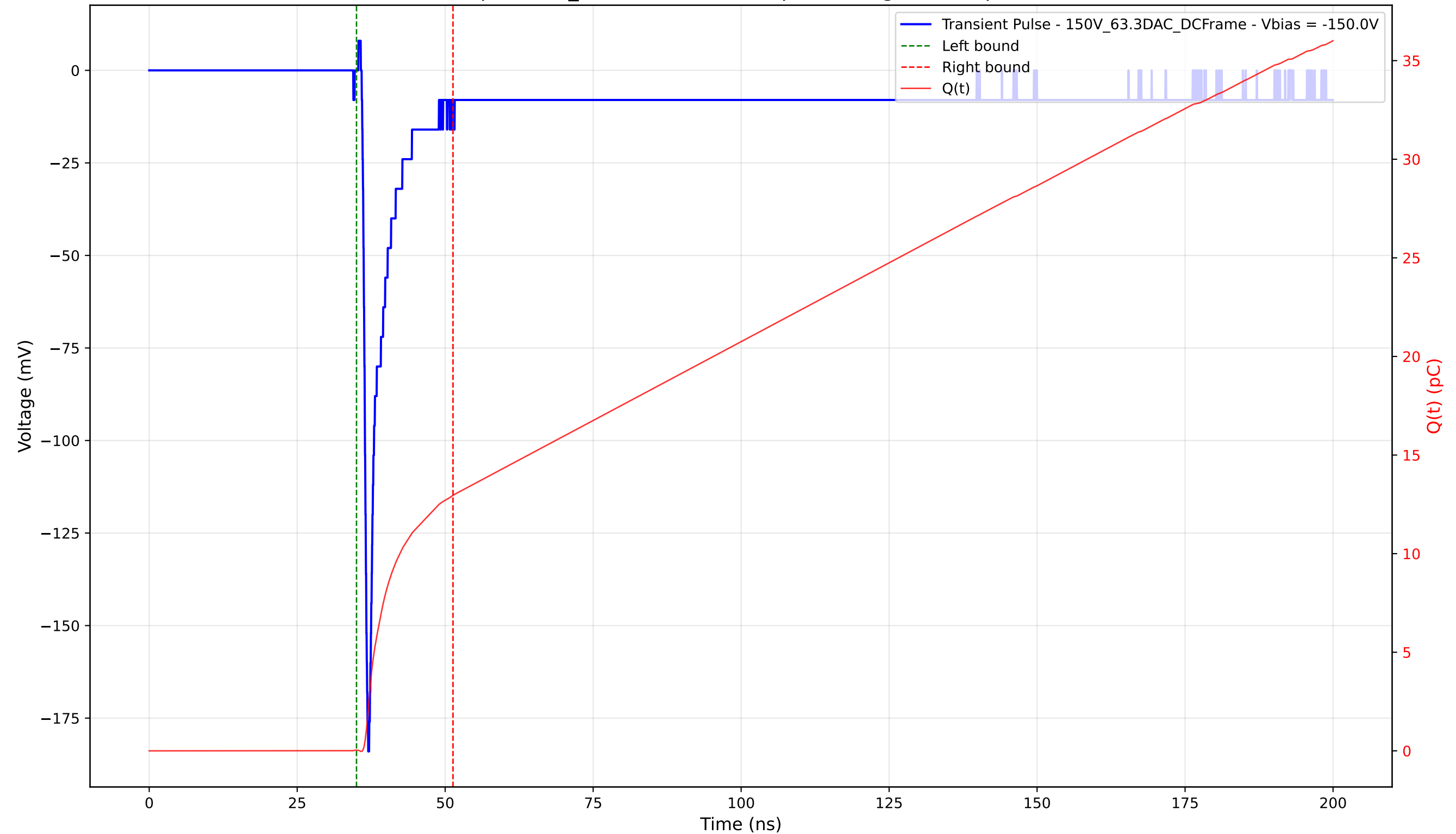
Transient Pulse - Sample: 1cm_42 - Position: 395.0 \mu\text{m} - Charge: 12.92 pC - Rise Time: 0.77 ns
