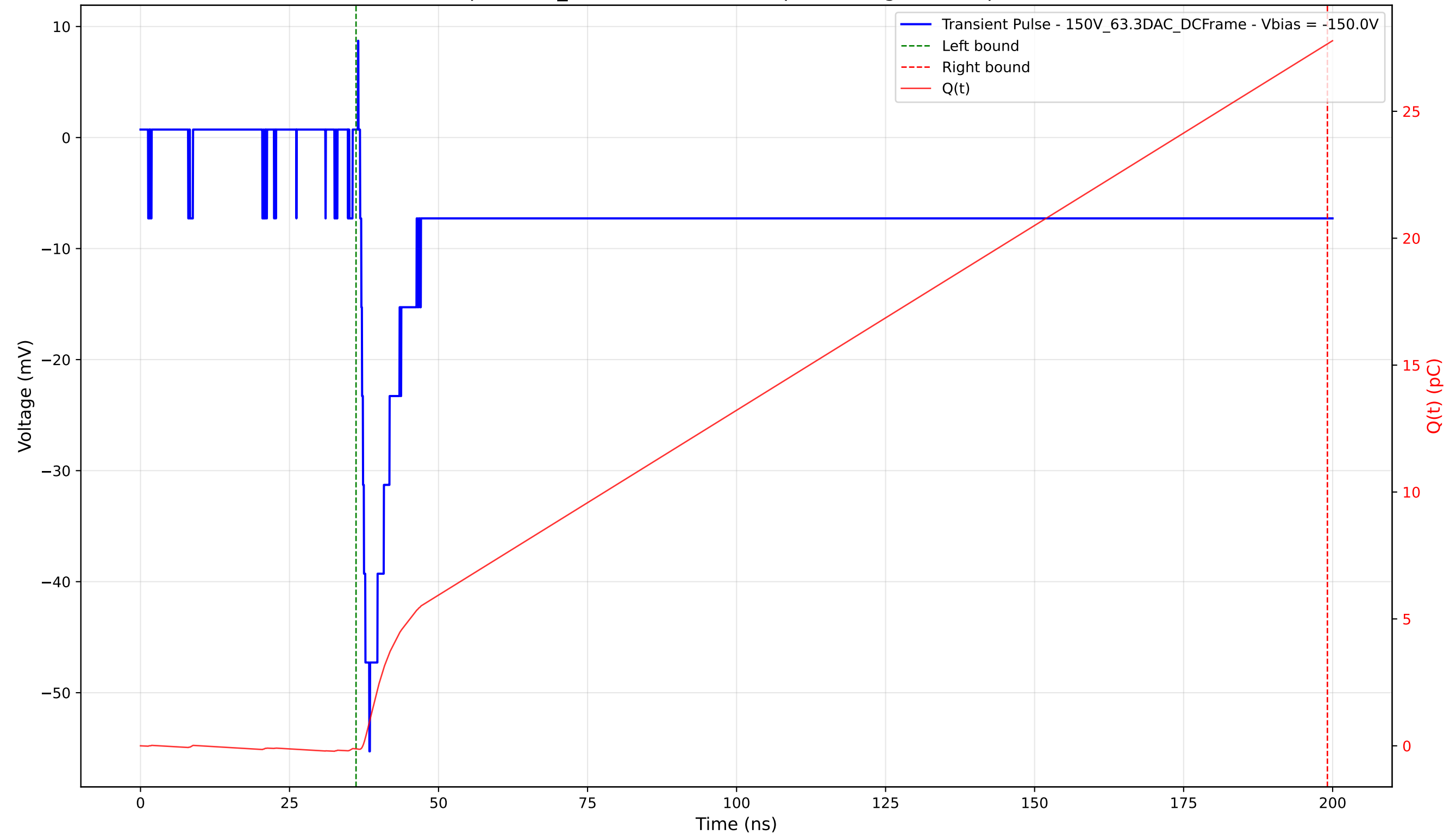
Transient Pulse - Sample: 1cm_42 - Position: 3935.0 \mu\text{m} - Charge: 27.77 pC - Rise Time: 1.55 ns
