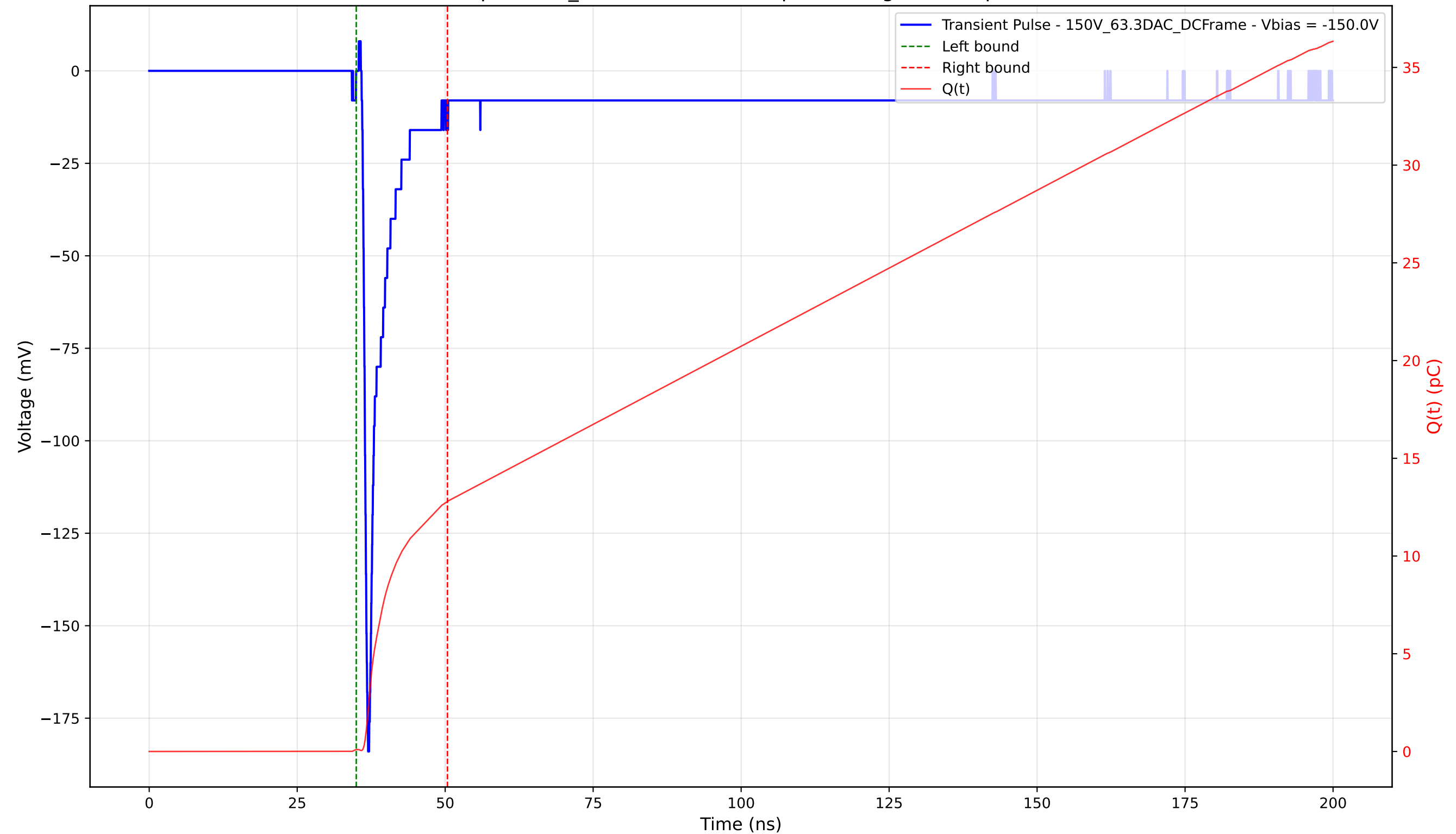
Transient Pulse - Sample: 1cm_42 - Position: 390.0 \mu\text{m} - Charge: 12.68 pC - Rise Time: 0.75 ns
