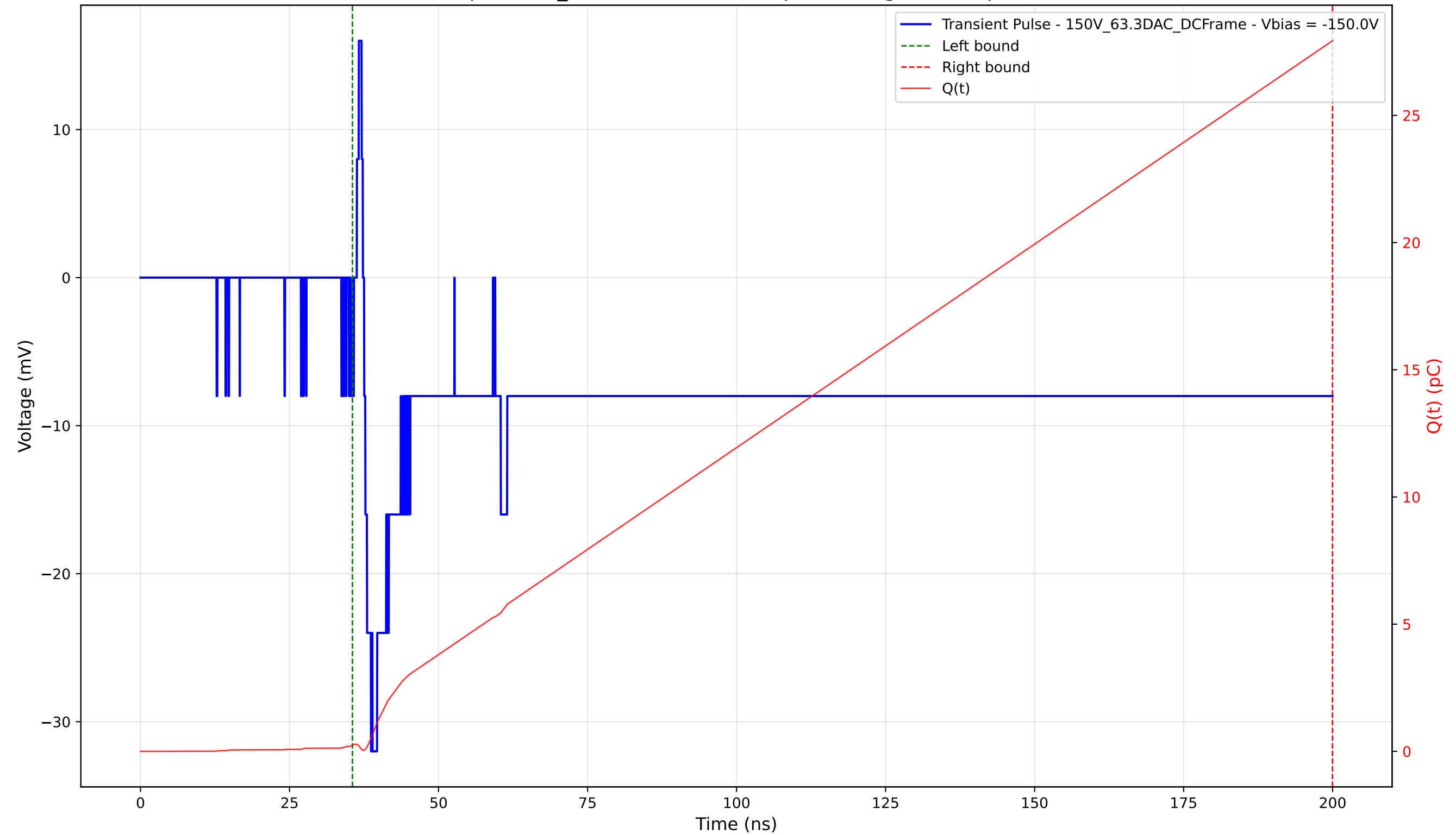
Transient Pulse - Sample: 1cm_42 - Position: 2895.0 \mu\text{m} - Charge: 27.68 pC - Rise Time: 1.15 ns
