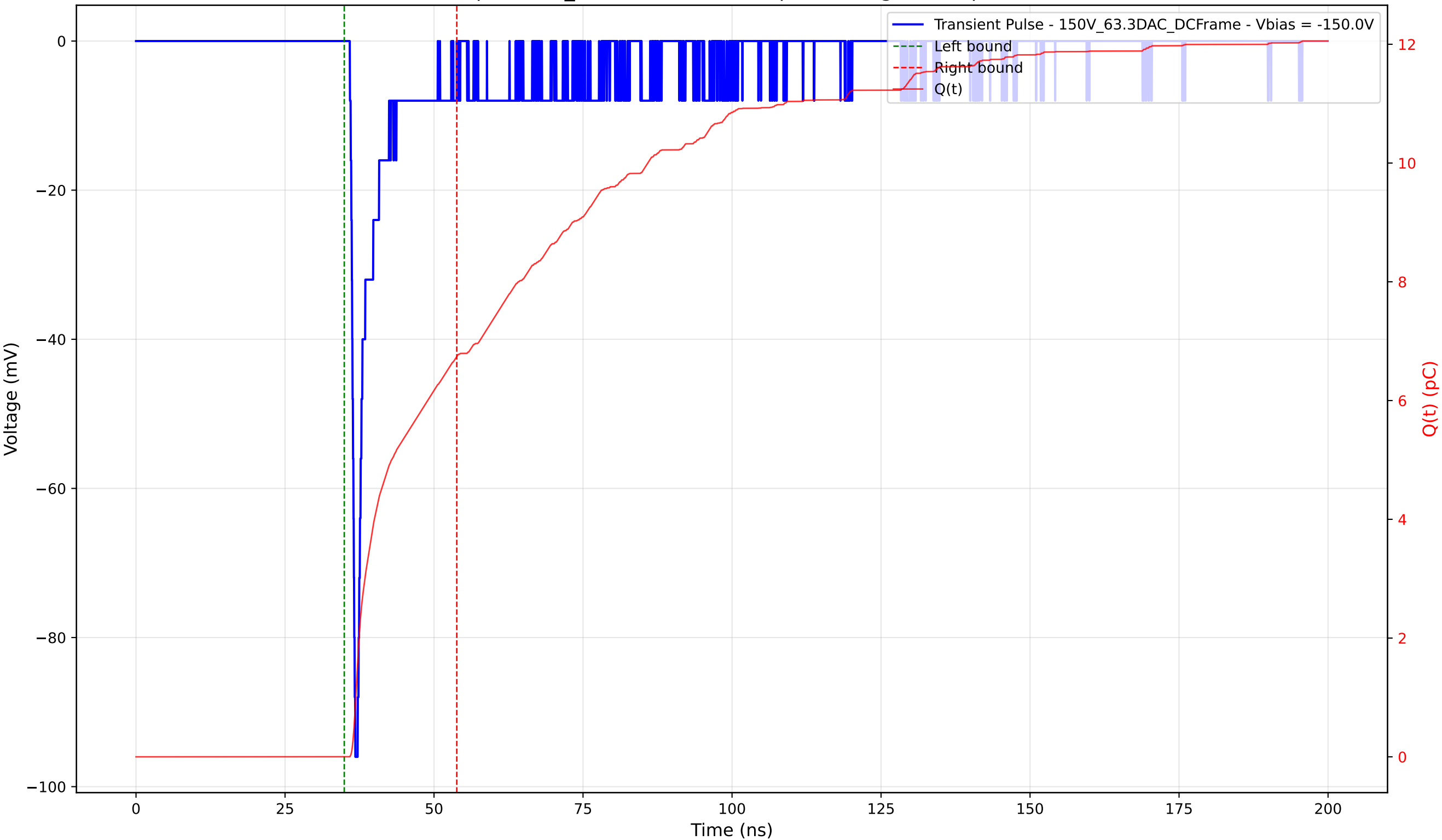
Transient Pulse - Sample: 1cm_42 - Position: 125.0 \mu\text{m} - Charge: 6.74 pC - Rise Time: 0.68 ns
