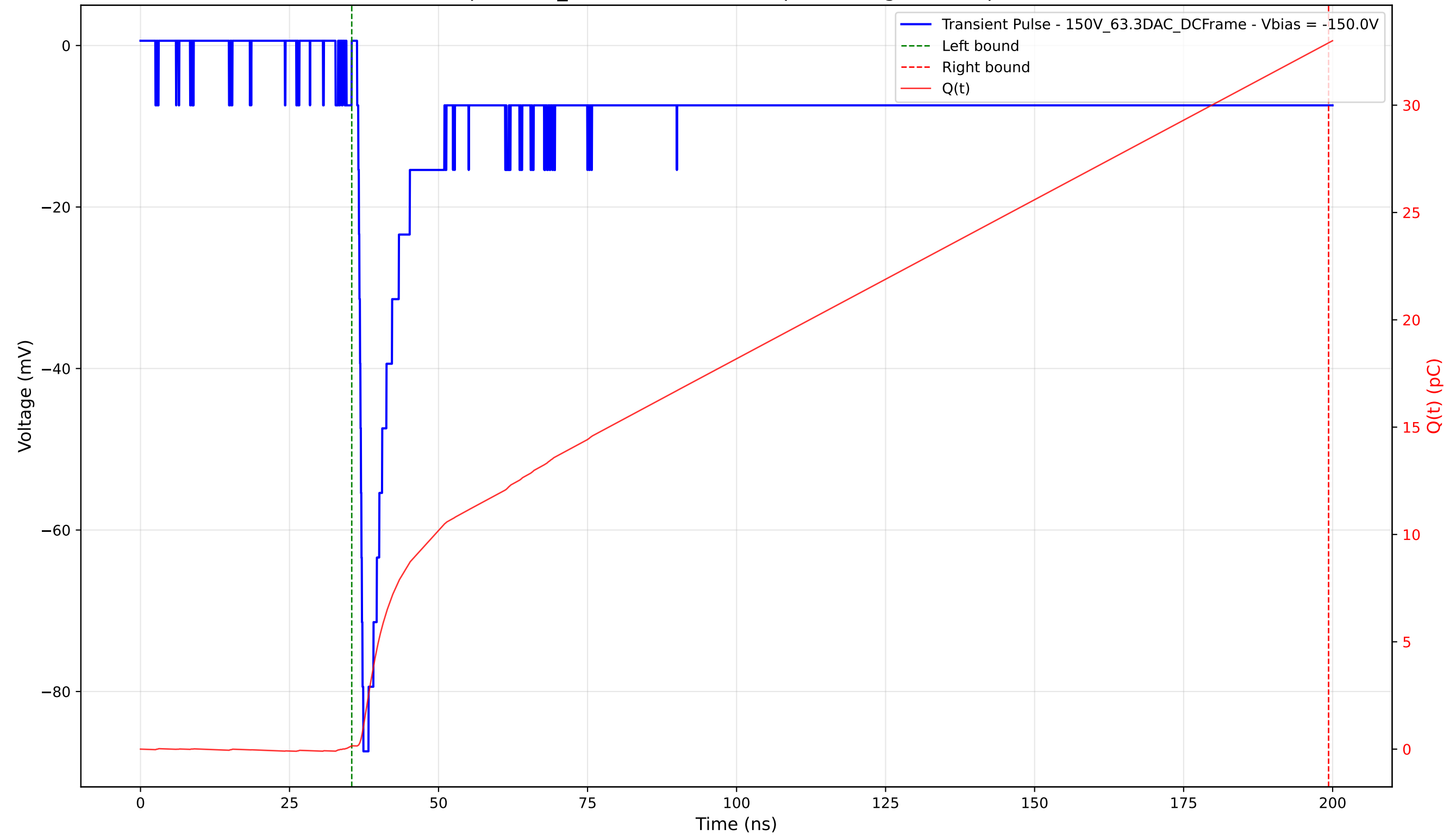
Transient Pulse - Sample: 1cm_42 - Position: 4235.0 \mu\text{m} - Charge: 32.75 pC - Rise Time: 0.72 ns
