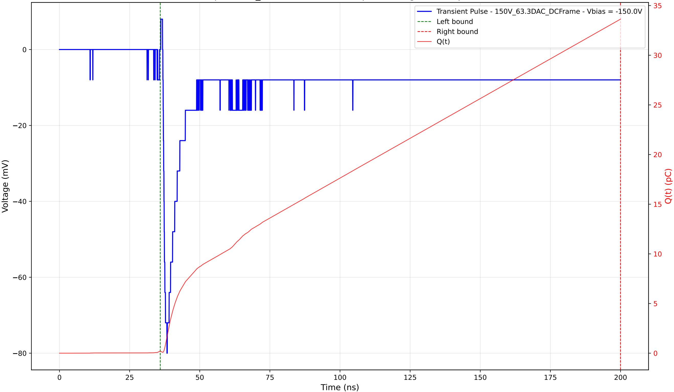
Transient Pulse - Sample: 1cm_42 - Position: 1190.0 \mu\text{m} - Charge: 33.44 pC - Rise Time: 0.84 ns
