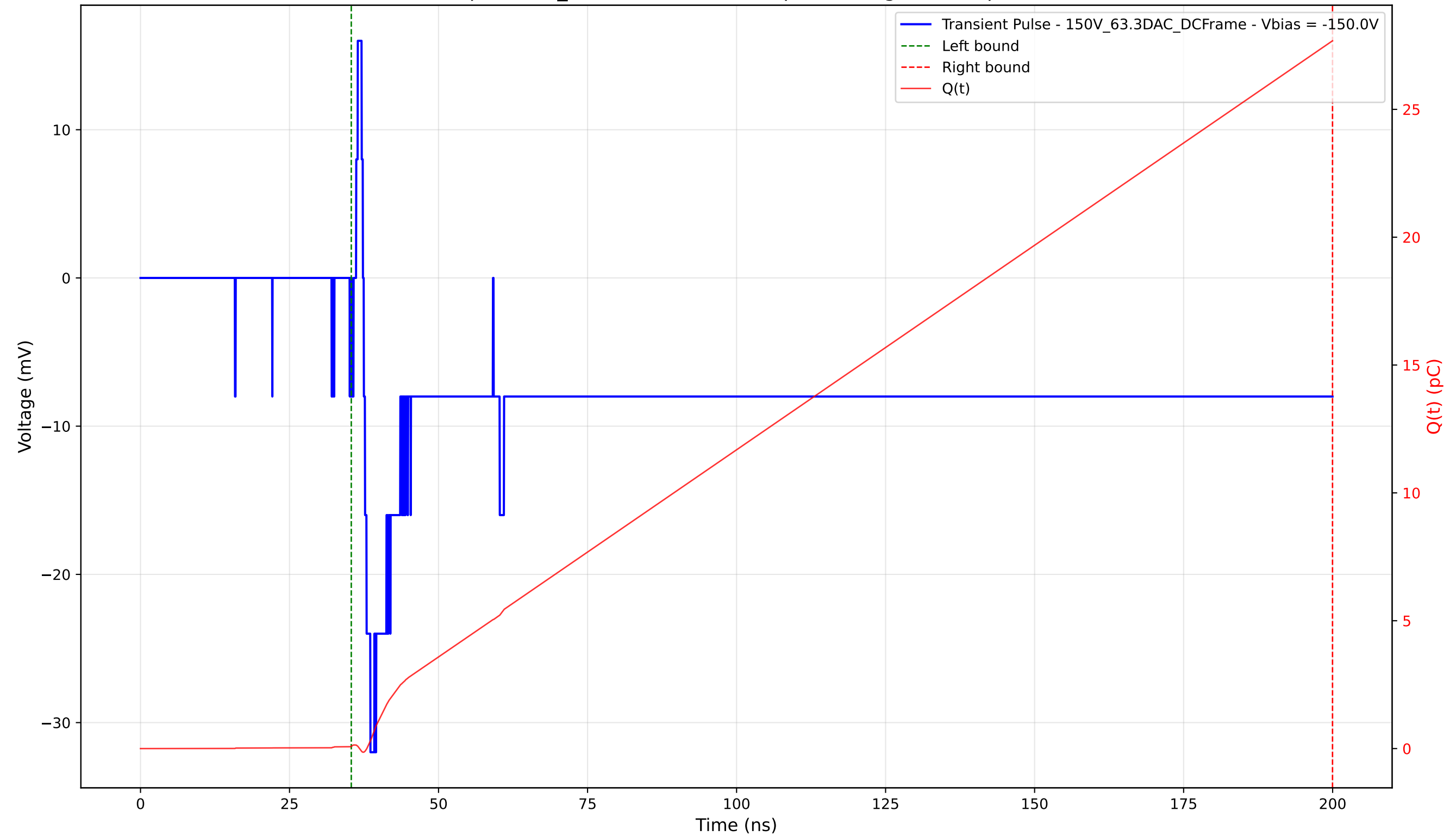
Transient Pulse - Sample: 1cm_42 - Position: 2480.0 \mu\text{m} - Charge: 27.59 pC - Rise Time: 1.11 ns
