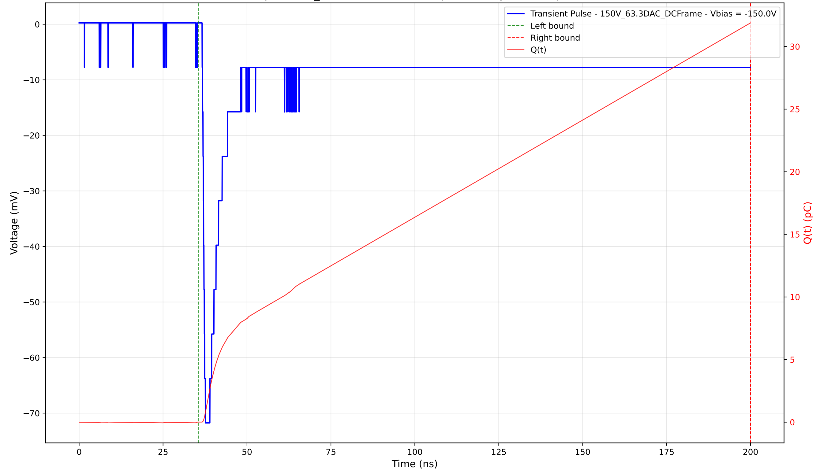
Transient Pulse - Sample: 1cm_42 - Position: 1050.0 \mu\text{m} - Charge: 31.88 pC - Rise Time: 0.96 ns
