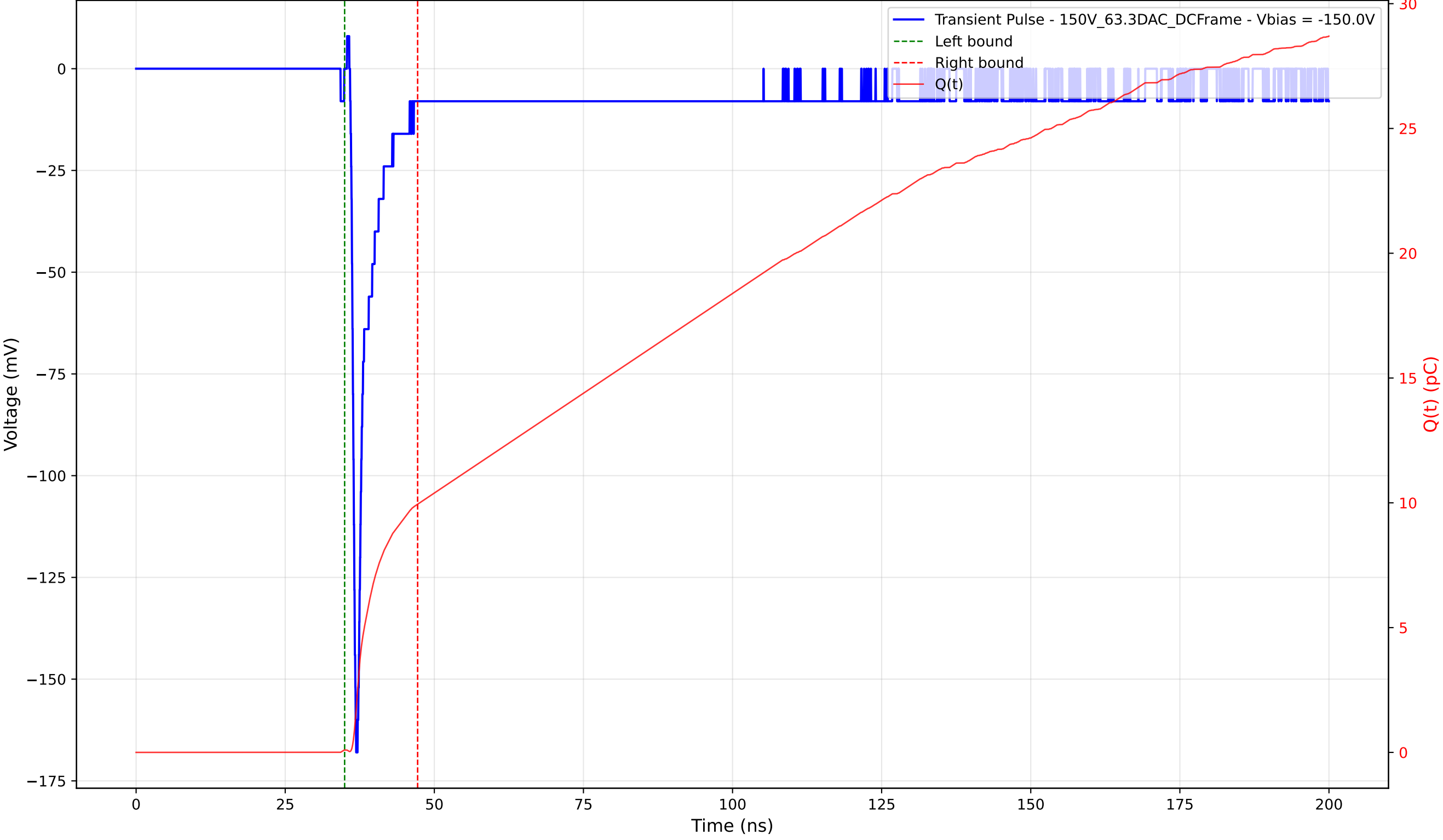
Transient Pulse - Sample: 1cm_42 - Position: 260.0 \mu\text{m} - Charge: 9.85 pC - Rise Time: 0.72 ns
