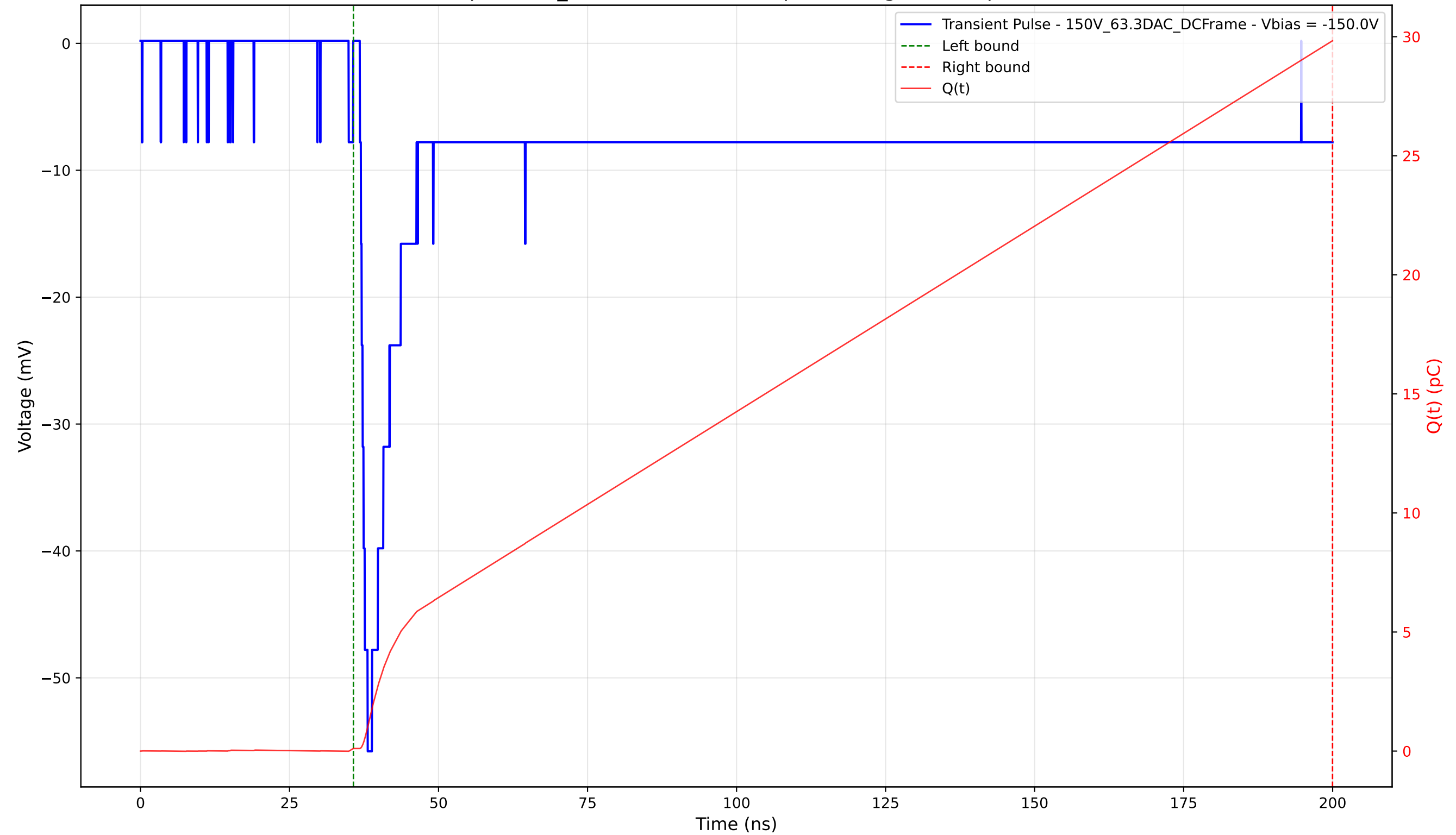
Transient Pulse - Sample: 1cm_42 - Position: 3965.0 \mu\text{m} - Charge: 29.72 pC - Rise Time: 1.31 ns
