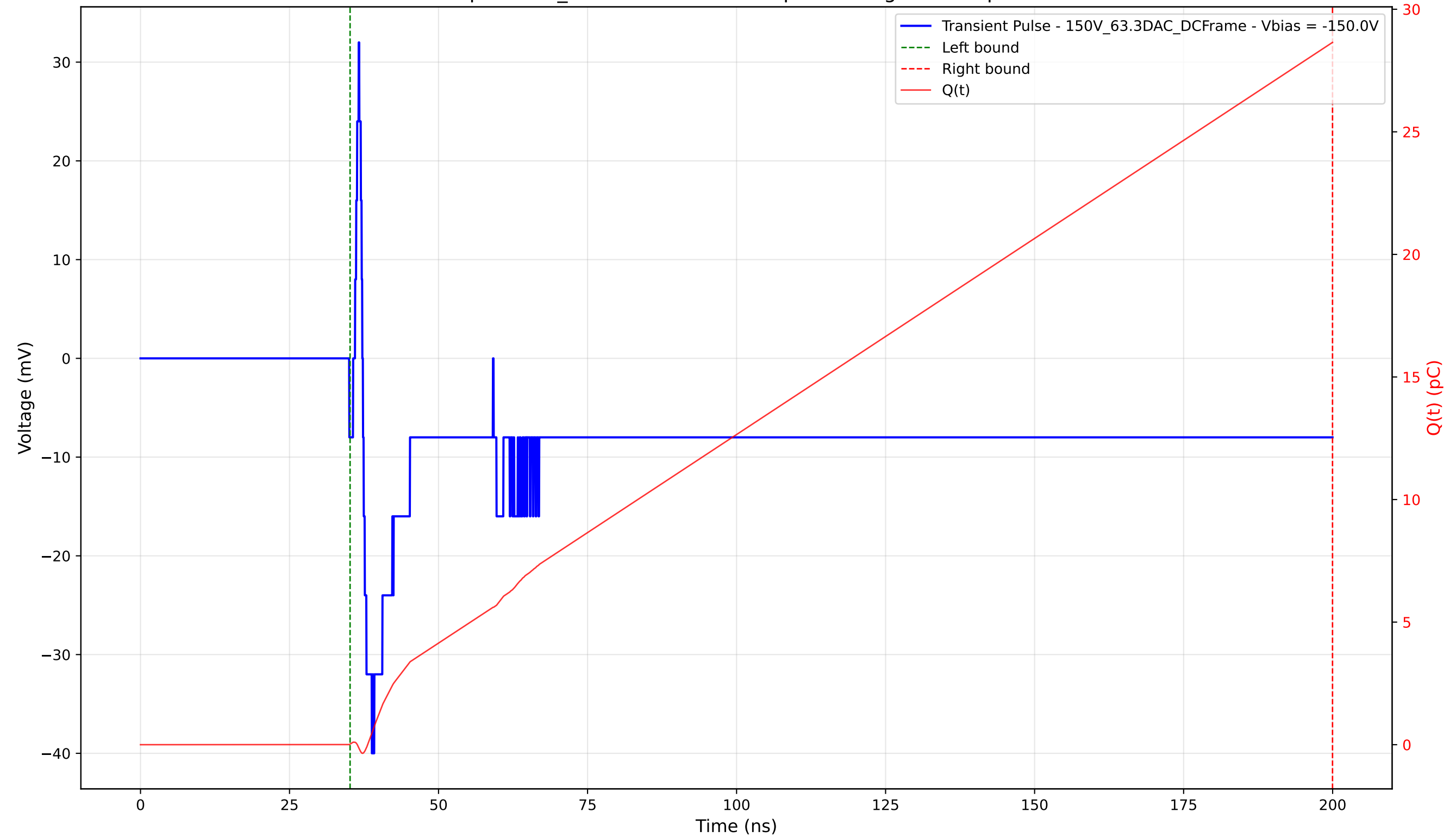
Transient Pulse - Sample: 1cm_42 - Position: 2205.0 \mu\text{m} - Charge: 28.62 pC - Rise Time: 1.49 ns
