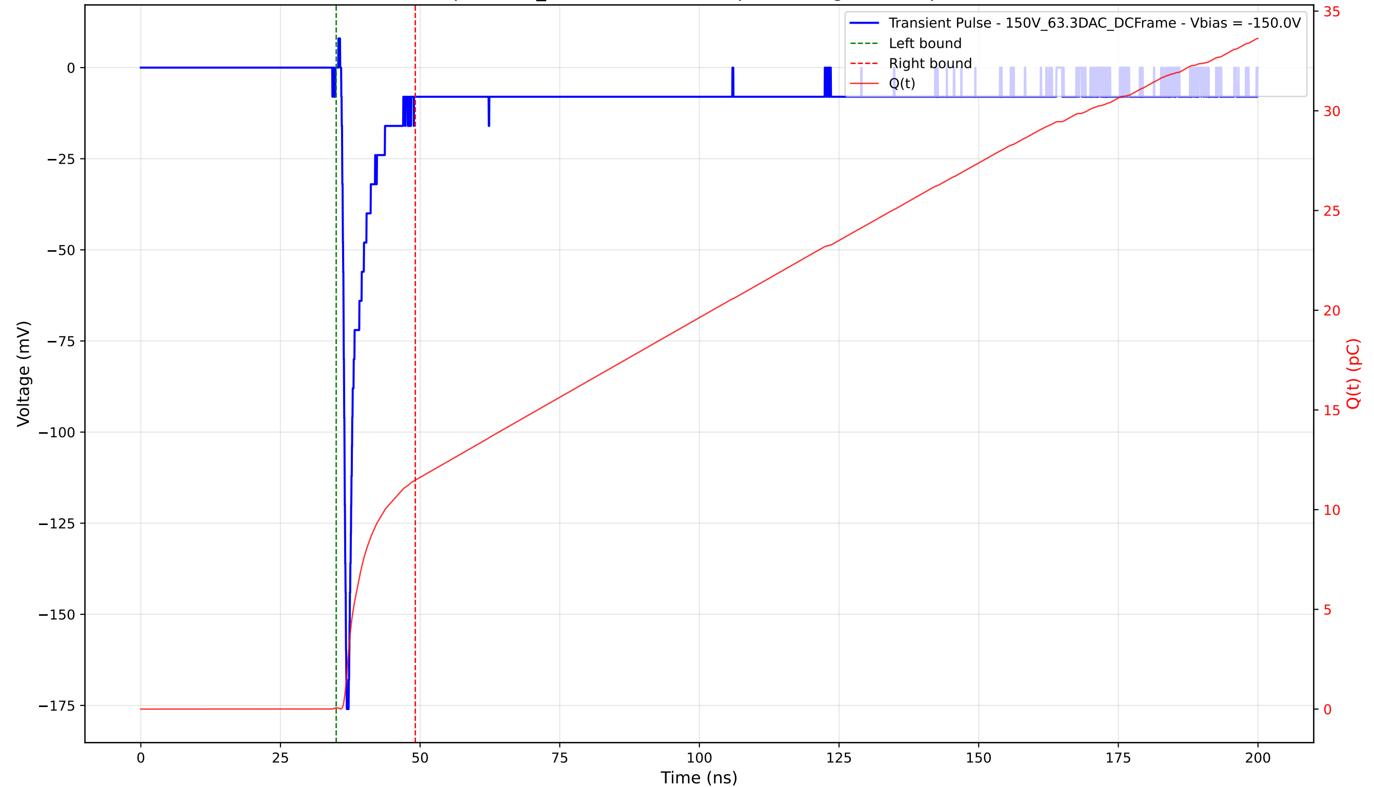
Transient Pulse - Sample: 1cm_42 - Position: 335.0 \mu\text{m} - Charge: 11.42 pC - Rise Time: 0.72 ns
