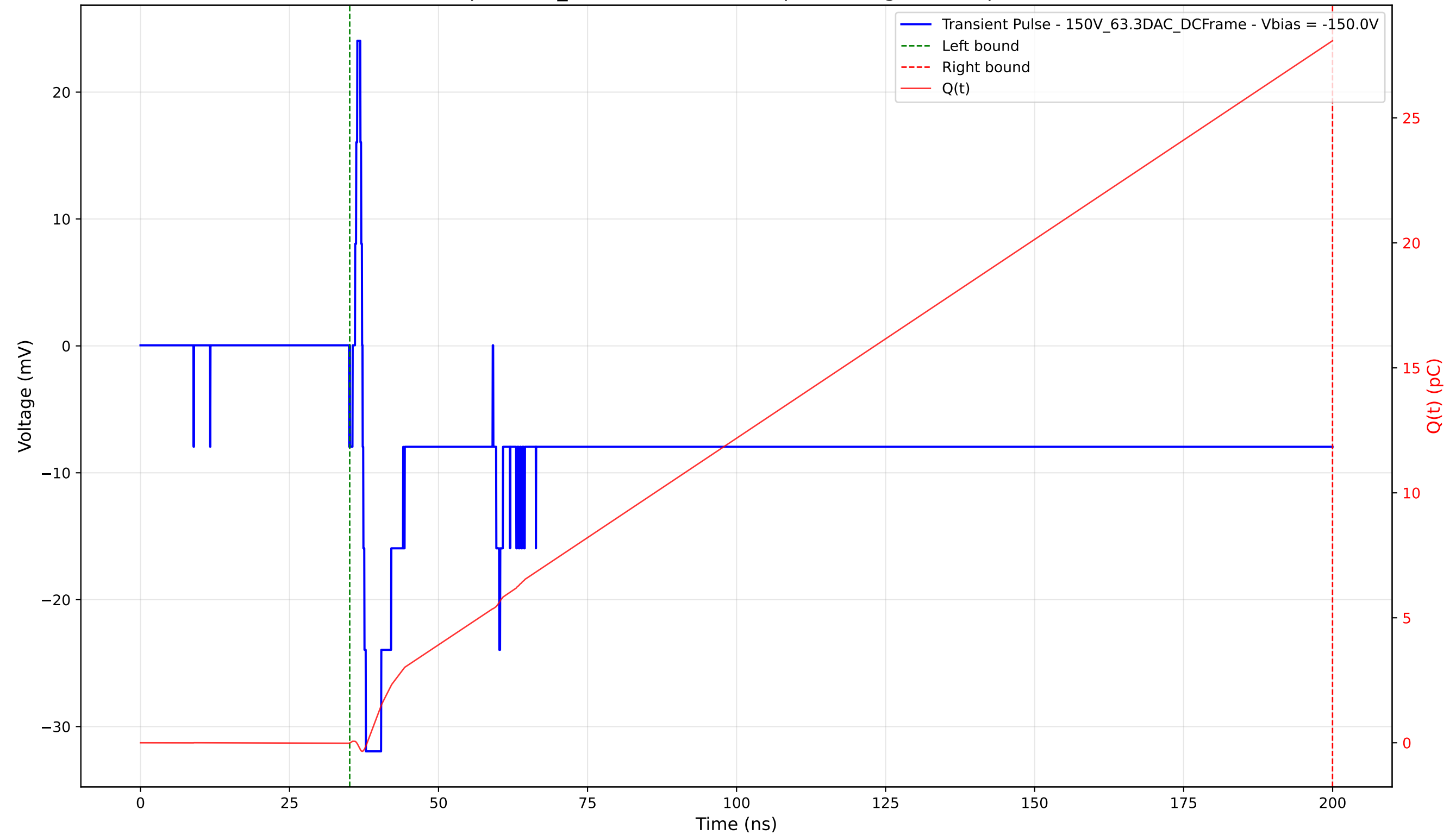
Transient Pulse - Sample: 1cm_42 - Position: 2110.0 \mu\text{m} - Charge: 28.10 pC - Rise Time: 0.55 ns
