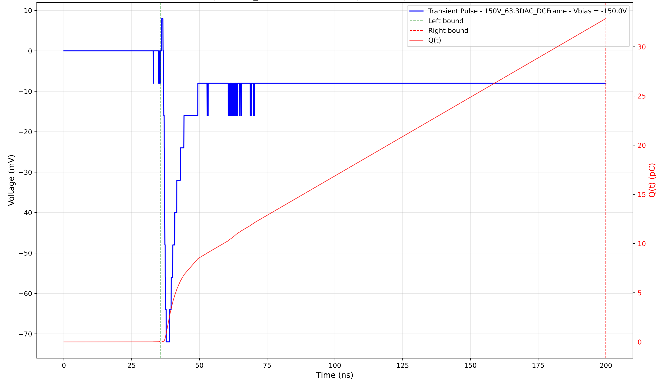
Transient Pulse - Sample: 1cm_42 - Position: 1105.0 \mu\text{m} - Charge: 32.78 pC - Rise Time: 1.00 ns
