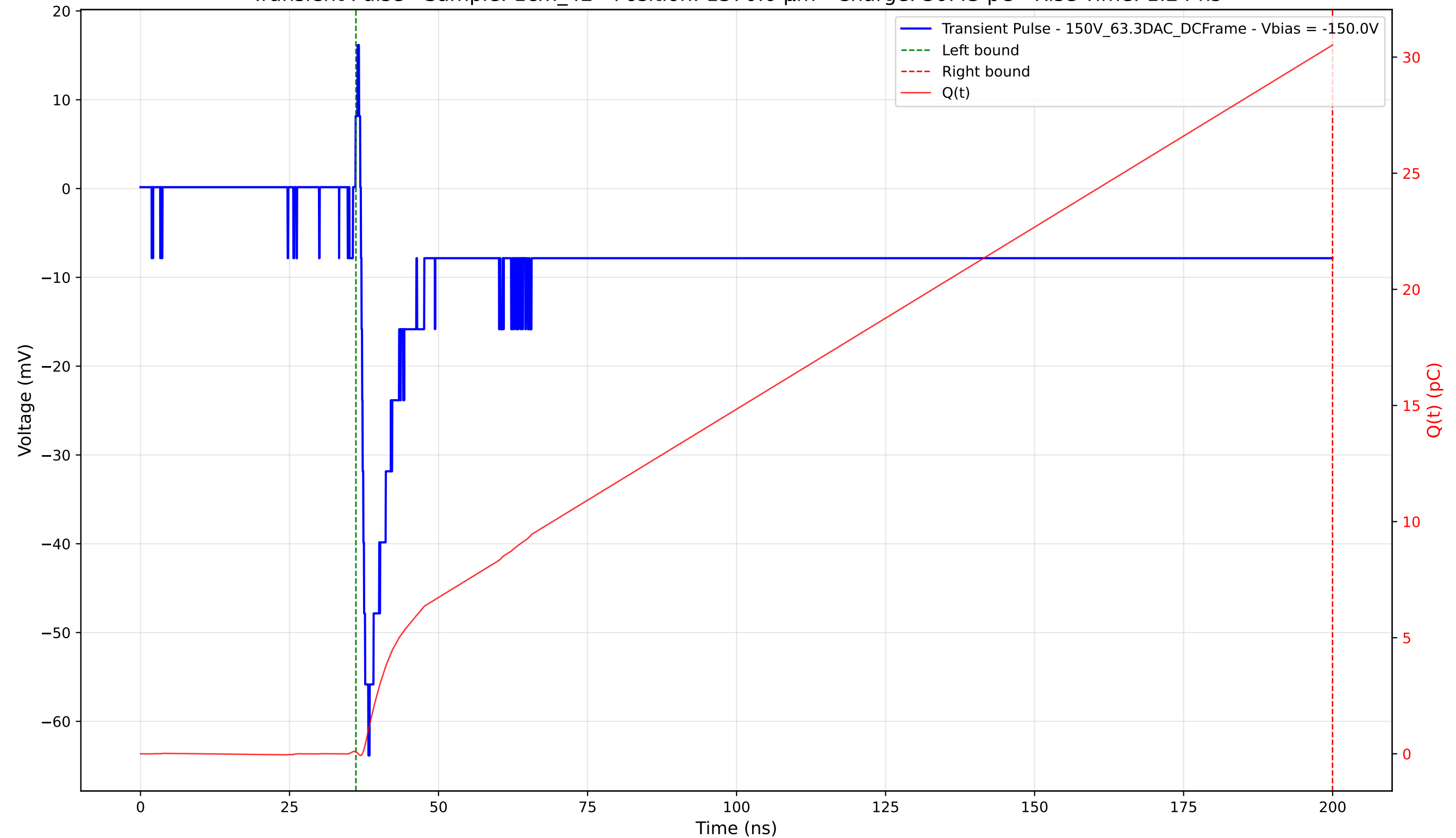
Transient Pulse - Sample: 1cm_42 - Position: 1370.0 \mu\text{m} - Charge: 30.43 pC - Rise Time: 1.24 ns
