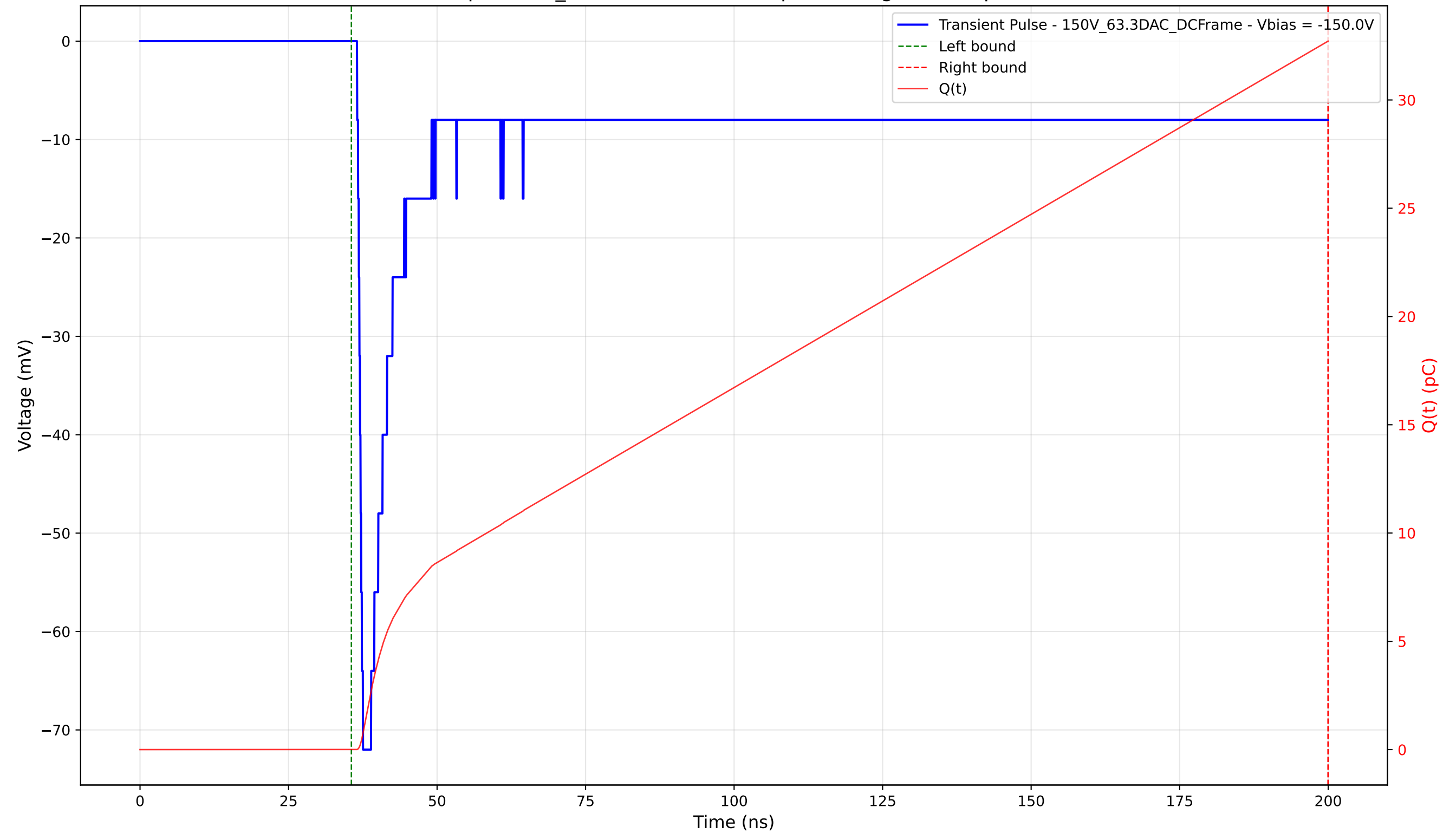
Transient Pulse - Sample: 1cm_42 - Position: 1020.0 \mu\text{m} - Charge: 32.72 pC - Rise Time: 0.98 ns
