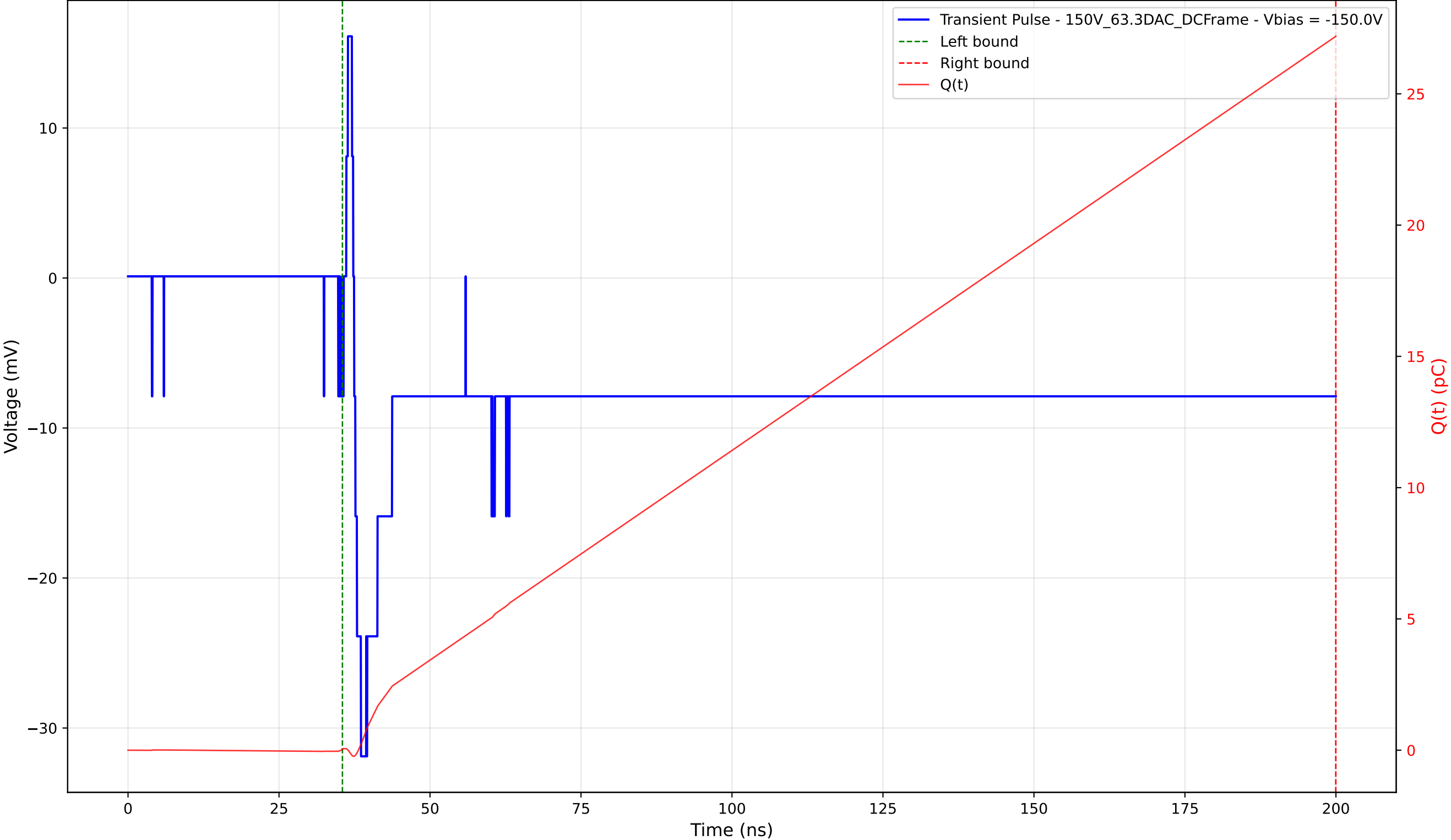
Transient Pulse - Sample: 1cm_42 - Position: 2475.0 \mu\text{m} - Charge: 27.16 pC - Rise Time: 1.13 ns
