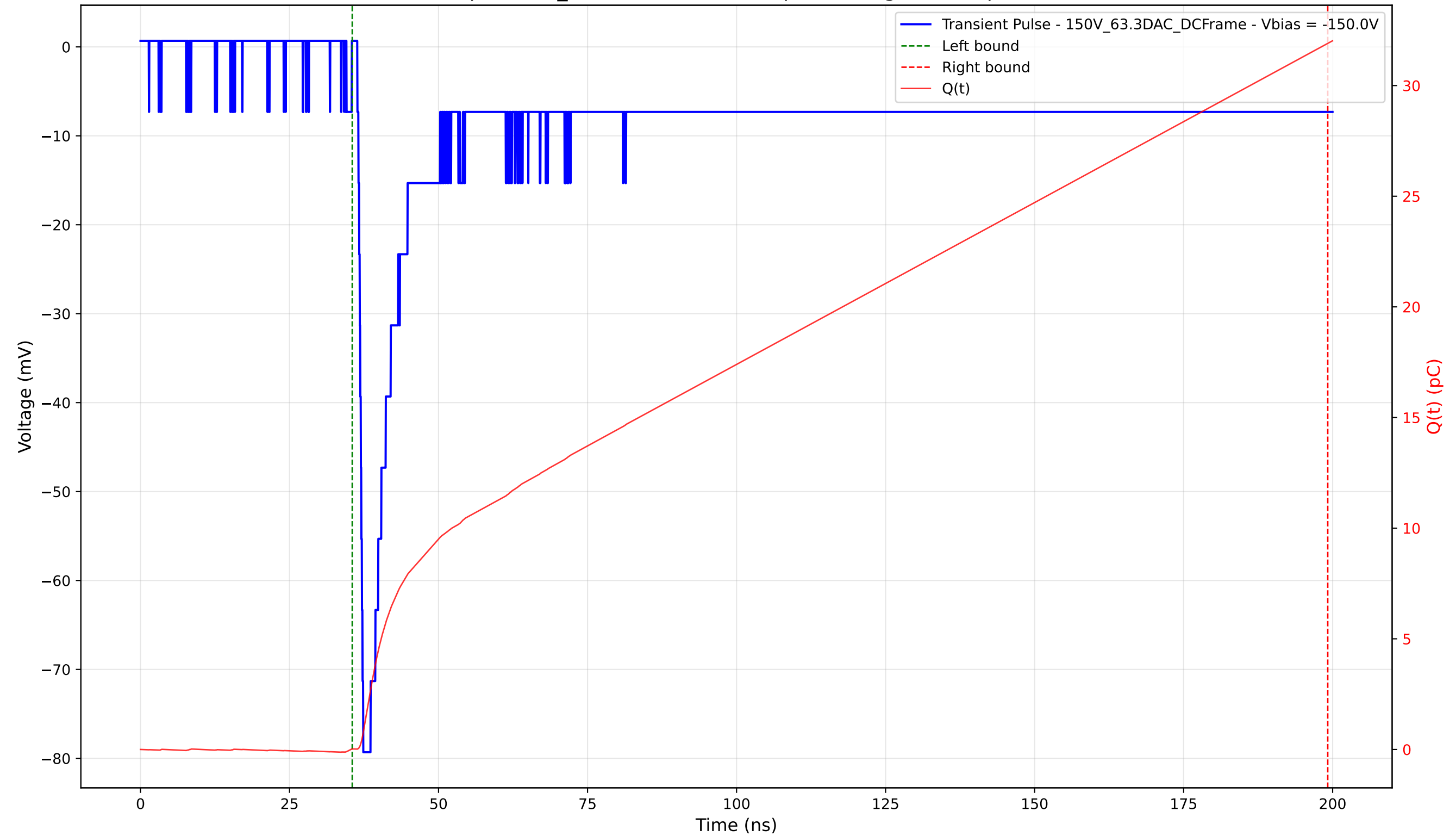
Transient Pulse - Sample: 1cm_42 - Position: 4195.0 \mu\text{m} - Charge: 31.88 pC - Rise Time: 0.82 ns
