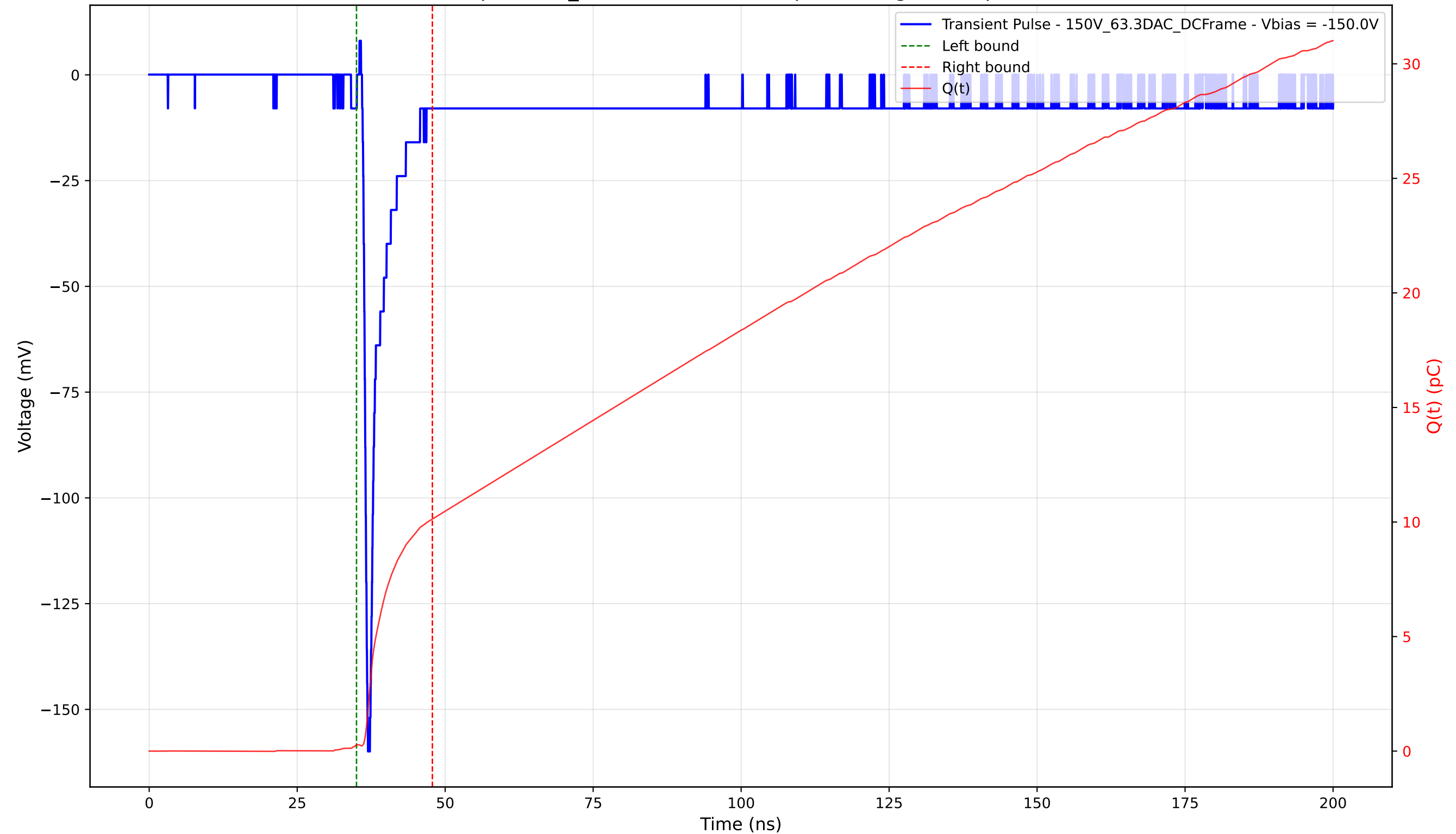
Transient Pulse - Sample: 1cm_42 - Position: 4965.0 \mu\text{m} - Charge: 9.86 pC - Rise Time: 0.74 ns
