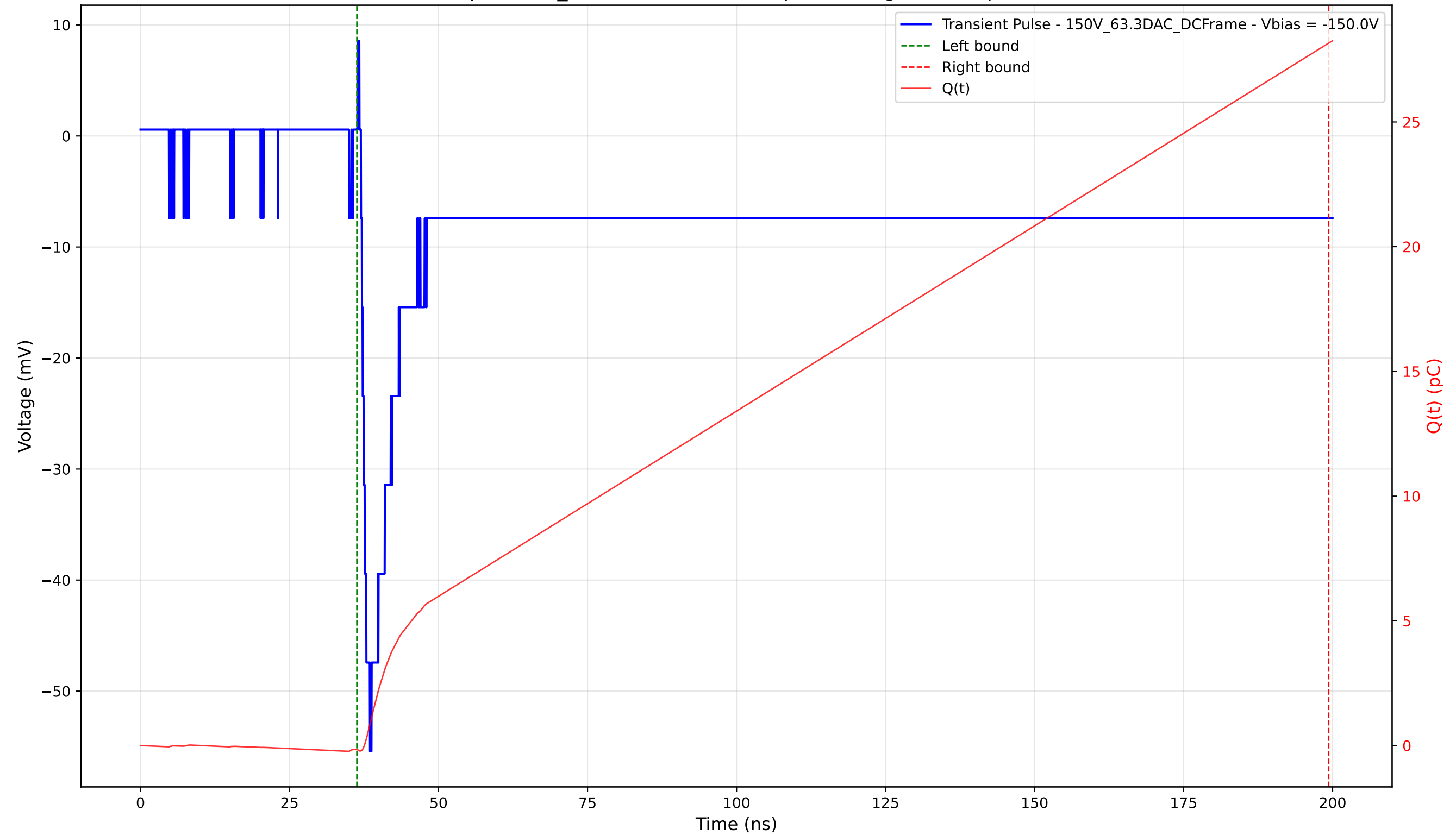
Transient Pulse - Sample: 1cm_42 - Position: 3845.0 \mu\text{m} - Charge: 28.32 pC - Rise Time: 1.51 ns
