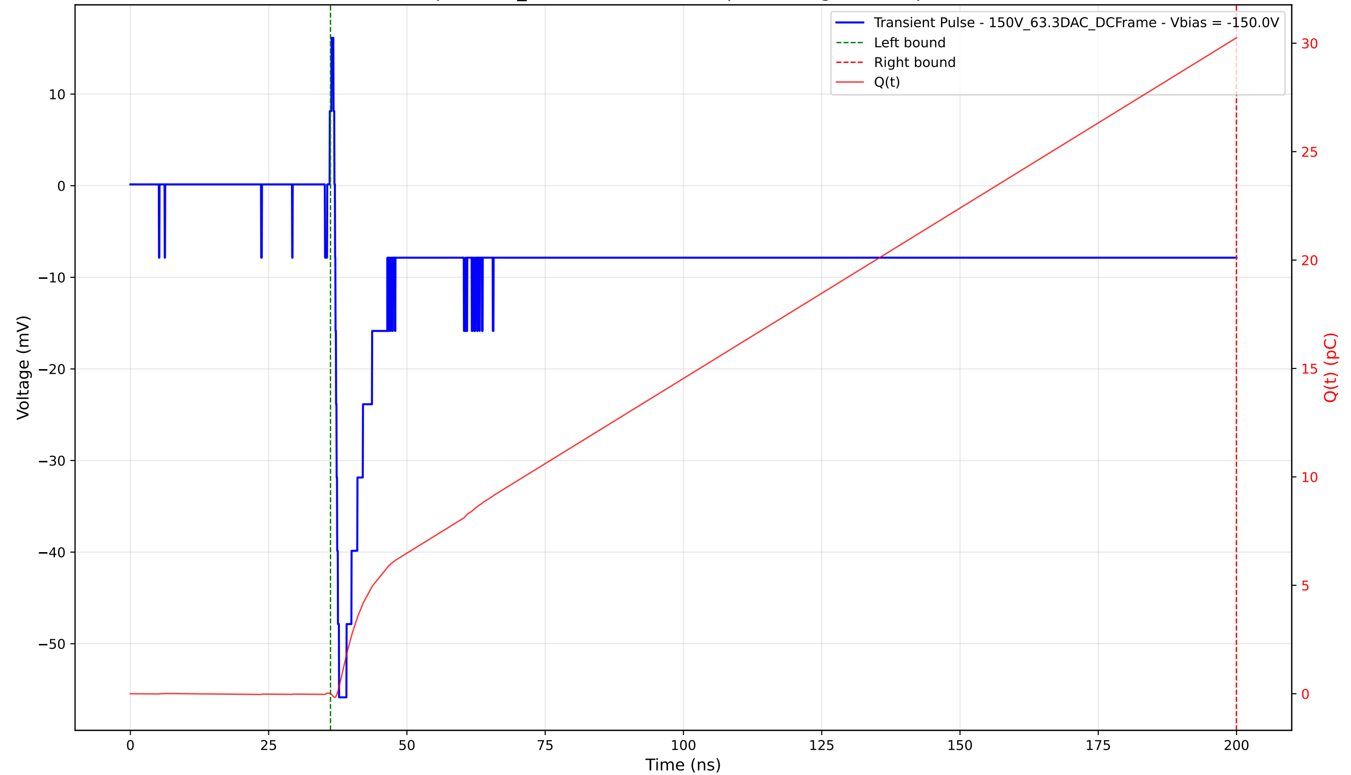
Transient Pulse - Sample: 1cm_42 - Position: 1385.0 \mu\text{m} - Charge: 30.25 pC - Rise Time: 0.73 ns
