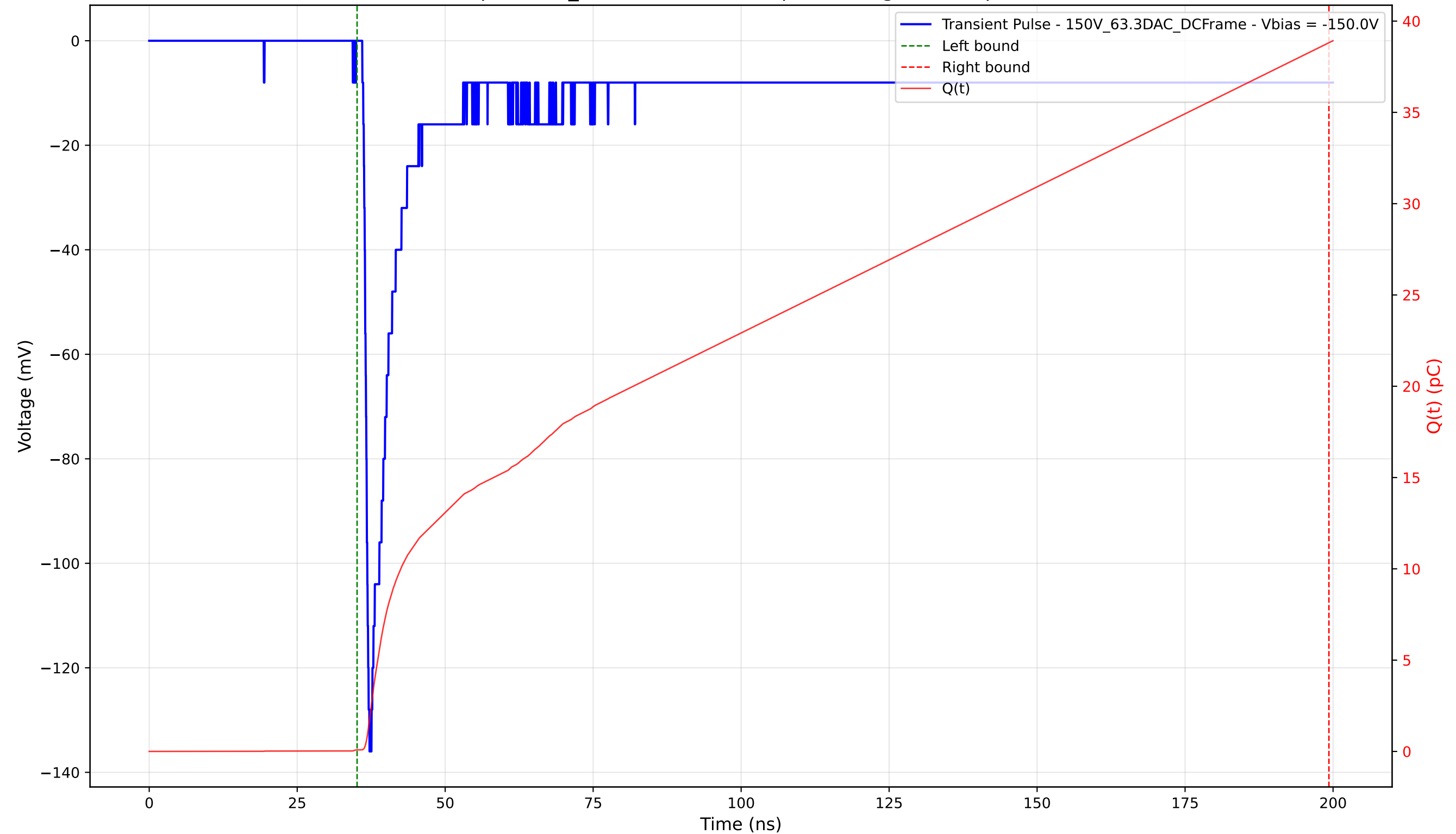
Transient Pulse - Sample: 1cm_42 - Position: 655.0 \mu\text{m} - Charge: 38.73 pC - Rise Time: 0.91 ns
