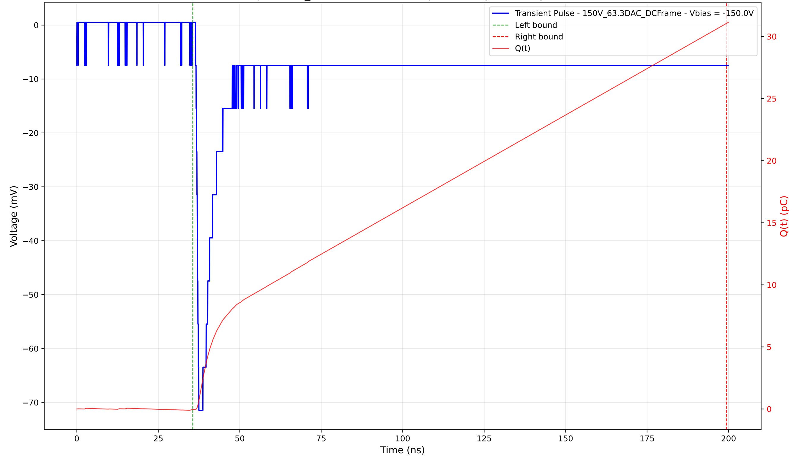
Transient Pulse - Sample: 1cm_42 - Position: 4150.0 \mu\text{m} - Charge: 31.10 pC - Rise Time: 1.00 ns
