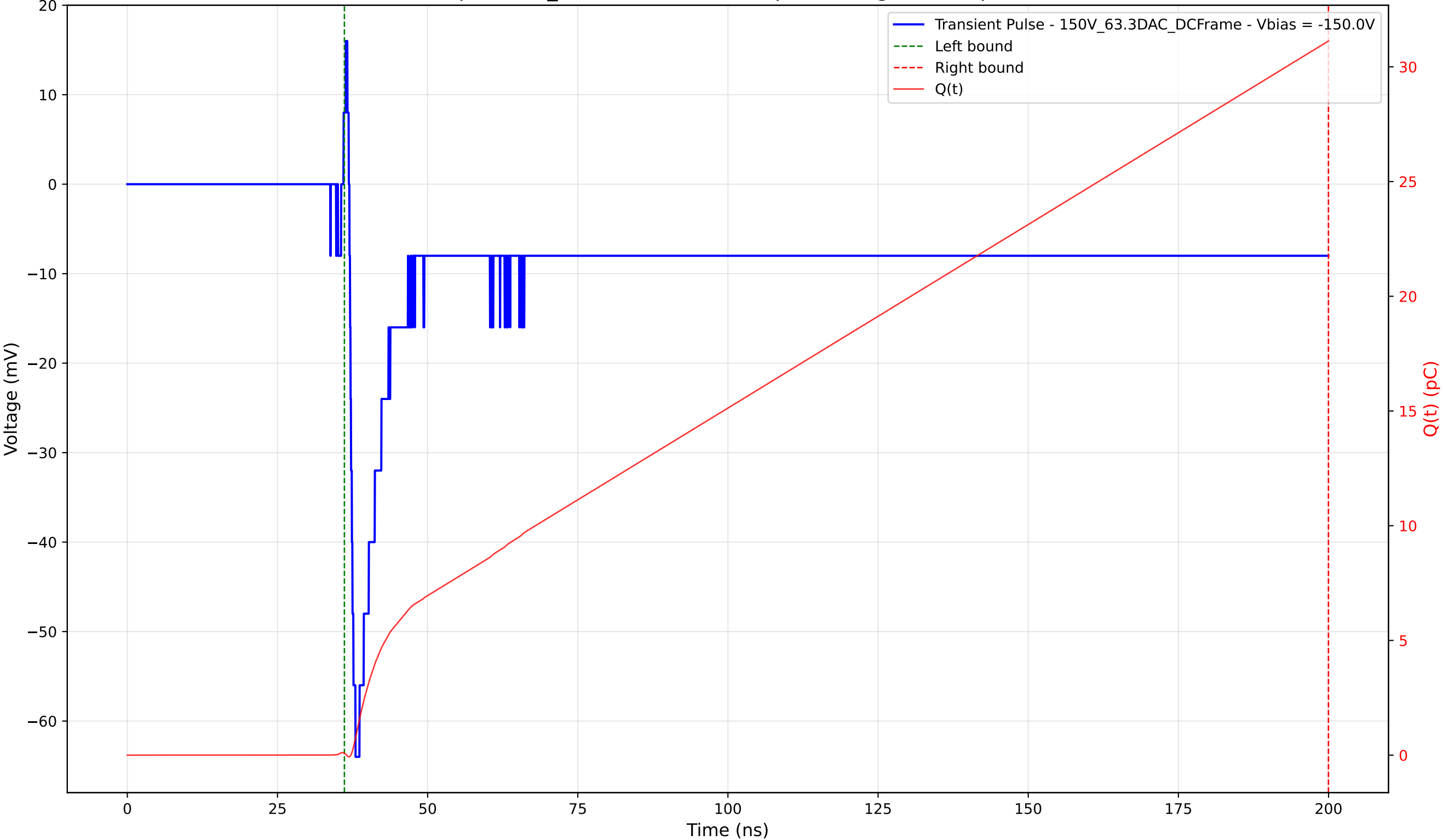
Transient Pulse - Sample: 1cm_42 - Position: 1350.0 \mu\text{m} - Charge: 31.04 pC - Rise Time: 1.00 ns
