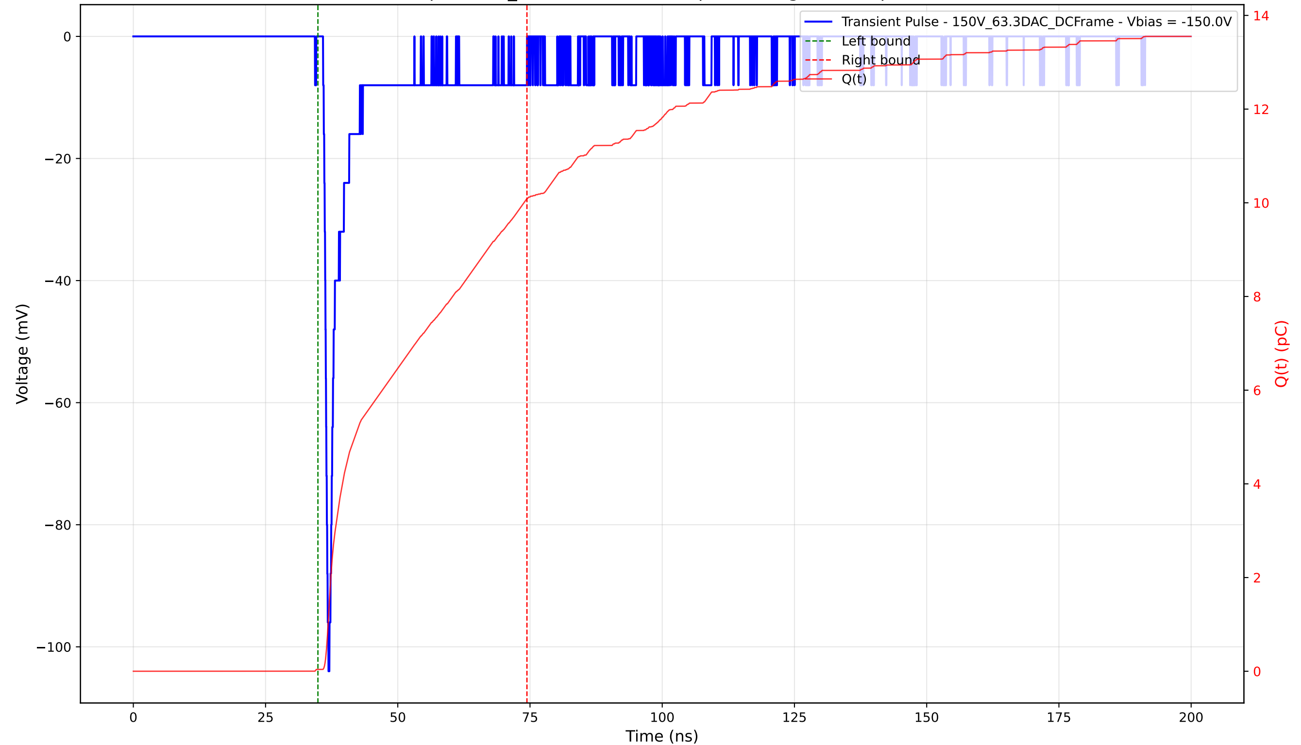
Transient Pulse - Sample: 1cm_42 - Position: 130.0 \mu\text{m} - Charge: 10.05 pC - Rise Time: 0.75 ns
