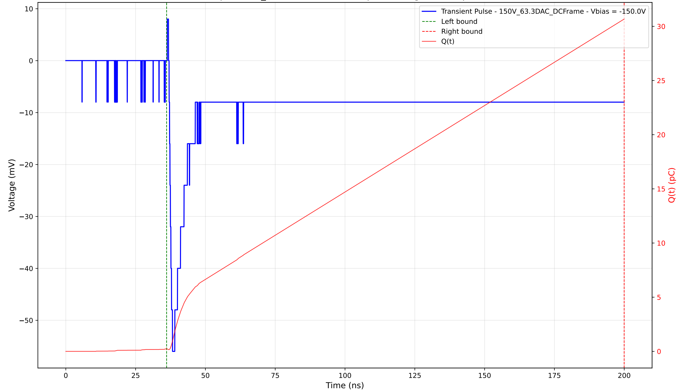
Transient Pulse - Sample: 1cm_42 - Position: 3800.0 \mu\text{m} - Charge: 30.45 pC - Rise Time: 1.21 ns
