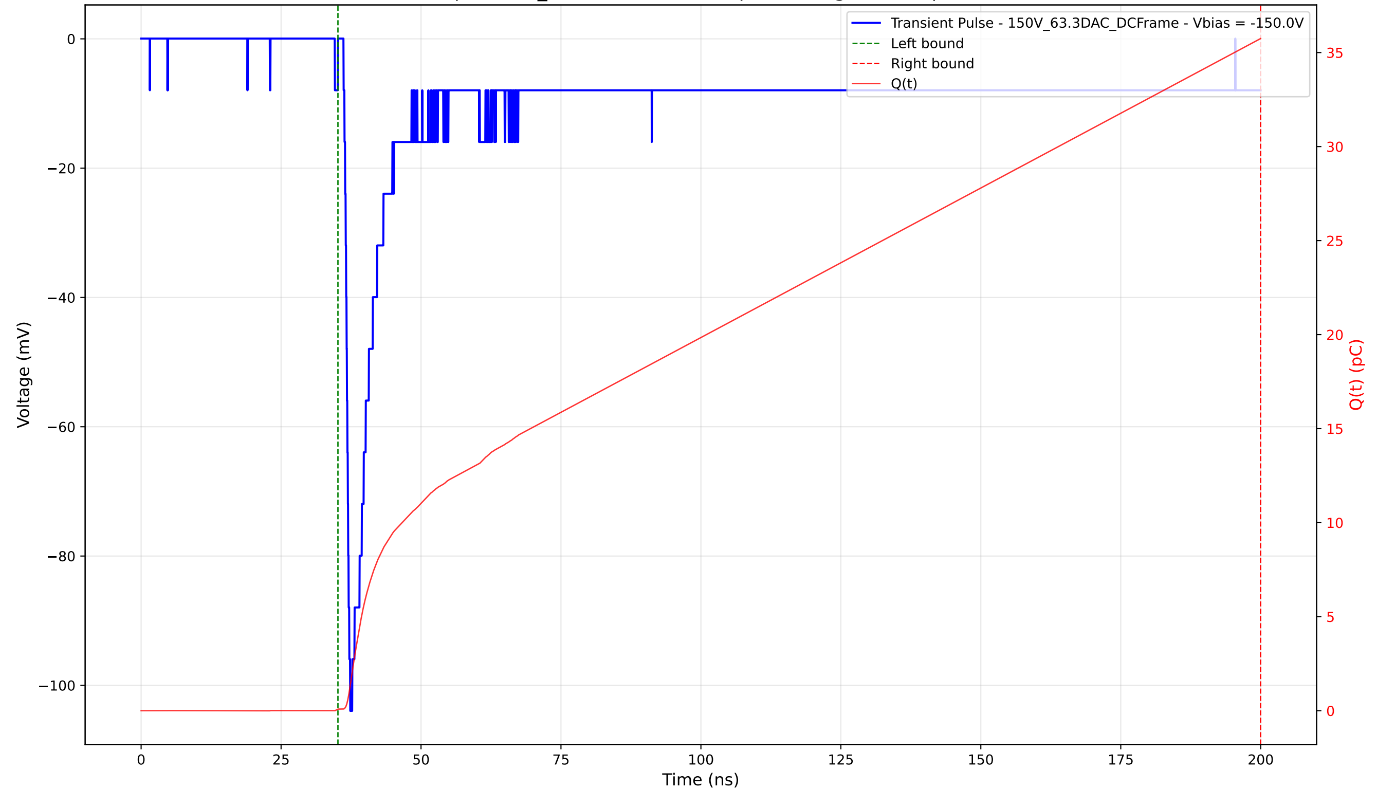
Transient Pulse - Sample: 1cm_42 - Position: 850.0 \mu\text{m} - Charge: 35.66 pC - Rise Time: 0.87 ns
