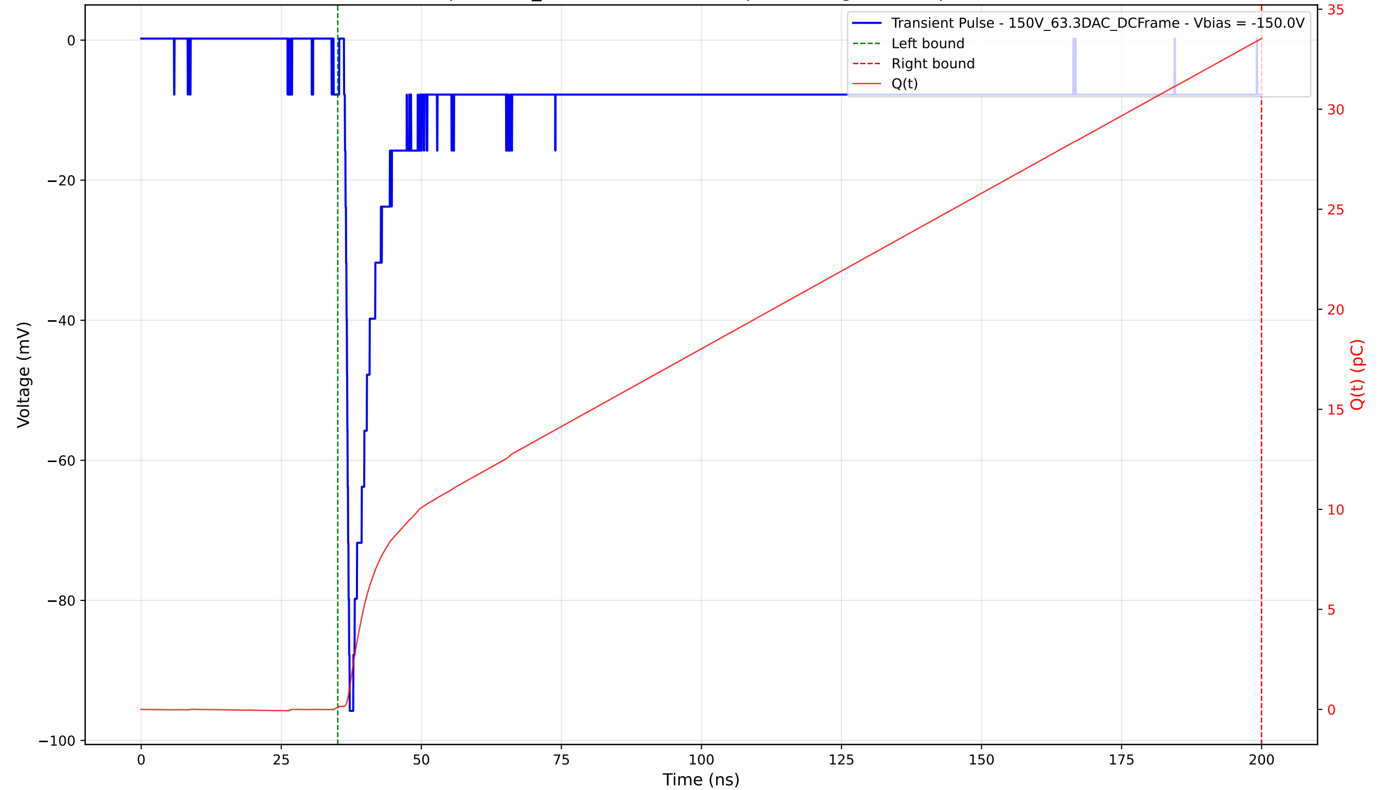
Transient Pulse - Sample: 1cm_42 - Position: 4435.0 \mu\text{m} - Charge: 33.42 pC - Rise Time: 0.76 ns
