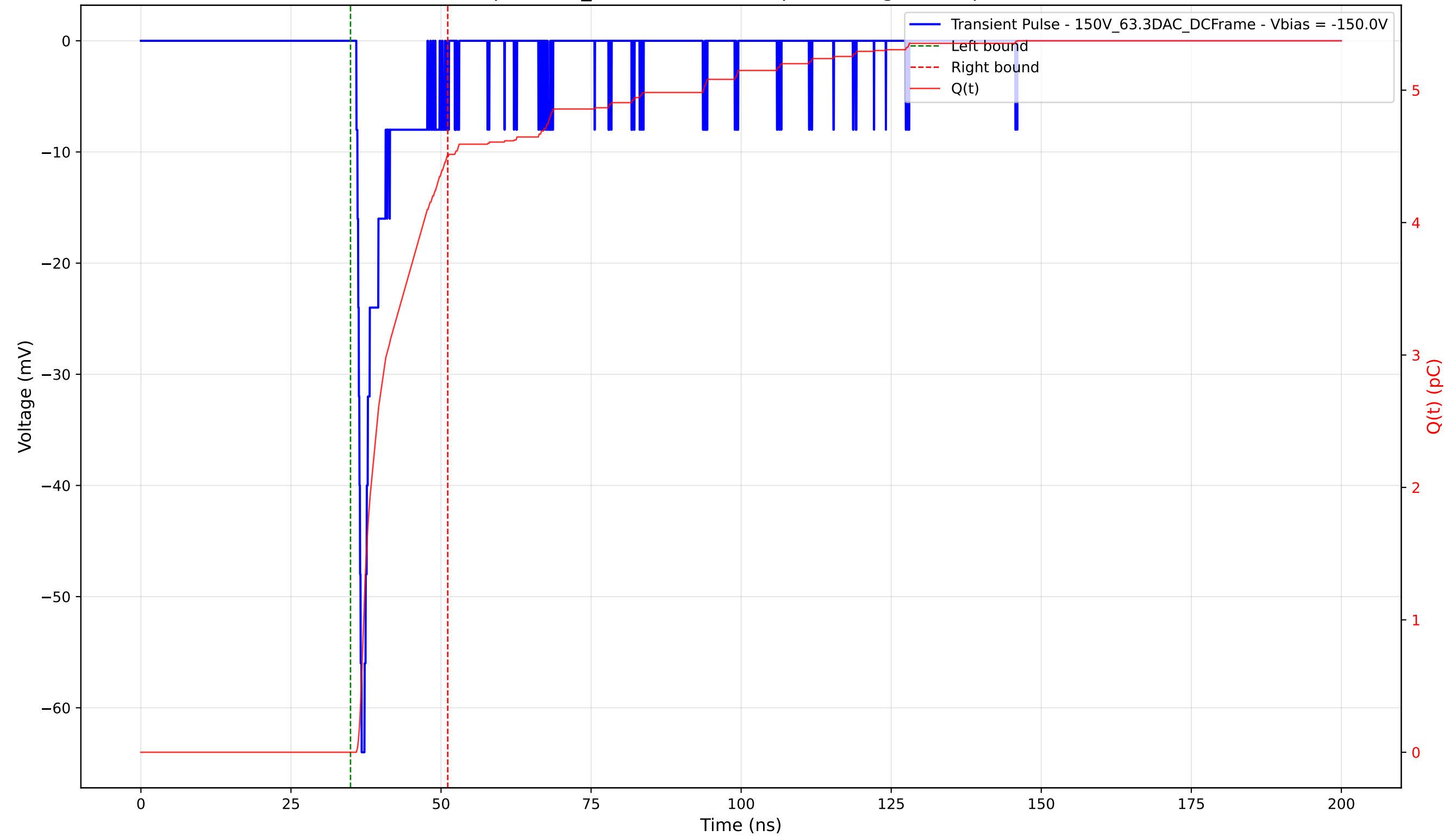
Transient Pulse - Sample: 1cm_42 - Position: 75.0 \mu\text{m} - Charge: 4.50 pC - Rise Time: 0.86 ns
