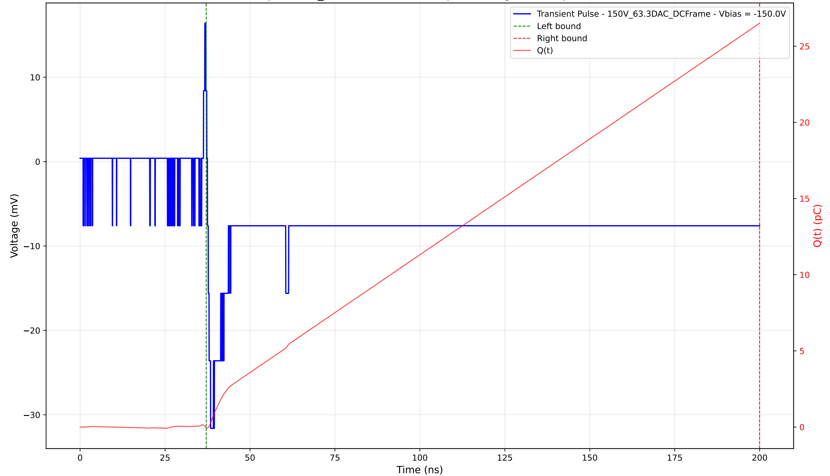
Transient Pulse - Sample: 1cm_42 - Position: 3030.0 \mu\text{m} - Charge: 26.56 pC - Rise Time: 0.93 ns
