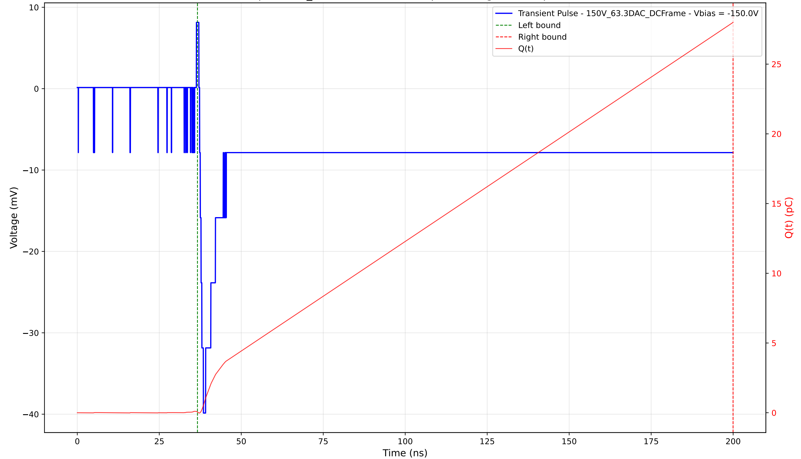
Transient Pulse - Sample: 1cm_42 - Position: 3470.0 \mu\text{m} - Charge: 27.94 pC - Rise Time: 1.15 ns
