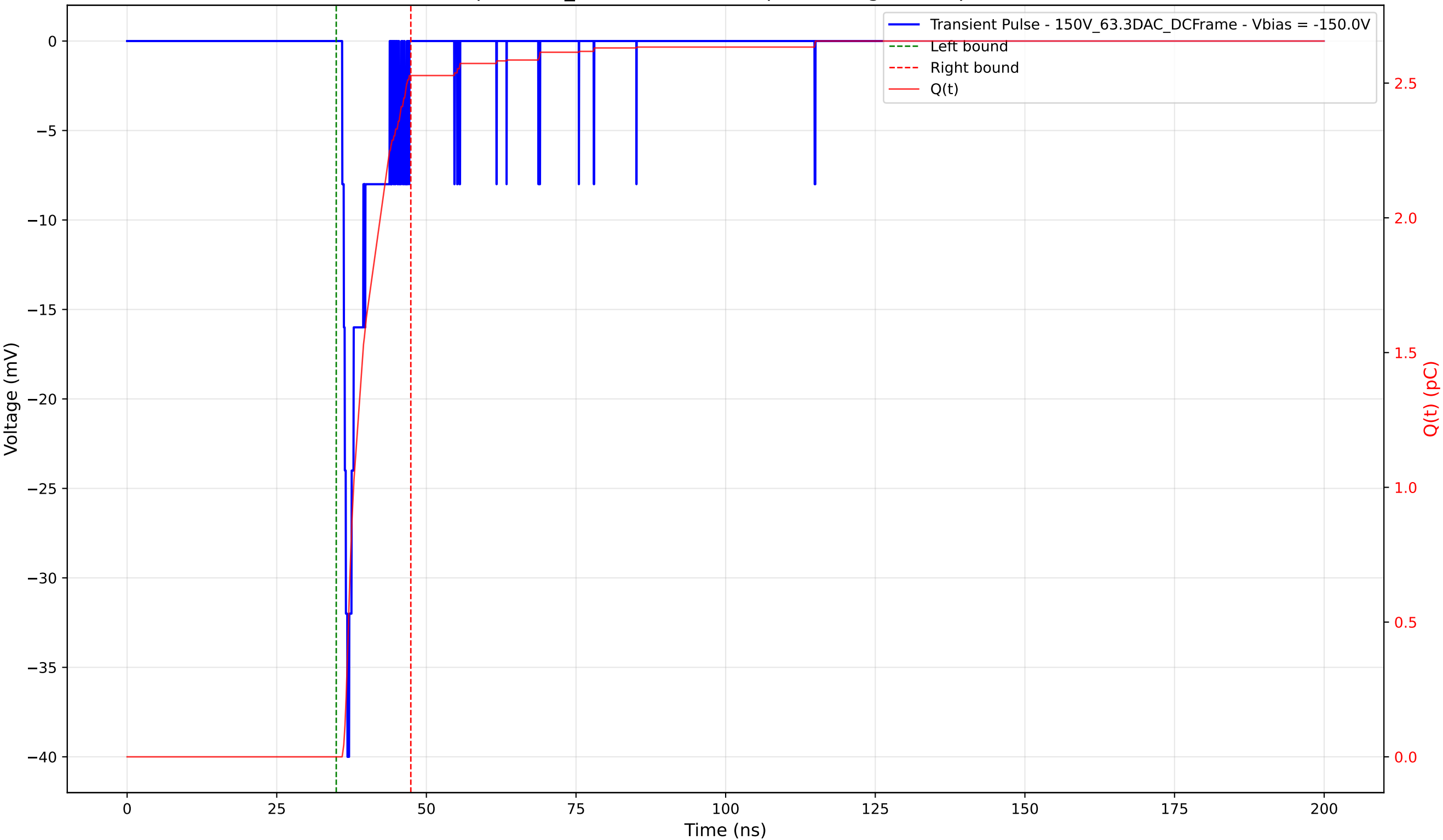
Transient Pulse - Sample: 1cm_42 - Position: 30.0 \mu\text{m} - Charge: 2.53 pC - Rise Time: 0.87 ns
