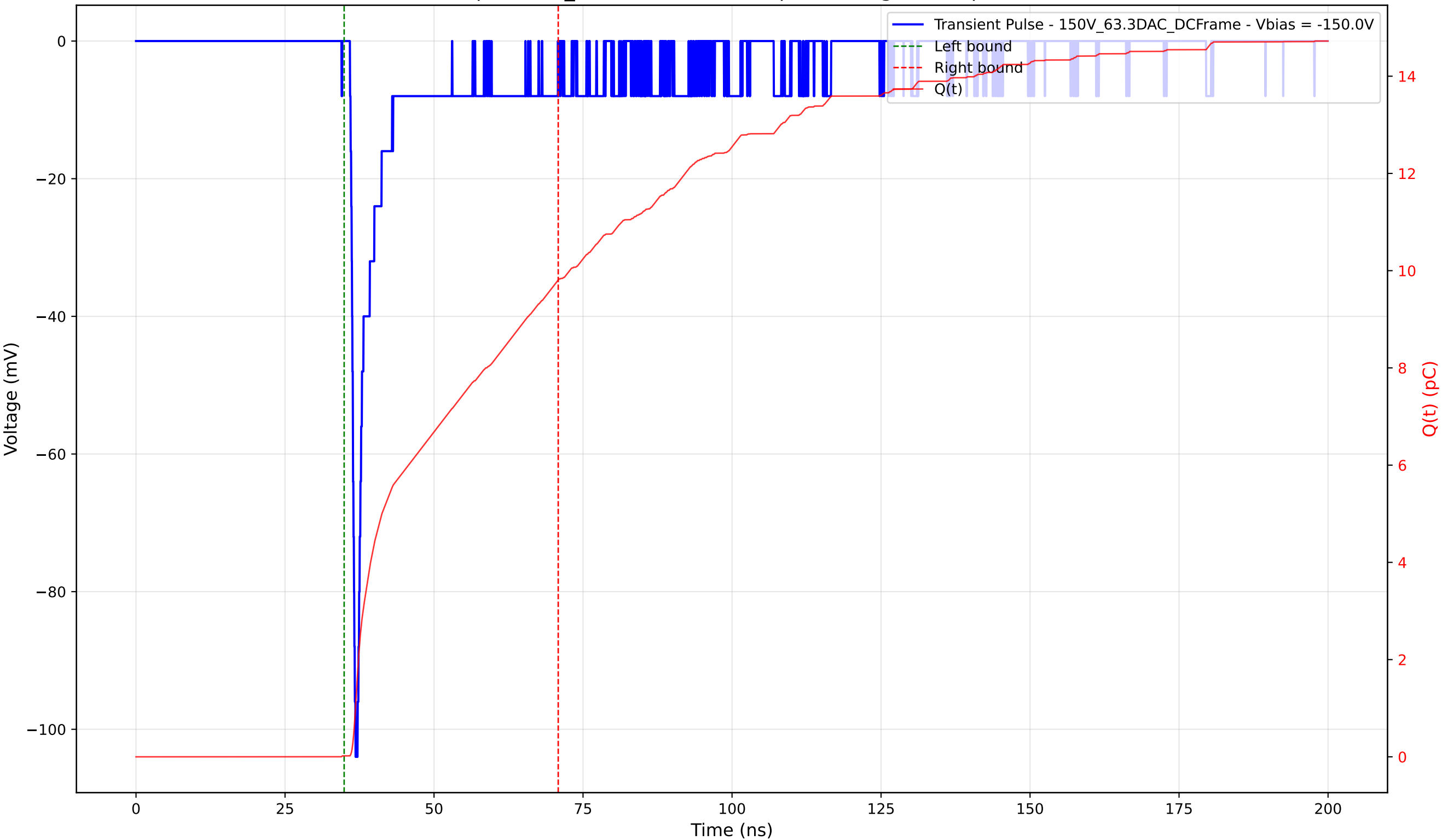
Transient Pulse - Sample: 1cm_42 - Position: 135.0 \mu\text{m} - Charge: 9.79 pC - Rise Time: 0.71 ns
