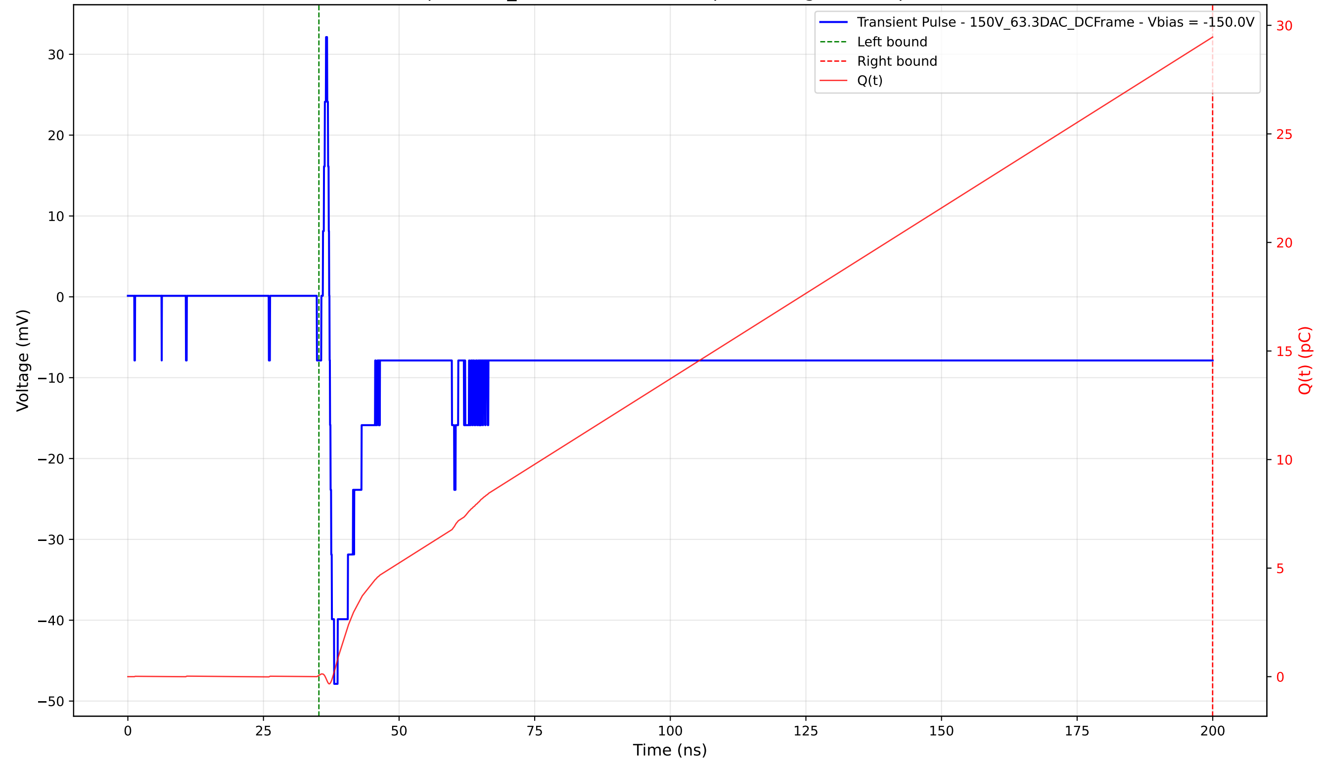
Transient Pulse - Sample: 1cm_42 - Position: 1780.0 \mu\text{m} - Charge: 29.40 pC - Rise Time: 0.85 ns
