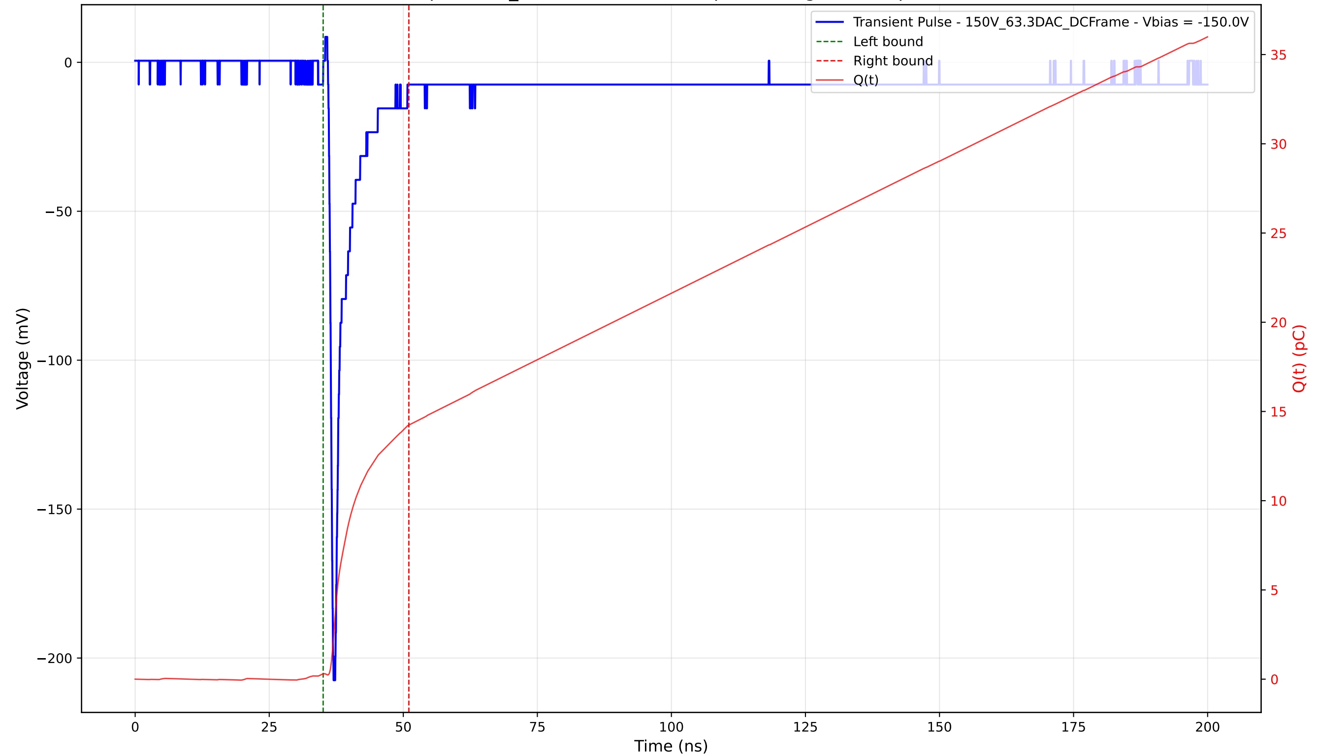
Transient Pulse - Sample: 1cm_42 - Position: 4895.0 \mu\text{m} - Charge: 13.93 pC - Rise Time: 0.75 ns
