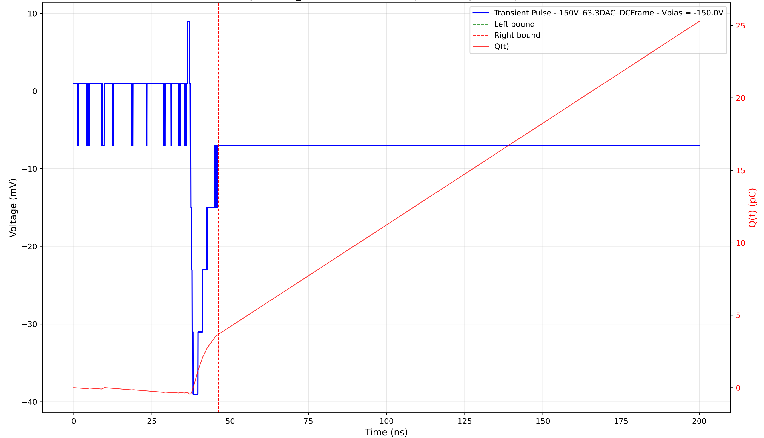
Transient Pulse - Sample: 1cm_42 - Position: 3540.0 \mu\text{m} - Charge: 4.10 pC - Rise Time: 0.95 ns
