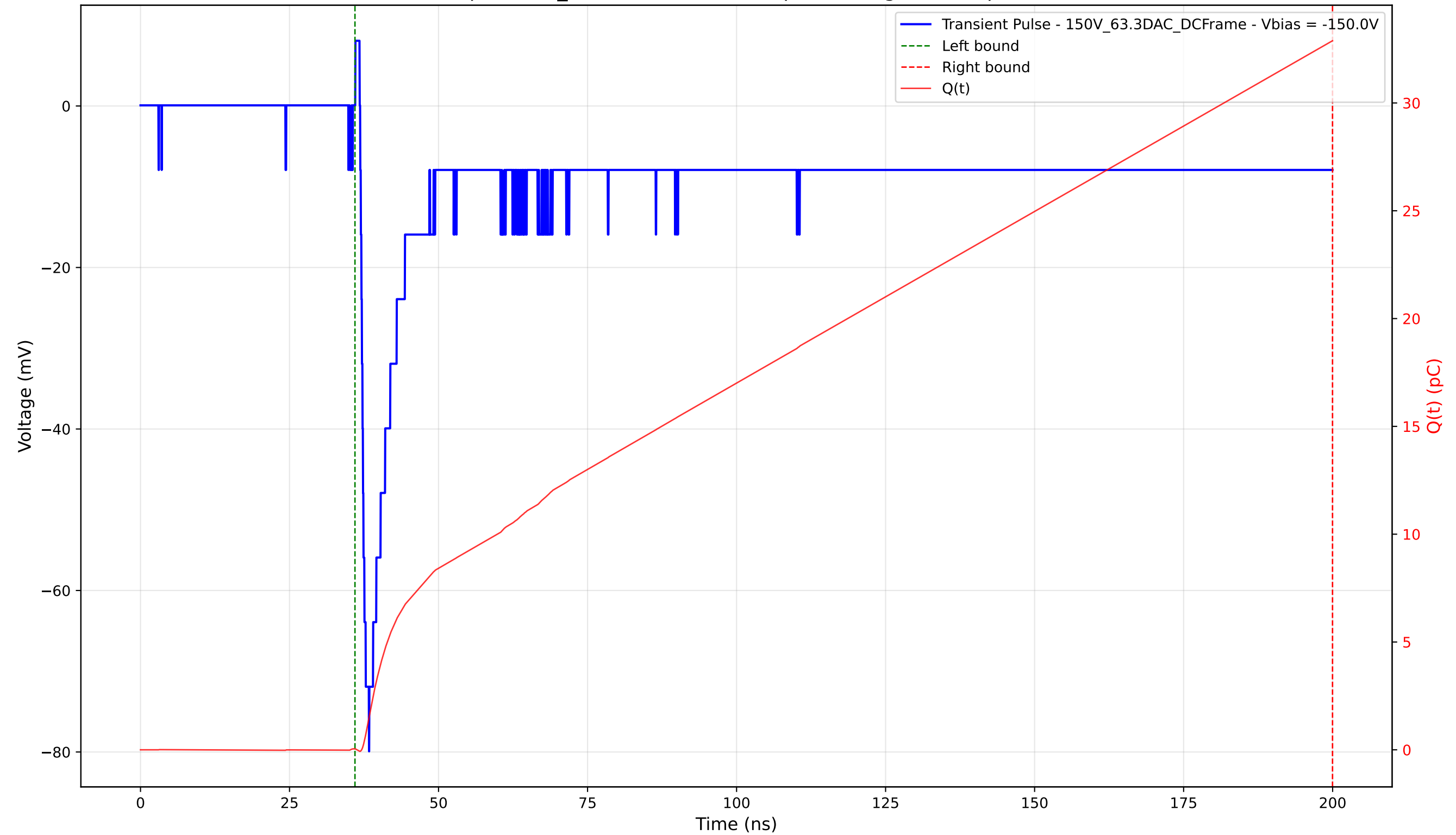
Transient Pulse - Sample: 1cm_42 - Position: 1200.0 \mu\text{m} - Charge: 32.84 pC - Rise Time: 1.38 ns
