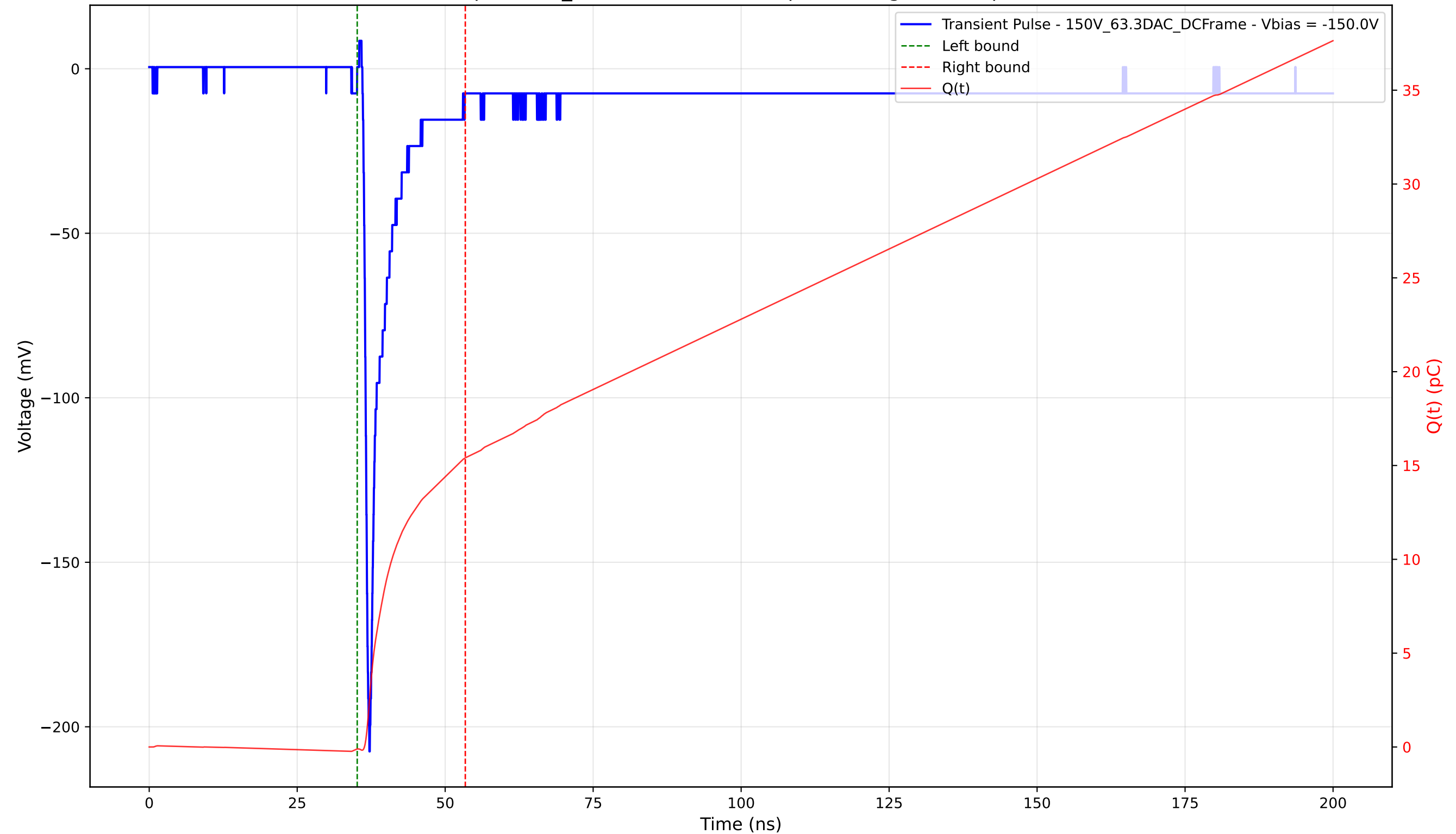
Transient Pulse - Sample: 1cm_42 - Position: 4680.0 \mu\text{m} - Charge: 15.51 pC - Rise Time: 0.81 ns
