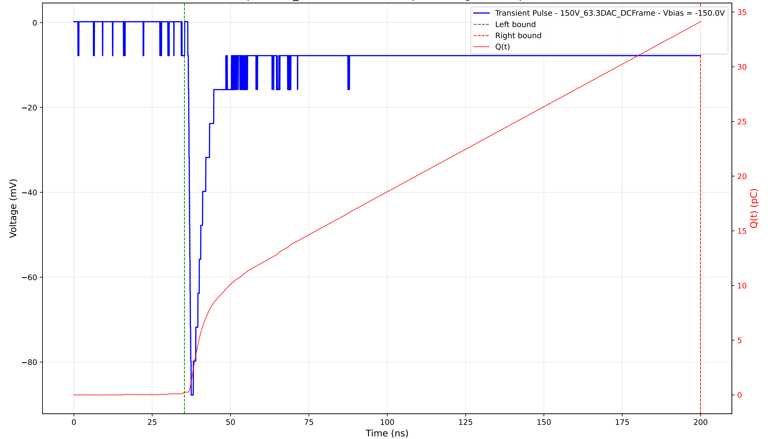
Transient Pulse - Sample: 1cm_42 - Position: 4225.0 \mu\text{m} - Charge: 33.88 pC - Rise Time: 0.76 ns
