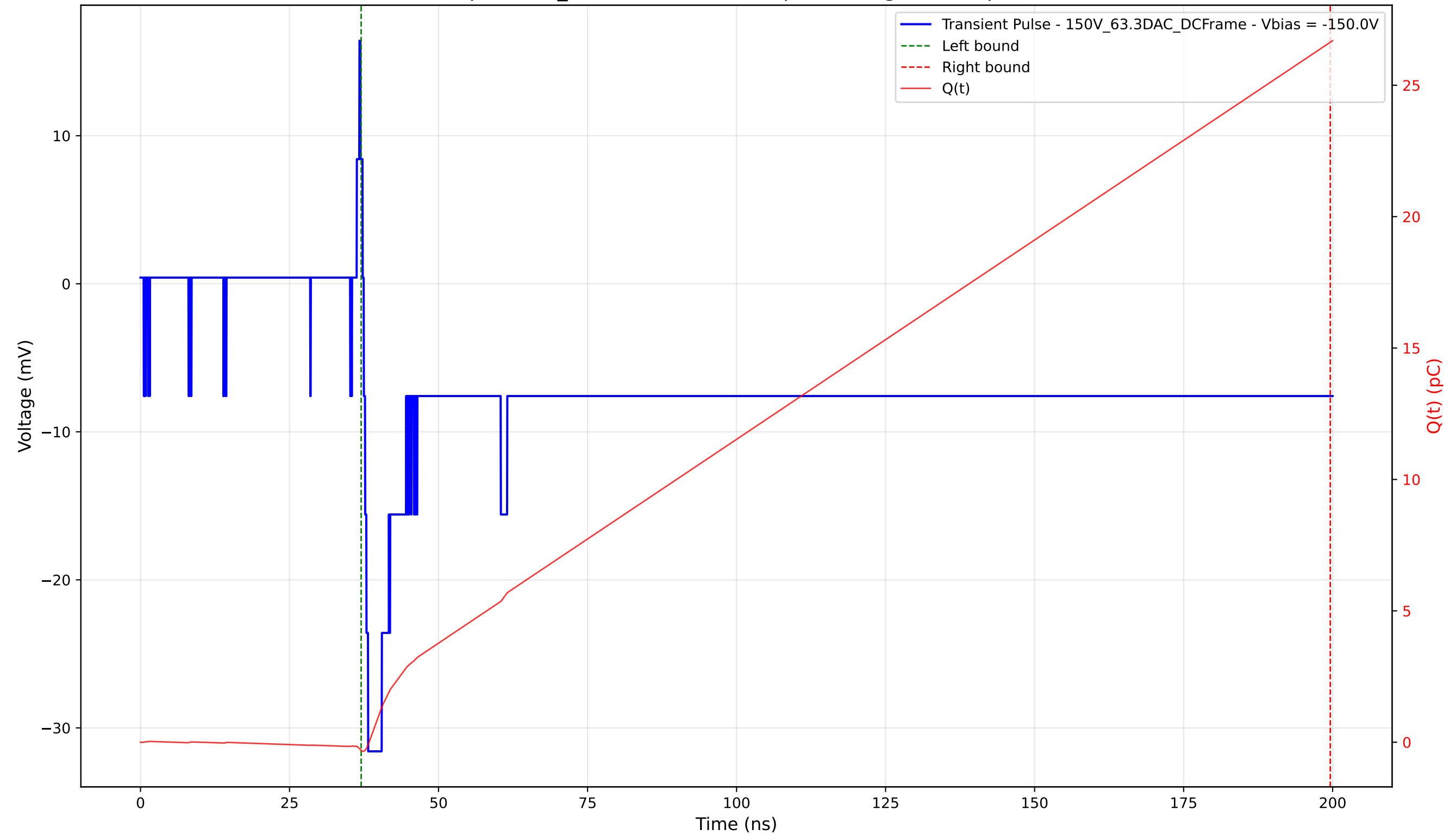
Transient Pulse - Sample: 1cm_42 - Position: 3135.0 \mu\text{m} - Charge: 26.94 pC - Rise Time: 0.73 ns
