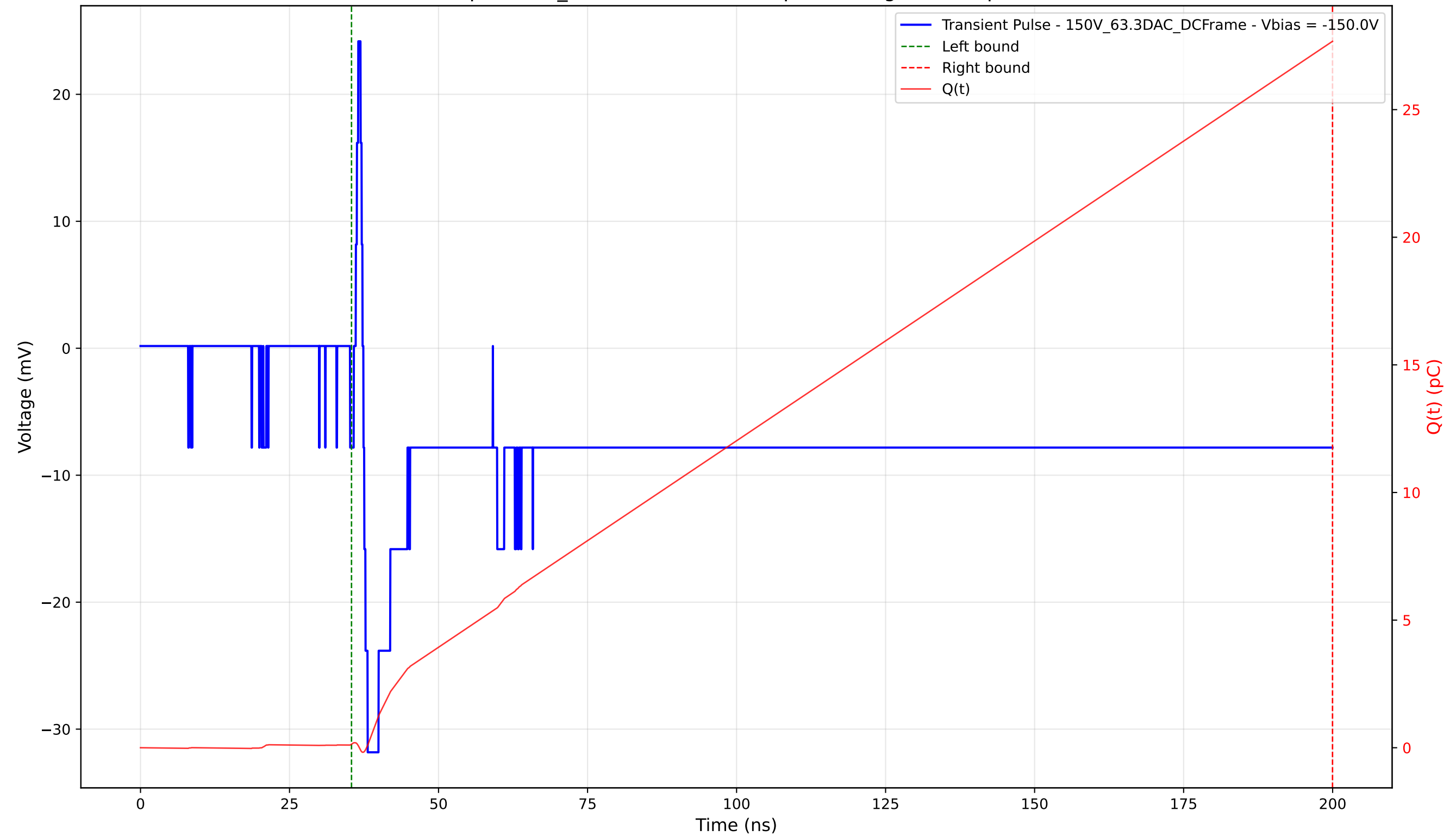
Transient Pulse - Sample: 1cm_42 - Position: 2365.0 \mu\text{m} - Charge: 27.54 pC - Rise Time: 0.71 ns
