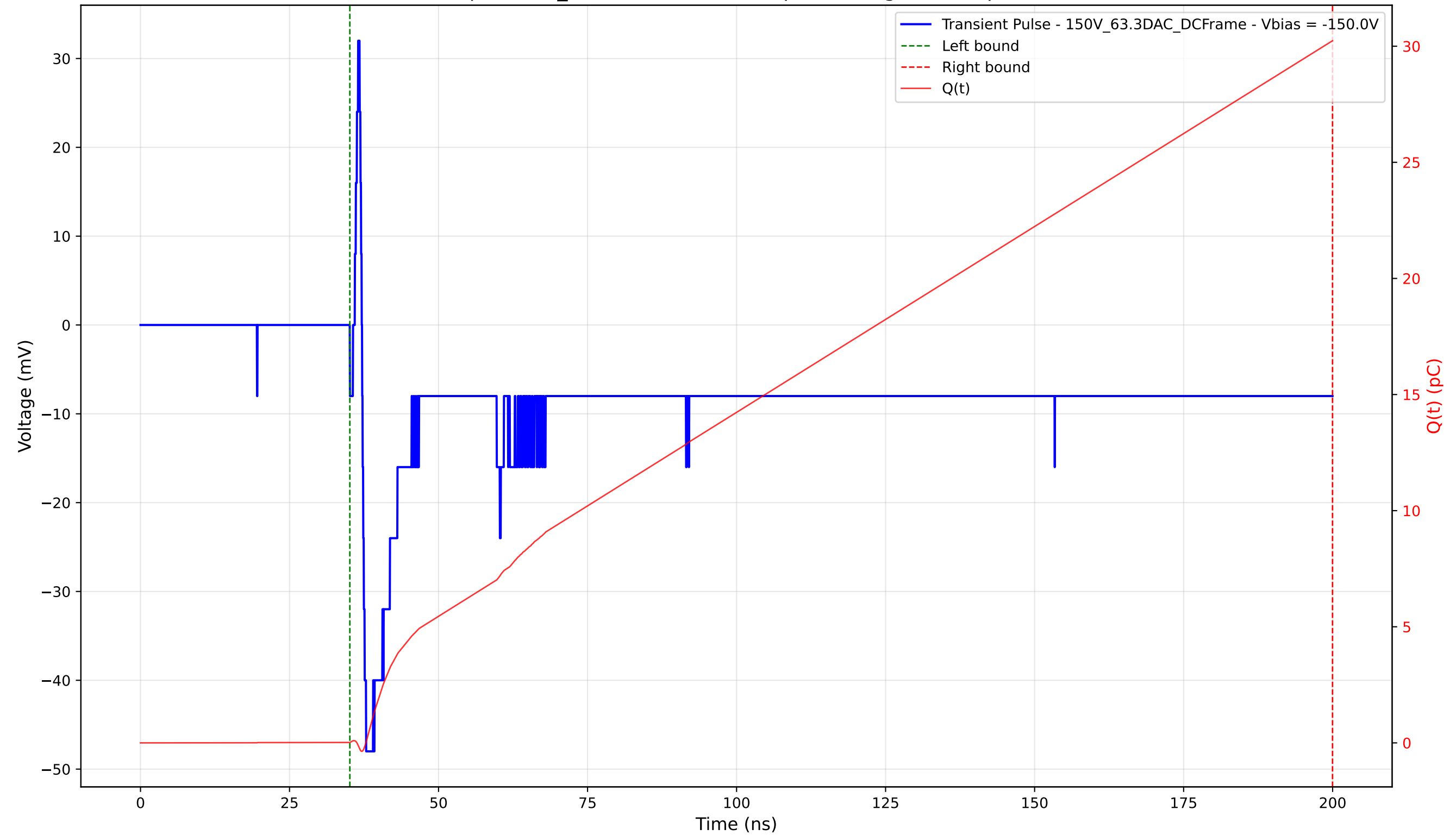
Transient Pulse - Sample: 1cm_42 - Position: 1705.0 \mu\text{m} - Charge: 30.22 pC - Rise Time: 0.67 ns
