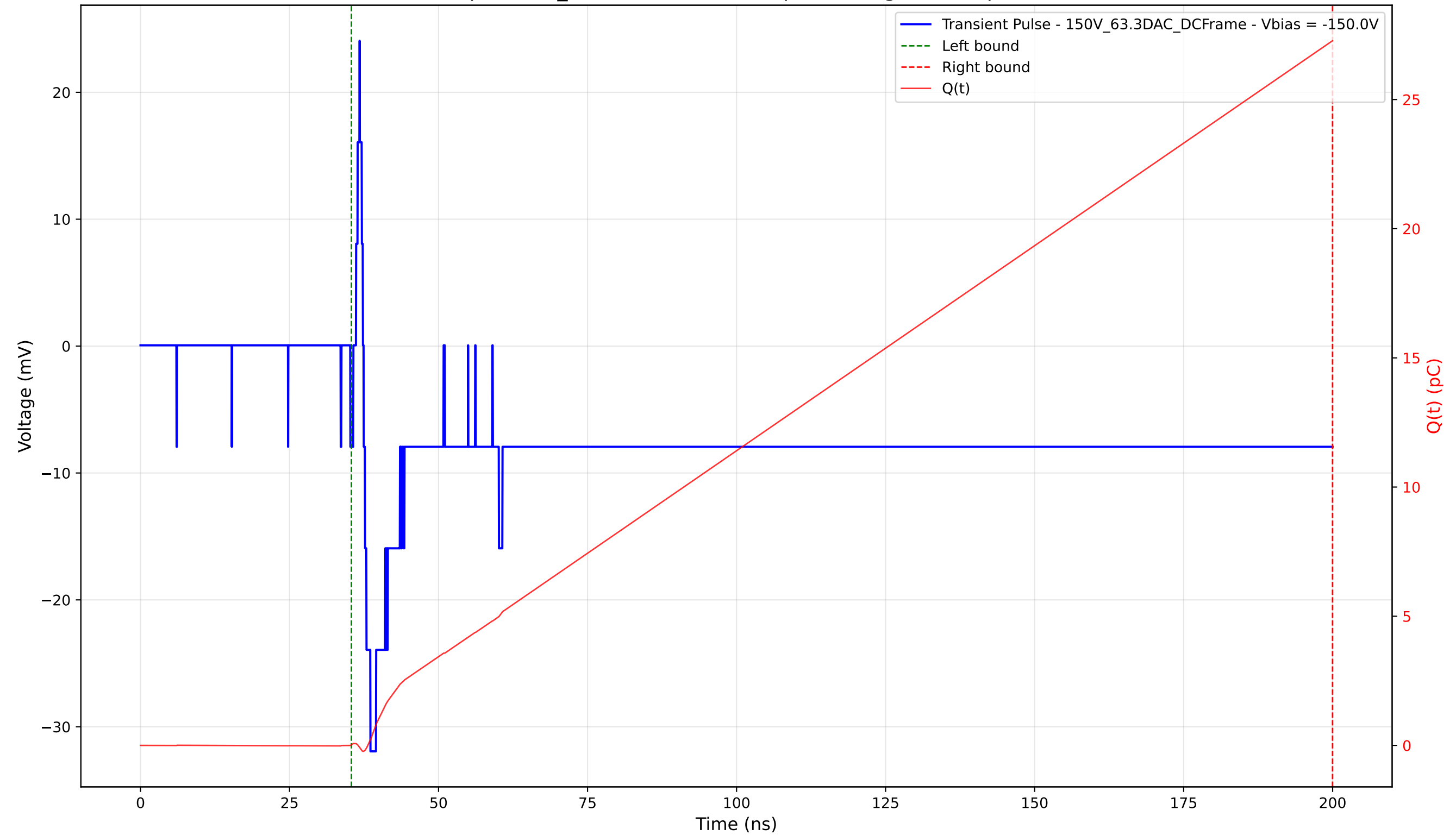
Transient Pulse - Sample: 1cm_42 - Position: 2465.0 \mu\text{m} - Charge: 27.25 pC - Rise Time: 1.13 ns
