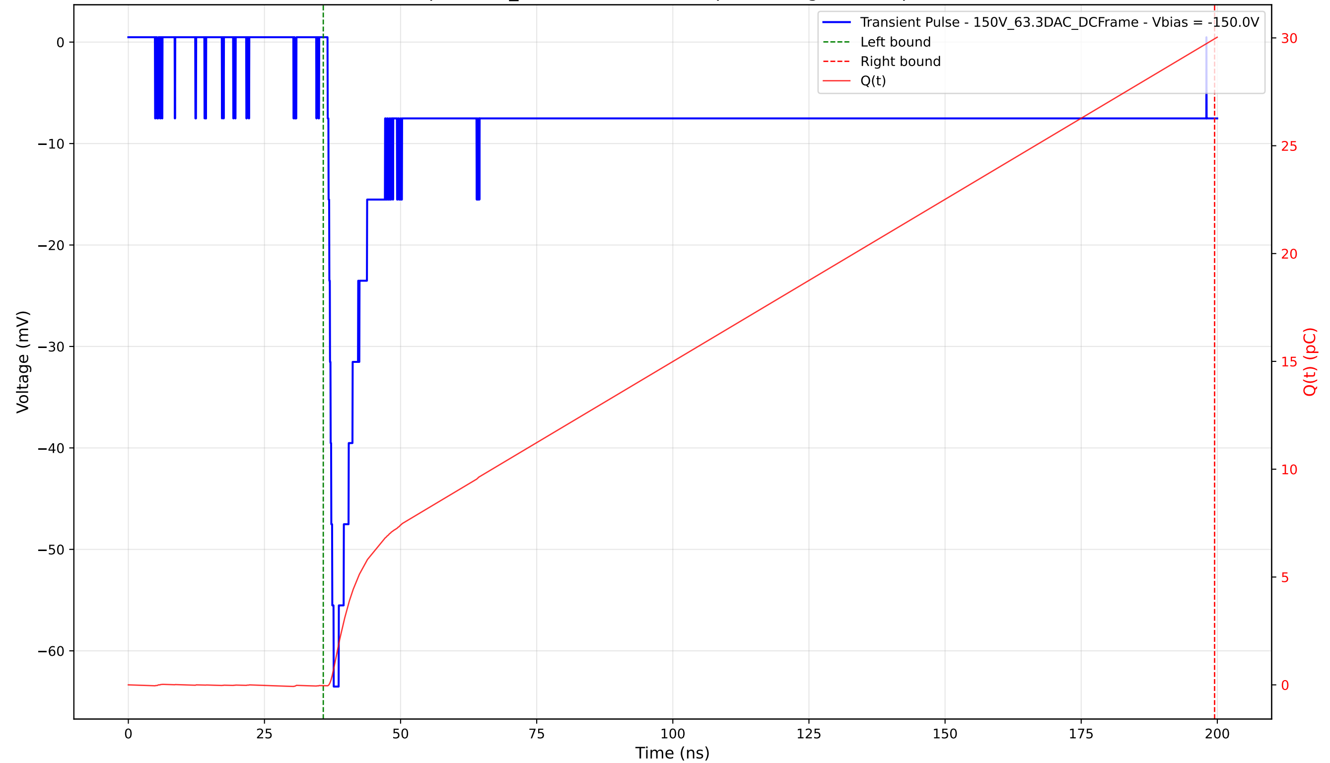
Transient Pulse - Sample: 1cm_42 - Position: 4070.0 \mu\text{m} - Charge: 30.00 pC - Rise Time: 1.10 ns
