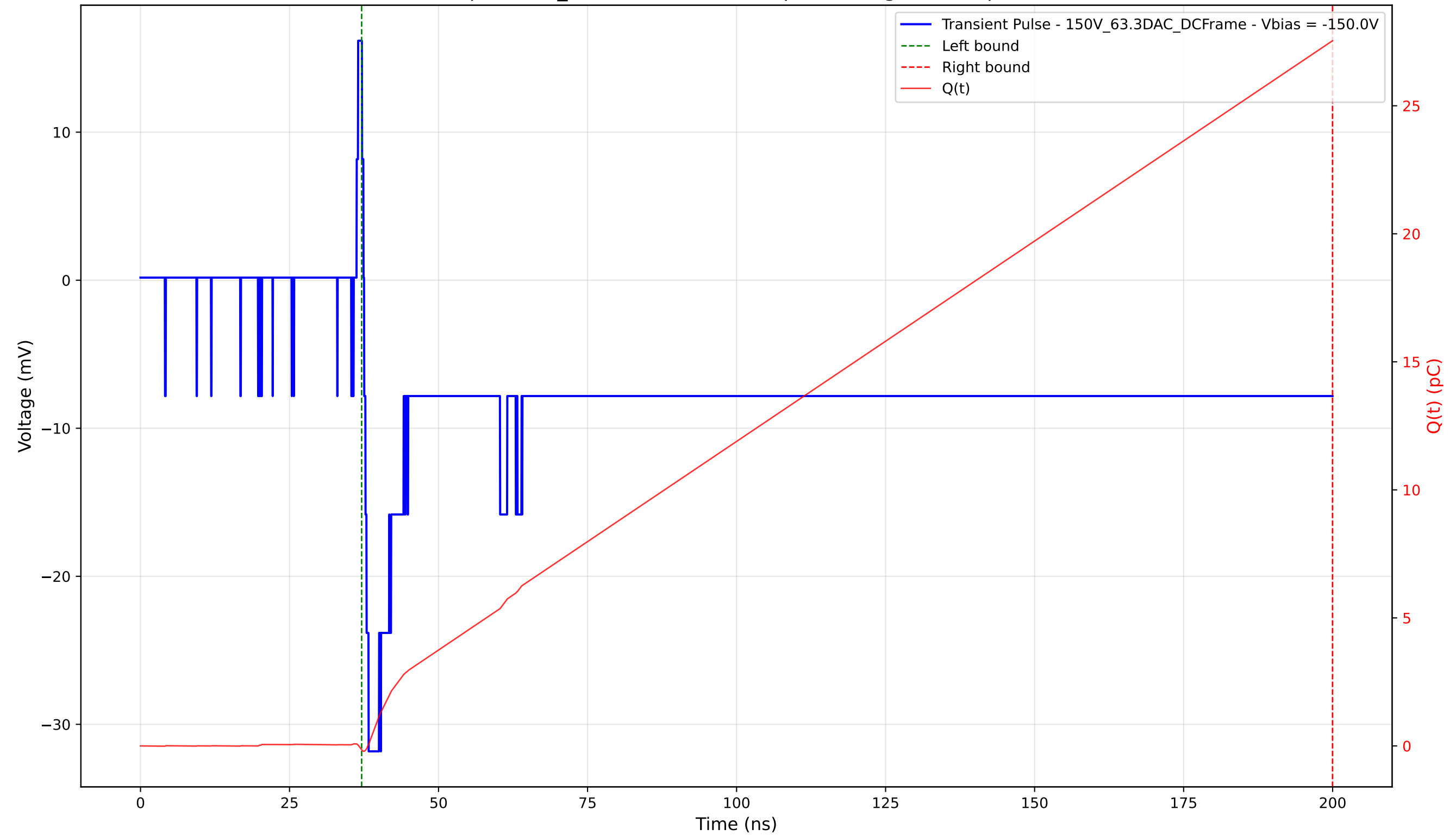
Transient Pulse - Sample: 1cm_42 - Position: 2755.0 \mu\text{m} - Charge: 27.70 pC - Rise Time: 0.75 ns
