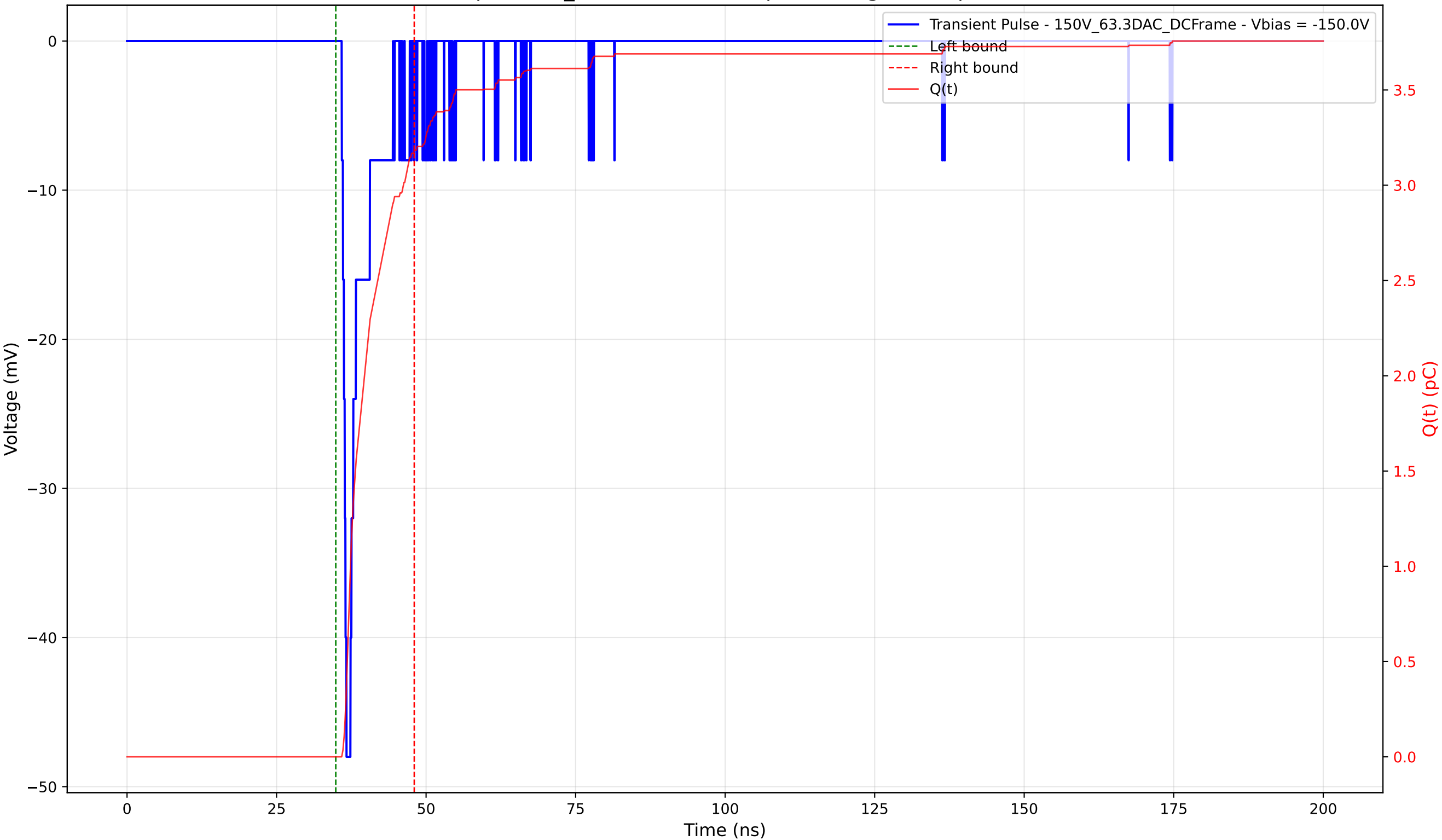
Transient Pulse - Sample: 1cm_42 - Position: 55.0 \mu\text{m} - Charge: 3.18 pC - Rise Time: 0.79 ns
