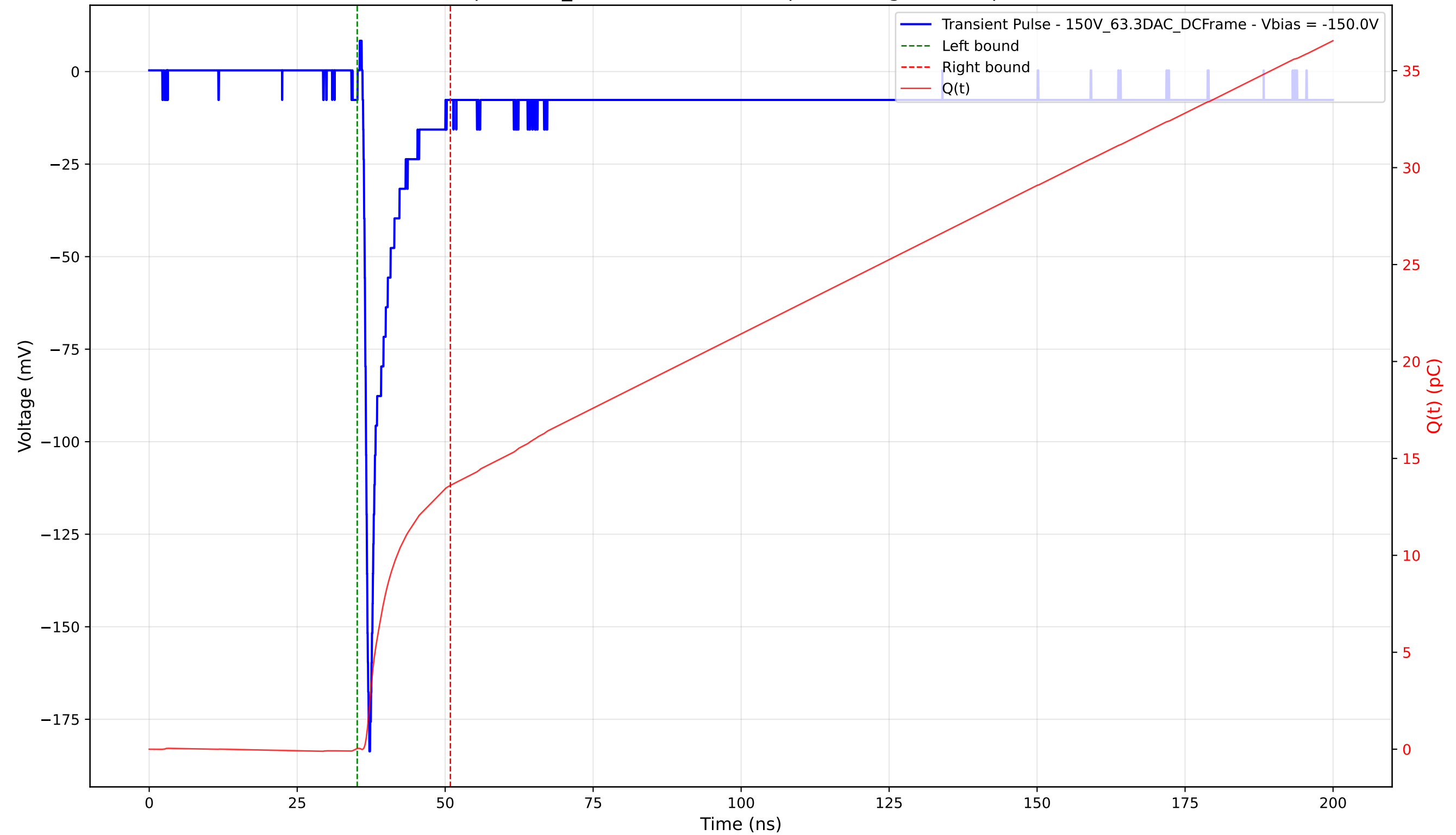
Transient Pulse - Sample: 1cm_42 - Position: 4645.0 \mu\text{m} - Charge: 13.56 pC - Rise Time: 0.79 ns
