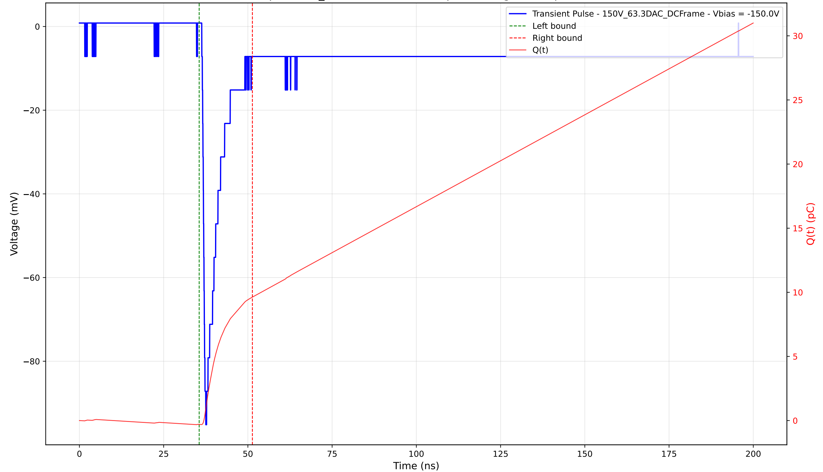
Transient Pulse - Sample: 1cm_42 - Position: 4350.0 \mu\text{m} - Charge: 9.93 pC - Rise Time: 0.79 ns
