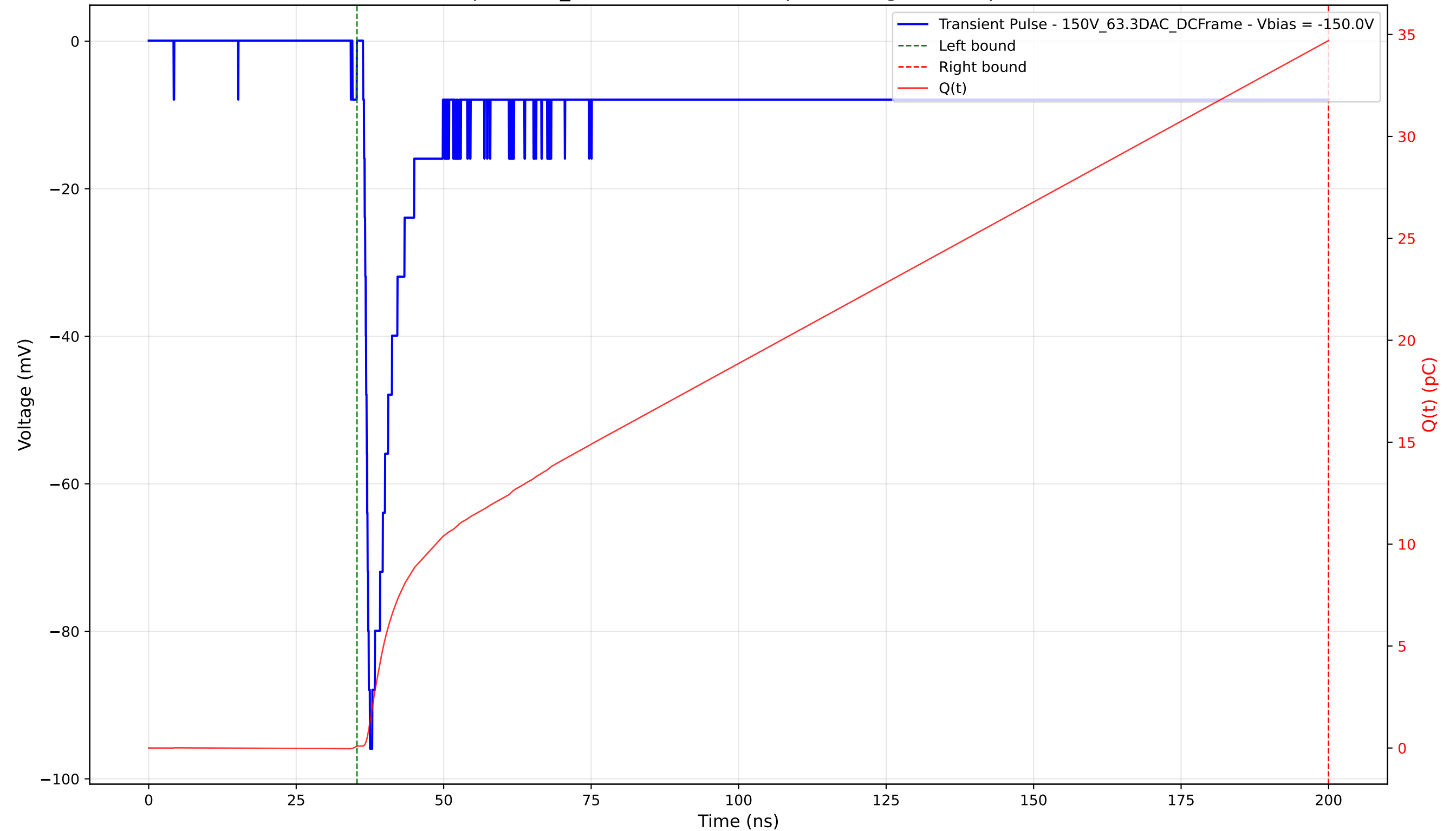
Transient Pulse - Sample: 1cm_42 - Position: 4290.0 \mu\text{m} - Charge: 34.61 pC - Rise Time: 0.82 ns
