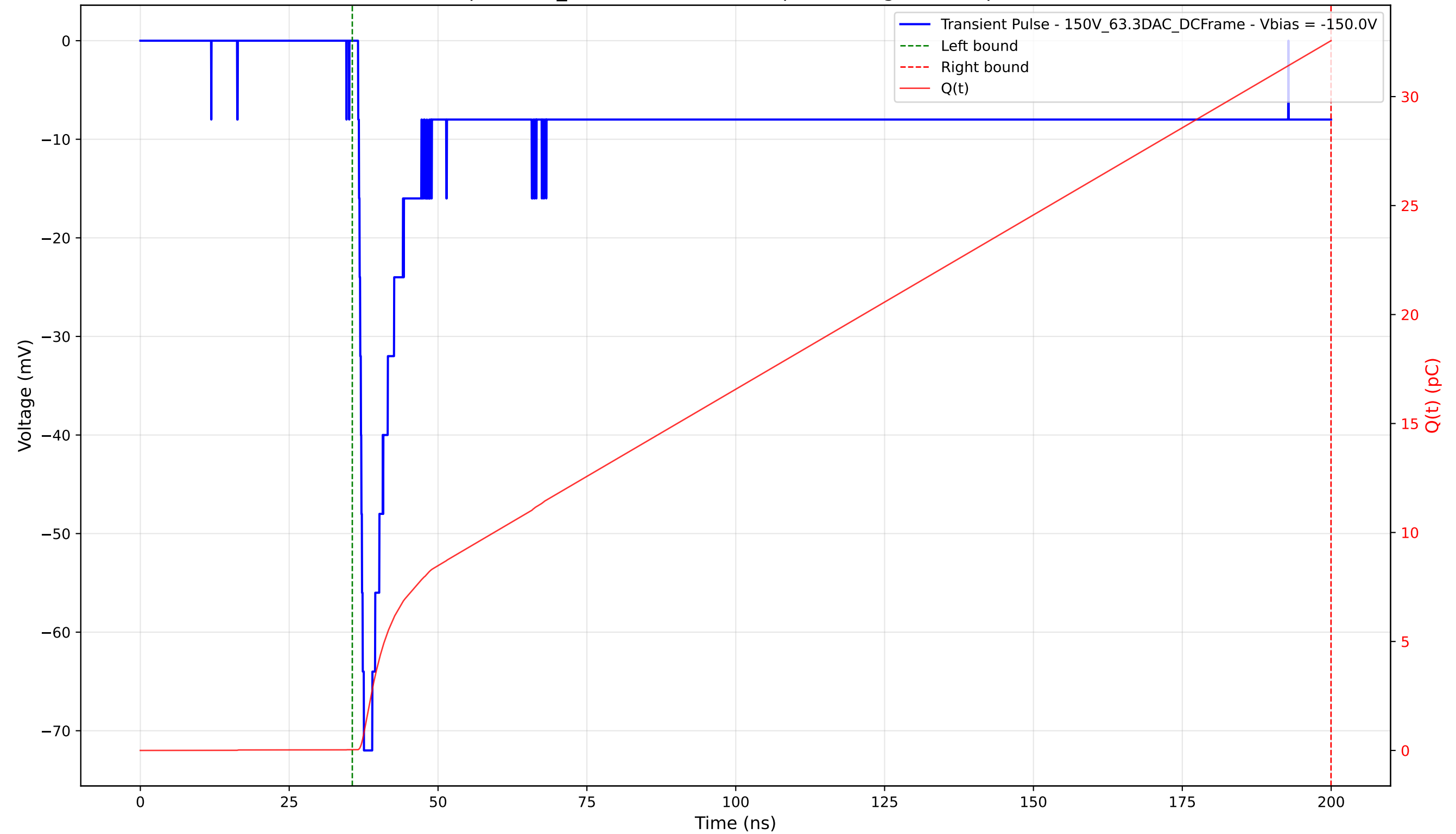
Transient Pulse - Sample: 1cm_42 - Position: 1025.0 \mu\text{m} - Charge: 32.53 pC - Rise Time: 0.96 ns
