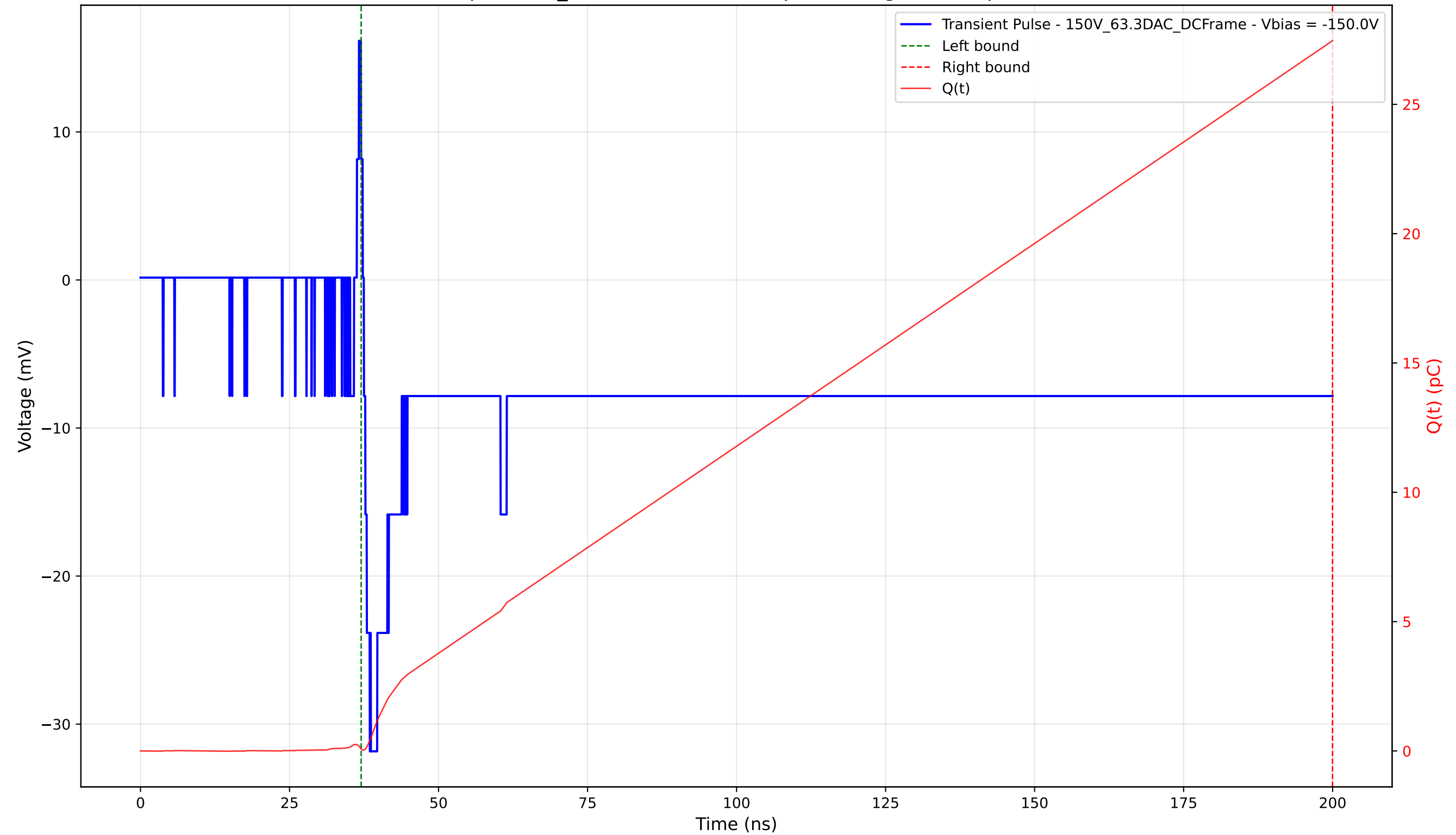
Transient Pulse - Sample: 1cm_42 - Position: 3045.0 \mu\text{m} - Charge: 27.39 pC - Rise Time: 0.99 ns
