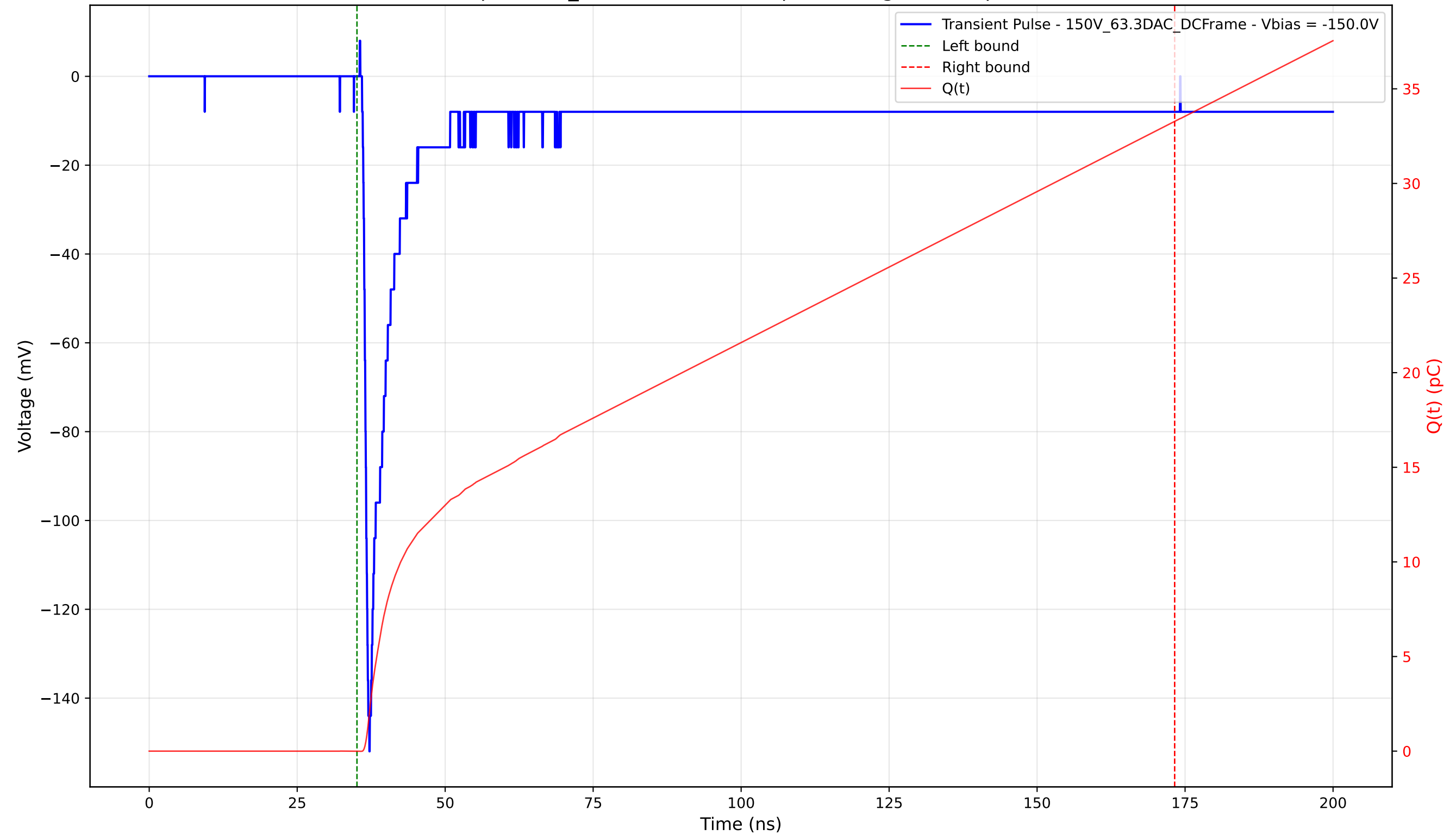
Transient Pulse - Sample: 1cm_42 - Position: 565.0 \mu\text{m} - Charge: 33.28 pC - Rise Time: 0.92 ns
