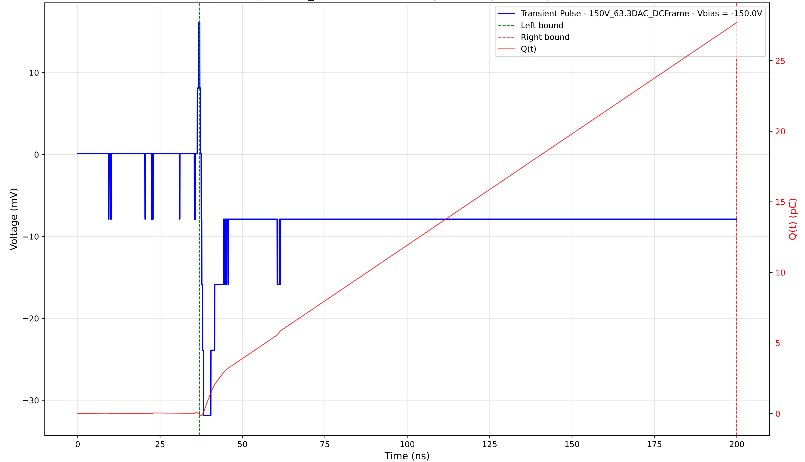
Transient Pulse - Sample: 1cm_42 - Position: 3105.0 \mu\text{m} - Charge: 27.77 pC - Rise Time: 0.73 ns
