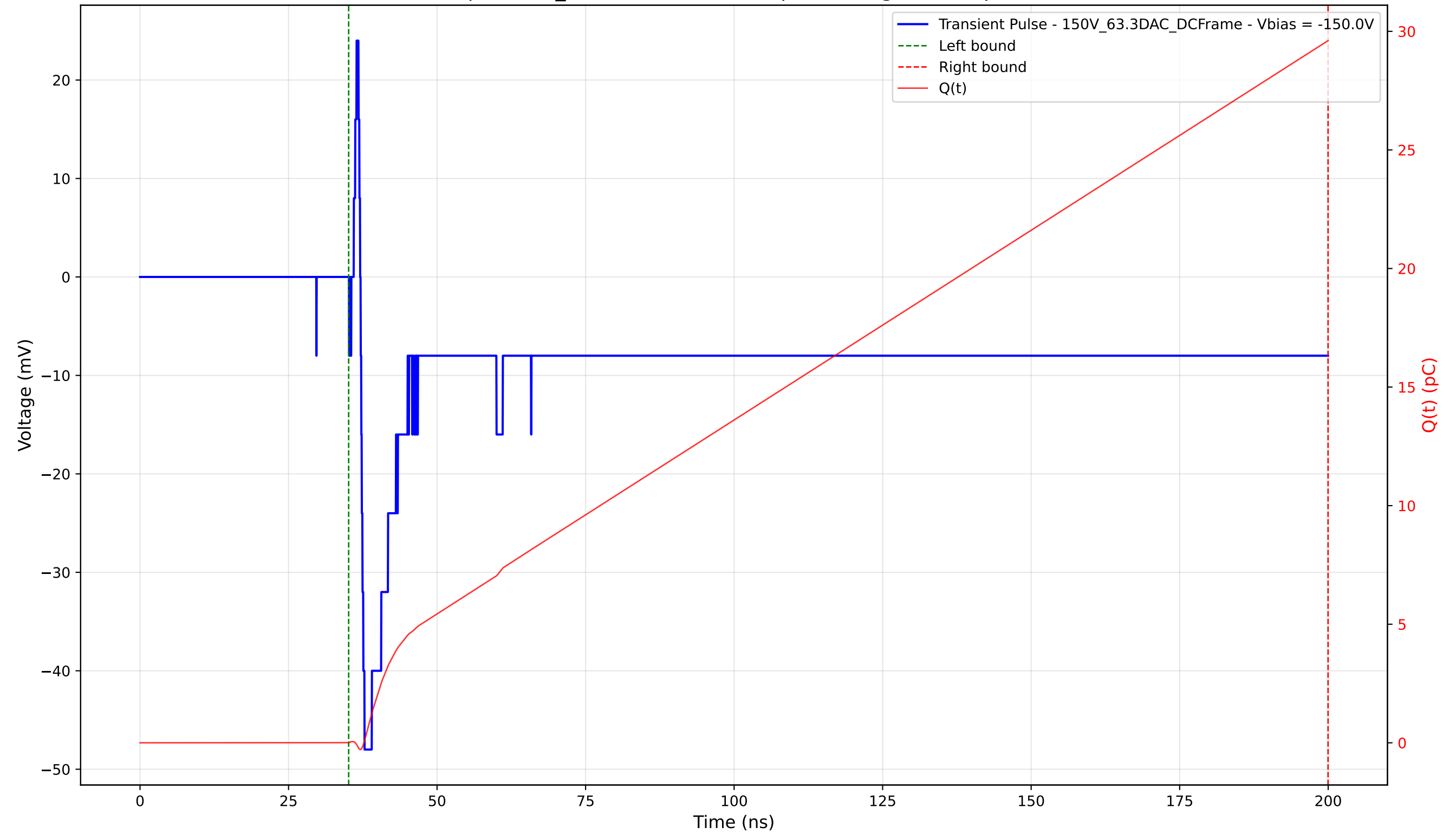
Transient Pulse - Sample: 1cm_42 - Position: 1565.0 \mu\text{m} - Charge: 29.60 pC - Rise Time: 0.65 ns
