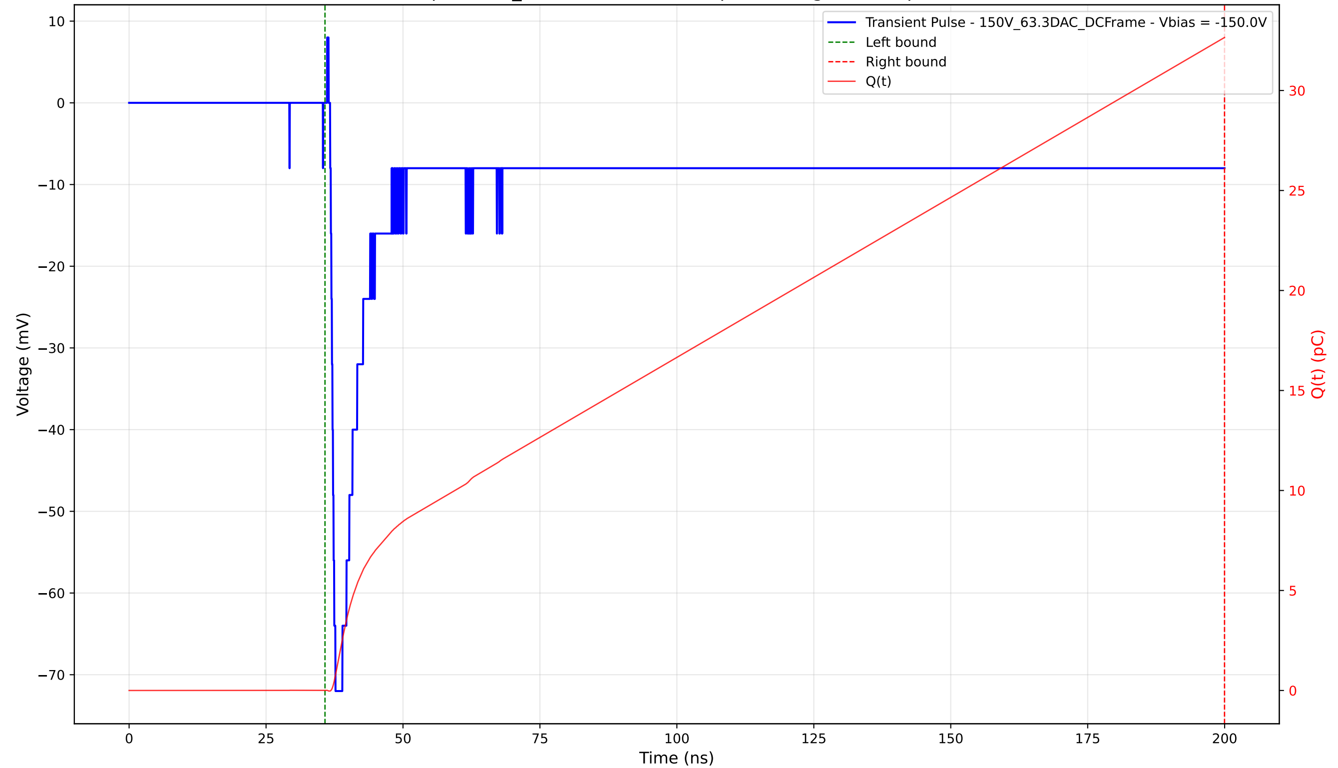
Transient Pulse - Sample: 1cm_42 - Position: 1080.0 \mu\text{m} - Charge: 32.64 pC - Rise Time: 0.96 ns
