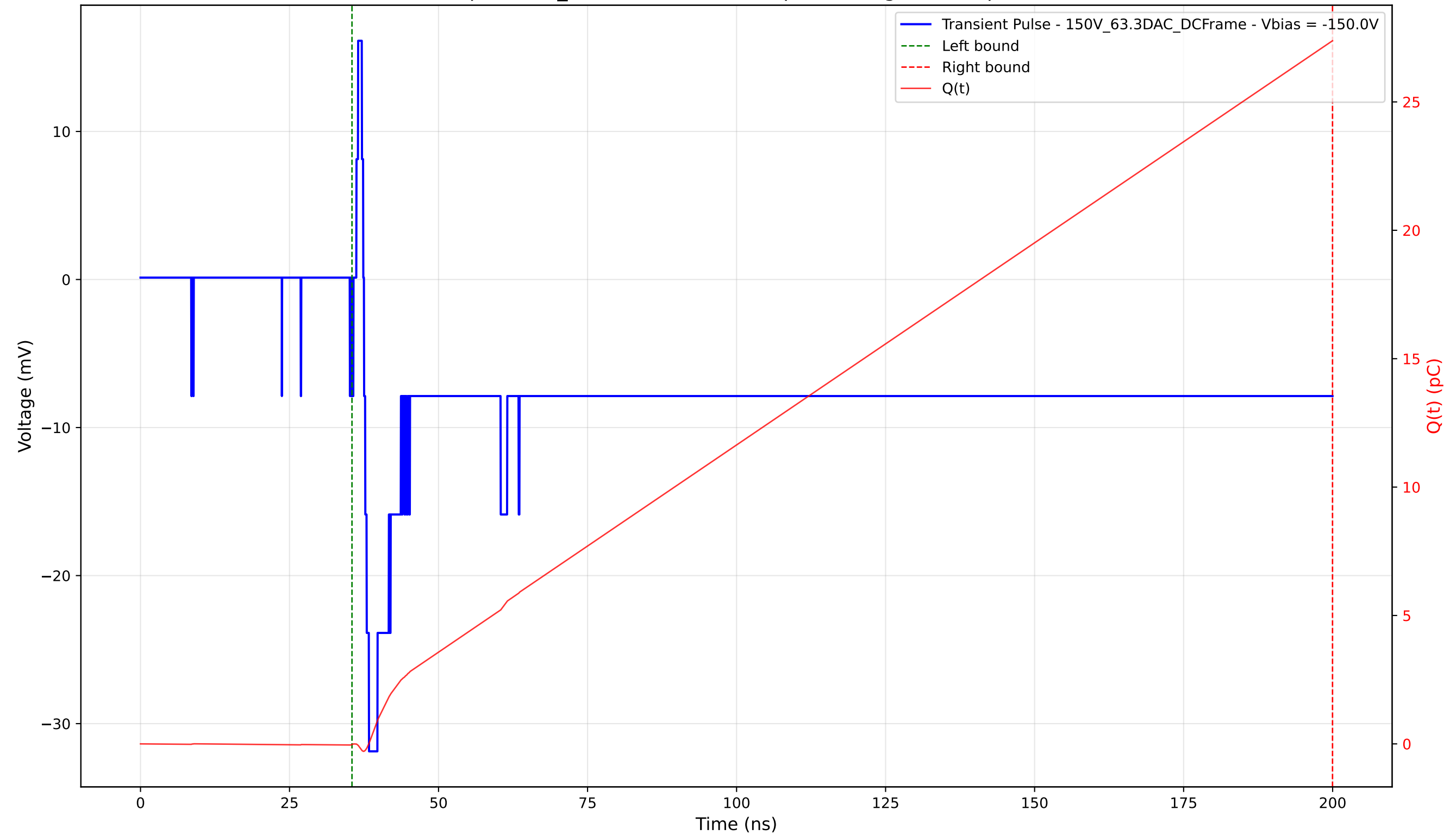
Transient Pulse - Sample: 1cm_42 - Position: 2625.0 \mu\text{m} - Charge: 27.41 pC - Rise Time: 0.83 ns
