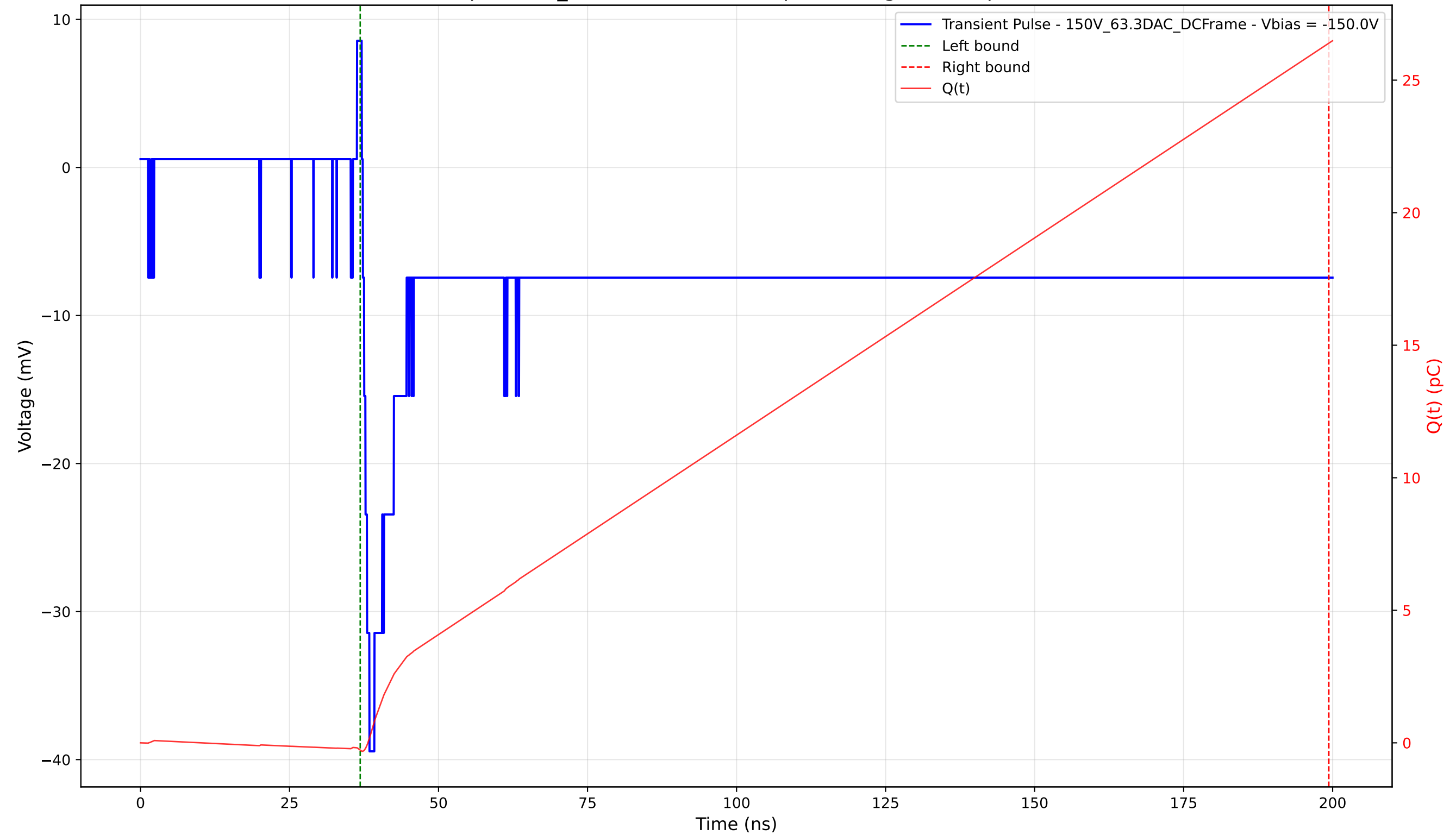
Transient Pulse - Sample: 1cm_42 - Position: 3430.0 \mu\text{m} - Charge: 26.67 pC - Rise Time: 1.11 ns
