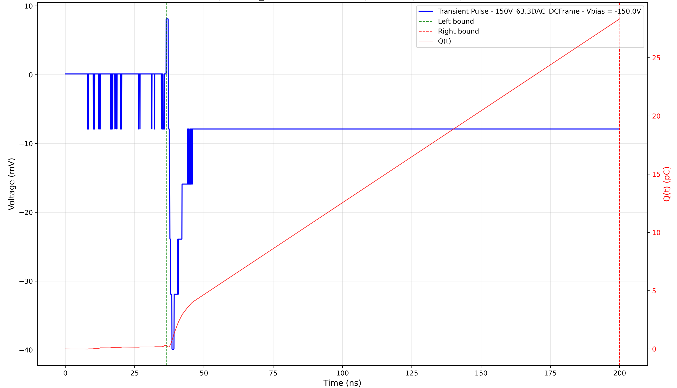
Transient Pulse - Sample: 1cm_42 - Position: 3460.0 \mu\text{m} - Charge: 28.08 pC - Rise Time: 1.17 ns
