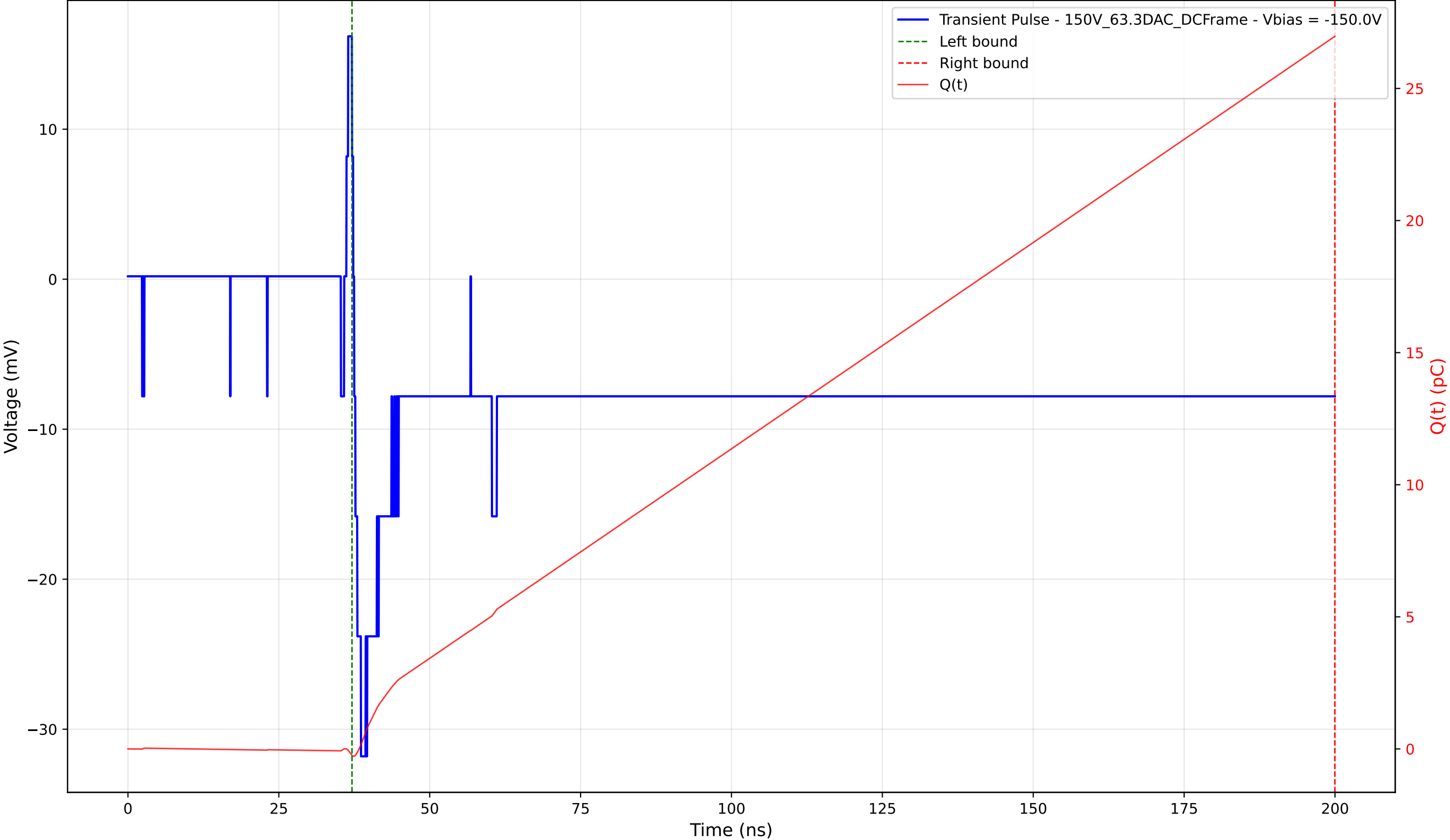
Transient Pulse - Sample: 1cm_42 - Position: 2520.0 \mu\text{m} - Charge: 27.22 pC - Rise Time: 1.13 ns
