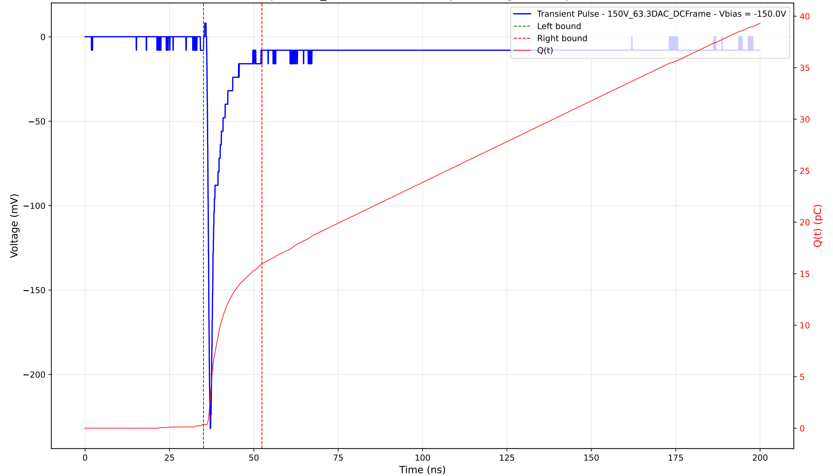
Transient Pulse - Sample: 1cm_42 - Position: 4860.0 \mu\text{m} - Charge: 15.59 pC - Rise Time: 0.82 ns
