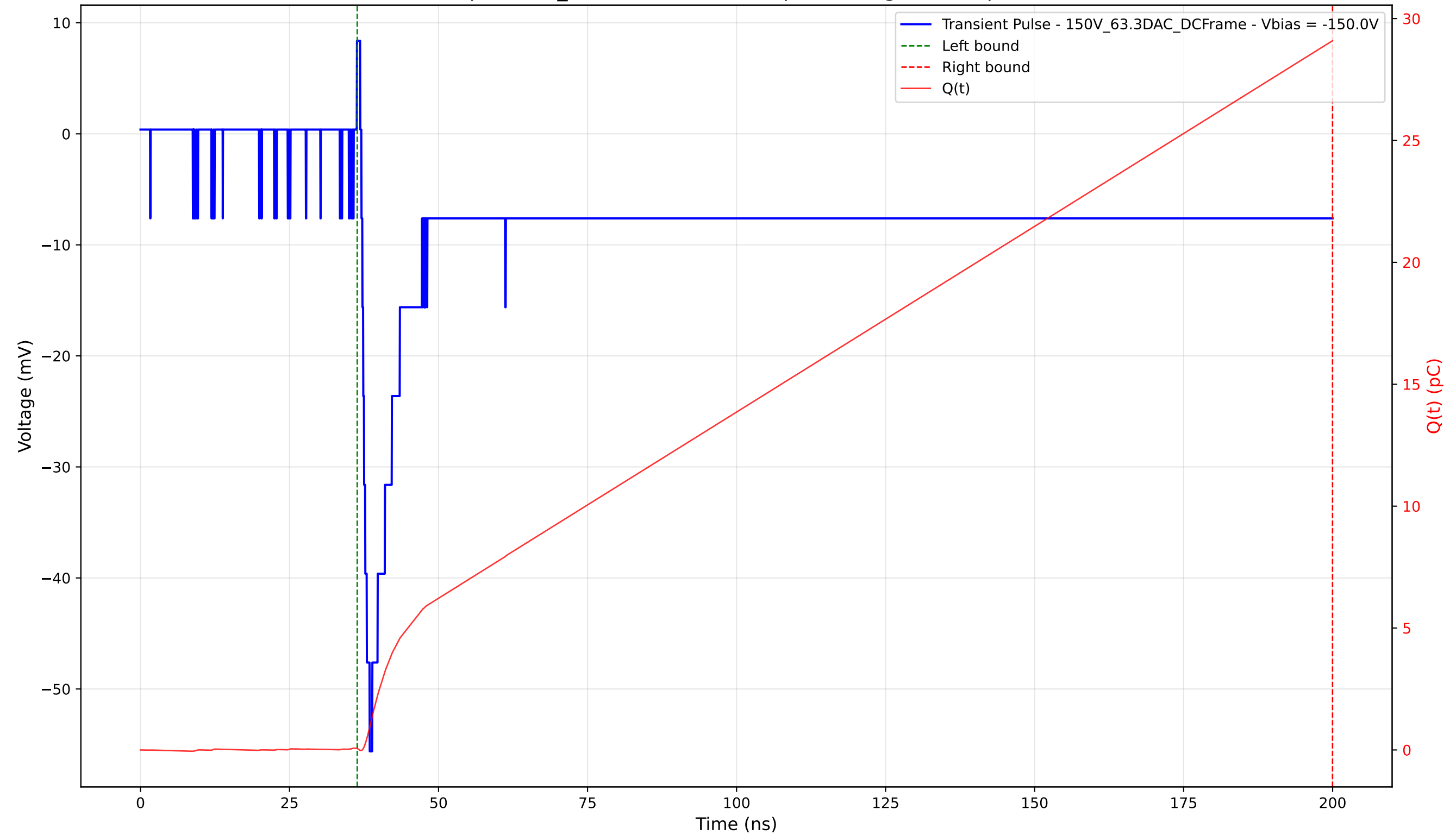
Transient Pulse - Sample: 1cm_42 - Position: 3710.0 \mu\text{m} - Charge: 29.03 pC - Rise Time: 1.39 ns
