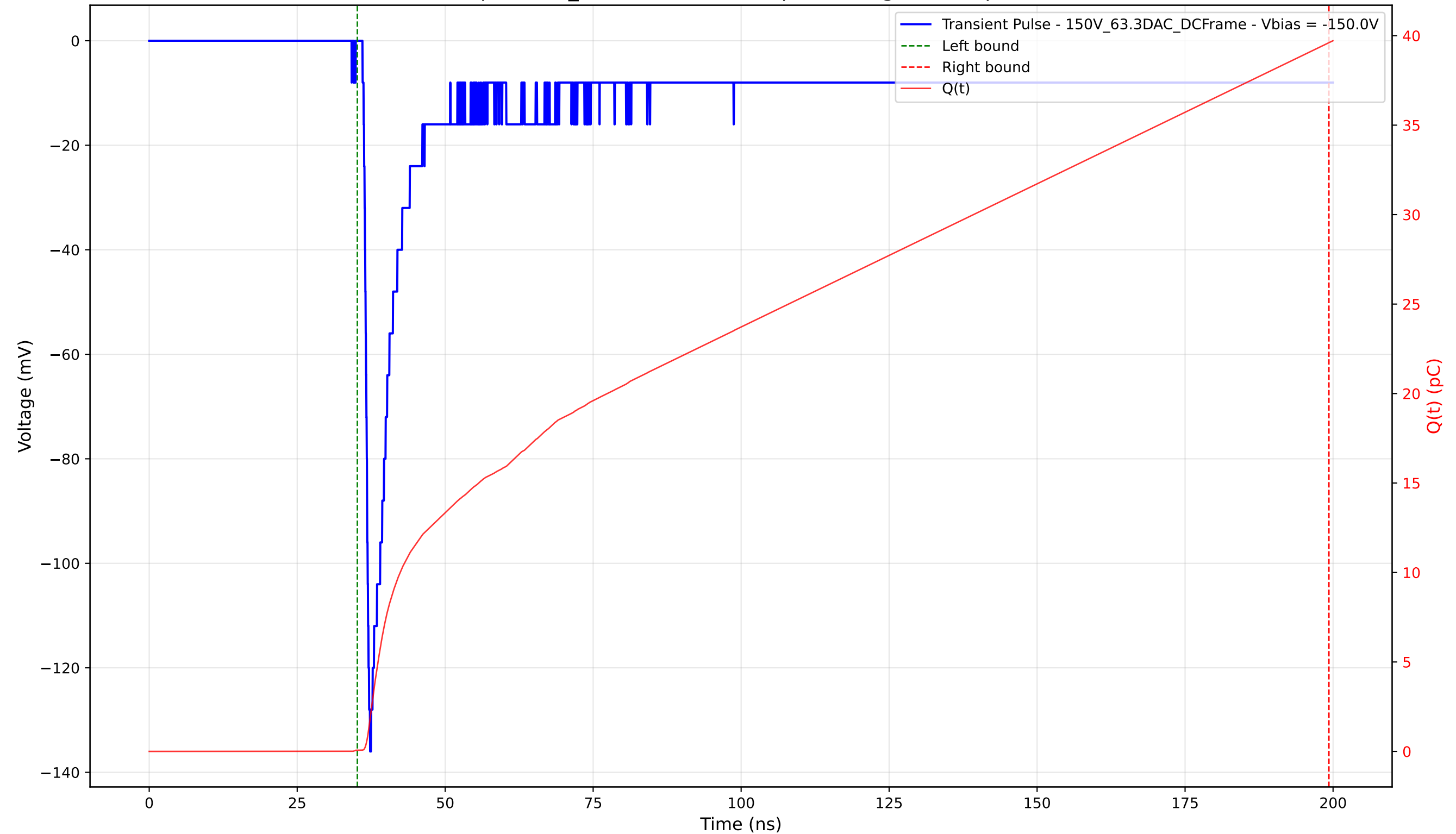
Transient Pulse - Sample: 1cm_42 - Position: 720.0 \mu\text{m} - Charge: 39.54 pC - Rise Time: 0.93 ns
