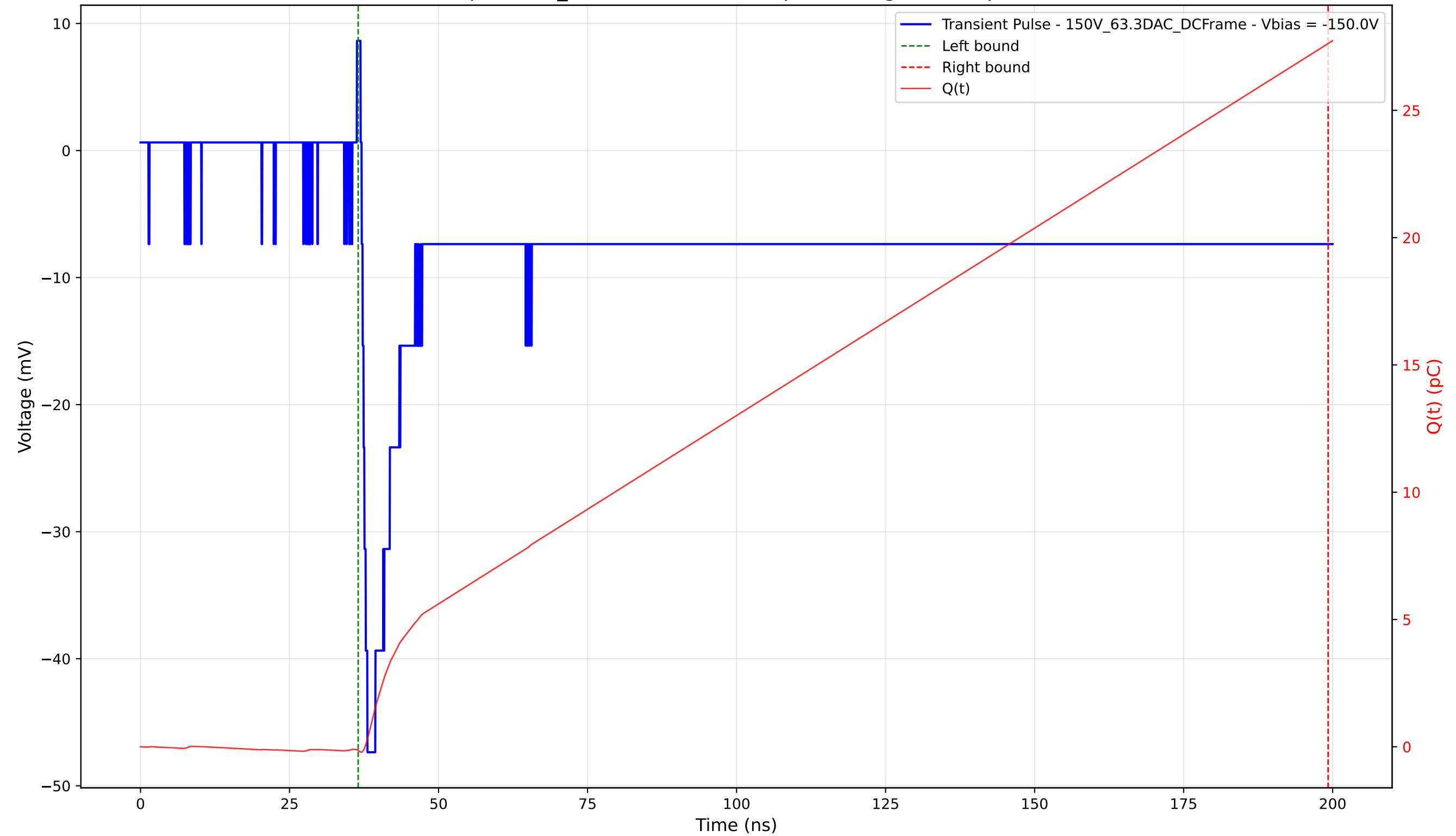
Transient Pulse - Sample: 1cm_42 - Position: 3670.0 \mu\text{m} - Charge: 27.77 pC - Rise Time: 0.97 ns
