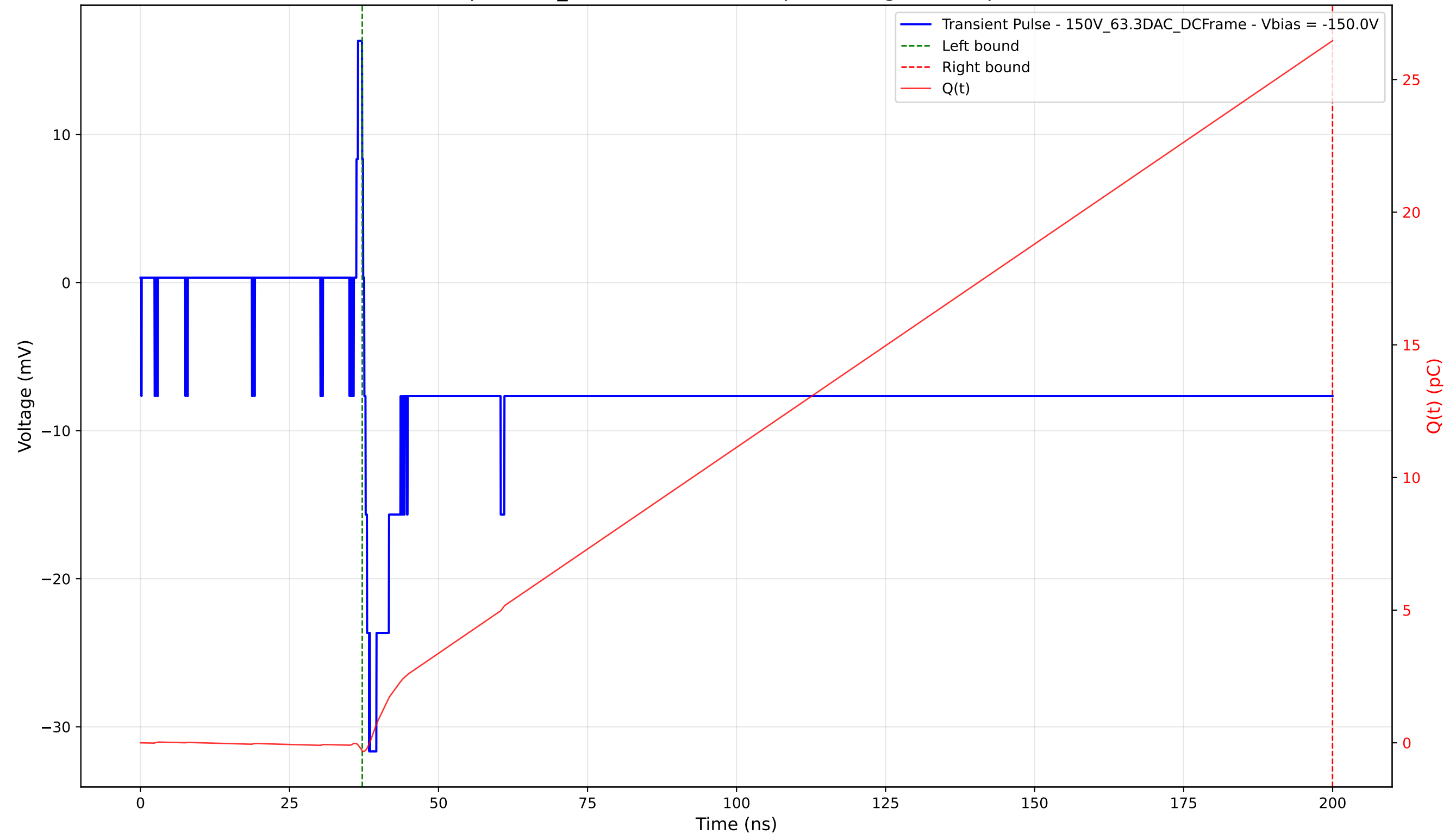
Transient Pulse - Sample: 1cm_42 - Position: 2605.0 \mu\text{m} - Charge: 26.76 pC - Rise Time: 0.85 ns
