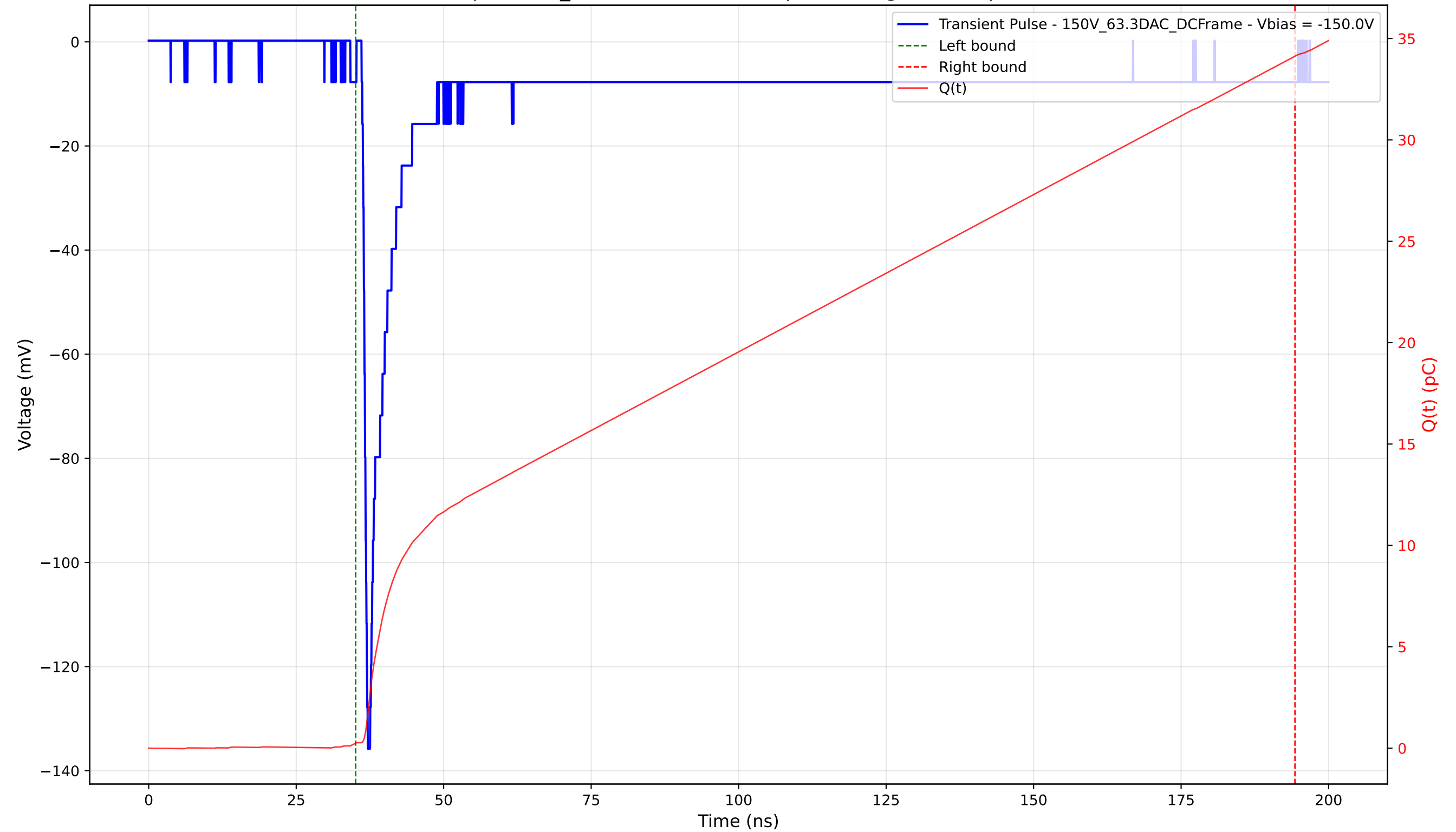
Transient Pulse - Sample: 1cm_42 - Position: 4560.0 \mu\text{m} - Charge: 33.88 pC - Rise Time: 0.83 ns
