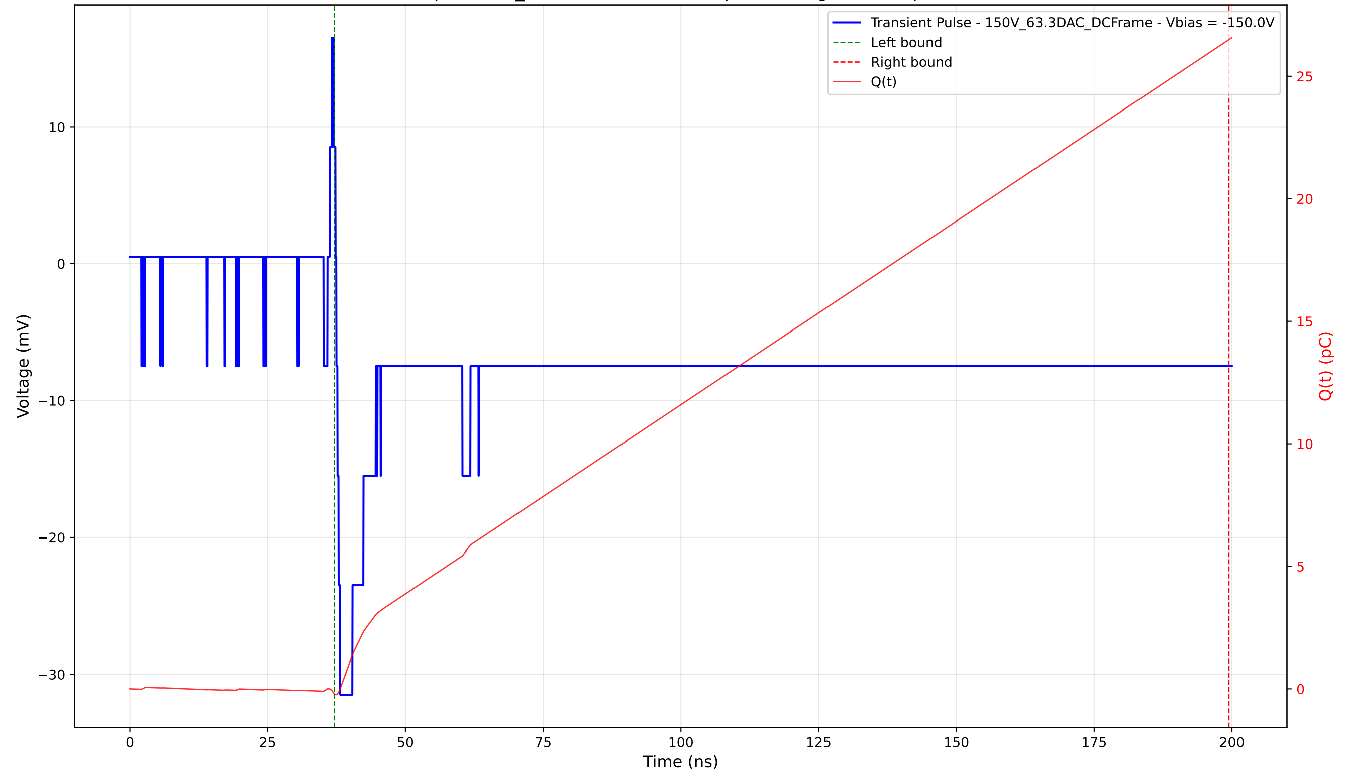
Transient Pulse - Sample: 1cm_42 - Position: 3125.0 \mu\text{m} - Charge: 26.70 pC - Rise Time: 0.69 ns
