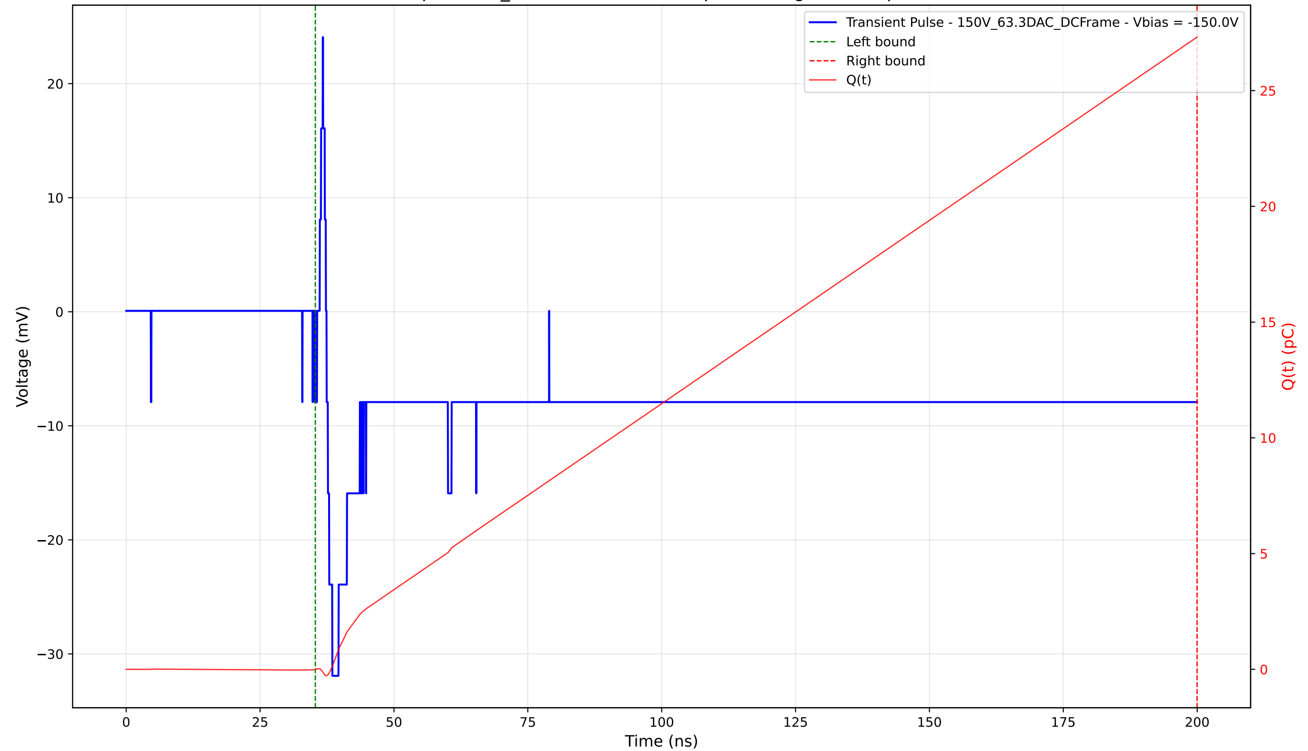
Transient Pulse - Sample: 1cm_42 - Position: 2450.0 \mu\text{m} - Charge: 27.31 pC - Rise Time: 1.07 ns
