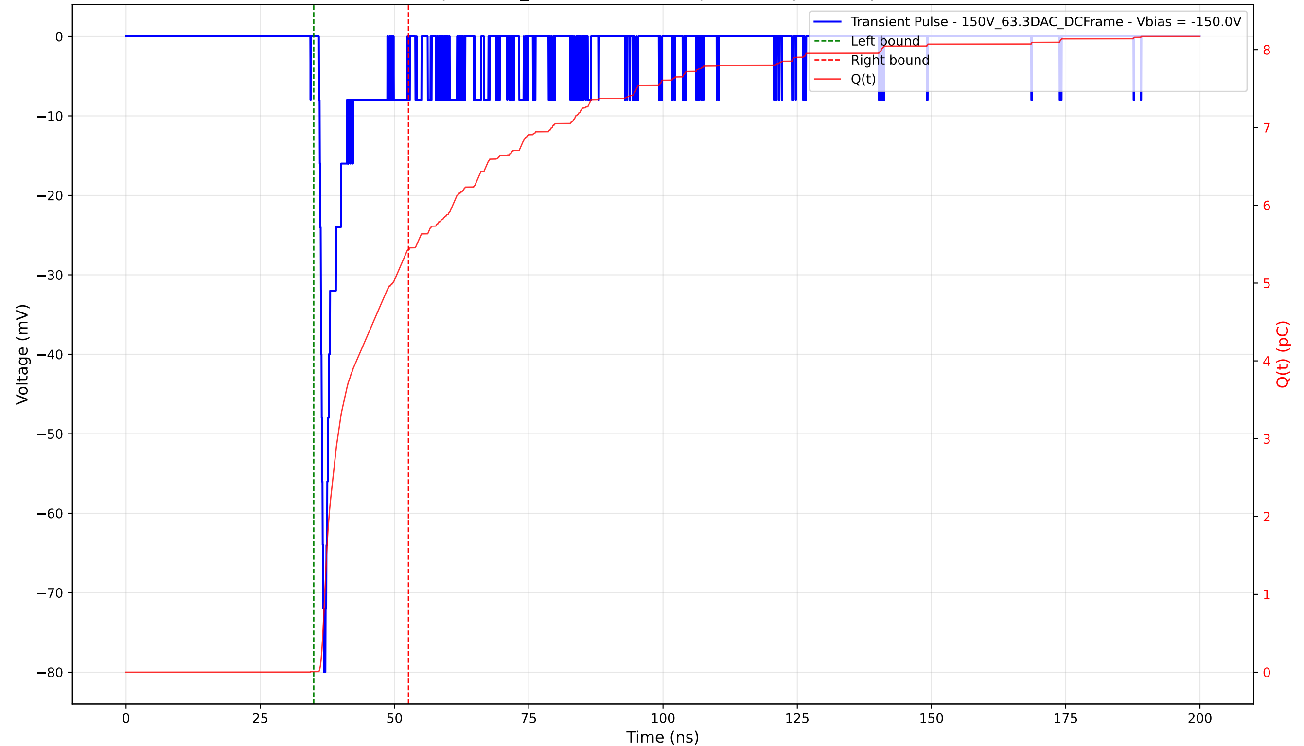
Transient Pulse - Sample: 1cm_42 - Position: 95.0 \mu\text{m} - Charge: 5.42 pC - Rise Time: 0.66 ns
