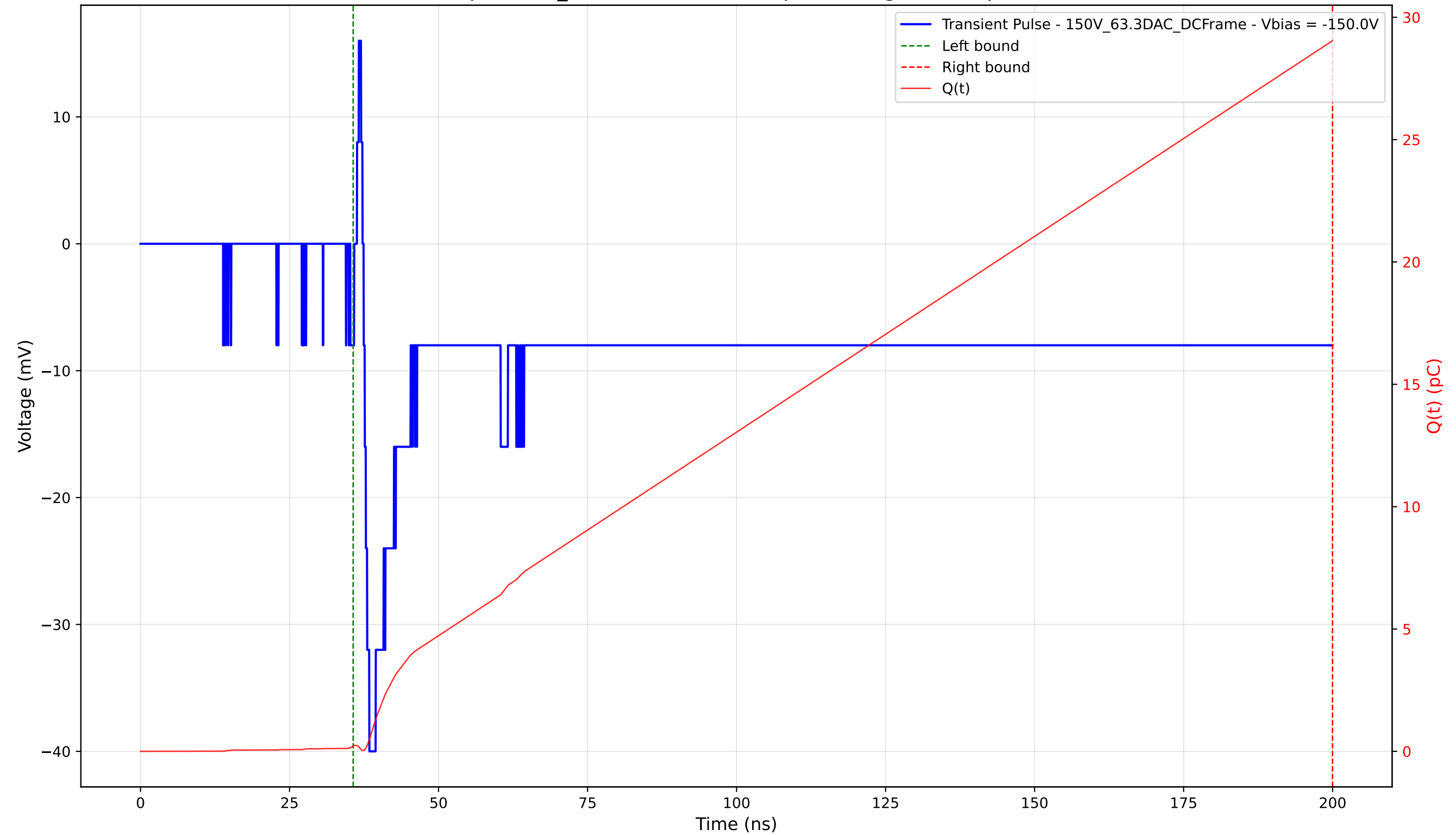
Transient Pulse - Sample: 1cm_42 - Position: 3225.0 \mu\text{m} - Charge: 28.82 pC - Rise Time: 0.95 ns
