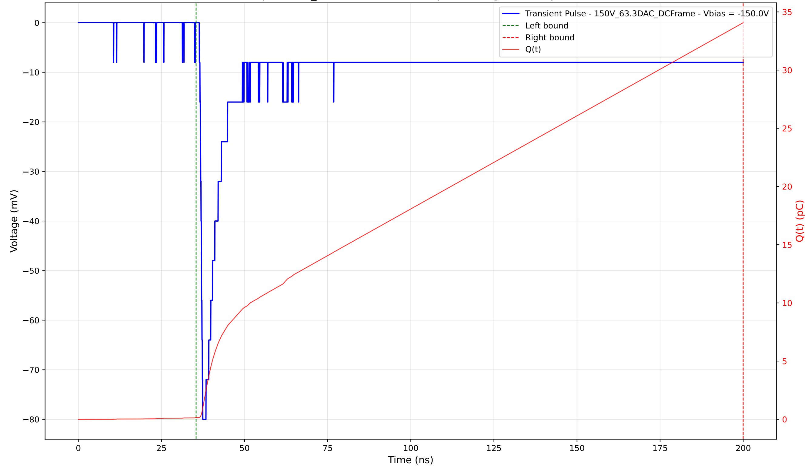
Transient Pulse - Sample: 1cm_42 - Position: 4180.0 \mu\text{m} - Charge: 33.92 pC - Rise Time: 0.72 ns
