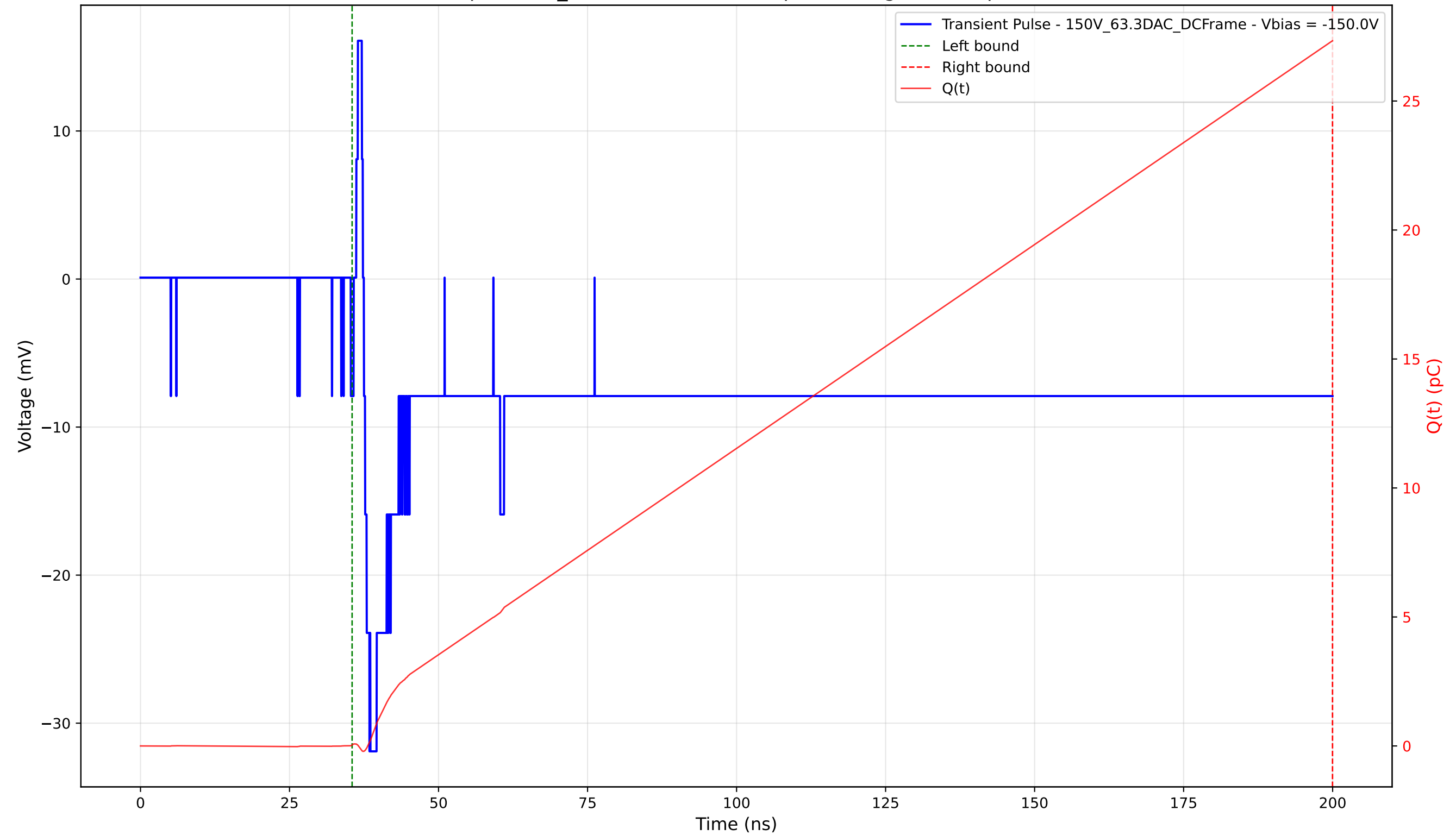
Transient Pulse - Sample: 1cm_42 - Position: 2545.0 \mu\text{m} - Charge: 27.30 pC - Rise Time: 0.95 ns
