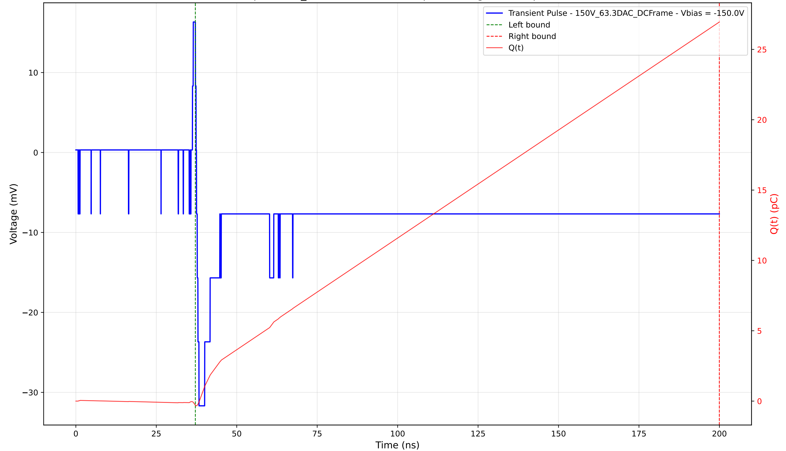
Transient Pulse - Sample: 1cm_42 - Position: 2670.0 \mu\text{m} - Charge: 27.25 pC - Rise Time: 0.77 ns
