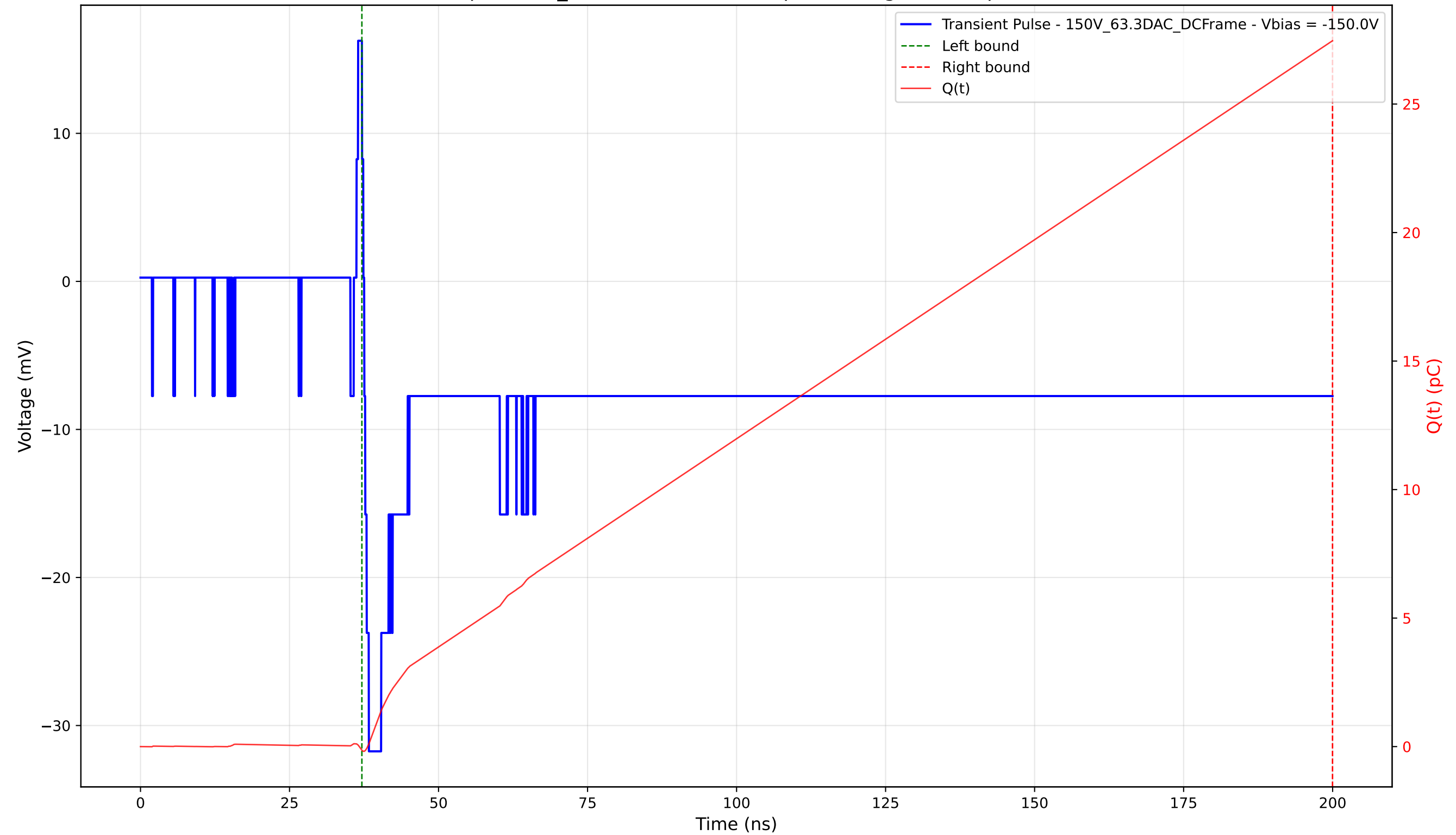
Transient Pulse - Sample: 1cm_42 - Position: 2700.0 \mu\text{m} - Charge: 27.61 pC - Rise Time: 0.77 ns
