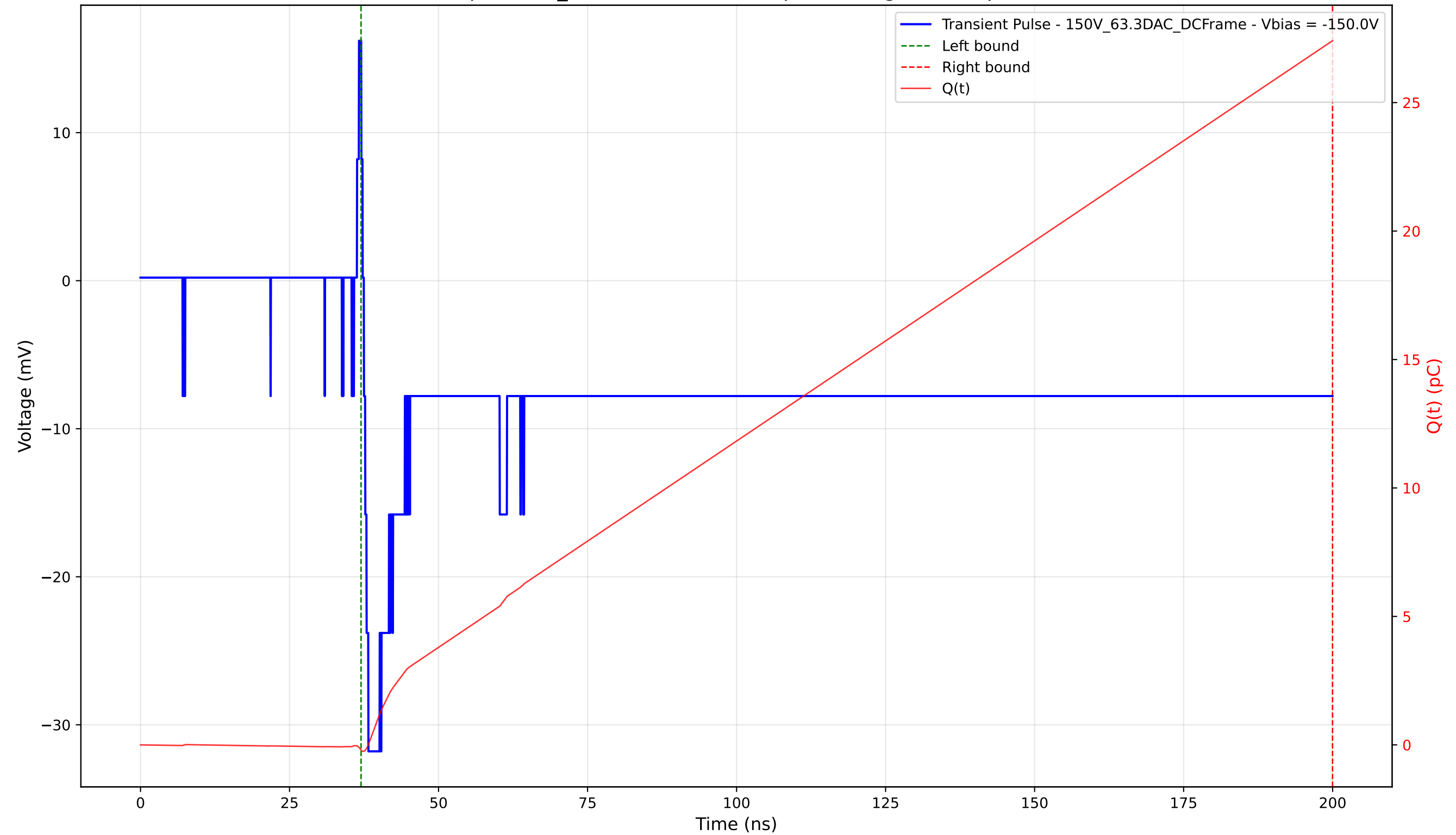
Transient Pulse - Sample: 1cm_42 - Position: 3120.0 \mu\text{m} - Charge: 27.61 pC - Rise Time: 0.75 ns
