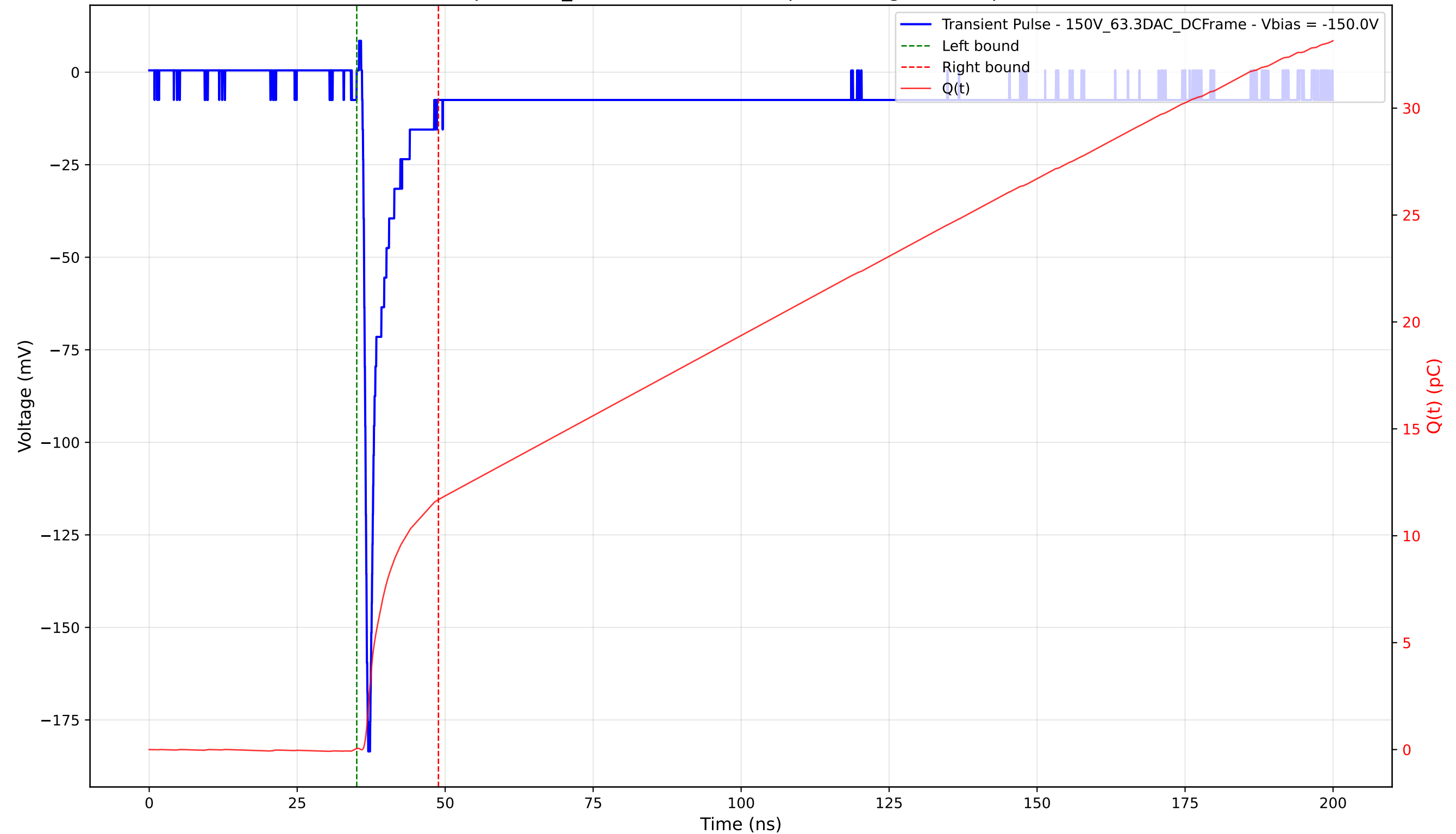
Transient Pulse - Sample: 1cm_42 - Position: 4930.0 \mu\text{m} - Charge: 11.63 pC - Rise Time: 0.73 ns
