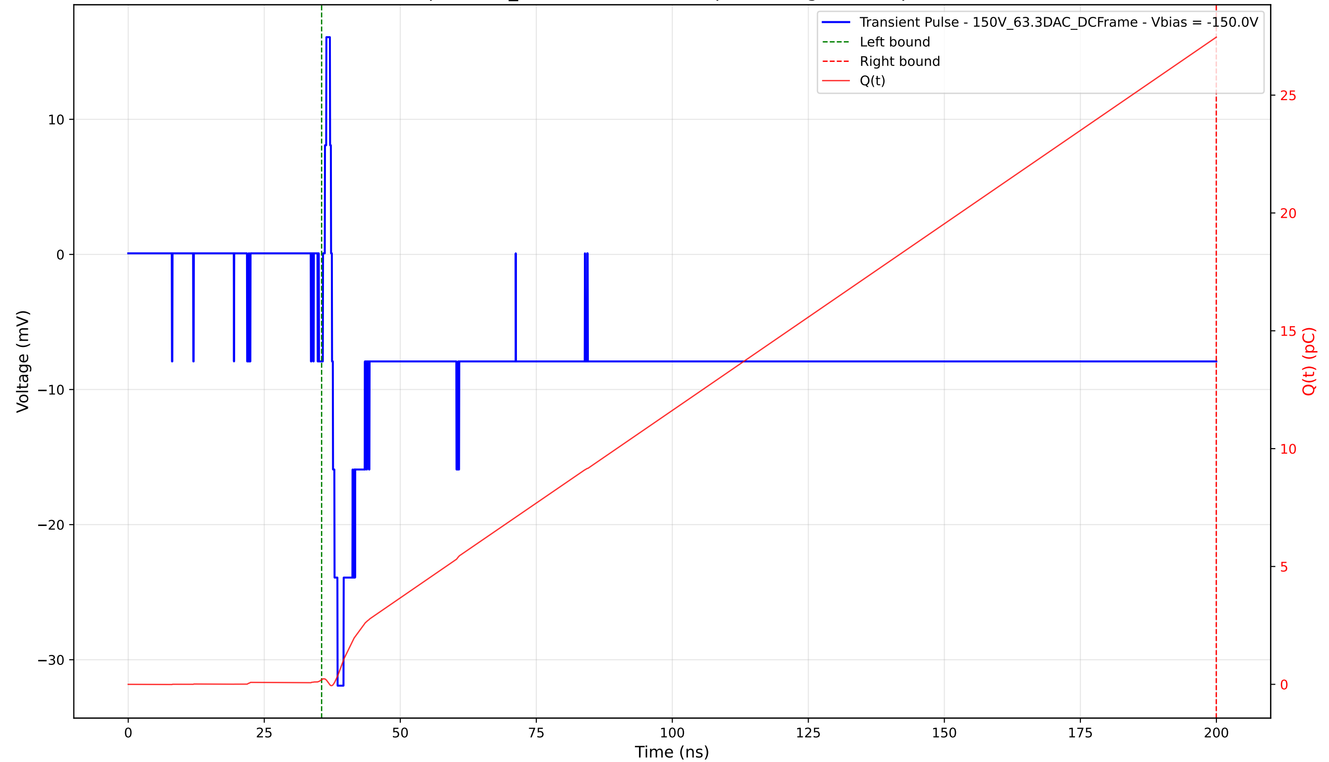
Transient Pulse - Sample: 1cm_42 - Position: 2455.0 \mu\text{m} - Charge: 27.26 pC - Rise Time: 1.03 ns
