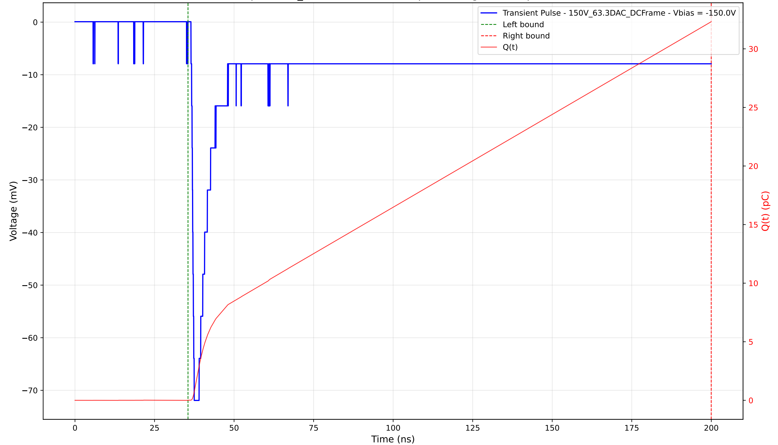
Transient Pulse - Sample: 1cm_42 - Position: 1005.0 \mu\text{m} - Charge: 32.31 pC - Rise Time: 1.00 ns
