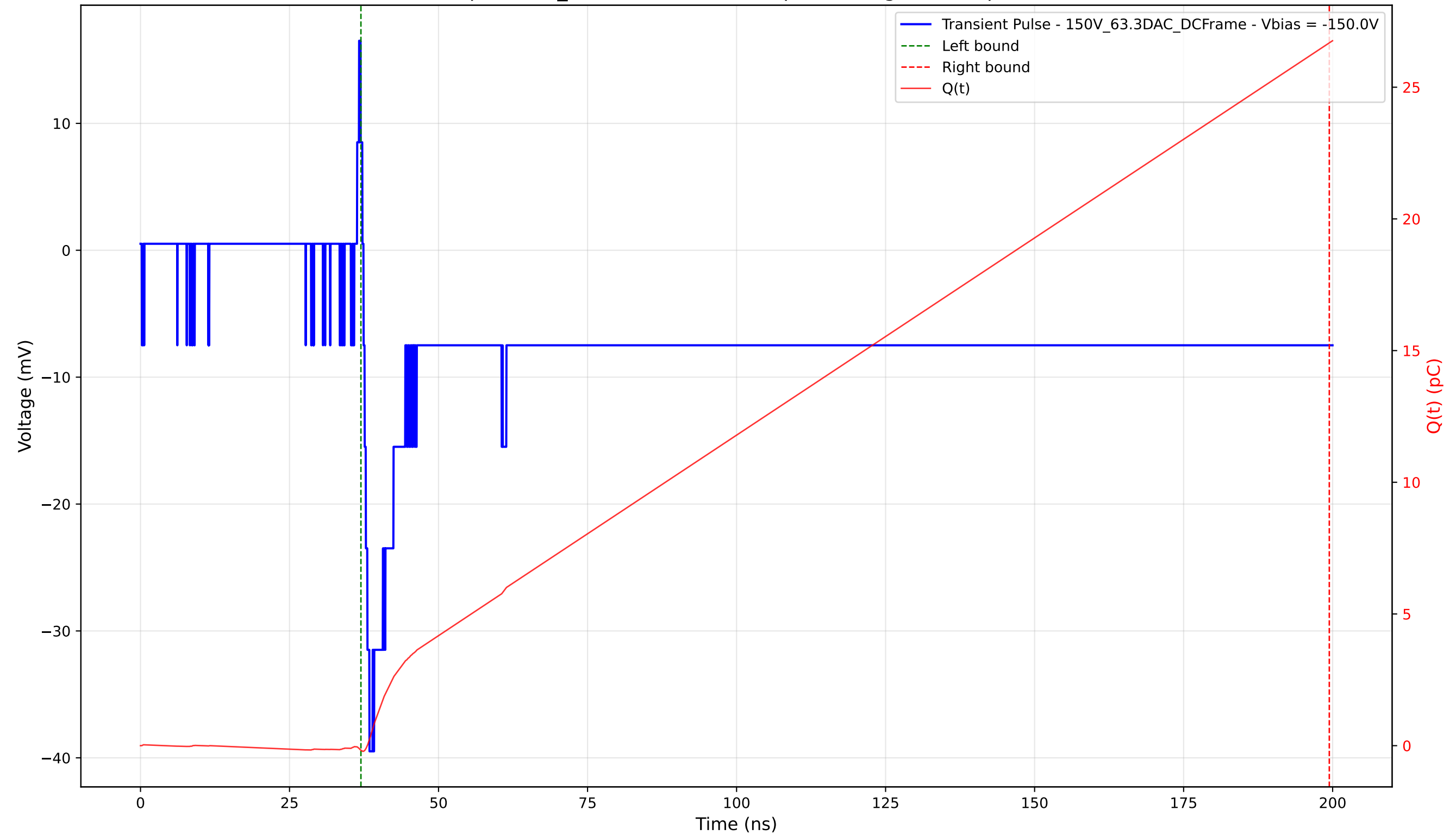
Transient Pulse - Sample: 1cm_42 - Position: 3340.0 \mu\text{m} - Charge: 26.86 pC - Rise Time: 0.99 ns
