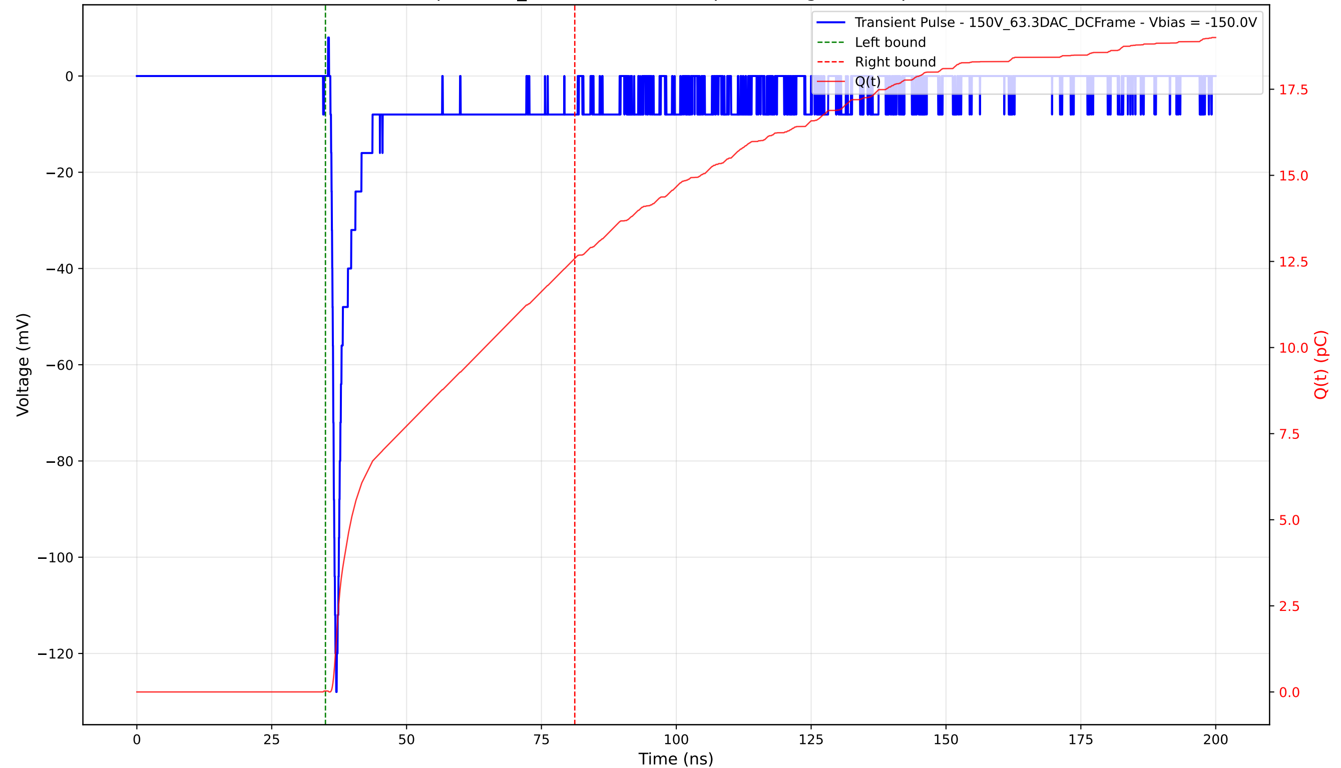
Transient Pulse - Sample: 1cm_42 - Position: 165.0 \mu\text{m} - Charge: 12.56 pC - Rise Time: 0.81 ns
