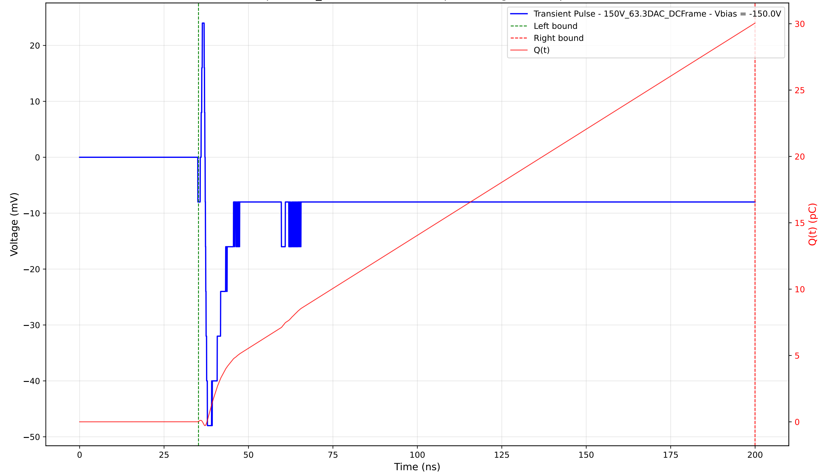
Transient Pulse - Sample: 1cm_42 - Position: 1655.0 \mu\text{m} - Charge: 30.02 pC - Rise Time: 0.65 ns
