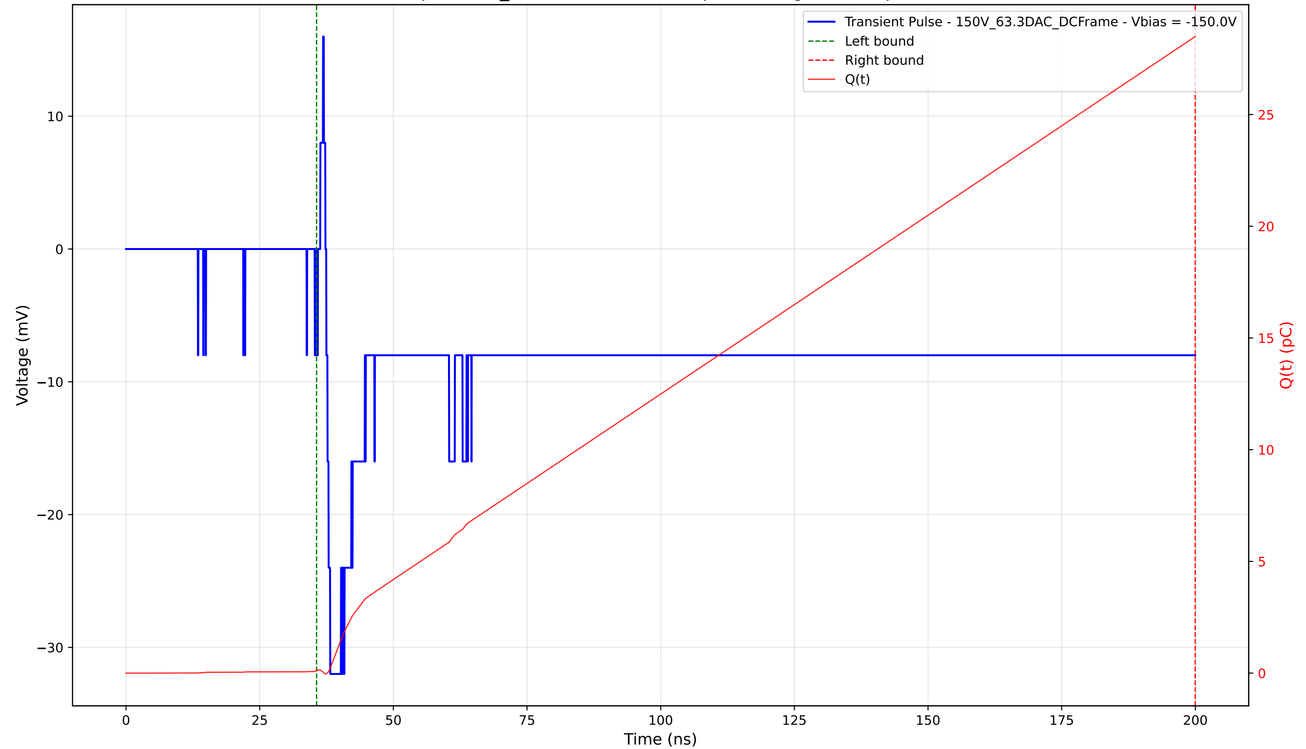
Transient Pulse - Sample: 1cm_42 - Position: 3140.0 \mu\text{m} - Charge: 28.38 pC - Rise Time: 0.73 ns
