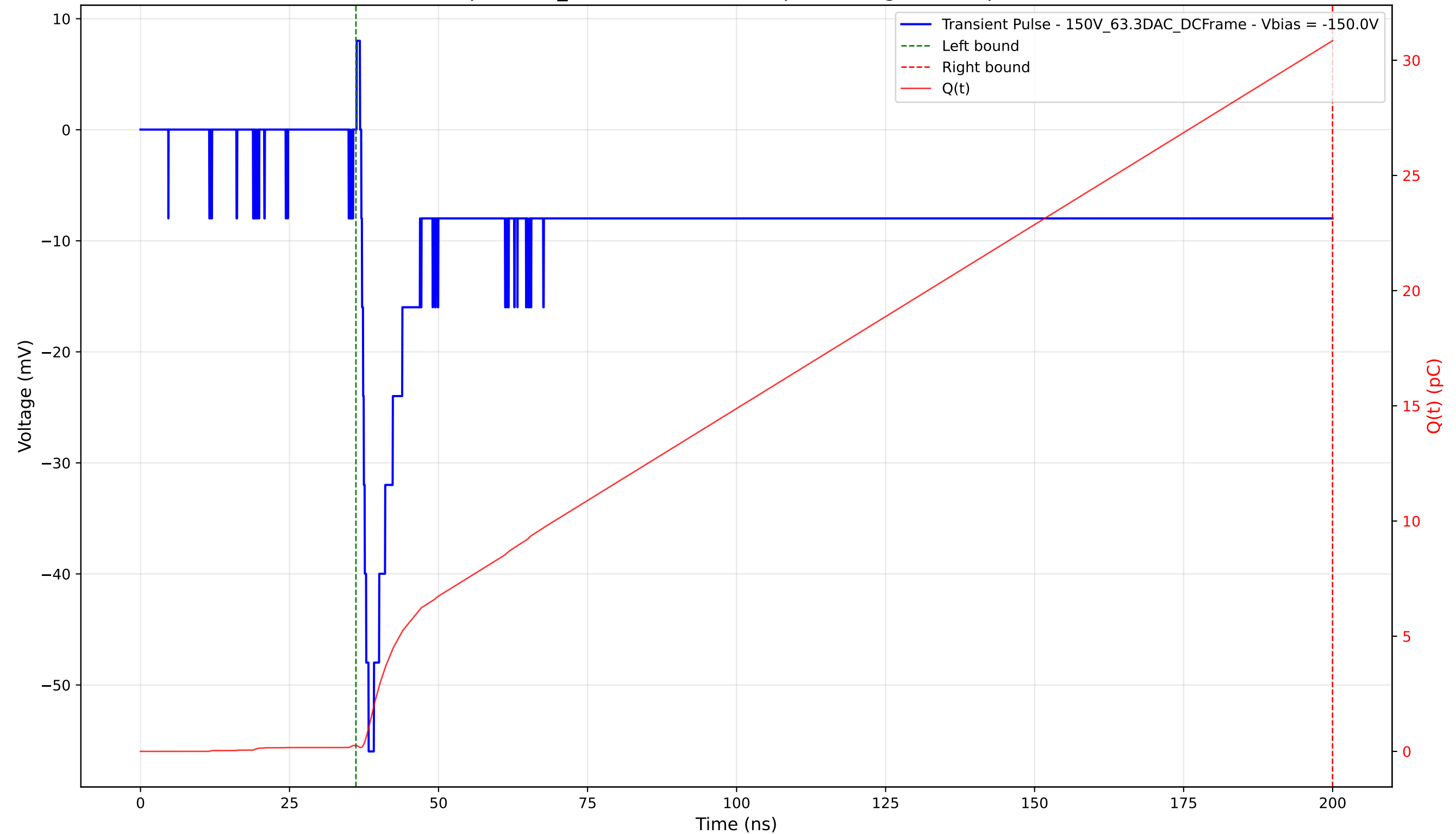
Transient Pulse - Sample: 1cm_42 - Position: 3770.0 \mu\text{m} - Charge: 30.59 pC - Rise Time: 1.23 ns
