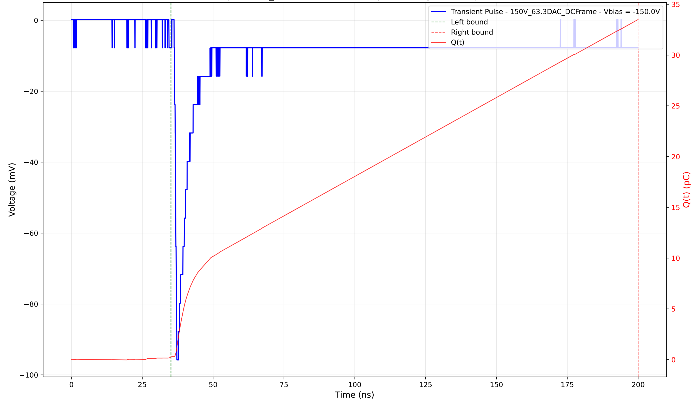
Transient Pulse - Sample: 1cm_42 - Position: 4425.0 \mu\text{m} - Charge: 33.24 pC - Rise Time: 0.76 ns
