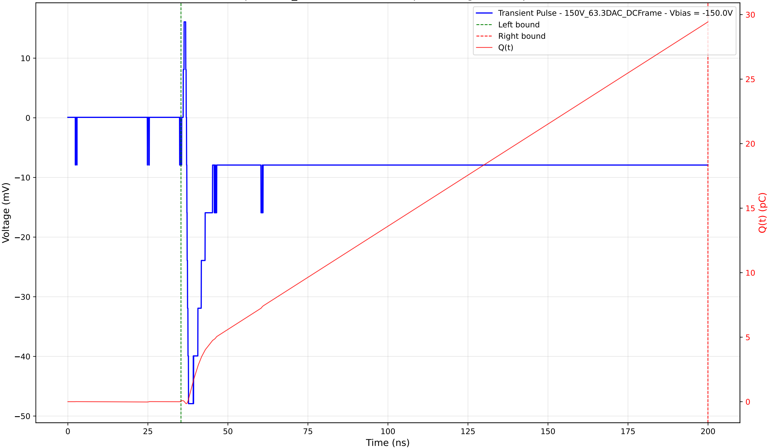
Transient Pulse - Sample: 1cm_42 - Position: 1470.0 \mu\text{m} - Charge: 29.39 pC - Rise Time: 0.61 ns
