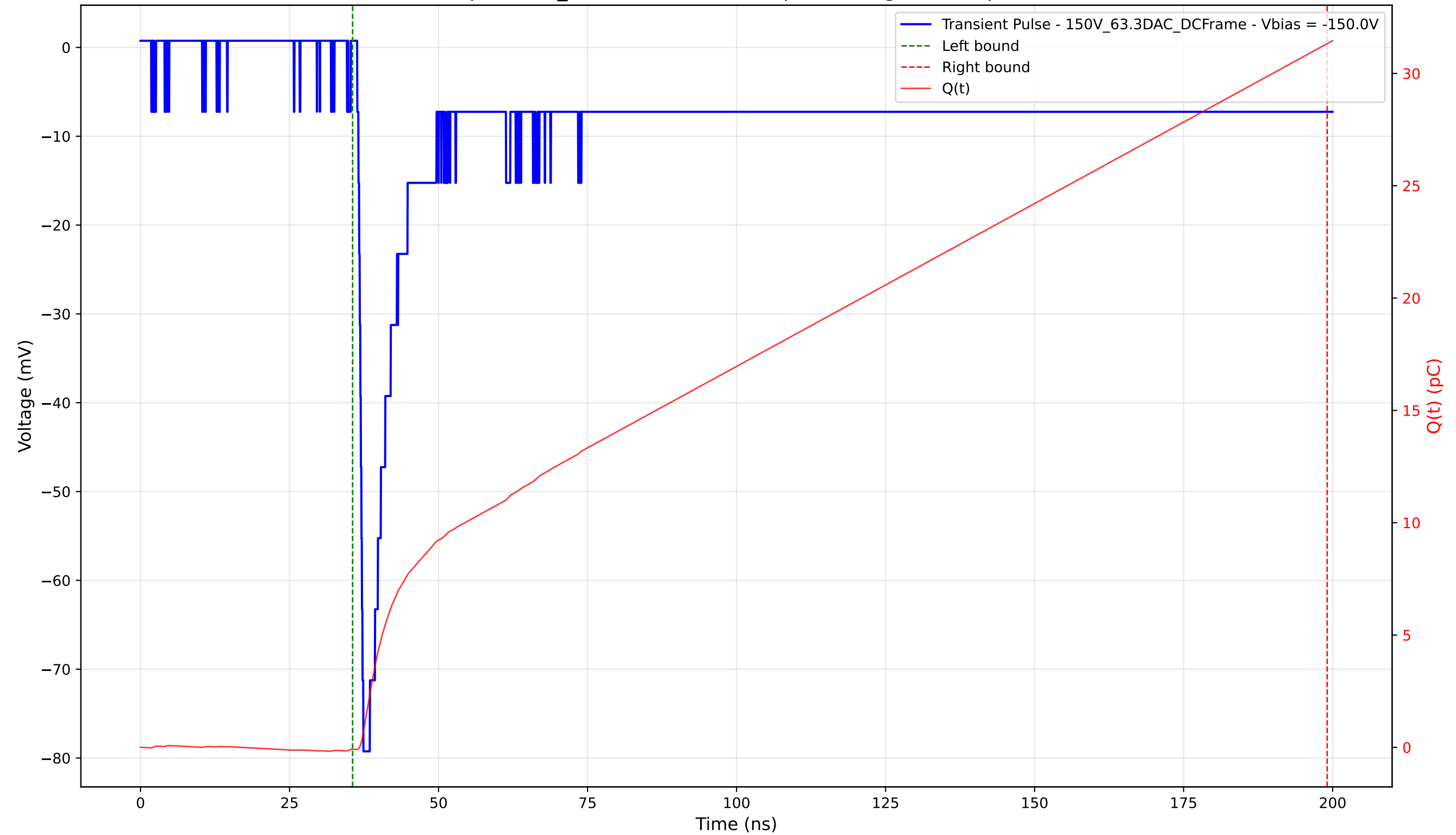
Transient Pulse - Sample: 1cm_42 - Position: 4190.0 \mu\text{m} - Charge: 31.41 pC - Rise Time: 0.84 ns
