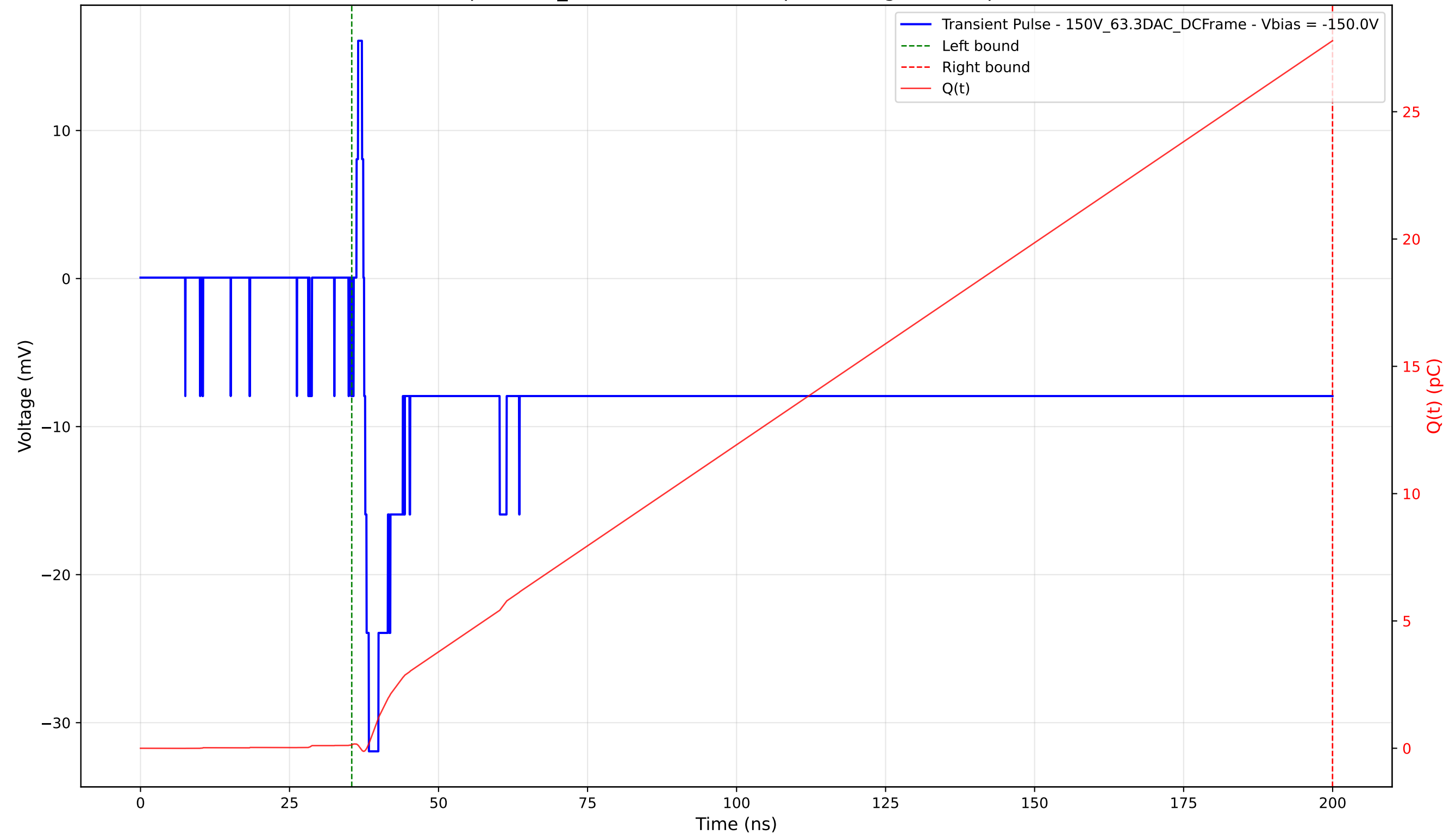
Transient Pulse - Sample: 1cm_42 - Position: 2650.0 \mu\text{m} - Charge: 27.65 pC - Rise Time: 0.79 ns
