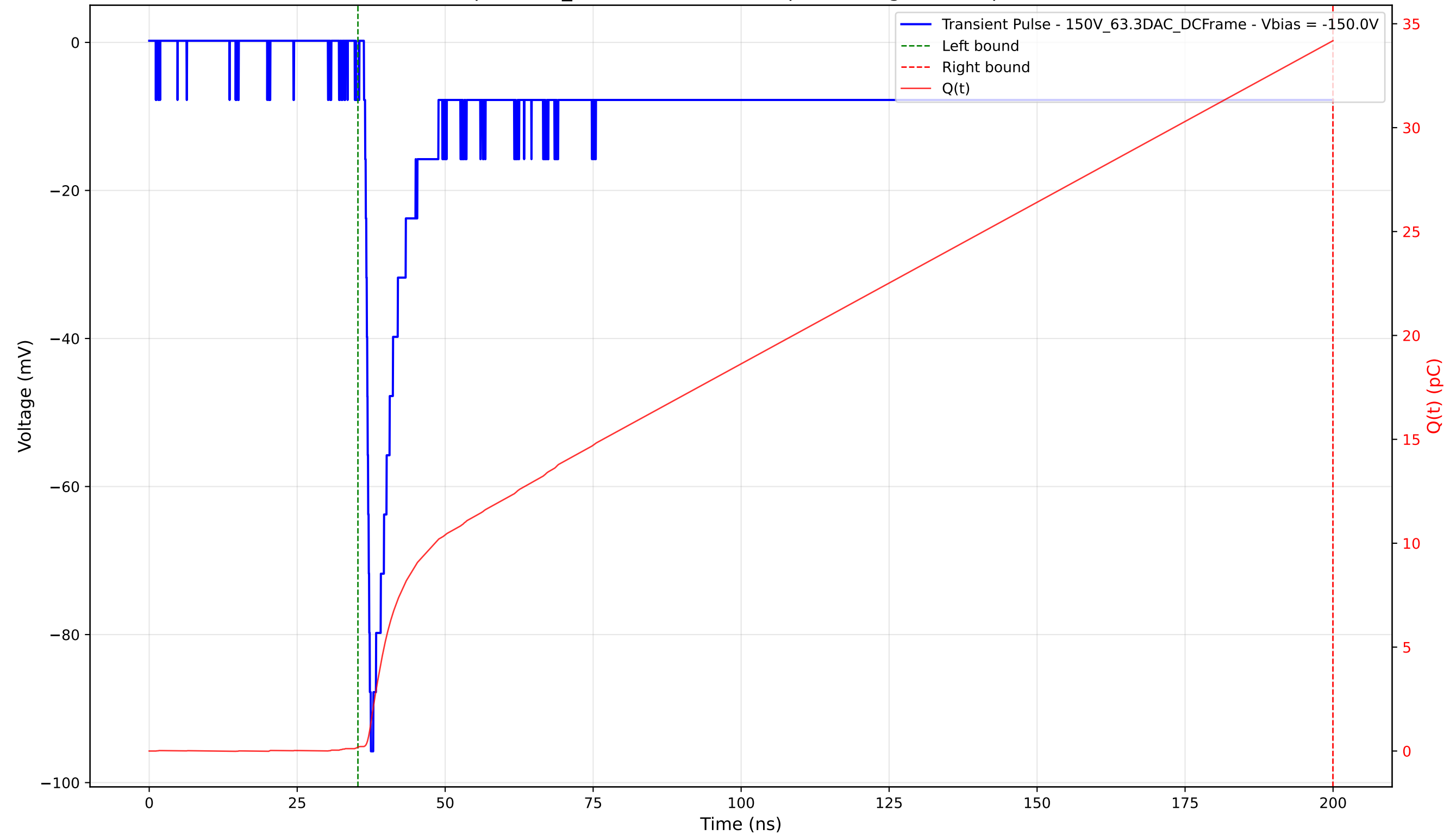
Transient Pulse - Sample: 1cm_42 - Position: 4320.0 \mu\text{m} - Charge: 33.99 pC - Rise Time: 0.80 ns
