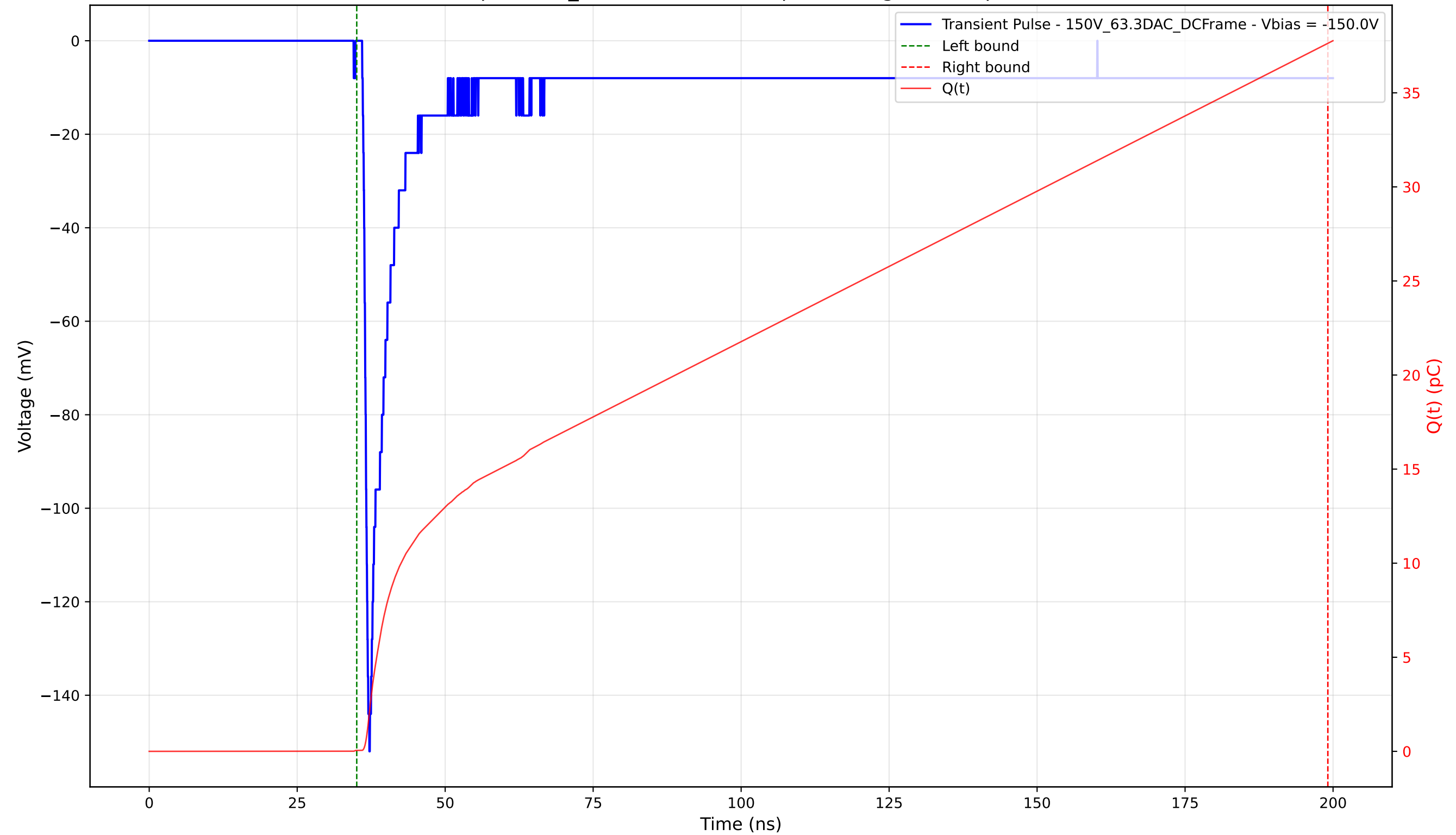
Transient Pulse - Sample: 1cm_42 - Position: 560.0 \mu\text{m} - Charge: 37.58 pC - Rise Time: 0.92 ns
