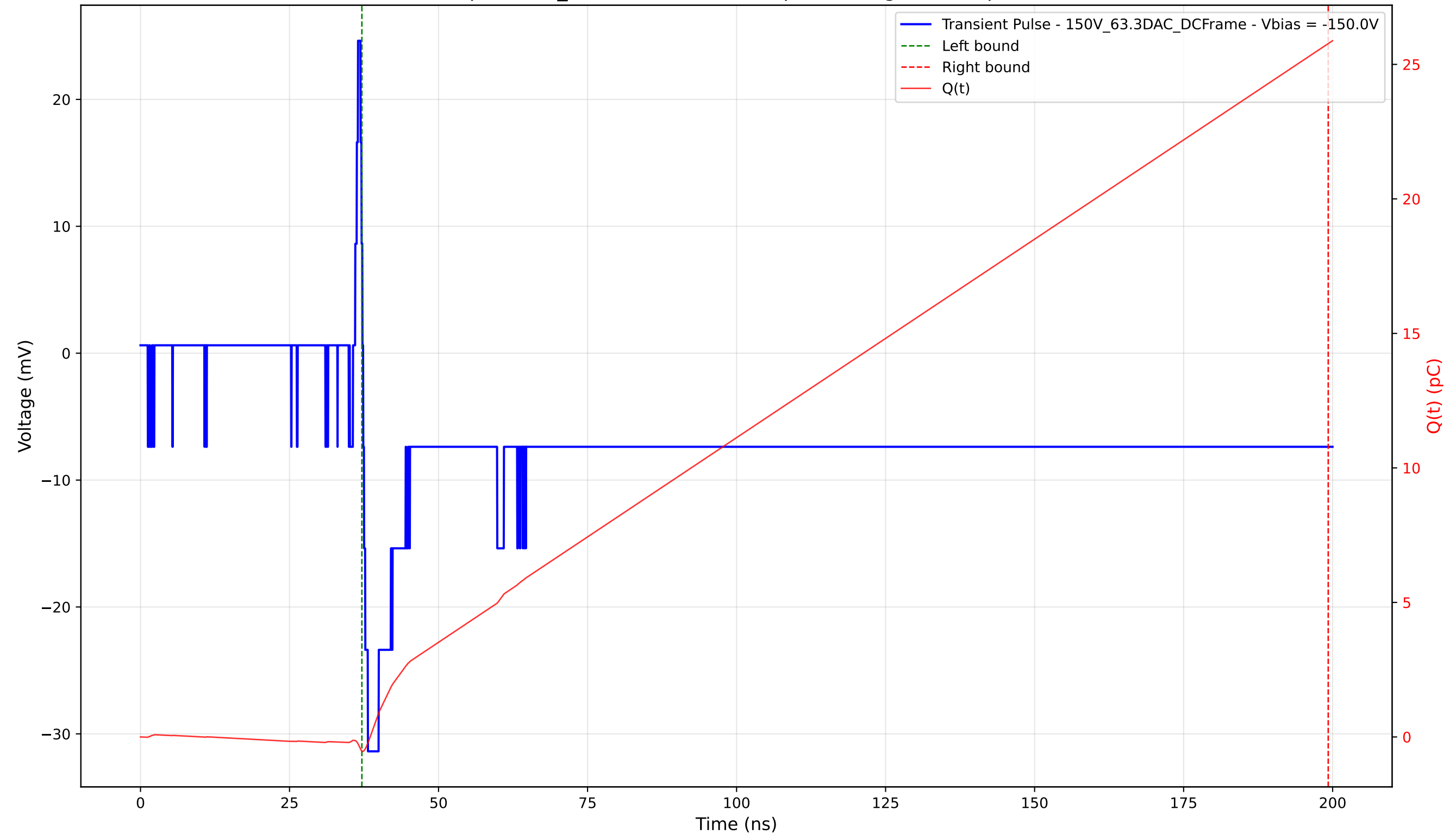
Transient Pulse - Sample: 1cm_42 - Position: 2335.0 \mu\text{m} - Charge: 26.29 pC - Rise Time: 0.79 ns
