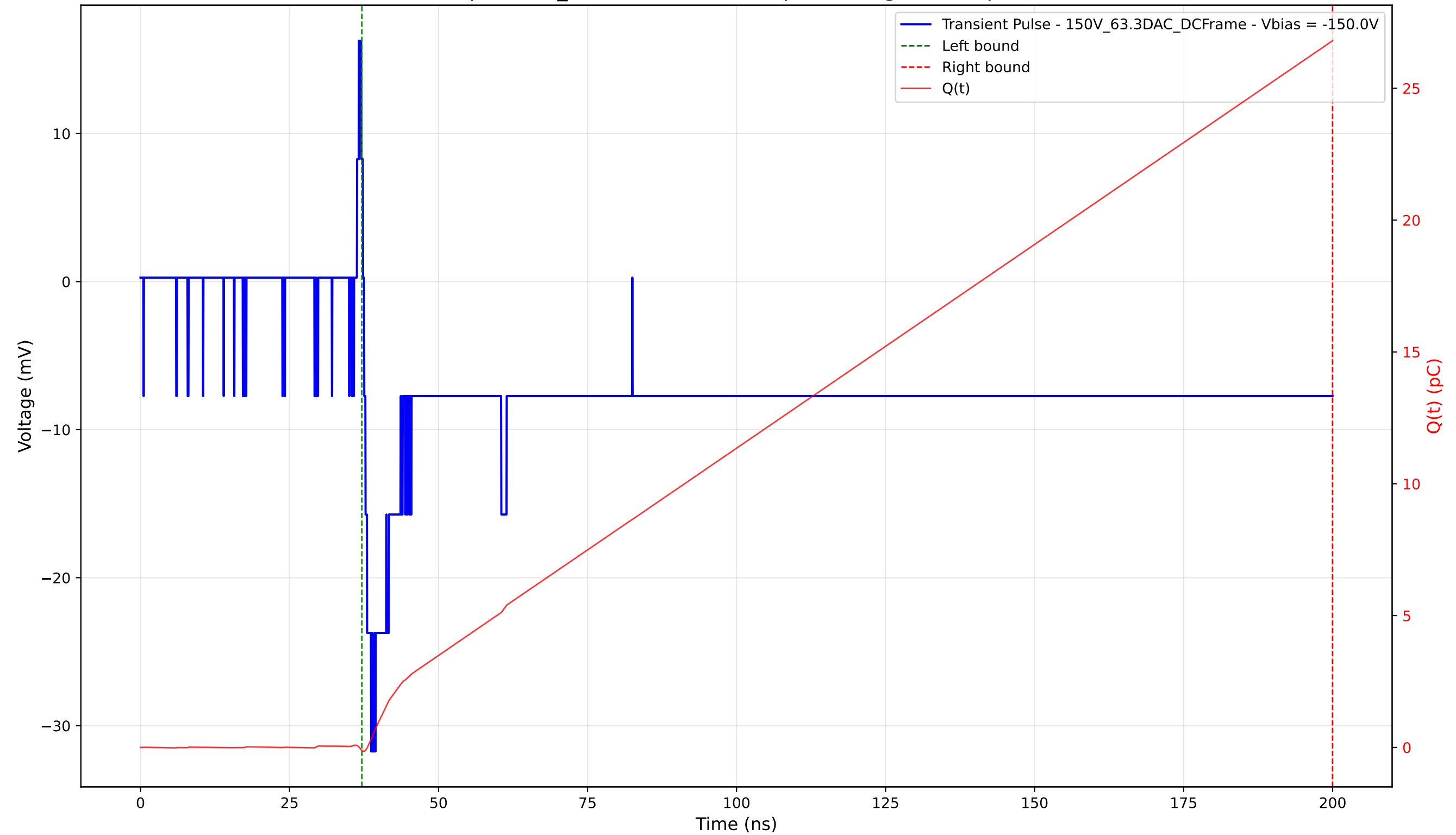
Transient Pulse - Sample: 1cm_42 - Position: 2945.0 \mu\text{m} - Charge: 26.92 pC - Rise Time: 1.17 ns
