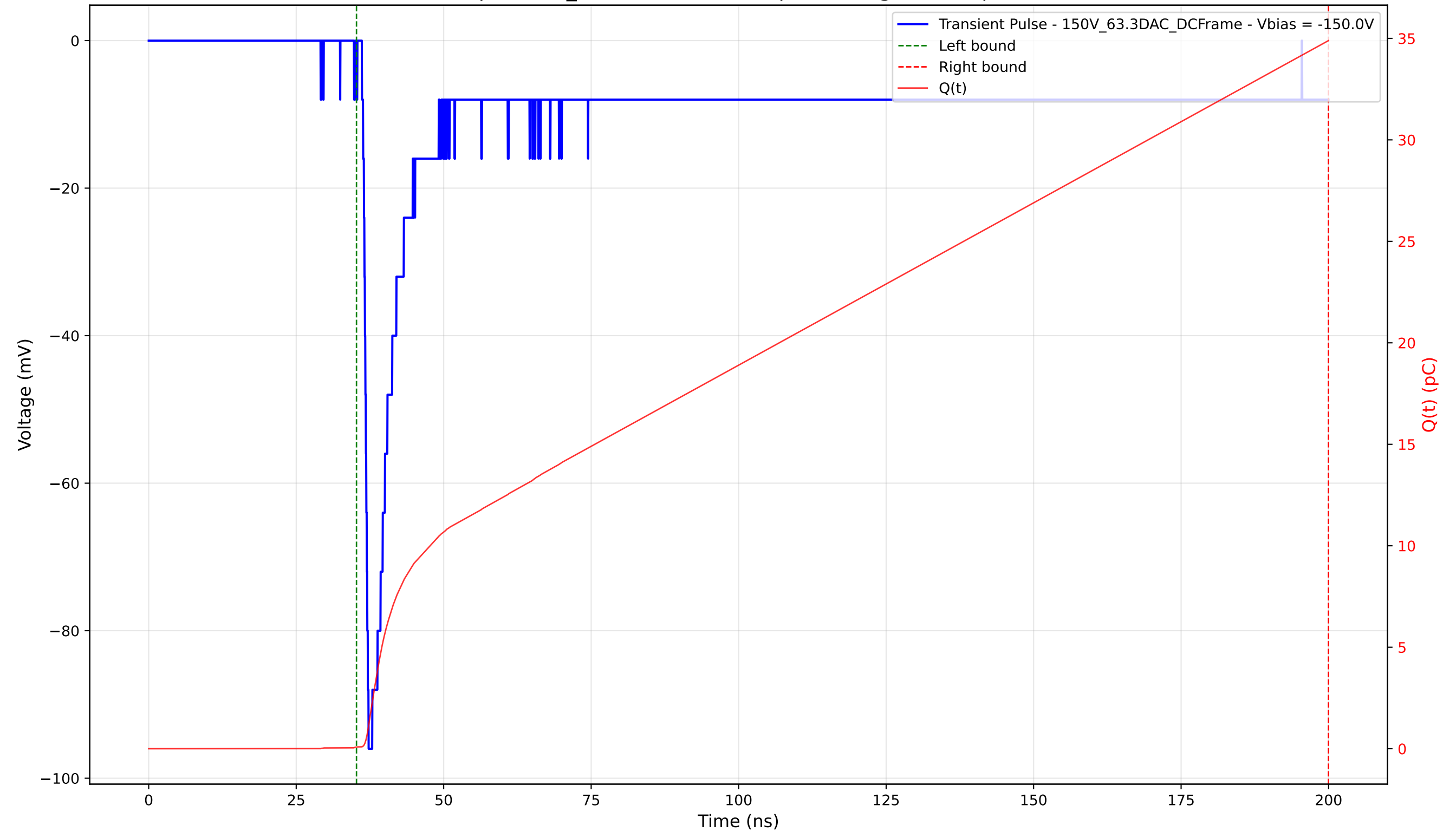
Transient Pulse - Sample: 1cm_42 - Position: 865.0 \mu\text{m} - Charge: 34.81 pC - Rise Time: 0.82 ns
