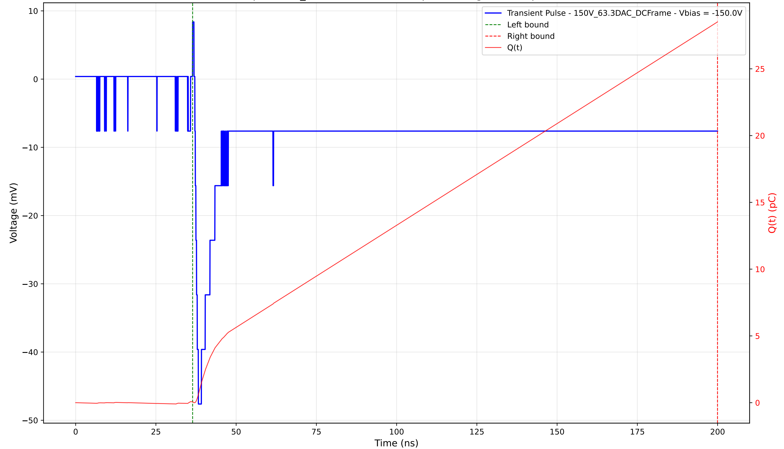
Transient Pulse - Sample: 1cm_42 - Position: 3630.0 \mu\text{m} - Charge: 28.45 pC - Rise Time: 1.09 ns
