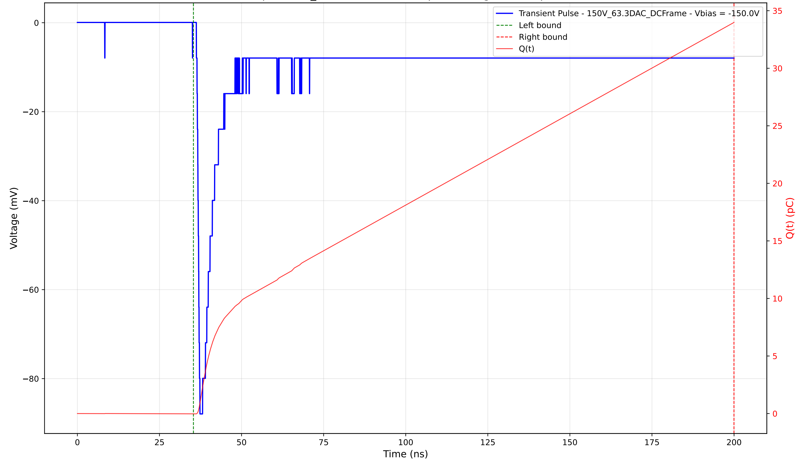
Transient Pulse - Sample: 1cm_42 - Position: 900.0 \mu\text{m} - Charge: 34.01 pC - Rise Time: 0.76 ns
