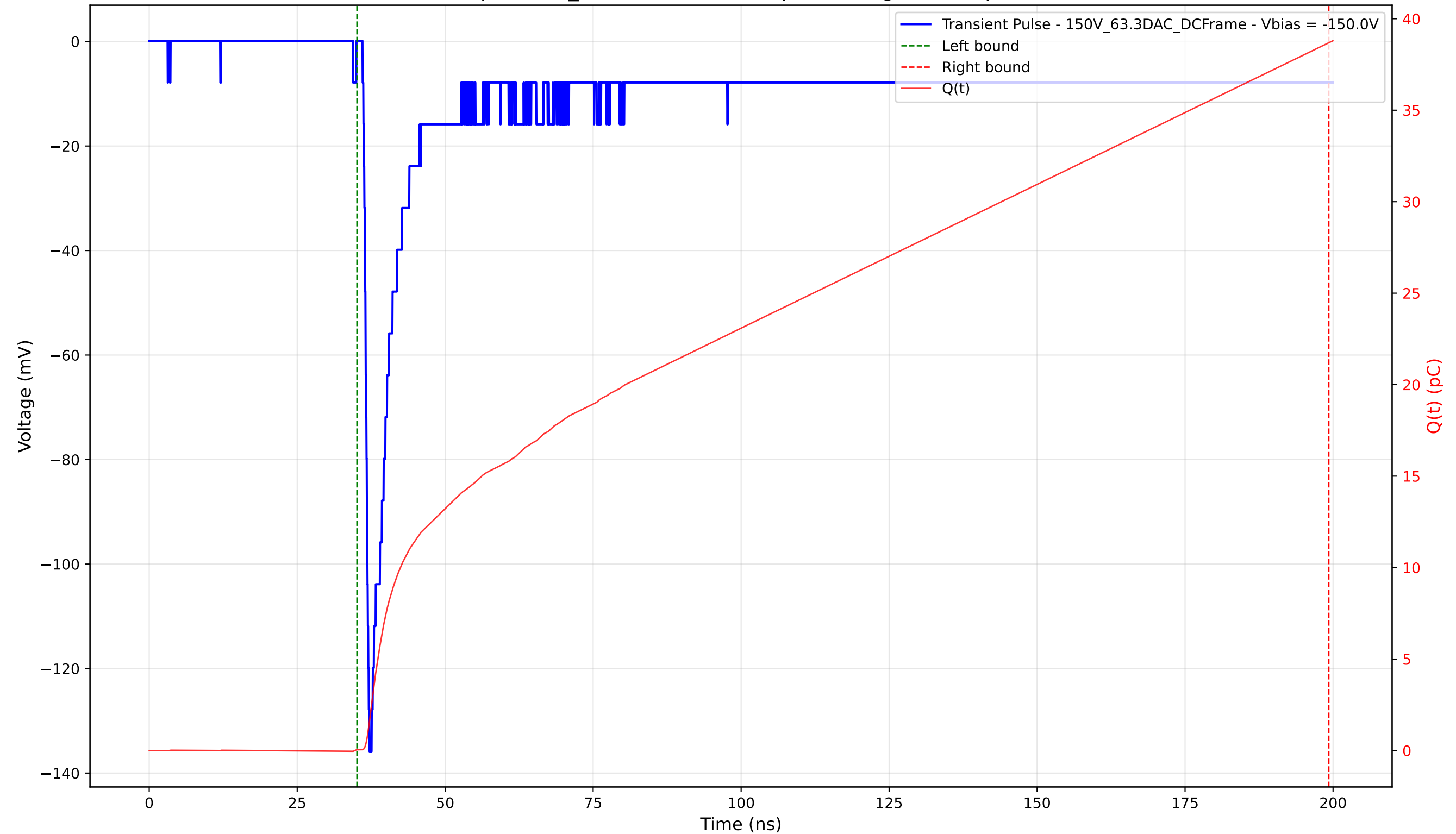
Transient Pulse - Sample: 1cm_42 - Position: 685.0 \mu\text{m} - Charge: 38.64 pC - Rise Time: 0.91 ns
