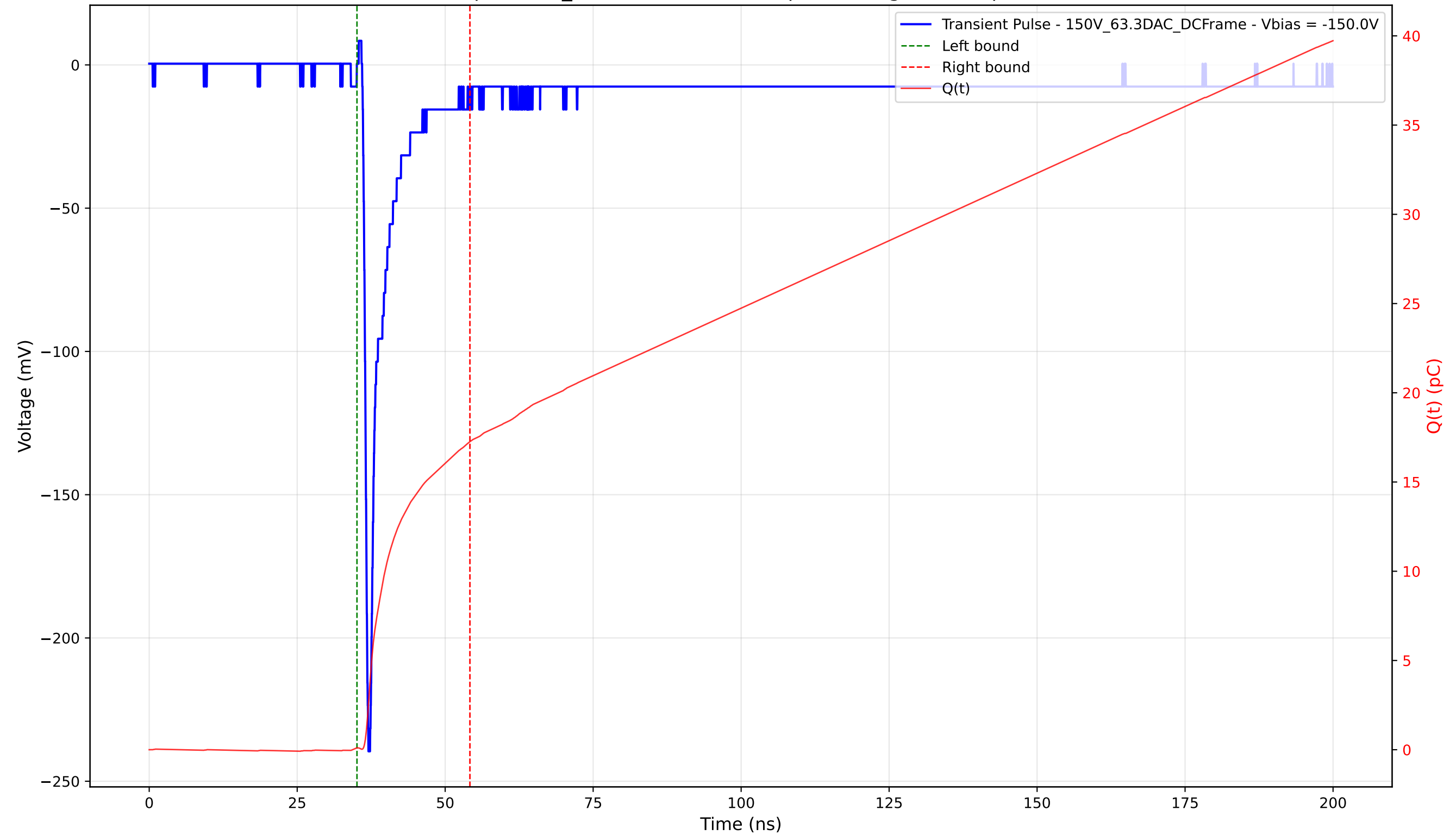
Transient Pulse - Sample: 1cm_42 - Position: 4810.0 \mu\text{m} - Charge: 17.16 pC - Rise Time: 0.76 ns
