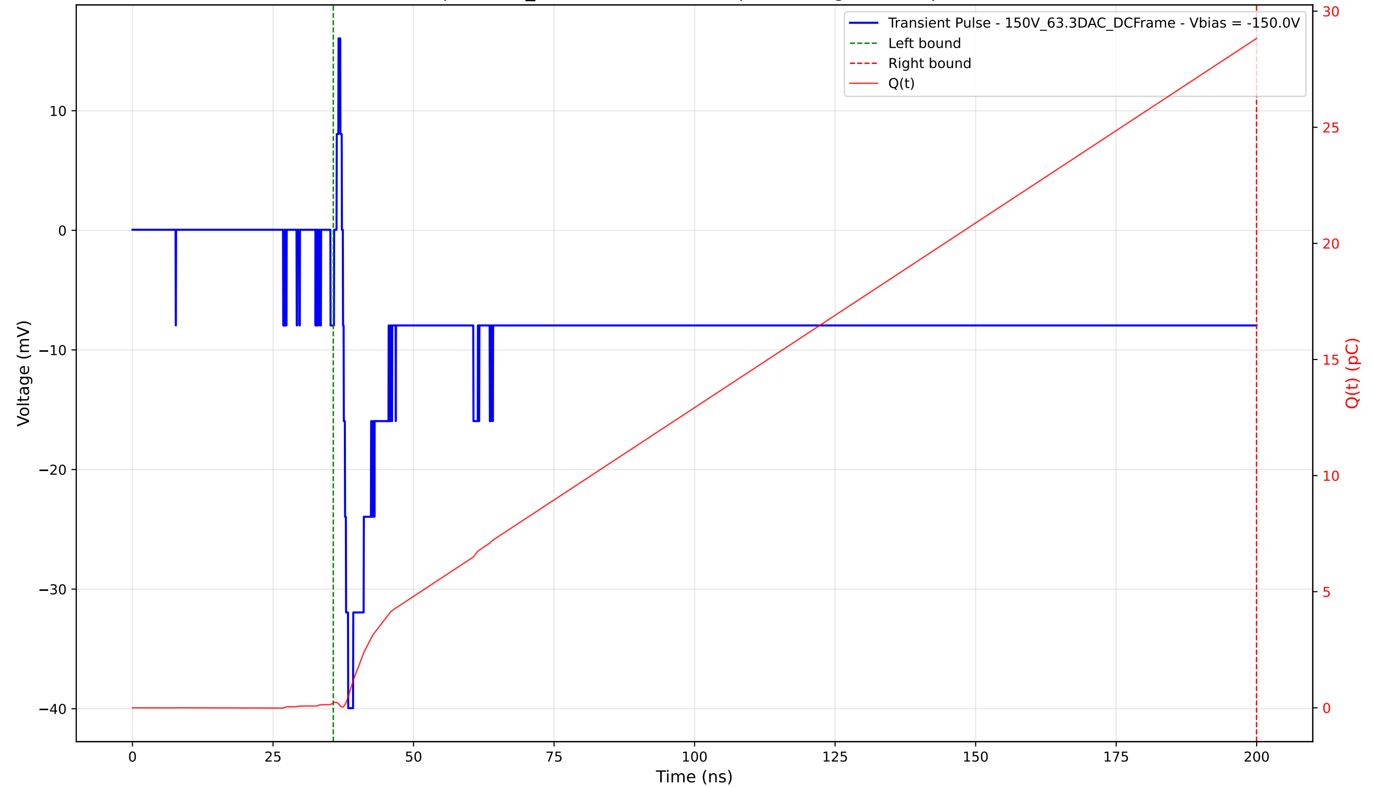
Transient Pulse - Sample: 1cm_42 - Position: 3280.0 \mu\text{m} - Charge: 28.61 pC - Rise Time: 0.93 ns
