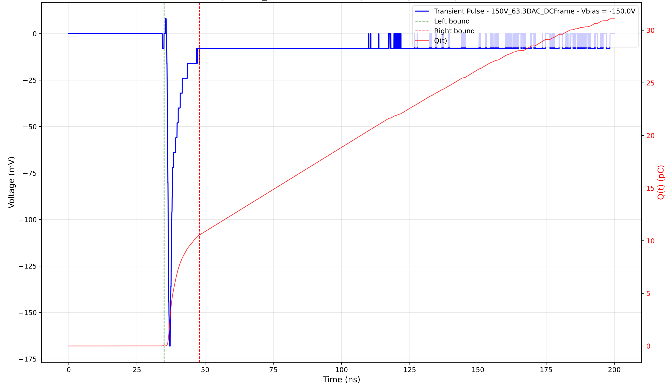
Transient Pulse - Sample: 1cm_42 - Position: 275.0 \mu\text{m} - Charge: 10.46 pC - Rise Time: 0.72 ns
