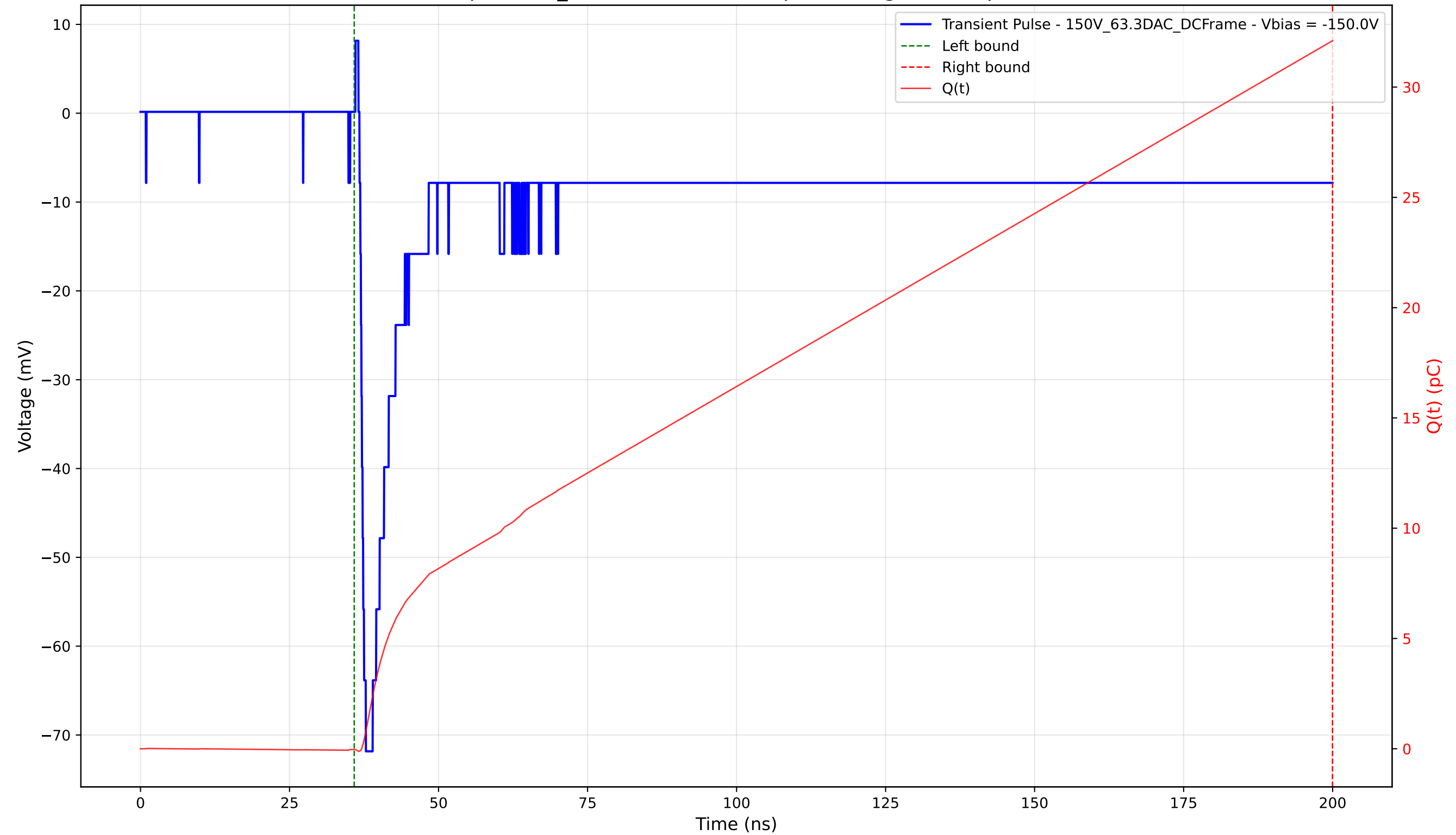
Transient Pulse - Sample: 1cm_42 - Position: 1115.0 \mu\text{m} - Charge: 32.14 pC - Rise Time: 1.06 ns
