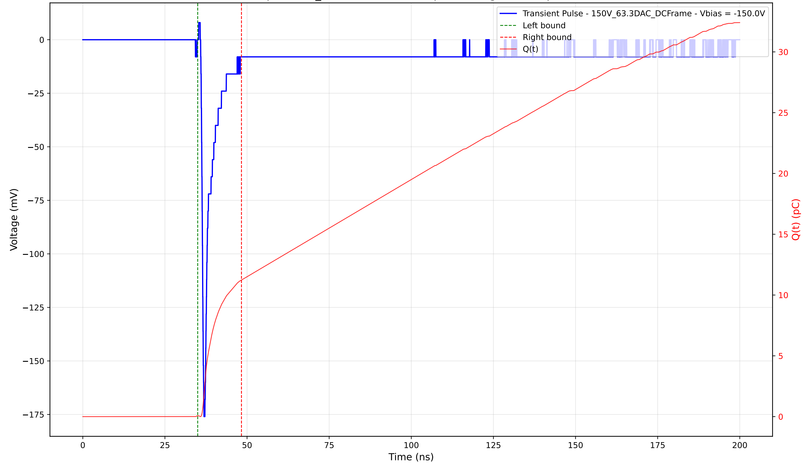
Transient Pulse - Sample: 1cm_42 - Position: 325.0 \mu\text{m} - Charge: 11.17 pC - Rise Time: 0.72 ns
