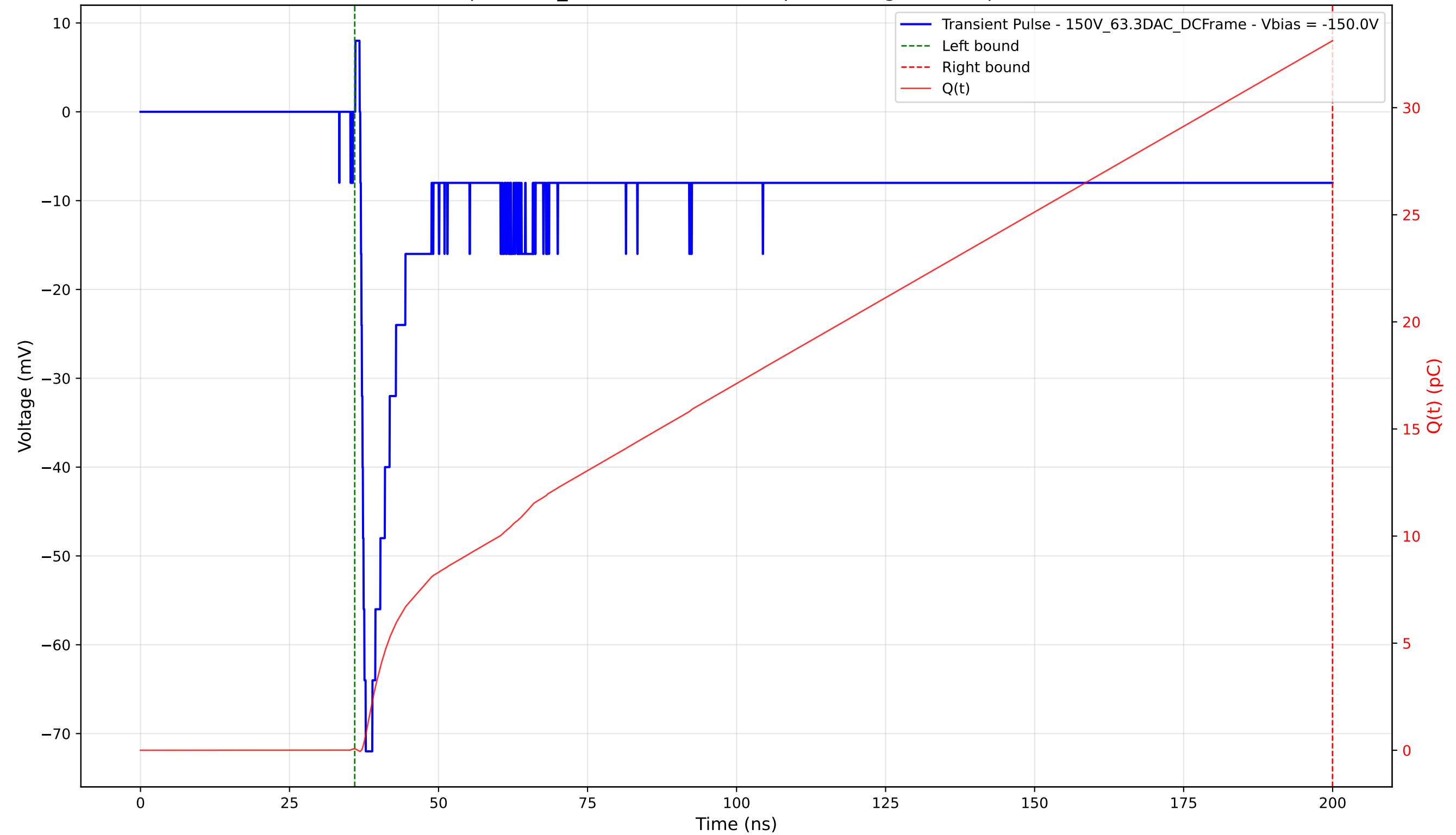
Transient Pulse - Sample: 1cm_42 - Position: 1215.0 \mu\text{m} - Charge: 33.06 pC - Rise Time: 0.90 ns
