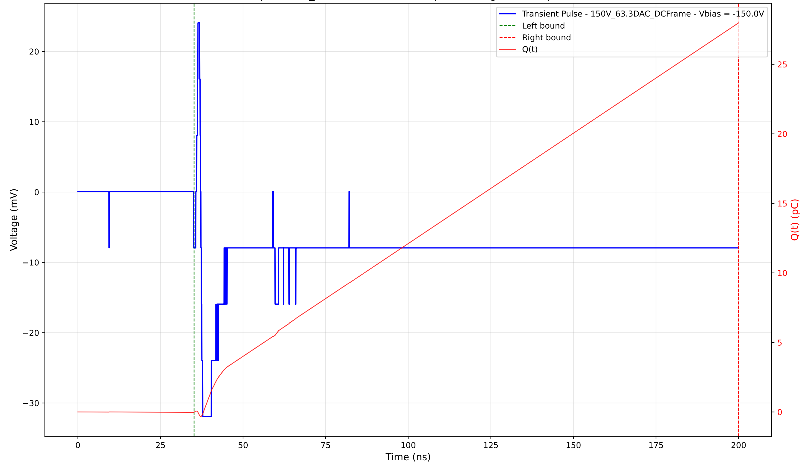
Transient Pulse - Sample: 1cm_42 - Position: 2060.0 \mu\text{m} - Charge: 27.99 pC - Rise Time: 0.57 ns
