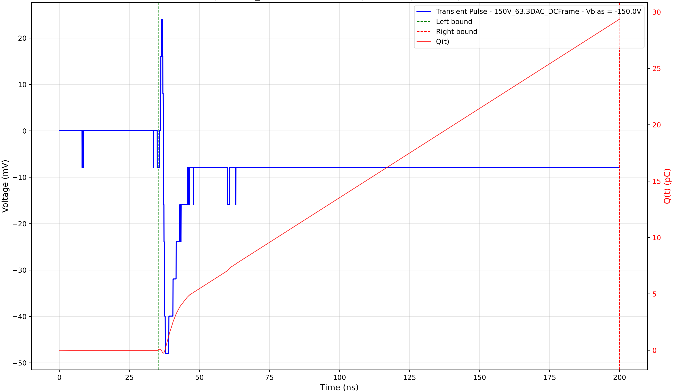
Transient Pulse - Sample: 1cm_42 - Position: 1570.0 \mu\text{m} - Charge: 29.34 pC - Rise Time: 0.63 ns
