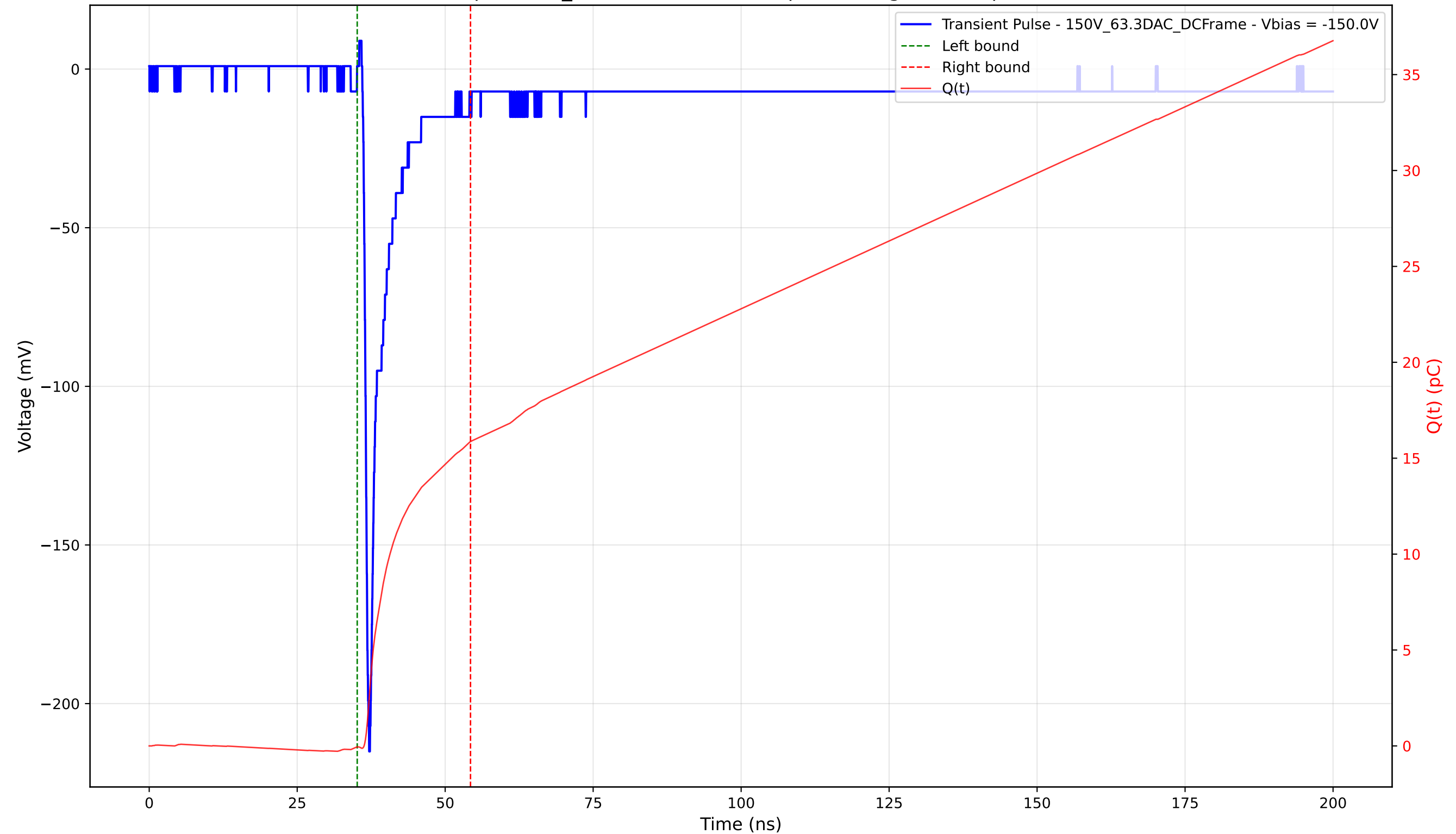
Transient Pulse - Sample: 1cm_42 - Position: 4700.0 \mu\text{m} - Charge: 15.91 pC - Rise Time: 0.80 ns
