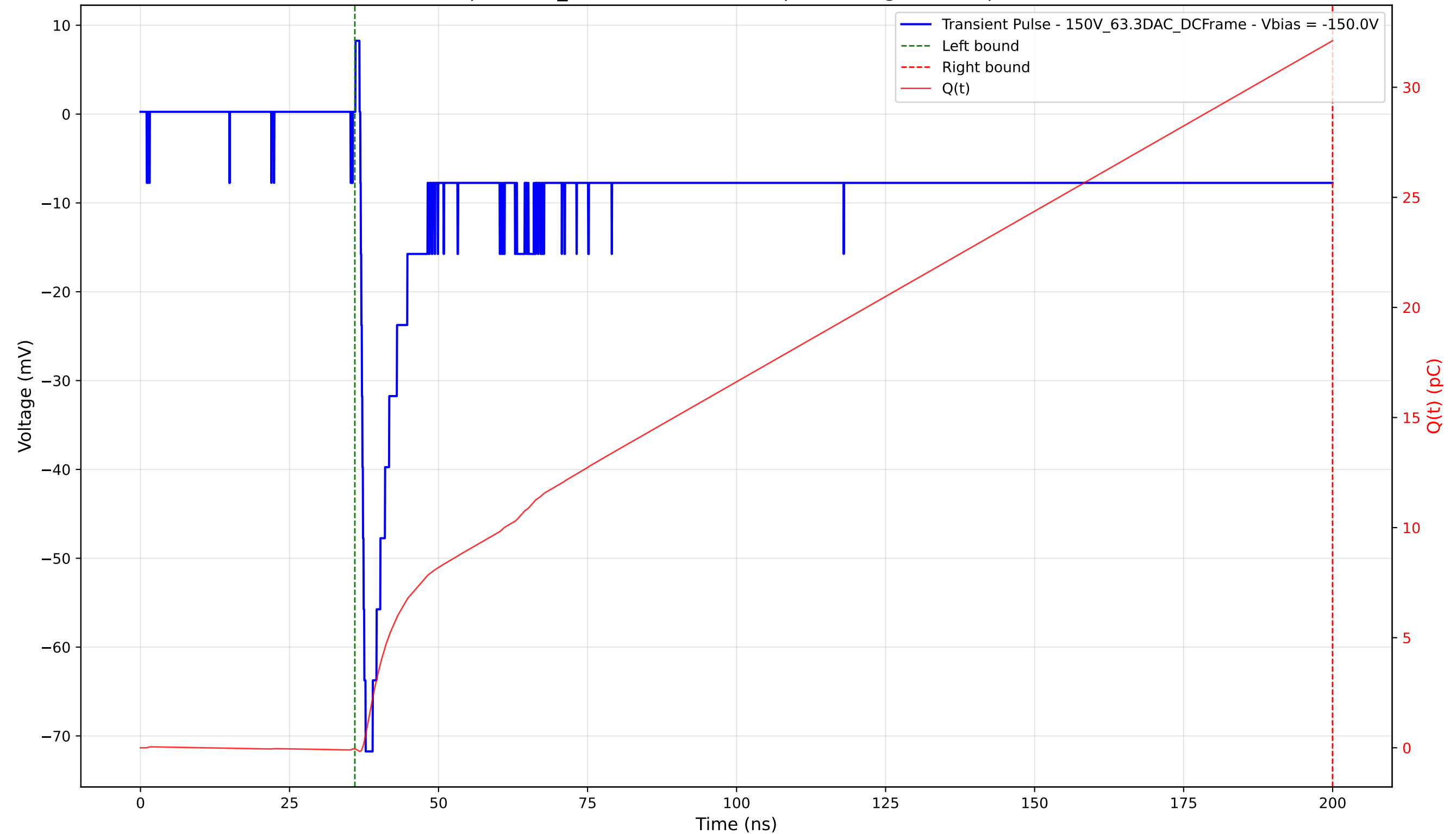
Transient Pulse - Sample: 1cm_42 - Position: 1205.0 \mu\text{m} - Charge: 32.17 pC - Rise Time: 0.88 ns
