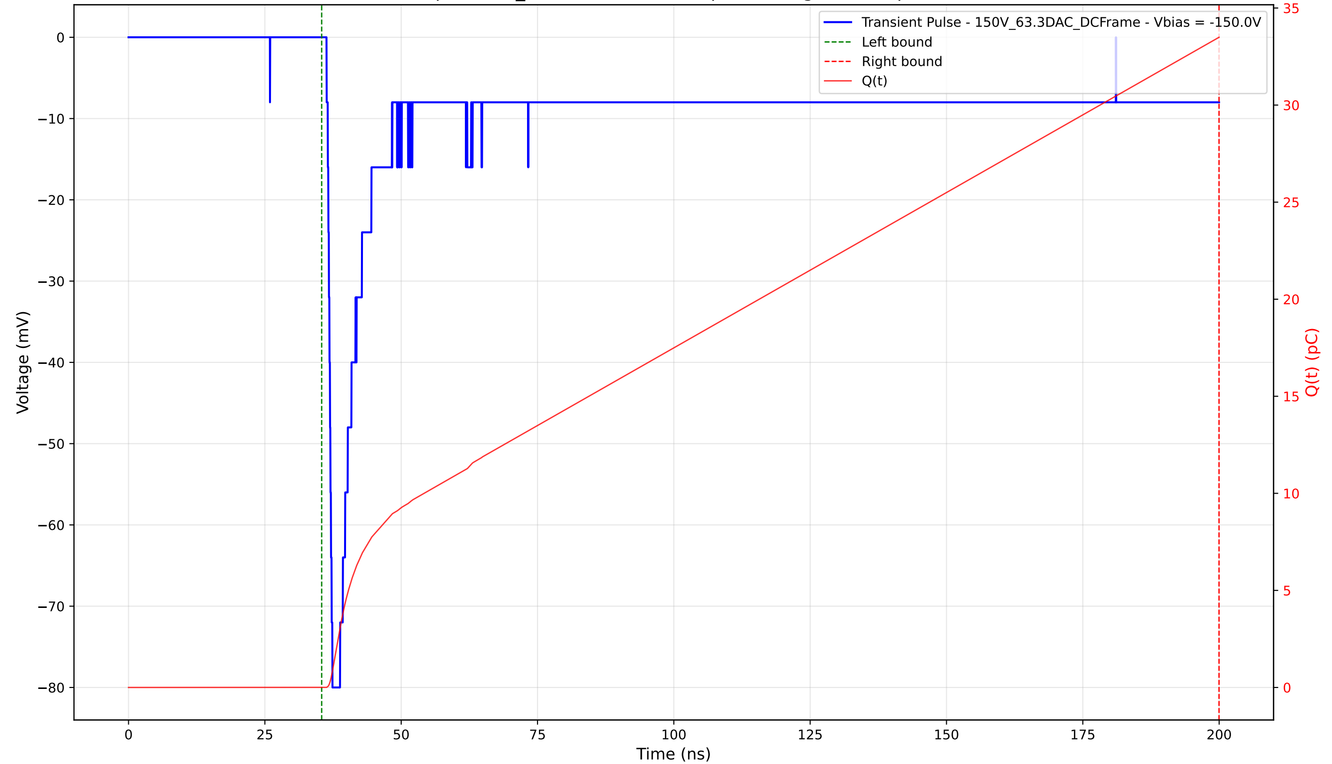
Transient Pulse - Sample: 1cm_42 - Position: 940.0 \mu\text{m} - Charge: 33.49 pC - Rise Time: 0.72 ns
