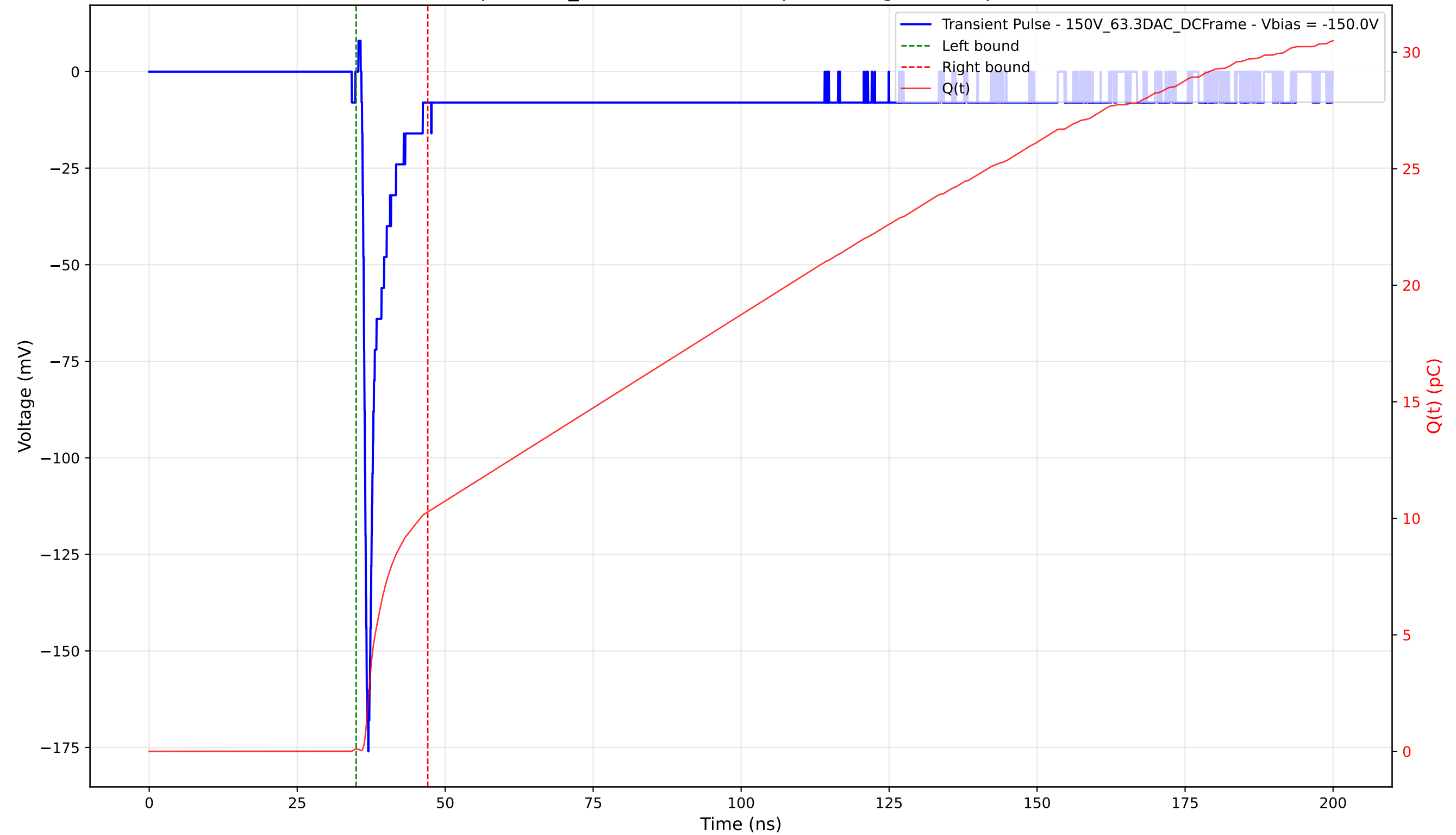
Transient Pulse - Sample: 1cm_42 - Position: 285.0 \mu\text{m} - Charge: 10.17 pC - Rise Time: 0.74 ns
