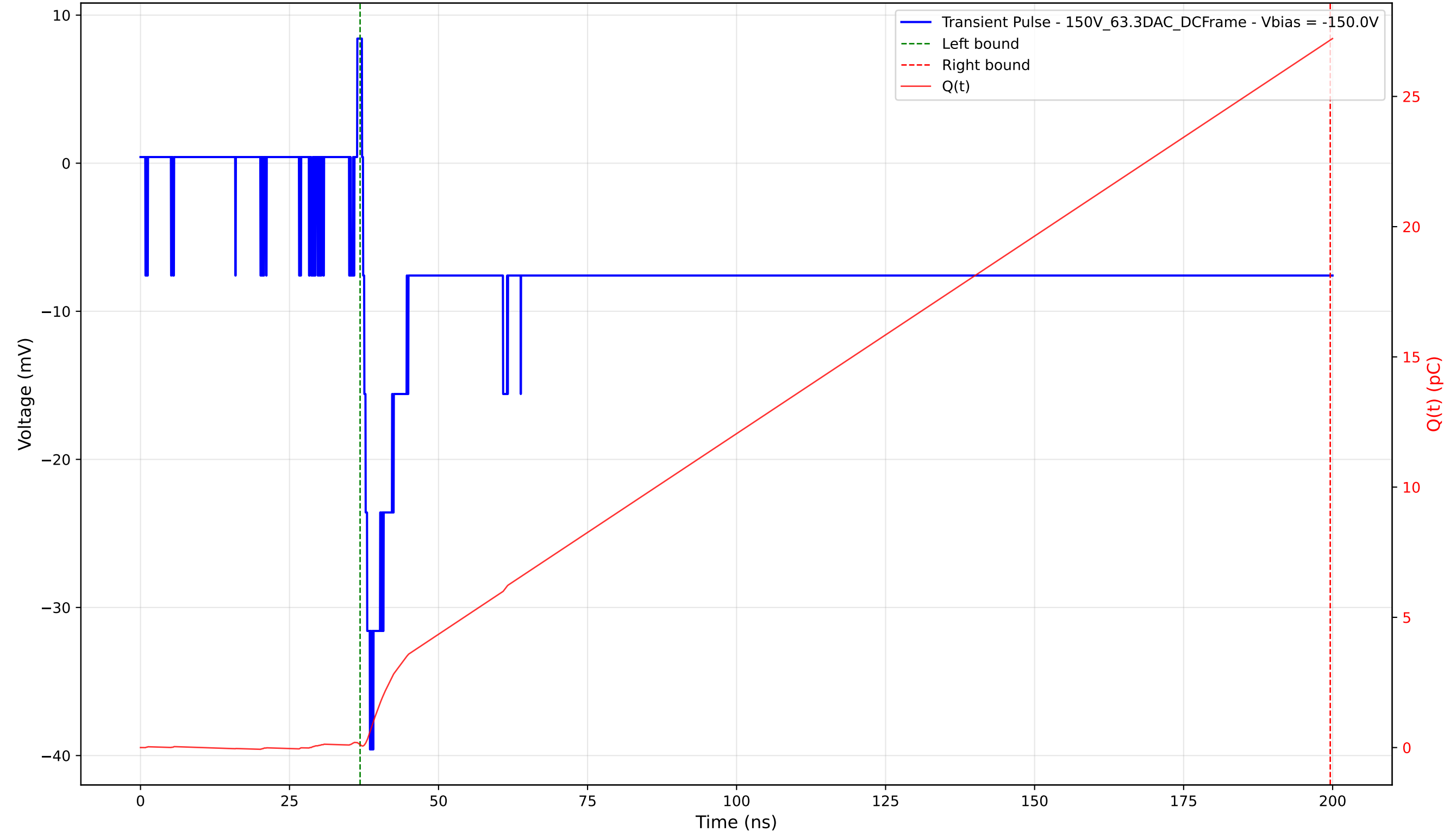
Transient Pulse - Sample: 1cm_42 - Position: 3415.0 \mu\text{m} - Charge: 27.05 pC - Rise Time: 1.15 ns
