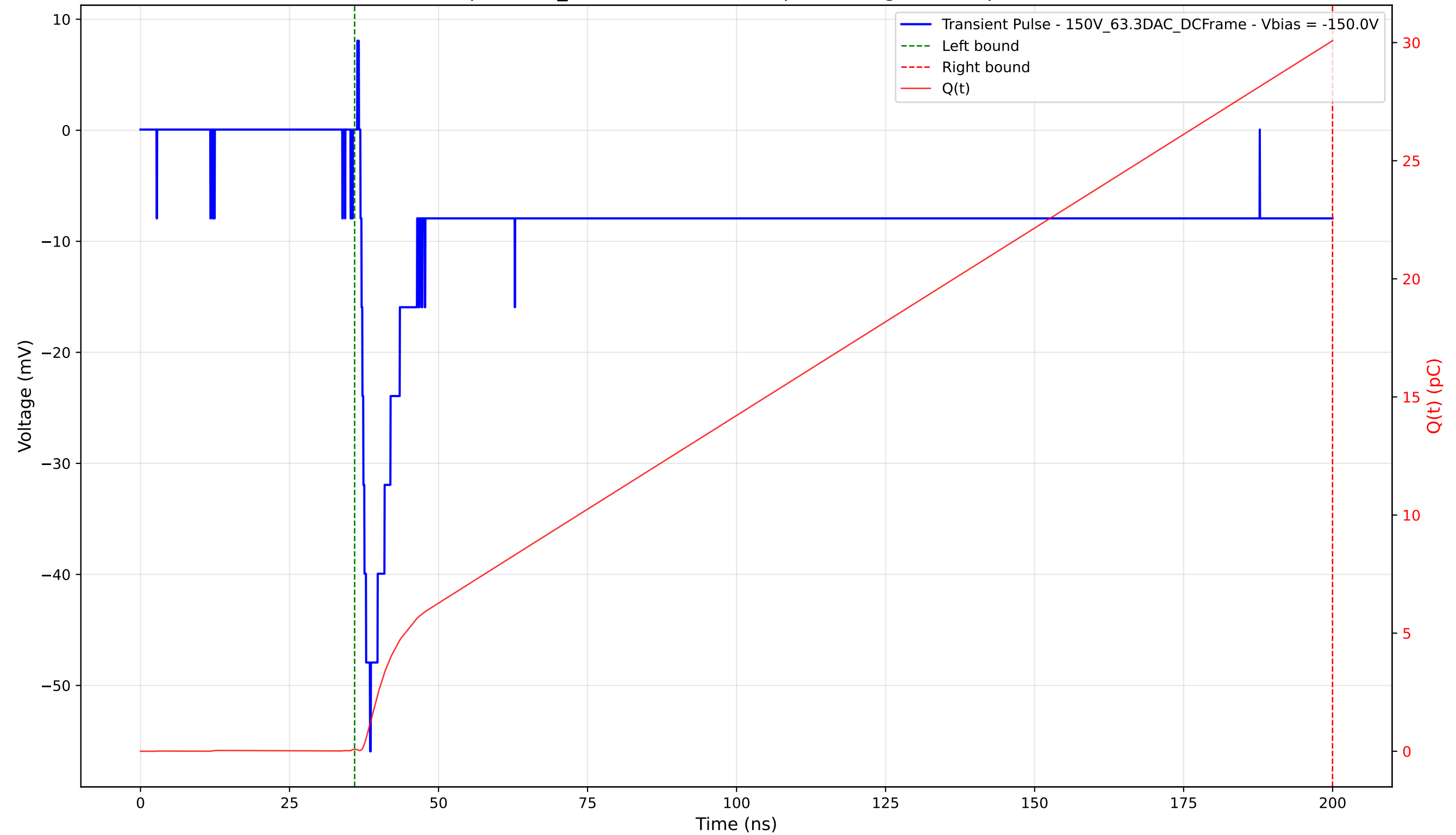
Transient Pulse - Sample: 1cm_42 - Position: 3890.0 \mu\text{m} - Charge: 30.00 pC - Rise Time: 1.61 ns
