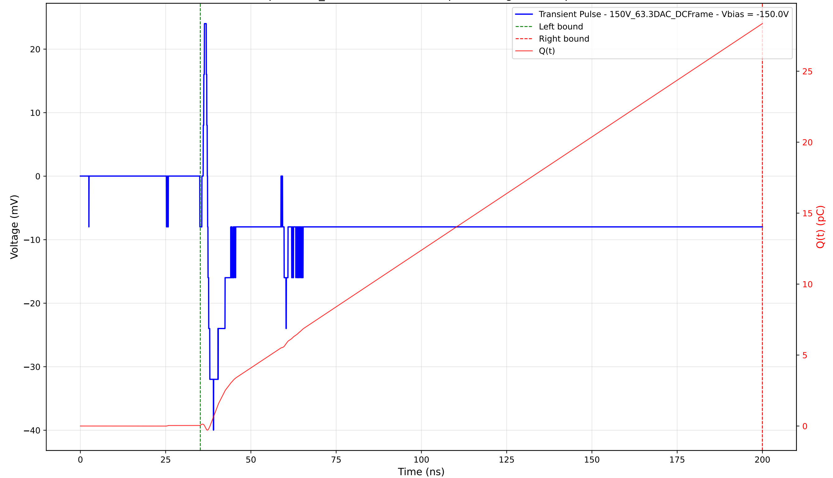
Transient Pulse - Sample: 1cm_42 - Position: 2175.0 \mu\text{m} - Charge: 28.30 pC - Rise Time: 1.73 ns
