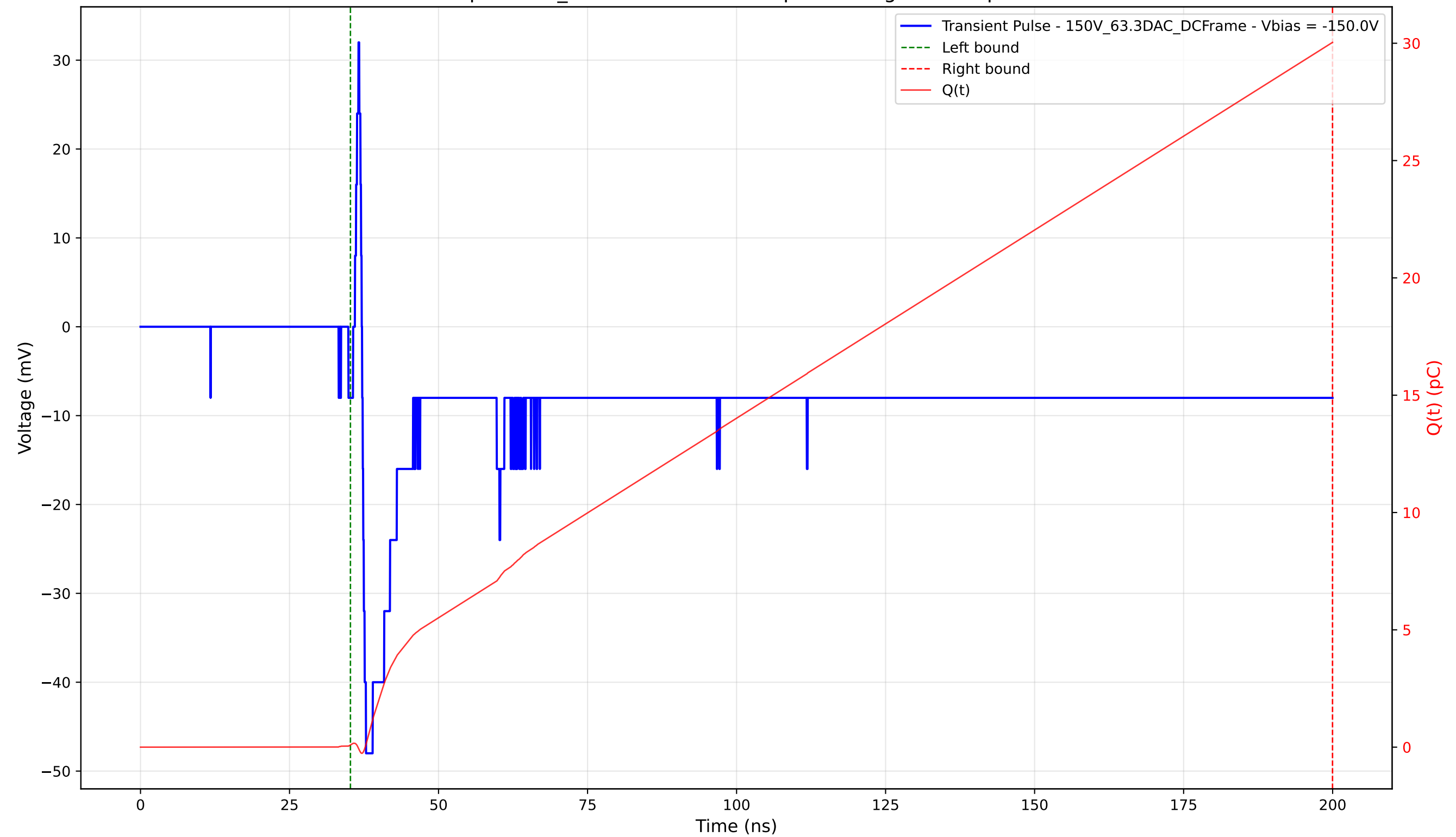
Transient Pulse - Sample: 1cm_42 - Position: 1690.0 \mu\text{m} - Charge: 29.94 pC - Rise Time: 0.65 ns
