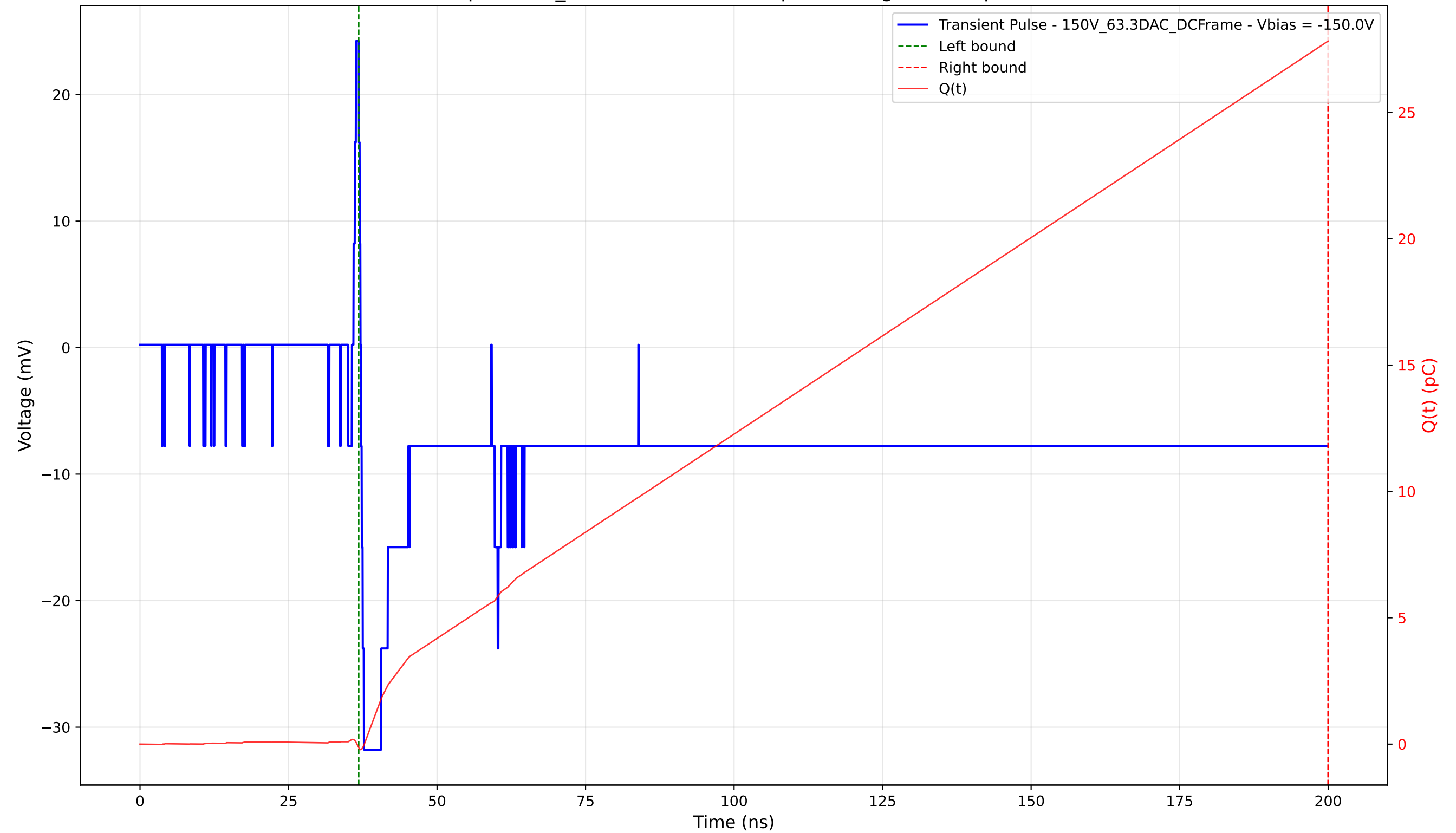
Transient Pulse - Sample: 1cm_42 - Position: 1980.0 \mu\text{m} - Charge: 27.96 pC - Rise Time: 0.49 ns
