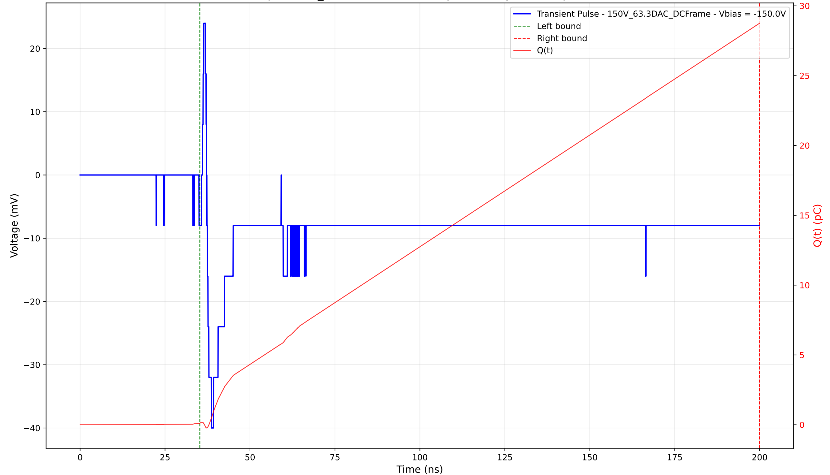
Transient Pulse - Sample: 1cm_42 - Position: 2255.0 \mu\text{m} - Charge: 28.65 pC - Rise Time: 1.31 ns
