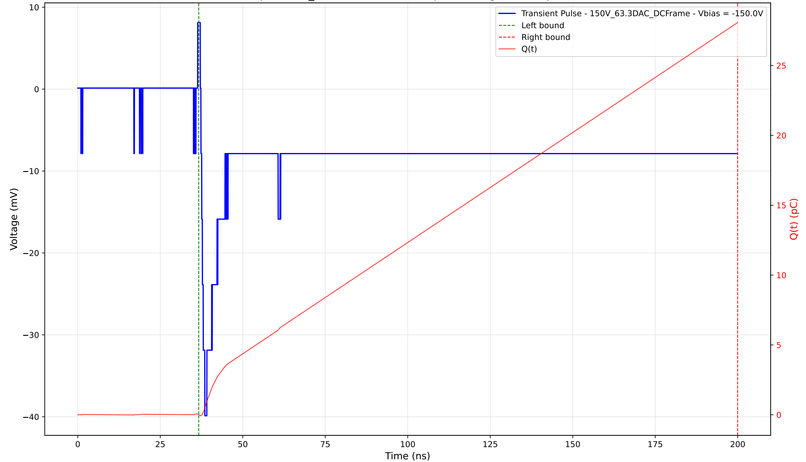
Transient Pulse - Sample: 1cm_42 - Position: 3425.0 \mu\text{m} - Charge: 28.07 pC - Rise Time: 1.19 ns
