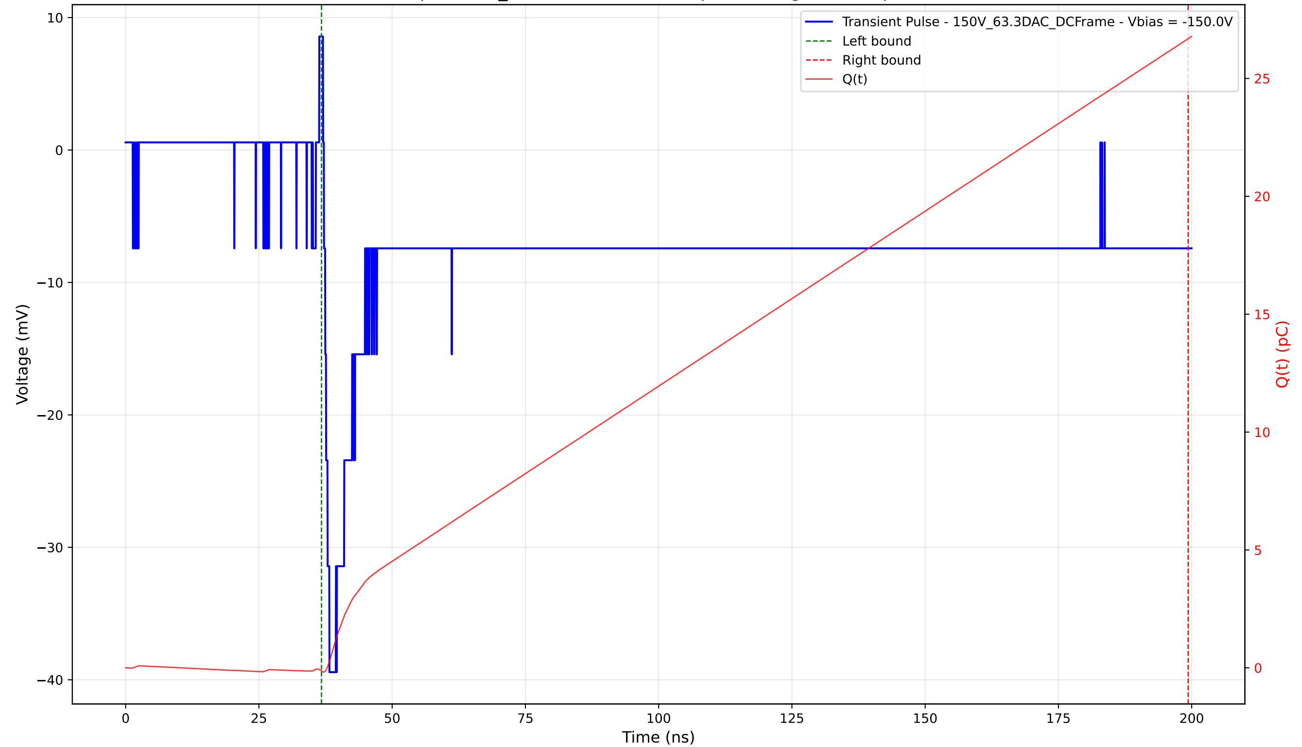
Transient Pulse - Sample: 1cm_42 - Position: 3535.0 \mu\text{m} - Charge: 26.82 pC - Rise Time: 1.03 ns
