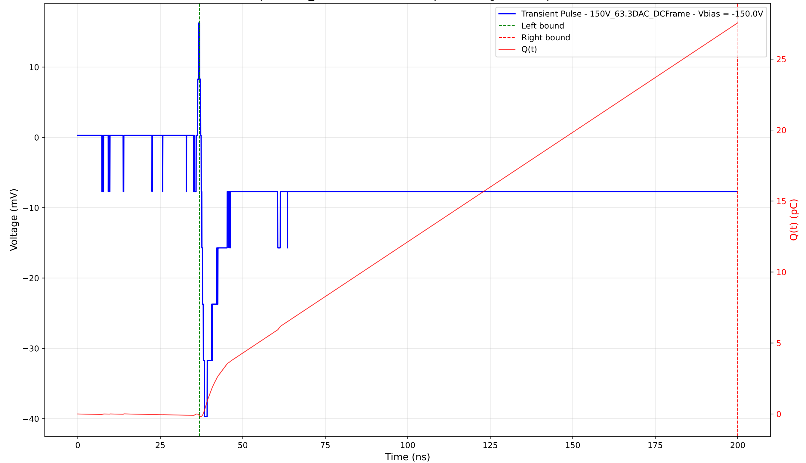
Transient Pulse - Sample: 1cm_42 - Position: 3345.0 \mu\text{m} - Charge: 27.68 pC - Rise Time: 0.97 ns
