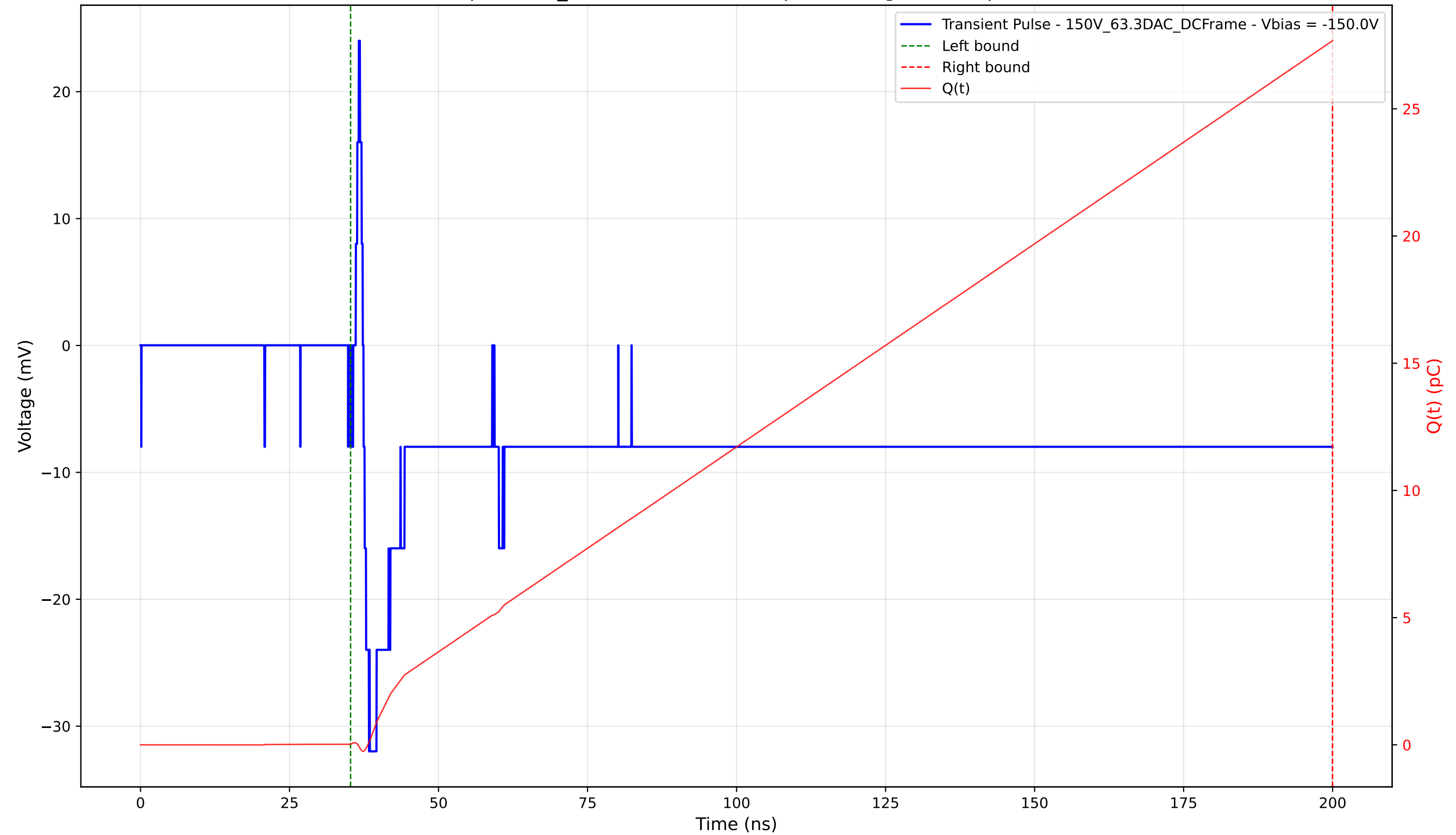
Transient Pulse - Sample: 1cm_42 - Position: 2425.0 \mu\text{m} - Charge: 27.65 pC - Rise Time: 0.91 ns
