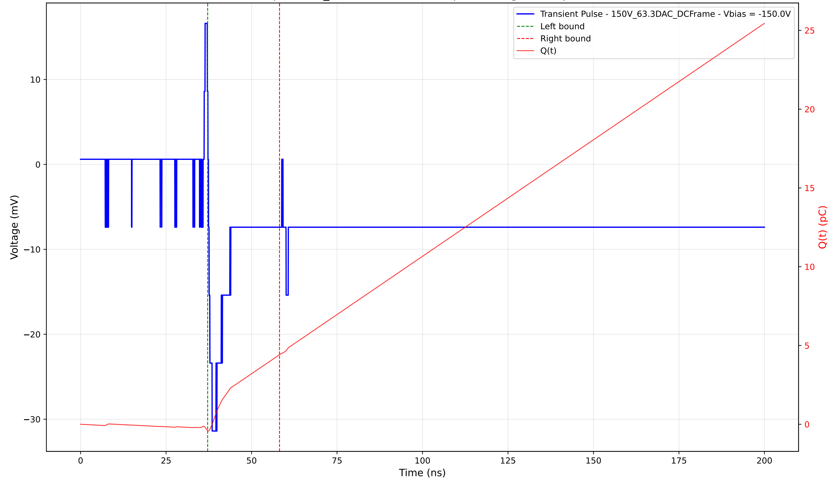
Transient Pulse - Sample: 1cm_42 - Position: 2440.0 \mu\text{m} - Charge: 4.83 pC - Rise Time: 1.07 ns
