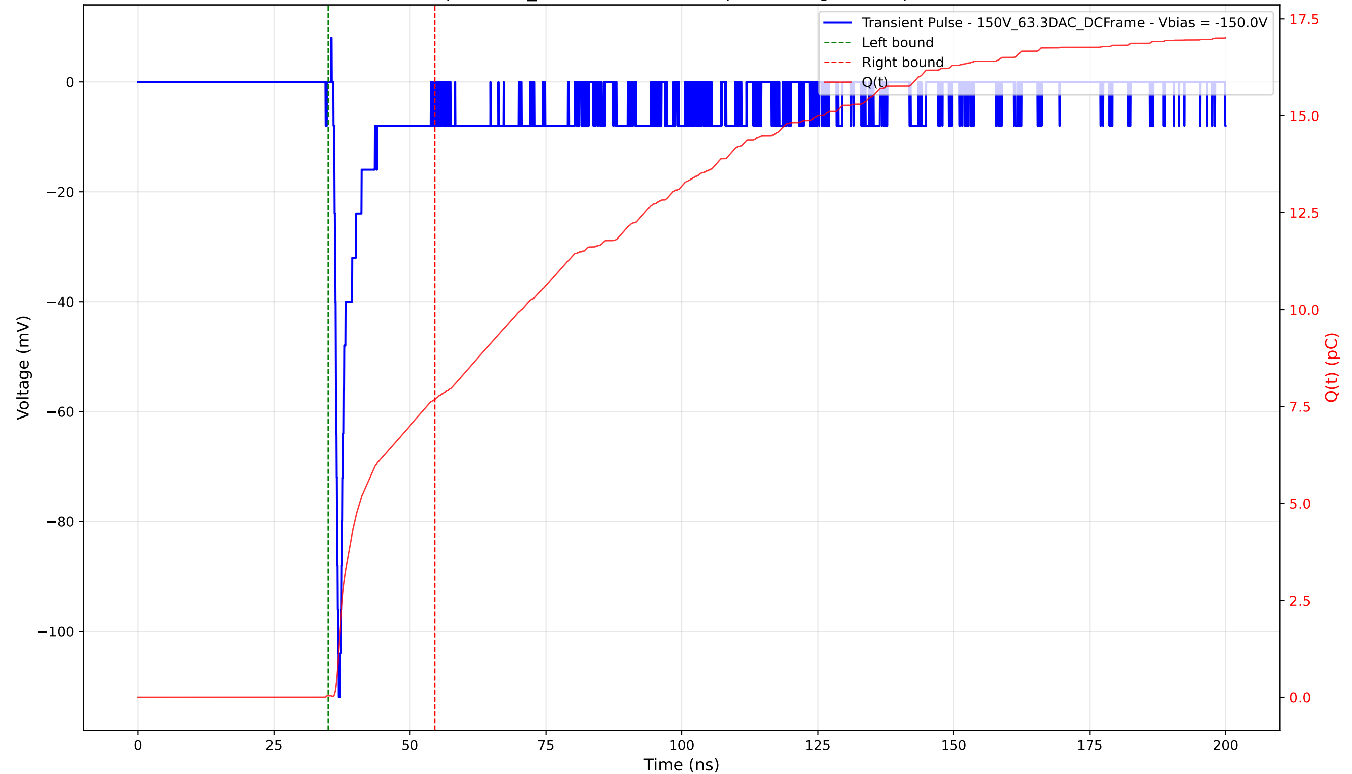
Transient Pulse - Sample: 1cm_42 - Position: 145.0 \mu\text{m} - Charge: 7.65 pC - Rise Time: 0.75 ns
