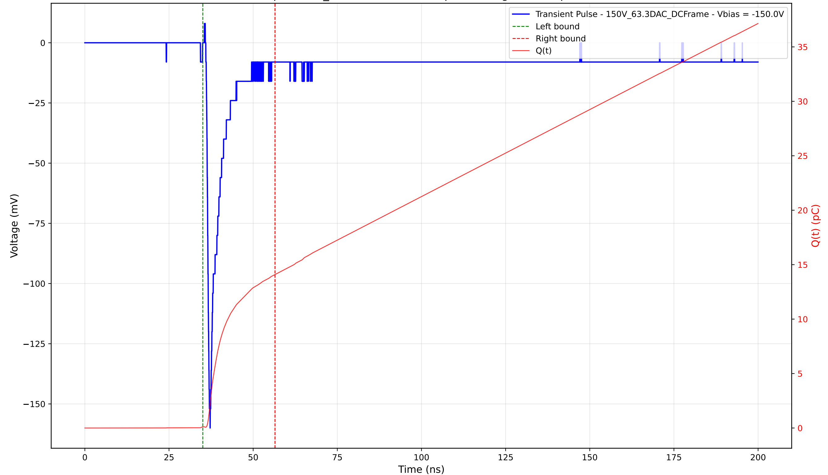
Transient Pulse - Sample: 1cm_42 - Position: 525.0 \mu\text{m} - Charge: 13.98 pC - Rise Time: 0.78 ns
