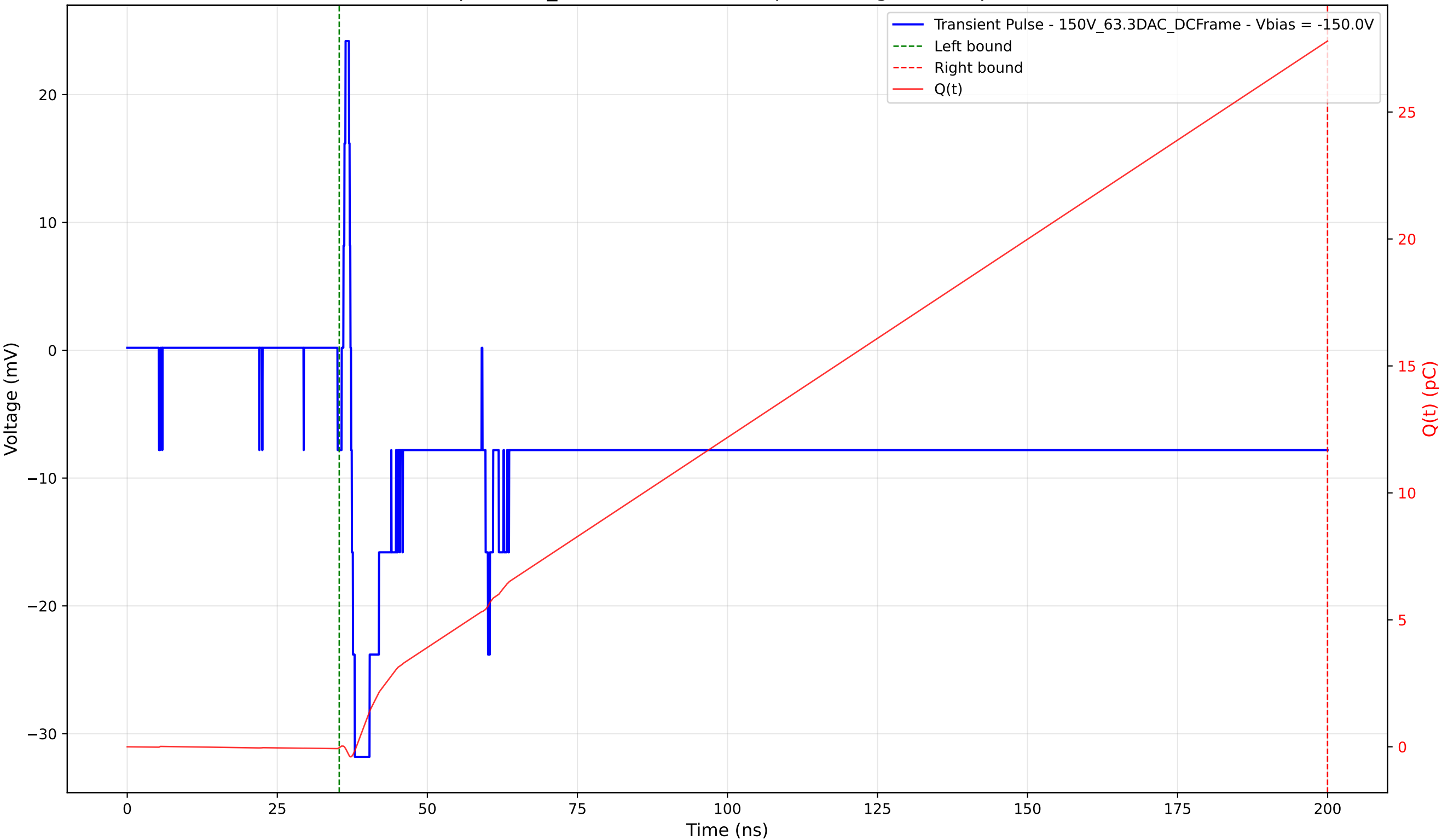
Transient Pulse - Sample: 1cm_42 - Position: 2160.0 \mu\text{m} - Charge: 27.83 pC - Rise Time: 0.61 ns
