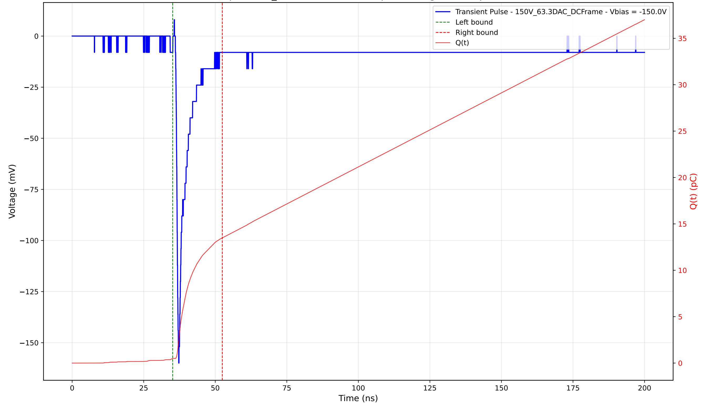
Transient Pulse - Sample: 1cm_42 - Position: 4595.0 \mu\text{m} - Charge: 12.99 pC - Rise Time: 0.86 ns
