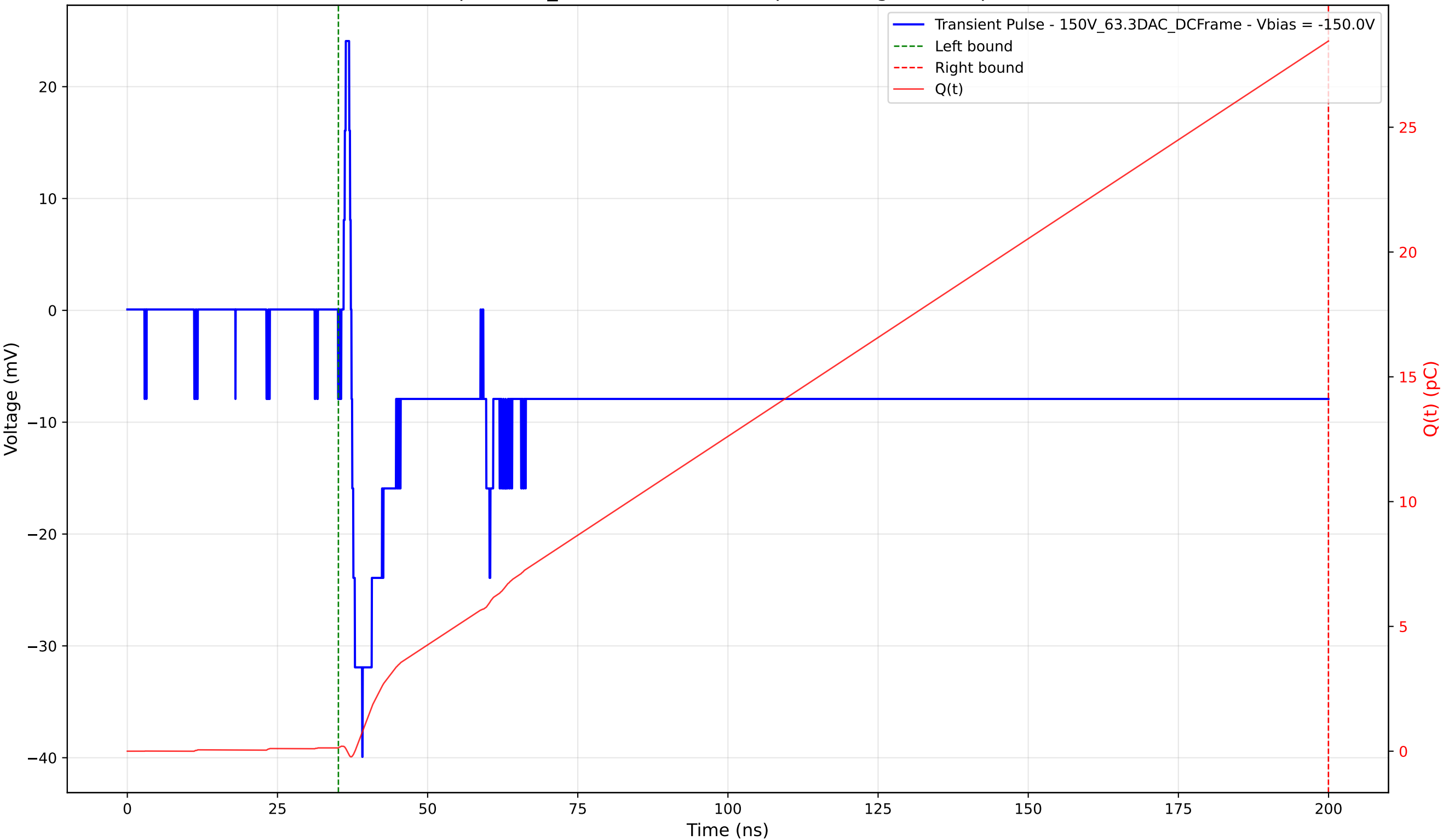
Transient Pulse - Sample: 1cm_42 - Position: 2230.0 \mu\text{m} - Charge: 28.32 pC - Rise Time: 1.79 ns
