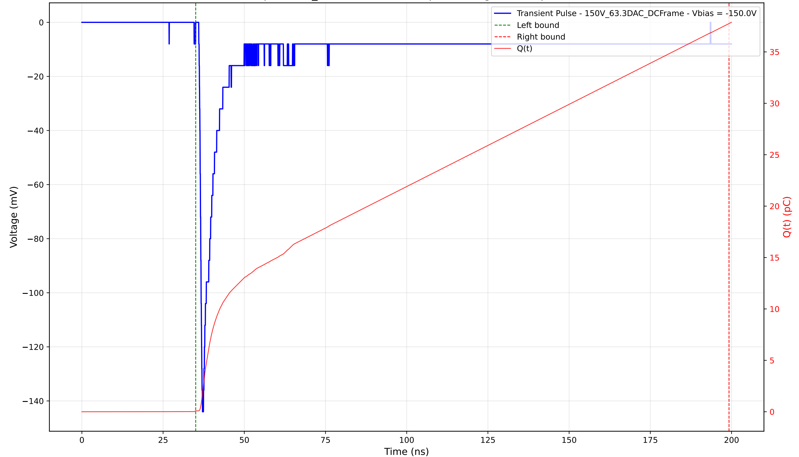
Transient Pulse - Sample: 1cm_42 - Position: 585.0 \mu\text{m} - Charge: 37.67 pC - Rise Time: 0.88 ns
