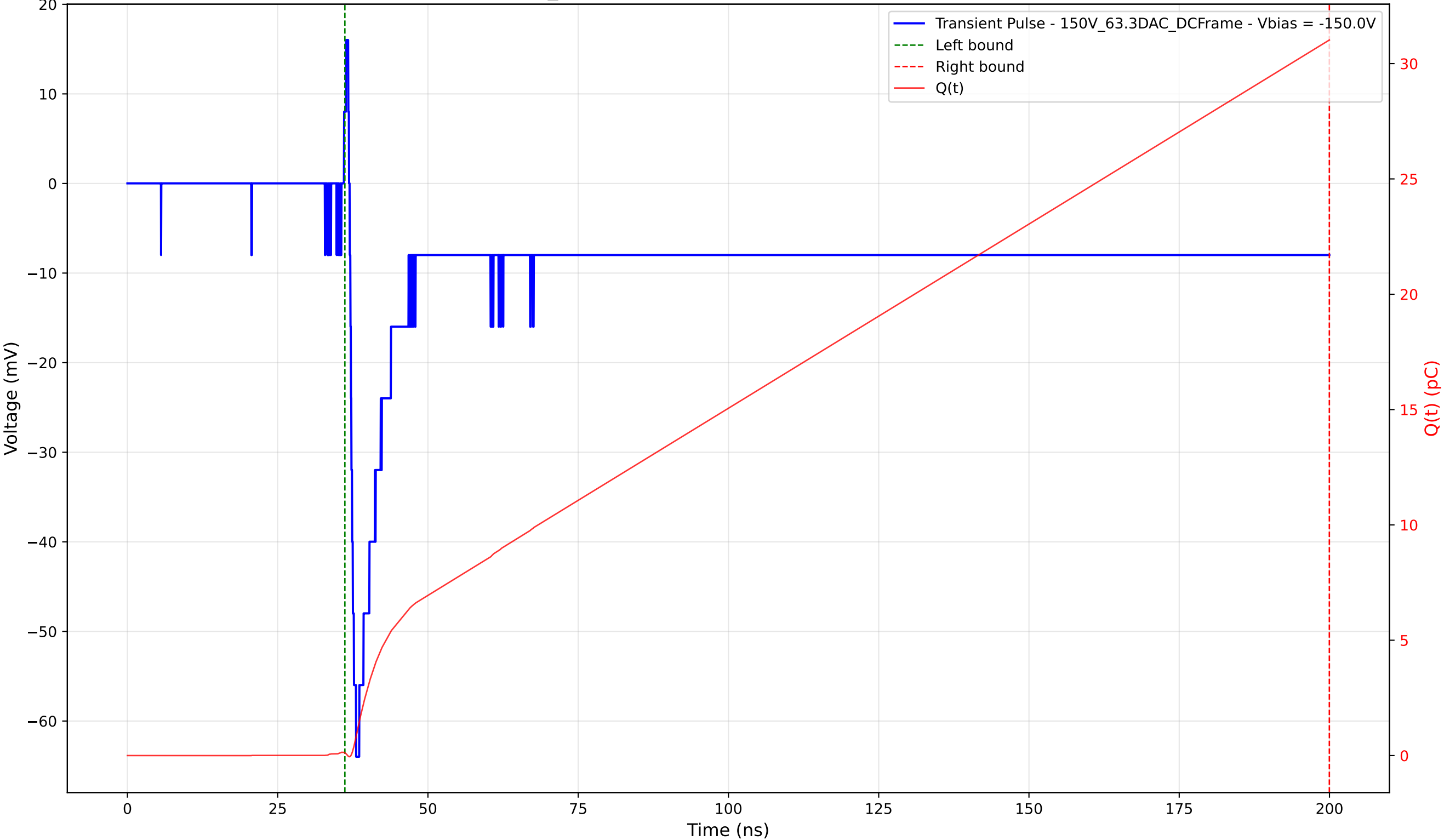
Transient Pulse - Sample: 1cm_42 - Position: 1360.0 \mu\text{m} - Charge: 30.90 pC - Rise Time: 1.06 ns
