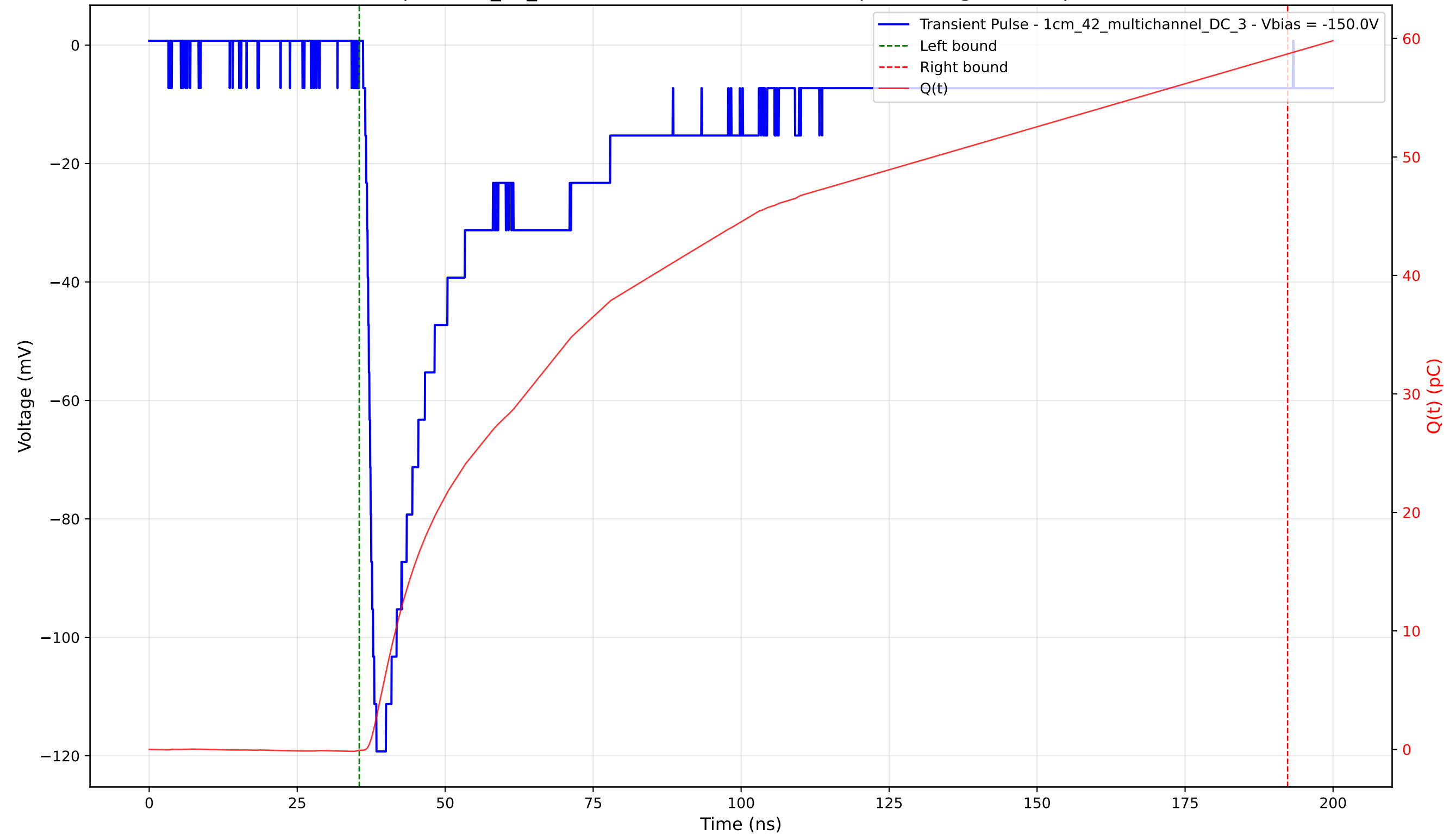
Transient Pulse - Sample: 1cm_42_multichannel - Position: 1650.0 \mu\text{m} - Charge: 58.79 pC - Rise Time: 1.53 ns
