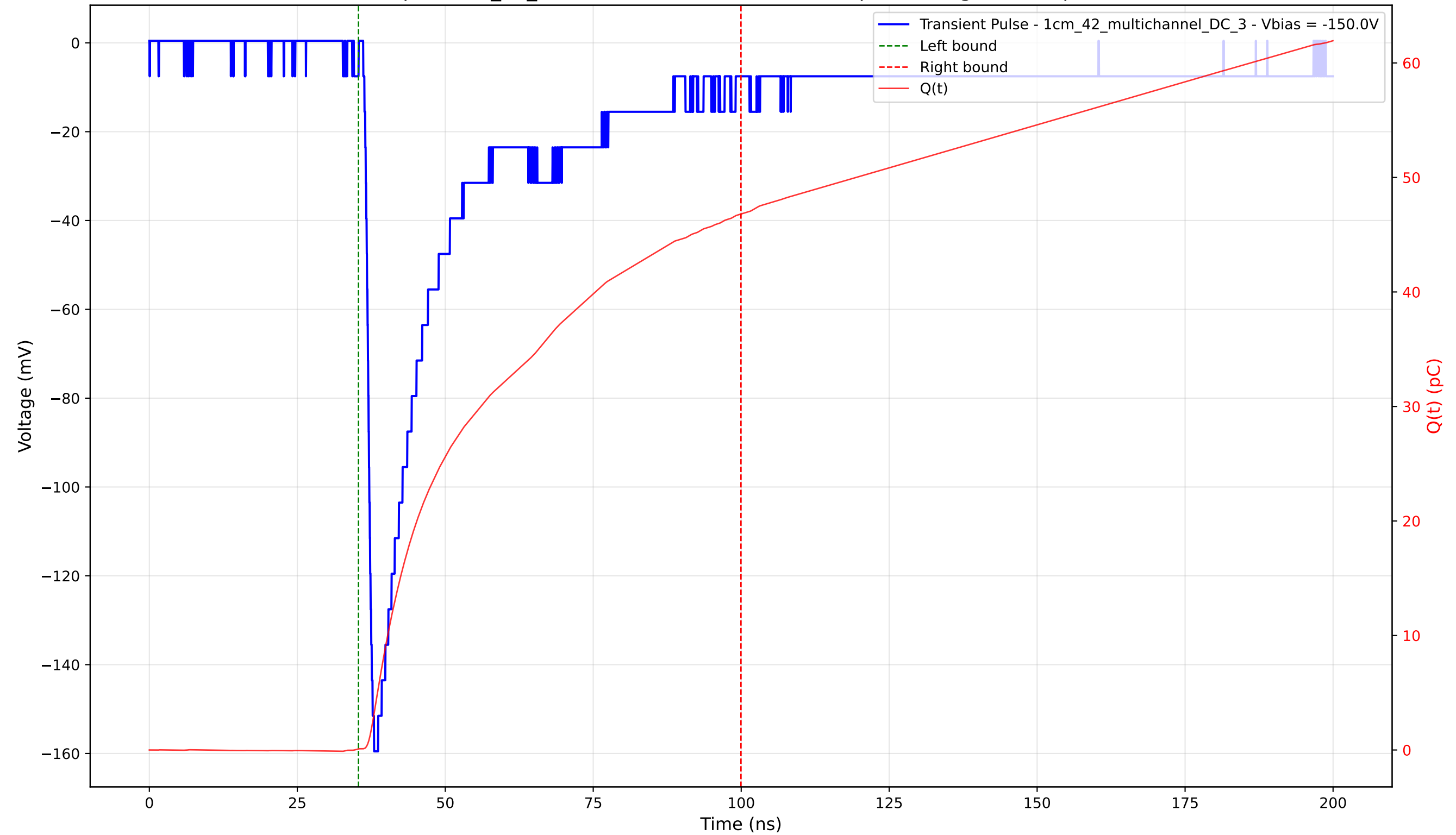
Transient Pulse - Sample: 1cm_42_multichannel - Position: 1150.0 \mu\text{m} - Charge: 46.70 pC - Rise Time: 1.26 ns
