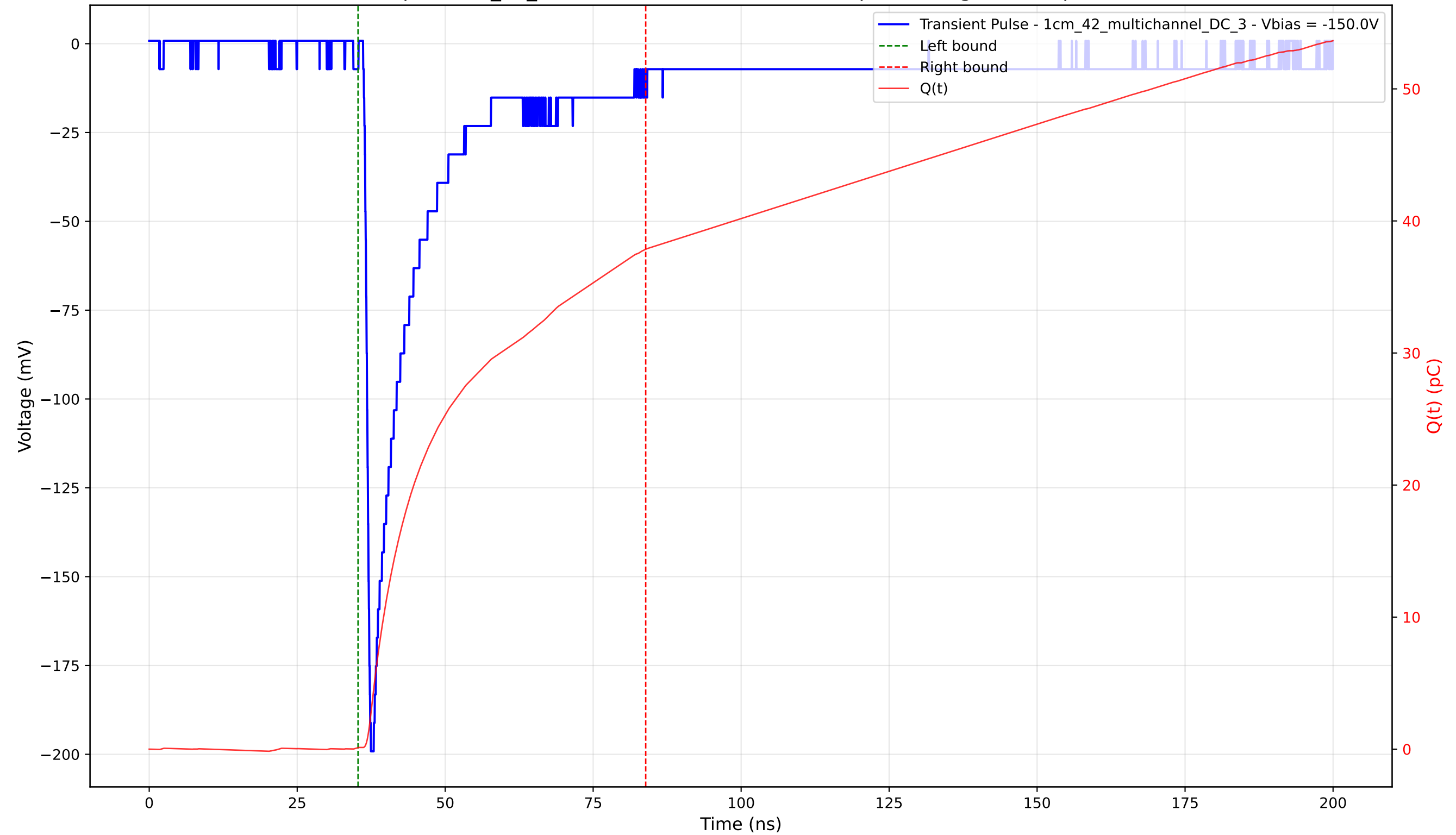
Transient Pulse - Sample: 1cm_42_multichannel - Position: 4275.0 \mu\text{m} - Charge: 37.73 pC - Rise Time: 0.93 ns
