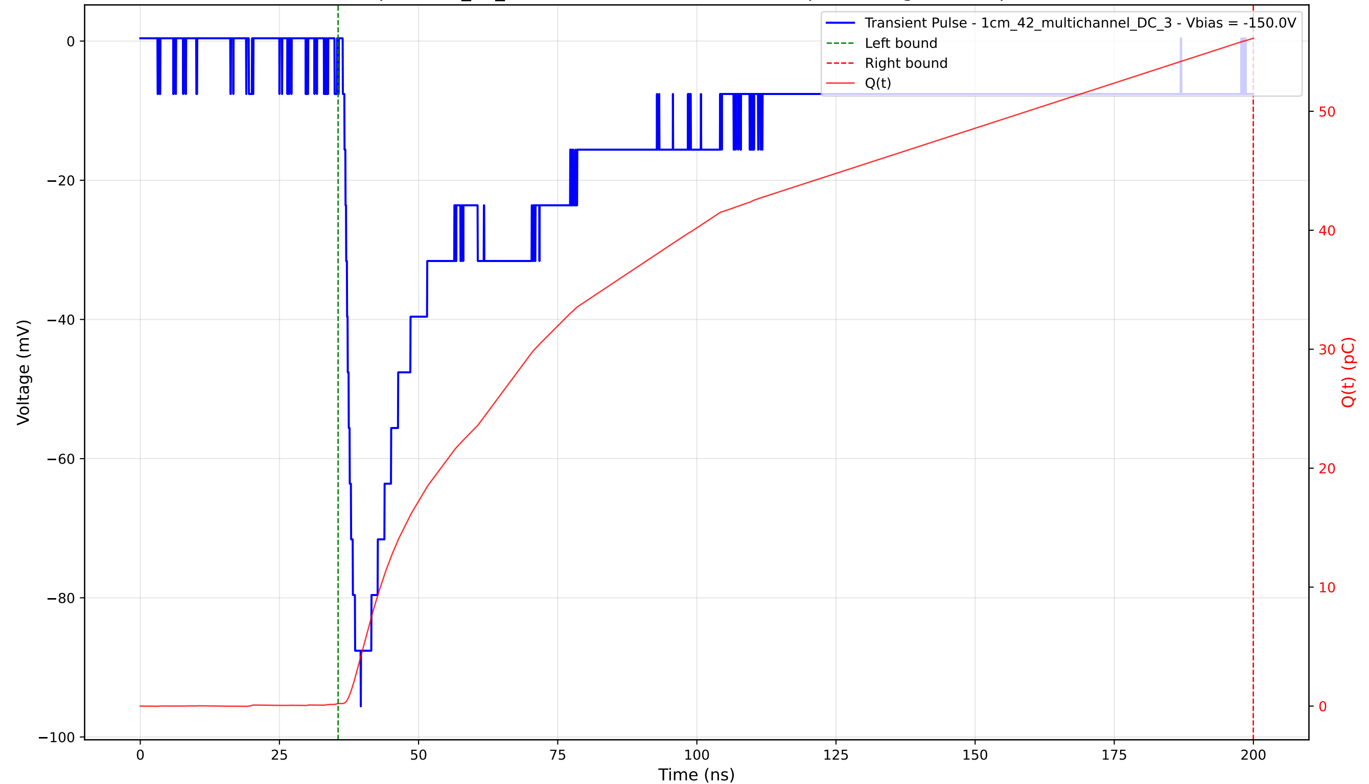
Transient Pulse - Sample: 1cm_42_multichannel - Position: 2775.0 \mu\text{m} - Charge: 55.94 pC - Rise Time: 1.92 ns
