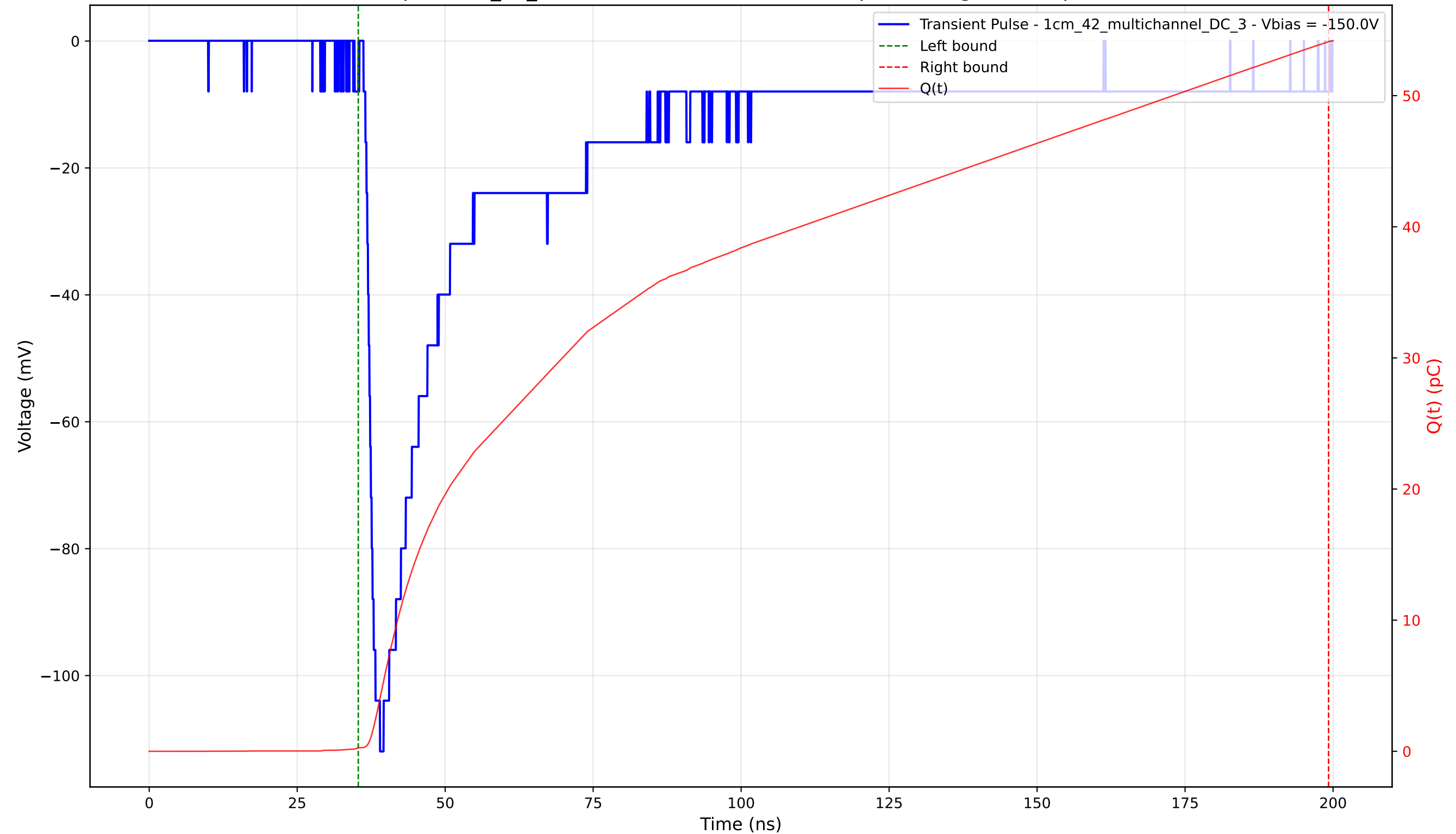
Transient Pulse - Sample: 1cm_42_multichannel - Position: 3305.0 \mu\text{m} - Charge: 53.85 pC - Rise Time: 1.71 ns
