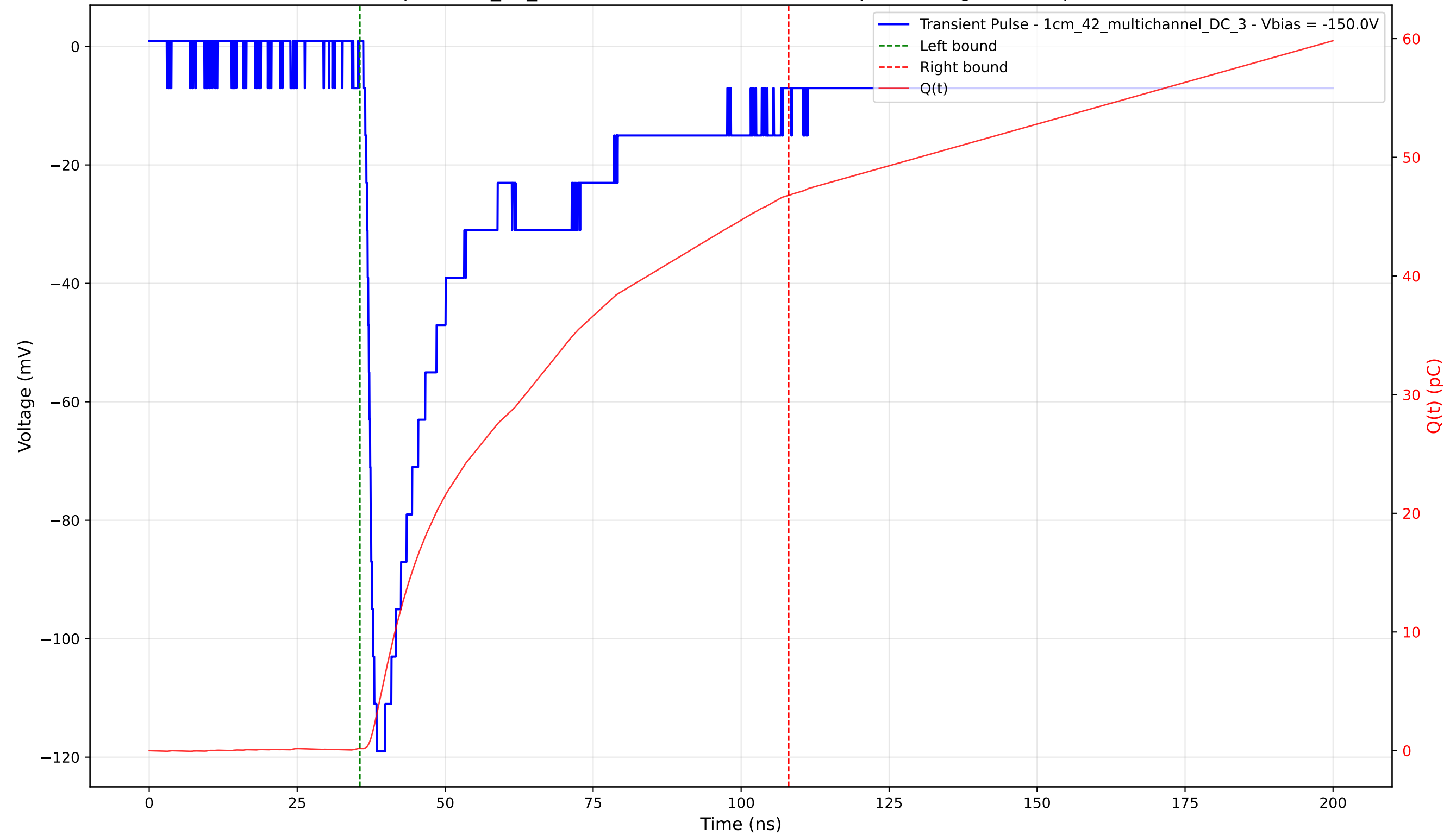
Transient Pulse - Sample: 1cm_42_multichannel - Position: 1660.0 \mu\text{m} - Charge: 46.60 pC - Rise Time: 1.53 ns
