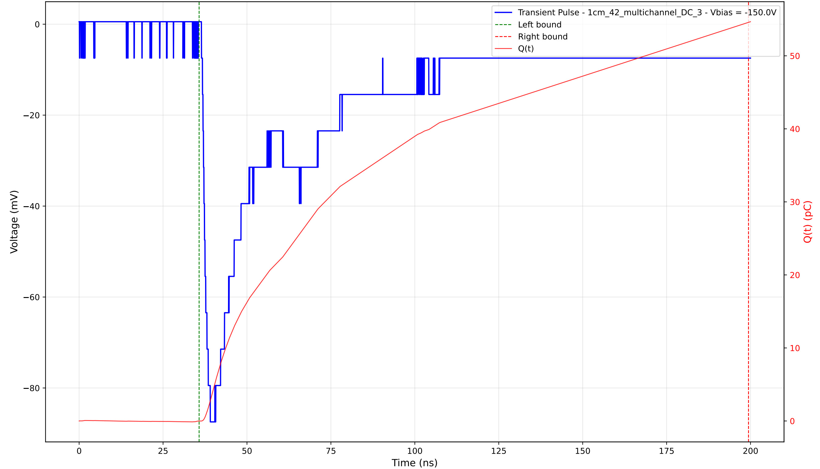
Transient Pulse - Sample: 1cm_42_multichannel - Position: 2670.0 \mu\text{m} - Charge: 54.59 pC - Rise Time: 1.74 ns
