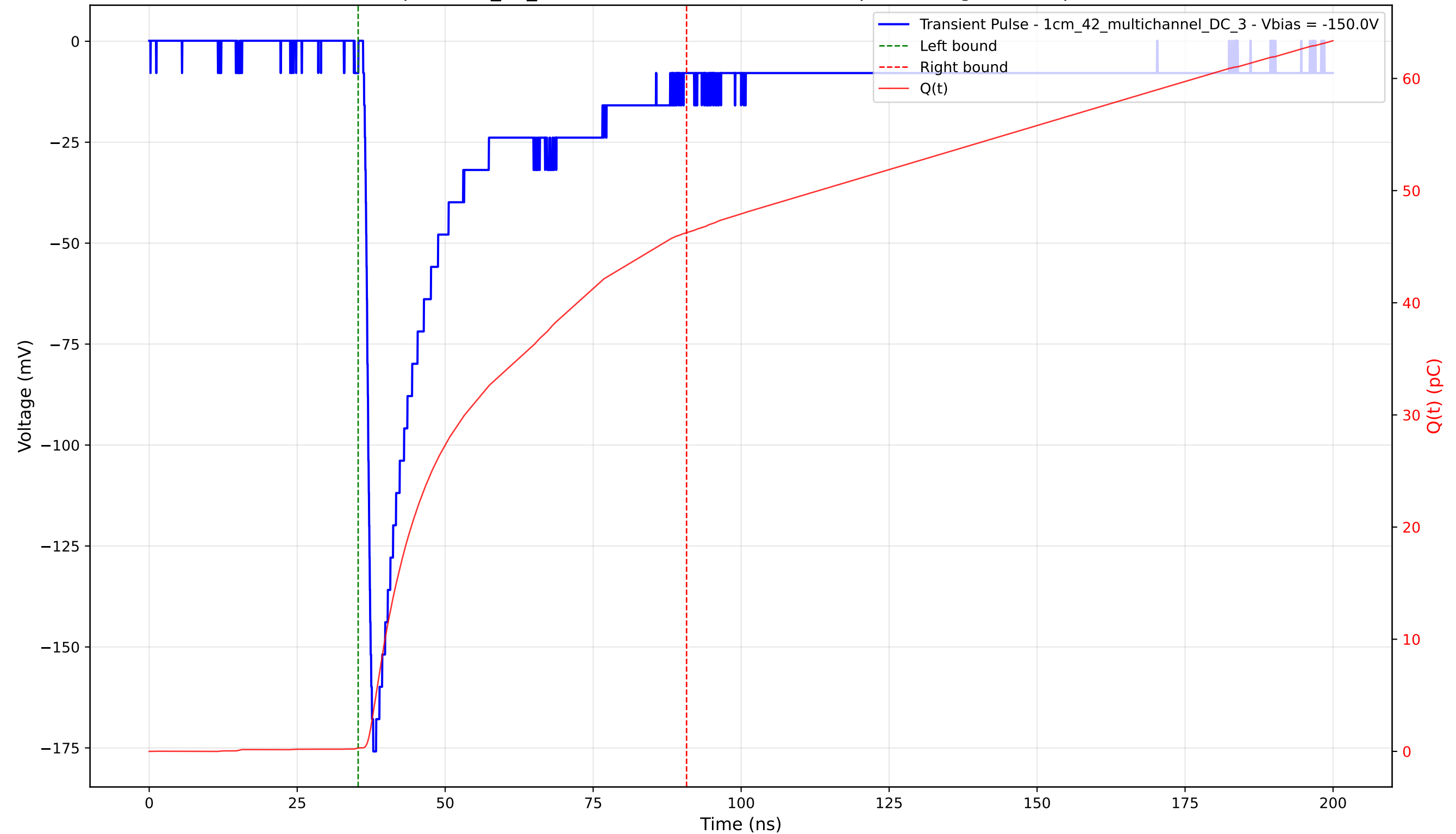
Transient Pulse - Sample: 1cm_42_multichannel - Position: 1020.0 \mu\text{m} - Charge: 45.95 pC - Rise Time: 1.10 ns
