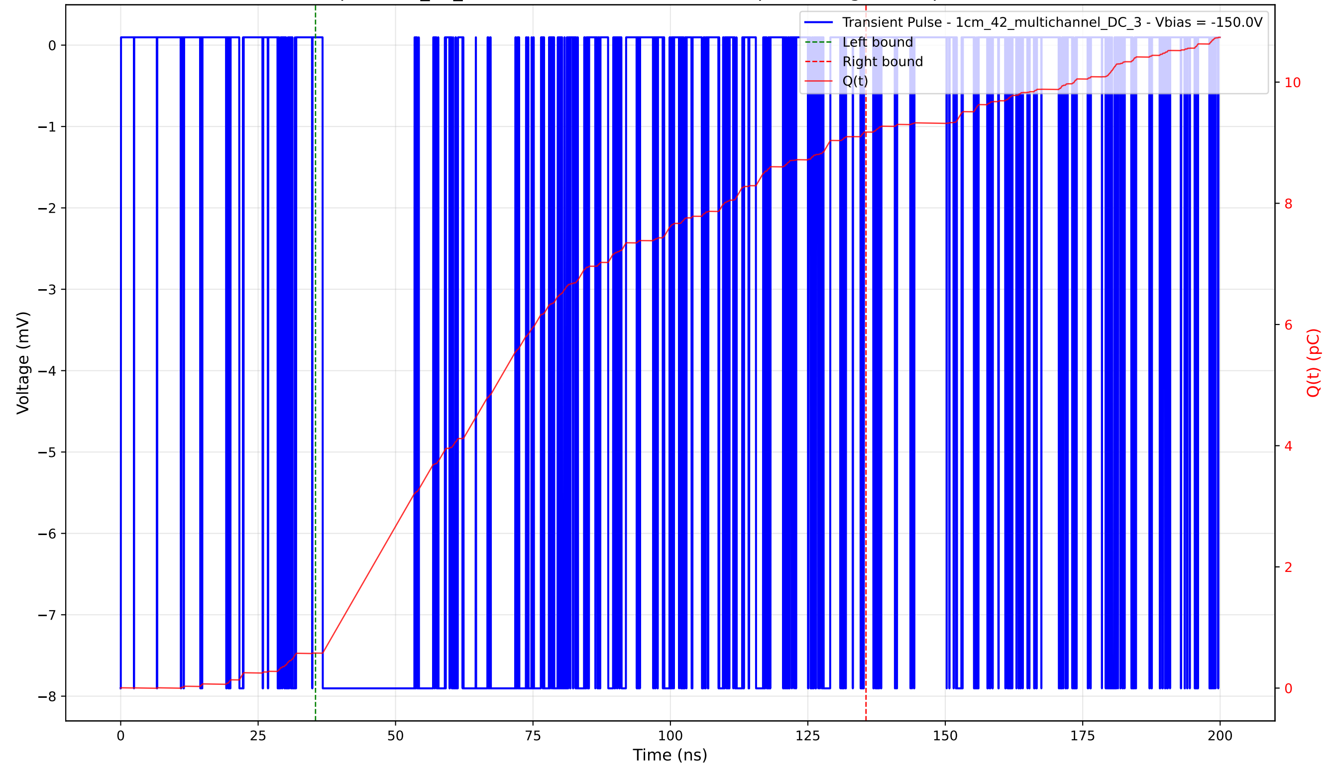
Transient Pulse - Sample: 1cm_42_multichannel - Position: 1875.0 \mu\text{m} - Charge: 8.60 pC - Rise Time: 0.00 ns (N/A)
