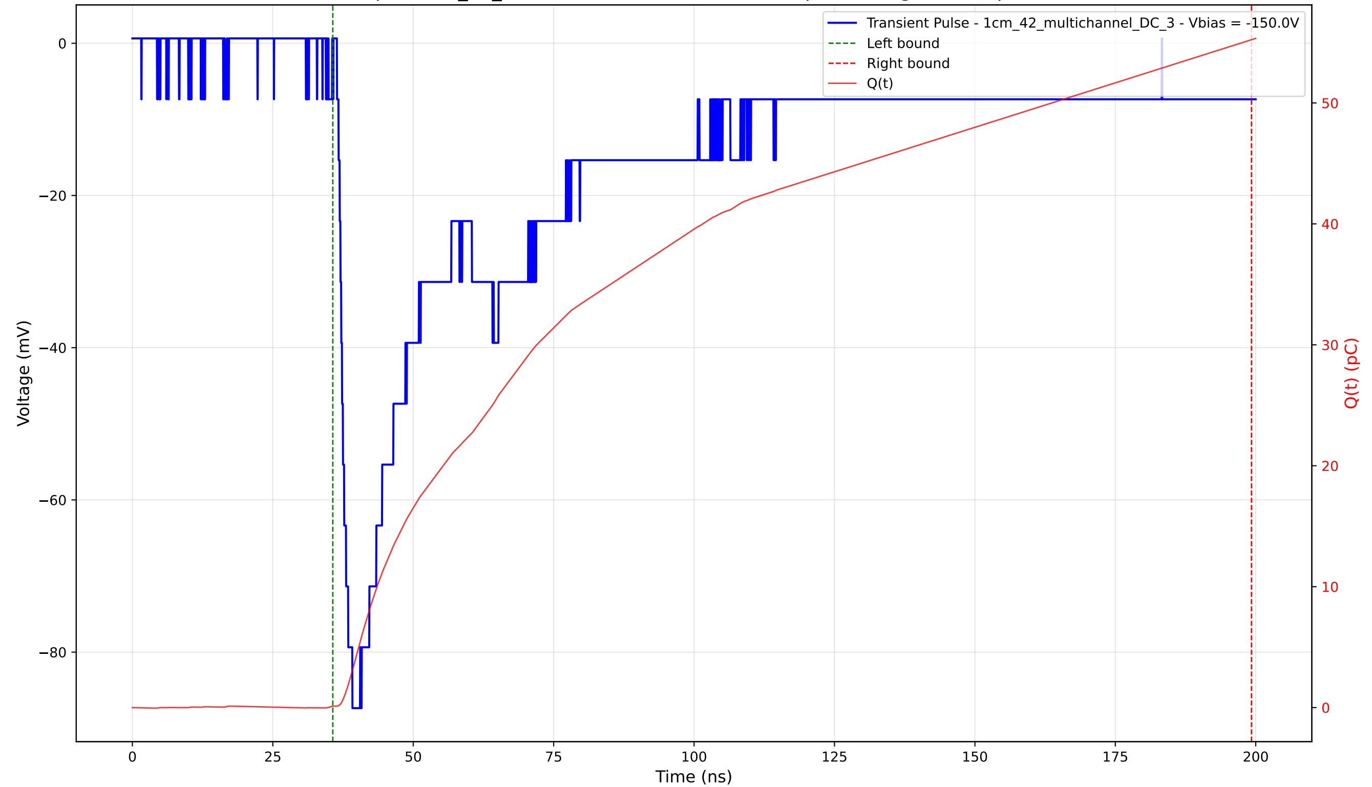
Transient Pulse - Sample: 1cm_42_multichannel - Position: 2665.0 \mu\text{m} - Charge: 55.12 pC - Rise Time: 1.74 ns
