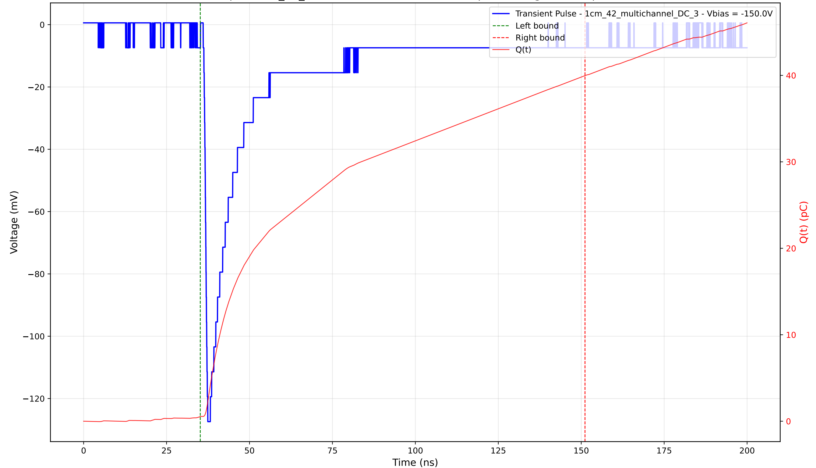
Transient Pulse - Sample: 1cm_42_multichannel - Position: 800.0 \mu\text{m} - Charge: 39.43 pC - Rise Time: 1.03 ns
