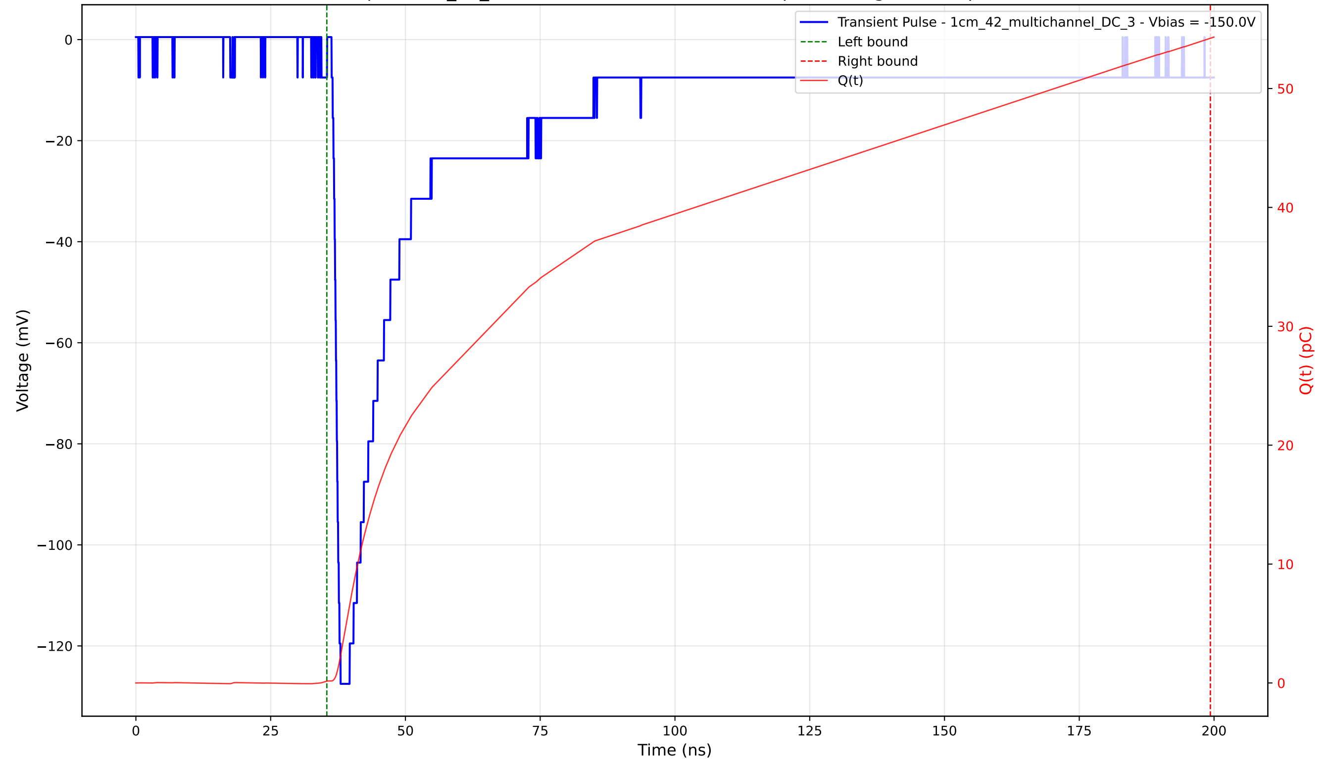
Transient Pulse - Sample: 1cm_42_multichannel - Position: 3650.0 \mu\text{m} - Charge: 54.06 pC - Rise Time: 1.27 ns
