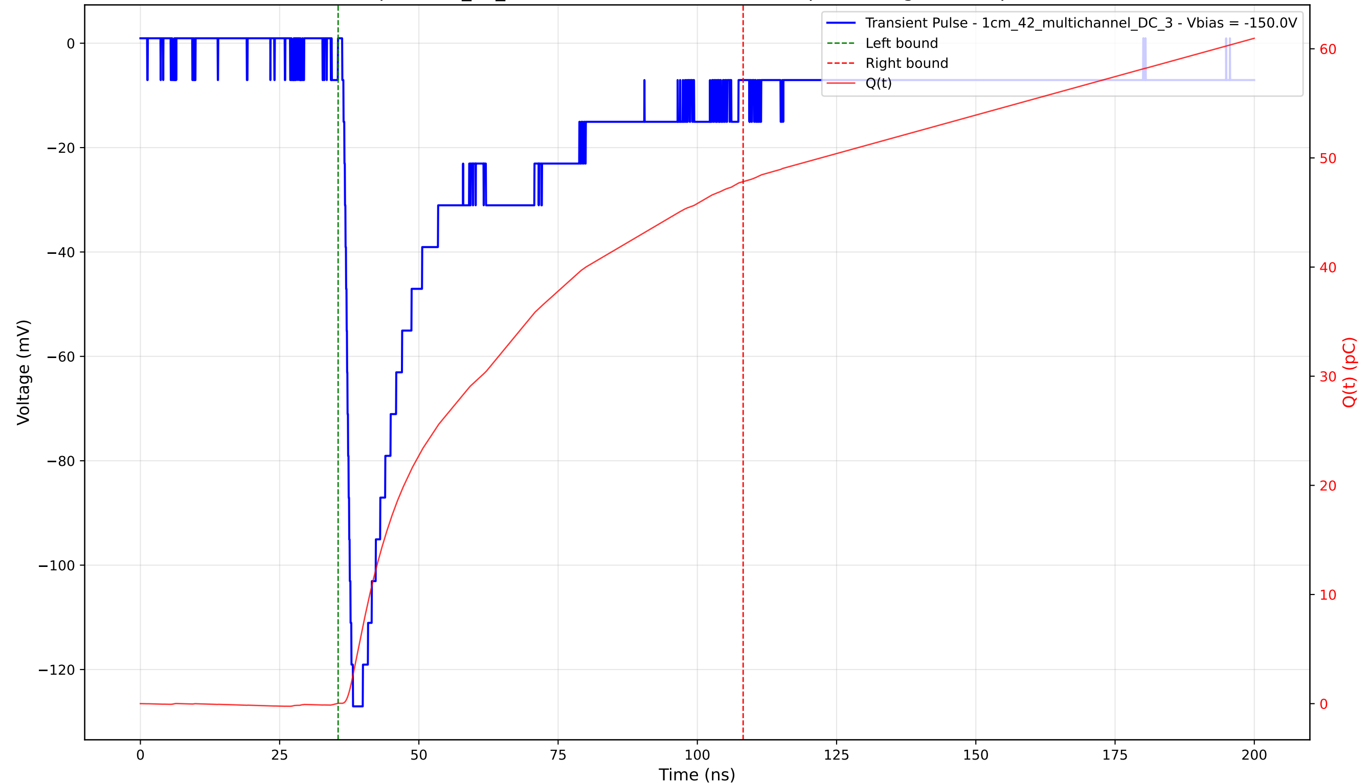
Transient Pulse - Sample: 1cm_42_multichannel - Position: 1530.0 \mu\text{m} - Charge: 47.79 pC - Rise Time: 1.43 ns
