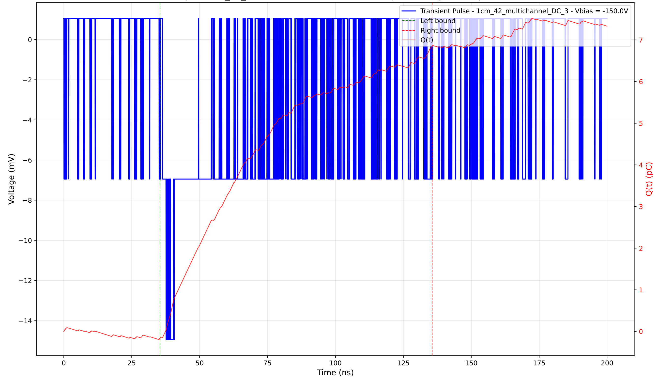
Transient Pulse - Sample: 1cm_42_multichannel - Position: 3875.0 \mu\text{m} - Charge: 7.01 pC - Rise Time: 1.30 ns
