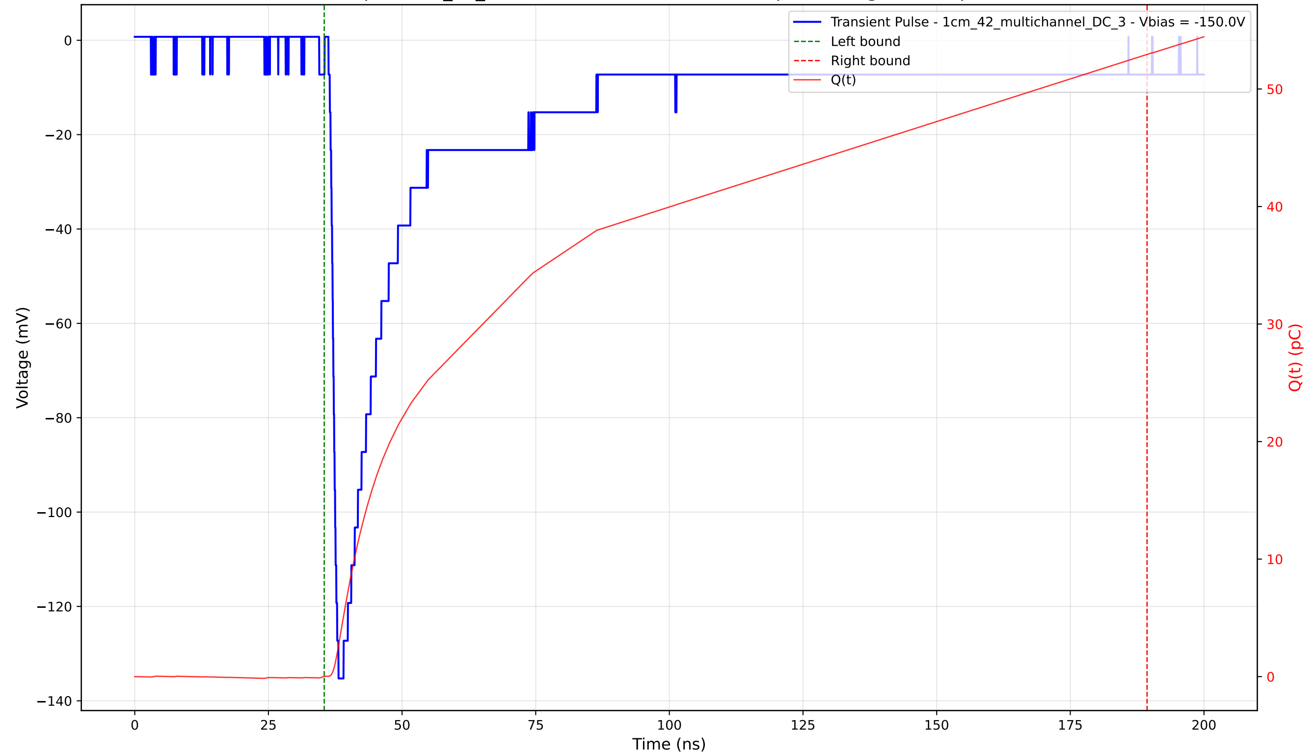
Transient Pulse - Sample: 1cm_42_multichannel - Position: 3685.0 \mu\text{m} - Charge: 52.93 pC - Rise Time: 1.38 ns
