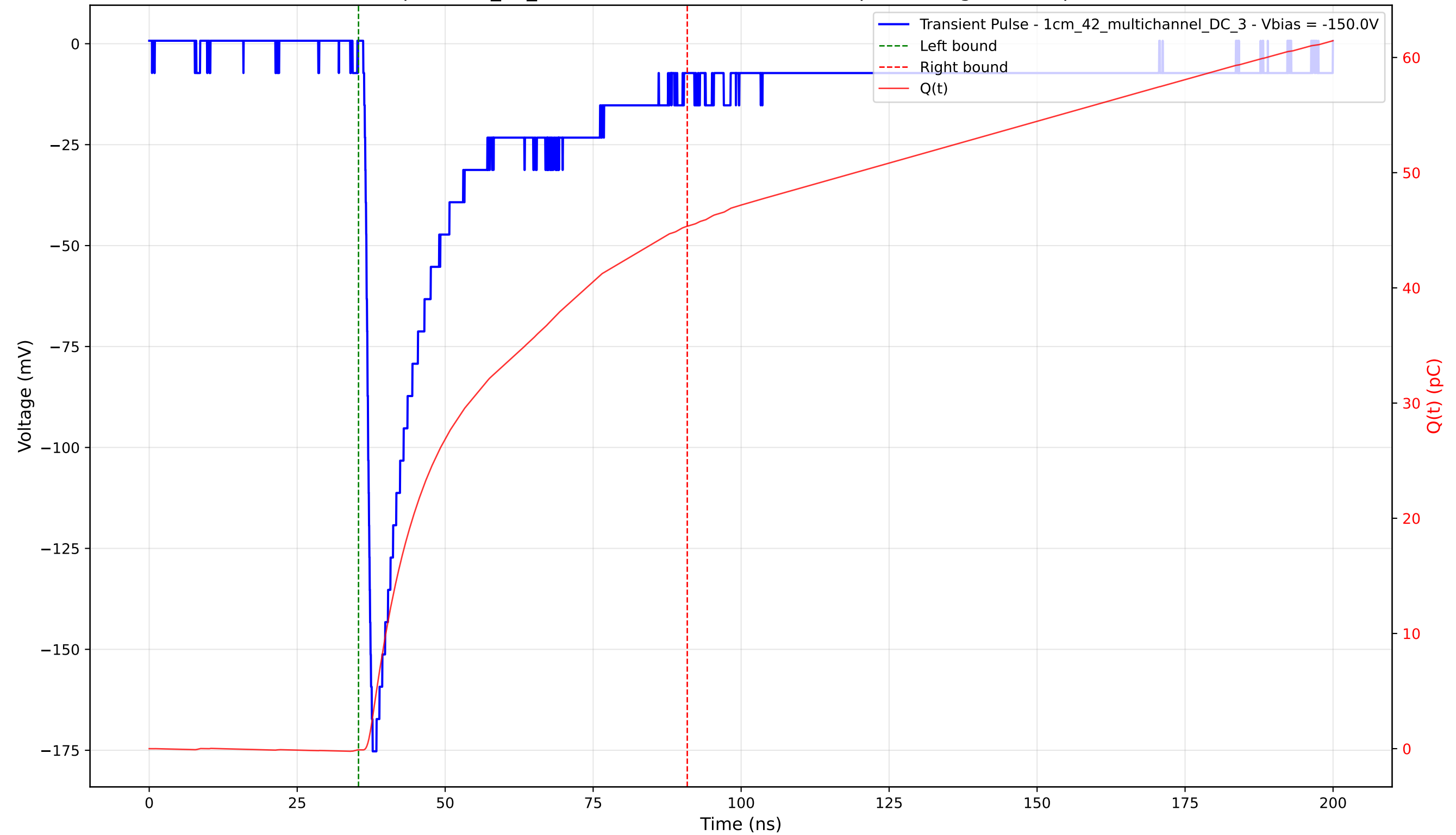
Transient Pulse - Sample: 1cm_42_multichannel - Position: 1010.0 \mu\text{m} - Charge: 45.45 pC - Rise Time: 1.05 ns
