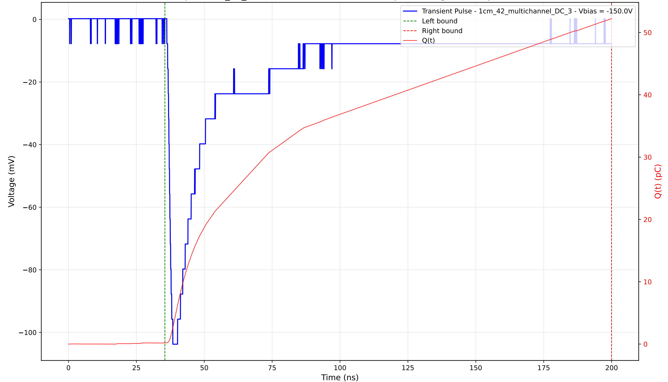
Transient Pulse - Sample: 1cm_42_multichannel - Position: 3310.0 \mu\text{m} - Charge: 52.02 pC - Rise Time: 1.51 ns
