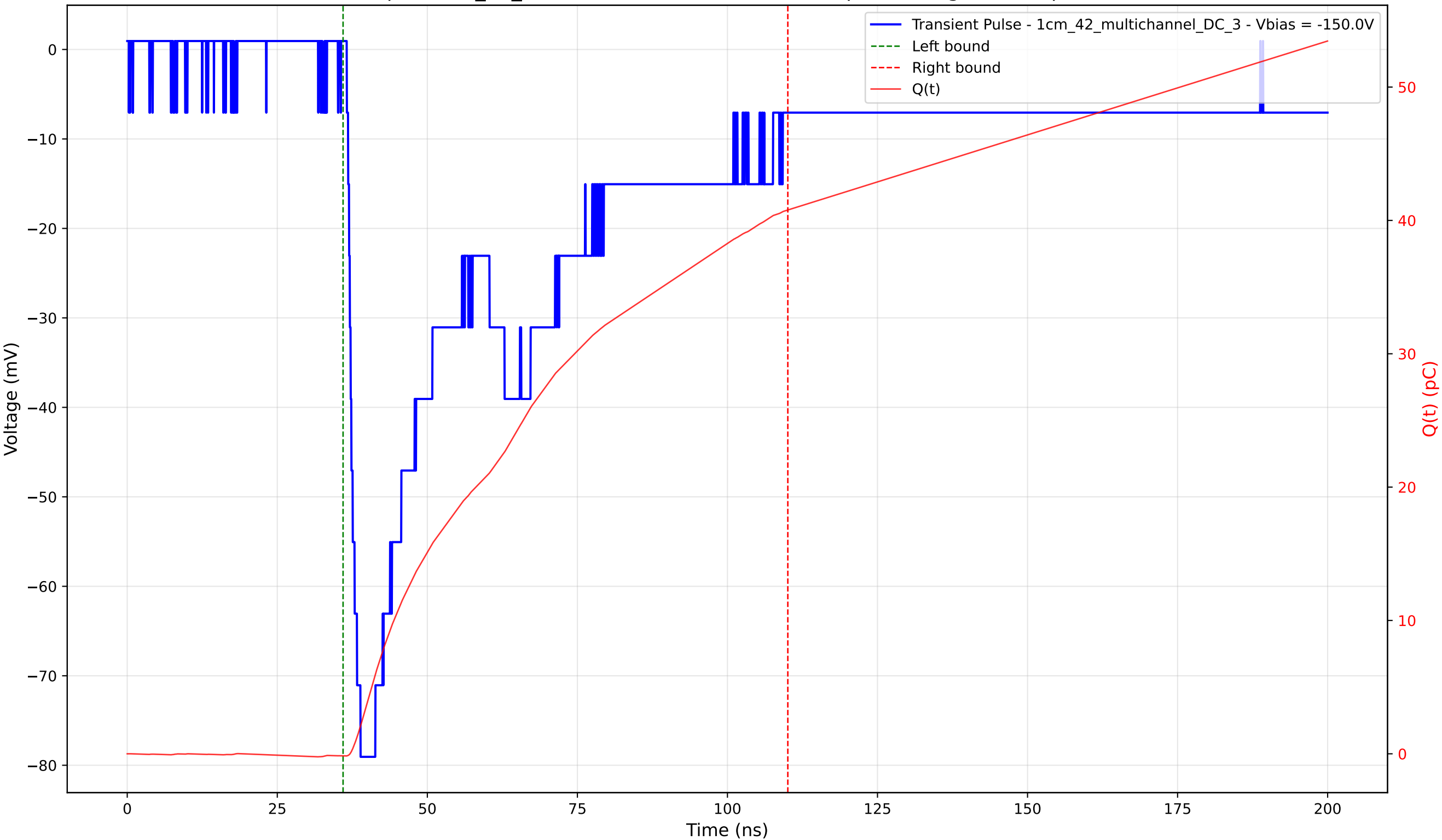
Transient Pulse - Sample: 1cm_42_multichannel - Position: 2520.0 \mu\text{m} - Charge: 40.93 pC - Rise Time: 2.08 ns
