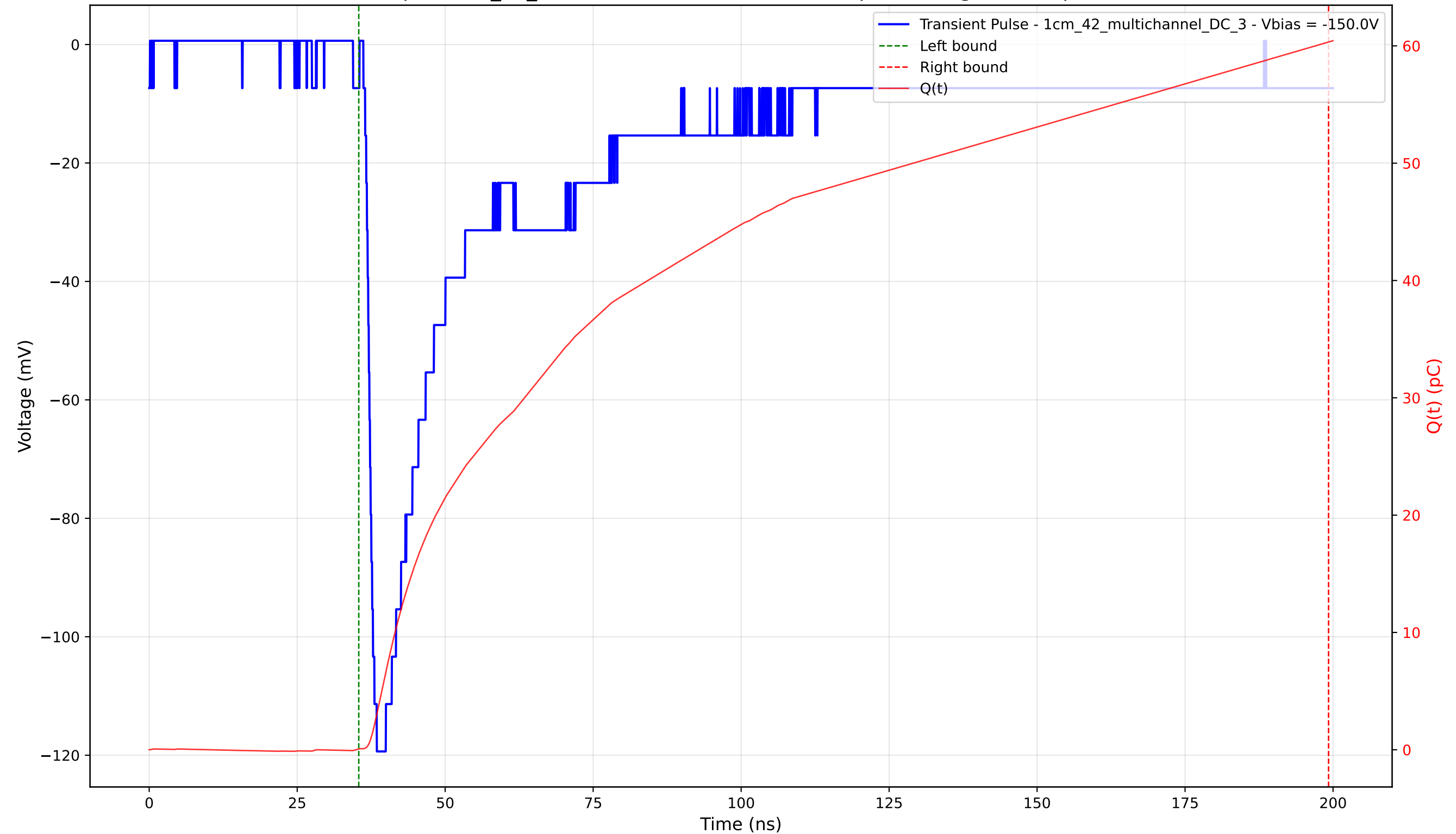
Transient Pulse - Sample: 1cm_42_multichannel - Position: 1645.0 \mu\text{m} - Charge: 60.26 pC - Rise Time: 1.57 ns
