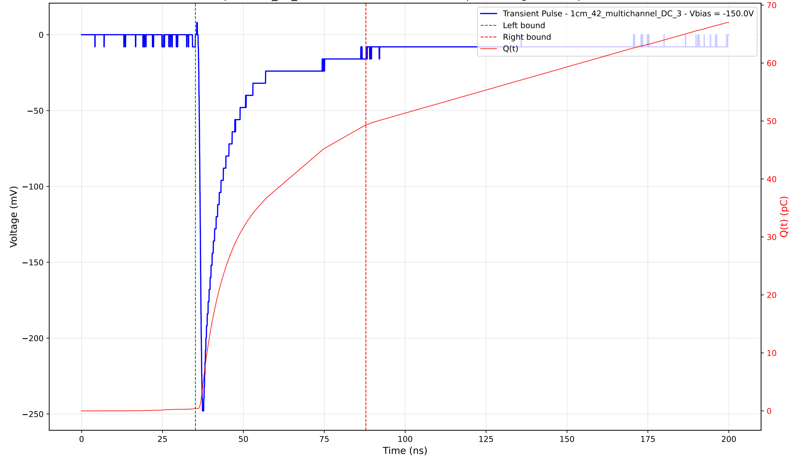
Transient Pulse - Sample: 1cm_42_multichannel - Position: 580.0 \mu\text{m} - Charge: 48.89 pC - Rise Time: 0.90 ns
