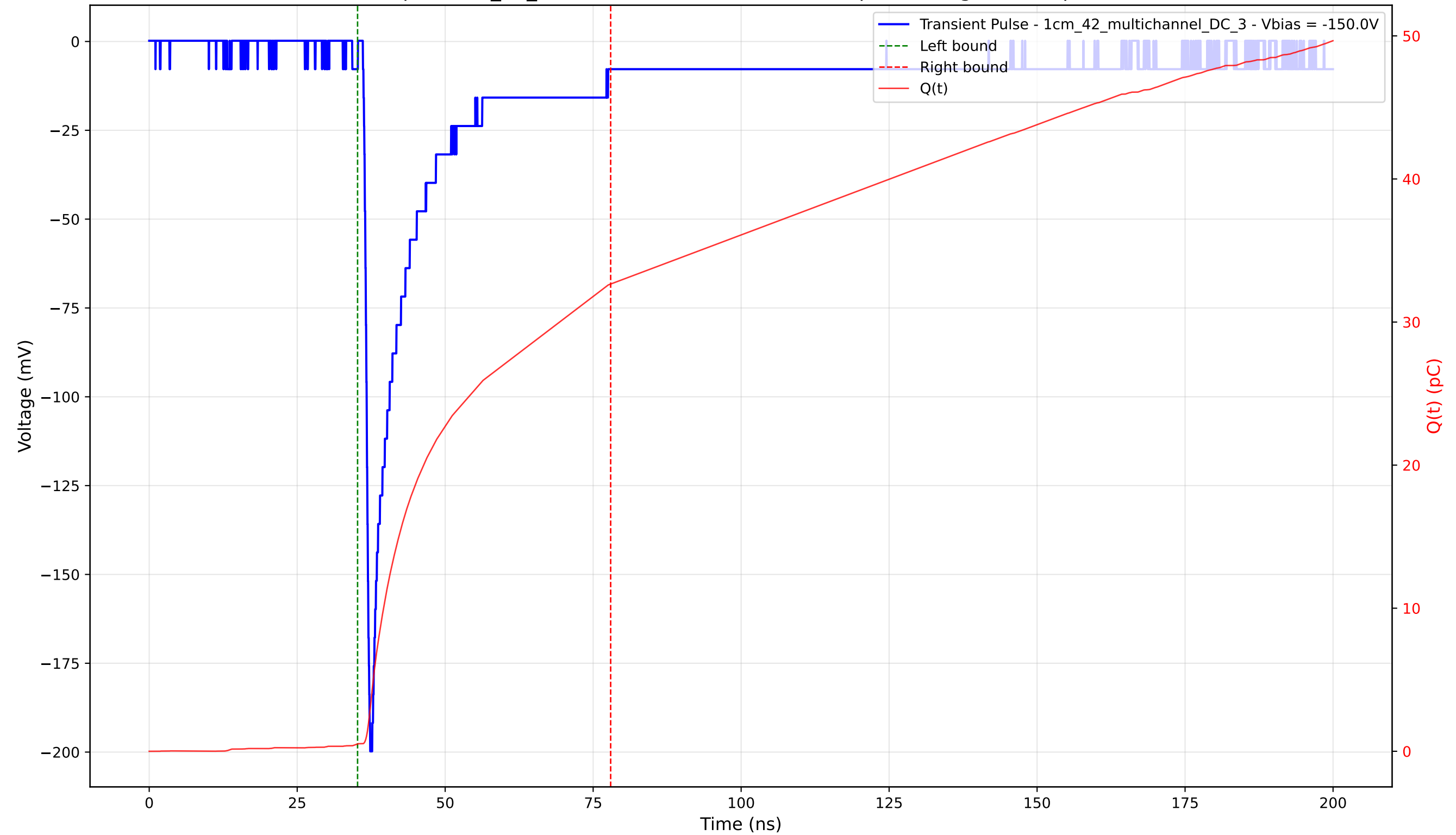
Transient Pulse - Sample: 1cm_42_multichannel - Position: 4460.0 \mu\text{m} - Charge: 32.14 pC - Rise Time: 0.89 ns
