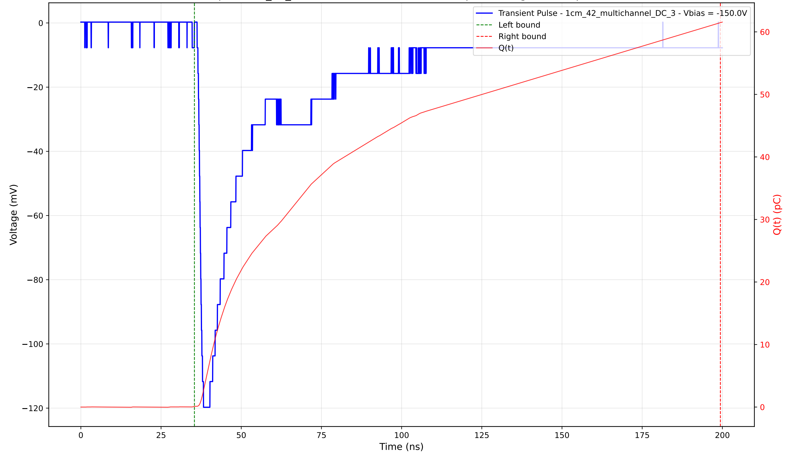
Transient Pulse - Sample: 1cm_42_multichannel - Position: 1600.0 \mu\text{m} - Charge: 61.35 pC - Rise Time: 1.43 ns
