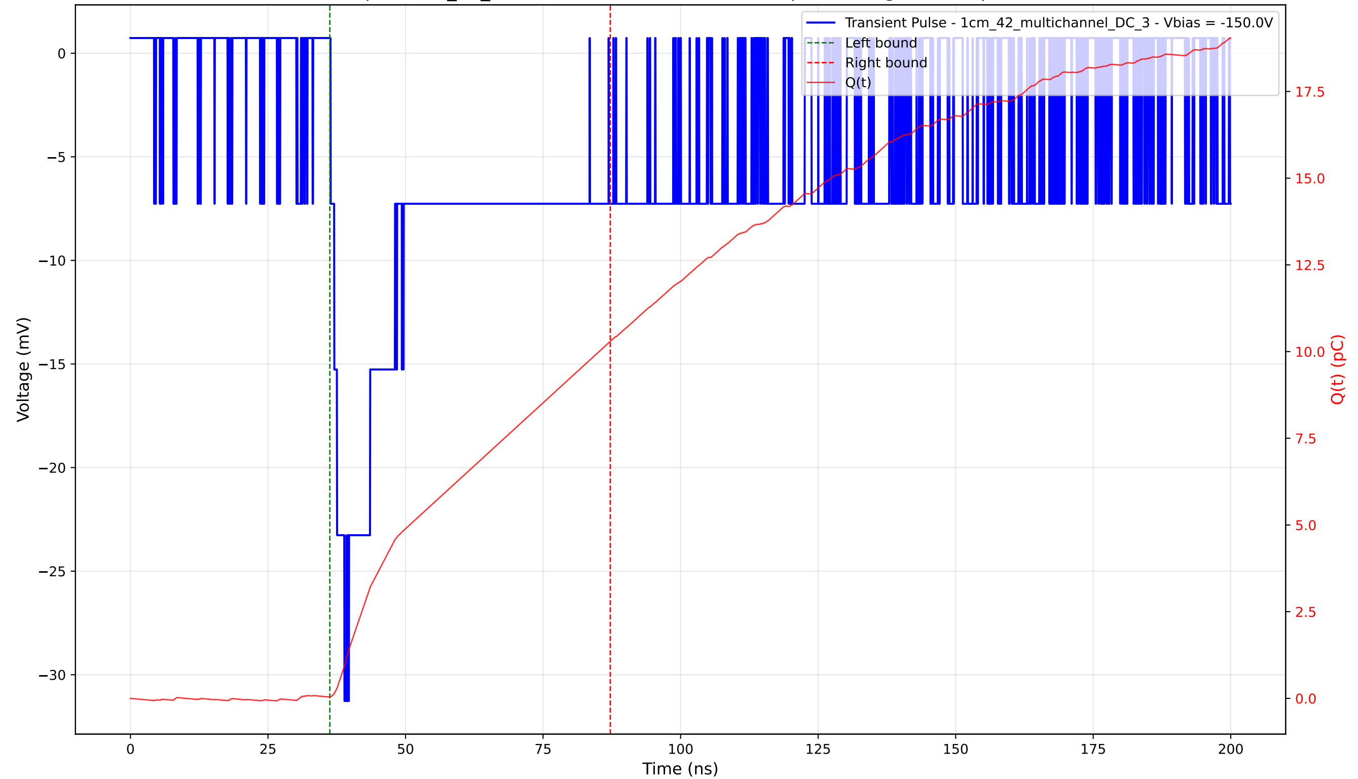
Transient Pulse - Sample: 1cm_42_multichannel - Position: 3350.0 \mu\text{m} - Charge: 10.26 pC - Rise Time: 2.51 ns
