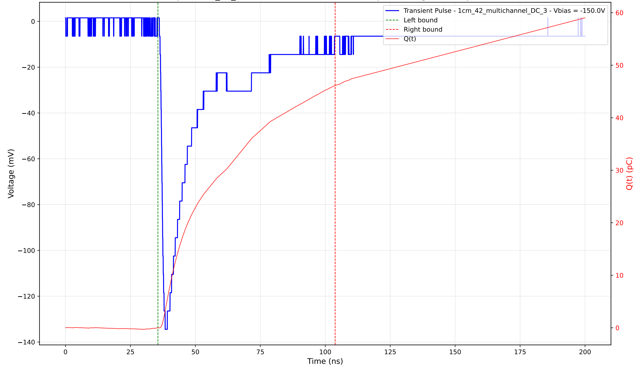
Transient Pulse - Sample: 1cm_42_multichannel - Position: 1455.0 \mu\text{m} - Charge: 46.17 pC - Rise Time: 1.54 ns
