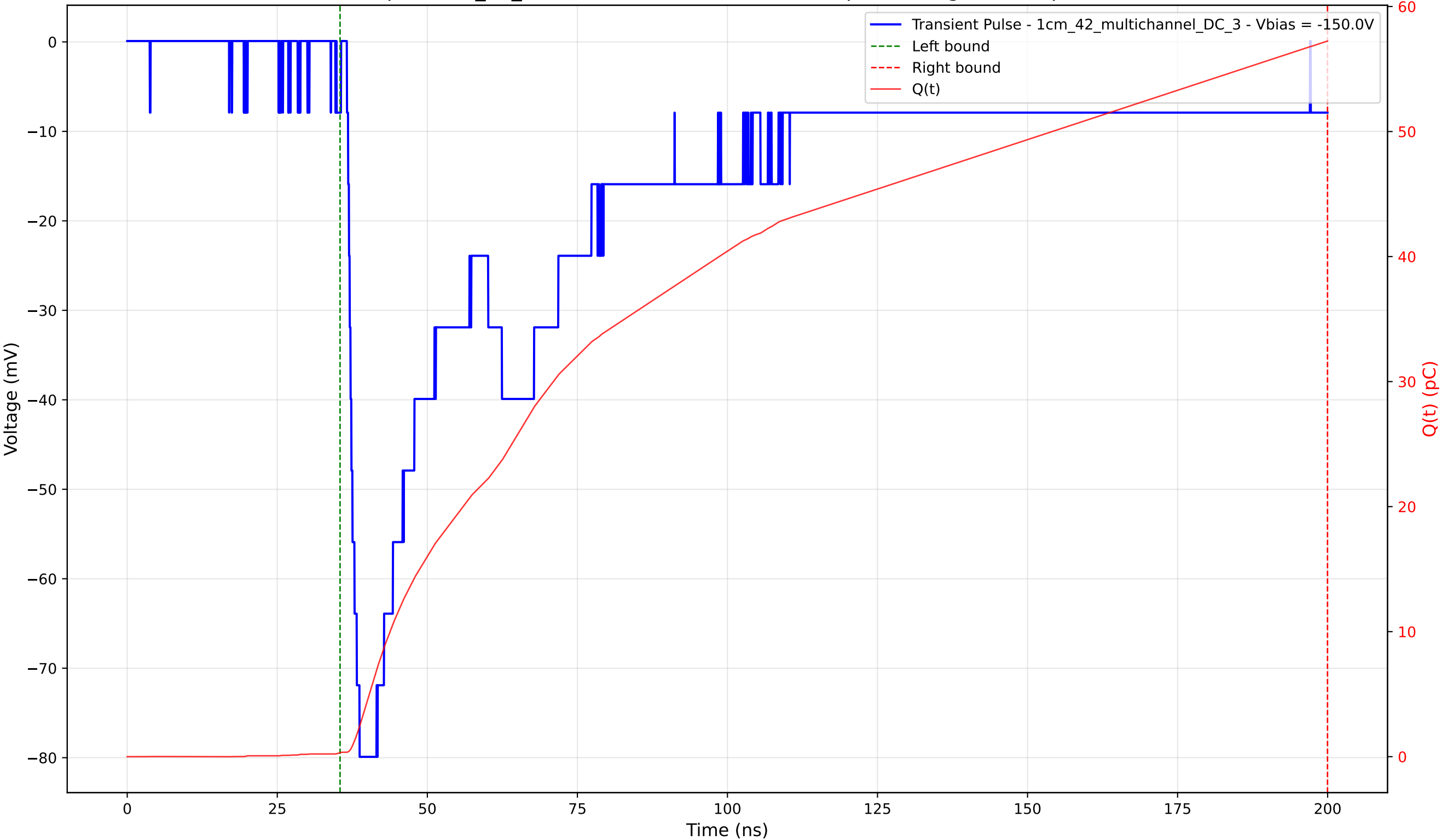
Transient Pulse - Sample: 1cm_42_multichannel - Position: 2495.0 \mu\text{m} - Charge: 56.91 pC - Rise Time: 1.92 ns
