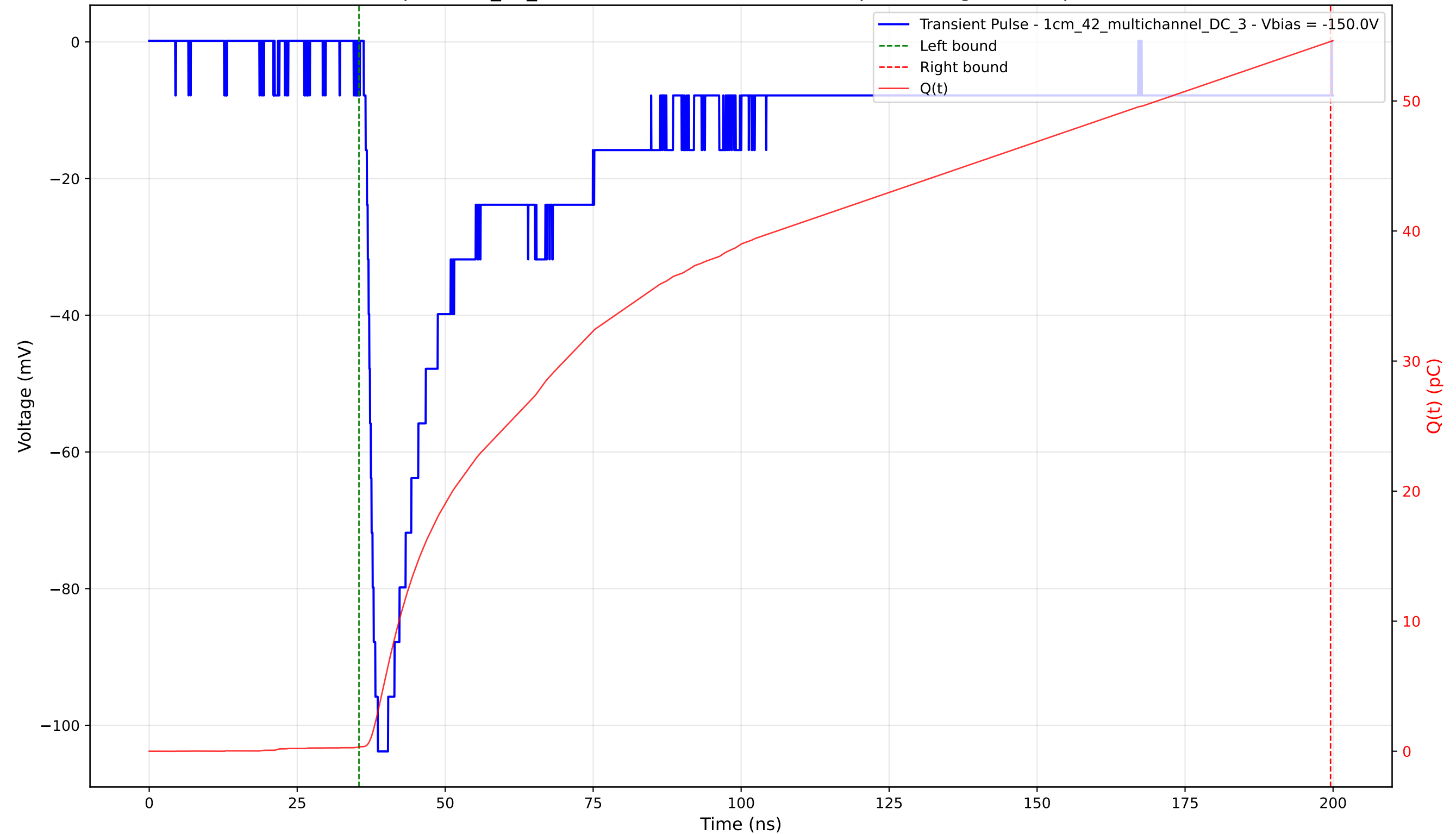
Transient Pulse - Sample: 1cm_42_multichannel - Position: 3160.0 \mu\text{m} - Charge: 54.25 pC - Rise Time: 1.65 ns
