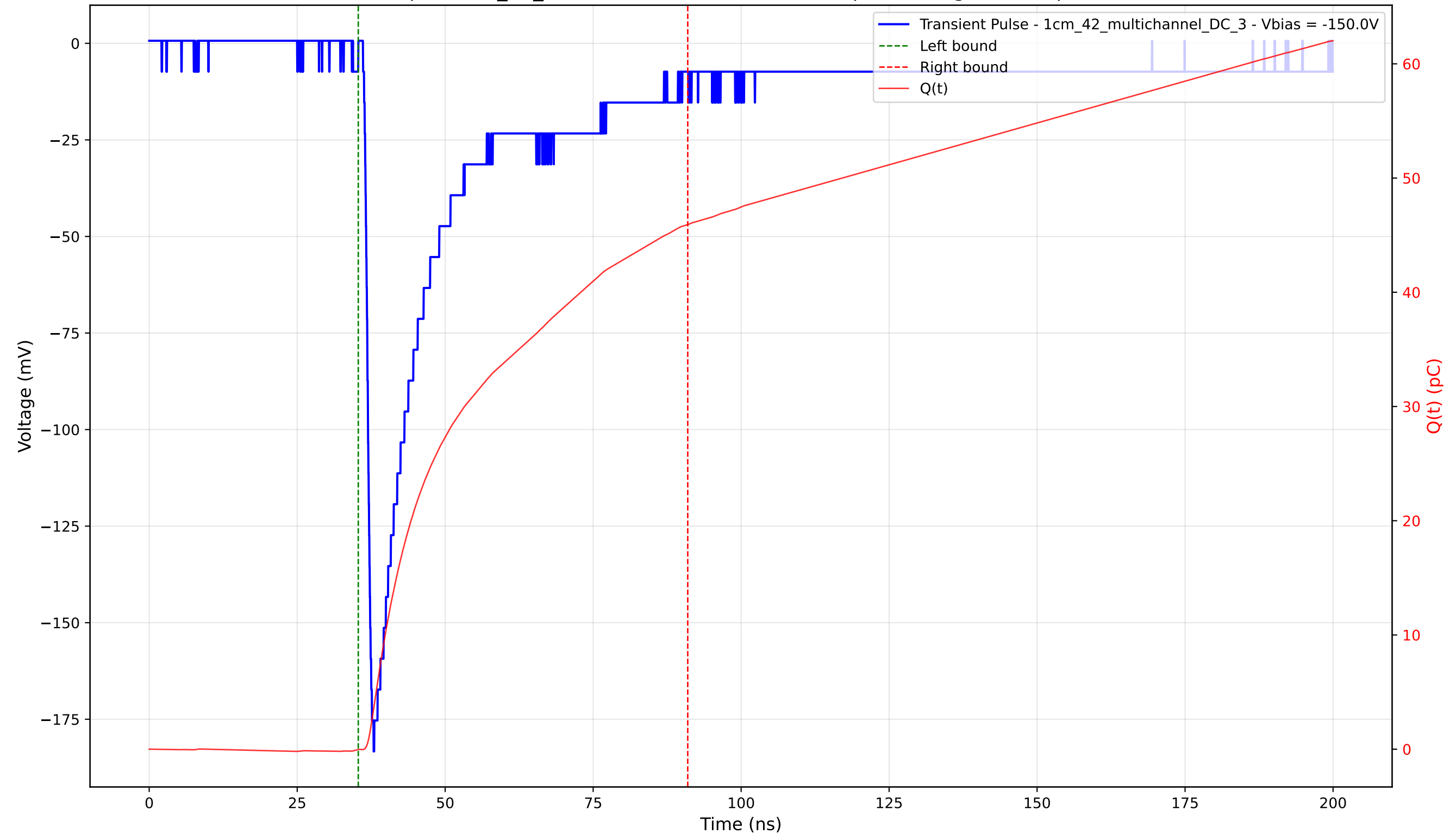
Transient Pulse - Sample: 1cm_42_multichannel - Position: 985.0 \mu\text{m} - Charge: 45.94 pC - Rise Time: 1.11 ns
