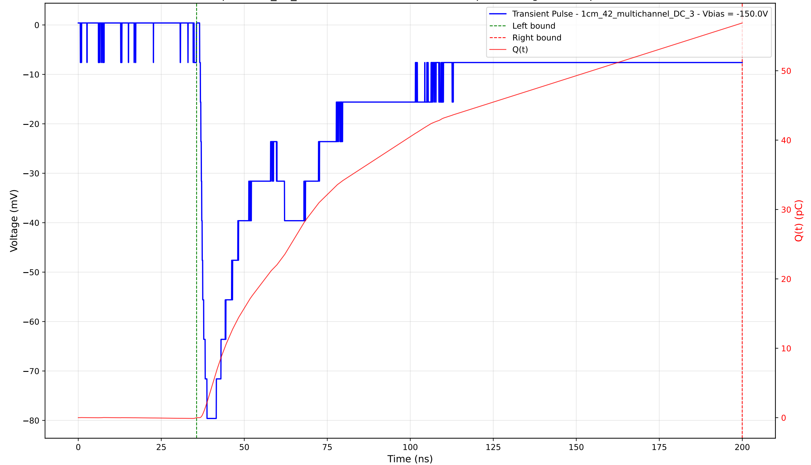
Transient Pulse - Sample: 1cm_42_multichannel - Position: 2280.0 \mu\text{m} - Charge: 56.89 pC - Rise Time: 2.00 ns
