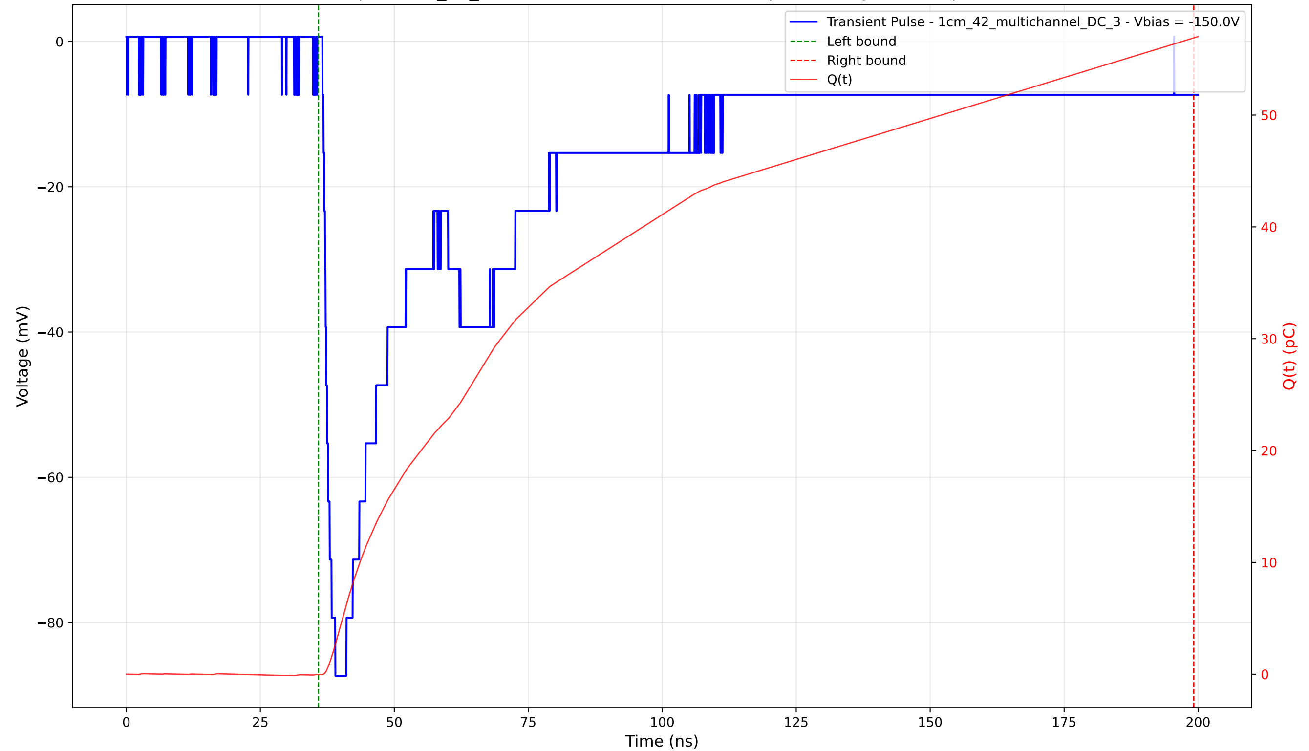
Transient Pulse - Sample: 1cm_42_multichannel - Position: 2200.0 \mu\text{m} - Charge: 56.92 pC - Rise Time: 1.52 ns
