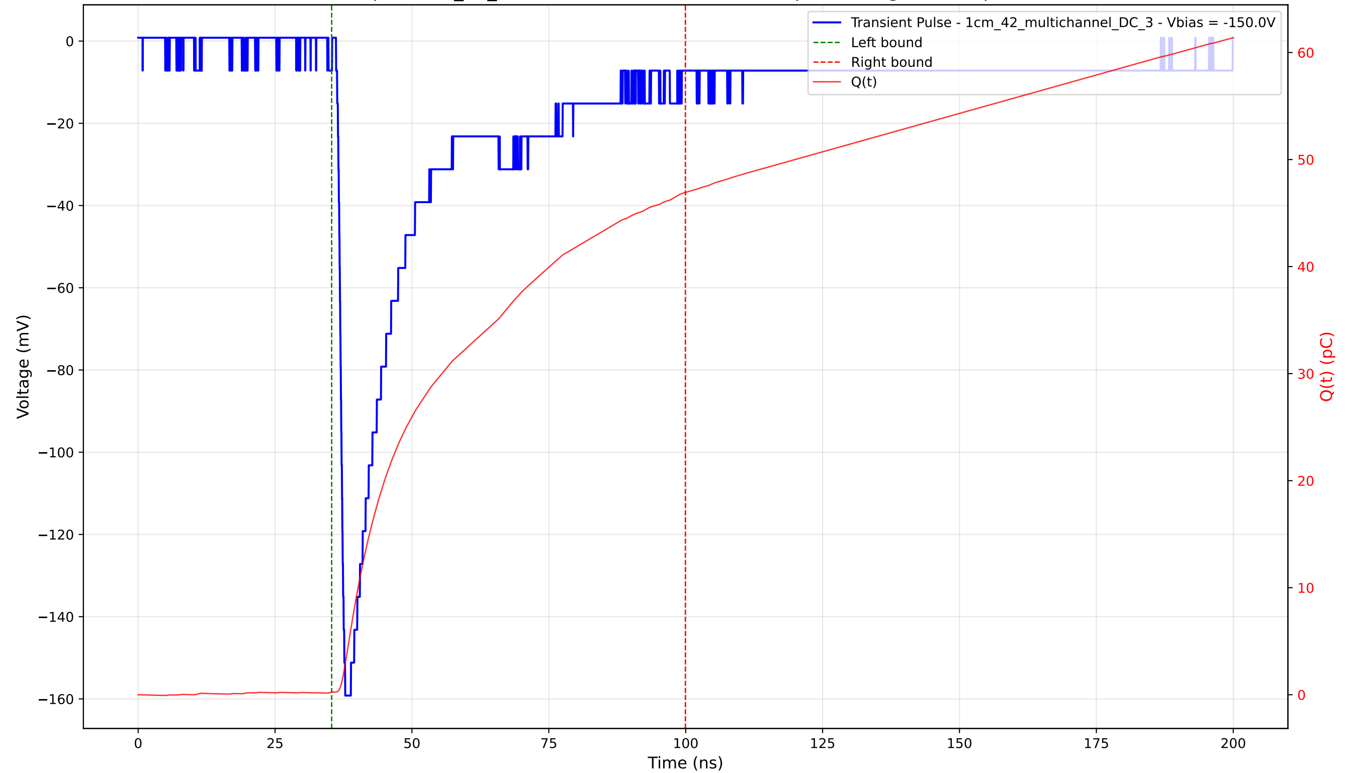
Transient Pulse - Sample: 1cm_42_multichannel - Position: 1125.0 \mu\text{m} - Charge: 46.68 pC - Rise Time: 1.18 ns
