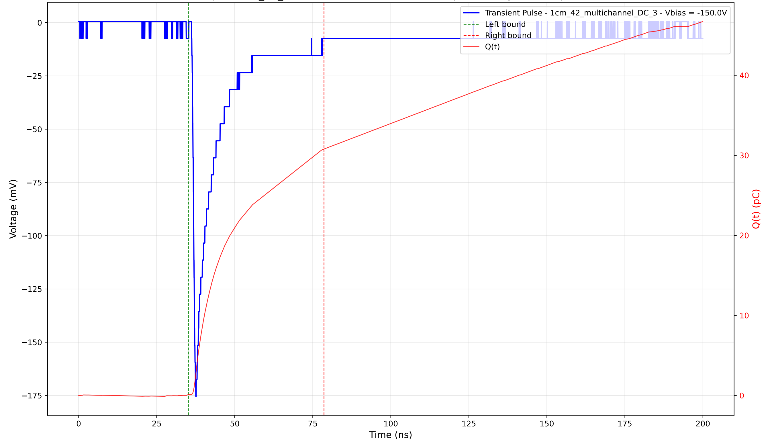
Transient Pulse - Sample: 1cm_42_multichannel - Position: 4320.0 \mu\text{m} - Charge: 30.66 pC - Rise Time: 0.91 ns
