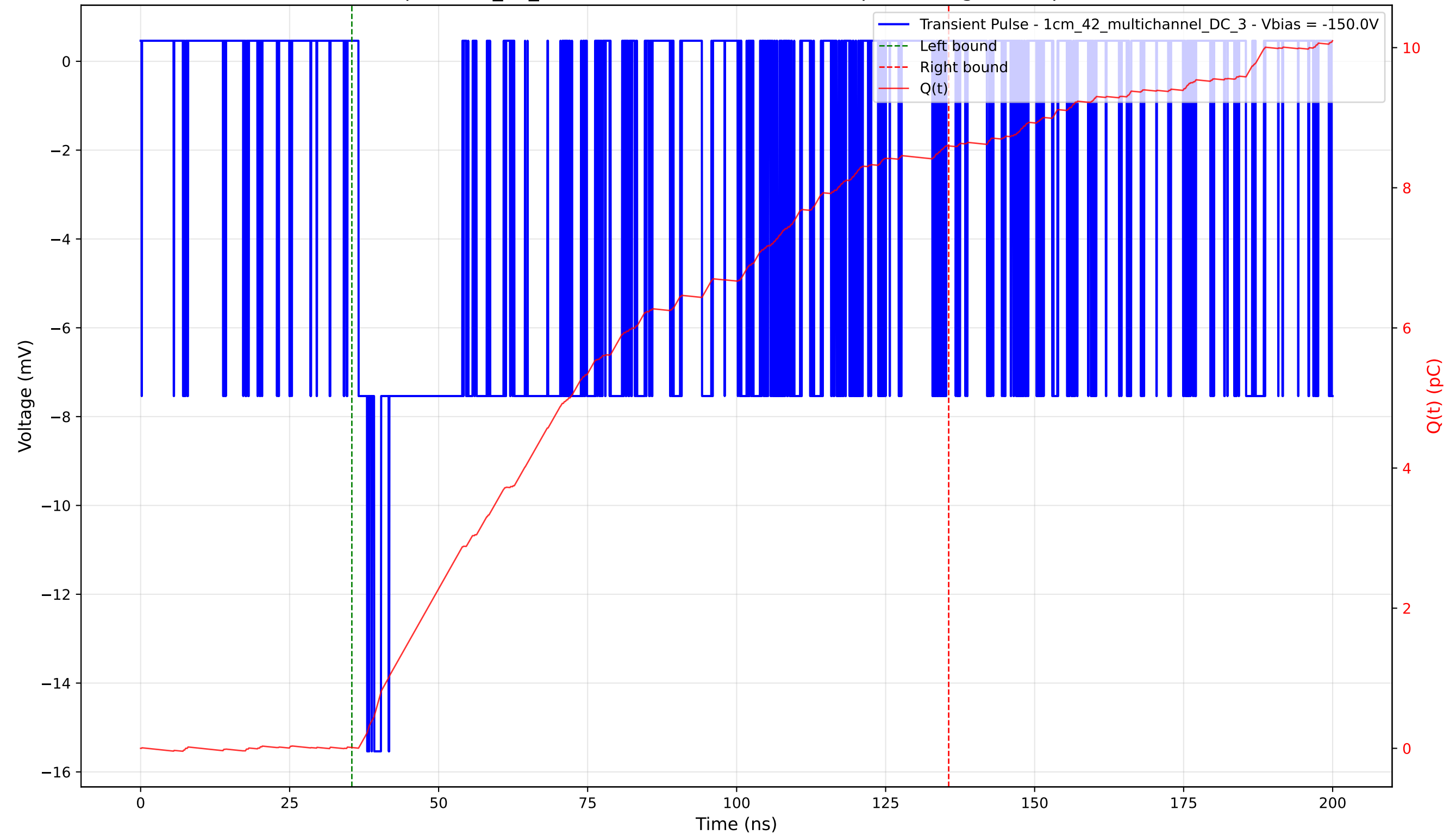
Transient Pulse - Sample: 1cm_42_multichannel - Position: 1375.0 \mu\text{m} - Charge: 8.59 pC - Rise Time: 1.46 ns
