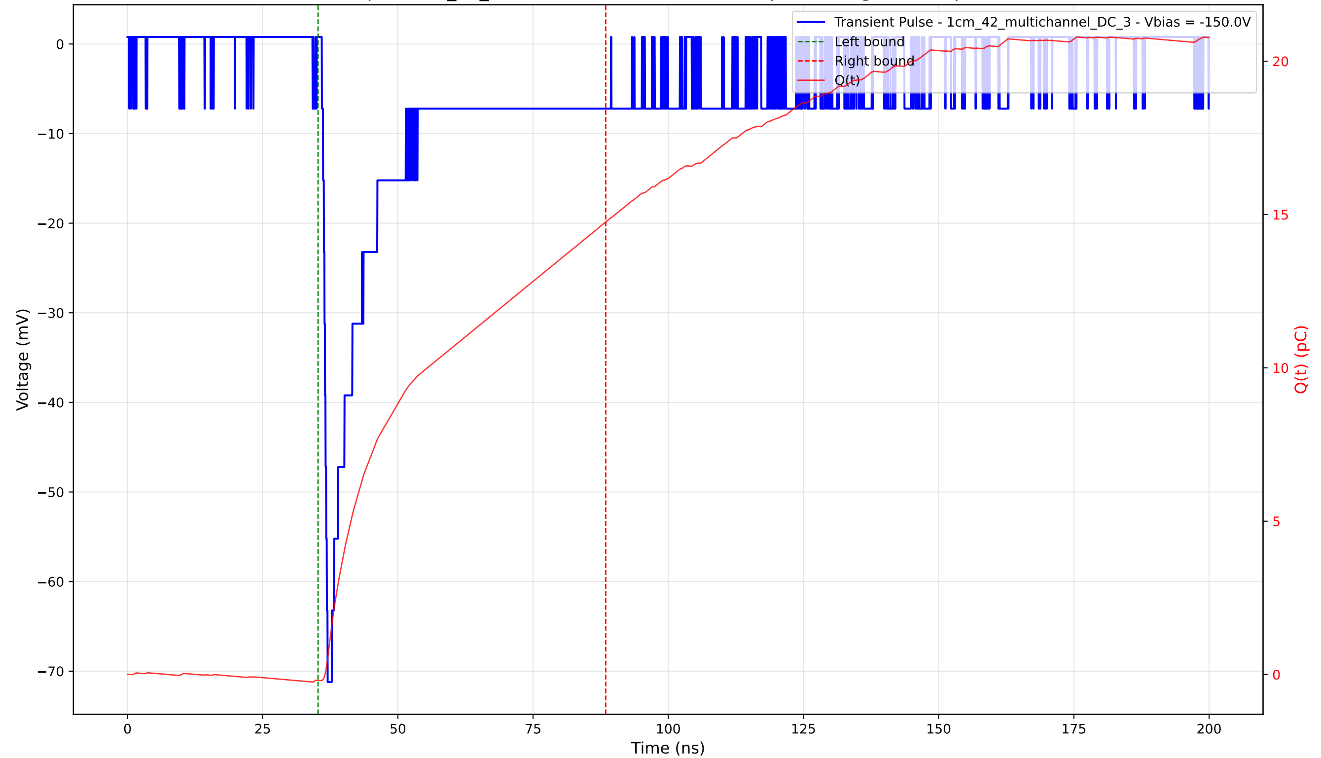
Transient Pulse - Sample: 1cm_42_multichannel - Position: 390.0 \mu\text{m} - Charge: 14.95 pC - Rise Time: 1.06 ns
