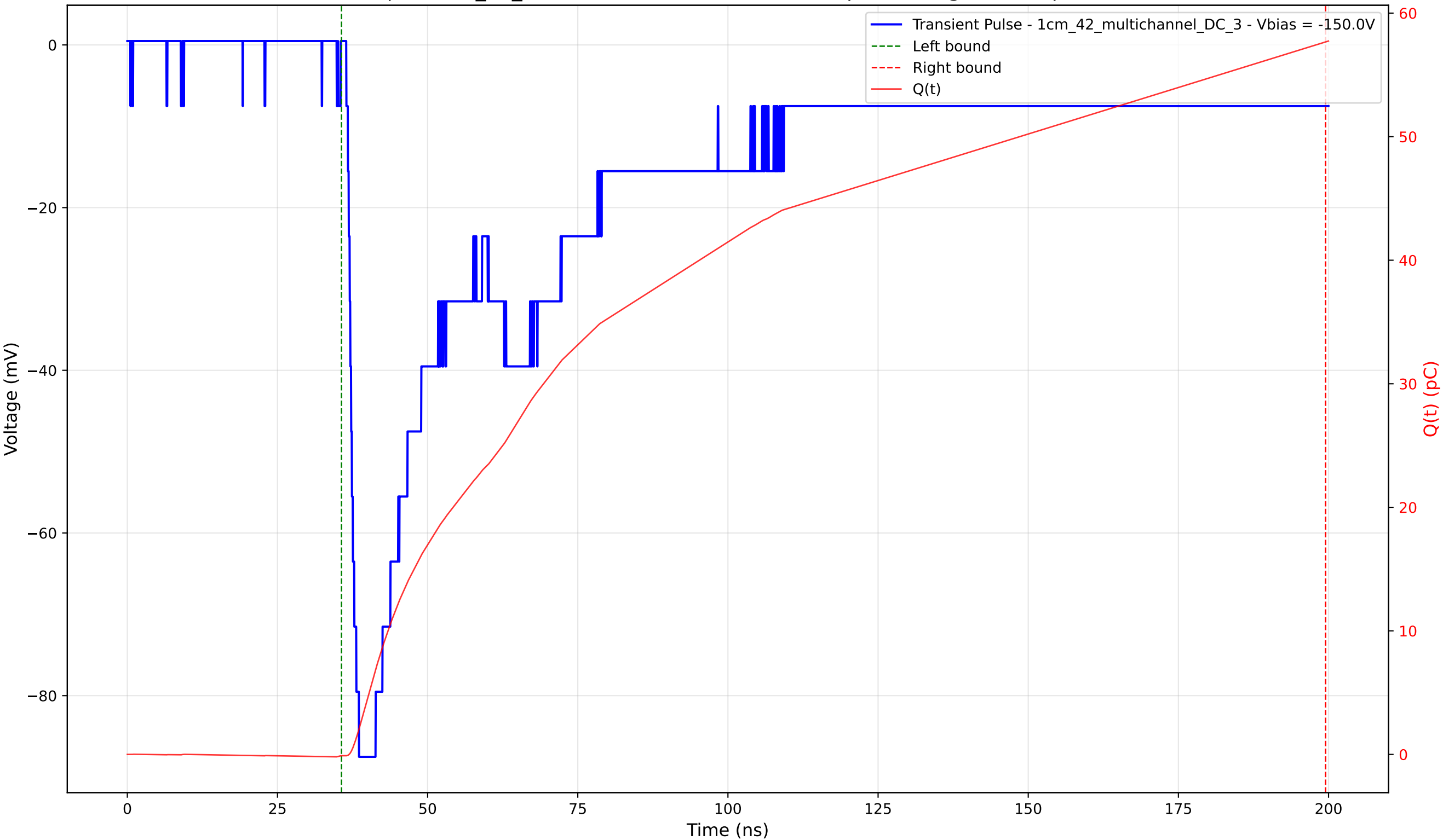
Transient Pulse - Sample: 1cm_42_multichannel - Position: 2115.0 \mu\text{m} - Charge: 57.78 pC - Rise Time: 1.42 ns
