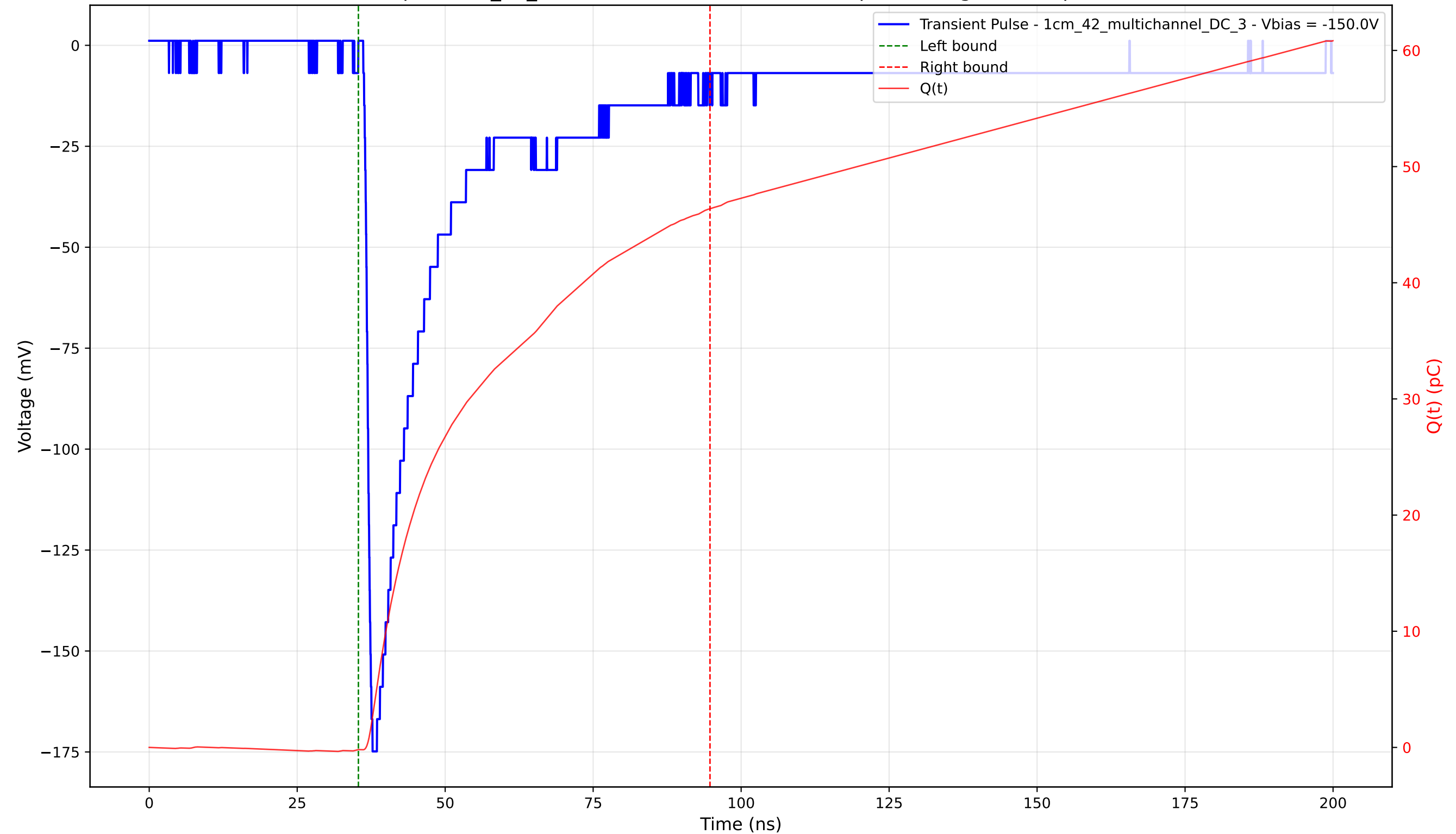
Transient Pulse - Sample: 1cm_42_multichannel - Position: 1000.0 \mu\text{m} - Charge: 46.57 pC - Rise Time: 1.05 ns
