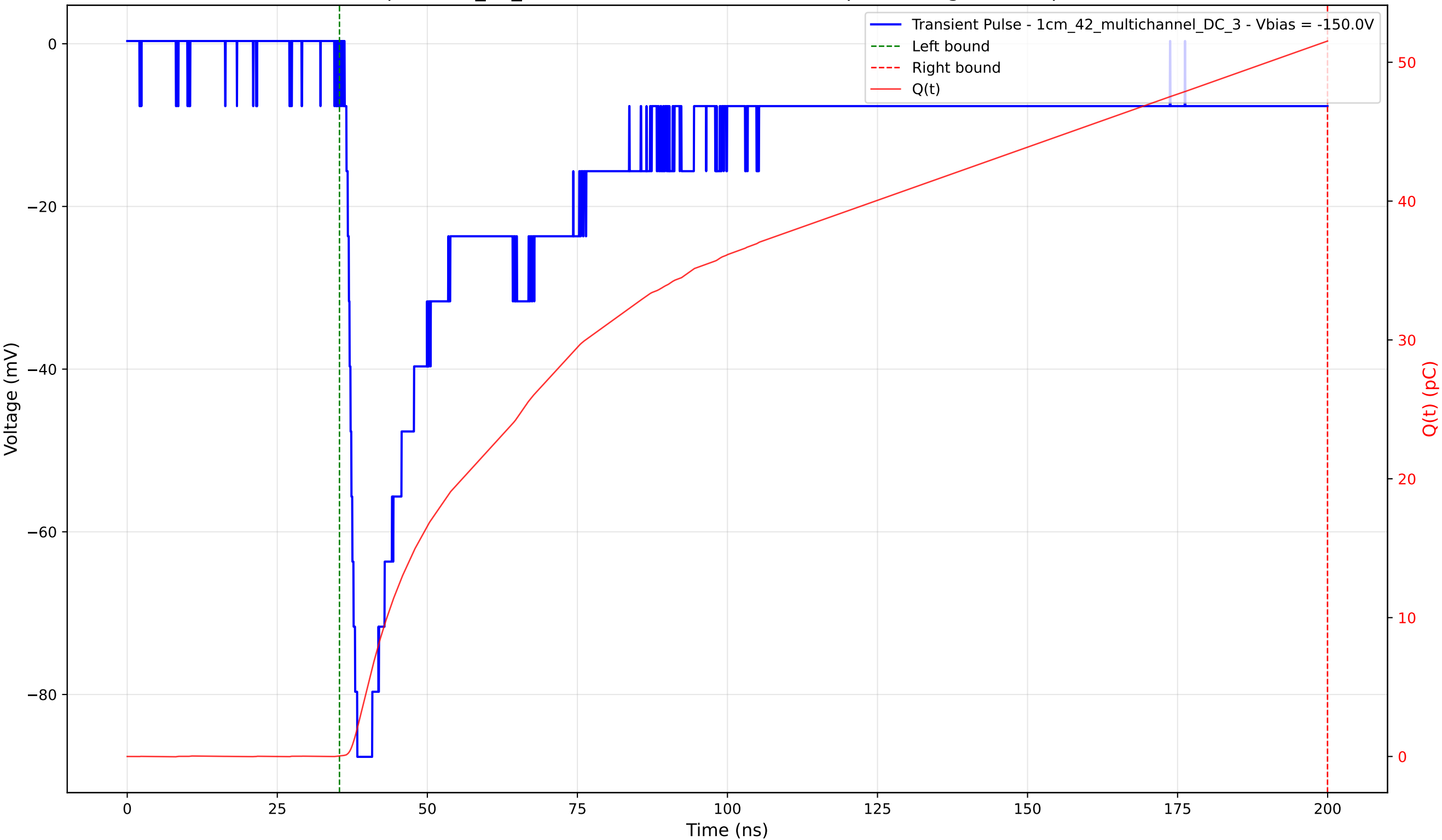
Transient Pulse - Sample: 1cm_42_multichannel - Position: 1800.0 \mu\text{m} - Charge: 51.48 pC - Rise Time: 1.46 ns
