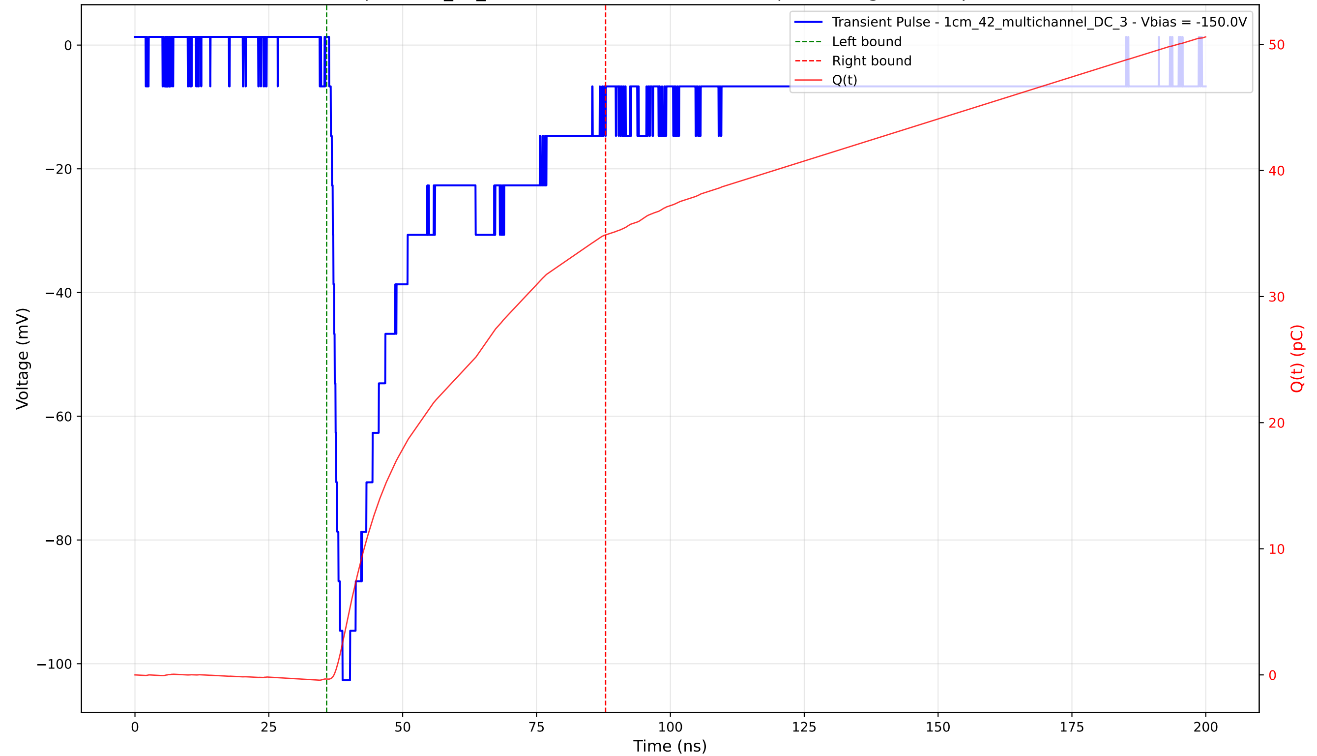
Transient Pulse - Sample: 1cm_42_multichannel - Position: 3125.0 \mu\text{m} - Charge: 35.22 pC - Rise Time: 1.71 ns
