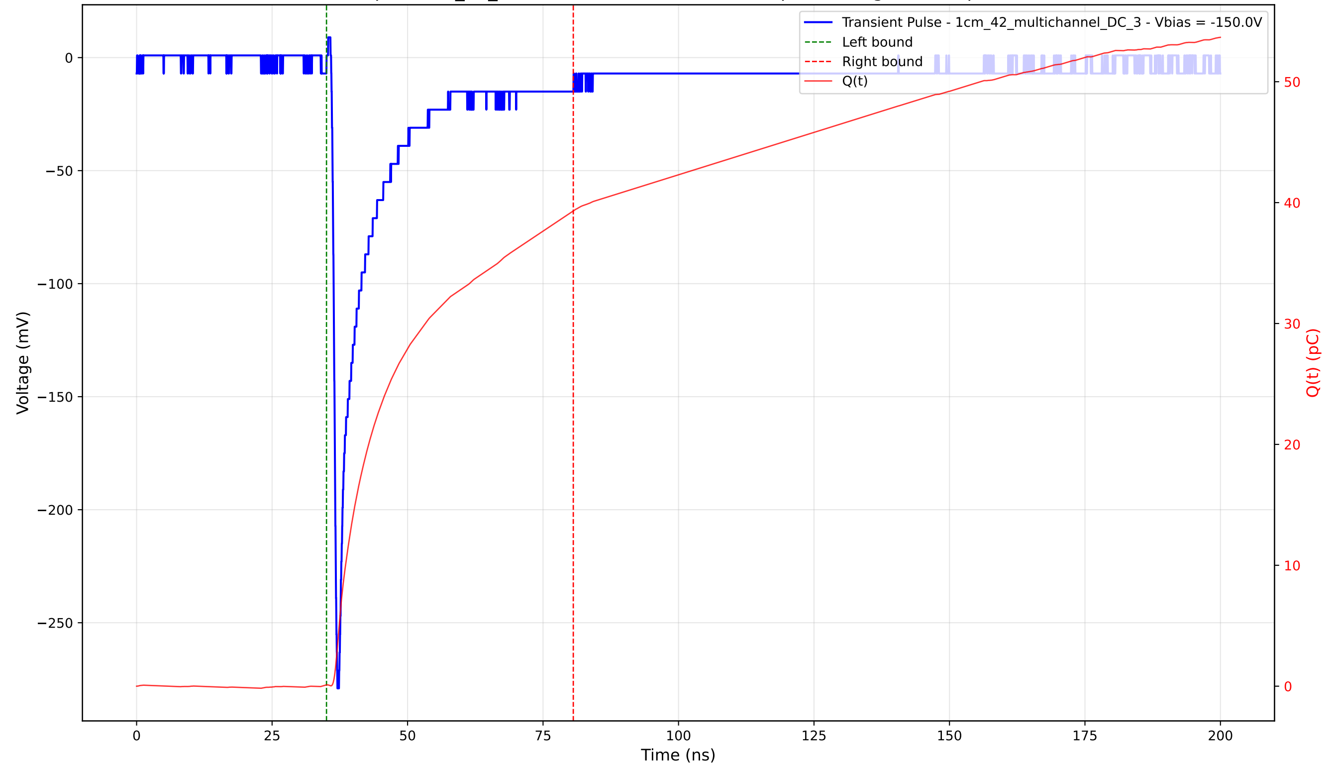
Transient Pulse - Sample: 1cm_42_multichannel - Position: 275.0 \mu\text{m} - Charge: 39.22 pC - Rise Time: 0.83 ns
