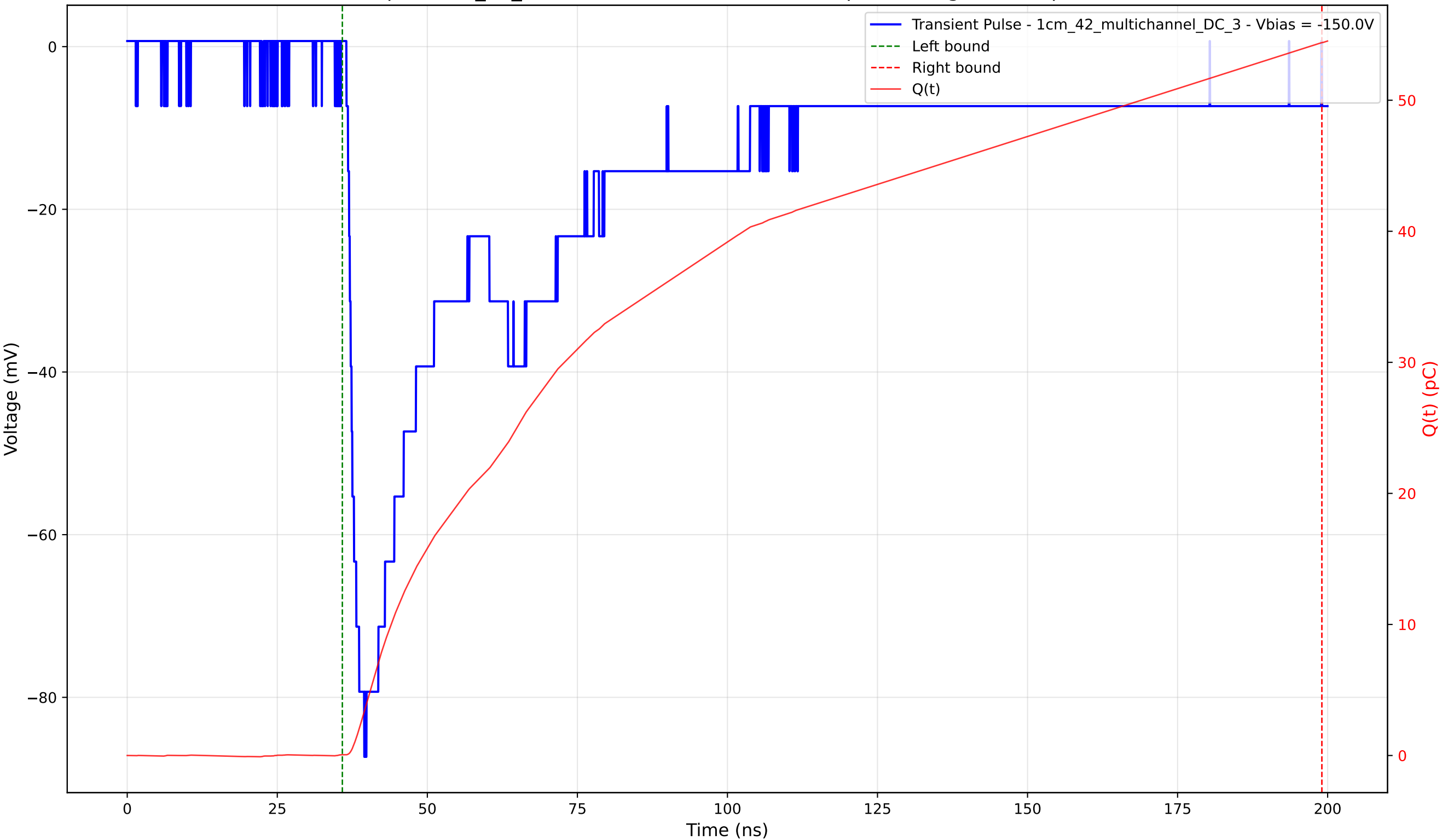
Transient Pulse - Sample: 1cm_42_multichannel - Position: 2605.0 \mu\text{m} - Charge: 54.32 pC - Rise Time: 1.88 ns
