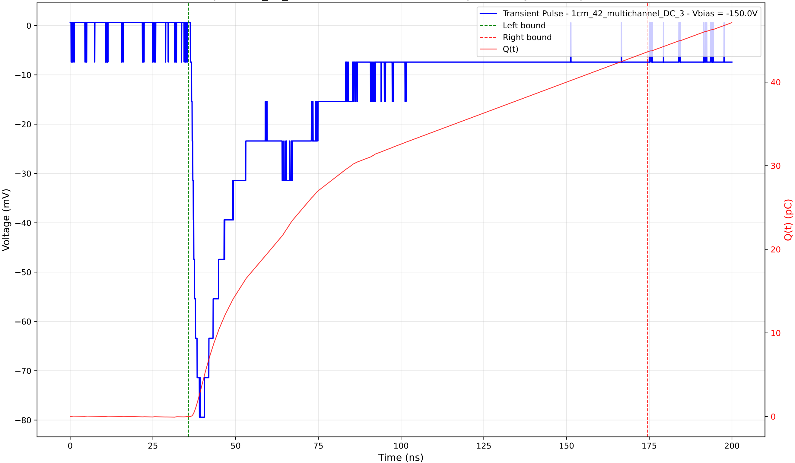
Transient Pulse - Sample: 1cm_42_multichannel - Position: 2810.0 \mu\text{m} - Charge: 43.63 pC - Rise Time: 2.36 ns
