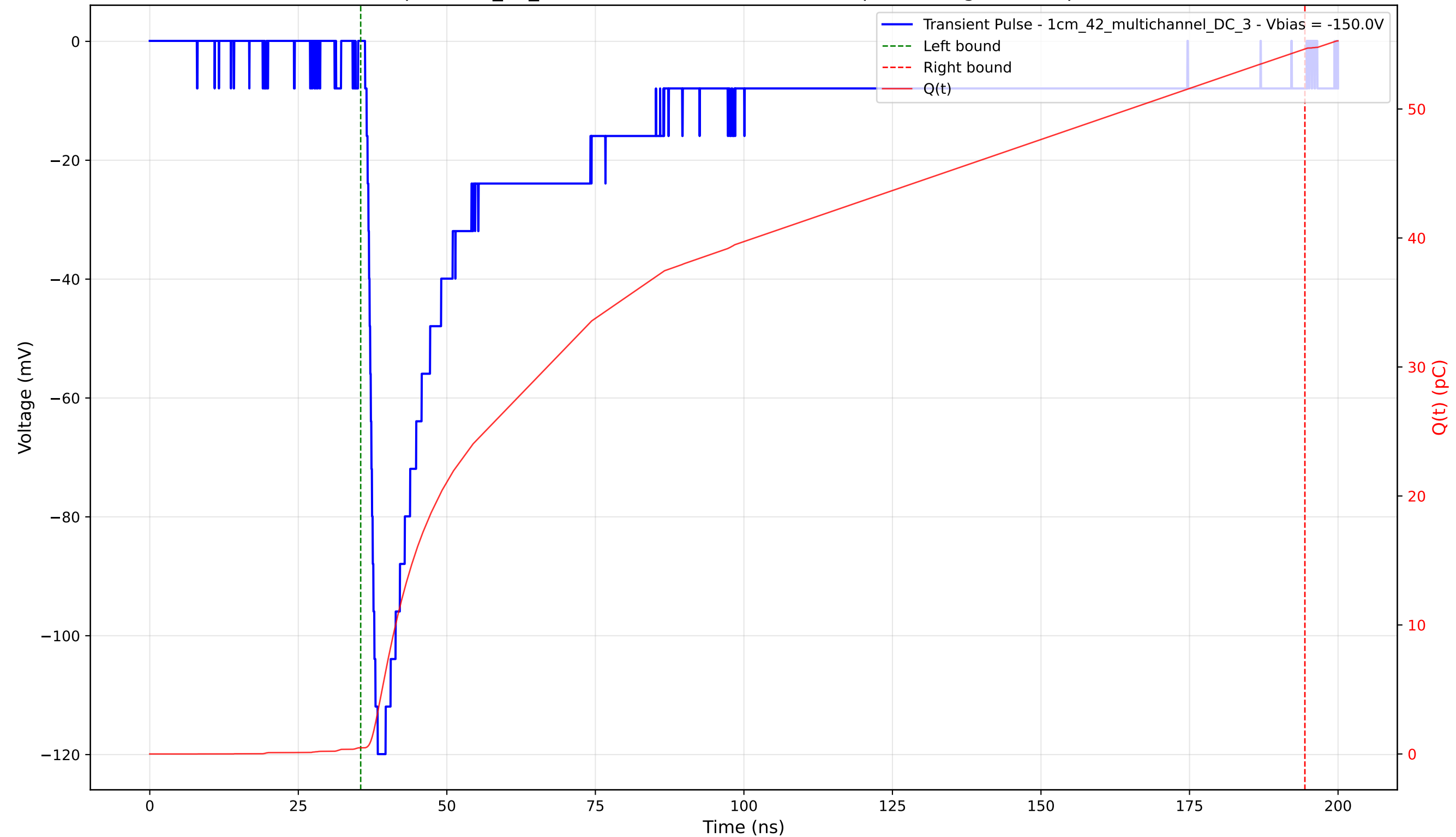
Transient Pulse - Sample: 1cm_42_multichannel - Position: 3470.0 \mu\text{m} - Charge: 54.18 pC - Rise Time: 1.49 ns
