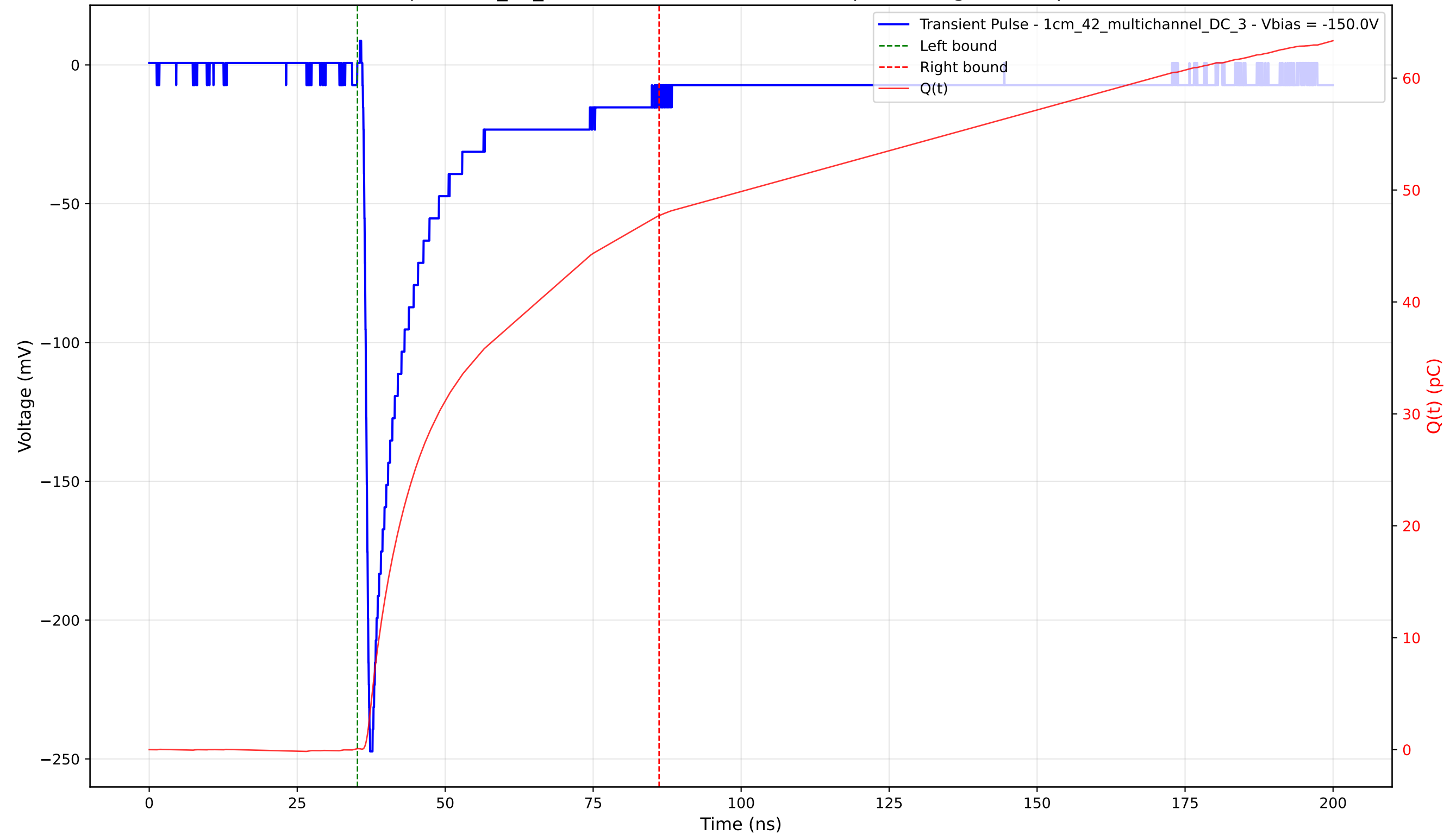
Transient Pulse - Sample: 1cm_42_multichannel - Position: 570.0 \mu\text{m} - Charge: 47.62 pC - Rise Time: 0.86 ns
