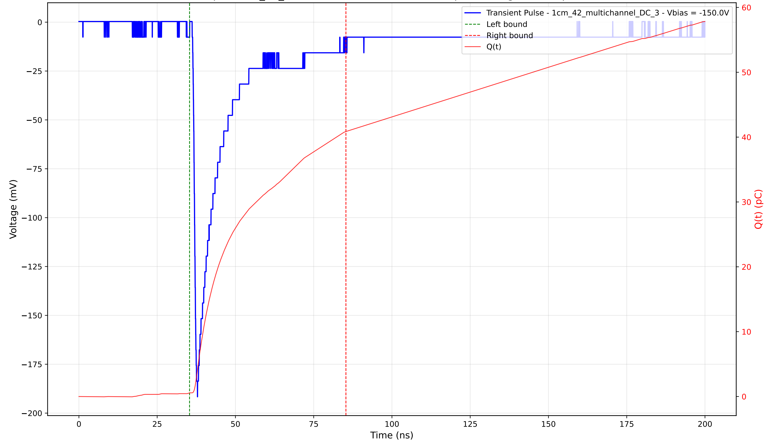
Transient Pulse - Sample: 1cm_42_multichannel - Position: 4135.0 \mu\text{m} - Charge: 40.29 pC - Rise Time: 1.05 ns
