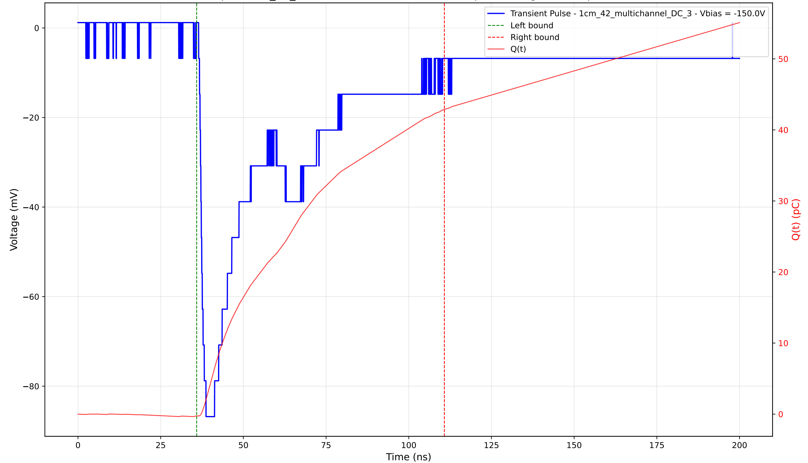
Transient Pulse - Sample: 1cm_42_multichannel - Position: 2135.0 \mu\text{m} - Charge: 43.13 pC - Rise Time: 1.46 ns
