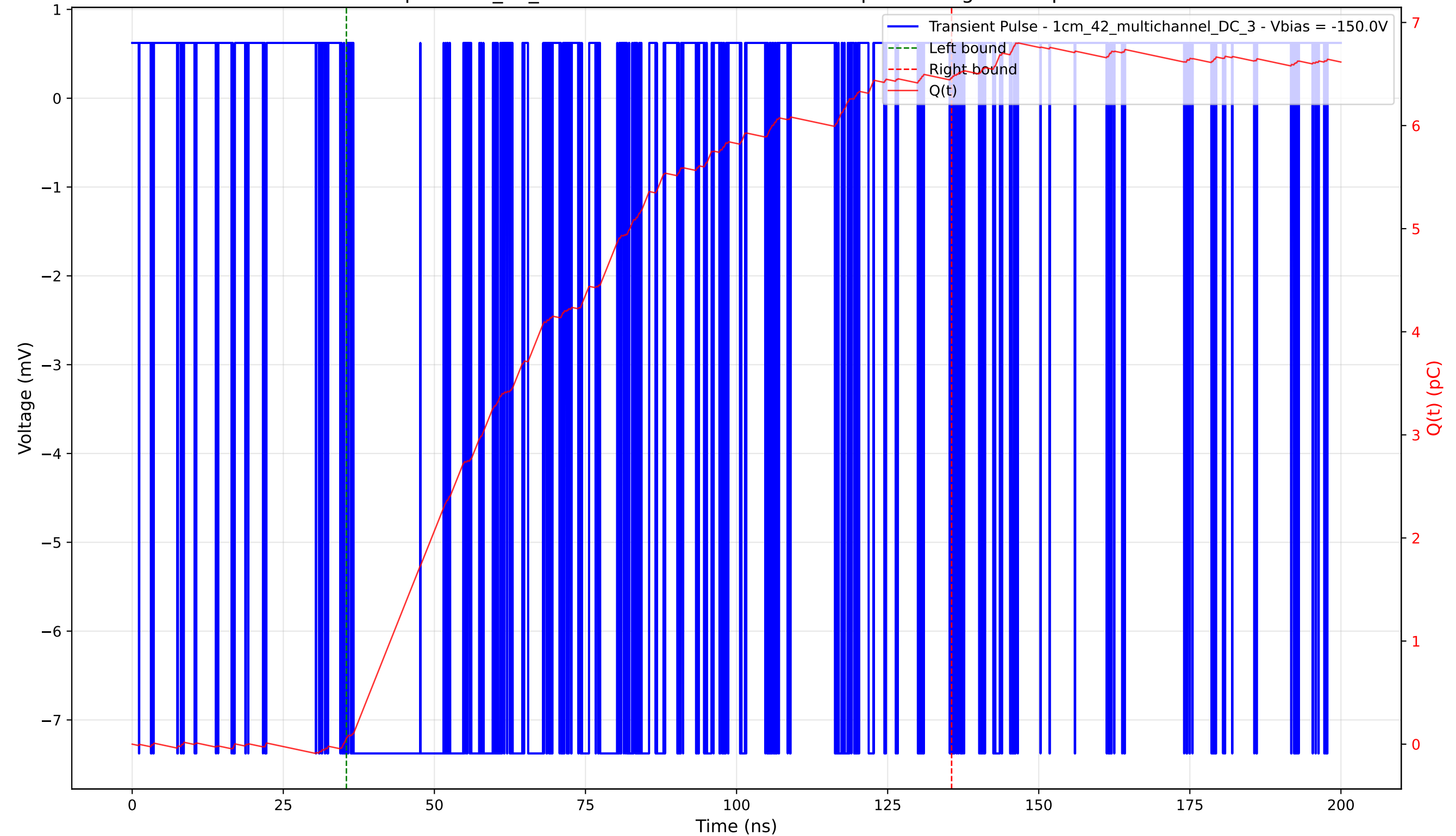
Transient Pulse - Sample: 1cm_42_multichannel - Position: 3885.0 \mu\text{m} - Charge: 6.40 pC - Rise Time: 0.02 ns
