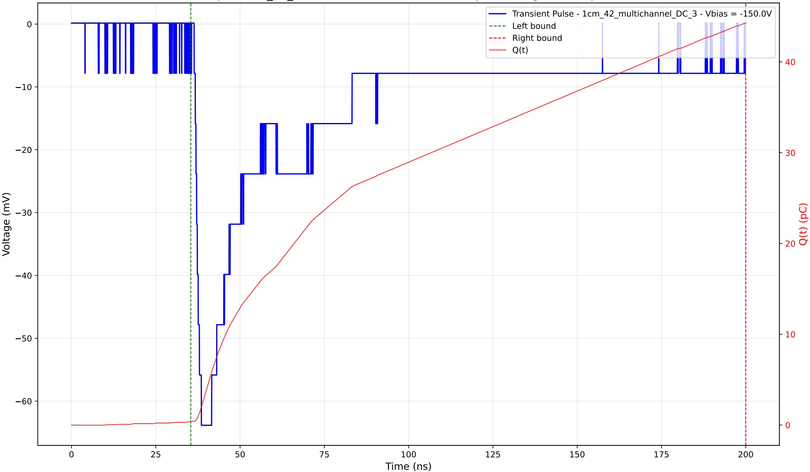
Transient Pulse - Sample: 1cm_42_multichannel - Position: 2820.0 \mu\text{m} - Charge: 43.87 pC - Rise Time: 2.14 ns
