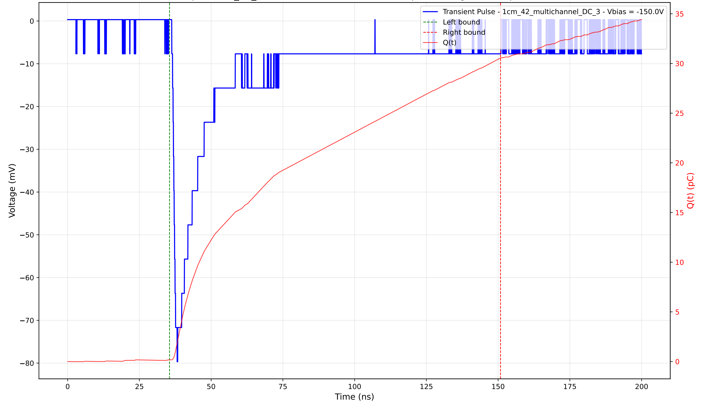
Transient Pulse - Sample: 1cm_42_multichannel - Position: 3840.0 \mu\text{m} - Charge: 30.38 pC - Rise Time: 1.60 ns
