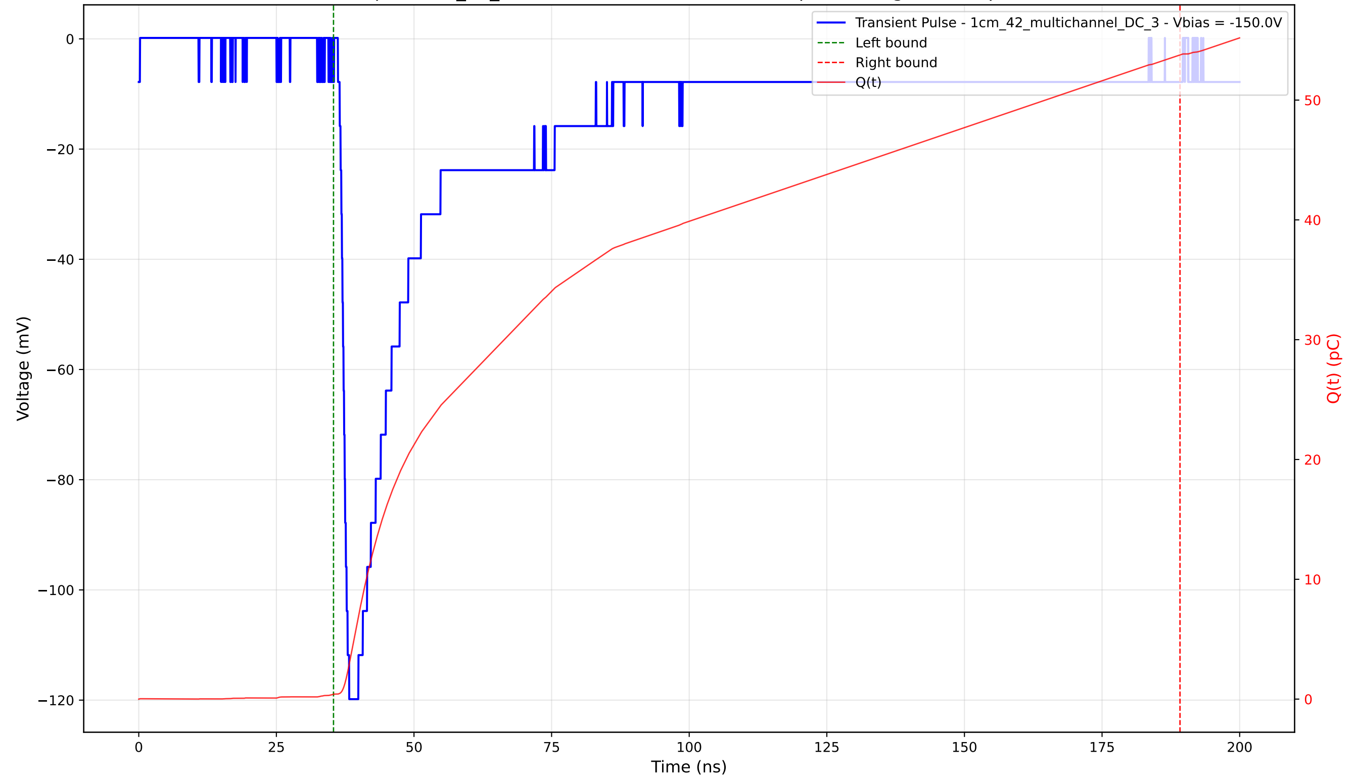
Transient Pulse - Sample: 1cm_42_multichannel - Position: 3475.0 \mu\text{m} - Charge: 53.37 pC - Rise Time: 1.45 ns
