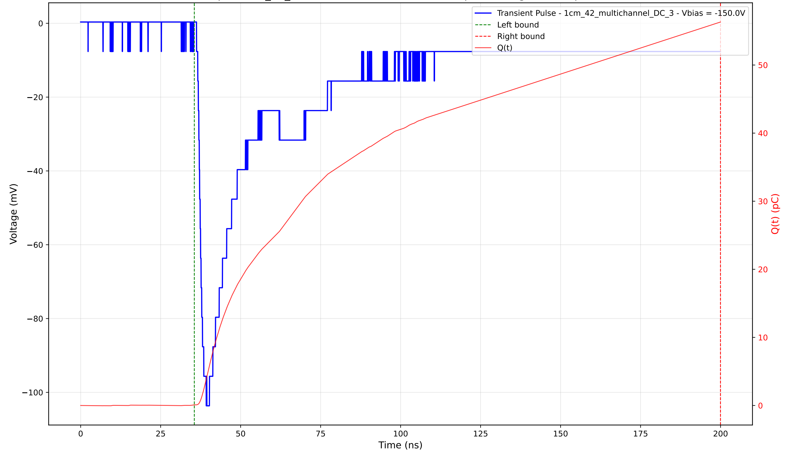
Transient Pulse - Sample: 1cm_42_multichannel - Position: 2980.0 \mu\text{m} - Charge: 56.23 pC - Rise Time: 1.89 ns
