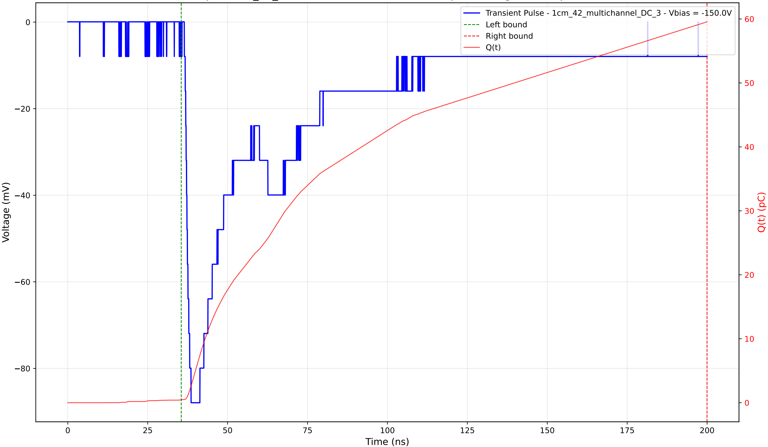
Transient Pulse - Sample: 1cm_42_multichannel - Position: 2110.0 \mu\text{m} - Charge: 59.08 pC - Rise Time: 1.42 ns
