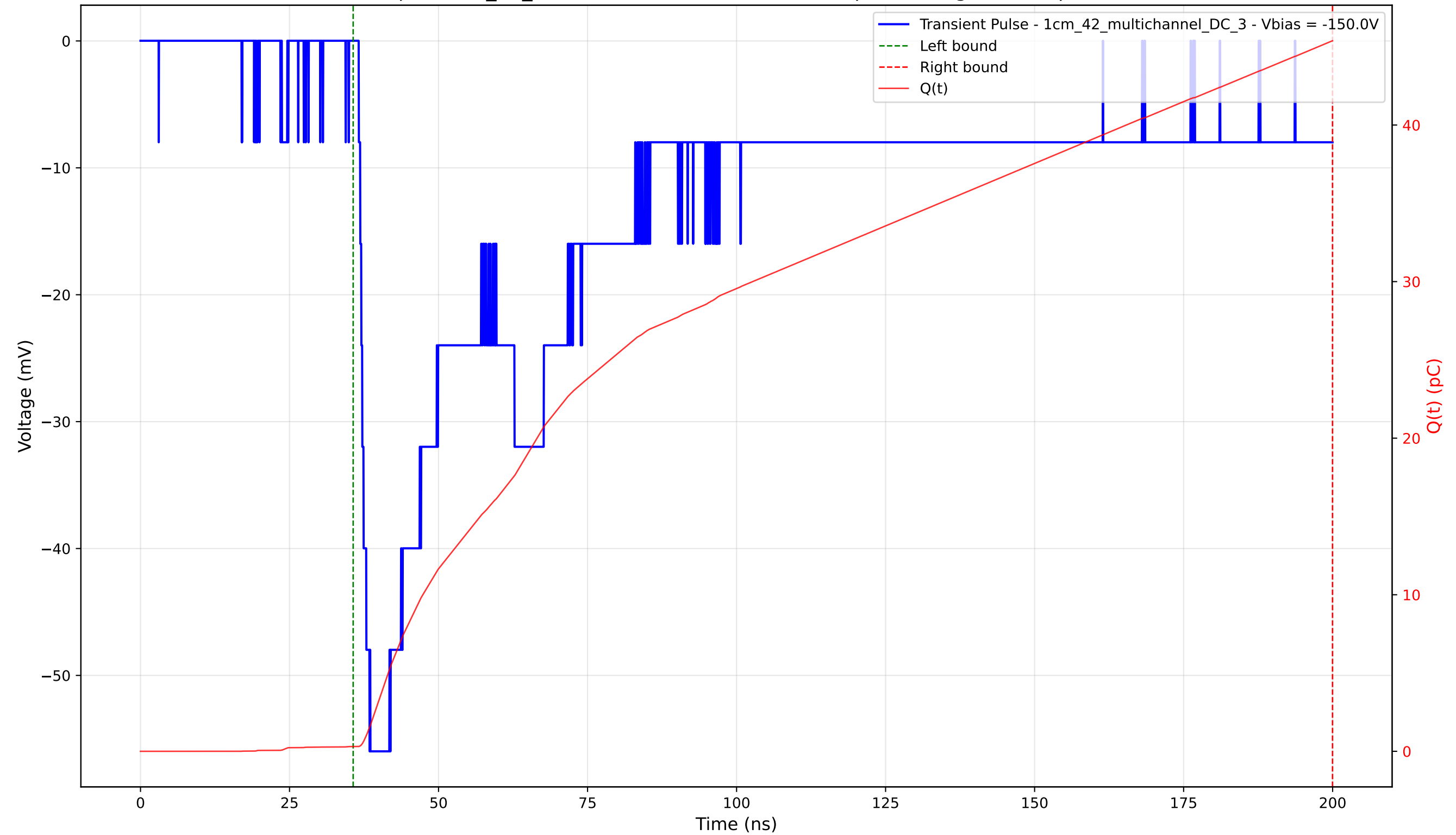
Transient Pulse - Sample: 1cm_42_multichannel - Position: 2315.0 \mu\text{m} - Charge: 45.08 pC - Rise Time: 1.81 ns
