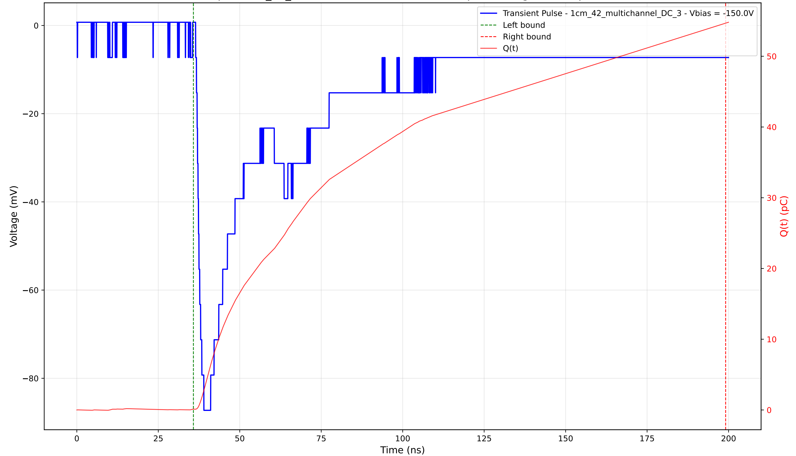
Transient Pulse - Sample: 1cm_42_multichannel - Position: 2680.0 \mu\text{m} - Charge: 54.57 pC - Rise Time: 1.66 ns
