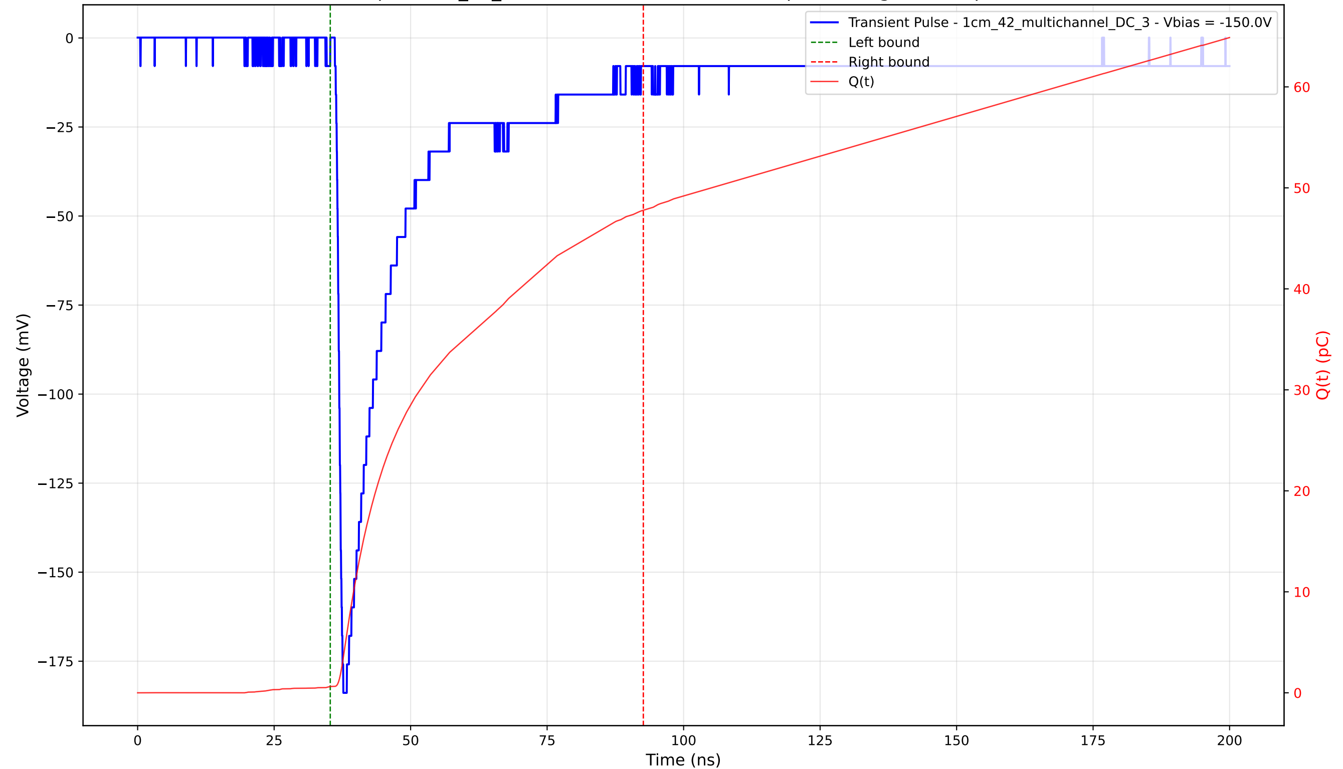
Transient Pulse - Sample: 1cm_42_multichannel - Position: 950.0 \mu\text{m} - Charge: 47.15 pC - Rise Time: 1.05 ns
