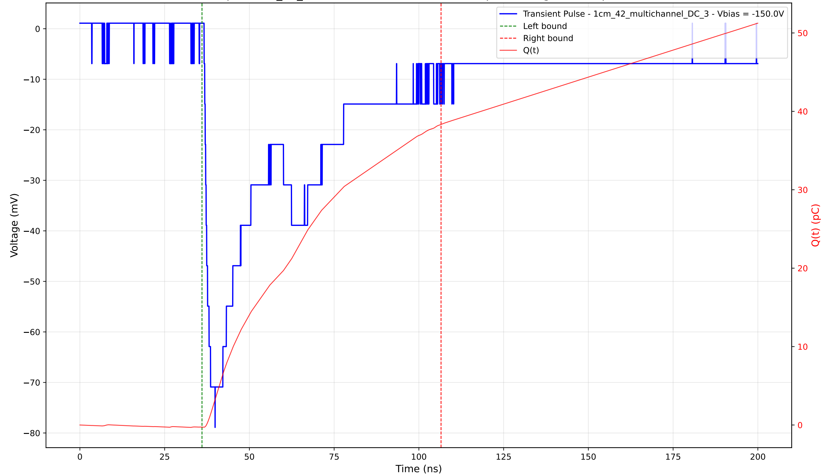
Transient Pulse - Sample: 1cm_42_multichannel - Position: 2450.0 \mu\text{m} - Charge: 38.61 pC - Rise Time: 3.08 ns
