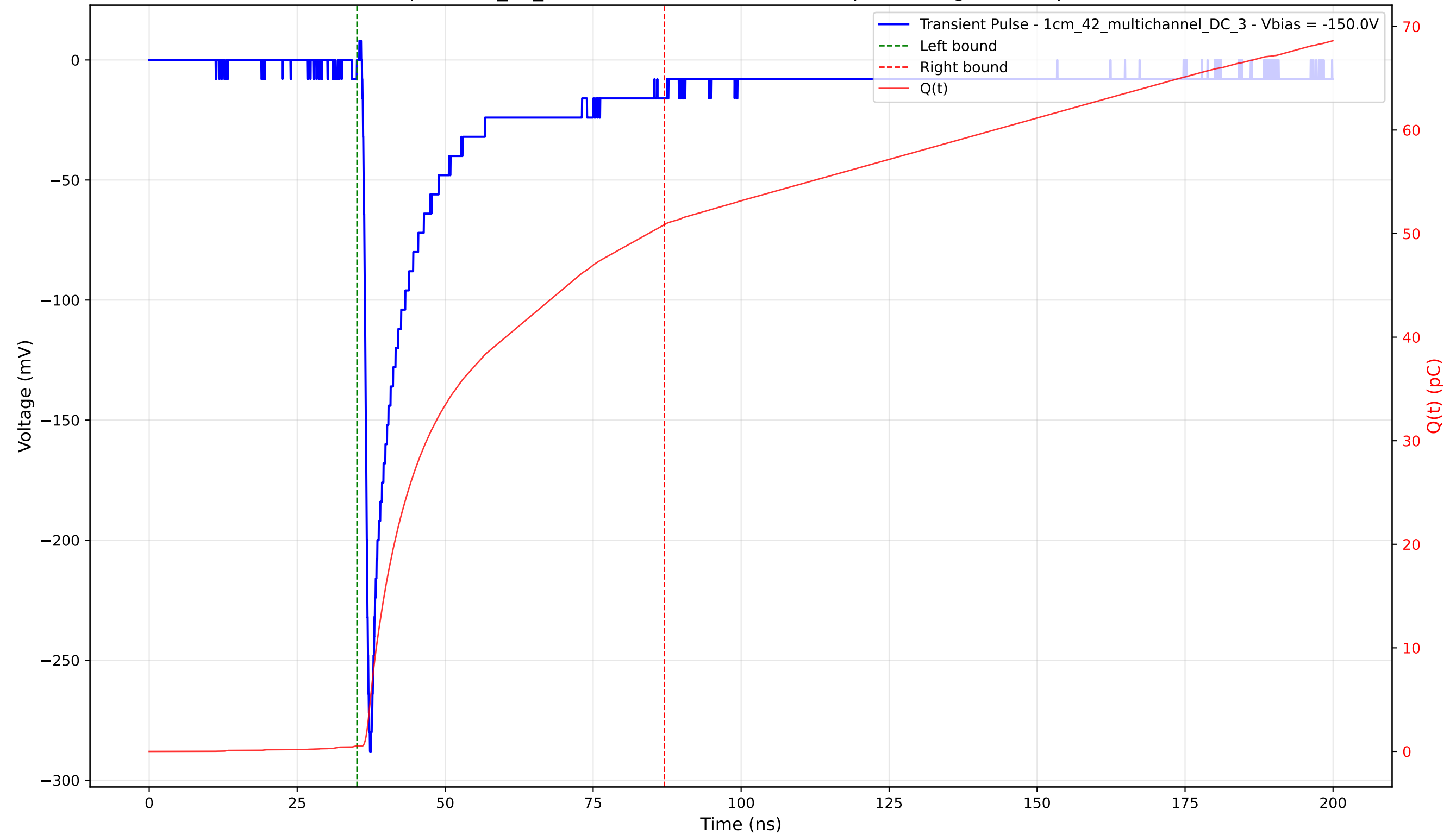
Transient Pulse - Sample: 1cm_42_multichannel - Position: 455.0 \mu\text{m} - Charge: 50.31 pC - Rise Time: 0.91 ns
