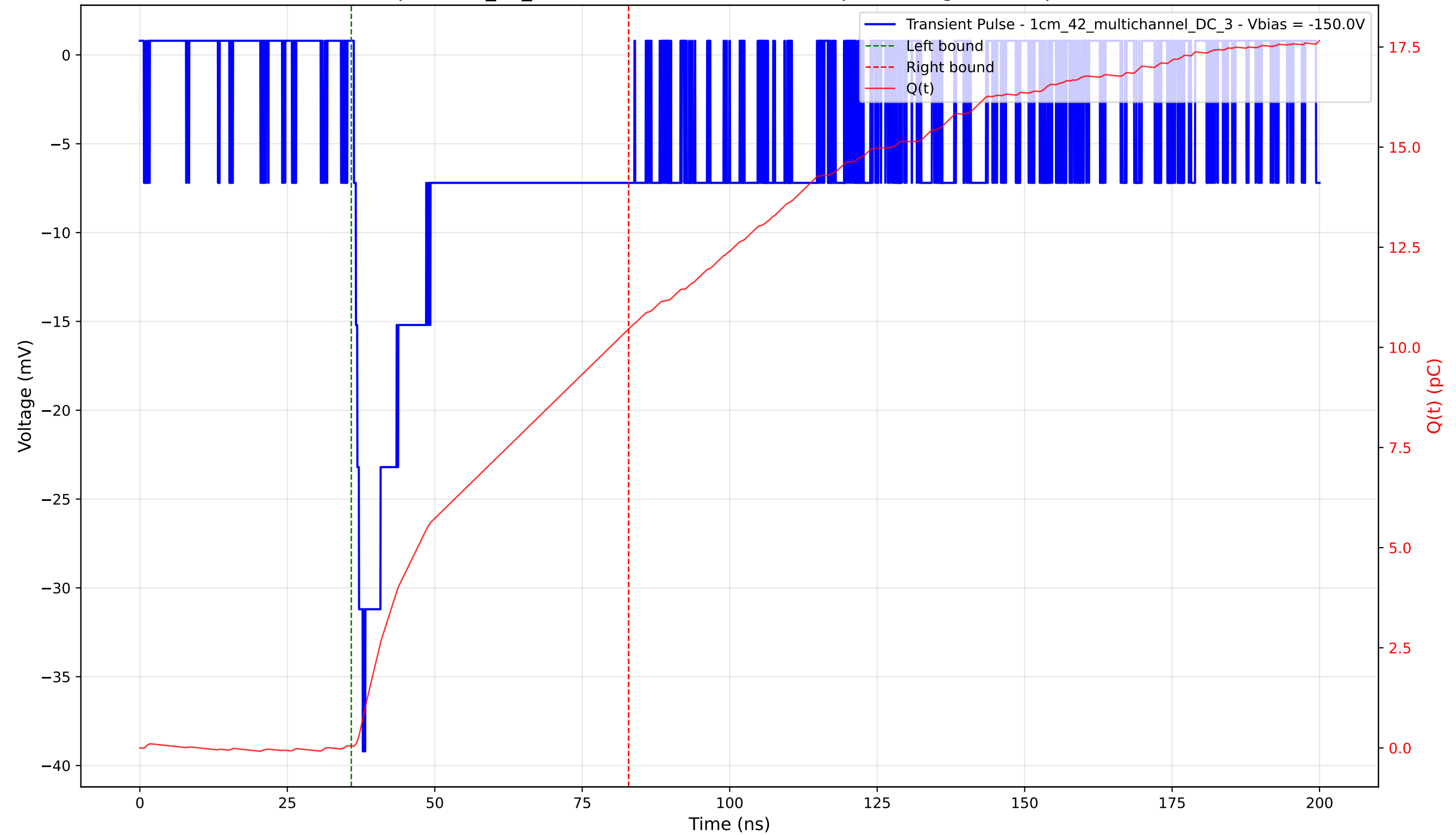
Transient Pulse - Sample: 1cm_42_multichannel - Position: 890.0 \mu\text{m} - Charge: 10.42 pC - Rise Time: 1.51 ns
