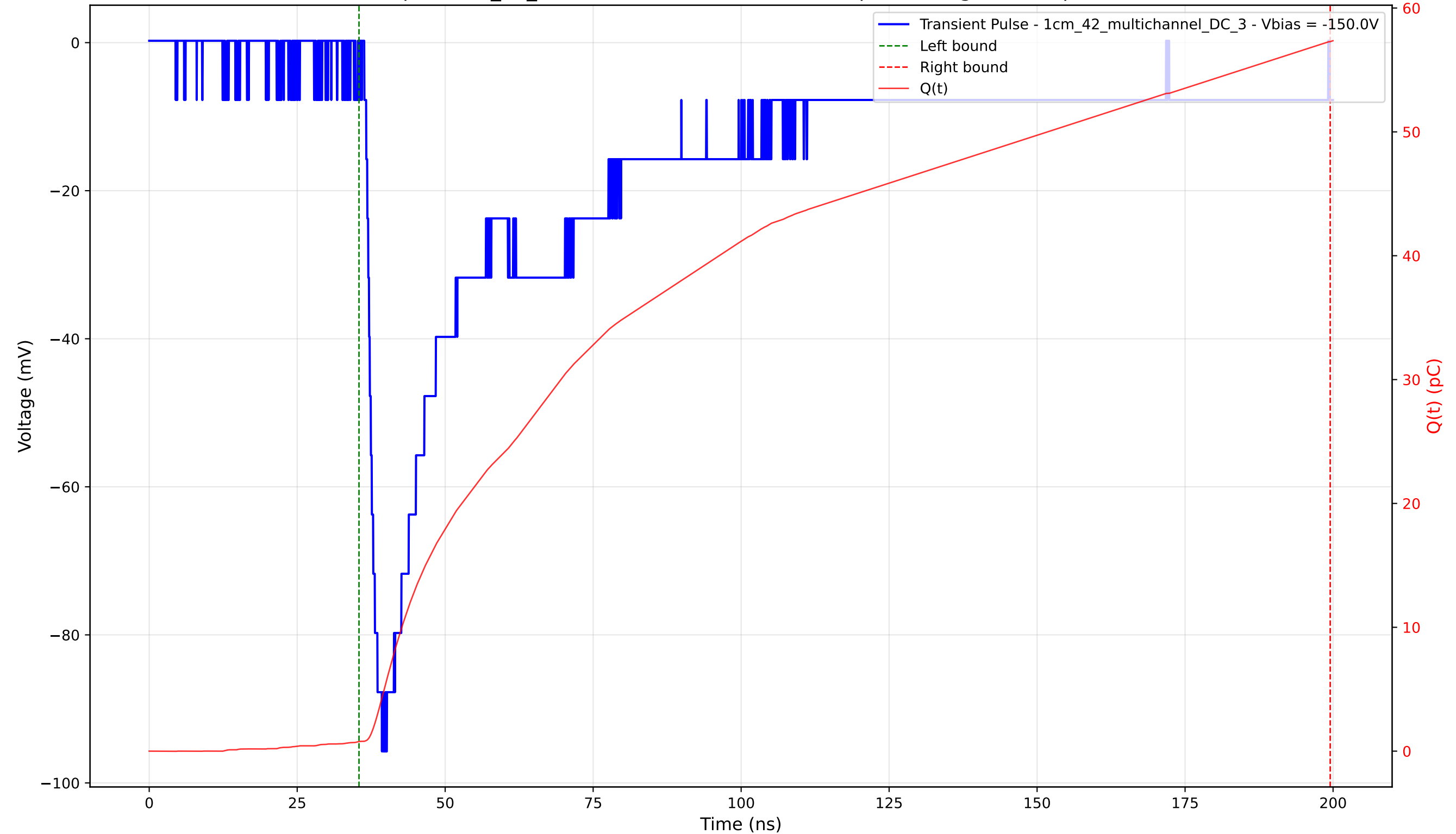
Transient Pulse - Sample: 1cm_42_multichannel - Position: 2785.0 \mu\text{m} - Charge: 56.52 pC - Rise Time: 1.92 ns
