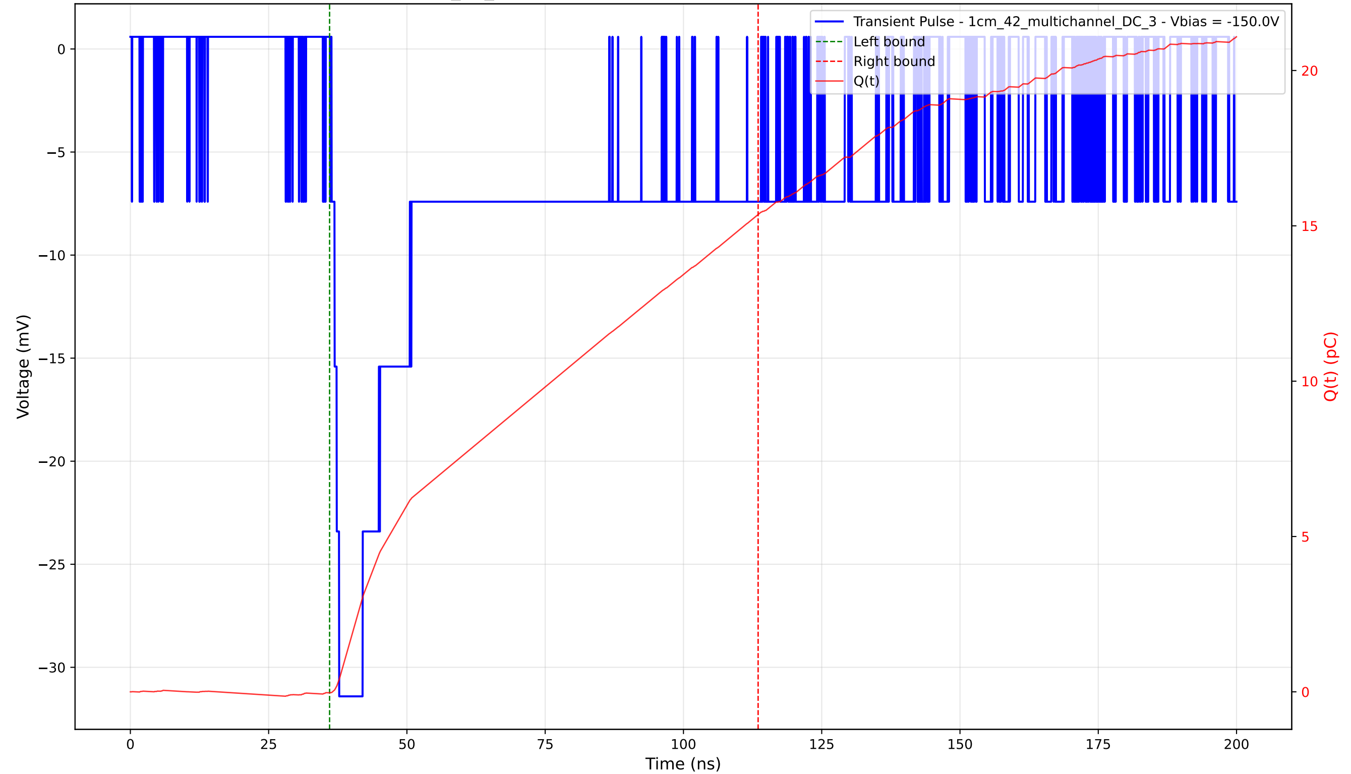
Transient Pulse - Sample: 1cm_42_multichannel - Position: 3425.0 \mu\text{m} - Charge: 15.40 pC - Rise Time: 1.37 ns
