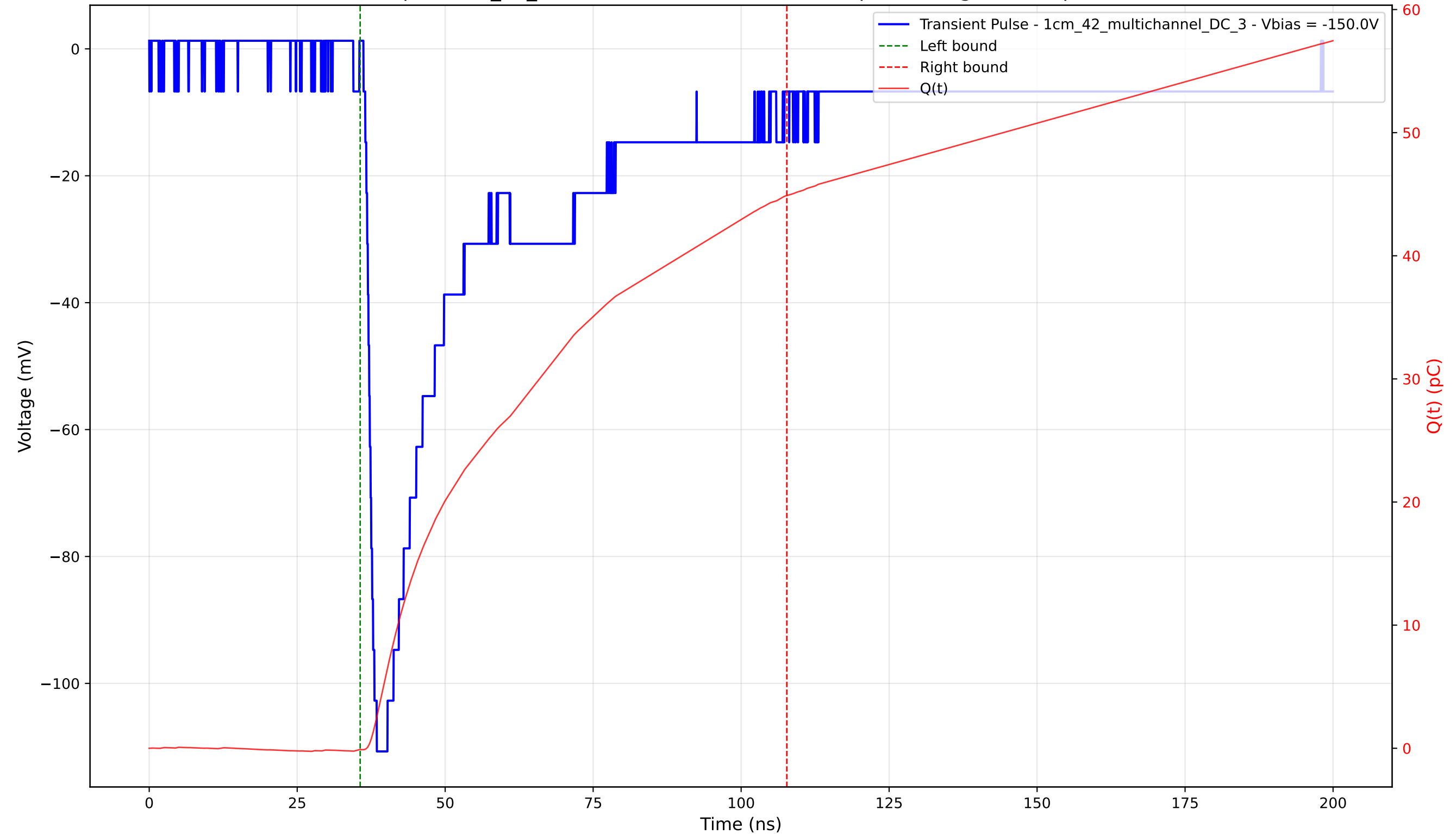
Transient Pulse - Sample: 1cm_42_multichannel - Position: 1760.0 \mu\text{m} - Charge: 45.00 pC - Rise Time: 1.55 ns
