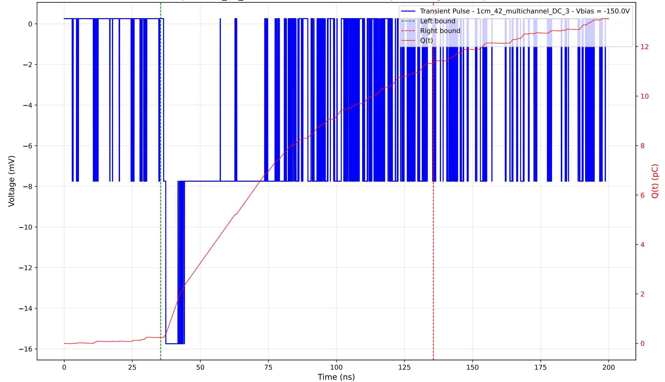
Transient Pulse - Sample: 1cm_42_multichannel - Position: 1340.0 \mu\text{m} - Charge: 11.10 pC - Rise Time: 0.82 ns
