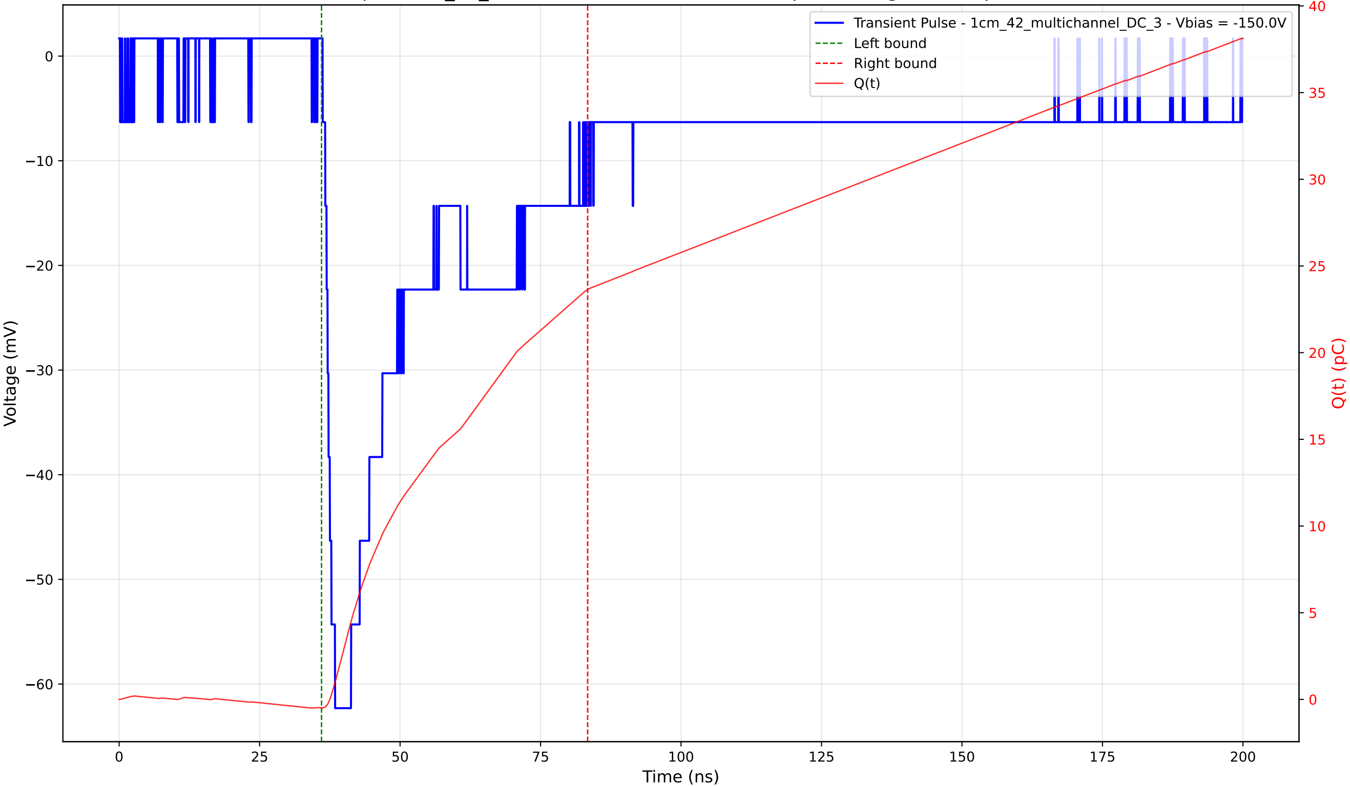
Transient Pulse - Sample: 1cm_42_multichannel - Position: 1925.0 \mu\text{m} - Charge: 24.13 pC - Rise Time: 2.20 ns
