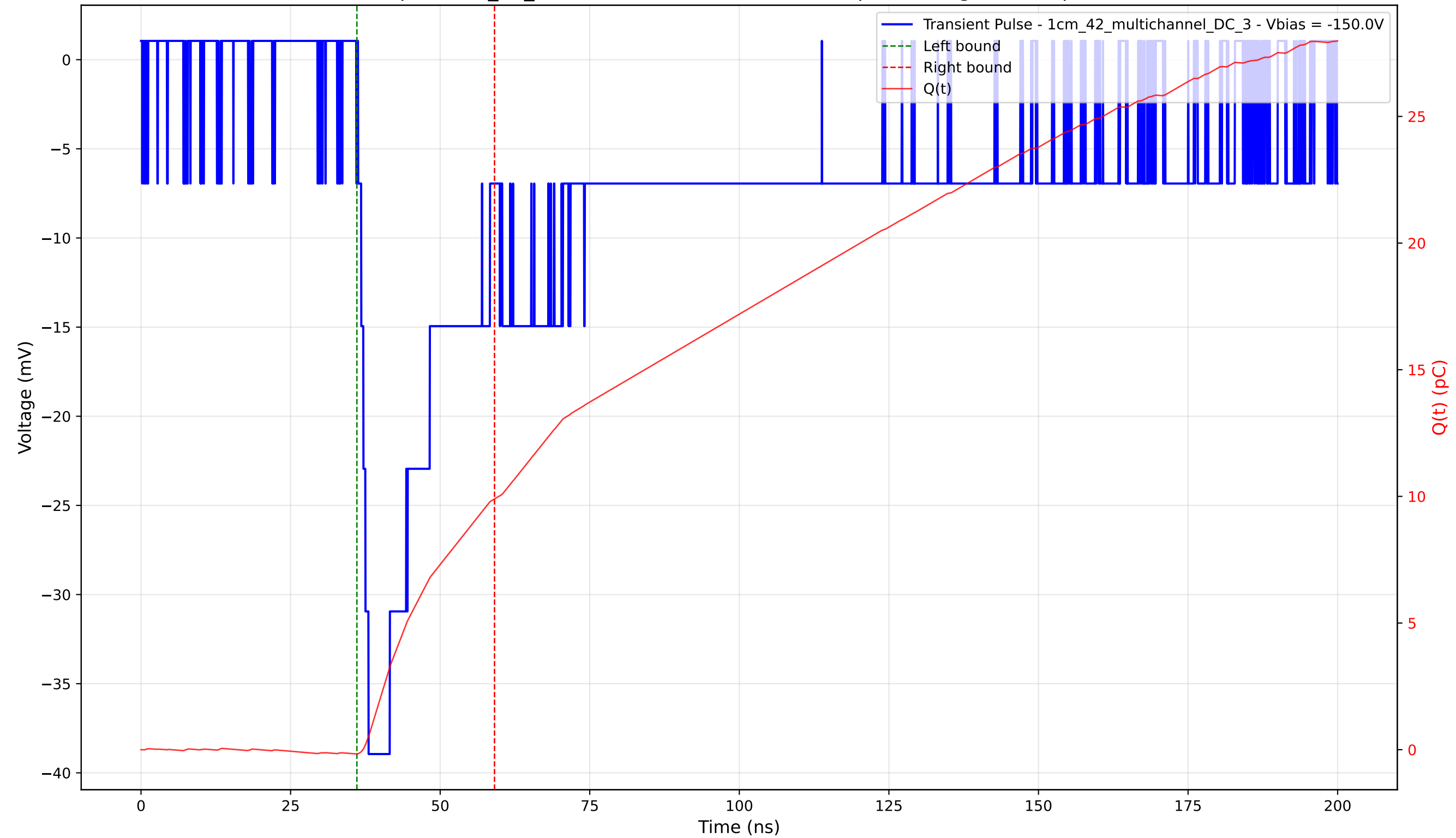
Transient Pulse - Sample: 1cm_42_multichannel - Position: 1825.0 \mu\text{m} - Charge: 10.05 pC - Rise Time: 1.75 ns
