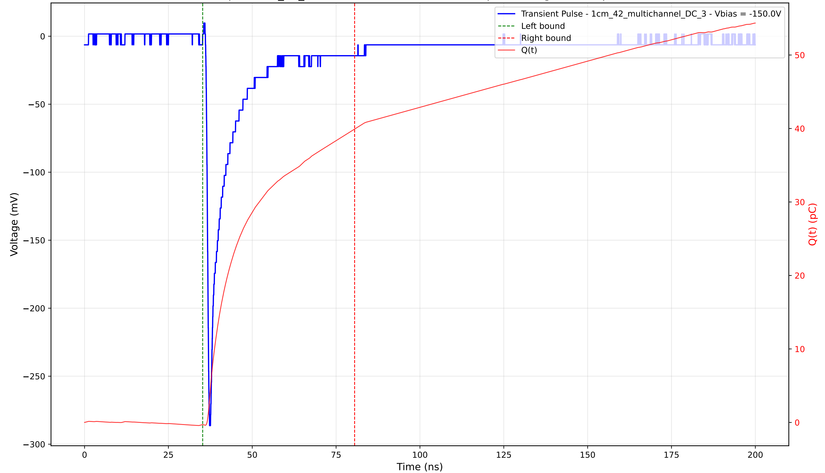
Transient Pulse - Sample: 1cm_42_multichannel - Position: 4565.0 \mu\text{m} - Charge: 40.23 pC - Rise Time: 0.84 ns
