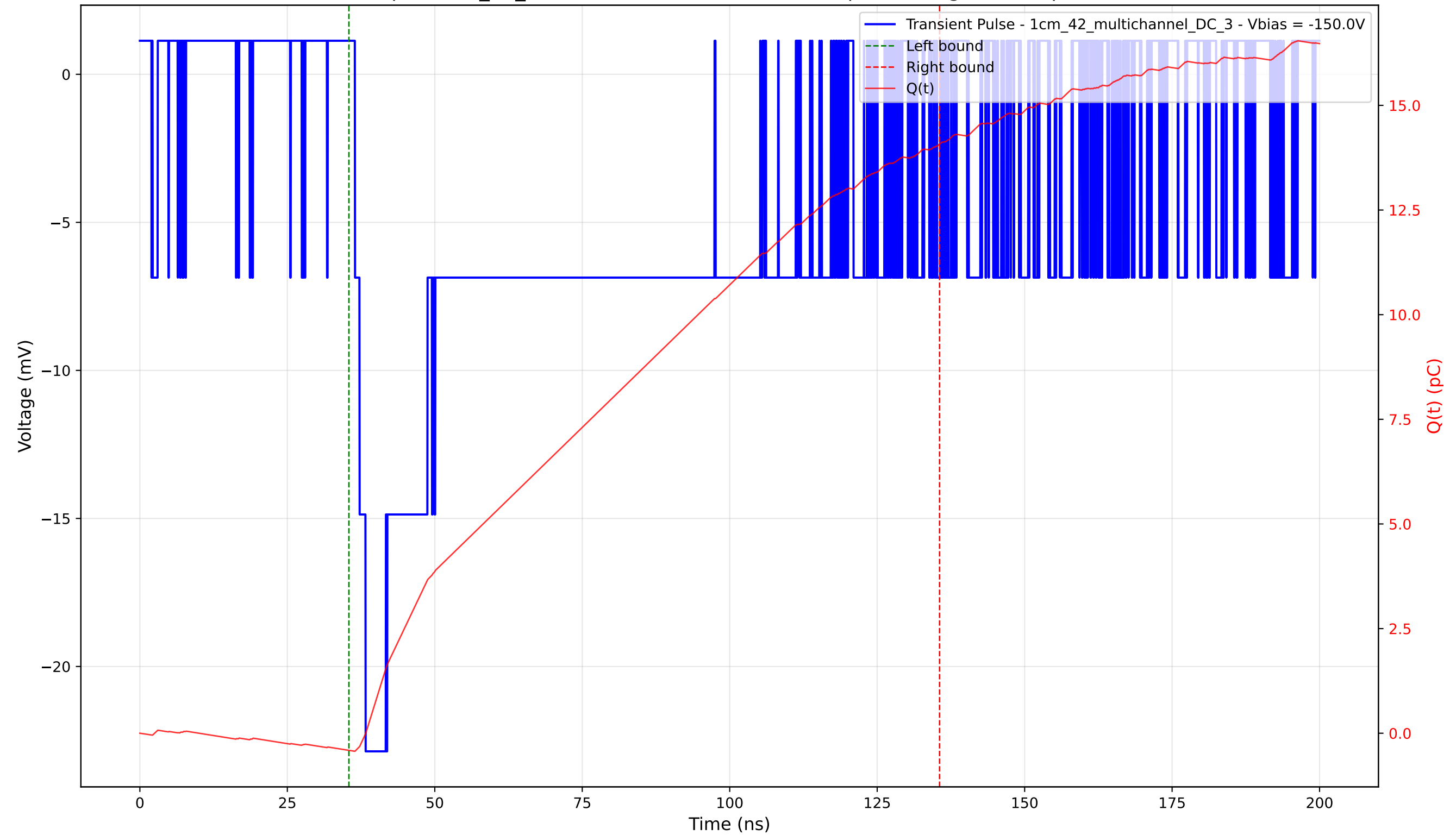
Transient Pulse - Sample: 1cm_42_multichannel - Position: 2915.0 \mu\text{m} - Charge: 14.49 pC - Rise Time: 1.82 ns
