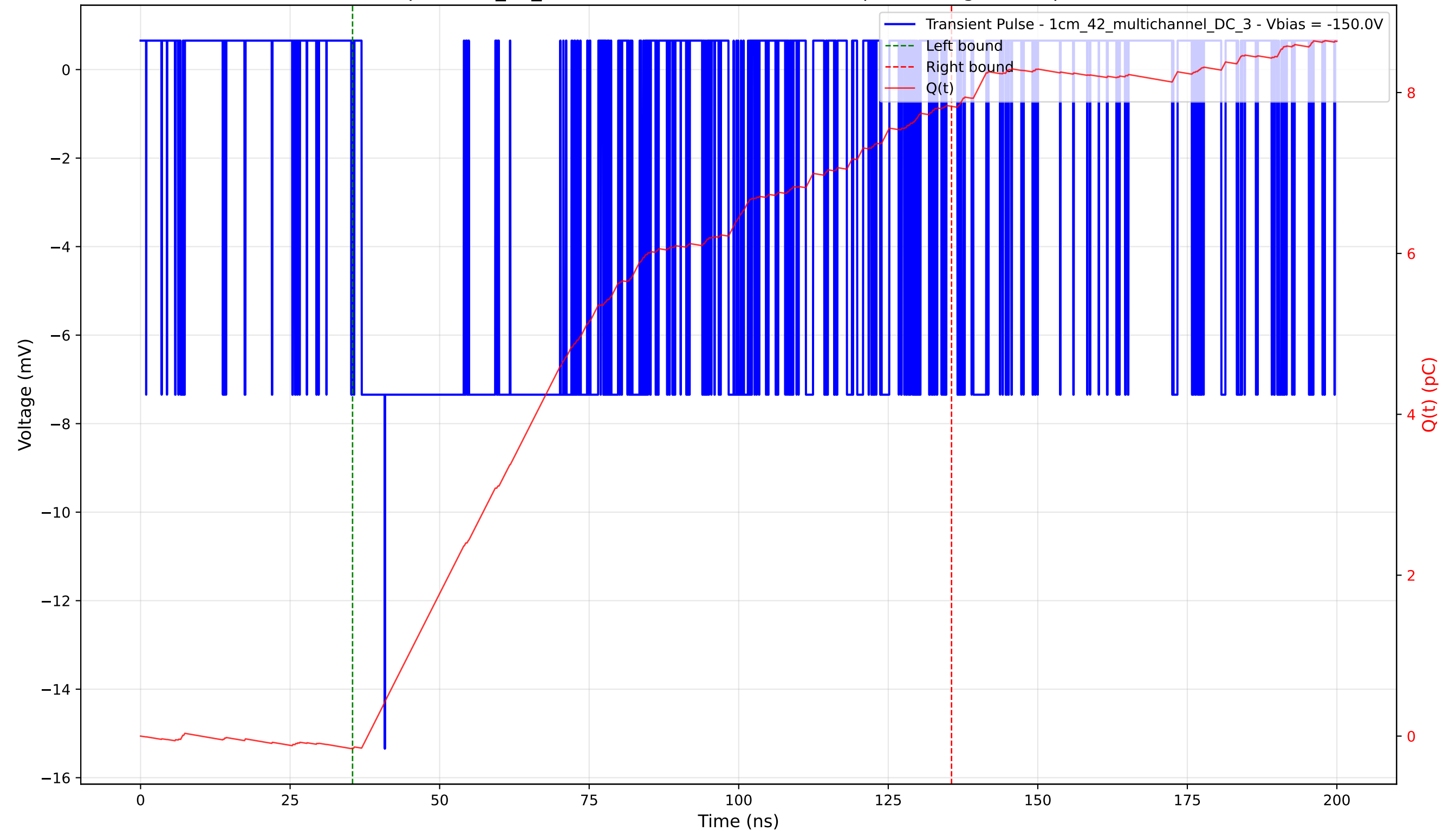
Transient Pulse - Sample: 1cm_42_multichannel - Position: 2860.0 \mu\text{m} - Charge: 7.98 pC - Rise Time: 3.88 ns
