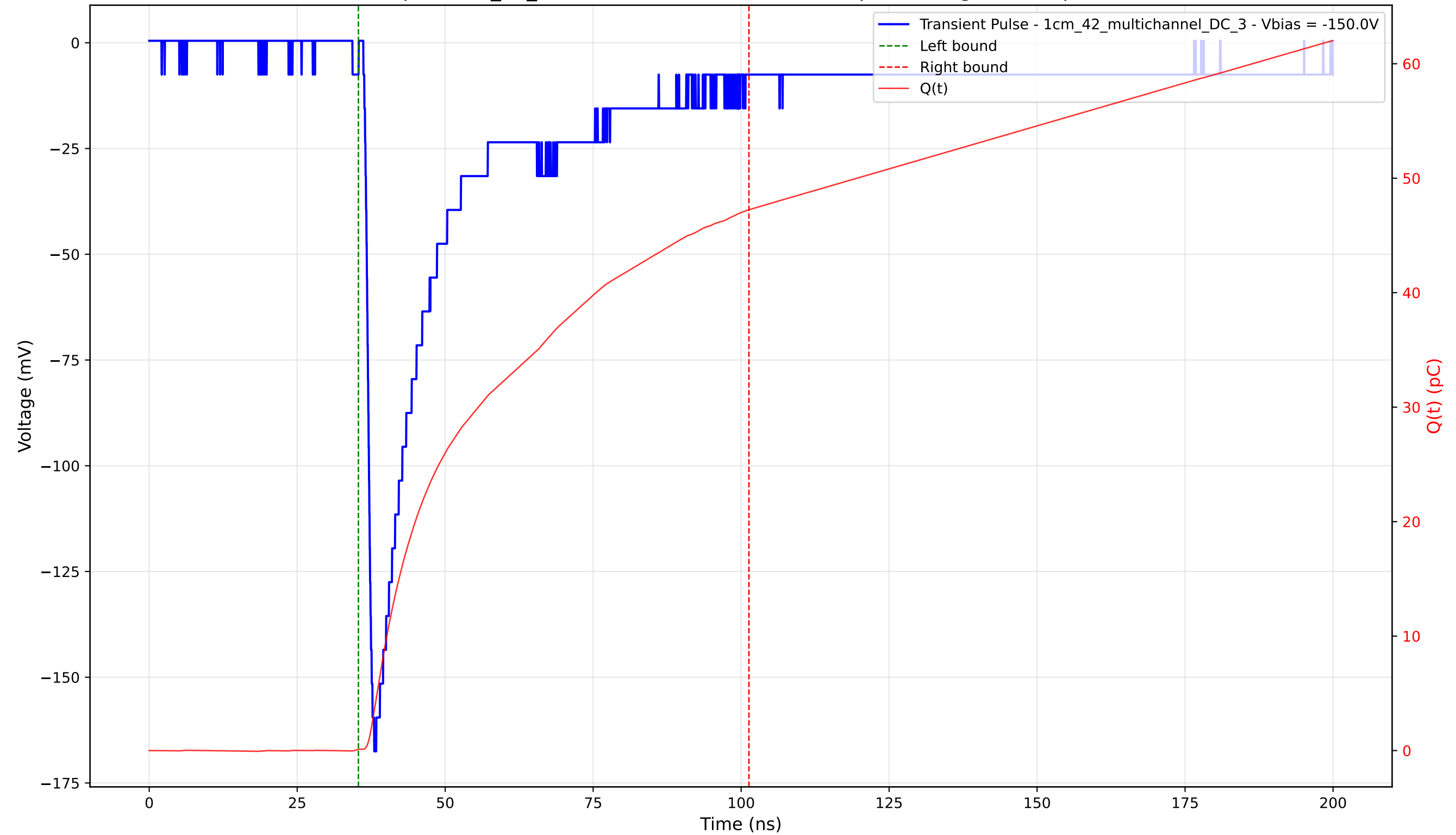
Transient Pulse - Sample: 1cm_42_multichannel - Position: 1085.0 \mu\text{m} - Charge: 47.13 pC - Rise Time: 1.14 ns
