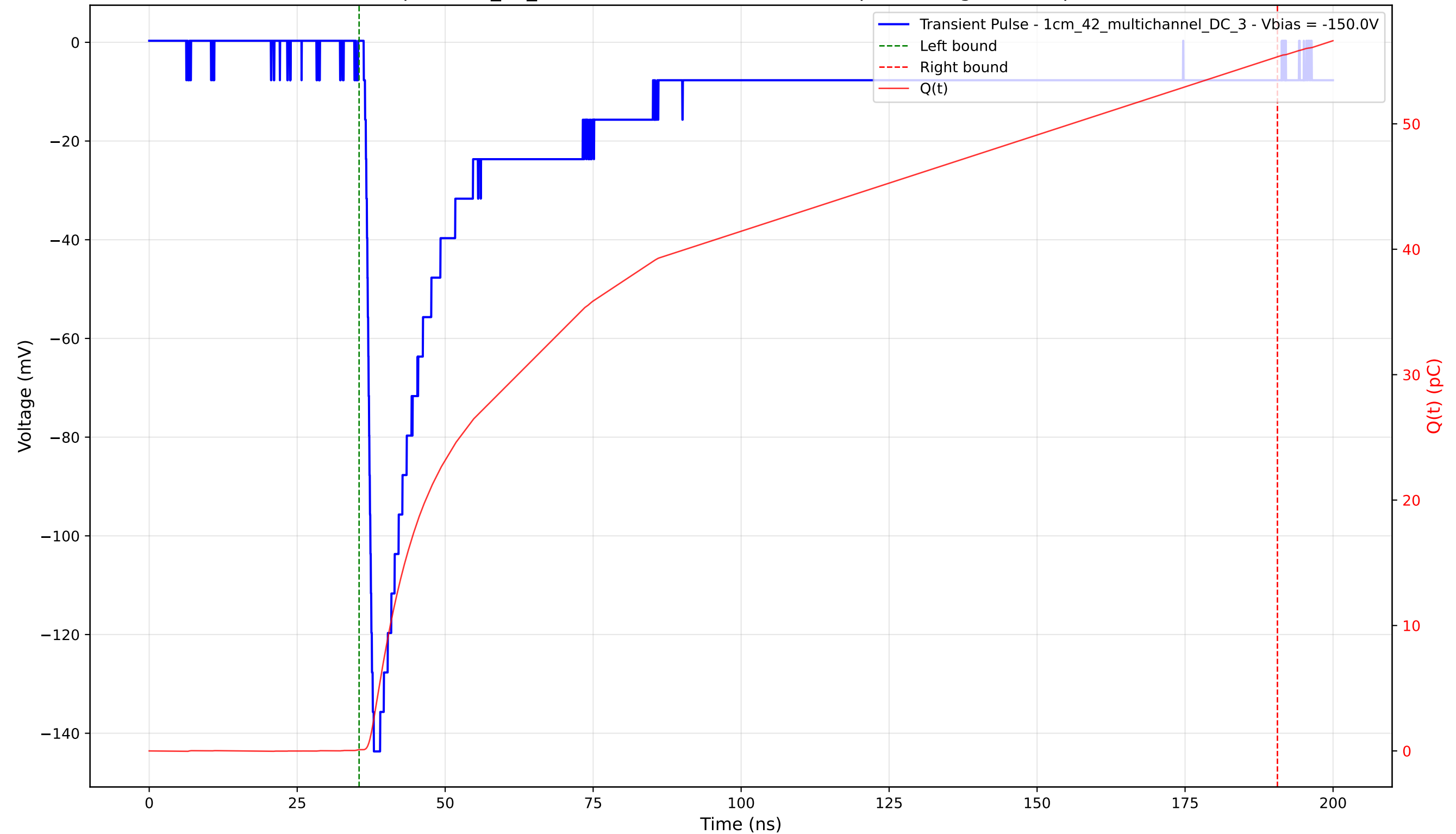
Transient Pulse - Sample: 1cm_42_multichannel - Position: 3750.0 \mu\text{m} - Charge: 55.26 pC - Rise Time: 1.30 ns
