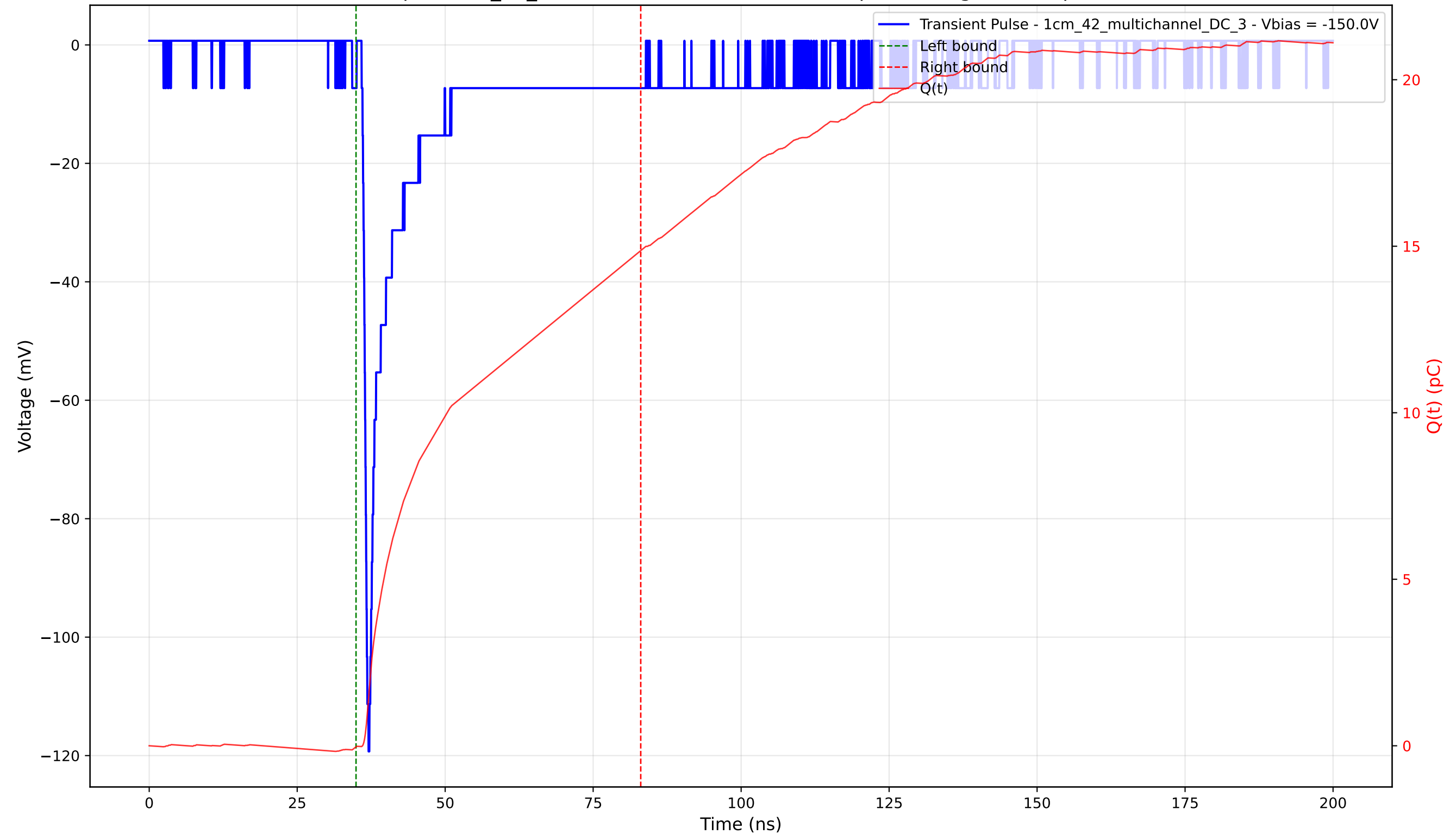
Transient Pulse - Sample: 1cm_42_multichannel - Position: 4860.0 \mu\text{m} - Charge: 14.90 pC - Rise Time: 0.81 ns
