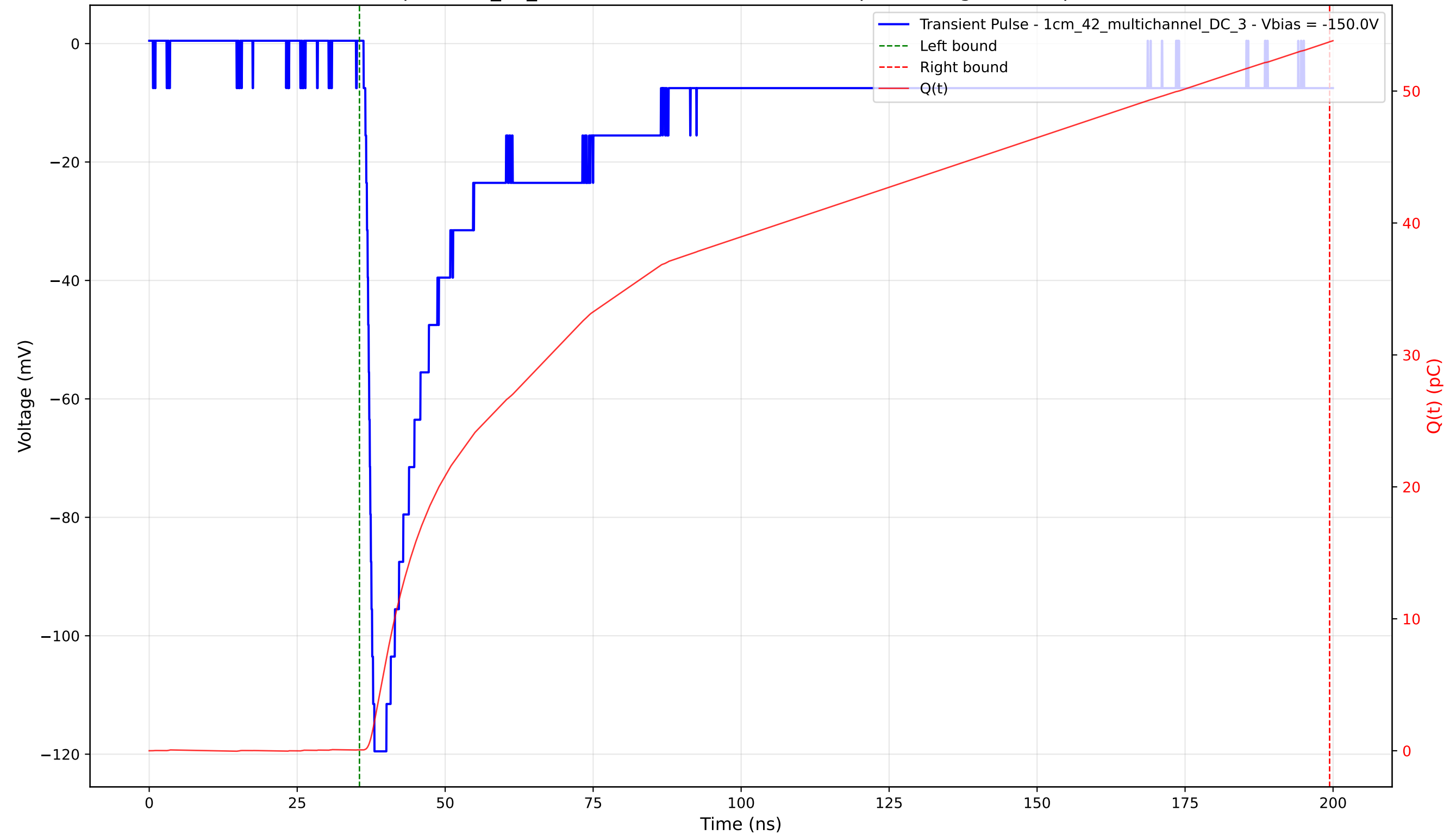
Transient Pulse - Sample: 1cm_42_multichannel - Position: 3565.0 \mu\text{m} - Charge: 53.67 pC - Rise Time: 1.31 ns
