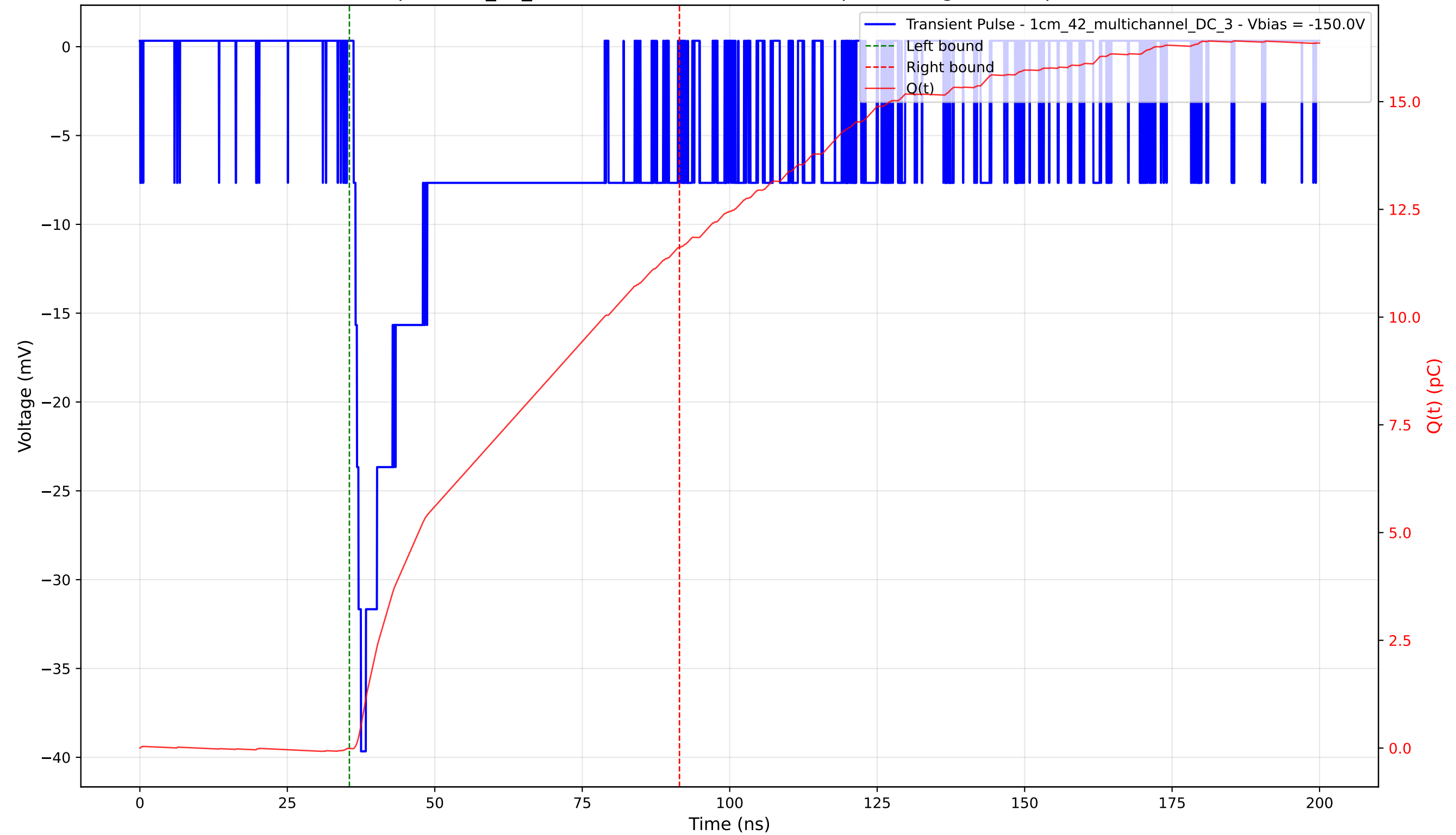
Transient Pulse - Sample: 1cm_42_multichannel - Position: 825.0 \mu\text{m} - Charge: 11.63 pC - Rise Time: 1.25 ns
