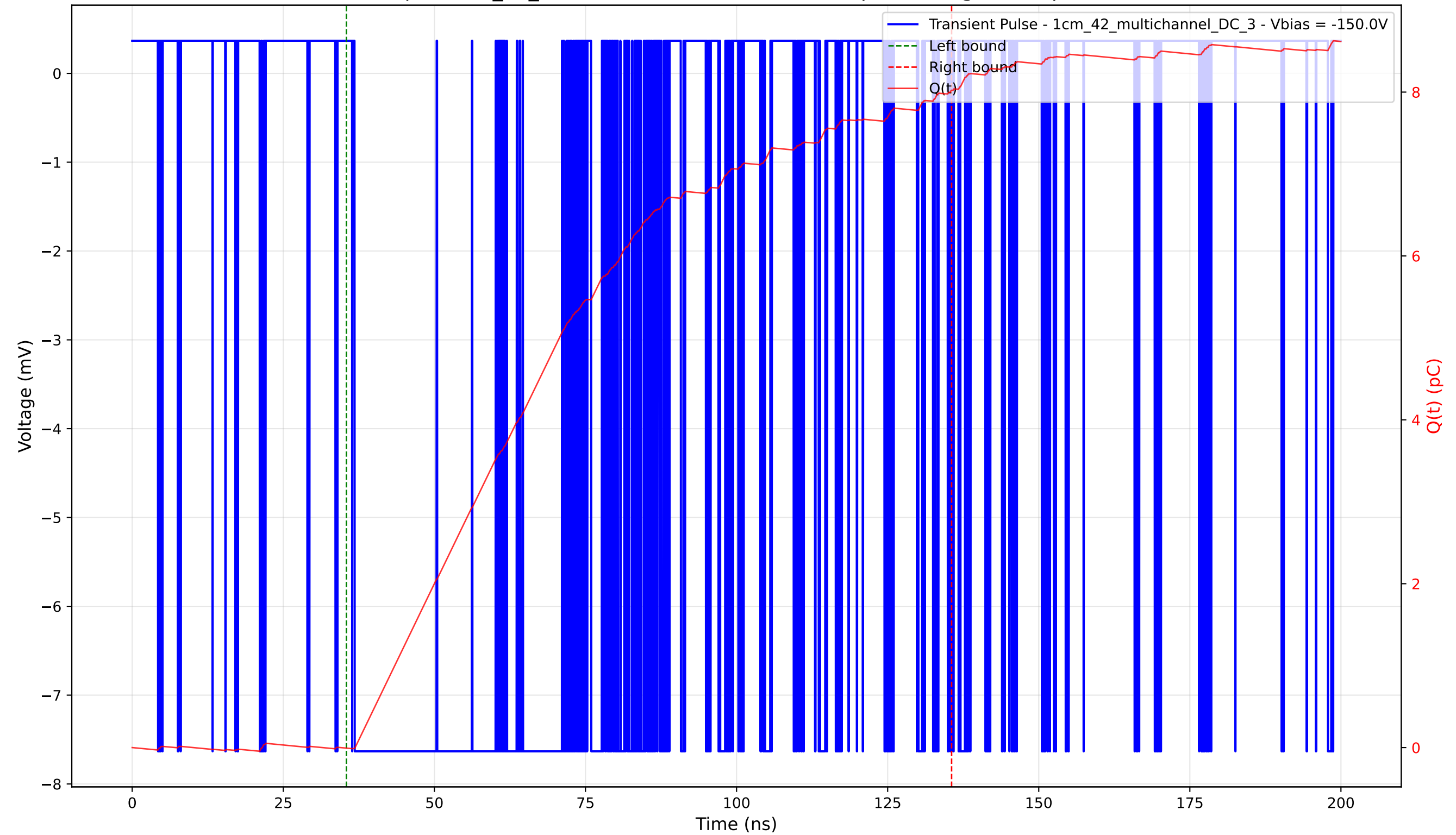
Transient Pulse - Sample: 1cm_42_multichannel - Position: 2865.0 \mu\text{m} - Charge: 8.03 pC - Rise Time: 0.02 ns
