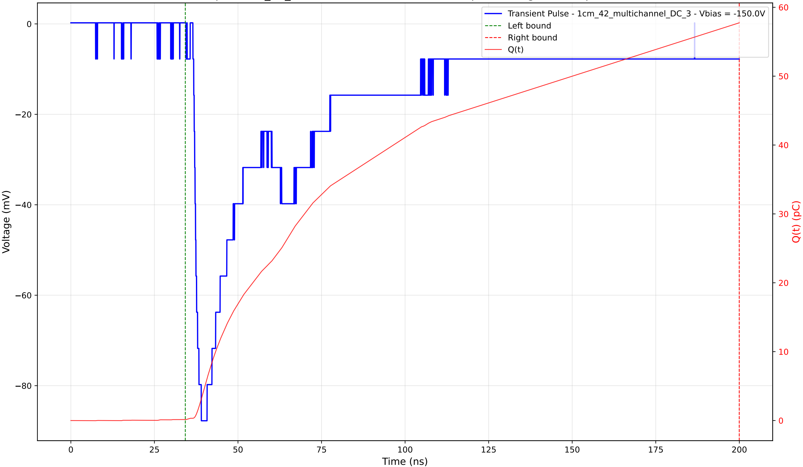
Transient Pulse - Sample: 1cm_42_multichannel - Position: 2160.0 \mu\text{m} - Charge: 57.61 pC - Rise Time: 1.58 ns
