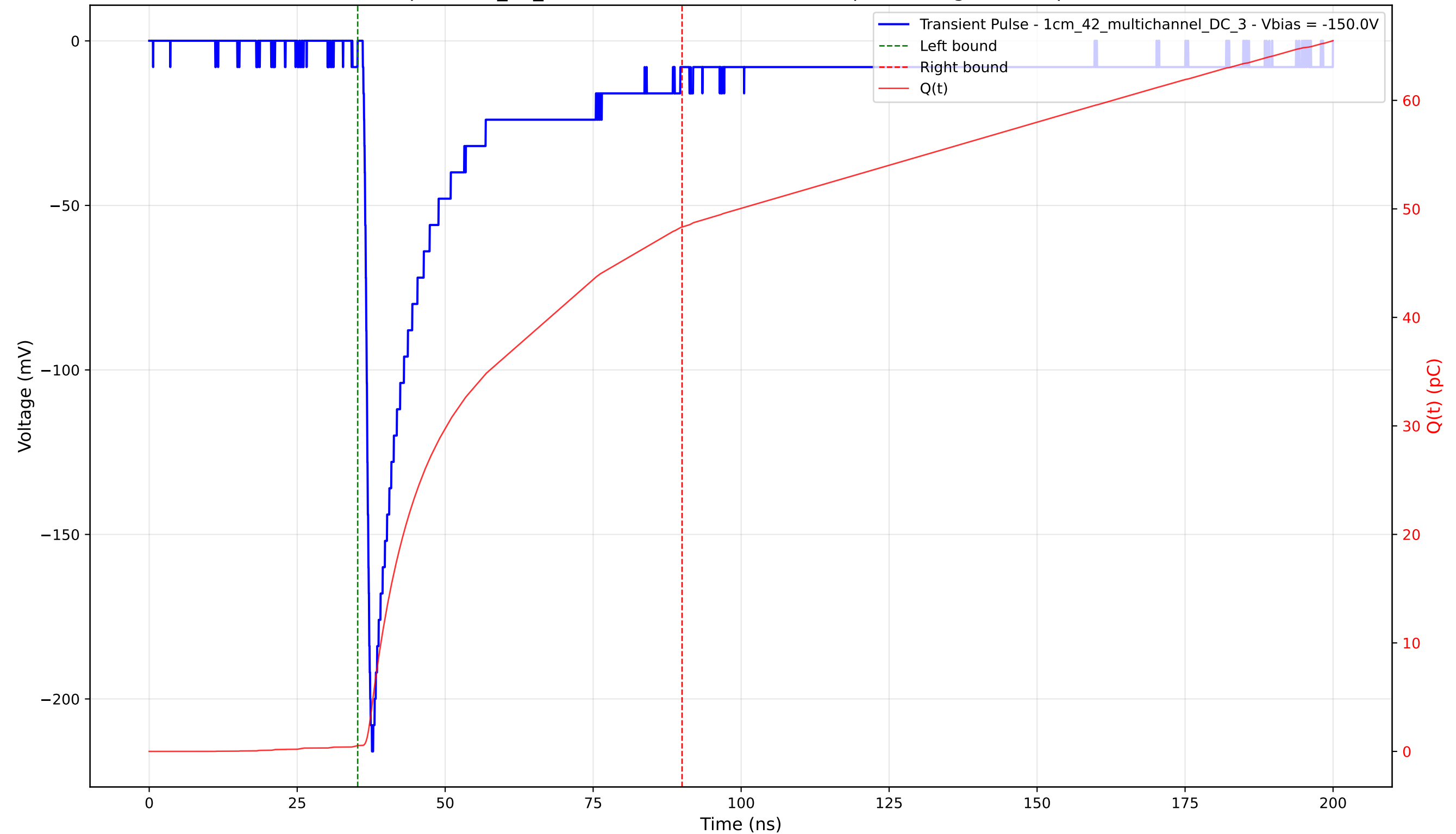
Transient Pulse - Sample: 1cm_42_multichannel - Position: 740.0 \mu\text{m} - Charge: 47.78 pC - Rise Time: 1.05 ns
