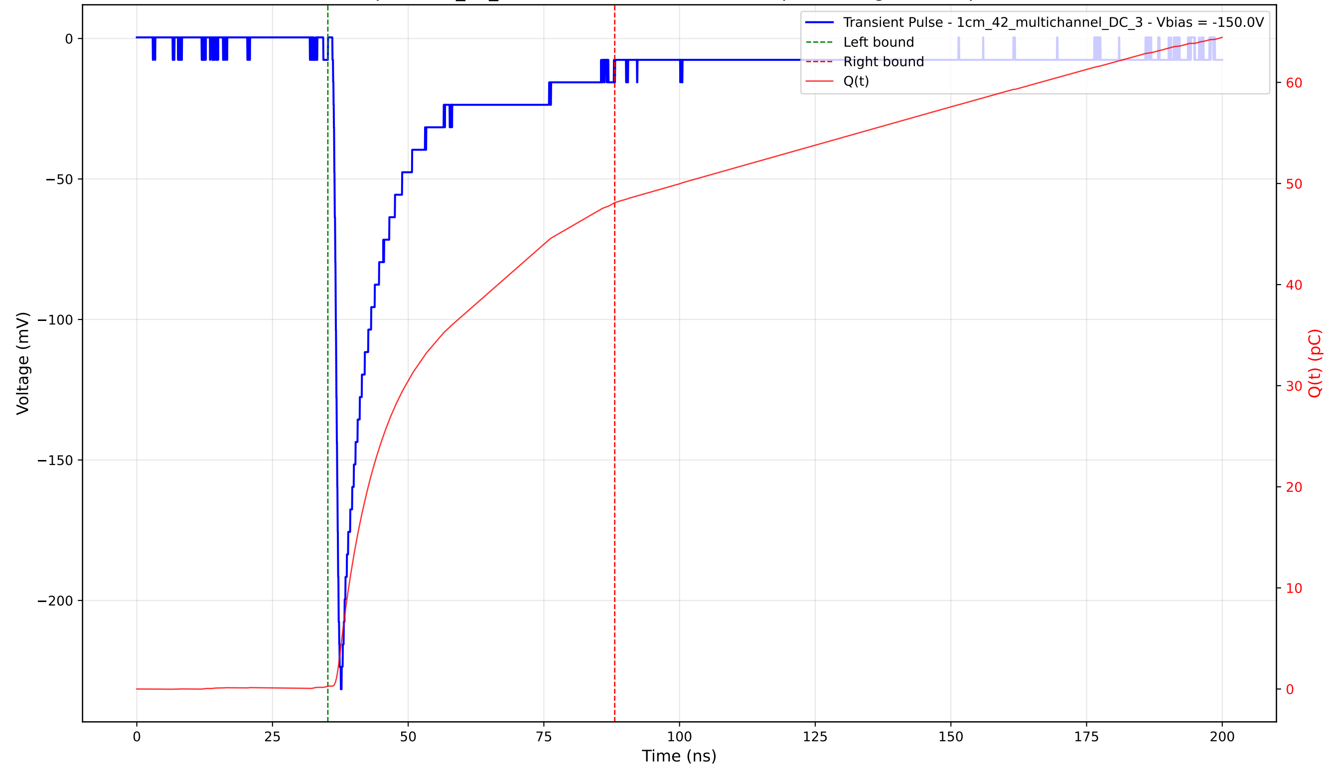
Transient Pulse - Sample: 1cm_42_multichannel - Position: 680.0 \mu\text{m} - Charge: 47.82 pC - Rise Time: 1.04 ns
