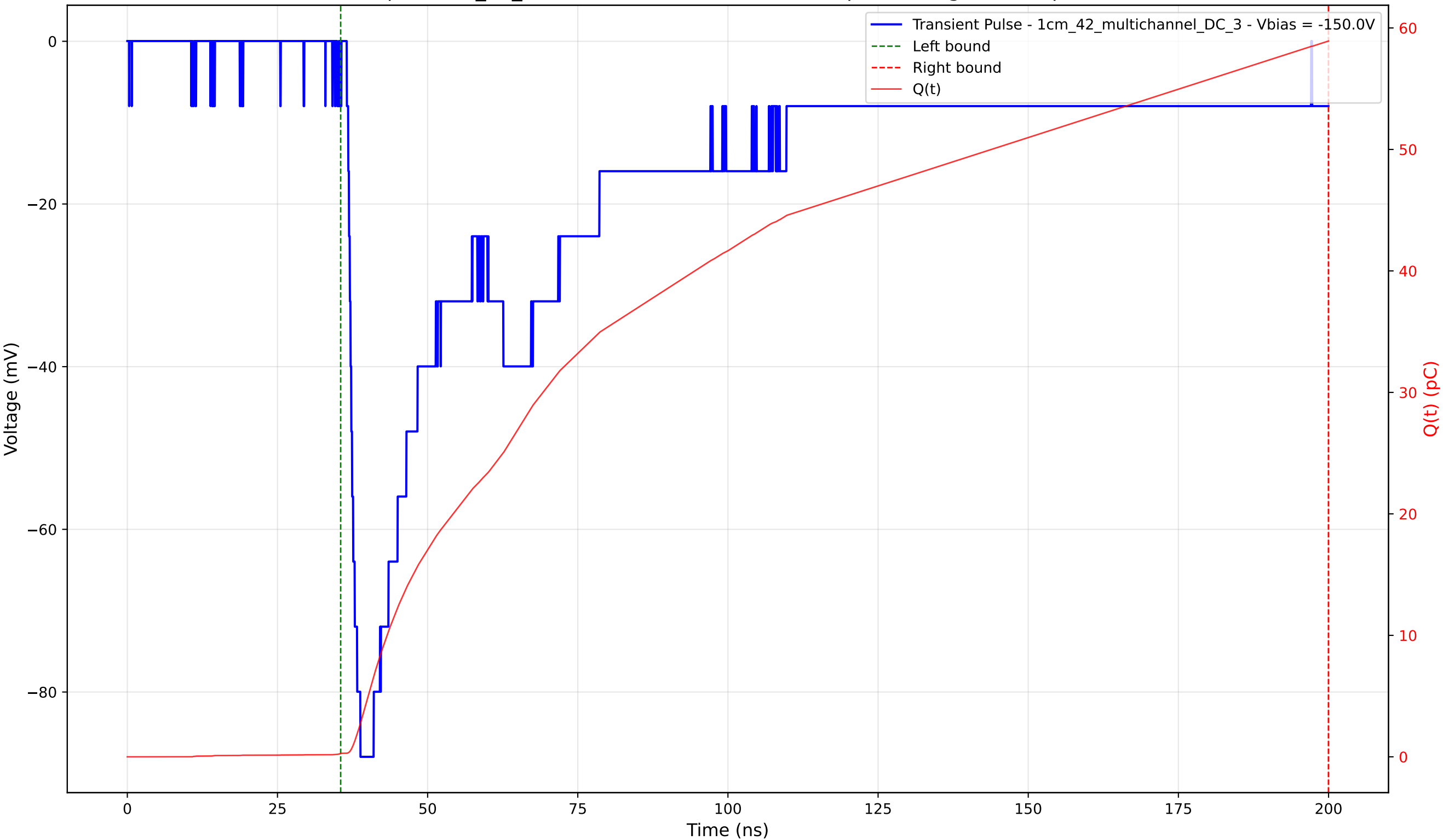
Transient Pulse - Sample: 1cm_42_multichannel - Position: 2165.0 \mu\text{m} - Charge: 58.65 pC - Rise Time: 1.50 ns
