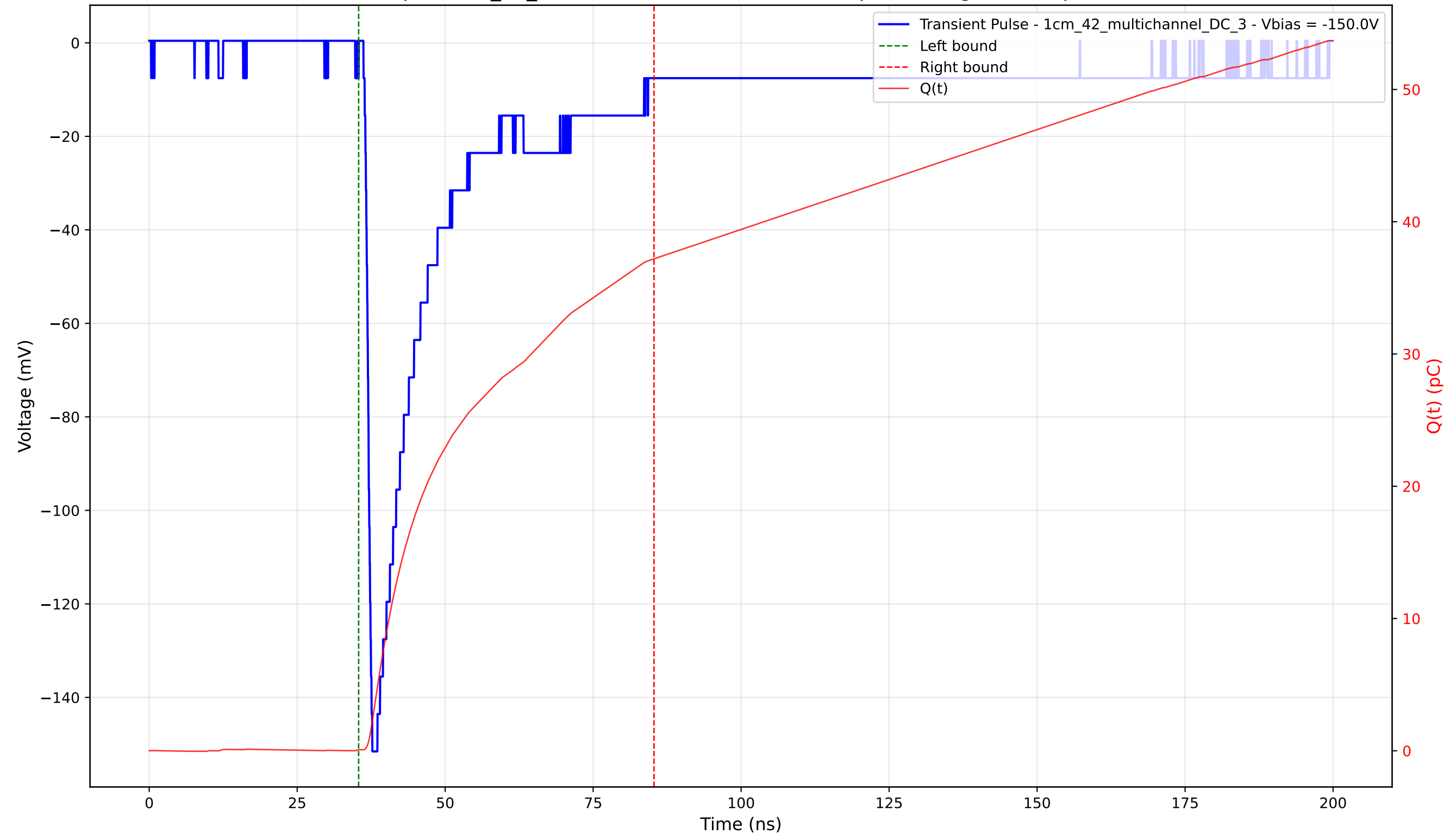
Transient Pulse - Sample: 1cm_42_multichannel - Position: 3965.0 \mu\text{m} - Charge: 37.12 pC - Rise Time: 1.16 ns
