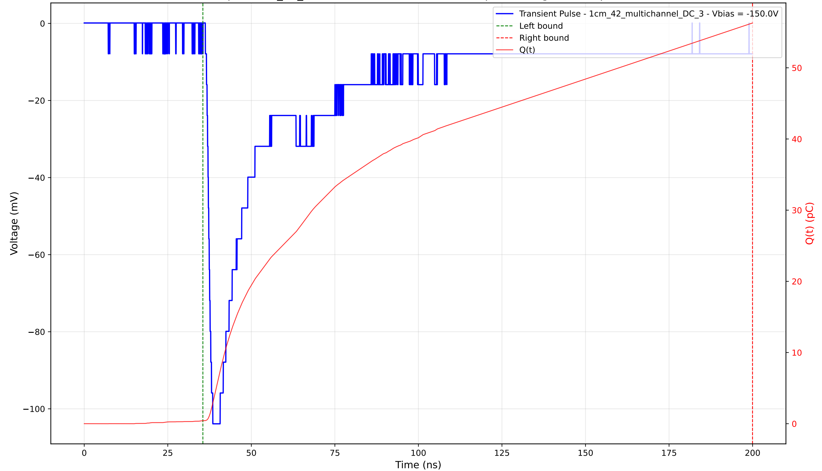
Transient Pulse - Sample: 1cm_42_multichannel - Position: 3175.0 \mu\text{m} - Charge: 55.87 pC - Rise Time: 1.51 ns
