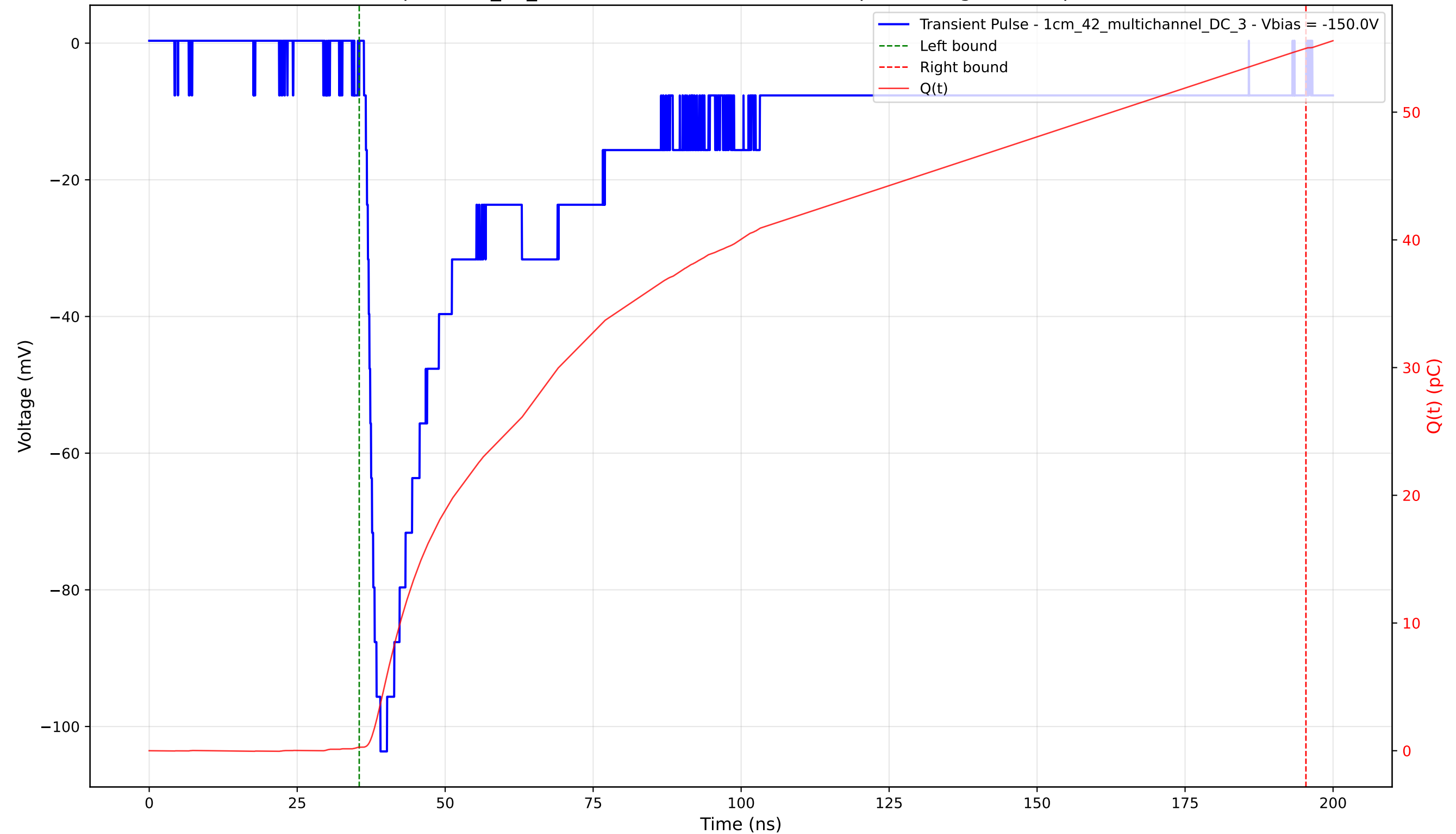
Transient Pulse - Sample: 1cm_42_multichannel - Position: 3045.0 \mu\text{m} - Charge: 54.73 pC - Rise Time: 1.81 ns
