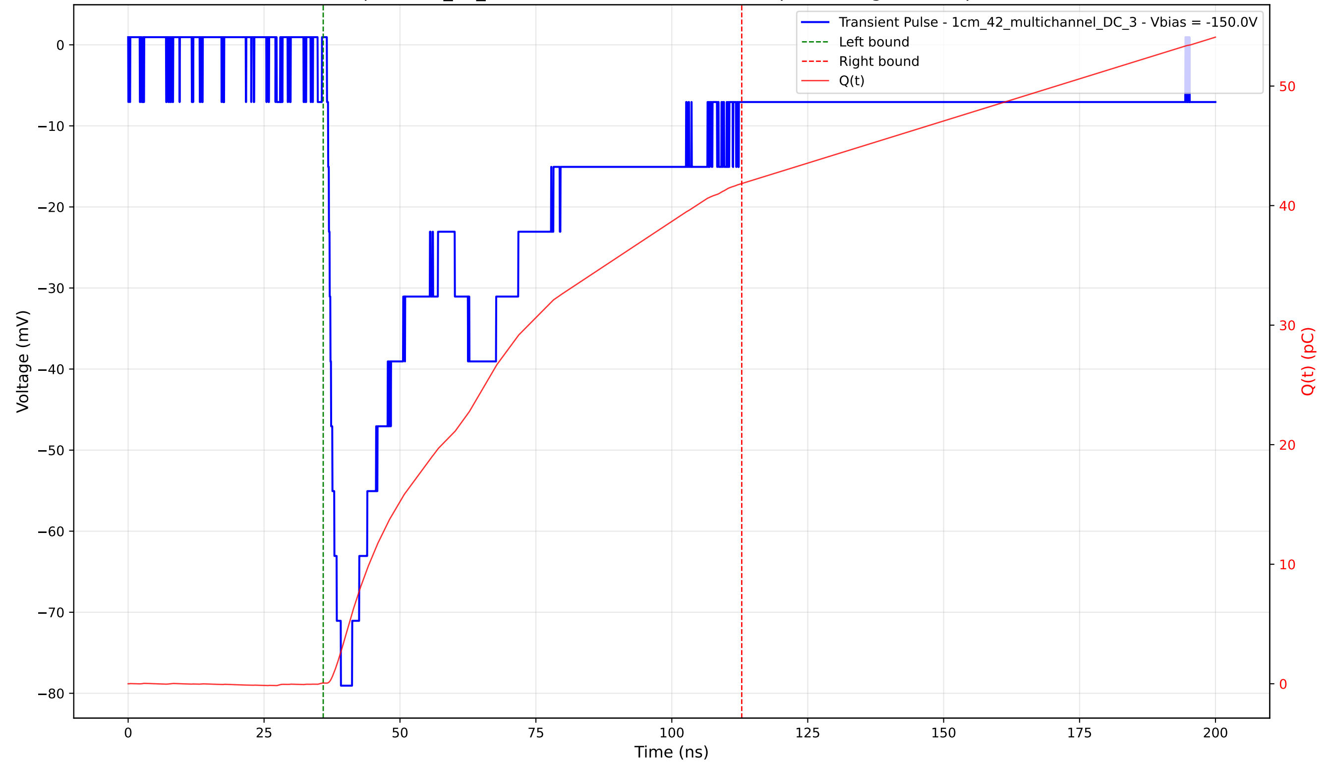
Transient Pulse - Sample: 1cm_42_multichannel - Position: 2460.0 \mu\text{m} - Charge: 41.80 pC - Rise Time: 2.36 ns
