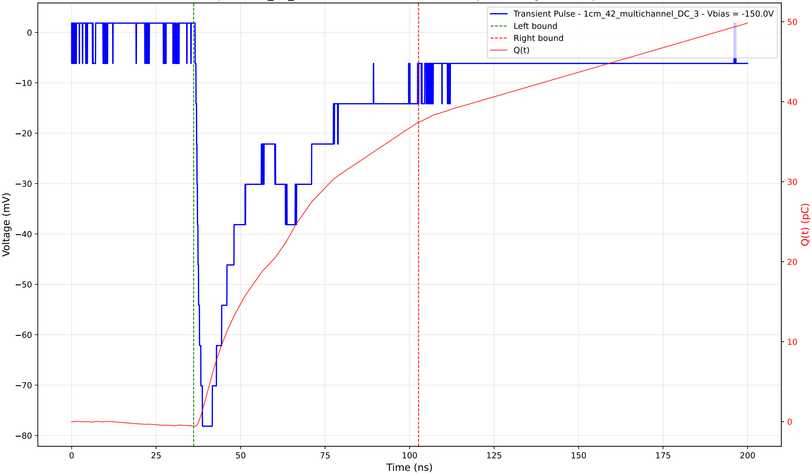
Transient Pulse - Sample: 1cm_42_multichannel - Position: 2595.0 \mu\text{m} - Charge: 38.00 pC - Rise Time: 1.92 ns
