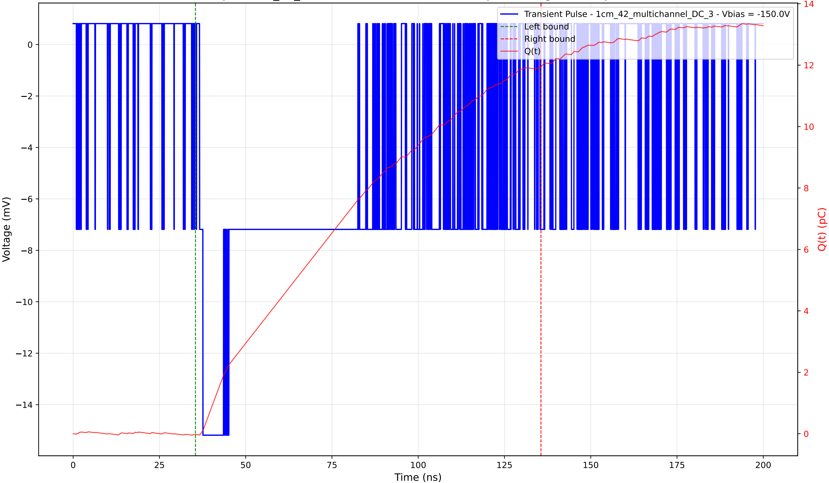
Transient Pulse - Sample: 1cm_42_multichannel - Position: 2850.0 \mu\text{m} - Charge: 11.96 pC - Rise Time: 0.98 ns
