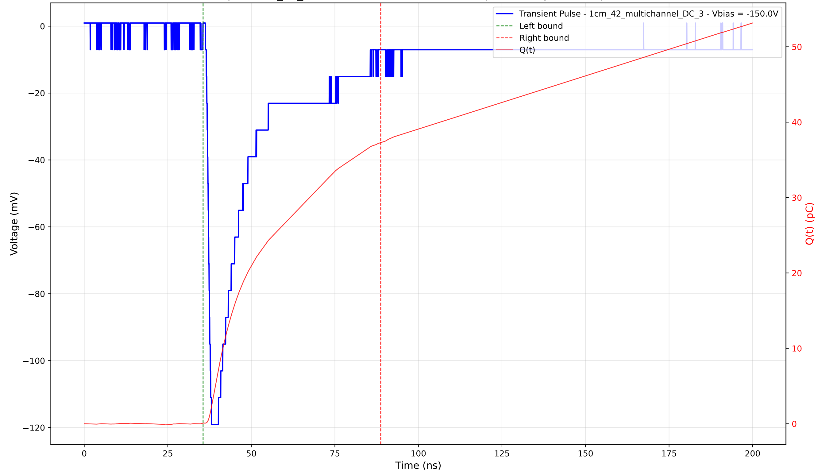
Transient Pulse - Sample: 1cm_42_multichannel - Position: 3525.0 \mu\text{m} - Charge: 37.20 pC - Rise Time: 1.33 ns
