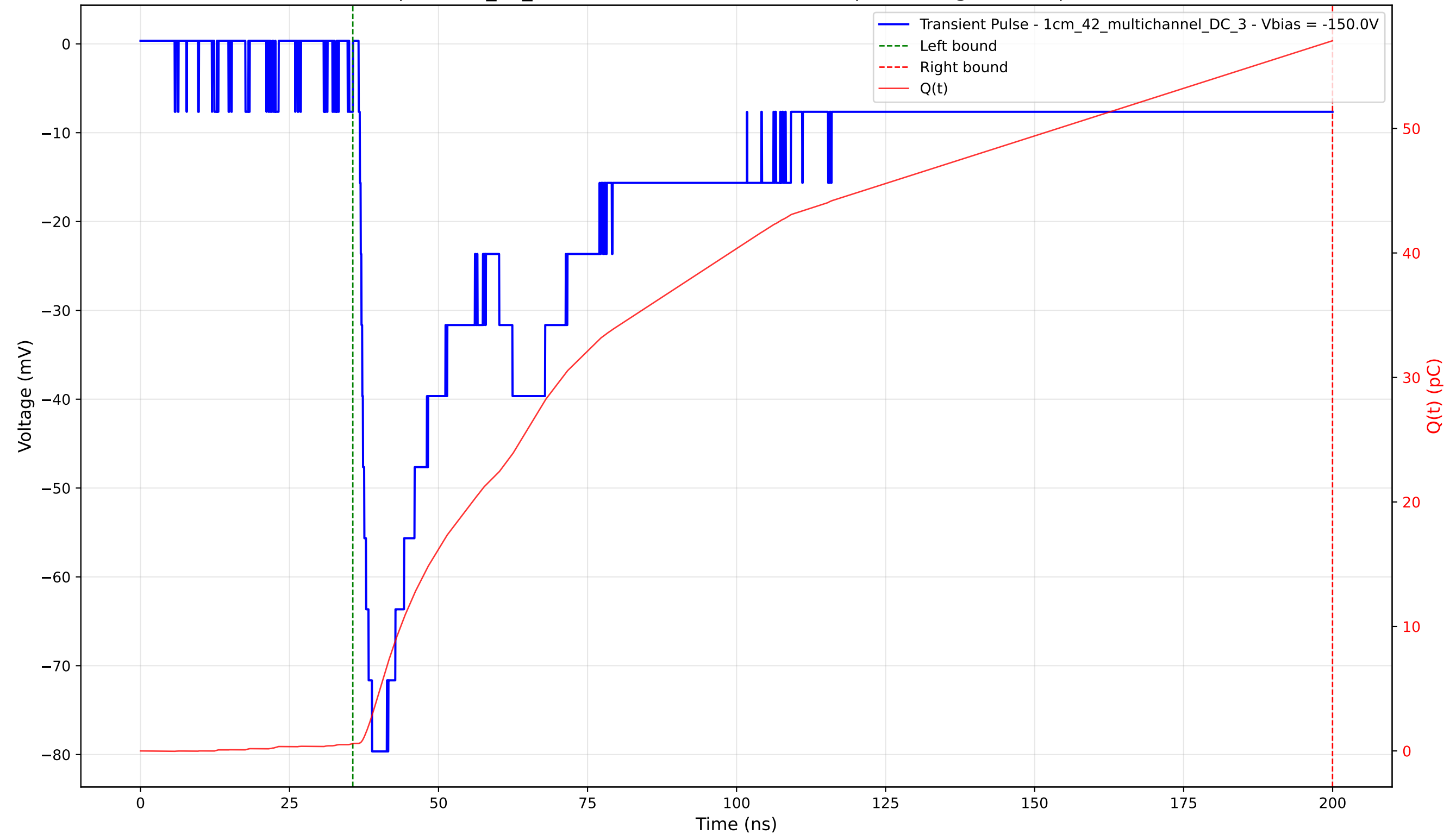
Transient Pulse - Sample: 1cm_42_multichannel - Position: 2505.0 \mu\text{m} - Charge: 56.45 pC - Rise Time: 2.06 ns
