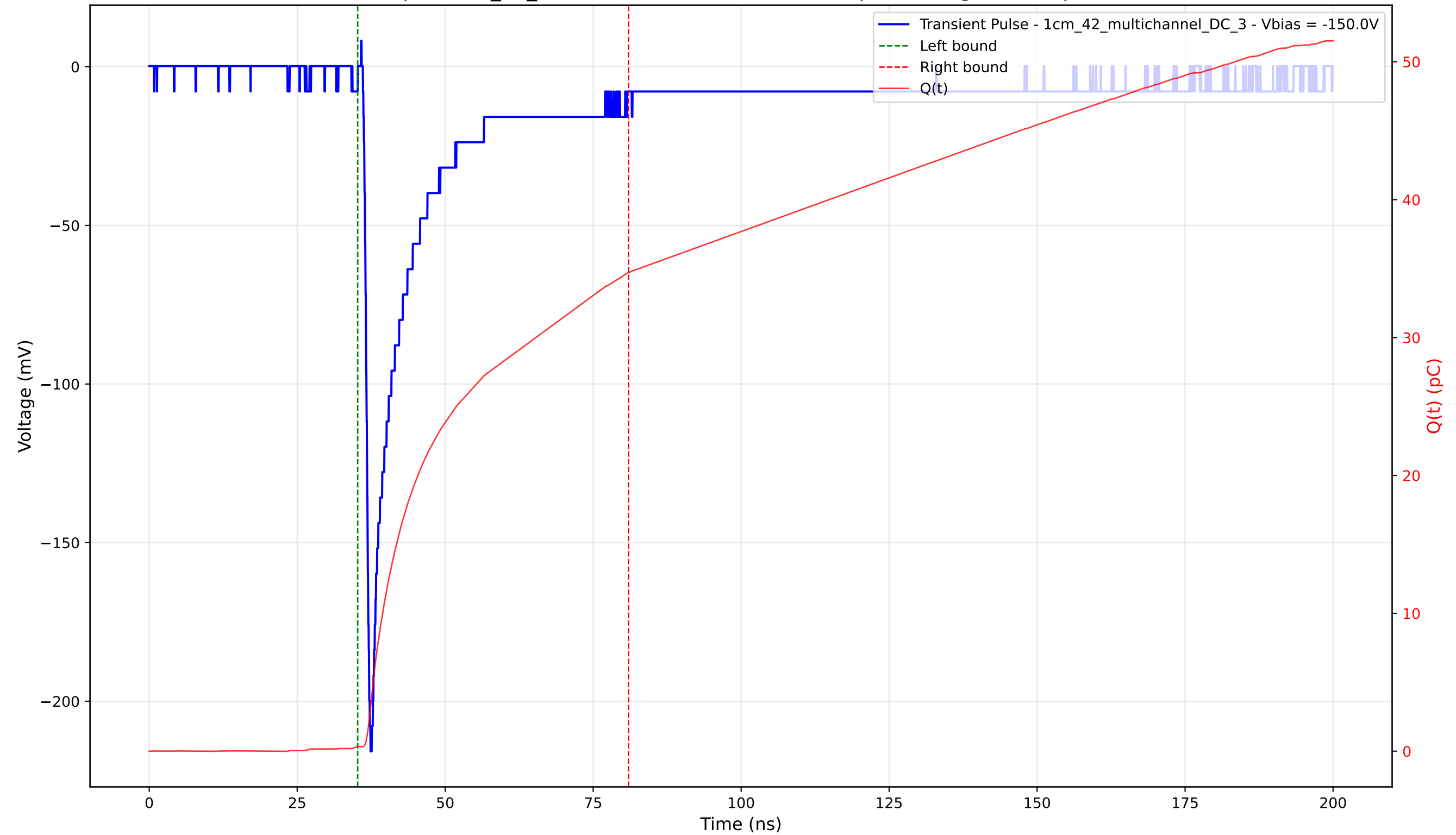
Transient Pulse - Sample: 1cm_42_multichannel - Position: 4465.0 \mu\text{m} - Charge: 34.37 pC - Rise Time: 0.93 ns
