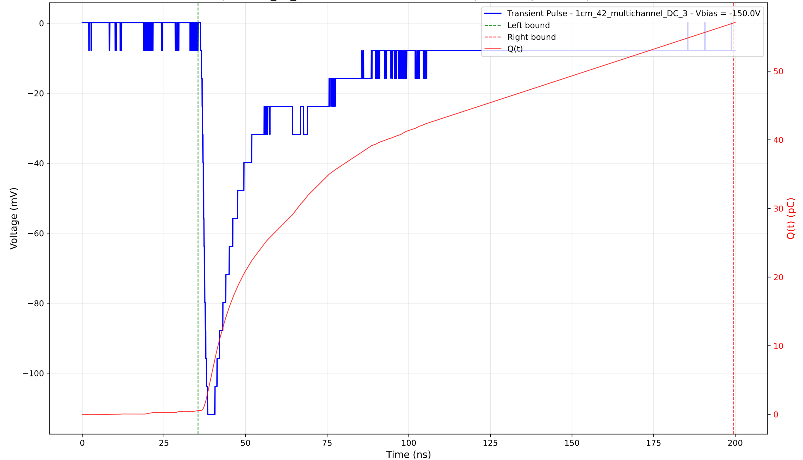
Transient Pulse - Sample: 1cm_42_multichannel - Position: 3270.0 \mu\text{m} - Charge: 56.49 pC - Rise Time: 1.53 ns
