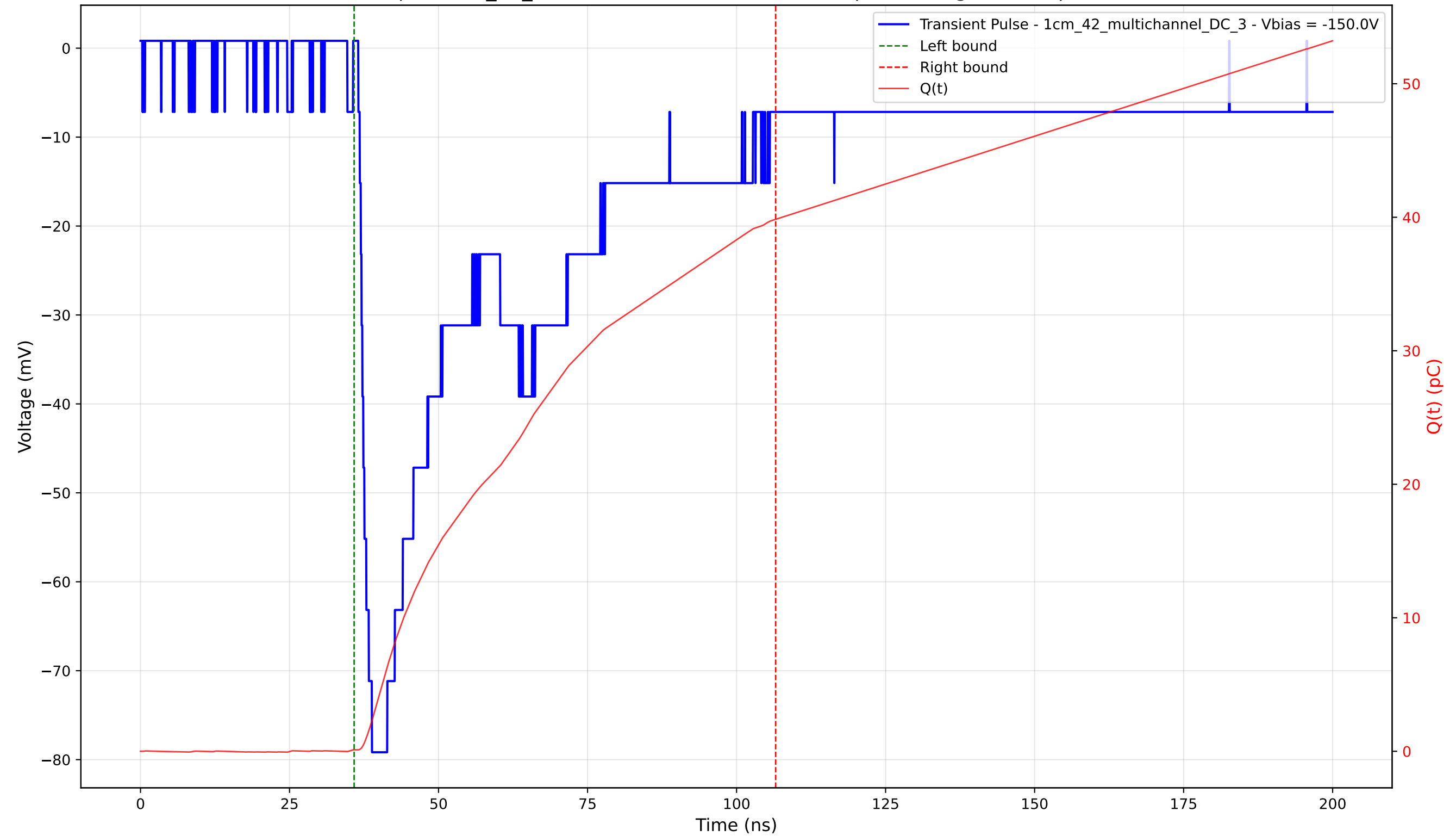
Transient Pulse - Sample: 1cm_42_multichannel - Position: 2580.0 \mu\text{m} - Charge: 39.74 pC - Rise Time: 2.06 ns
