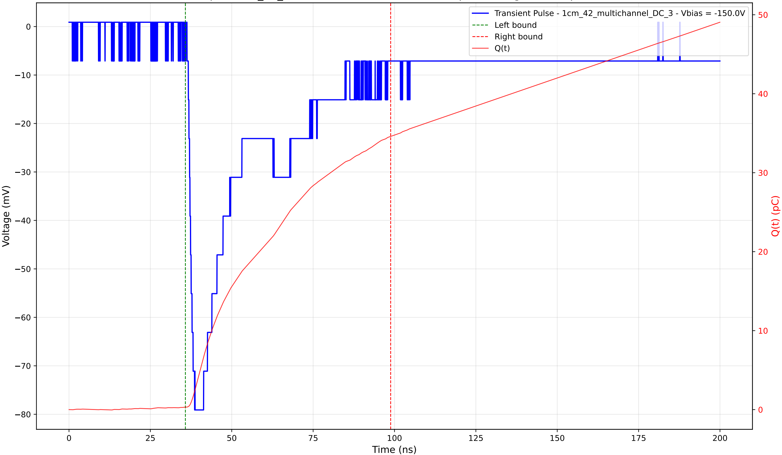
Transient Pulse - Sample: 1cm_42_multichannel - Position: 2805.0 \mu\text{m} - Charge: 34.28 pC - Rise Time: 1.94 ns
