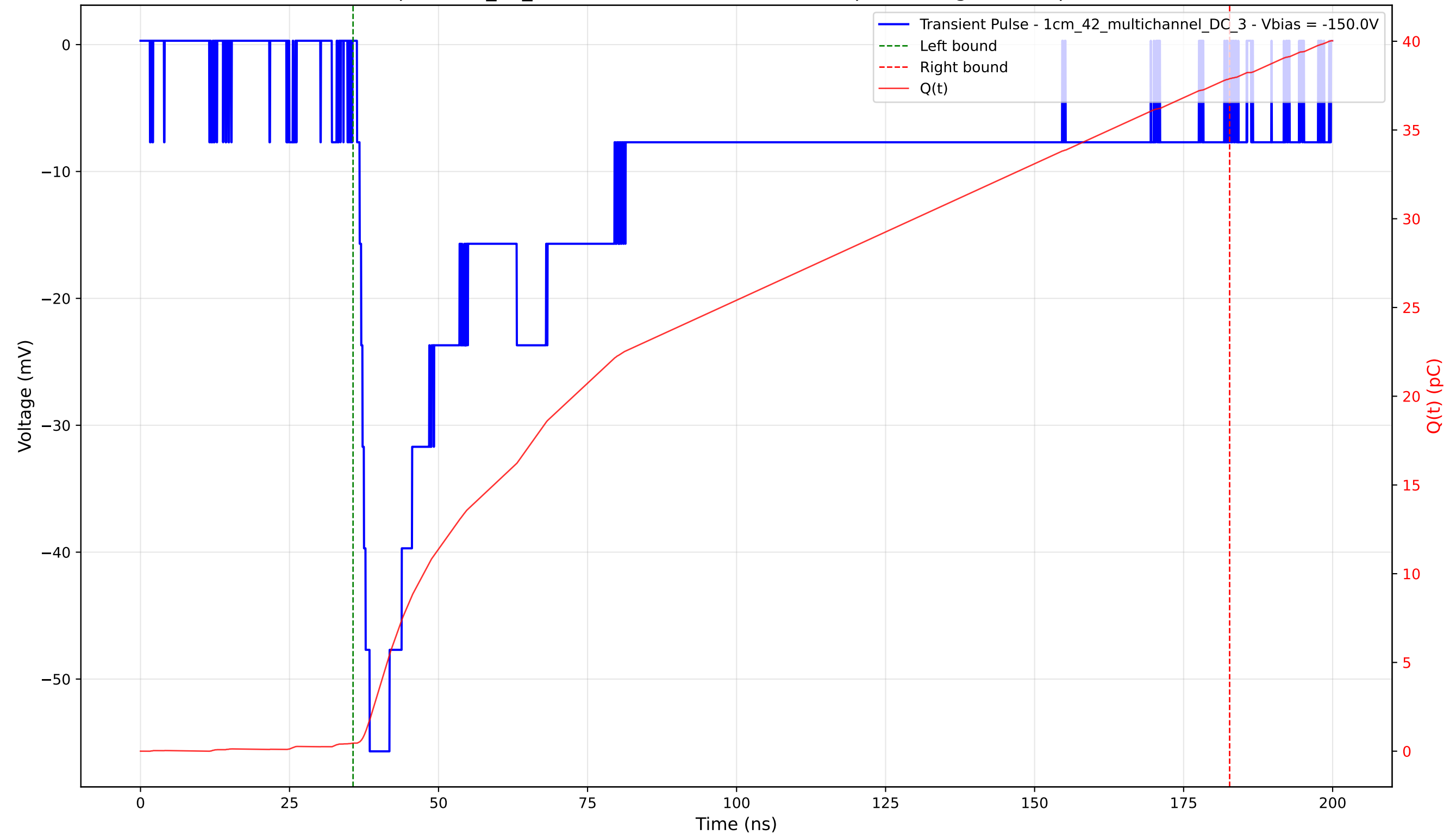
Transient Pulse - Sample: 1cm_42_multichannel - Position: 2825.0 \mu\text{m} - Charge: 37.45 pC - Rise Time: 2.13 ns
