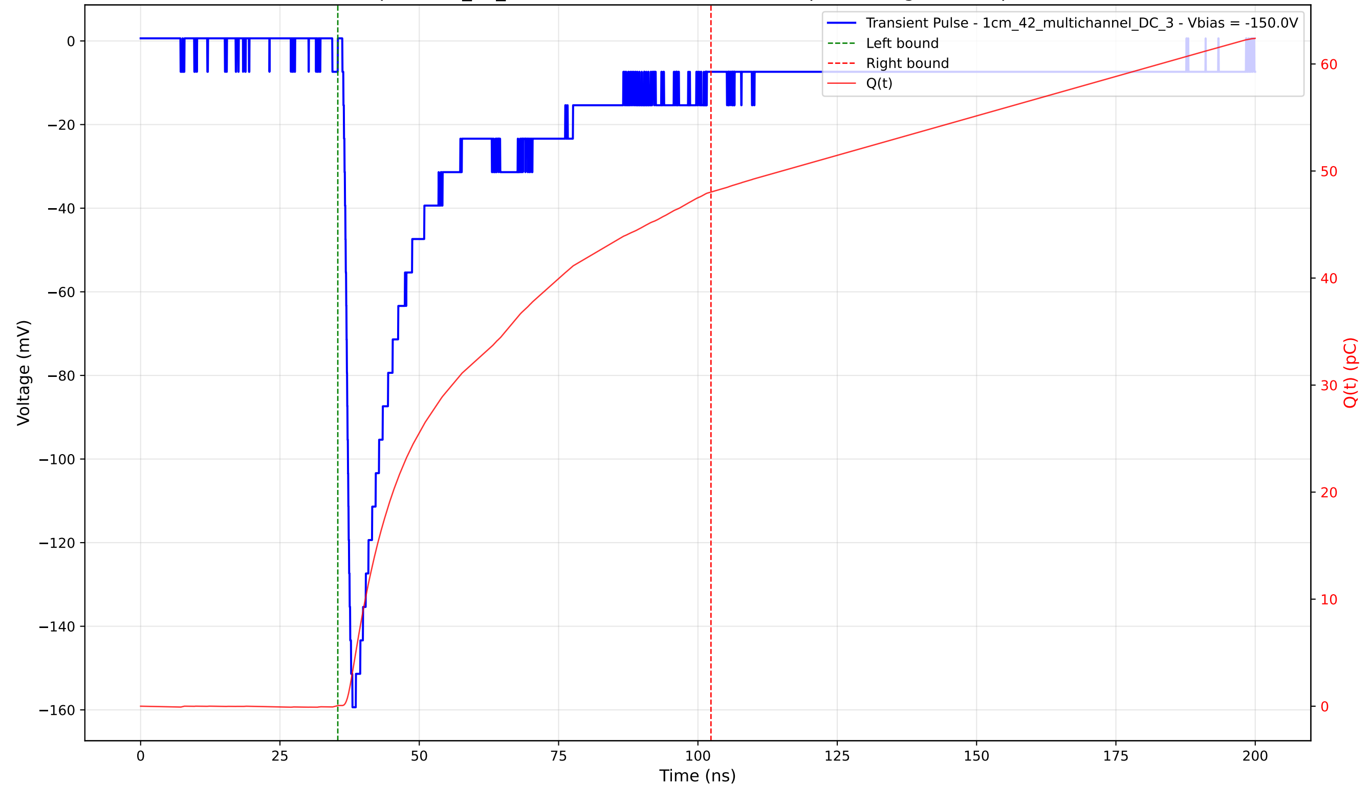
Transient Pulse - Sample: 1cm_42_multichannel - Position: 1170.0 \mu\text{m} - Charge: 47.97 pC - Rise Time: 1.30 ns
