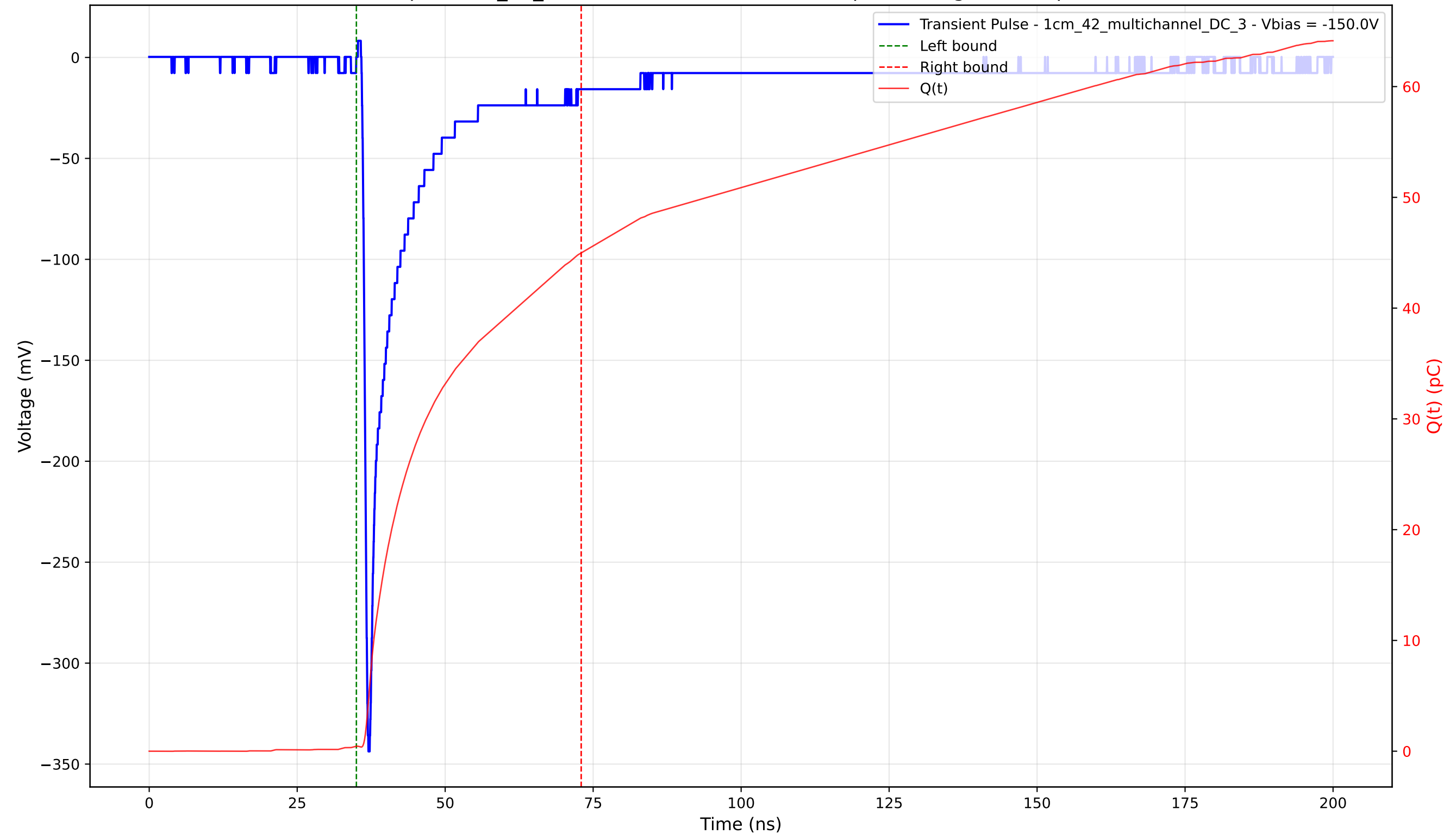
Transient Pulse - Sample: 1cm_42_multichannel - Position: 215.0 \mu\text{m} - Charge: 44.53 pC - Rise Time: 0.79 ns
