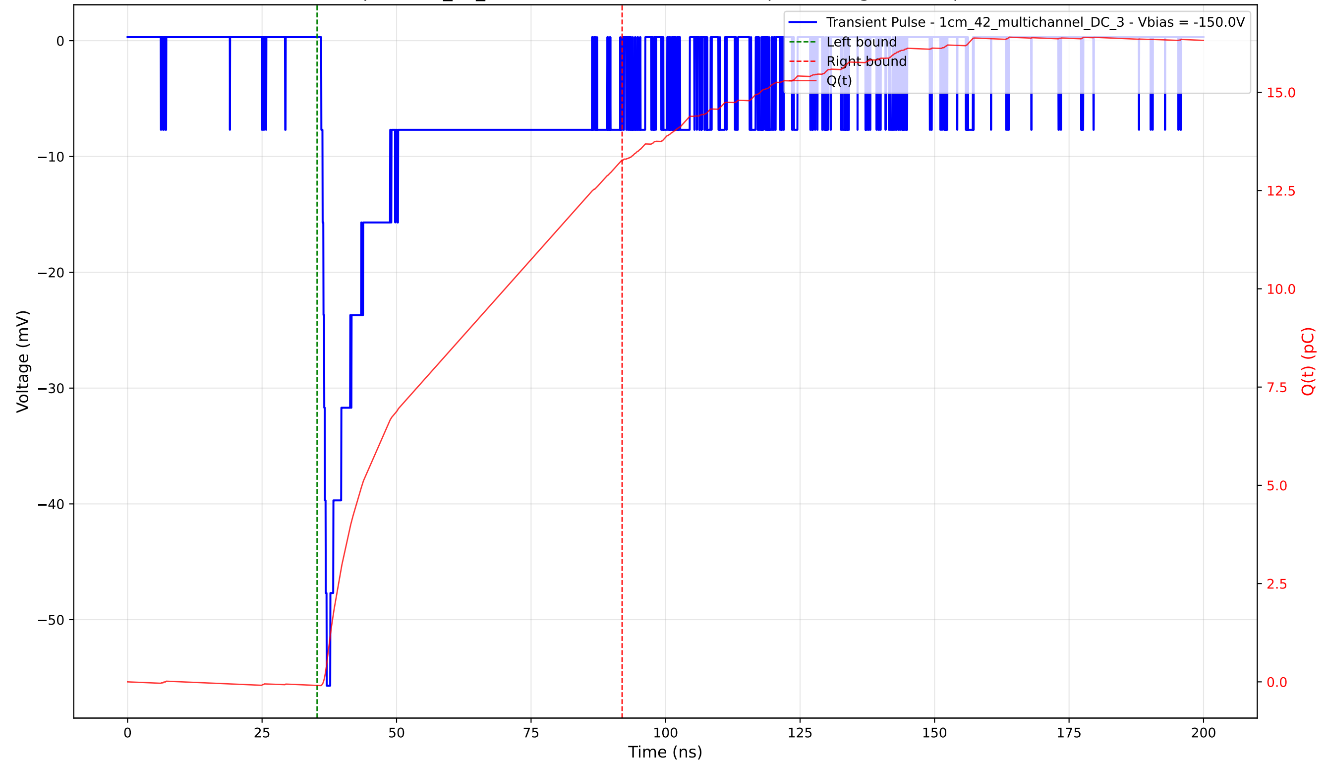
Transient Pulse - Sample: 1cm_42_multichannel - Position: 385.0 \mu\text{m} - Charge: 13.37 pC - Rise Time: 1.01 ns
