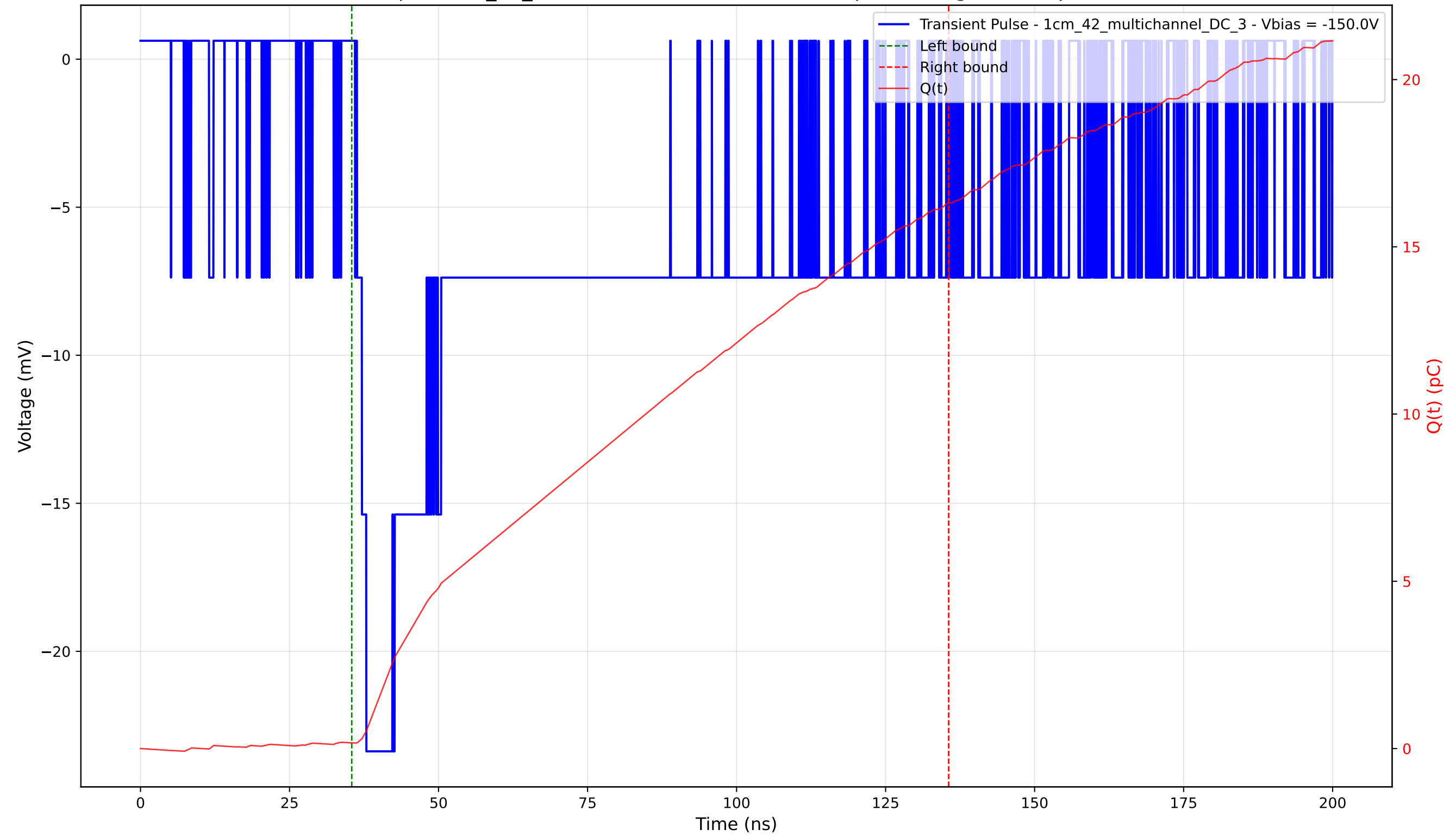
Transient Pulse - Sample: 1cm_42_multichannel - Position: 1835.0 \mu\text{m} - Charge: 16.15 pC - Rise Time: 1.57 ns
