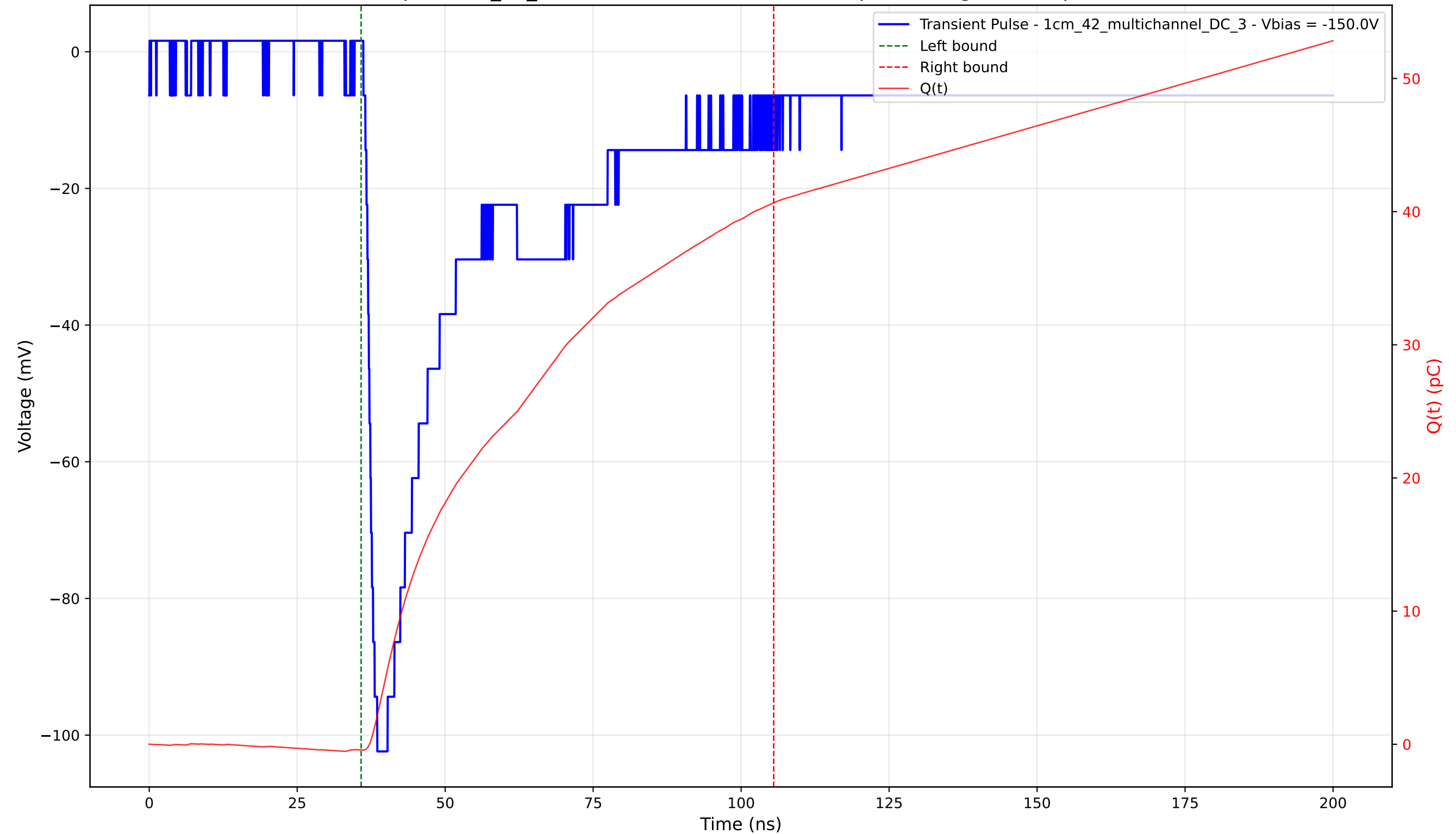
Transient Pulse - Sample: 1cm_42_multichannel - Position: 1785.0 \mu\text{m} - Charge: 41.10 pC - Rise Time: 1.57 ns
