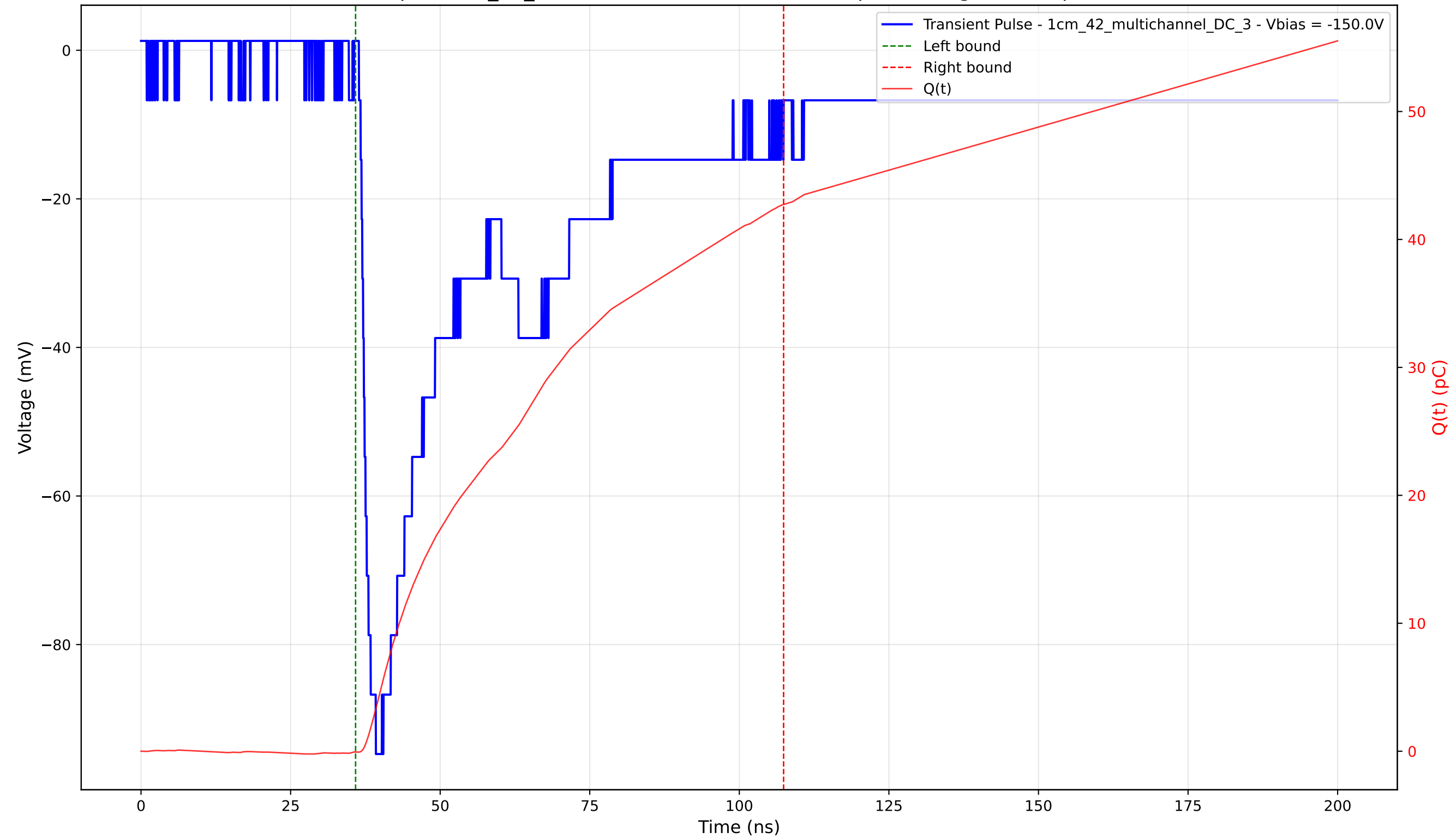
Transient Pulse - Sample: 1cm_42_multichannel - Position: 2065.0 \mu\text{m} - Charge: 42.81 pC - Rise Time: 1.69 ns
