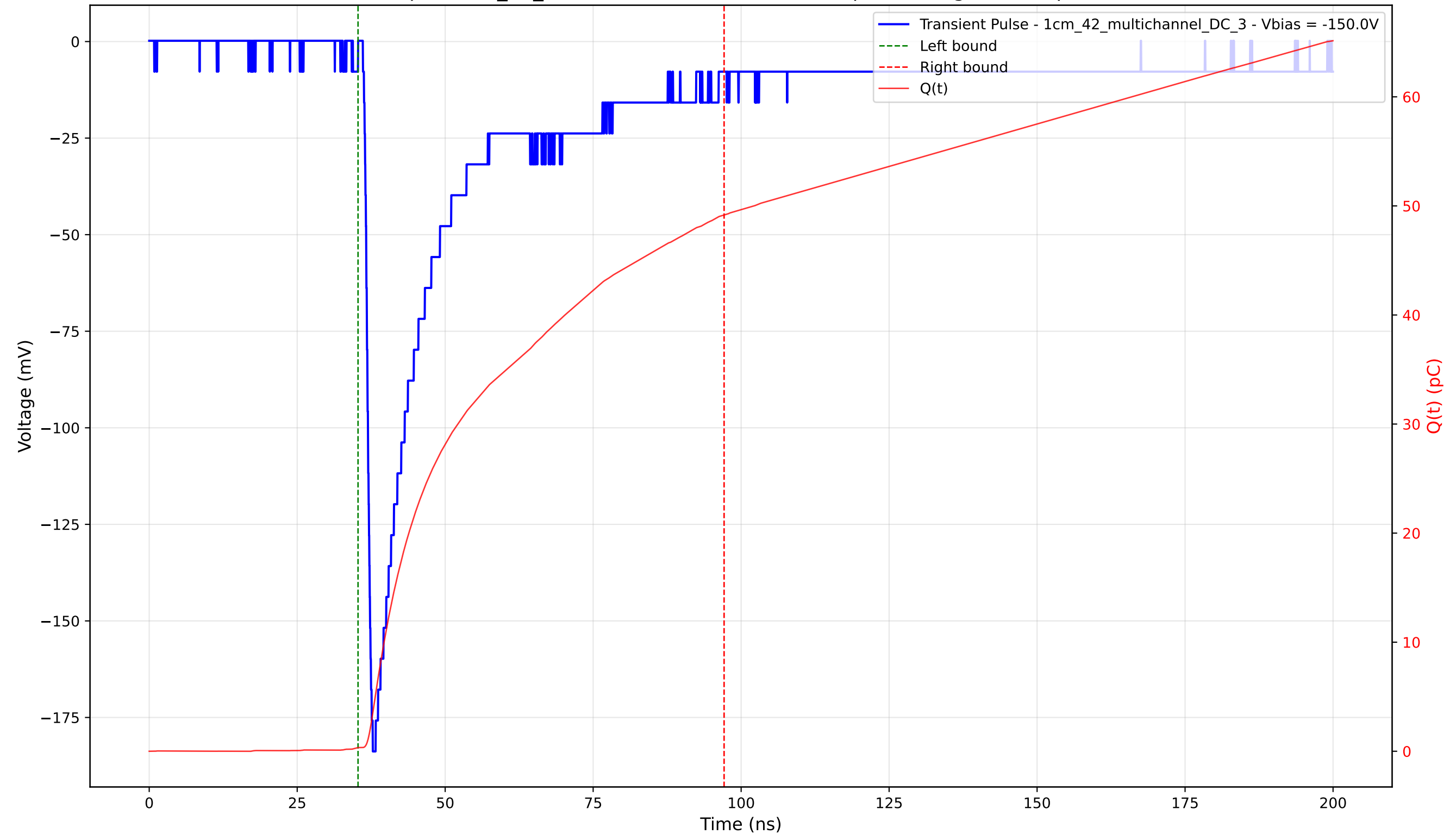
Transient Pulse - Sample: 1cm_42_multichannel - Position: 975.0 \mu\text{m} - Charge: 48.82 pC - Rise Time: 1.09 ns
