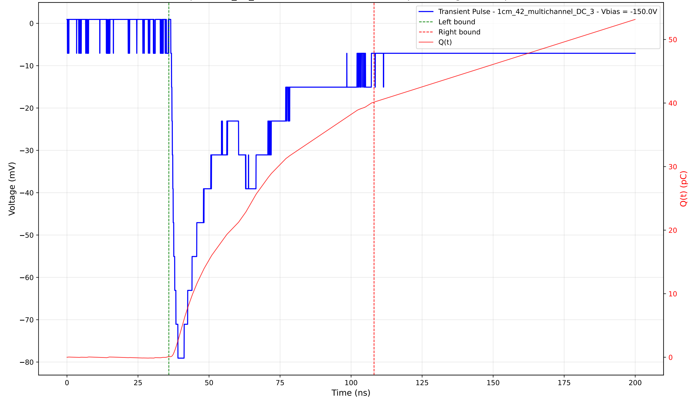
Transient Pulse - Sample: 1cm_42_multichannel - Position: 2550.0 \mu\text{m} - Charge: 40.03 pC - Rise Time: 2.26 ns
