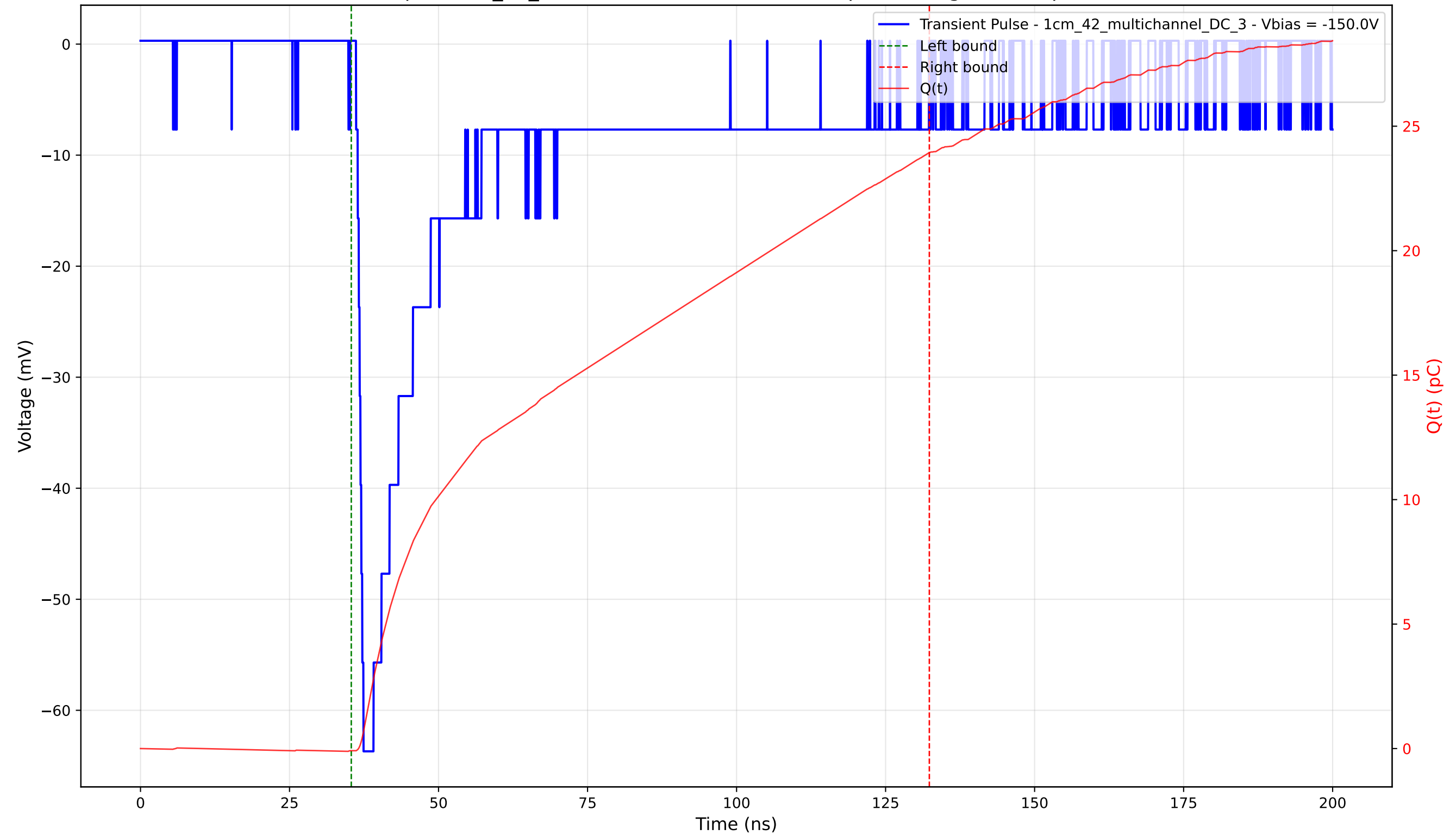
Transient Pulse - Sample: 1cm_42_multichannel - Position: 900.0 \mu\text{m} - Charge: 24.02 pC - Rise Time: 1.24 ns
