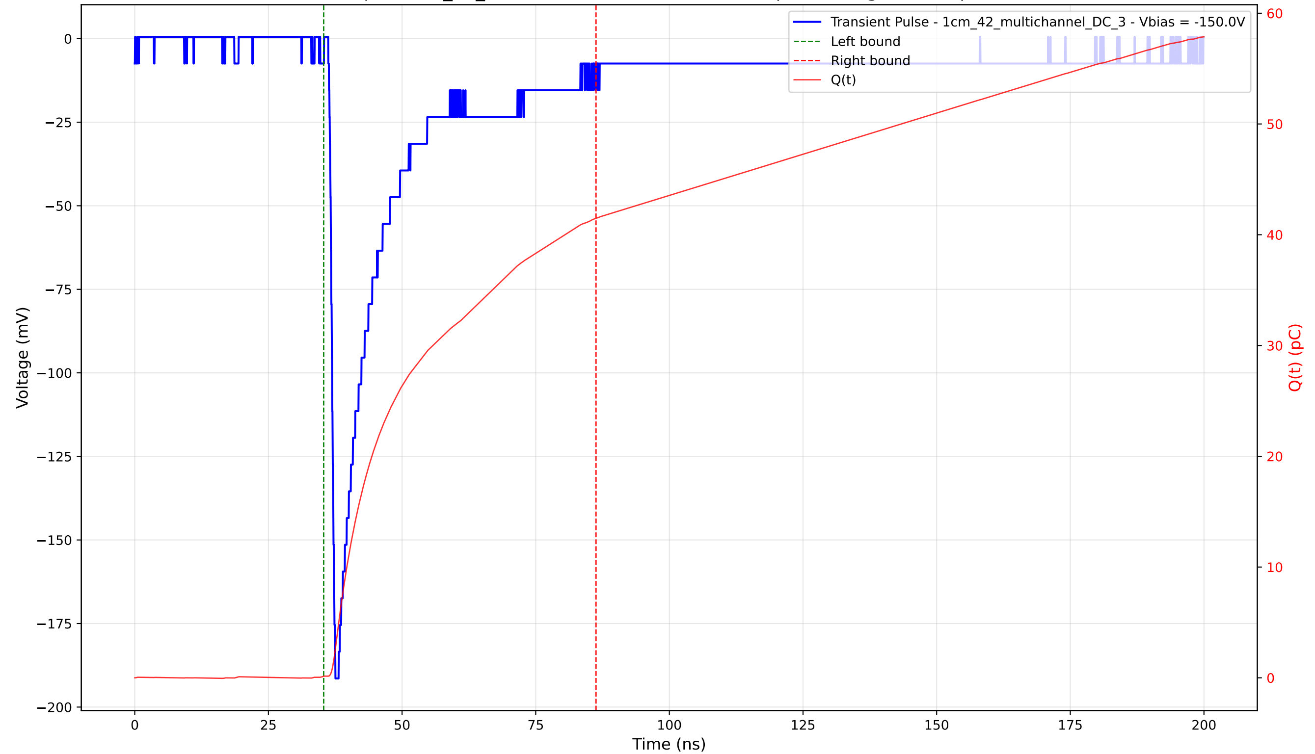
Transient Pulse - Sample: 1cm_42_multichannel - Position: 4160.0 \mu\text{m} - Charge: 41.35 pC - Rise Time: 0.93 ns
