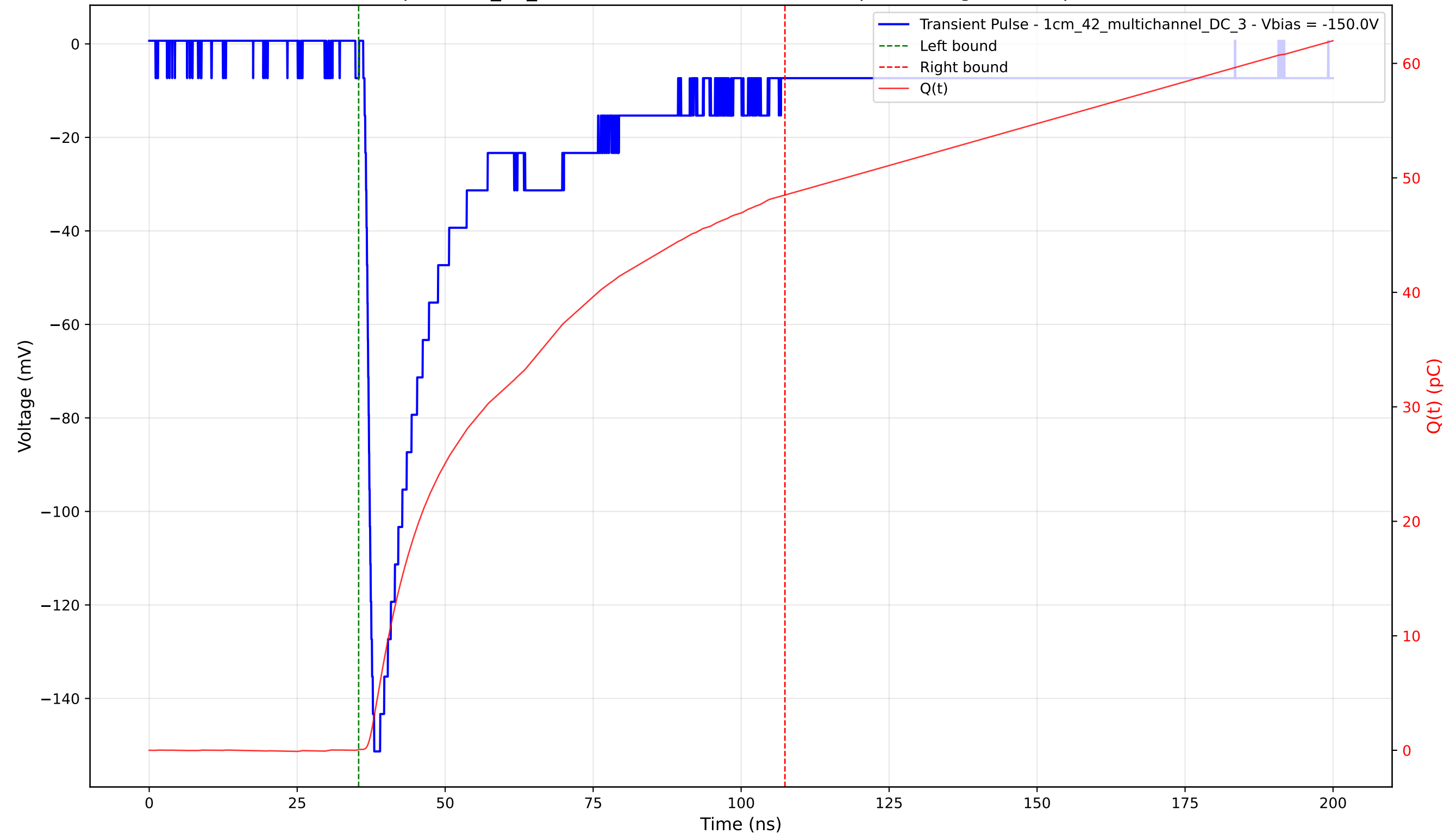
Transient Pulse - Sample: 1cm_42_multichannel - Position: 1260.0 \mu\text{m} - Charge: 48.45 pC - Rise Time: 1.40 ns
