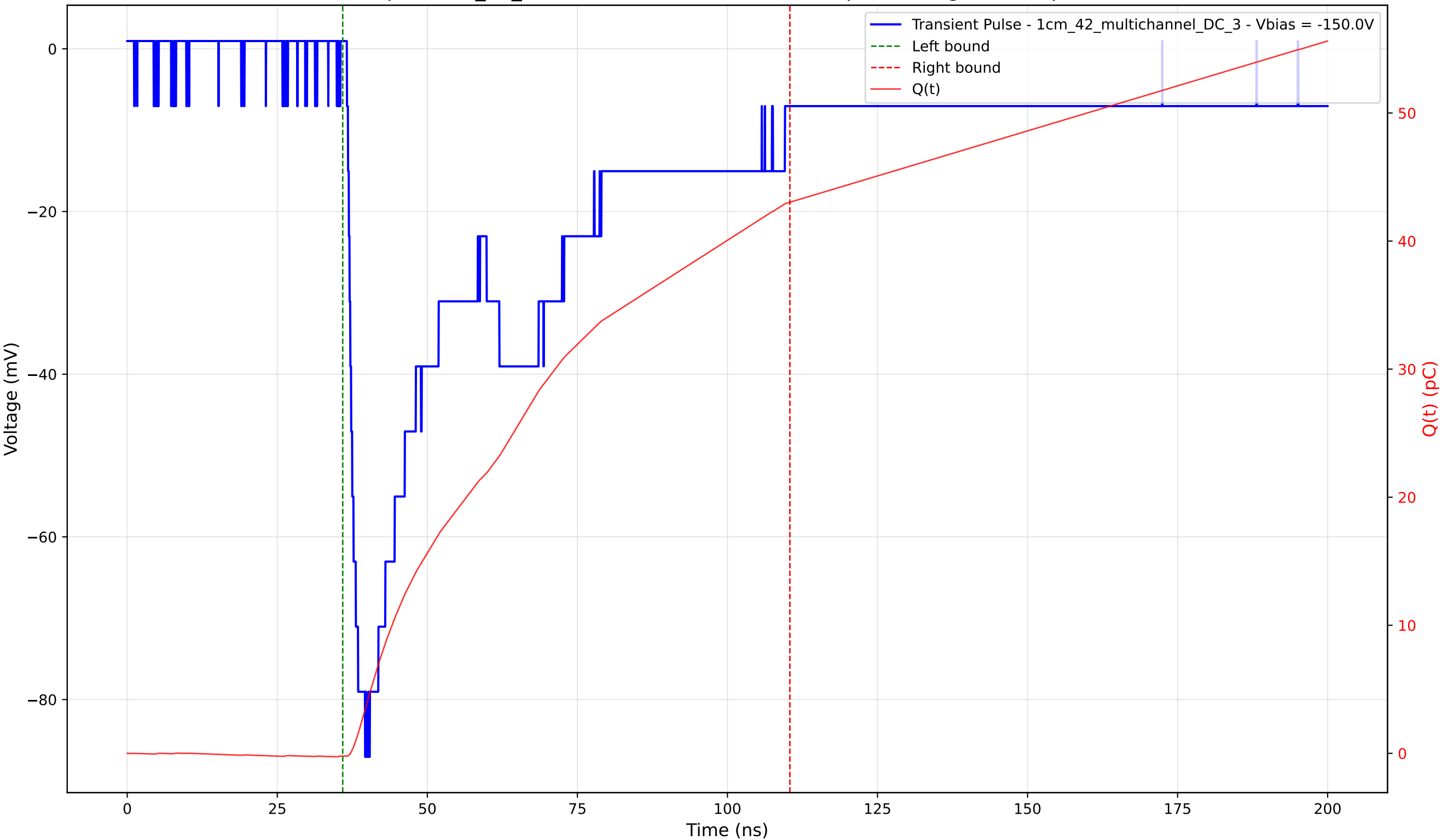
Transient Pulse - Sample: 1cm_42_multichannel - Position: 2265.0 \mu\text{m} - Charge: 43.25 pC - Rise Time: 1.70 ns
