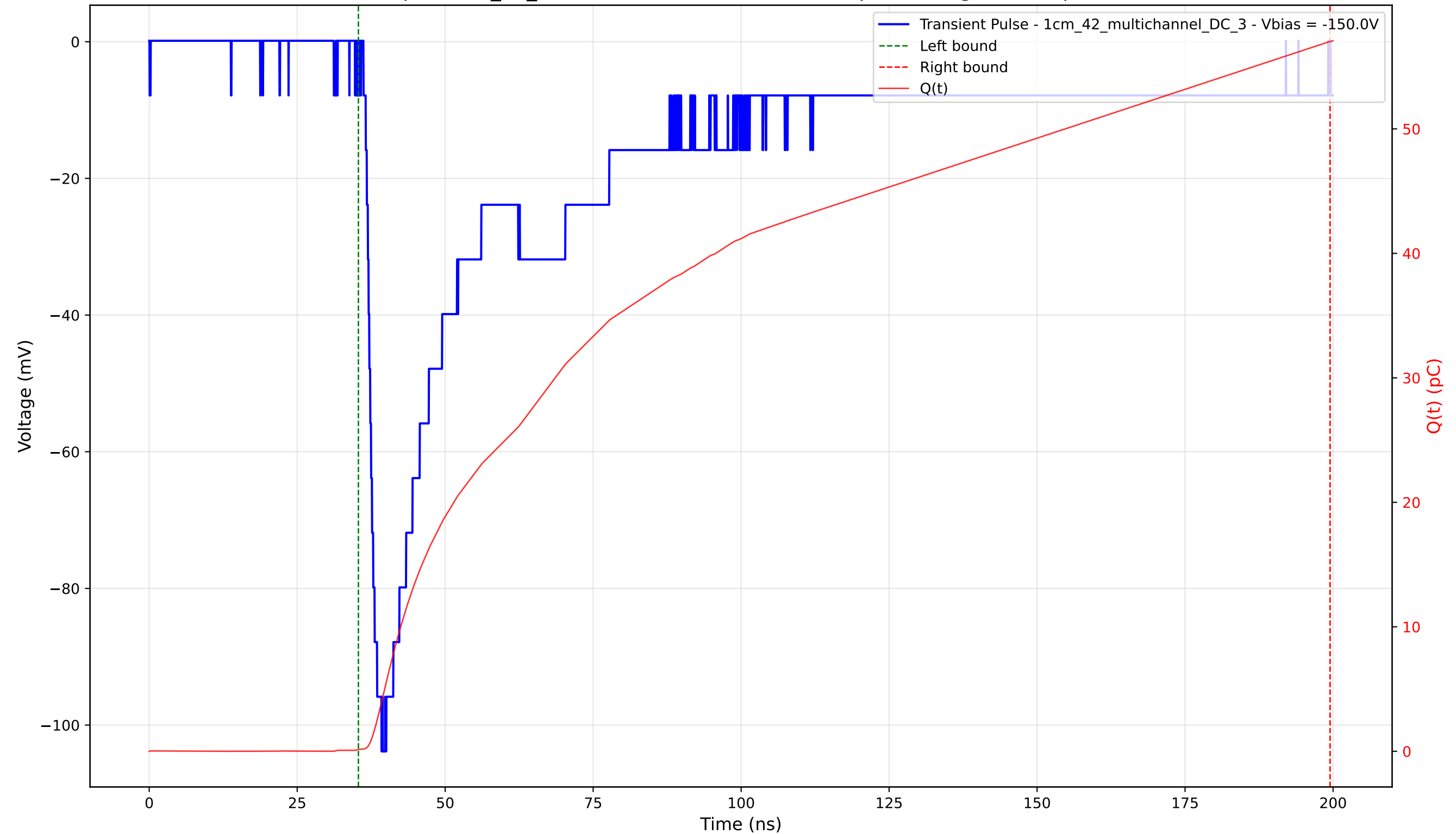
Transient Pulse - Sample: 1cm_42_multichannel - Position: 2985.0 \mu\text{m} - Charge: 56.87 pC - Rise Time: 1.93 ns
