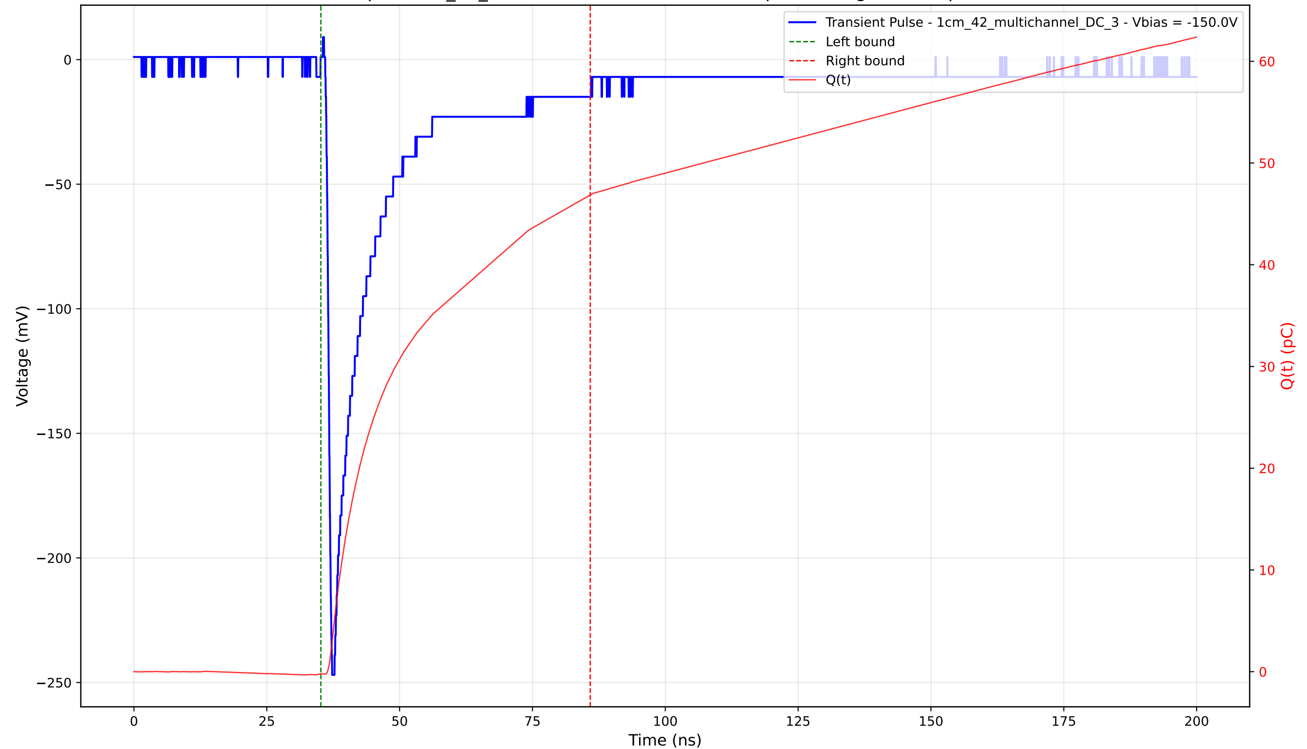
Transient Pulse - Sample: 1cm_42_multichannel - Position: 565.0 \mu\text{m} - Charge: 47.09 pC - Rise Time: 0.88 ns
