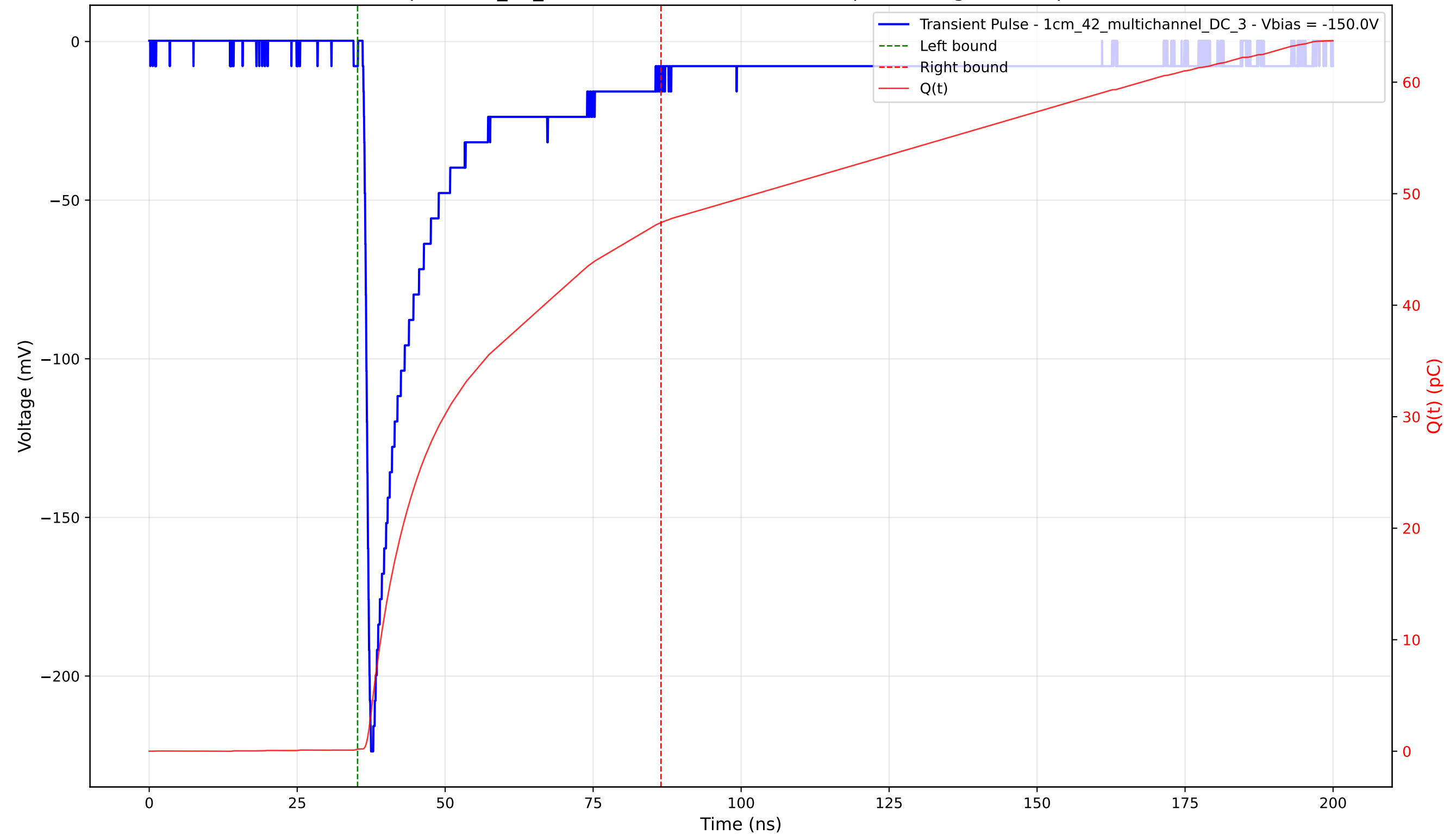
Transient Pulse - Sample: 1cm_42_multichannel - Position: 705.0 \mu\text{m} - Charge: 47.21 pC - Rise Time: 1.00 ns
