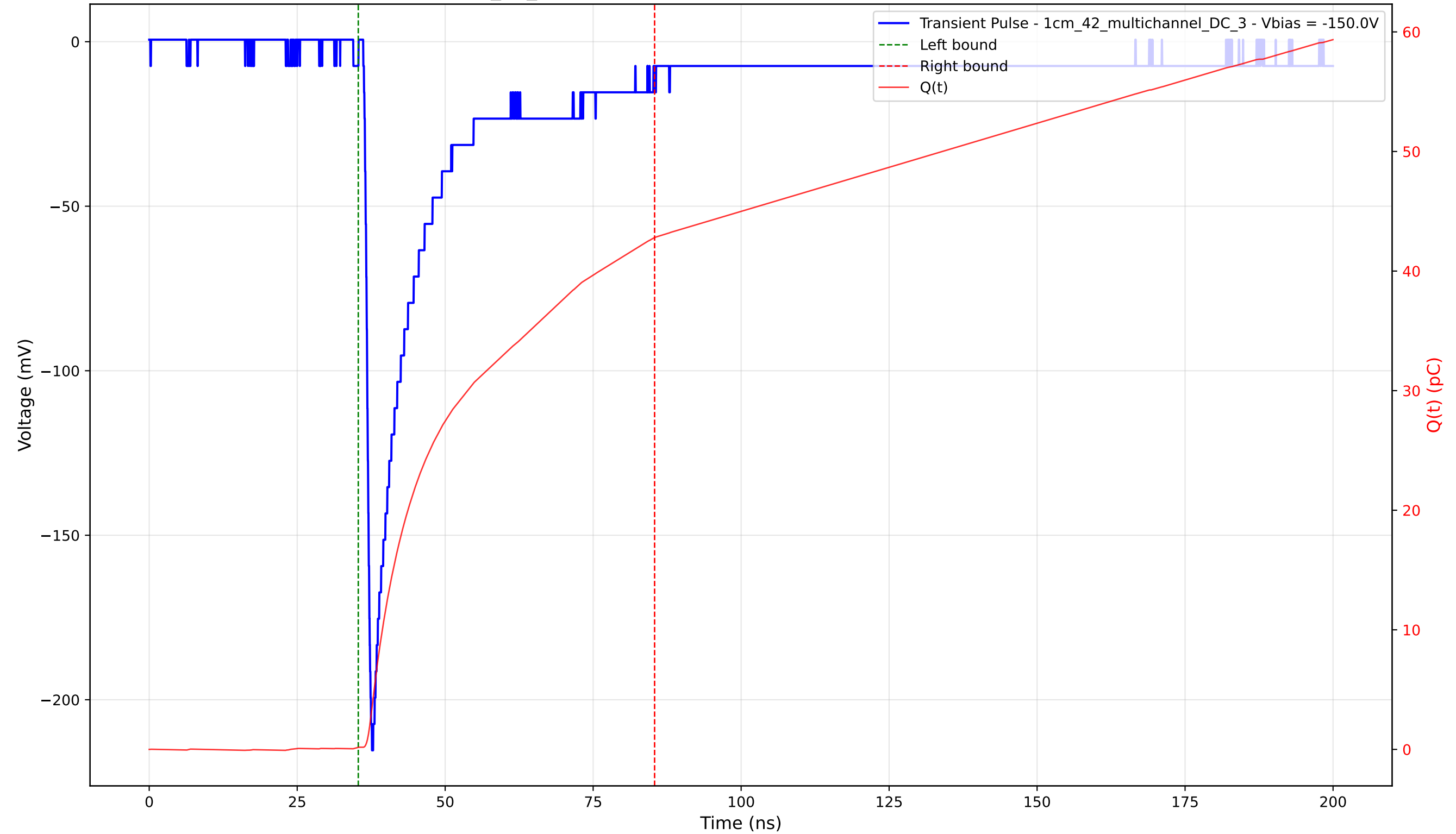
Transient Pulse - Sample: 1cm_42_multichannel - Position: 4225.0 \mu\text{m} - Charge: 42.61 pC - Rise Time: 1.02 ns
