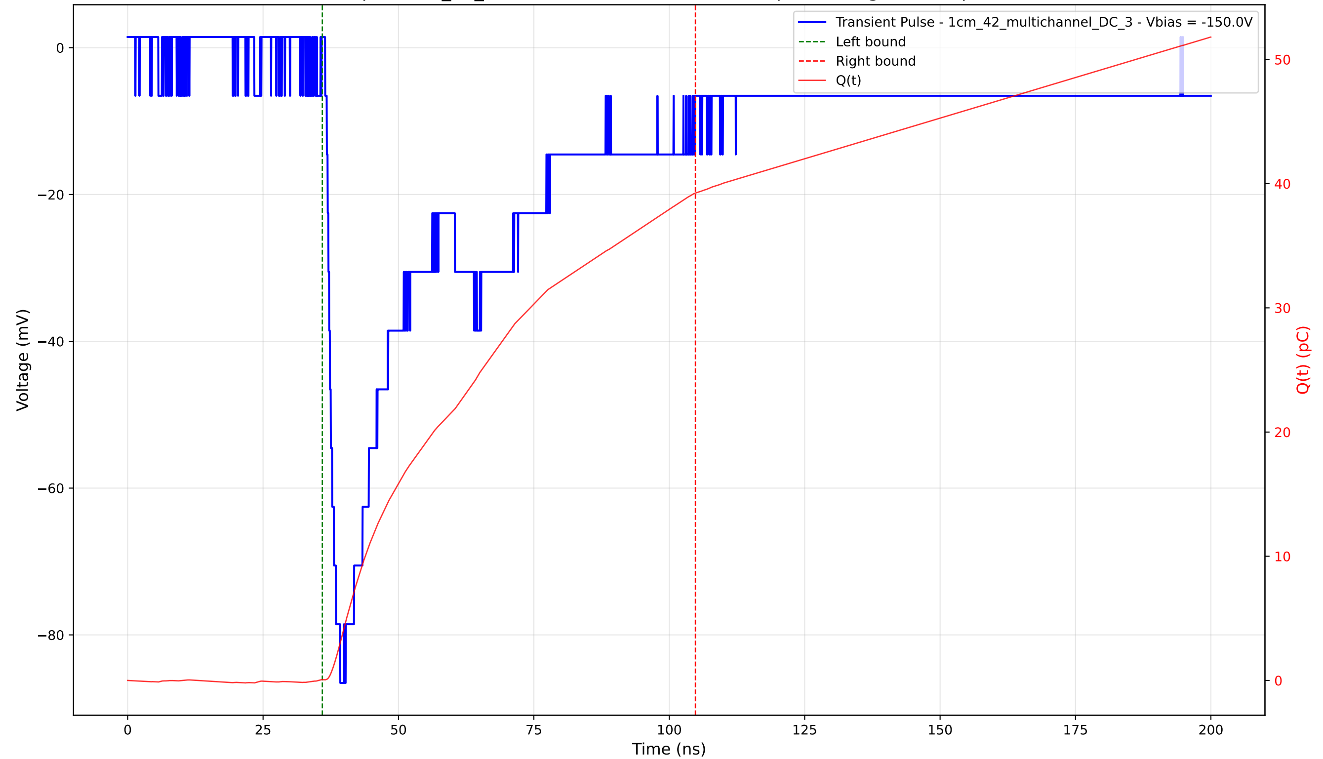
Transient Pulse - Sample: 1cm_42_multichannel - Position: 2645.0 \mu\text{m} - Charge: 39.18 pC - Rise Time: 1.71 ns
