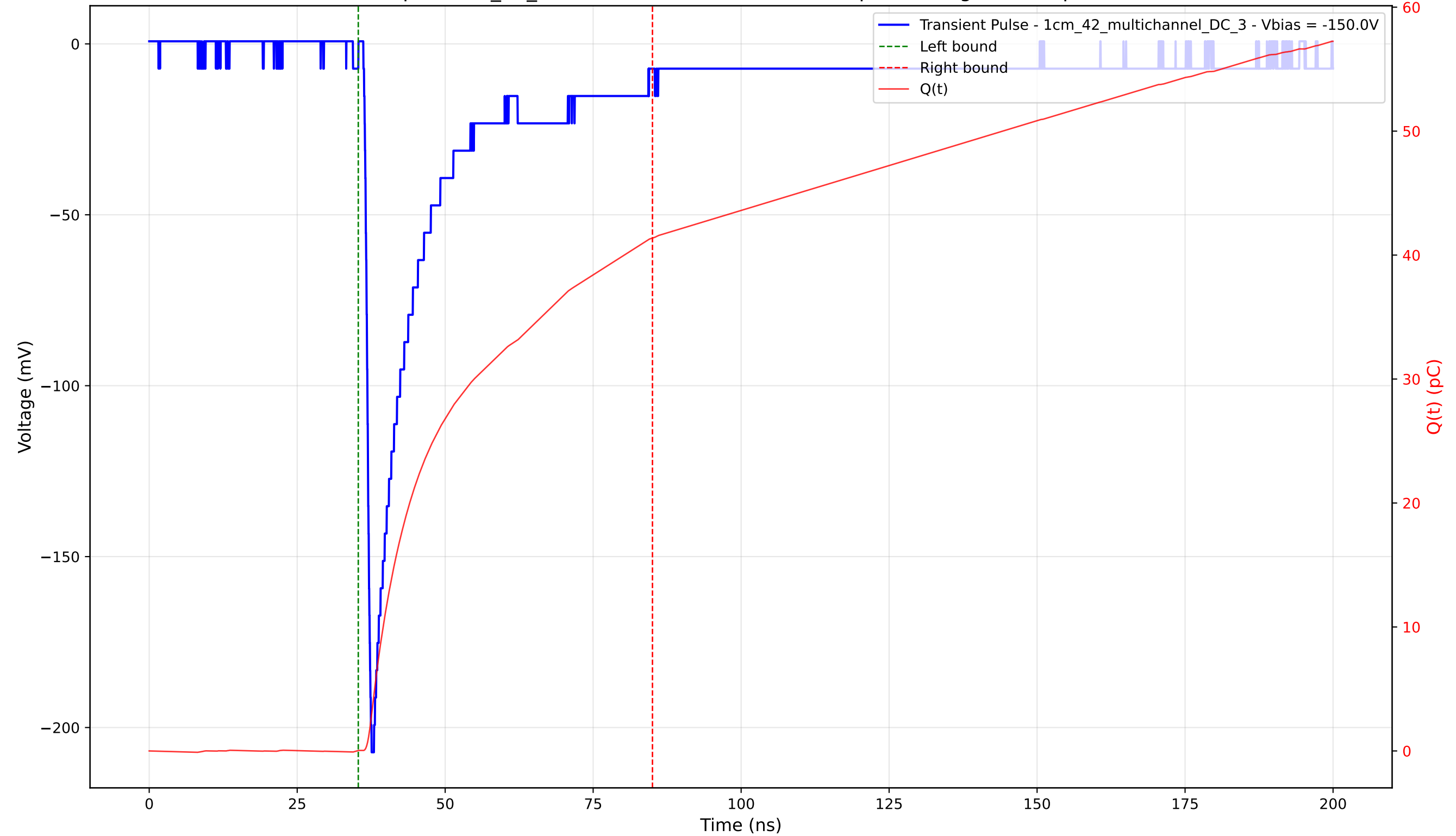
Transient Pulse - Sample: 1cm_42_multichannel - Position: 4210.0 \mu\text{m} - Charge: 41.33 pC - Rise Time: 0.99 ns
