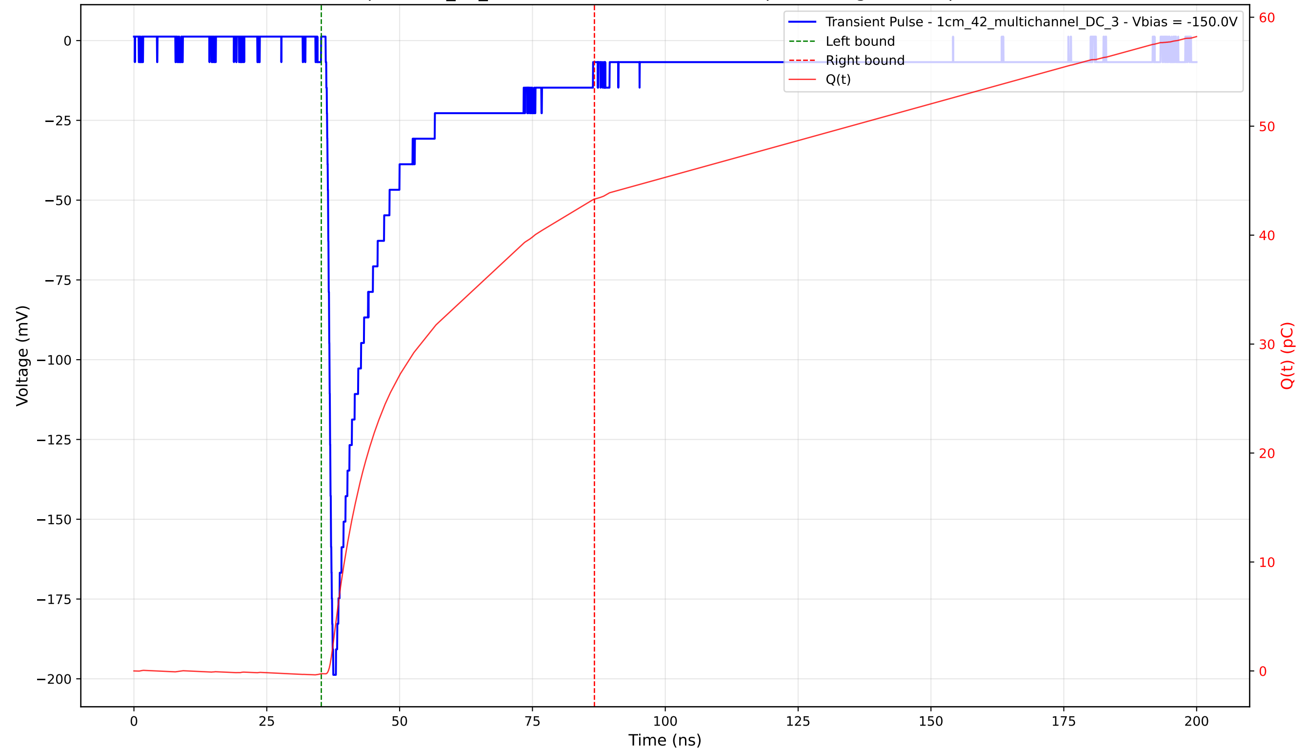
Transient Pulse - Sample: 1cm_42_multichannel - Position: 765.0 \mu\text{m} - Charge: 43.55 pC - Rise Time: 1.01 ns
