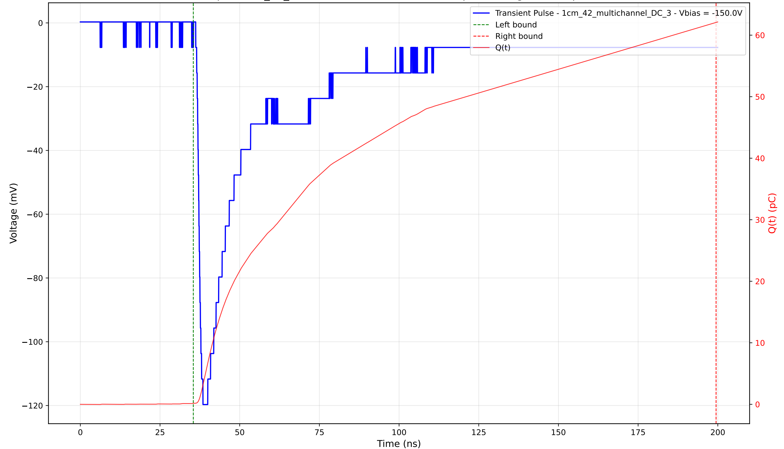
Transient Pulse - Sample: 1cm_42_multichannel - Position: 1670.0 \mu\text{m} - Charge: 61.90 pC - Rise Time: 1.55 ns
