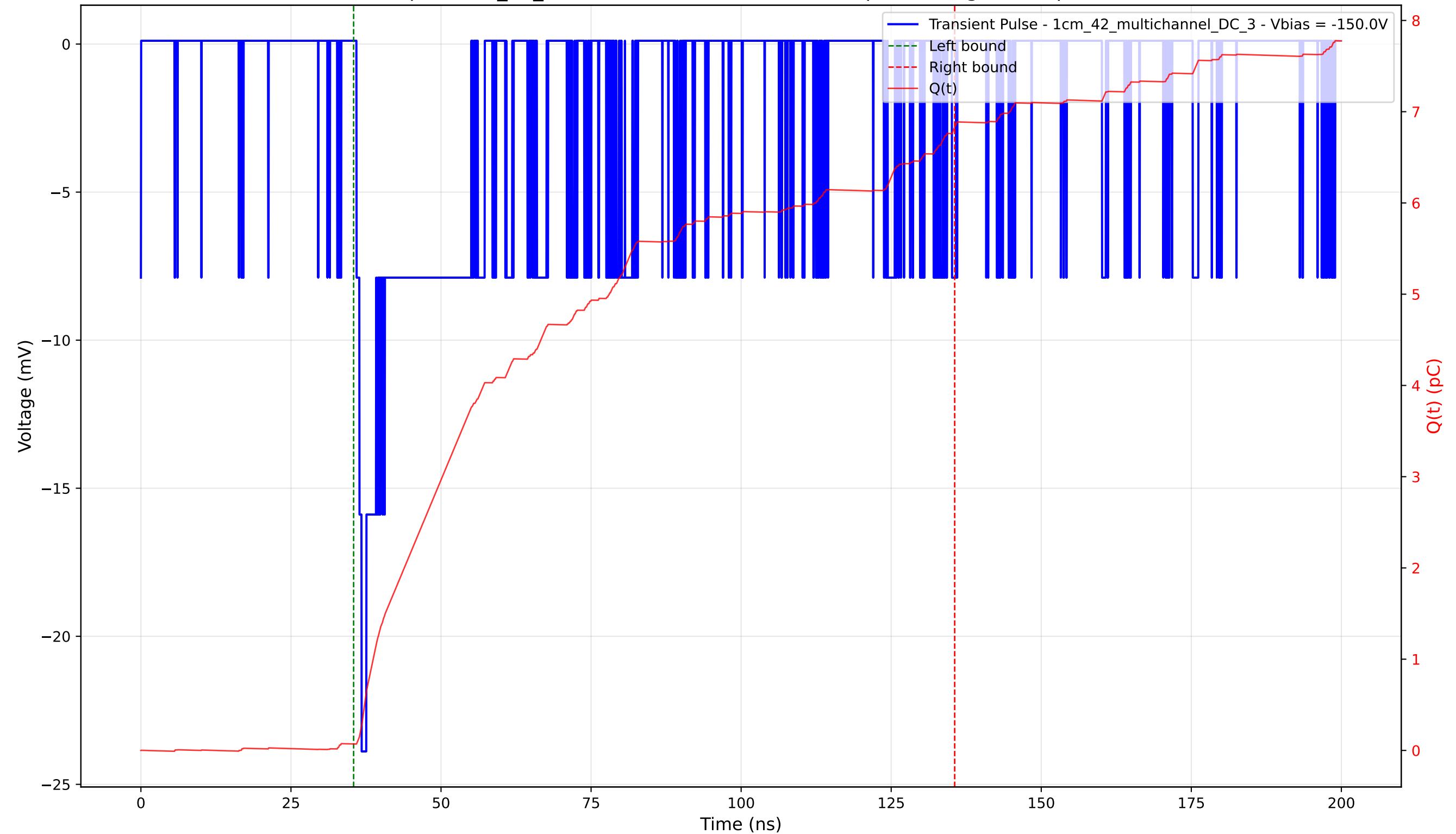
Transient Pulse - Sample: 1cm_42_multichannel - Position: 4885.0 \mu\text{m} - Charge: 6.76 pC - Rise Time: 0.85 ns
