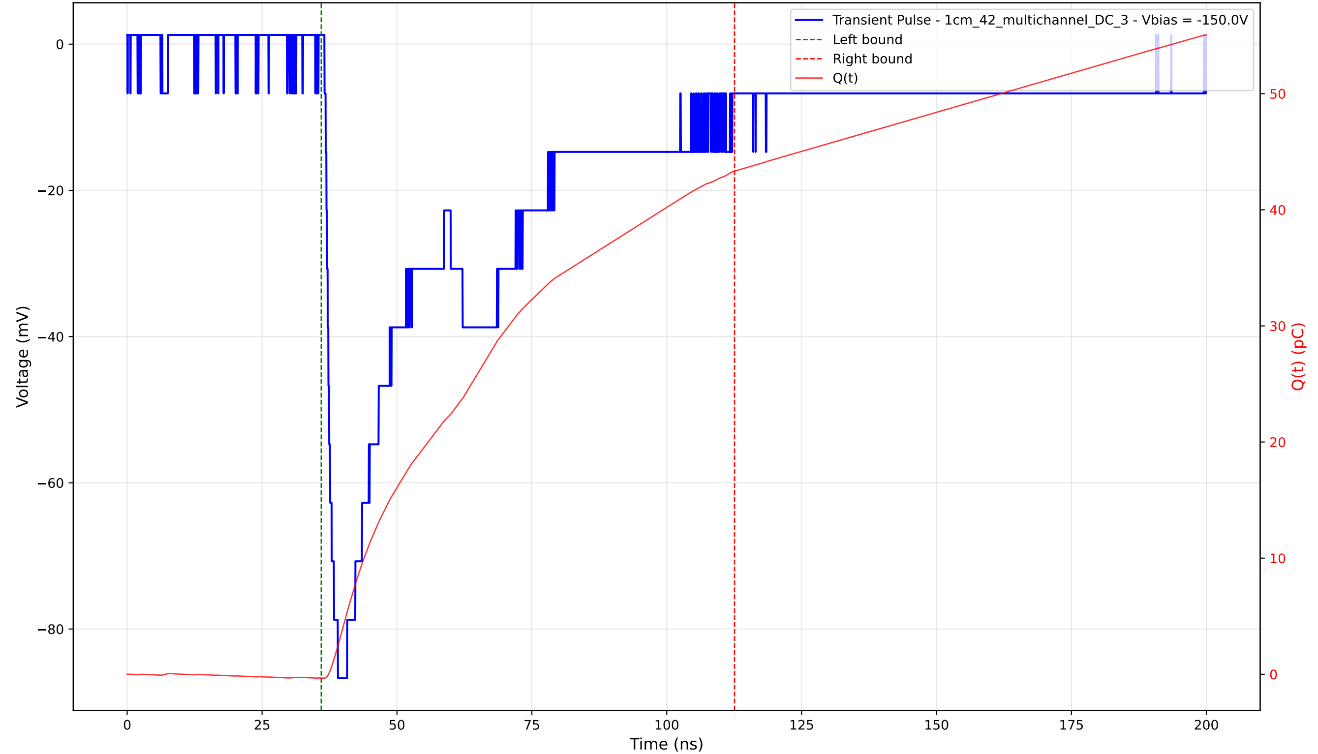
Transient Pulse - Sample: 1cm_42_multichannel - Position: 2220.0 \mu\text{m} - Charge: 43.66 pC - Rise Time: 1.56 ns
