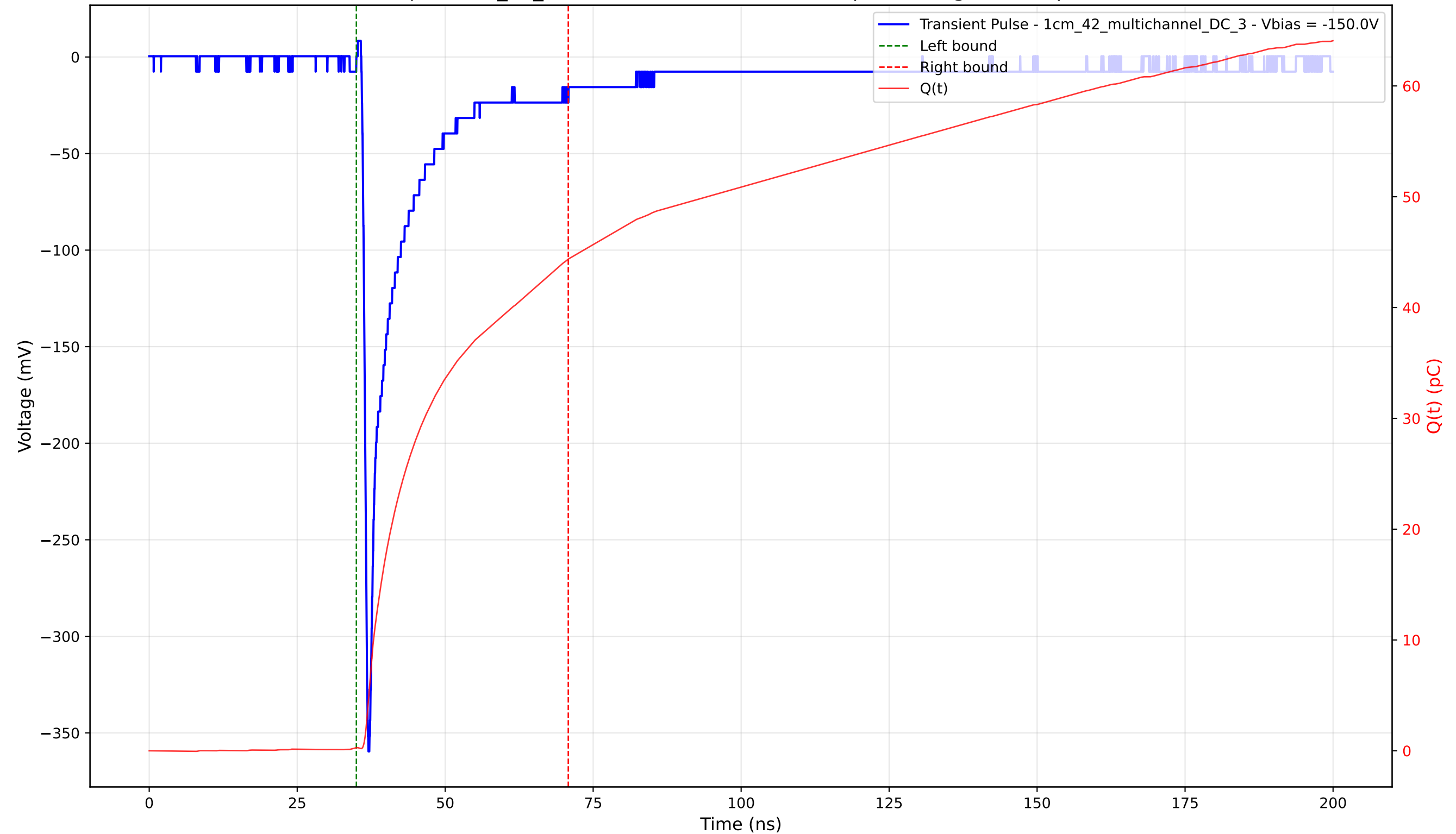
Transient Pulse - Sample: 1cm_42_multichannel - Position: 190.0 \mu\text{m} - Charge: 44.09 pC - Rise Time: 0.81 ns
