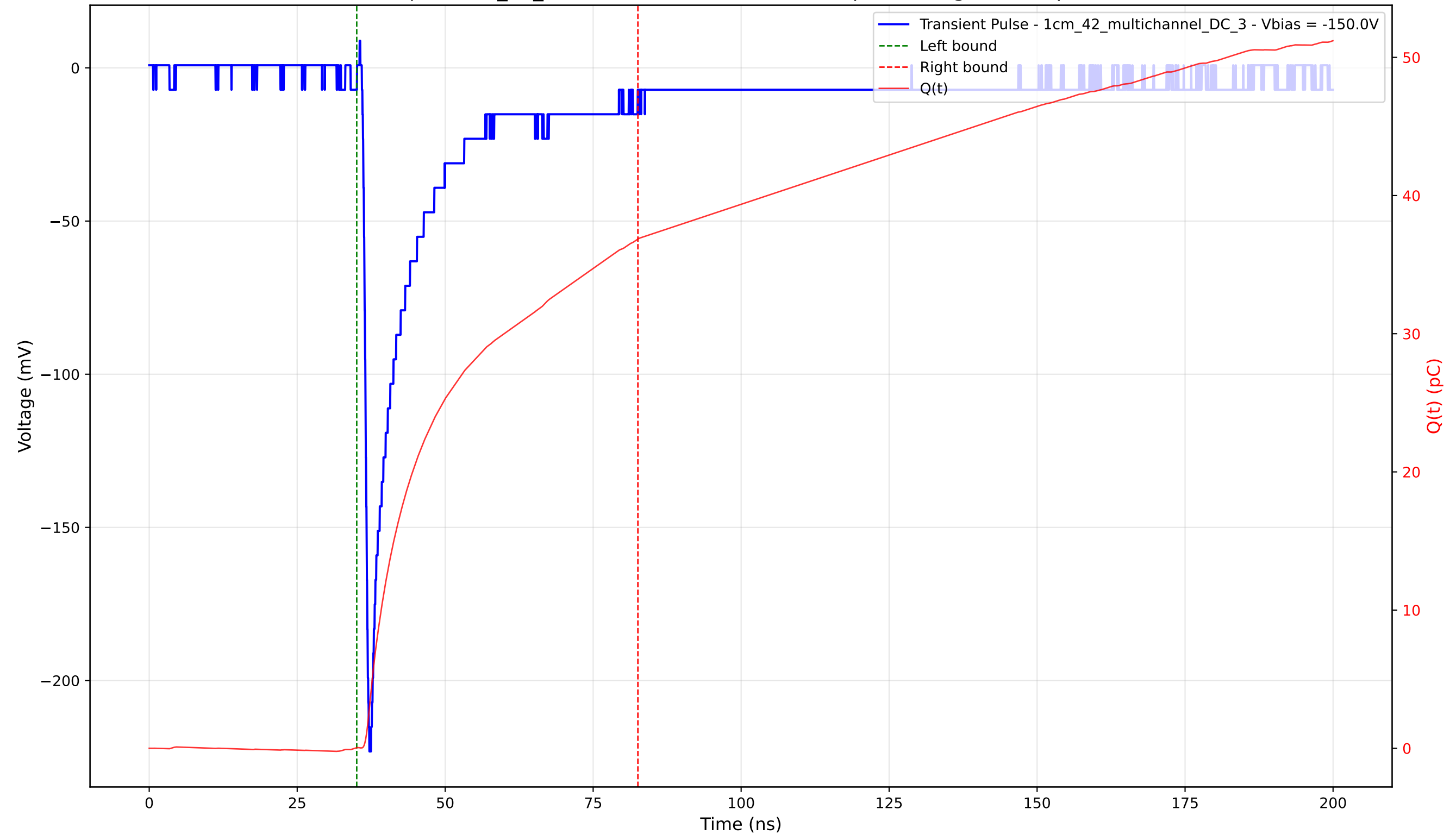
Transient Pulse - Sample: 1cm_42_multichannel - Position: 415.0 \mu\text{m} - Charge: 36.80 pC - Rise Time: 0.90 ns
