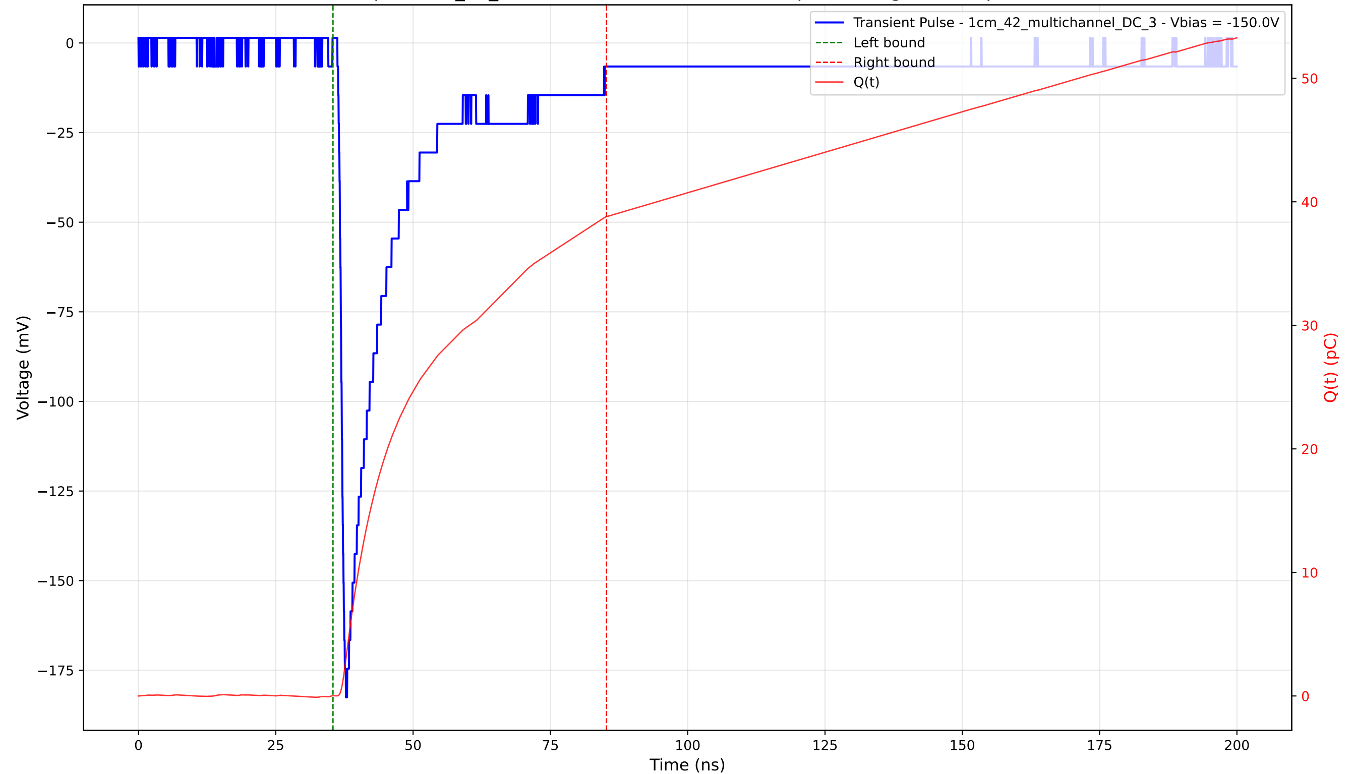
Transient Pulse - Sample: 1cm_42_multichannel - Position: 4105.0 \mu\text{m} - Charge: 38.78 pC - Rise Time: 1.03 ns
