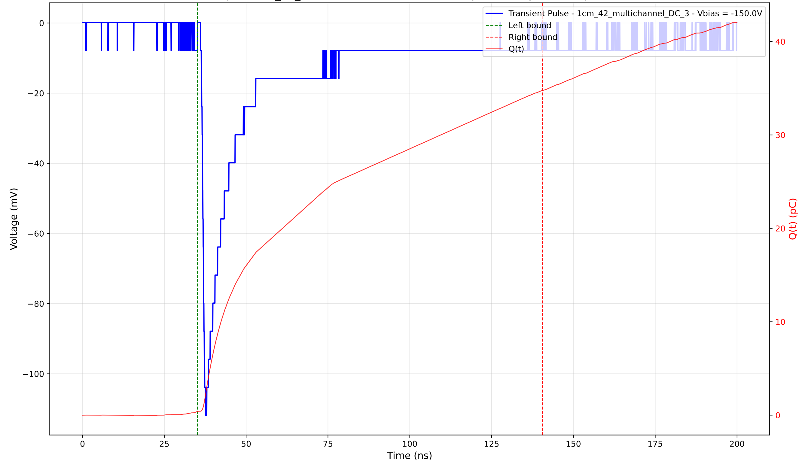
Transient Pulse - Sample: 1cm_42_multichannel - Position: 805.0 \mu\text{m} - Charge: 34.36 pC - Rise Time: 1.05 ns
