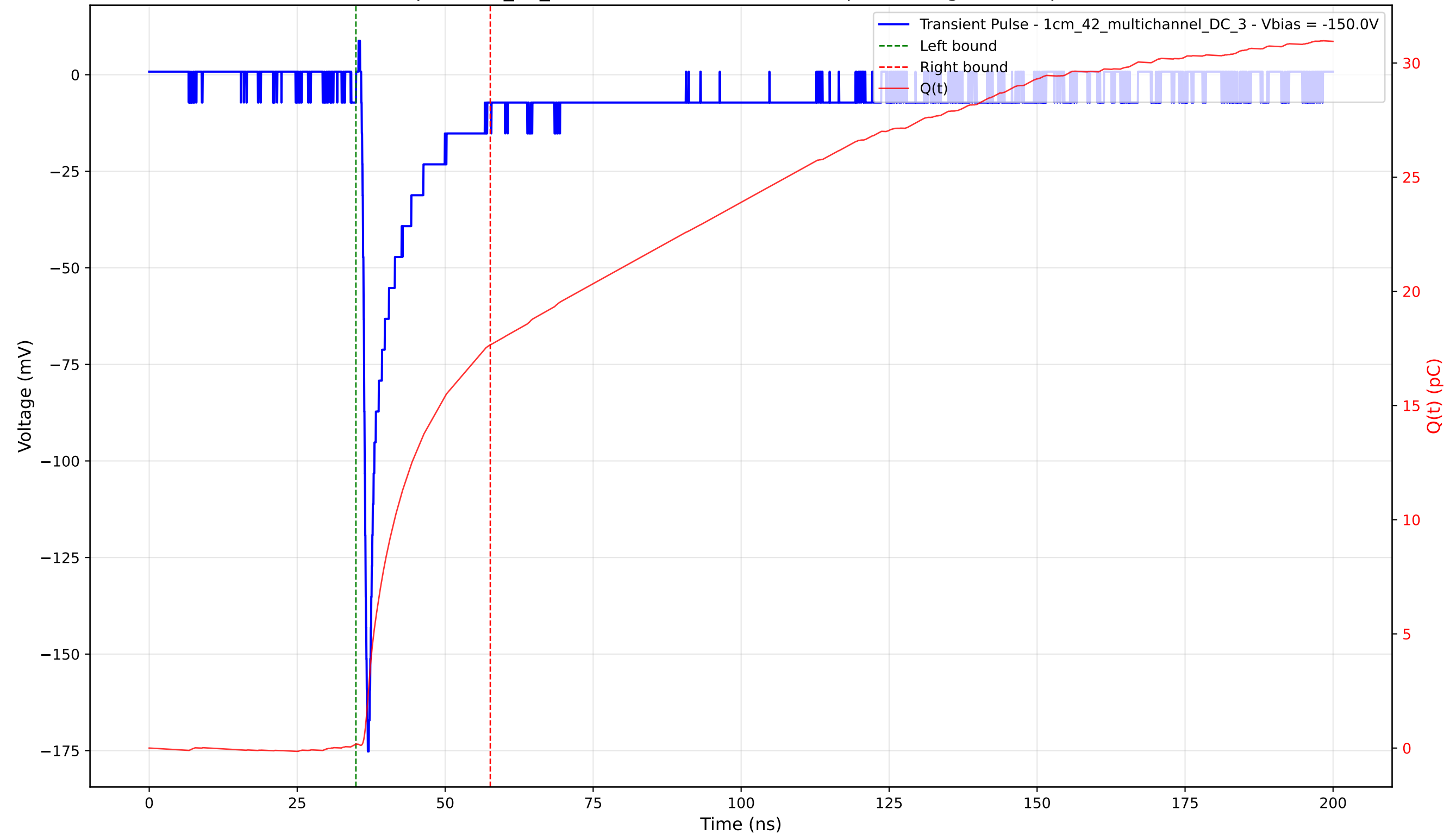
Transient Pulse - Sample: 1cm_42_multichannel - Position: 75.0 \mu\text{m} - Charge: 17.48 pC - Rise Time: 0.77 ns
