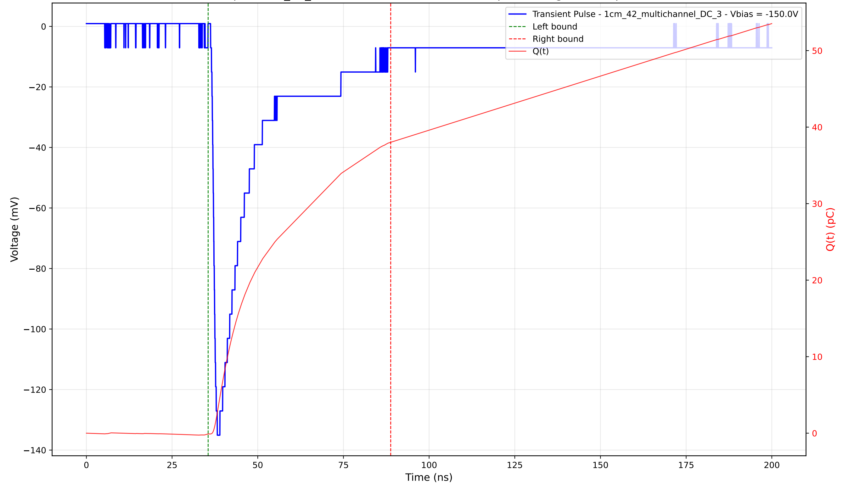
Transient Pulse - Sample: 1cm_42_multichannel - Position: 3665.0 \mu\text{m} - Charge: 38.12 pC - Rise Time: 1.38 ns
