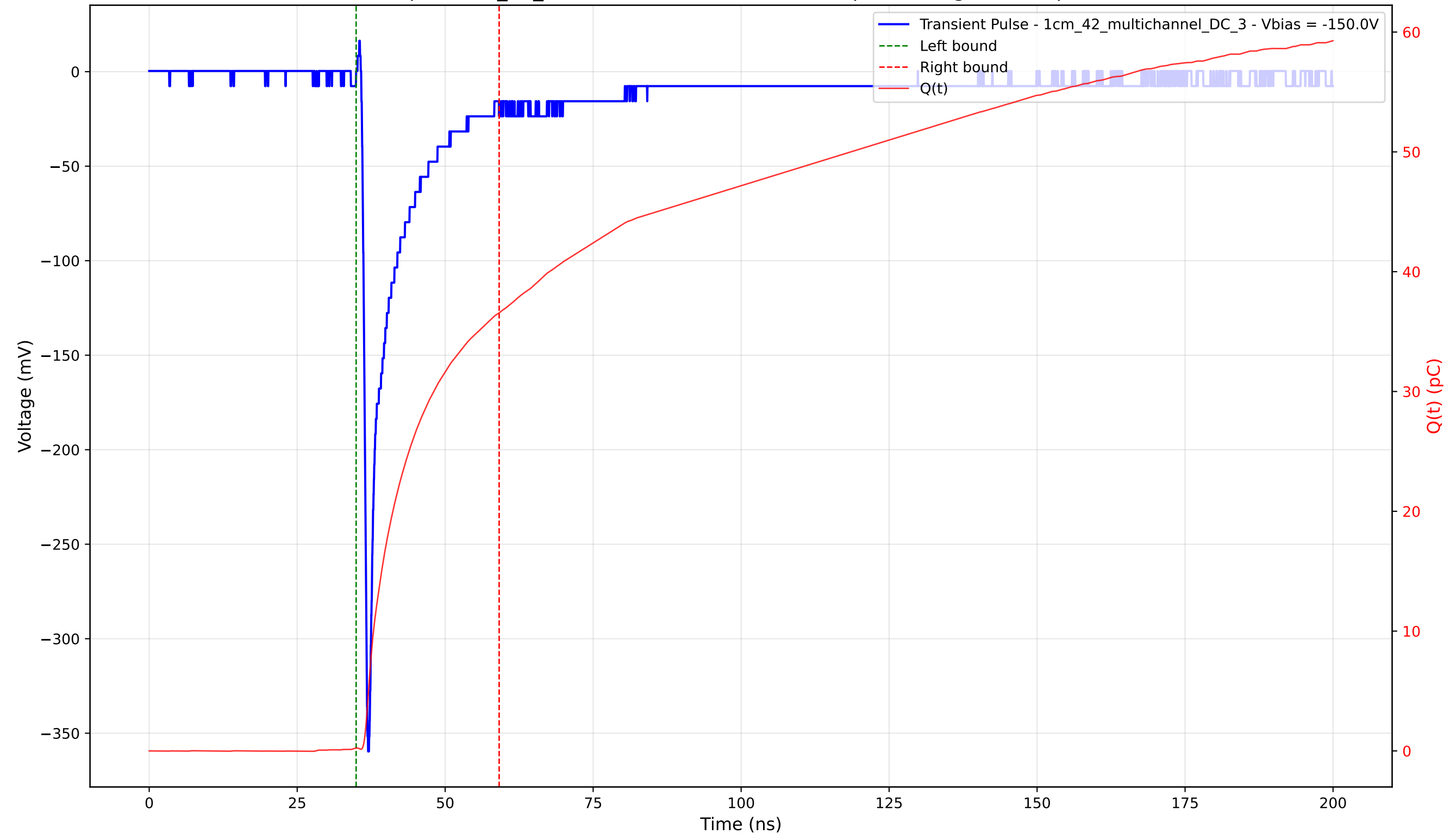
Transient Pulse - Sample: 1cm_42_multichannel - Position: 125.0 \mu\text{m} - Charge: 36.30 pC - Rise Time: 0.80 ns
