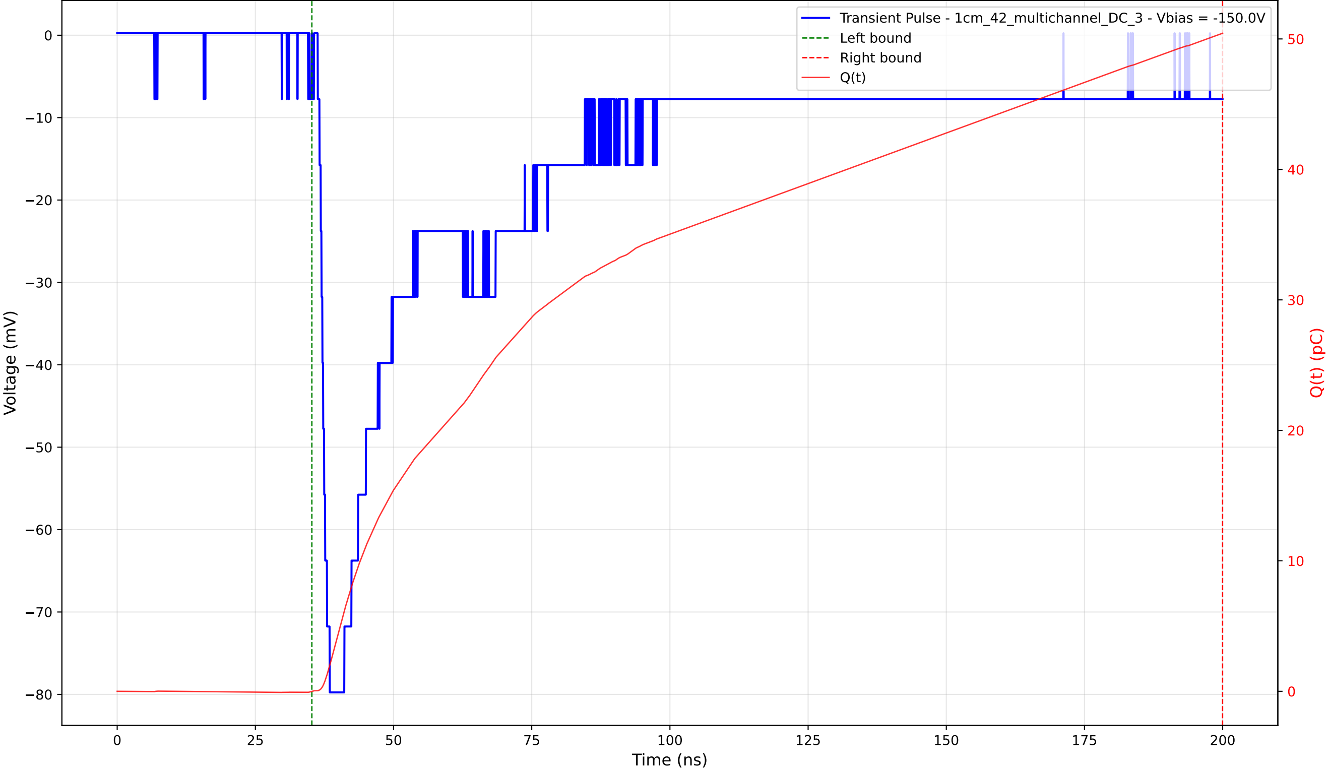
Transient Pulse - Sample: 1cm_42_multichannel - Position: 1935.0 \mu\text{m} - Charge: 50.44 pC - Rise Time: 1.86 ns
