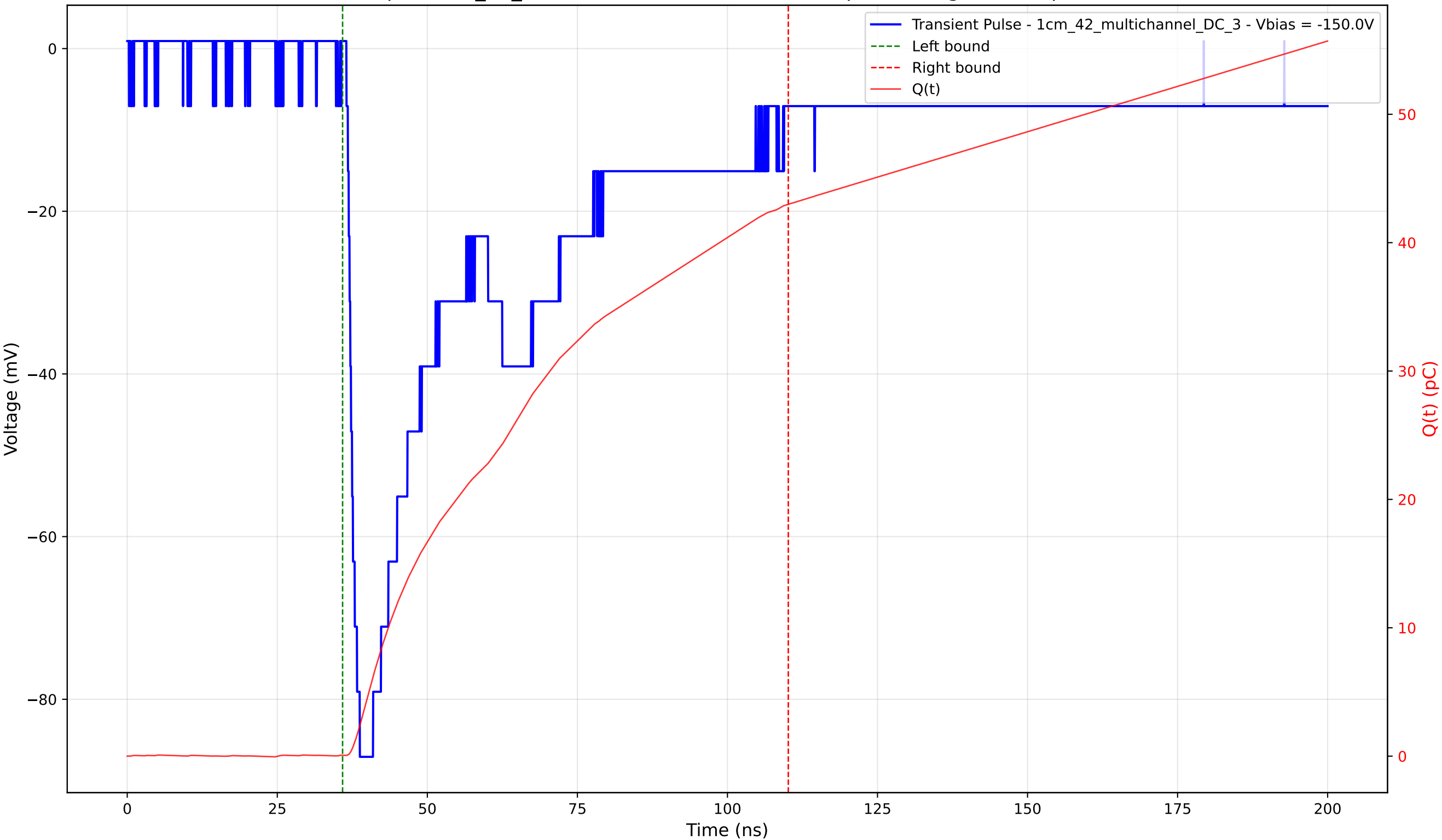
Transient Pulse - Sample: 1cm_42_multichannel - Position: 2145.0 \mu\text{m} - Charge: 42.92 pC - Rise Time: 1.54 ns
