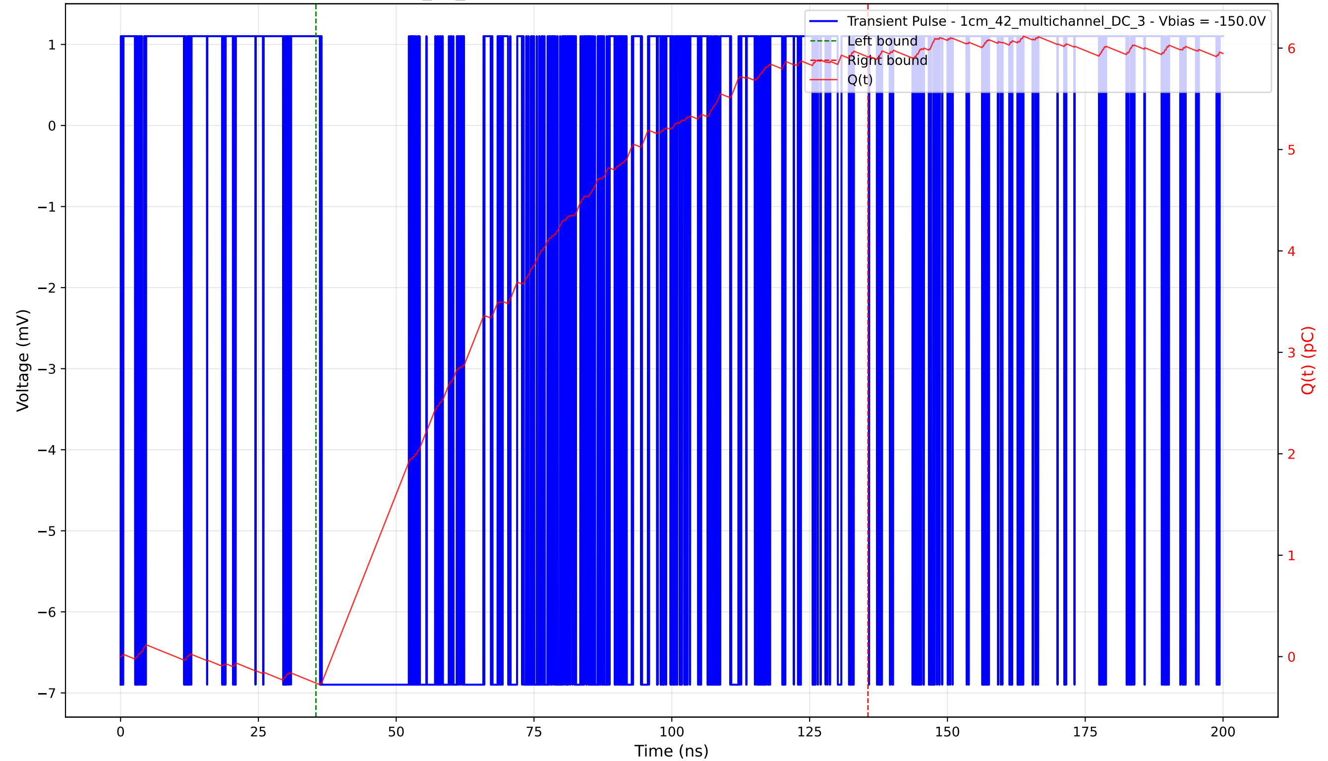
Transient Pulse - Sample: 1cm_42_multichannel - Position: 1365.0 \mu\text{m} - Charge: 6.17 pC - Rise Time: 0.00 ns (N/A)
