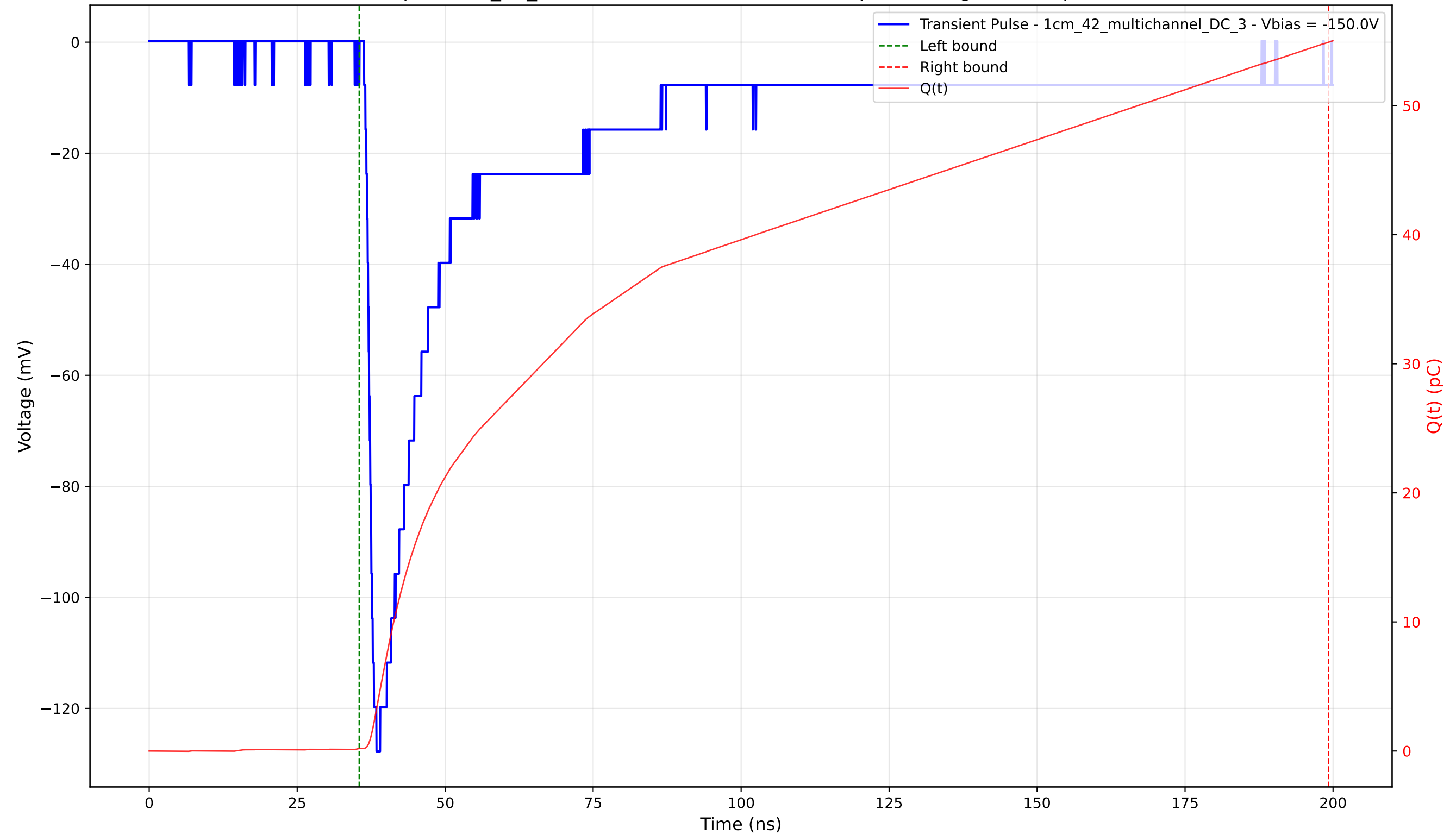
Transient Pulse - Sample: 1cm_42_multichannel - Position: 3570.0 \mu\text{m} - Charge: 54.72 pC - Rise Time: 1.45 ns
