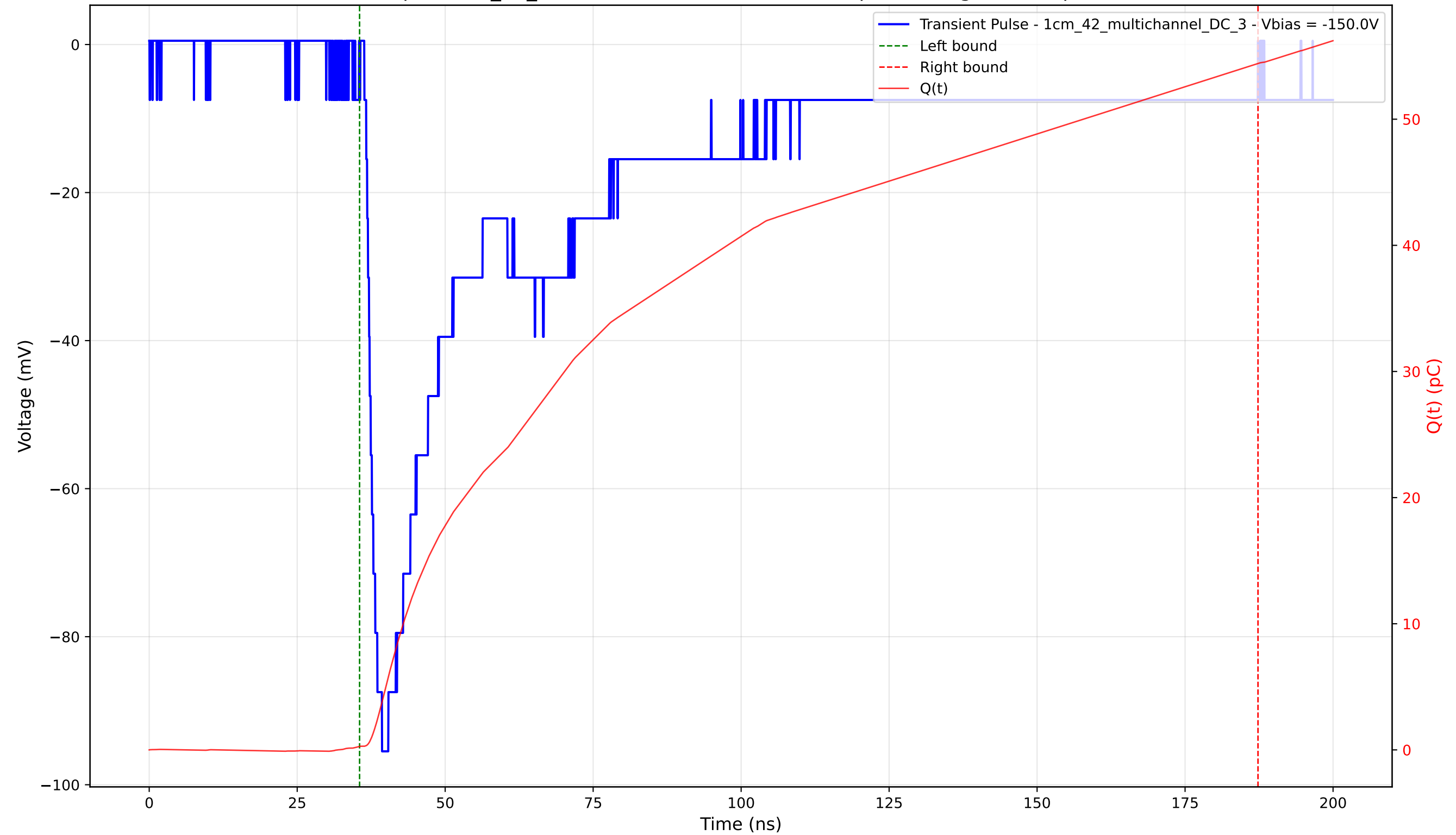
Transient Pulse - Sample: 1cm_42_multichannel - Position: 2765.0 \mu\text{m} - Charge: 54.16 pC - Rise Time: 1.89 ns
