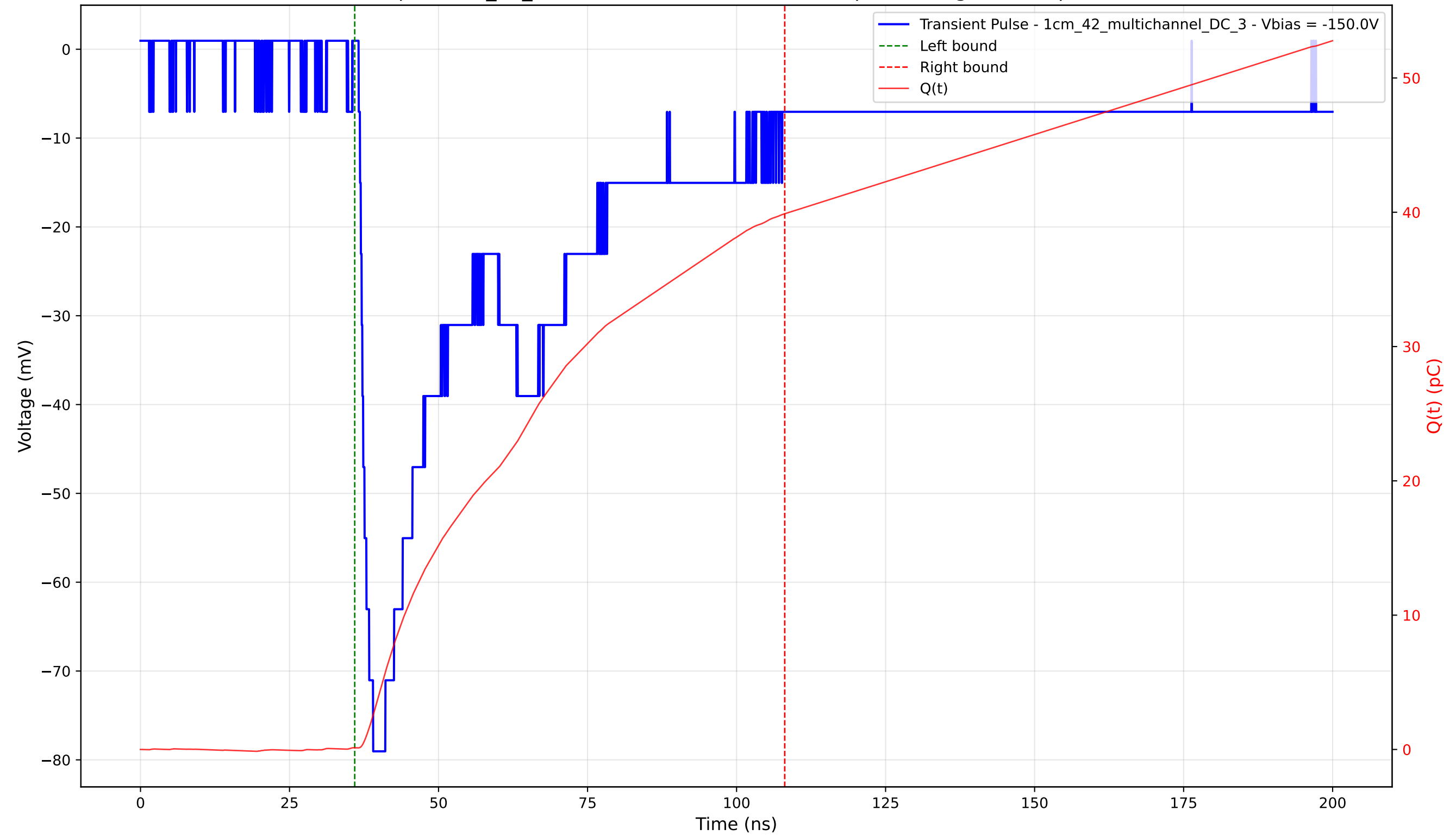
Transient Pulse - Sample: 1cm_42_multichannel - Position: 2530.0 \mu\text{m} - Charge: 39.77 pC - Rise Time: 2.22 ns
