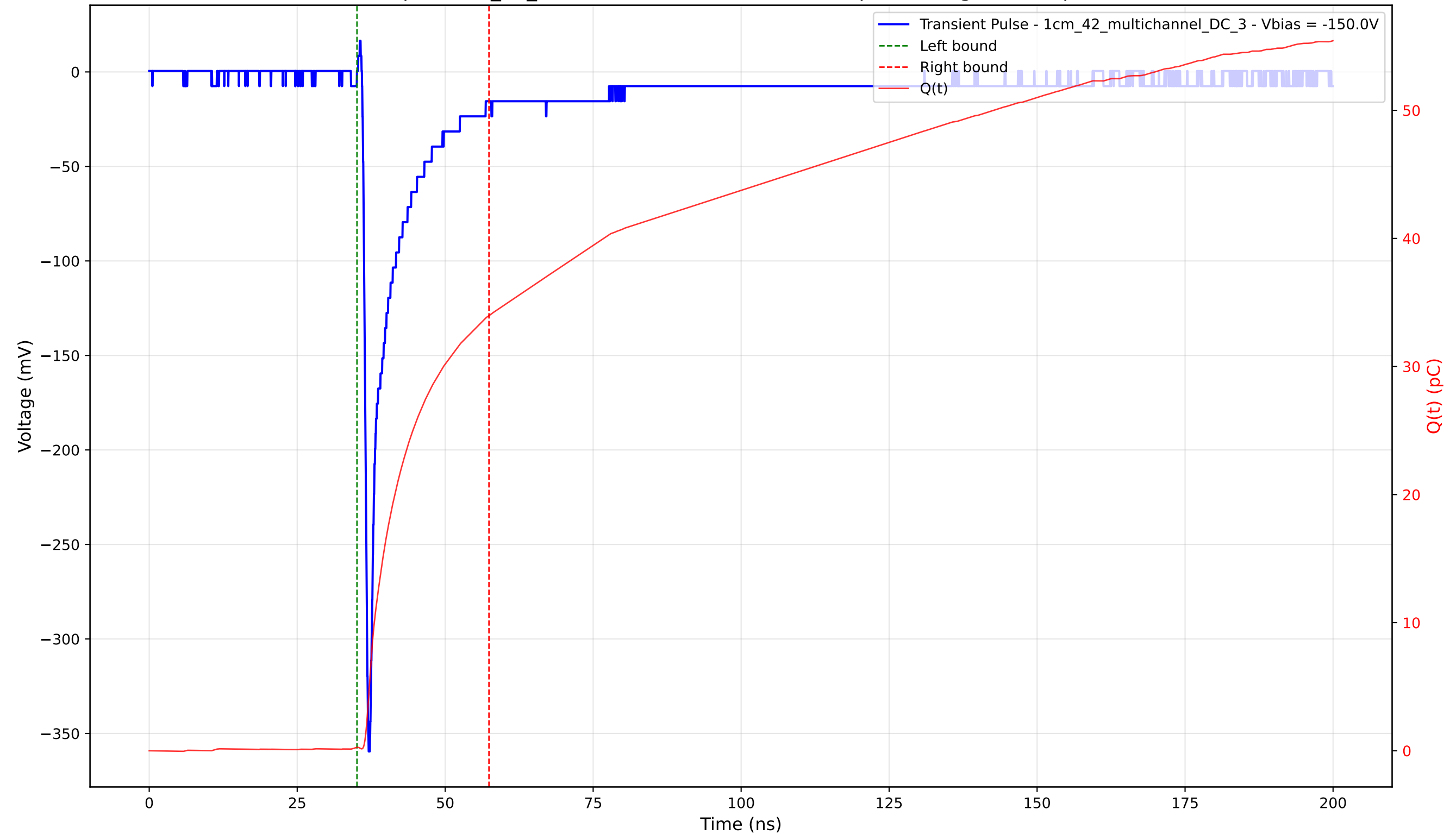
Transient Pulse - Sample: 1cm_42_multichannel - Position: 4790.0 \mu\text{m} - Charge: 33.69 pC - Rise Time: 0.78 ns
