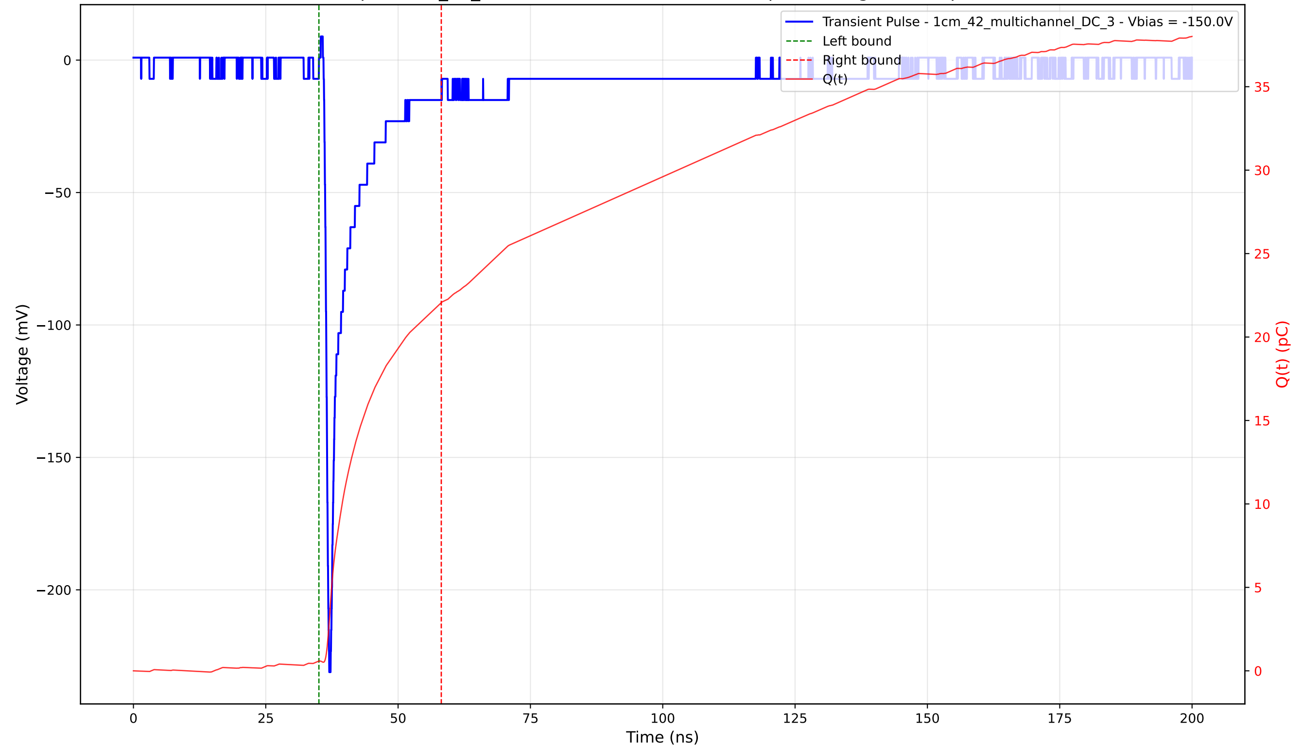
Transient Pulse - Sample: 1cm_42_multichannel - Position: 4845.0 \mu\text{m} - Charge: 21.48 pC - Rise Time: 0.78 ns
