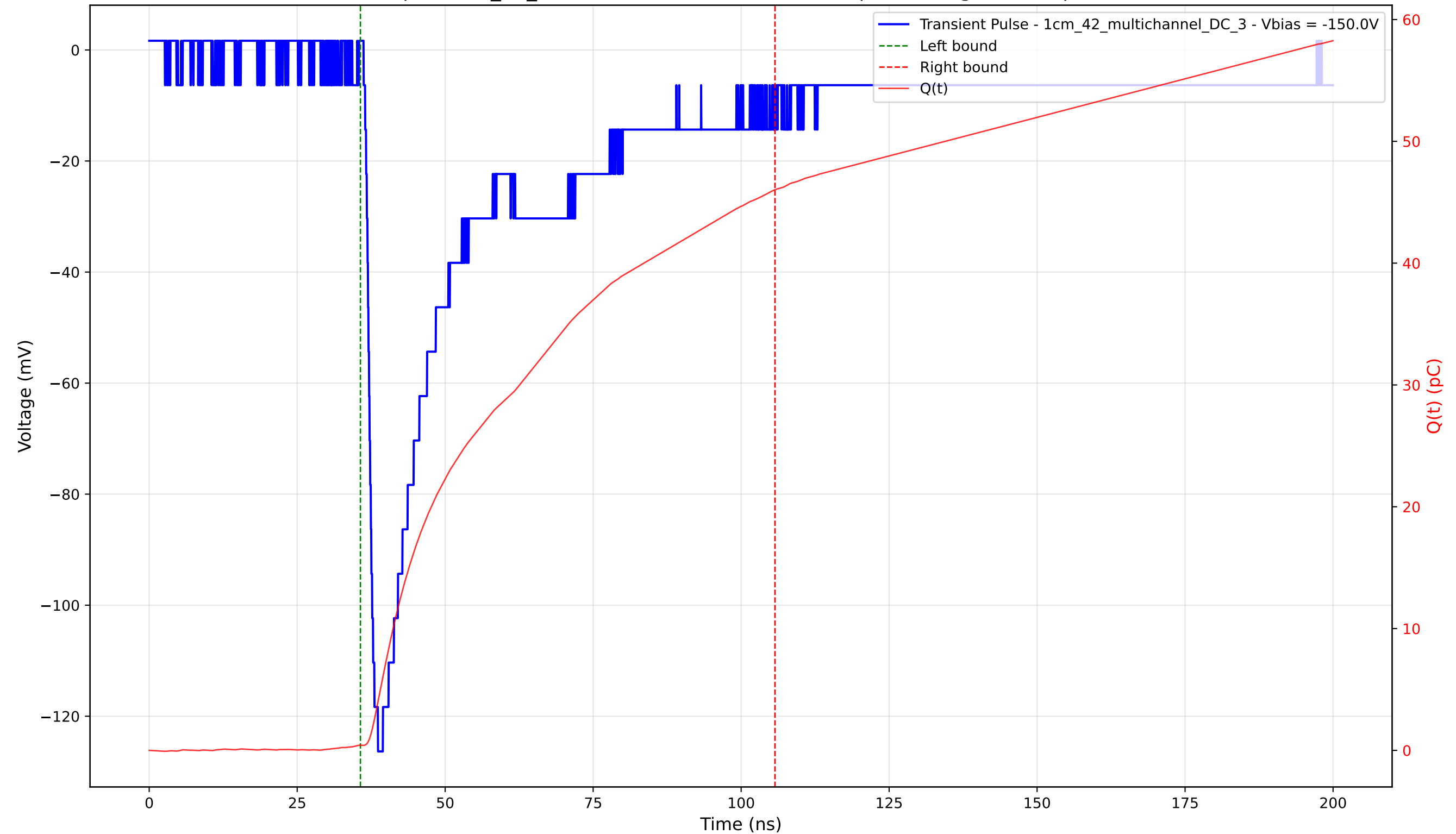
Transient Pulse - Sample: 1cm_42_multichannel - Position: 1565.0 \mu\text{m} - Charge: 45.60 pC - Rise Time: 1.56 ns
