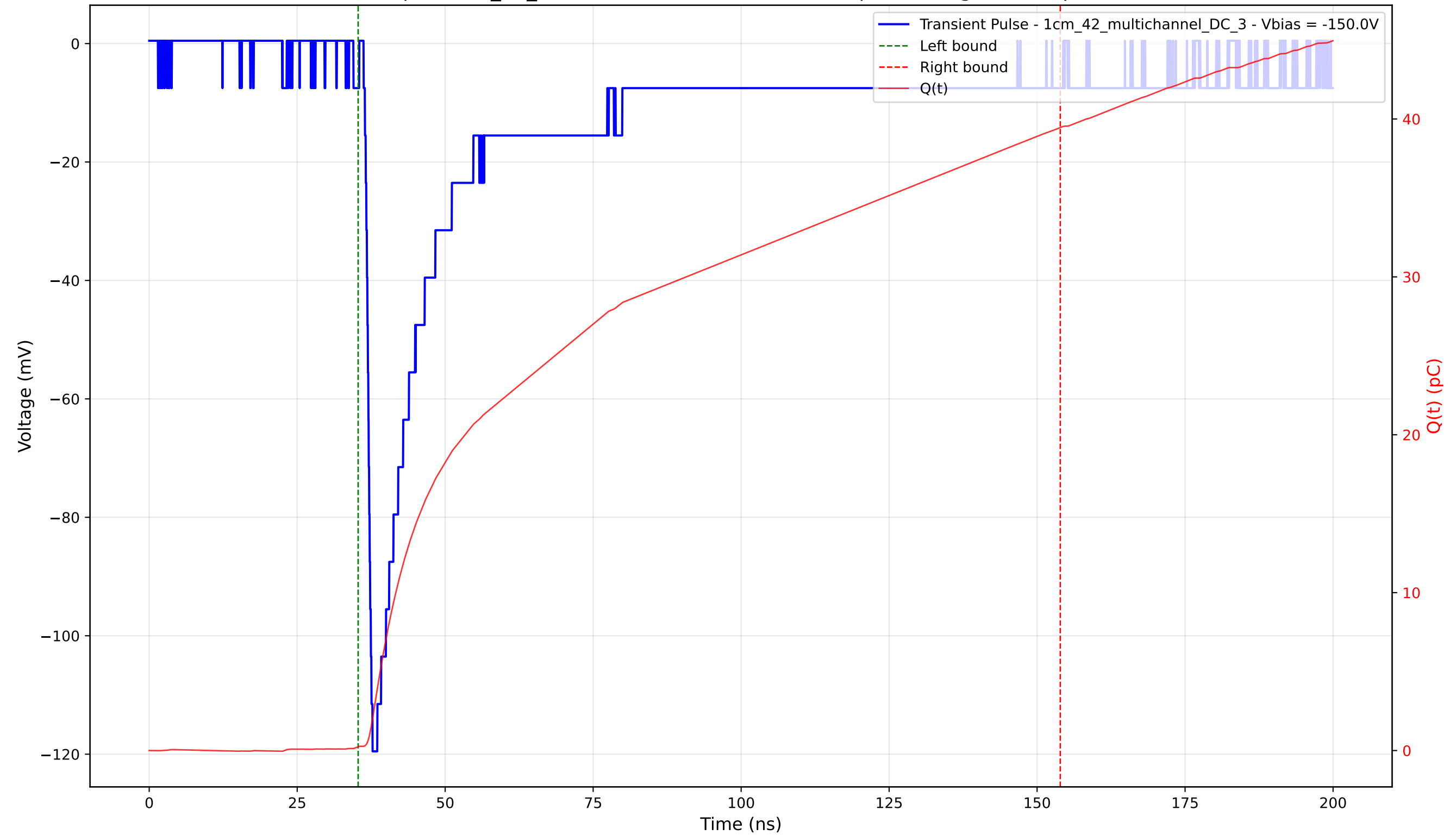
Transient Pulse - Sample: 1cm_42_multichannel - Position: 3950.0 \mu\text{m} - Charge: 39.22 pC - Rise Time: 1.11 ns
