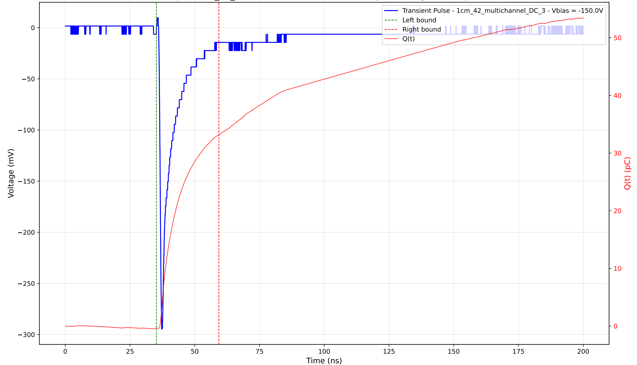
Transient Pulse - Sample: 1cm_42_multichannel - Position: 4600.0 \mu\text{m} - Charge: 33.54 pC - Rise Time: 0.84 ns
