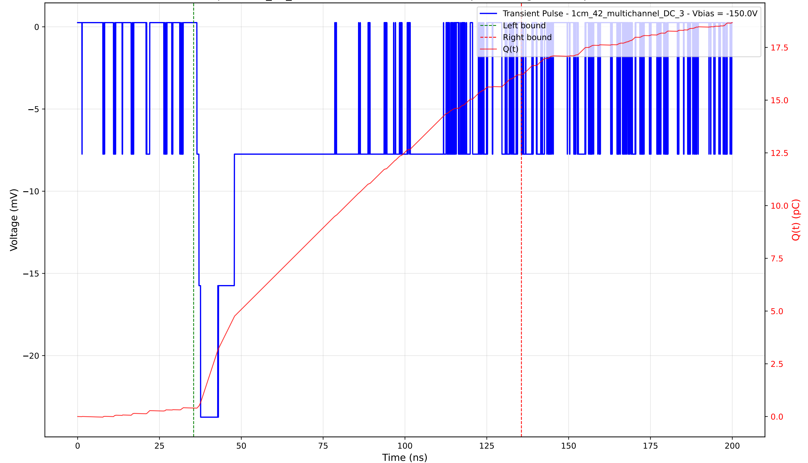
Transient Pulse - Sample: 1cm_42_multichannel - Position: 3420.0 \mu\text{m} - Charge: 15.80 pC - Rise Time: 1.13 ns
