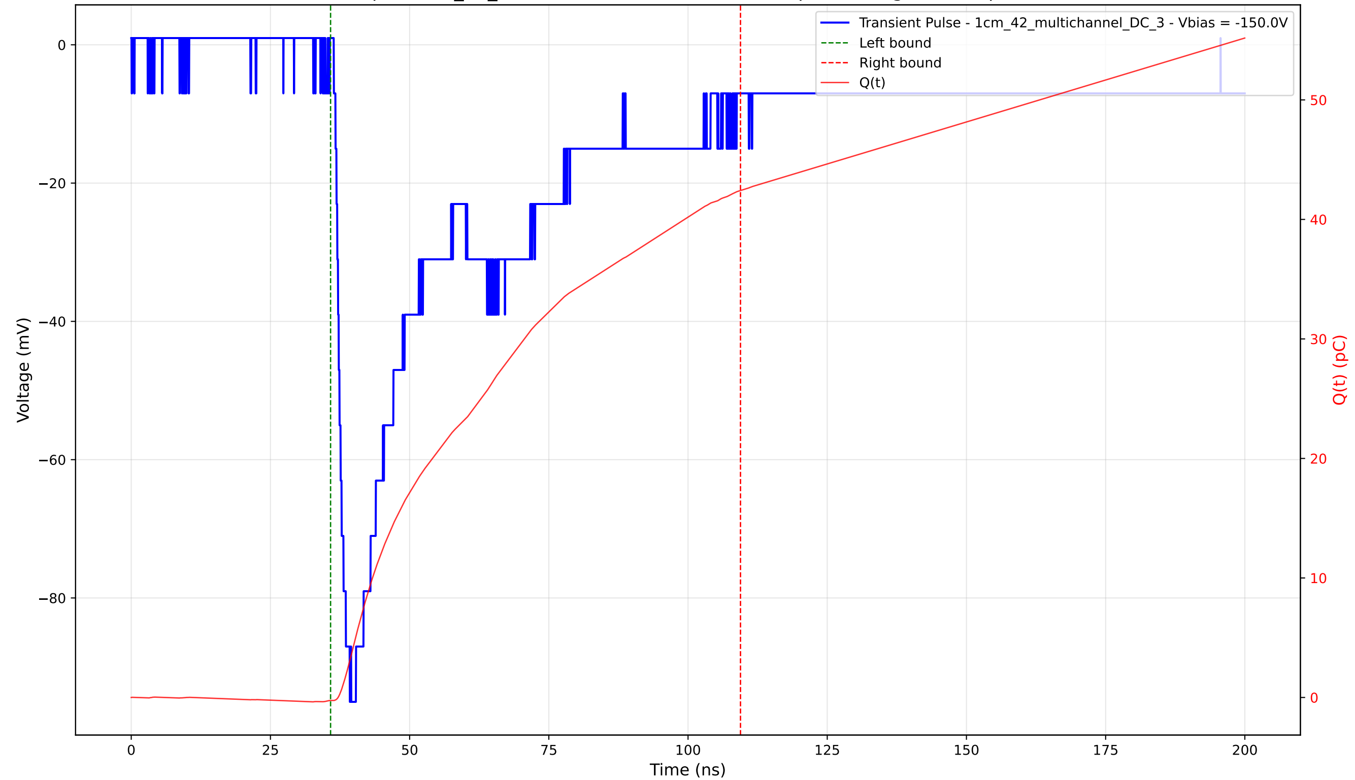
Transient Pulse - Sample: 1cm_42_multichannel - Position: 2740.0 \mu\text{m} - Charge: 42.66 pC - Rise Time: 1.87 ns
