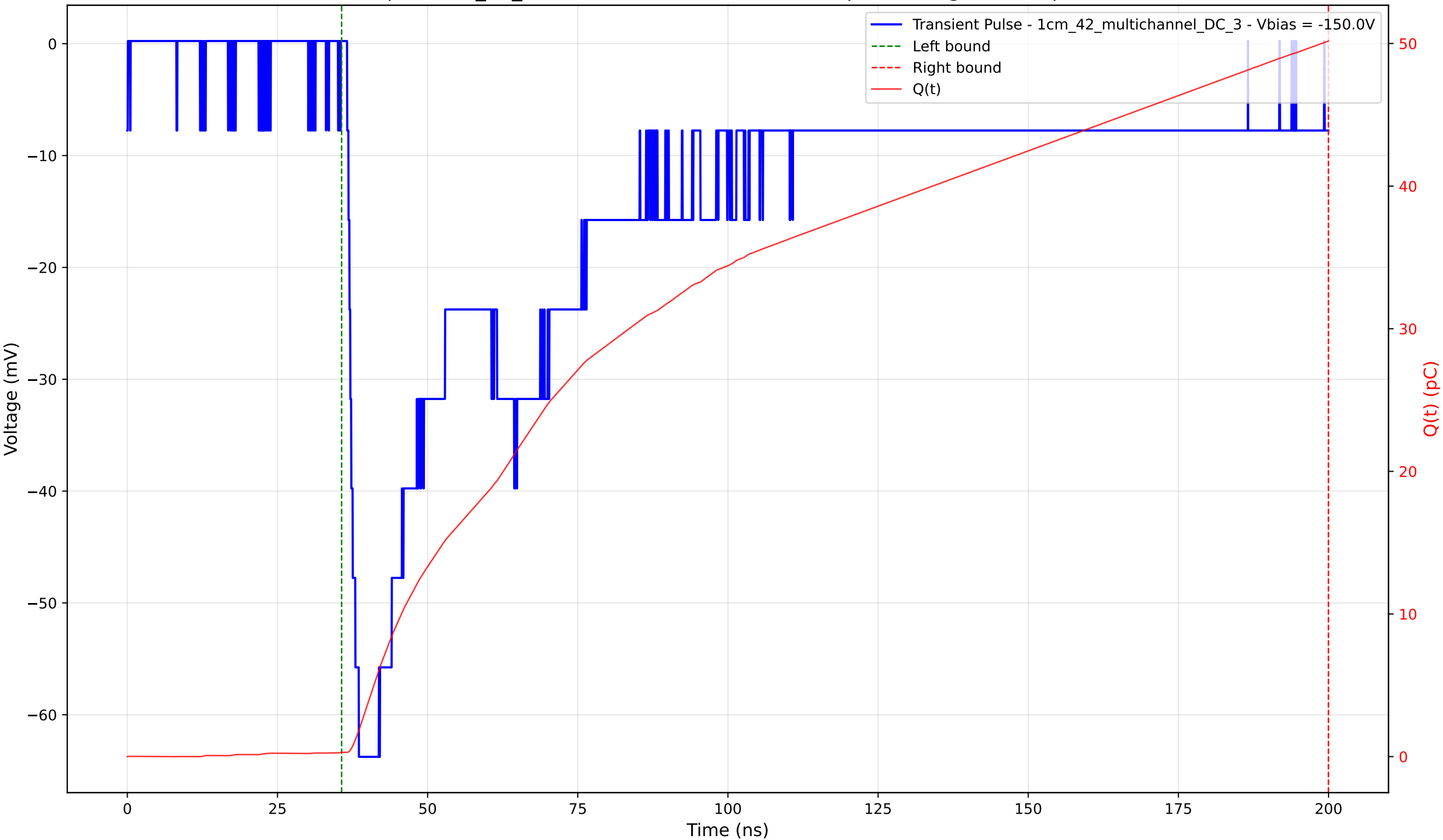
Transient Pulse - Sample: 1cm_42_multichannel - Position: 2440.0 \mu\text{m} - Charge: 49.88 pC - Rise Time: 1.94 ns
