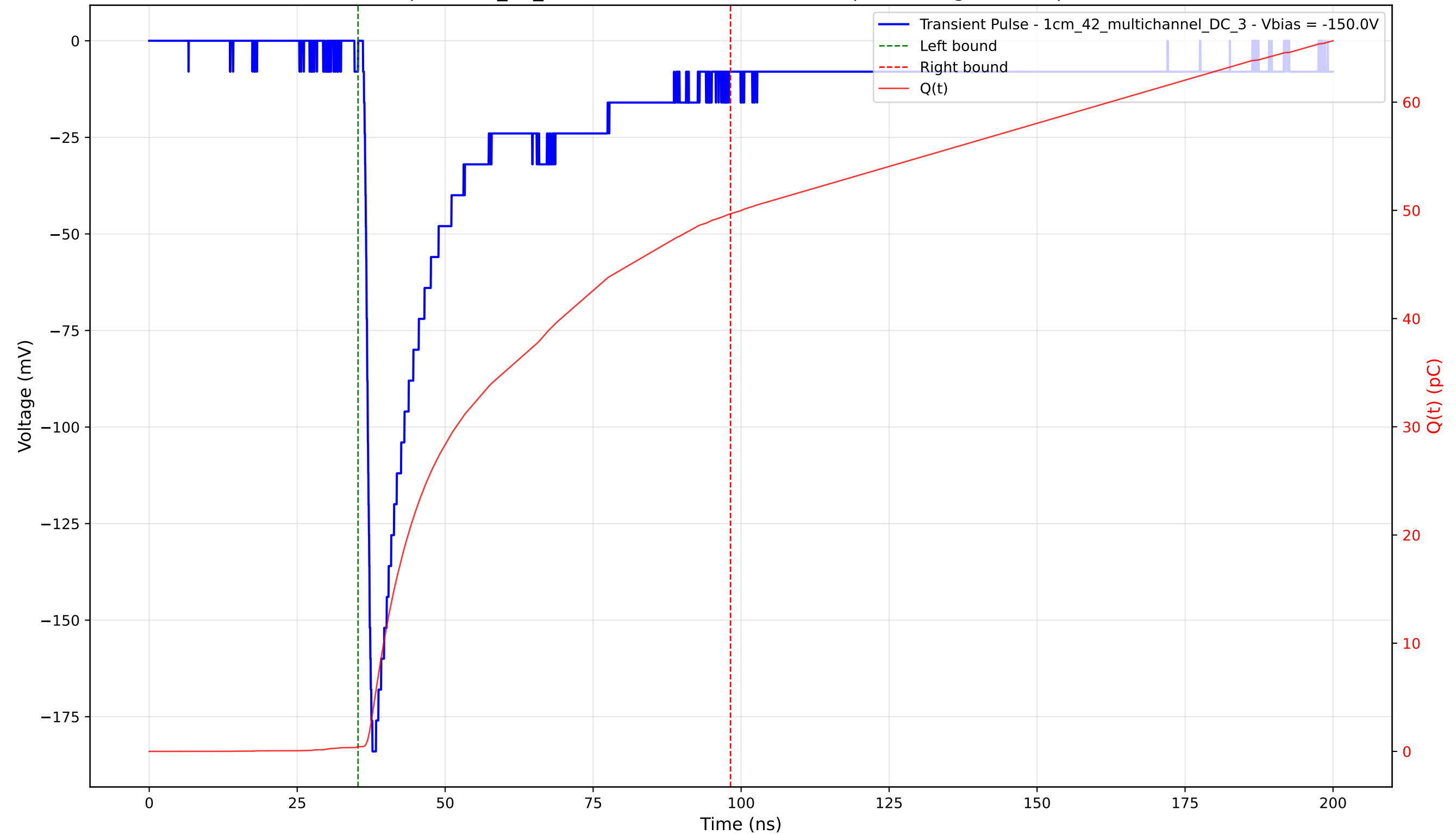
Transient Pulse - Sample: 1cm_42_multichannel - Position: 955.0 \mu\text{m} - Charge: 49.25 pC - Rise Time: 1.05 ns
