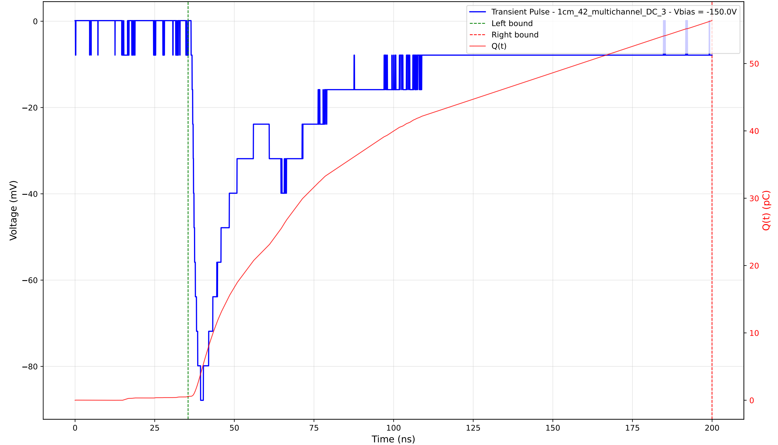
Transient Pulse - Sample: 1cm_42_multichannel - Position: 2640.0 \mu\text{m} - Charge: 55.81 pC - Rise Time: 1.78 ns
