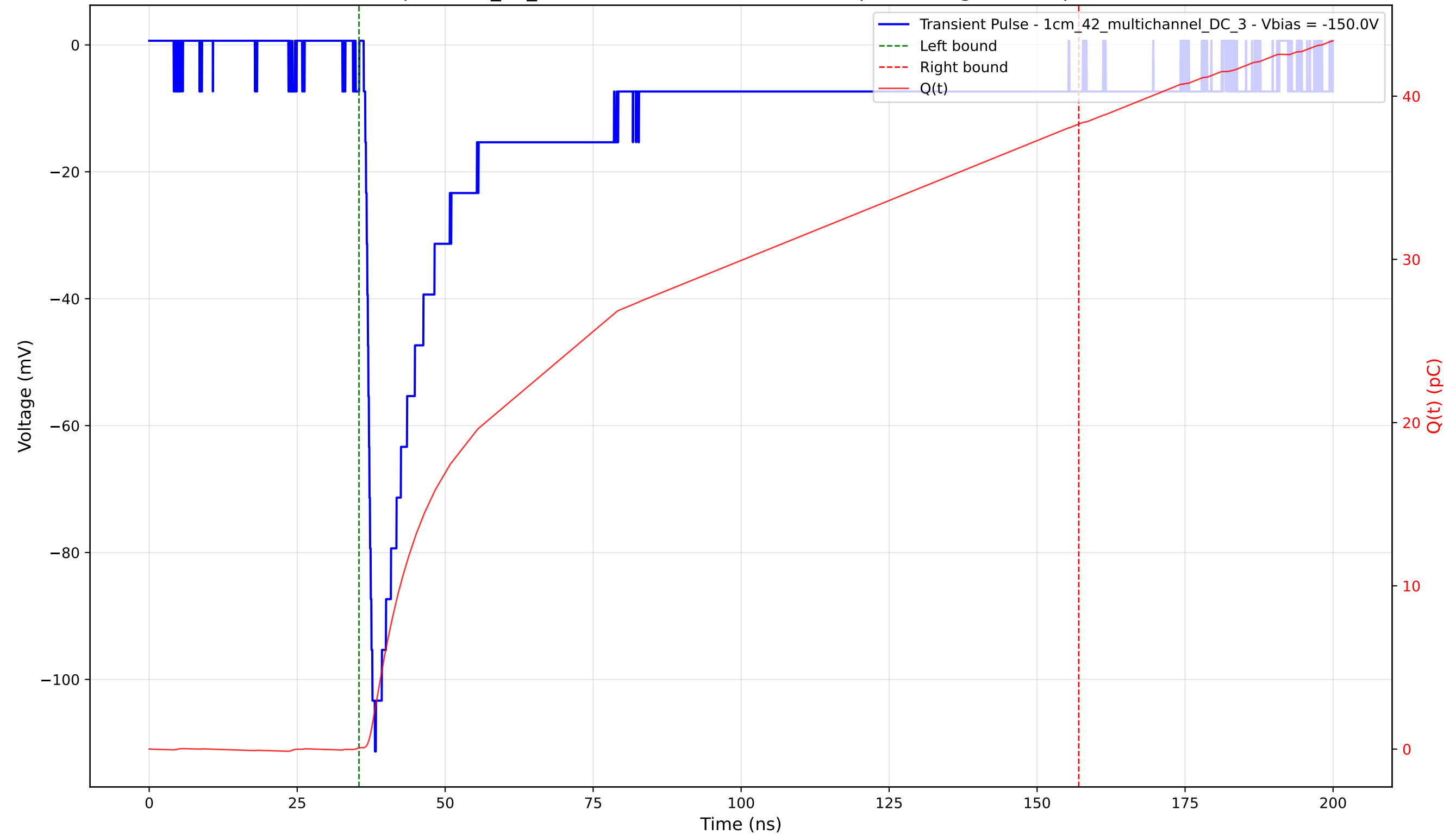
Transient Pulse - Sample: 1cm_42_multichannel - Position: 3830.0 \mu\text{m} - Charge: 38.21 pC - Rise Time: 1.21 ns
