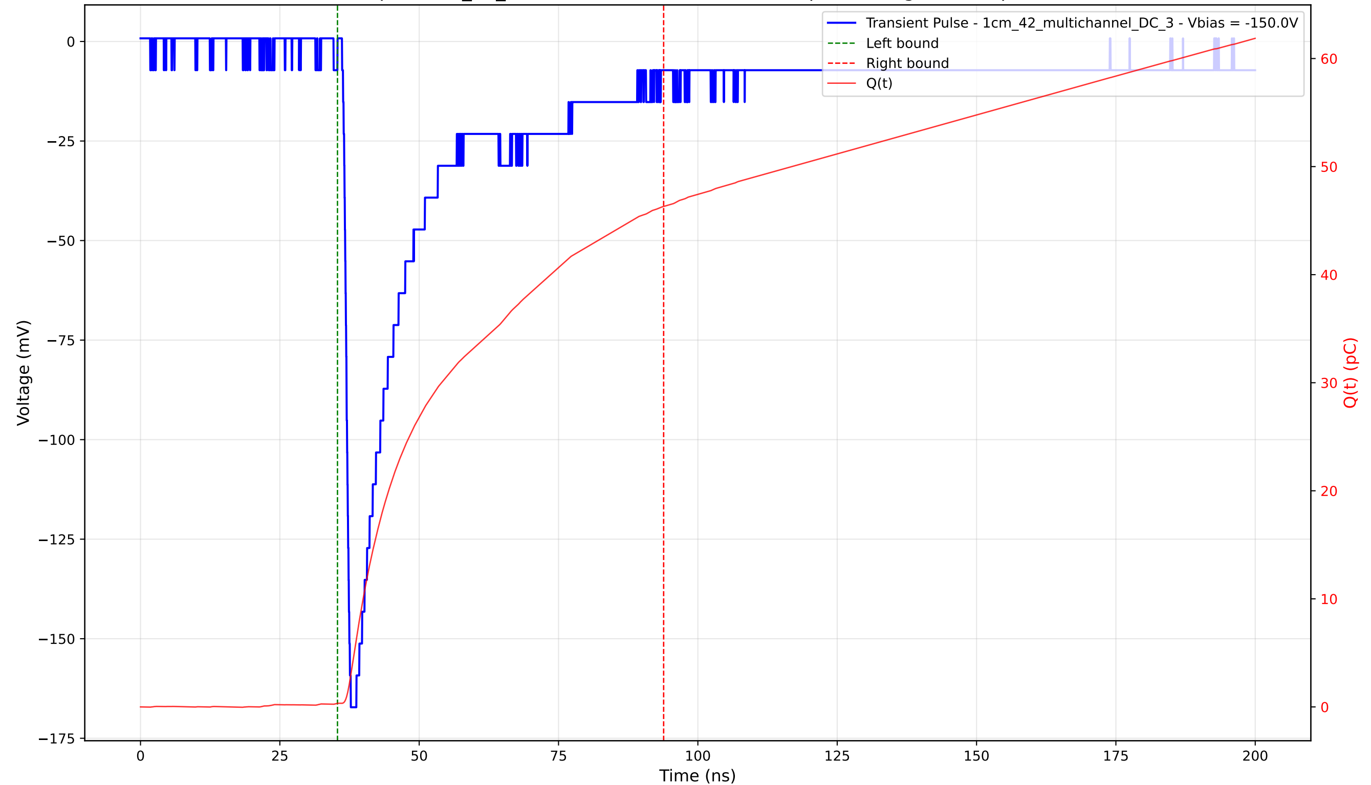
Transient Pulse - Sample: 1cm_42_multichannel - Position: 1045.0 \mu\text{m} - Charge: 45.97 pC - Rise Time: 1.04 ns
