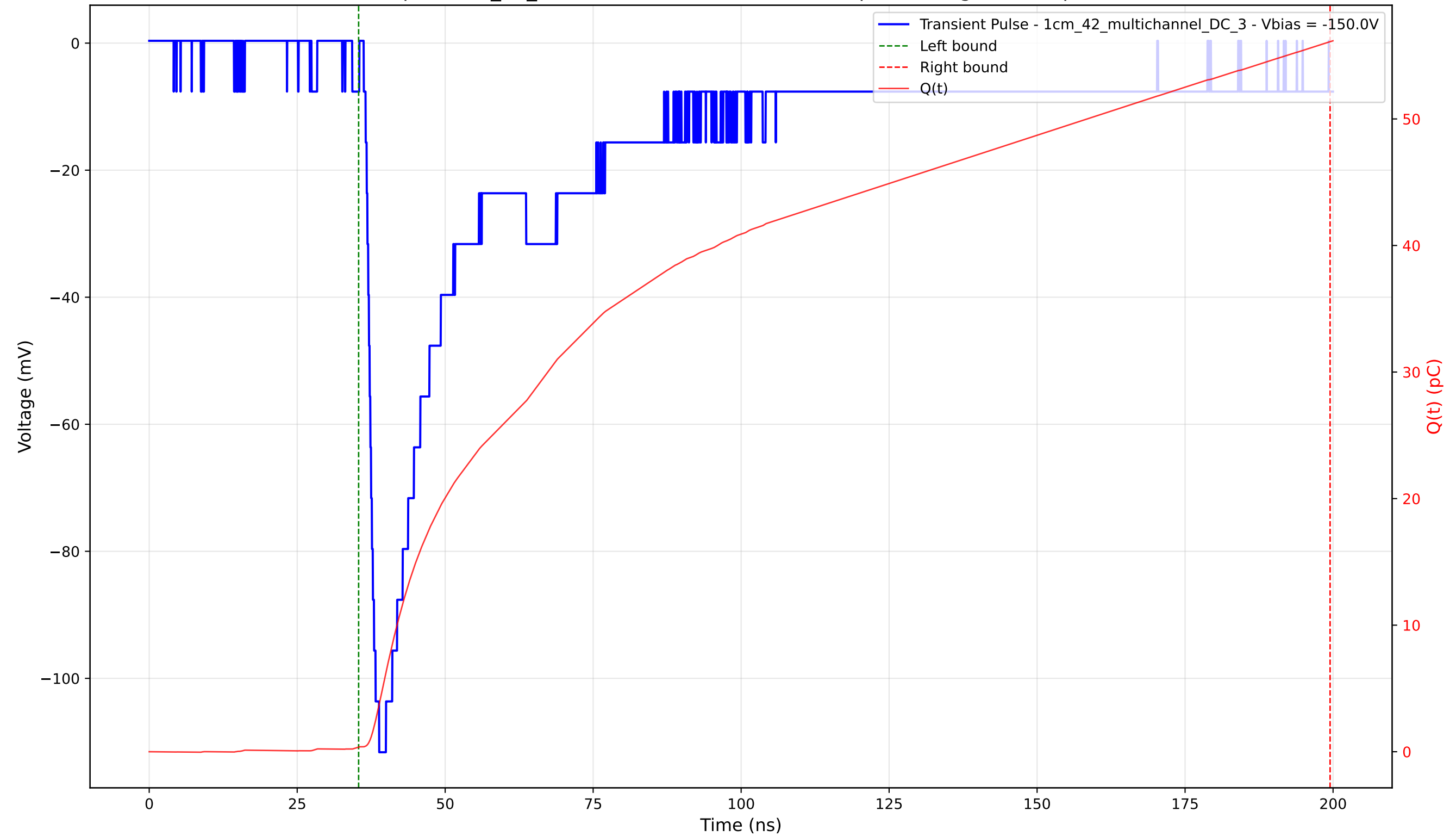
Transient Pulse - Sample: 1cm_42_multichannel - Position: 3200.0 \mu\text{m} - Charge: 55.73 pC - Rise Time: 1.69 ns
