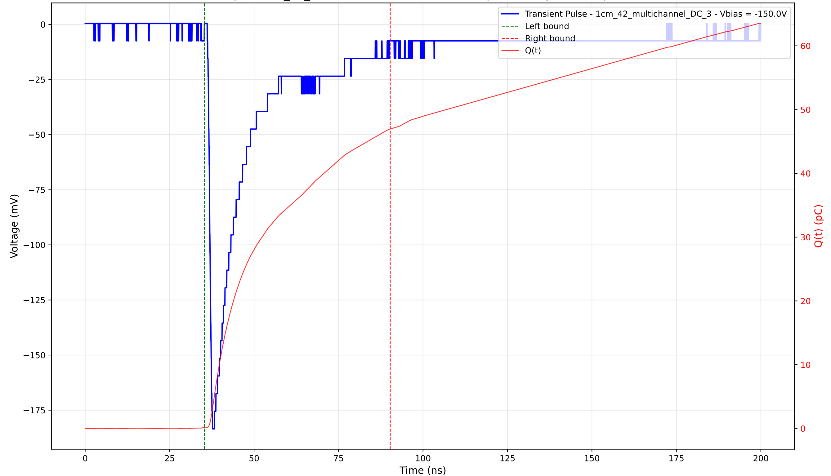
Transient Pulse - Sample: 1cm_42_multichannel - Position: 960.0 \mu\text{m} - Charge: 46.77 pC - Rise Time: 1.05 ns
