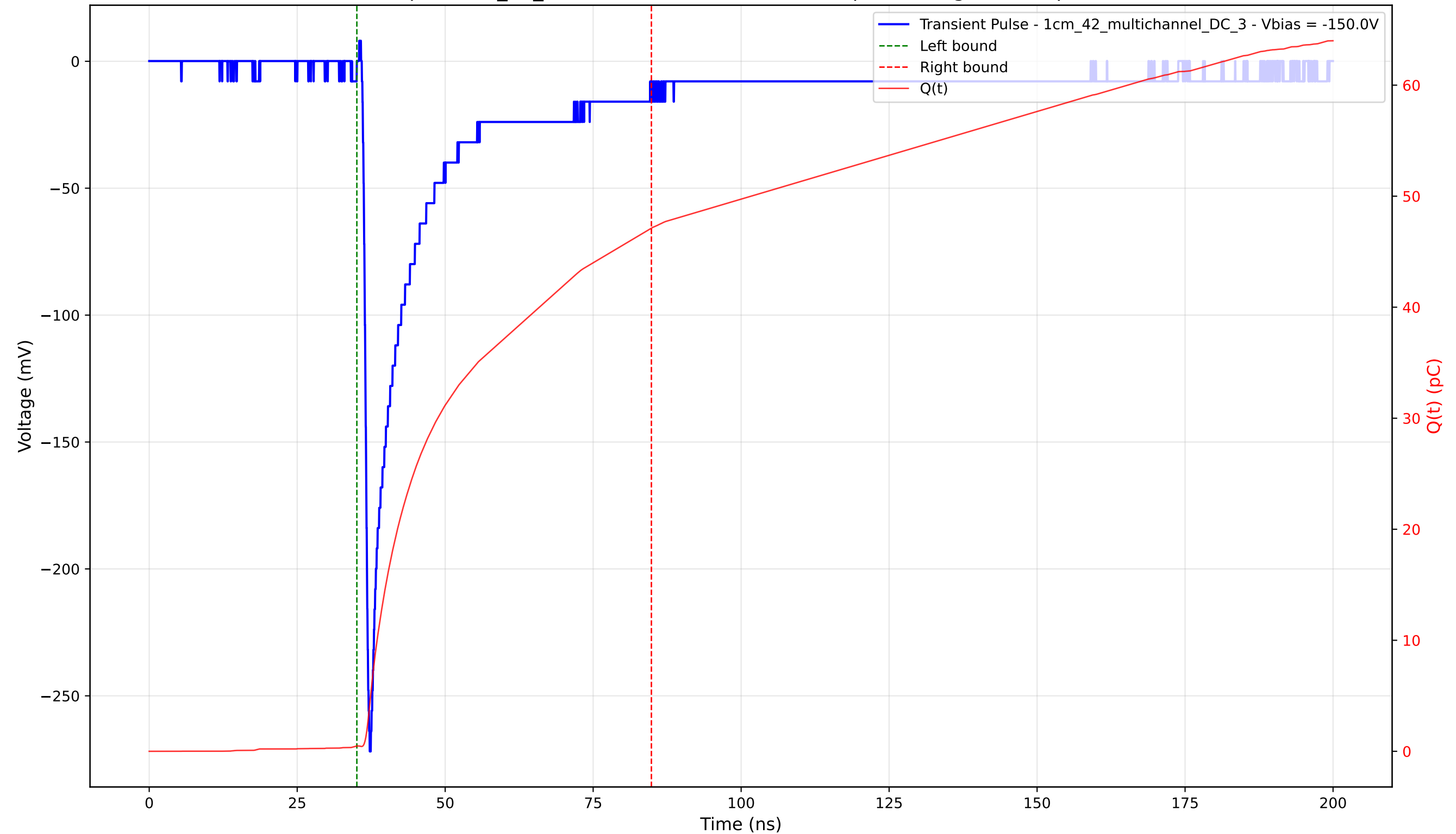
Transient Pulse - Sample: 1cm_42_multichannel - Position: 430.0 \mu\text{m} - Charge: 46.65 pC - Rise Time: 0.89 ns
