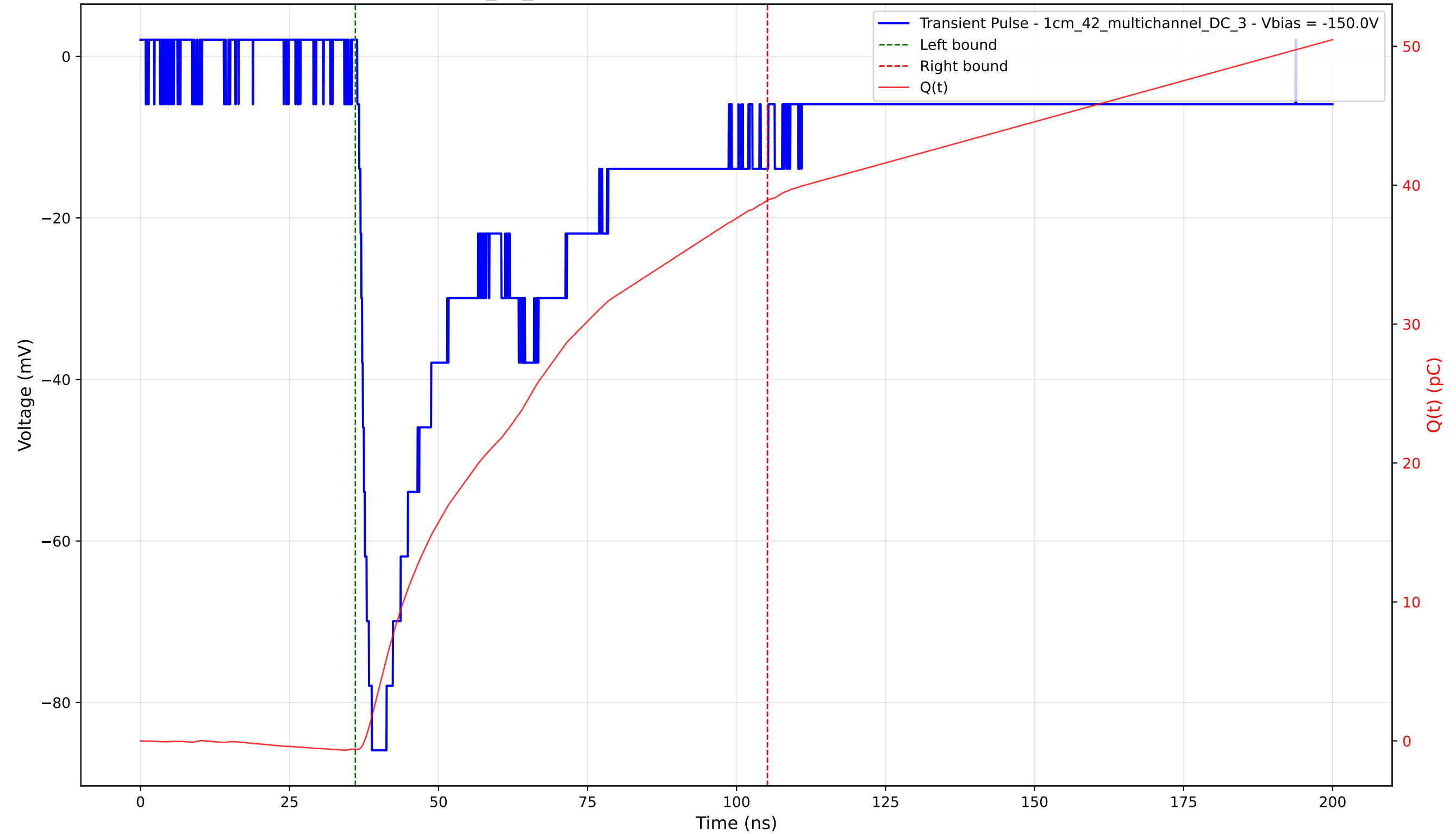
Transient Pulse - Sample: 1cm_42_multichannel - Position: 2690.0 \mu\text{m} - Charge: 39.53 pC - Rise Time: 1.65 ns
