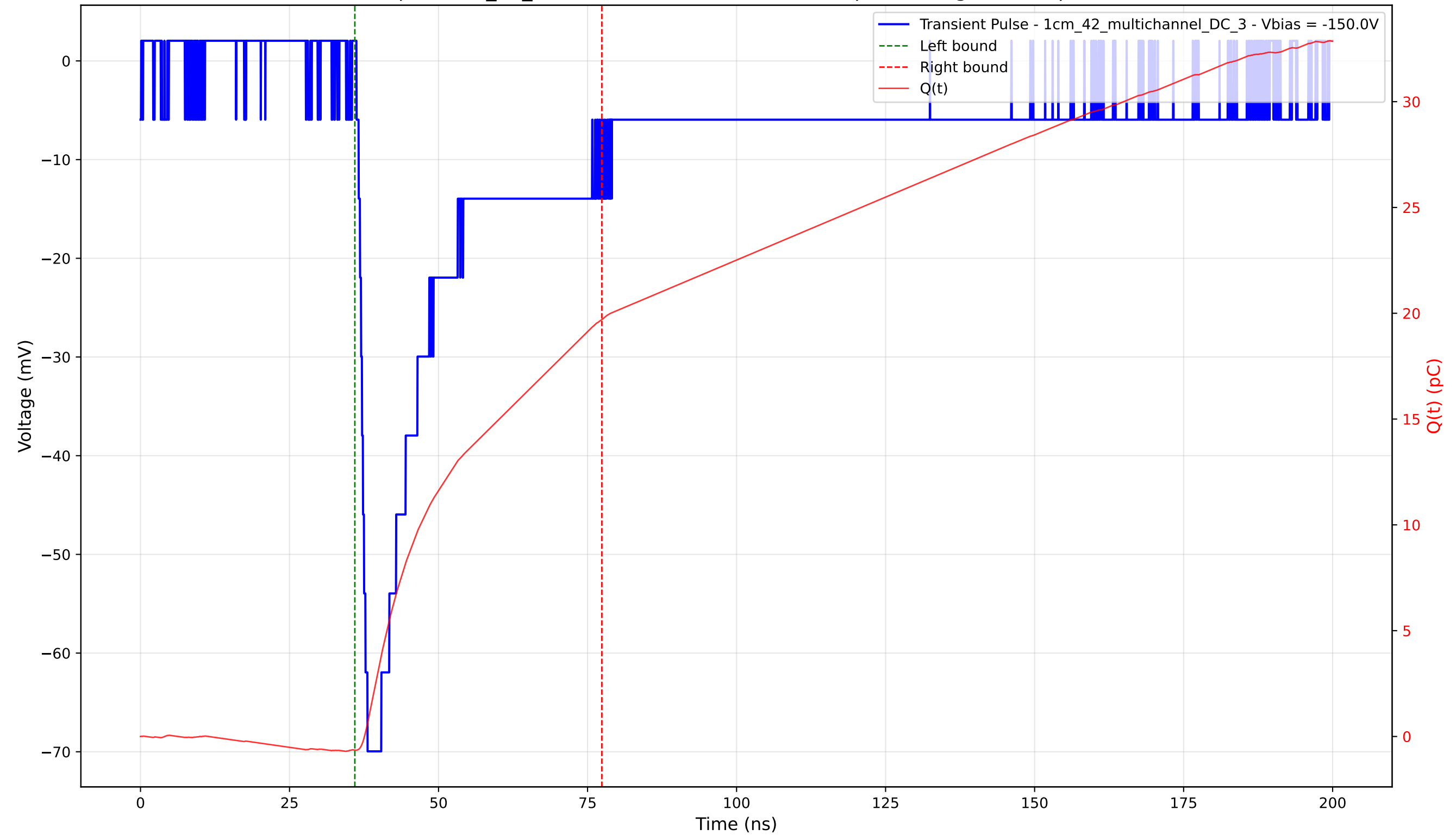
Transient Pulse - Sample: 1cm_42_multichannel - Position: 3440.0 \mu\text{m} - Charge: 20.35 pC - Rise Time: 1.50 ns
