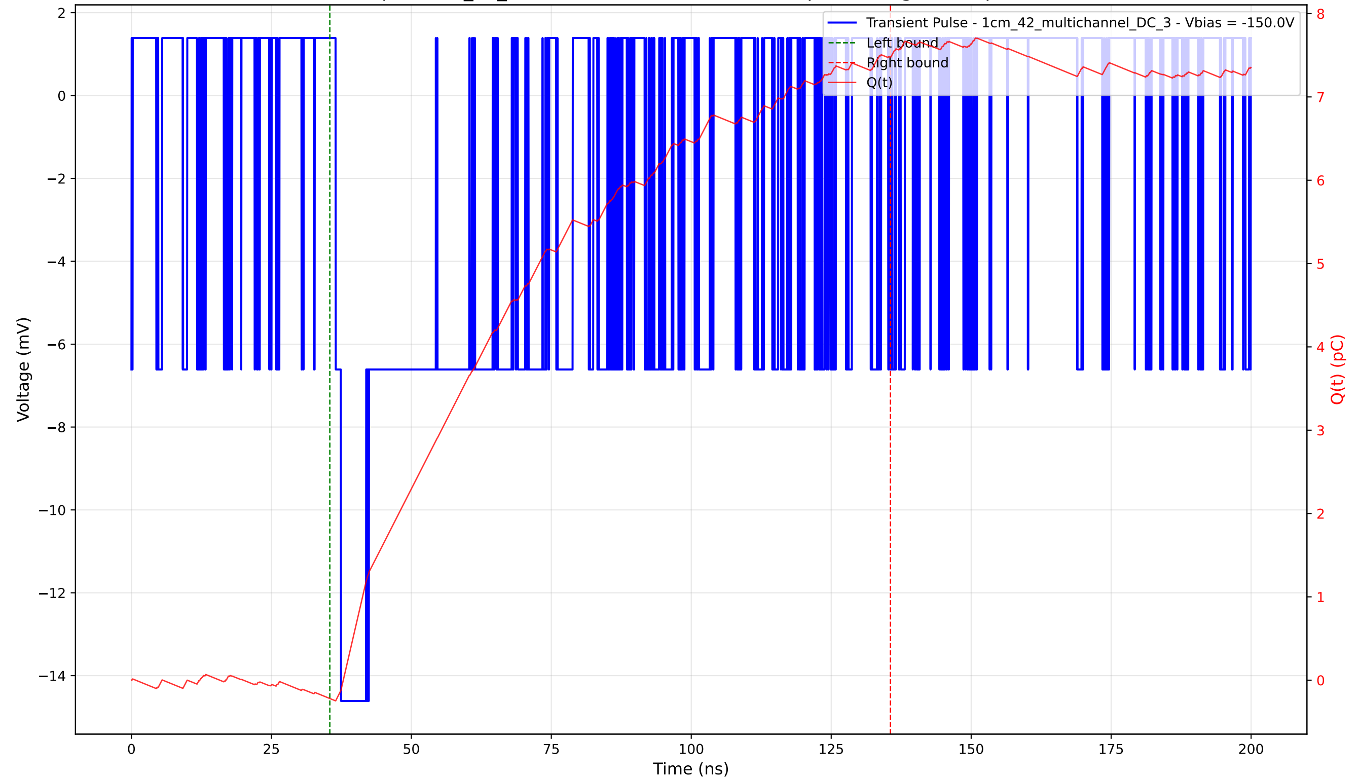
Transient Pulse - Sample: 1cm_42_multichannel - Position: 3910.0 \mu\text{m} - Charge: 7.70 pC - Rise Time: 0.96 ns
