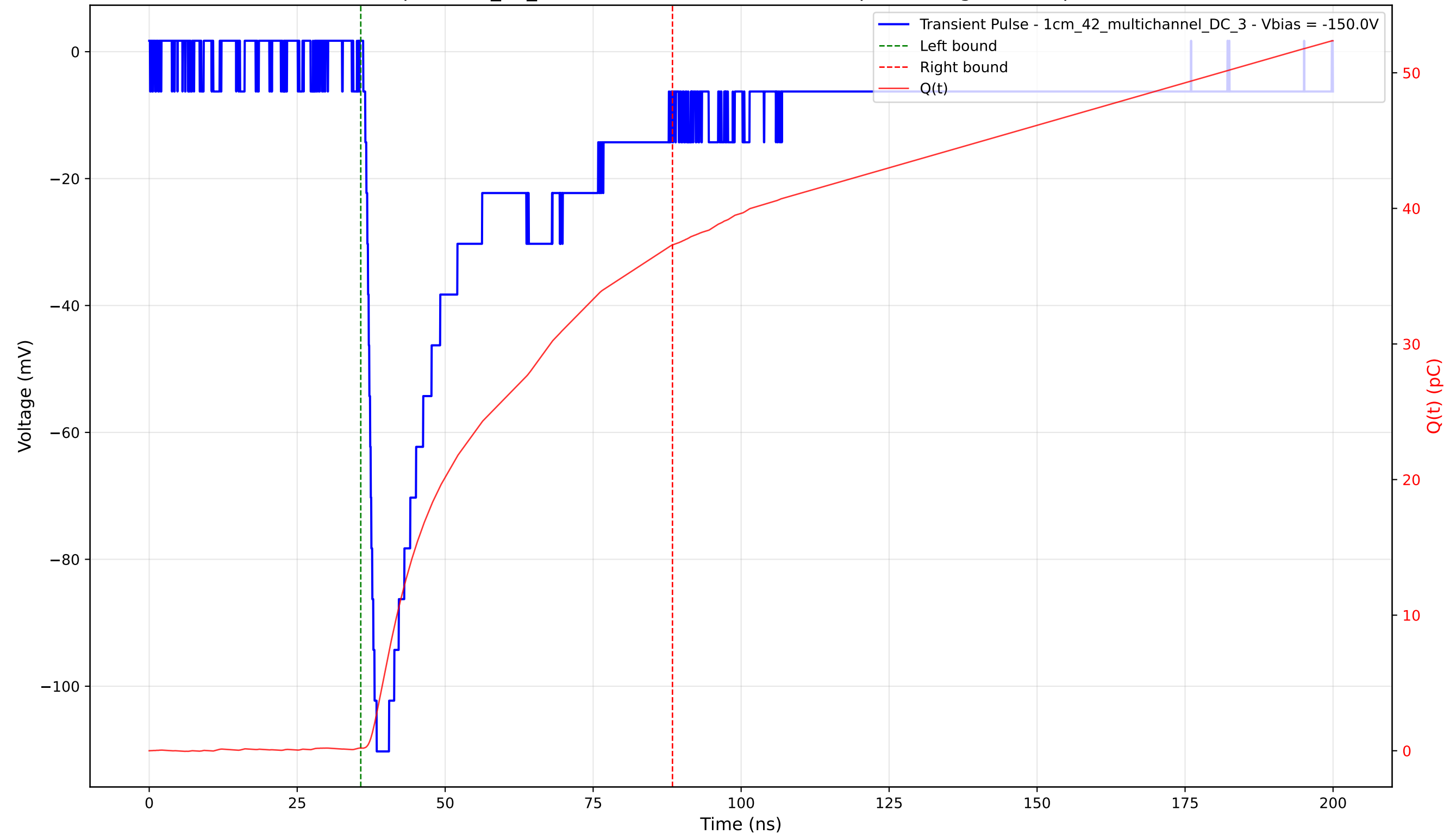
Transient Pulse - Sample: 1cm_42_multichannel - Position: 3255.0 \mu\text{m} - Charge: 37.09 pC - Rise Time: 1.57 ns
