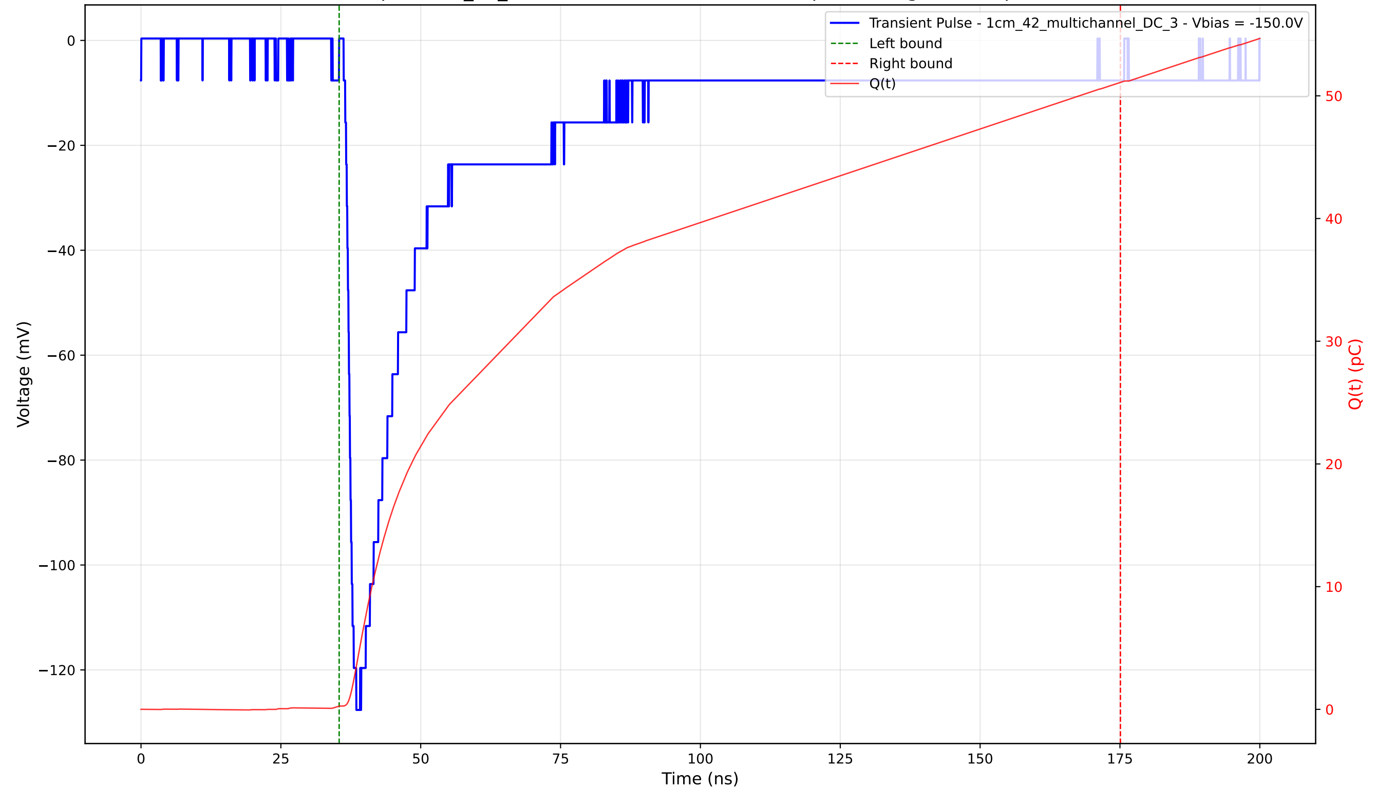
Transient Pulse - Sample: 1cm_42_multichannel - Position: 3550.0 \mu\text{m} - Charge: 50.83 pC - Rise Time: 1.53 ns
