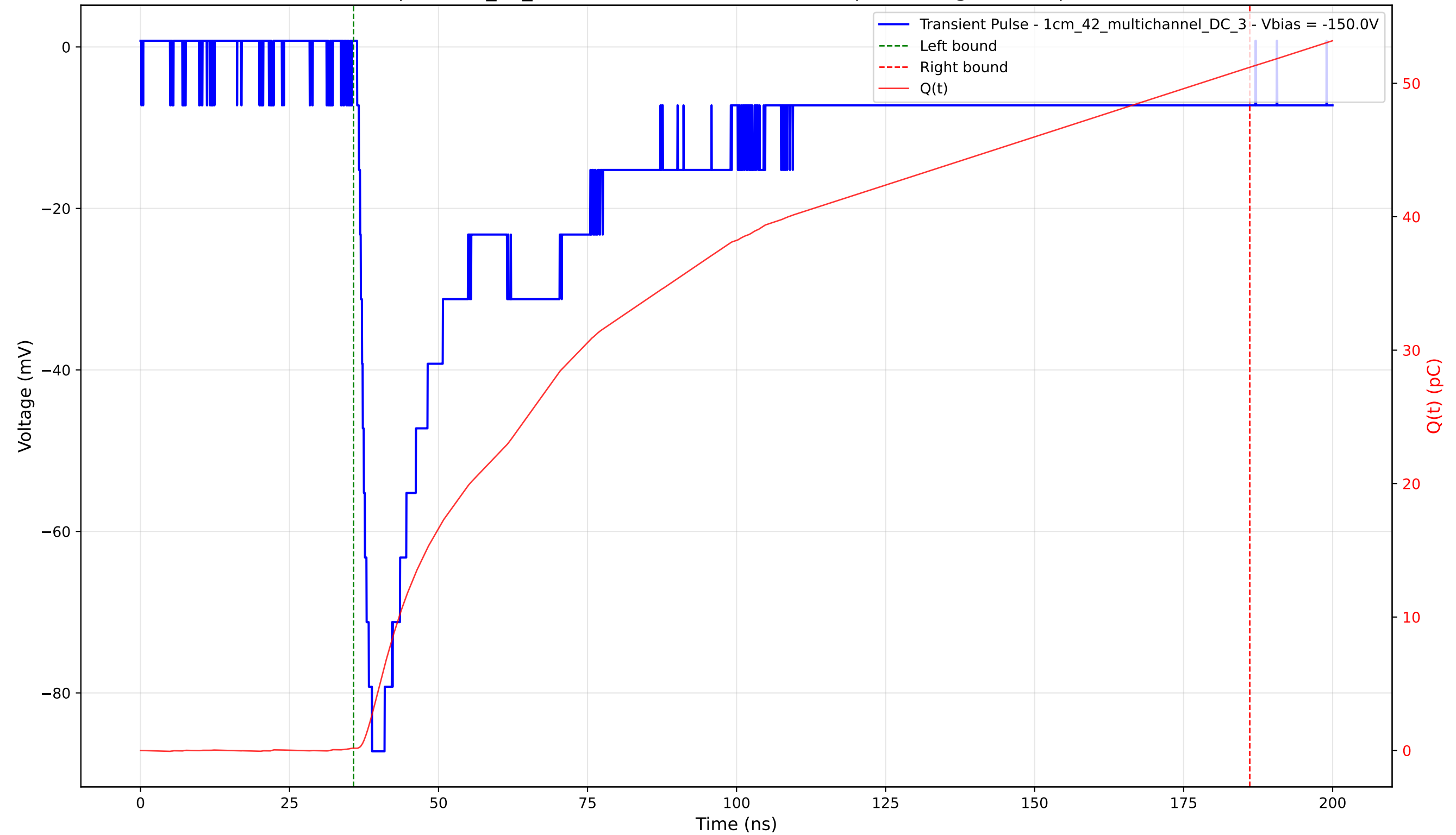
Transient Pulse - Sample: 1cm_42_multichannel - Position: 2795.0 \mu\text{m} - Charge: 51.05 pC - Rise Time: 1.68 ns
