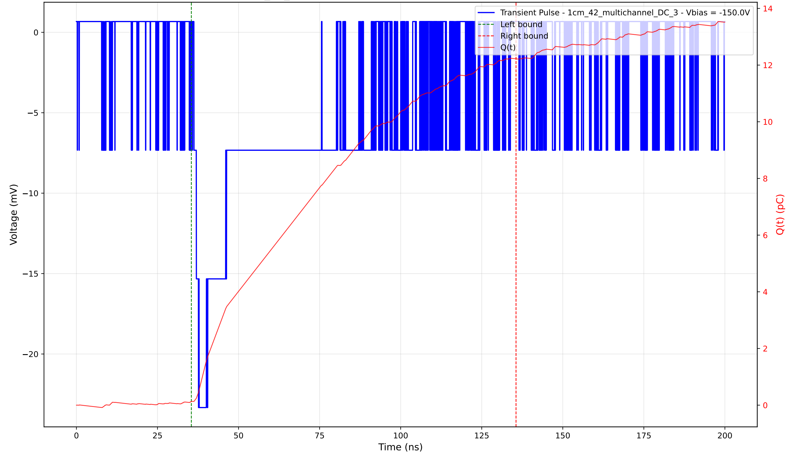
Transient Pulse - Sample: 1cm_42_multichannel - Position: 1335.0 \mu\text{m} - Charge: 12.08 pC - Rise Time: 1.42 ns
