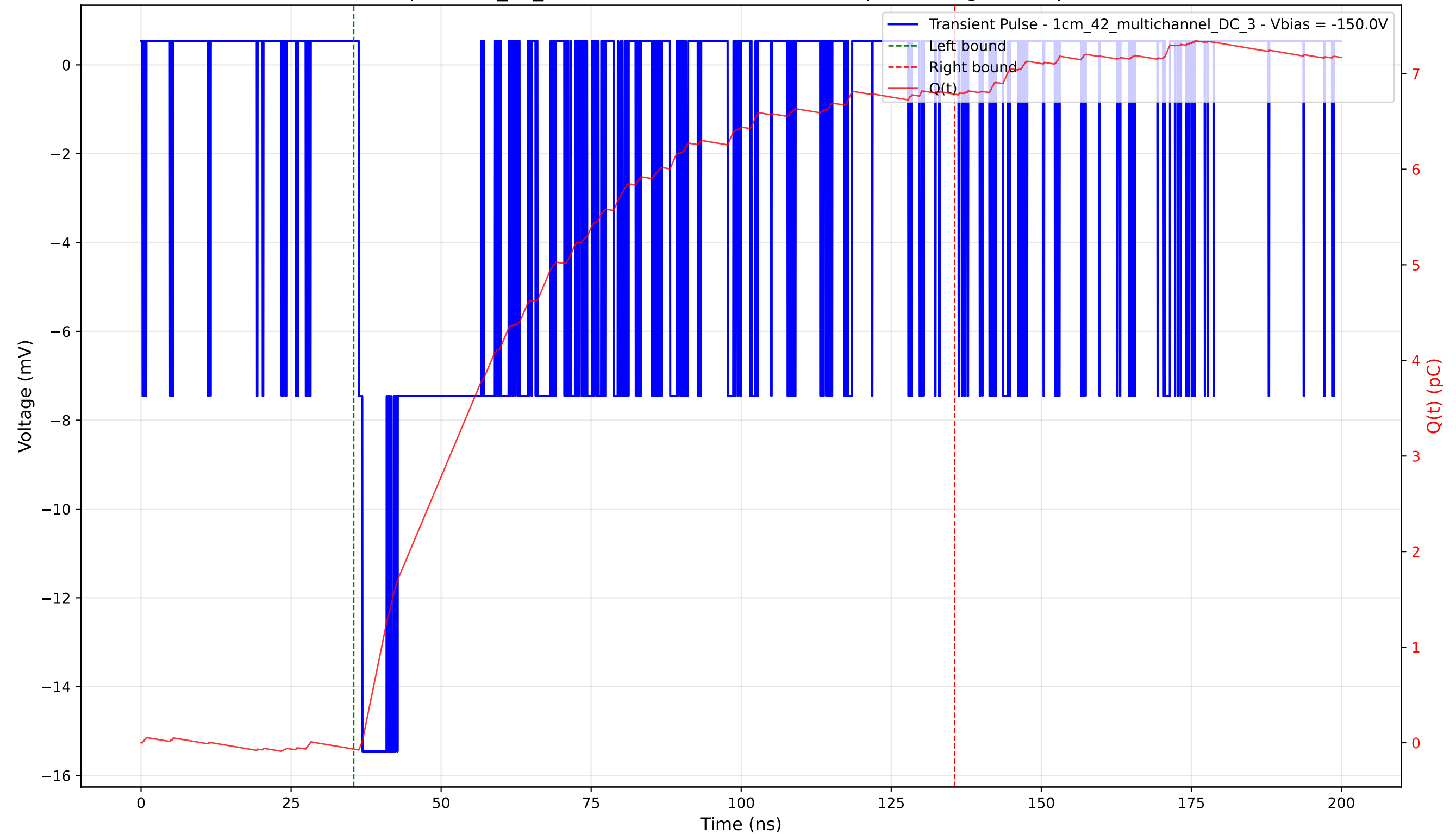
Transient Pulse - Sample: 1cm_42_multichannel - Position: 4370.0 \mu\text{m} - Charge: 6.85 pC - Rise Time: 0.62 ns
