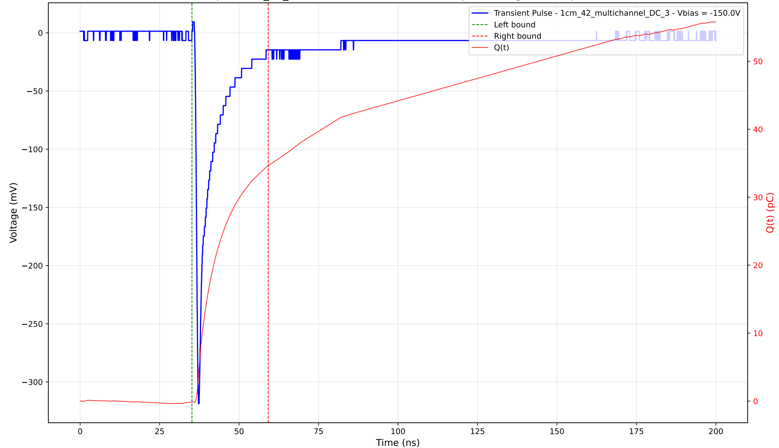
Transient Pulse - Sample: 1cm_42_multichannel - Position: 4650.0 \mu\text{m} - Charge: 34.73 pC - Rise Time: 0.82 ns
