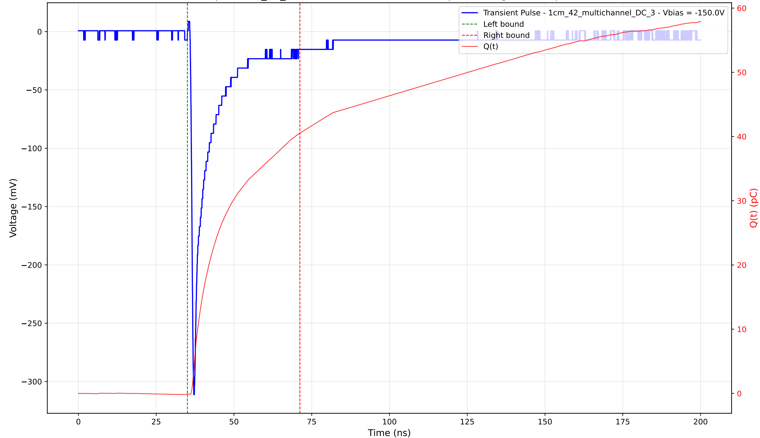
Transient Pulse - Sample: 1cm_42_multichannel - Position: 260.0 \mu\text{m} - Charge: 40.60 pC - Rise Time: 0.86 ns
