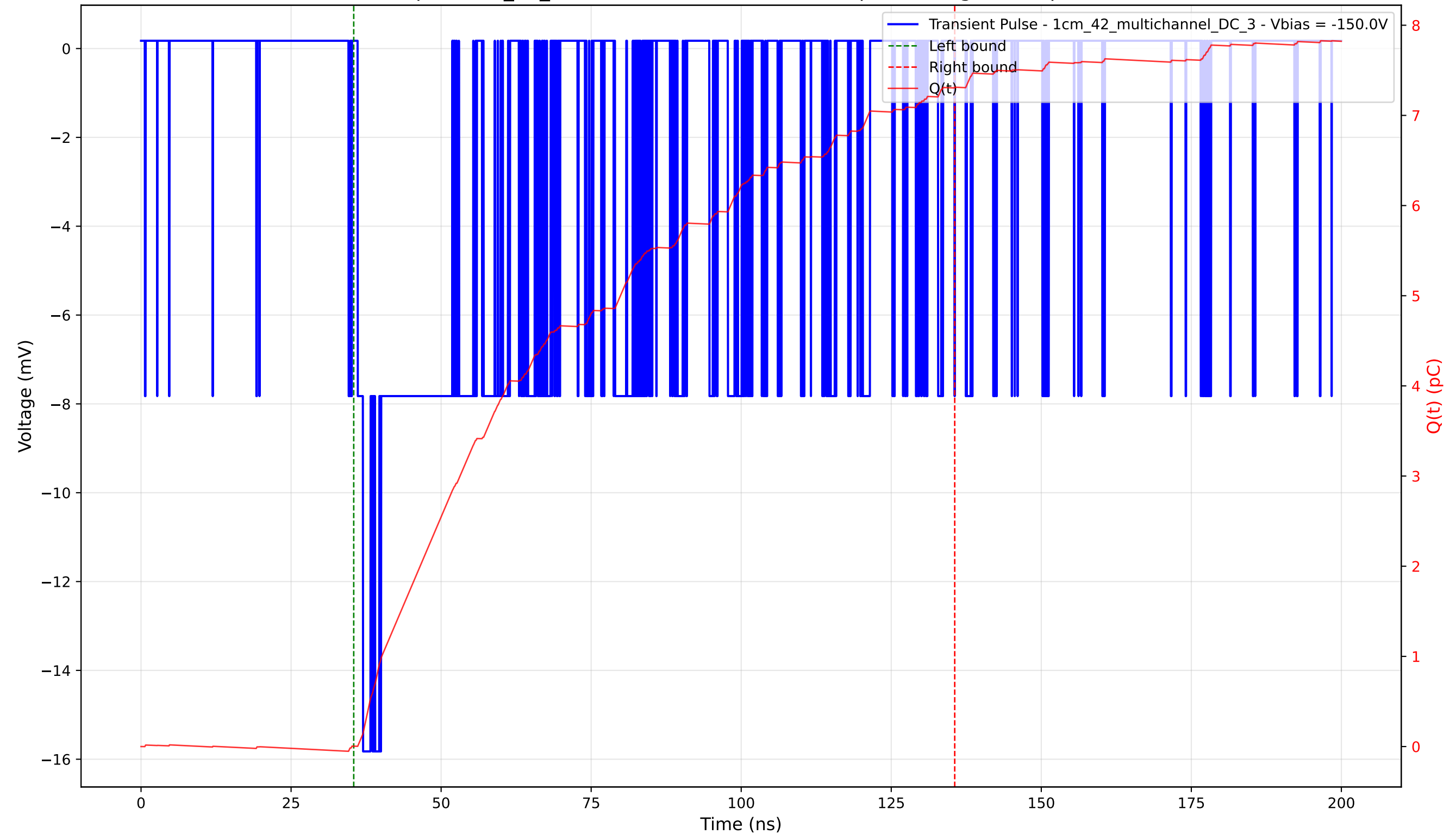
Transient Pulse - Sample: 1cm_42_multichannel - Position: 355.0 \mu\text{m} - Charge: 7.30 pC - Rise Time: 0.90 ns
