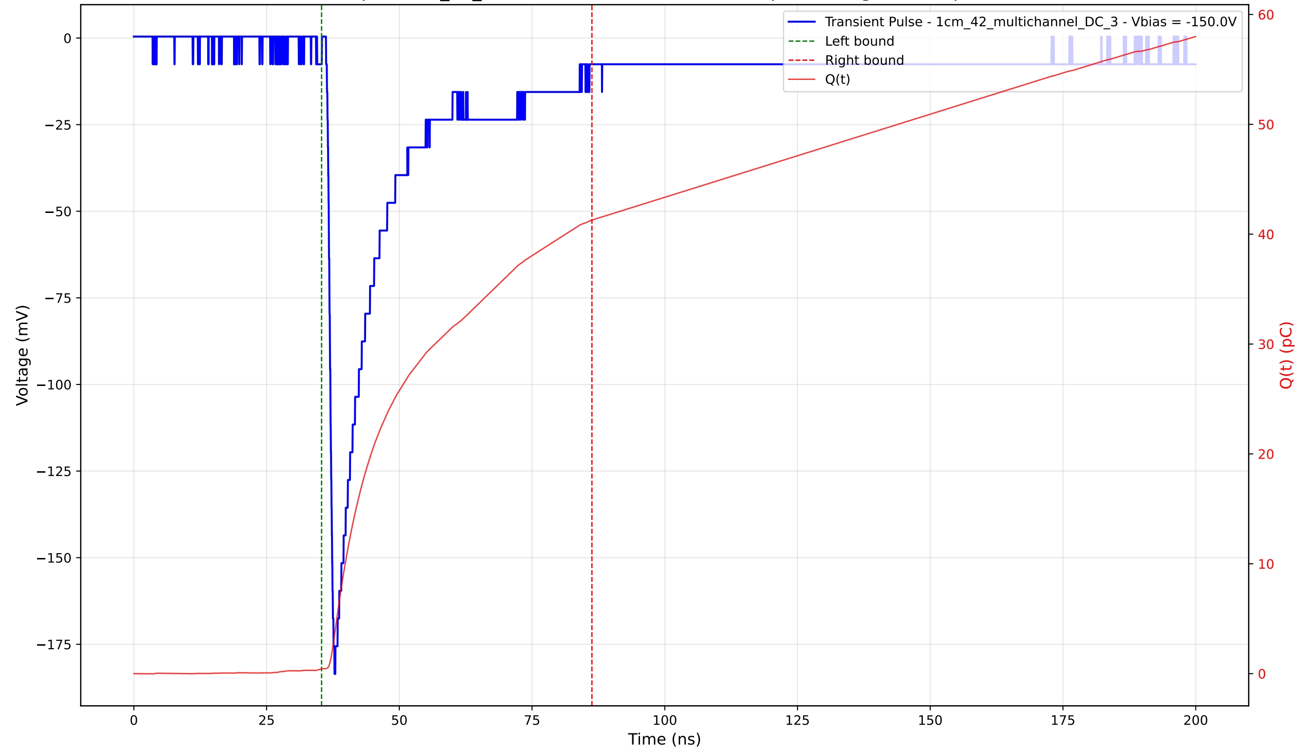
Transient Pulse - Sample: 1cm_42_multichannel - Position: 4070.0 \mu\text{m} - Charge: 40.84 pC - Rise Time: 1.03 ns
