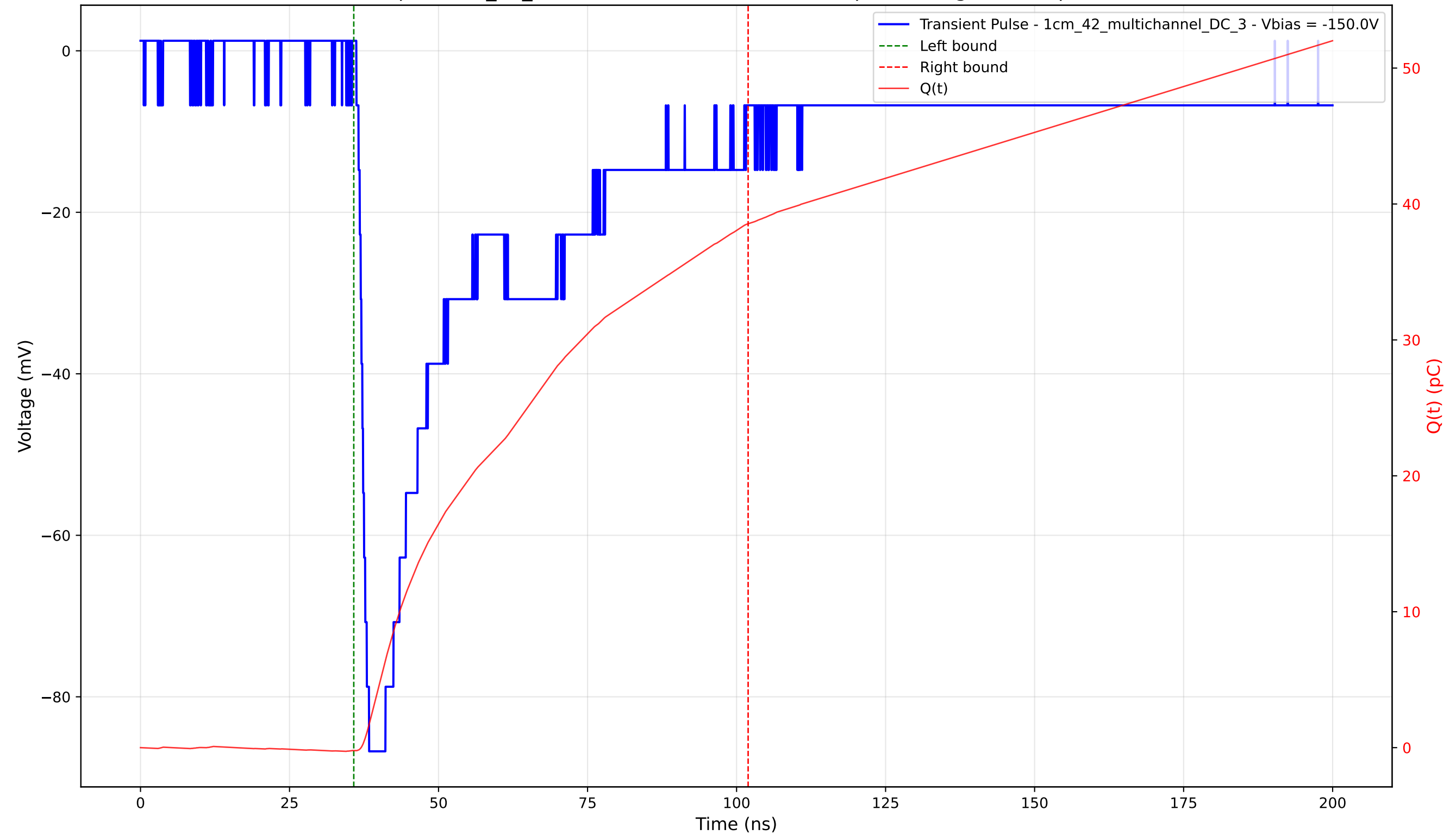
Transient Pulse - Sample: 1cm_42_multichannel - Position: 1945.0 \mu\text{m} - Charge: 38.76 pC - Rise Time: 1.40 ns
