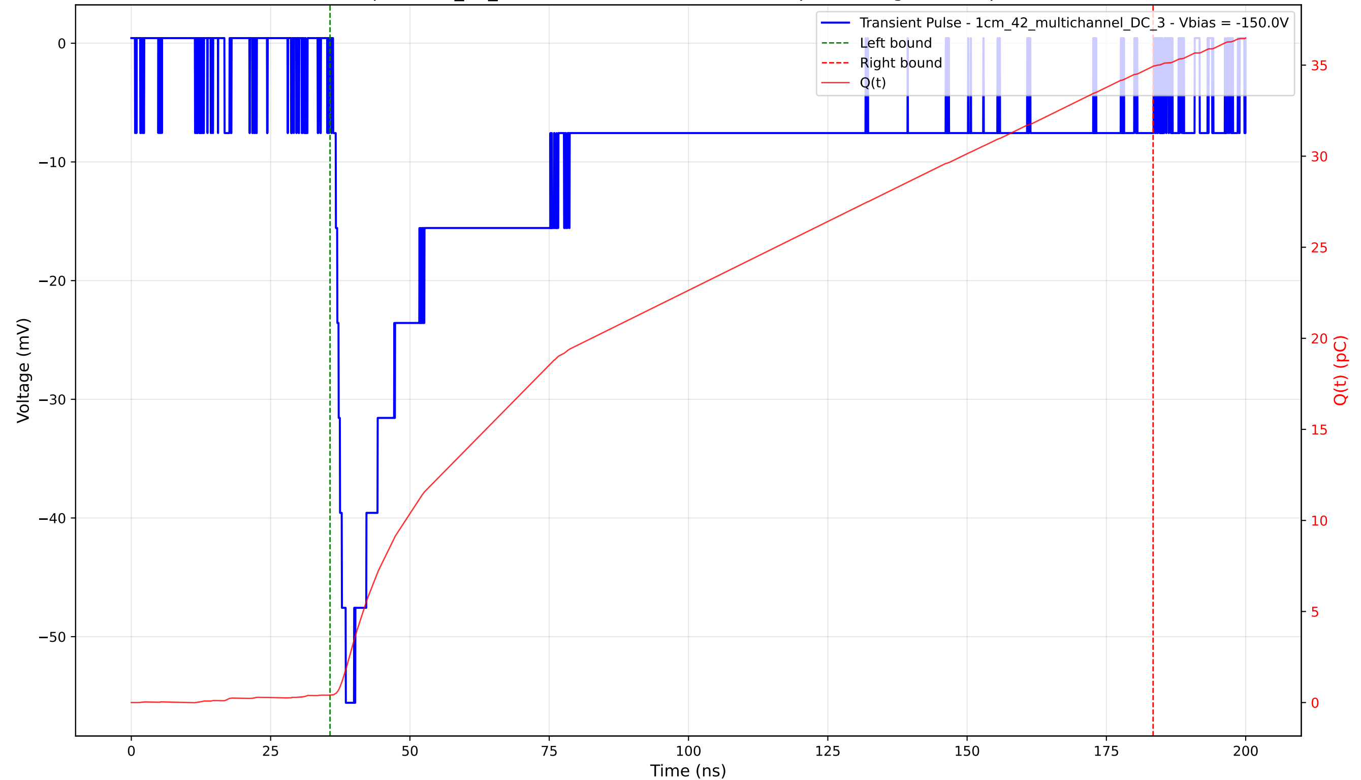
Transient Pulse - Sample: 1cm_42_multichannel - Position: 1820.0 \mu\text{m} - Charge: 34.53 pC - Rise Time: 2.27 ns
