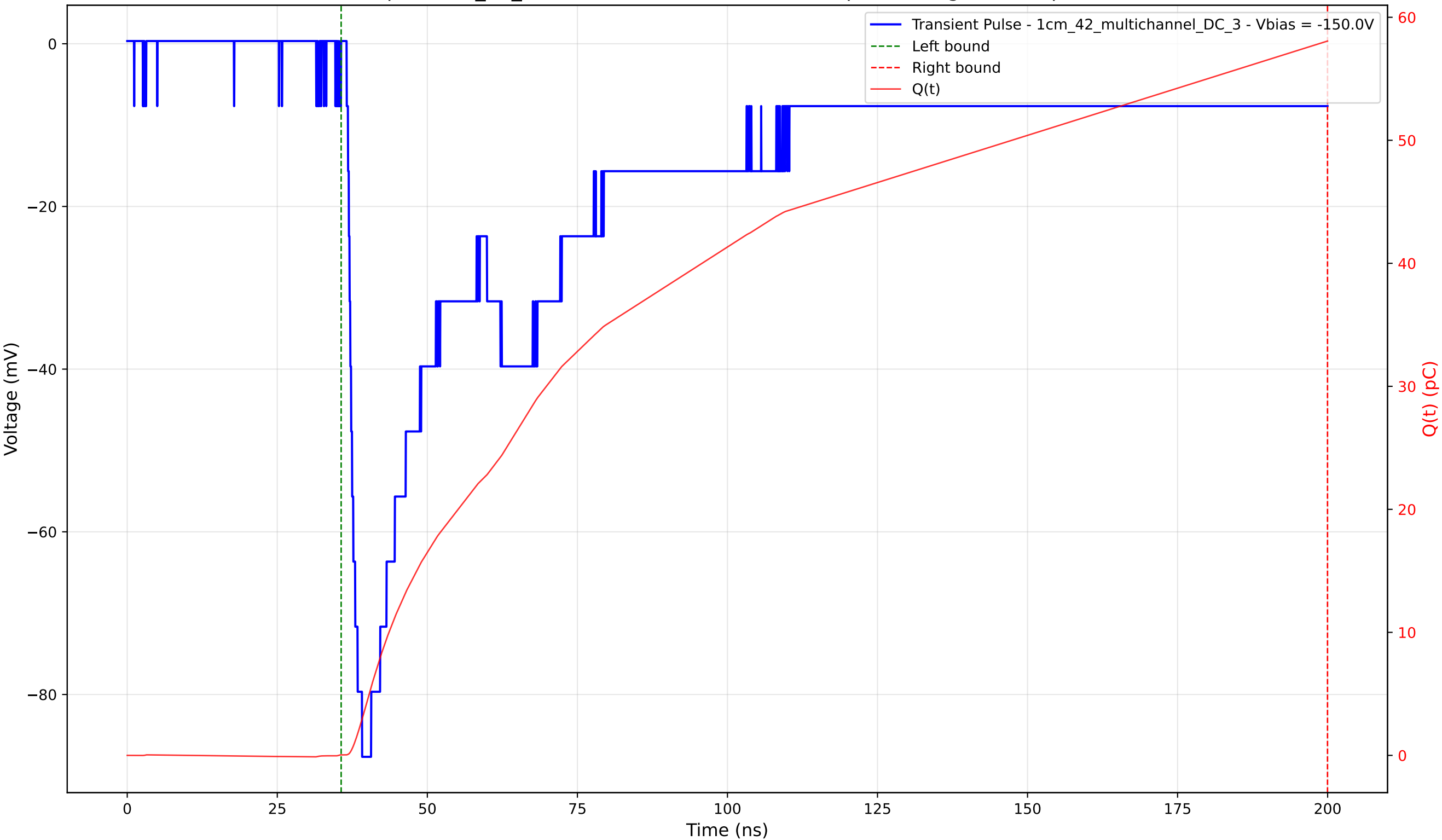
Transient Pulse - Sample: 1cm_42_multichannel - Position: 2205.0 \mu\text{m} - Charge: 58.02 pC - Rise Time: 1.62 ns
