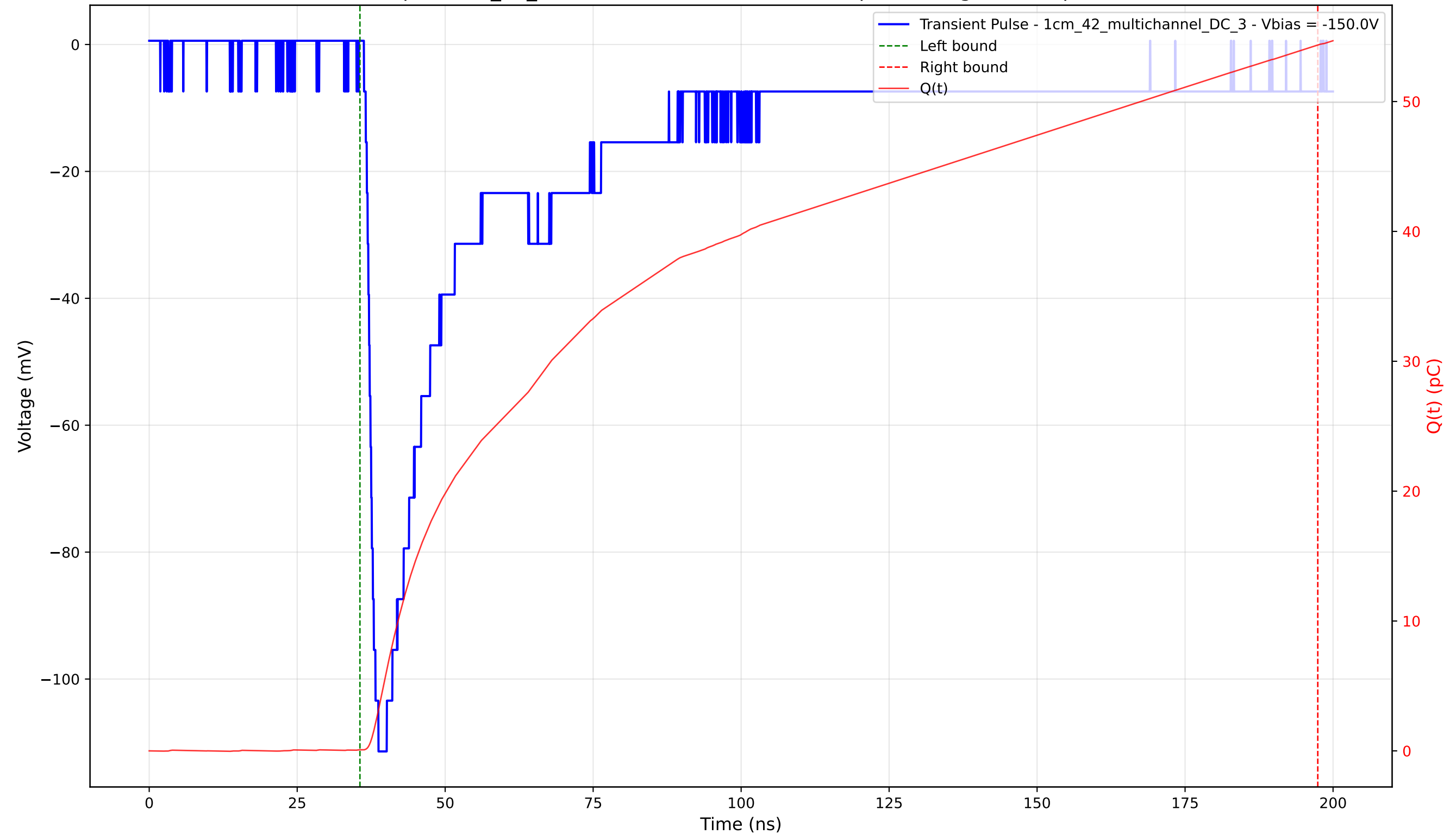
Transient Pulse - Sample: 1cm_42_multichannel - Position: 3215.0 \mu\text{m} - Charge: 54.27 pC - Rise Time: 1.65 ns
