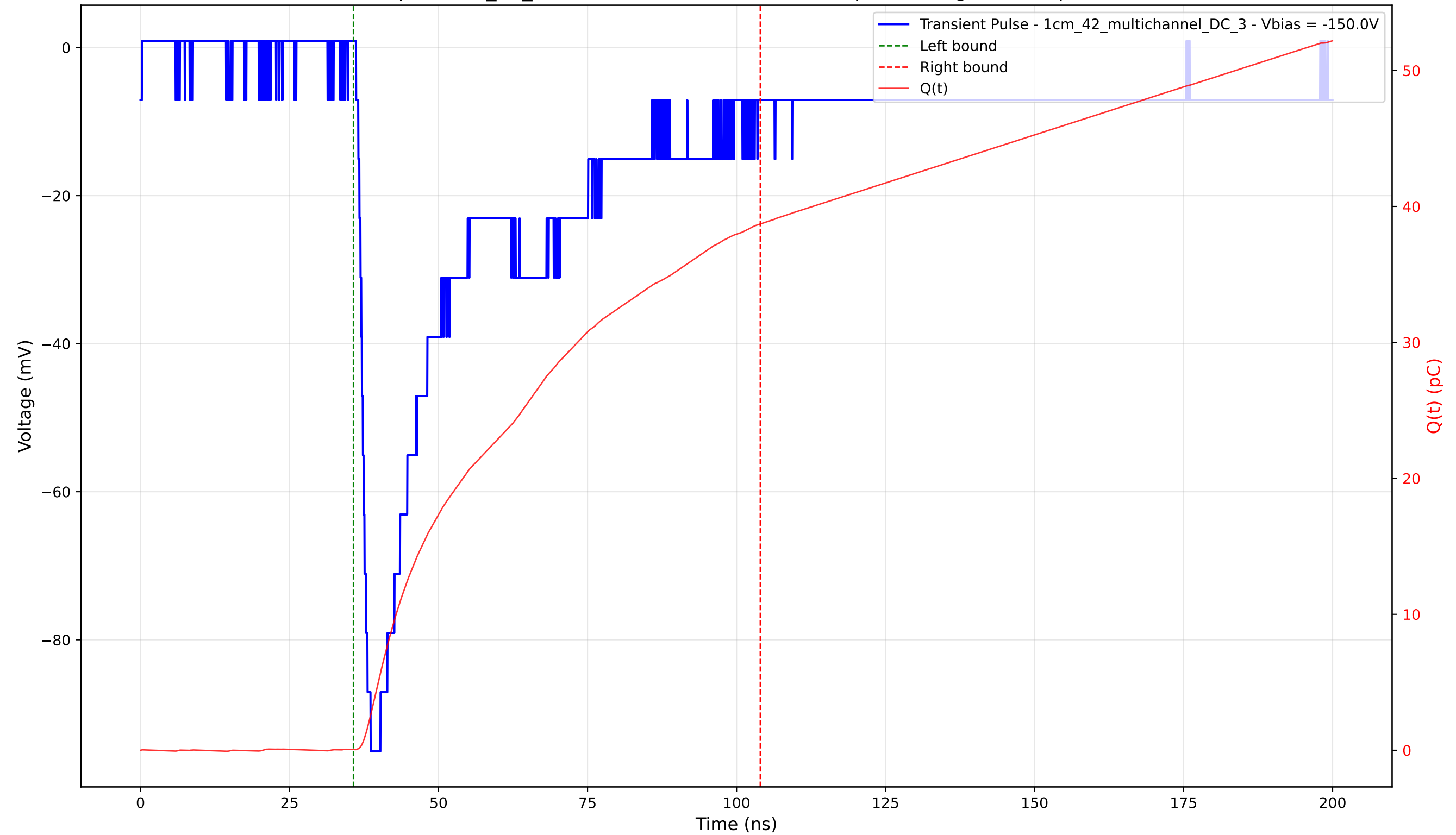
Transient Pulse - Sample: 1cm_42_multichannel - Position: 1795.0 \mu\text{m} - Charge: 38.66 pC - Rise Time: 1.55 ns
