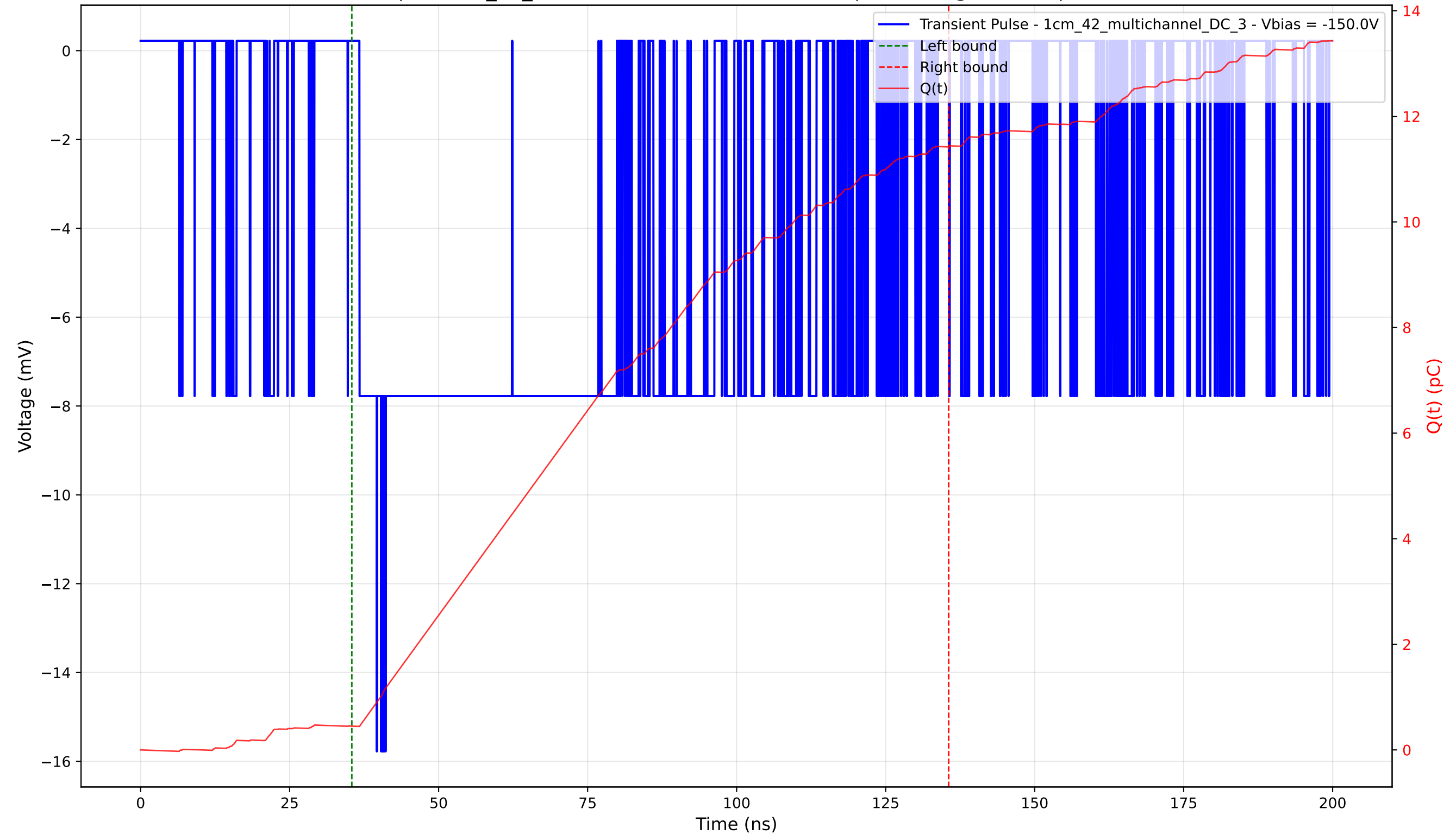
Transient Pulse - Sample: 1cm_42_multichannel - Position: 2900.0 \mu\text{m} - Charge: 10.97 pC - Rise Time: 2.94 ns
