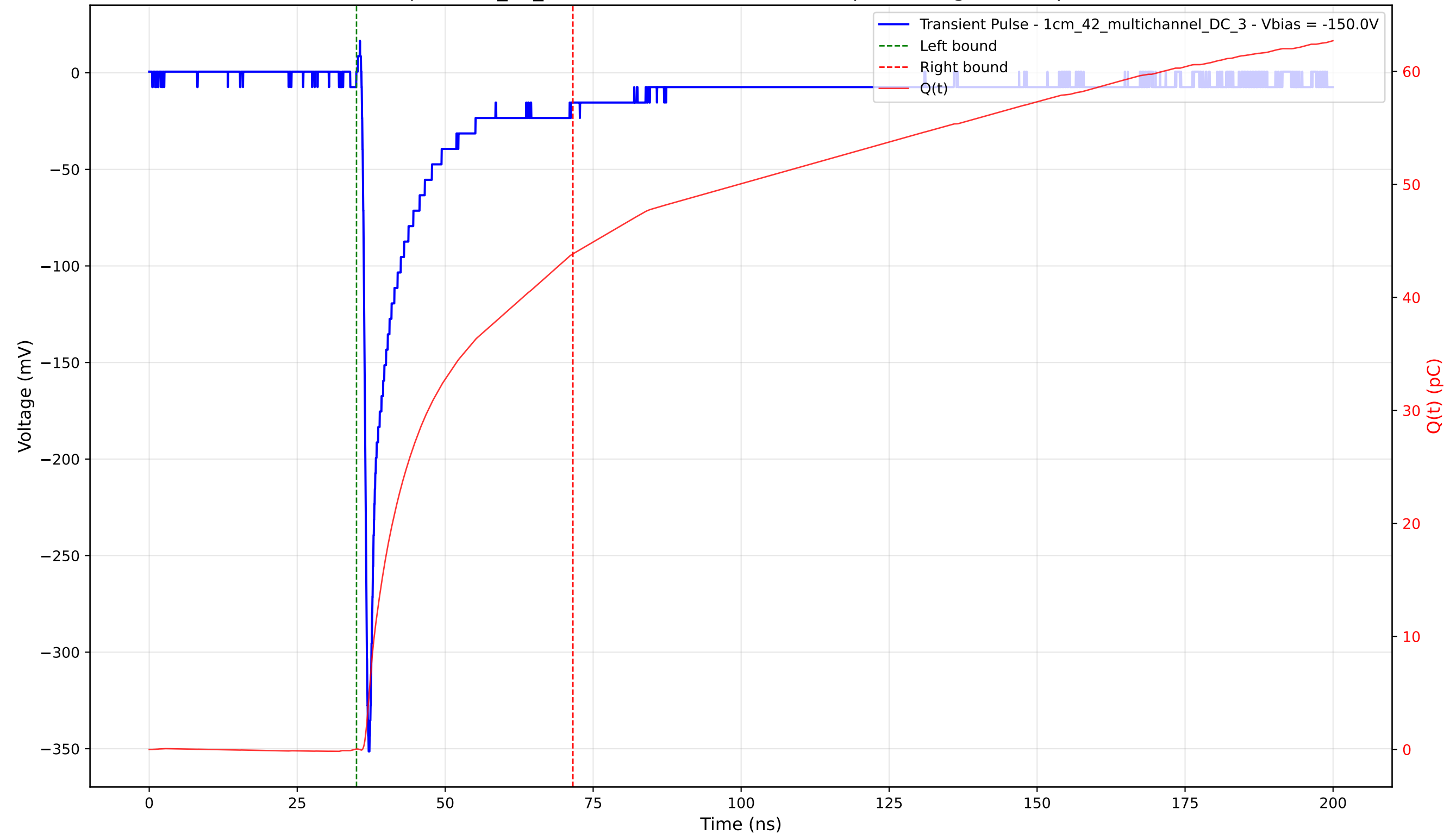
Transient Pulse - Sample: 1cm_42_multichannel - Position: 210.0 \mu\text{m} - Charge: 43.81 pC - Rise Time: 0.82 ns
