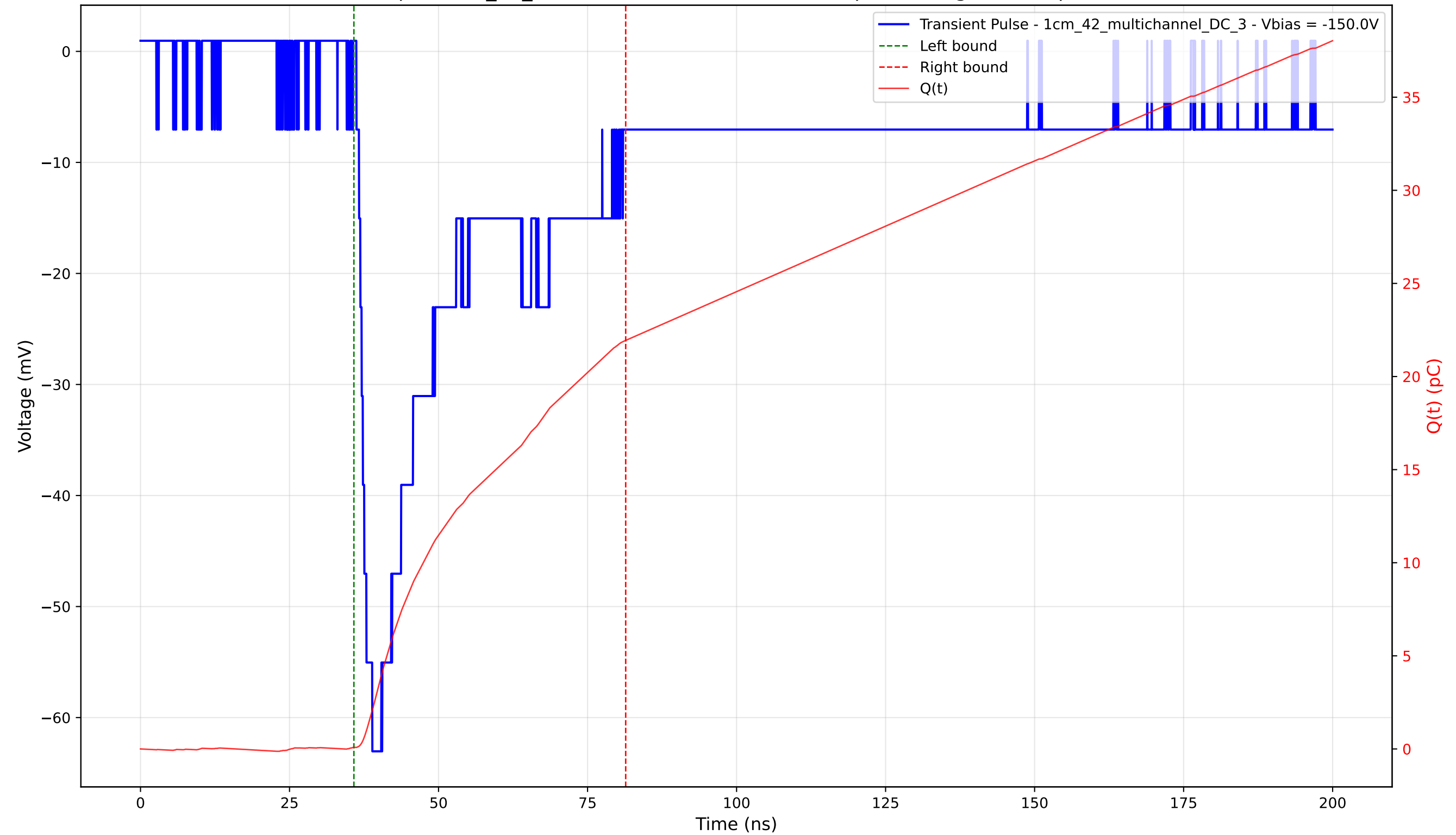
Transient Pulse - Sample: 1cm_42_multichannel - Position: 1815.0 \mu\text{m} - Charge: 21.86 pC - Rise Time: 2.66 ns
