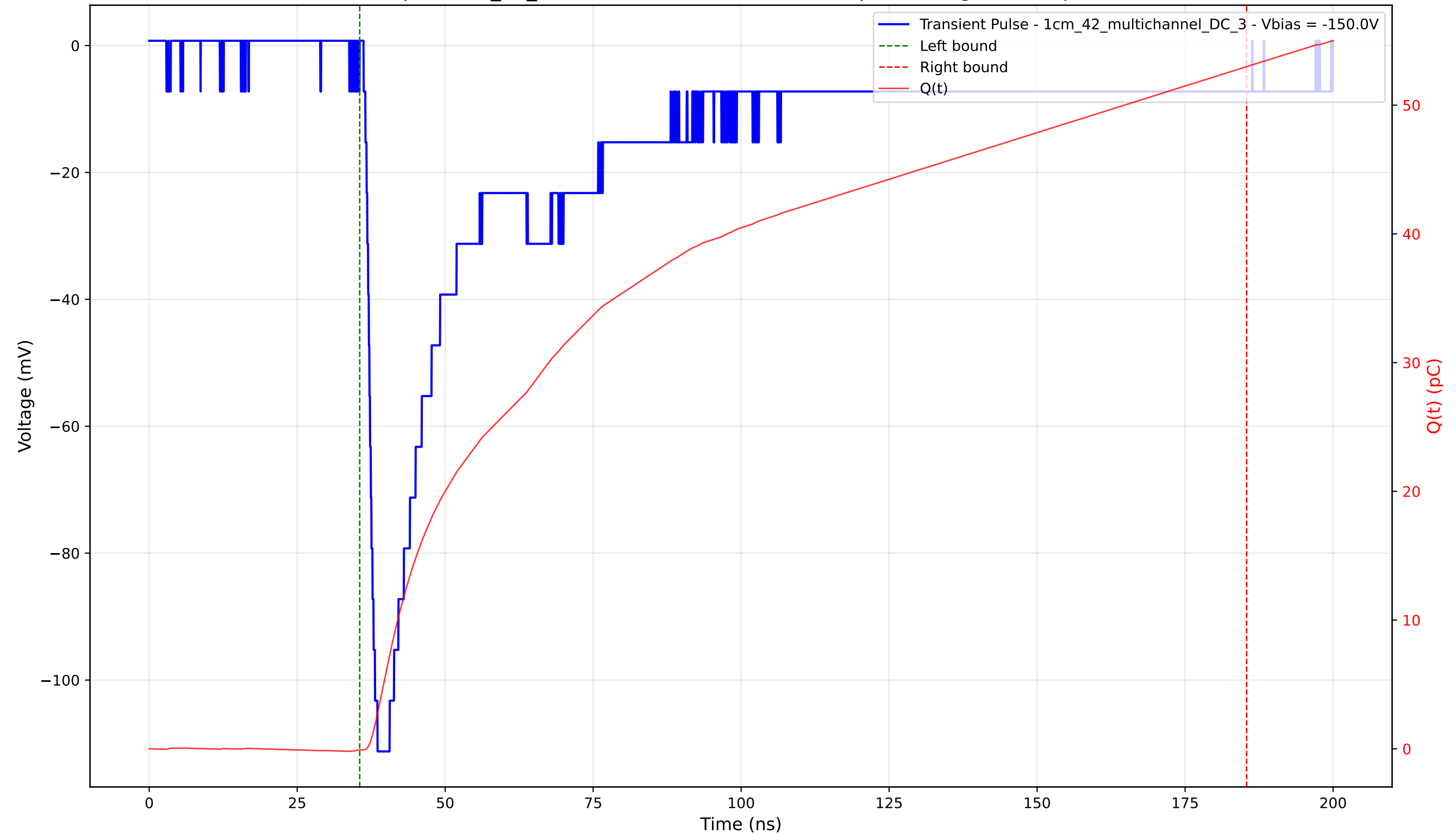
Transient Pulse - Sample: 1cm_42_multichannel - Position: 3240.0 \mu\text{m} - Charge: 53.10 pC - Rise Time: 1.63 ns
