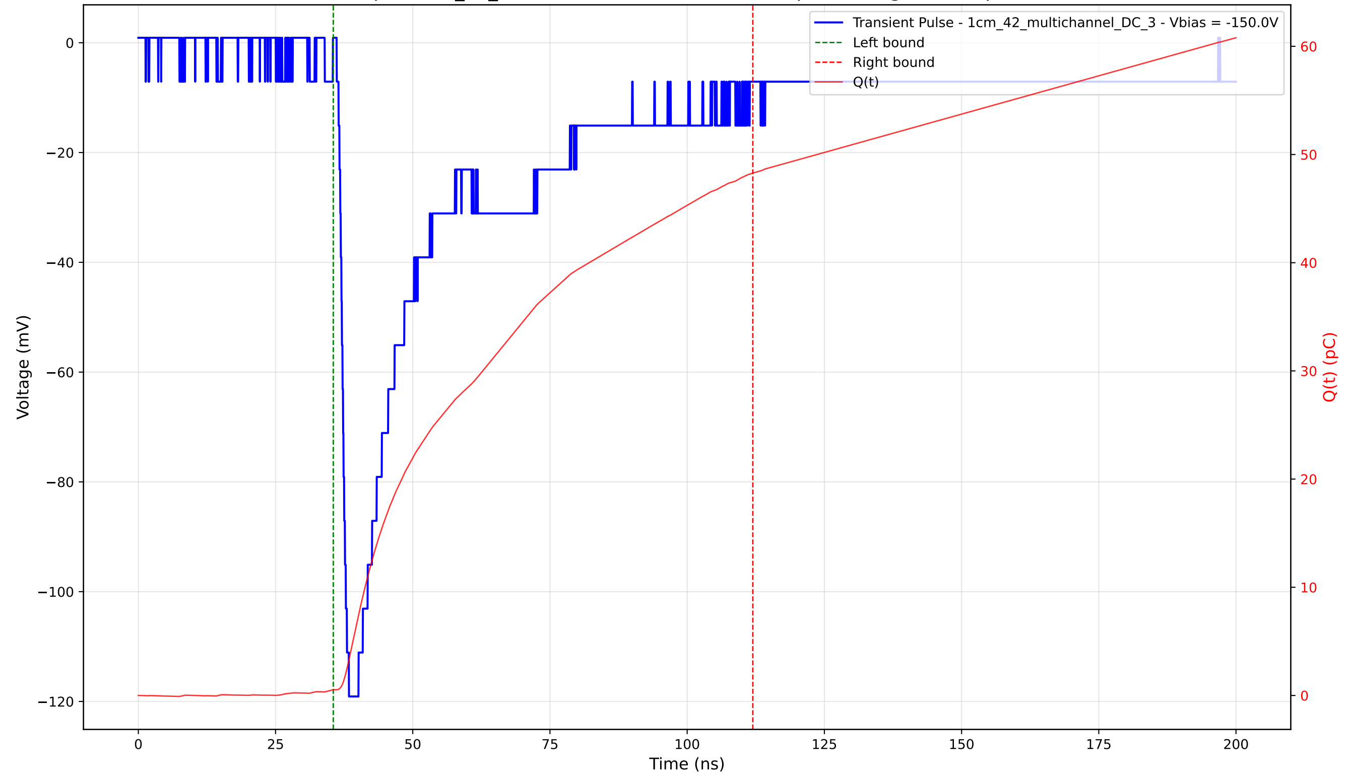
Transient Pulse - Sample: 1cm_42_multichannel - Position: 1655.0 \mu\text{m} - Charge: 47.75 pC - Rise Time: 1.53 ns
