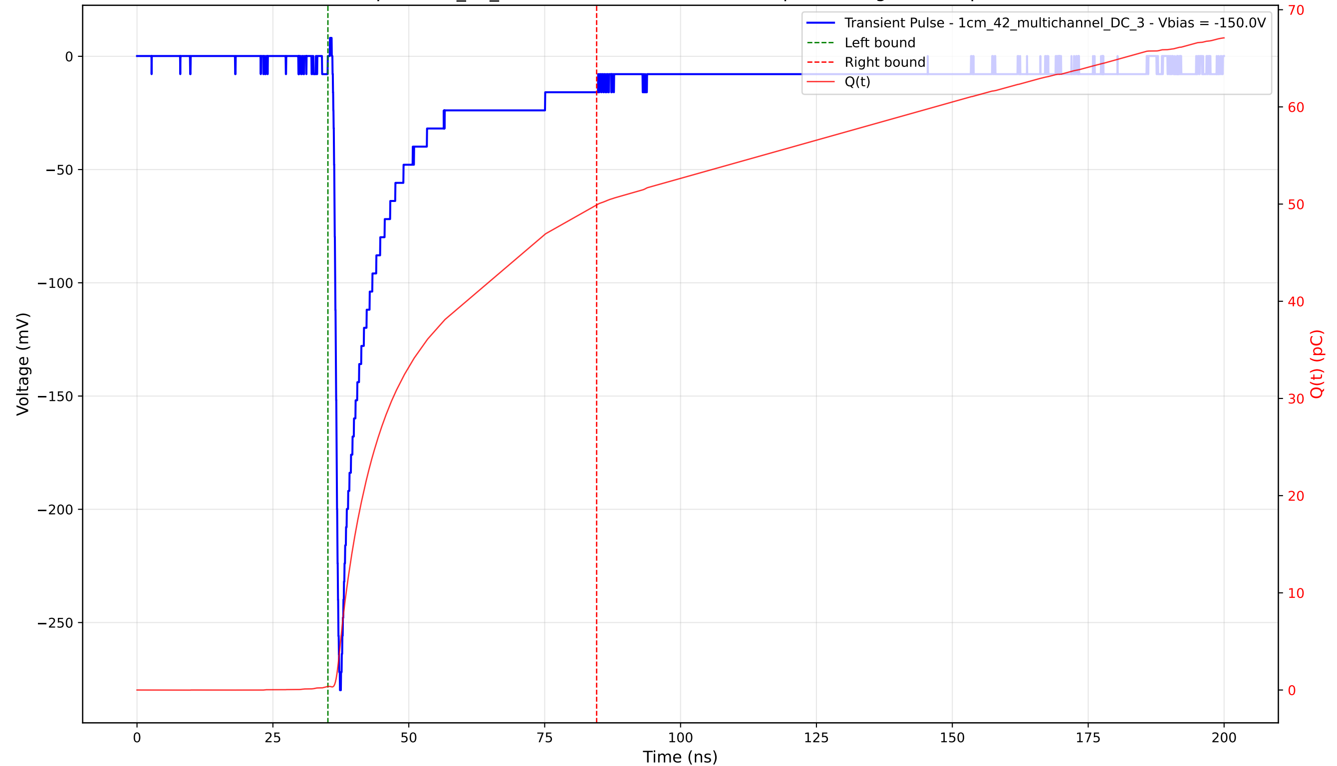
Transient Pulse - Sample: 1cm_42_multichannel - Position: 490.0 \mu\text{m} - Charge: 49.55 pC - Rise Time: 0.91 ns
