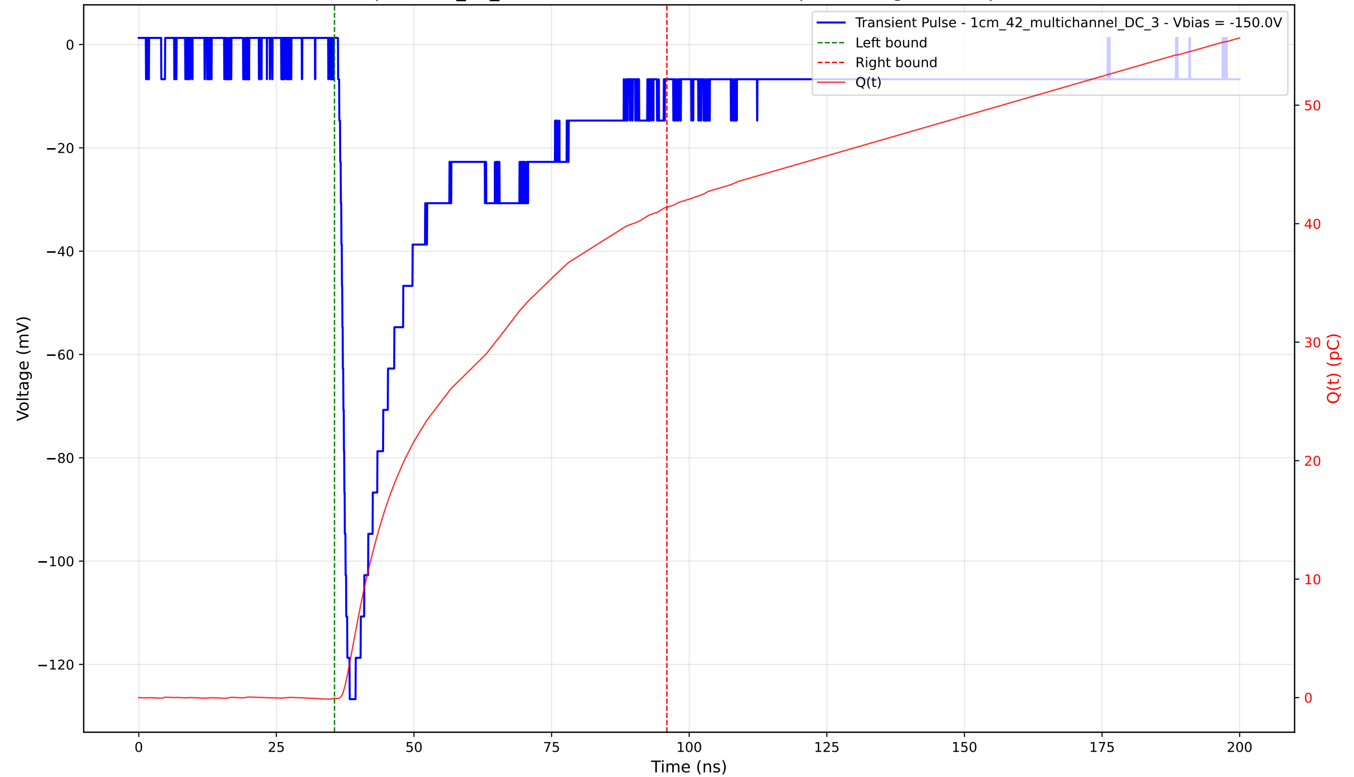
Transient Pulse - Sample: 1cm_42_multichannel - Position: 1440.0 \mu\text{m} - Charge: 41.46 pC - Rise Time: 1.47 ns
