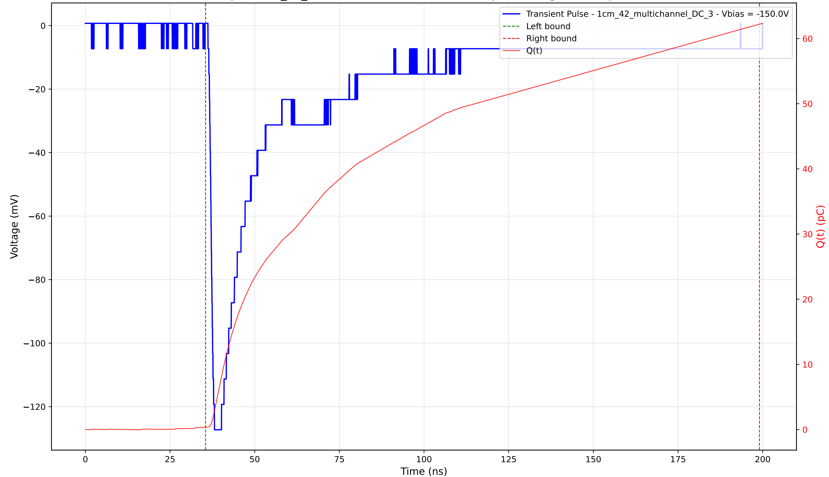
Transient Pulse - Sample: 1cm_42_multichannel - Position: 1515.0 \mu\text{m} - Charge: 61.83 pC - Rise Time: 1.41 ns
