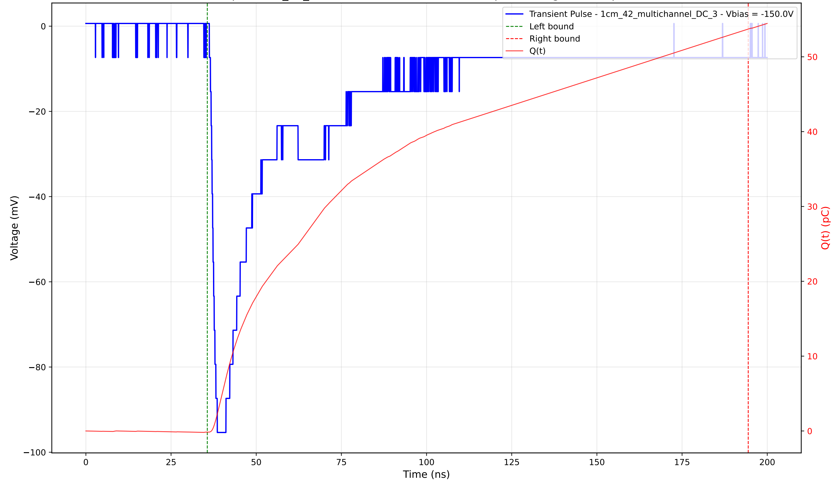
Transient Pulse - Sample: 1cm_42_multichannel - Position: 2970.0 \mu\text{m} - Charge: 53.87 pC - Rise Time: 1.61 ns
