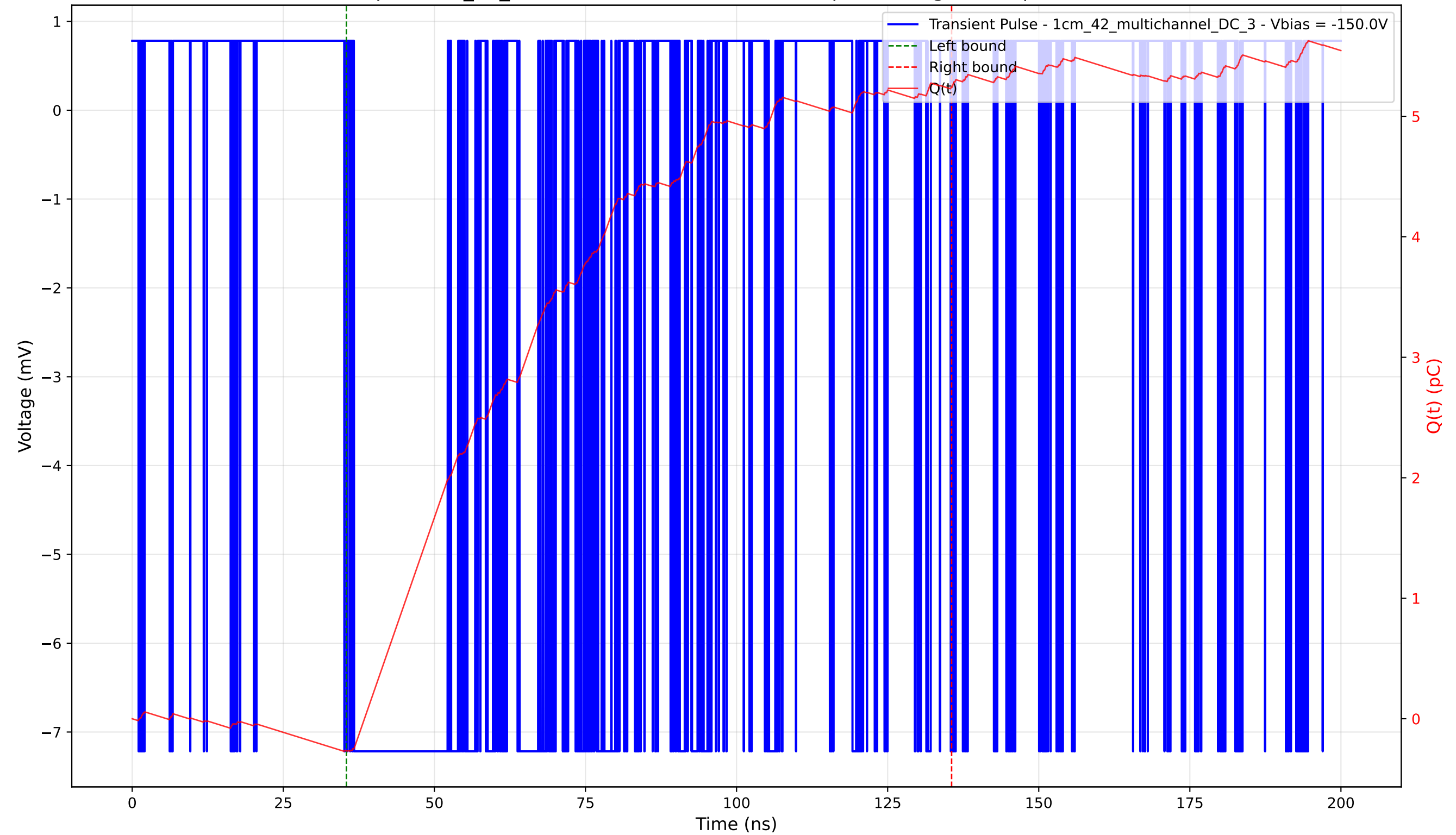
Transient Pulse - Sample: 1cm_42_multichannel - Position: 2870.0 \mu\text{m} - Charge: 5.51 pC - Rise Time: 0.00 ns (N/A)
