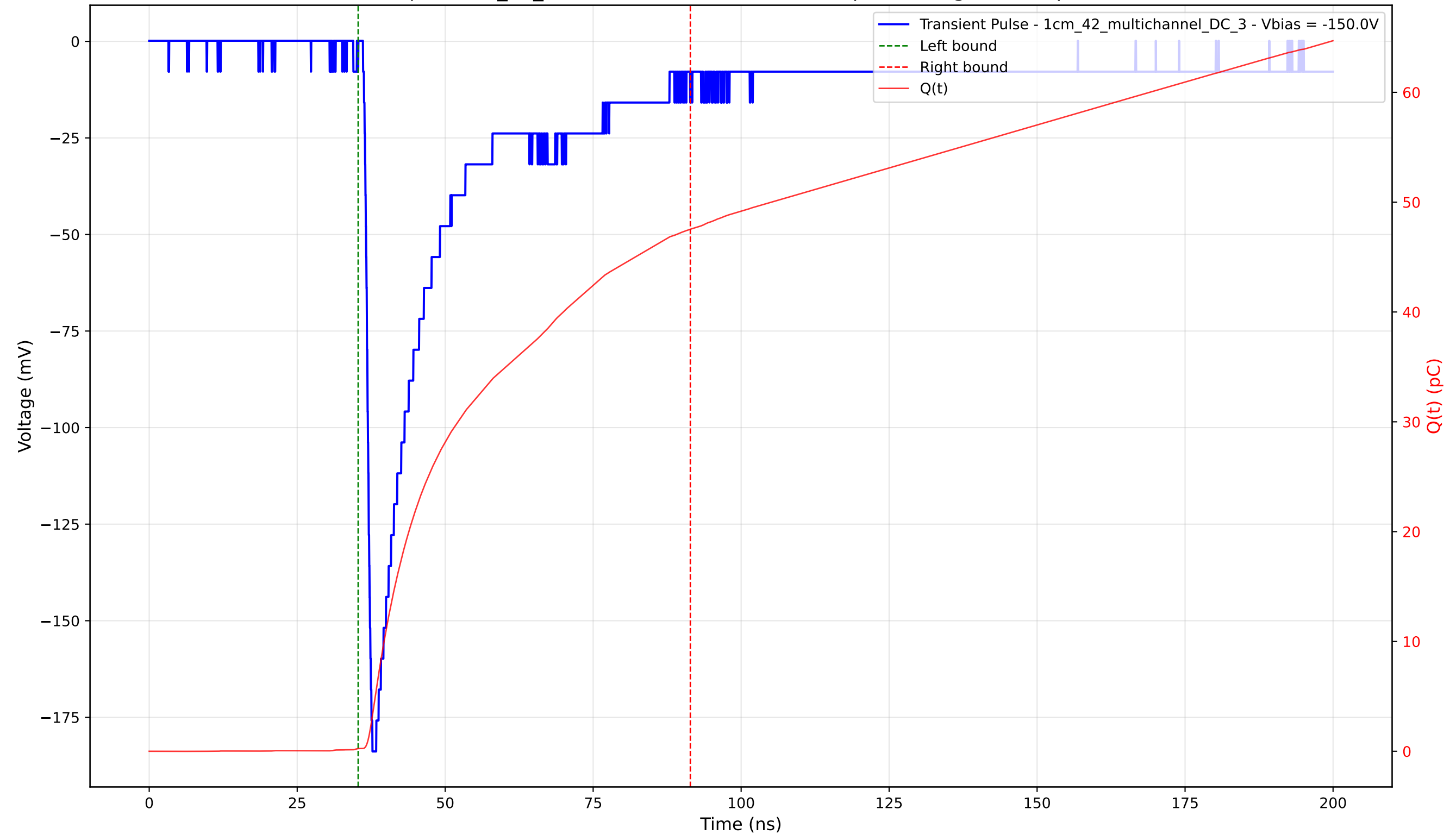
Transient Pulse - Sample: 1cm_42_multichannel - Position: 965.0 \mu\text{m} - Charge: 47.28 pC - Rise Time: 1.07 ns
