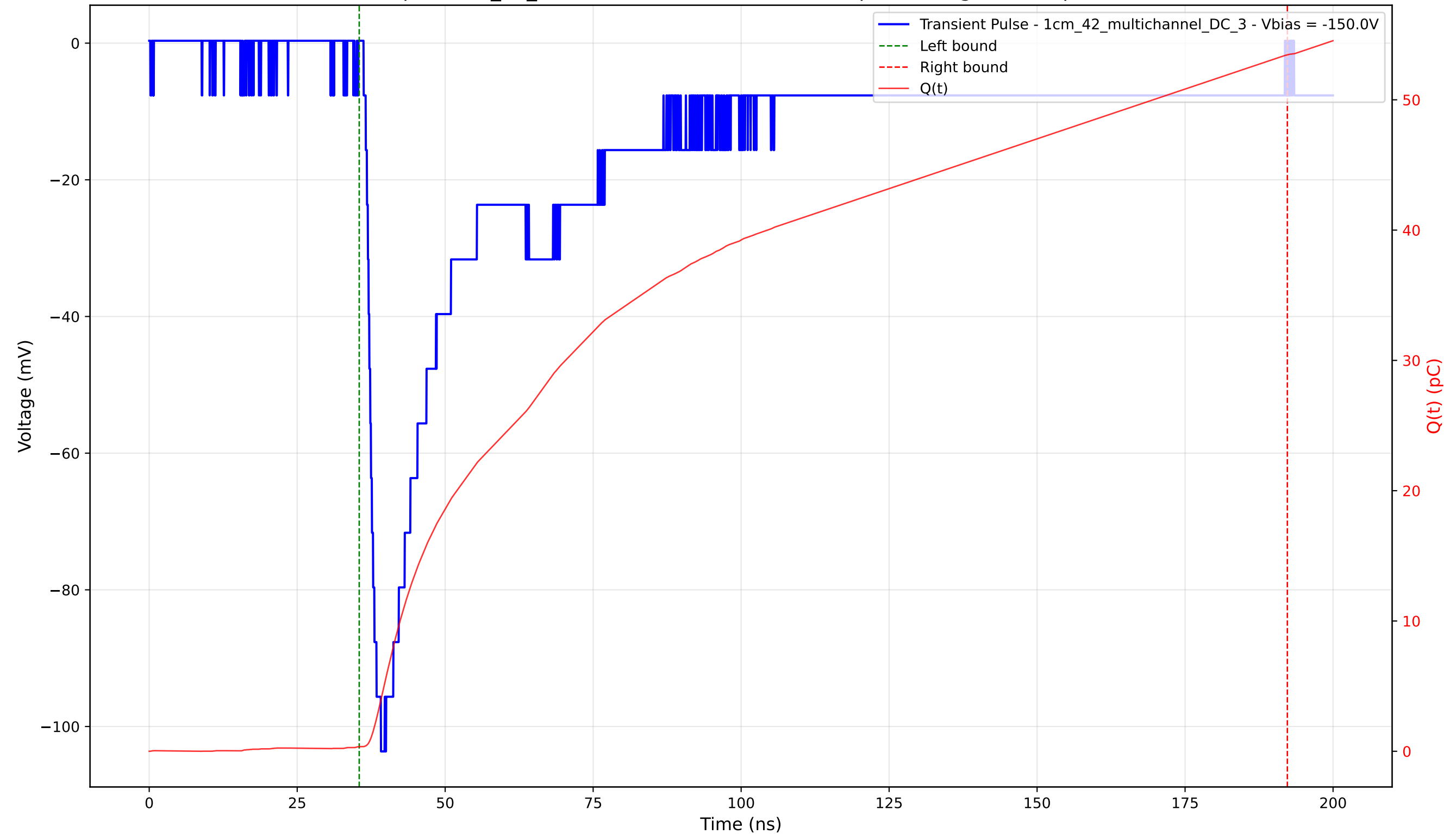
Transient Pulse - Sample: 1cm_42_multichannel - Position: 3085.0 \mu\text{m} - Charge: 53.10 pC - Rise Time: 1.83 ns
