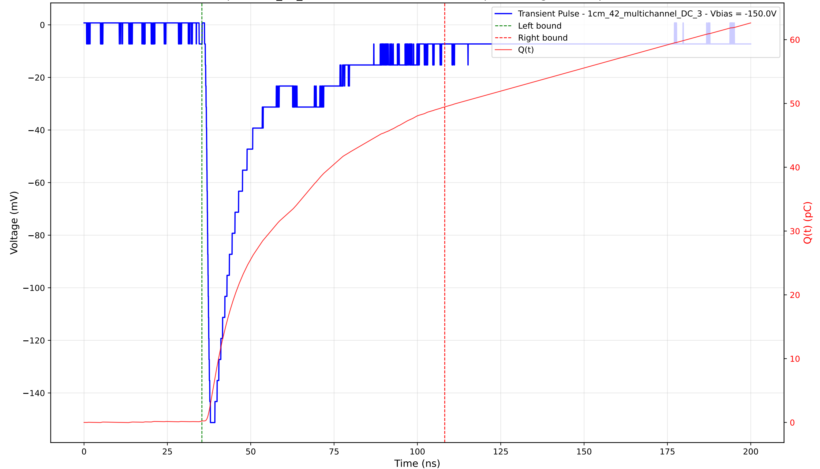
Transient Pulse - Sample: 1cm_42_multichannel - Position: 1245.0 \mu\text{m} - Charge: 49.23 pC - Rise Time: 1.34 ns
