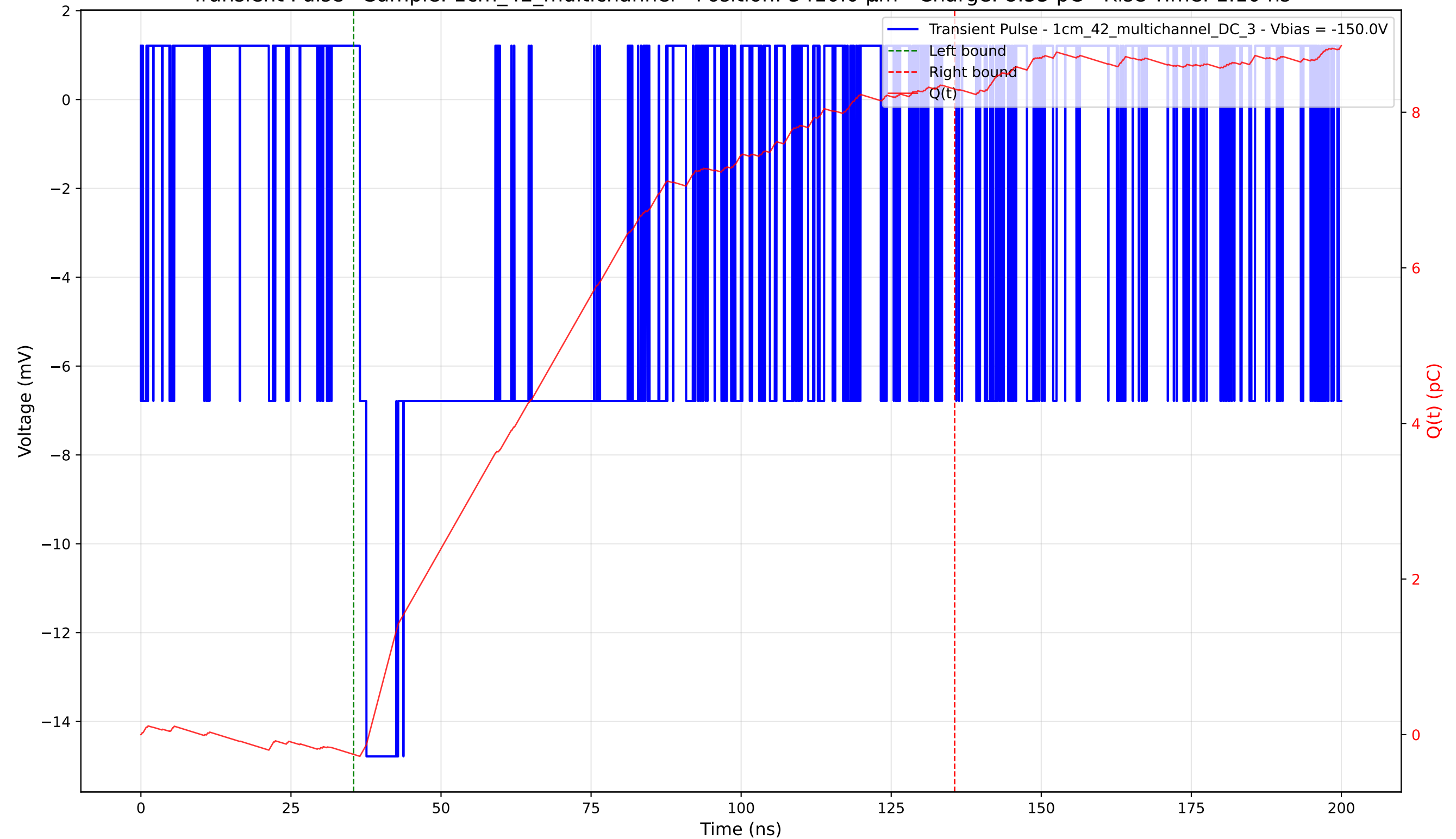
Transient Pulse - Sample: 1cm_42_multichannel - Position: 3410.0 \mu\text{m} - Charge: 8.55 pC - Rise Time: 1.10 ns
