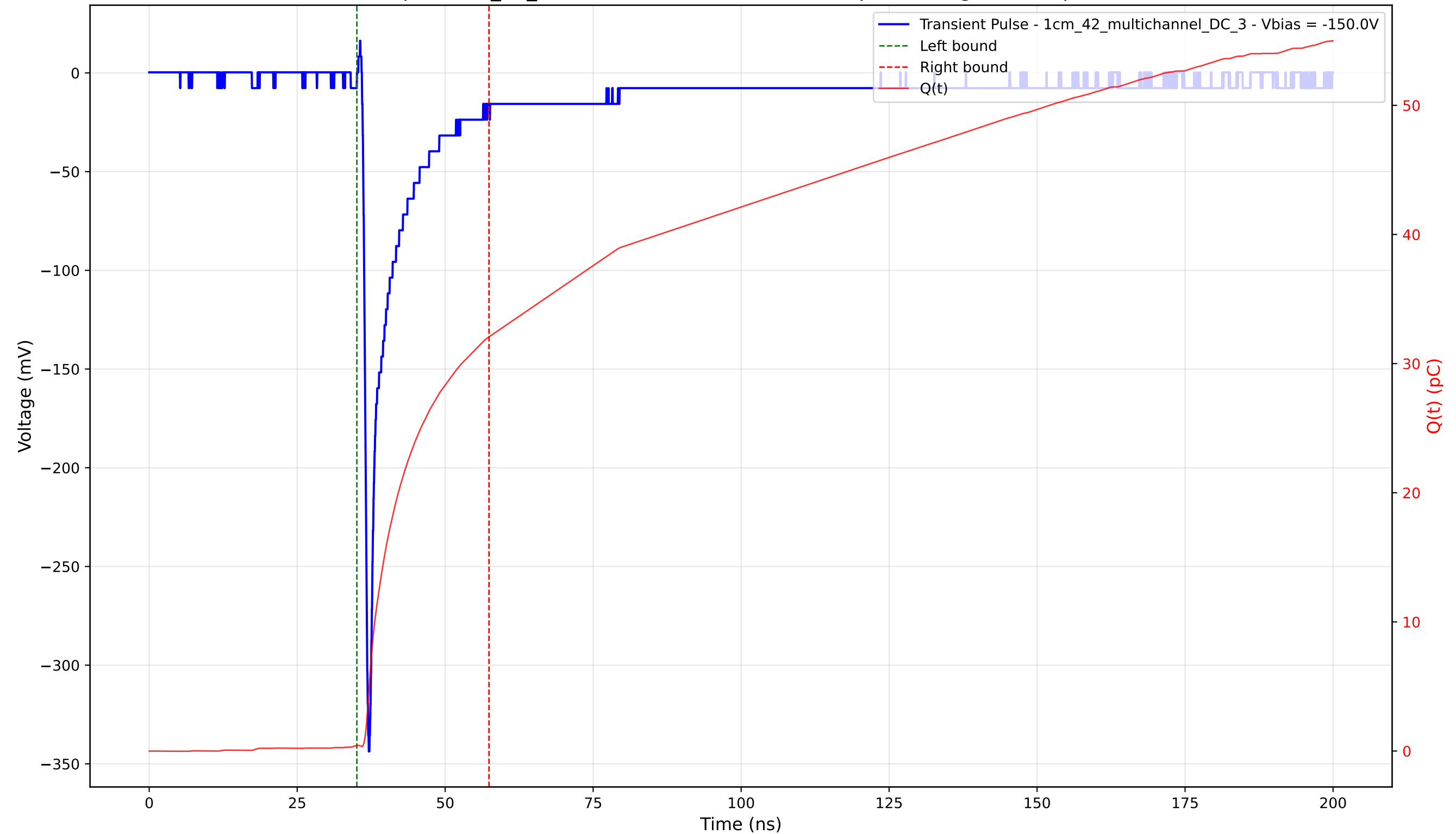
Transient Pulse - Sample: 1cm_42_multichannel - Position: 4815.0 \mu\text{m} - Charge: 31.62 pC - Rise Time: 0.77 ns
