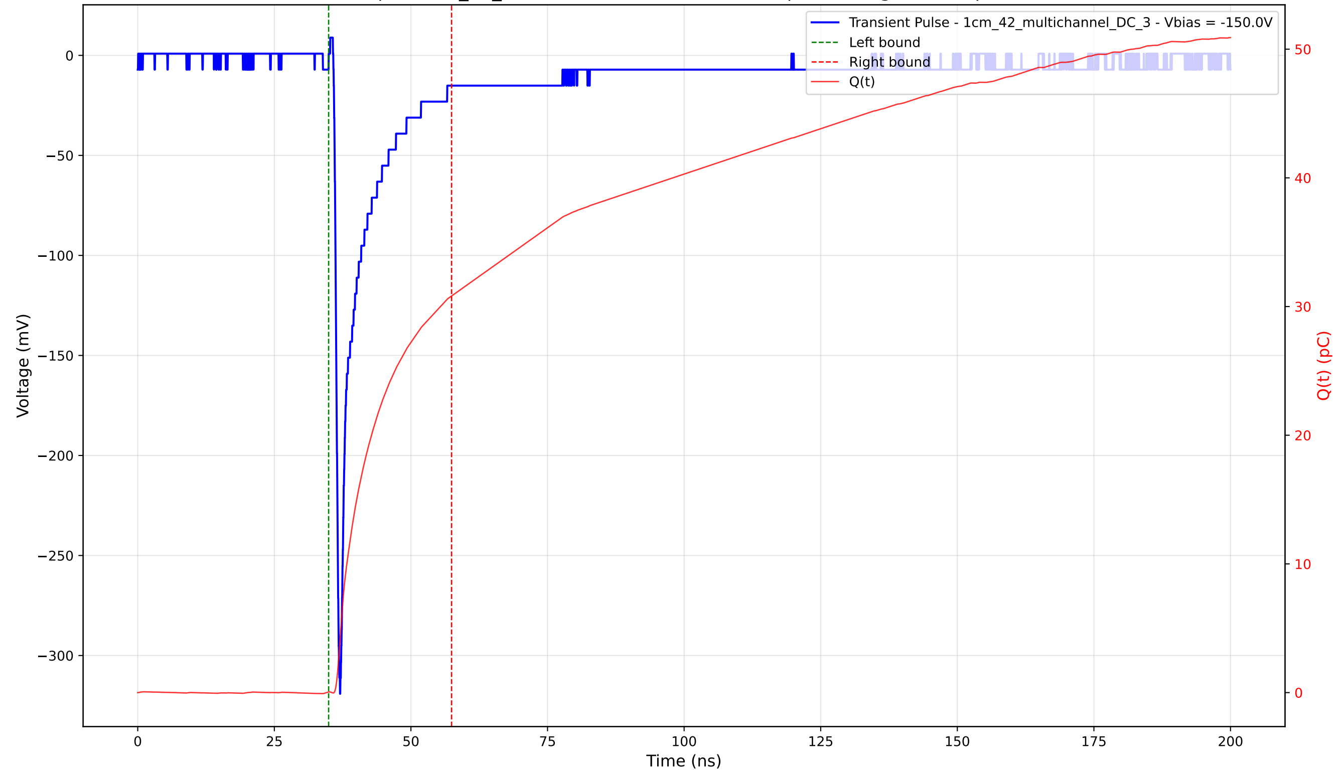
Transient Pulse - Sample: 1cm_42_multichannel - Position: 100.0 \mu\text{m} - Charge: 30.76 pC - Rise Time: 0.80 ns
