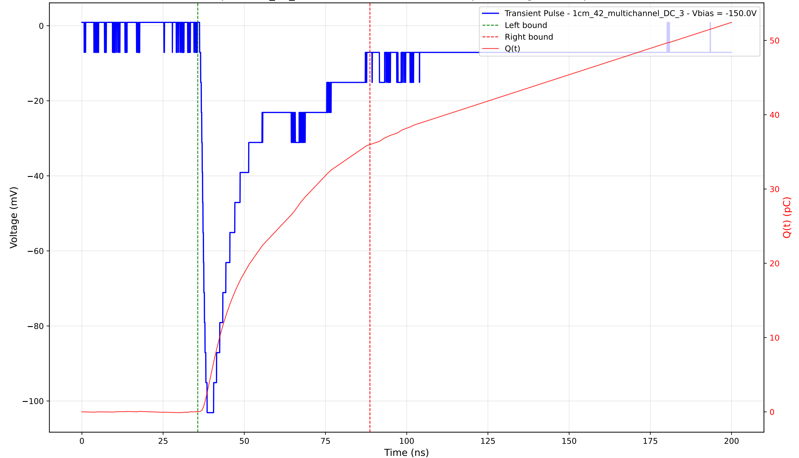
Transient Pulse - Sample: 1cm_42_multichannel - Position: 3170.0 \mu\text{m} - Charge: 35.93 pC - Rise Time: 1.61 ns
