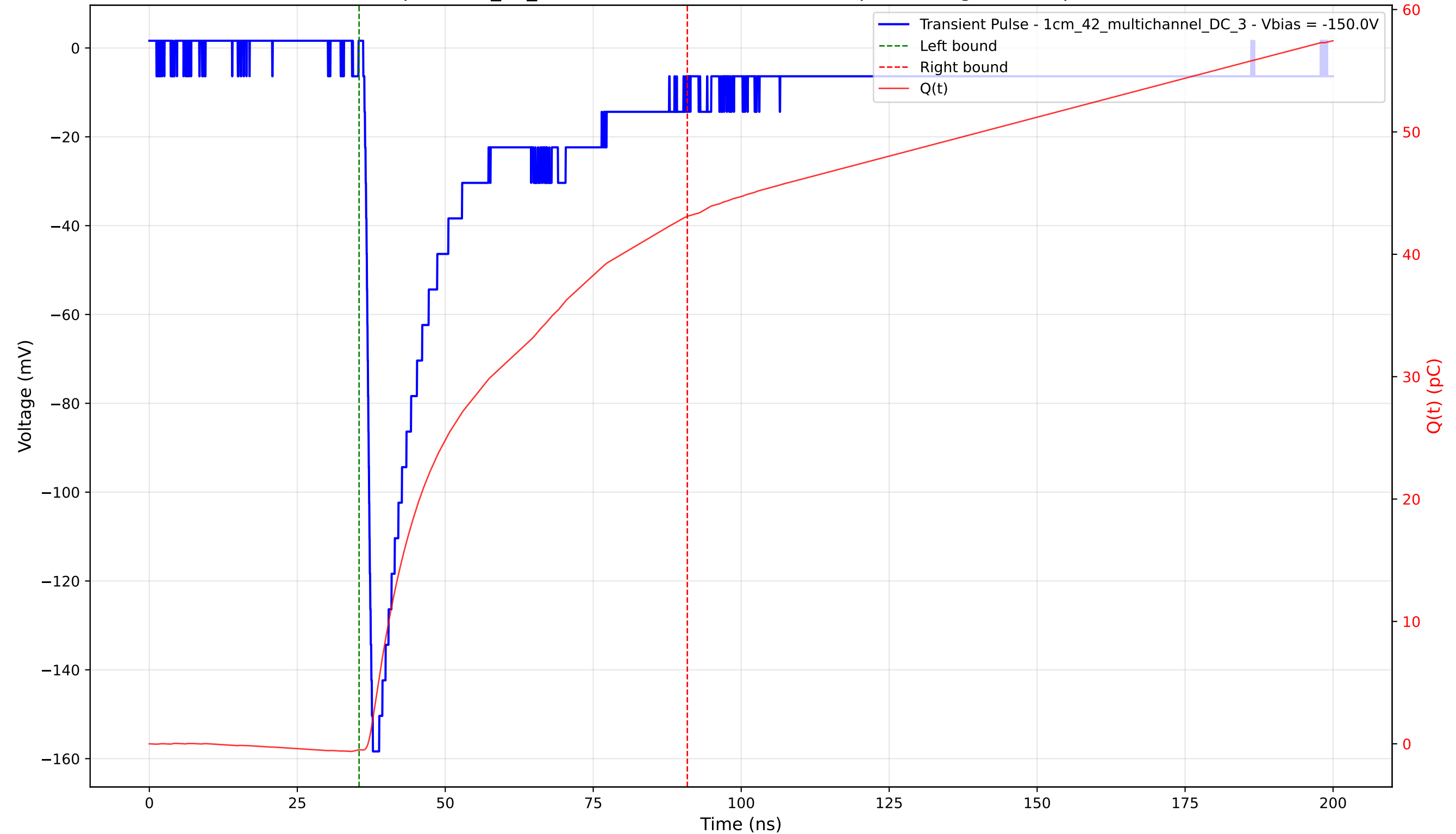
Transient Pulse - Sample: 1cm_42_multichannel - Position: 1095.0 \mu\text{m} - Charge: 43.59 pC - Rise Time: 1.18 ns
