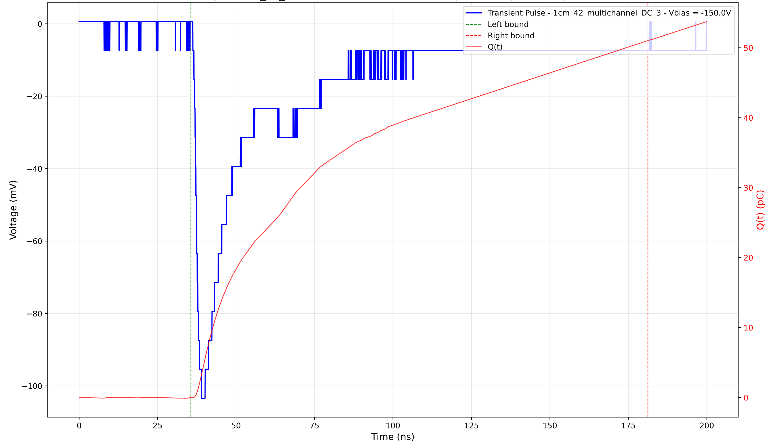
Transient Pulse - Sample: 1cm_42_multichannel - Position: 3065.0 \mu\text{m} - Charge: 51.06 pC - Rise Time: 1.79 ns
