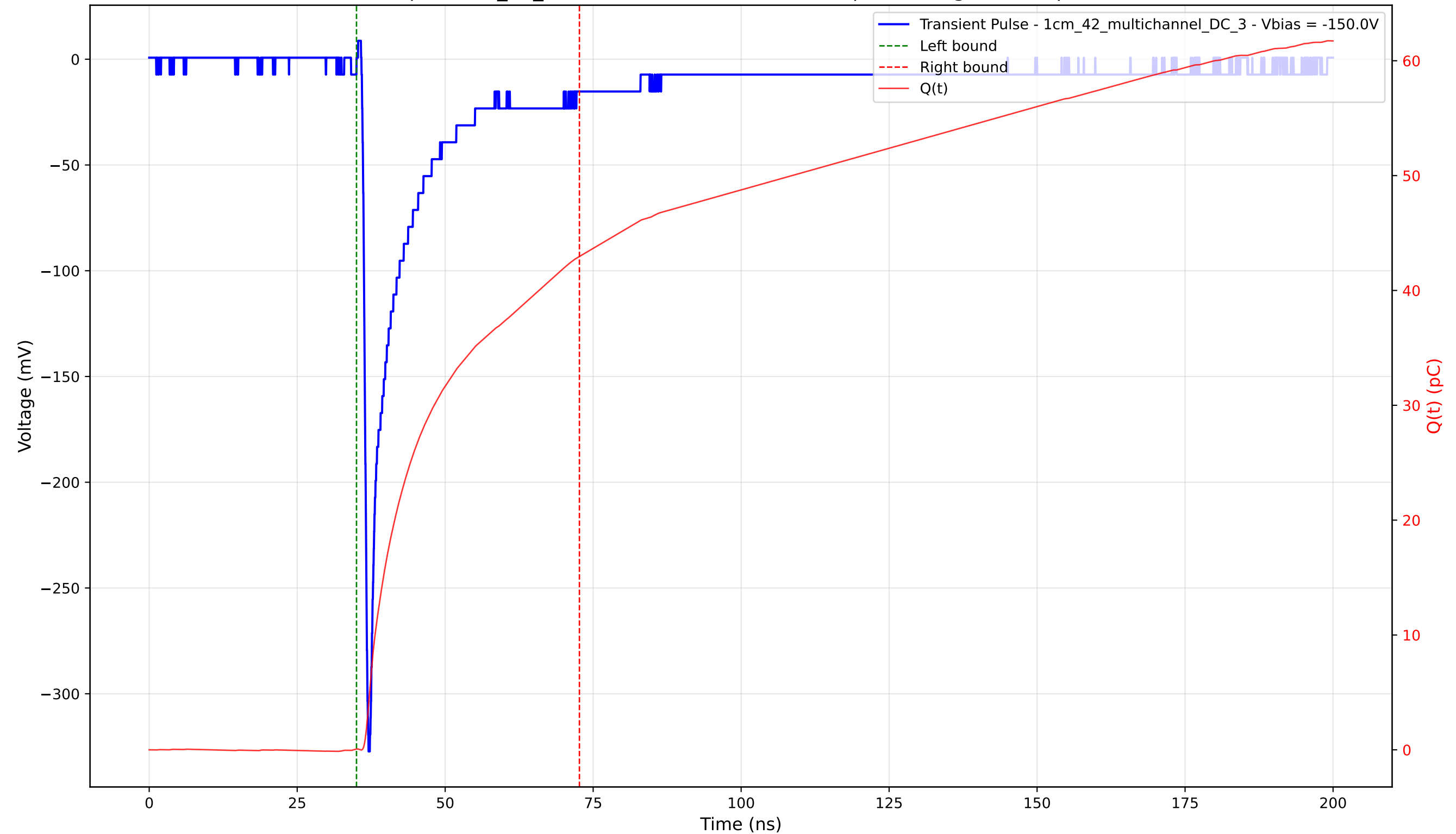
Transient Pulse - Sample: 1cm_42_multichannel - Position: 240.0 \mu\text{m} - Charge: 42.89 pC - Rise Time: 0.80 ns
