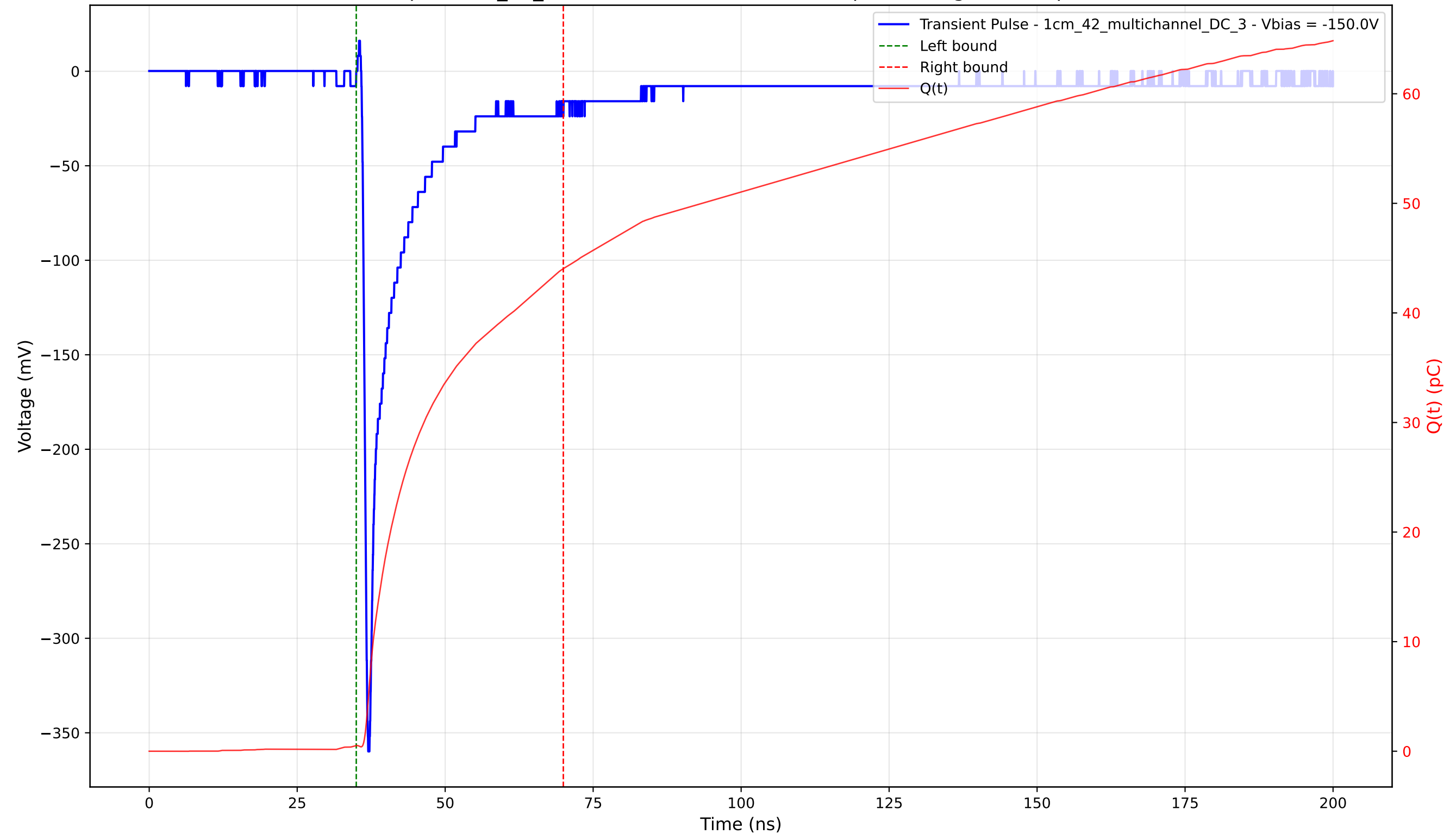
Transient Pulse - Sample: 1cm_42_multichannel - Position: 175.0 \mu\text{m} - Charge: 43.51 pC - Rise Time: 0.79 ns
