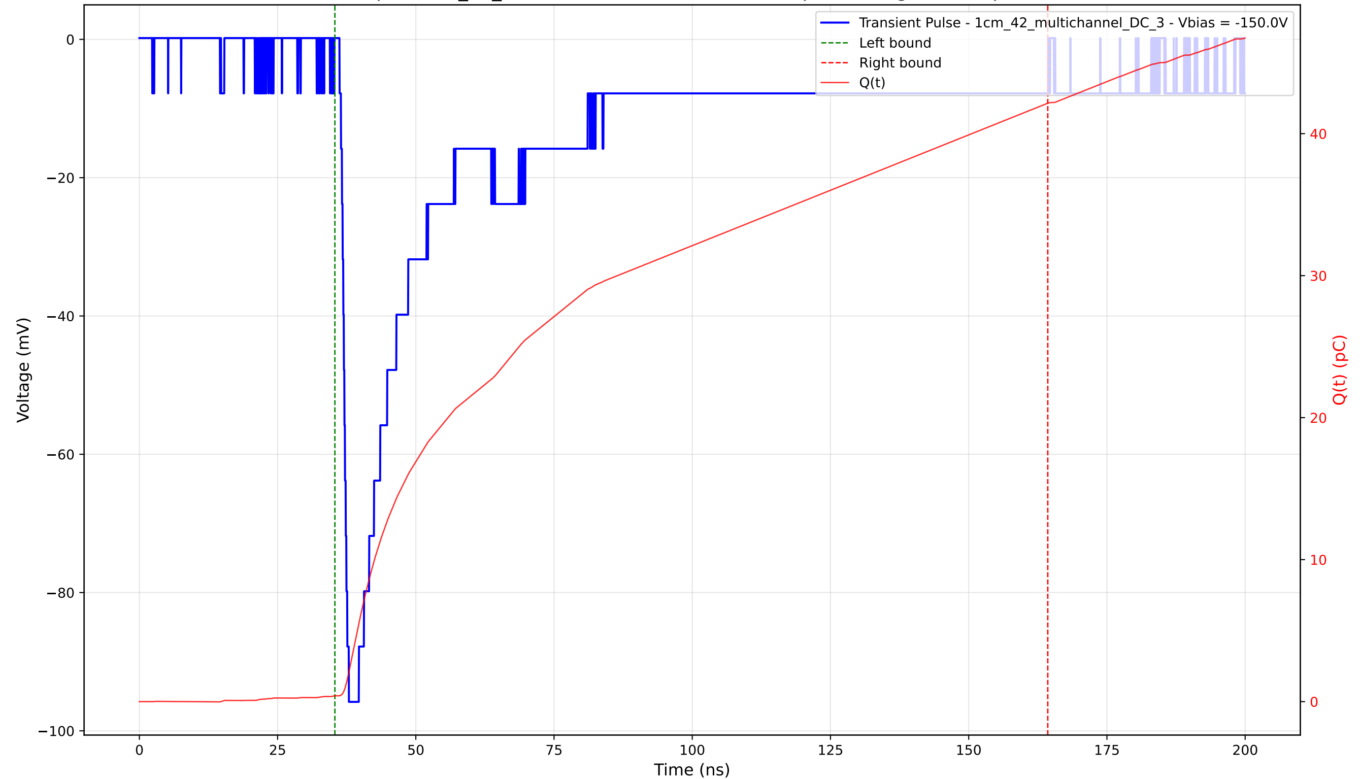
Transient Pulse - Sample: 1cm_42_multichannel - Position: 1305.0 \mu\text{m} - Charge: 41.75 pC - Rise Time: 1.16 ns
