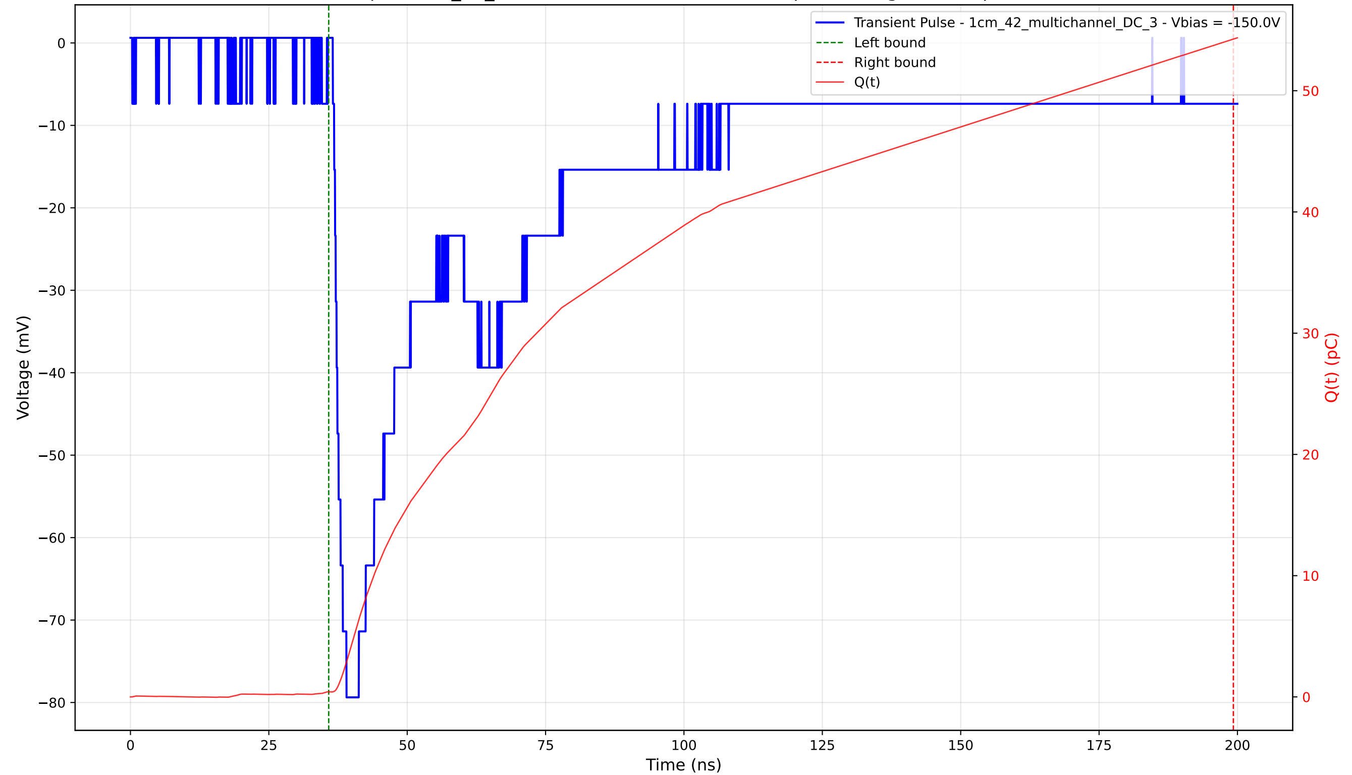
Transient Pulse - Sample: 1cm_42_multichannel - Position: 2535.0 \mu\text{m} - Charge: 53.83 pC - Rise Time: 2.24 ns
