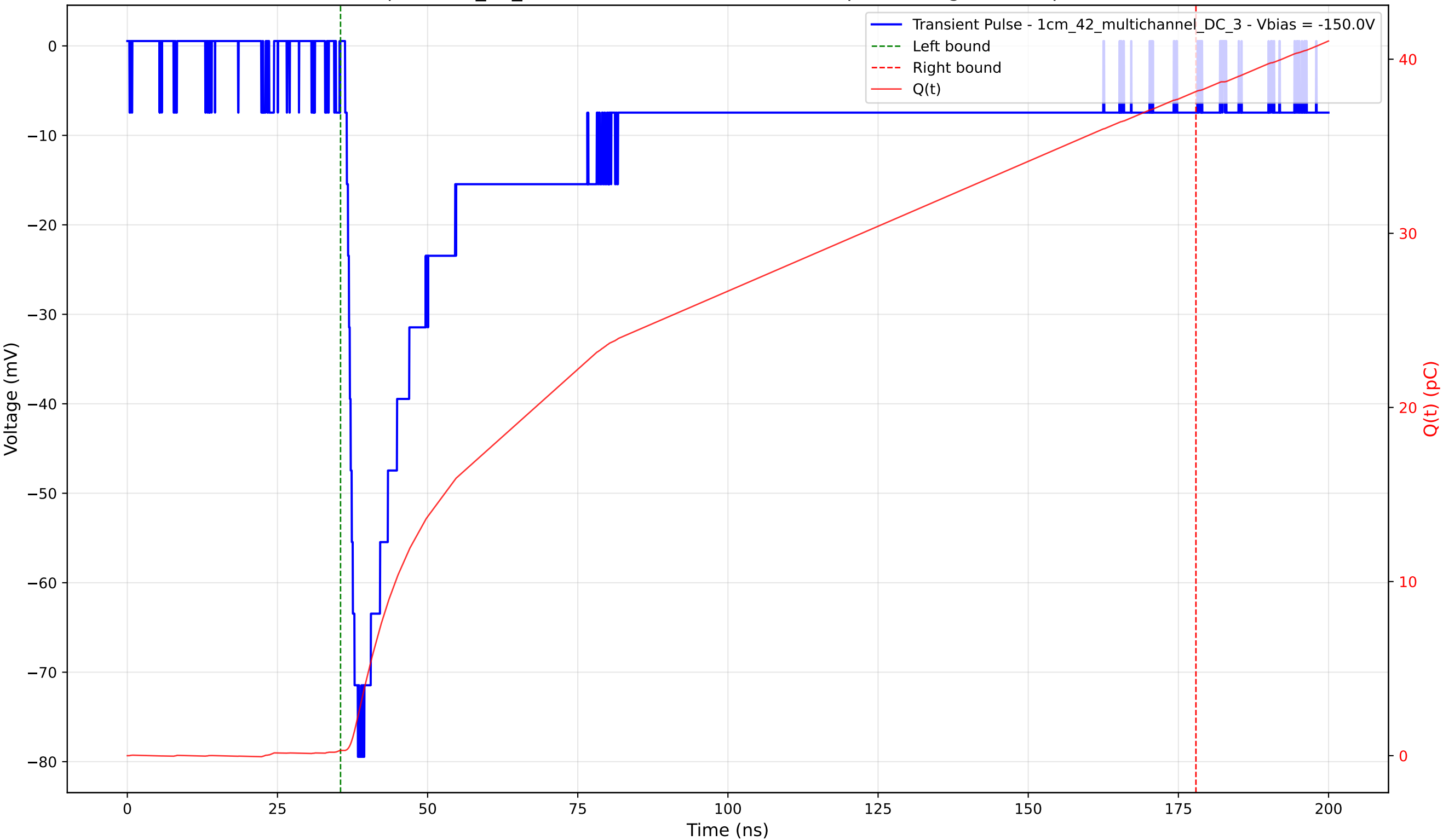
Transient Pulse - Sample: 1cm_42_multichannel - Position: 1415.0 \mu\text{m} - Charge: 37.85 pC - Rise Time: 1.86 ns
