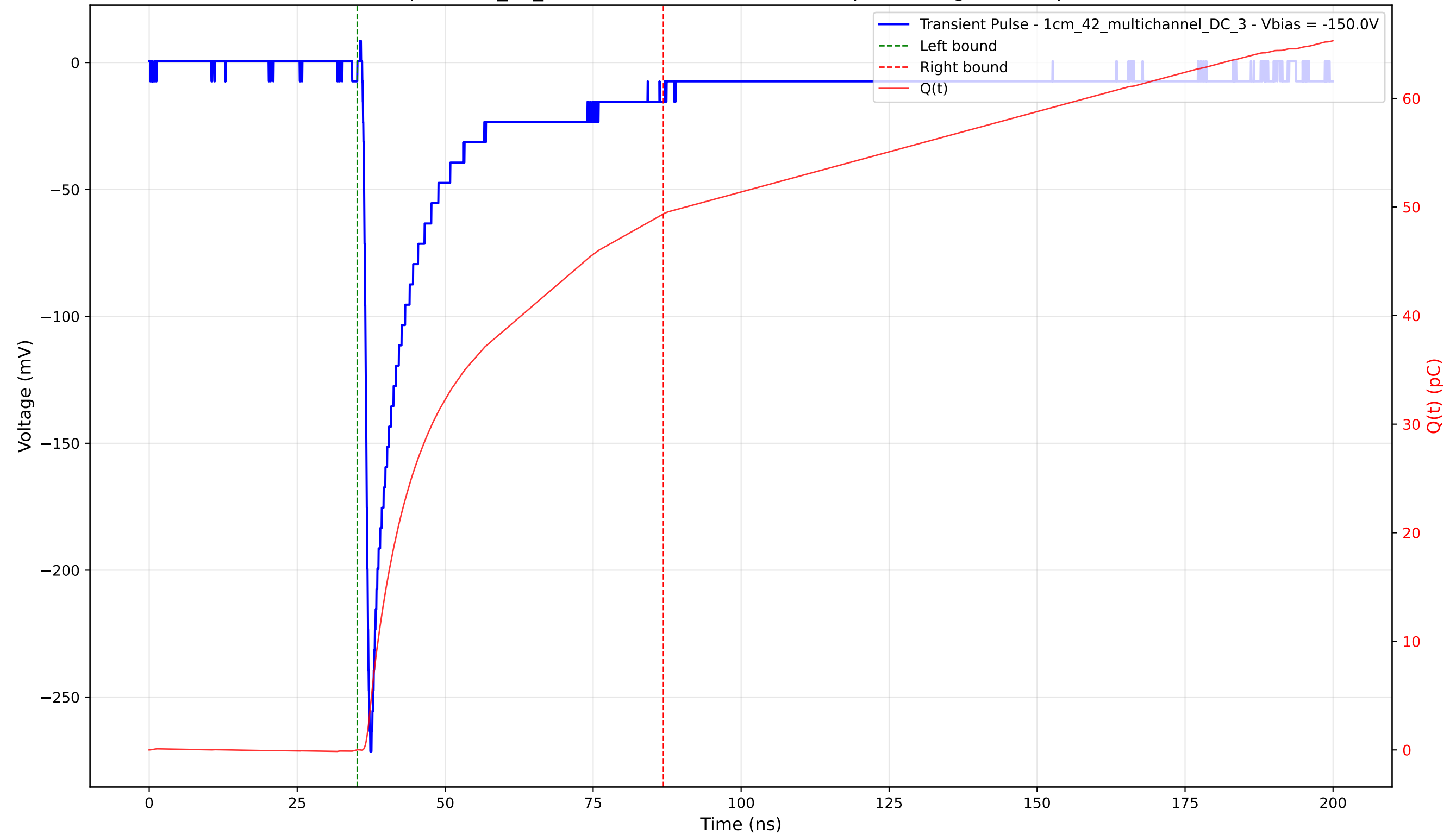
Transient Pulse - Sample: 1cm_42_multichannel - Position: 515.0 \mu\text{m} - Charge: 49.31 pC - Rise Time: 0.91 ns
