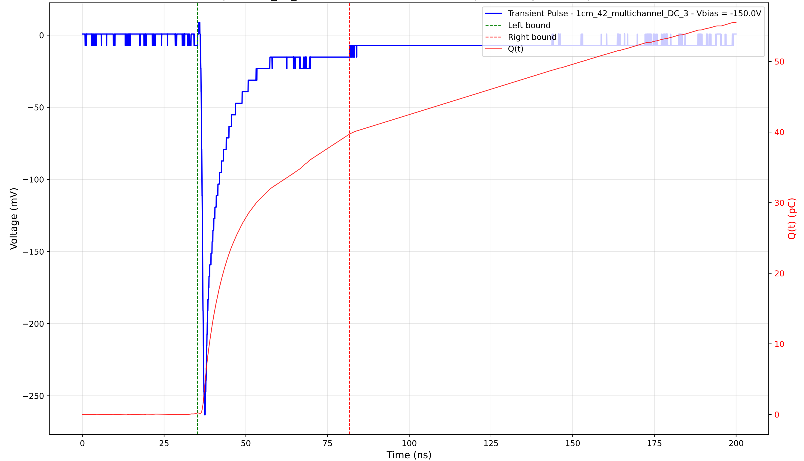
Transient Pulse - Sample: 1cm_42_multichannel - Position: 4505.0 \mu\text{m} - Charge: 39.49 pC - Rise Time: 0.87 ns
