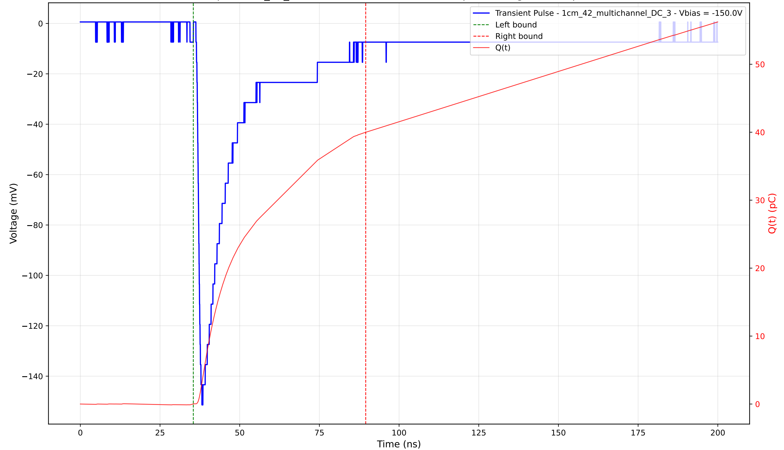
Transient Pulse - Sample: 1cm_42_multichannel - Position: 3780.0 \mu\text{m} - Charge: 39.96 pC - Rise Time: 1.40 ns
