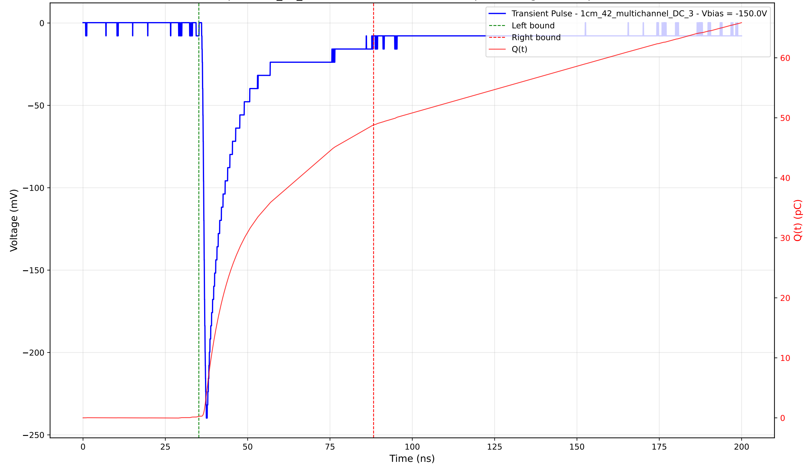
Transient Pulse - Sample: 1cm_42_multichannel - Position: 630.0 \mu\text{m} - Charge: 48.54 pC - Rise Time: 0.98 ns
