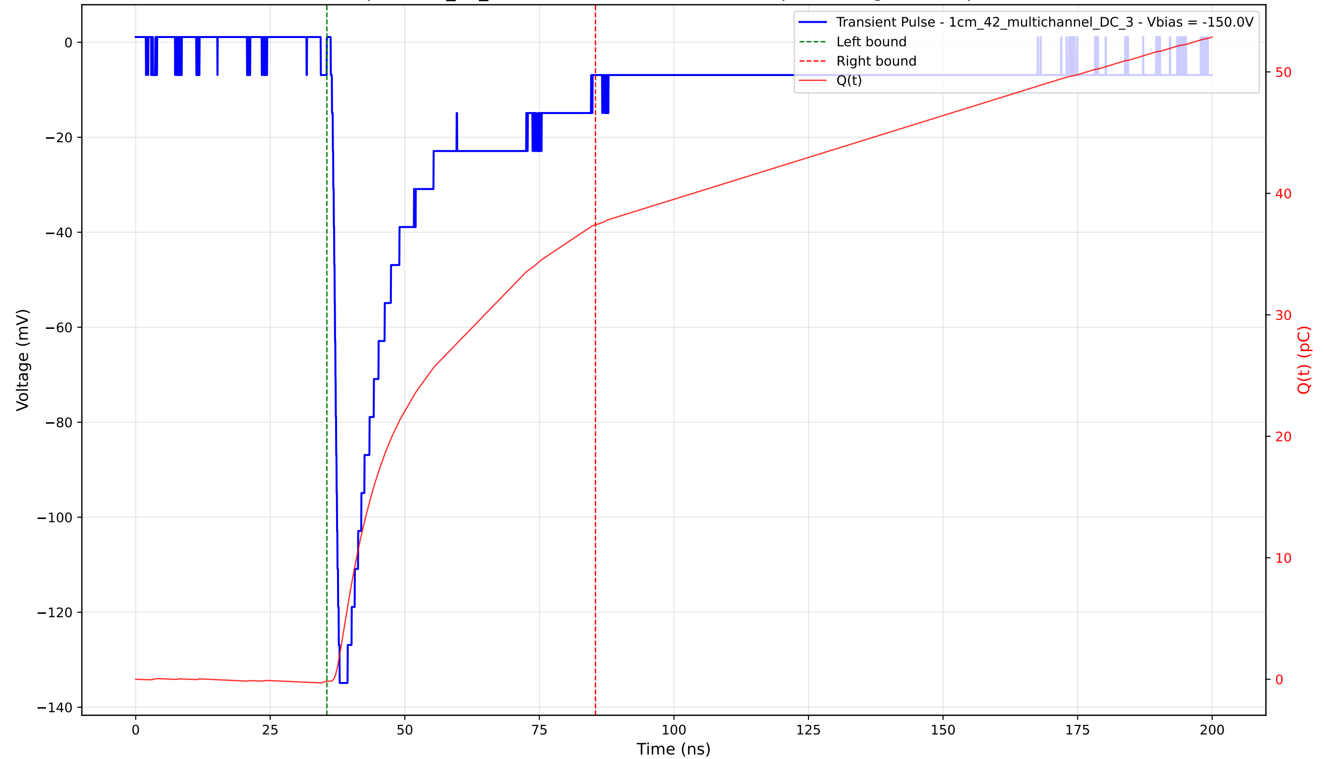
Transient Pulse - Sample: 1cm_42_multichannel - Position: 3725.0 \mu\text{m} - Charge: 37.56 pC - Rise Time: 1.26 ns
