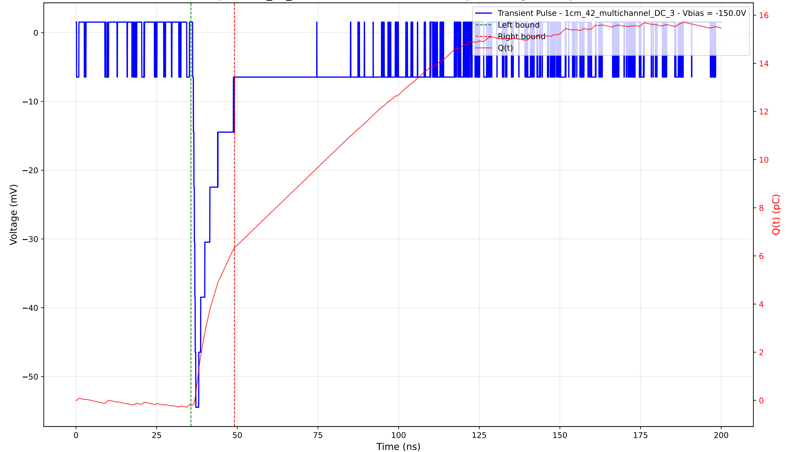
Transient Pulse - Sample: 1cm_42_multichannel - Position: 4430.0 \mu\text{m} - Charge: 6.53 pC - Rise Time: 0.98 ns
