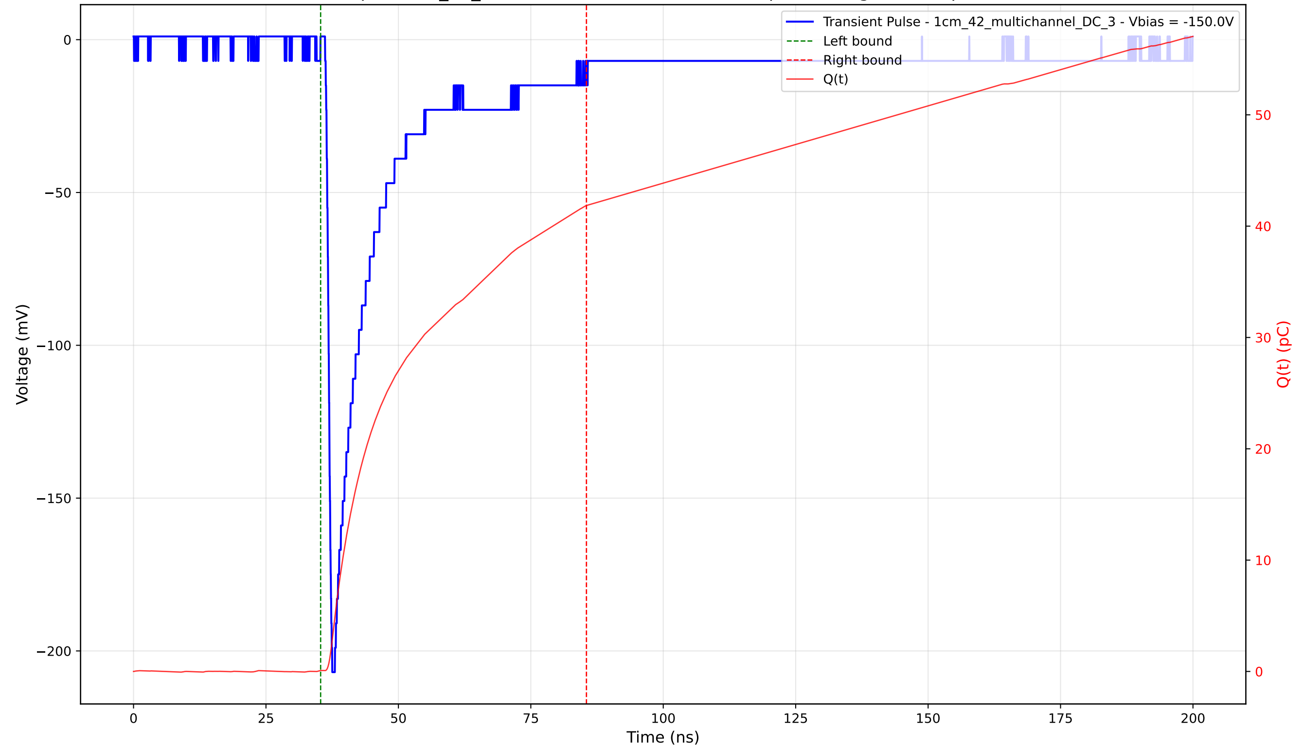
Transient Pulse - Sample: 1cm_42_multichannel - Position: 4220.0 \mu\text{m} - Charge: 41.76 pC - Rise Time: 0.97 ns
