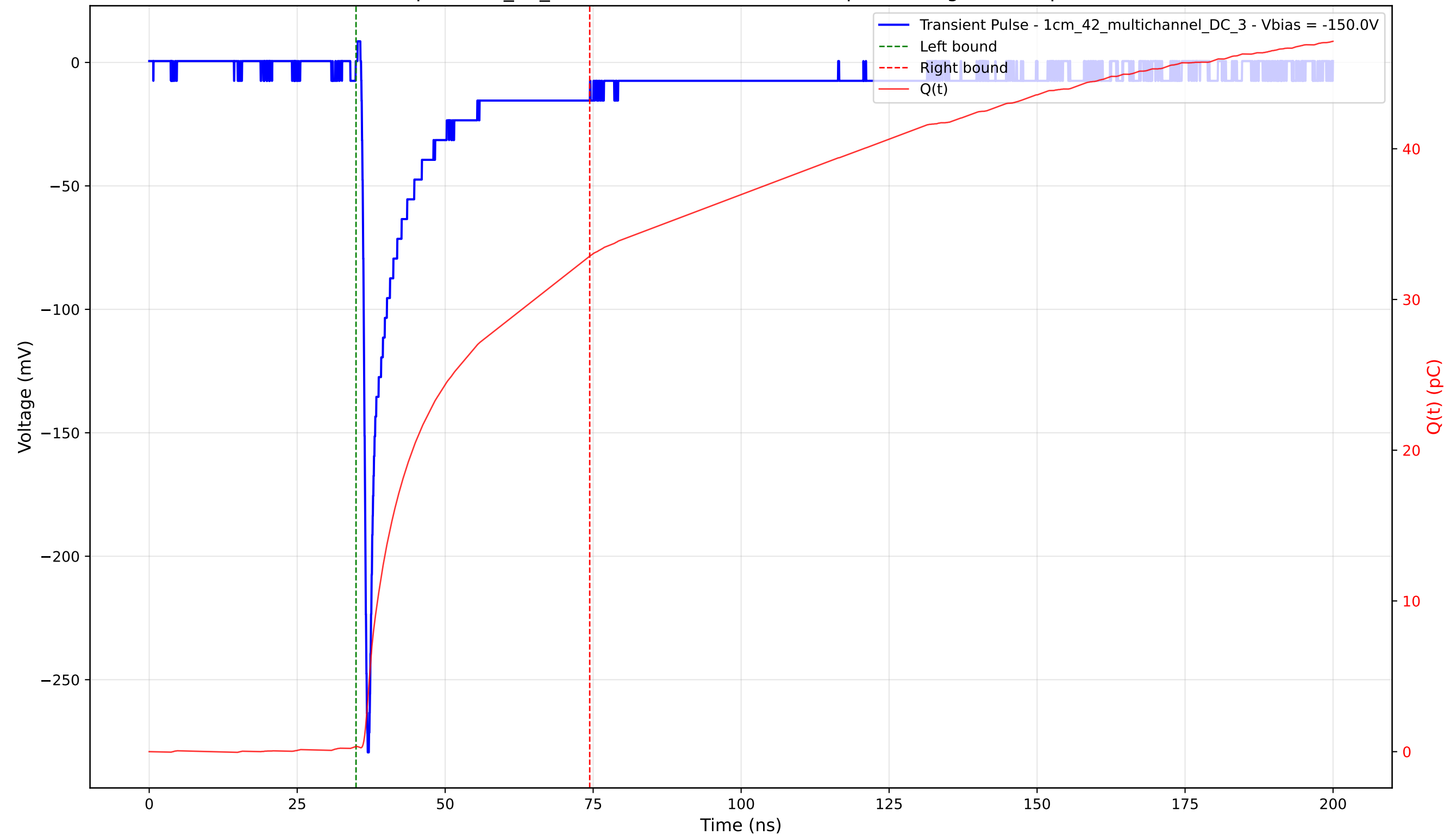
Transient Pulse - Sample: 1cm_42_multichannel - Position: 90.0 \mu\text{m} - Charge: 32.54 pC - Rise Time: 0.79 ns
