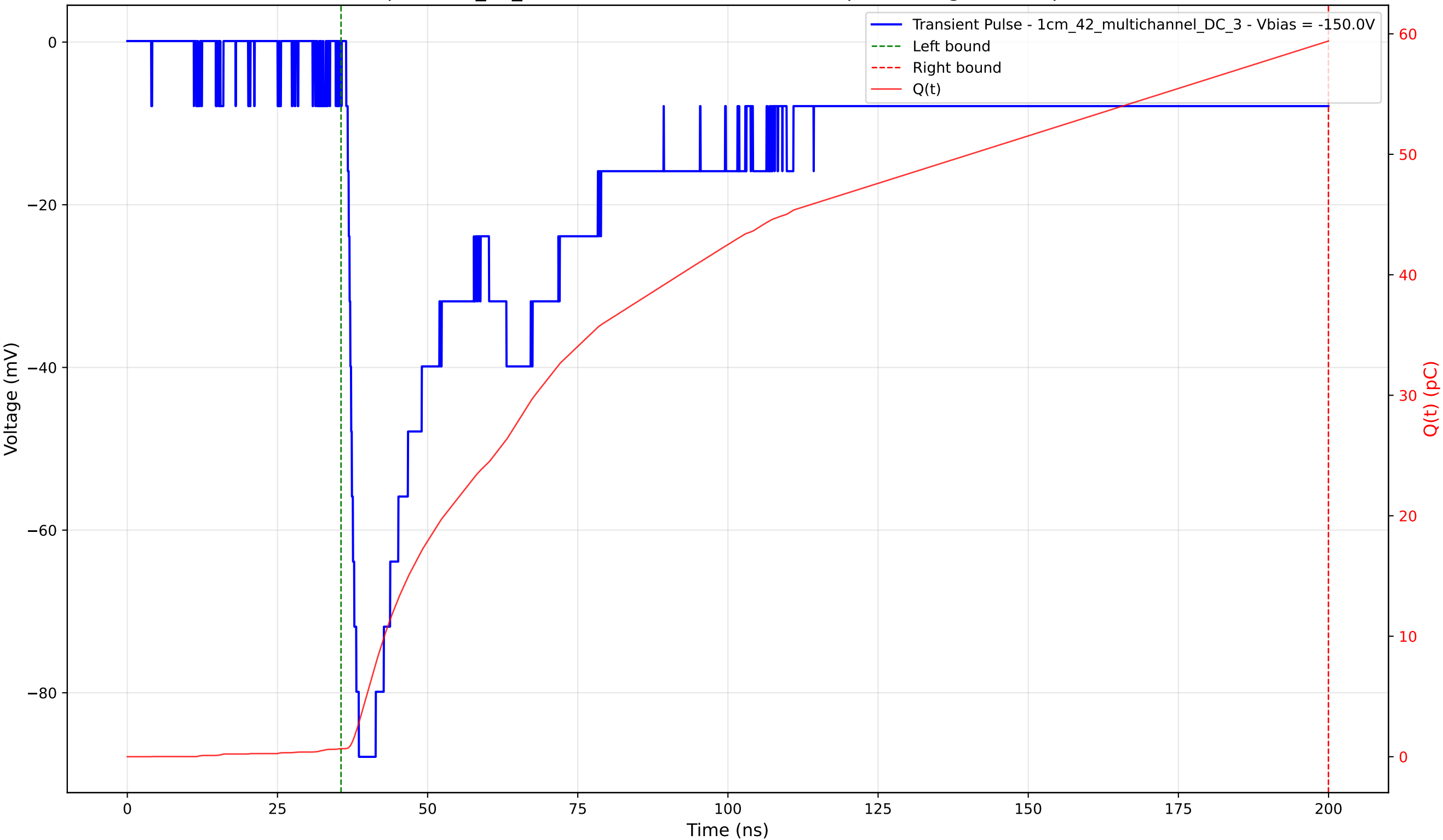
Transient Pulse - Sample: 1cm_42_multichannel - Position: 2080.0 \mu\text{m} - Charge: 58.74 pC - Rise Time: 1.44 ns
