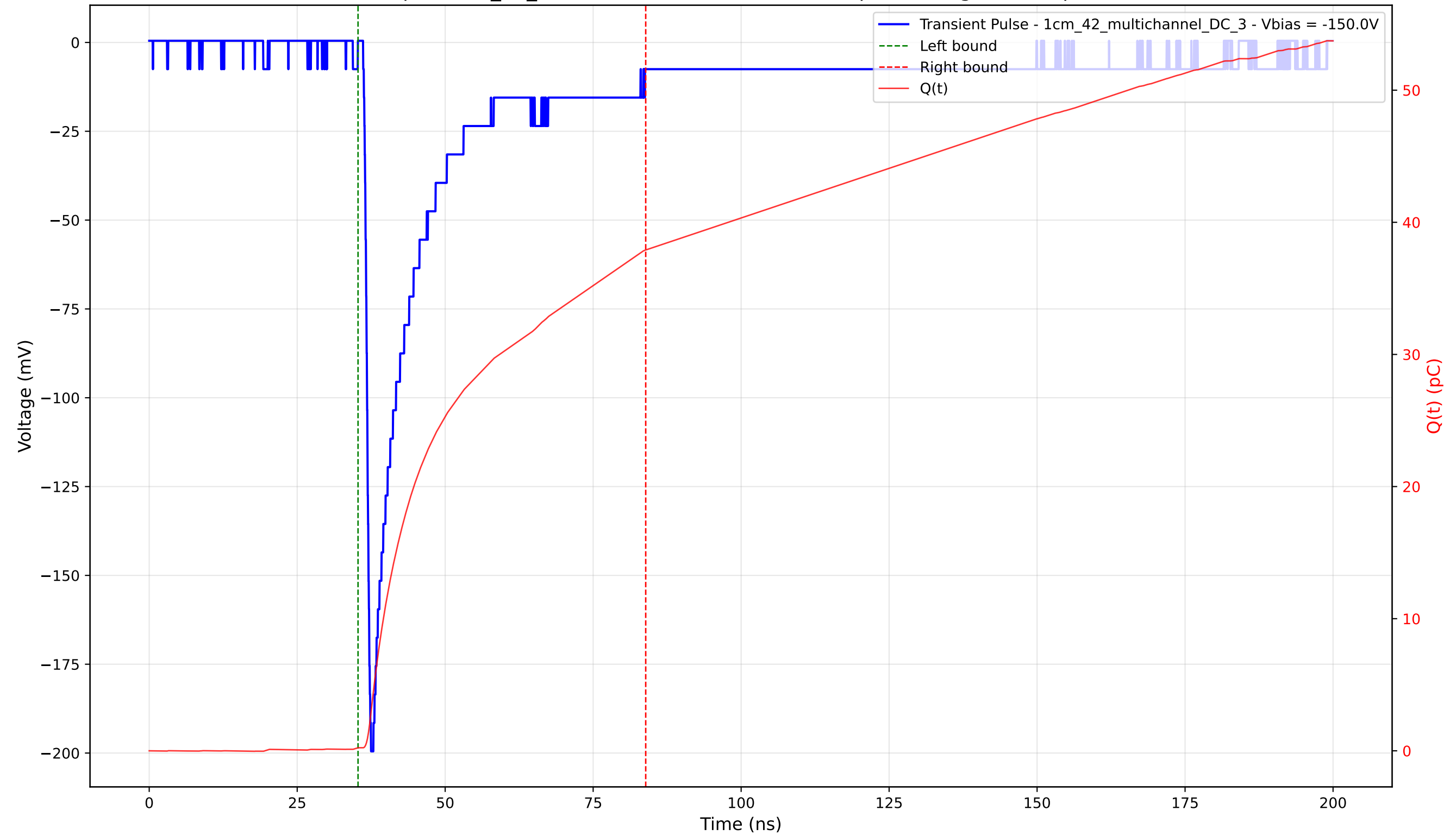
Transient Pulse - Sample: 1cm_42_multichannel - Position: 4280.0 \mu\text{m} - Charge: 37.67 pC - Rise Time: 0.93 ns
