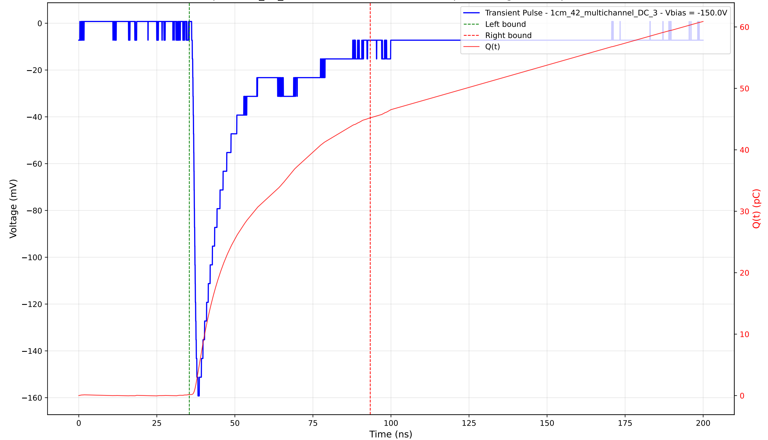
Transient Pulse - Sample: 1cm_42_multichannel - Position: 1180.0 \mu\text{m} - Charge: 45.02 pC - Rise Time: 1.34 ns
