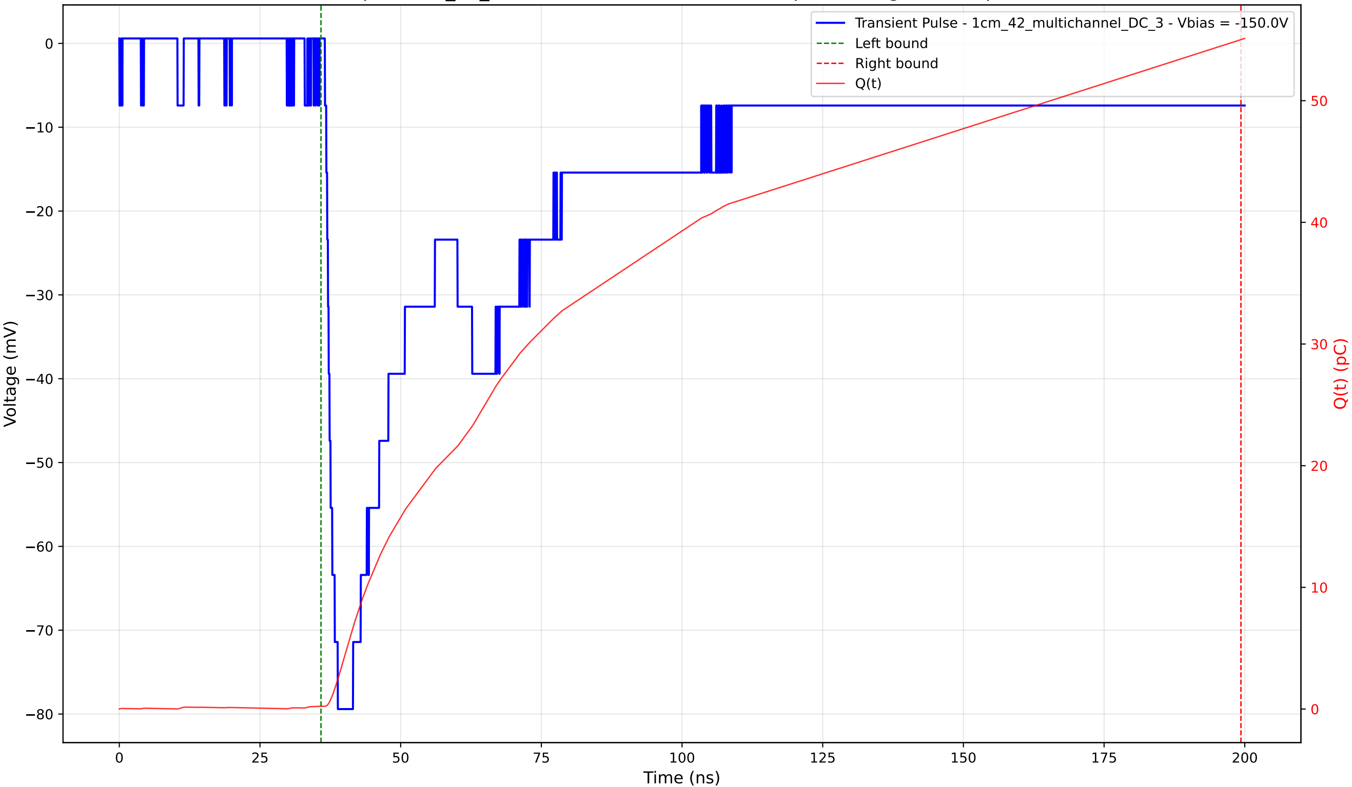
Transient Pulse - Sample: 1cm_42_multichannel - Position: 2515.0 \mu\text{m} - Charge: 54.79 pC - Rise Time: 2.06 ns
