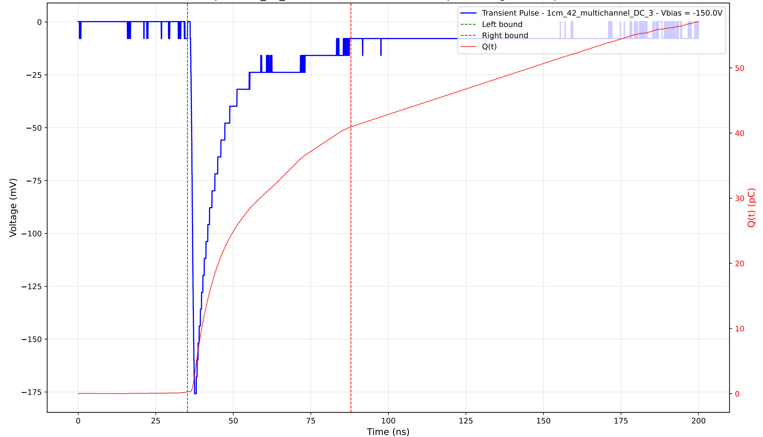
Transient Pulse - Sample: 1cm_42_multichannel - Position: 785.0 \mu\text{m} - Charge: 40.66 pC - Rise Time: 0.98 ns
