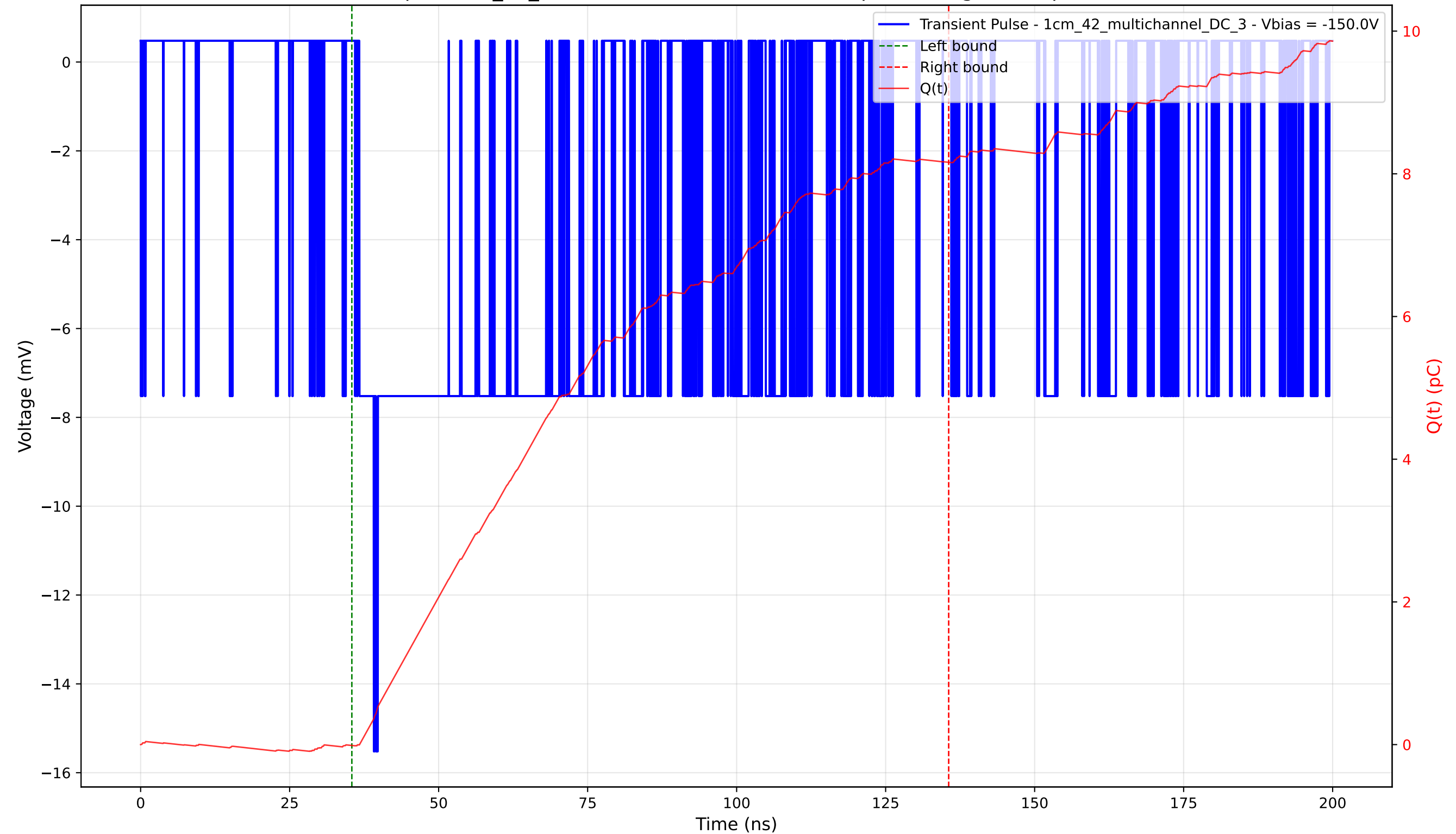
Transient Pulse - Sample: 1cm_42_multichannel - Position: 3370.0 \mu\text{m} - Charge: 8.17 pC - Rise Time: 2.44 ns
