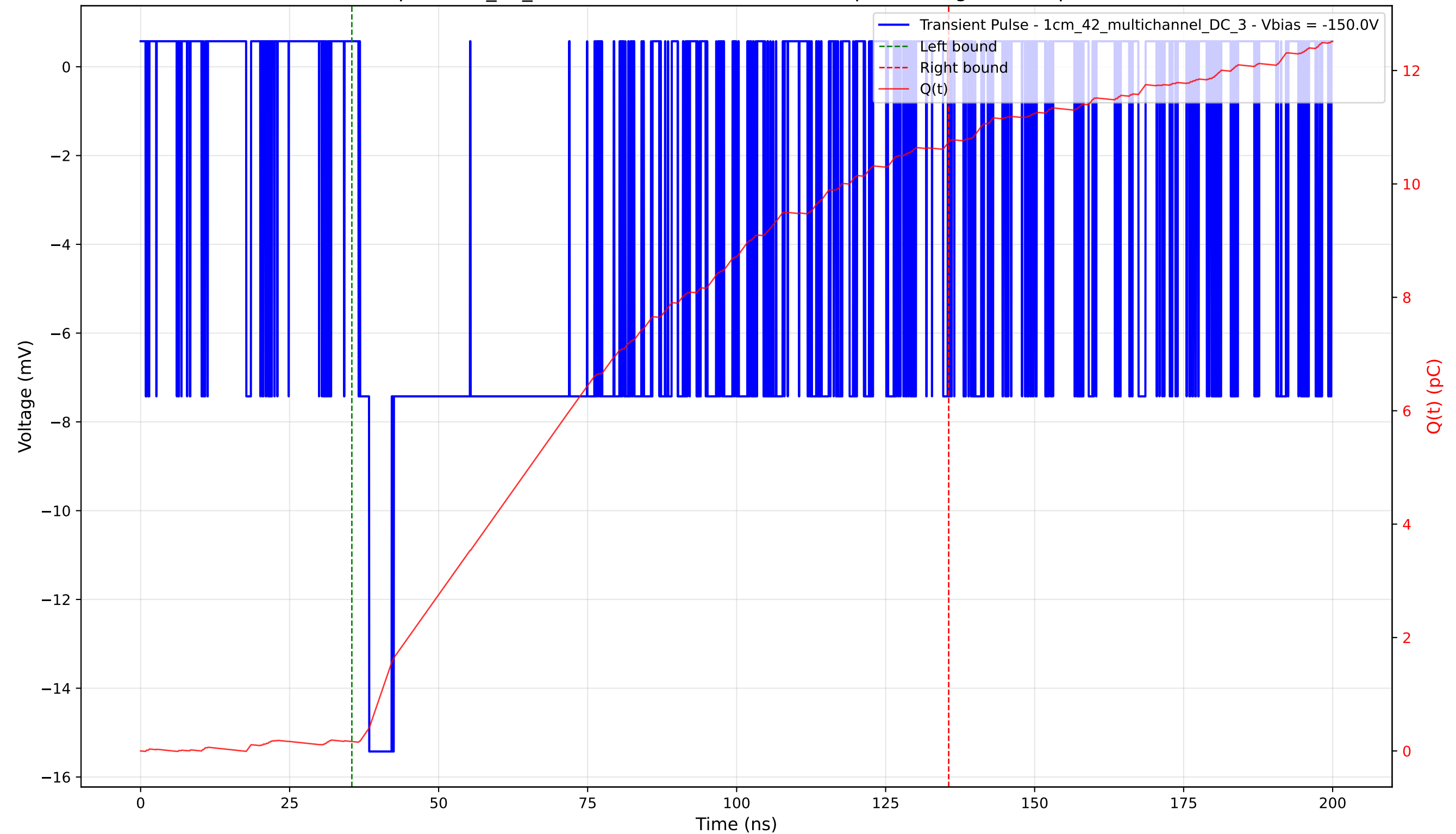
Transient Pulse - Sample: 1cm_42_multichannel - Position: 2855.0 \mu\text{m} - Charge: 10.57 pC - Rise Time: 1.54 ns
