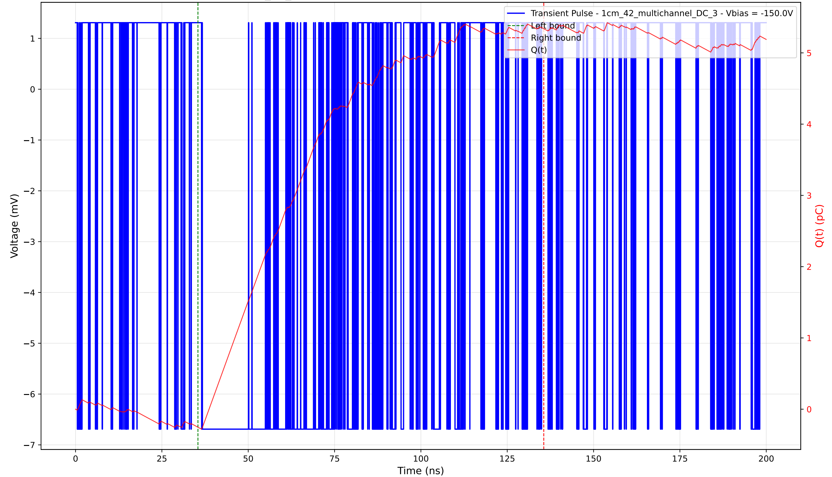
Transient Pulse - Sample: 1cm_42_multichannel - Position: 1870.0 \mu\text{m} - Charge: 5.59 pC - Rise Time: 0.00 ns (N/A)
