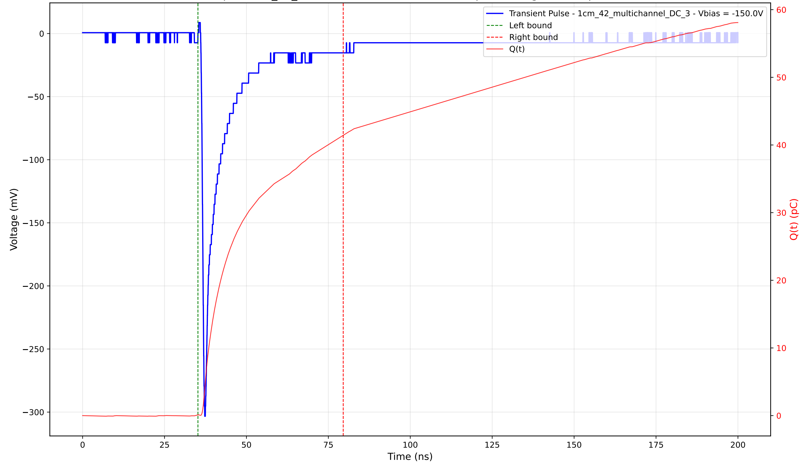
Transient Pulse - Sample: 1cm_42_multichannel - Position: 4605.0 \mu\text{m} - Charge: 41.32 pC - Rise Time: 0.86 ns
