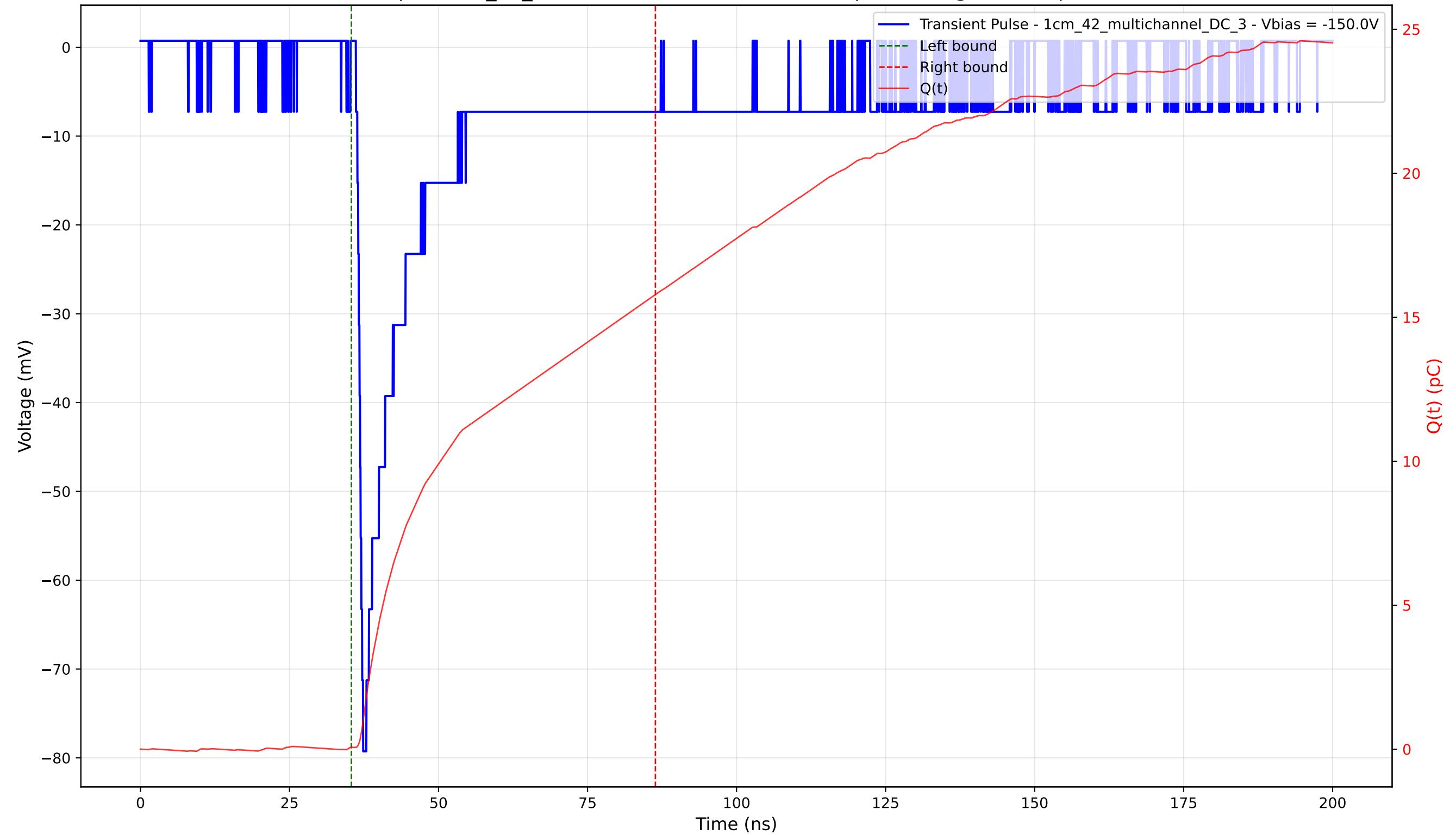
Transient Pulse - Sample: 1cm_42_multichannel - Position: 4345.0 \mu\text{m} - Charge: 15.73 pC - Rise Time: 0.98 ns
