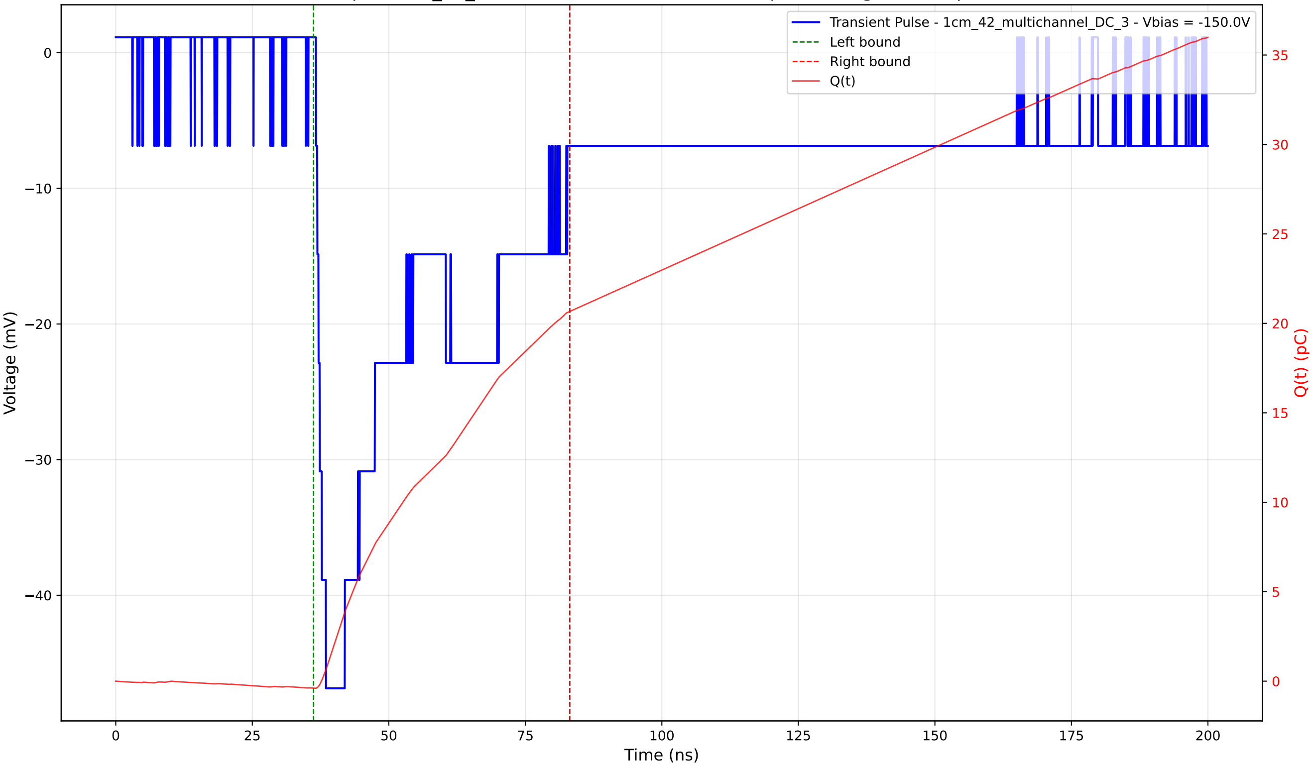
Transient Pulse - Sample: 1cm_42_multichannel - Position: 2320.0 \mu\text{m} - Charge: 21.06 pC - Rise Time: 1.83 ns
