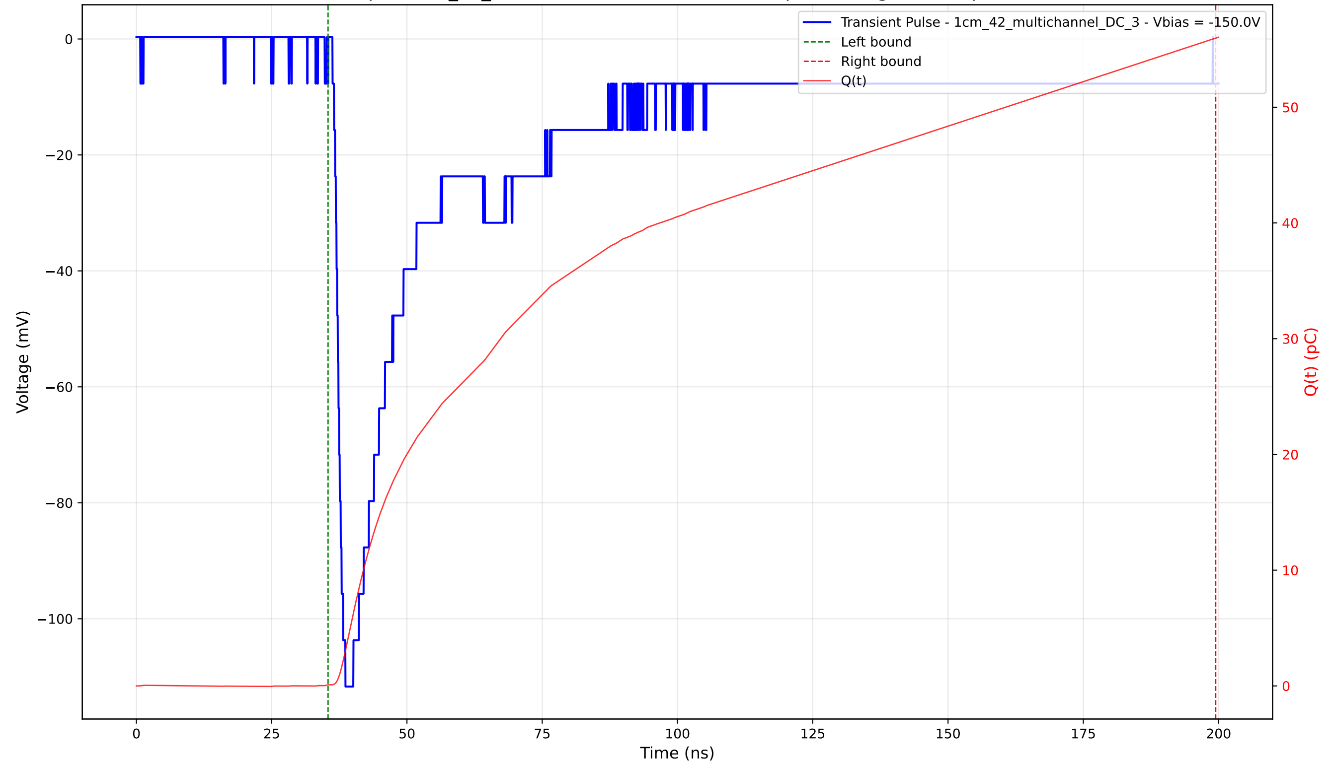
Transient Pulse - Sample: 1cm_42_multichannel - Position: 3210.0 \mu\text{m} - Charge: 55.88 pC - Rise Time: 1.69 ns
