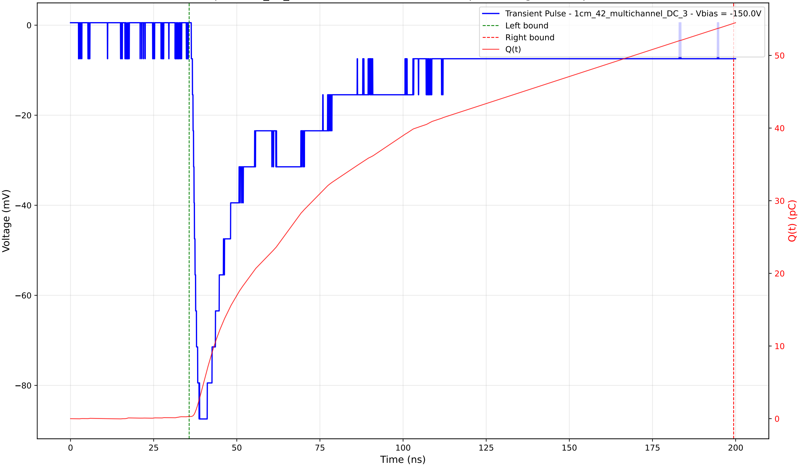
Transient Pulse - Sample: 1cm_42_multichannel - Position: 2790.0 \mu\text{m} - Charge: 54.12 pC - Rise Time: 1.60 ns
