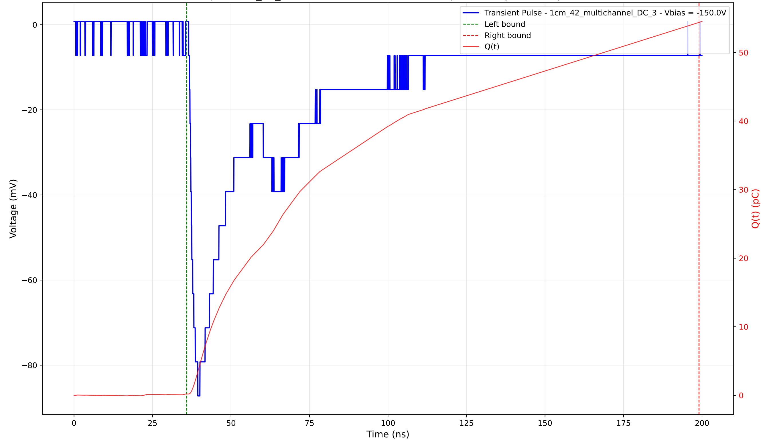
Transient Pulse - Sample: 1cm_42_multichannel - Position: 2615.0 \mu\text{m} - Charge: 54.20 pC - Rise Time: 1.84 ns
