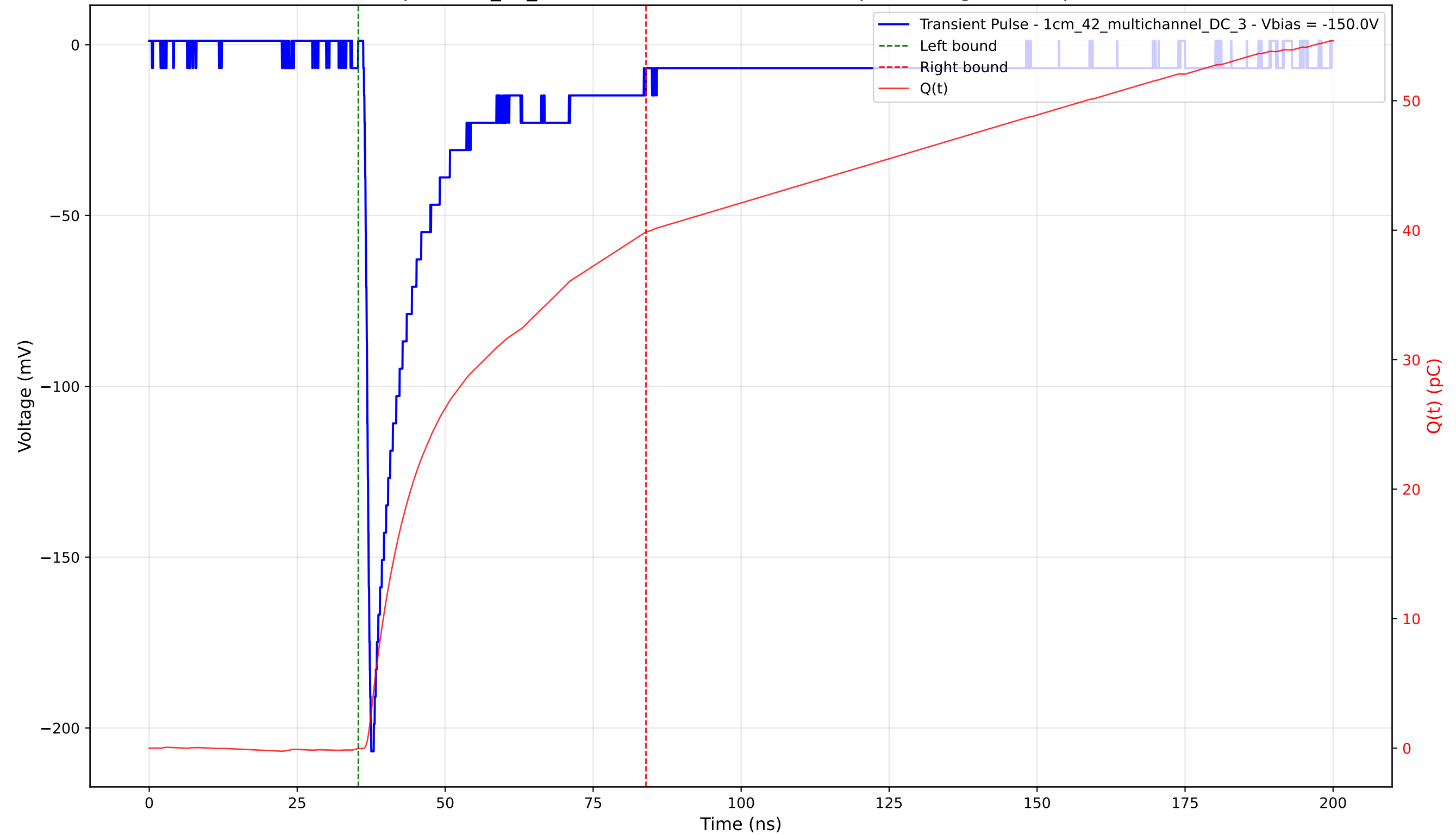
Transient Pulse - Sample: 1cm_42_multichannel - Position: 4245.0 \mu\text{m} - Charge: 39.87 pC - Rise Time: 0.97 ns
