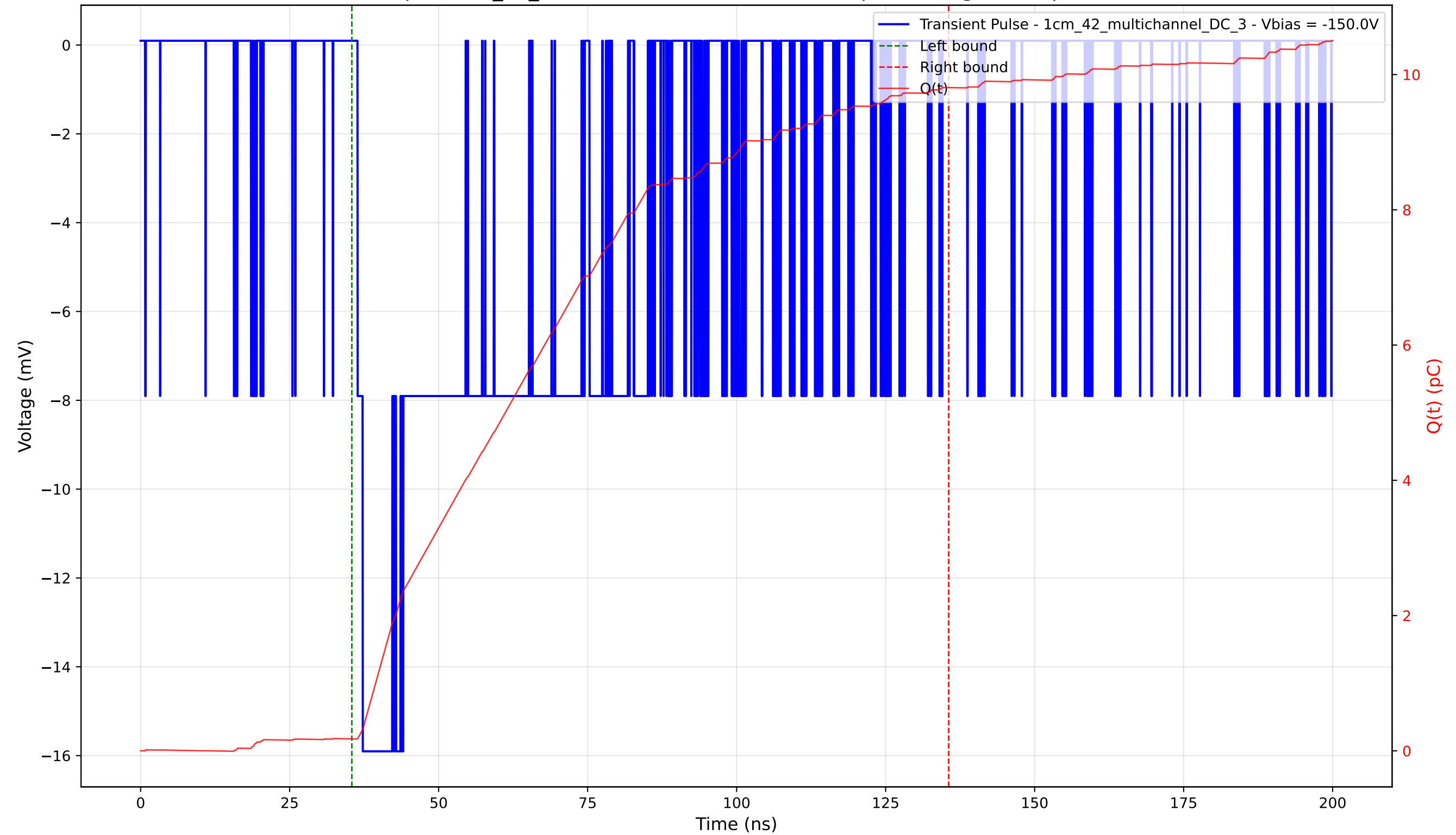
Transient Pulse - Sample: 1cm_42_multichannel - Position: 3865.0 \mu\text{m} - Charge: 9.63 pC - Rise Time: 0.88 ns
