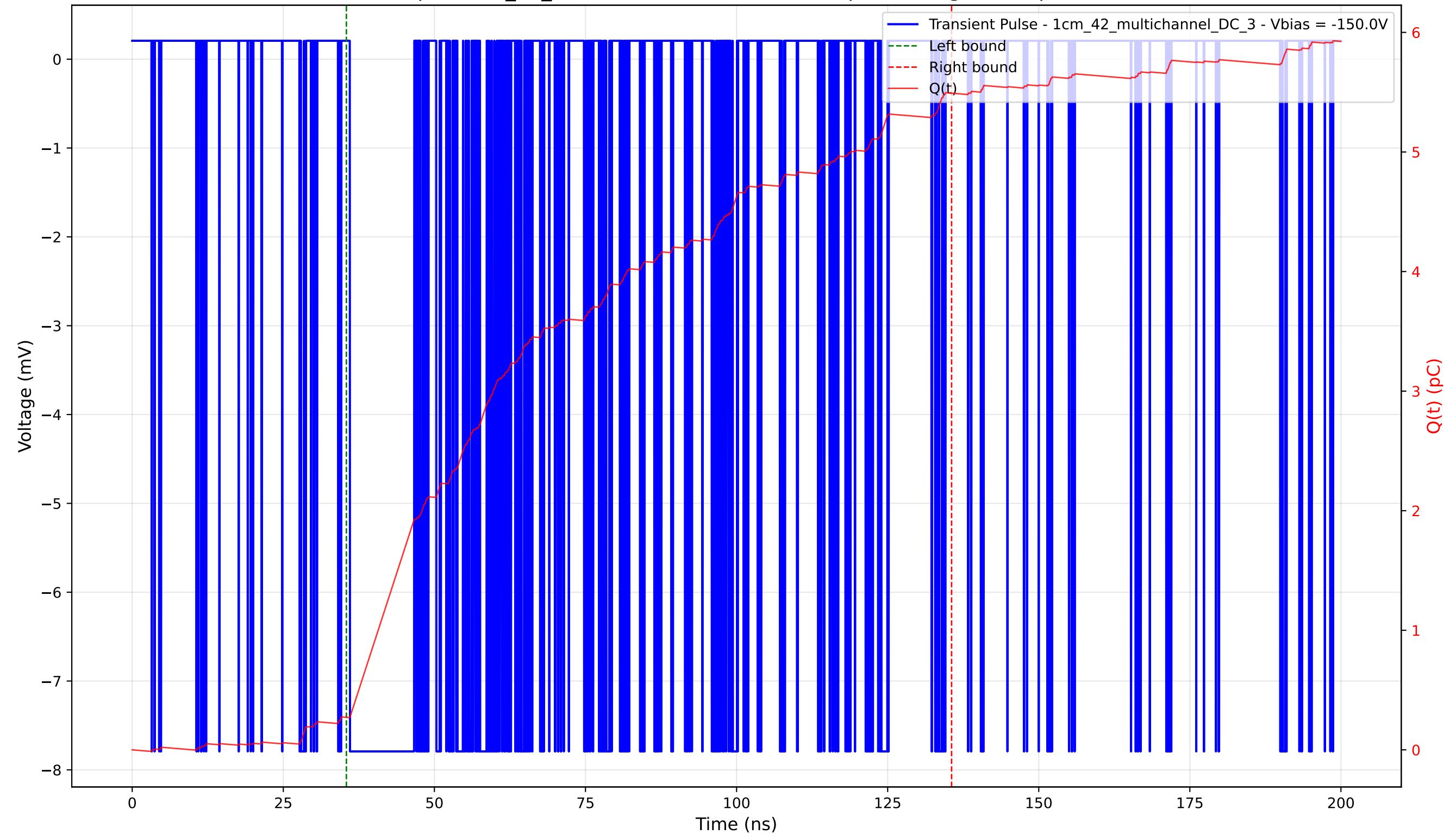
Transient Pulse - Sample: 1cm_42_multichannel - Position: 25.0 \mu\text{m} - Charge: 5.22 pC - Rise Time: 0.02 ns
