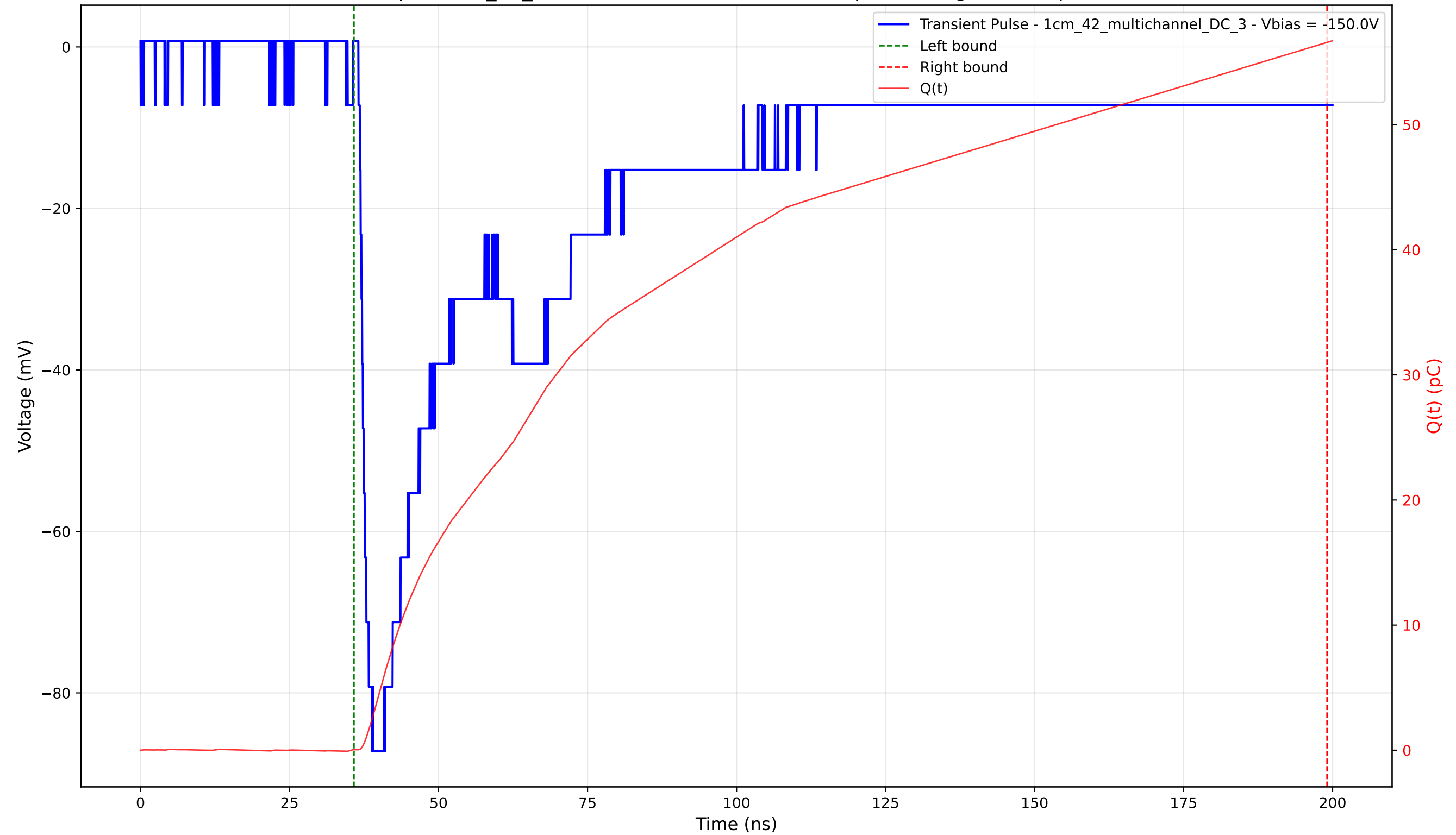
Transient Pulse - Sample: 1cm_42_multichannel - Position: 2190.0 \mu\text{m} - Charge: 56.53 pC - Rise Time: 1.50 ns
