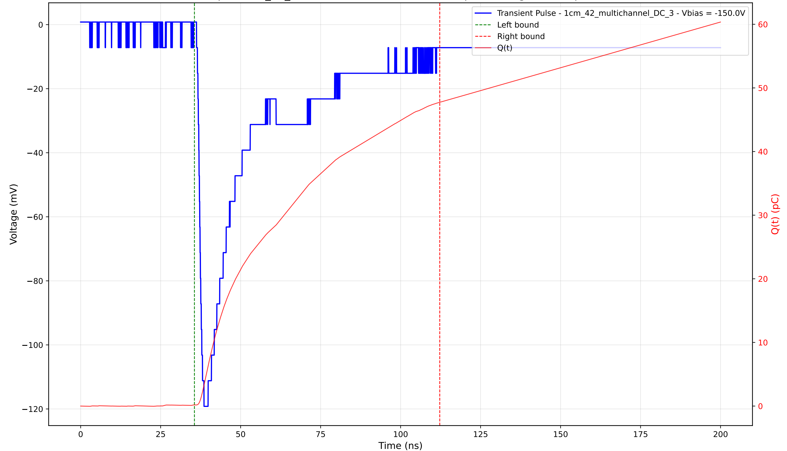
Transient Pulse - Sample: 1cm_42_multichannel - Position: 1675.0 \mu\text{m} - Charge: 47.57 pC - Rise Time: 1.59 ns
