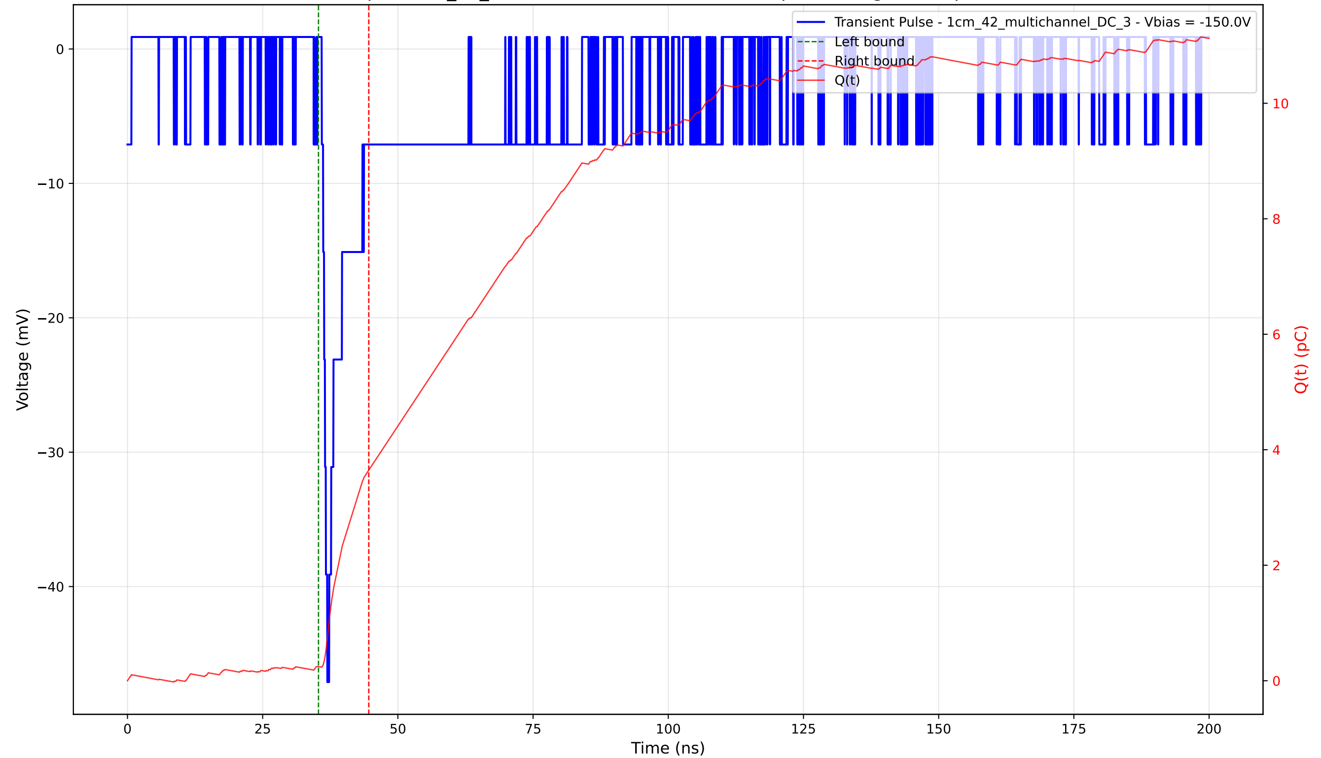
Transient Pulse - Sample: 1cm_42_multichannel - Position: 4875.0 \mu\text{m} - Charge: 3.40 pC - Rise Time: 1.03 ns
