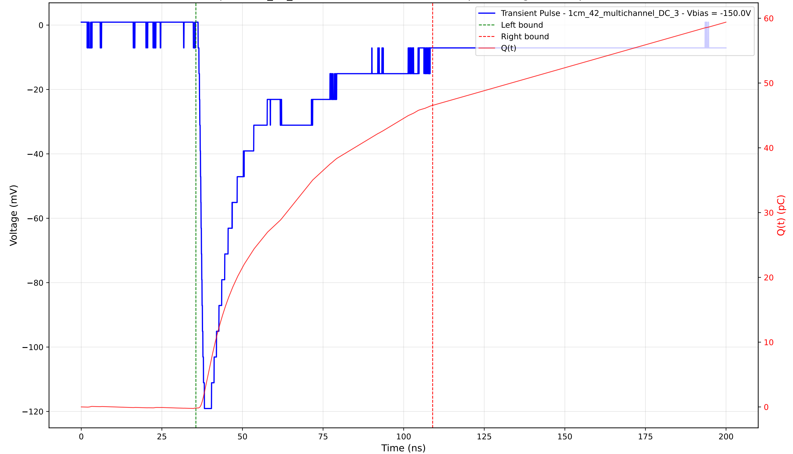
Transient Pulse - Sample: 1cm_42_multichannel - Position: 1585.0 \mu\text{m} - Charge: 46.71 pC - Rise Time: 1.41 ns
