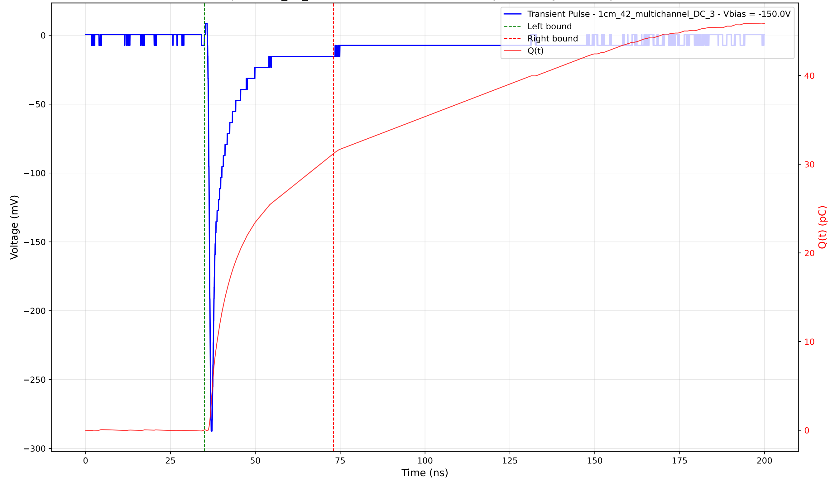
Transient Pulse - Sample: 1cm_42_multichannel - Position: 4835.0 \mu\text{m} - Charge: 31.18 pC - Rise Time: 0.79 ns
