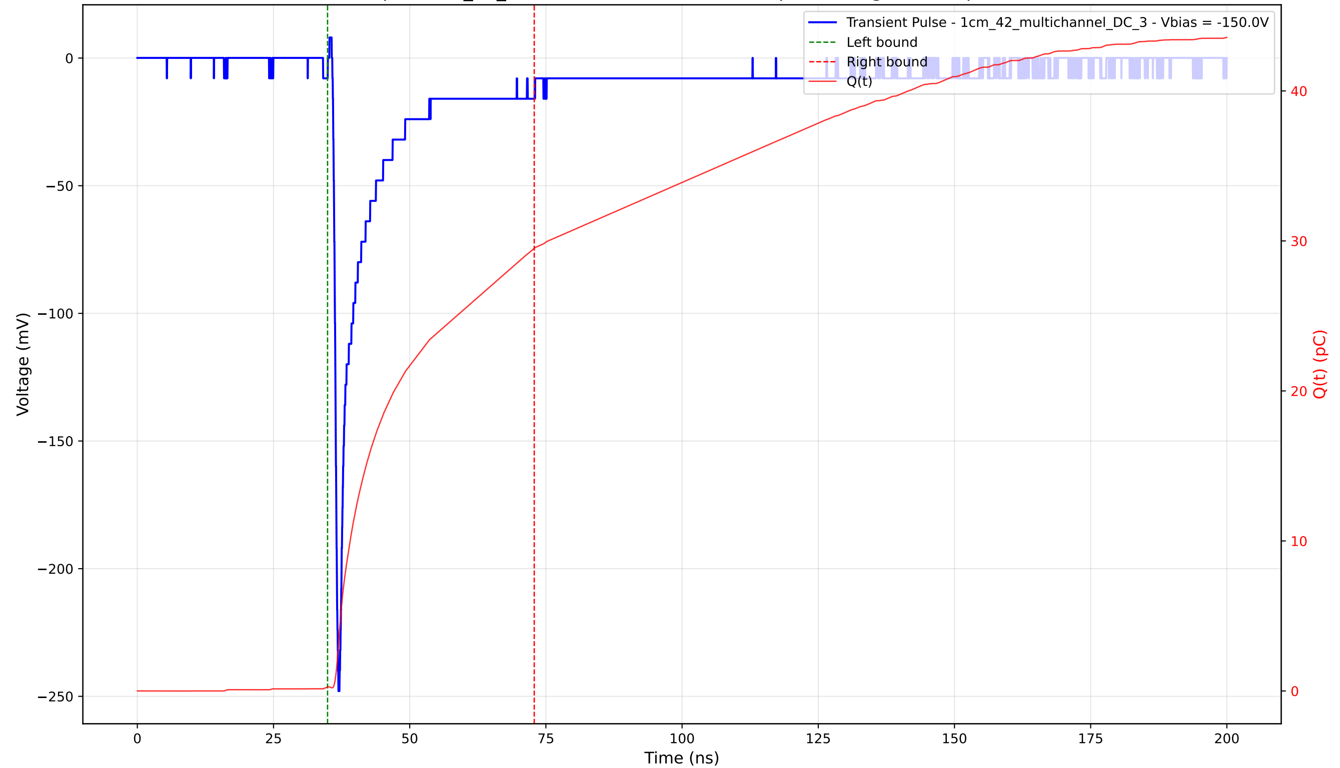
Transient Pulse - Sample: 1cm_42_multichannel - Position: 85.0 \mu\text{m} - Charge: 29.25 pC - Rise Time: 0.76 ns
