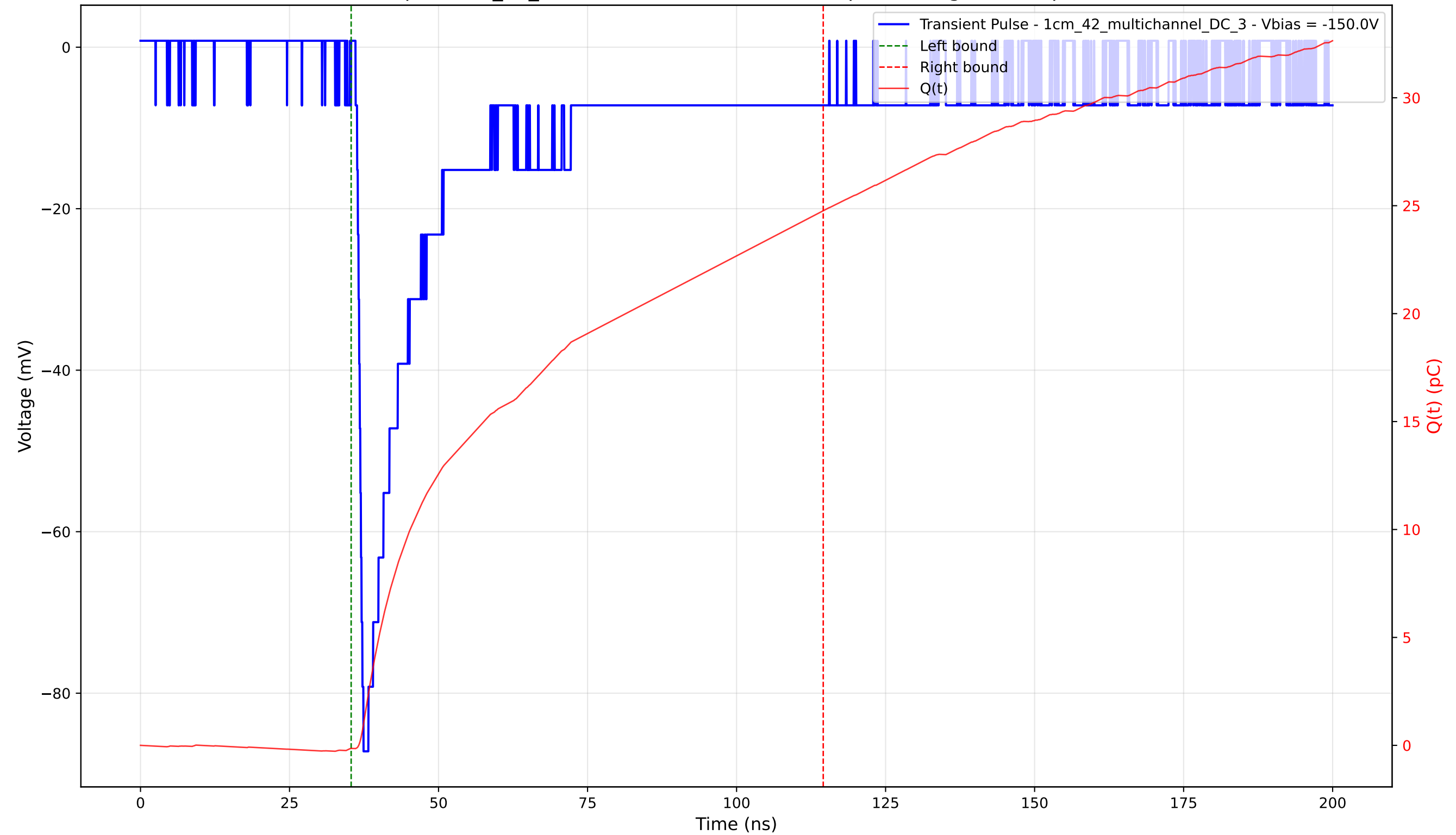
Transient Pulse - Sample: 1cm_42_multichannel - Position: 810.0 \mu\text{m} - Charge: 24.92 pC - Rise Time: 0.90 ns
