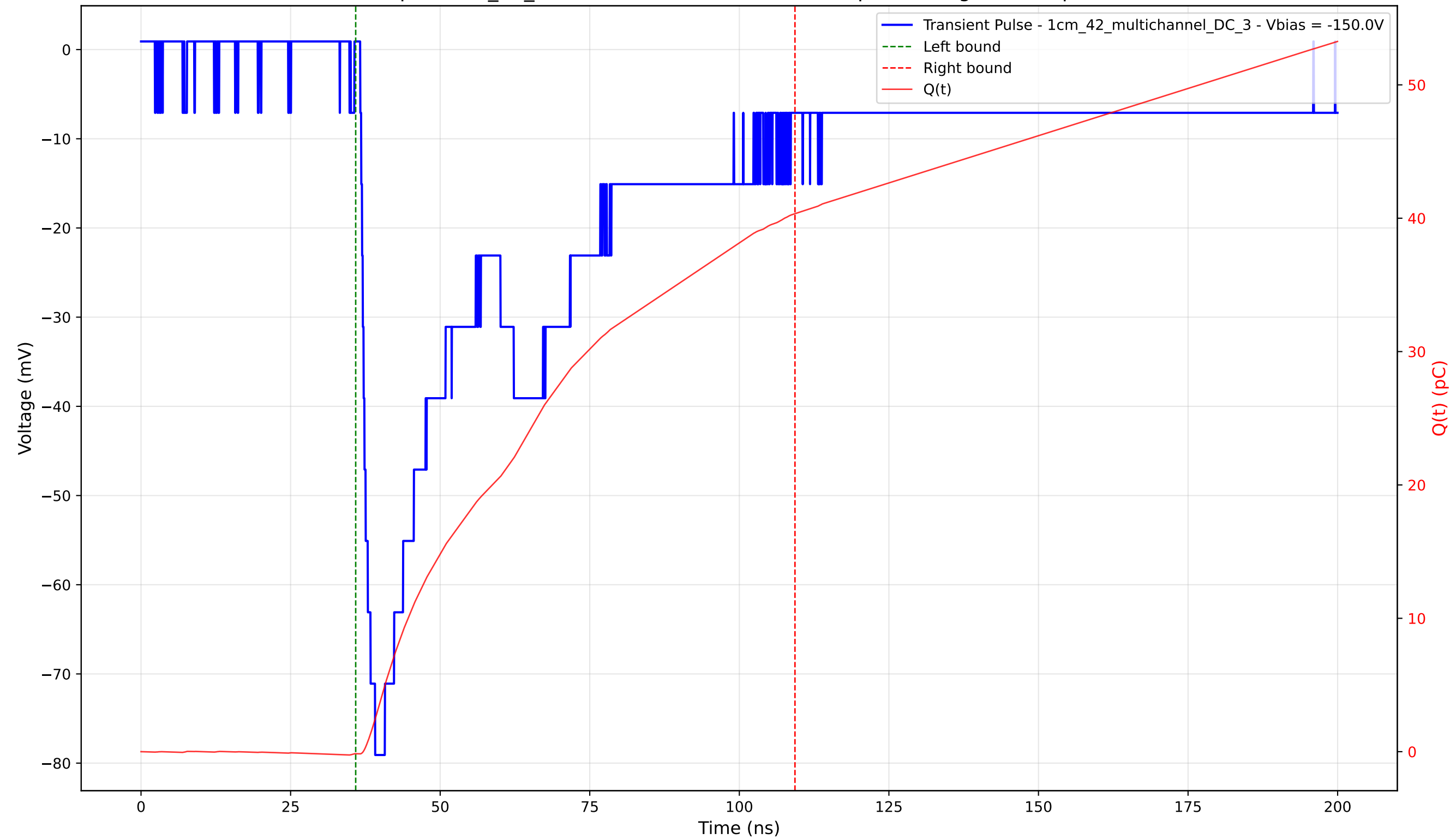
Transient Pulse - Sample: 1cm_42_multichannel - Position: 2290.0 \mu\text{m} - Charge: 40.49 pC - Rise Time: 2.34 ns
