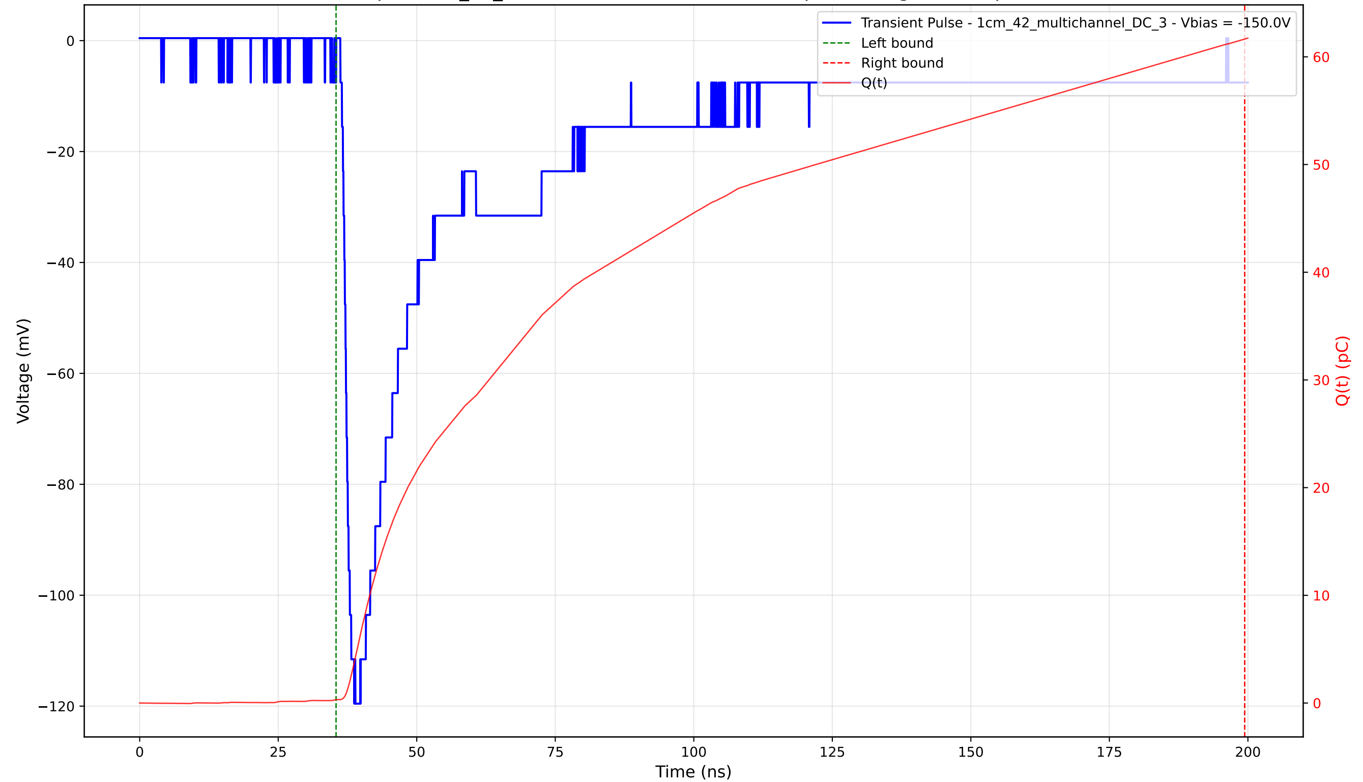
Transient Pulse - Sample: 1cm_42_multichannel - Position: 1715.0 \mu\text{m} - Charge: 61.33 pC - Rise Time: 1.69 ns
