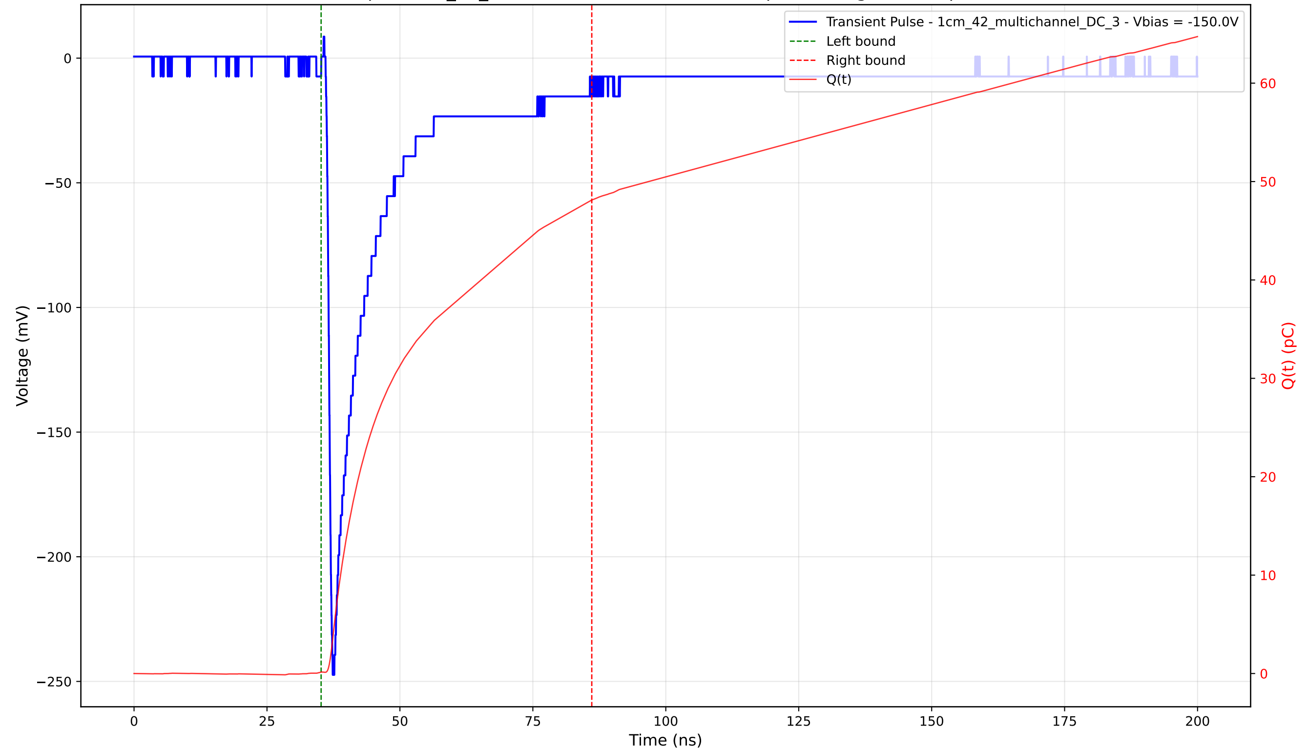
Transient Pulse - Sample: 1cm_42_multichannel - Position: 585.0 \mu\text{m} - Charge: 47.97 pC - Rise Time: 0.90 ns
