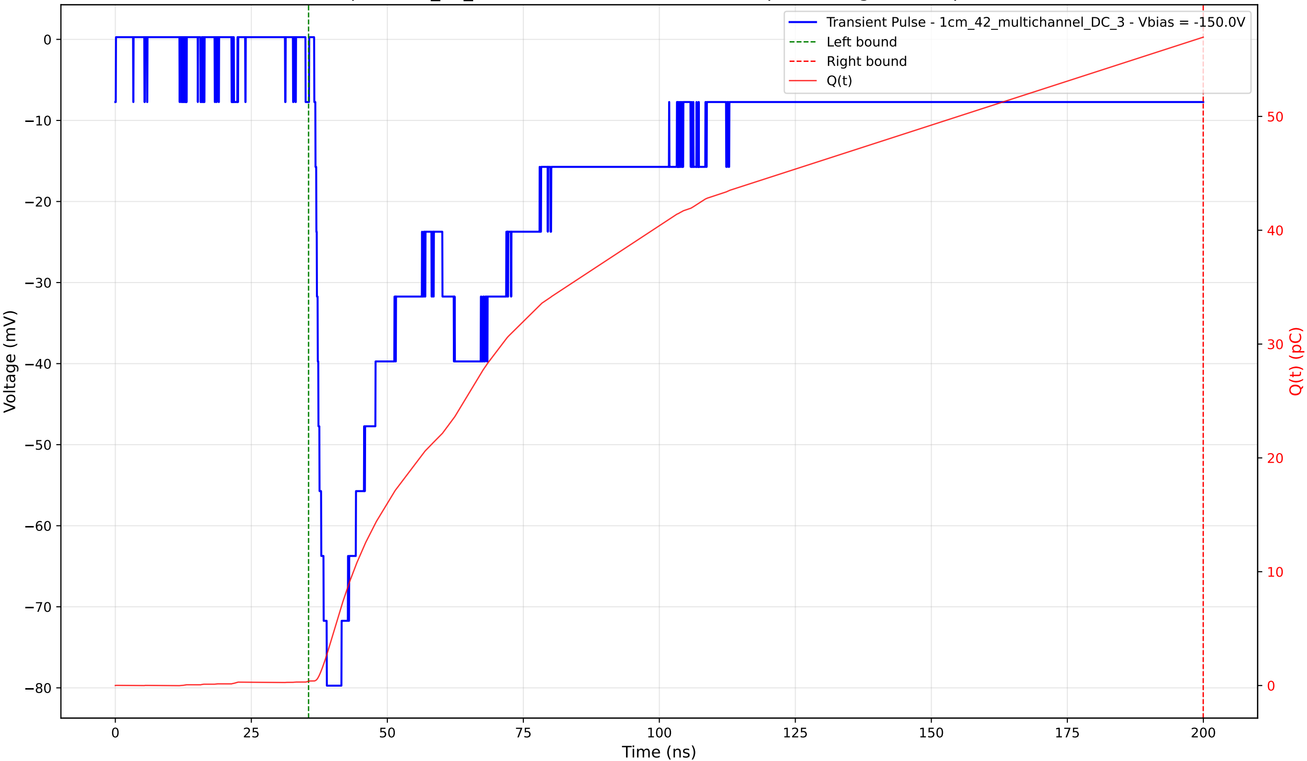
Transient Pulse - Sample: 1cm_42_multichannel - Position: 2480.0 \mu\text{m} - Charge: 56.58 pC - Rise Time: 2.10 ns
