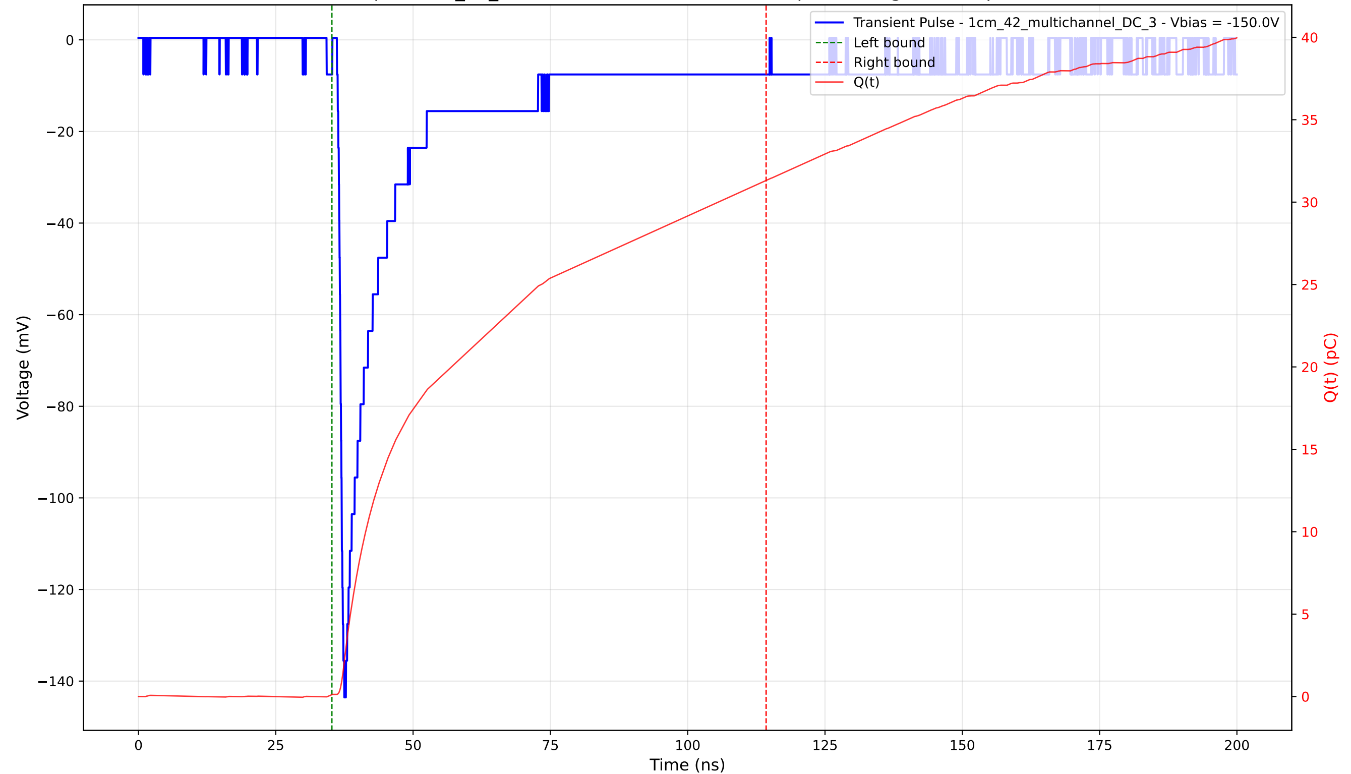
Transient Pulse - Sample: 1cm_42_multichannel - Position: 4330.0 \mu\text{m} - Charge: 31.20 pC - Rise Time: 1.02 ns
