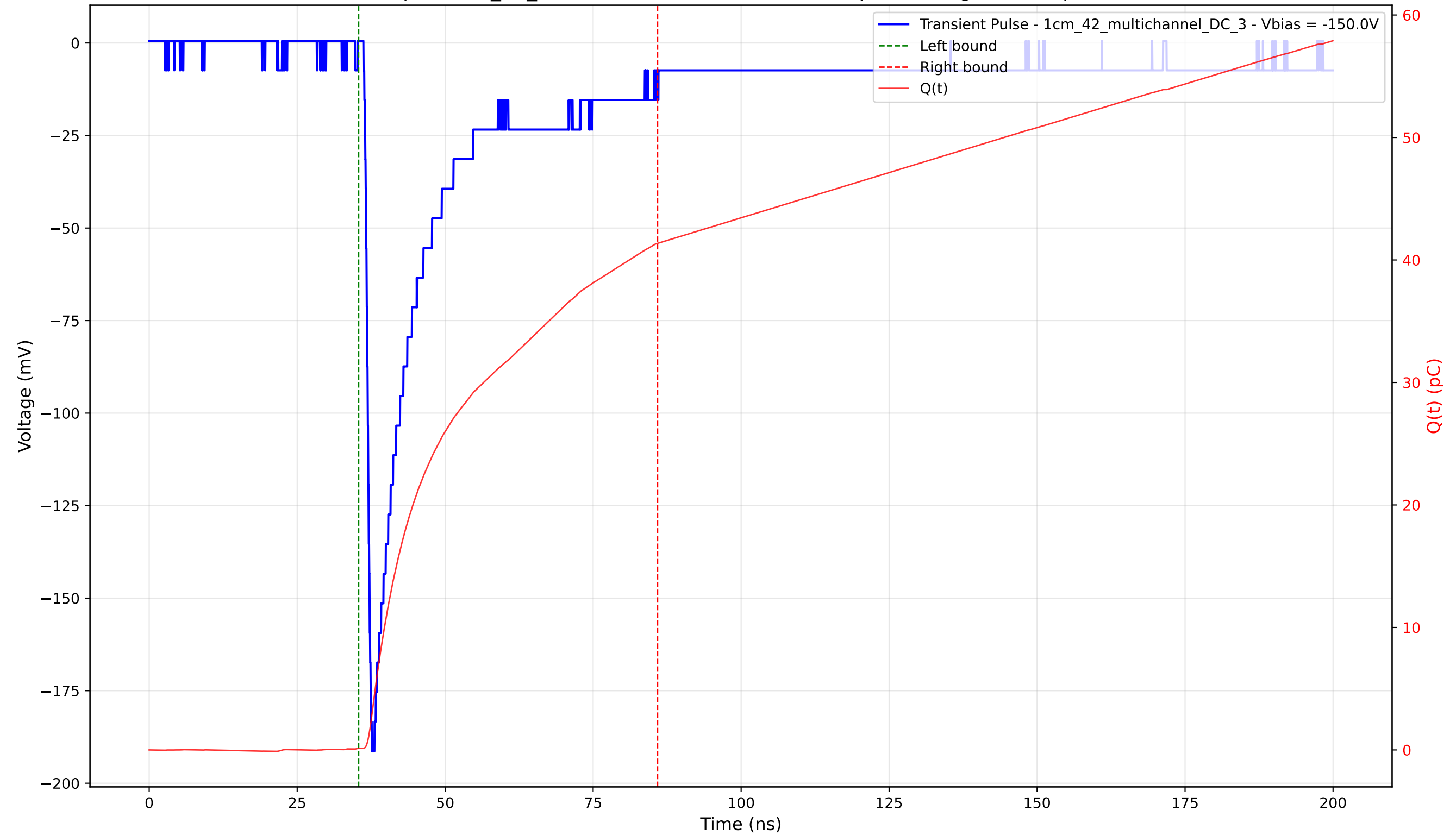
Transient Pulse - Sample: 1cm_42_multichannel - Position: 4145.0 \mu\text{m} - Charge: 41.22 pC - Rise Time: 0.99 ns
