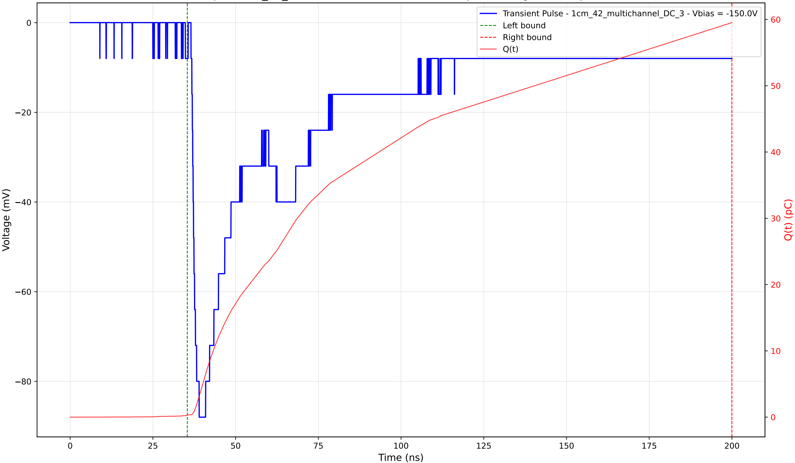
Transient Pulse - Sample: 1cm_42_multichannel - Position: 2185.0 \mu\text{m} - Charge: 59.21 pC - Rise Time: 1.46 ns
