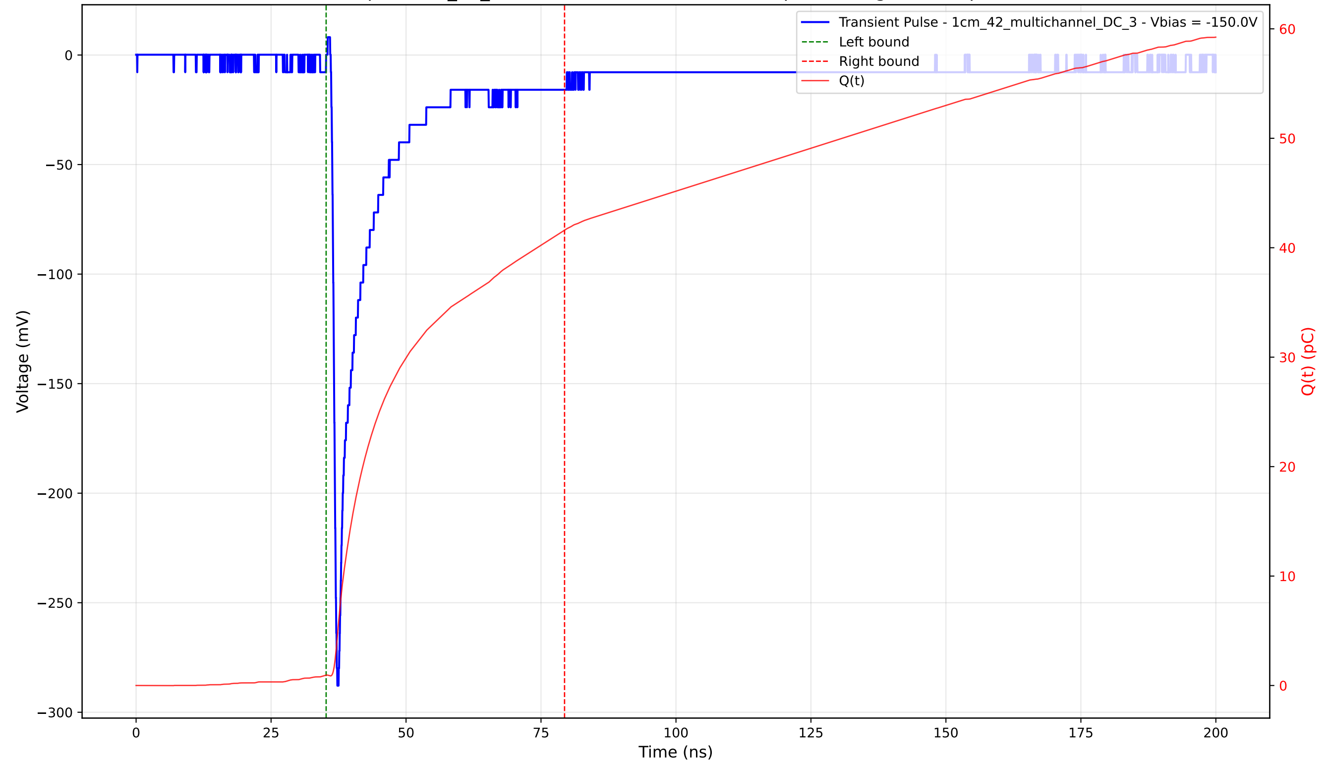
Transient Pulse - Sample: 1cm_42_multichannel - Position: 4570.0 \mu\text{m} - Charge: 40.66 pC - Rise Time: 0.85 ns
