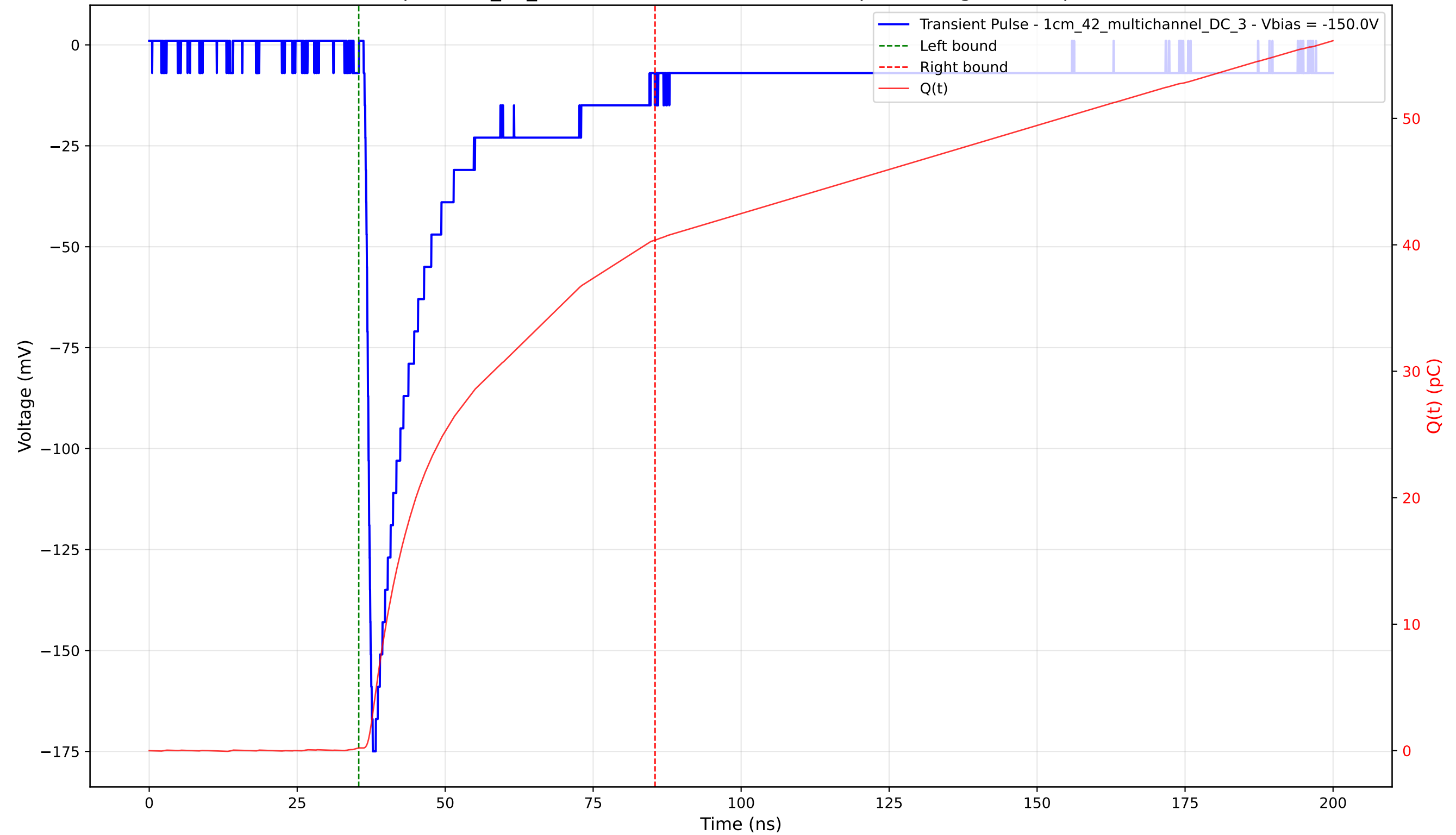
Transient Pulse - Sample: 1cm_42_multichannel - Position: 4020.0 \mu\text{m} - Charge: 40.15 pC - Rise Time: 1.01 ns
