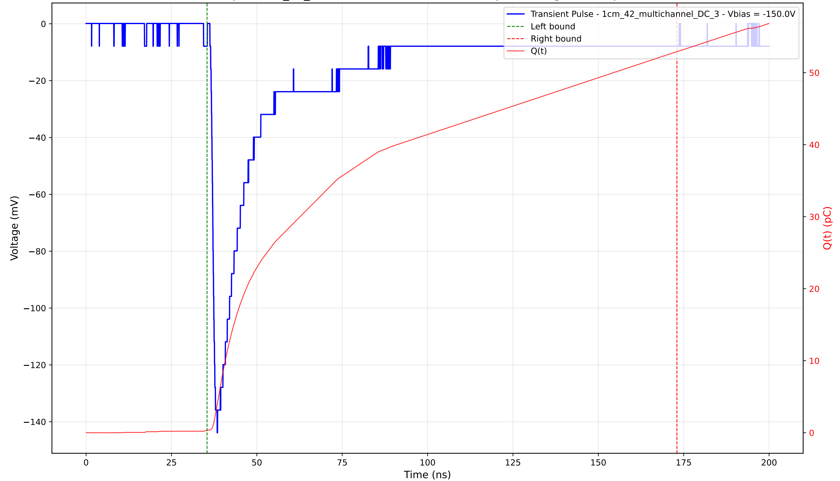
Transient Pulse - Sample: 1cm_42_multichannel - Position: 3720.0 \mu\text{m} - Charge: 52.57 pC - Rise Time: 1.40 ns
