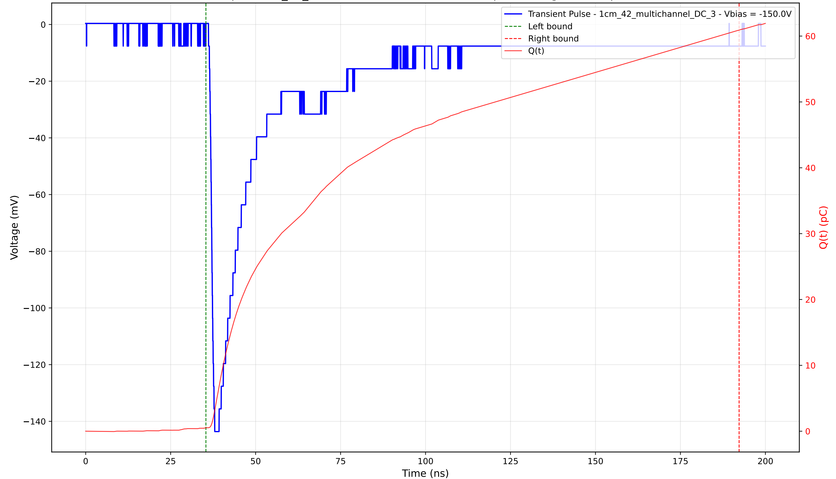
Transient Pulse - Sample: 1cm_42_multichannel - Position: 1275.0 \mu\text{m} - Charge: 60.40 pC - Rise Time: 1.36 ns
