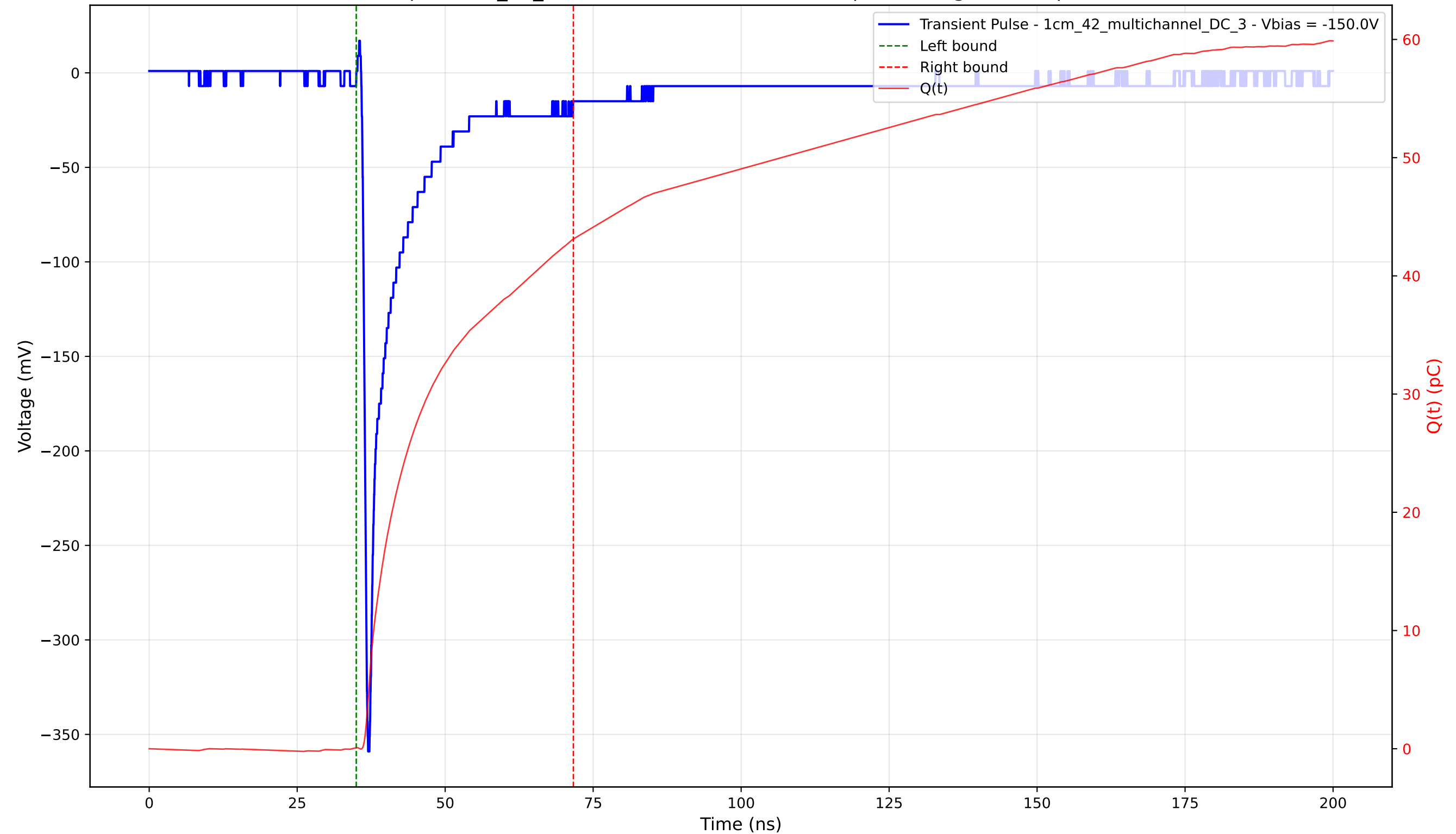
Transient Pulse - Sample: 1cm_42_multichannel - Position: 160.0 \mu\text{m} - Charge: 43.02 pC - Rise Time: 0.79 ns
