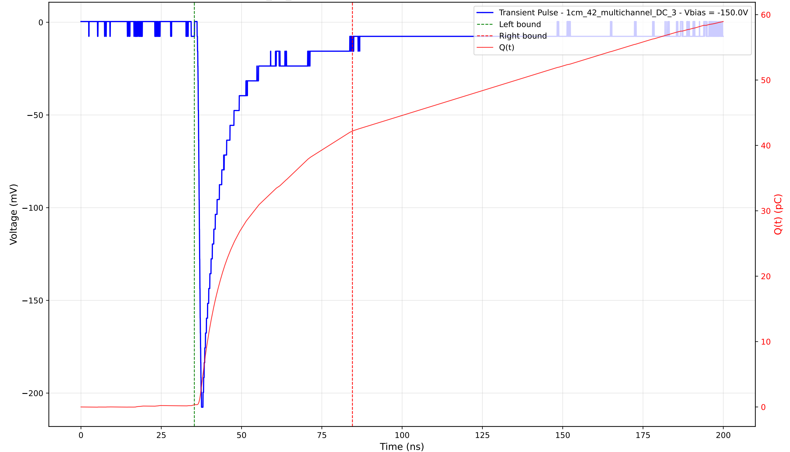
Transient Pulse - Sample: 1cm_42_multichannel - Position: 4215.0 \mu\text{m} - Charge: 41.84 pC - Rise Time: 0.97 ns
