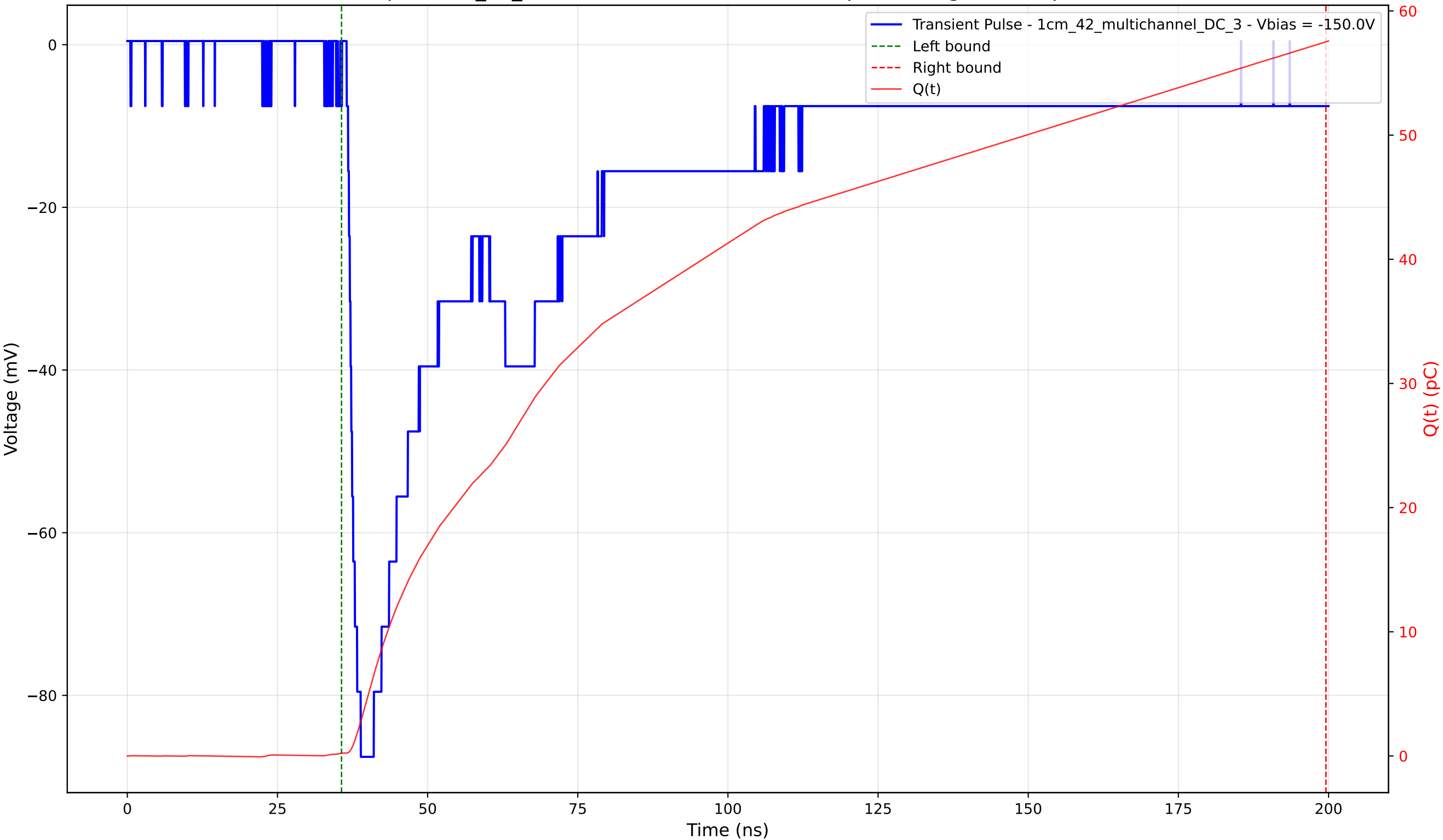
Transient Pulse - Sample: 1cm_42_multichannel - Position: 2140.0 \mu\text{m} - Charge: 57.30 pC - Rise Time: 1.52 ns
