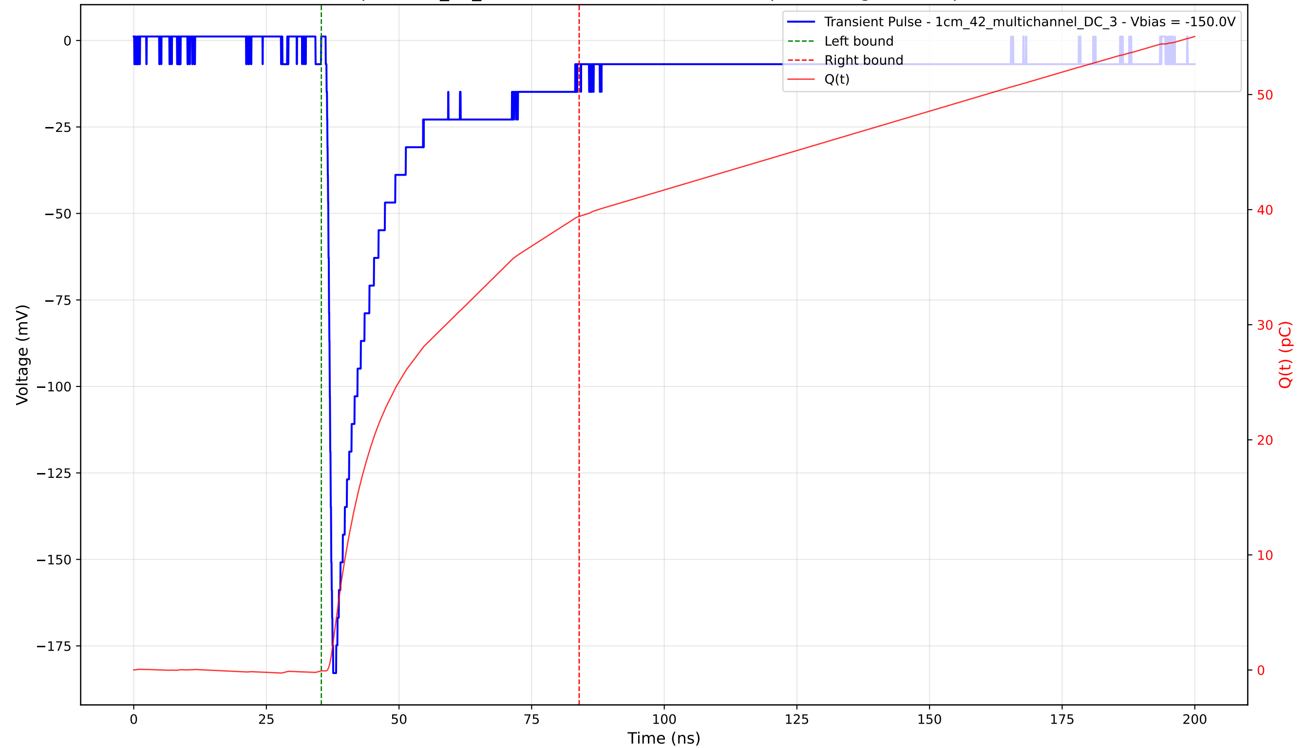
Transient Pulse - Sample: 1cm_42_multichannel - Position: 4130.0 \mu\text{m} - Charge: 39.48 pC - Rise Time: 0.95 ns
