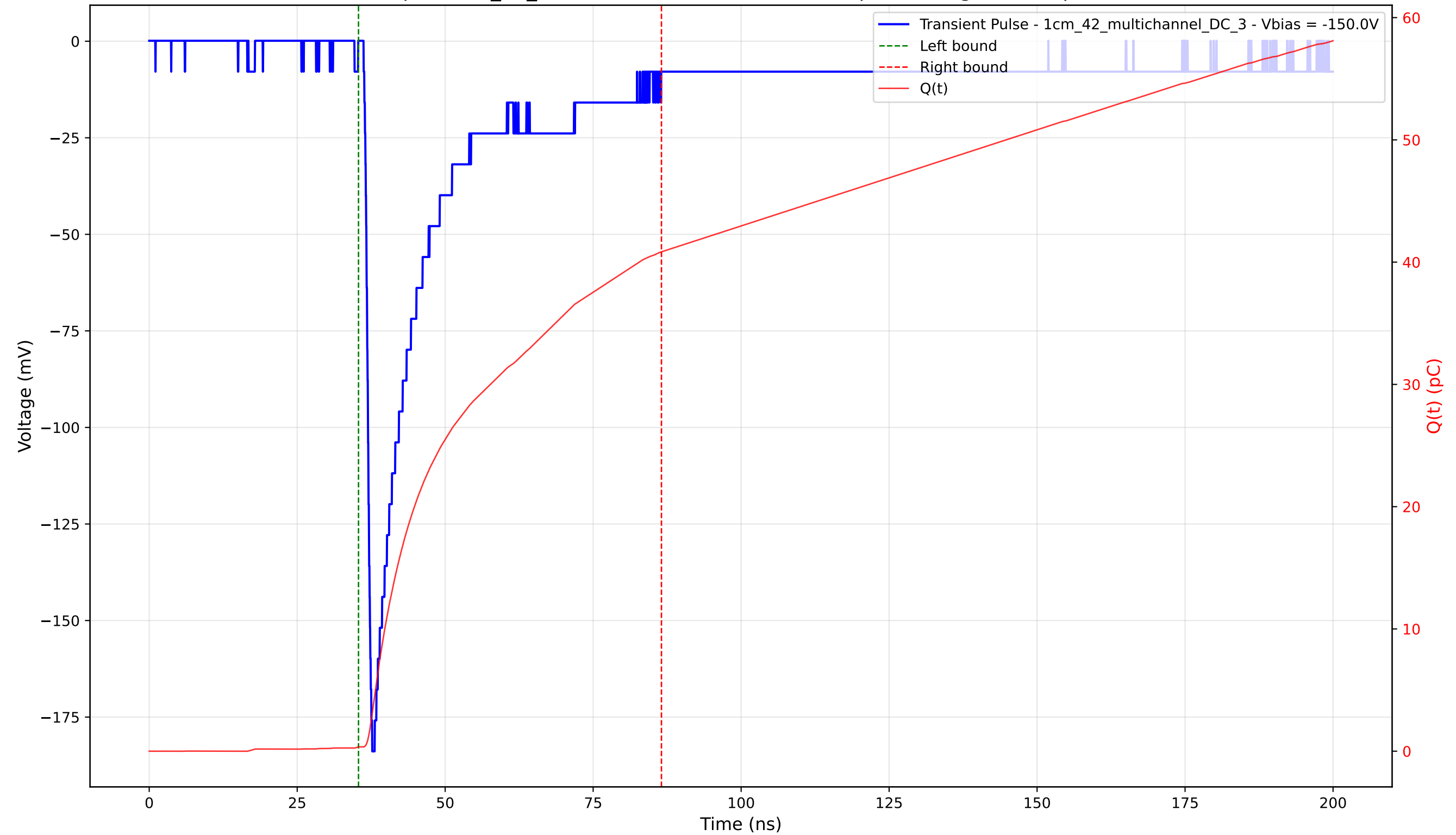
Transient Pulse - Sample: 1cm_42_multichannel - Position: 4120.0 \mu\text{m} - Charge: 40.50 pC - Rise Time: 0.99 ns
