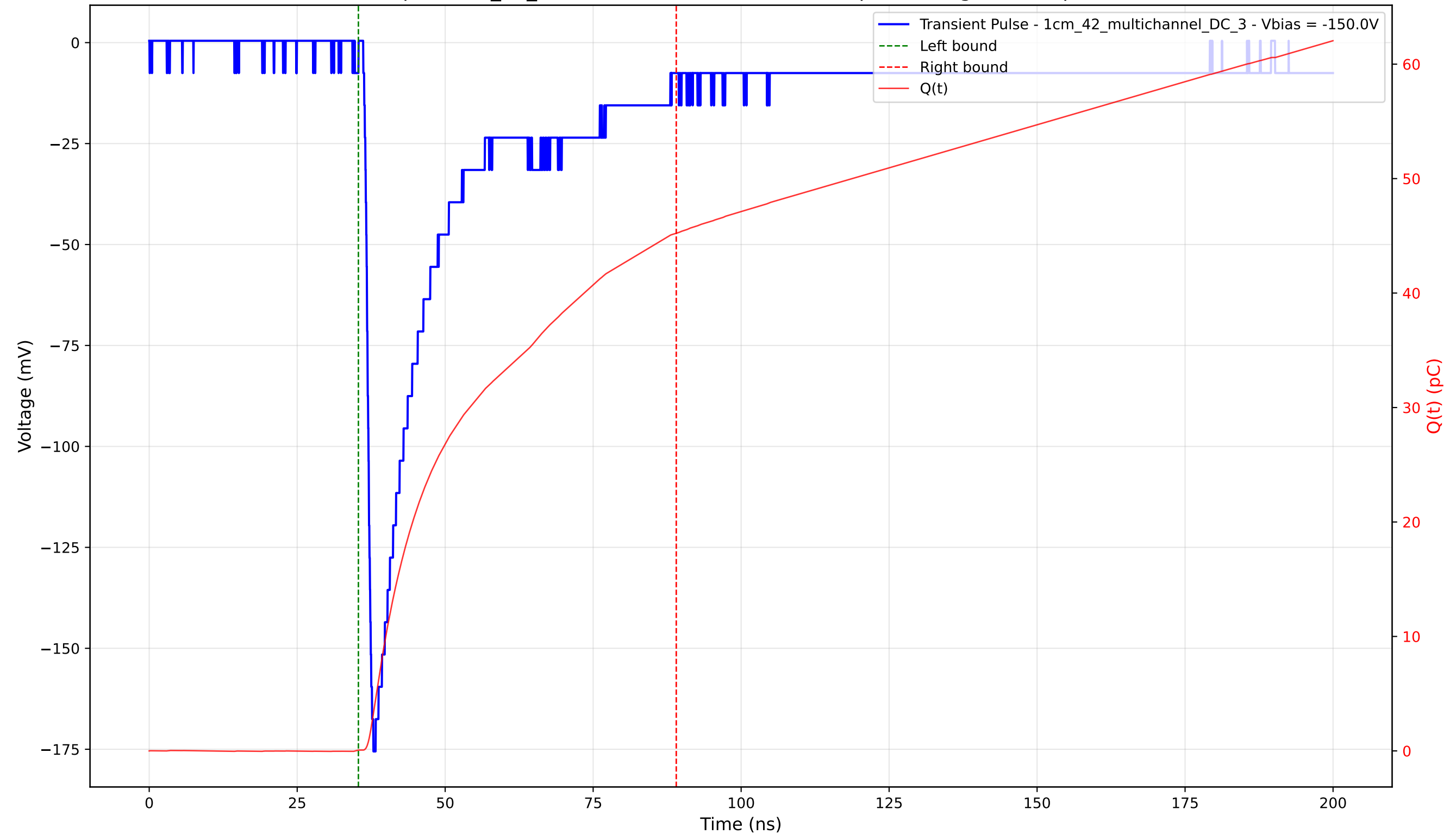
Transient Pulse - Sample: 1cm_42_multichannel - Position: 1025.0 \mu\text{m} - Charge: 45.15 pC - Rise Time: 1.09 ns
