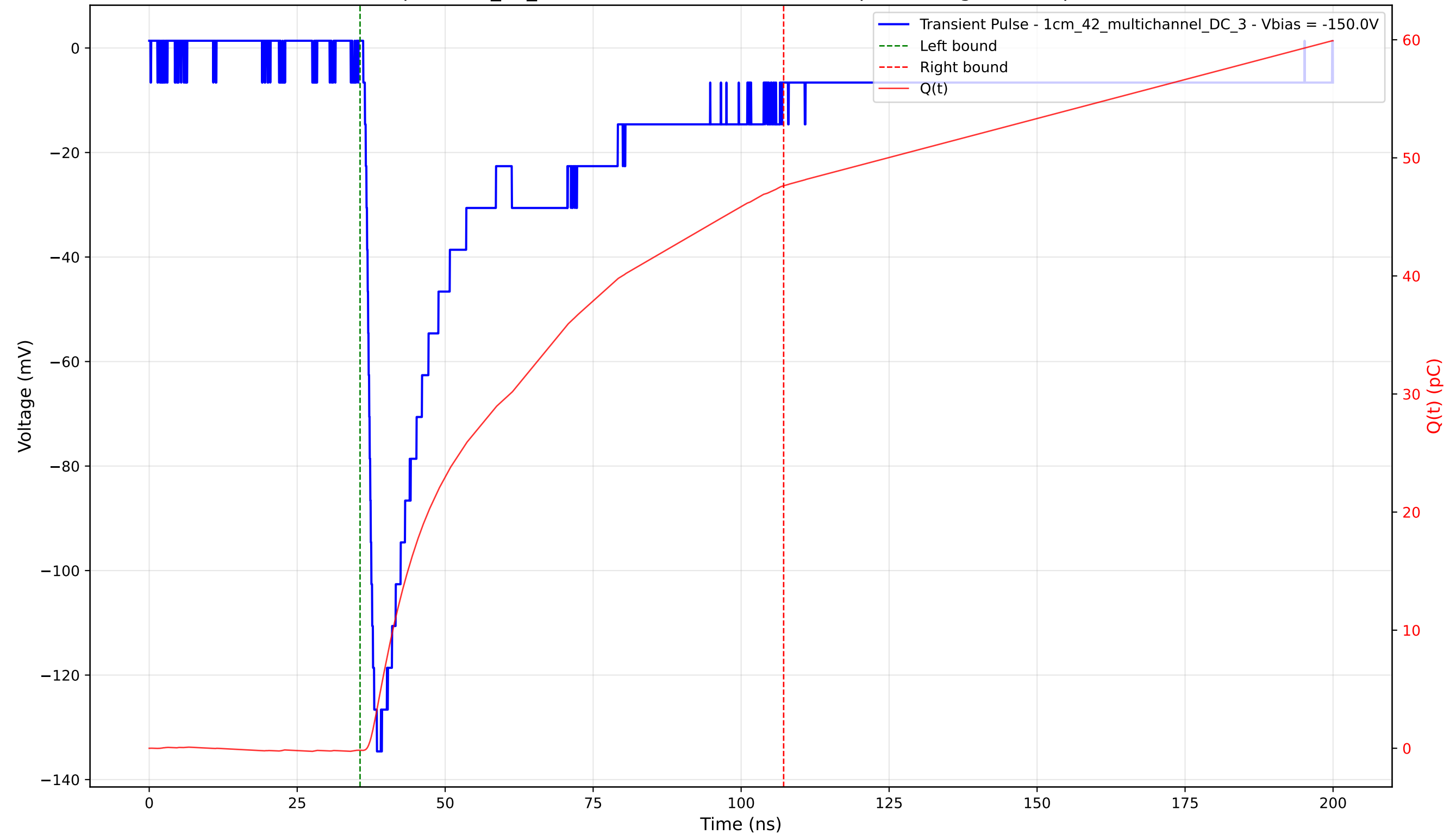
Transient Pulse - Sample: 1cm_42_multichannel - Position: 1505.0 \mu\text{m} - Charge: 47.81 pC - Rise Time: 1.56 ns
