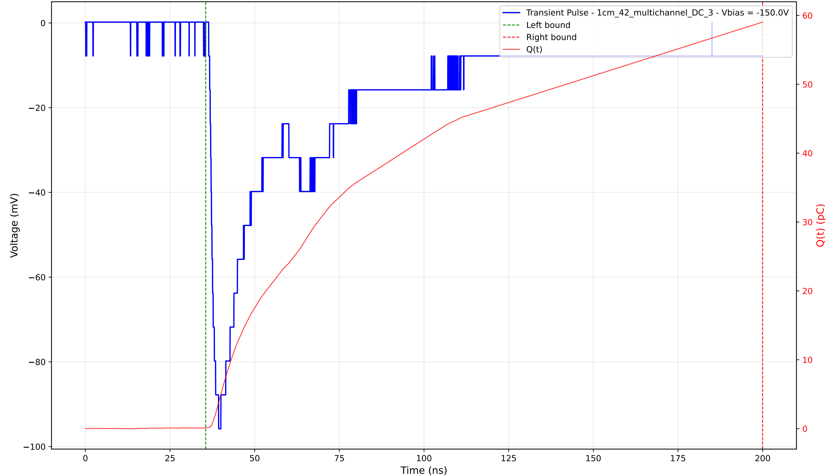
Transient Pulse - Sample: 1cm_42_multichannel - Position: 2075.0 \mu\text{m} - Charge: 58.87 pC - Rise Time: 1.78 ns
