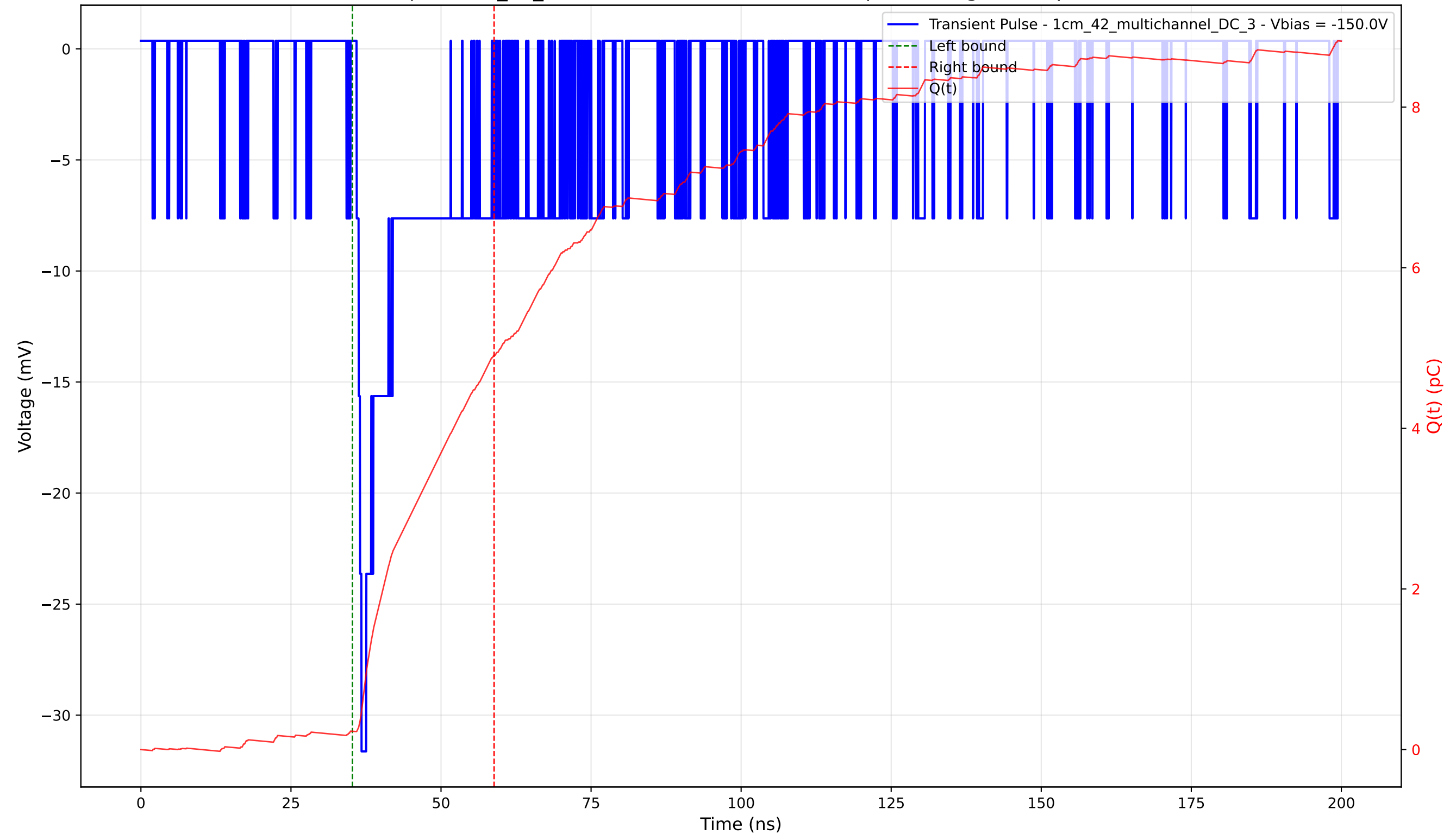
Transient Pulse - Sample: 1cm_42_multichannel - Position: 4880.0 \mu\text{m} - Charge: 4.68 pC - Rise Time: 0.81 ns
