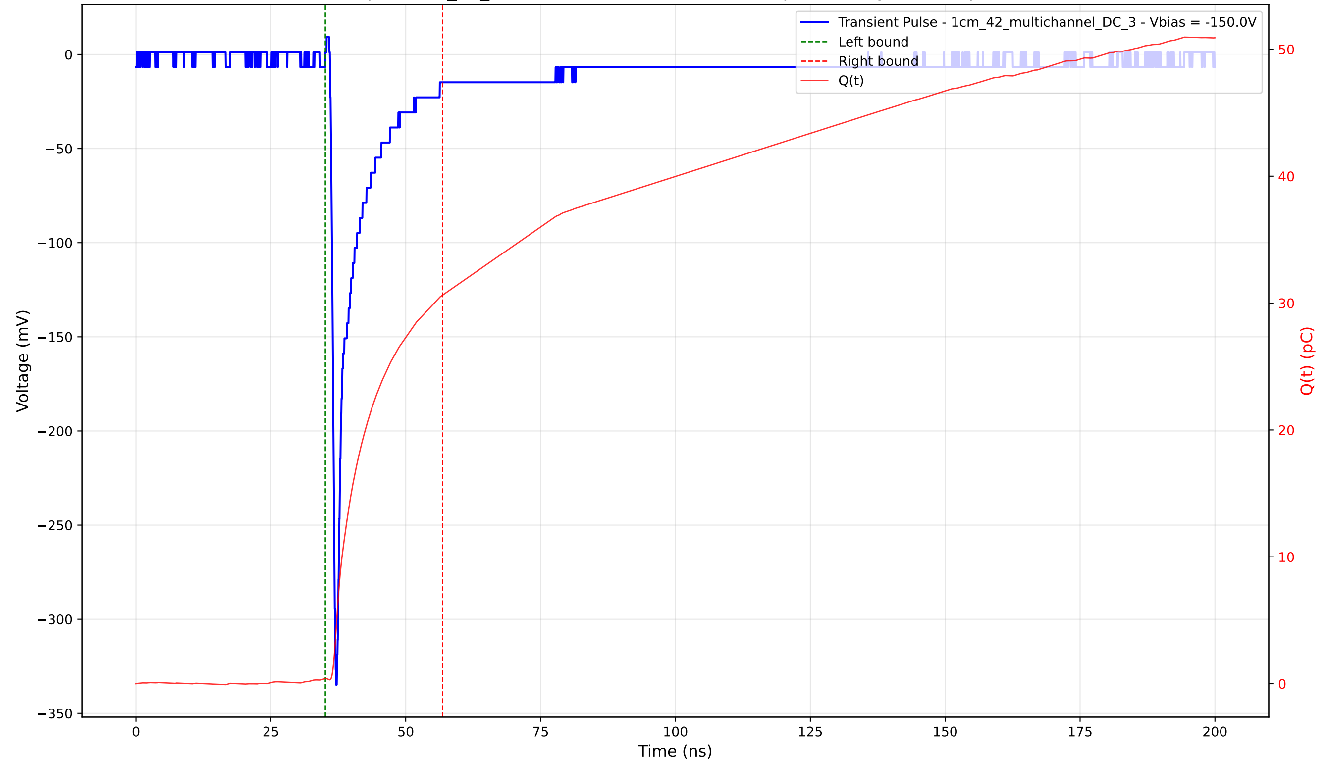
Transient Pulse - Sample: 1cm_42_multichannel - Position: 4820.0 \mu\text{m} - Charge: 30.21 pC - Rise Time: 0.77 ns
