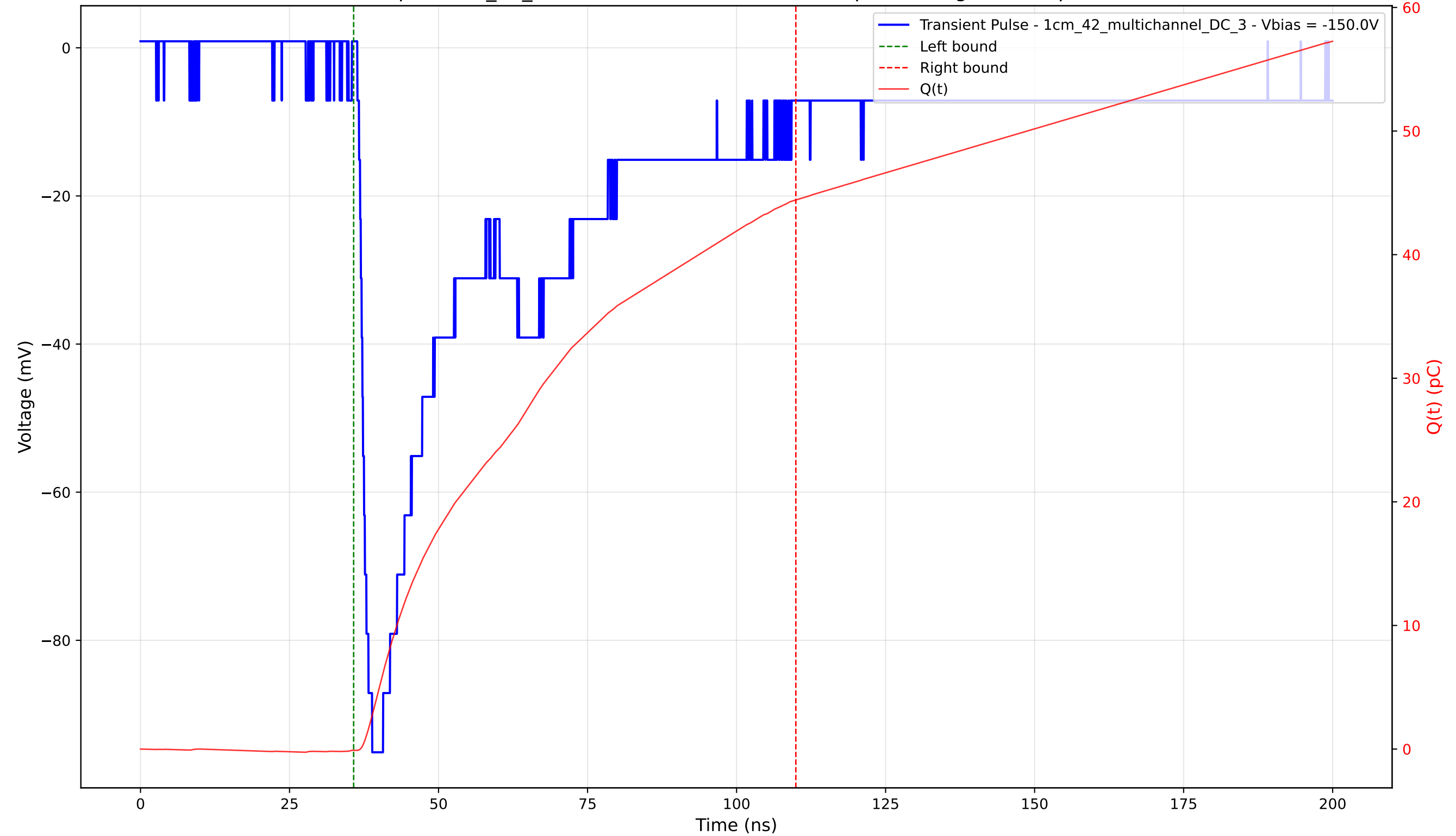
Transient Pulse - Sample: 1cm_42_multichannel - Position: 2045.0 \mu\text{m} - Charge: 44.53 pC - Rise Time: 1.59 ns
