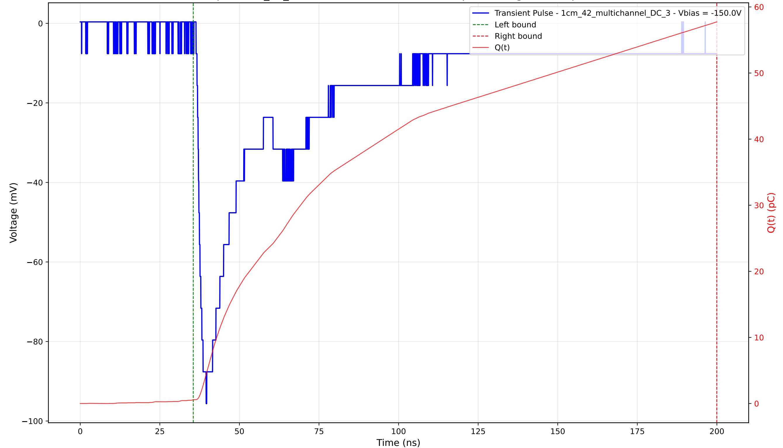
Transient Pulse - Sample: 1cm_42_multichannel - Position: 2715.0 \mu\text{m} - Charge: 57.17 pC - Rise Time: 1.92 ns
