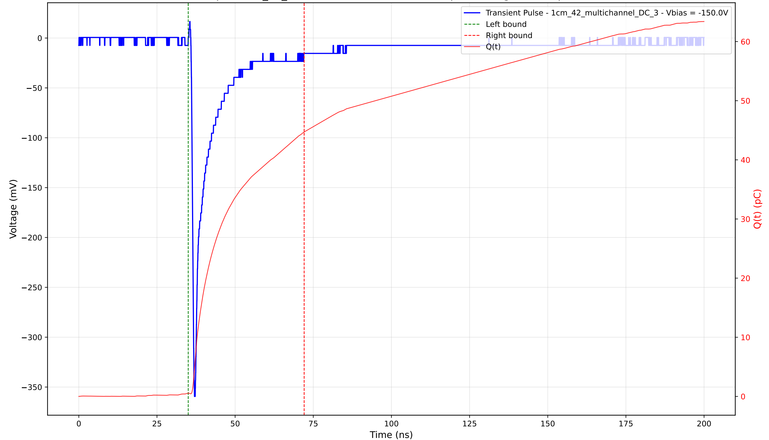
Transient Pulse - Sample: 1cm_42_multichannel - Position: 180.0 \mu\text{m} - Charge: 44.16 pC - Rise Time: 0.79 ns
