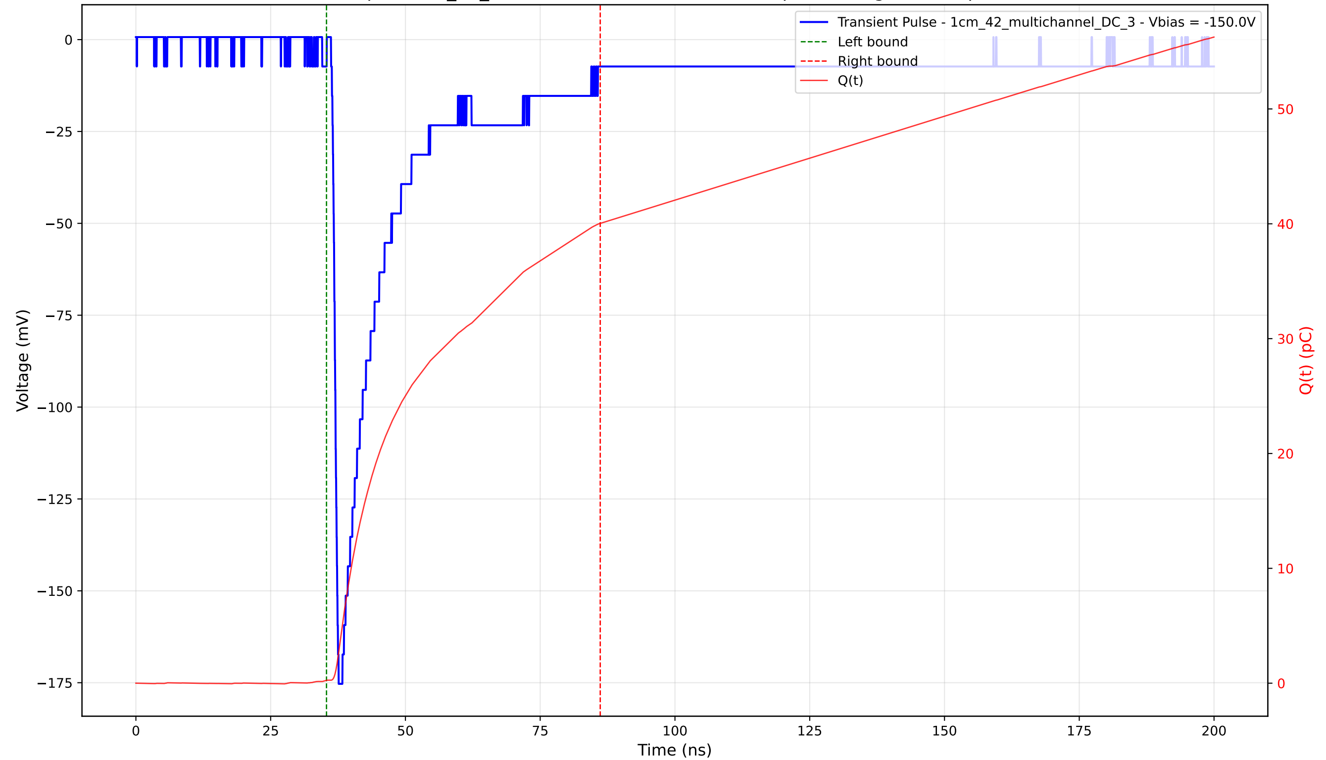
Transient Pulse - Sample: 1cm_42_multichannel - Position: 4085.0 \mu\text{m} - Charge: 39.78 pC - Rise Time: 0.95 ns
