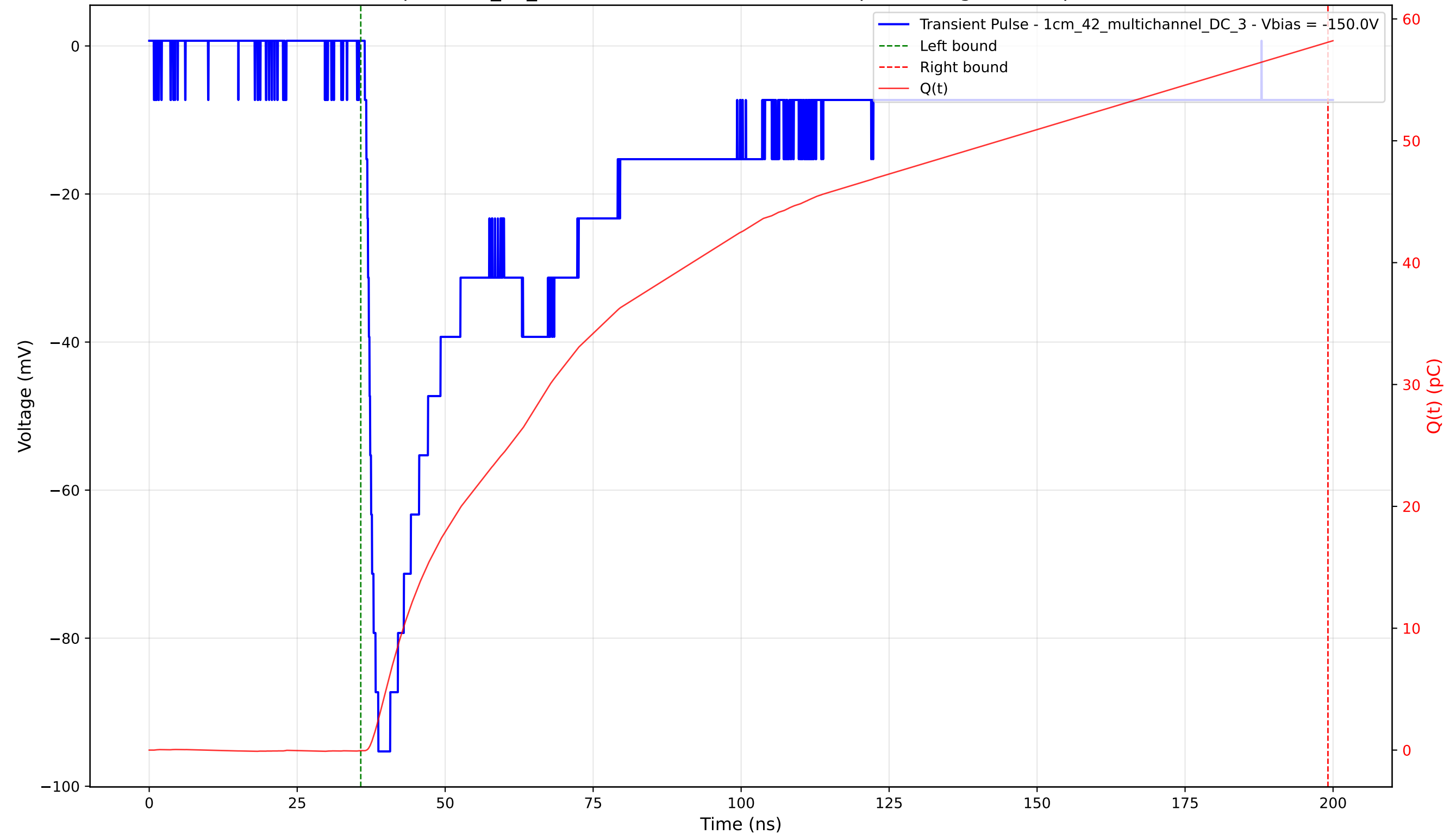
Transient Pulse - Sample: 1cm_42_multichannel - Position: 2040.0 \mu\text{m} - Charge: 58.13 pC - Rise Time: 1.57 ns
