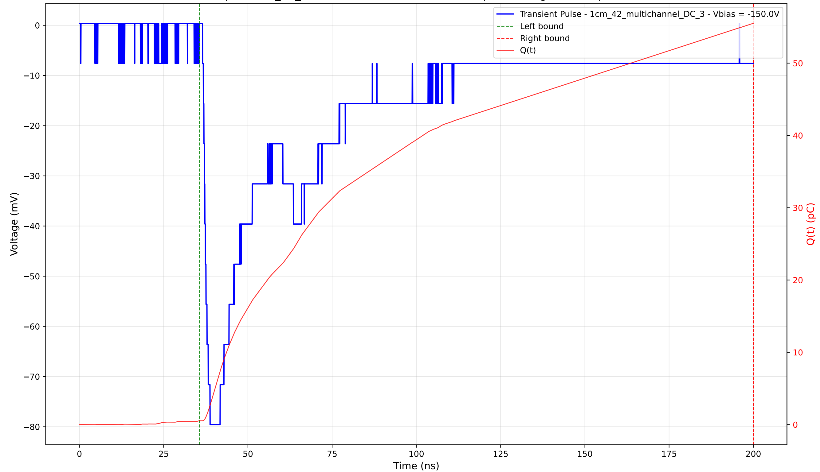
Transient Pulse - Sample: 1cm_42_multichannel - Position: 2590.0 \mu\text{m} - Charge: 54.98 pC - Rise Time: 2.00 ns
