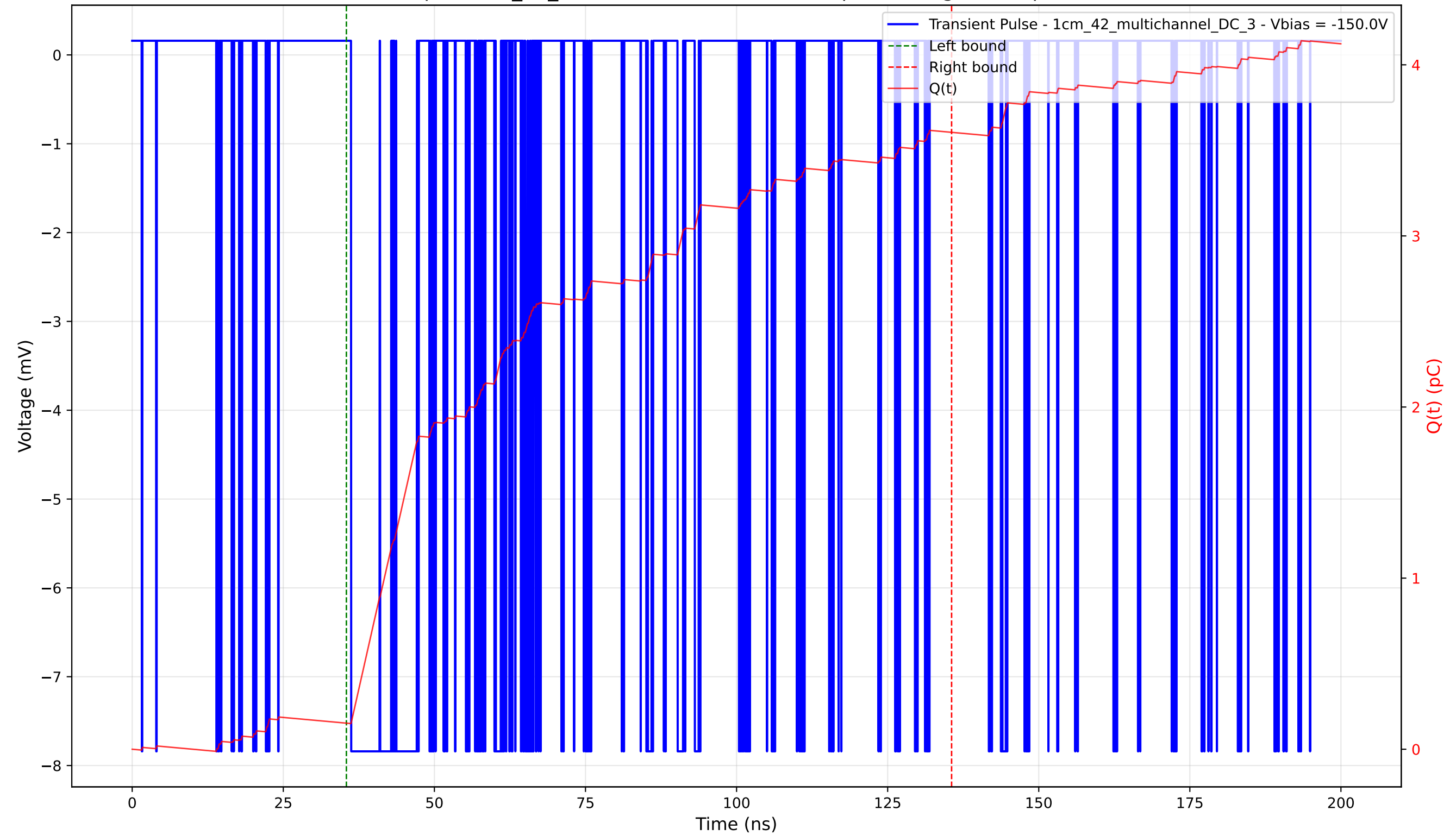
Transient Pulse - Sample: 1cm_42_multichannel - Position: 0.0 \mu\text{m} - Charge: 3.45 pC - Rise Time: 0.02 ns
