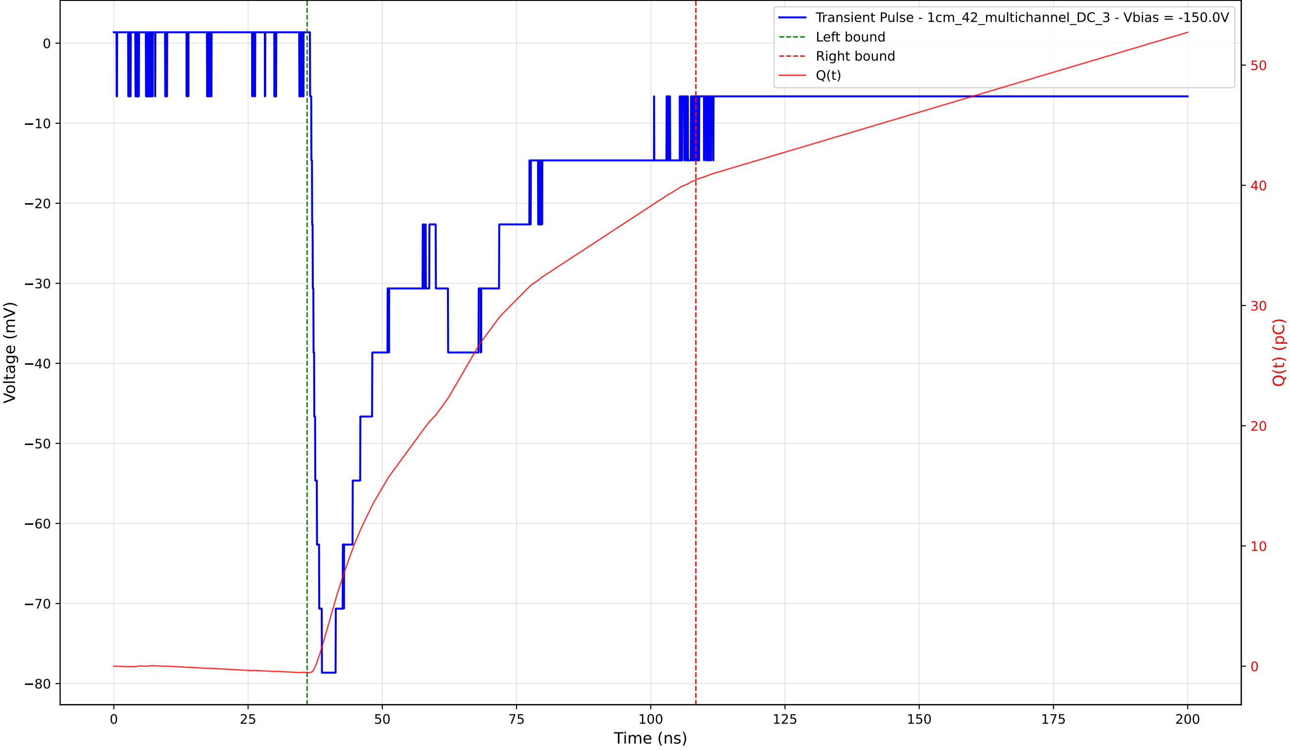
Transient Pulse - Sample: 1cm_42_multichannel - Position: 2285.0 \mu\text{m} - Charge: 40.98 pC - Rise Time: 1.98 ns
