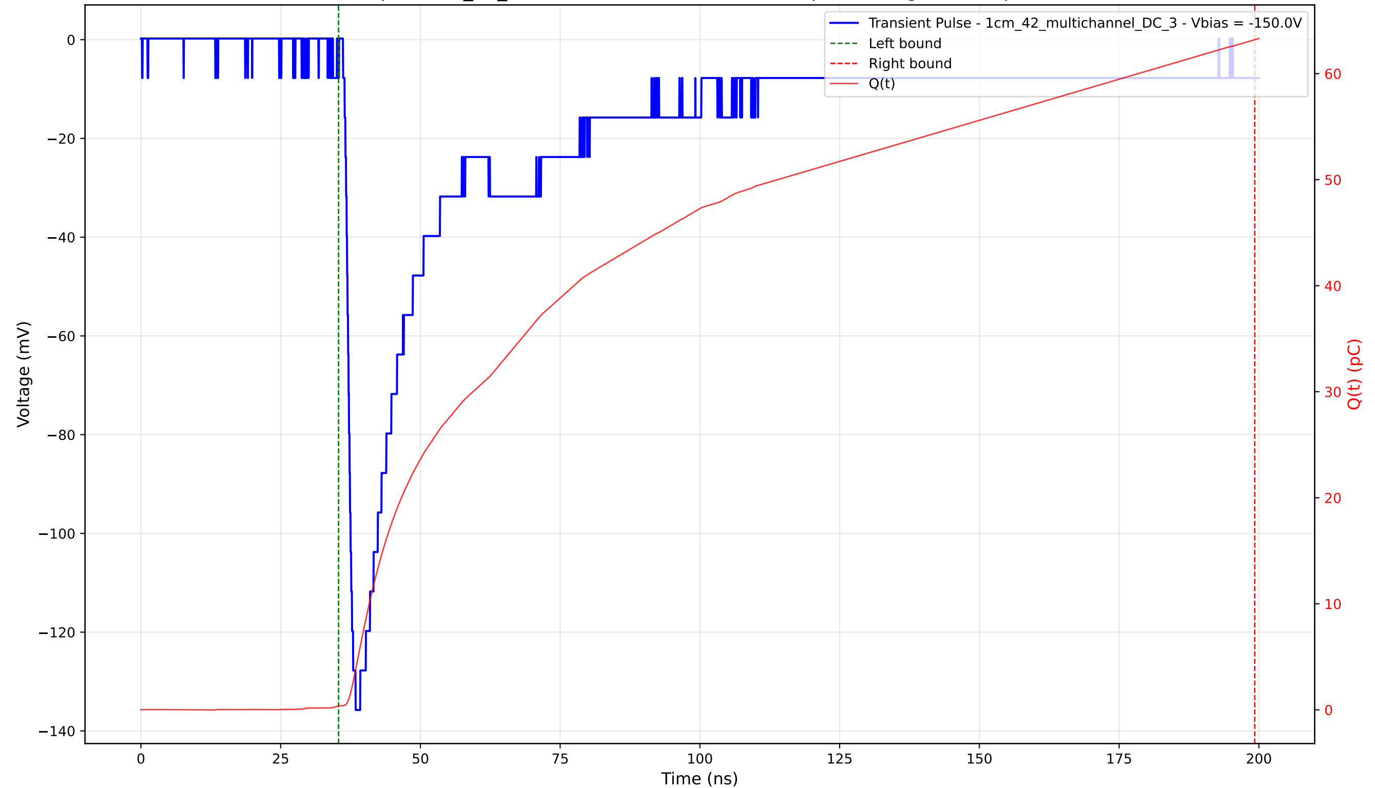
Transient Pulse - Sample: 1cm_42_multichannel - Position: 1465.0 \mu\text{m} - Charge: 62.83 pC - Rise Time: 1.53 ns
