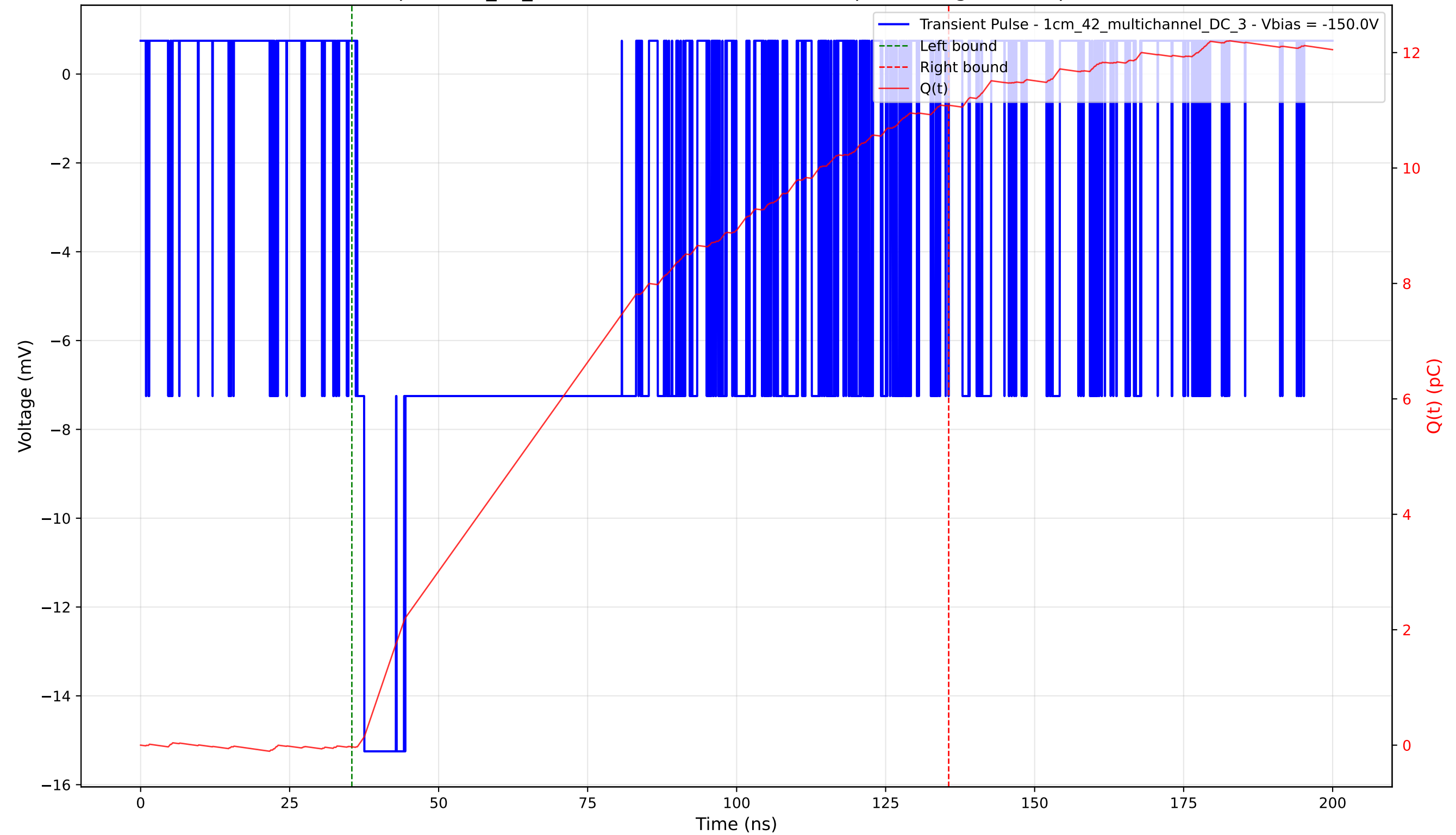
Transient Pulse - Sample: 1cm_42_multichannel - Position: 3360.0 \mu\text{m} - Charge: 11.11 pC - Rise Time: 1.18 ns
