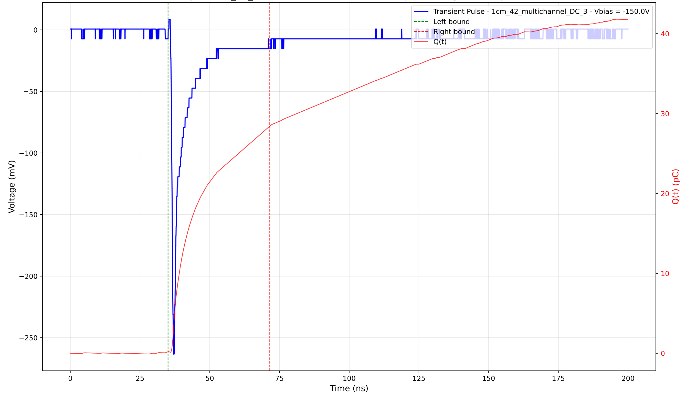
Transient Pulse - Sample: 1cm_42_multichannel - Position: 4840.0 \mu\text{m} - Charge: 28.23 pC - Rise Time: 0.77 ns
