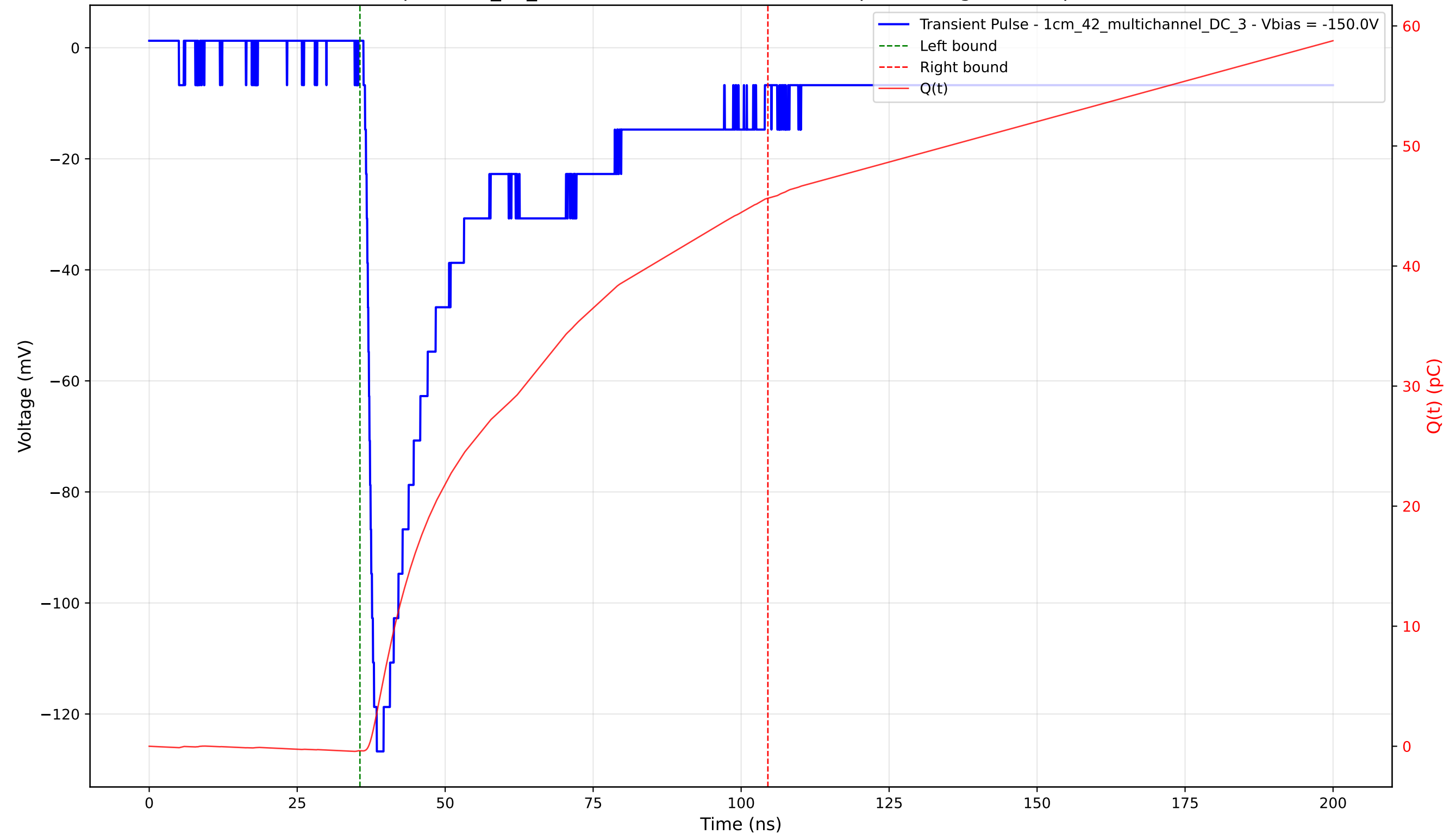
Transient Pulse - Sample: 1cm_42_multichannel - Position: 1560.0 \mu\text{m} - Charge: 46.02 pC - Rise Time: 1.53 ns
