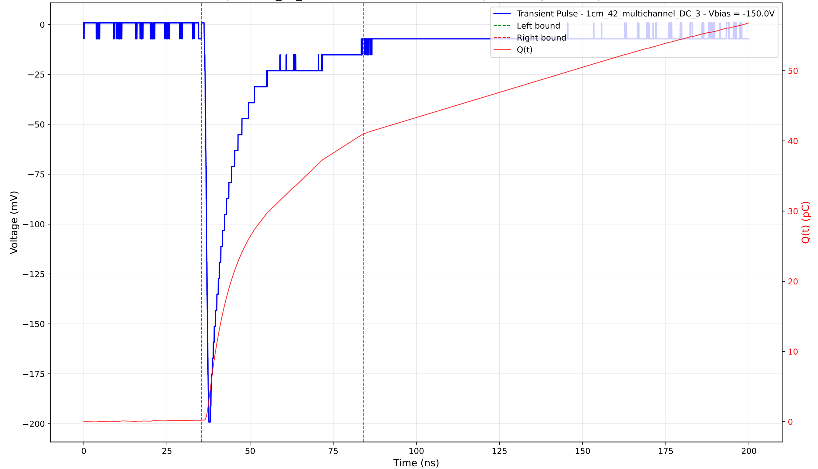
Transient Pulse - Sample: 1cm_42_multichannel - Position: 4180.0 \mu\text{m} - Charge: 40.77 pC - Rise Time: 0.99 ns
