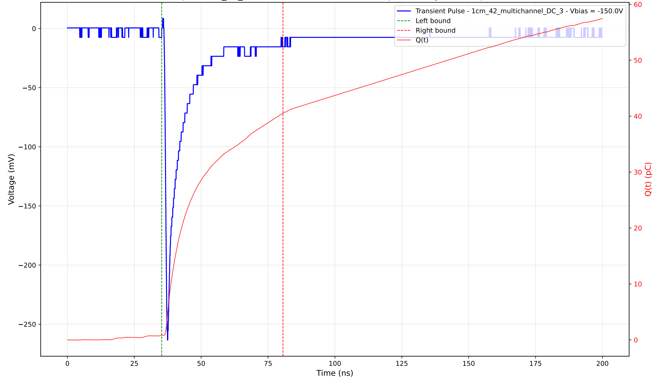
Transient Pulse - Sample: 1cm_42_multichannel - Position: 4500.0 \mu\text{m} - Charge: 39.66 pC - Rise Time: 0.87 ns
