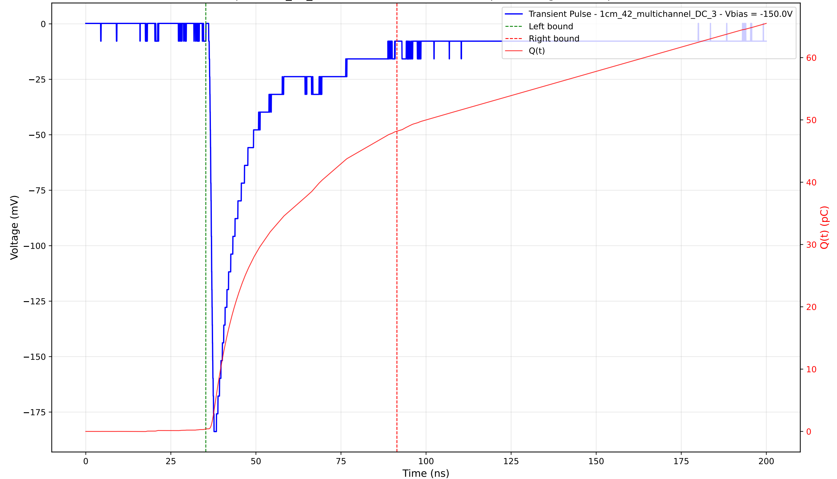
Transient Pulse - Sample: 1cm_42_multichannel - Position: 970.0 \mu\text{m} - Charge: 47.78 pC - Rise Time: 1.07 ns
