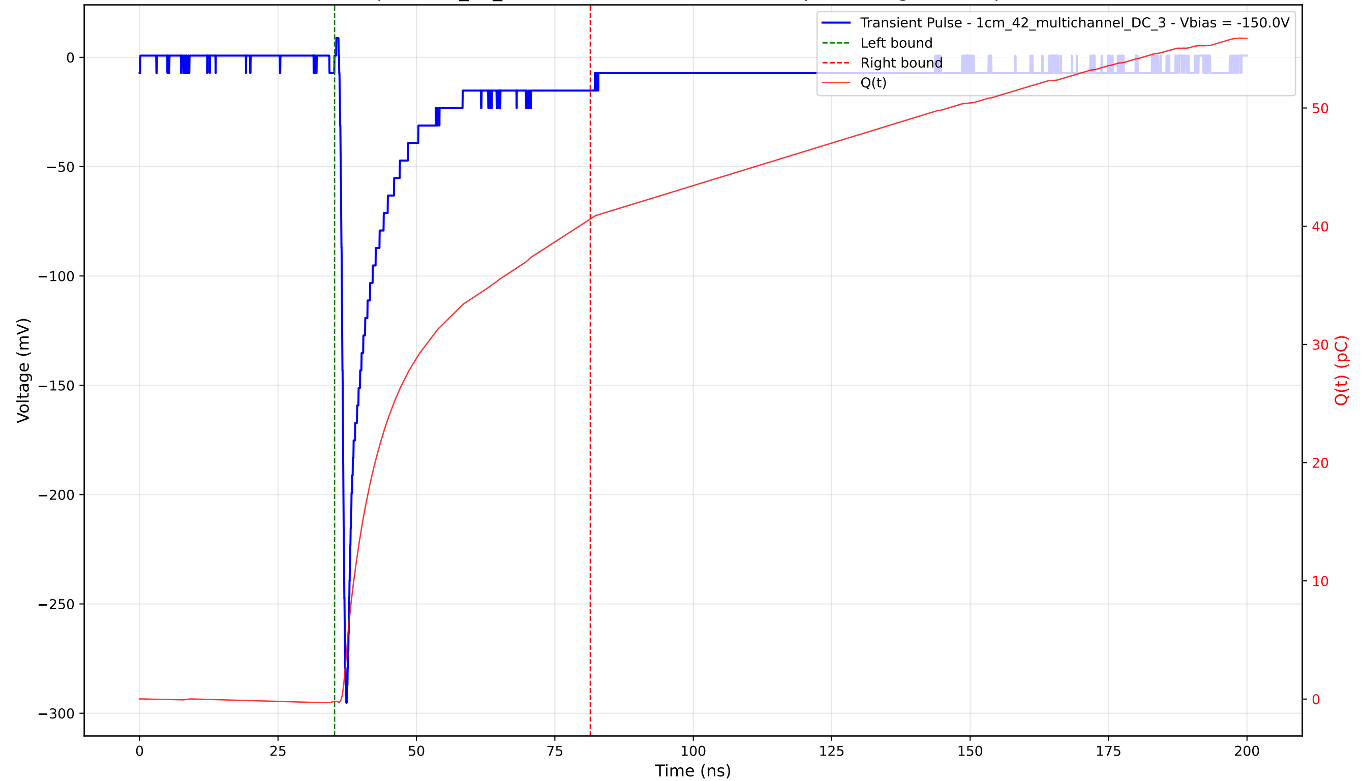
Transient Pulse - Sample: 1cm_42_multichannel - Position: 4580.0 \mu\text{m} - Charge: 40.80 pC - Rise Time: 0.88 ns
