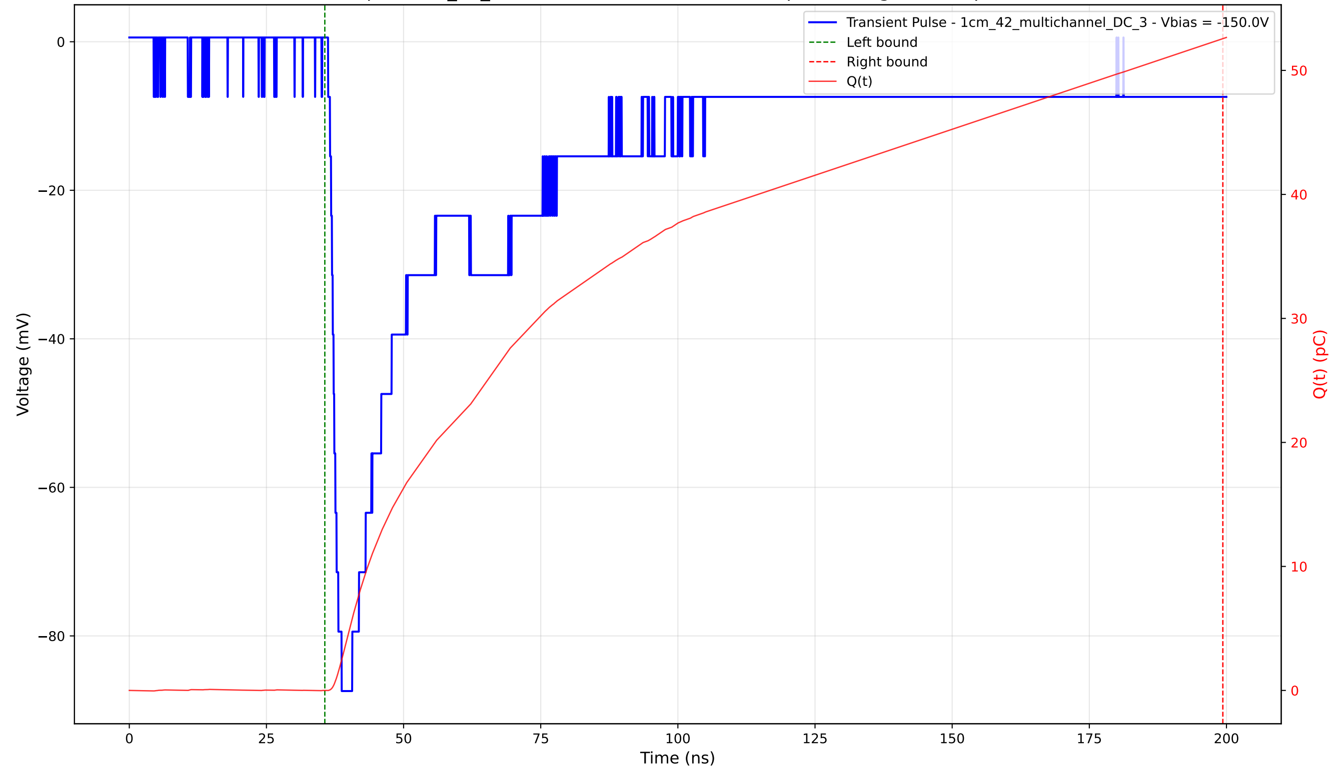
Transient Pulse - Sample: 1cm_42_multichannel - Position: 1940.0 \mu\text{m} - Charge: 52.57 pC - Rise Time: 1.54 ns
