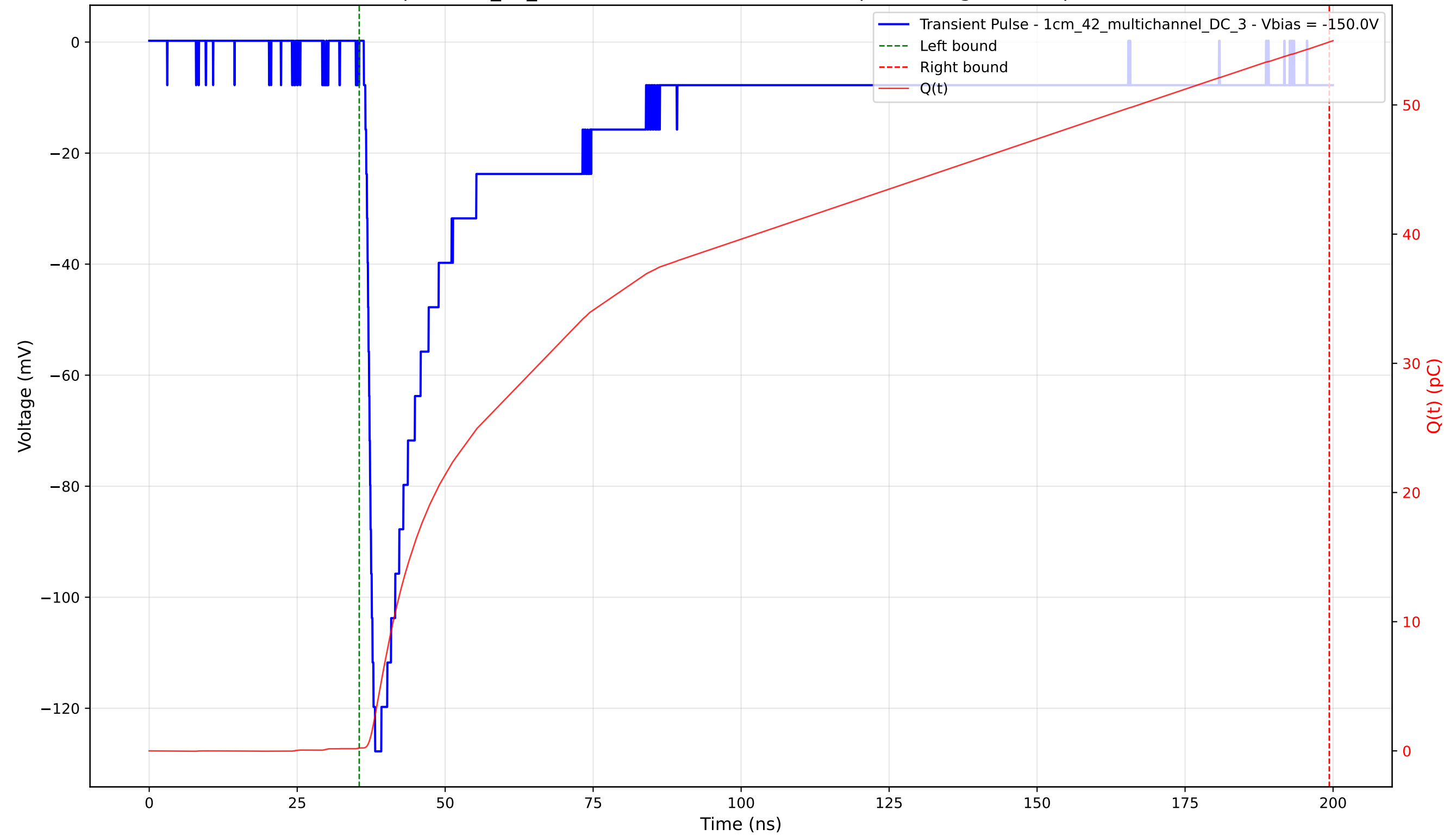
Transient Pulse - Sample: 1cm_42_multichannel - Position: 3620.0 \mu\text{m} - Charge: 54.65 pC - Rise Time: 1.37 ns
