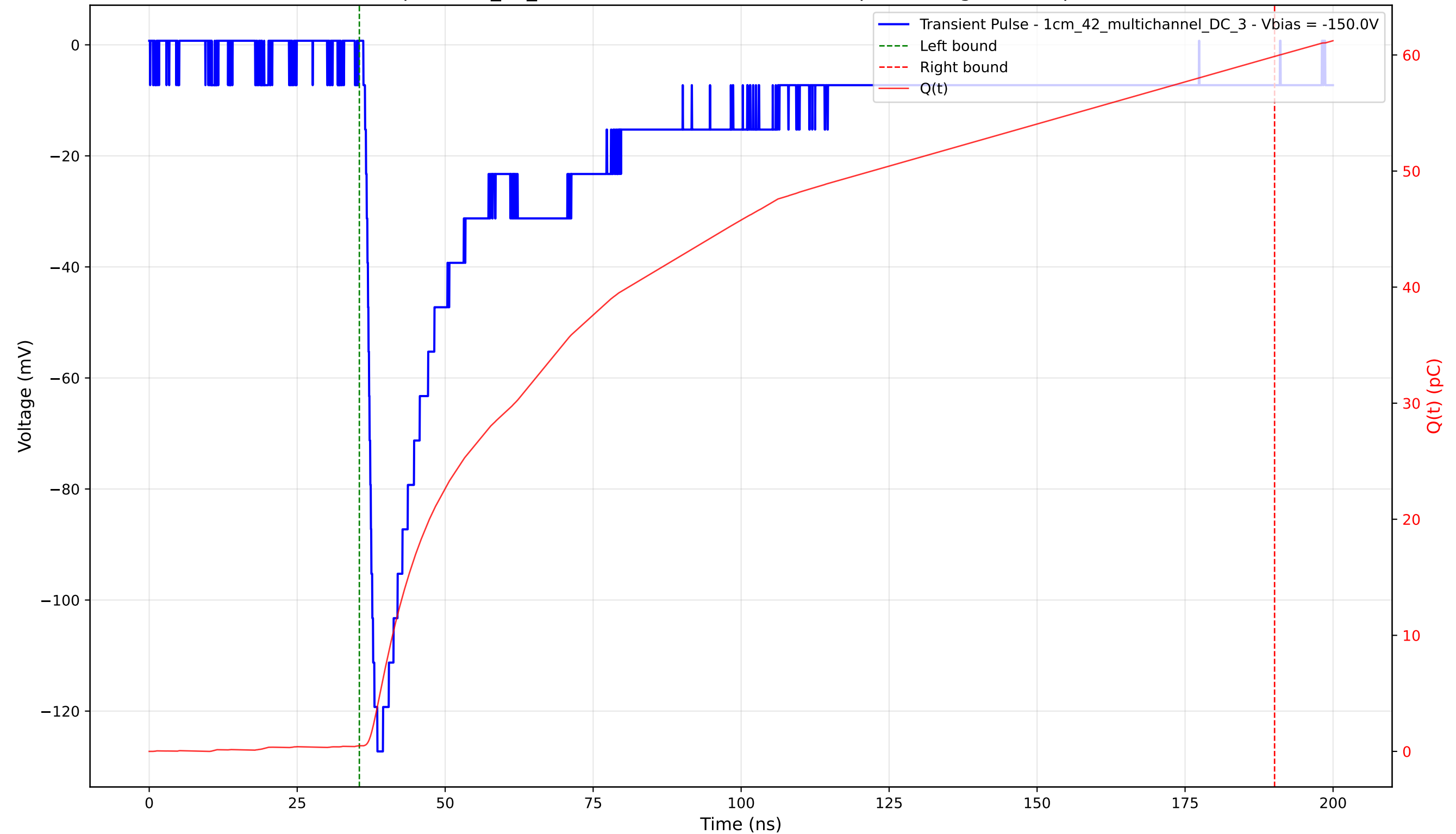
Transient Pulse - Sample: 1cm_42_multichannel - Position: 1570.0 \mu\text{m} - Charge: 59.40 pC - Rise Time: 1.59 ns
