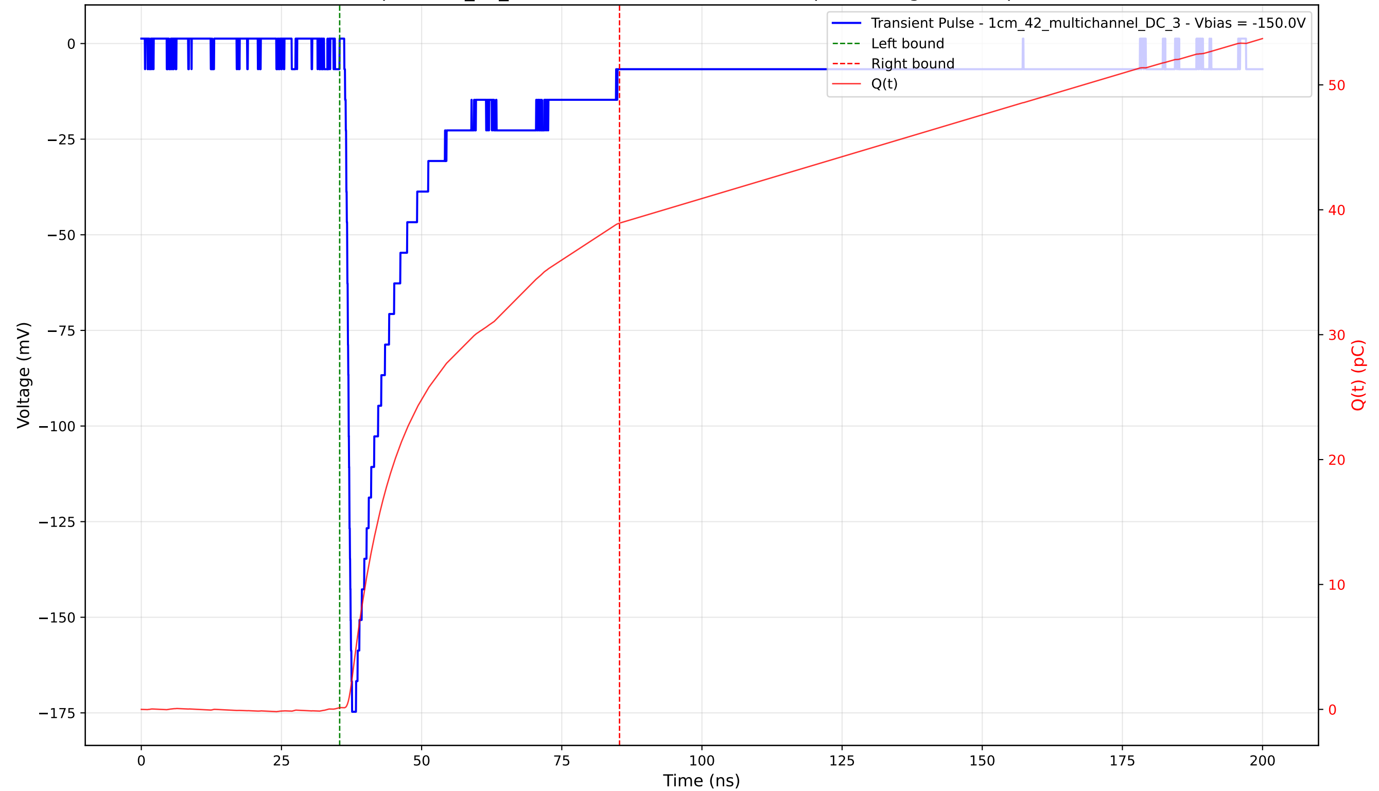
Transient Pulse - Sample: 1cm_42_multichannel - Position: 4090.0 \mu\text{m} - Charge: 38.79 pC - Rise Time: 0.93 ns
