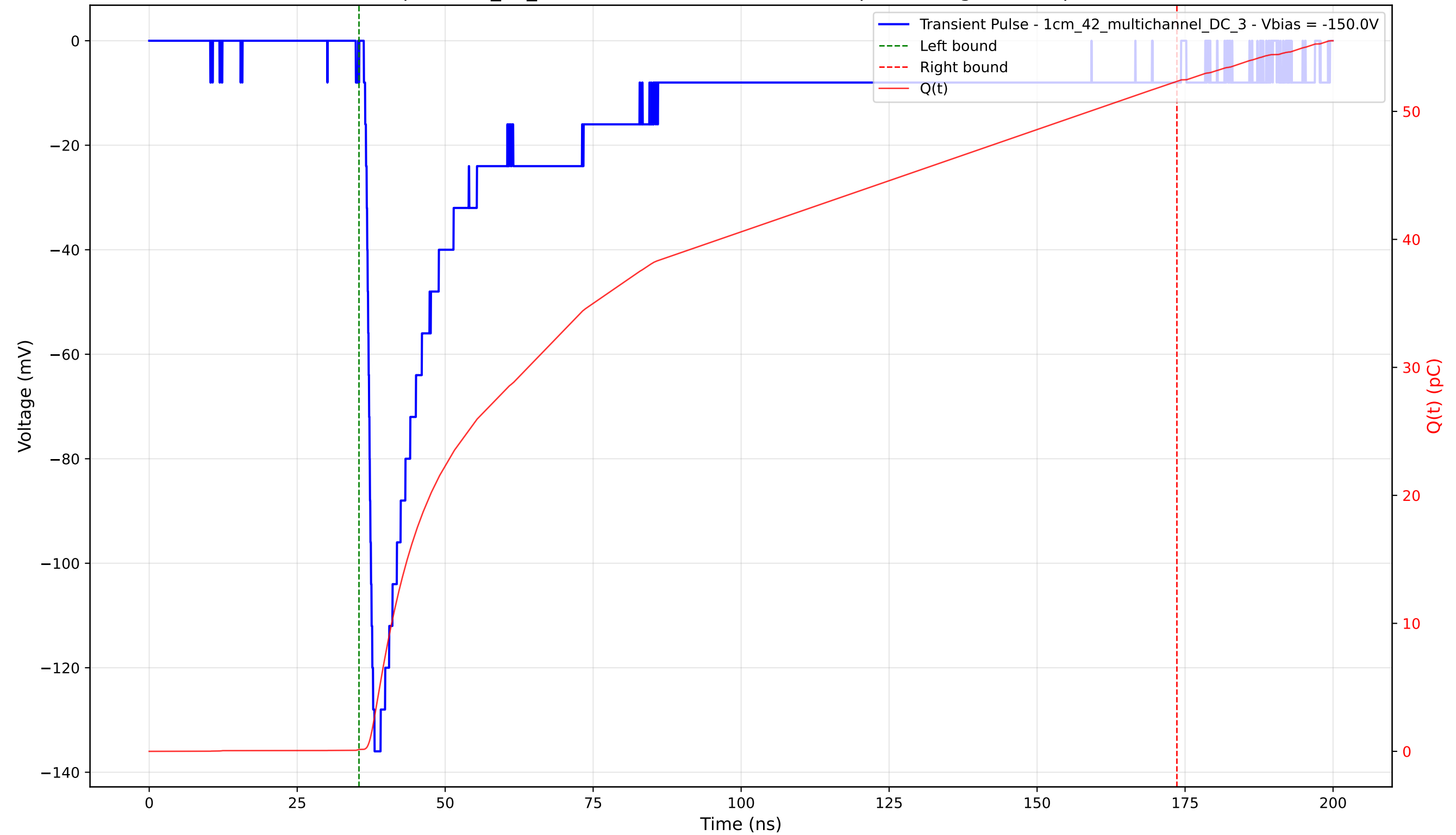
Transient Pulse - Sample: 1cm_42_multichannel - Position: 3700.0 \mu\text{m} - Charge: 52.21 pC - Rise Time: 1.35 ns
