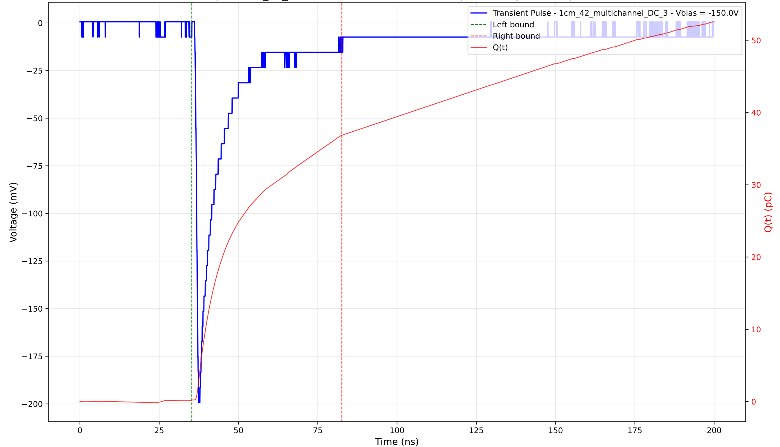
Transient Pulse - Sample: 1cm_42_multichannel - Position: 4290.0 \mu\text{m} - Charge: 36.63 pC - Rise Time: 0.93 ns
