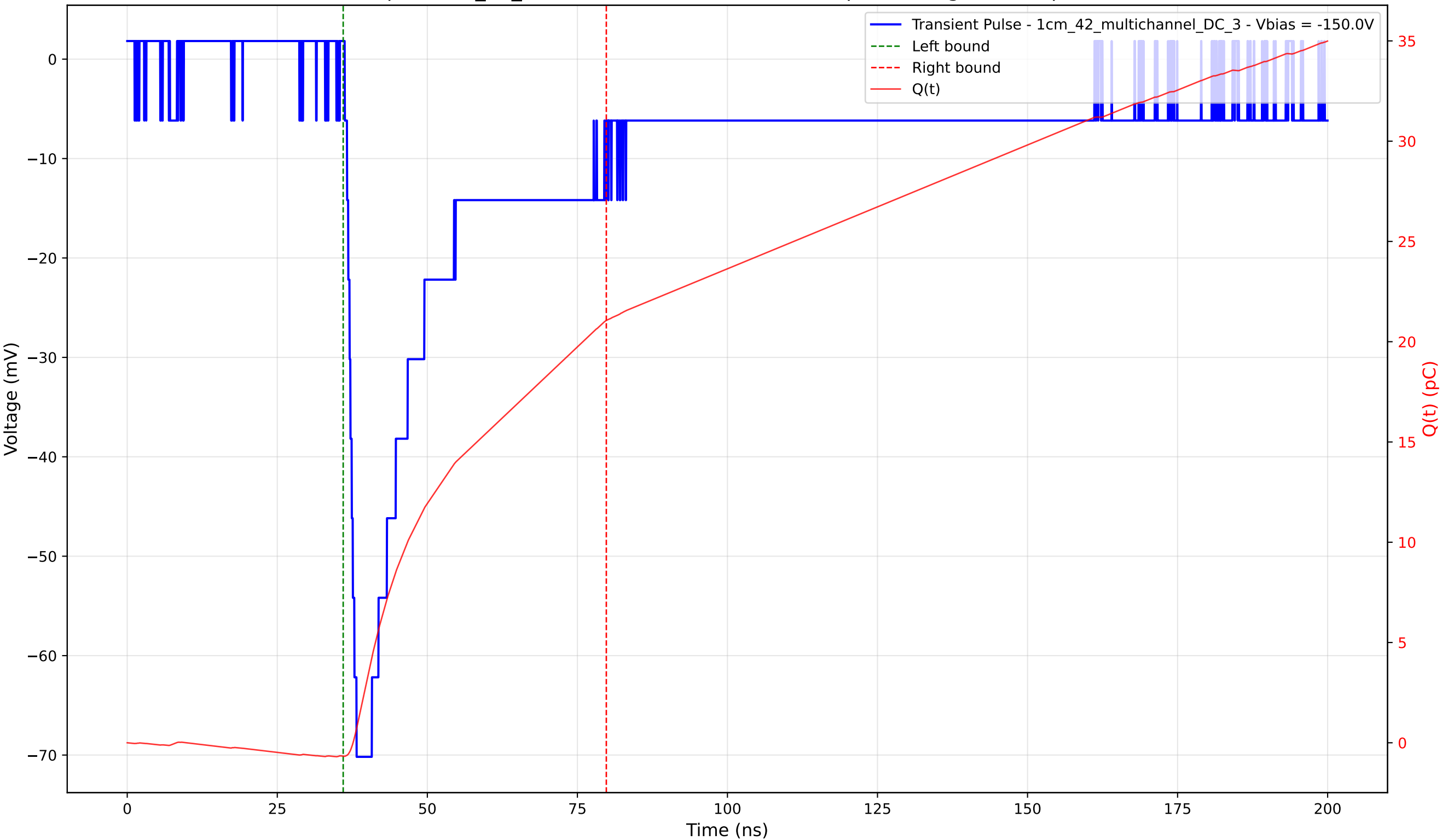
Transient Pulse - Sample: 1cm_42_multichannel - Position: 3330.0 \mu\text{m} - Charge: 21.73 pC - Rise Time: 1.60 ns
