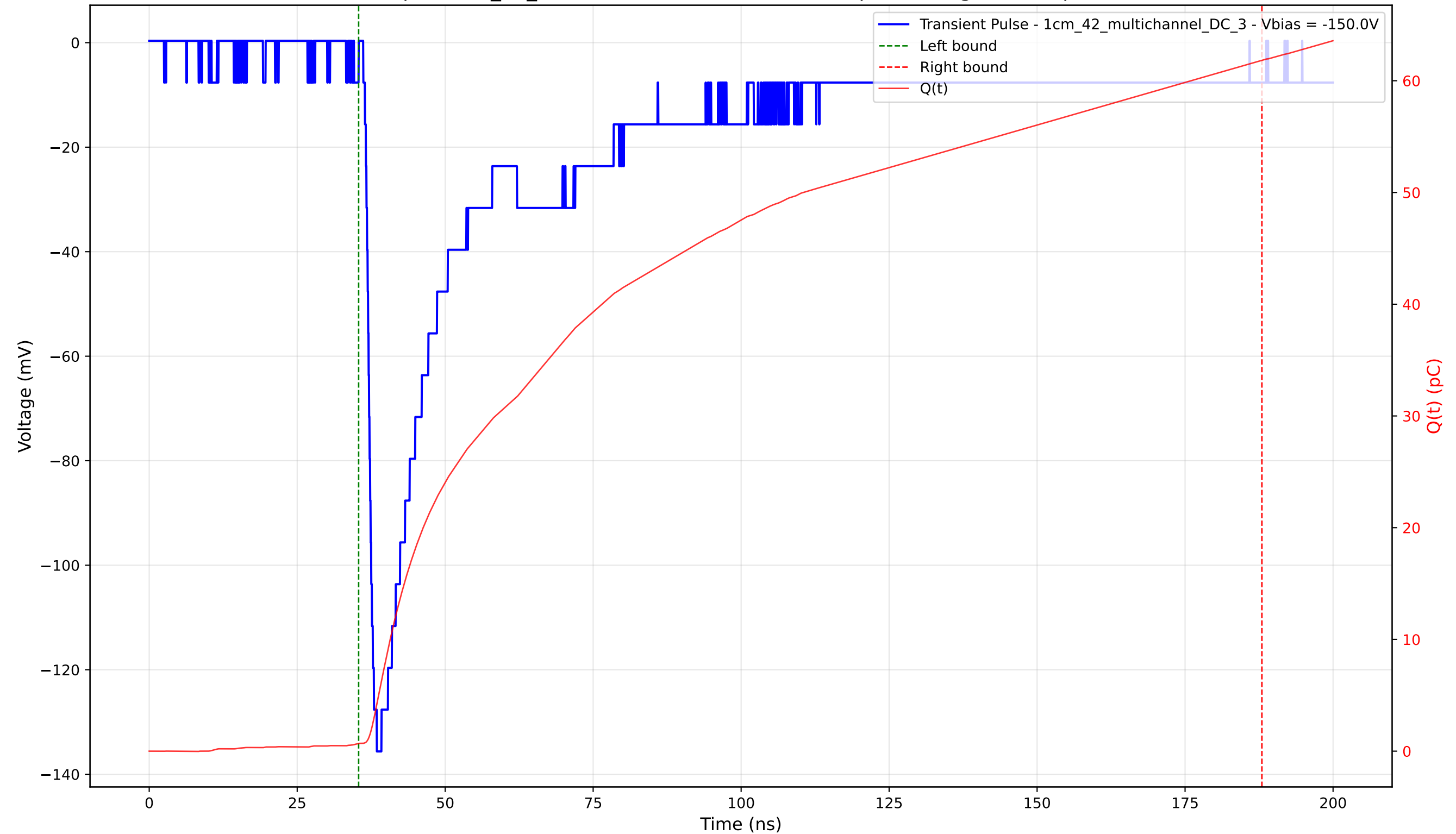
Transient Pulse - Sample: 1cm_42_multichannel - Position: 1480.0 \mu\text{m} - Charge: 61.14 pC - Rise Time: 1.53 ns
