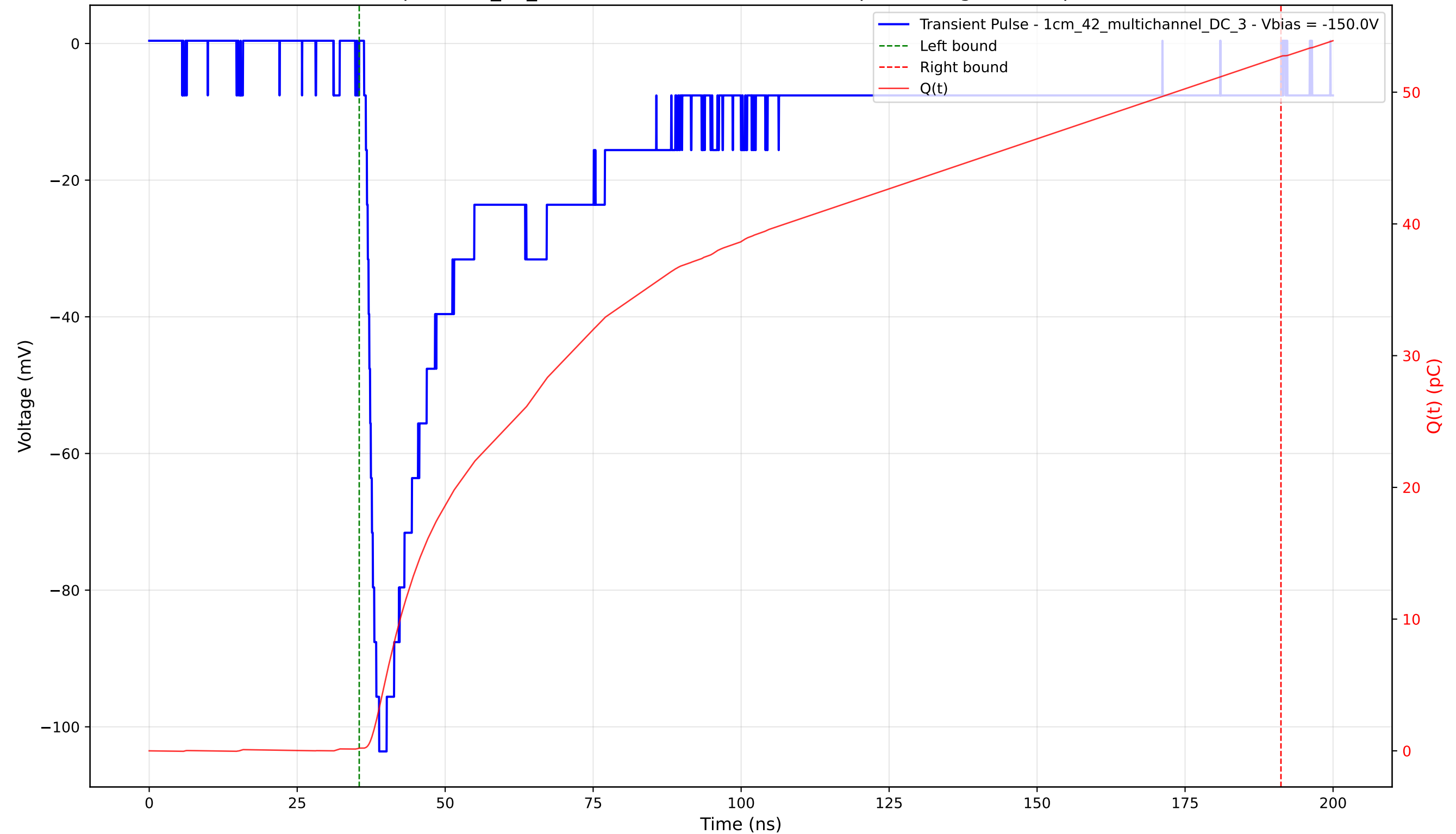
Transient Pulse - Sample: 1cm_42_multichannel - Position: 3110.0 \mu\text{m} - Charge: 52.52 pC - Rise Time: 1.77 ns
