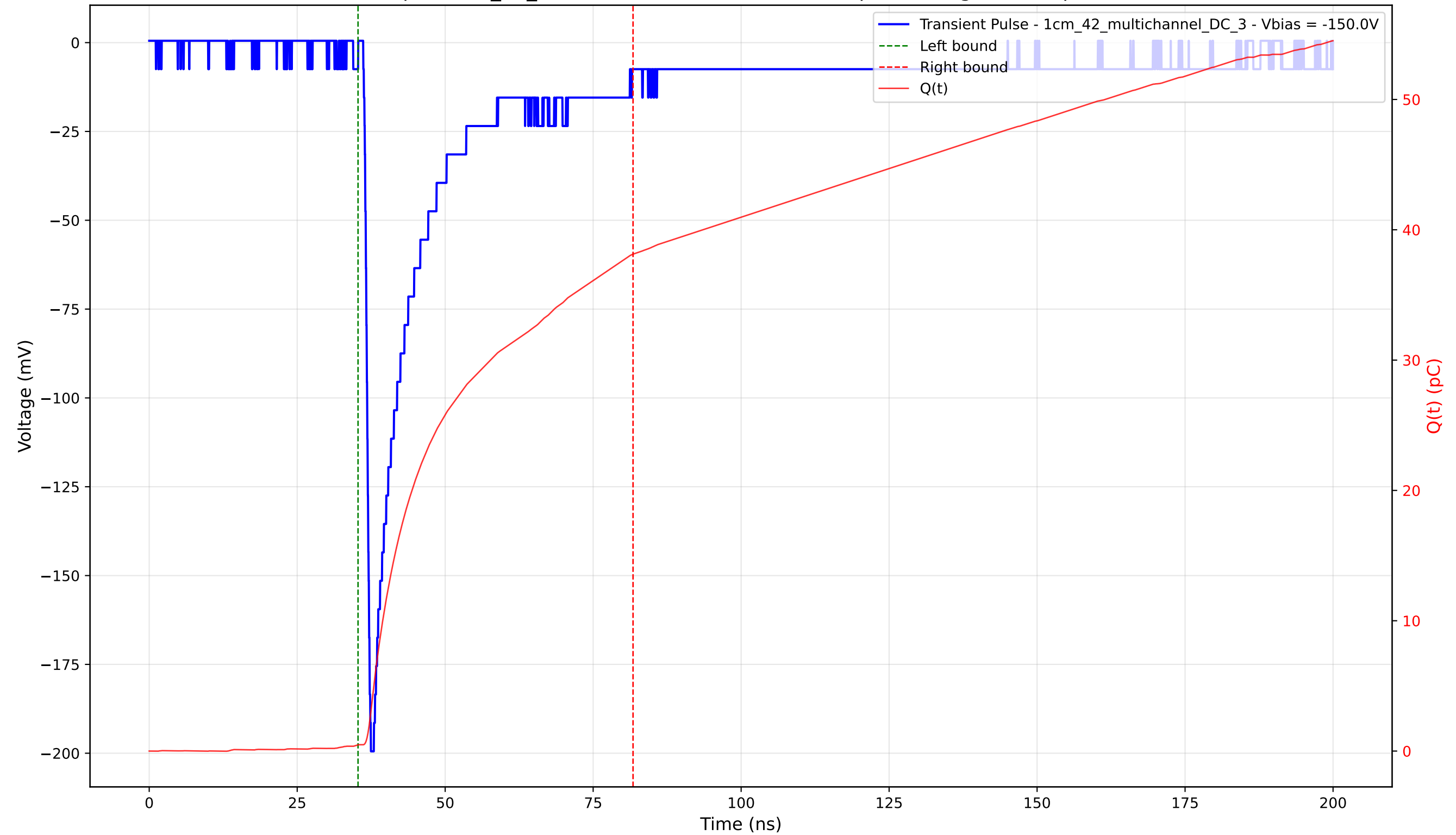
Transient Pulse - Sample: 1cm_42_multichannel - Position: 4270.0 \mu\text{m} - Charge: 37.64 pC - Rise Time: 0.91 ns
