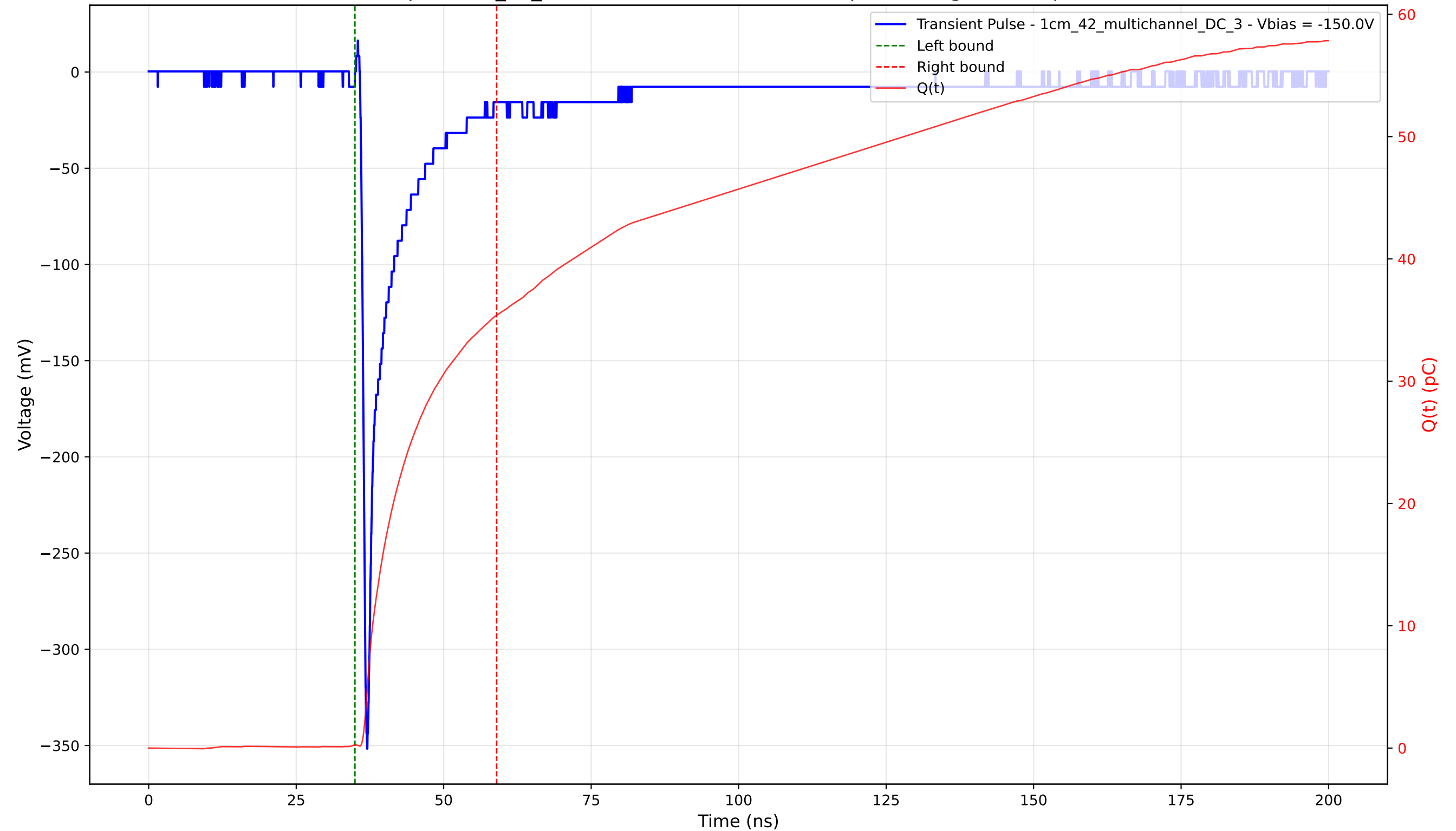
Transient Pulse - Sample: 1cm_42_multichannel - Position: 115.0 \mu\text{m} - Charge: 35.12 pC - Rise Time: 0.79 ns
