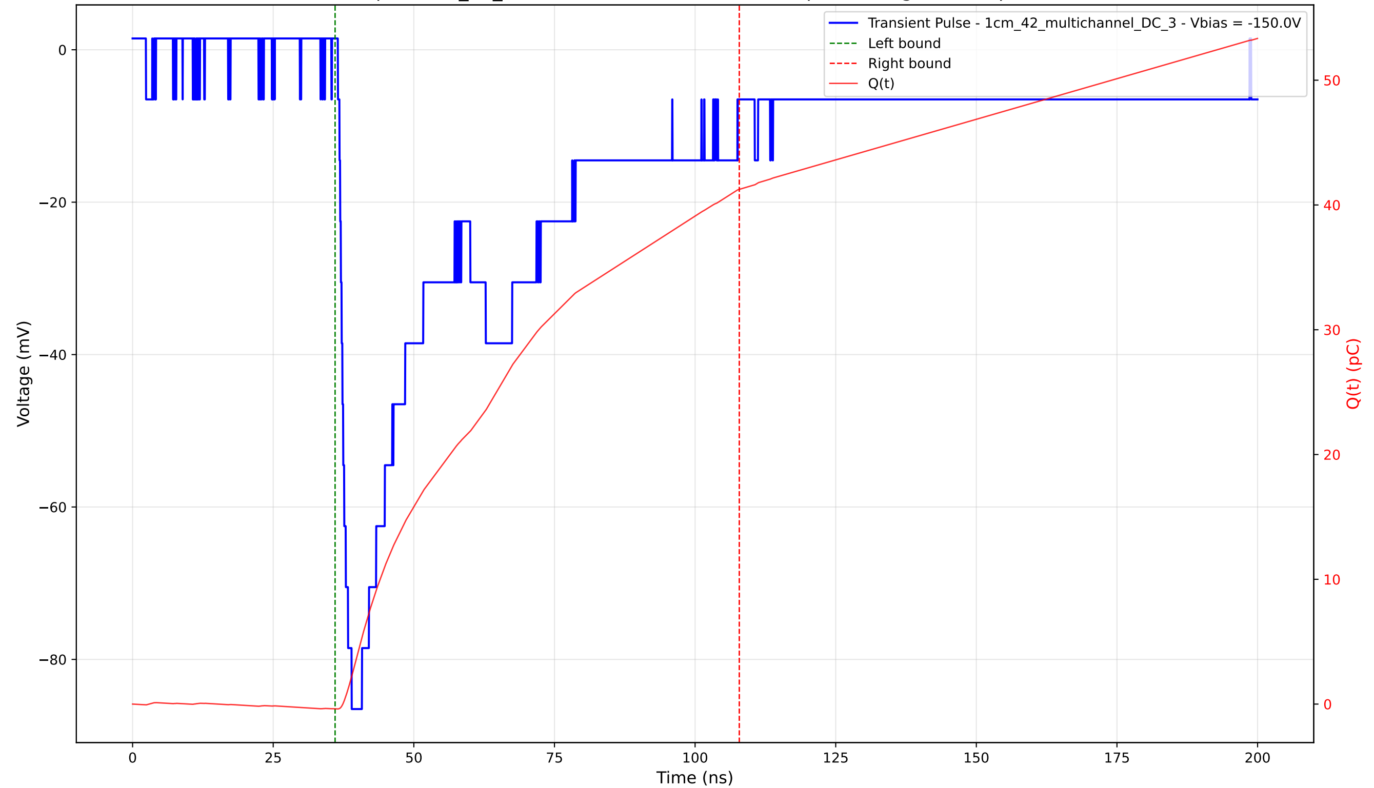
Transient Pulse - Sample: 1cm_42_multichannel - Position: 2150.0 \mu\text{m} - Charge: 41.63 pC - Rise Time: 1.53 ns
