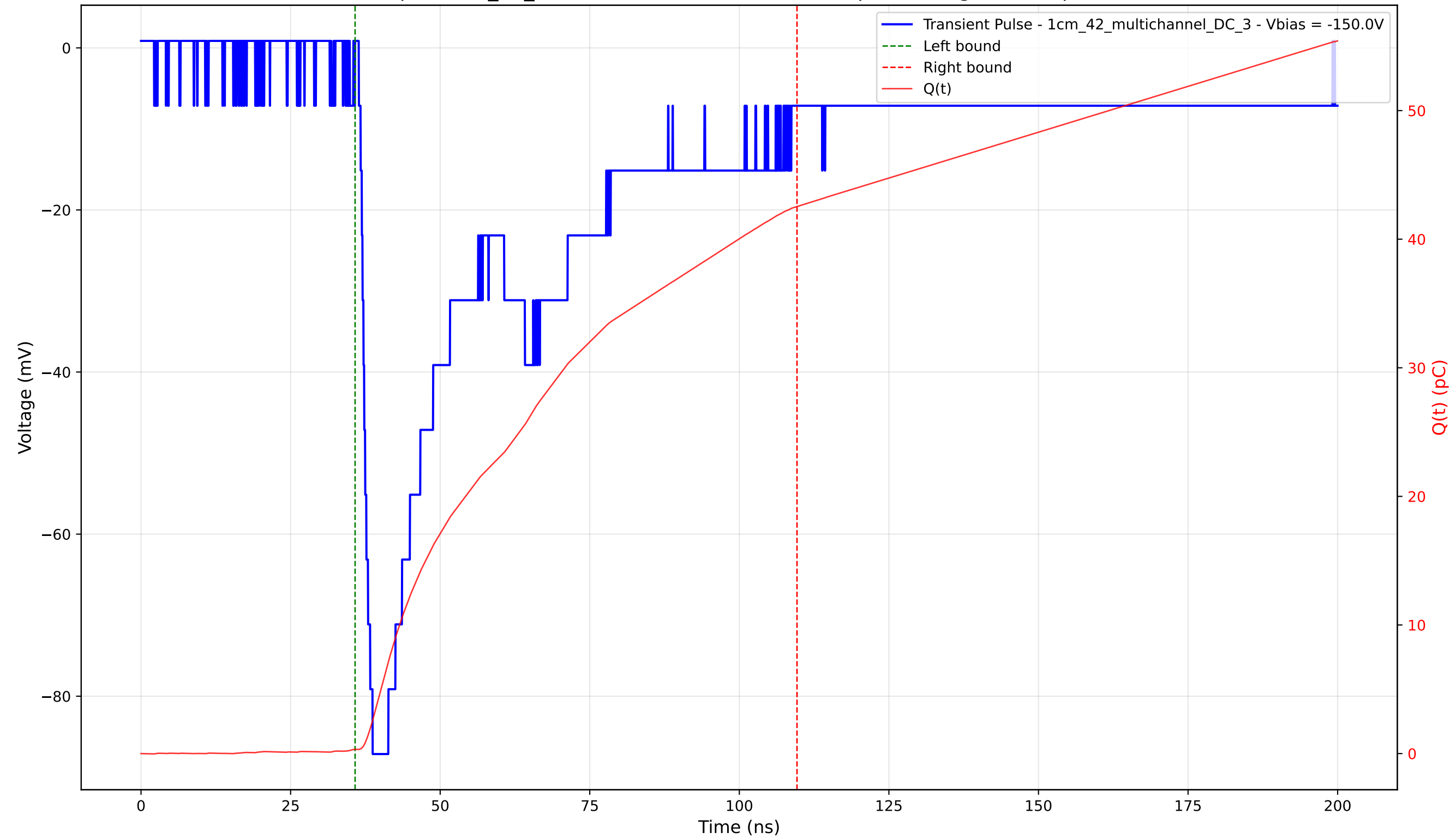
Transient Pulse - Sample: 1cm_42_multichannel - Position: 2695.0 \mu\text{m} - Charge: 42.21 pC - Rise Time: 1.62 ns
