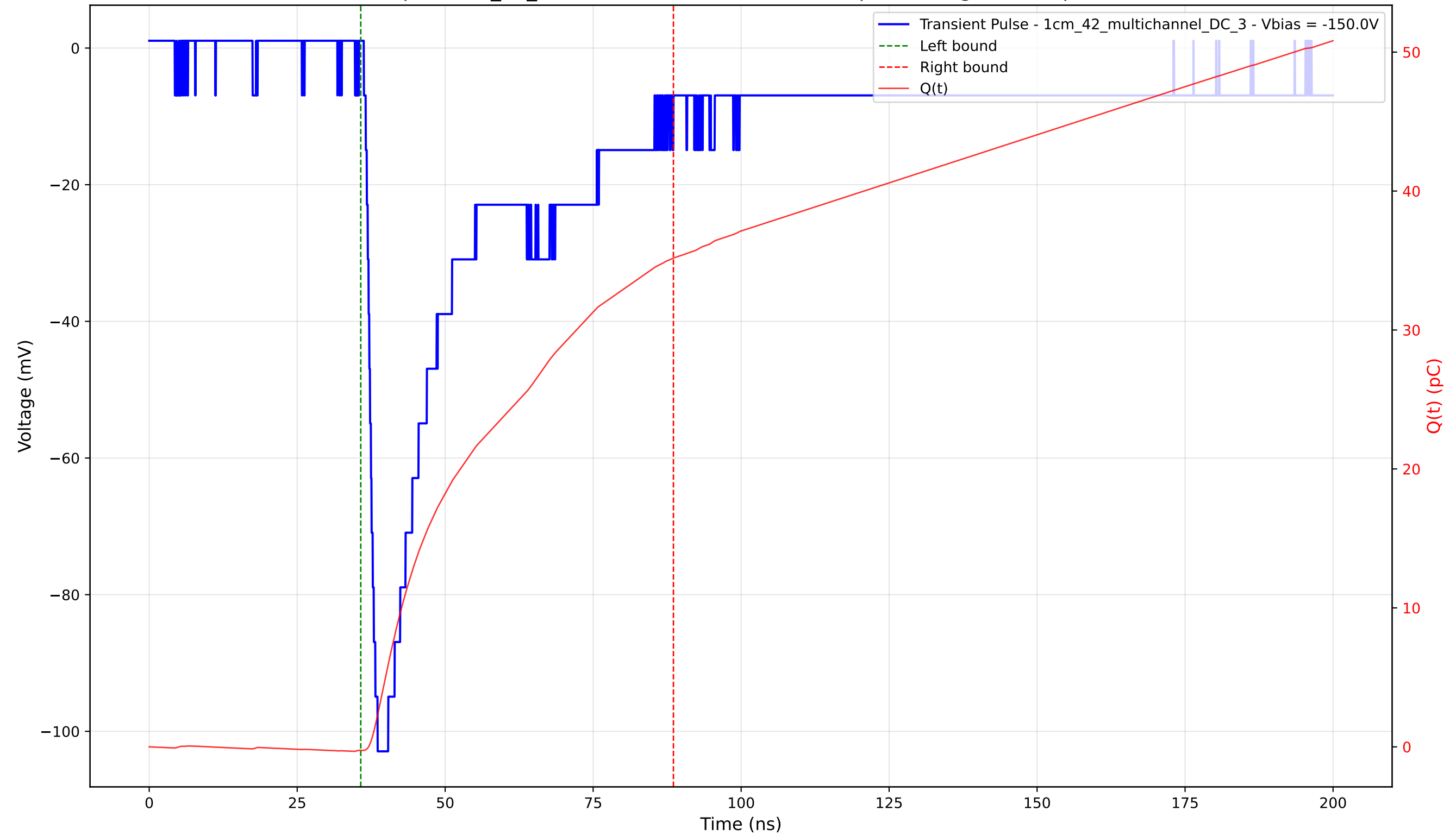
Transient Pulse - Sample: 1cm_42_multichannel - Position: 3145.0 \mu\text{m} - Charge: 35.43 pC - Rise Time: 1.63 ns
