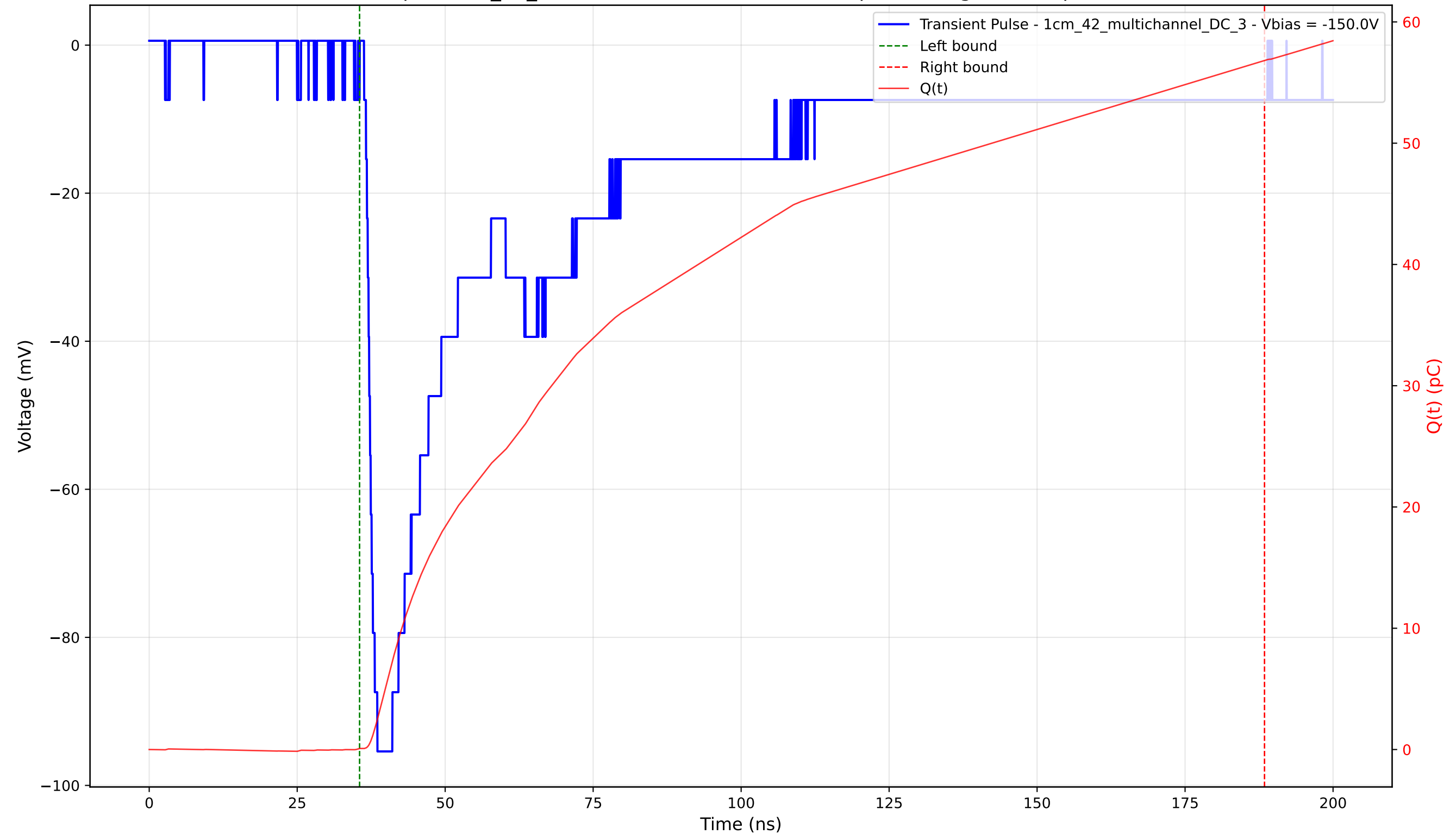
Transient Pulse - Sample: 1cm_42_multichannel - Position: 1975.0 \mu\text{m} - Charge: 56.74 pC - Rise Time: 1.49 ns
