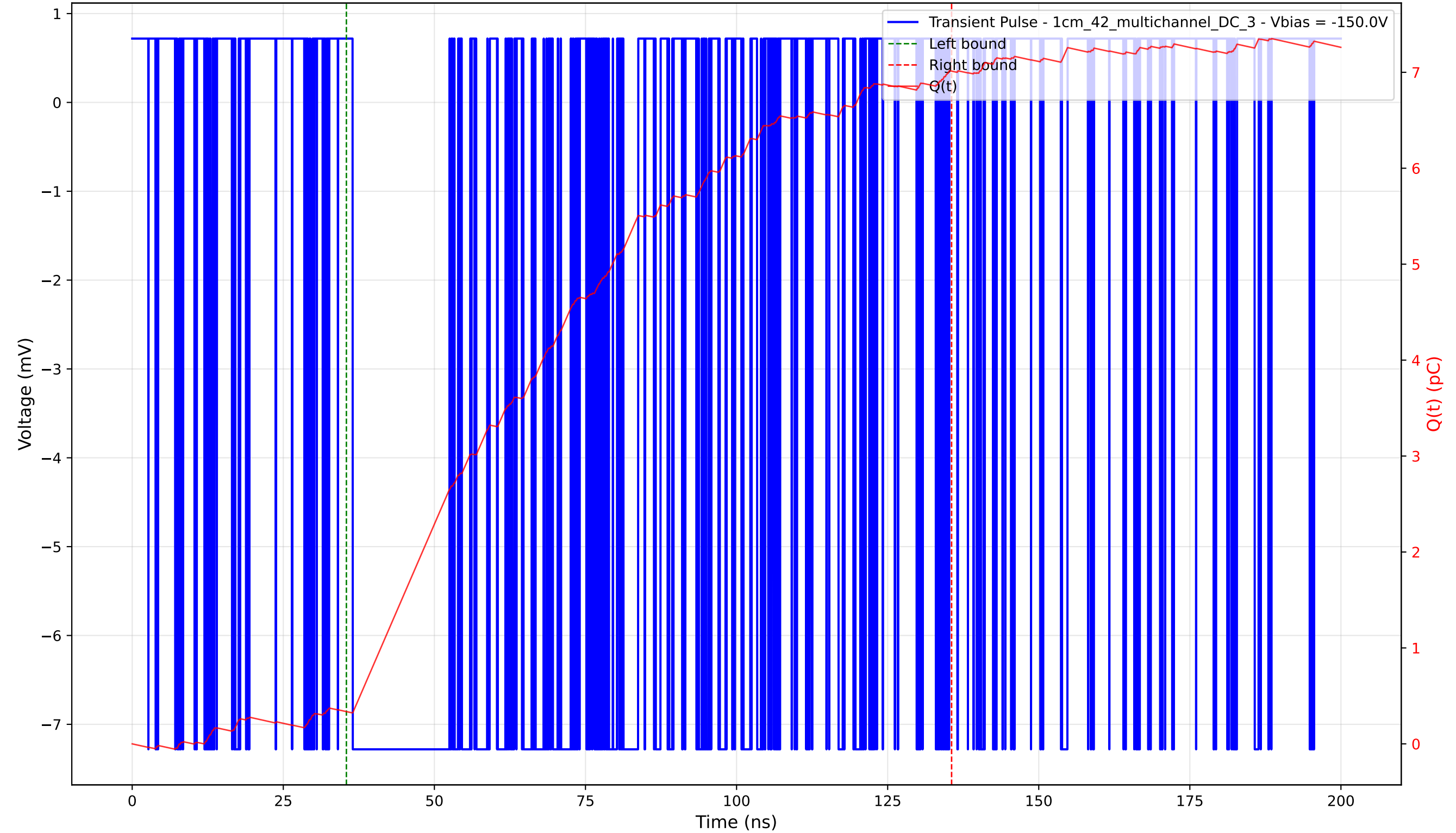
Transient Pulse - Sample: 1cm_42_multichannel - Position: 3390.0 \mu\text{m} - Charge: 6.68 pC - Rise Time: 0.02 ns
