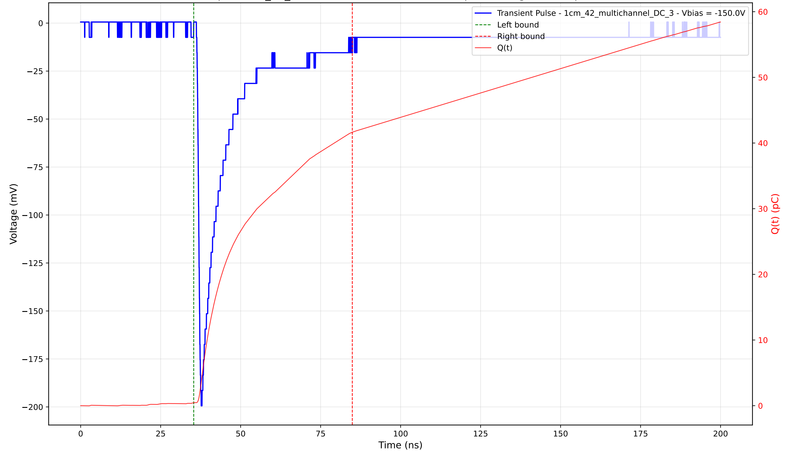
Transient Pulse - Sample: 1cm_42_multichannel - Position: 4170.0 \mu\text{m} - Charge: 41.19 pC - Rise Time: 1.01 ns
