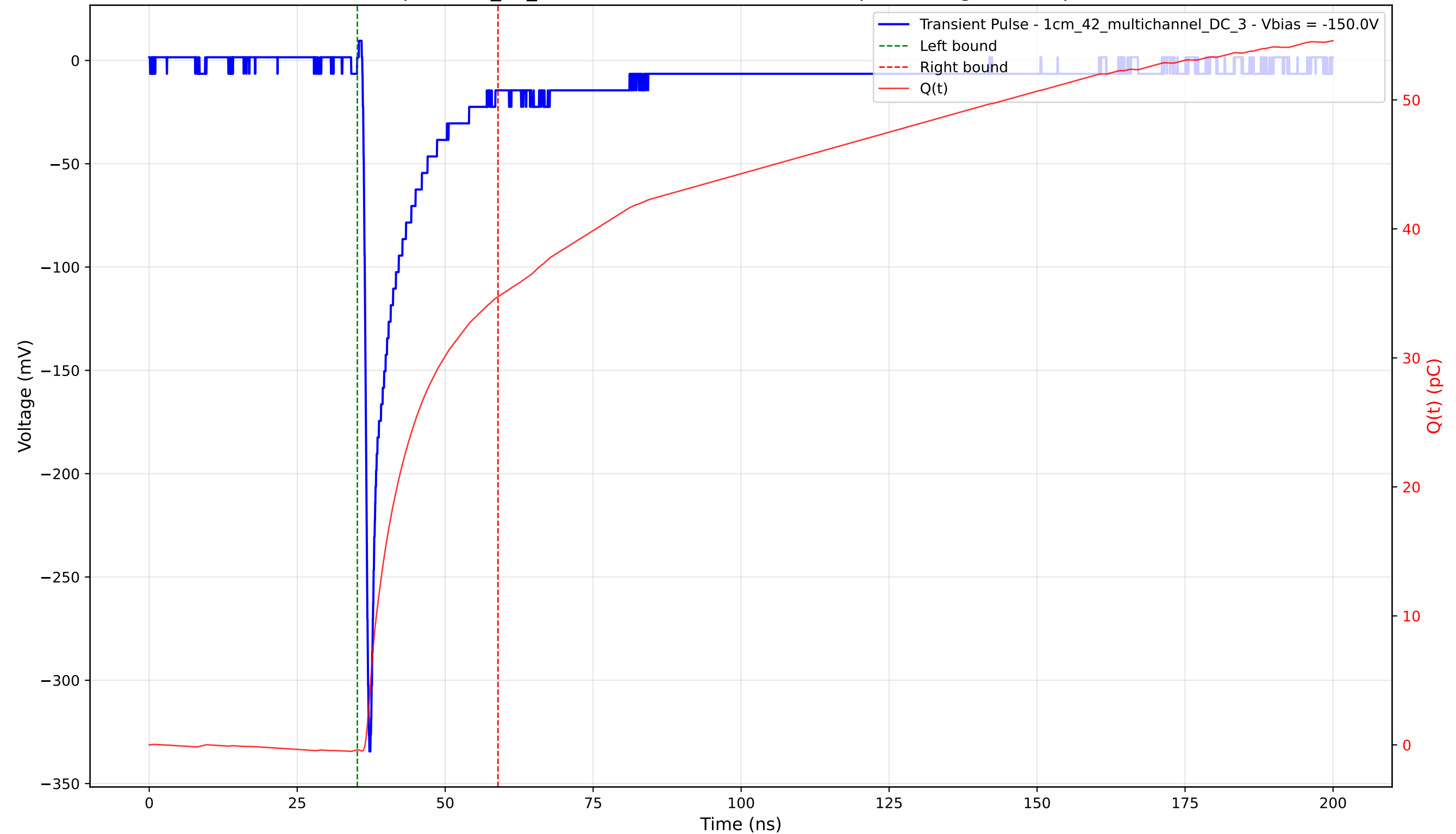
Transient Pulse - Sample: 1cm_42_multichannel - Position: 4675.0 \mu\text{m} - Charge: 35.12 pC - Rise Time: 0.81 ns
