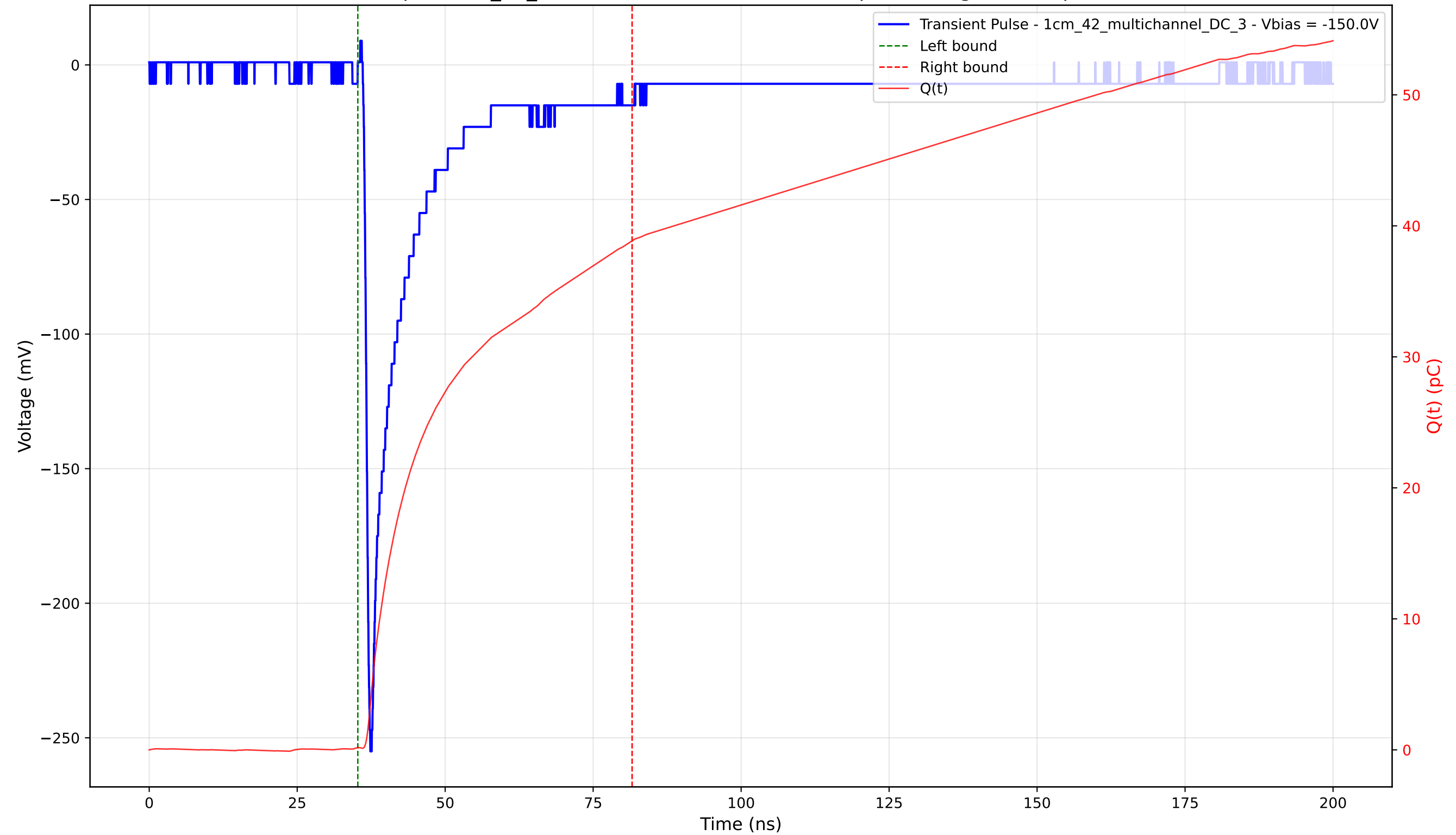
Transient Pulse - Sample: 1cm_42_multichannel - Position: 4495.0 \mu\text{m} - Charge: 38.68 pC - Rise Time: 0.83 ns
