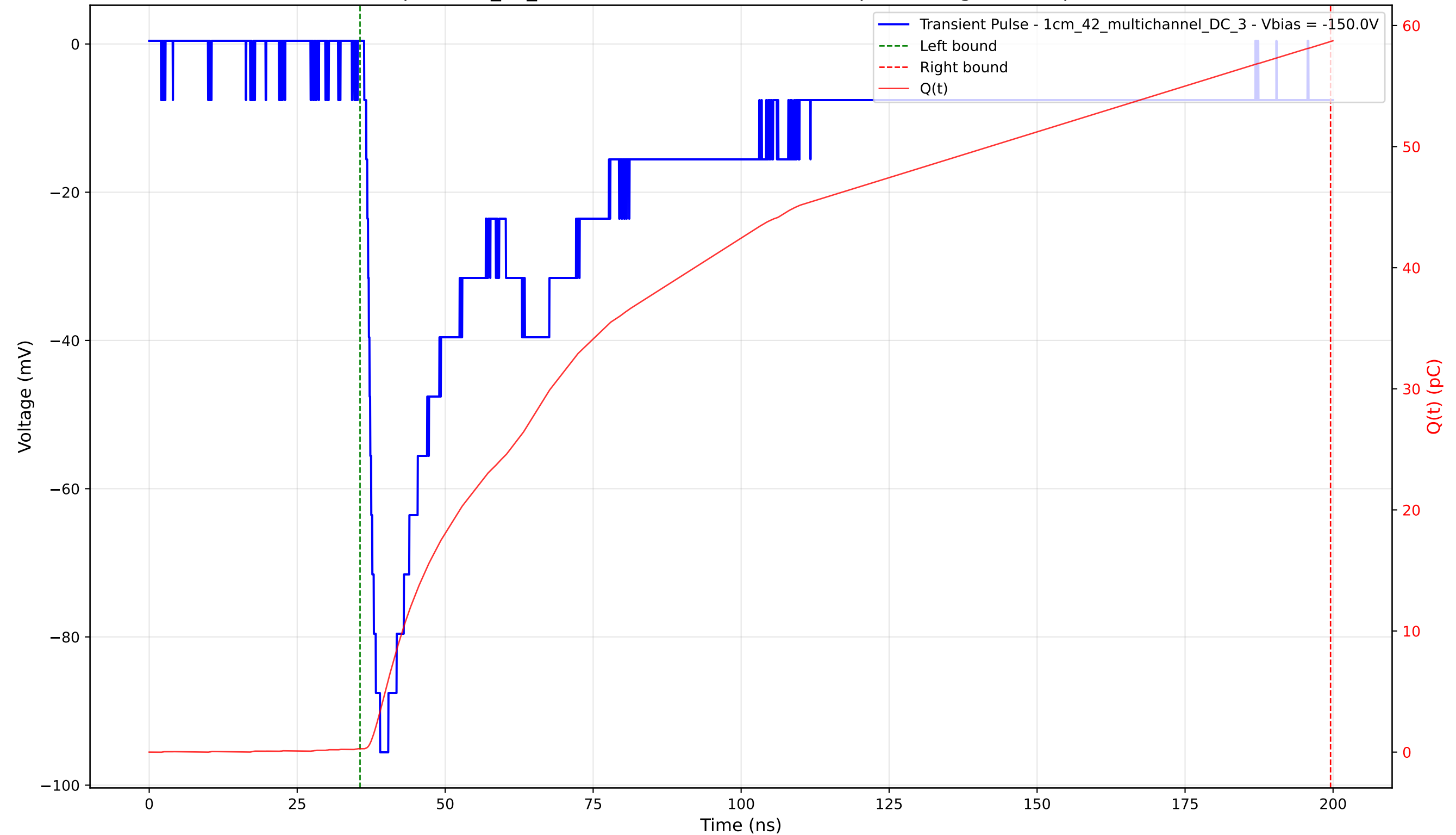
Transient Pulse - Sample: 1cm_42_multichannel - Position: 2050.0 \mu\text{m} - Charge: 58.40 pC - Rise Time: 1.64 ns
