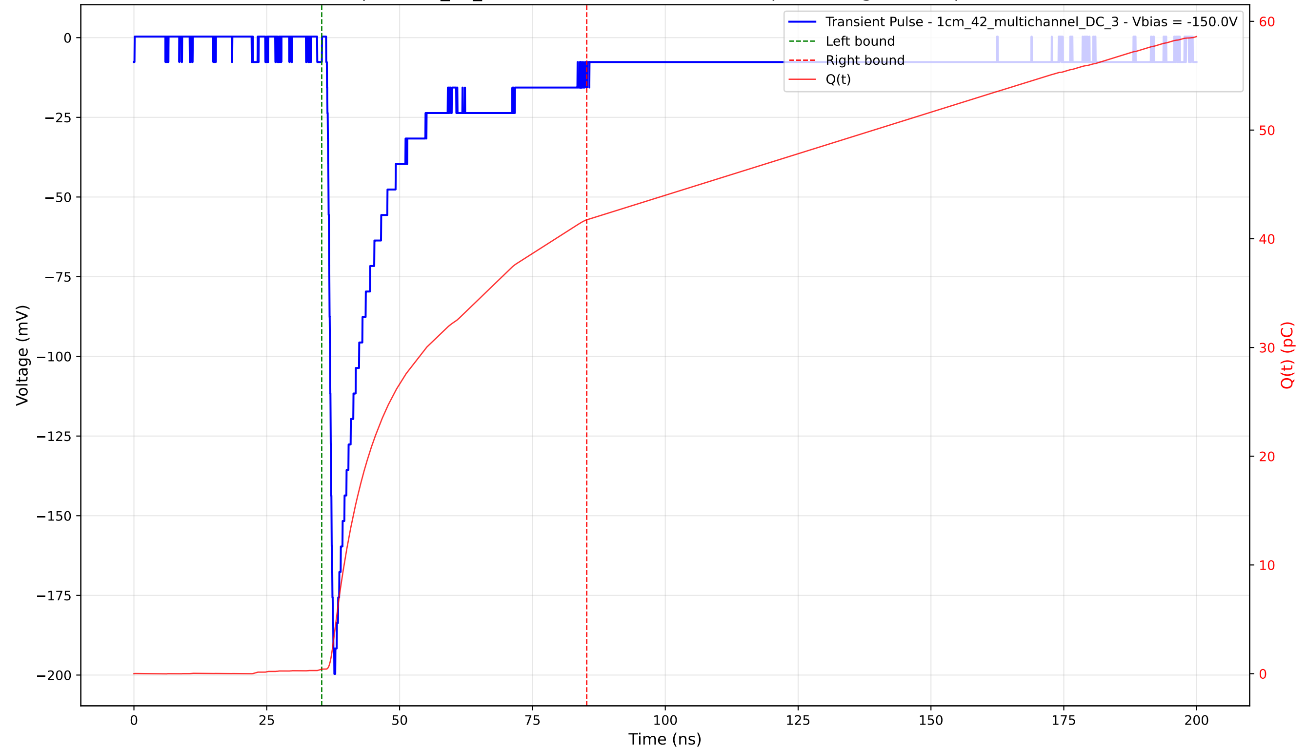
Transient Pulse - Sample: 1cm_42_multichannel - Position: 4165.0 \mu\text{m} - Charge: 41.33 pC - Rise Time: 1.03 ns
