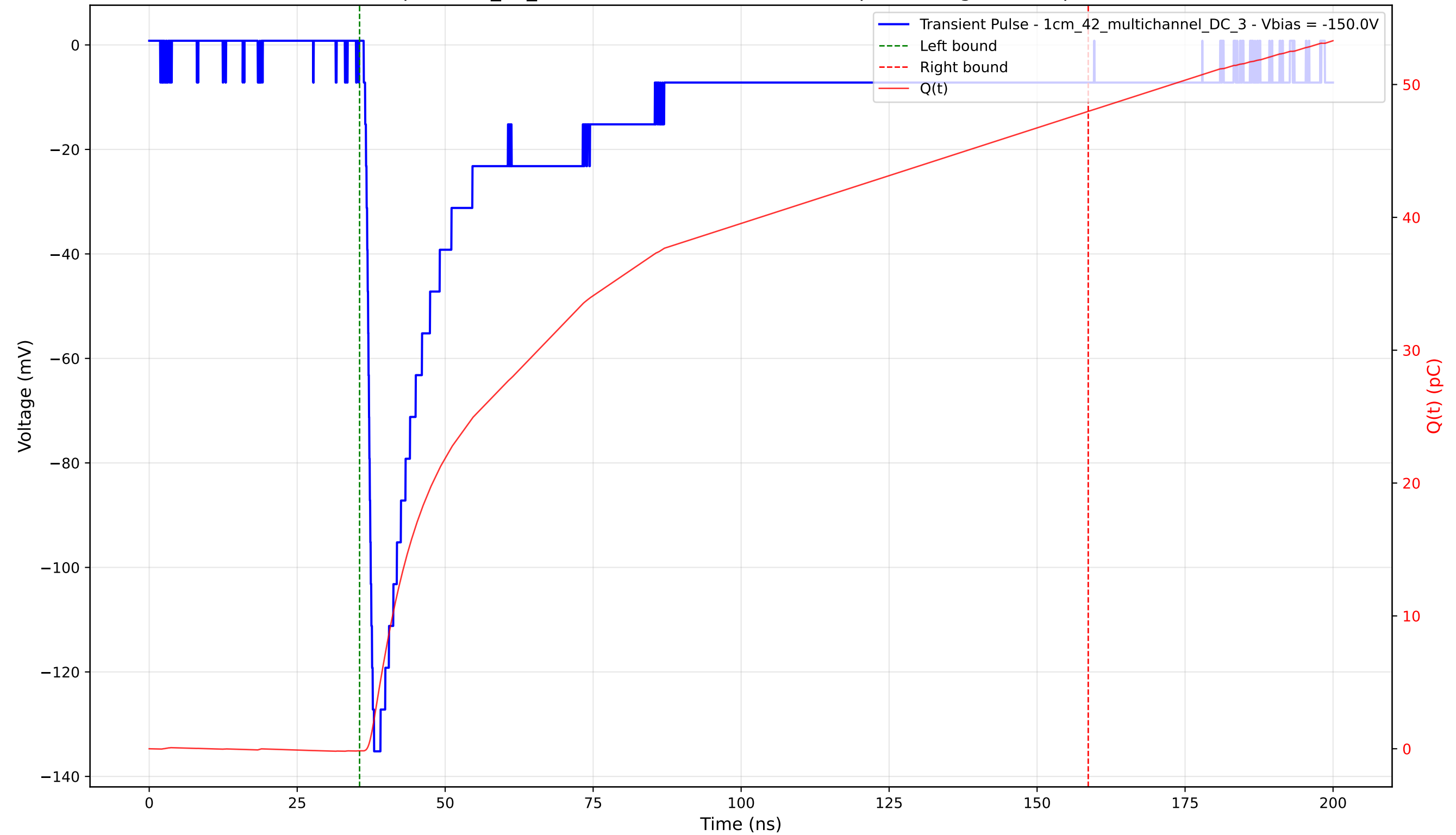
Transient Pulse - Sample: 1cm_42_multichannel - Position: 3710.0 \mu\text{m} - Charge: 48.14 pC - Rise Time: 1.28 ns
