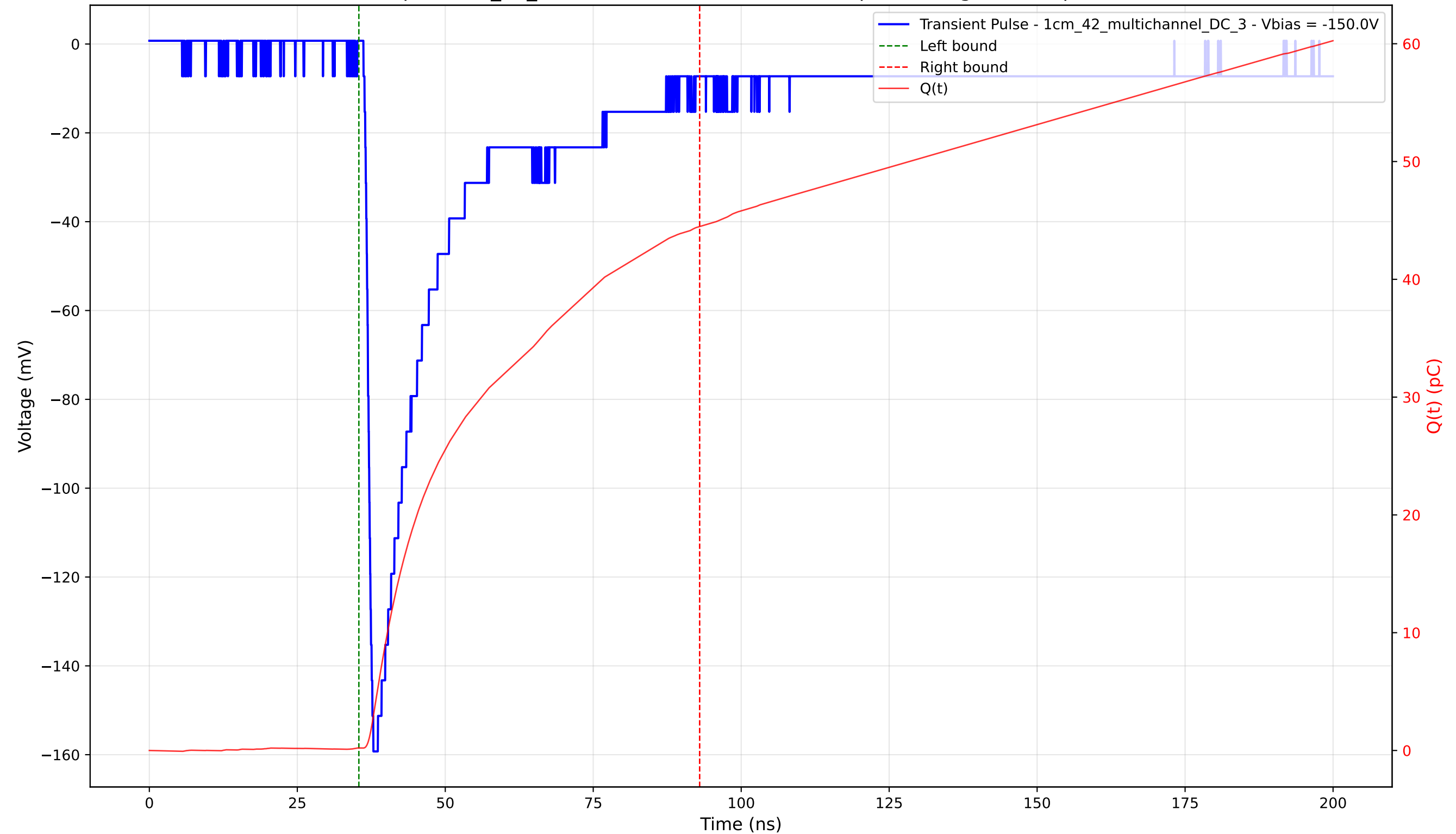
Transient Pulse - Sample: 1cm_42_multichannel - Position: 1120.0 \mu\text{m} - Charge: 44.27 pC - Rise Time: 1.22 ns
