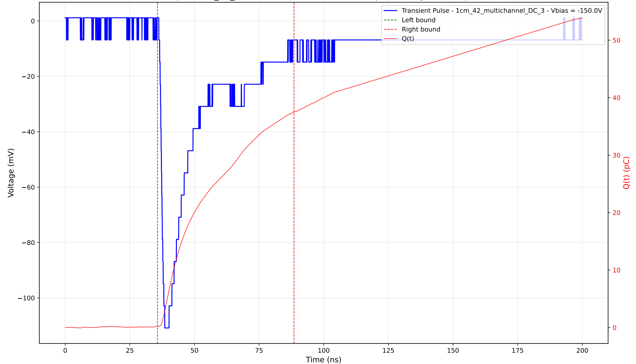
Transient Pulse - Sample: 1cm_42_multichannel - Position: 3230.0 \mu\text{m} - Charge: 37.27 pC - Rise Time: 1.63 ns
