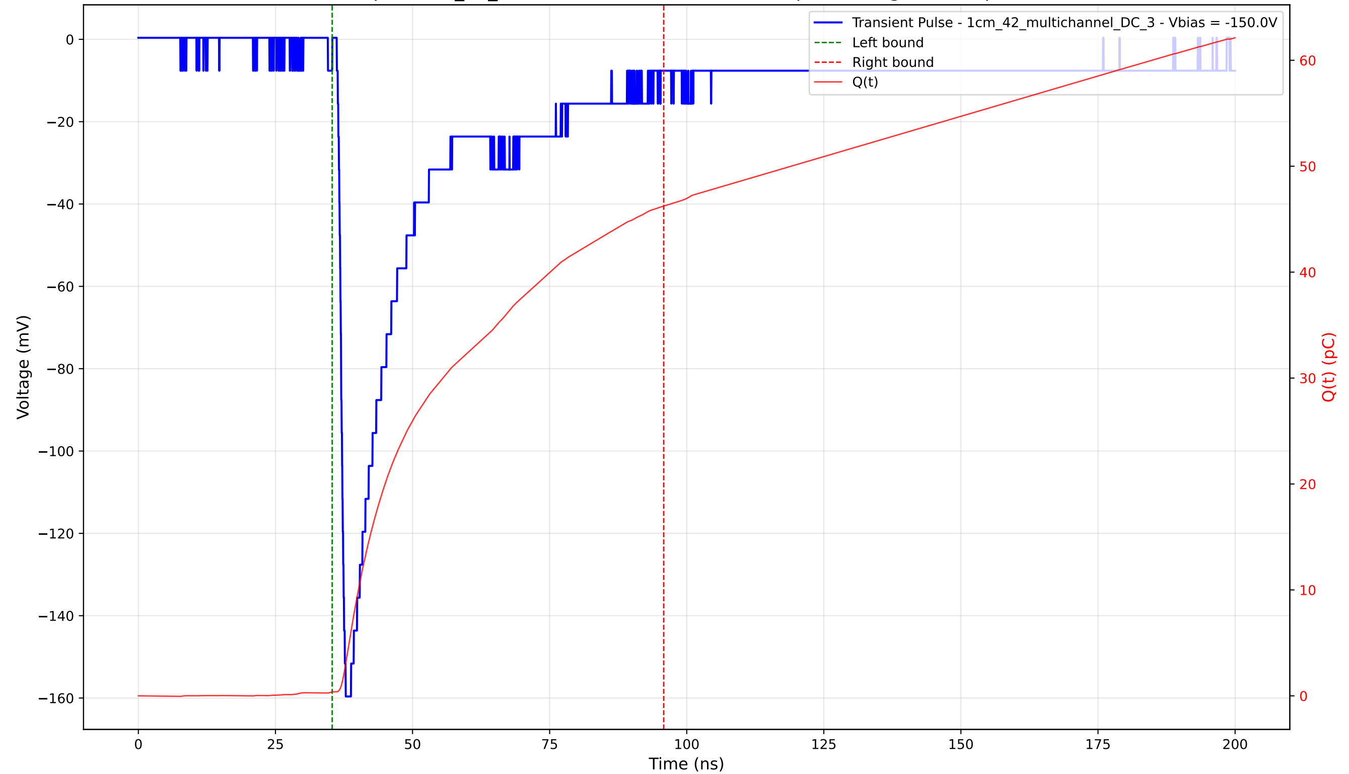
Transient Pulse - Sample: 1cm_42_multichannel - Position: 1100.0 \mu\text{m} - Charge: 45.87 pC - Rise Time: 1.20 ns
