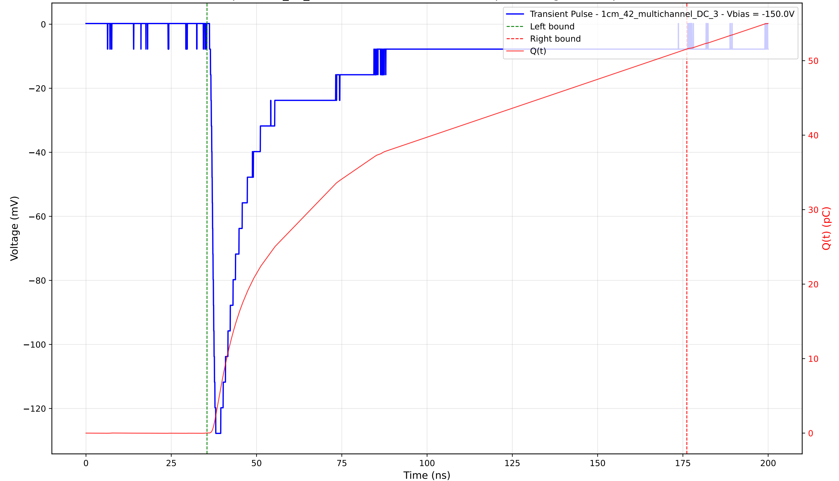
Transient Pulse - Sample: 1cm_42_multichannel - Position: 3645.0 \mu\text{m} - Charge: 51.56 pC - Rise Time: 1.31 ns
