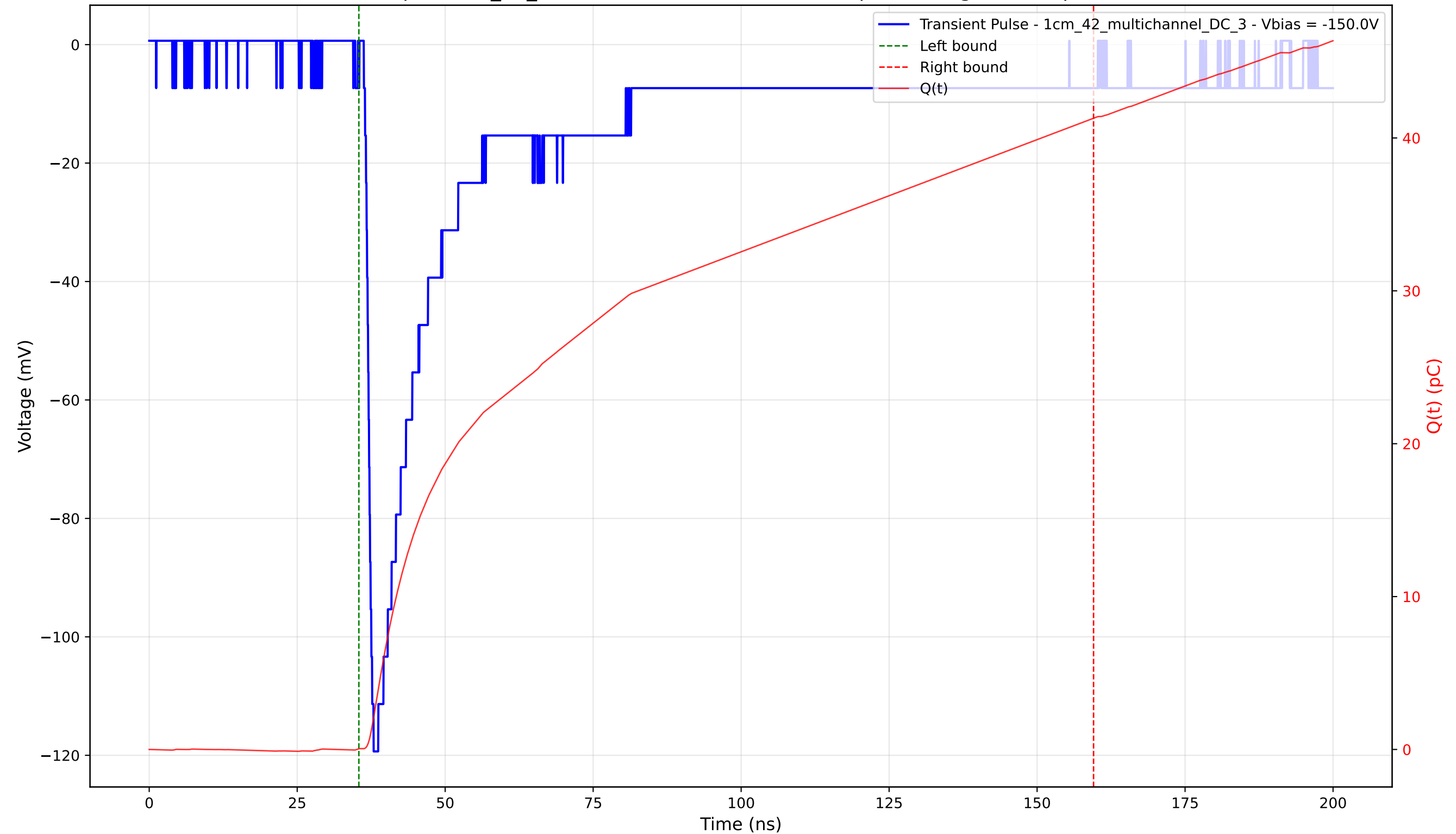
Transient Pulse - Sample: 1cm_42_multichannel - Position: 3825.0 \mu\text{m} - Charge: 41.25 pC - Rise Time: 1.21 ns
