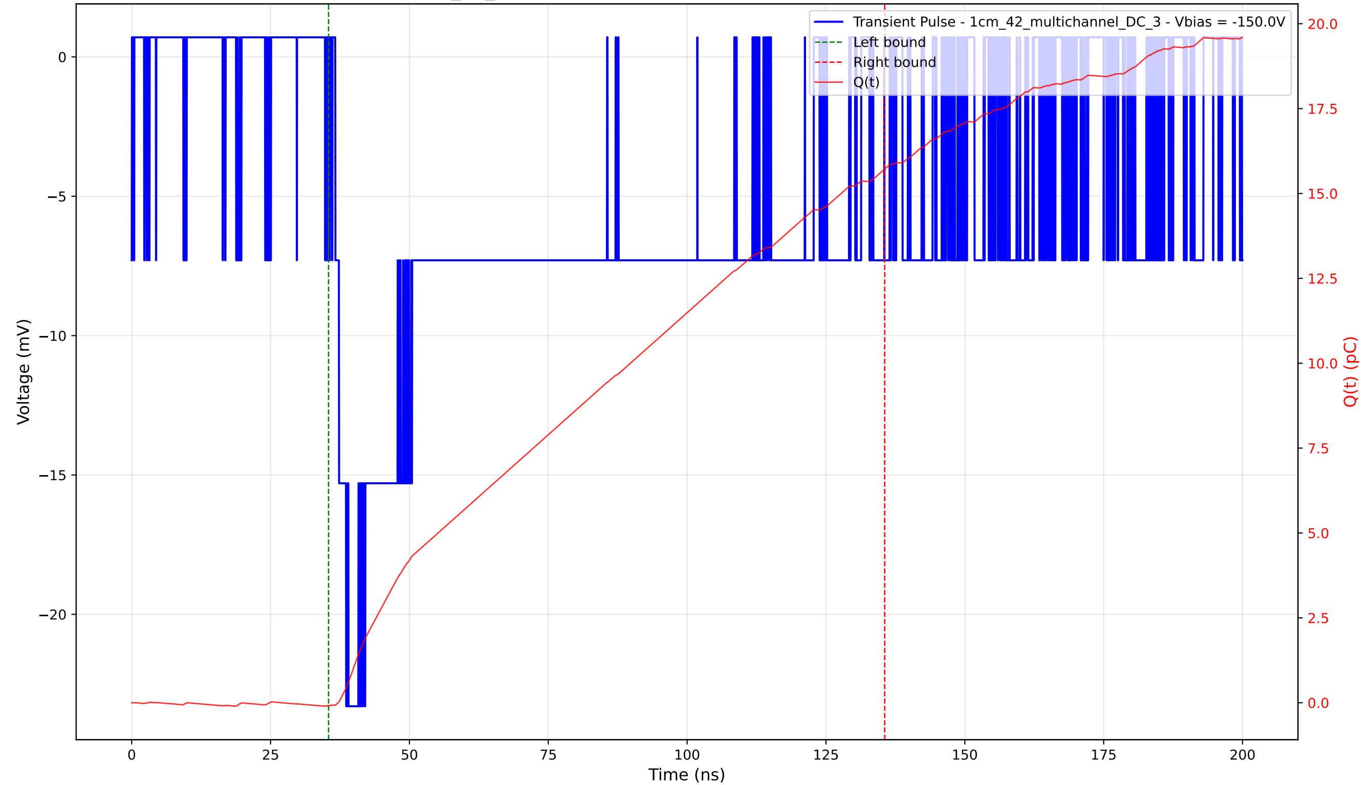
Transient Pulse - Sample: 1cm_42_multichannel - Position: 2410.0 \mu\text{m} - Charge: 15.80 pC - Rise Time: 1.96 ns
