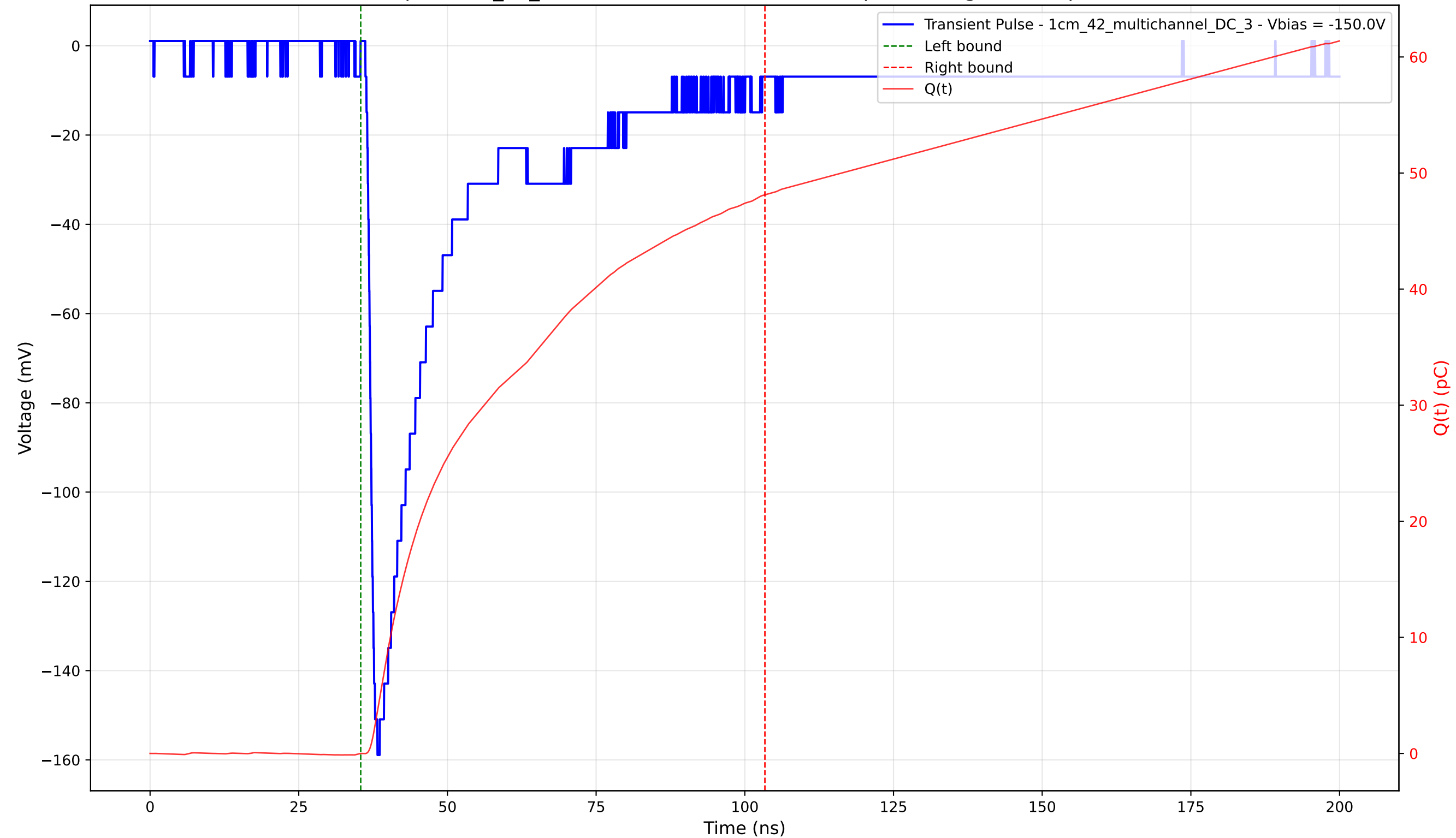
Transient Pulse - Sample: 1cm_42_multichannel - Position: 1225.0 \mu\text{m} - Charge: 48.12 pC - Rise Time: 1.32 ns
