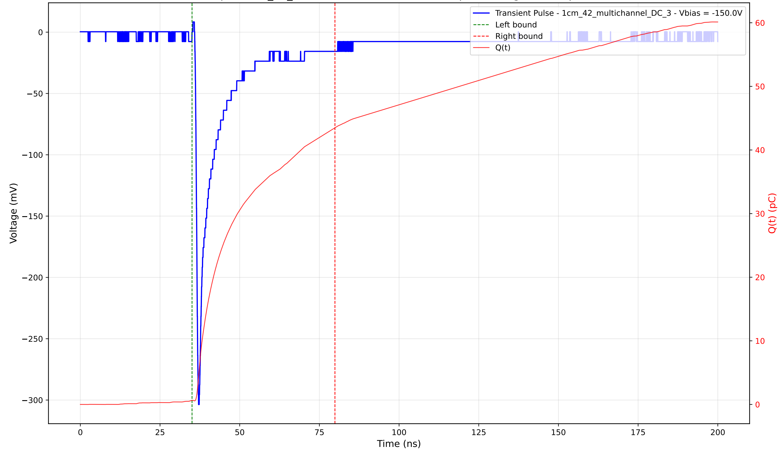
Transient Pulse - Sample: 1cm_42_multichannel - Position: 265.0 \mu\text{m} - Charge: 42.86 pC - Rise Time: 0.84 ns
