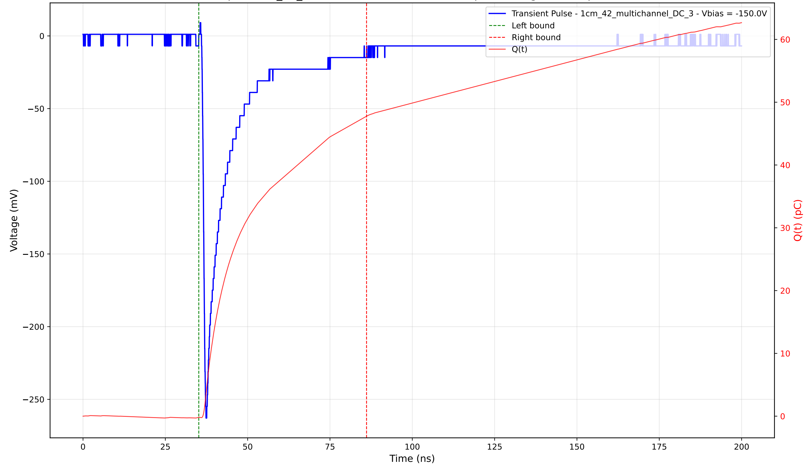
Transient Pulse - Sample: 1cm_42_multichannel - Position: 535.0 \mu\text{m} - Charge: 47.95 pC - Rise Time: 0.91 ns
