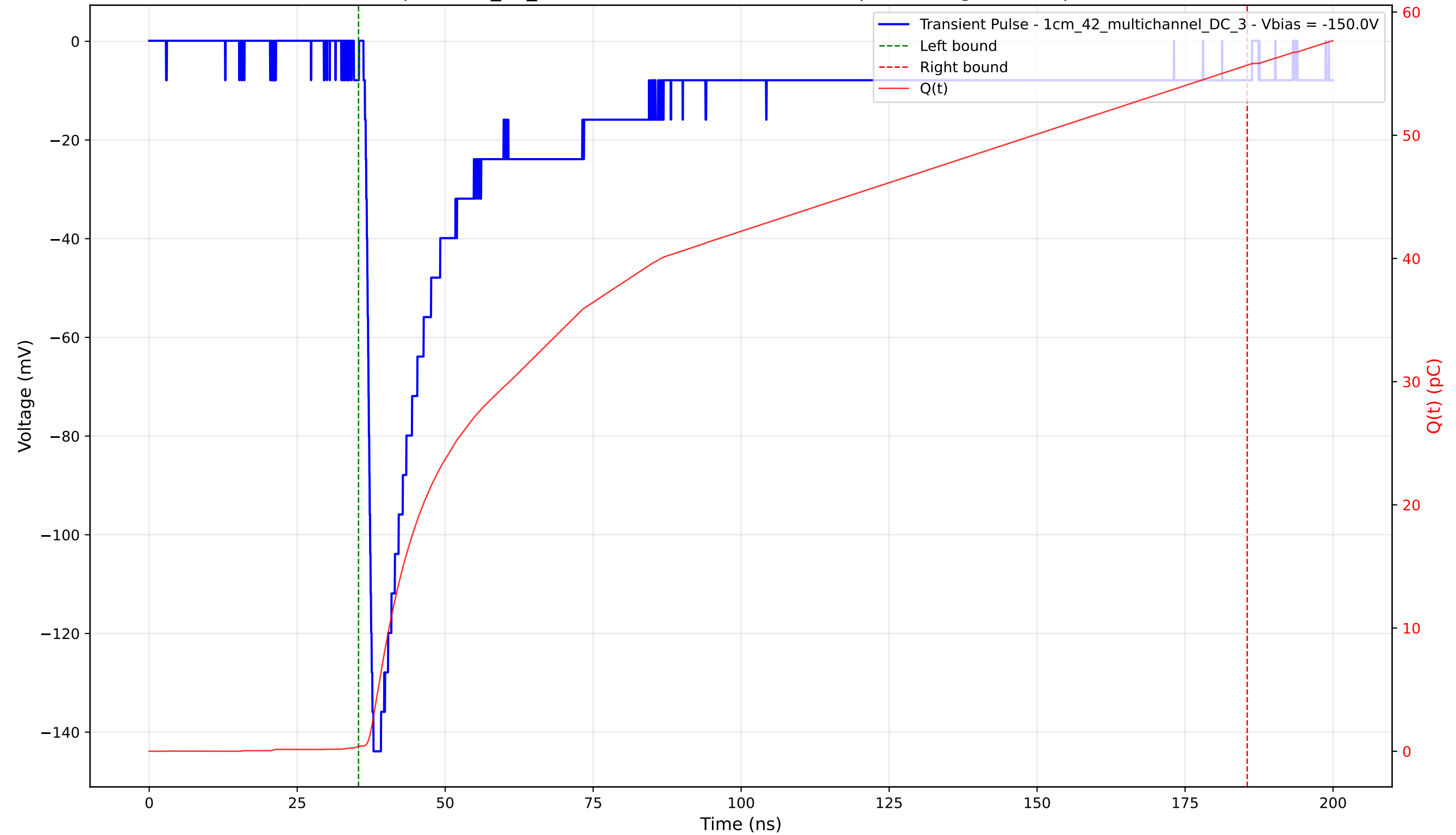
Transient Pulse - Sample: 1cm_42_multichannel - Position: 3775.0 \mu\text{m} - Charge: 55.30 pC - Rise Time: 1.26 ns
