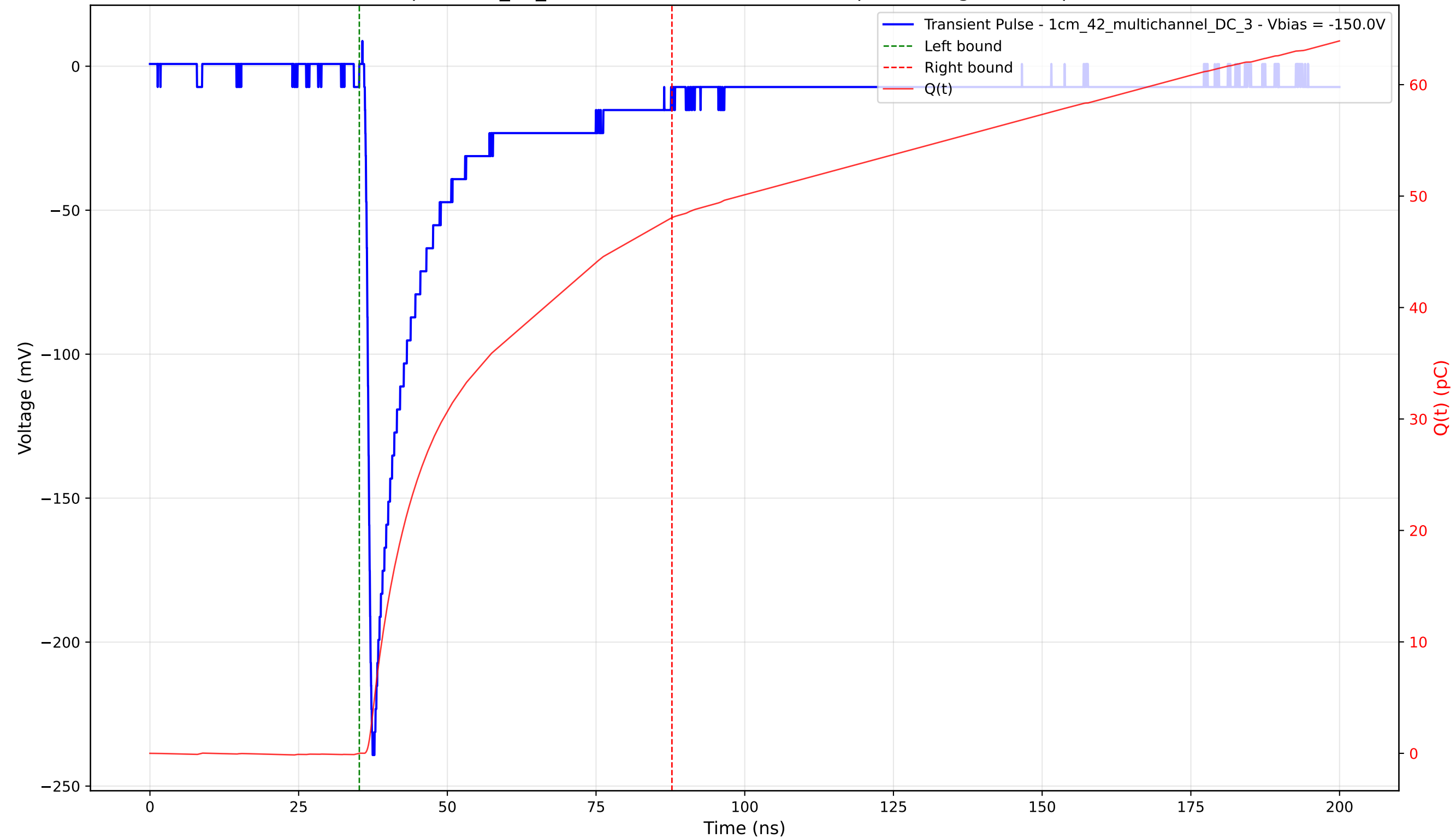
Transient Pulse - Sample: 1cm_42_multichannel - Position: 625.0 \mu\text{m} - Charge: 48.05 pC - Rise Time: 0.98 ns
