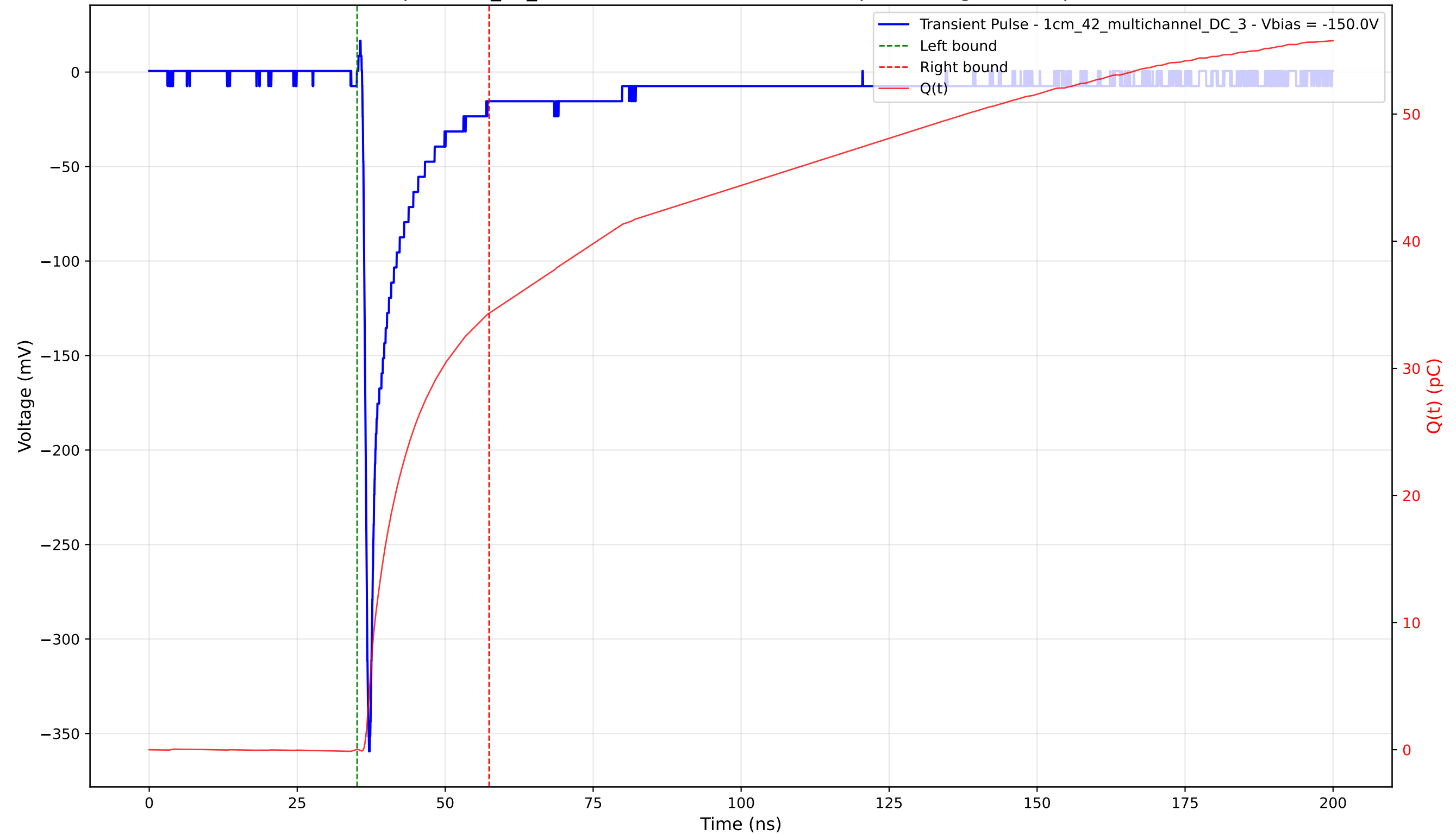
Transient Pulse - Sample: 1cm_42_multichannel - Position: 4765.0 \mu\text{m} - Charge: 34.31 pC - Rise Time: 0.79 ns
