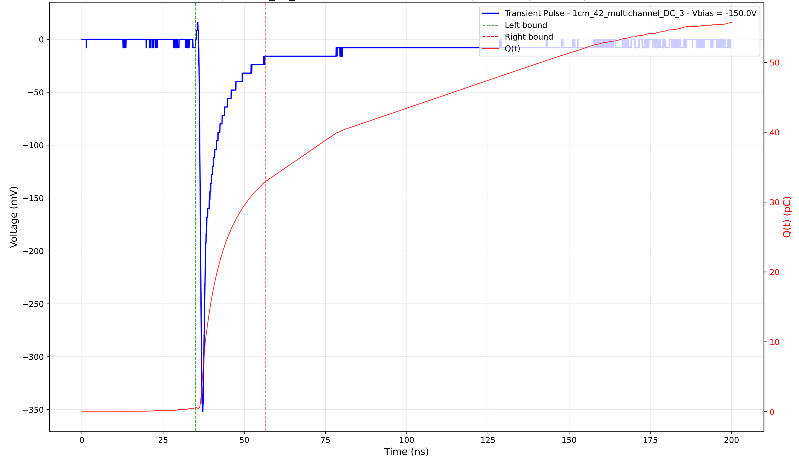
Transient Pulse - Sample: 1cm_42_multichannel - Position: 4805.0 \mu\text{m} - Charge: 32.41 pC - Rise Time: 0.77 ns
