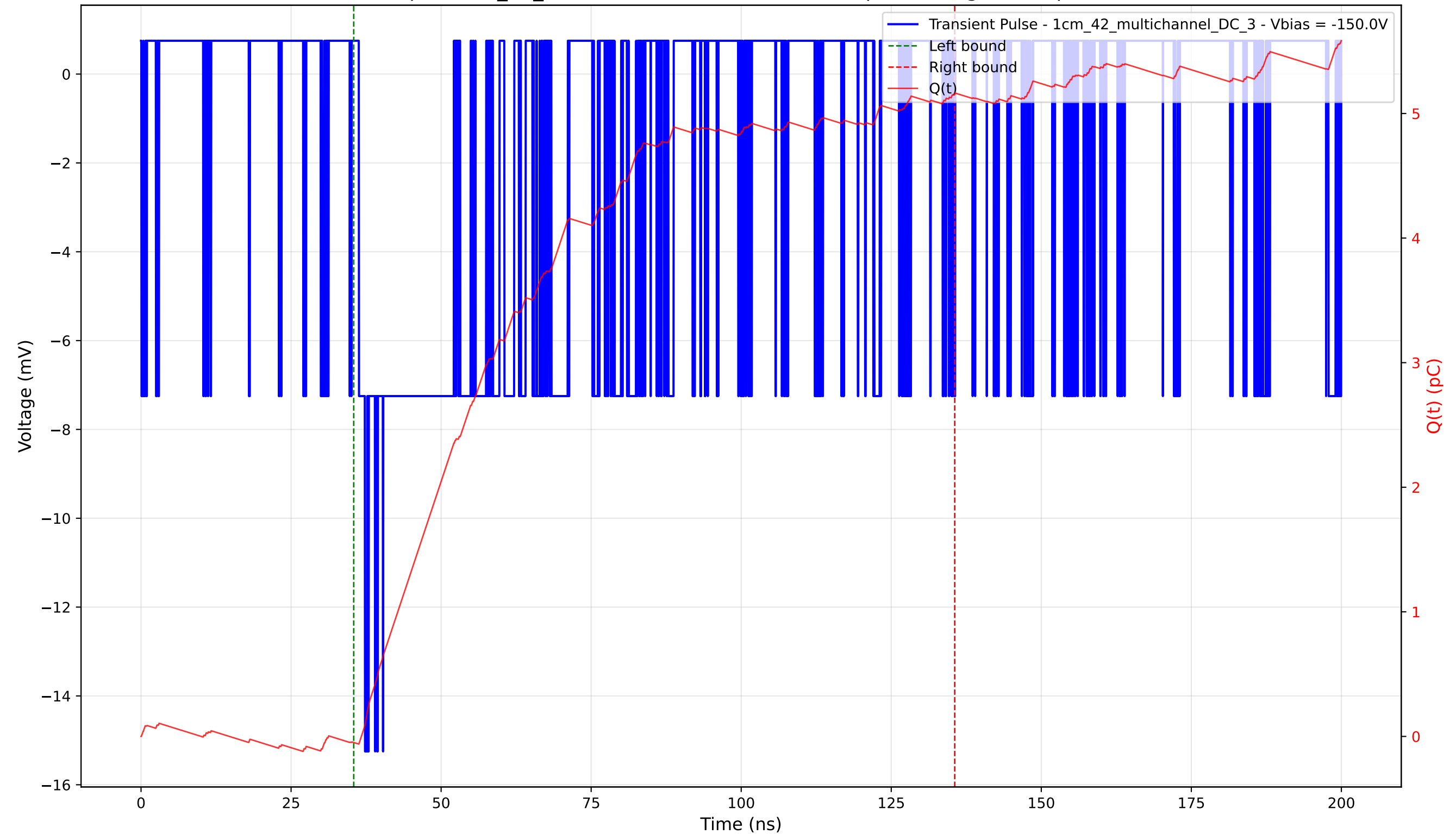
Transient Pulse - Sample: 1cm_42_multichannel - Position: 4390.0 \mu\text{m} - Charge: 5.20 pC - Rise Time: 1.02 ns
