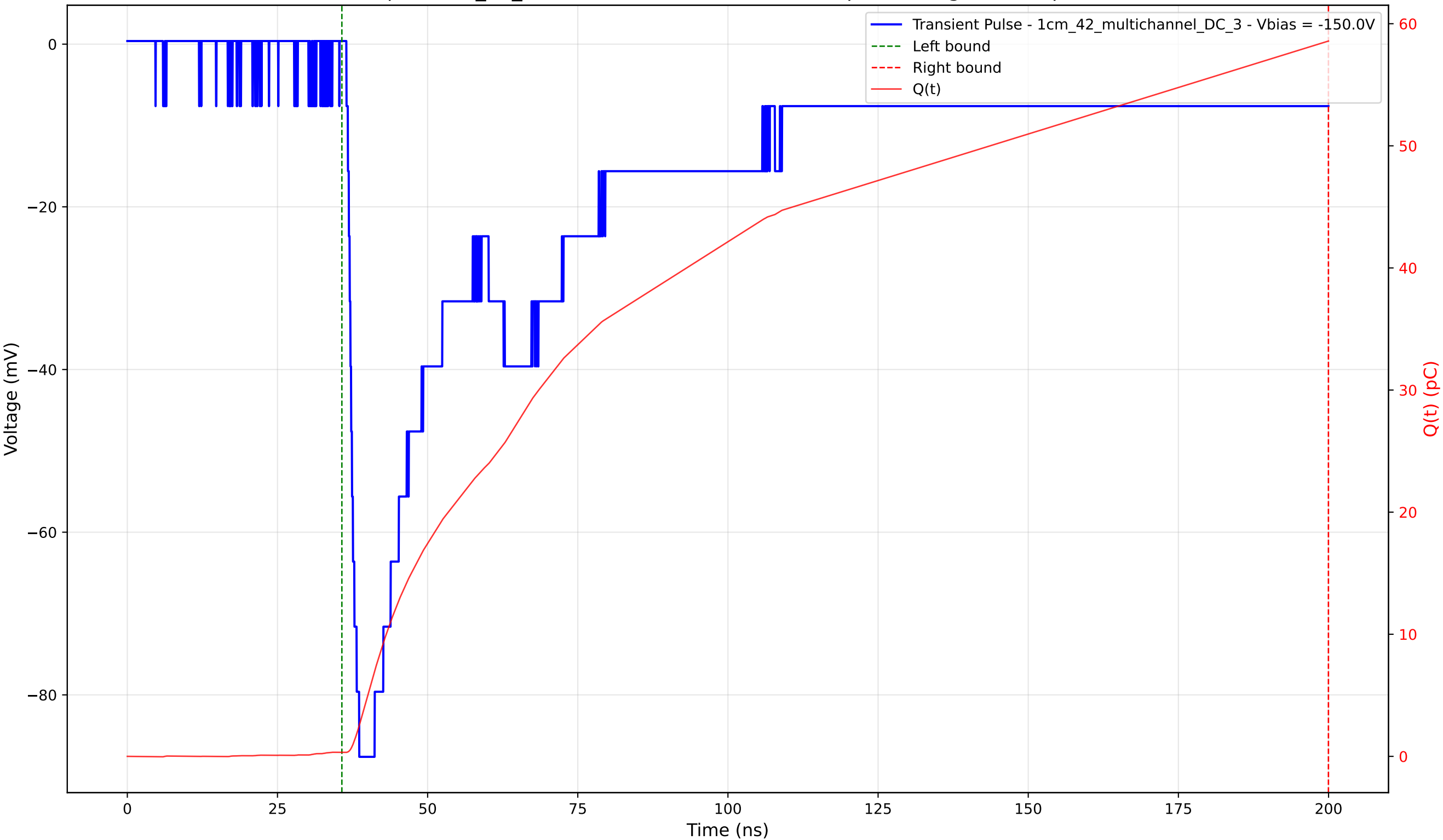
Transient Pulse - Sample: 1cm_42_multichannel - Position: 2130.0 \mu\text{m} - Charge: 58.26 pC - Rise Time: 1.48 ns
