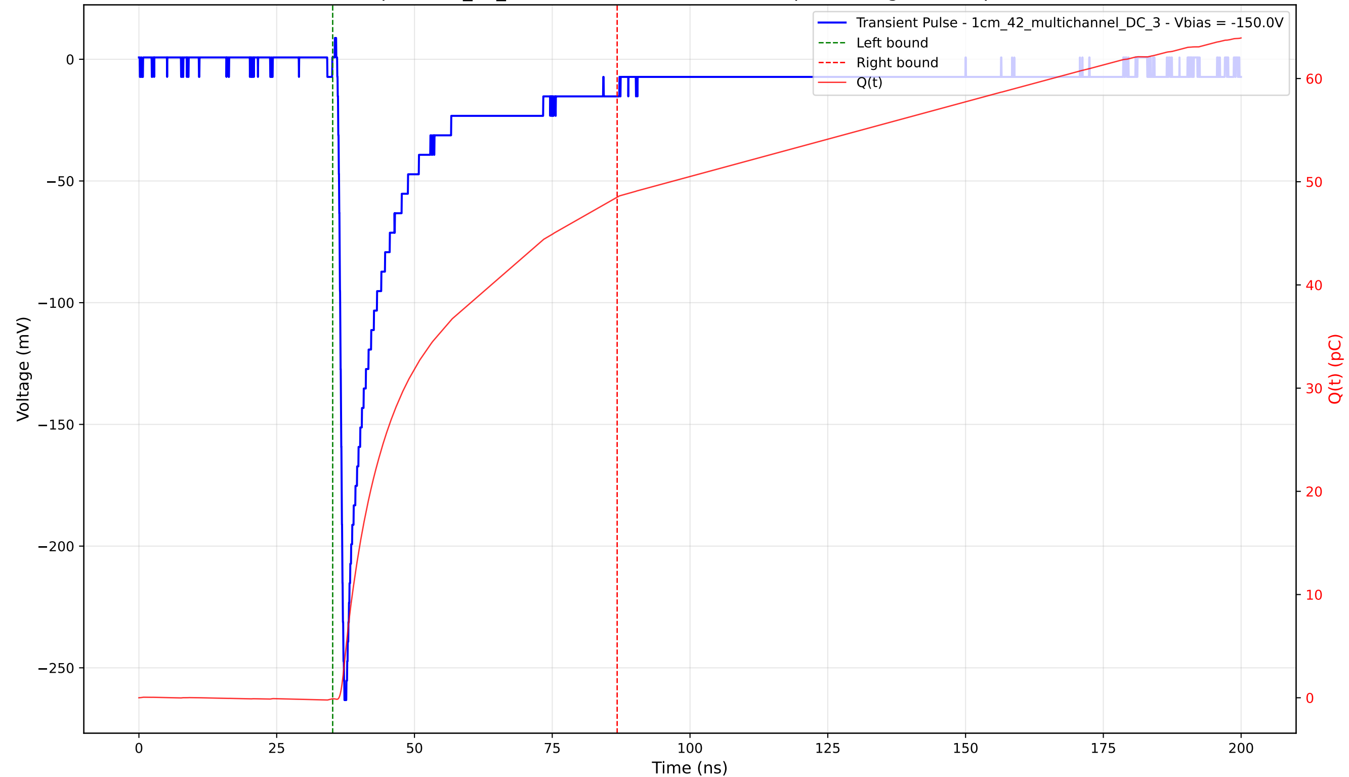
Transient Pulse - Sample: 1cm_42_multichannel - Position: 525.0 \mu\text{m} - Charge: 48.60 pC - Rise Time: 0.91 ns
