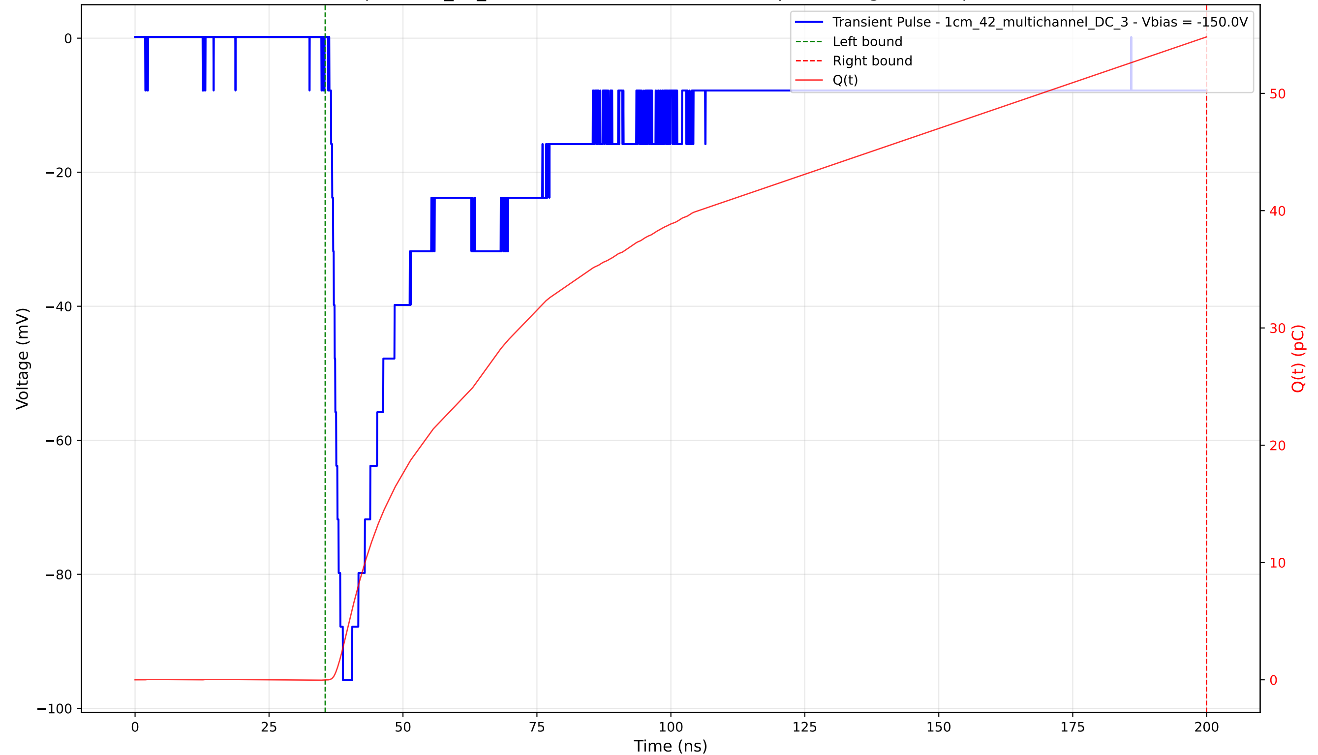
Transient Pulse - Sample: 1cm_42_multichannel - Position: 2960.0 \mu\text{m} - Charge: 54.83 pC - Rise Time: 1.74 ns
