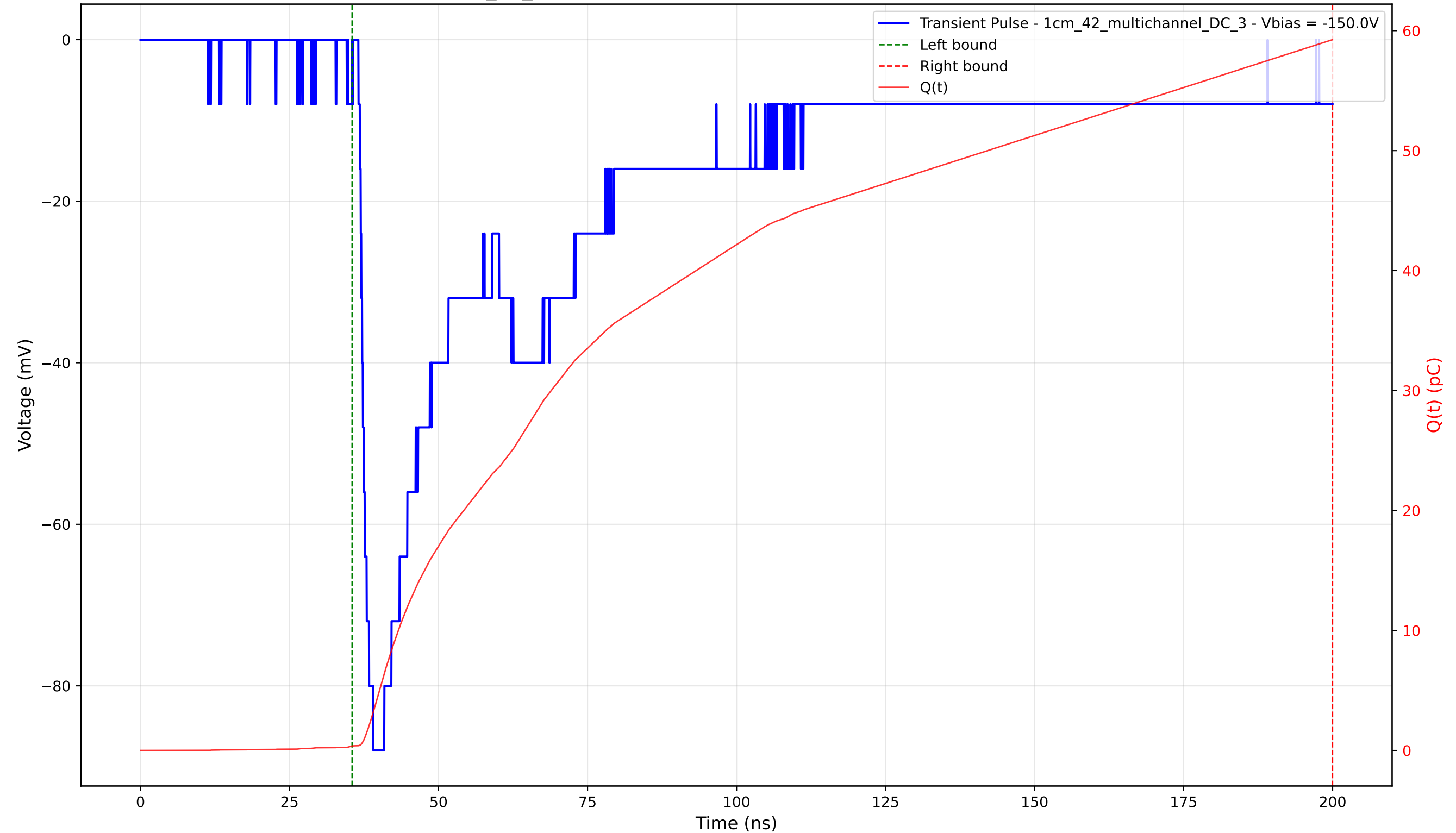
Transient Pulse - Sample: 1cm_42_multichannel - Position: 2195.0 \mu\text{m} - Charge: 58.88 pC - Rise Time: 1.56 ns
