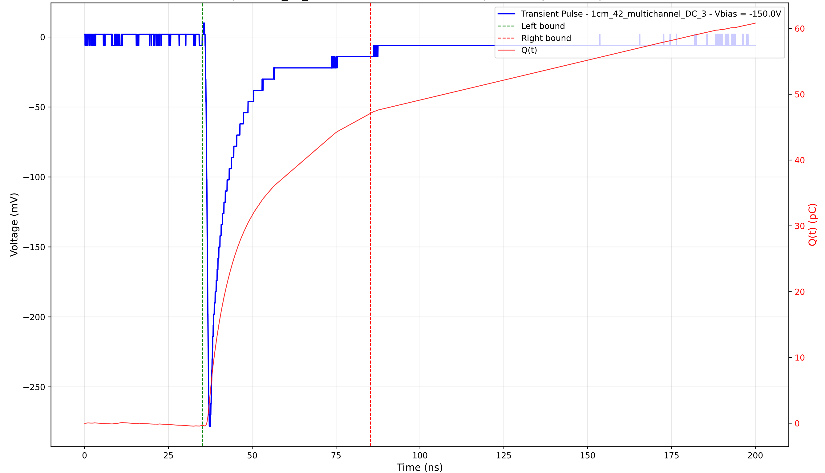
Transient Pulse - Sample: 1cm_42_multichannel - Position: 445.0 \mu\text{m} - Charge: 47.45 pC - Rise Time: 0.89 ns
