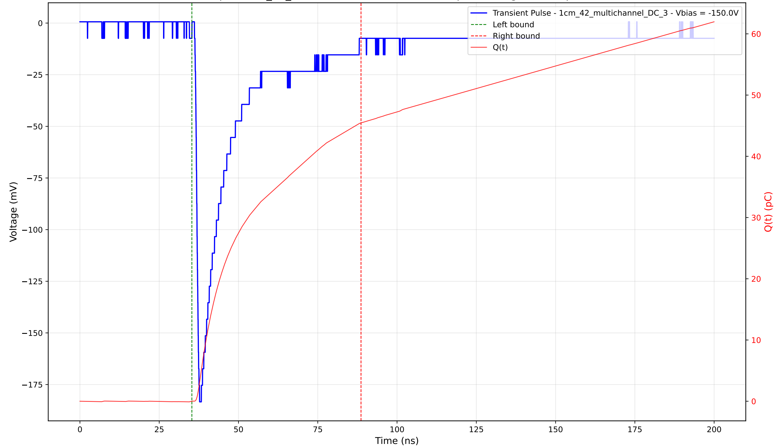
Transient Pulse - Sample: 1cm_42_multichannel - Position: 945.0 \mu\text{m} - Charge: 45.43 pC - Rise Time: 1.07 ns
