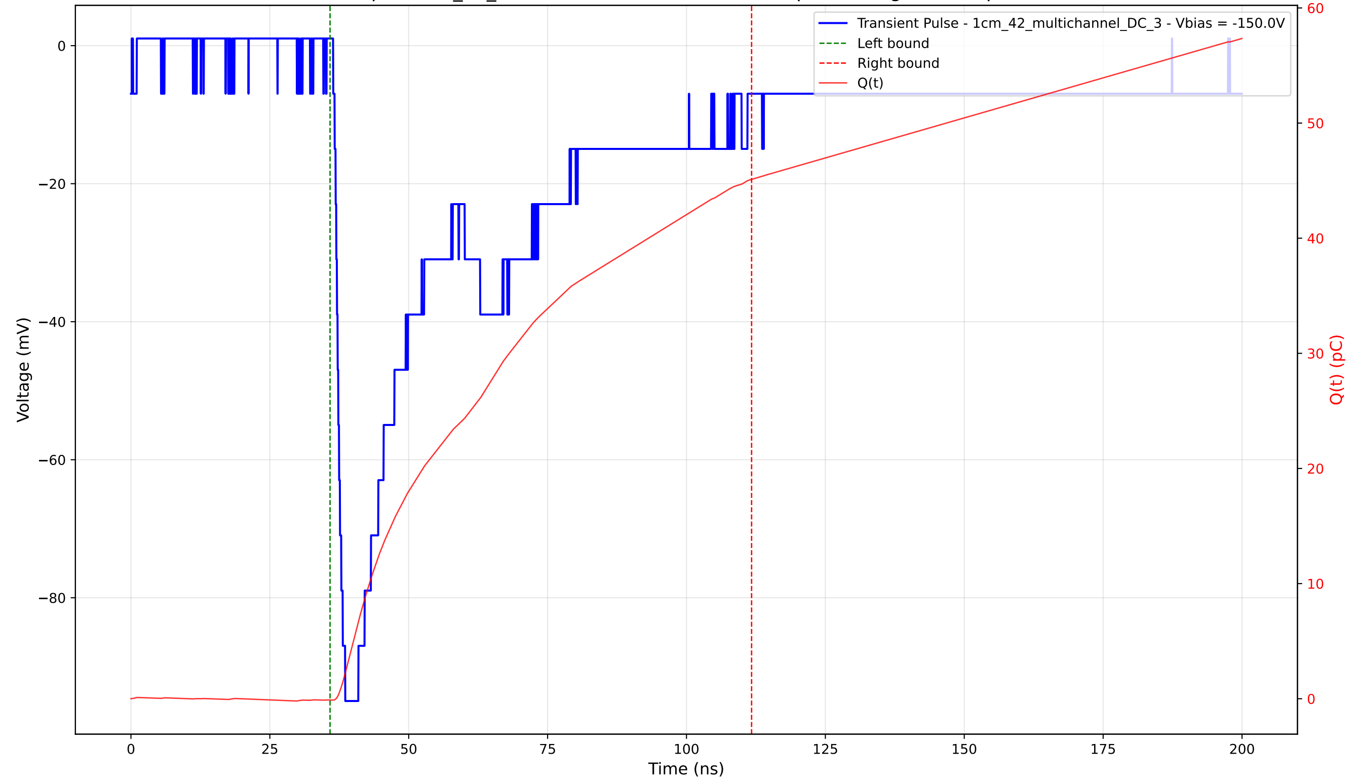
Transient Pulse - Sample: 1cm_42_multichannel - Position: 2020.0 \mu\text{m} - Charge: 45.22 pC - Rise Time: 1.47 ns
