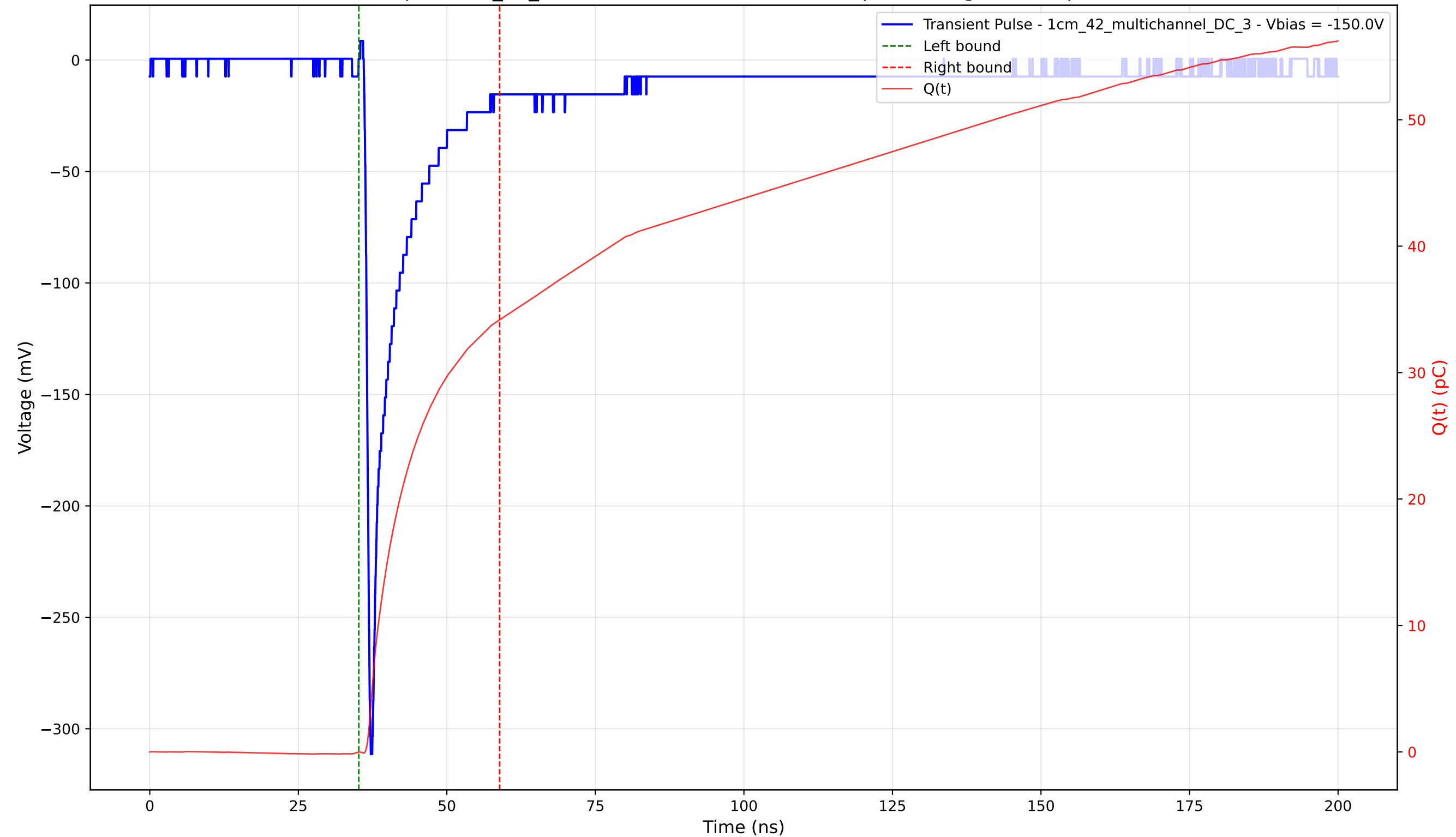
Transient Pulse - Sample: 1cm_42_multichannel - Position: 4640.0 \mu\text{m} - Charge: 34.18 pC - Rise Time: 0.84 ns
