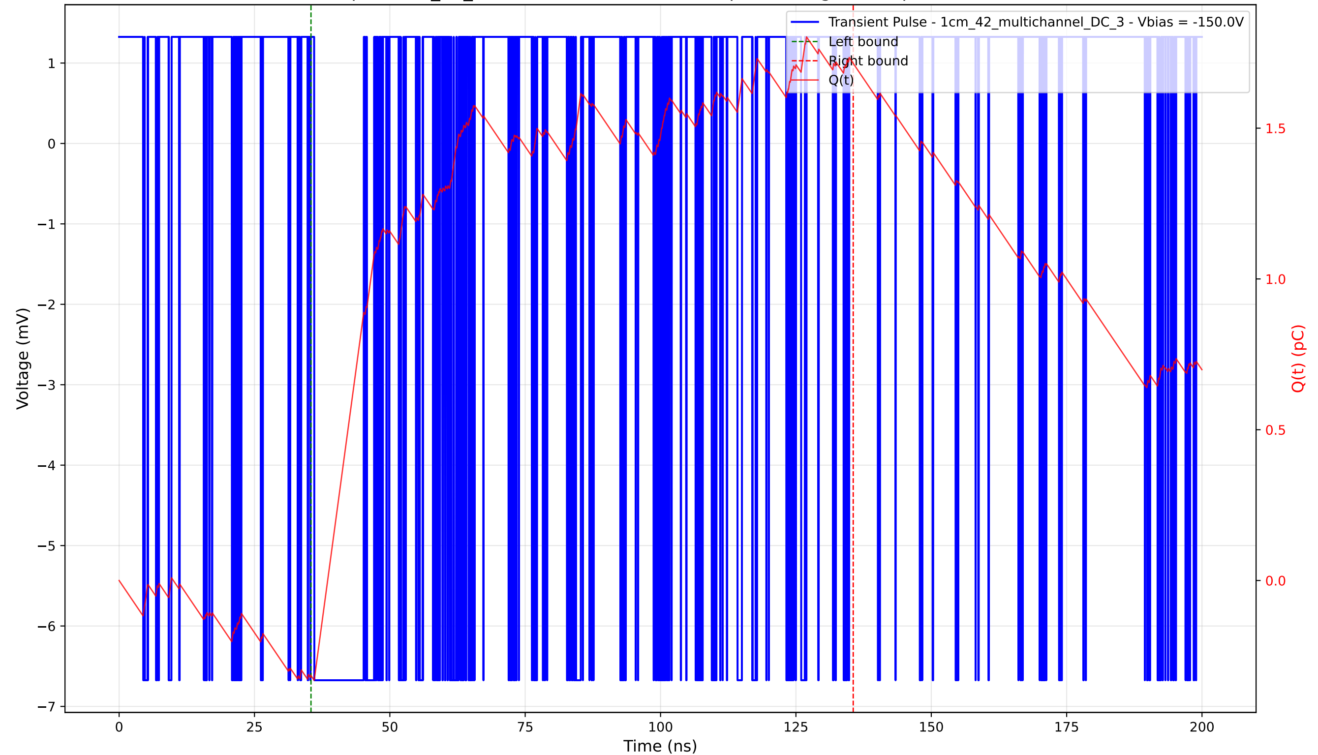
Transient Pulse - Sample: 1cm_42_multichannel - Position: 5.0 \mu\text{m} - Charge: 2.03 pC - Rise Time: 0.00 ns (N/A)
