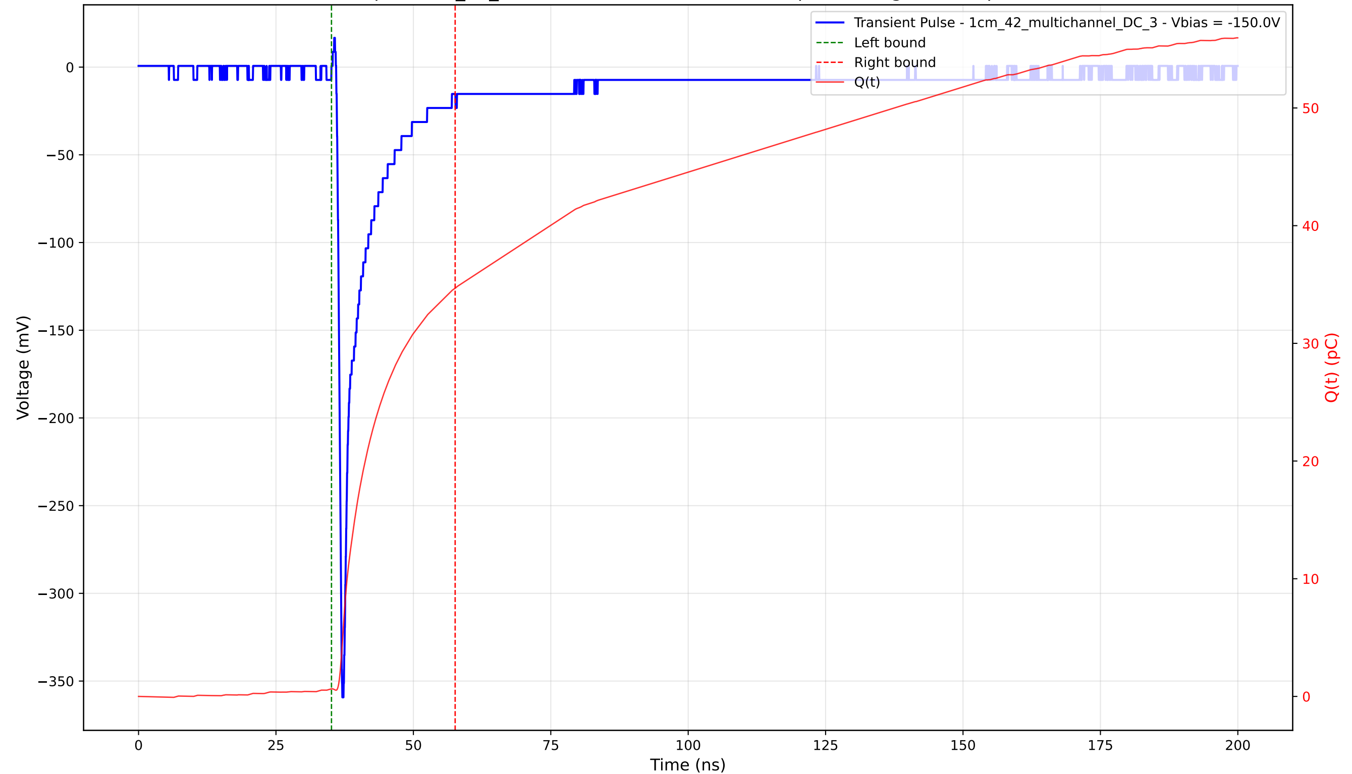
Transient Pulse - Sample: 1cm_42_multichannel - Position: 4780.0 \mu\text{m} - Charge: 34.02 pC - Rise Time: 0.79 ns
