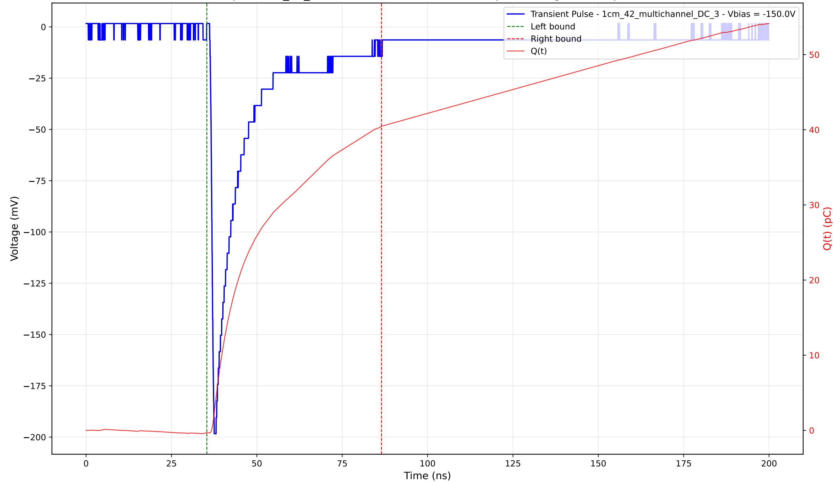
Transient Pulse - Sample: 1cm_42_multichannel - Position: 4200.0 \mu\text{m} - Charge: 40.78 pC - Rise Time: 0.95 ns
