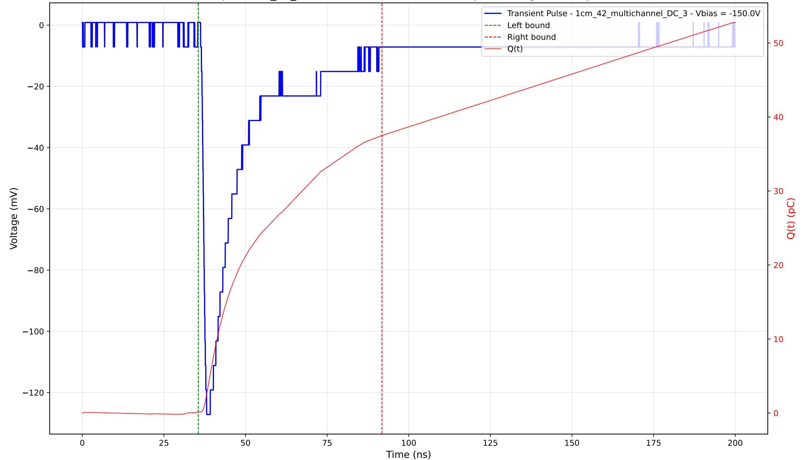
Transient Pulse - Sample: 1cm_42_multichannel - Position: 3625.0 \mu\text{m} - Charge: 37.36 pC - Rise Time: 1.35 ns
