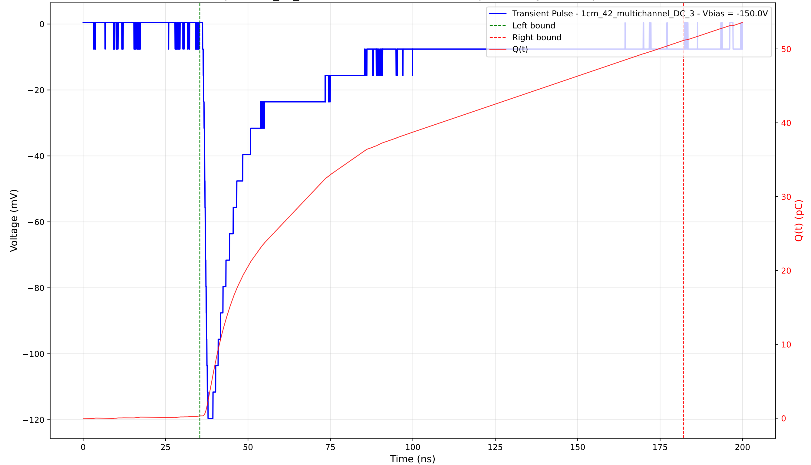
Transient Pulse - Sample: 1cm_42_multichannel - Position: 1295.0 \mu\text{m} - Charge: 50.84 pC - Rise Time: 1.25 ns
