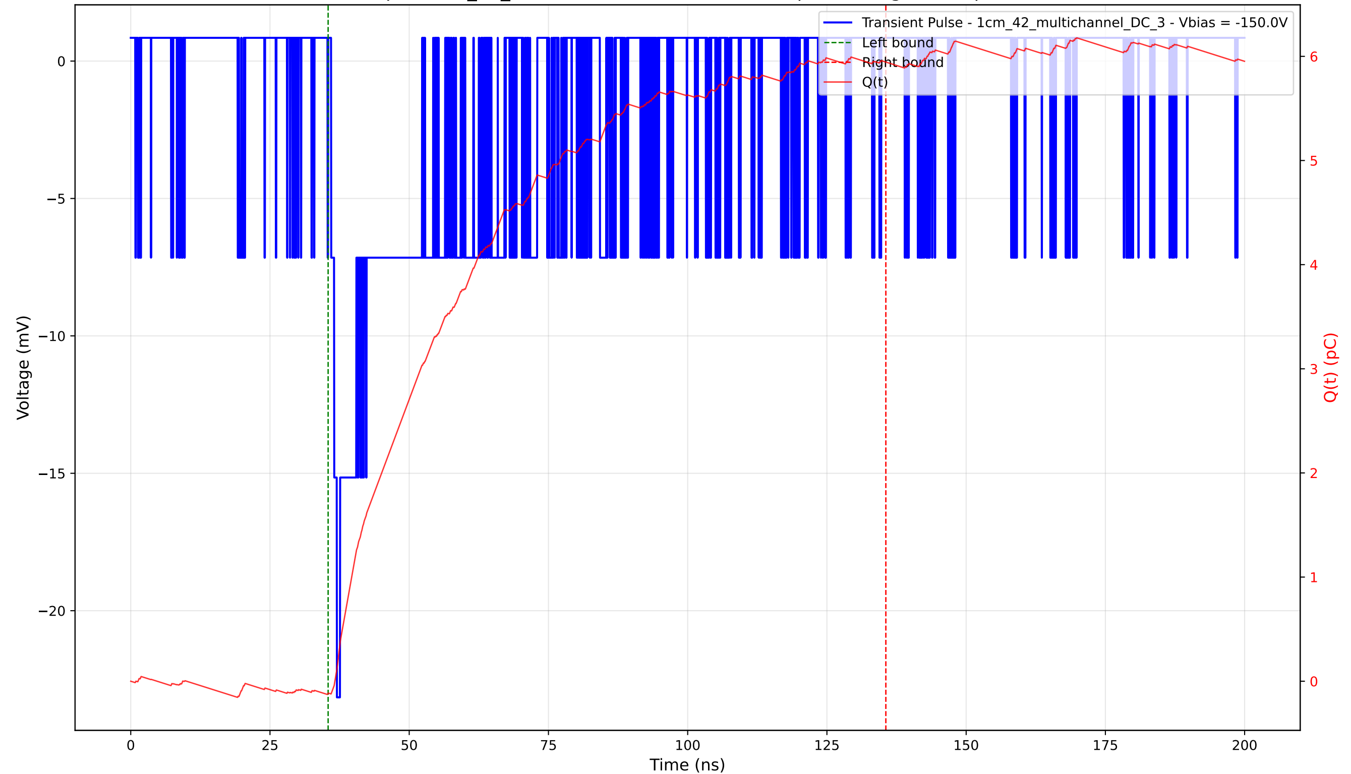
Transient Pulse - Sample: 1cm_42_multichannel - Position: 335.0 \mu\text{m} - Charge: 6.06 pC - Rise Time: 1.04 ns
