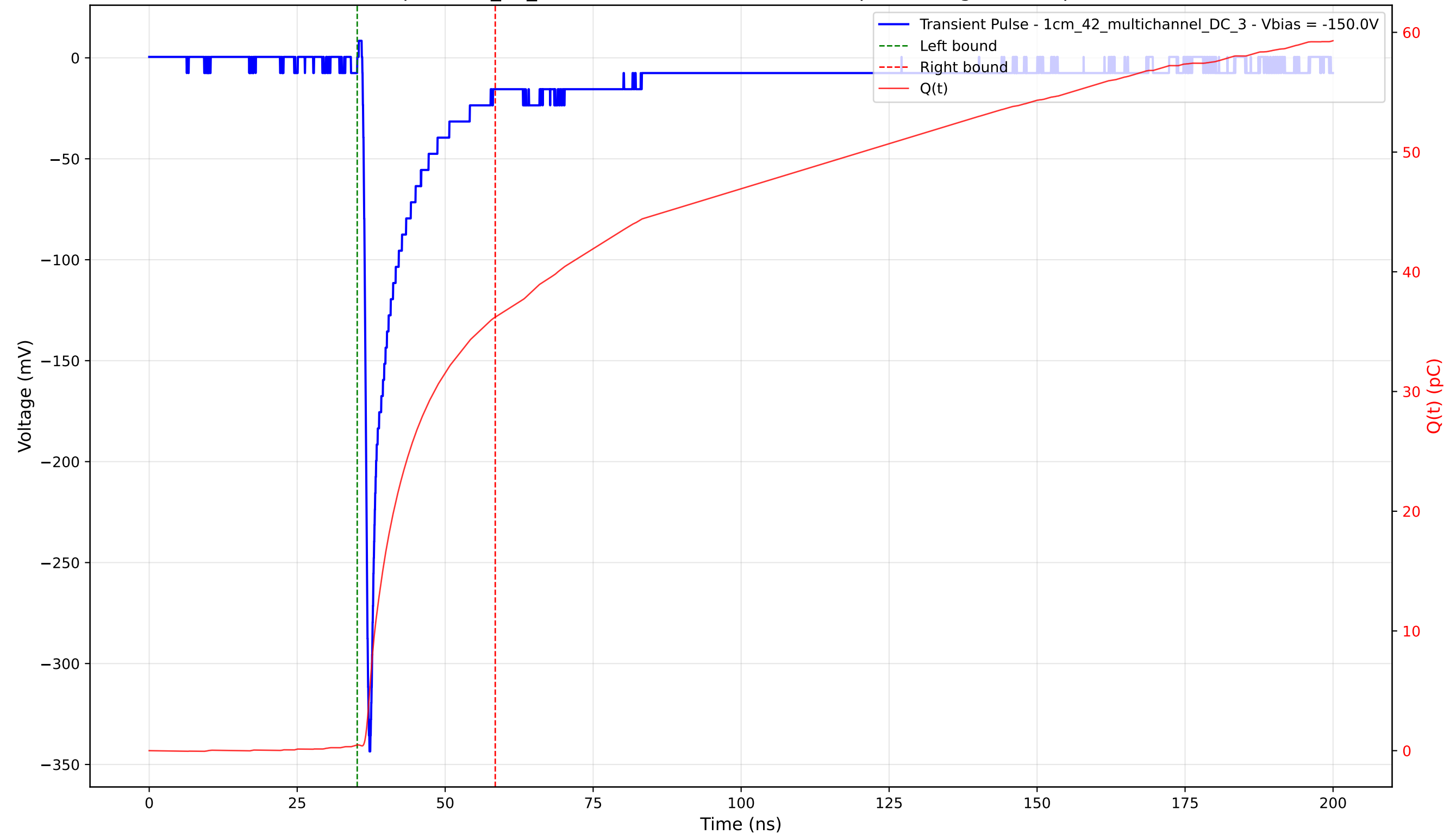
Transient Pulse - Sample: 1cm_42_multichannel - Position: 4690.0 \mu\text{m} - Charge: 35.73 pC - Rise Time: 0.81 ns
