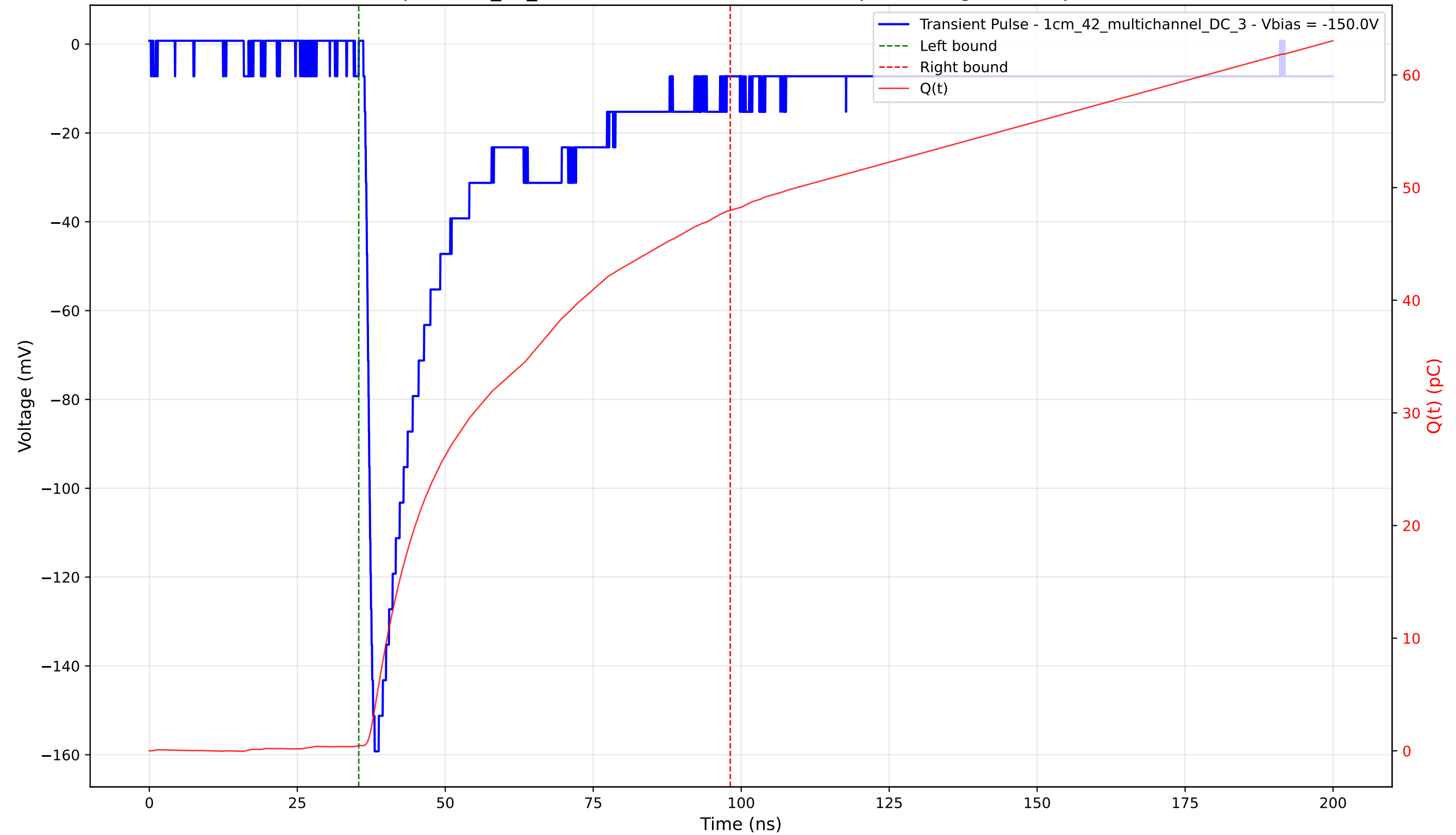
Transient Pulse - Sample: 1cm_42_multichannel - Position: 1215.0 \mu\text{m} - Charge: 47.51 pC - Rise Time: 1.32 ns
