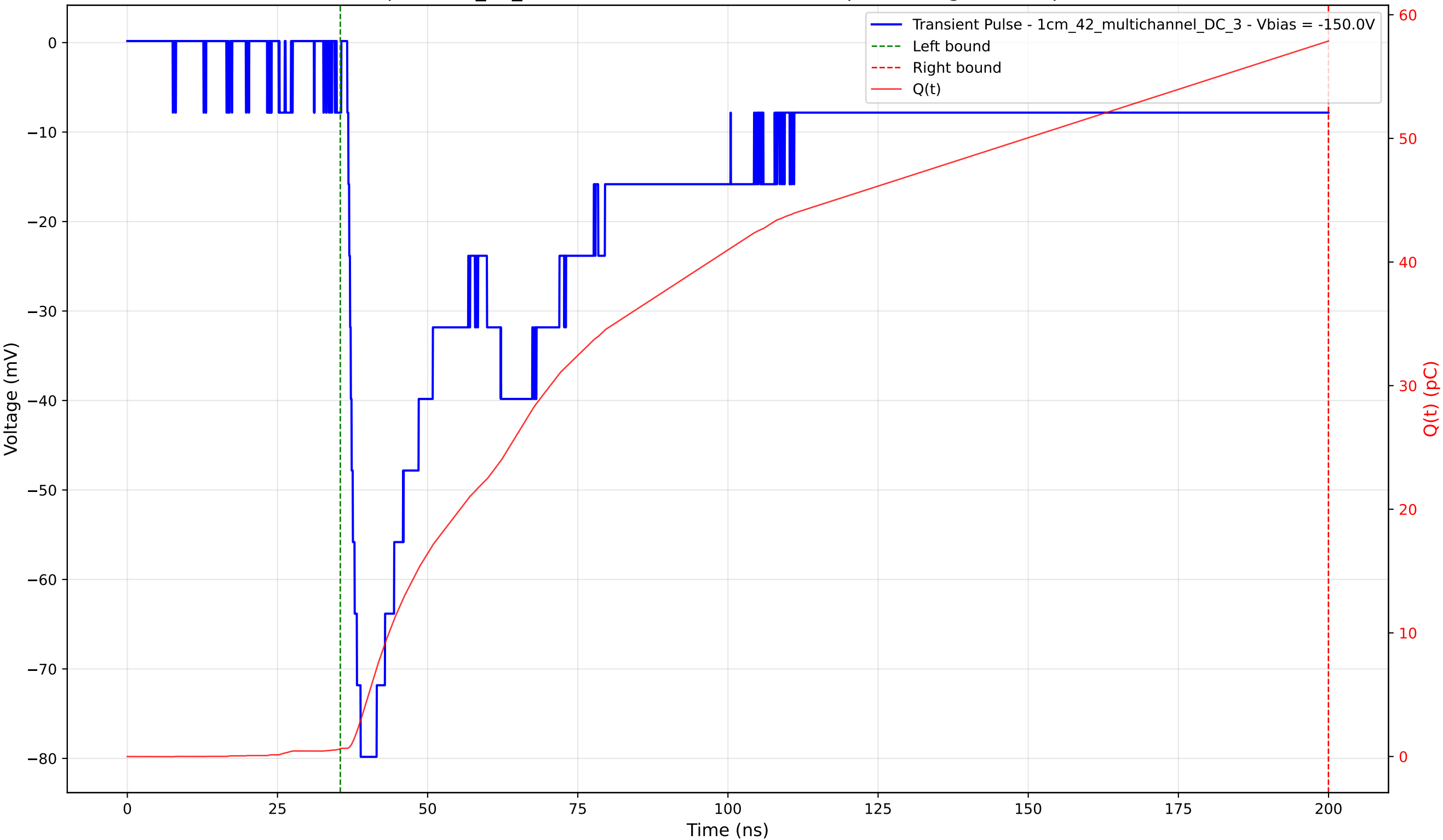
Transient Pulse - Sample: 1cm_42_multichannel - Position: 2475.0 \mu\text{m} - Charge: 57.24 pC - Rise Time: 2.06 ns
