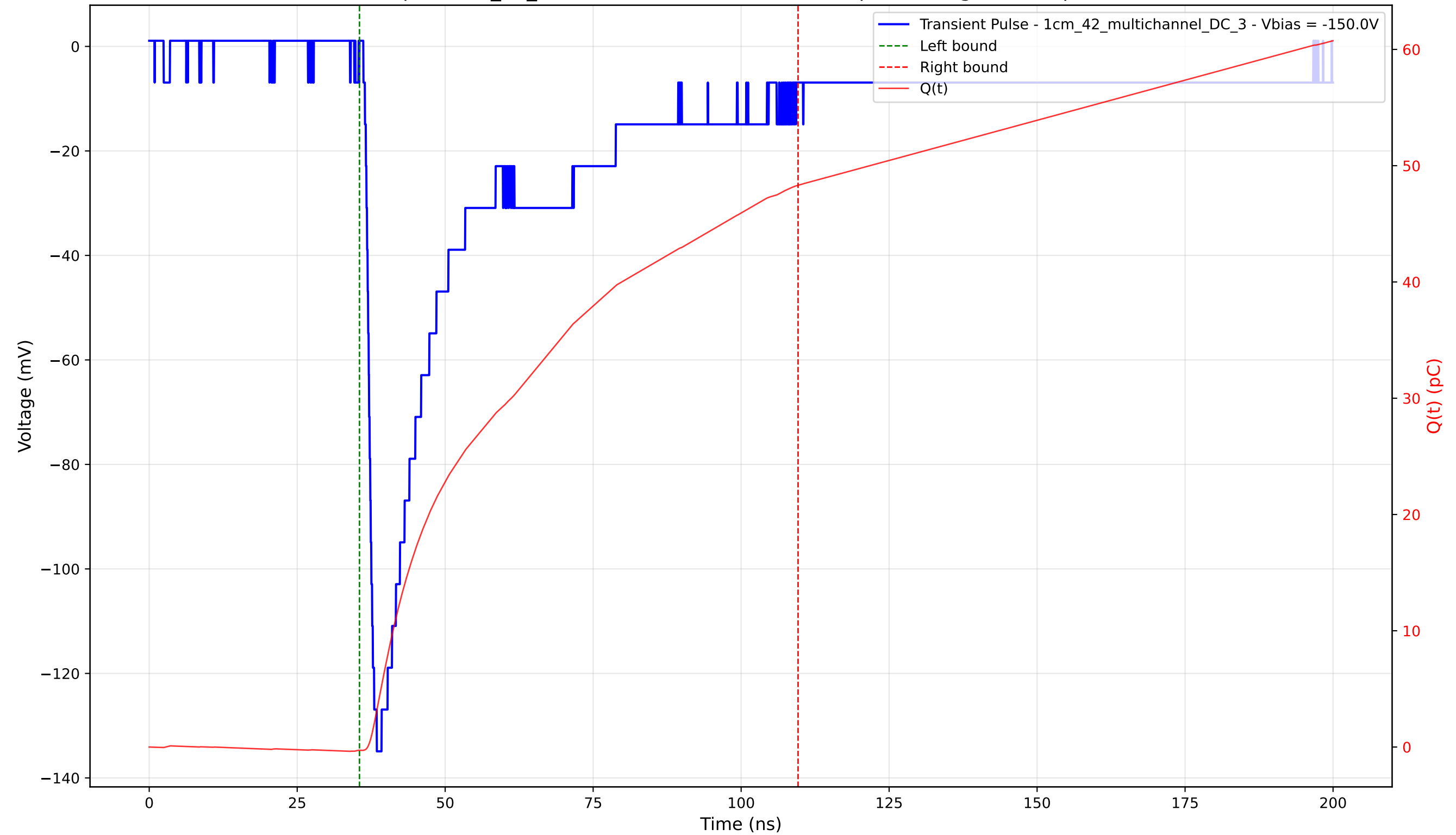
Transient Pulse - Sample: 1cm_42_multichannel - Position: 1500.0 \mu\text{m} - Charge: 48.58 pC - Rise Time: 1.56 ns
