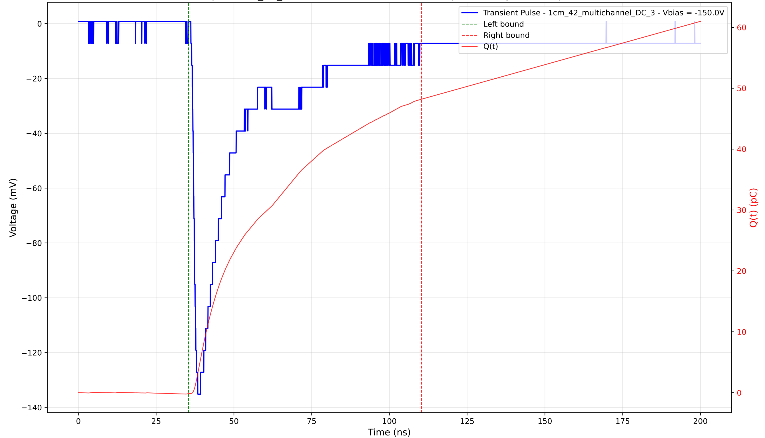
Transient Pulse - Sample: 1cm_42_multichannel - Position: 1475.0 \mu\text{m} - Charge: 48.35 pC - Rise Time: 1.54 ns
