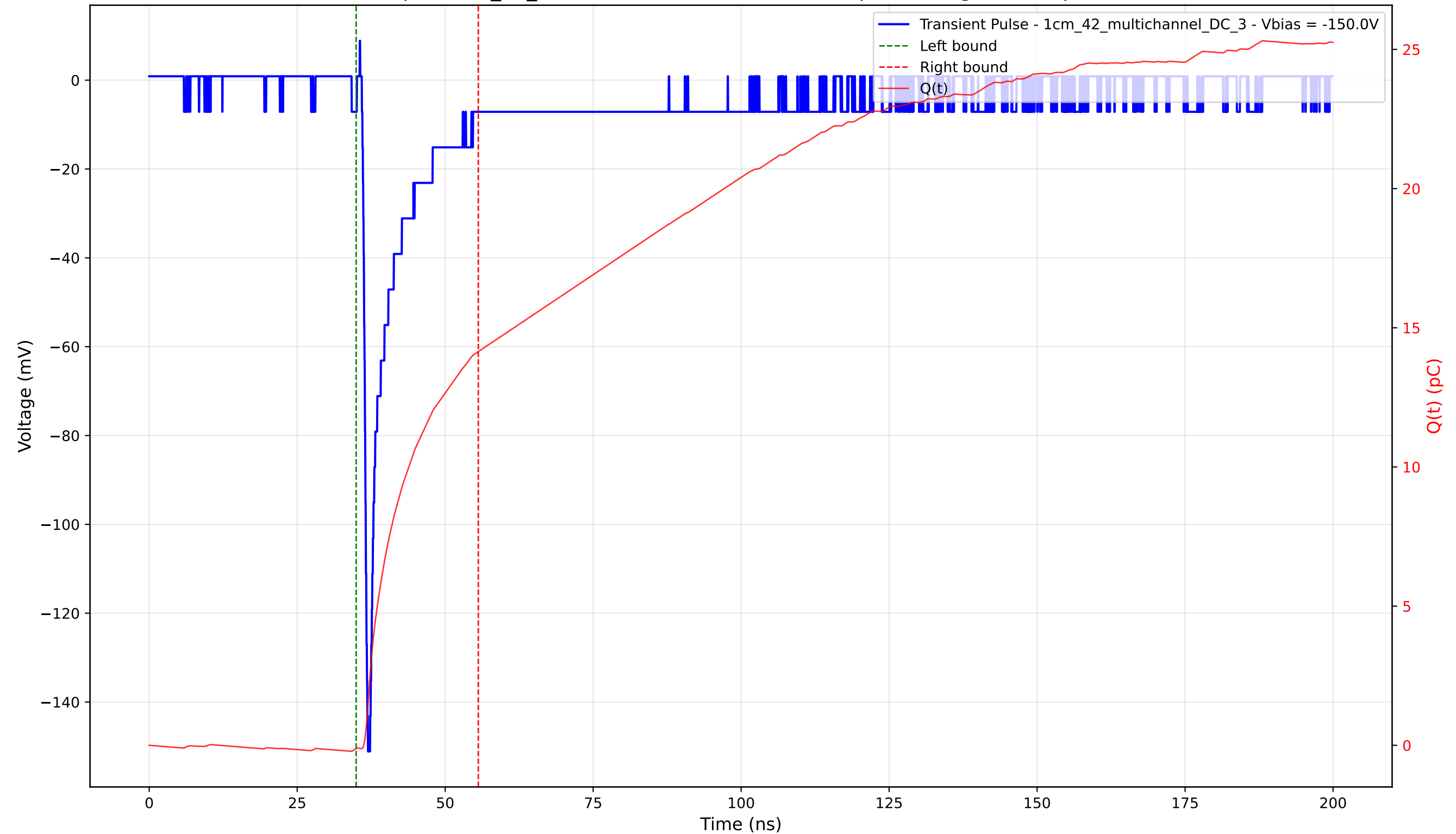
Transient Pulse - Sample: 1cm_42_multichannel - Position: 4855.0 \mu\text{m} - Charge: 14.26 pC - Rise Time: 0.82 ns
