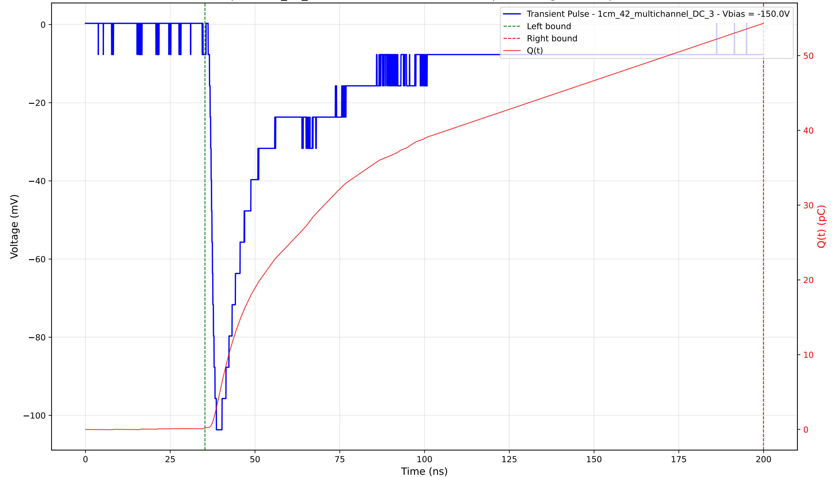
Transient Pulse - Sample: 1cm_42_multichannel - Position: 3165.0 \mu\text{m} - Charge: 54.12 pC - Rise Time: 1.63 ns
