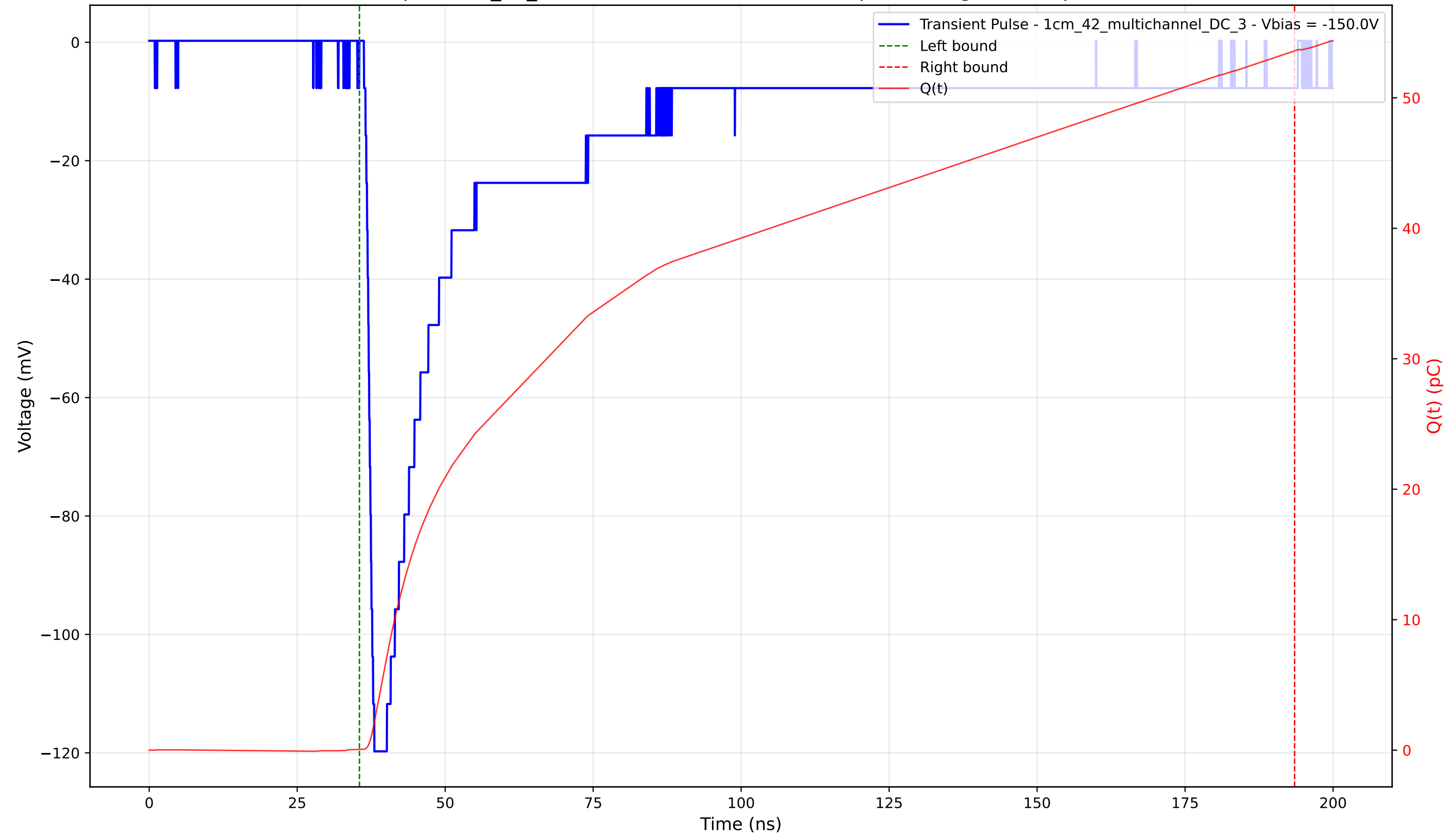
Transient Pulse - Sample: 1cm_42_multichannel - Position: 3545.0 \mu\text{m} - Charge: 53.54 pC - Rise Time: 1.29 ns
