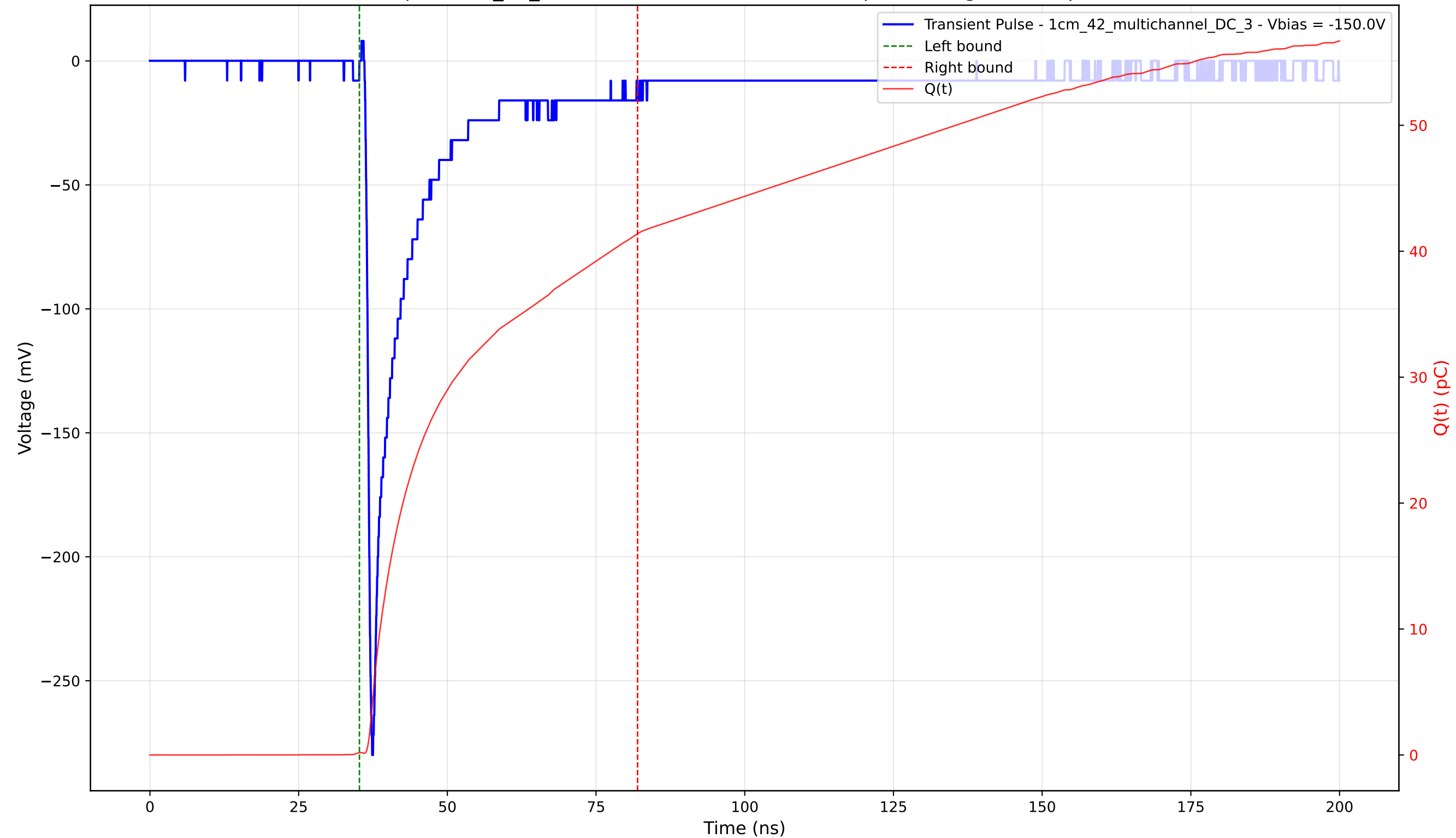
Transient Pulse - Sample: 1cm_42_multichannel - Position: 4535.0 \mu\text{m} - Charge: 41.19 pC - Rise Time: 0.87 ns
