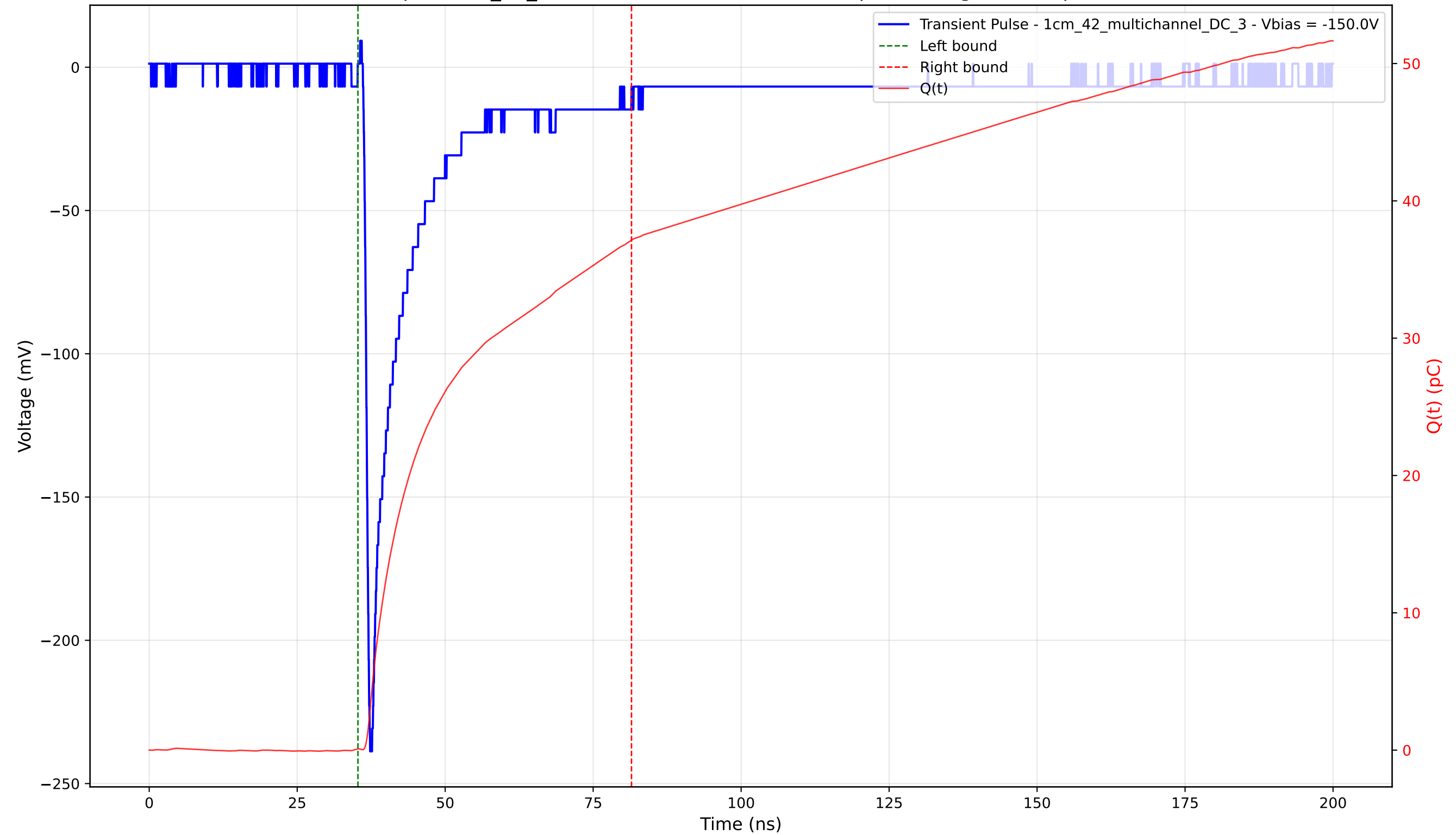
Transient Pulse - Sample: 1cm_42_multichannel - Position: 4480.0 \mu\text{m} - Charge: 37.04 pC - Rise Time: 0.88 ns
