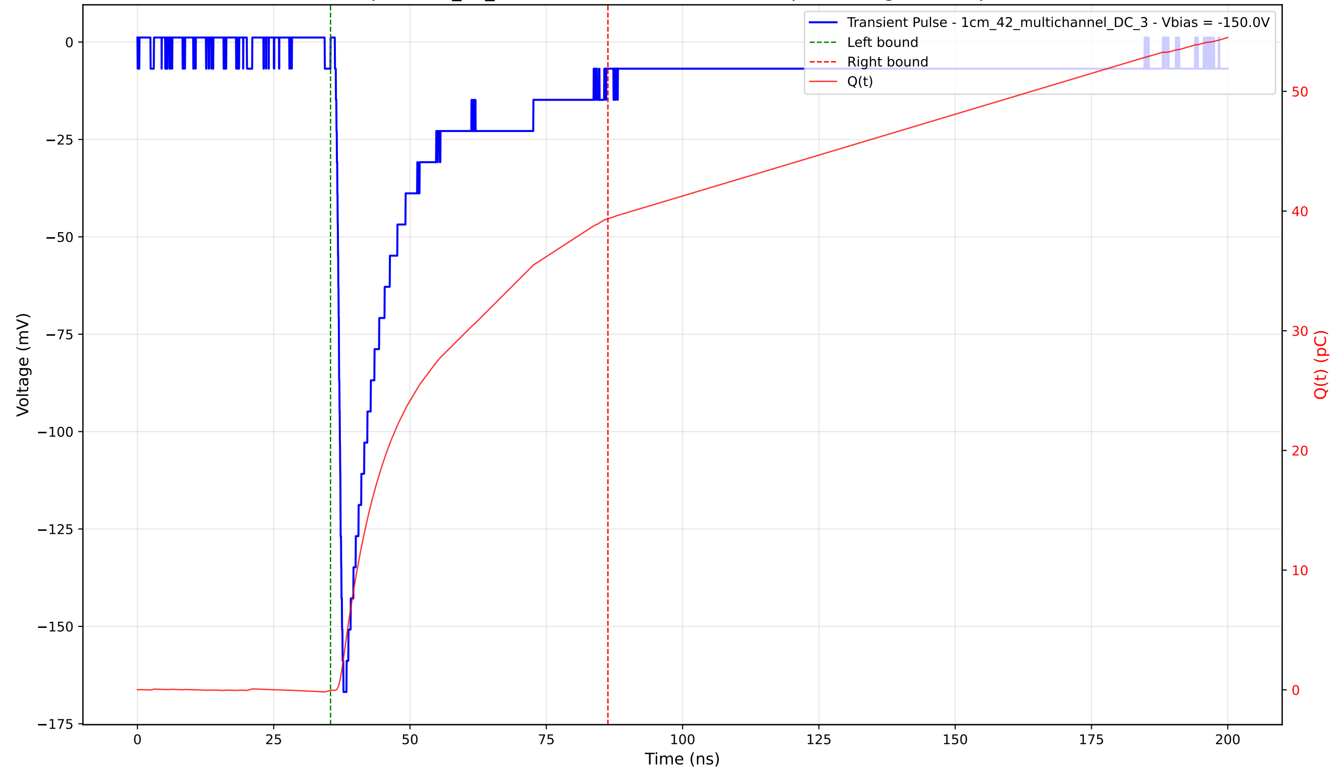
Transient Pulse - Sample: 1cm_42_multichannel - Position: 3980.0 \mu\text{m} - Charge: 39.40 pC - Rise Time: 1.04 ns
