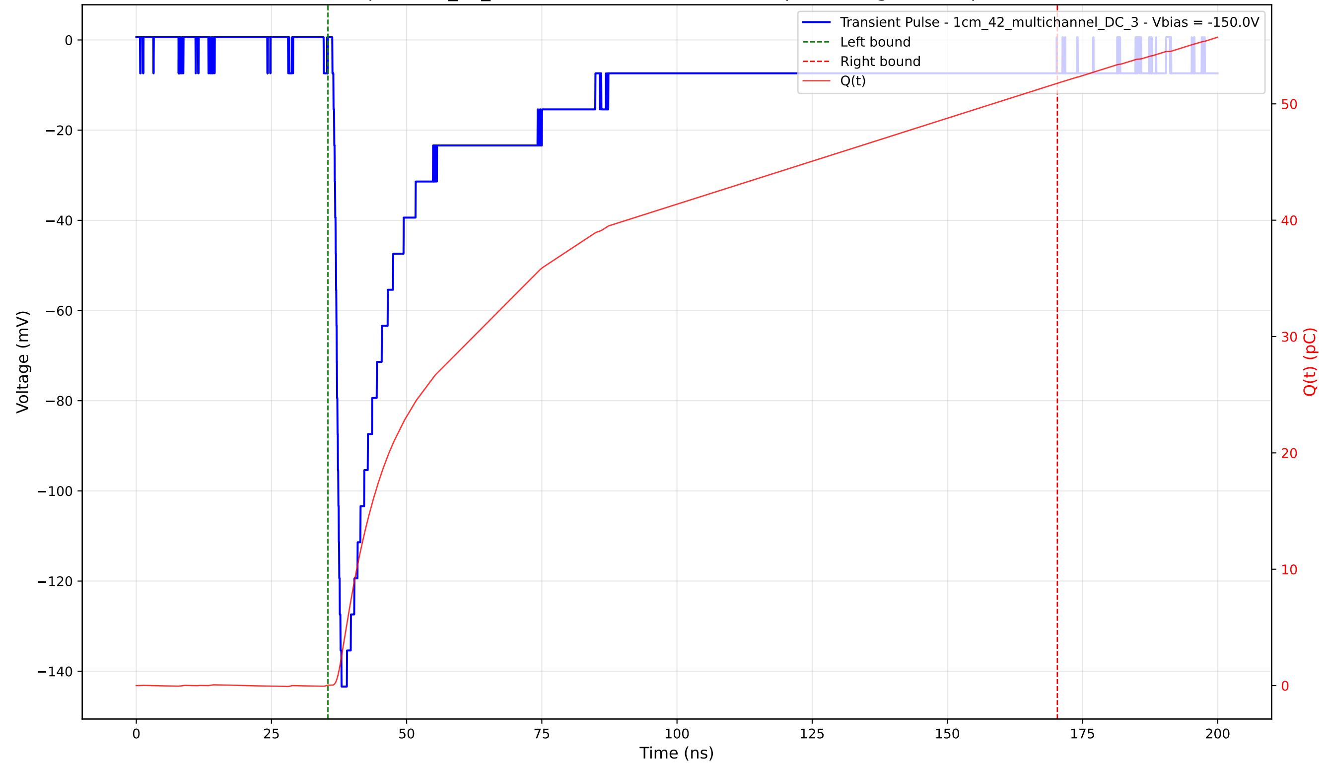
Transient Pulse - Sample: 1cm_42_multichannel - Position: 3745.0 \mu\text{m} - Charge: 51.74 pC - Rise Time: 1.30 ns
