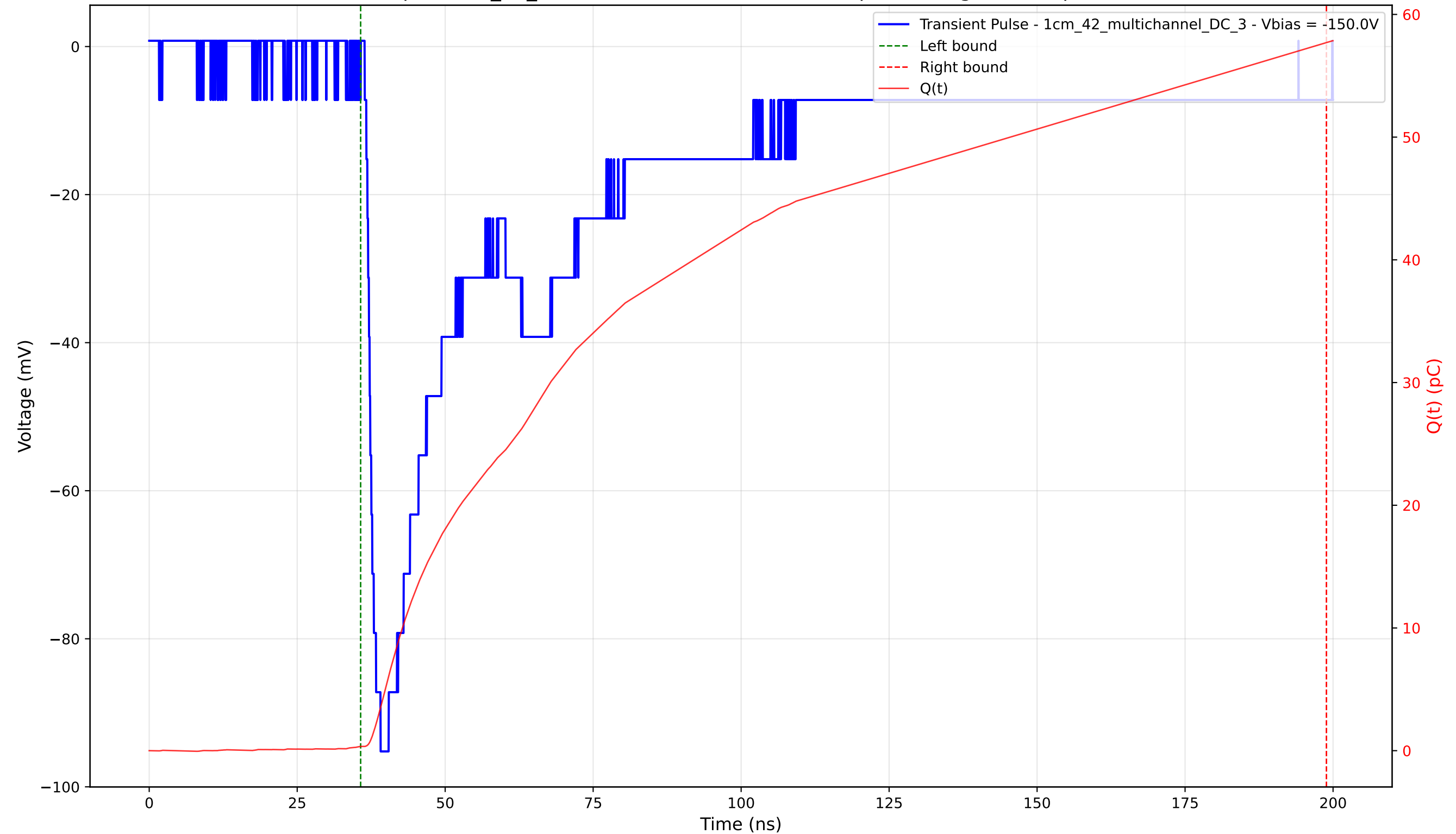
Transient Pulse - Sample: 1cm_42_multichannel - Position: 2055.0 \mu\text{m} - Charge: 57.37 pC - Rise Time: 1.65 ns
