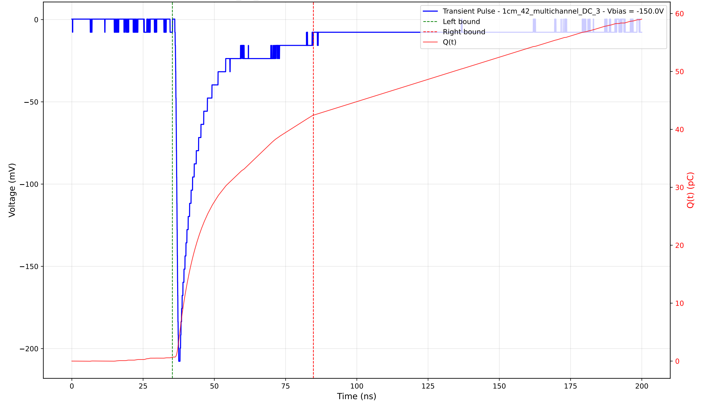
Transient Pulse - Sample: 1cm_42_multichannel - Position: 4235.0 \mu\text{m} - Charge: 41.76 pC - Rise Time: 0.95 ns
