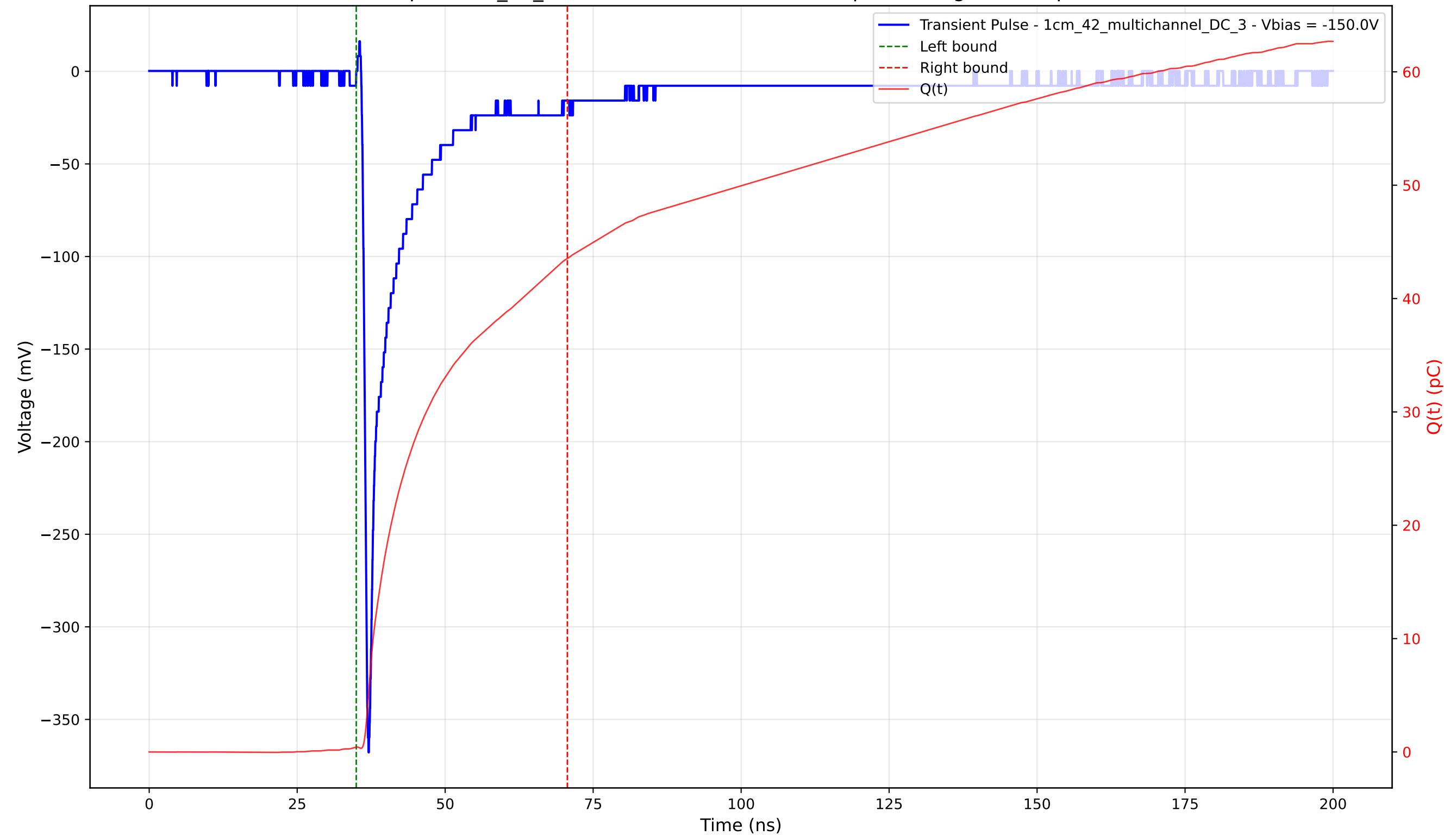
Transient Pulse - Sample: 1cm_42_multichannel - Position: 155.0 \mu\text{m} - Charge: 43.09 pC - Rise Time: 0.82 ns
