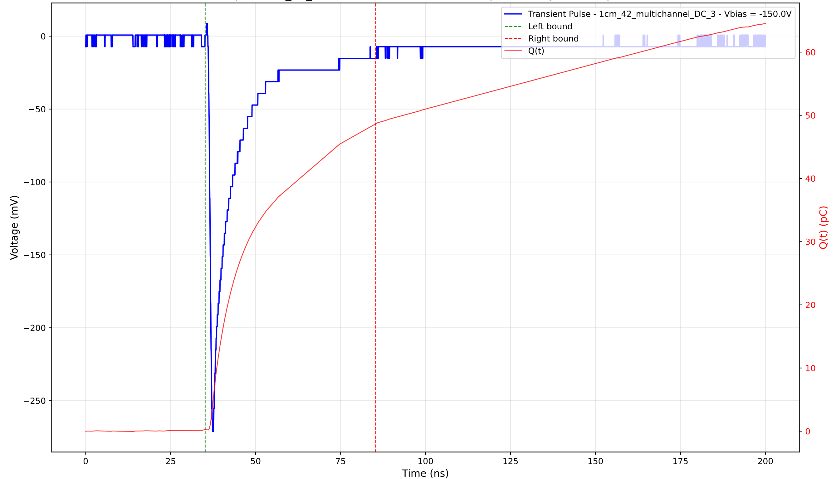
Transient Pulse - Sample: 1cm_42_multichannel - Position: 505.0 \mu\text{m} - Charge: 48.40 pC - Rise Time: 0.91 ns
