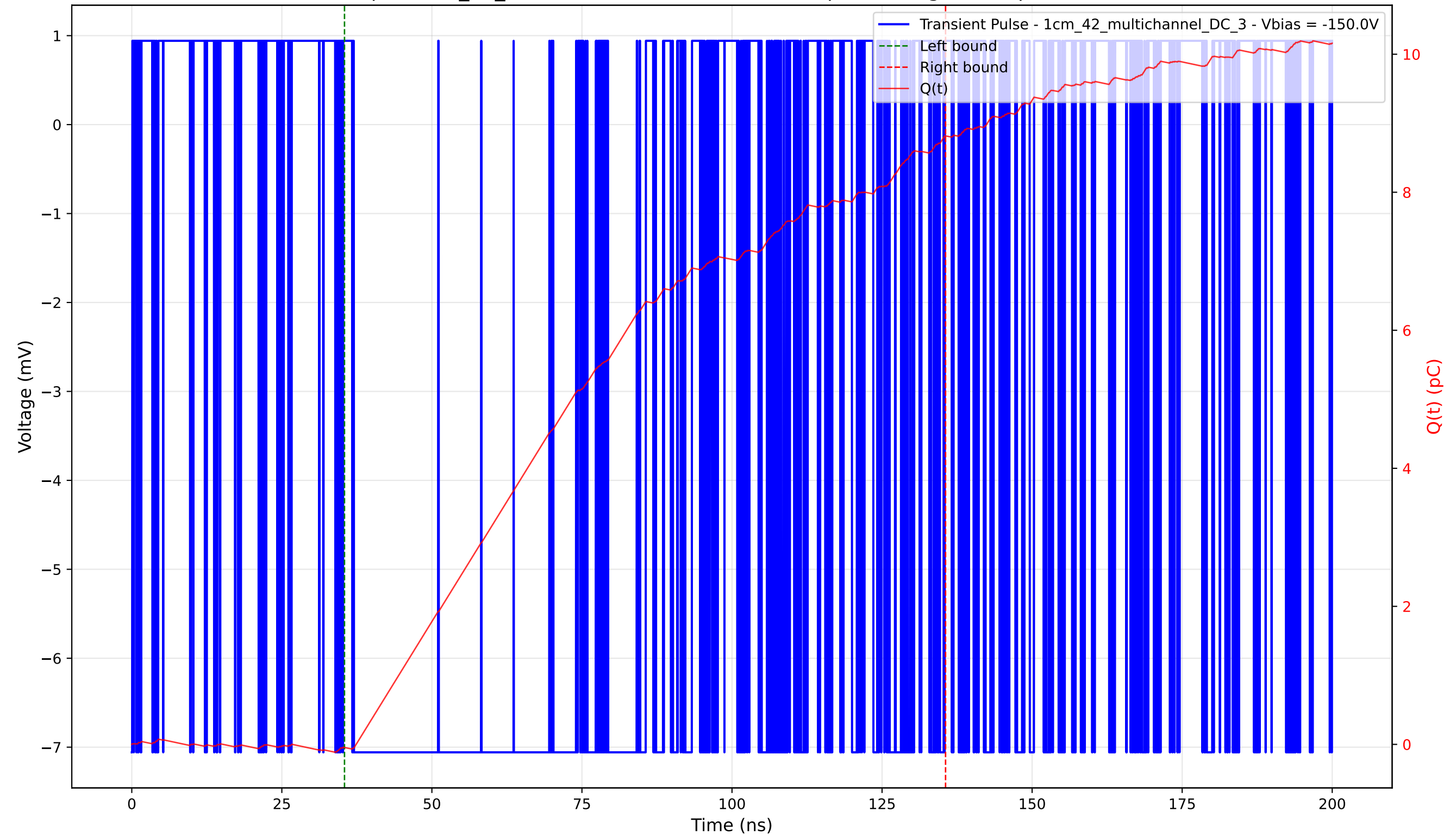
Transient Pulse - Sample: 1cm_42_multichannel - Position: 1855.0 \mu\text{m} - Charge: 8.86 pC - Rise Time: 0.00 ns (N/A)
