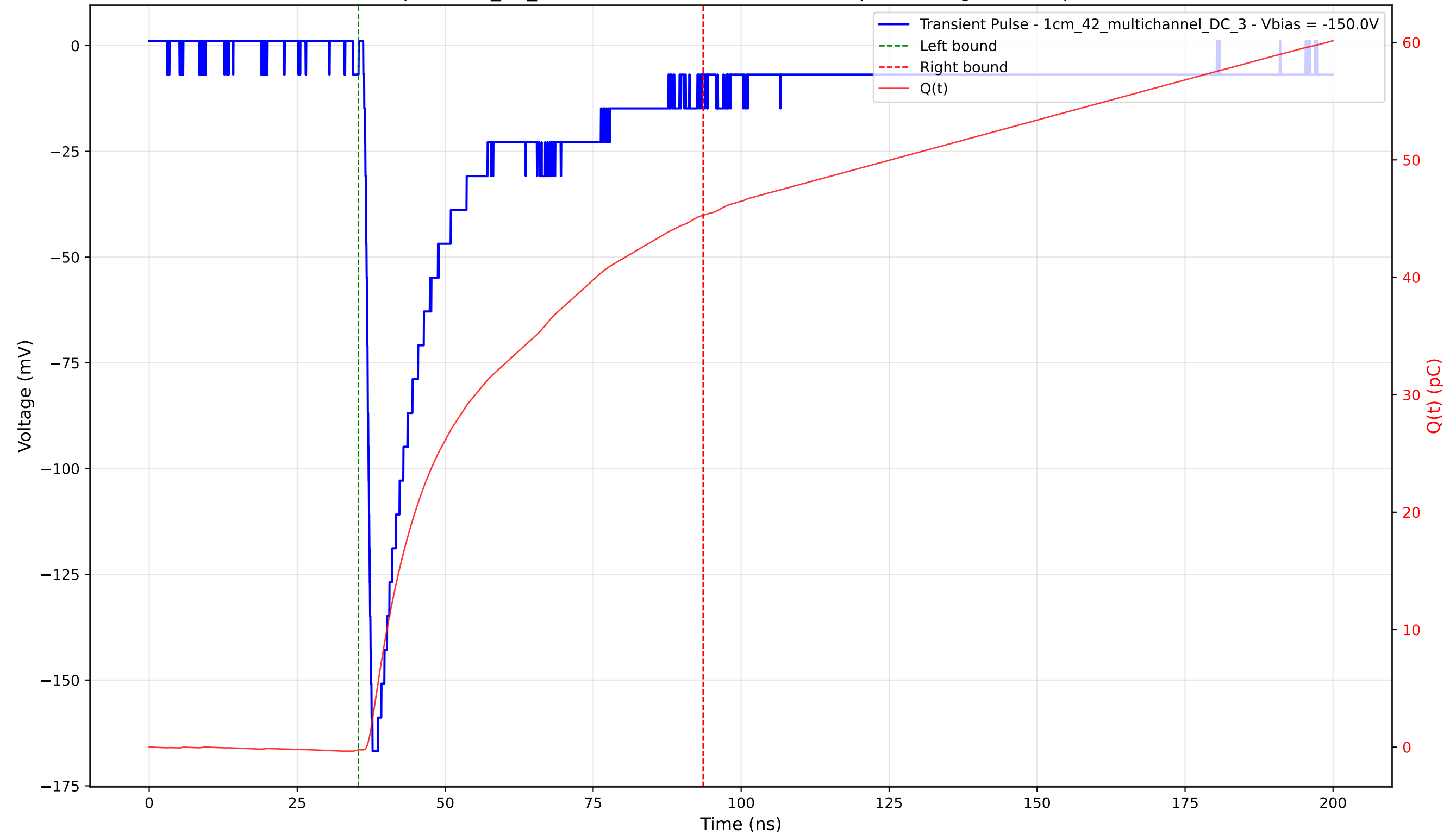
Transient Pulse - Sample: 1cm_42_multichannel - Position: 1055.0 \mu\text{m} - Charge: 45.51 pC - Rise Time: 1.04 ns
