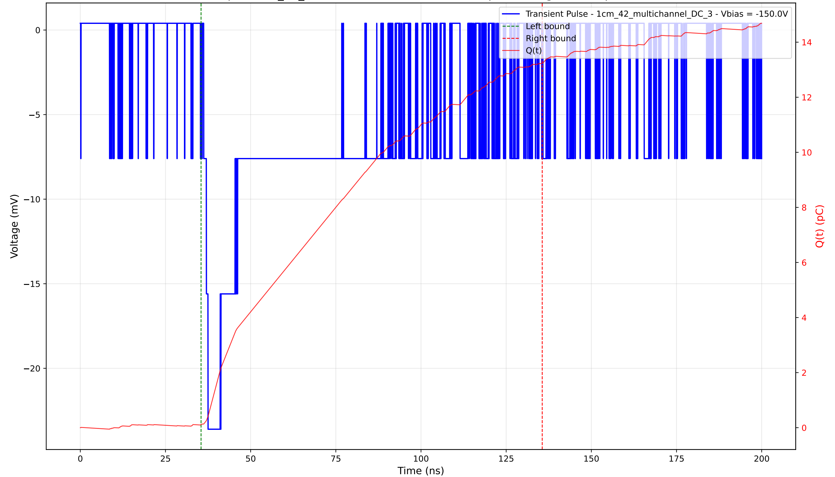
Transient Pulse - Sample: 1cm_42_multichannel - Position: 3860.0 \mu\text{m} - Charge: 13.12 pC - Rise Time: 1.27 ns
