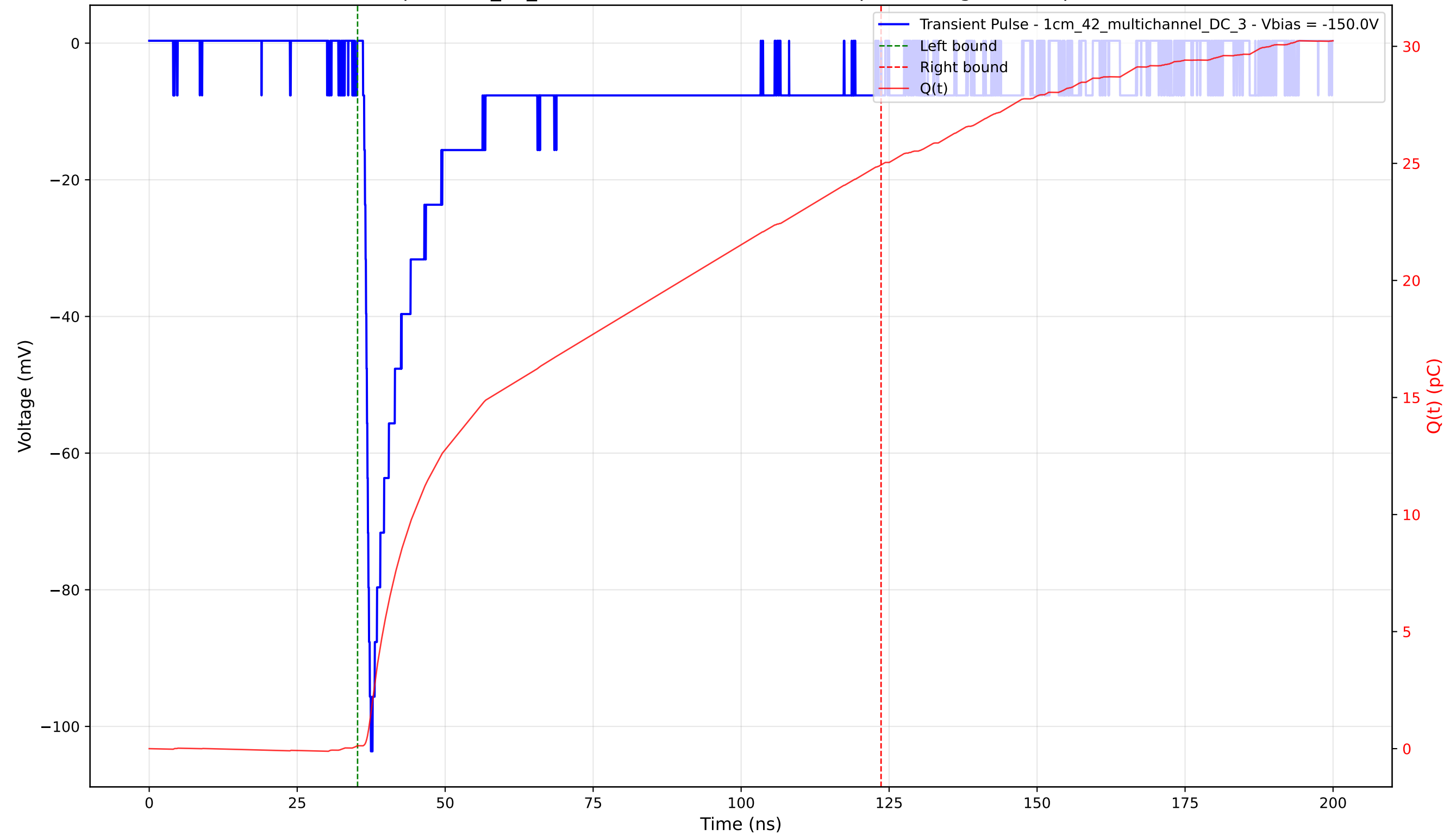
Transient Pulse - Sample: 1cm_42_multichannel - Position: 4340.0 \mu\text{m} - Charge: 24.81 pC - Rise Time: 0.95 ns
