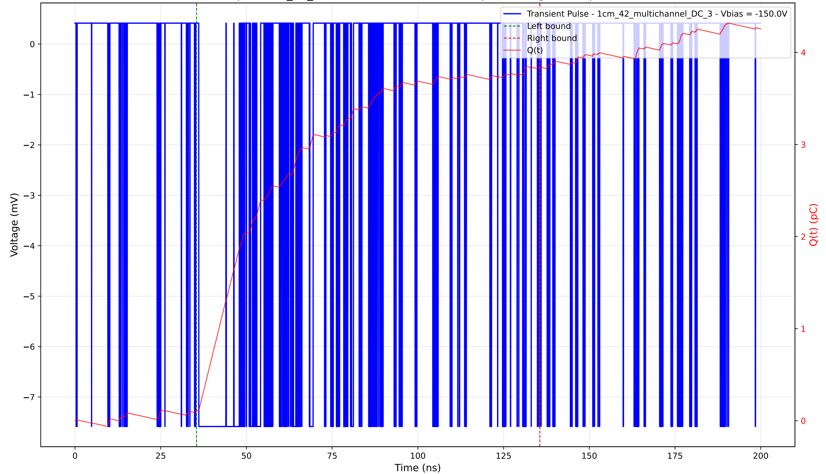
Transient Pulse - Sample: 1cm_42_multichannel - Position: 20.0 \mu\text{m} - Charge: 3.73 pC - Rise Time: 0.02 ns
