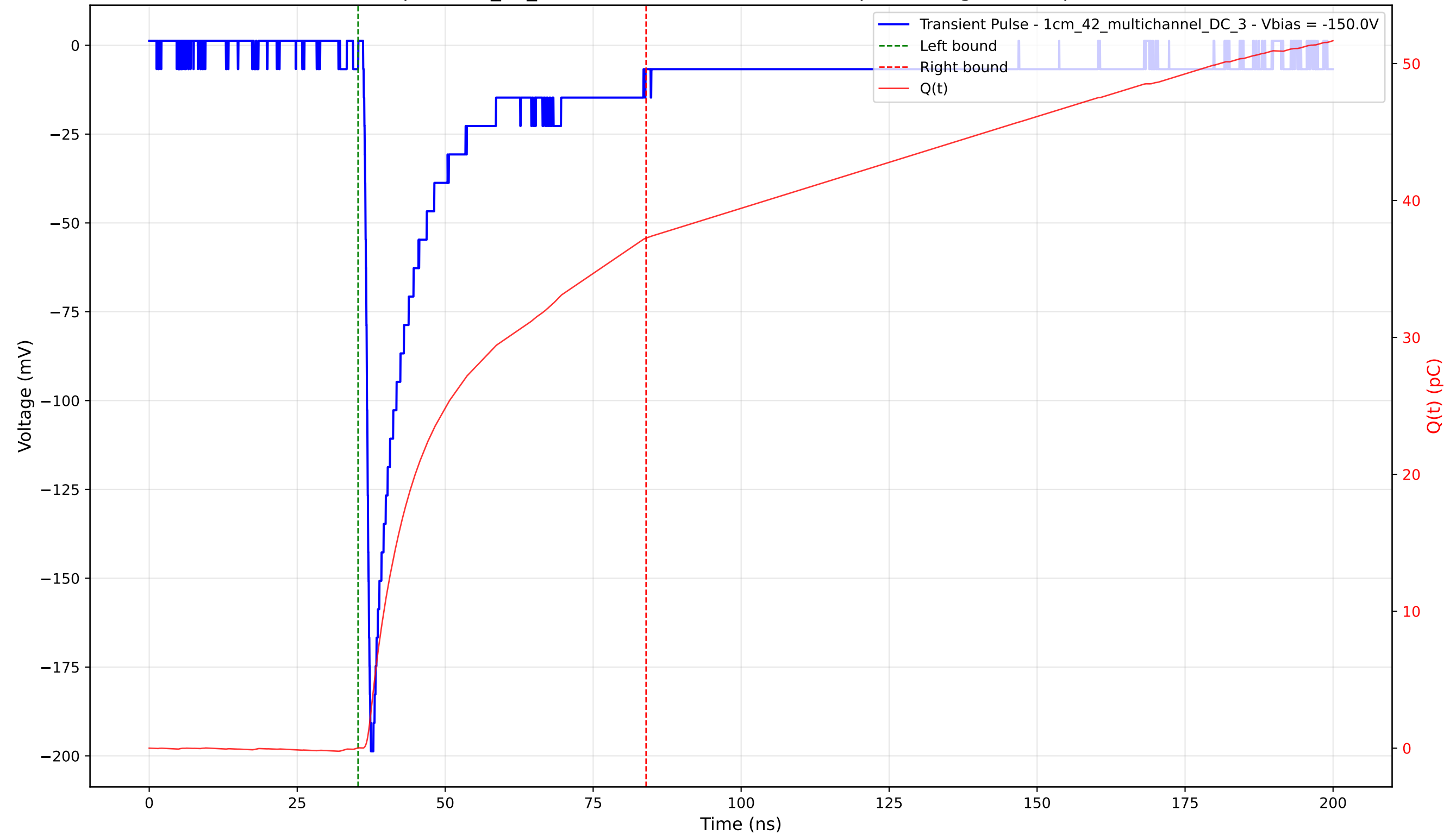
Transient Pulse - Sample: 1cm_42_multichannel - Position: 4285.0 \mu\text{m} - Charge: 37.23 pC - Rise Time: 0.93 ns
