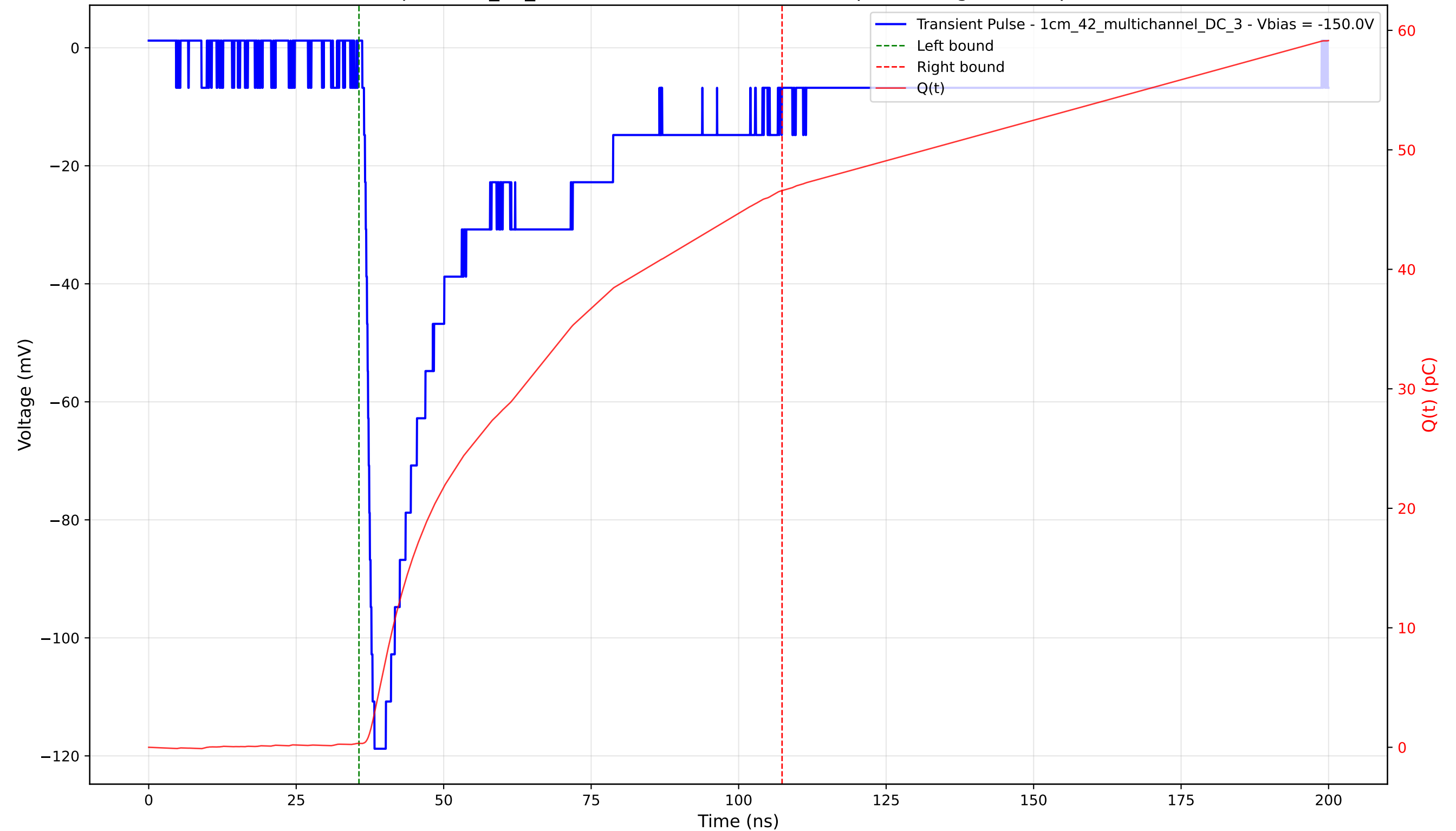
Transient Pulse - Sample: 1cm_42_multichannel - Position: 1615.0 \mu\text{m} - Charge: 46.27 pC - Rise Time: 1.45 ns
