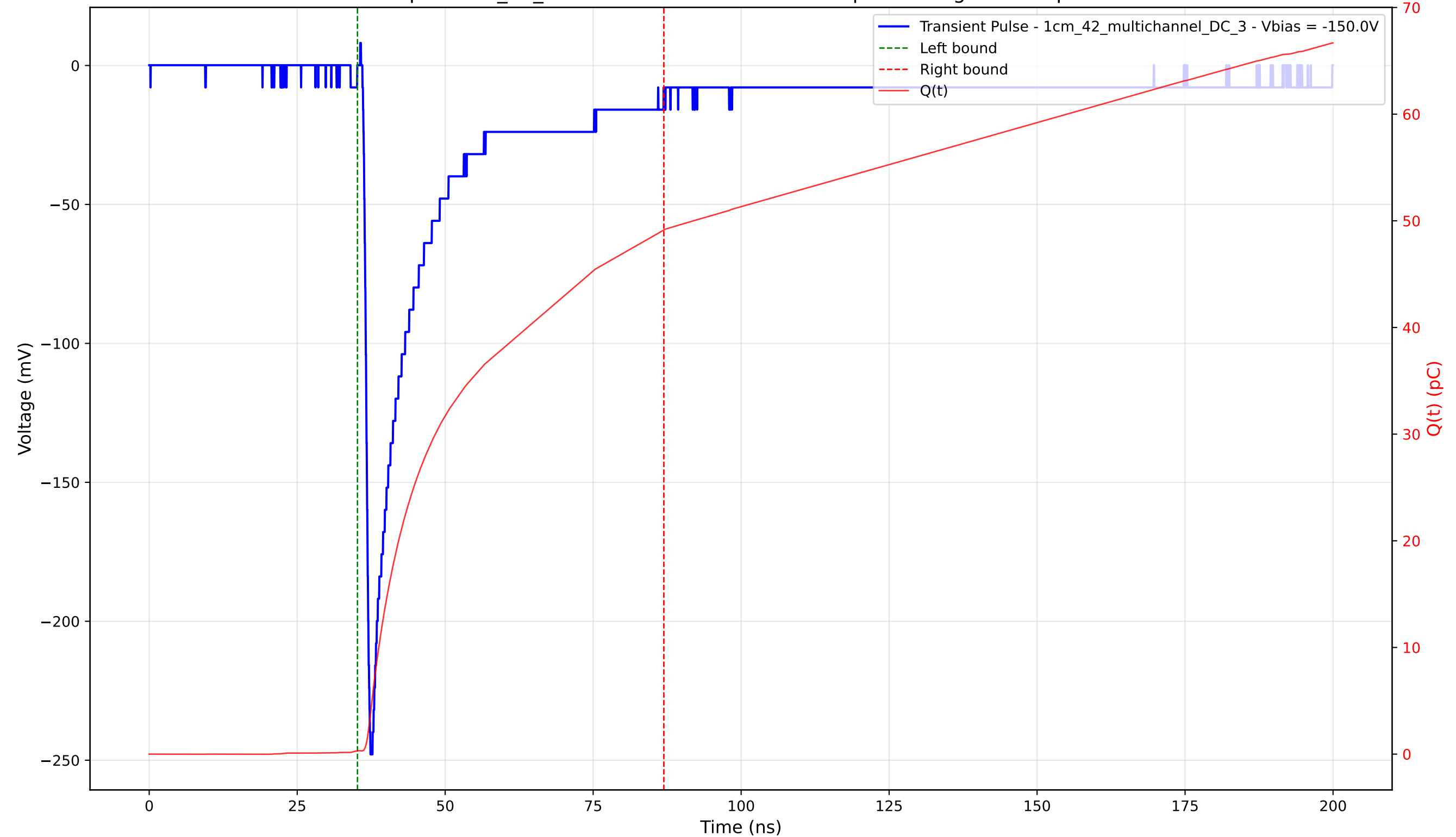
Transient Pulse - Sample: 1cm_42_multichannel - Position: 595.0 \mu\text{m} - Charge: 48.81 pC - Rise Time: 0.92 ns
