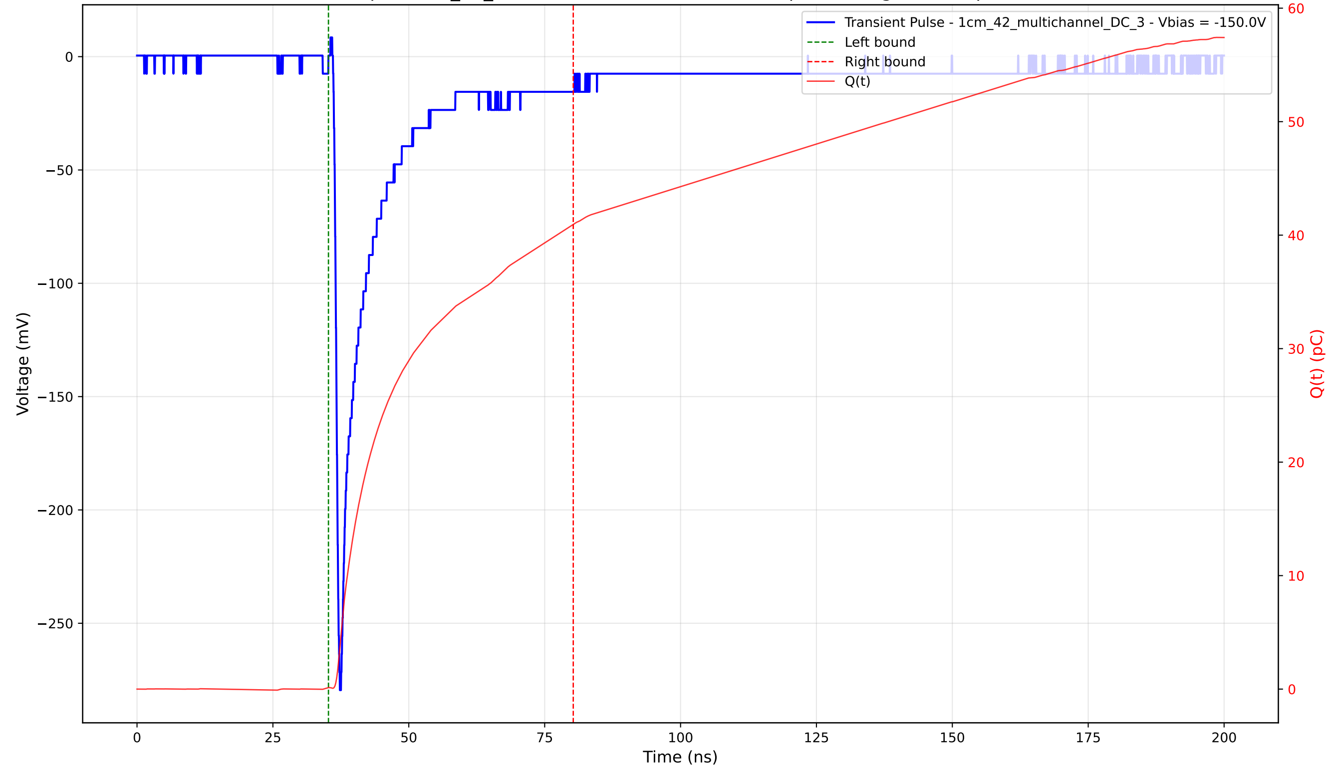
Transient Pulse - Sample: 1cm_42_multichannel - Position: 4540.0 \mu\text{m} - Charge: 40.83 pC - Rise Time: 0.87 ns
