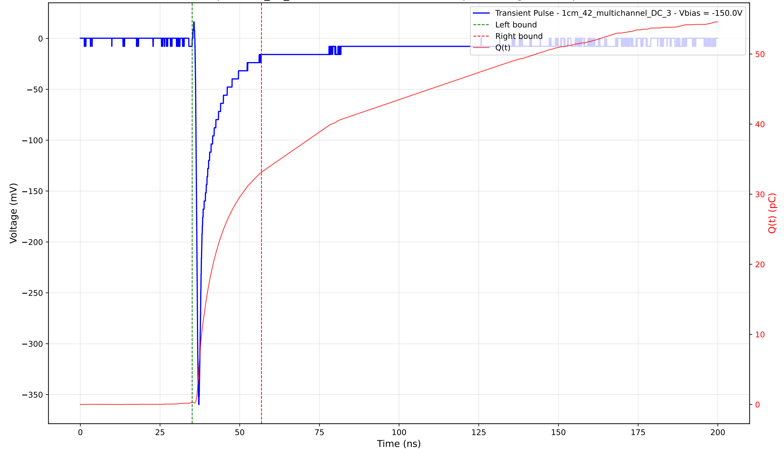
Transient Pulse - Sample: 1cm_42_multichannel - Position: 4800.0 \mu\text{m} - Charge: 32.82 pC - Rise Time: 0.79 ns
