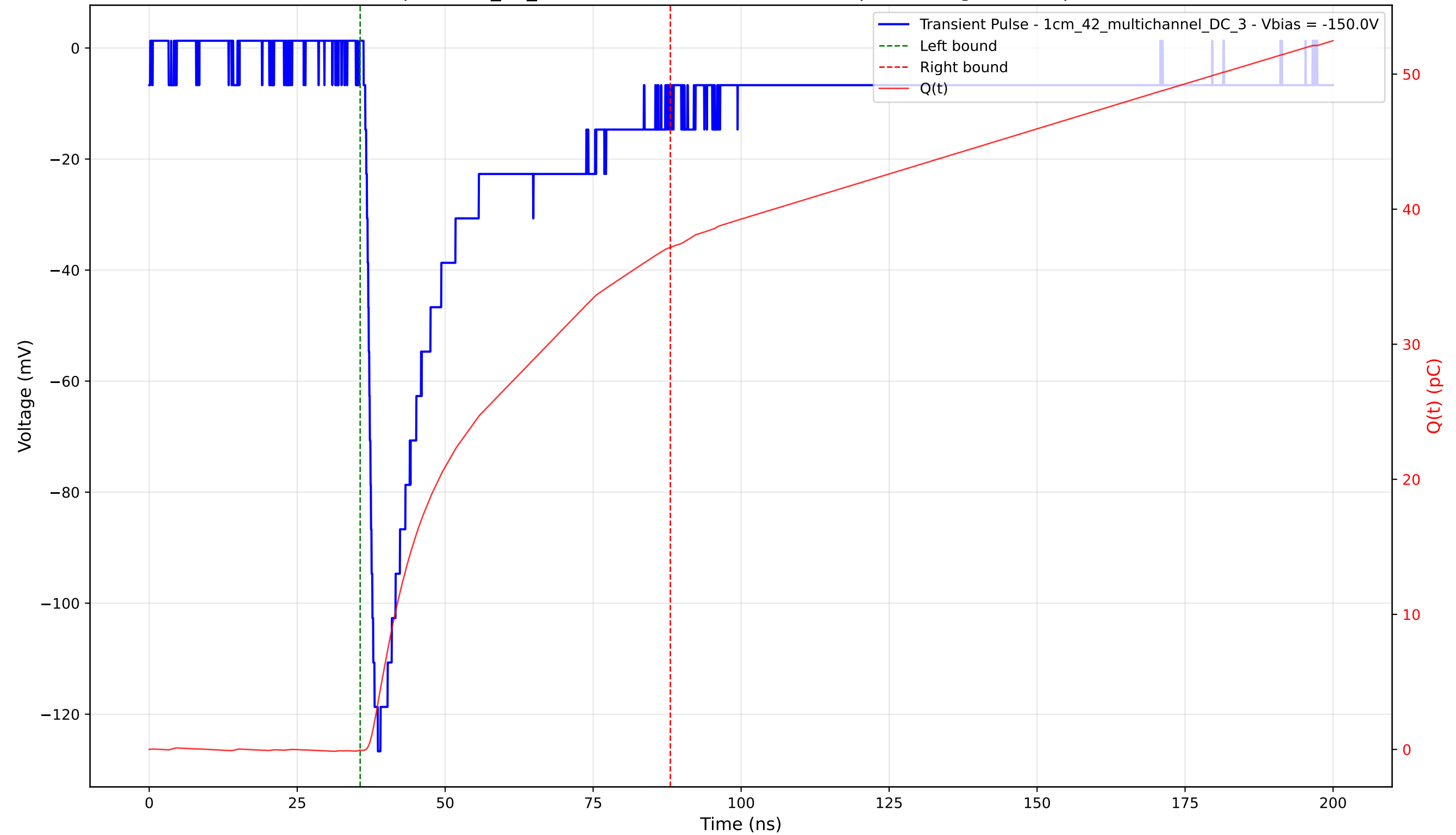
Transient Pulse - Sample: 1cm_42_multichannel - Position: 3505.0 \mu\text{m} - Charge: 37.23 pC - Rise Time: 1.57 ns
