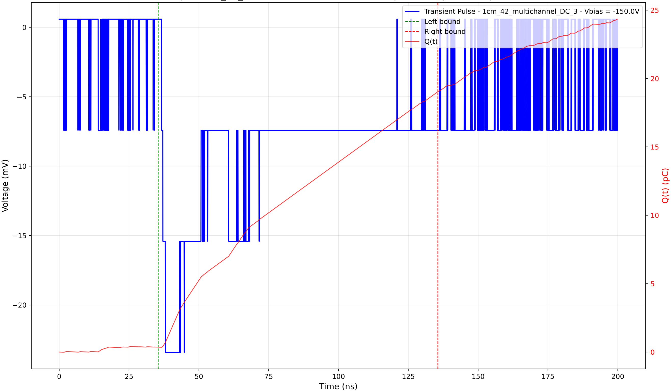
Transient Pulse - Sample: 1cm_42_multichannel - Position: 2335.0 \mu\text{m} - Charge: 18.68 pC - Rise Time: 1.35 ns
