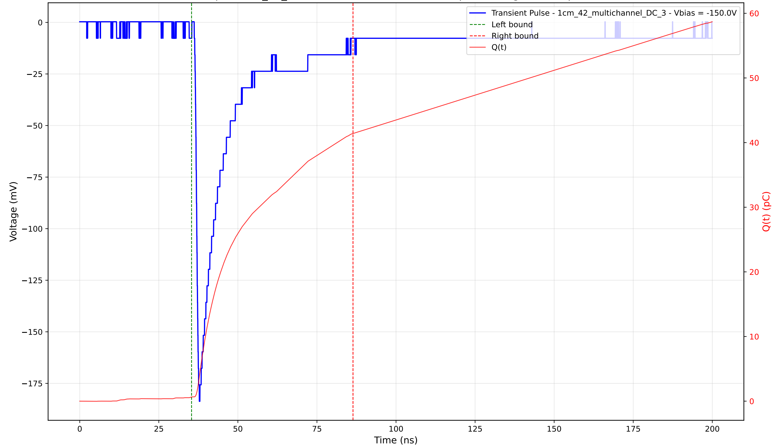
Transient Pulse - Sample: 1cm_42_multichannel - Position: 4065.0 \mu\text{m} - Charge: 40.76 pC - Rise Time: 1.03 ns
