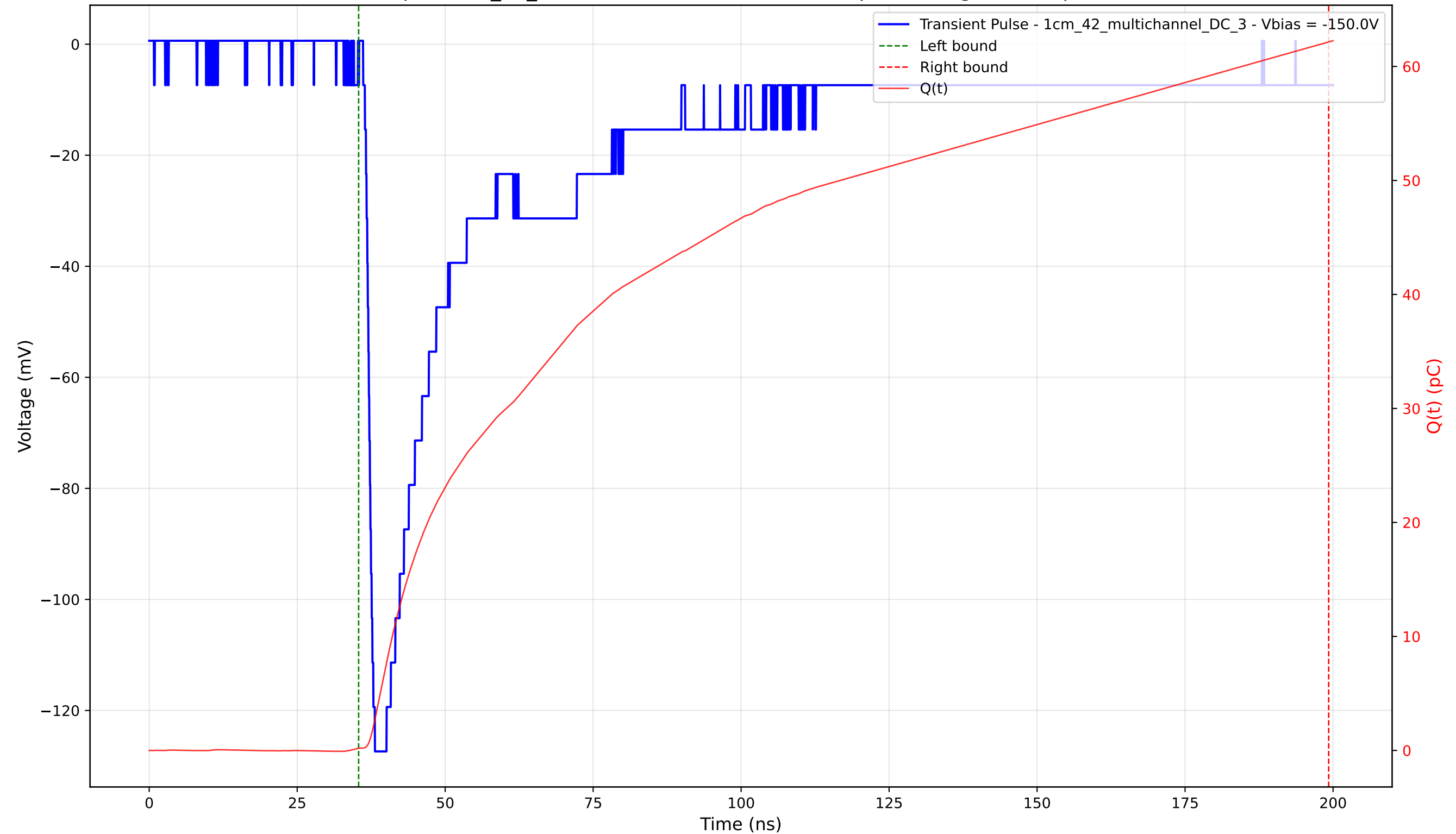
Transient Pulse - Sample: 1cm_42_multichannel - Position: 1525.0 \mu\text{m} - Charge: 61.96 pC - Rise Time: 1.43 ns
