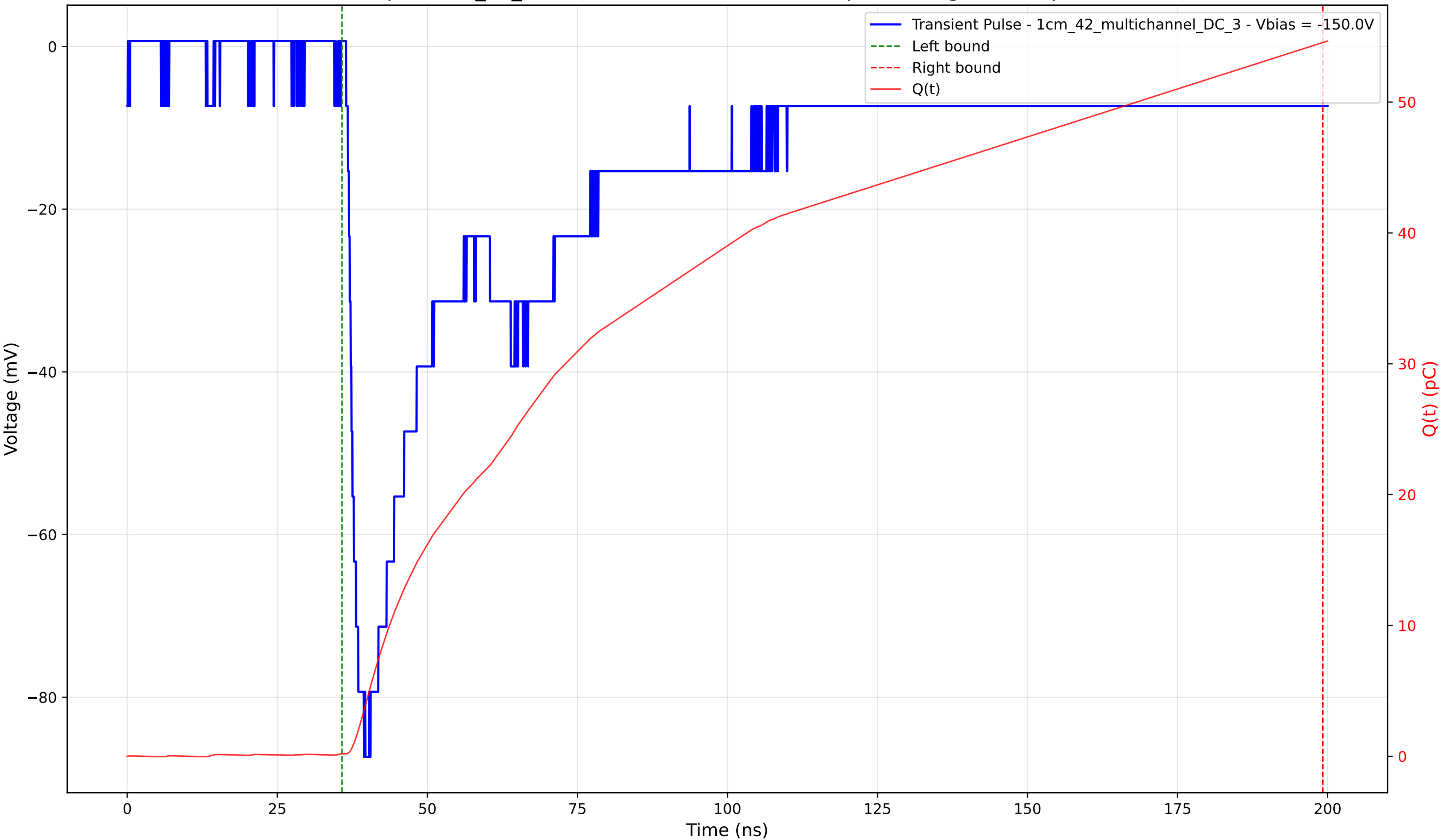
Transient Pulse - Sample: 1cm_42_multichannel - Position: 2650.0 \mu\text{m} - Charge: 54.36 pC - Rise Time: 1.74 ns
