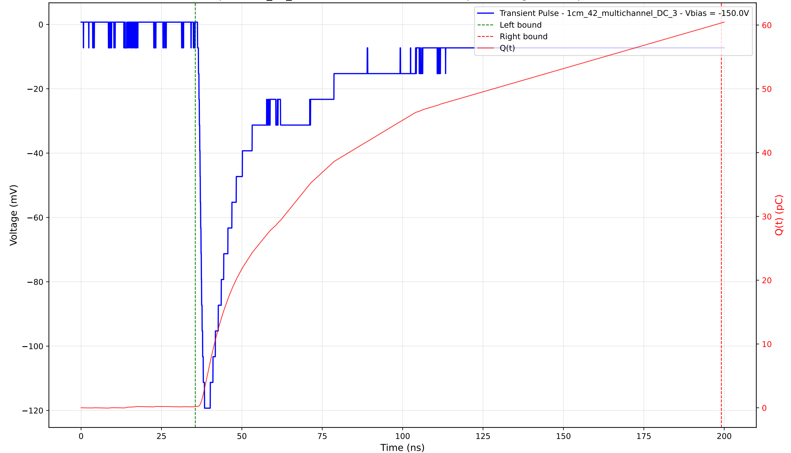
Transient Pulse - Sample: 1cm_42_multichannel - Position: 1630.0 \mu\text{m} - Charge: 60.12 pC - Rise Time: 1.51 ns
