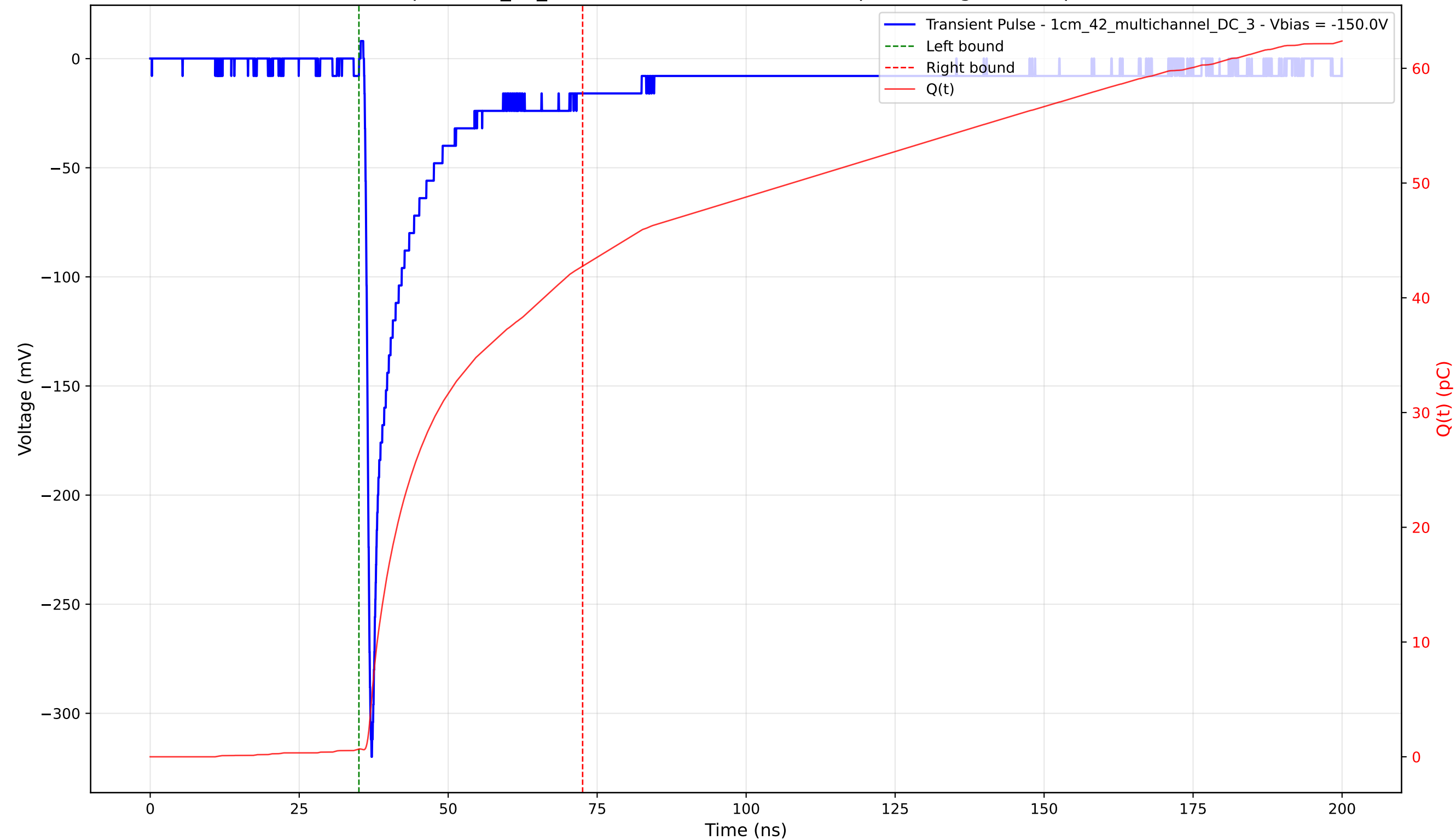
Transient Pulse - Sample: 1cm_42_multichannel - Position: 255.0 \mu\text{m} - Charge: 42.09 pC - Rise Time: 0.86 ns
