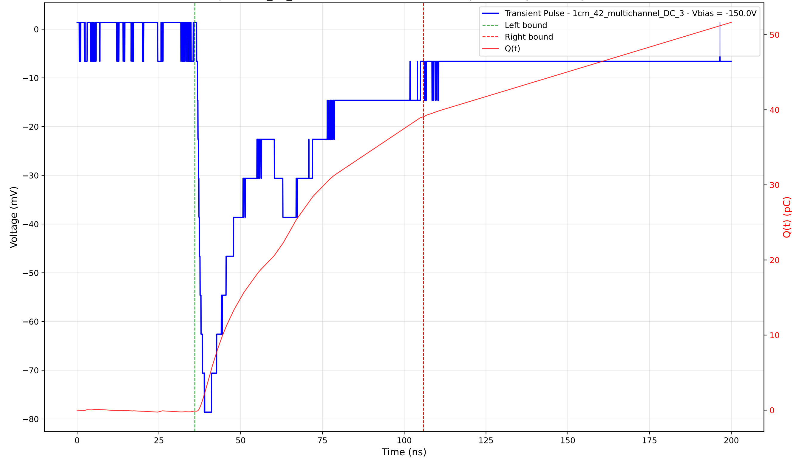
Transient Pulse - Sample: 1cm_42_multichannel - Position: 2560.0 \mu\text{m} - Charge: 39.20 pC - Rise Time: 2.10 ns
