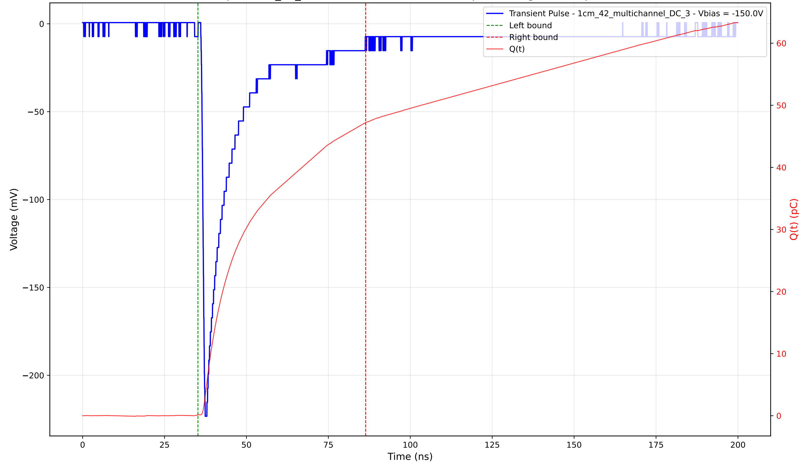
Transient Pulse - Sample: 1cm_42_multichannel - Position: 690.0 \mu\text{m} - Charge: 47.08 pC - Rise Time: 0.98 ns
