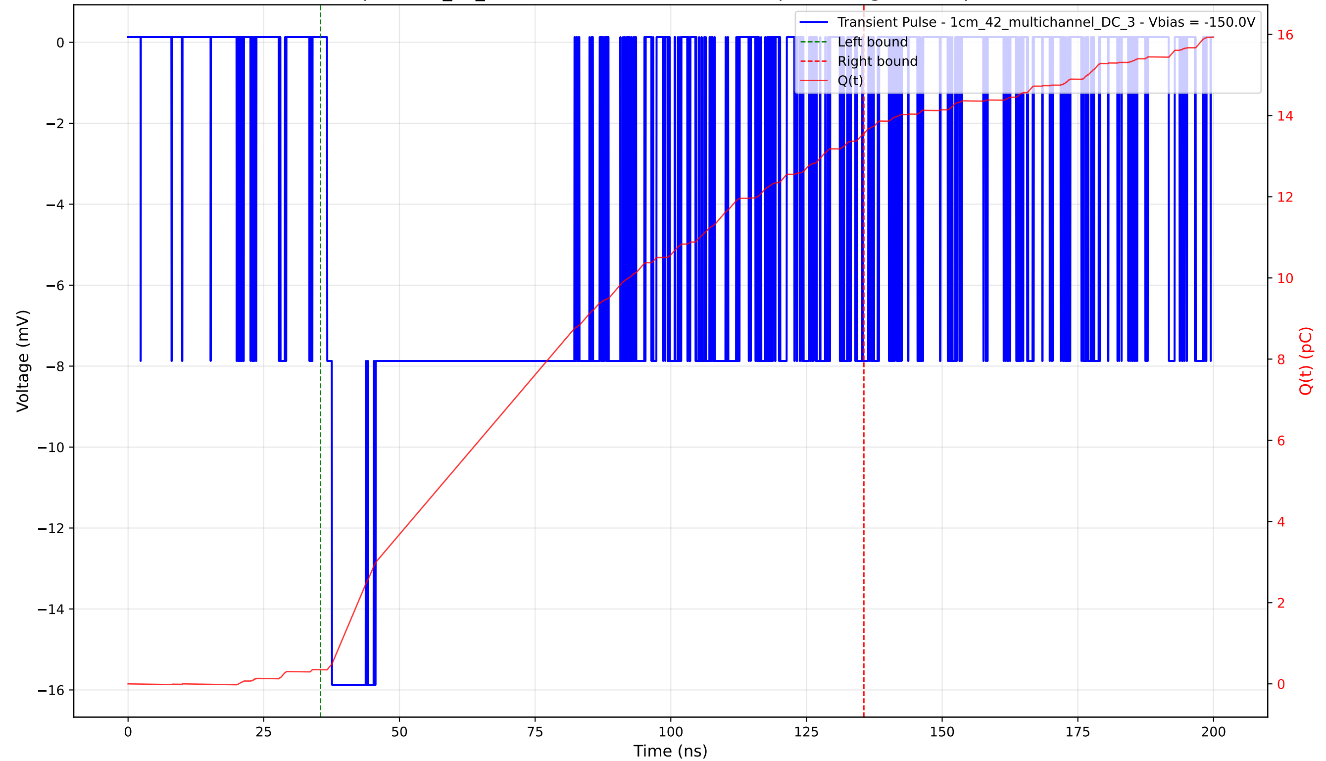
Transient Pulse - Sample: 1cm_42_multichannel - Position: 2910.0 \mu\text{m} - Charge: 13.21 pC - Rise Time: 0.90 ns
