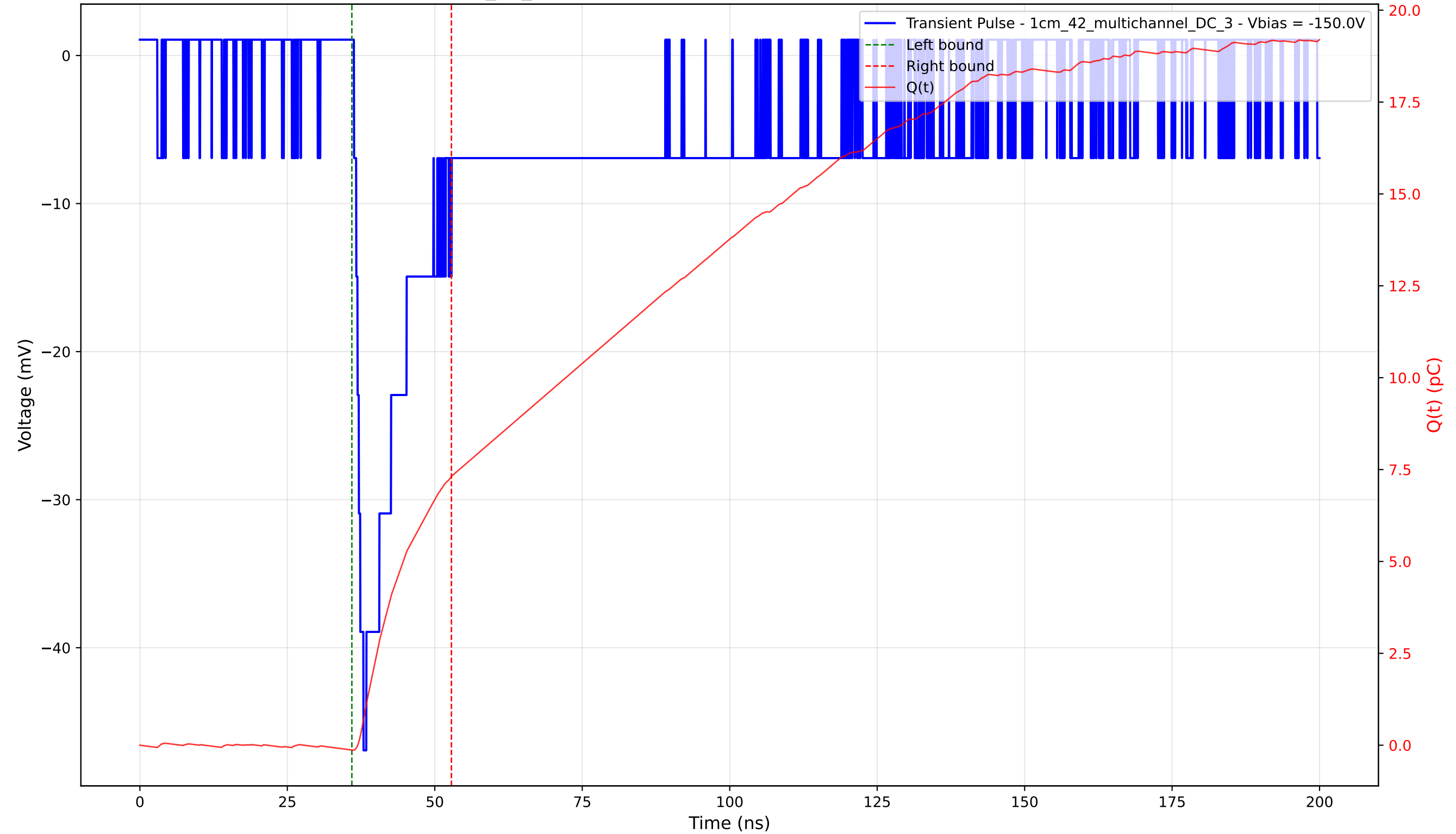
Transient Pulse - Sample: 1cm_42_multichannel - Position: 3930.0 \mu\text{m} - Charge: 7.44 pC - Rise Time: 1.61 ns
