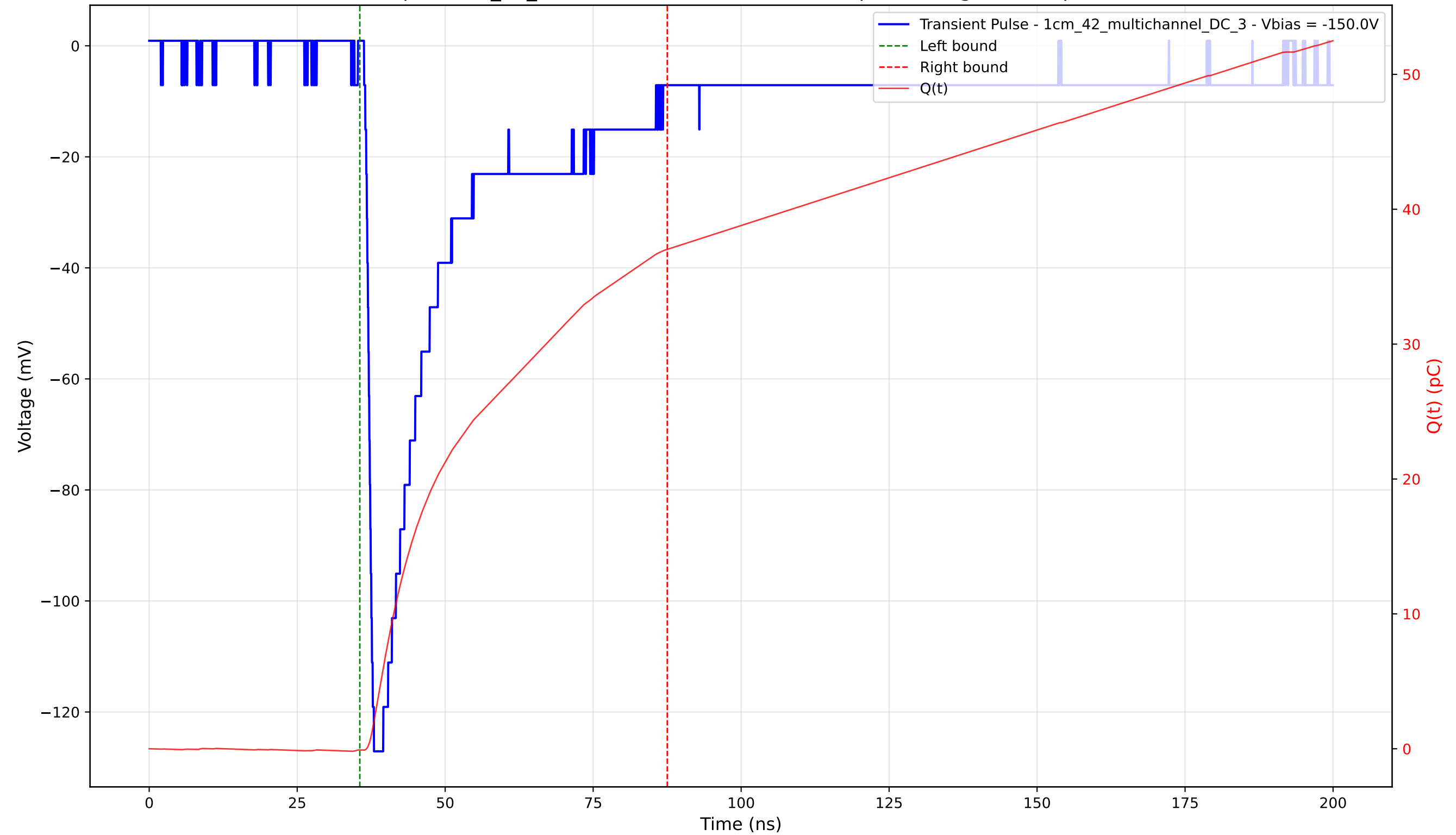
Transient Pulse - Sample: 1cm_42_multichannel - Position: 3655.0 \mu\text{m} - Charge: 37.12 pC - Rise Time: 1.27 ns
