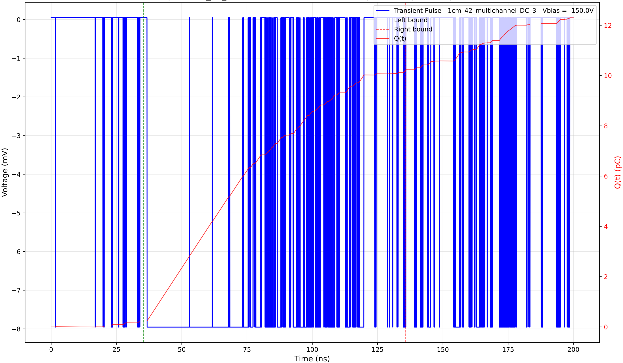
Transient Pulse - Sample: 1cm_42_multichannel - Position: 2355.0 \mu\text{m} - Charge: 9.96 pC - Rise Time: 0.02 ns
