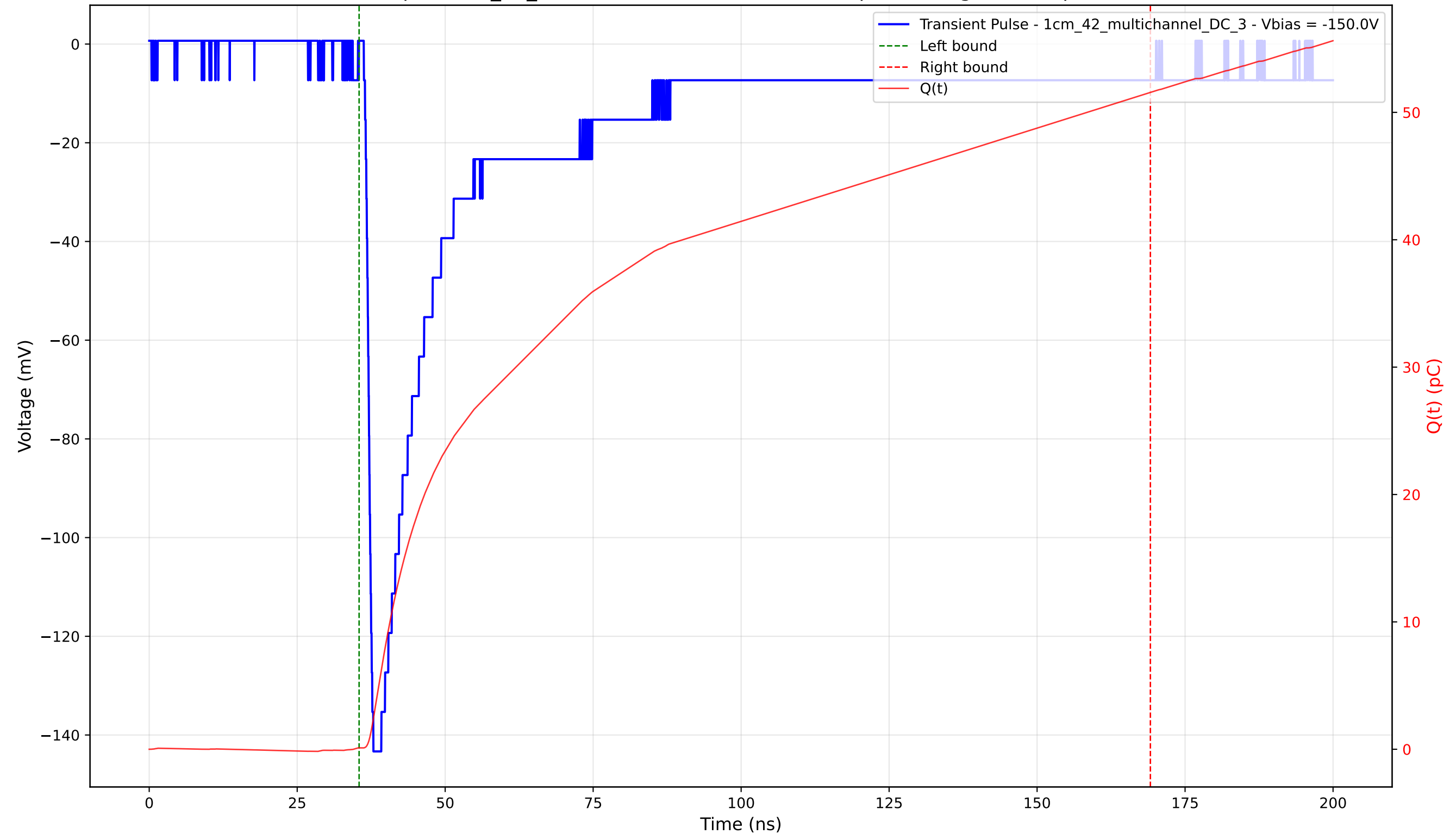
Transient Pulse - Sample: 1cm_42_multichannel - Position: 3765.0 \mu\text{m} - Charge: 51.47 pC - Rise Time: 1.22 ns
