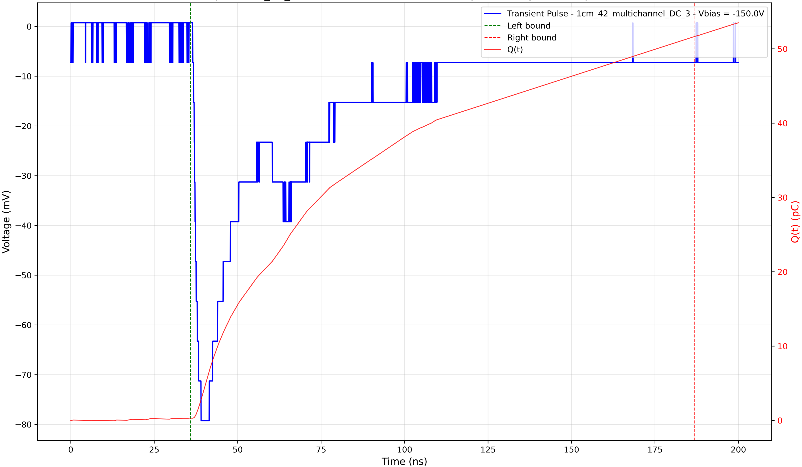
Transient Pulse - Sample: 1cm_42_multichannel - Position: 2565.0 \mu\text{m} - Charge: 51.34 pC - Rise Time: 2.24 ns
