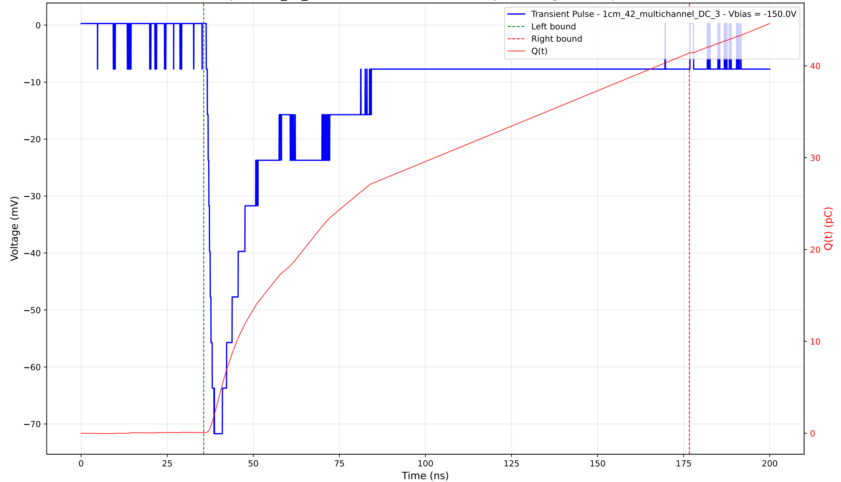
Transient Pulse - Sample: 1cm_42_multichannel - Position: 2940.0 \mu\text{m} - Charge: 41.31 pC - Rise Time: 2.26 ns
