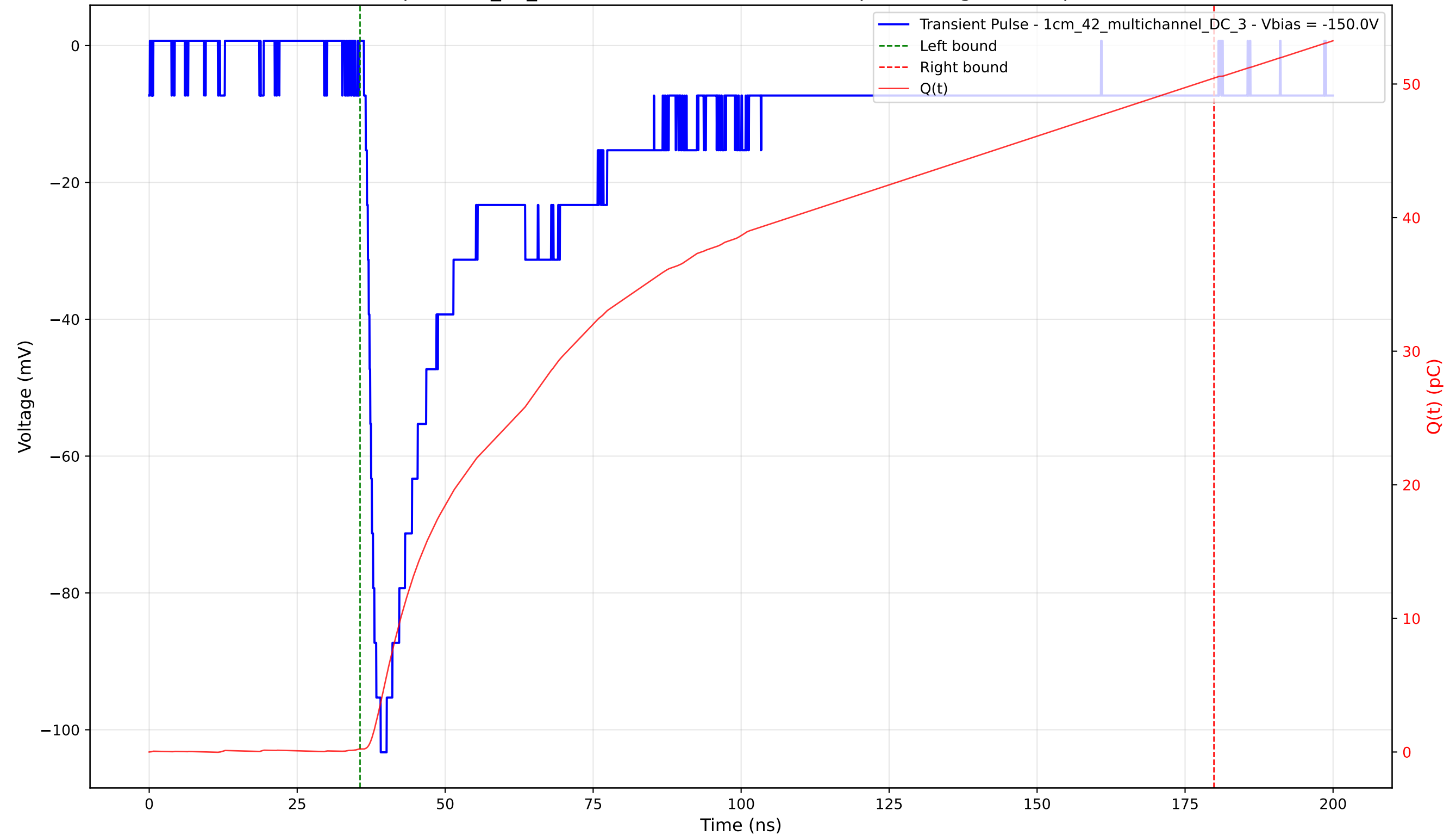
Transient Pulse - Sample: 1cm_42_multichannel - Position: 3095.0 \mu\text{m} - Charge: 50.22 pC - Rise Time: 1.79 ns
