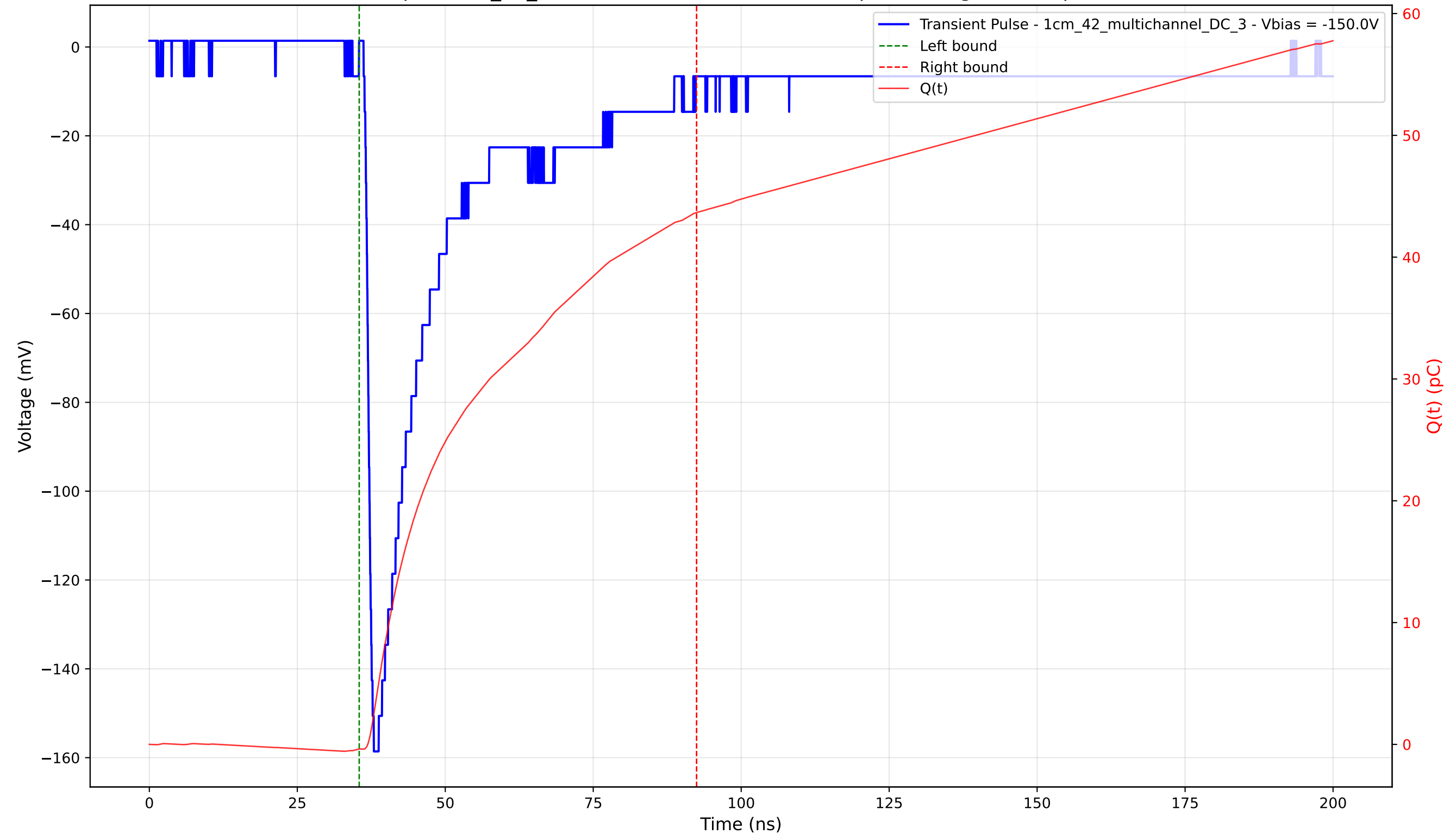
Transient Pulse - Sample: 1cm_42_multichannel - Position: 1135.0 \mu\text{m} - Charge: 44.04 pC - Rise Time: 1.24 ns
