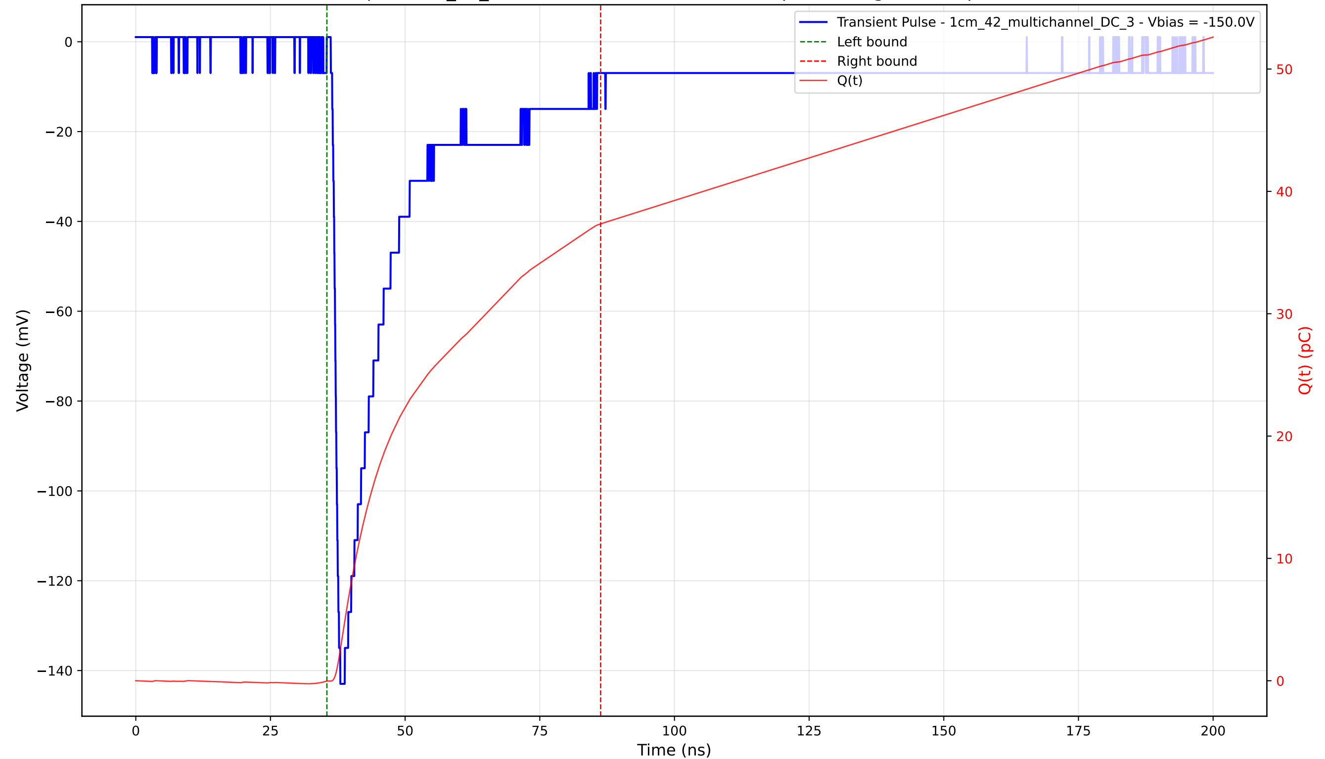
Transient Pulse - Sample: 1cm_42_multichannel - Position: 3805.0 \mu\text{m} - Charge: 37.36 pC - Rise Time: 1.26 ns
