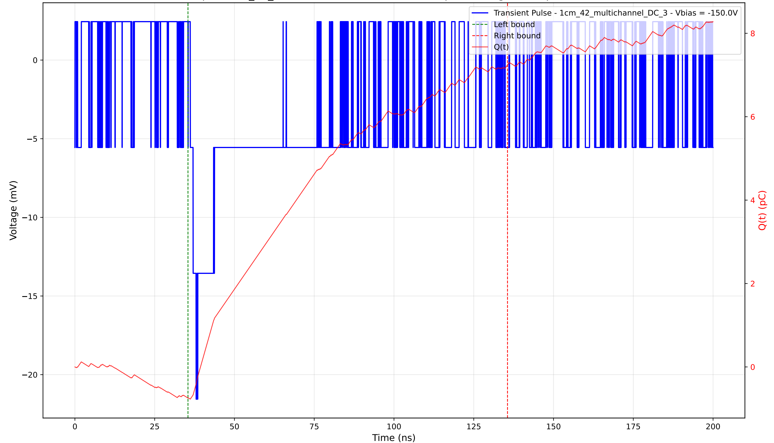
Transient Pulse - Sample: 1cm_42_multichannel - Position: 3915.0 \mu\text{m} - Charge: 7.99 pC - Rise Time: 0.00 ns (N/A)
