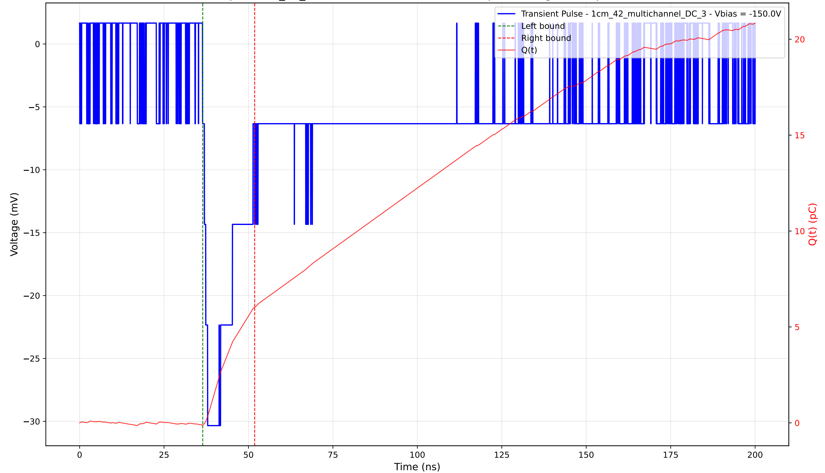
Transient Pulse - Sample: 1cm_42_multichannel - Position: 1830.0 \mu\text{m} - Charge: 6.13 pC - Rise Time: 1.51 ns
