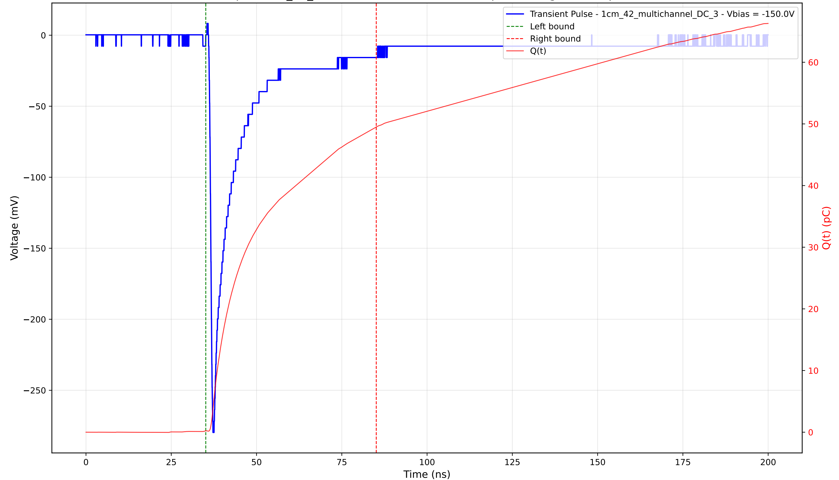
Transient Pulse - Sample: 1cm_42_multichannel - Position: 465.0 \mu\text{m} - Charge: 49.28 pC - Rise Time: 0.89 ns
