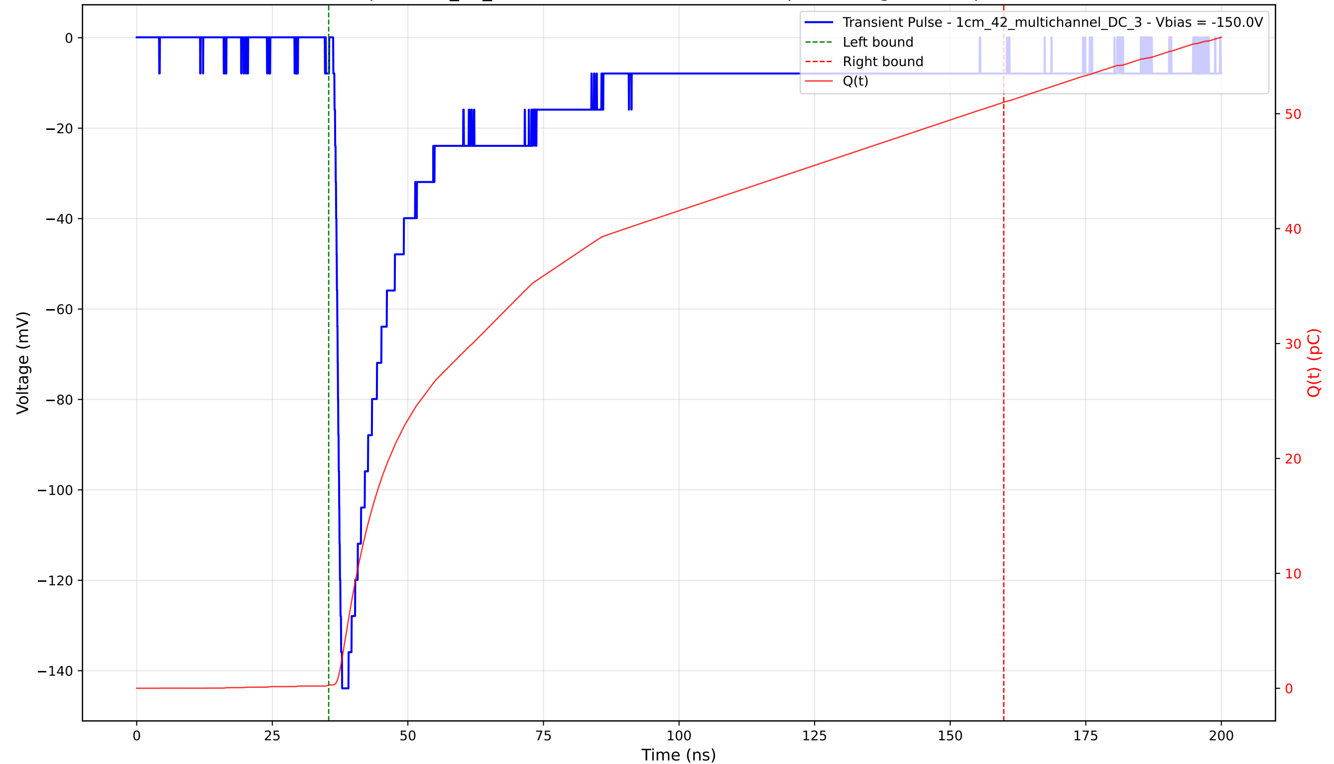
Transient Pulse - Sample: 1cm_42_multichannel - Position: 3800.0 \mu\text{m} - Charge: 50.73 pC - Rise Time: 1.22 ns
