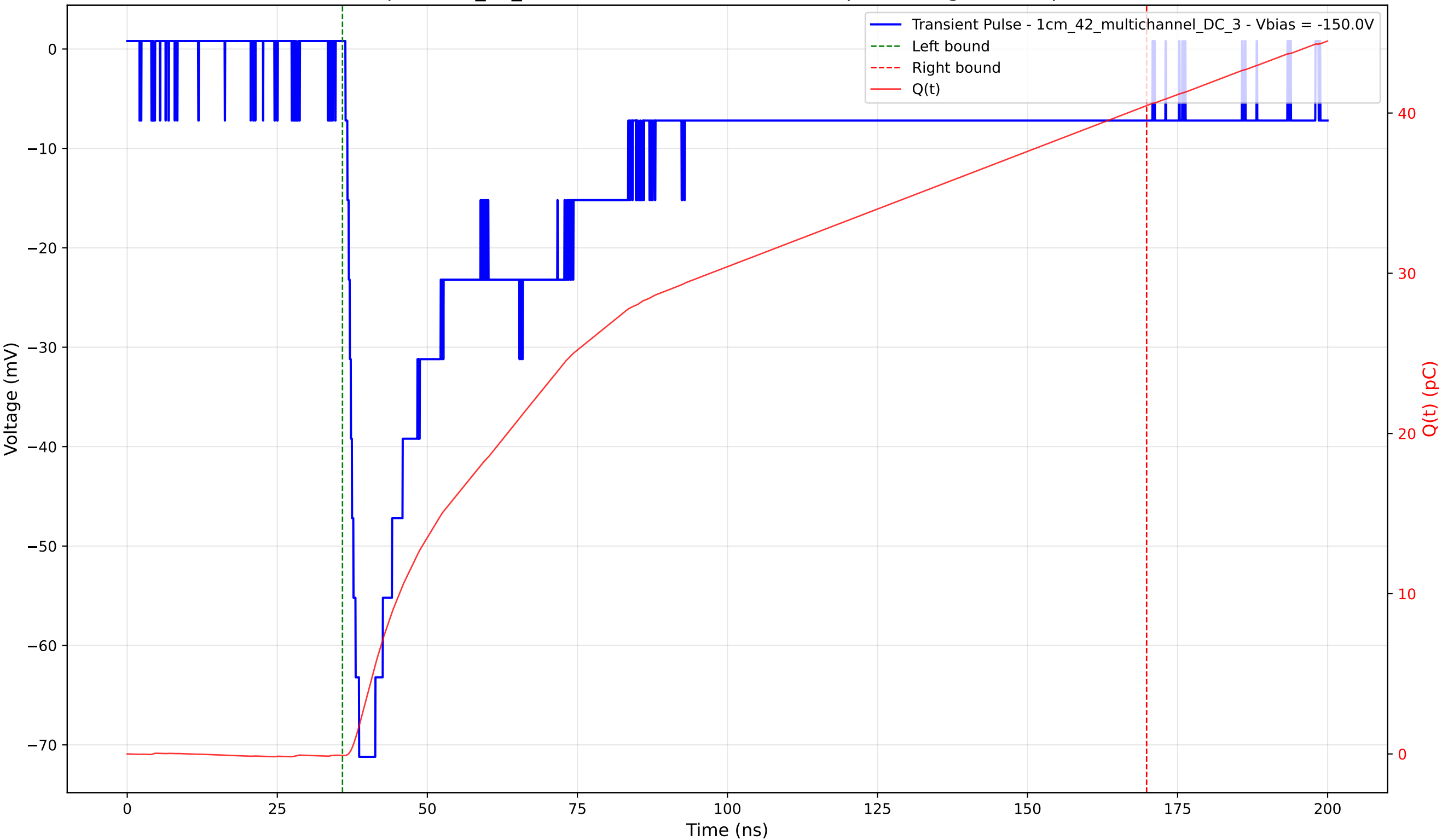
Transient Pulse - Sample: 1cm_42_multichannel - Position: 2815.0 \mu\text{m} - Charge: 40.57 pC - Rise Time: 2.26 ns
