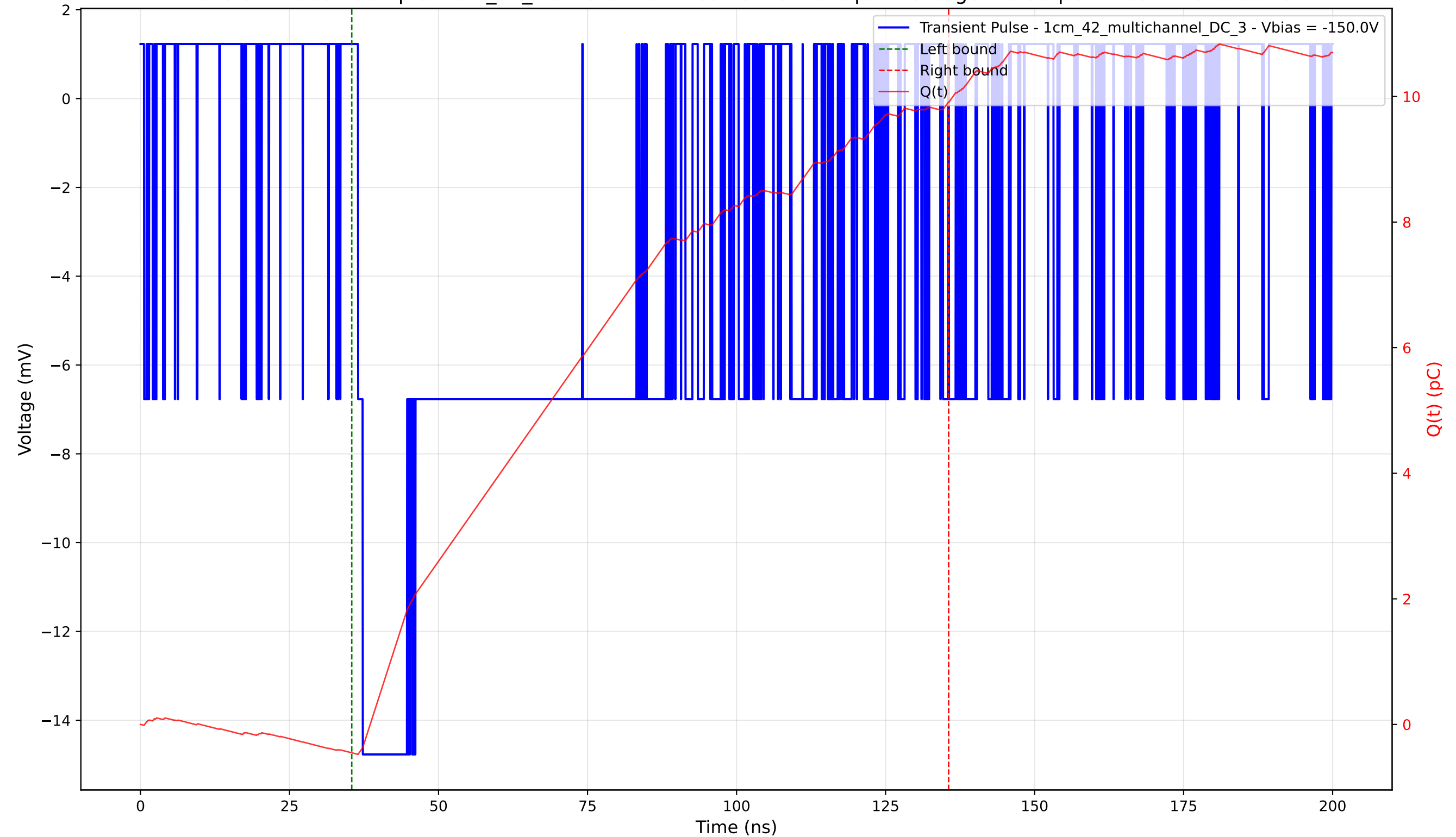
Transient Pulse - Sample: 1cm_42_multichannel - Position: 3415.0 \mu\text{m} - Charge: 10.36 pC - Rise Time: 0.80 ns
