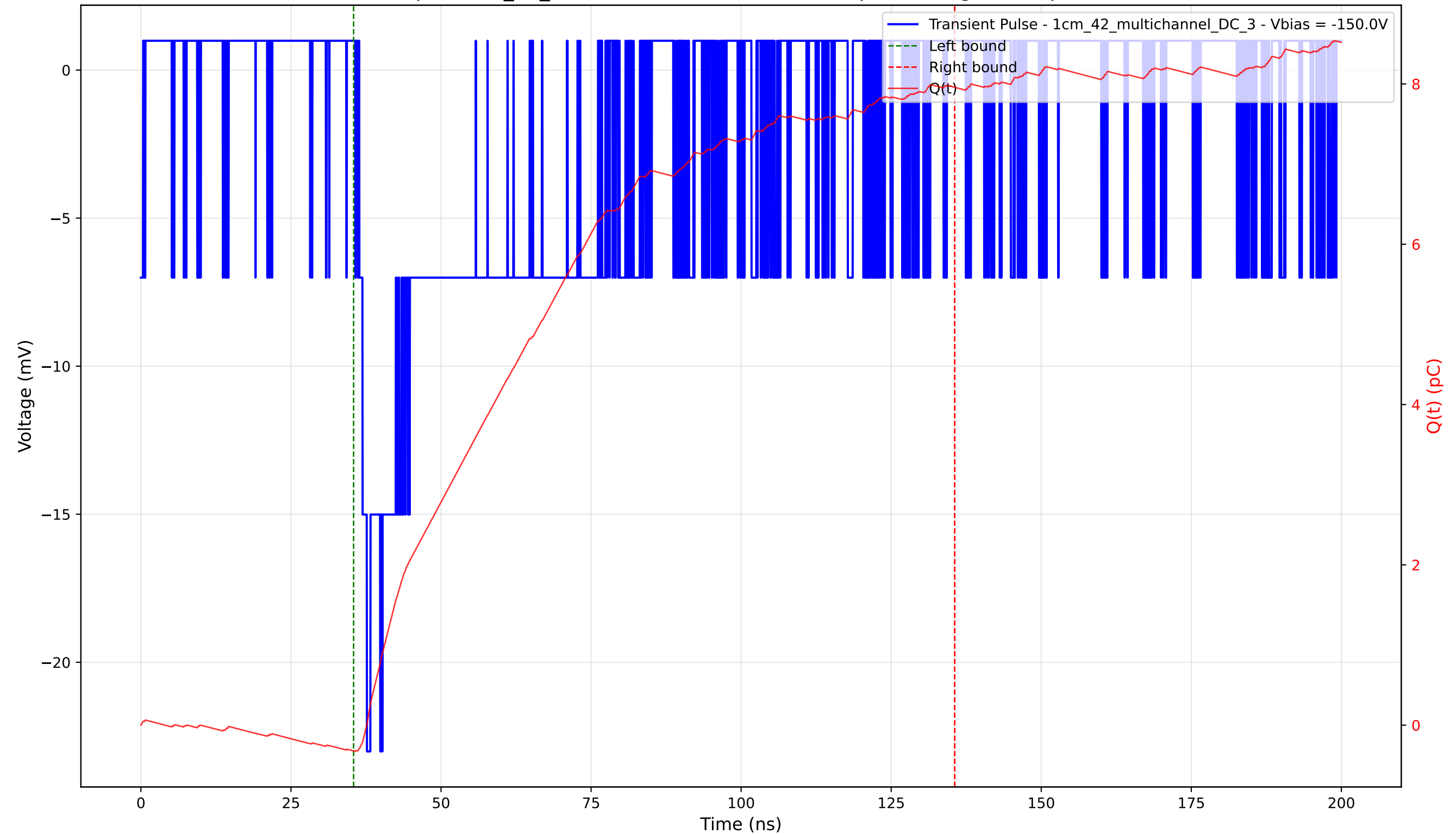
Transient Pulse - Sample: 1cm_42_multichannel - Position: 880.0 \mu\text{m} - Charge: 8.28 pC - Rise Time: 1.28 ns
