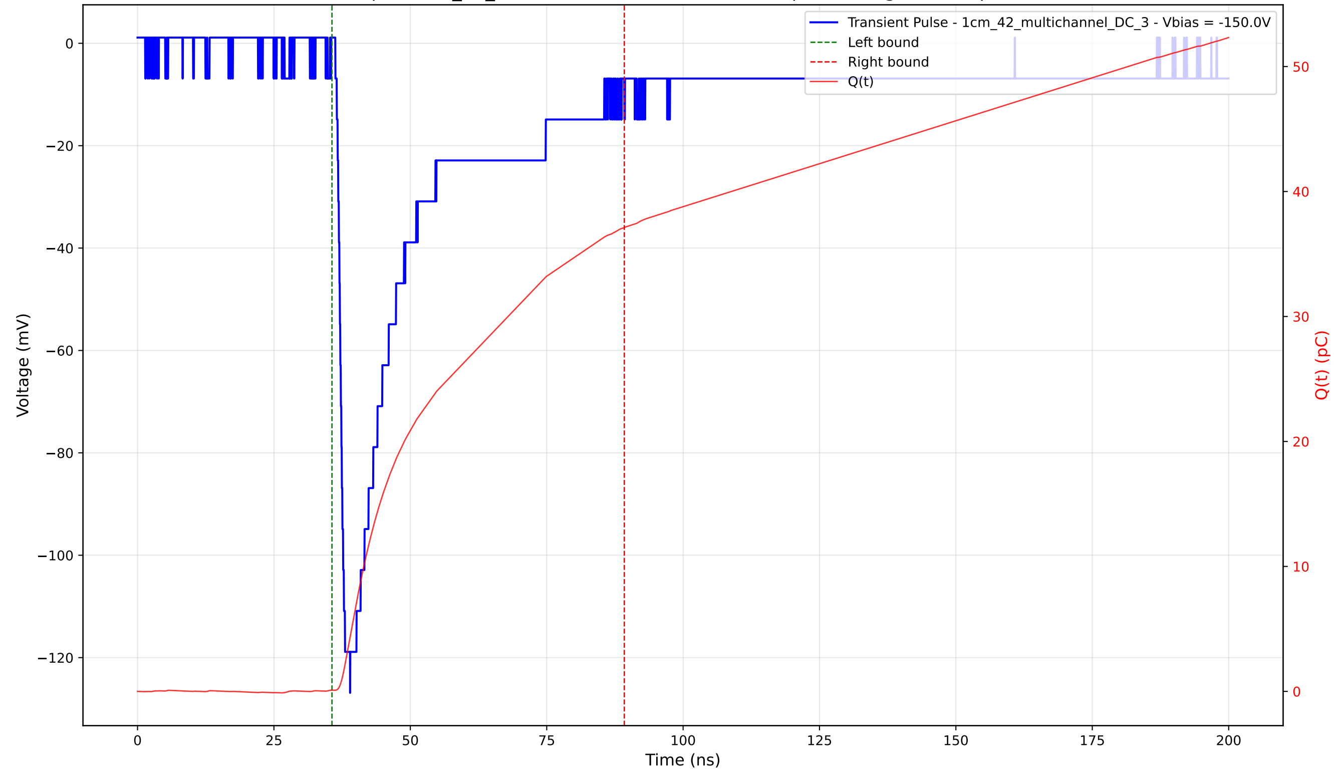
Transient Pulse - Sample: 1cm_42_multichannel - Position: 3520.0 \mu\text{m} - Charge: 37.02 pC - Rise Time: 1.51 ns
