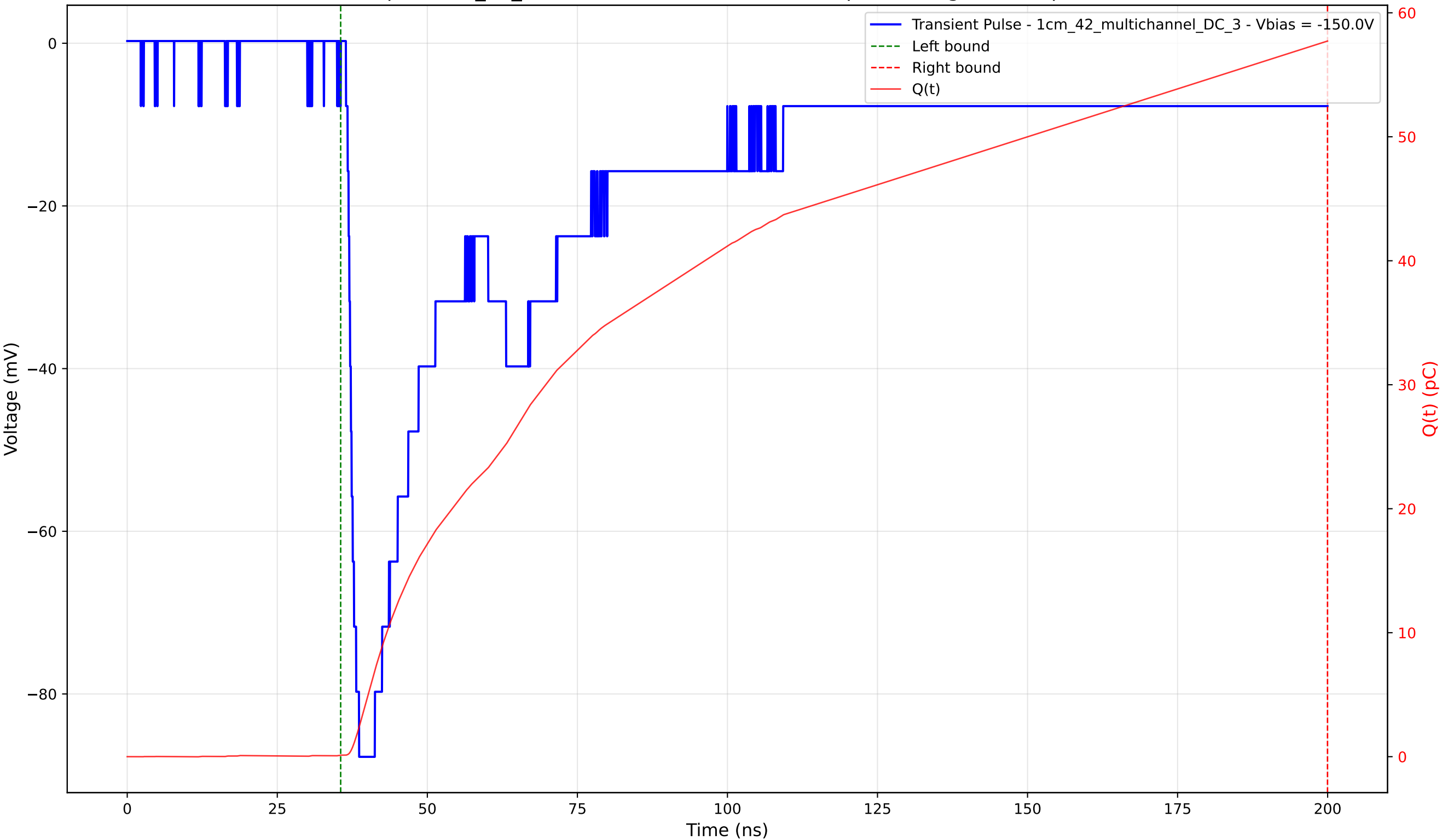
Transient Pulse - Sample: 1cm_42_multichannel - Position: 2085.0 \mu\text{m} - Charge: 57.60 pC - Rise Time: 1.44 ns
