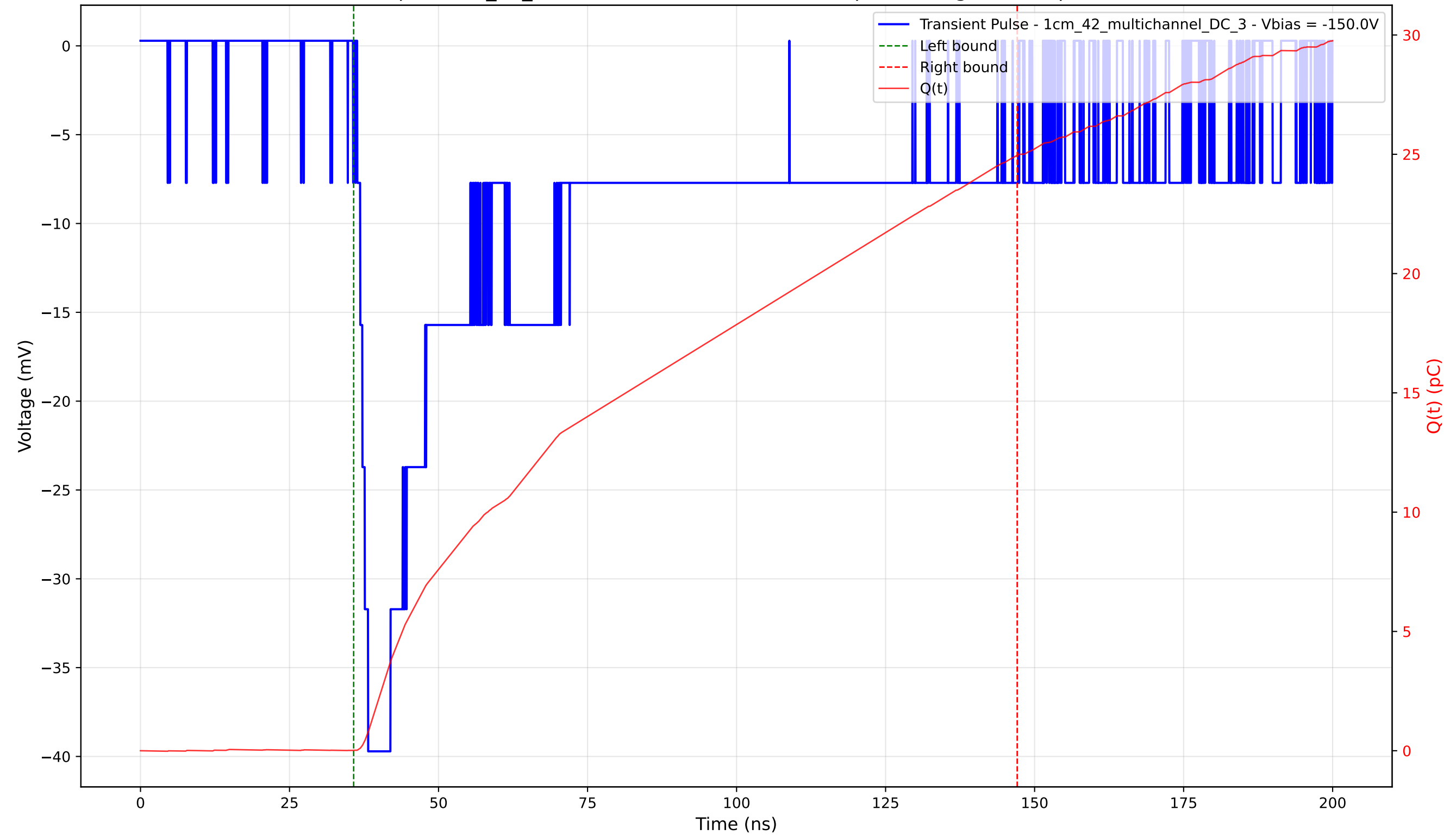
Transient Pulse - Sample: 1cm_42_multichannel - Position: 2925.0 \mu\text{m} - Charge: 24.95 pC - Rise Time: 1.83 ns
