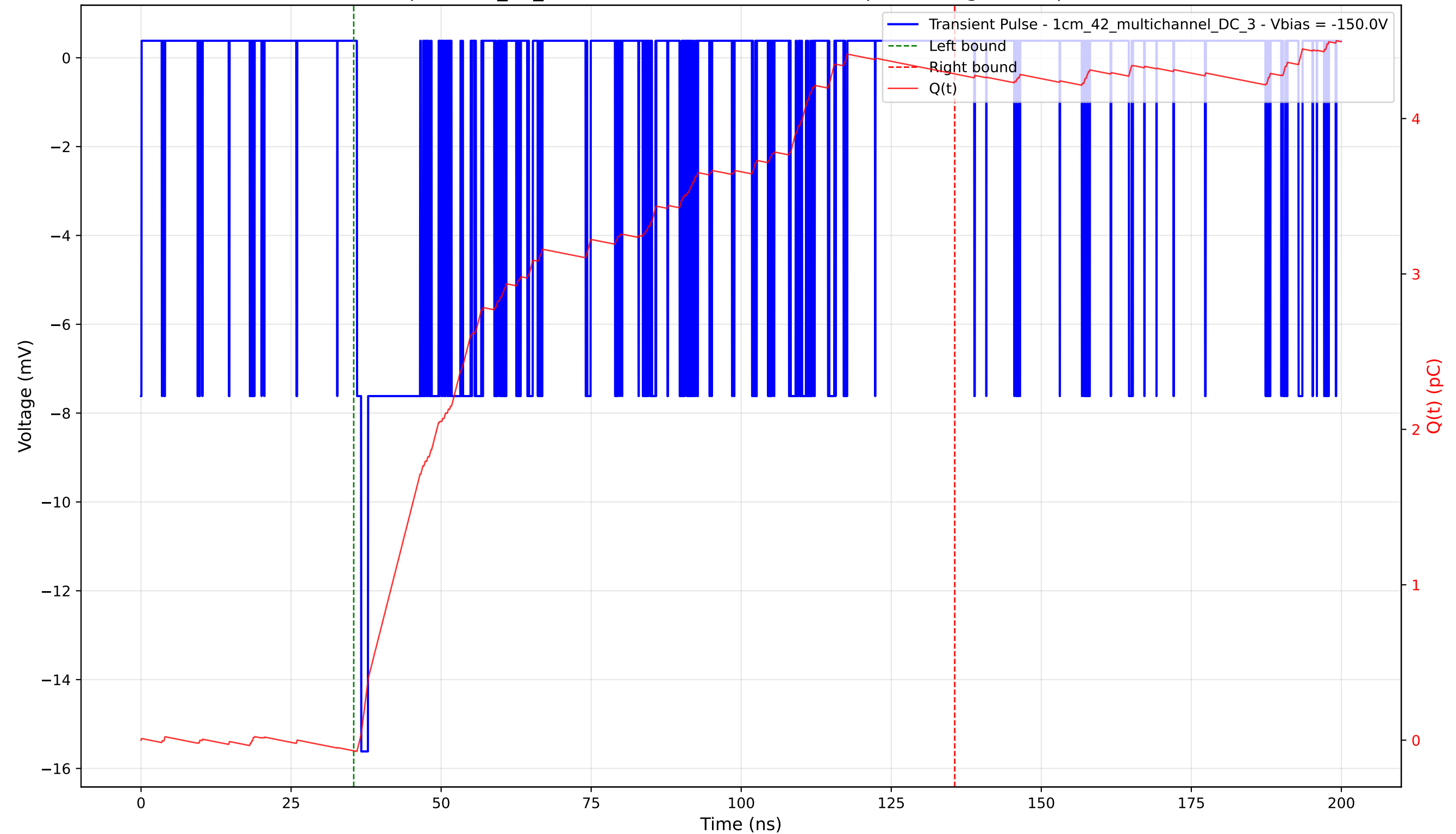
Transient Pulse - Sample: 1cm_42_multichannel - Position: 4895.0 \mu\text{m} - Charge: 4.36 pC - Rise Time: 0.72 ns
