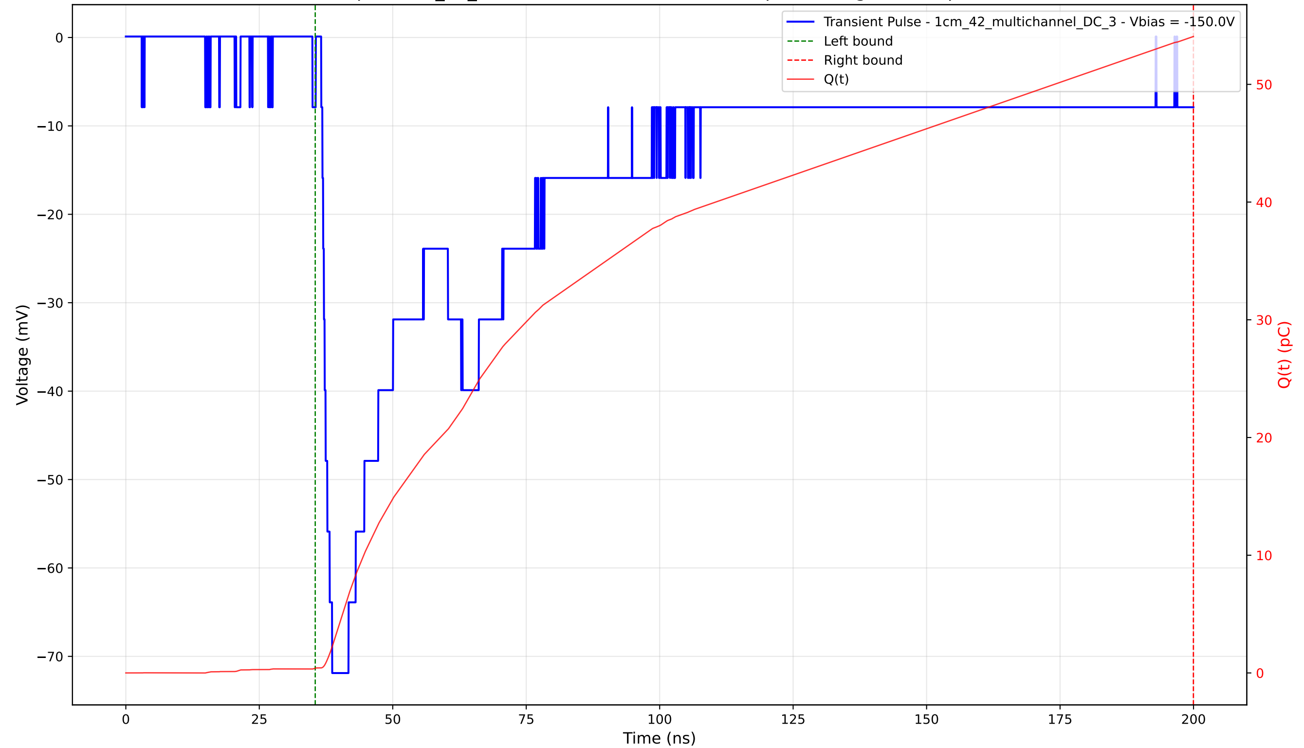
Transient Pulse - Sample: 1cm_42_multichannel - Position: 2300.0 \mu\text{m} - Charge: 53.66 pC - Rise Time: 2.04 ns
