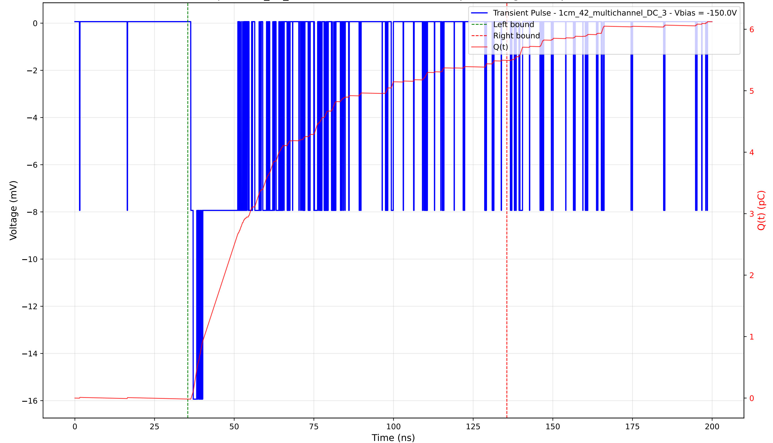
Transient Pulse - Sample: 1cm_42_multichannel - Position: 4380.0 \mu\text{m} - Charge: 5.51 pC - Rise Time: 0.76 ns
