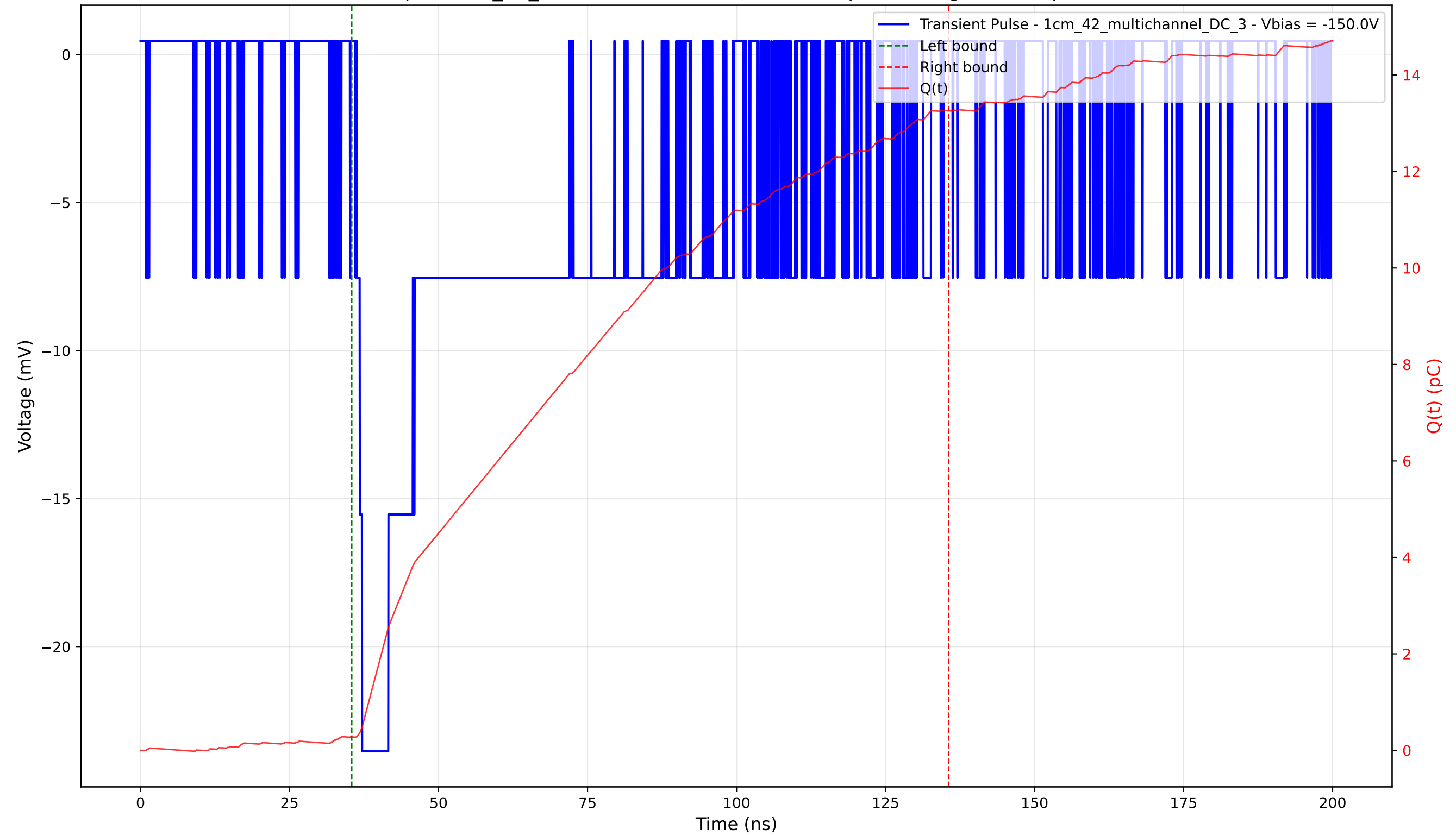
Transient Pulse - Sample: 1cm_42_multichannel - Position: 885.0 \mu\text{m} - Charge: 12.98 pC - Rise Time: 0.89 ns
