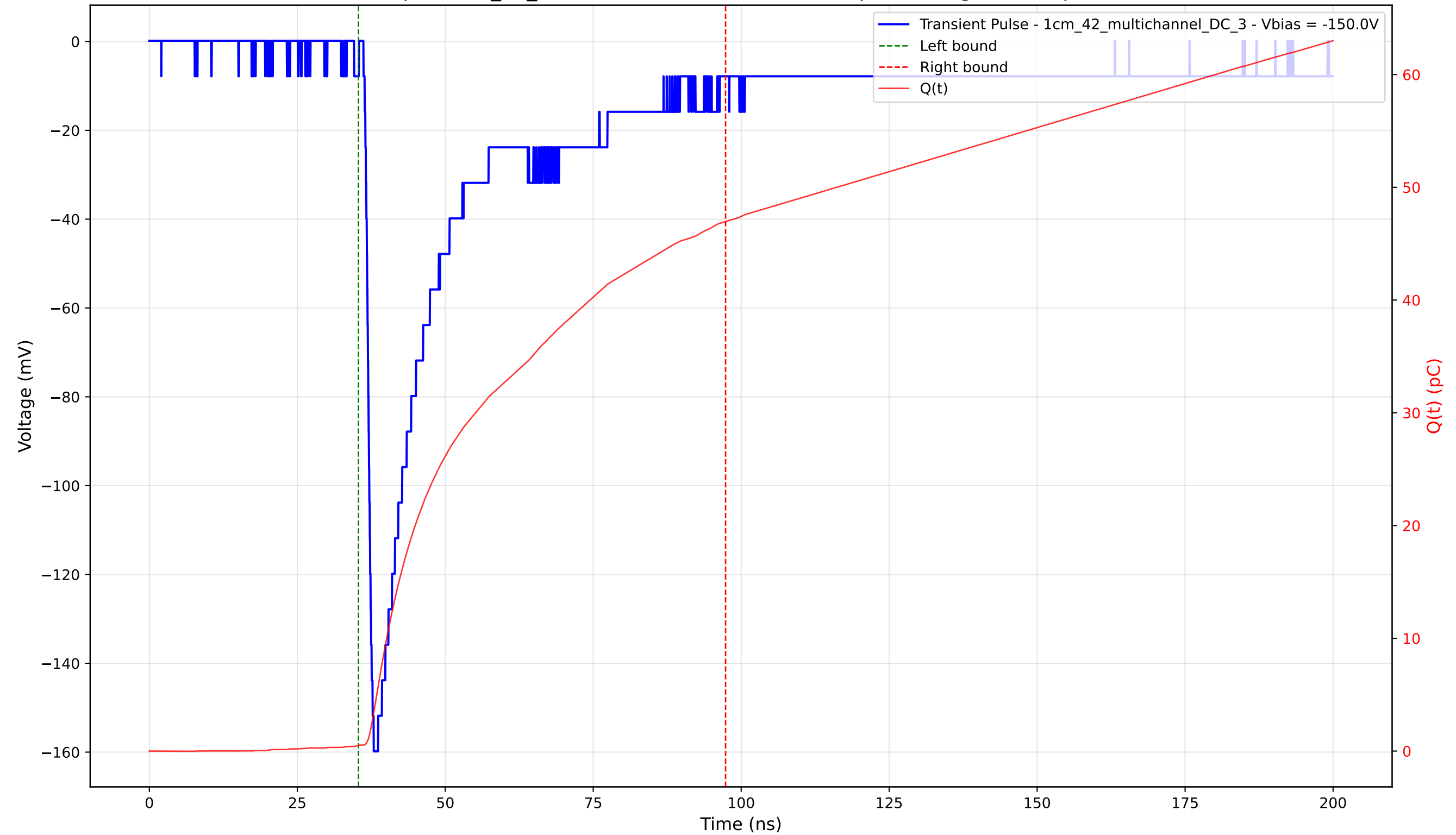
Transient Pulse - Sample: 1cm_42_multichannel - Position: 1140.0 \mu\text{m} - Charge: 46.45 pC - Rise Time: 1.24 ns
