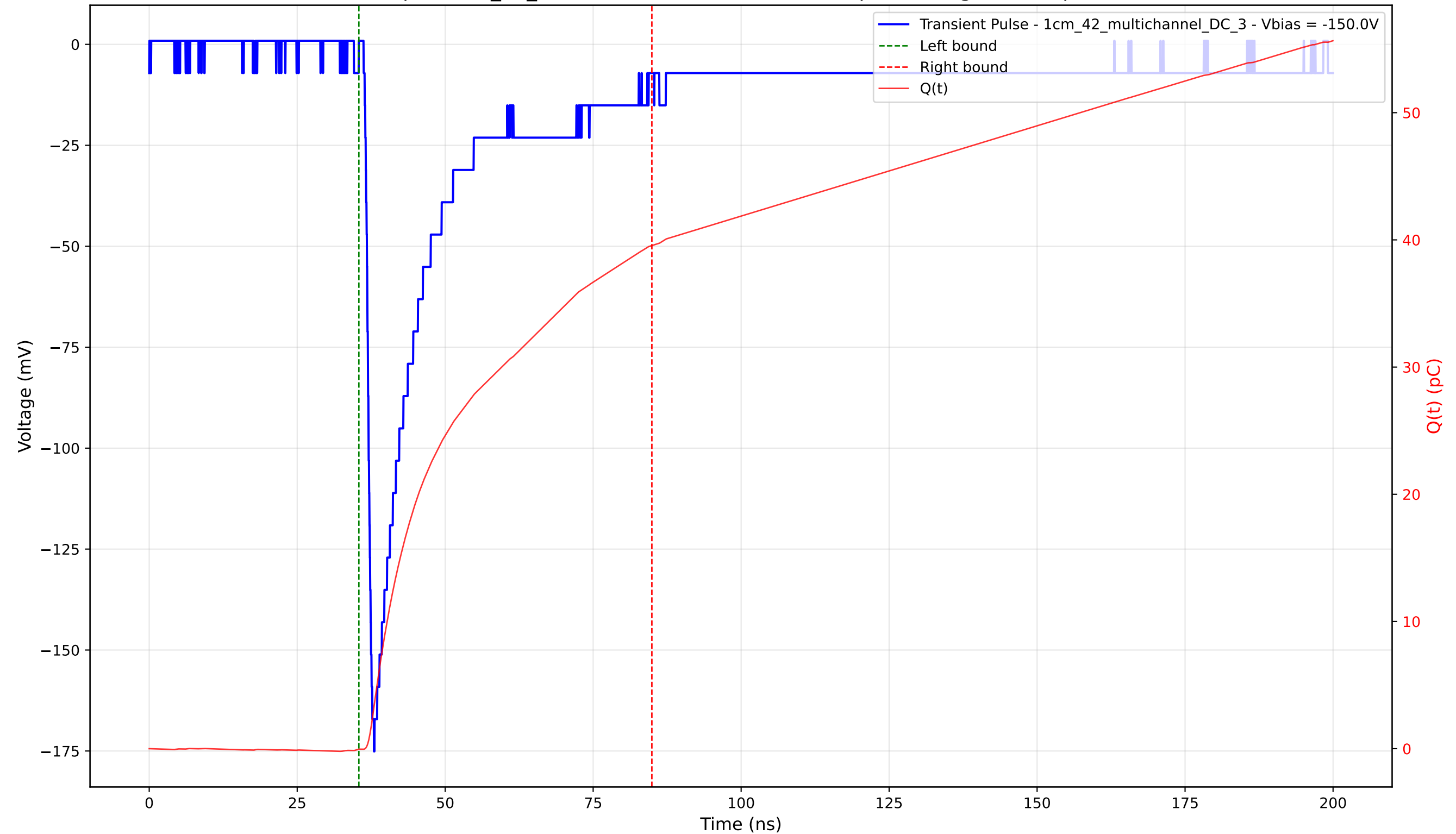
Transient Pulse - Sample: 1cm_42_multichannel - Position: 3995.0 \mu\text{m} - Charge: 39.59 pC - Rise Time: 1.07 ns
