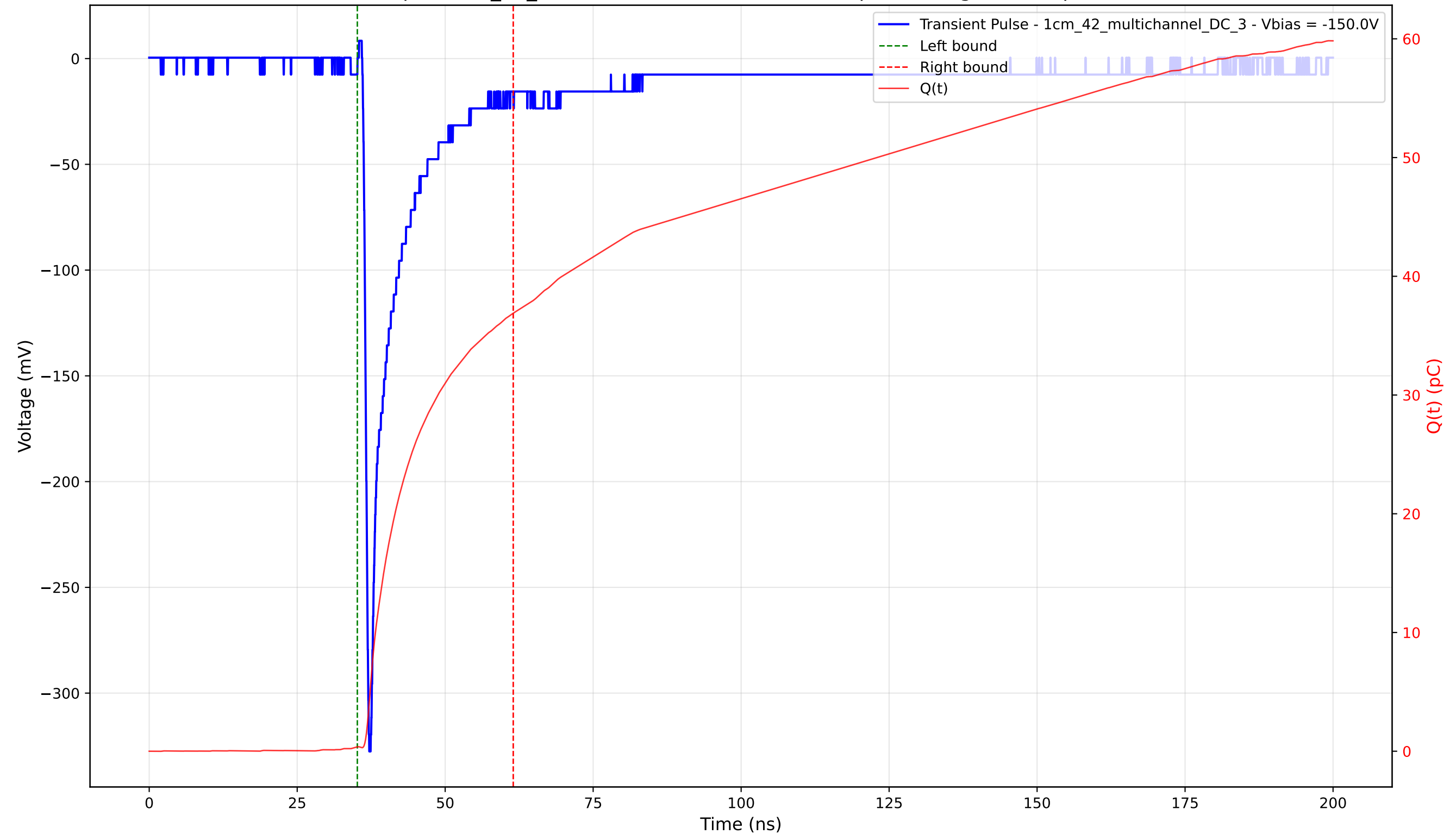
Transient Pulse - Sample: 1cm_42_multichannel - Position: 4665.0 \mu\text{m} - Charge: 36.50 pC - Rise Time: 0.80 ns
