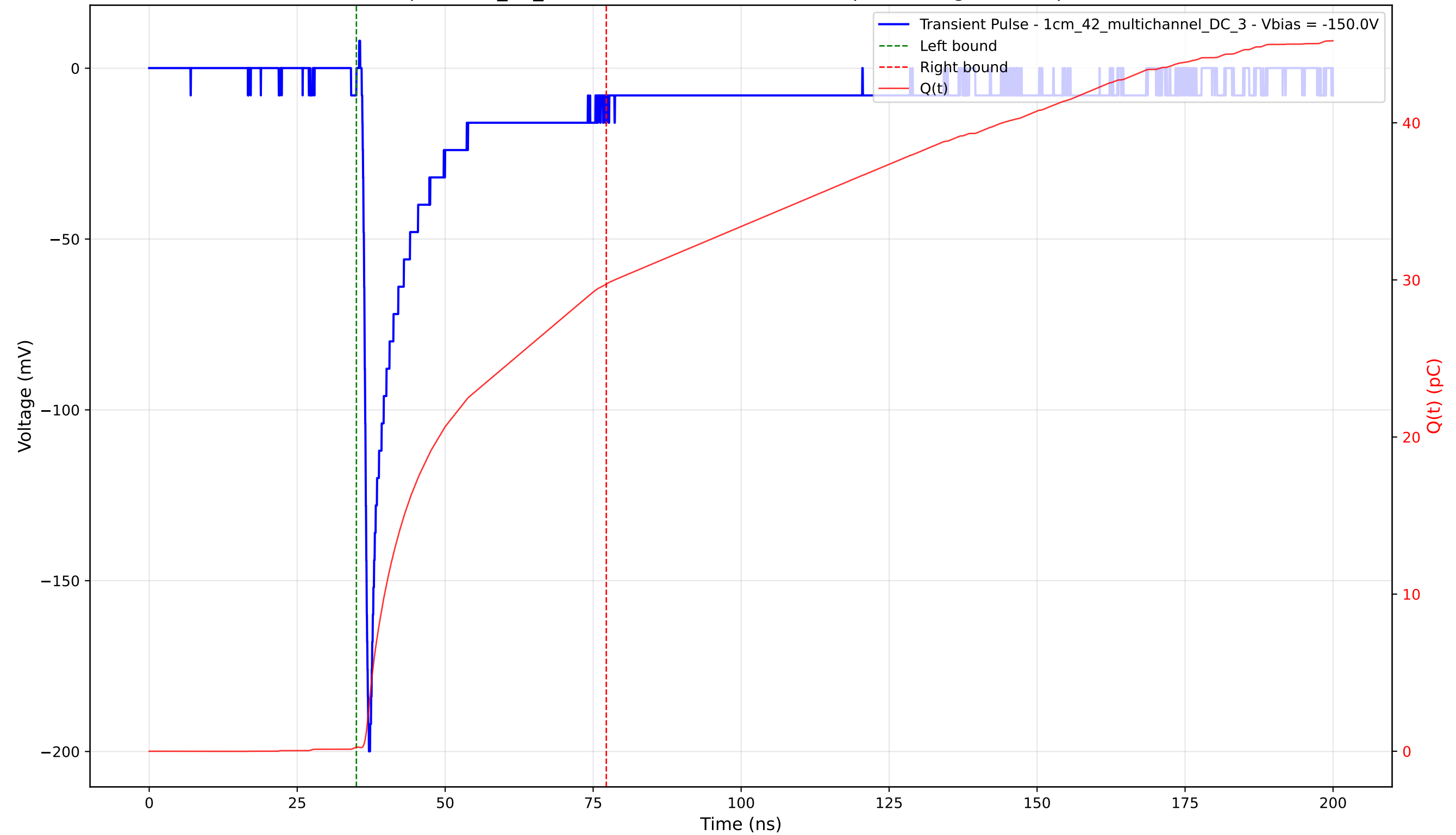
Transient Pulse - Sample: 1cm_42_multichannel - Position: 295.0 \mu\text{m} - Charge: 29.48 pC - Rise Time: 0.87 ns
