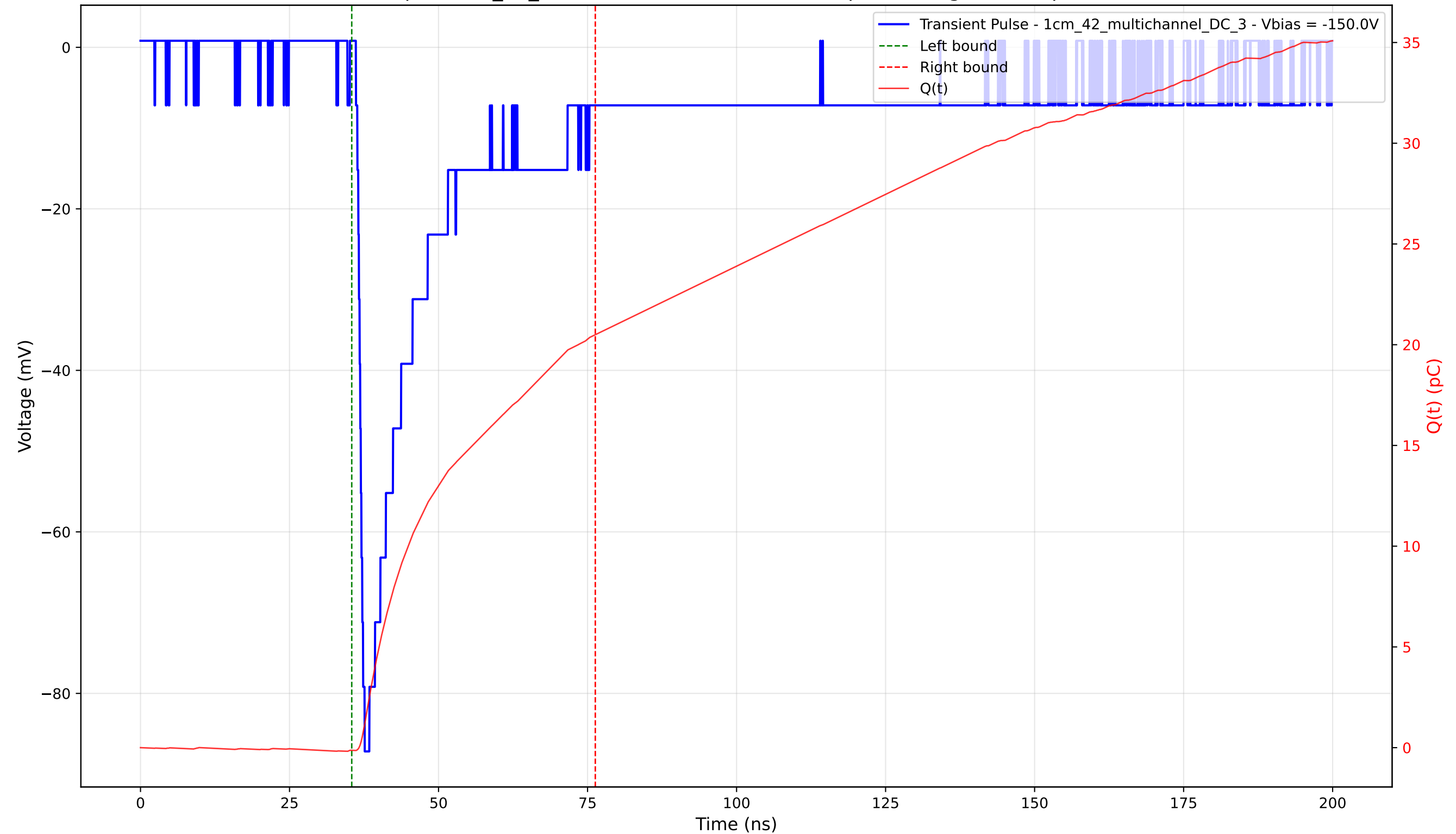
Transient Pulse - Sample: 1cm_42_multichannel - Position: 905.0 \mu\text{m} - Charge: 20.63 pC - Rise Time: 0.98 ns
