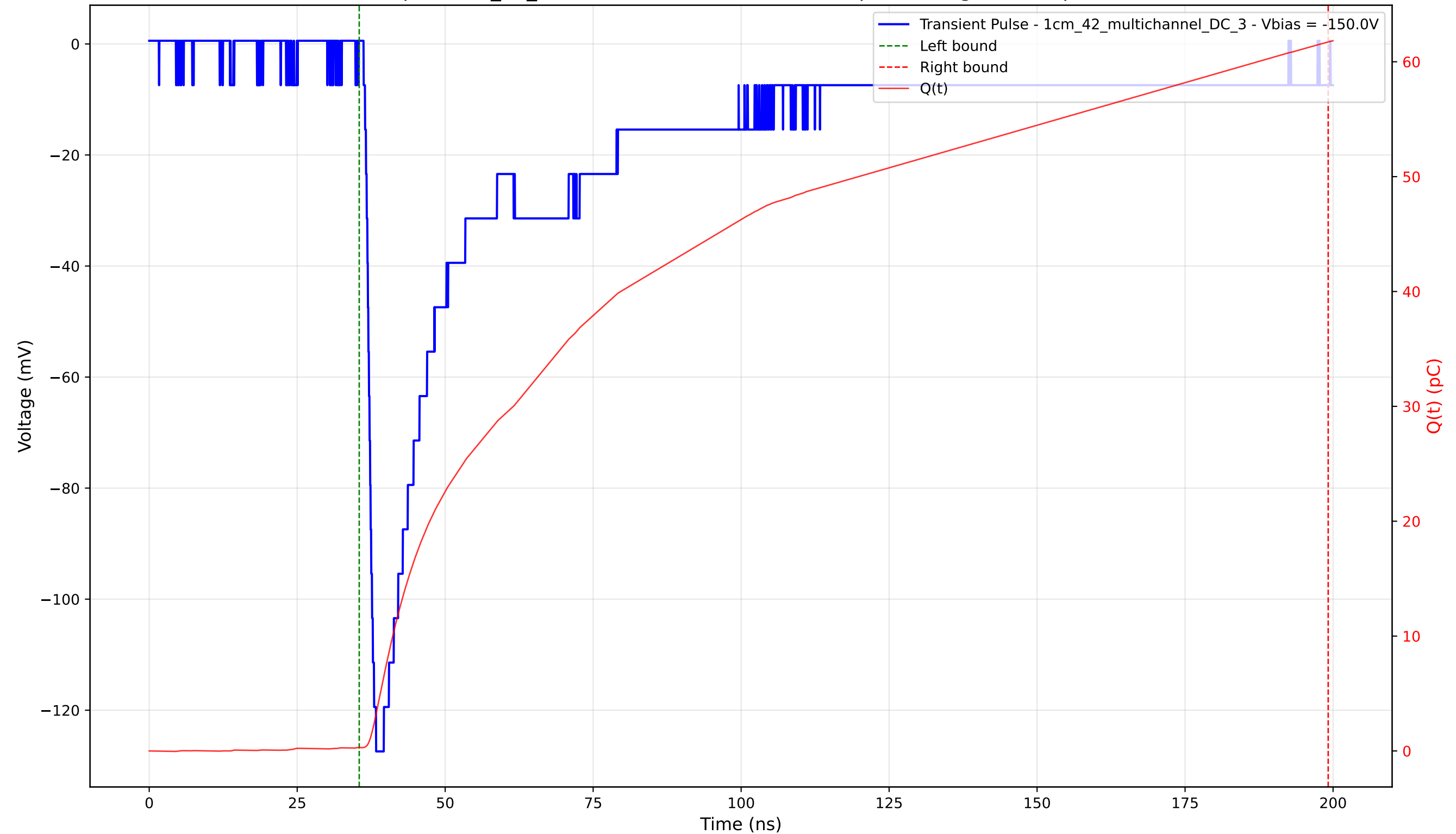
Transient Pulse - Sample: 1cm_42_multichannel - Position: 1555.0 \mu\text{m} - Charge: 61.43 pC - Rise Time: 1.53 ns
