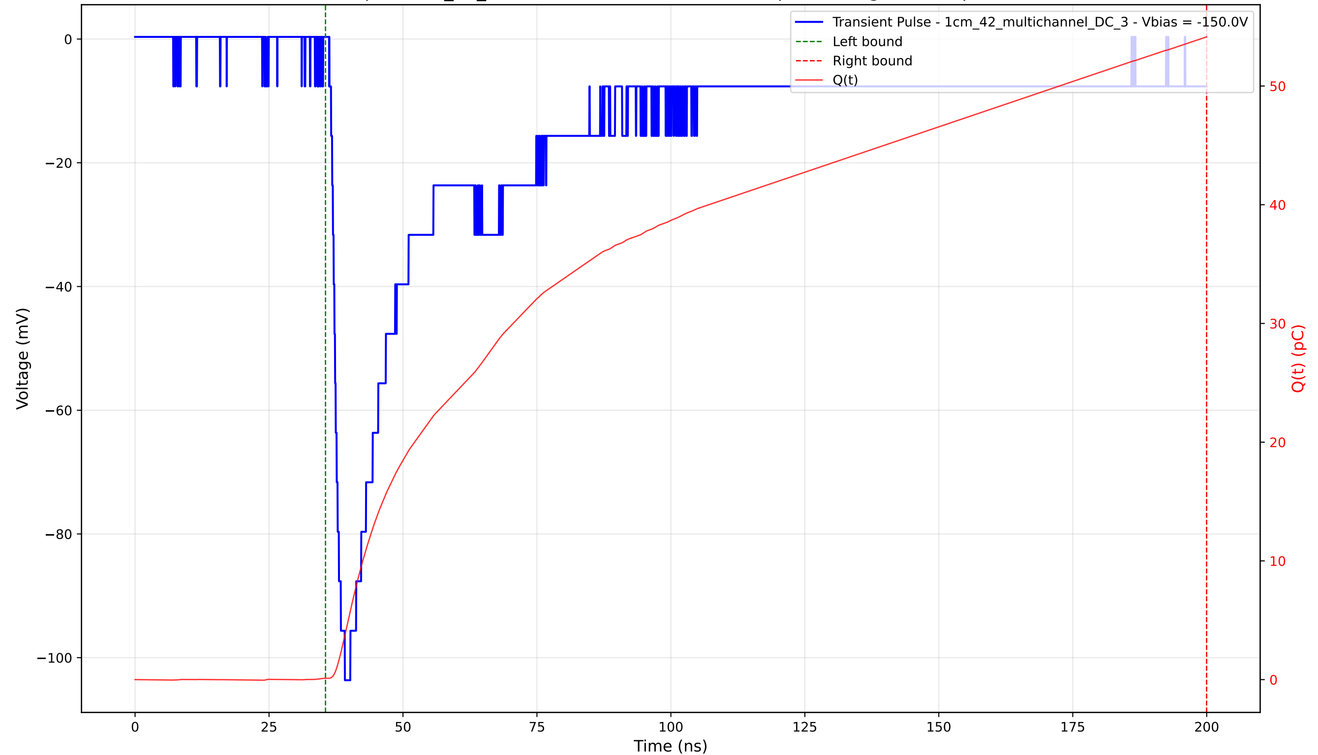
Transient Pulse - Sample: 1cm_42_multichannel - Position: 3080.0 \mu\text{m} - Charge: 54.03 pC - Rise Time: 1.83 ns
