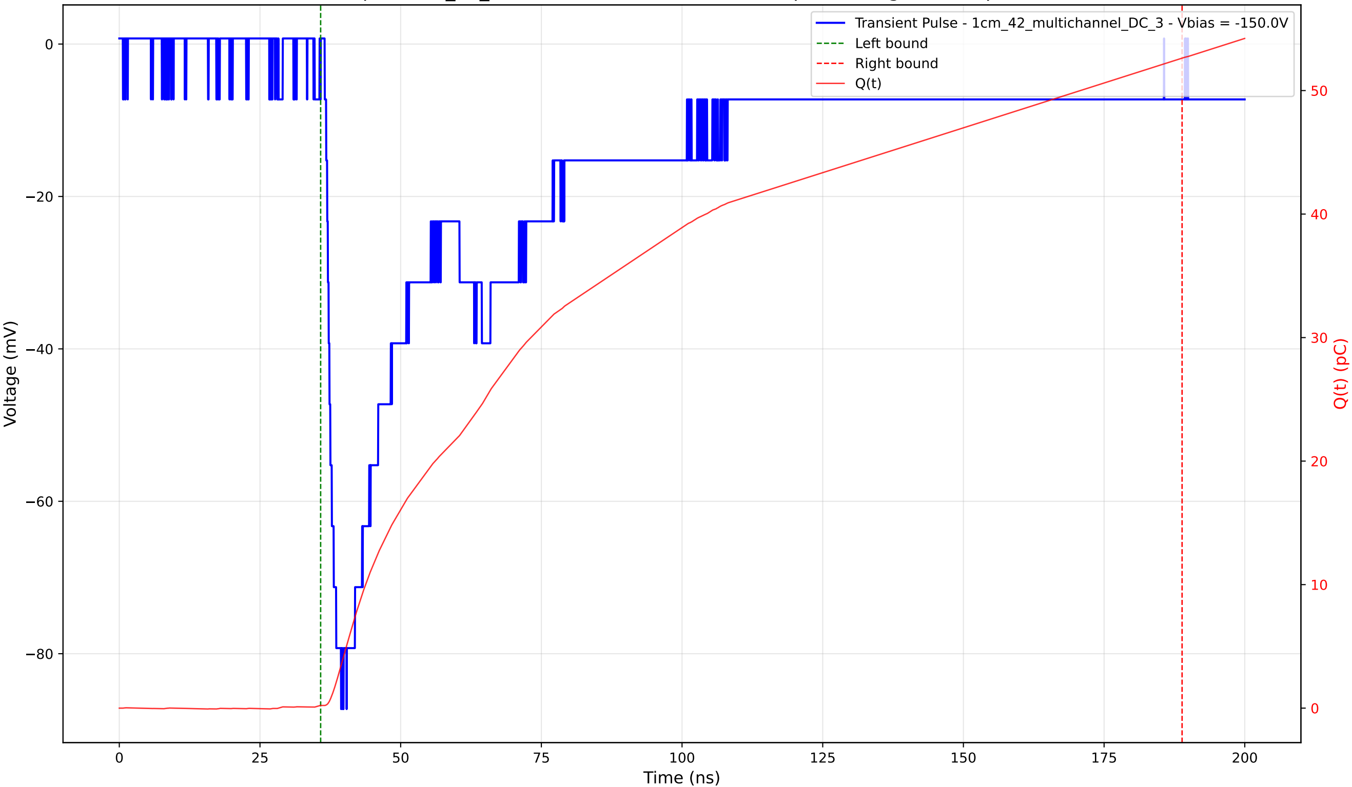
Transient Pulse - Sample: 1cm_42_multichannel - Position: 2630.0 \mu\text{m} - Charge: 52.41 pC - Rise Time: 1.80 ns
