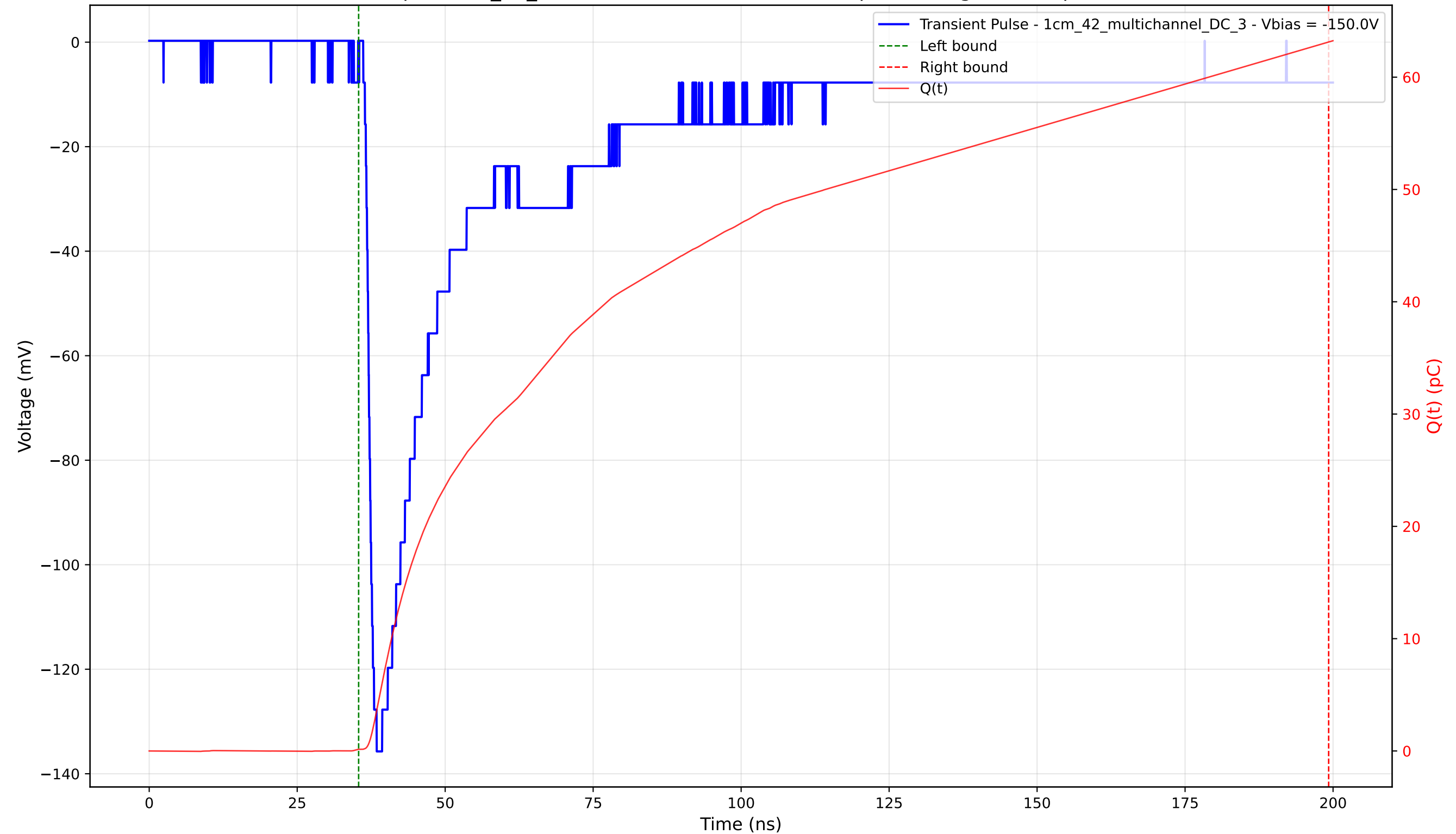
Transient Pulse - Sample: 1cm_42_multichannel - Position: 1485.0 \mu\text{m} - Charge: 62.98 pC - Rise Time: 1.55 ns
