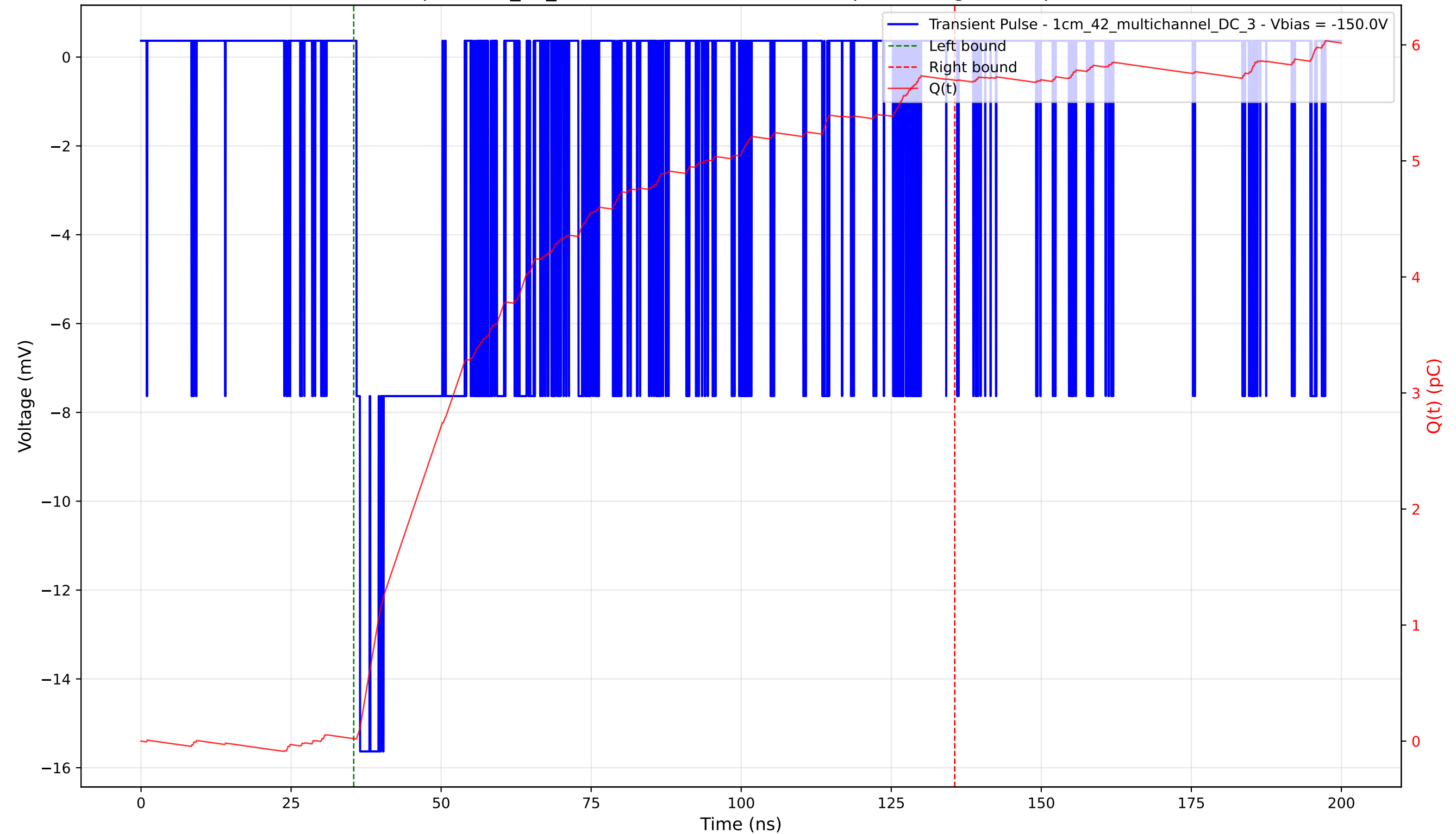
Transient Pulse - Sample: 1cm_42_multichannel - Position: 40.0 \mu\text{m} - Charge: 5.67 pC - Rise Time: 0.60 ns
