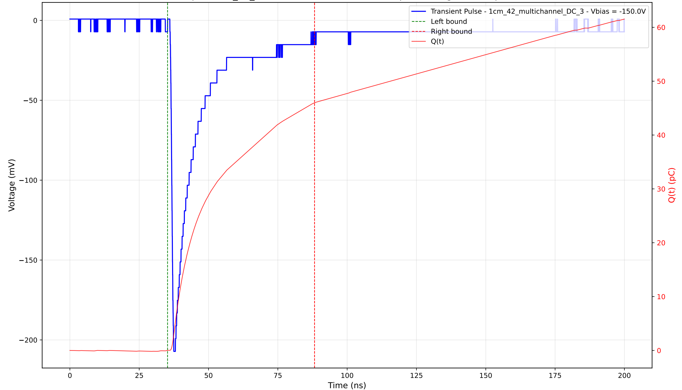
Transient Pulse - Sample: 1cm_42_multichannel - Position: 745.0 \mu\text{m} - Charge: 45.95 pC - Rise Time: 0.99 ns
