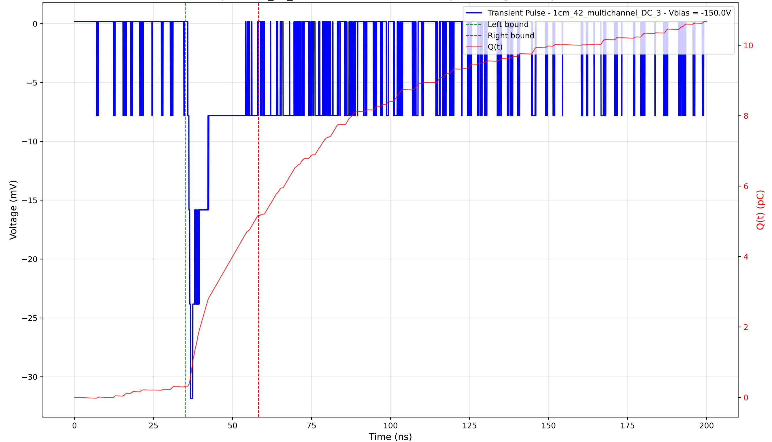
Transient Pulse - Sample: 1cm_42_multichannel - Position: 50.0 \mu\text{m} - Charge: 4.85 pC - Rise Time: 0.85 ns
