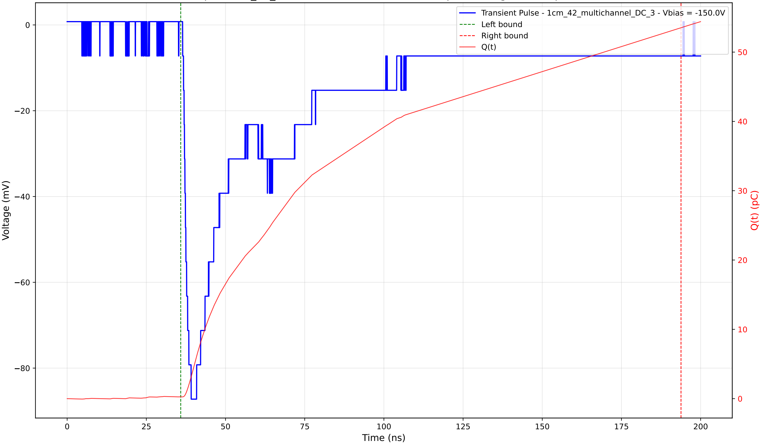
Transient Pulse - Sample: 1cm_42_multichannel - Position: 2675.0 \mu\text{m} - Charge: 53.28 pC - Rise Time: 1.70 ns
