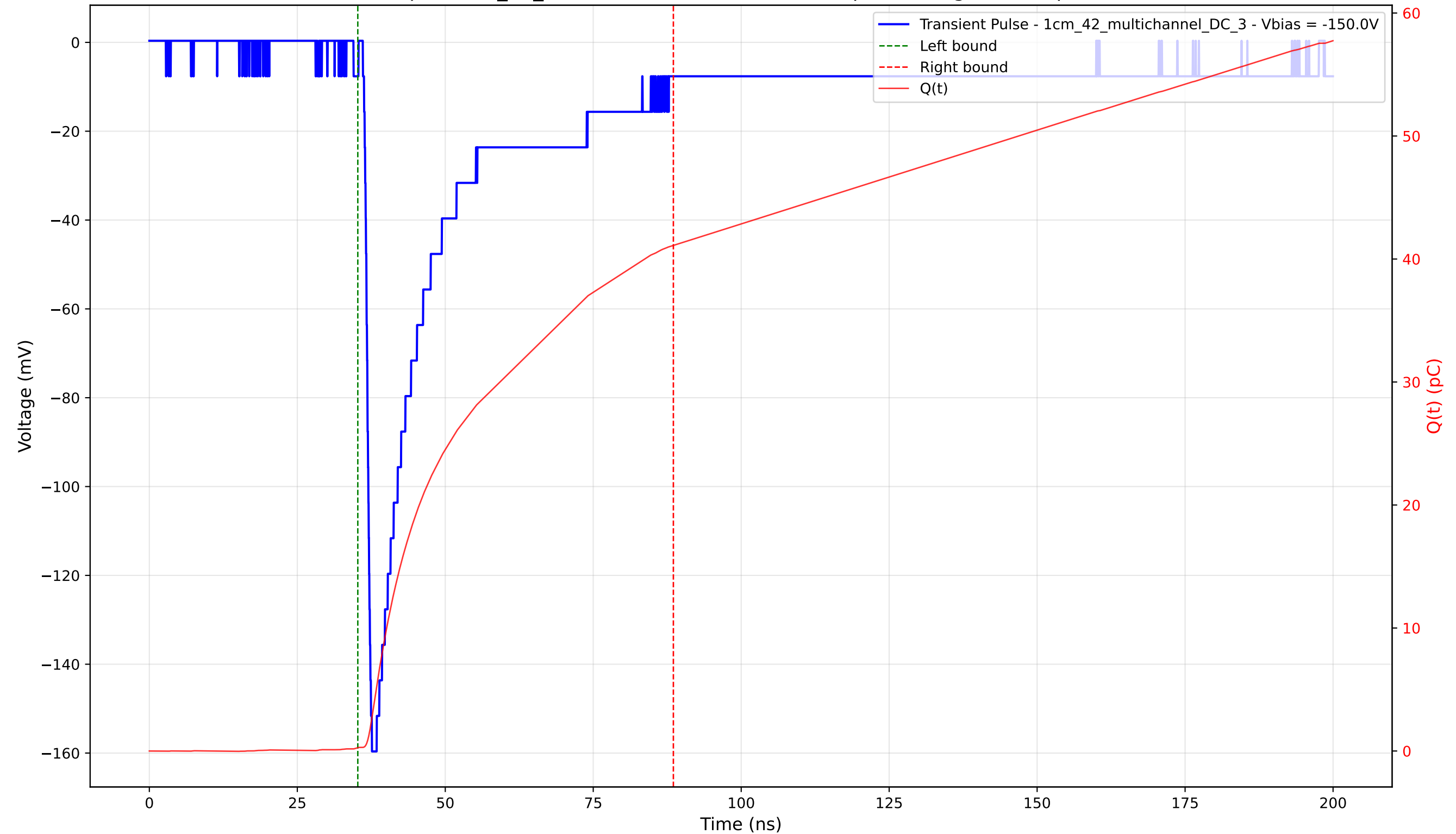
Transient Pulse - Sample: 1cm_42_multichannel - Position: 925.0 \mu\text{m} - Charge: 40.84 pC - Rise Time: 1.08 ns
