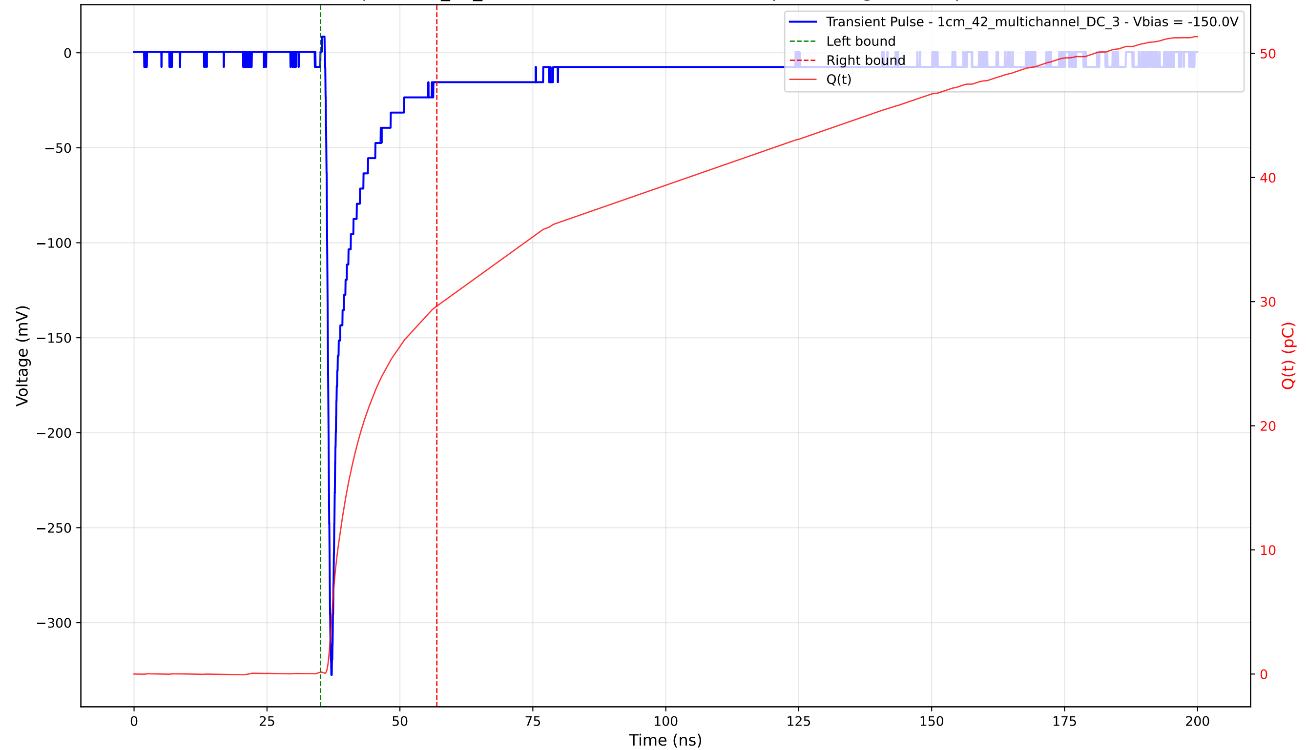
Transient Pulse - Sample: 1cm_42_multichannel - Position: 4825.0 \mu\text{m} - Charge: 29.48 pC - Rise Time: 0.78 ns
