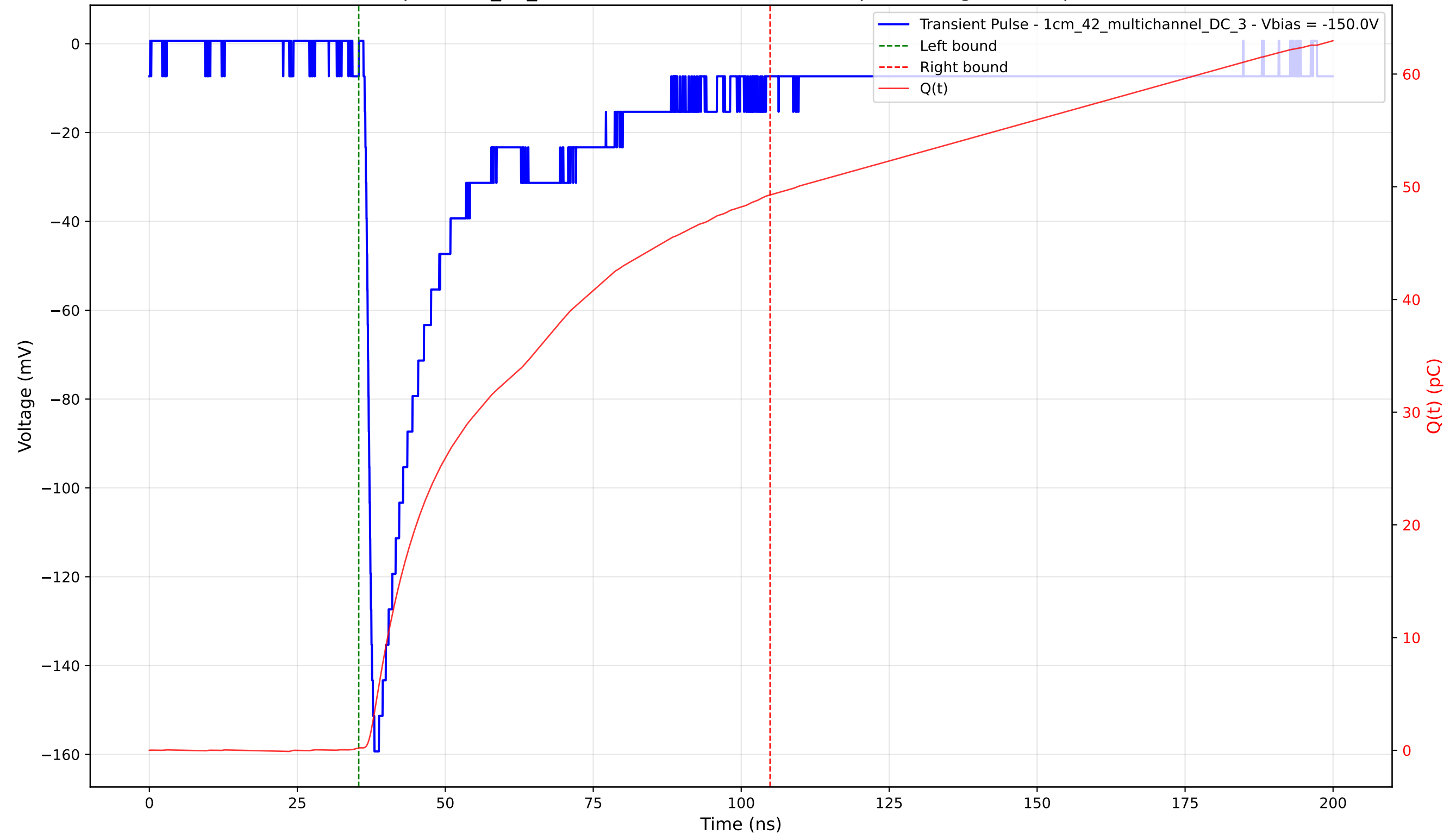
Transient Pulse - Sample: 1cm_42_multichannel - Position: 1205.0 \mu\text{m} - Charge: 49.05 pC - Rise Time: 1.30 ns
