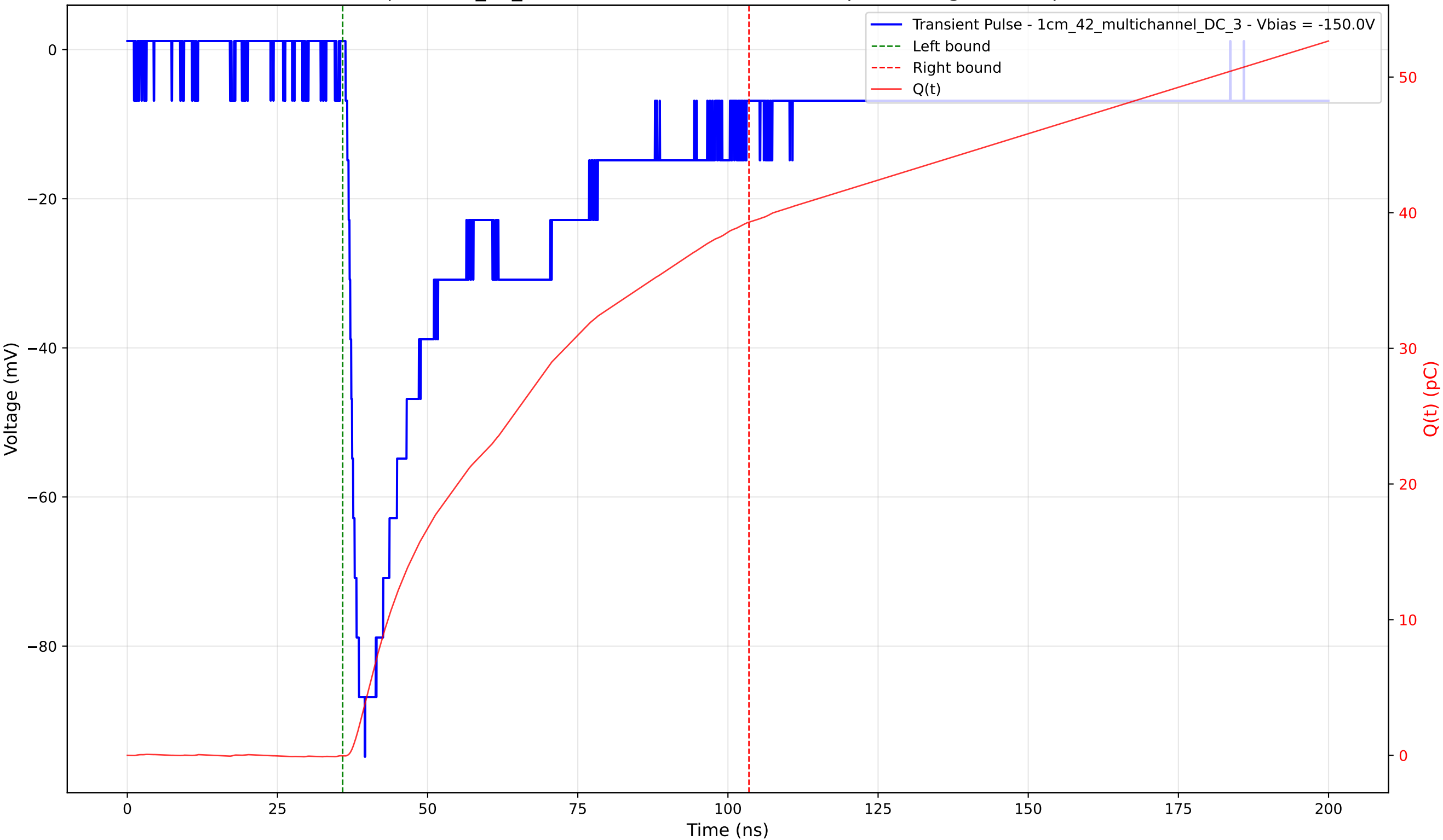
Transient Pulse - Sample: 1cm_42_multichannel - Position: 2780.0 \mu\text{m} - Charge: 39.34 pC - Rise Time: 1.95 ns
