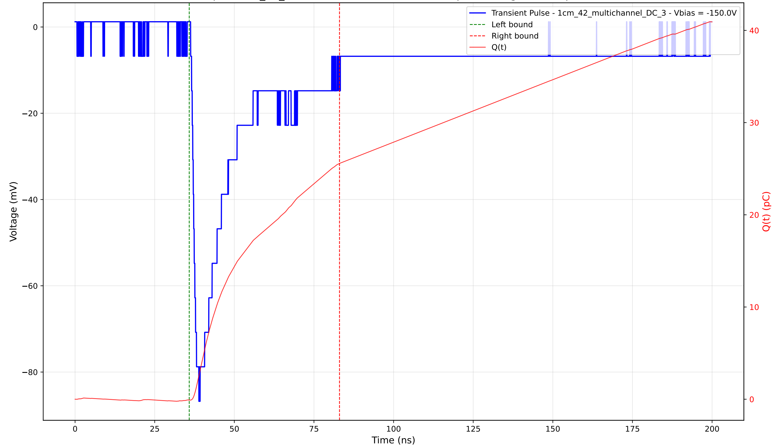
Transient Pulse - Sample: 1cm_42_multichannel - Position: 3325.0 \mu\text{m} - Charge: 25.67 pC - Rise Time: 1.56 ns
