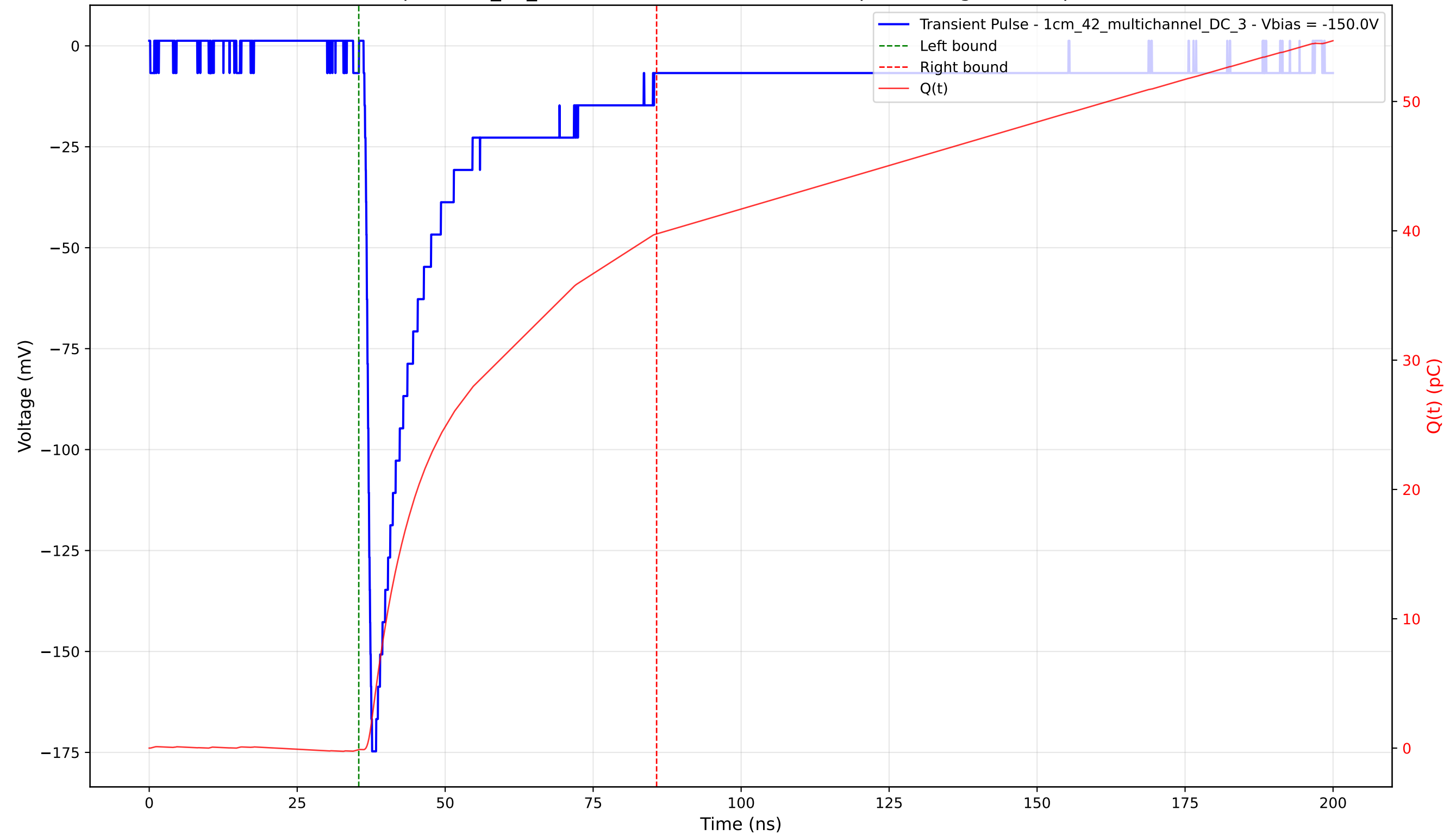
Transient Pulse - Sample: 1cm_42_multichannel - Position: 4050.0 \mu\text{m} - Charge: 39.87 pC - Rise Time: 0.99 ns
