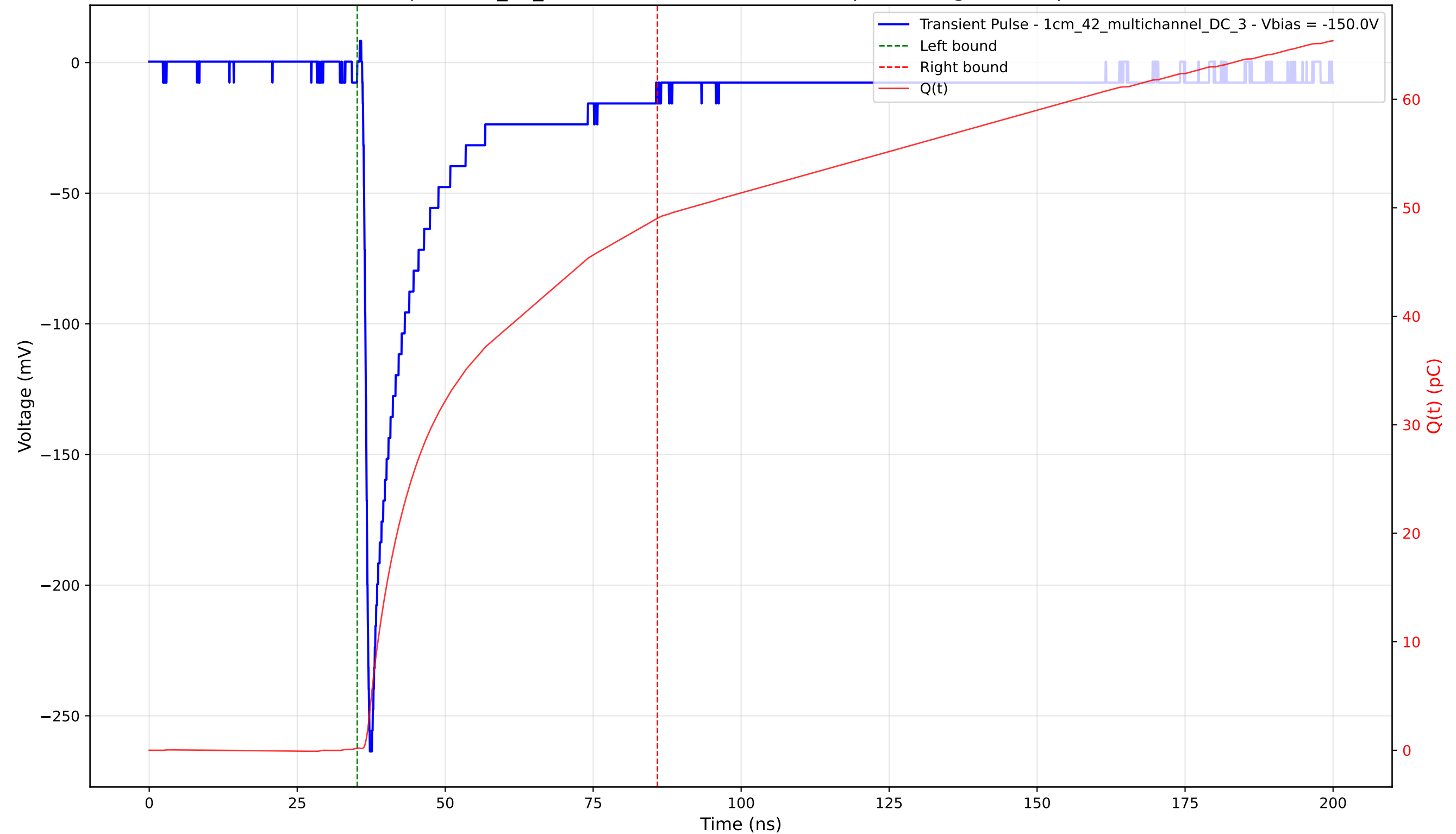
Transient Pulse - Sample: 1cm_42_multichannel - Position: 520.0 \mu\text{m} - Charge: 48.83 pC - Rise Time: 0.89 ns
