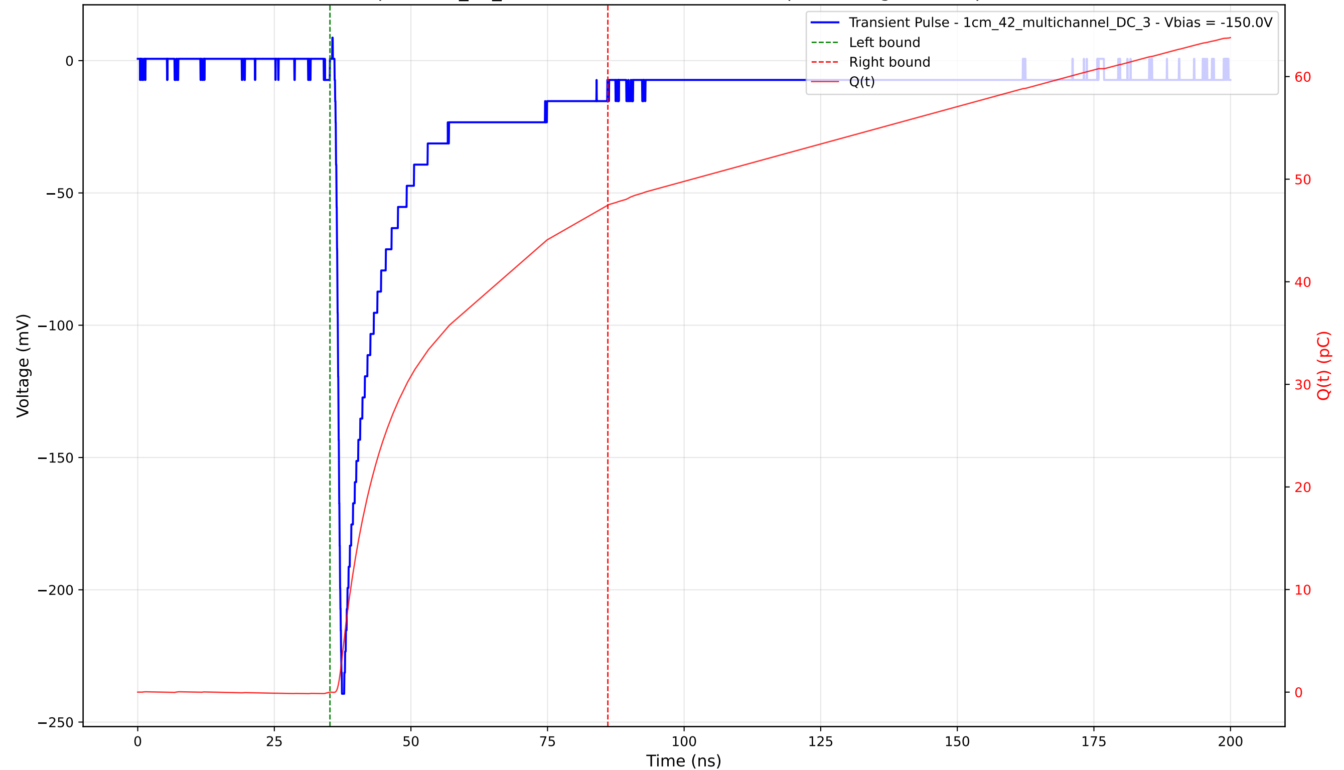
Transient Pulse - Sample: 1cm_42_multichannel - Position: 615.0 \mu\text{m} - Charge: 47.46 pC - Rise Time: 0.96 ns
