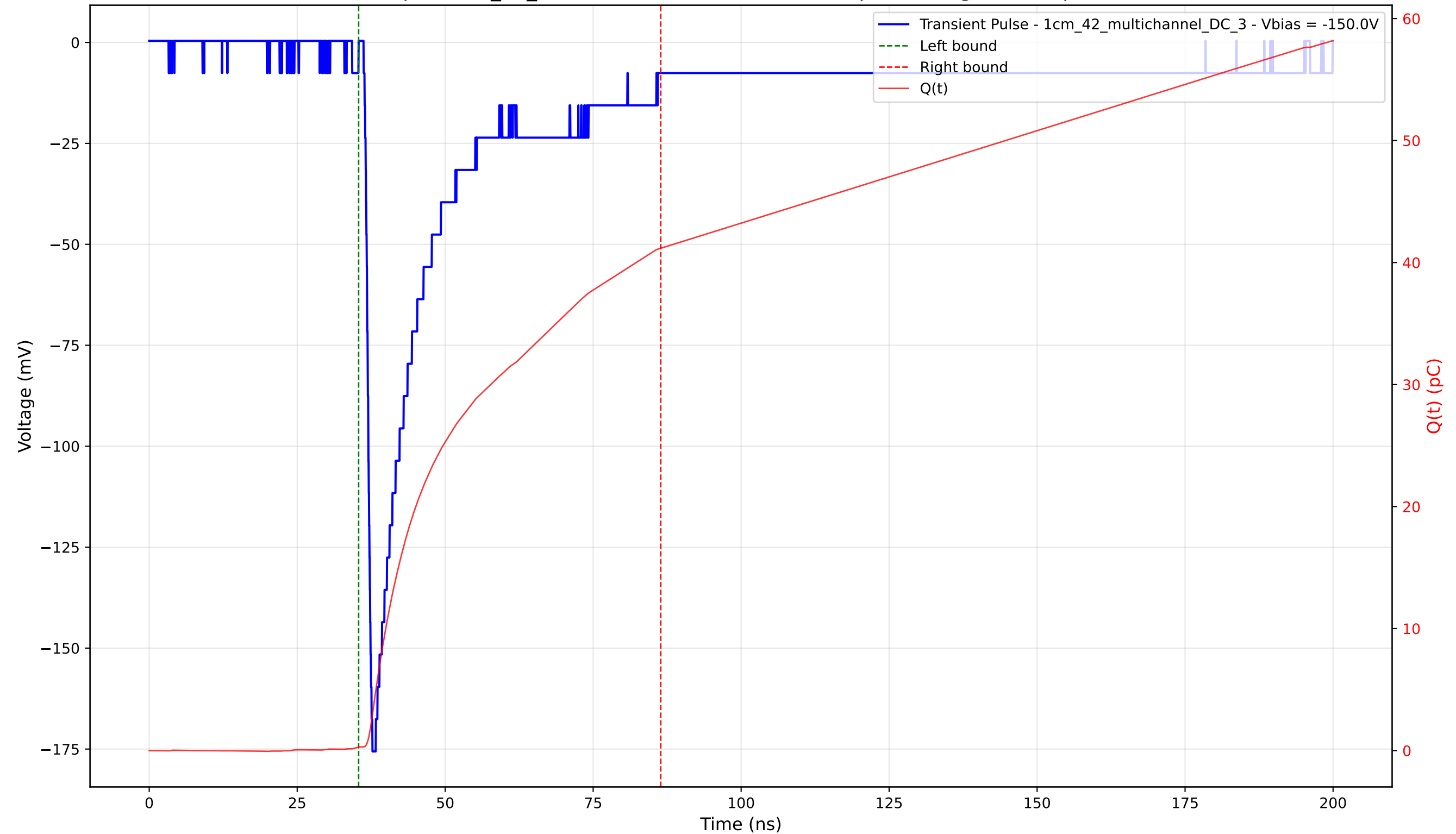
Transient Pulse - Sample: 1cm_42_multichannel - Position: 4045.0 \mu\text{m} - Charge: 40.88 pC - Rise Time: 1.00 ns
