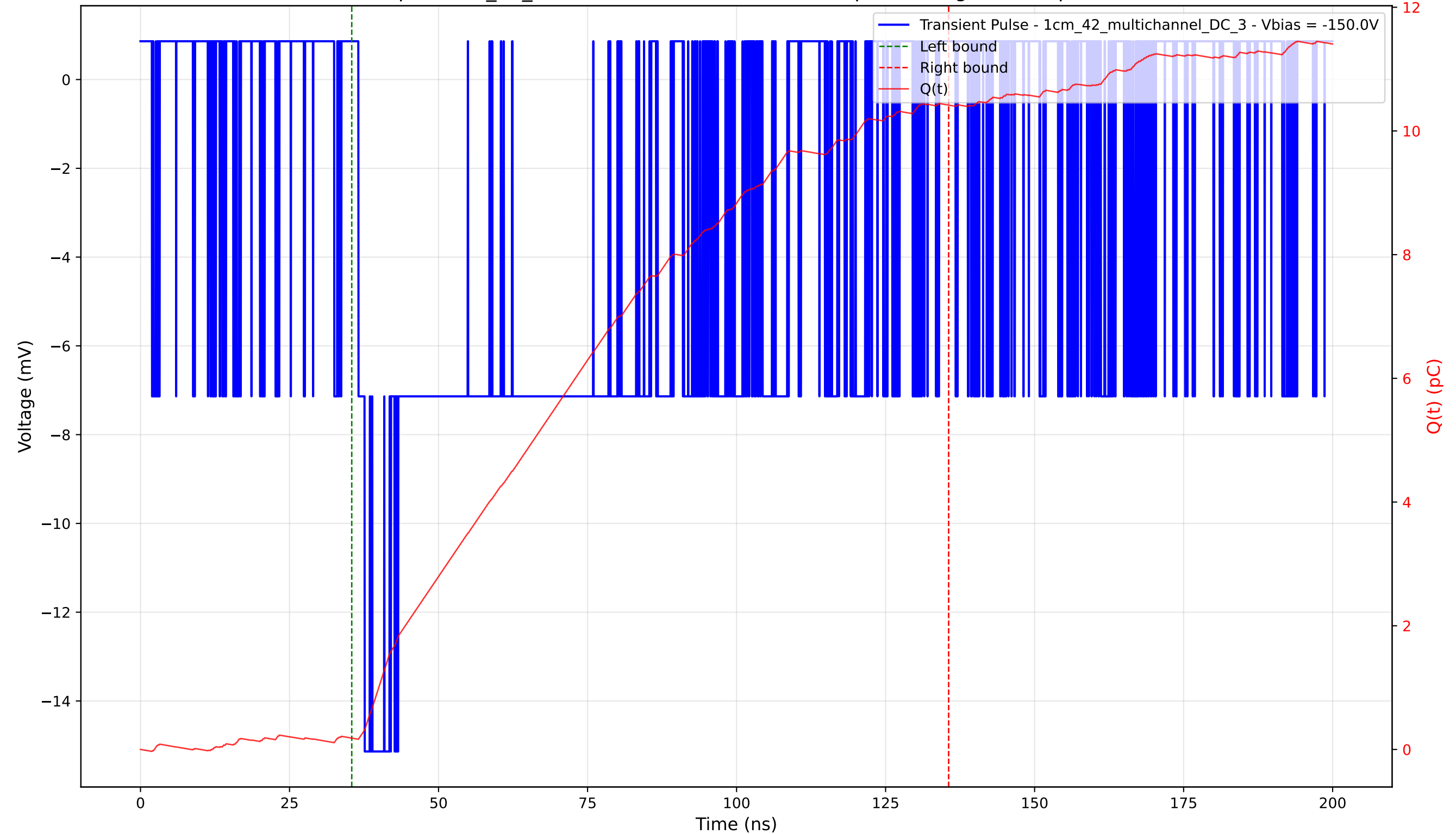
Transient Pulse - Sample: 1cm_42_multichannel - Position: 1845.0 \mu\text{m} - Charge: 10.23 pC - Rise Time: 1.06 ns
