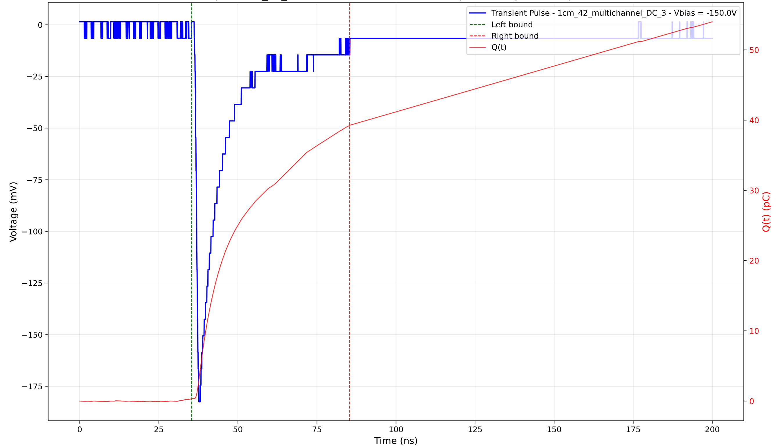
Transient Pulse - Sample: 1cm_42_multichannel - Position: 4125.0 \mu\text{m} - Charge: 38.92 pC - Rise Time: 0.99 ns
