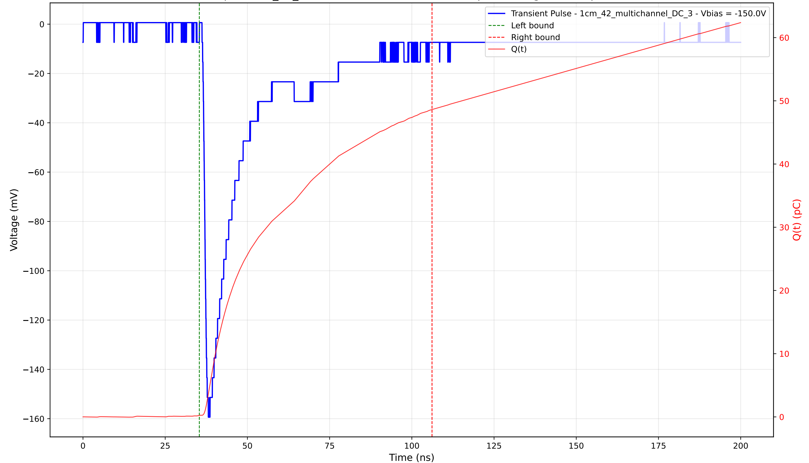
Transient Pulse - Sample: 1cm_42_multichannel - Position: 1195.0 \mu\text{m} - Charge: 48.36 pC - Rise Time: 1.30 ns
