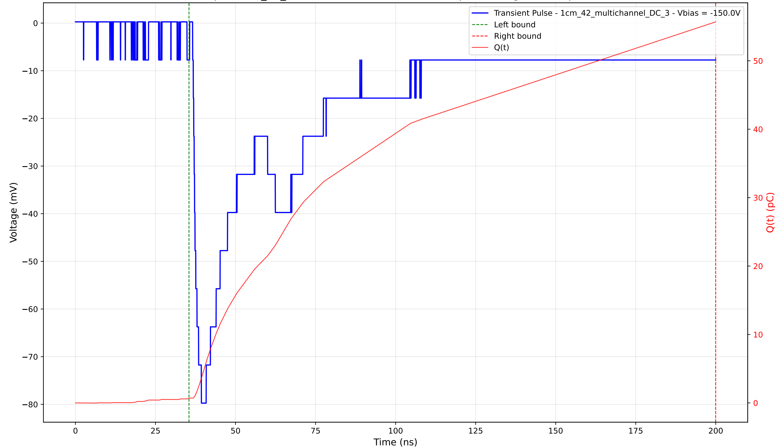
Transient Pulse - Sample: 1cm_42_multichannel - Position: 2455.0 \mu\text{m} - Charge: 55.02 pC - Rise Time: 2.54 ns
