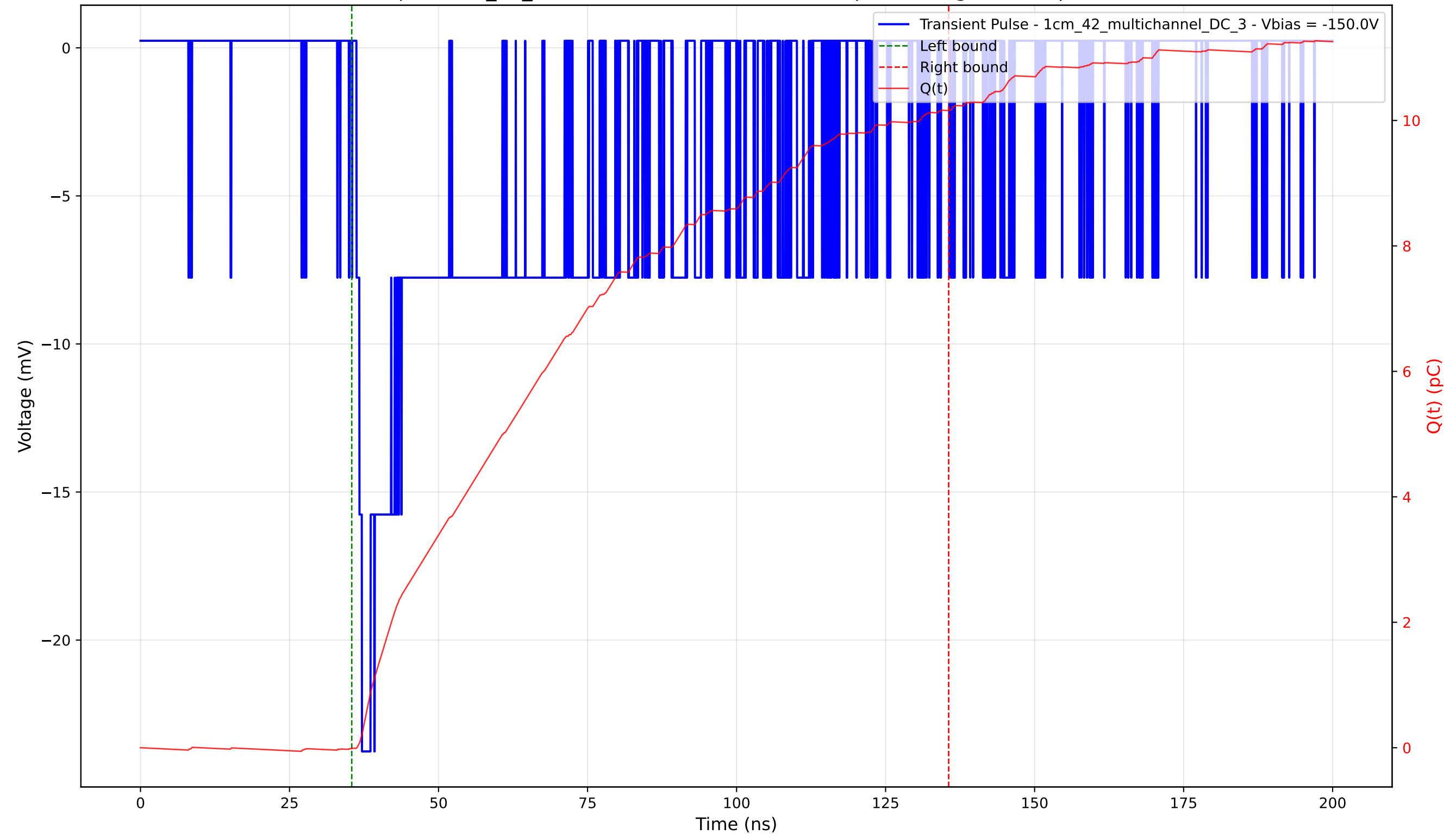
Transient Pulse - Sample: 1cm_42_multichannel - Position: 4365.0 \mu\text{m} - Charge: 10.17 pC - Rise Time: 0.91 ns
