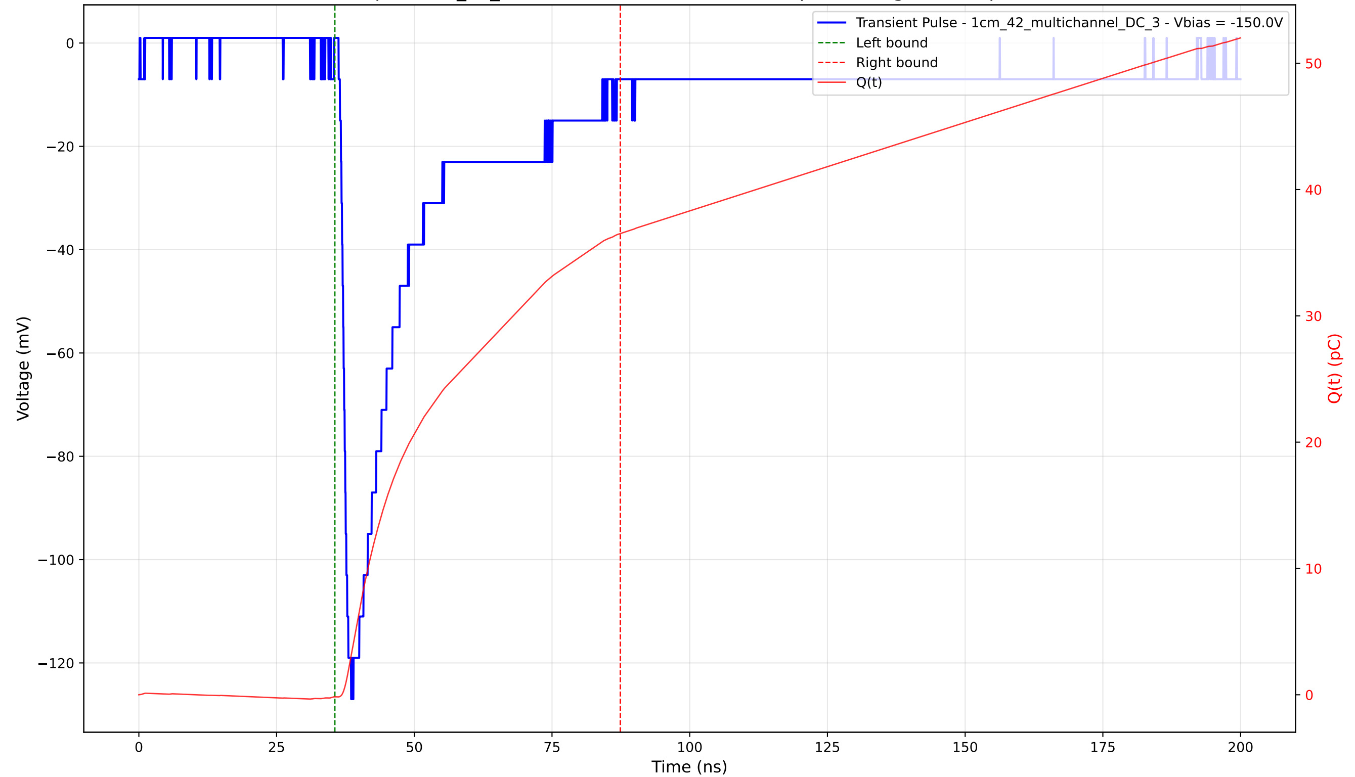
Transient Pulse - Sample: 1cm_42_multichannel - Position: 3540.0 \mu\text{m} - Charge: 36.68 pC - Rise Time: 1.53 ns
