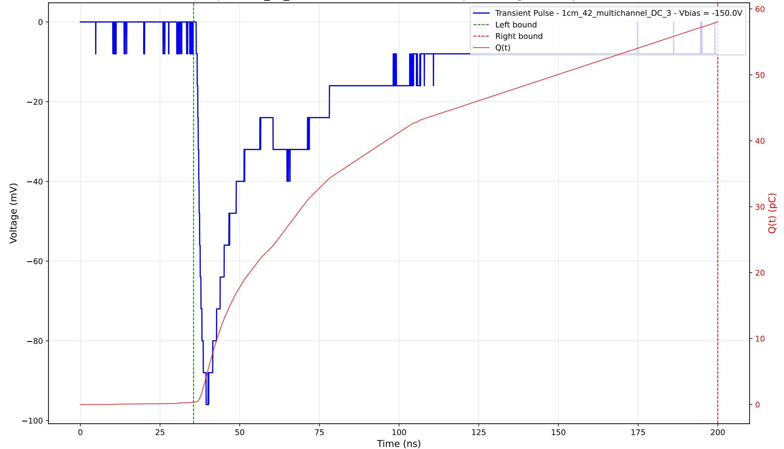
Transient Pulse - Sample: 1cm_42_multichannel - Position: 2755.0 \mu\text{m} - Charge: 57.65 pC - Rise Time: 1.92 ns
