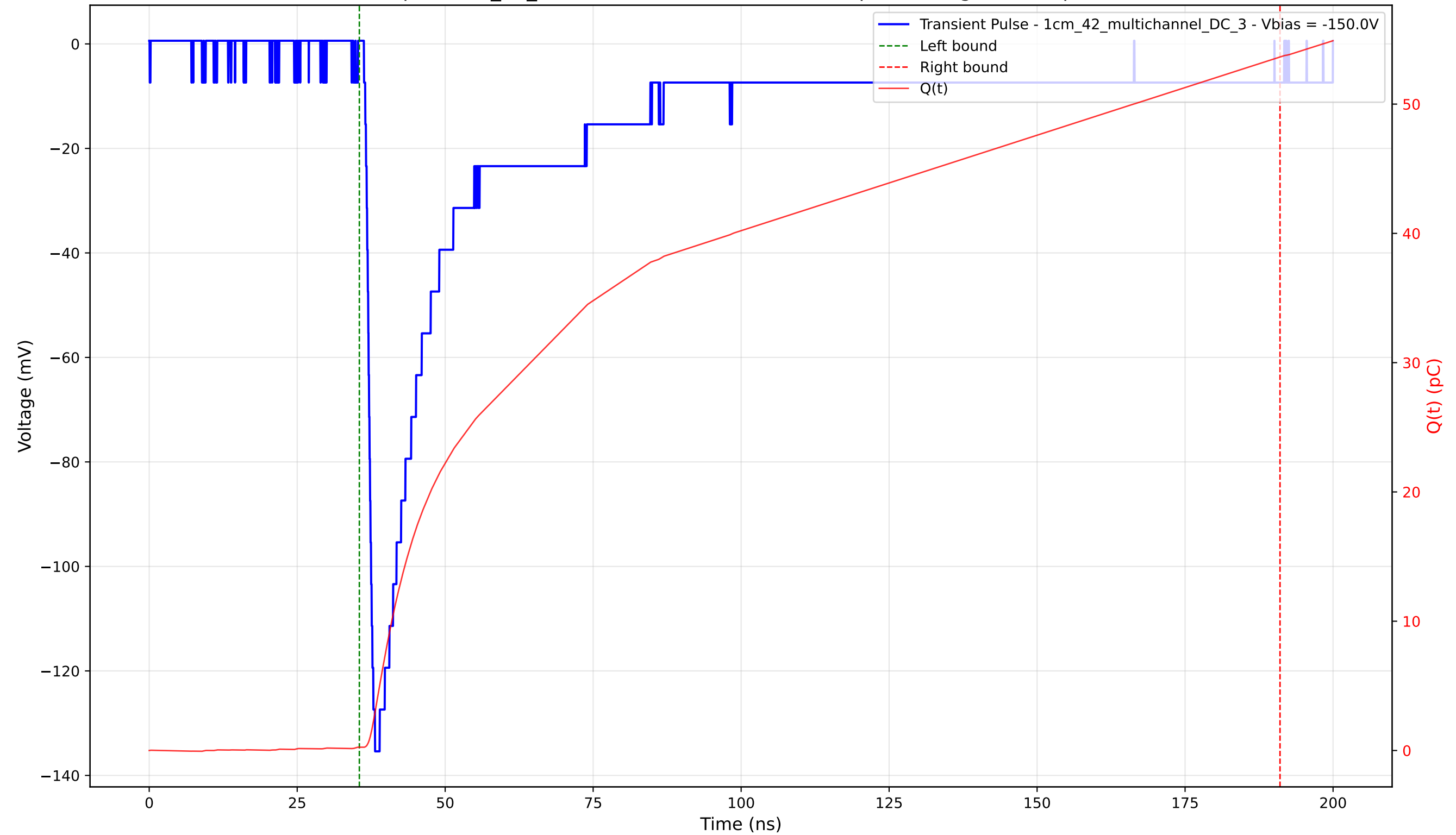
Transient Pulse - Sample: 1cm_42_multichannel - Position: 3675.0 \mu\text{m} - Charge: 53.40 pC - Rise Time: 1.36 ns
