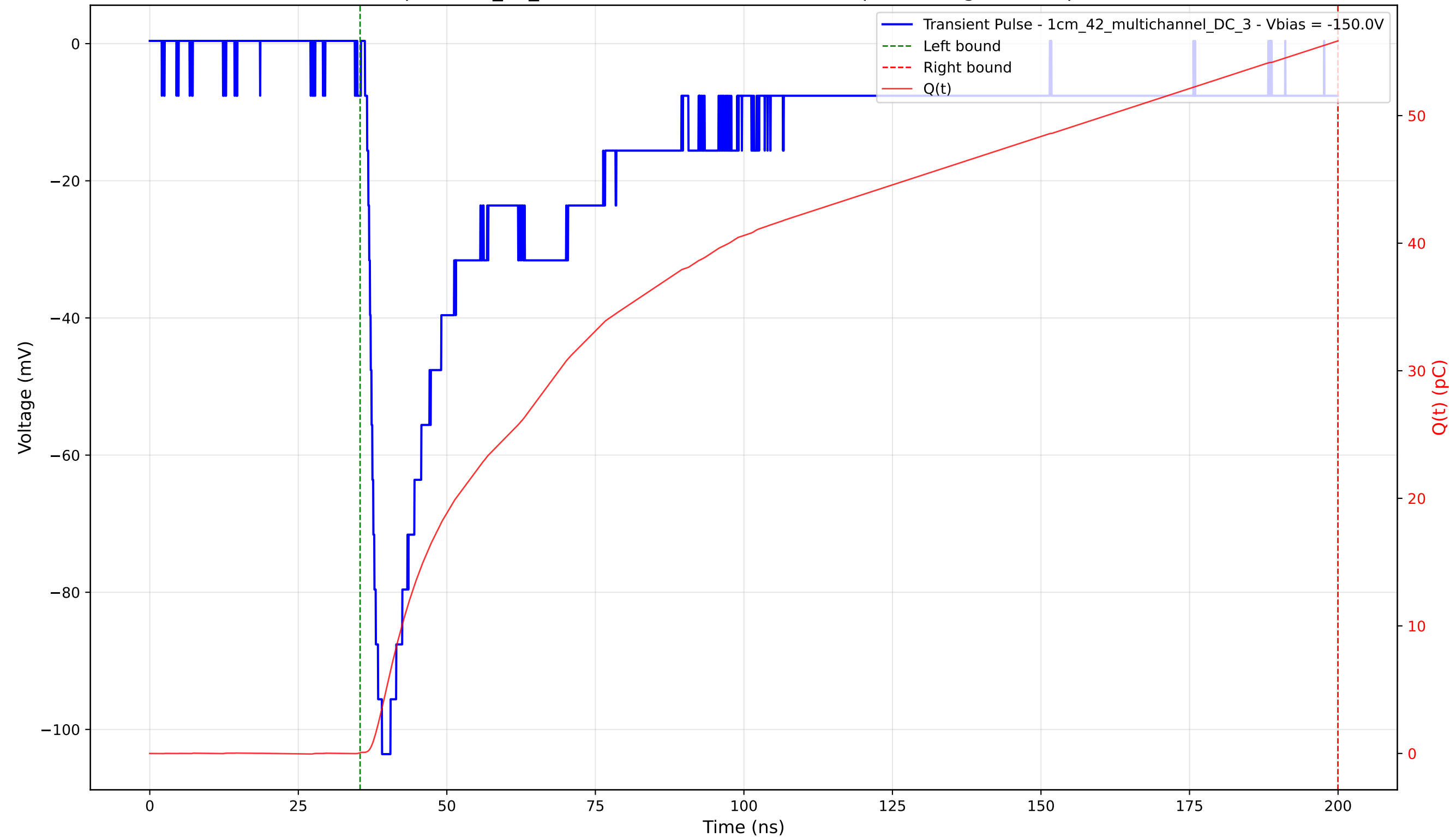
Transient Pulse - Sample: 1cm_42_multichannel - Position: 3000.0 \mu\text{m} - Charge: 55.79 pC - Rise Time: 1.85 ns
