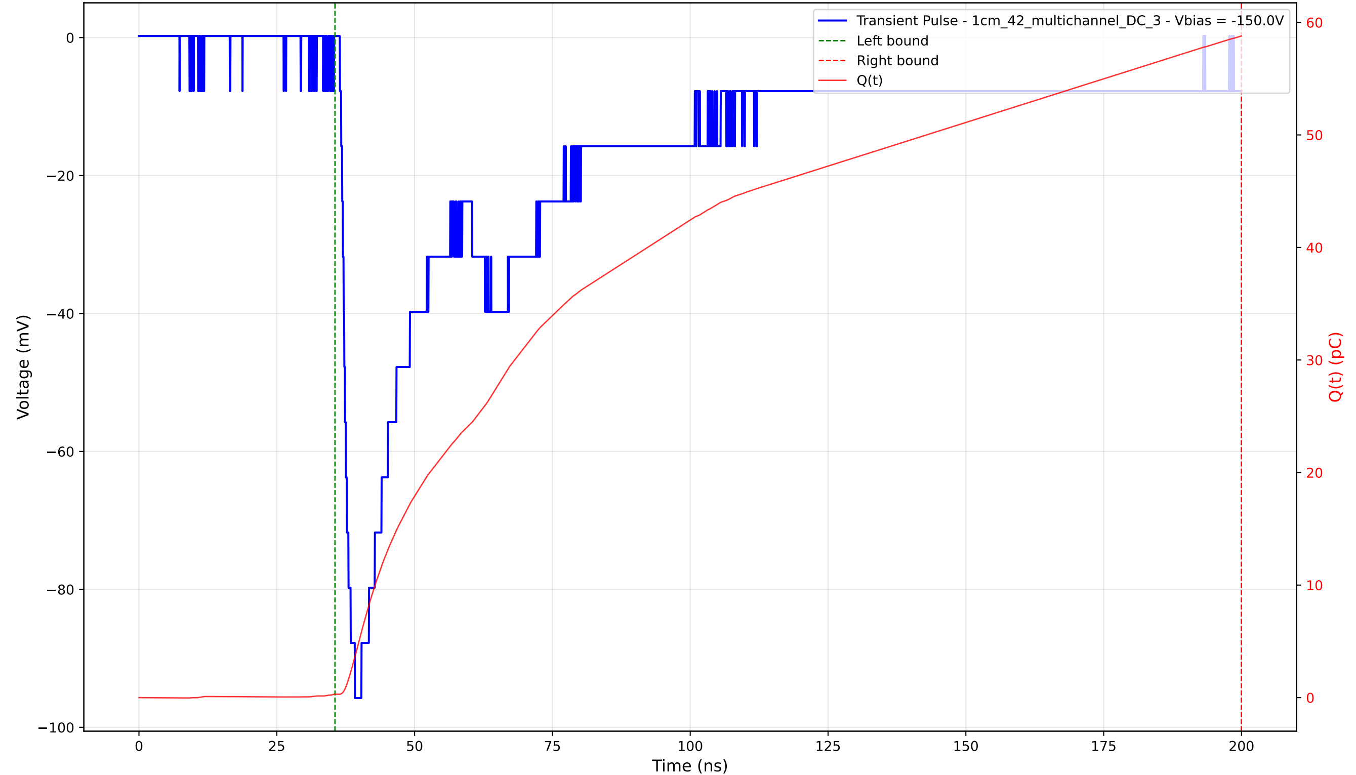
Transient Pulse - Sample: 1cm_42_multichannel - Position: 2060.0 \mu\text{m} - Charge: 58.50 pC - Rise Time: 1.74 ns
