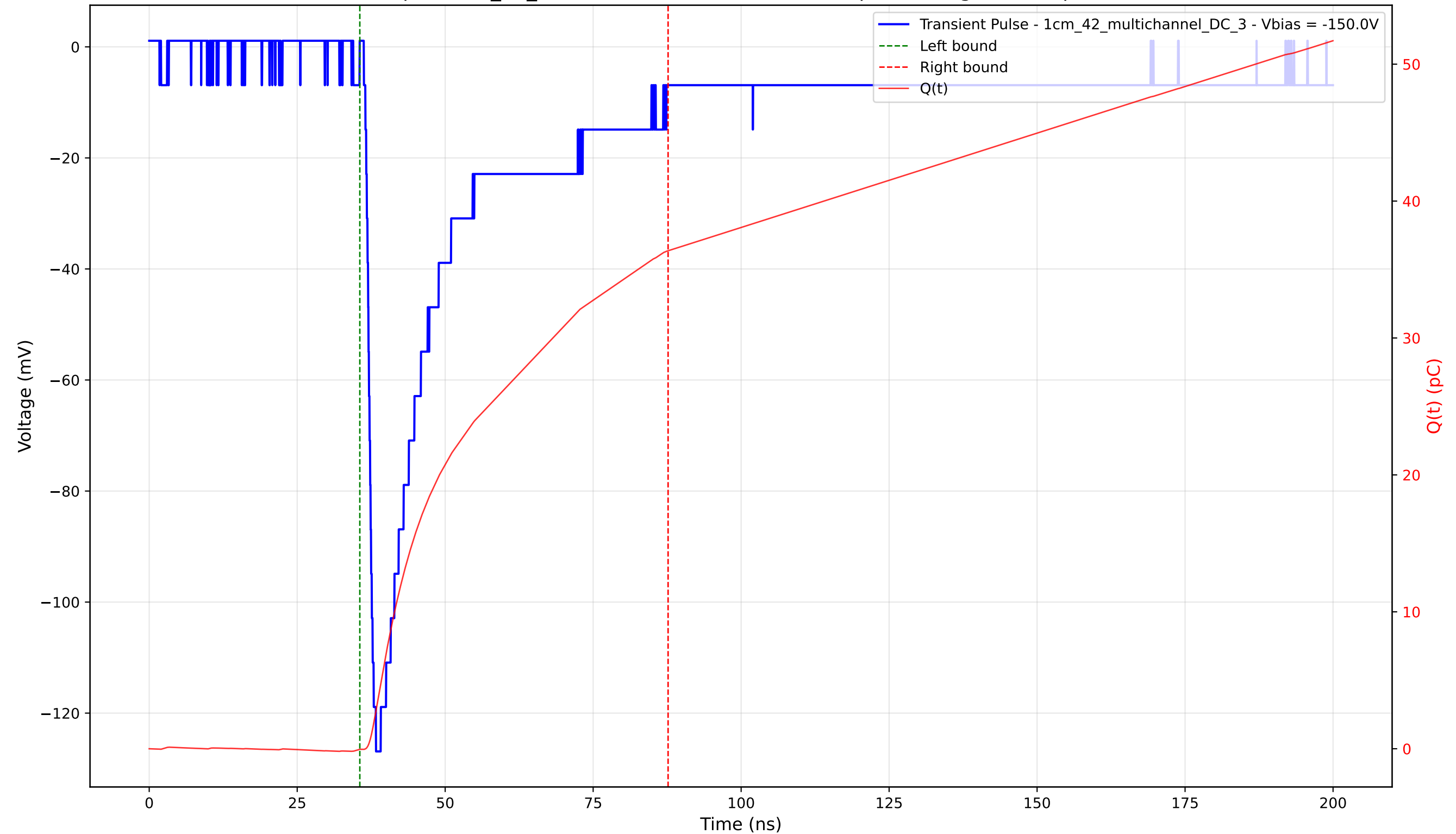
Transient Pulse - Sample: 1cm_42_multichannel - Position: 3605.0 \mu\text{m} - Charge: 36.41 pC - Rise Time: 1.41 ns
