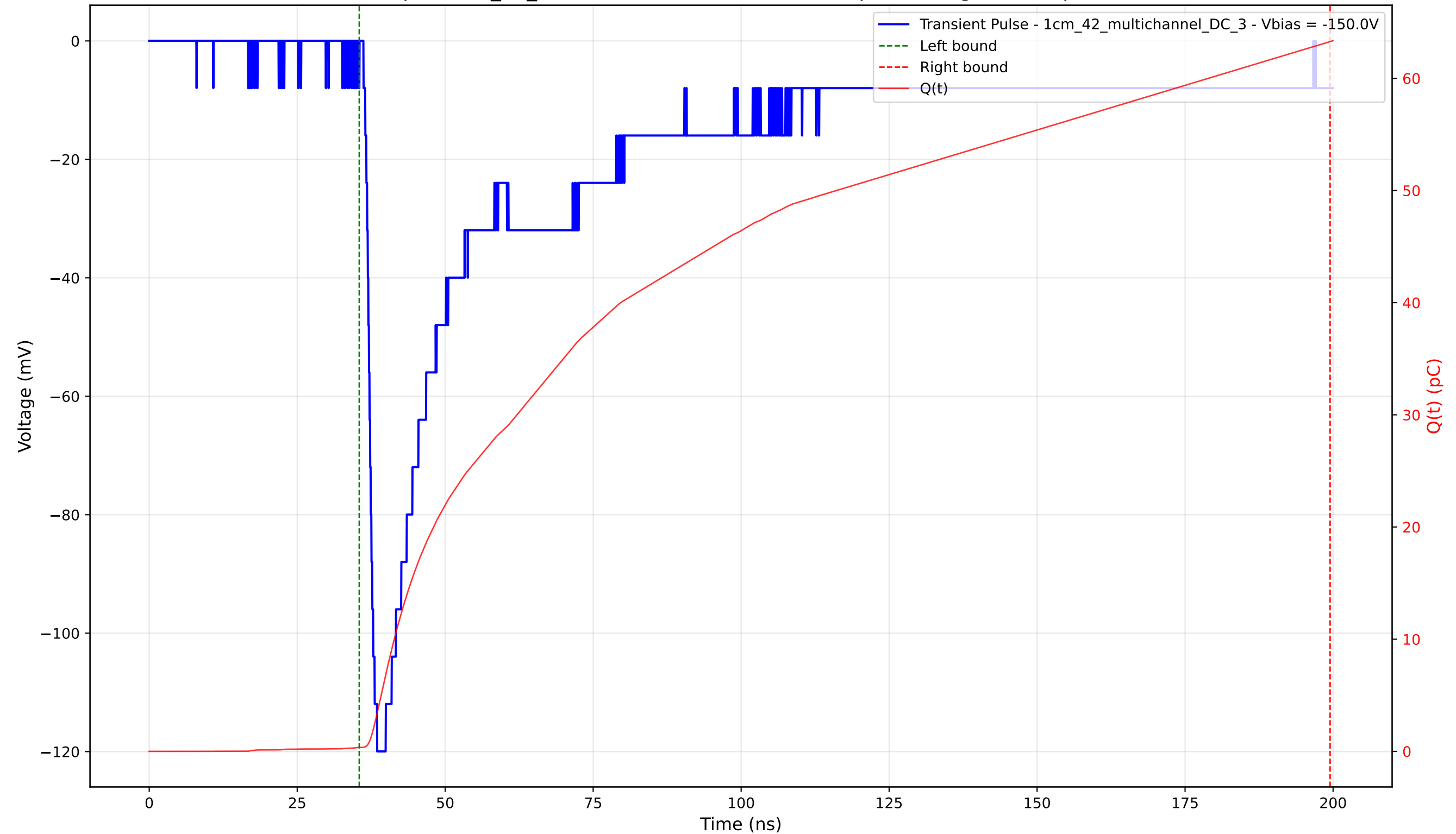
Transient Pulse - Sample: 1cm_42_multichannel - Position: 1685.0 \mu\text{m} - Charge: 62.92 pC - Rise Time: 1.59 ns
