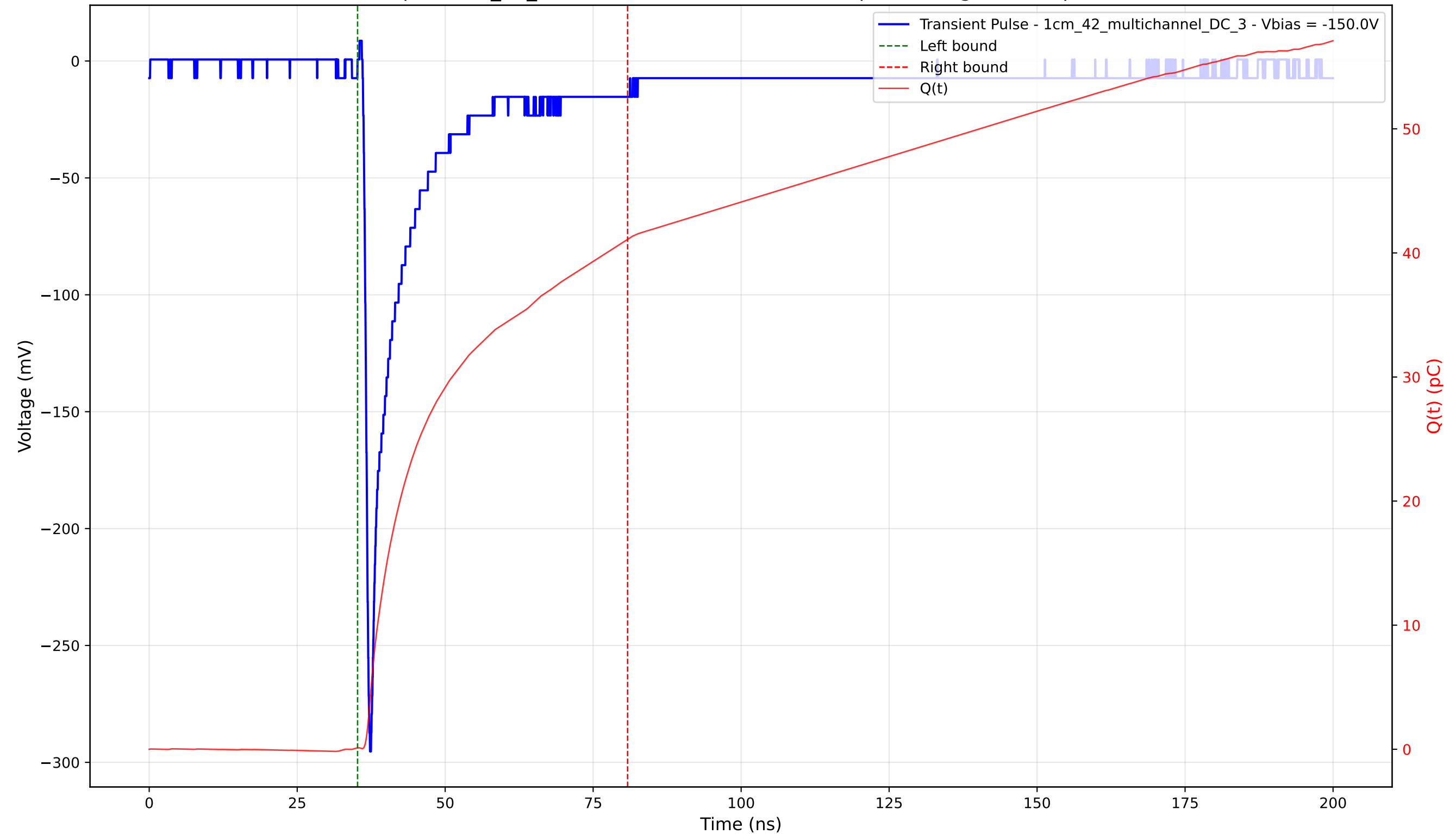
Transient Pulse - Sample: 1cm_42_multichannel - Position: 4590.0 \mu\text{m} - Charge: 40.98 pC - Rise Time: 0.86 ns
