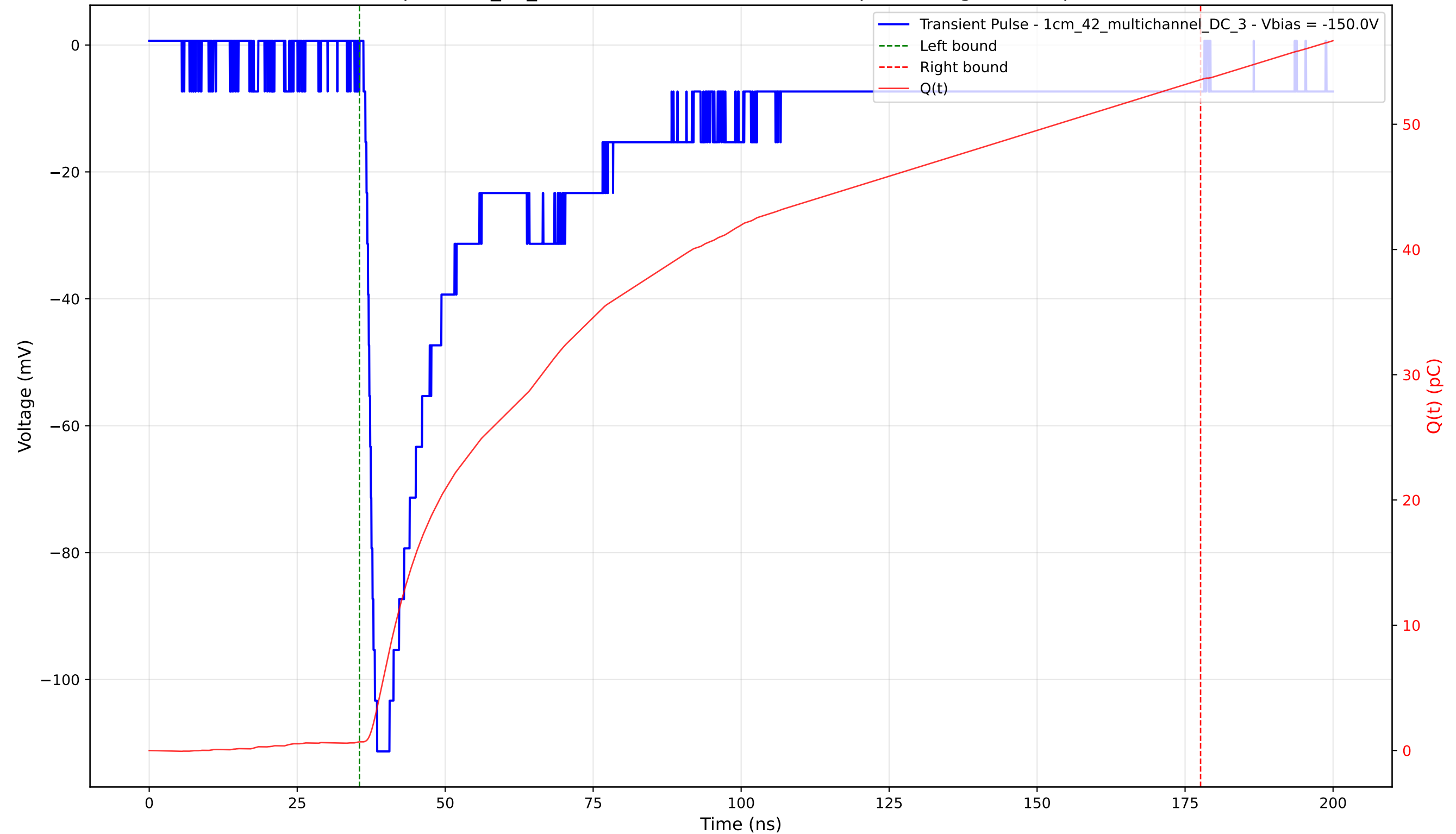
Transient Pulse - Sample: 1cm_42_multichannel - Position: 3235.0 \mu\text{m} - Charge: 52.87 pC - Rise Time: 1.61 ns
