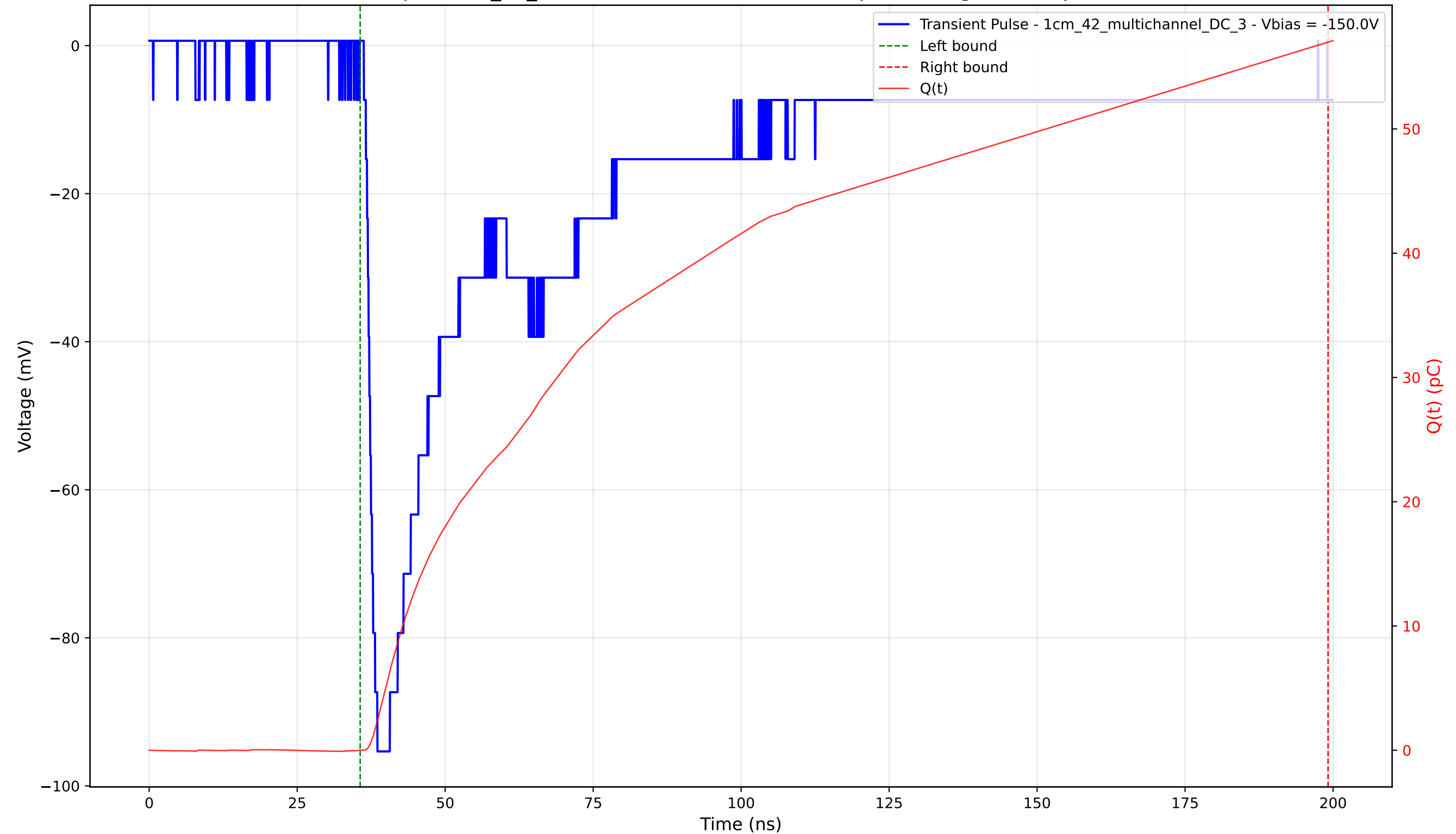
Transient Pulse - Sample: 1cm_42_multichannel - Position: 1970.0 \mu\text{m} - Charge: 56.97 pC - Rise Time: 1.57 ns
