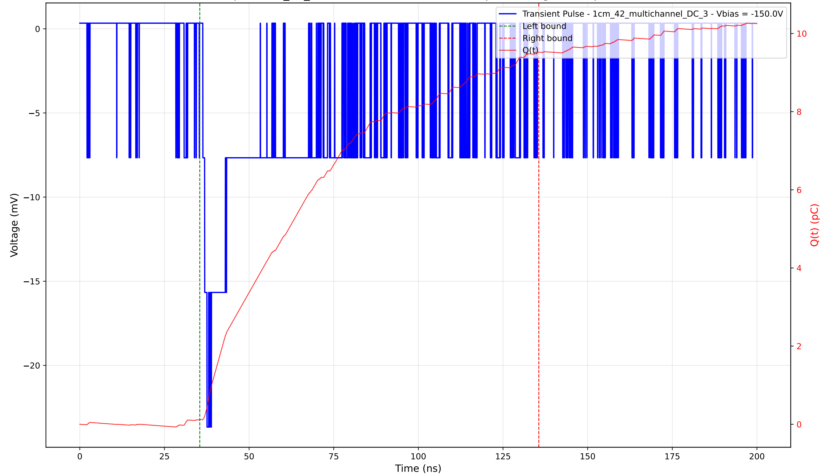
Transient Pulse - Sample: 1cm_42_multichannel - Position: 835.0 \mu\text{m} - Charge: 9.40 pC - Rise Time: 1.23 ns
