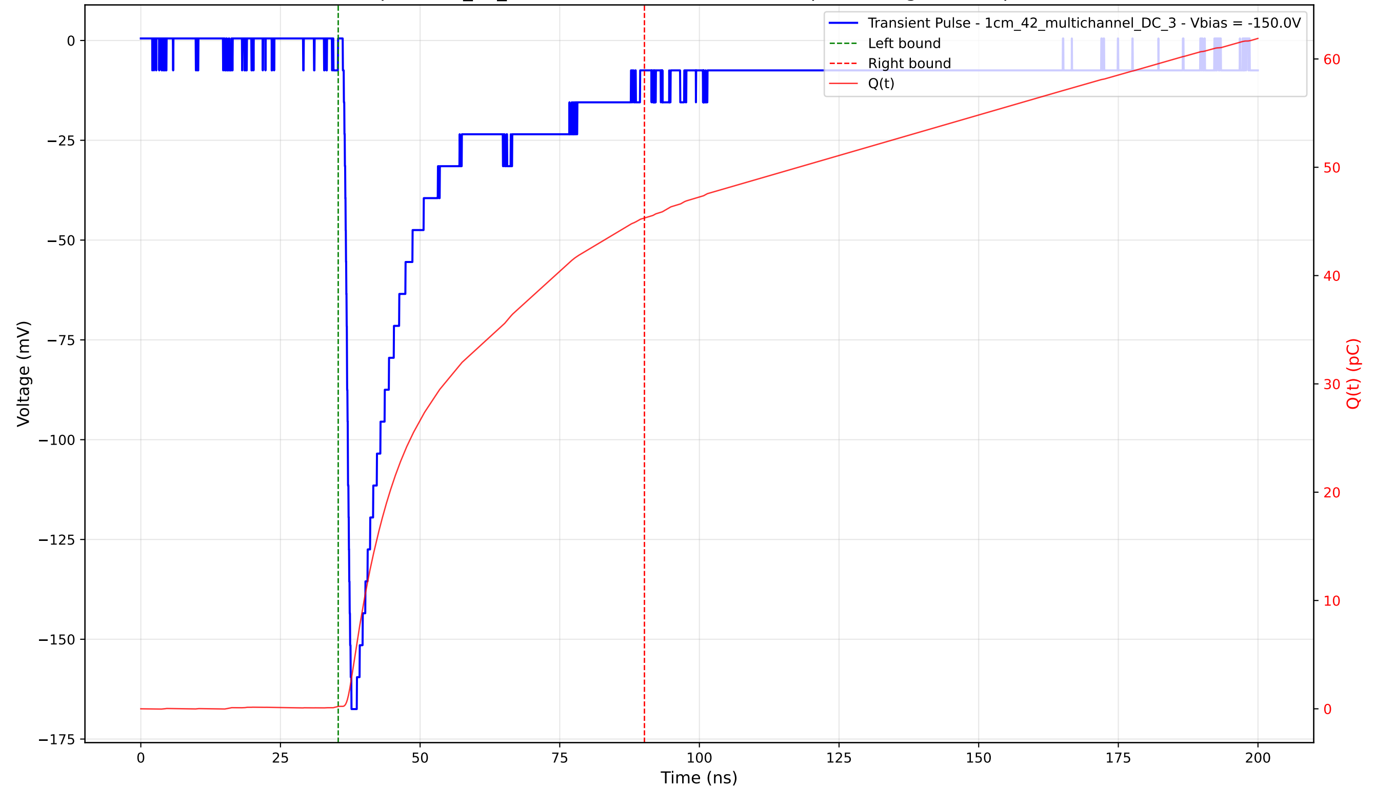
Transient Pulse - Sample: 1cm_42_multichannel - Position: 1040.0 \mu\text{m} - Charge: 45.09 pC - Rise Time: 1.04 ns
