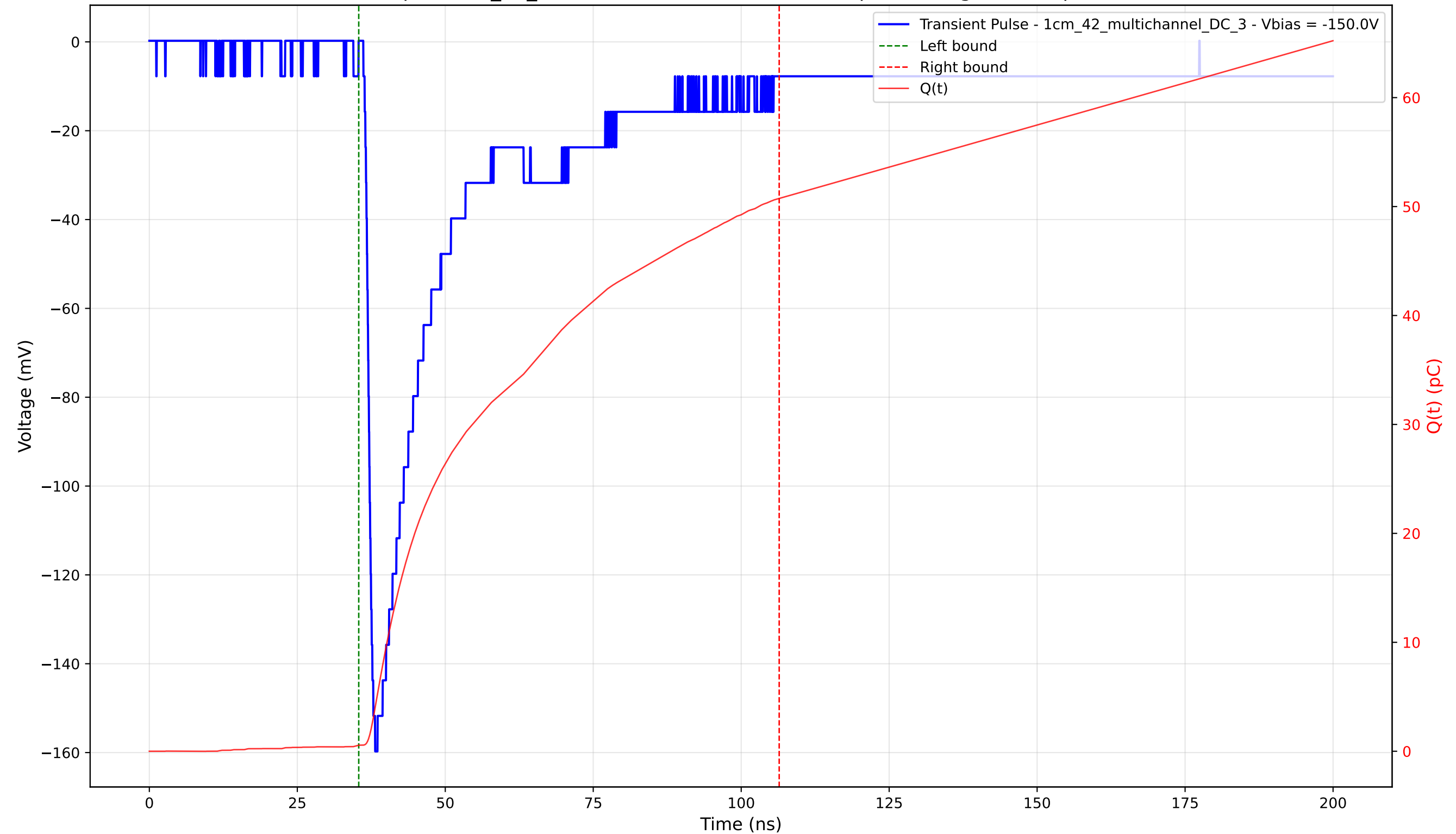
Transient Pulse - Sample: 1cm_42_multichannel - Position: 1230.0 \mu\text{m} - Charge: 50.19 pC - Rise Time: 1.36 ns
