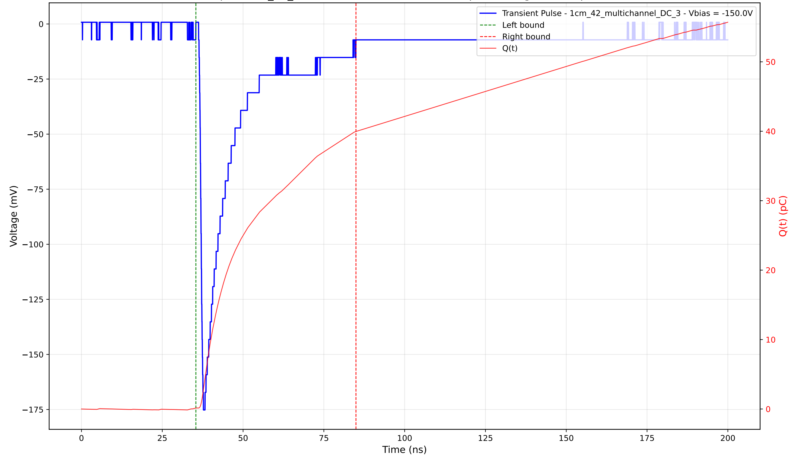
Transient Pulse - Sample: 1cm_42_multichannel - Position: 4040.0 \mu\text{m} - Charge: 39.82 pC - Rise Time: 1.01 ns
