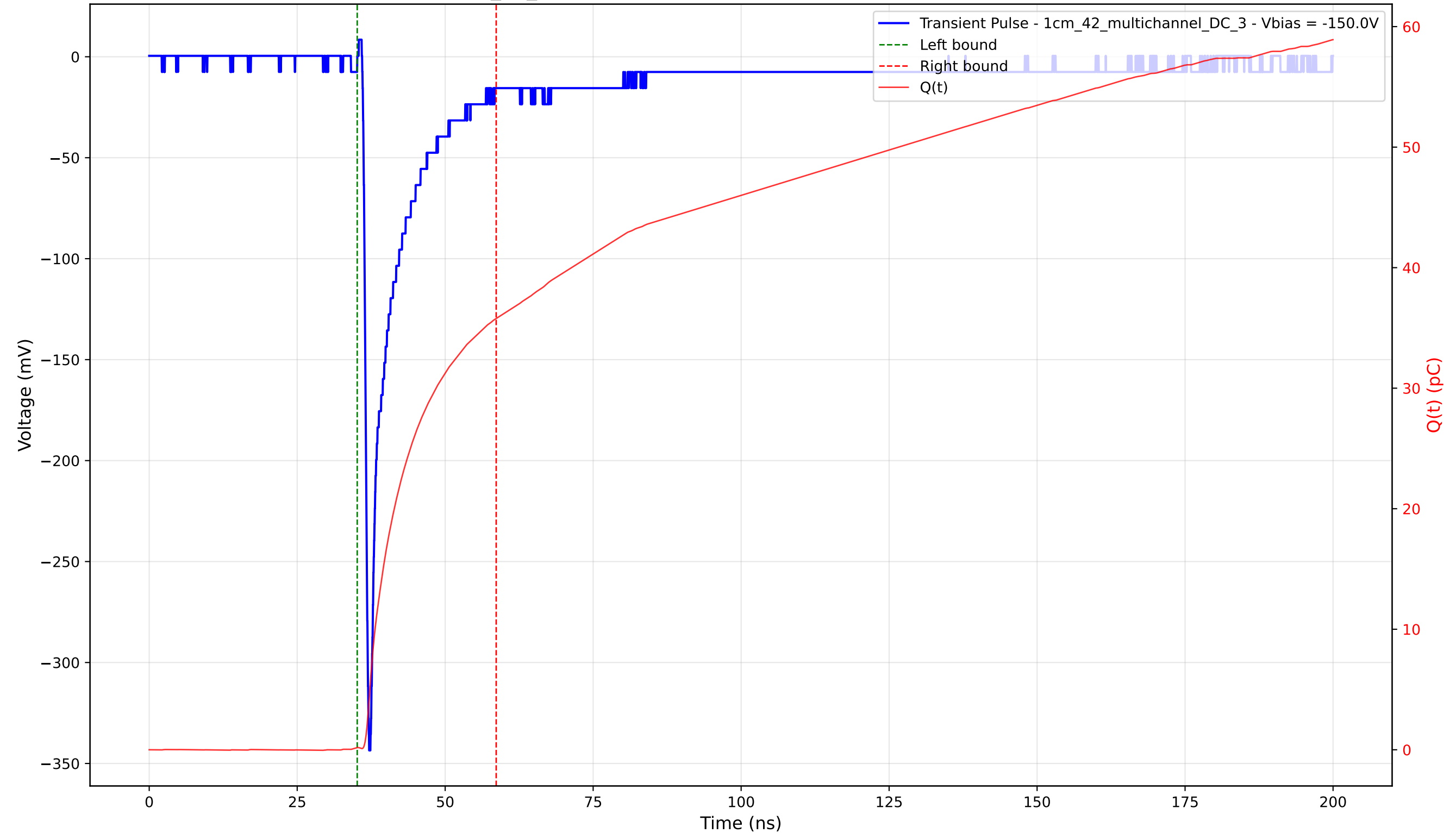
Transient Pulse - Sample: 1cm_42_multichannel - Position: 4700.0 \mu\text{m} - Charge: 35.61 pC - Rise Time: 0.79 ns
