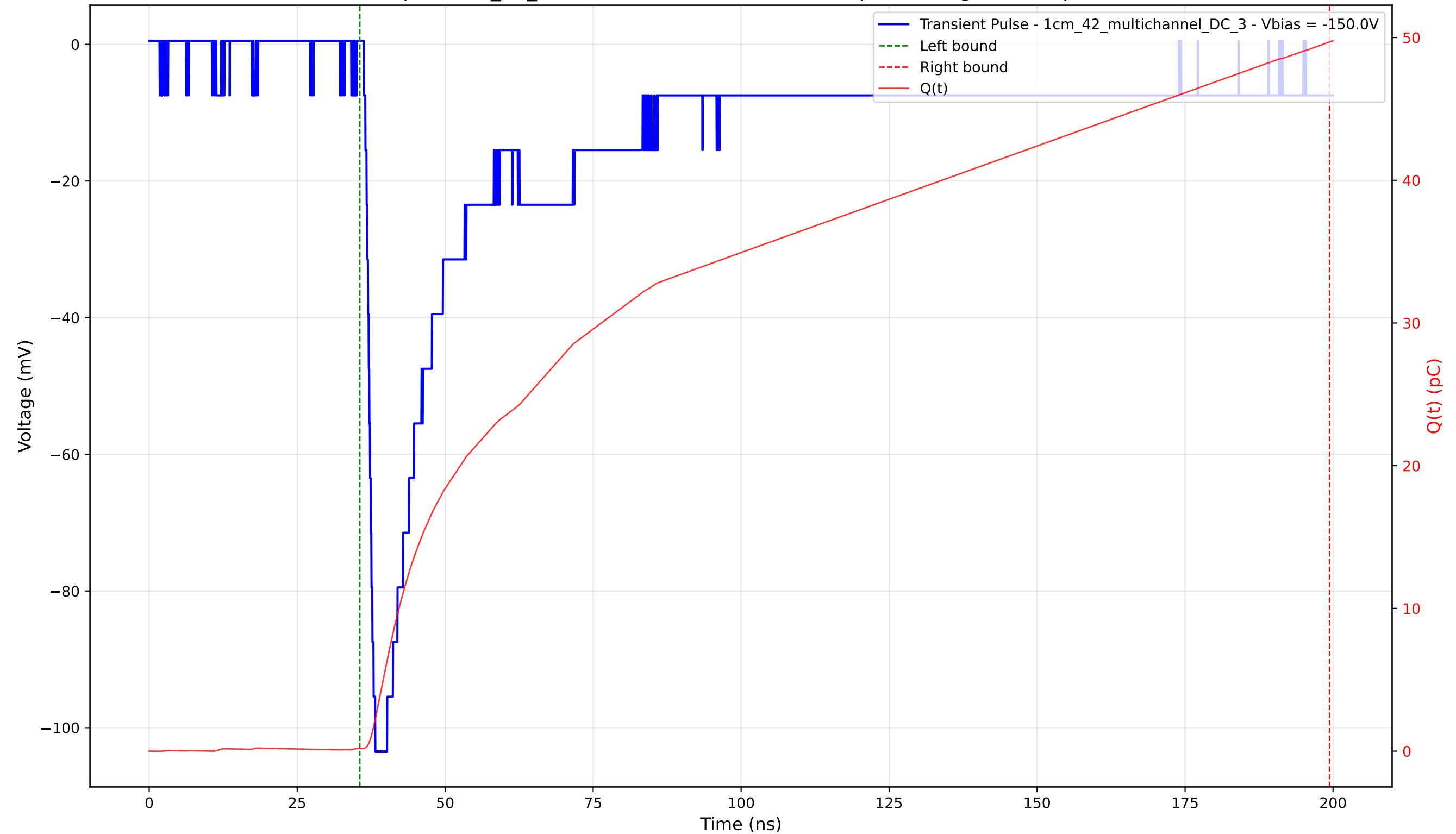
Transient Pulse - Sample: 1cm_42_multichannel - Position: 3455.0 \mu\text{m} - Charge: 49.50 pC - Rise Time: 1.39 ns
