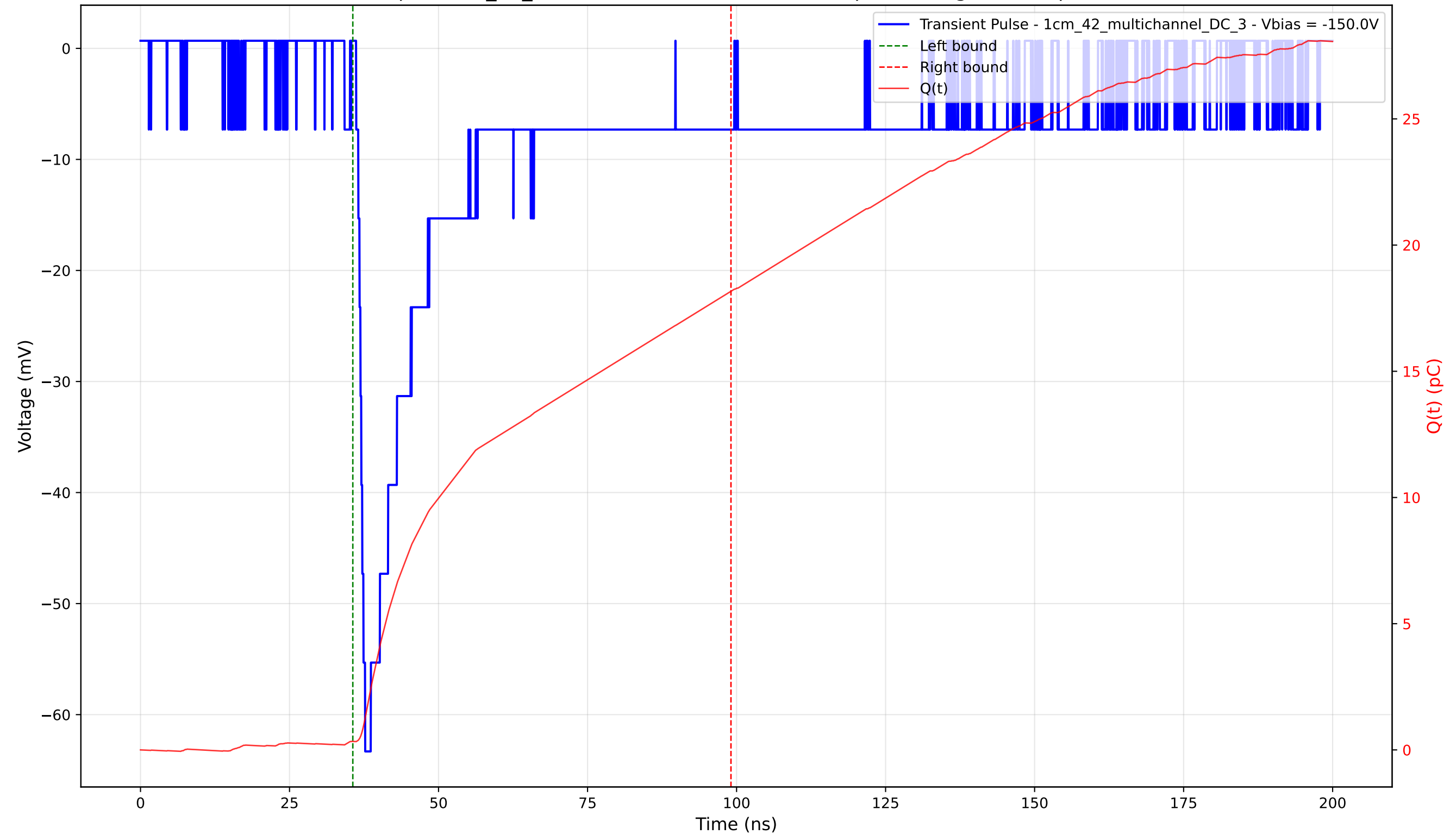
Transient Pulse - Sample: 1cm_42_multichannel - Position: 3935.0 \mu\text{m} - Charge: 17.84 pC - Rise Time: 1.50 ns
