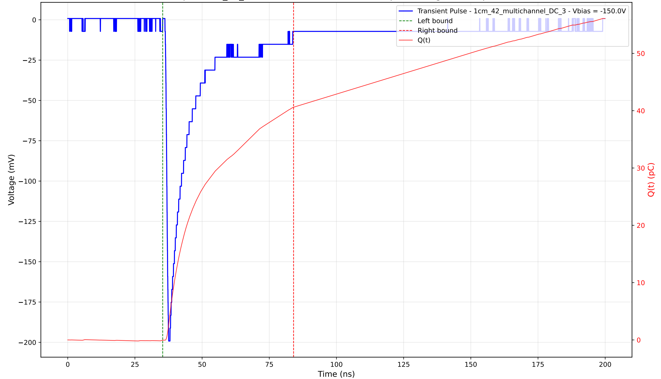
Transient Pulse - Sample: 1cm_42_multichannel - Position: 4185.0 \mu\text{m} - Charge: 40.64 pC - Rise Time: 0.97 ns
