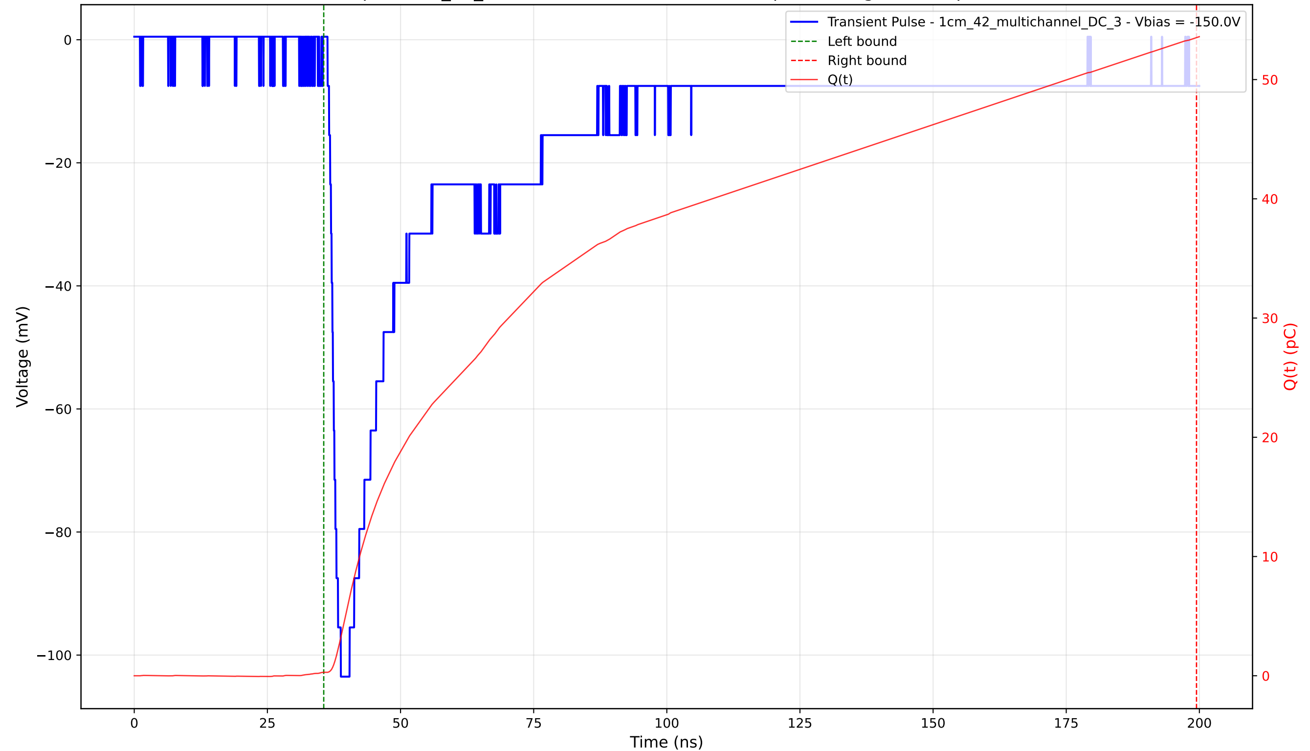
Transient Pulse - Sample: 1cm_42_multichannel - Position: 3135.0 \mu\text{m} - Charge: 53.23 pC - Rise Time: 1.69 ns
