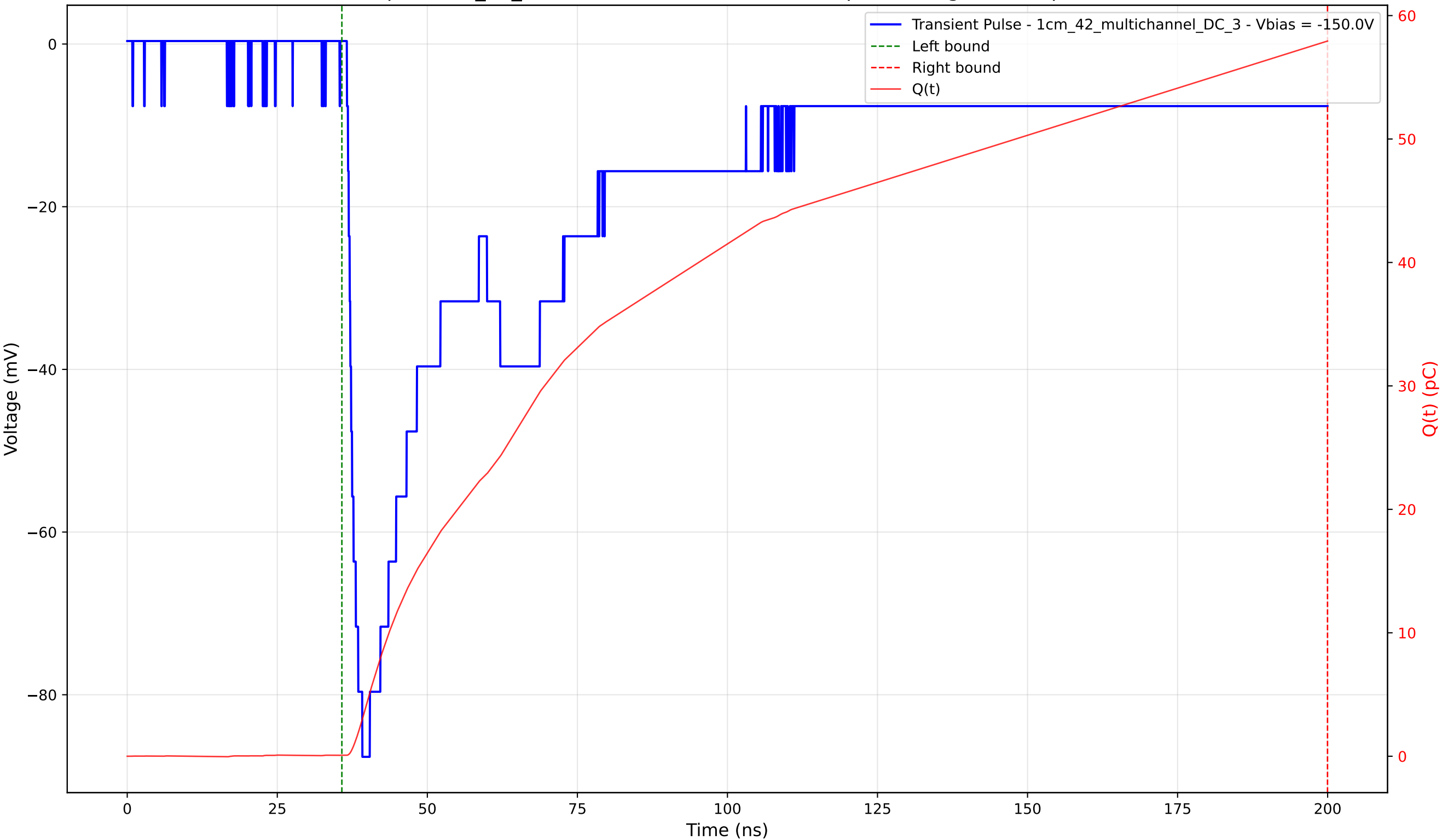
Transient Pulse - Sample: 1cm_42_multichannel - Position: 2245.0 \mu\text{m} - Charge: 57.86 pC - Rise Time: 1.72 ns
