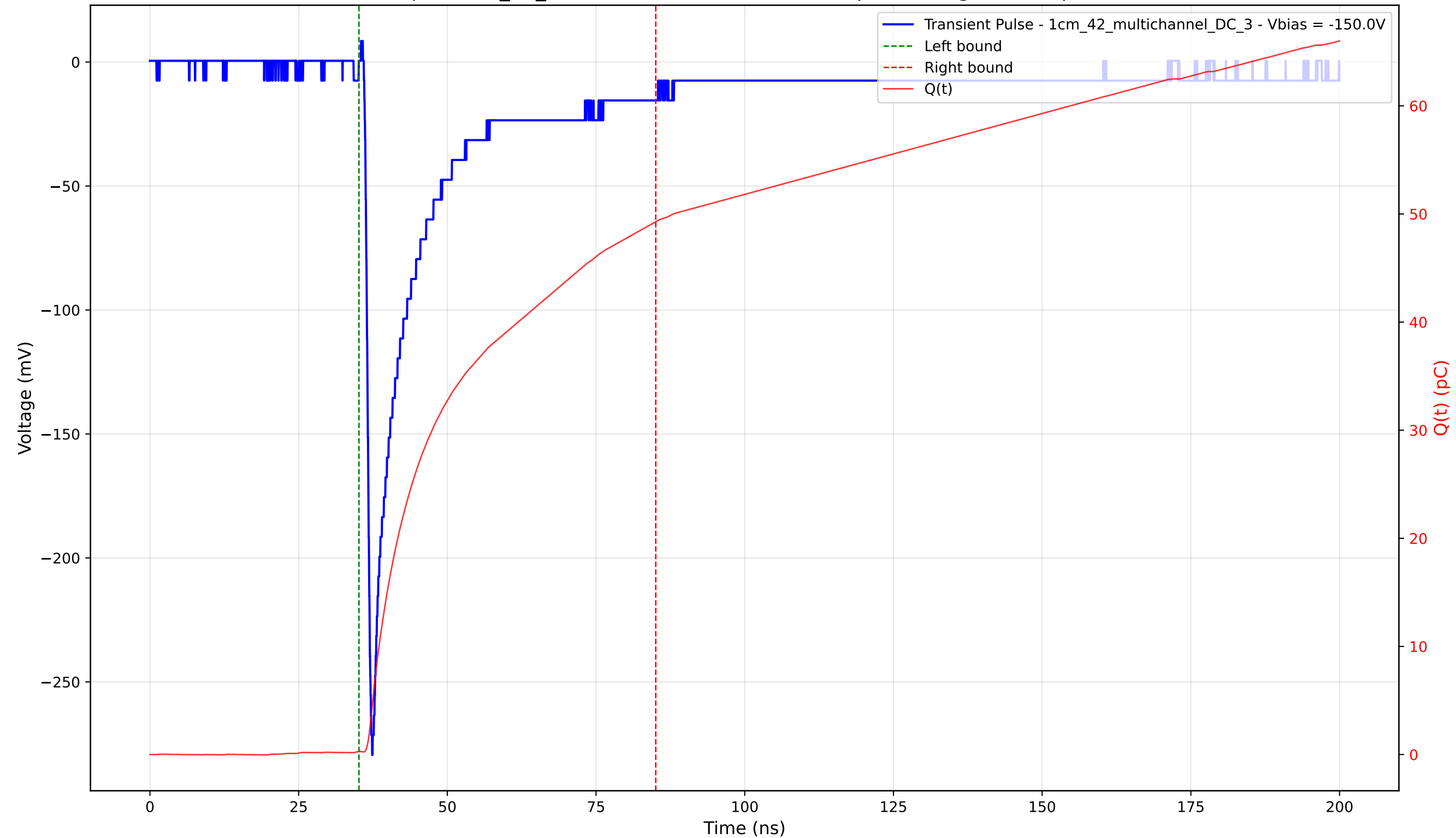
Transient Pulse - Sample: 1cm_42_multichannel - Position: 485.0 \mu\text{m} - Charge: 49.00 pC - Rise Time: 0.93 ns
