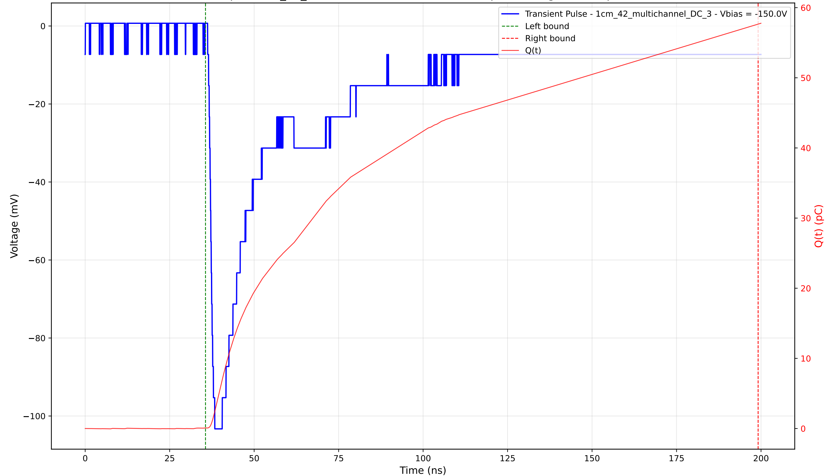
Transient Pulse - Sample: 1cm_42_multichannel - Position: 1780.0 \mu\text{m} - Charge: 57.57 pC - Rise Time: 1.43 ns
