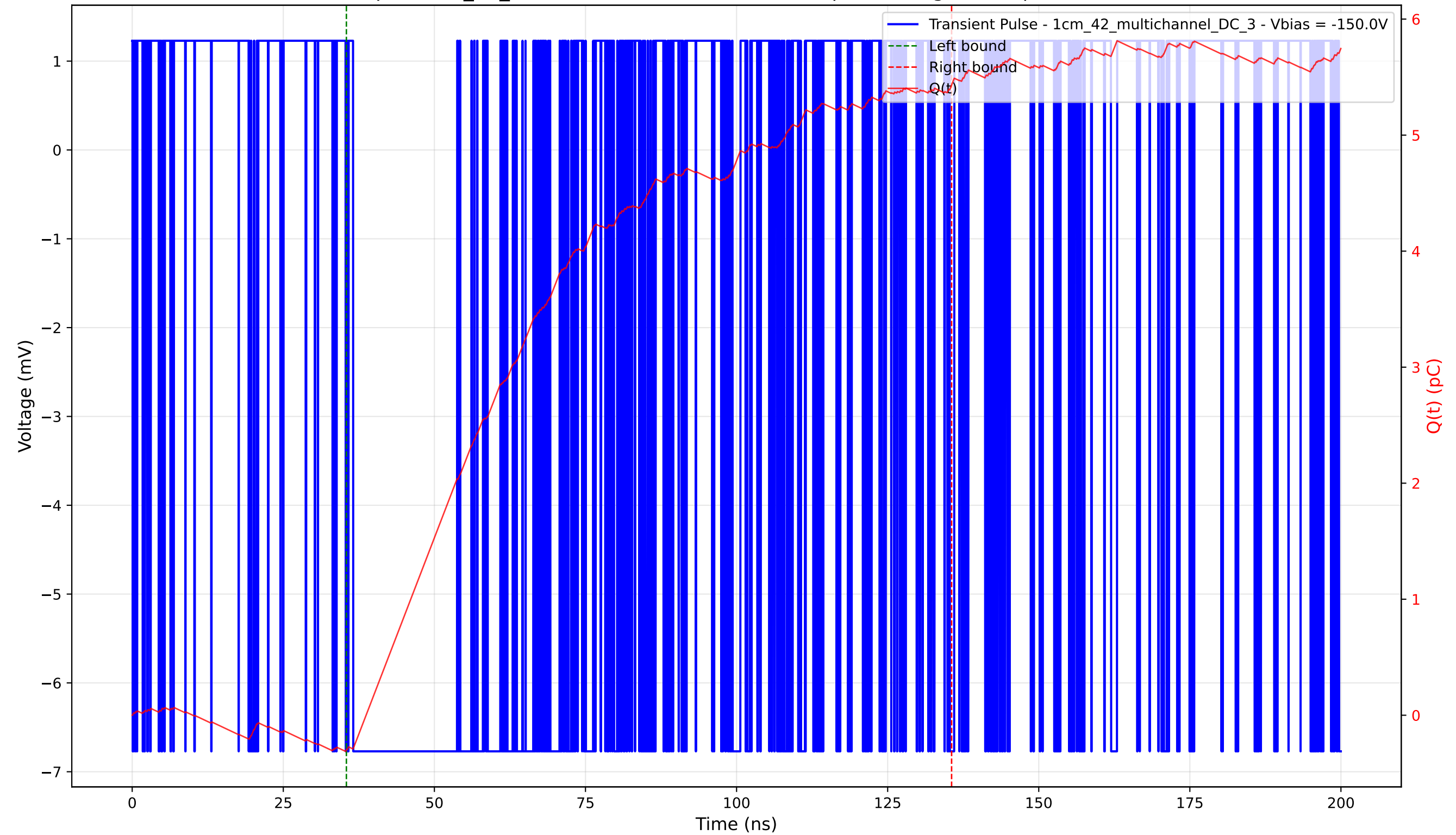
Transient Pulse - Sample: 1cm_42_multichannel - Position: 3375.0 \mu\text{m} - Charge: 5.72 pC - Rise Time: 0.00 ns (N/A)
