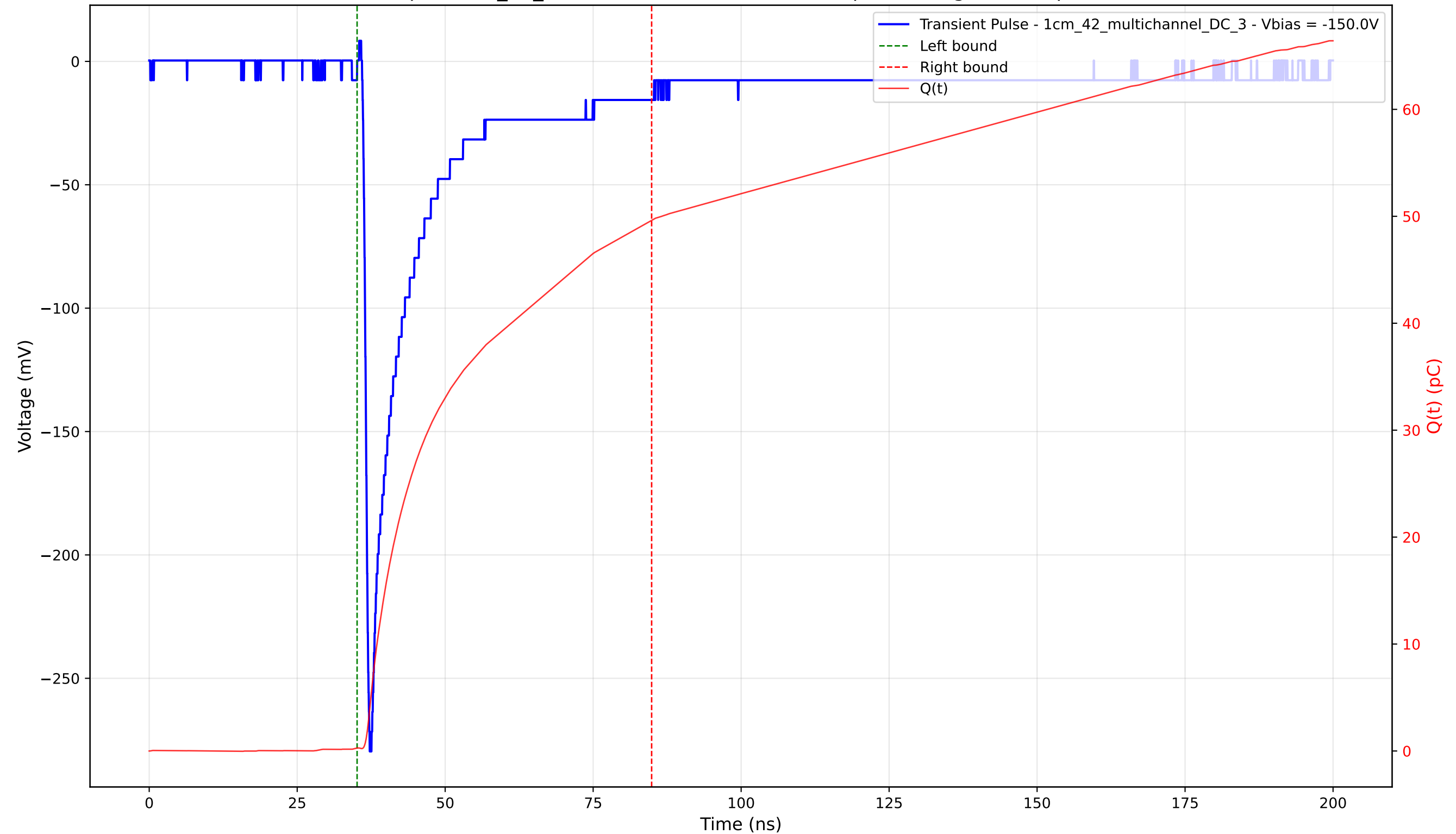
Transient Pulse - Sample: 1cm_42_multichannel - Position: 480.0 \mu\text{m} - Charge: 49.34 pC - Rise Time: 0.89 ns
