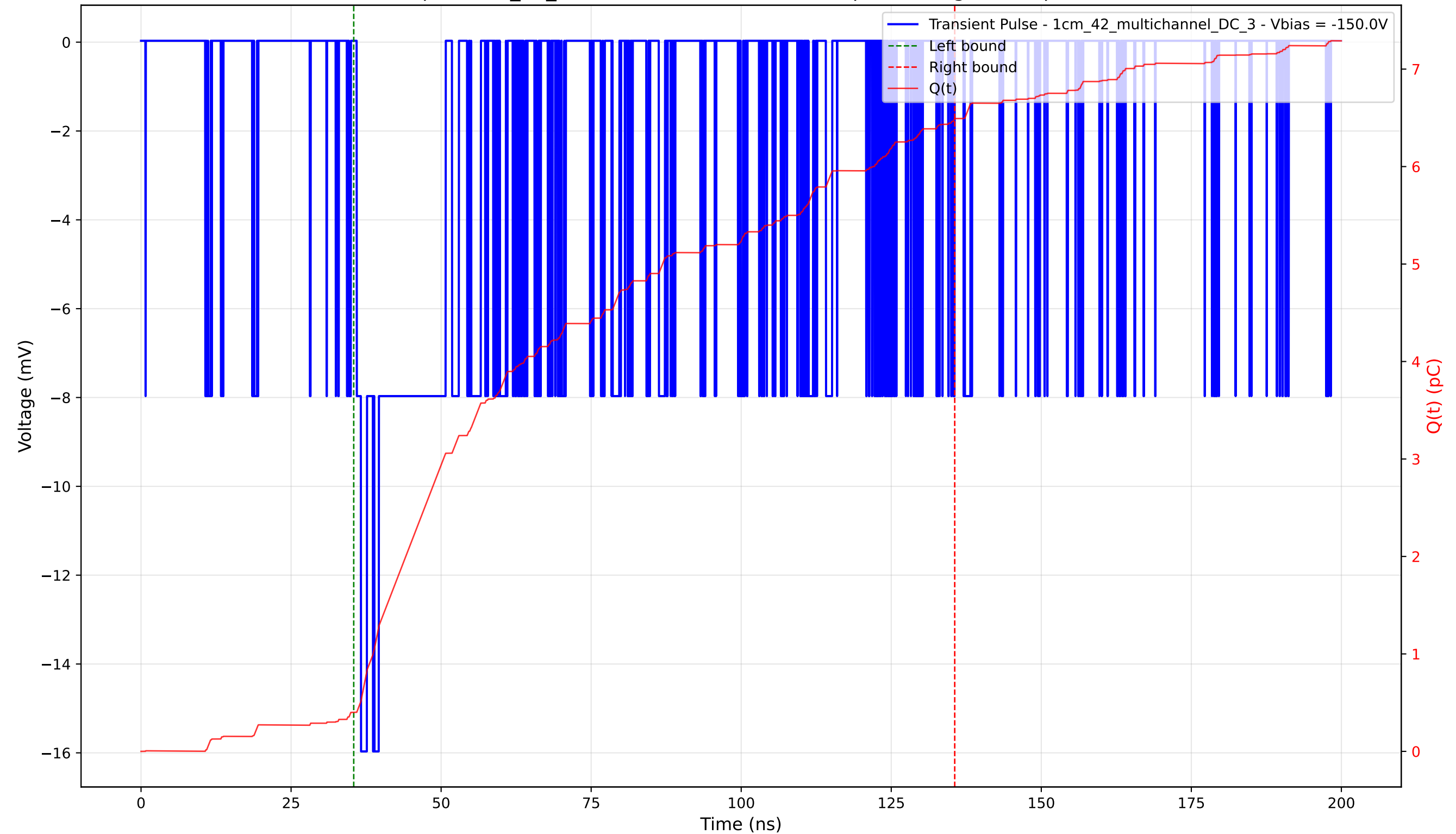
Transient Pulse - Sample: 1cm_42_multichannel - Position: 35.0 \mu\text{m} - Charge: 6.09 pC - Rise Time: 0.72 ns
