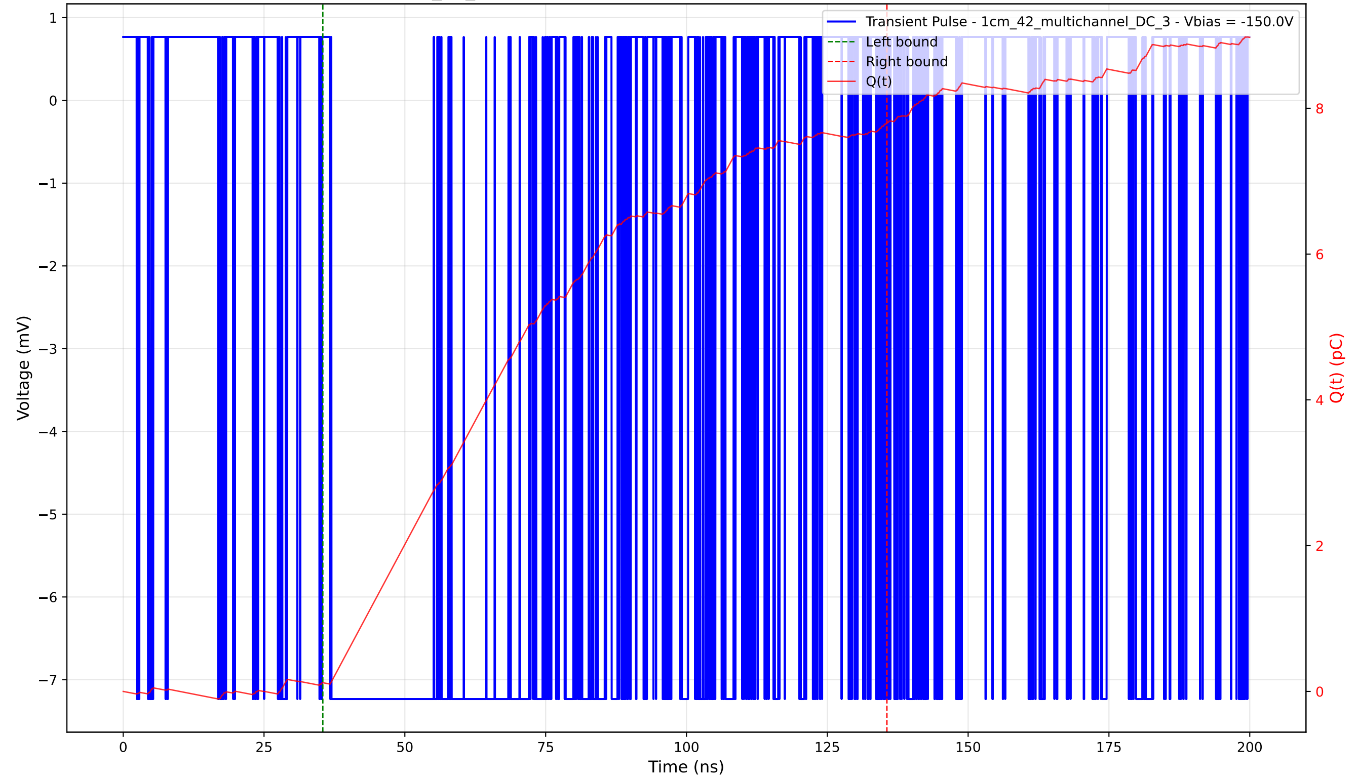
Transient Pulse - Sample: 1cm_42_multichannel - Position: 2895.0 \mu\text{m} - Charge: 7.69 pC - Rise Time: 0.00 ns (N/A)
