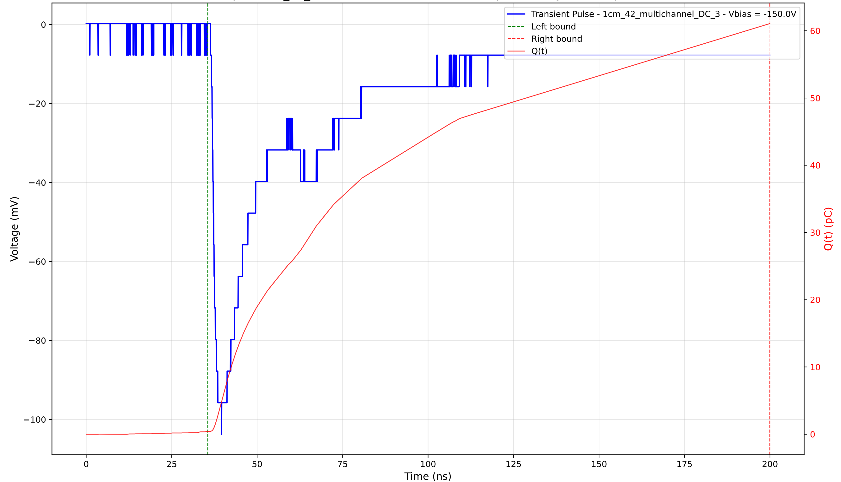
Transient Pulse - Sample: 1cm_42_multichannel - Position: 2000.0 \mu\text{m} - Charge: 60.64 pC - Rise Time: 1.87 ns
