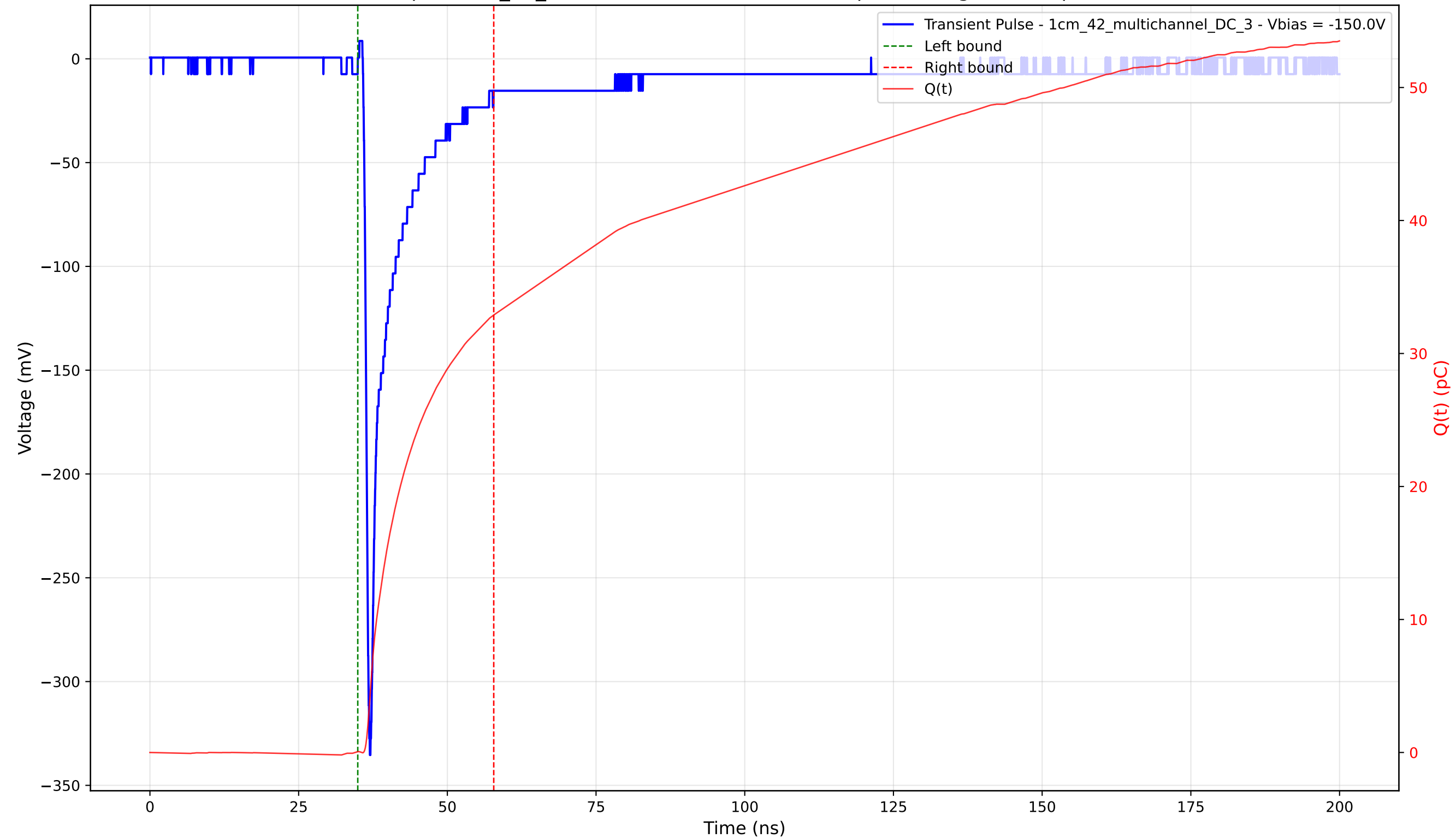
Transient Pulse - Sample: 1cm_42_multichannel - Position: 105.0 \mu\text{m} - Charge: 32.82 pC - Rise Time: 0.79 ns
