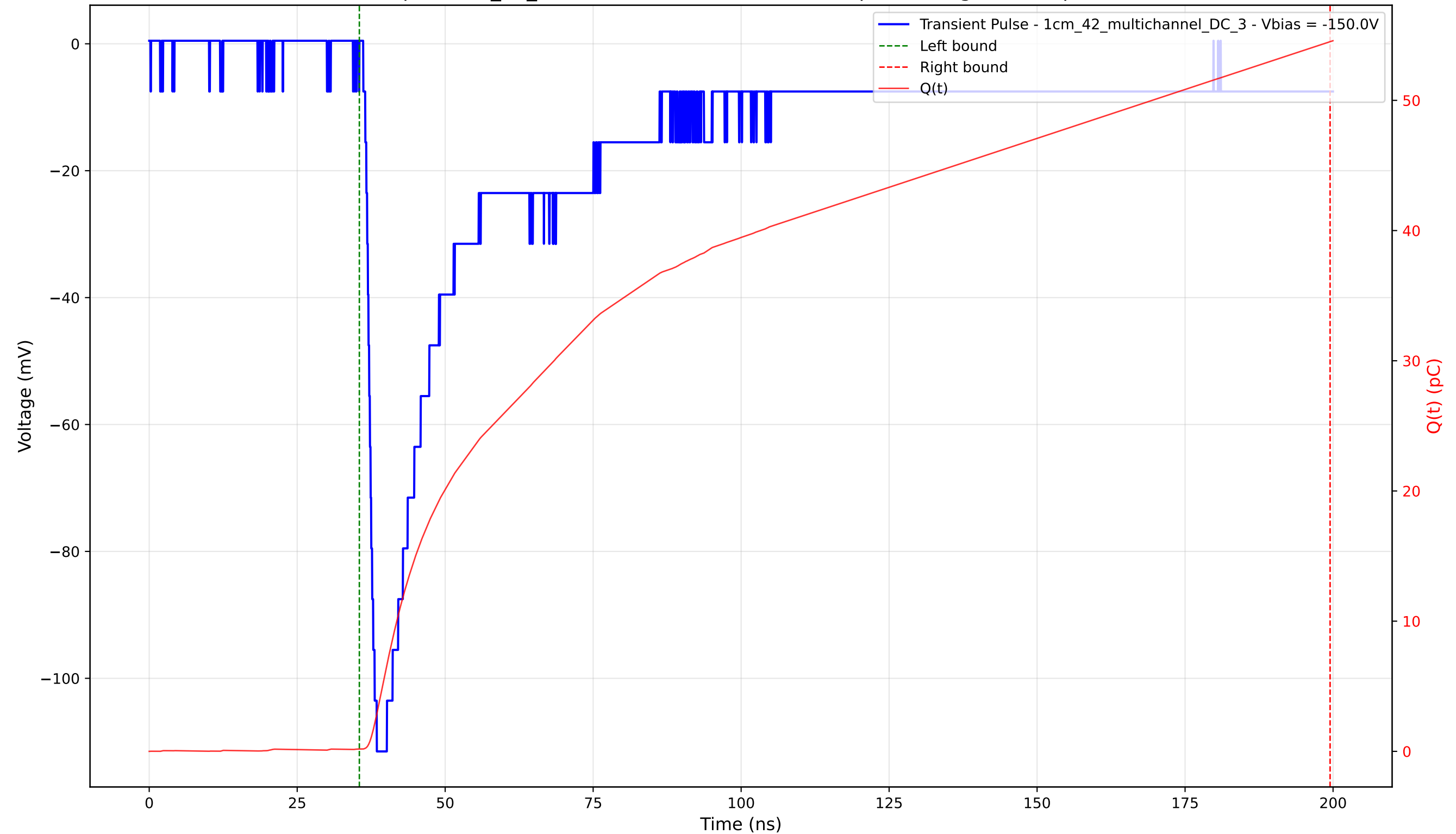
Transient Pulse - Sample: 1cm_42_multichannel - Position: 3295.0 \mu\text{m} - Charge: 54.32 pC - Rise Time: 1.59 ns
