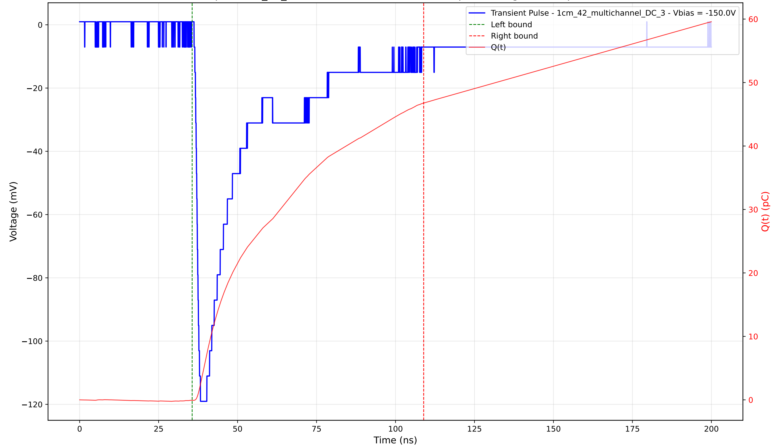
Transient Pulse - Sample: 1cm_42_multichannel - Position: 1620.0 \mu\text{m} - Charge: 46.84 pC - Rise Time: 1.47 ns
