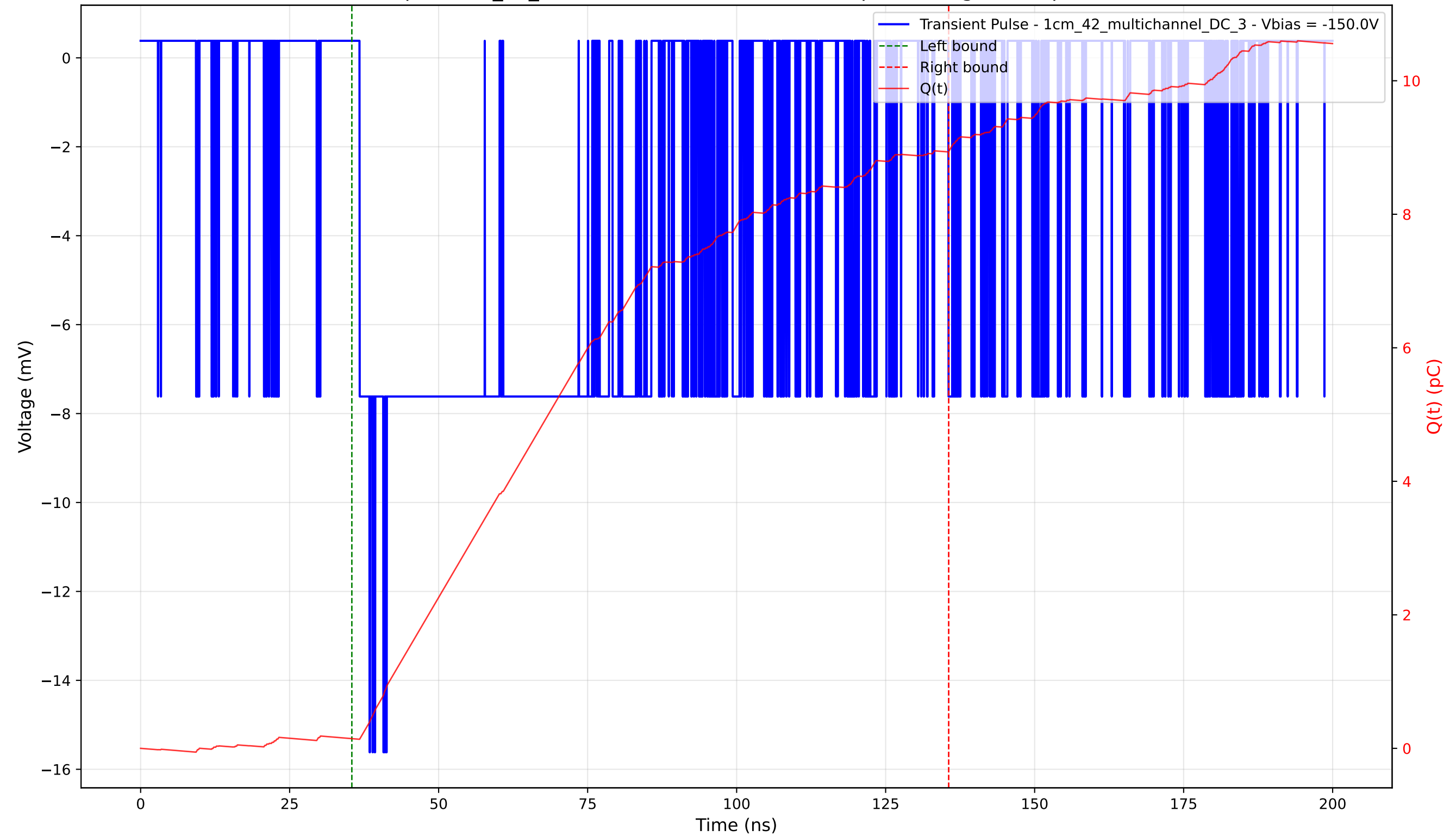
Transient Pulse - Sample: 1cm_42_multichannel - Position: 1850.0 \mu\text{m} - Charge: 8.79 pC - Rise Time: 1.68 ns
