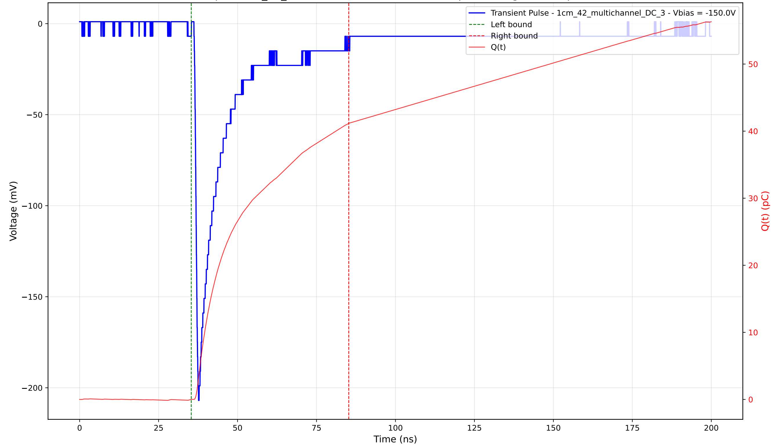
Transient Pulse - Sample: 1cm_42_multichannel - Position: 4195.0 \mu\text{m} - Charge: 41.15 pC - Rise Time: 1.03 ns
