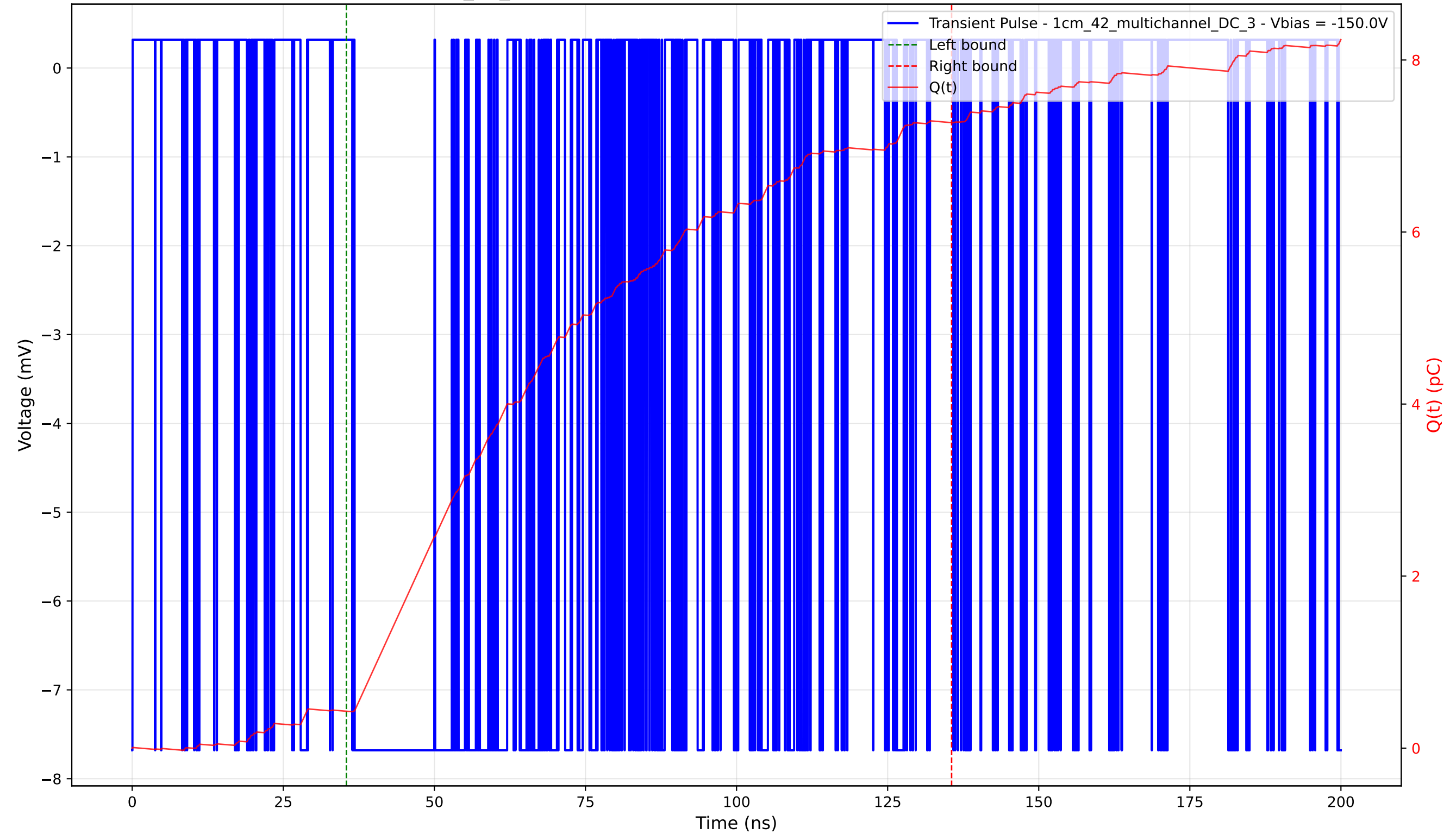
Transient Pulse - Sample: 1cm_42_multichannel - Position: 1360.0 \mu\text{m} - Charge: 6.84 pC - Rise Time: 0.00 ns (N/A)
