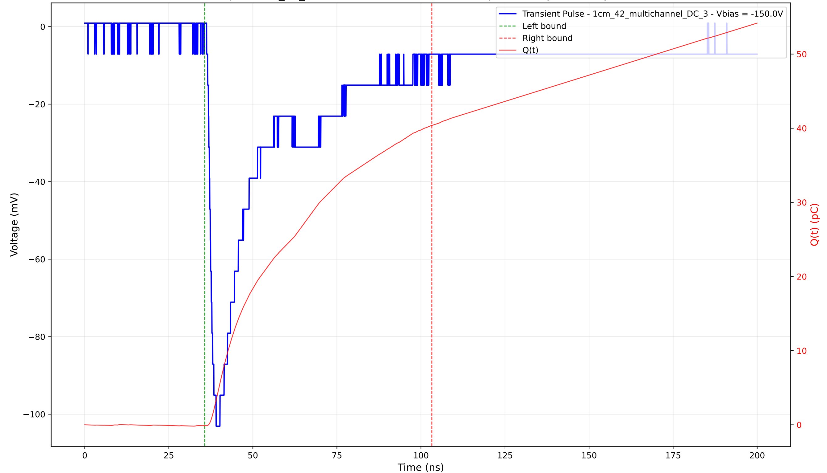
Transient Pulse - Sample: 1cm_42_multichannel - Position: 2990.0 \mu\text{m} - Charge: 40.49 pC - Rise Time: 1.83 ns
