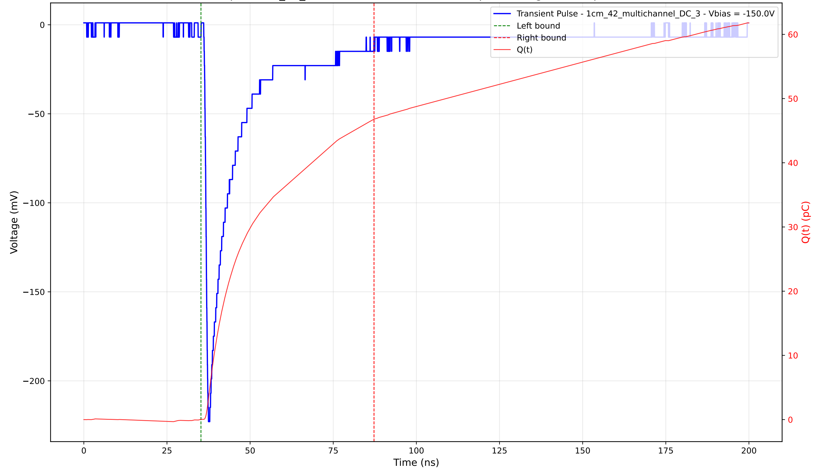
Transient Pulse - Sample: 1cm_42_multichannel - Position: 700.0 \mu\text{m} - Charge: 46.75 pC - Rise Time: 1.02 ns
