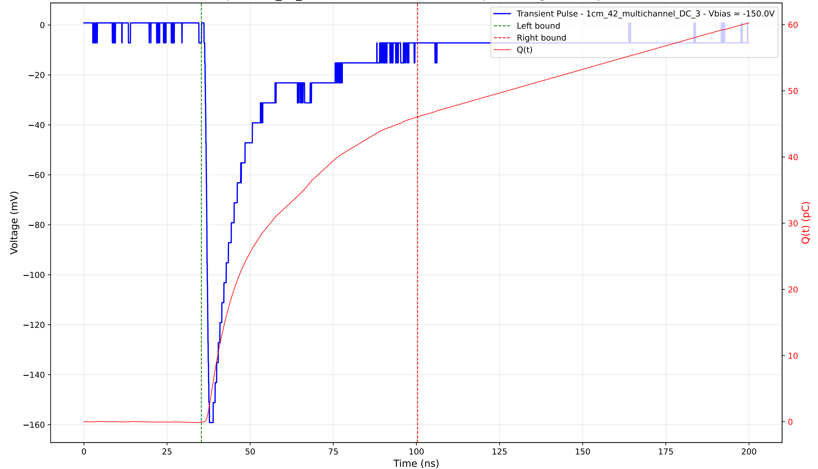
Transient Pulse - Sample: 1cm_42_multichannel - Position: 1090.0 \mu\text{m} - Charge: 46.11 pC - Rise Time: 1.14 ns
