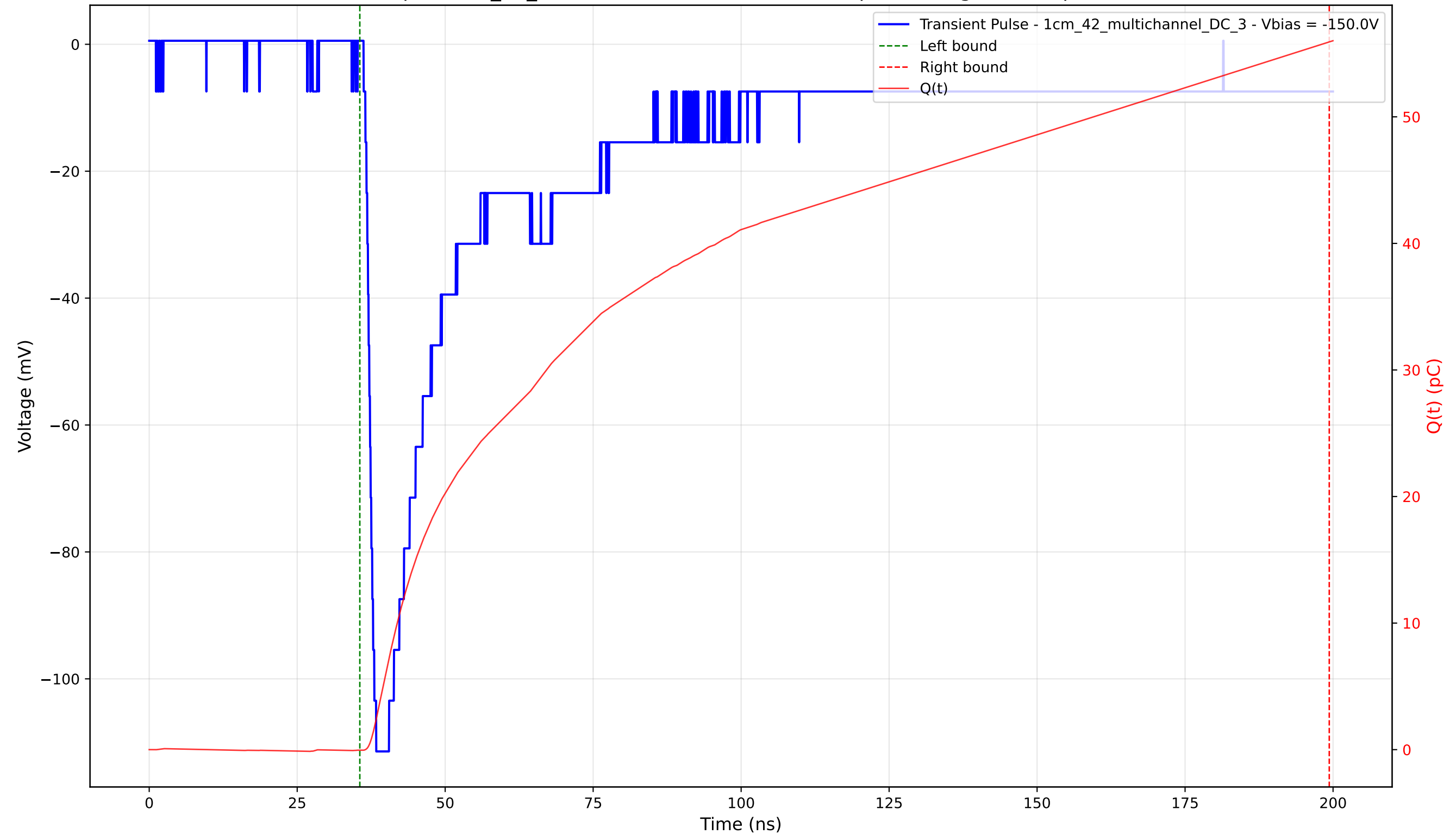
Transient Pulse - Sample: 1cm_42_multichannel - Position: 3275.0 \mu\text{m} - Charge: 55.97 pC - Rise Time: 1.51 ns
