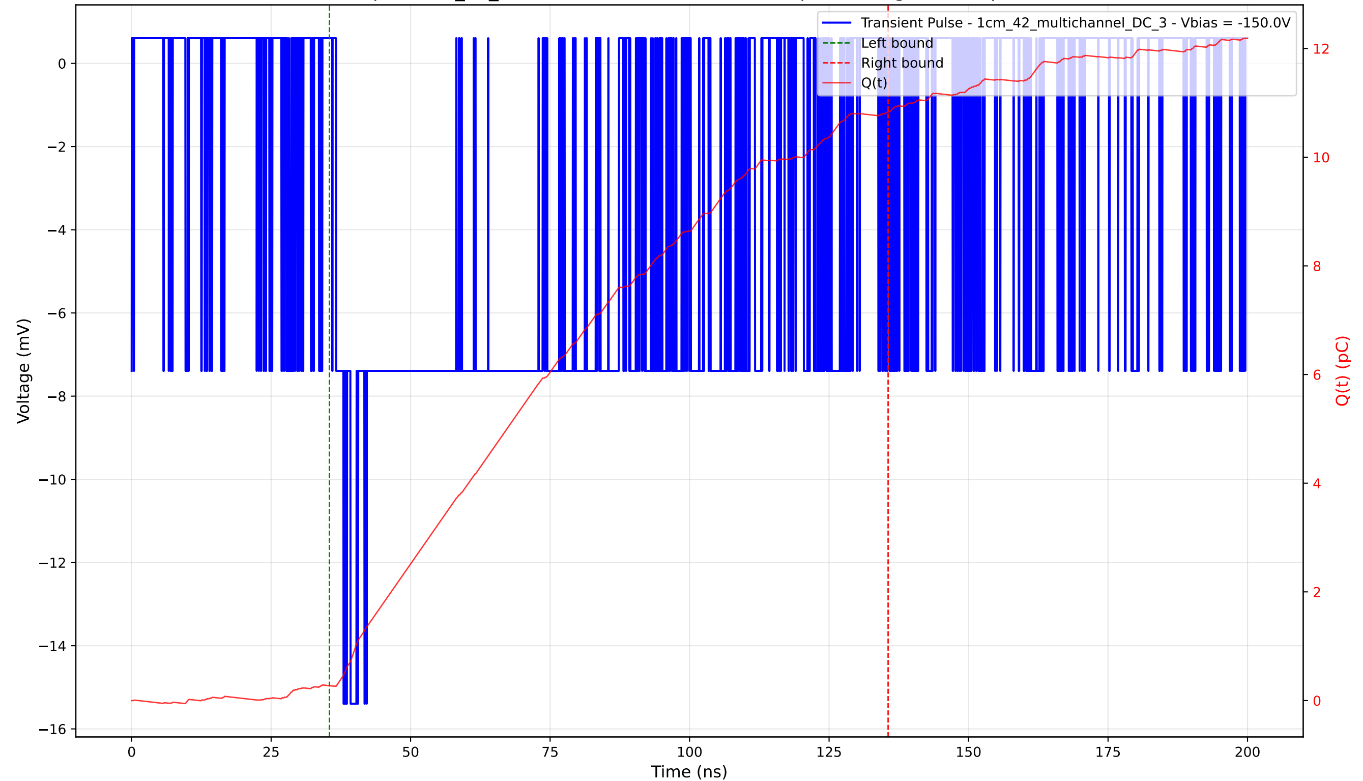
Transient Pulse - Sample: 1cm_42_multichannel - Position: 1890.0 \mu\text{m} - Charge: 10.56 pC - Rise Time: 1.34 ns
