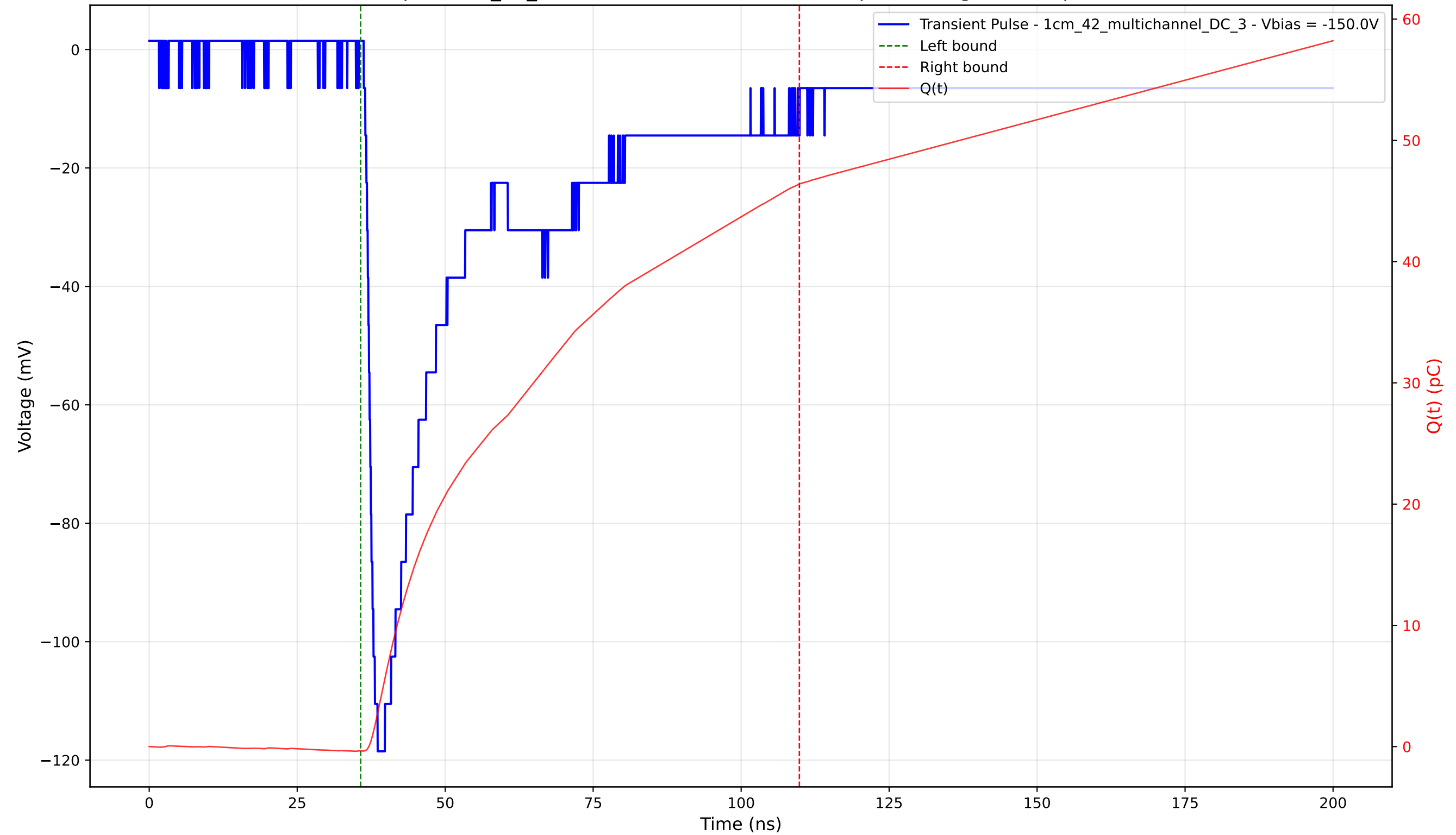
Transient Pulse - Sample: 1cm_42_multichannel - Position: 1705.0 \mu\text{m} - Charge: 46.76 pC - Rise Time: 1.63 ns
