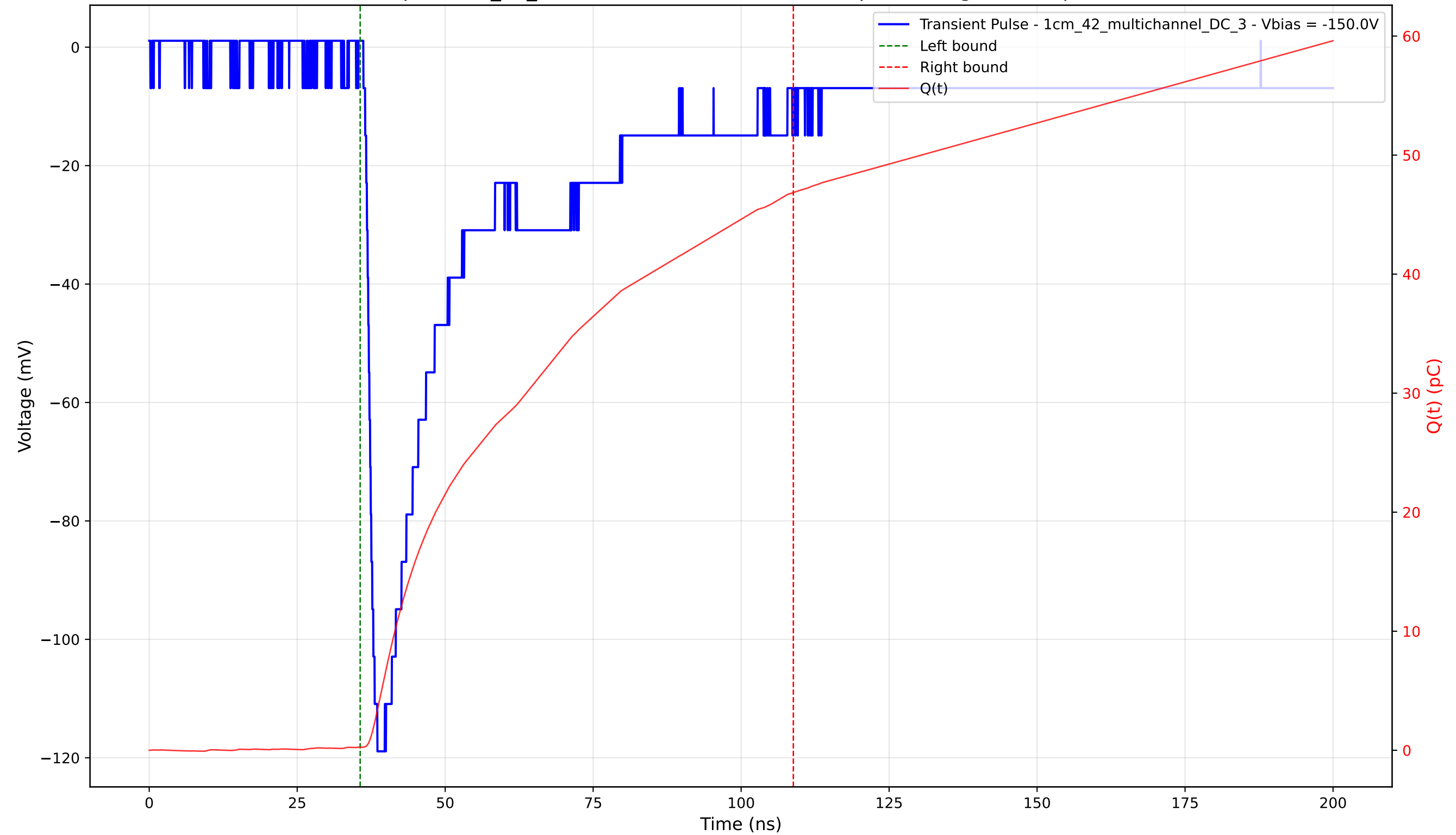
Transient Pulse - Sample: 1cm_42_multichannel - Position: 1680.0 \mu\text{m} - Charge: 46.60 pC - Rise Time: 1.61 ns
