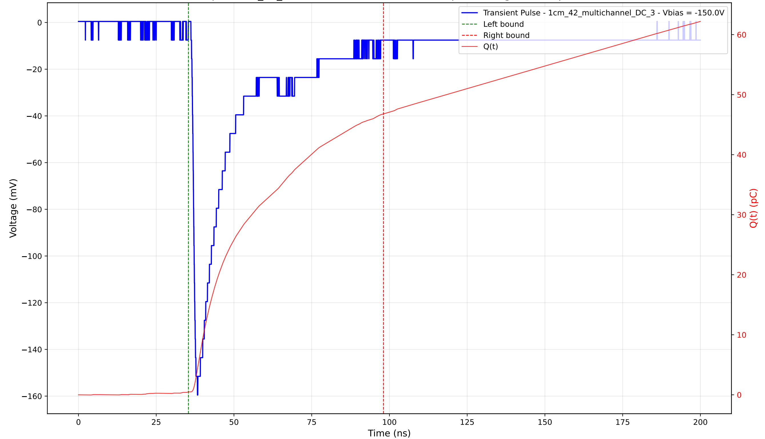
Transient Pulse - Sample: 1cm_42_multichannel - Position: 1175.0 \mu\text{m} - Charge: 46.30 pC - Rise Time: 1.30 ns
