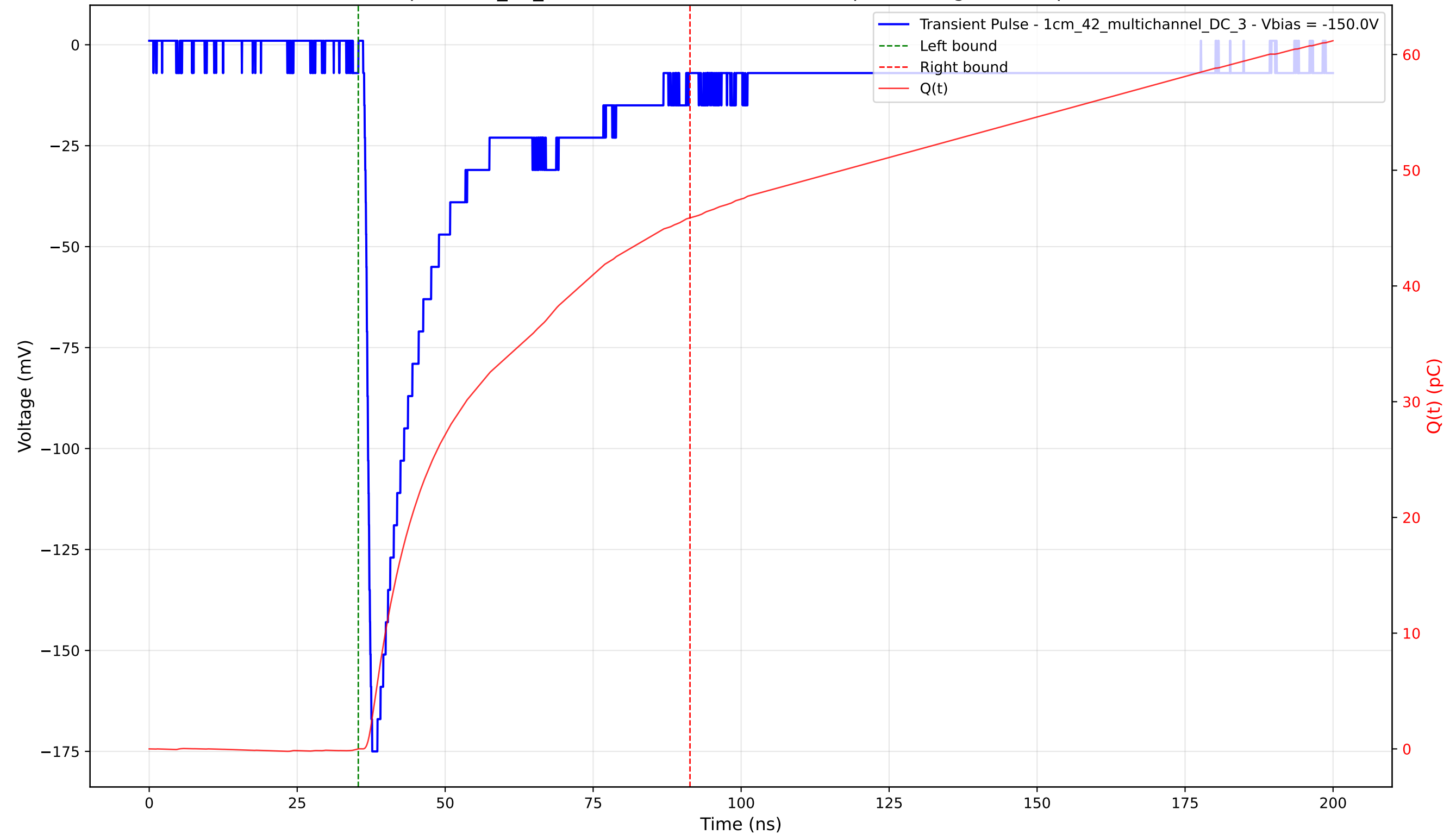
Transient Pulse - Sample: 1cm_42_multichannel - Position: 995.0 \mu\text{m} - Charge: 45.88 pC - Rise Time: 1.03 ns
