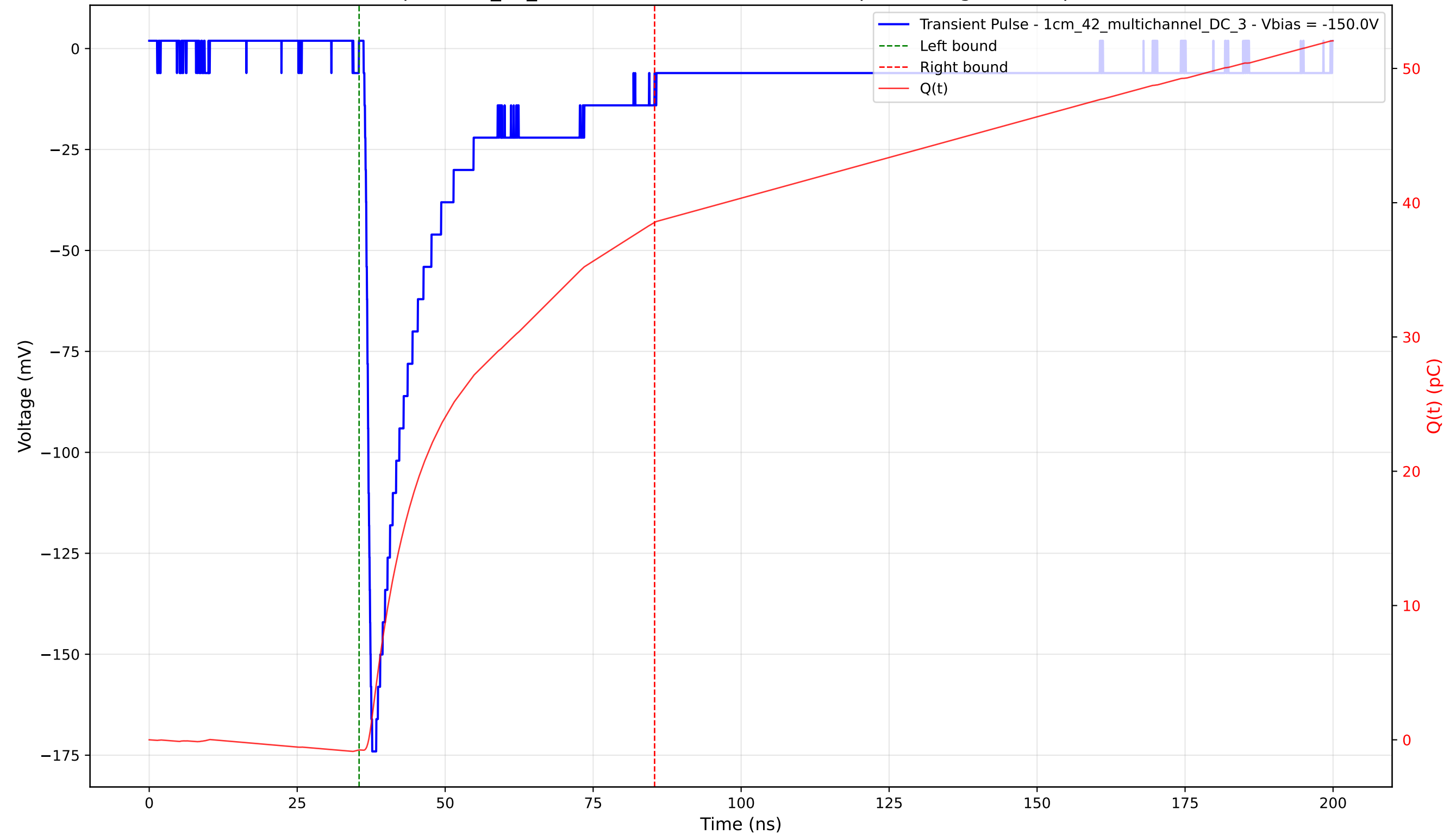
Transient Pulse - Sample: 1cm_42_multichannel - Position: 4055.0 \mu\text{m} - Charge: 39.29 pC - Rise Time: 0.97 ns
