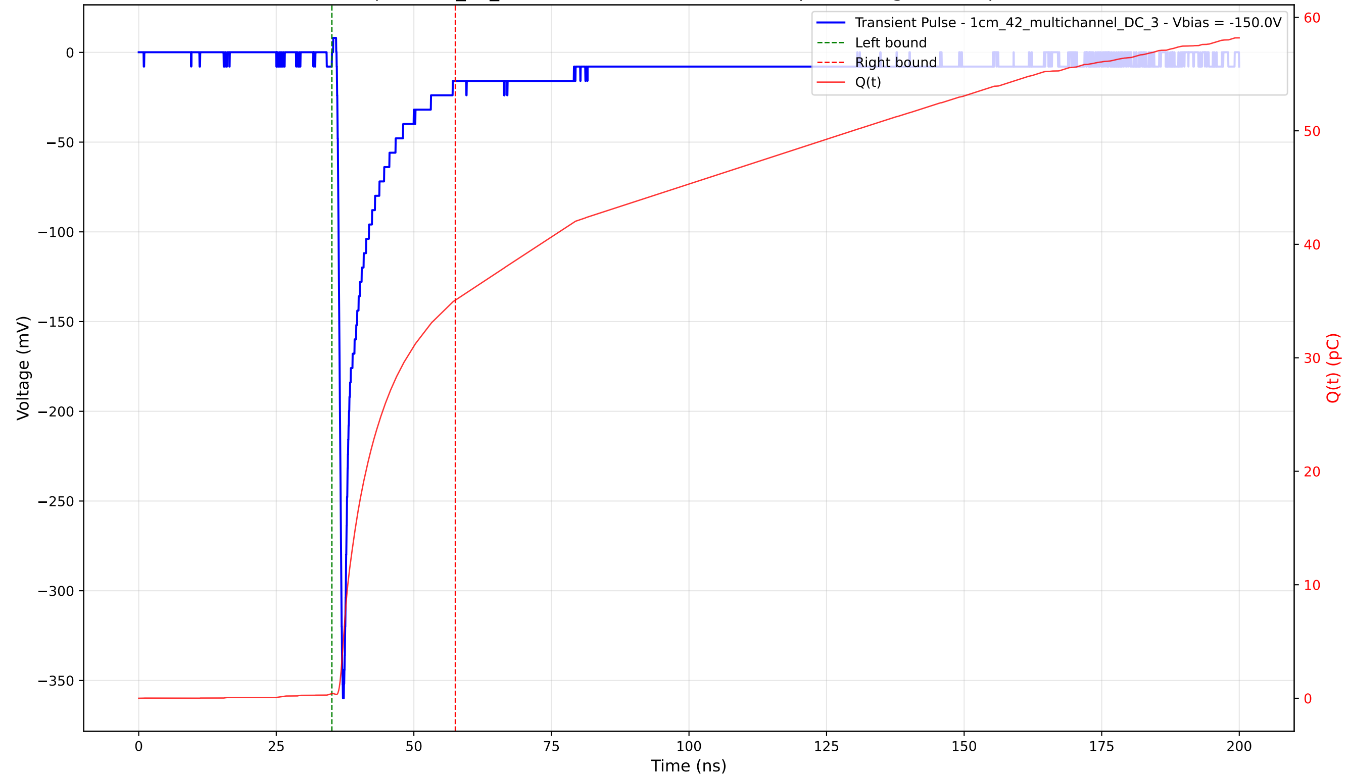
Transient Pulse - Sample: 1cm_42_multichannel - Position: 4770.0 \mu\text{m} - Charge: 34.66 pC - Rise Time: 0.80 ns
