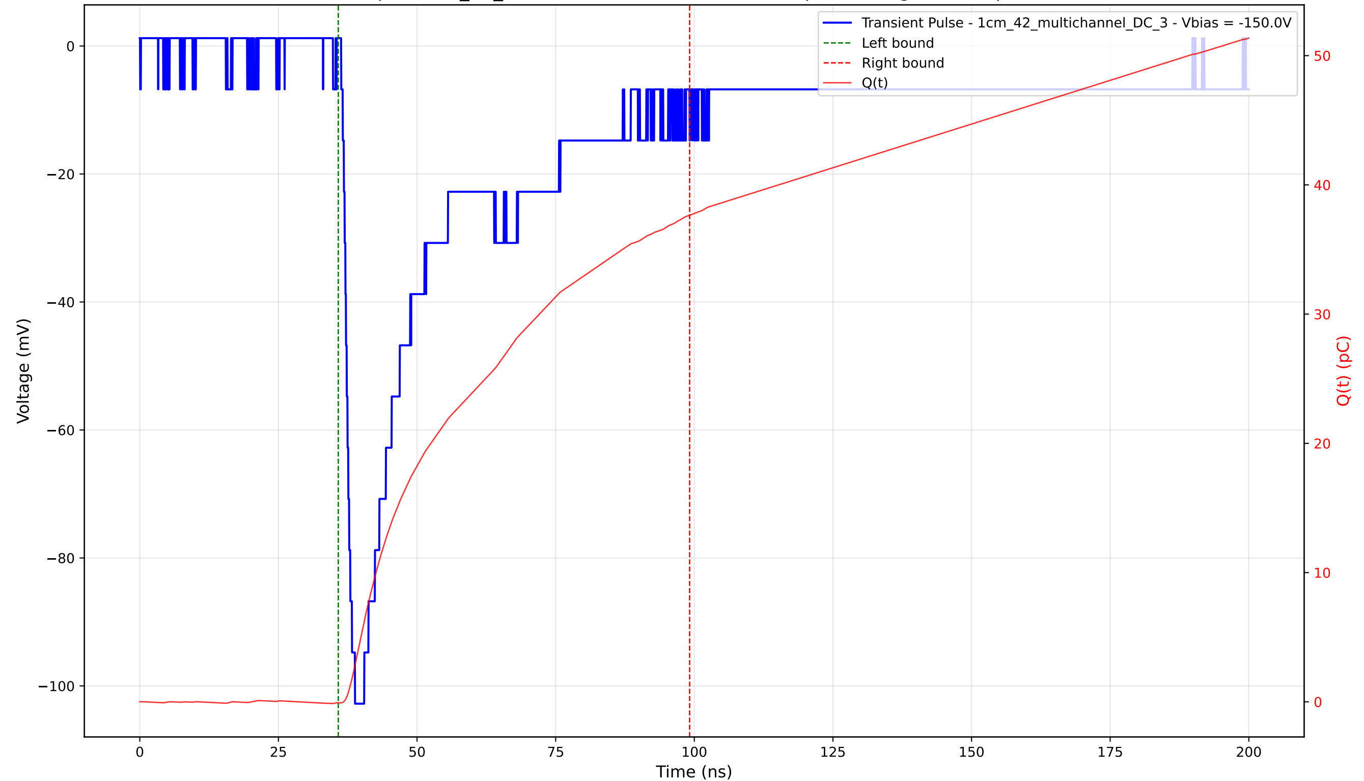
Transient Pulse - Sample: 1cm_42_multichannel - Position: 3115.0 \mu\text{m} - Charge: 37.73 pC - Rise Time: 1.67 ns
