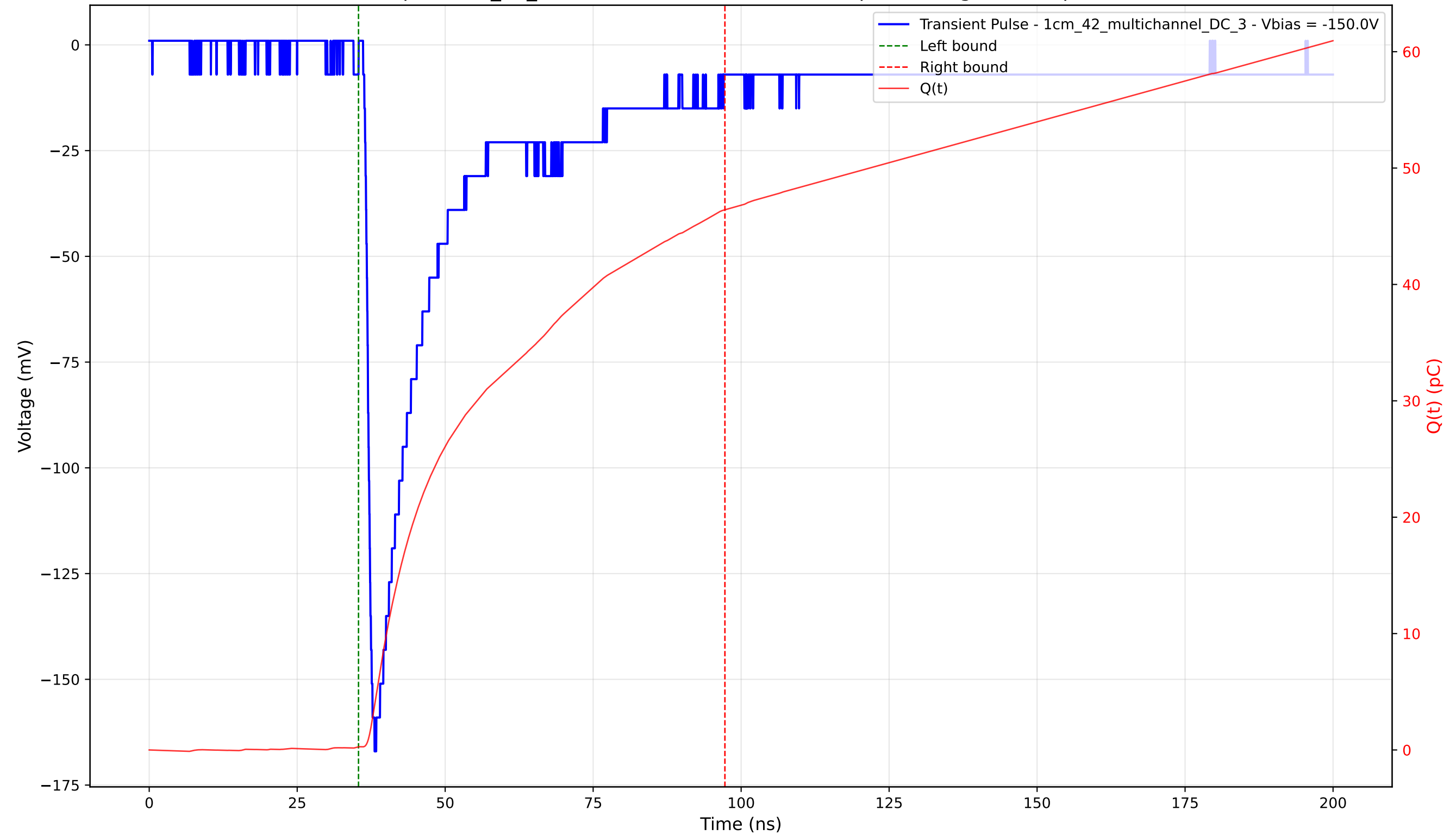
Transient Pulse - Sample: 1cm_42_multichannel - Position: 1080.0 \mu\text{m} - Charge: 46.14 pC - Rise Time: 1.14 ns
