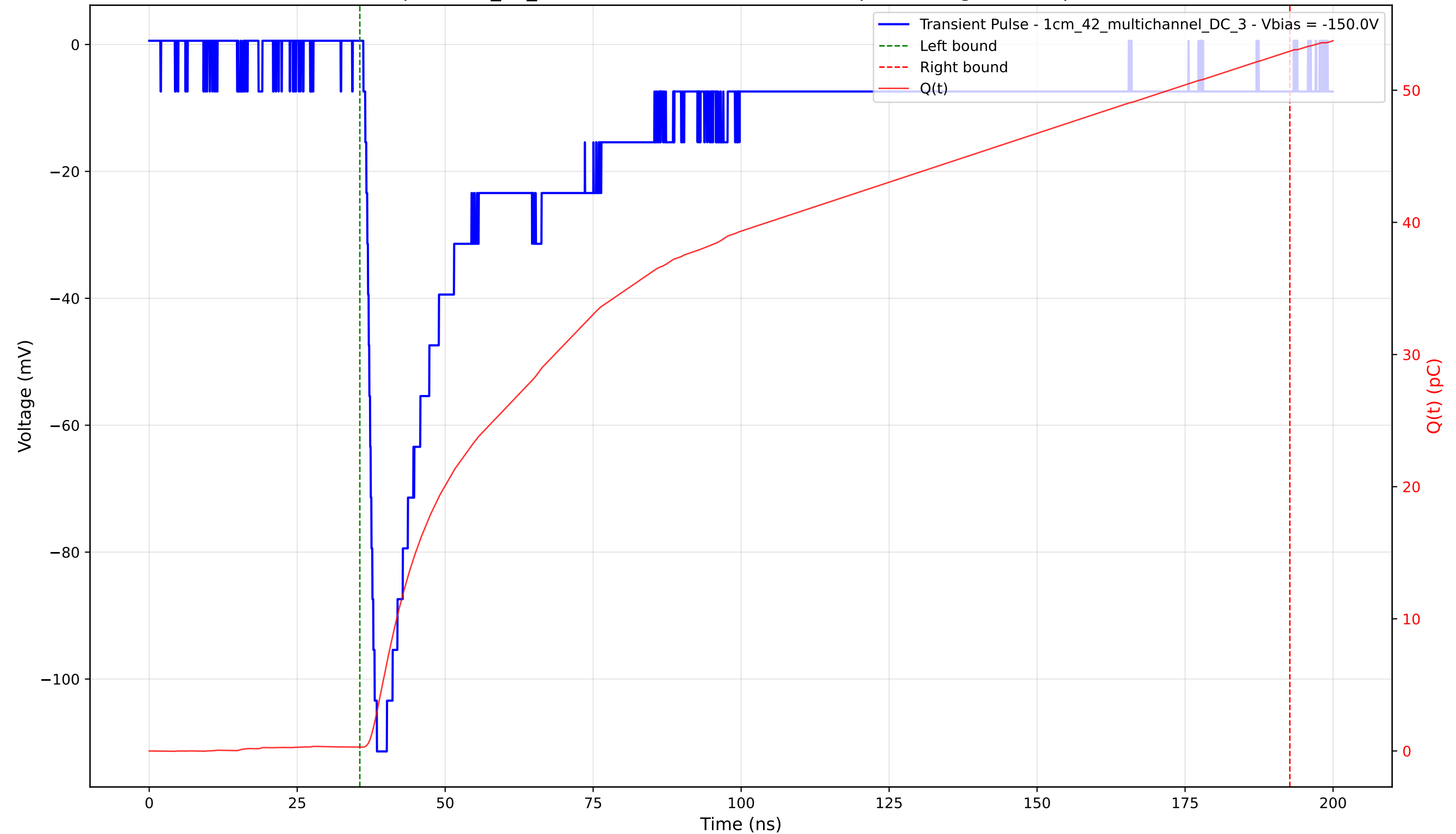
Transient Pulse - Sample: 1cm_42_multichannel - Position: 3300.0 \mu\text{m} - Charge: 52.68 pC - Rise Time: 1.59 ns
