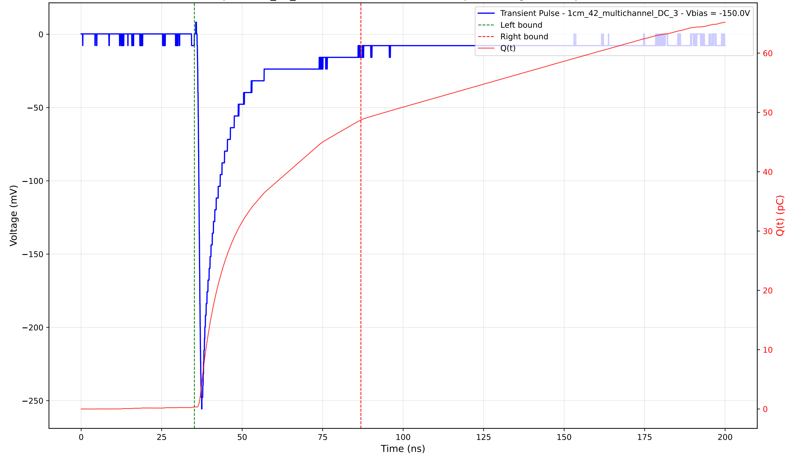
Transient Pulse - Sample: 1cm_42_multichannel - Position: 560.0 \mu\text{m} - Charge: 48.34 pC - Rise Time: 0.94 ns
