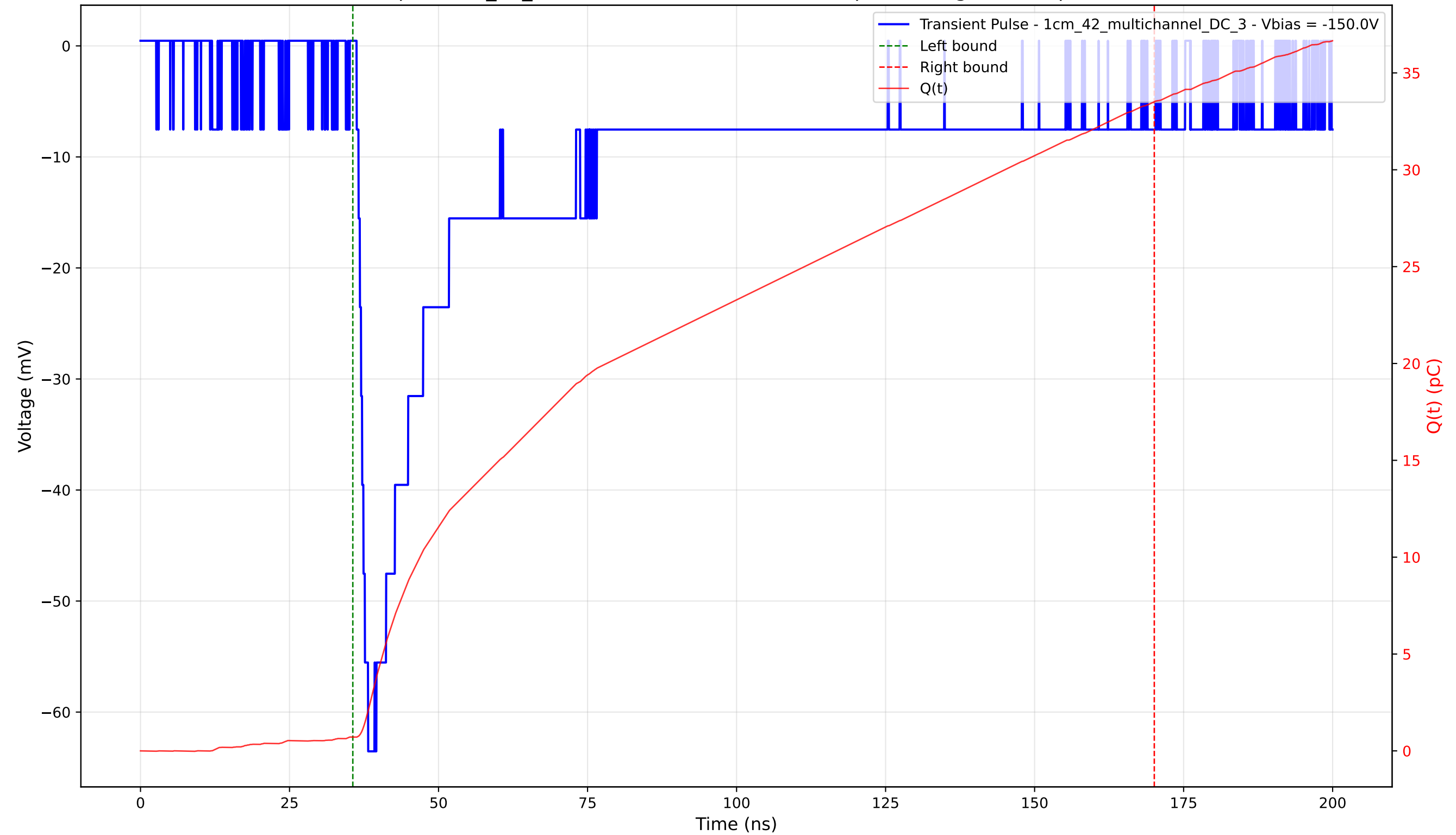
Transient Pulse - Sample: 1cm_42_multichannel - Position: 1410.0 \mu\text{m} - Charge: 32.81 pC - Rise Time: 1.92 ns
