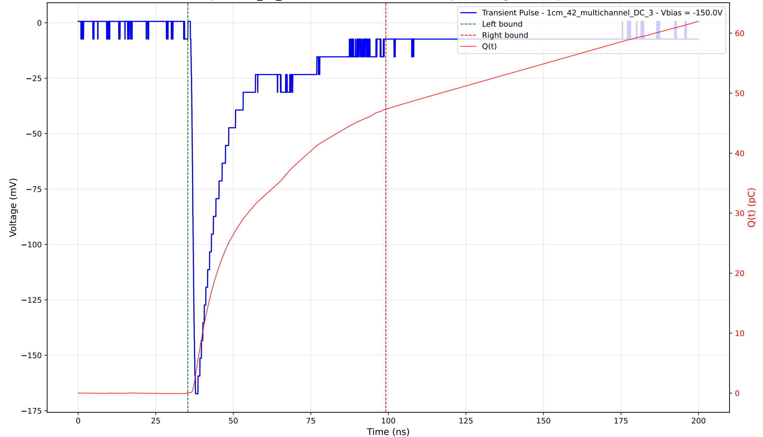
Transient Pulse - Sample: 1cm_42_multichannel - Position: 1060.0 \mu\text{m} - Charge: 47.27 pC - Rise Time: 1.08 ns
