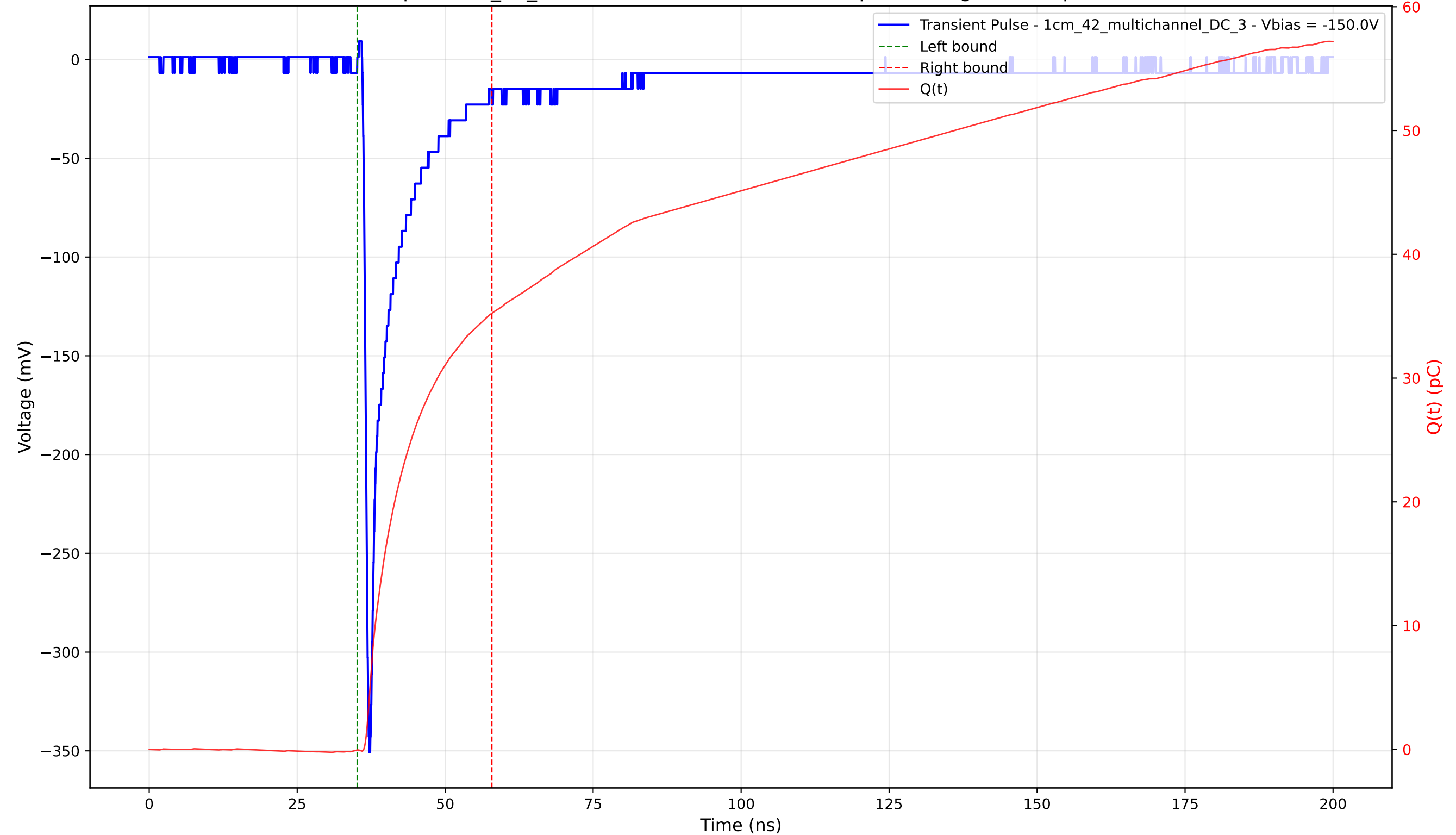
Transient Pulse - Sample: 1cm_42_multichannel - Position: 4715.0 \mu\text{m} - Charge: 35.26 pC - Rise Time: 0.81 ns
