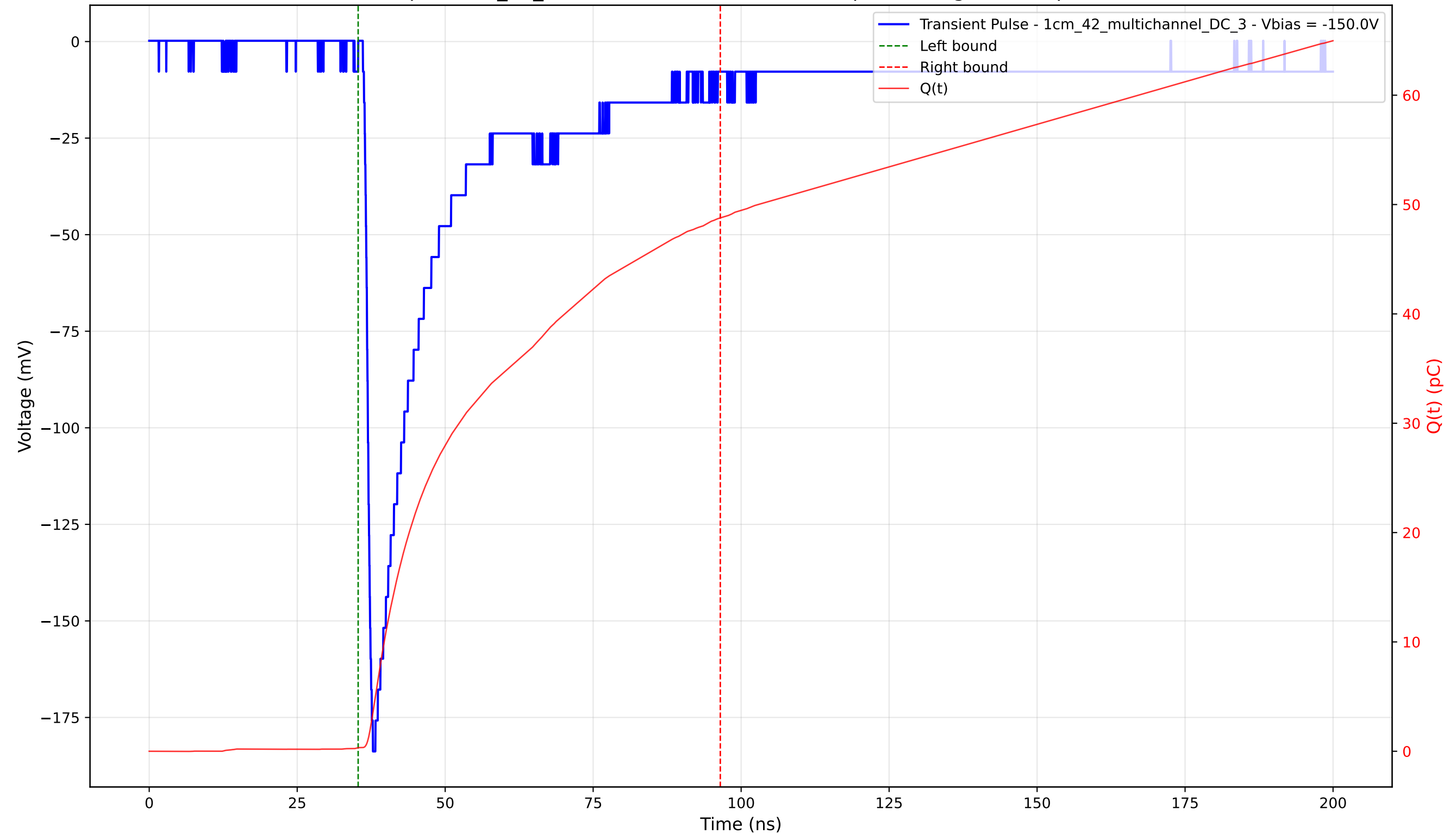
Transient Pulse - Sample: 1cm_42_multichannel - Position: 980.0 \mu\text{m} - Charge: 48.44 pC - Rise Time: 1.09 ns
