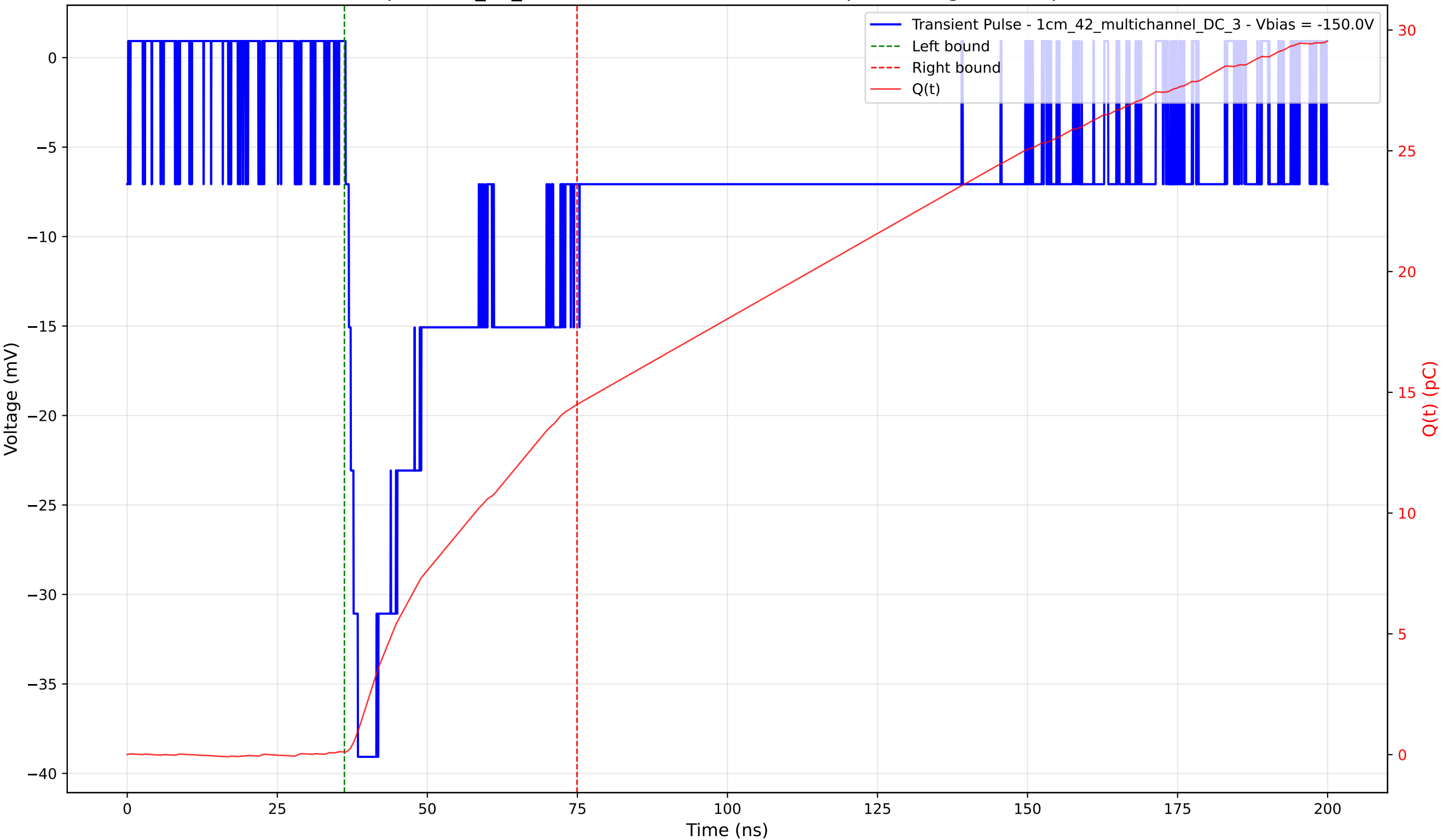
Transient Pulse - Sample: 1cm_42_multichannel - Position: 2835.0 \mu\text{m} - Charge: 14.39 pC - Rise Time: 2.05 ns
