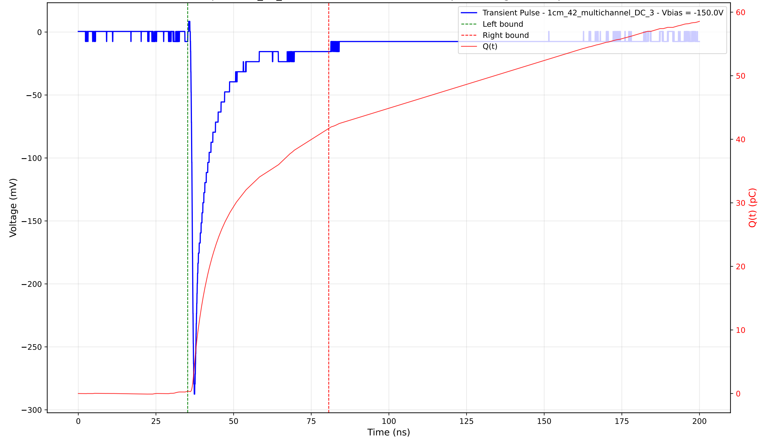
Transient Pulse - Sample: 1cm_42_multichannel - Position: 4560.0 \mu\text{m} - Charge: 41.36 pC - Rise Time: 0.87 ns
