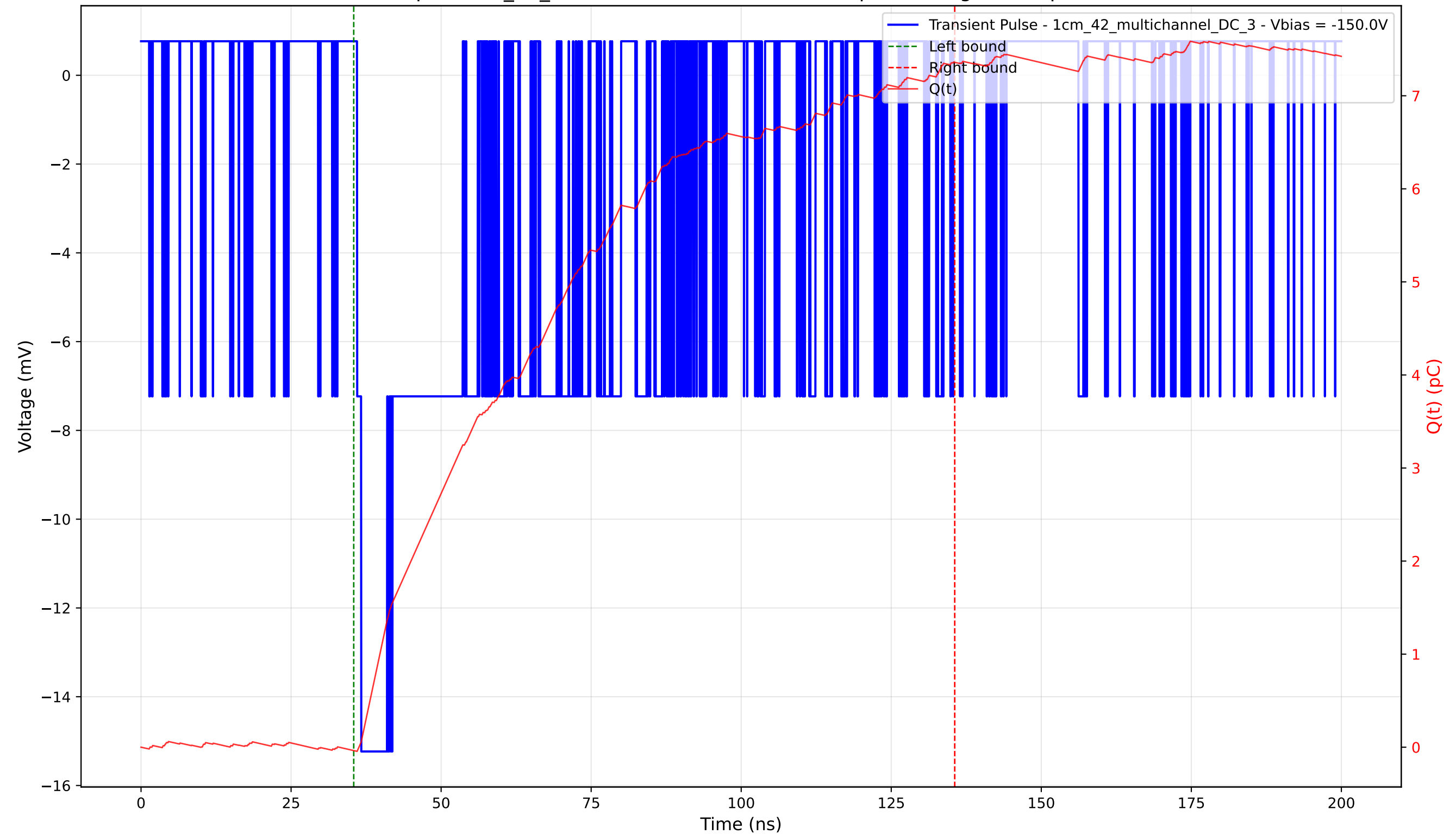
Transient Pulse - Sample: 1cm_42_multichannel - Position: 365.0 \mu\text{m} - Charge: 7.40 pC - Rise Time: 0.70 ns
