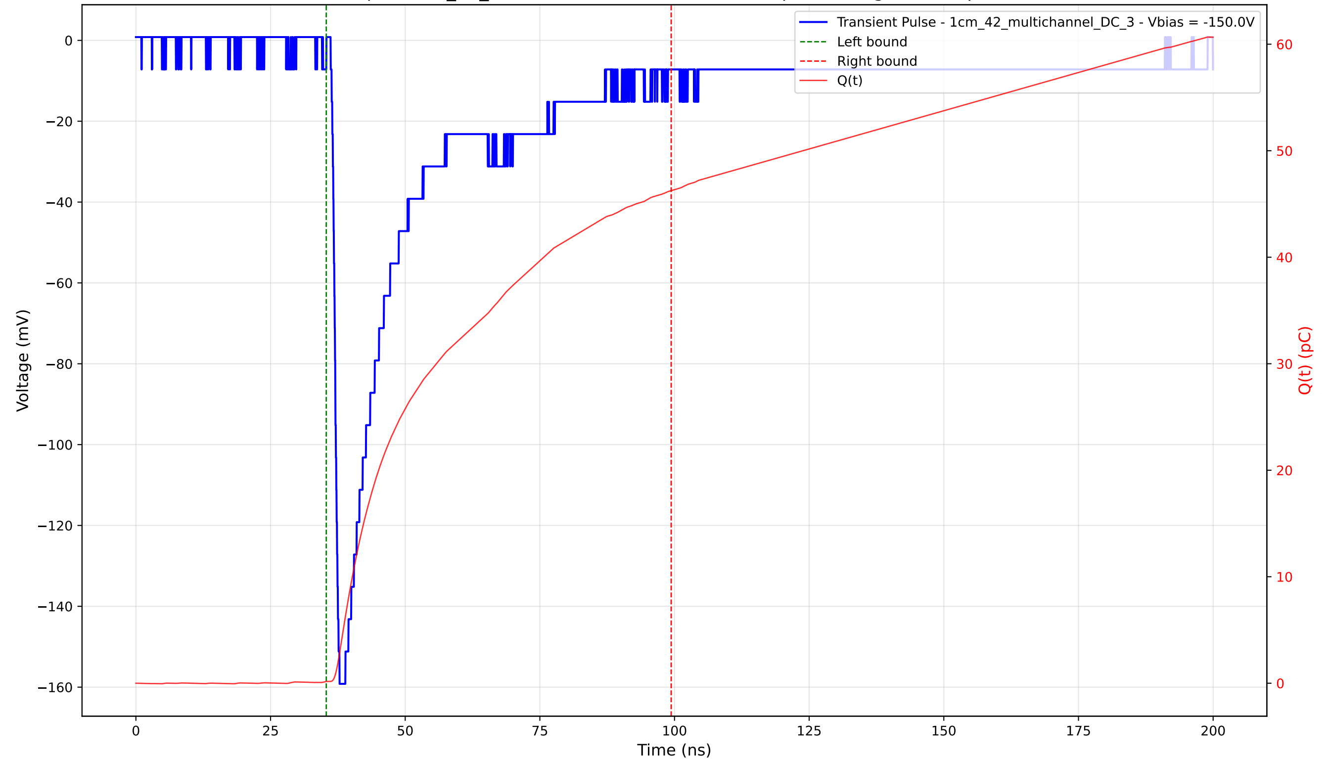
Transient Pulse - Sample: 1cm_42_multichannel - Position: 1105.0 \mu\text{m} - Charge: 46.08 pC - Rise Time: 1.18 ns
