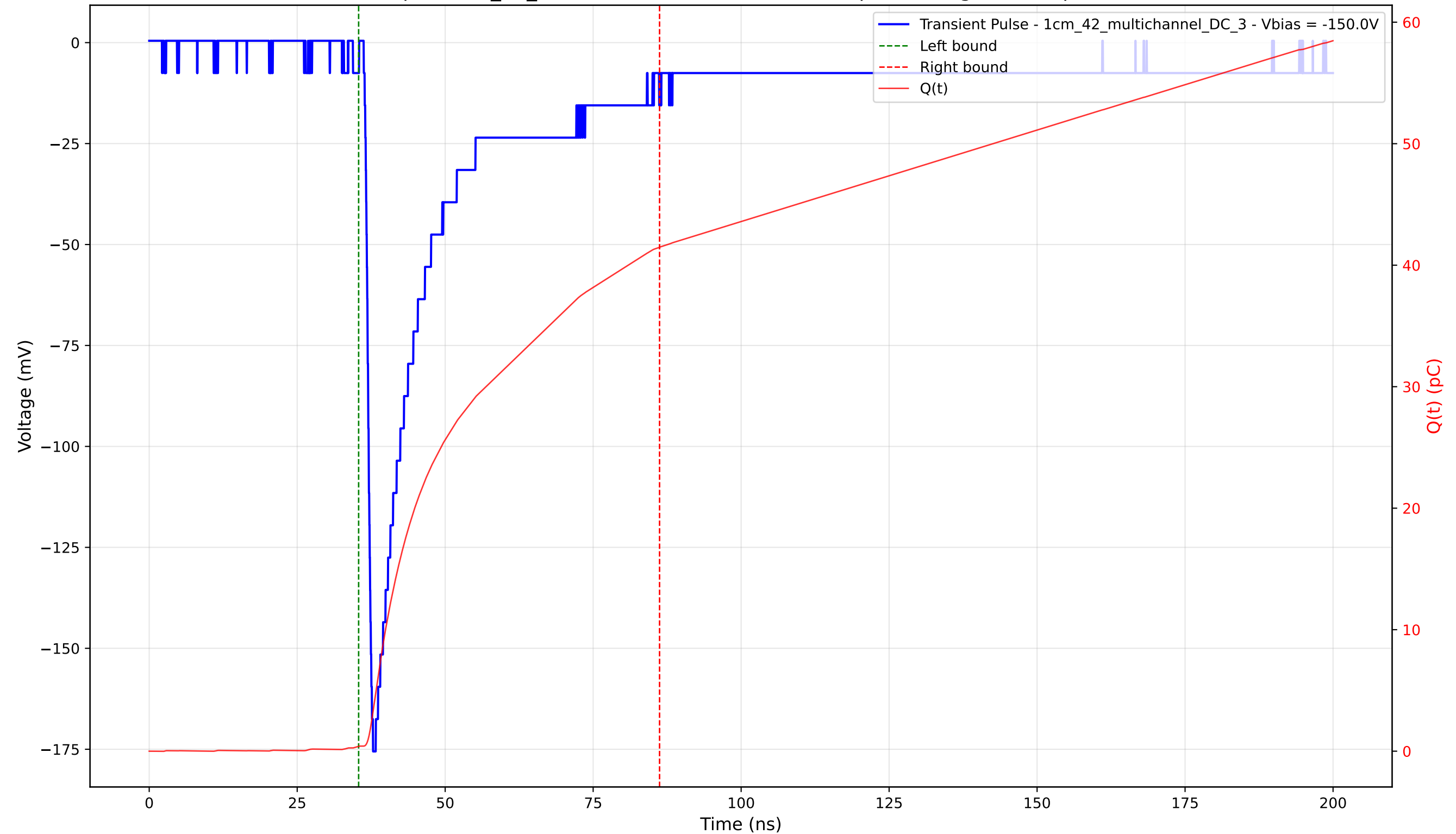
Transient Pulse - Sample: 1cm_42_multichannel - Position: 4000.0 \mu\text{m} - Charge: 41.07 pC - Rise Time: 1.03 ns
