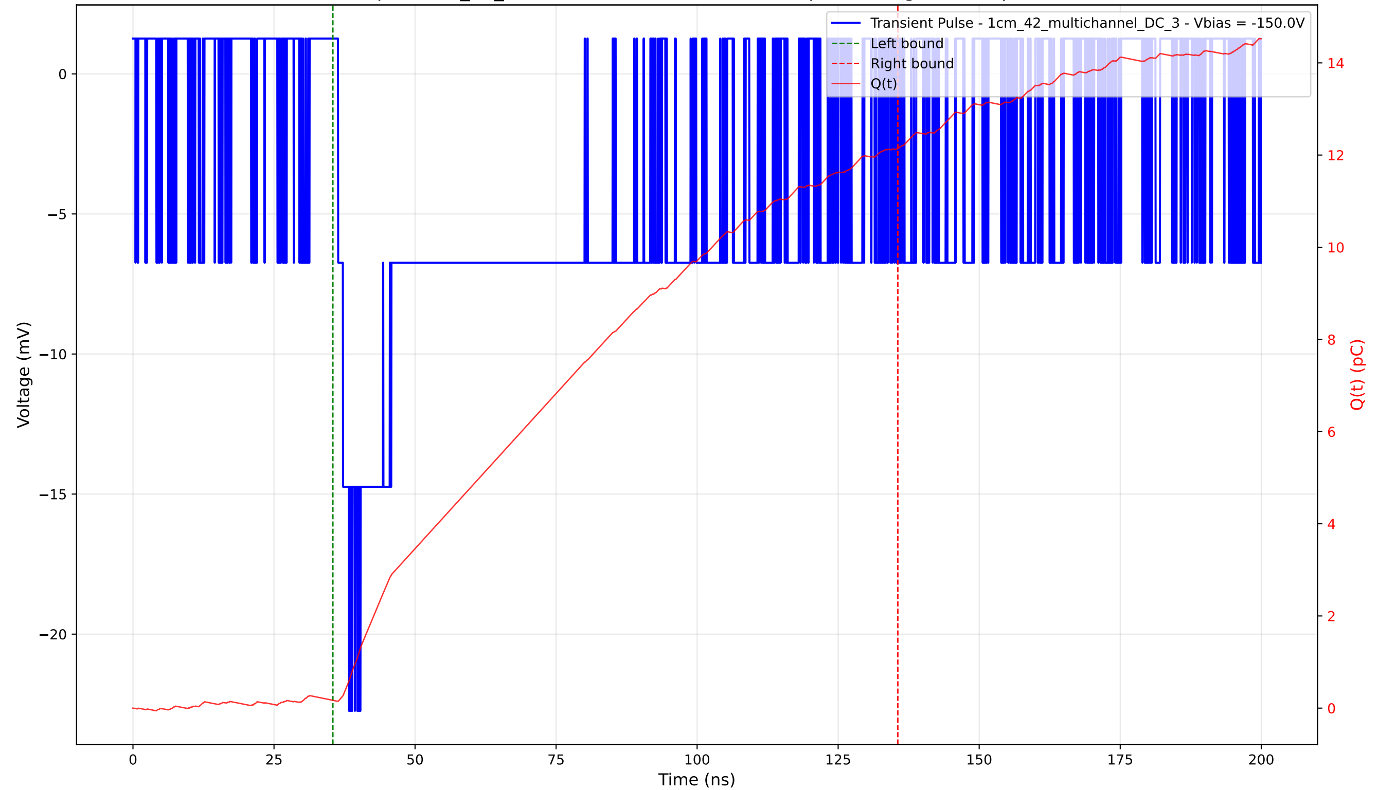
Transient Pulse - Sample: 1cm_42_multichannel - Position: 1390.0 \mu\text{m} - Charge: 11.97 pC - Rise Time: 1.94 ns
