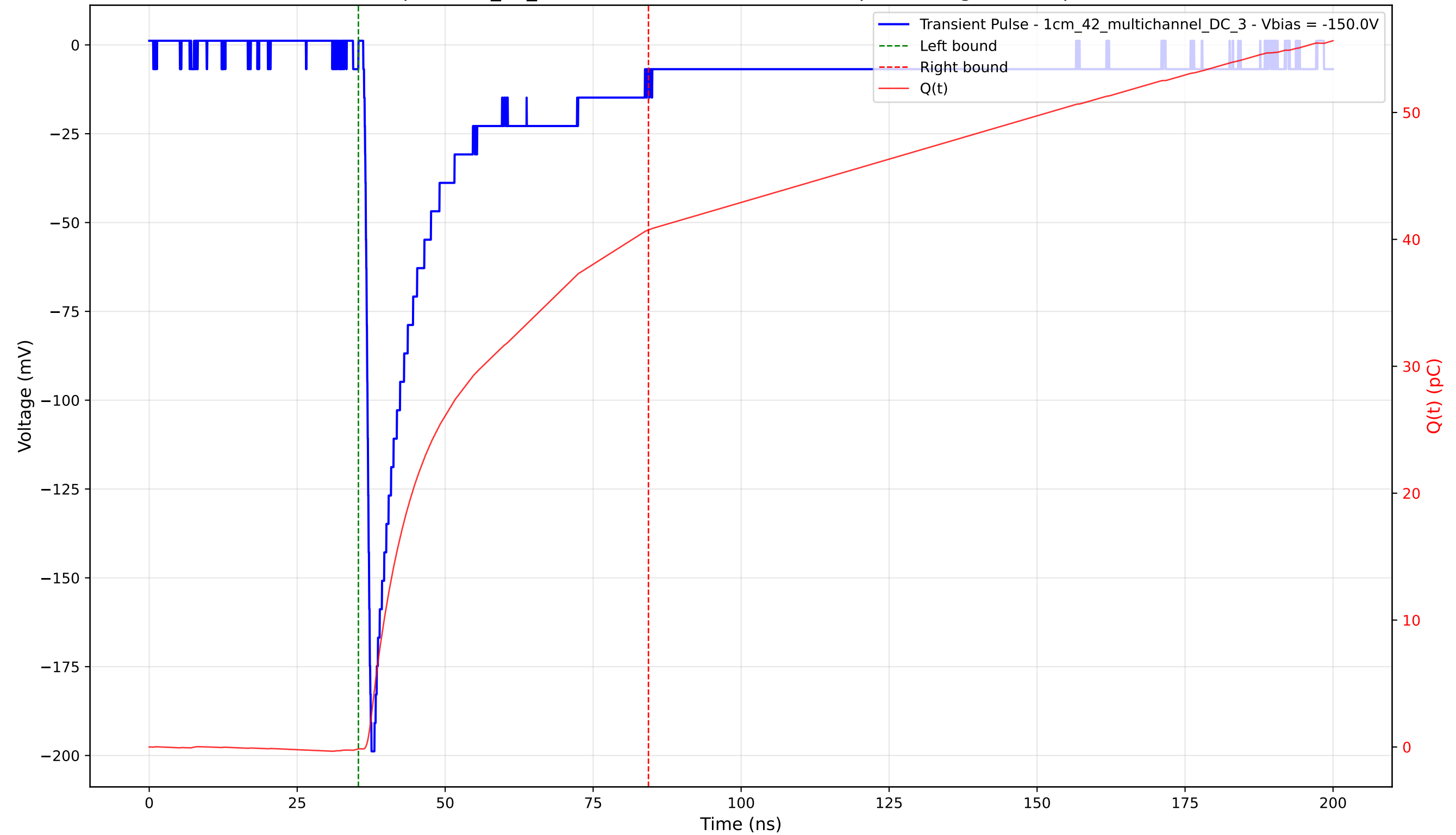
Transient Pulse - Sample: 1cm_42_multichannel - Position: 4190.0 \mu\text{m} - Charge: 40.88 pC - Rise Time: 0.95 ns
