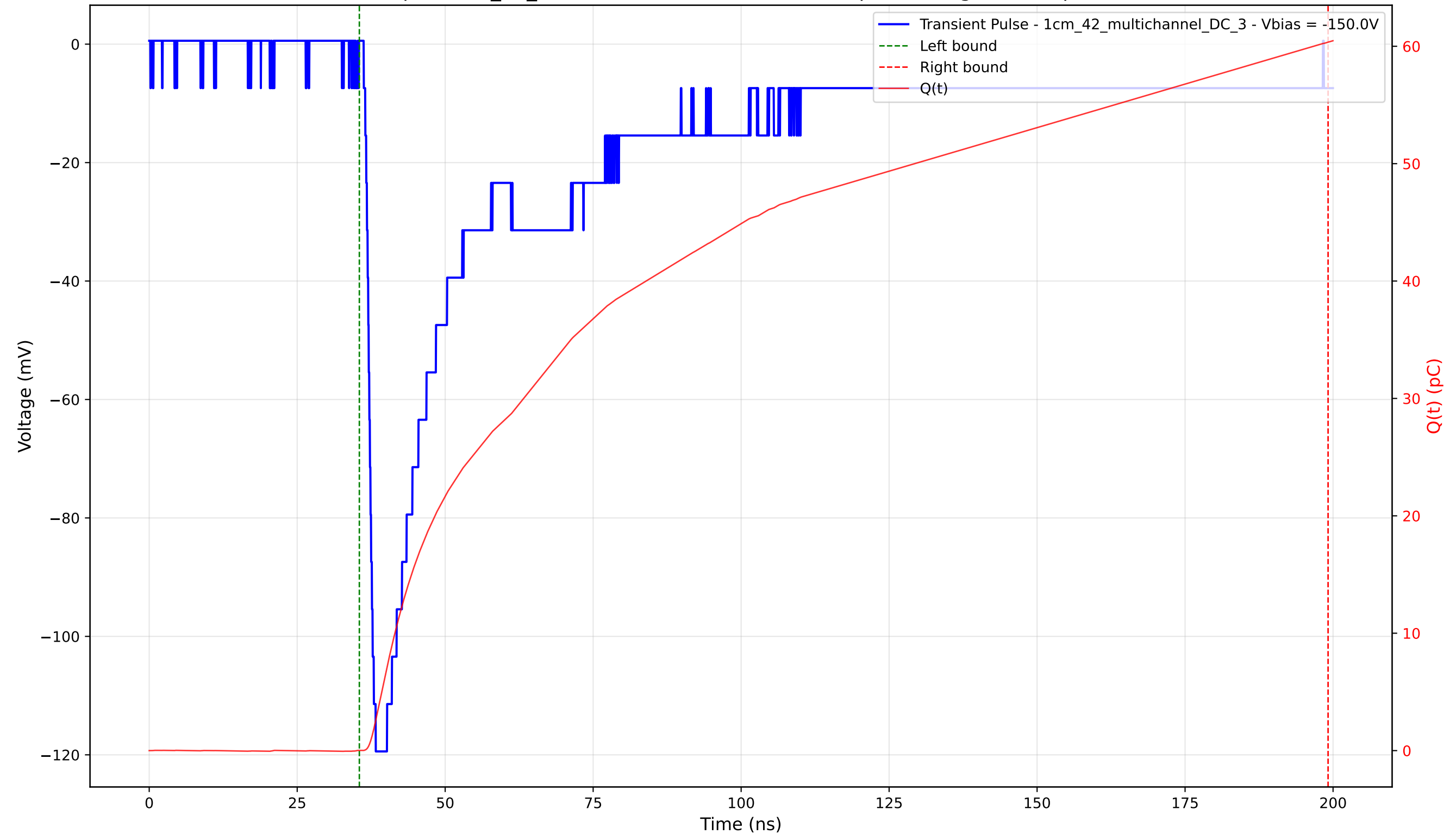
Transient Pulse - Sample: 1cm_42_multichannel - Position: 1625.0 \mu\text{m} - Charge: 60.33 pC - Rise Time: 1.45 ns
