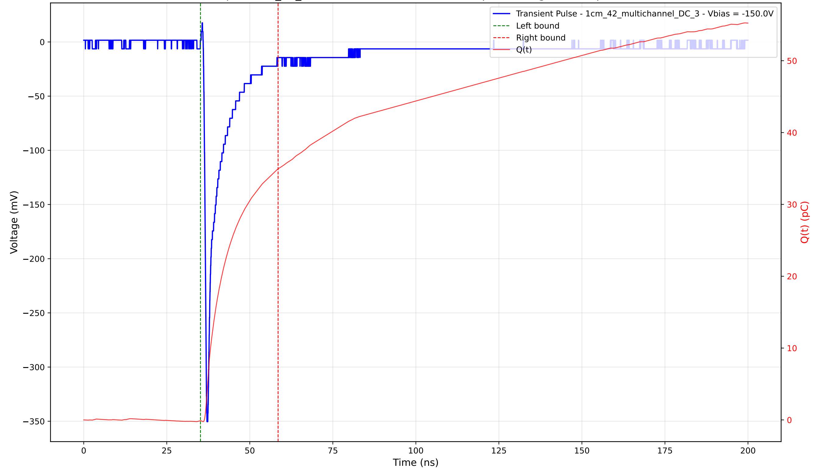
Transient Pulse - Sample: 1cm_42_multichannel - Position: 4735.0 \mu\text{m} - Charge: 35.06 pC - Rise Time: 0.77 ns
