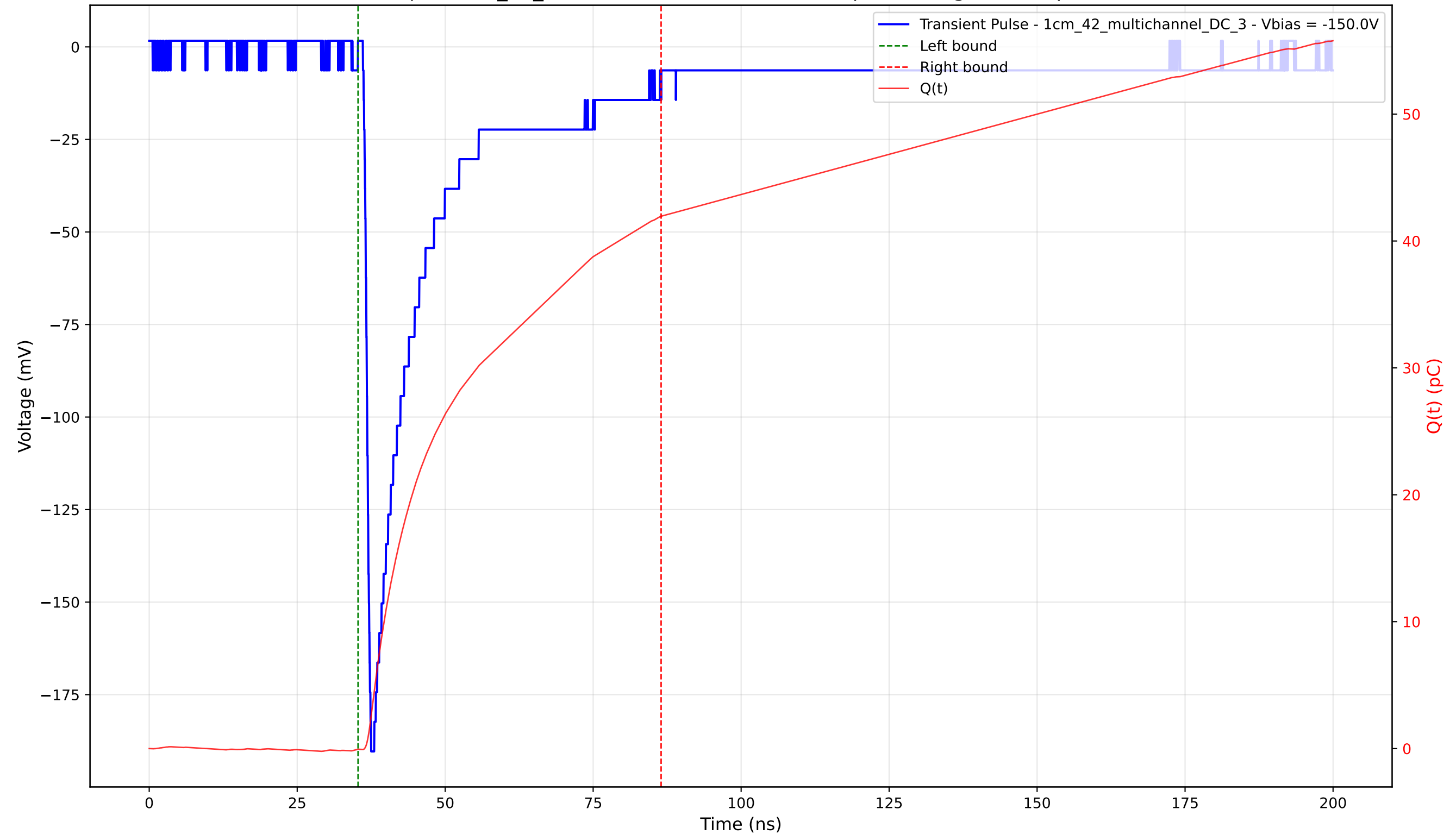
Transient Pulse - Sample: 1cm_42_multichannel - Position: 775.0 \mu\text{m} - Charge: 42.01 pC - Rise Time: 0.99 ns
