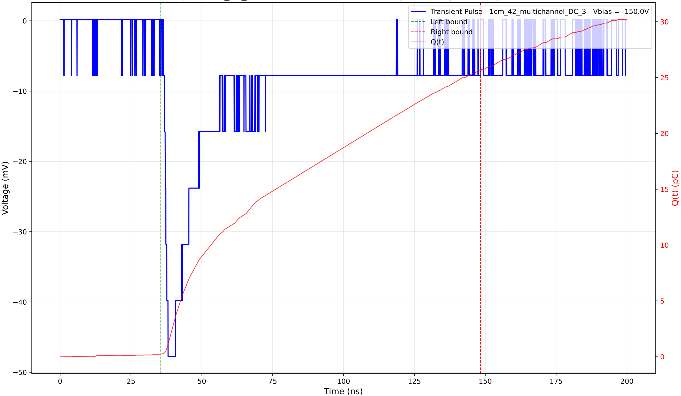
Transient Pulse - Sample: 1cm_42_multichannel - Position: 3340.0 \mu\text{m} - Charge: 25.48 pC - Rise Time: 1.69 ns
