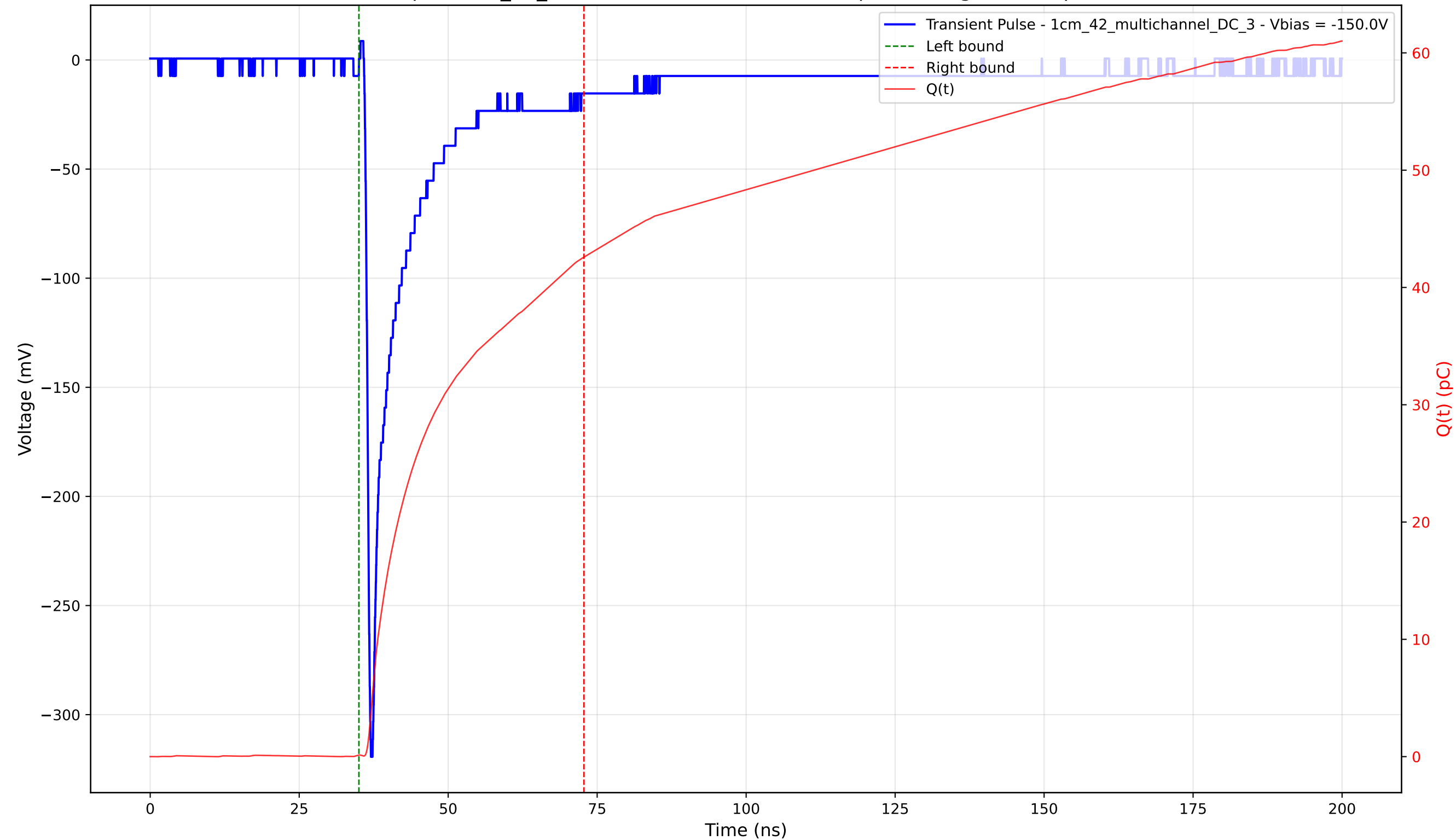
Transient Pulse - Sample: 1cm_42_multichannel - Position: 245.0 \mu\text{m} - Charge: 42.45 pC - Rise Time: 0.82 ns
