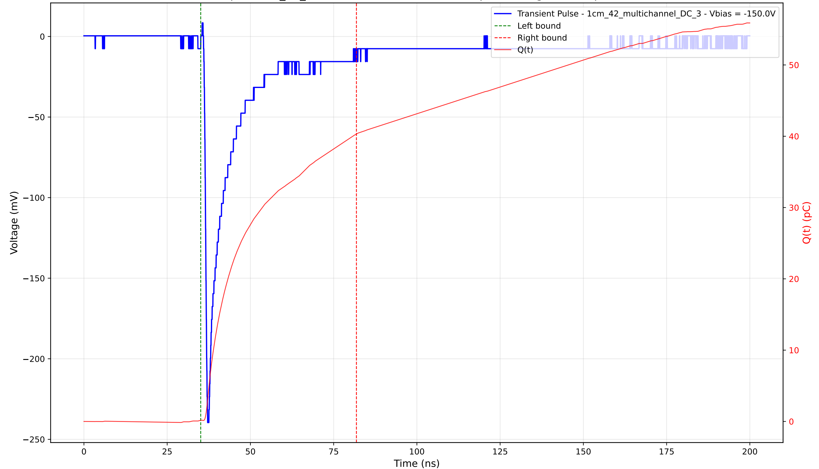
Transient Pulse - Sample: 1cm_42_multichannel - Position: 420.0 \mu\text{m} - Charge: 40.13 pC - Rise Time: 0.88 ns
