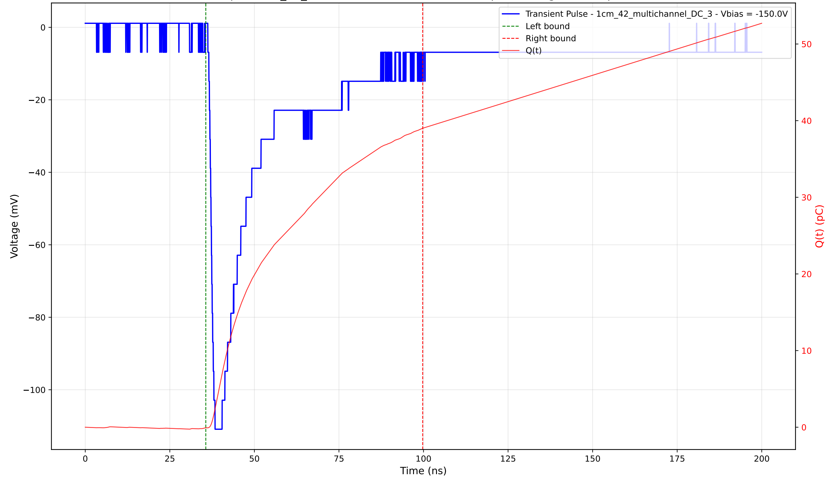
Transient Pulse - Sample: 1cm_42_multichannel - Position: 3285.0 \mu\text{m} - Charge: 39.07 pC - Rise Time: 1.49 ns
