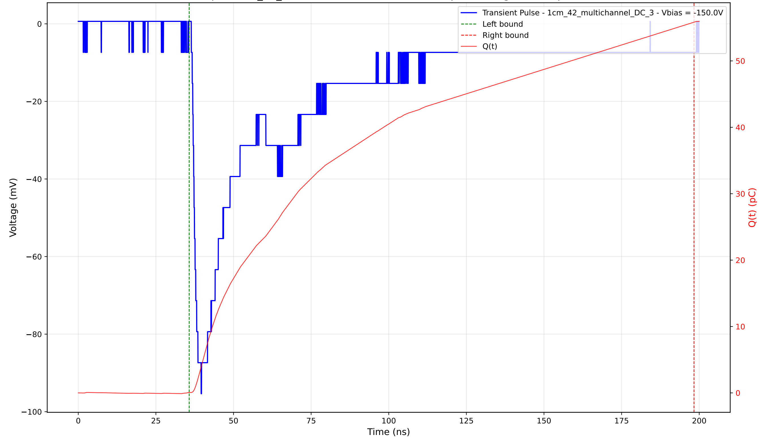
Transient Pulse - Sample: 1cm_42_multichannel - Position: 2730.0 \mu\text{m} - Charge: 55.77 pC - Rise Time: 1.85 ns
