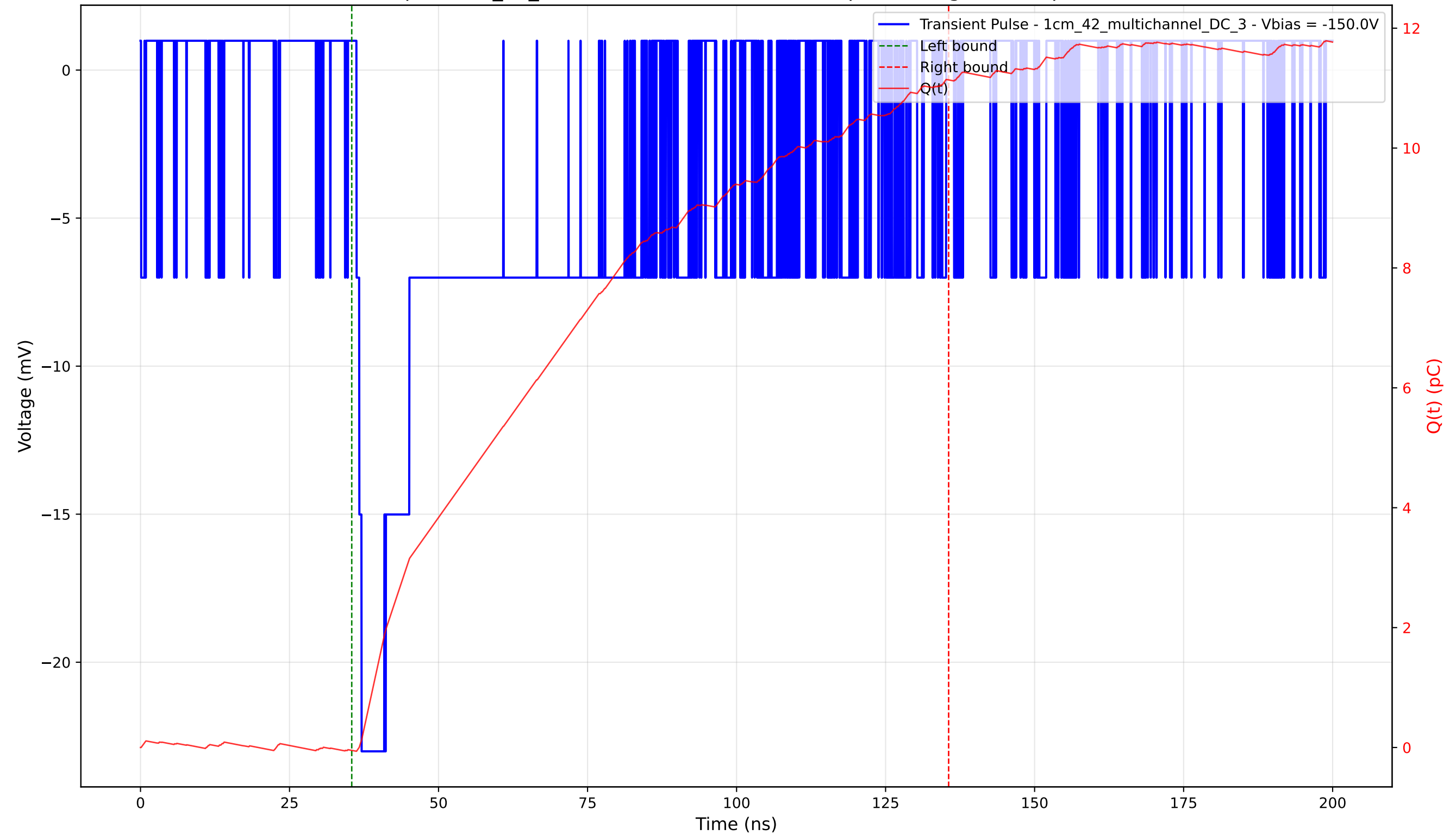
Transient Pulse - Sample: 1cm_42_multichannel - Position: 830.0 \mu\text{m} - Charge: 11.19 pC - Rise Time: 0.86 ns
