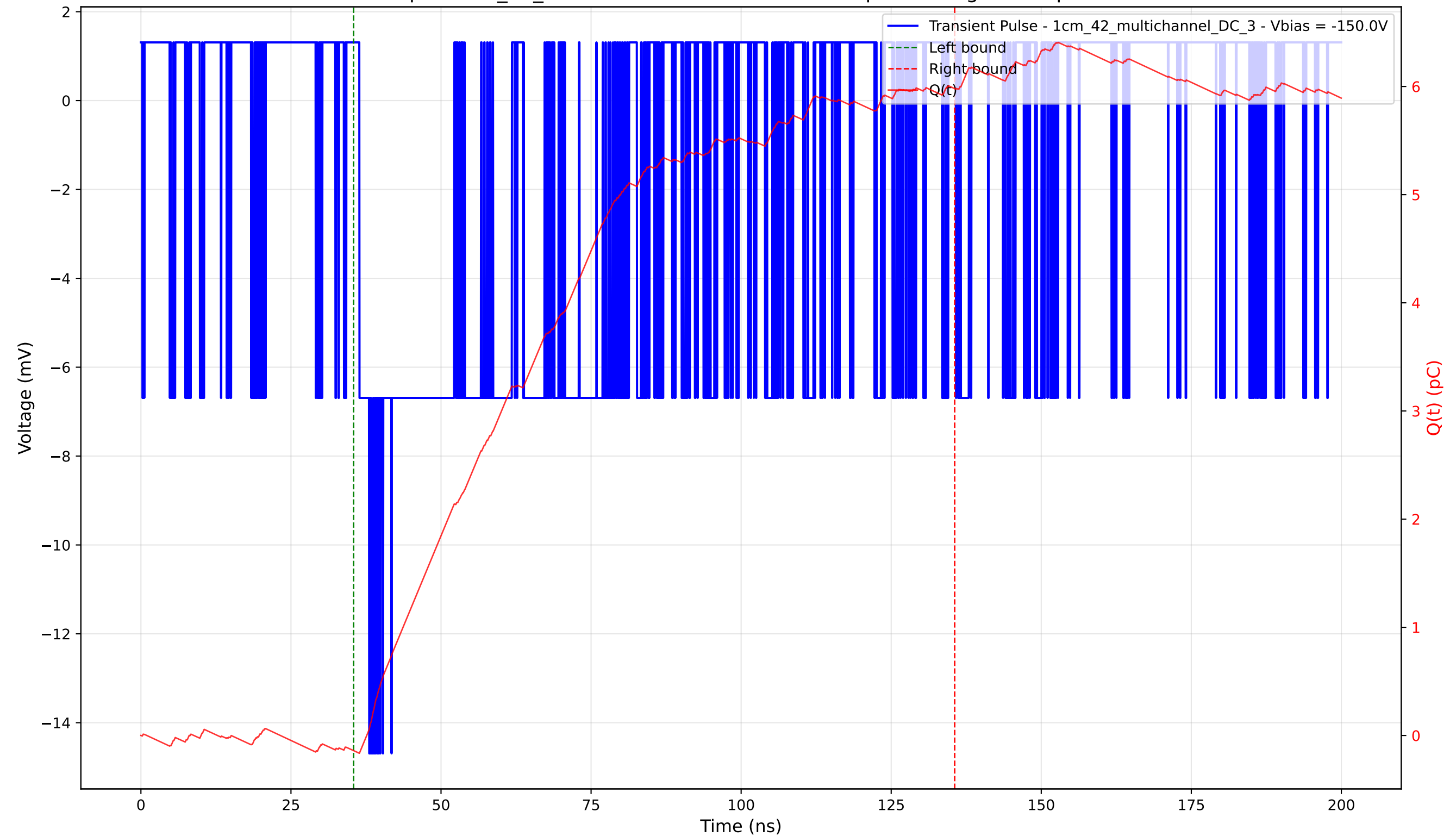
Transient Pulse - Sample: 1cm_42_multichannel - Position: 1350.0 \mu\text{m} - Charge: 6.12 pC - Rise Time: 1.64 ns
