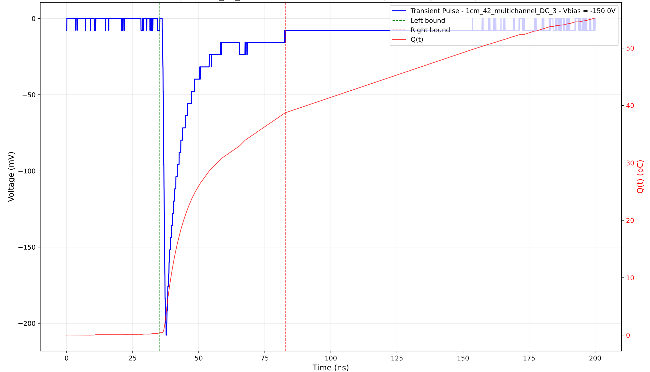
Transient Pulse - Sample: 1cm_42_multichannel - Position: 4265.0 \mu\text{m} - Charge: 38.33 pC - Rise Time: 0.99 ns
