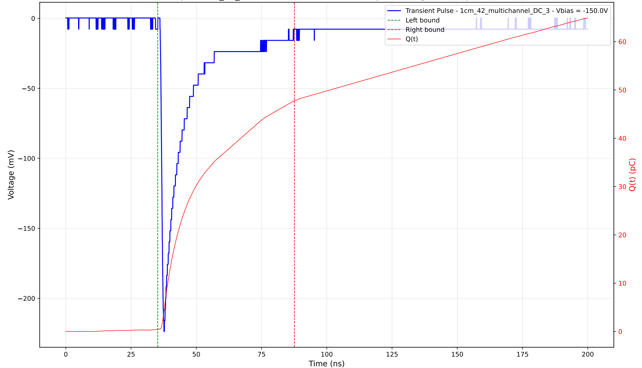
Transient Pulse - Sample: 1cm_42_multichannel - Position: 710.0 \mu\text{m} - Charge: 47.26 pC - Rise Time: 1.04 ns
