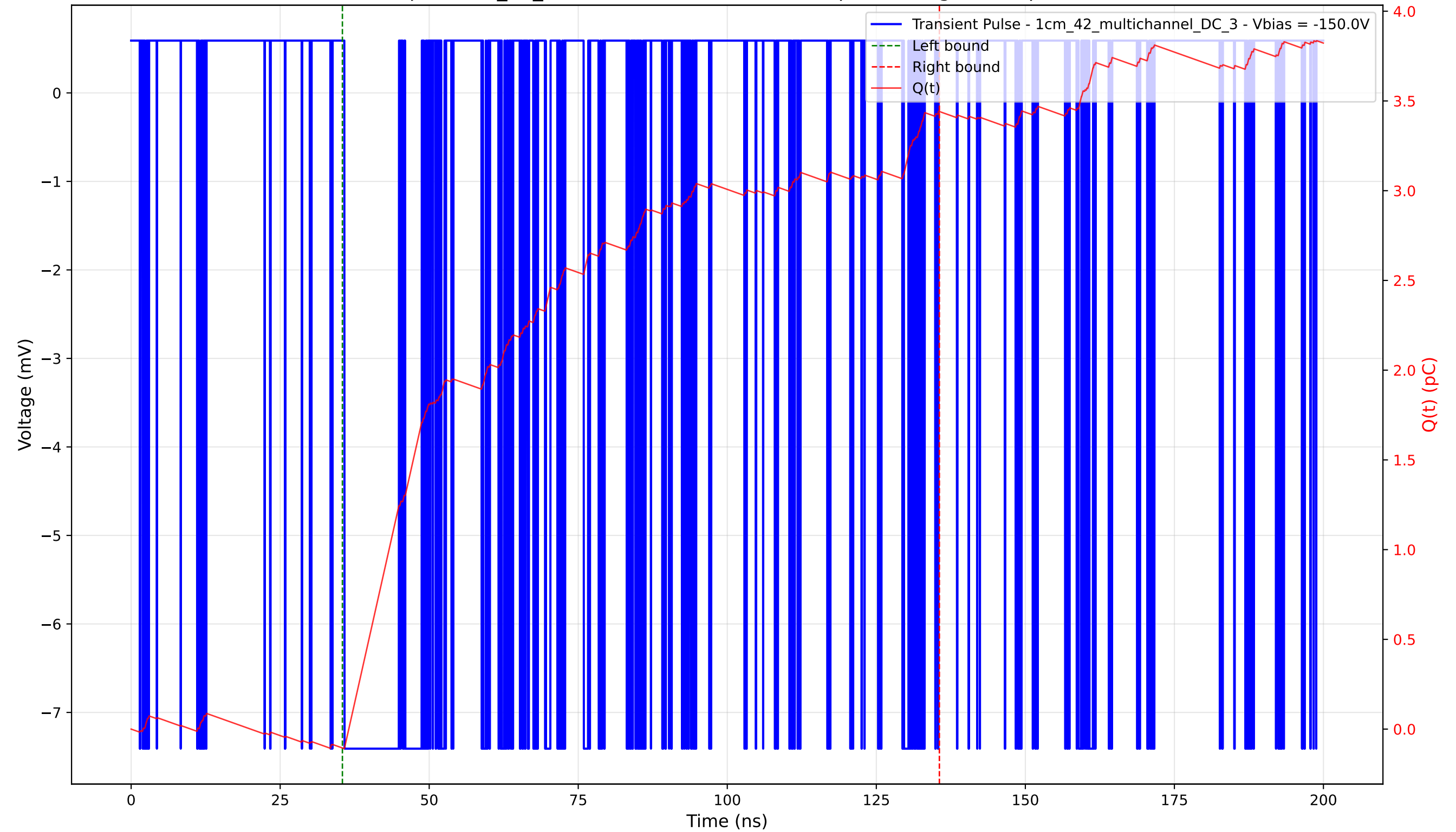
Transient Pulse - Sample: 1cm_42_multichannel - Position: 15.0 \mu\text{m} - Charge: 3.55 pC - Rise Time: 0.02 ns
