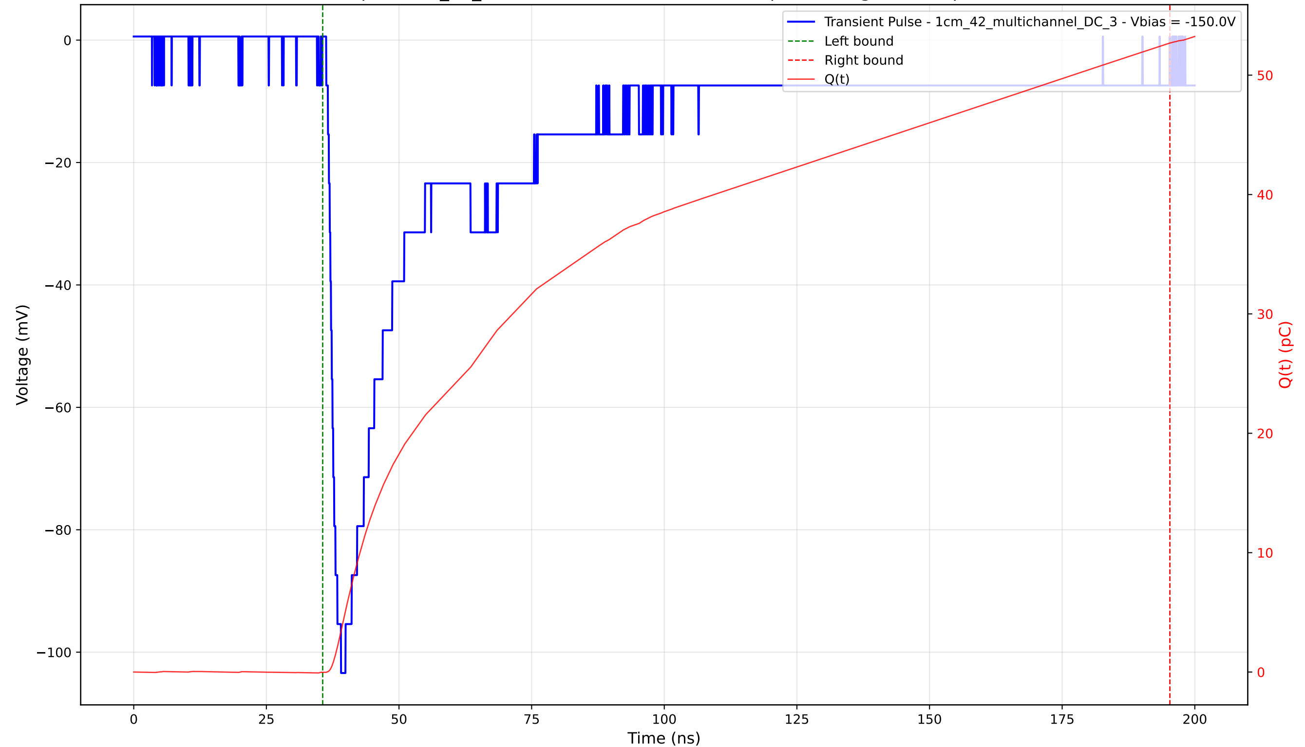
Transient Pulse - Sample: 1cm_42_multichannel - Position: 3090.0 \mu\text{m} - Charge: 52.71 pC - Rise Time: 1.79 ns
