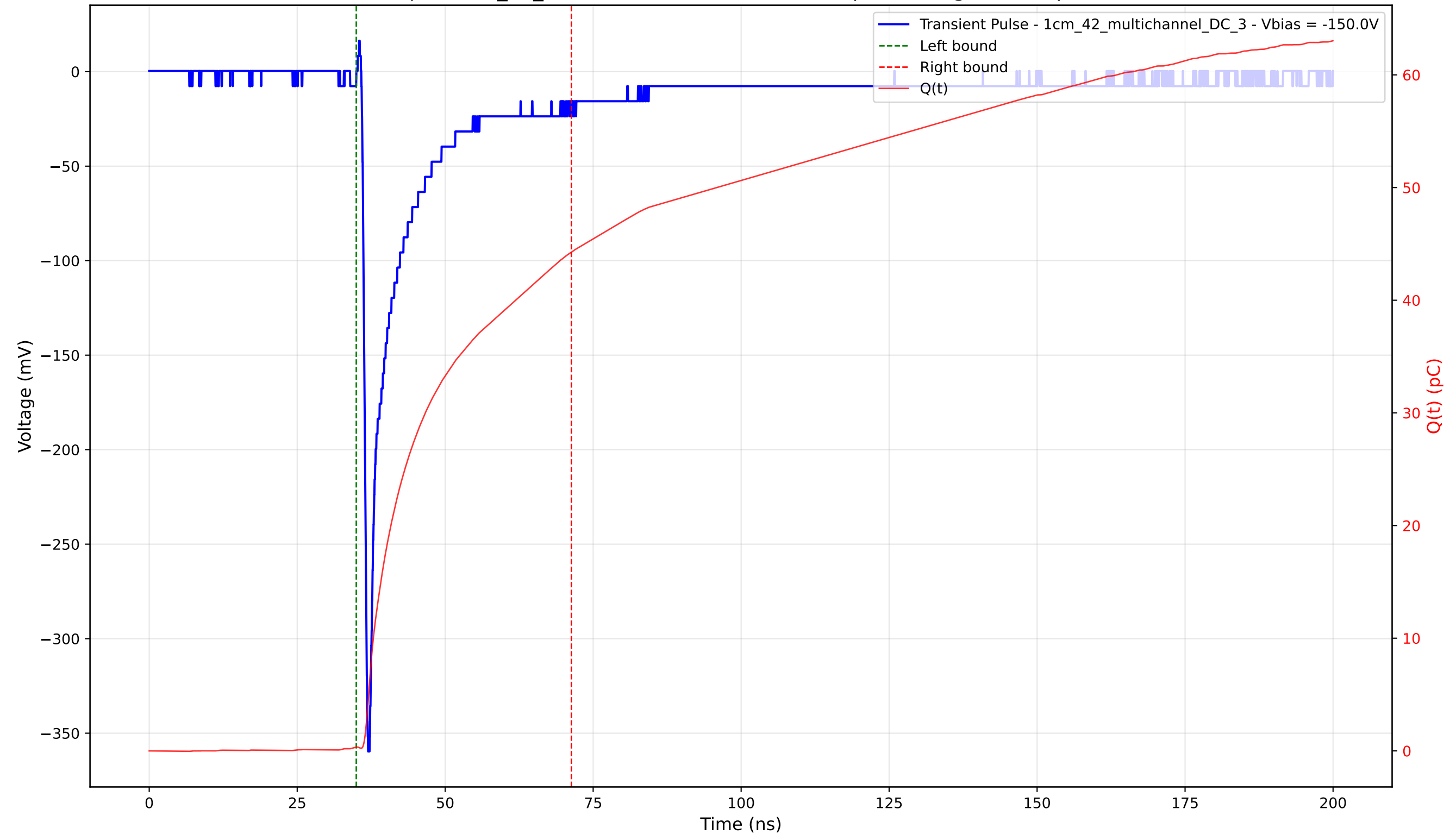
Transient Pulse - Sample: 1cm_42_multichannel - Position: 170.0 \mu\text{m} - Charge: 43.91 pC - Rise Time: 0.78 ns
