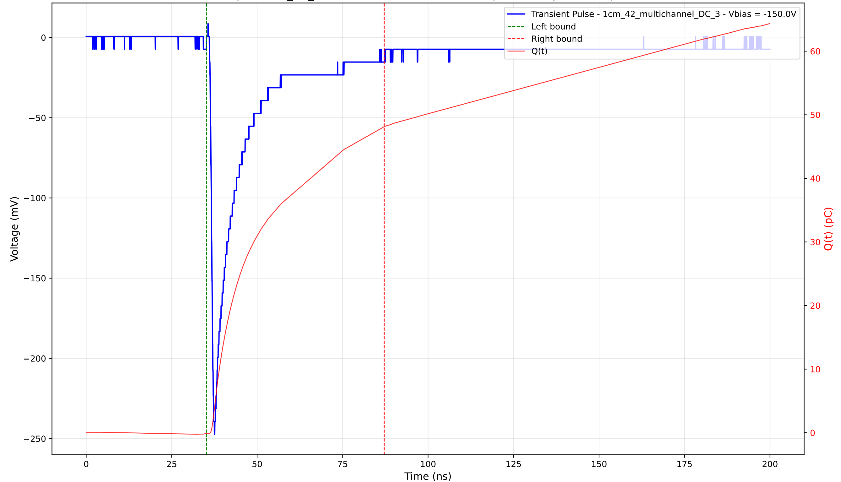
Transient Pulse - Sample: 1cm_42_multichannel - Position: 610.0 \mu\text{m} - Charge: 48.22 pC - Rise Time: 0.92 ns
