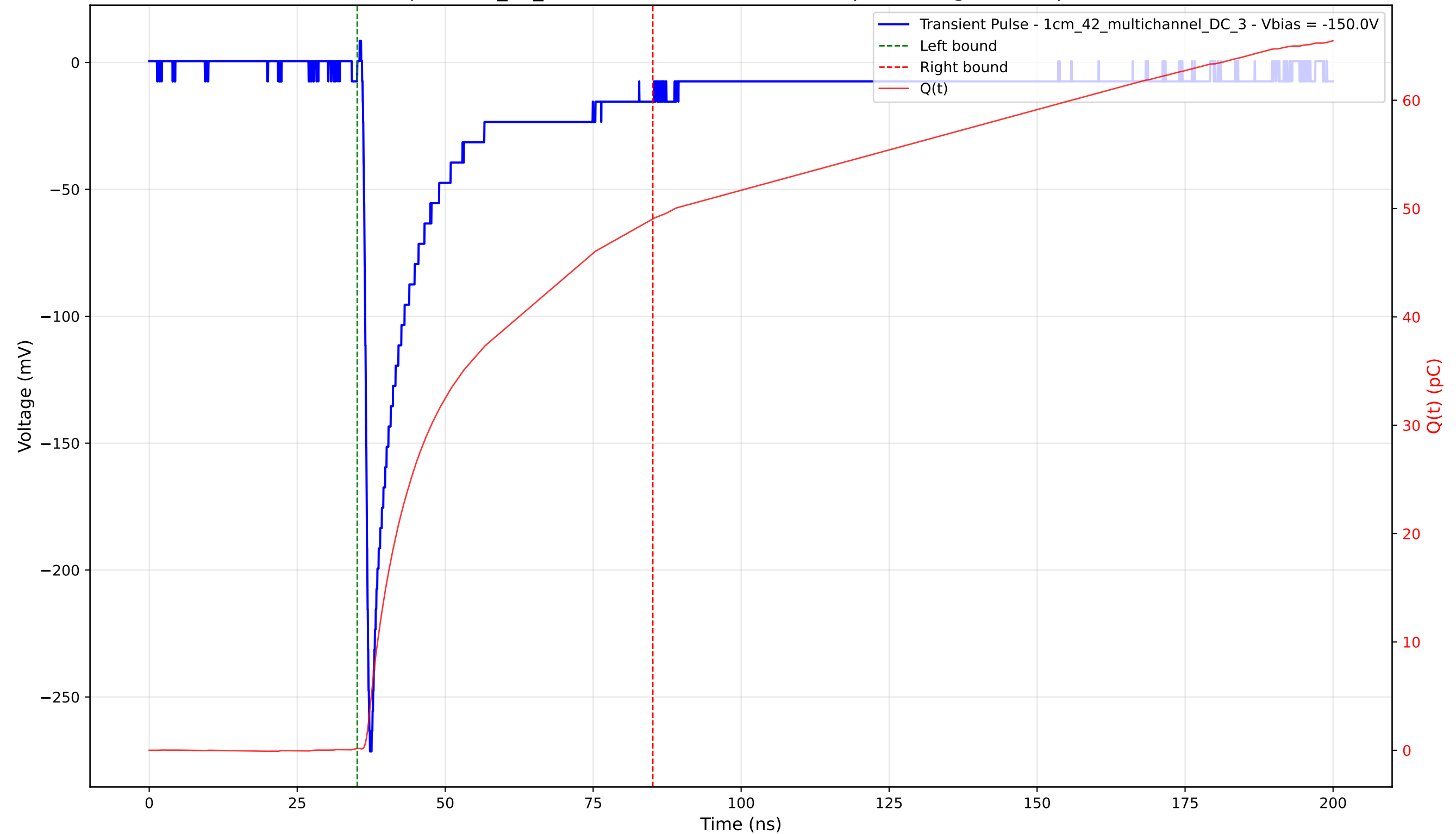
Transient Pulse - Sample: 1cm_42_multichannel - Position: 500.0 \mu\text{m} - Charge: 48.88 pC - Rise Time: 0.89 ns
