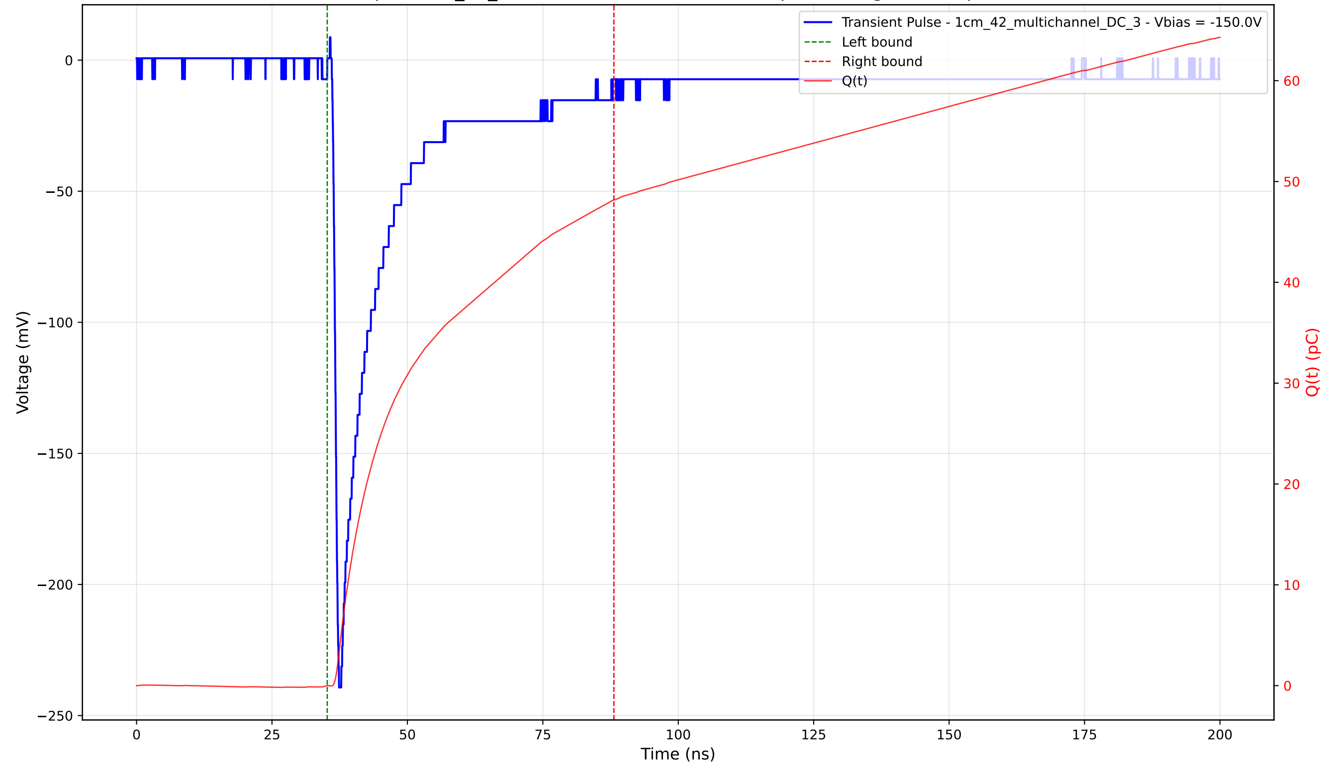
Transient Pulse - Sample: 1cm_42_multichannel - Position: 620.0 \mu\text{m} - Charge: 48.17 pC - Rise Time: 0.96 ns
