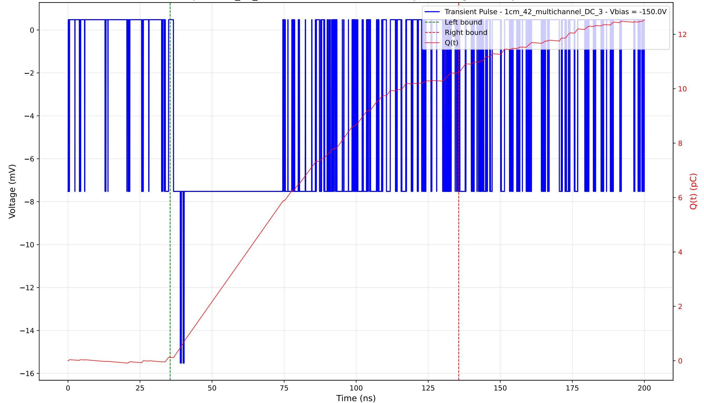
Transient Pulse - Sample: 1cm_42_multichannel - Position: 2350.0 \mu\text{m} - Charge: 10.47 pC - Rise Time: 2.40 ns
