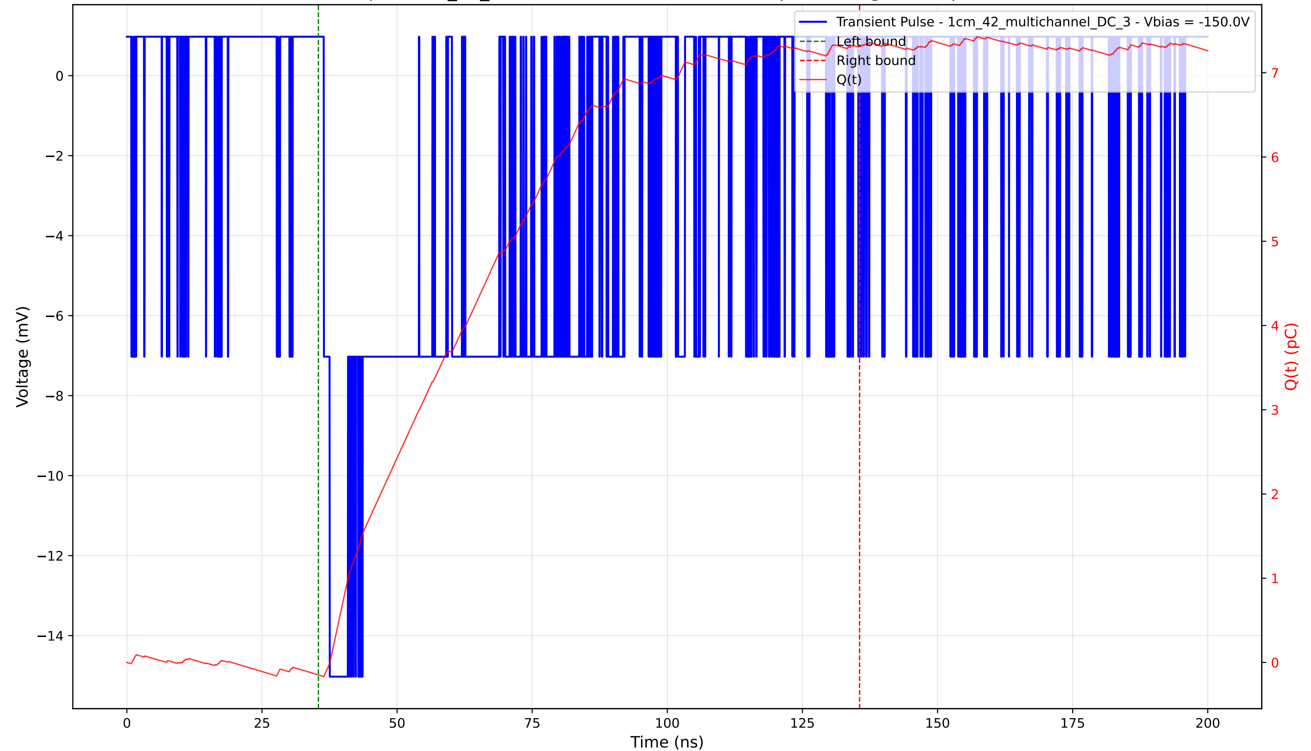
Transient Pulse - Sample: 1cm_42_multichannel - Position: 1345.0 \mu\text{m} - Charge: 7.46 pC - Rise Time: 1.10 ns
