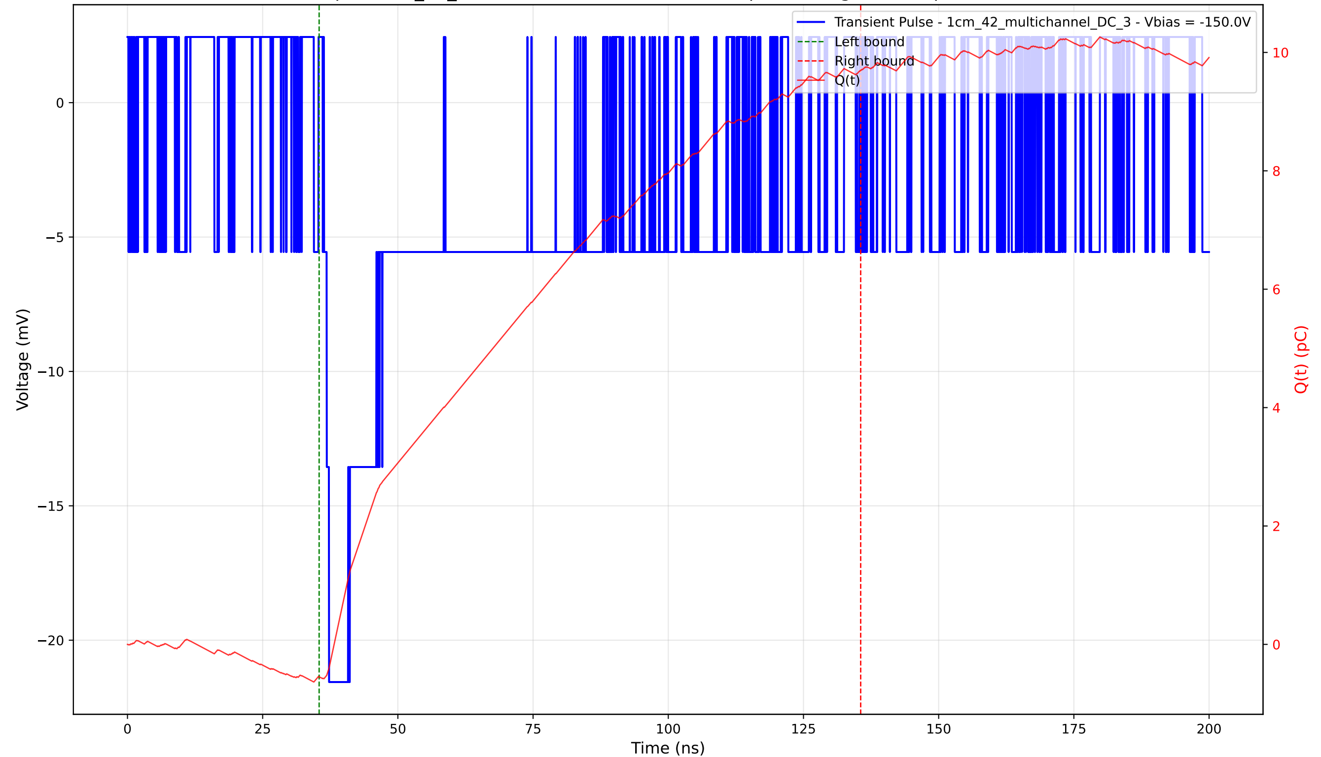
Transient Pulse - Sample: 1cm_42_multichannel - Position: 3920.0 \mu\text{m} - Charge: 10.24 pC - Rise Time: 0.00 ns (N/A)
