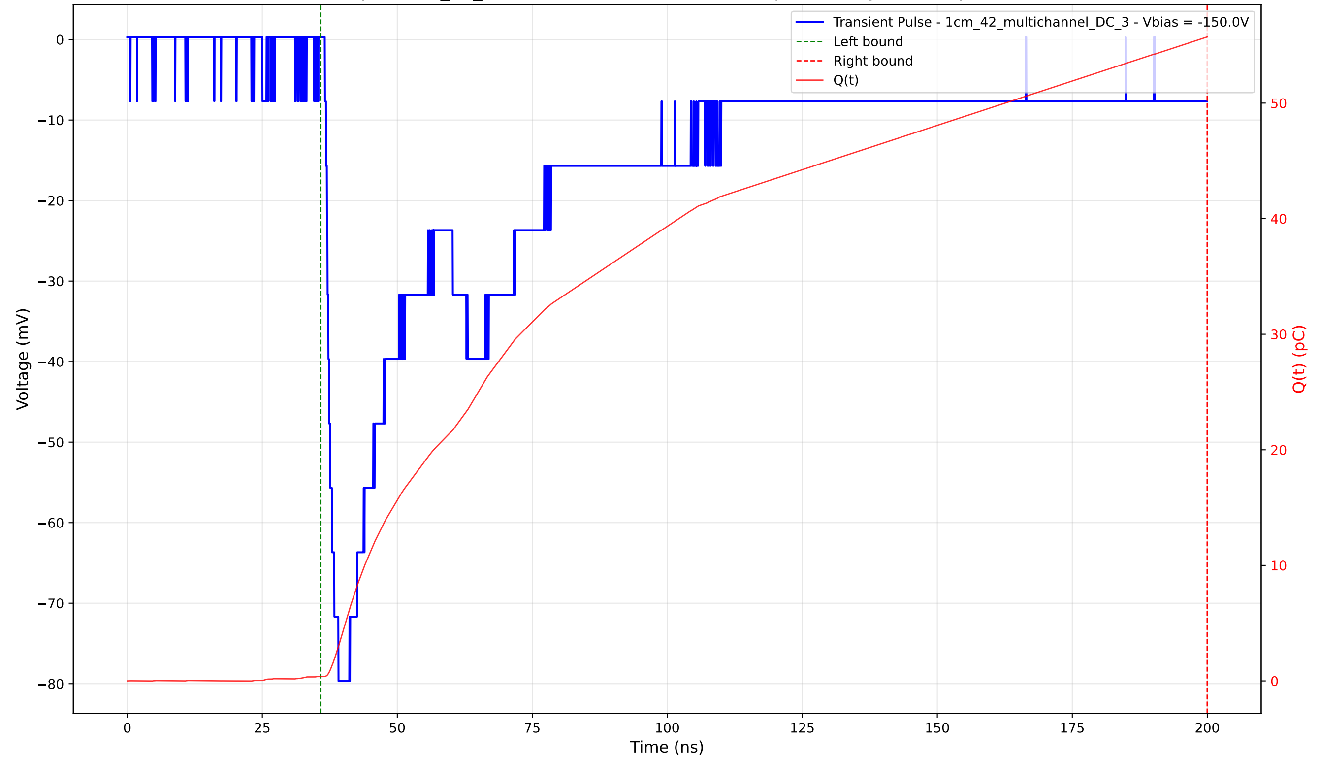
Transient Pulse - Sample: 1cm_42_multichannel - Position: 2525.0 \mu\text{m} - Charge: 55.34 pC - Rise Time: 2.32 ns
