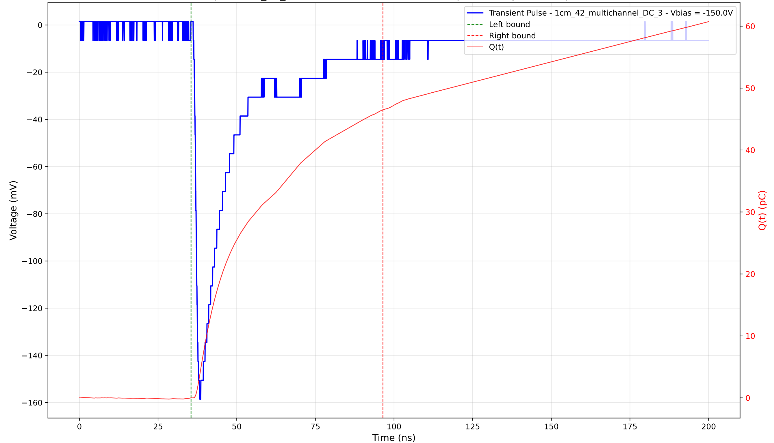
Transient Pulse - Sample: 1cm_42_multichannel - Position: 1240.0 \mu\text{m} - Charge: 46.49 pC - Rise Time: 1.36 ns
