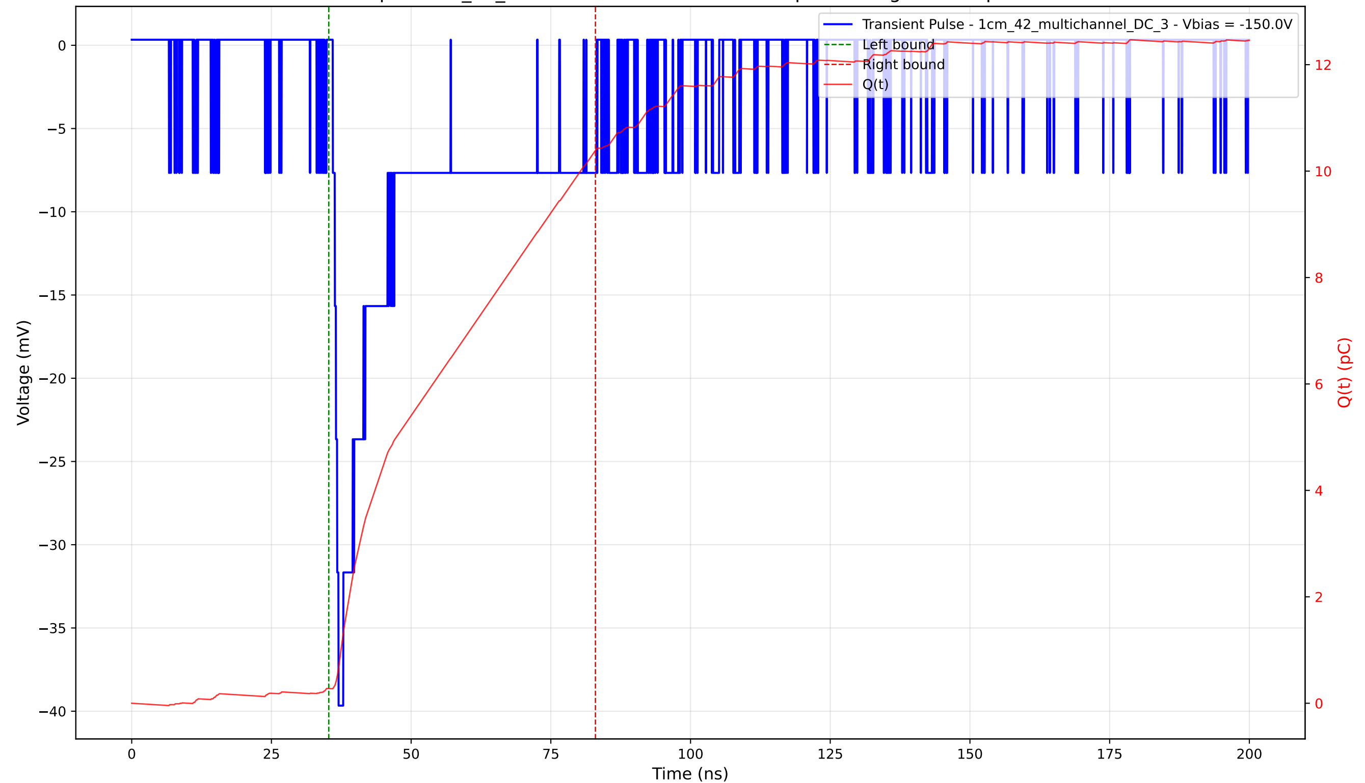
Transient Pulse - Sample: 1cm_42_multichannel - Position: 380.0 \mu\text{m} - Charge: 10.12 pC - Rise Time: 1.03 ns
