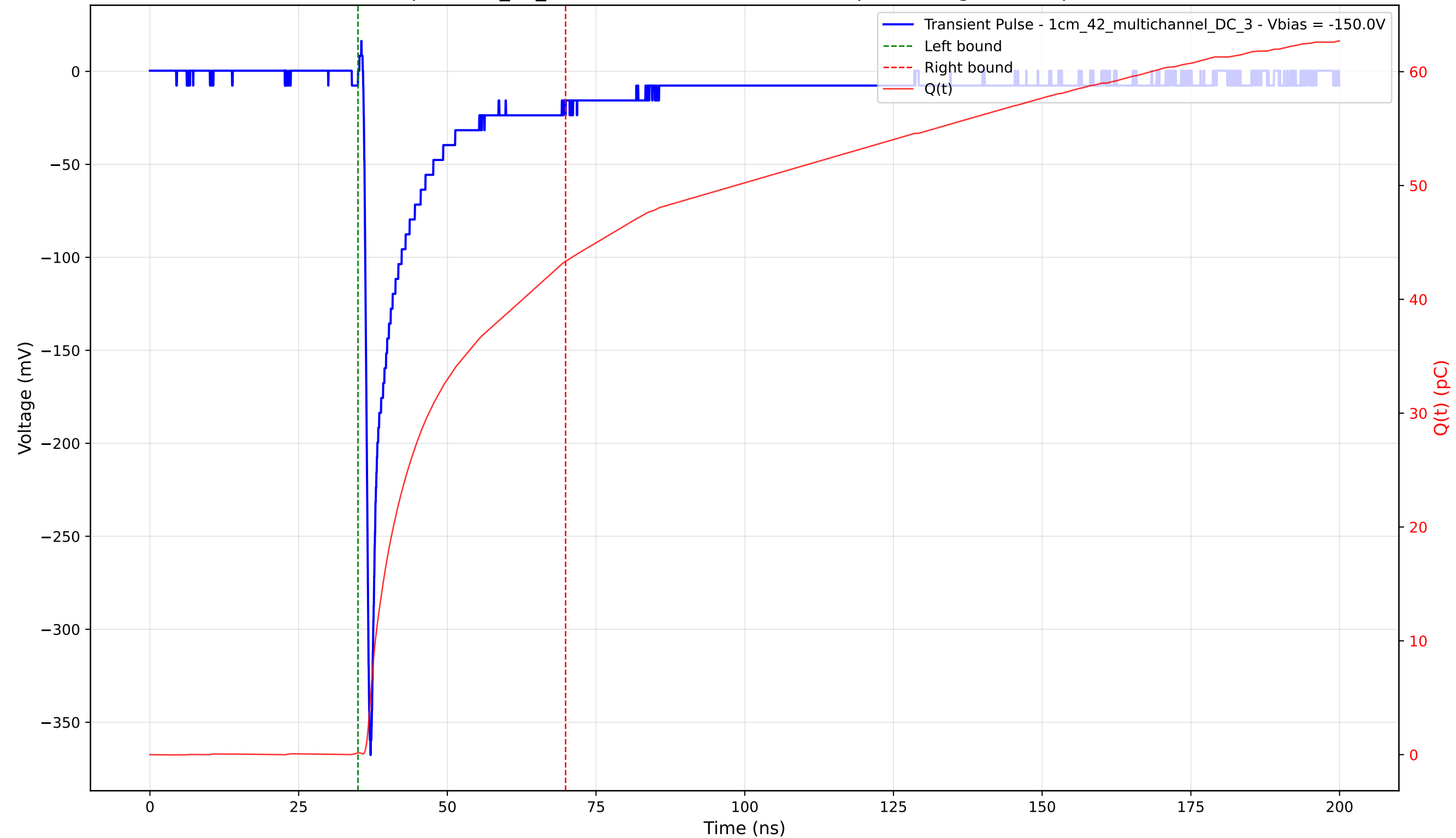
Transient Pulse - Sample: 1cm_42_multichannel - Position: 165.0 \mu\text{m} - Charge: 43.18 pC - Rise Time: 0.83 ns
