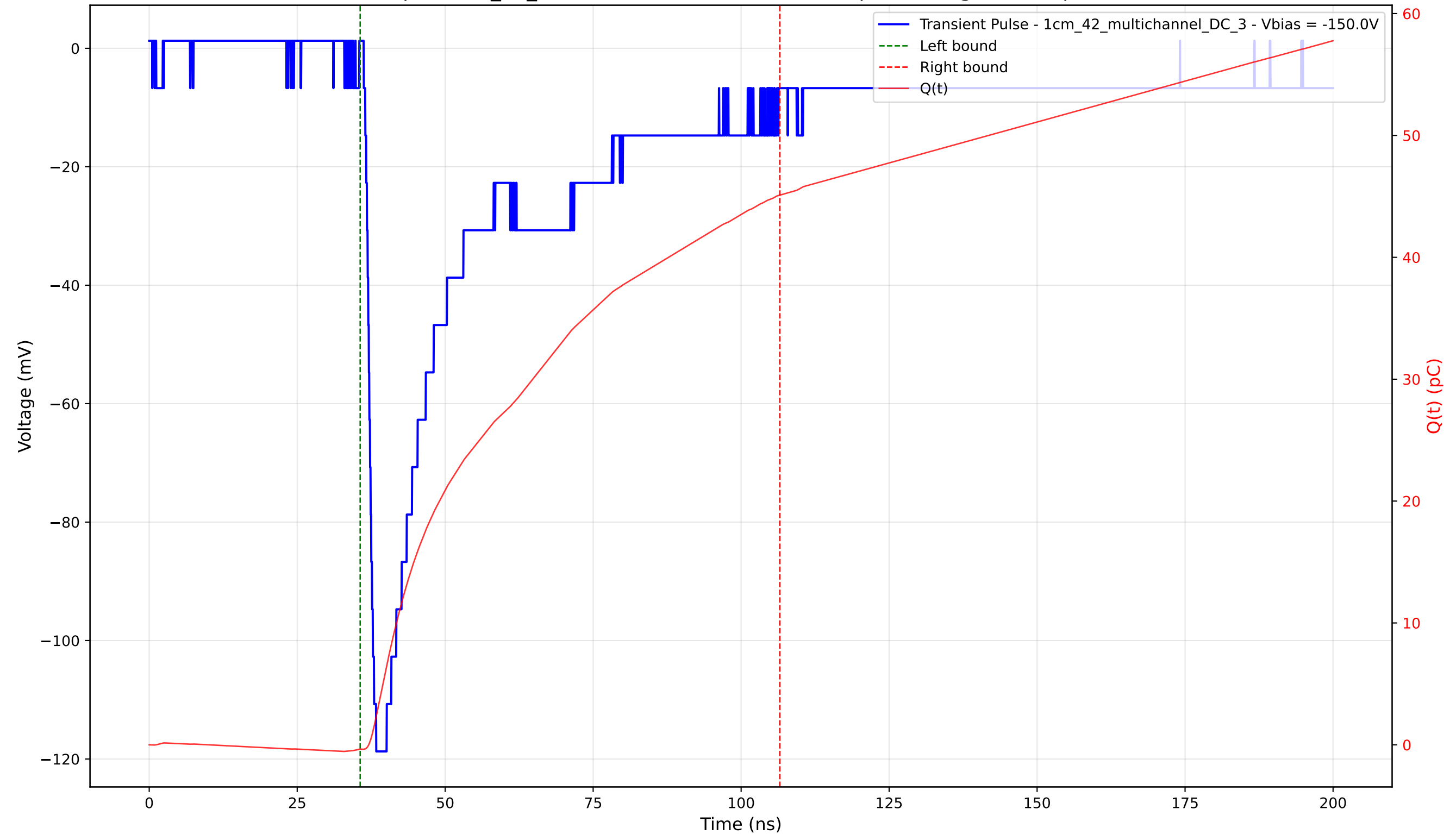
Transient Pulse - Sample: 1cm_42_multichannel - Position: 1640.0 \mu\text{m} - Charge: 45.47 pC - Rise Time: 1.49 ns
