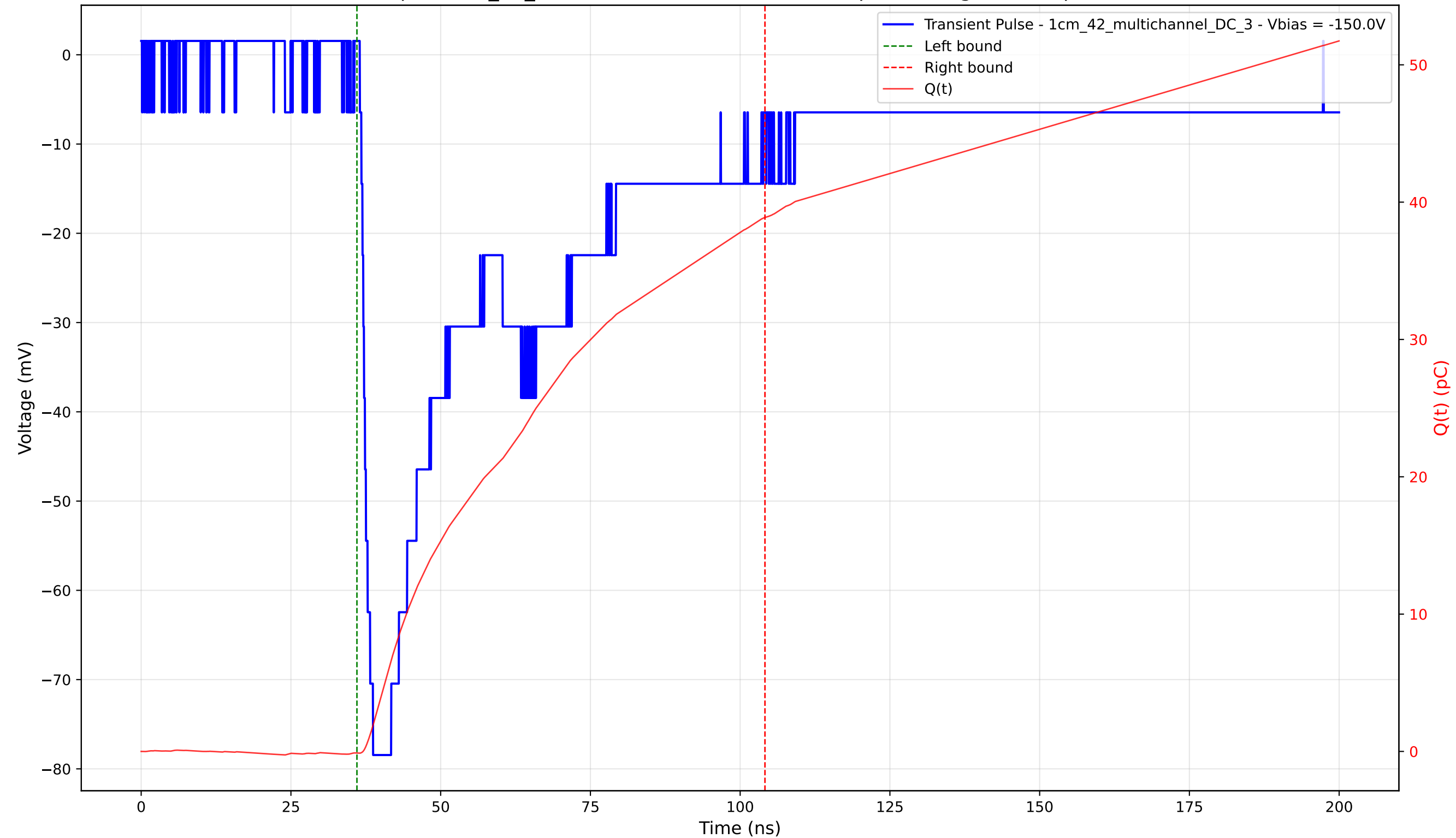
Transient Pulse - Sample: 1cm_42_multichannel - Position: 2610.0 \mu\text{m} - Charge: 39.00 pC - Rise Time: 1.96 ns
