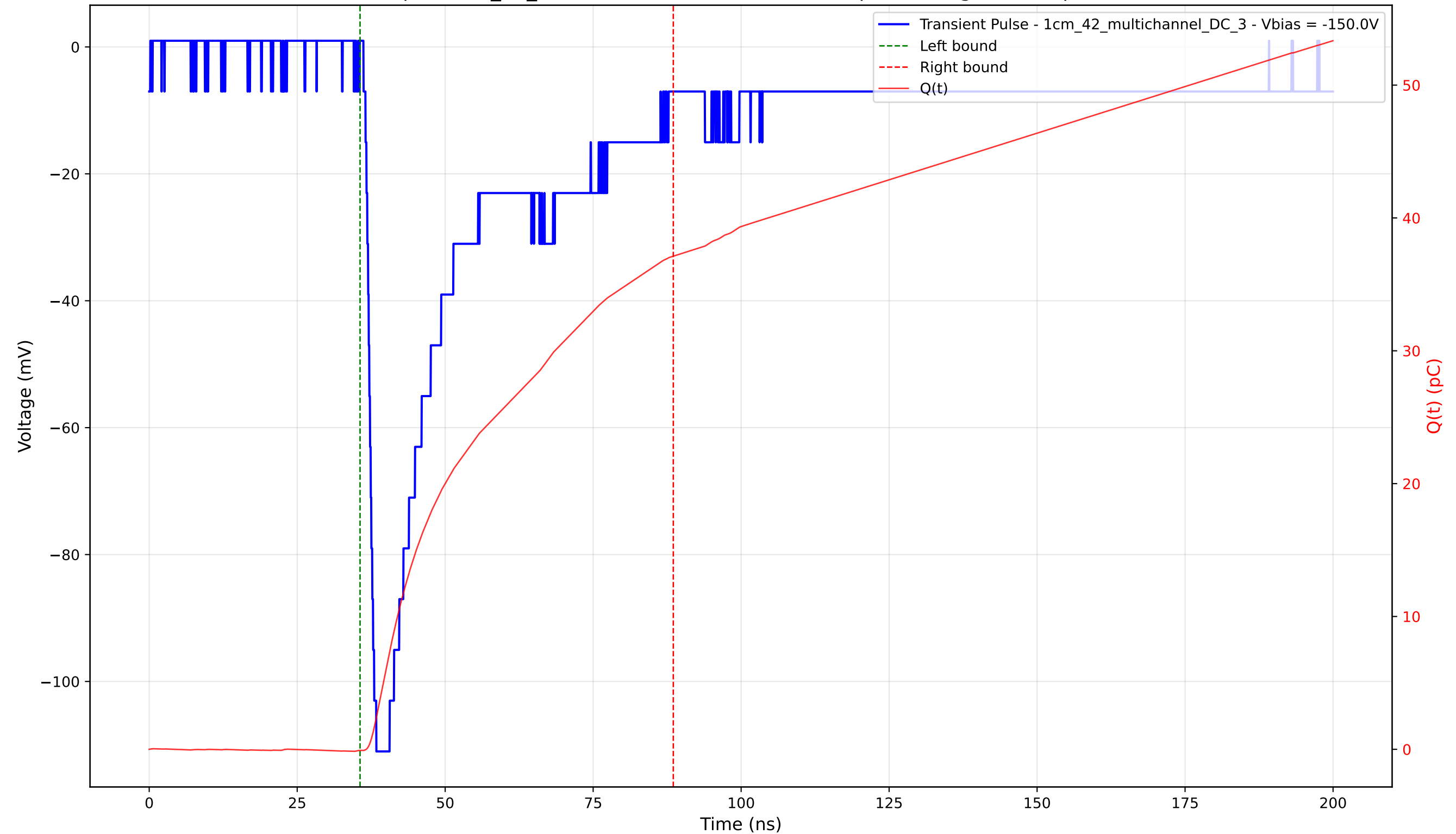
Transient Pulse - Sample: 1cm_42_multichannel - Position: 3290.0 \mu\text{m} - Charge: 37.20 pC - Rise Time: 1.47 ns
