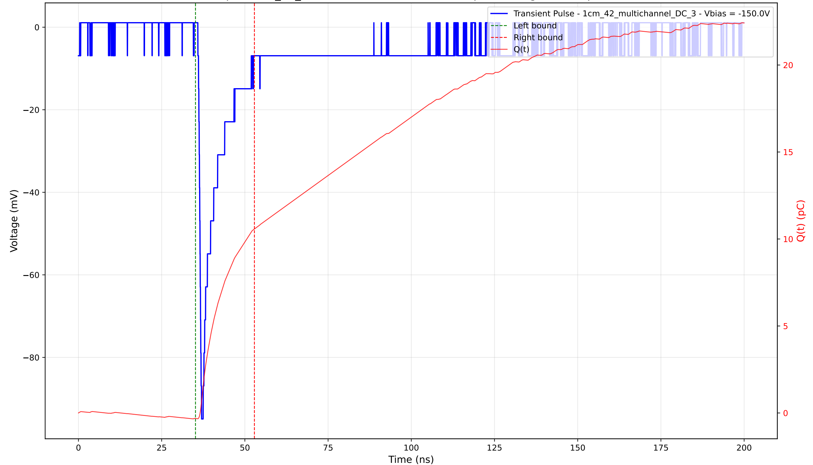
Transient Pulse - Sample: 1cm_42_multichannel - Position: 310.0 \mu\text{m} - Charge: 10.89 pC - Rise Time: 0.77 ns
