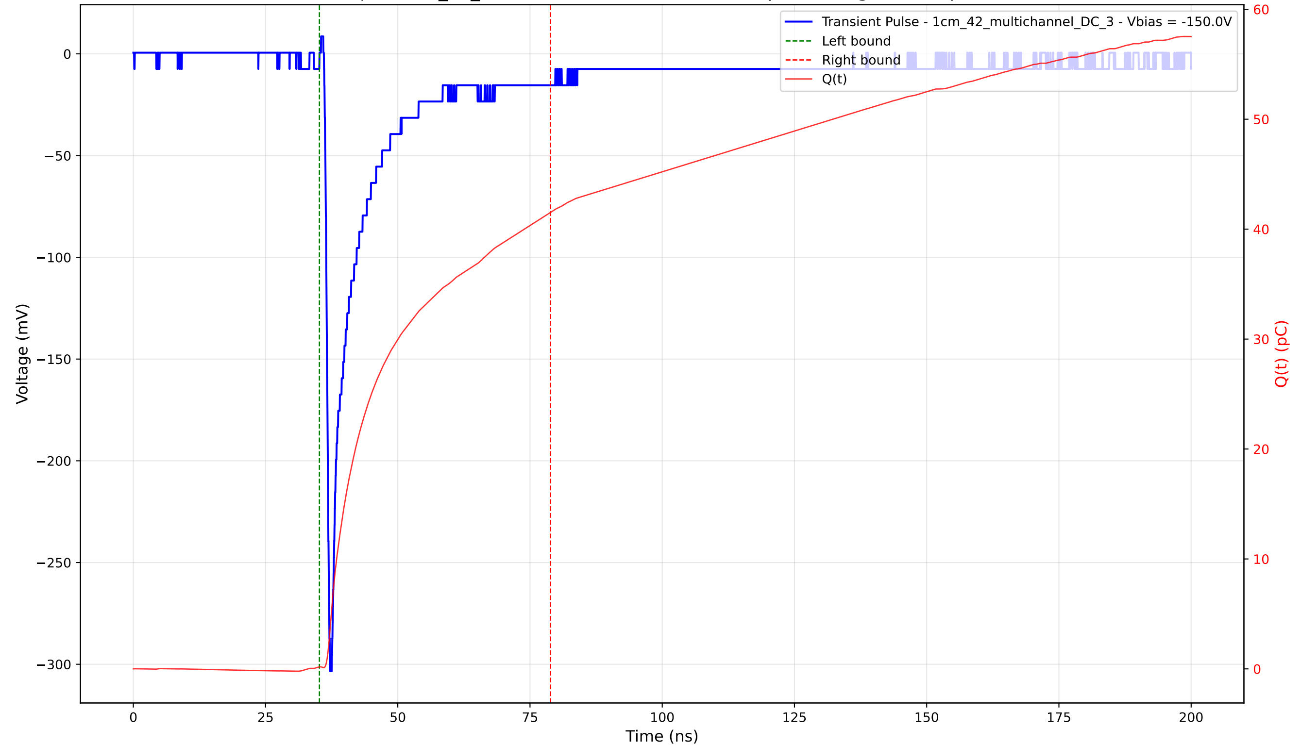
Transient Pulse - Sample: 1cm_42_multichannel - Position: 4610.0 \mu\text{m} - Charge: 41.33 pC - Rise Time: 0.84 ns
