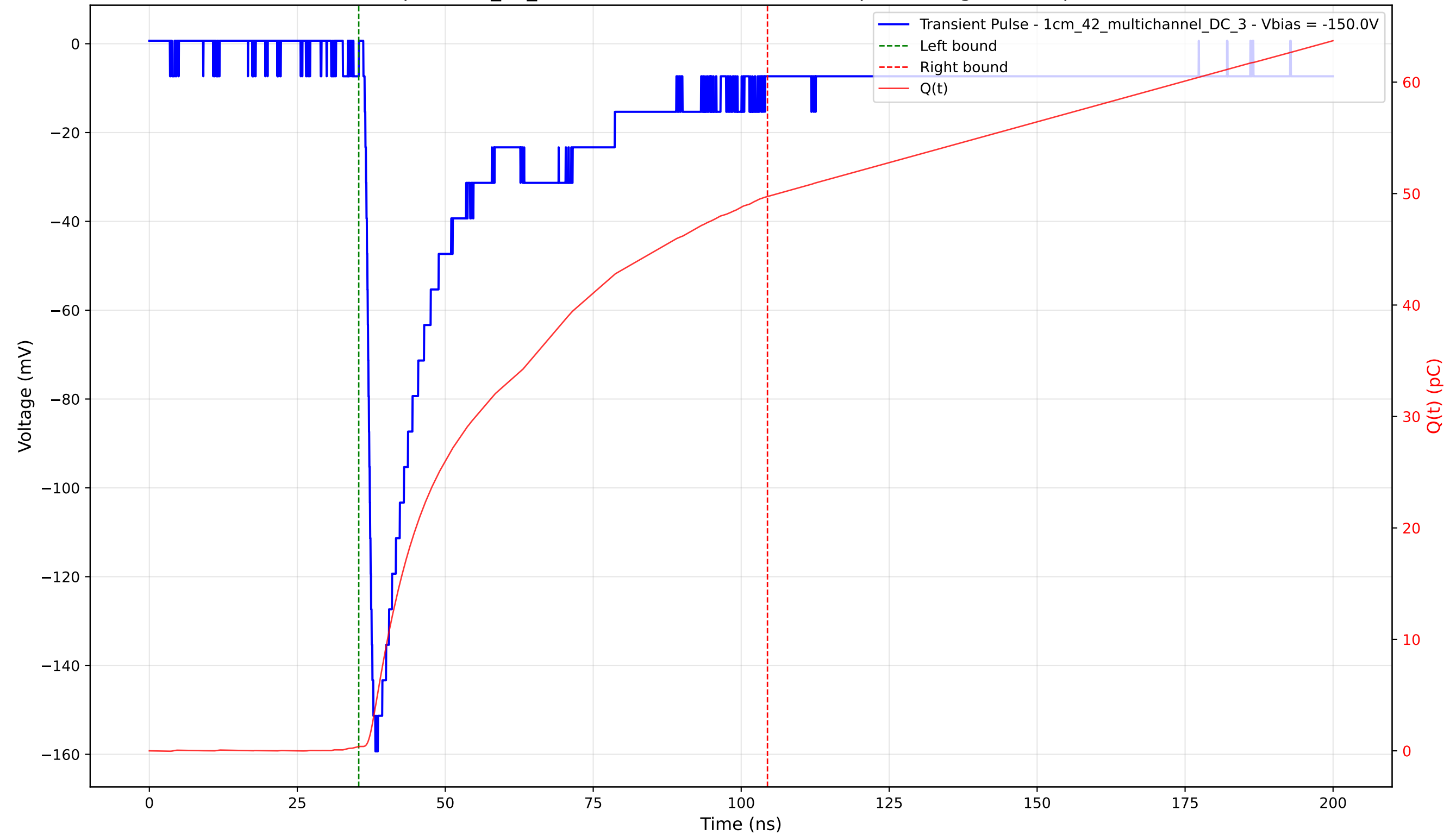
Transient Pulse - Sample: 1cm_42_multichannel - Position: 1235.0 \mu\text{m} - Charge: 49.35 pC - Rise Time: 1.36 ns
