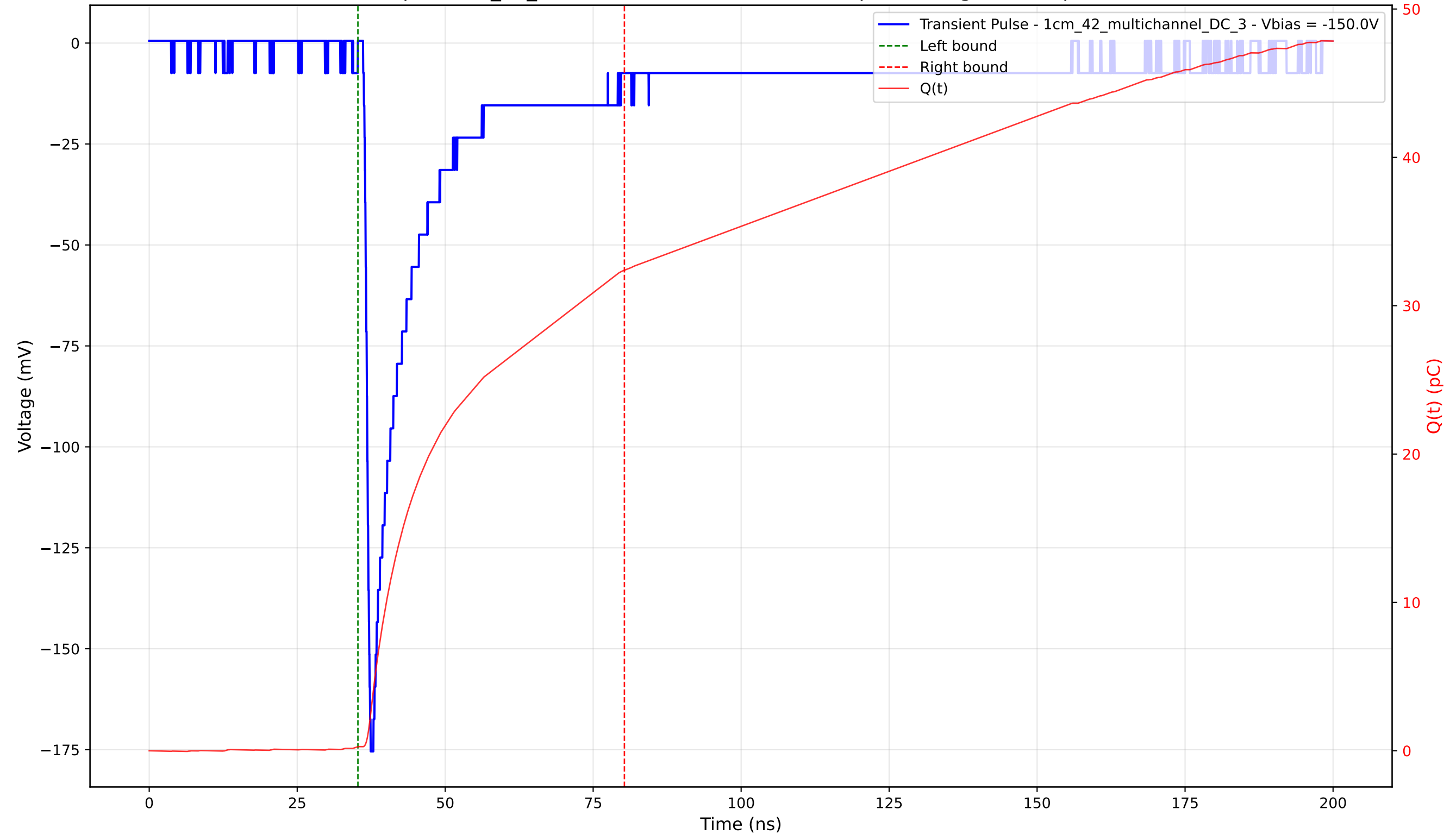
Transient Pulse - Sample: 1cm_42_multichannel - Position: 4315.0 \mu\text{m} - Charge: 32.11 pC - Rise Time: 0.87 ns
