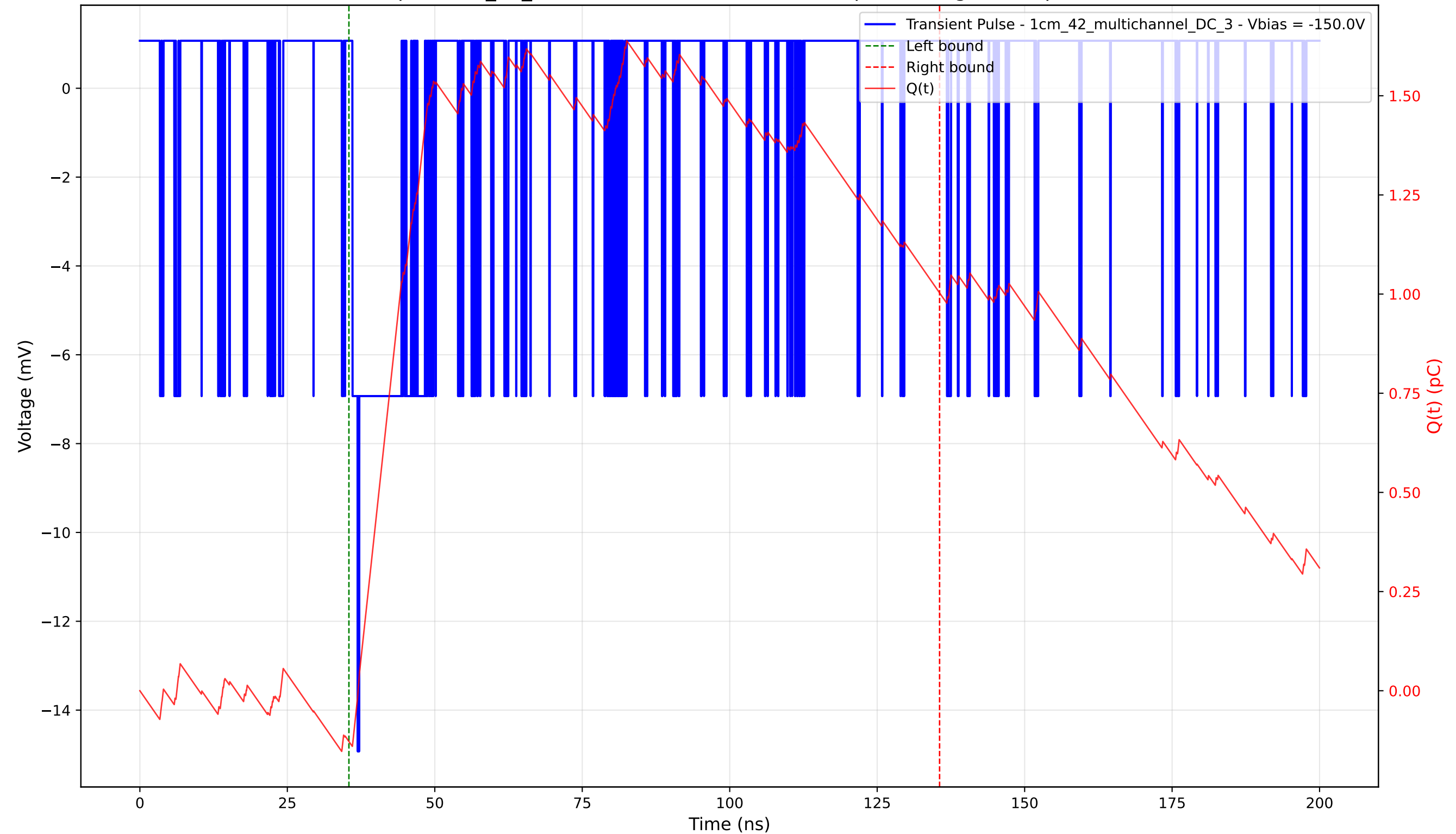
Transient Pulse - Sample: 1cm_42_multichannel - Position: 4915.0 \mu\text{m} - Charge: 1.13 pC - Rise Time: 0.90 ns
