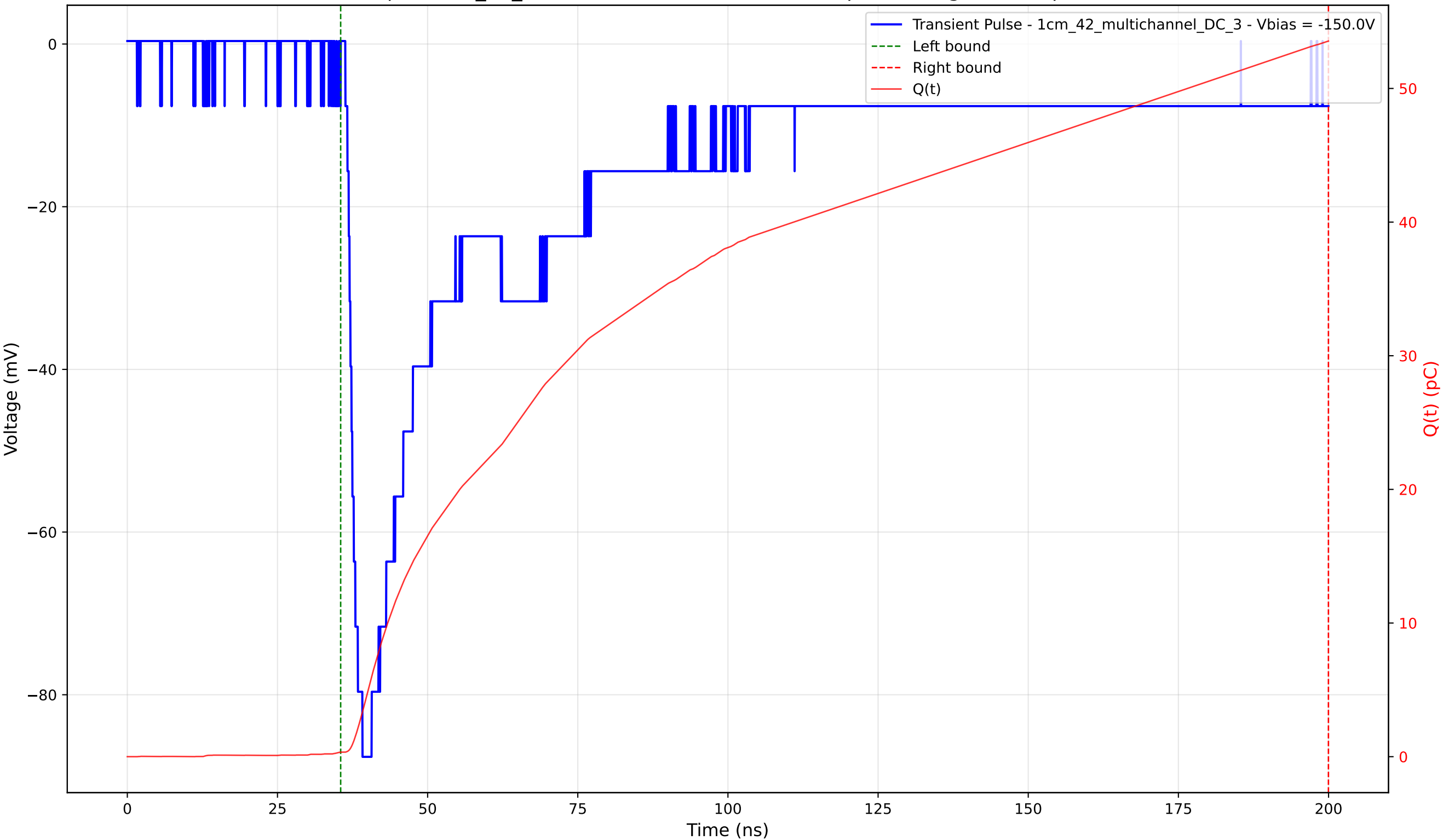
Transient Pulse - Sample: 1cm_42_multichannel - Position: 2800.0 \mu\text{m} - Charge: 53.21 pC - Rise Time: 1.76 ns
