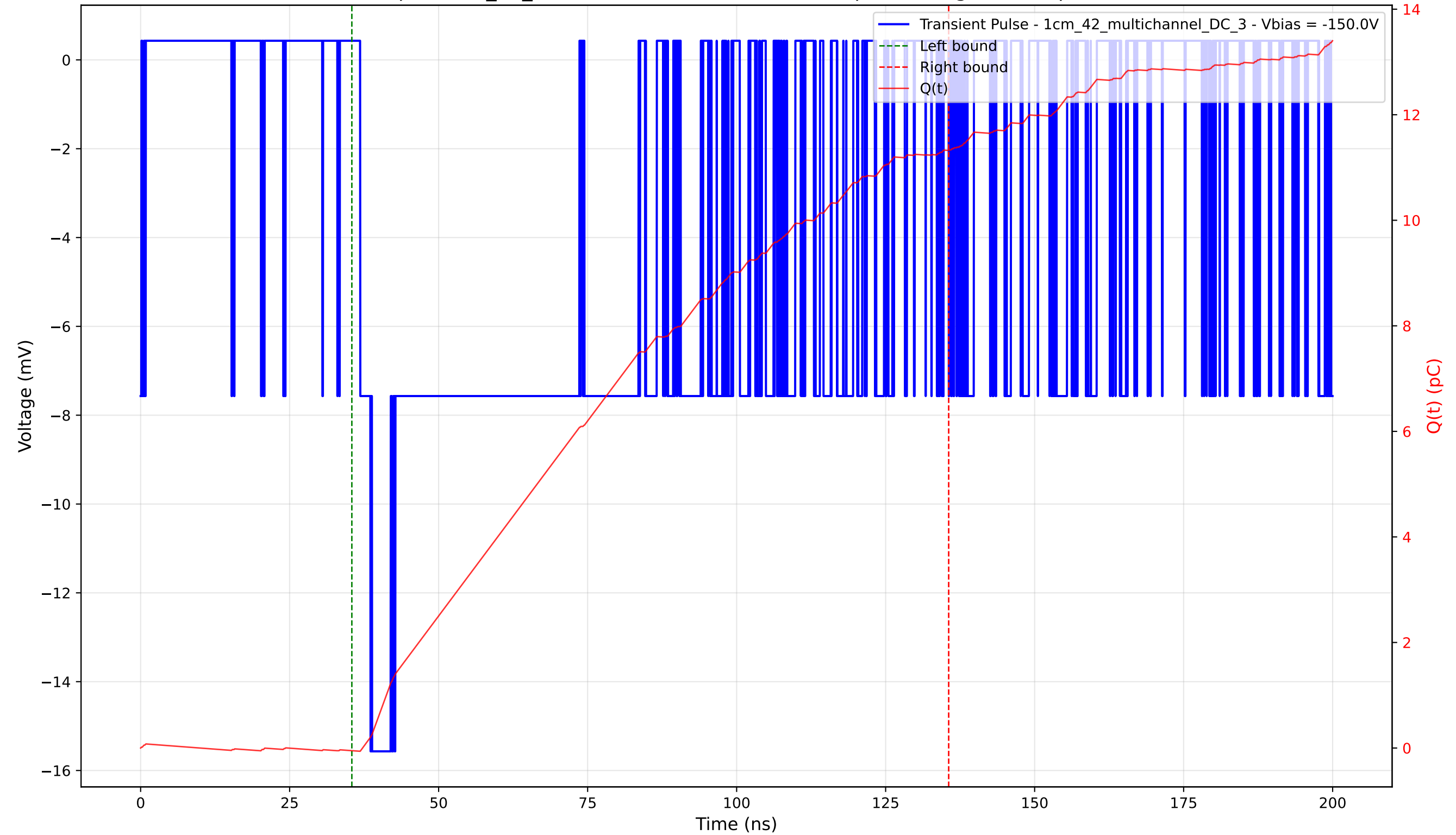
Transient Pulse - Sample: 1cm_42_multichannel - Position: 2400.0 \mu\text{m} - Charge: 11.37 pC - Rise Time: 1.74 ns
