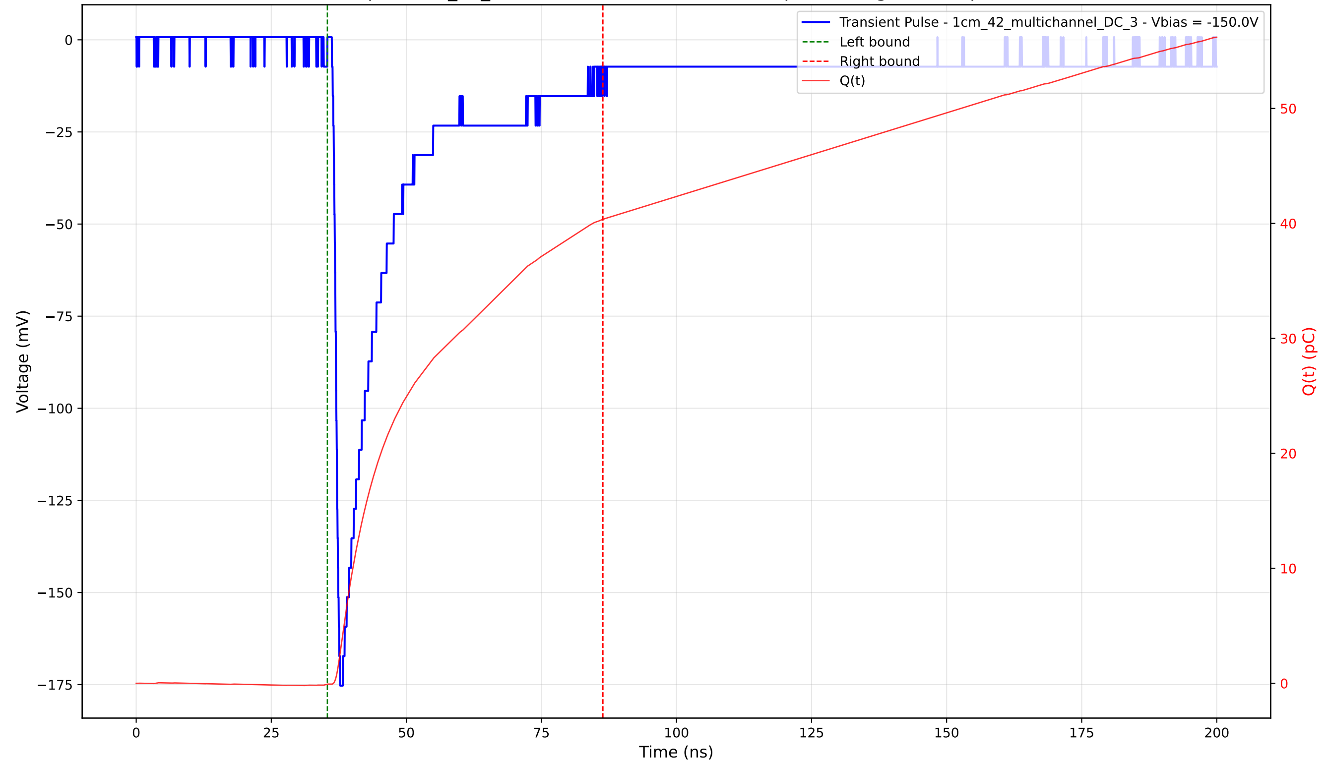
Transient Pulse - Sample: 1cm_42_multichannel - Position: 4030.0 \mu\text{m} - Charge: 40.42 pC - Rise Time: 1.01 ns
