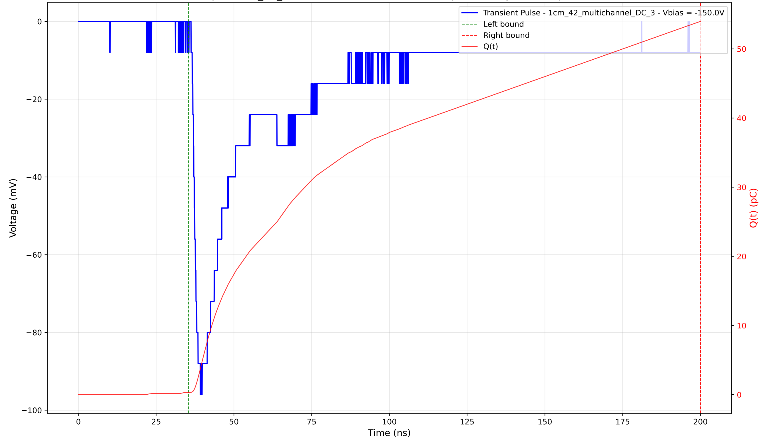
Transient Pulse - Sample: 1cm_42_multichannel - Position: 2955.0 \mu\text{m} - Charge: 53.67 pC - Rise Time: 1.90 ns
