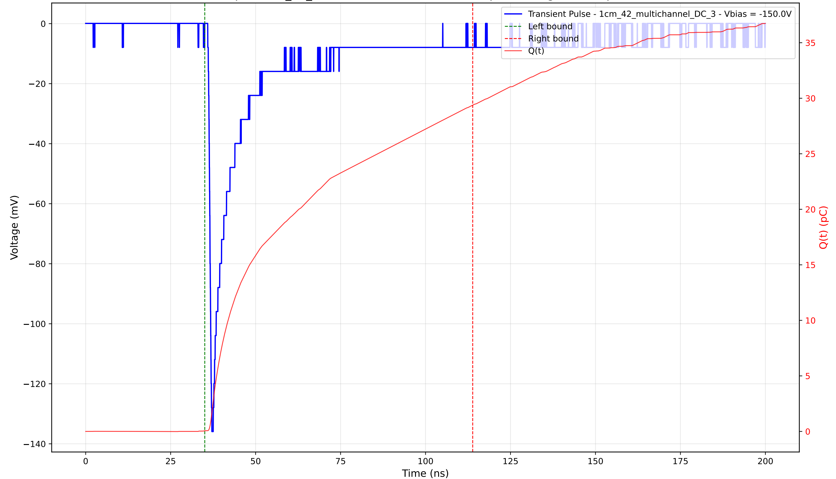
Transient Pulse - Sample: 1cm_42_multichannel - Position: 400.0 \mu\text{m} - Charge: 29.32 pC - Rise Time: 0.93 ns
