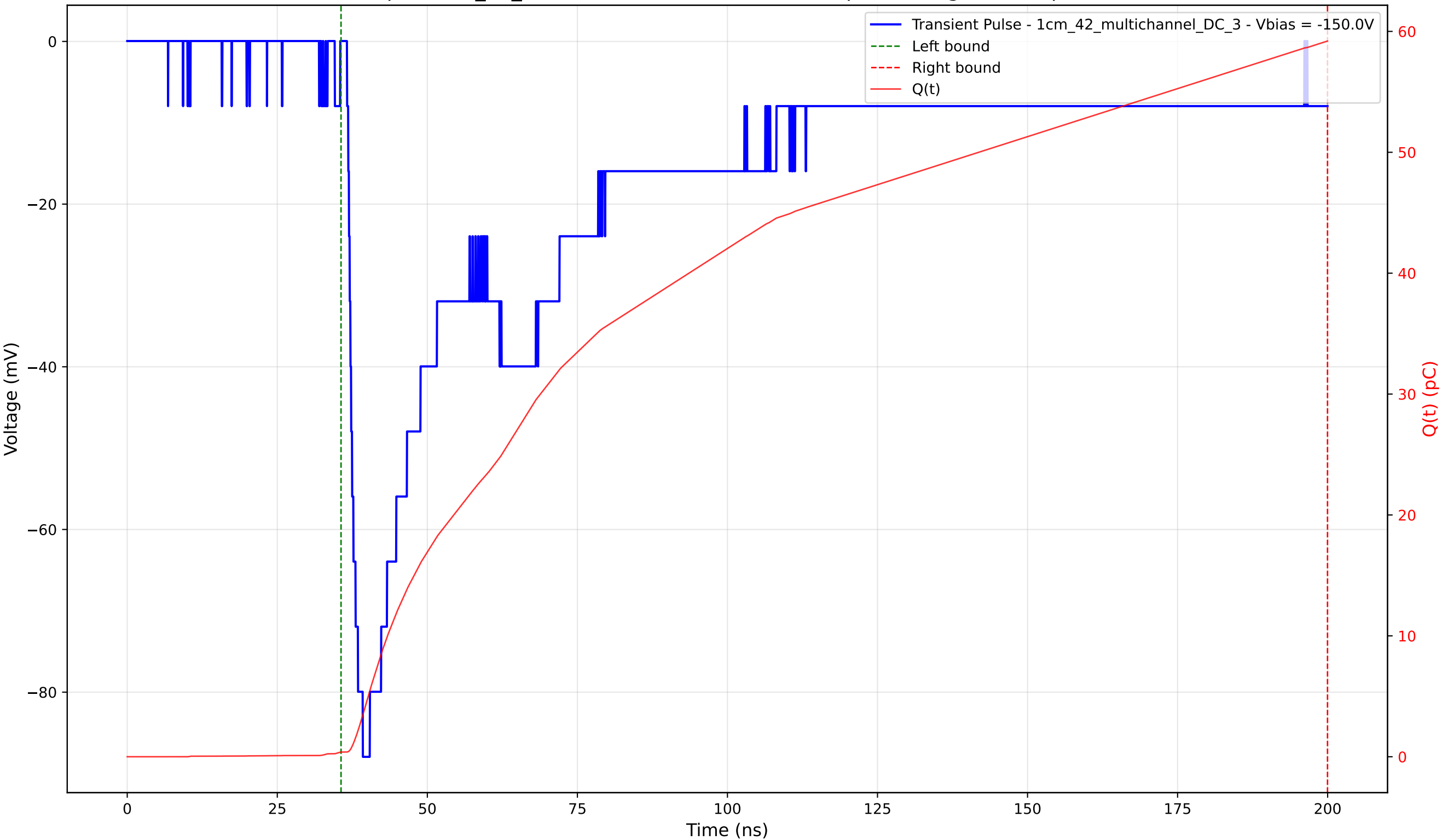
Transient Pulse - Sample: 1cm_42_multichannel - Position: 2250.0 \mu\text{m} - Charge: 58.82 pC - Rise Time: 1.64 ns
