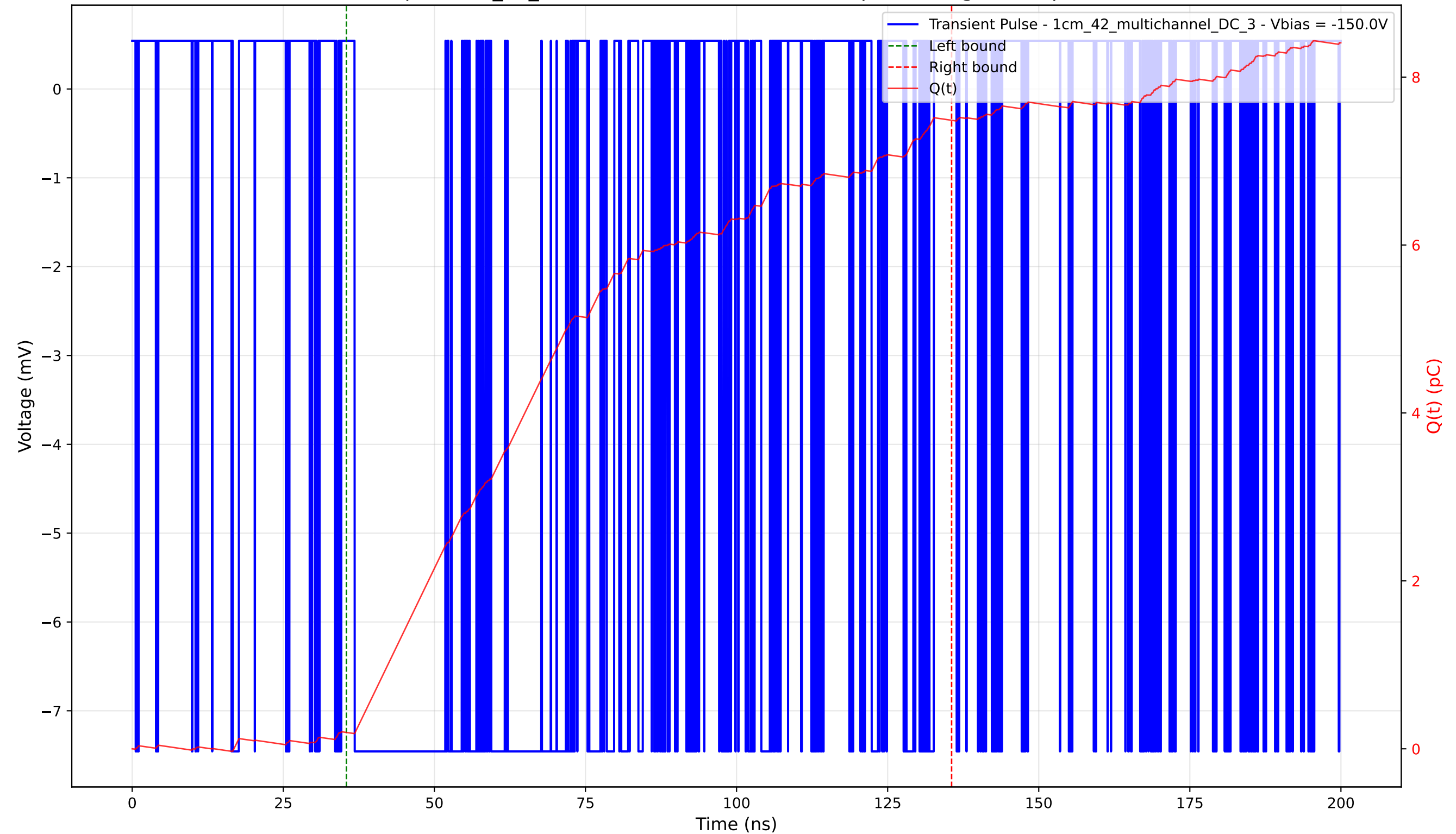
Transient Pulse - Sample: 1cm_42_multichannel - Position: 1355.0 \mu\text{m} - Charge: 7.29 pC - Rise Time: 0.02 ns
