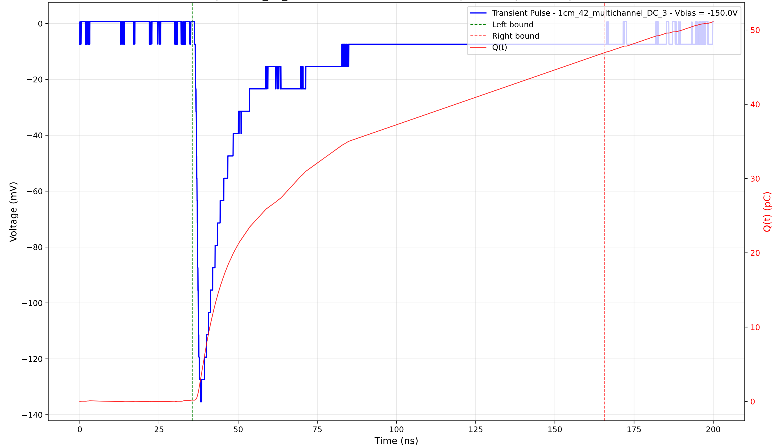
Transient Pulse - Sample: 1cm_42_multichannel - Position: 3815.0 \mu\text{m} - Charge: 46.77 pC - Rise Time: 1.28 ns
