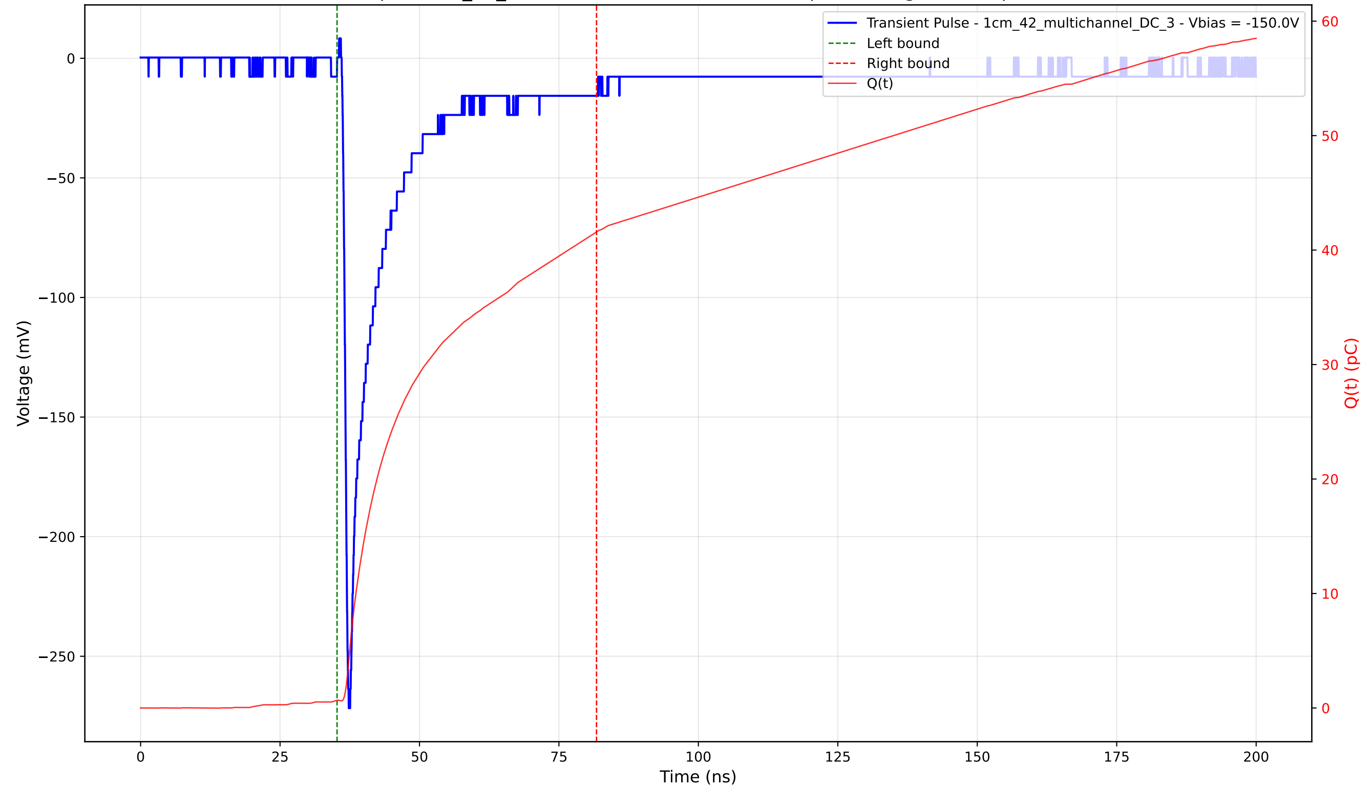
Transient Pulse - Sample: 1cm_42_multichannel - Position: 4525.0 \mu\text{m} - Charge: 40.92 pC - Rise Time: 0.85 ns
