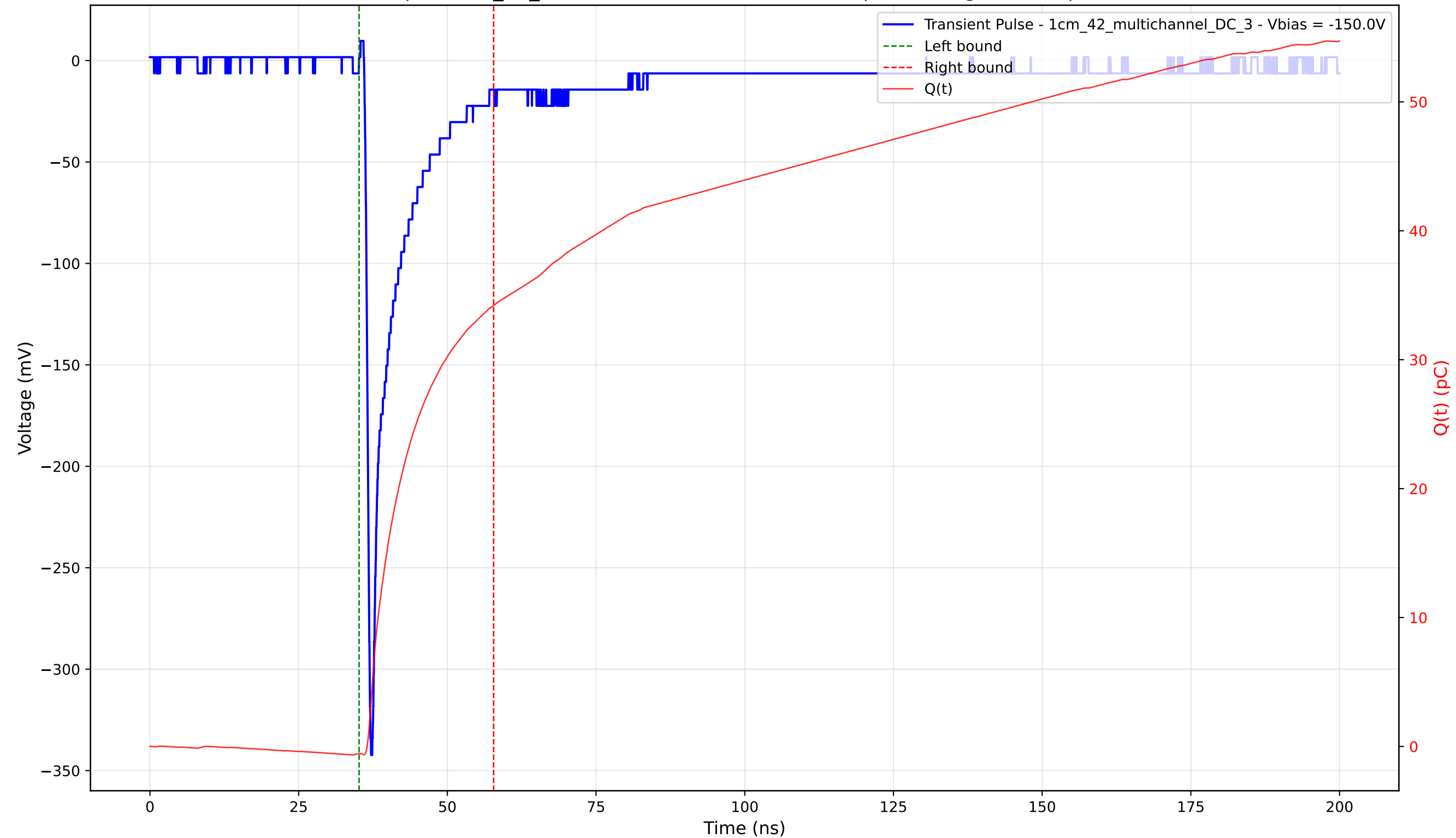
Transient Pulse - Sample: 1cm_42_multichannel - Position: 4695.0 \mu\text{m} - Charge: 34.73 pC - Rise Time: 0.80 ns
