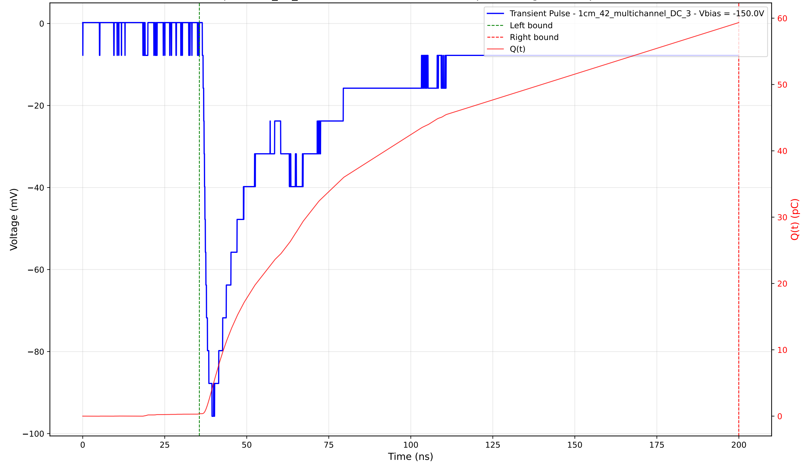
Transient Pulse - Sample: 1cm_42_multichannel - Position: 2070.0 \mu\text{m} - Charge: 58.97 pC - Rise Time: 1.76 ns
