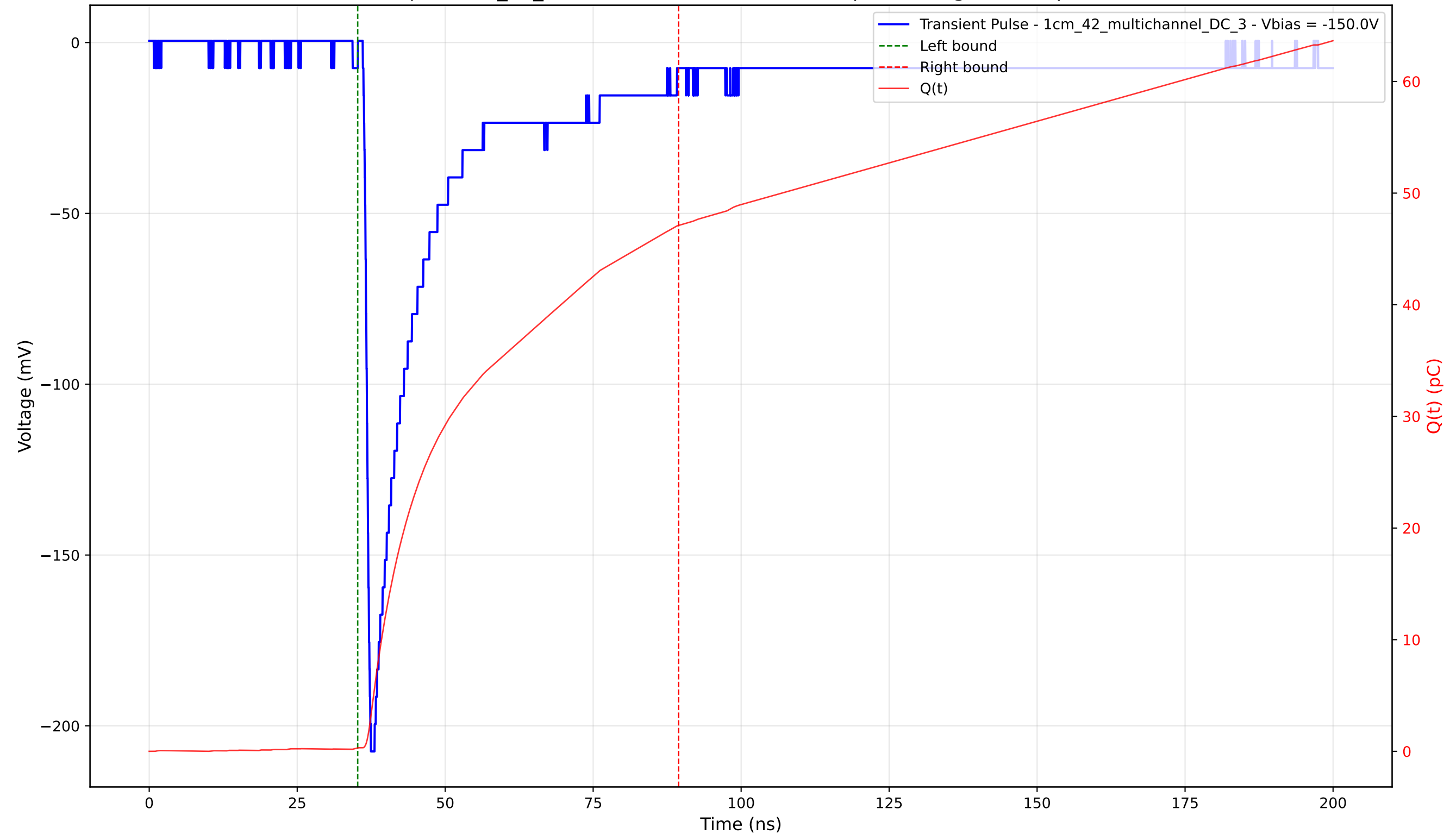
Transient Pulse - Sample: 1cm_42_multichannel - Position: 750.0 \mu\text{m} - Charge: 46.79 pC - Rise Time: 0.99 ns
