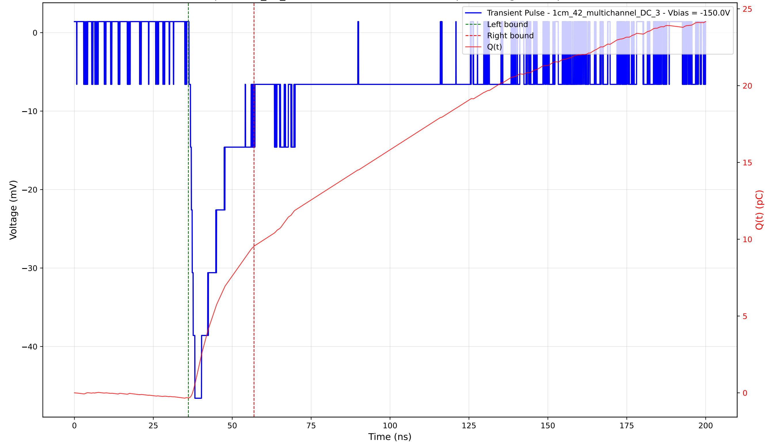
Transient Pulse - Sample: 1cm_42_multichannel - Position: 3430.0 \mu\text{m} - Charge: 9.88 pC - Rise Time: 1.87 ns
