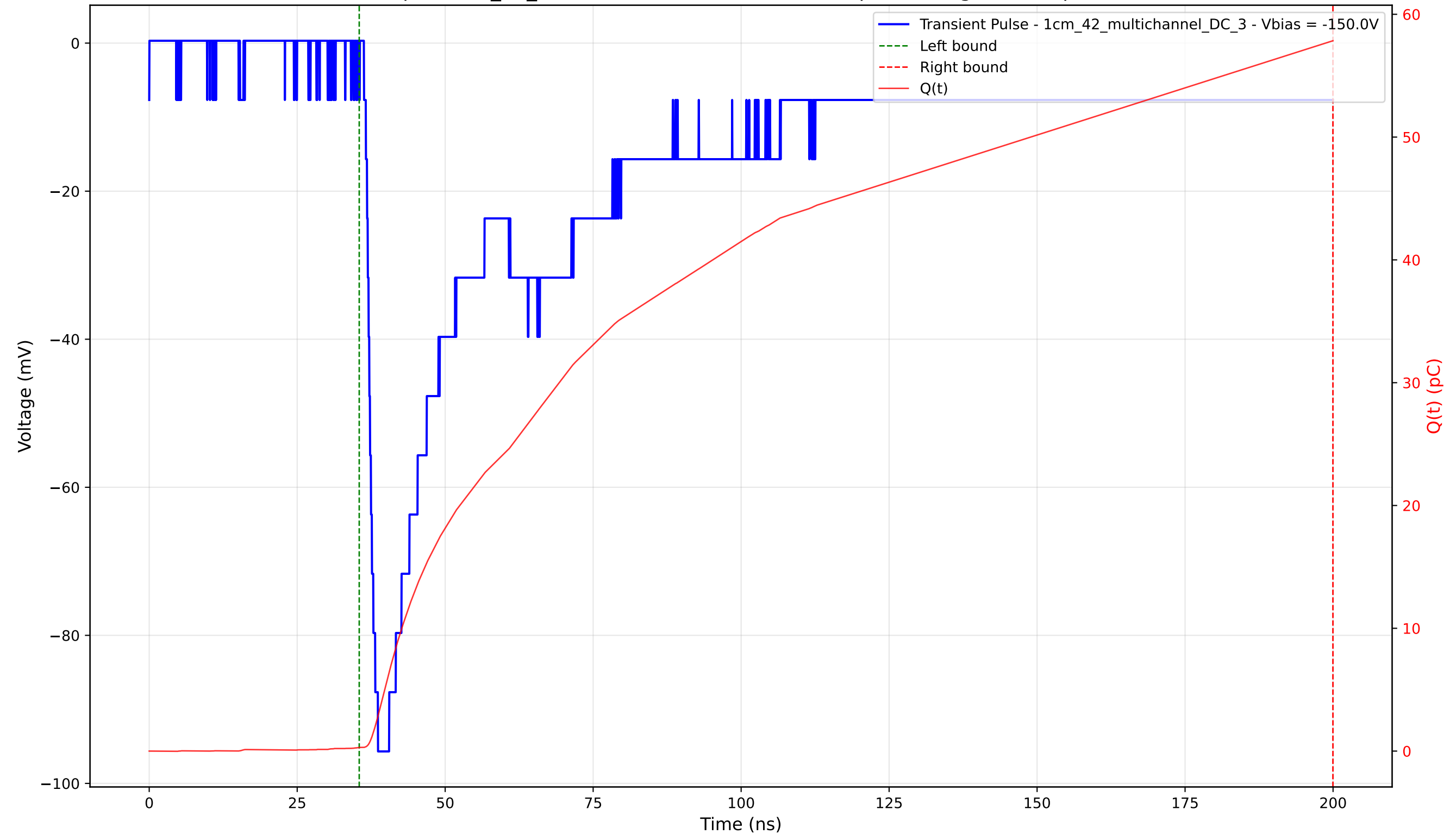
Transient Pulse - Sample: 1cm_42_multichannel - Position: 1955.0 \mu\text{m} - Charge: 57.56 pC - Rise Time: 1.60 ns
