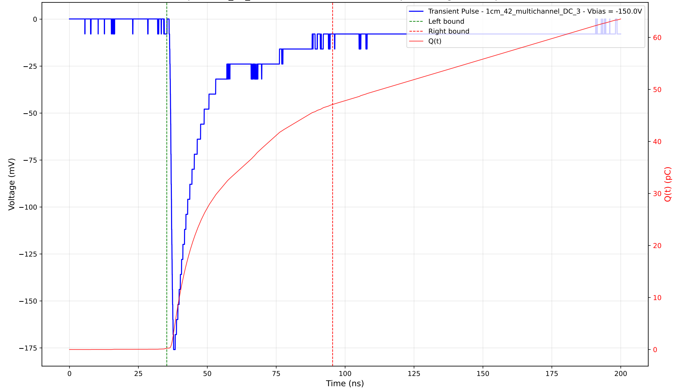
Transient Pulse - Sample: 1cm_42_multichannel - Position: 1005.0 \mu\text{m} - Charge: 46.84 pC - Rise Time: 1.08 ns
