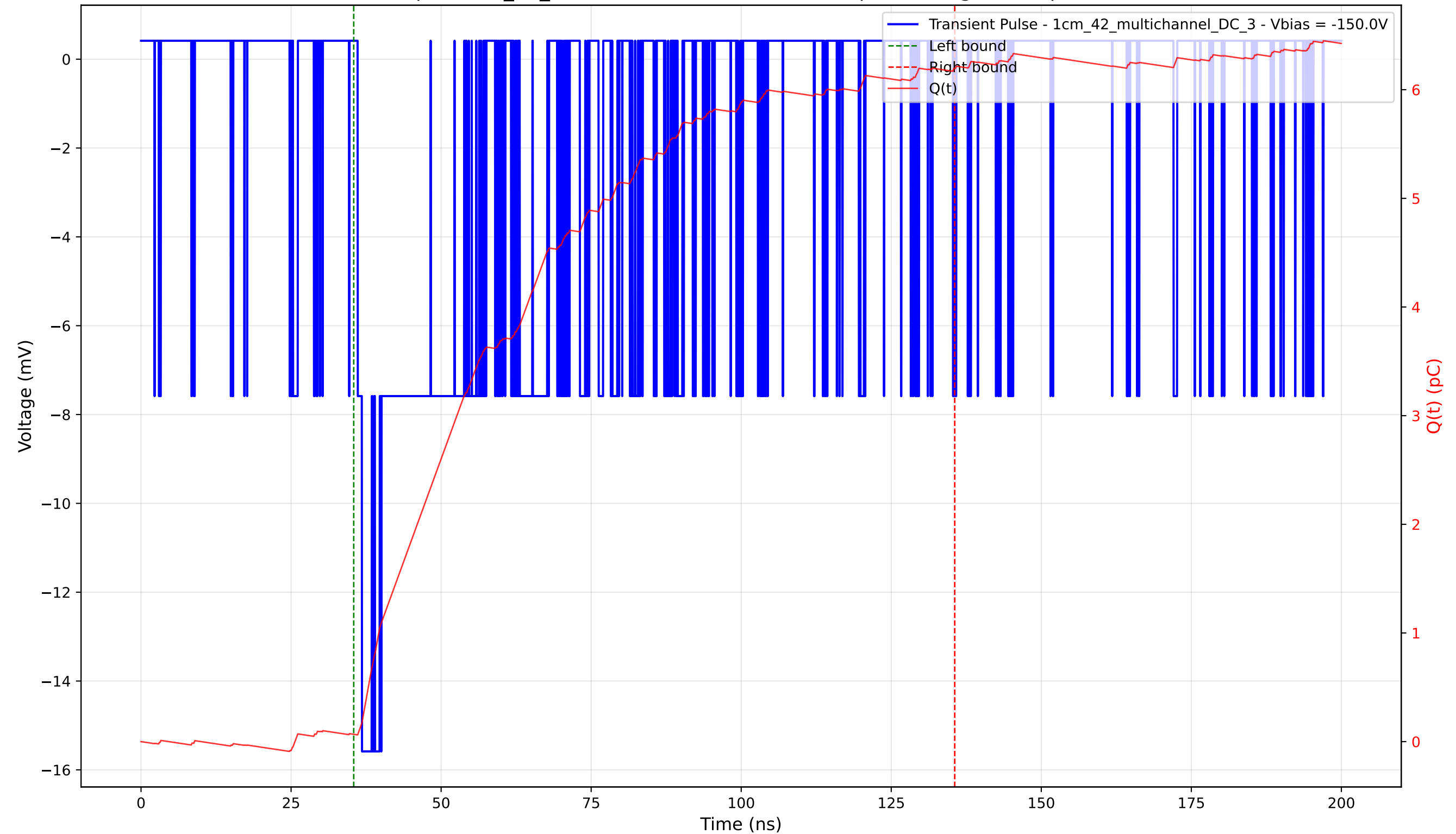
Transient Pulse - Sample: 1cm_42_multichannel - Position: 345.0 \mu\text{m} - Charge: 6.13 pC - Rise Time: 0.72 ns
