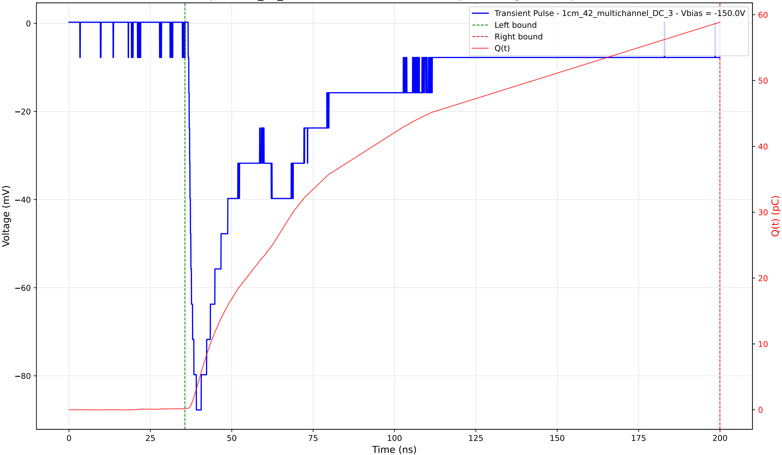
Transient Pulse - Sample: 1cm_42_multichannel - Position: 2240.0 \mu\text{m} - Charge: 58.63 pC - Rise Time: 1.58 ns
