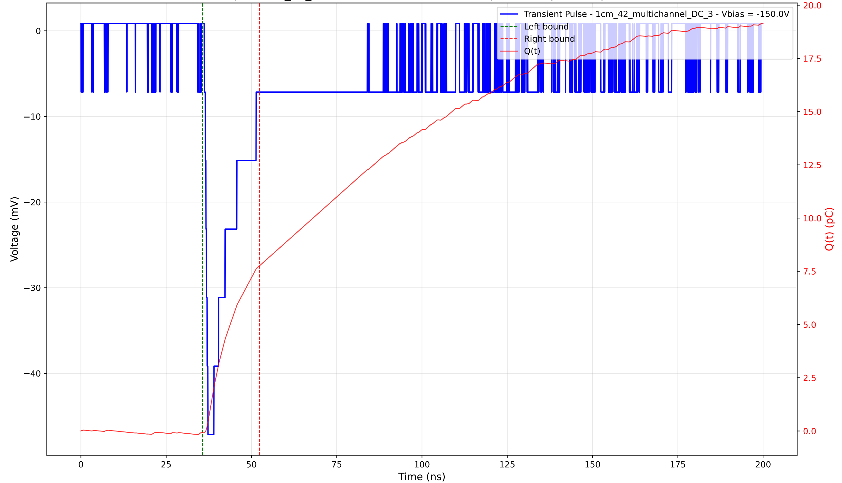
Transient Pulse - Sample: 1cm_42_multichannel - Position: 820.0 \mu\text{m} - Charge: 7.83 pC - Rise Time: 1.09 ns
