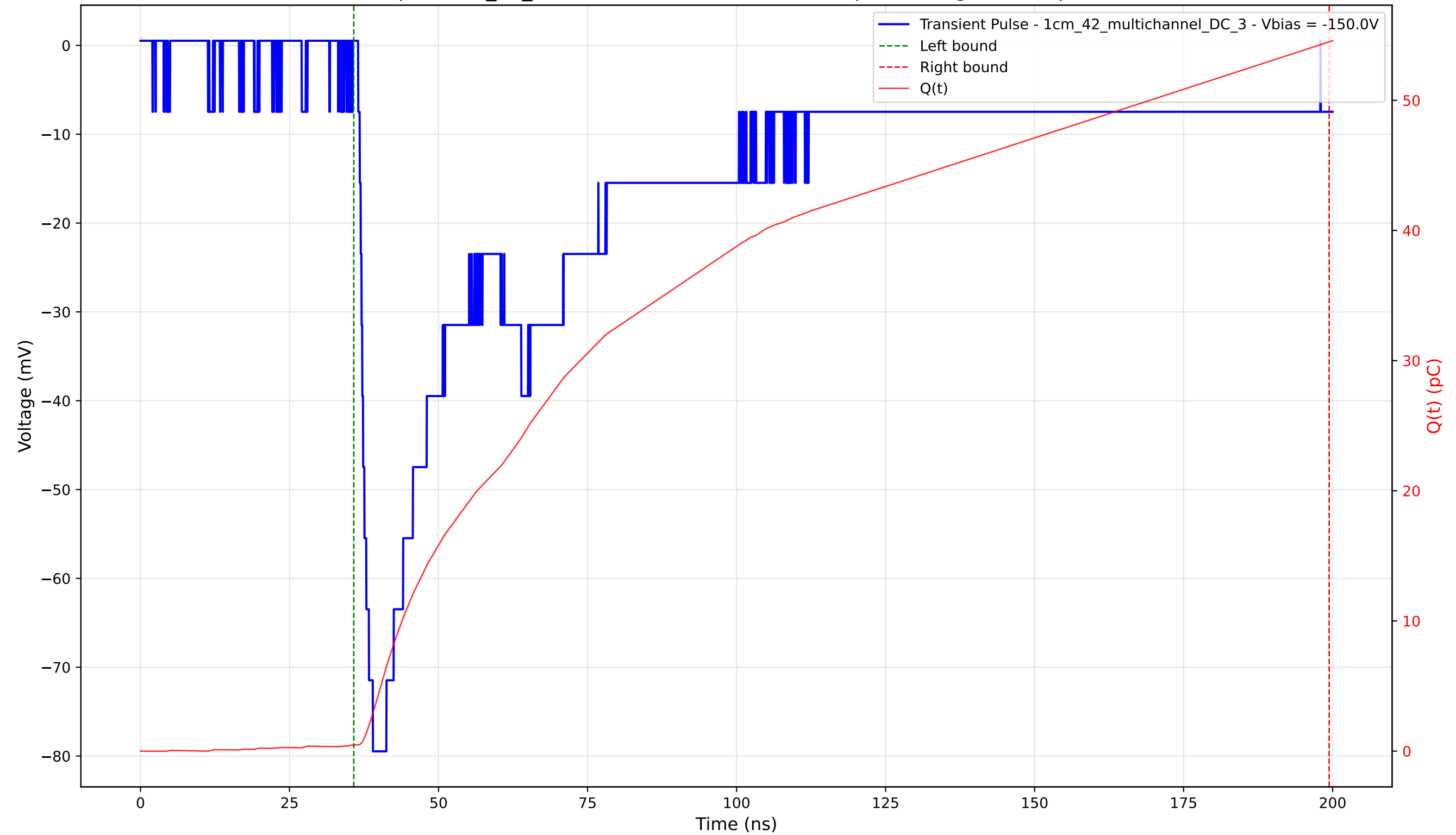
Transient Pulse - Sample: 1cm_42_multichannel - Position: 2575.0 \mu\text{m} - Charge: 54.02 pC - Rise Time: 2.22 ns
