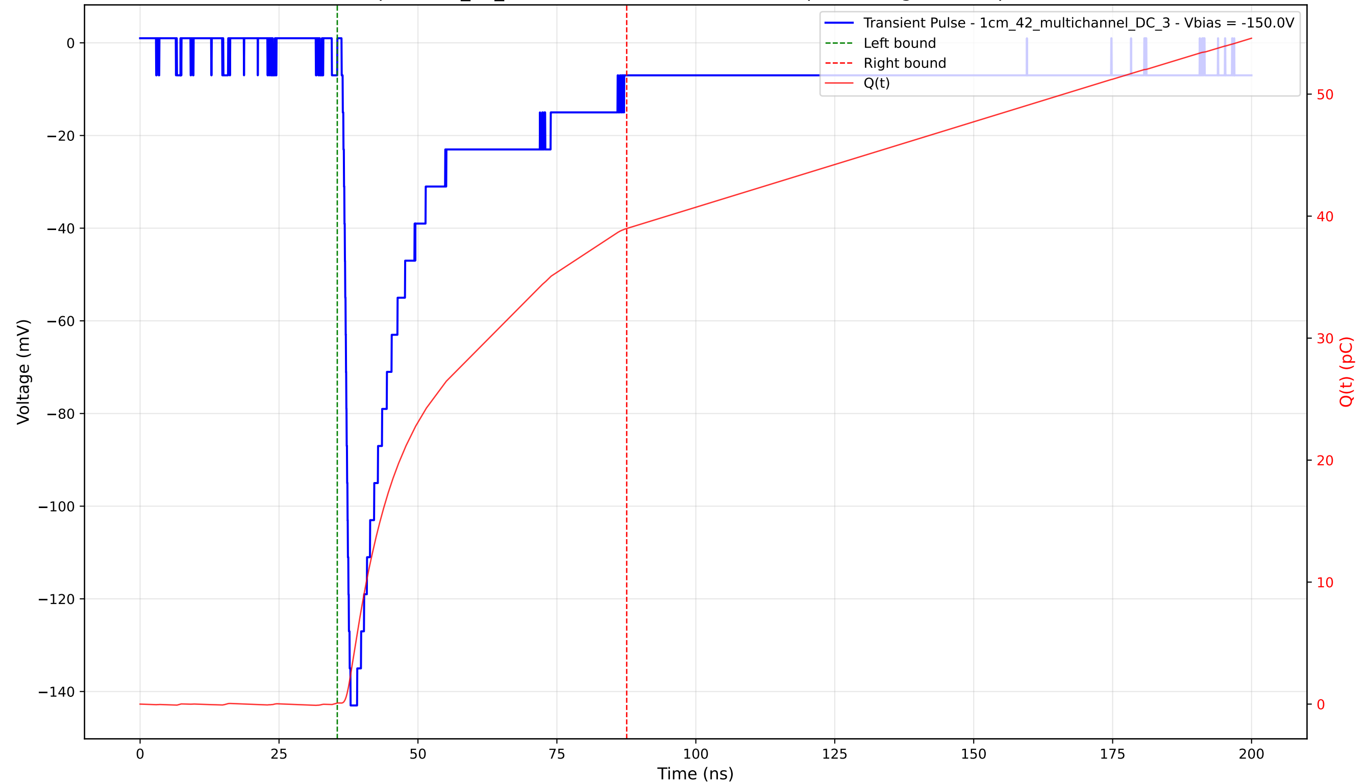
Transient Pulse - Sample: 1cm_42_multichannel - Position: 3790.0 \mu\text{m} - Charge: 38.89 pC - Rise Time: 1.24 ns
