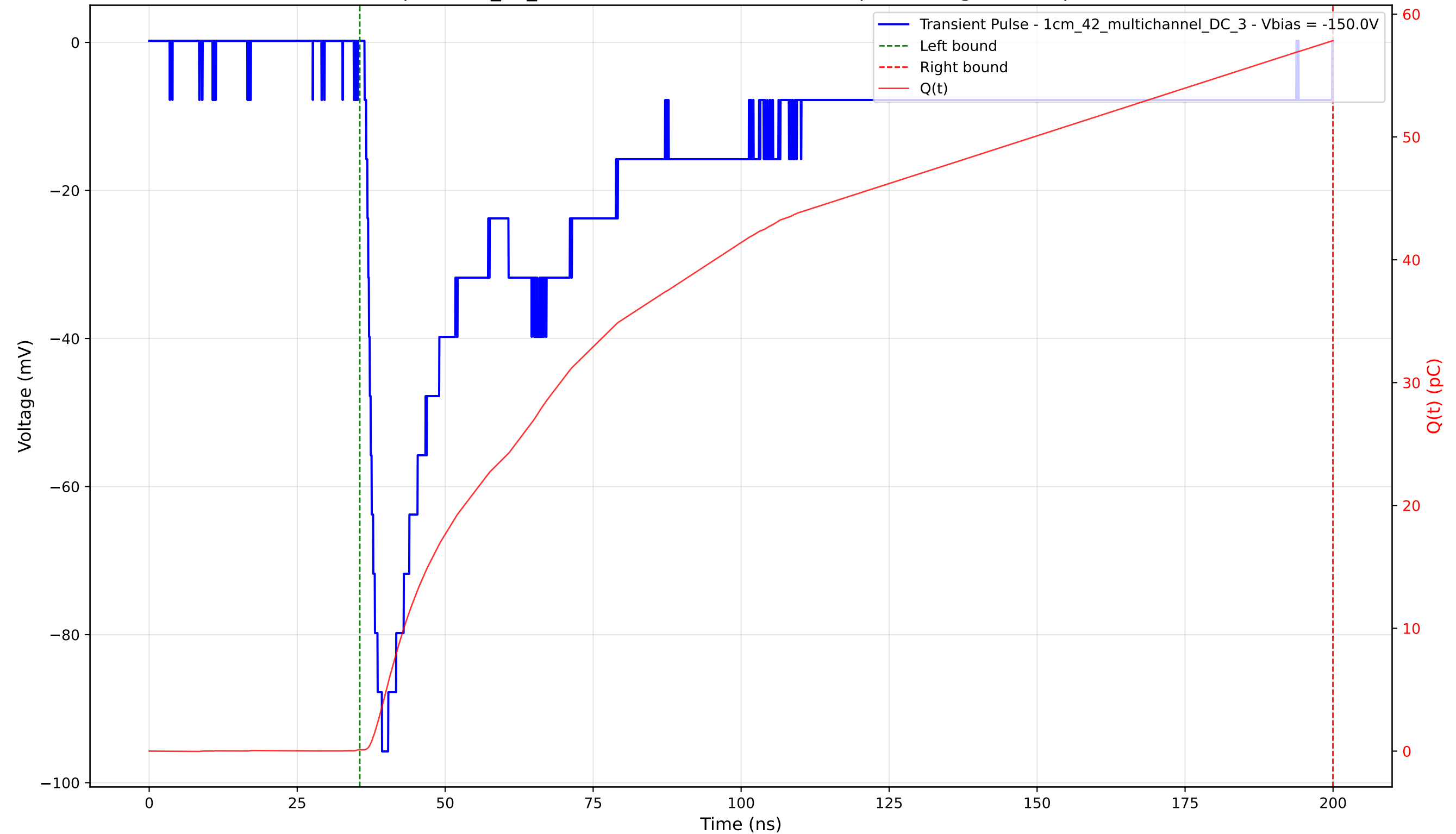
Transient Pulse - Sample: 1cm_42_multichannel - Position: 2745.0 \mu\text{m} - Charge: 57.73 pC - Rise Time: 1.94 ns
