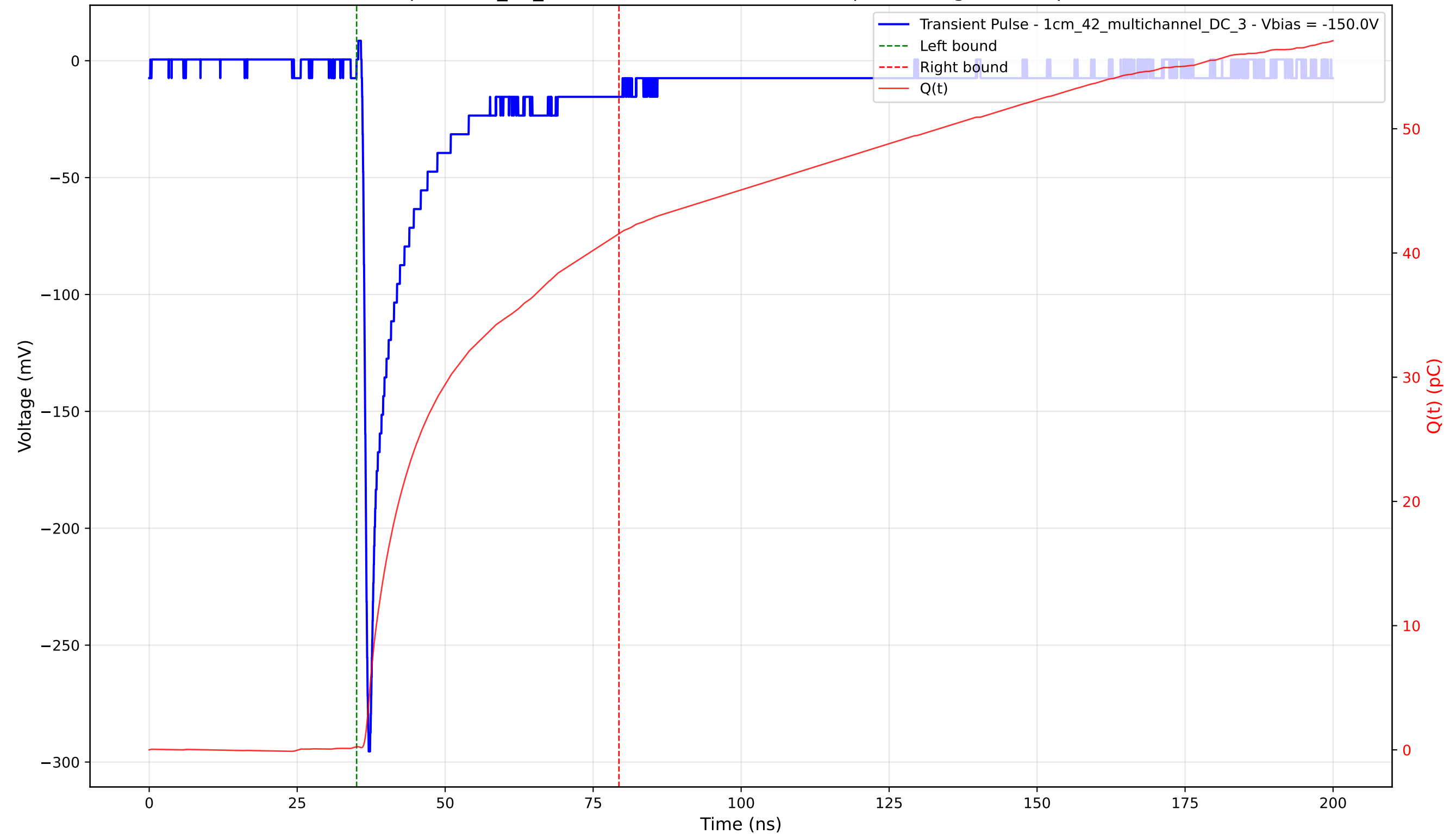
Transient Pulse - Sample: 1cm_42_multichannel - Position: 270.0 \mu\text{m} - Charge: 41.30 pC - Rise Time: 0.84 ns
