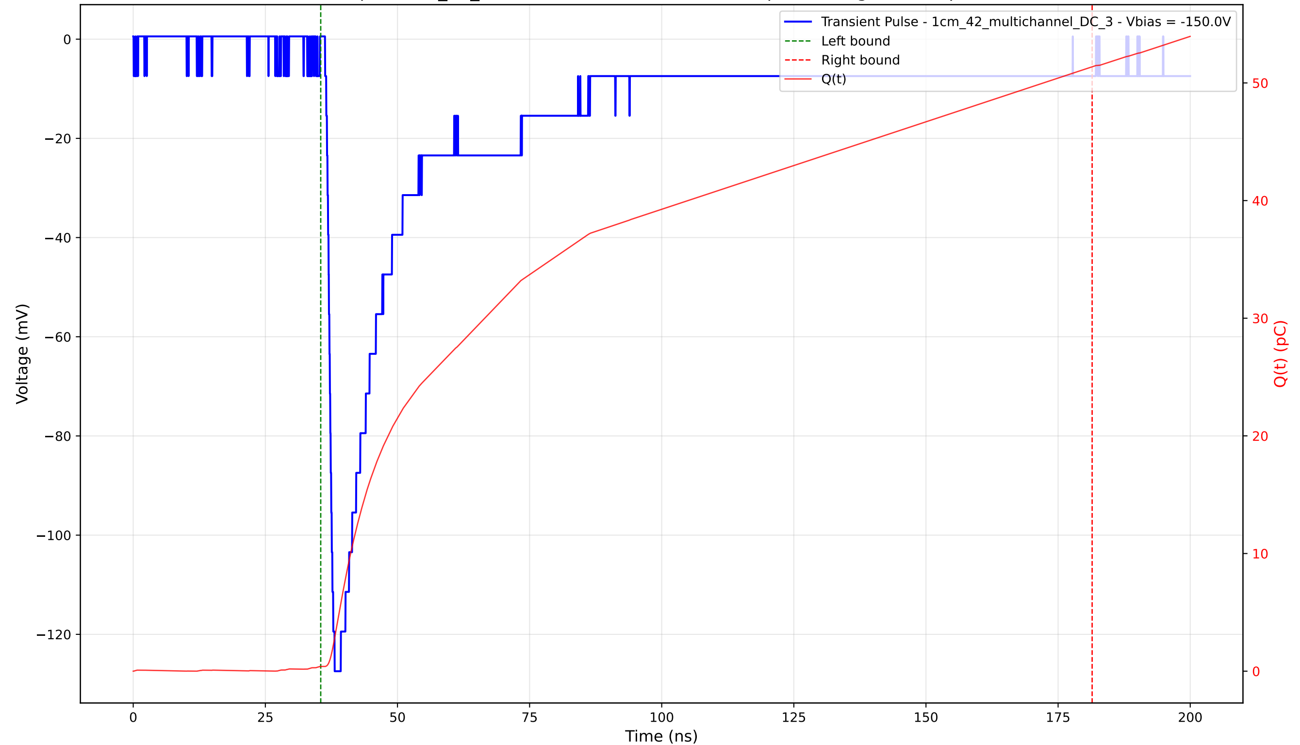
Transient Pulse - Sample: 1cm_42_multichannel - Position: 3630.0 \mu\text{m} - Charge: 50.97 pC - Rise Time: 1.33 ns
