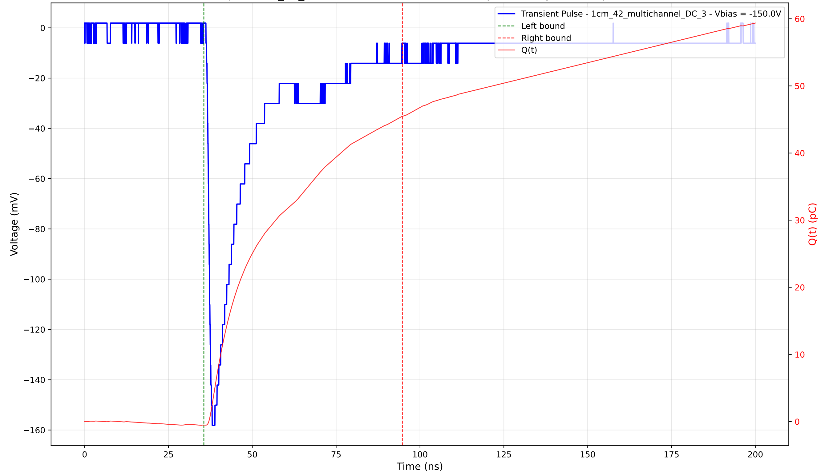
Transient Pulse - Sample: 1cm_42_multichannel - Position: 1220.0 \mu\text{m} - Charge: 45.99 pC - Rise Time: 1.30 ns
