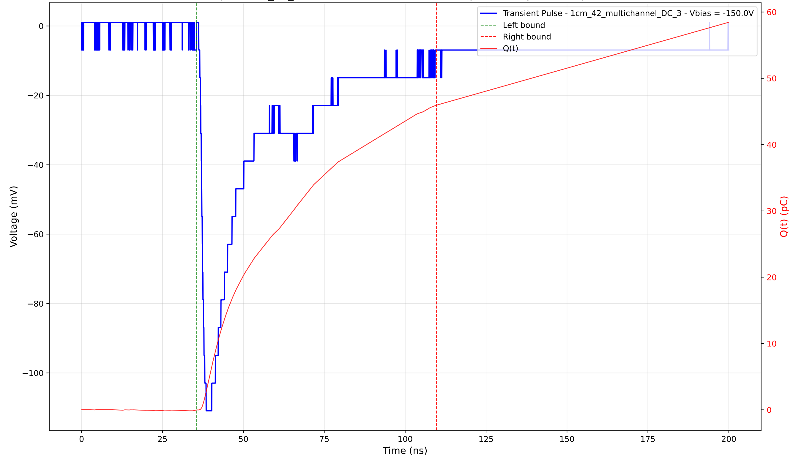
Transient Pulse - Sample: 1cm_42_multichannel - Position: 1755.0 \mu\text{m} - Charge: 45.96 pC - Rise Time: 1.55 ns
