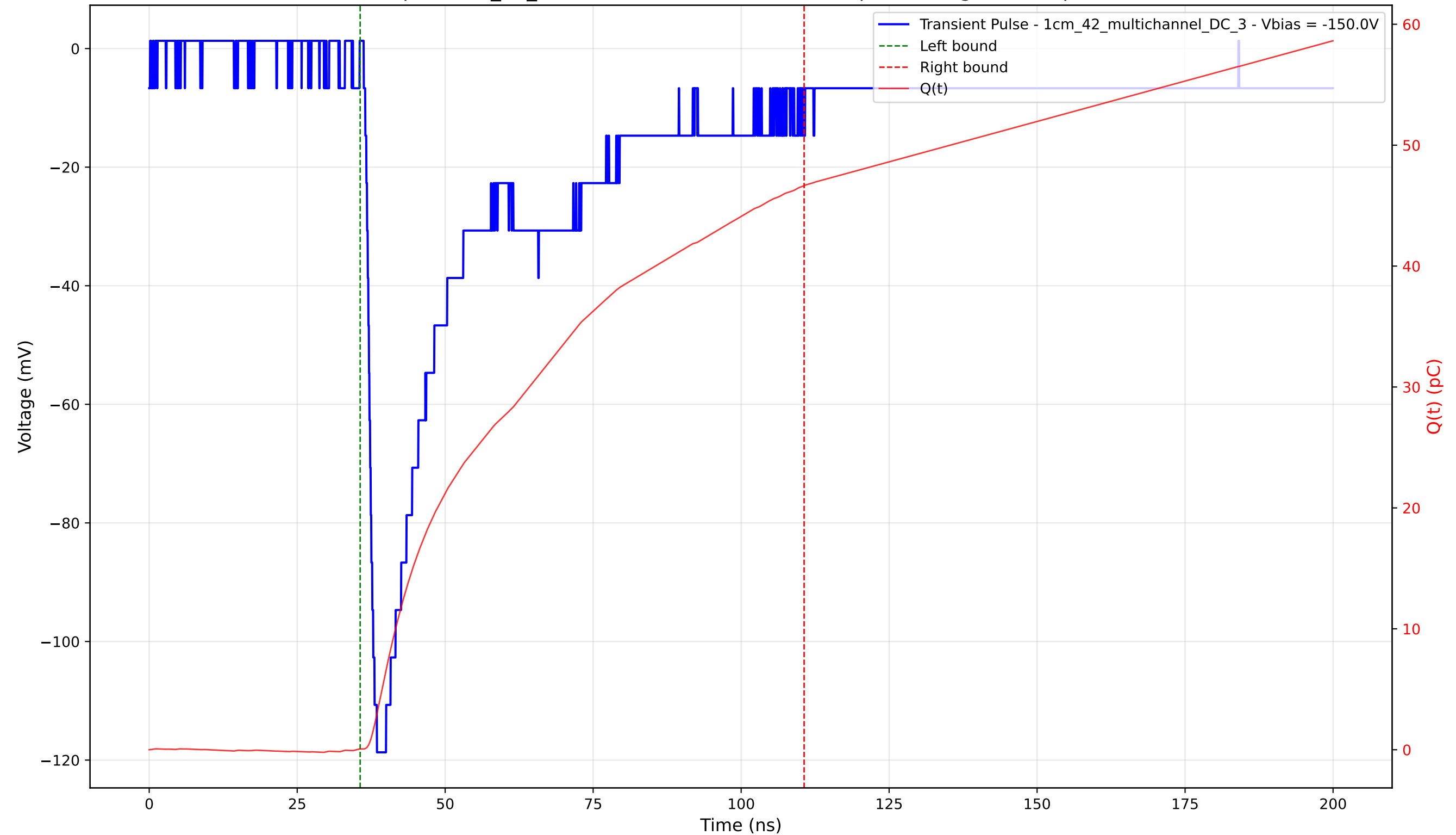
Transient Pulse - Sample: 1cm_42_multichannel - Position: 1665.0 \mu\text{m} - Charge: 46.58 pC - Rise Time: 1.57 ns
