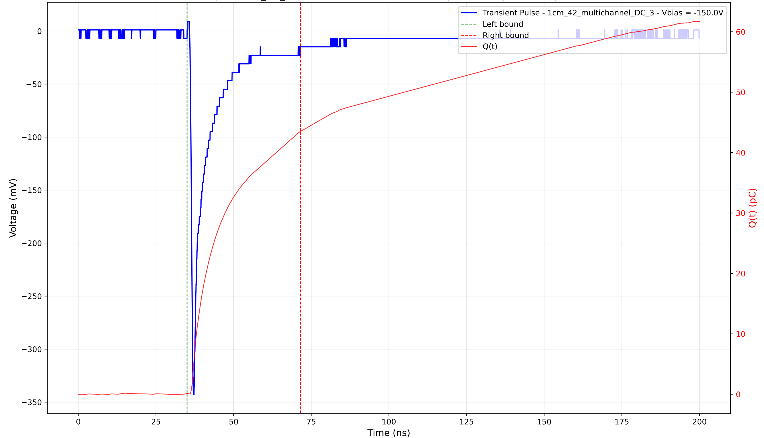
Transient Pulse - Sample: 1cm_42_multichannel - Position: 220.0 \mu\text{m} - Charge: 43.37 pC - Rise Time: 0.81 ns
