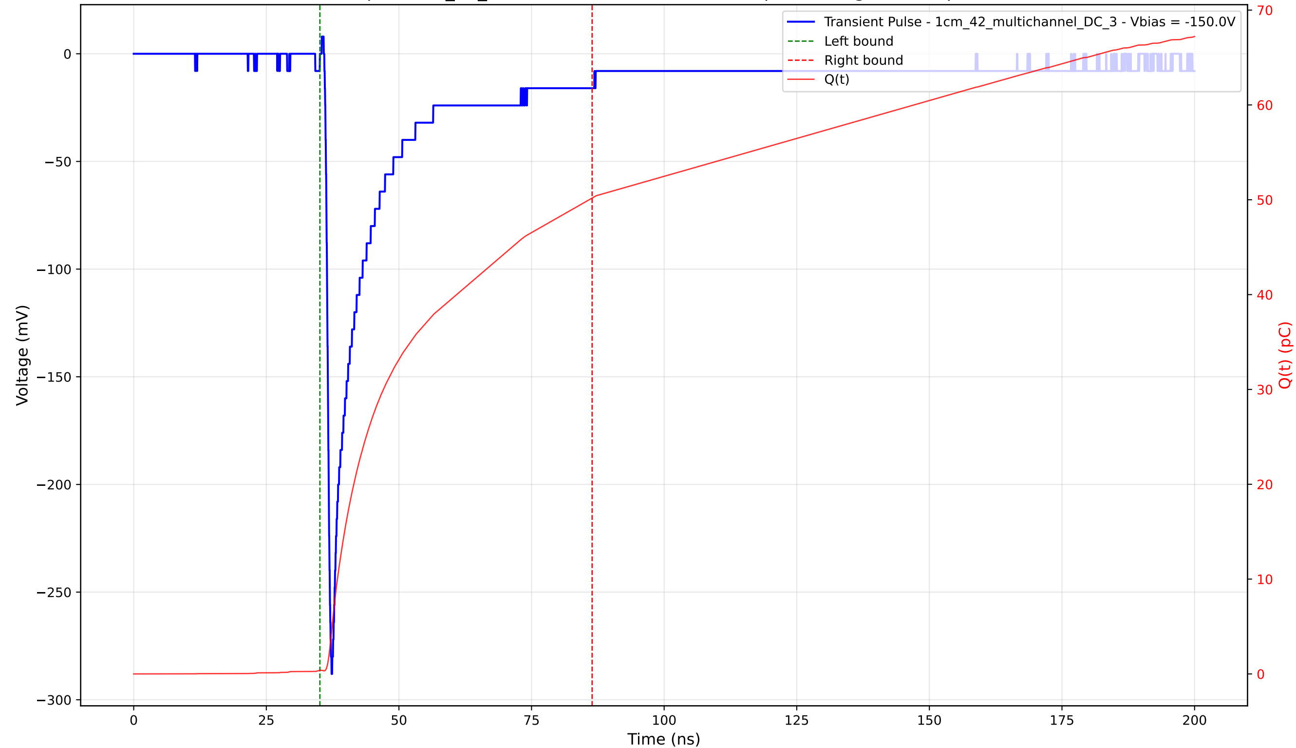
Transient Pulse - Sample: 1cm_42_multichannel - Position: 450.0 \mu\text{m} - Charge: 49.82 pC - Rise Time: 0.91 ns
