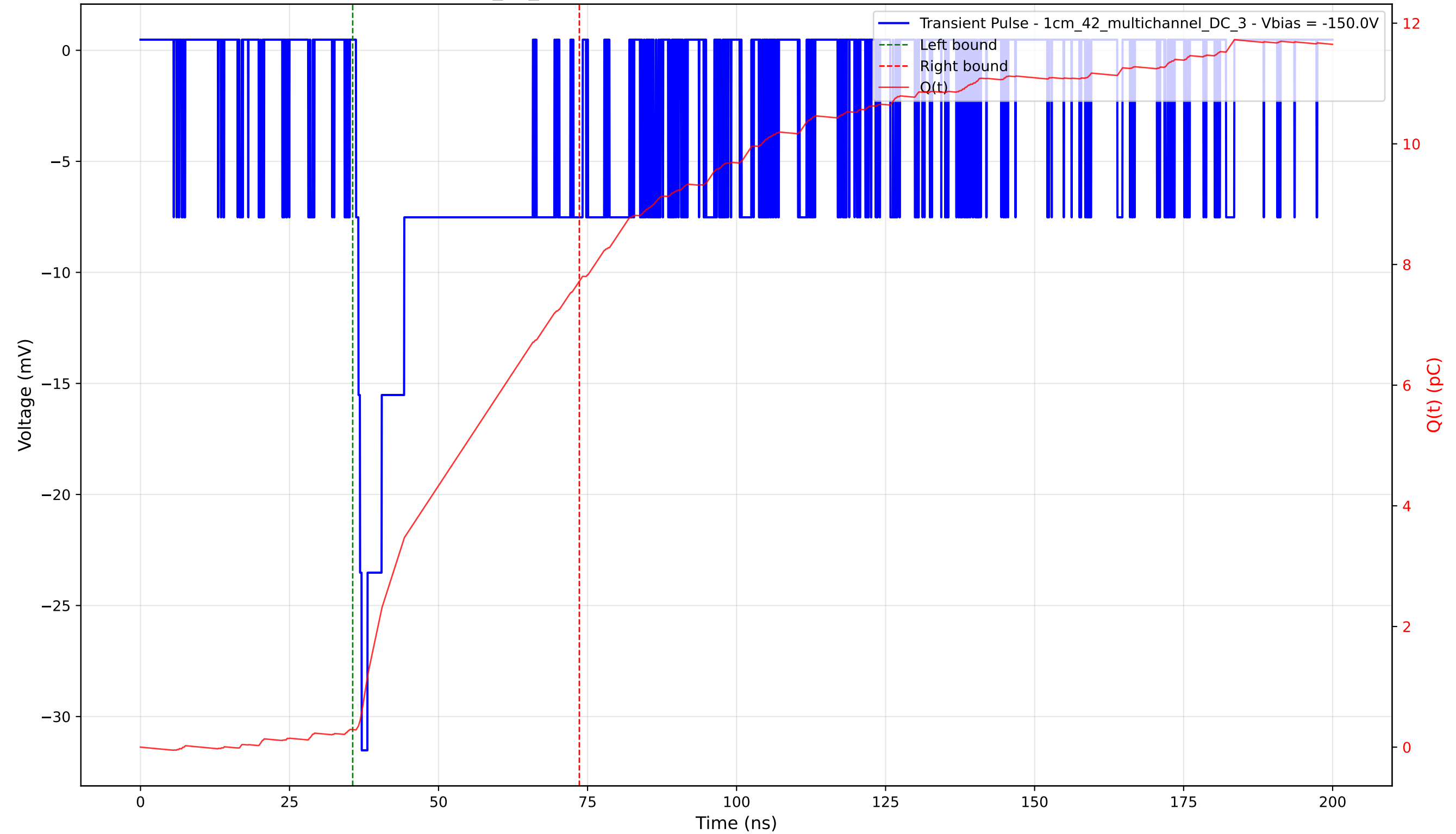
Transient Pulse - Sample: 1cm_42_multichannel - Position: 4420.0 \mu\text{m} - Charge: 7.43 pC - Rise Time: 0.95 ns
