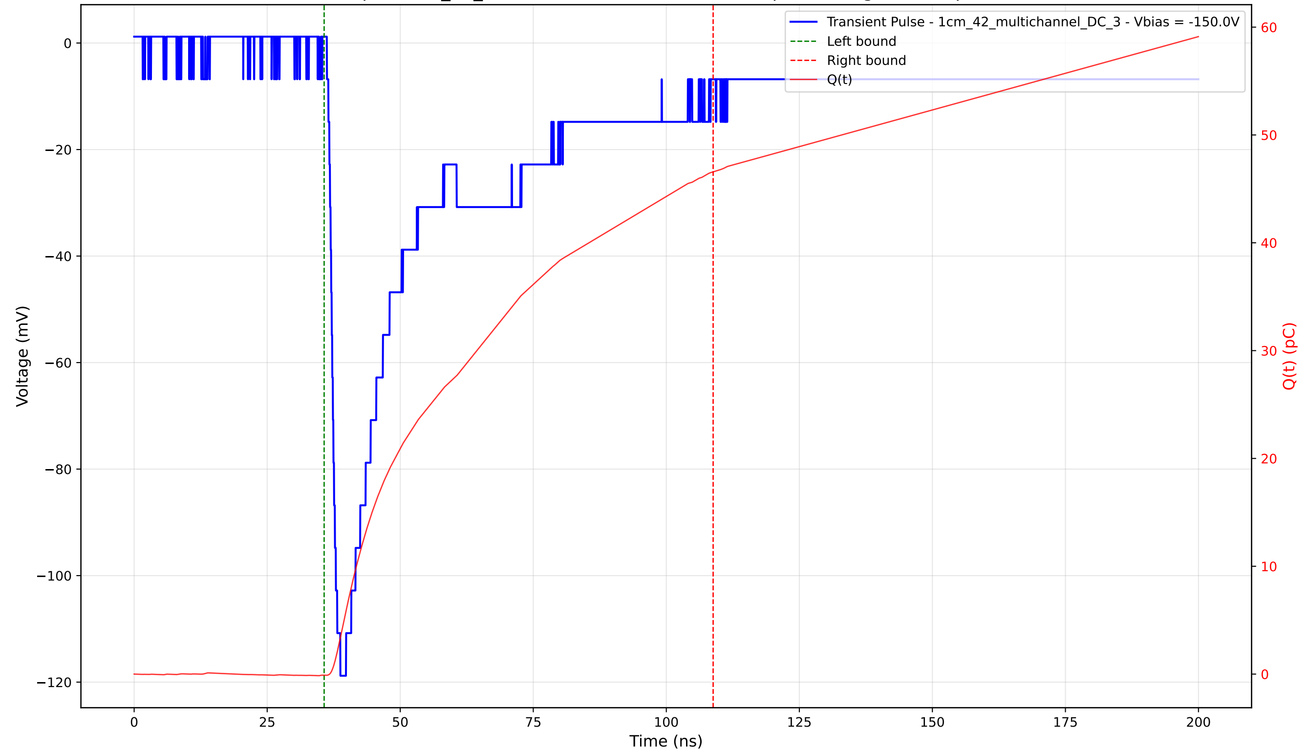
Transient Pulse - Sample: 1cm_42_multichannel - Position: 1720.0 \mu\text{m} - Charge: 46.68 pC - Rise Time: 1.67 ns
