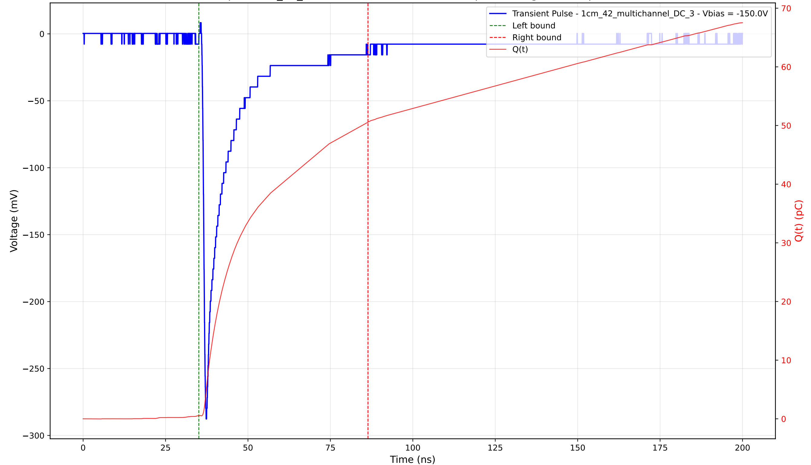
Transient Pulse - Sample: 1cm_42_multichannel - Position: 460.0 \mu\text{m} - Charge: 50.01 pC - Rise Time: 0.91 ns
