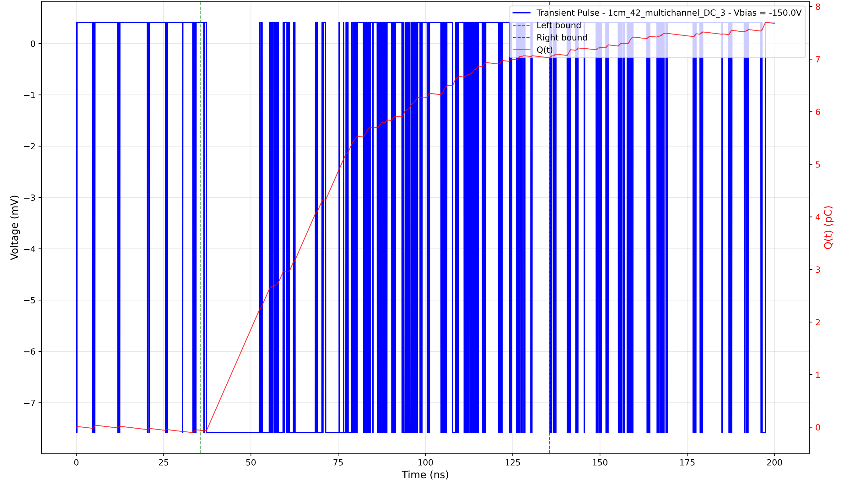
Transient Pulse - Sample: 1cm_42_multichannel - Position: 2365.0 \mu\text{m} - Charge: 7.08 pC - Rise Time: 0.02 ns
