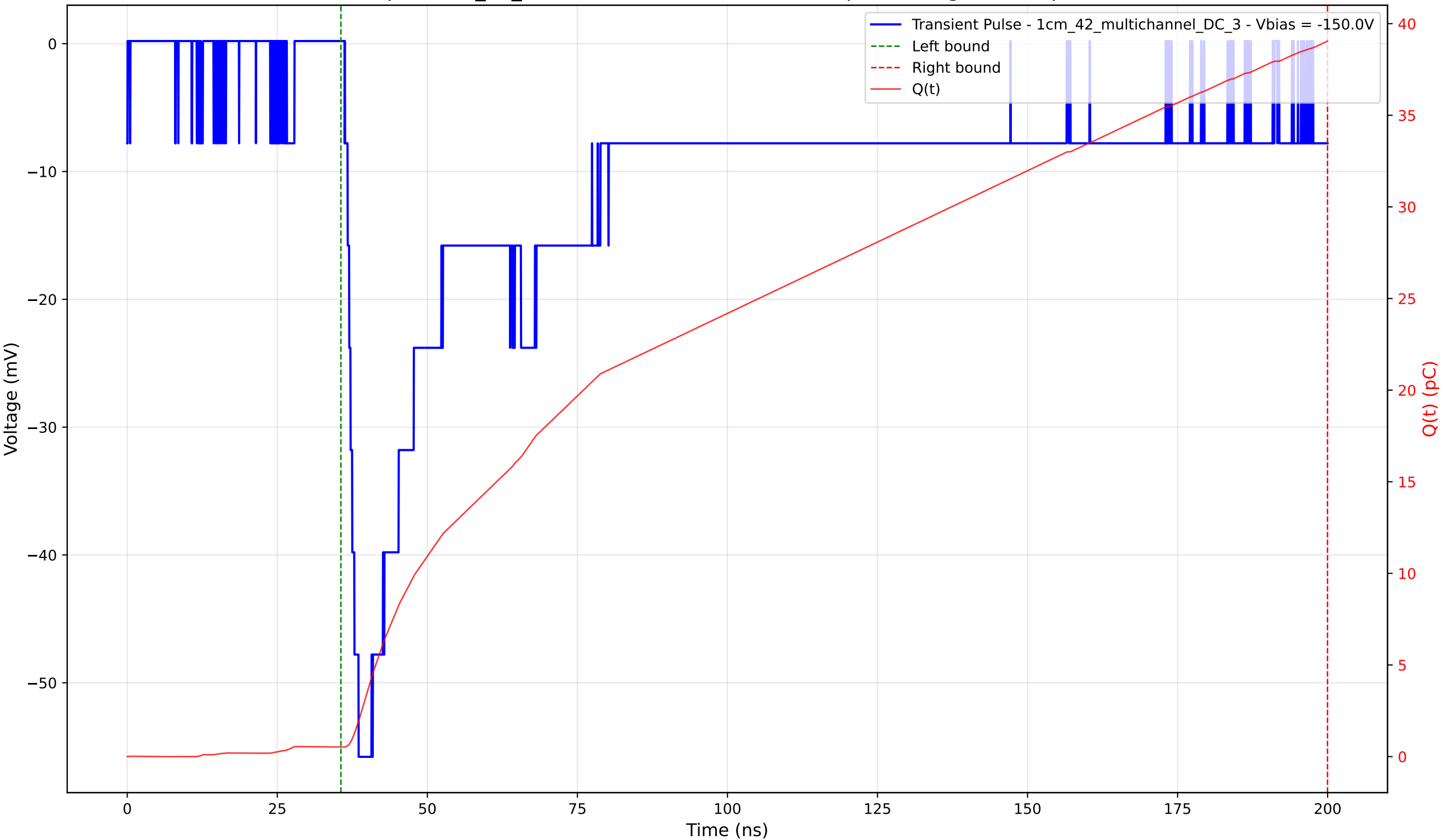
Transient Pulse - Sample: 1cm_42_multichannel - Position: 1920.0 \mu\text{m} - Charge: 38.54 pC - Rise Time: 2.27 ns
