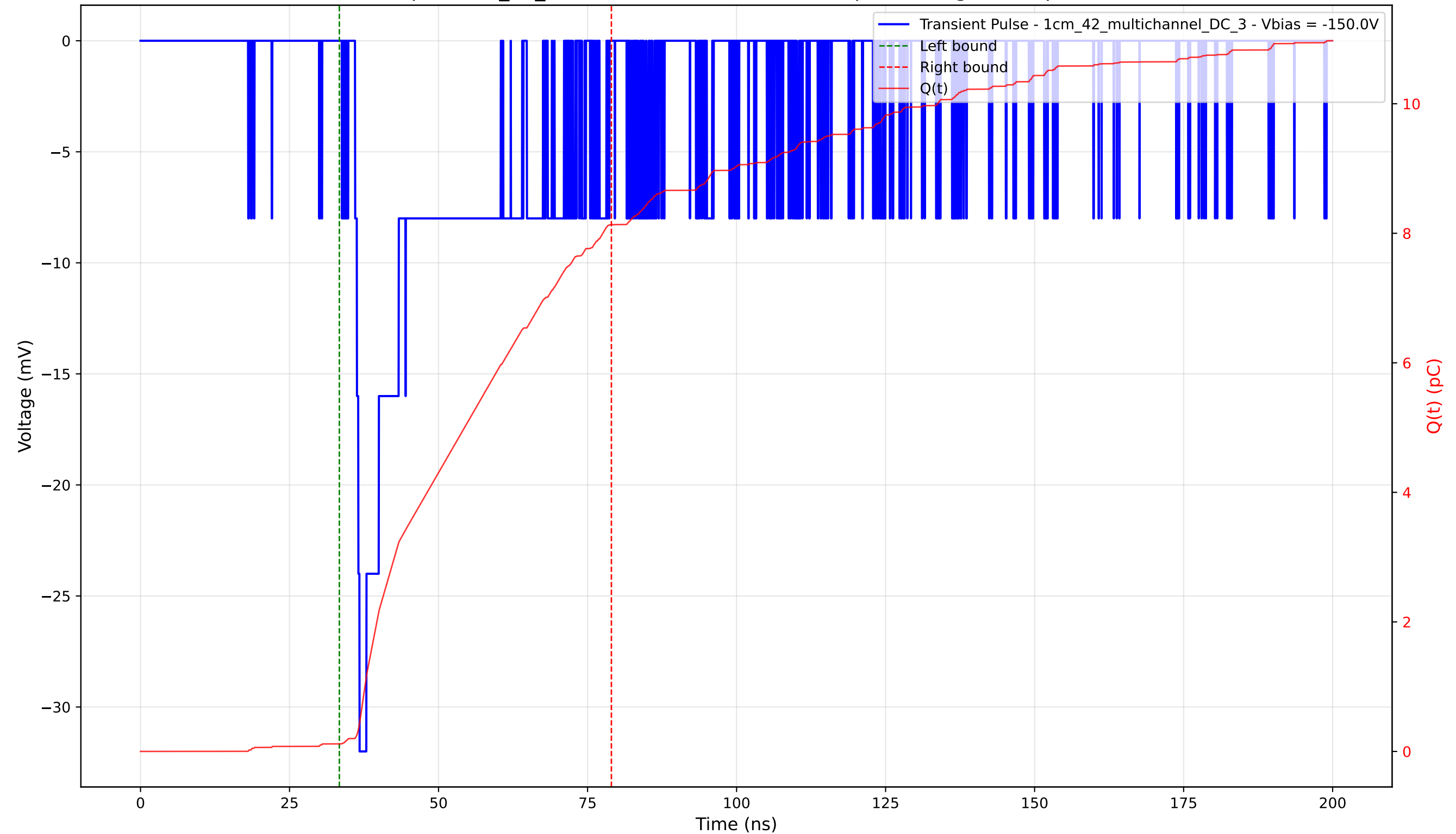
Transient Pulse - Sample: 1cm_42_multichannel - Position: 325.0 \mu\text{m} - Charge: 8.02 pC - Rise Time: 0.75 ns
