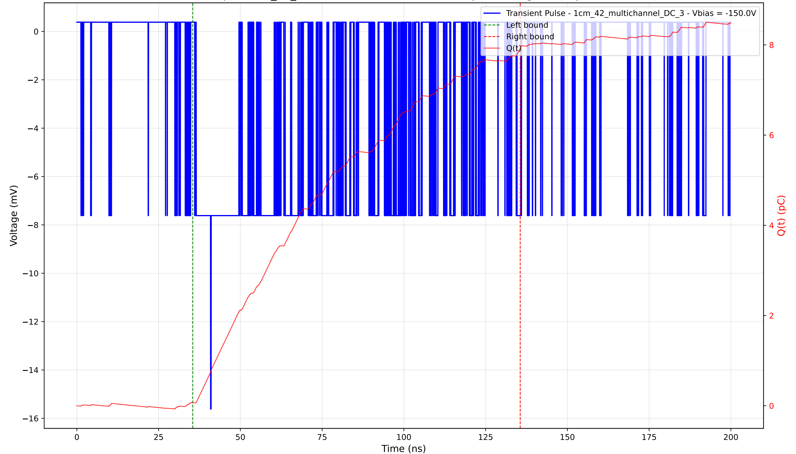
Transient Pulse - Sample: 1cm_42_multichannel - Position: 3400.0 \mu\text{m} - Charge: 7.86 pC - Rise Time: 4.42 ns
