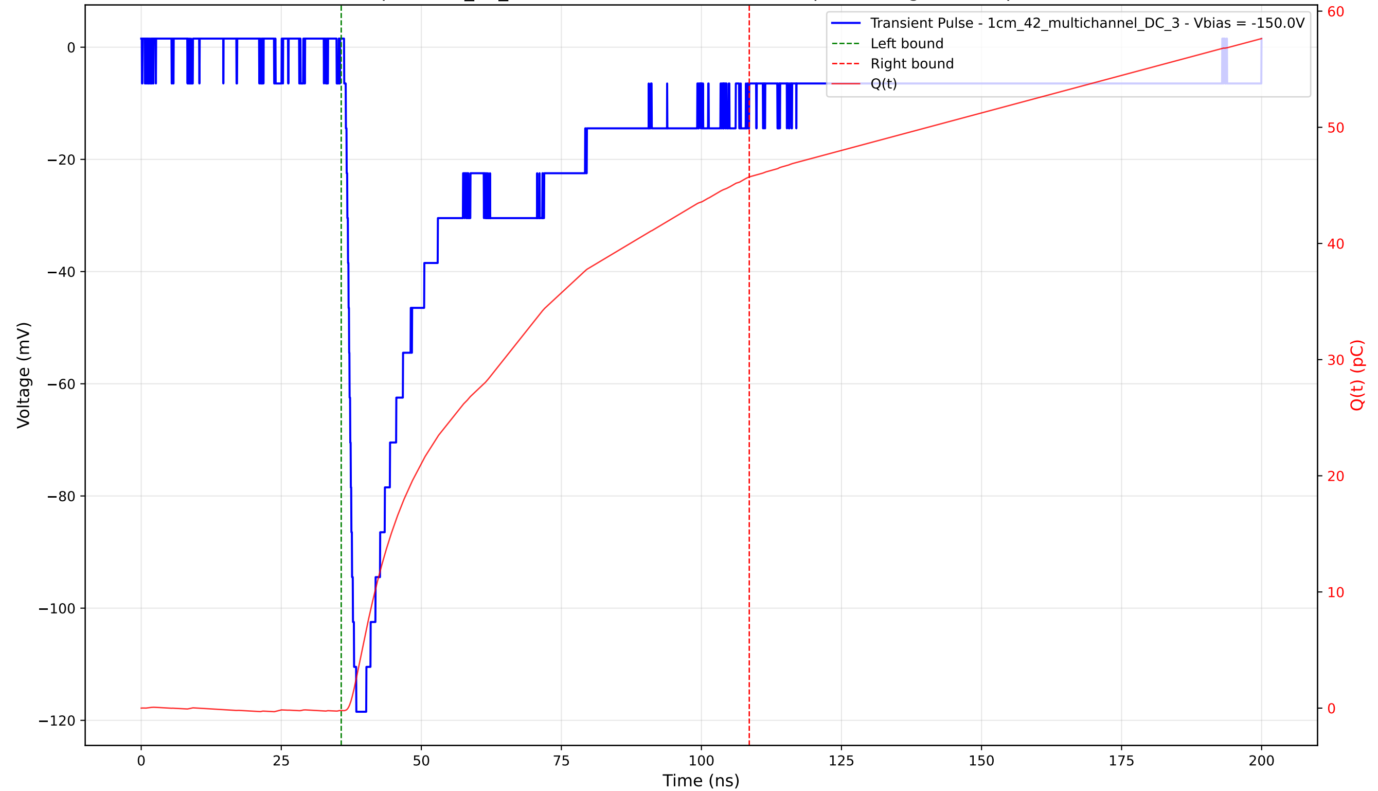
Transient Pulse - Sample: 1cm_42_multichannel - Position: 1635.0 \mu\text{m} - Charge: 45.94 pC - Rise Time: 1.47 ns
