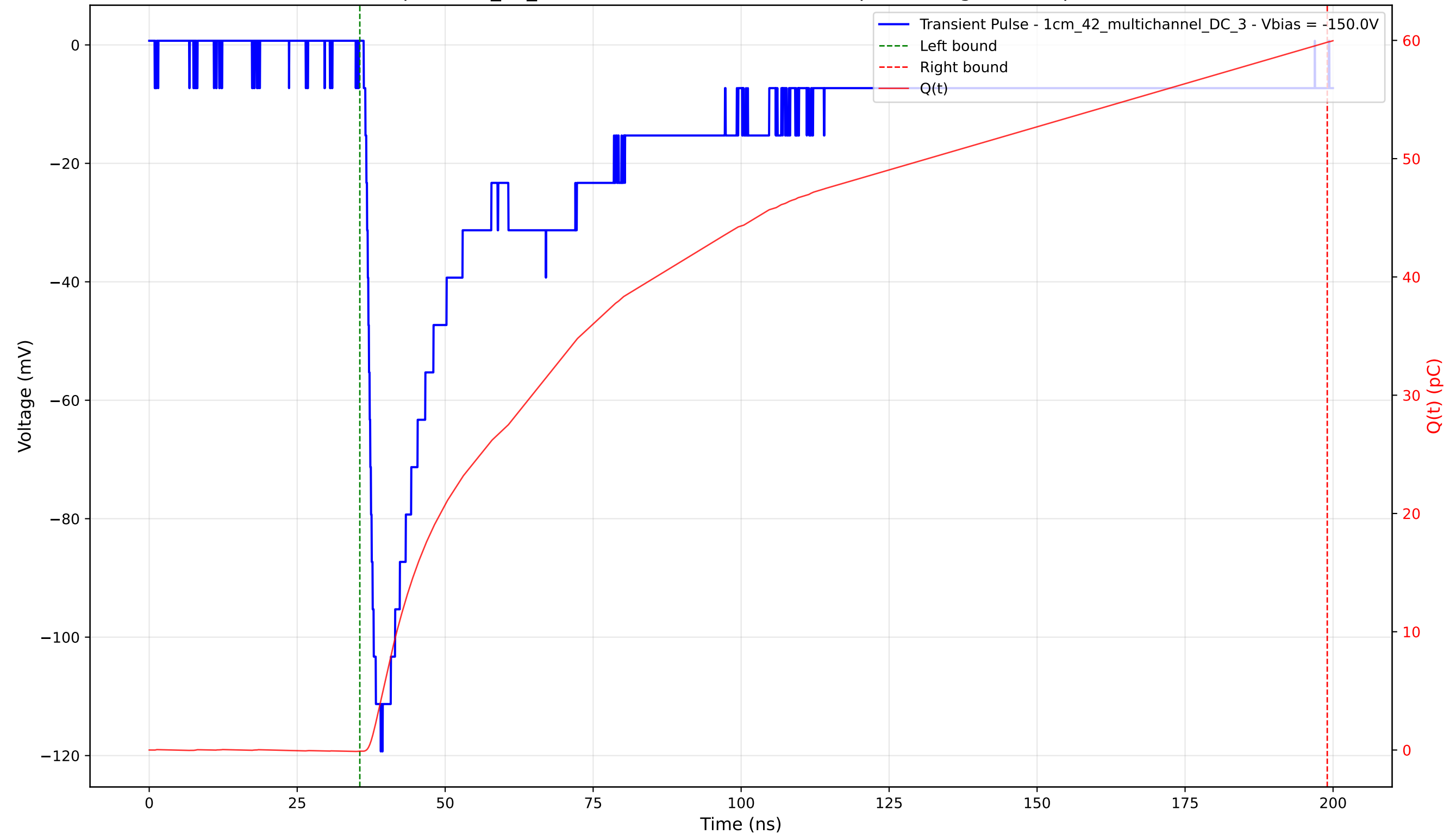
Transient Pulse - Sample: 1cm_42_multichannel - Position: 1730.0 \mu\text{m} - Charge: 59.94 pC - Rise Time: 1.77 ns
