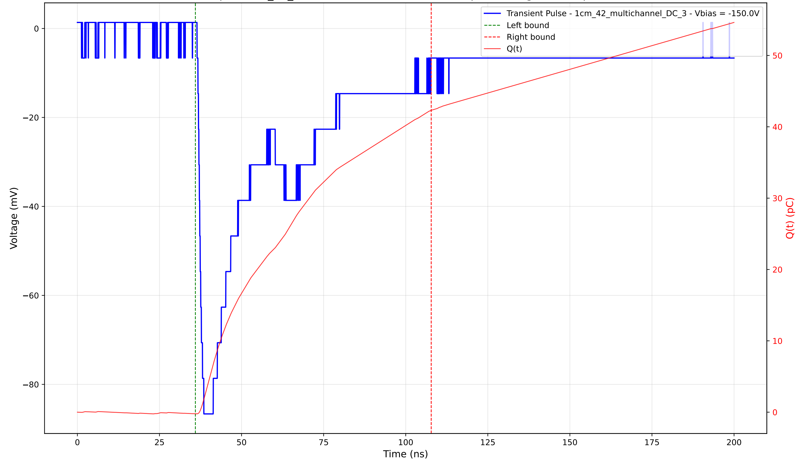
Transient Pulse - Sample: 1cm_42_multichannel - Position: 2090.0 \mu\text{m} - Charge: 42.54 pC - Rise Time: 1.39 ns
