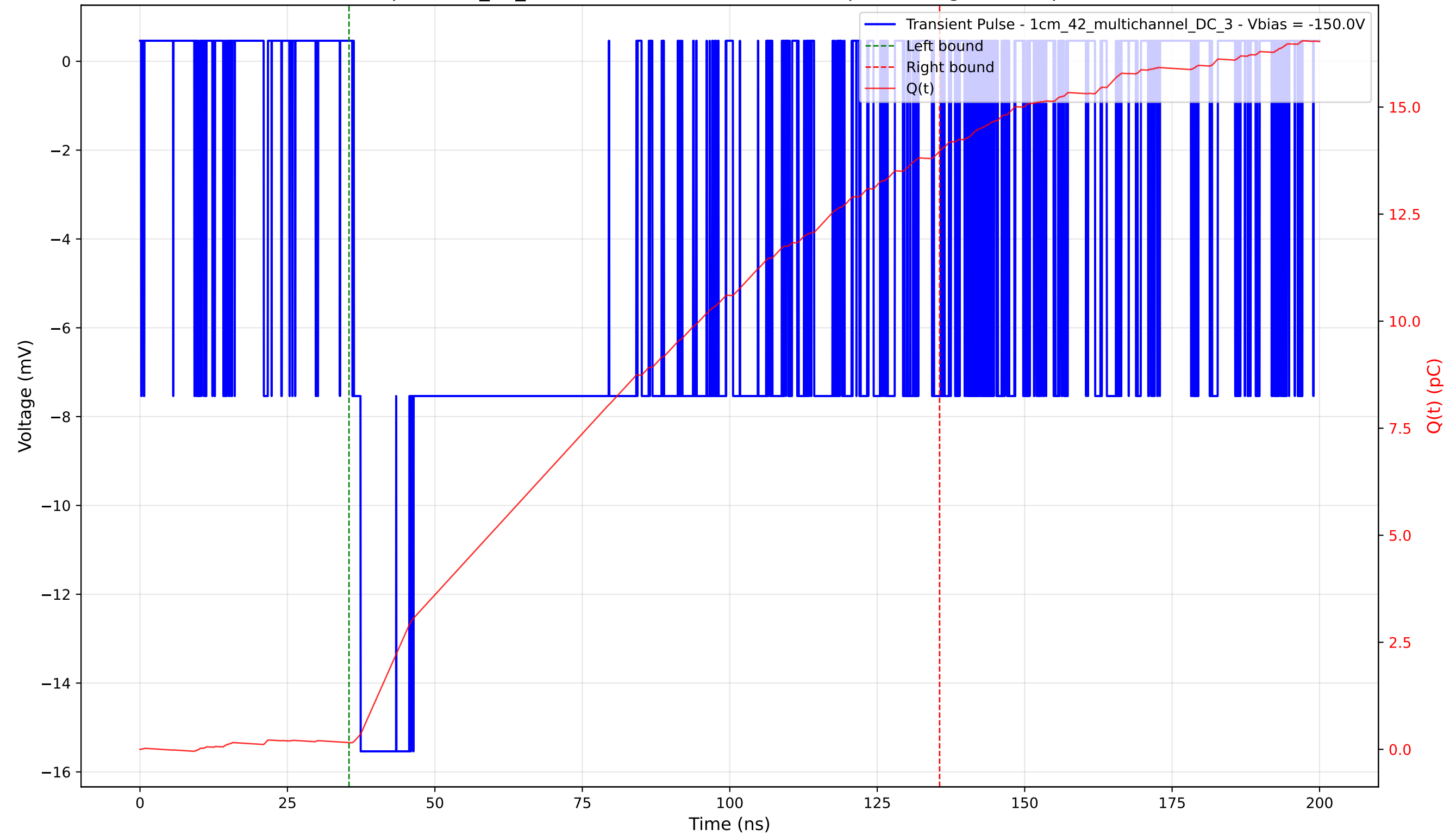
Transient Pulse - Sample: 1cm_42_multichannel - Position: 1840.0 \mu\text{m} - Charge: 13.81 pC - Rise Time: 1.16 ns
