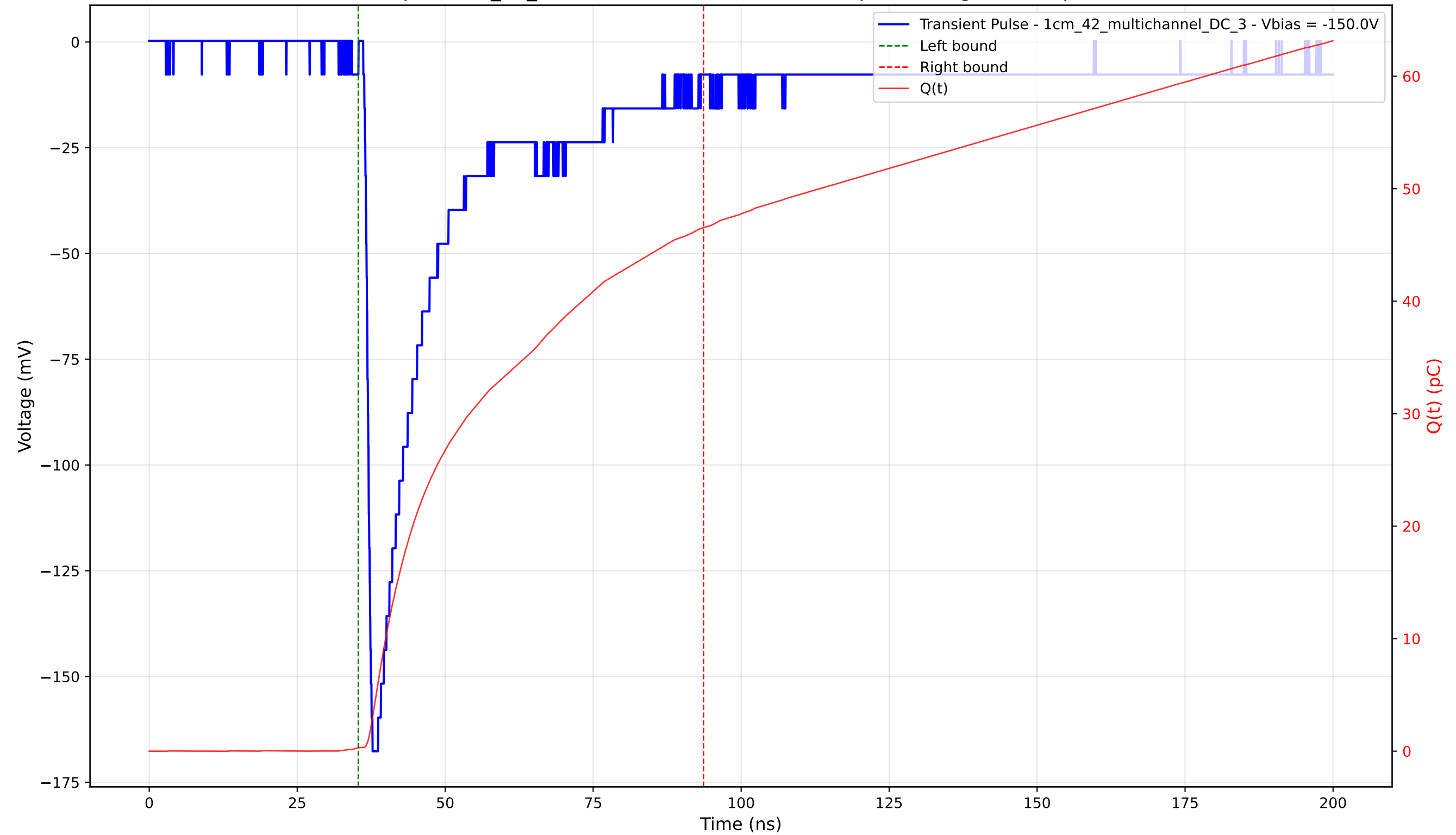
Transient Pulse - Sample: 1cm_42_multichannel - Position: 1035.0 \mu\text{m} - Charge: 46.22 pC - Rise Time: 1.02 ns
