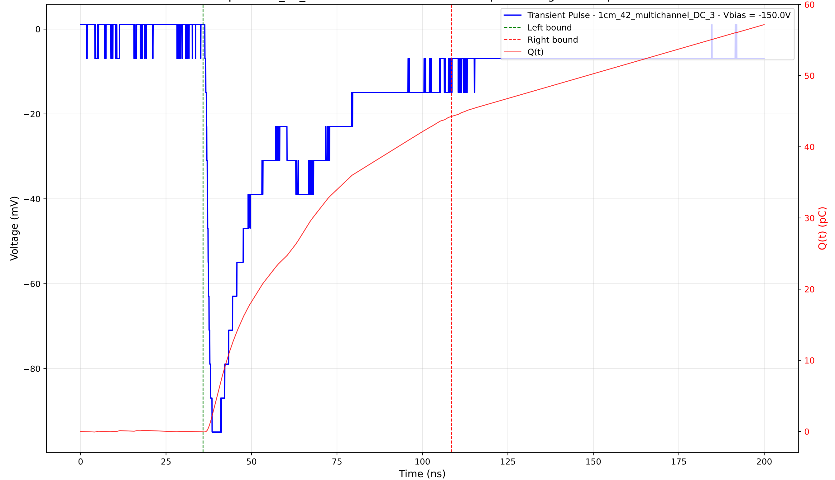
Transient Pulse - Sample: 1cm_42_multichannel - Position: 1985.0 \mu\text{m} - Charge: 44.32 pC - Rise Time: 1.43 ns
