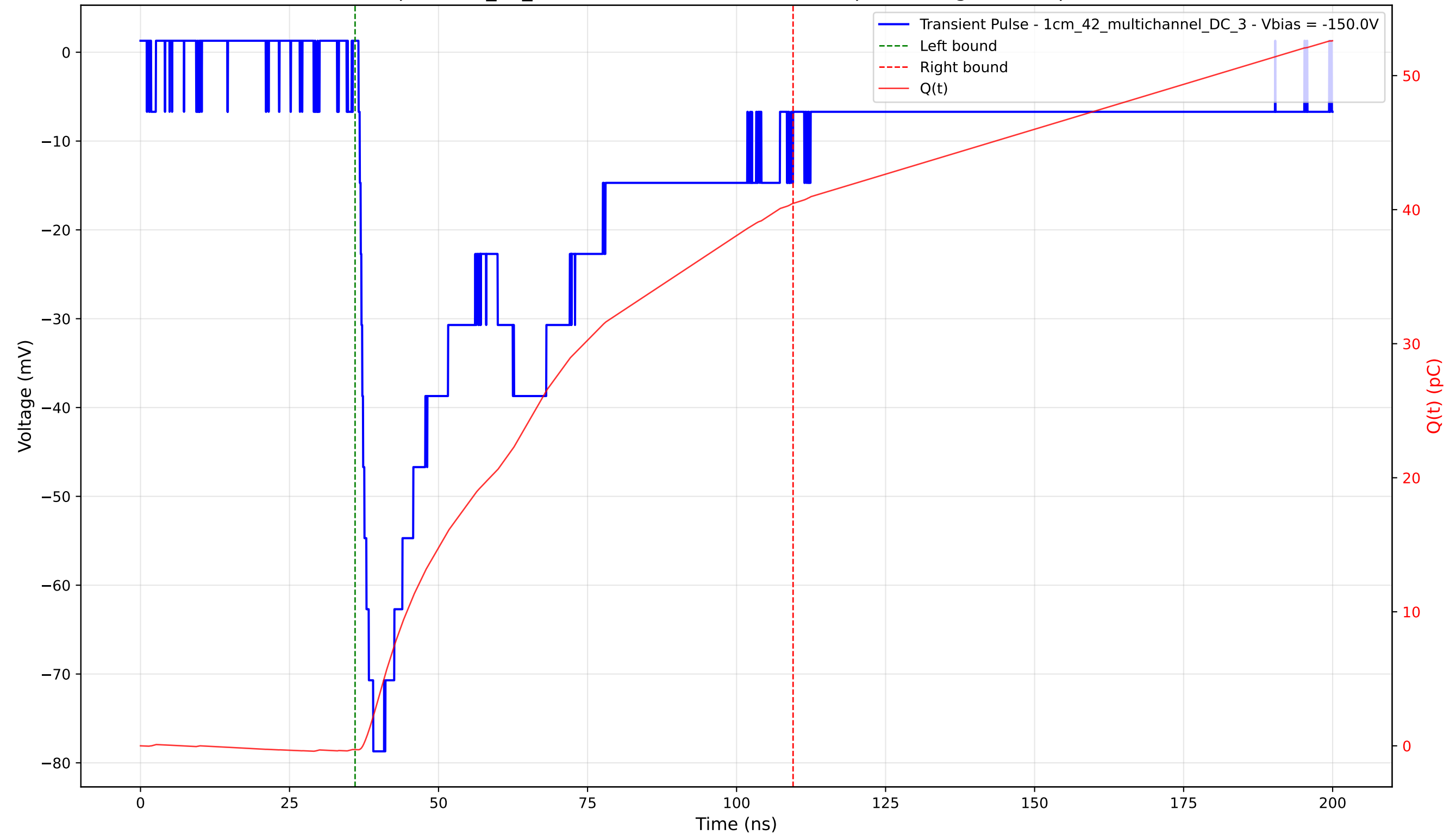
Transient Pulse - Sample: 1cm_42_multichannel - Position: 2465.0 \mu\text{m} - Charge: 40.75 pC - Rise Time: 2.28 ns
