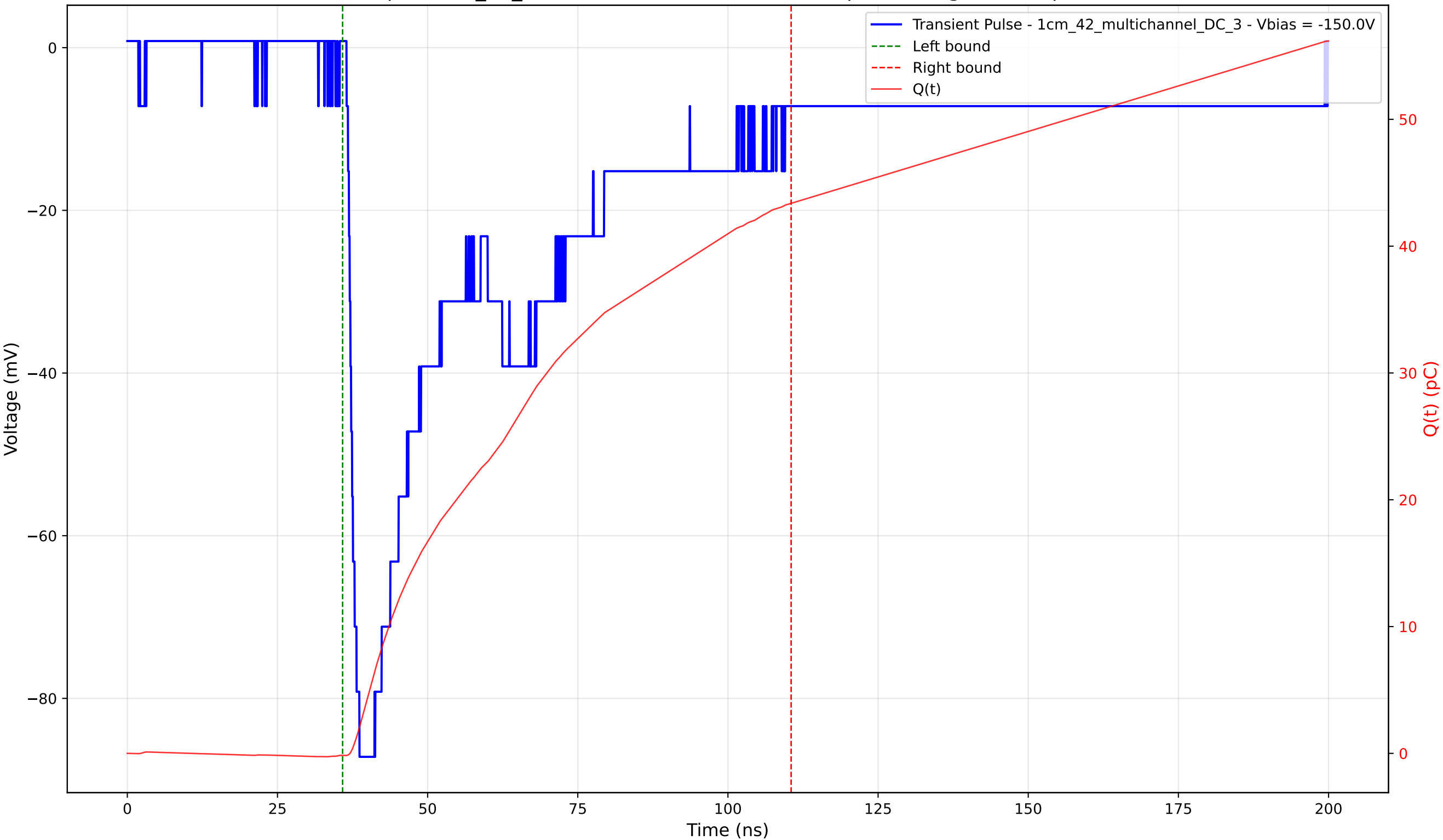
Transient Pulse - Sample: 1cm_42_multichannel - Position: 2120.0 \mu\text{m} - Charge: 43.54 pC - Rise Time: 1.44 ns
