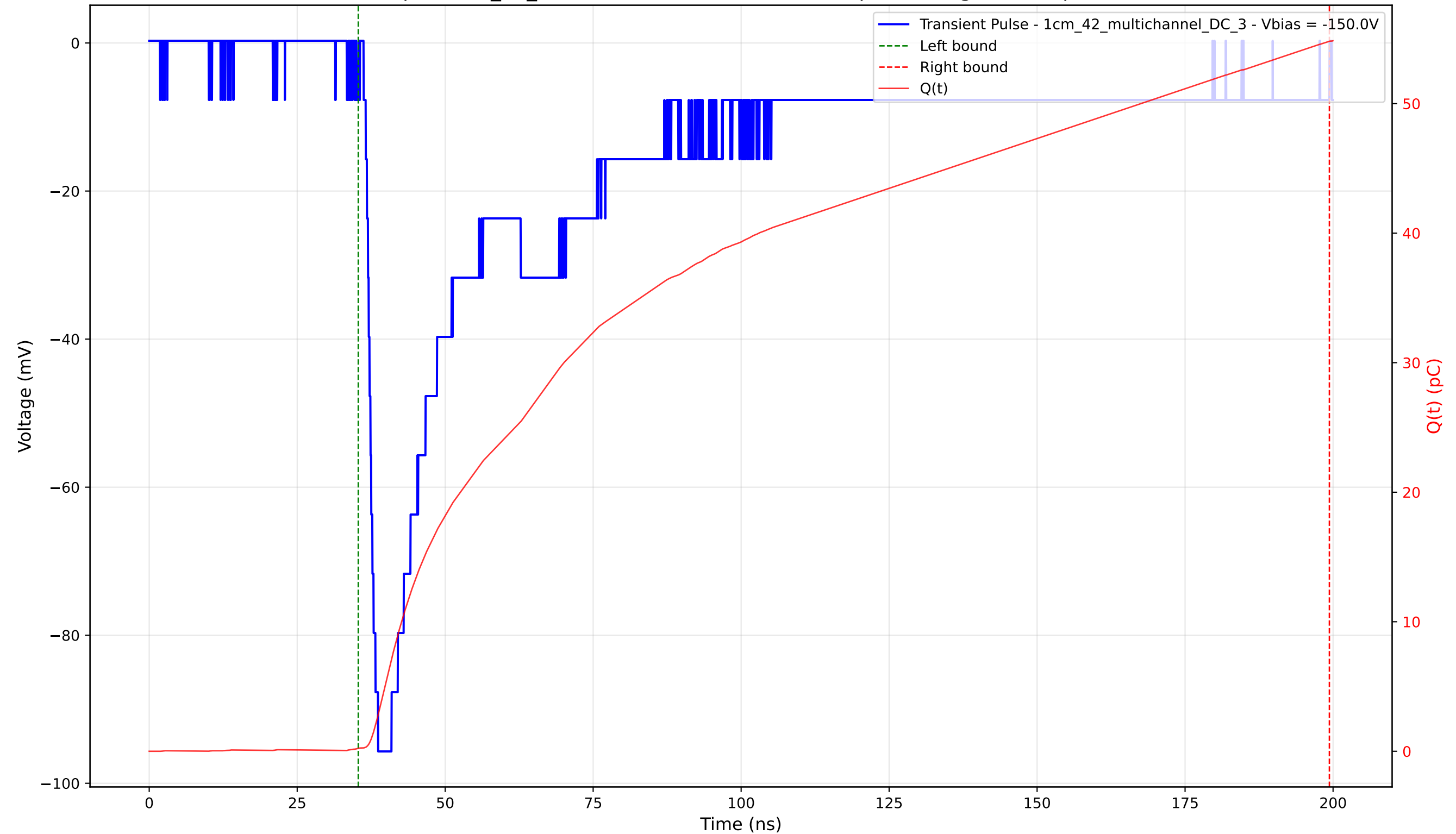
Transient Pulse - Sample: 1cm_42_multichannel - Position: 2965.0 \mu\text{m} - Charge: 54.59 pC - Rise Time: 1.66 ns
