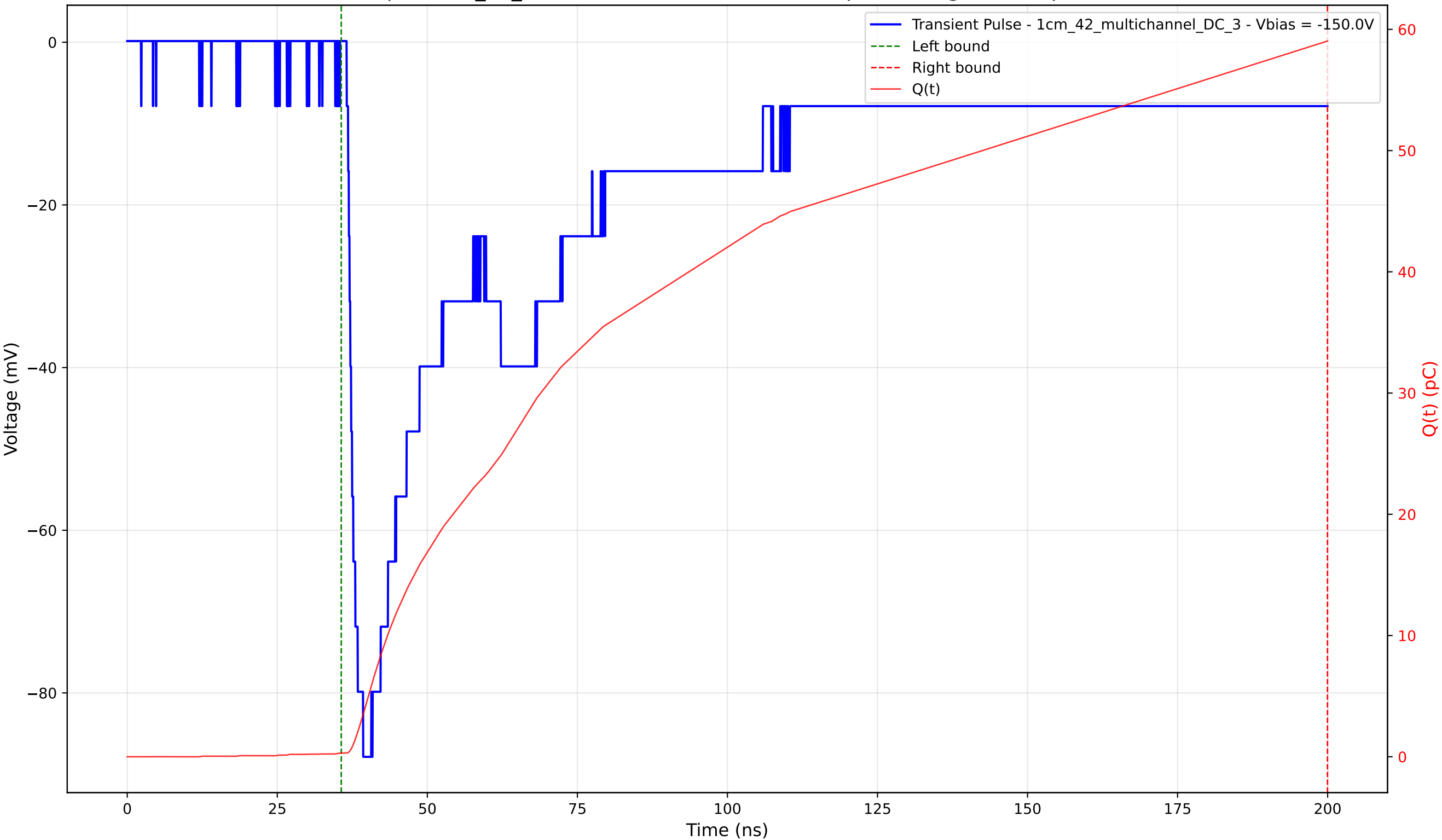
Transient Pulse - Sample: 1cm_42_multichannel - Position: 2235.0 \mu\text{m} - Charge: 58.73 pC - Rise Time: 1.62 ns
