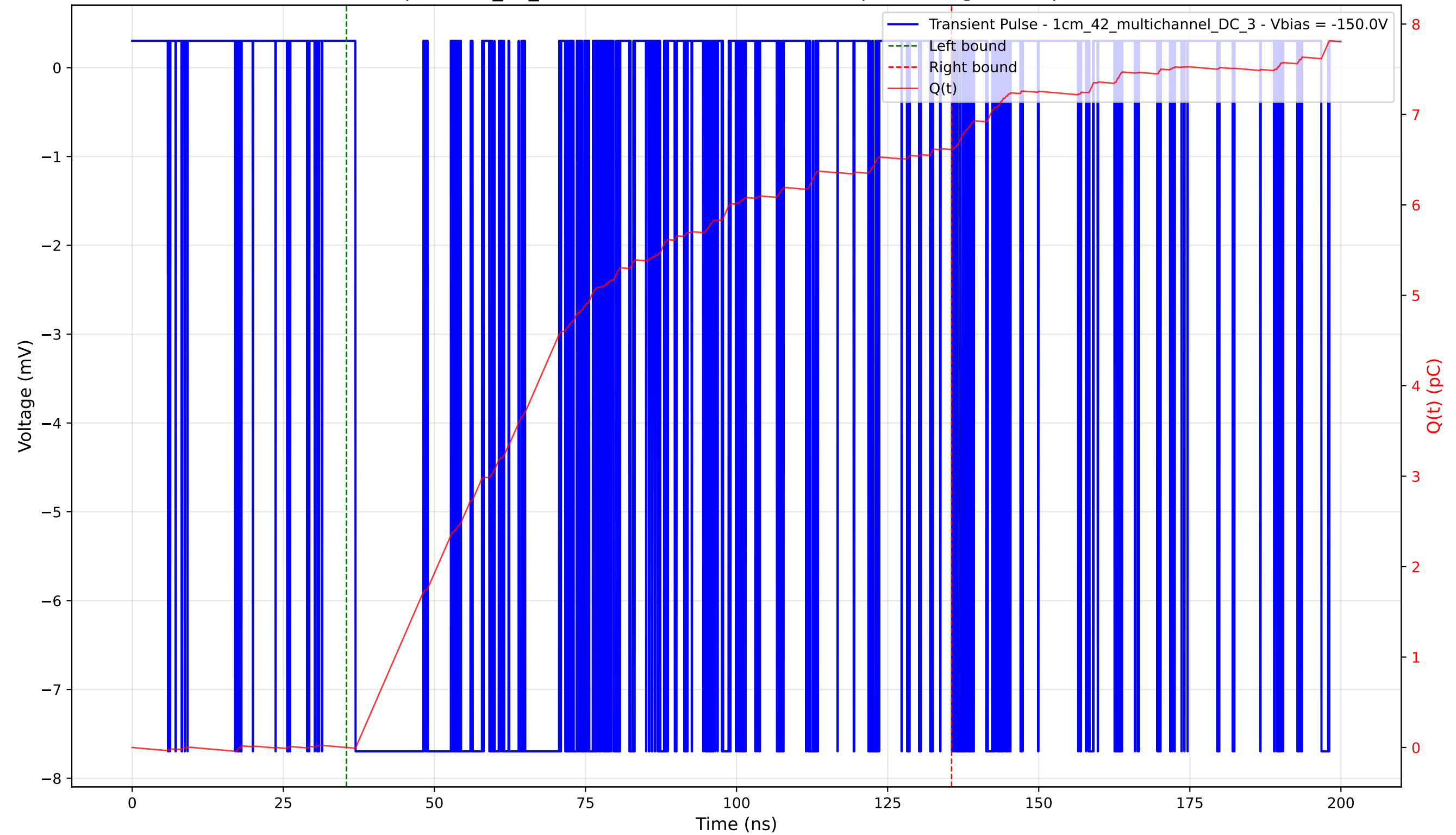
Transient Pulse - Sample: 1cm_42_multichannel - Position: 2370.0 \mu\text{m} - Charge: 6.61 pC - Rise Time: 0.02 ns
