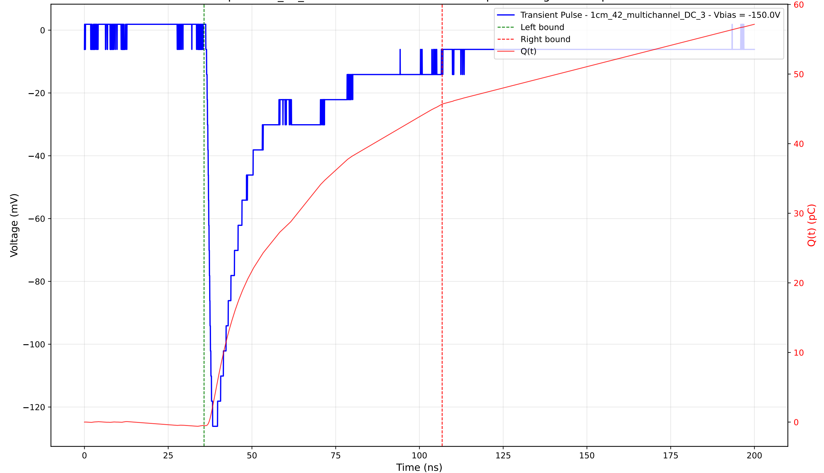
Transient Pulse - Sample: 1cm_42_multichannel - Position: 1535.0 \mu\text{m} - Charge: 46.18 pC - Rise Time: 1.46 ns
