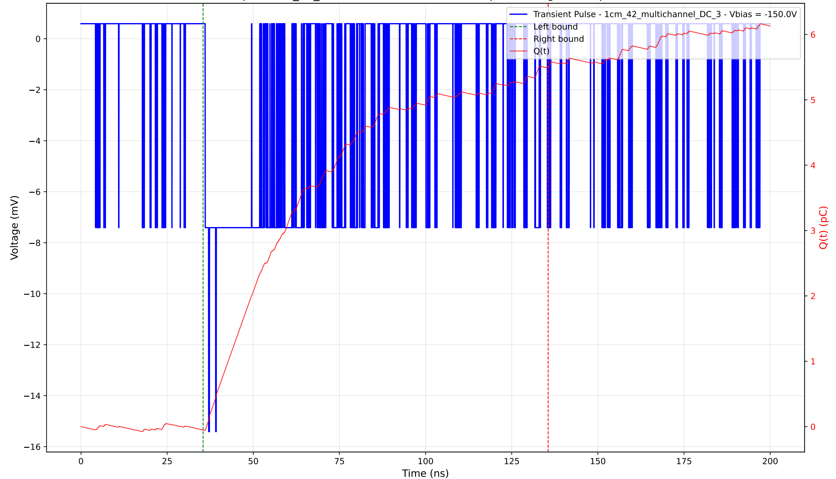
Transient Pulse - Sample: 1cm_42_multichannel - Position: 30.0 \mu\text{m} - Charge: 5.55 pC - Rise Time: 1.02 ns
