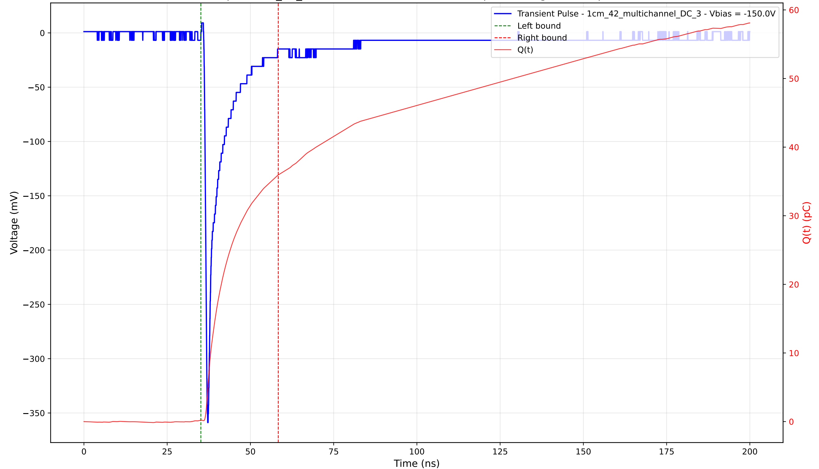
Transient Pulse - Sample: 1cm_42_multichannel - Position: 4730.0 \mu\text{m} - Charge: 35.72 pC - Rise Time: 0.80 ns
