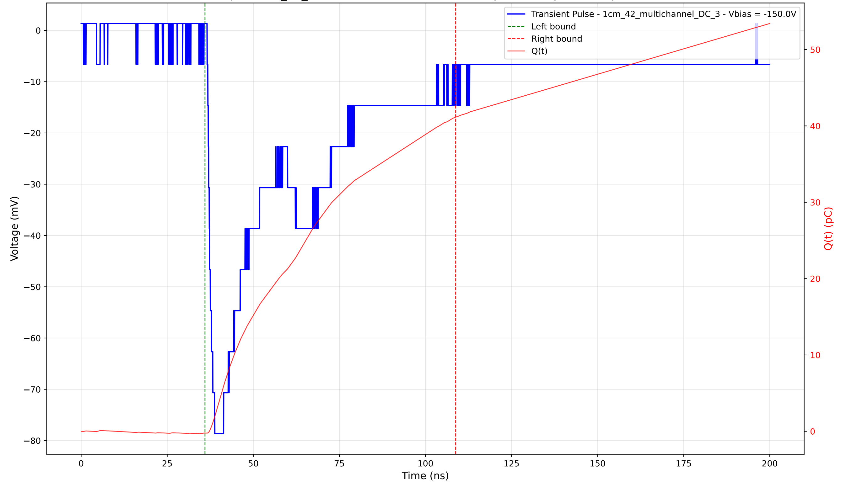
Transient Pulse - Sample: 1cm_42_multichannel - Position: 2470.0 \mu\text{m} - Charge: 41.38 pC - Rise Time: 2.02 ns
