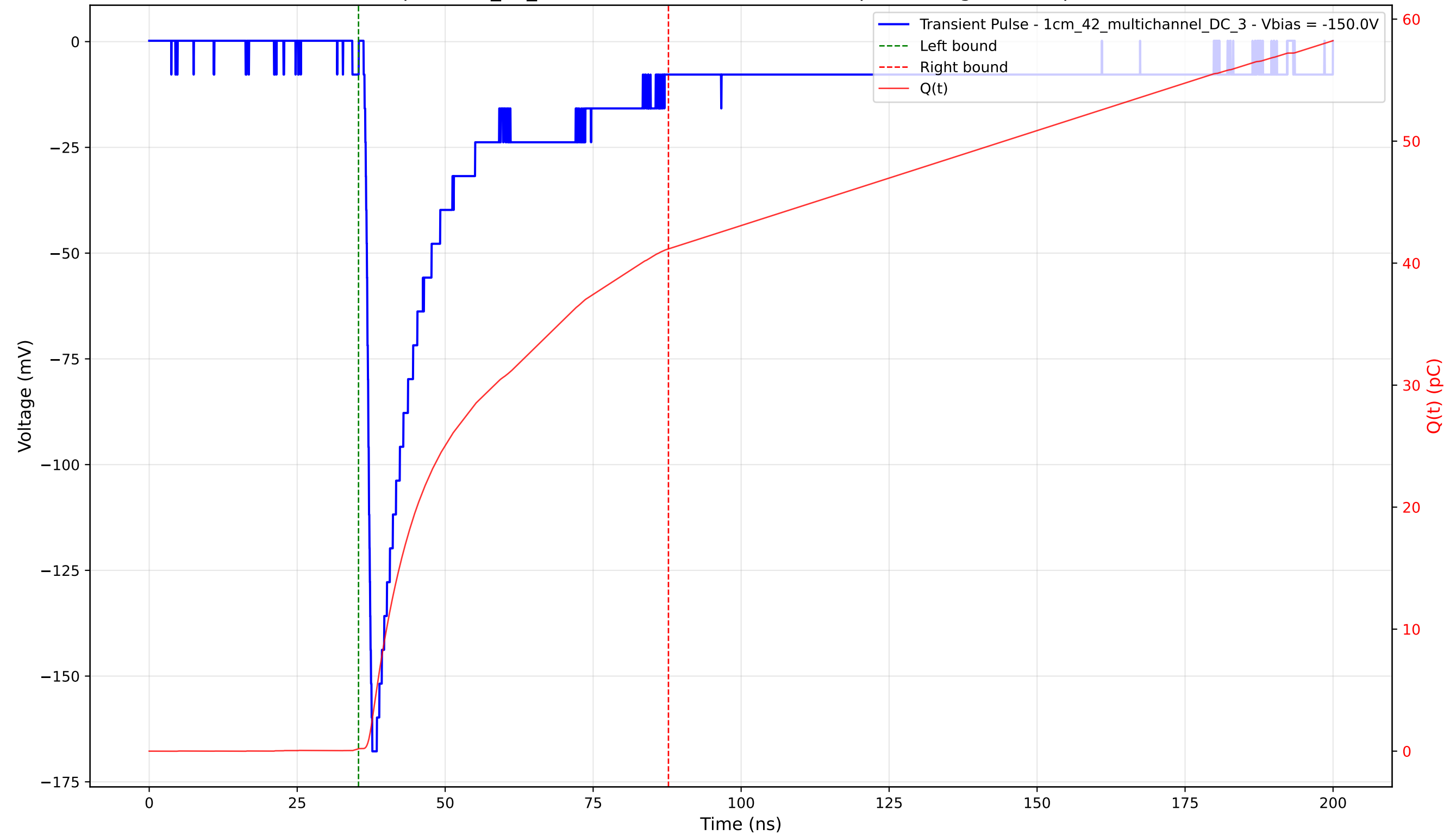
Transient Pulse - Sample: 1cm_42_multichannel - Position: 3985.0 \mu\text{m} - Charge: 40.96 pC - Rise Time: 0.98 ns
