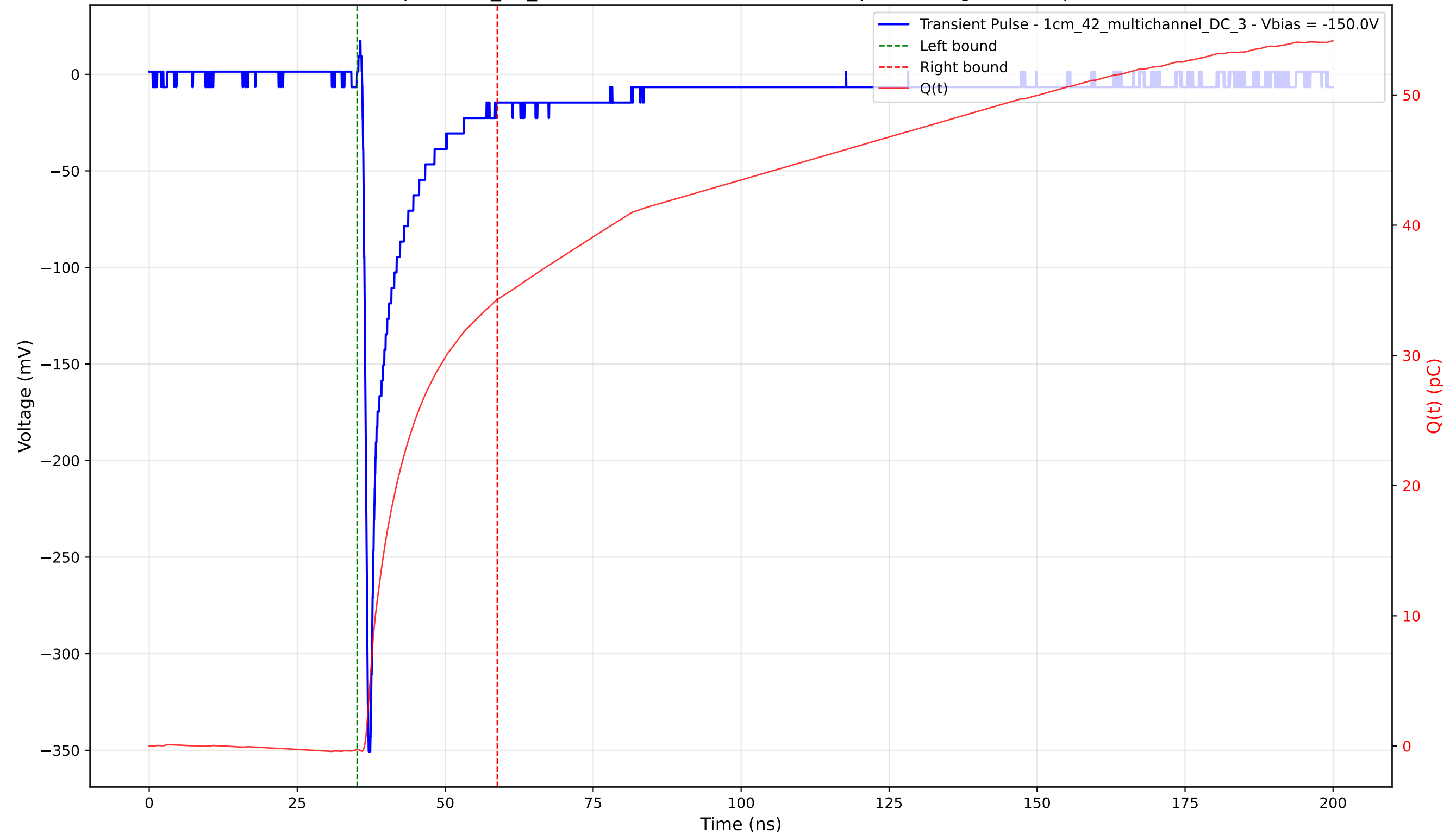
Transient Pulse - Sample: 1cm_42_multichannel - Position: 4760.0 \mu\text{m} - Charge: 34.56 pC - Rise Time: 0.78 ns
