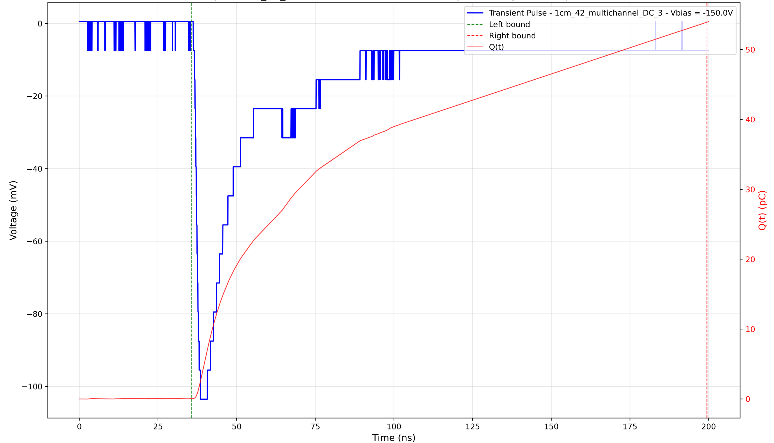
Transient Pulse - Sample: 1cm_42_multichannel - Position: 3185.0 \mu\text{m} - Charge: 53.86 pC - Rise Time: 1.51 ns
