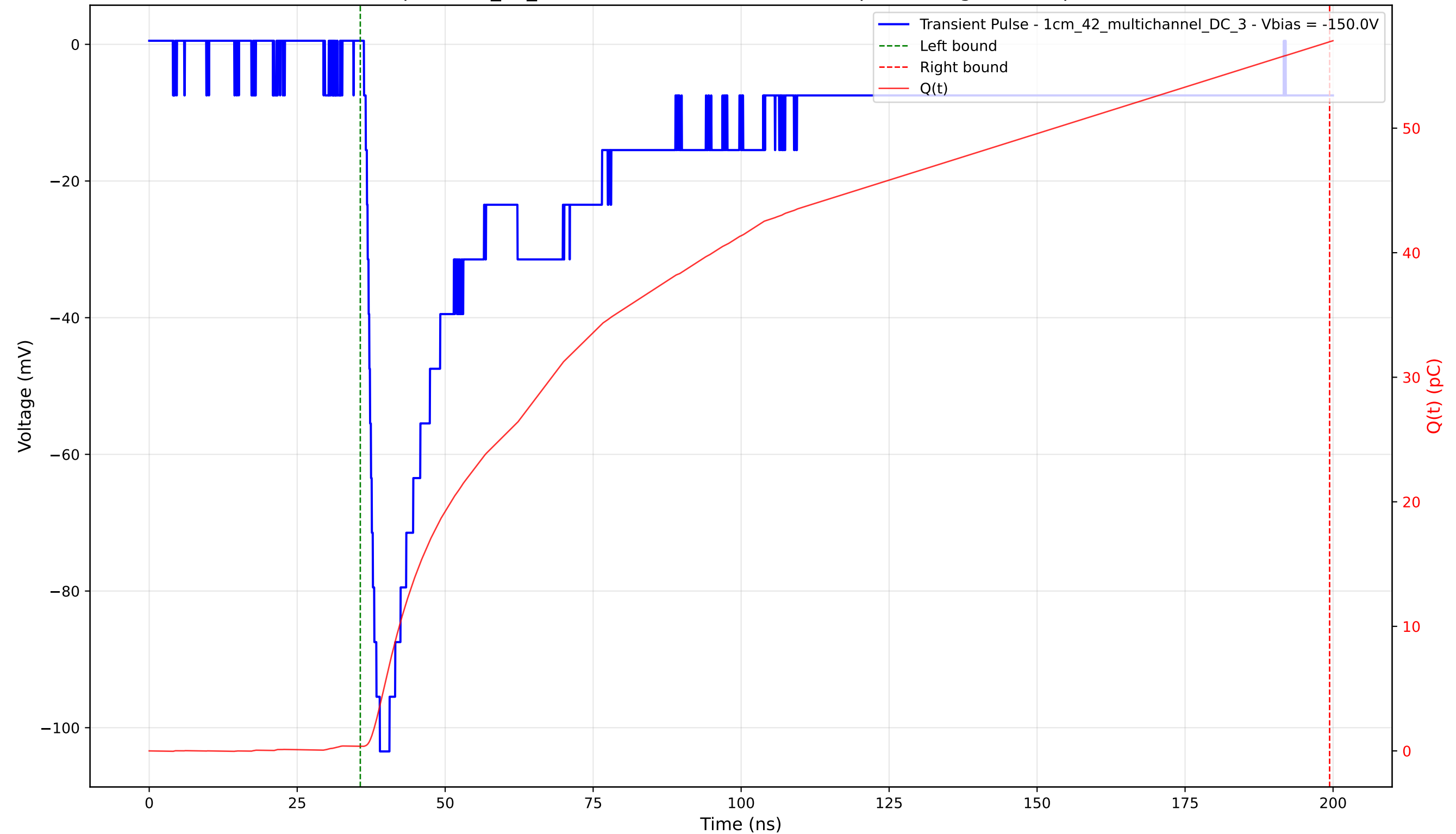
Transient Pulse - Sample: 1cm_42_multichannel - Position: 3010.0 \mu\text{m} - Charge: 56.56 pC - Rise Time: 1.81 ns
