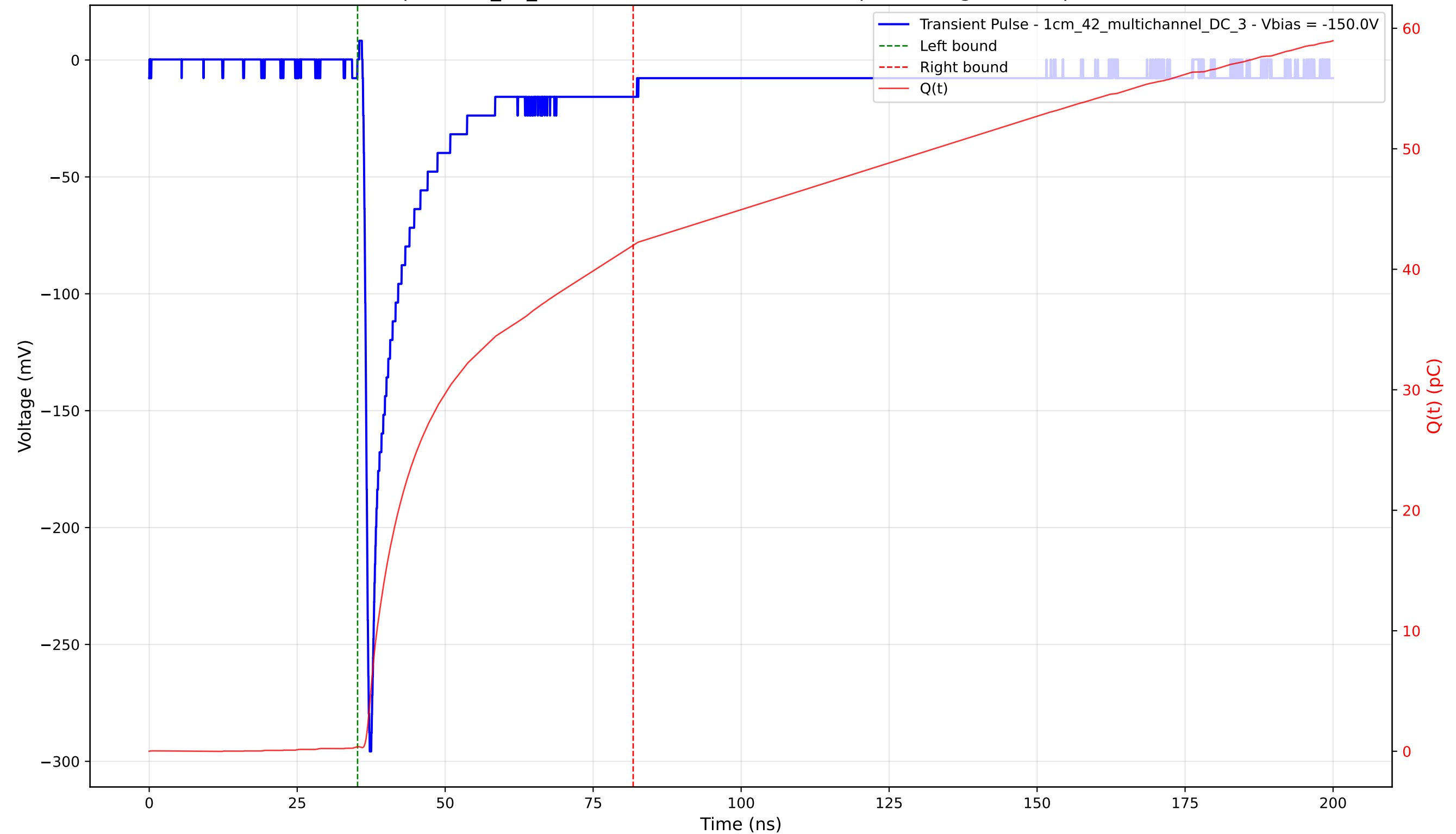
Transient Pulse - Sample: 1cm_42_multichannel - Position: 4595.0 \mu\text{m} - Charge: 41.62 pC - Rise Time: 0.85 ns
