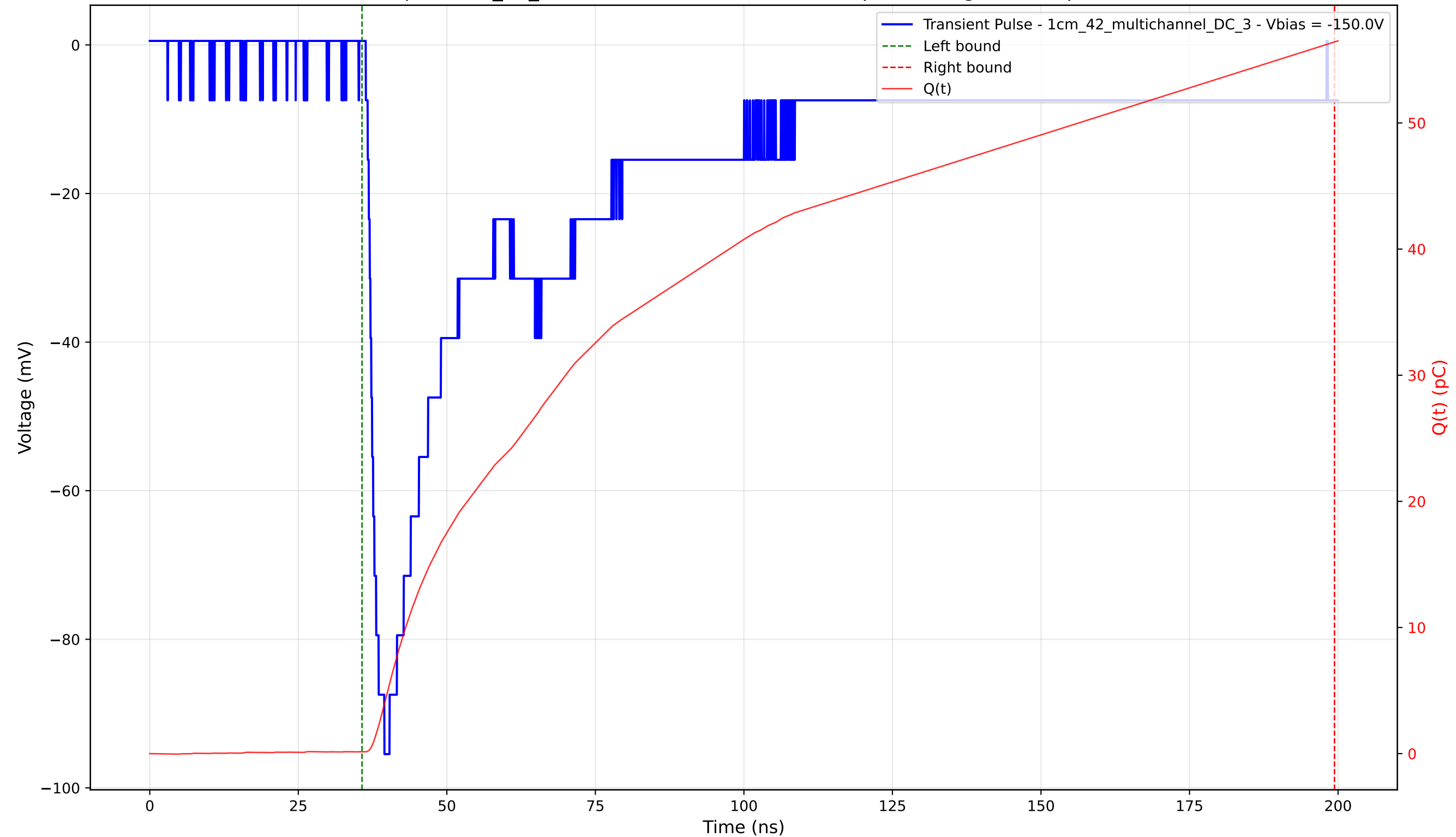
Transient Pulse - Sample: 1cm_42_multichannel - Position: 2750.0 \mu\text{m} - Charge: 56.28 pC - Rise Time: 1.85 ns
