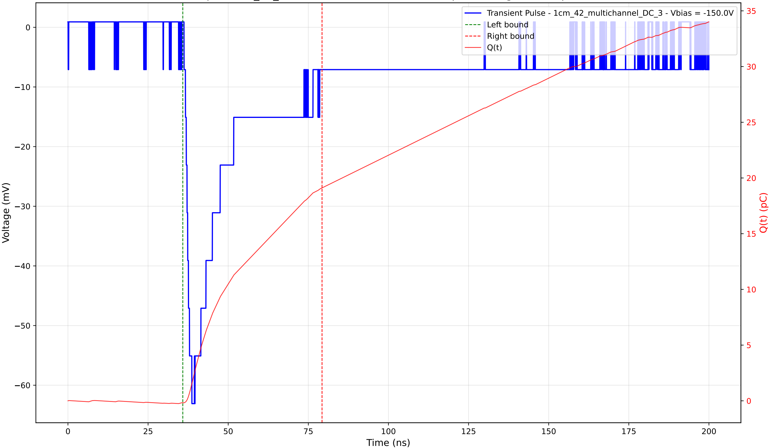
Transient Pulse - Sample: 1cm_42_multichannel - Position: 3335.0 \mu\text{m} - Charge: 19.28 pC - Rise Time: 2.44 ns
