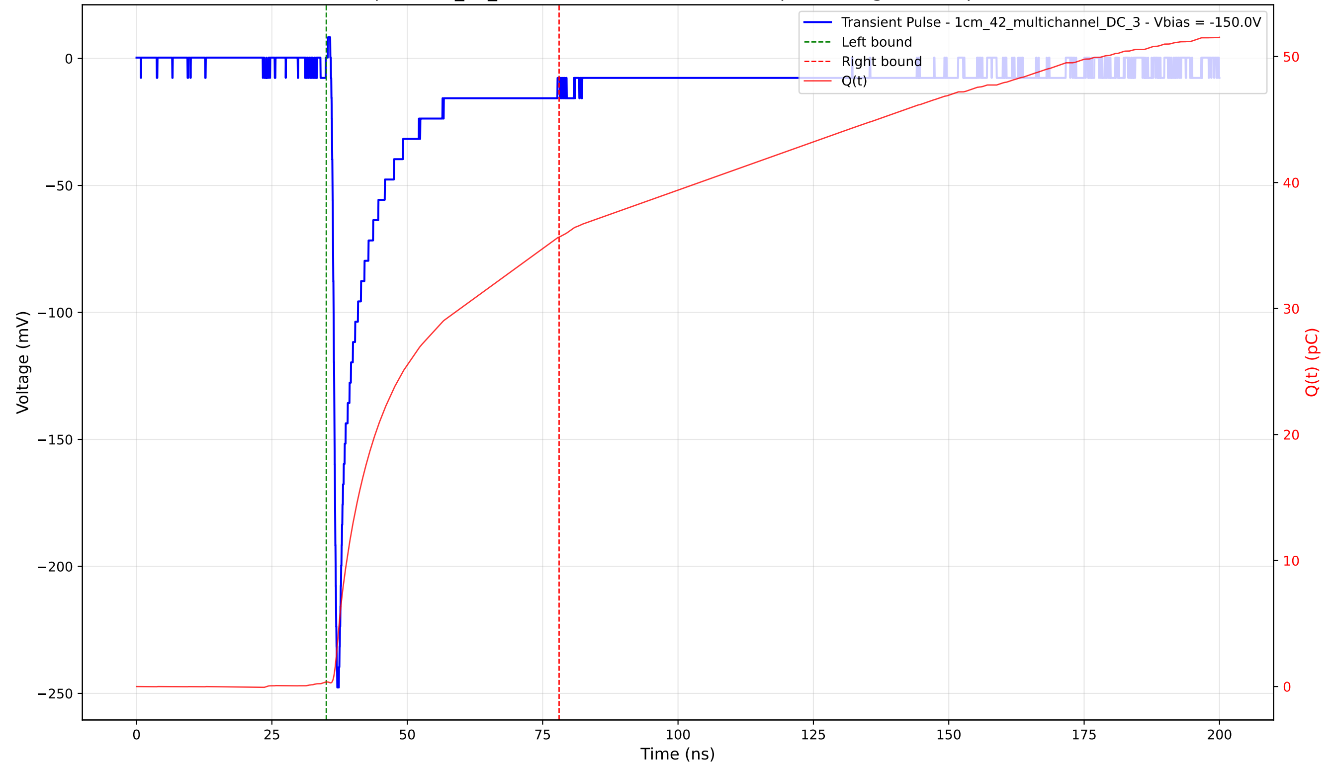
Transient Pulse - Sample: 1cm_42_multichannel - Position: 285.0 \mu\text{m} - Charge: 35.30 pC - Rise Time: 0.80 ns
