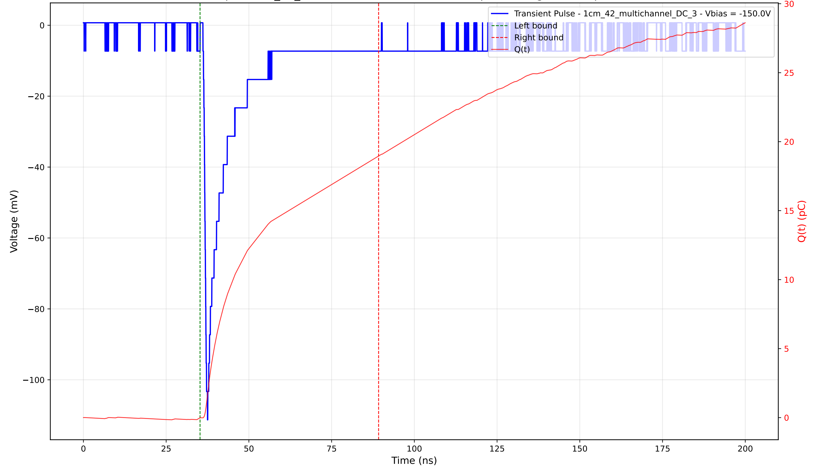
Transient Pulse - Sample: 1cm_42_multichannel - Position: 4440.0 \mu\text{m} - Charge: 18.98 pC - Rise Time: 0.93 ns
