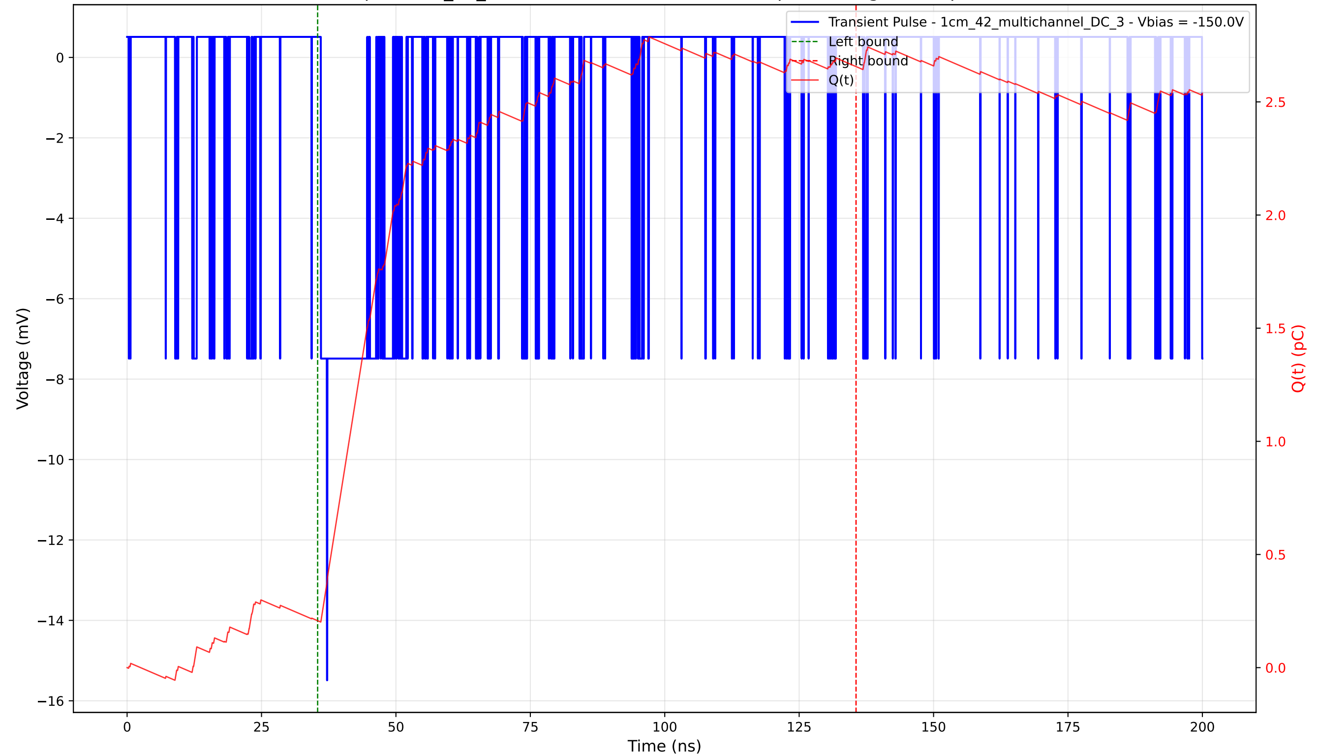
Transient Pulse - Sample: 1cm_42_multichannel - Position: 4910.0 \mu\text{m} - Charge: 2.45 pC - Rise Time: 1.14 ns
