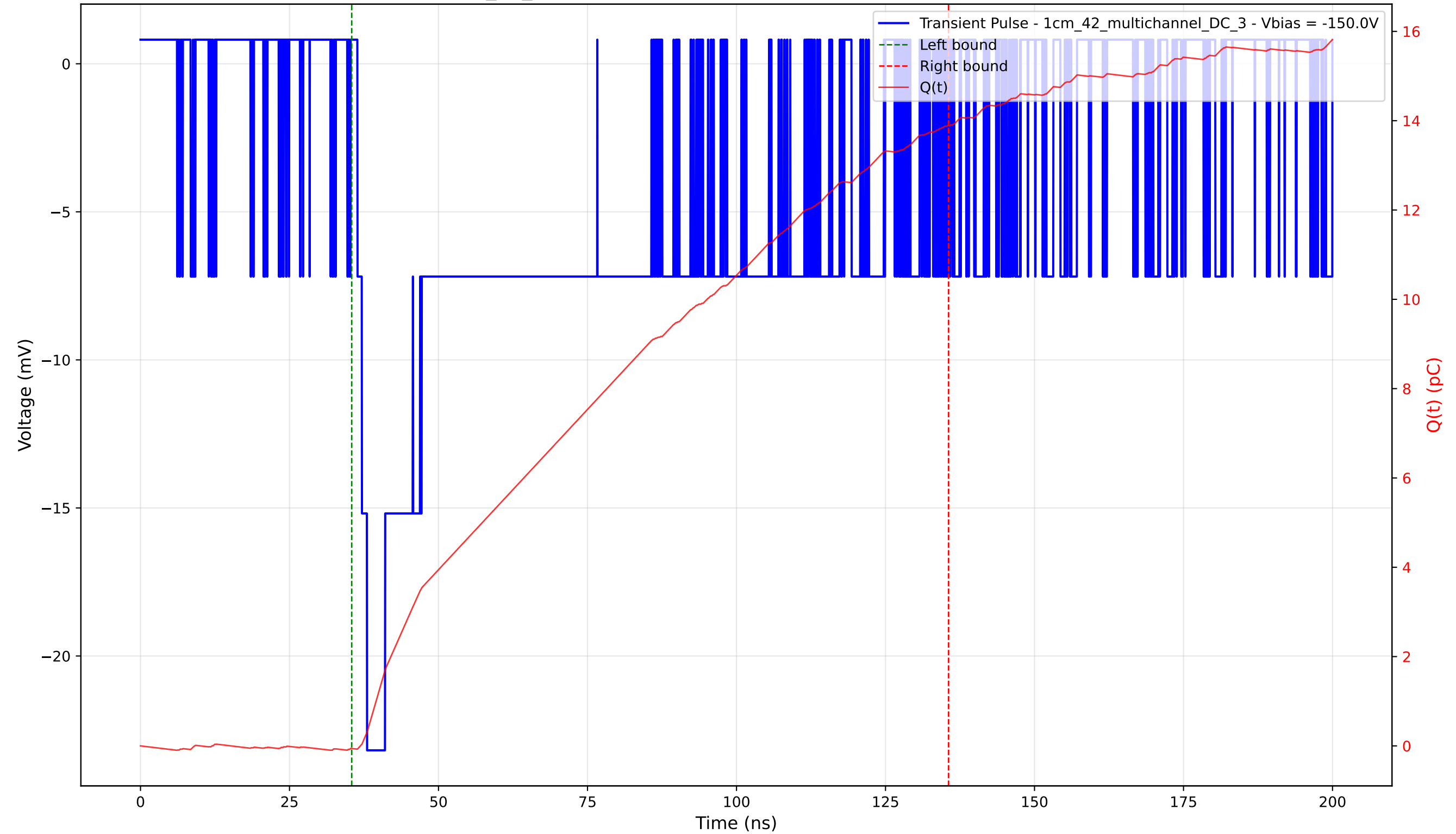
Transient Pulse - Sample: 1cm_42_multichannel - Position: 3355.0 \mu\text{m} - Charge: 13.95 pC - Rise Time: 1.62 ns
