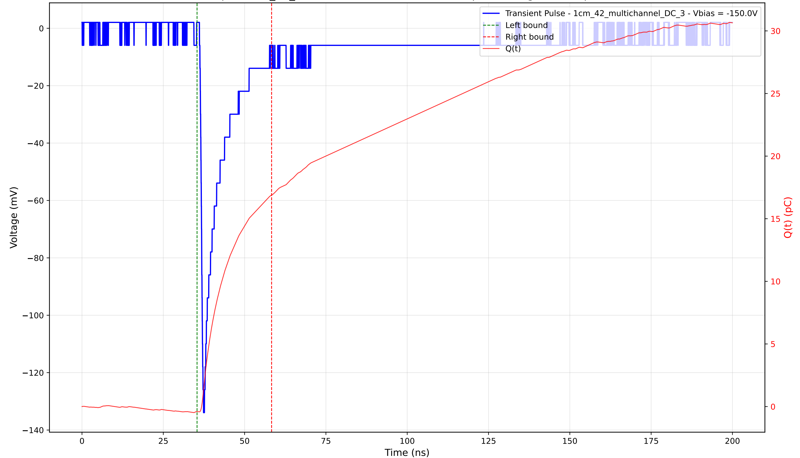
Transient Pulse - Sample: 1cm_42_multichannel - Position: 4445.0 \mu\text{m} - Charge: 17.28 pC - Rise Time: 0.94 ns
