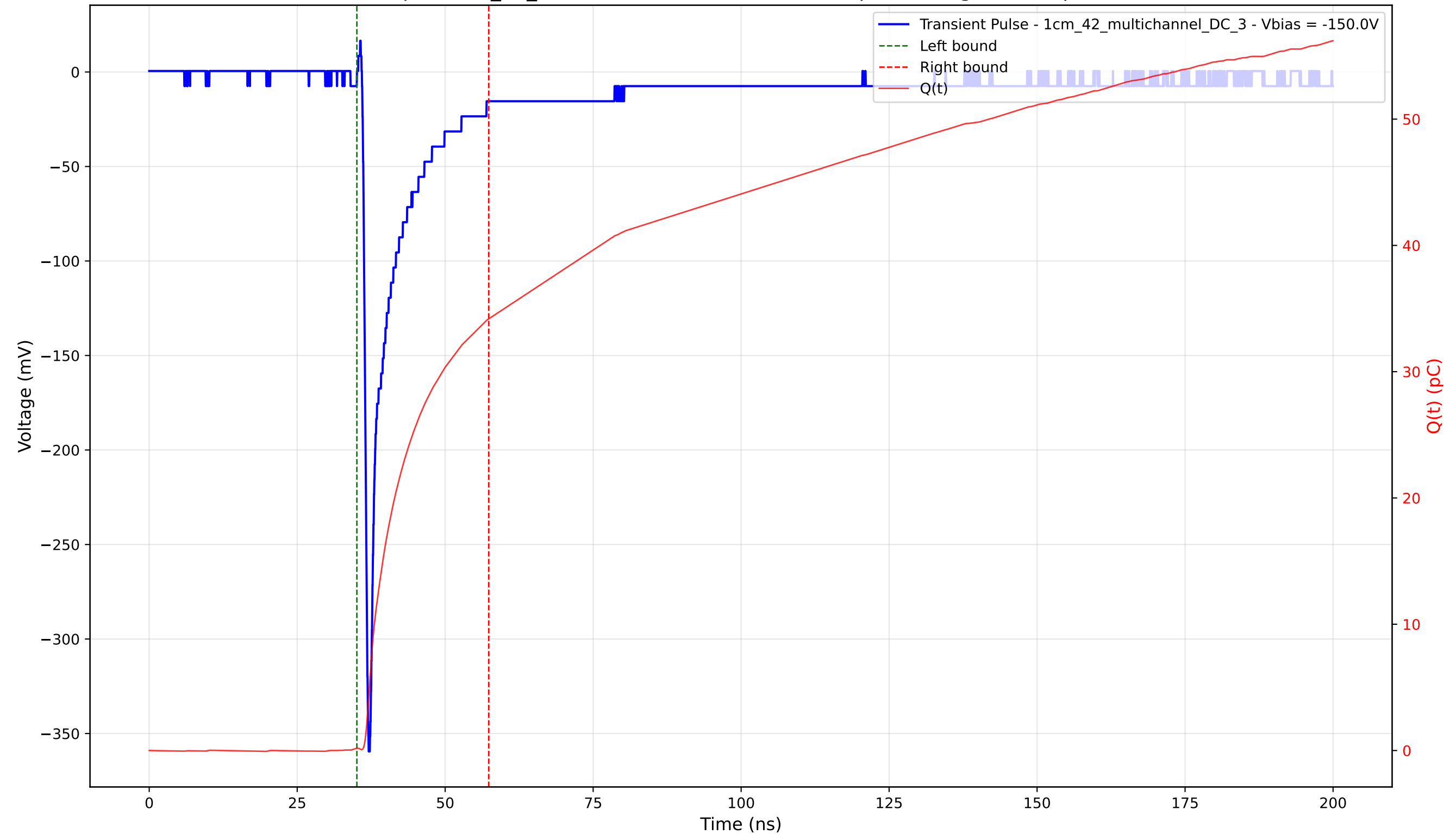
Transient Pulse - Sample: 1cm_42_multichannel - Position: 4785.0 \mu\text{m} - Charge: 34.00 pC - Rise Time: 0.78 ns
