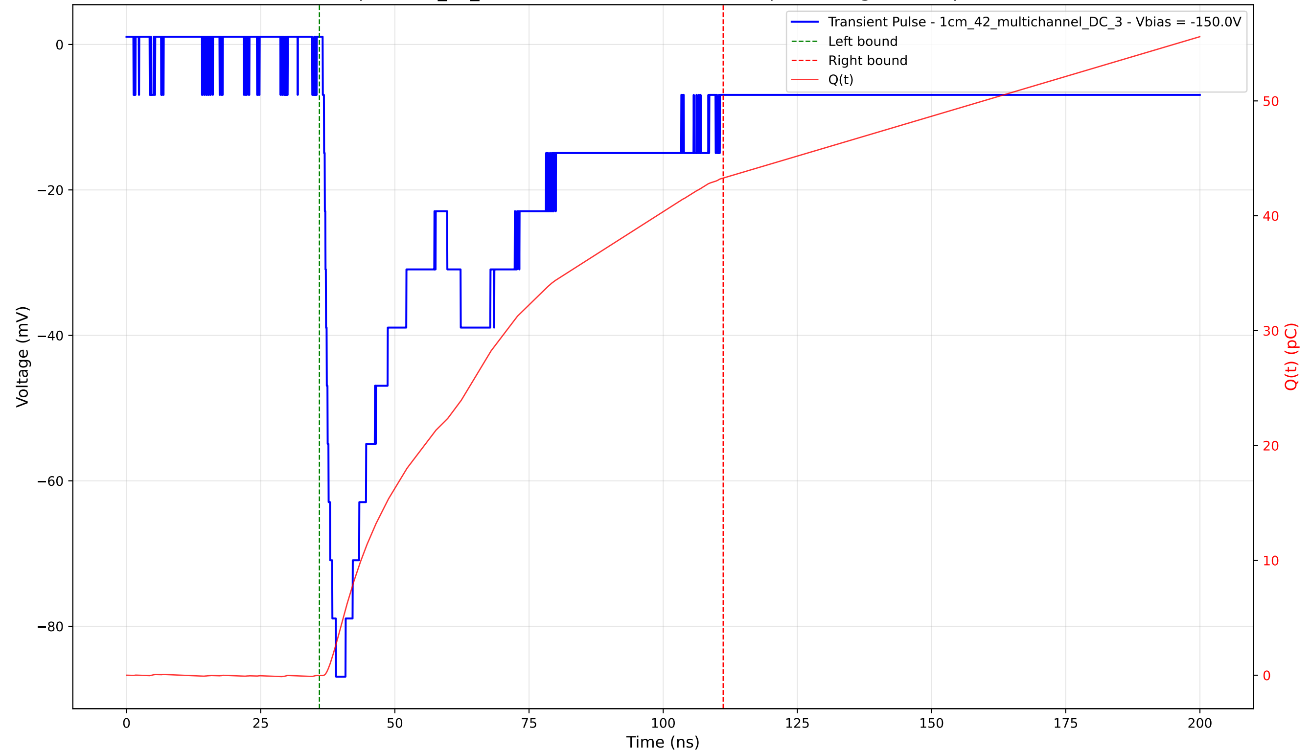
Transient Pulse - Sample: 1cm_42_multichannel - Position: 2215.0 \mu\text{m} - Charge: 43.31 pC - Rise Time: 1.56 ns
