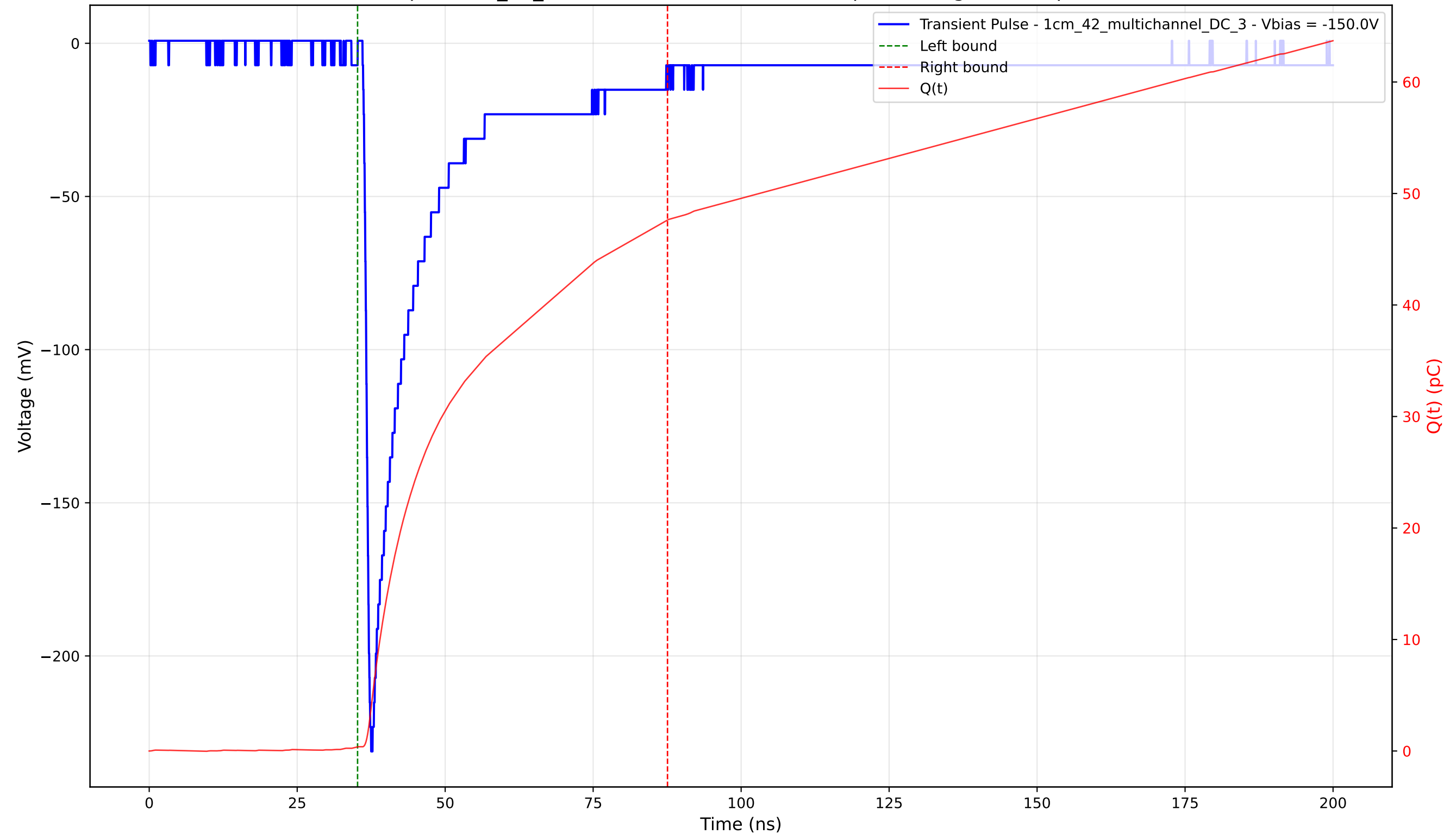
Transient Pulse - Sample: 1cm_42_multichannel - Position: 660.0 \mu\text{m} - Charge: 47.24 pC - Rise Time: 1.02 ns
