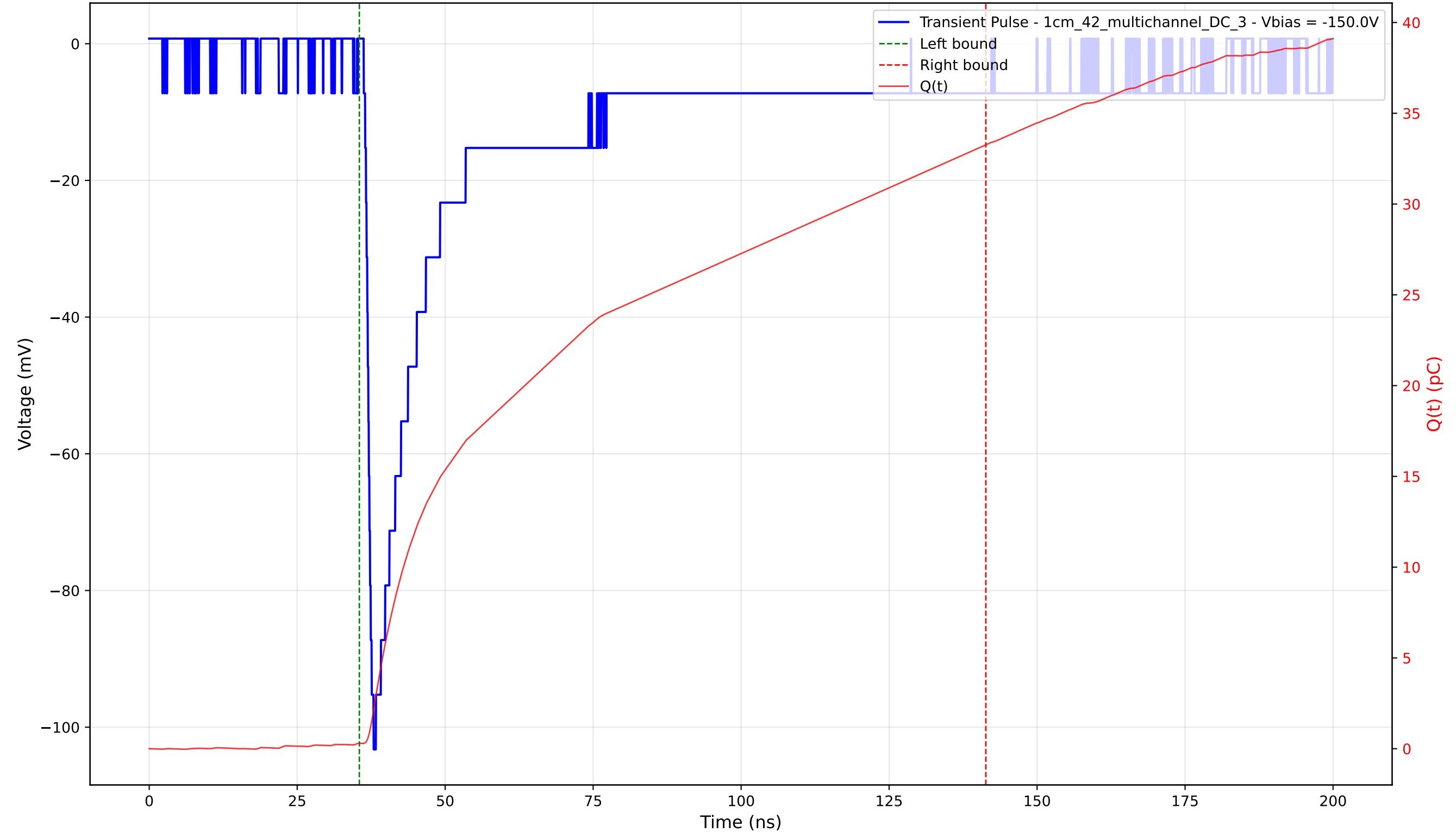
Transient Pulse - Sample: 1cm_42_multichannel - Position: 3945.0 \mu\text{m} - Charge: 32.97 pC - Rise Time: 1.11 ns
