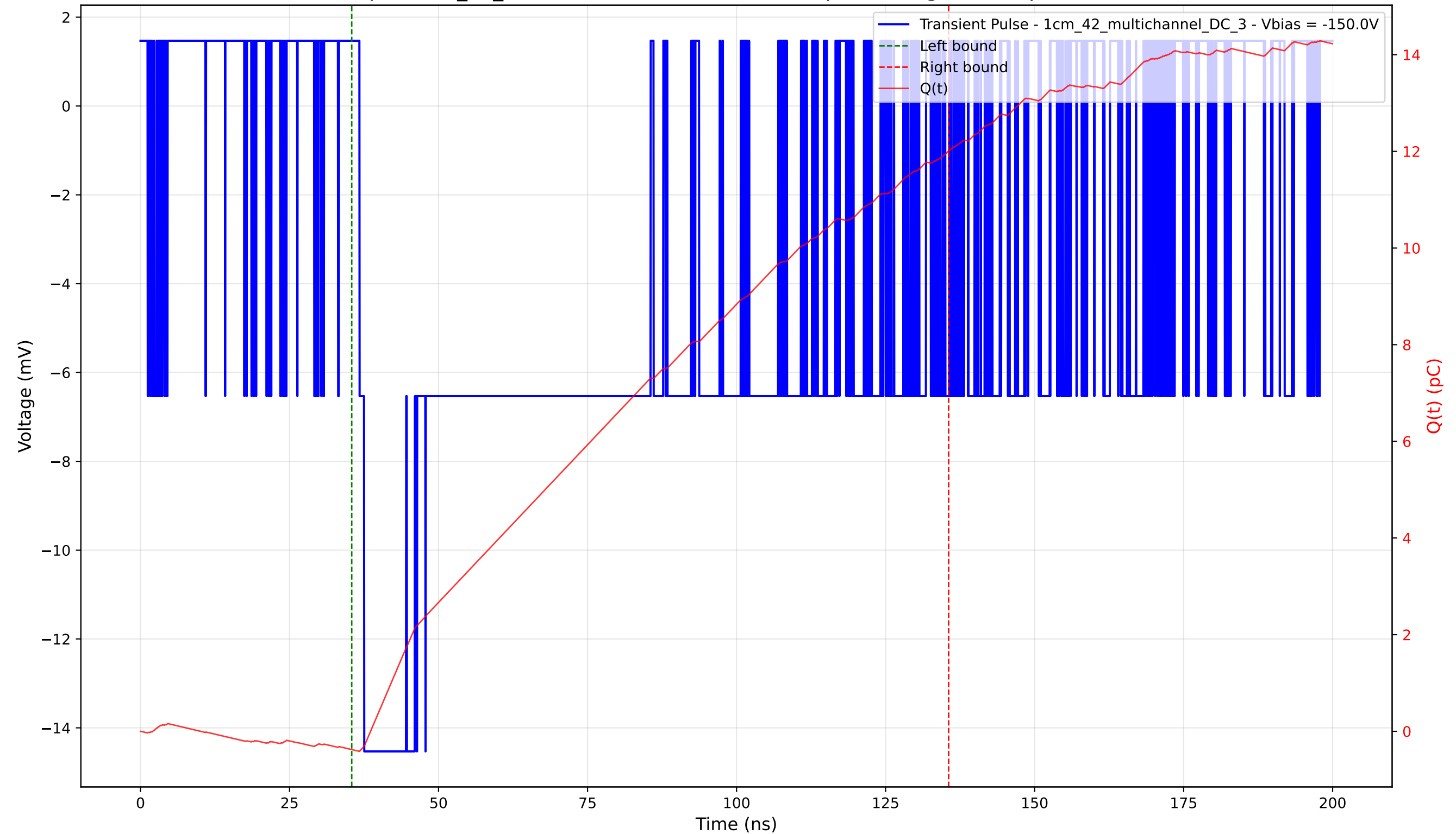
Transient Pulse - Sample: 1cm_42_multichannel - Position: 2405.0 \mu\text{m} - Charge: 12.39 pC - Rise Time: 0.00 ns (N/A)
