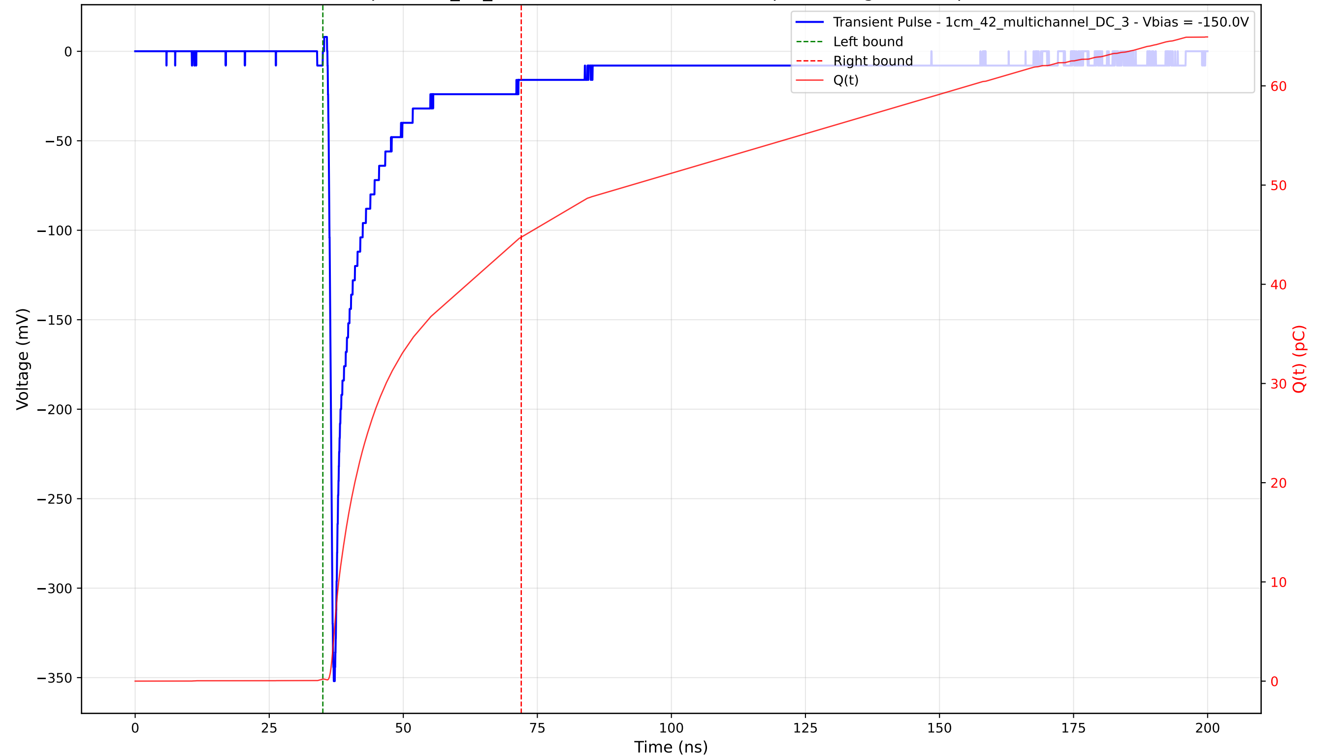
Transient Pulse - Sample: 1cm_42_multichannel - Position: 205.0 \mu\text{m} - Charge: 44.54 pC - Rise Time: 0.79 ns
