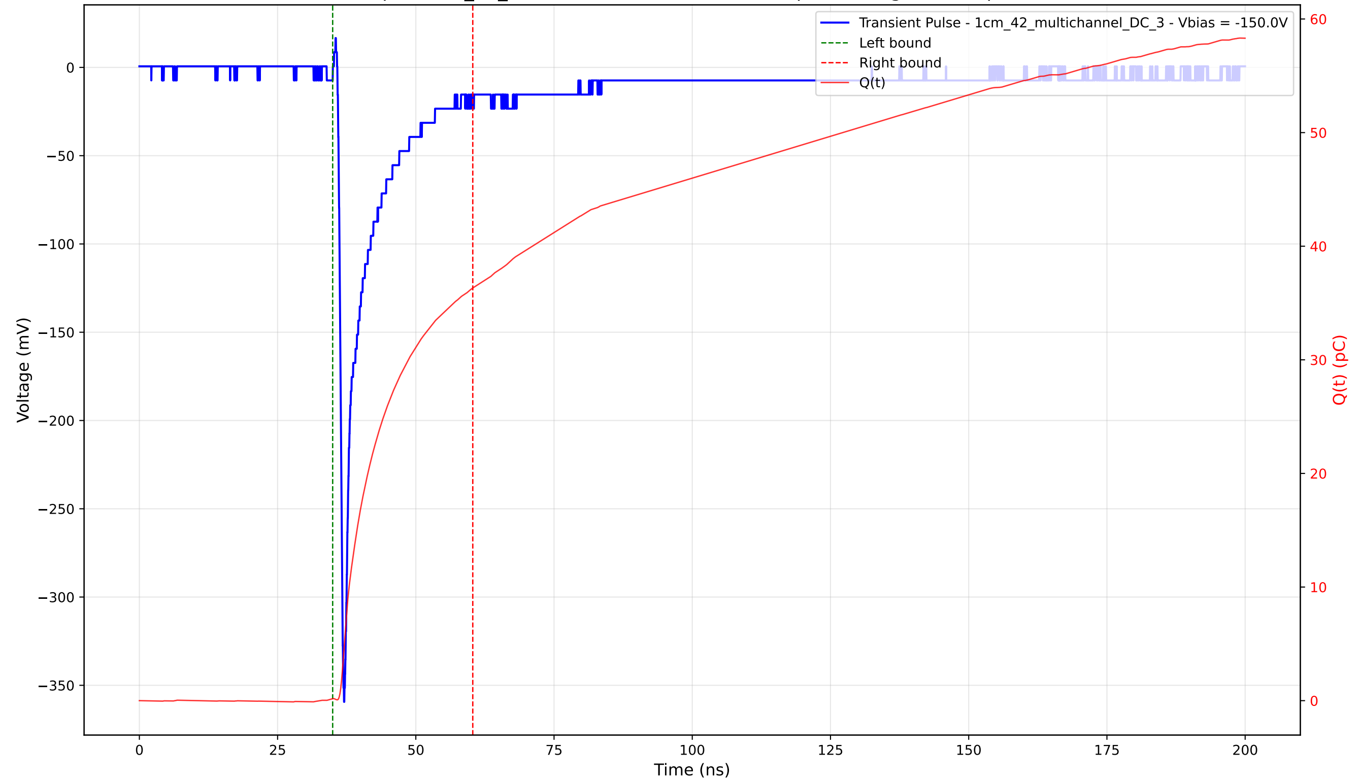
Transient Pulse - Sample: 1cm_42_multichannel - Position: 120.0 \mu\text{m} - Charge: 36.14 pC - Rise Time: 0.81 ns
