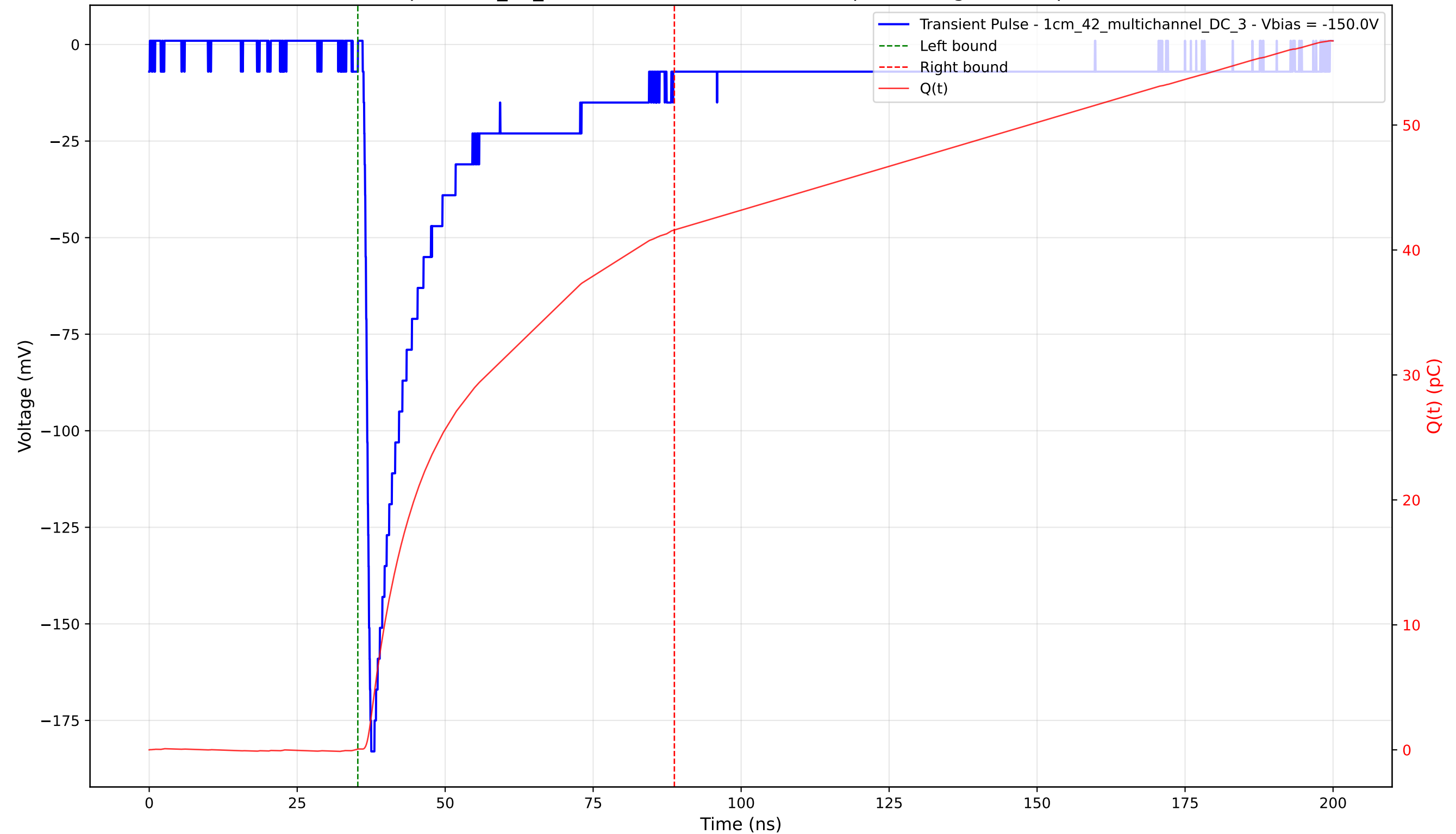
Transient Pulse - Sample: 1cm_42_multichannel - Position: 780.0 \mu\text{m} - Charge: 41.54 pC - Rise Time: 0.97 ns
