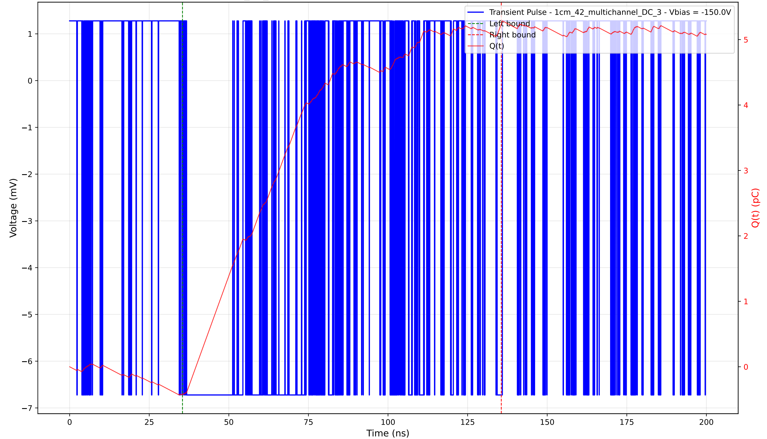
Transient Pulse - Sample: 1cm_42_multichannel - Position: 3395.0 \mu\text{m} - Charge: 5.66 pC - Rise Time: 0.00 ns (N/A)
