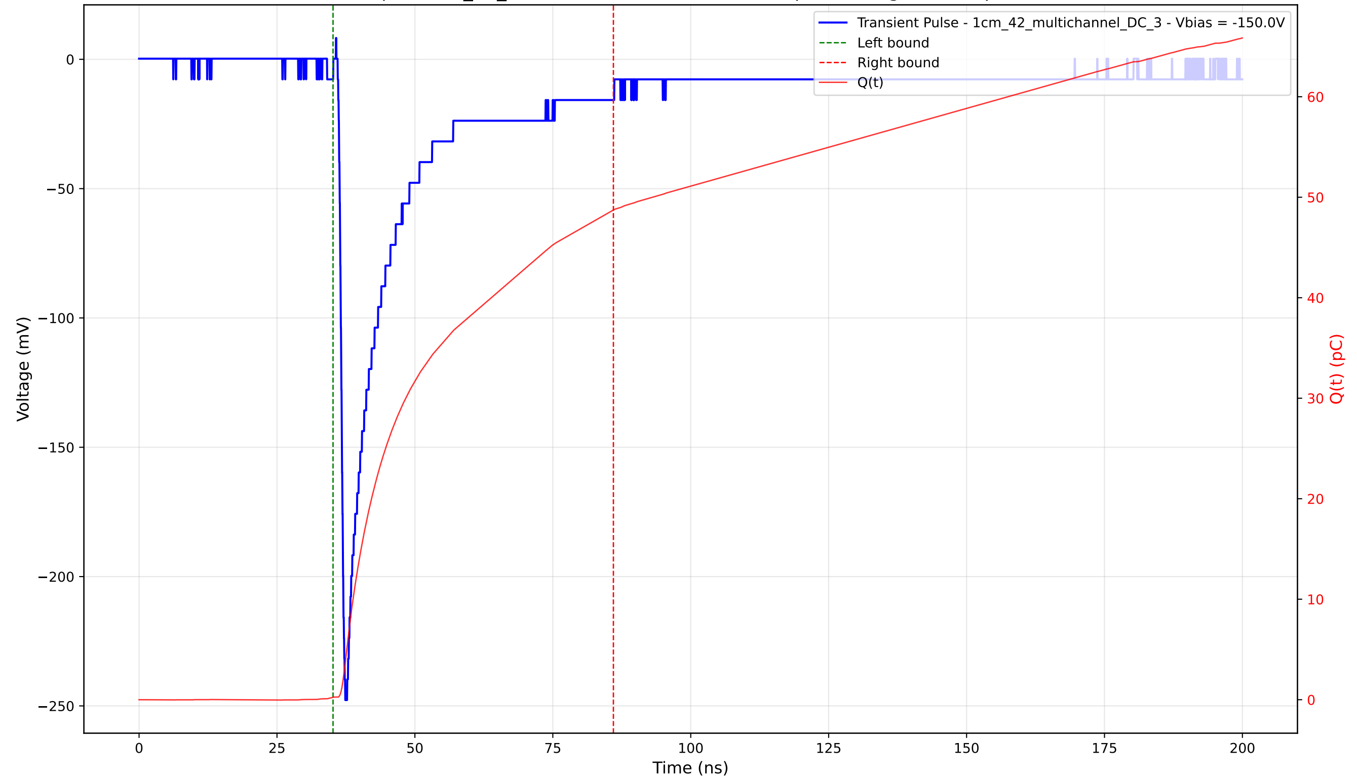
Transient Pulse - Sample: 1cm_42_multichannel - Position: 590.0 \mu\text{m} - Charge: 48.49 pC - Rise Time: 0.90 ns
