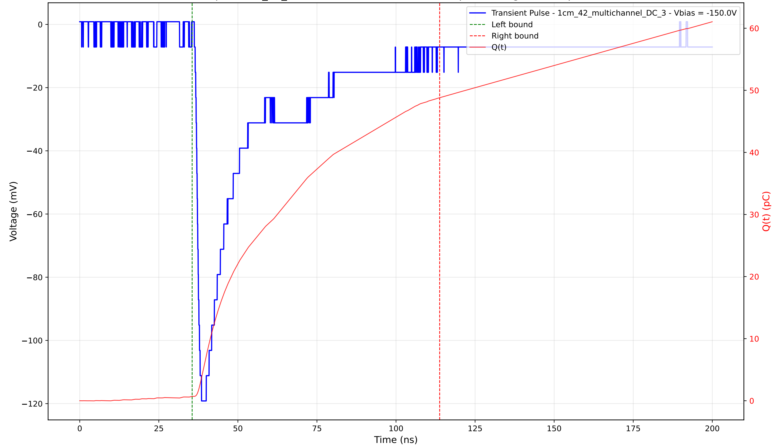
Transient Pulse - Sample: 1cm_42_multichannel - Position: 1695.0 \mu\text{m} - Charge: 48.11 pC - Rise Time: 1.57 ns
