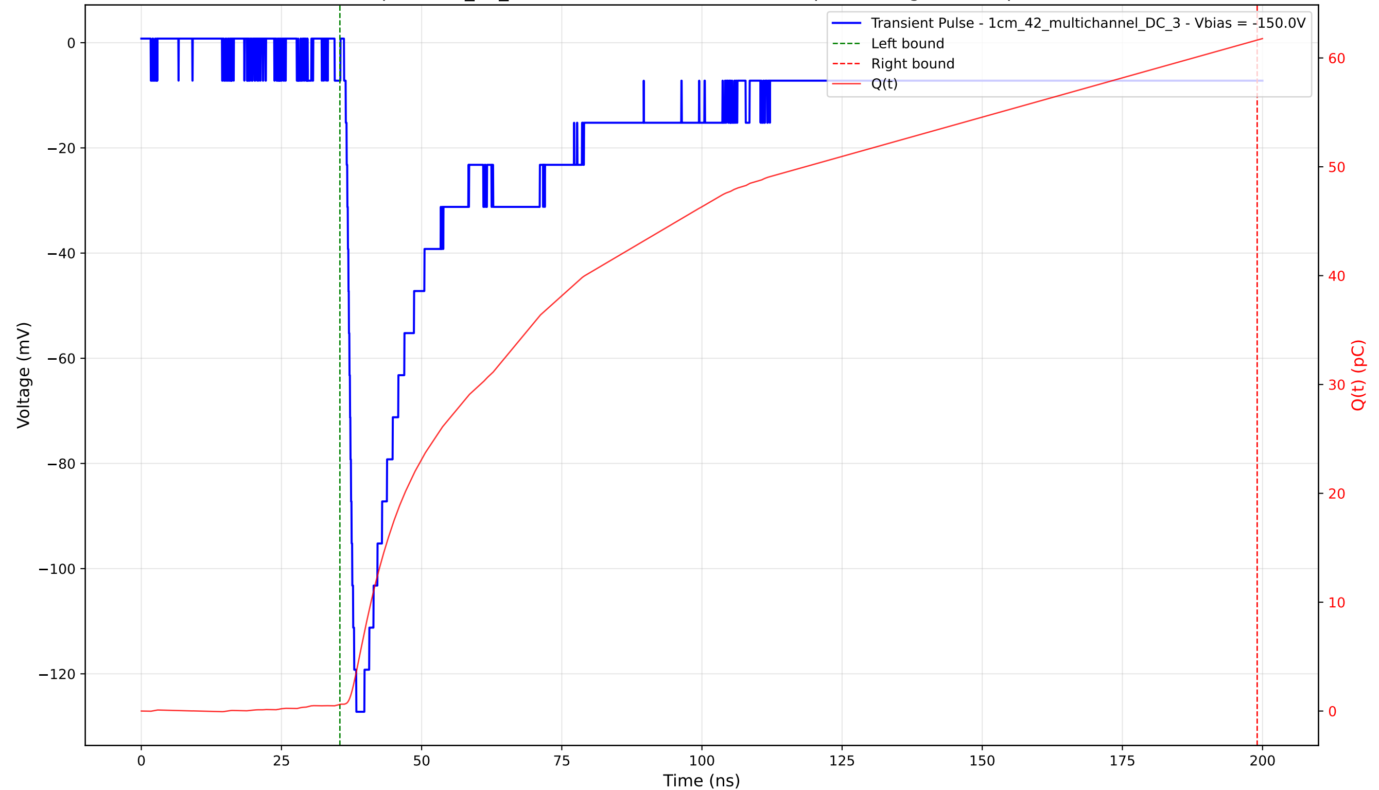
Transient Pulse - Sample: 1cm_42_multichannel - Position: 1545.0 \mu\text{m} - Charge: 61.02 pC - Rise Time: 1.51 ns
