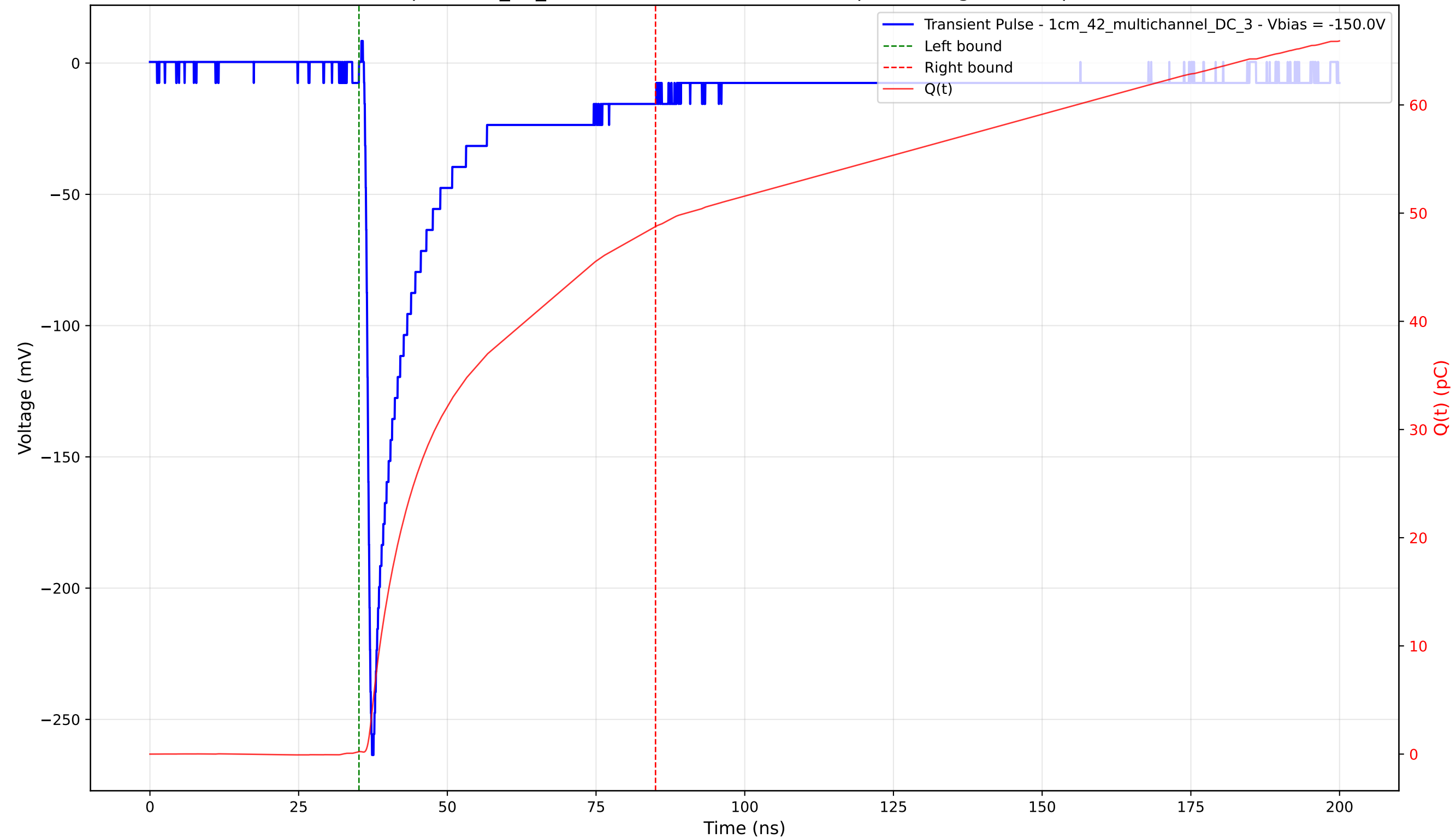
Transient Pulse - Sample: 1cm_42_multichannel - Position: 530.0 \mu\text{m} - Charge: 48.55 pC - Rise Time: 0.91 ns
