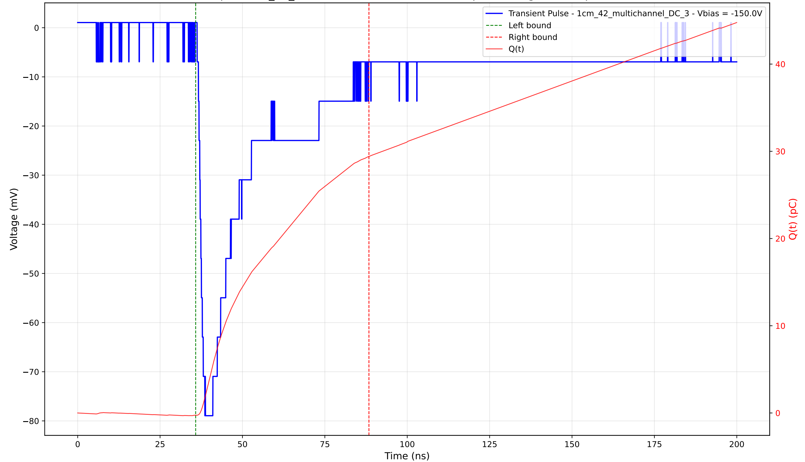
Transient Pulse - Sample: 1cm_42_multichannel - Position: 2945.0 \mu\text{m} - Charge: 29.67 pC - Rise Time: 1.96 ns
