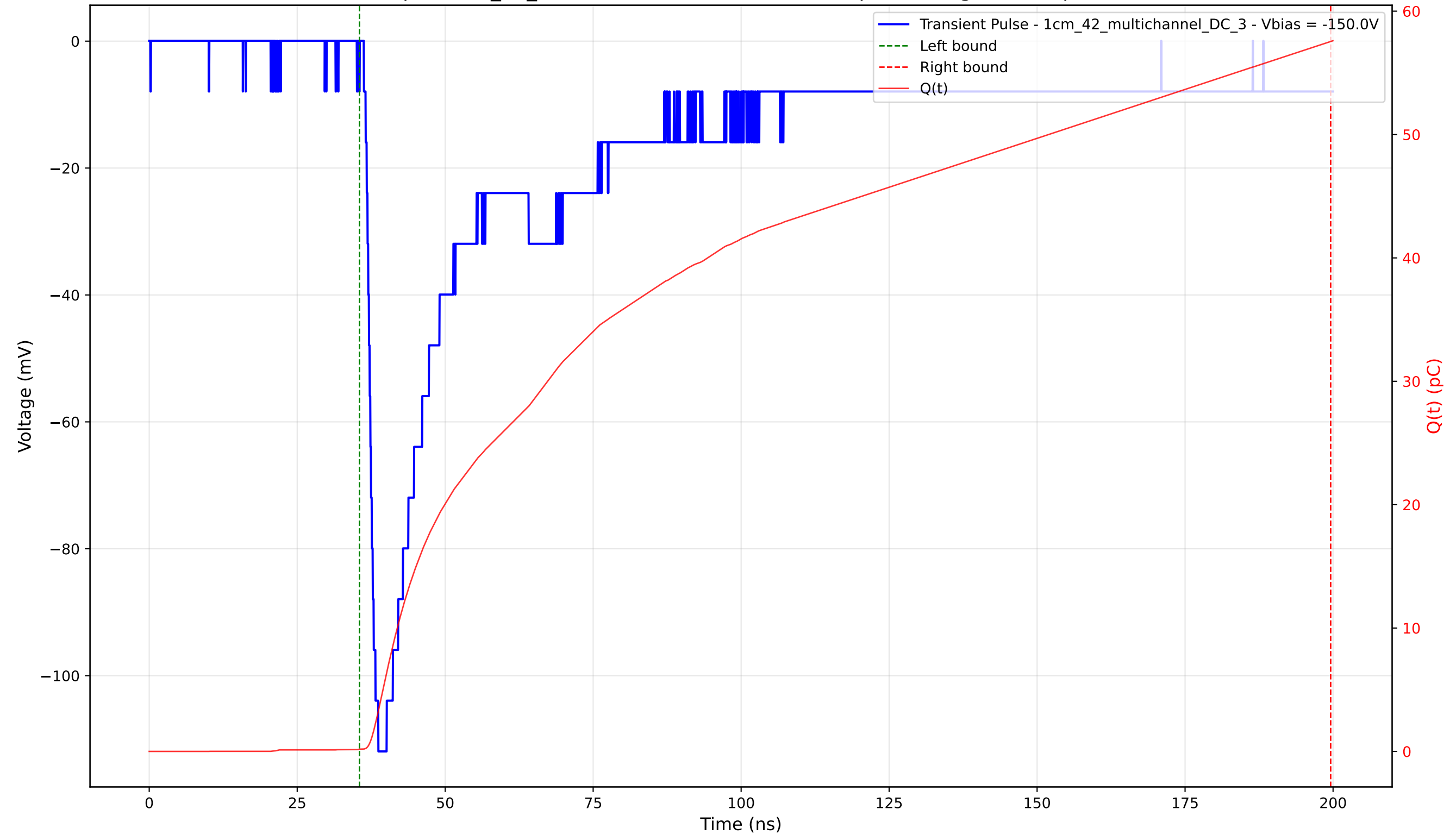
Transient Pulse - Sample: 1cm_42_multichannel - Position: 3205.0 \mu\text{m} - Charge: 57.36 pC - Rise Time: 1.67 ns
