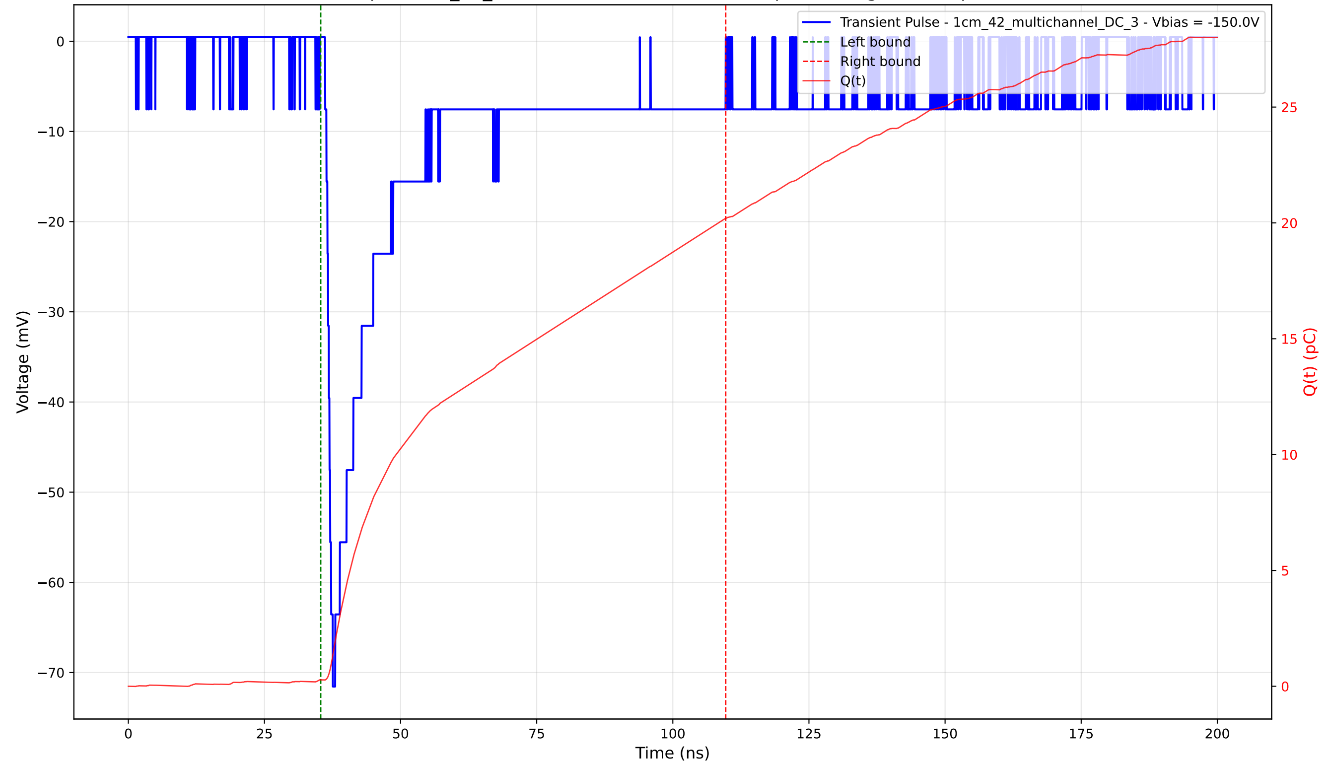
Transient Pulse - Sample: 1cm_42_multichannel - Position: 815.0 \mu\text{m} - Charge: 19.93 pC - Rise Time: 1.40 ns
