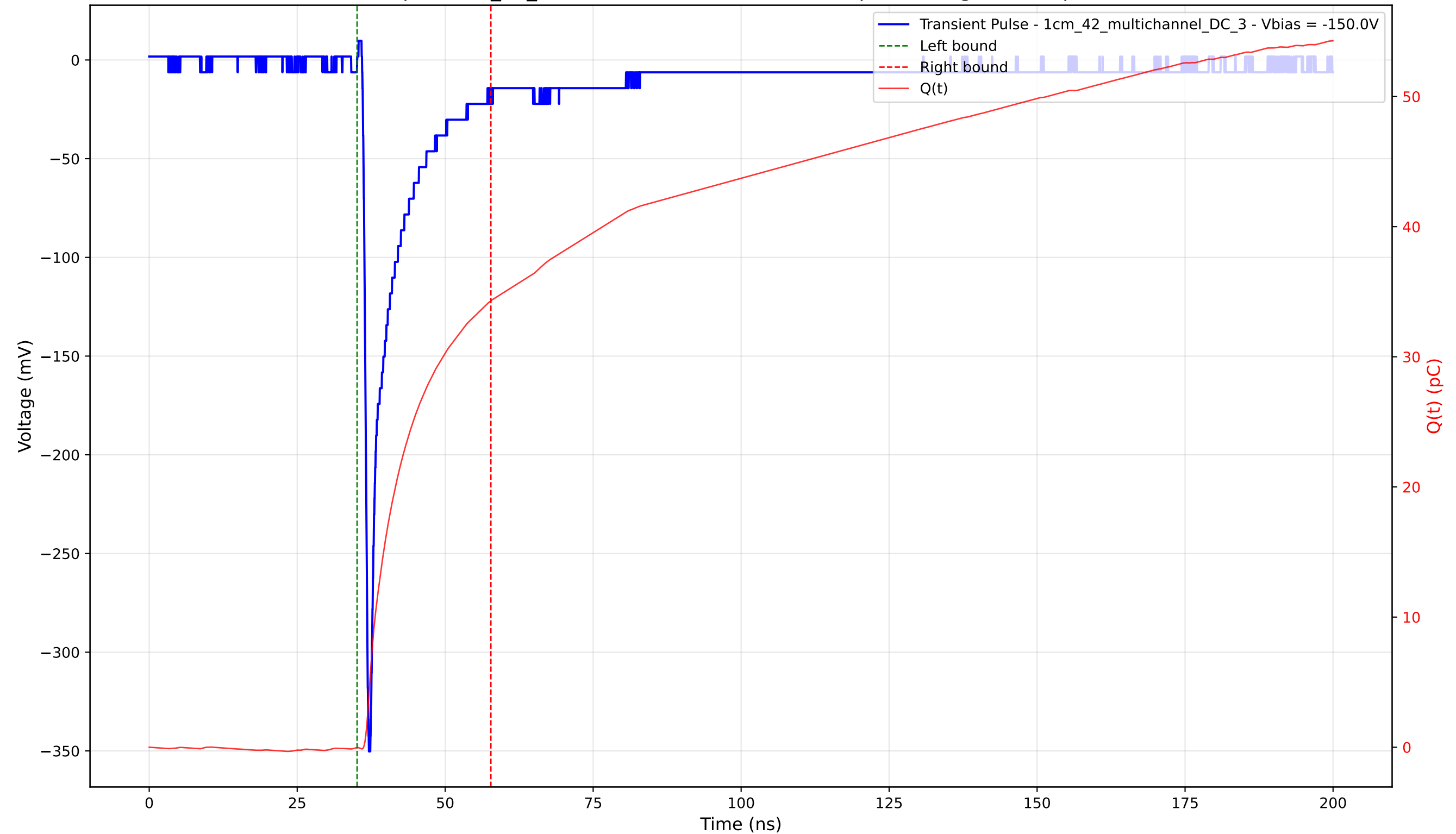
Transient Pulse - Sample: 1cm_42_multichannel - Position: 4745.0 \mu\text{m} - Charge: 34.32 pC - Rise Time: 0.79 ns
