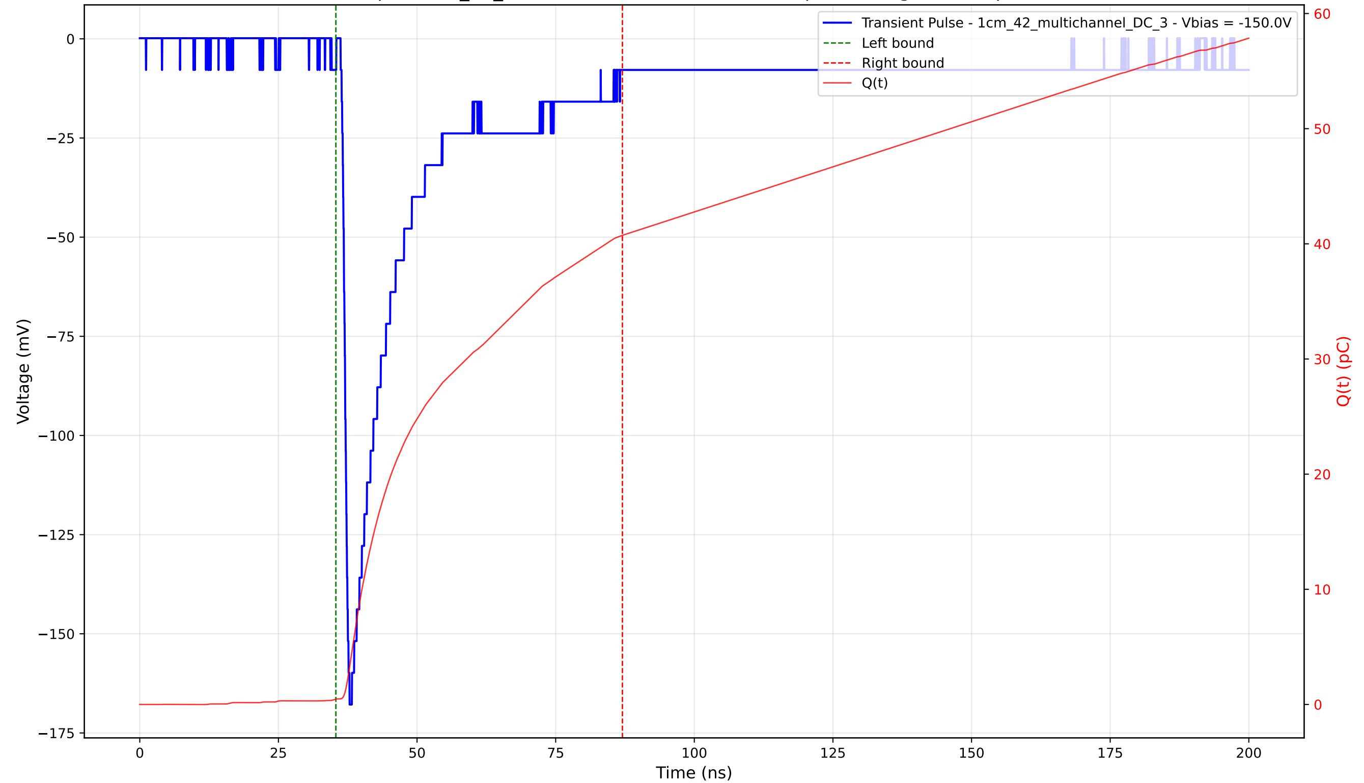
Transient Pulse - Sample: 1cm_42_multichannel - Position: 3975.0 \mu\text{m} - Charge: 40.27 pC - Rise Time: 1.04 ns
