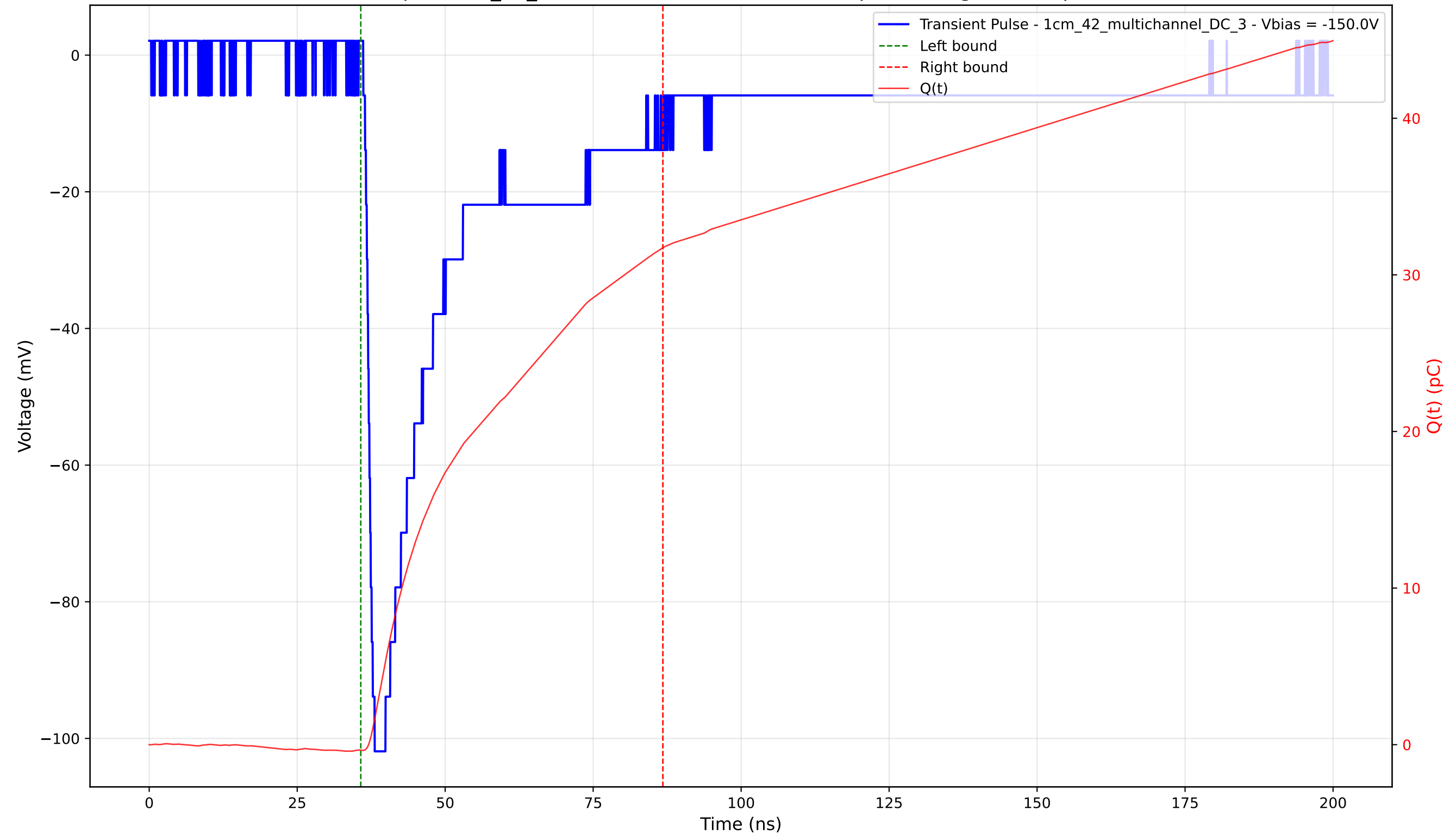
Transient Pulse - Sample: 1cm_42_multichannel - Position: 1425.0 \mu\text{m} - Charge: 32.09 pC - Rise Time: 1.31 ns
