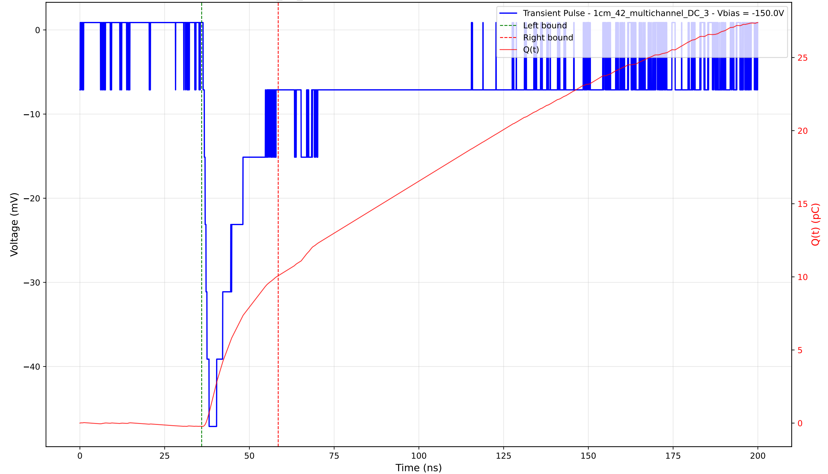
Transient Pulse - Sample: 1cm_42_multichannel - Position: 1405.0 \mu\text{m} - Charge: 10.30 pC - Rise Time: 1.77 ns
