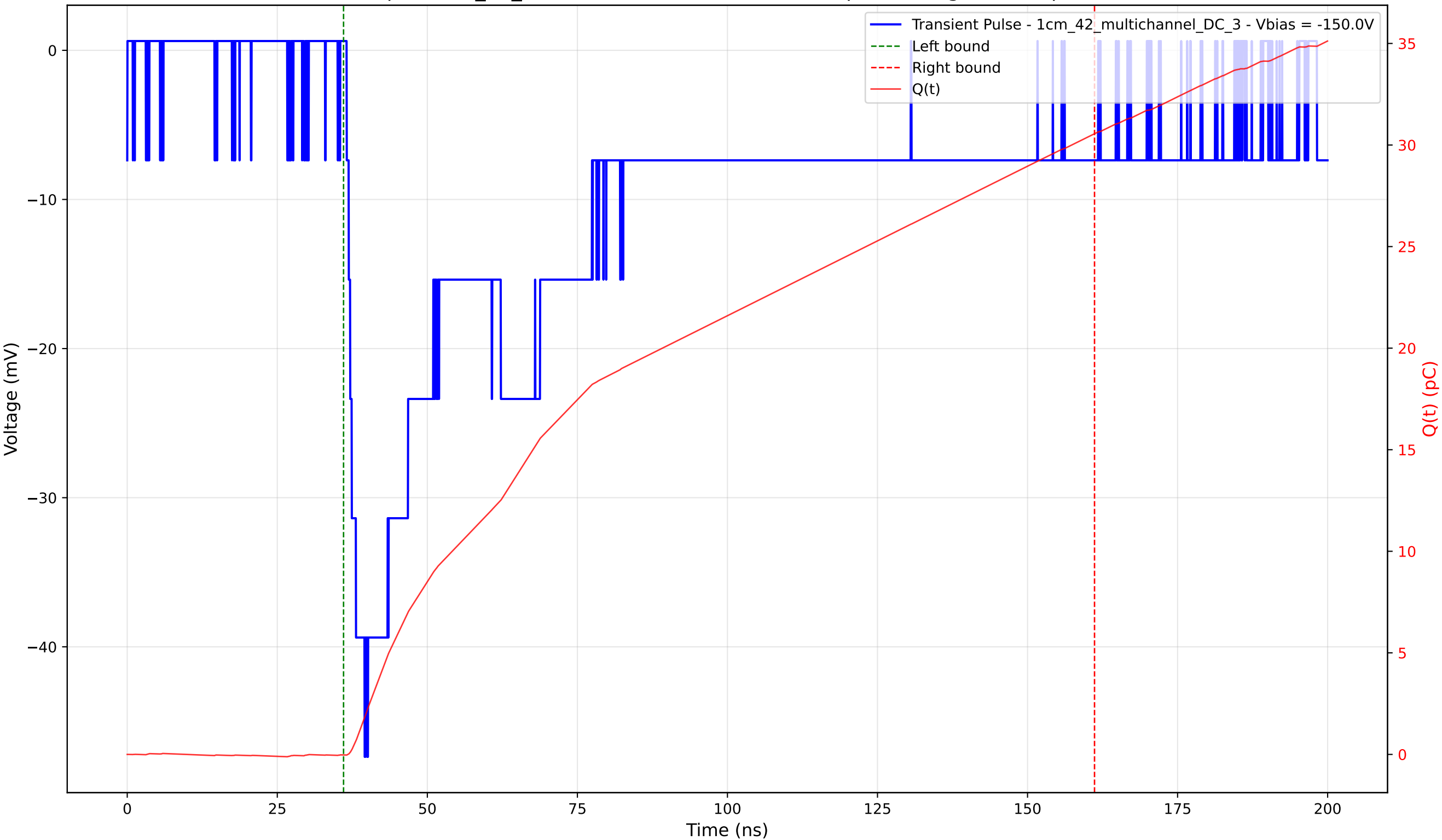
Transient Pulse - Sample: 1cm_42_multichannel - Position: 2425.0 \mu\text{m} - Charge: 30.59 pC - Rise Time: 2.99 ns
