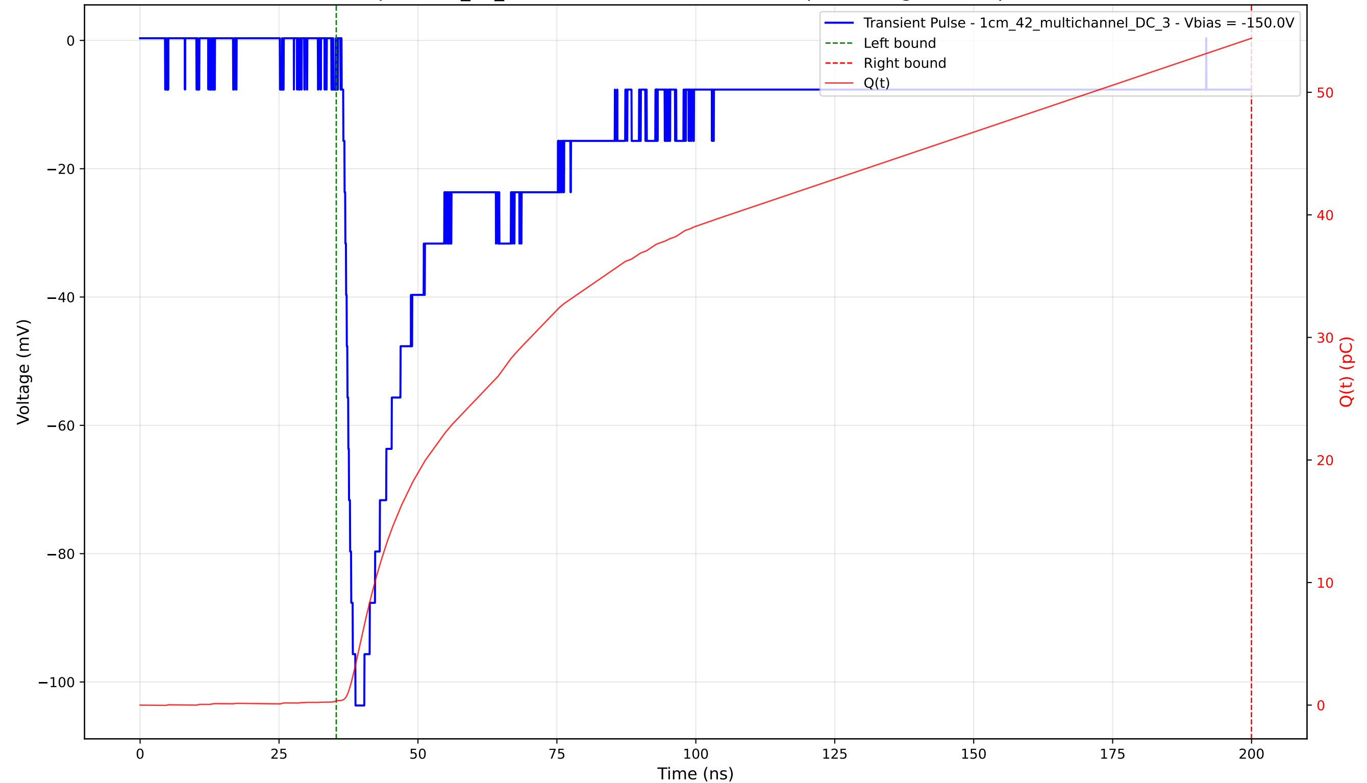
Transient Pulse - Sample: 1cm_42_multichannel - Position: 3130.0 \mu\text{m} - Charge: 54.07 pC - Rise Time: 1.71 ns
