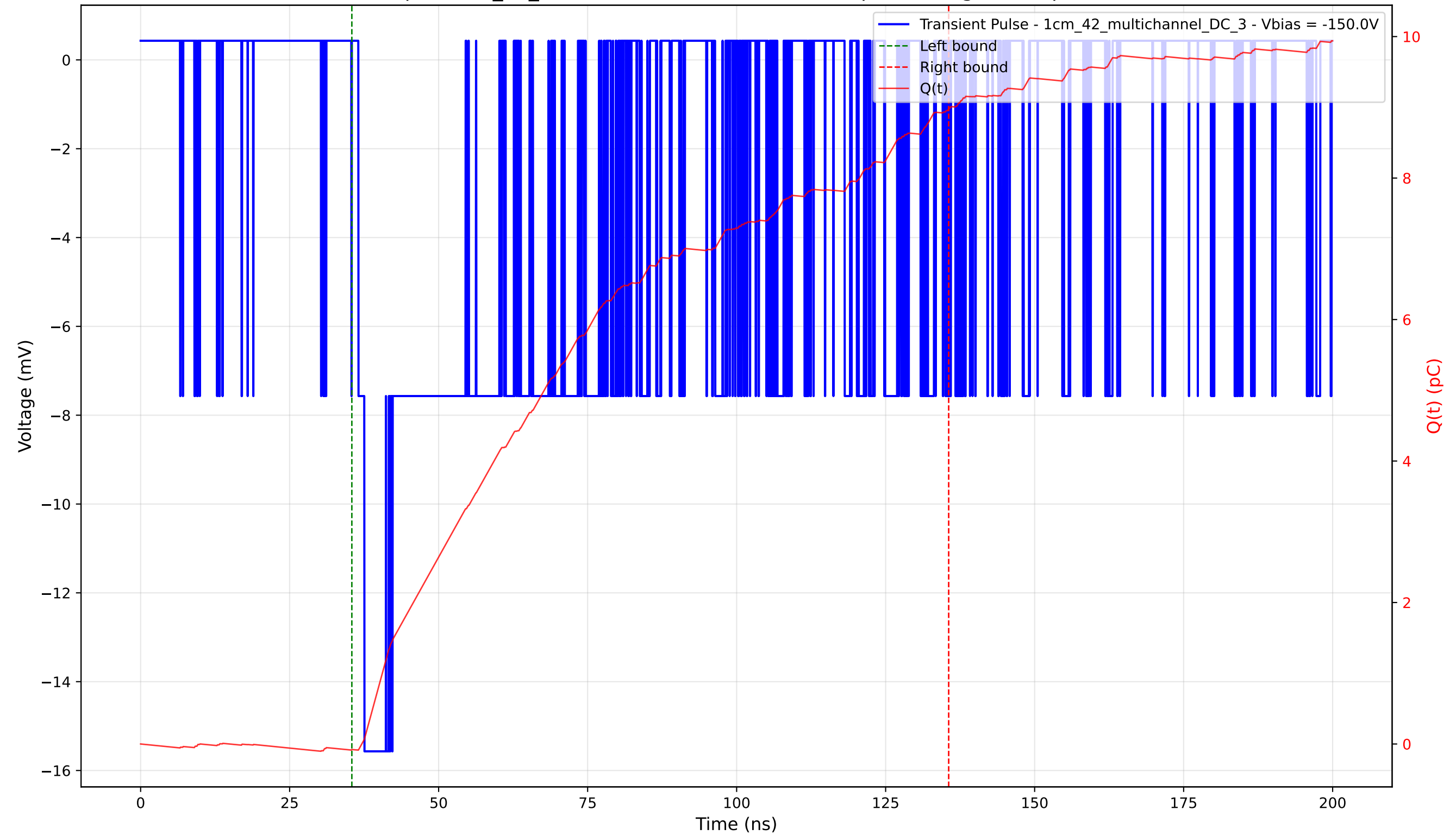
Transient Pulse - Sample: 1cm_42_multichannel - Position: 3870.0 \mu\text{m} - Charge: 9.06 pC - Rise Time: 1.02 ns
