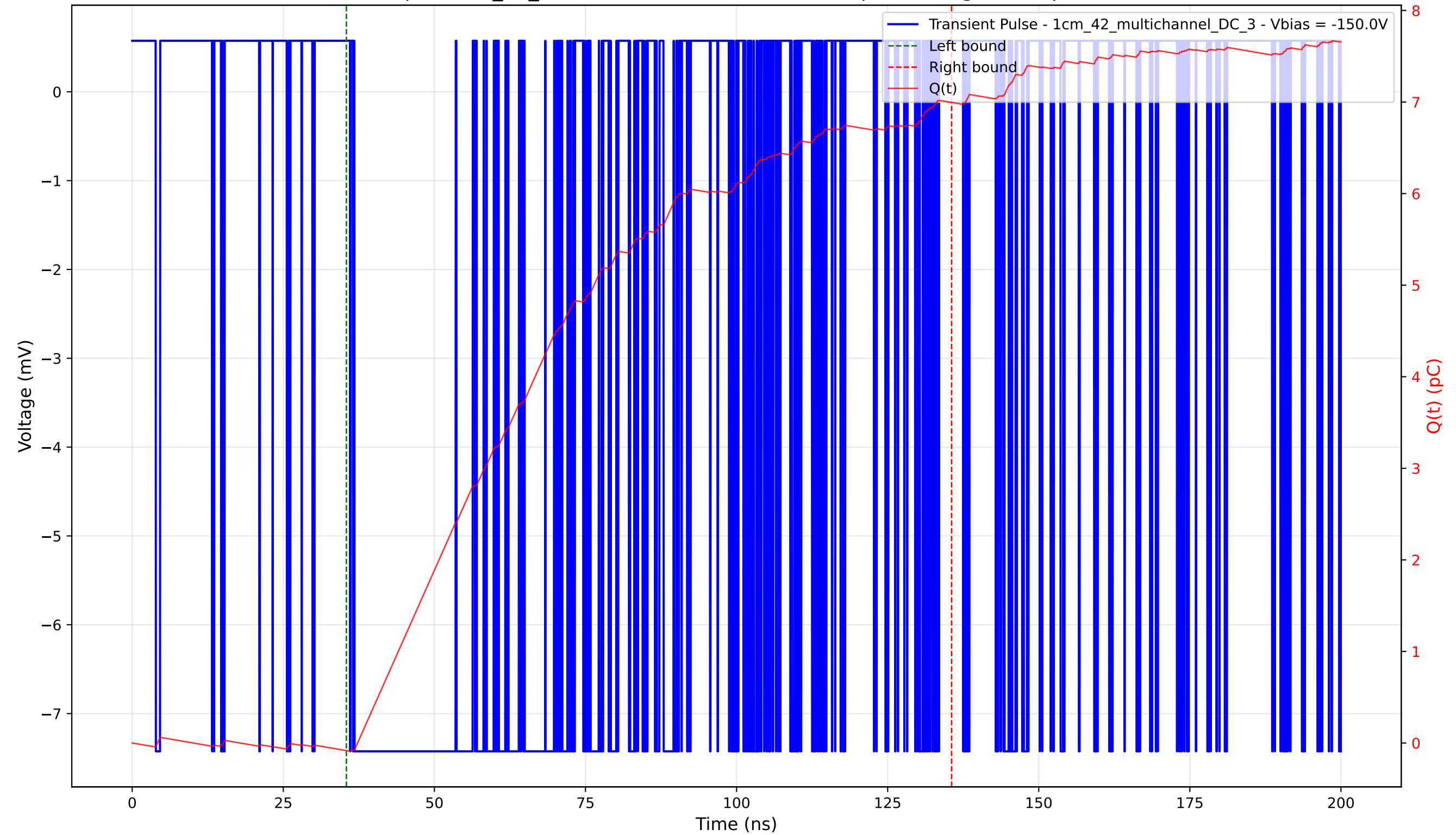
Transient Pulse - Sample: 1cm_42_multichannel - Position: 2375.0 \mu\text{m} - Charge: 7.08 pC - Rise Time: 0.02 ns
