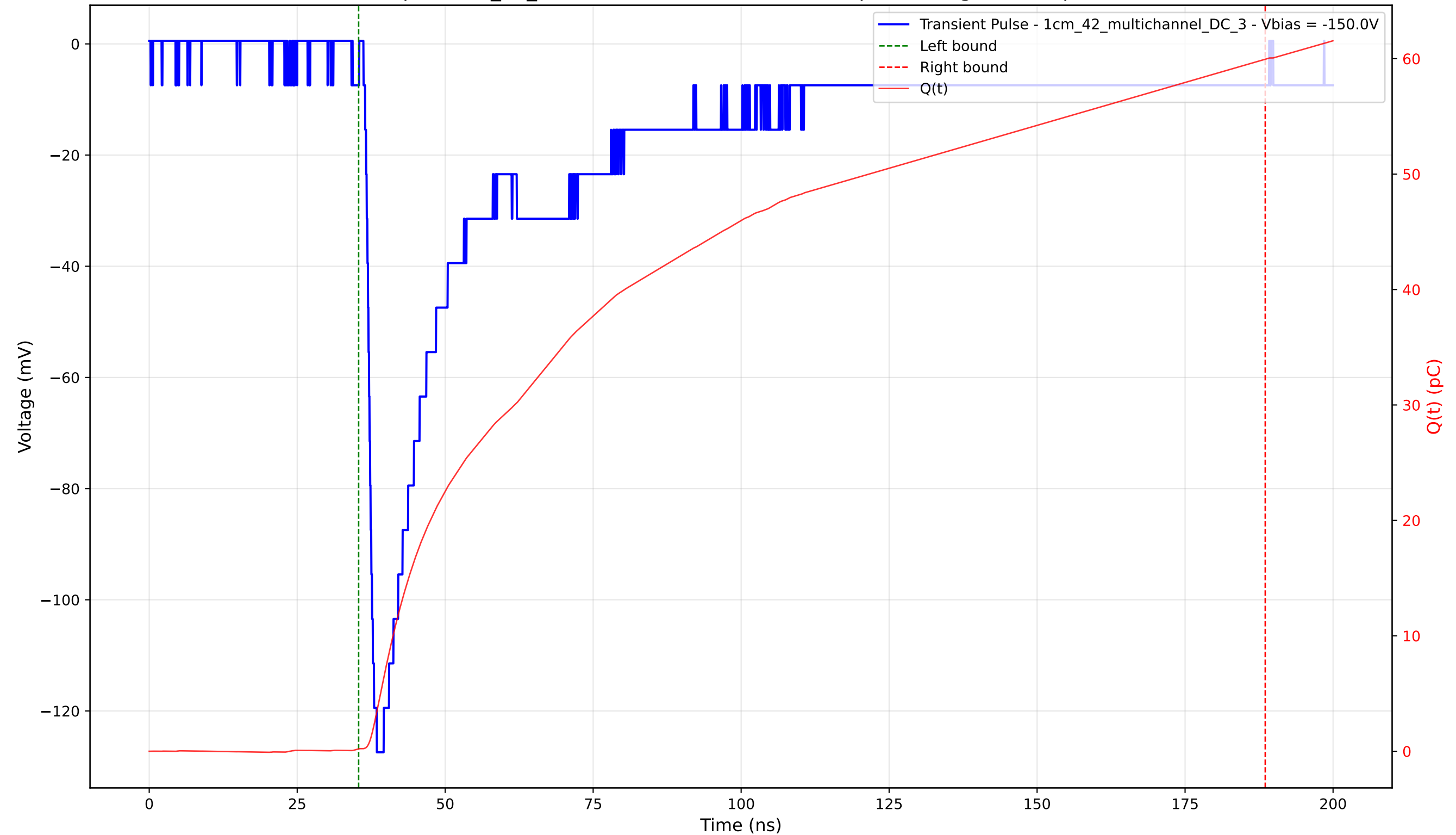
Transient Pulse - Sample: 1cm_42_multichannel - Position: 1550.0 \mu\text{m} - Charge: 59.75 pC - Rise Time: 1.51 ns
