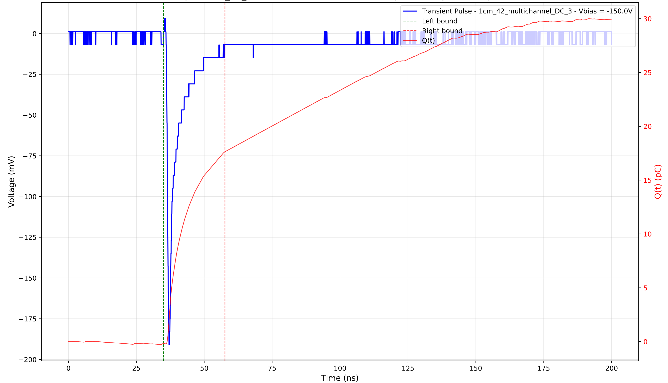
Transient Pulse - Sample: 1cm_42_multichannel - Position: 4850.0 \mu\text{m} - Charge: 17.79 pC - Rise Time: 0.77 ns
