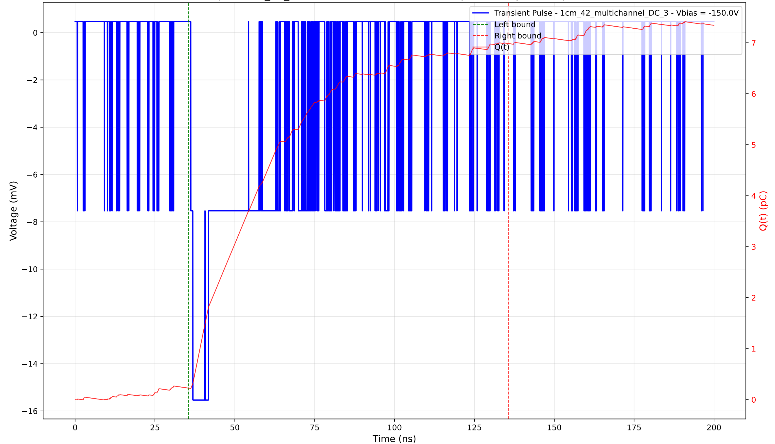
Transient Pulse - Sample: 1cm_42_multichannel - Position: 4410.0 \mu\text{m} - Charge: 6.76 pC - Rise Time: 0.66 ns
