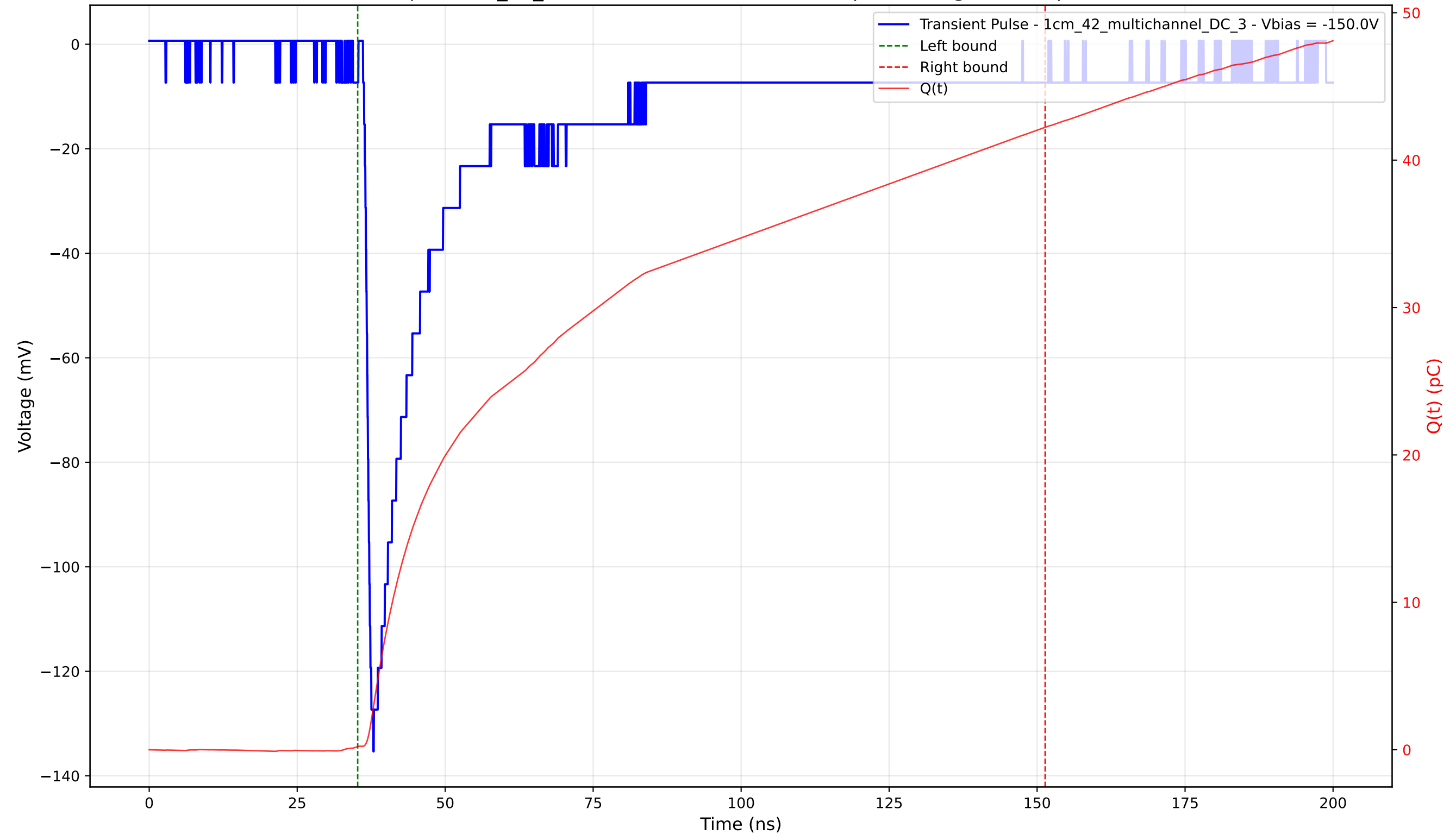
Transient Pulse - Sample: 1cm_42_multichannel - Position: 915.0 \mu\text{m} - Charge: 42.01 pC - Rise Time: 1.22 ns
