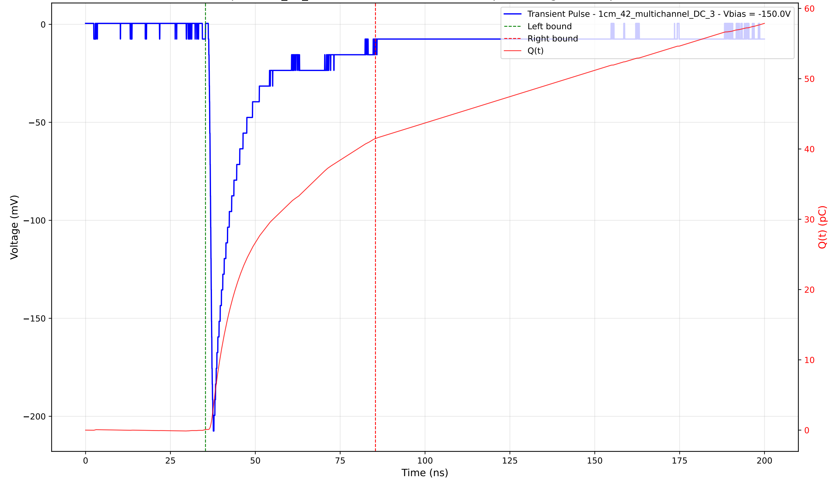
Transient Pulse - Sample: 1cm_42_multichannel - Position: 4205.0 \mu\text{m} - Charge: 41.40 pC - Rise Time: 1.01 ns
