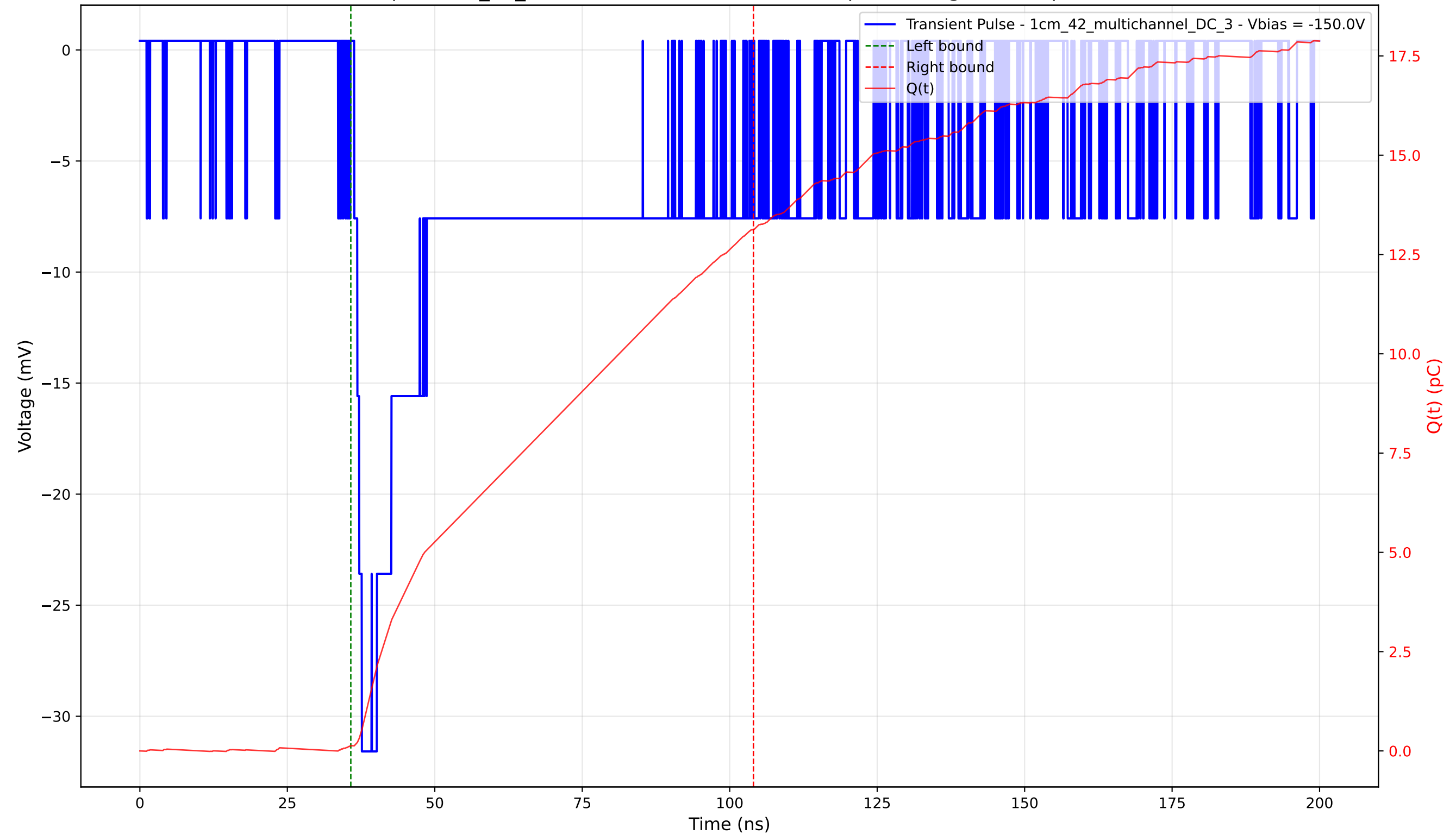
Transient Pulse - Sample: 1cm_42_multichannel - Position: 3855.0 \mu\text{m} - Charge: 13.00 pC - Rise Time: 1.29 ns
