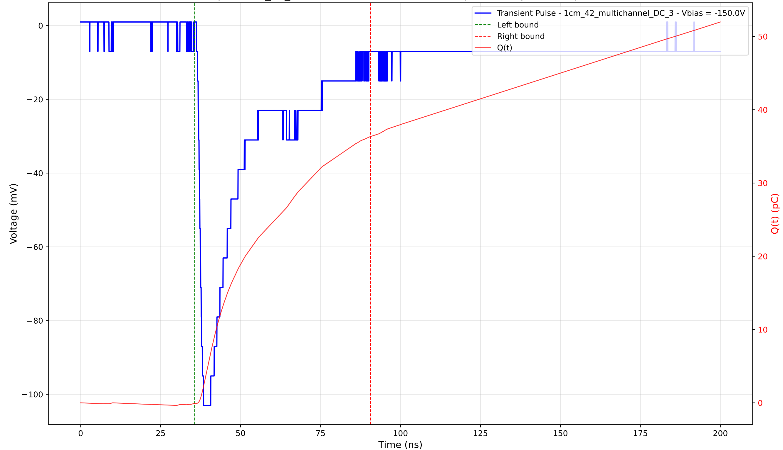
Transient Pulse - Sample: 1cm_42_multichannel - Position: 3180.0 \mu\text{m} - Charge: 36.42 pC - Rise Time: 1.51 ns
