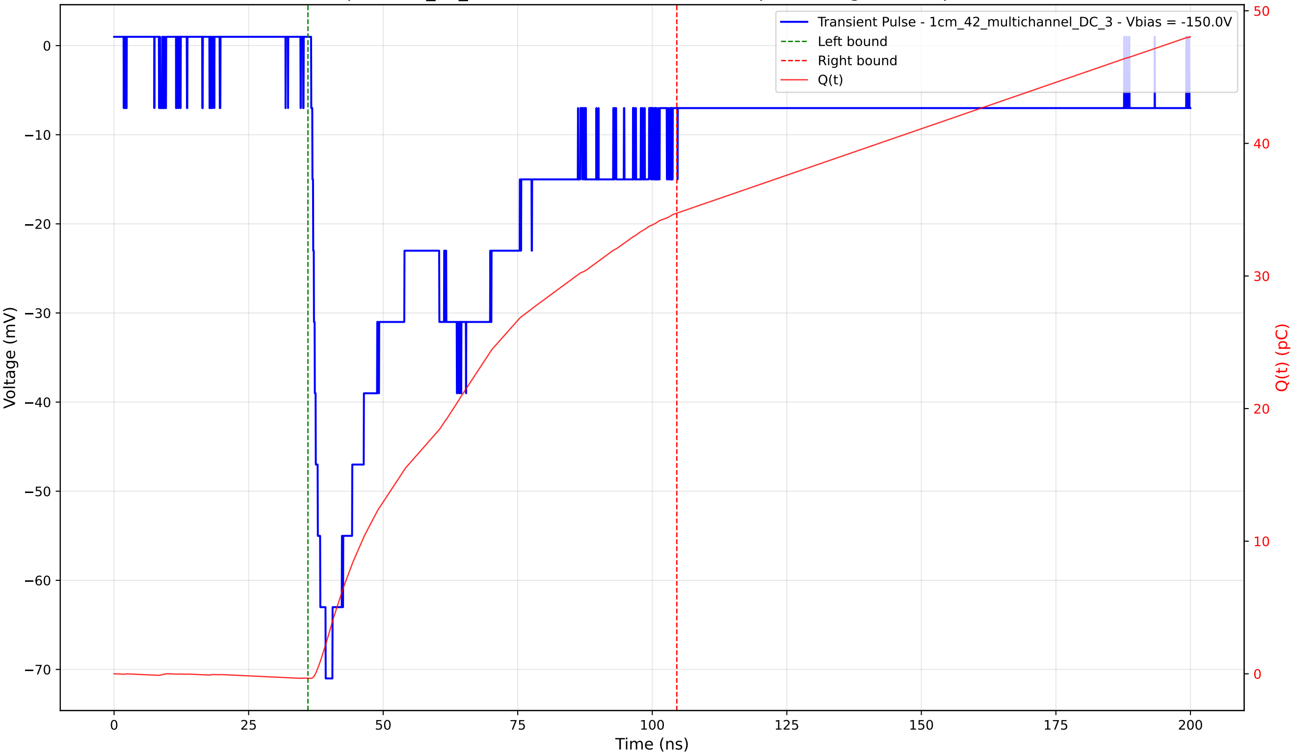
Transient Pulse - Sample: 1cm_42_multichannel - Position: 2305.0 \mu\text{m} - Charge: 35.08 pC - Rise Time: 2.48 ns
