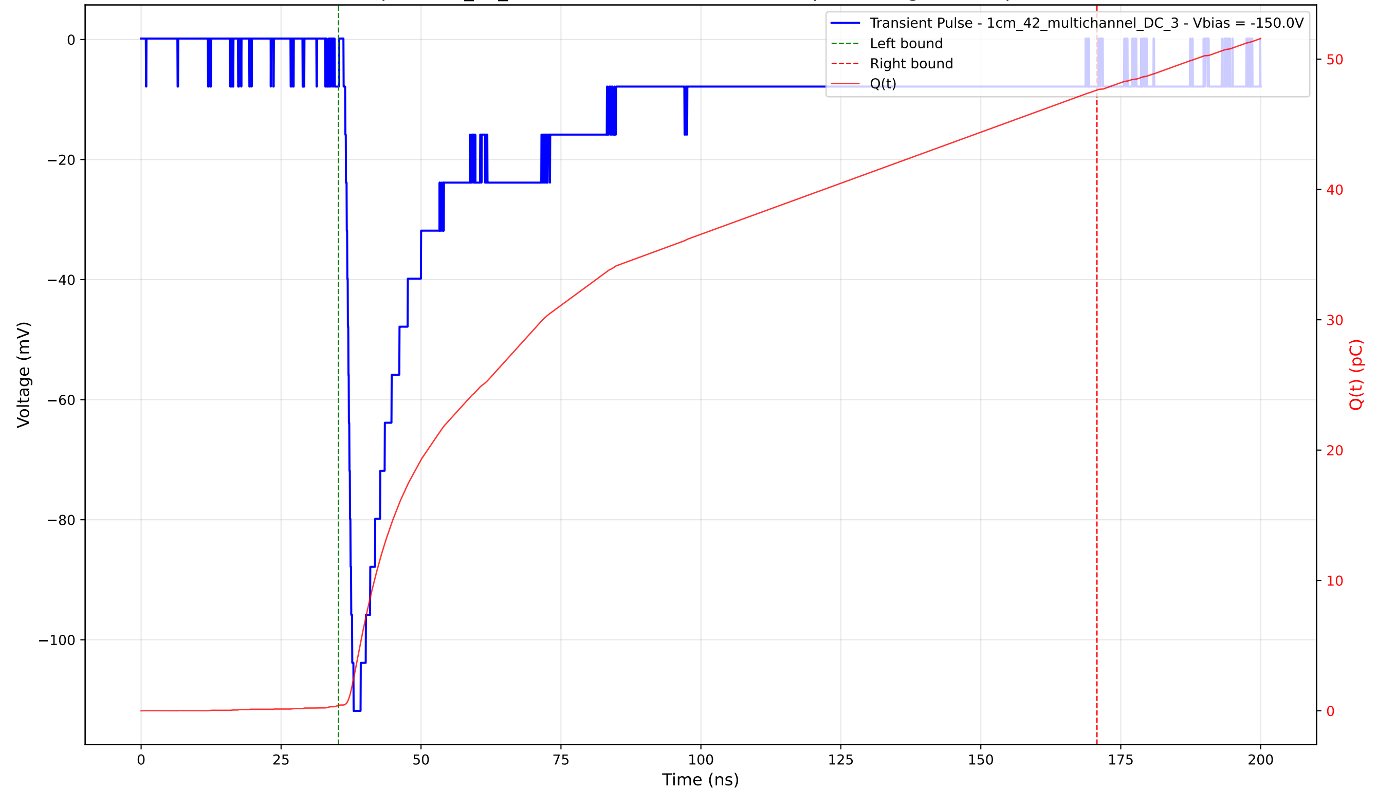
Transient Pulse - Sample: 1cm_42_multichannel - Position: 1300.0 \mu\text{m} - Charge: 47.21 pC - Rise Time: 1.25 ns
