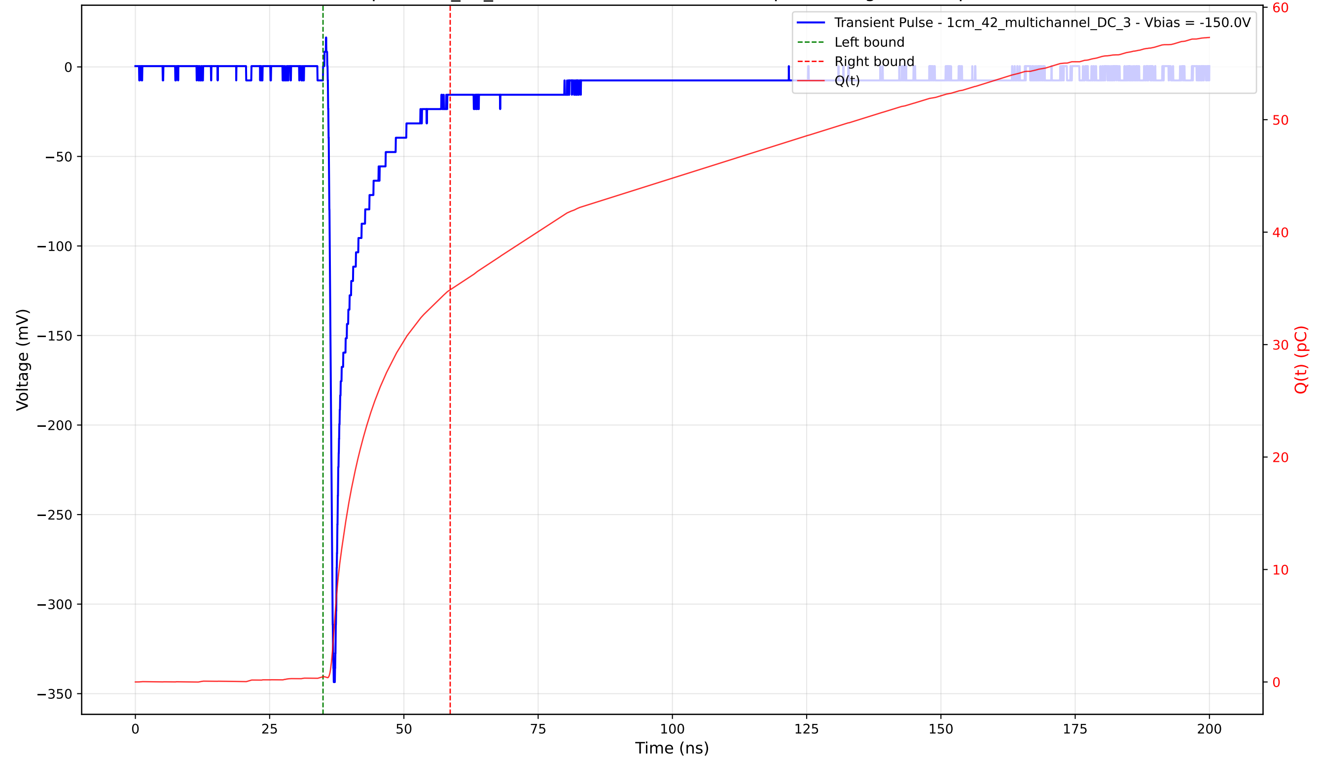
Transient Pulse - Sample: 1cm_42_multichannel - Position: 110.0 \mu\text{m} - Charge: 34.40 pC - Rise Time: 0.77 ns
