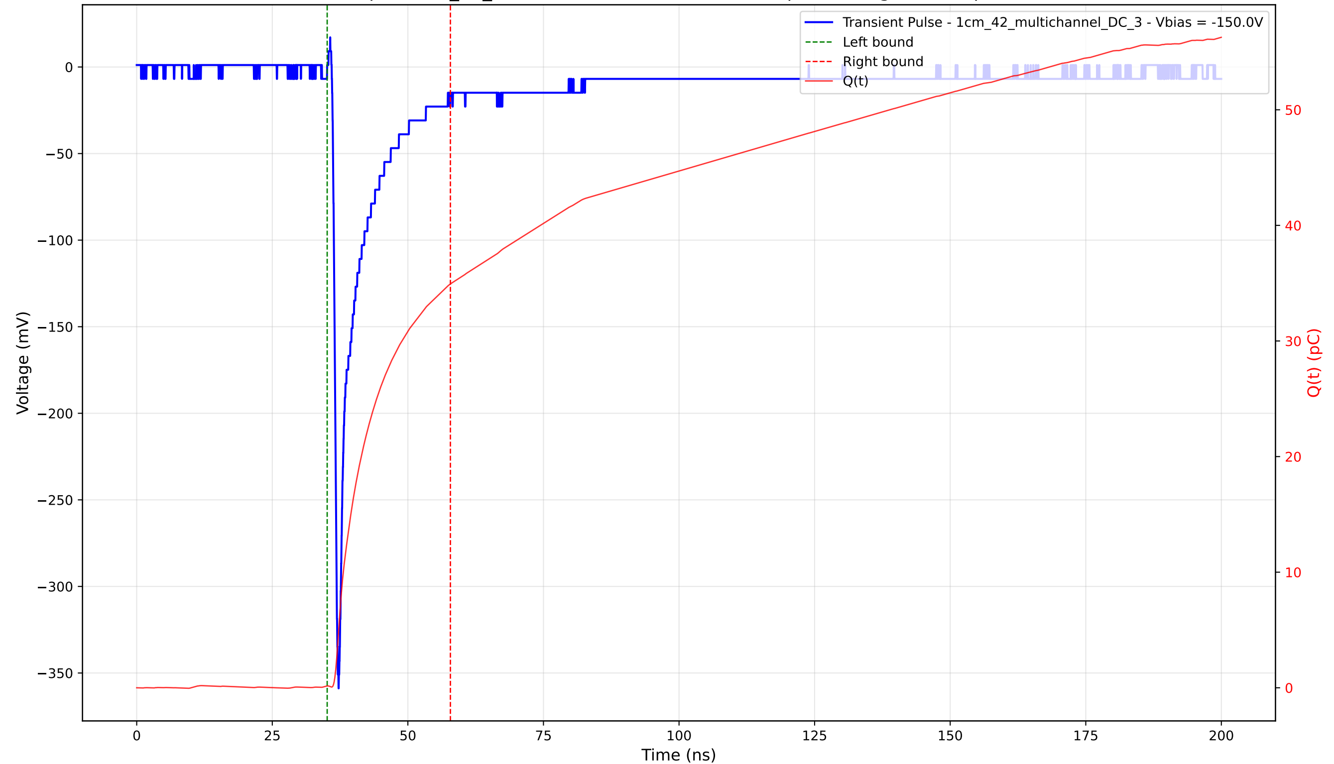
Transient Pulse - Sample: 1cm_42_multichannel - Position: 4740.0 \mu\text{m} - Charge: 34.77 pC - Rise Time: 0.80 ns
