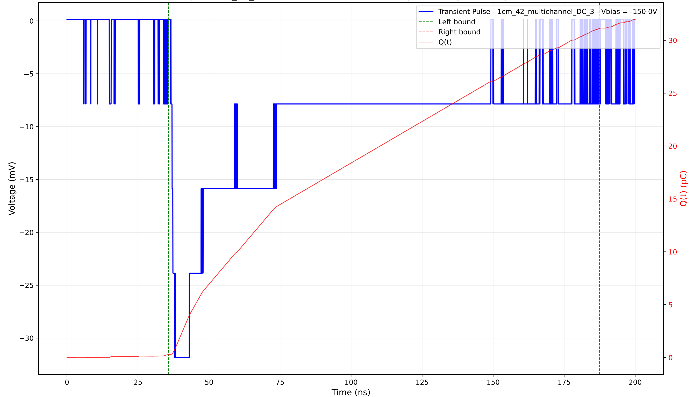
Transient Pulse - Sample: 1cm_42_multichannel - Position: 2330.0 \mu\text{m} - Charge: 30.86 pC - Rise Time: 1.35 ns
