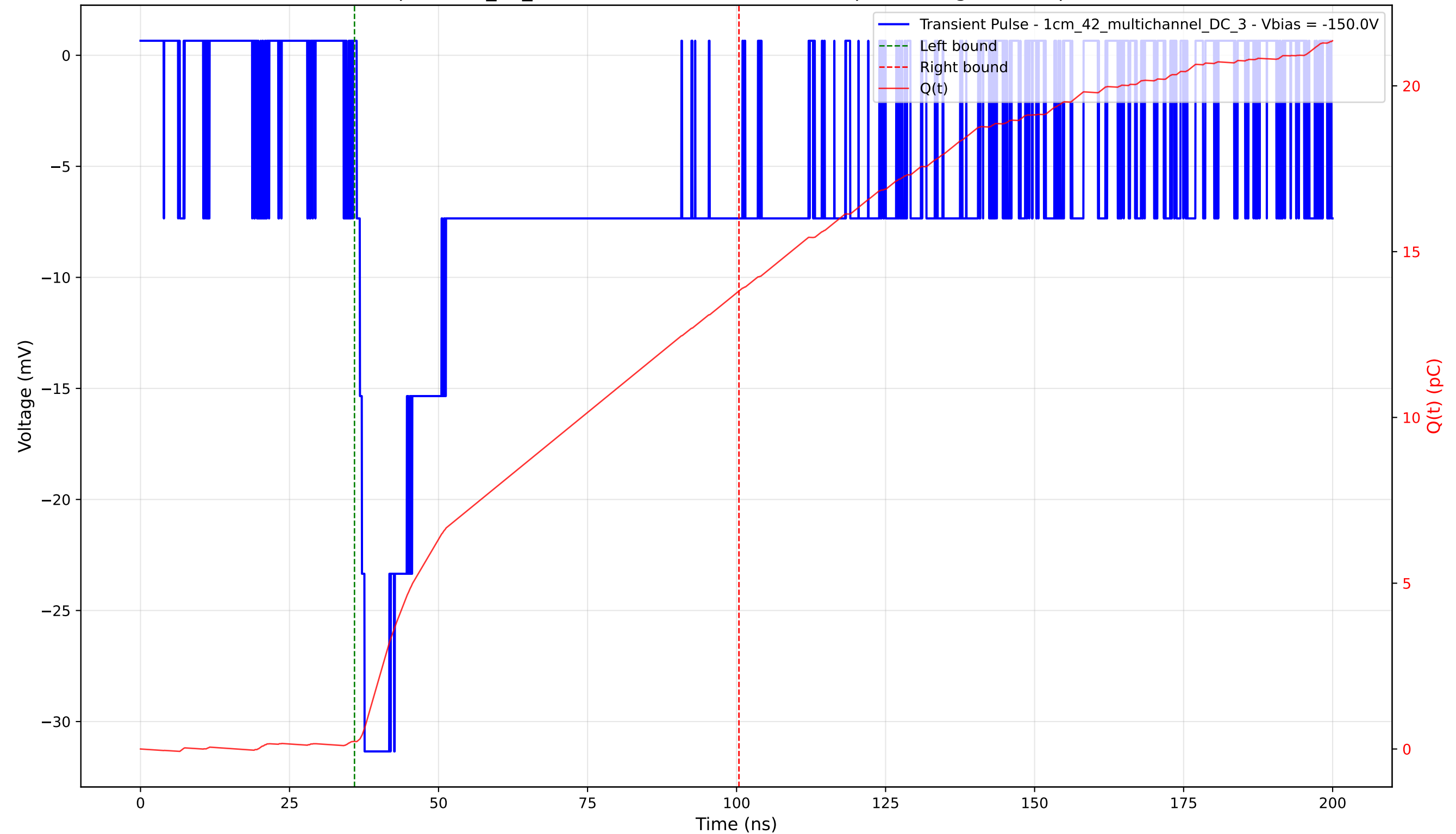
Transient Pulse - Sample: 1cm_42_multichannel - Position: 1400.0 \mu\text{m} - Charge: 13.59 pC - Rise Time: 1.31 ns
