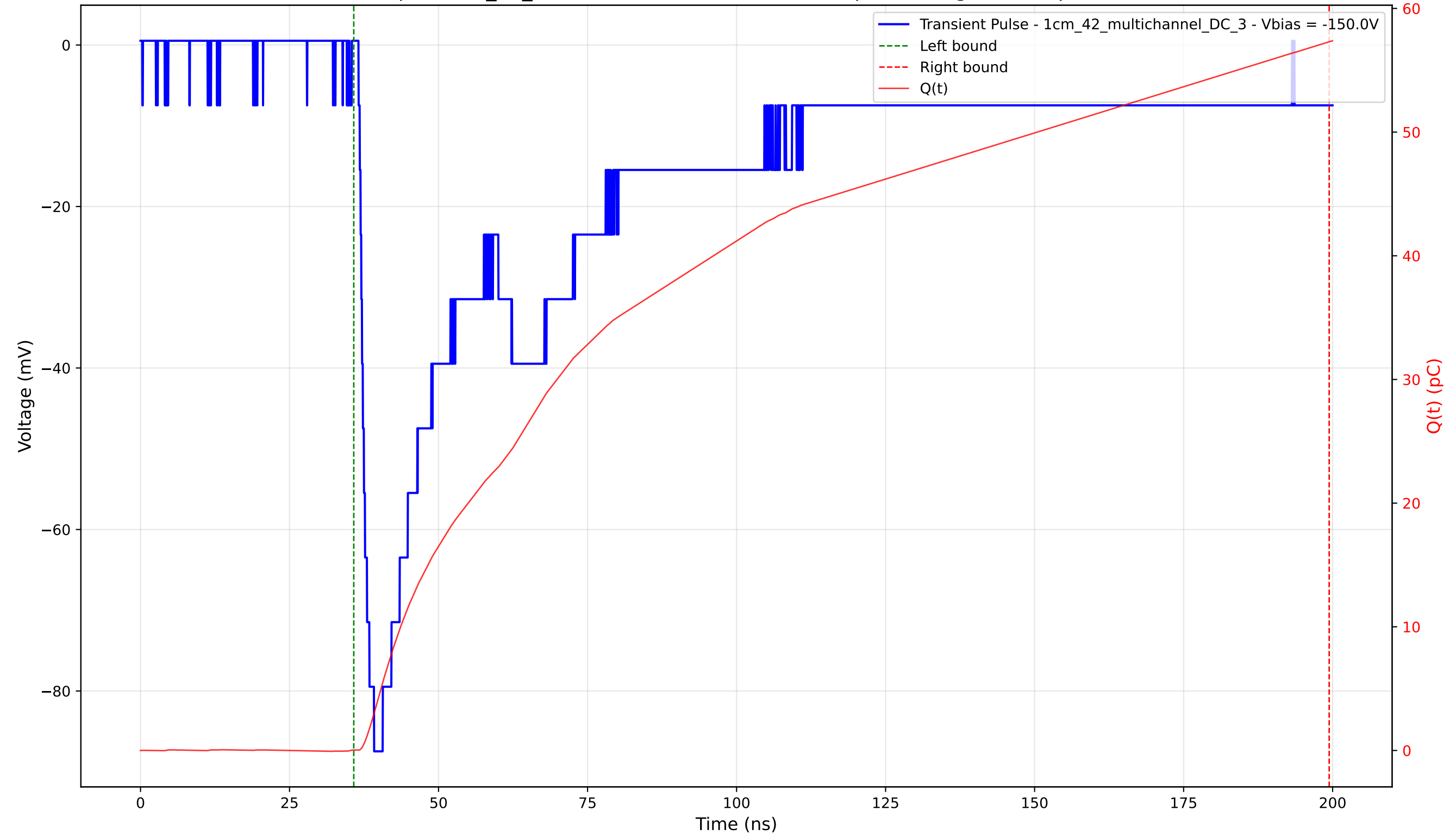
Transient Pulse - Sample: 1cm_42_multichannel - Position: 2230.0 \mu\text{m} - Charge: 57.28 pC - Rise Time: 1.64 ns
