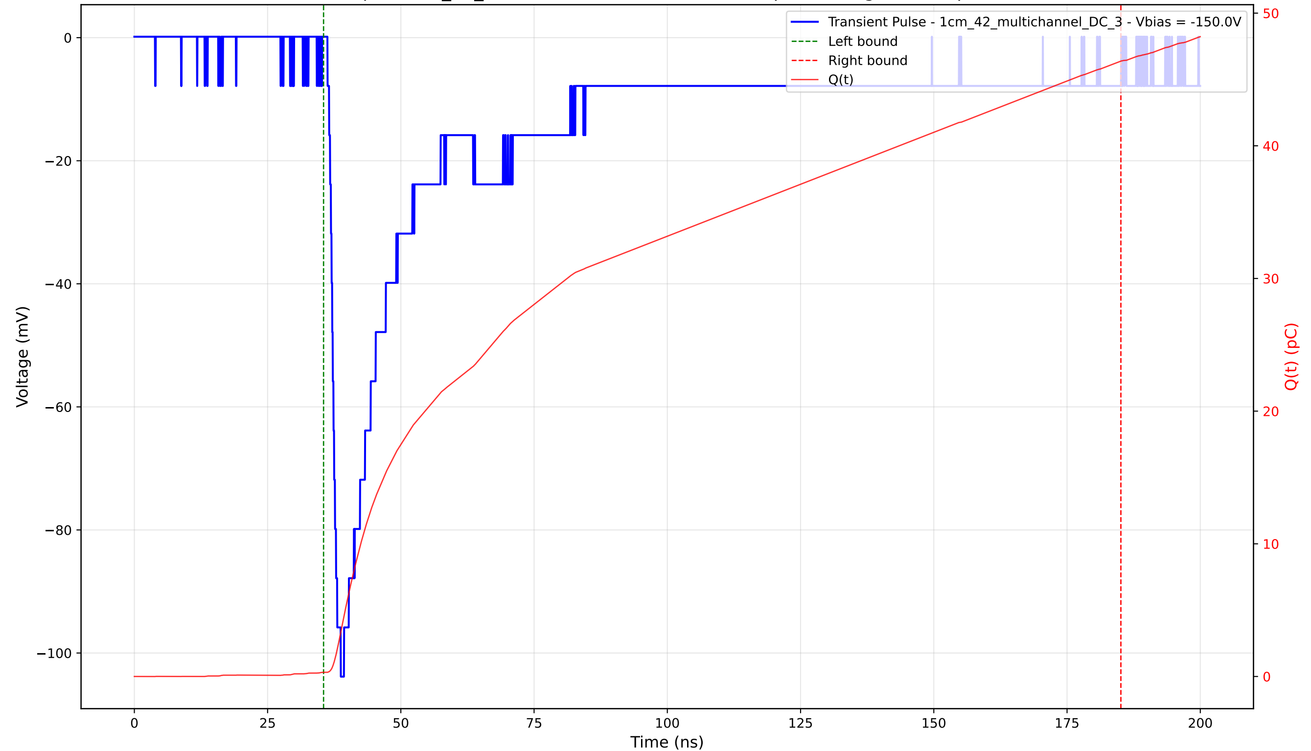
Transient Pulse - Sample: 1cm_42_multichannel - Position: 3450.0 \mu\text{m} - Charge: 46.08 pC - Rise Time: 1.53 ns
