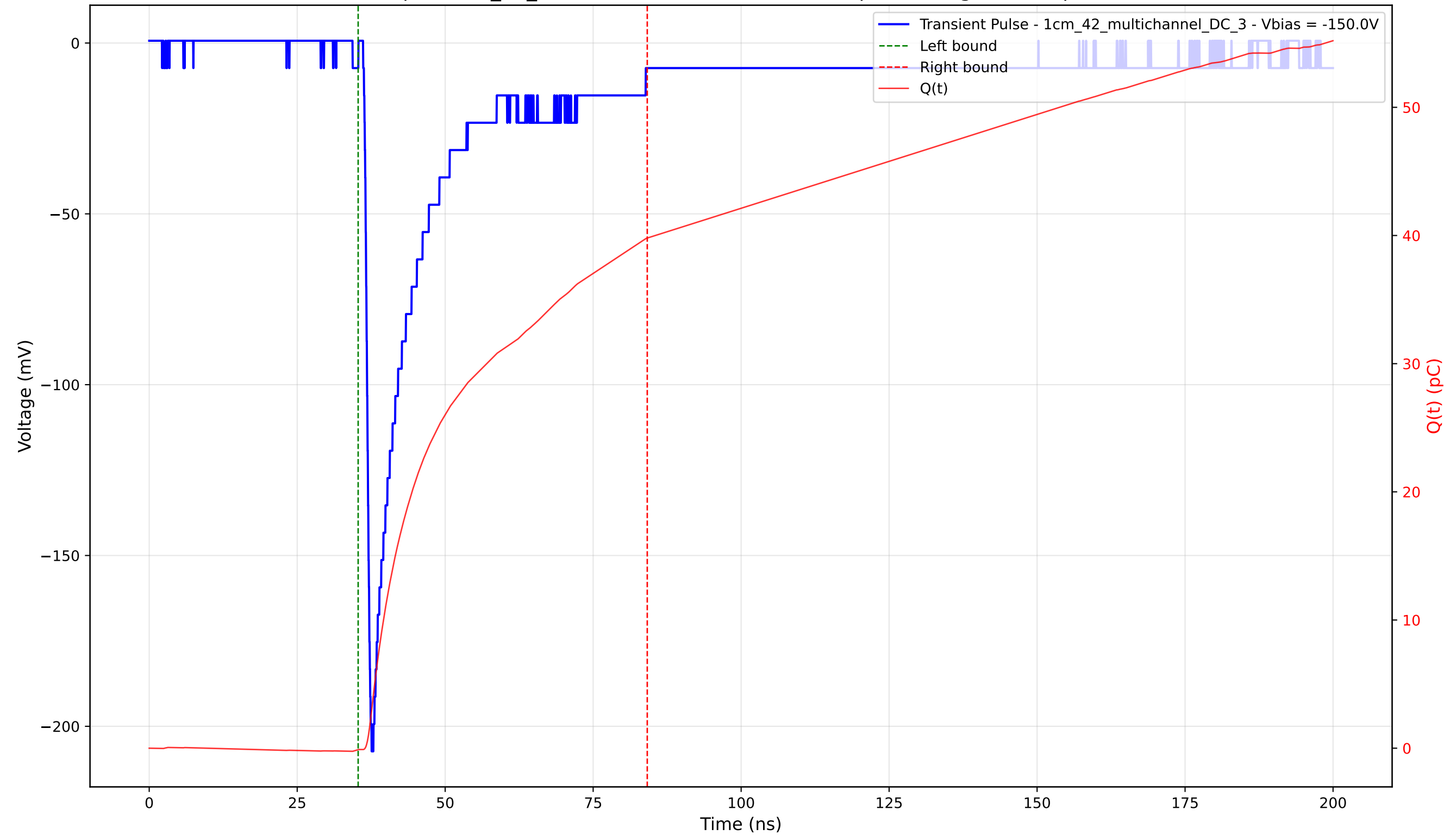
Transient Pulse - Sample: 1cm_42_multichannel - Position: 4250.0 \mu\text{m} - Charge: 39.91 pC - Rise Time: 0.97 ns
