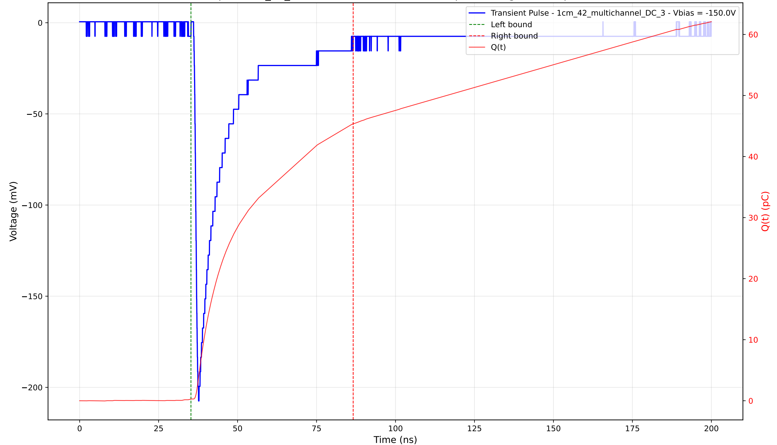
Transient Pulse - Sample: 1cm_42_multichannel - Position: 760.0 \mu\text{m} - Charge: 45.07 pC - Rise Time: 1.07 ns
