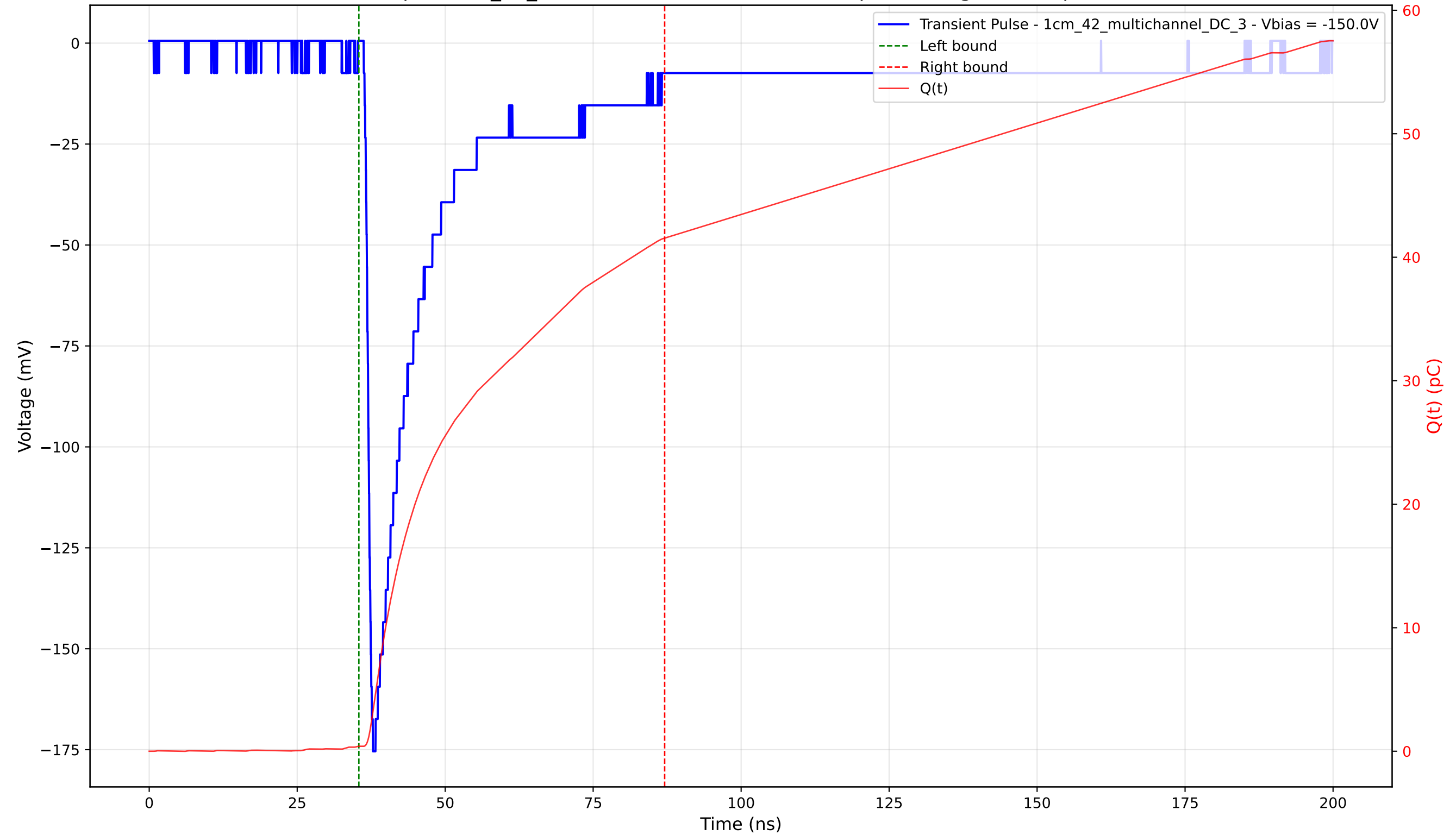
Transient Pulse - Sample: 1cm_42_multichannel - Position: 4010.0 \mu\text{m} - Charge: 41.15 pC - Rise Time: 1.03 ns
