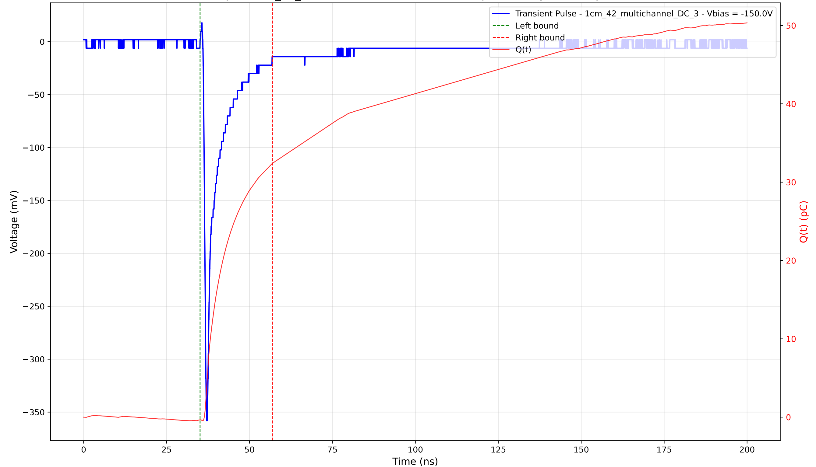
Transient Pulse - Sample: 1cm_42_multichannel - Position: 4795.0 \mu\text{m} - Charge: 32.72 pC - Rise Time: 0.78 ns
