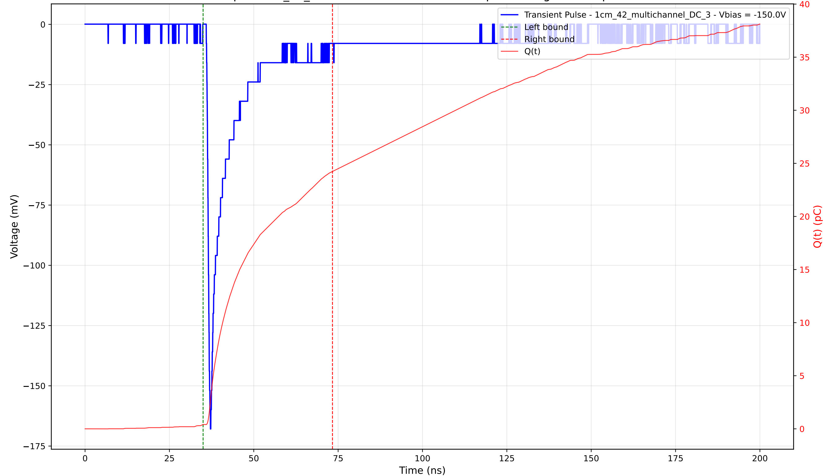
Transient Pulse - Sample: 1cm_42_multichannel - Position: 300.0 \mu\text{m} - Charge: 23.84 pC - Rise Time: 0.82 ns
