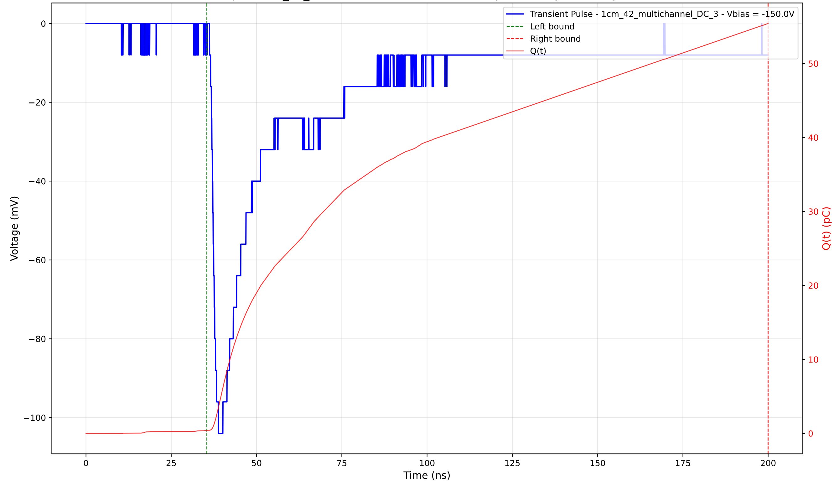
Transient Pulse - Sample: 1cm_42_multichannel - Position: 3140.0 \mu\text{m} - Charge: 55.00 pC - Rise Time: 1.73 ns
