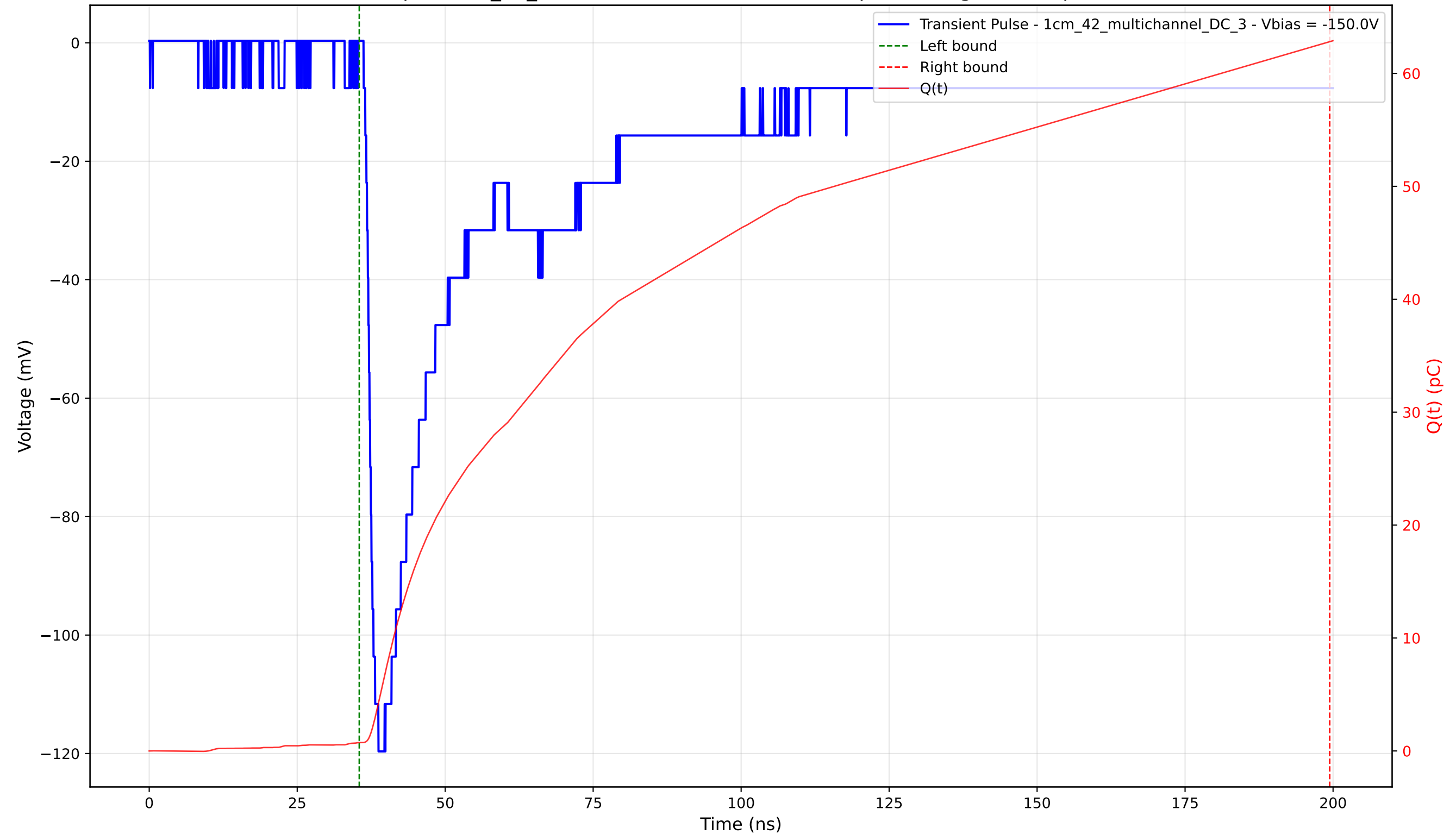
Transient Pulse - Sample: 1cm_42_multichannel - Position: 1700.0 \mu\text{m} - Charge: 62.07 pC - Rise Time: 1.67 ns
