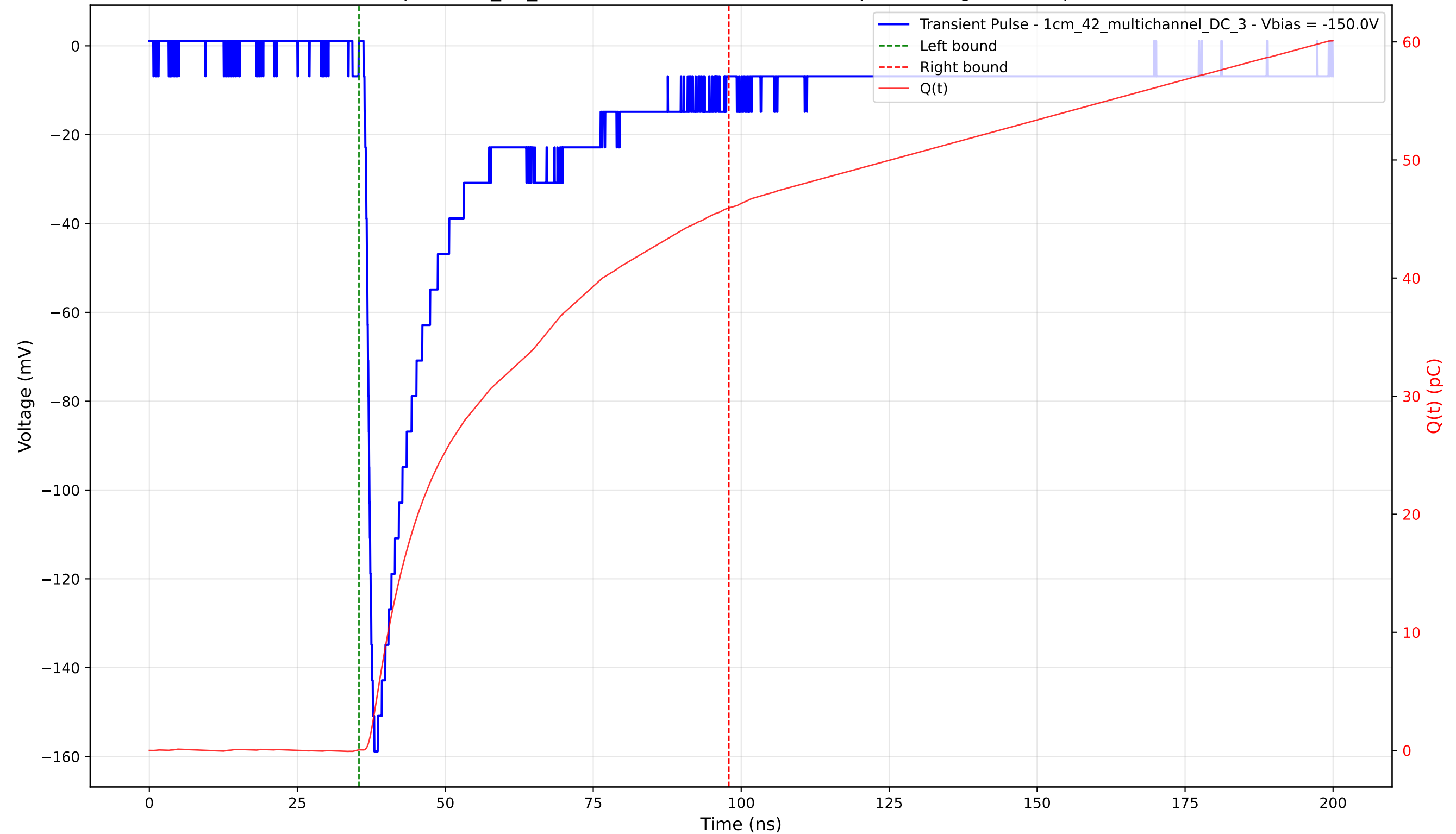
Transient Pulse - Sample: 1cm_42_multichannel - Position: 1160.0 \mu\text{m} - Charge: 45.89 pC - Rise Time: 1.30 ns
