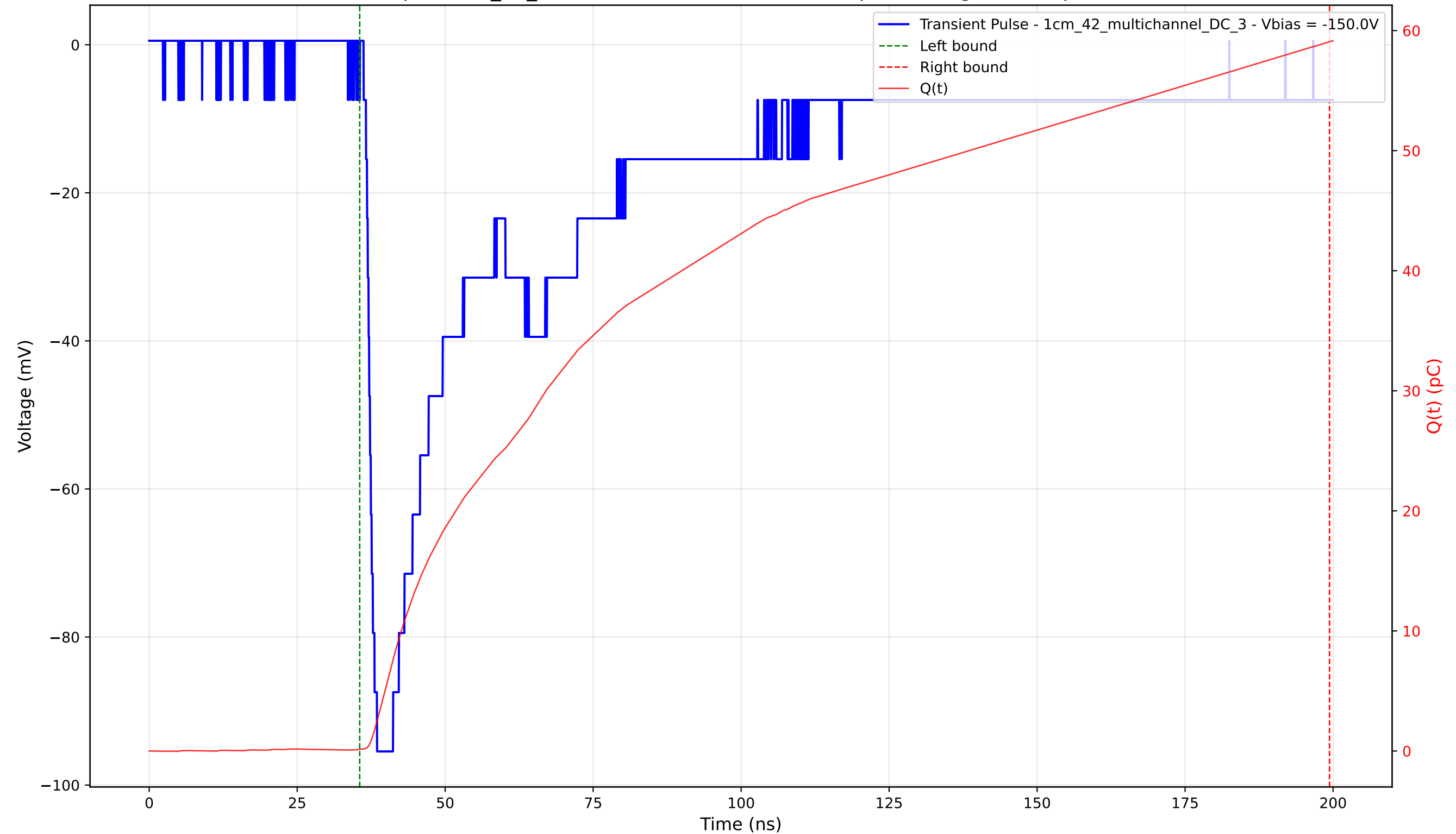
Transient Pulse - Sample: 1cm_42_multichannel - Position: 1995.0 \mu\text{m} - Charge: 58.91 pC - Rise Time: 1.45 ns
