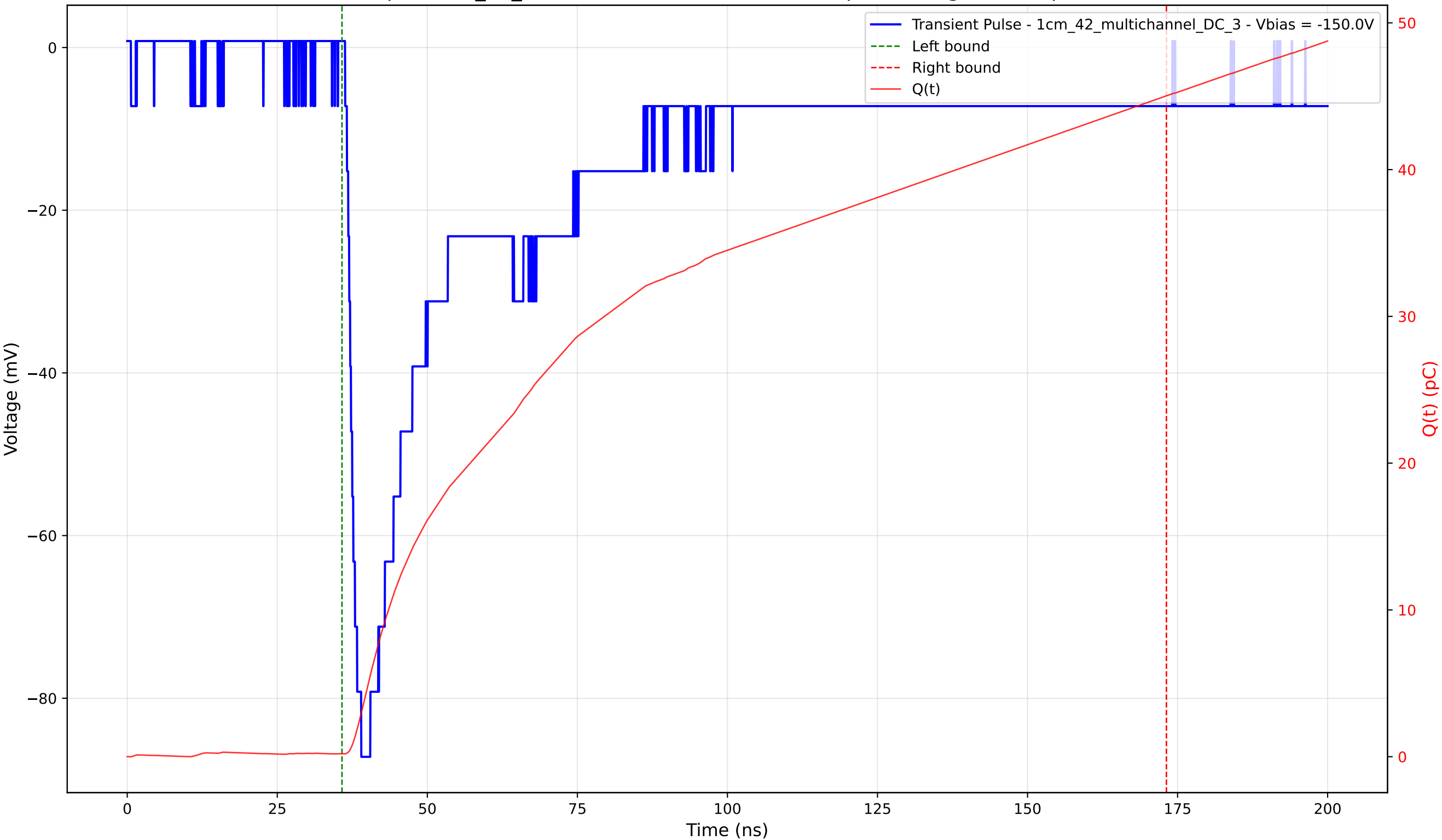
Transient Pulse - Sample: 1cm_42_multichannel - Position: 2950.0 \mu\text{m} - Charge: 44.85 pC - Rise Time: 1.72 ns
