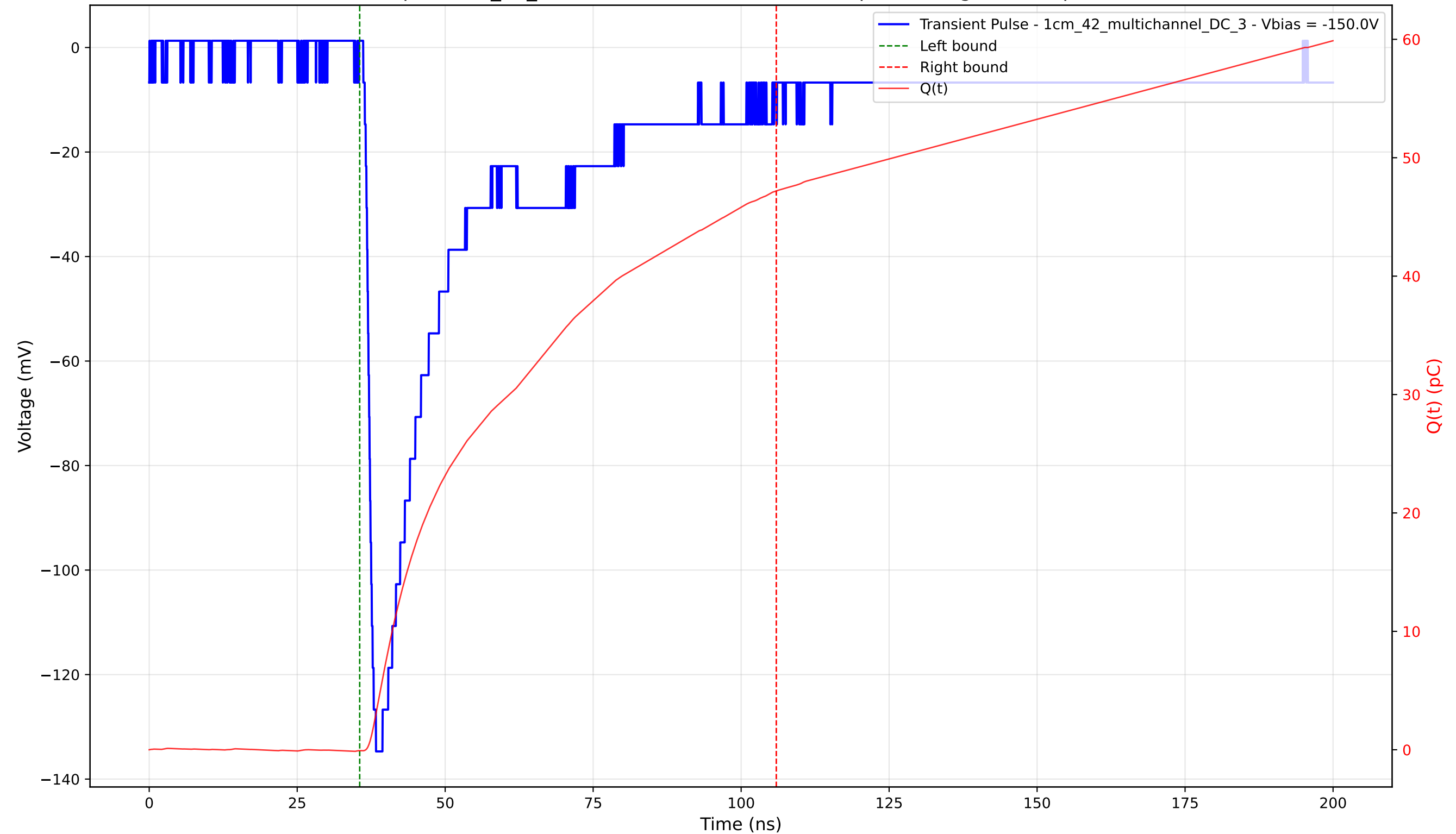
Transient Pulse - Sample: 1cm_42_multichannel - Position: 1470.0 \mu\text{m} - Charge: 47.27 pC - Rise Time: 1.50 ns
