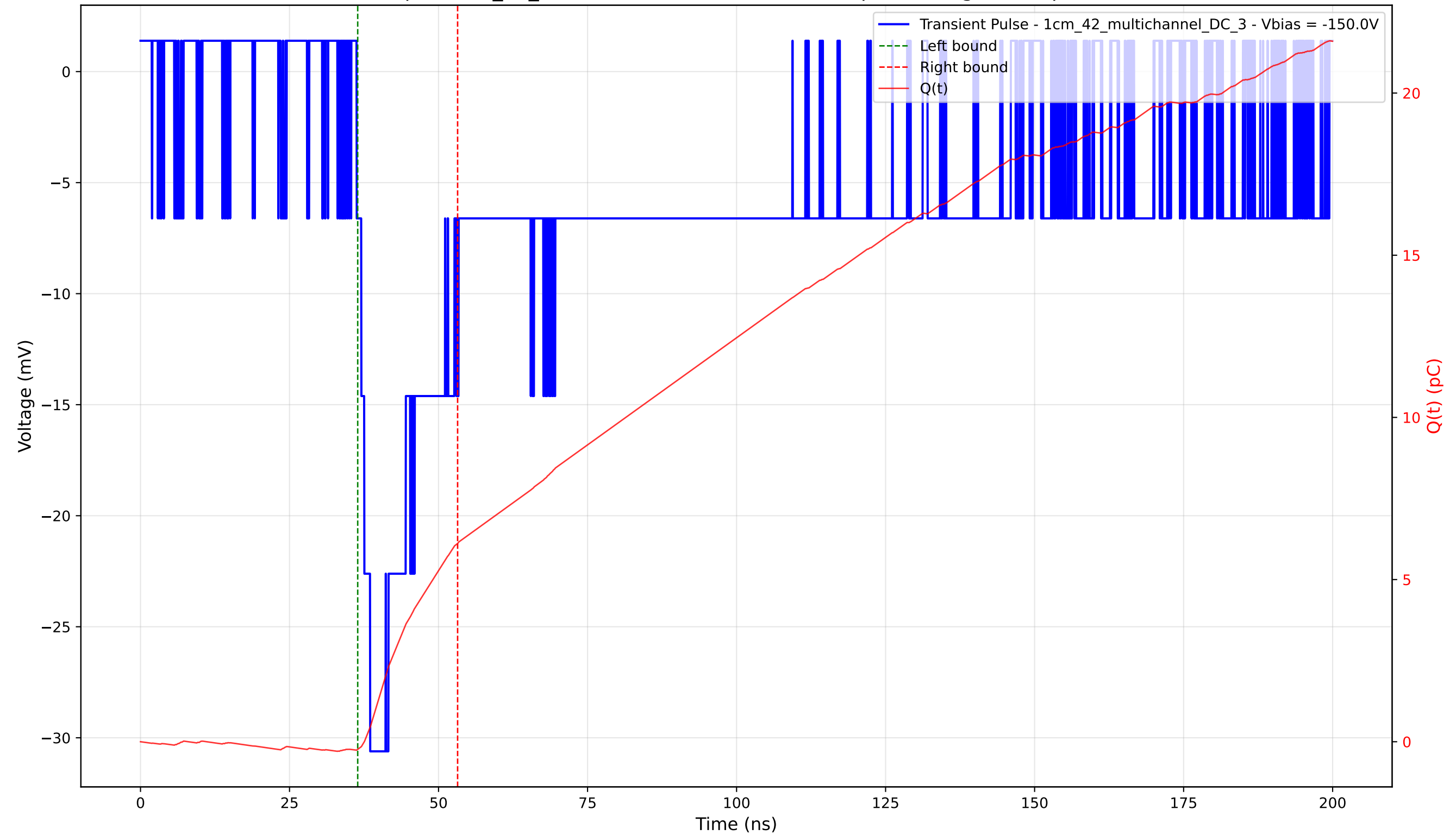
Transient Pulse - Sample: 1cm_42_multichannel - Position: 2840.0 \mu\text{m} - Charge: 6.35 pC - Rise Time: 2.27 ns
