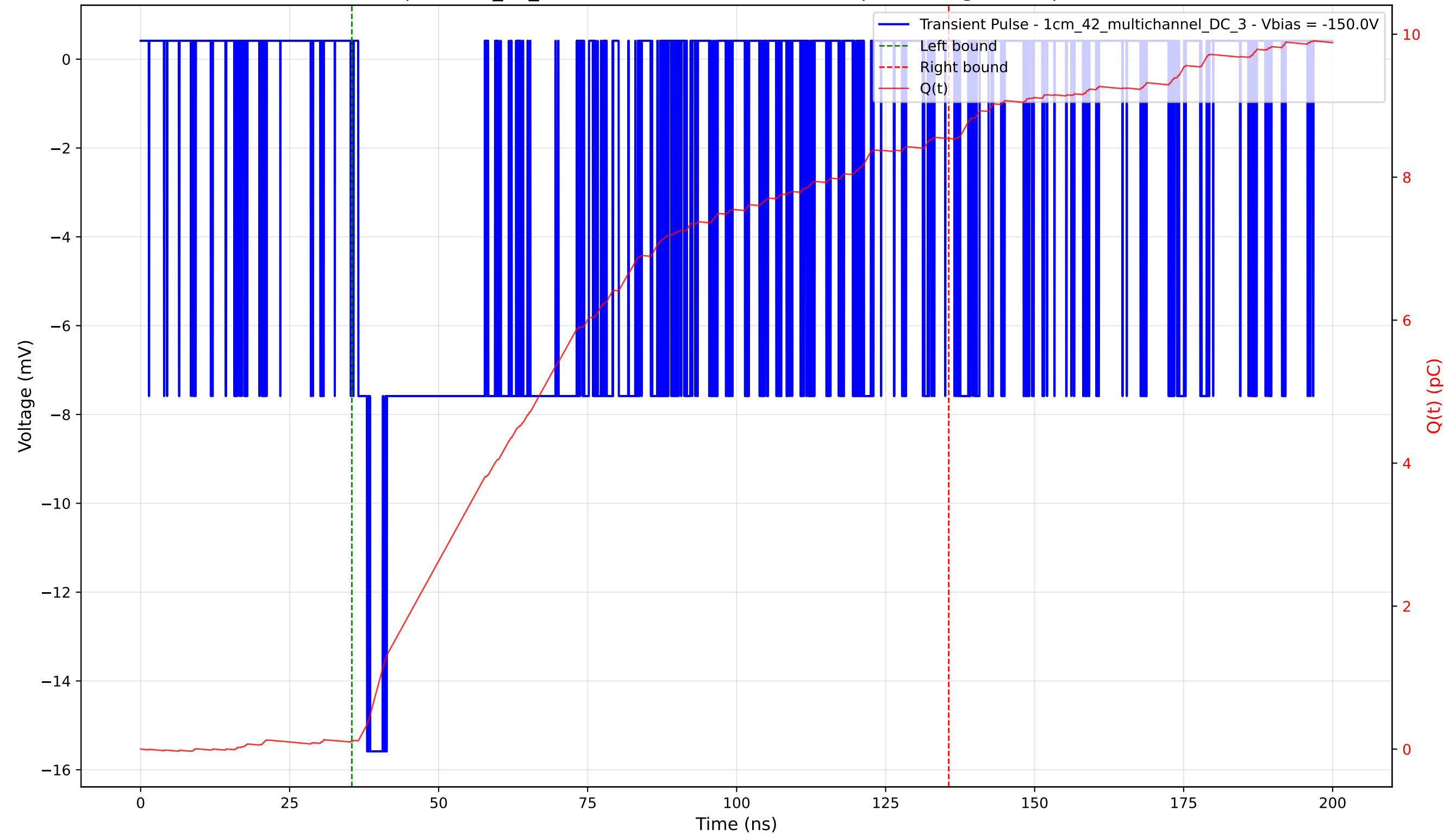
Transient Pulse - Sample: 1cm_42_multichannel - Position: 1380.0 \mu\text{m} - Charge: 8.43 pC - Rise Time: 1.48 ns
