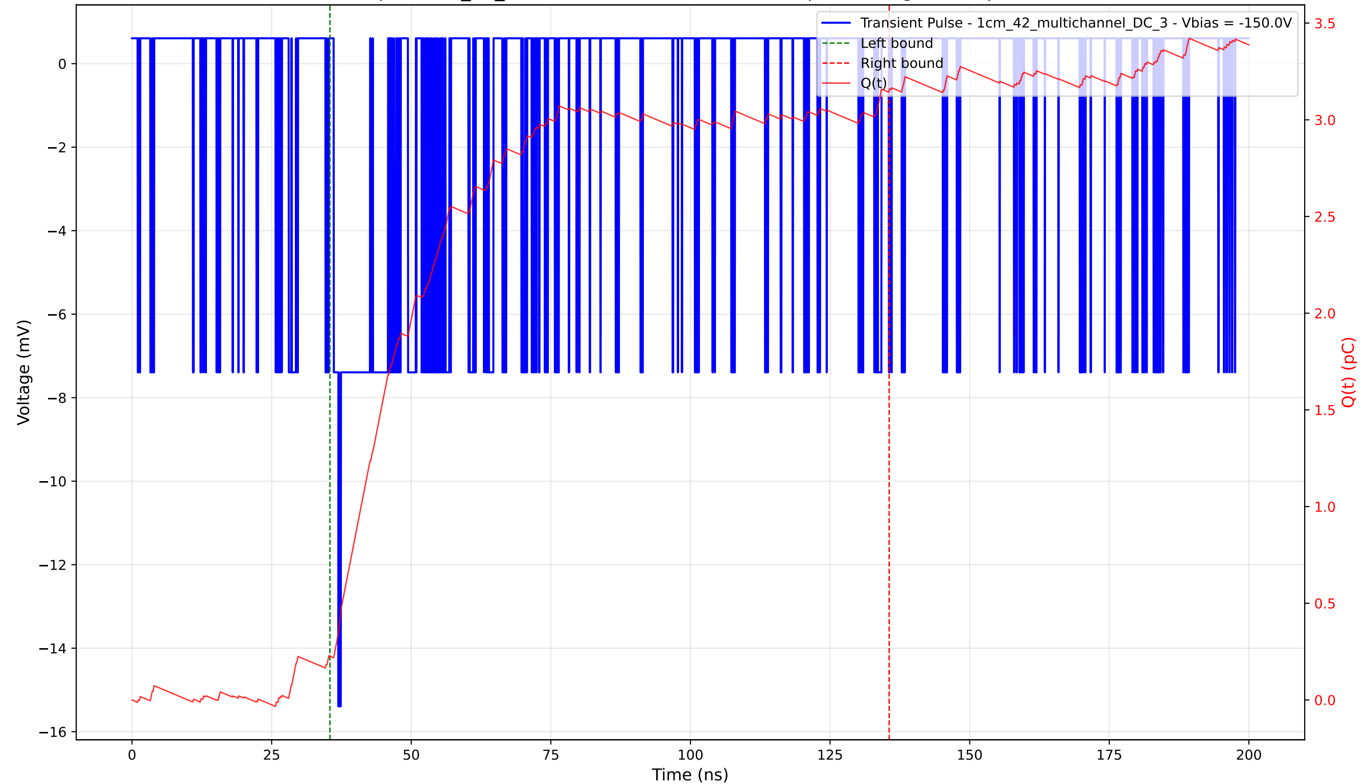
Transient Pulse - Sample: 1cm_42_multichannel - Position: 4905.0 \mu\text{m} - Charge: 2.92 pC - Rise Time: 0.88 ns
