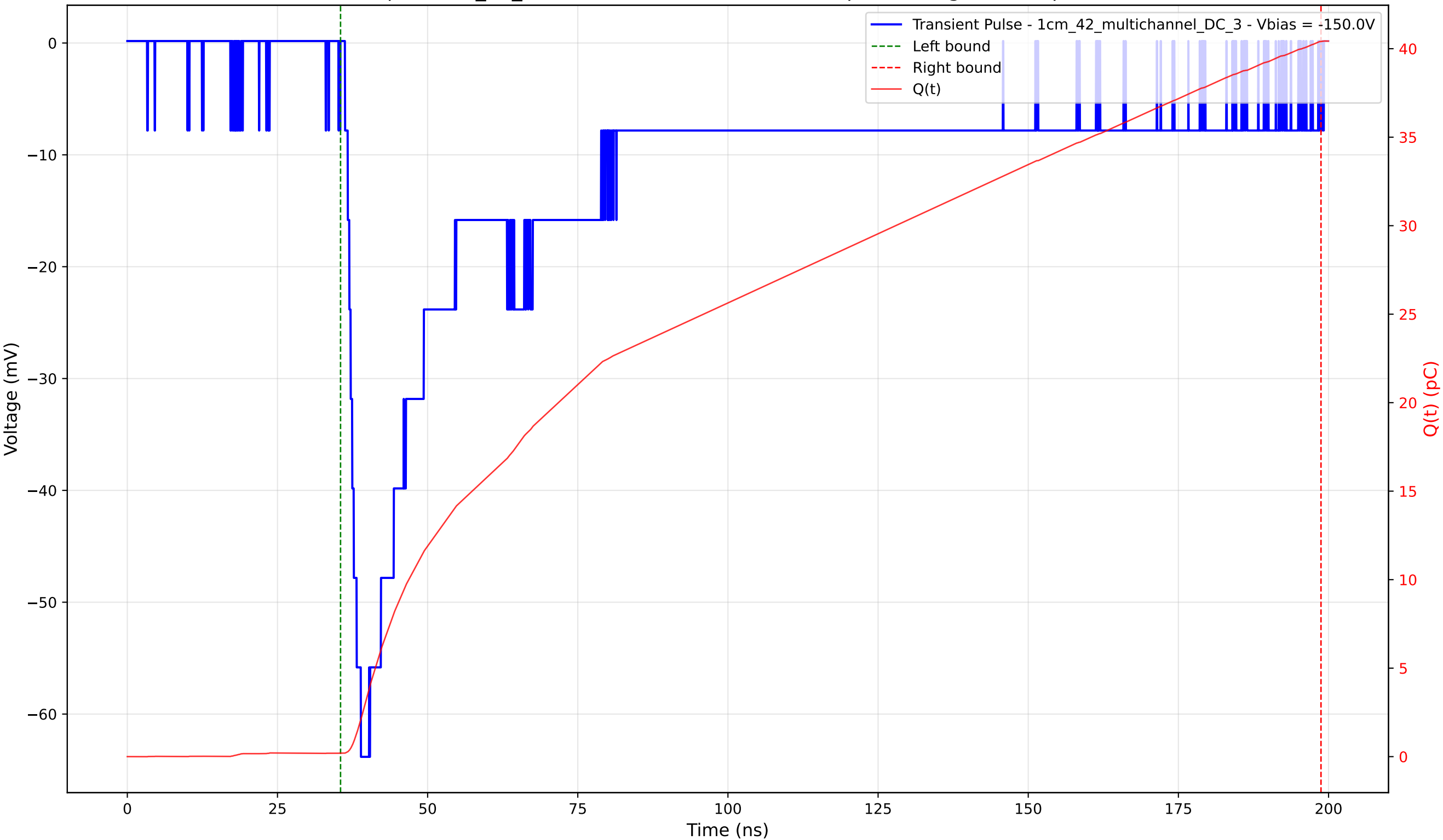
Transient Pulse - Sample: 1cm_42_multichannel - Position: 2935.0 \mu\text{m} - Charge: 40.20 pC - Rise Time: 2.64 ns
