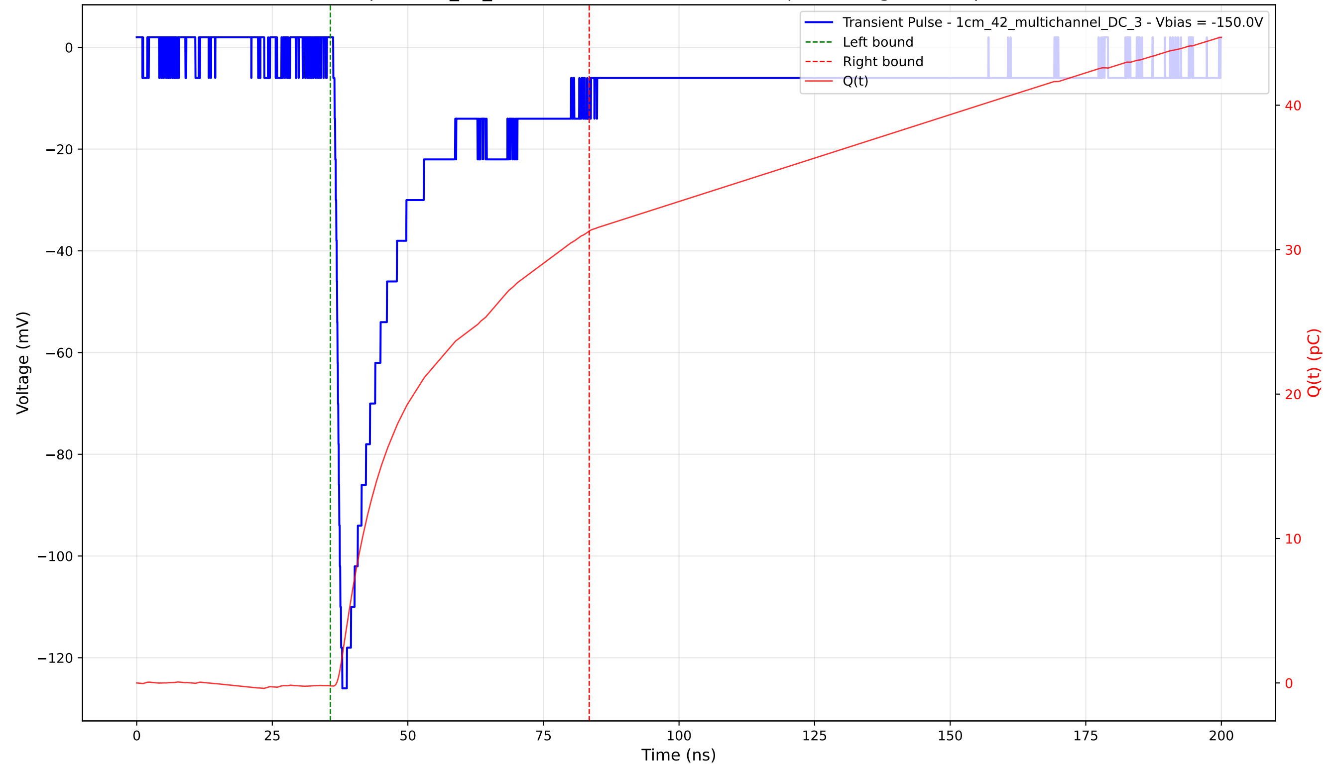
Transient Pulse - Sample: 1cm_42_multichannel - Position: 3820.0 \mu\text{m} - Charge: 31.49 pC - Rise Time: 1.20 ns
