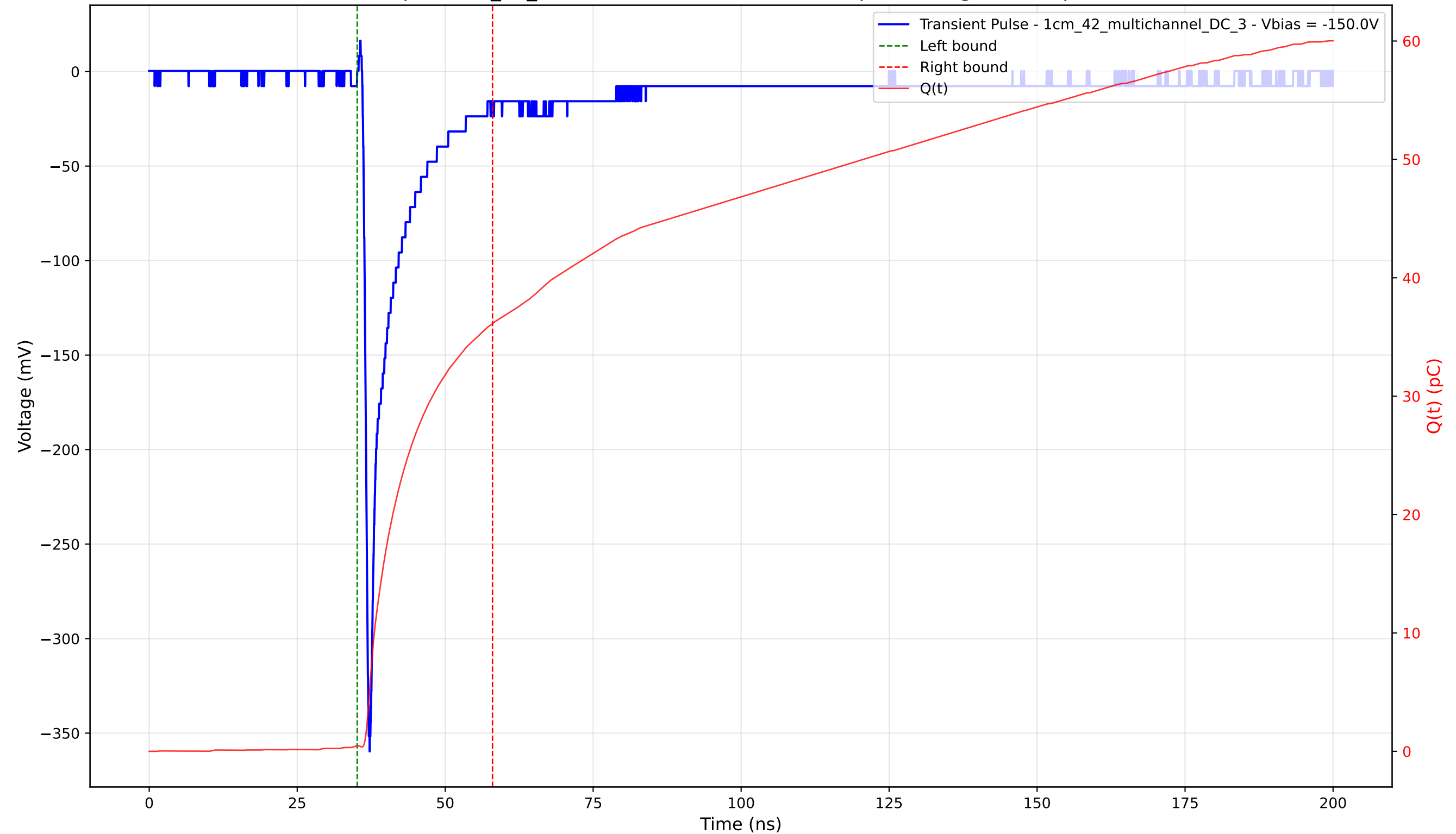
Transient Pulse - Sample: 1cm_42_multichannel - Position: 4725.0 \mu\text{m} - Charge: 35.65 pC - Rise Time: 0.82 ns
