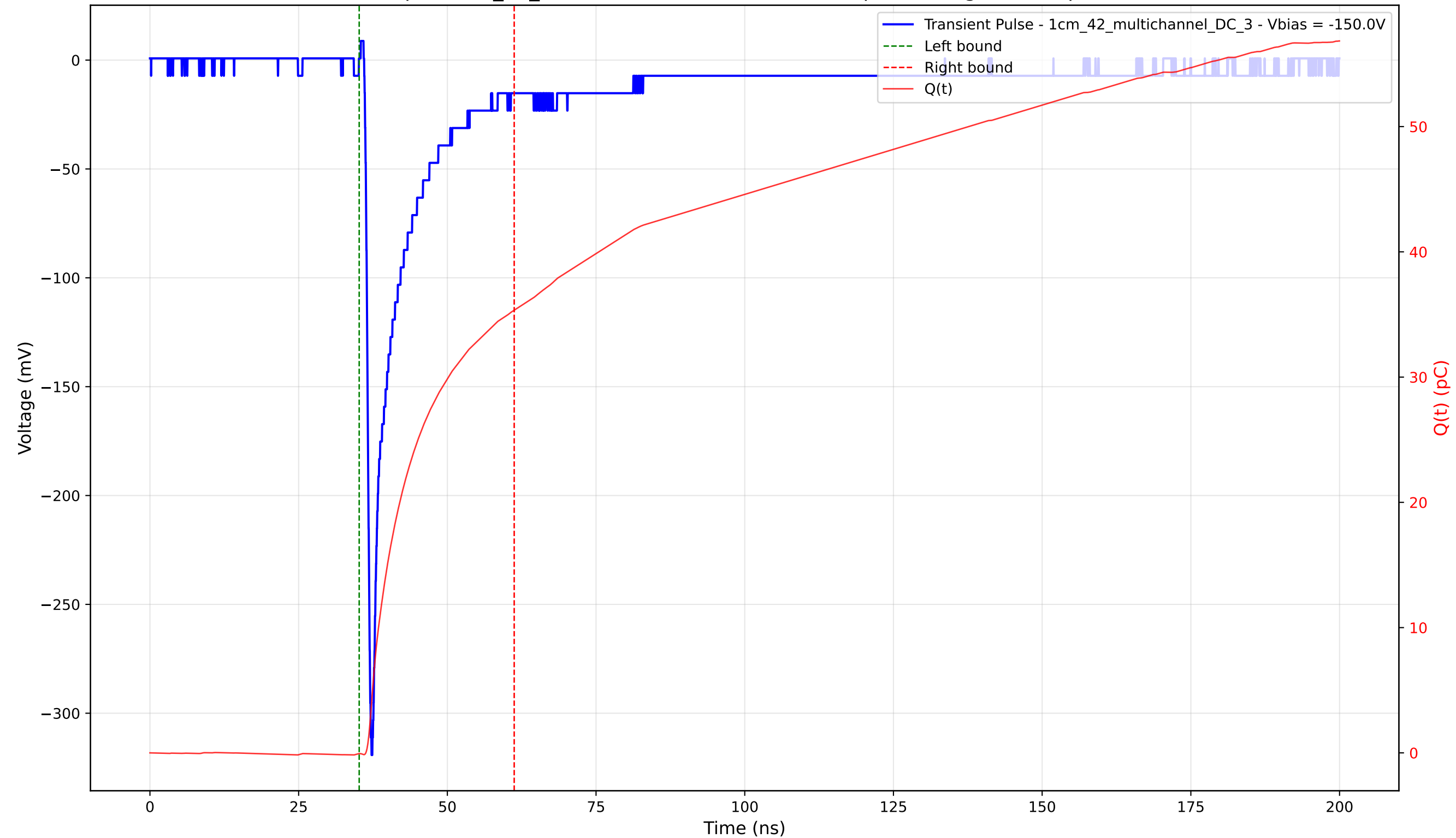
Transient Pulse - Sample: 1cm_42_multichannel - Position: 4645.0 \mu\text{m} - Charge: 35.39 pC - Rise Time: 0.84 ns
