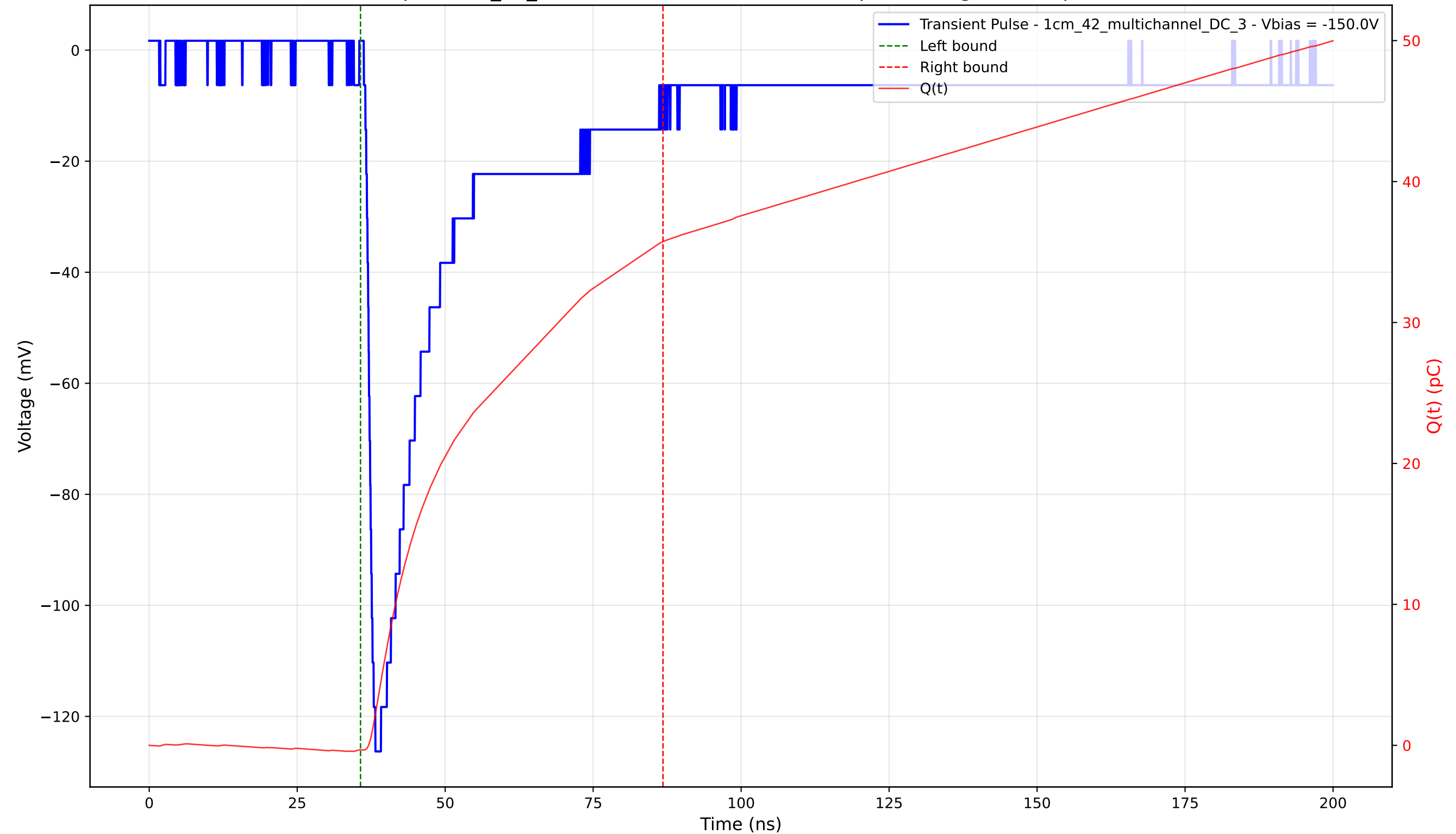
Transient Pulse - Sample: 1cm_42_multichannel - Position: 3585.0 \mu\text{m} - Charge: 36.06 pC - Rise Time: 1.40 ns
