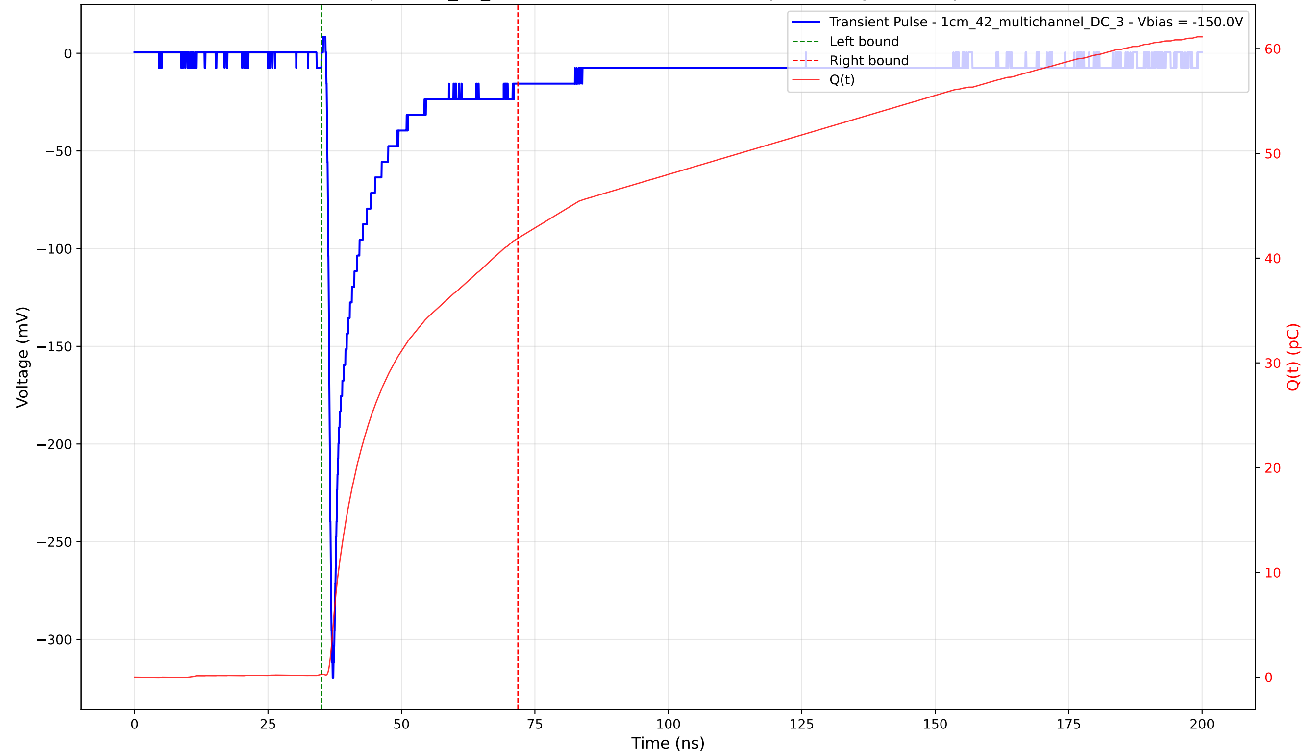
Transient Pulse - Sample: 1cm_42_multichannel - Position: 250.0 \mu\text{m} - Charge: 41.63 pC - Rise Time: 0.84 ns
