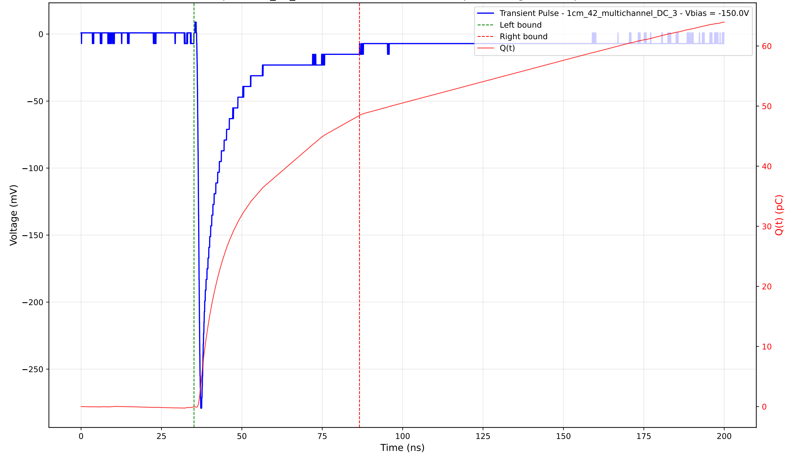
Transient Pulse - Sample: 1cm_42_multichannel - Position: 440.0 \mu\text{m} - Charge: 48.49 pC - Rise Time: 0.87 ns
