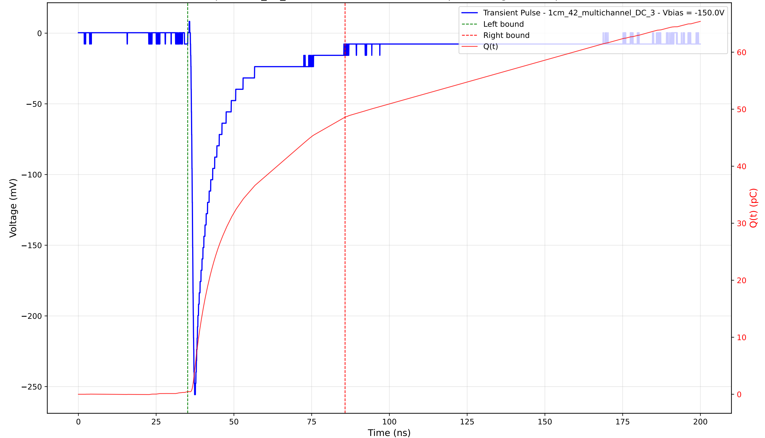
Transient Pulse - Sample: 1cm_42_multichannel - Position: 550.0 \mu\text{m} - Charge: 48.12 pC - Rise Time: 0.92 ns
