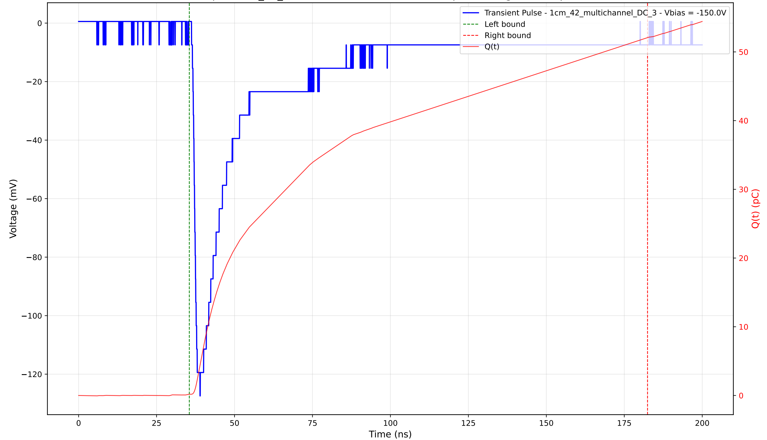
Transient Pulse - Sample: 1cm_42_multichannel - Position: 3495.0 \mu\text{m} - Charge: 51.90 pC - Rise Time: 1.55 ns
