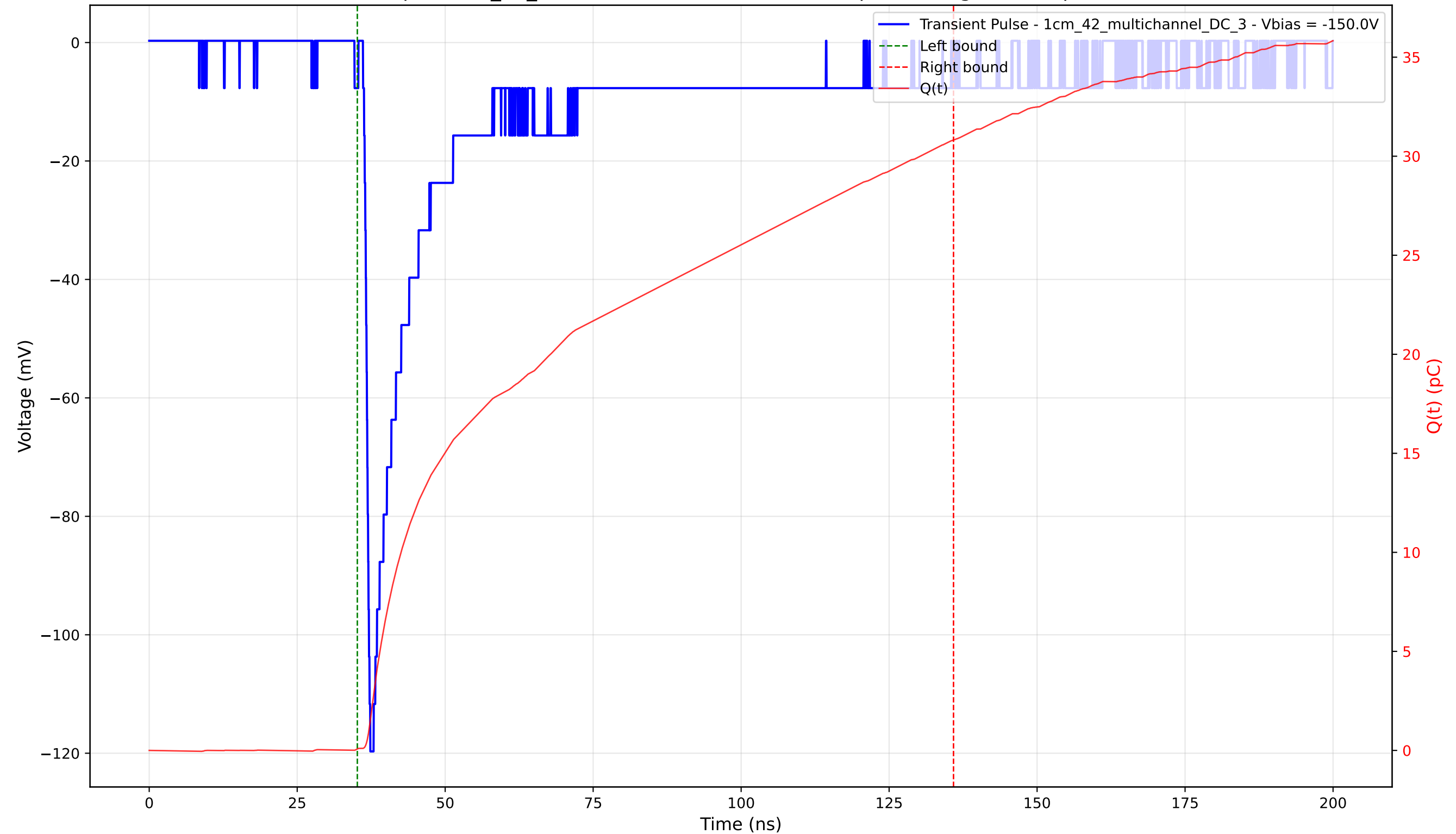
Transient Pulse - Sample: 1cm_42_multichannel - Position: 4335.0 \mu\text{m} - Charge: 30.75 pC - Rise Time: 0.93 ns
