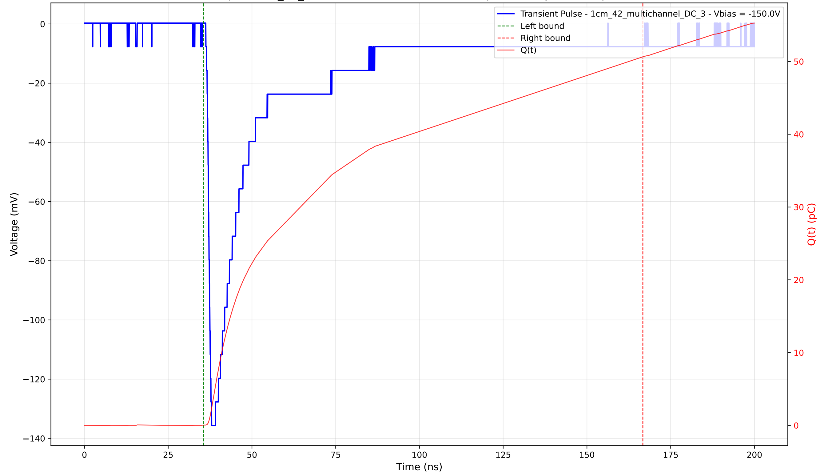
Transient Pulse - Sample: 1cm_42_multichannel - Position: 3705.0 \mu\text{m} - Charge: 50.60 pC - Rise Time: 1.29 ns
