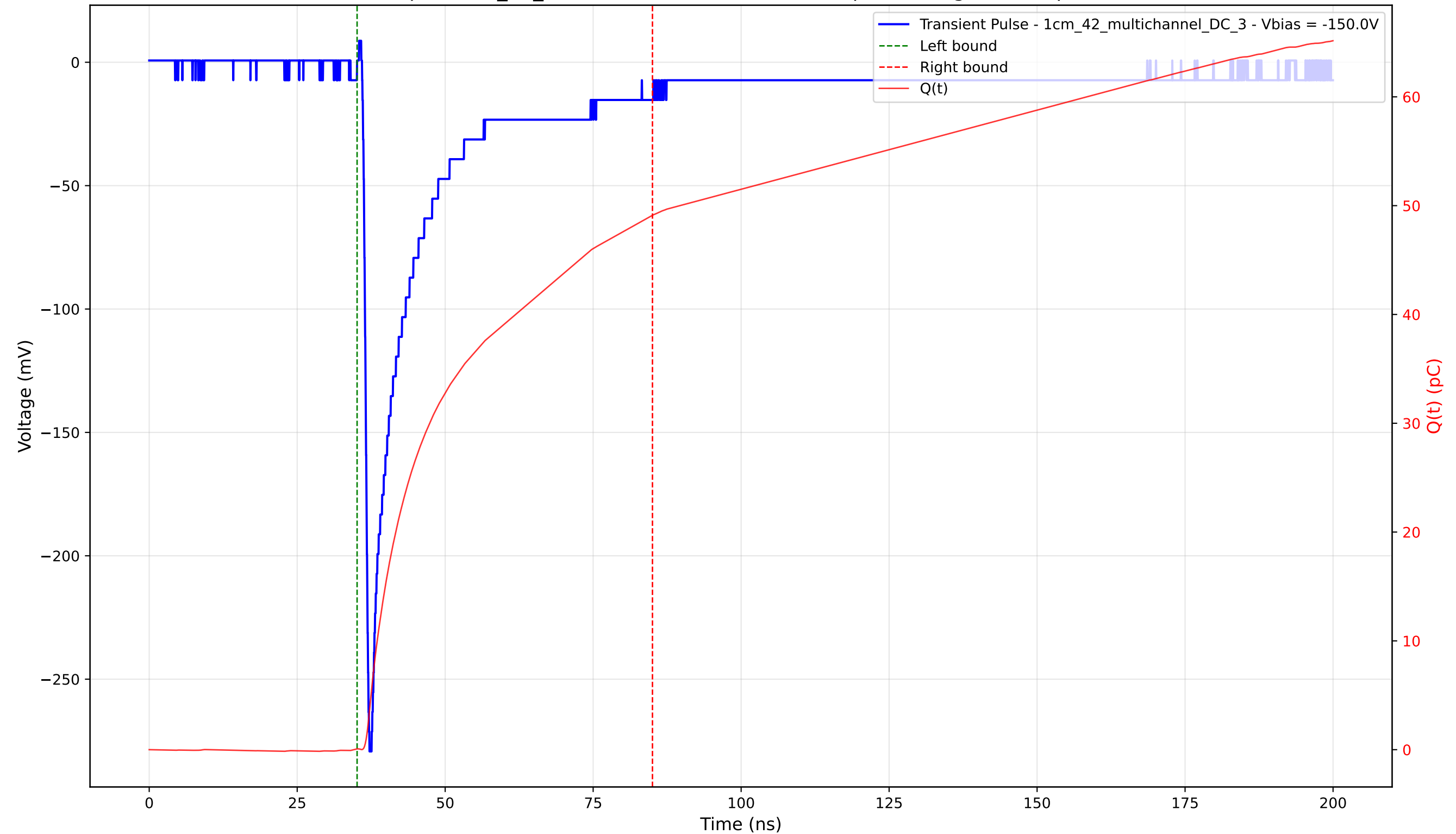
Transient Pulse - Sample: 1cm_42_multichannel - Position: 470.0 \mu\text{m} - Charge: 49.04 pC - Rise Time: 0.89 ns
