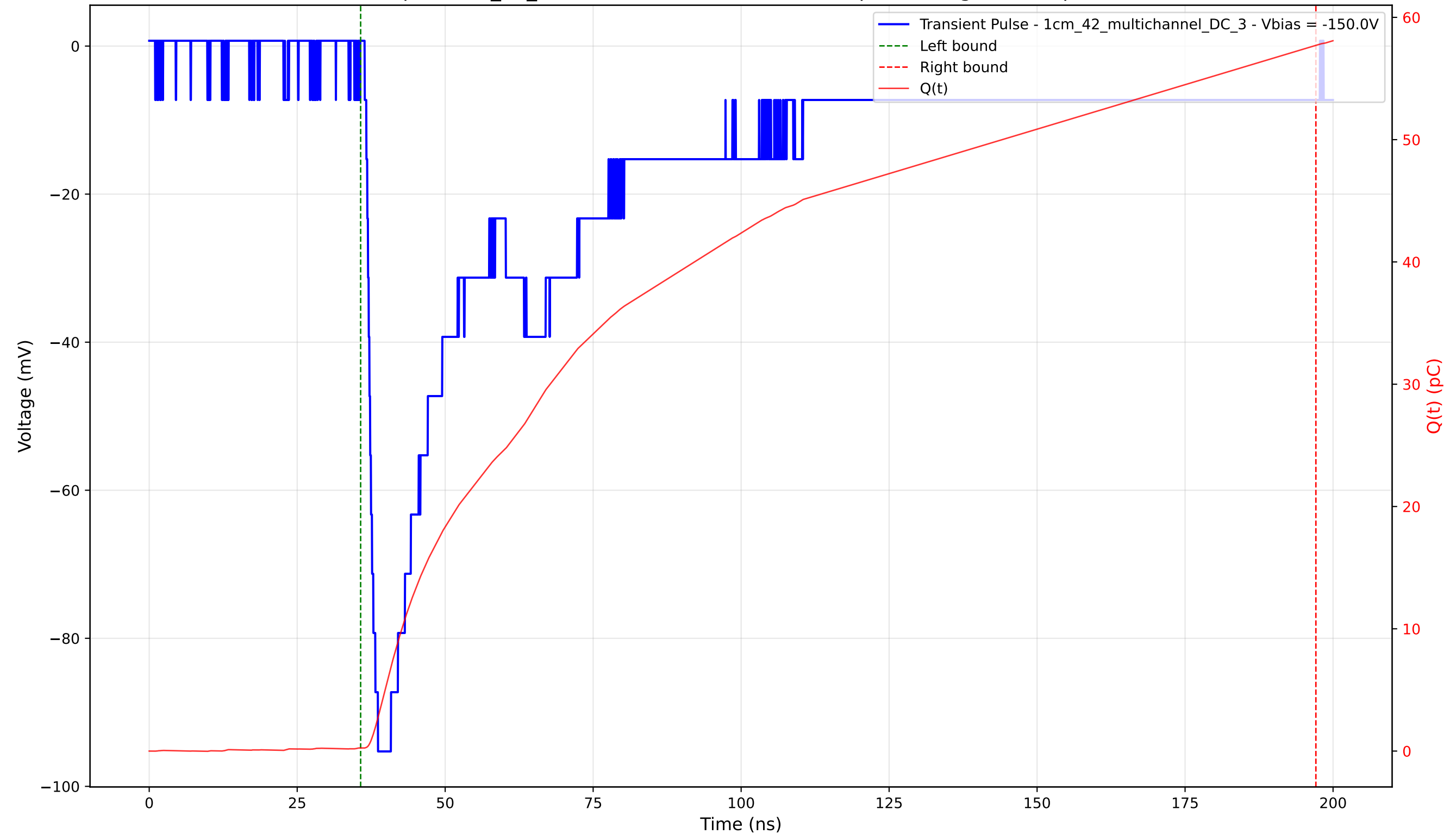
Transient Pulse - Sample: 1cm_42_multichannel - Position: 2025.0 \mu\text{m} - Charge: 57.46 pC - Rise Time: 1.53 ns
