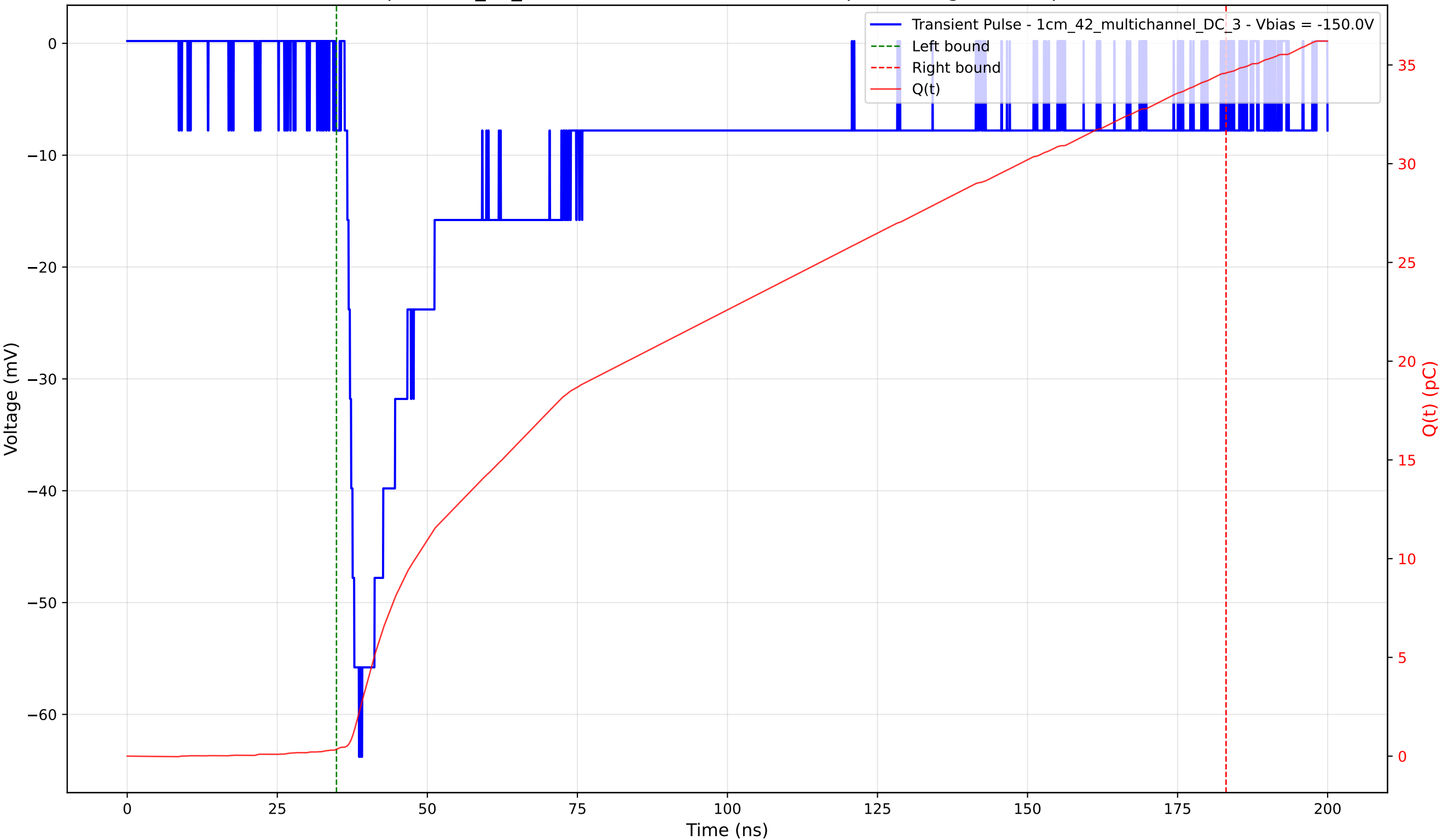
Transient Pulse - Sample: 1cm_42_multichannel - Position: 3435.0 \mu\text{m} - Charge: 34.25 pC - Rise Time: 2.38 ns
