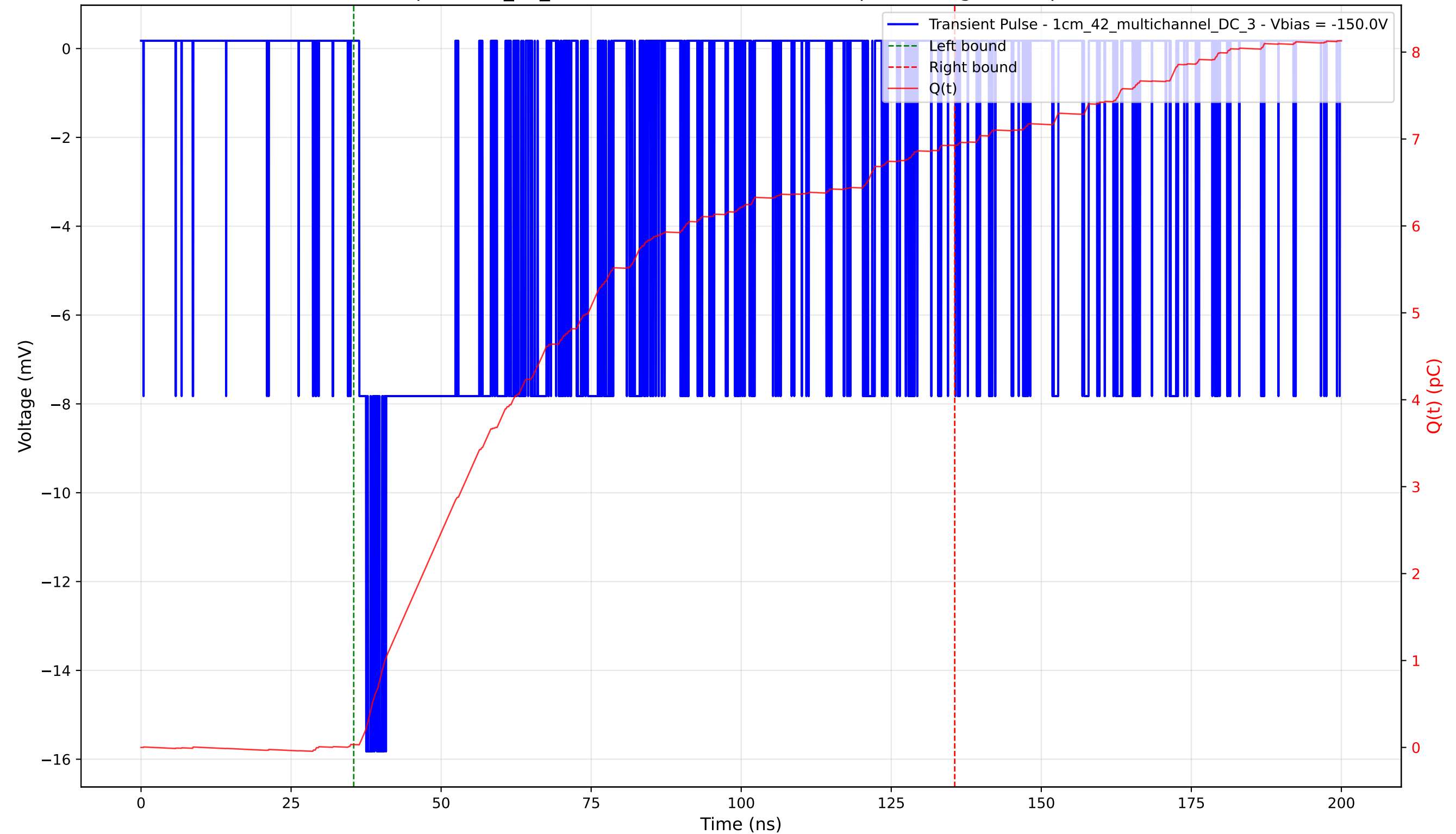
Transient Pulse - Sample: 1cm_42_multichannel - Position: 855.0 \mu\text{m} - Charge: 6.89 pC - Rise Time: 1.16 ns
