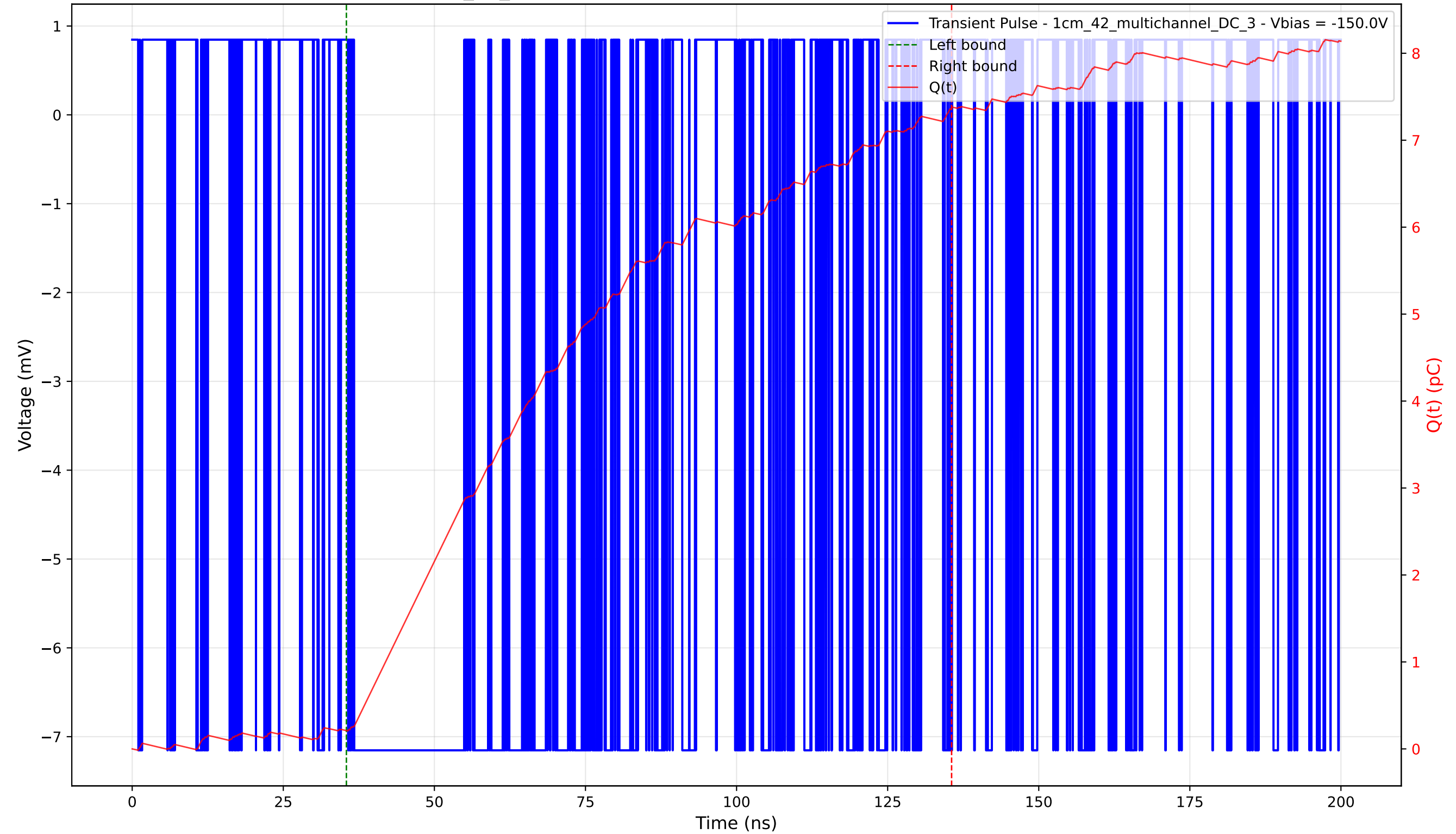
Transient Pulse - Sample: 1cm_42_multichannel - Position: 1865.0 \mu\text{m} - Charge: 7.16 pC - Rise Time: 0.00 ns (N/A)
