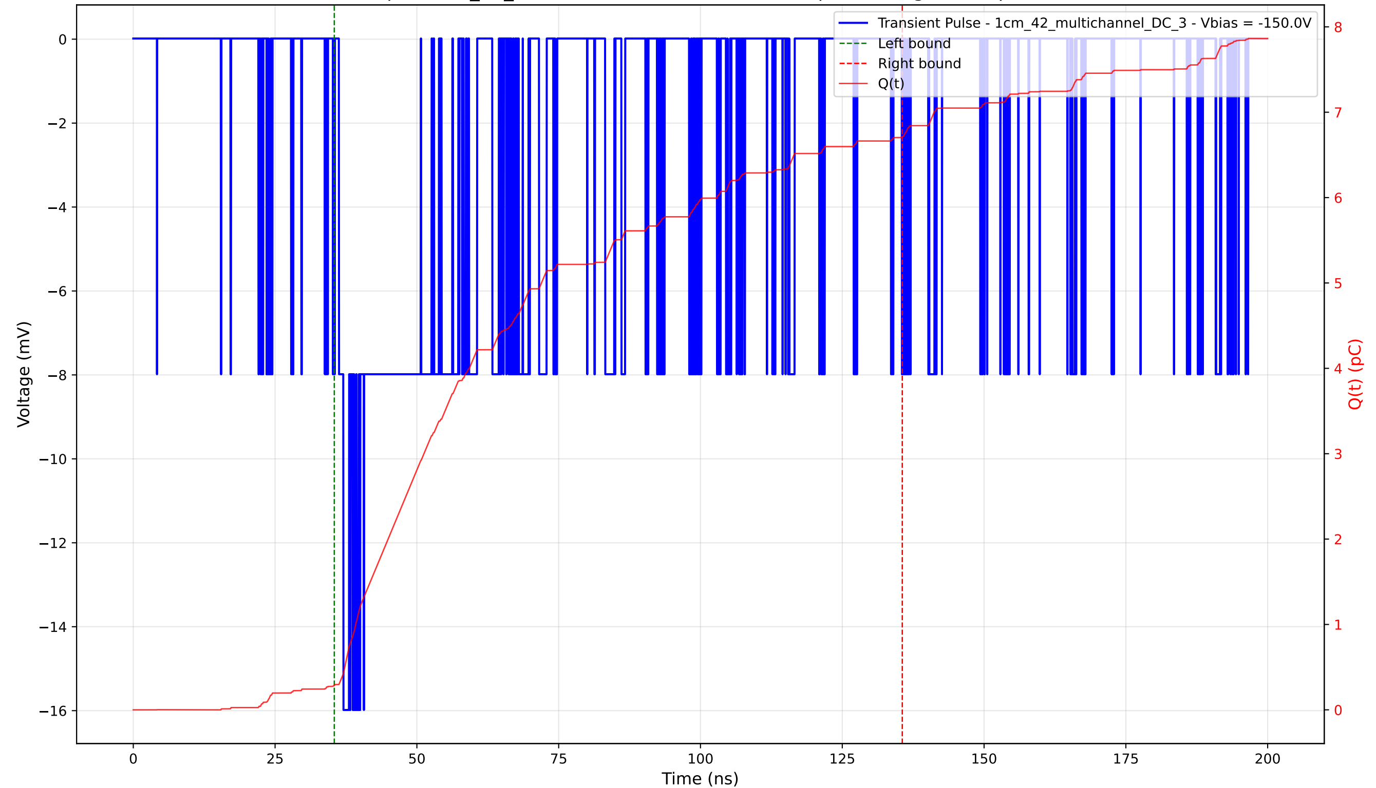
Transient Pulse - Sample: 1cm_42_multichannel - Position: 4400.0 \mu\text{m} - Charge: 6.43 pC - Rise Time: 0.80 ns
