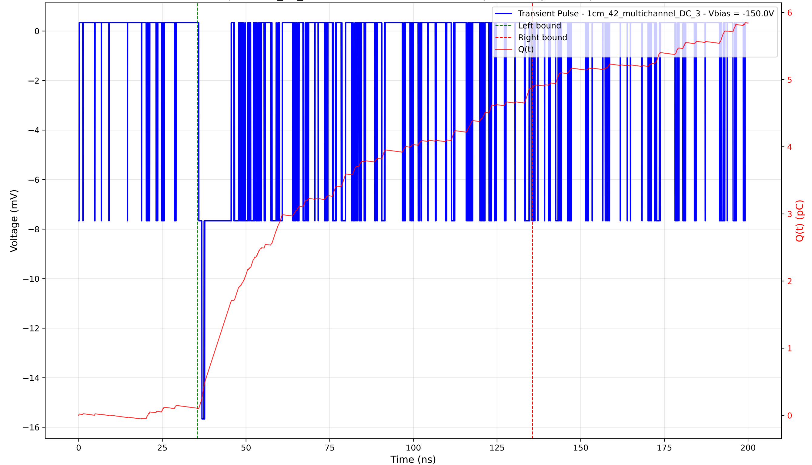
Transient Pulse - Sample: 1cm_42_multichannel - Position: 4925.0 \mu\text{m} - Charge: 4.77 pC - Rise Time: 0.94 ns
