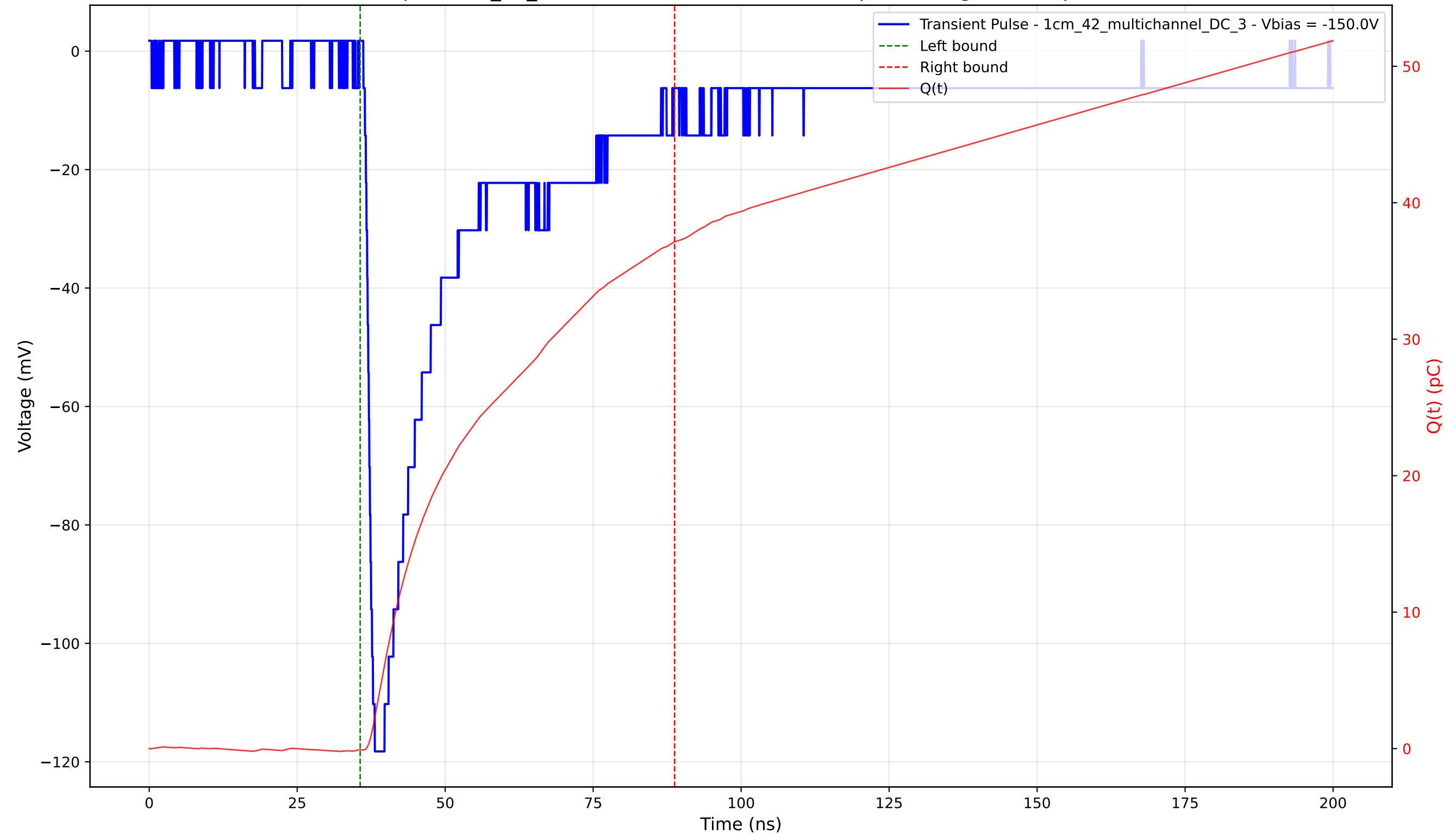
Transient Pulse - Sample: 1cm_42_multichannel - Position: 1435.0 \mu\text{m} - Charge: 37.23 pC - Rise Time: 1.37 ns
