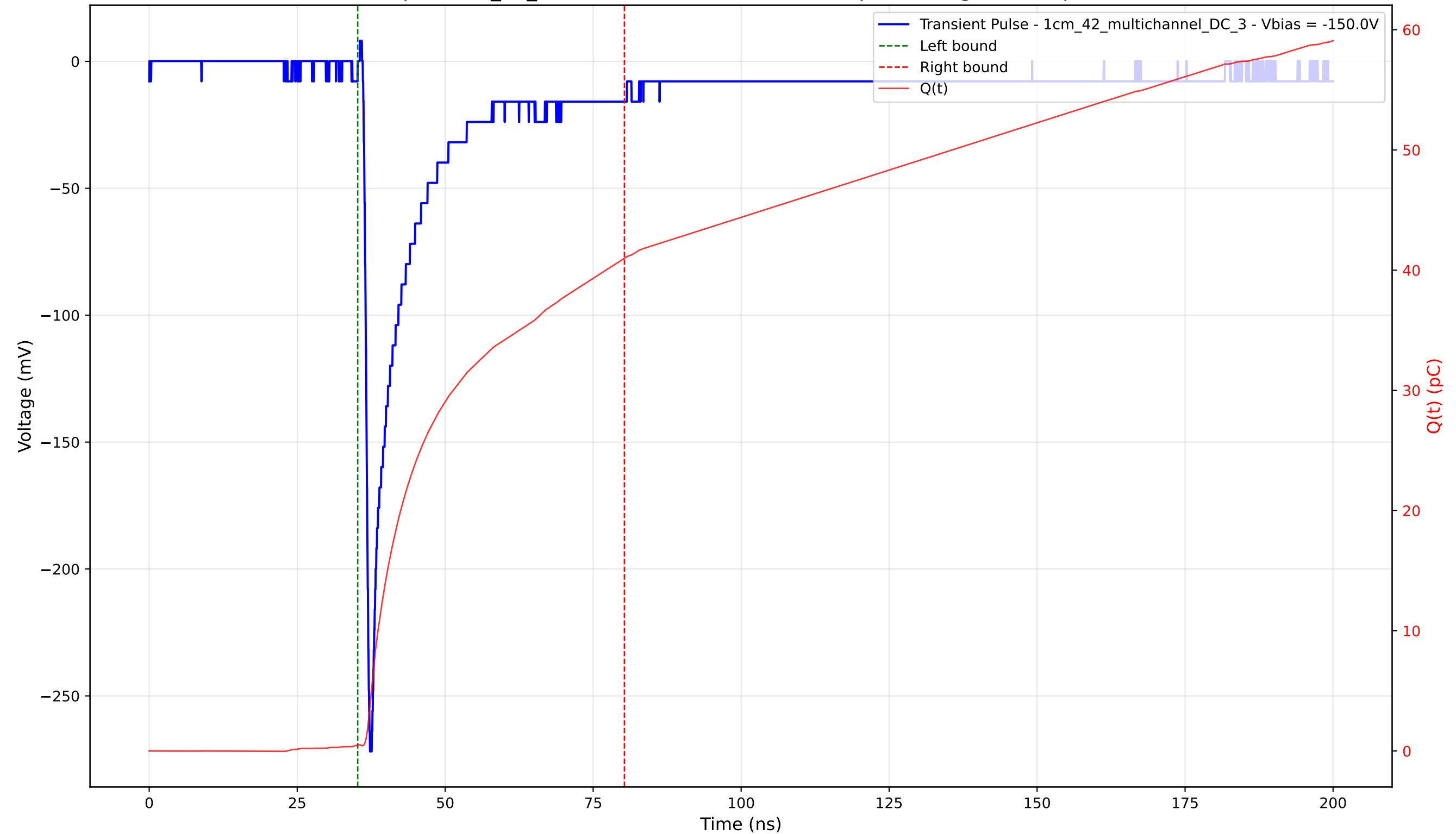
Transient Pulse - Sample: 1cm_42_multichannel - Position: 4530.0 \mu\text{m} - Charge: 40.50 pC - Rise Time: 0.85 ns
