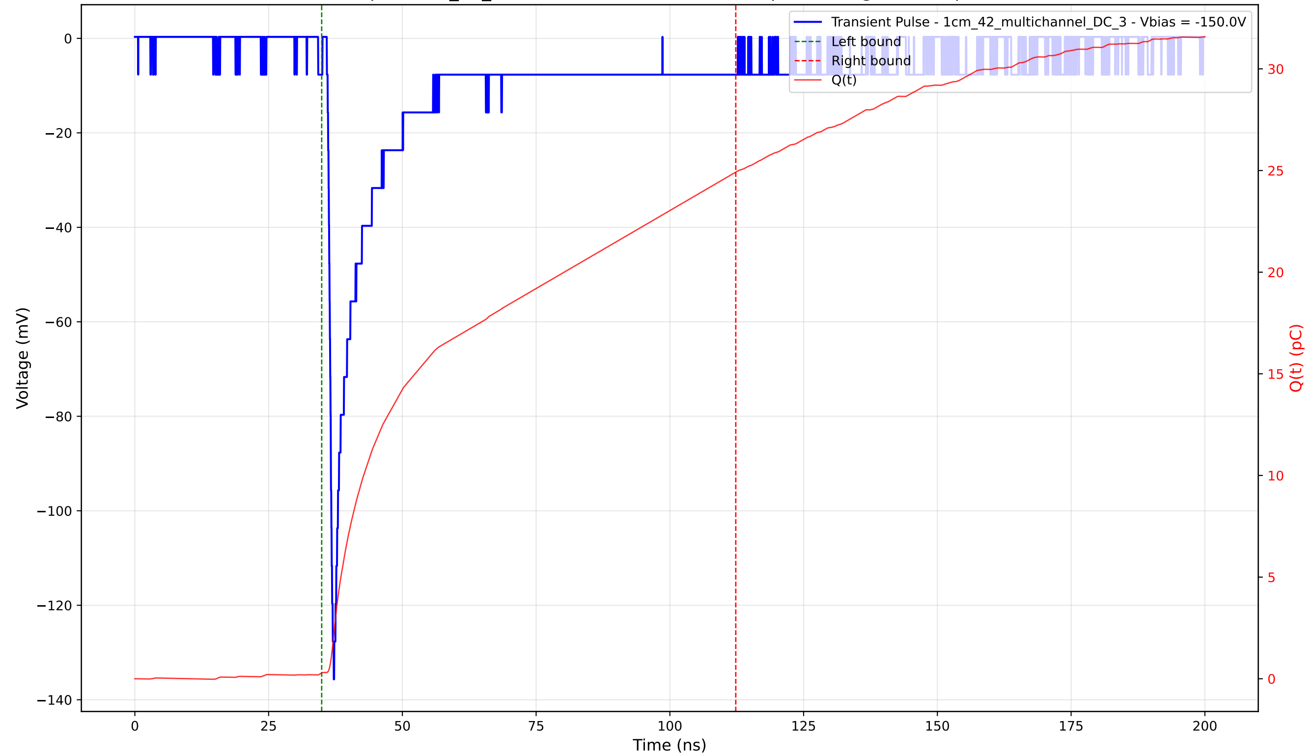
Transient Pulse - Sample: 1cm_42_multichannel - Position: 305.0 \mu\text{m} - Charge: 24.64 pC - Rise Time: 0.95 ns
