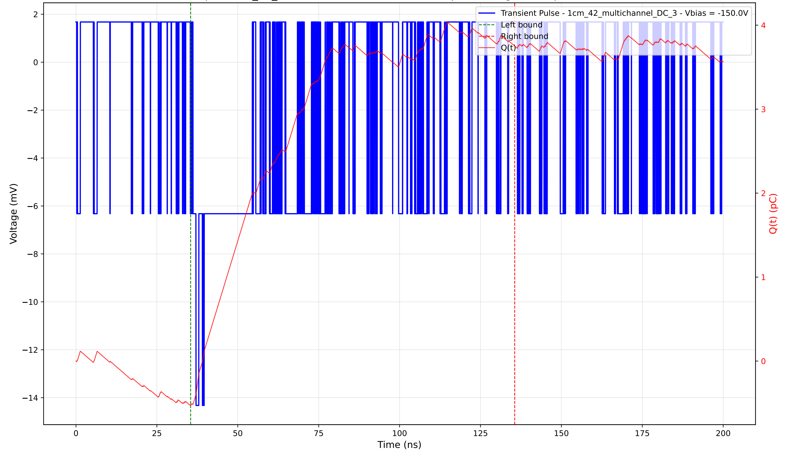
Transient Pulse - Sample: 1cm_42_multichannel - Position: 4395.0 \mu\text{m} - Charge: 4.27 pC - Rise Time: 0.00 ns (N/A)
