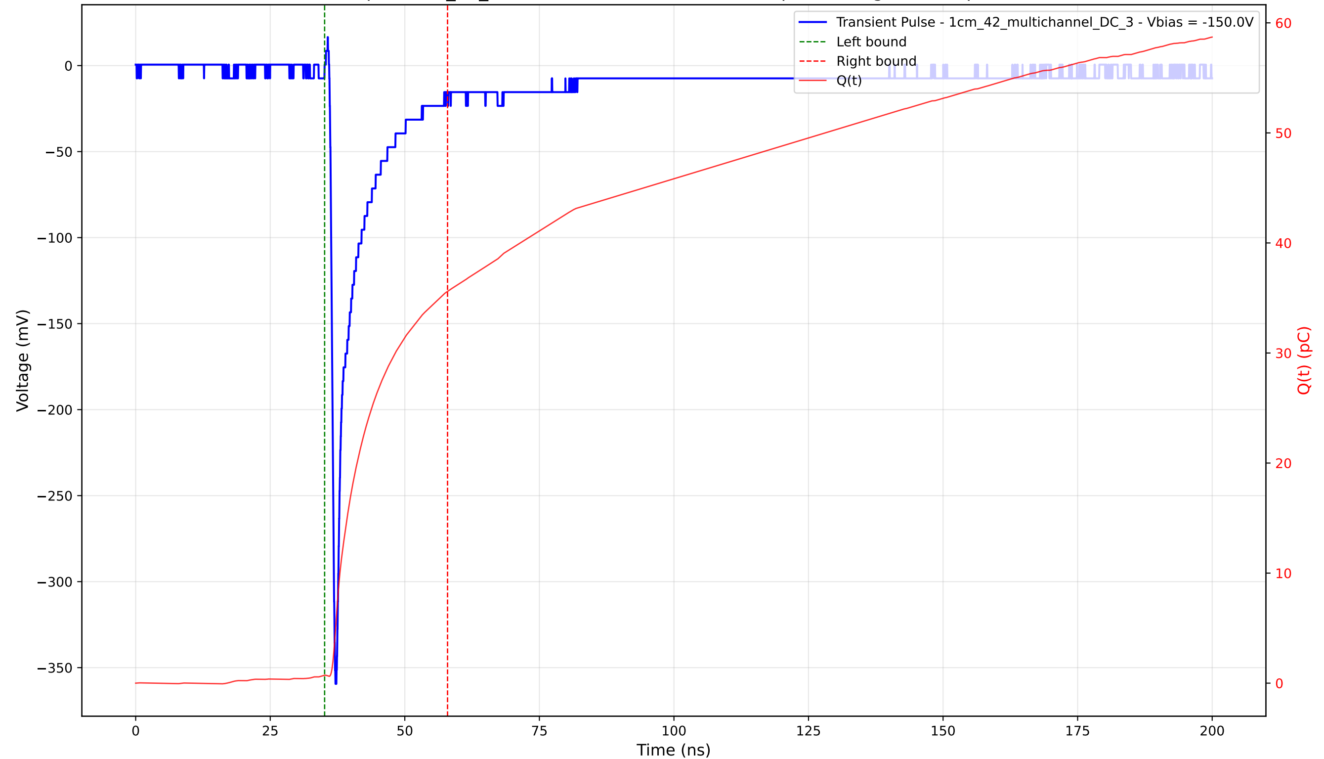
Transient Pulse - Sample: 1cm_42_multichannel - Position: 4755.0 \mu\text{m} - Charge: 34.87 pC - Rise Time: 0.79 ns
