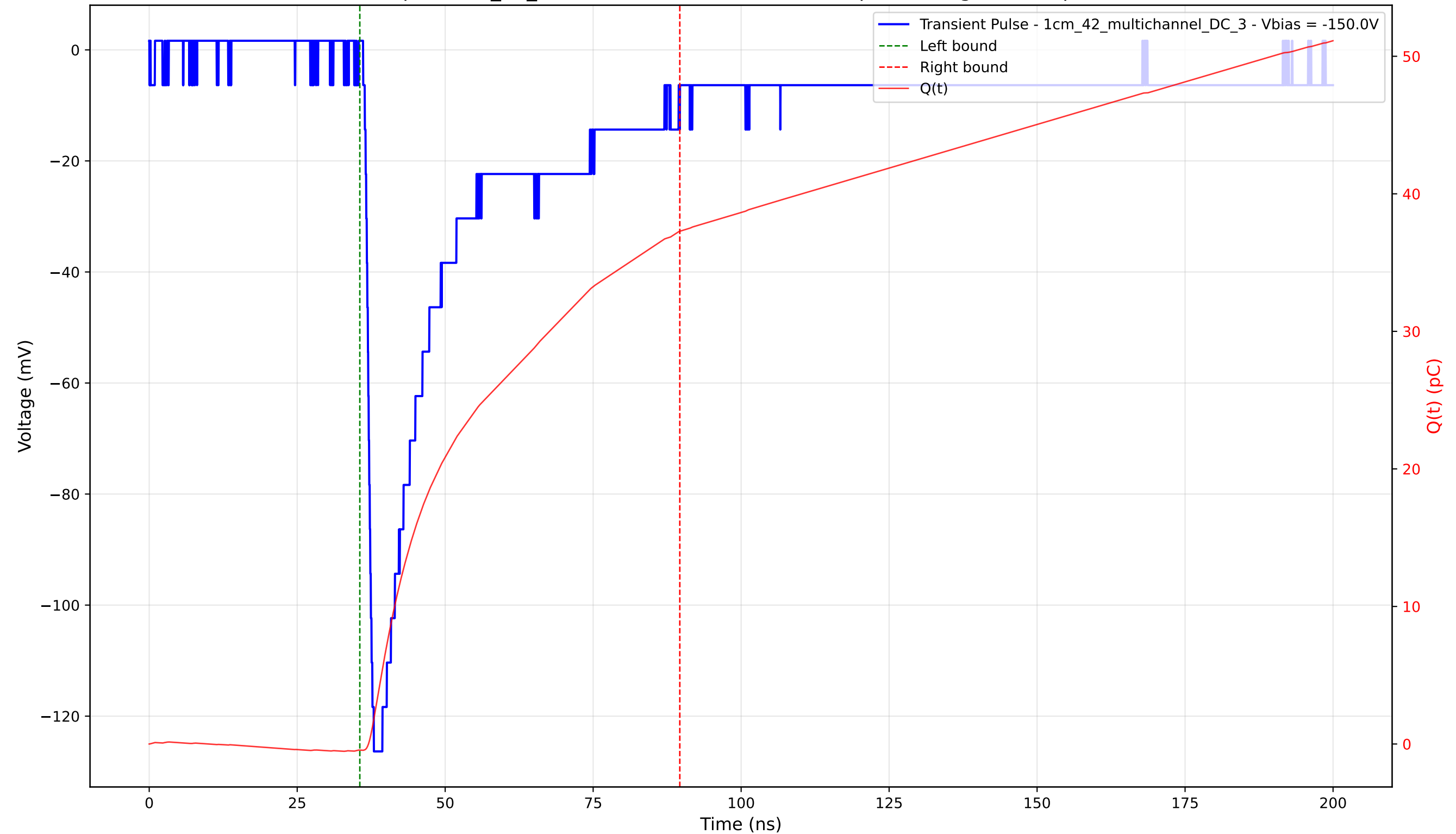
Transient Pulse - Sample: 1cm_42_multichannel - Position: 1290.0 \mu\text{m} - Charge: 37.73 pC - Rise Time: 1.28 ns
