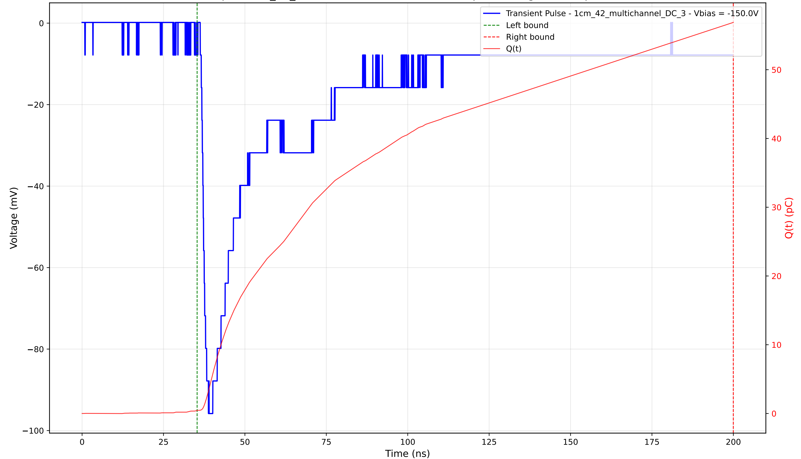
Transient Pulse - Sample: 1cm_42_multichannel - Position: 1950.0 \mu\text{m} - Charge: 56.43 pC - Rise Time: 1.68 ns
