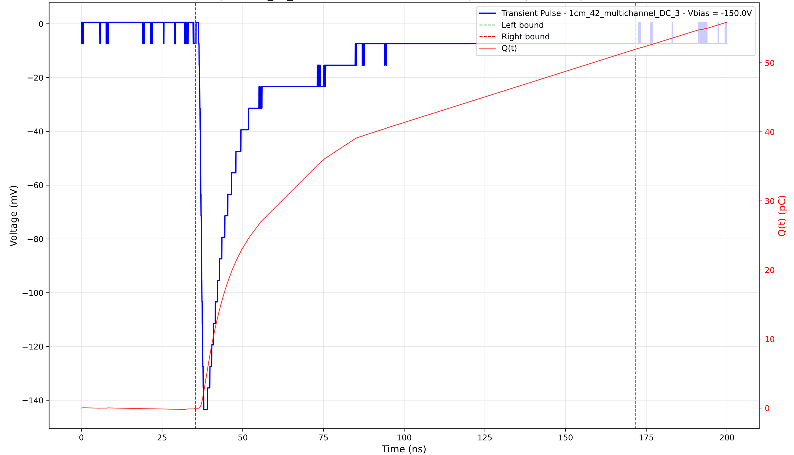
Transient Pulse - Sample: 1cm_42_multichannel - Position: 3755.0 \mu\text{m} - Charge: 52.04 pC - Rise Time: 1.26 ns
