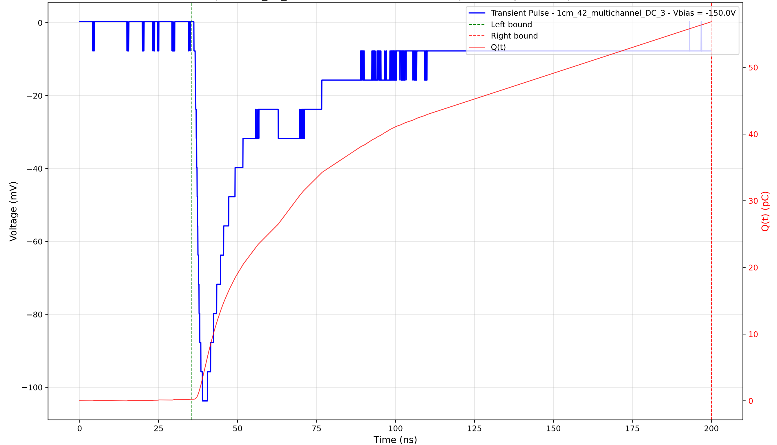
Transient Pulse - Sample: 1cm_42_multichannel - Position: 3005.0 \mu\text{m} - Charge: 56.62 pC - Rise Time: 1.81 ns
