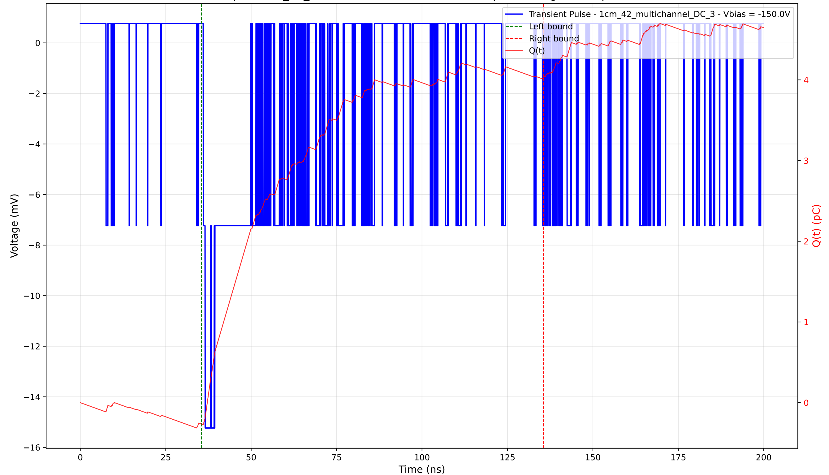
Transient Pulse - Sample: 1cm_42_multichannel - Position: 4890.0 \mu\text{m} - Charge: 4.28 pC - Rise Time: 0.56 ns
