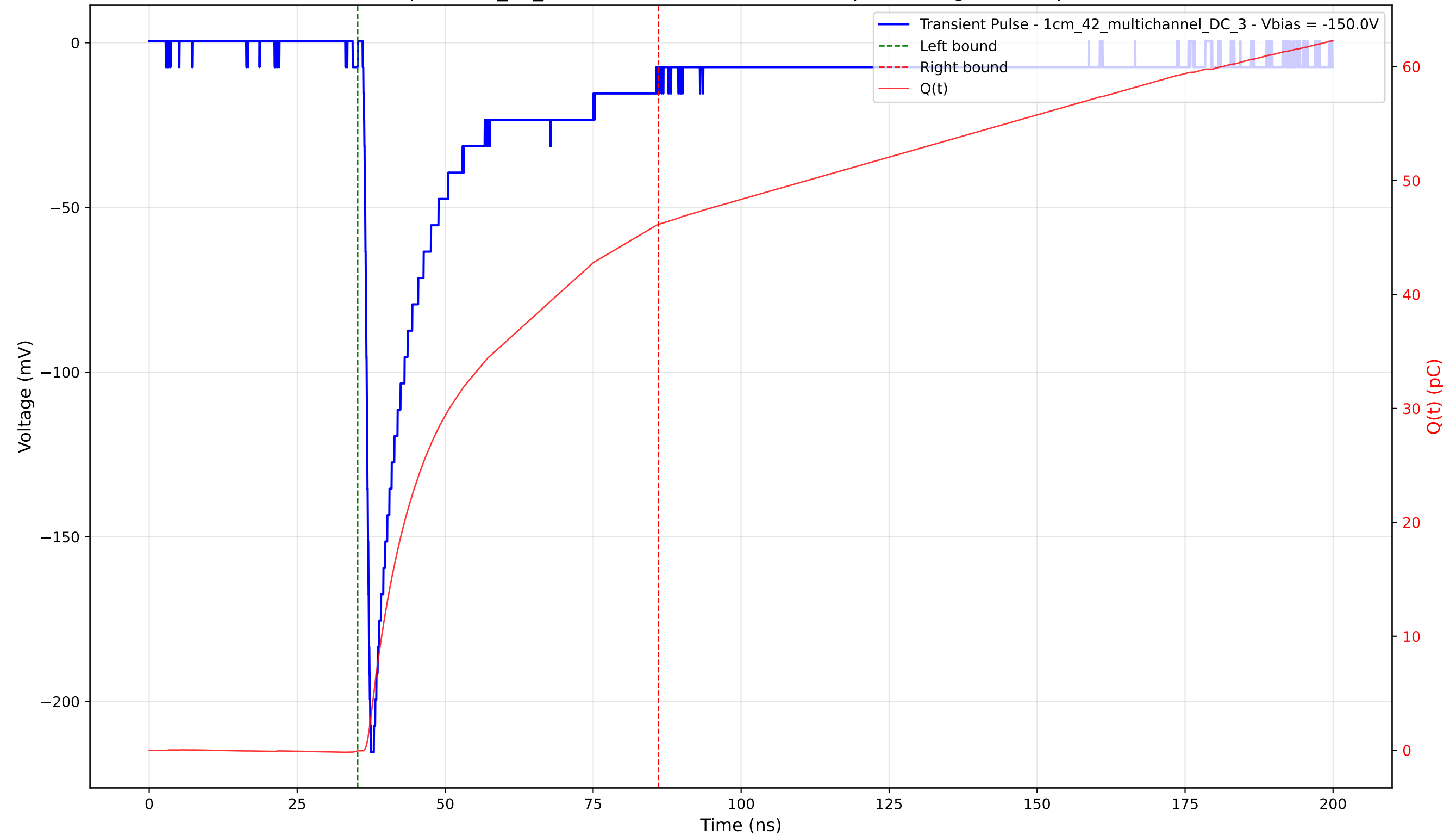
Transient Pulse - Sample: 1cm_42_multichannel - Position: 725.0 \mu\text{m} - Charge: 46.19 pC - Rise Time: 1.00 ns
