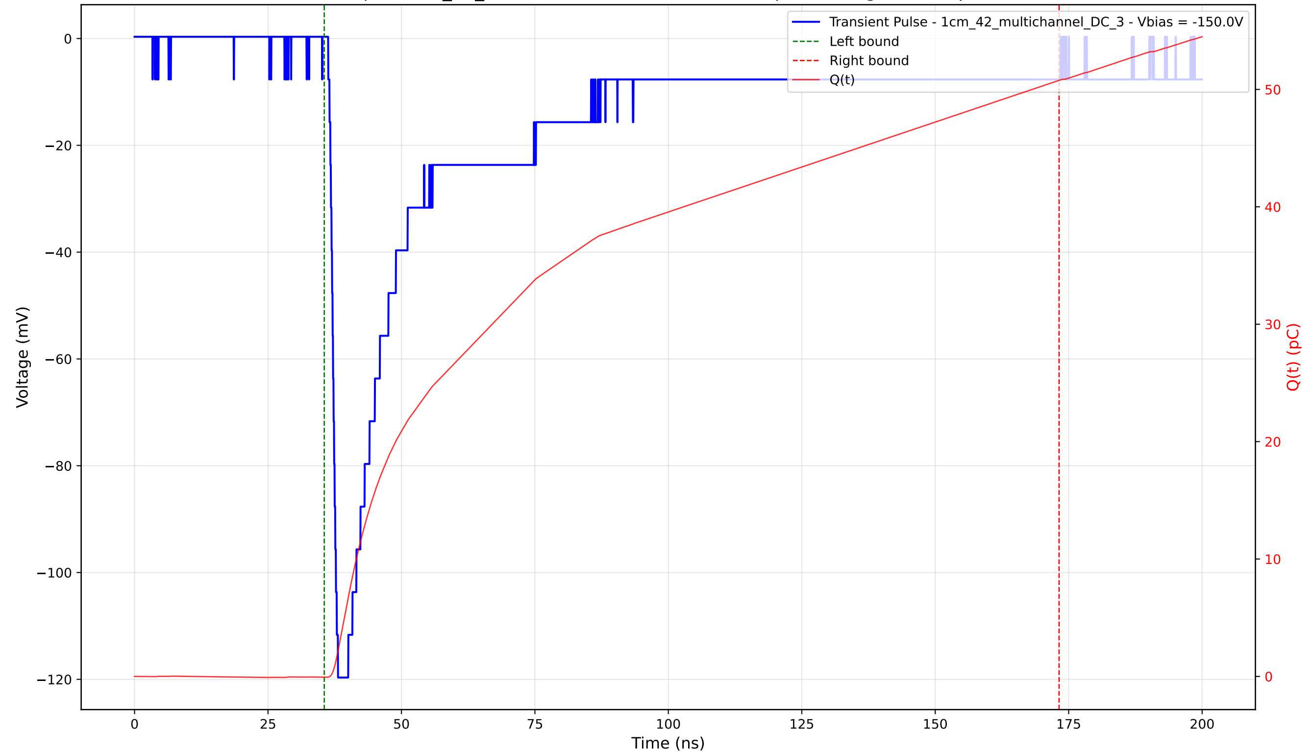
Transient Pulse - Sample: 1cm_42_multichannel - Position: 3485.0 \mu\text{m} - Charge: 50.84 pC - Rise Time: 1.37 ns
