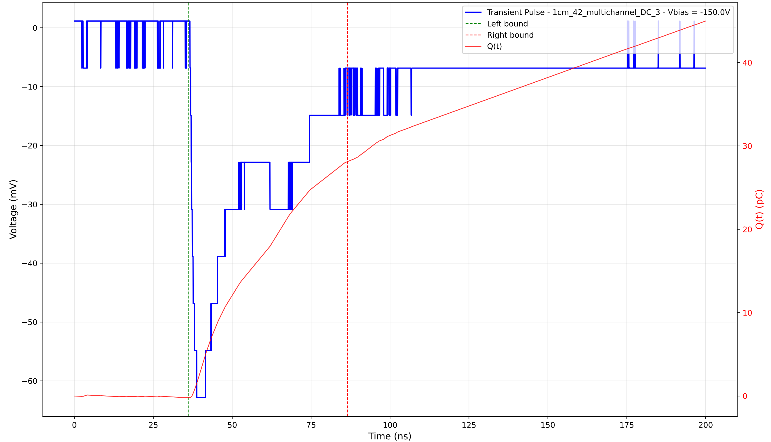
Transient Pulse - Sample: 1cm_42_multichannel - Position: 2310.0 \mu\text{m} - Charge: 28.28 pC - Rise Time: 2.16 ns
