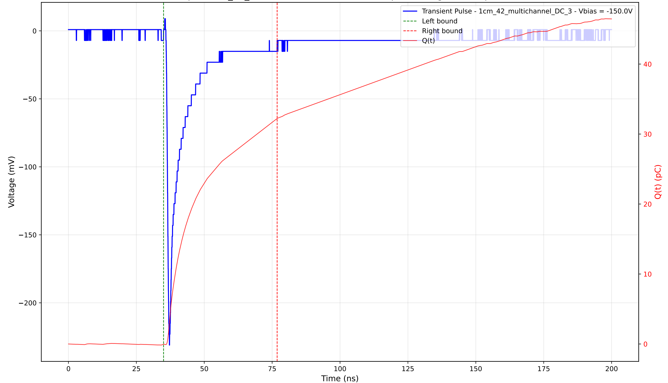
Transient Pulse - Sample: 1cm_42_multichannel - Position: 290.0 \mu\text{m} - Charge: 32.26 pC - Rise Time: 0.86 ns
