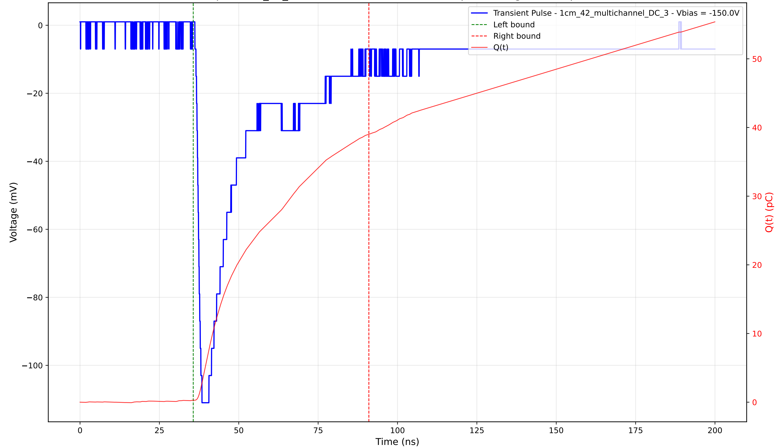
Transient Pulse - Sample: 1cm_42_multichannel - Position: 3250.0 \mu\text{m} - Charge: 38.73 pC - Rise Time: 1.55 ns
