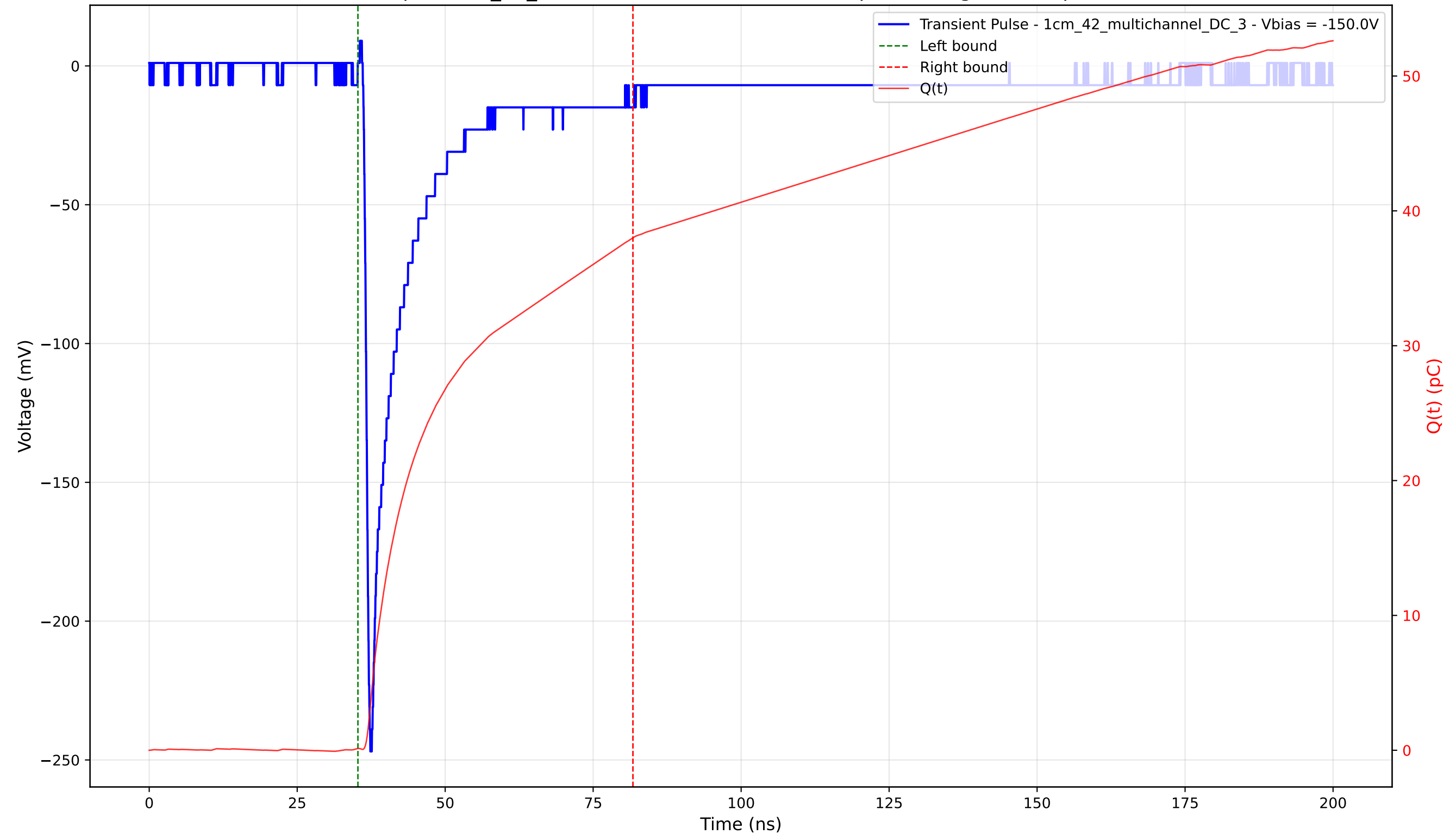
Transient Pulse - Sample: 1cm_42_multichannel - Position: 4485.0 \mu\text{m} - Charge: 37.86 pC - Rise Time: 0.84 ns
