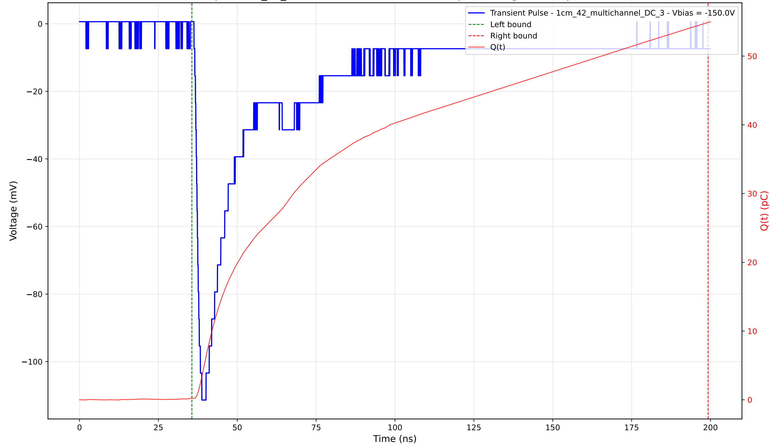
Transient Pulse - Sample: 1cm_42_multichannel - Position: 3195.0 \mu\text{m} - Charge: 54.68 pC - Rise Time: 1.77 ns
