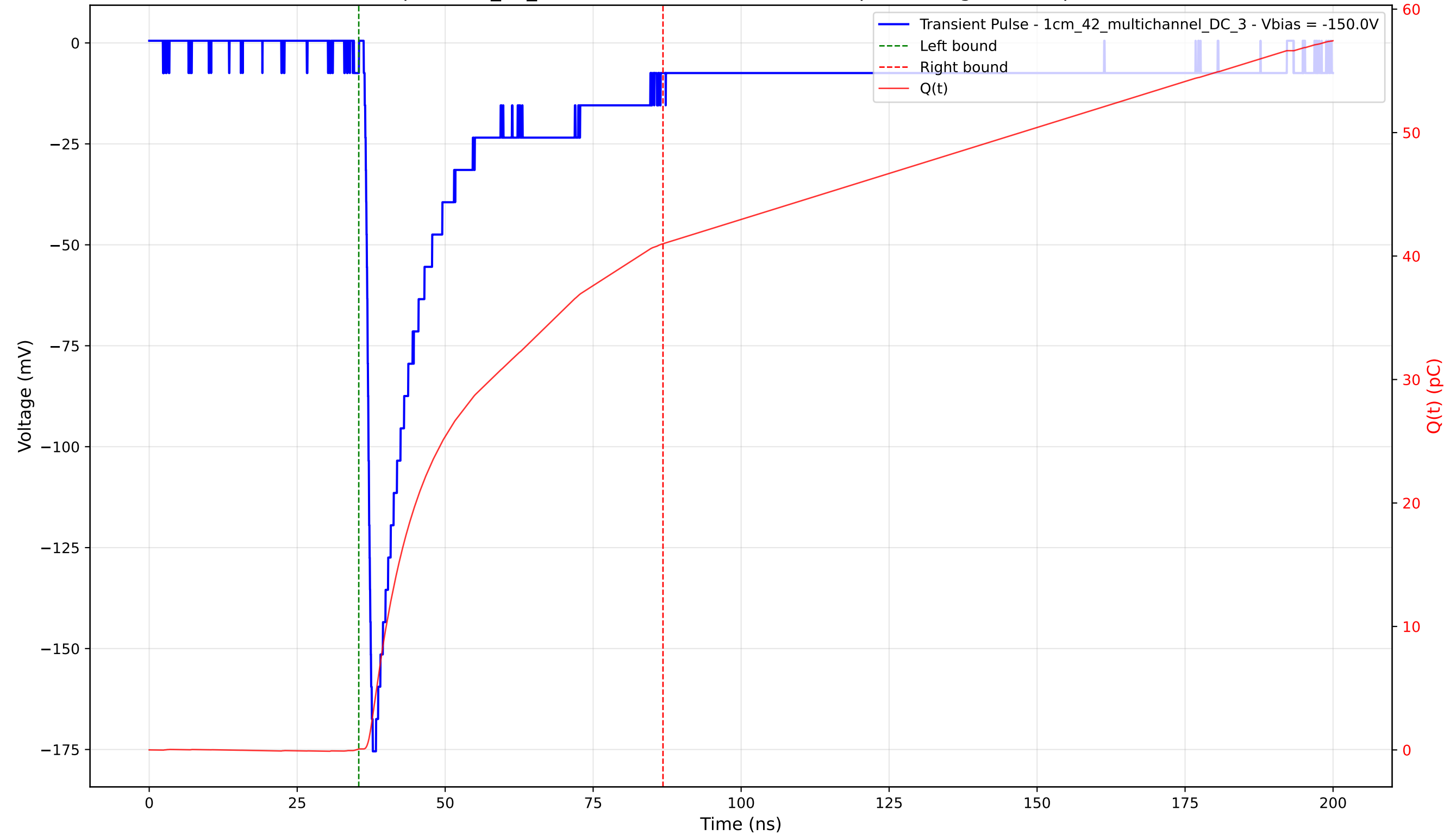
Transient Pulse - Sample: 1cm_42_multichannel - Position: 4015.0 \mu\text{m} - Charge: 40.92 pC - Rise Time: 0.99 ns
