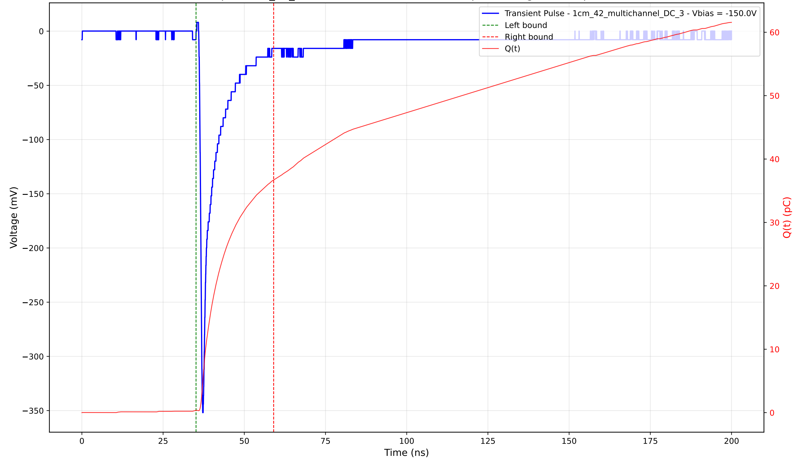
Transient Pulse - Sample: 1cm_42_multichannel - Position: 4705.0 \mu\text{m} - Charge: 36.31 pC - Rise Time: 0.80 ns
