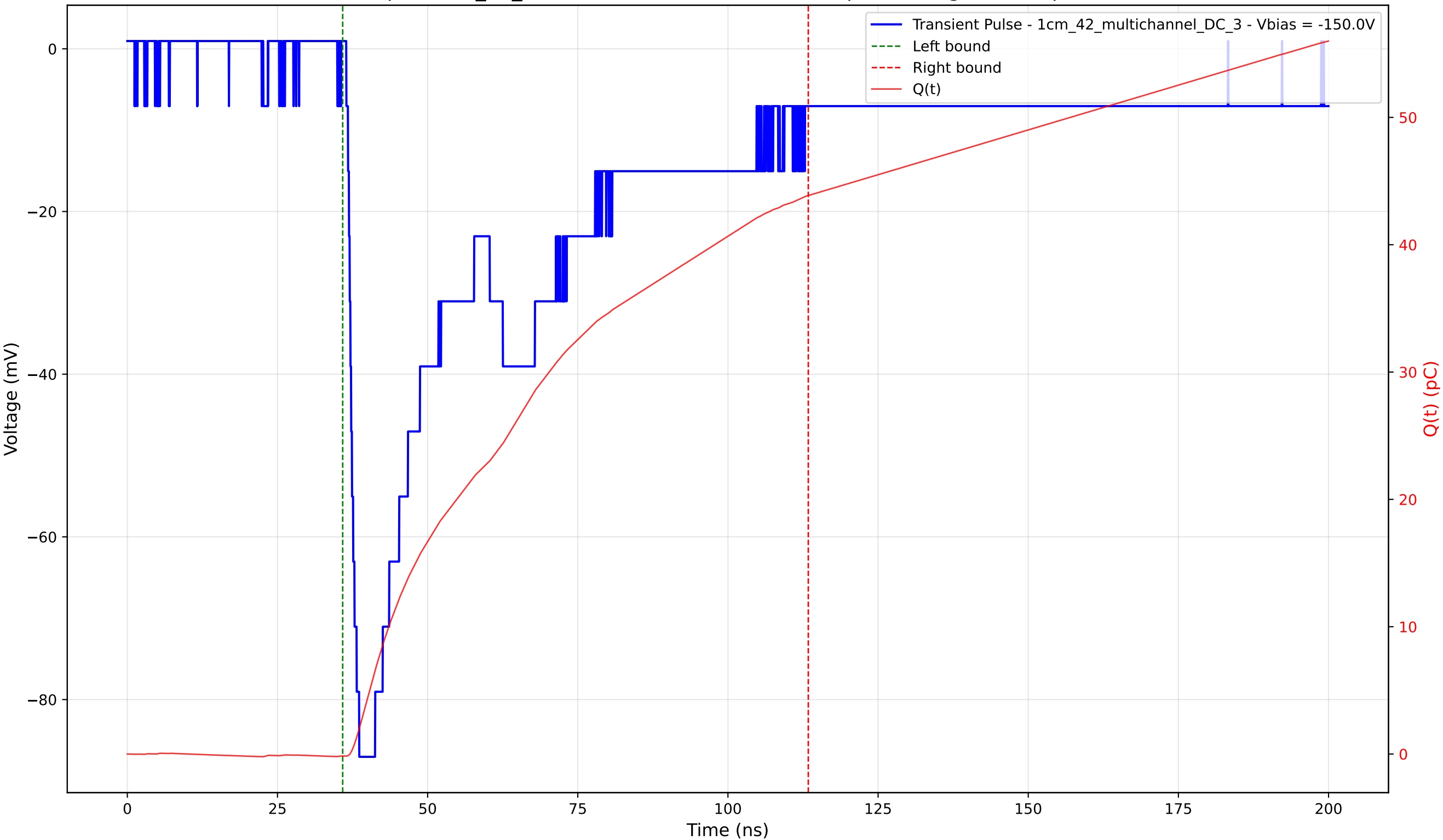
Transient Pulse - Sample: 1cm_42_multichannel - Position: 2125.0 \mu\text{m} - Charge: 44.02 pC - Rise Time: 1.46 ns
