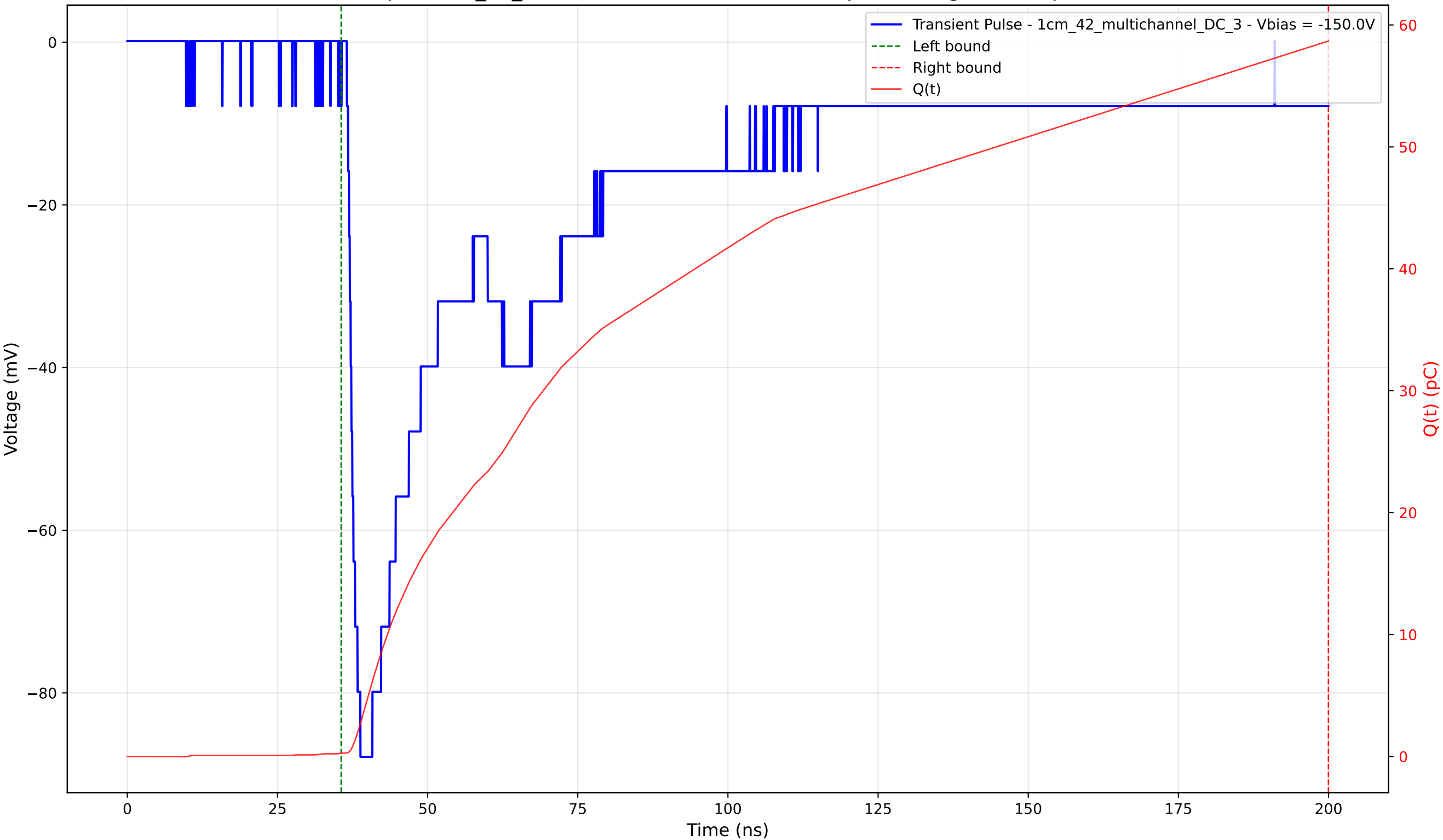
Transient Pulse - Sample: 1cm_42_multichannel - Position: 2180.0 \mu\text{m} - Charge: 58.40 pC - Rise Time: 1.58 ns
