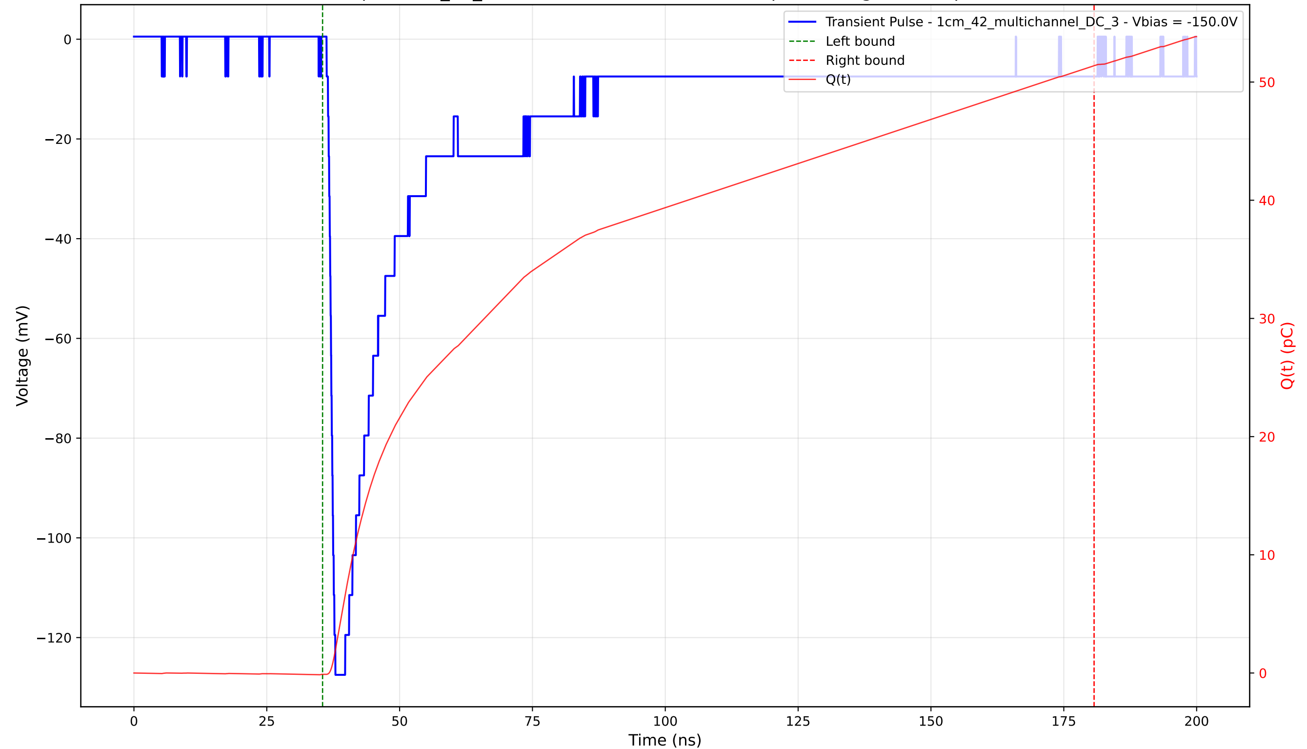
Transient Pulse - Sample: 1cm_42_multichannel - Position: 3660.0 \mu\text{m} - Charge: 51.50 pC - Rise Time: 1.21 ns
