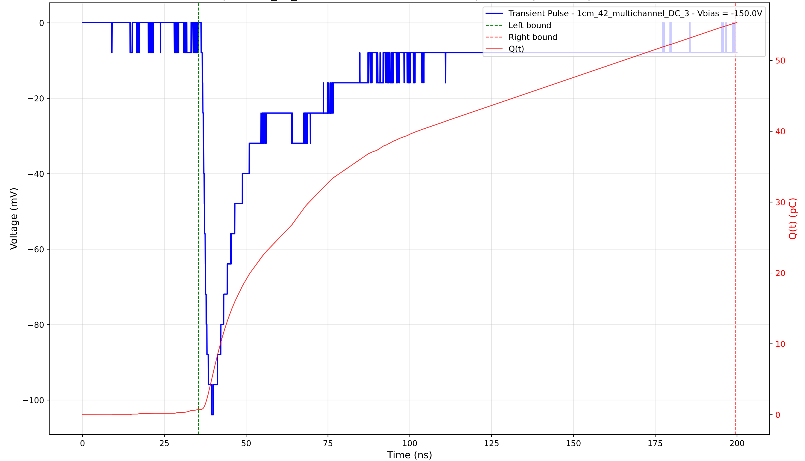
Transient Pulse - Sample: 1cm_42_multichannel - Position: 3100.0 \mu\text{m} - Charge: 54.53 pC - Rise Time: 1.85 ns
