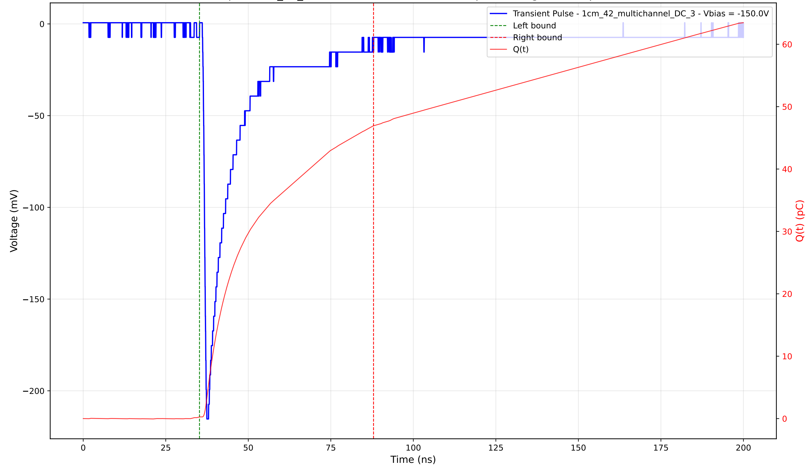
Transient Pulse - Sample: 1cm_42_multichannel - Position: 720.0 \mu\text{m} - Charge: 46.66 pC - Rise Time: 0.98 ns
