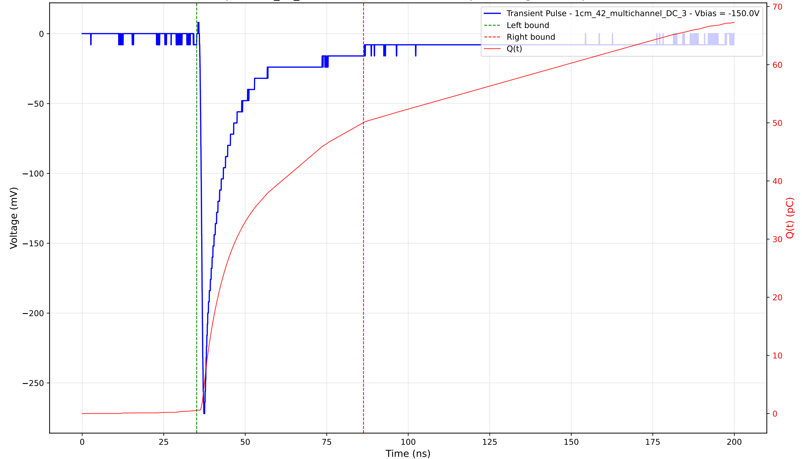
Transient Pulse - Sample: 1cm_42_multichannel - Position: 510.0 \mu\text{m} - Charge: 49.46 pC - Rise Time: 0.91 ns
