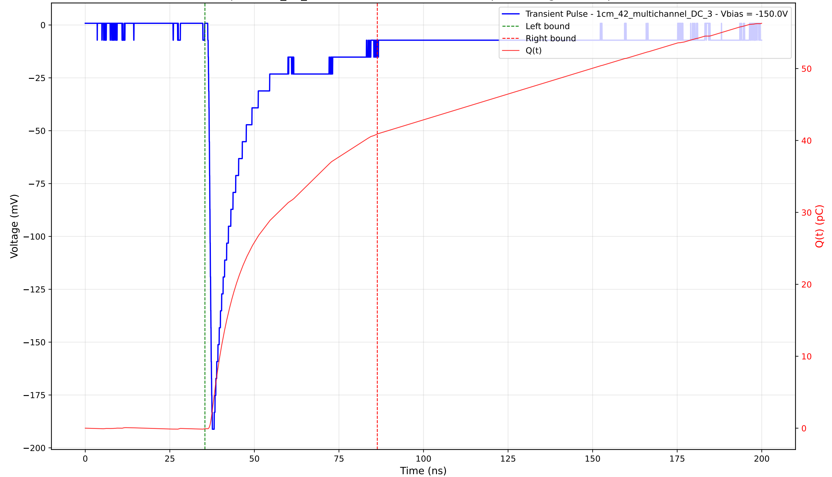
Transient Pulse - Sample: 1cm_42_multichannel - Position: 4155.0 \mu\text{m} - Charge: 40.98 pC - Rise Time: 0.95 ns
