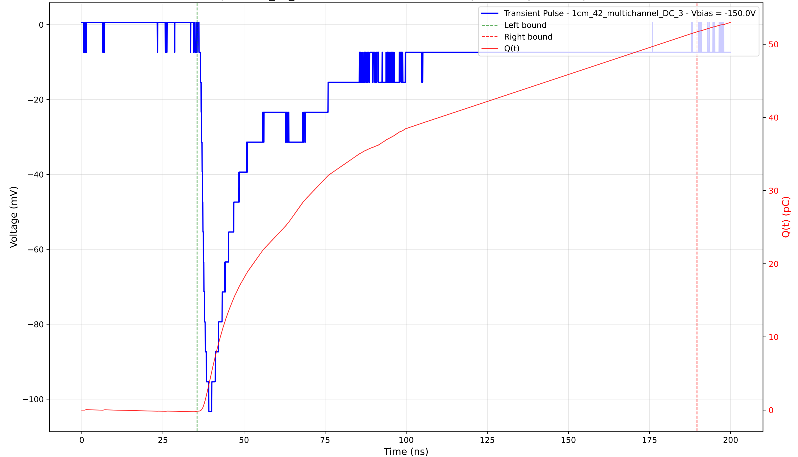
Transient Pulse - Sample: 1cm_42_multichannel - Position: 3070.0 \mu\text{m} - Charge: 51.86 pC - Rise Time: 1.83 ns
