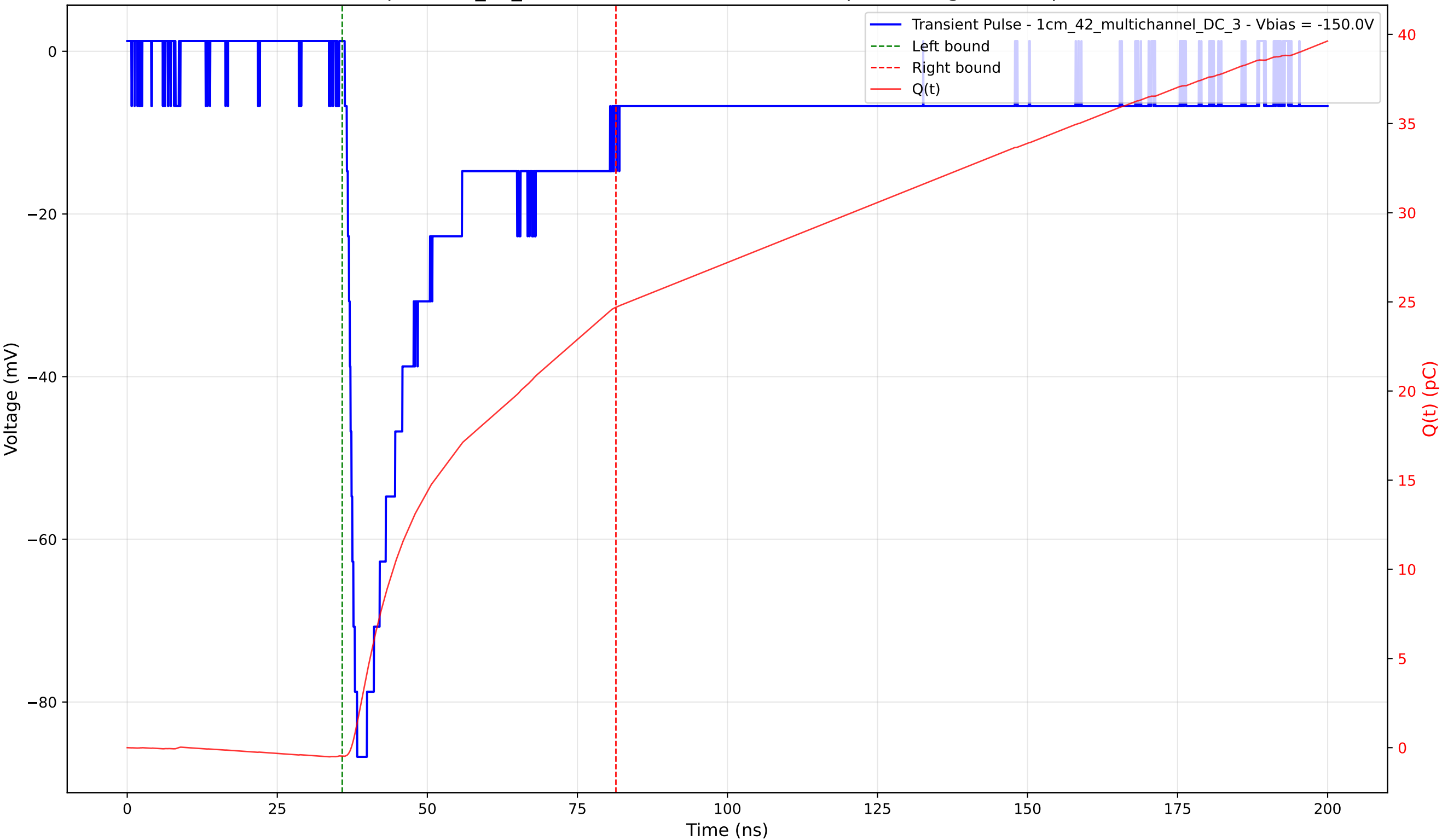
Transient Pulse - Sample: 1cm_42_multichannel - Position: 3445.0 \mu\text{m} - Charge: 25.17 pC - Rise Time: 1.36 ns
