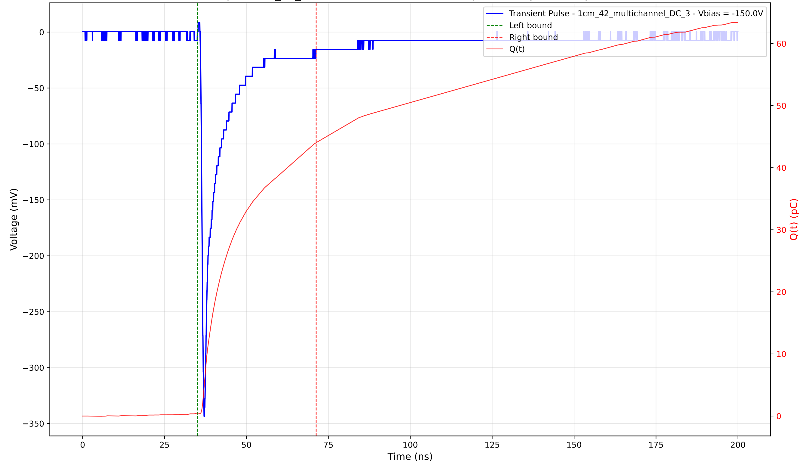
Transient Pulse - Sample: 1cm_42_multichannel - Position: 225.0 \mu\text{m} - Charge: 43.54 pC - Rise Time: 0.81 ns
