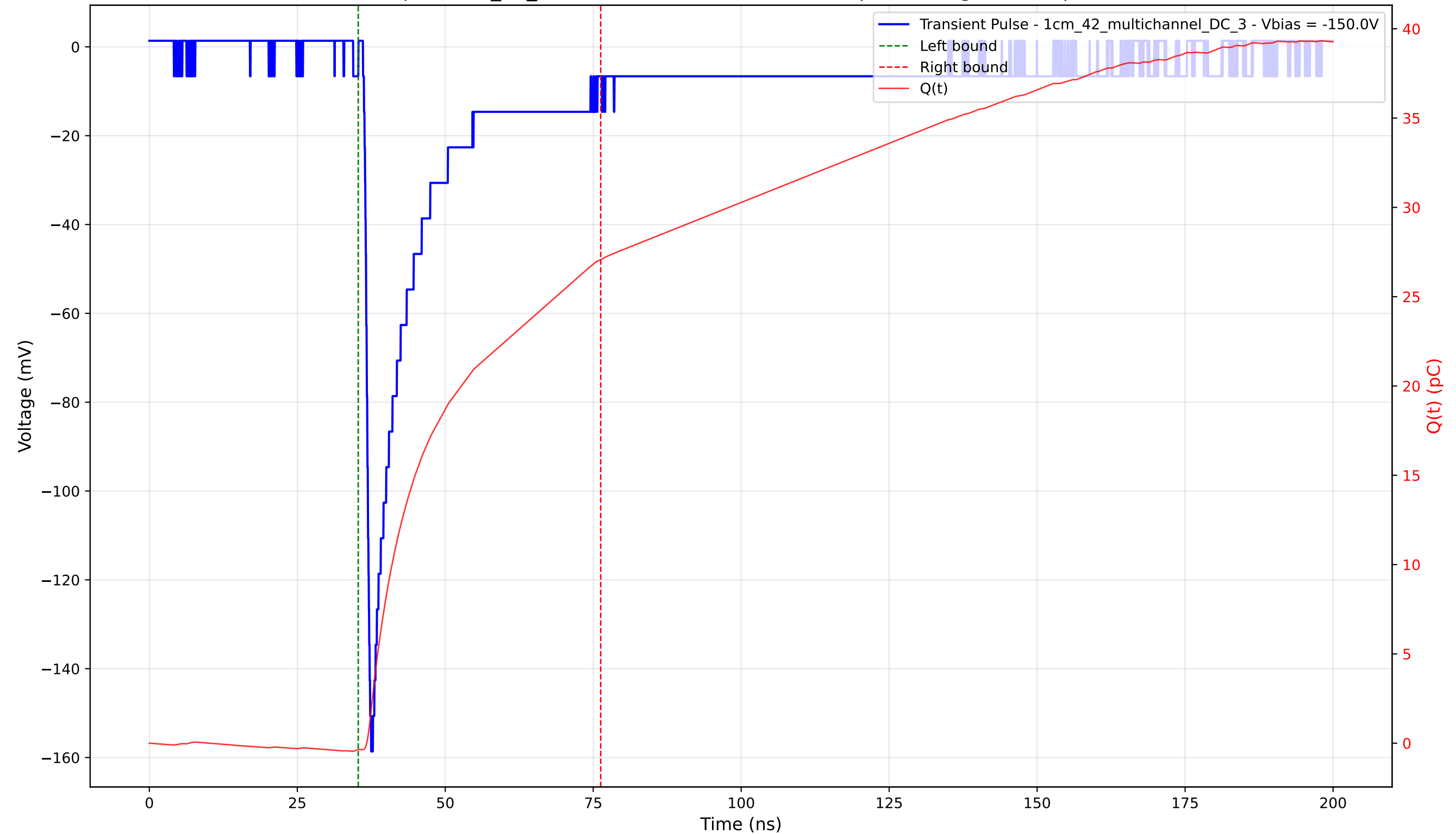
Transient Pulse - Sample: 1cm_42_multichannel - Position: 4325.0 \mu\text{m} - Charge: 27.41 pC - Rise Time: 0.96 ns
