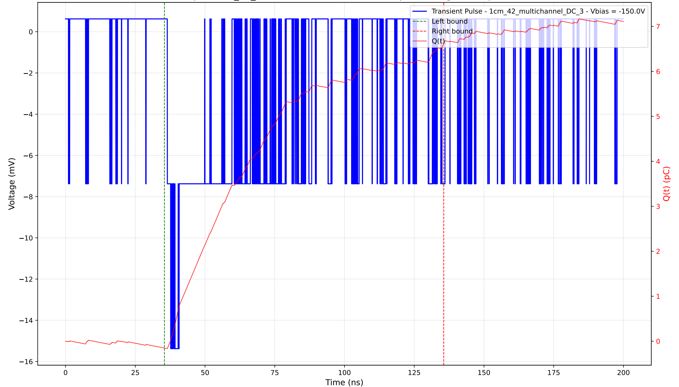
Transient Pulse - Sample: 1cm_42_multichannel - Position: 865.0 \mu\text{m} - Charge: 6.76 pC - Rise Time: 1.22 ns
