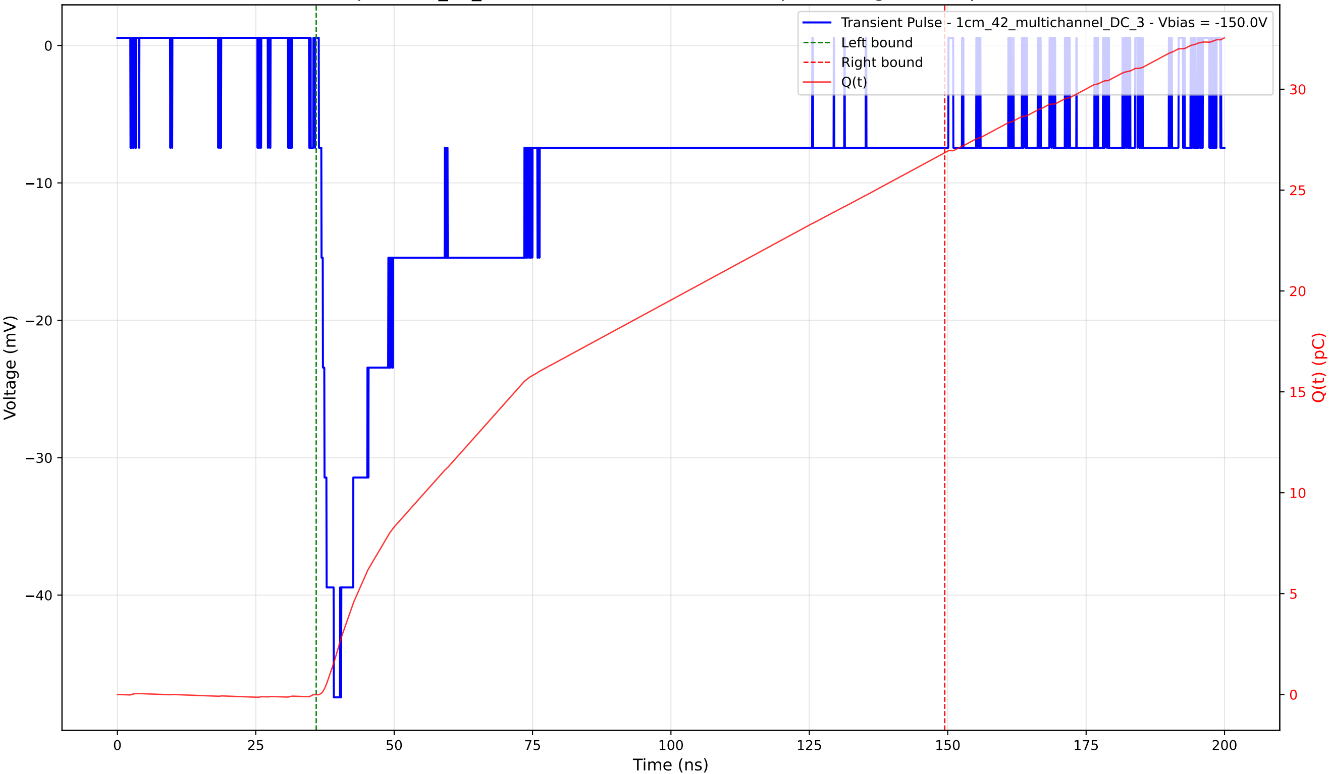
Transient Pulse - Sample: 1cm_42_multichannel - Position: 1915.0 \mu\text{m} - Charge: 26.87 pC - Rise Time: 2.69 ns
