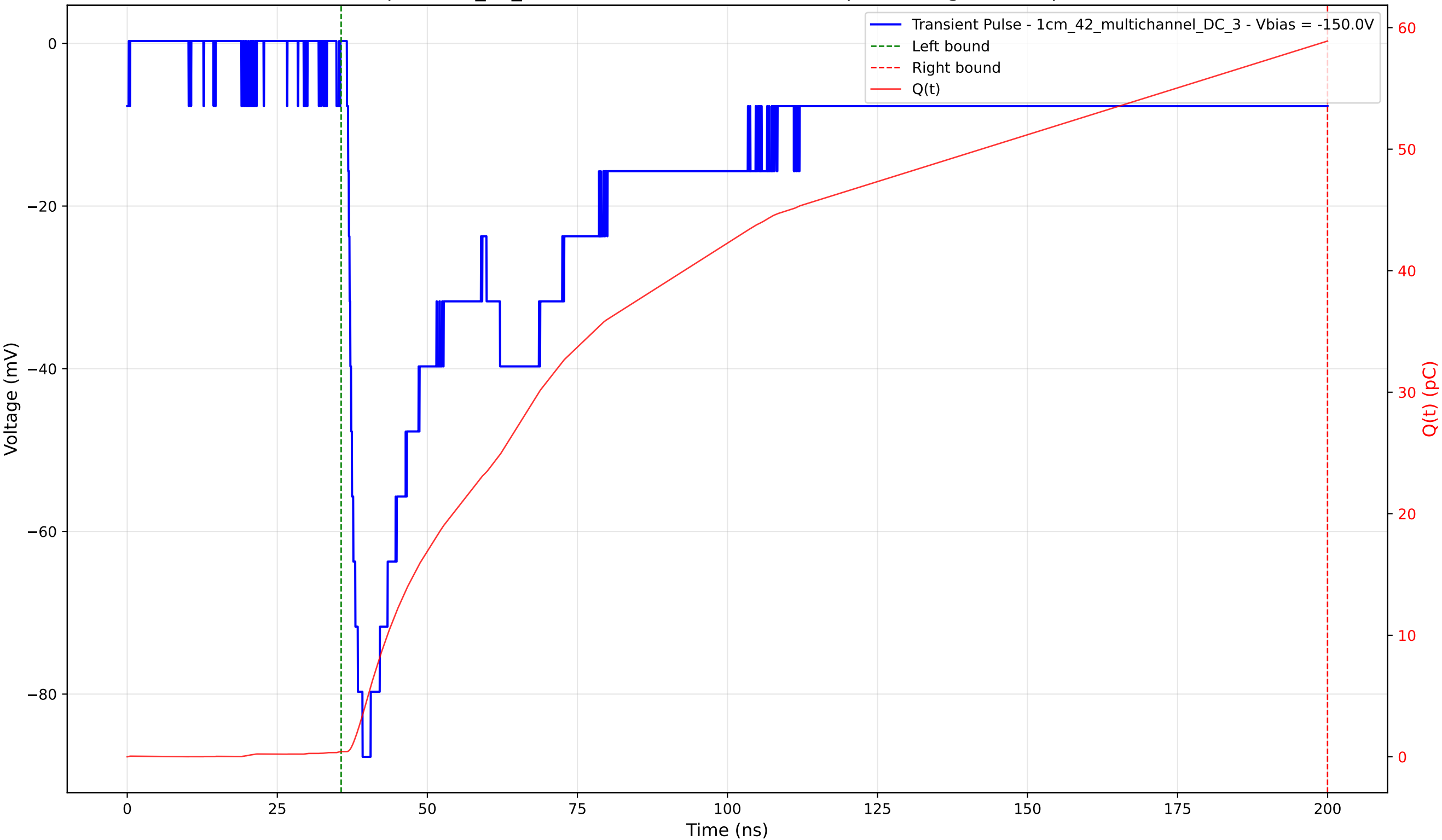
Transient Pulse - Sample: 1cm_42_multichannel - Position: 2255.0 \mu\text{m} - Charge: 58.47 pC - Rise Time: 1.64 ns
