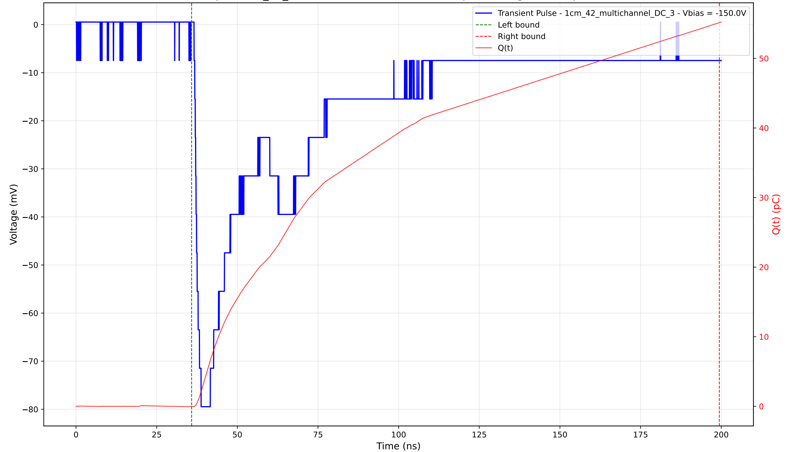
Transient Pulse - Sample: 1cm_42_multichannel - Position: 2510.0 \mu\text{m} - Charge: 55.15 pC - Rise Time: 1.98 ns
