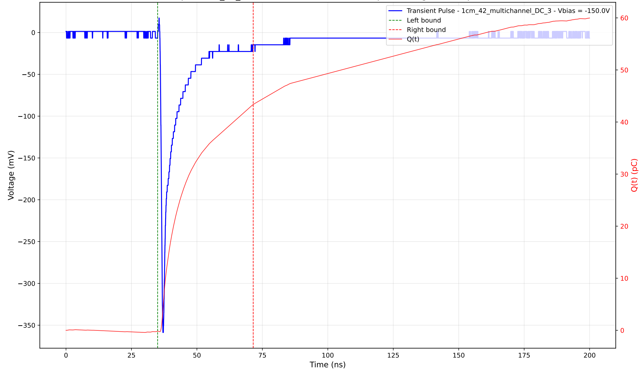
Transient Pulse - Sample: 1cm_42_multichannel - Position: 185.0 \mu\text{m} - Charge: 43.53 pC - Rise Time: 0.81 ns
