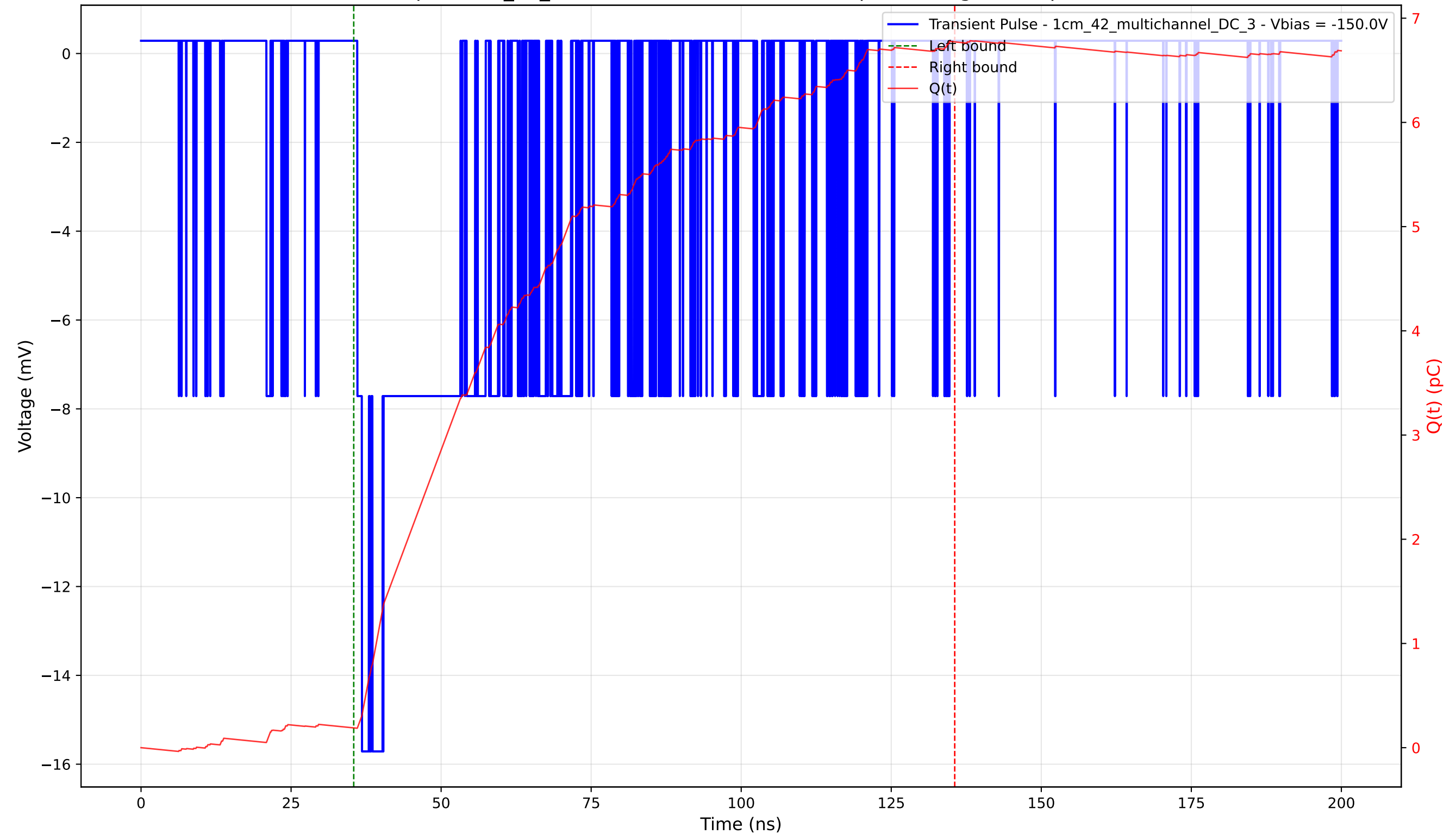
Transient Pulse - Sample: 1cm_42_multichannel - Position: 360.0 \mu\text{m} - Charge: 6.58 pC - Rise Time: 0.78 ns
