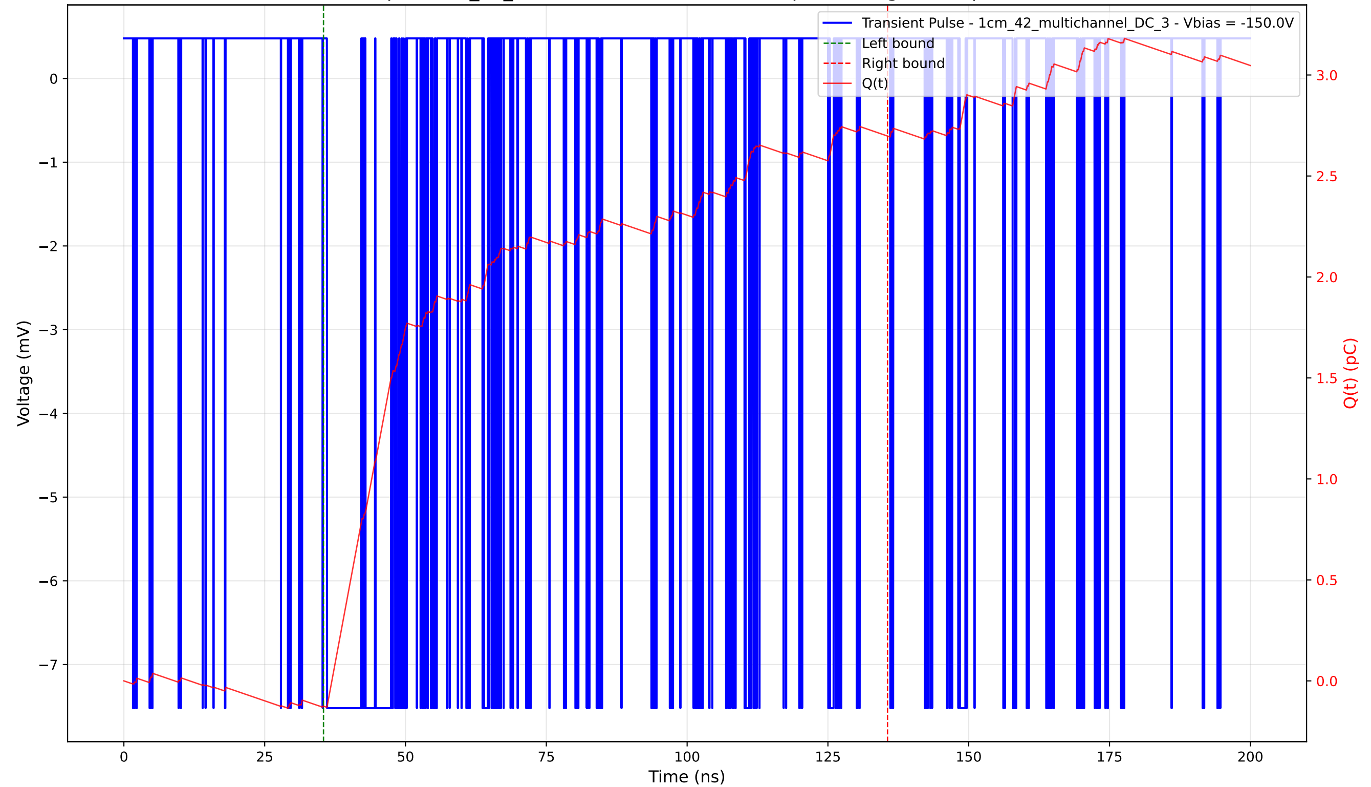
Transient Pulse - Sample: 1cm_42_multichannel - Position: 10.0 \mu\text{m} - Charge: 2.82 pC - Rise Time: 0.02 ns
