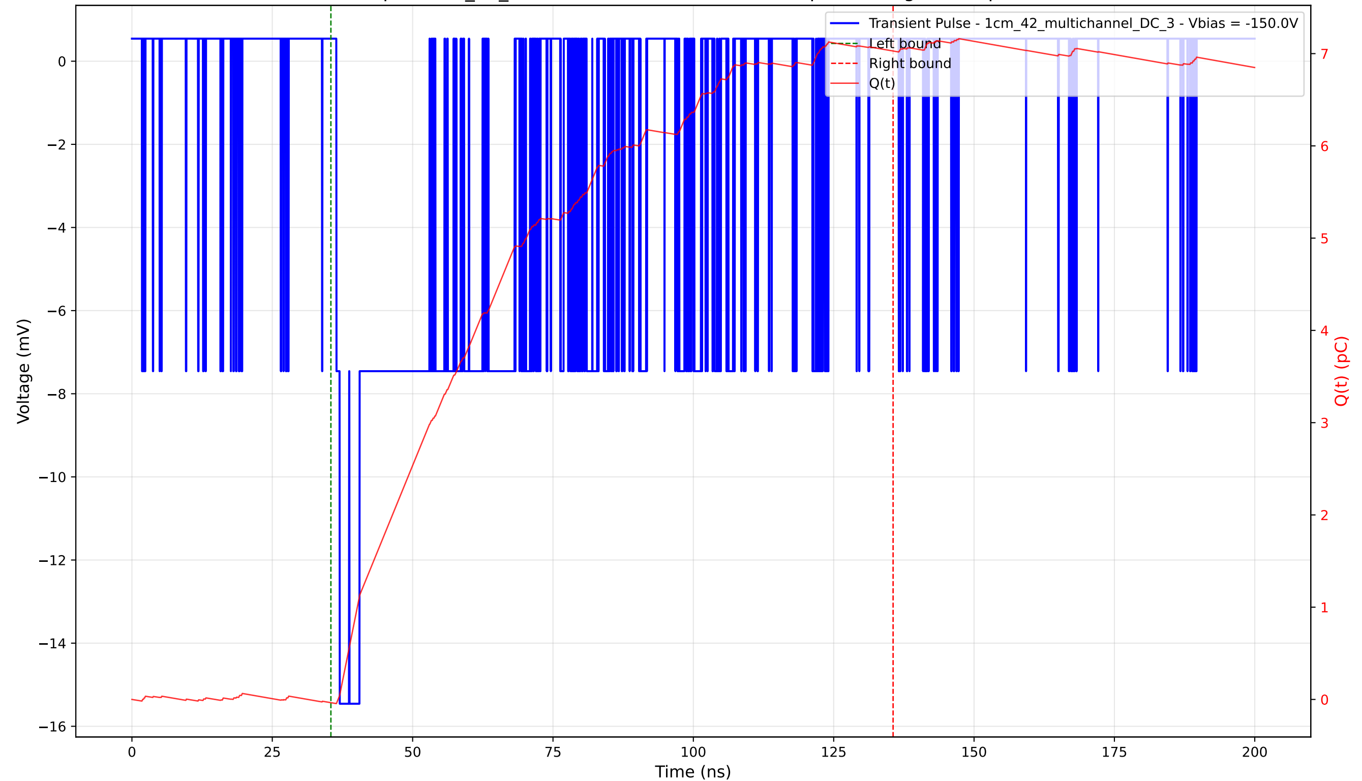
Transient Pulse - Sample: 1cm_42_multichannel - Position: 4375.0 \mu\text{m} - Charge: 7.06 pC - Rise Time: 0.60 ns
