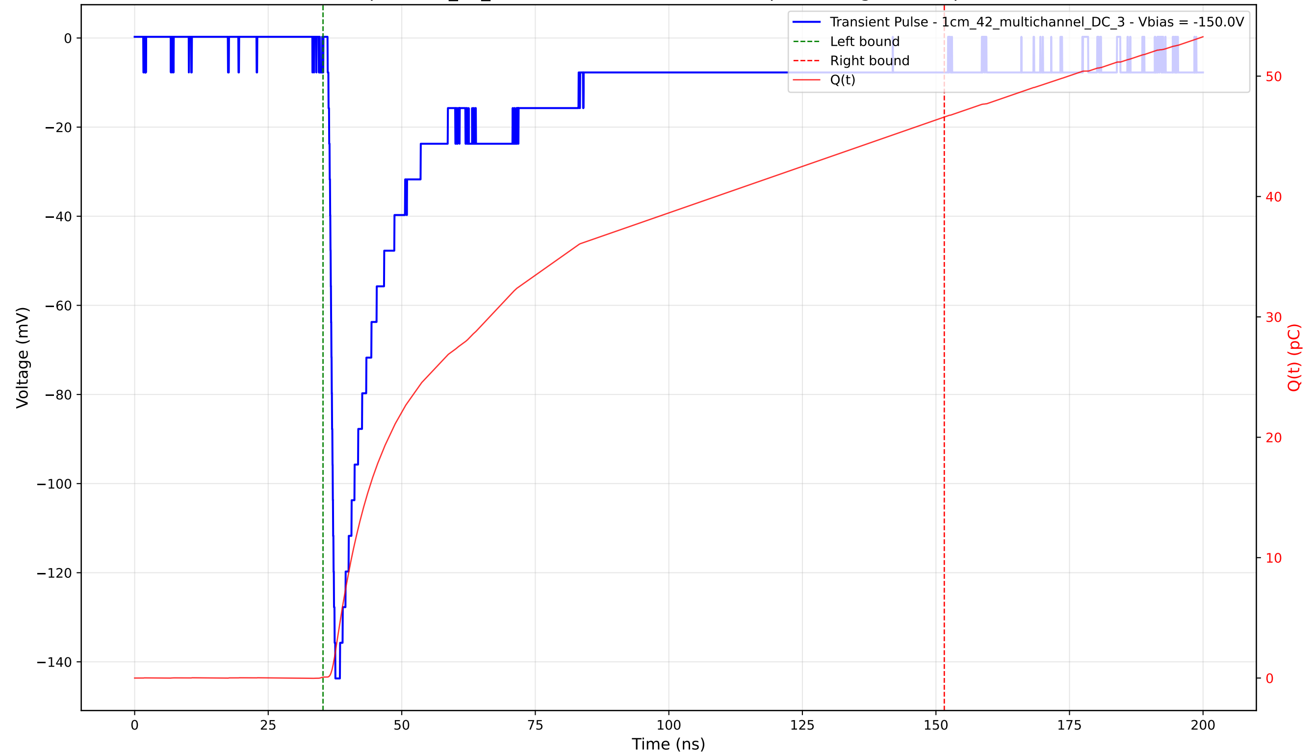
Transient Pulse - Sample: 1cm_42_multichannel - Position: 920.0 \mu\text{m} - Charge: 46.55 pC - Rise Time: 1.14 ns
