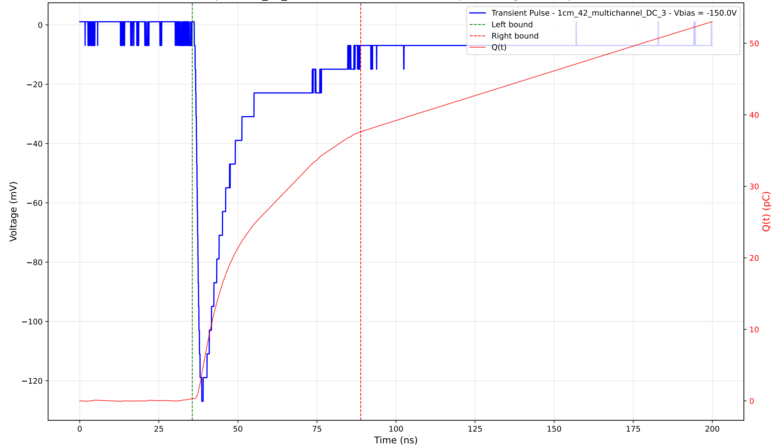
Transient Pulse - Sample: 1cm_42_multichannel - Position: 3510.0 \mu\text{m} - Charge: 37.32 pC - Rise Time: 1.57 ns
