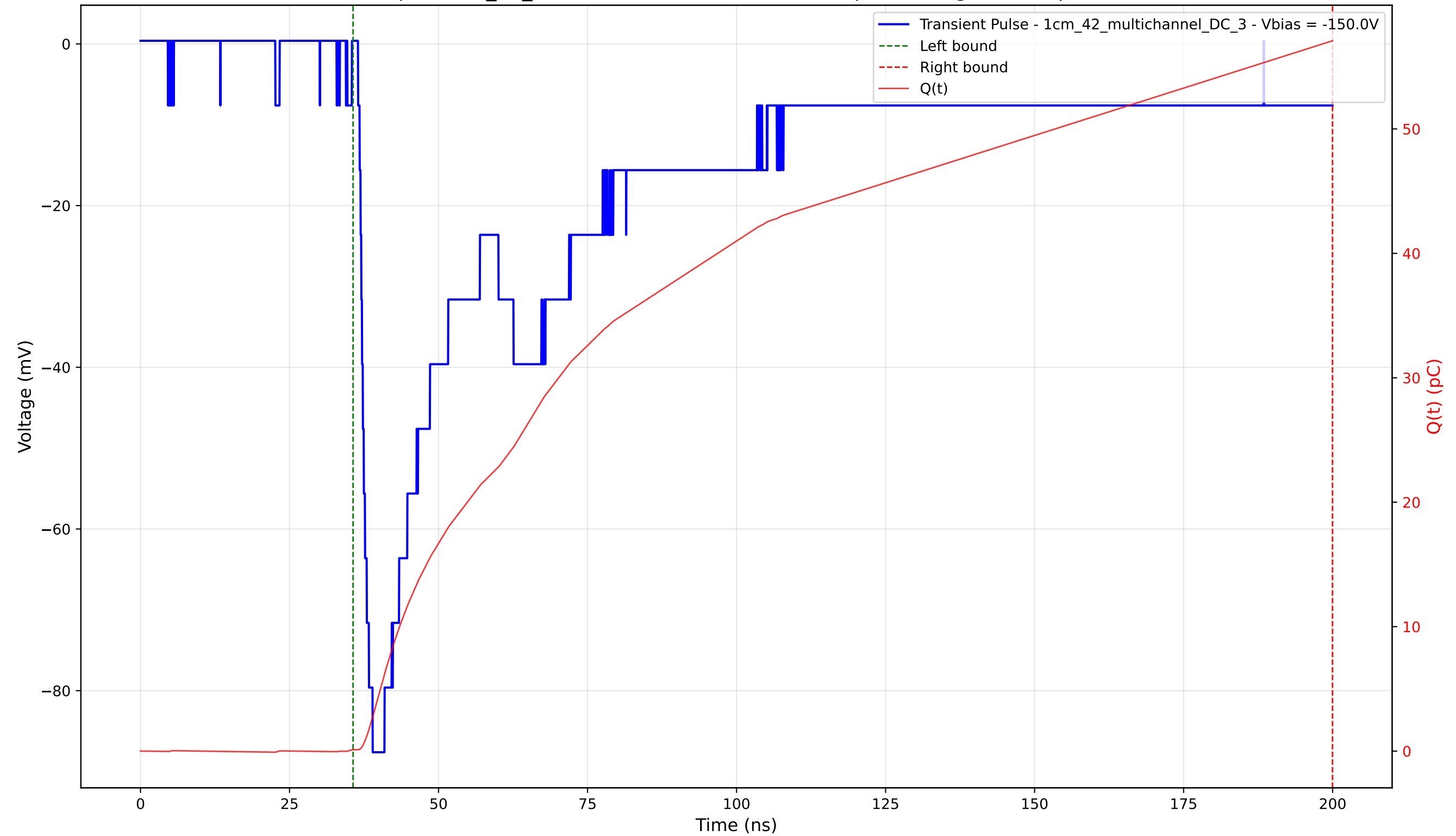
Transient Pulse - Sample: 1cm_42_multichannel - Position: 2170.0 \mu\text{m} - Charge: 56.98 pC - Rise Time: 1.58 ns
