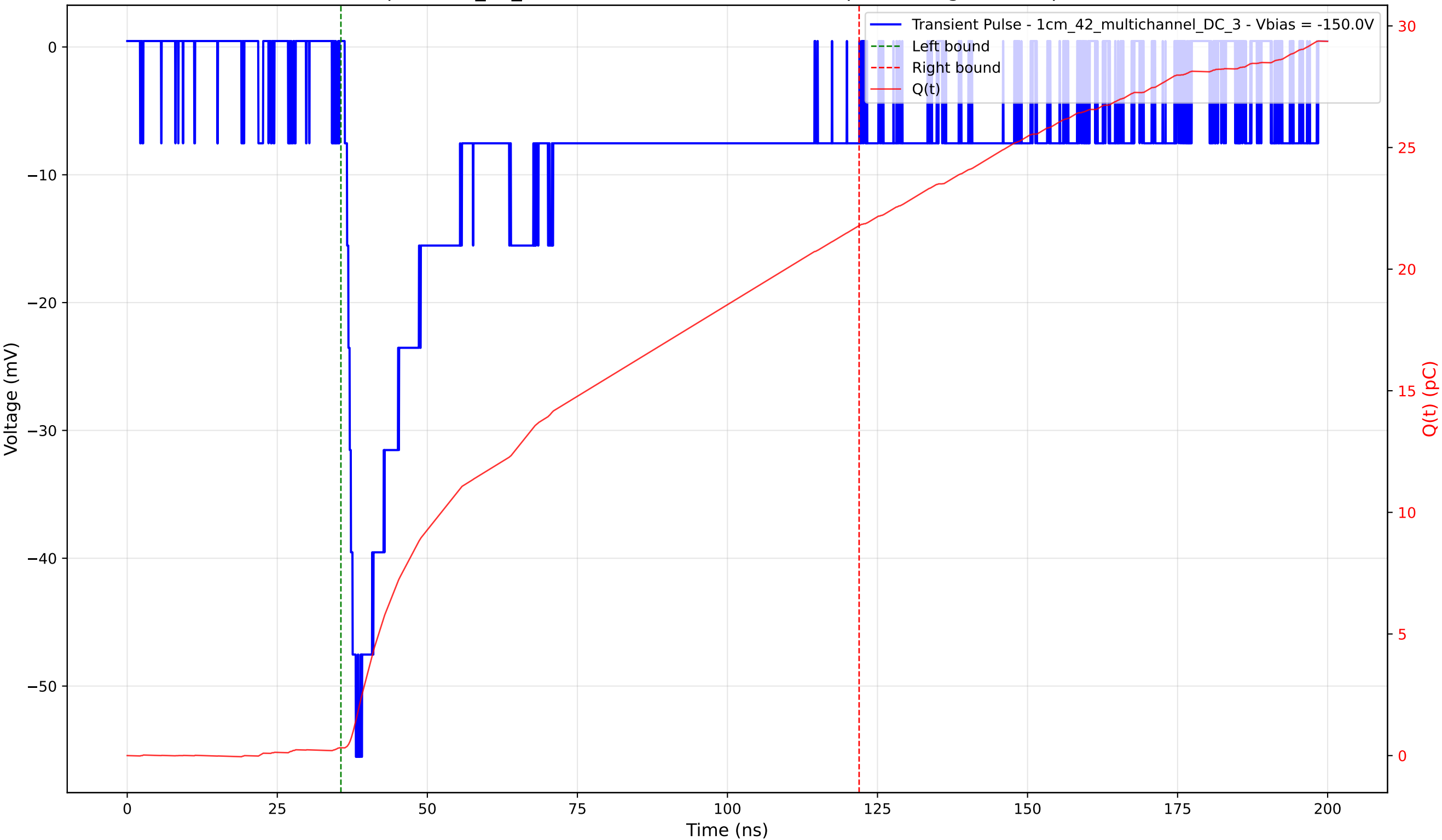
Transient Pulse - Sample: 1cm_42_multichannel - Position: 1320.0 \mu\text{m} - Charge: 21.47 pC - Rise Time: 1.85 ns
