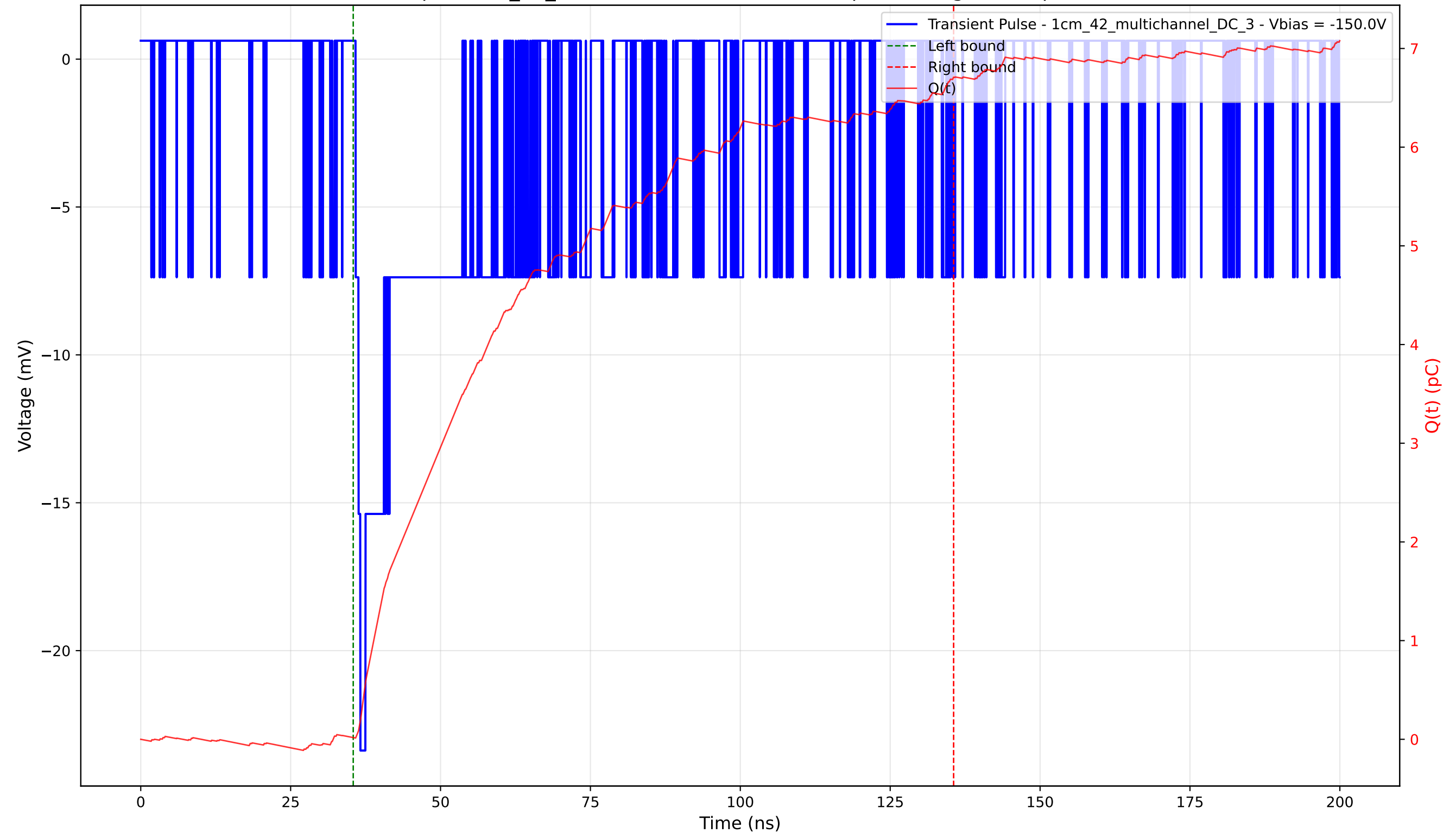
Transient Pulse - Sample: 1cm_42_multichannel - Position: 45.0 \mu\text{m} - Charge: 6.69 pC - Rise Time: 0.79 ns
