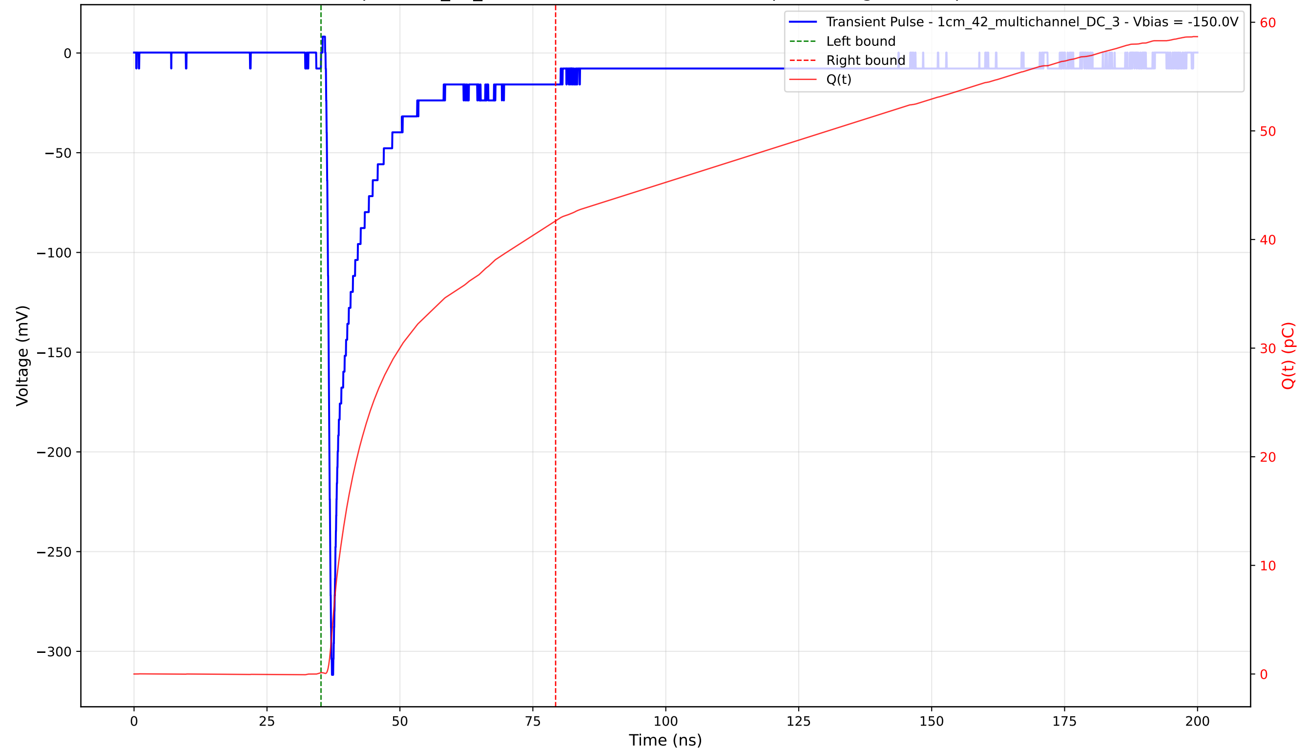
Transient Pulse - Sample: 1cm_42_multichannel - Position: 4635.0 \mu\text{m} - Charge: 41.60 pC - Rise Time: 0.86 ns
