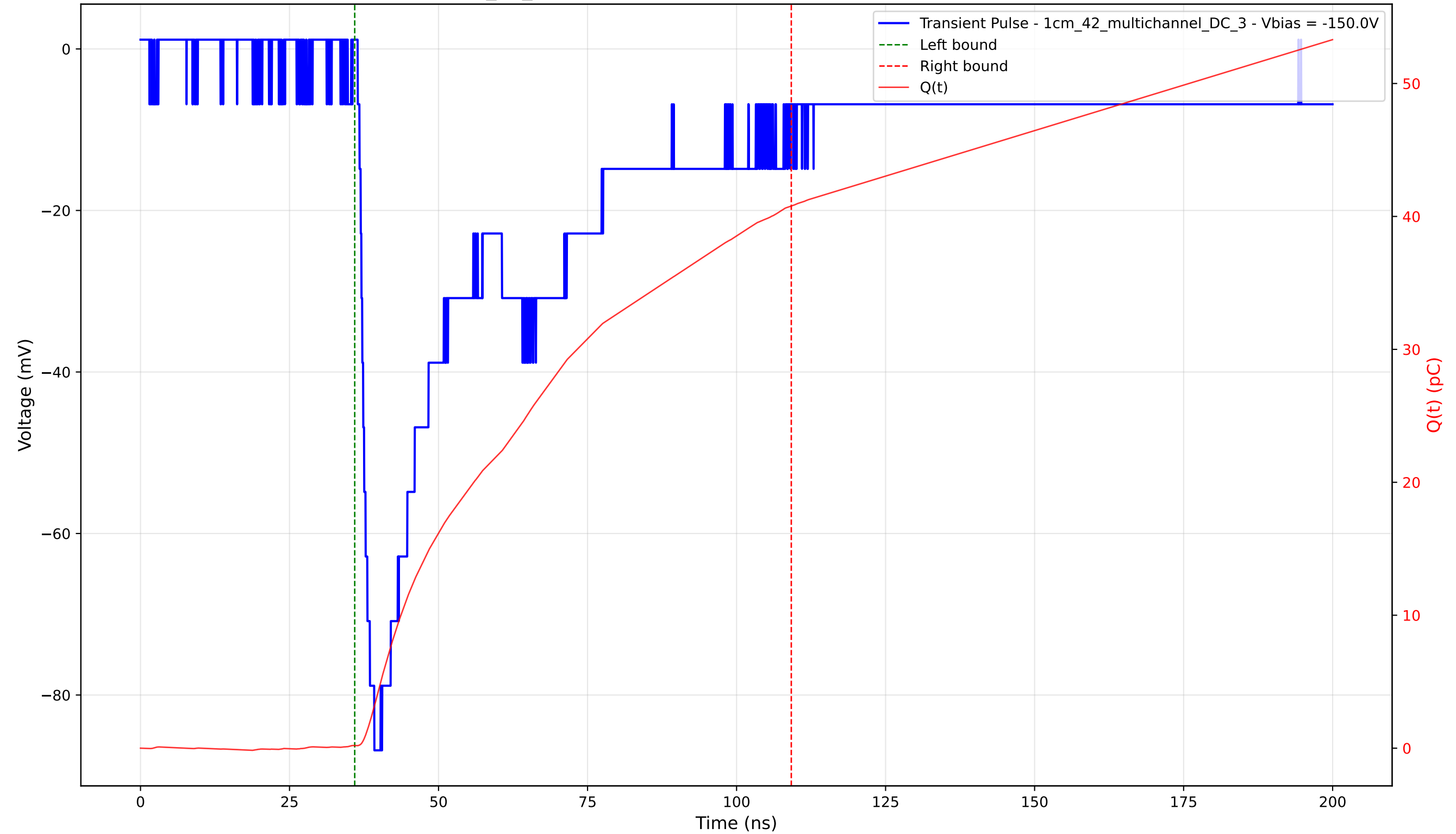
Transient Pulse - Sample: 1cm_42_multichannel - Position: 2655.0 \mu\text{m} - Charge: 40.59 pC - Rise Time: 1.76 ns
