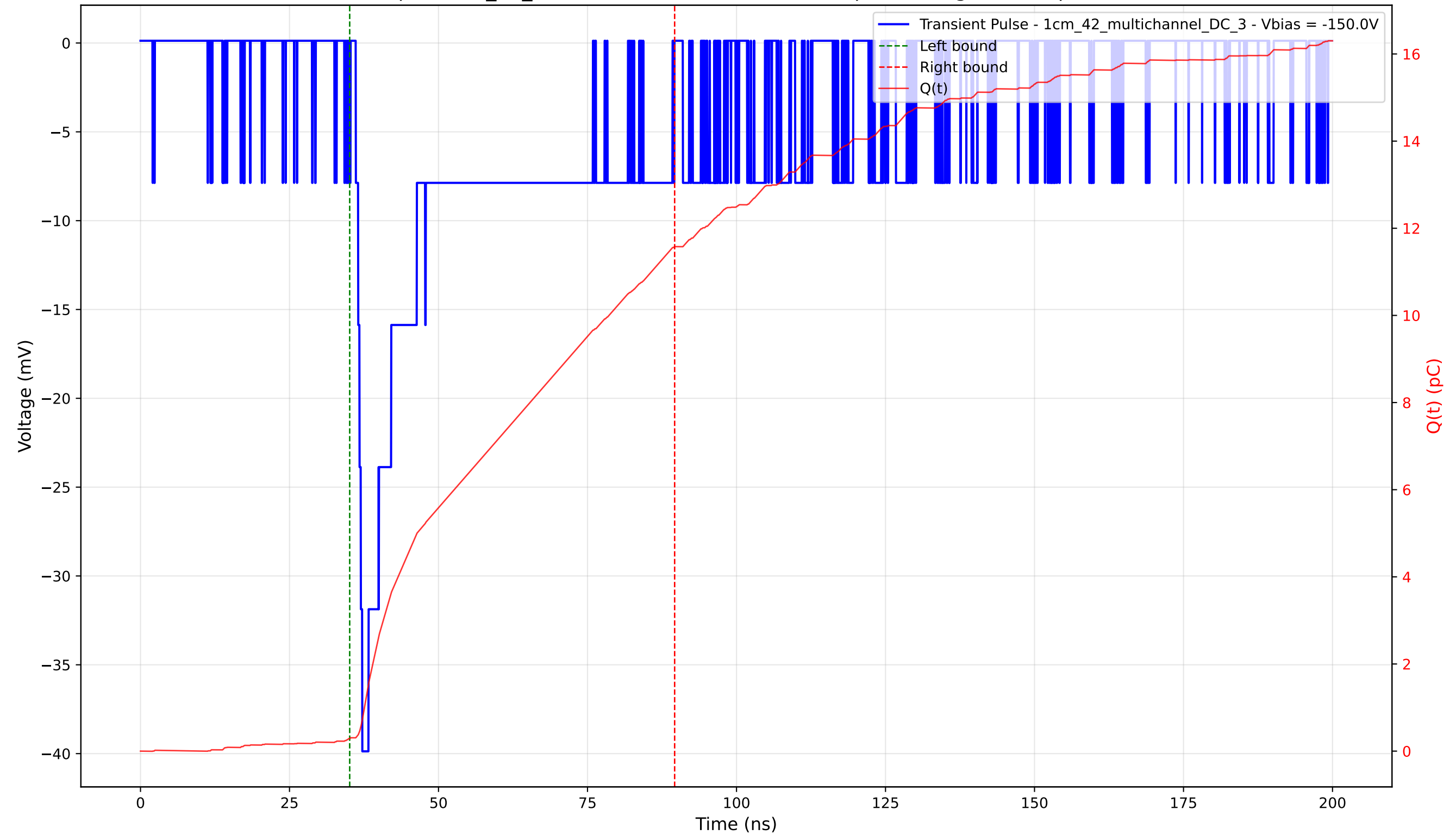
Transient Pulse - Sample: 1cm_42_multichannel - Position: 4355.0 \mu\text{m} - Charge: 11.29 pC - Rise Time: 1.09 ns
