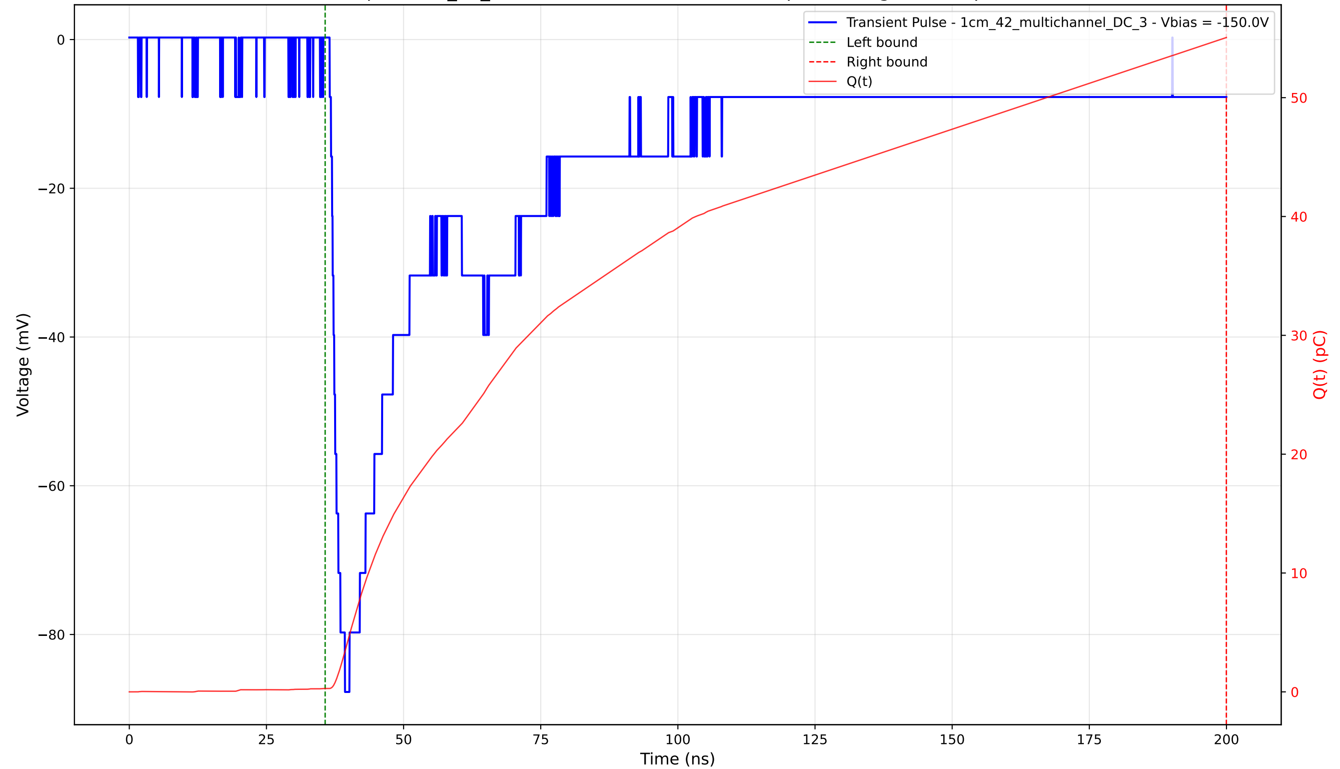
Transient Pulse - Sample: 1cm_42_multichannel - Position: 2660.0 \mu\text{m} - Charge: 54.78 pC - Rise Time: 1.74 ns
