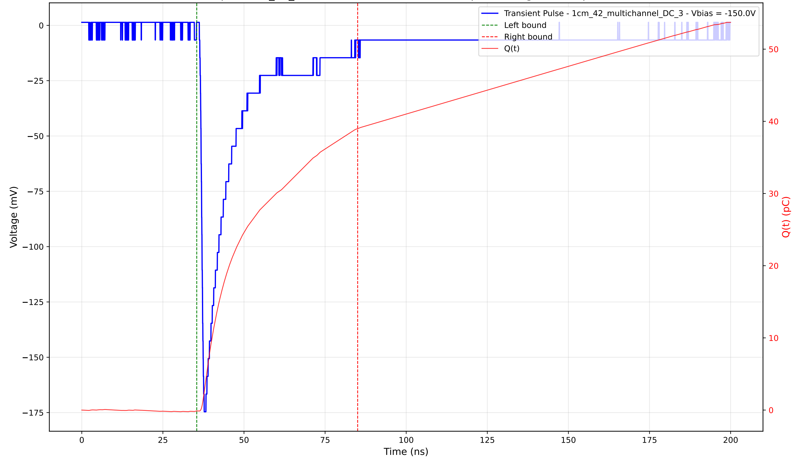
Transient Pulse - Sample: 1cm_42_multichannel - Position: 4035.0 \mu\text{m} - Charge: 39.10 pC - Rise Time: 0.99 ns
