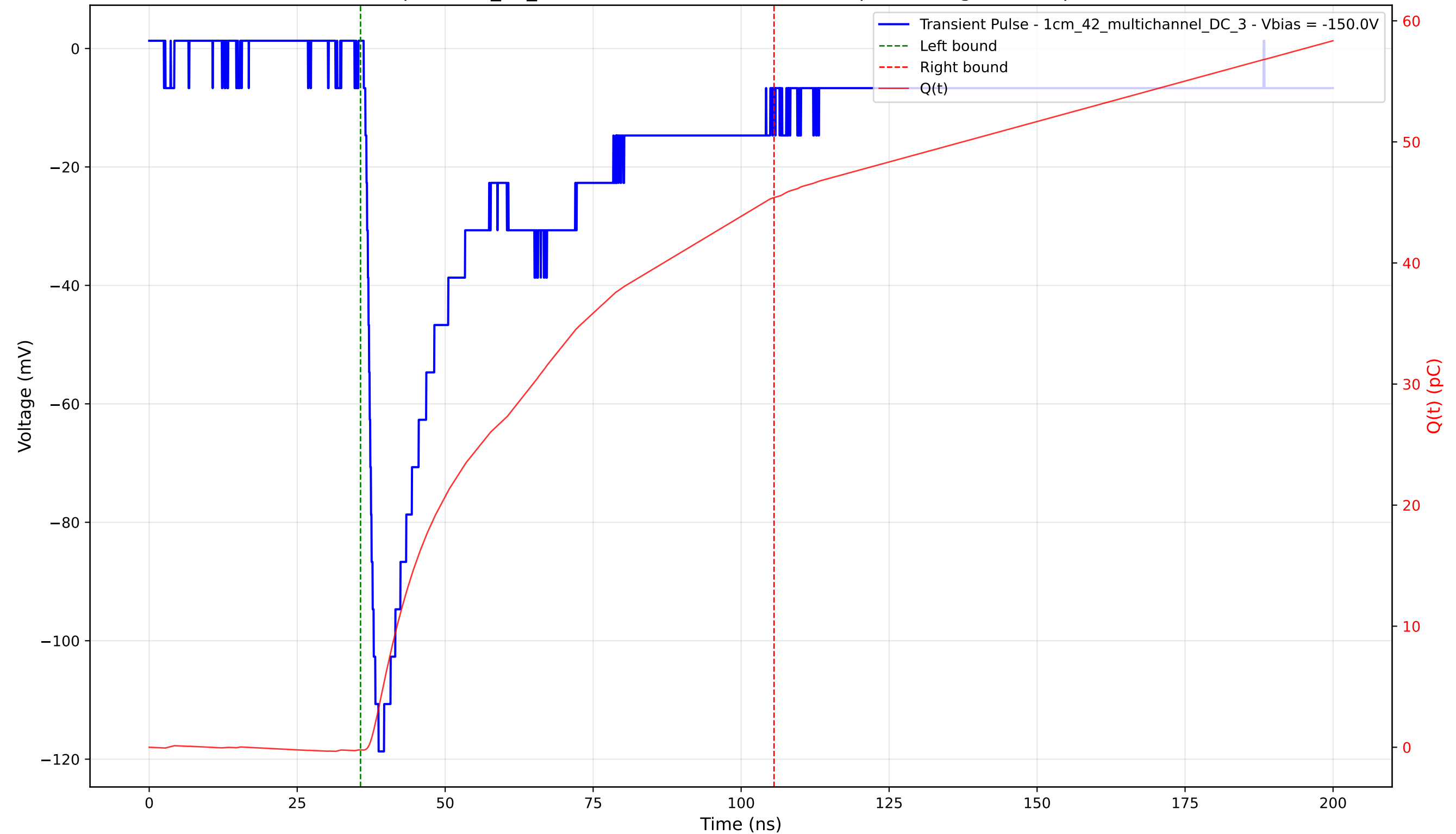
Transient Pulse - Sample: 1cm_42_multichannel - Position: 1710.0 \mu\text{m} - Charge: 45.62 pC - Rise Time: 1.69 ns
