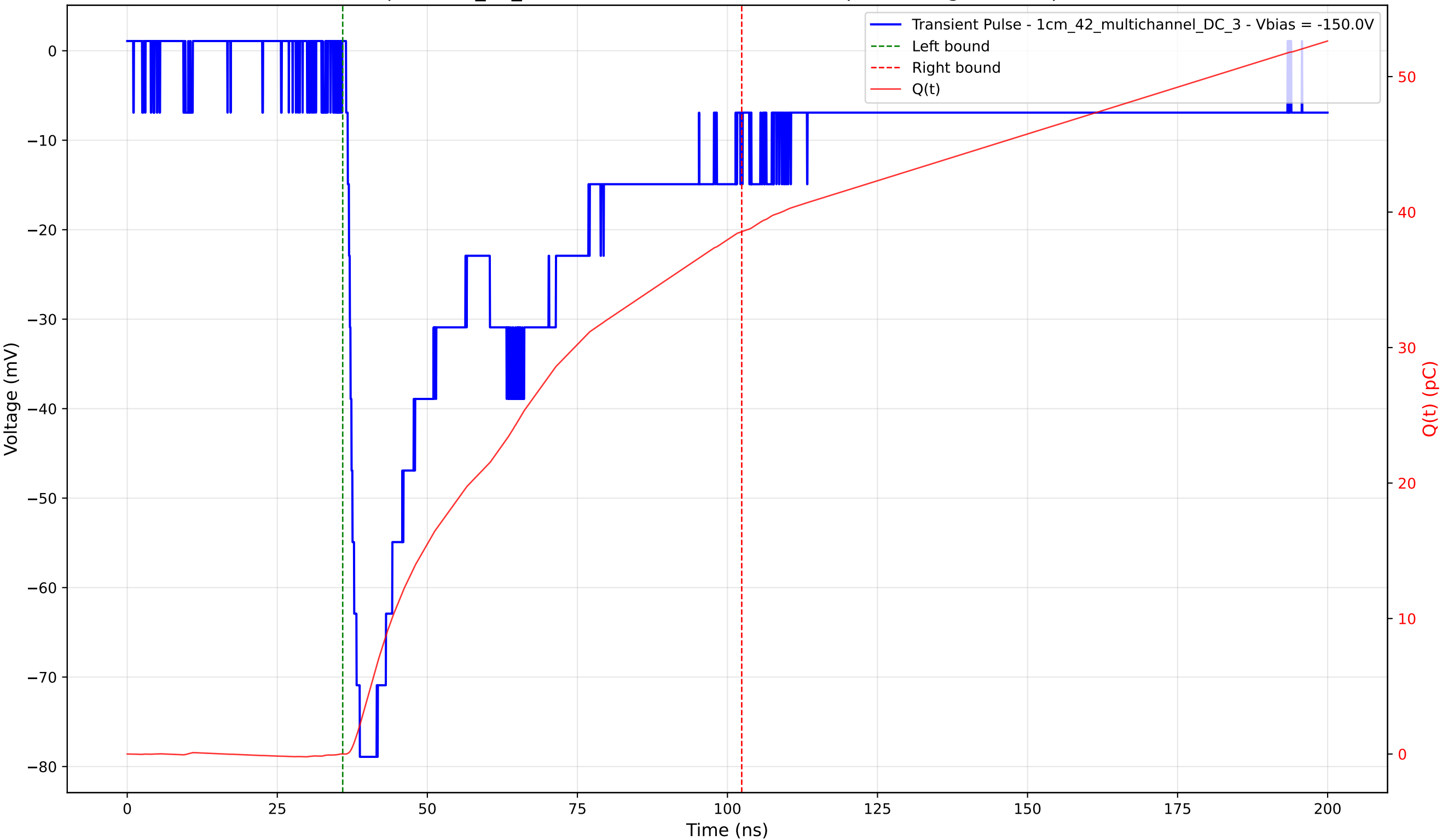
Transient Pulse - Sample: 1cm_42_multichannel - Position: 2600.0 \mu\text{m} - Charge: 38.54 pC - Rise Time: 2.02 ns
