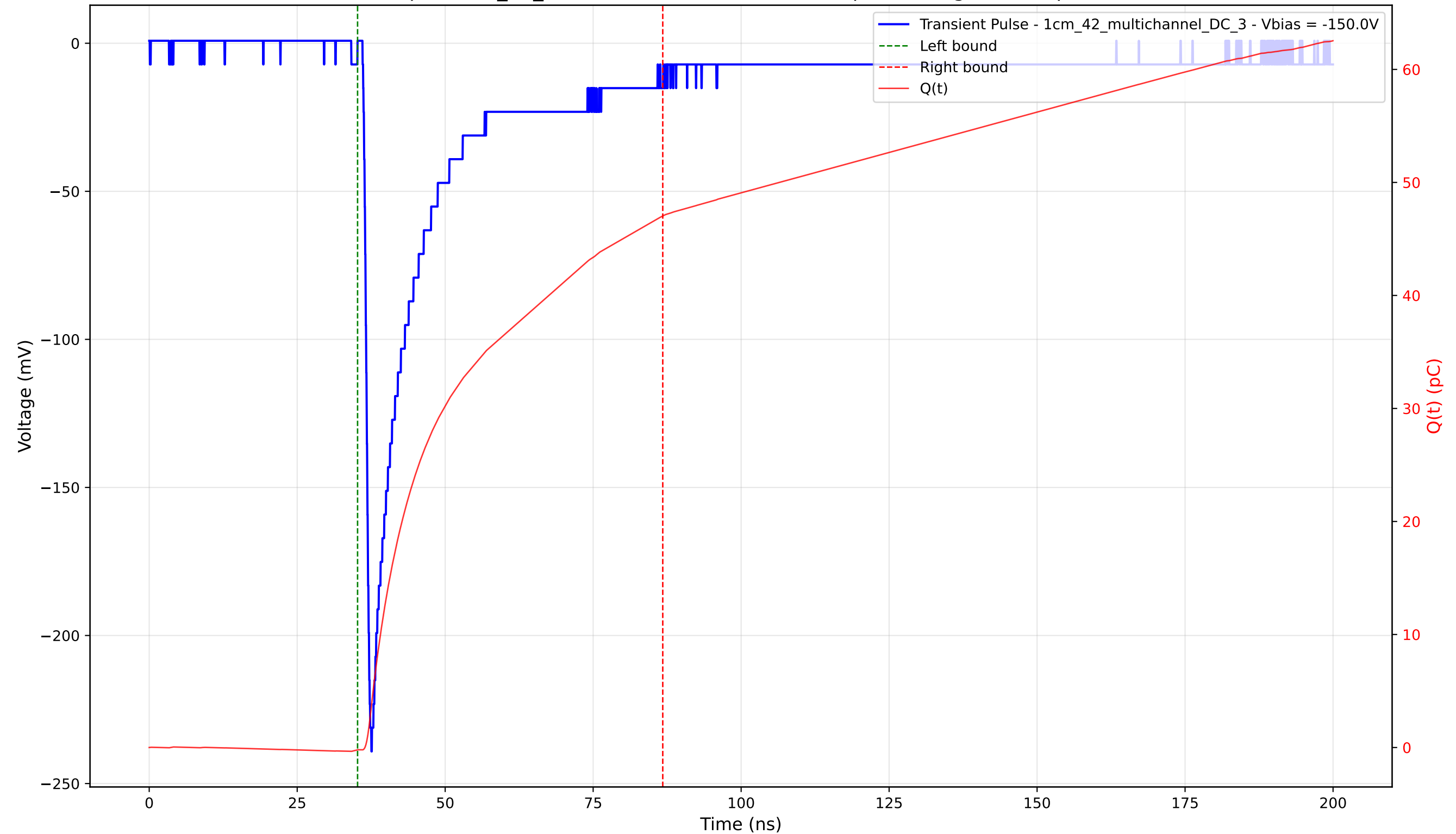
Transient Pulse - Sample: 1cm_42_multichannel - Position: 635.0 \mu\text{m} - Charge: 47.24 pC - Rise Time: 0.98 ns
