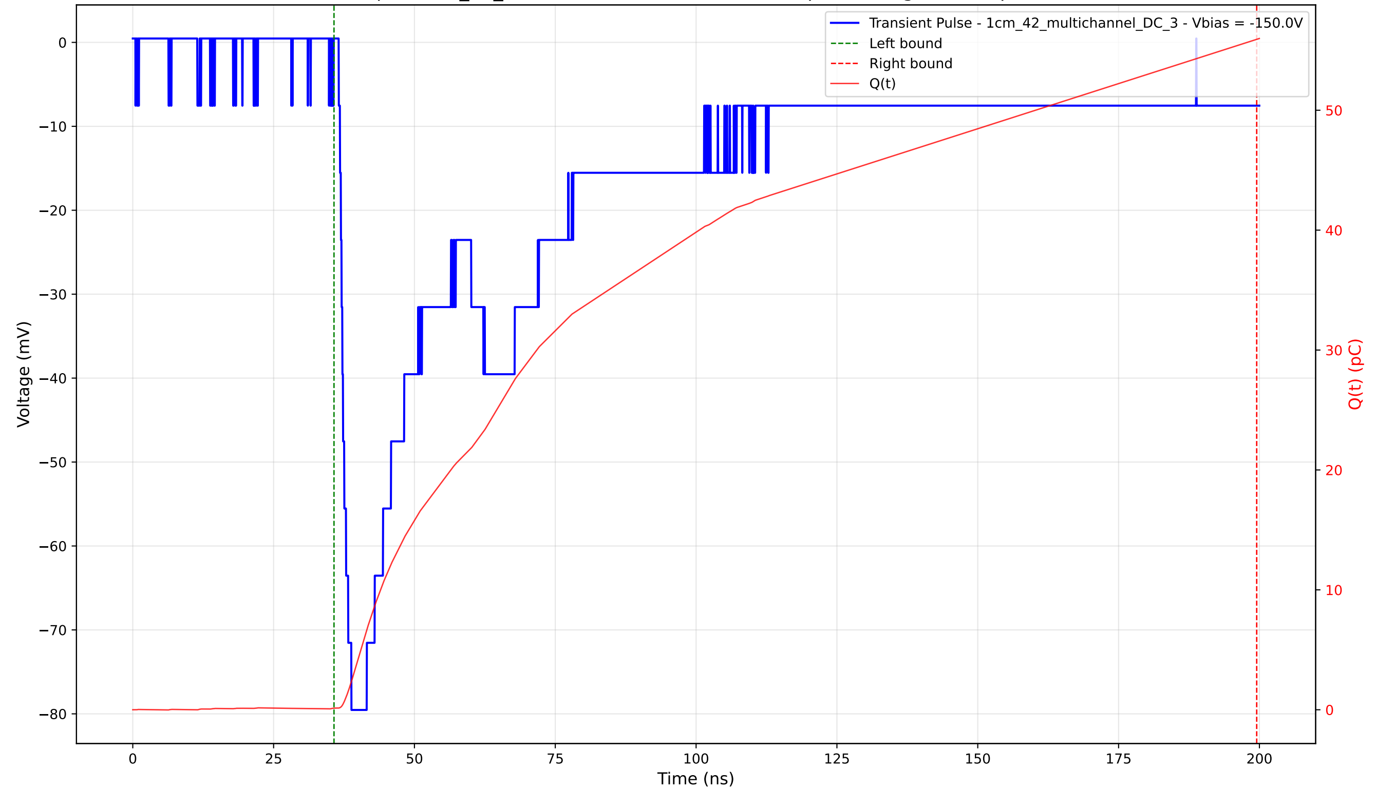
Transient Pulse - Sample: 1cm_42_multichannel - Position: 2500.0 \mu\text{m} - Charge: 55.77 pC - Rise Time: 2.04 ns
