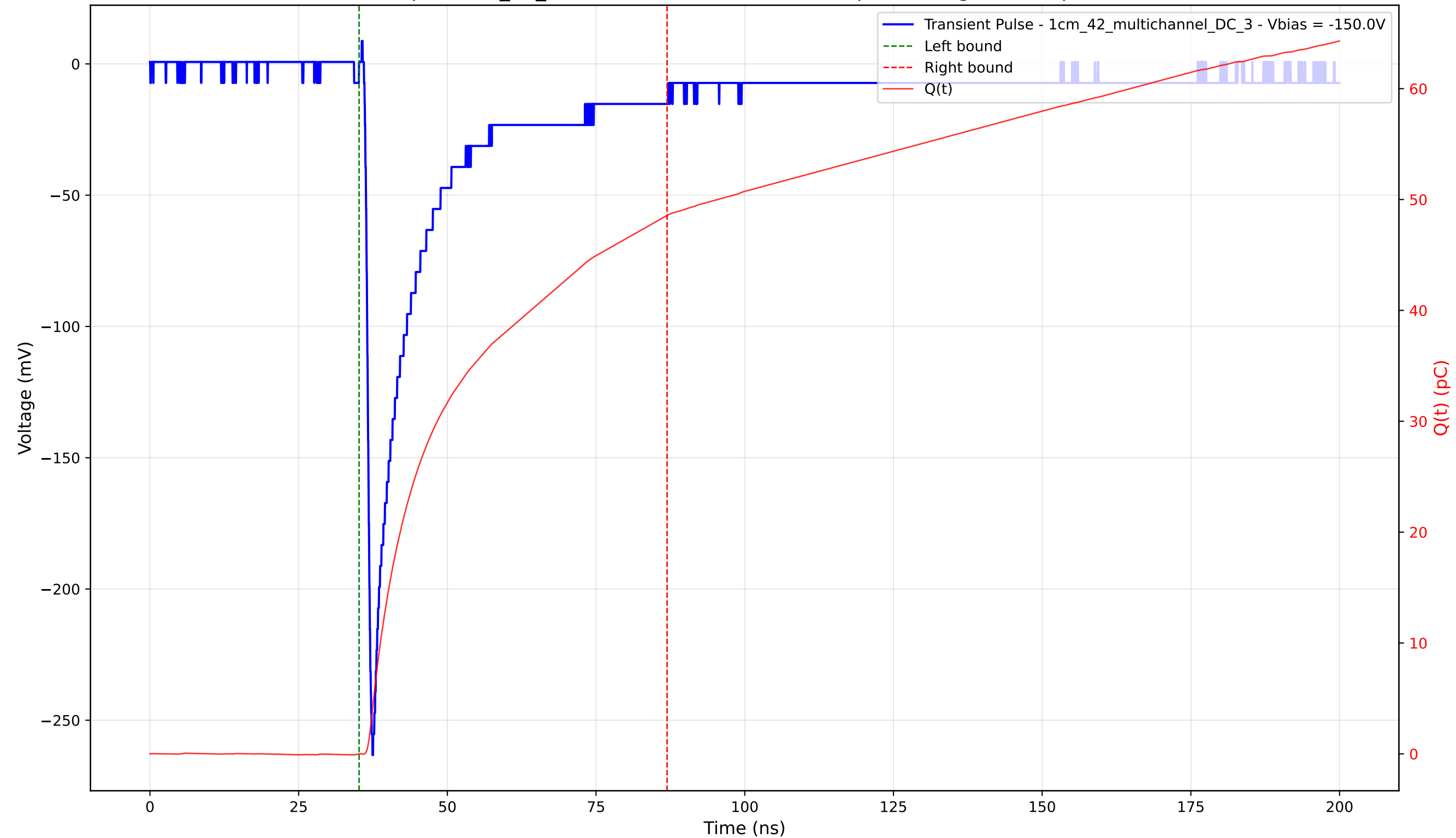
Transient Pulse - Sample: 1cm_42_multichannel - Position: 540.0 \mu\text{m} - Charge: 48.57 pC - Rise Time: 0.93 ns
