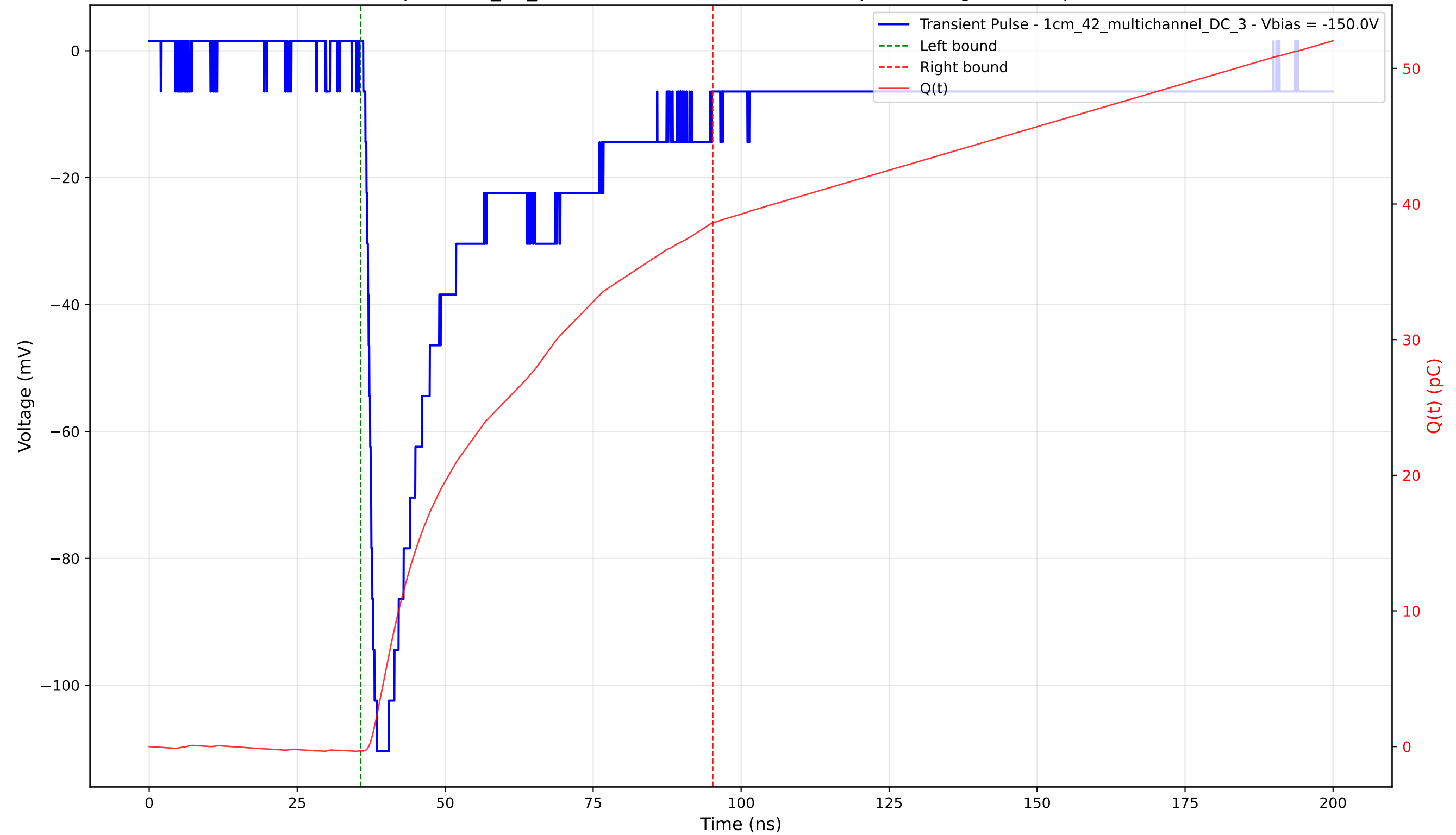
Transient Pulse - Sample: 1cm_42_multichannel - Position: 3245.0 \mu\text{m} - Charge: 38.93 pC - Rise Time: 1.55 ns
