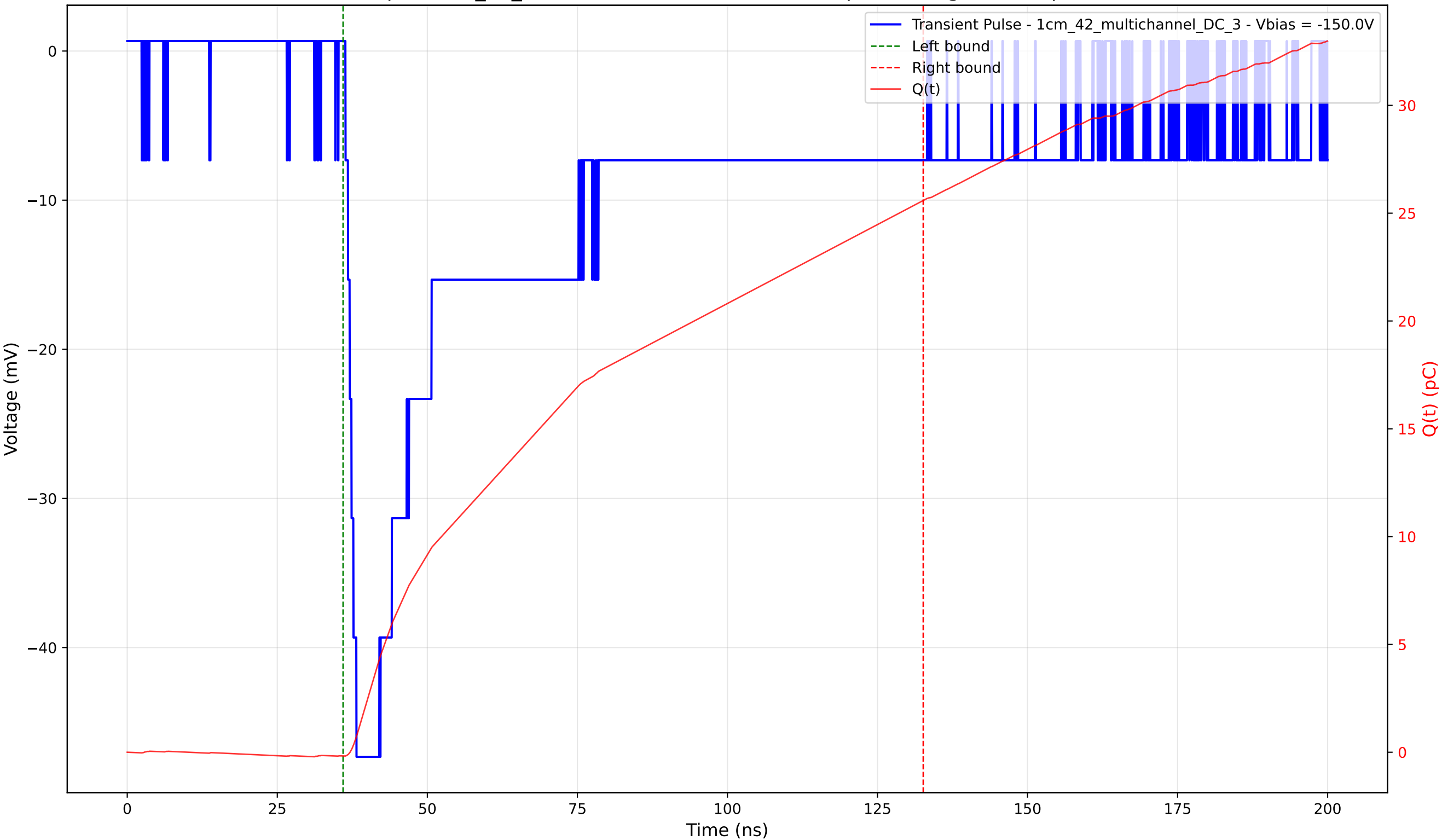
Transient Pulse - Sample: 1cm_42_multichannel - Position: 2930.0 \mu\text{m} - Charge: 25.77 pC - Rise Time: 1.83 ns
