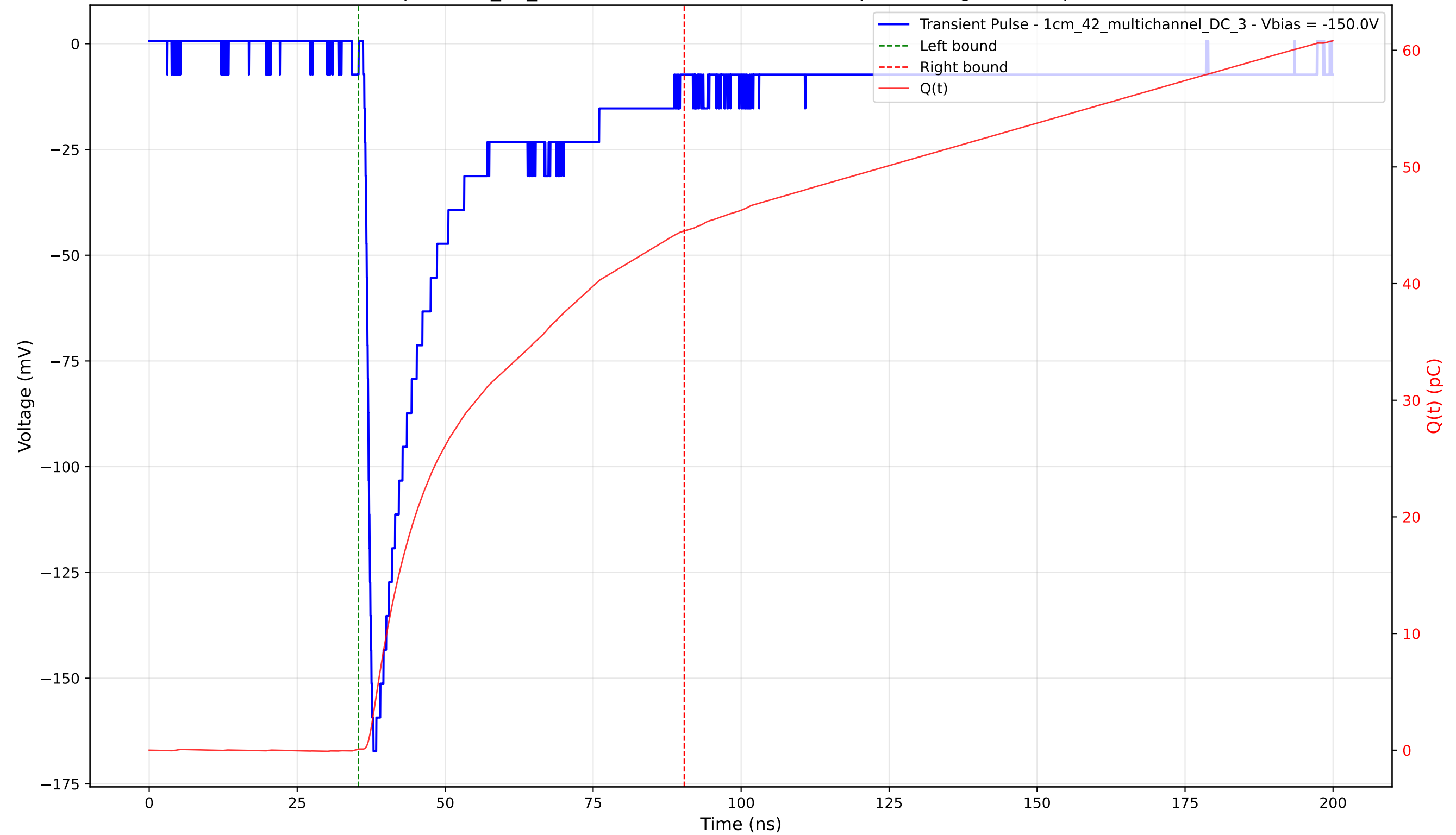
Transient Pulse - Sample: 1cm_42_multichannel - Position: 1075.0 \mu\text{m} - Charge: 44.42 pC - Rise Time: 1.12 ns
