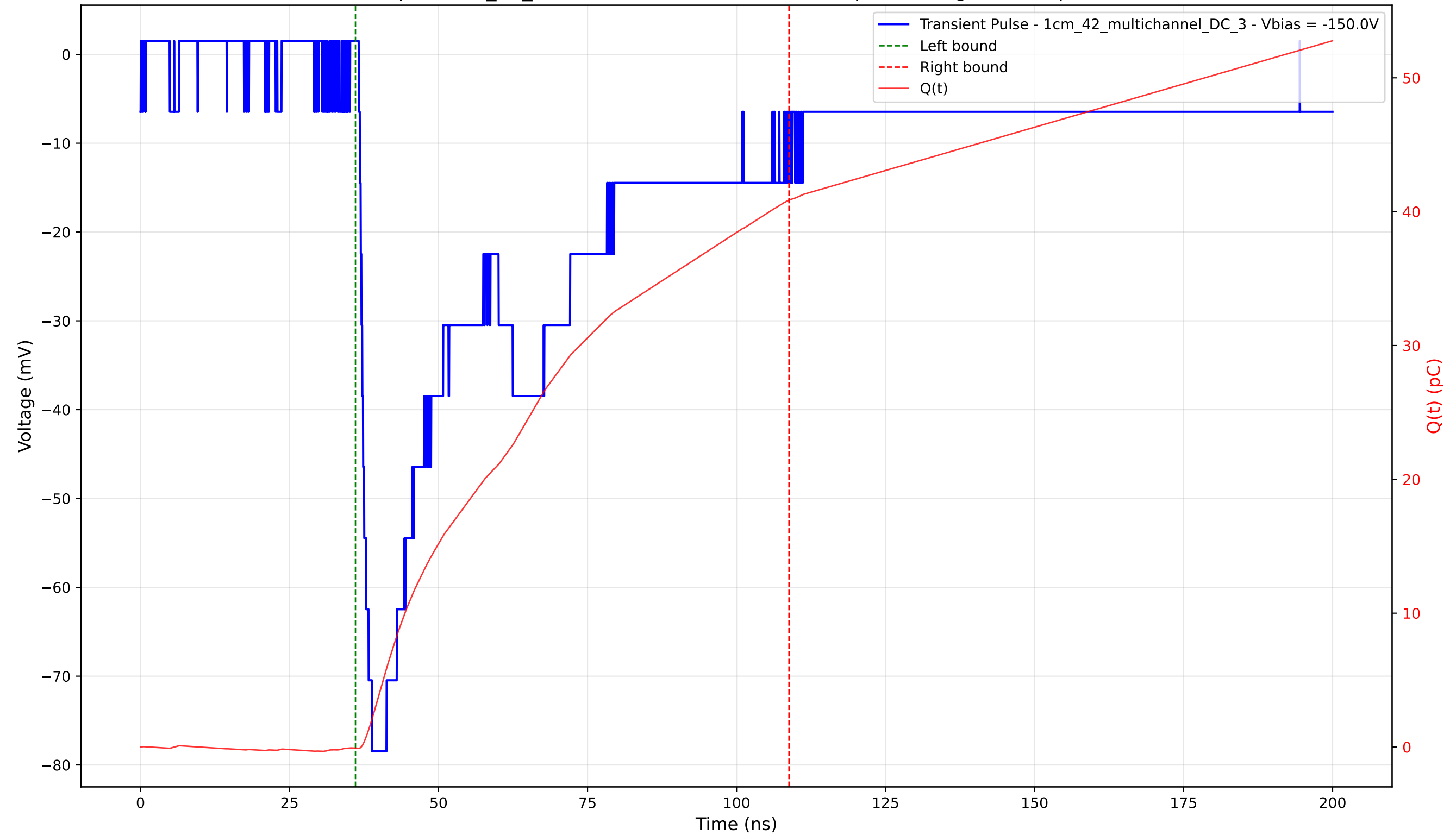
Transient Pulse - Sample: 1cm_42_multichannel - Position: 2490.0 \mu\text{m} - Charge: 40.96 pC - Rise Time: 2.06 ns
