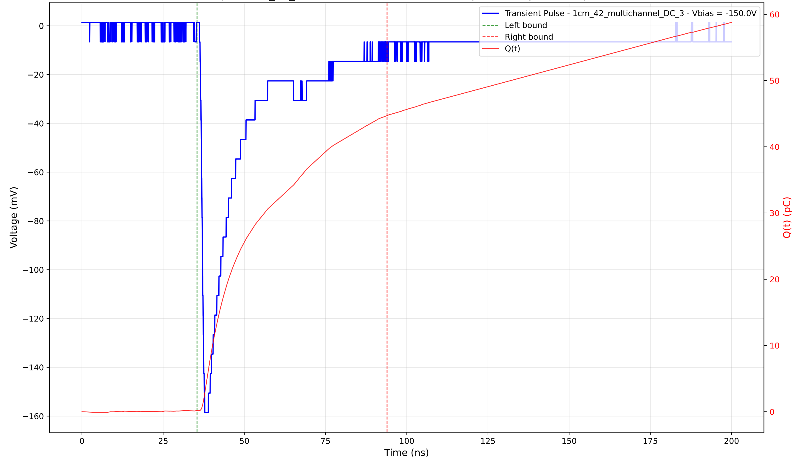
Transient Pulse - Sample: 1cm_42_multichannel - Position: 1110.0 \mu\text{m} - Charge: 44.53 pC - Rise Time: 1.20 ns
