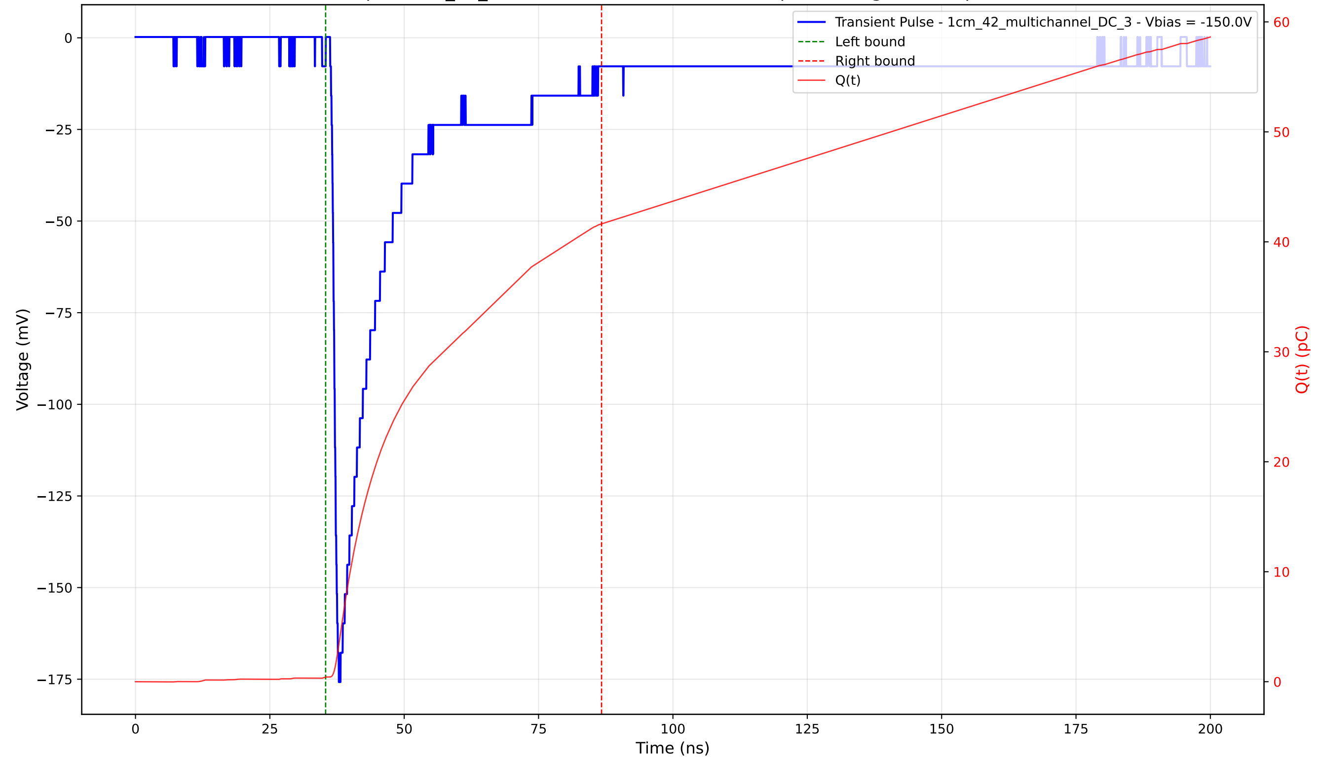
Transient Pulse - Sample: 1cm_42_multichannel - Position: 4005.0 \mu\text{m} - Charge: 41.21 pC - Rise Time: 1.06 ns
