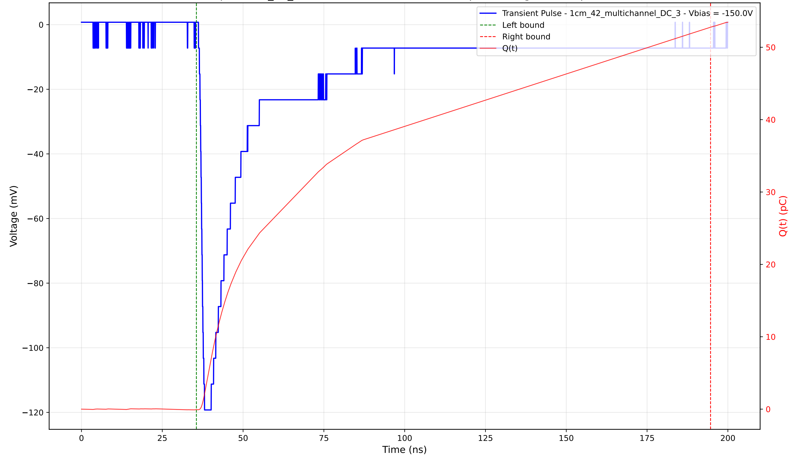
Transient Pulse - Sample: 1cm_42_multichannel - Position: 3500.0 \mu\text{m} - Charge: 52.86 pC - Rise Time: 1.39 ns
