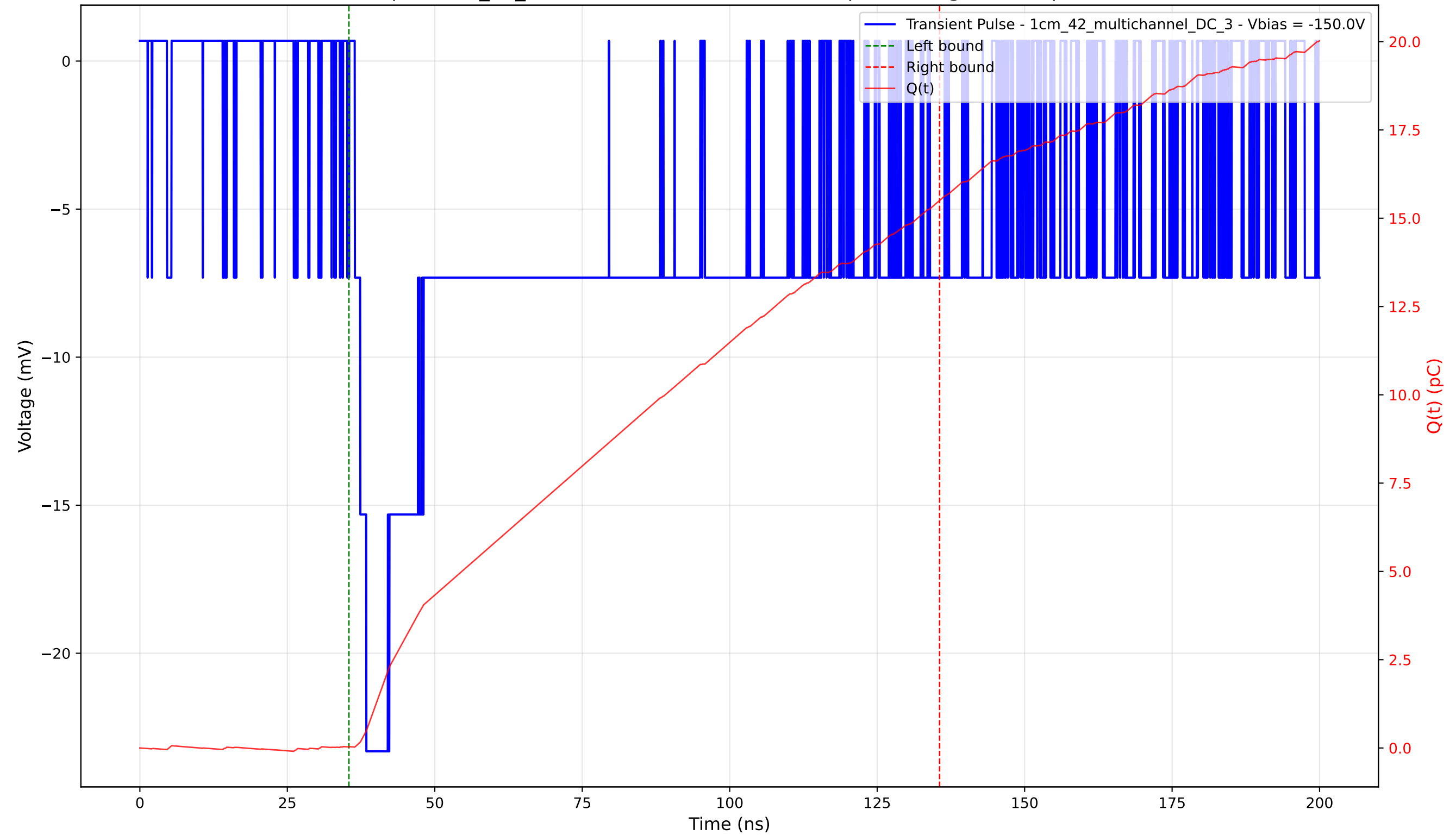
Transient Pulse - Sample: 1cm_42_multichannel - Position: 2845.0 \mu\text{m} - Charge: 15.47 pC - Rise Time: 1.96 ns
