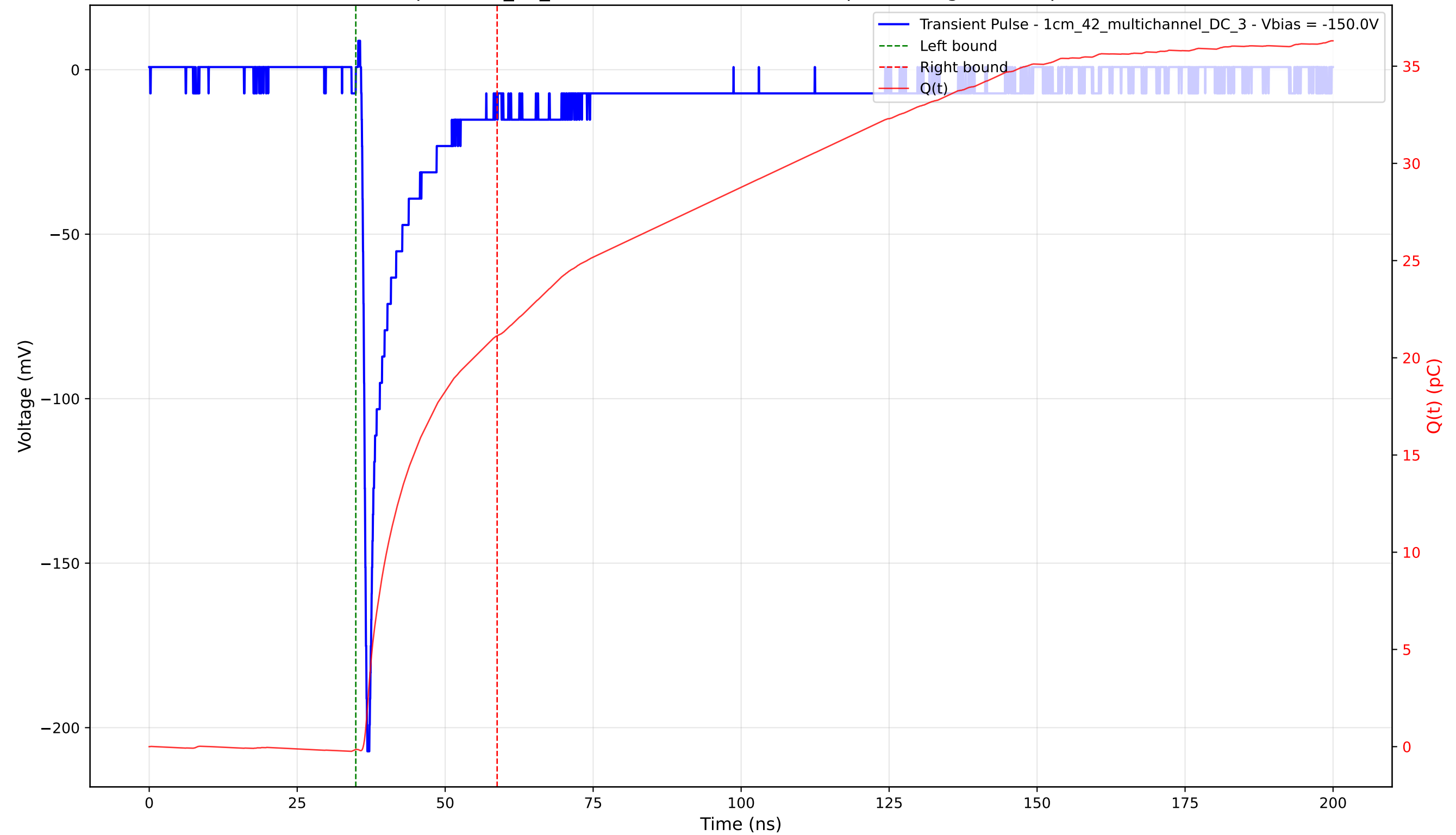
Transient Pulse - Sample: 1cm_42_multichannel - Position: 80.0 \mu\text{m} - Charge: 21.27 pC - Rise Time: 0.79 ns
