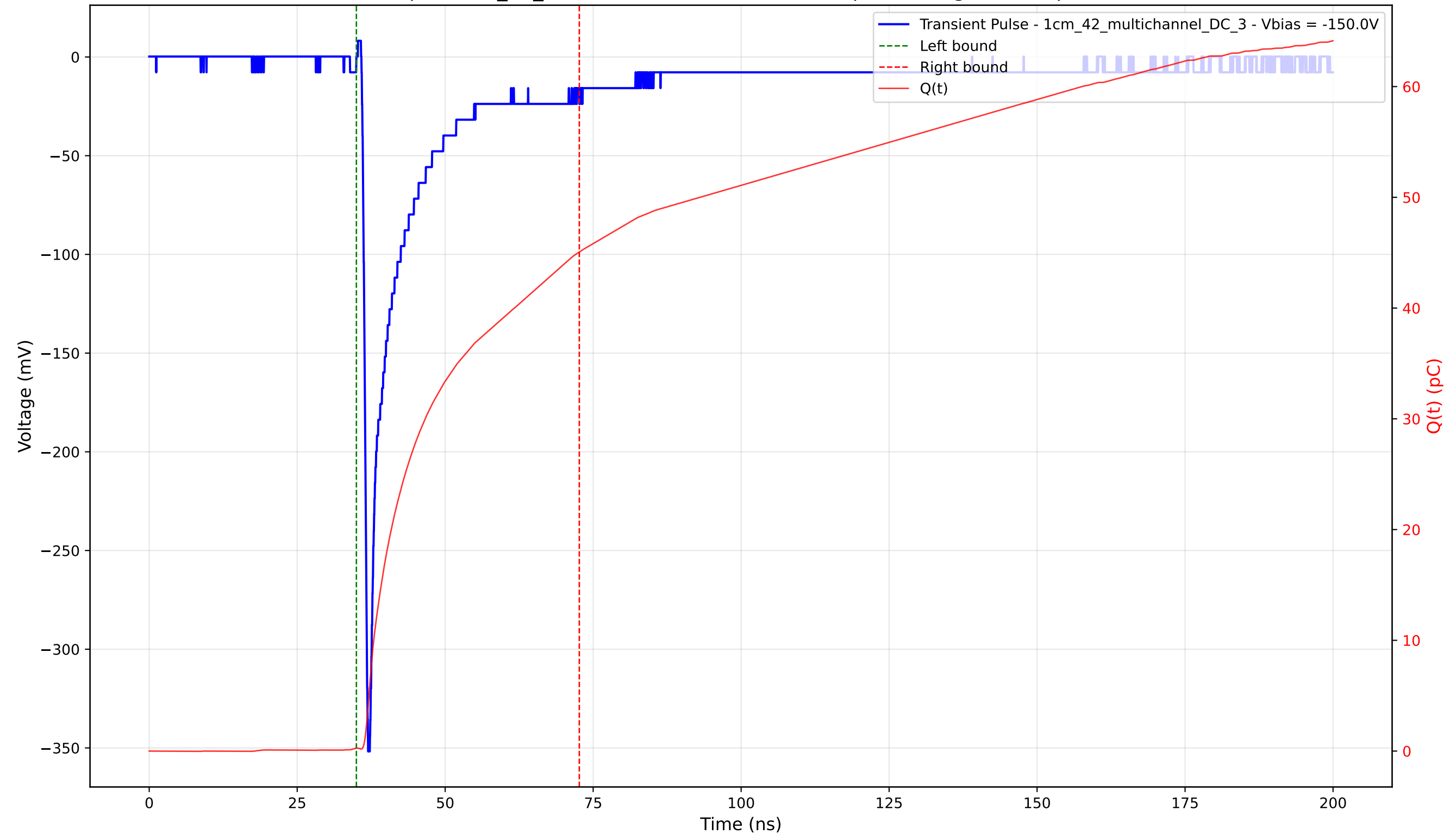
Transient Pulse - Sample: 1cm_42_multichannel - Position: 200.0 \mu\text{m} - Charge: 44.79 pC - Rise Time: 0.79 ns
