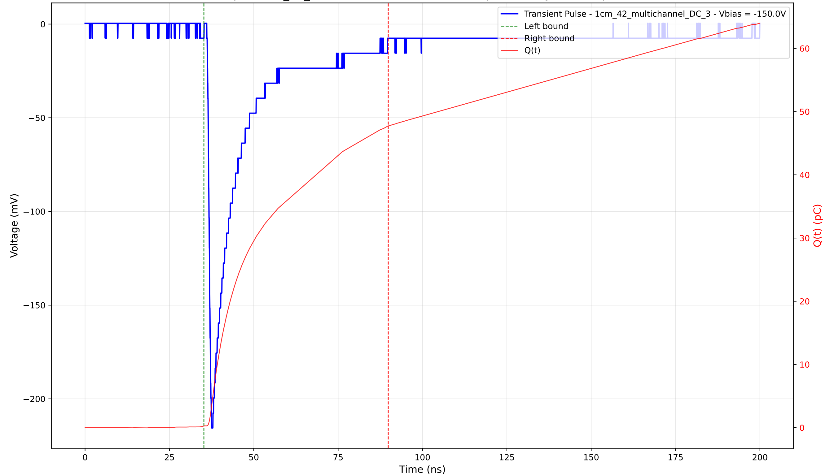
Transient Pulse - Sample: 1cm_42_multichannel - Position: 735.0 \mu\text{m} - Charge: 47.45 pC - Rise Time: 1.02 ns
