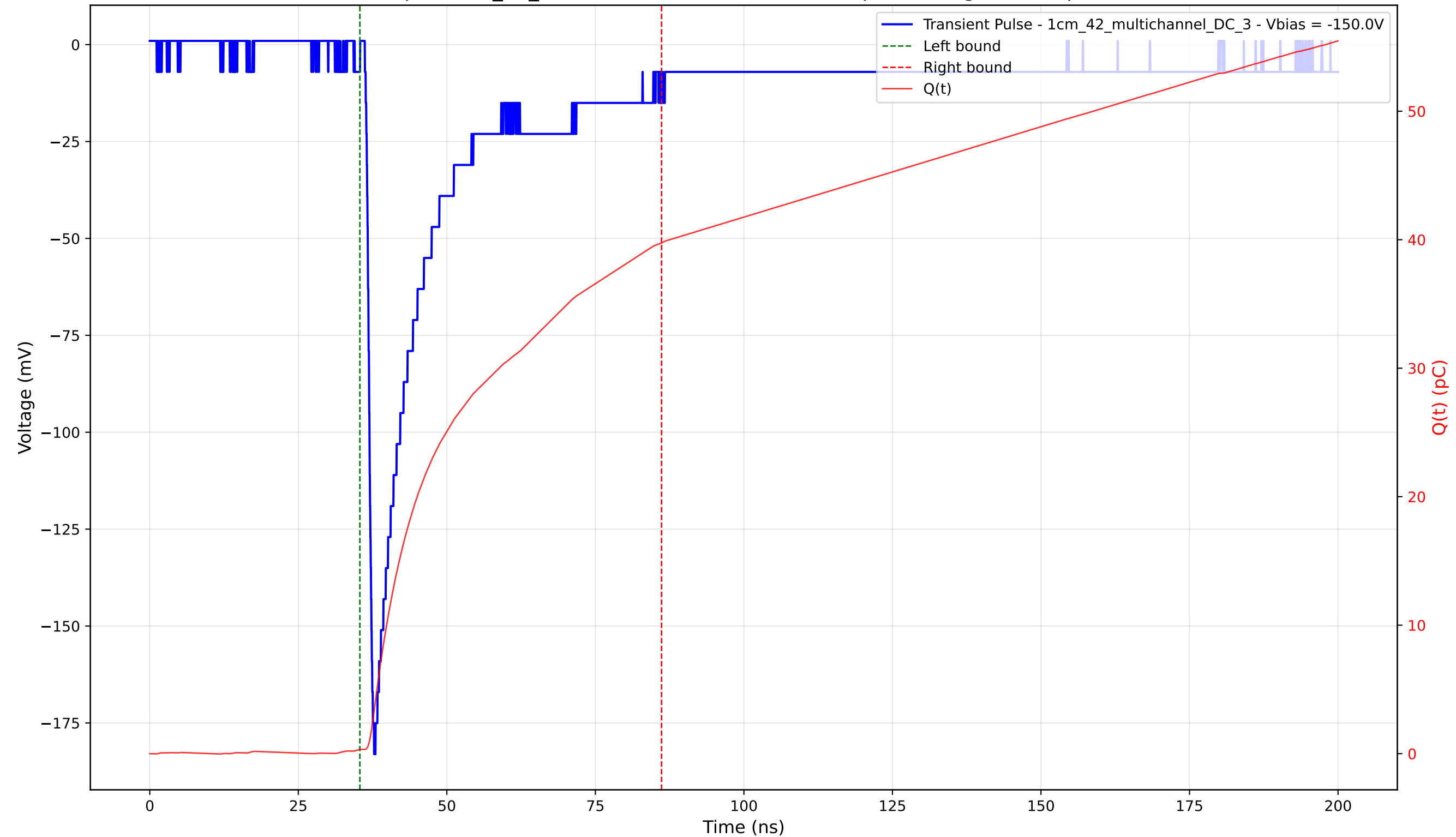
Transient Pulse - Sample: 1cm_42_multichannel - Position: 4115.0 \mu\text{m} - Charge: 39.42 pC - Rise Time: 1.01 ns
