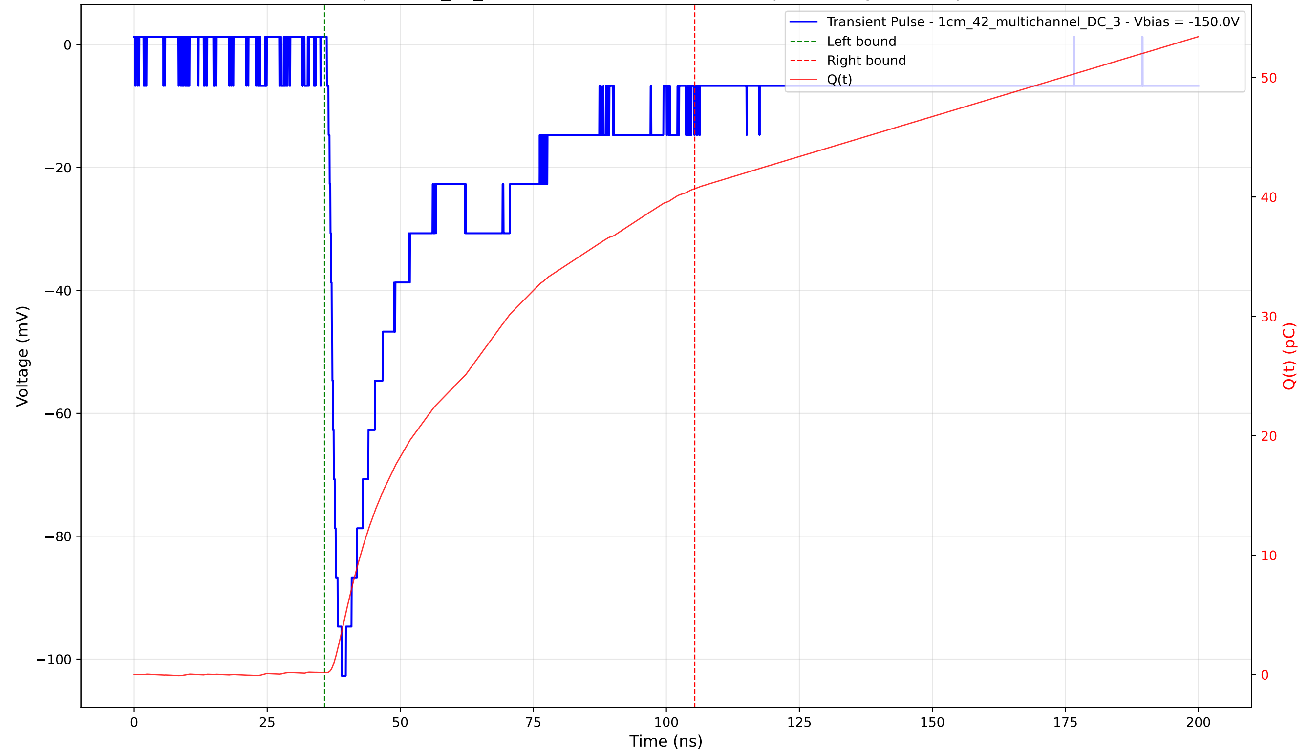
Transient Pulse - Sample: 1cm_42_multichannel - Position: 1790.0 \mu\text{m} - Charge: 40.53 pC - Rise Time: 1.73 ns
