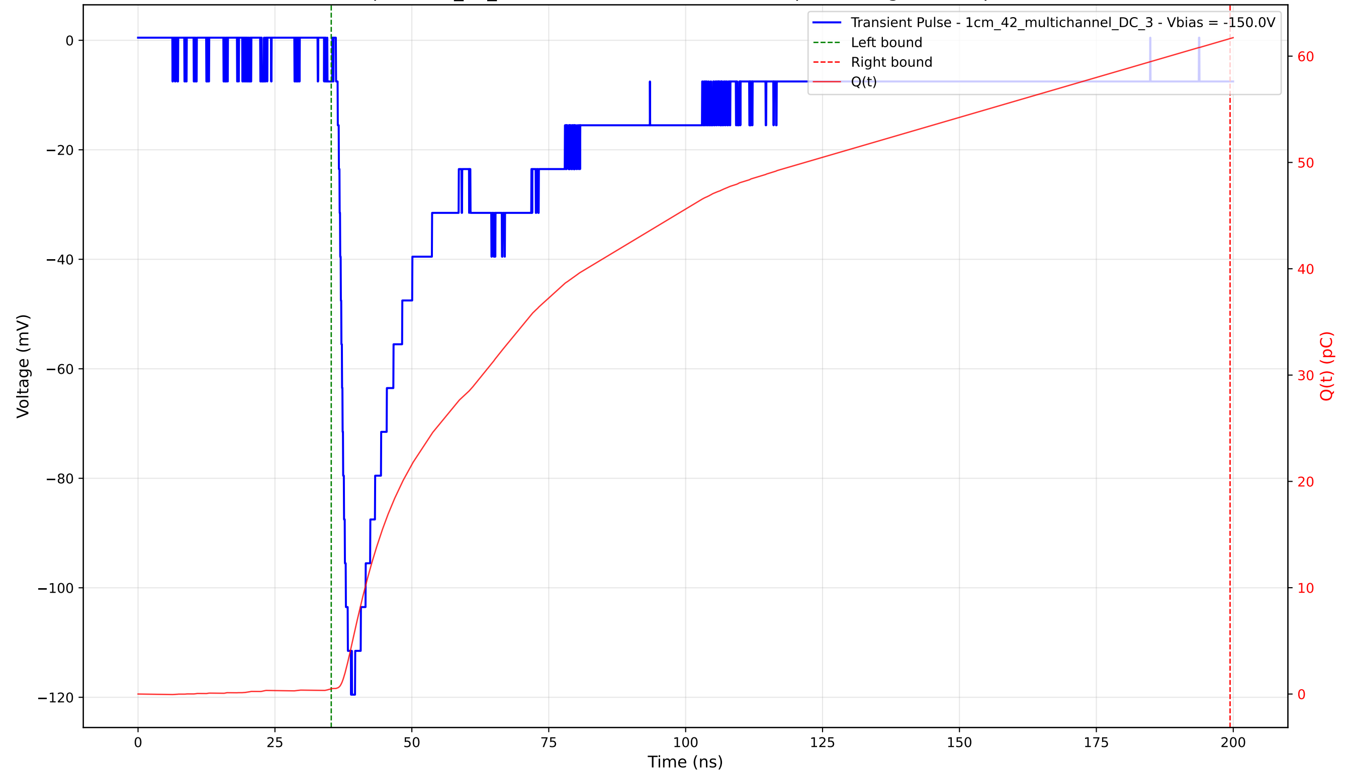
Transient Pulse - Sample: 1cm_42_multichannel - Position: 1735.0 \mu\text{m} - Charge: 61.16 pC - Rise Time: 1.85 ns
