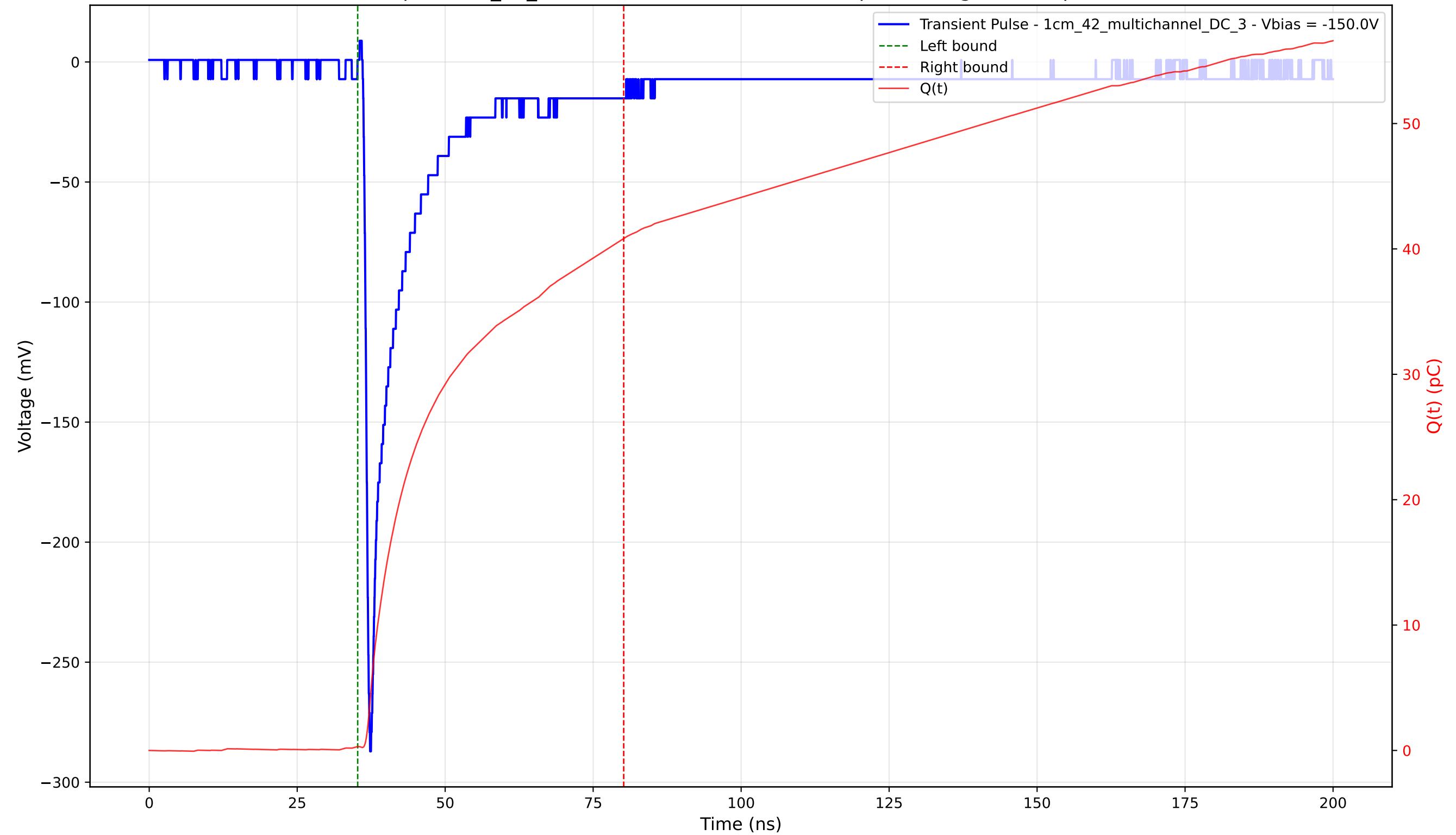
Transient Pulse - Sample: 1cm_42_multichannel - Position: 4555.0 \mu\text{m} - Charge: 40.53 pC - Rise Time: 0.87 ns
