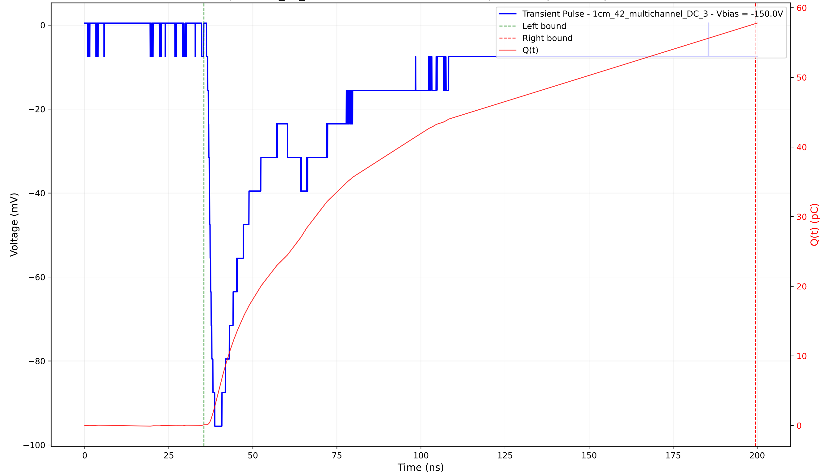
Transient Pulse - Sample: 1cm_42_multichannel - Position: 1965.0 \mu\text{m} - Charge: 57.61 pC - Rise Time: 1.55 ns
