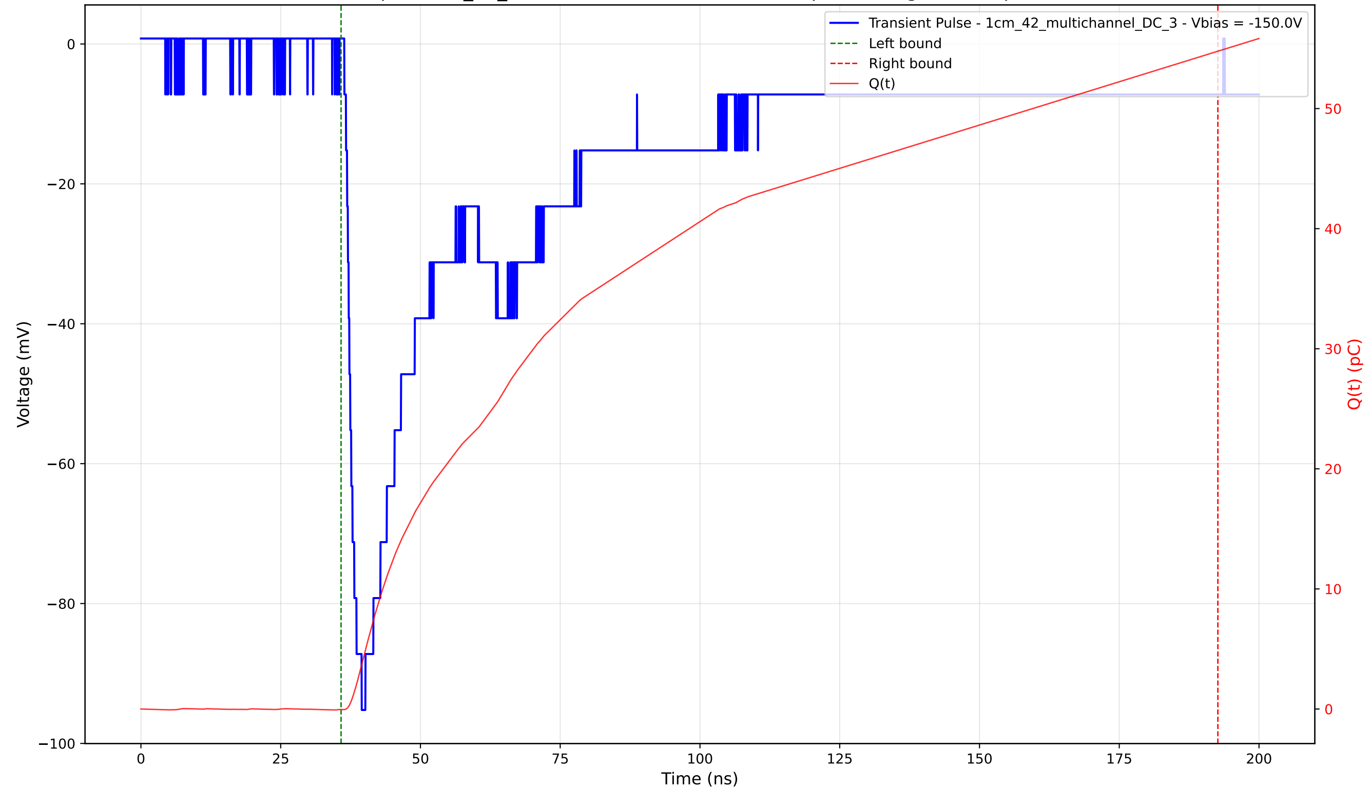
Transient Pulse - Sample: 1cm_42_multichannel - Position: 2720.0 \mu\text{m} - Charge: 54.84 pC - Rise Time: 1.89 ns
