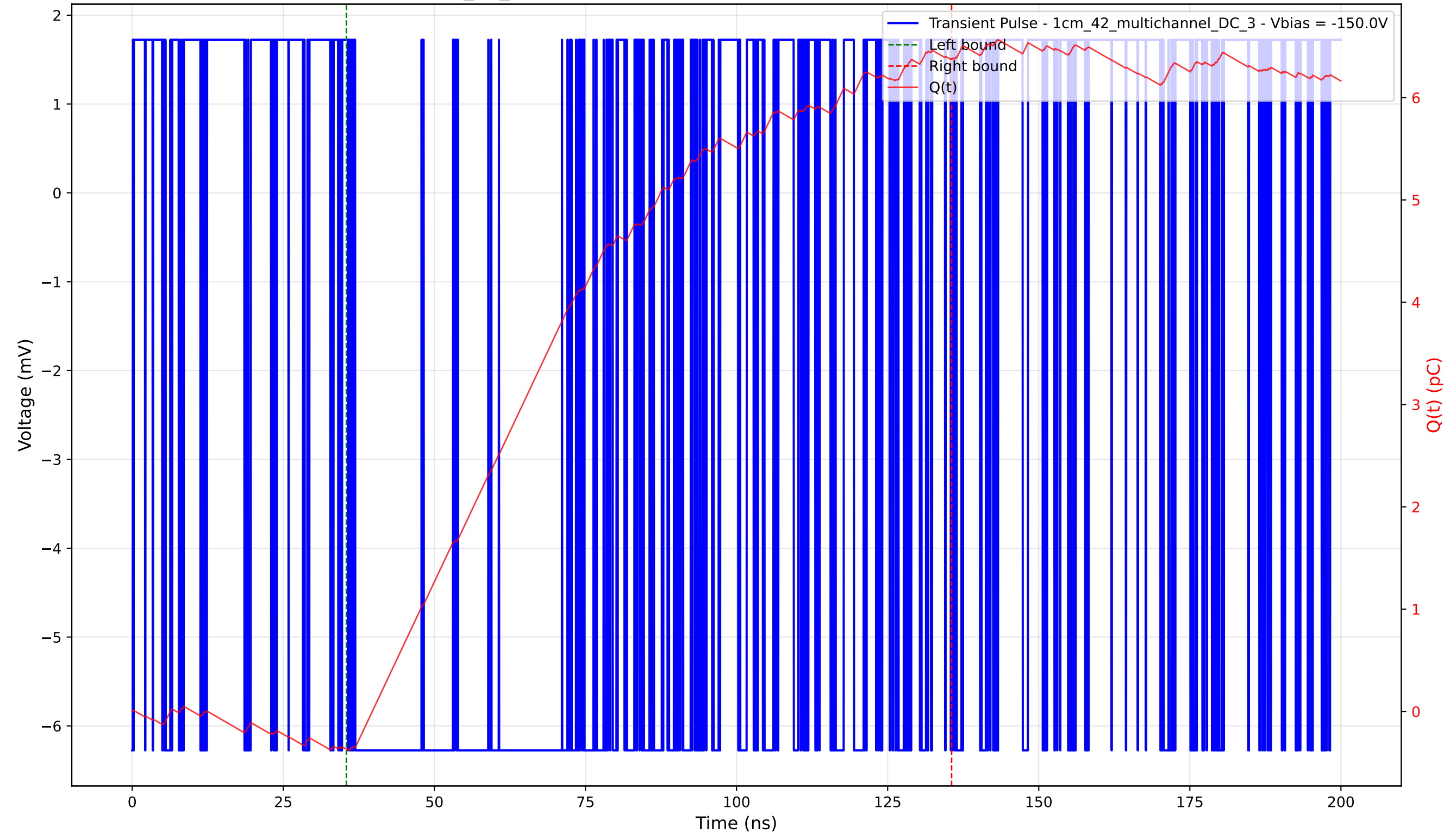
Transient Pulse - Sample: 1cm_42_multichannel - Position: 2360.0 \mu\text{m} - Charge: 6.75 pC - Rise Time: 0.00 ns (N/A)
