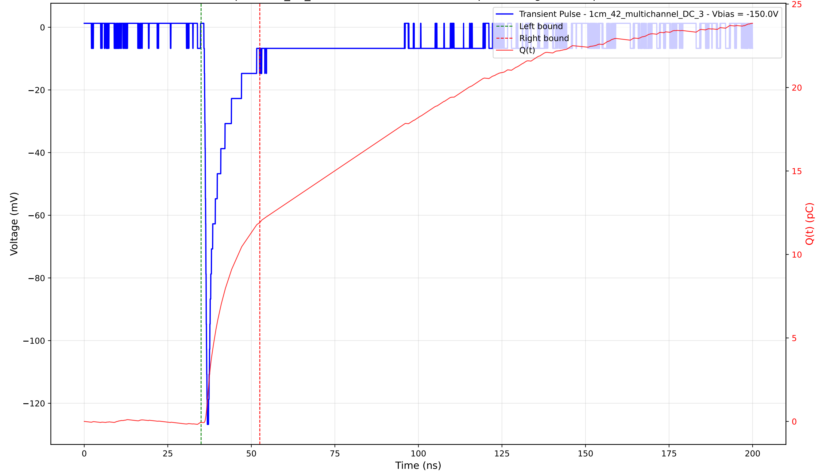
Transient Pulse - Sample: 1cm_42_multichannel - Position: 70.0 \mu\text{m} - Charge: 11.98 pC - Rise Time: 0.79 ns
