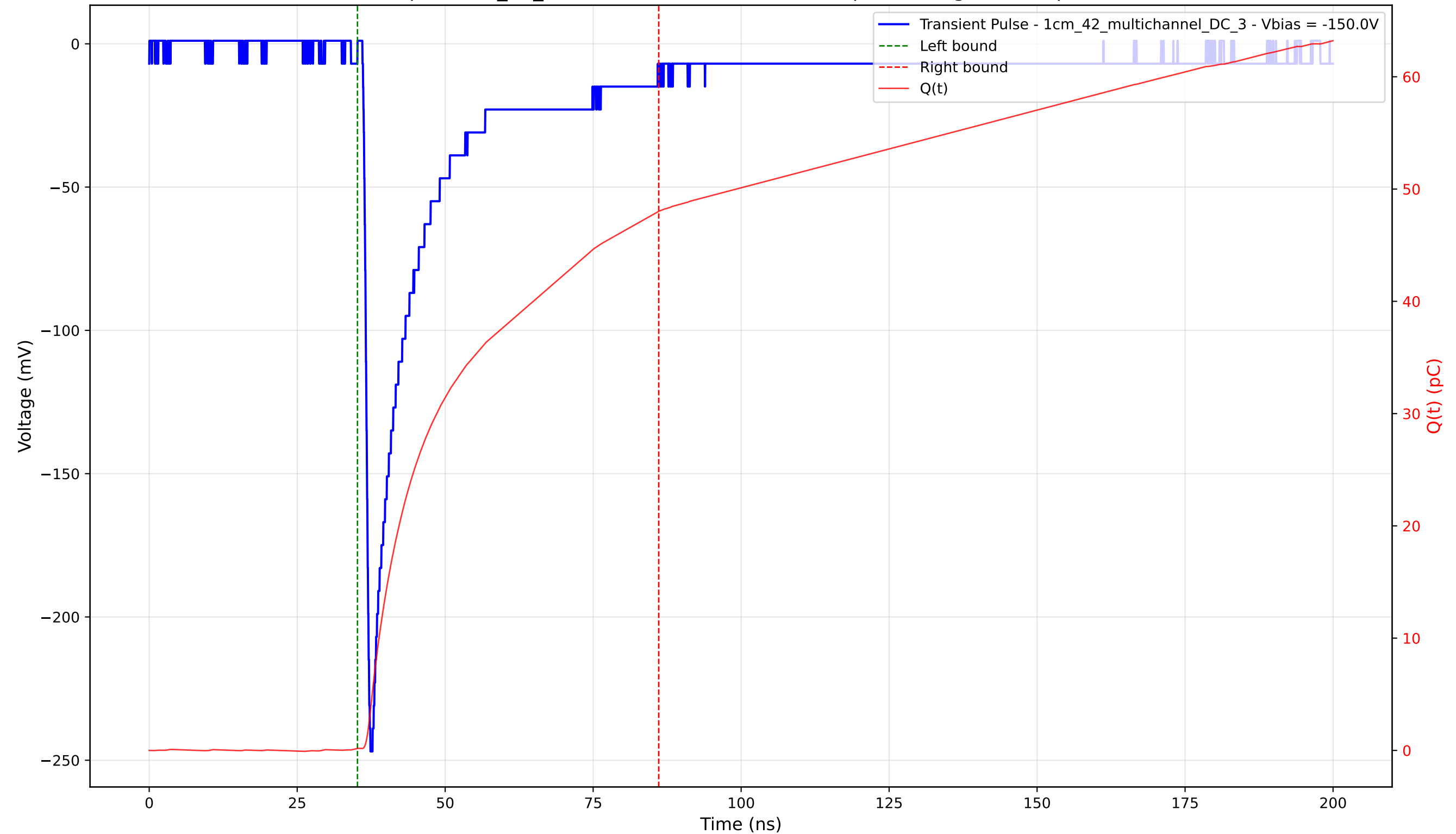
Transient Pulse - Sample: 1cm_42_multichannel - Position: 600.0 \mu\text{m} - Charge: 47.84 pC - Rise Time: 0.92 ns
