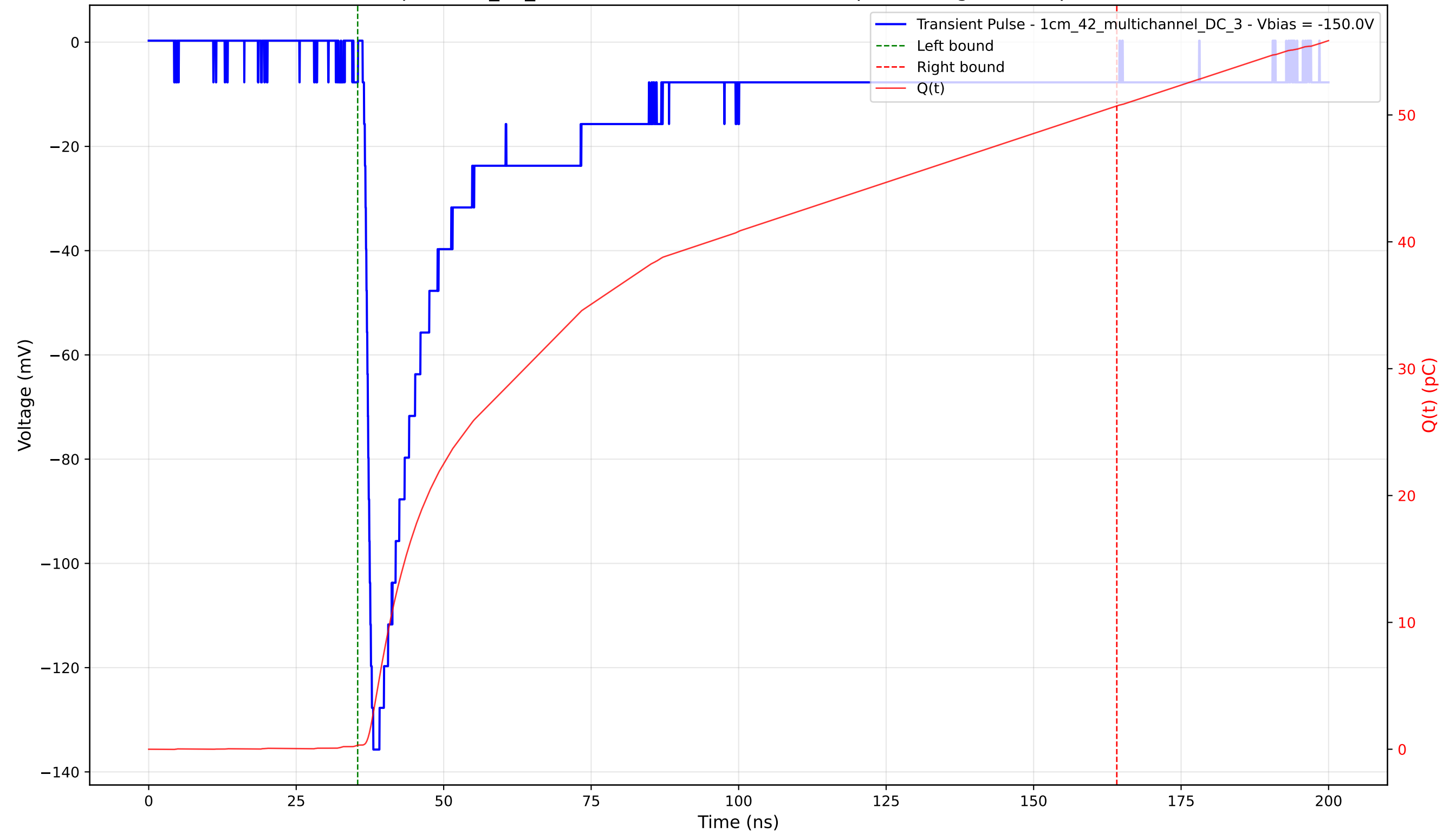
Transient Pulse - Sample: 1cm_42_multichannel - Position: 3690.0 \mu\text{m} - Charge: 50.40 pC - Rise Time: 1.33 ns
