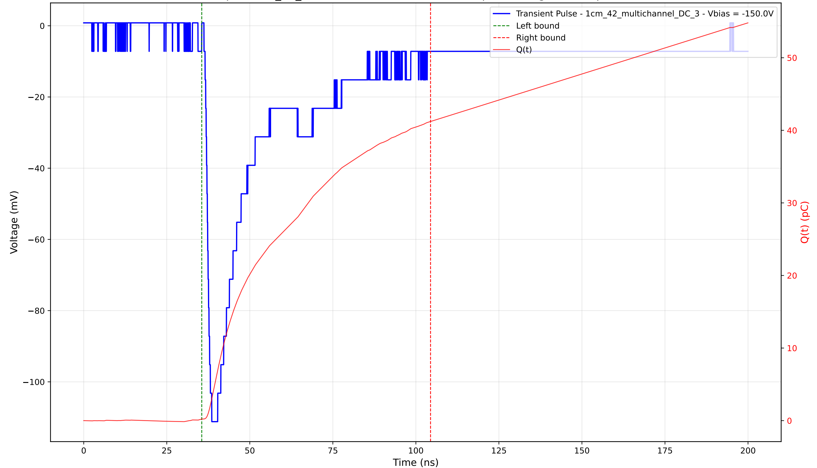
Transient Pulse - Sample: 1cm_42_multichannel - Position: 3225.0 \mu\text{m} - Charge: 40.99 pC - Rise Time: 1.59 ns
