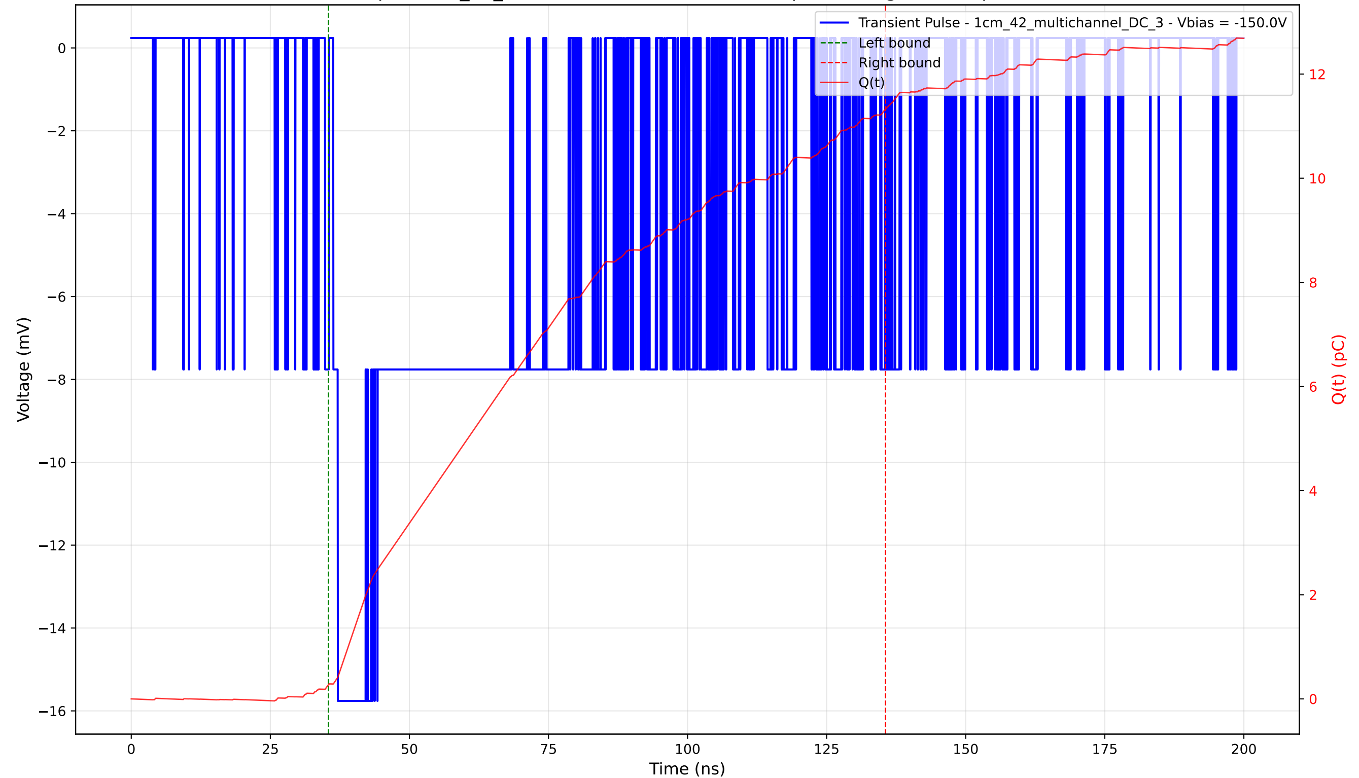
Transient Pulse - Sample: 1cm_42_multichannel - Position: 875.0 \mu\text{m} - Charge: 11.05 pC - Rise Time: 0.82 ns
