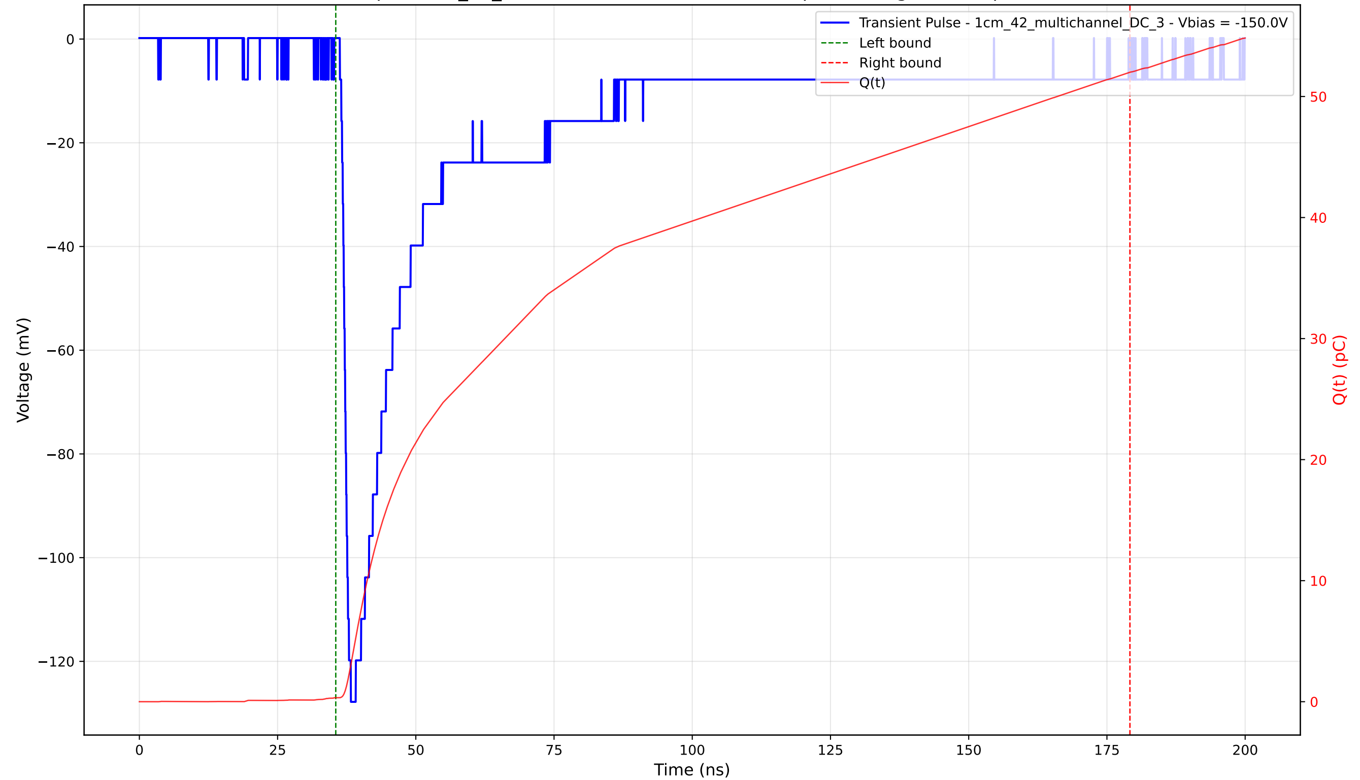
Transient Pulse - Sample: 1cm_42_multichannel - Position: 3610.0 \mu\text{m} - Charge: 51.68 pC - Rise Time: 1.39 ns
