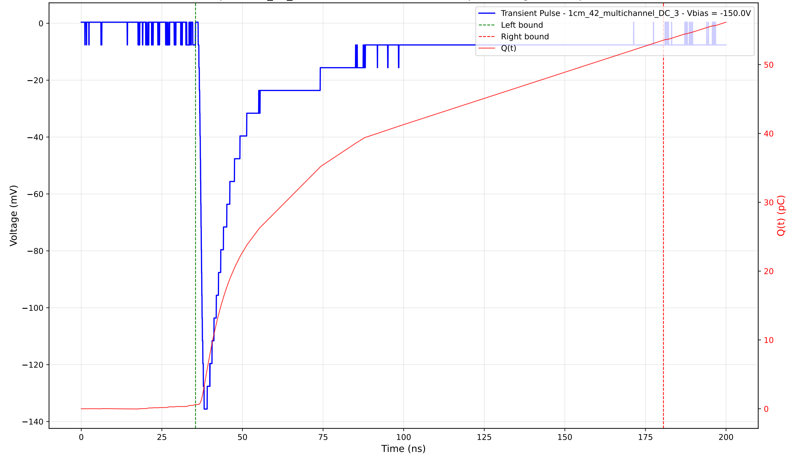
Transient Pulse - Sample: 1cm_42_multichannel - Position: 3680.0 \mu\text{m} - Charge: 52.94 pC - Rise Time: 1.39 ns
