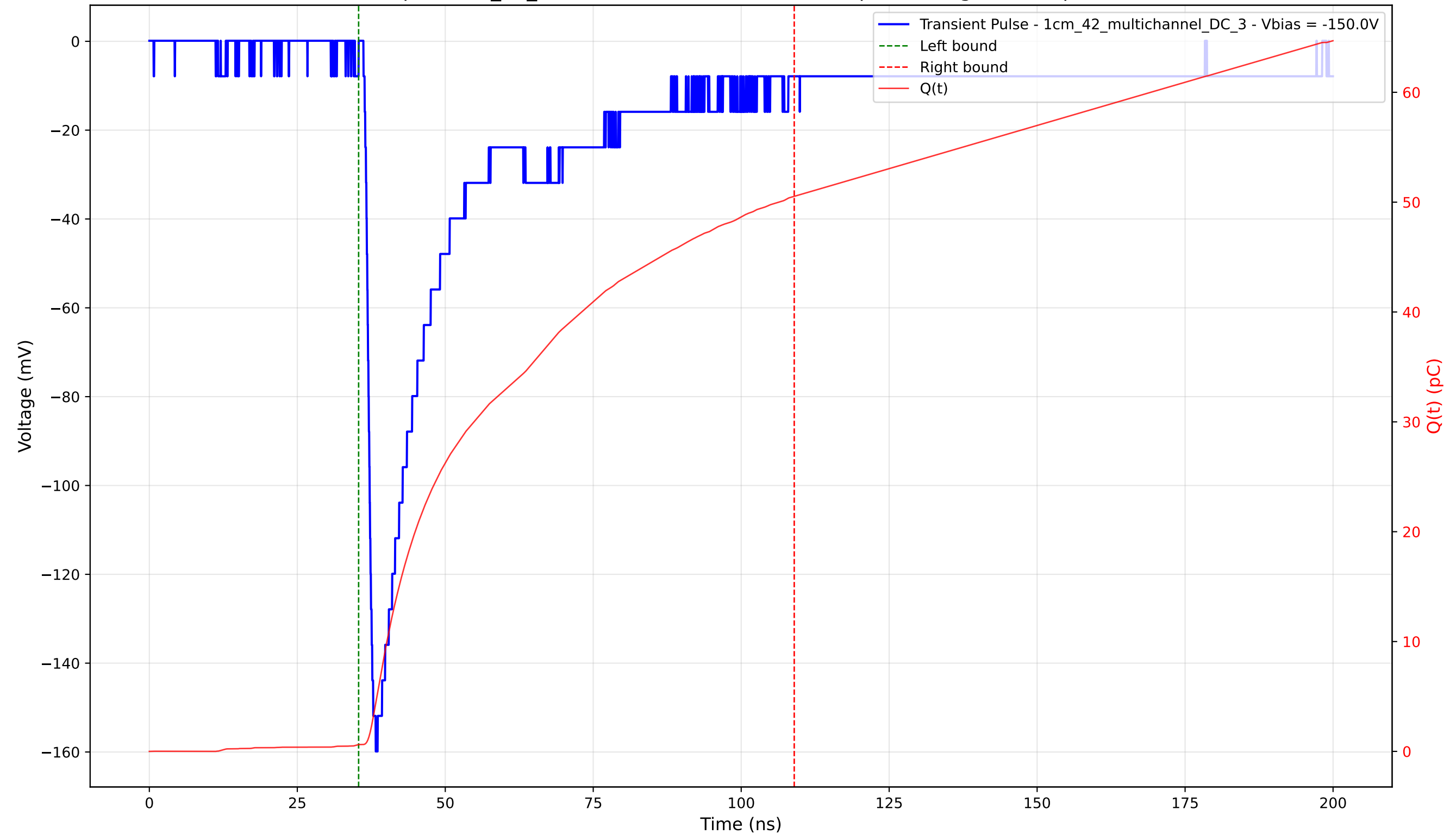
Transient Pulse - Sample: 1cm_42_multichannel - Position: 1210.0 \mu\text{m} - Charge: 49.91 pC - Rise Time: 1.36 ns
