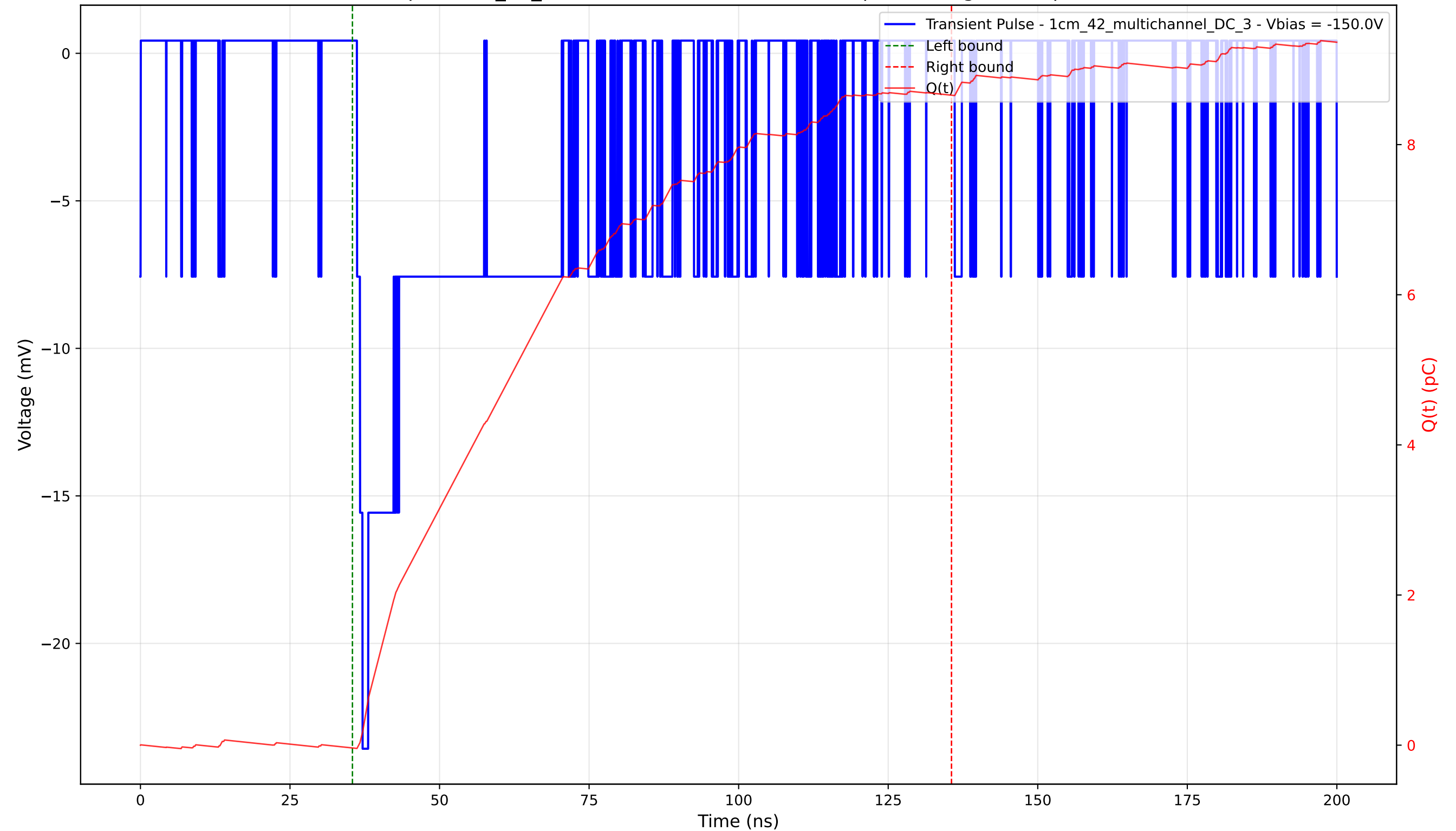
Transient Pulse - Sample: 1cm_42_multichannel - Position: 4415.0 \mu\text{m} - Charge: 8.70 pC - Rise Time: 0.93 ns
