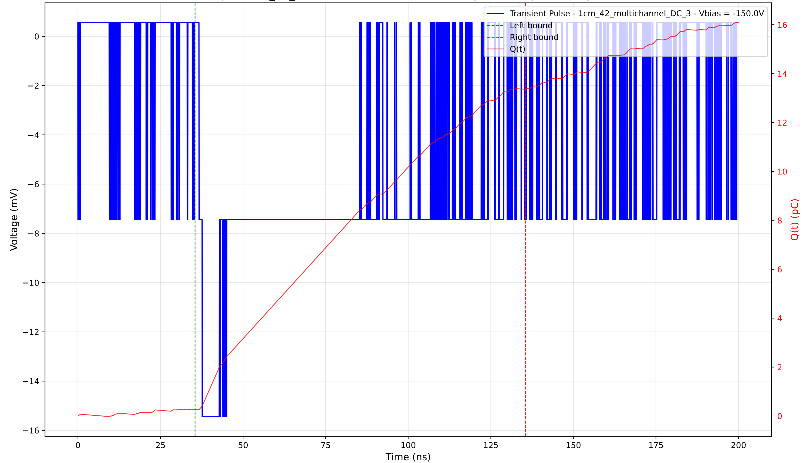
Transient Pulse - Sample: 1cm_42_multichannel - Position: 2345.0 \mu\text{m} - Charge: 13.11 pC - Rise Time: 0.96 ns
