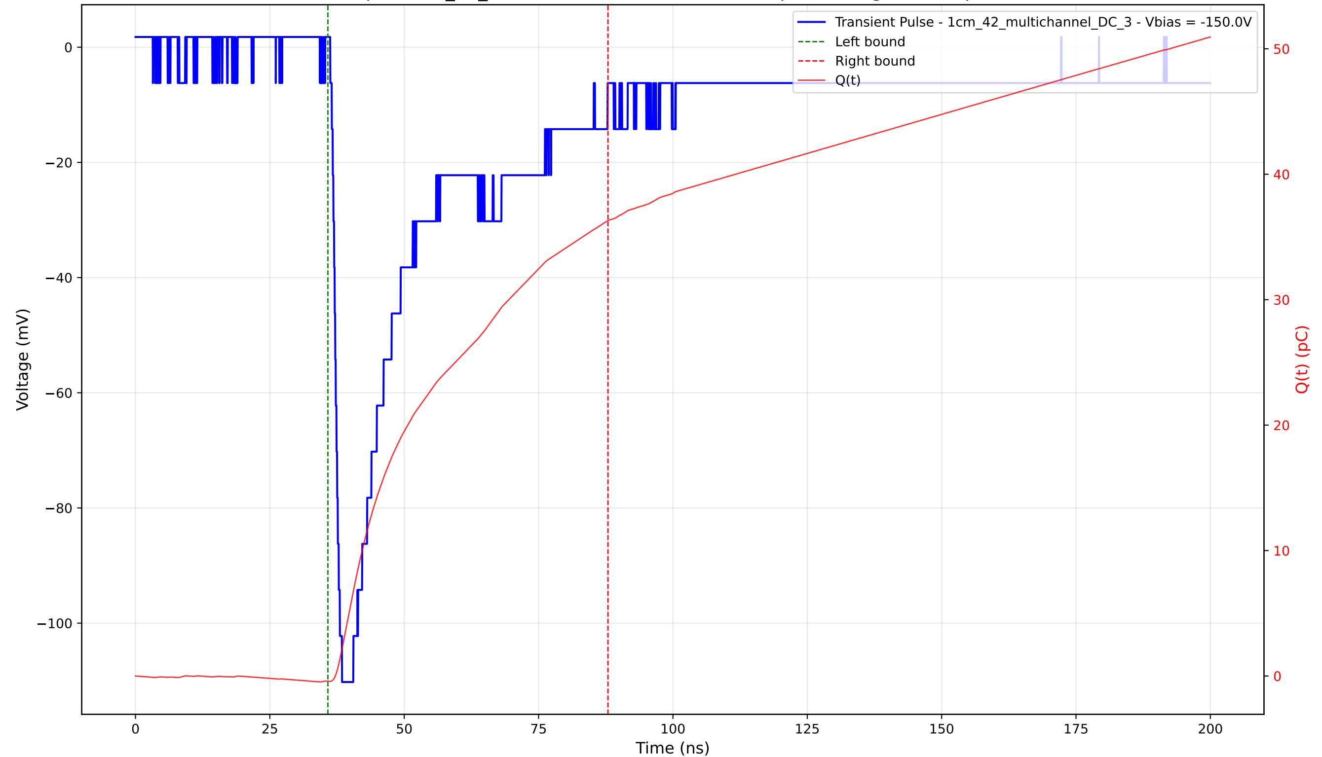
Transient Pulse - Sample: 1cm_42_multichannel - Position: 3265.0 \mu\text{m} - Charge: 36.73 pC - Rise Time: 1.51 ns
