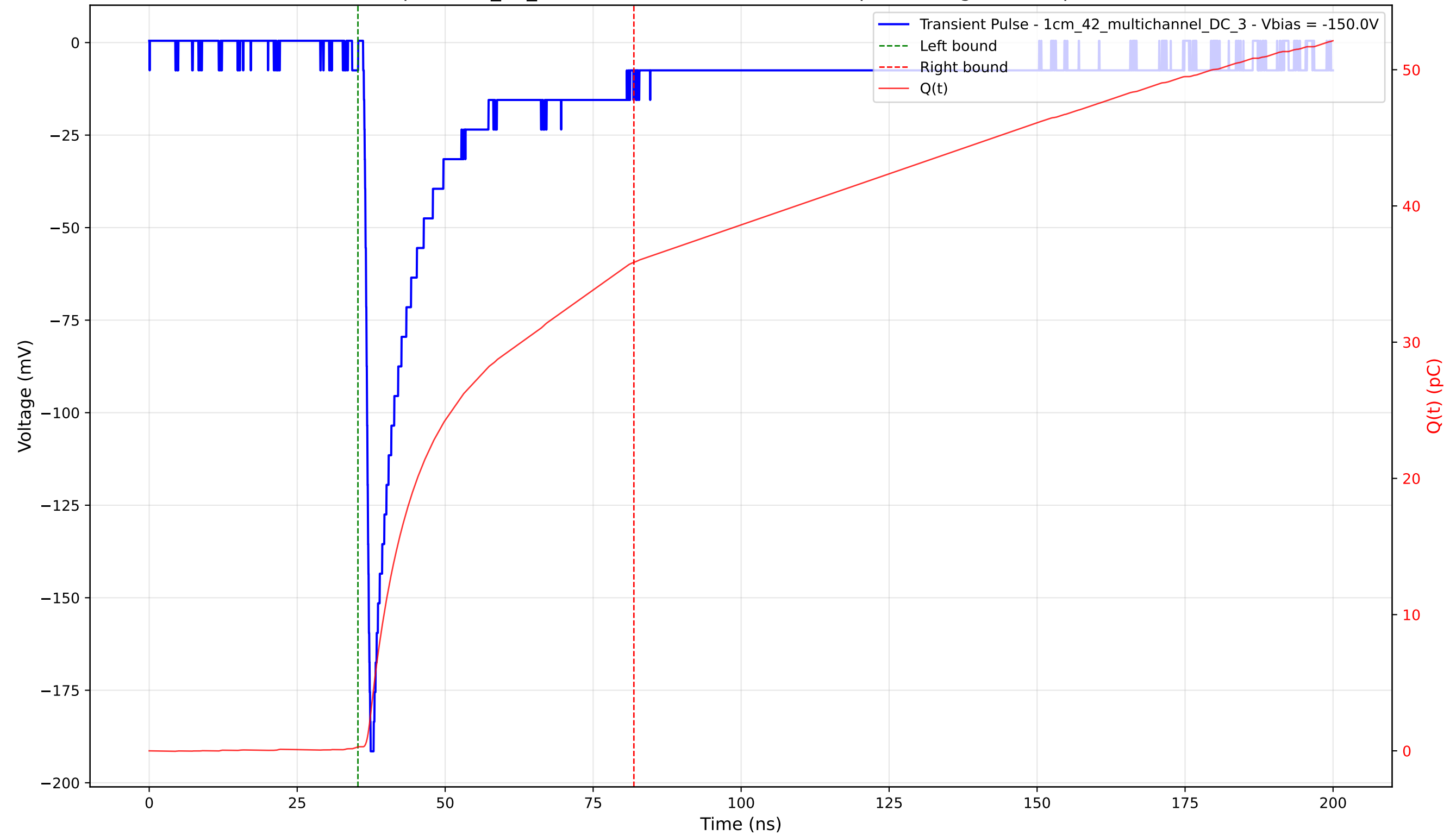
Transient Pulse - Sample: 1cm_42_multichannel - Position: 4300.0 \mu\text{m} - Charge: 35.56 pC - Rise Time: 0.91 ns
