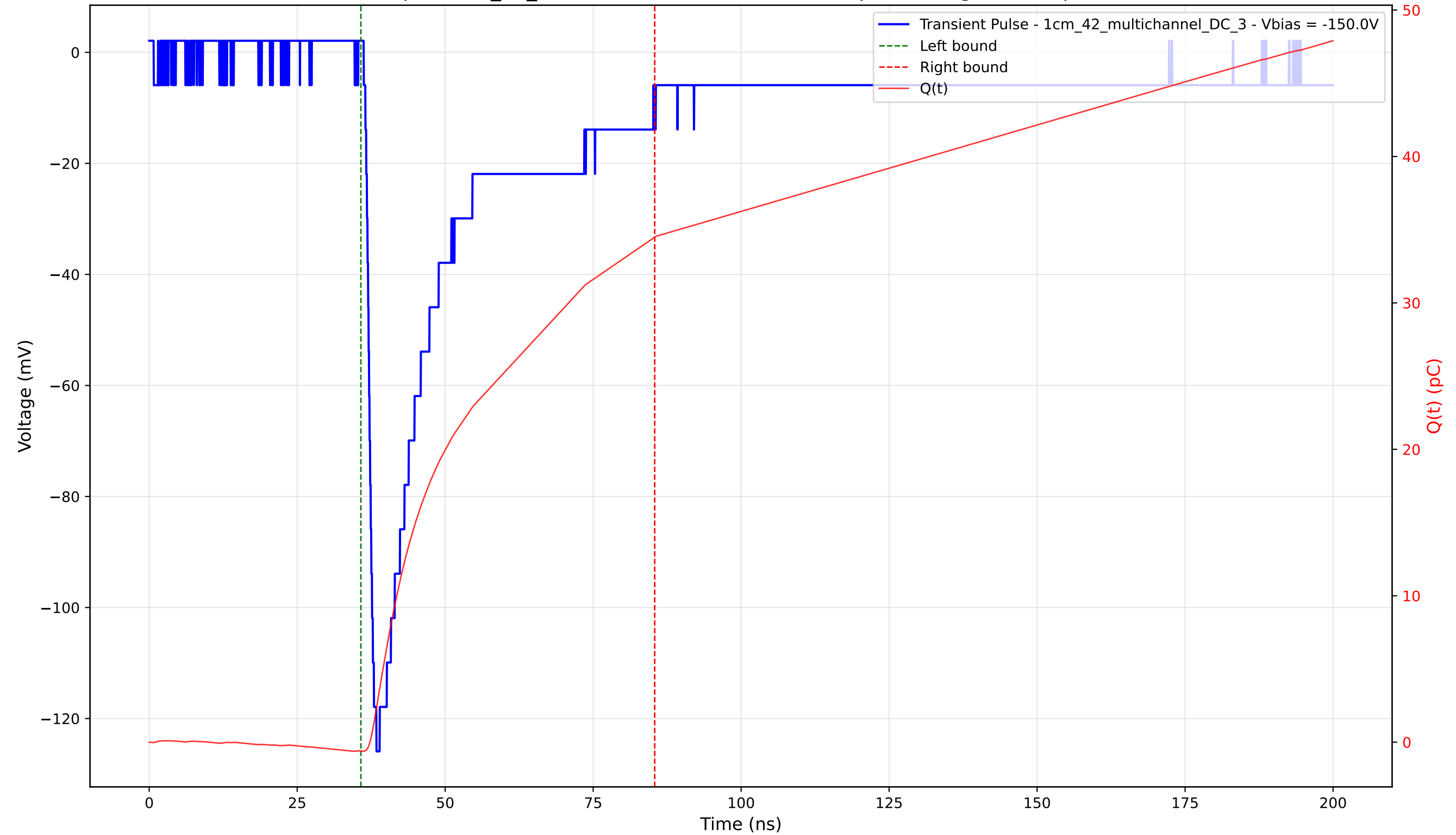
Transient Pulse - Sample: 1cm_42_multichannel - Position: 3575.0 \mu\text{m} - Charge: 35.10 pC - Rise Time: 1.44 ns
