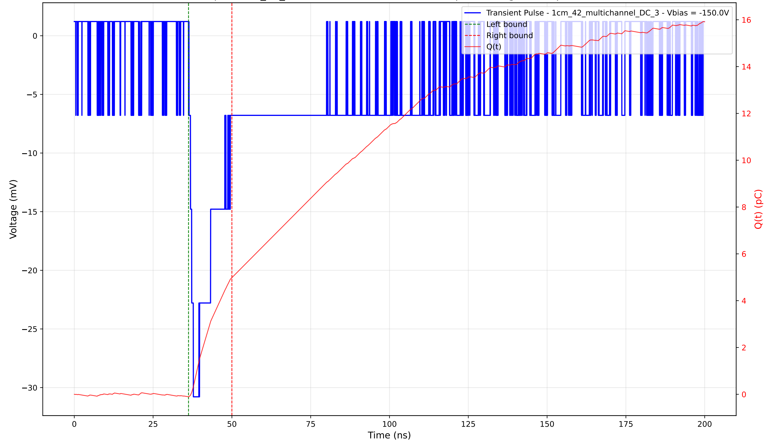
Transient Pulse - Sample: 1cm_42_multichannel - Position: 1330.0 \mu\text{m} - Charge: 5.09 pC - Rise Time: 1.37 ns
