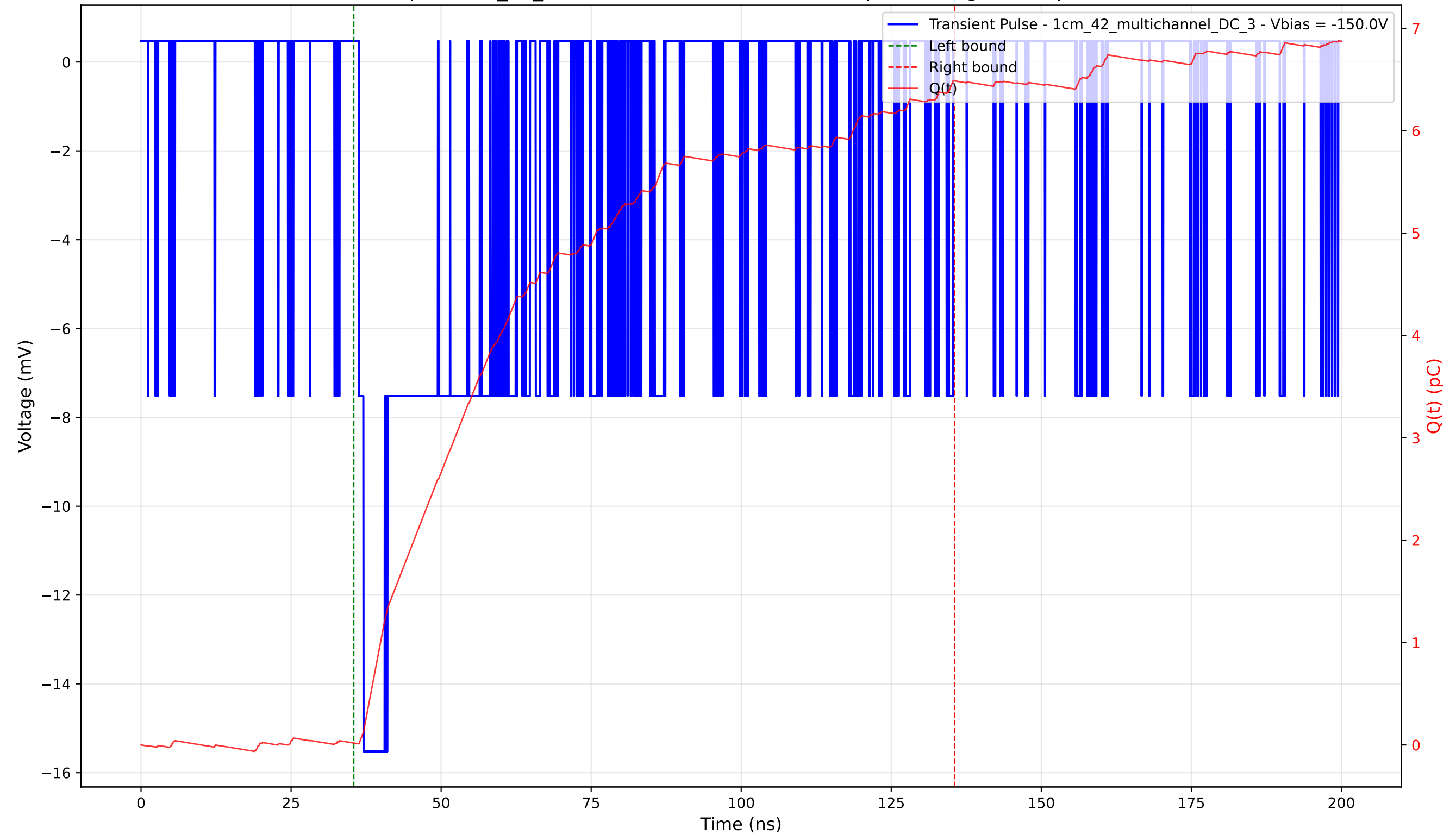
Transient Pulse - Sample: 1cm_42_multichannel - Position: 4405.0 \mu\text{m} - Charge: 6.47 pC - Rise Time: 0.76 ns
