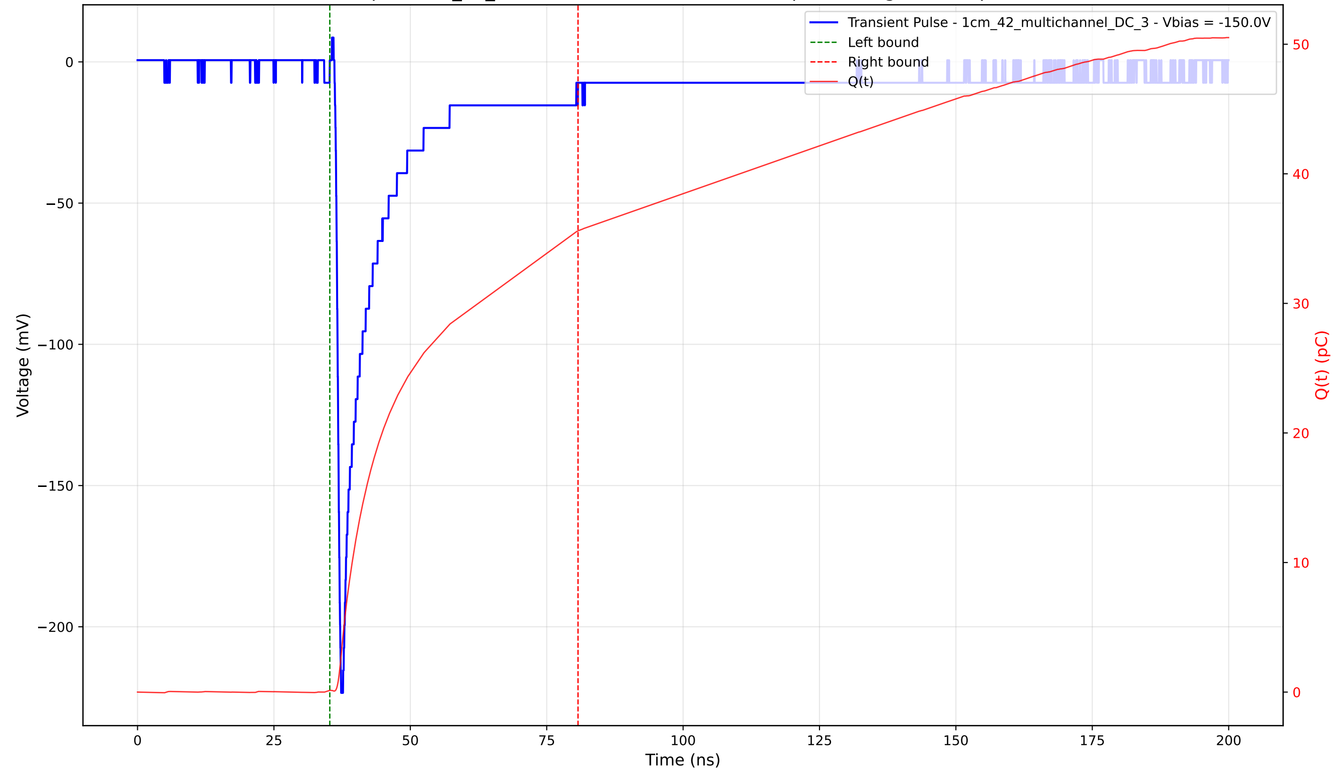
Transient Pulse - Sample: 1cm_42_multichannel - Position: 4470.0 \mu\text{m} - Charge: 35.46 pC - Rise Time: 0.90 ns
