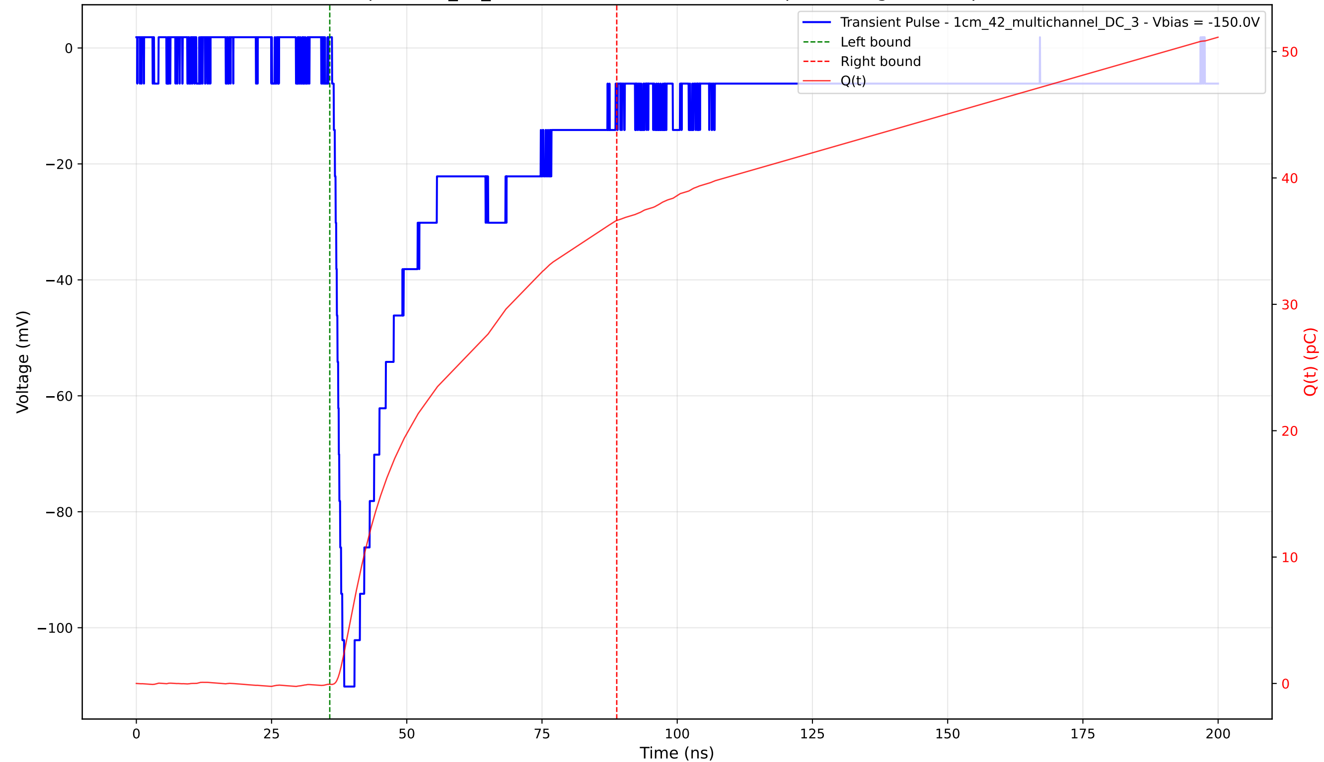
Transient Pulse - Sample: 1cm_42_multichannel - Position: 3260.0 \mu\text{m} - Charge: 36.70 pC - Rise Time: 1.59 ns
