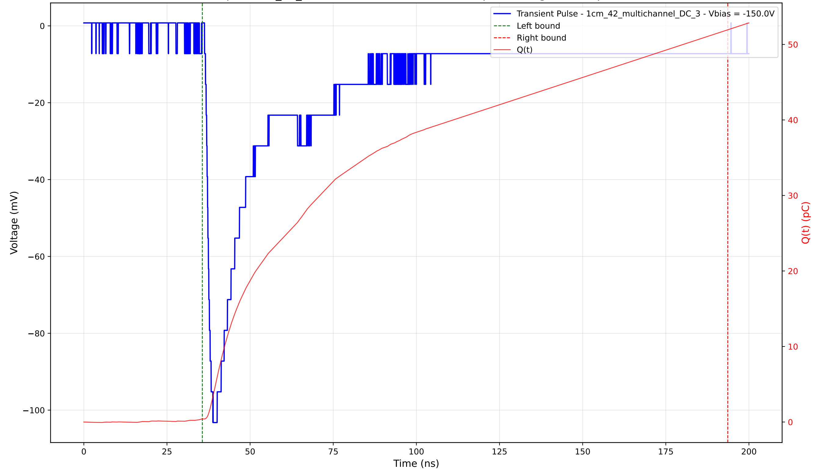
Transient Pulse - Sample: 1cm_42_multichannel - Position: 3120.0 \mu\text{m} - Charge: 51.55 pC - Rise Time: 1.71 ns
