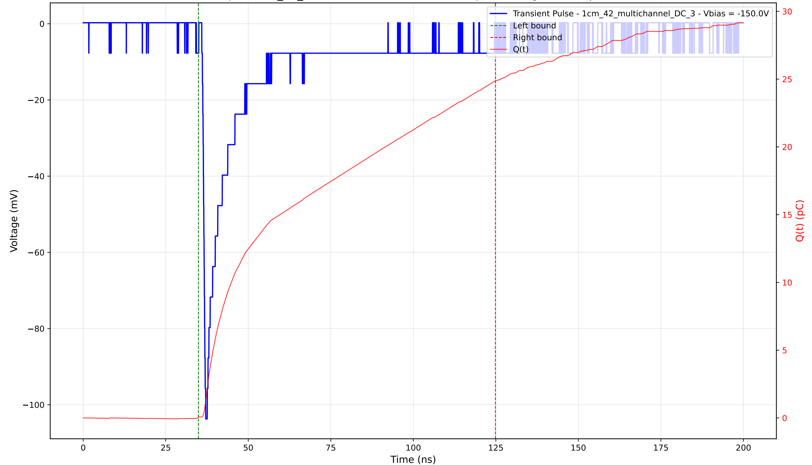
Transient Pulse - Sample: 1cm_42_multichannel - Position: 395.0 \mu\text{m} - Charge: 24.83 pC - Rise Time: 0.85 ns
