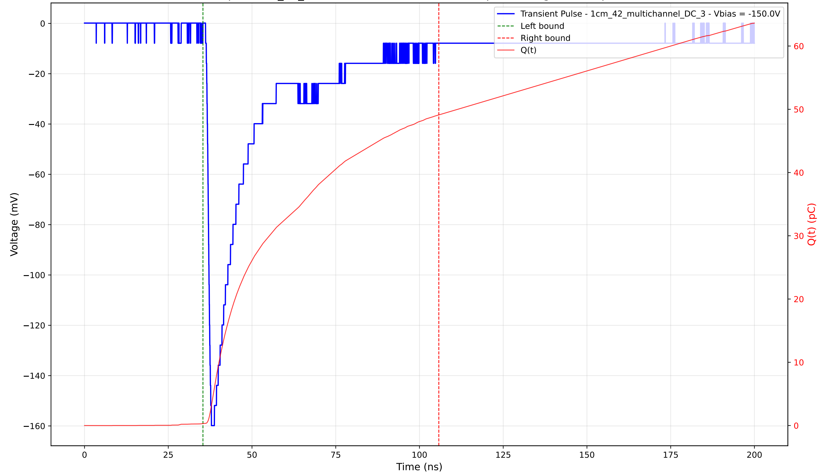
Transient Pulse - Sample: 1cm_42_multichannel - Position: 1145.0 \mu\text{m} - Charge: 48.79 pC - Rise Time: 1.22 ns
