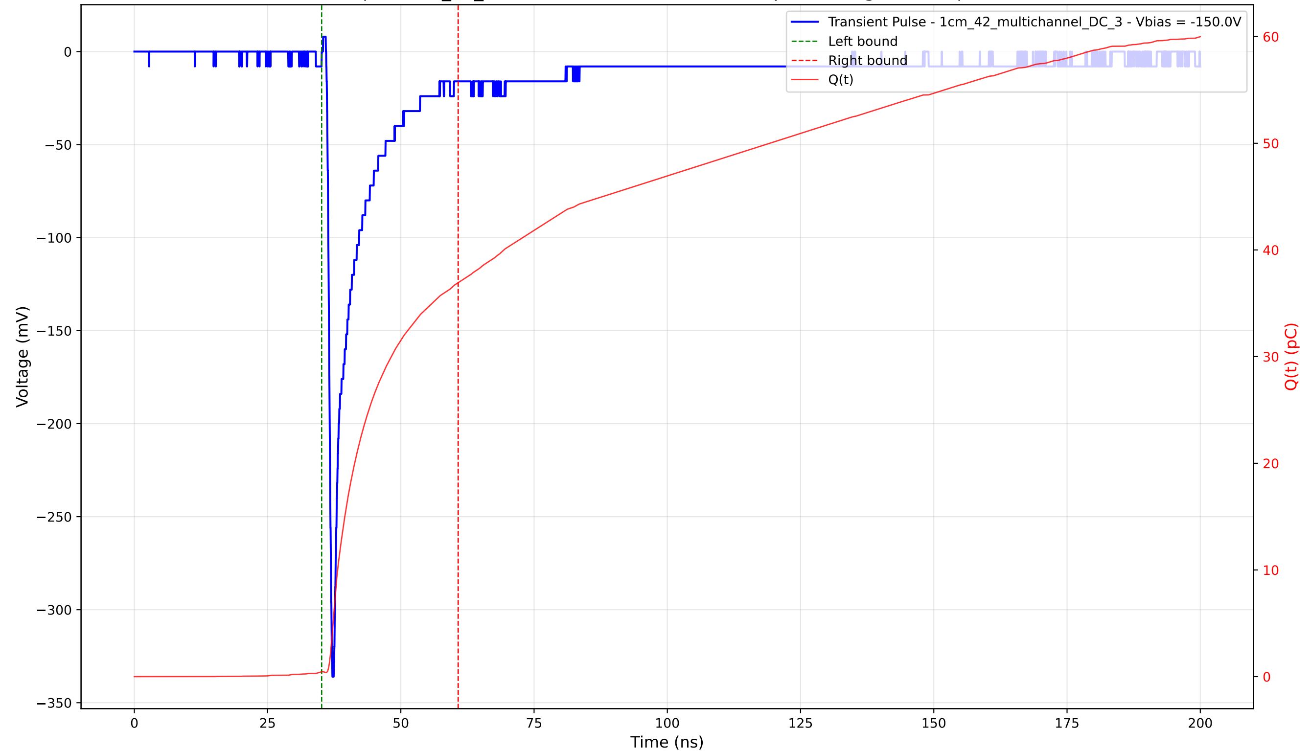
Transient Pulse - Sample: 1cm_42_multichannel - Position: 4685.0 \mu\text{m} - Charge: 36.46 pC - Rise Time: 0.79 ns
