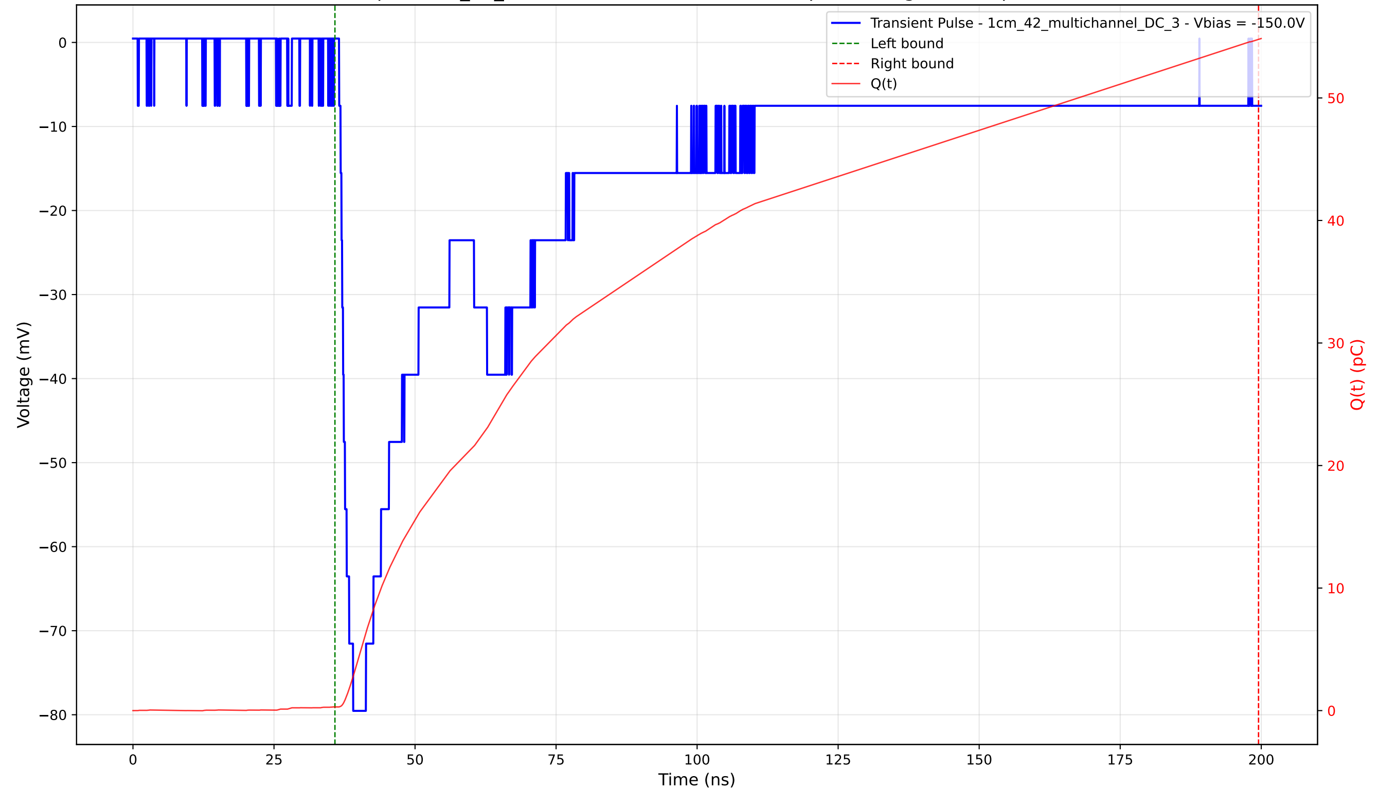
Transient Pulse - Sample: 1cm_42_multichannel - Position: 2540.0 \mu\text{m} - Charge: 54.47 pC - Rise Time: 2.24 ns
