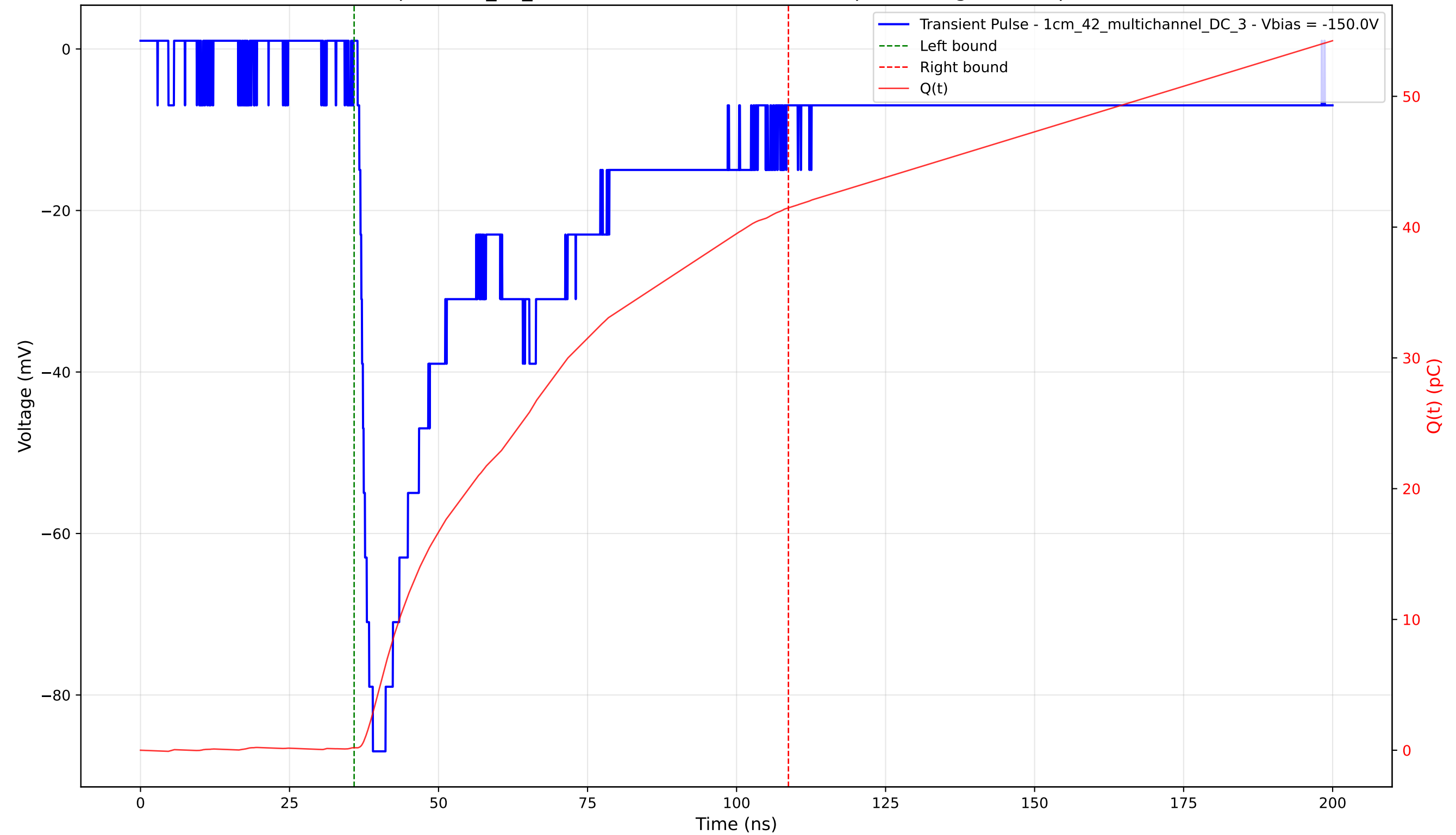
Transient Pulse - Sample: 1cm_42_multichannel - Position: 2685.0 \mu\text{m} - Charge: 41.28 pC - Rise Time: 1.68 ns
