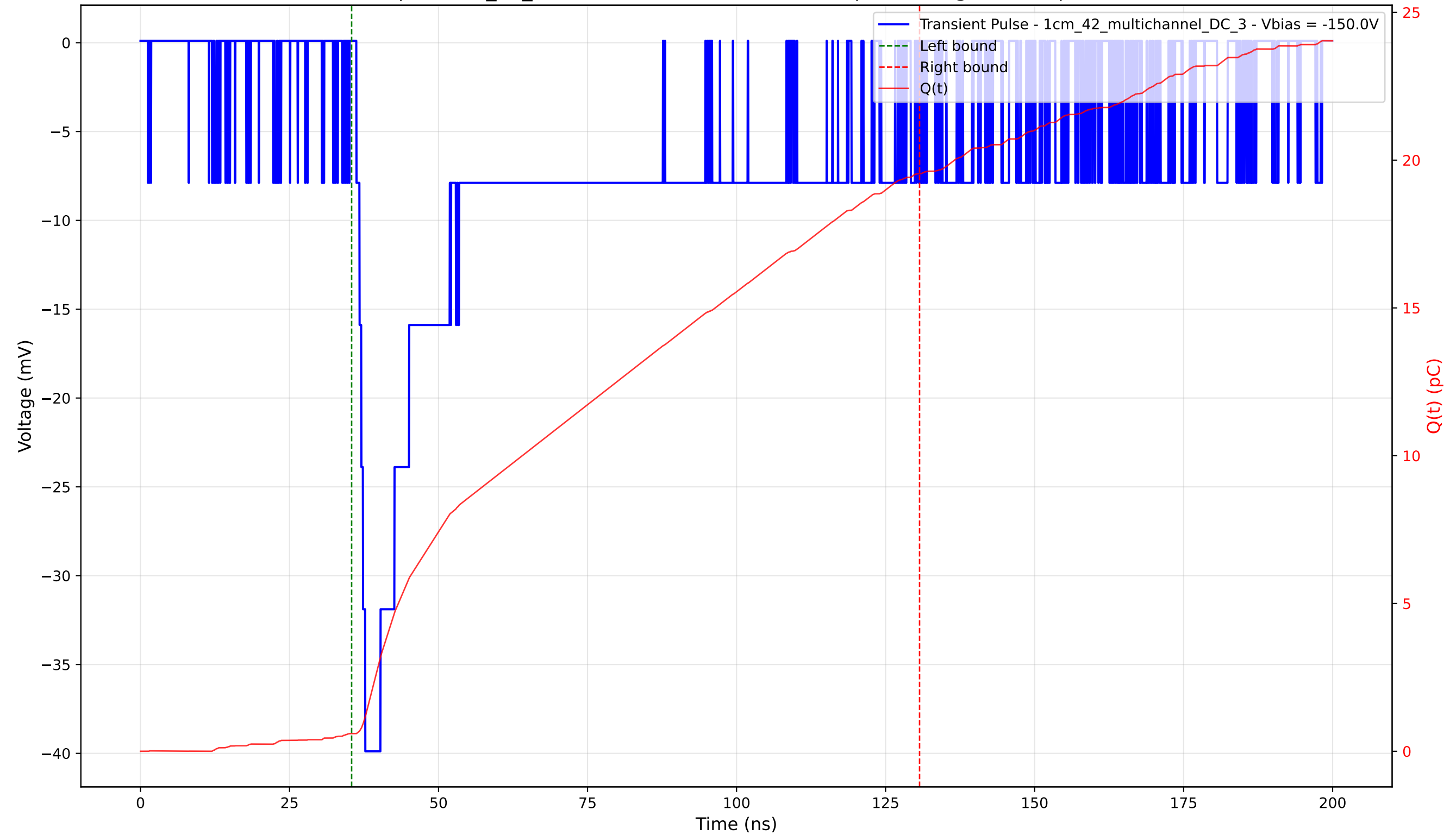
Transient Pulse - Sample: 1cm_42_multichannel - Position: 1325.0 \mu\text{m} - Charge: 18.94 pC - Rise Time: 1.49 ns
