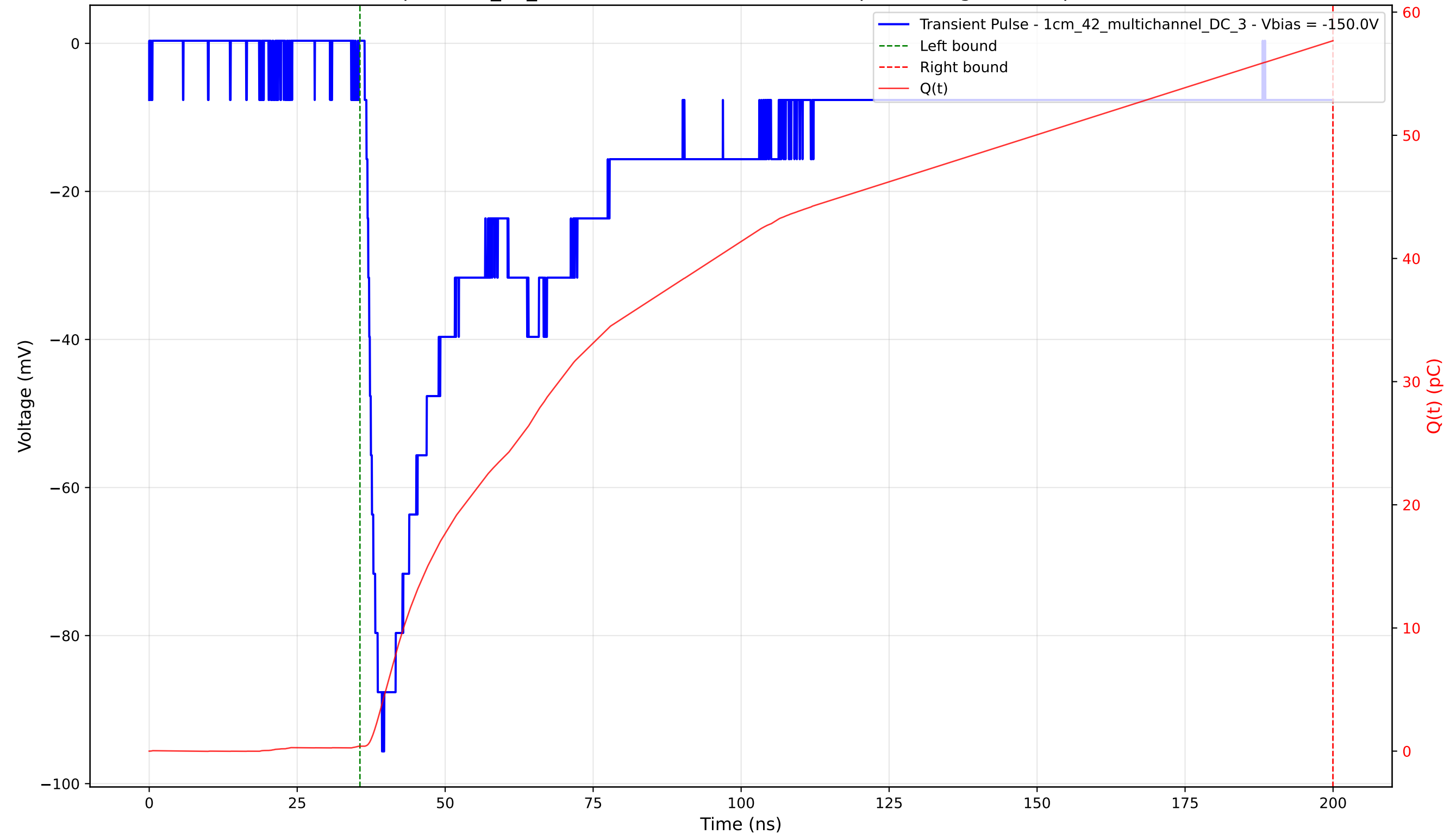
Transient Pulse - Sample: 1cm_42_multichannel - Position: 2725.0 \mu\text{m} - Charge: 57.28 pC - Rise Time: 1.92 ns
