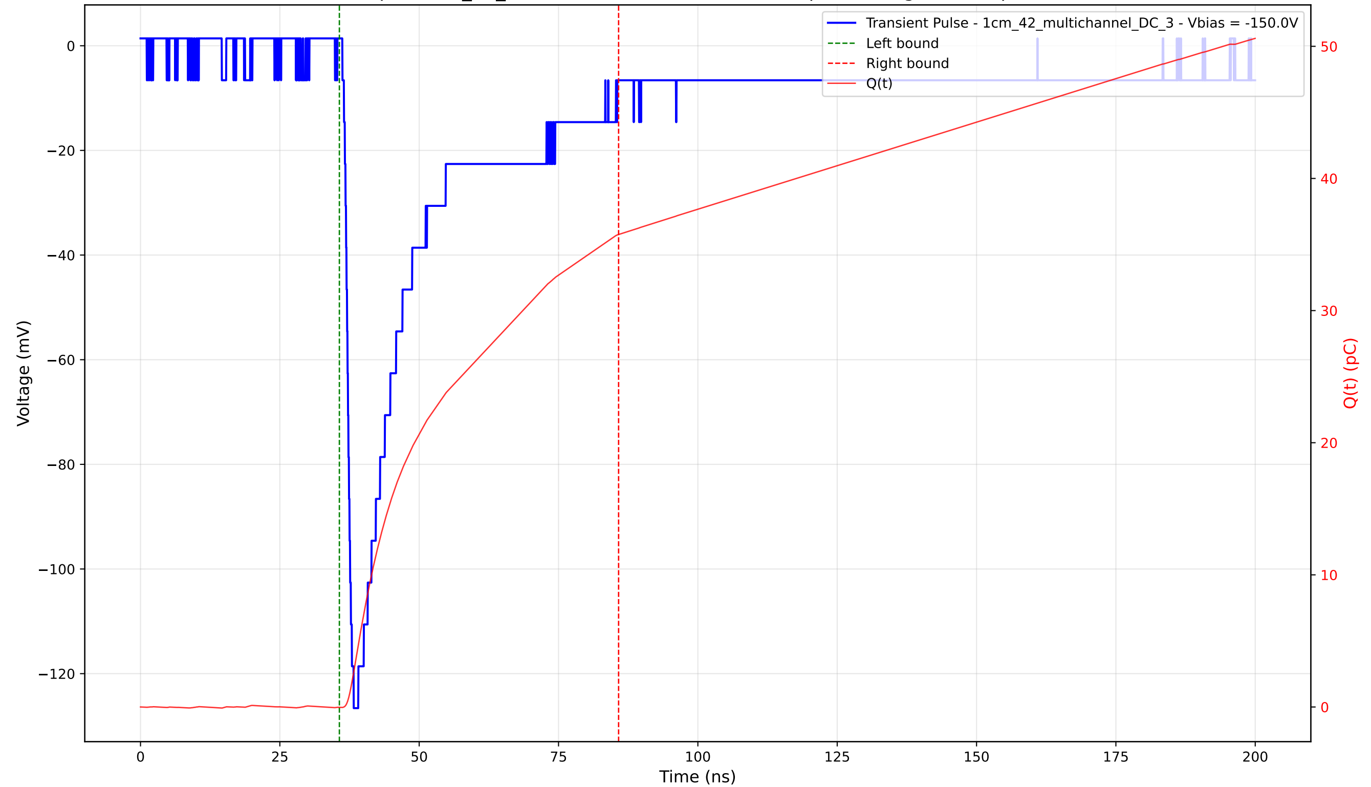
Transient Pulse - Sample: 1cm_42_multichannel - Position: 3615.0 \mu\text{m} - Charge: 35.79 pC - Rise Time: 1.42 ns
