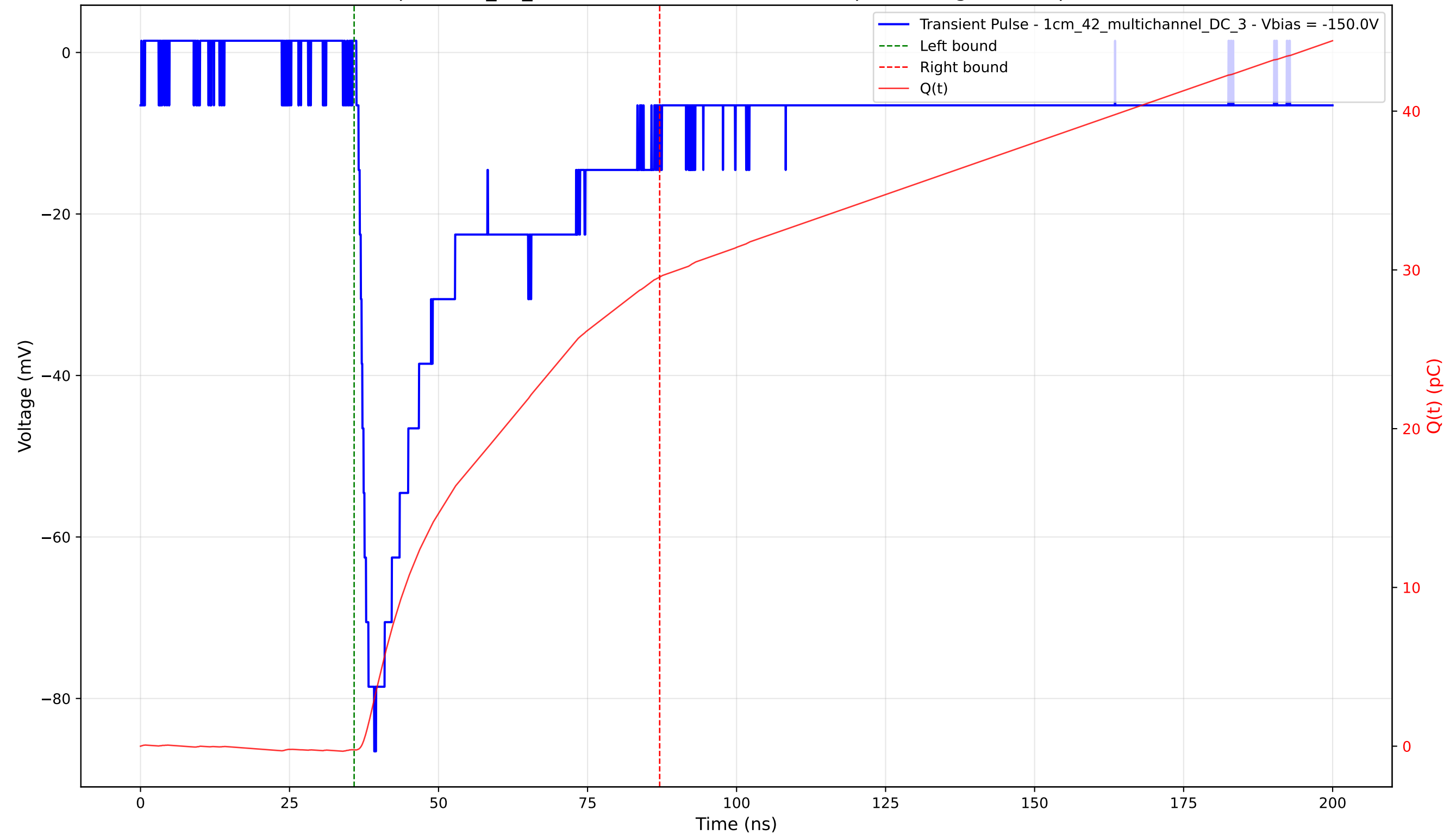
Transient Pulse - Sample: 1cm_42_multichannel - Position: 1805.0 \mu\text{m} - Charge: 29.78 pC - Rise Time: 1.67 ns
