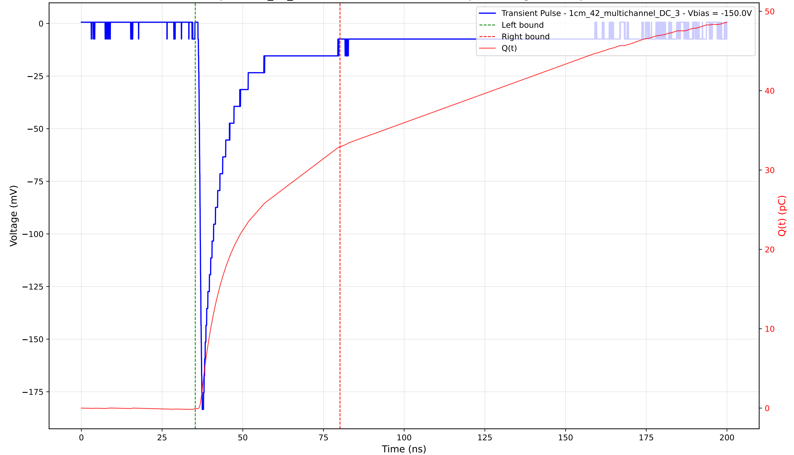
Transient Pulse - Sample: 1cm_42_multichannel - Position: 4310.0 \mu\text{m} - Charge: 32.99 pC - Rise Time: 0.91 ns
