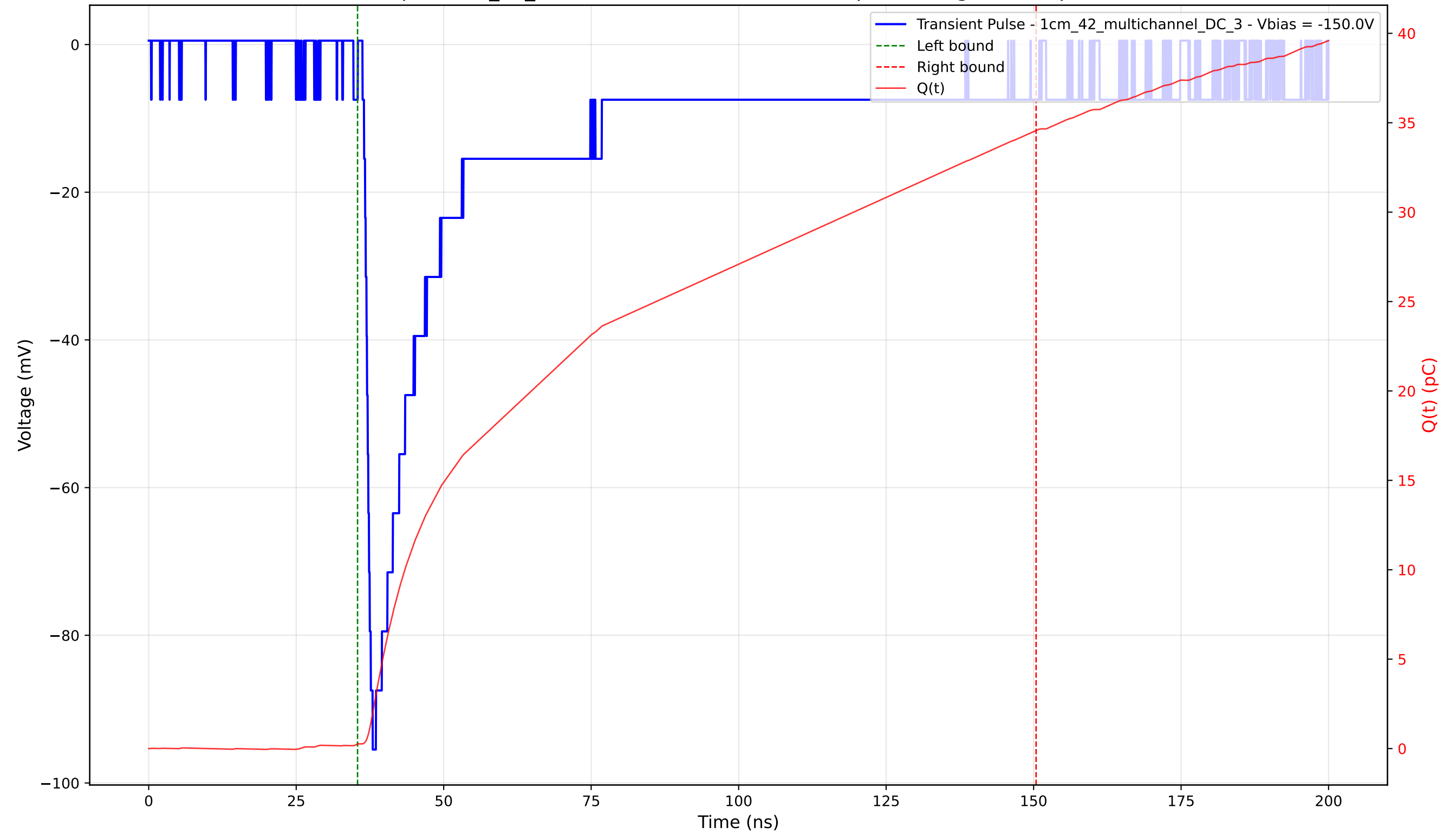
Transient Pulse - Sample: 1cm_42_multichannel - Position: 3835.0 \mu\text{m} - Charge: 34.30 pC - Rise Time: 1.15 ns
