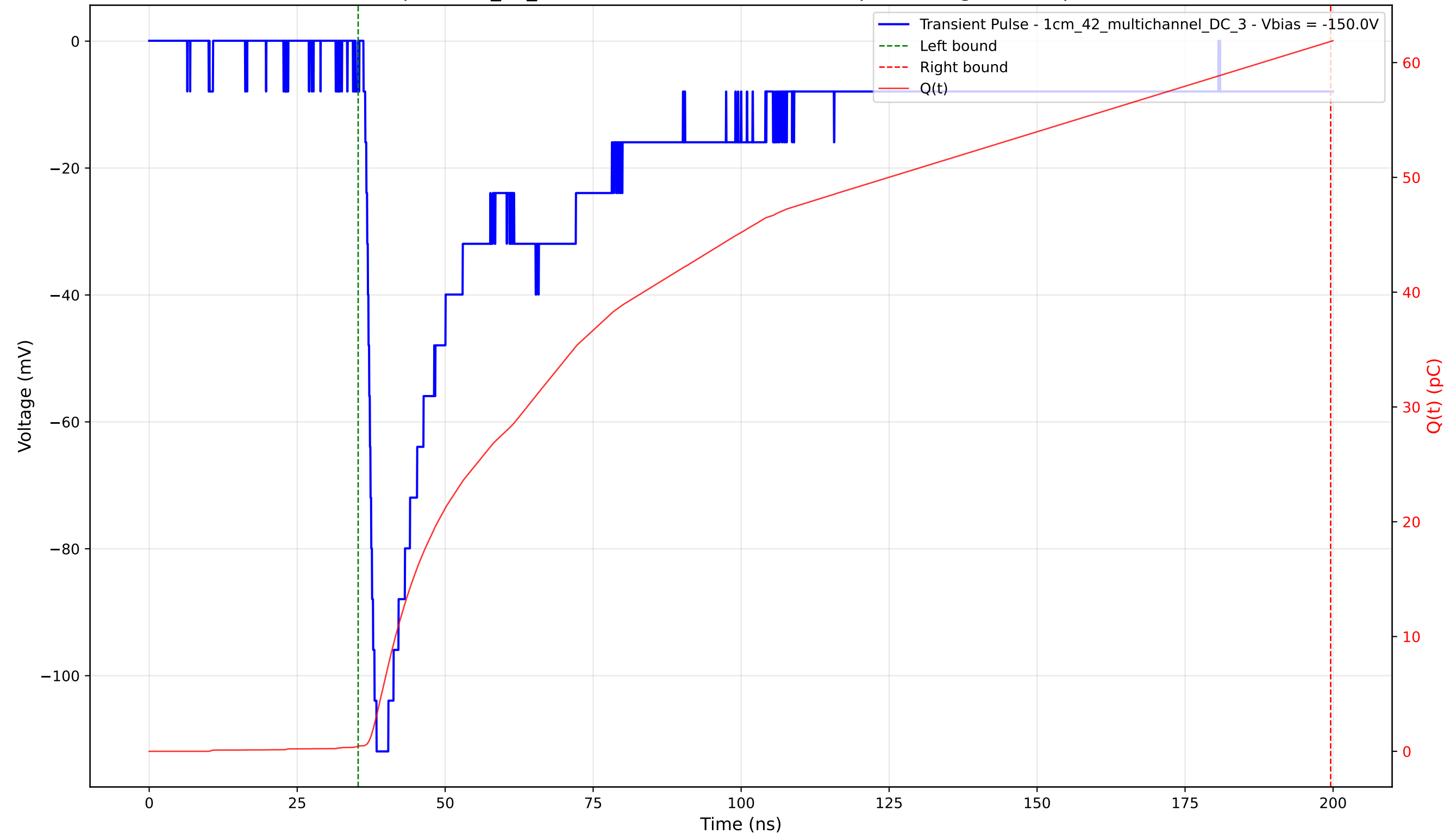
Transient Pulse - Sample: 1cm_42_multichannel - Position: 1750.0 \mu\text{m} - Charge: 61.40 pC - Rise Time: 1.57 ns
