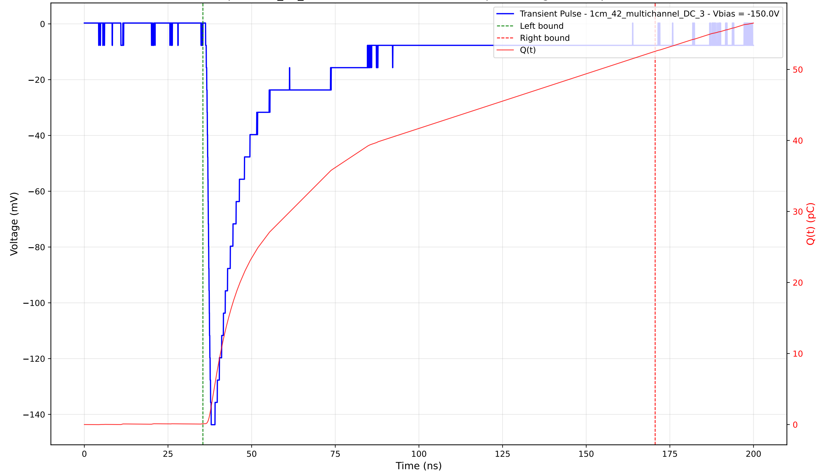
Transient Pulse - Sample: 1cm_42_multichannel - Position: 3760.0 \mu\text{m} - Charge: 52.44 pC - Rise Time: 1.28 ns
