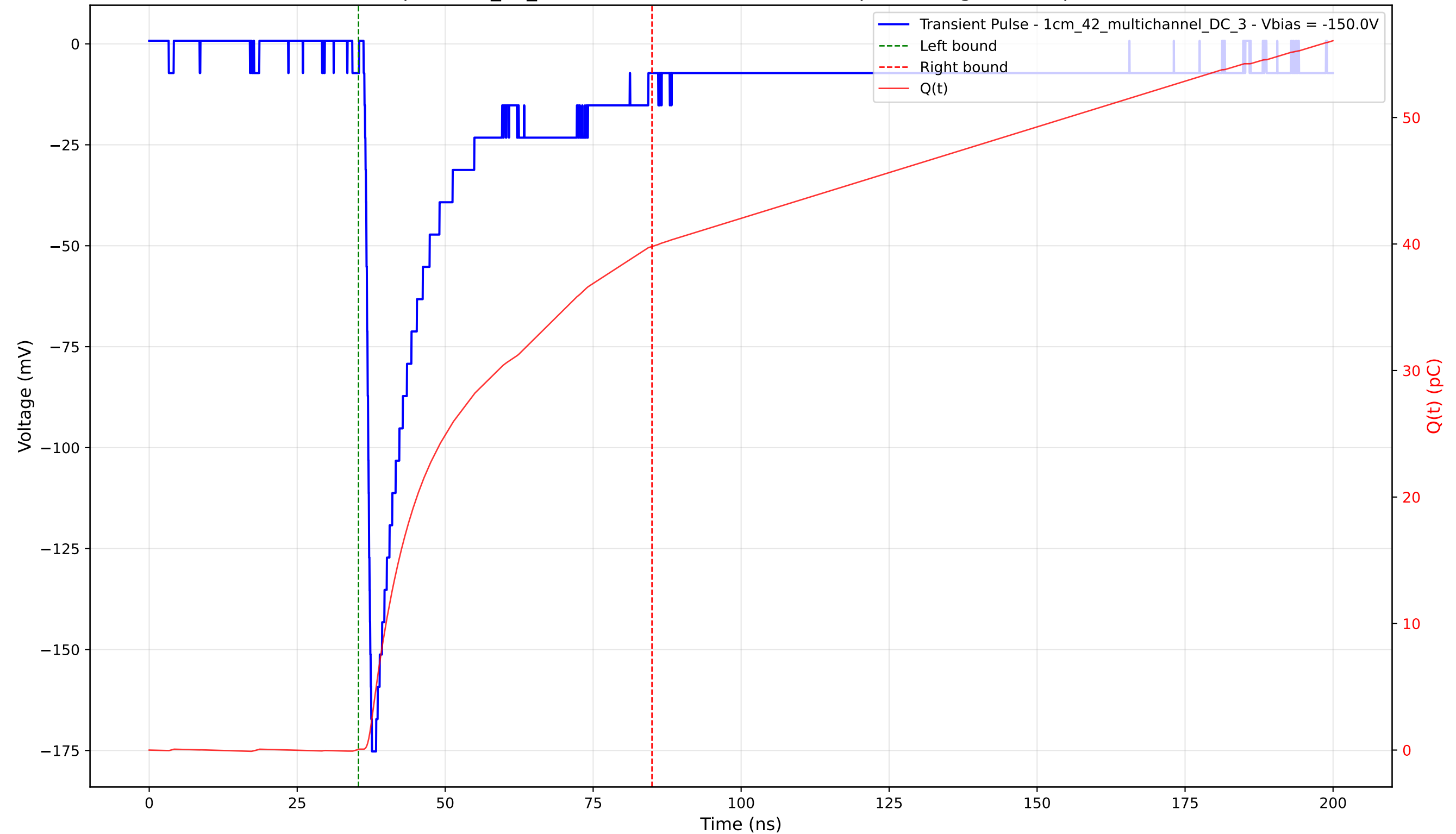
Transient Pulse - Sample: 1cm_42_multichannel - Position: 4080.0 \mu\text{m} - Charge: 39.74 pC - Rise Time: 0.97 ns
