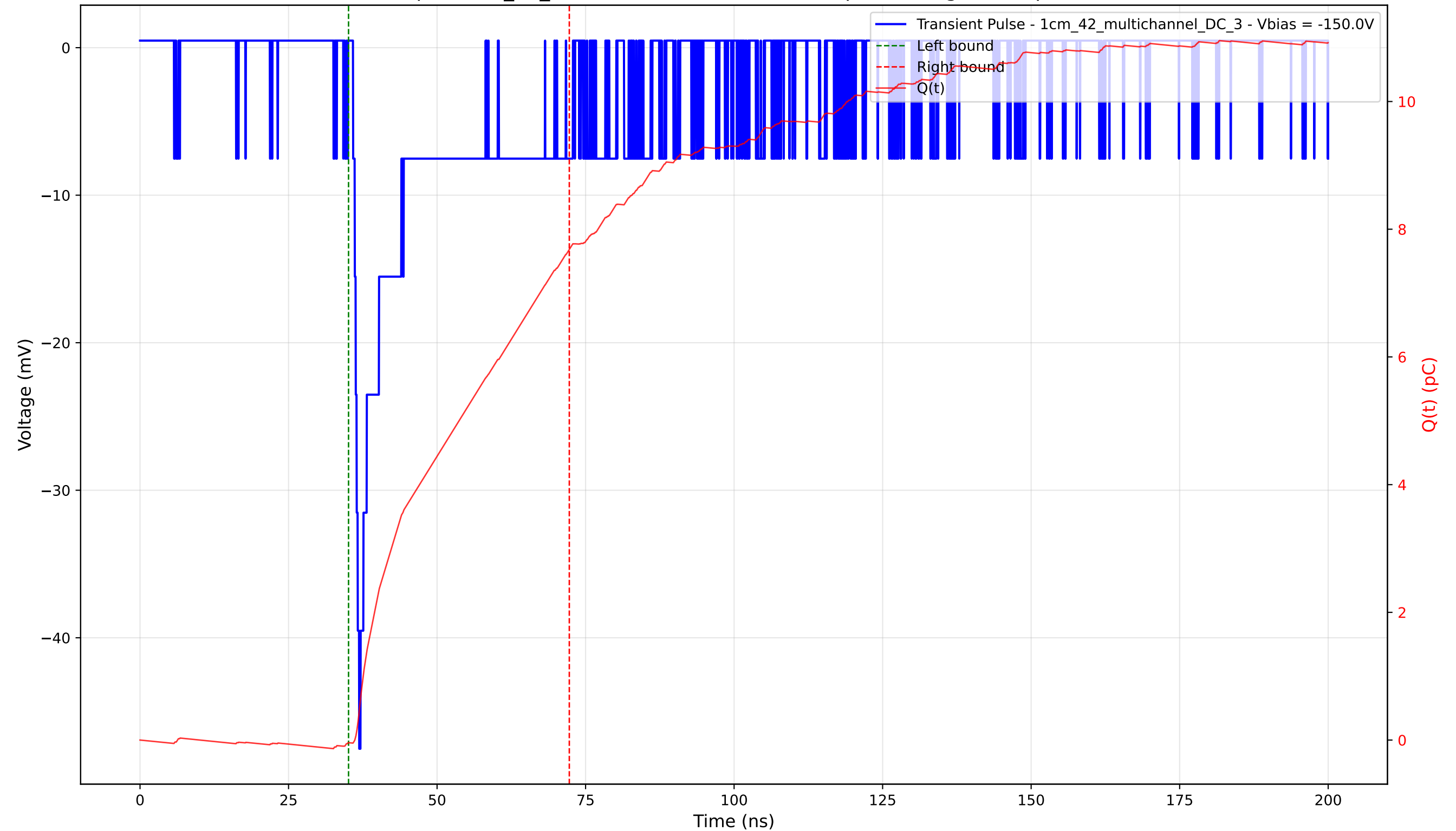
Transient Pulse - Sample: 1cm_42_multichannel - Position: 55.0 \mu\text{m} - Charge: 7.73 pC - Rise Time: 1.03 ns
