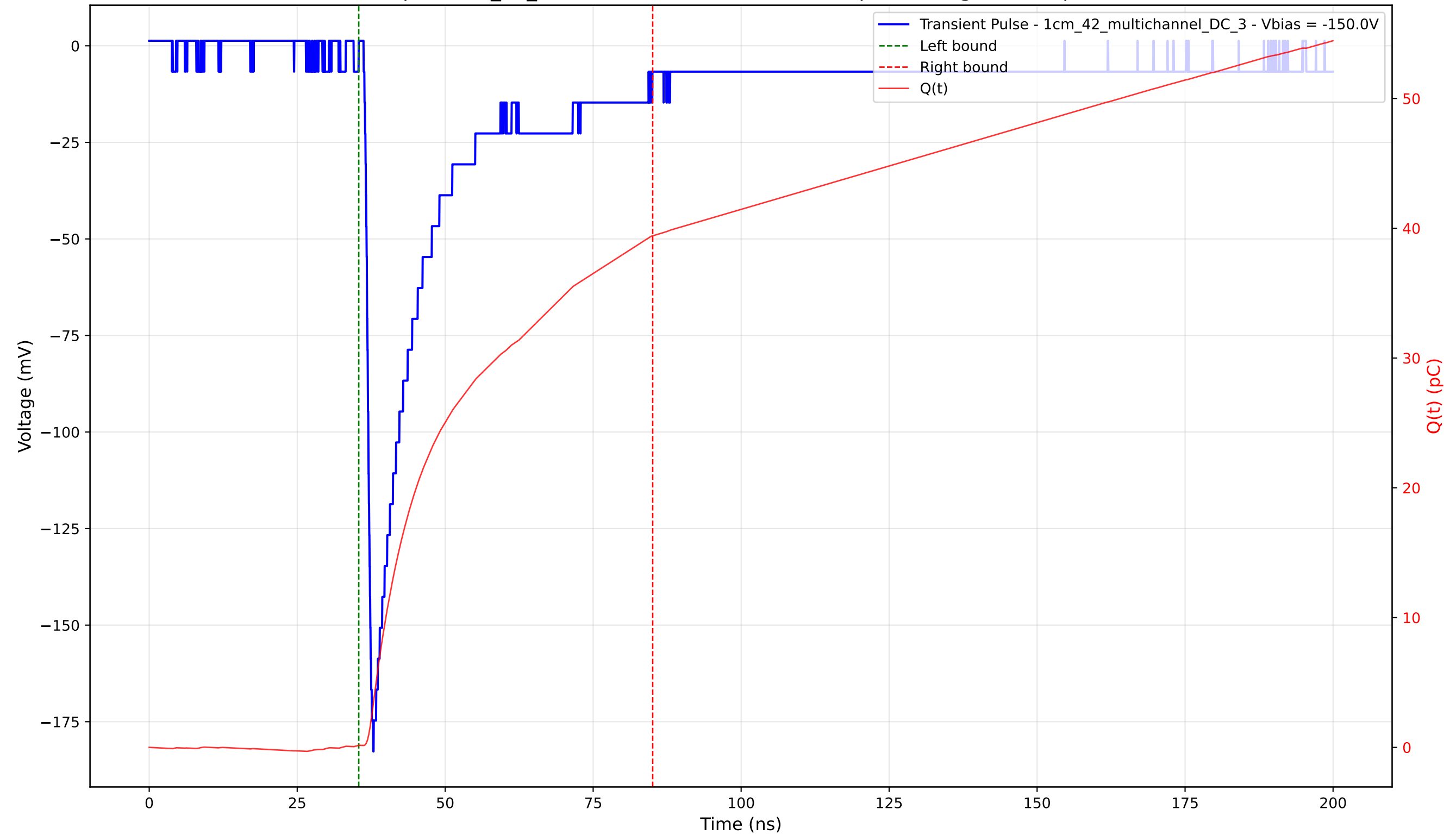
Transient Pulse - Sample: 1cm_42_multichannel - Position: 4075.0 \mu\text{m} - Charge: 39.26 pC - Rise Time: 1.03 ns
