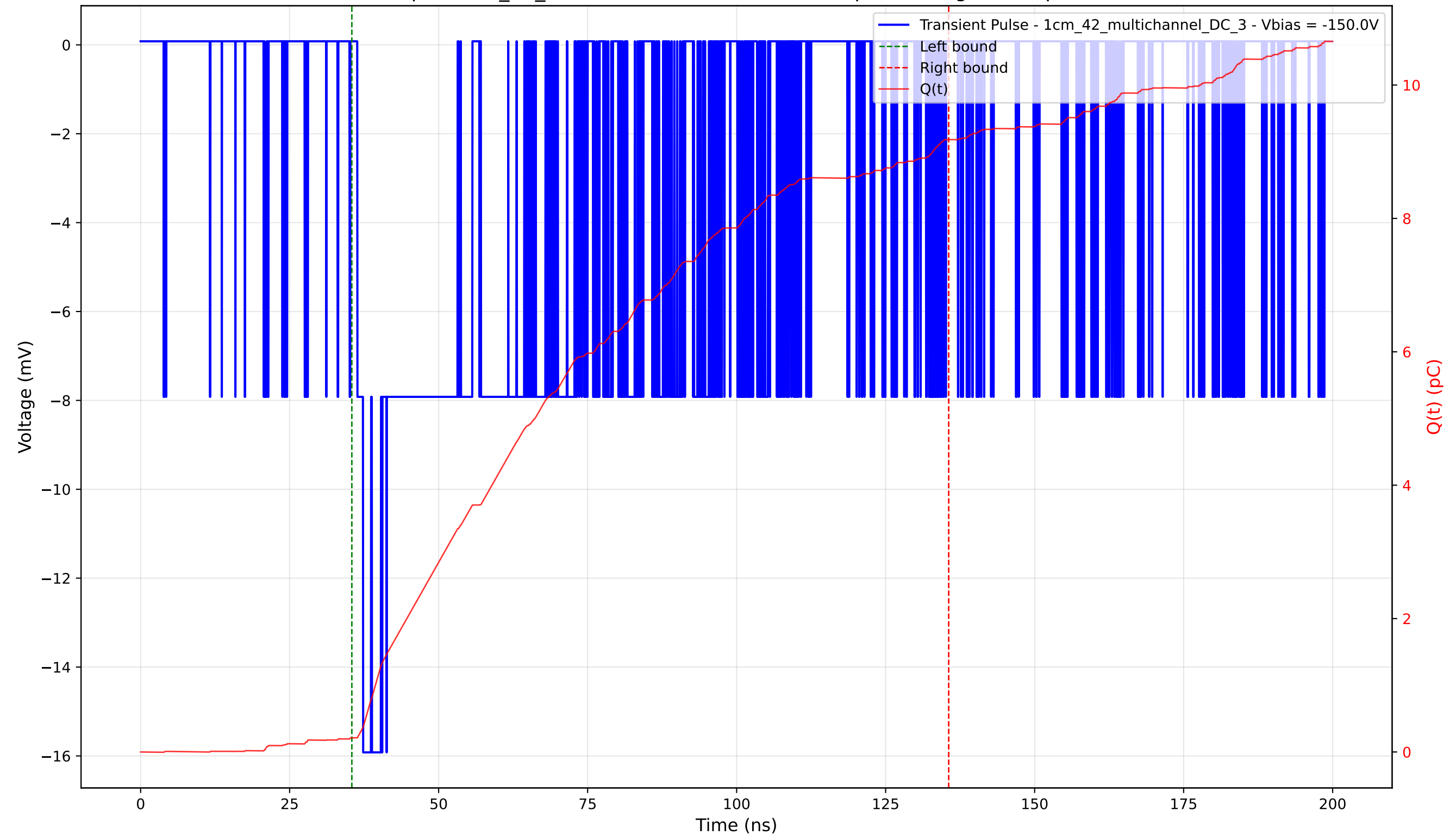
Transient Pulse - Sample: 1cm_42_multichannel - Position: 850.0 \mu\text{m} - Charge: 8.97 pC - Rise Time: 0.98 ns
