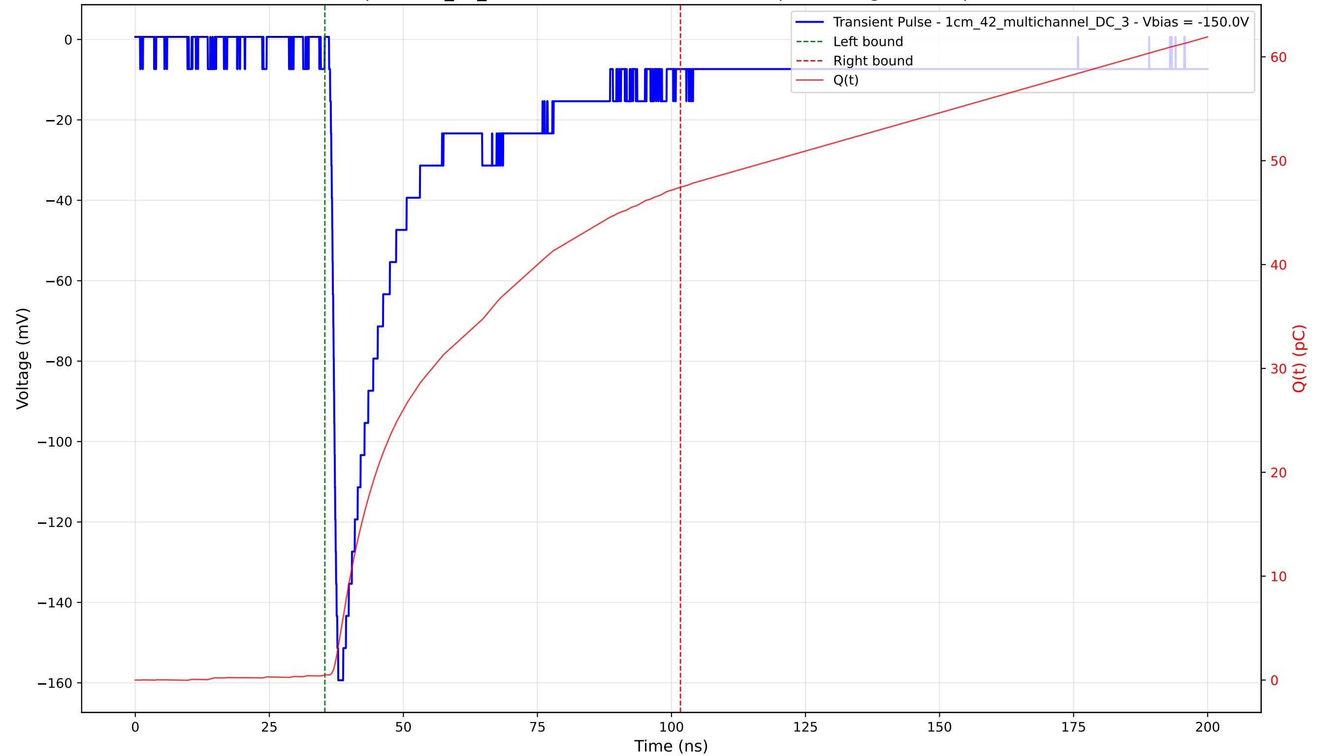
Transient Pulse - Sample: 1cm_42_multichannel - Position: 1130.0 \mu\text{m} - Charge: 46.94 pC - Rise Time: 1.22 ns
