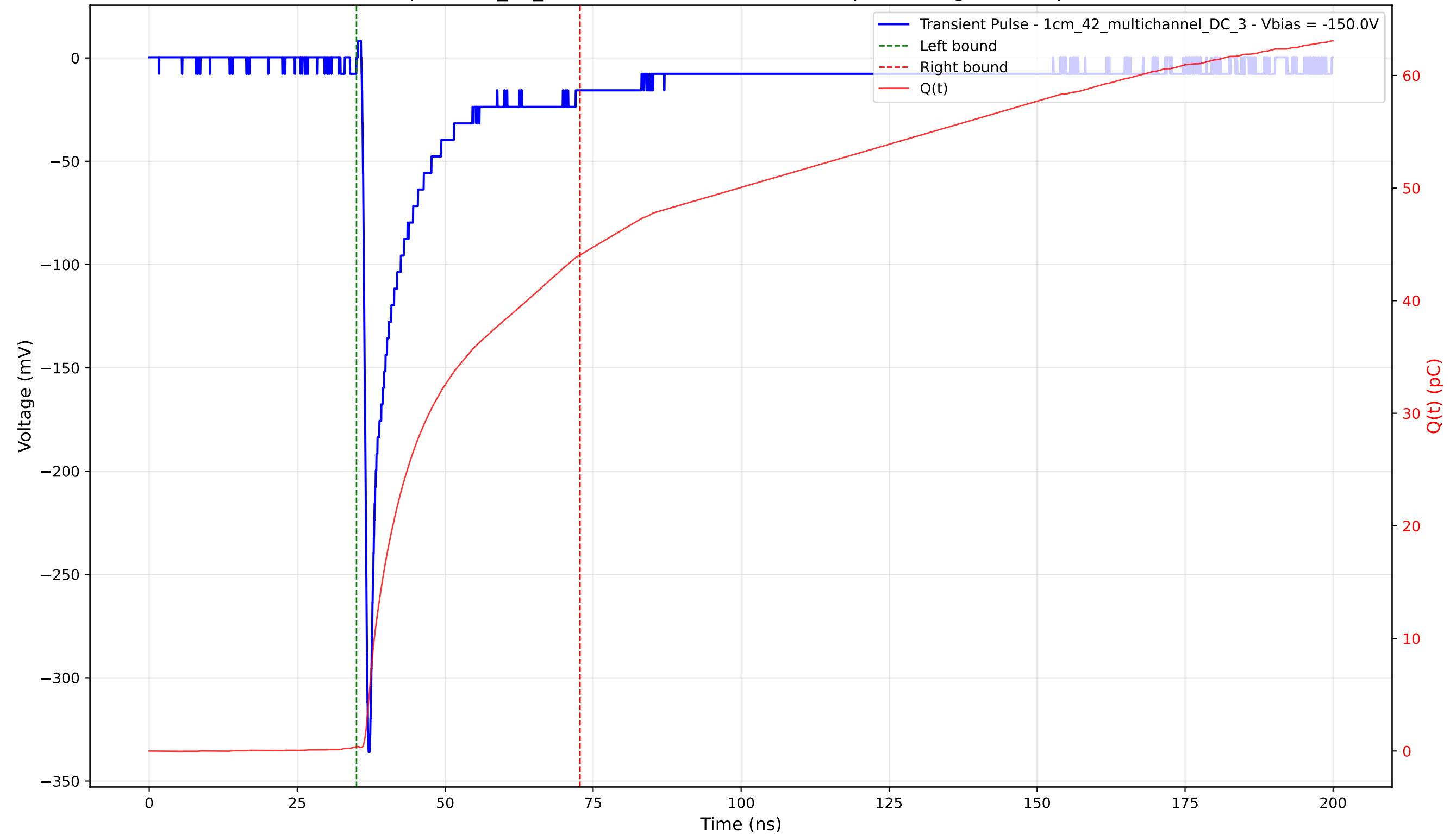
Transient Pulse - Sample: 1cm_42_multichannel - Position: 230.0 \mu\text{m} - Charge: 43.66 pC - Rise Time: 0.80 ns
