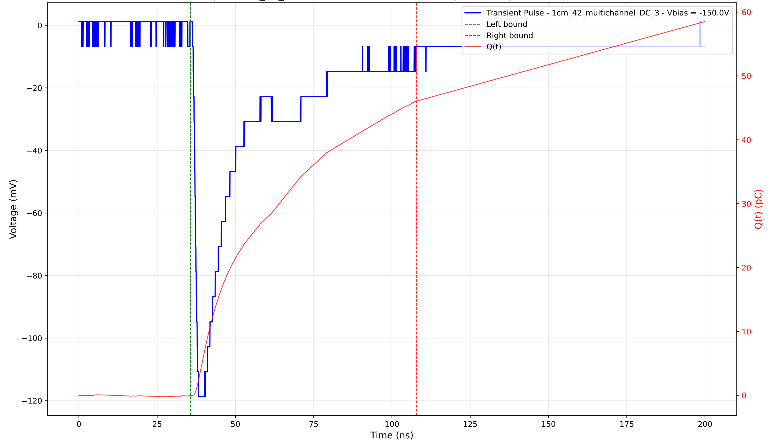
Transient Pulse - Sample: 1cm_42_multichannel - Position: 1610.0 \mu\text{m} - Charge: 46.09 pC - Rise Time: 1.41 ns
