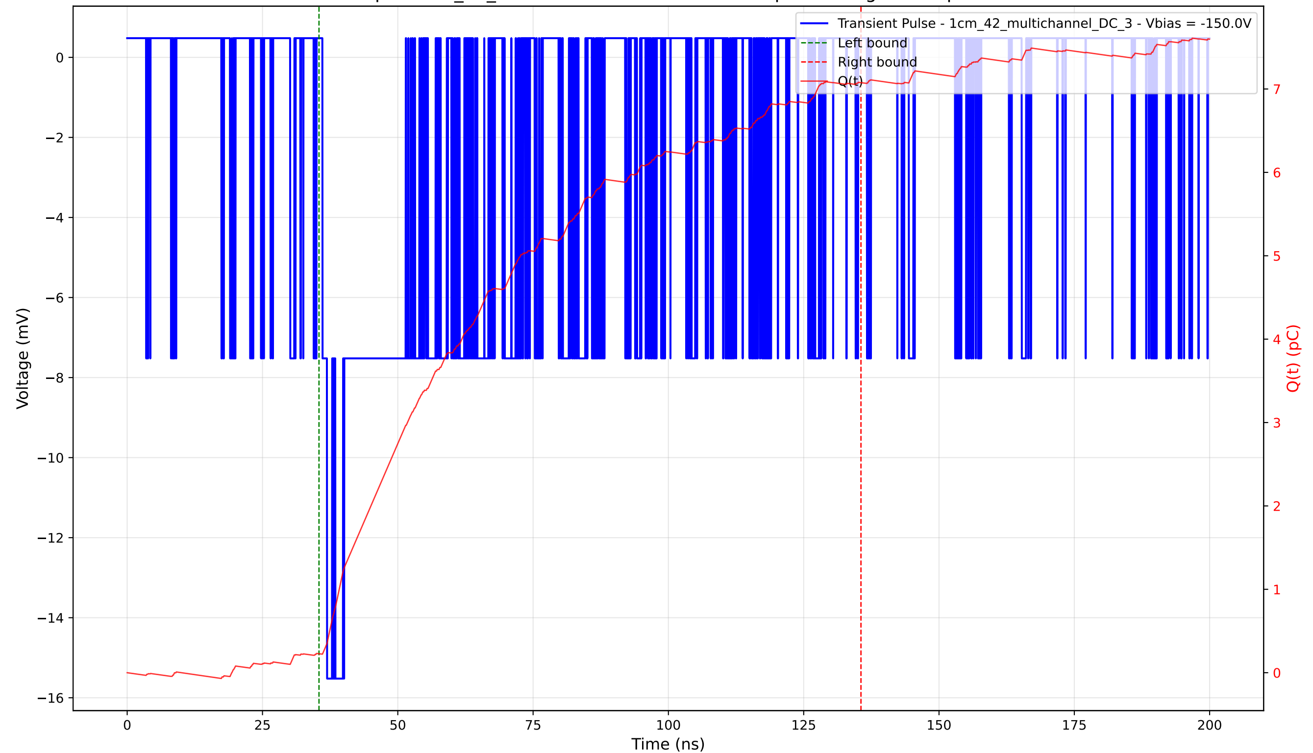
Transient Pulse - Sample: 1cm_42_multichannel - Position: 350.0 \mu\text{m} - Charge: 6.85 pC - Rise Time: 0.86 ns
