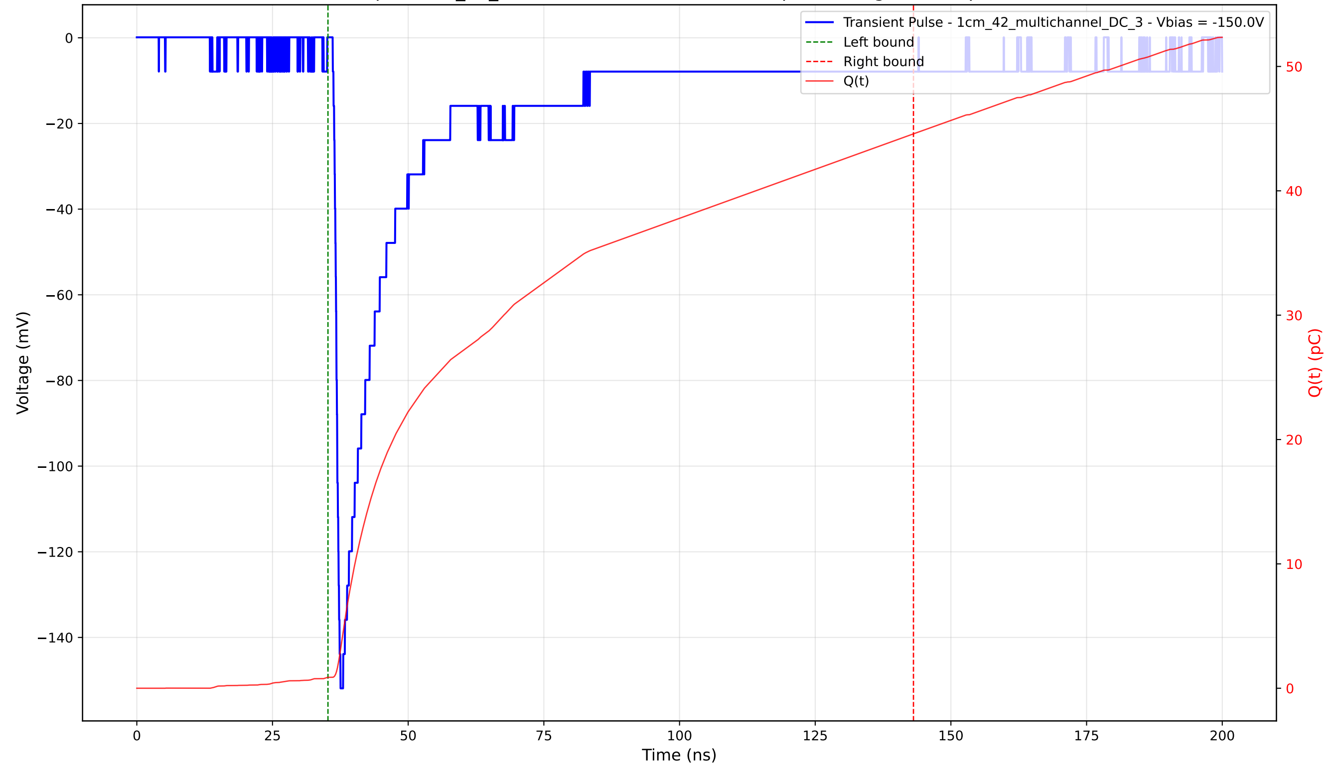
Transient Pulse - Sample: 1cm_42_multichannel - Position: 795.0 \mu\text{m} - Charge: 43.72 pC - Rise Time: 1.12 ns
