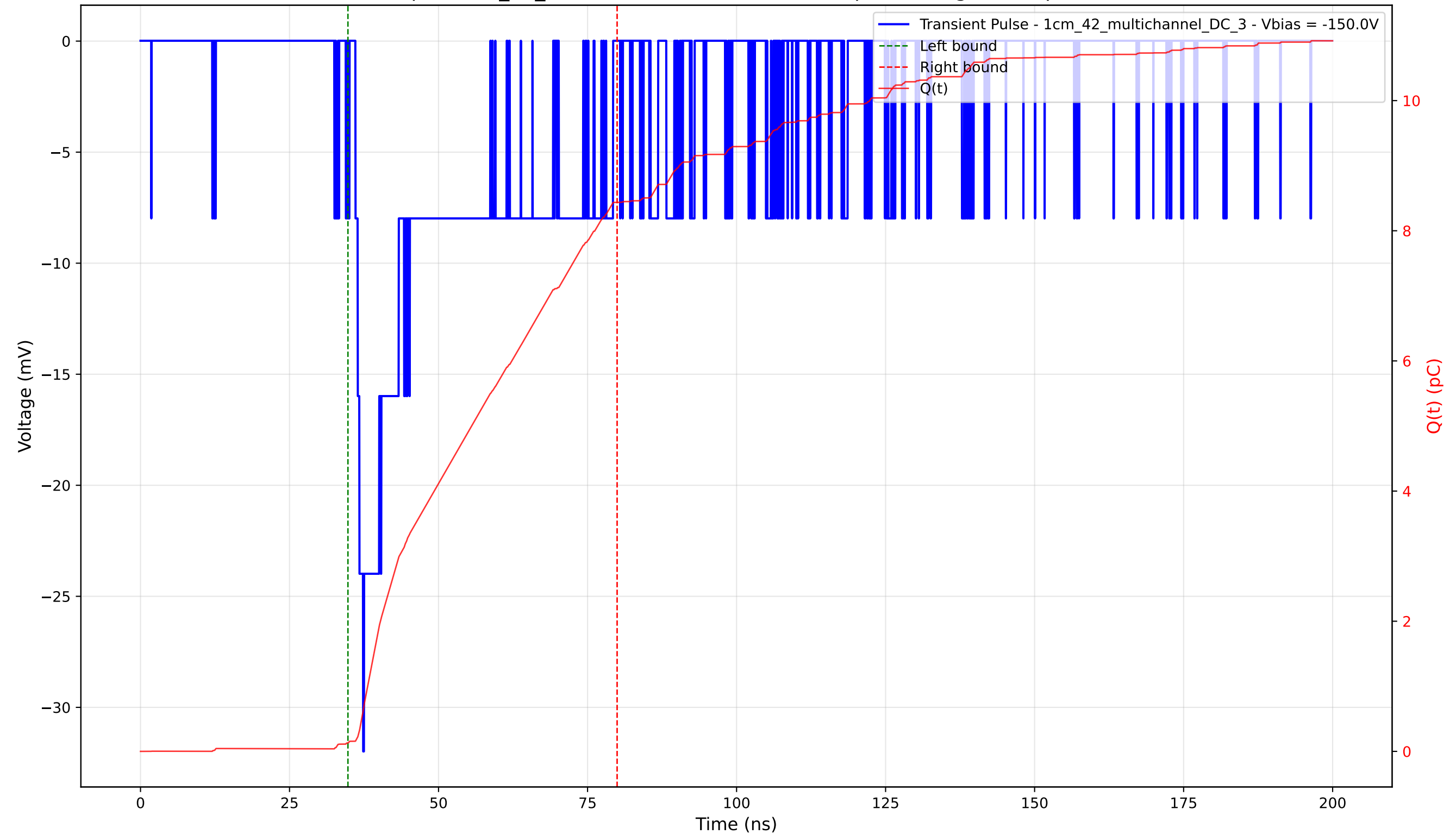
Transient Pulse - Sample: 1cm_42_multichannel - Position: 375.0 \mu\text{m} - Charge: 8.30 pC - Rise Time: 1.29 ns
