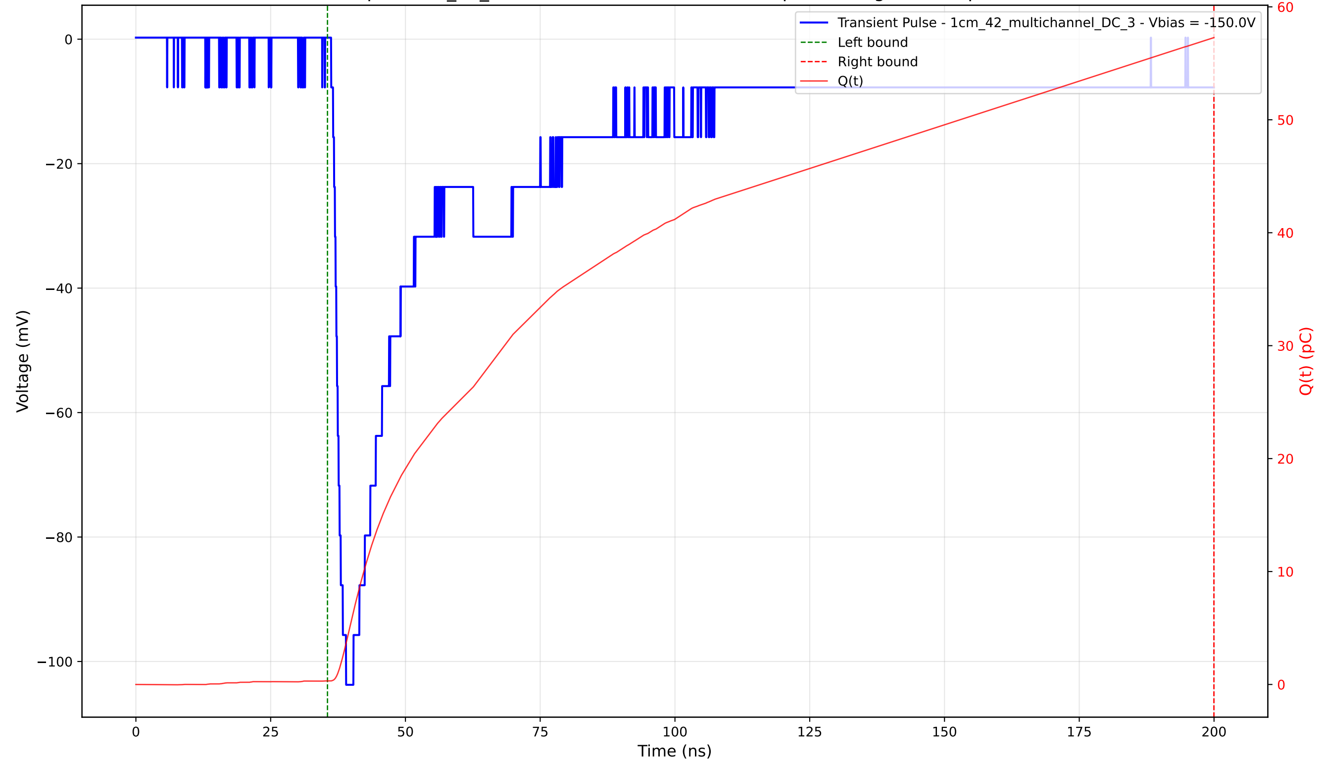
Transient Pulse - Sample: 1cm_42_multichannel - Position: 3015.0 \mu\text{m} - Charge: 56.97 pC - Rise Time: 1.81 ns
