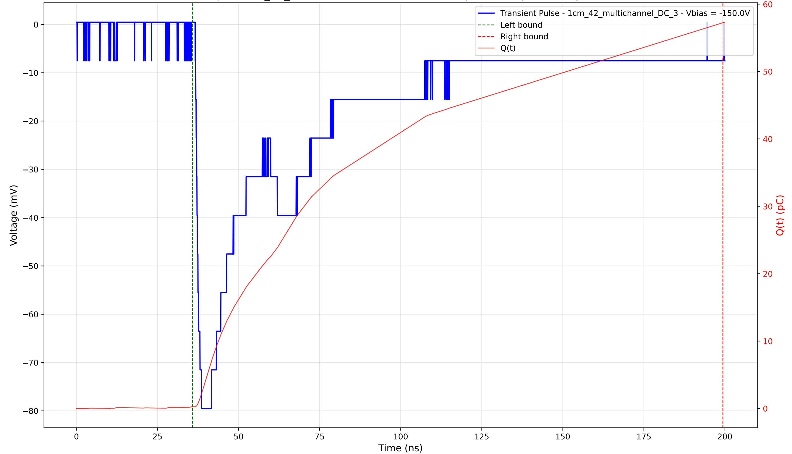
Transient Pulse - Sample: 1cm_42_multichannel - Position: 2275.0 \mu\text{m} - Charge: 57.00 pC - Rise Time: 1.82 ns
