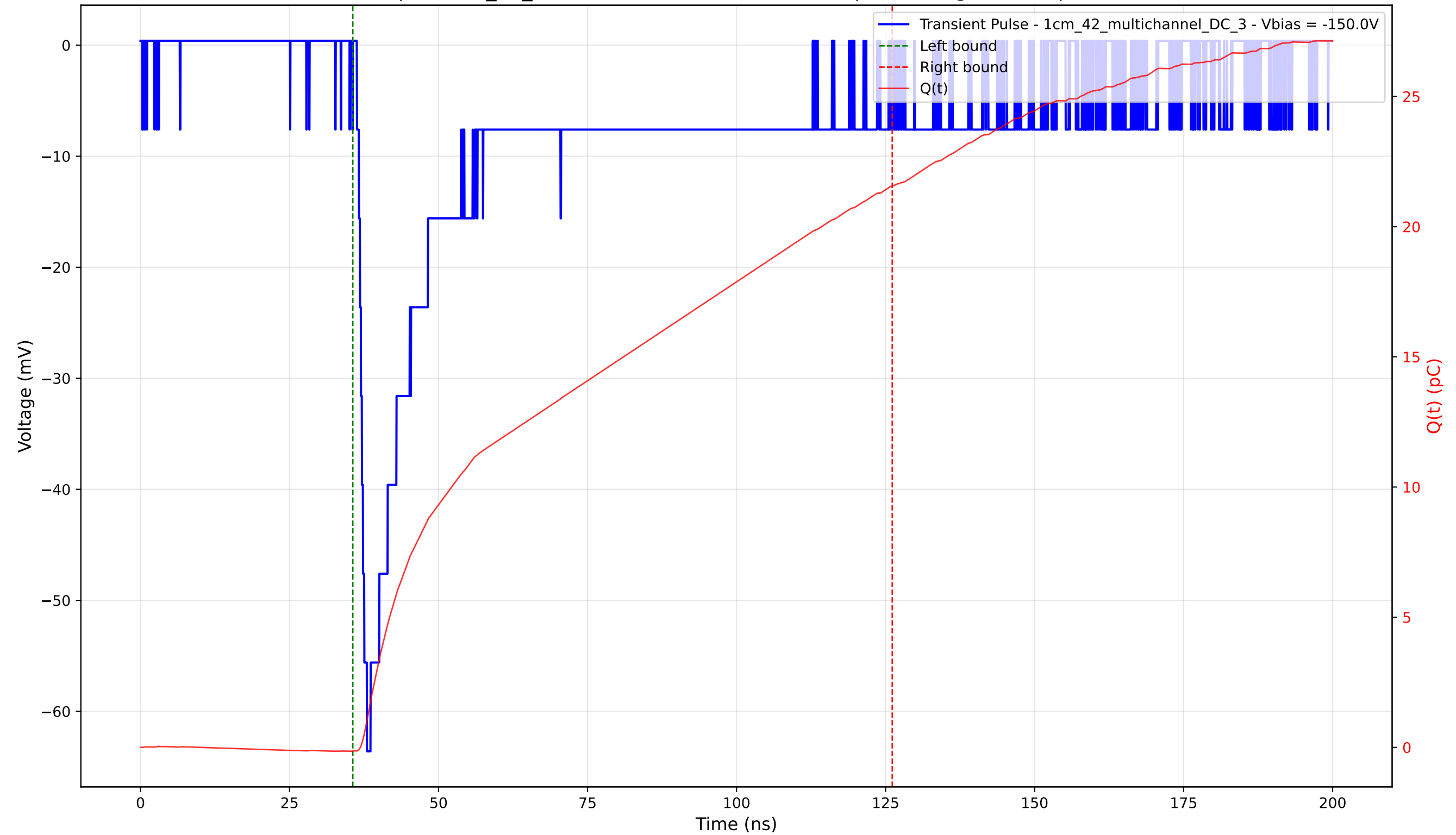
Transient Pulse - Sample: 1cm_42_multichannel - Position: 3845.0 \mu\text{m} - Charge: 21.69 pC - Rise Time: 1.68 ns
