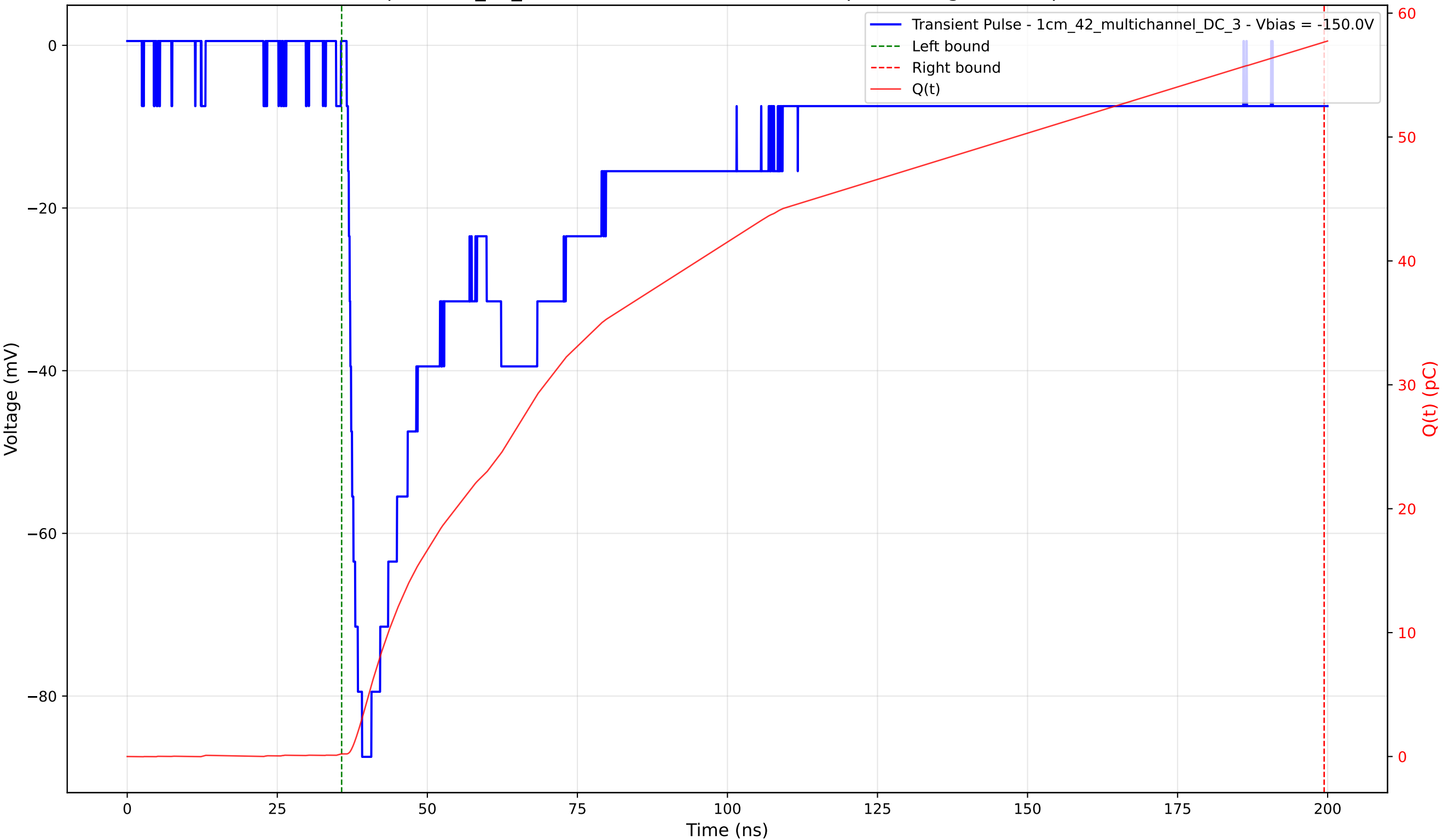
Transient Pulse - Sample: 1cm_42_multichannel - Position: 2225.0 \mu\text{m} - Charge: 57.45 pC - Rise Time: 1.66 ns
