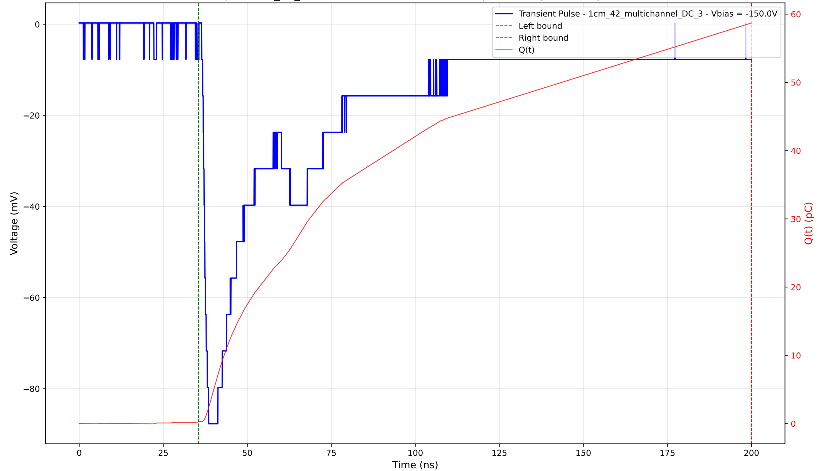
Transient Pulse - Sample: 1cm_42_multichannel - Position: 2100.0 \mu\text{m} - Charge: 58.45 pC - Rise Time: 1.40 ns
