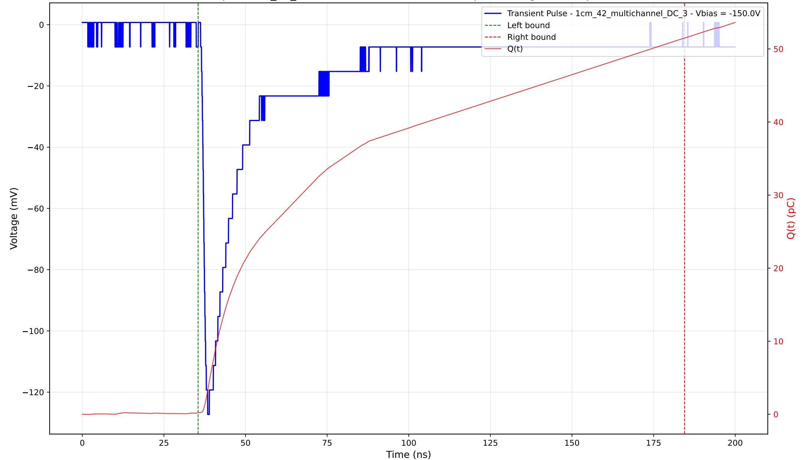
Transient Pulse - Sample: 1cm_42_multichannel - Position: 3555.0 \mu\text{m} - Charge: 51.26 pC - Rise Time: 1.47 ns
