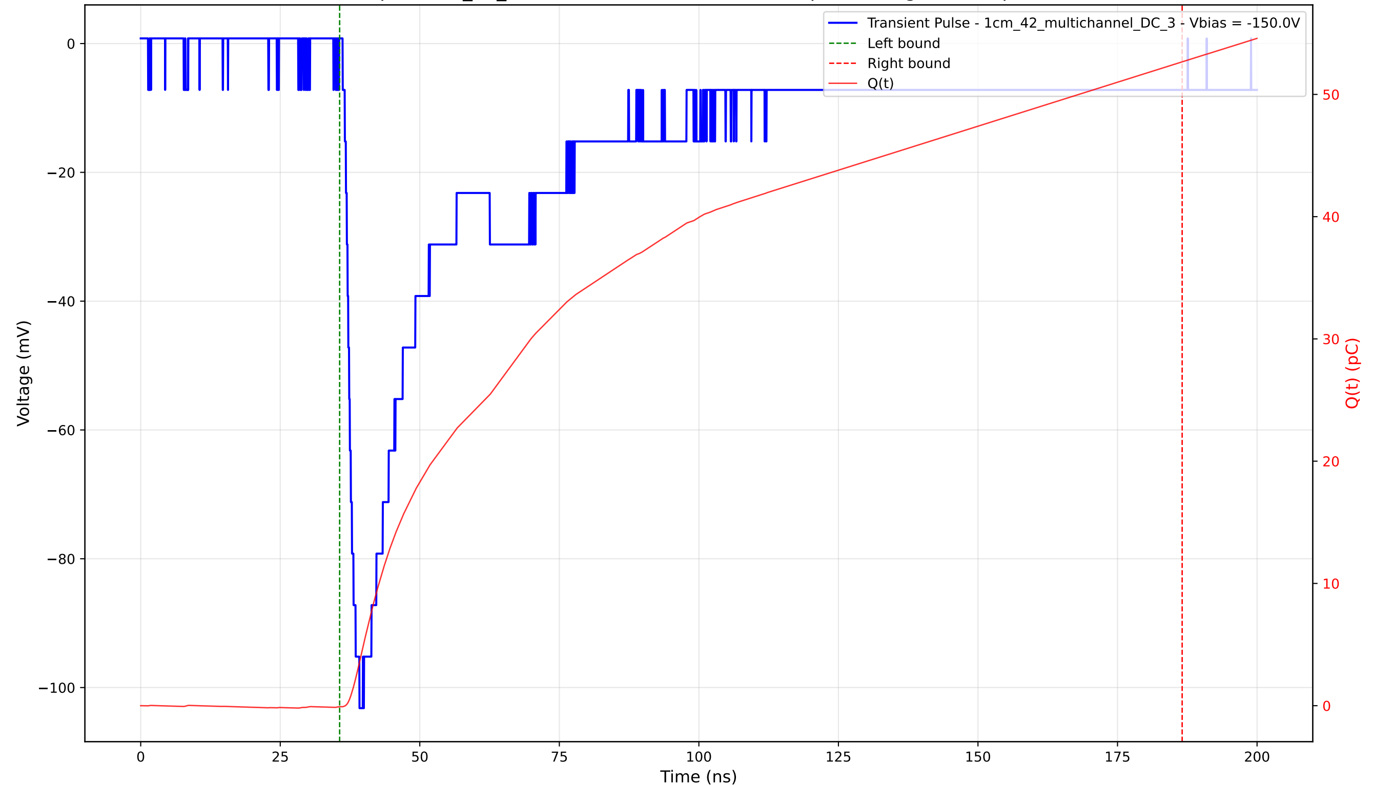
Transient Pulse - Sample: 1cm_42_multichannel - Position: 2975.0 \mu\text{m} - Charge: 52.76 pC - Rise Time: 1.95 ns
