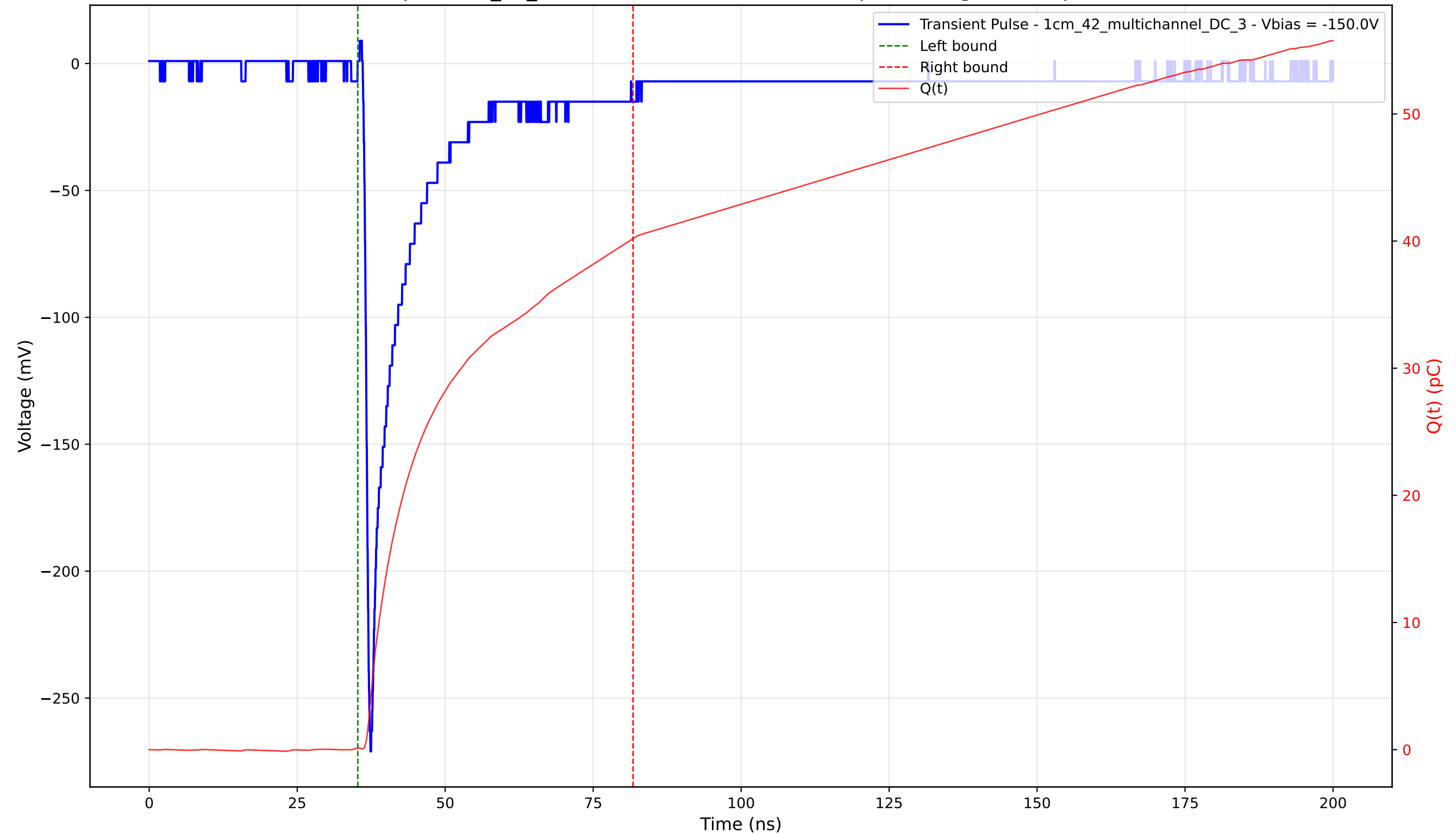
Transient Pulse - Sample: 1cm_42_multichannel - Position: 4520.0 \mu\text{m} - Charge: 40.07 pC - Rise Time: 0.87 ns
