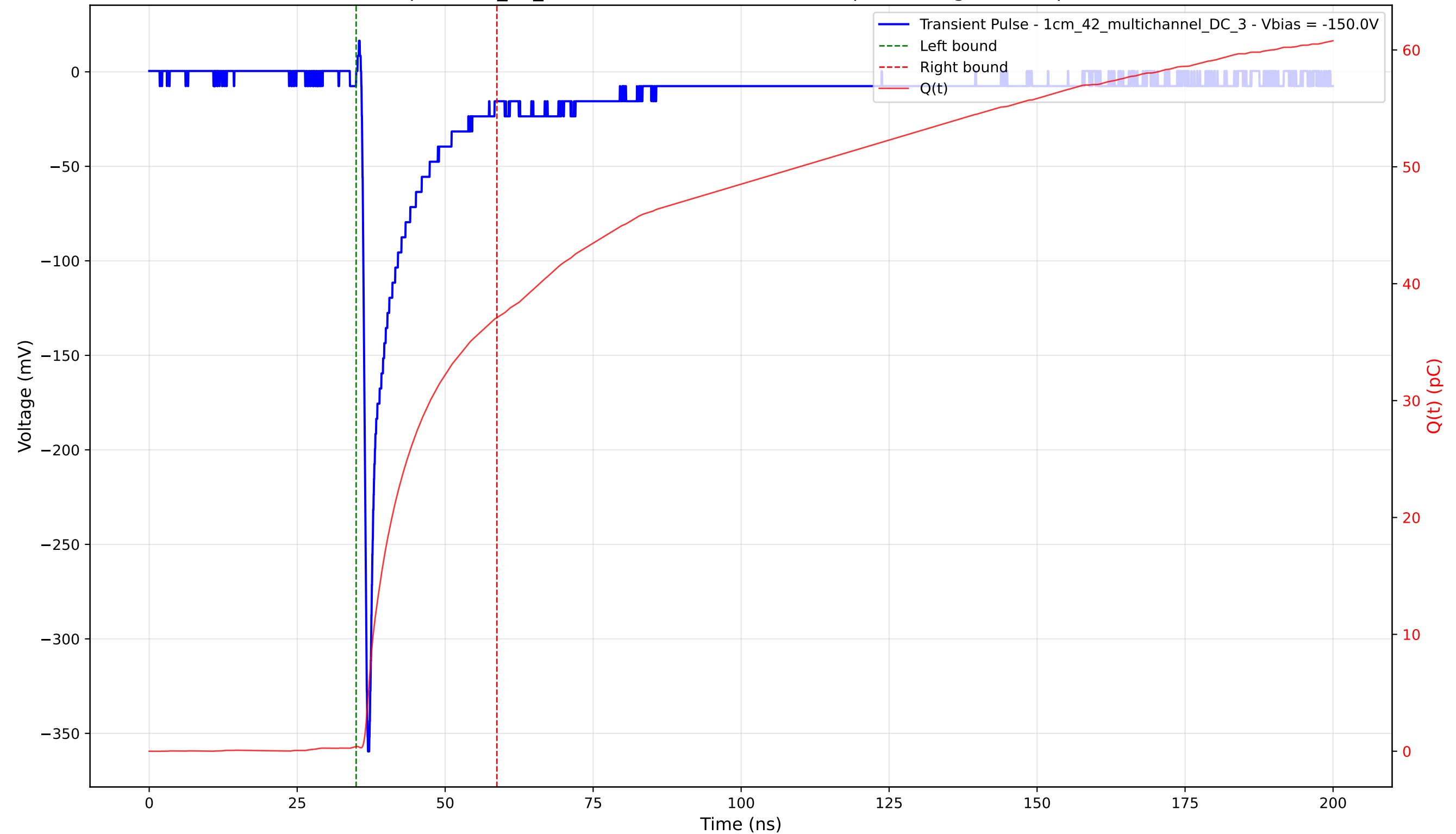
Transient Pulse - Sample: 1cm_42_multichannel - Position: 135.0 \mu\text{m} - Charge: 36.68 pC - Rise Time: 0.79 ns
