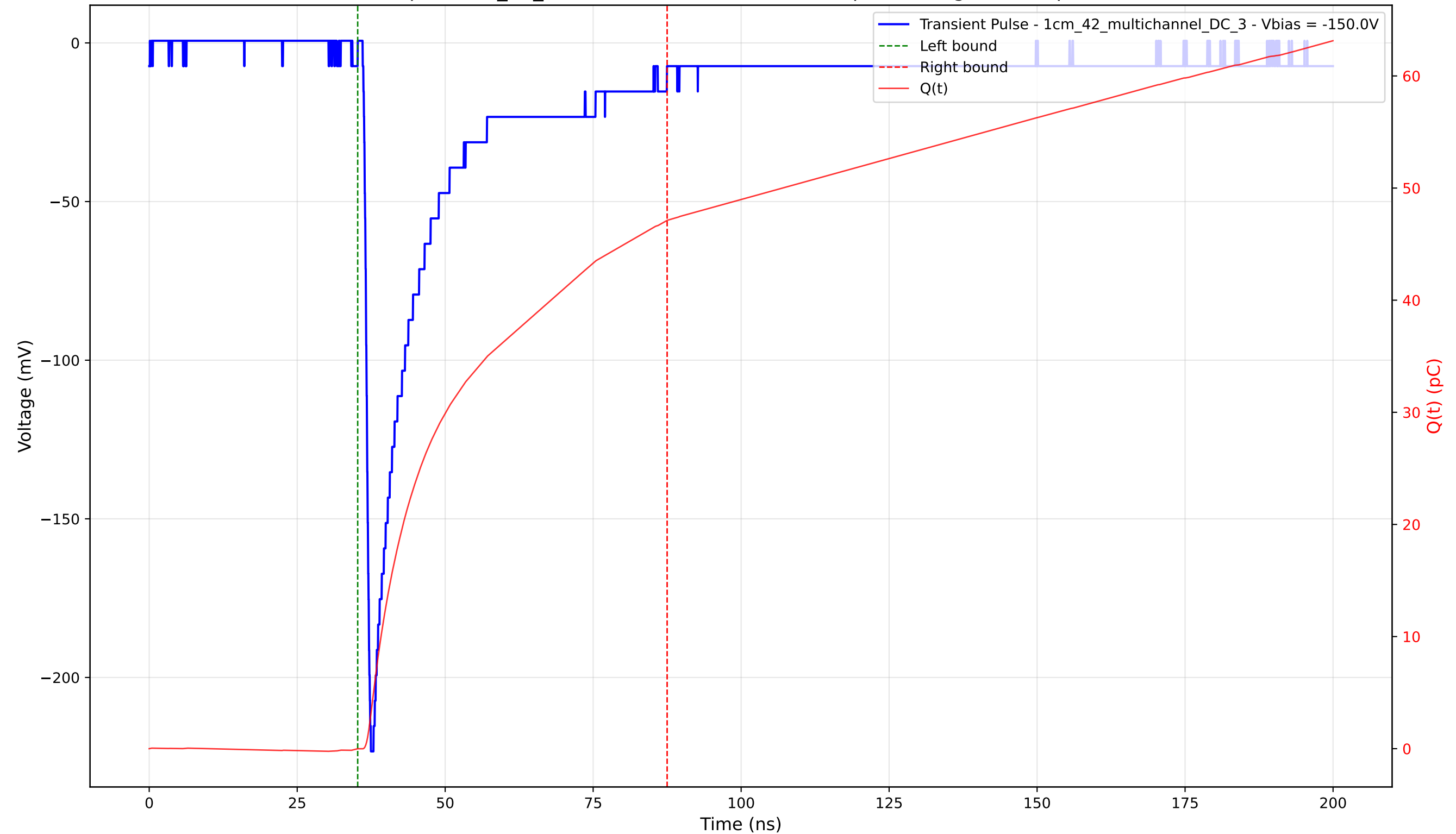
Transient Pulse - Sample: 1cm_42_multichannel - Position: 695.0 \mu\text{m} - Charge: 47.13 pC - Rise Time: 1.00 ns
