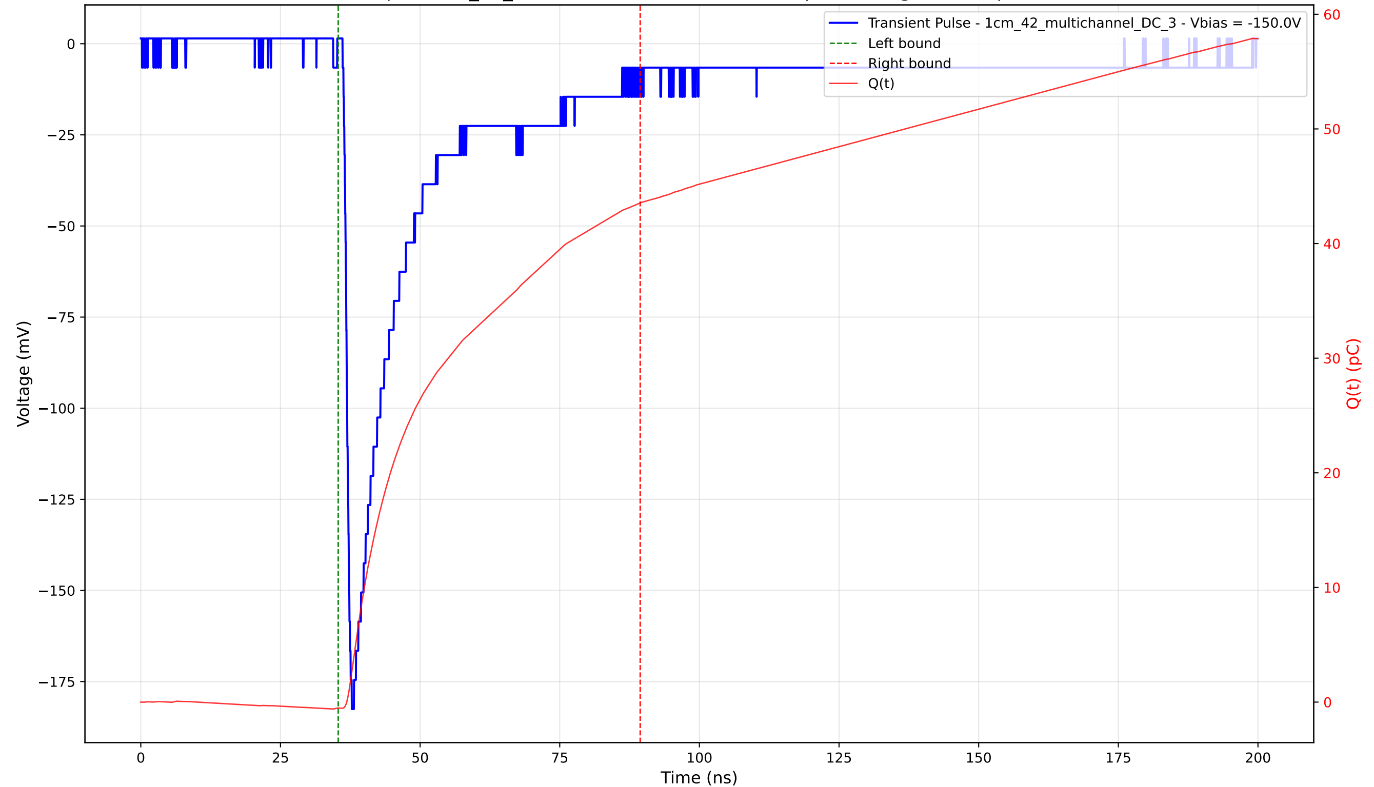
Transient Pulse - Sample: 1cm_42_multichannel - Position: 940.0 \mu\text{m} - Charge: 44.07 pC - Rise Time: 1.09 ns
