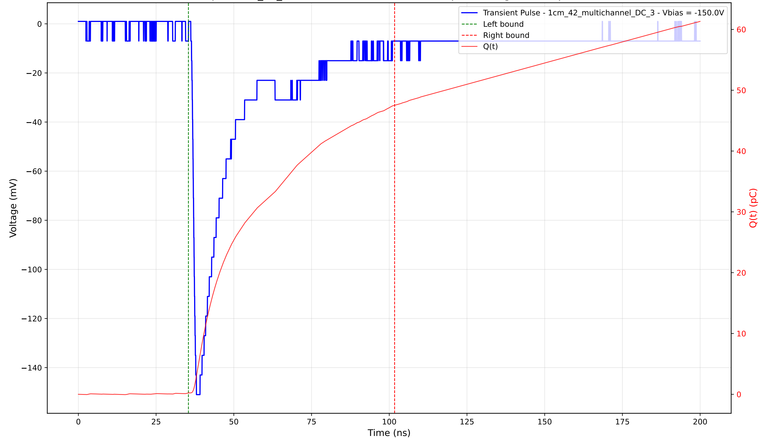
Transient Pulse - Sample: 1cm_42_multichannel - Position: 1255.0 \mu\text{m} - Charge: 47.28 pC - Rise Time: 1.26 ns
