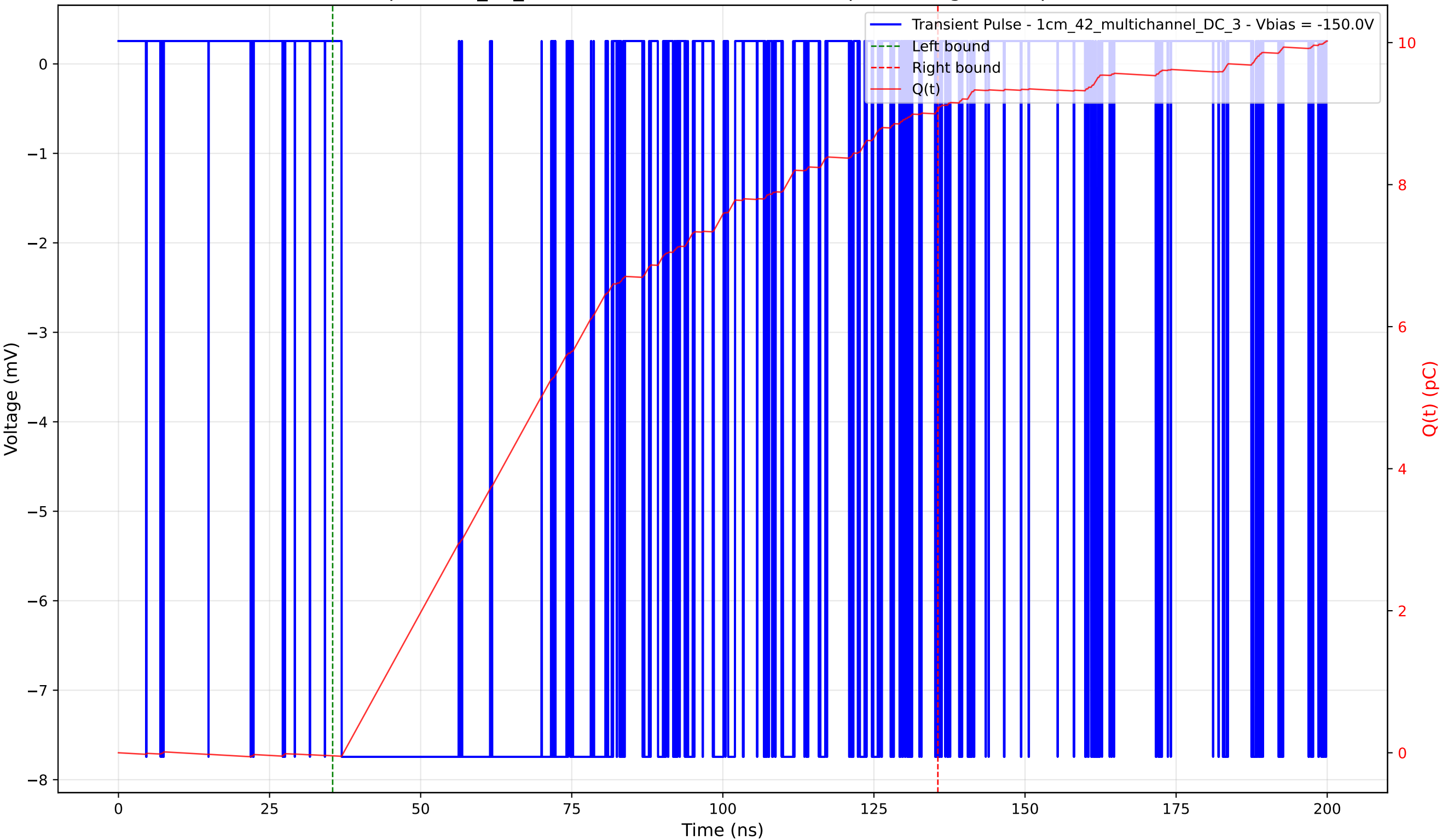
Transient Pulse - Sample: 1cm_42_multichannel - Position: 2390.0 \mu\text{m} - Charge: 9.09 pC - Rise Time: 0.02 ns
