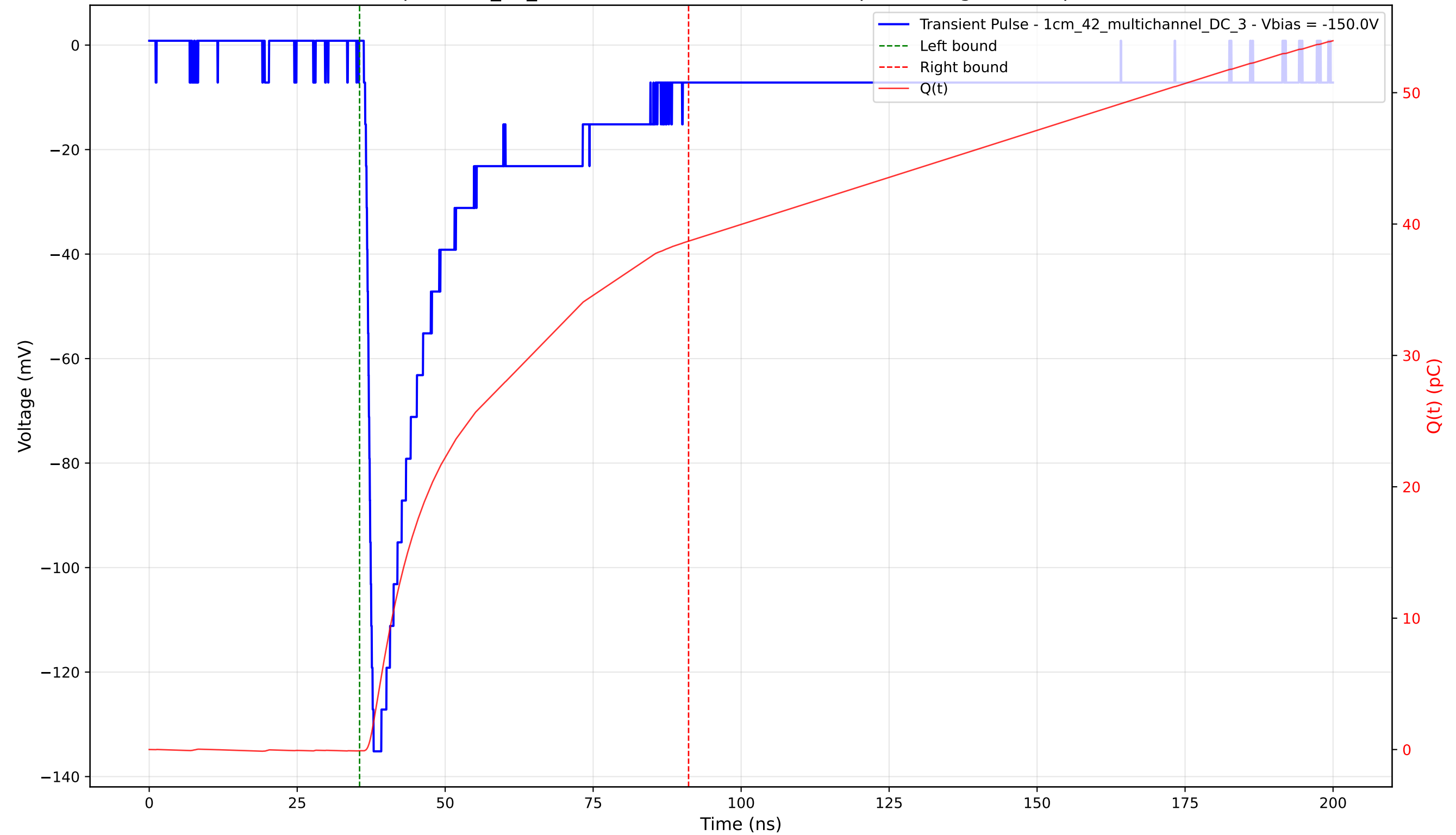
Transient Pulse - Sample: 1cm_42_multichannel - Position: 3715.0 \mu\text{m} - Charge: 38.79 pC - Rise Time: 1.26 ns
