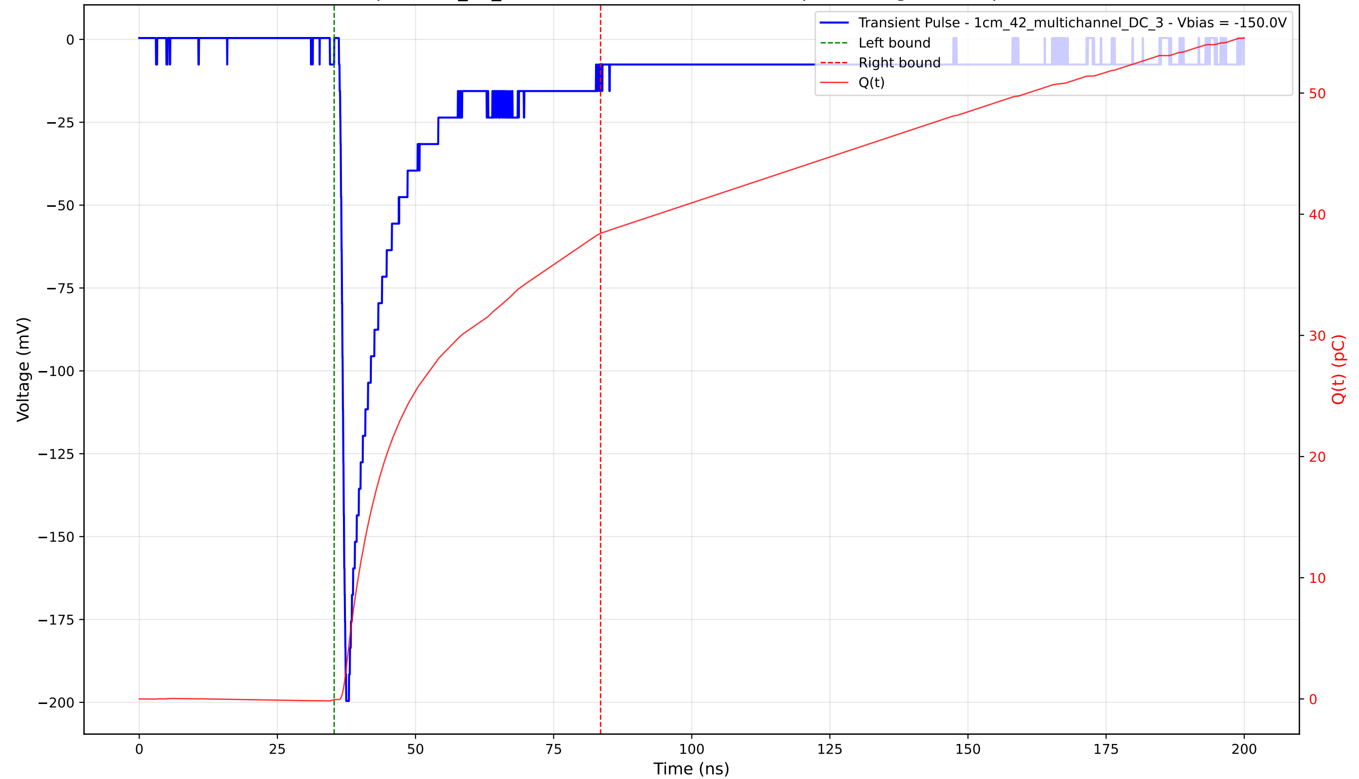
Transient Pulse - Sample: 1cm_42_multichannel - Position: 4260.0 \mu\text{m} - Charge: 38.47 pC - Rise Time: 0.93 ns
