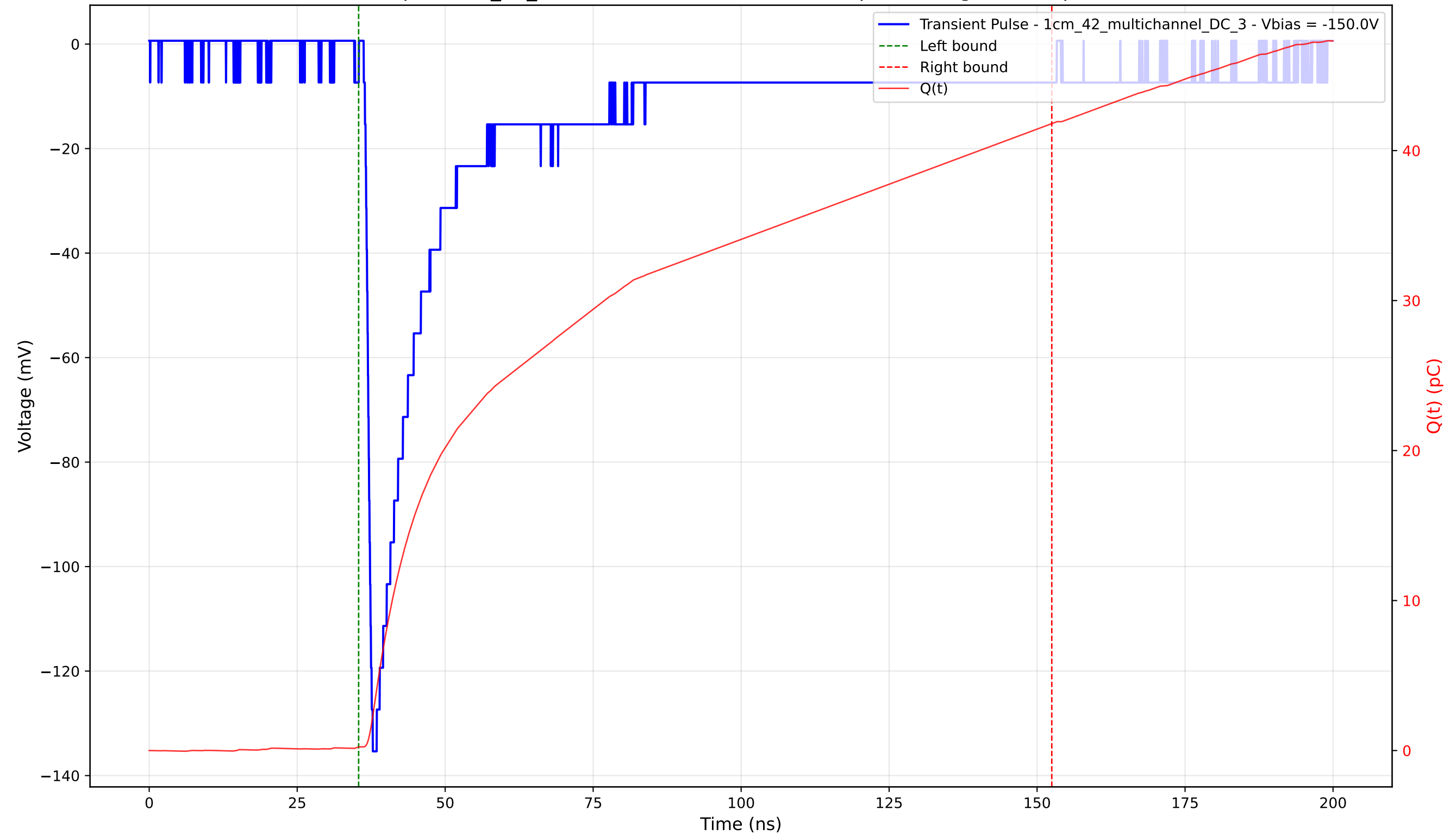
Transient Pulse - Sample: 1cm_42_multichannel - Position: 3955.0 \mu\text{m} - Charge: 41.57 pC - Rise Time: 1.14 ns
