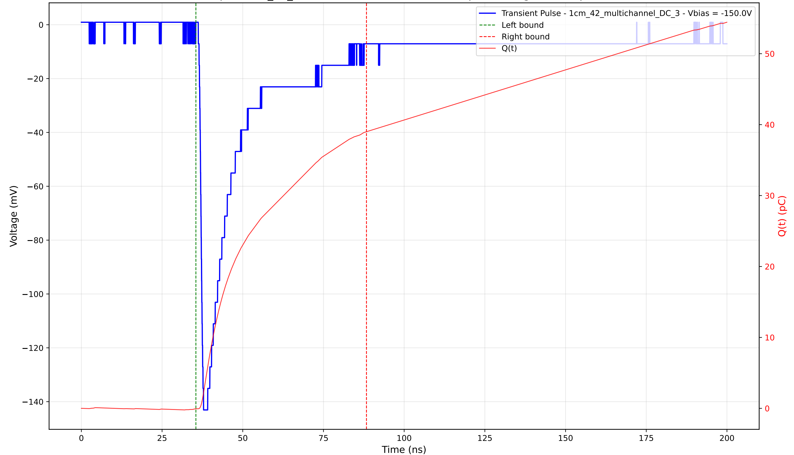
Transient Pulse - Sample: 1cm_42_multichannel - Position: 3785.0 \mu\text{m} - Charge: 39.06 pC - Rise Time: 1.22 ns
