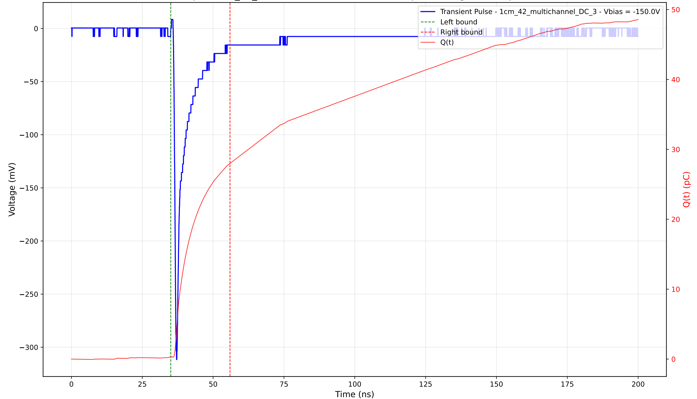
Transient Pulse - Sample: 1cm_42_multichannel - Position: 4830.0 \mu\text{m} - Charge: 27.64 pC - Rise Time: 0.80 ns
