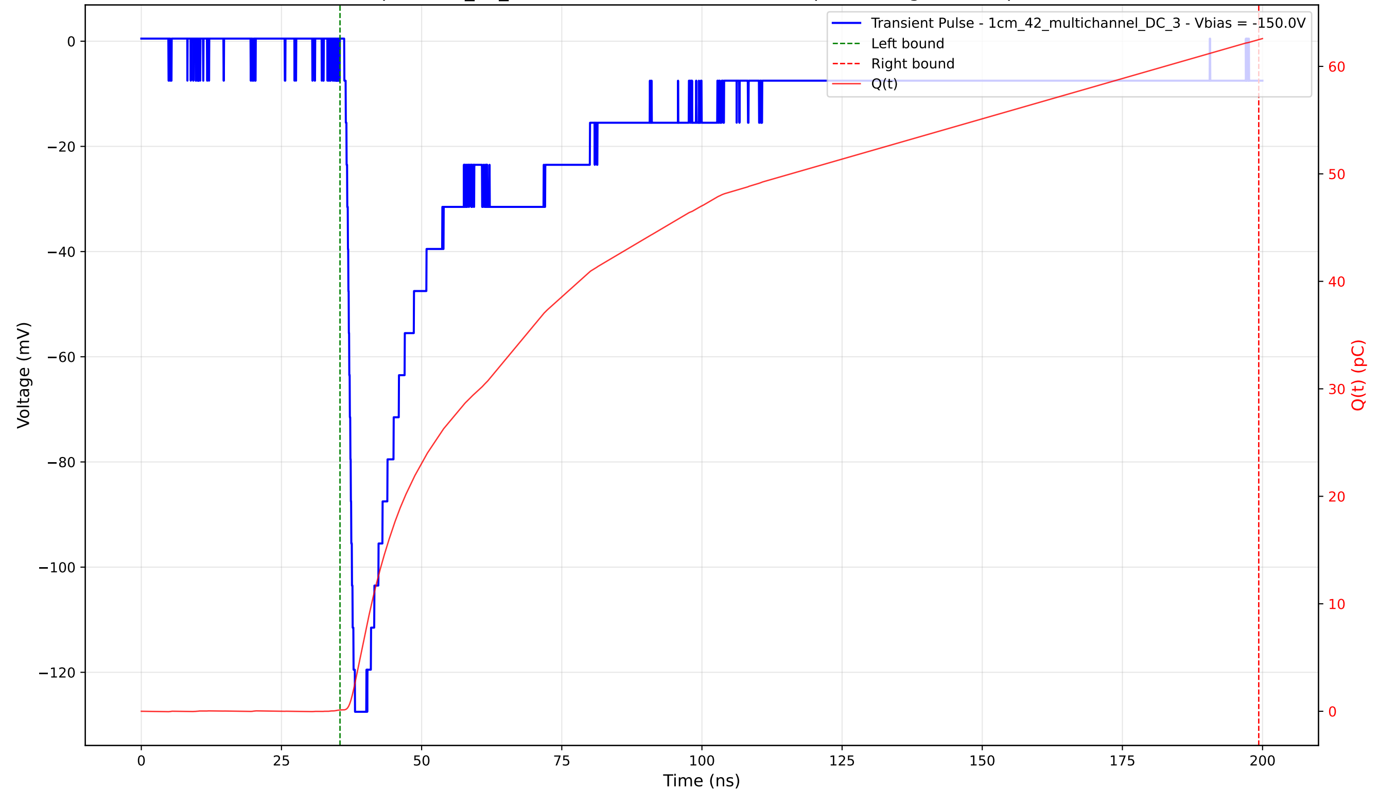
Transient Pulse - Sample: 1cm_42_multichannel - Position: 1520.0 \mu\text{m} - Charge: 62.35 pC - Rise Time: 1.39 ns
