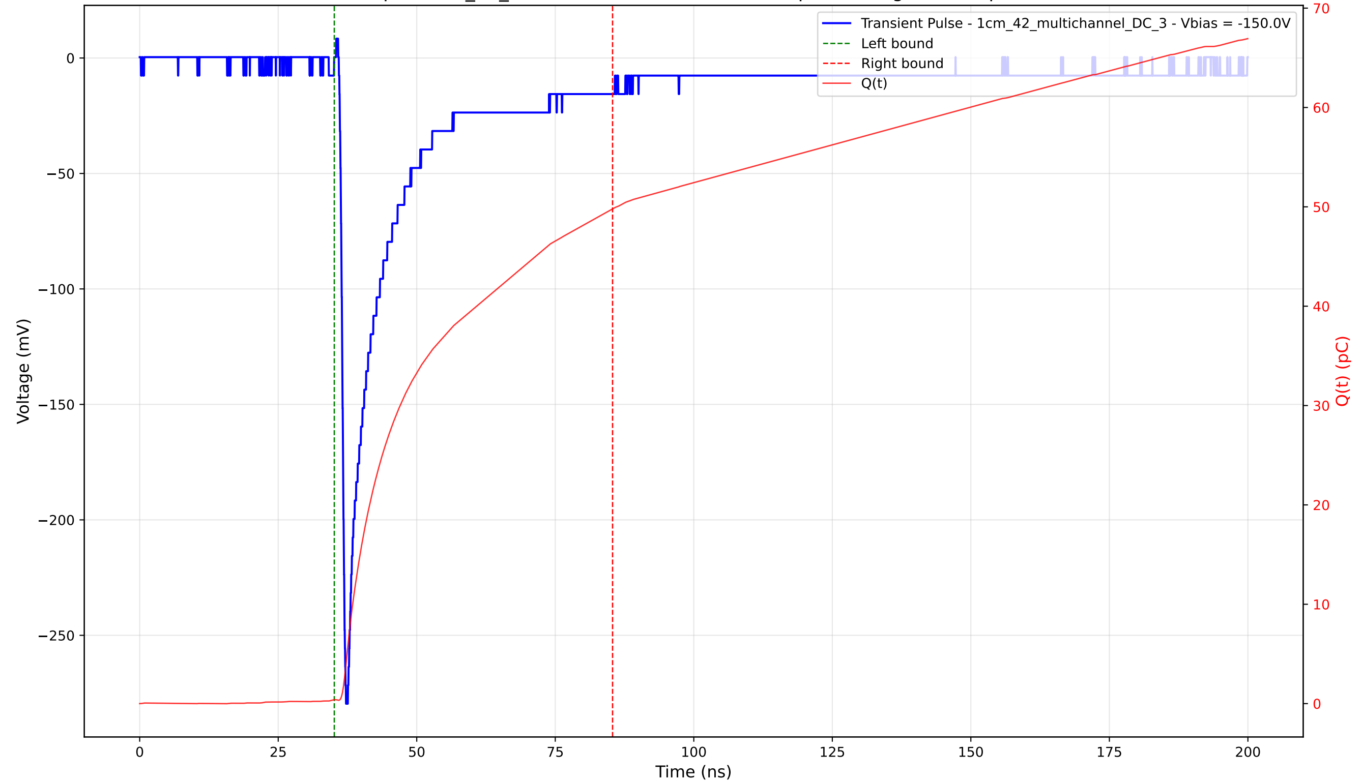
Transient Pulse - Sample: 1cm_42_multichannel - Position: 475.0 \mu\text{m} - Charge: 49.40 pC - Rise Time: 0.89 ns
