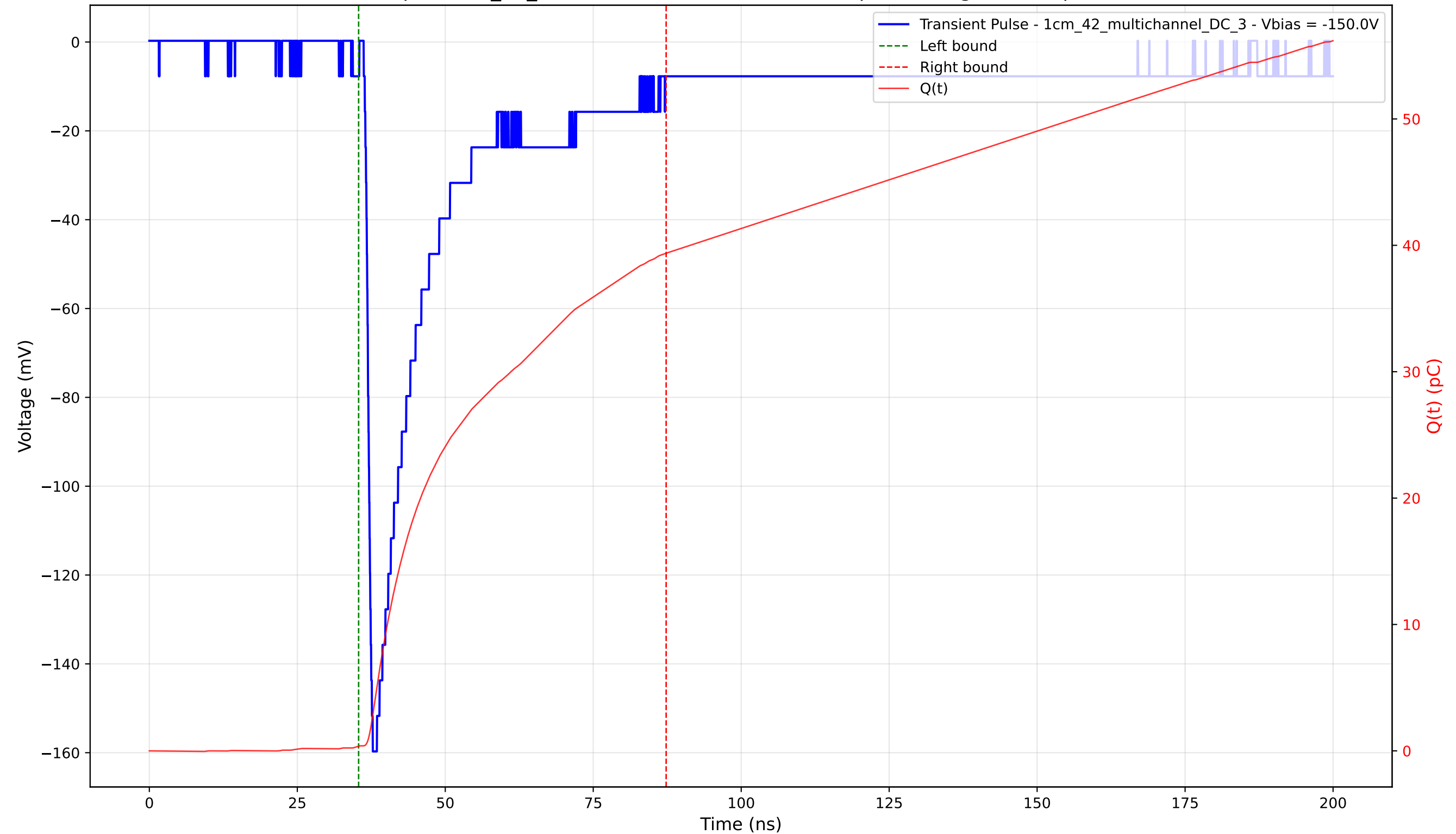
Transient Pulse - Sample: 1cm_42_multichannel - Position: 3970.0 \mu\text{m} - Charge: 39.00 pC - Rise Time: 1.12 ns
