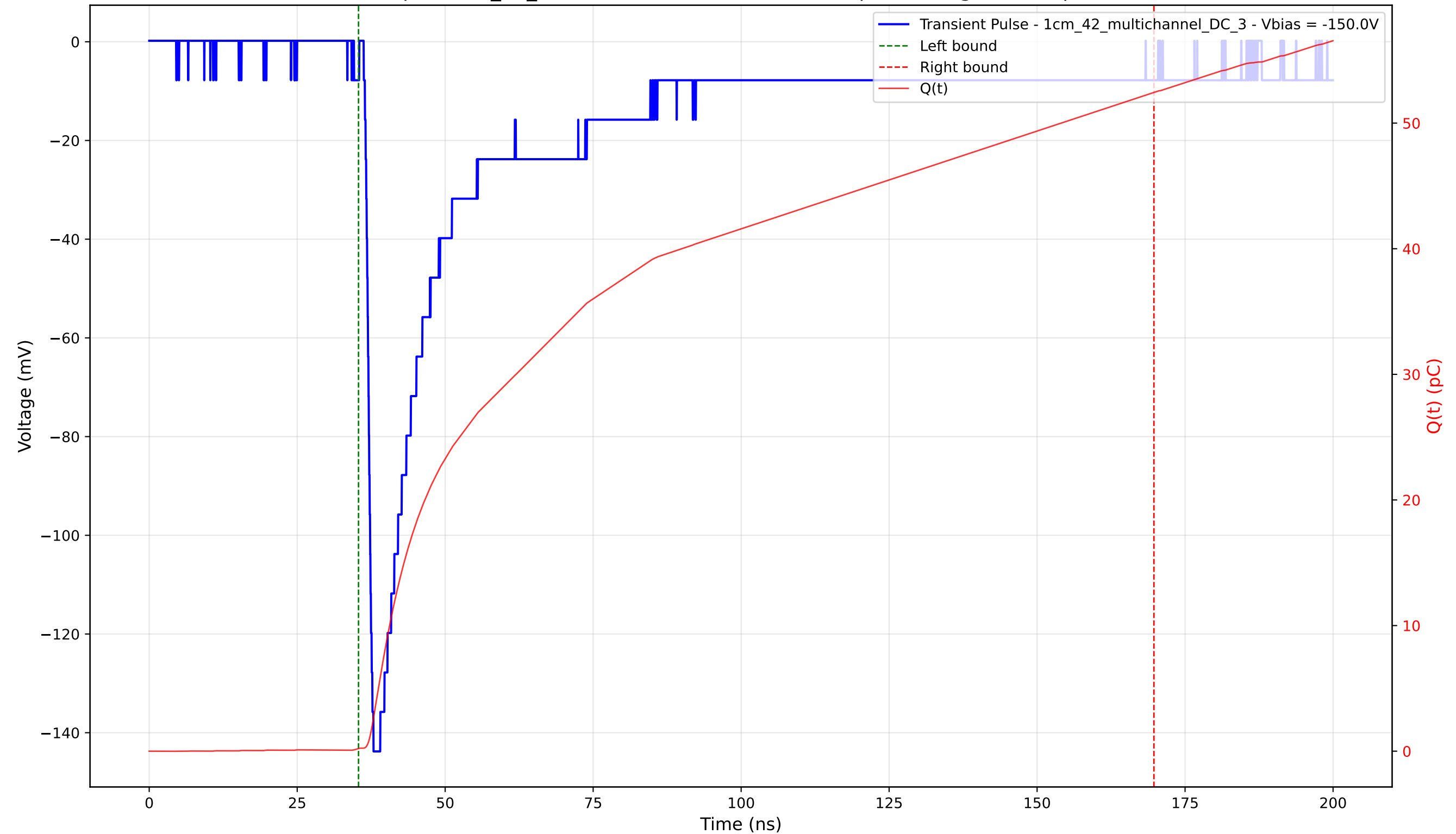
Transient Pulse - Sample: 1cm_42_multichannel - Position: 3795.0 \mu\text{m} - Charge: 52.23 pC - Rise Time: 1.26 ns
