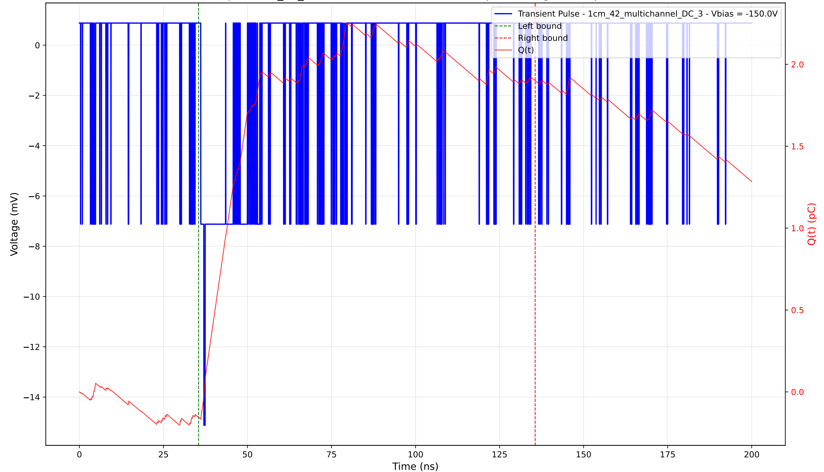
Transient Pulse - Sample: 1cm_42_multichannel - Position: 4900.0 \mu\text{m} - Charge: 2.06 pC - Rise Time: 0.94 ns
