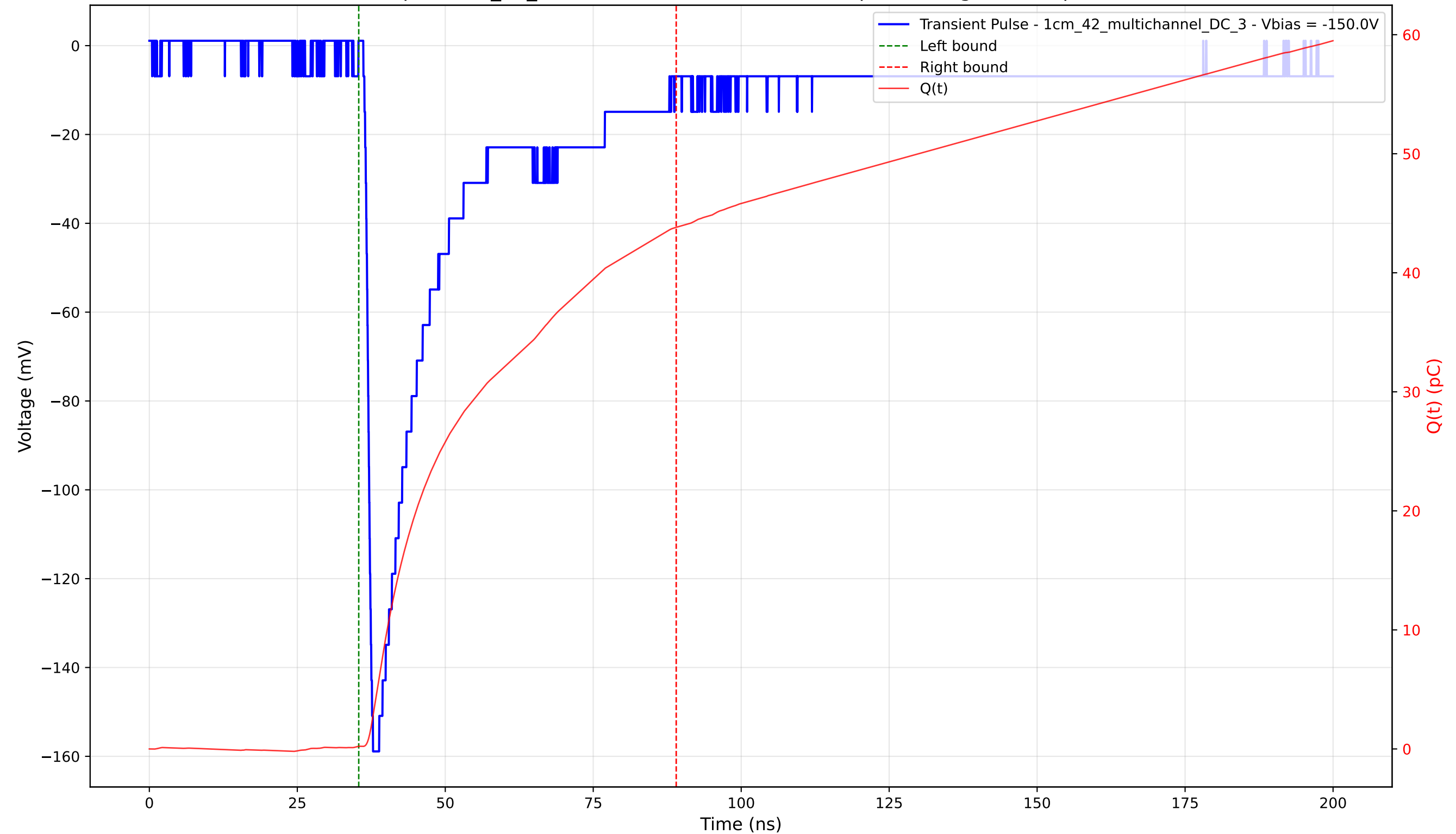
Transient Pulse - Sample: 1cm_42_multichannel - Position: 1115.0 \mu\text{m} - Charge: 43.59 pC - Rise Time: 1.18 ns
