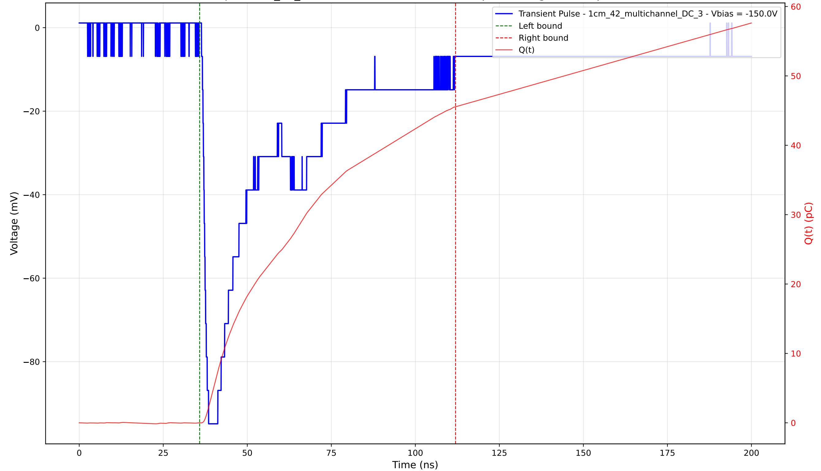
Transient Pulse - Sample: 1cm_42_multichannel - Position: 2010.0 \mu\text{m} - Charge: 45.56 pC - Rise Time: 1.43 ns
