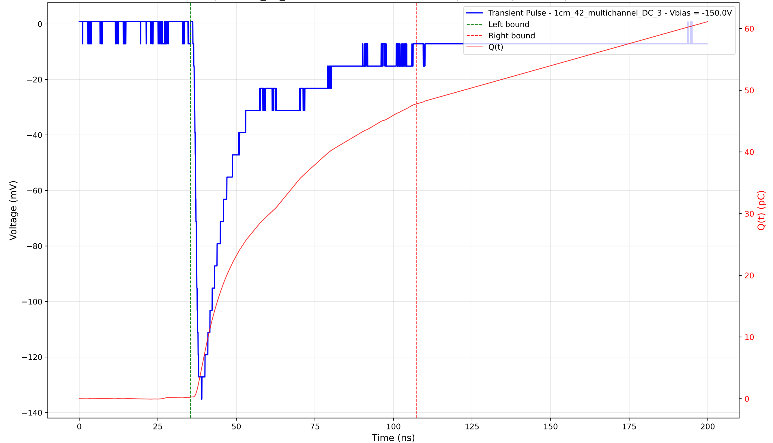
Transient Pulse - Sample: 1cm_42_multichannel - Position: 1495.0 \mu\text{m} - Charge: 47.49 pC - Rise Time: 1.58 ns
