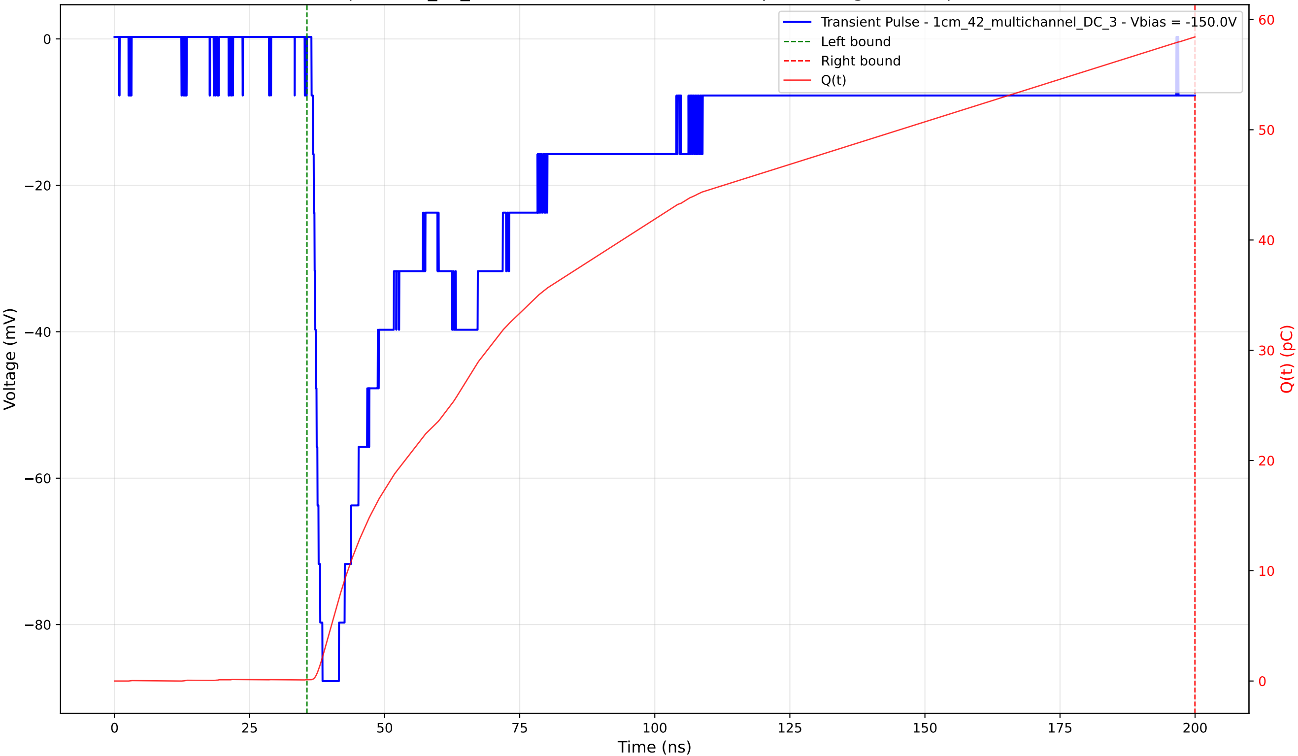
Transient Pulse - Sample: 1cm_42_multichannel - Position: 2105.0 \mu\text{m} - Charge: 58.29 pC - Rise Time: 1.36 ns
