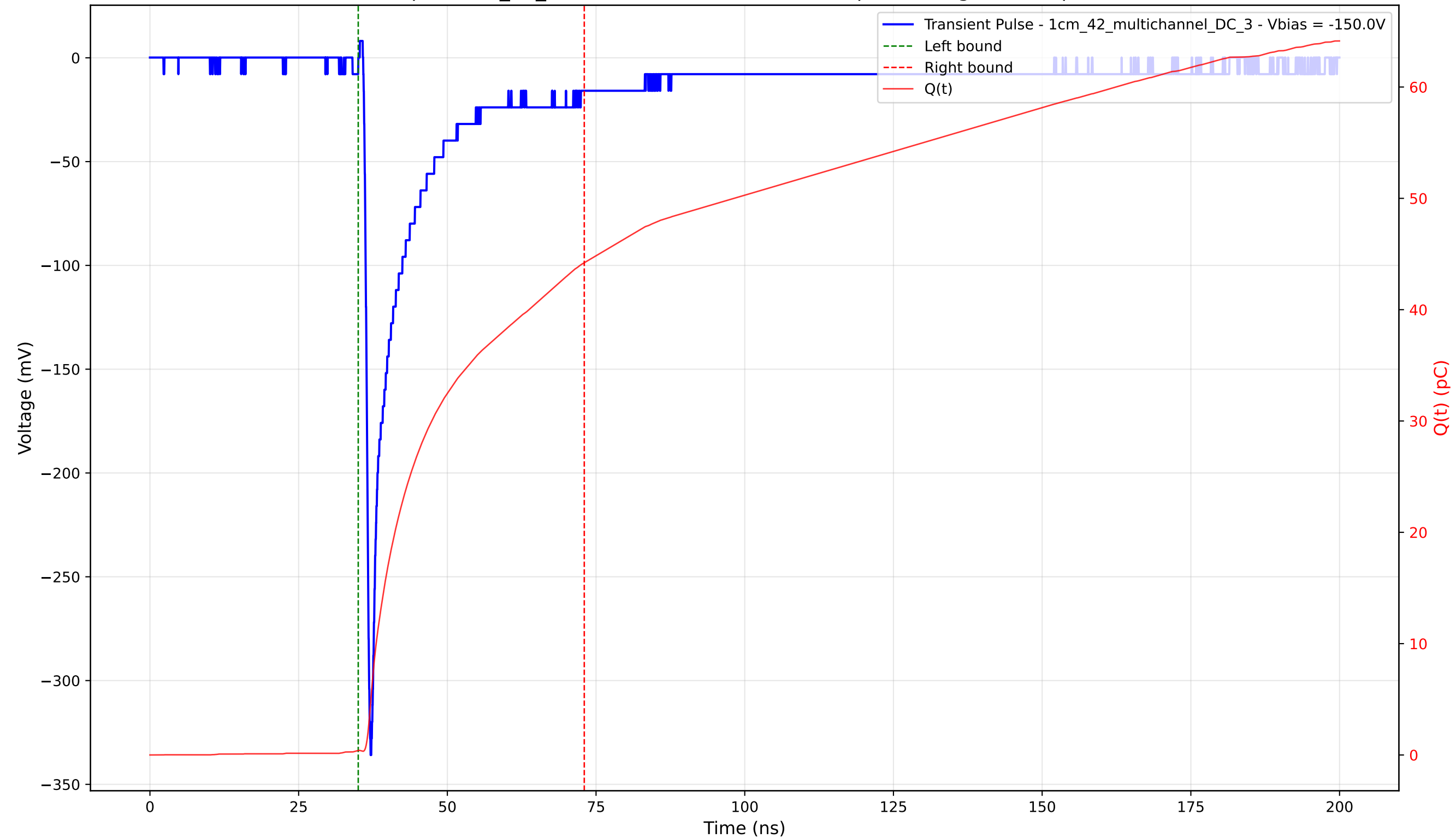
Transient Pulse - Sample: 1cm_42_multichannel - Position: 235.0 \mu\text{m} - Charge: 43.80 pC - Rise Time: 0.82 ns
