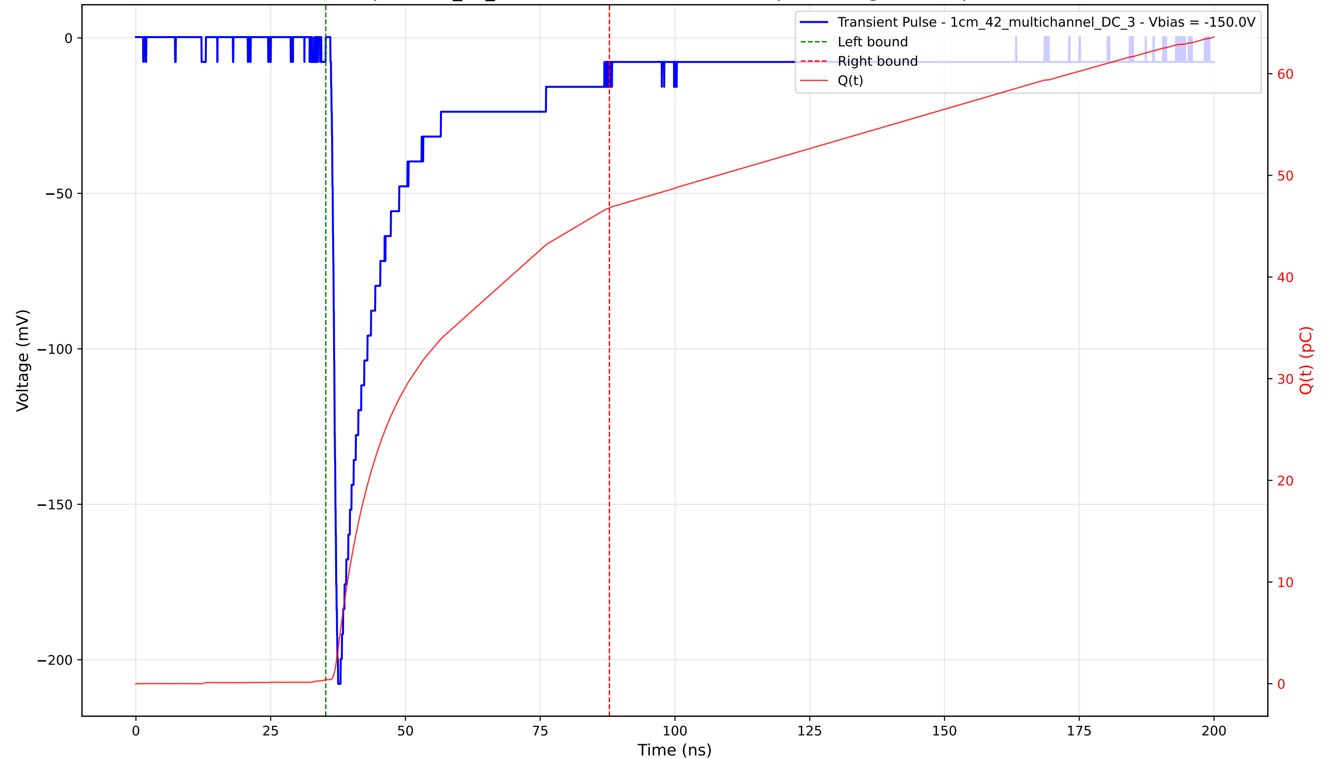
Transient Pulse - Sample: 1cm_42_multichannel - Position: 755.0 \mu\text{m} - Charge: 46.40 pC - Rise Time: 1.03 ns
