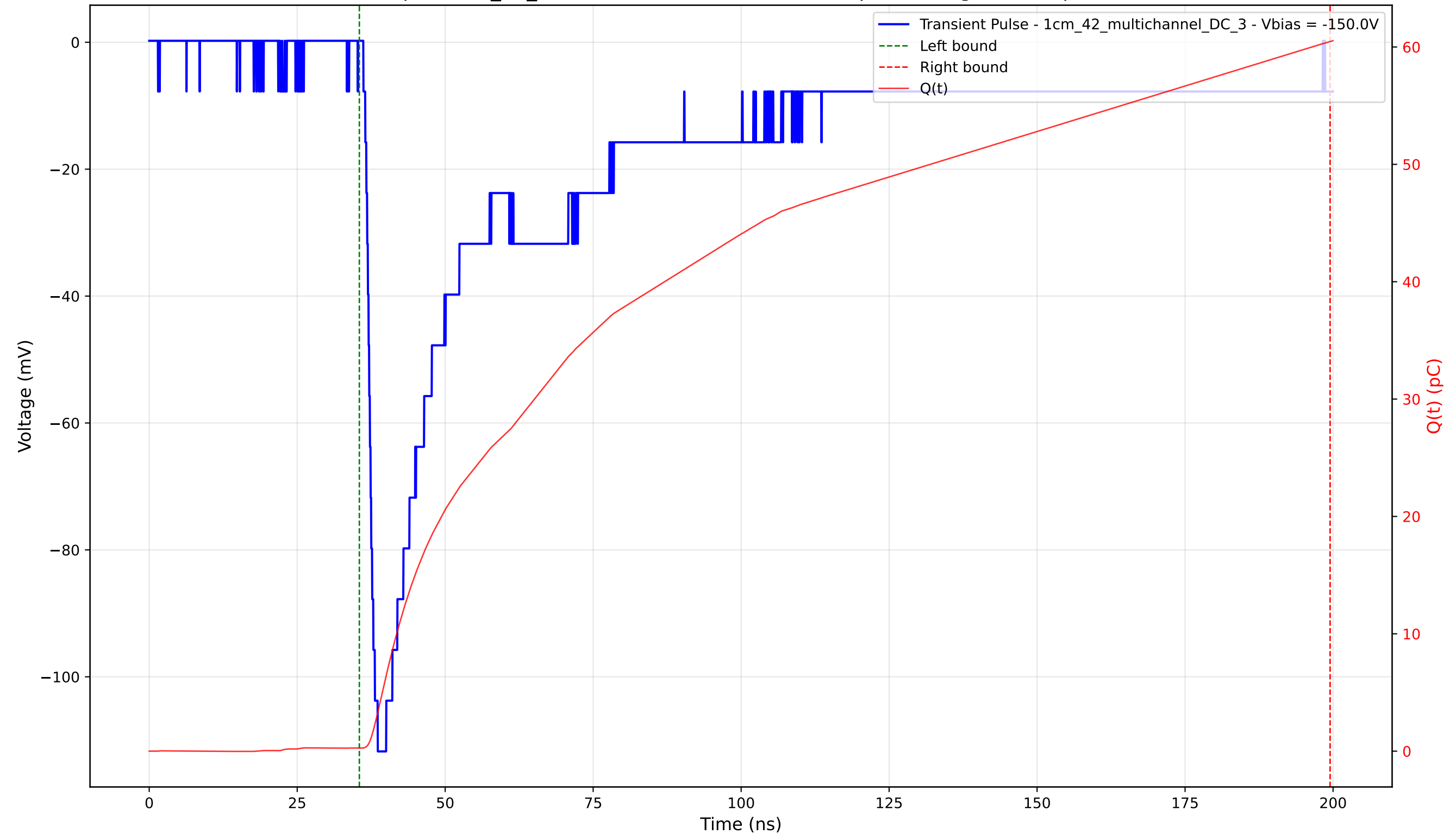
Transient Pulse - Sample: 1cm_42_multichannel - Position: 1765.0 \mu\text{m} - Charge: 60.19 pC - Rise Time: 1.63 ns
