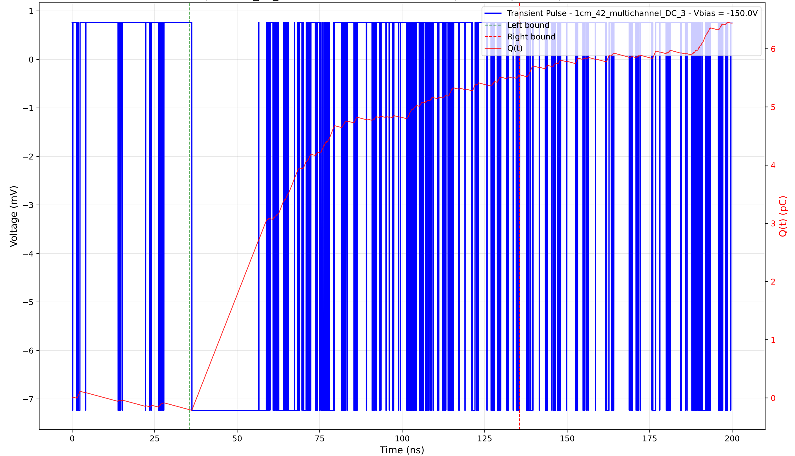
Transient Pulse - Sample: 1cm_42_multichannel - Position: 3880.0 \mu\text{m} - Charge: 5.75 pC - Rise Time: 0.00 ns (N/A)
