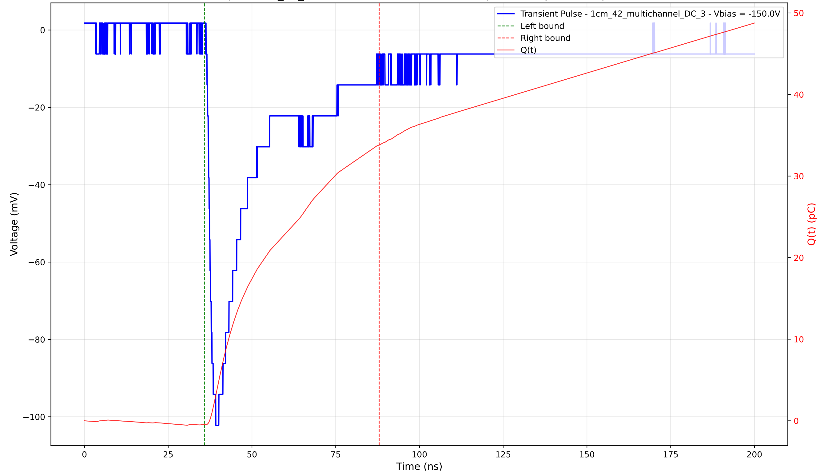
Transient Pulse - Sample: 1cm_42_multichannel - Position: 3075.0 \mu\text{m} - Charge: 34.29 pC - Rise Time: 1.85 ns
