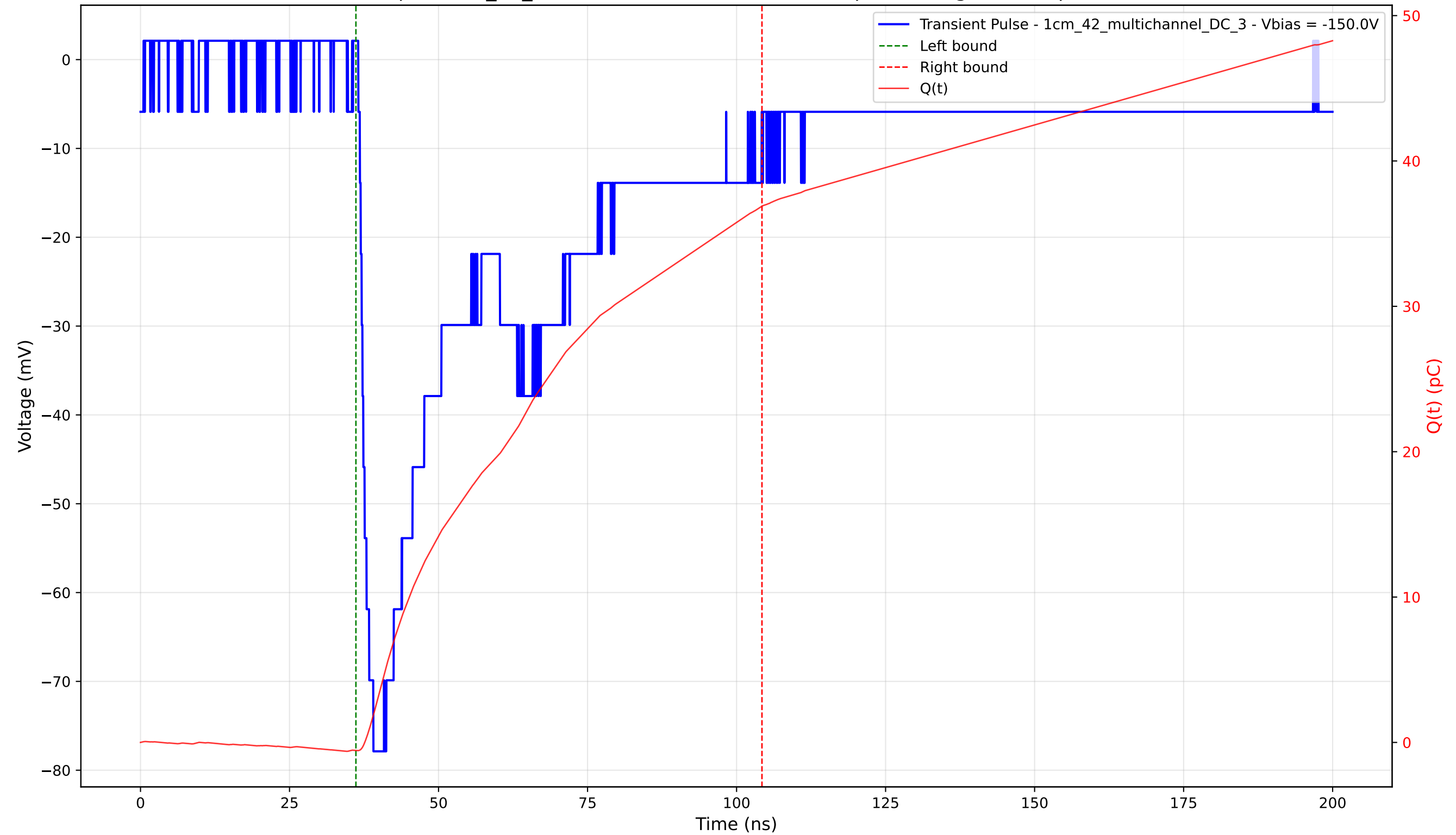
Transient Pulse - Sample: 1cm_42_multichannel - Position: 2555.0 \mu\text{m} - Charge: 37.44 pC - Rise Time: 2.28 ns
