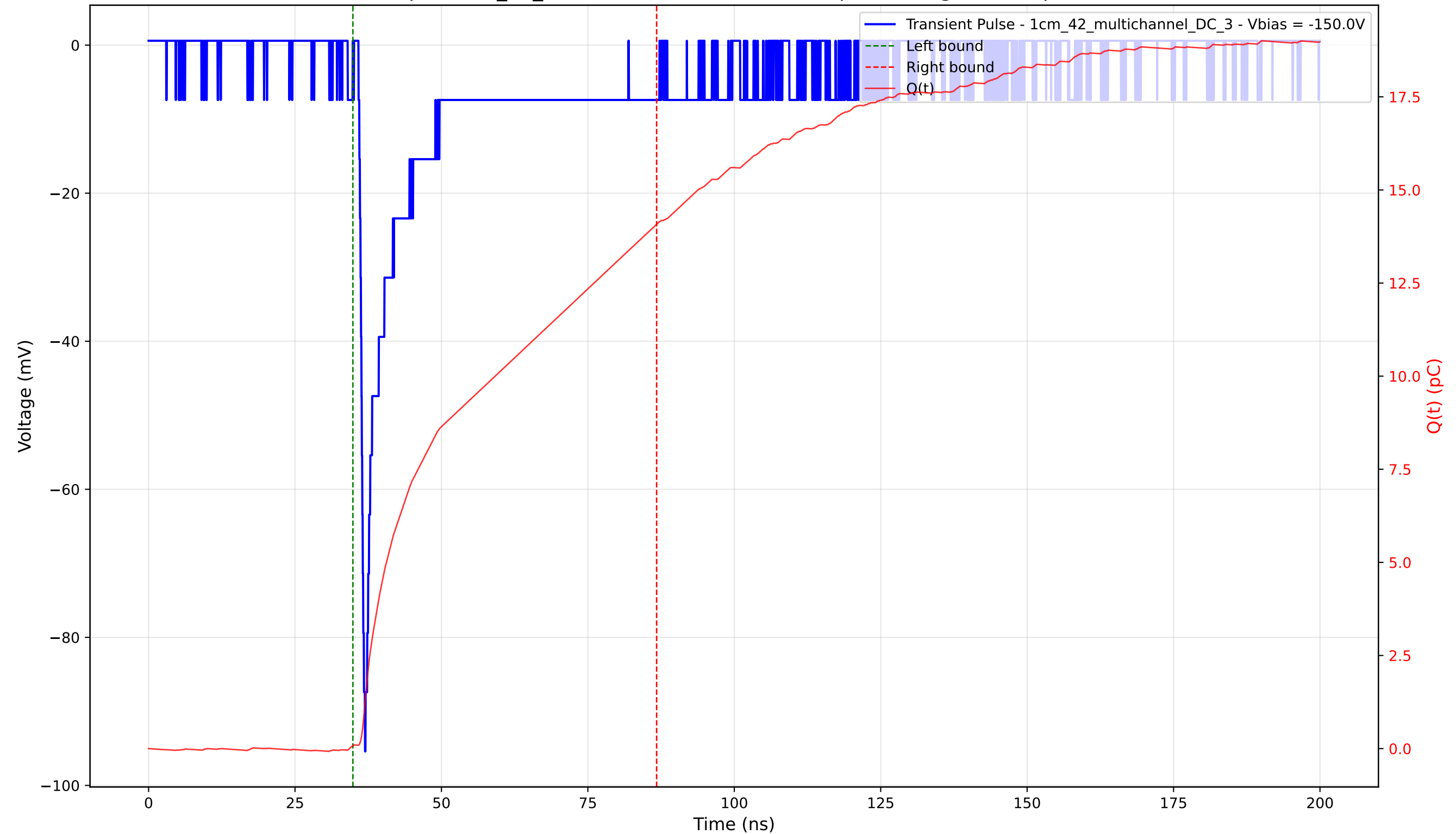
Transient Pulse - Sample: 1cm_42_multichannel - Position: 65.0 \mu\text{m} - Charge: 14.00 pC - Rise Time: 0.79 ns
