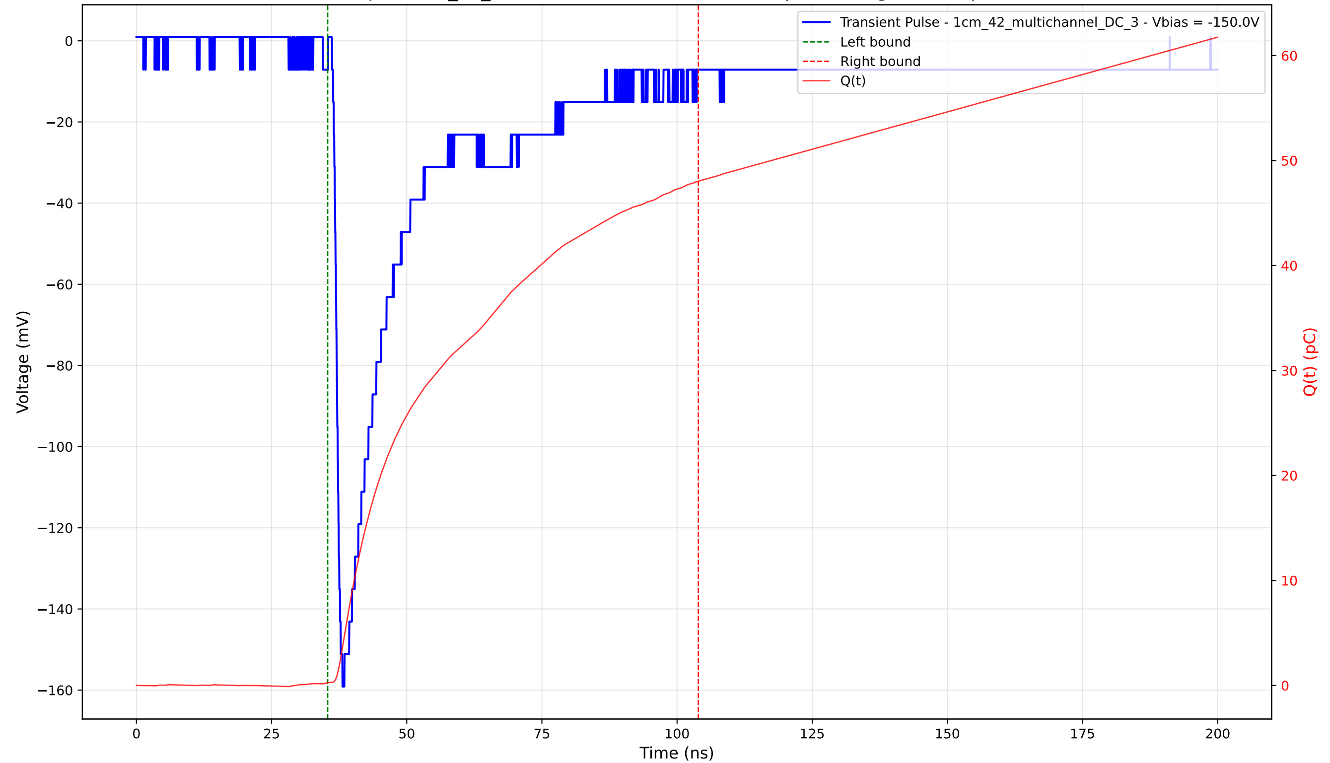
Transient Pulse - Sample: 1cm_42_multichannel - Position: 1200.0 \mu\text{m} - Charge: 47.76 pC - Rise Time: 1.30 ns
