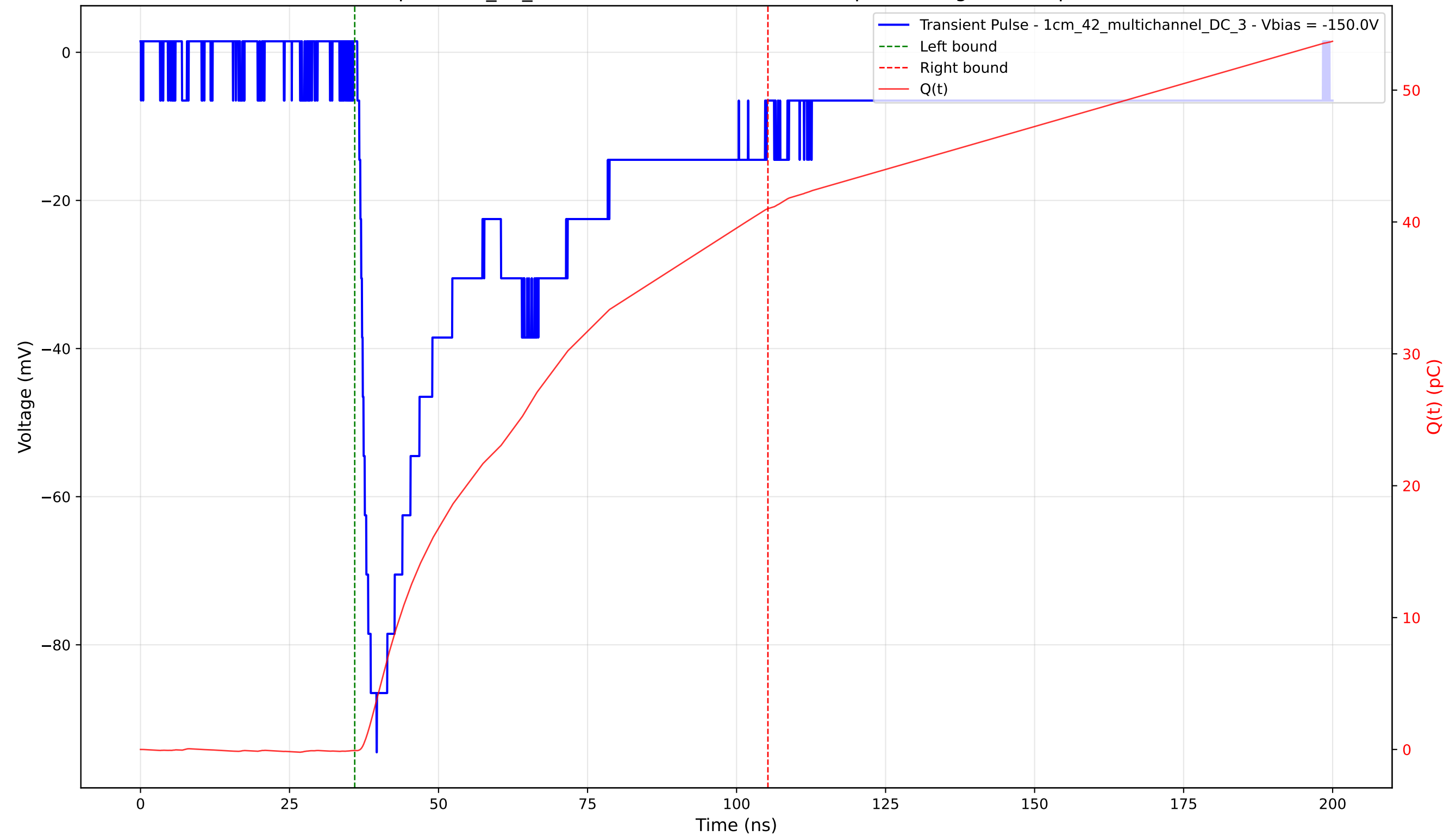
Transient Pulse - Sample: 1cm_42_multichannel - Position: 2710.0 \mu\text{m} - Charge: 41.09 pC - Rise Time: 1.93 ns
