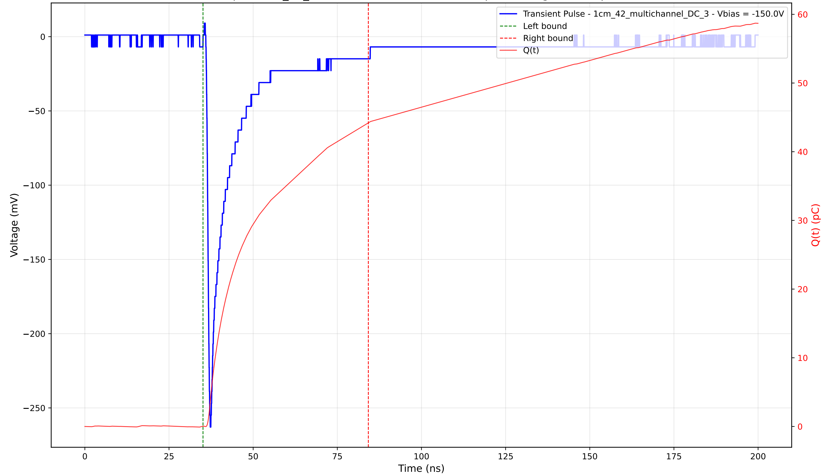
Transient Pulse - Sample: 1cm_42_multichannel - Position: 425.0 \mu\text{m} - Charge: 44.17 pC - Rise Time: 0.87 ns
