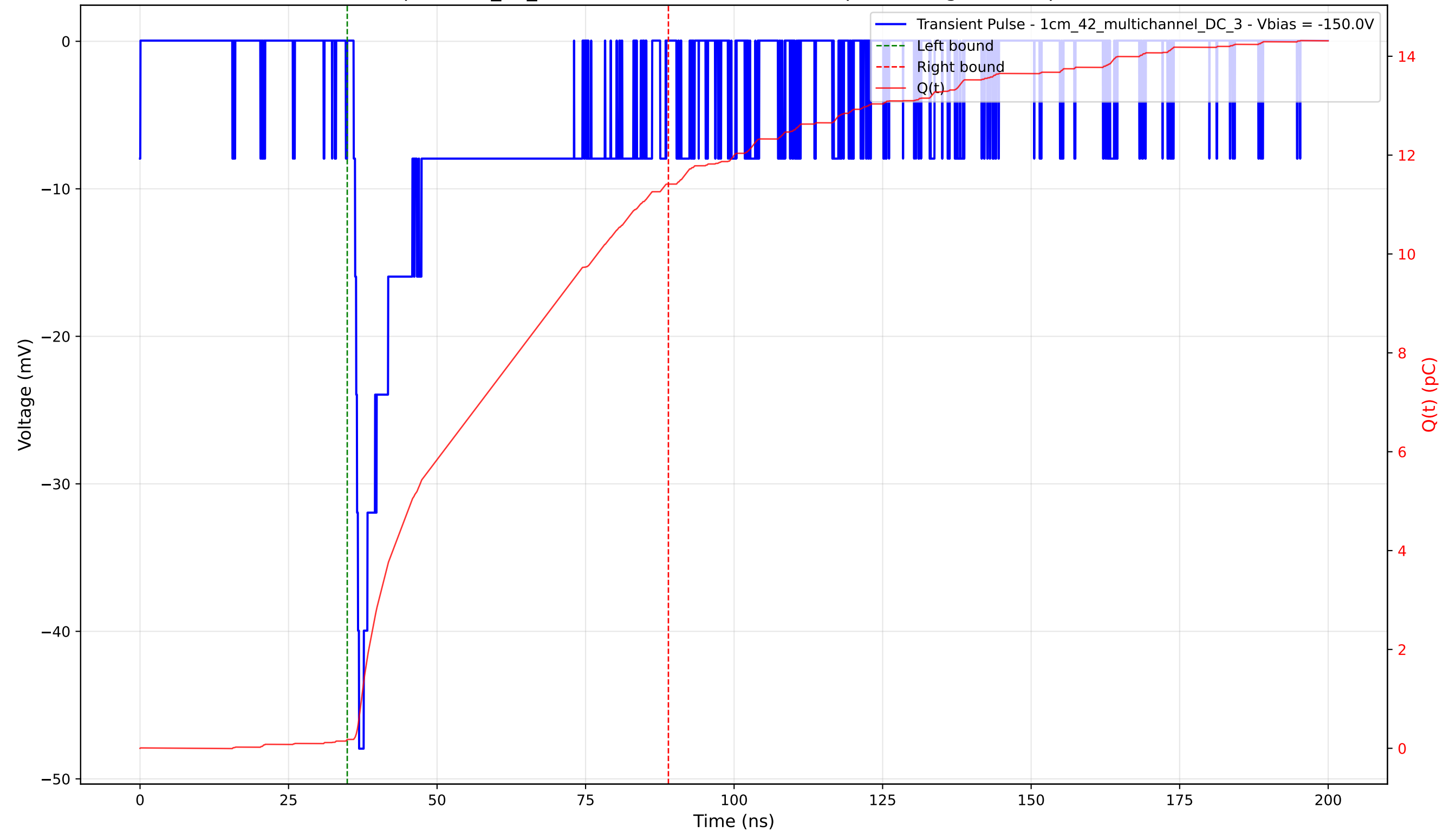
Transient Pulse - Sample: 1cm_42_multichannel - Position: 320.0 \mu\text{m} - Charge: 11.23 pC - Rise Time: 0.91 ns
