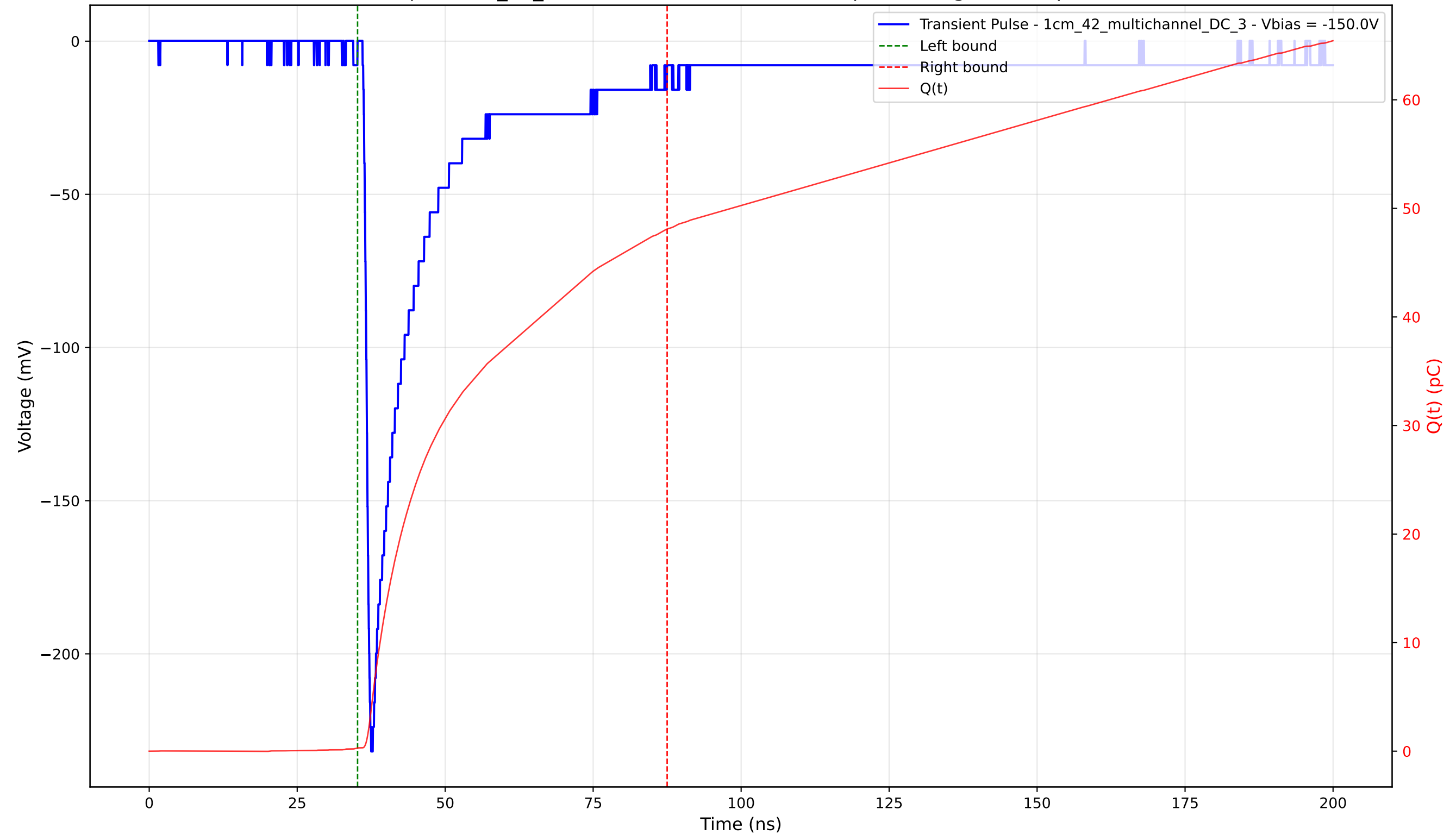
Transient Pulse - Sample: 1cm_42_multichannel - Position: 670.0 \mu\text{m} - Charge: 47.79 pC - Rise Time: 1.02 ns
