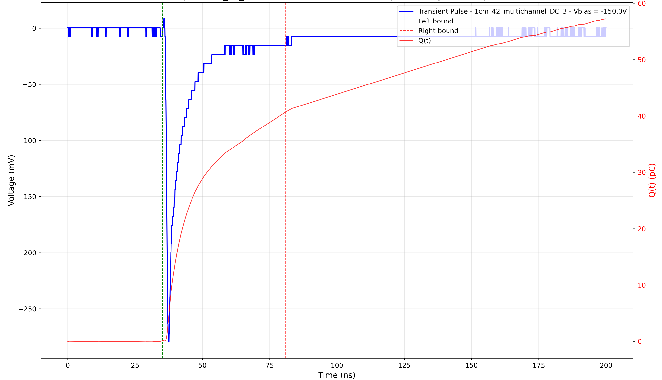
Transient Pulse - Sample: 1cm_42_multichannel - Position: 4545.0 \mu\text{m} - Charge: 40.62 pC - Rise Time: 0.85 ns
