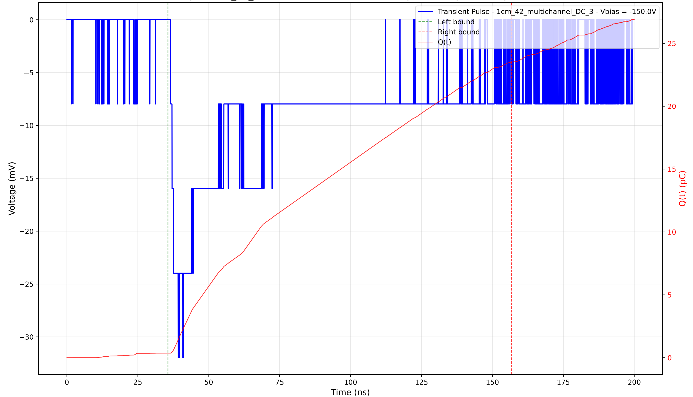
Transient Pulse - Sample: 1cm_42_multichannel - Position: 2415.0 \mu\text{m} - Charge: 23.14 pC - Rise Time: 2.63 ns
