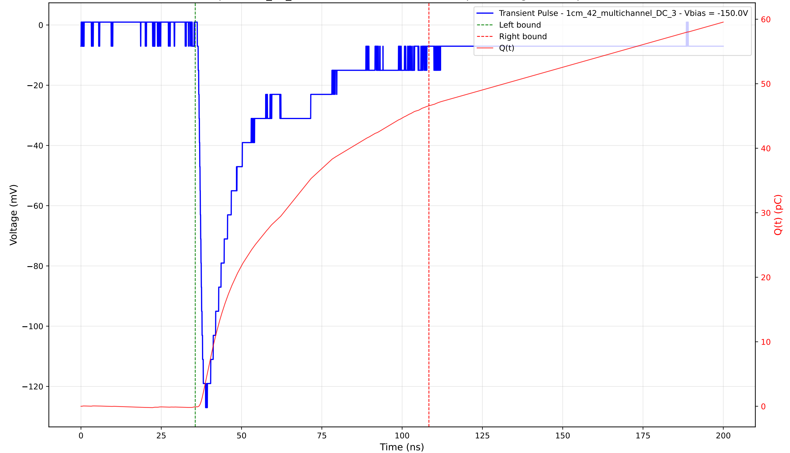
Transient Pulse - Sample: 1cm_42_multichannel - Position: 1580.0 \mu\text{m} - Charge: 46.66 pC - Rise Time: 1.59 ns
