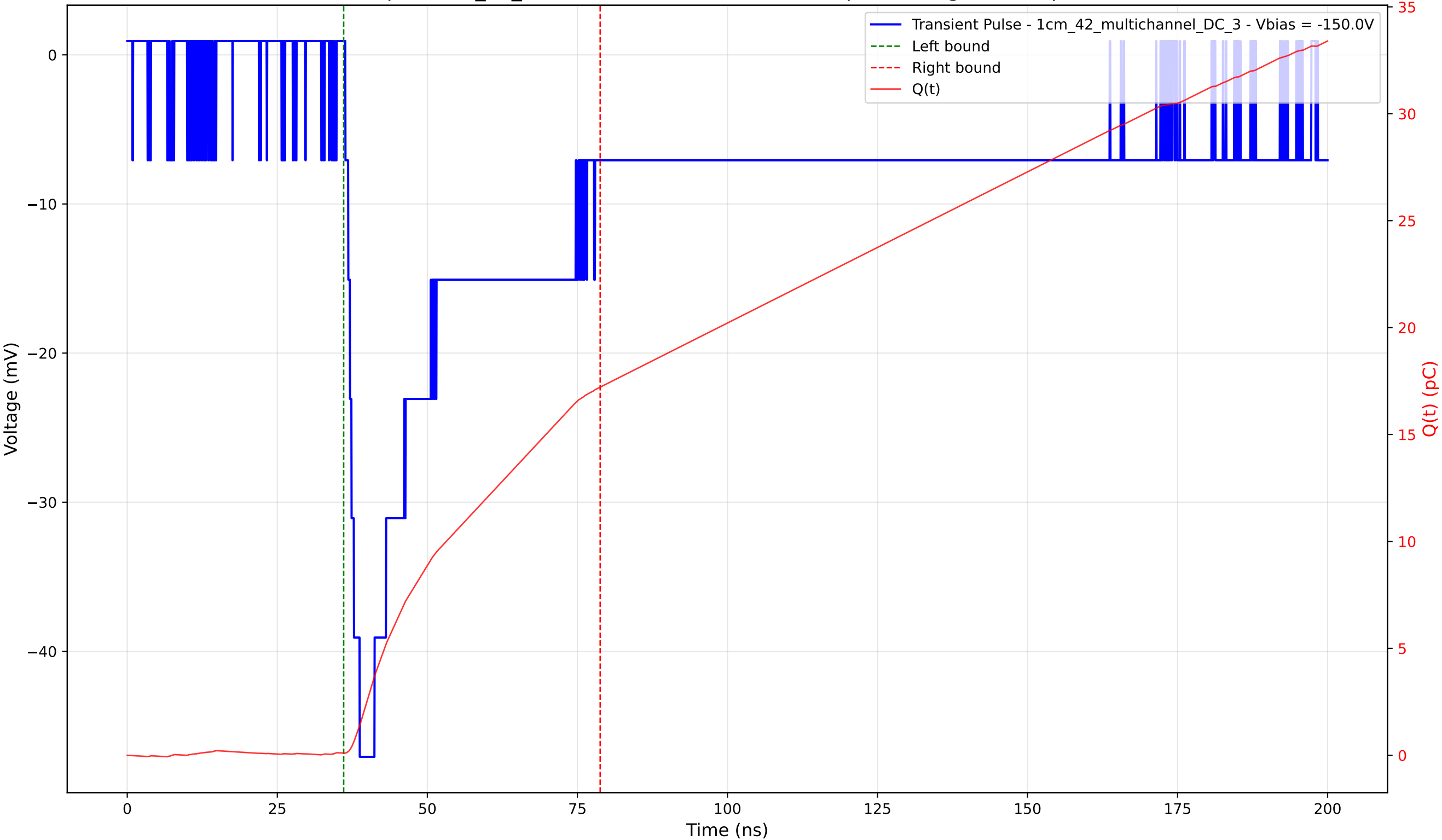
Transient Pulse - Sample: 1cm_42_multichannel - Position: 2830.0 \mu\text{m} - Charge: 17.12 pC - Rise Time: 2.39 ns
