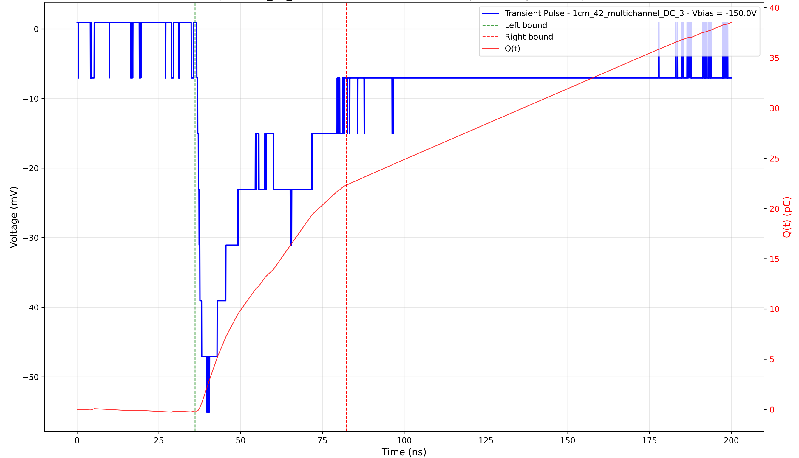
Transient Pulse - Sample: 1cm_42_multichannel - Position: 2430.0 \mu\text{m} - Charge: 22.48 pC - Rise Time: 3.01 ns
