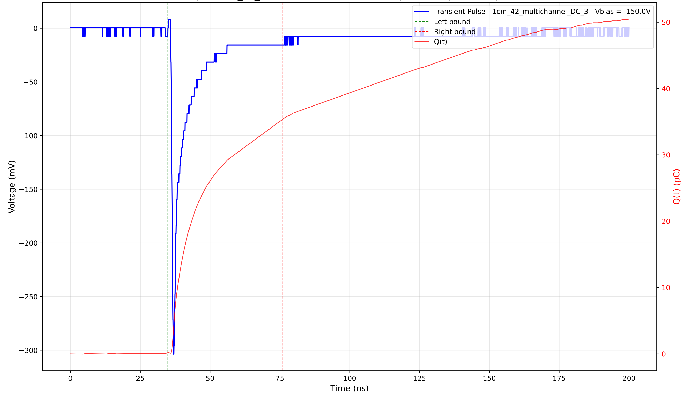
Transient Pulse - Sample: 1cm_42_multichannel - Position: 95.0 \mu\text{m} - Charge: 35.12 pC - Rise Time: 0.80 ns
