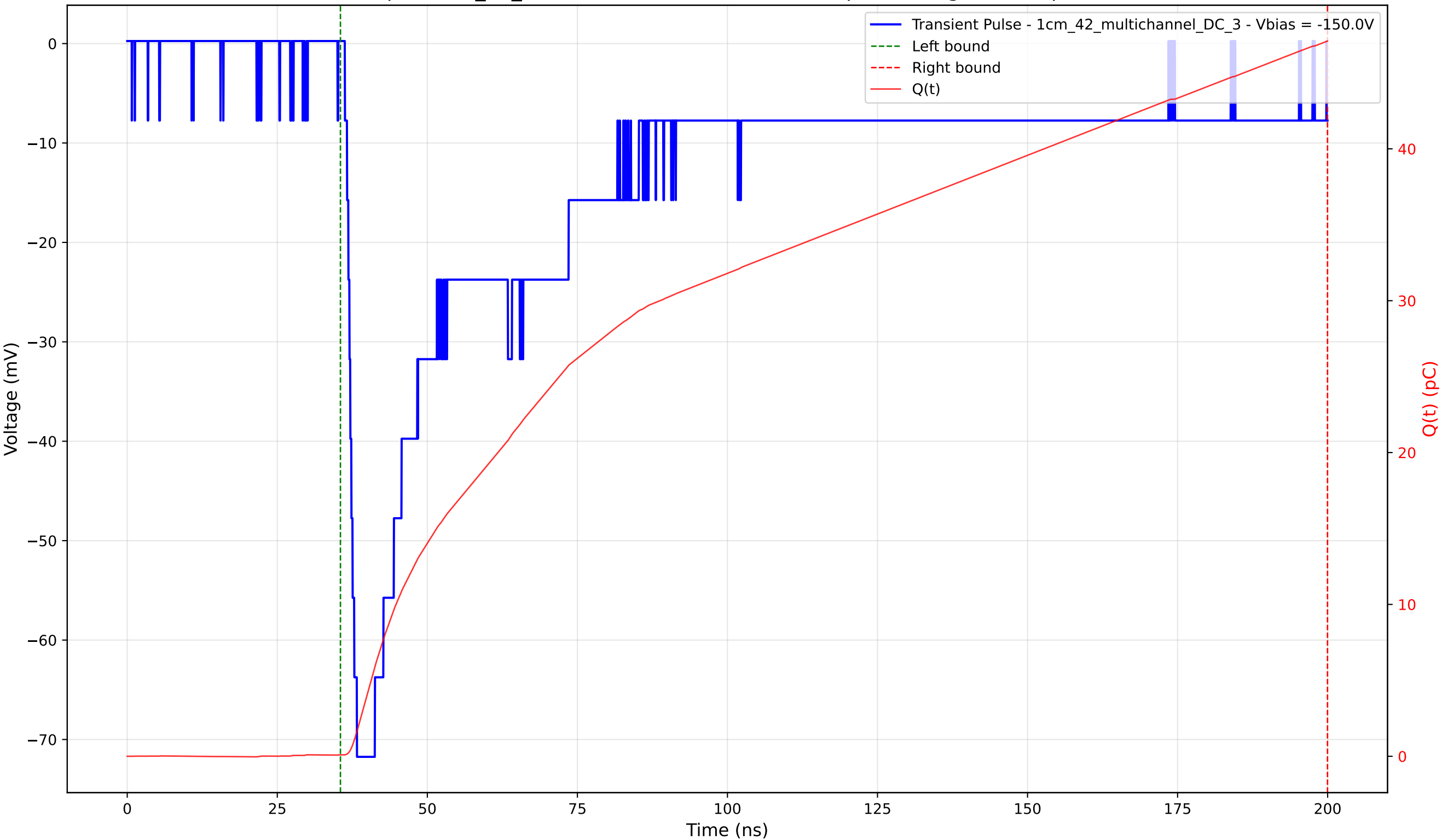
Transient Pulse - Sample: 1cm_42_multichannel - Position: 1930.0 \mu\text{m} - Charge: 47.01 pC - Rise Time: 2.00 ns
