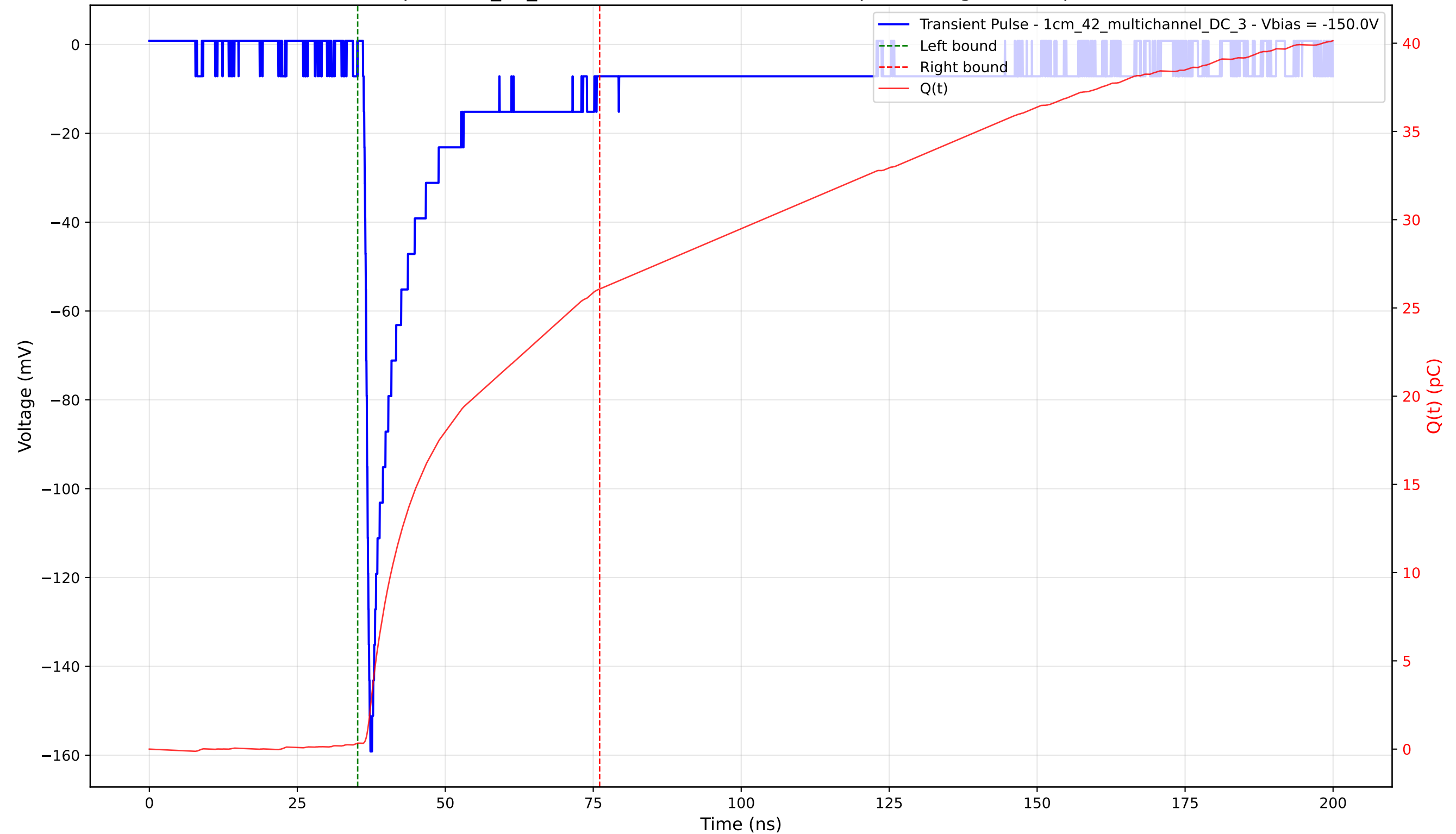
Transient Pulse - Sample: 1cm_42_multichannel - Position: 4450.0 \mu\text{m} - Charge: 25.73 pC - Rise Time: 0.92 ns
