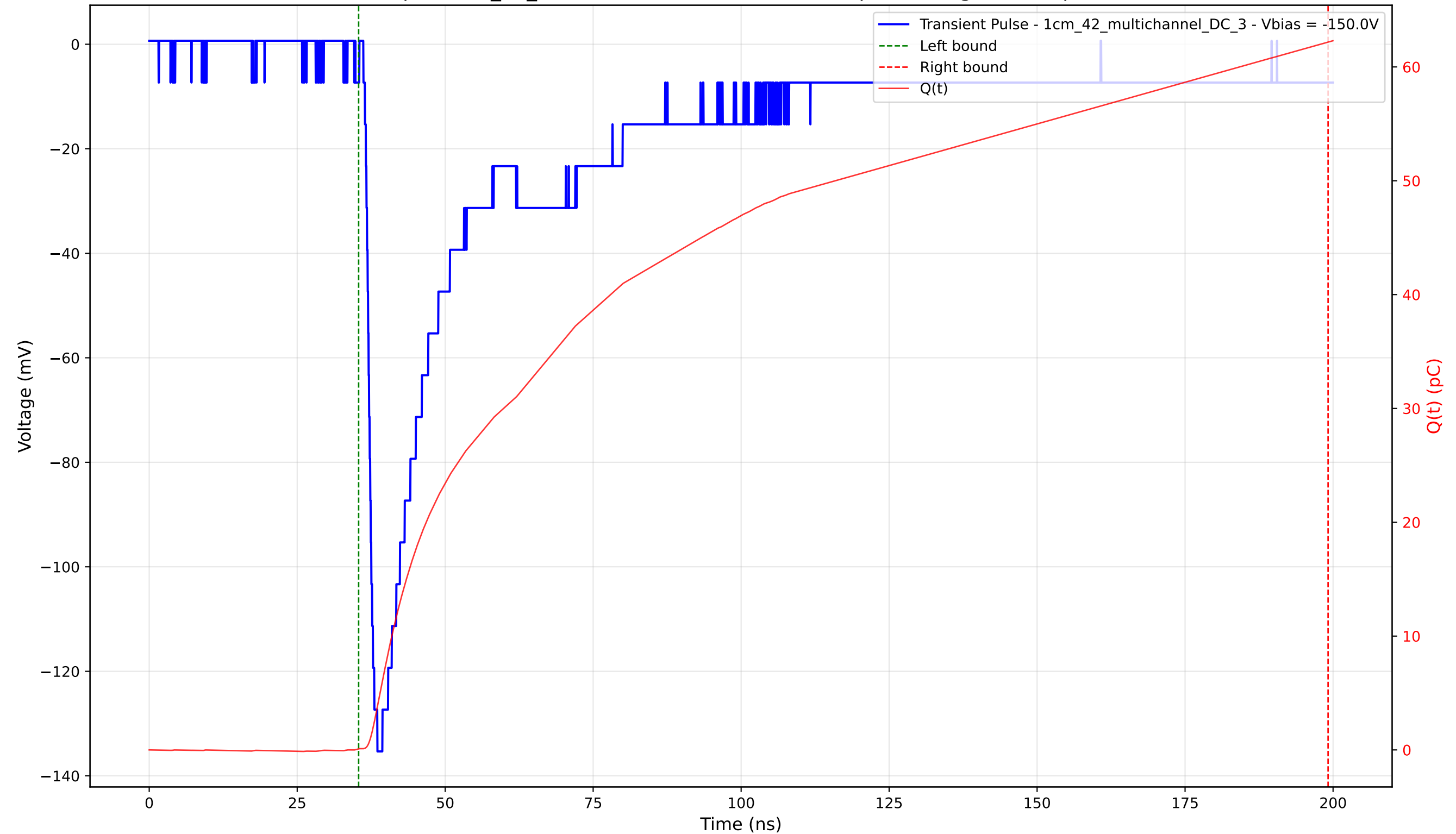
Transient Pulse - Sample: 1cm_42_multichannel - Position: 1490.0 \mu\text{m} - Charge: 62.09 pC - Rise Time: 1.58 ns
