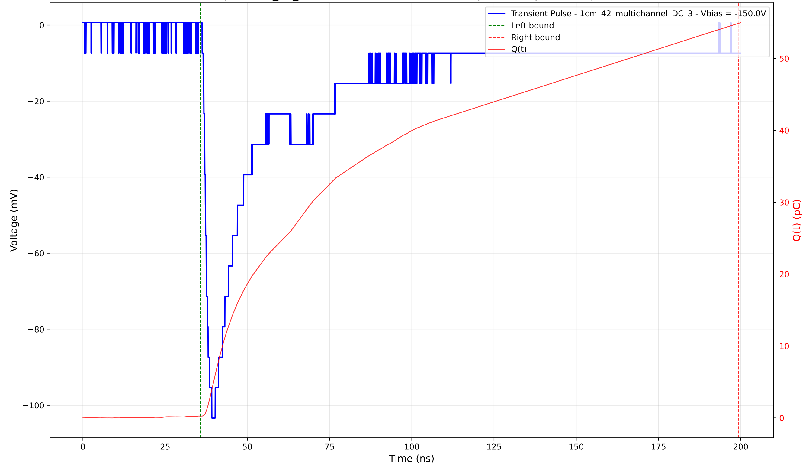
Transient Pulse - Sample: 1cm_42_multichannel - Position: 3025.0 \mu\text{m} - Charge: 54.61 pC - Rise Time: 1.87 ns
