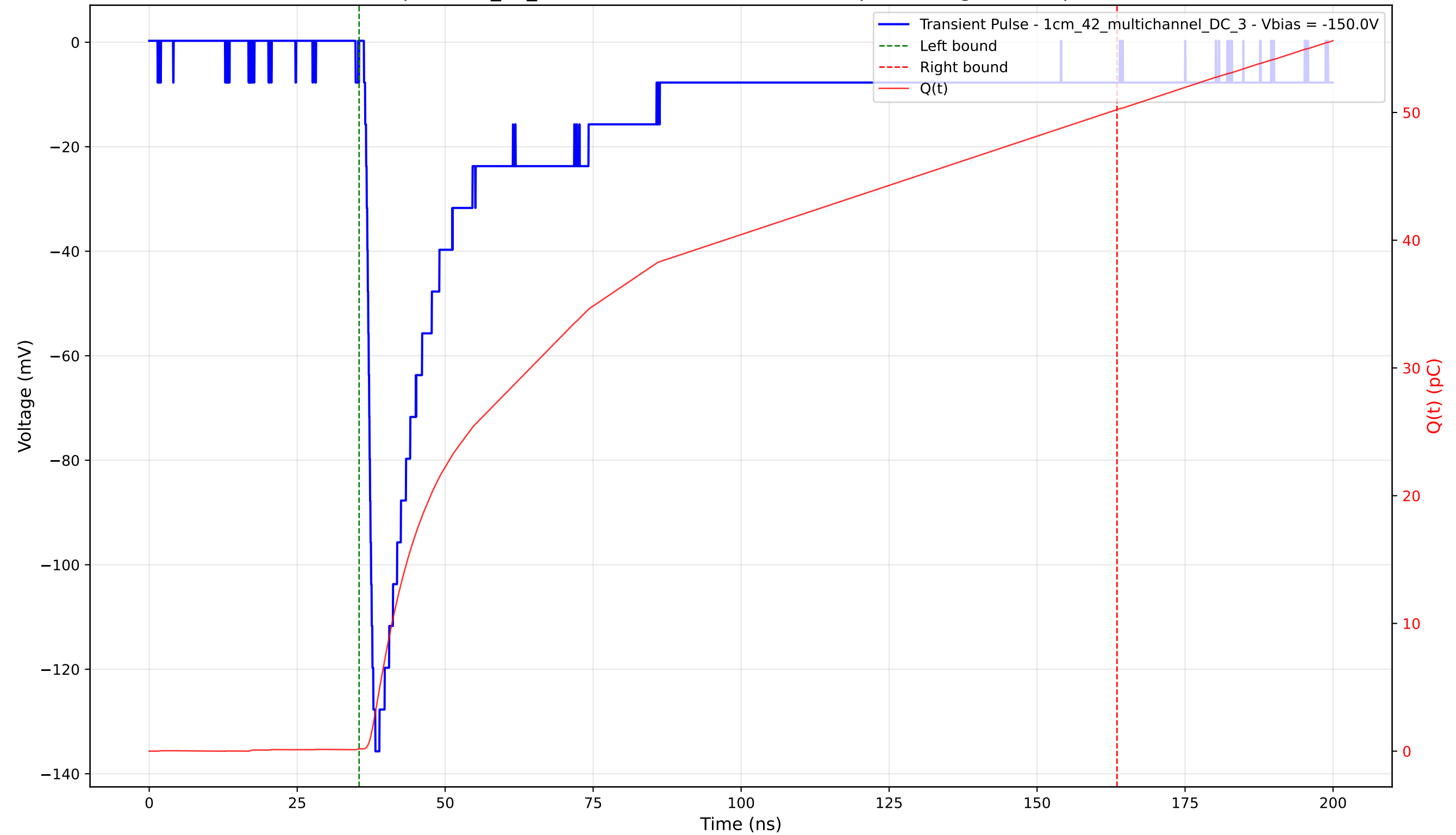
Transient Pulse - Sample: 1cm_42_multichannel - Position: 3670.0 \mu\text{m} - Charge: 50.06 pC - Rise Time: 1.39 ns
