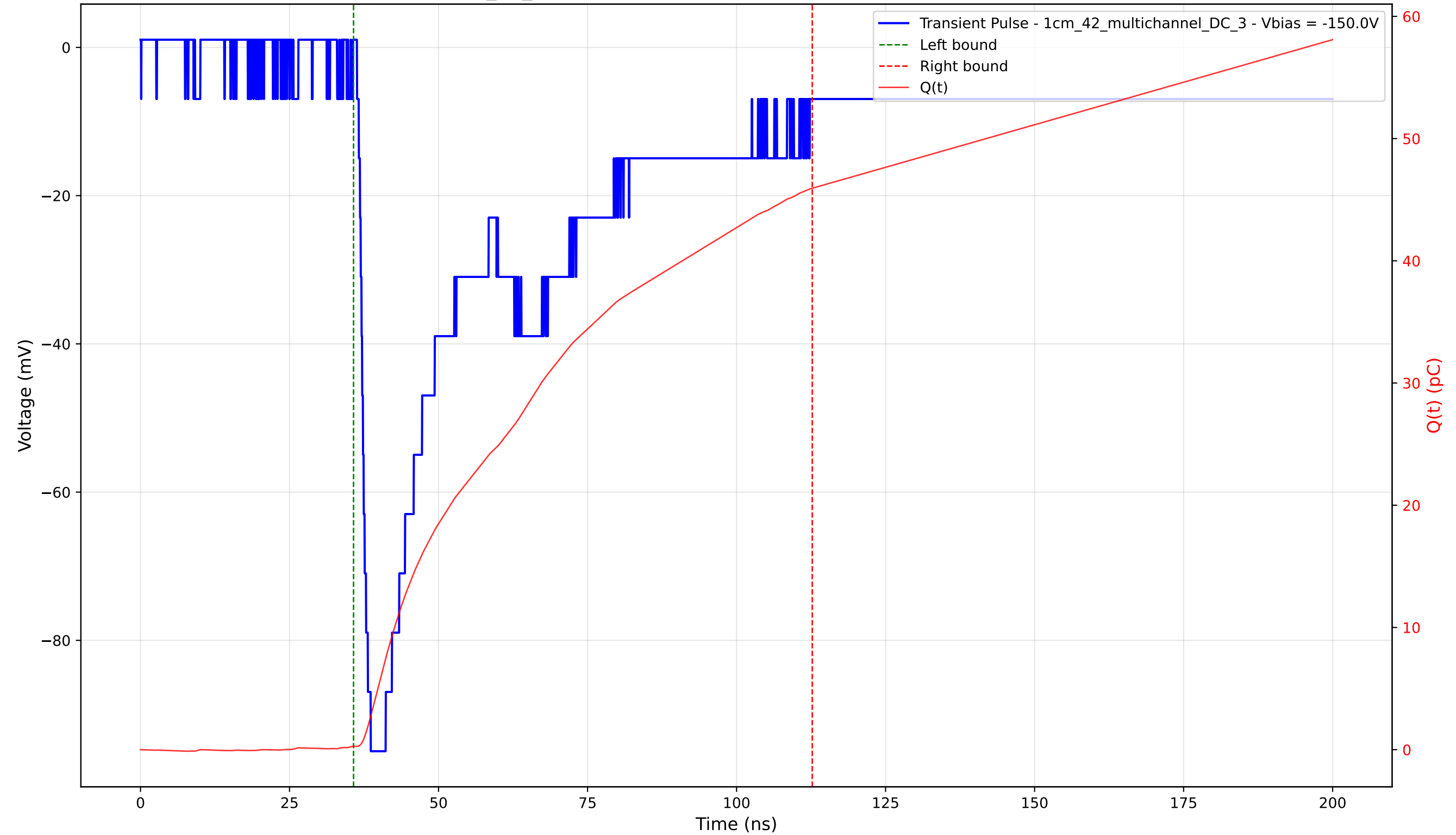
Transient Pulse - Sample: 1cm_42_multichannel - Position: 2015.0 \mu\text{m} - Charge: 45.66 pC - Rise Time: 1.53 ns
