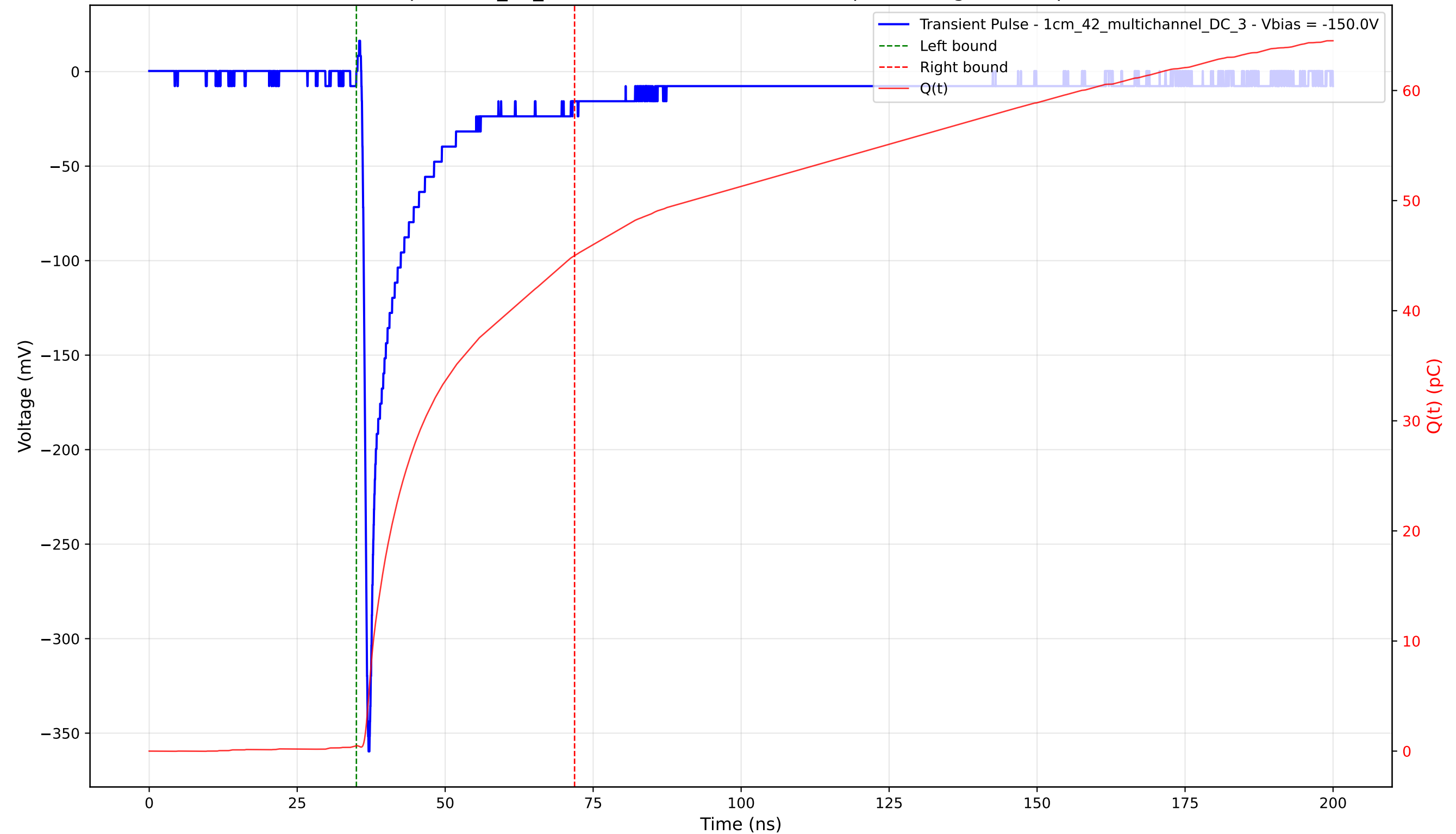
Transient Pulse - Sample: 1cm_42_multichannel - Position: 195.0 \mu\text{m} - Charge: 44.50 pC - Rise Time: 0.82 ns
