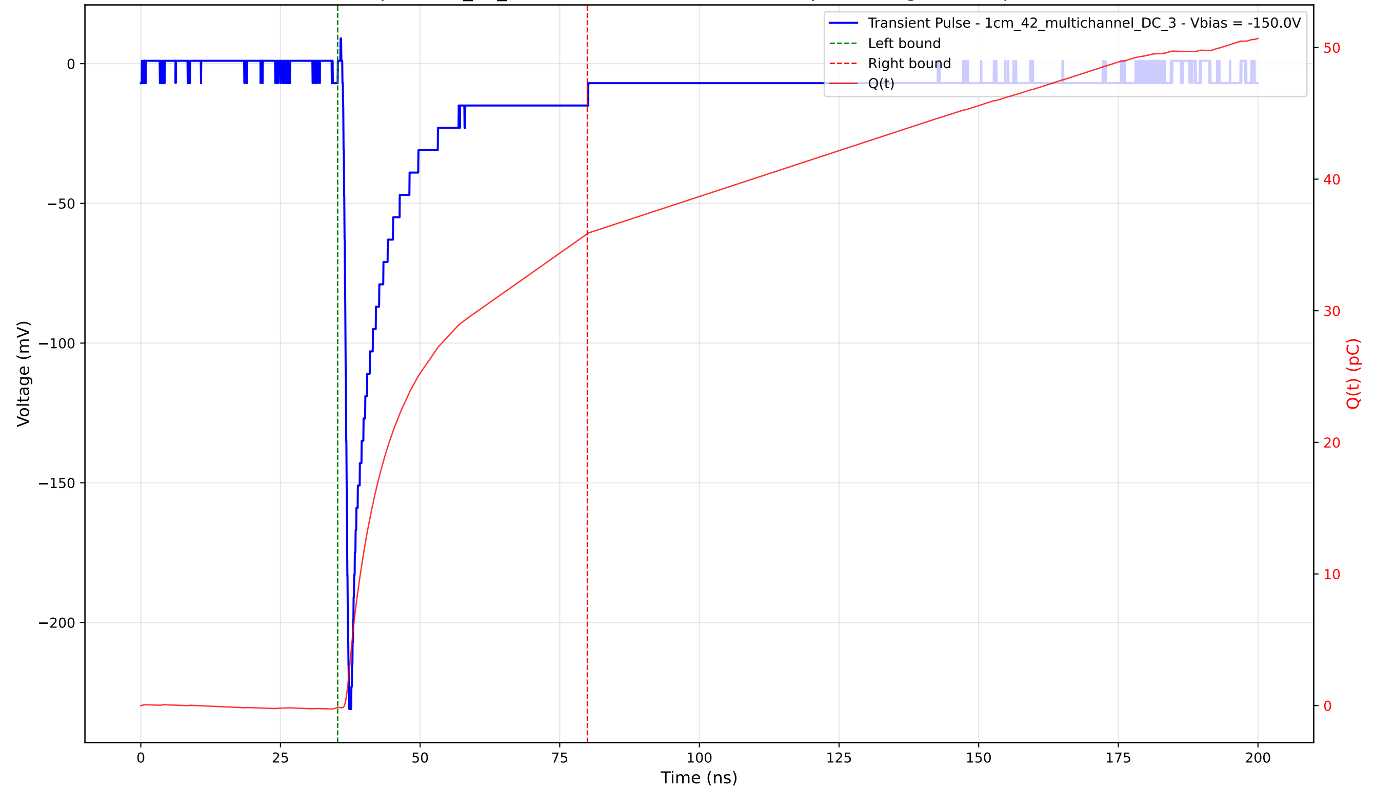
Transient Pulse - Sample: 1cm_42_multichannel - Position: 4475.0 \mu\text{m} - Charge: 36.00 pC - Rise Time: 0.88 ns
