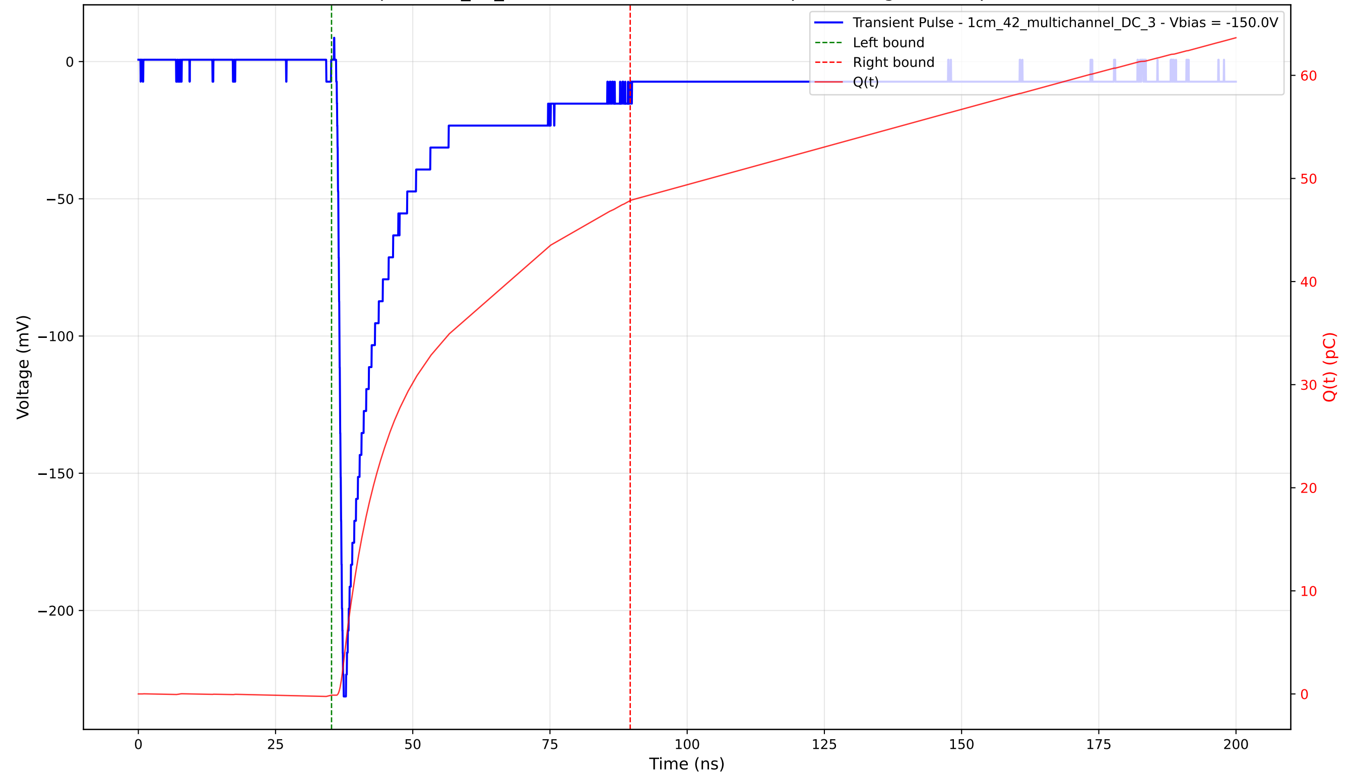
Transient Pulse - Sample: 1cm_42_multichannel - Position: 640.0 \mu\text{m} - Charge: 47.97 pC - Rise Time: 1.00 ns
