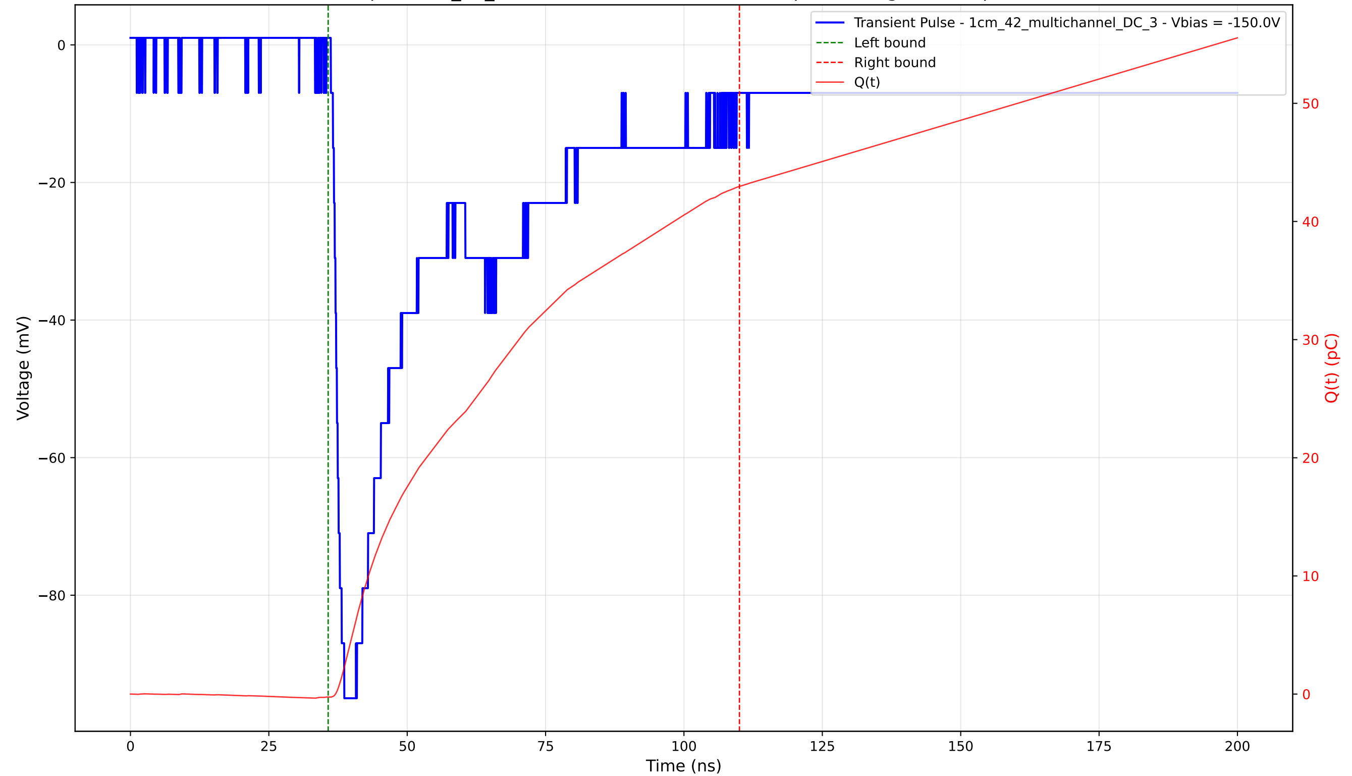
Transient Pulse - Sample: 1cm_42_multichannel - Position: 1960.0 \mu\text{m} - Charge: 43.22 pC - Rise Time: 1.59 ns
