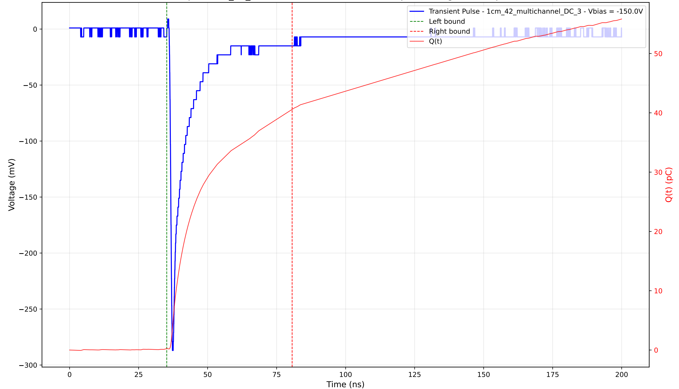
Transient Pulse - Sample: 1cm_42_multichannel - Position: 4575.0 \mu\text{m} - Charge: 40.34 pC - Rise Time: 0.85 ns
