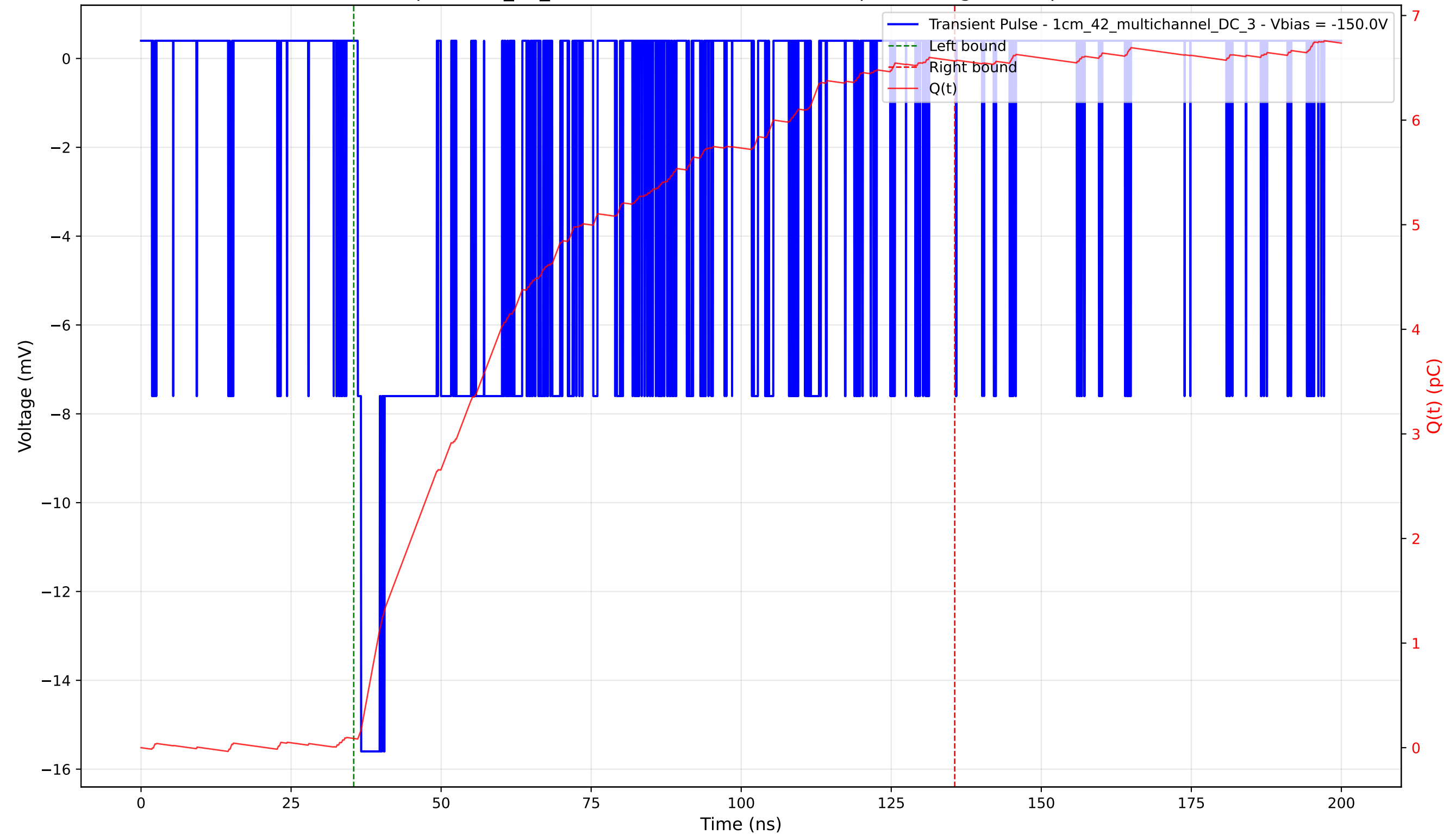
Transient Pulse - Sample: 1cm_42_multichannel - Position: 340.0 \mu\text{m} - Charge: 6.48 pC - Rise Time: 0.56 ns
