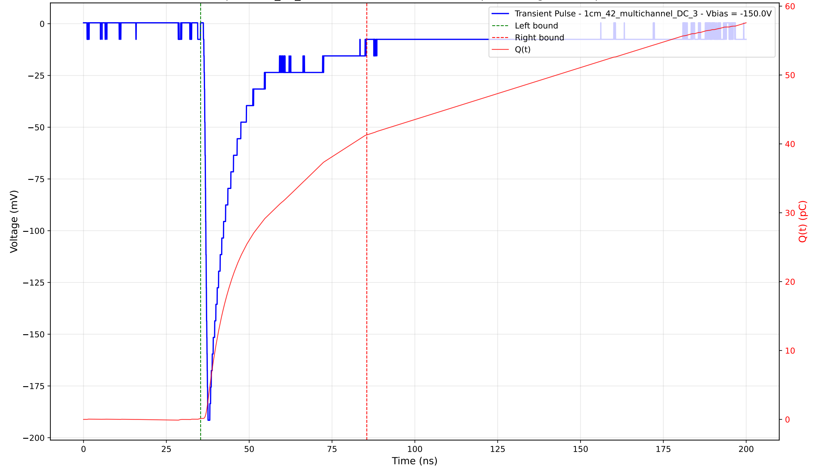
Transient Pulse - Sample: 1cm_42_multichannel - Position: 4150.0 \mu\text{m} - Charge: 41.17 pC - Rise Time: 0.99 ns
