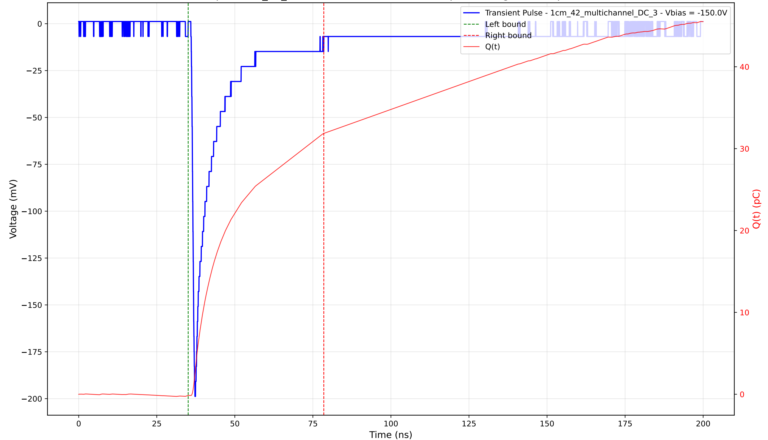
Transient Pulse - Sample: 1cm_42_multichannel - Position: 410.0 \mu\text{m} - Charge: 32.00 pC - Rise Time: 0.91 ns
