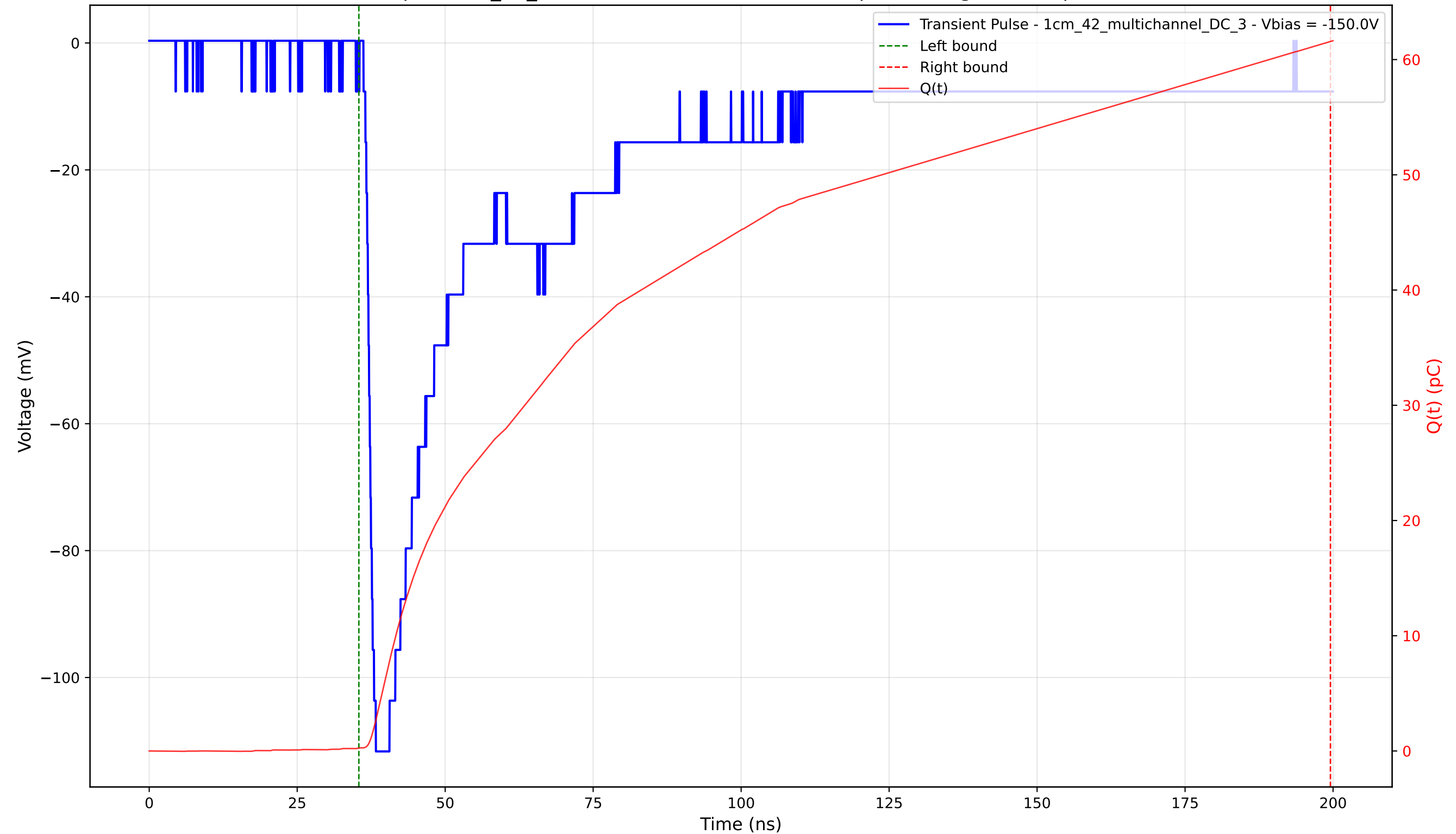
Transient Pulse - Sample: 1cm_42_multichannel - Position: 1740.0 \mu\text{m} - Charge: 61.31 pC - Rise Time: 1.47 ns
