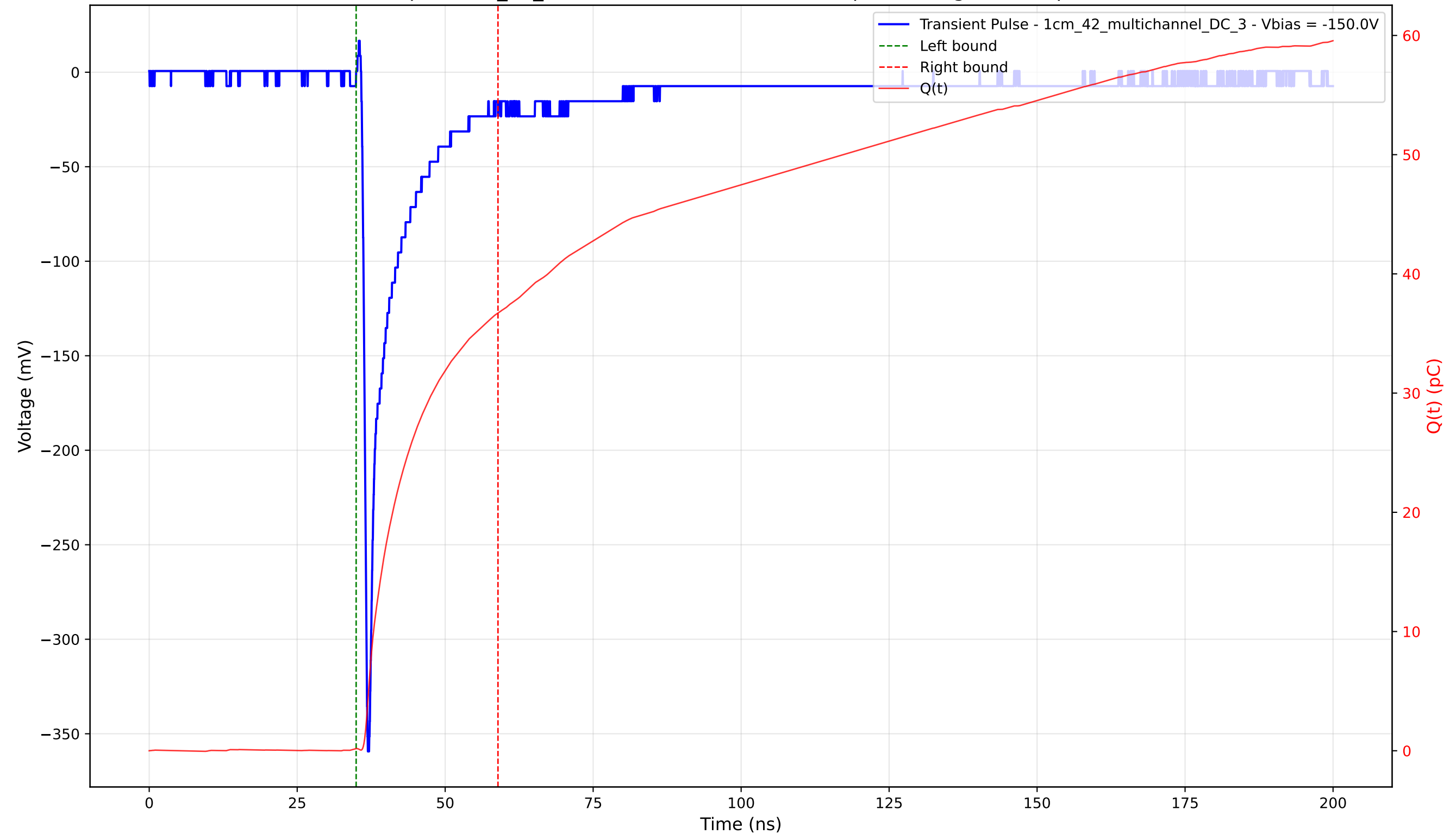
Transient Pulse - Sample: 1cm_42_multichannel - Position: 130.0 \mu\text{m} - Charge: 36.53 pC - Rise Time: 0.79 ns
