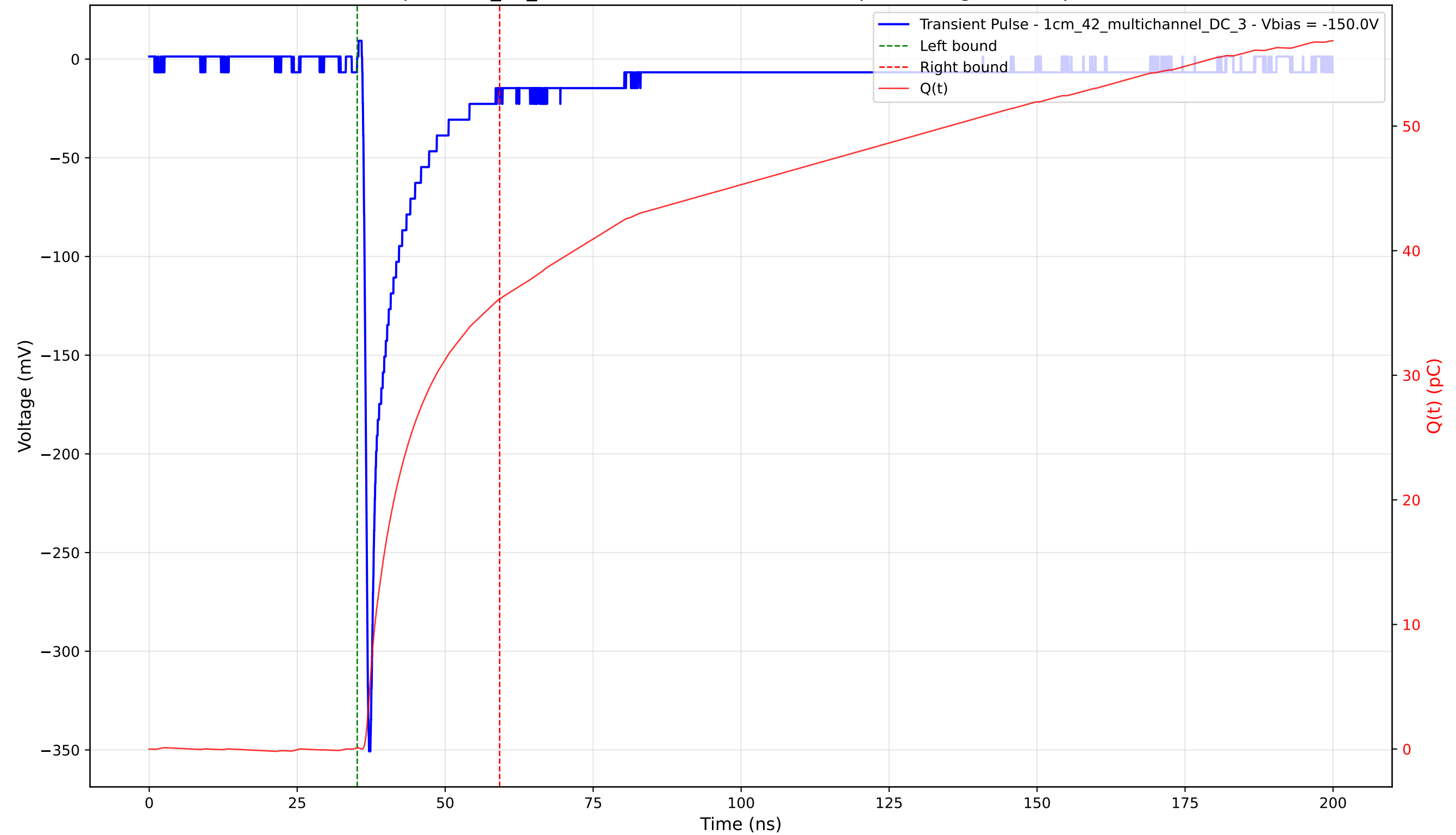
Transient Pulse - Sample: 1cm_42_multichannel - Position: 4720.0 \mu\text{m} - Charge: 36.02 pC - Rise Time: 0.79 ns
