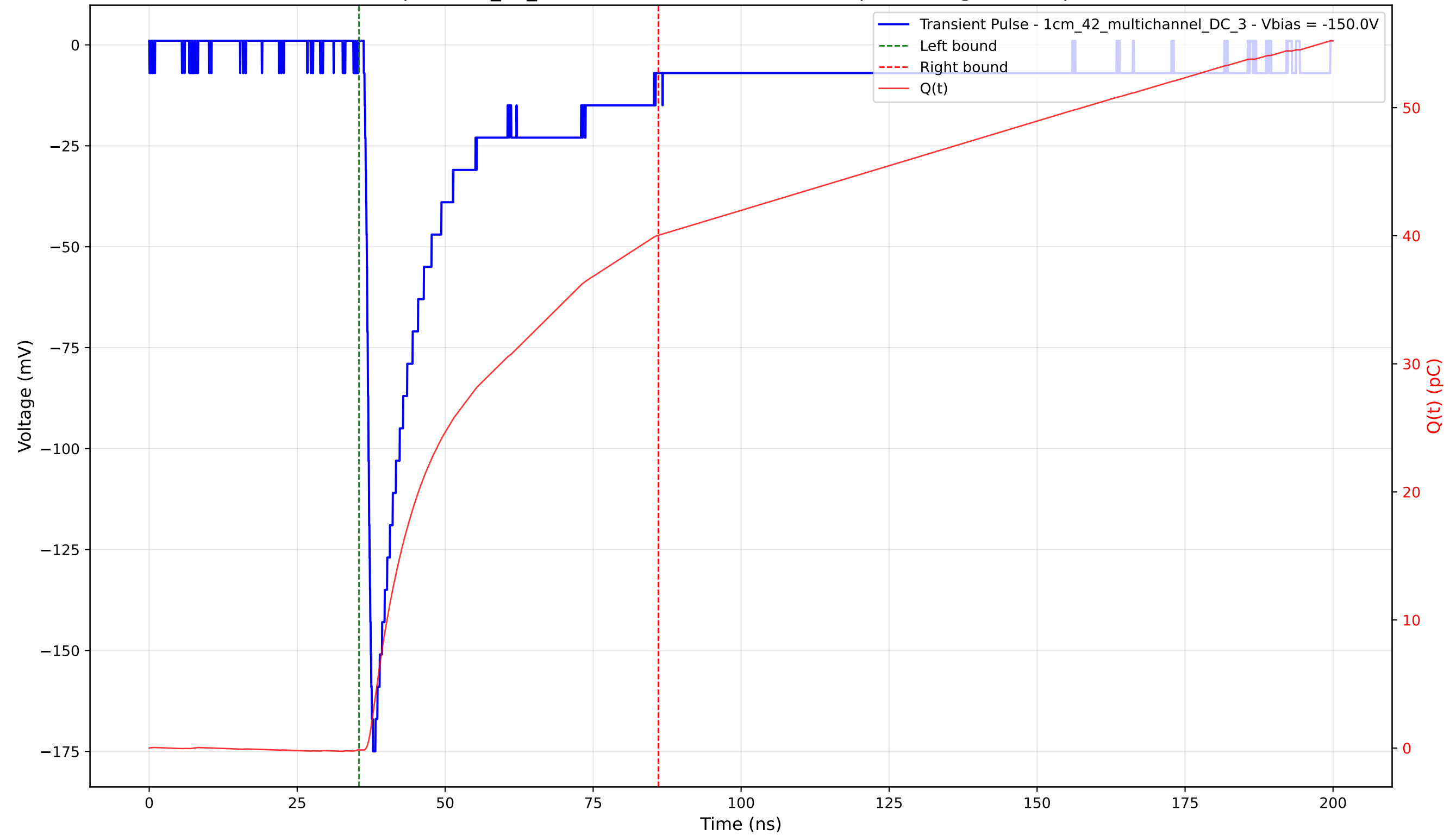
Transient Pulse - Sample: 1cm_42_multichannel - Position: 4025.0 \mu\text{m} - Charge: 40.18 pC - Rise Time: 1.03 ns
