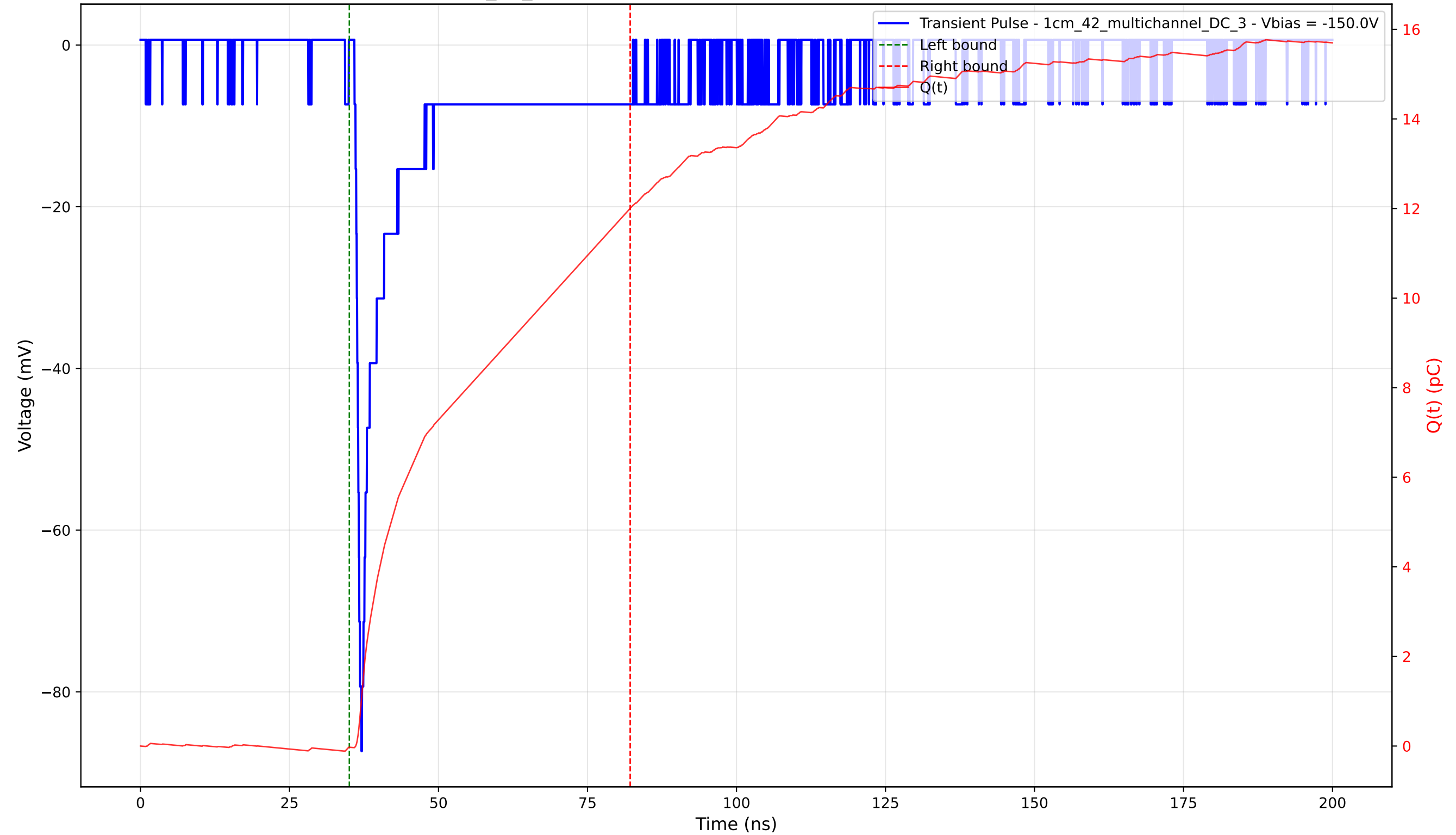
Transient Pulse - Sample: 1cm_42_multichannel - Position: 4865.0 \mu\text{m} - Charge: 12.03 pC - Rise Time: 0.76 ns
