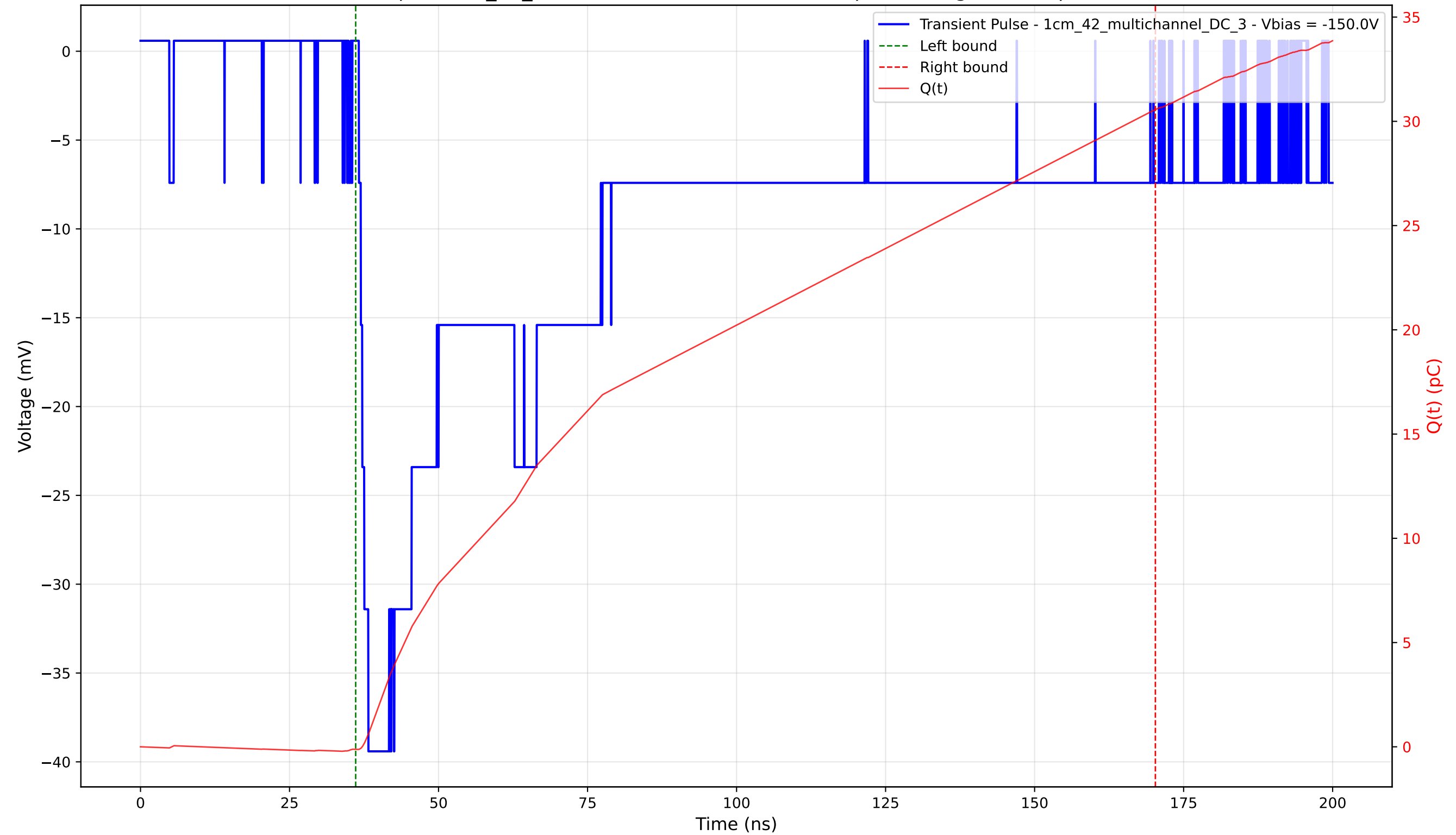
Transient Pulse - Sample: 1cm_42_multichannel - Position: 2325.0 \mu\text{m} - Charge: 30.69 pC - Rise Time: 1.59 ns
