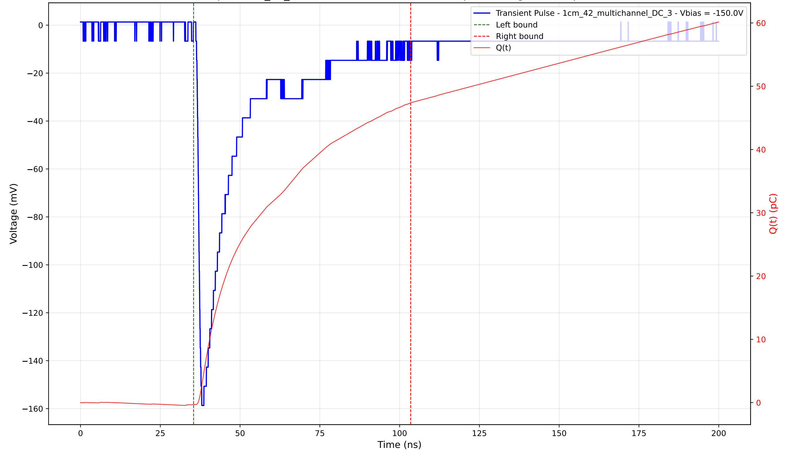
Transient Pulse - Sample: 1cm_42_multichannel - Position: 1185.0 \mu\text{m} - Charge: 47.66 pC - Rise Time: 1.28 ns
