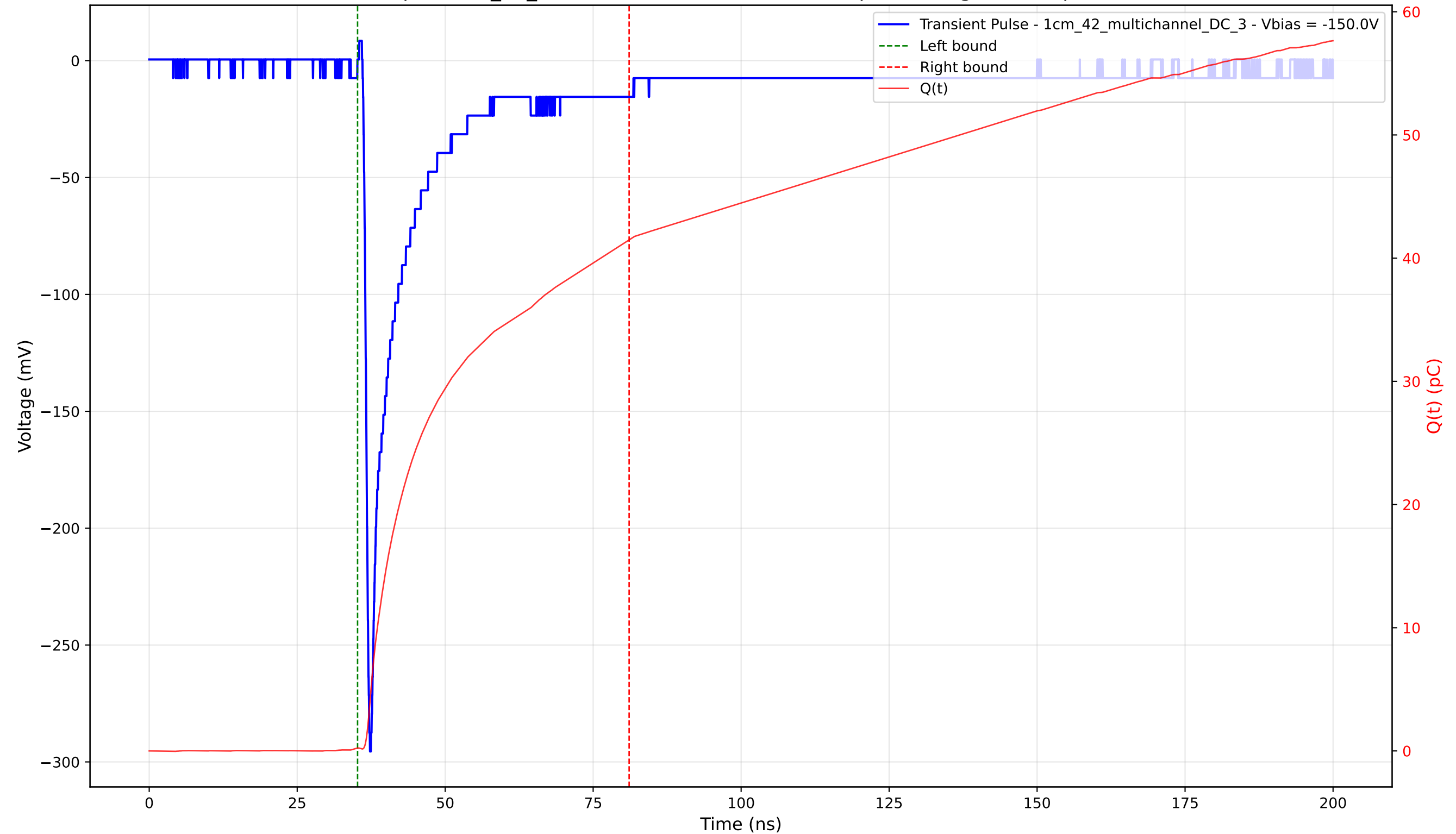
Transient Pulse - Sample: 1cm_42_multichannel - Position: 4585.0 \mu\text{m} - Charge: 41.26 pC - Rise Time: 0.86 ns
