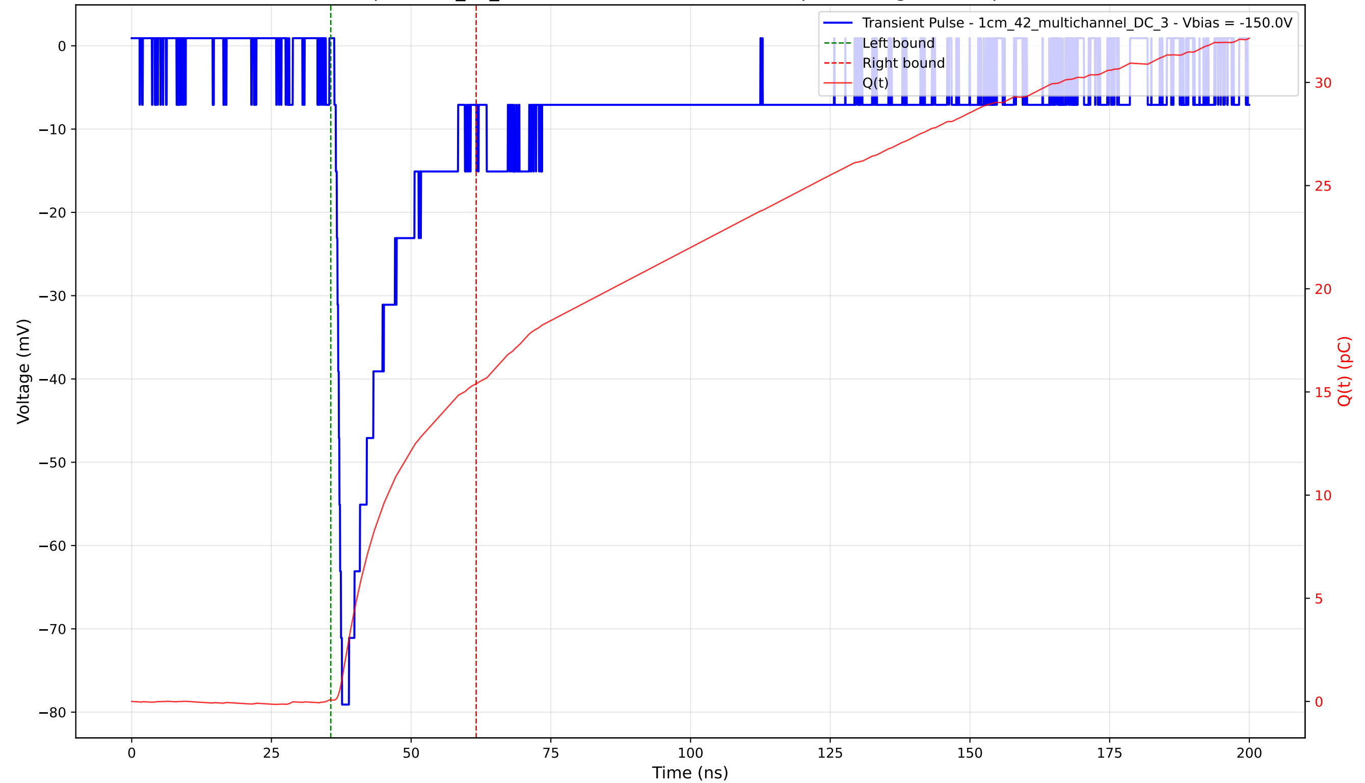
Transient Pulse - Sample: 1cm_42_multichannel - Position: 3940.0 \mu\text{m} - Charge: 15.32 pC - Rise Time: 1.12 ns
