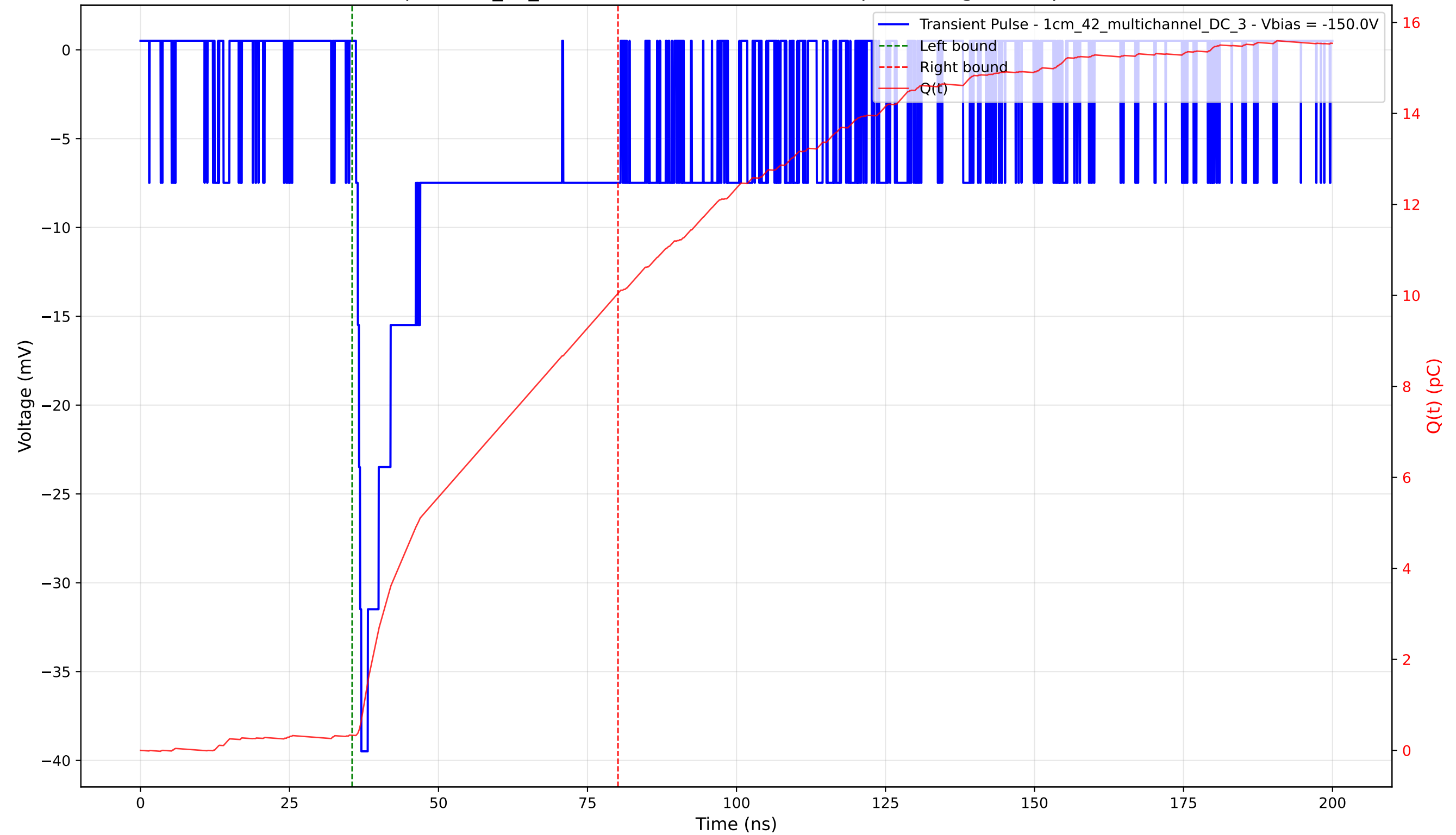
Transient Pulse - Sample: 1cm_42_multichannel - Position: 4425.0 \mu\text{m} - Charge: 9.72 pC - Rise Time: 0.89 ns
