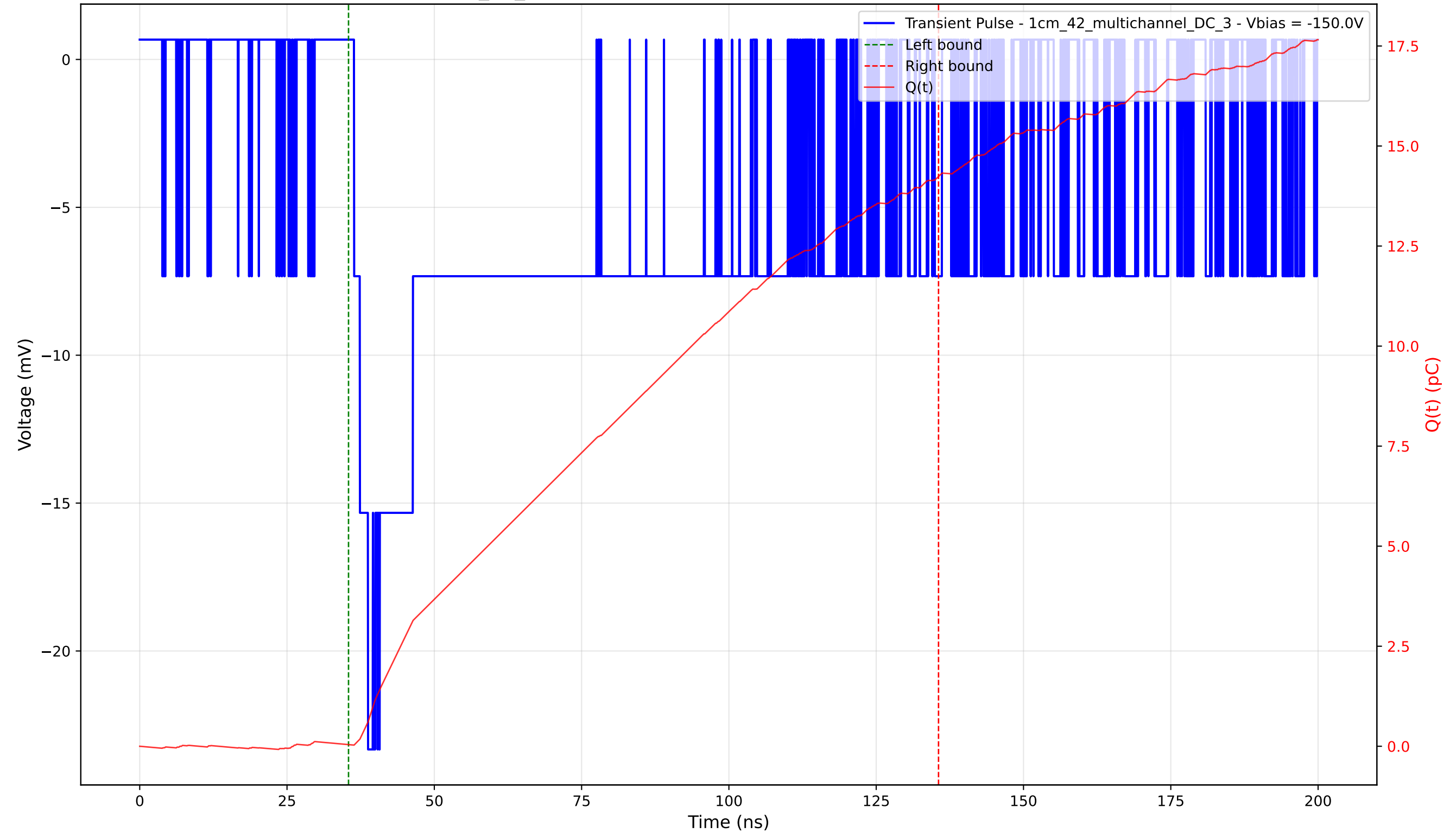
Transient Pulse - Sample: 1cm_42_multichannel - Position: 1900.0 \mu\text{m} - Charge: 14.20 pC - Rise Time: 2.38 ns
