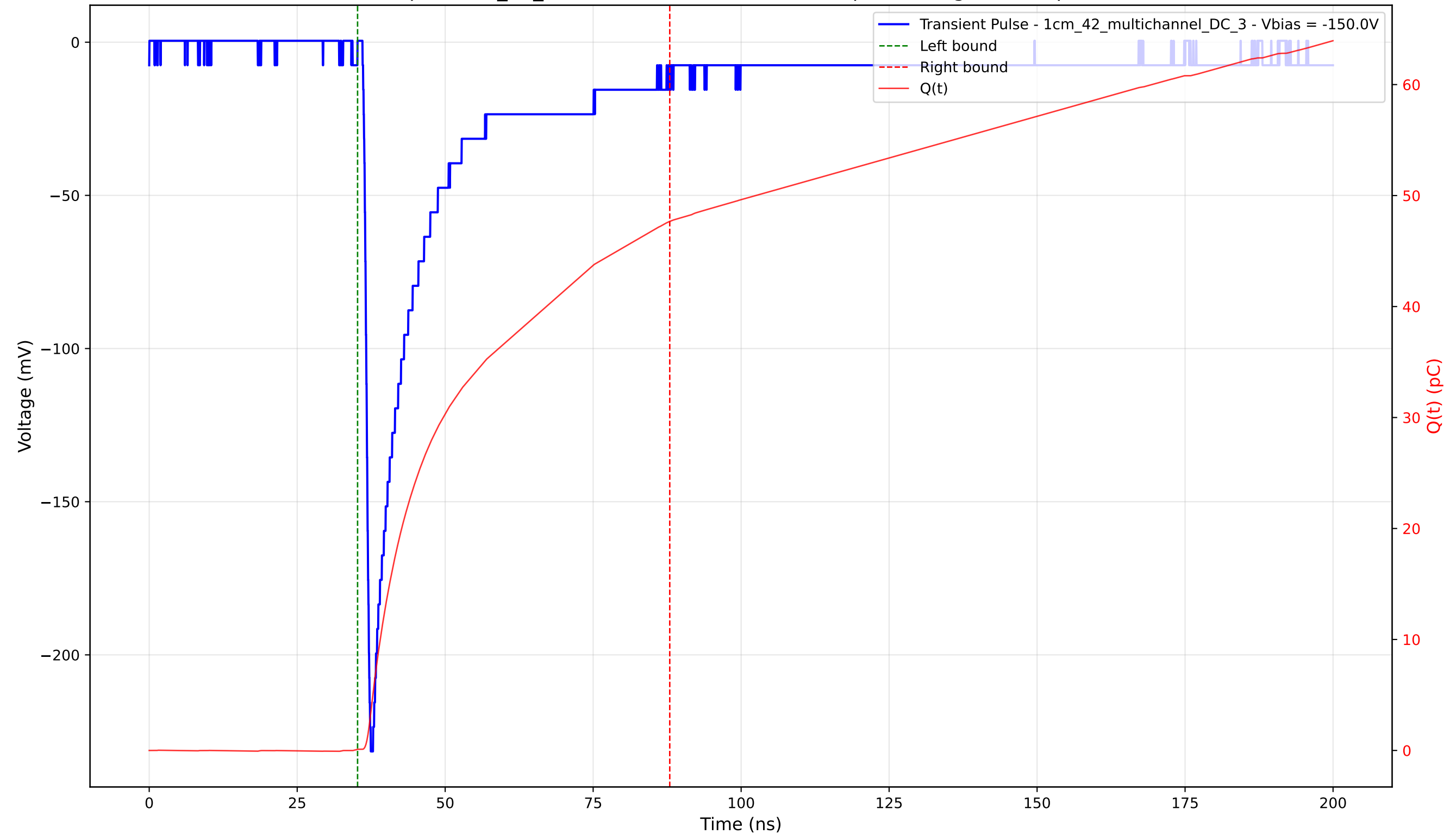
Transient Pulse - Sample: 1cm_42_multichannel - Position: 655.0 \mu\text{m} - Charge: 47.56 pC - Rise Time: 1.00 ns
