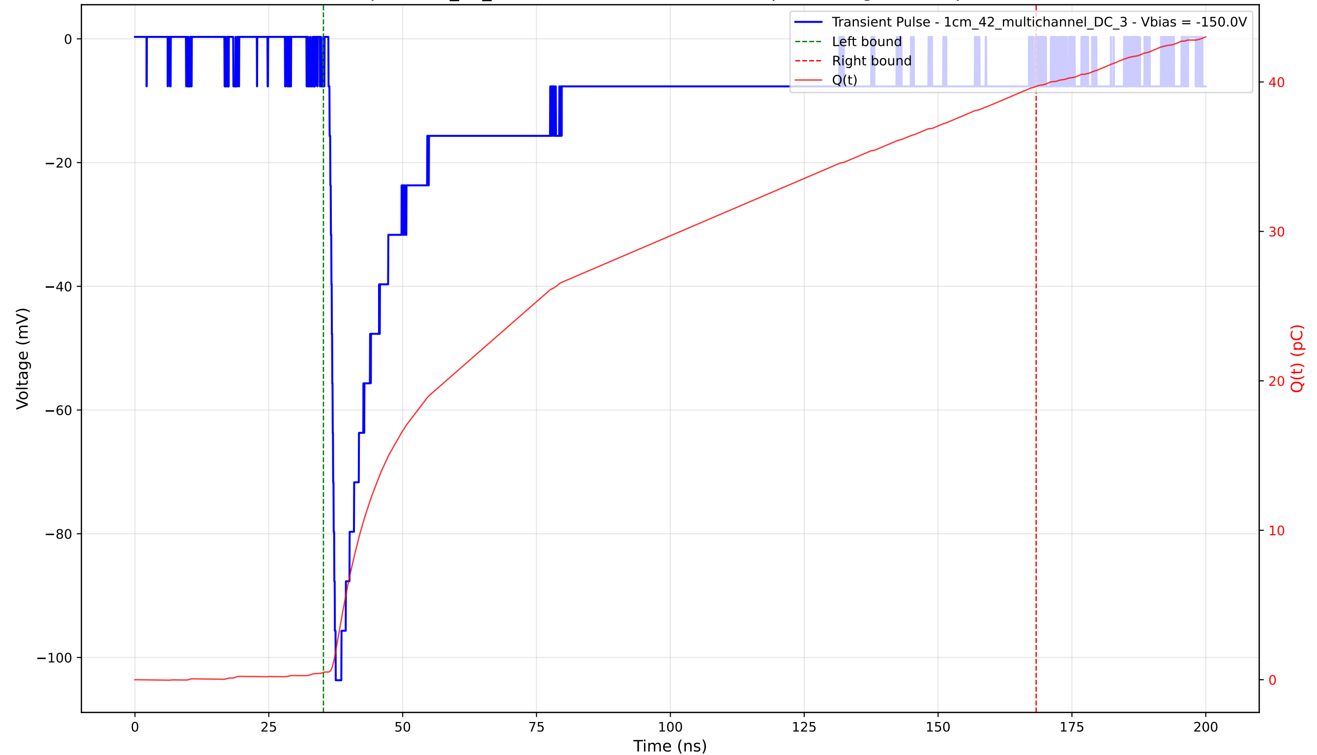
Transient Pulse - Sample: 1cm_42_multichannel - Position: 910.0 \mu\text{m} - Charge: 39.22 pC - Rise Time: 0.99 ns
