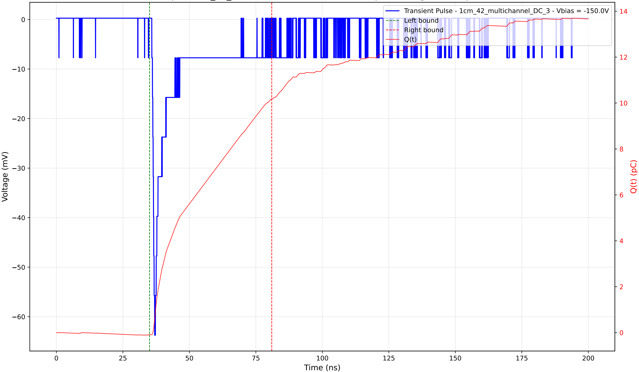
Transient Pulse - Sample: 1cm_42_multichannel - Position: 4870.0 \mu\text{m} - Charge: 10.27 pC - Rise Time: 1.06 ns
