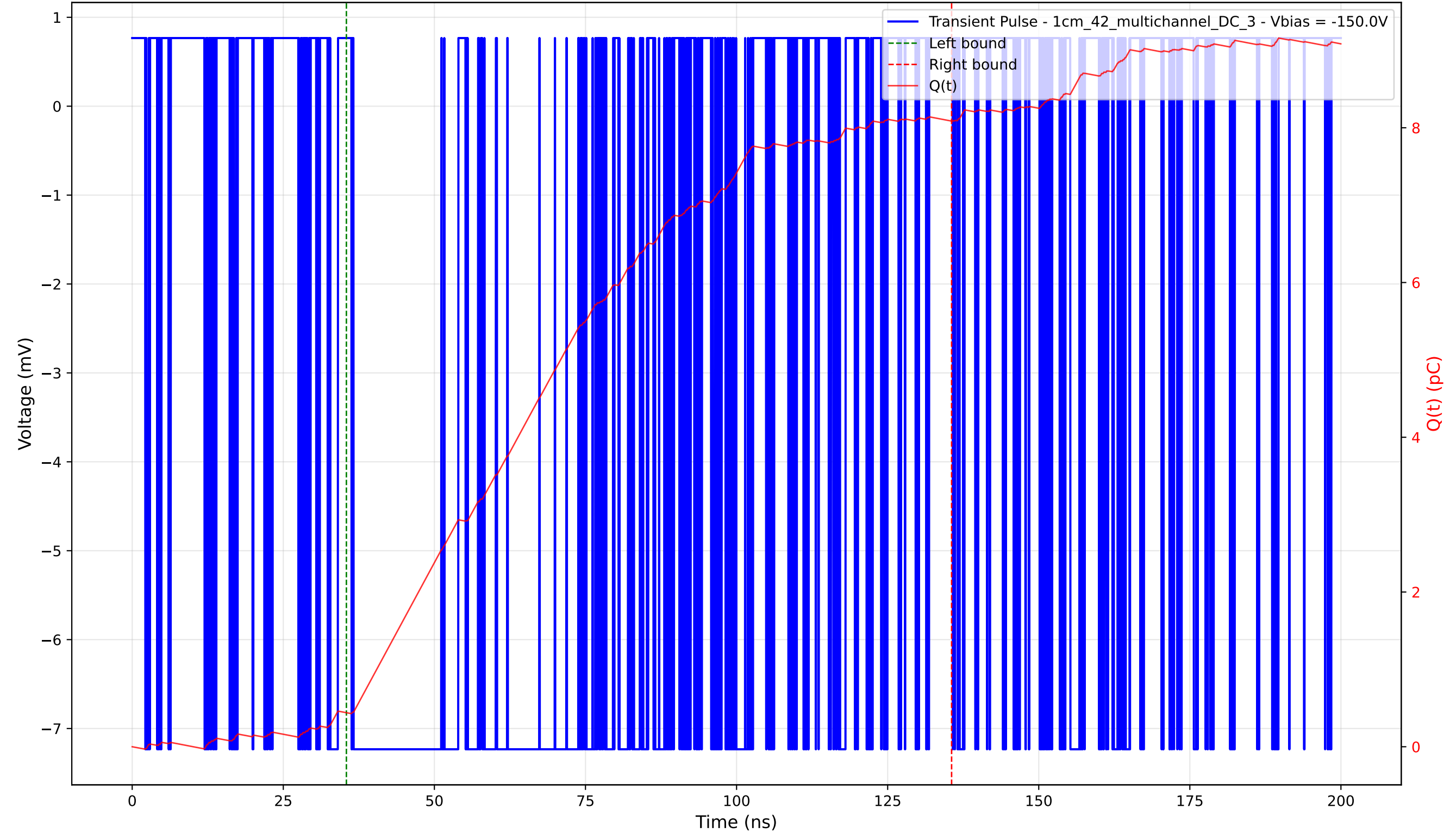
Transient Pulse - Sample: 1cm_42_multichannel - Position: 1880.0 \mu\text{m} - Charge: 7.65 pC - Rise Time: 0.00 ns (N/A)
