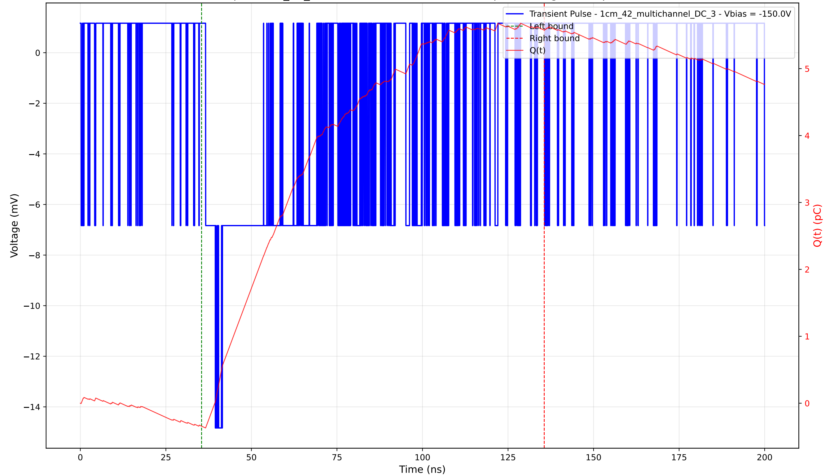
Transient Pulse - Sample: 1cm_42_multichannel - Position: 3405.0 \mu\text{m} - Charge: 5.92 pC - Rise Time: 2.86 ns
