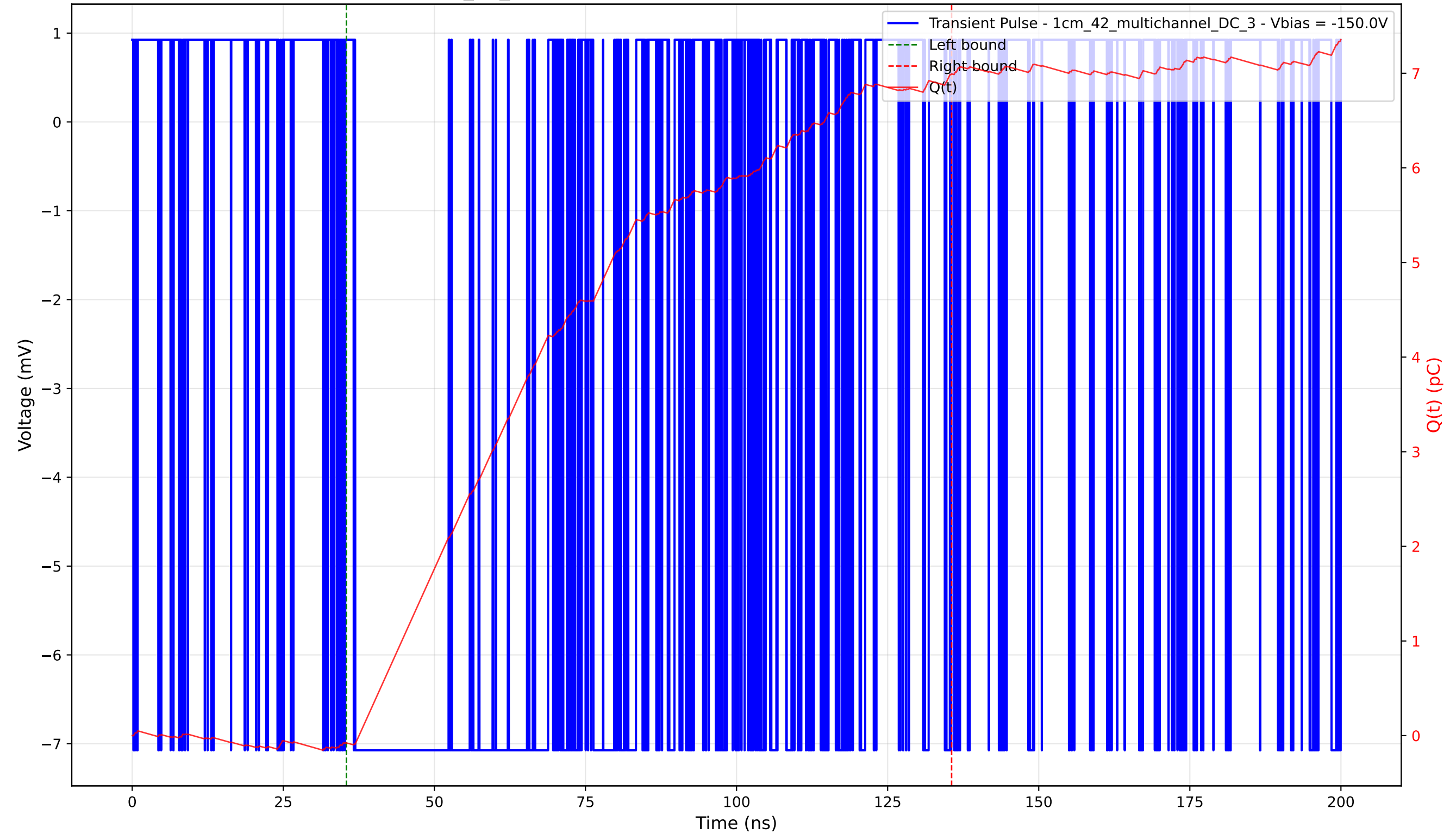
Transient Pulse - Sample: 1cm_42_multichannel - Position: 3380.0 \mu\text{m} - Charge: 7.07 pC - Rise Time: 0.00 ns (N/A)
