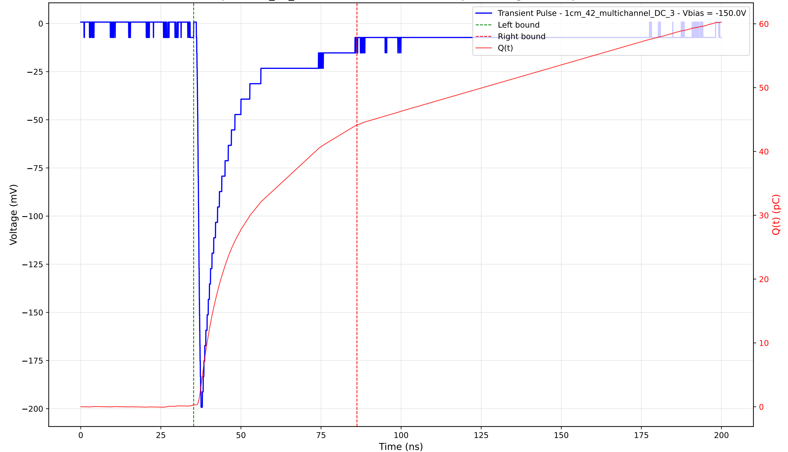
Transient Pulse - Sample: 1cm_42_multichannel - Position: 770.0 \mu\text{m} - Charge: 43.85 pC - Rise Time: 1.05 ns
