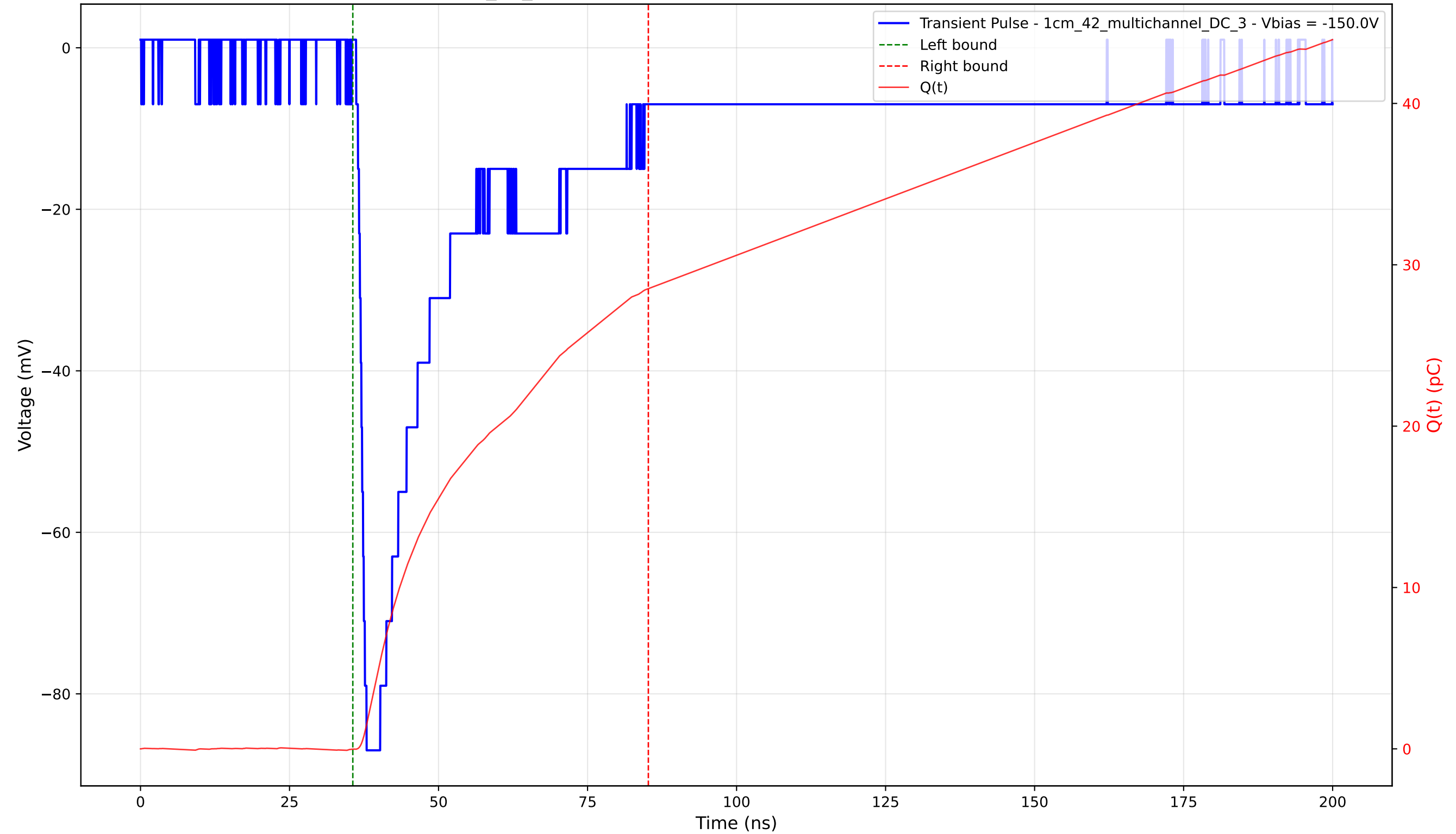
Transient Pulse - Sample: 1cm_42_multichannel - Position: 1420.0 \mu\text{m} - Charge: 28.54 pC - Rise Time: 1.18 ns
