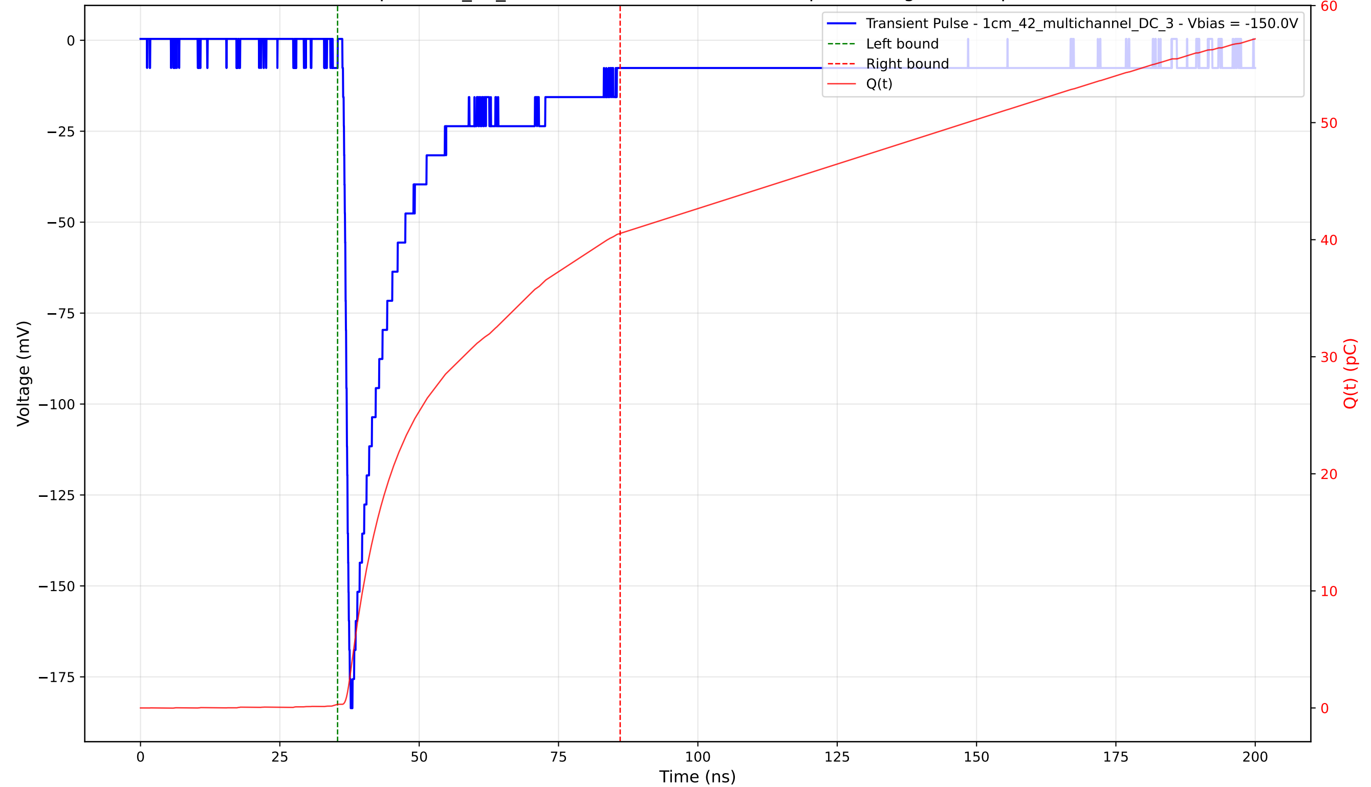
Transient Pulse - Sample: 1cm_42_multichannel - Position: 4110.0 \mu\text{m} - Charge: 40.23 pC - Rise Time: 0.99 ns
