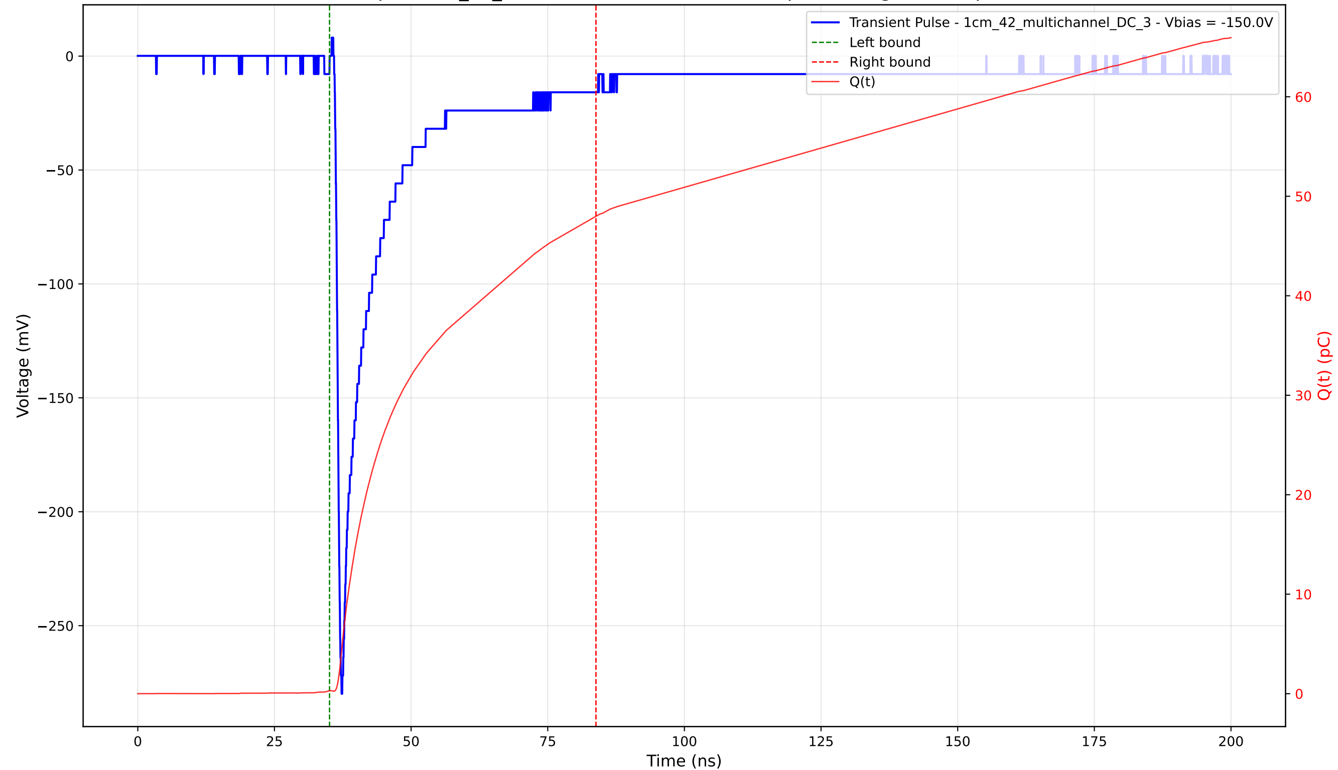
Transient Pulse - Sample: 1cm_42_multichannel - Position: 435.0 \mu\text{m} - Charge: 47.70 pC - Rise Time: 0.91 ns
