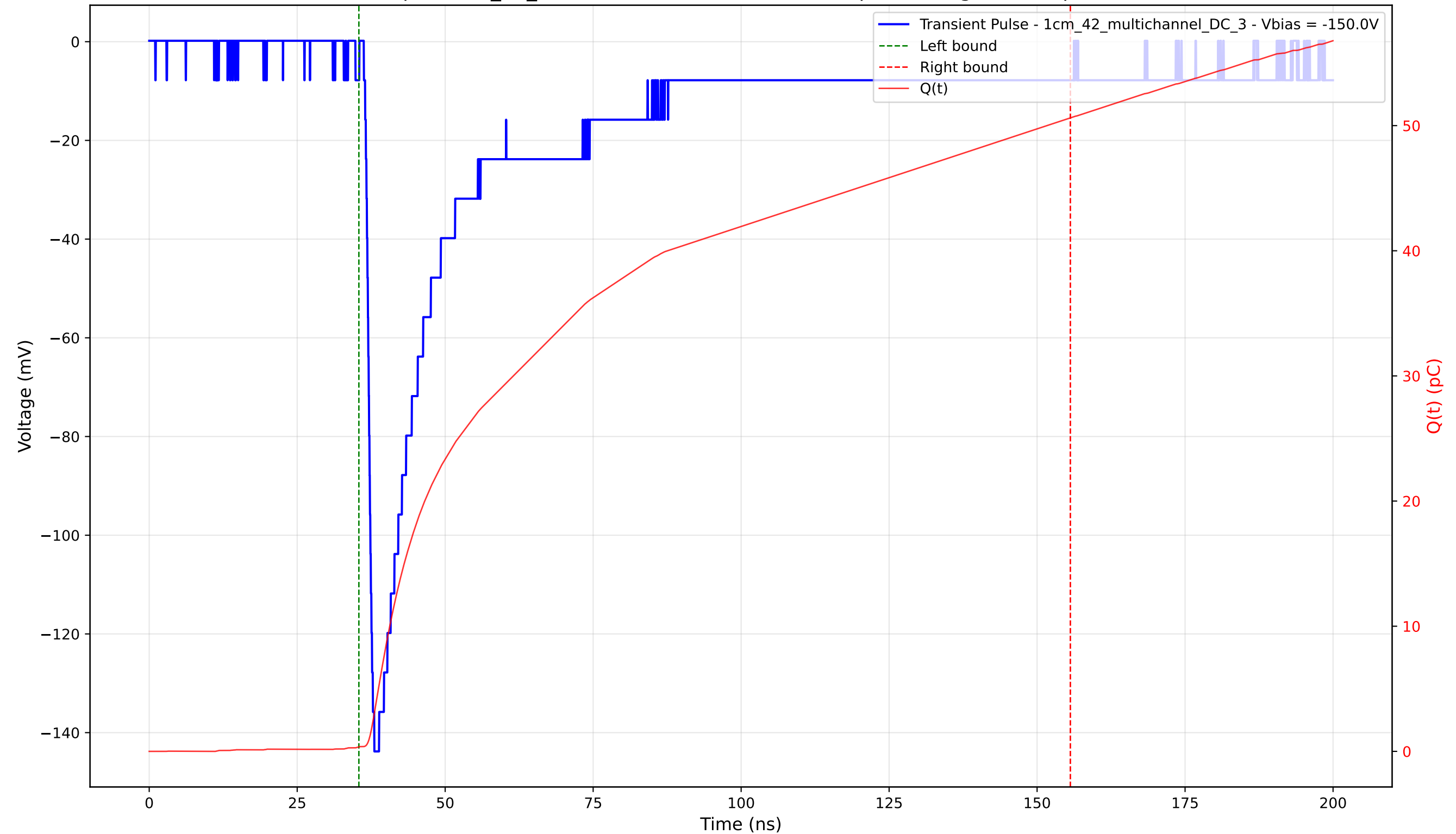
Transient Pulse - Sample: 1cm_42_multichannel - Position: 3735.0 \mu\text{m} - Charge: 50.26 pC - Rise Time: 1.30 ns
