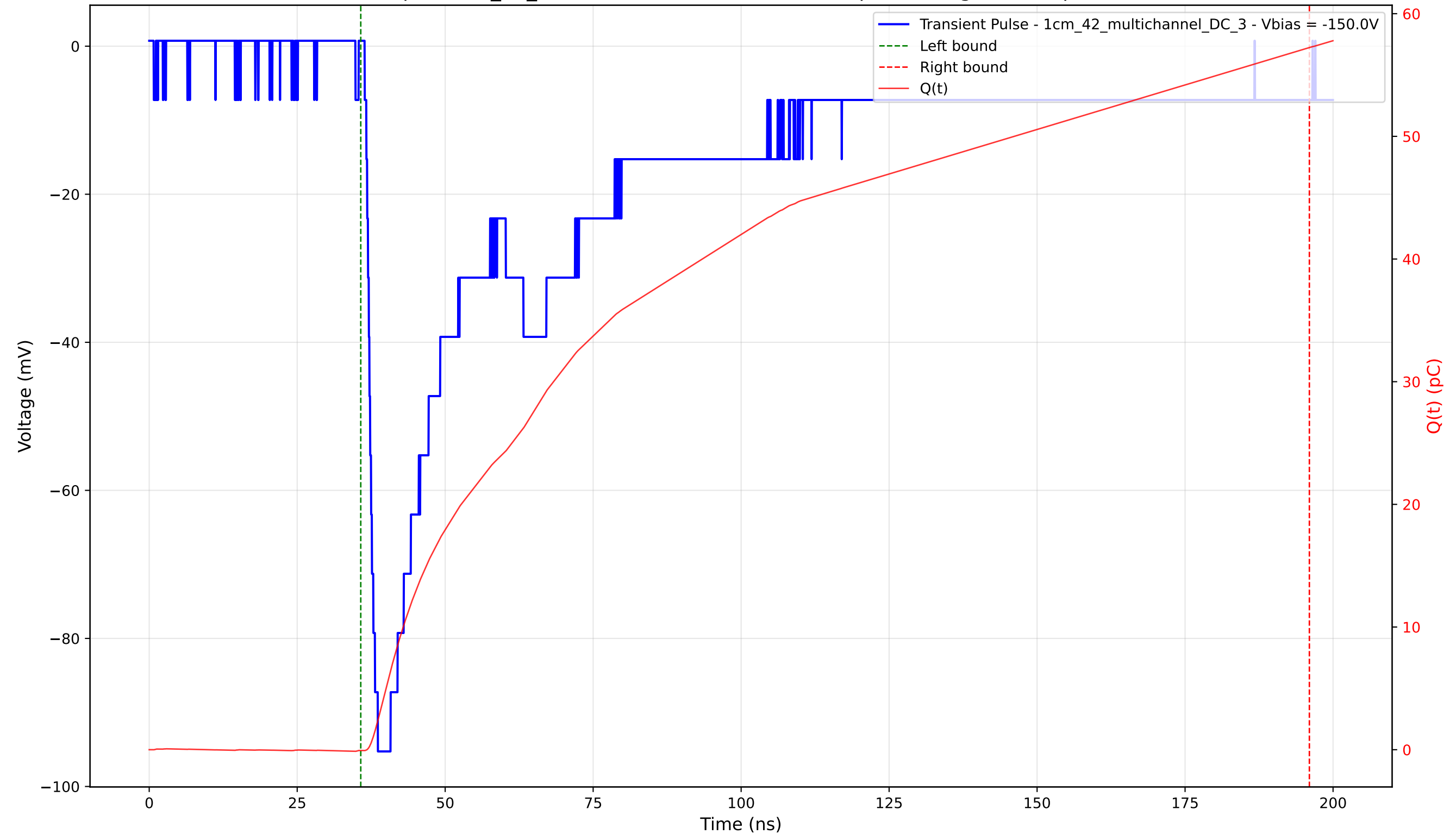
Transient Pulse - Sample: 1cm_42_multichannel - Position: 2030.0 \mu\text{m} - Charge: 57.30 pC - Rise Time: 1.47 ns
