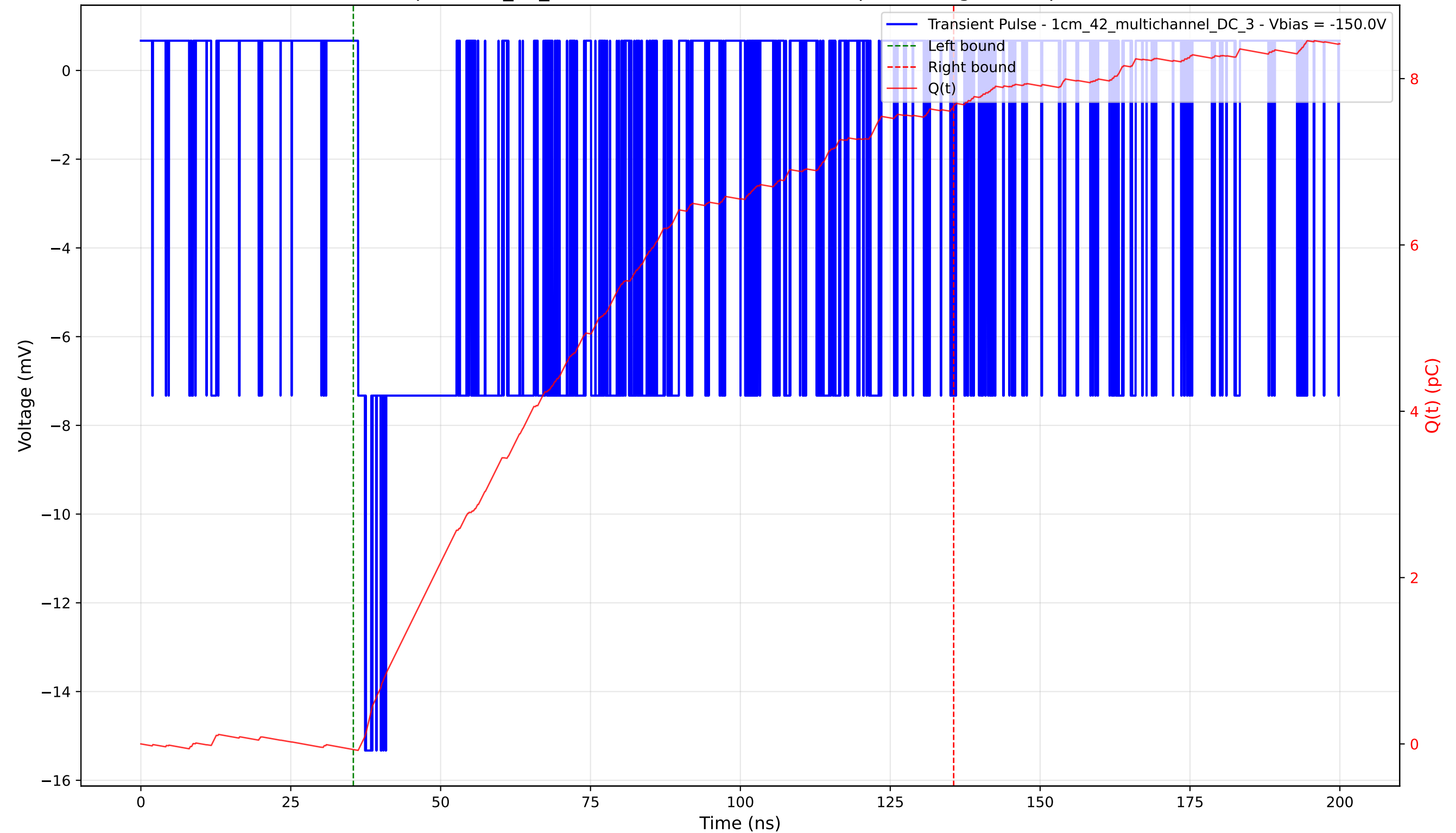
Transient Pulse - Sample: 1cm_42_multichannel - Position: 860.0 \mu\text{m} - Charge: 7.73 pC - Rise Time: 1.16 ns
