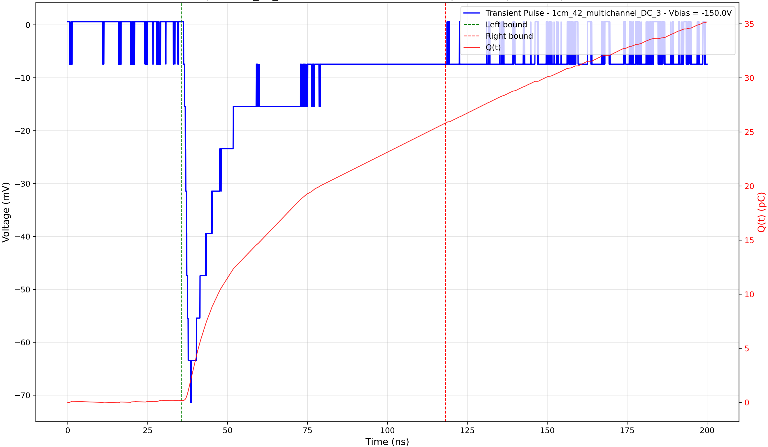
Transient Pulse - Sample: 1cm_42_multichannel - Position: 1315.0 \mu\text{m} - Charge: 25.66 pC - Rise Time: 2.18 ns
