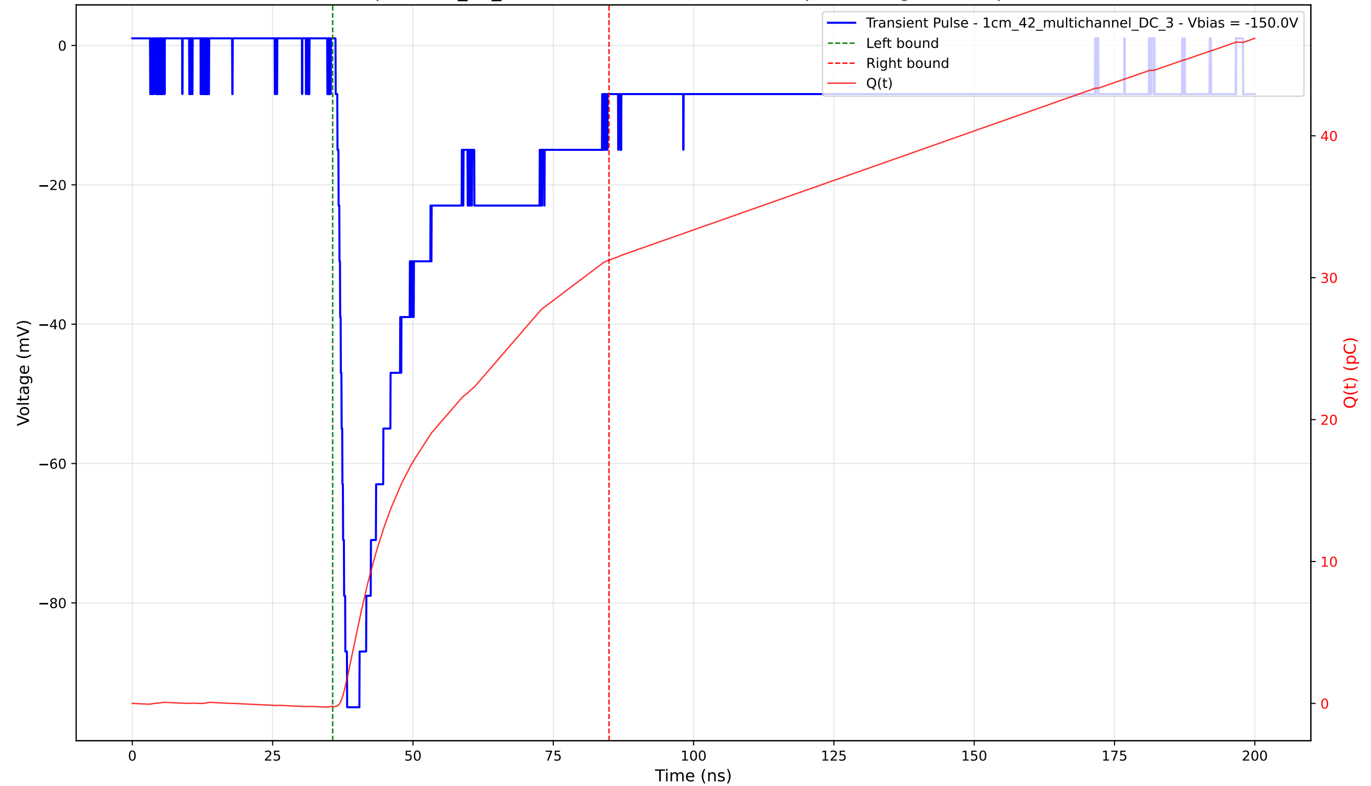
Transient Pulse - Sample: 1cm_42_multichannel - Position: 3315.0 \mu\text{m} - Charge: 31.45 pC - Rise Time: 1.41 ns
