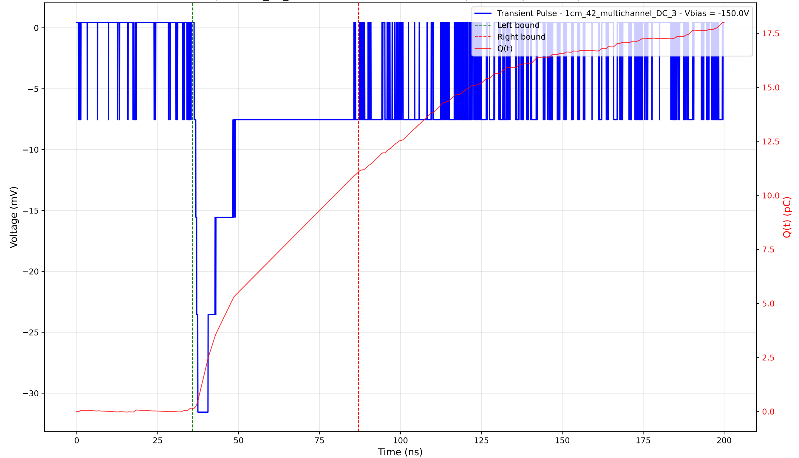
Transient Pulse - Sample: 1cm_42_multichannel - Position: 3925.0 \mu\text{m} - Charge: 10.94 pC - Rise Time: 1.15 ns
