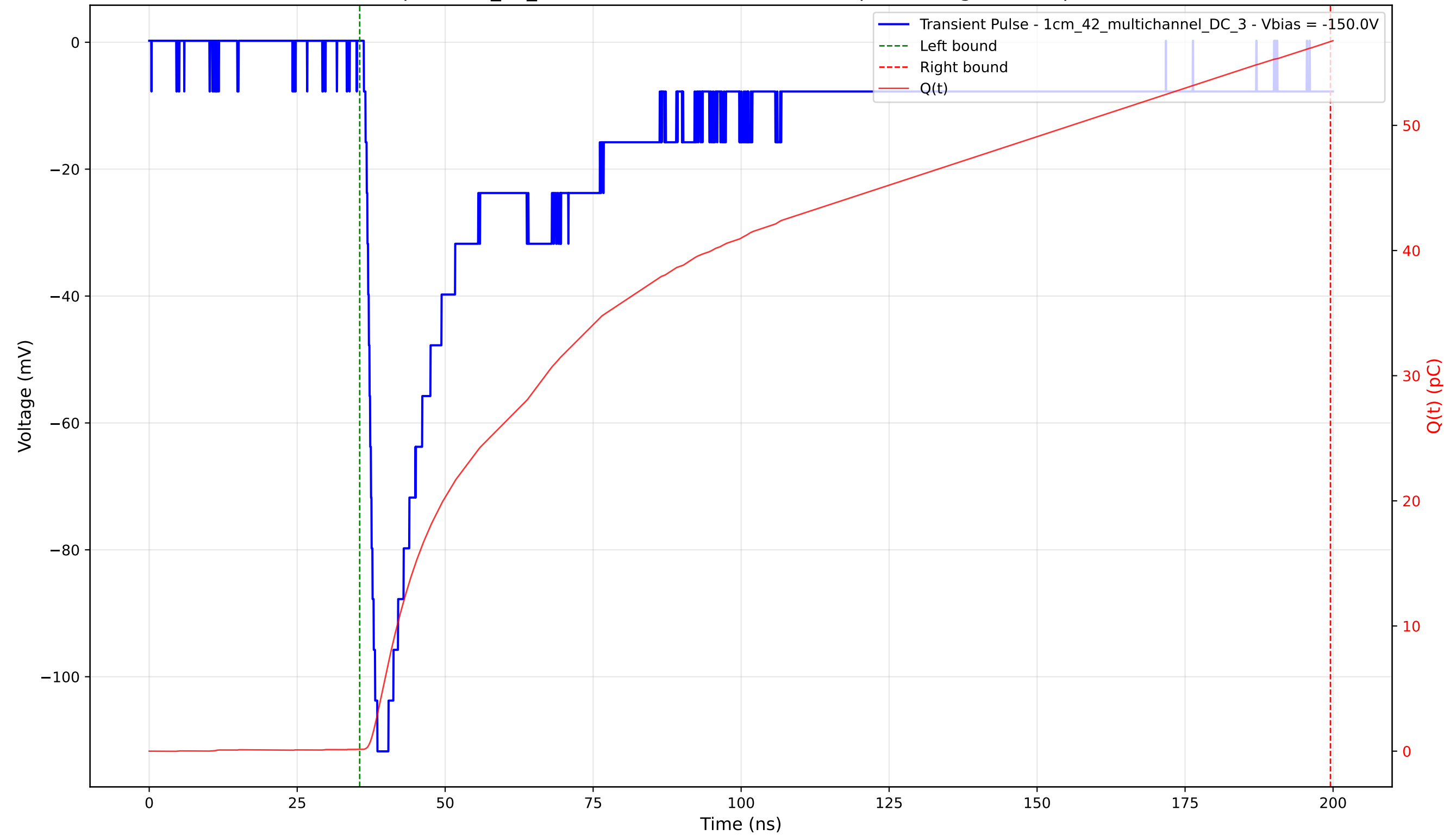
Transient Pulse - Sample: 1cm_42_multichannel - Position: 3220.0 \mu\text{m} - Charge: 56.55 pC - Rise Time: 1.63 ns
