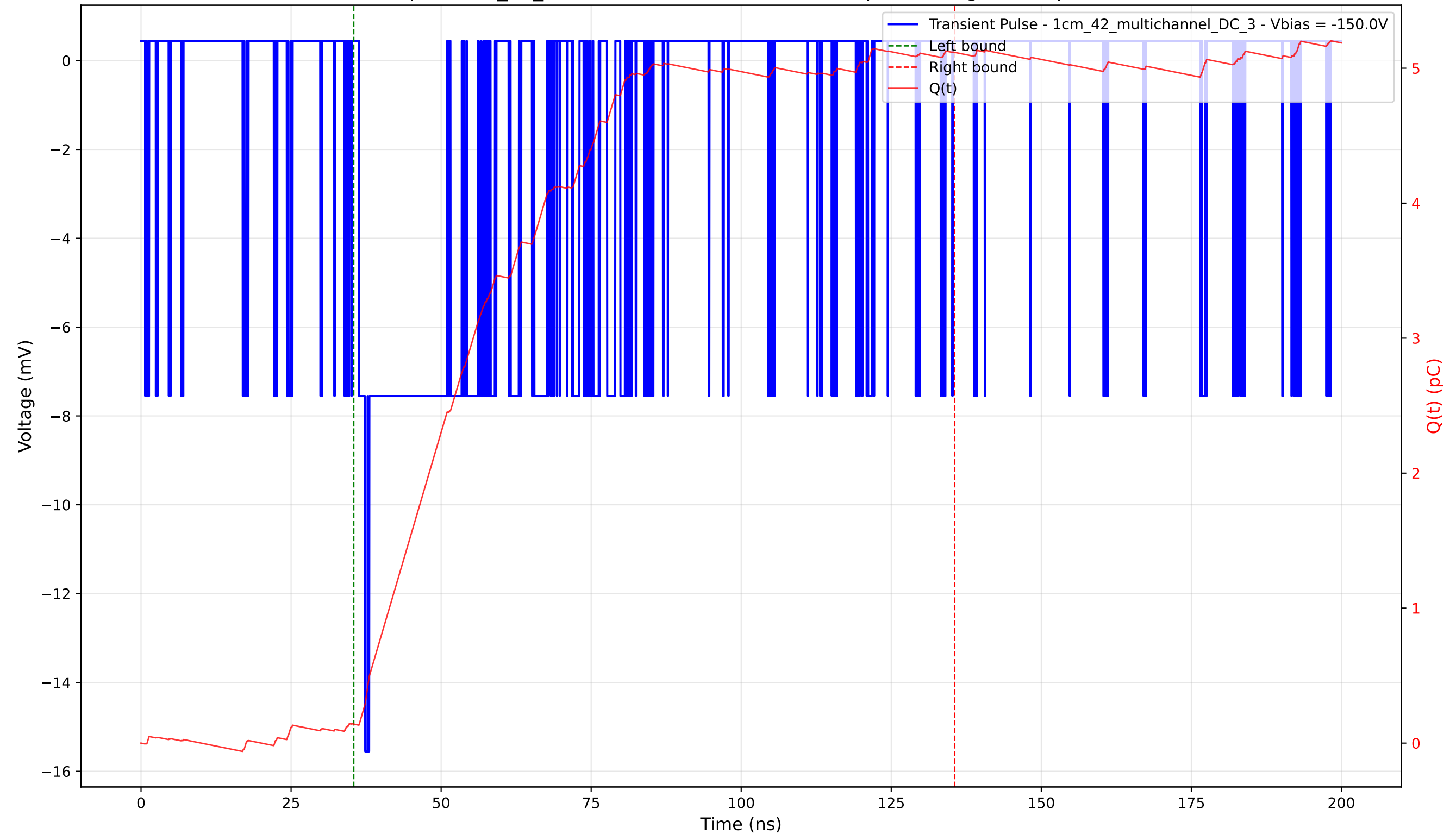
Transient Pulse - Sample: 1cm_42_multichannel - Position: 4385.0 \mu\text{m} - Charge: 4.98 pC - Rise Time: 1.04 ns
