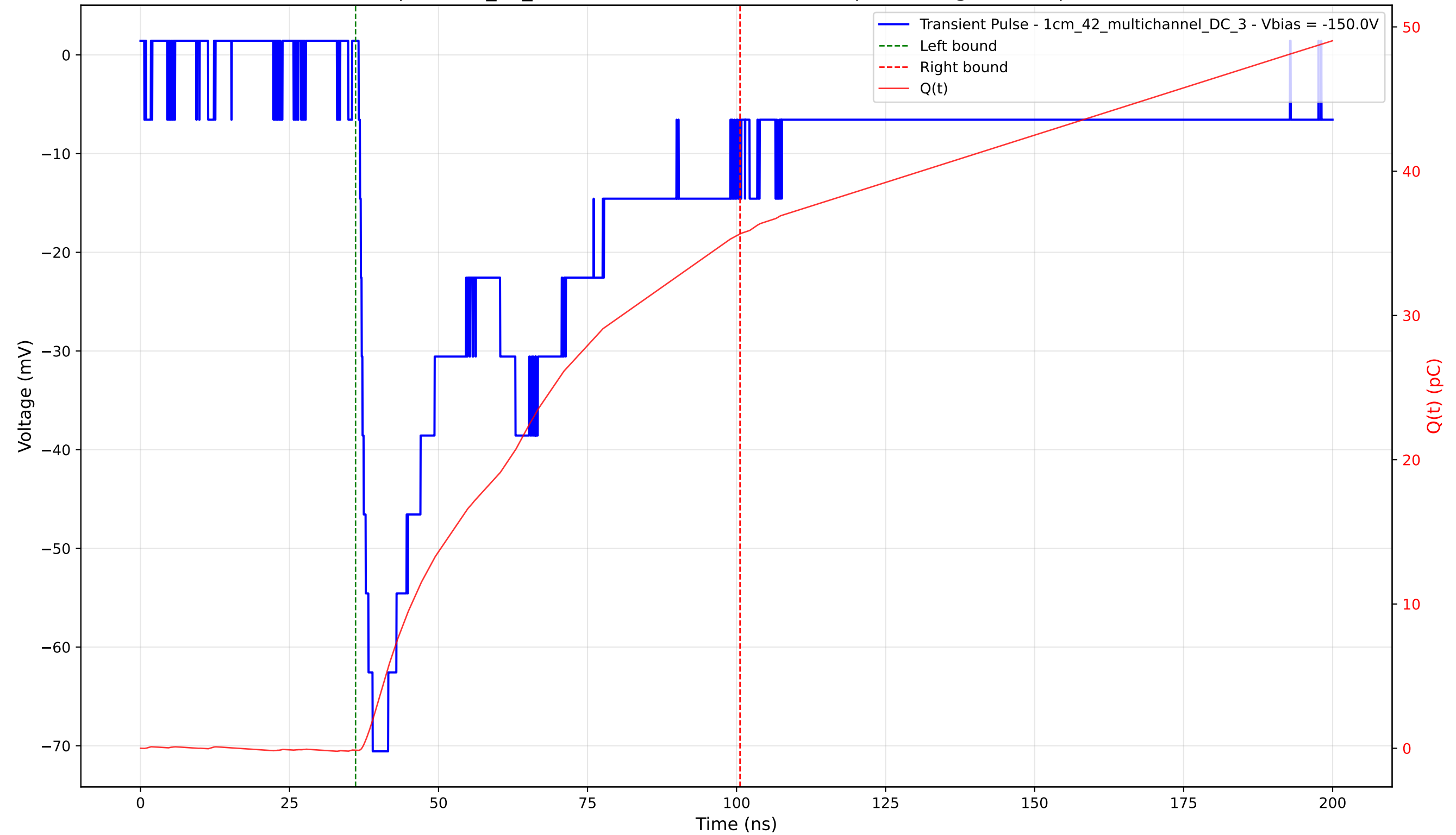
Transient Pulse - Sample: 1cm_42_multichannel - Position: 2445.0 \mu\text{m} - Charge: 35.78 pC - Rise Time: 2.14 ns
