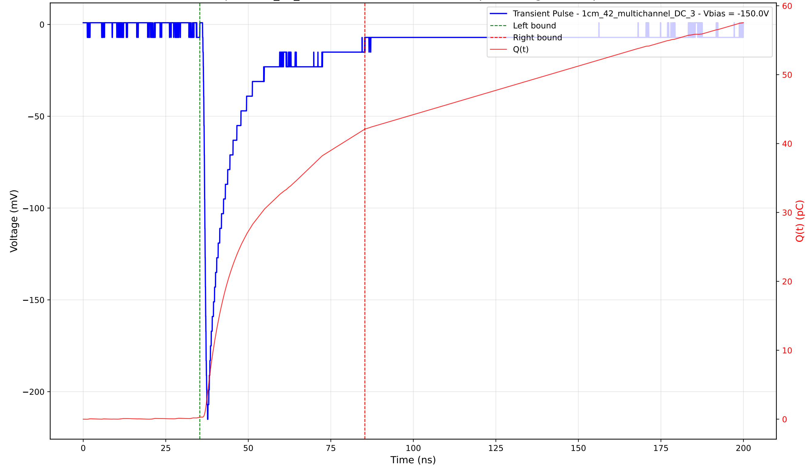
Transient Pulse - Sample: 1cm_42_multichannel - Position: 4230.0 \mu\text{m} - Charge: 41.79 pC - Rise Time: 1.02 ns
