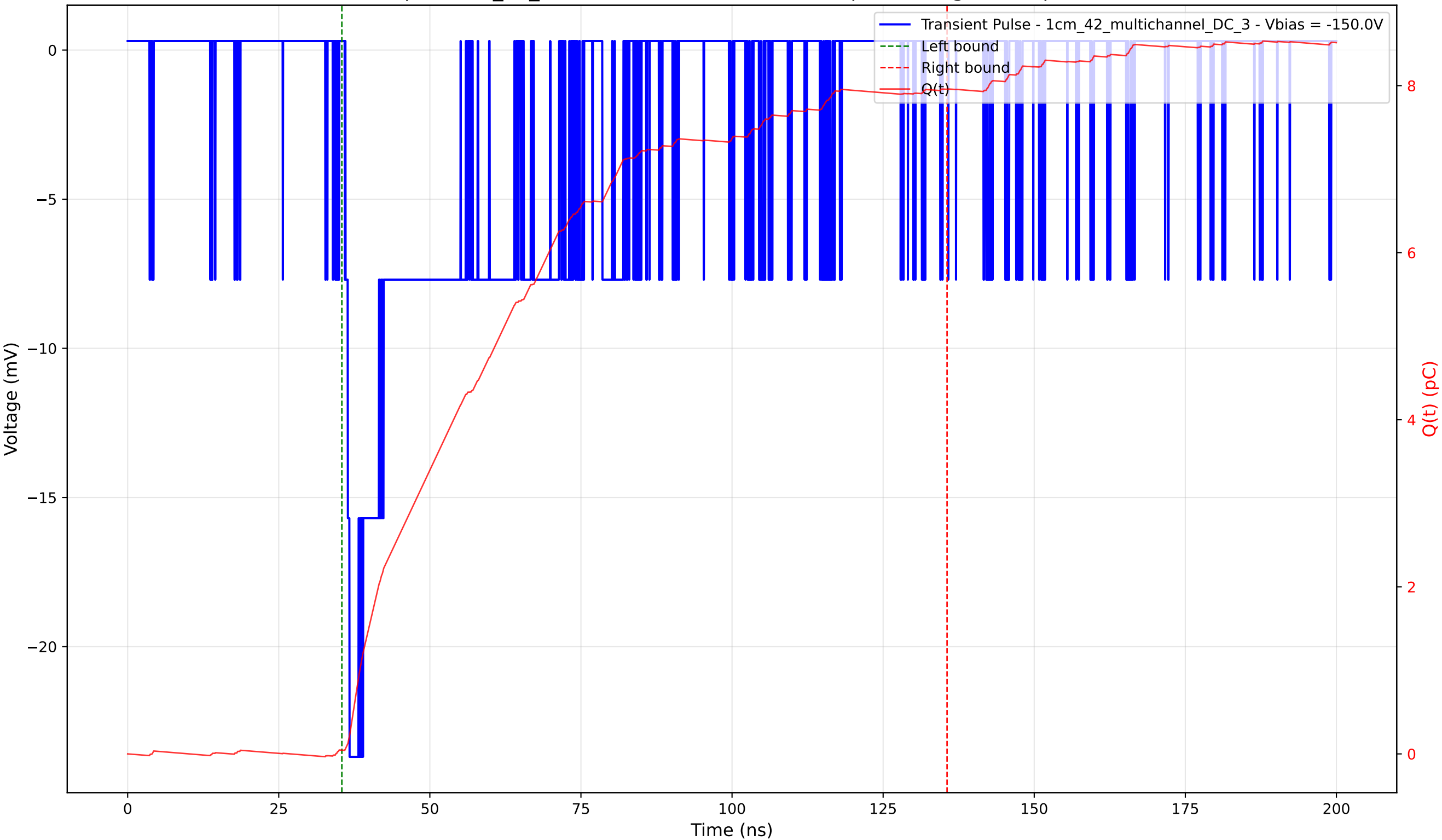
Transient Pulse - Sample: 1cm_42_multichannel - Position: 330.0 \mu\text{m} - Charge: 7.91 pC - Rise Time: 0.67 ns
