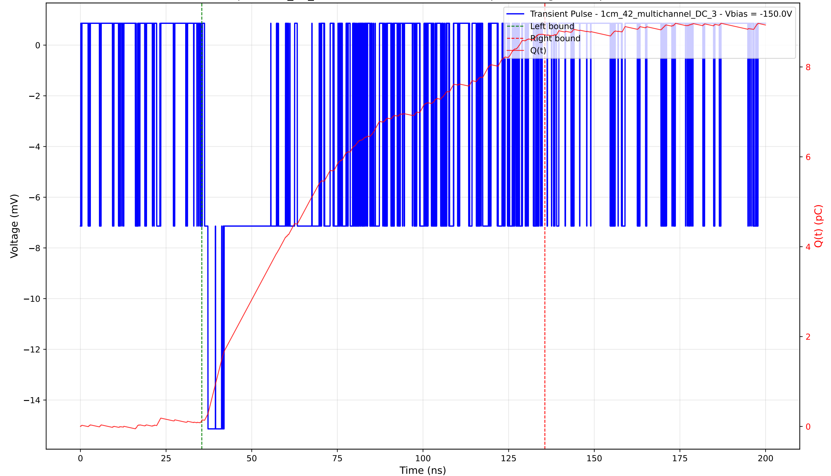
Transient Pulse - Sample: 1cm_42_multichannel - Position: 870.0 \mu\text{m} - Charge: 8.59 pC - Rise Time: 1.00 ns
