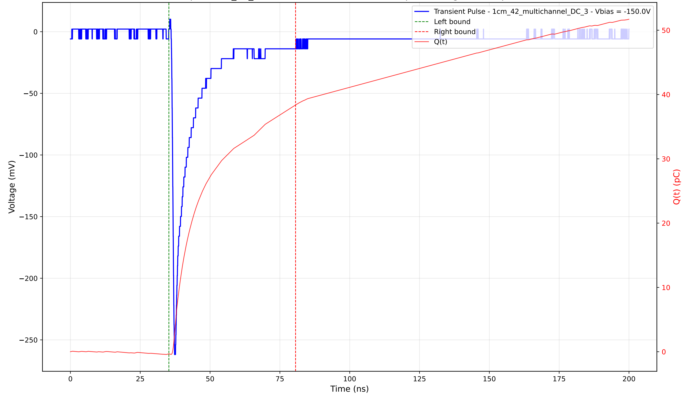
Transient Pulse - Sample: 1cm_42_multichannel - Position: 4515.0 \mu\text{m} - Charge: 38.72 pC - Rise Time: 0.83 ns
