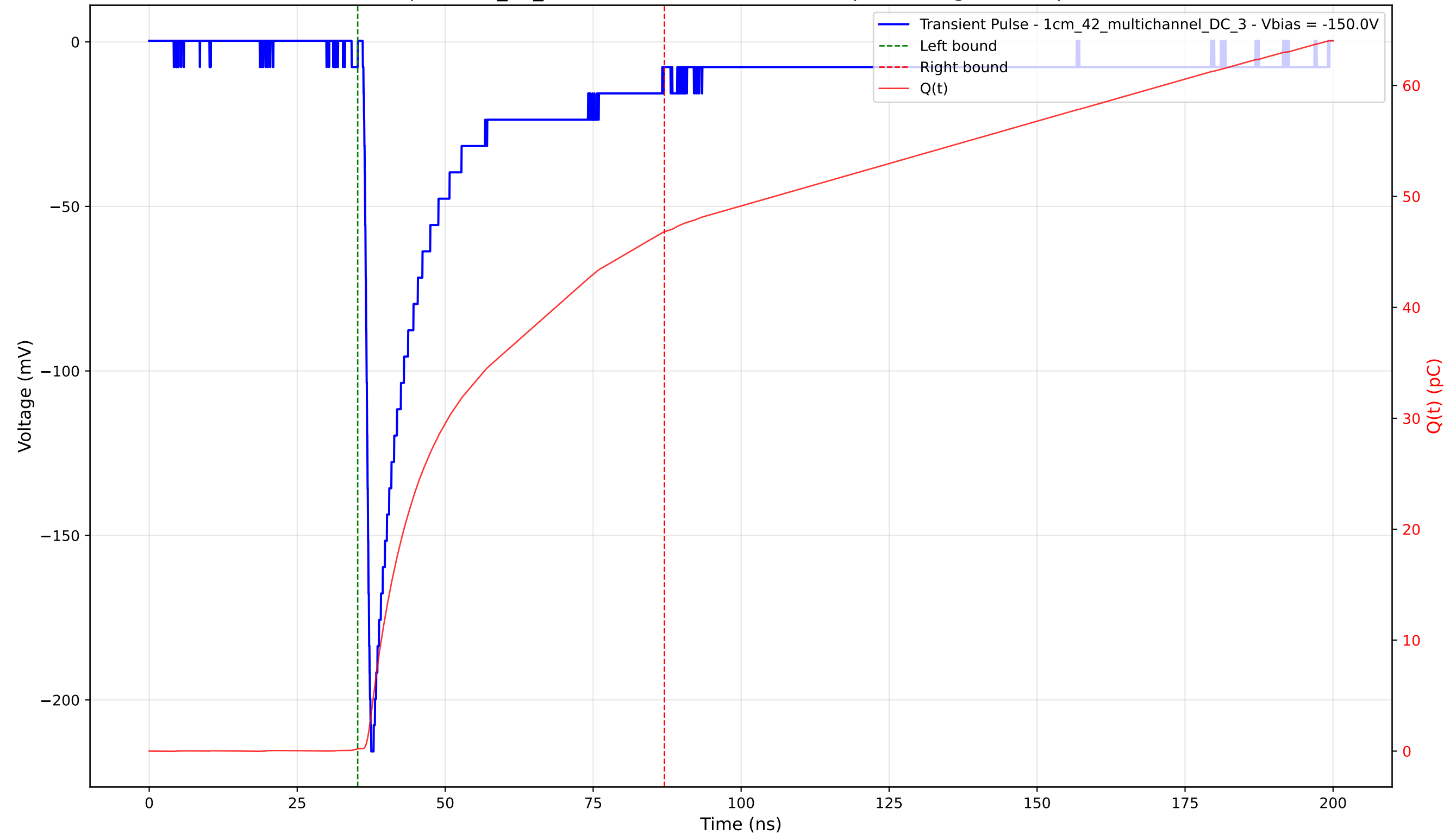
Transient Pulse - Sample: 1cm_42_multichannel - Position: 730.0 \mu\text{m} - Charge: 46.60 pC - Rise Time: 1.01 ns
