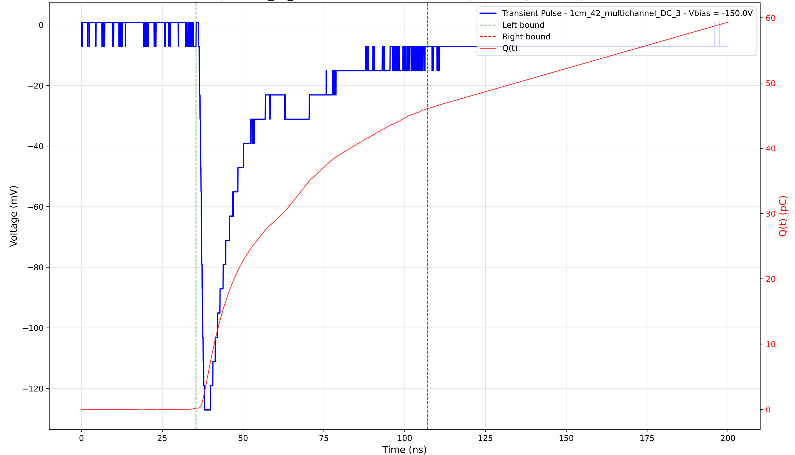
Transient Pulse - Sample: 1cm_42_multichannel - Position: 1450.0 \mu\text{m} - Charge: 45.87 pC - Rise Time: 1.39 ns
