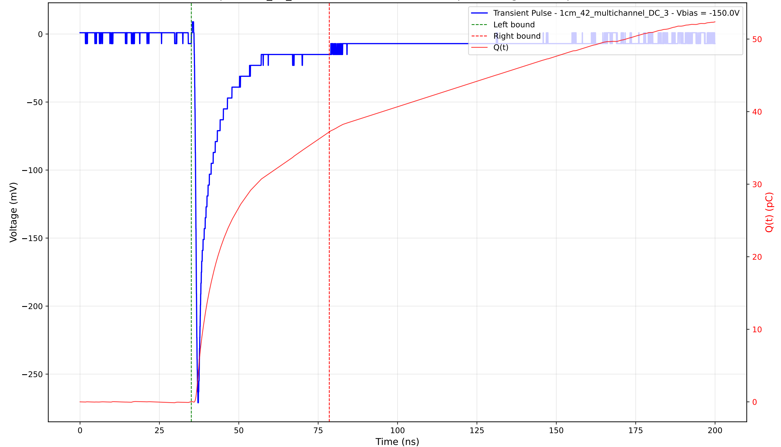
Transient Pulse - Sample: 1cm_42_multichannel - Position: 280.0 \mu\text{m} - Charge: 37.18 pC - Rise Time: 0.83 ns
