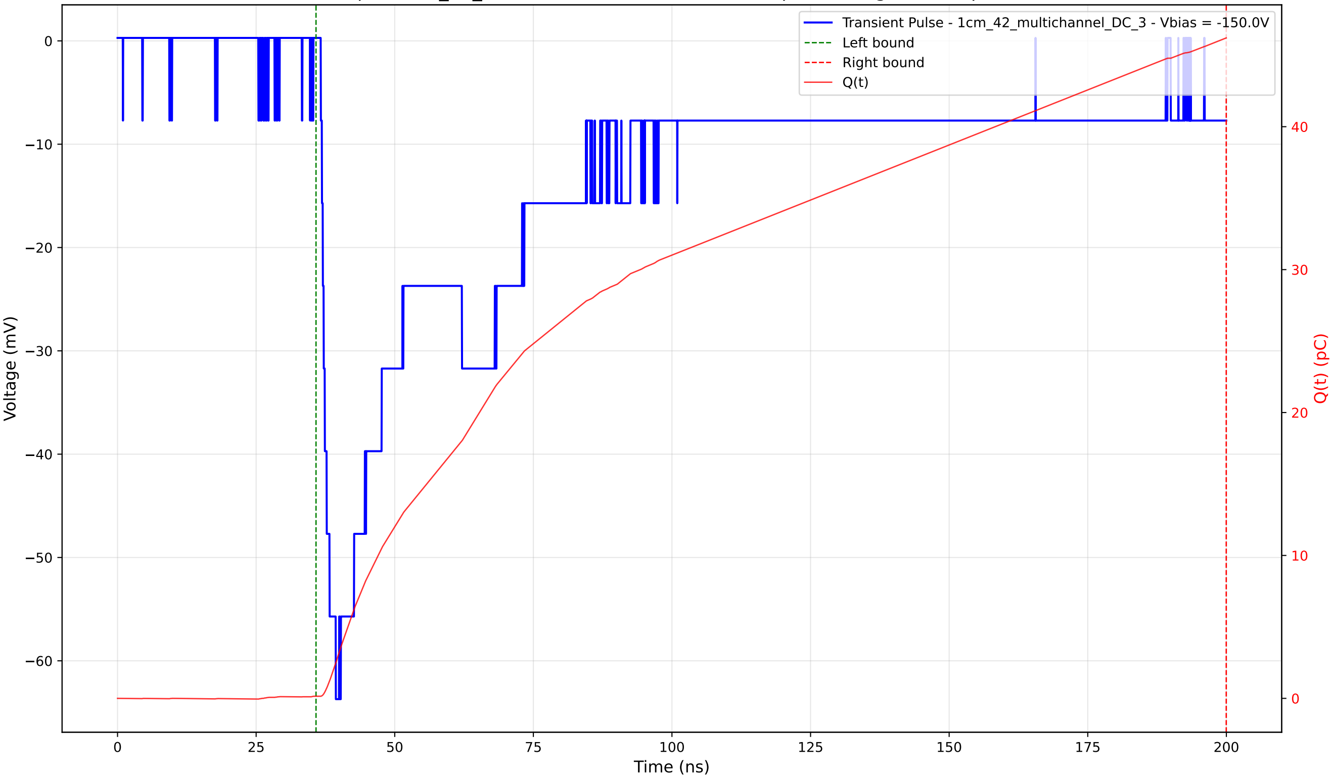
Transient Pulse - Sample: 1cm_42_multichannel - Position: 2435.0 \mu\text{m} - Charge: 46.07 pC - Rise Time: 2.70 ns
