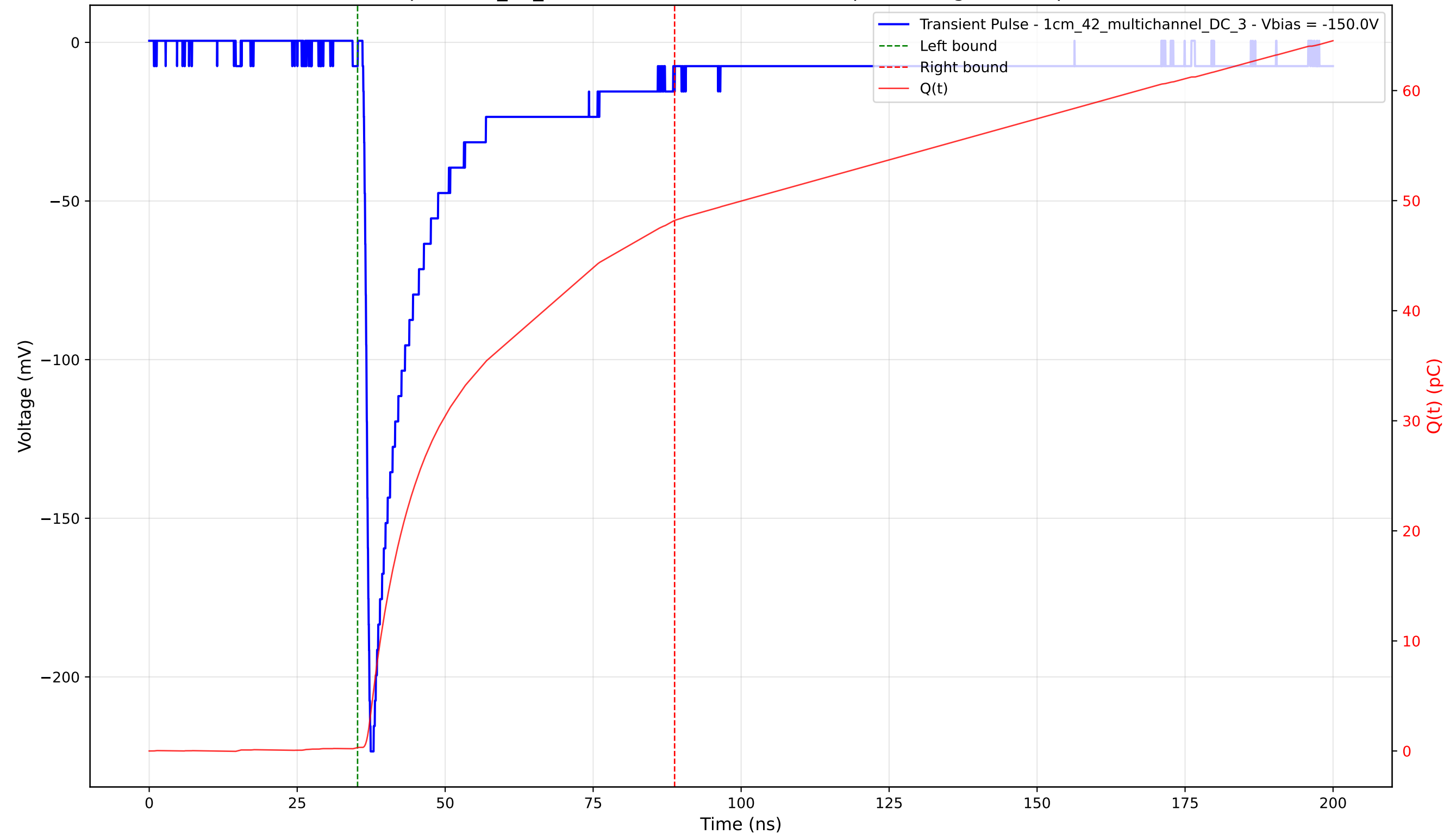
Transient Pulse - Sample: 1cm_42_multichannel - Position: 685.0 \mu\text{m} - Charge: 47.89 pC - Rise Time: 0.98 ns
