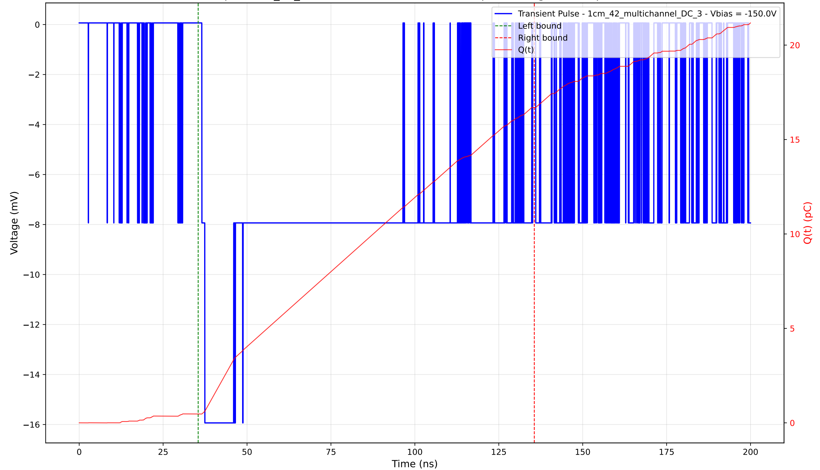
Transient Pulse - Sample: 1cm_42_multichannel - Position: 2340.0 \mu\text{m} - Charge: 16.23 pC - Rise Time: 0.90 ns
