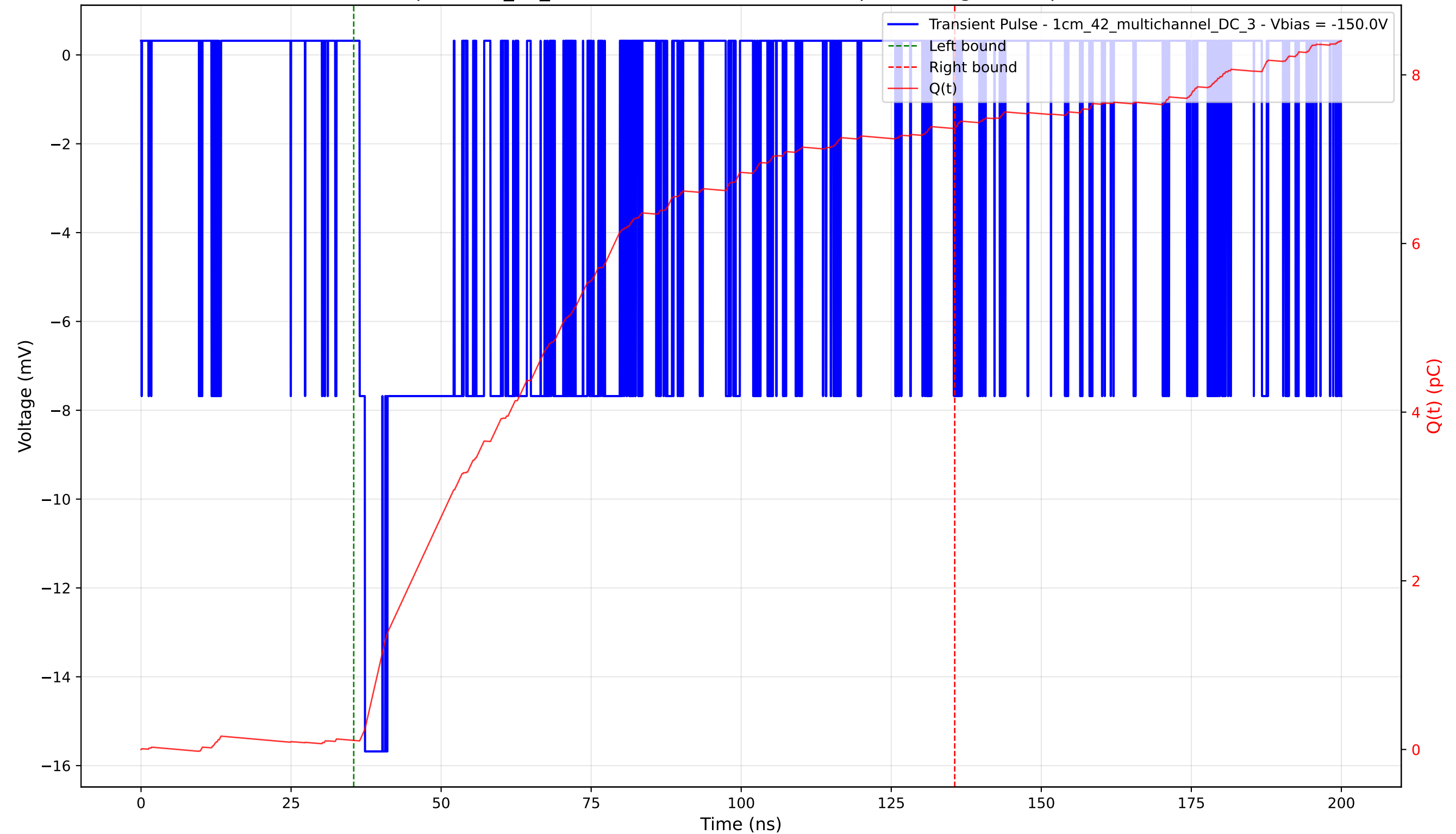
Transient Pulse - Sample: 1cm_42_multichannel - Position: 845.0 \mu\text{m} - Charge: 7.26 pC - Rise Time: 0.90 ns
