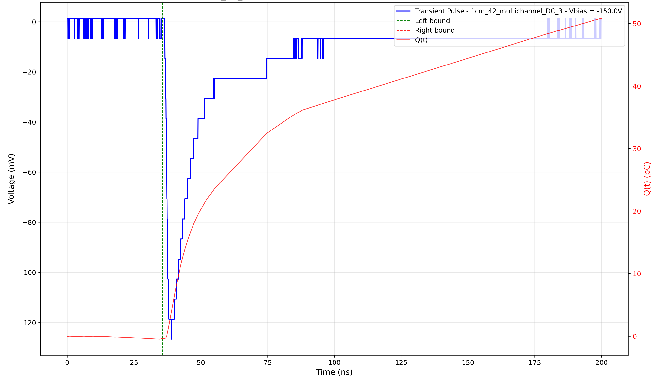
Transient Pulse - Sample: 1cm_42_multichannel - Position: 3530.0 \mu\text{m} - Charge: 36.58 pC - Rise Time: 1.54 ns
