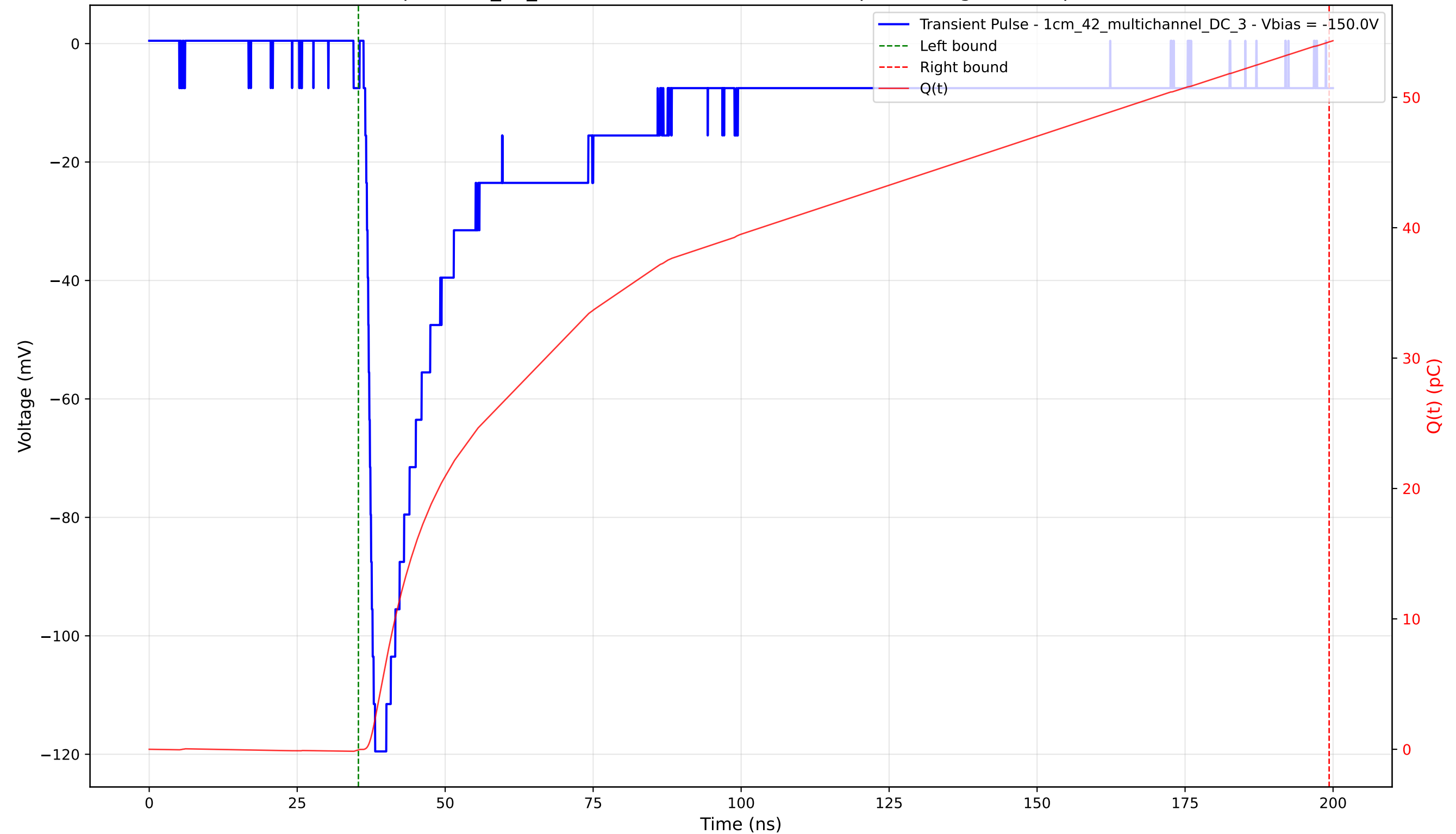
Transient Pulse - Sample: 1cm_42_multichannel - Position: 3480.0 \mu\text{m} - Charge: 54.28 pC - Rise Time: 1.43 ns
