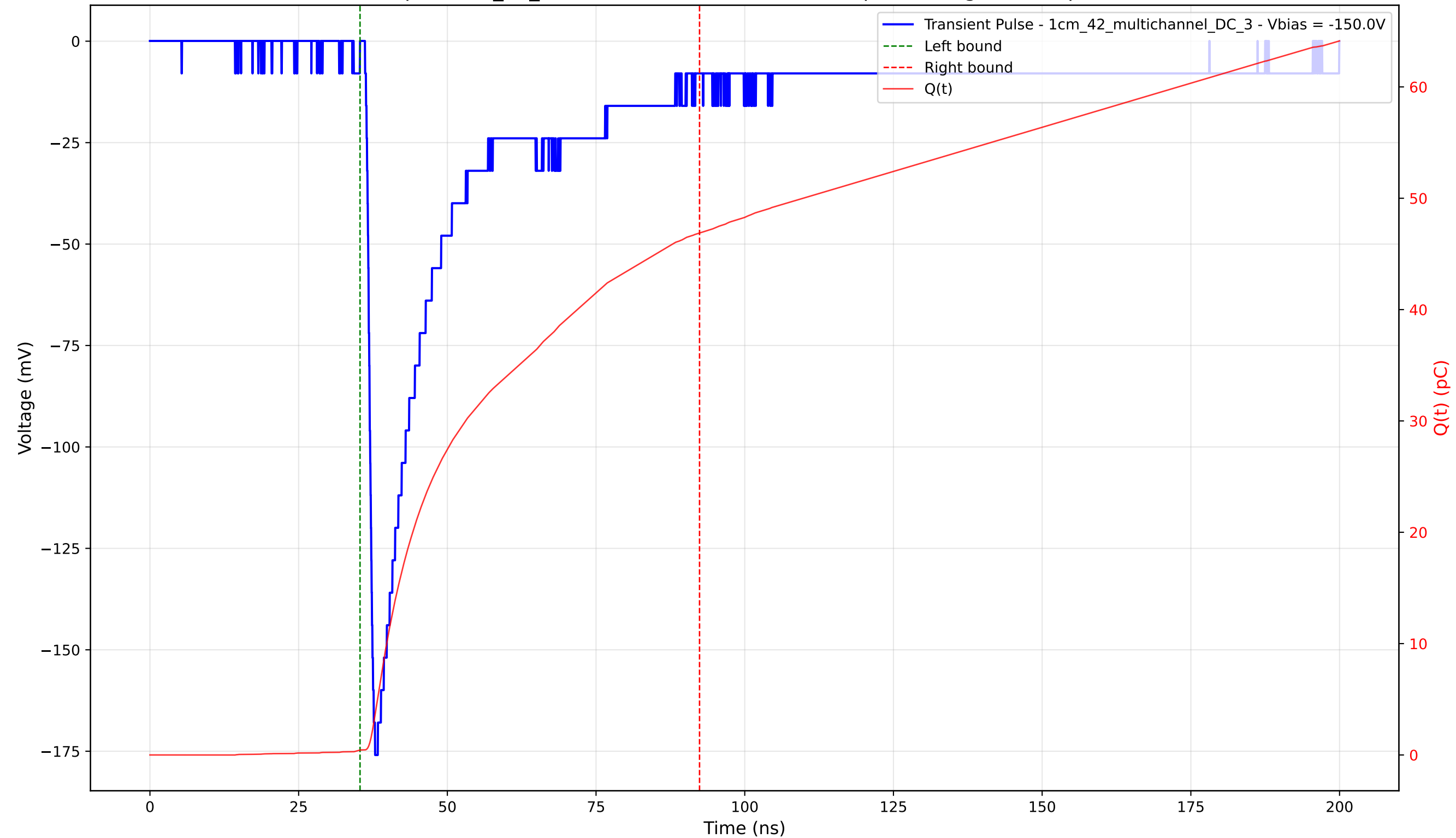
Transient Pulse - Sample: 1cm_42_multichannel - Position: 1015.0 \mu\text{m} - Charge: 46.43 pC - Rise Time: 1.10 ns
