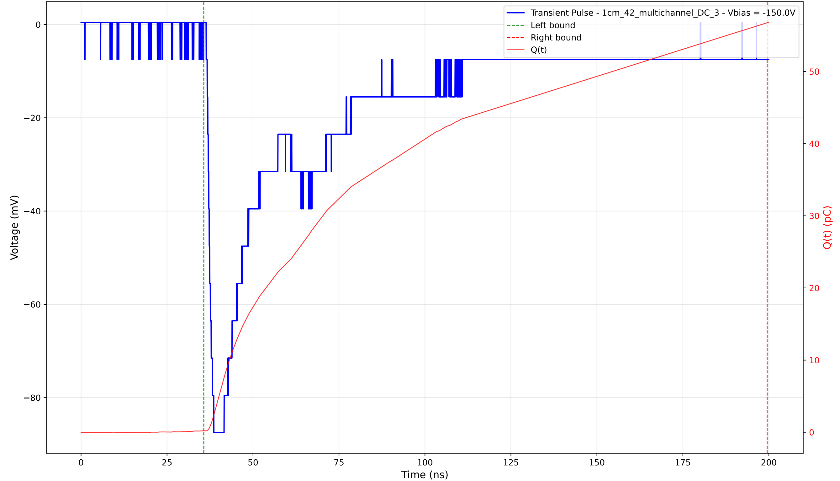
Transient Pulse - Sample: 1cm_42_multichannel - Position: 2735.0 \mu\text{m} - Charge: 56.56 pC - Rise Time: 1.52 ns
