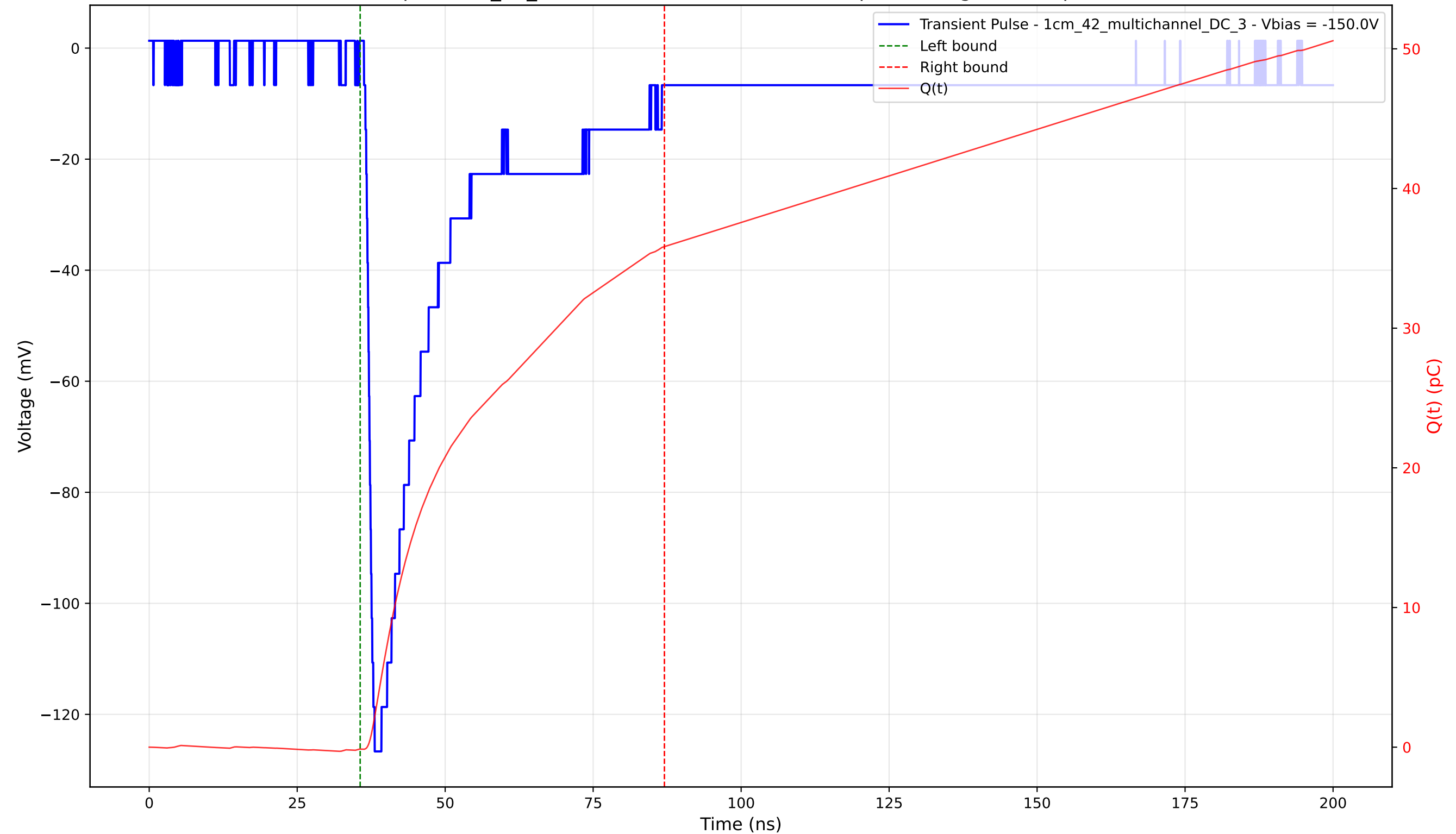
Transient Pulse - Sample: 1cm_42_multichannel - Position: 3635.0 \mu\text{m} - Charge: 35.98 pC - Rise Time: 1.35 ns
