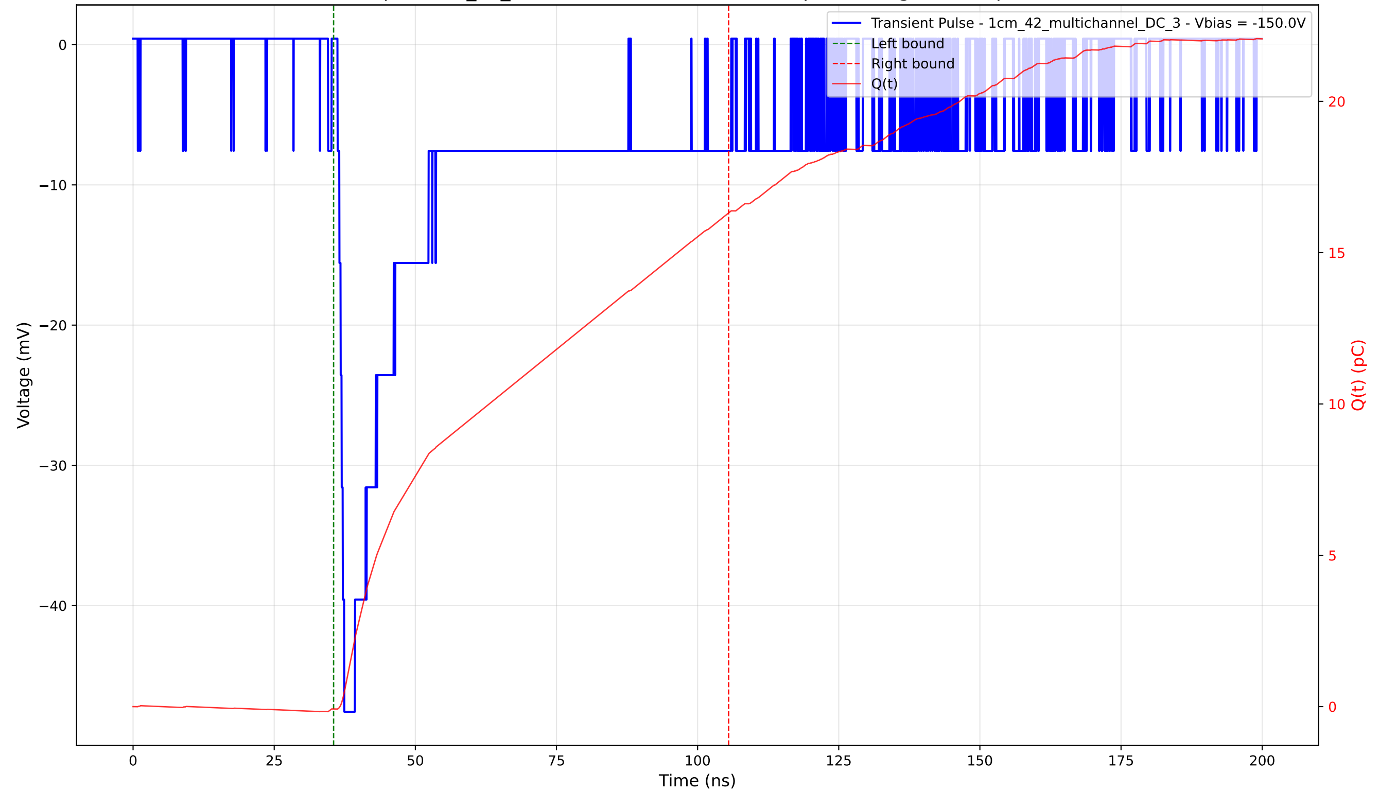
Transient Pulse - Sample: 1cm_42_multichannel - Position: 895.0 \mu\text{m} - Charge: 16.40 pC - Rise Time: 1.19 ns
