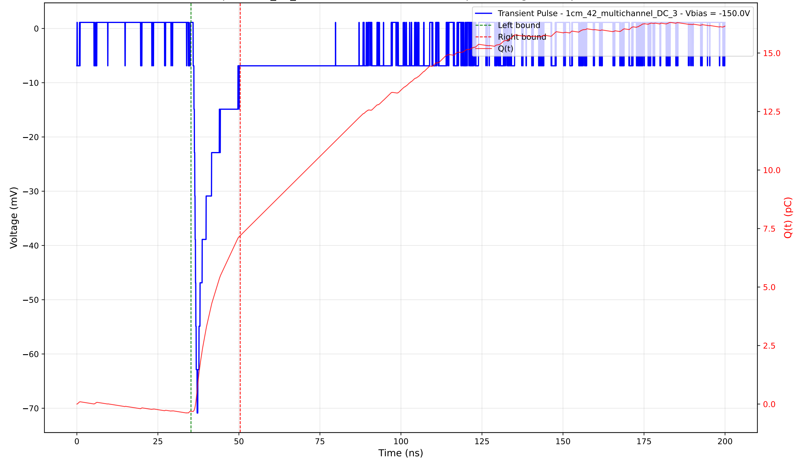
Transient Pulse - Sample: 1cm_42_multichannel - Position: 315.0 \mu\text{m} - Charge: 7.50 pC - Rise Time: 1.00 ns
