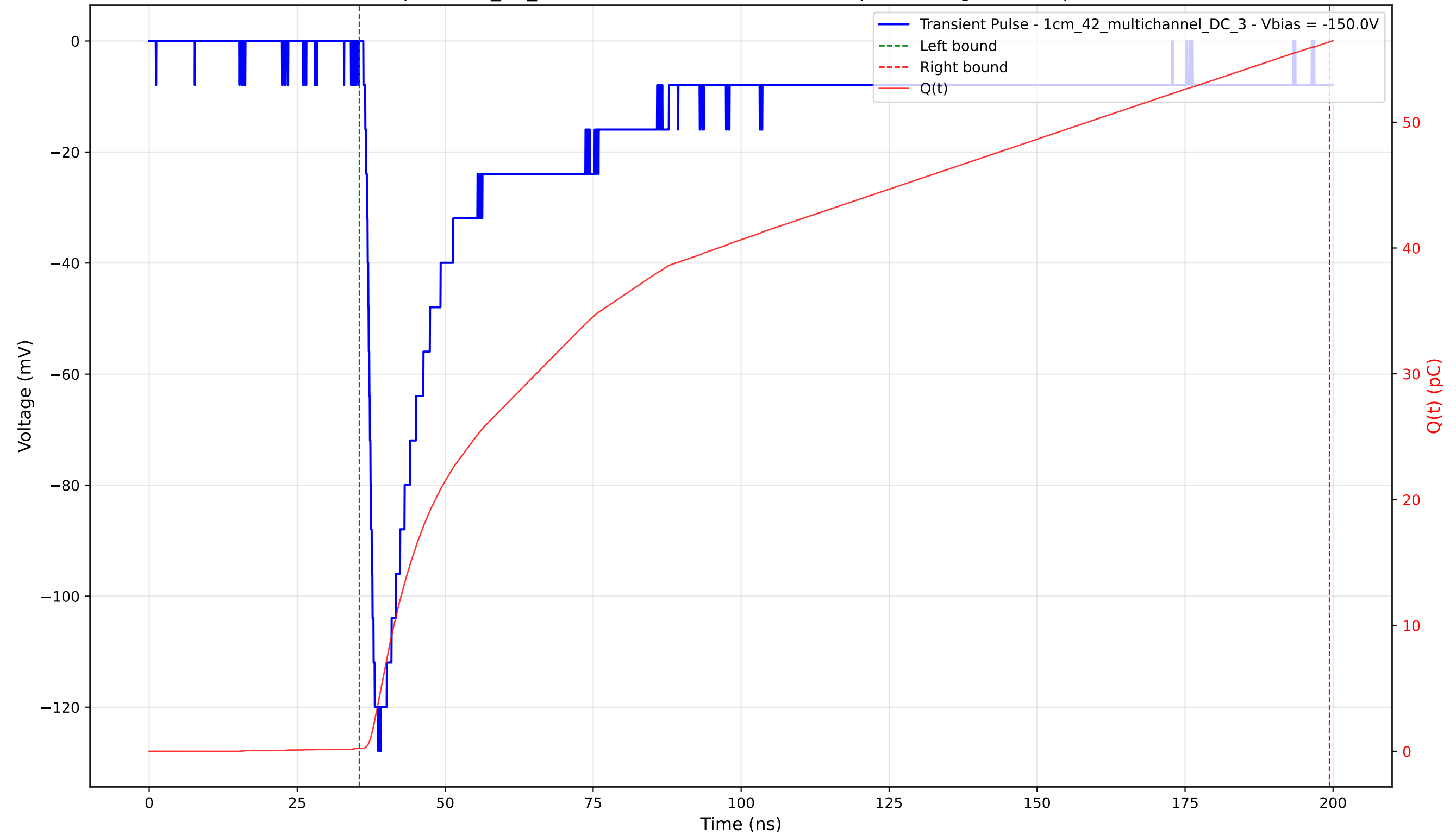
Transient Pulse - Sample: 1cm_42_multichannel - Position: 3490.0 \mu\text{m} - Charge: 56.15 pC - Rise Time: 1.61 ns
