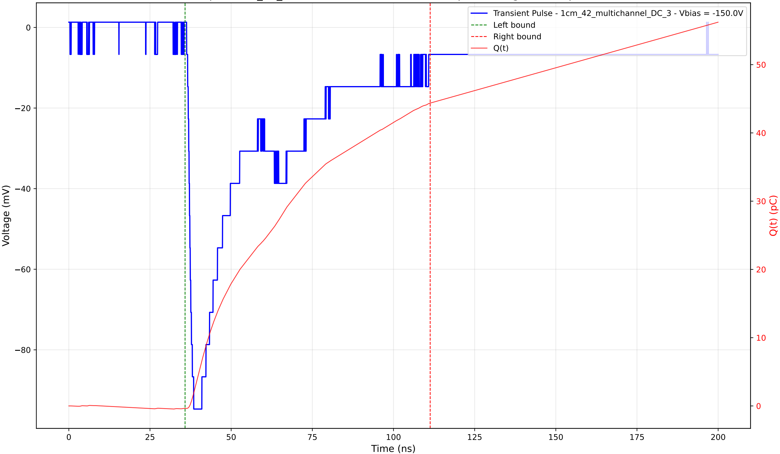
Transient Pulse - Sample: 1cm_42_multichannel - Position: 1980.0 \mu\text{m} - Charge: 44.73 pC - Rise Time: 1.45 ns
