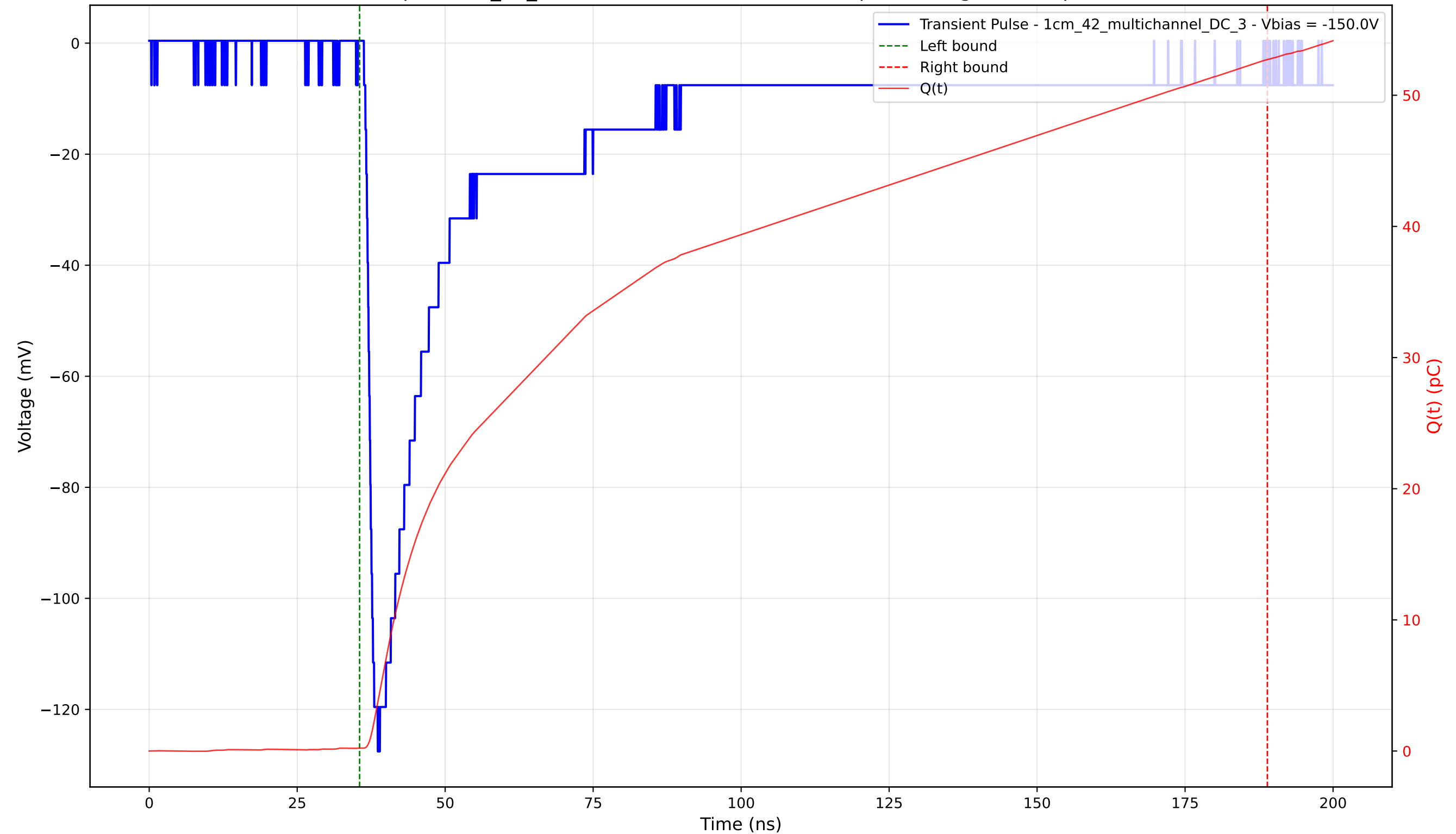
Transient Pulse - Sample: 1cm_42_multichannel - Position: 3560.0 \mu\text{m} - Charge: 52.50 pC - Rise Time: 1.49 ns
