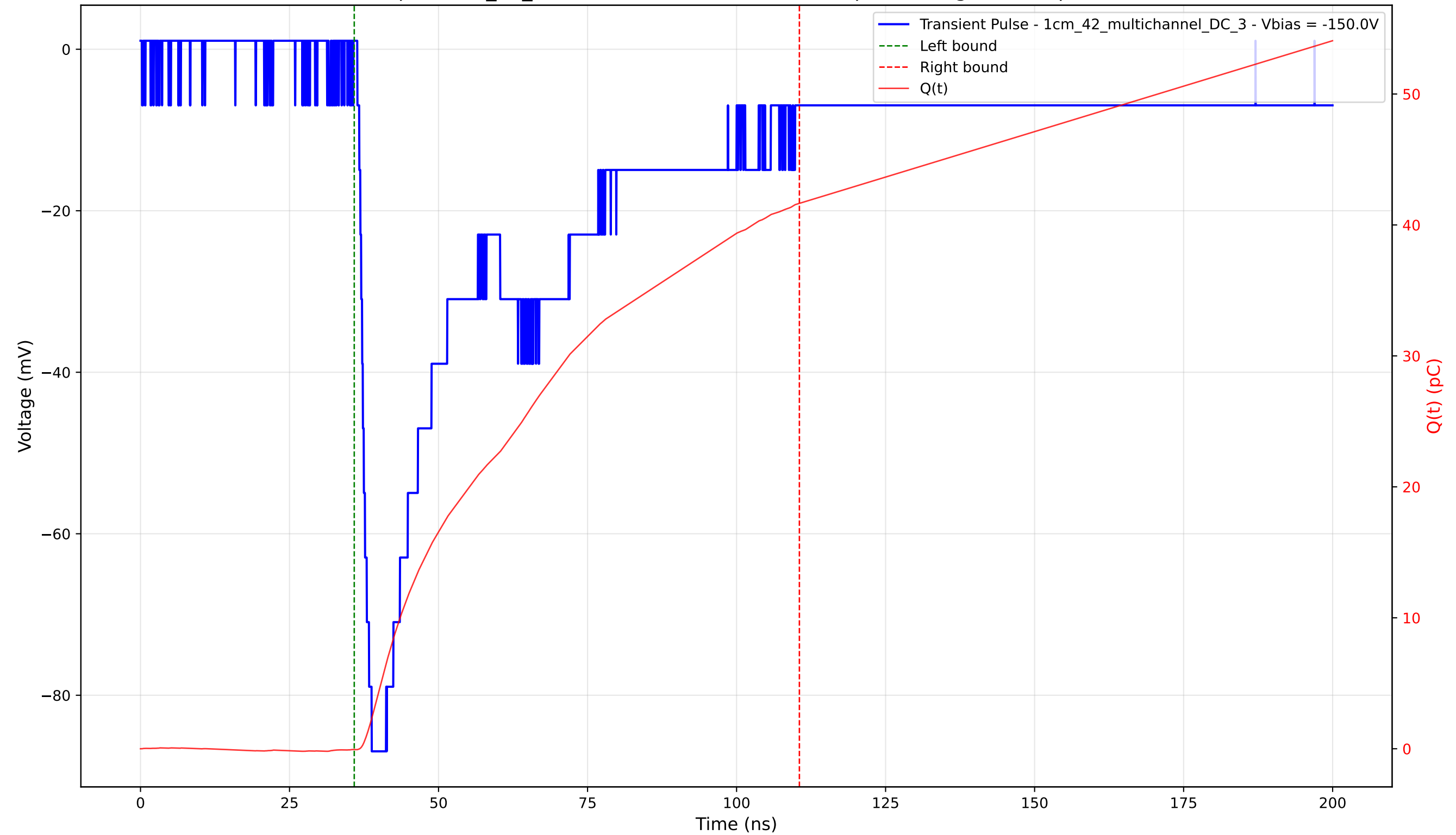
Transient Pulse - Sample: 1cm_42_multichannel - Position: 2700.0 \mu\text{m} - Charge: 41.71 pC - Rise Time: 1.66 ns
