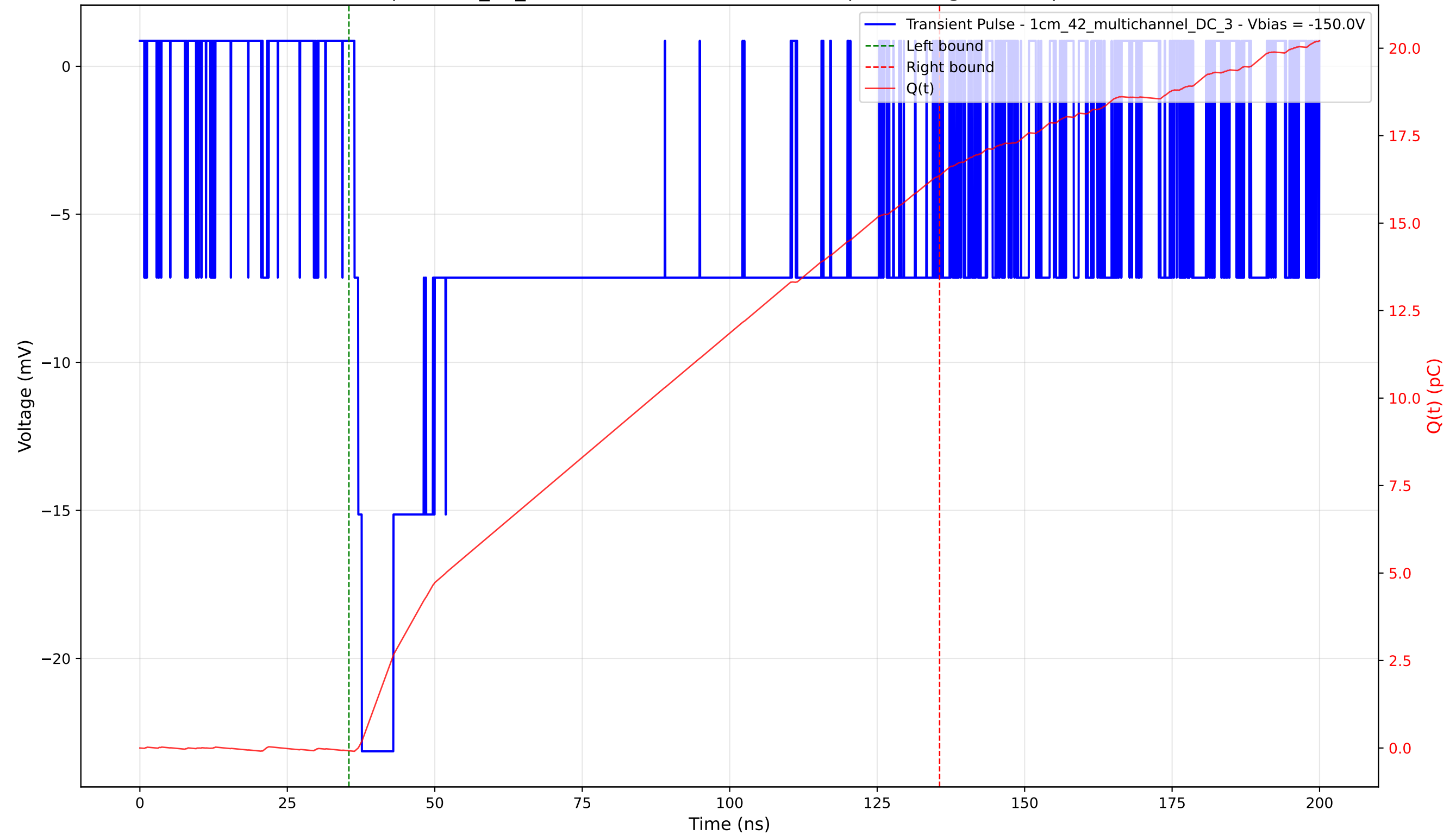
Transient Pulse - Sample: 1cm_42_multichannel - Position: 1905.0 \mu\text{m} - Charge: 16.45 pC - Rise Time: 1.26 ns
