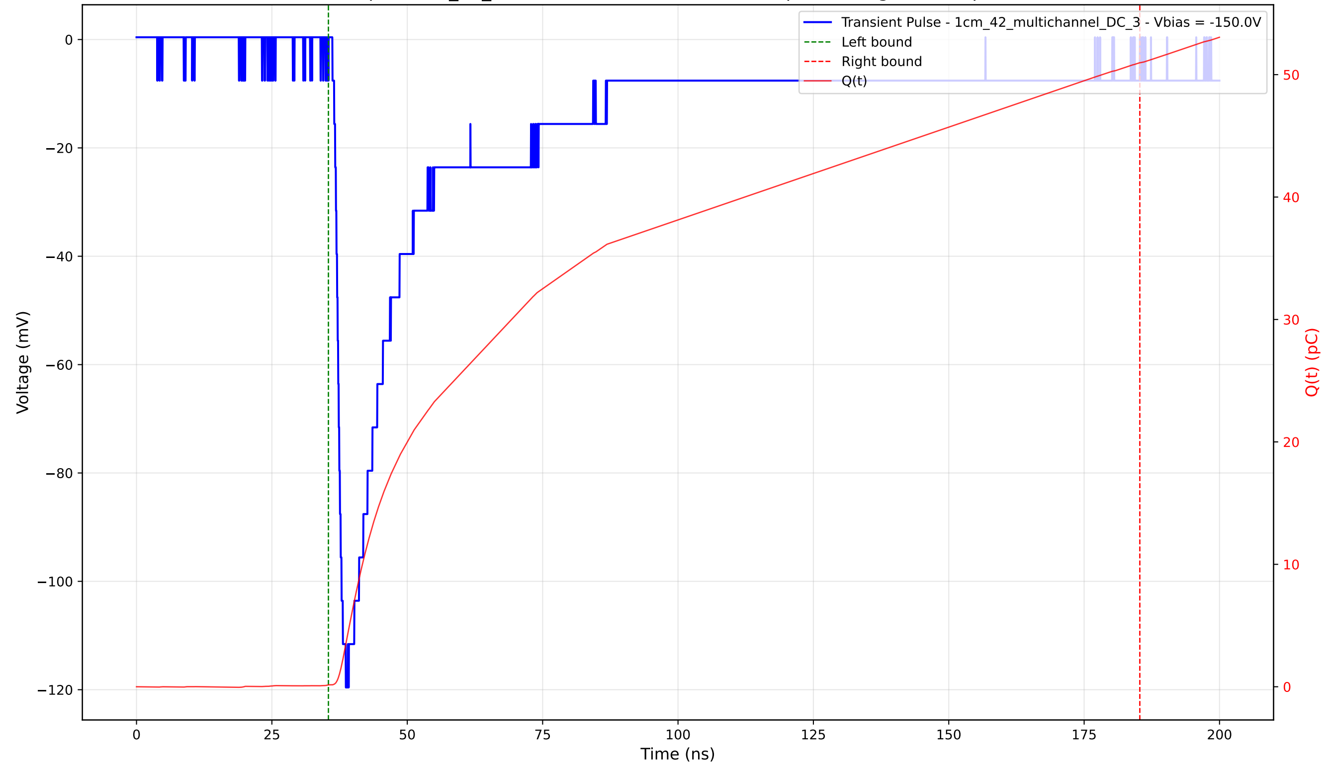
Transient Pulse - Sample: 1cm_42_multichannel - Position: 3465.0 \mu\text{m} - Charge: 50.82 pC - Rise Time: 1.61 ns
