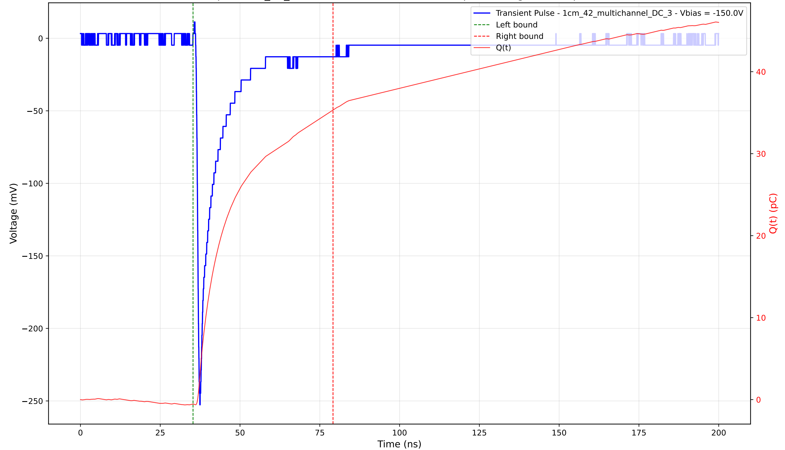
Transient Pulse - Sample: 1cm_42_multichannel - Position: 4490.0 \mu\text{m} - Charge: 35.87 pC - Rise Time: 0.87 ns
