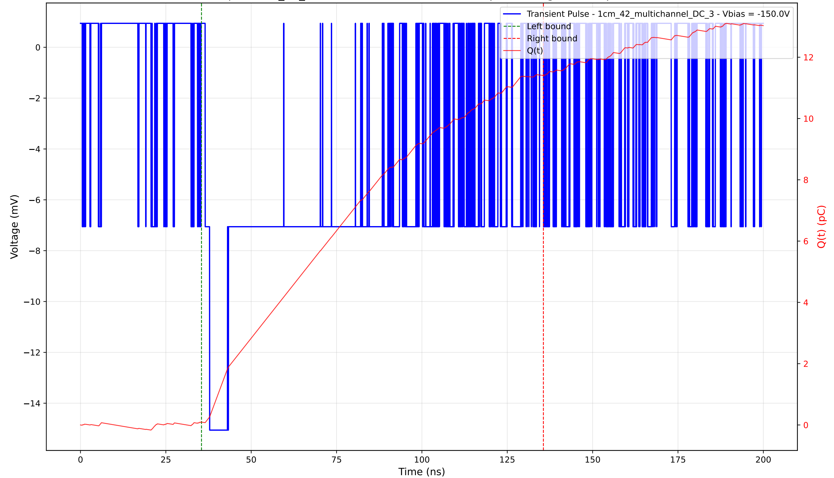
Transient Pulse - Sample: 1cm_42_multichannel - Position: 2905.0 \mu\text{m} - Charge: 11.31 pC - Rise Time: 1.32 ns
