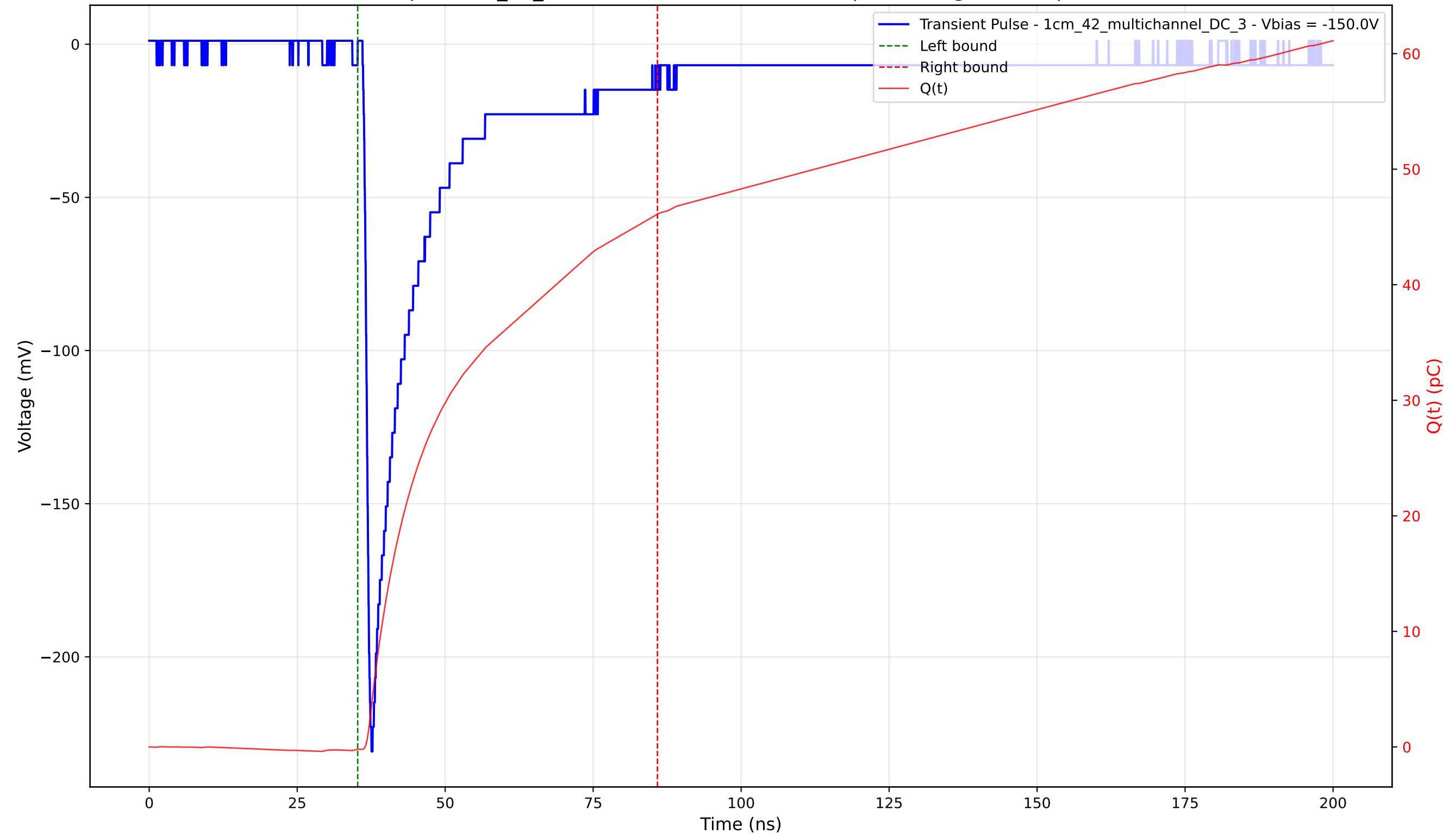
Transient Pulse - Sample: 1cm_42_multichannel - Position: 675.0 \mu\text{m} - Charge: 46.32 pC - Rise Time: 1.00 ns
