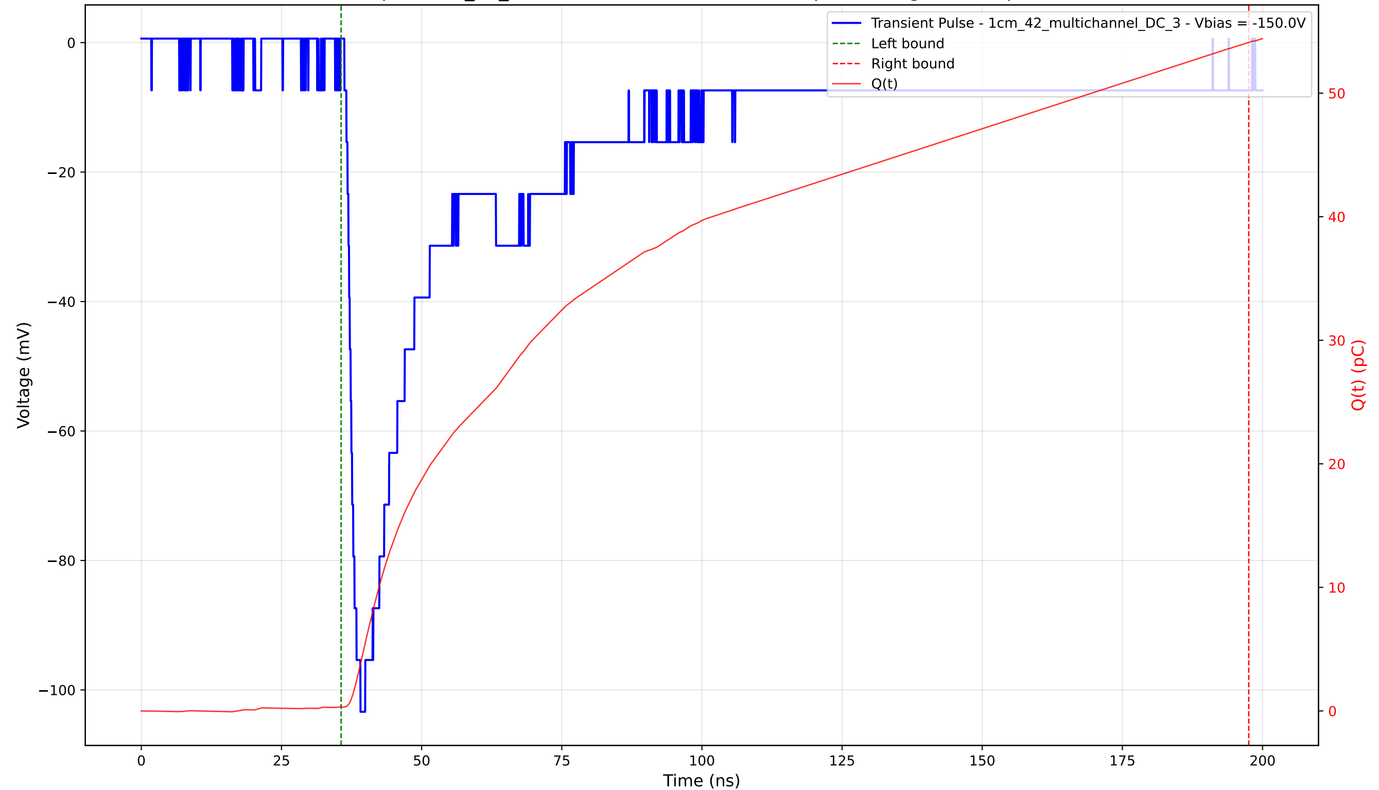
Transient Pulse - Sample: 1cm_42_multichannel - Position: 3060.0 \mu\text{m} - Charge: 53.80 pC - Rise Time: 1.81 ns
