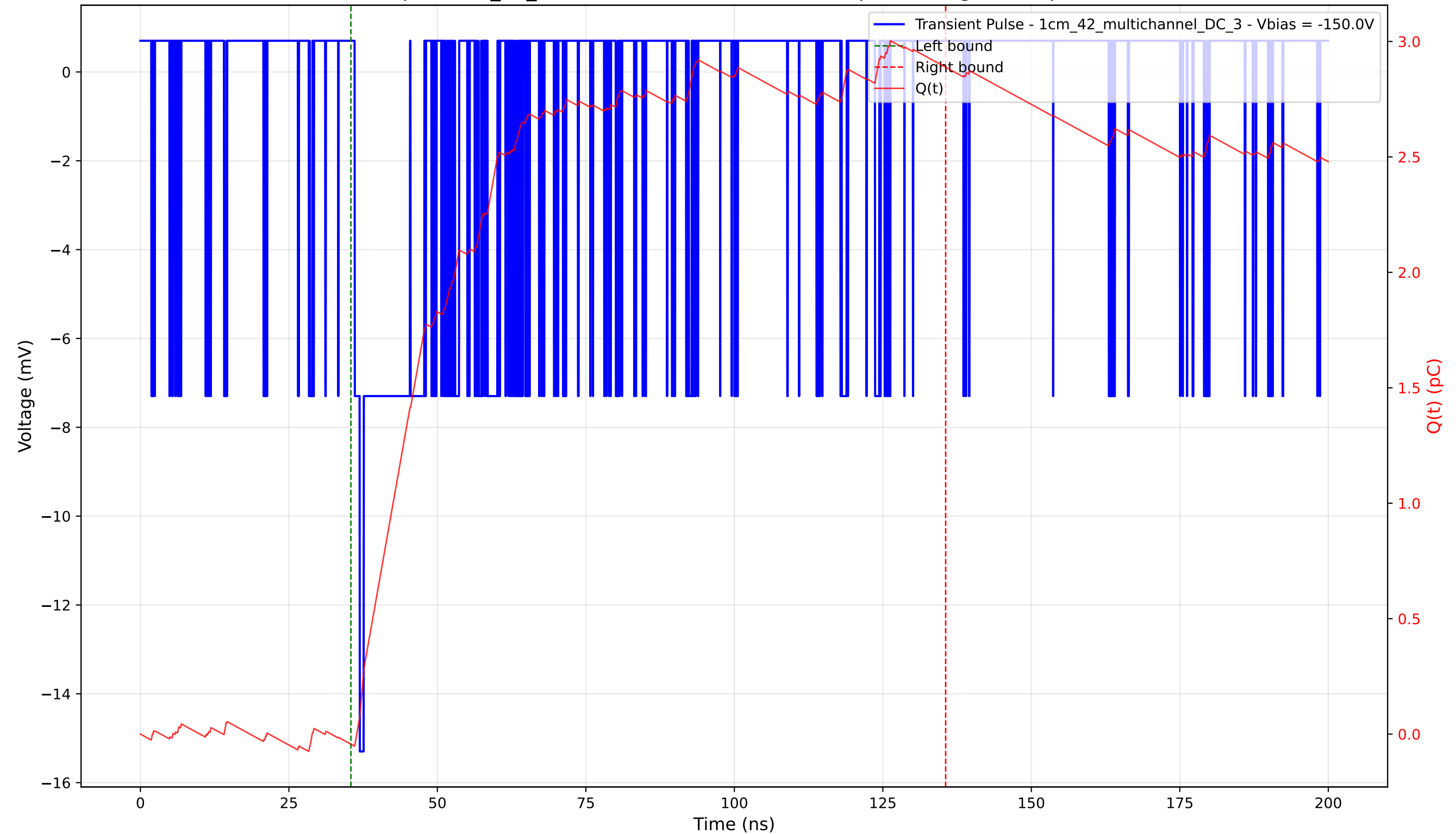
Transient Pulse - Sample: 1cm_42_multichannel - Position: 4920.0 \mu\text{m} - Charge: 2.93 pC - Rise Time: 0.86 ns
