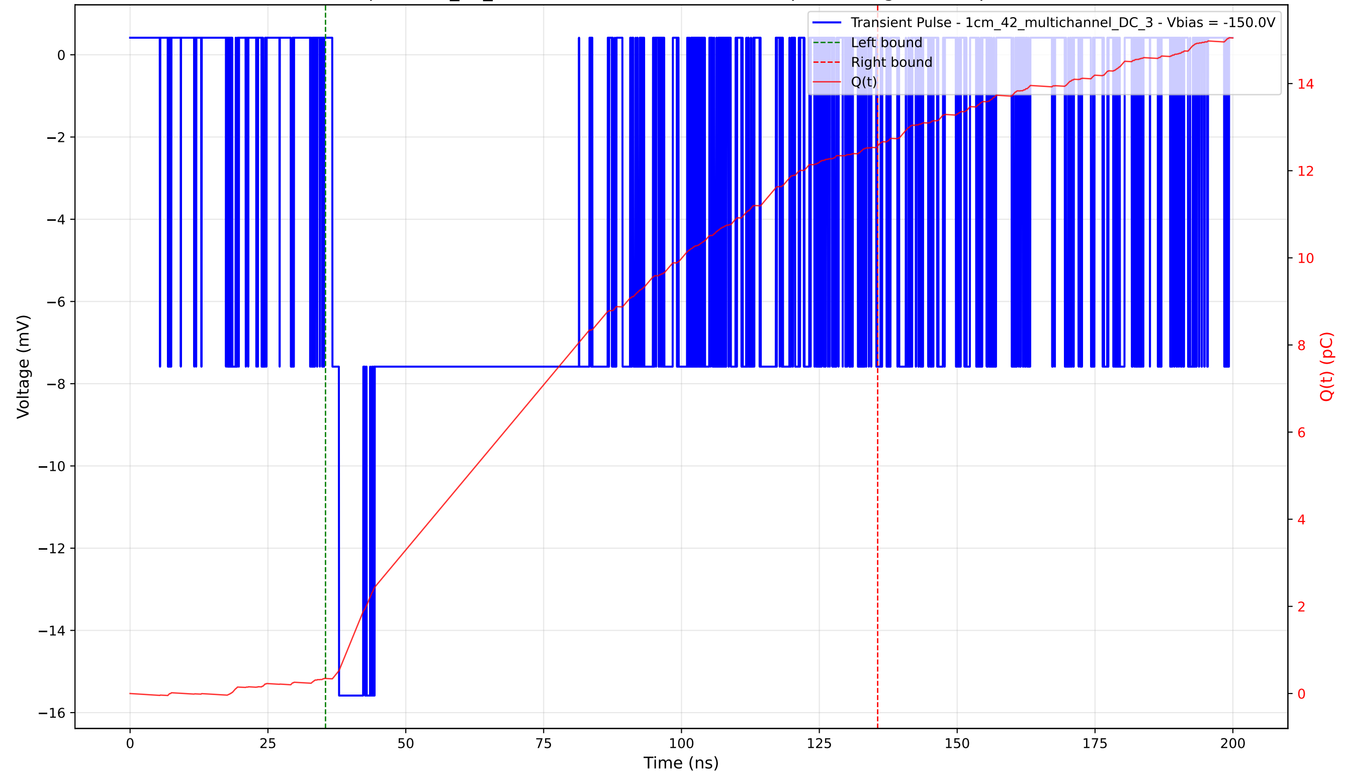
Transient Pulse - Sample: 1cm_42_multichannel - Position: 1895.0 \mu\text{m} - Charge: 12.22 pC - Rise Time: 1.22 ns
