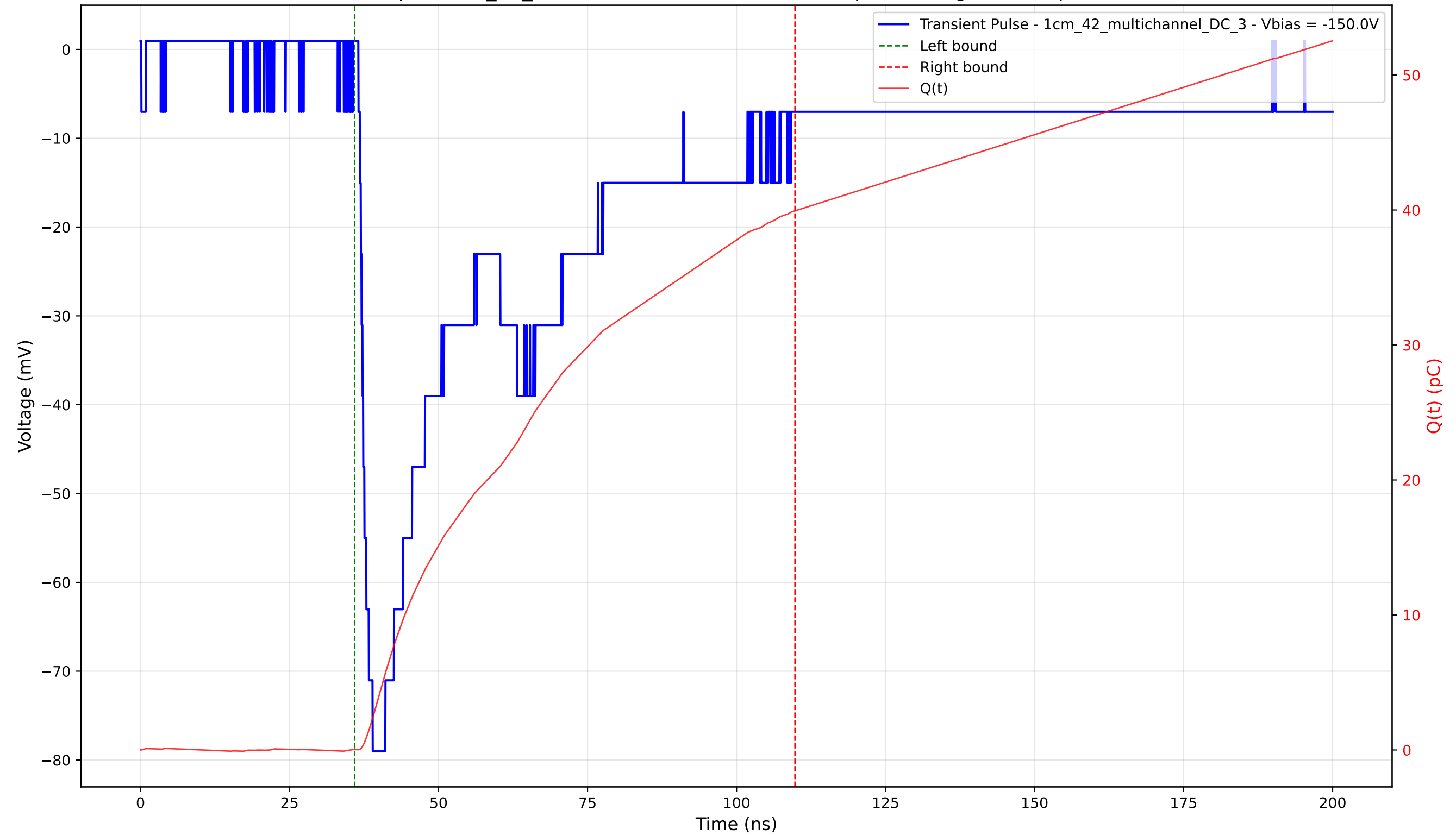
Transient Pulse - Sample: 1cm_42_multichannel - Position: 2570.0 \mu\text{m} - Charge: 39.91 pC - Rise Time: 2.16 ns
