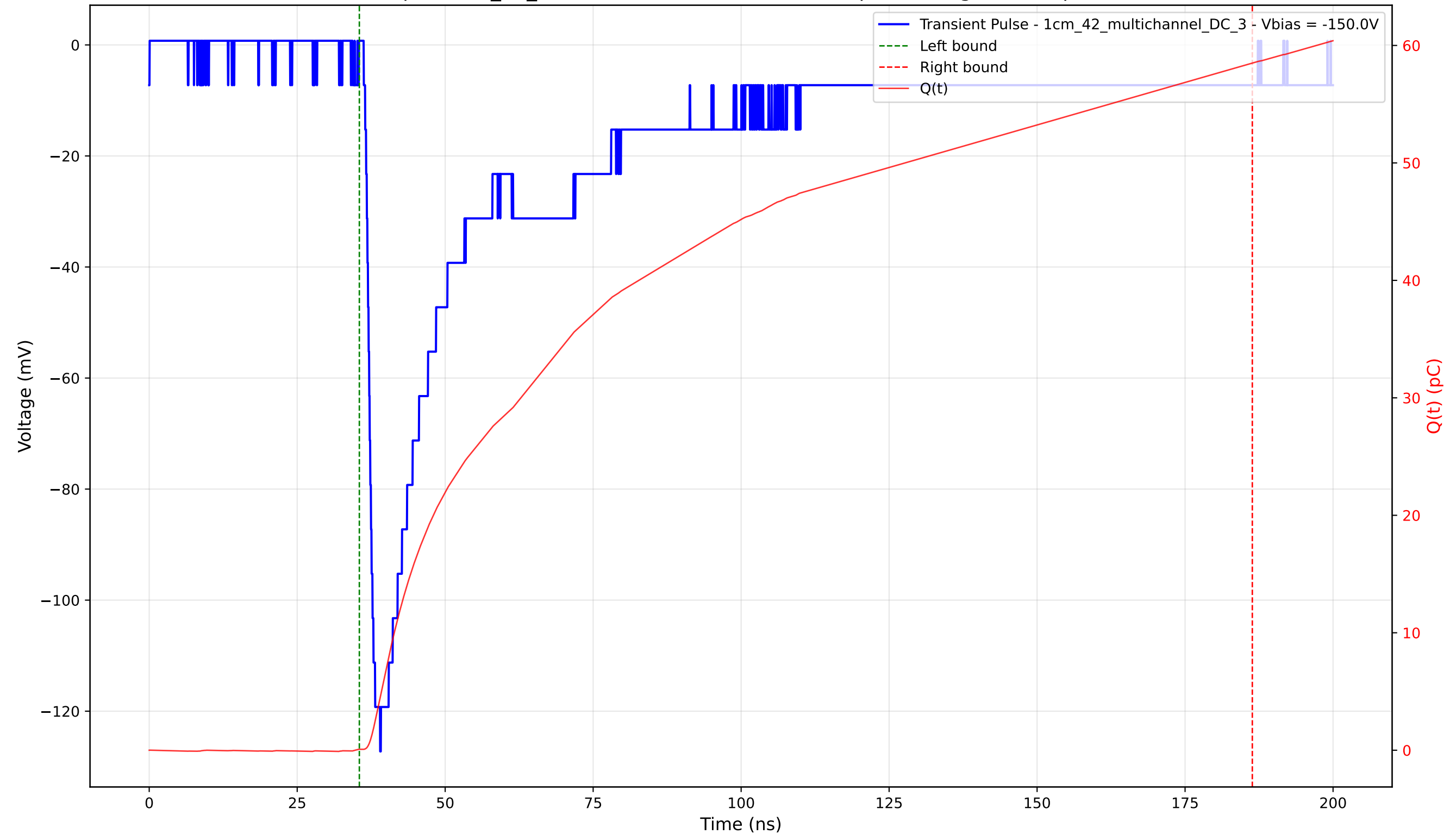
Transient Pulse - Sample: 1cm_42_multichannel - Position: 1590.0 \mu\text{m} - Charge: 58.43 pC - Rise Time: 1.69 ns
