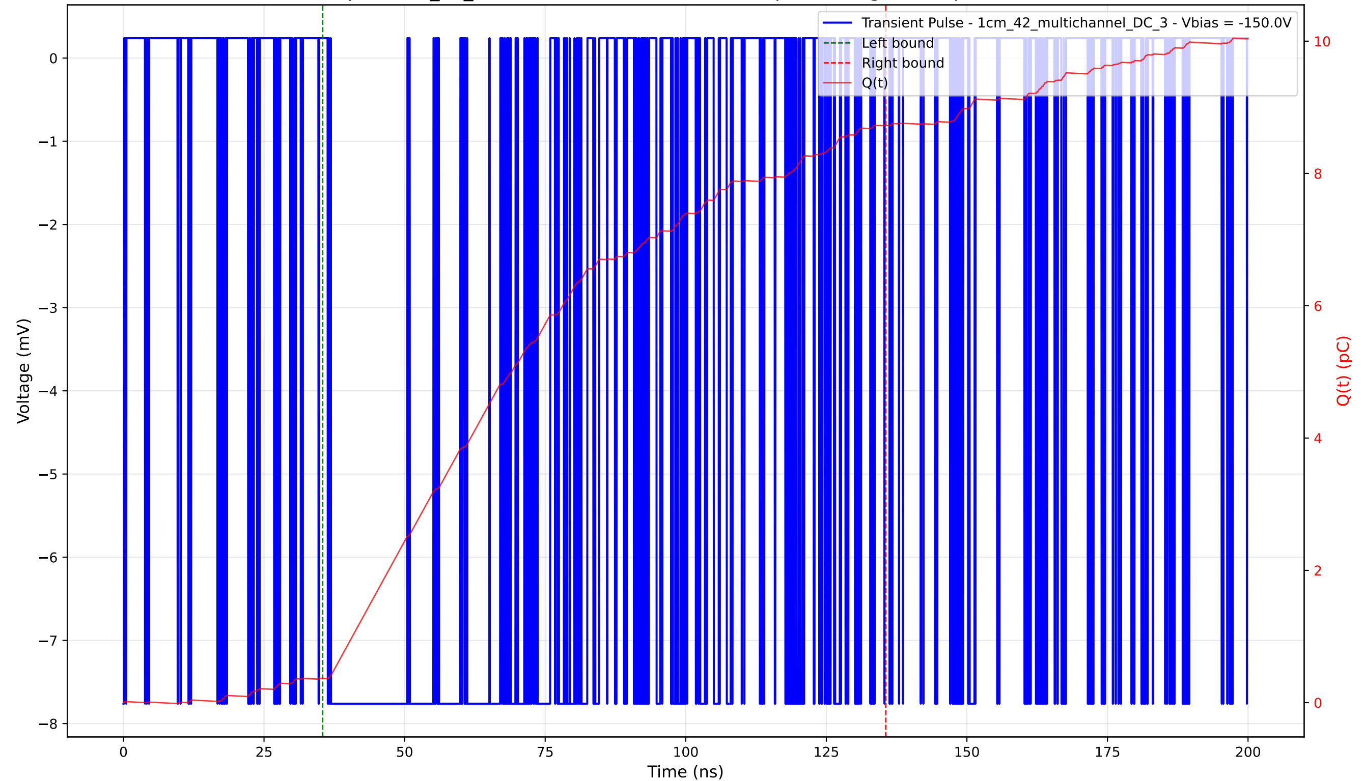
Transient Pulse - Sample: 1cm_42_multichannel - Position: 1860.0 \mu\text{m} - Charge: 8.36 pC - Rise Time: 0.00 ns (N/A)
