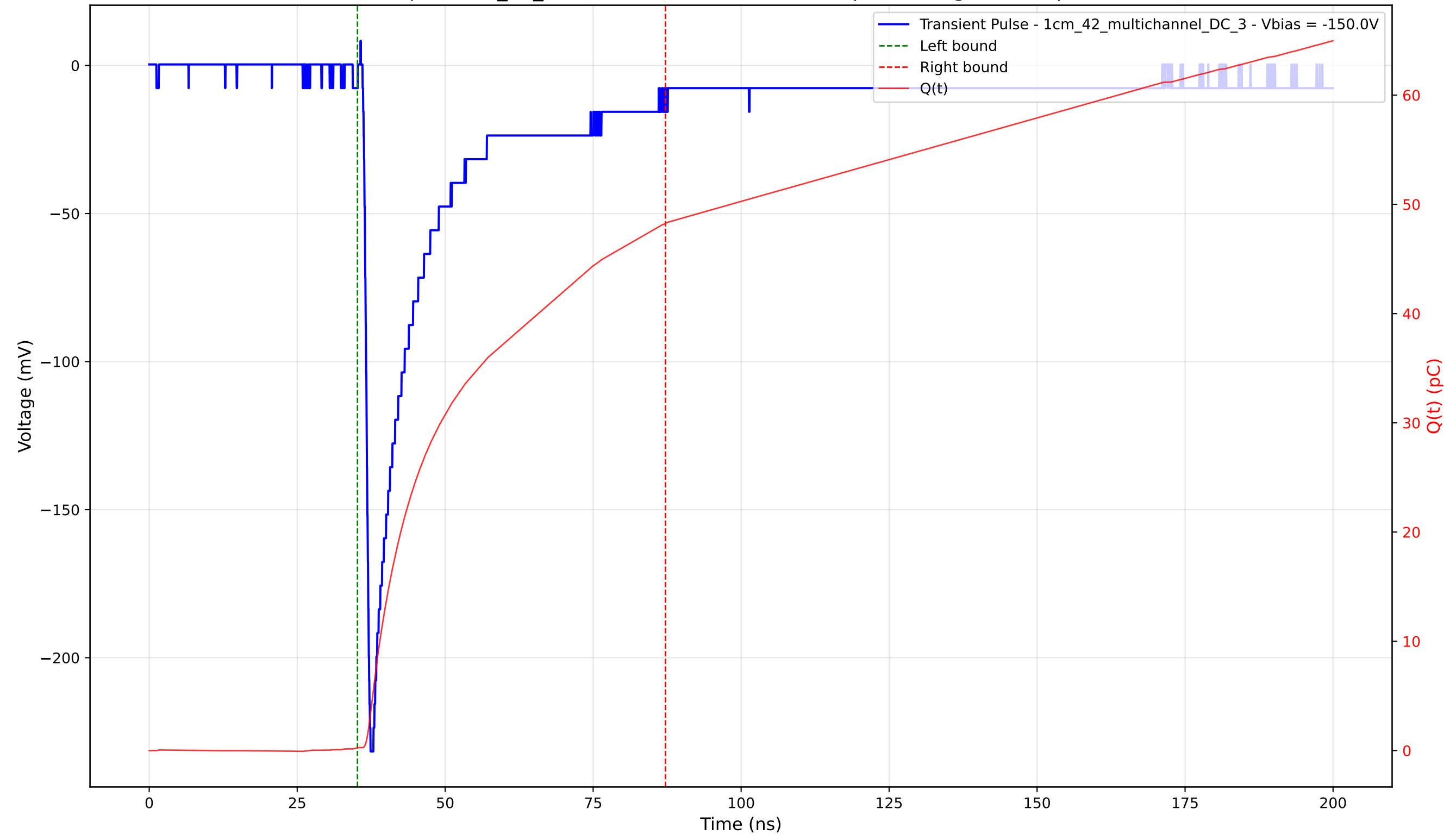
Transient Pulse - Sample: 1cm_42_multichannel - Position: 645.0 \mu\text{m} - Charge: 47.99 pC - Rise Time: 0.98 ns
