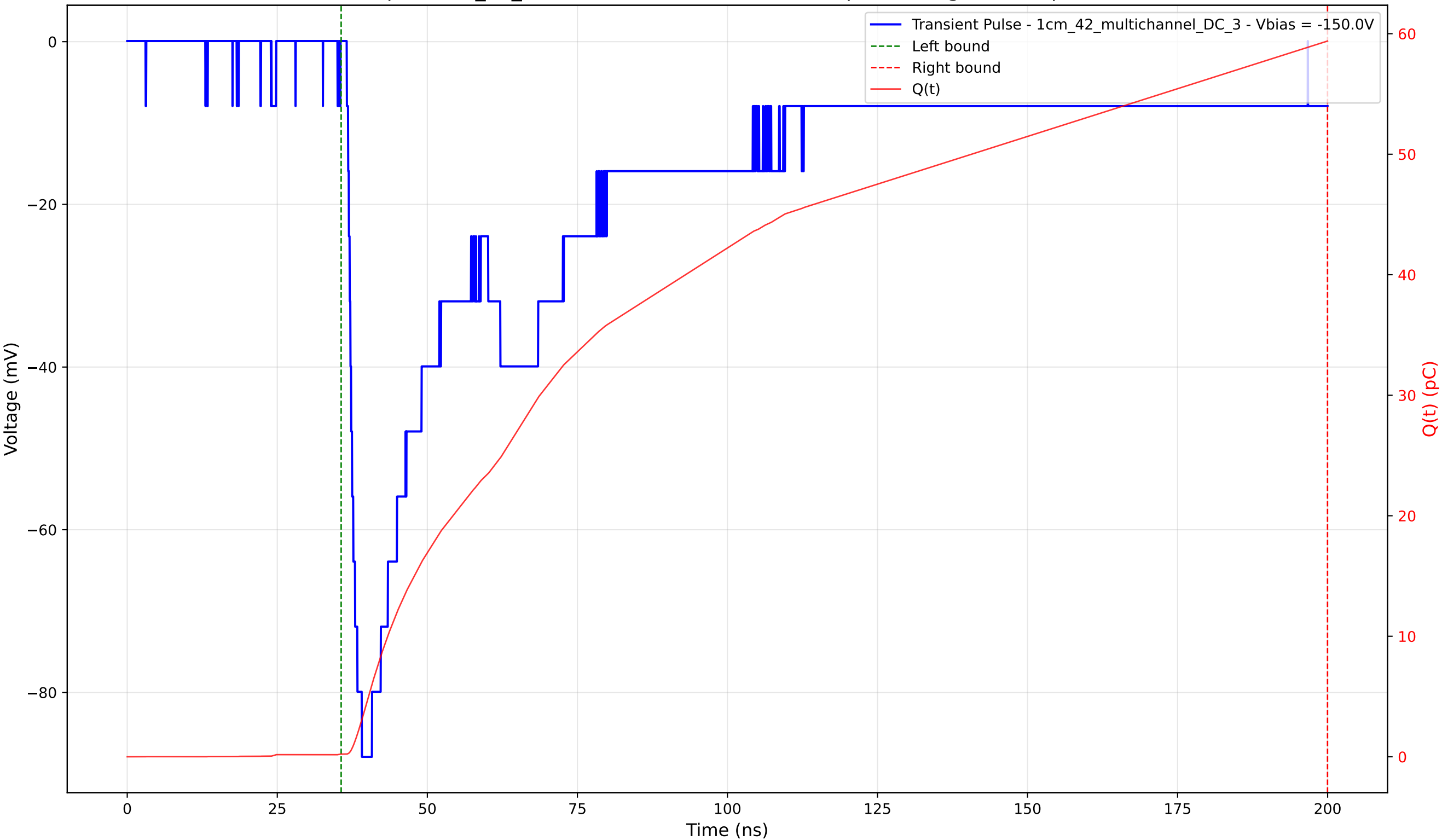
Transient Pulse - Sample: 1cm_42_multichannel - Position: 2210.0 \mu\text{m} - Charge: 59.17 pC - Rise Time: 1.56 ns
