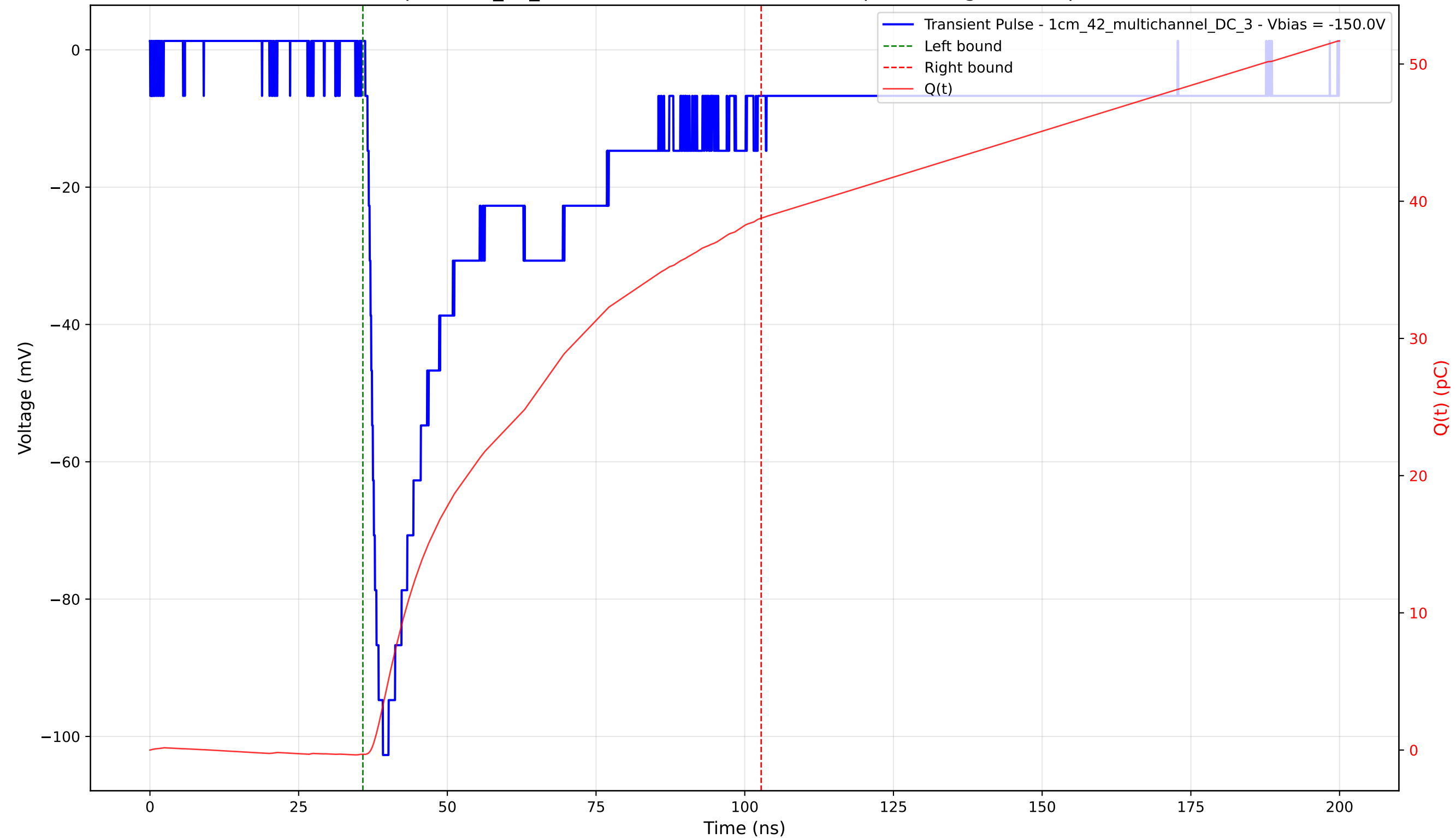
Transient Pulse - Sample: 1cm_42_multichannel - Position: 3040.0 \mu\text{m} - Charge: 39.07 pC - Rise Time: 1.87 ns
