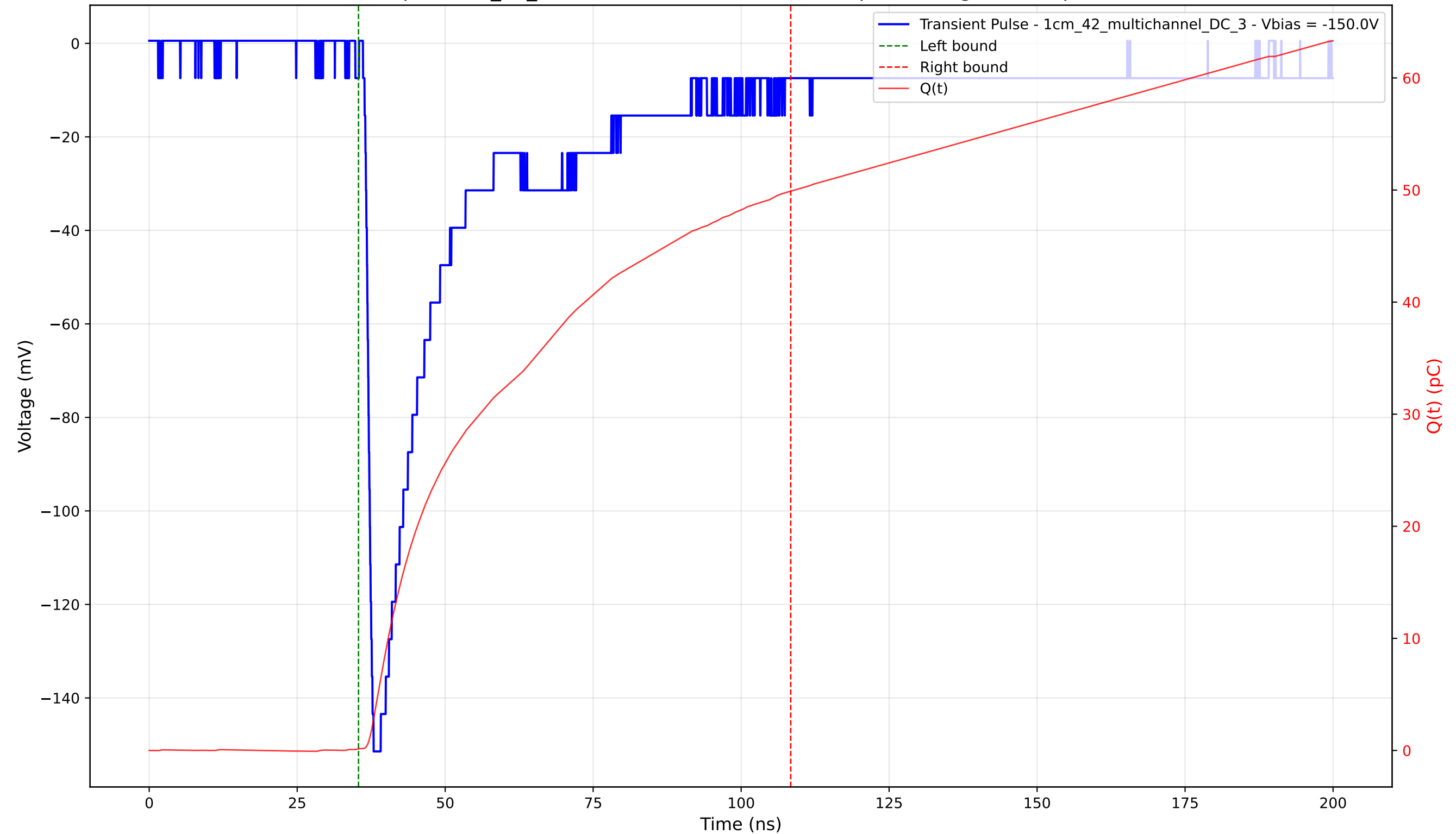
Transient Pulse - Sample: 1cm_42_multichannel - Position: 1250.0 \mu\text{m} - Charge: 49.74 pC - Rise Time: 1.34 ns
