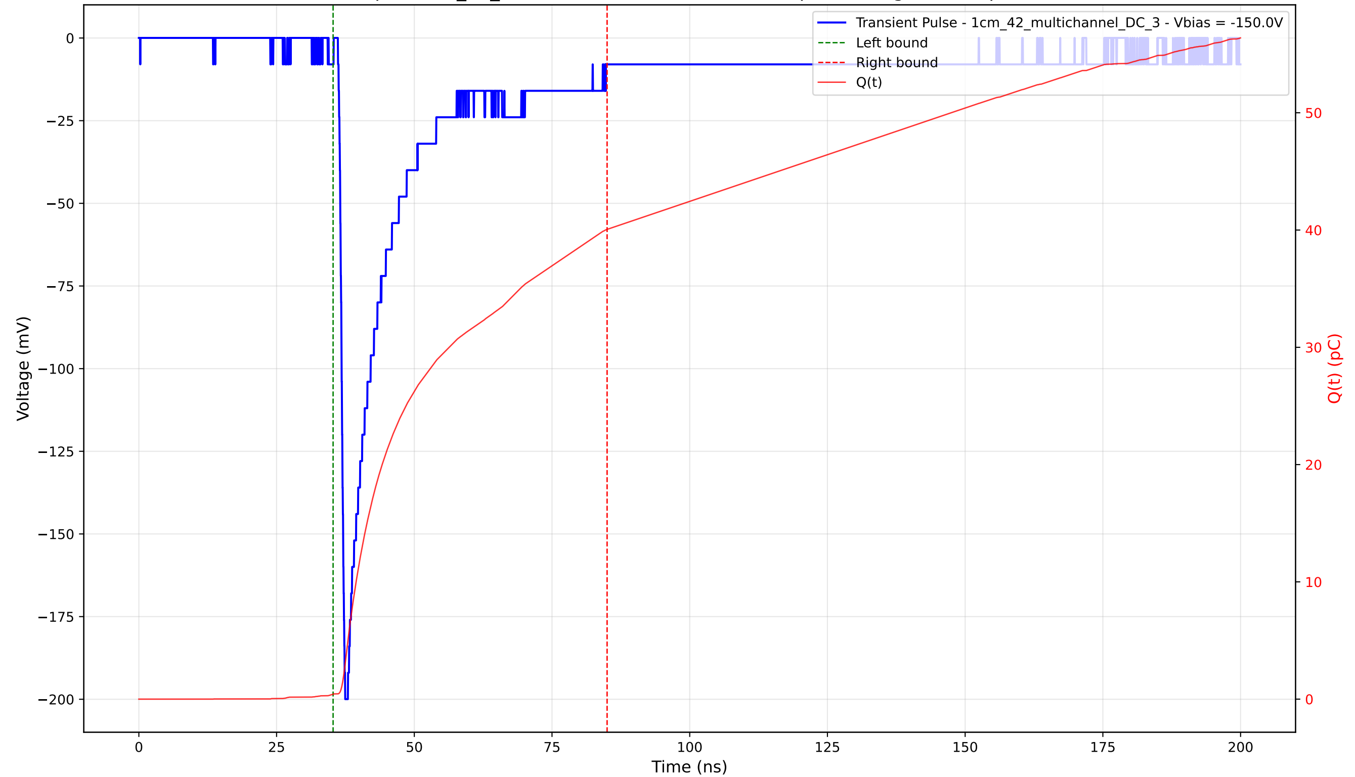
Transient Pulse - Sample: 1cm_42_multichannel - Position: 4255.0 \mu\text{m} - Charge: 39.63 pC - Rise Time: 0.95 ns
