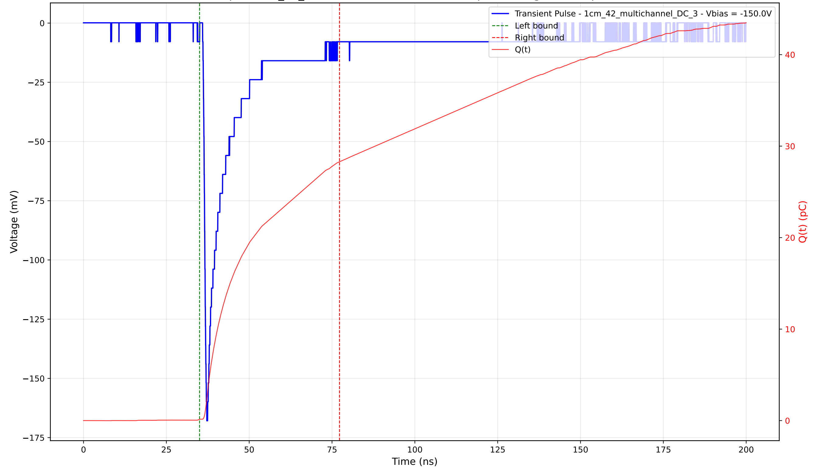
Transient Pulse - Sample: 1cm_42_multichannel - Position: 405.0 \mu\text{m} - Charge: 28.14 pC - Rise Time: 0.86 ns
