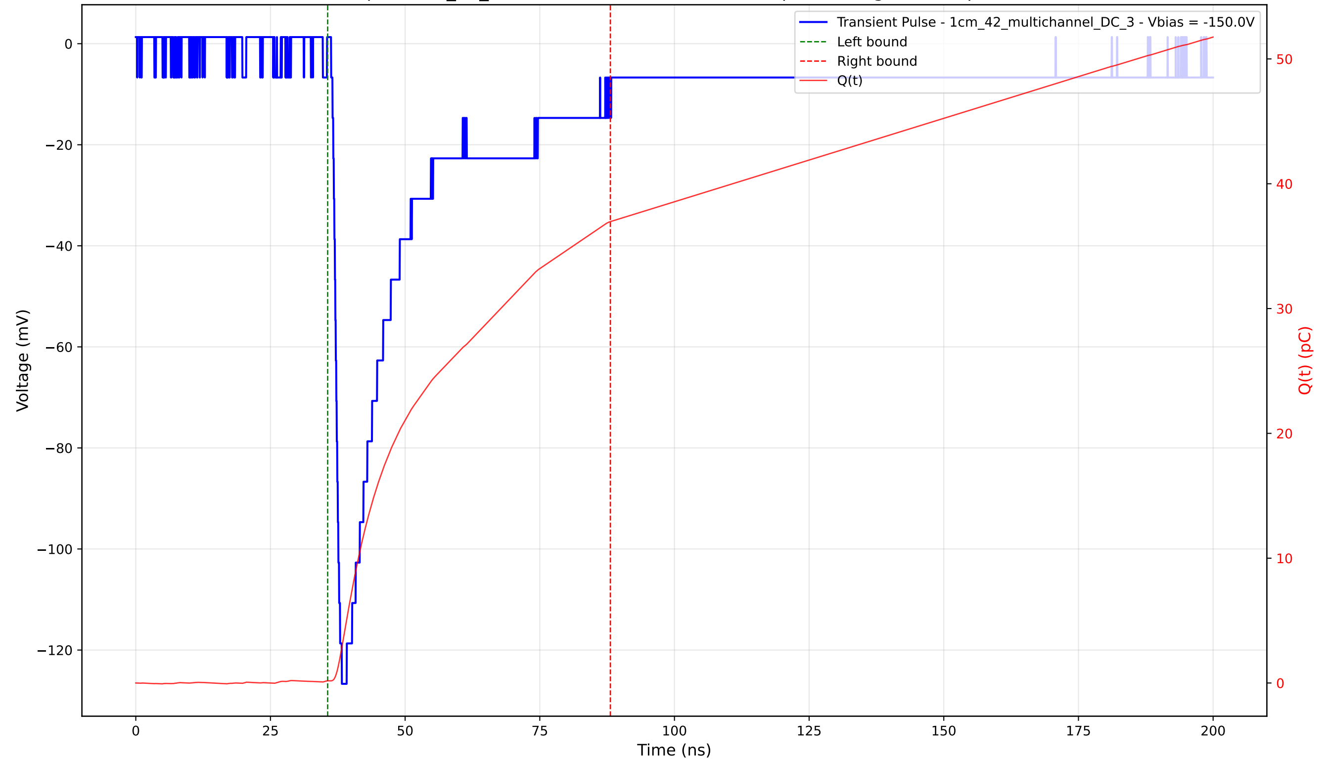
Transient Pulse - Sample: 1cm_42_multichannel - Position: 3600.0 \mu\text{m} - Charge: 36.79 pC - Rise Time: 1.41 ns
