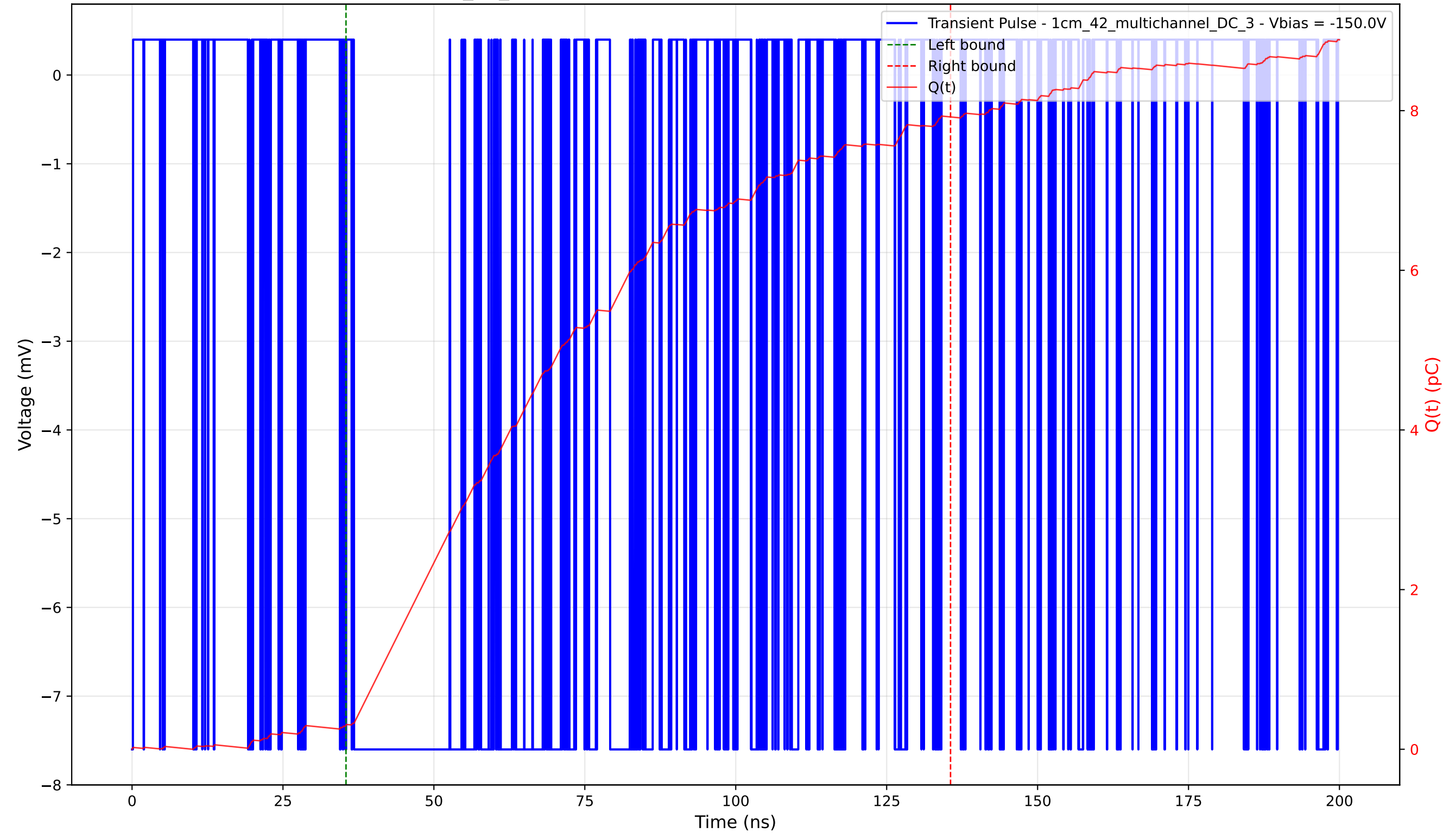
Transient Pulse - Sample: 1cm_42_multichannel - Position: 2880.0 \mu\text{m} - Charge: 7.62 pC - Rise Time: 0.00 ns (N/A)
