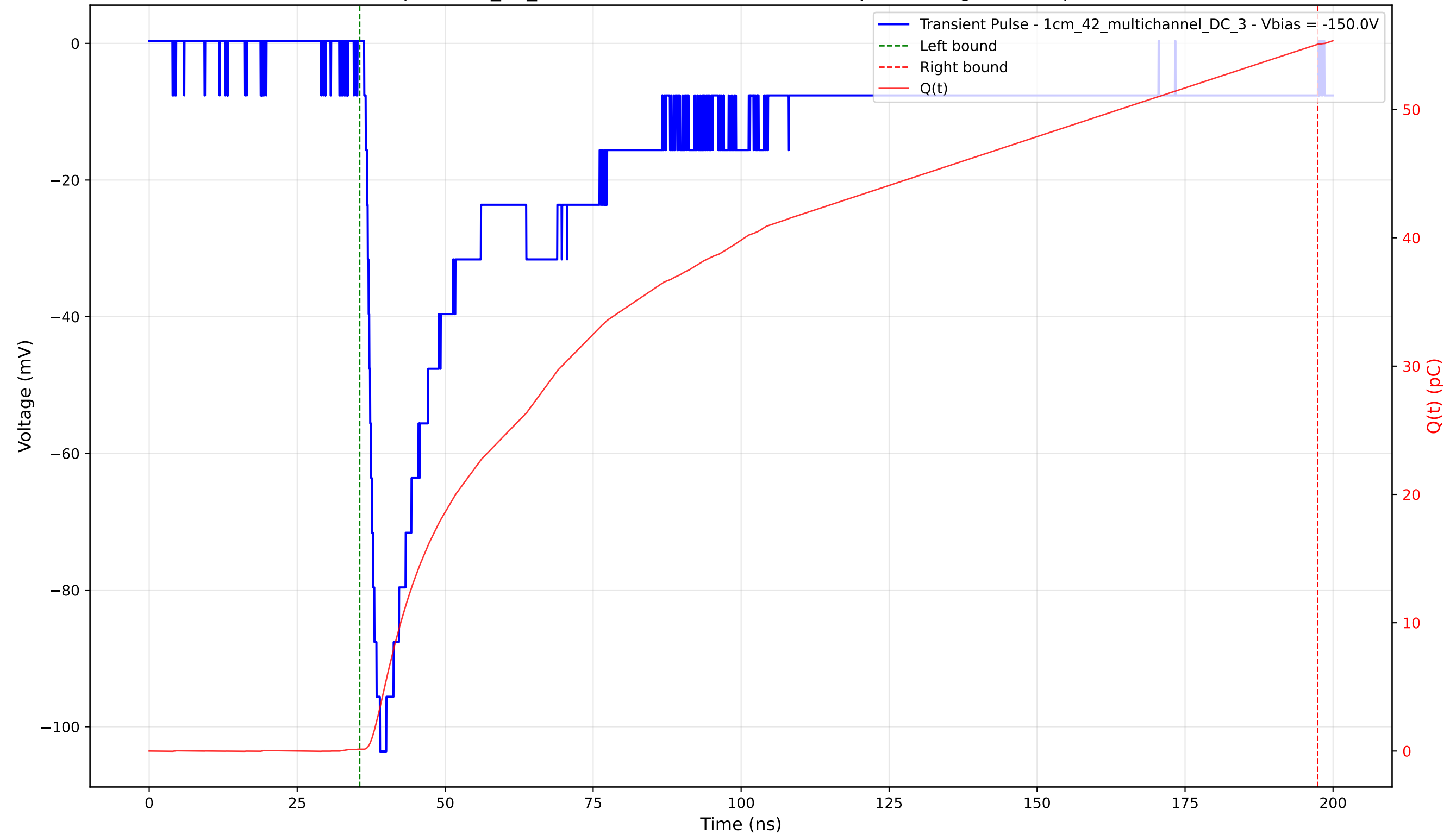
Transient Pulse - Sample: 1cm_42_multichannel - Position: 3035.0 \mu\text{m} - Charge: 54.95 pC - Rise Time: 1.83 ns
