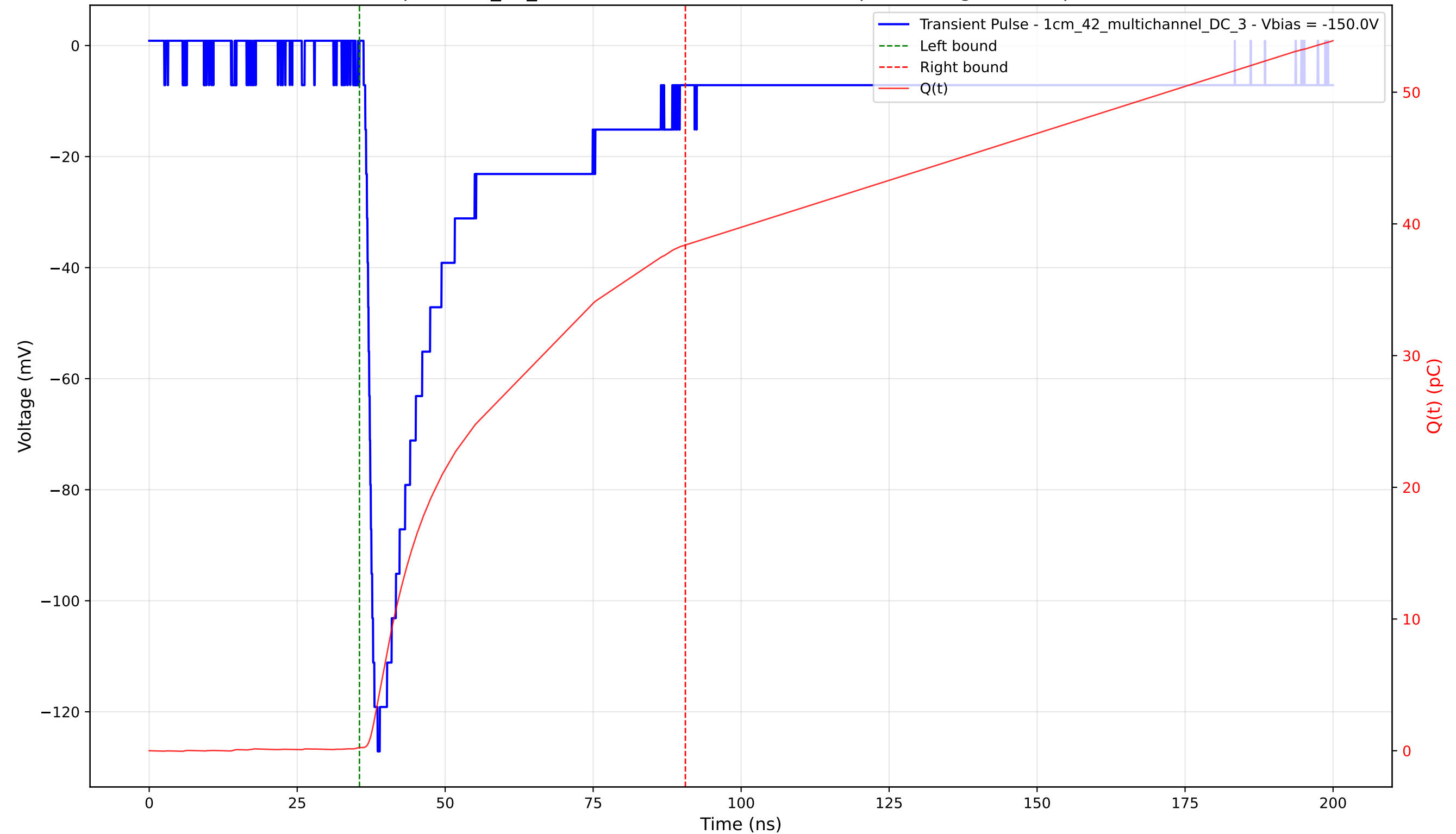
Transient Pulse - Sample: 1cm_42_multichannel - Position: 3515.0 \mu\text{m} - Charge: 38.15 pC - Rise Time: 1.55 ns
