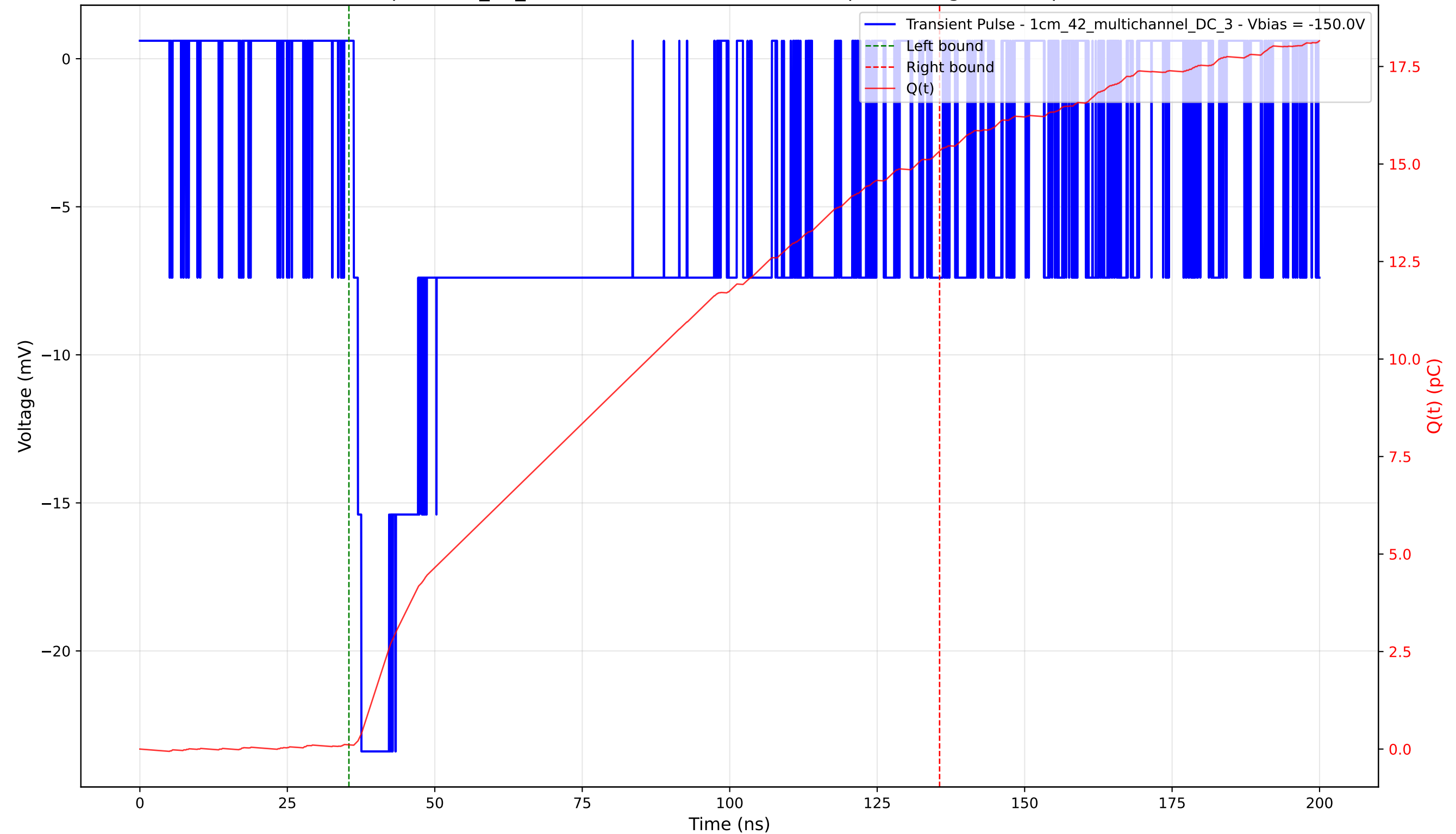
Transient Pulse - Sample: 1cm_42_multichannel - Position: 1395.0 \mu\text{m} - Charge: 15.22 pC - Rise Time: 1.29 ns
