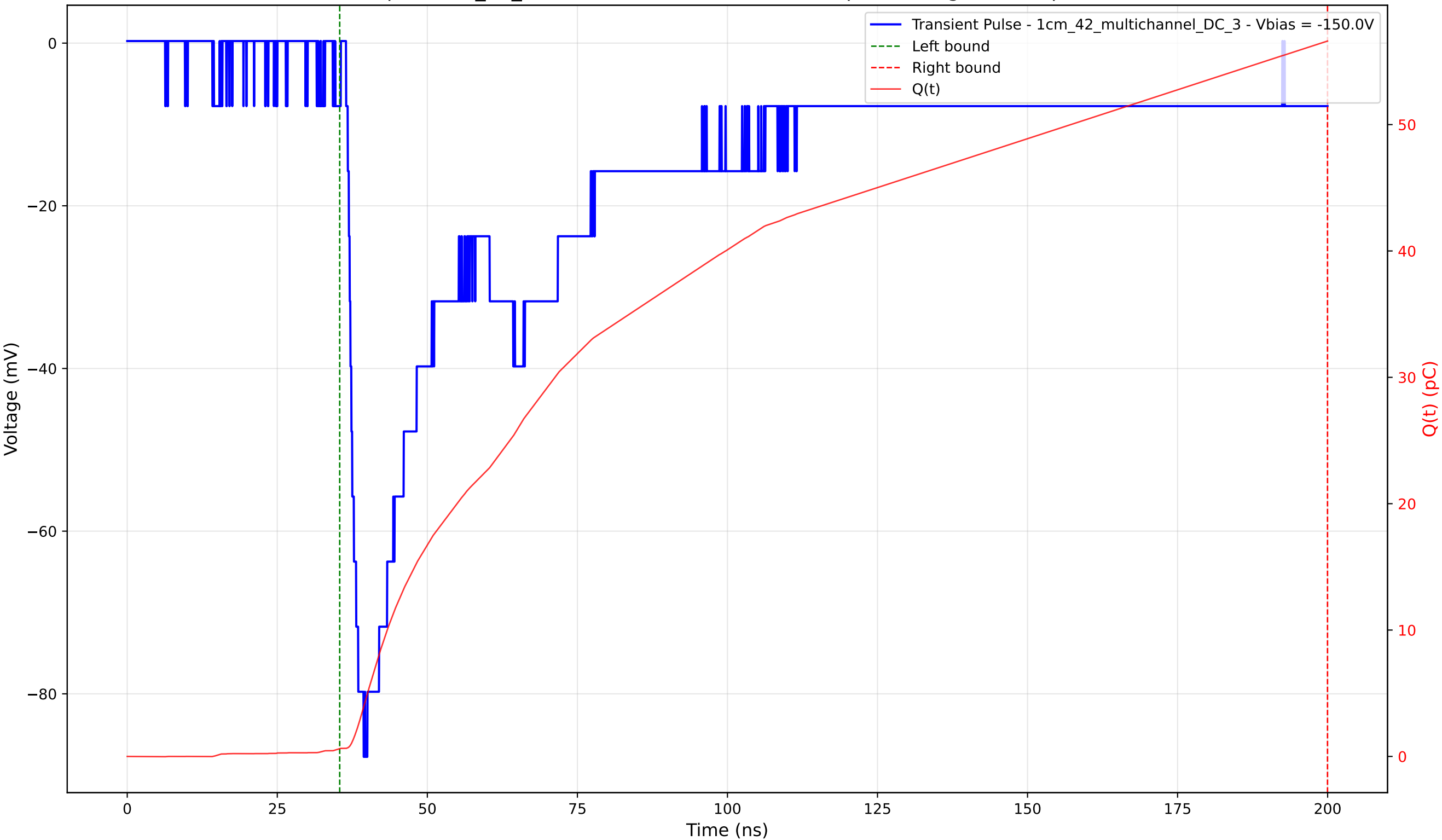
Transient Pulse - Sample: 1cm_42_multichannel - Position: 2635.0 \mu\text{m} - Charge: 56.00 pC - Rise Time: 1.76 ns
