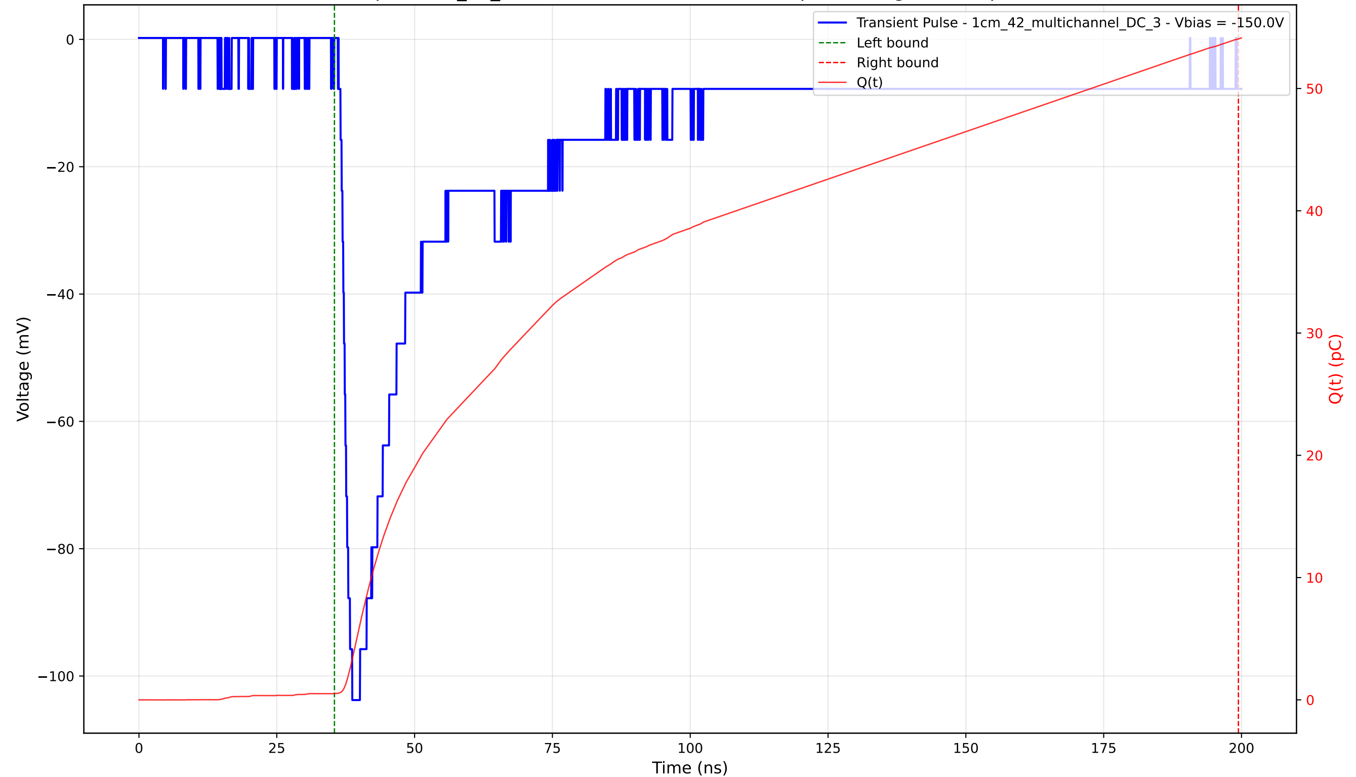
Transient Pulse - Sample: 1cm_42_multichannel - Position: 3150.0 \mu\text{m} - Charge: 53.53 pC - Rise Time: 1.73 ns
