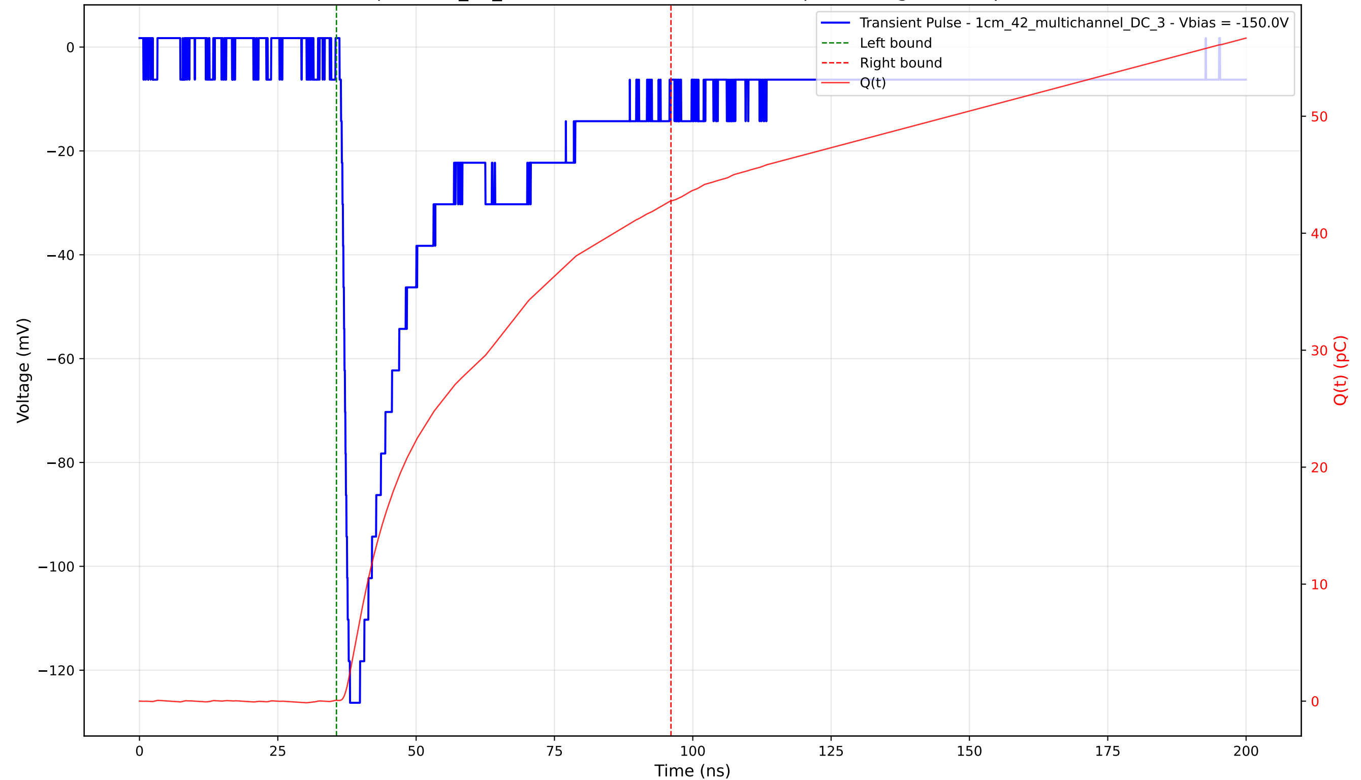
Transient Pulse - Sample: 1cm_42_multichannel - Position: 1445.0 \mu\text{m} - Charge: 42.70 pC - Rise Time: 1.38 ns
