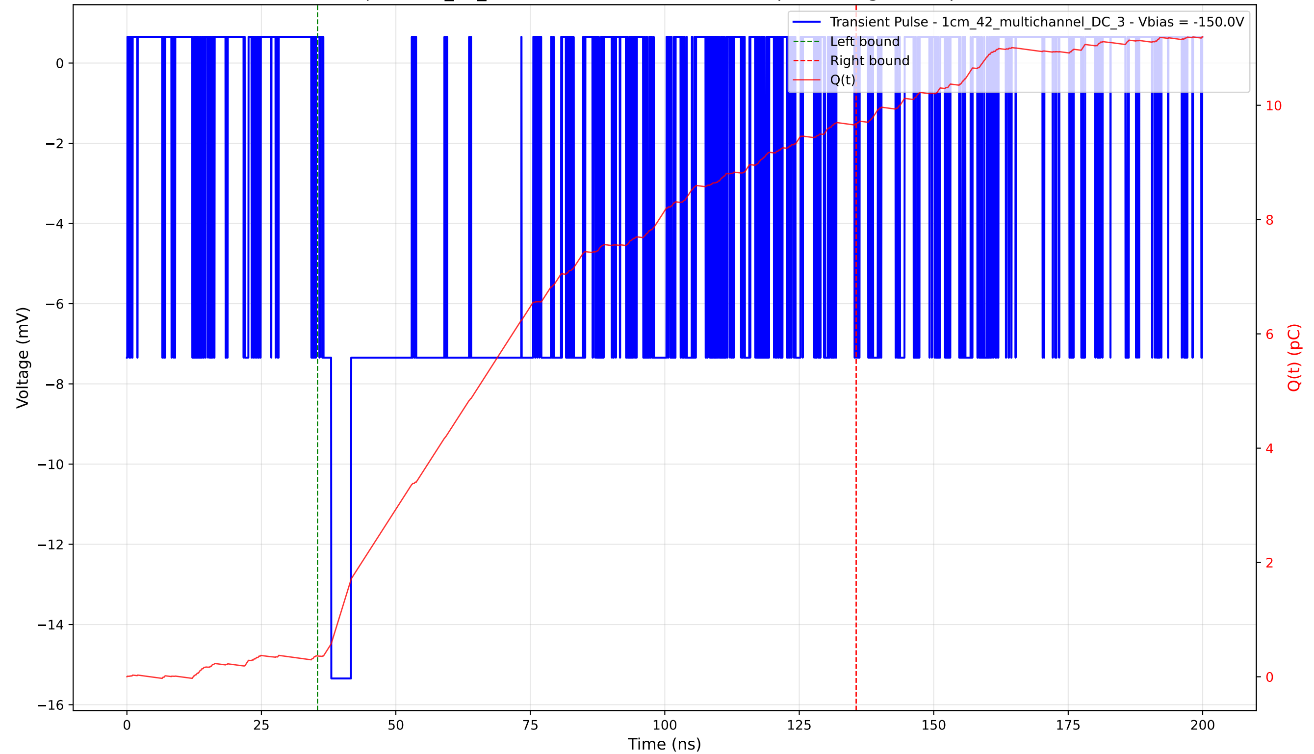
Transient Pulse - Sample: 1cm_42_multichannel - Position: 3365.0 \mu\text{m} - Charge: 9.31 pC - Rise Time: 1.46 ns
