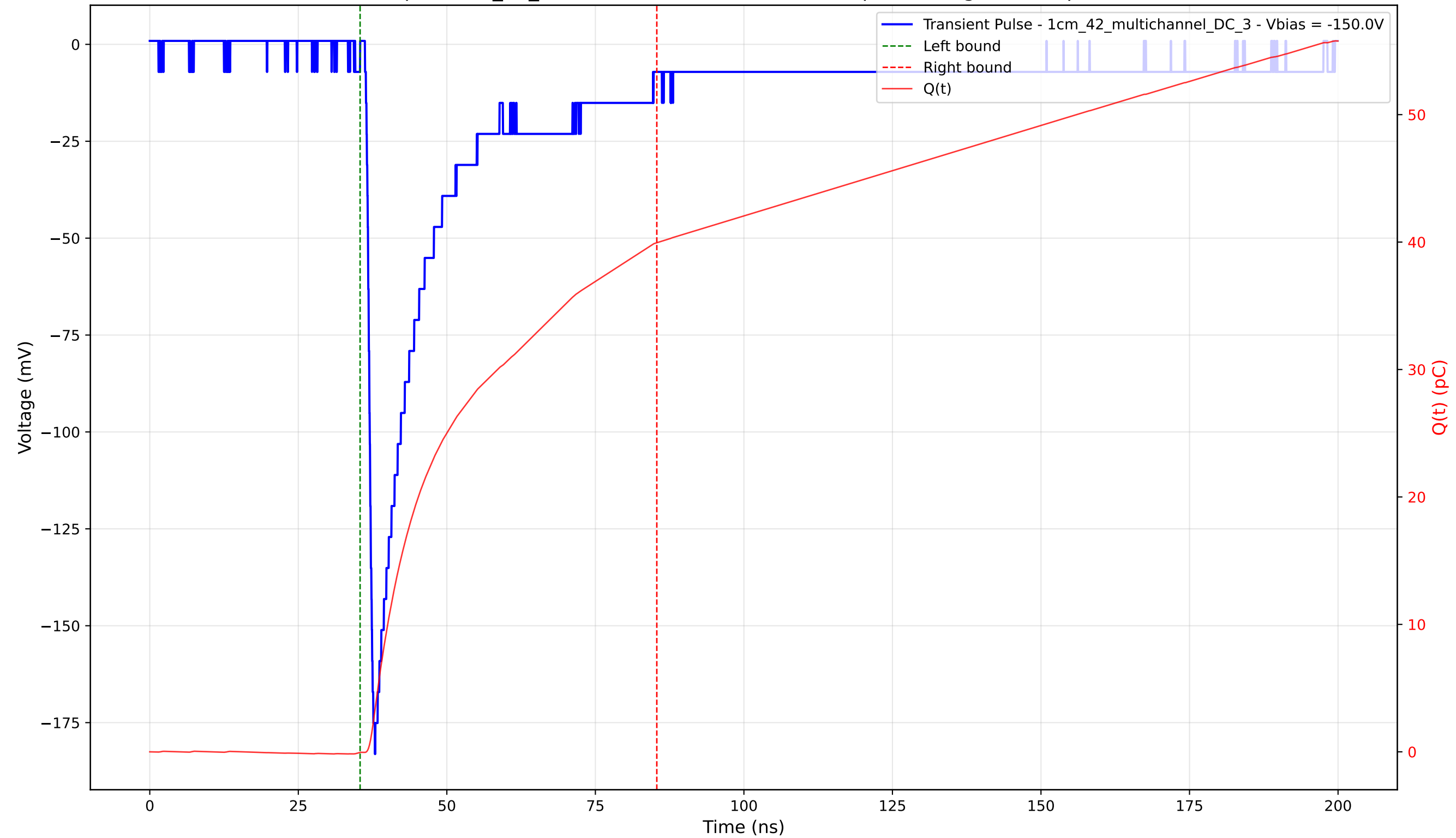
Transient Pulse - Sample: 1cm_42_multichannel - Position: 4060.0 \mu\text{m} - Charge: 39.98 pC - Rise Time: 1.03 ns
