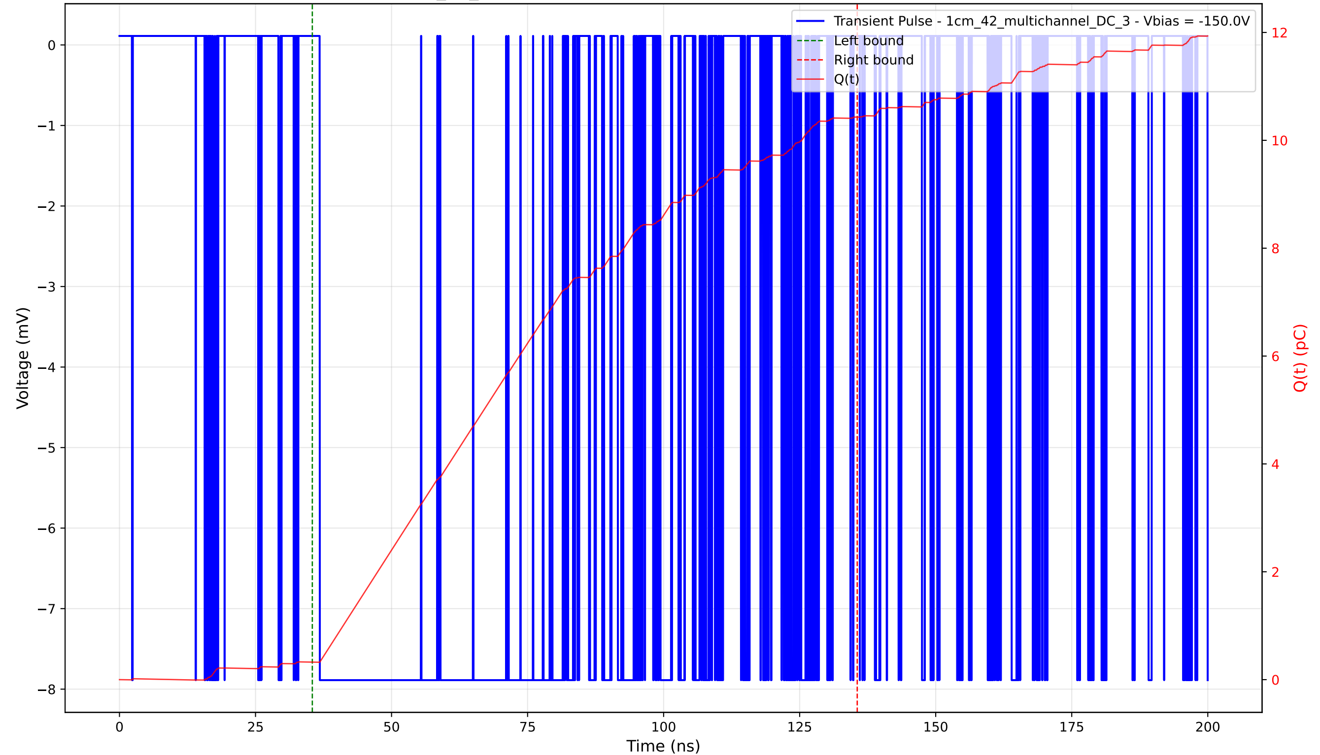
Transient Pulse - Sample: 1cm_42_multichannel - Position: 1885.0 \mu\text{m} - Charge: 10.11 pC - Rise Time: 0.02 ns
