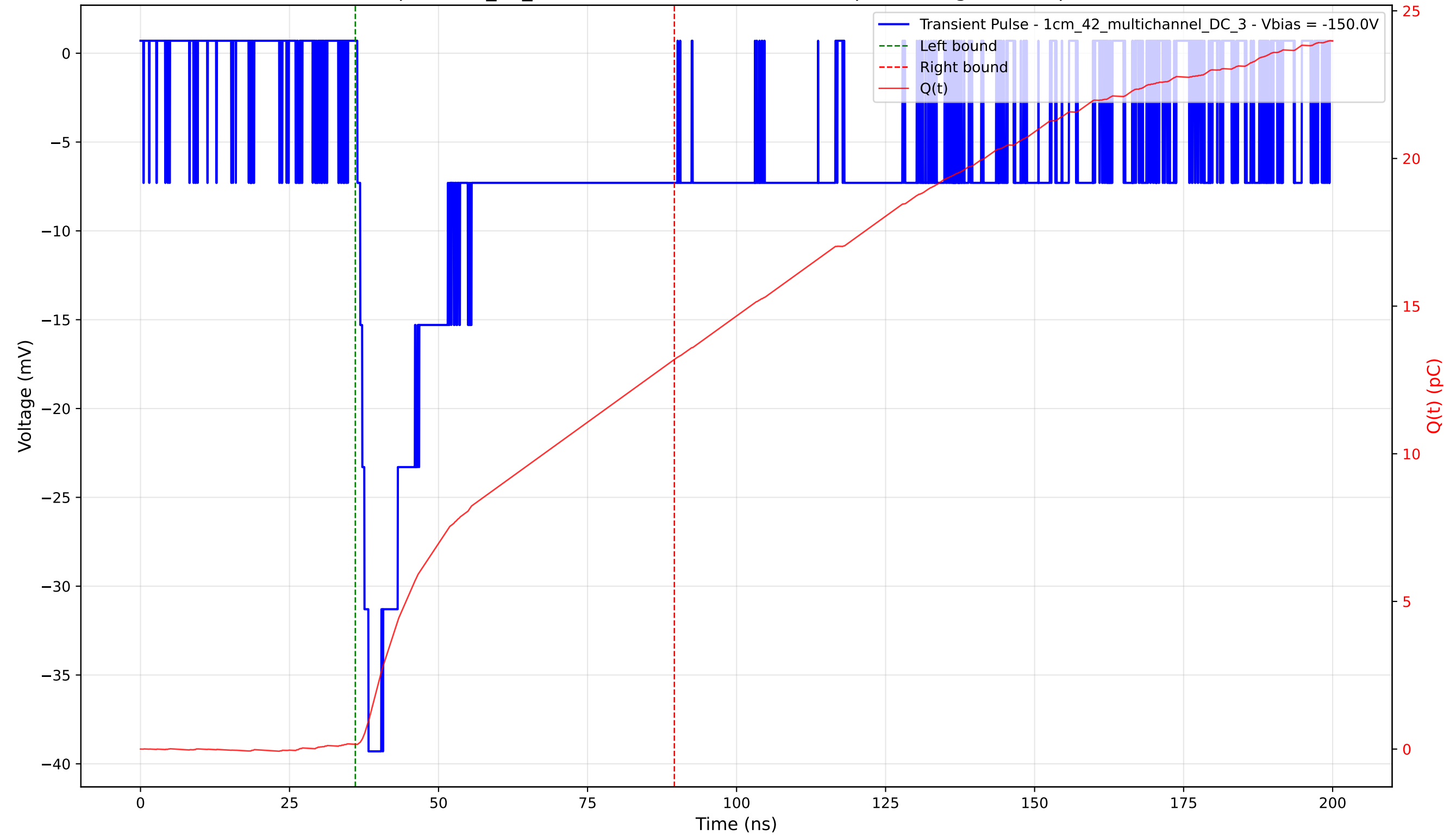
Transient Pulse - Sample: 1cm_42_multichannel - Position: 3345.0 \mu\text{m} - Charge: 13.04 pC - Rise Time: 1.87 ns
