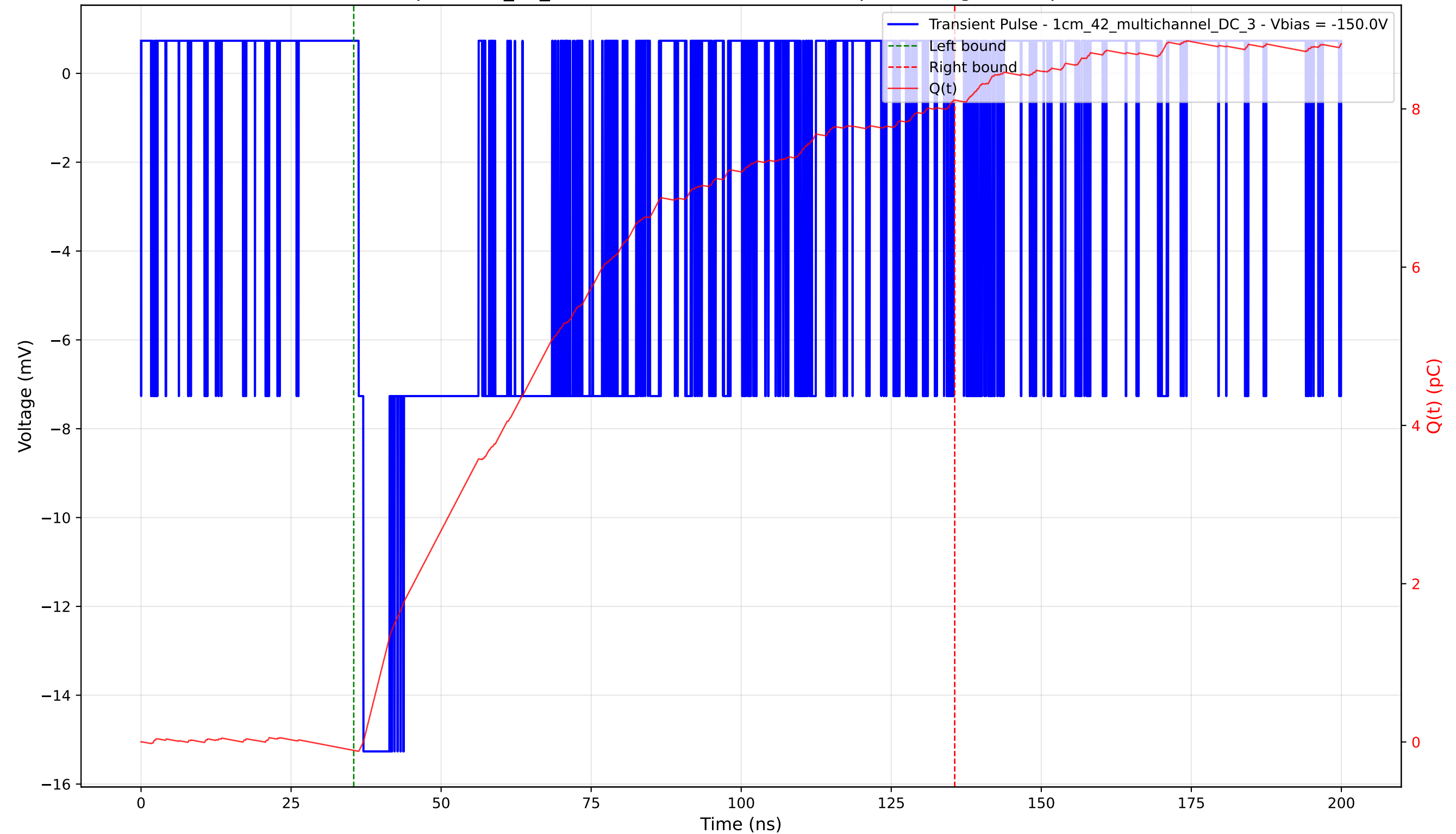
Transient Pulse - Sample: 1cm_42_multichannel - Position: 840.0 \mu\text{m} - Charge: 8.22 pC - Rise Time: 0.80 ns
