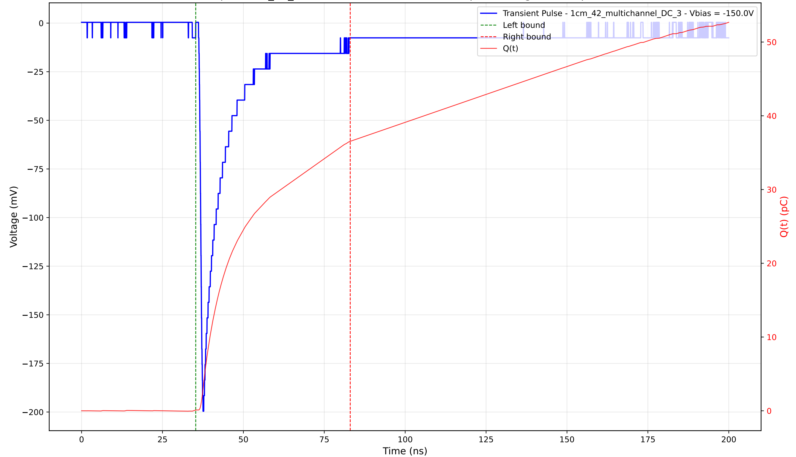
Transient Pulse - Sample: 1cm_42_multichannel - Position: 4295.0 \mu\text{m} - Charge: 36.43 pC - Rise Time: 0.97 ns
