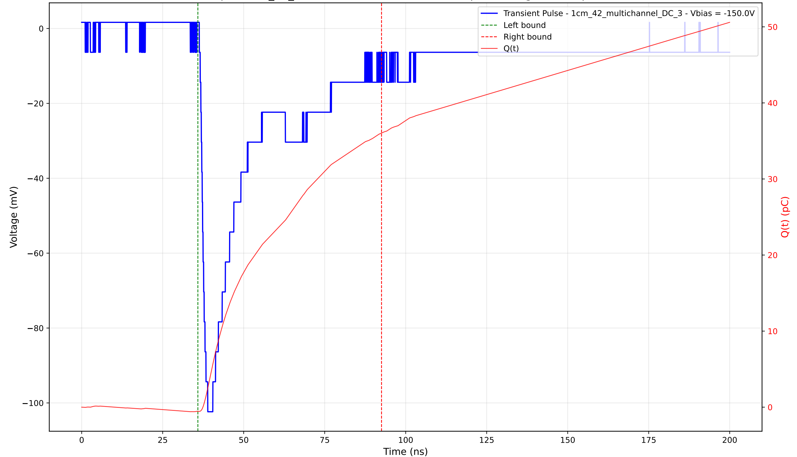
Transient Pulse - Sample: 1cm_42_multichannel - Position: 3030.0 \mu\text{m} - Charge: 36.59 pC - Rise Time: 1.79 ns
