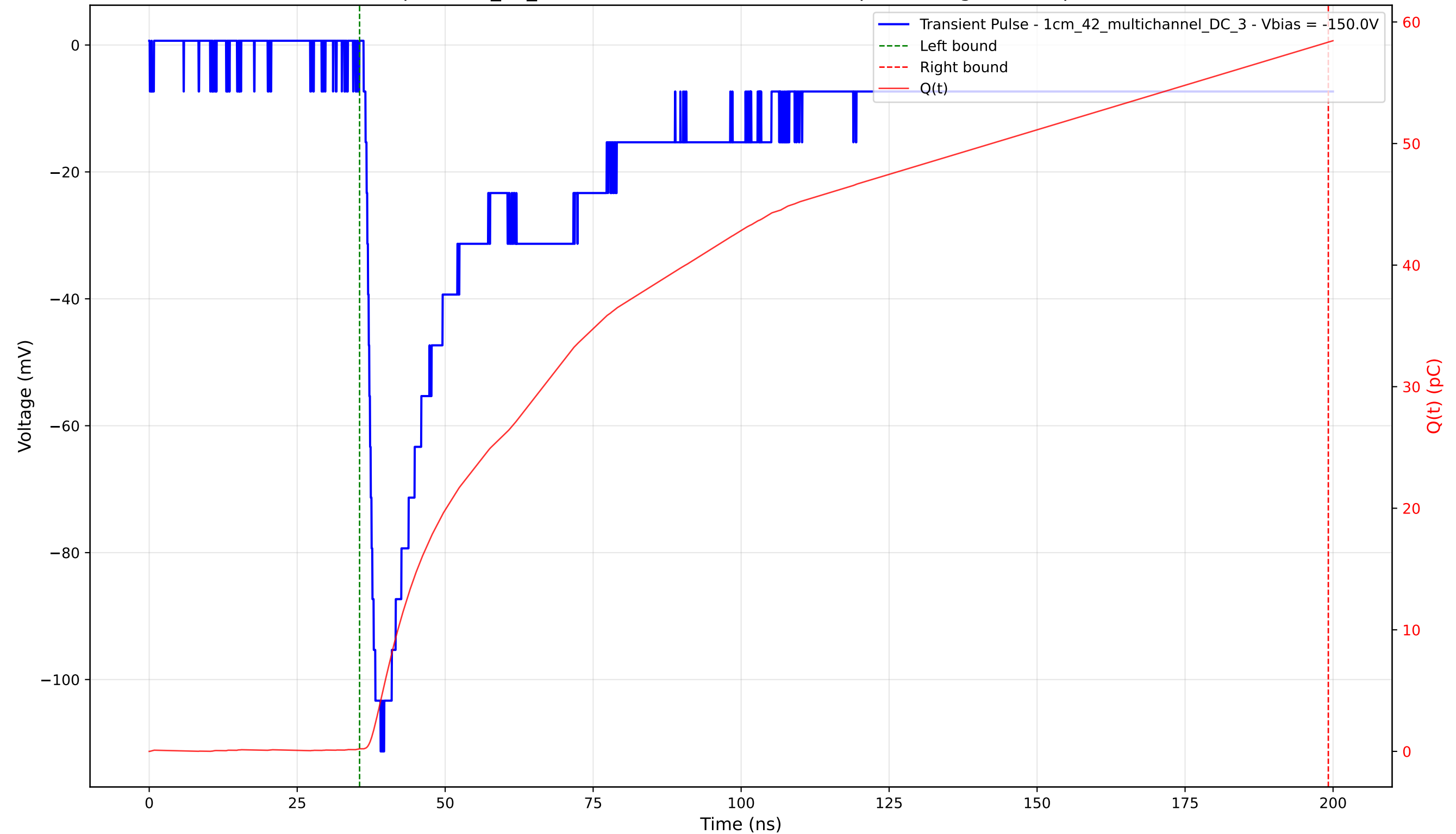
Transient Pulse - Sample: 1cm_42_multichannel - Position: 1775.0 \mu\text{m} - Charge: 58.13 pC - Rise Time: 1.67 ns
