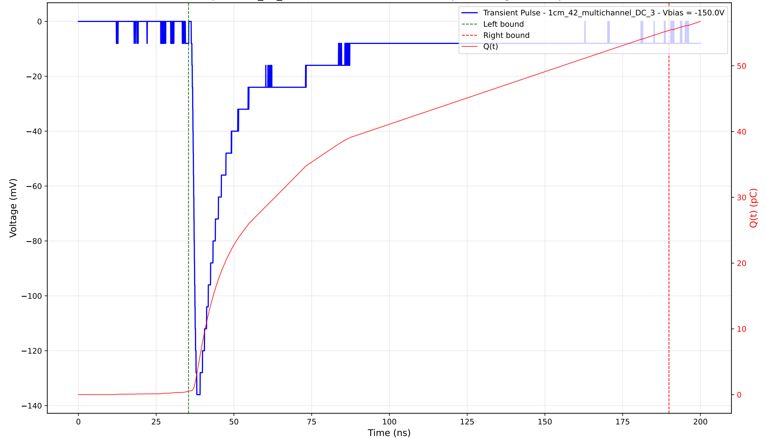
Transient Pulse - Sample: 1cm_42_multichannel - Position: 3695.0 \mu\text{m} - Charge: 54.83 pC - Rise Time: 1.33 ns
