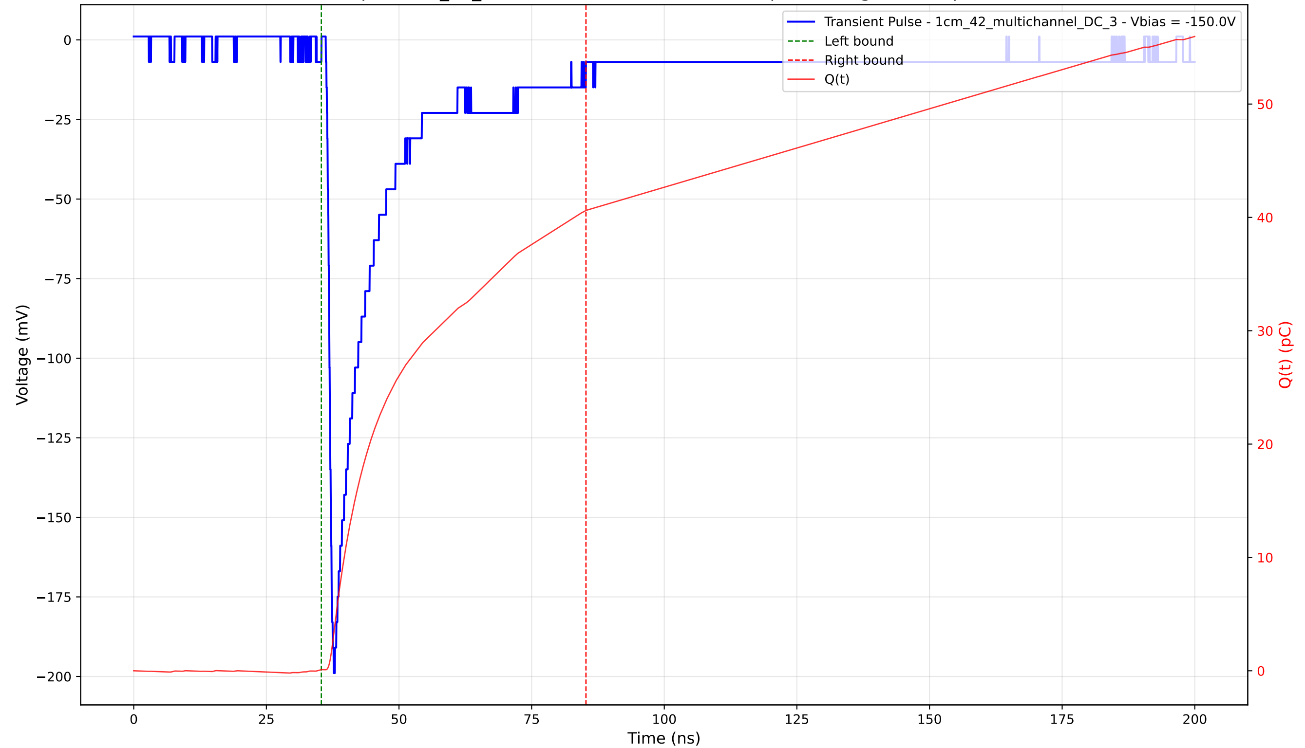
Transient Pulse - Sample: 1cm_42_multichannel - Position: 4175.0 \mu\text{m} - Charge: 40.52 pC - Rise Time: 1.01 ns
