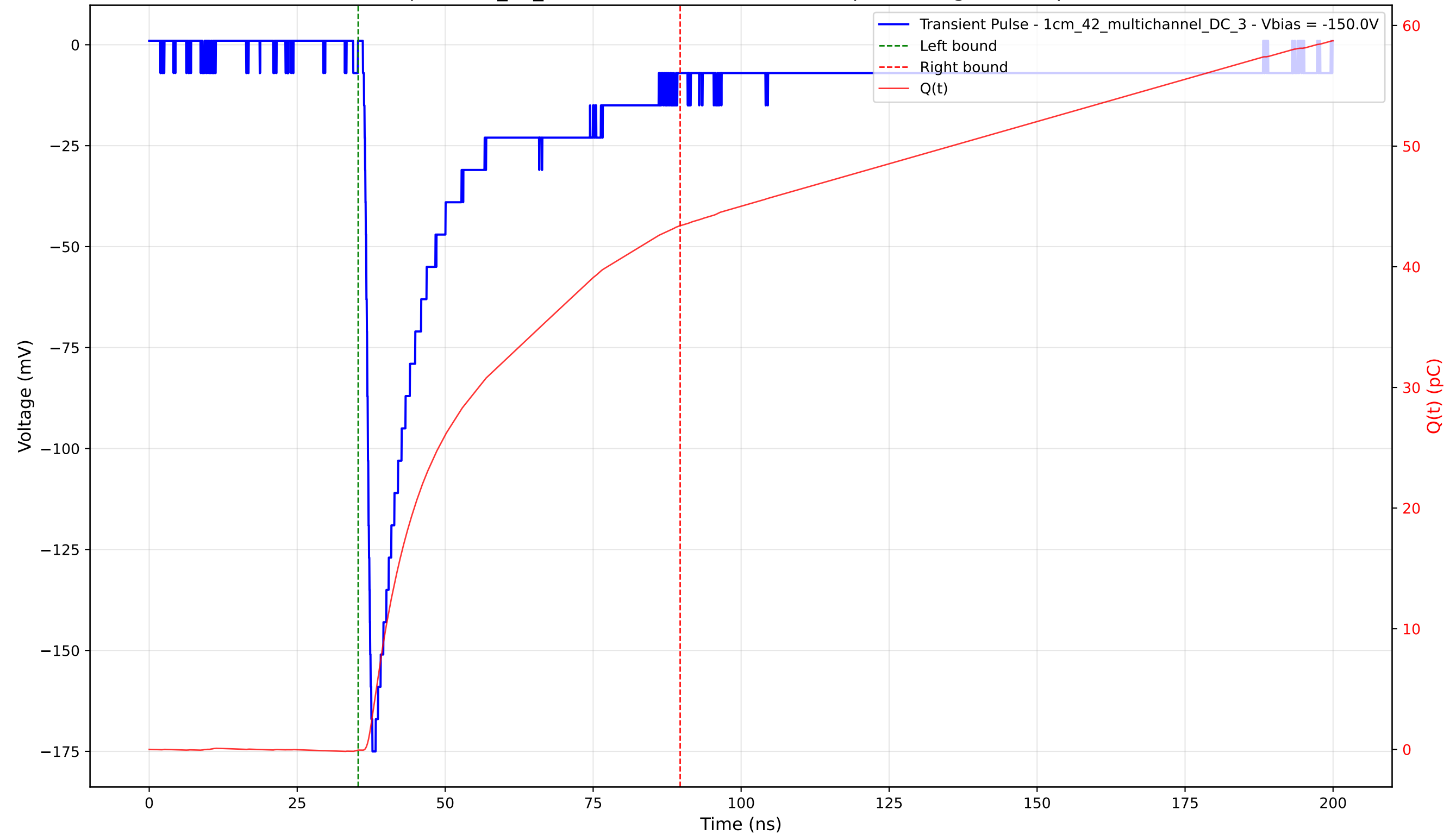
Transient Pulse - Sample: 1cm_42_multichannel - Position: 935.0 \mu\text{m} - Charge: 43.46 pC - Rise Time: 1.03 ns
