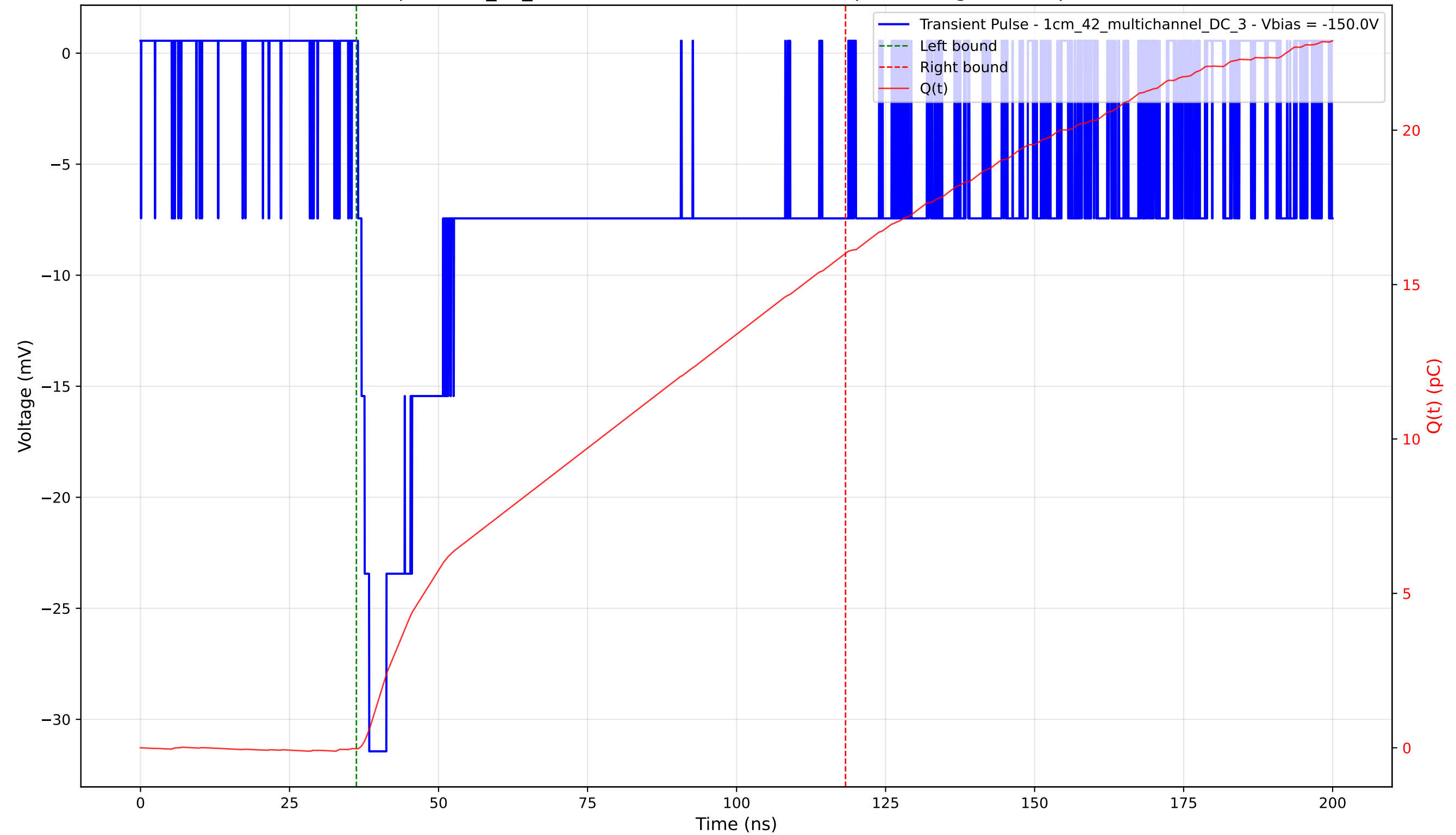
Transient Pulse - Sample: 1cm_42_multichannel - Position: 2920.0 \mu\text{m} - Charge: 16.05 pC - Rise Time: 1.87 ns
