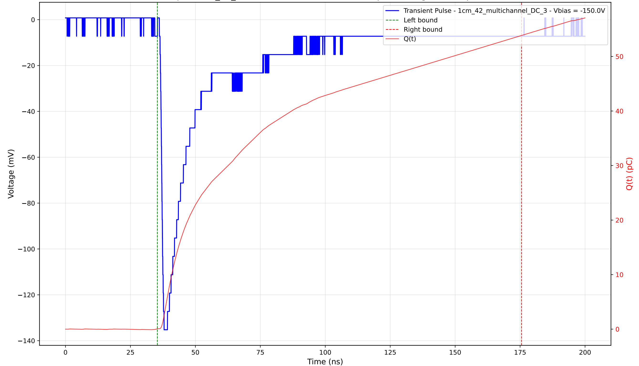
Transient Pulse - Sample: 1cm_42_multichannel - Position: 1285.0 \mu\text{m} - Charge: 53.79 pC - Rise Time: 1.32 ns
