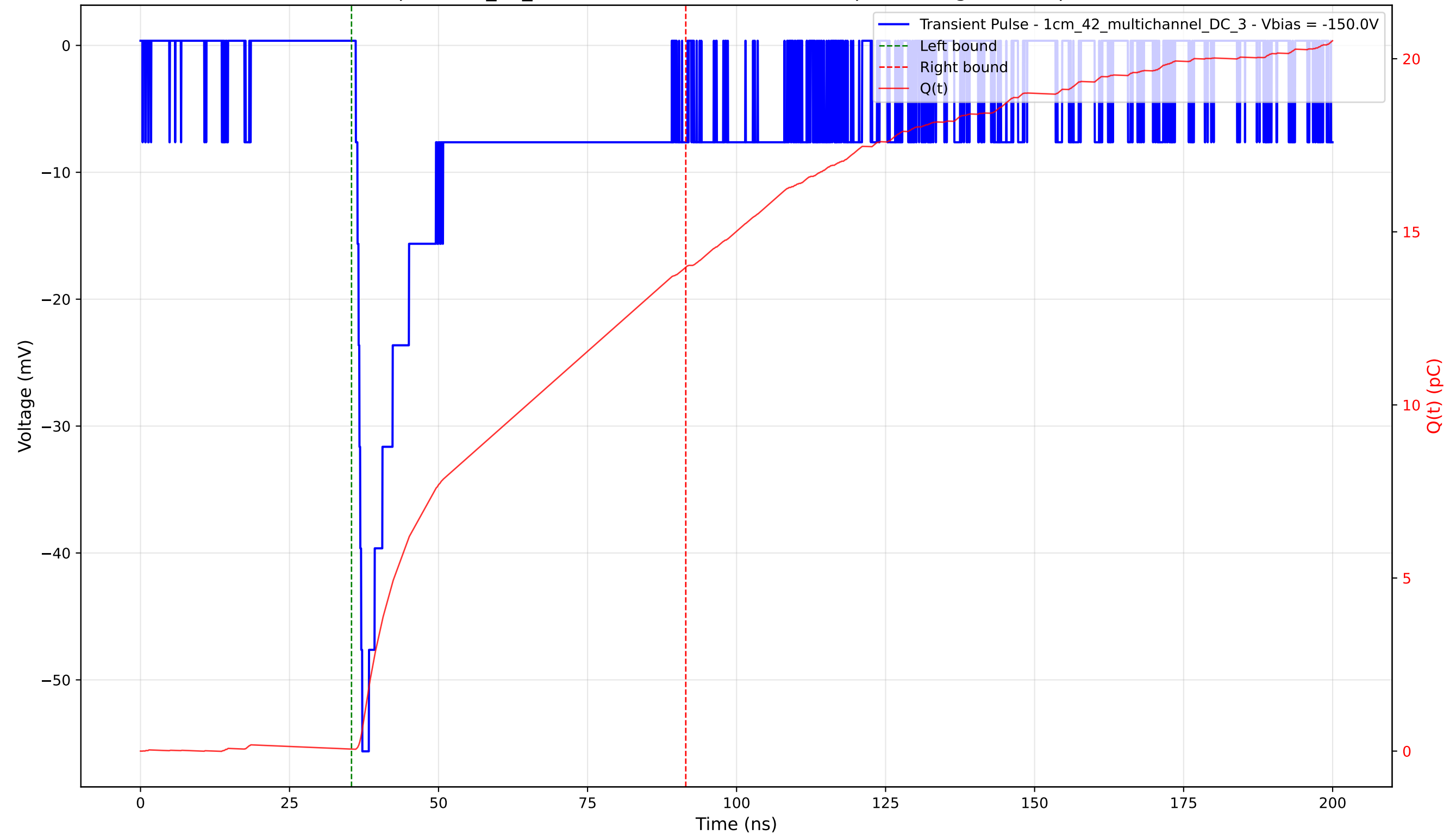
Transient Pulse - Sample: 1cm_42_multichannel - Position: 4350.0 \mu\text{m} - Charge: 13.92 pC - Rise Time: 1.09 ns
