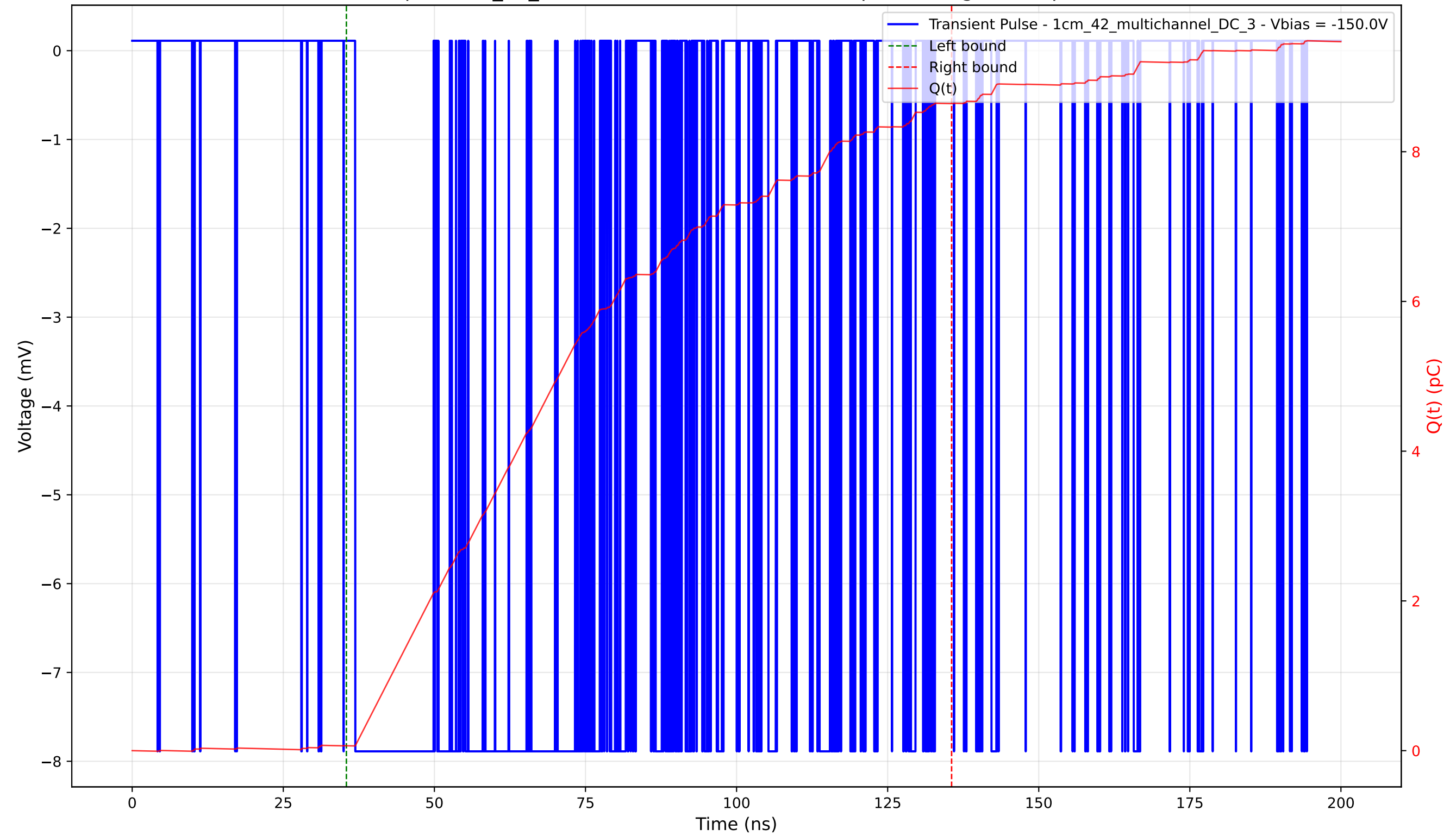
Transient Pulse - Sample: 1cm_42_multichannel - Position: 2380.0 \mu\text{m} - Charge: 8.58 pC - Rise Time: 0.02 ns
