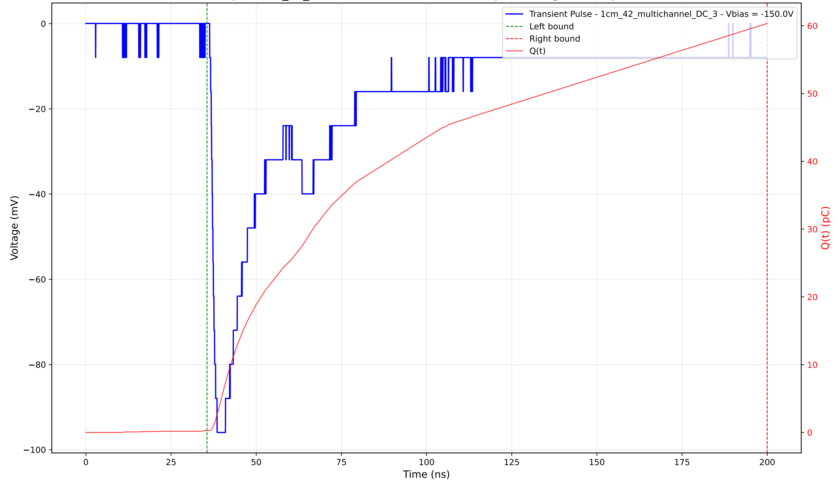
Transient Pulse - Sample: 1cm_42_multichannel - Position: 1990.0 \mu\text{m} - Charge: 60.05 pC - Rise Time: 1.48 ns
