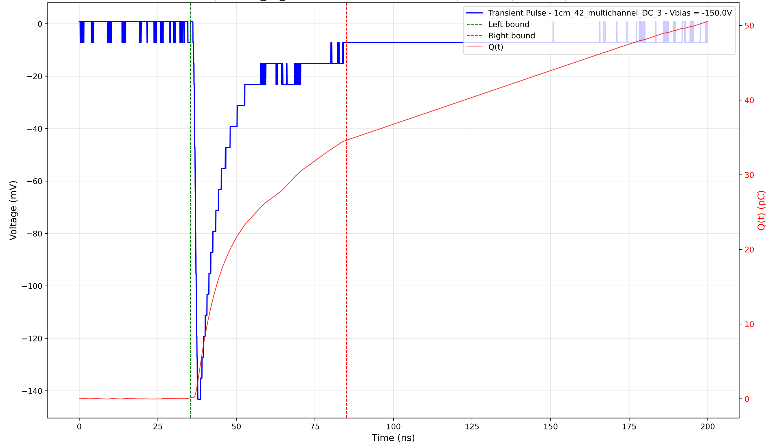
Transient Pulse - Sample: 1cm_42_multichannel - Position: 3960.0 \mu\text{m} - Charge: 34.50 pC - Rise Time: 1.16 ns
