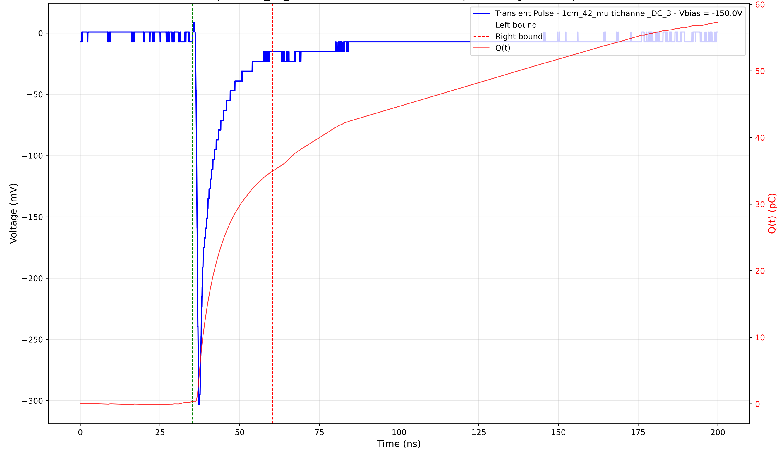
Transient Pulse - Sample: 1cm_42_multichannel - Position: 4615.0 \mu\text{m} - Charge: 34.60 pC - Rise Time: 0.84 ns
