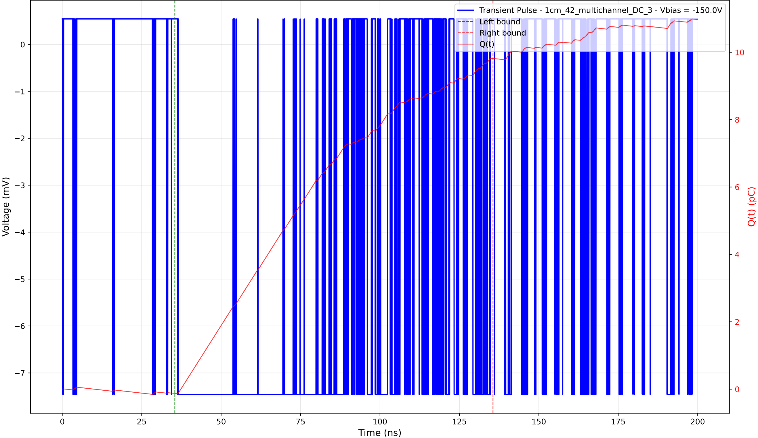
Transient Pulse - Sample: 1cm_42_multichannel - Position: 2395.0 \mu\text{m} - Charge: 9.94 pC - Rise Time: 0.02 ns
