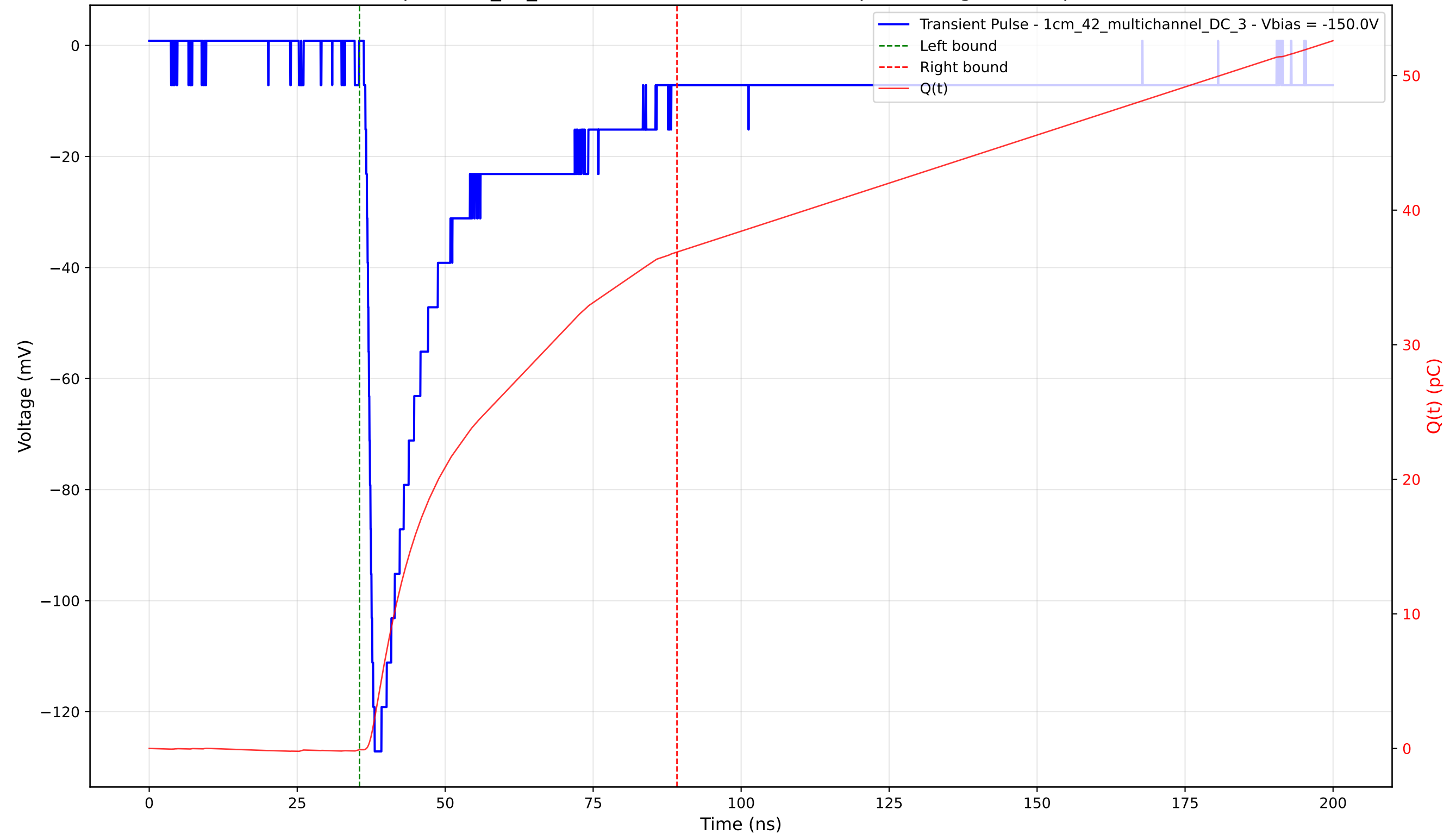
Transient Pulse - Sample: 1cm_42_multichannel - Position: 3640.0 \mu\text{m} - Charge: 36.98 pC - Rise Time: 1.33 ns
