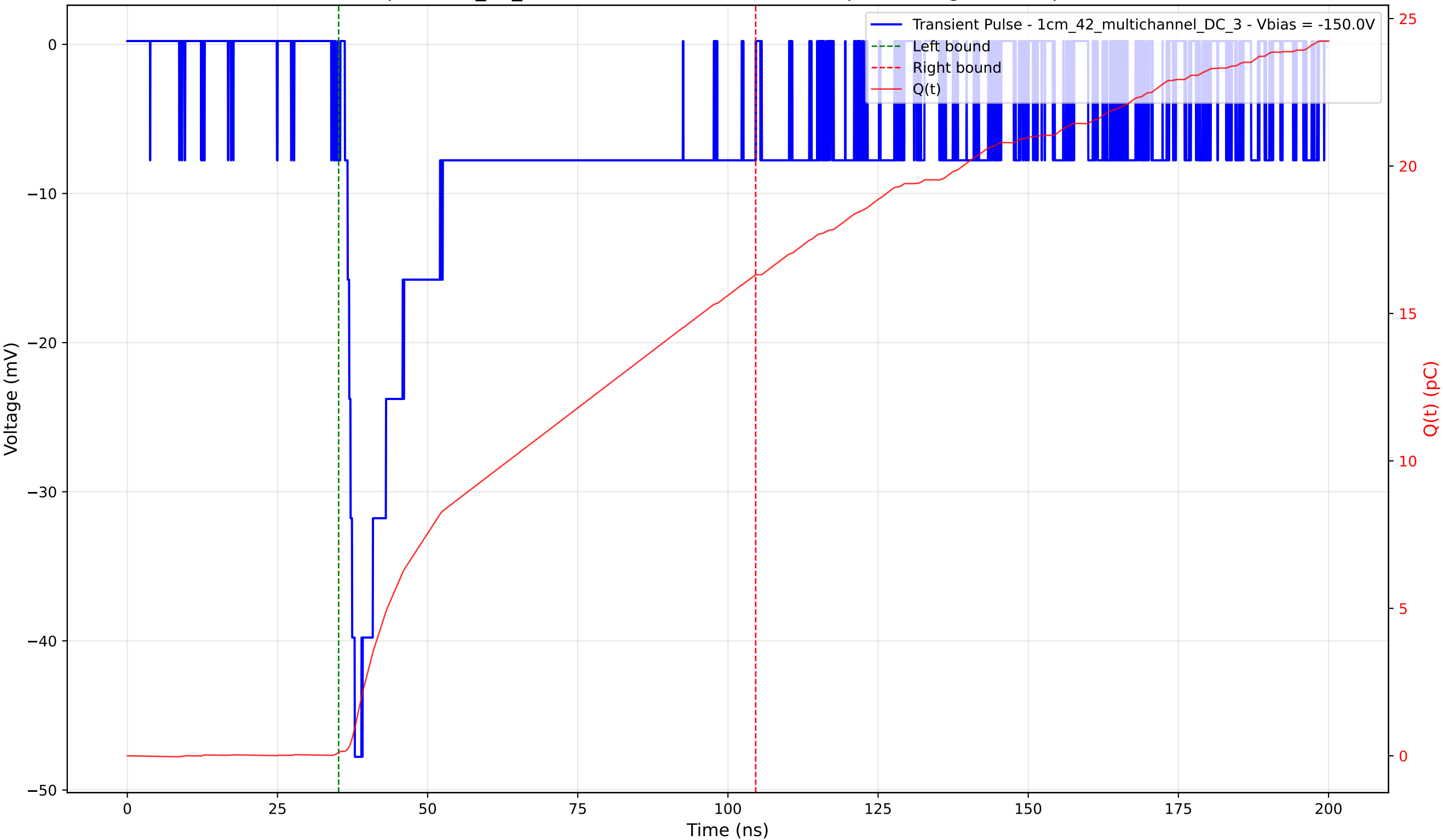
Transient Pulse - Sample: 1cm_42_multichannel - Position: 3850.0 \mu\text{m} - Charge: 16.20 pC - Rise Time: 1.65 ns
