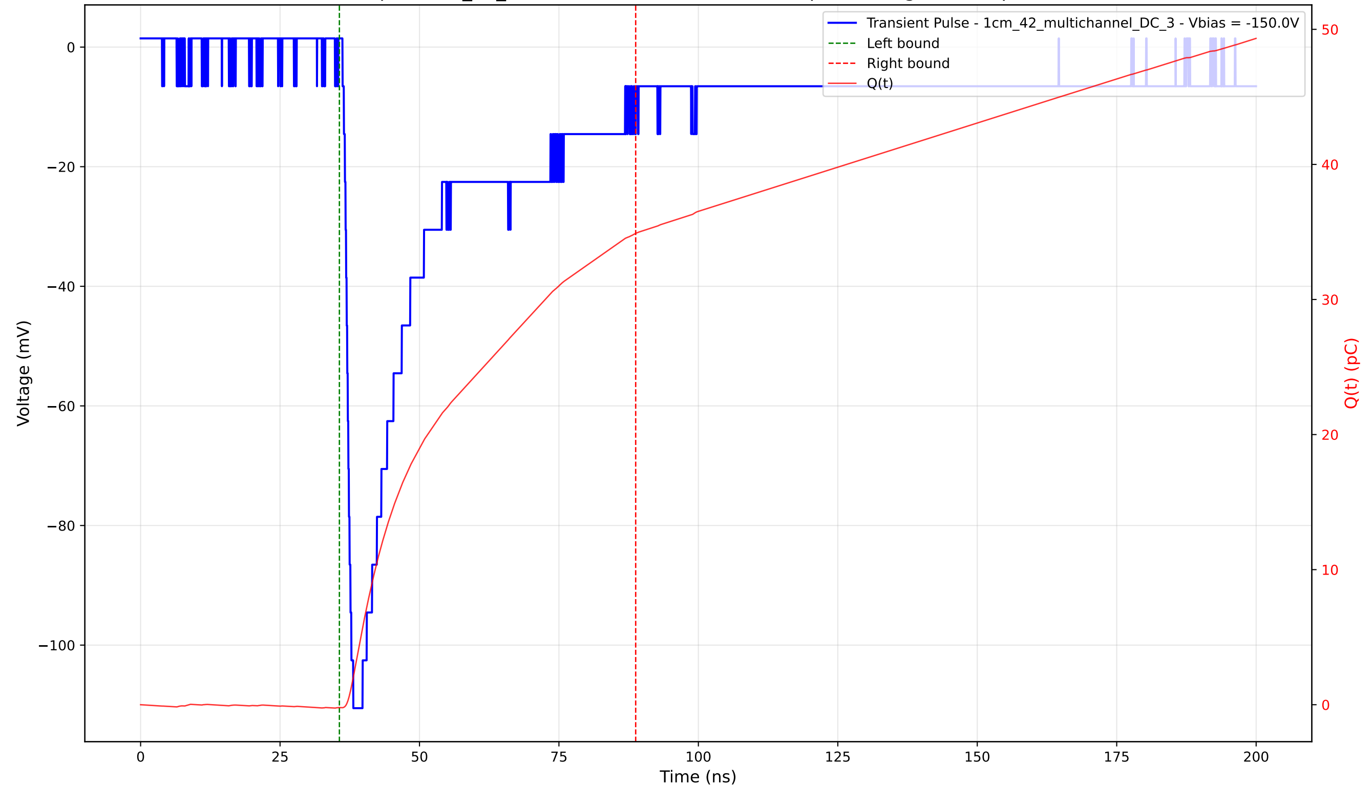
Transient Pulse - Sample: 1cm_42_multichannel - Position: 1430.0 \mu\text{m} - Charge: 35.11 pC - Rise Time: 1.35 ns
