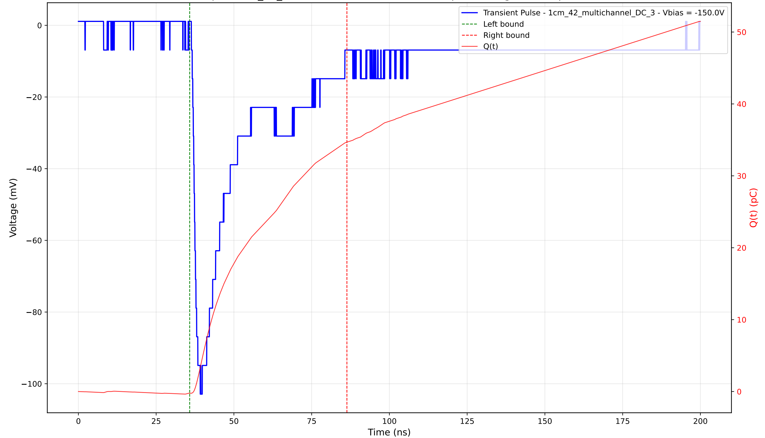
Transient Pulse - Sample: 1cm_42_multichannel - Position: 3050.0 \mu\text{m} - Charge: 34.91 pC - Rise Time: 1.81 ns
