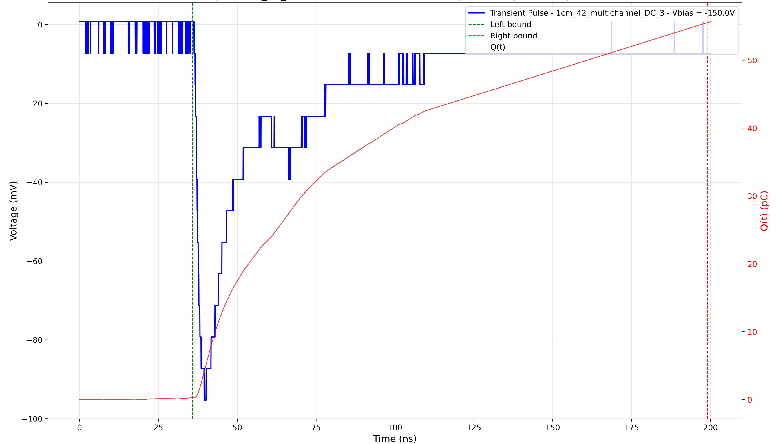
Transient Pulse - Sample: 1cm_42_multichannel - Position: 2770.0 \mu\text{m} - Charge: 55.29 pC - Rise Time: 1.93 ns
