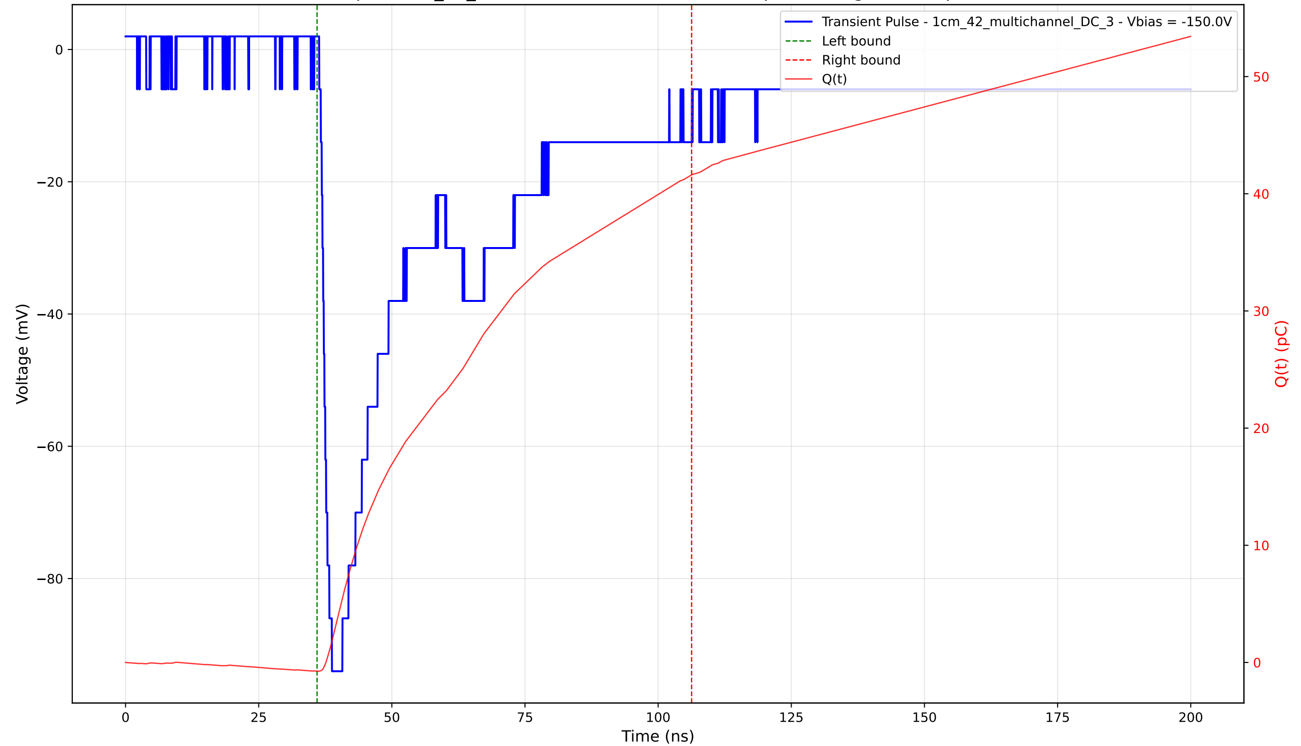
Transient Pulse - Sample: 1cm_42_multichannel - Position: 2035.0 \mu\text{m} - Charge: 42.36 pC - Rise Time: 1.61 ns
