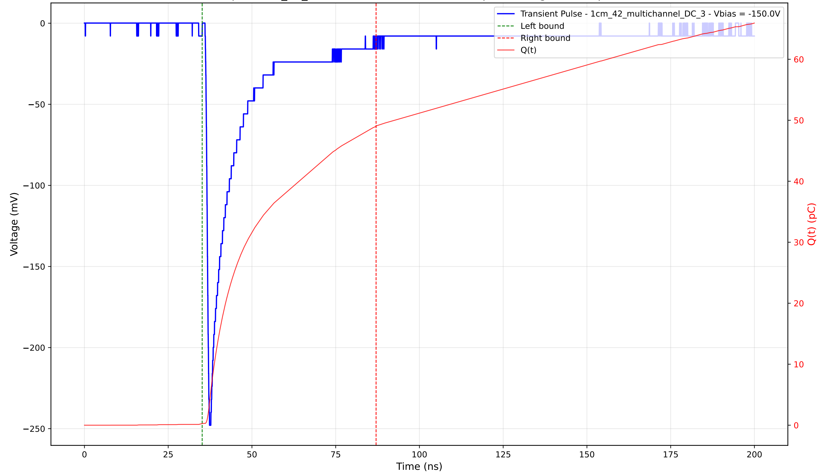
Transient Pulse - Sample: 1cm_42_multichannel - Position: 575.0 \mu\text{m} - Charge: 48.74 pC - Rise Time: 0.90 ns
