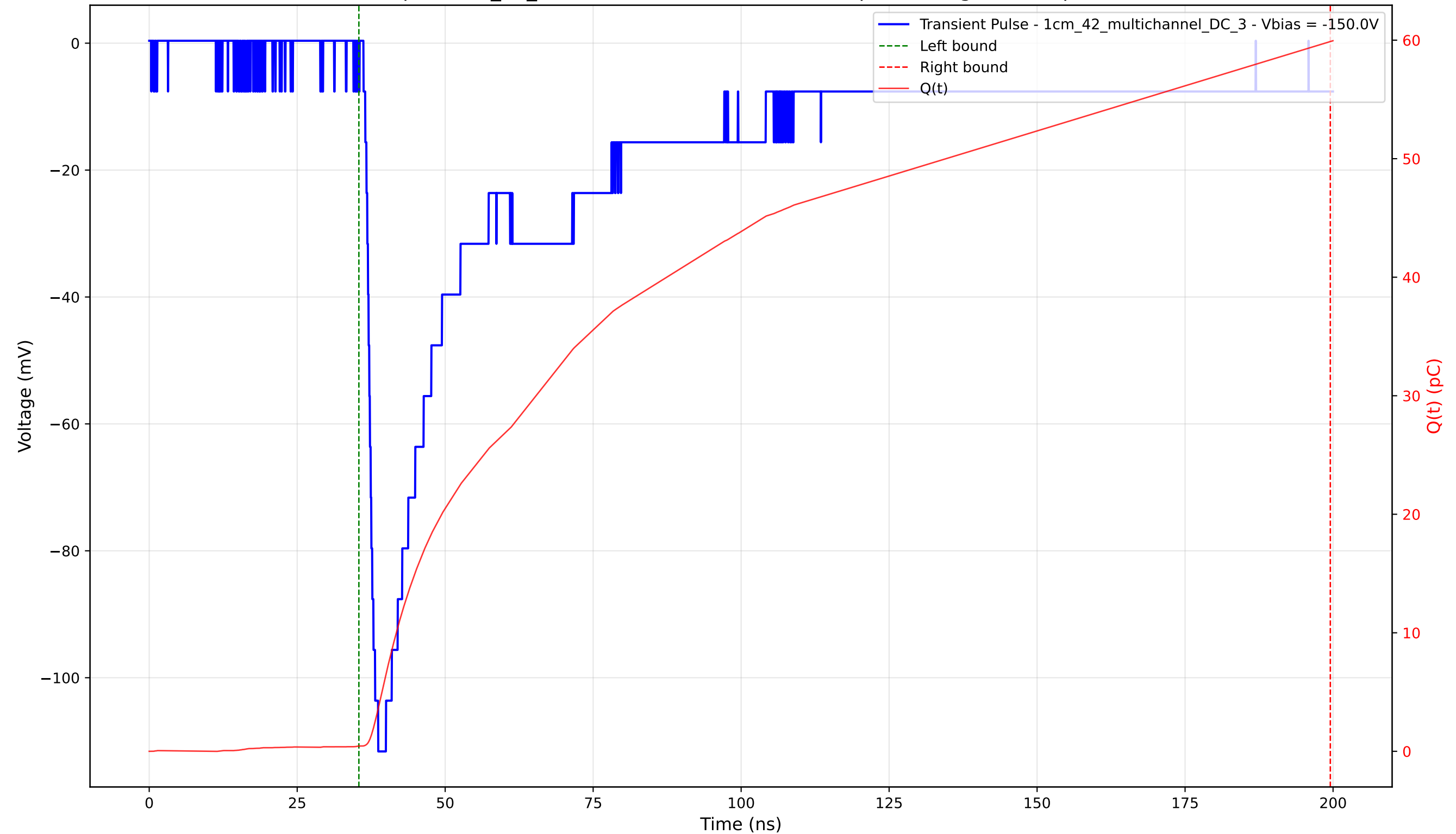
Transient Pulse - Sample: 1cm_42_multichannel - Position: 1770.0 \mu\text{m} - Charge: 59.44 pC - Rise Time: 1.67 ns
