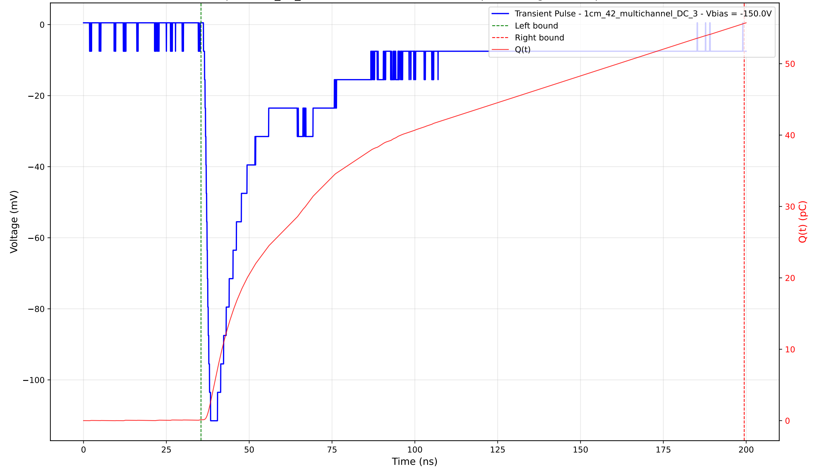
Transient Pulse - Sample: 1cm_42_multichannel - Position: 3280.0 \mu\text{m} - Charge: 55.52 pC - Rise Time: 1.51 ns
