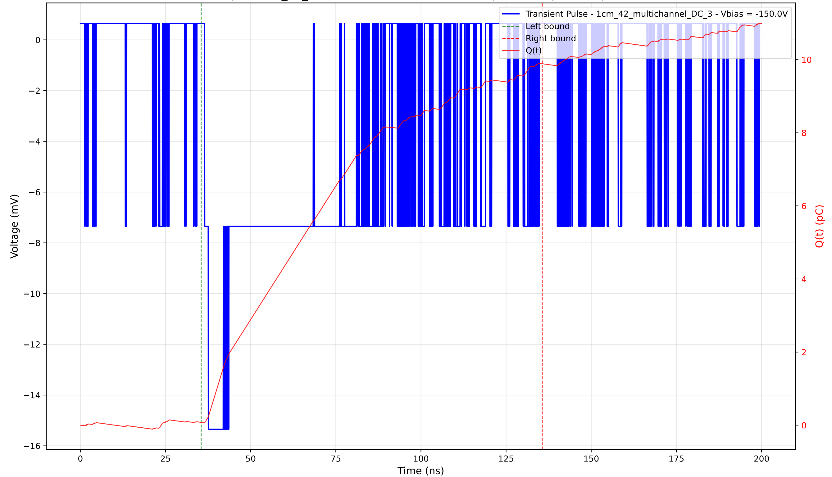
Transient Pulse - Sample: 1cm_42_multichannel - Position: 1385.0 \mu\text{m} - Charge: 9.81 pC - Rise Time: 1.08 ns
