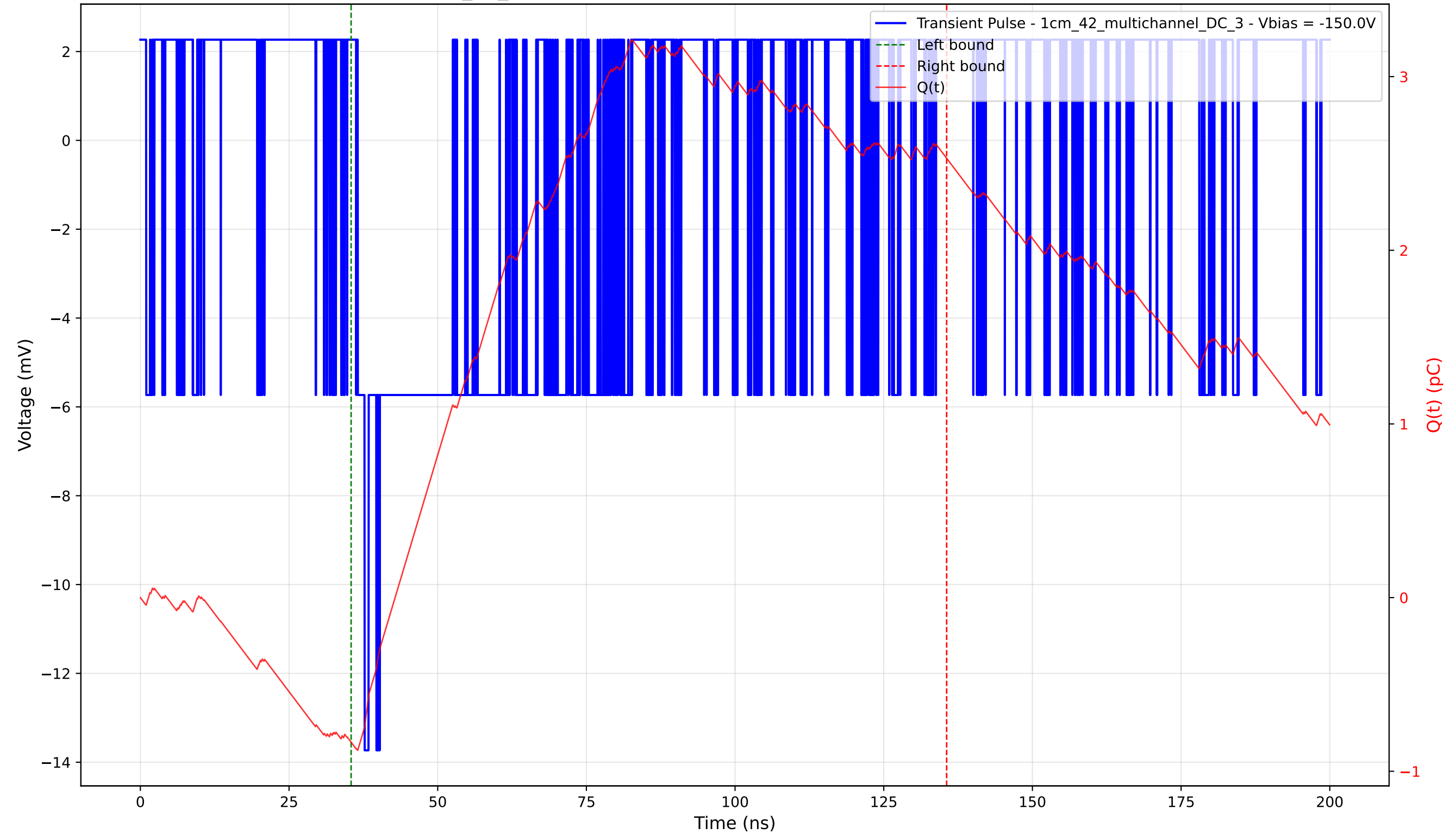
Transient Pulse - Sample: 1cm_42_multichannel - Position: 3905.0 \mu\text{m} - Charge: 3.36 pC - Rise Time: 0.00 ns (N/A)
