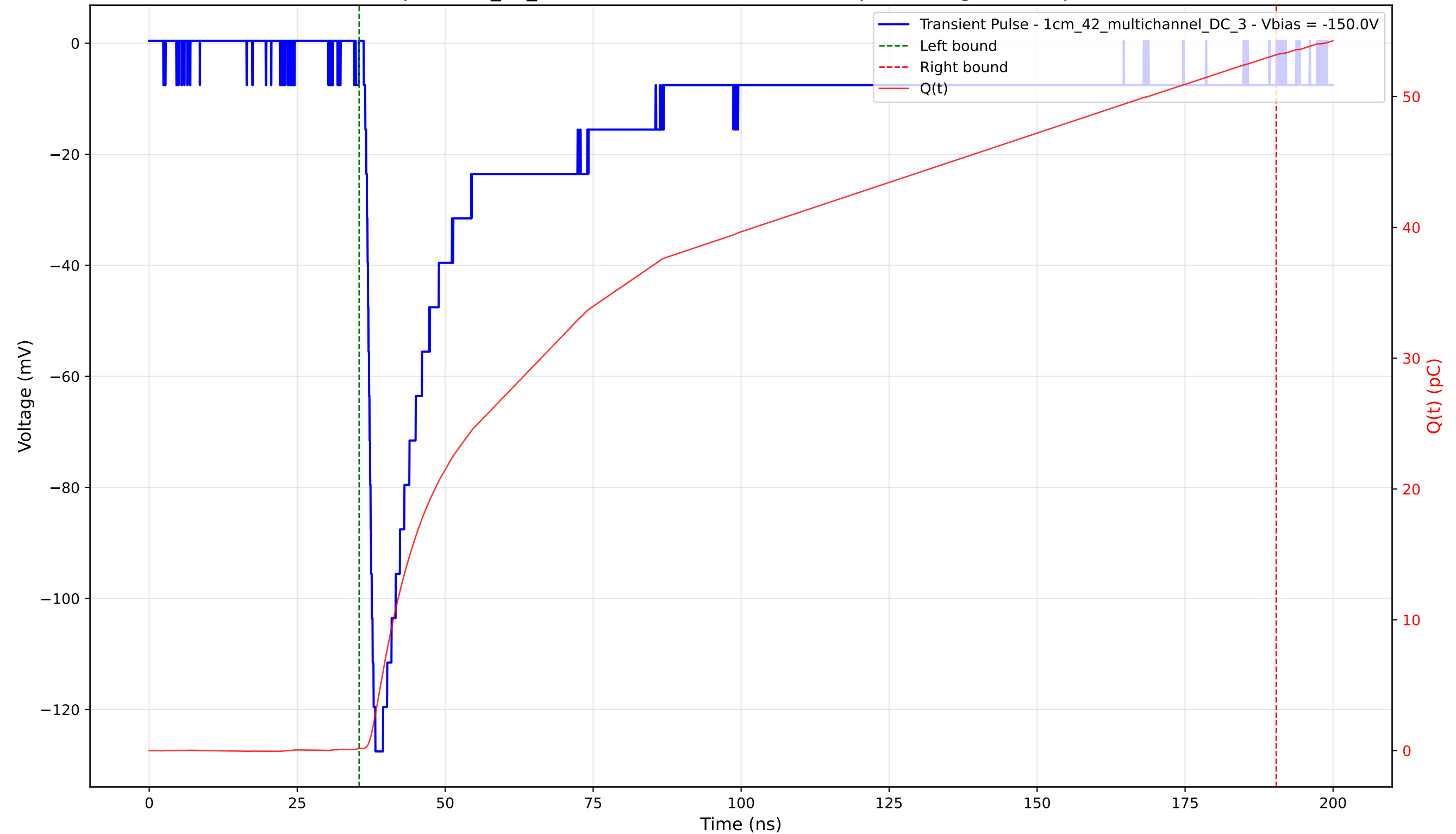
Transient Pulse - Sample: 1cm_42_multichannel - Position: 3580.0 \mu\text{m} - Charge: 53.03 pC - Rise Time: 1.41 ns
