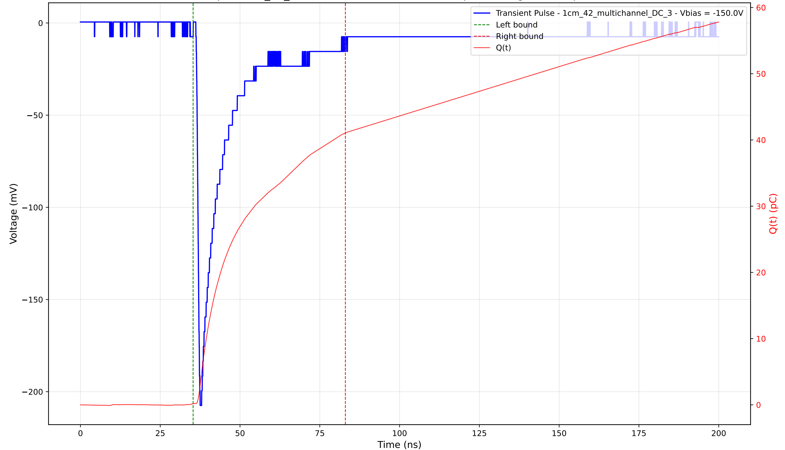
Transient Pulse - Sample: 1cm_42_multichannel - Position: 4240.0 \mu\text{m} - Charge: 40.87 pC - Rise Time: 0.95 ns
