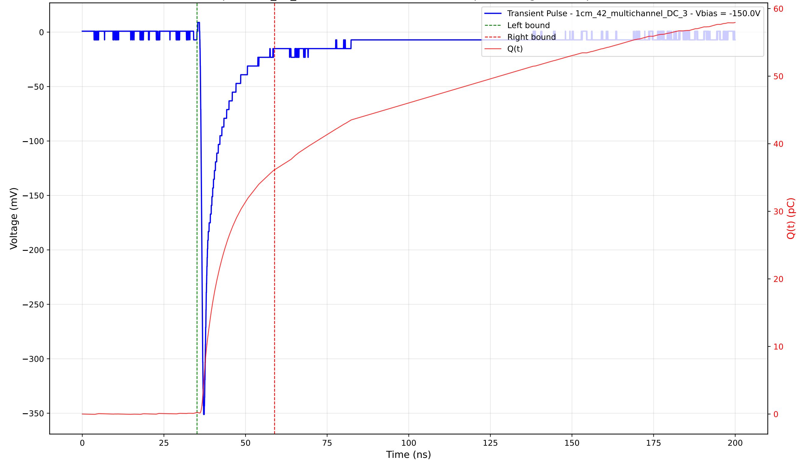
Transient Pulse - Sample: 1cm_42_multichannel - Position: 4710.0 \mu\text{m} - Charge: 35.91 pC - Rise Time: 0.79 ns
