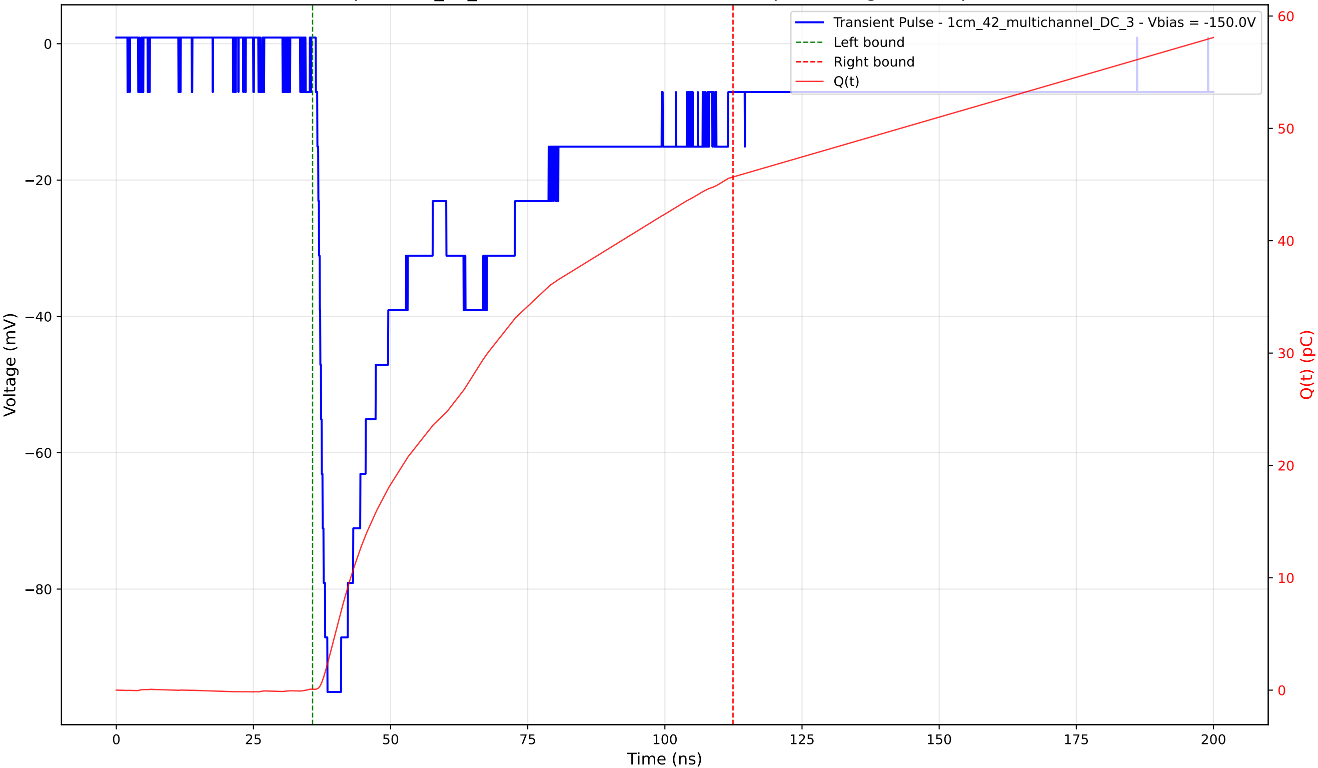
Transient Pulse - Sample: 1cm_42_multichannel - Position: 2005.0 \mu\text{m} - Charge: 45.59 pC - Rise Time: 1.43 ns
