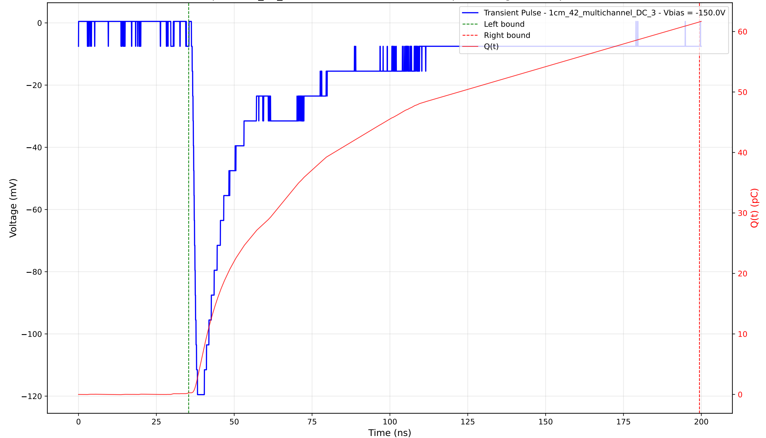
Transient Pulse - Sample: 1cm_42_multichannel - Position: 1605.0 \mu\text{m} - Charge: 61.33 pC - Rise Time: 1.41 ns
