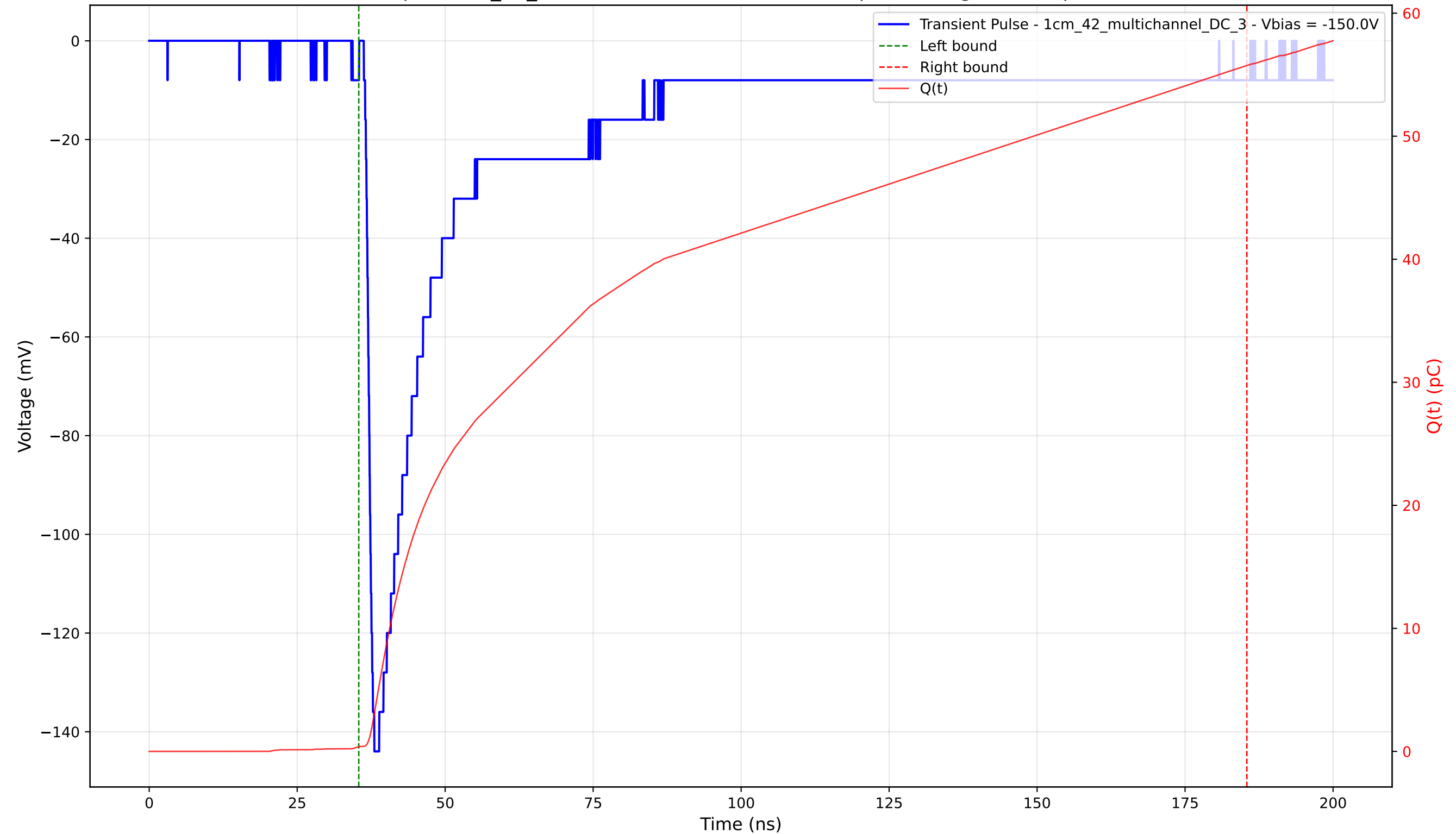
Transient Pulse - Sample: 1cm_42_multichannel - Position: 3740.0 \mu\text{m} - Charge: 55.36 pC - Rise Time: 1.30 ns
