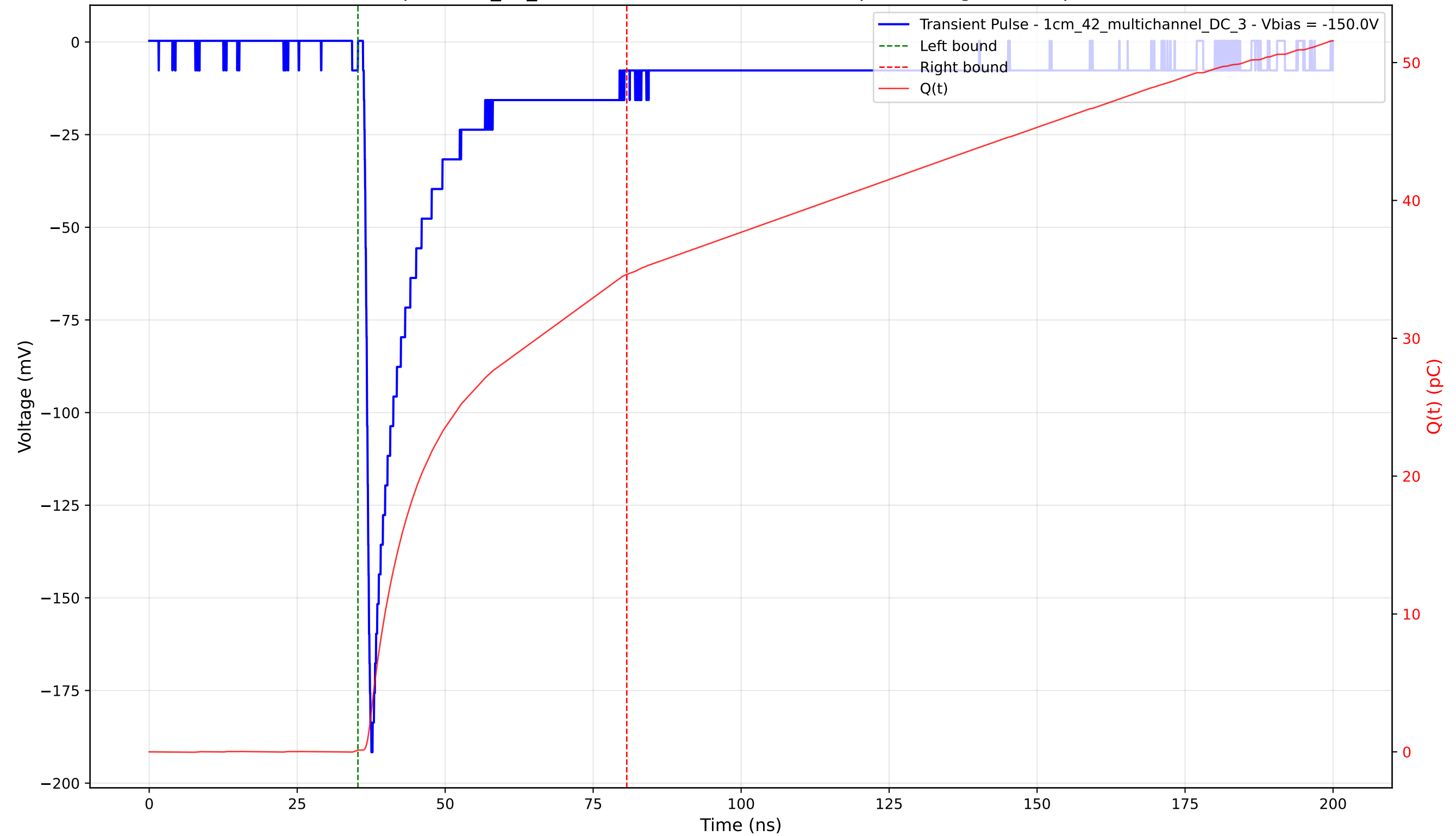
Transient Pulse - Sample: 1cm_42_multichannel - Position: 4305.0 \mu\text{m} - Charge: 34.50 pC - Rise Time: 0.95 ns
