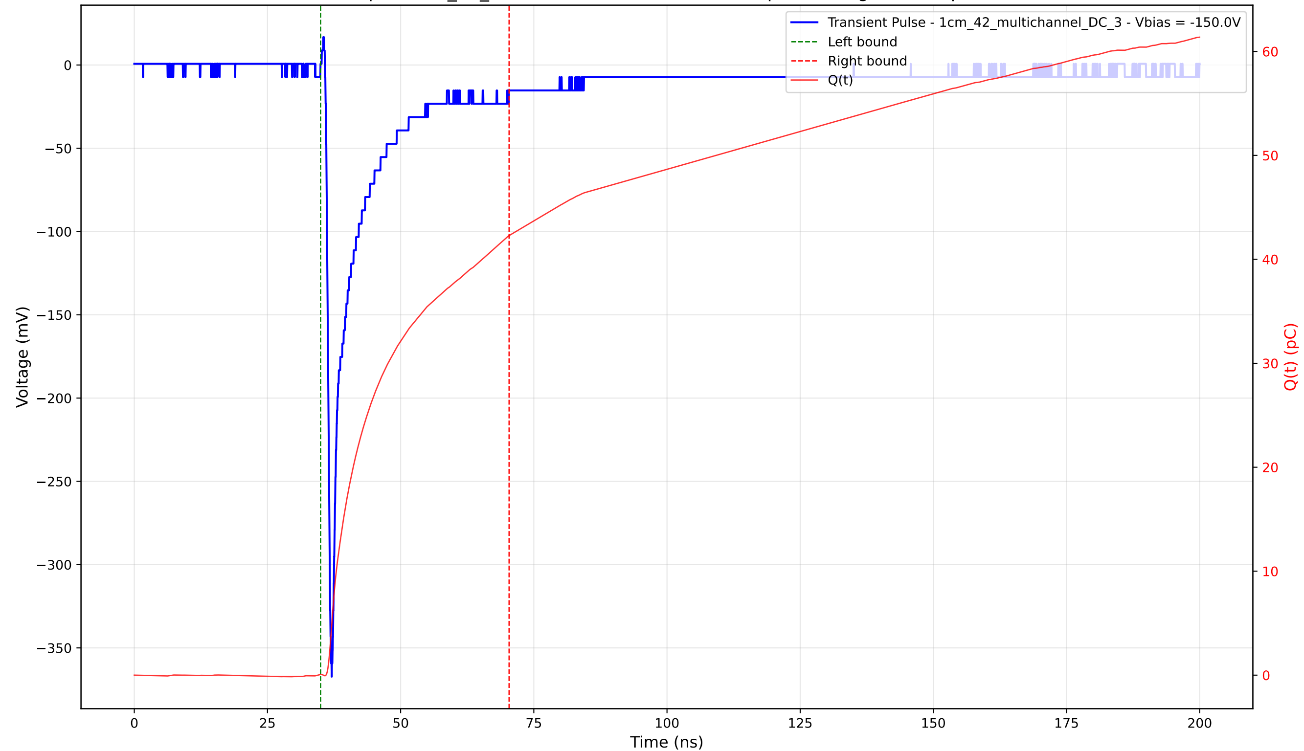
Transient Pulse - Sample: 1cm_42_multichannel - Position: 140.0 \mu\text{m} - Charge: 42.21 pC - Rise Time: 0.81 ns
