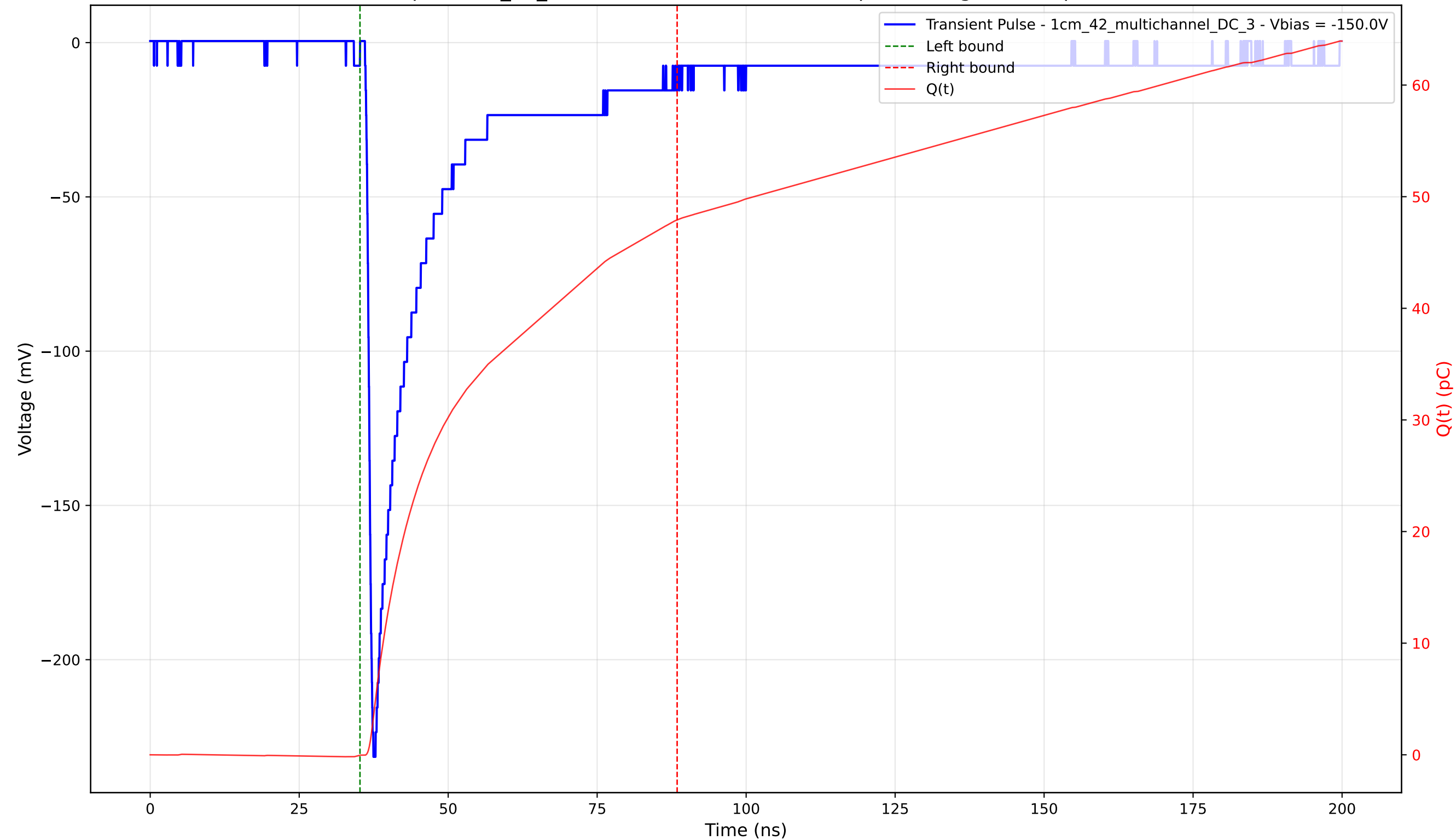
Transient Pulse - Sample: 1cm_42_multichannel - Position: 650.0 \mu\text{m} - Charge: 47.96 pC - Rise Time: 1.02 ns
