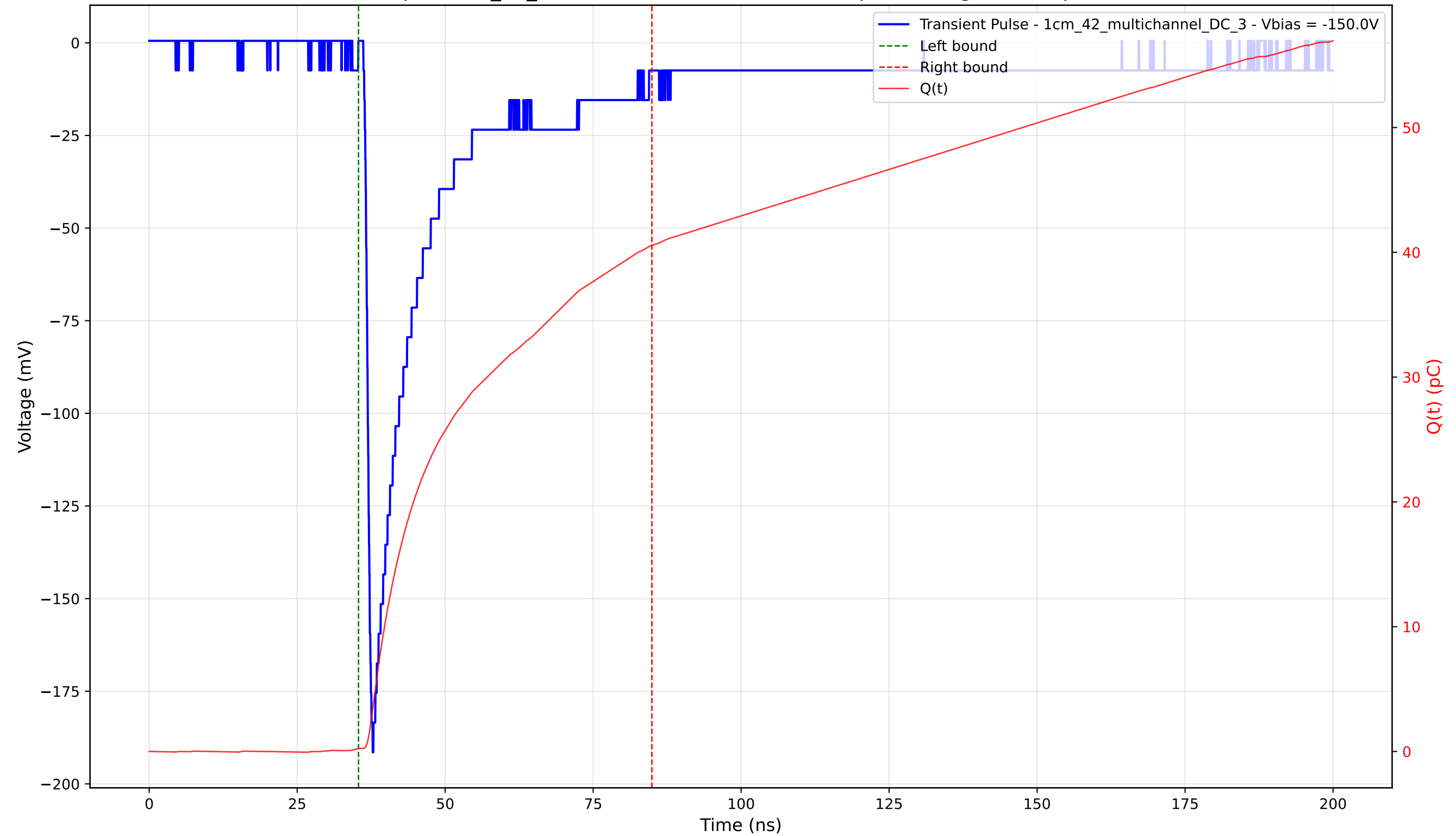
Transient Pulse - Sample: 1cm_42_multichannel - Position: 4140.0 \mu\text{m} - Charge: 40.30 pC - Rise Time: 1.03 ns
