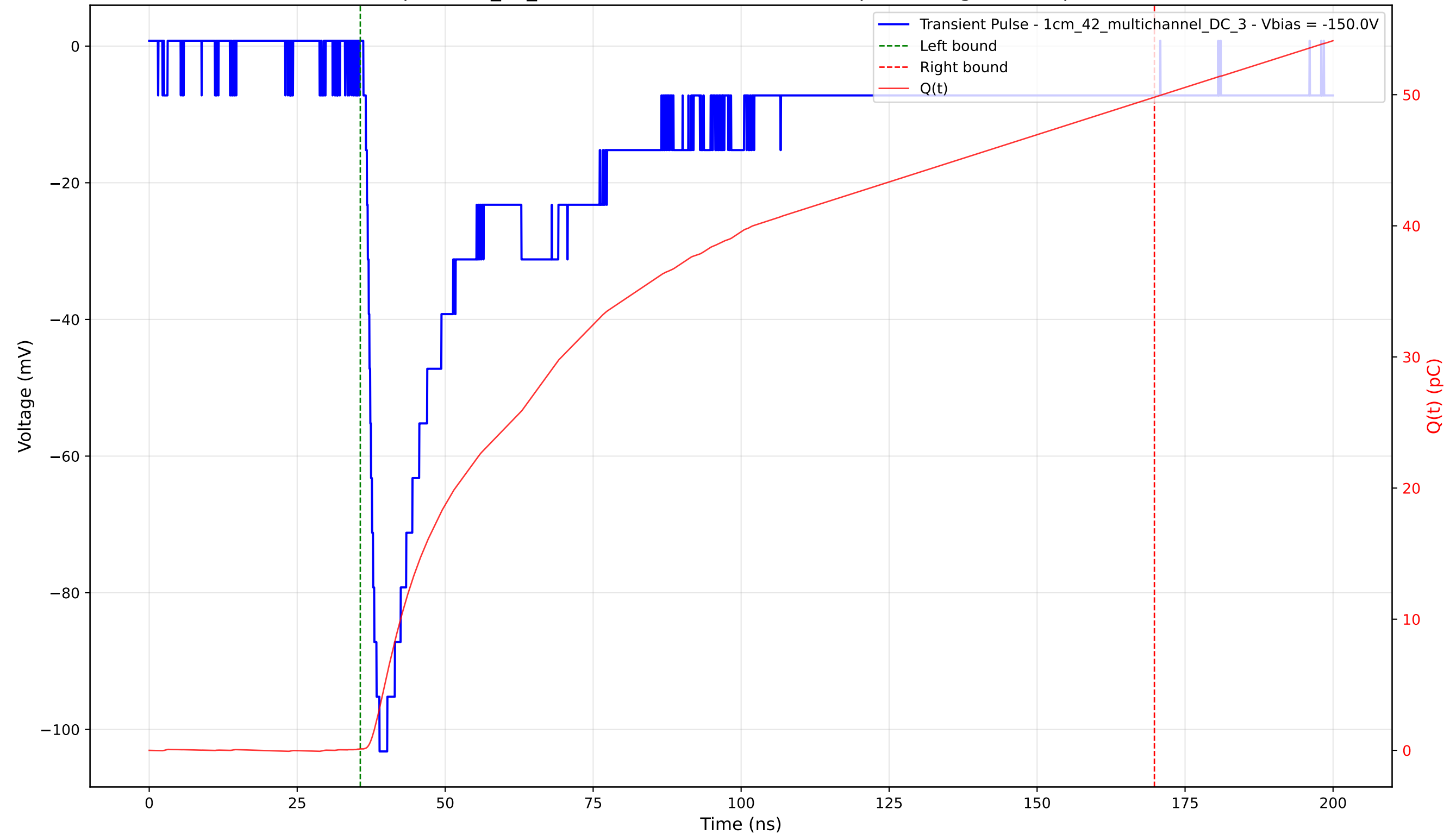
Transient Pulse - Sample: 1cm_42_multichannel - Position: 3020.0 \mu\text{m} - Charge: 49.71 pC - Rise Time: 1.81 ns
