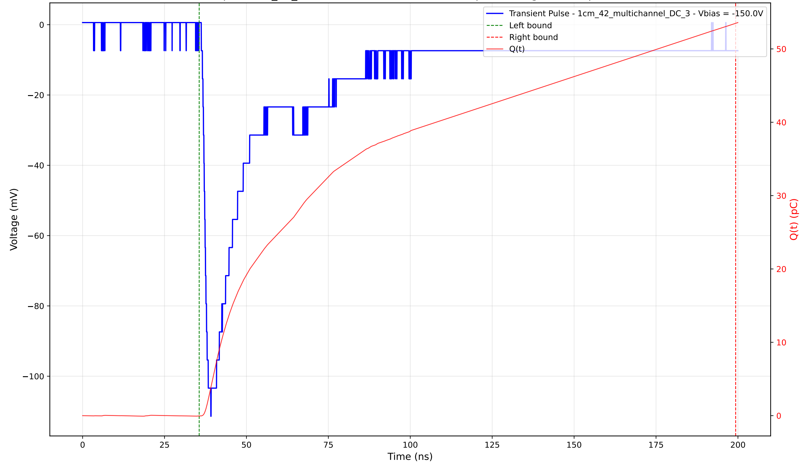
Transient Pulse - Sample: 1cm_42_multichannel - Position: 3190.0 \mu\text{m} - Charge: 53.53 pC - Rise Time: 1.79 ns
