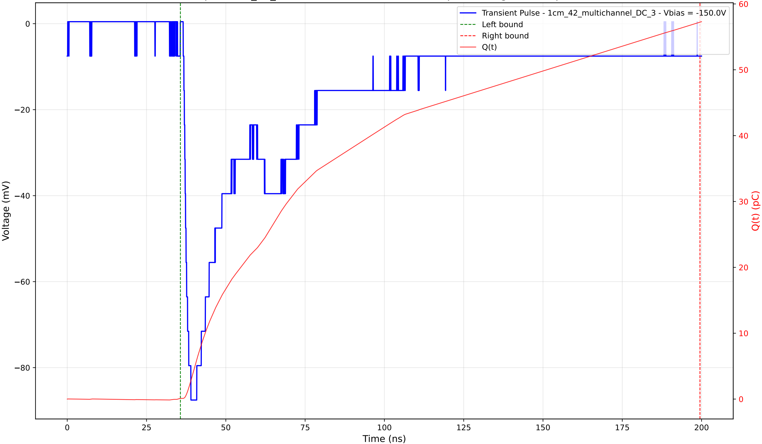
Transient Pulse - Sample: 1cm_42_multichannel - Position: 2175.0 \mu\text{m} - Charge: 57.12 pC - Rise Time: 1.54 ns
