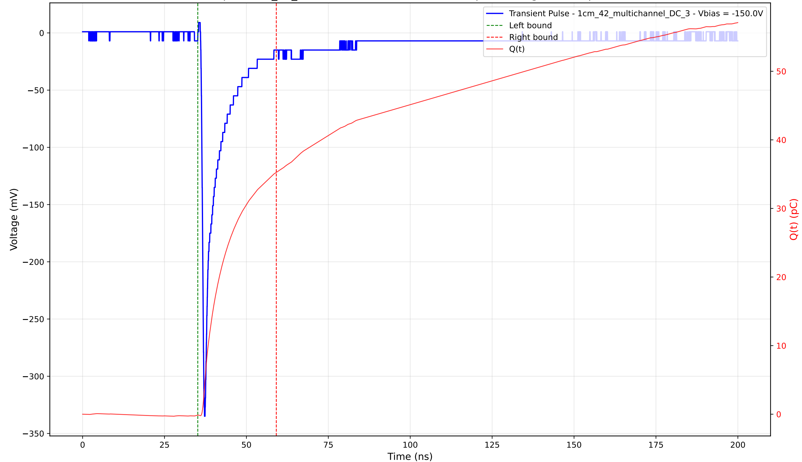
Transient Pulse - Sample: 1cm_42_multichannel - Position: 4670.0 \mu\text{m} - Charge: 35.37 pC - Rise Time: 0.81 ns
