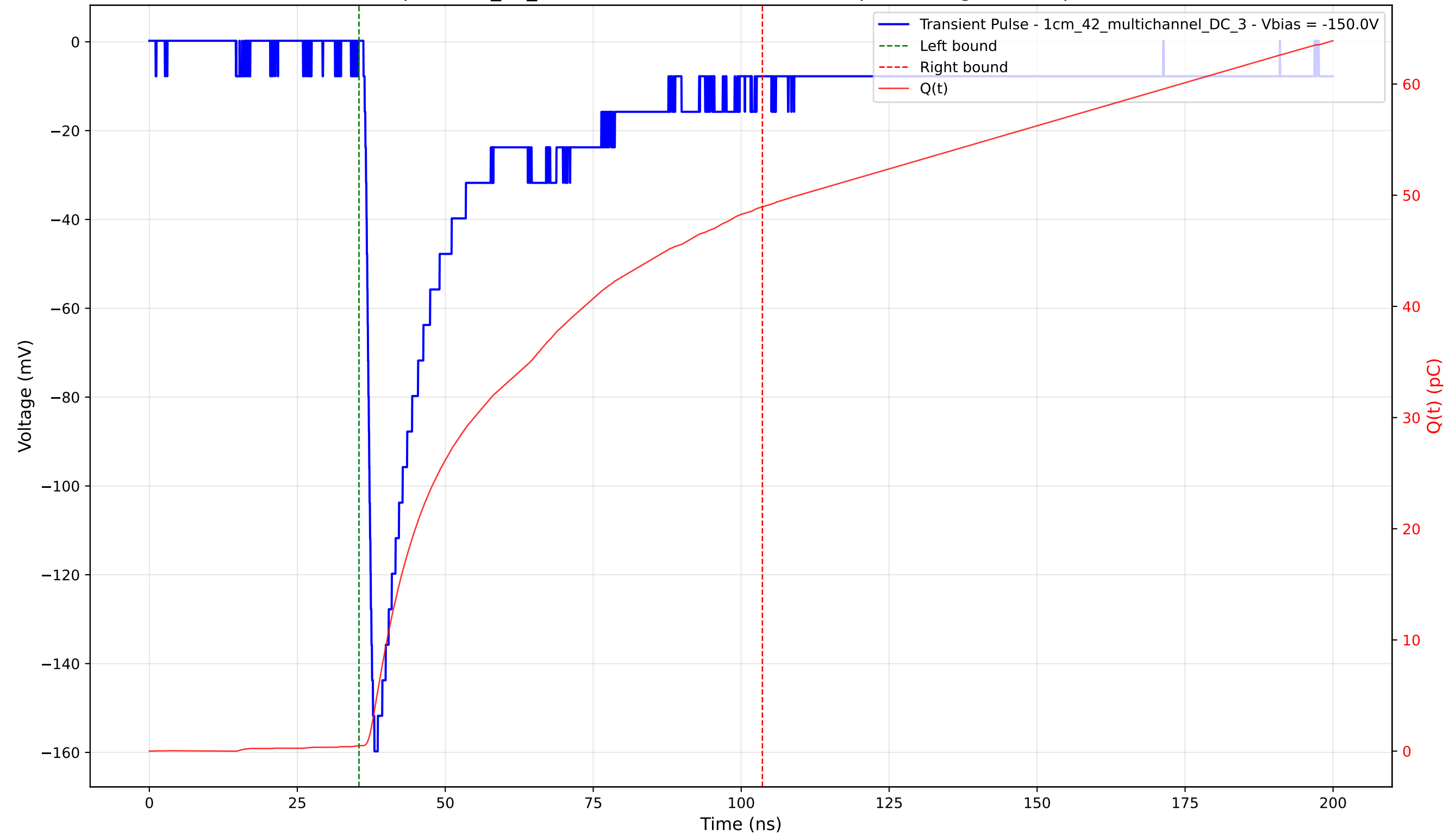
Transient Pulse - Sample: 1cm_42_multichannel - Position: 1190.0 \mu\text{m} - Charge: 48.46 pC - Rise Time: 1.30 ns
