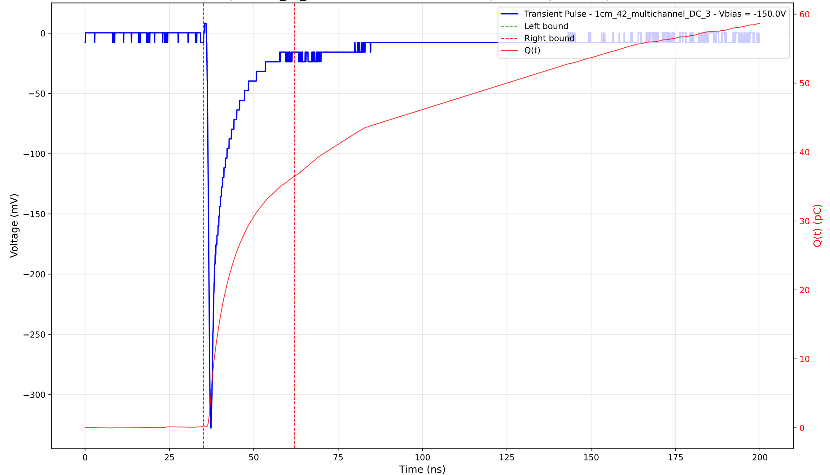
Transient Pulse - Sample: 1cm_42_multichannel - Position: 4660.0 \mu\text{m} - Charge: 36.20 pC - Rise Time: 0.82 ns
