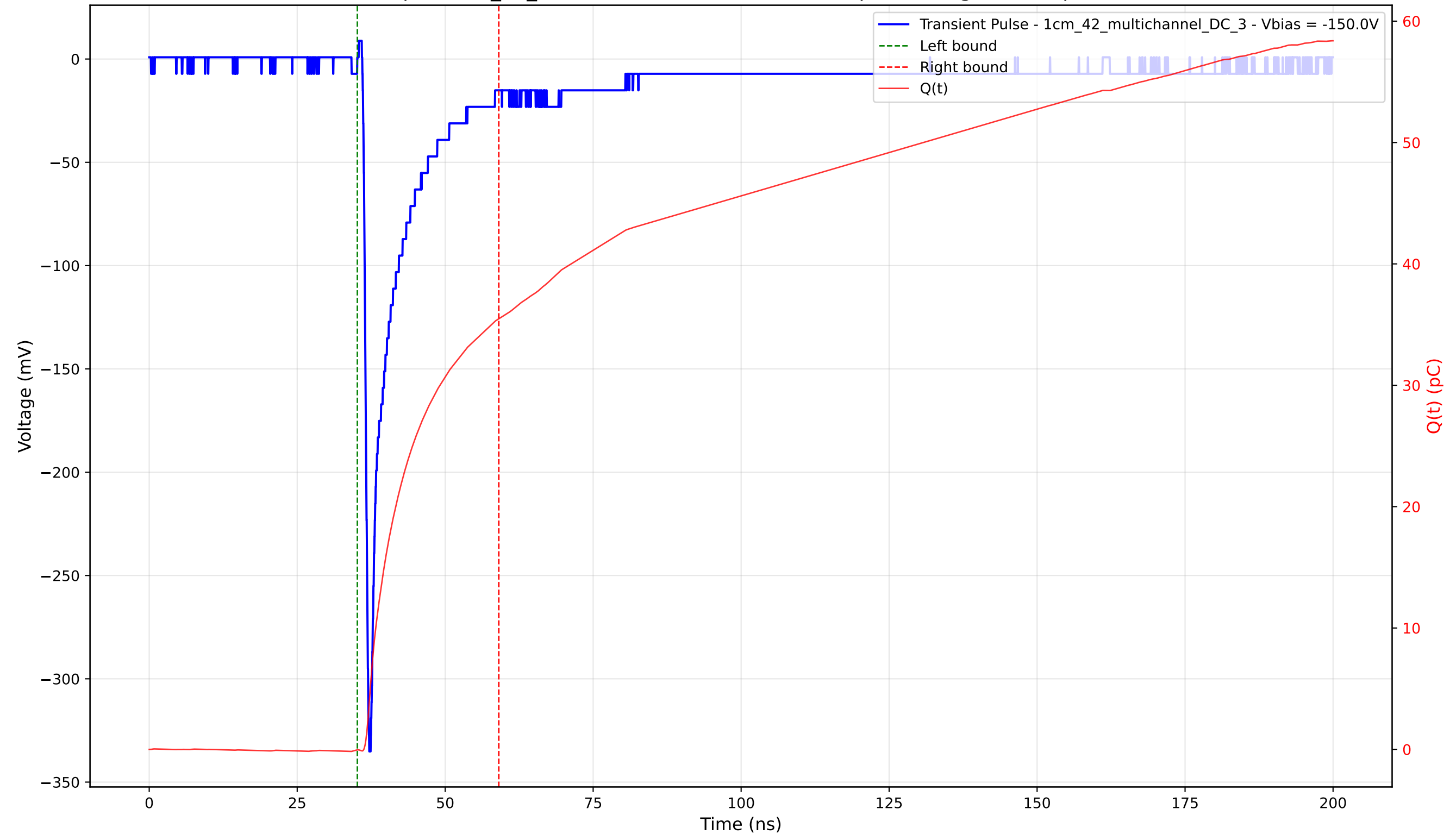
Transient Pulse - Sample: 1cm_42_multichannel - Position: 4680.0 \mu\text{m} - Charge: 35.51 pC - Rise Time: 0.79 ns
