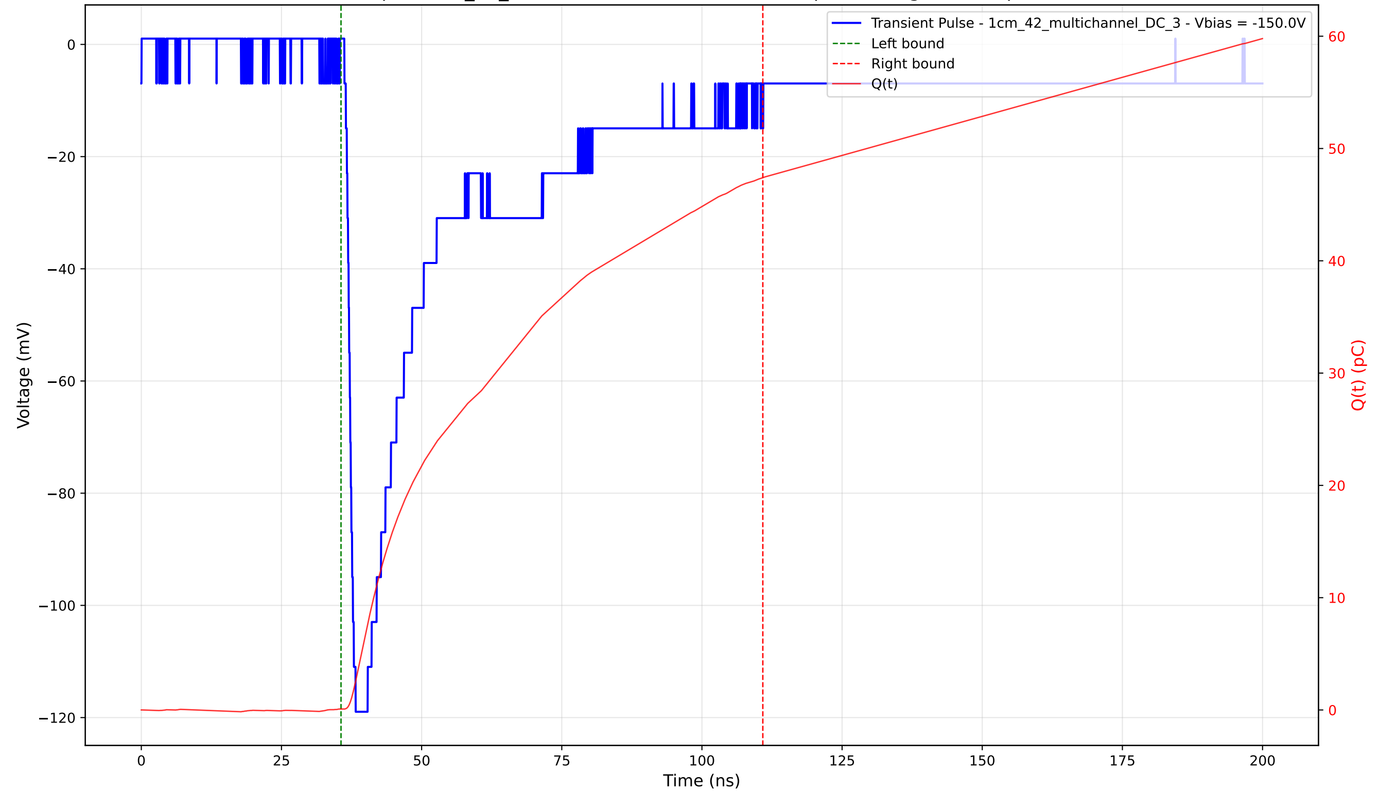
Transient Pulse - Sample: 1cm_42_multichannel - Position: 1595.0 \mu\text{m} - Charge: 47.32 pC - Rise Time: 1.43 ns
