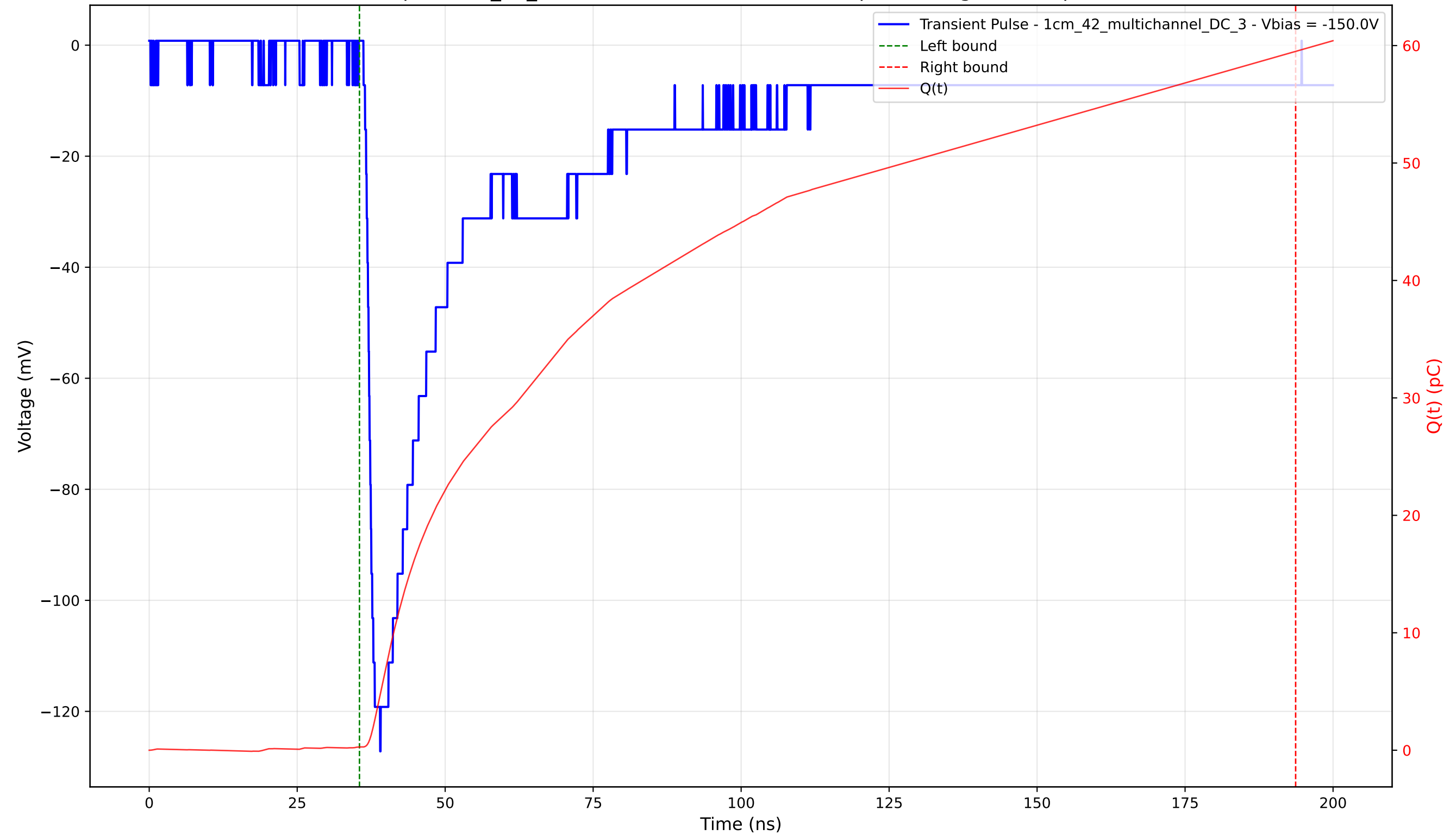
Transient Pulse - Sample: 1cm_42_multichannel - Position: 1575.0 \mu\text{m} - Charge: 59.24 pC - Rise Time: 1.65 ns
