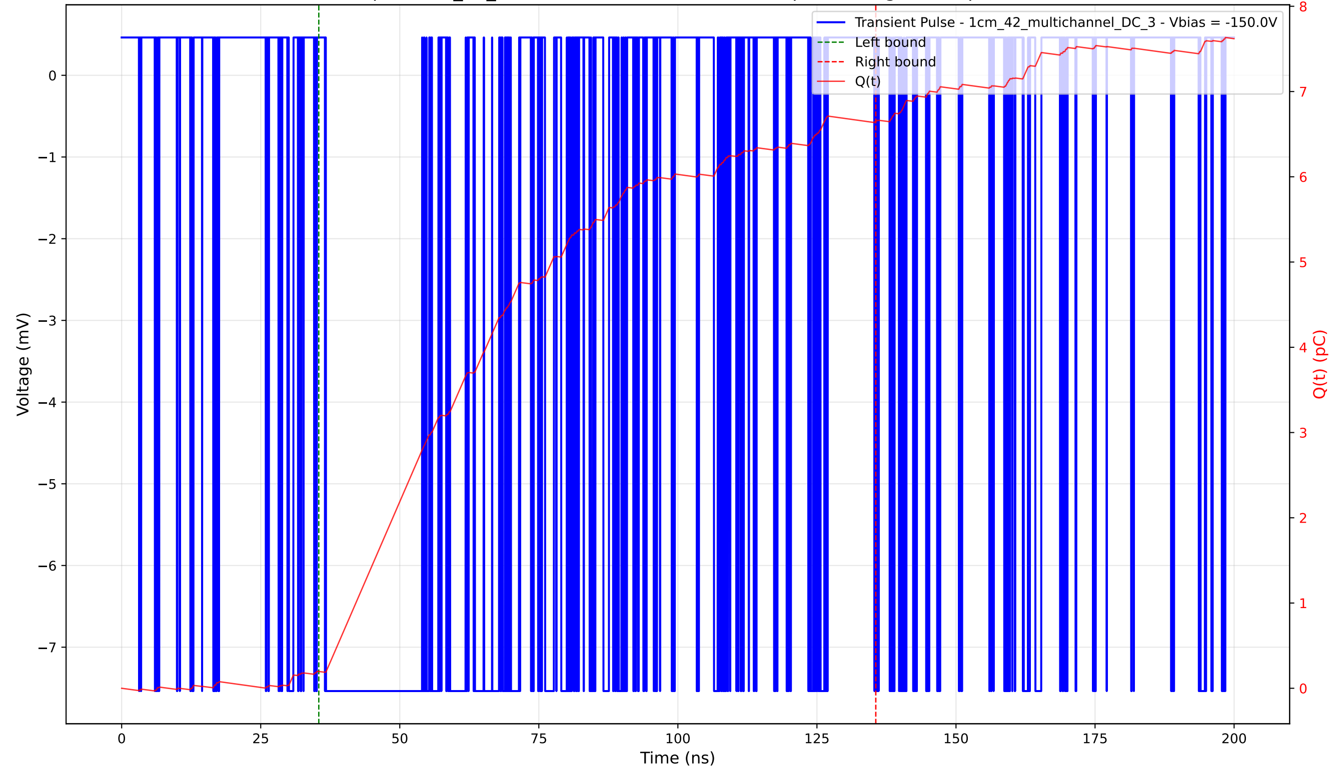
Transient Pulse - Sample: 1cm_42_multichannel - Position: 3895.0 \mu\text{m} - Charge: 6.45 pC - Rise Time: 0.02 ns
