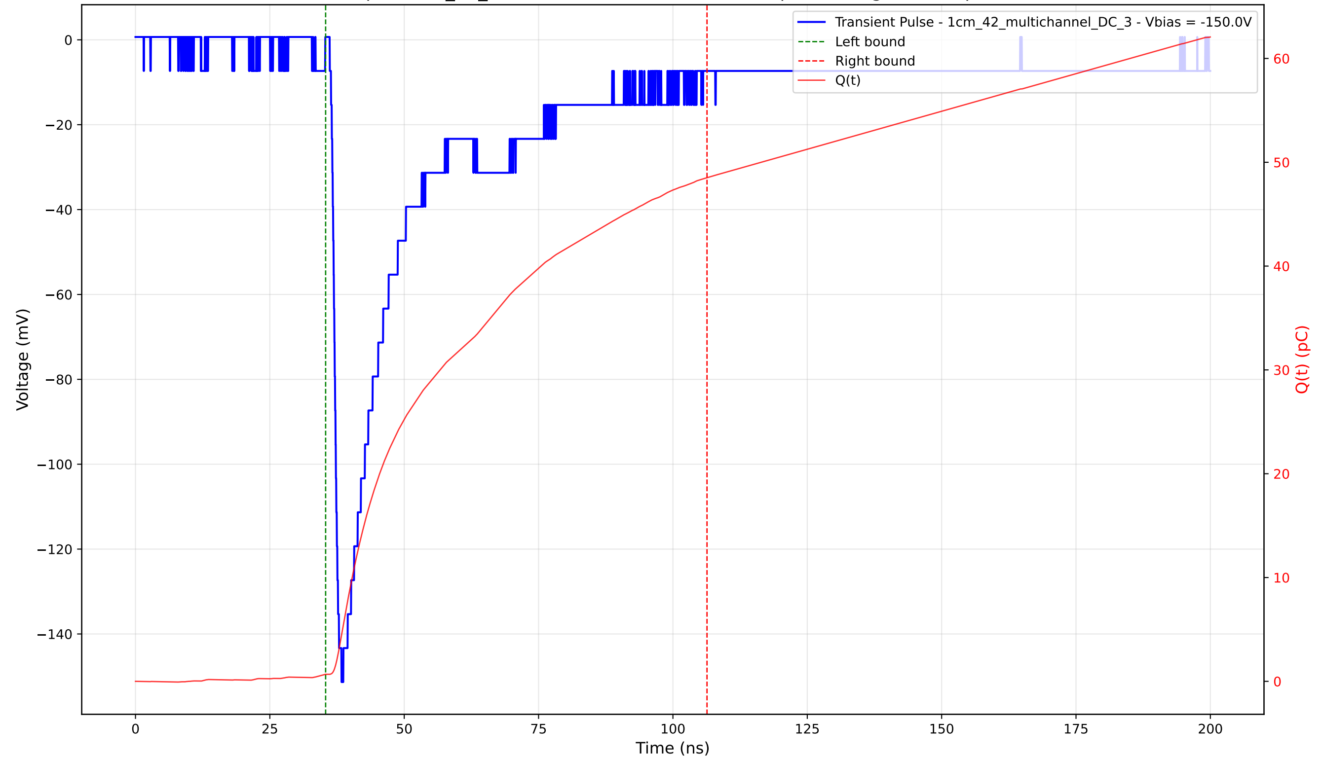
Transient Pulse - Sample: 1cm_42_multichannel - Position: 1270.0 \mu\text{m} - Charge: 47.83 pC - Rise Time: 1.48 ns
