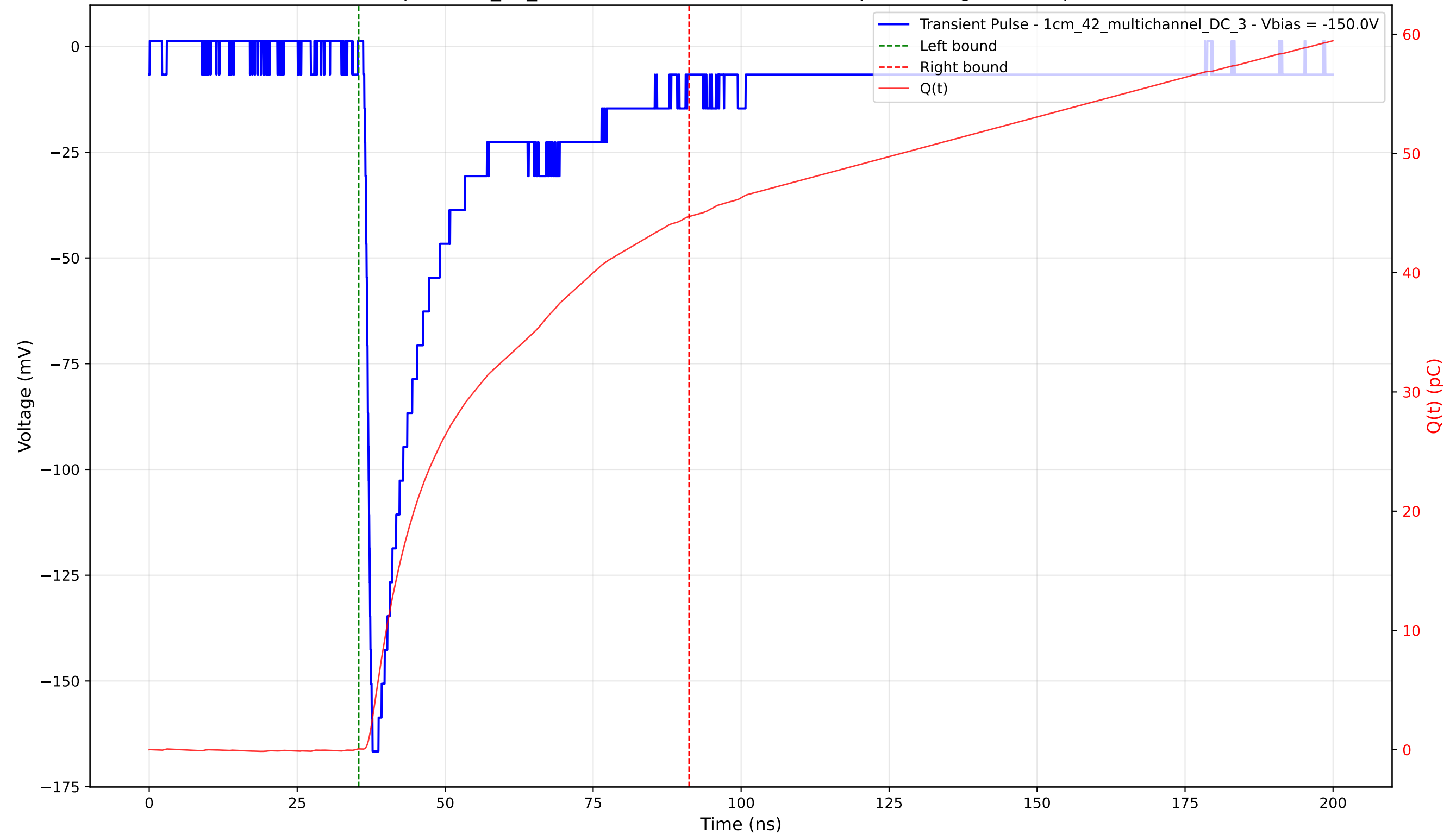
Transient Pulse - Sample: 1cm_42_multichannel - Position: 1050.0 \mu\text{m} - Charge: 44.65 pC - Rise Time: 1.03 ns
