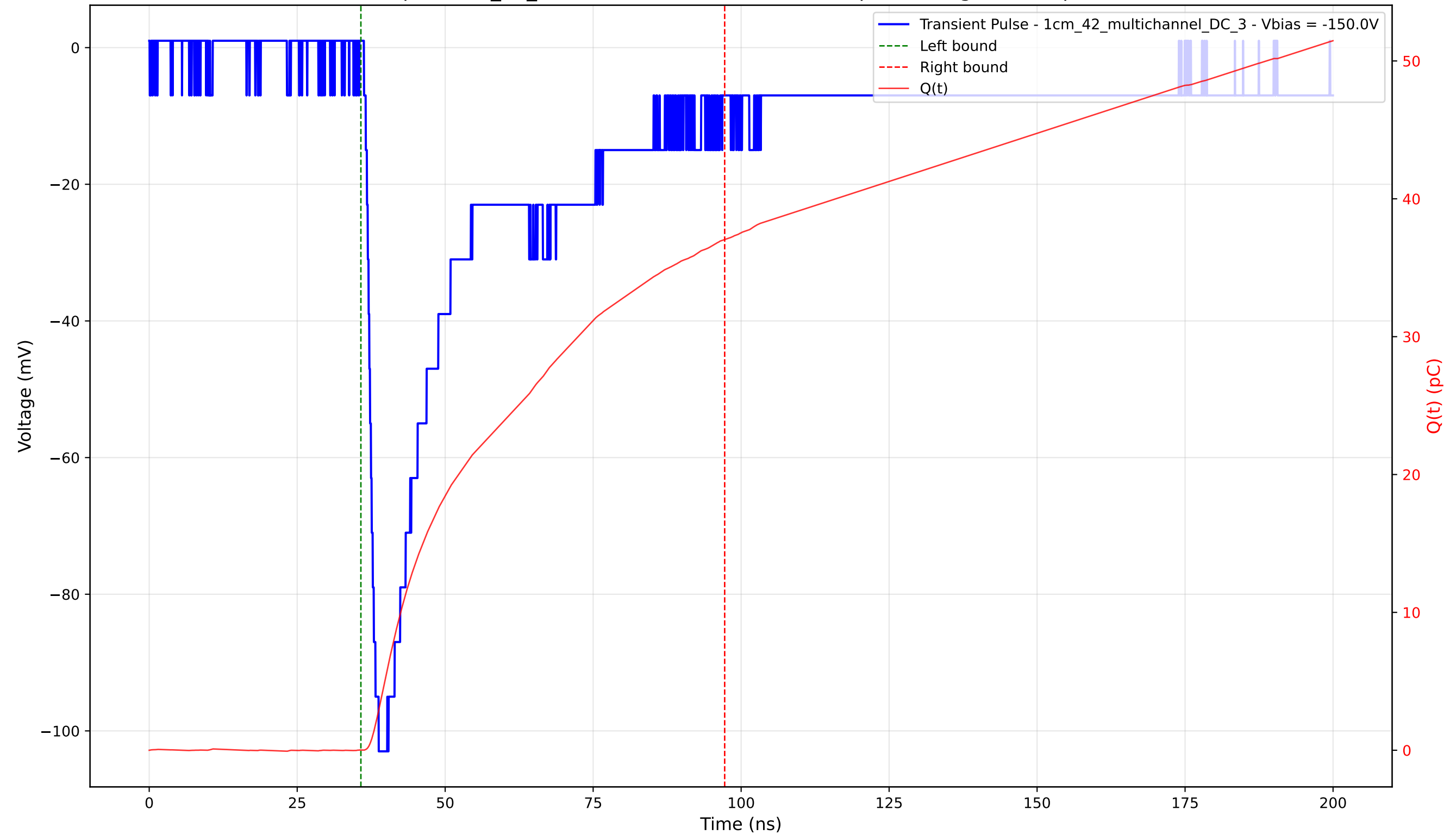
Transient Pulse - Sample: 1cm_42_multichannel - Position: 3155.0 \mu\text{m} - Charge: 37.03 pC - Rise Time: 1.65 ns
