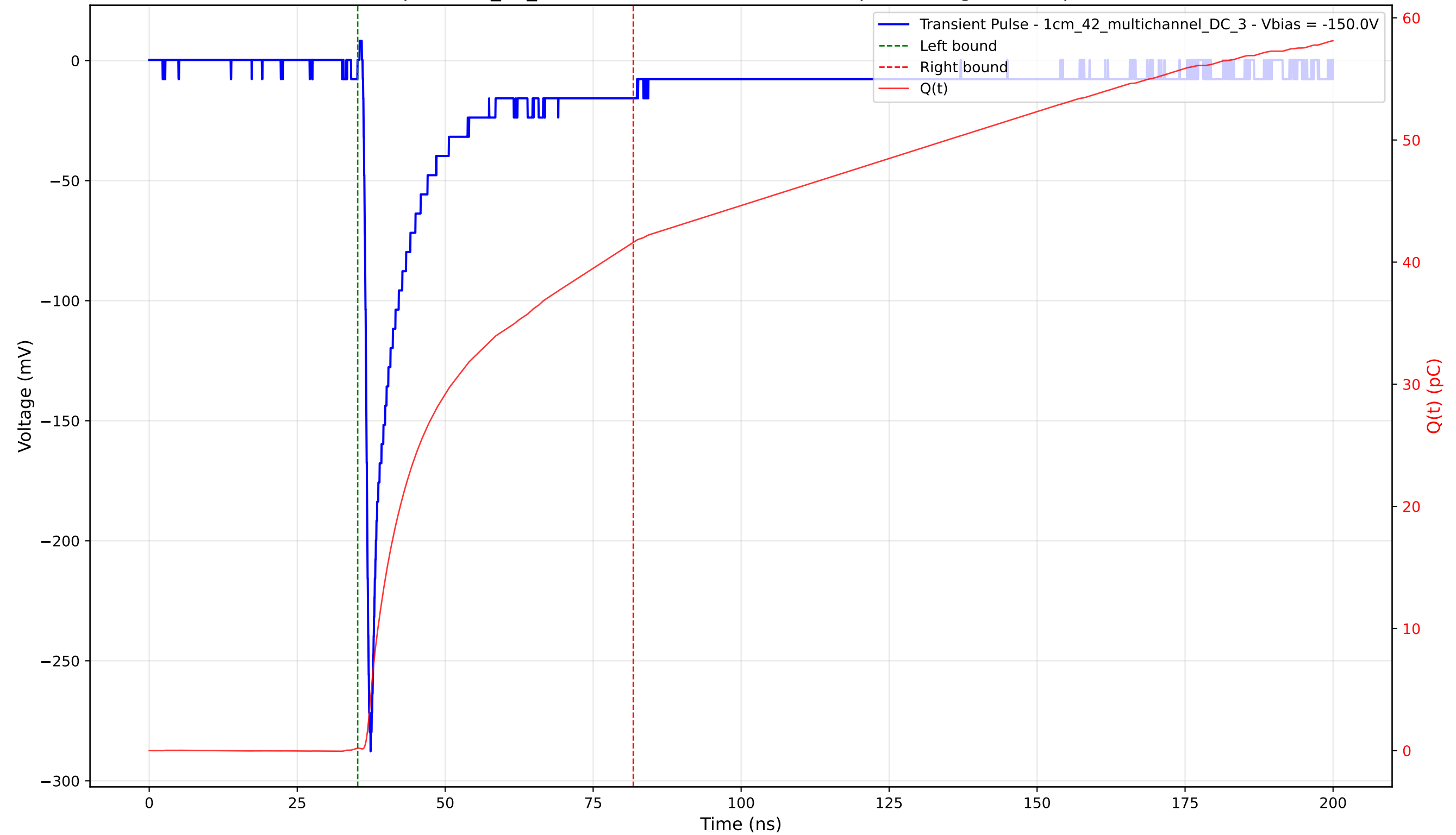
Transient Pulse - Sample: 1cm_42_multichannel - Position: 4550.0 \mu\text{m} - Charge: 41.43 pC - Rise Time: 0.89 ns
