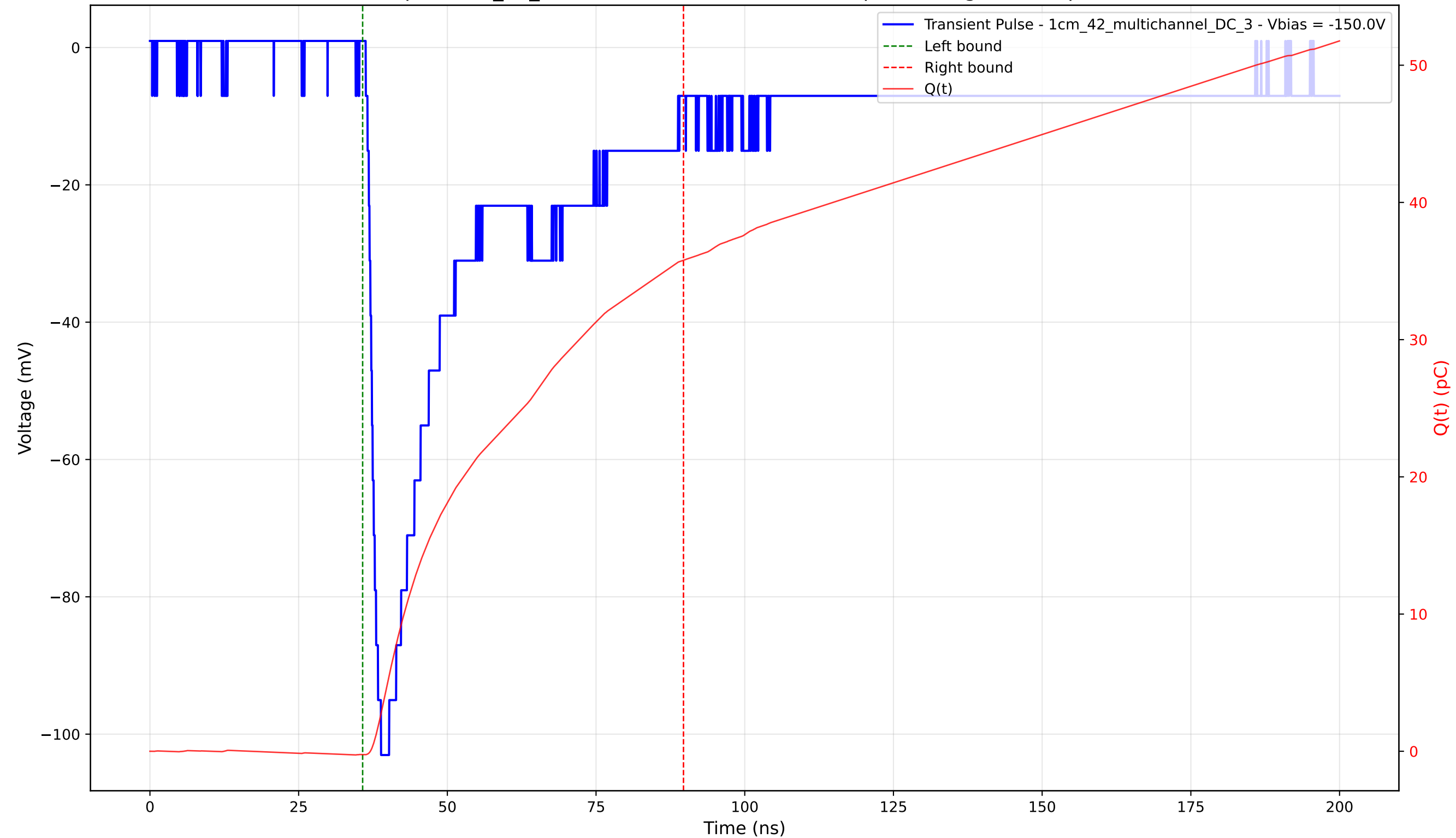
Transient Pulse - Sample: 1cm_42_multichannel - Position: 3105.0 \mu\text{m} - Charge: 36.03 pC - Rise Time: 1.77 ns
