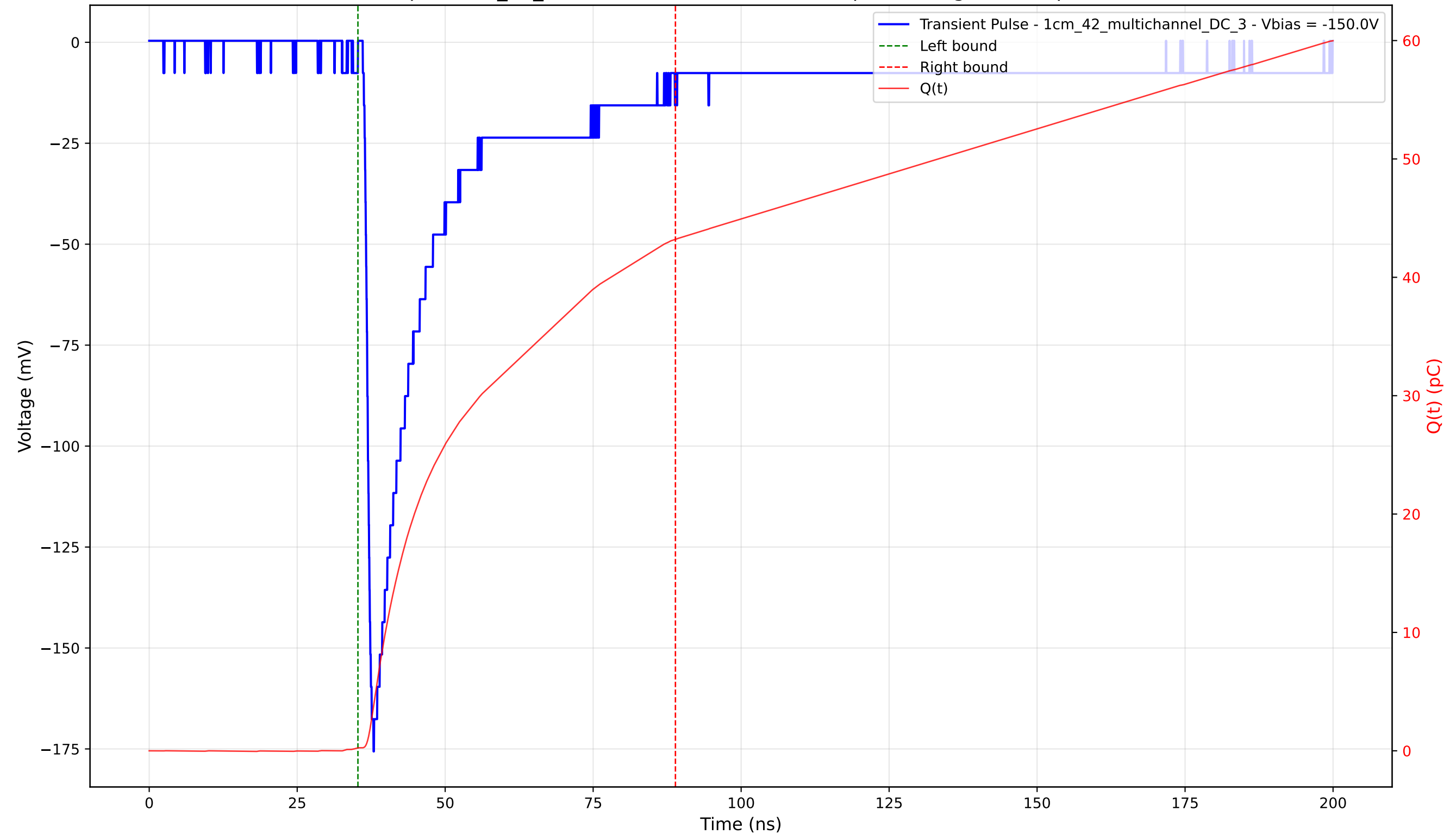
Transient Pulse - Sample: 1cm_42_multichannel - Position: 930.0 \mu\text{m} - Charge: 42.95 pC - Rise Time: 1.08 ns
