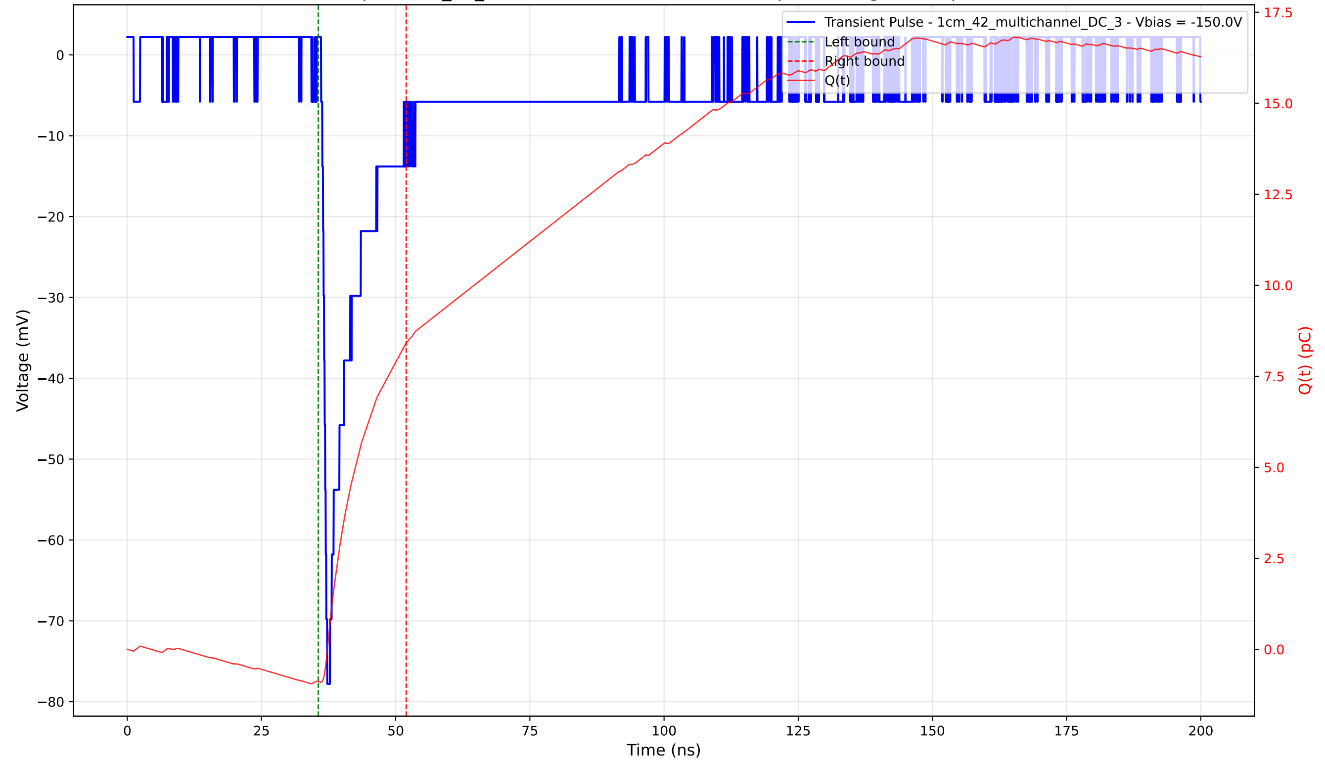
Transient Pulse - Sample: 1cm_42_multichannel - Position: 4435.0 \mu\text{m} - Charge: 9.30 pC - Rise Time: 0.94 ns
