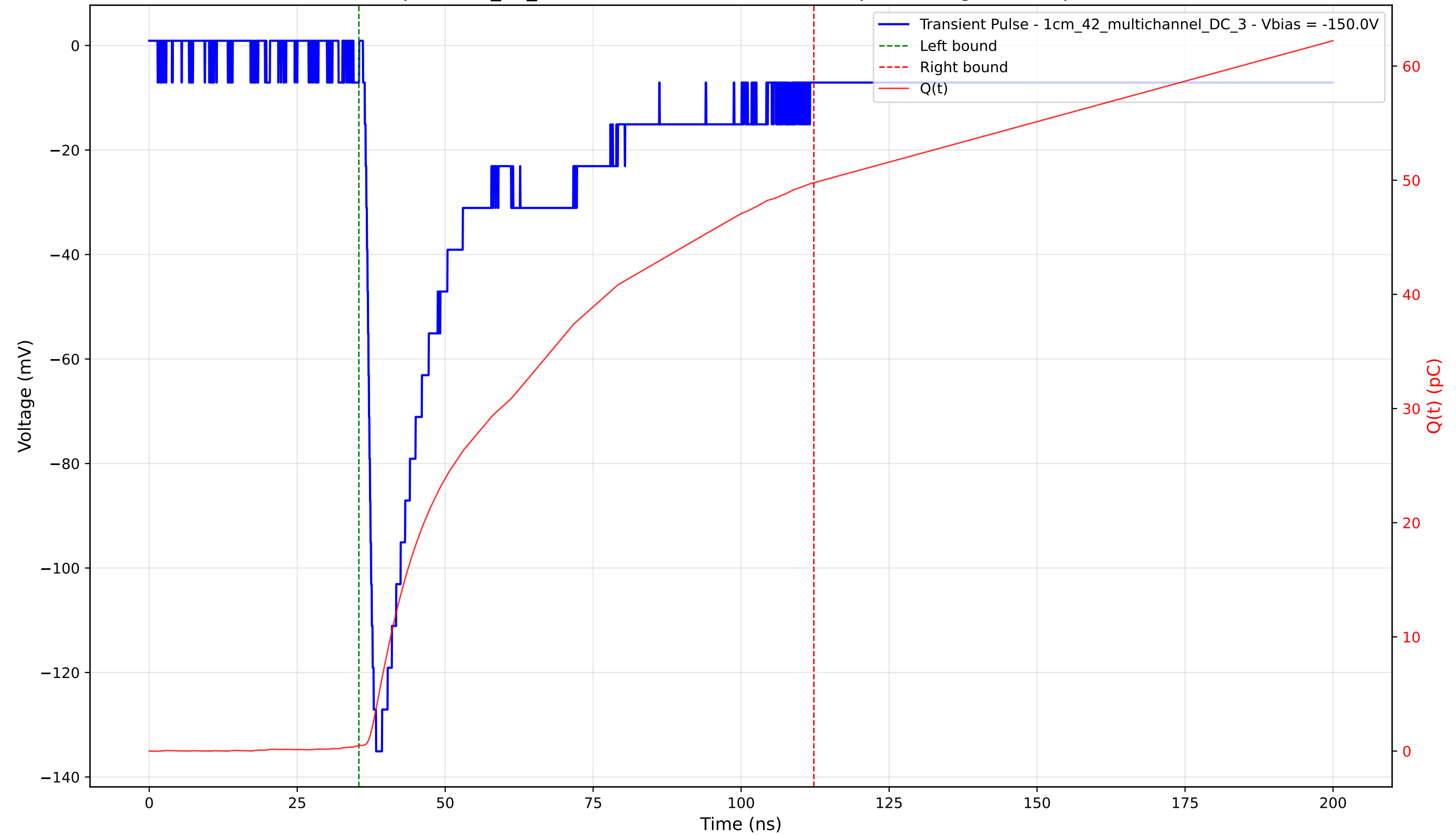
Transient Pulse - Sample: 1cm_42_multichannel - Position: 1460.0 \mu\text{m} - Charge: 49.29 pC - Rise Time: 1.50 ns
