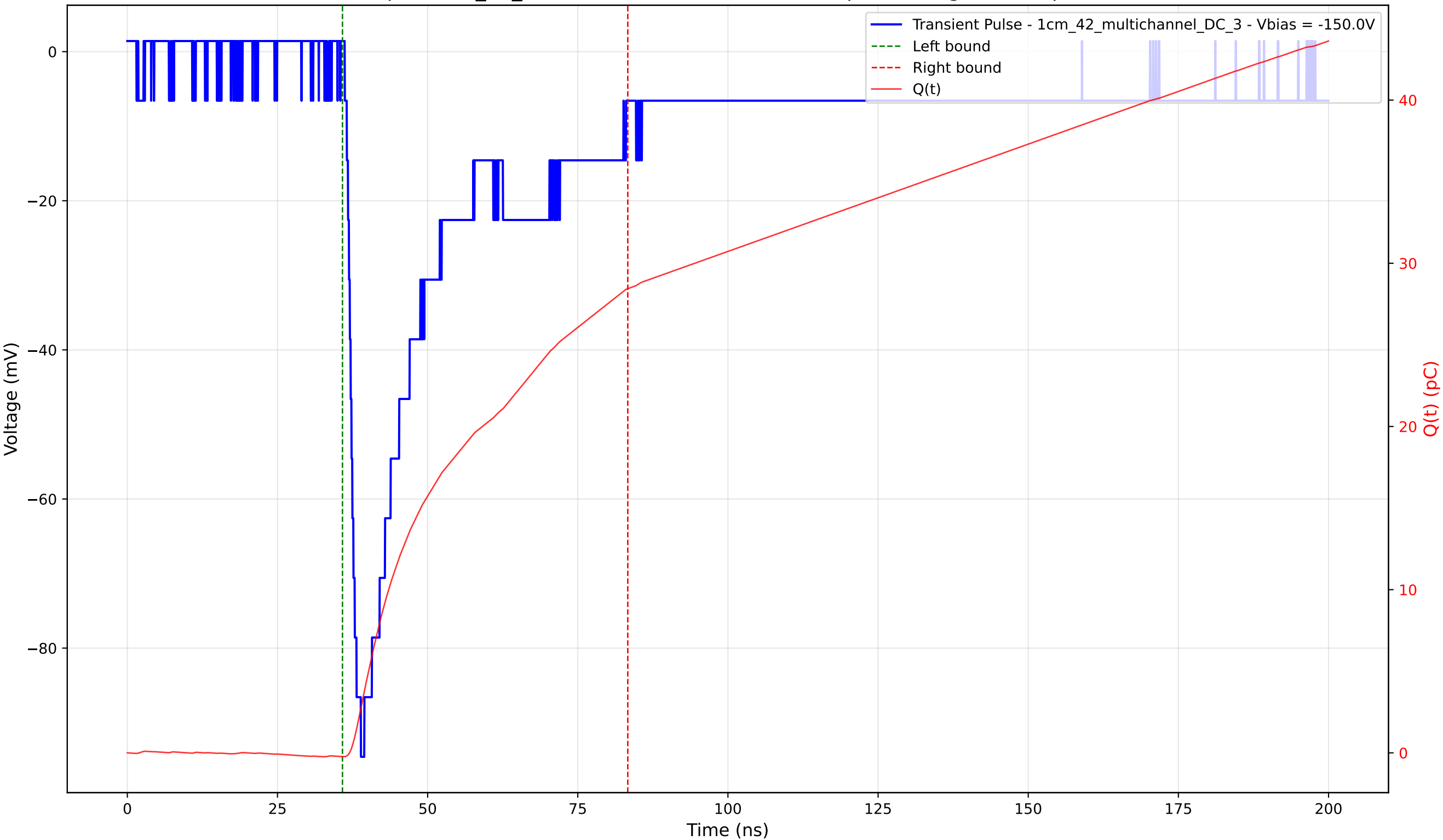
Transient Pulse - Sample: 1cm_42_multichannel - Position: 3320.0 \mu\text{m} - Charge: 28.67 pC - Rise Time: 1.63 ns
