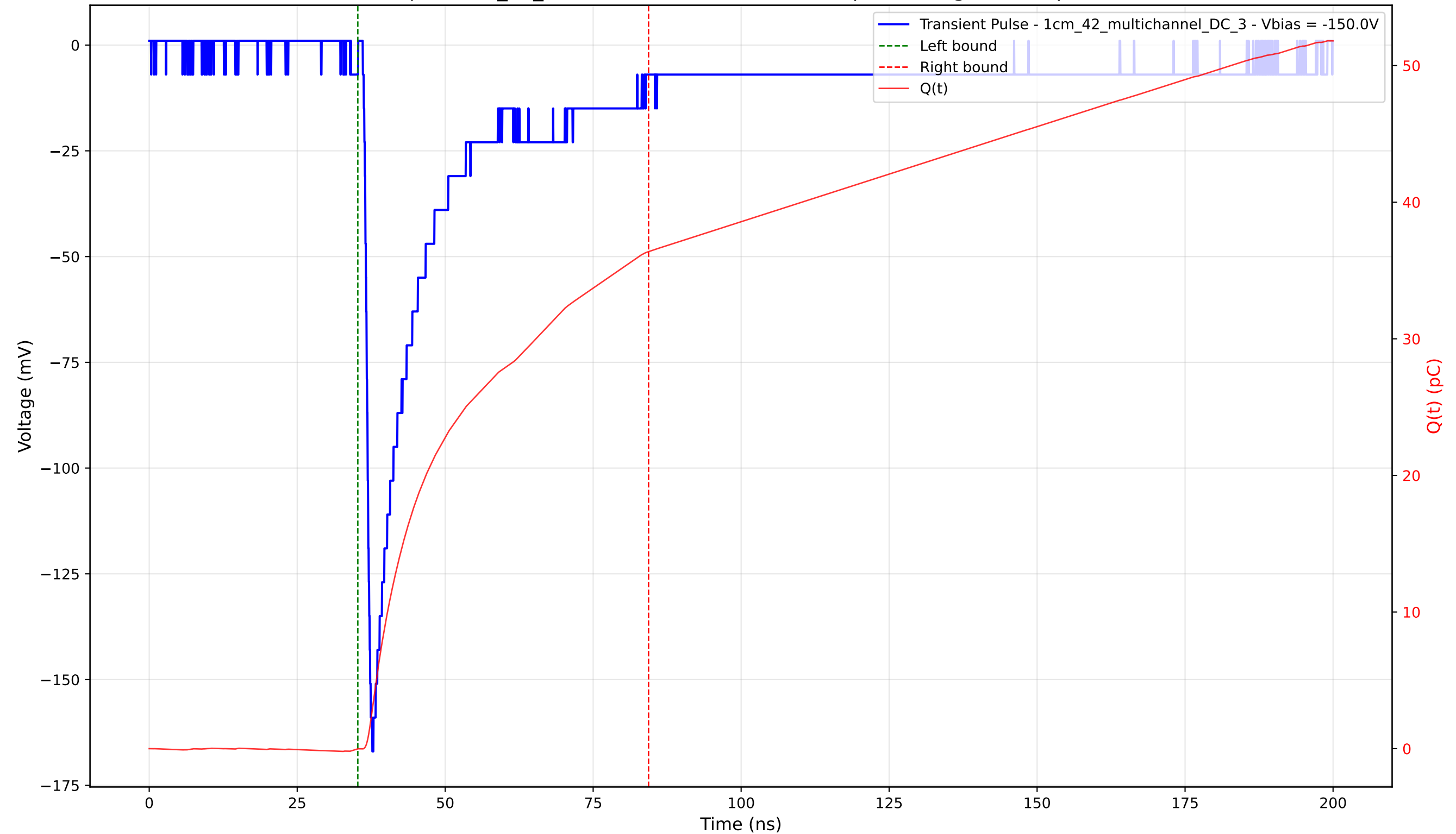
Transient Pulse - Sample: 1cm_42_multichannel - Position: 790.0 \mu\text{m} - Charge: 36.39 pC - Rise Time: 1.00 ns
