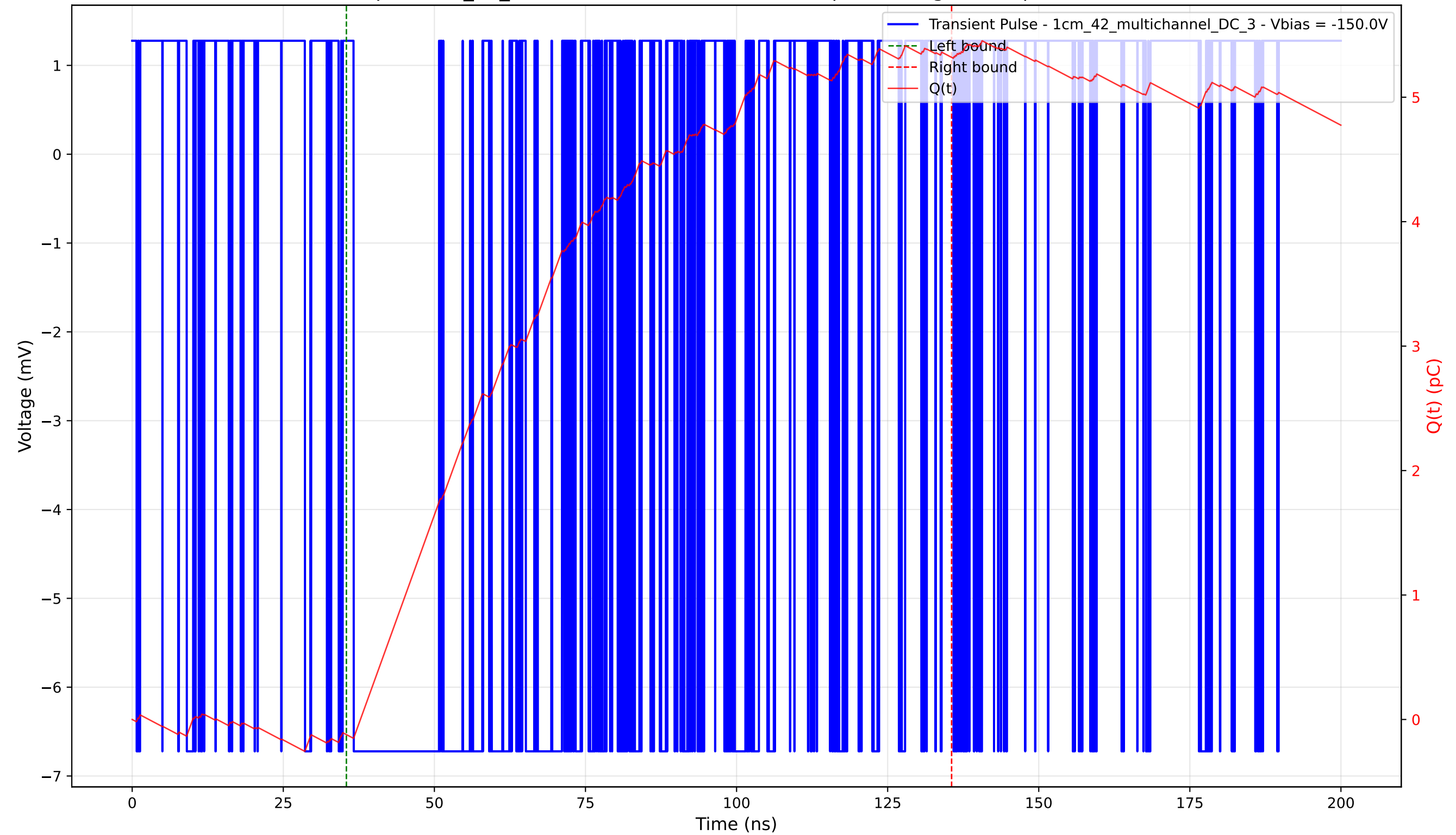
Transient Pulse - Sample: 1cm_42_multichannel - Position: 1370.0 \mu\text{m} - Charge: 5.44 pC - Rise Time: 0.00 ns (N/A)
