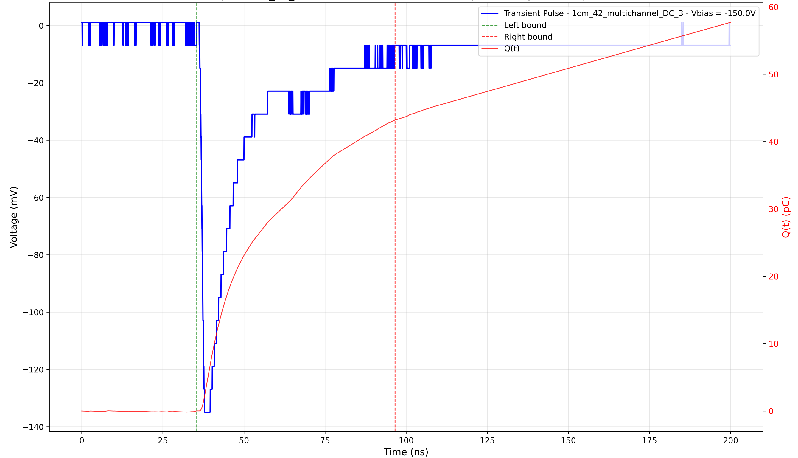
Transient Pulse - Sample: 1cm_42_multichannel - Position: 1280.0 \mu\text{m} - Charge: 43.18 pC - Rise Time: 1.26 ns
