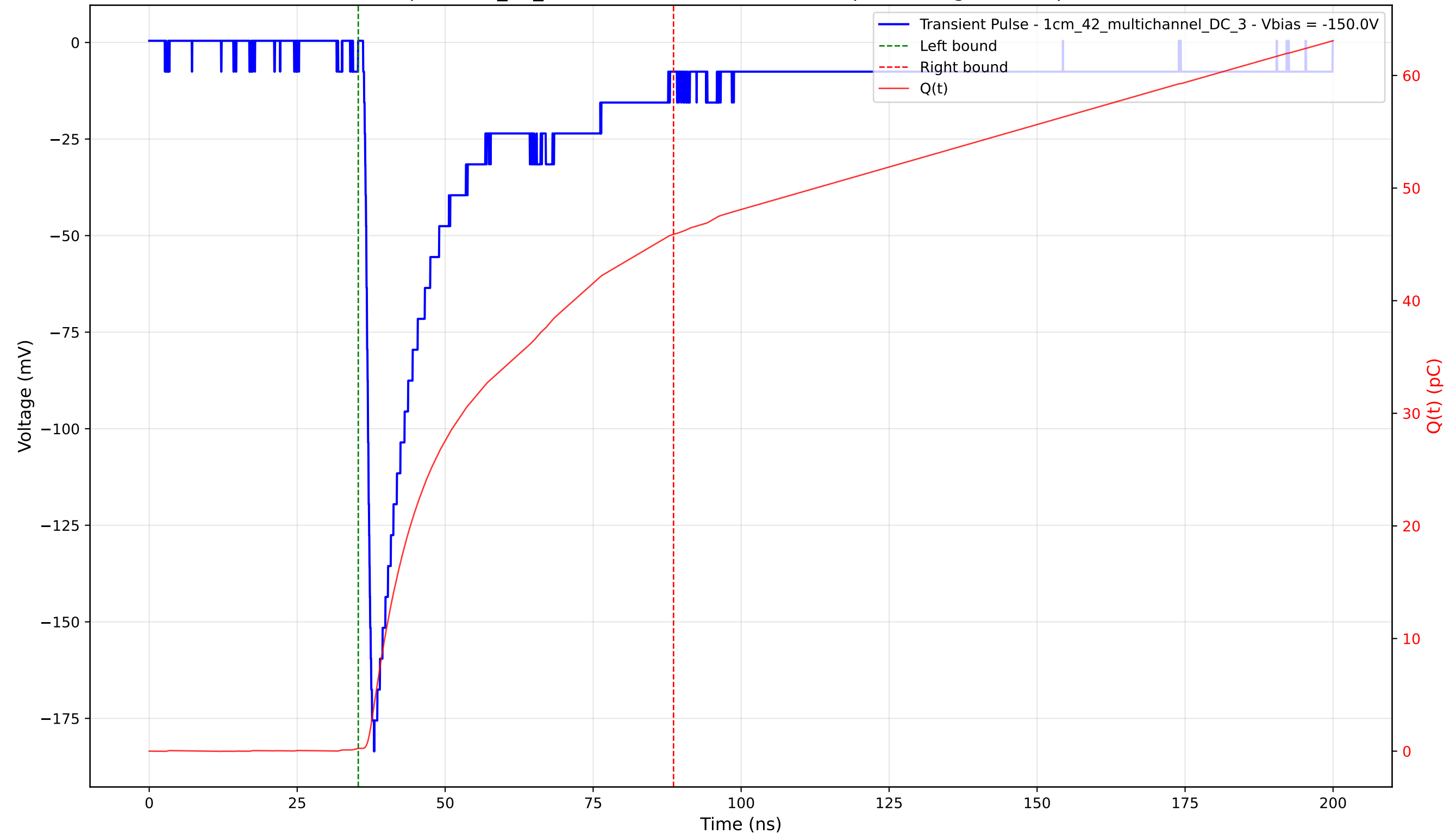
Transient Pulse - Sample: 1cm_42_multichannel - Position: 990.0 \mu\text{m} - Charge: 45.64 pC - Rise Time: 1.11 ns
