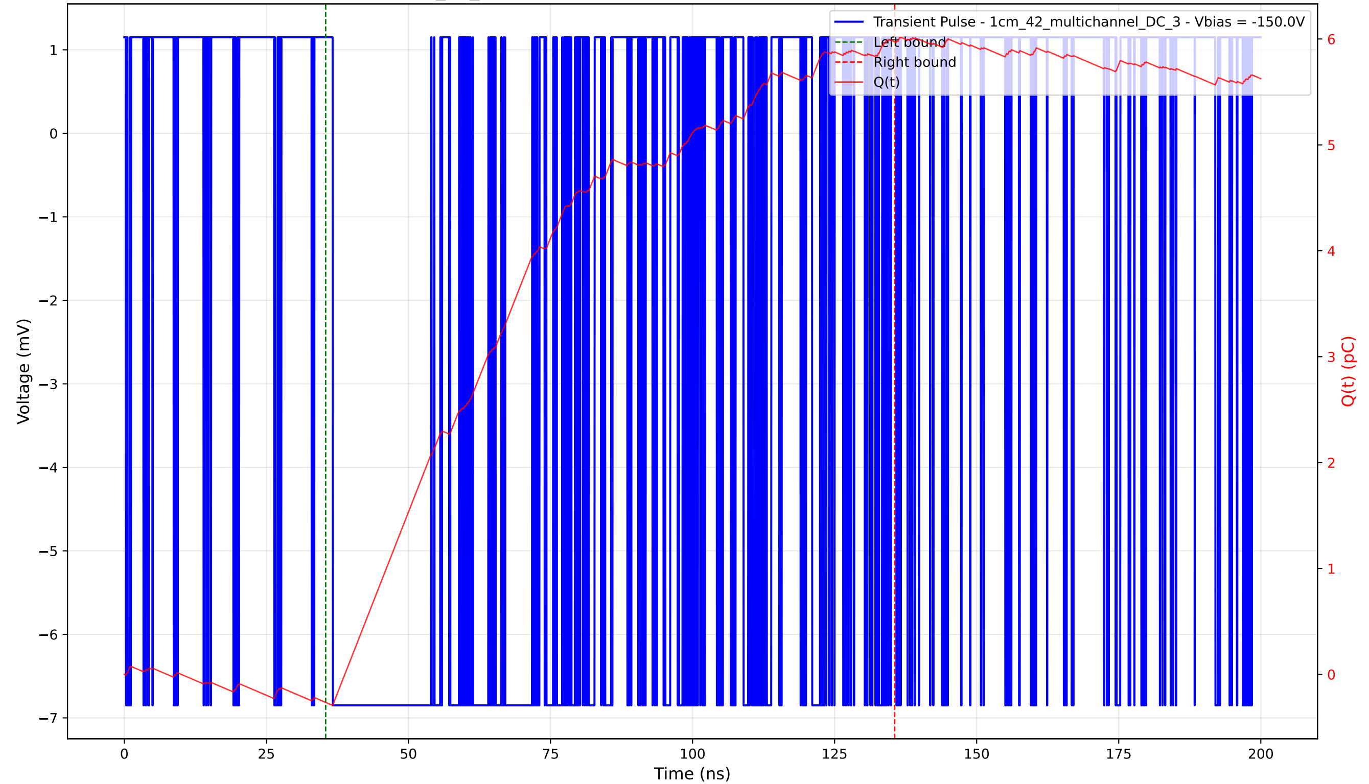
Transient Pulse - Sample: 1cm_42_multichannel - Position: 2885.0 \mu\text{m} - Charge: 6.24 pC - Rise Time: 0.00 ns (N/A)
