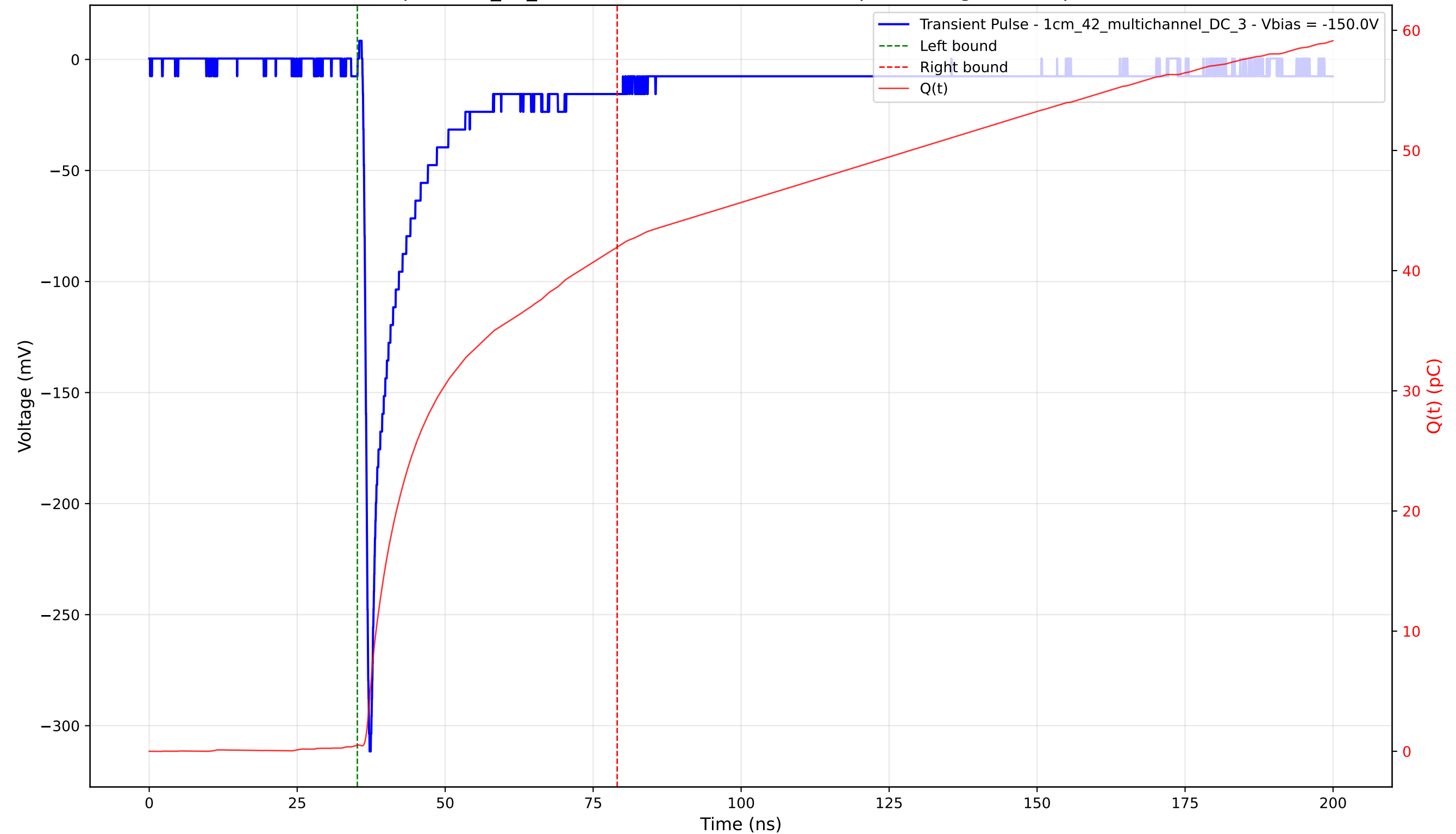
Transient Pulse - Sample: 1cm_42_multichannel - Position: 4625.0 \mu\text{m} - Charge: 41.45 pC - Rise Time: 0.86 ns
