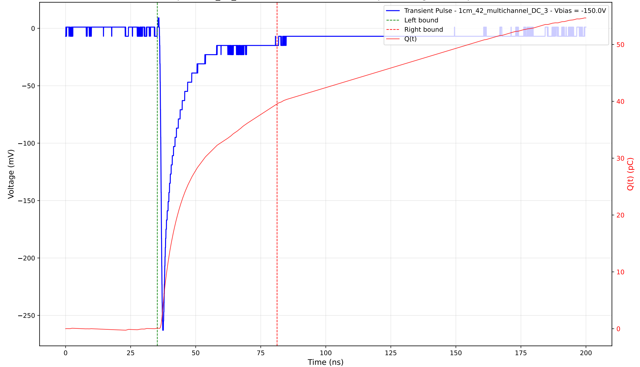
Transient Pulse - Sample: 1cm_42_multichannel - Position: 4510.0 \mu\text{m} - Charge: 39.44 pC - Rise Time: 0.87 ns
