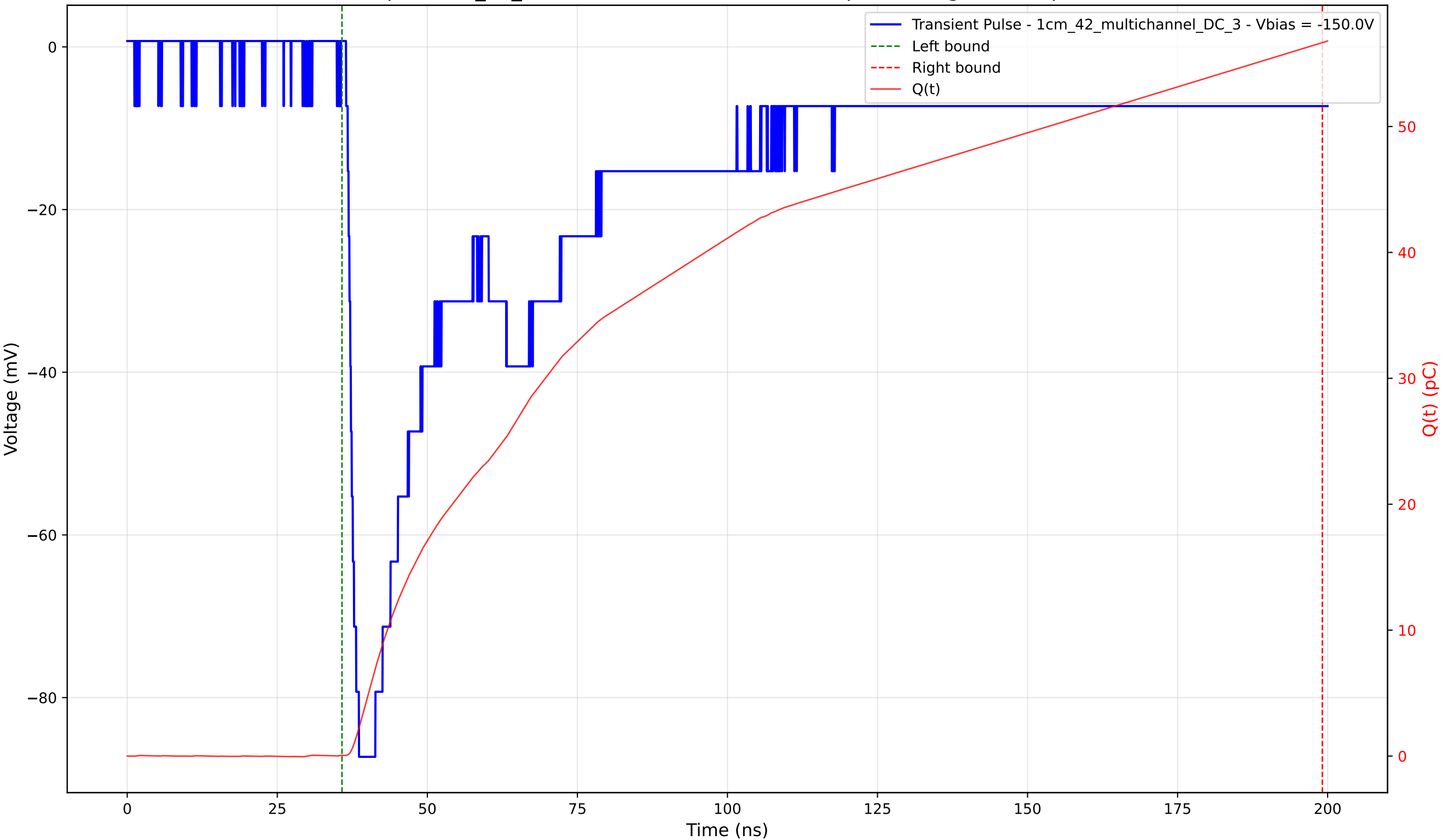
Transient Pulse - Sample: 1cm_42_multichannel - Position: 2095.0 \mu\text{m} - Charge: 56.61 pC - Rise Time: 1.42 ns
