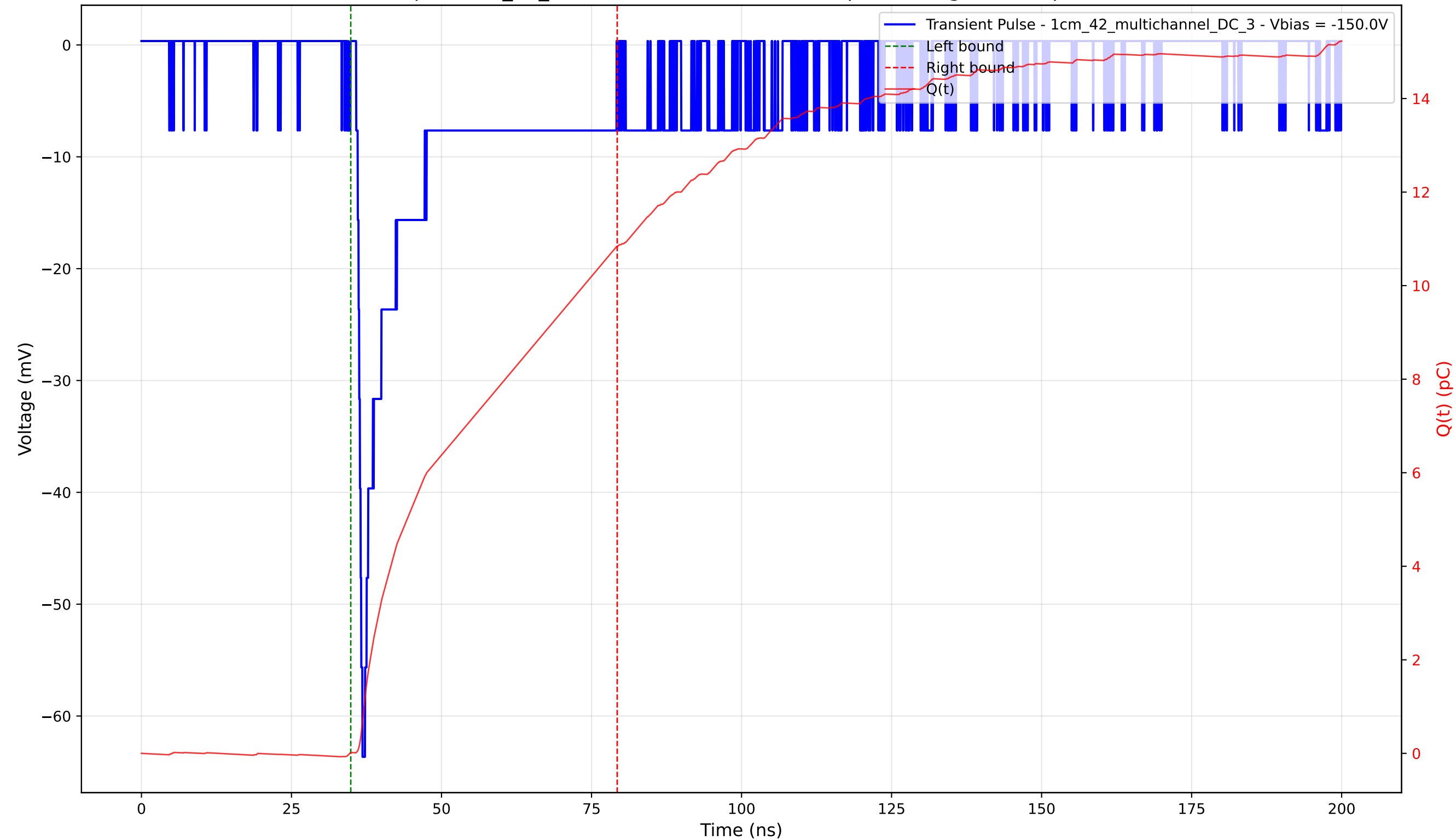
Transient Pulse - Sample: 1cm_42_multichannel - Position: 60.0 \mu\text{m} - Charge: 10.82 pC - Rise Time: 1.04 ns
