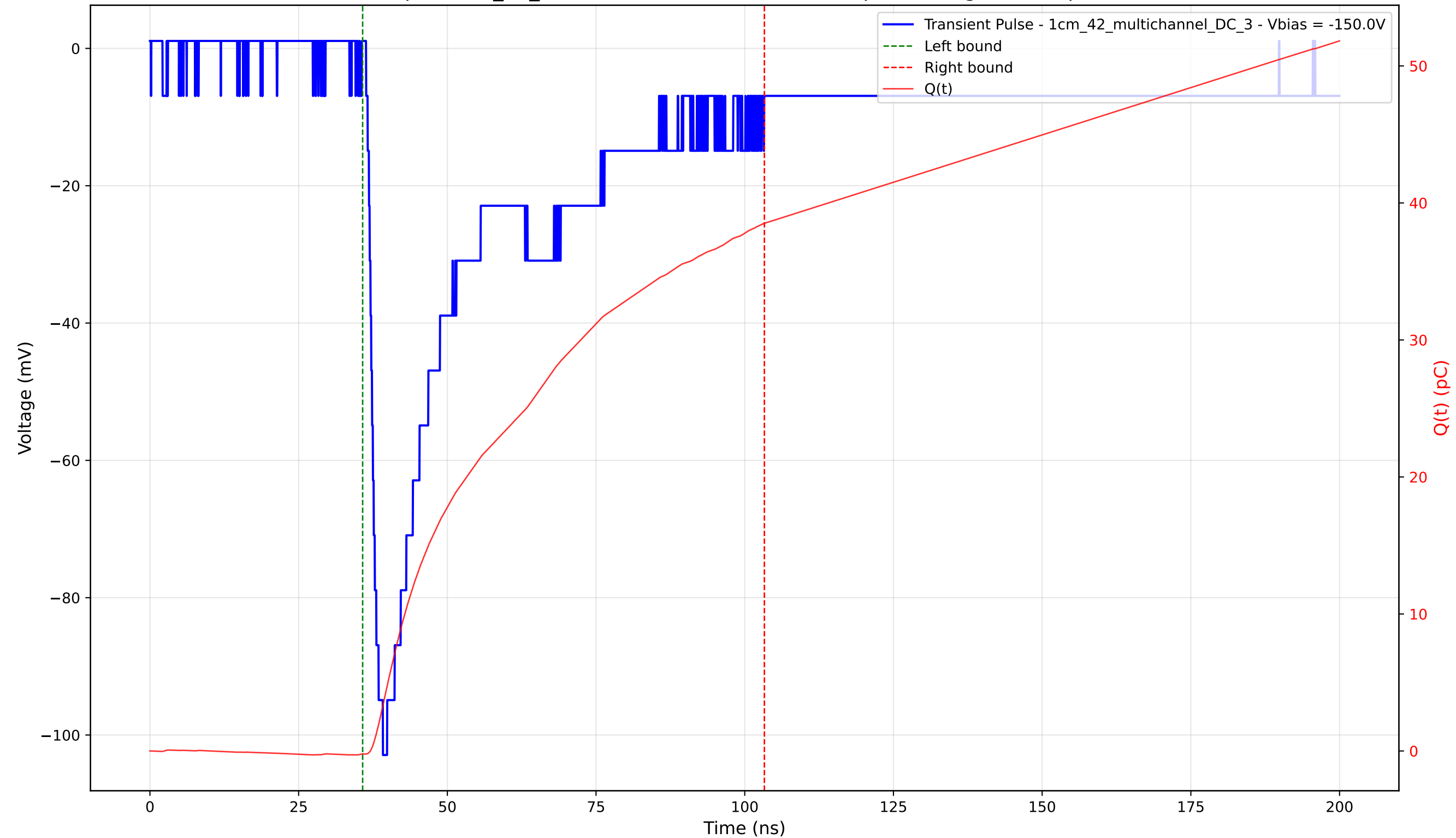
Transient Pulse - Sample: 1cm_42_multichannel - Position: 3055.0 \mu\text{m} - Charge: 38.73 pC - Rise Time: 1.85 ns
