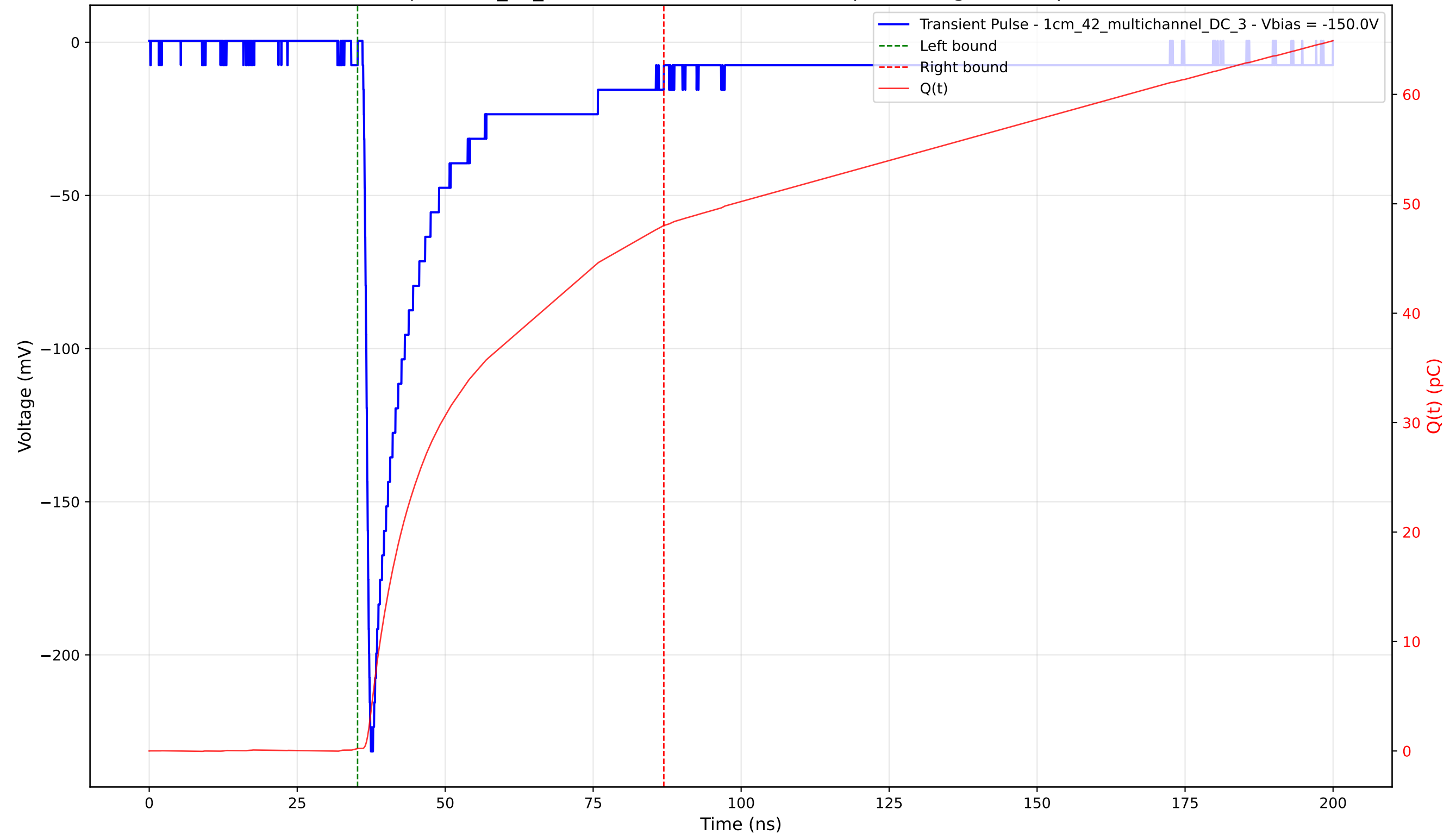
Transient Pulse - Sample: 1cm_42_multichannel - Position: 665.0 \mu\text{m} - Charge: 47.79 pC - Rise Time: 1.00 ns
