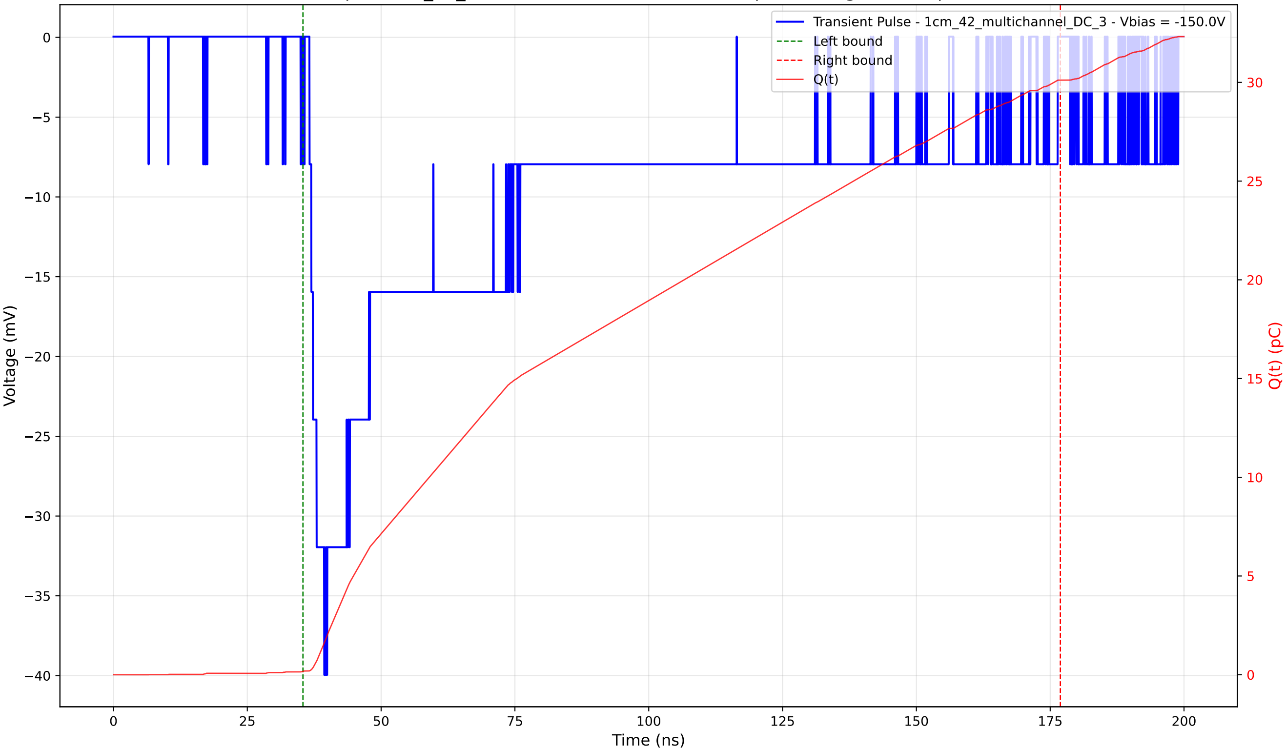
Transient Pulse - Sample: 1cm_42_multichannel - Position: 2420.0 \mu\text{m} - Charge: 29.95 pC - Rise Time: 2.75 ns
