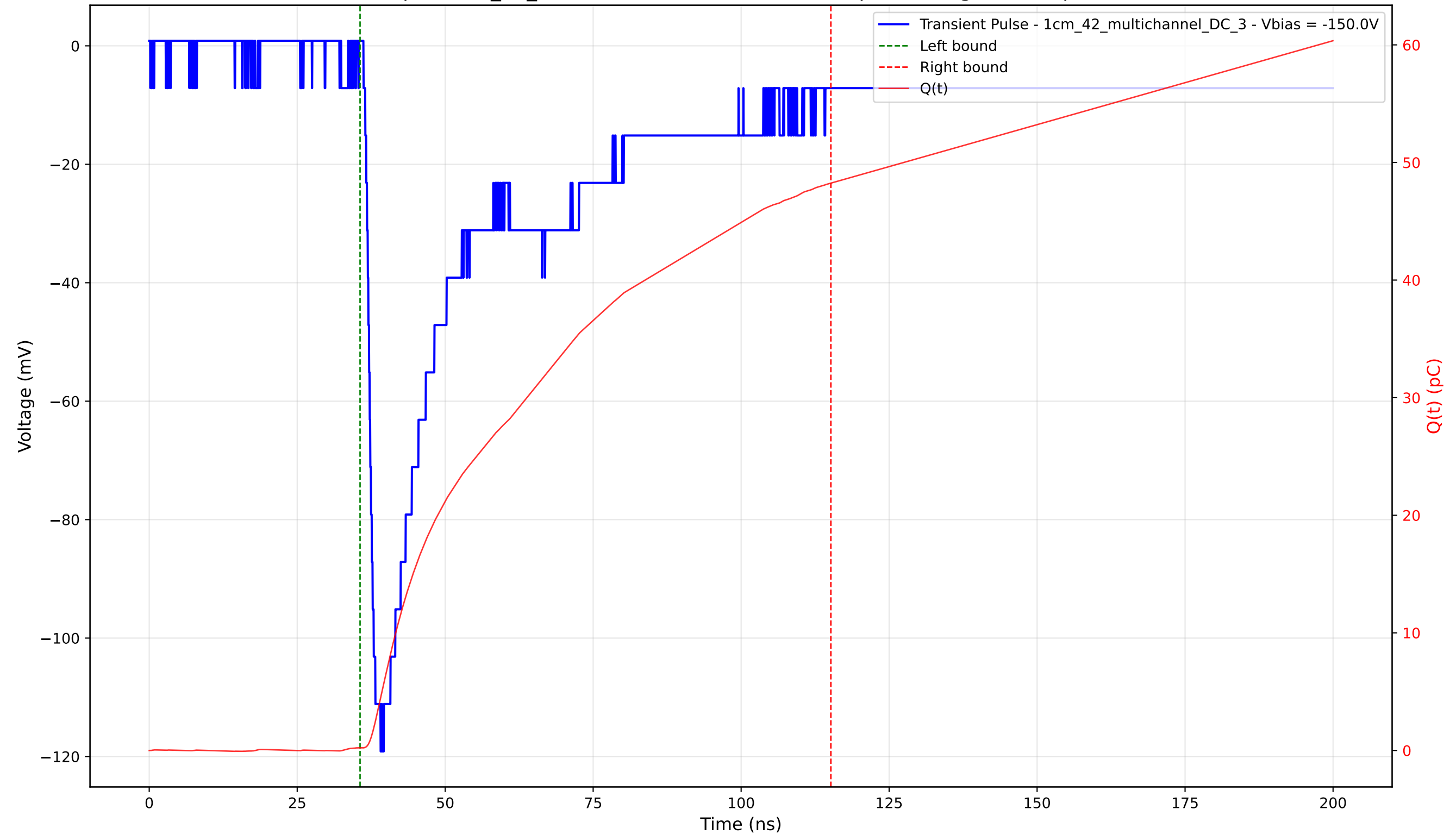
Transient Pulse - Sample: 1cm_42_multichannel - Position: 1725.0 \mu\text{m} - Charge: 48.02 pC - Rise Time: 1.71 ns
