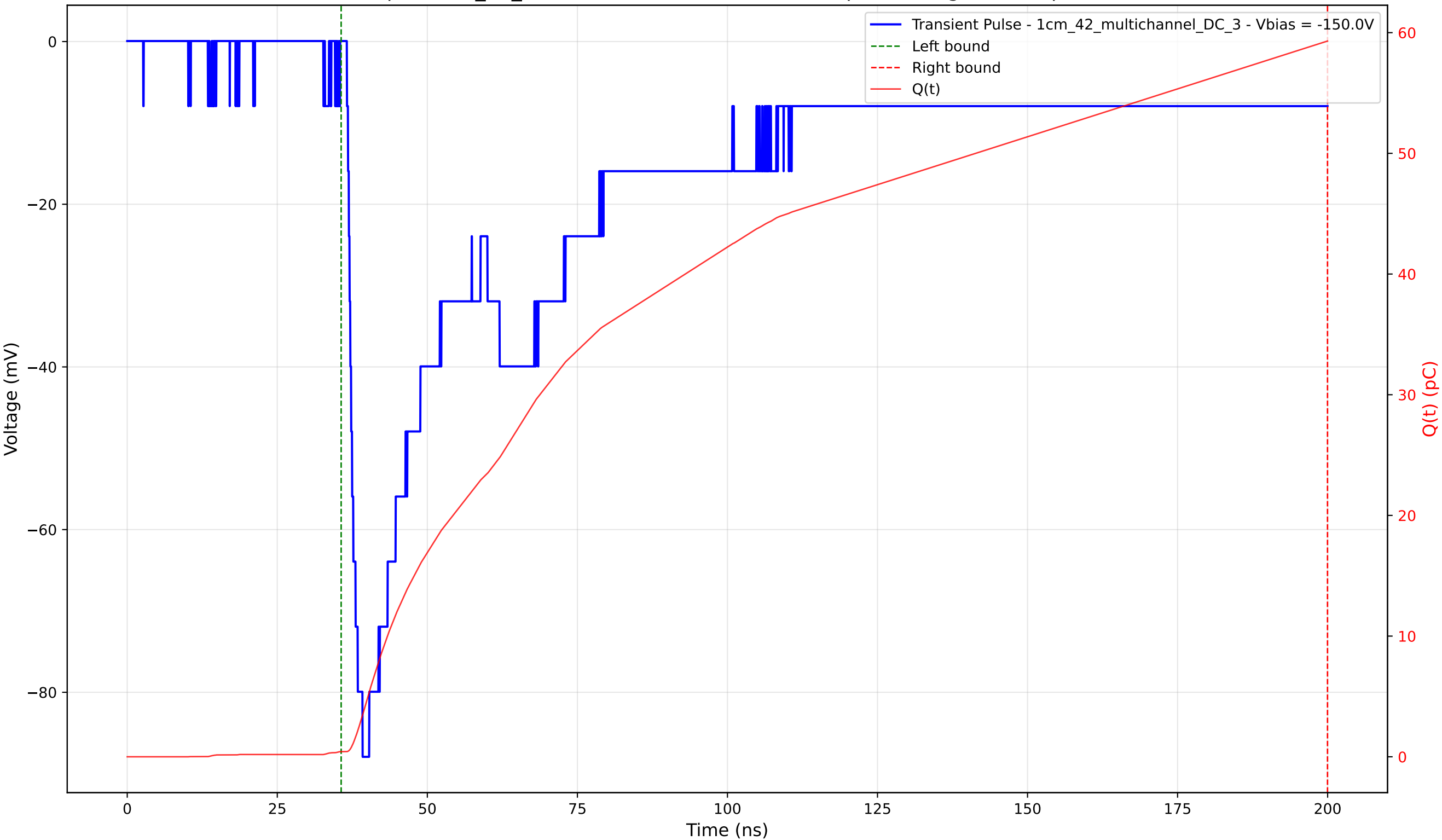
Transient Pulse - Sample: 1cm_42_multichannel - Position: 2260.0 \mu\text{m} - Charge: 58.88 pC - Rise Time: 1.64 ns
