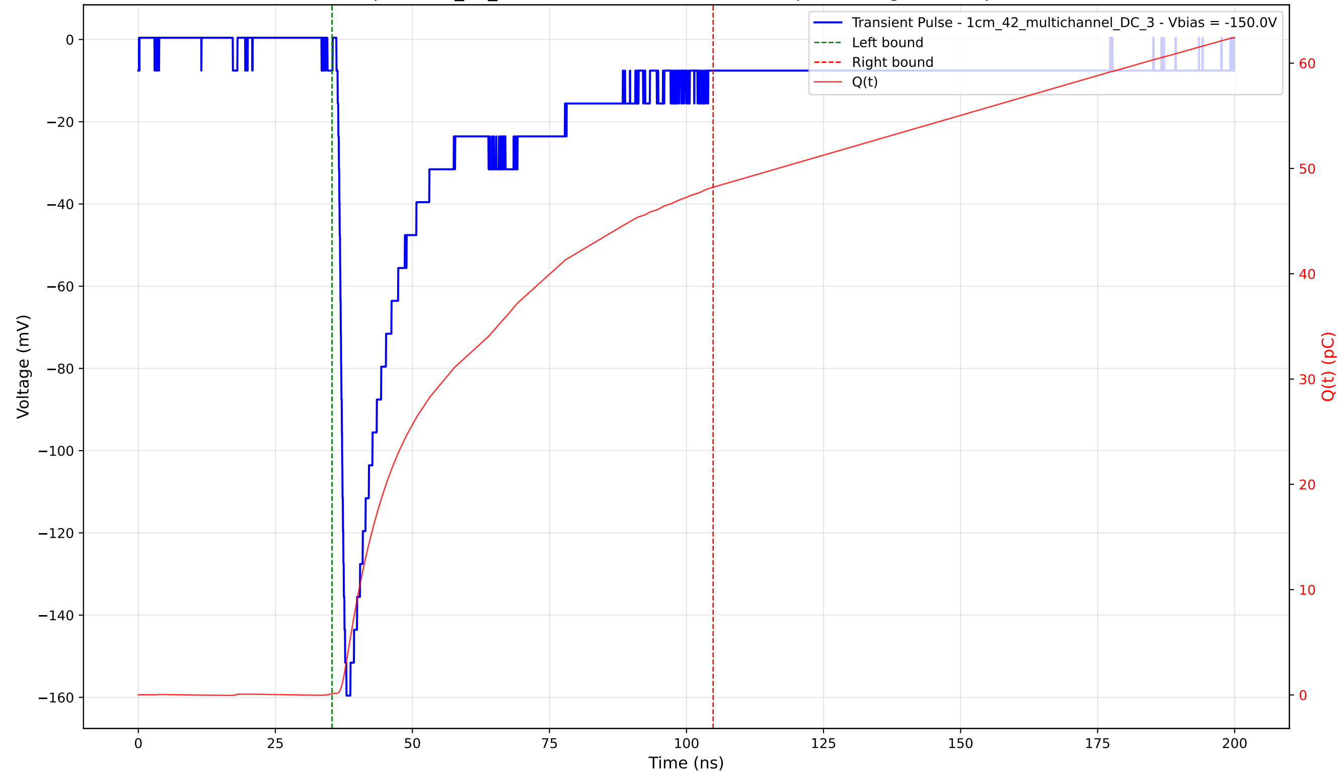
Transient Pulse - Sample: 1cm_42_multichannel - Position: 1155.0 \mu\text{m} - Charge: 48.09 pC - Rise Time: 1.26 ns
