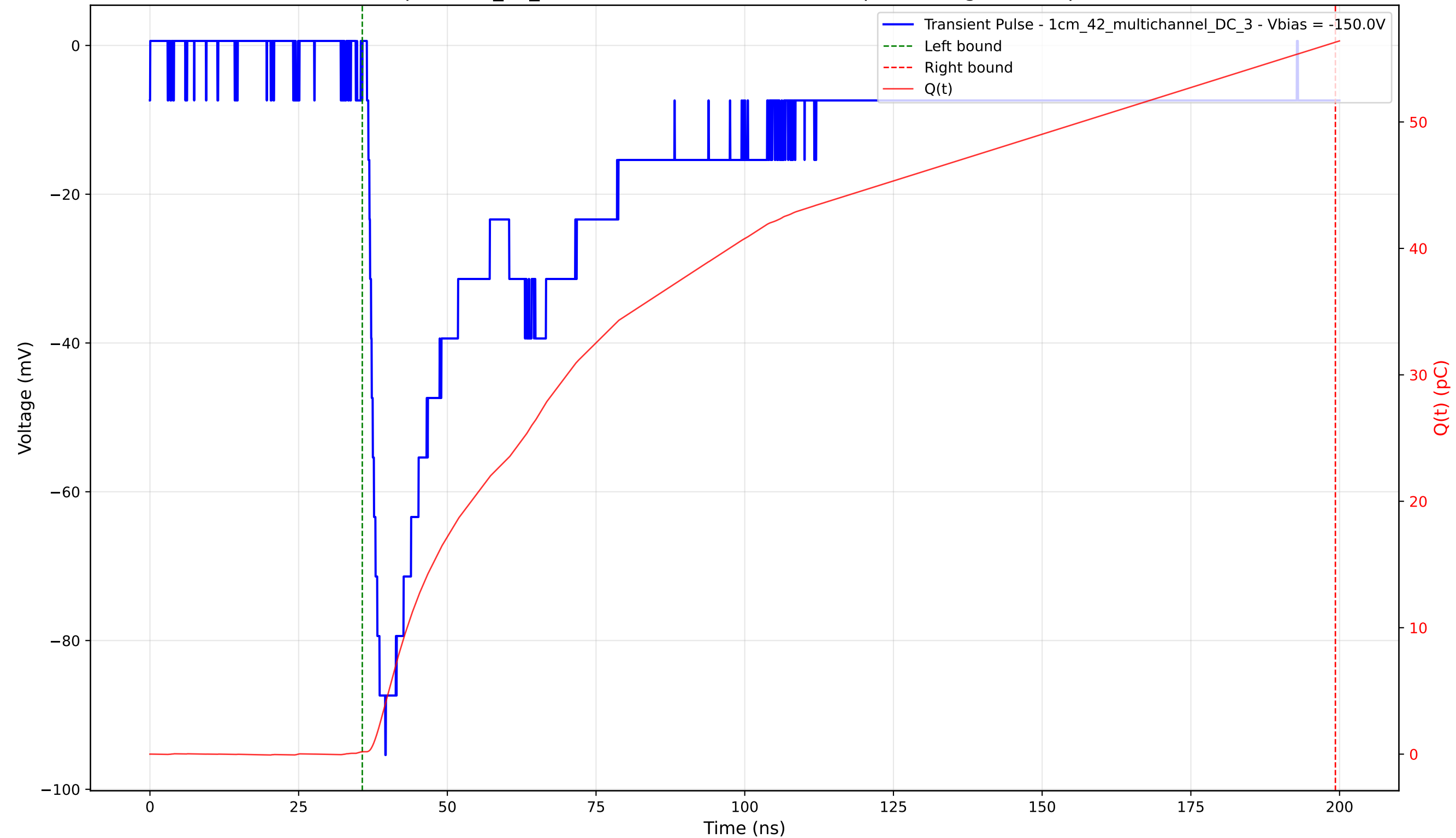
Transient Pulse - Sample: 1cm_42_multichannel - Position: 2705.0 \mu\text{m} - Charge: 56.12 pC - Rise Time: 1.89 ns
