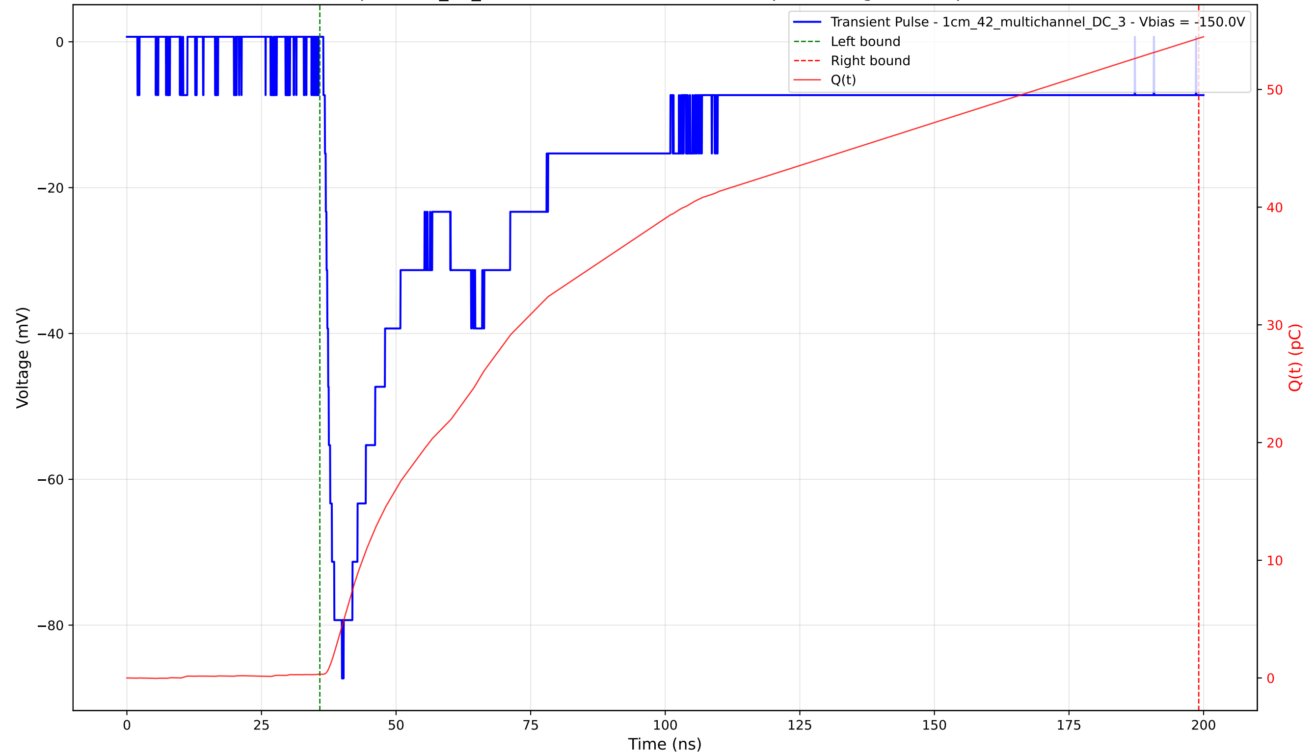
Transient Pulse - Sample: 1cm_42_multichannel - Position: 2625.0 \mu\text{m} - Charge: 54.03 pC - Rise Time: 1.76 ns
