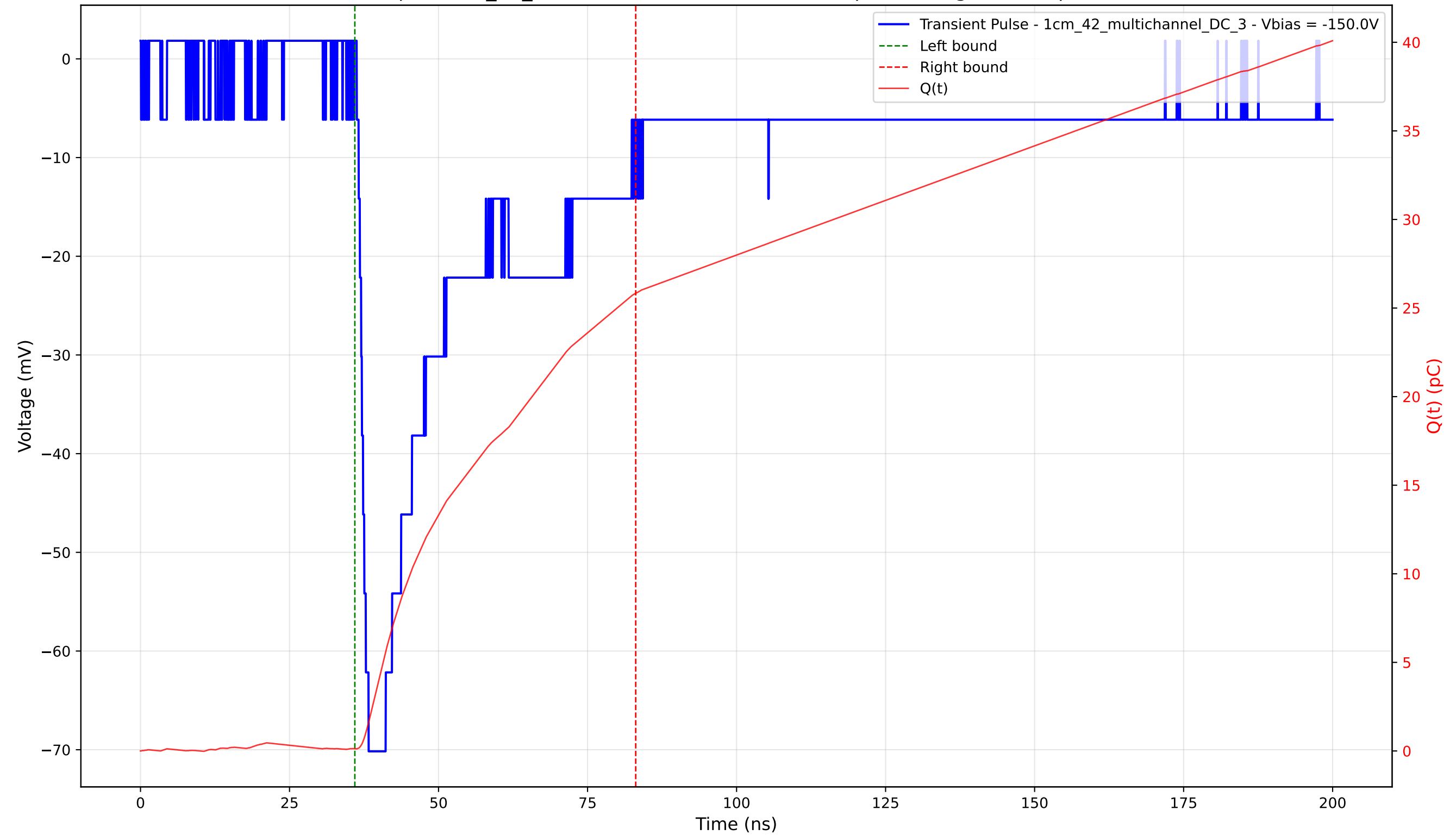
Transient Pulse - Sample: 1cm_42_multichannel - Position: 1810.0 \mu\text{m} - Charge: 25.70 pC - Rise Time: 1.68 ns
