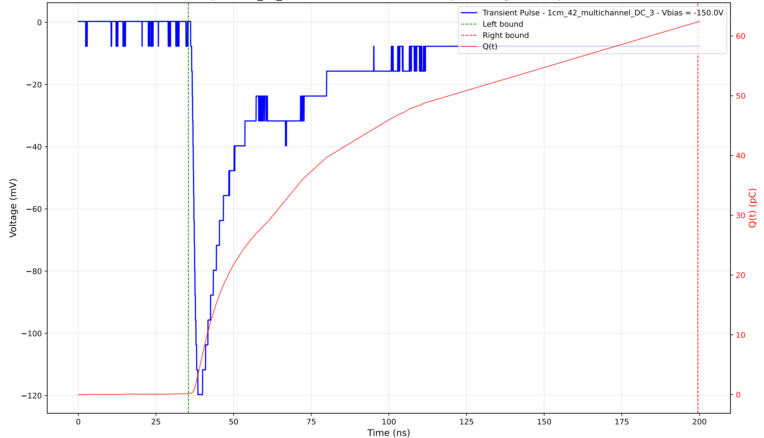
Transient Pulse - Sample: 1cm_42_multichannel - Position: 1690.0 \mu\text{m} - Charge: 62.14 pC - Rise Time: 1.61 ns
