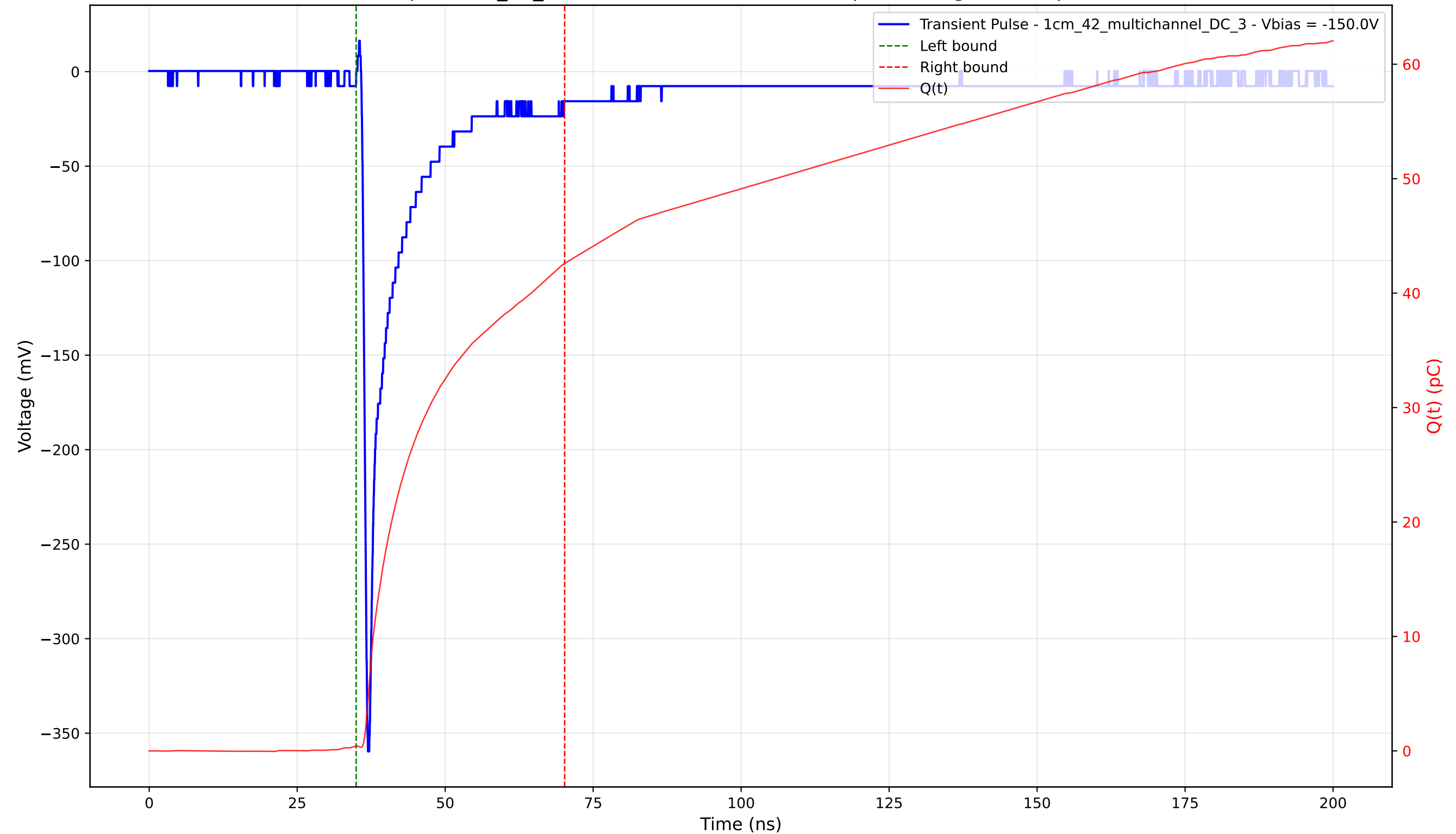
Transient Pulse - Sample: 1cm_42_multichannel - Position: 145.0 \mu\text{m} - Charge: 42.17 pC - Rise Time: 0.78 ns
