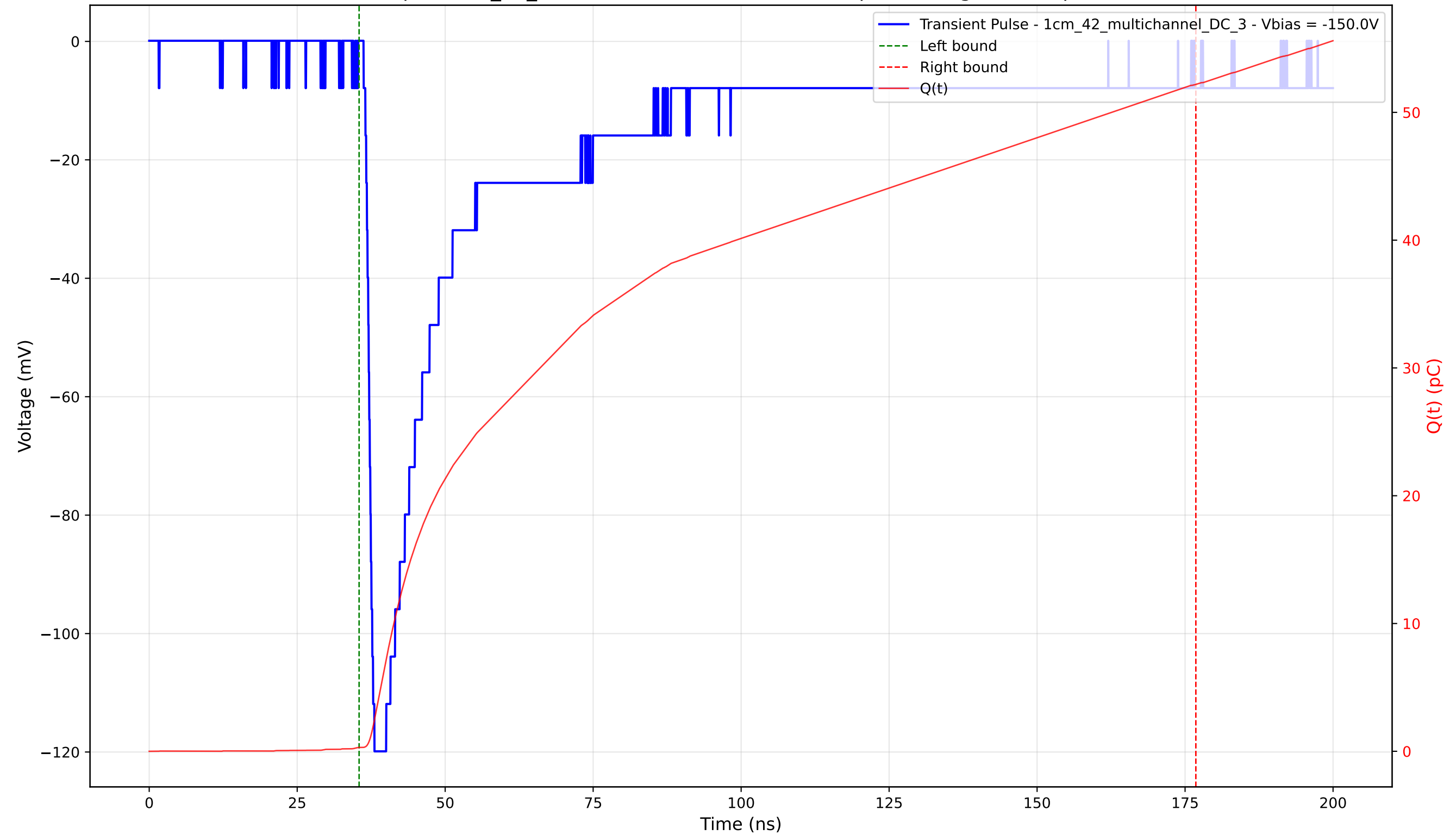
Transient Pulse - Sample: 1cm_42_multichannel - Position: 3535.0 \mu\text{m} - Charge: 51.89 pC - Rise Time: 1.31 ns
