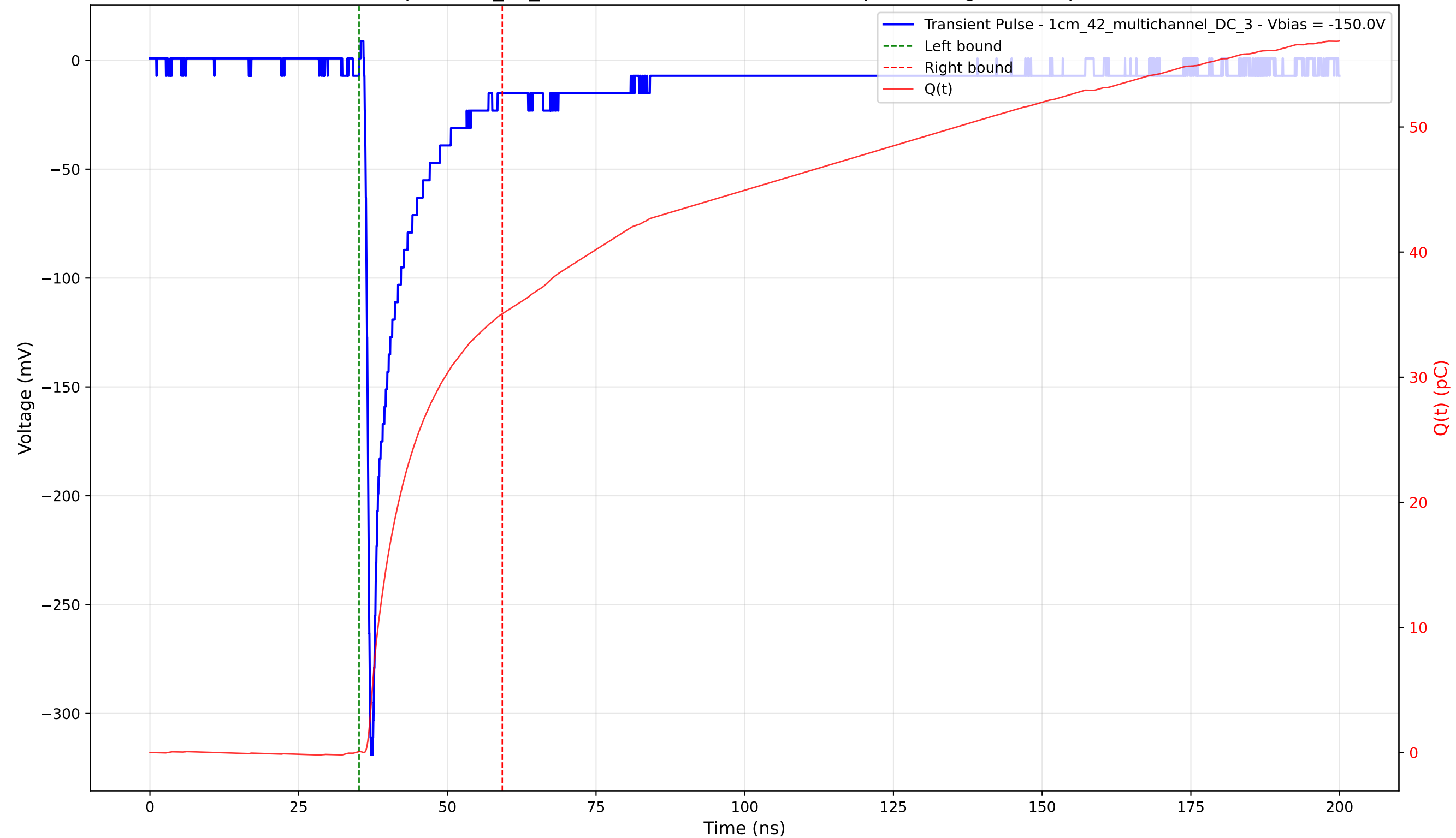
Transient Pulse - Sample: 1cm_42_multichannel - Position: 4655.0 \mu\text{m} - Charge: 34.99 pC - Rise Time: 0.82 ns
