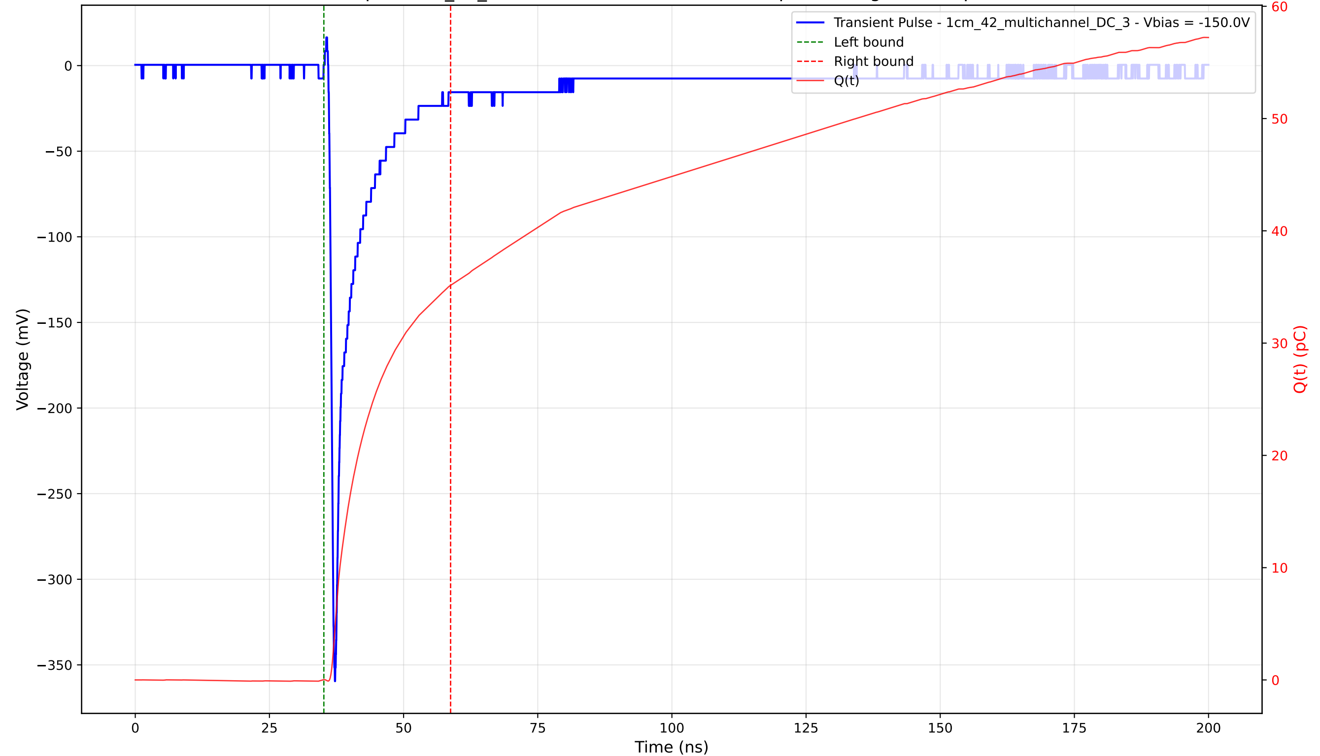
Transient Pulse - Sample: 1cm_42_multichannel - Position: 4750.0 \mu\text{m} - Charge: 35.11 pC - Rise Time: 0.81 ns
