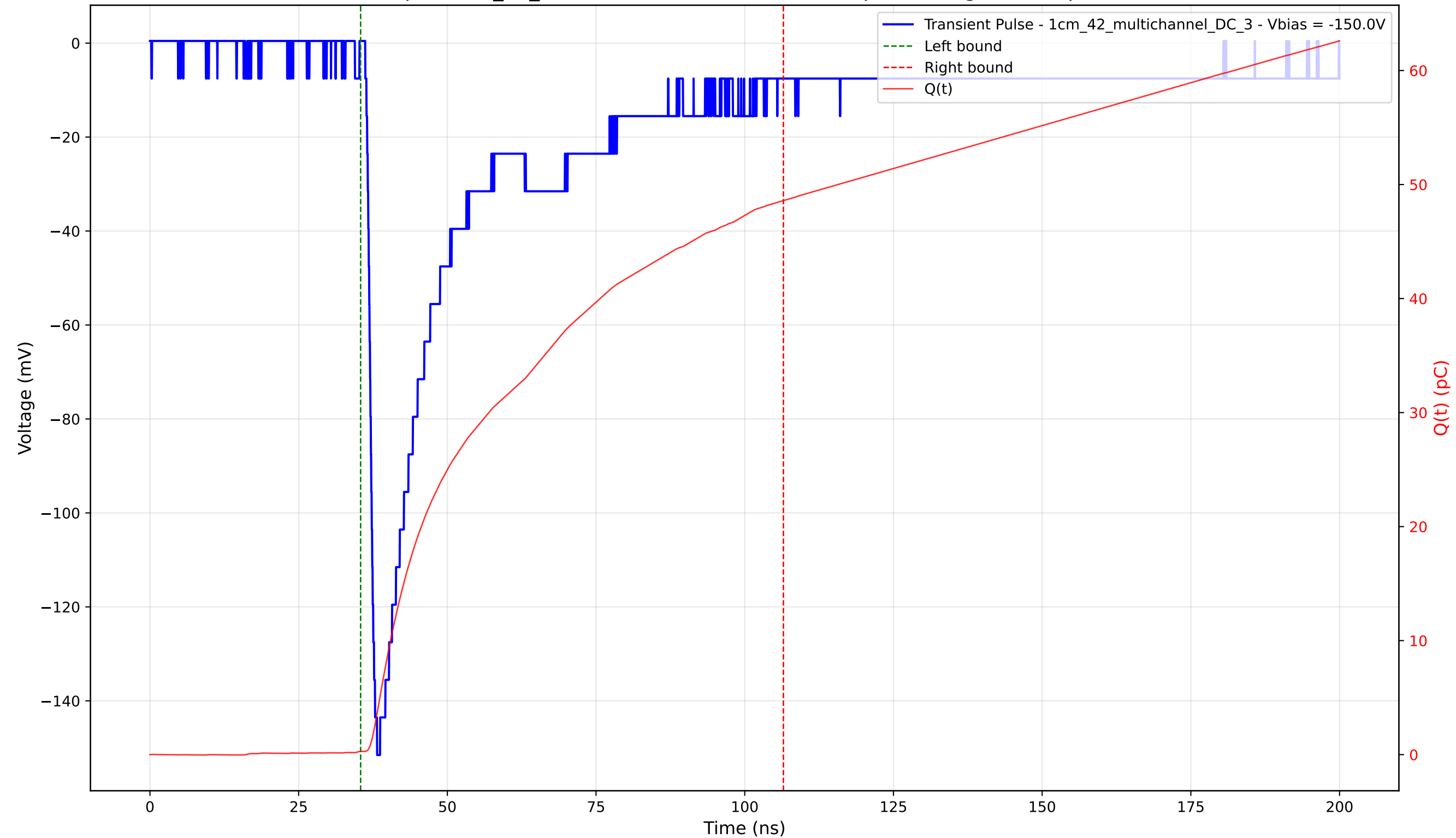
Transient Pulse - Sample: 1cm_42_multichannel - Position: 1265.0 \mu\text{m} - Charge: 48.30 pC - Rise Time: 1.44 ns
