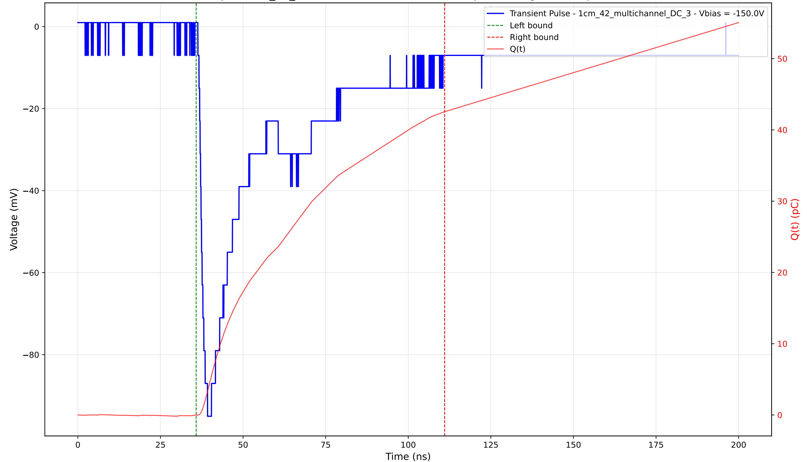
Transient Pulse - Sample: 1cm_42_multichannel - Position: 2760.0 \mu\text{m} - Charge: 42.57 pC - Rise Time: 1.87 ns
