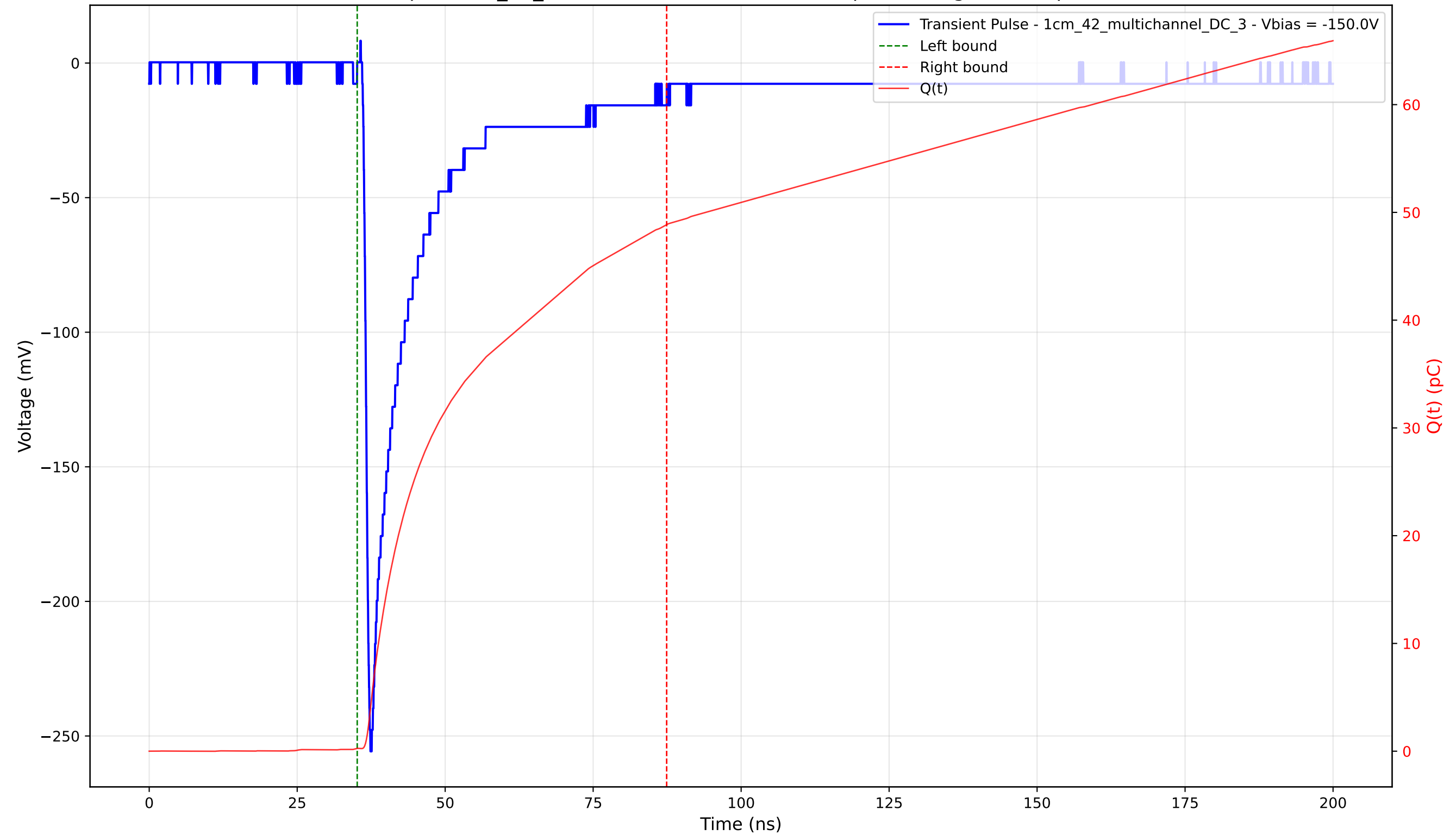
Transient Pulse - Sample: 1cm_42_multichannel - Position: 555.0 \mu\text{m} - Charge: 48.59 pC - Rise Time: 0.92 ns
