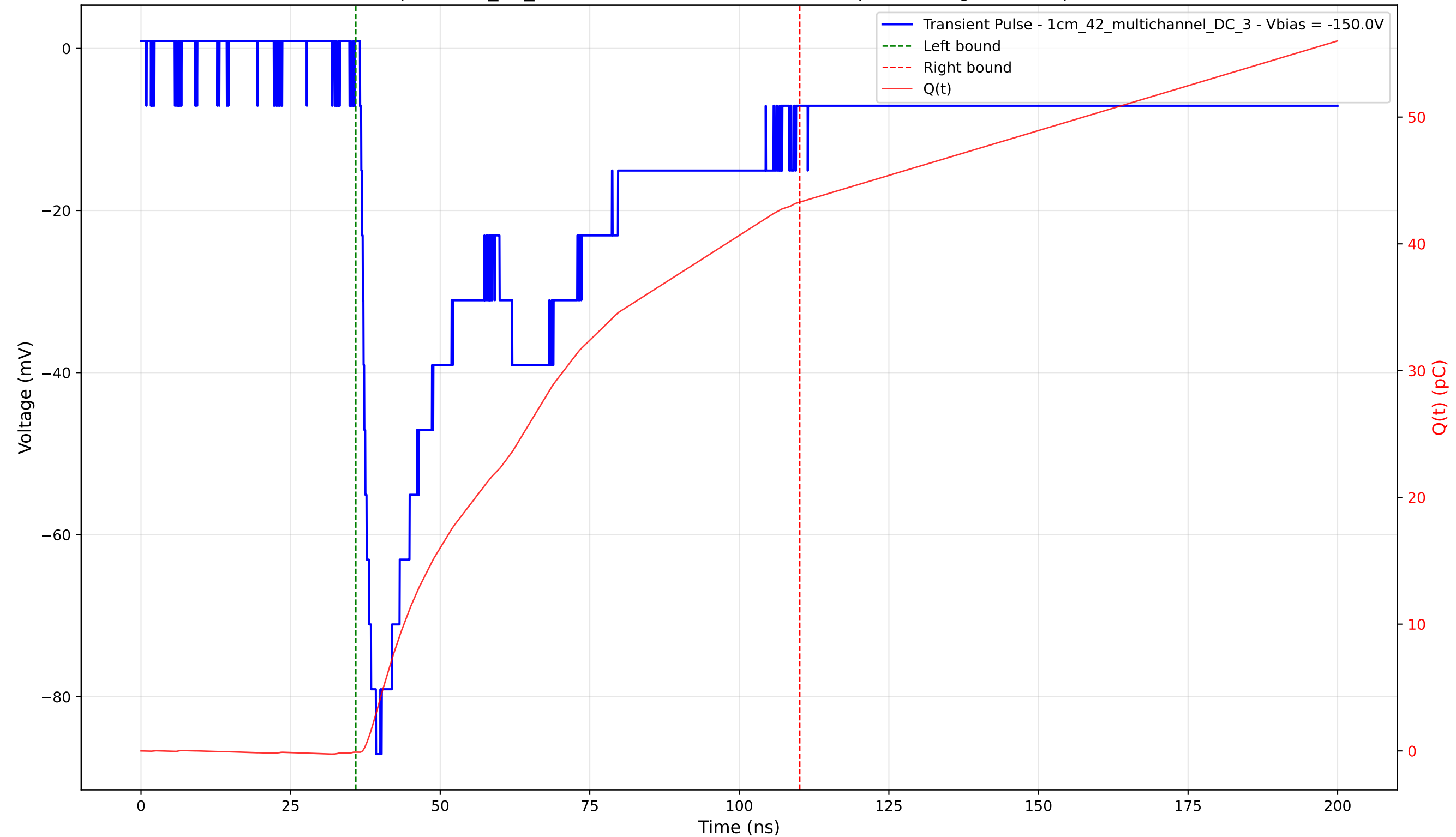
Transient Pulse - Sample: 1cm_42_multichannel - Position: 2270.0 \mu\text{m} - Charge: 43.39 pC - Rise Time: 1.66 ns
