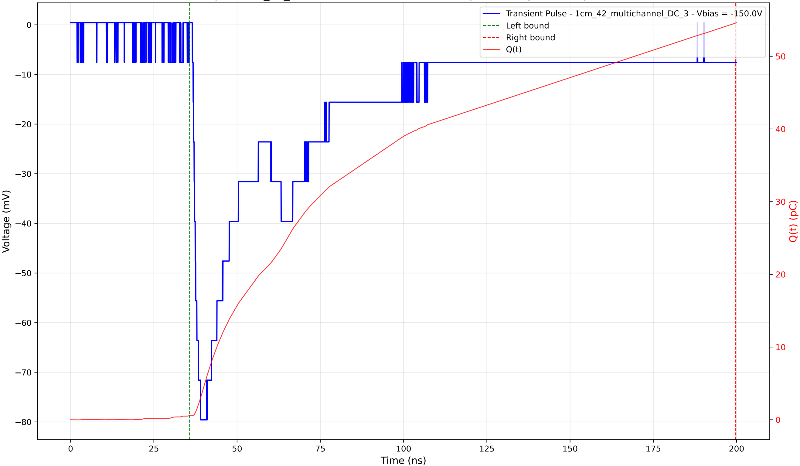
Transient Pulse - Sample: 1cm_42_multichannel - Position: 2545.0 \mu\text{m} - Charge: 54.01 pC - Rise Time: 2.26 ns
