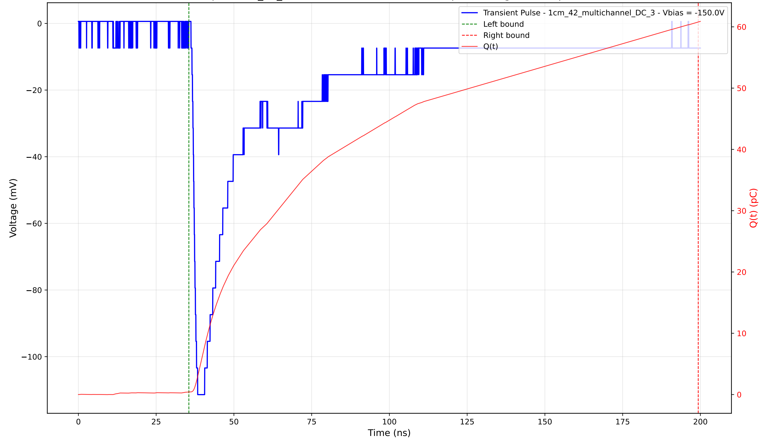
Transient Pulse - Sample: 1cm_42_multichannel - Position: 1745.0 \mu\text{m} - Charge: 60.36 pC - Rise Time: 1.47 ns
