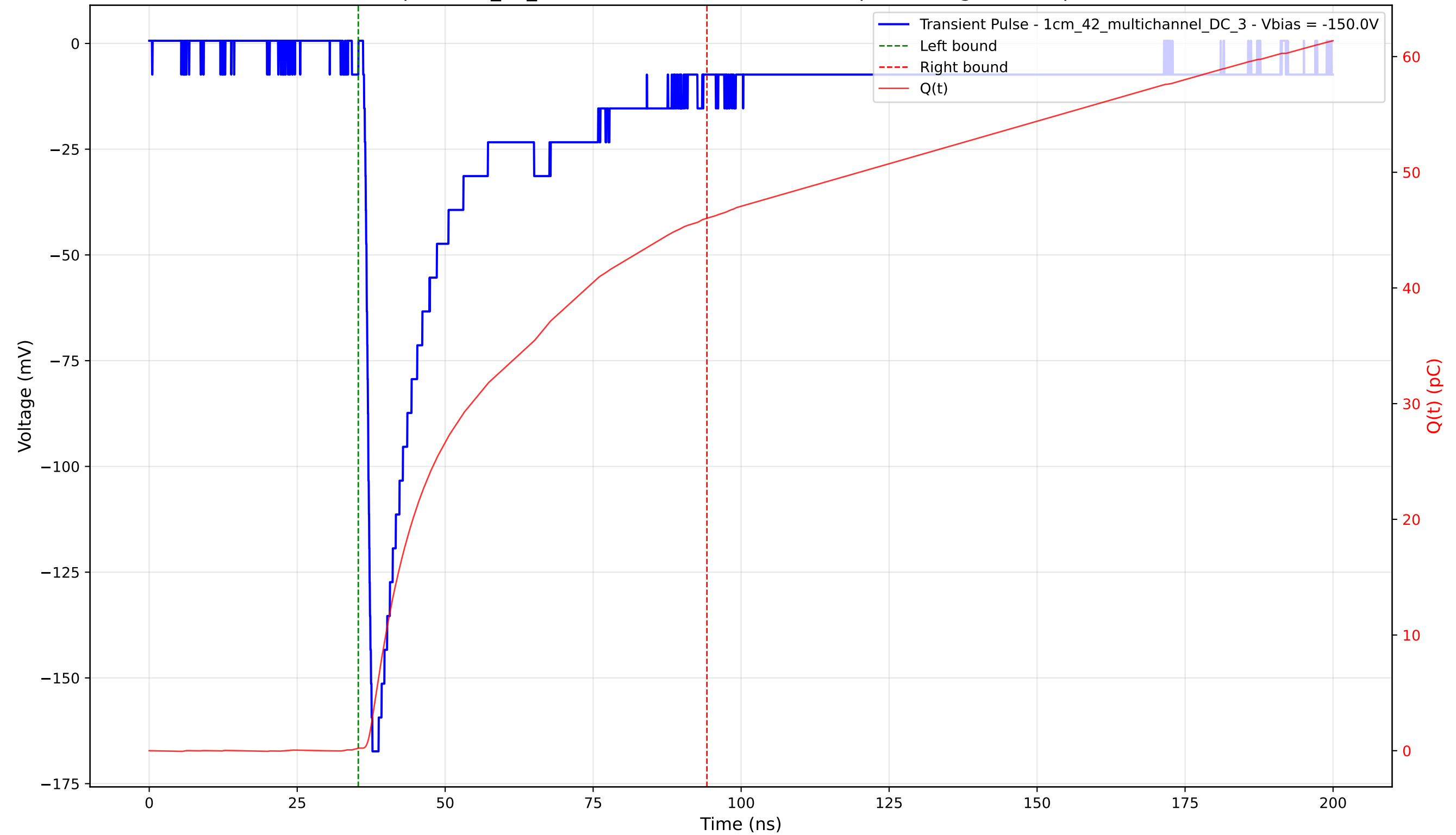
Transient Pulse - Sample: 1cm_42_multichannel - Position: 1030.0 \mu\text{m} - Charge: 45.80 pC - Rise Time: 1.06 ns
