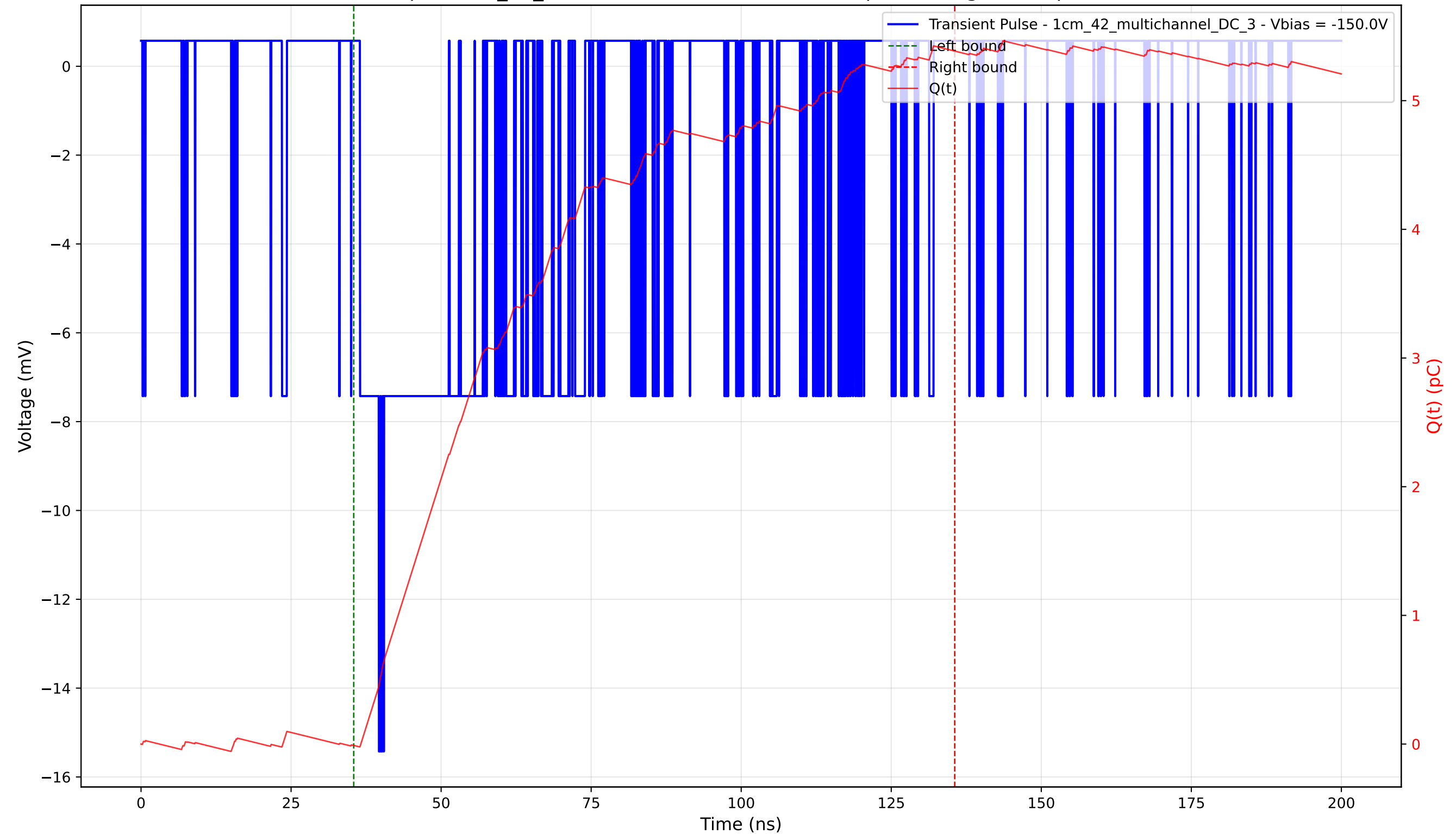
Transient Pulse - Sample: 1cm_42_multichannel - Position: 3900.0 \mu\text{m} - Charge: 5.40 pC - Rise Time: 3.16 ns
