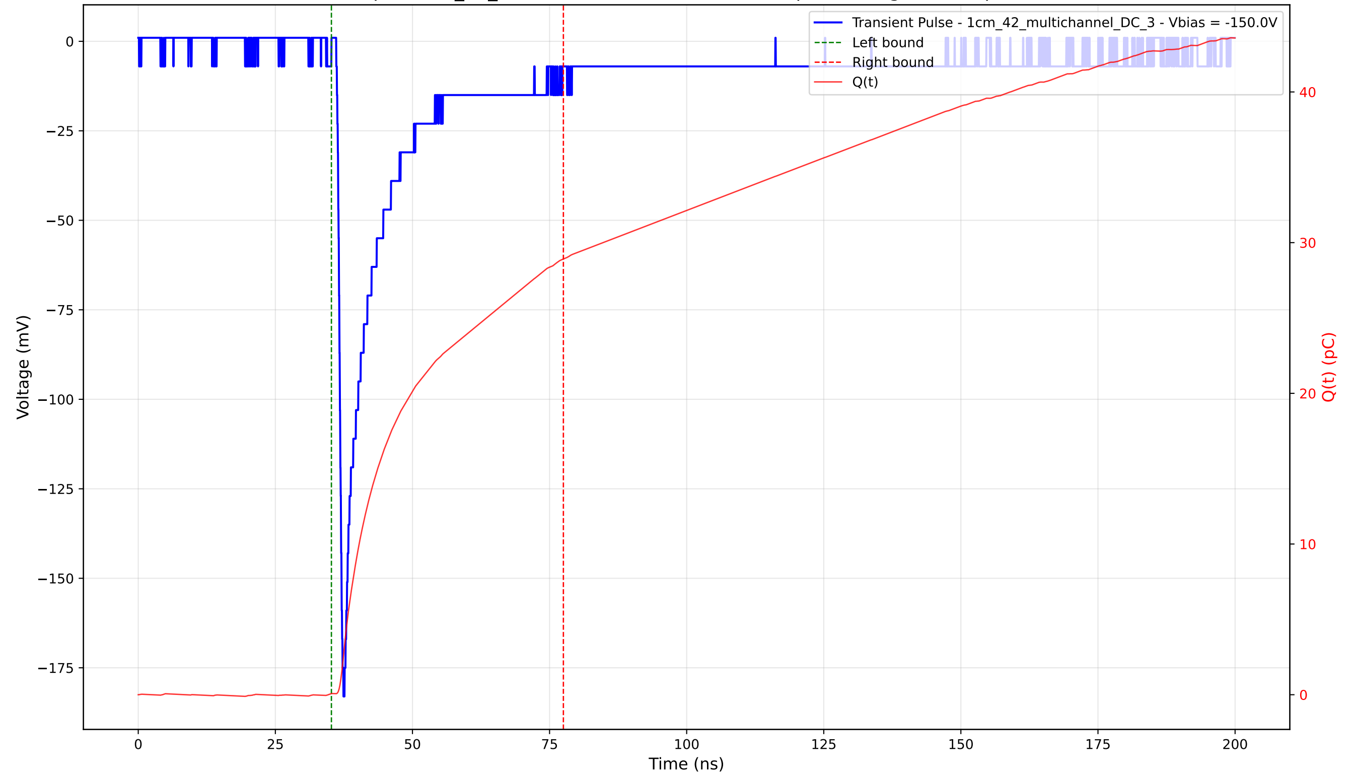
Transient Pulse - Sample: 1cm_42_multichannel - Position: 4455.0 \mu\text{m} - Charge: 28.83 pC - Rise Time: 0.87 ns
