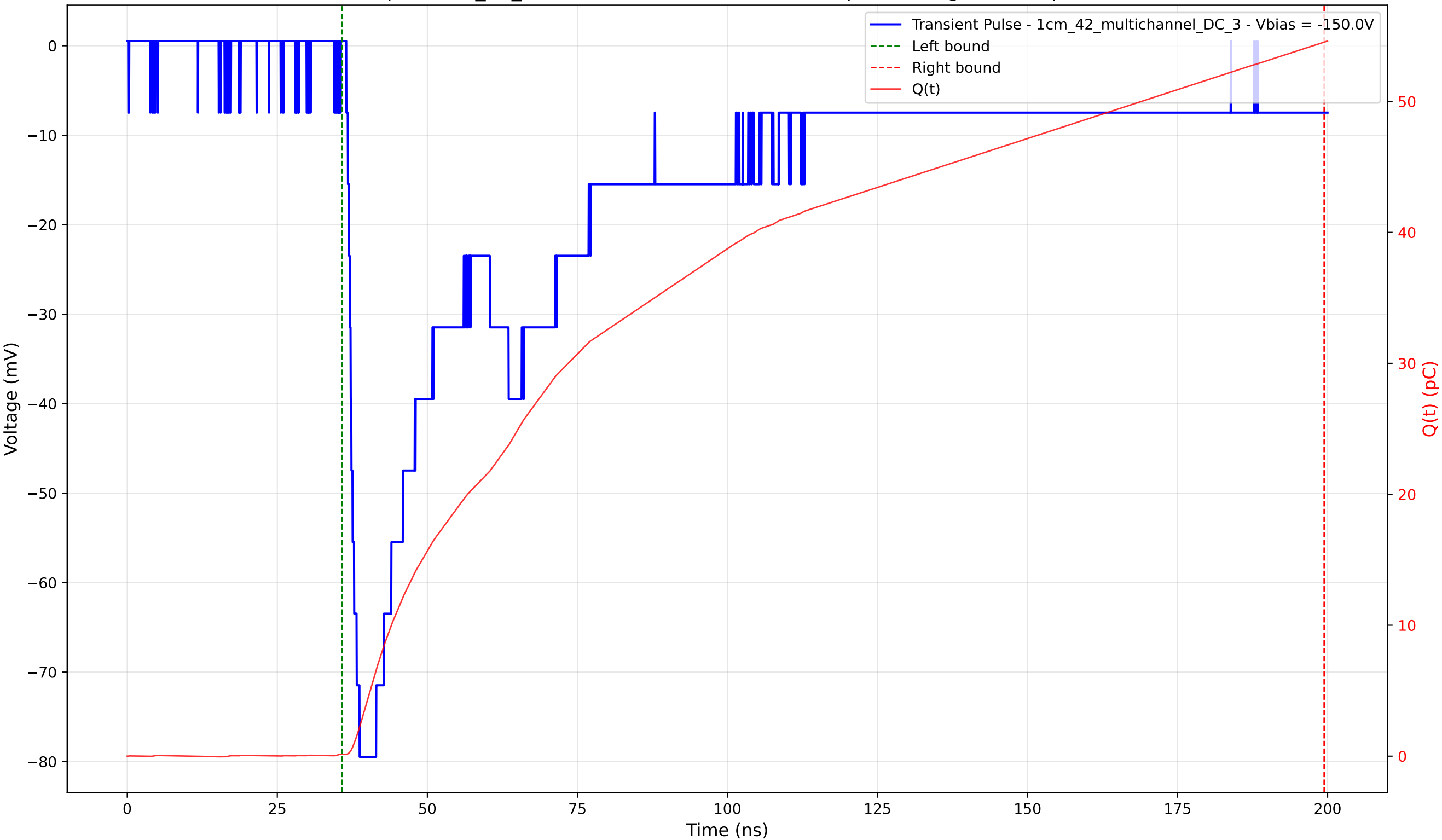
Transient Pulse - Sample: 1cm_42_multichannel - Position: 2585.0 \mu\text{m} - Charge: 54.39 pC - Rise Time: 1.96 ns
