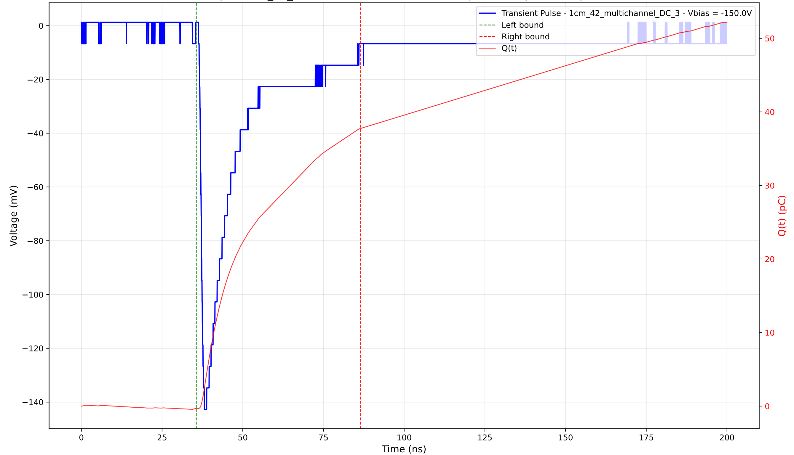
Transient Pulse - Sample: 1cm_42_multichannel - Position: 3730.0 \mu\text{m} - Charge: 38.04 pC - Rise Time: 1.34 ns
