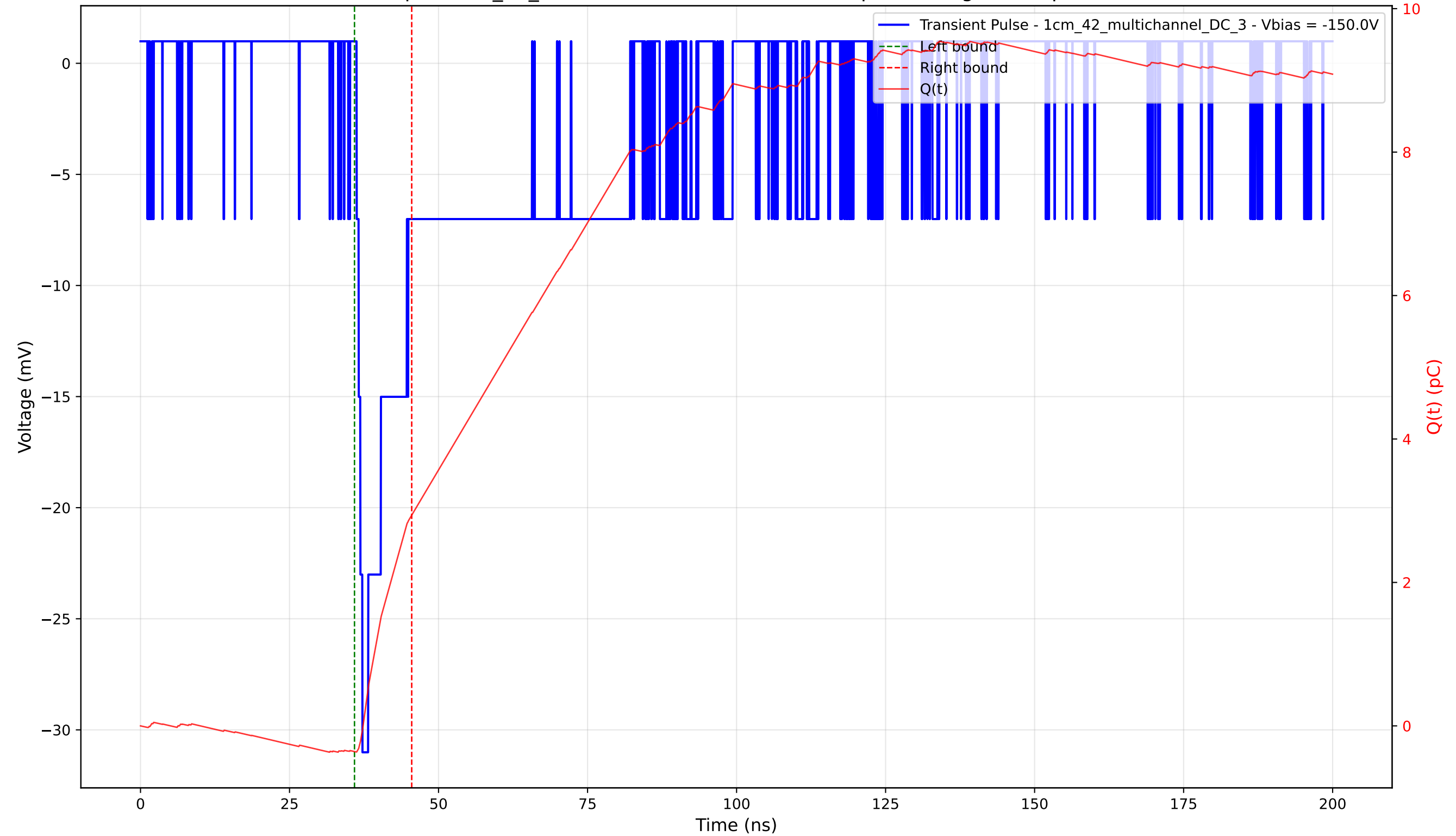
Transient Pulse - Sample: 1cm_42_multichannel - Position: 4360.0 \mu\text{m} - Charge: 3.30 pC - Rise Time: 0.97 ns
