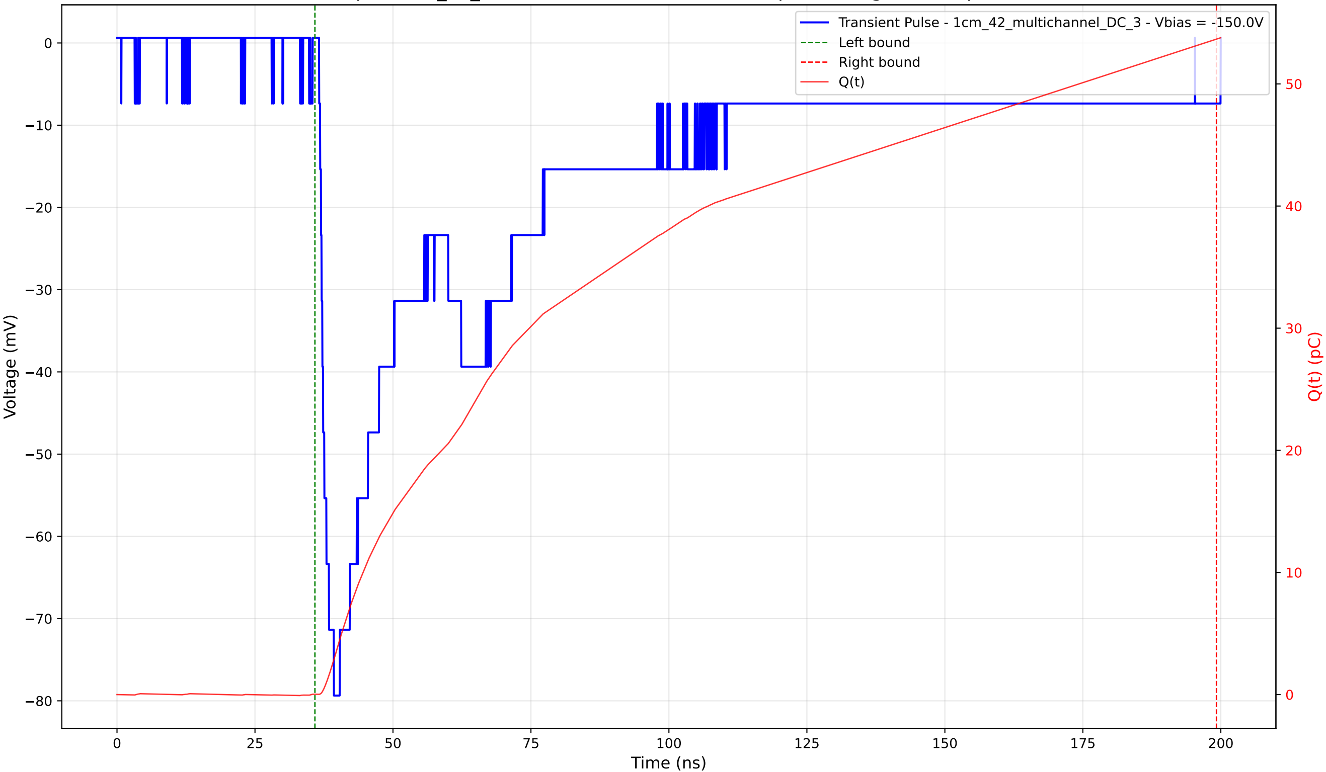
Transient Pulse - Sample: 1cm_42_multichannel - Position: 2295.0 \mu\text{m} - Charge: 53.65 pC - Rise Time: 2.50 ns
