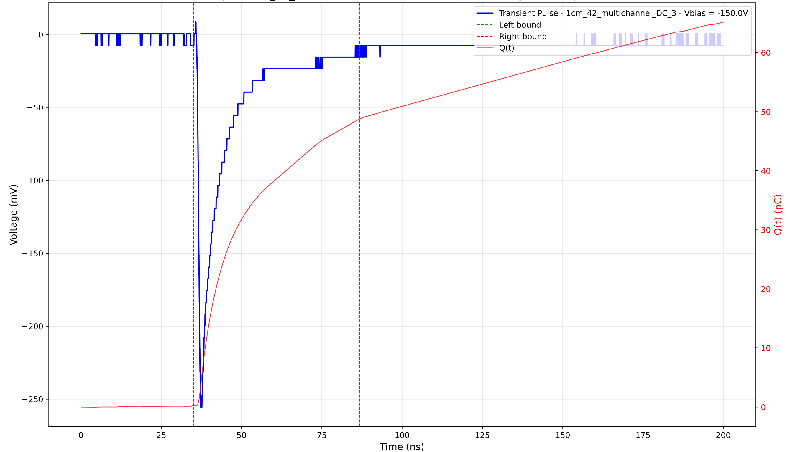
Transient Pulse - Sample: 1cm_42_multichannel - Position: 545.0 \mu\text{m} - Charge: 48.48 pC - Rise Time: 0.89 ns
