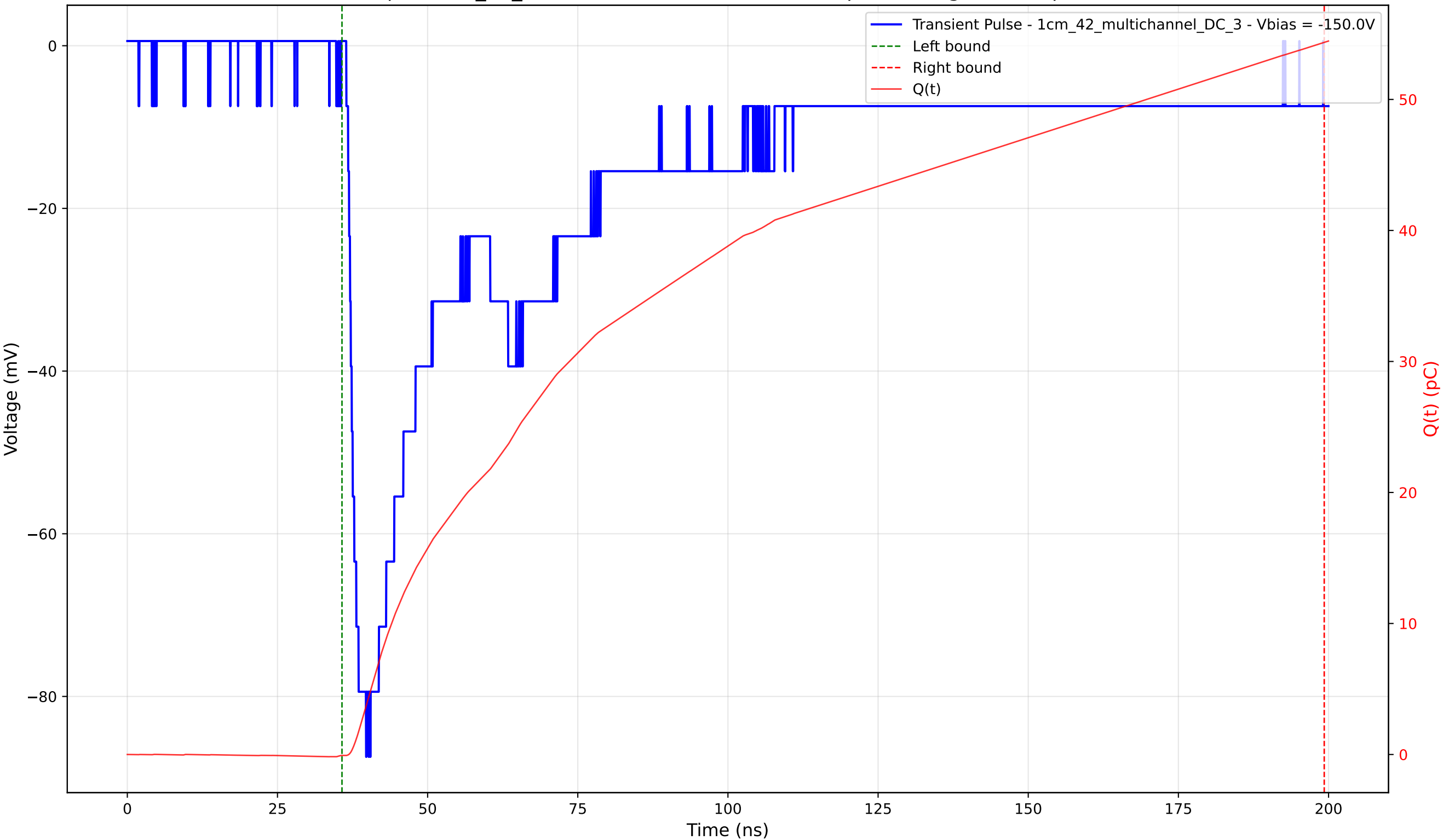
Transient Pulse - Sample: 1cm_42_multichannel - Position: 2620.0 \mu\text{m} - Charge: 54.43 pC - Rise Time: 1.76 ns
