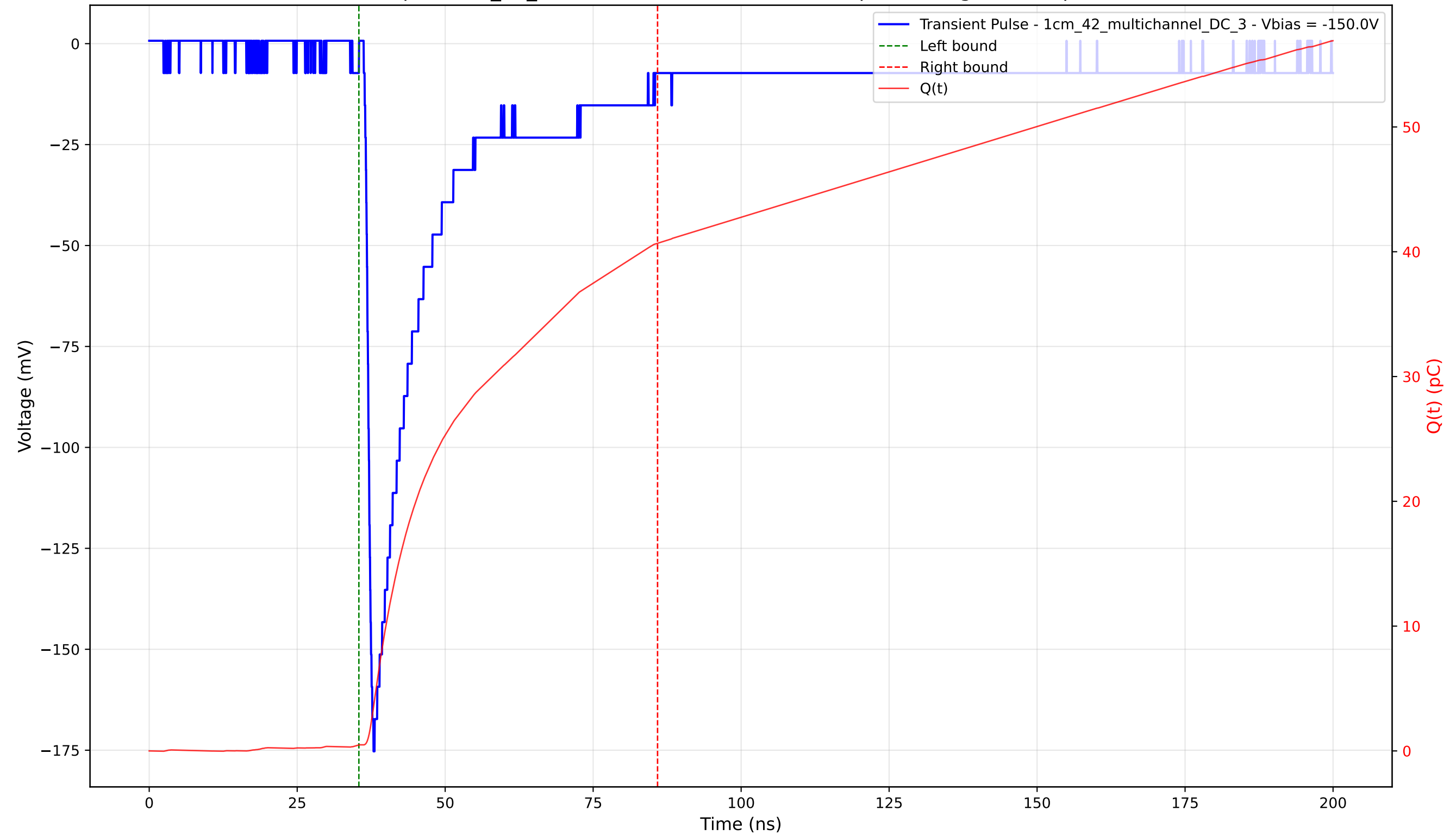
Transient Pulse - Sample: 1cm_42_multichannel - Position: 3990.0 \mu\text{m} - Charge: 40.20 pC - Rise Time: 1.07 ns
