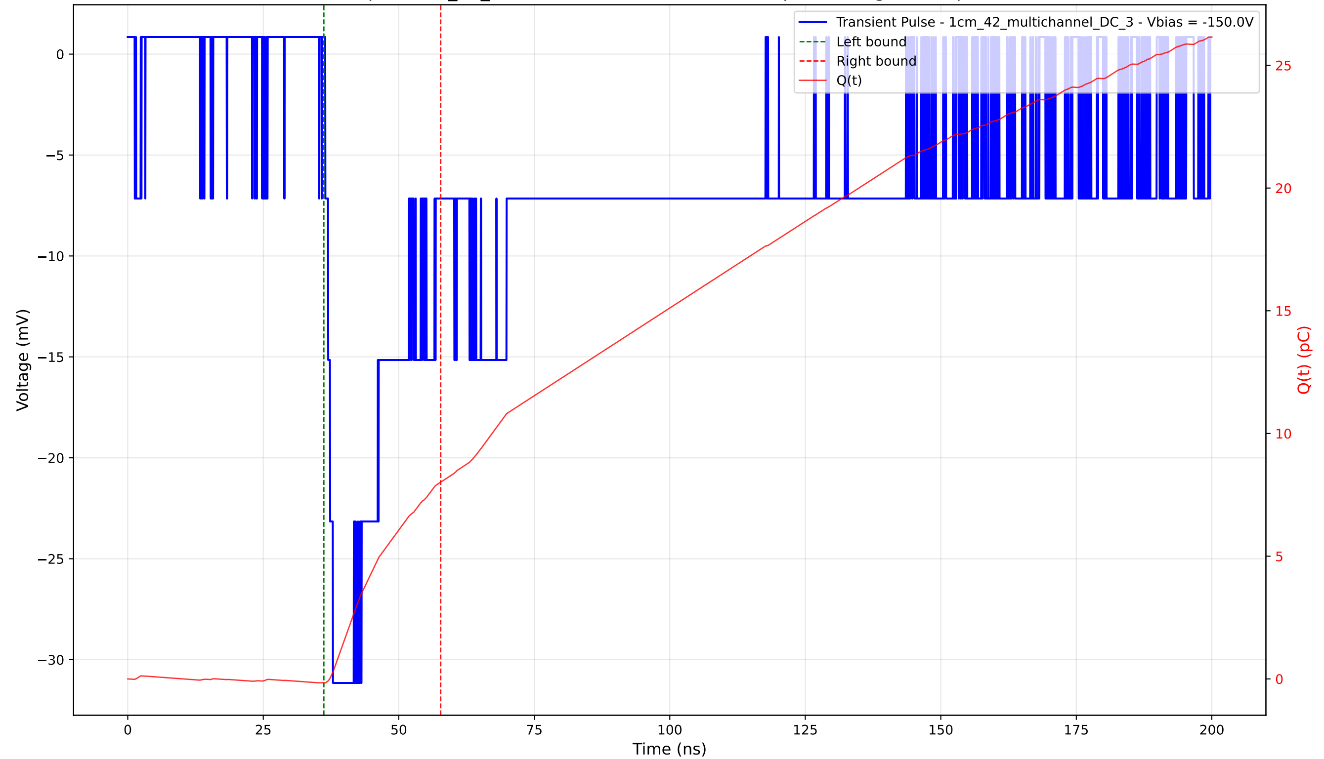
Transient Pulse - Sample: 1cm_42_multichannel - Position: 1910.0 \mu\text{m} - Charge: 8.18 pC - Rise Time: 1.41 ns
