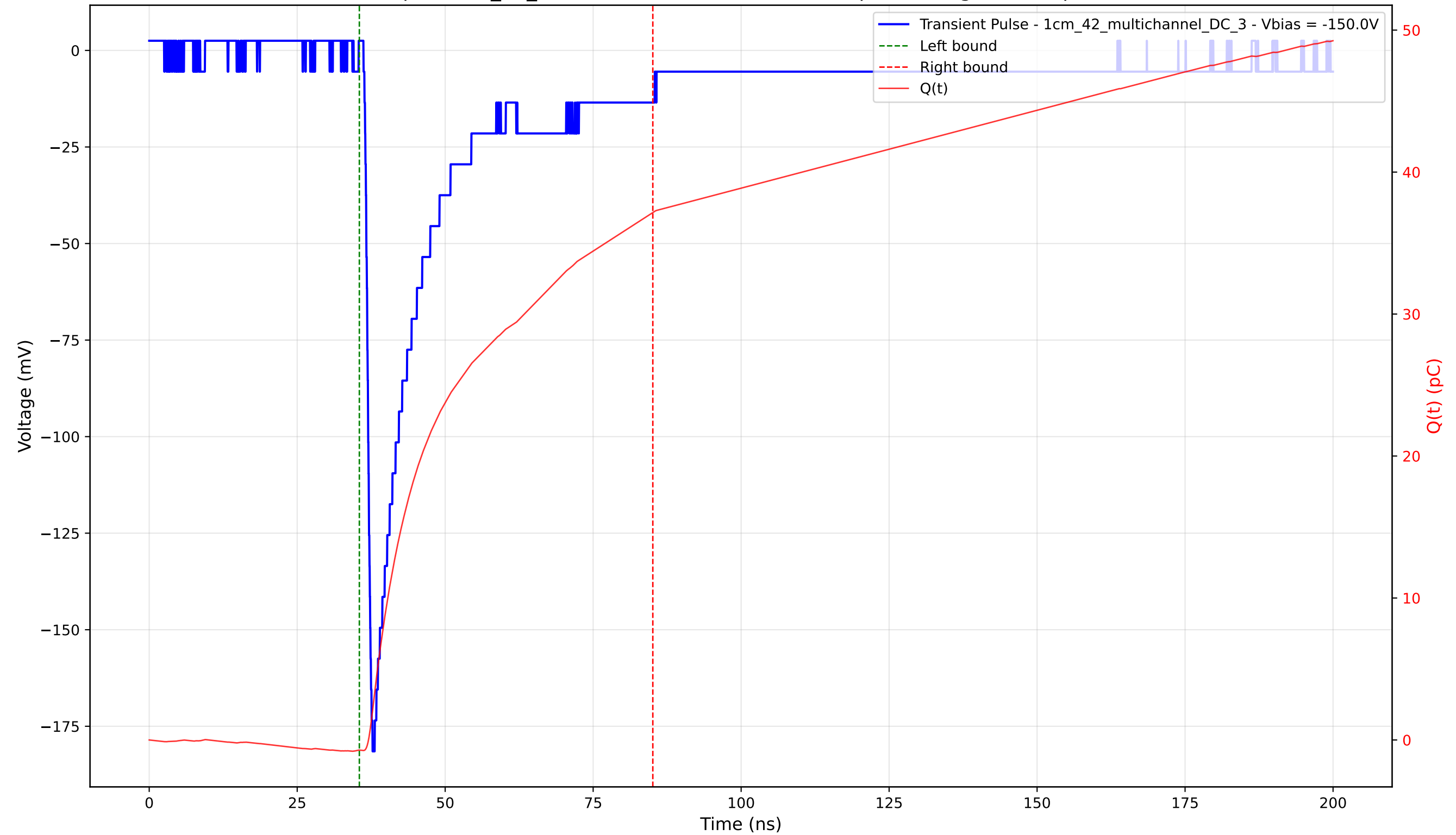
Transient Pulse - Sample: 1cm_42_multichannel - Position: 4100.0 \mu\text{m} - Charge: 37.88 pC - Rise Time: 1.01 ns
