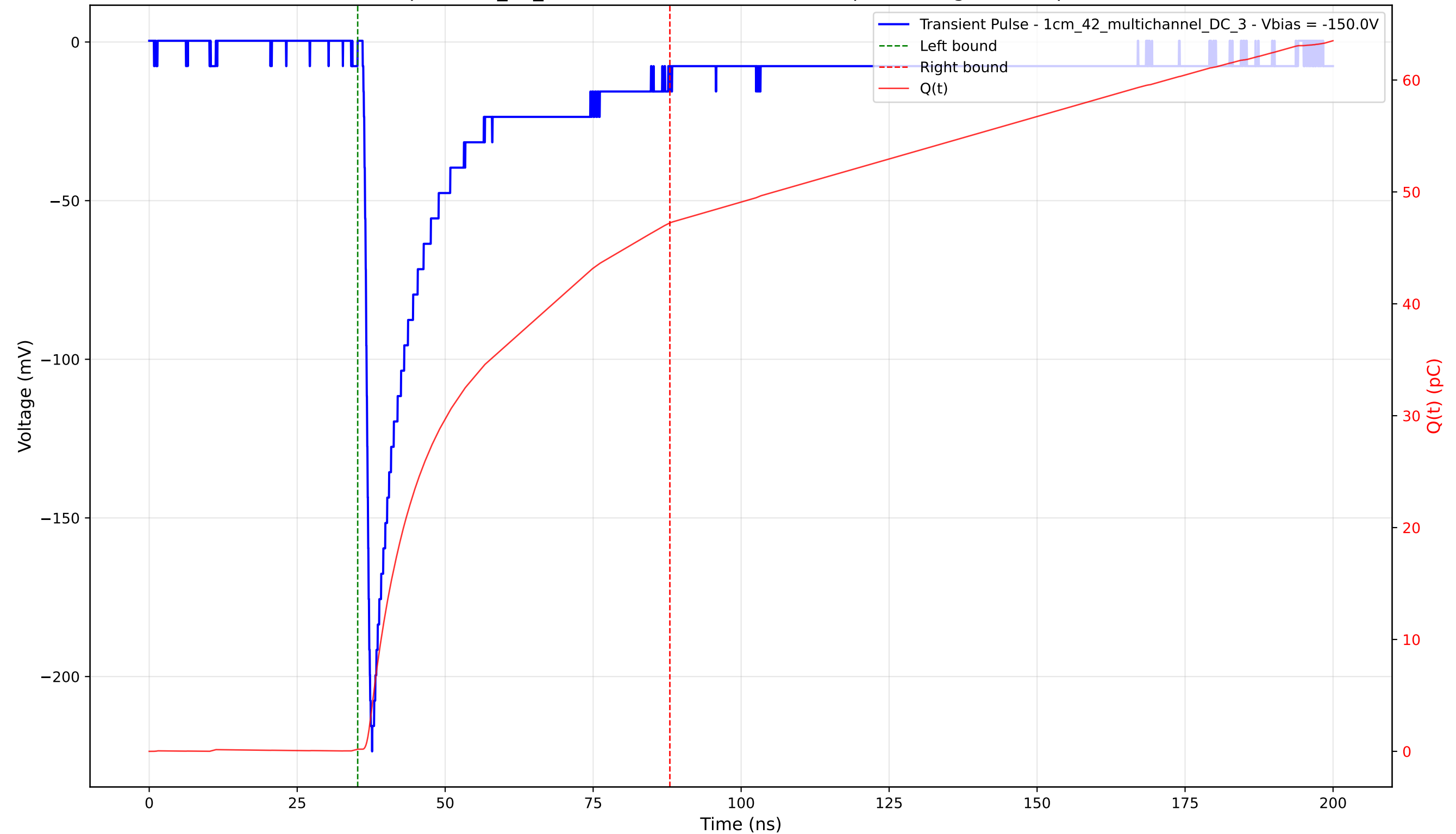
Transient Pulse - Sample: 1cm_42_multichannel - Position: 715.0 \mu\text{m} - Charge: 47.03 pC - Rise Time: 1.06 ns
