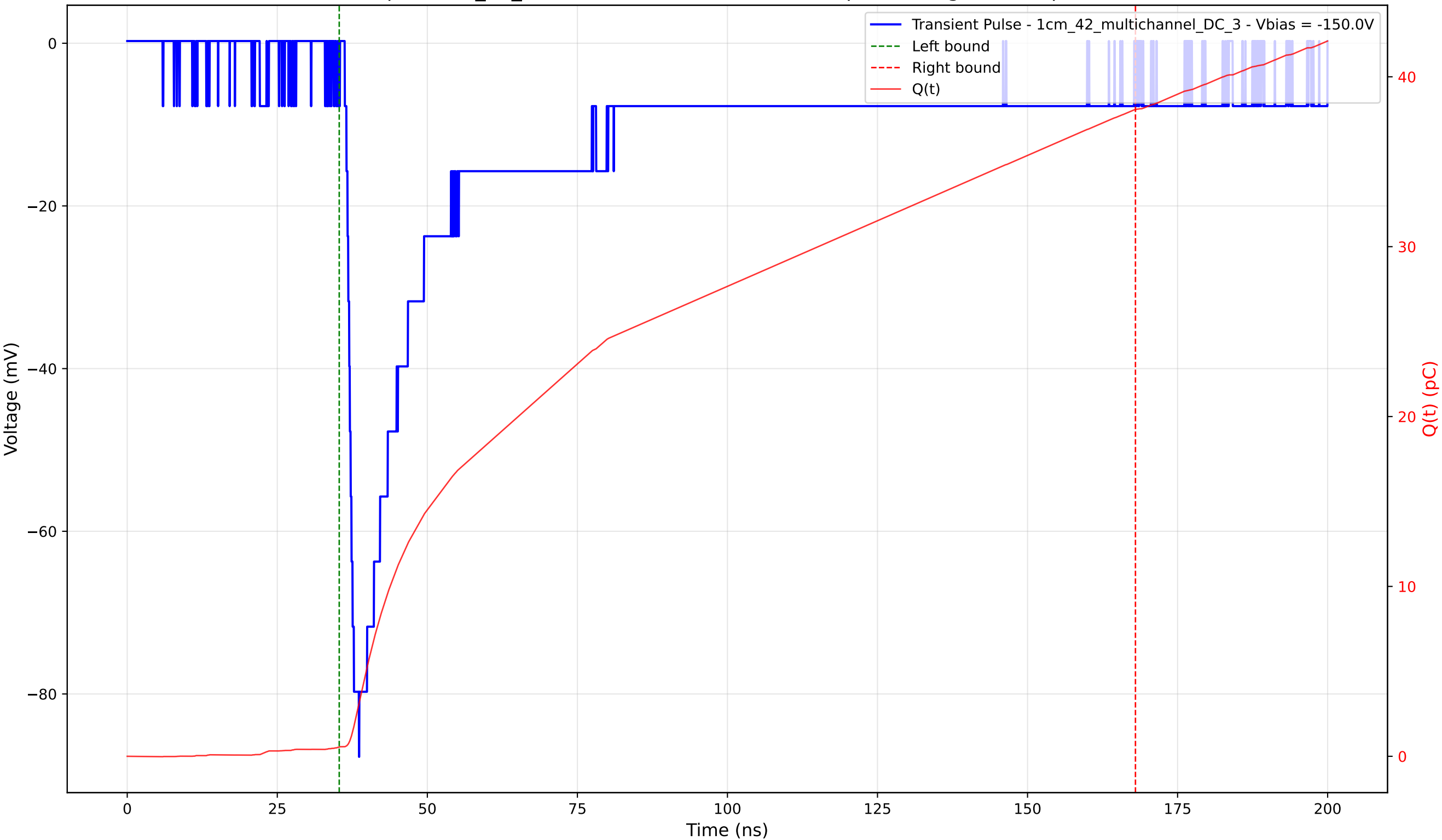
Transient Pulse - Sample: 1cm_42_multichannel - Position: 1310.0 \mu\text{m} - Charge: 37.53 pC - Rise Time: 1.26 ns
