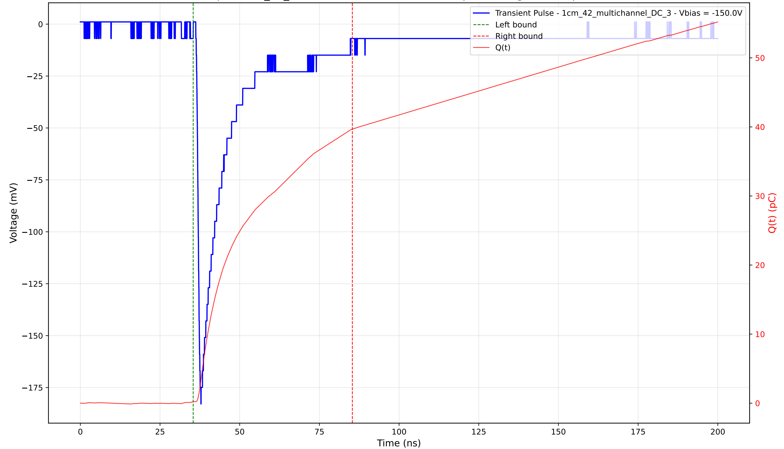
Transient Pulse - Sample: 1cm_42_multichannel - Position: 4095.0 \mu\text{m} - Charge: 39.45 pC - Rise Time: 1.03 ns
