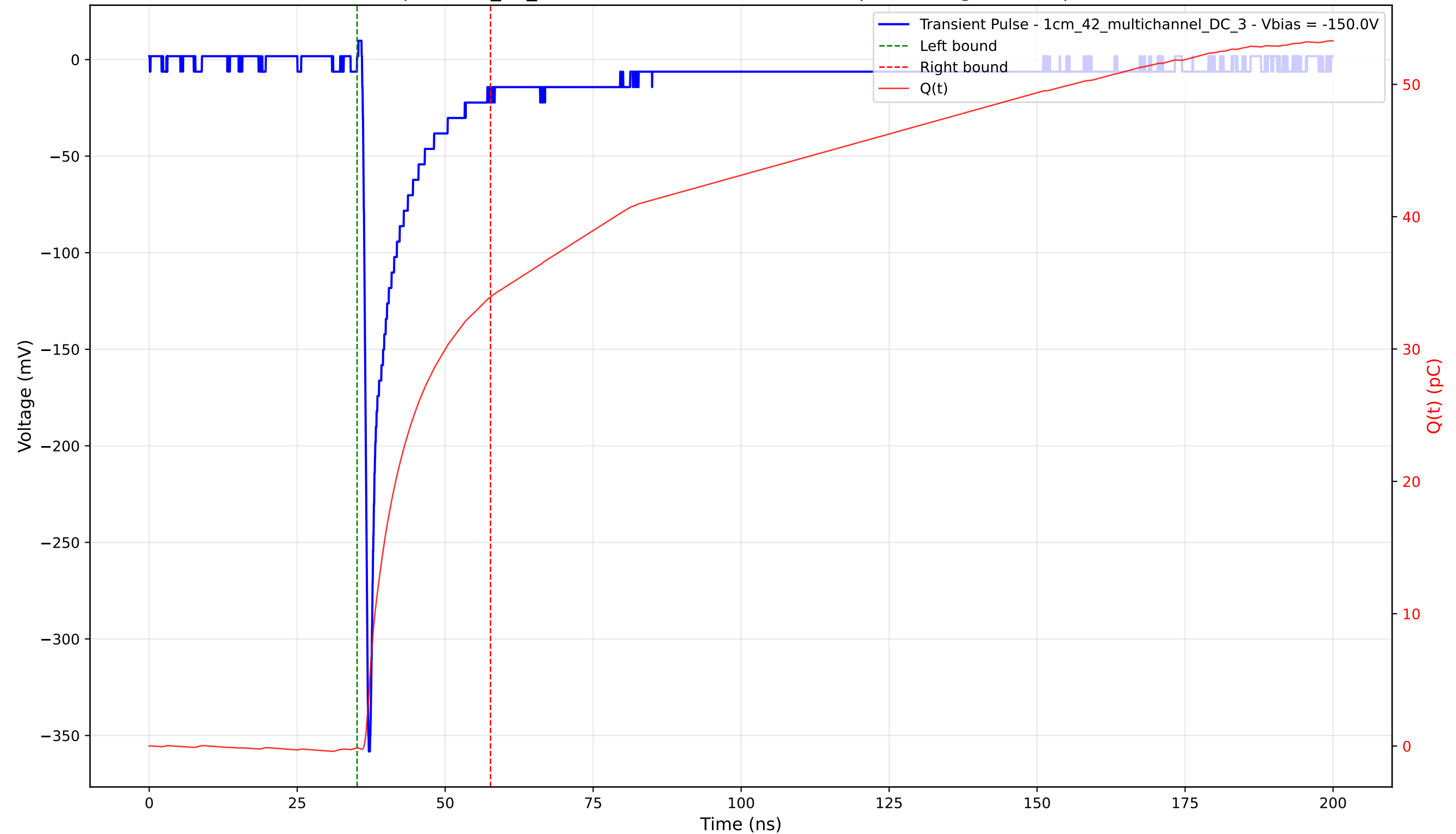
Transient Pulse - Sample: 1cm_42_multichannel - Position: 4775.0 \mu\text{m} - Charge: 34.07 pC - Rise Time: 0.78 ns
