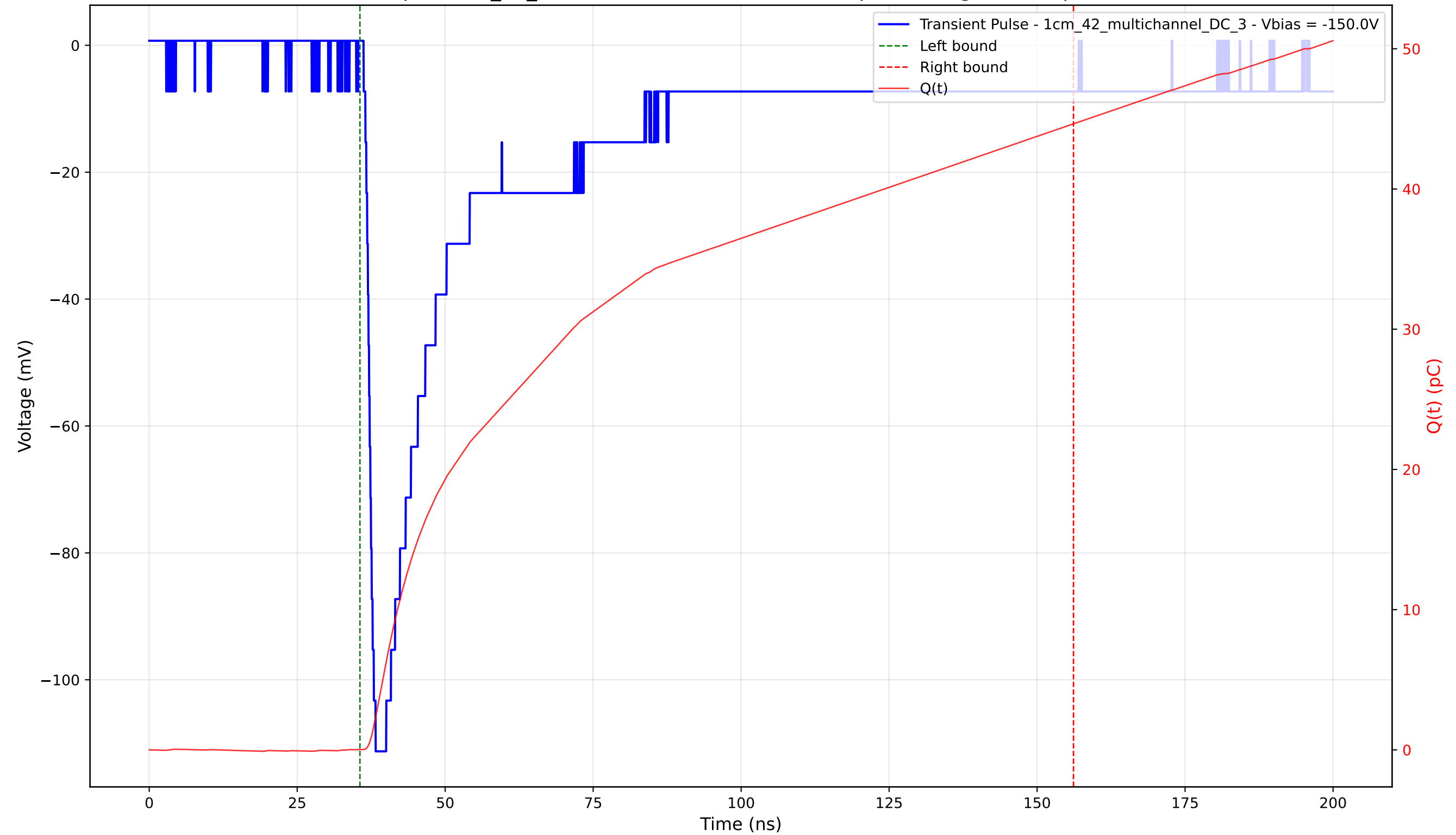
Transient Pulse - Sample: 1cm_42_multichannel - Position: 3460.0 \mu\text{m} - Charge: 44.64 pC - Rise Time: 1.43 ns
