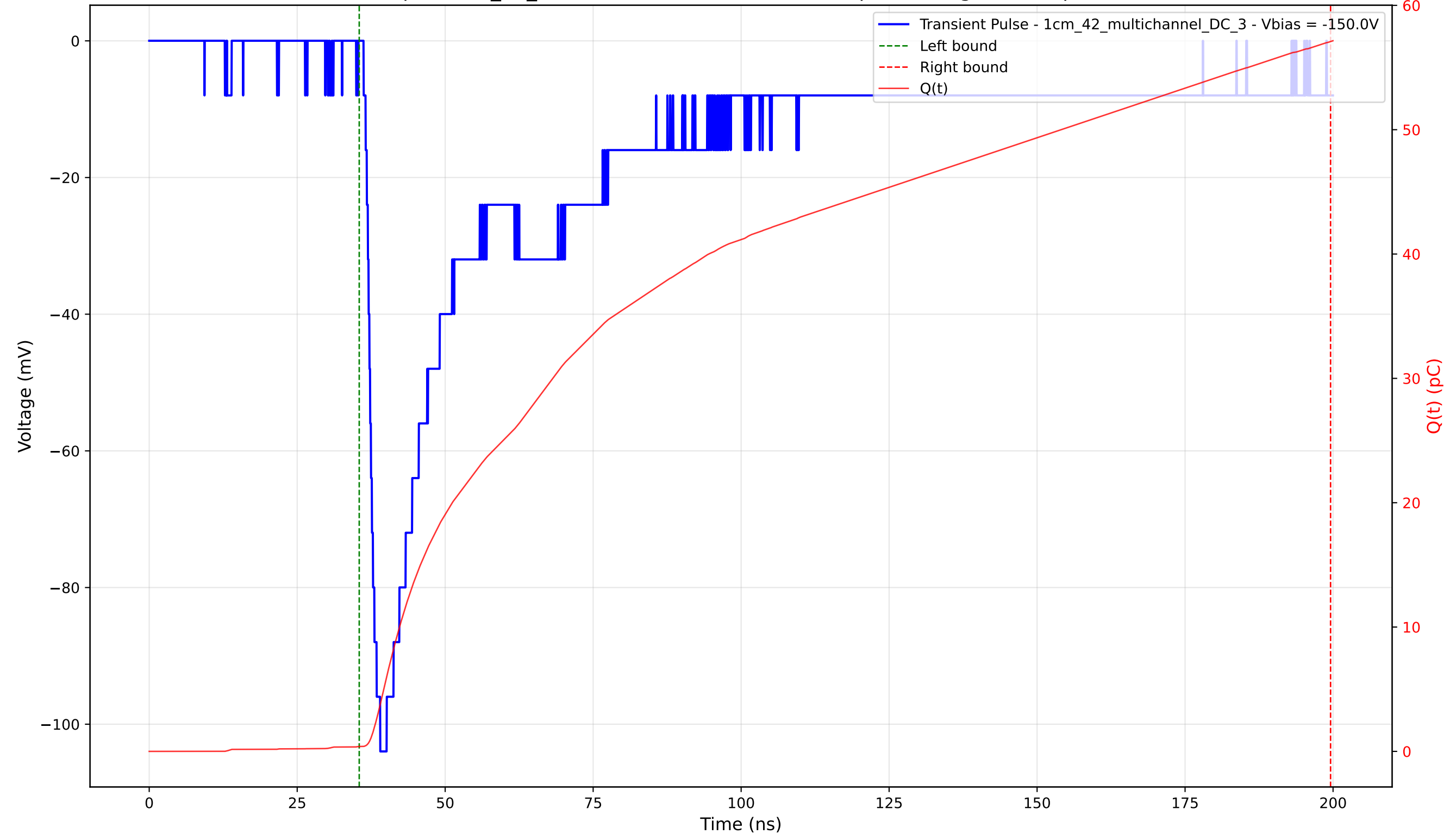
Transient Pulse - Sample: 1cm_42_multichannel - Position: 2995.0 \mu\text{m} - Charge: 56.70 pC - Rise Time: 1.87 ns
