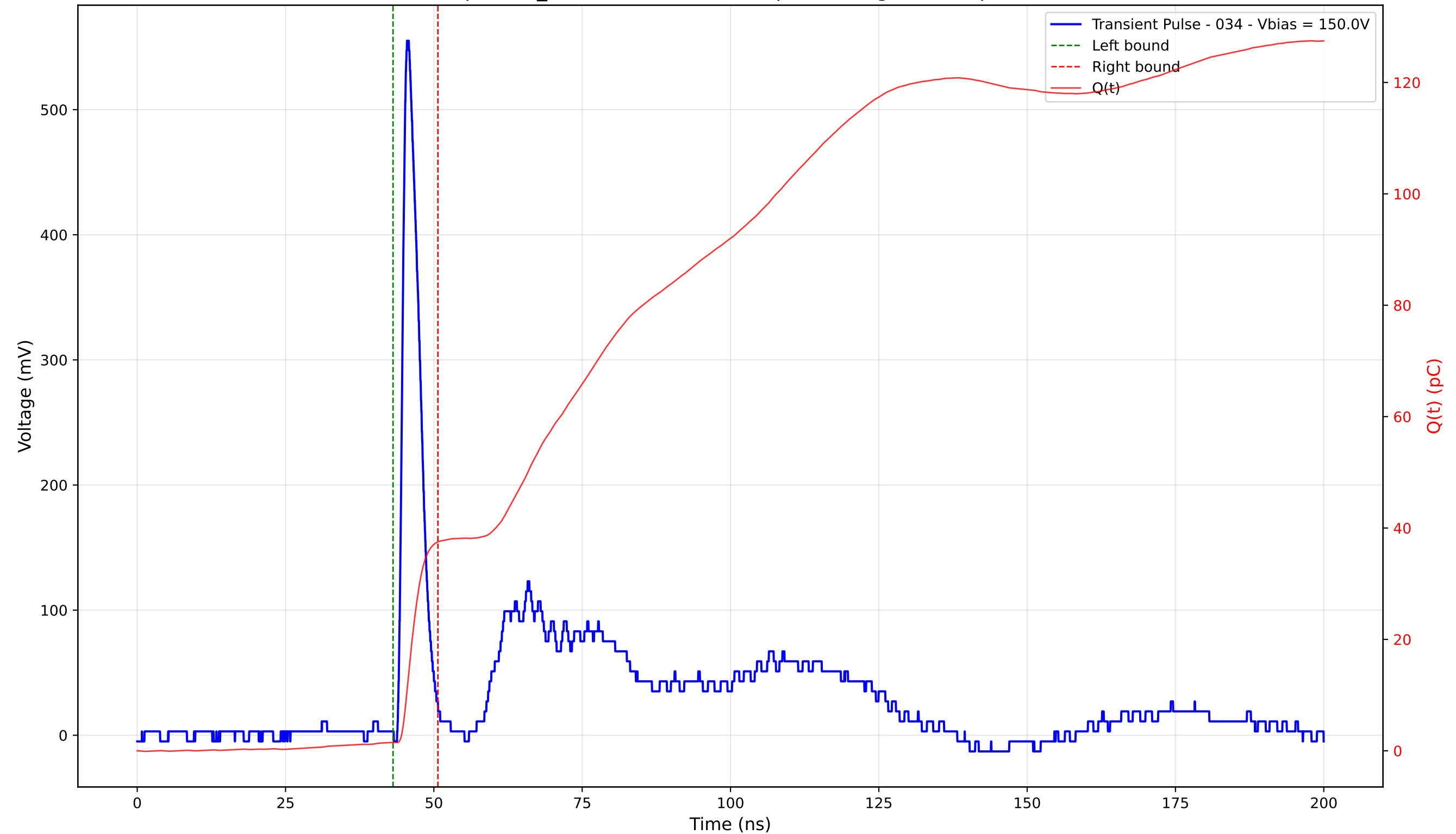
Transient Pulse - Sample: TD_4004 - Position: 300.0 \mu\text{m} - Charge: 36.00 pC - Rise Time: 1.07 ns
