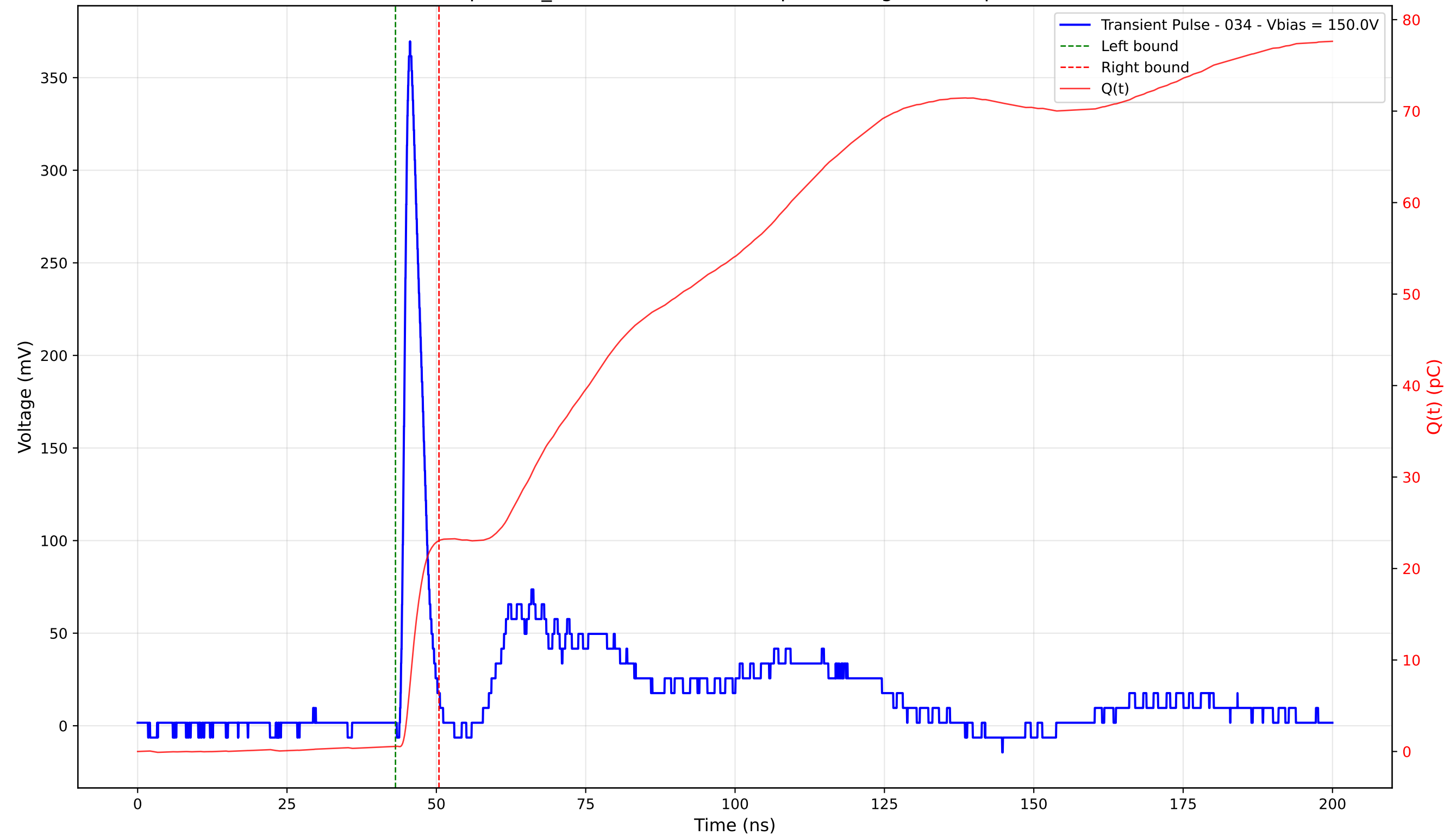
Transient Pulse - Sample: TD_4004 - Position: 335.0 \mu\text{m} - Charge: 22.48 pC - Rise Time: 1.07 ns
