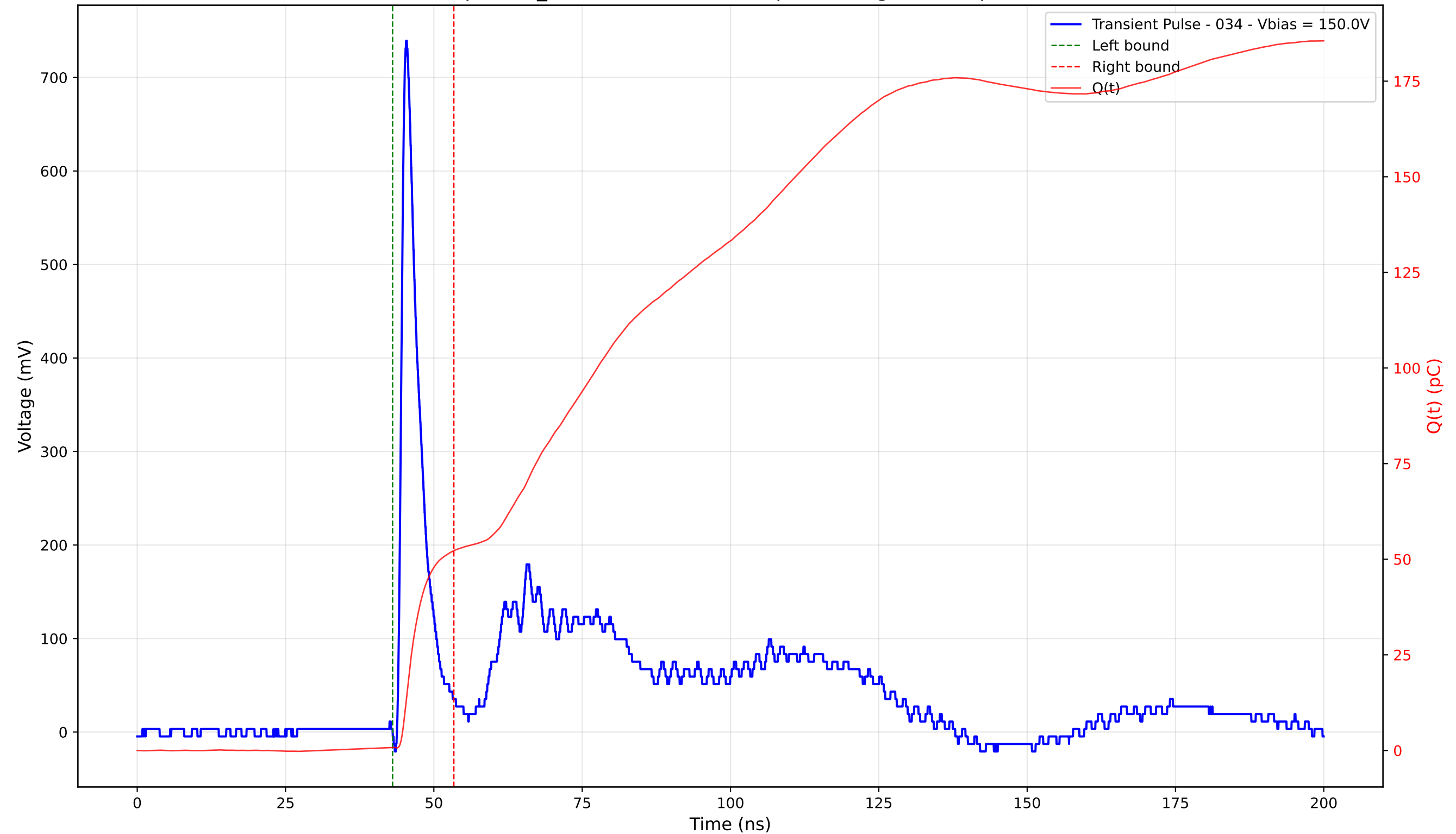
Transient Pulse - Sample: TD_4004 - Position: 120.0 \mu\text{m} - Charge: 51.40 pC - Rise Time: 0.94 ns
