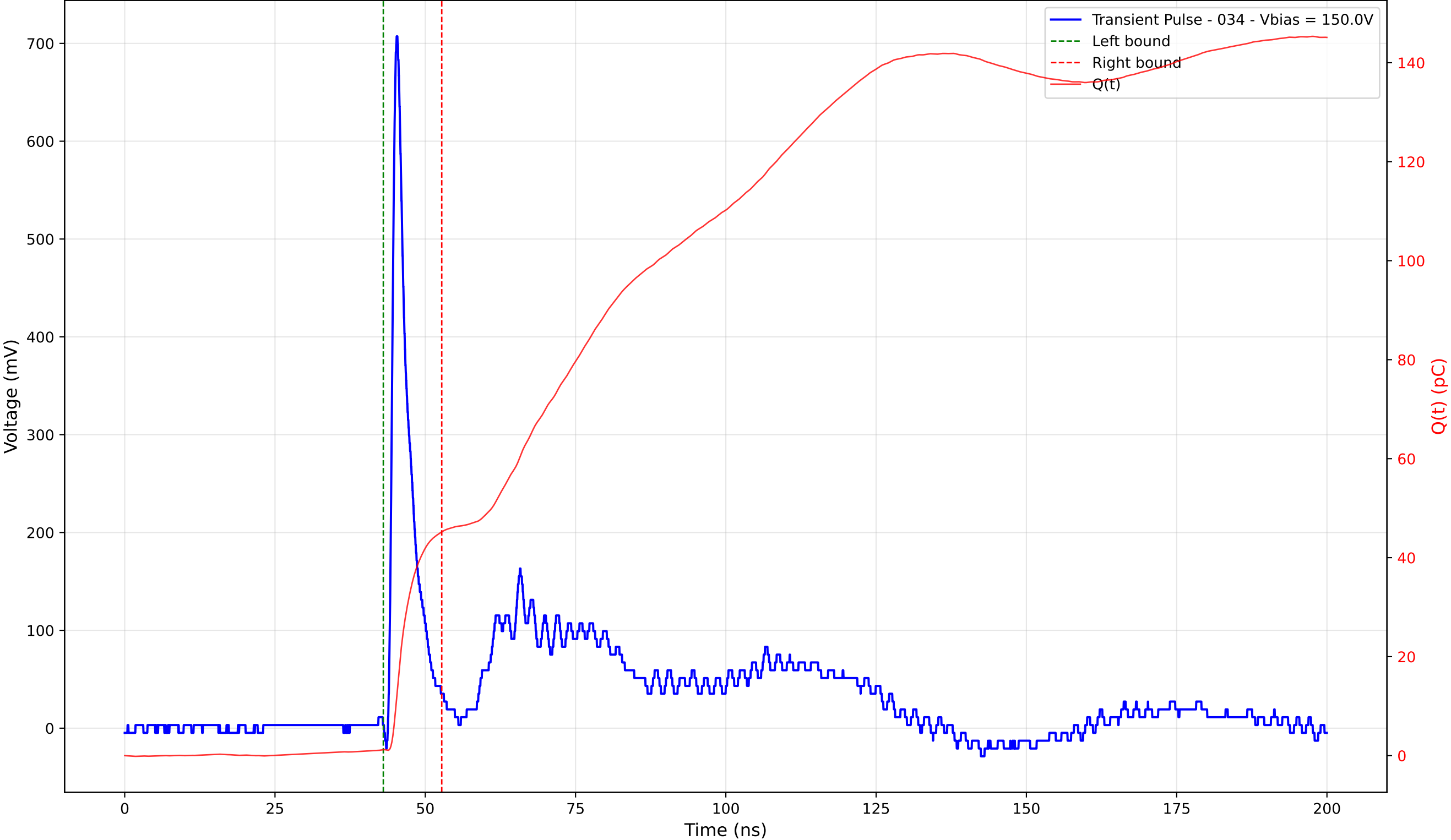
Transient Pulse - Sample: TD_4004 - Position: 90.0 \mu\text{m} - Charge: 44.01 pC - Rise Time: 0.91 ns
