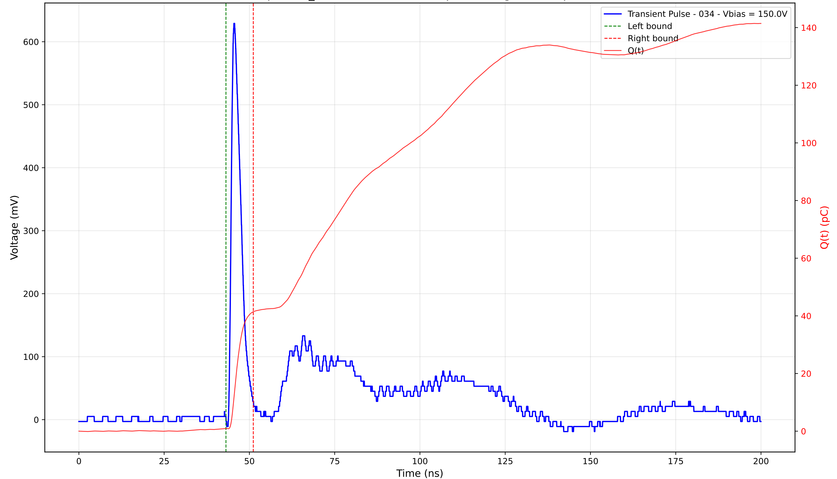
Transient Pulse - Sample: TD_4004 - Position: 255.0 \mu\text{m} - Charge: 40.50 pC - Rise Time: 1.02 ns
