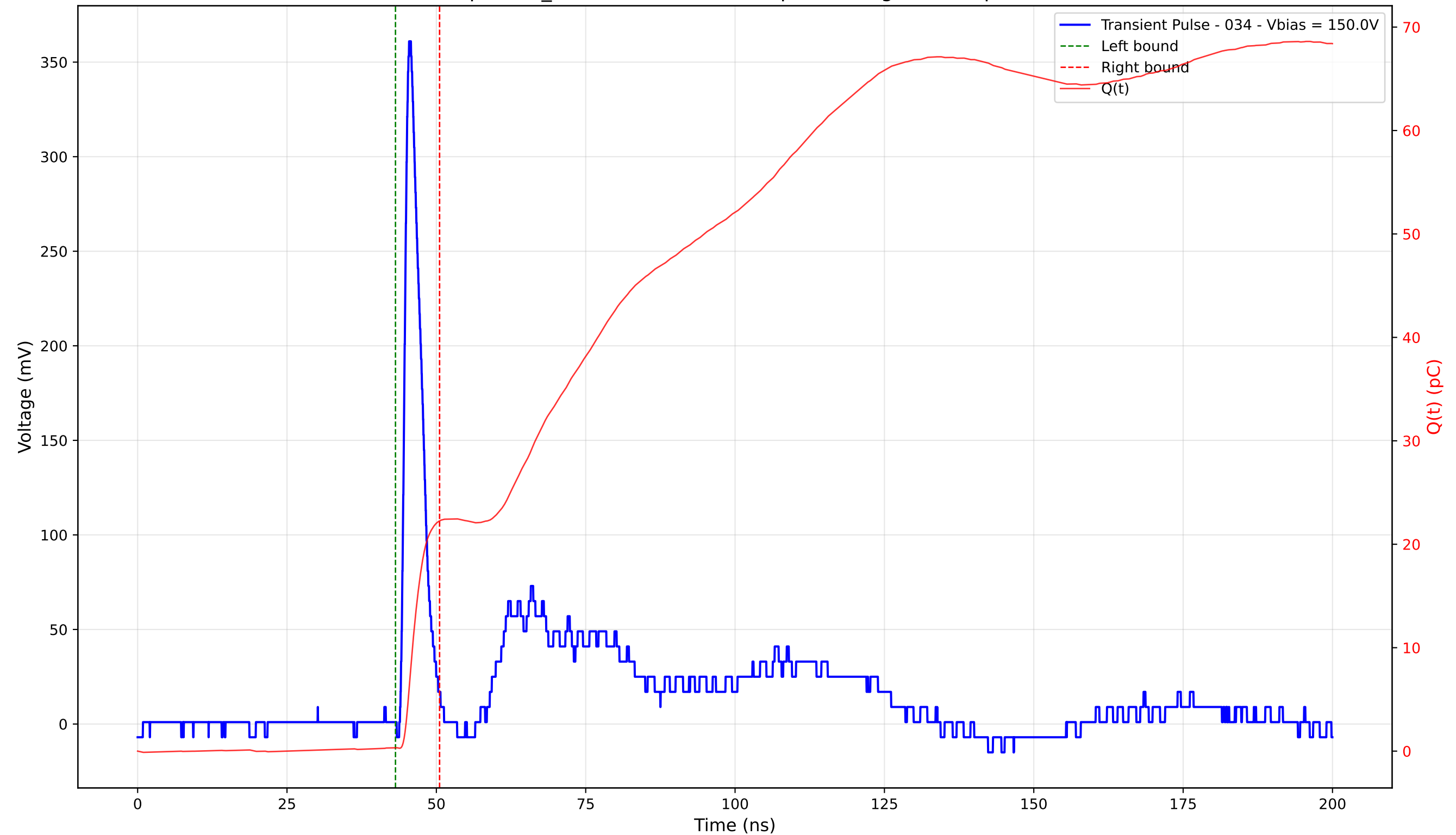
Transient Pulse - Sample: TD_4004 - Position: 340.0 \mu\text{m} - Charge: 21.93 pC - Rise Time: 1.01 ns
