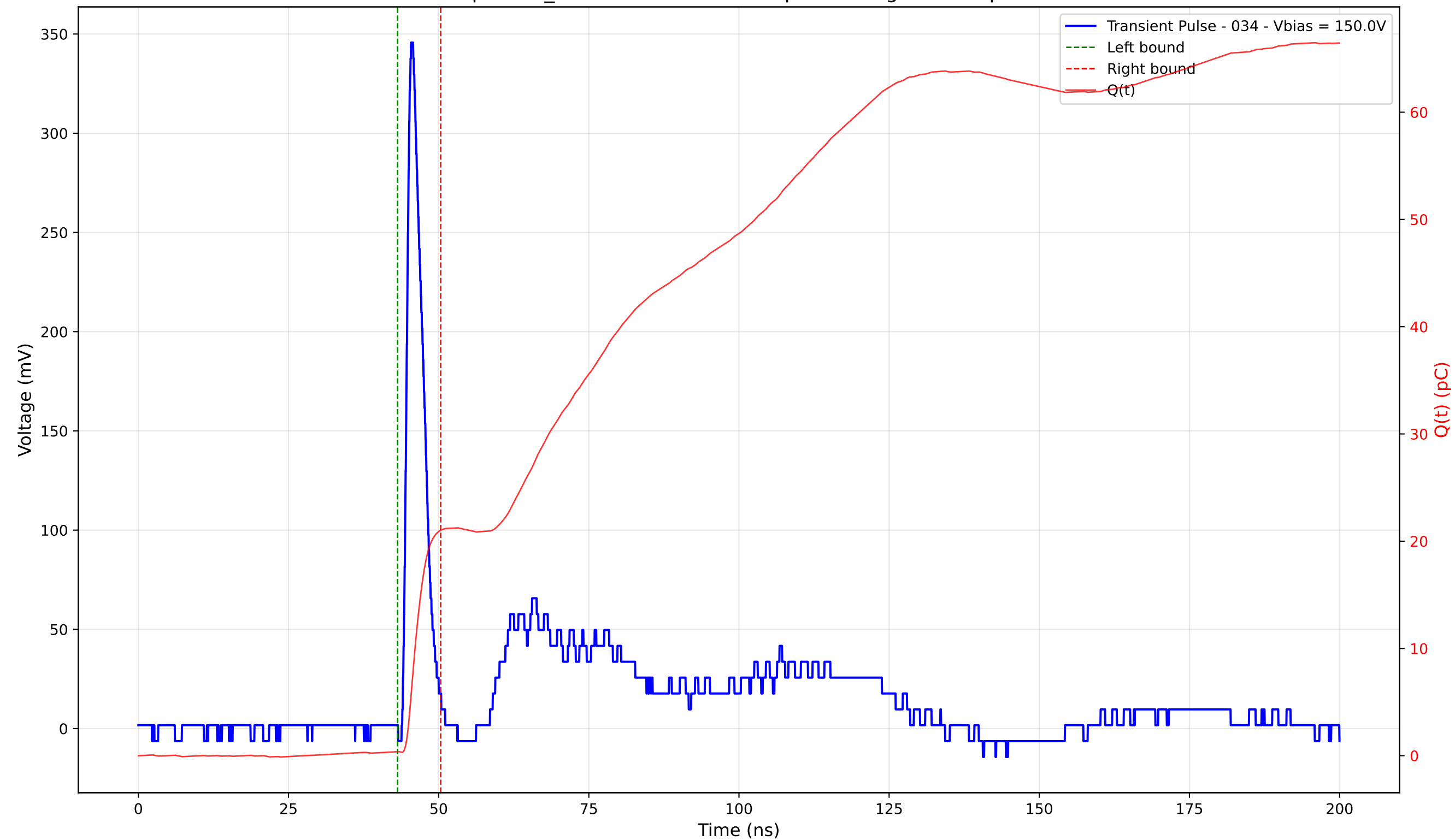
Transient Pulse - Sample: TD_4004 - Position: 355.0 \mu\text{m} - Charge: 20.64 pC - Rise Time: 1.00 ns
