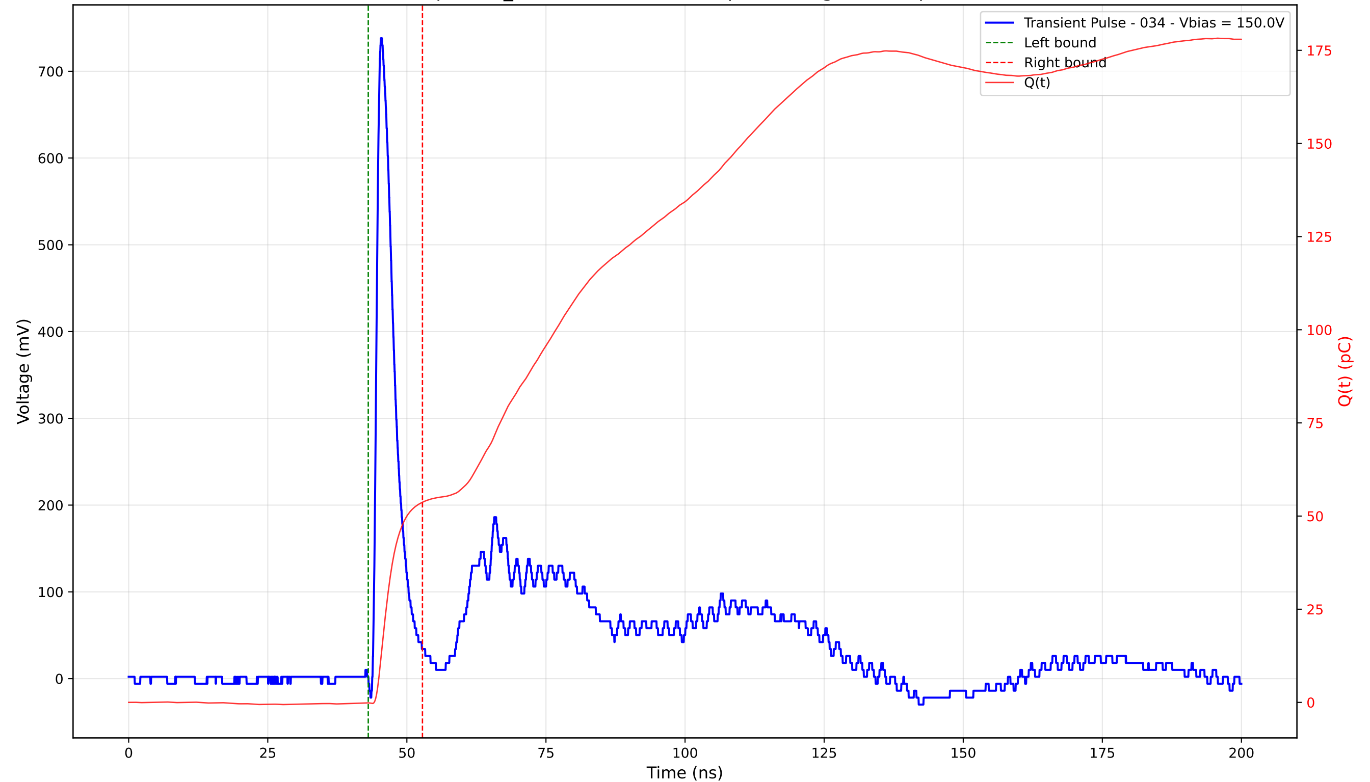
Transient Pulse - Sample: TD_4004 - Position: 180.0 \mu\text{m} - Charge: 53.85 pC - Rise Time: 0.94 ns
