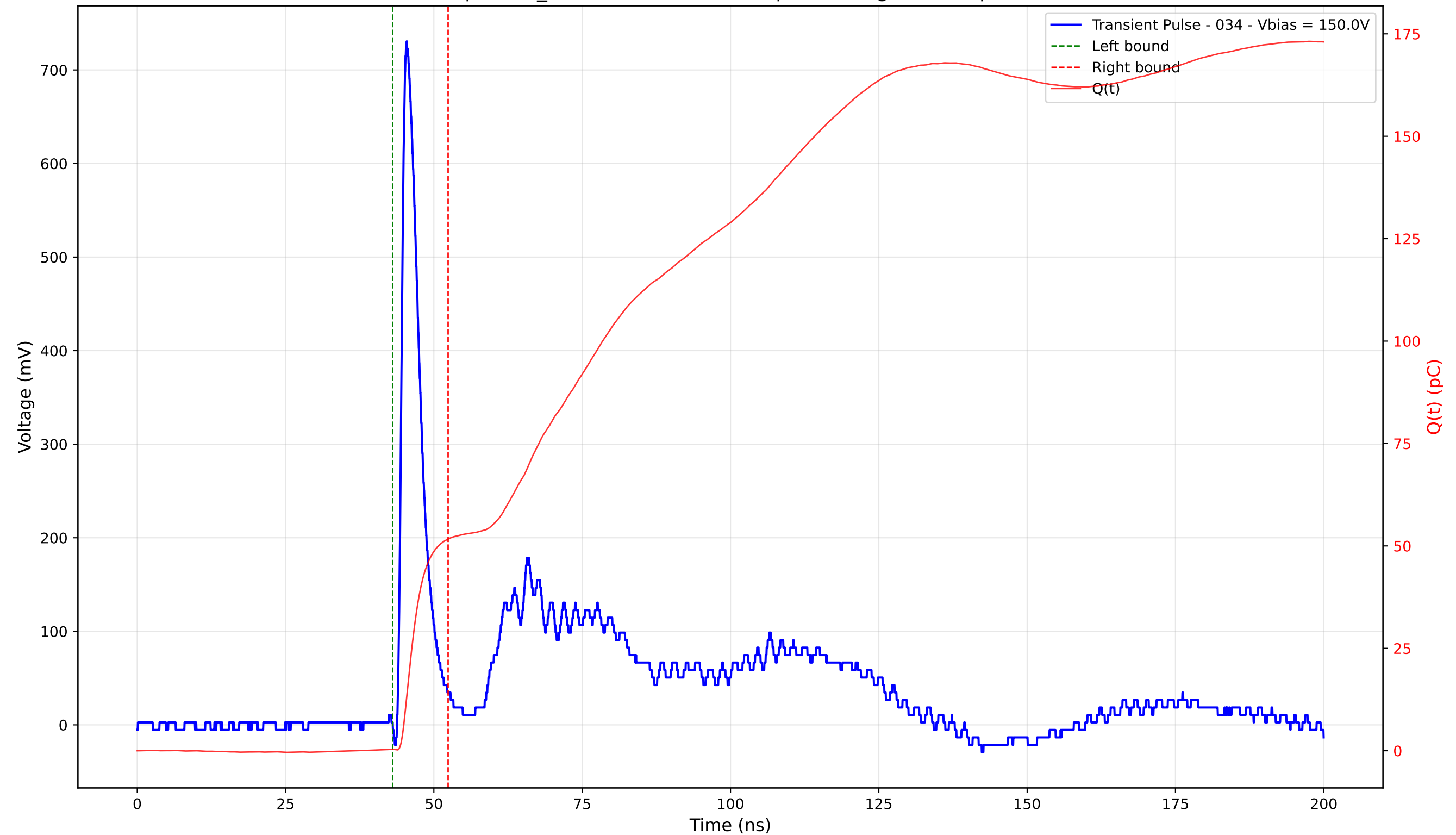
Transient Pulse - Sample: TD_4004 - Position: 205.0 \mu\text{m} - Charge: 51.31 pC - Rise Time: 0.96 ns
