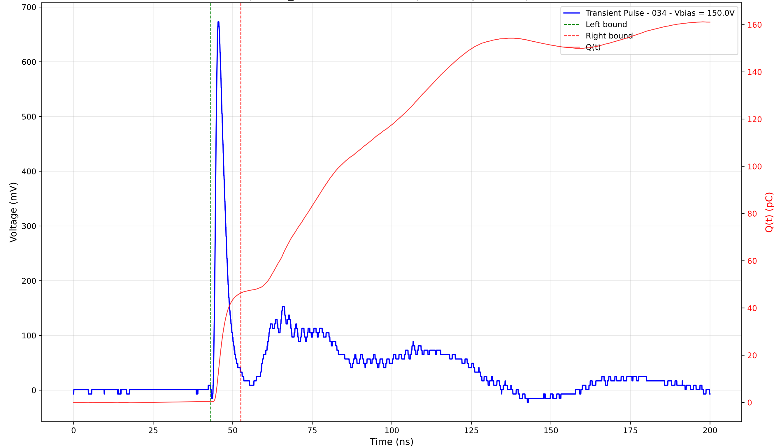
Transient Pulse - Sample: TD_4004 - Position: 155.0 \mu\text{m} - Charge: 45.89 pC - Rise Time: 0.99 ns
