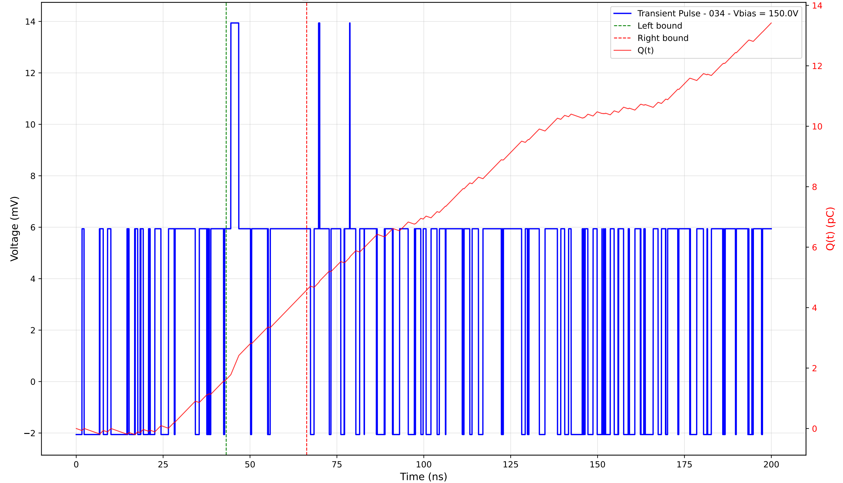
Transient Pulse - Sample: TD_4004 - Position: 15.0 \mu\text{m} - Charge: 2.96 pC - Rise Time: 0.00 ns (N/A)
