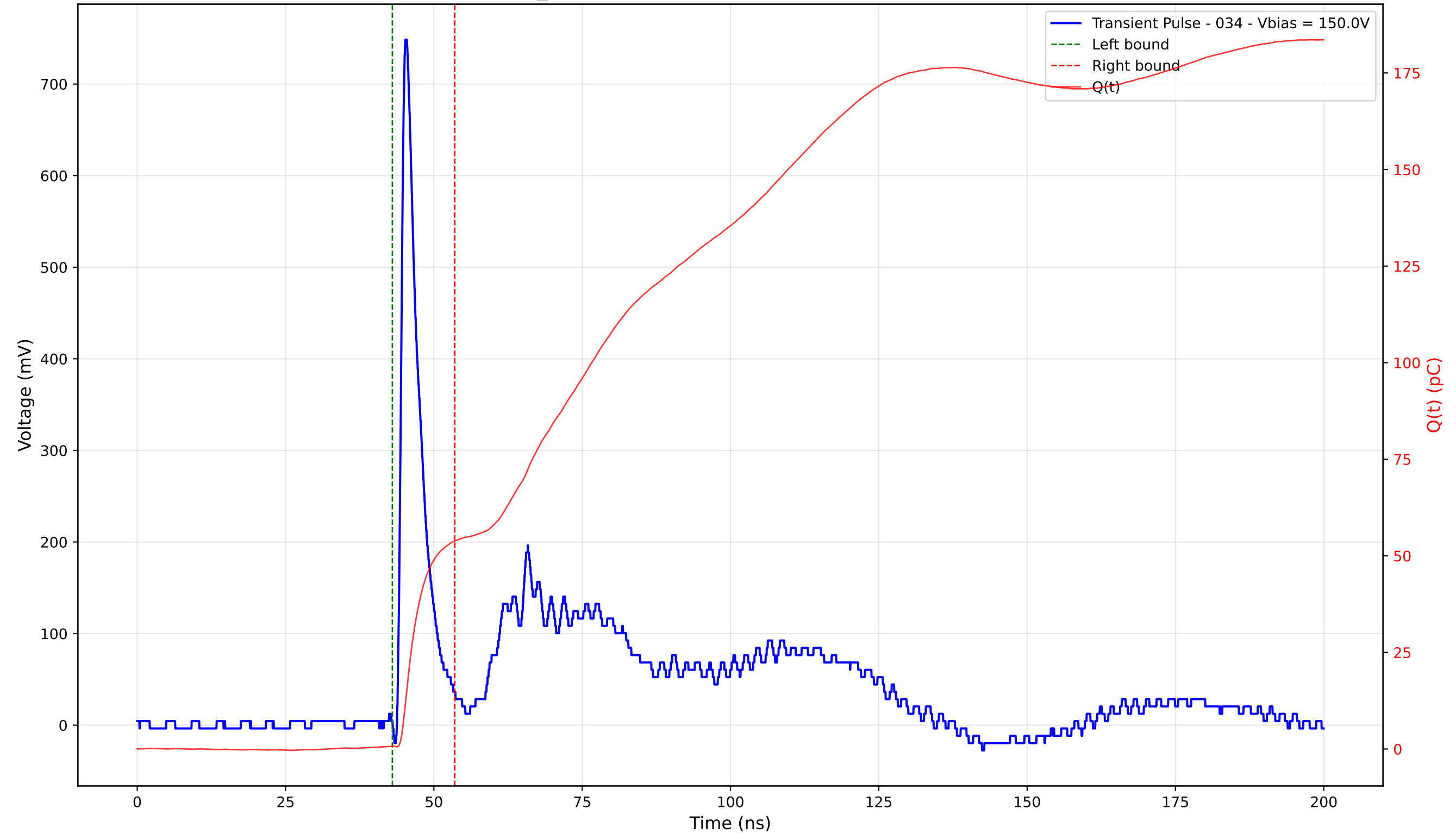
Transient Pulse - Sample: TD_4004 - Position: 110.0 \mu\text{m} - Charge: 53.13 pC - Rise Time: 0.90 ns
