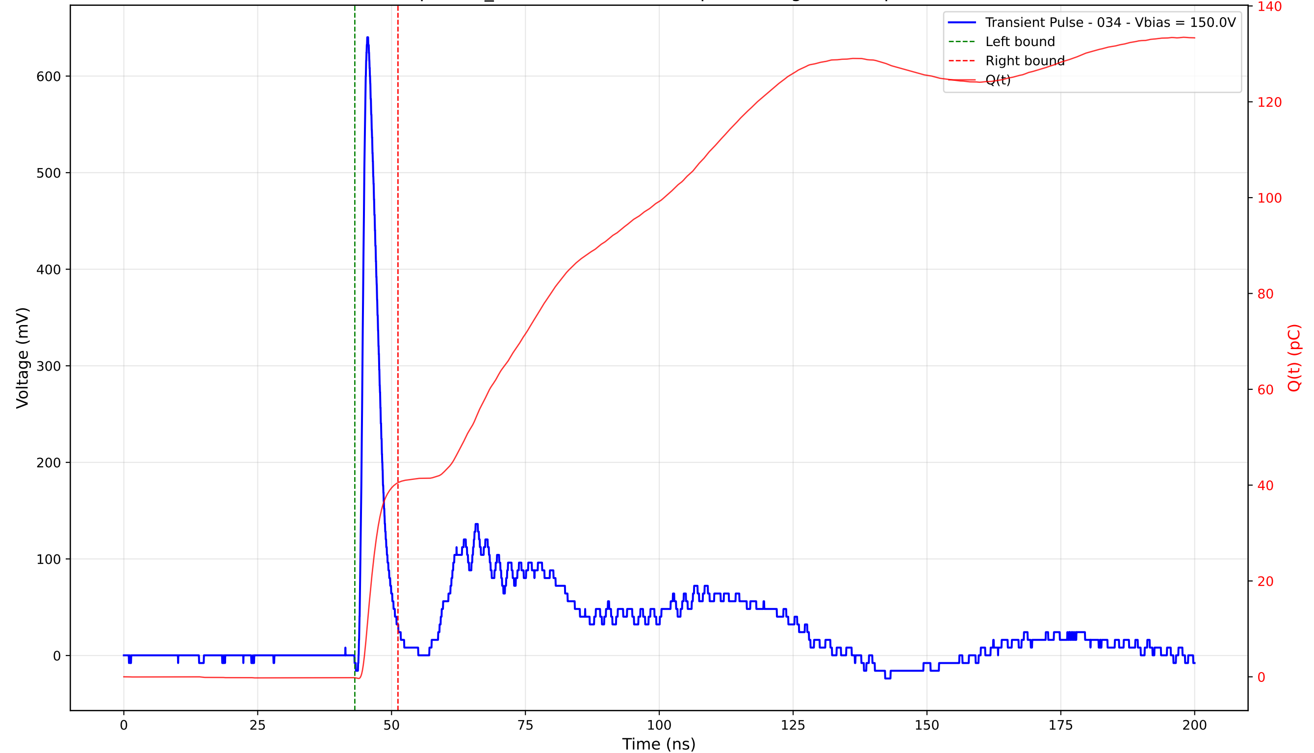
Transient Pulse - Sample: TD_4004 - Position: 240.0 \mu\text{m} - Charge: 40.70 pC - Rise Time: 1.00 ns
