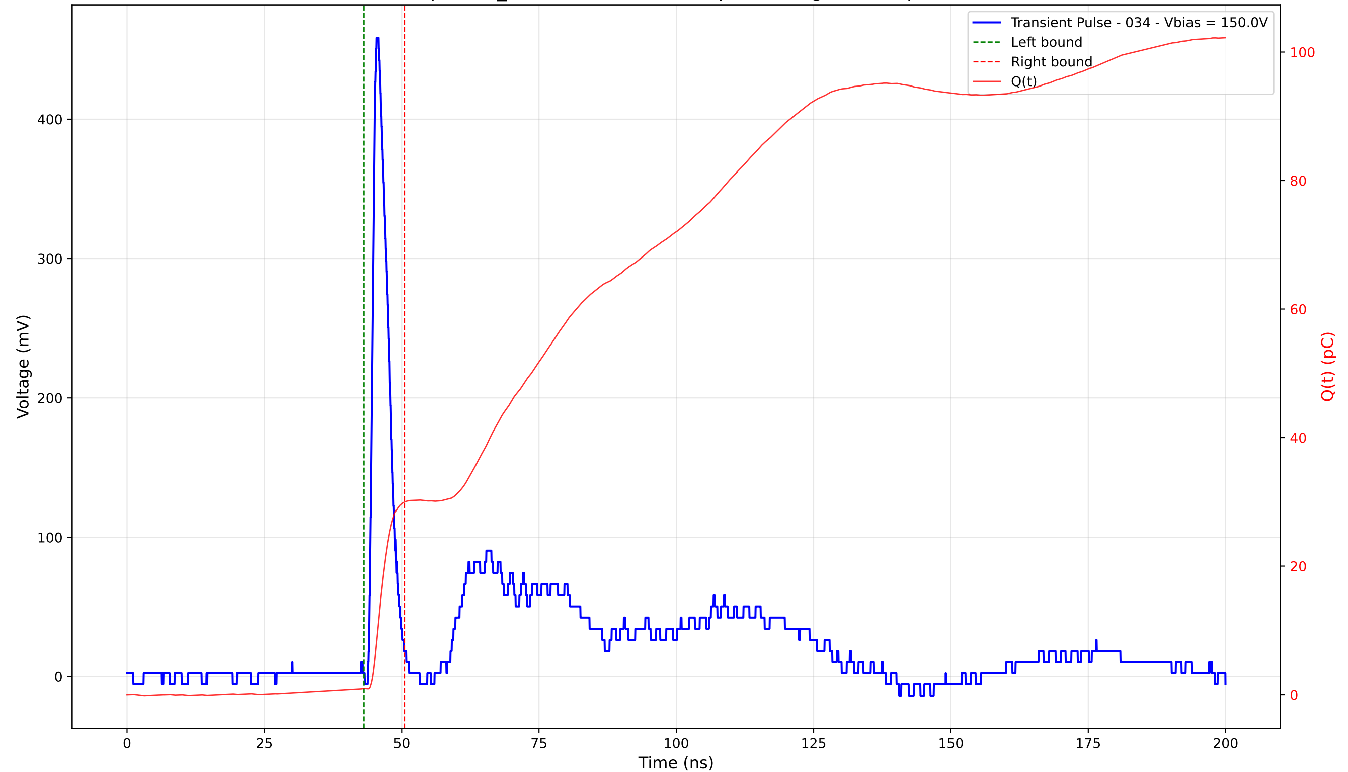
Transient Pulse - Sample: TD_4004 - Position: 320.0 \mu\text{m} - Charge: 28.99 pC - Rise Time: 1.05 ns
