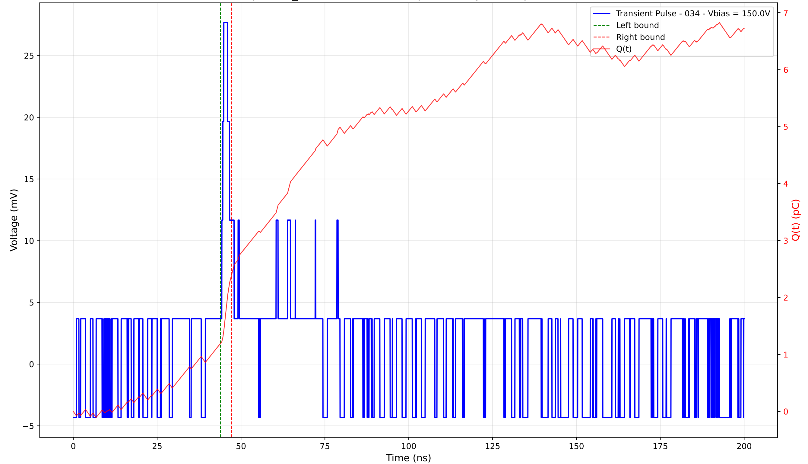
Transient Pulse - Sample: TD_4004 - Position: 35.0 \mu\text{m} - Charge: 1.22 pC - Rise Time: 0.00 ns (N/A)
