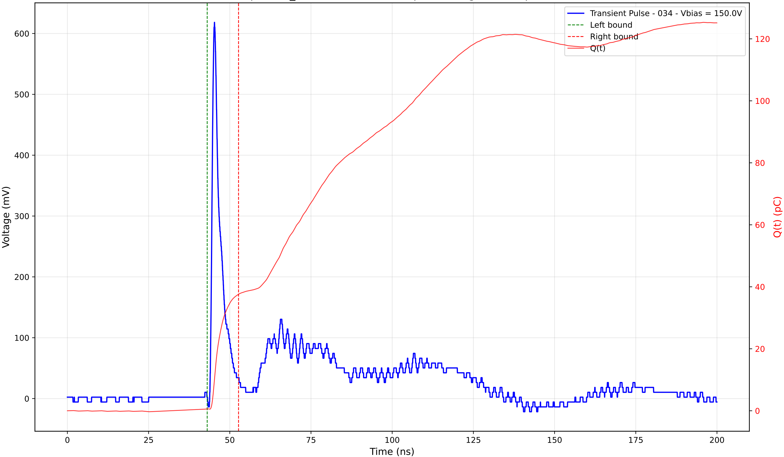
Transient Pulse - Sample: TD_4004 - Position: 80.0 \mu\text{m} - Charge: 36.97 pC - Rise Time: 0.92 ns
