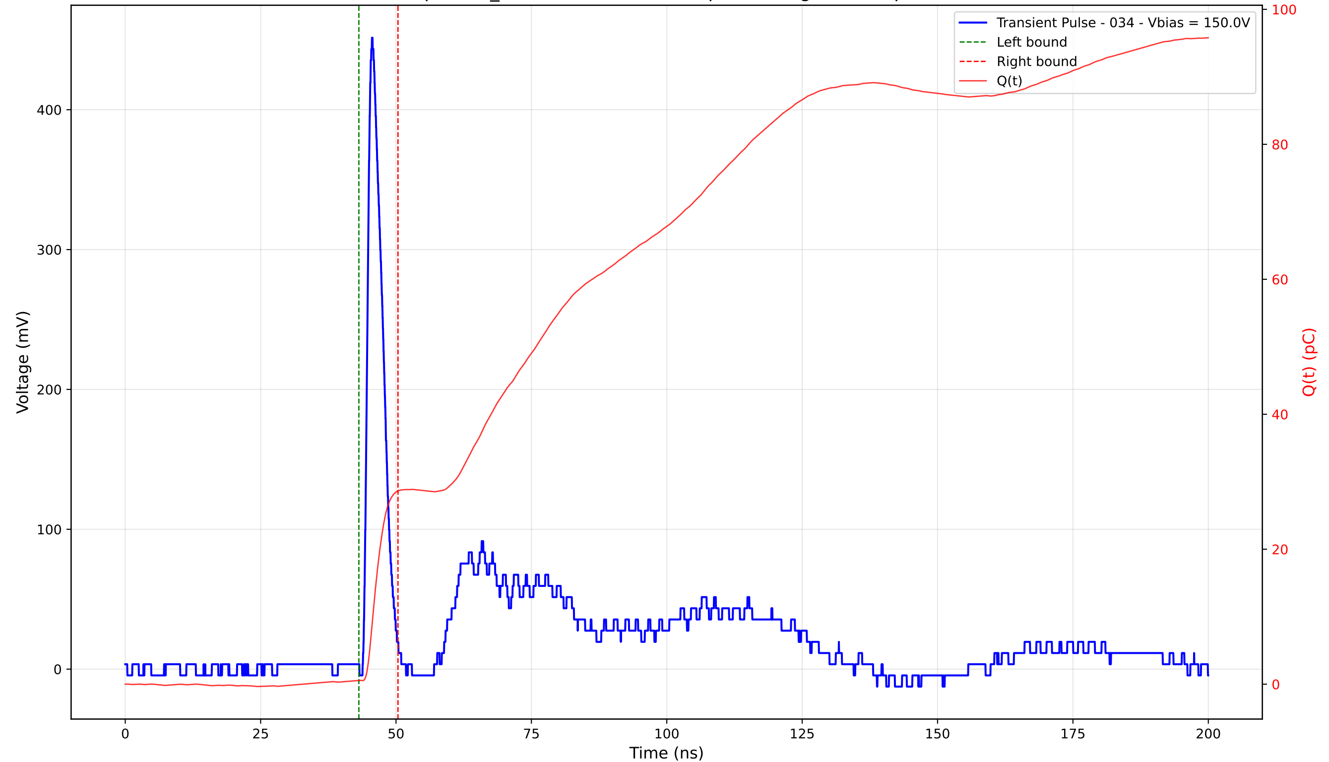
Transient Pulse - Sample: TD_4004 - Position: 325.0 \mu\text{m} - Charge: 28.07 pC - Rise Time: 1.06 ns
