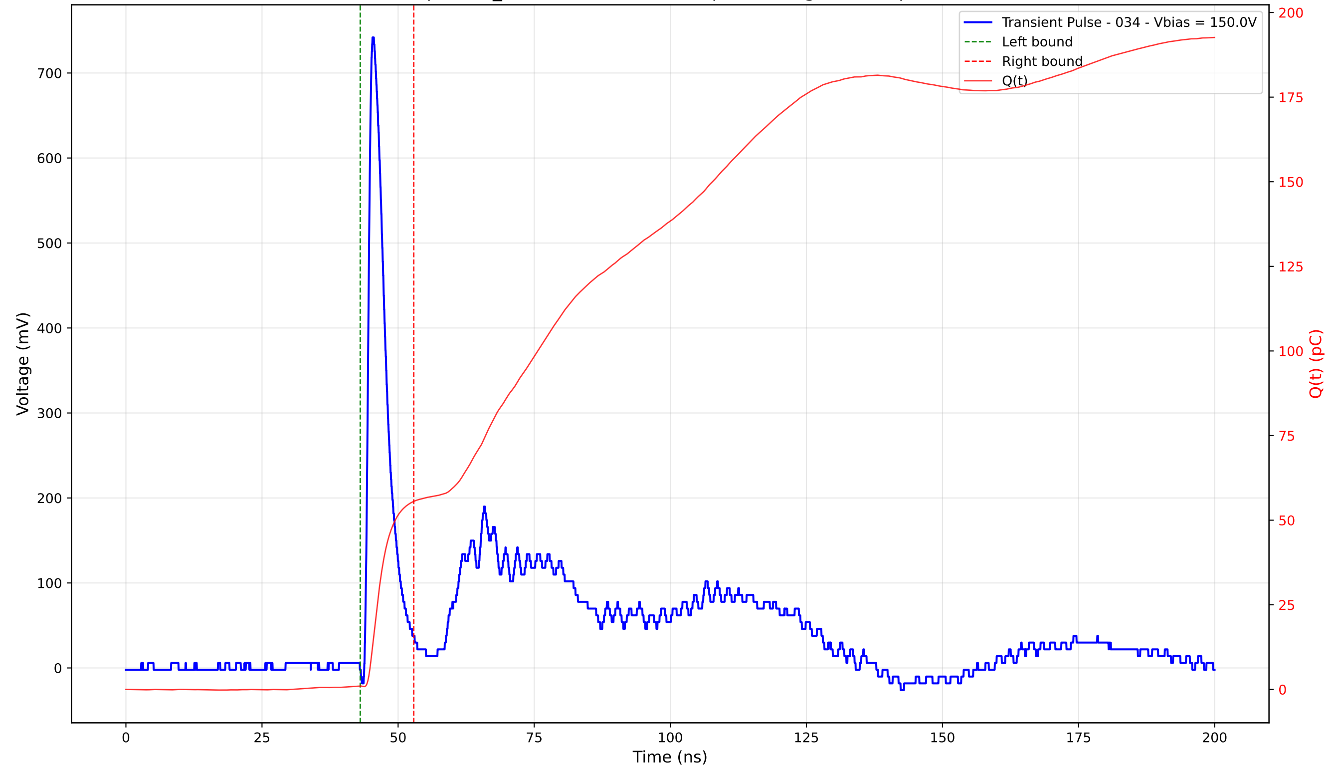
Transient Pulse - Sample: TD_4004 - Position: 190.0 \mu\text{m} - Charge: 54.55 pC - Rise Time: 0.94 ns
