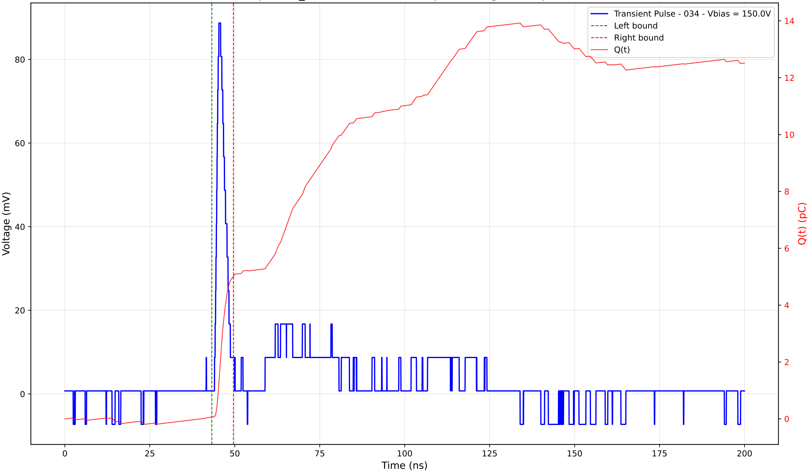
Transient Pulse - Sample: TD_4004 - Position: 415.0 \mu\text{m} - Charge: 4.96 pC - Rise Time: 0.92 ns
