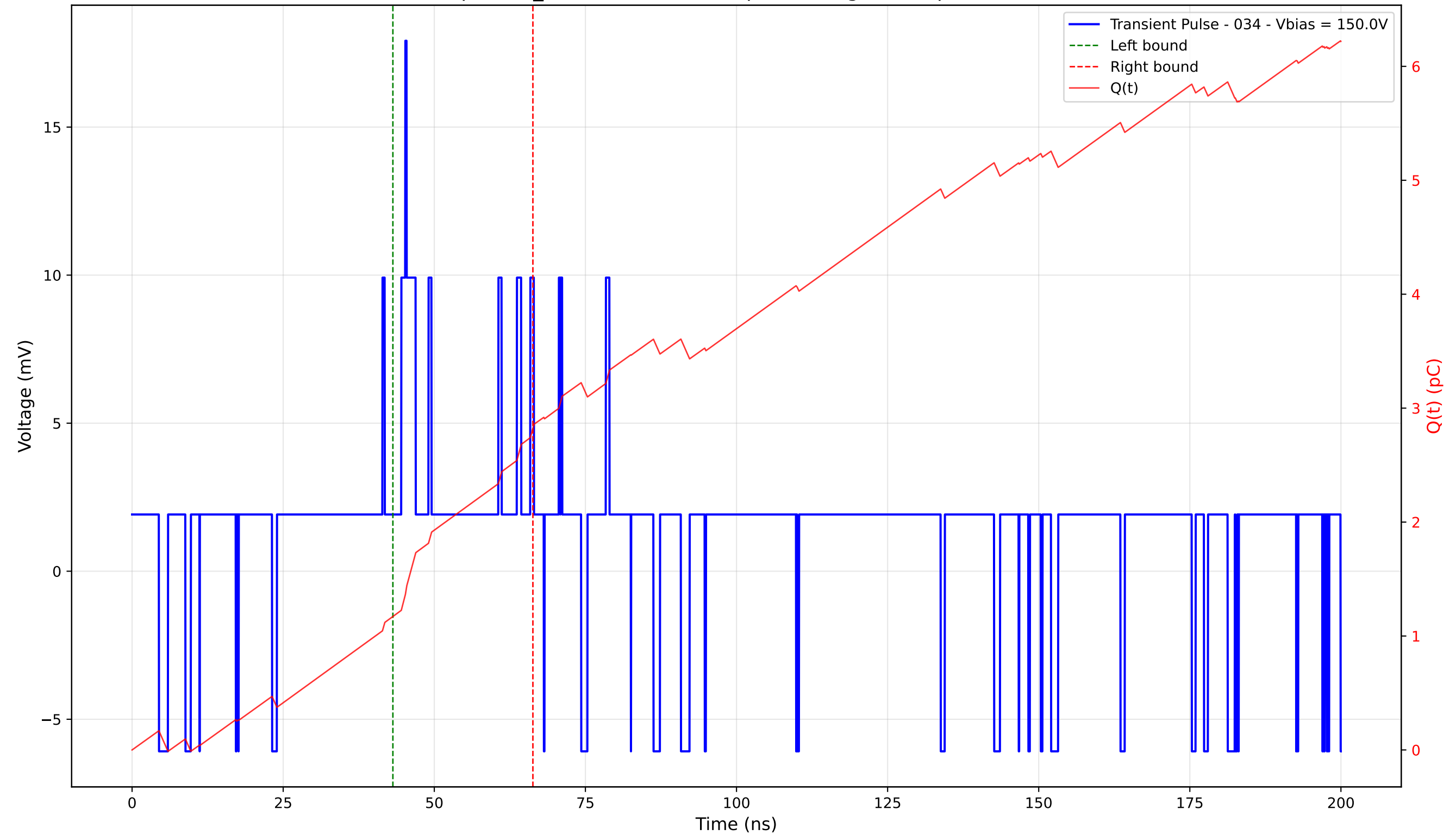
Transient Pulse - Sample: TD_4004 - Position: 5.0 \mu m - Charge: 1.65 pC - Rise Time: 0.00 ns (N/A)
