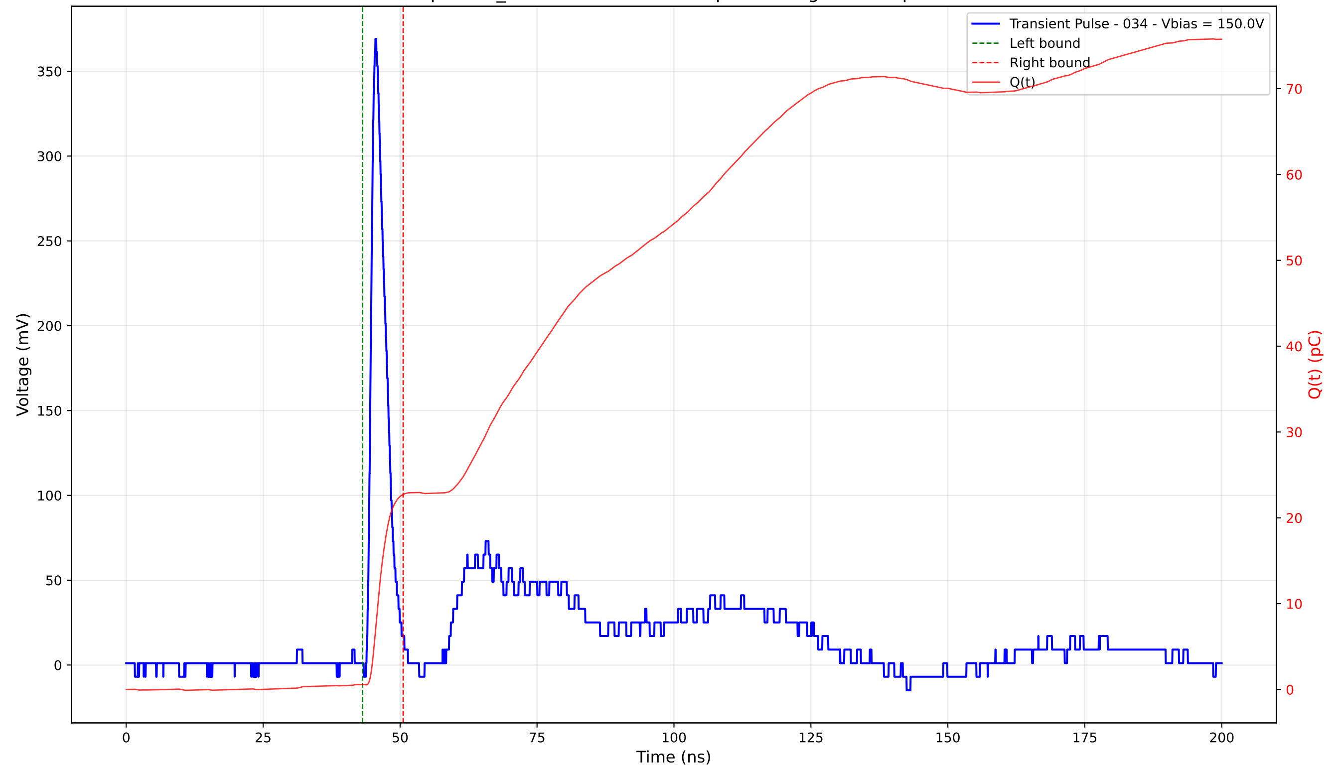
Transient Pulse - Sample: TD_4004 - Position: 345.0 \mu\text{m} - Charge: 22.13 pC - Rise Time: 1.05 ns
