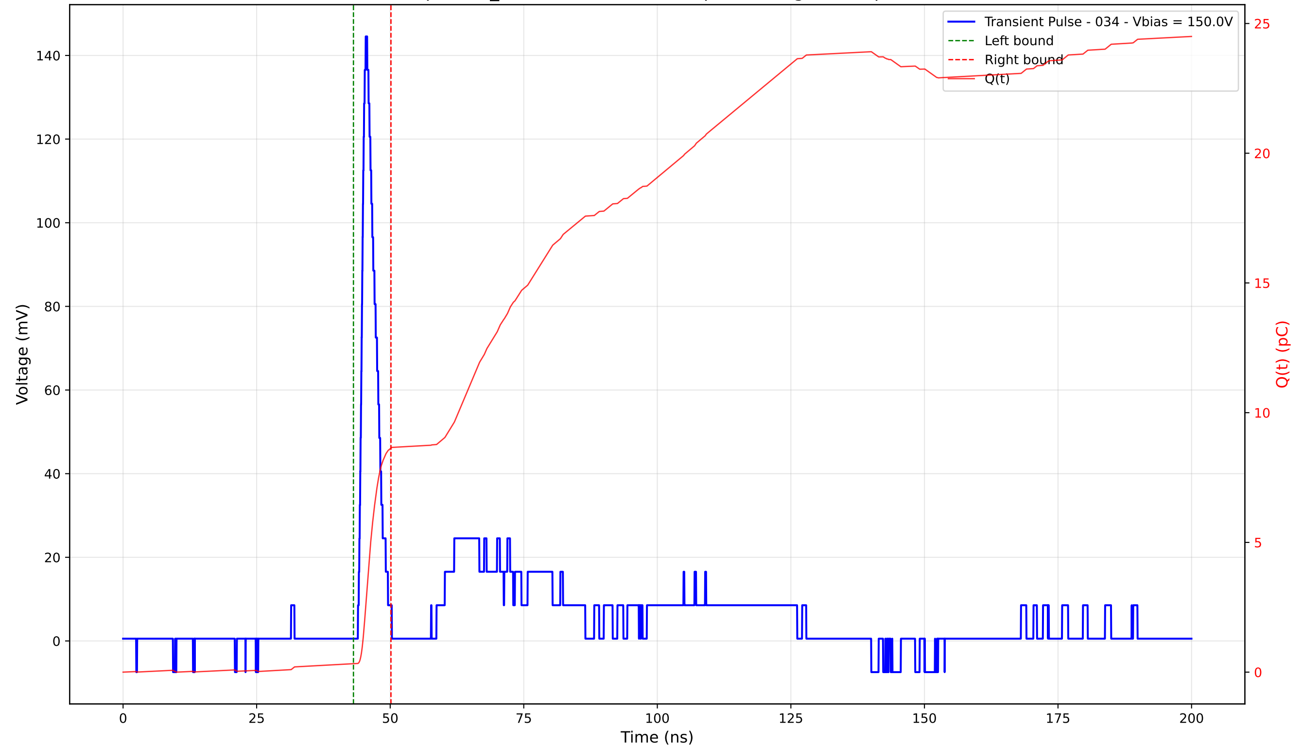
Transient Pulse - Sample: TD_4004 - Position: 405.0 \mu\text{m} - Charge: 8.31 pC - Rise Time: 1.11 ns
