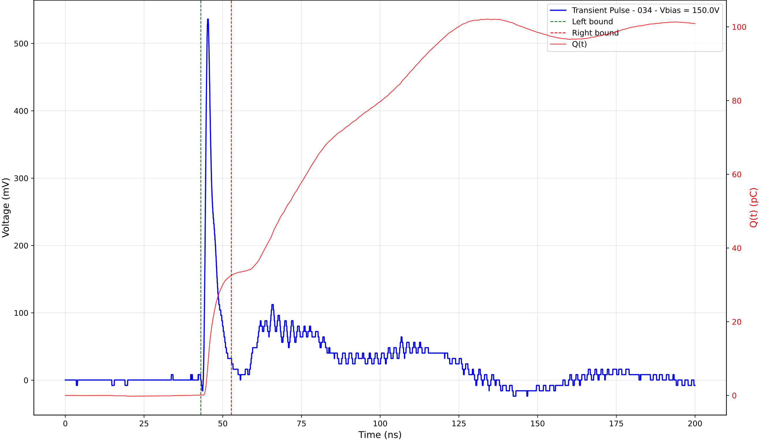
Transient Pulse - Sample: TD_4004 - Position: 75.0 \mu\text{m} - Charge: 32.40 pC - Rise Time: 0.89 ns
