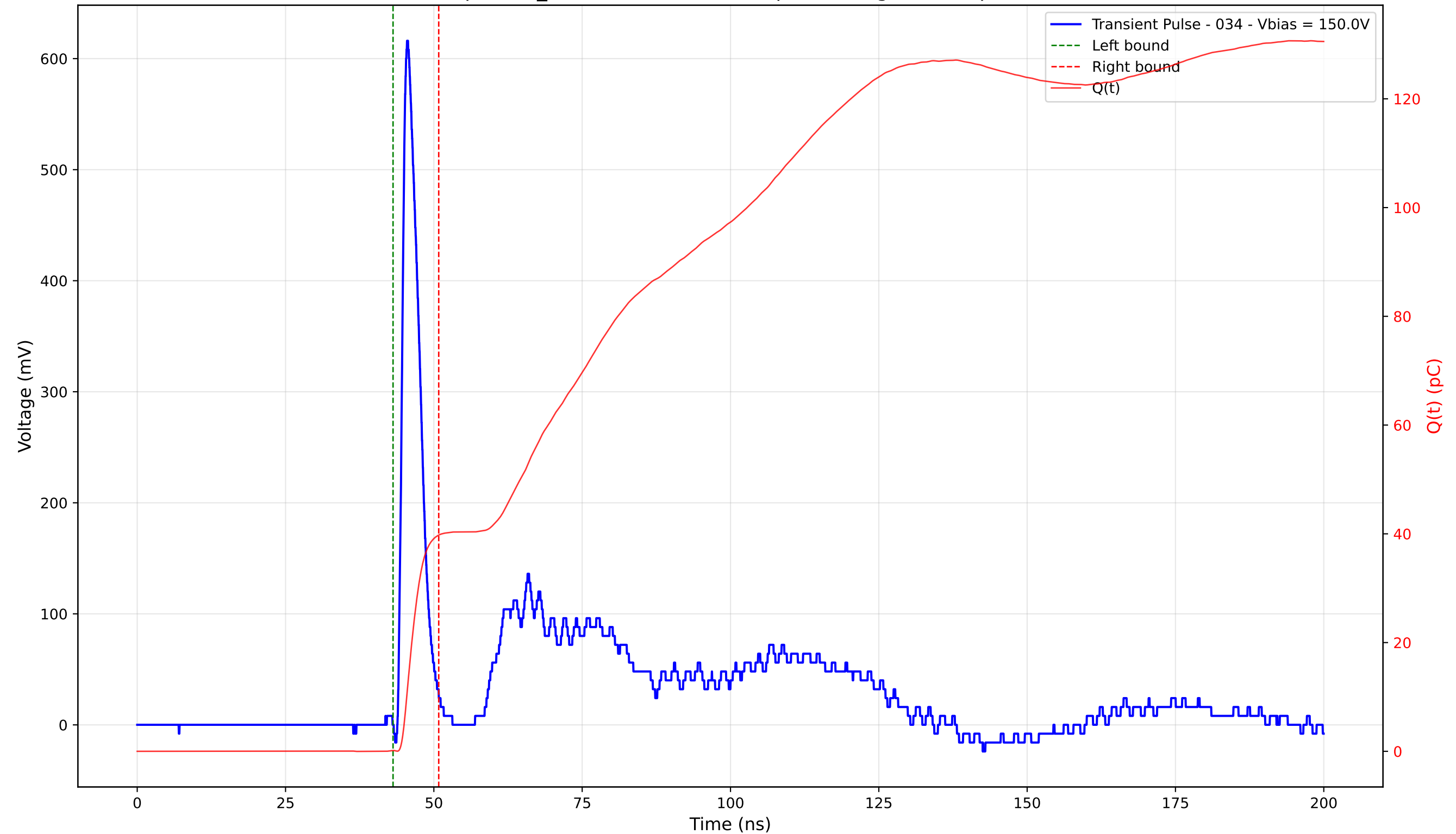
Transient Pulse - Sample: TD_4004 - Position: 275.0 \mu\text{m} - Charge: 39.62 pC - Rise Time: 1.01 ns
