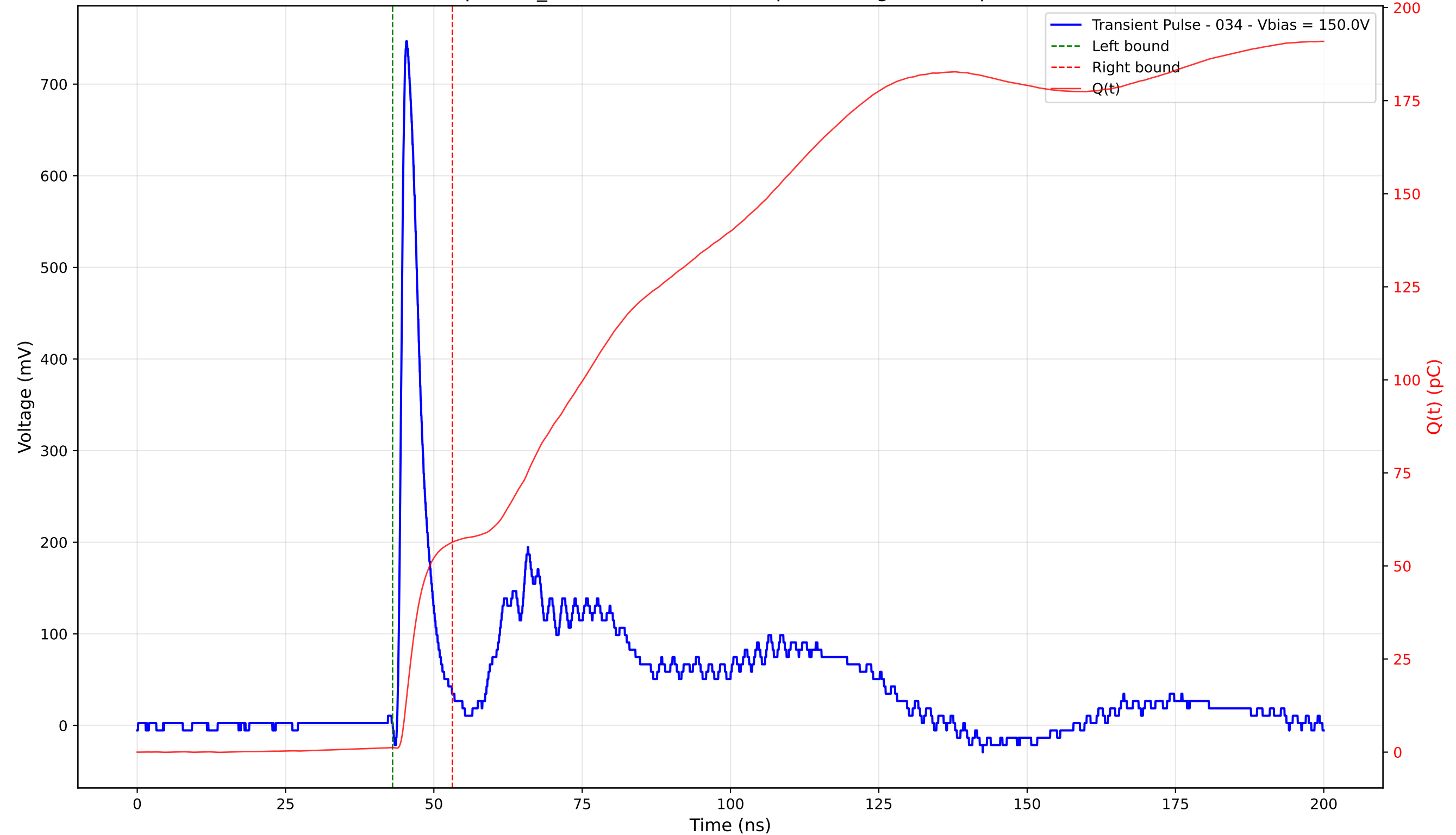
Transient Pulse - Sample: TD_4004 - Position: 185.0 \mu\text{m} - Charge: 55.16 pC - Rise Time: 0.94 ns
