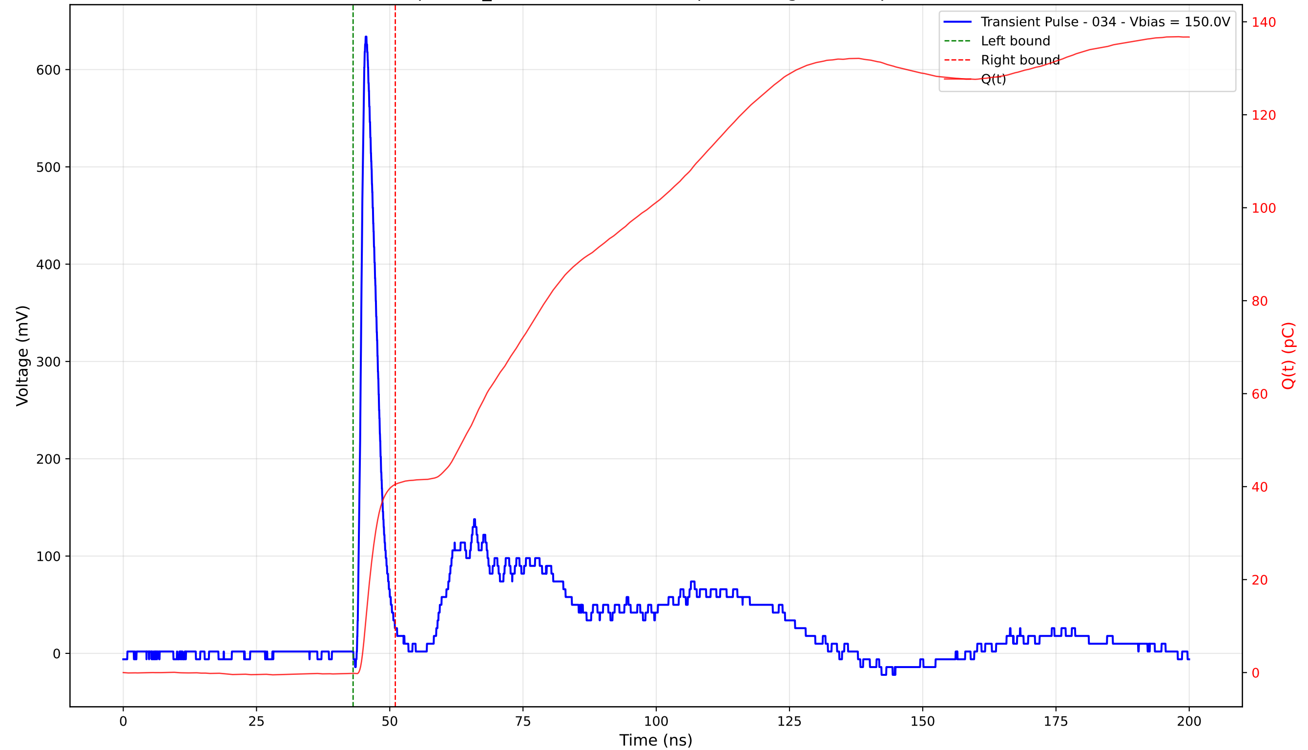
Transient Pulse - Sample: TD_4004 - Position: 250.0 \mu\text{m} - Charge: 40.65 pC - Rise Time: 1.03 ns
