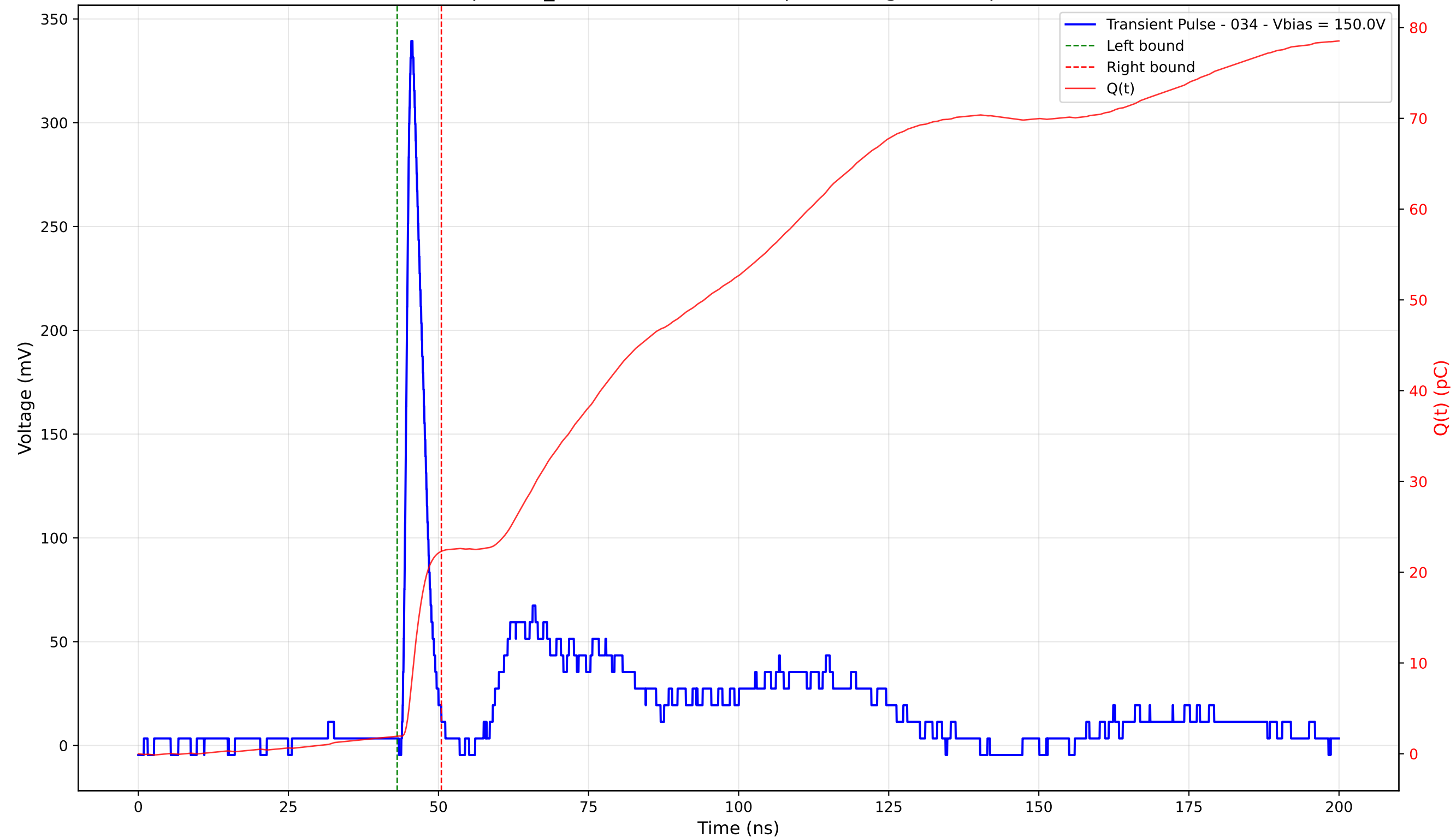
Transient Pulse - Sample: TD_4004 - Position: 360.0 \mu\text{m} - Charge: 20.36 pC - Rise Time: 1.04 ns
