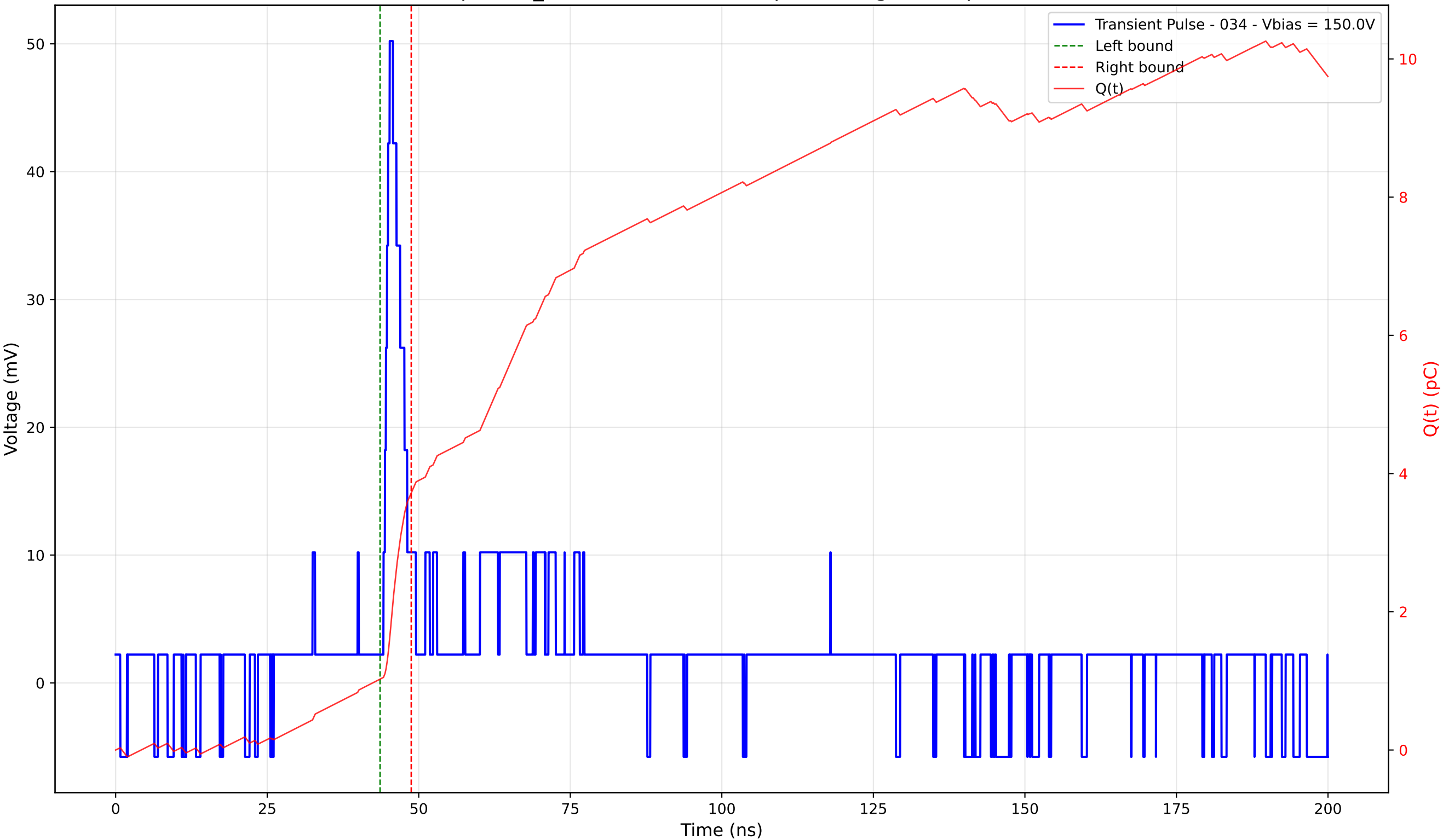
Transient Pulse - Sample: TD_4004 - Position: 425.0 \mu\text{m} - Charge: 2.70 pC - Rise Time: 1.03 ns
