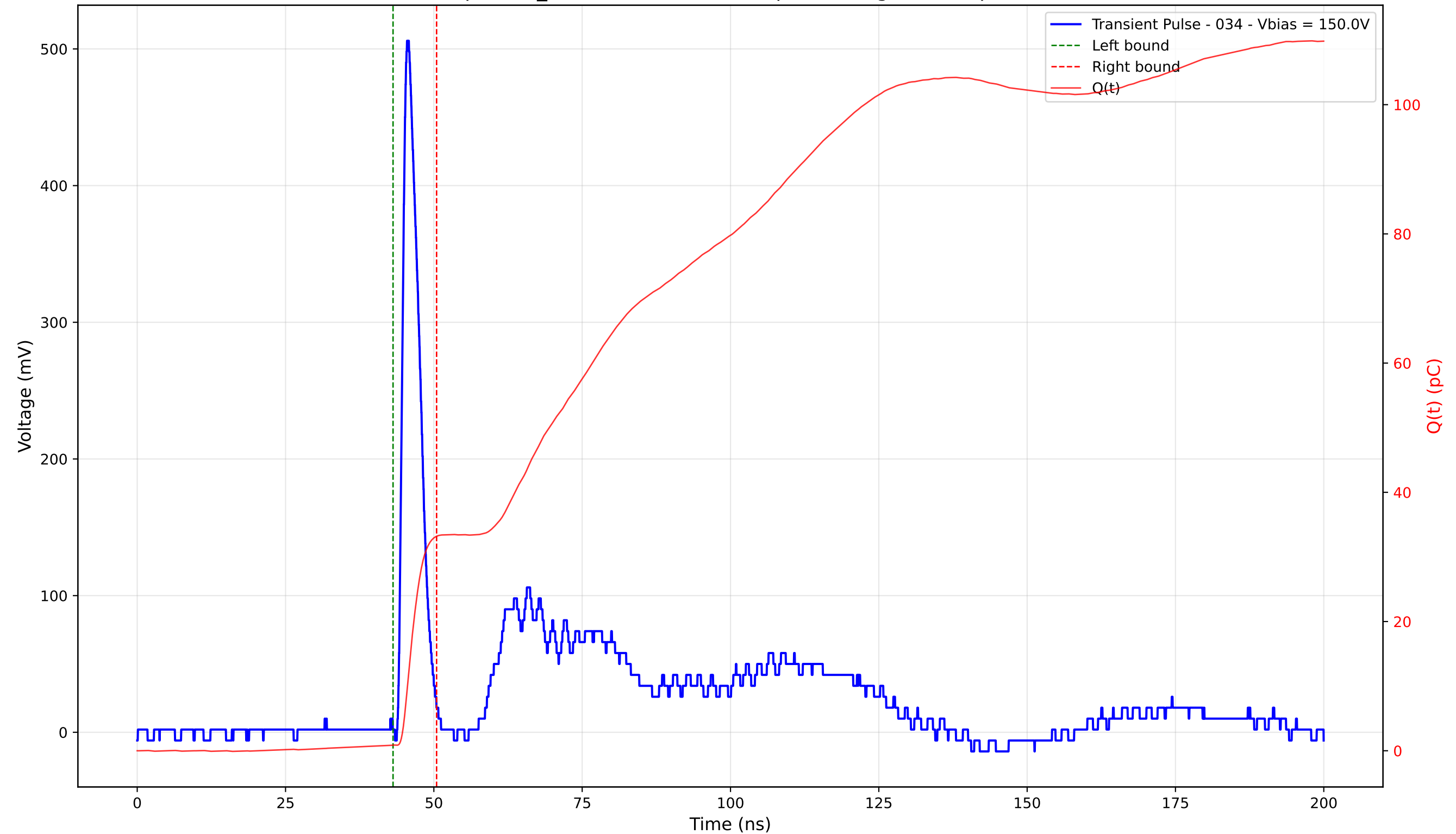
Transient Pulse - Sample: TD_4004 - Position: 310.0 \mu\text{m} - Charge: 32.32 pC - Rise Time: 1.05 ns
