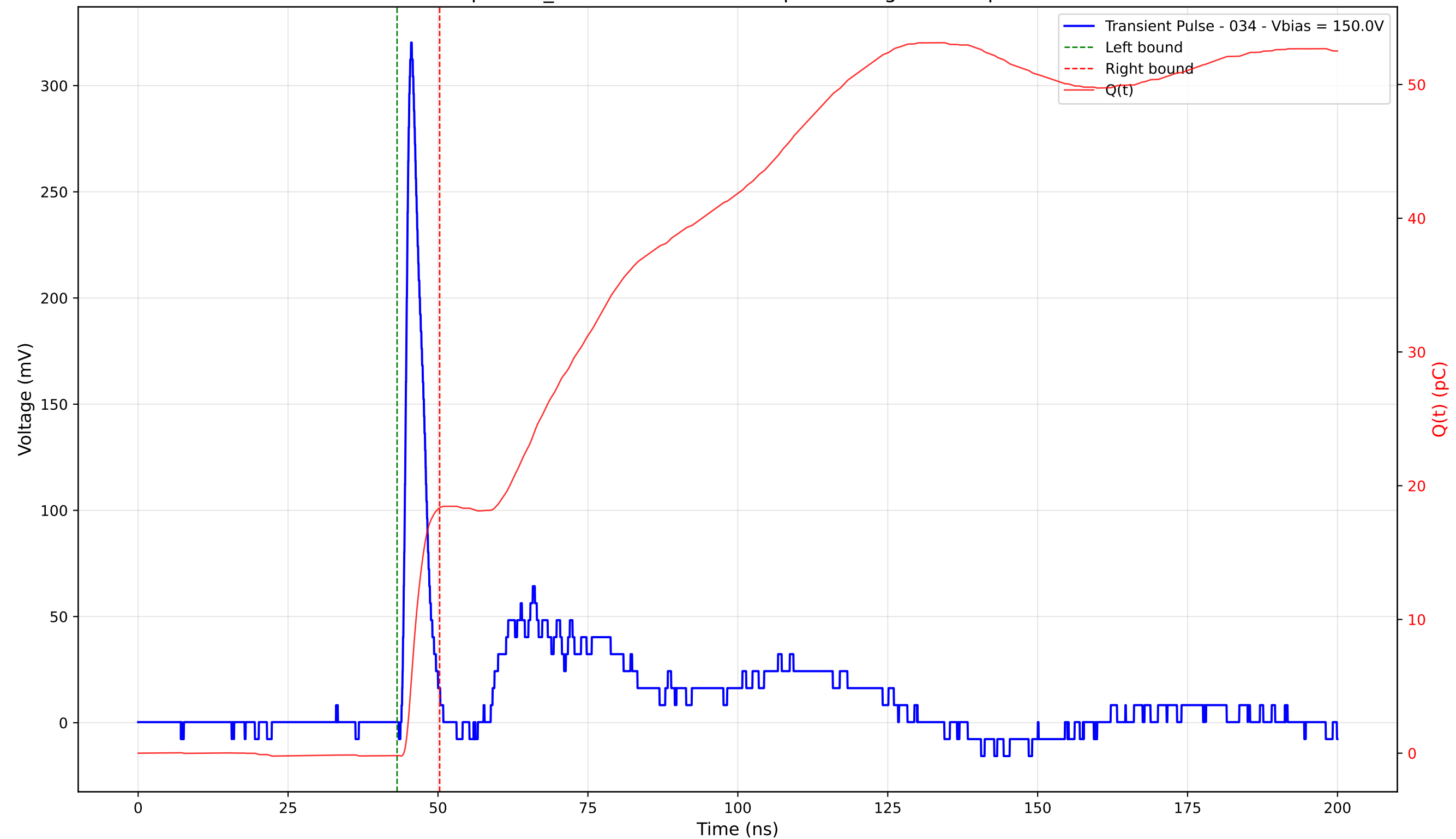
Transient Pulse - Sample: TD_4004 - Position: 375.0 \mu\text{m} - Charge: 18.52 pC - Rise Time: 1.04 ns
