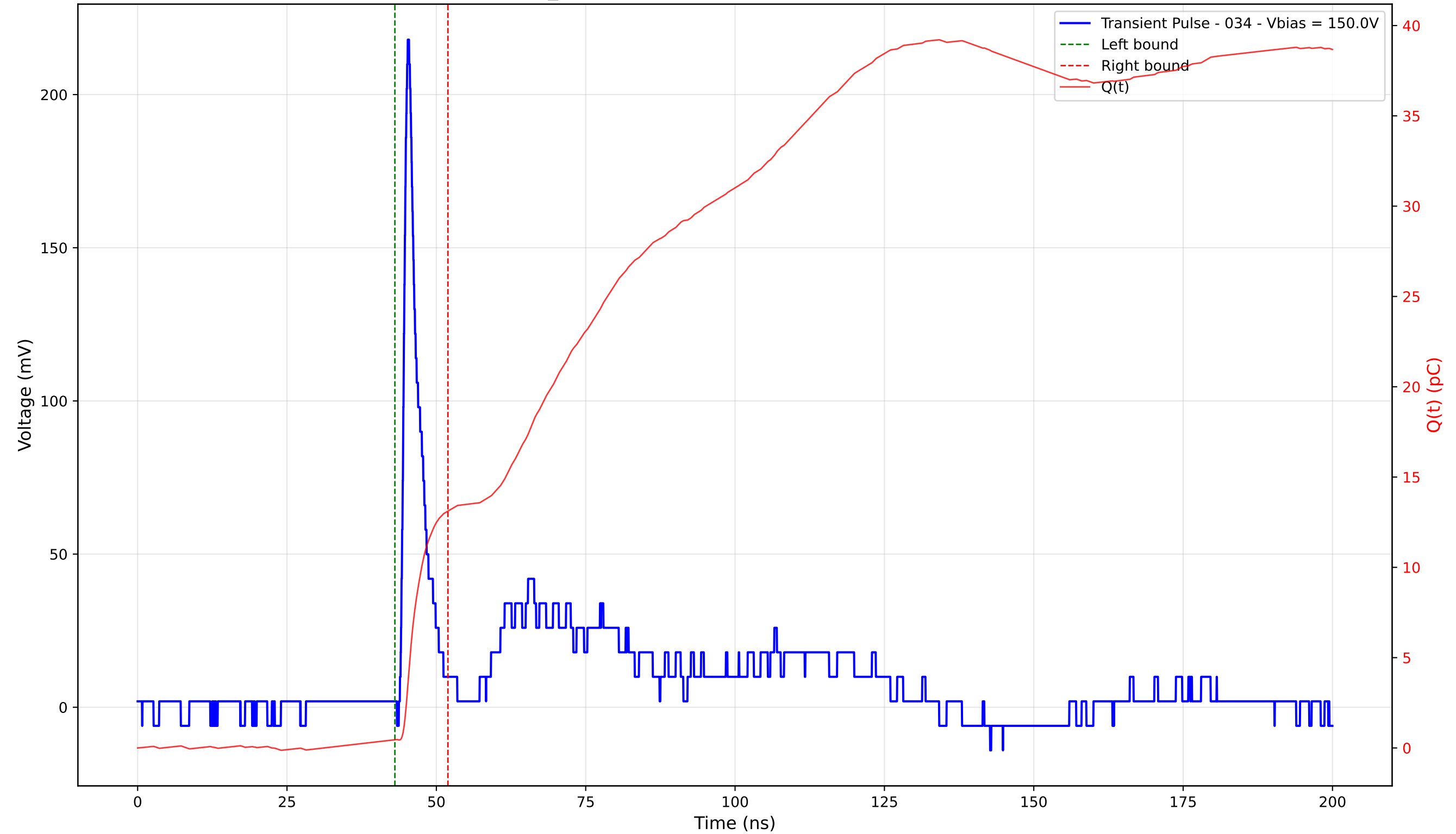
Transient Pulse - Sample: TD_4004 - Position: 60.0 \mu\text{m} - Charge: 12.66 pC - Rise Time: 0.95 ns
