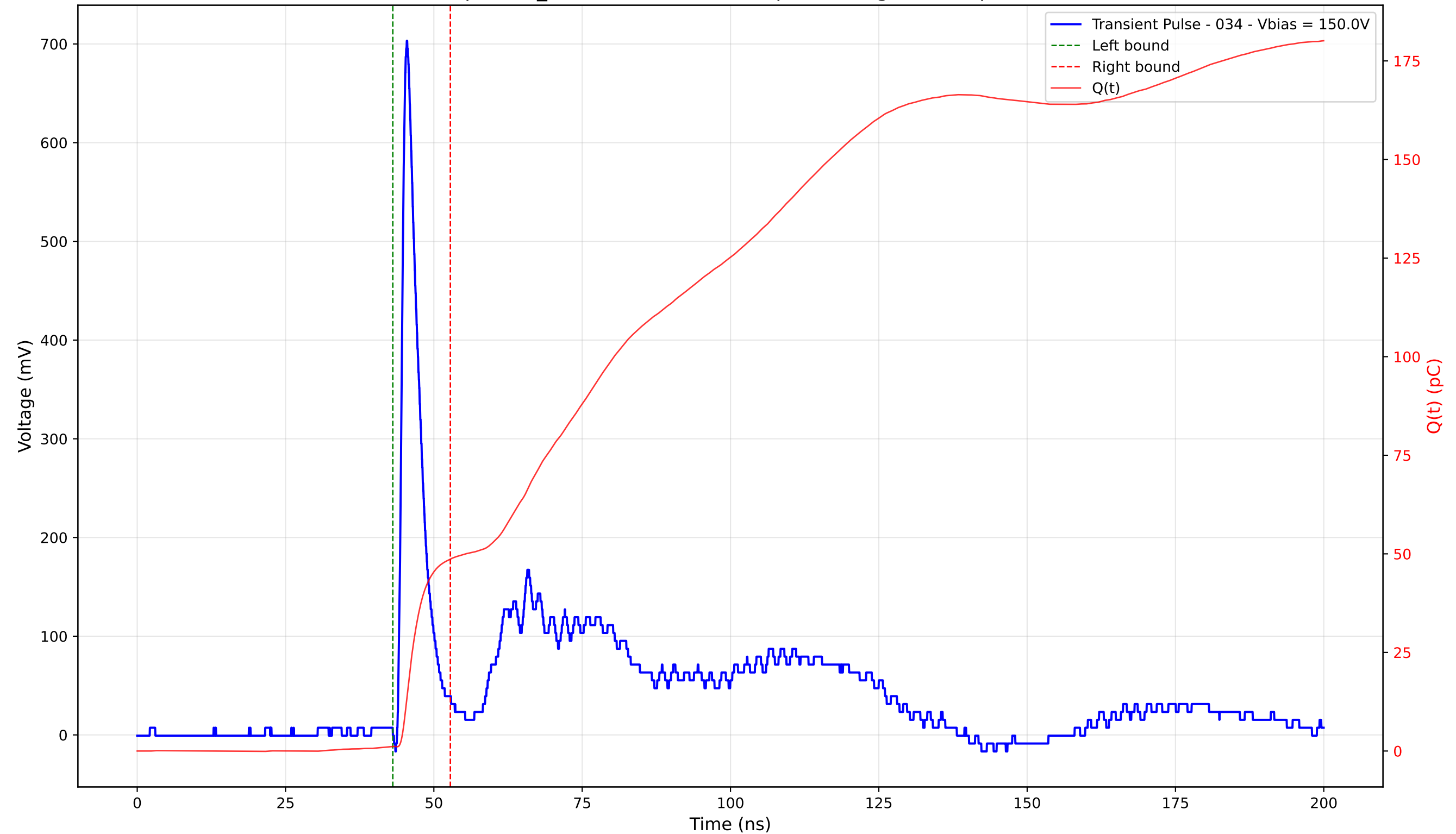
Transient Pulse - Sample: TD_4004 - Position: 130.0 \mu\text{m} - Charge: 47.52 pC - Rise Time: 0.99 ns
