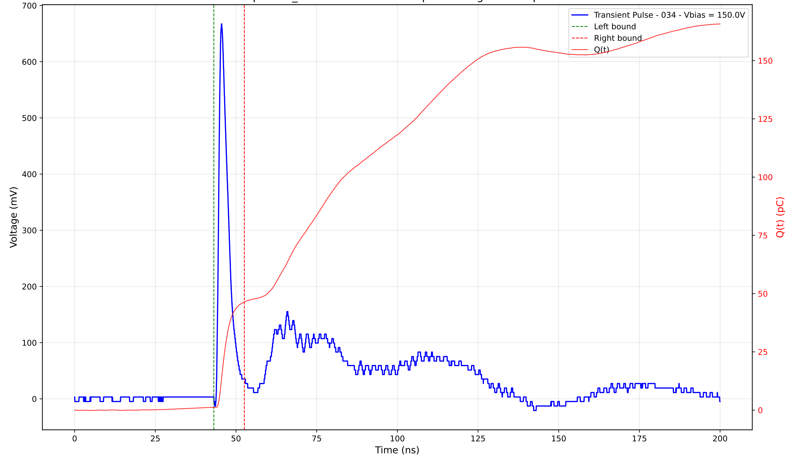
Transient Pulse - Sample: TD_4004 - Position: 140.0 \mu\text{m} - Charge: 45.15 pC - Rise Time: 1.01 ns
