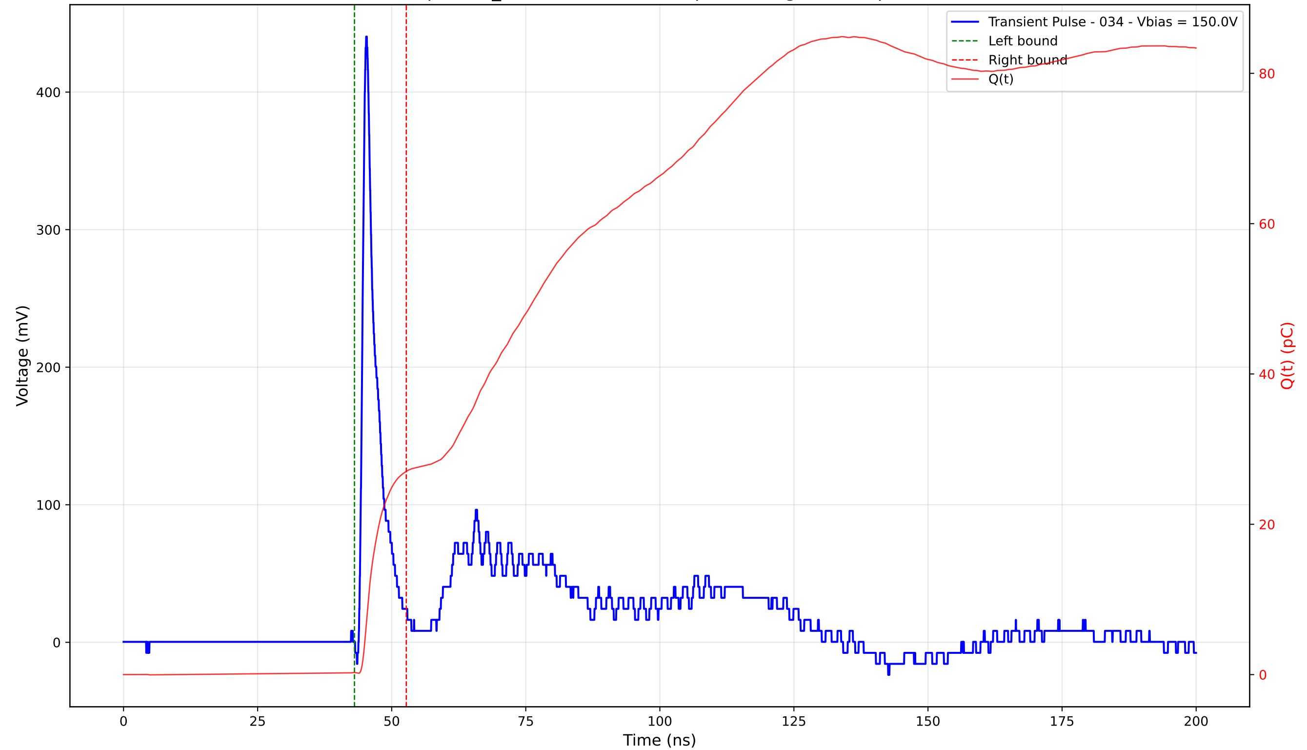
Transient Pulse - Sample: TD_4004 - Position: 70.0 \mu\text{m} - Charge: 26.77 pC - Rise Time: 0.93 ns
