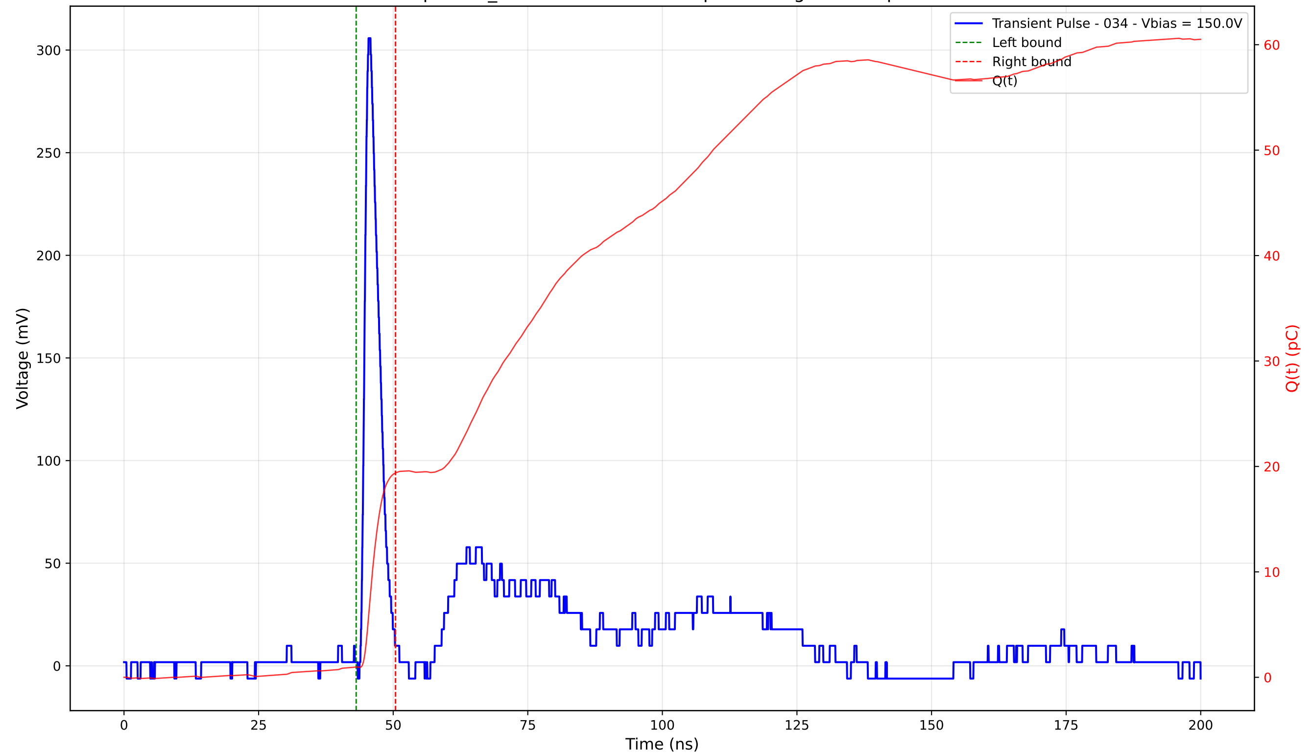
Transient Pulse - Sample: TD_4004 - Position: 370.0 \mu\text{m} - Charge: 18.41 pC - Rise Time: 1.05 ns
