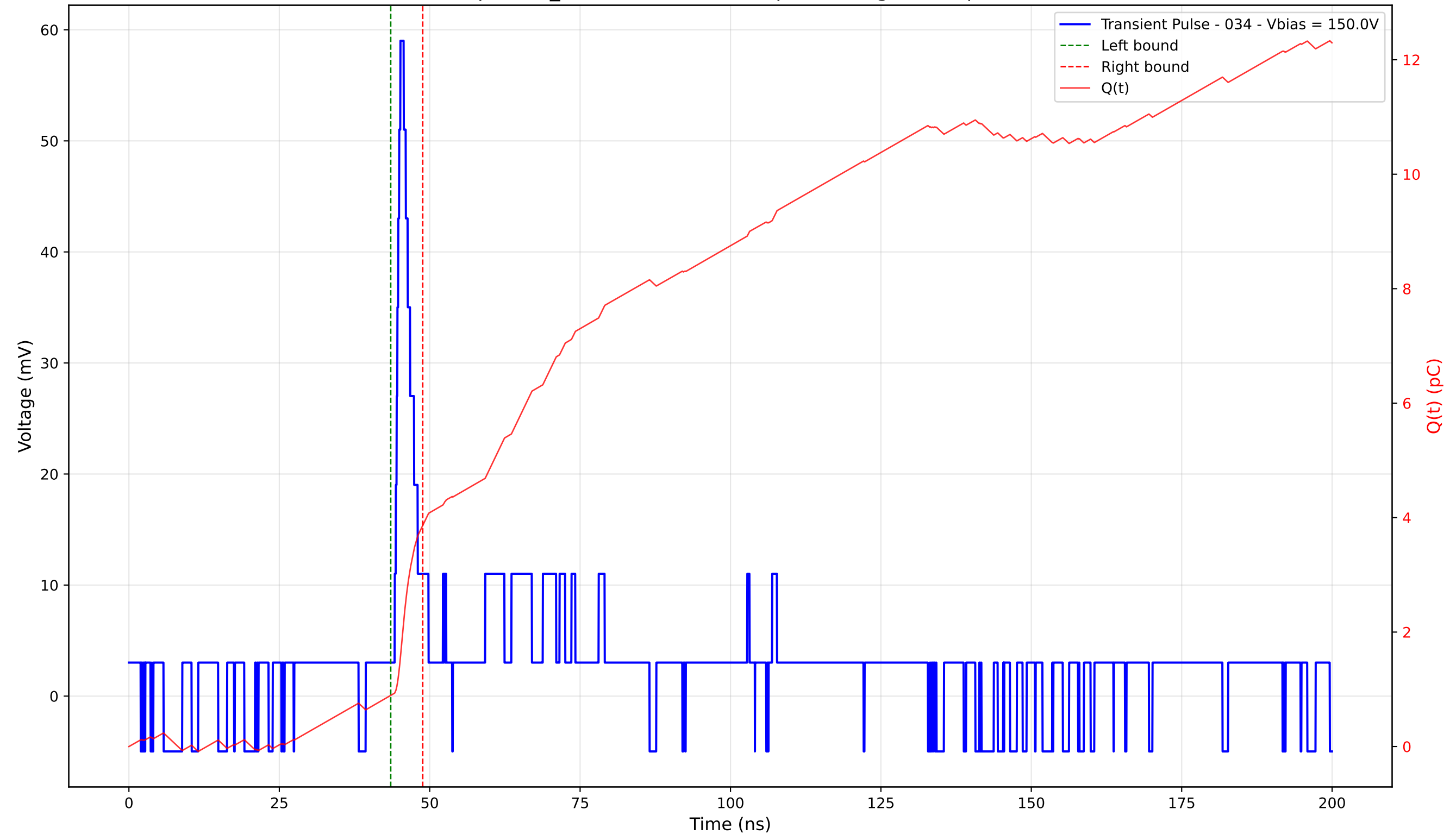
Transient Pulse - Sample: TD_4004 - Position: 45.0 \mu\text{m} - Charge: 2.97 pC - Rise Time: 0.95 ns
