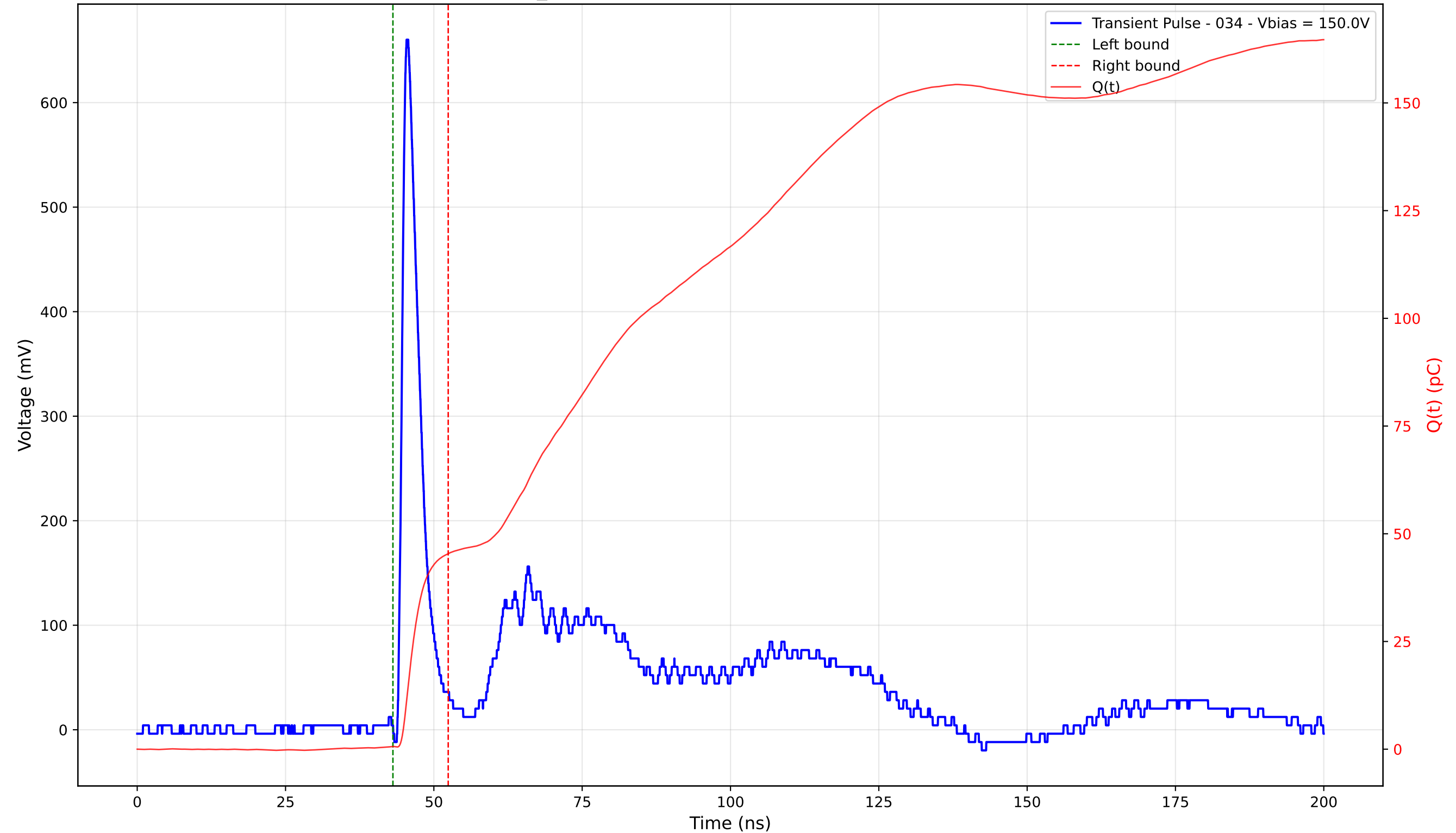
Transient Pulse - Sample: TD_4004 - Position: 145.0 \mu\text{m} - Charge: 44.77 pC - Rise Time: 1.00 ns
