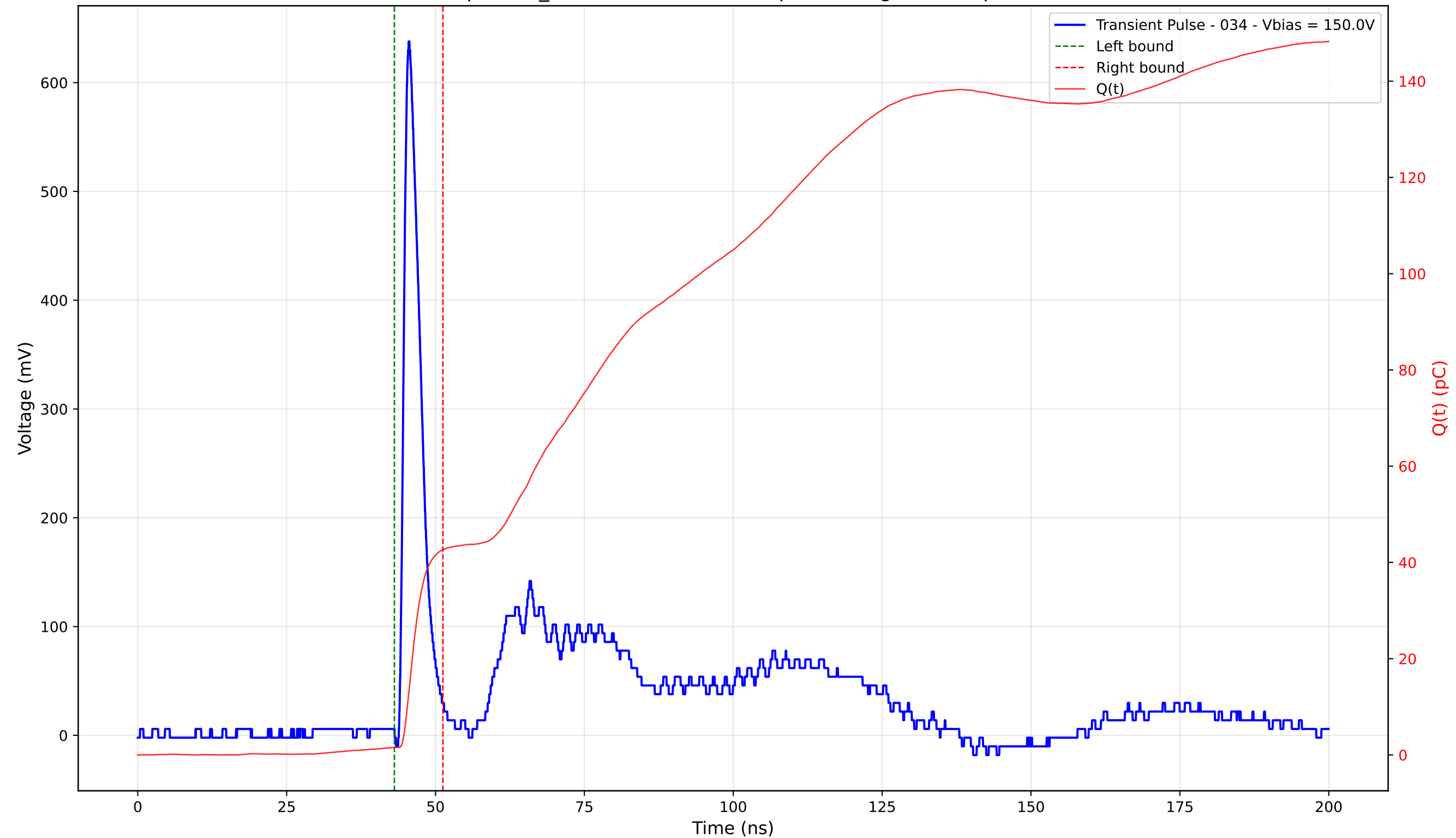
Transient Pulse - Sample: TD_4004 - Position: 245.0 \mu\text{m} - Charge: 41.06 pC - Rise Time: 1.04 ns
