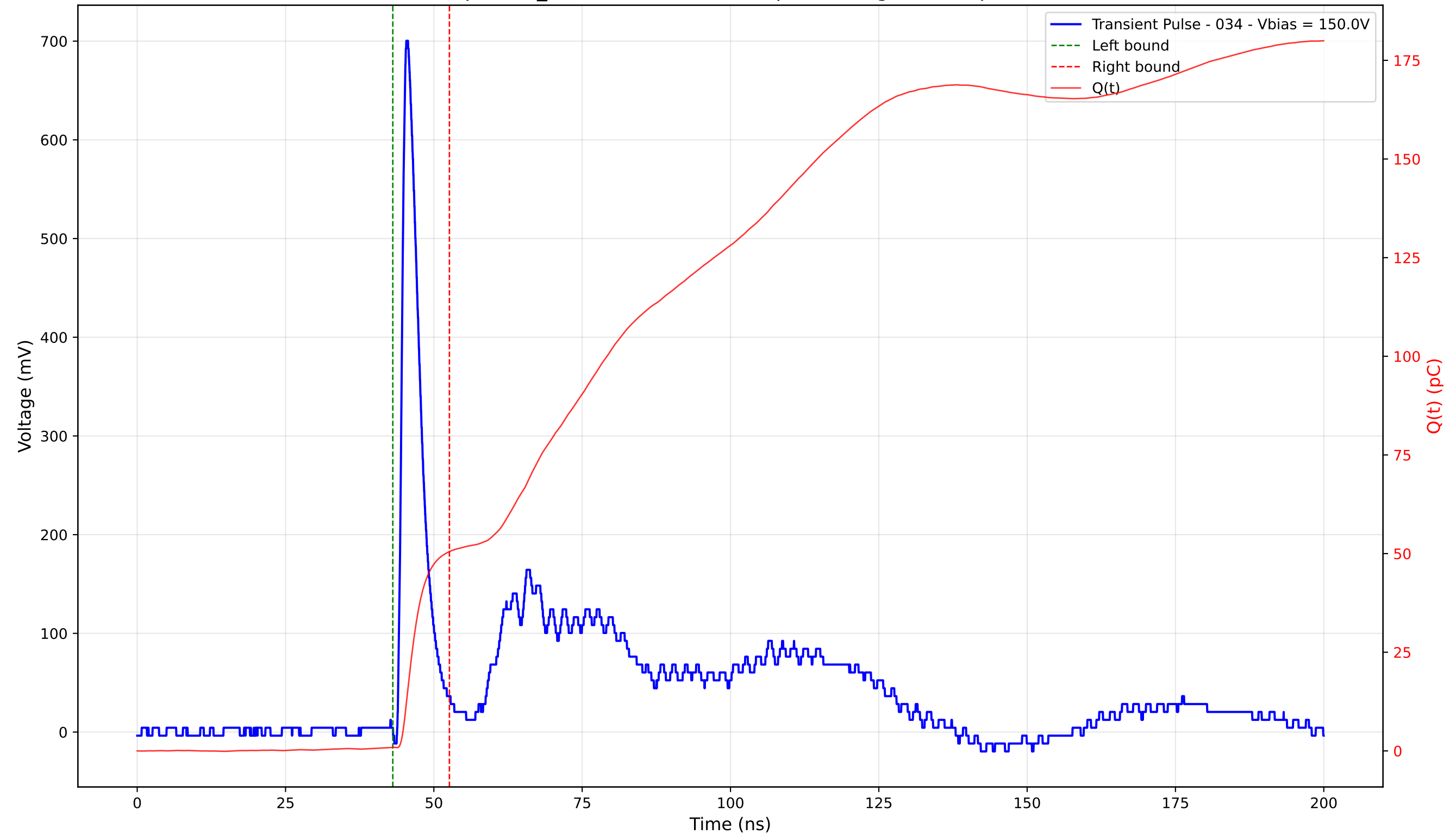
Transient Pulse - Sample: TD_4004 - Position: 165.0 \mu\text{m} - Charge: 49.59 pC - Rise Time: 0.98 ns
