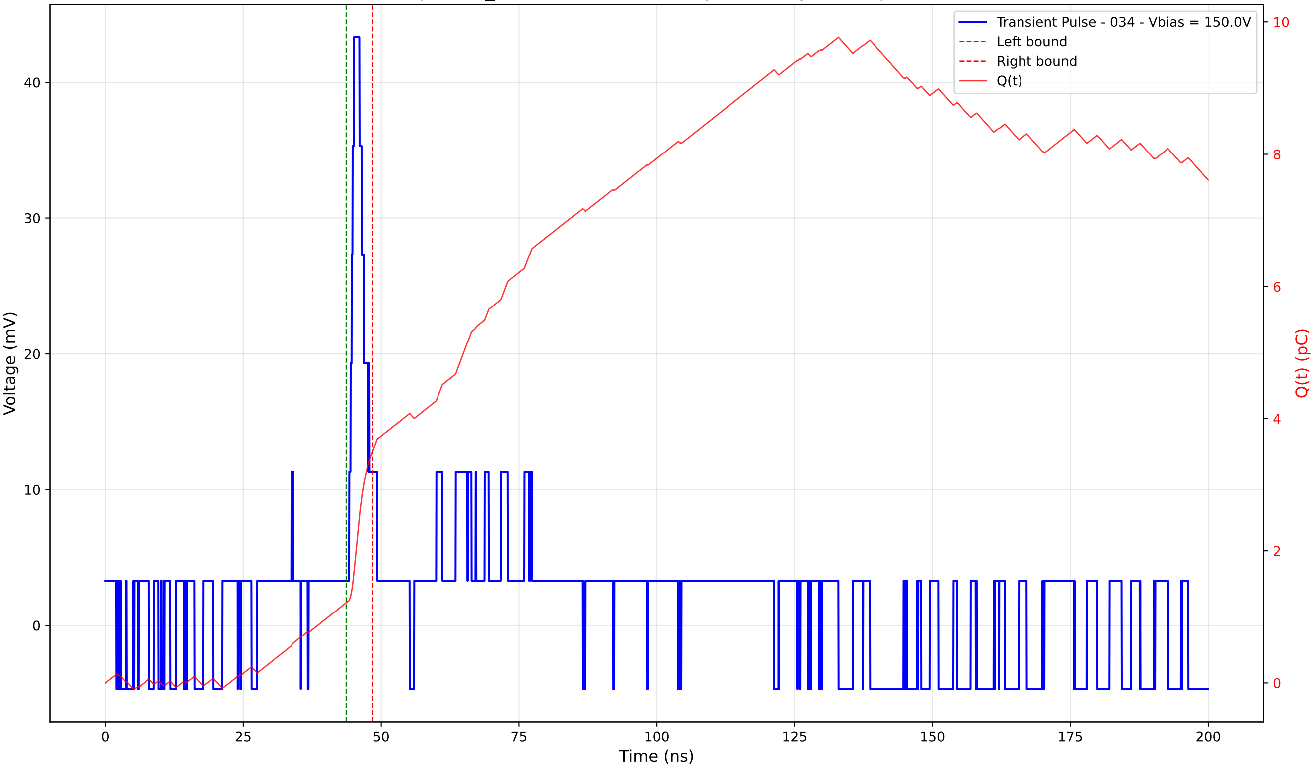
Transient Pulse - Sample: TD_4004 - Position: 430.0 \mu\text{m} - Charge: 2.30 pC - Rise Time: 0.84 ns
