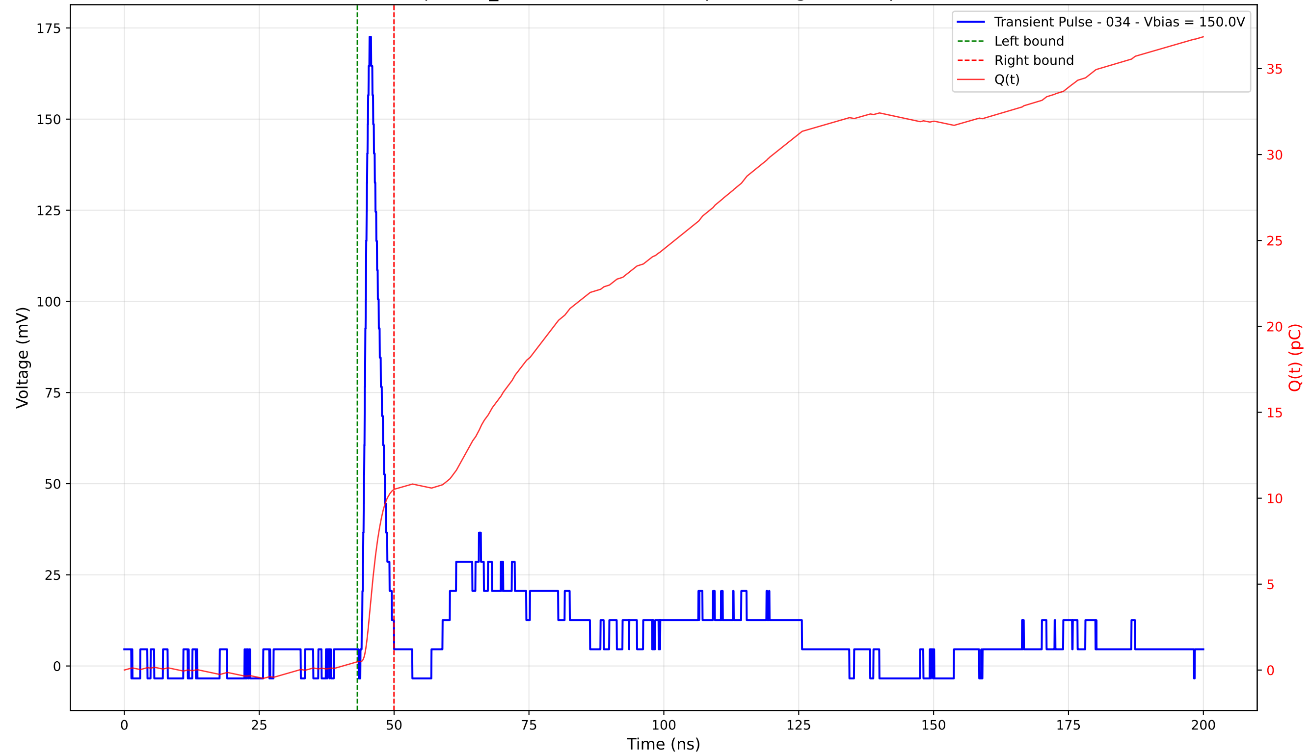
Transient Pulse - Sample: TD_4004 - Position: 400.0 \mu\text{m} - Charge: 10.03 pC - Rise Time: 1.07 ns
