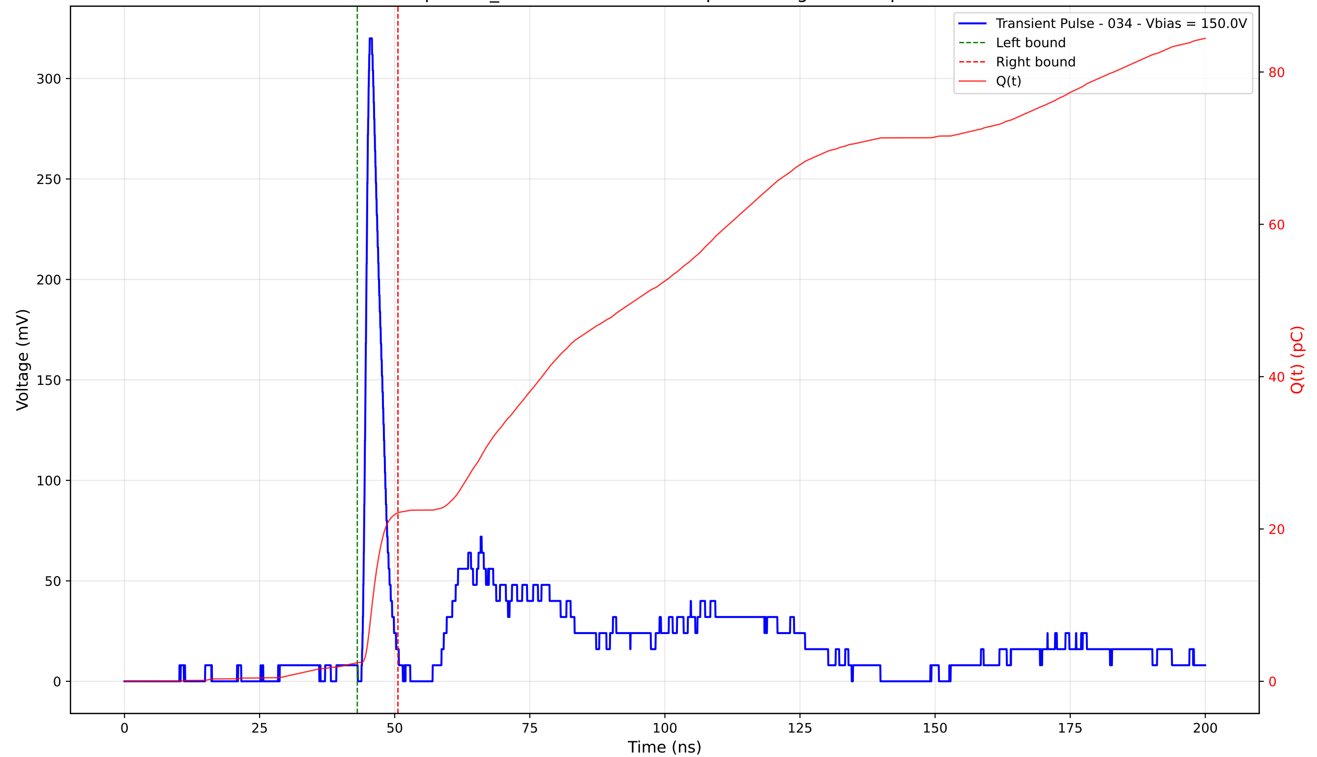
Transient Pulse - Sample: TD_4004 - Position: 365.0 \mu\text{m} - Charge: 19.67 pC - Rise Time: 1.00 ns
