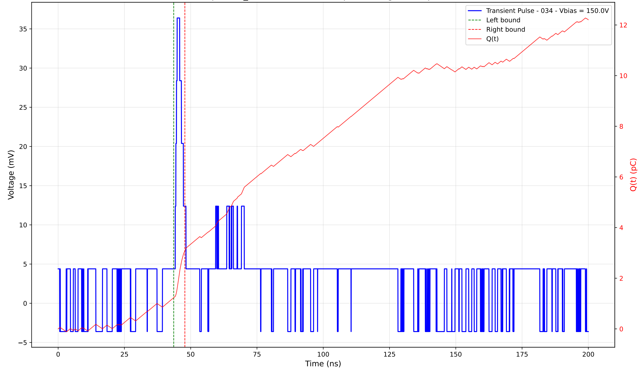
Transient Pulse - Sample: TD_4004 - Position: 40.0 \mu\text{m} - Charge: 1.86 pC - Rise Time: 5.56 ns
