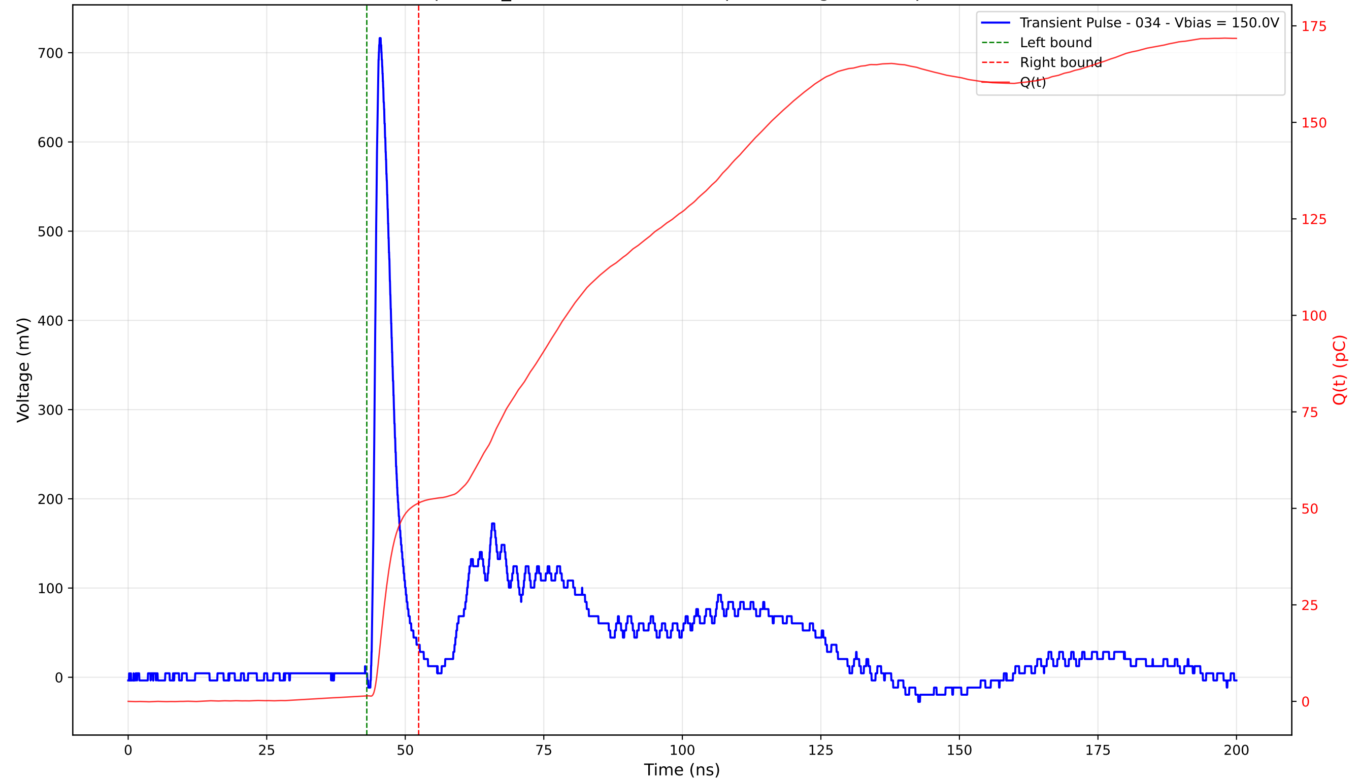
Transient Pulse - Sample: TD_4004 - Position: 210.0 \mu\text{m} - Charge: 49.95 pC - Rise Time: 0.97 ns
