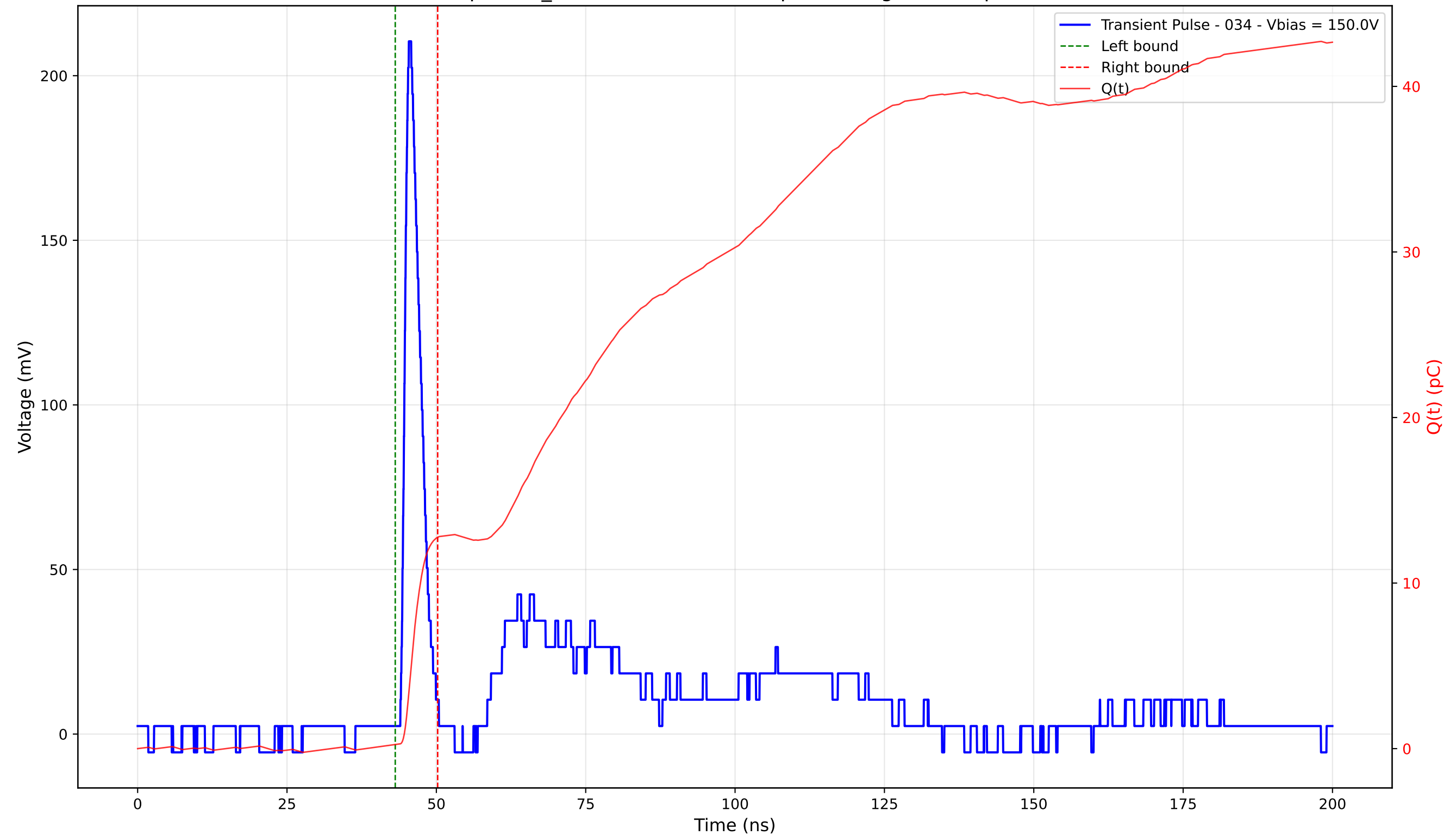
Transient Pulse - Sample: TD_4004 - Position: 395.0 \mu\text{m} - Charge: 12.52 pC - Rise Time: 1.03 ns
