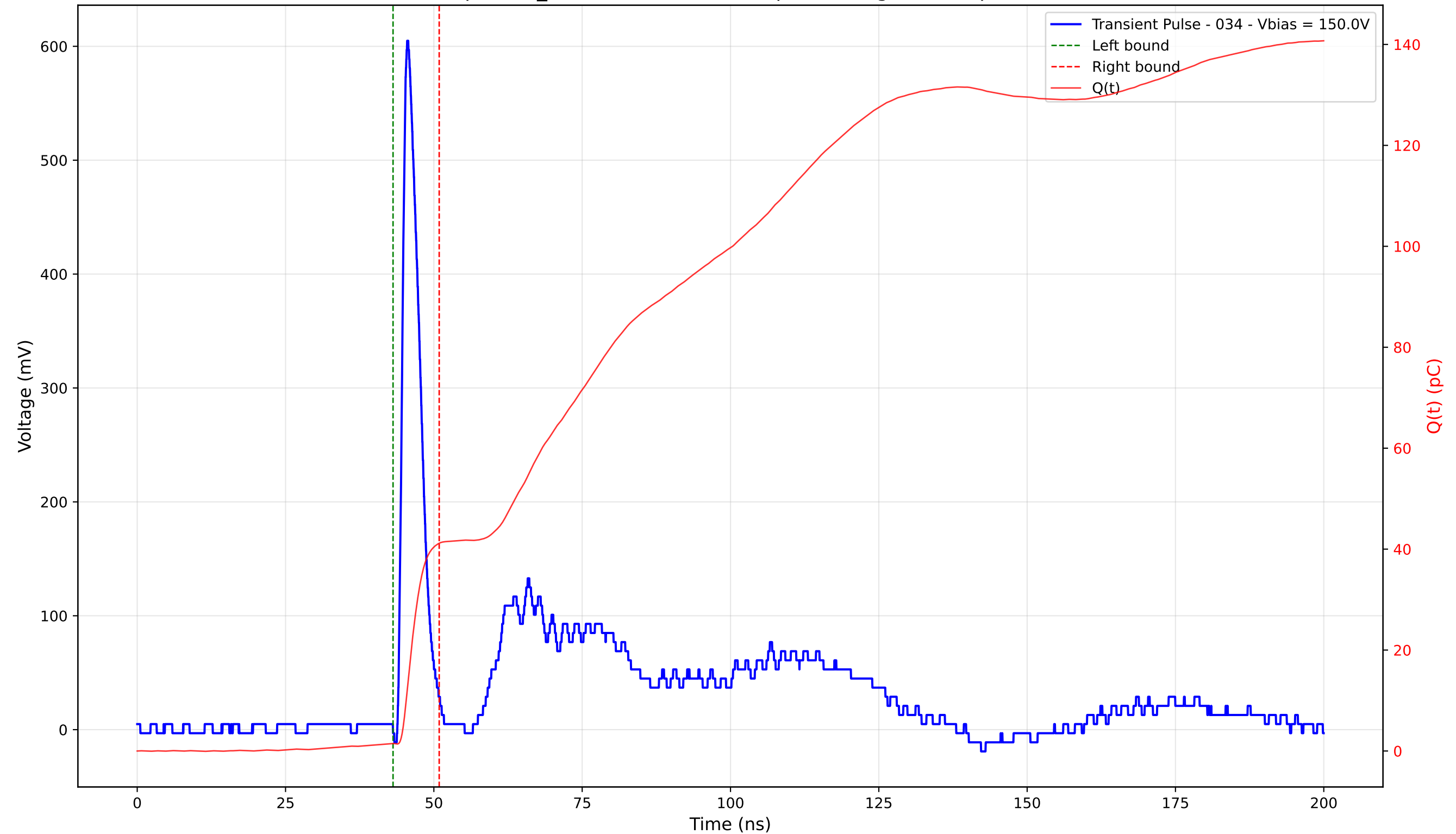
Transient Pulse - Sample: TD_4004 - Position: 285.0 \mu\text{m} - Charge: 39.67 pC - Rise Time: 1.03 ns
