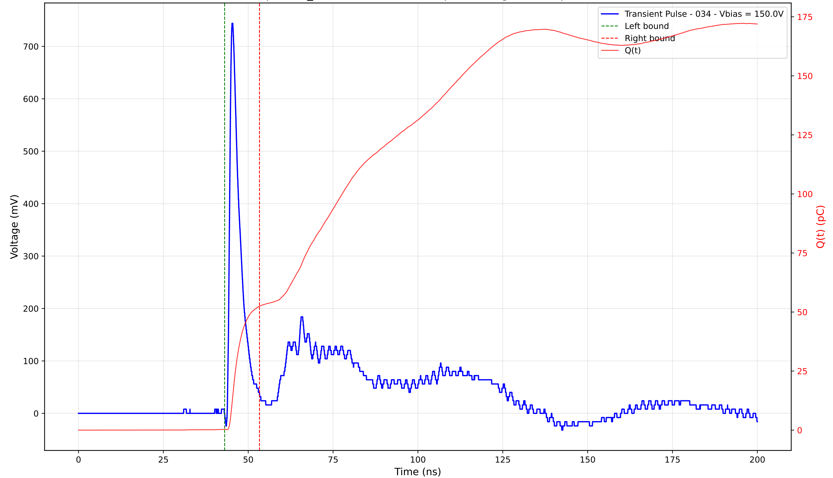
Transient Pulse - Sample: TD_4004 - Position: 115.0 \mu\text{m} - Charge: 52.11 pC - Rise Time: 0.91 ns
