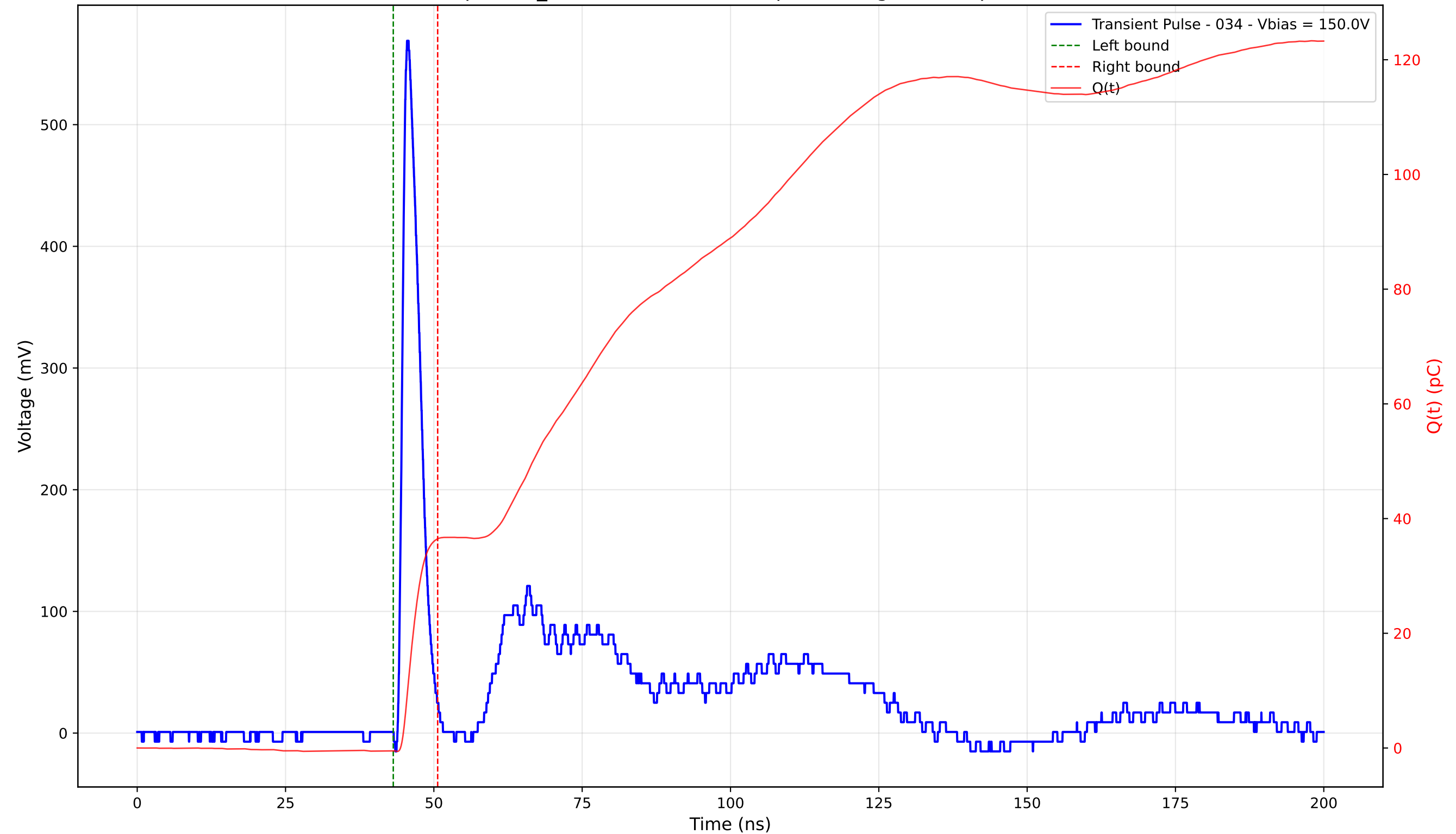
Transient Pulse - Sample: TD_4004 - Position: 290.0 \mu\text{m} - Charge: 36.95 pC - Rise Time: 1.02 ns
