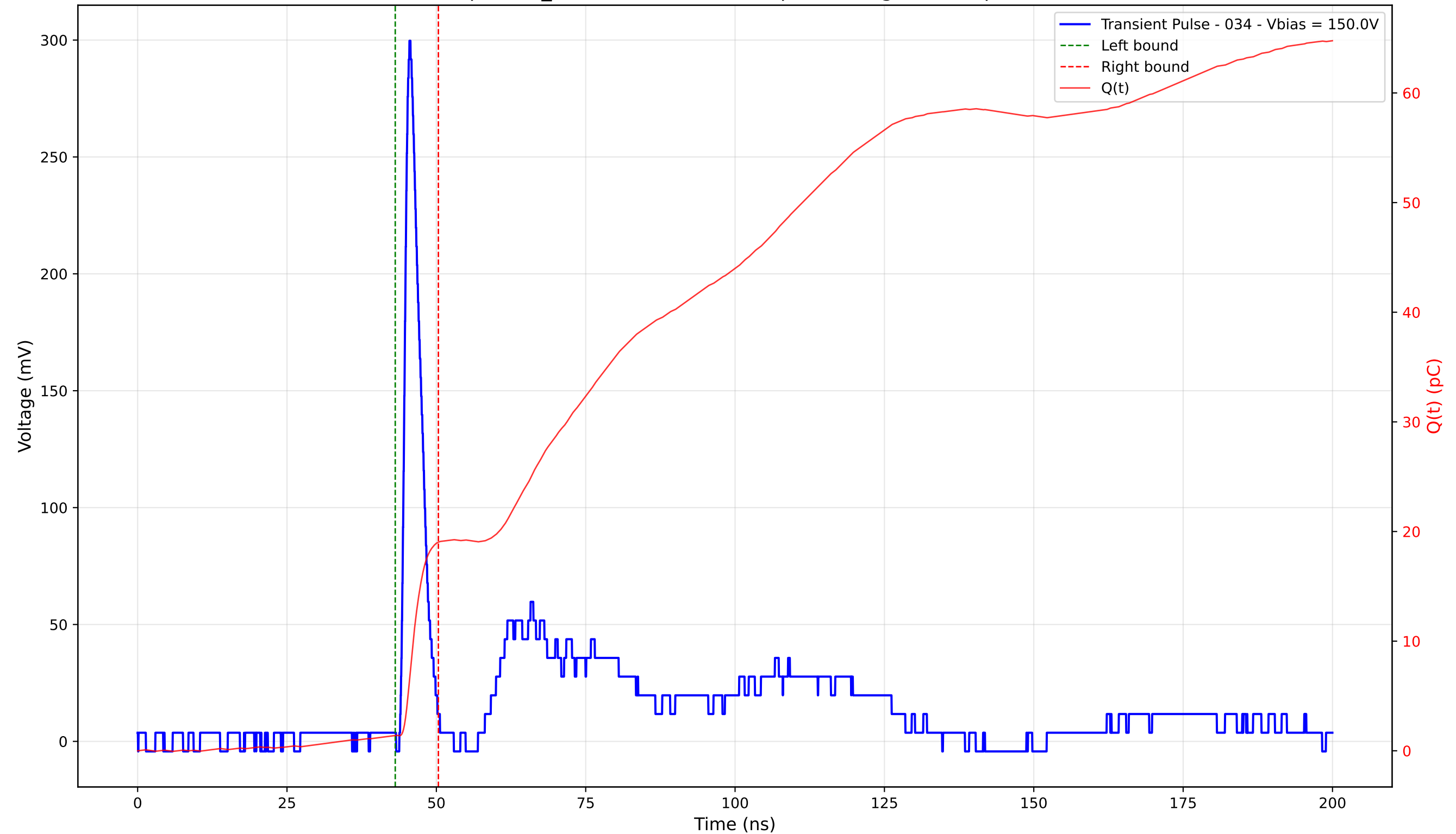
Transient Pulse - Sample: TD_4004 - Position: 385.0 \mu\text{m} - Charge: 17.62 pC - Rise Time: 1.07 ns
