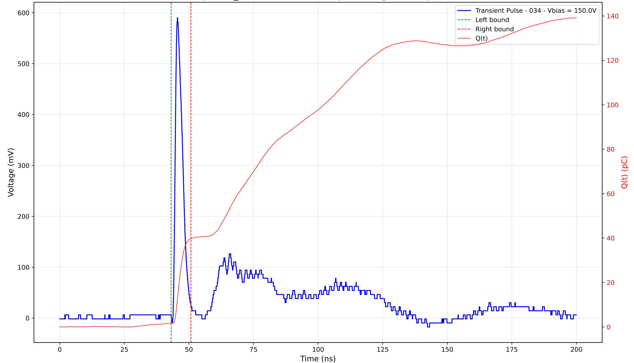
Transient Pulse - Sample: TD_4004 - Position: 265.0 \mu\text{m} - Charge: 38.03 pC - Rise Time: 1.04 ns
