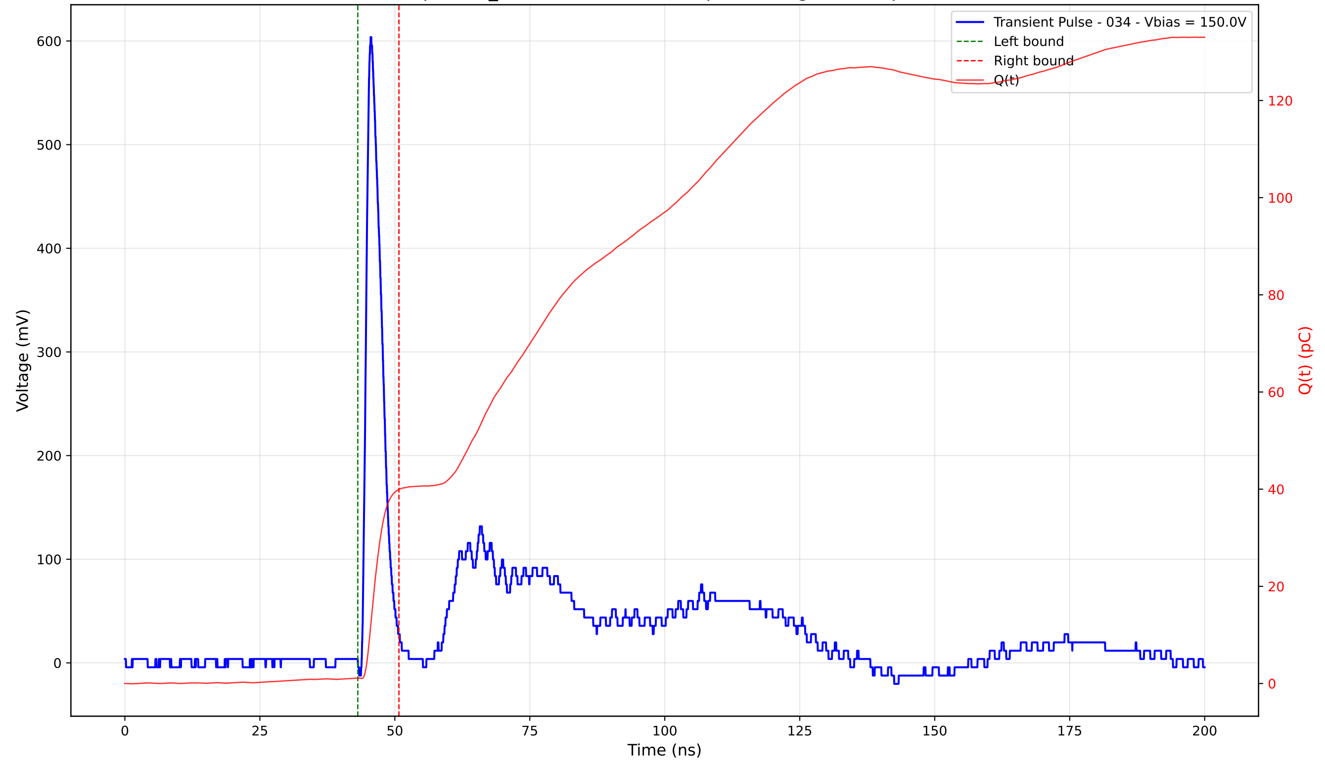
Transient Pulse - Sample: TD_4004 - Position: 270.0 \mu\text{m} - Charge: 38.81 pC - Rise Time: 1.03 ns
