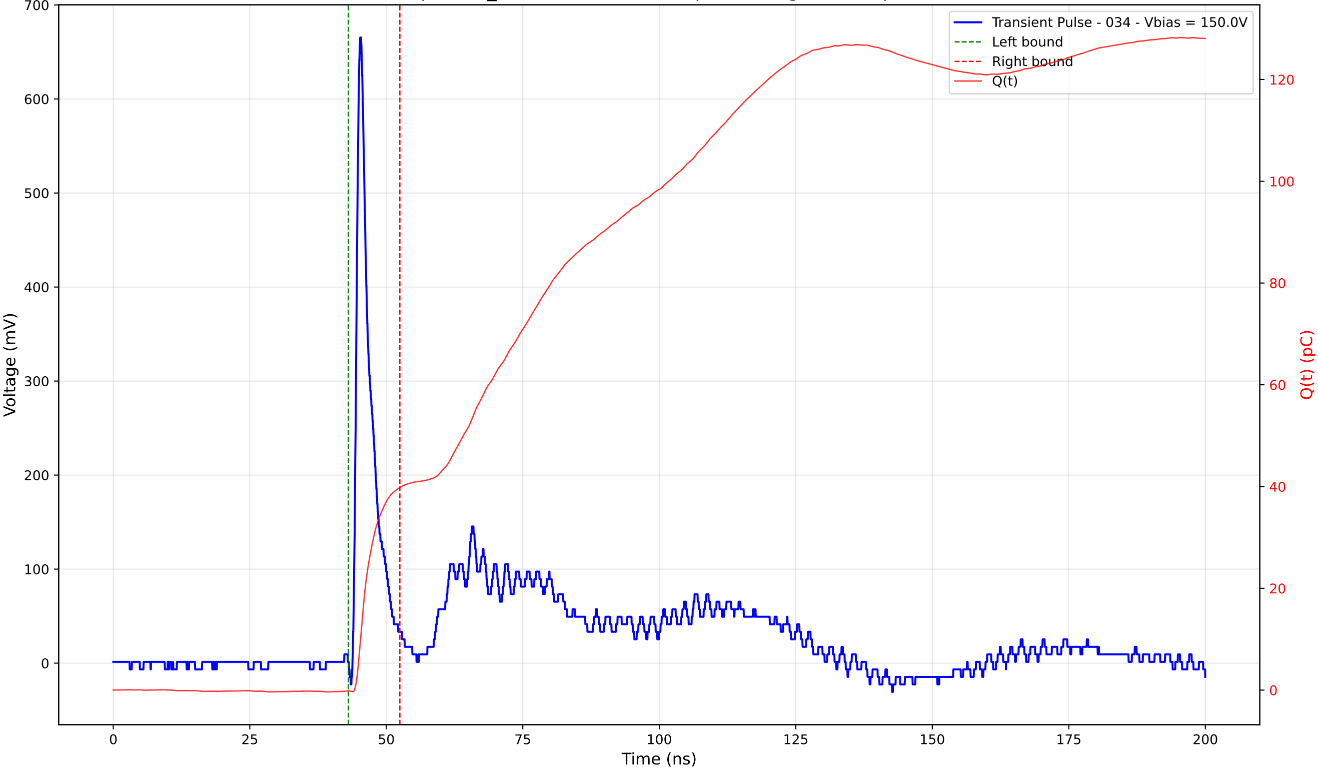
Transient Pulse - Sample: TD_4004 - Position: 85.0 \mu\text{m} - Charge: 39.97 pC - Rise Time: 0.89 ns
