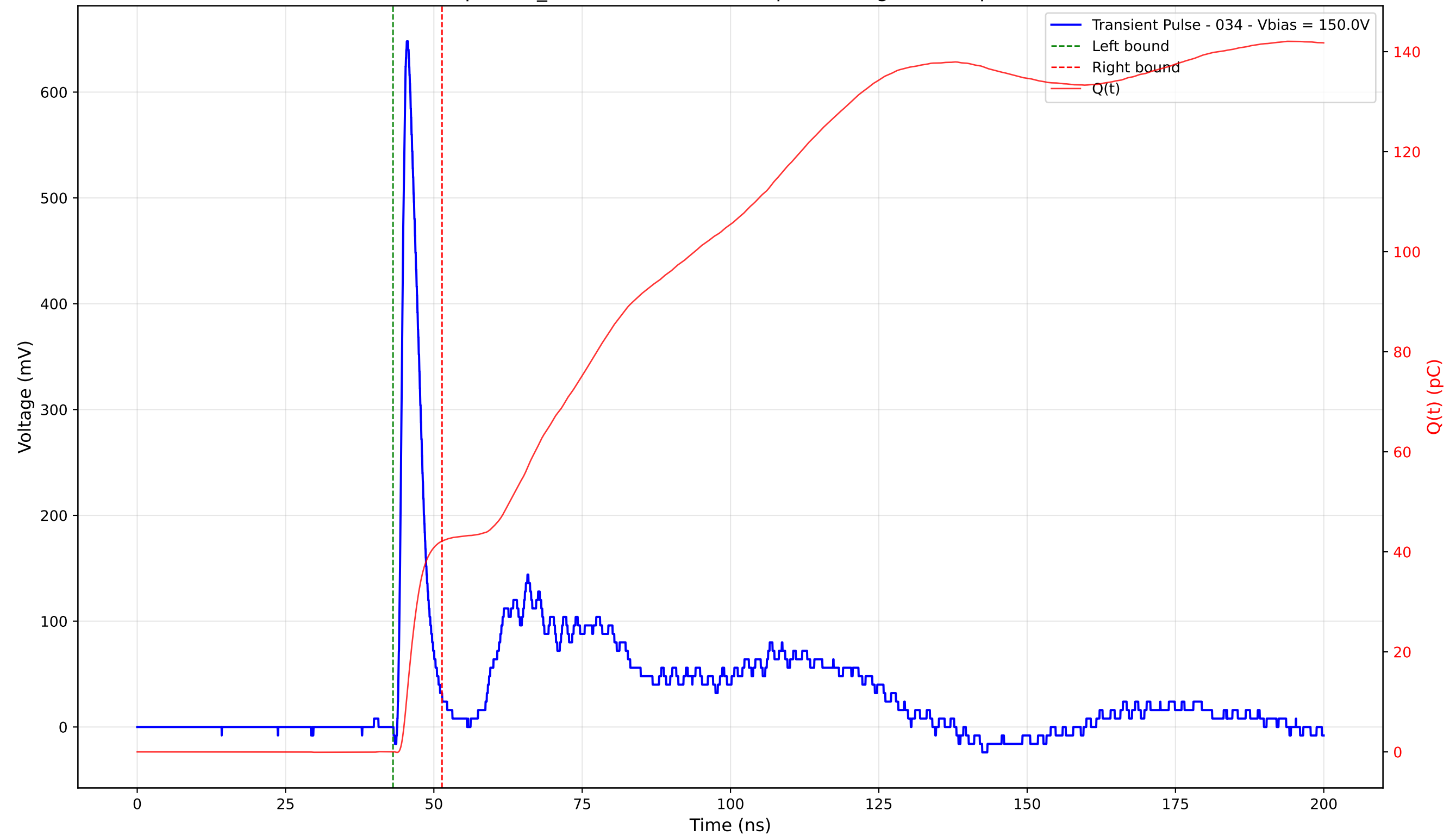
Transient Pulse - Sample: TD_4004 - Position: 235.0 \mu\text{m} - Charge: 42.12 pC - Rise Time: 1.02 ns
