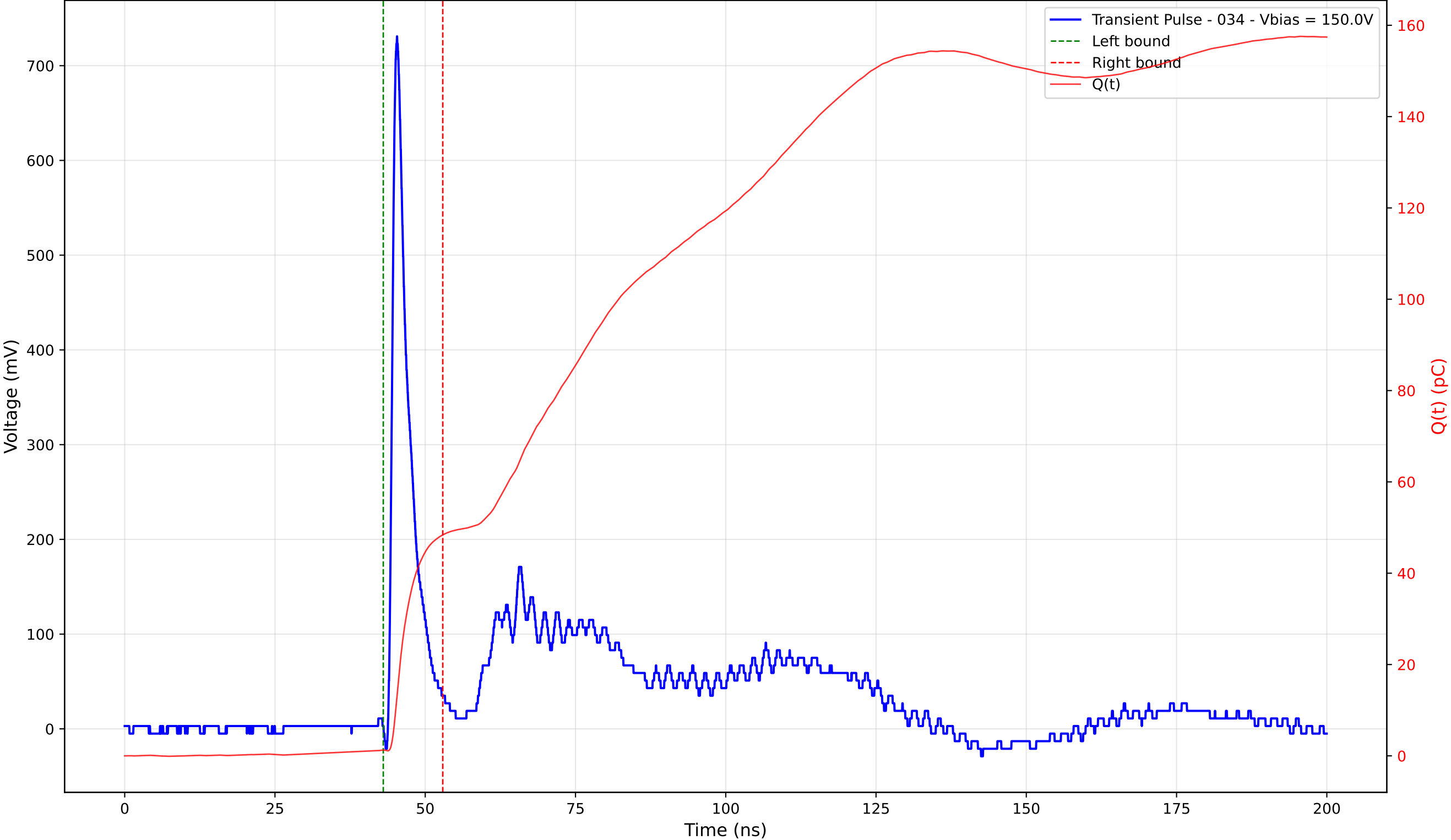
Transient Pulse - Sample: TD_4004 - Position: 95.0 \mu\text{m} - Charge: 47.12 pC - Rise Time: 0.91 ns
