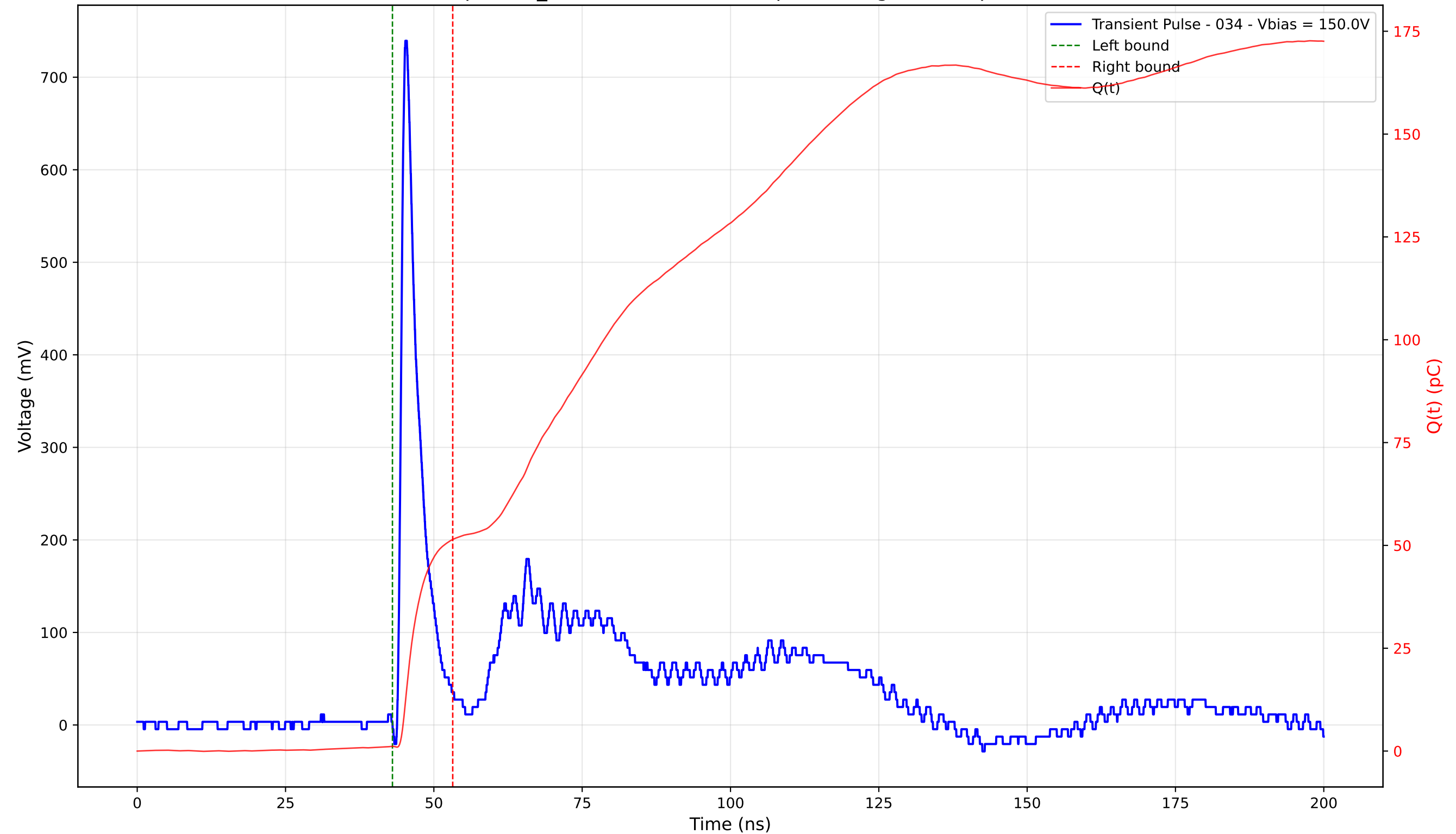
Transient Pulse - Sample: TD_4004 - Position: 100.0 \mu\text{m} - Charge: 50.29 pC - Rise Time: 0.90 ns
