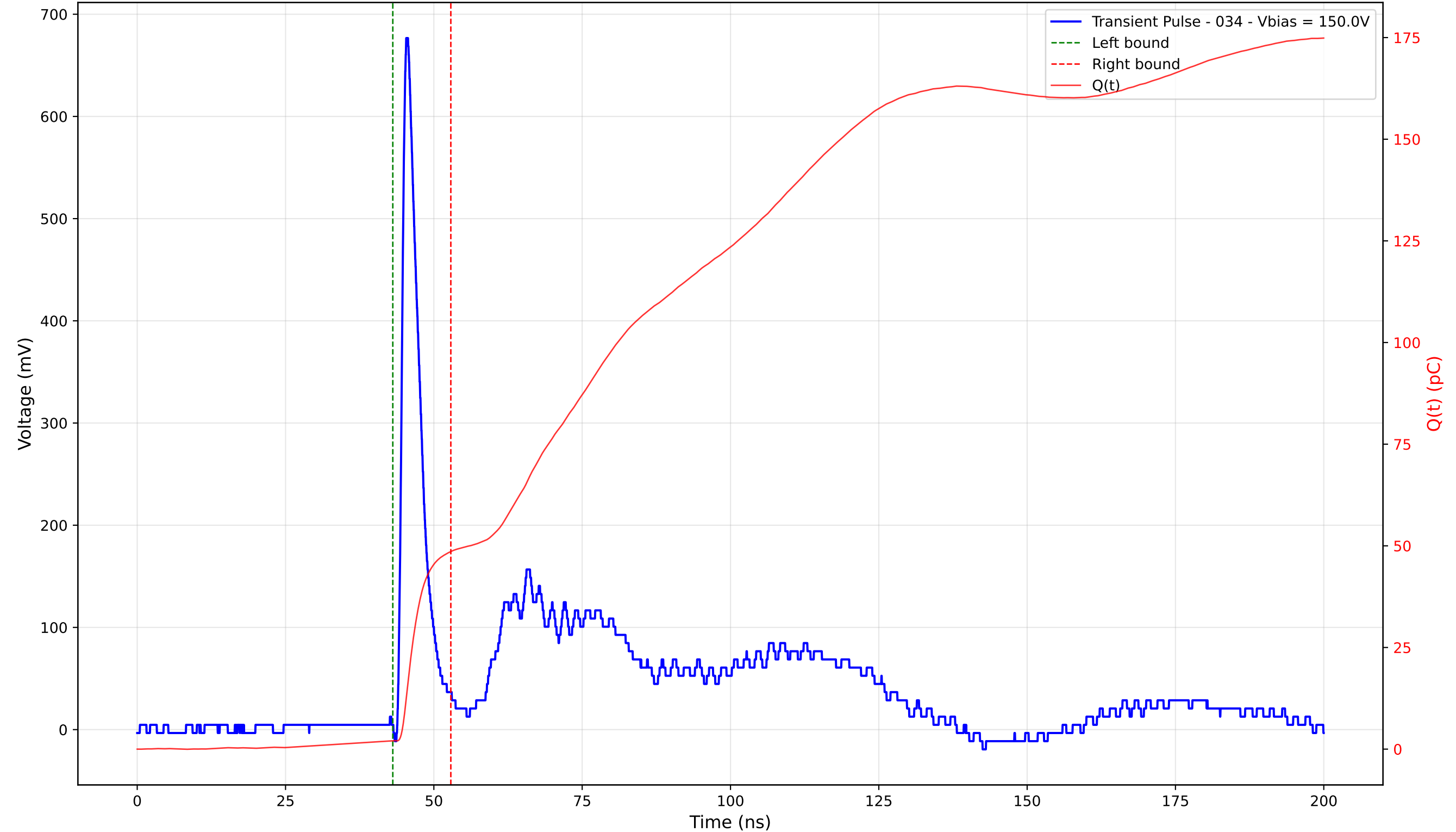
Transient Pulse - Sample: TD_4004 - Position: 135.0 \mu\text{m} - Charge: 46.49 pC - Rise Time: 0.99 ns
