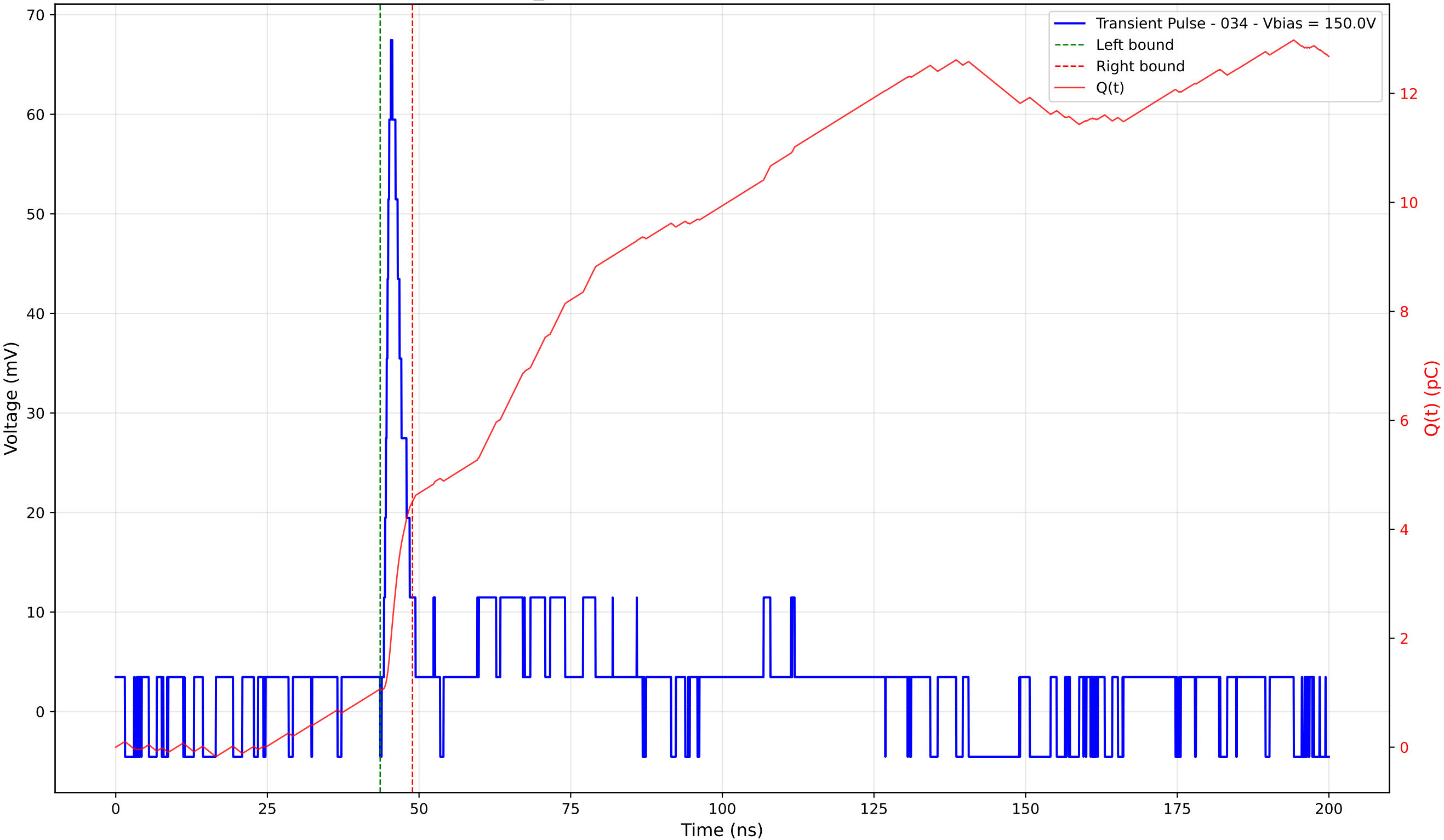
Transient Pulse - Sample: TD_4004 - Position: 420.0 \mu\text{m} - Charge: 3.44 pC - Rise Time: 1.15 ns
