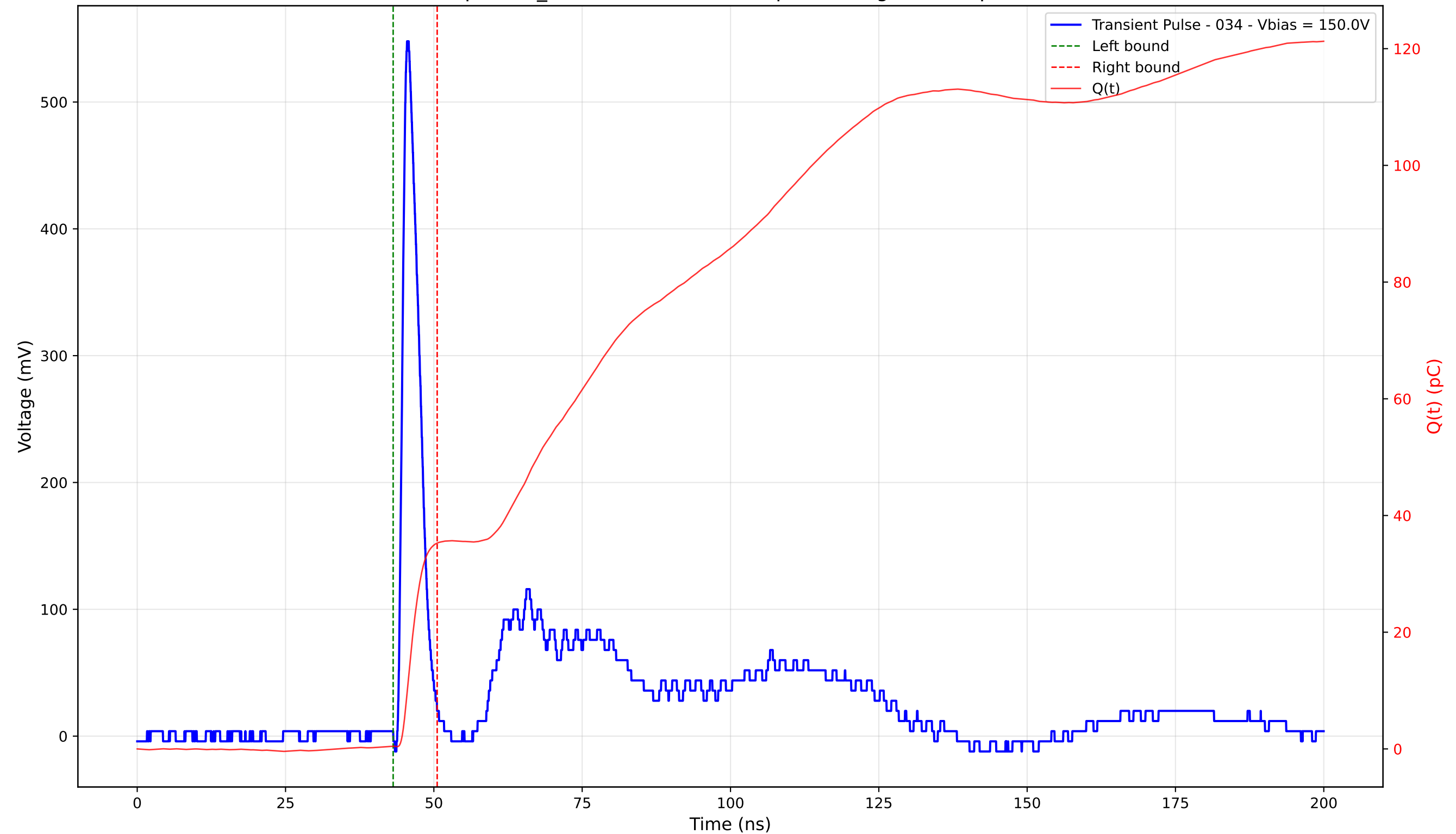
Transient Pulse - Sample: TD_4004 - Position: 305.0 \mu\text{m} - Charge: 34.80 pC - Rise Time: 1.05 ns
