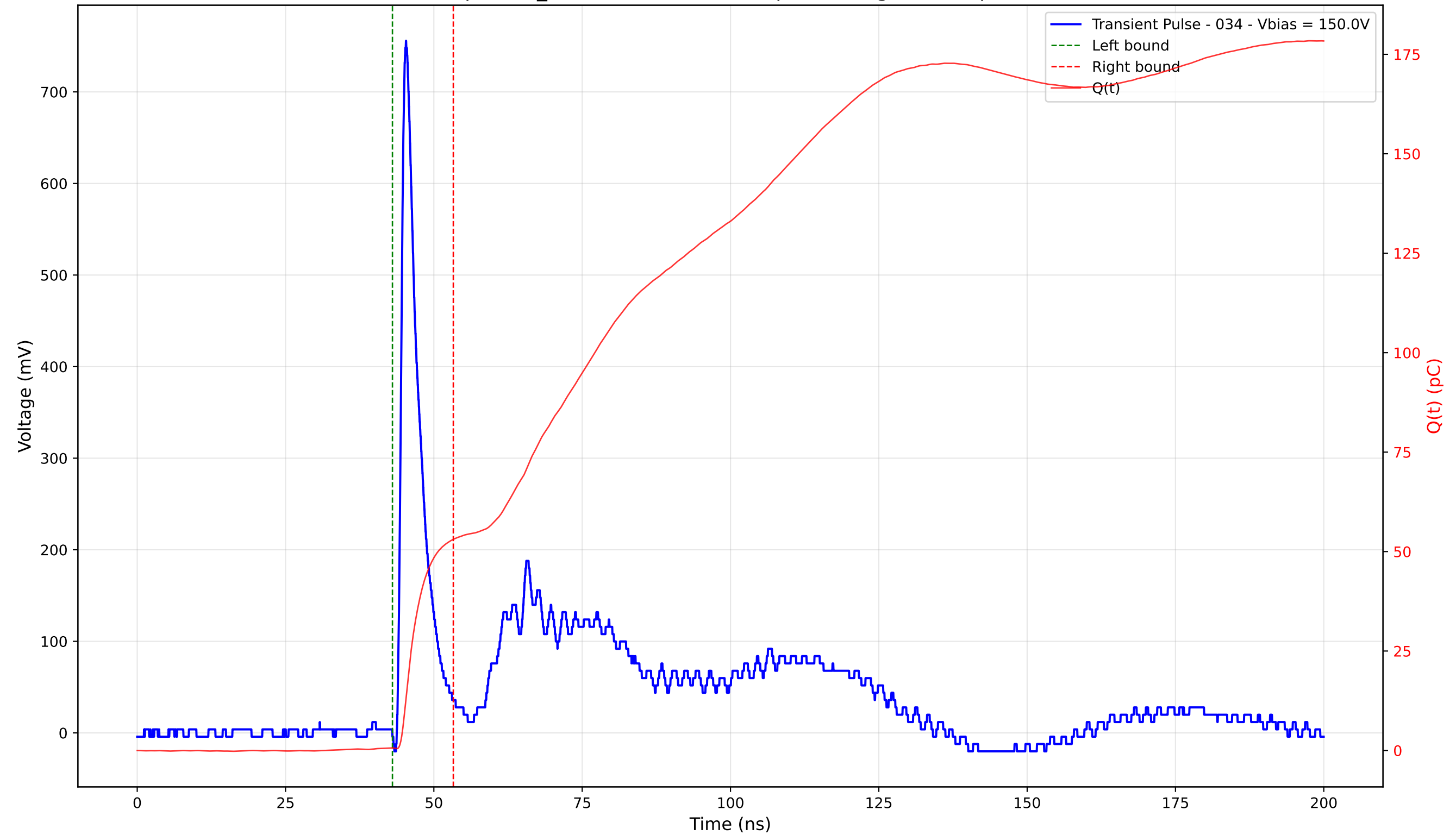
Transient Pulse - Sample: TD_4004 - Position: 105.0 \mu\text{m} - Charge: 52.41 pC - Rise Time: 0.93 ns
