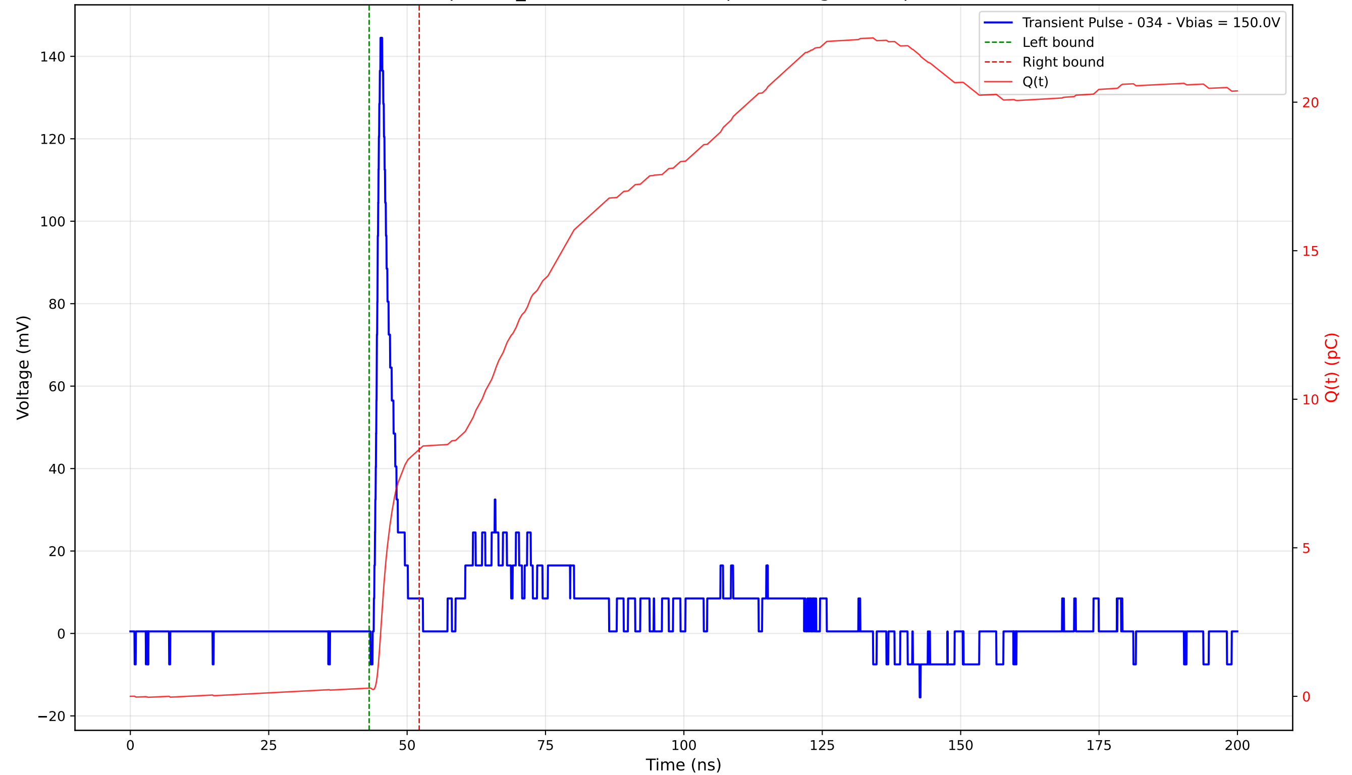
Transient Pulse - Sample: TD_4004 - Position: 55.0 \mu\text{m} - Charge: 8.03 pC - Rise Time: 0.99 ns
