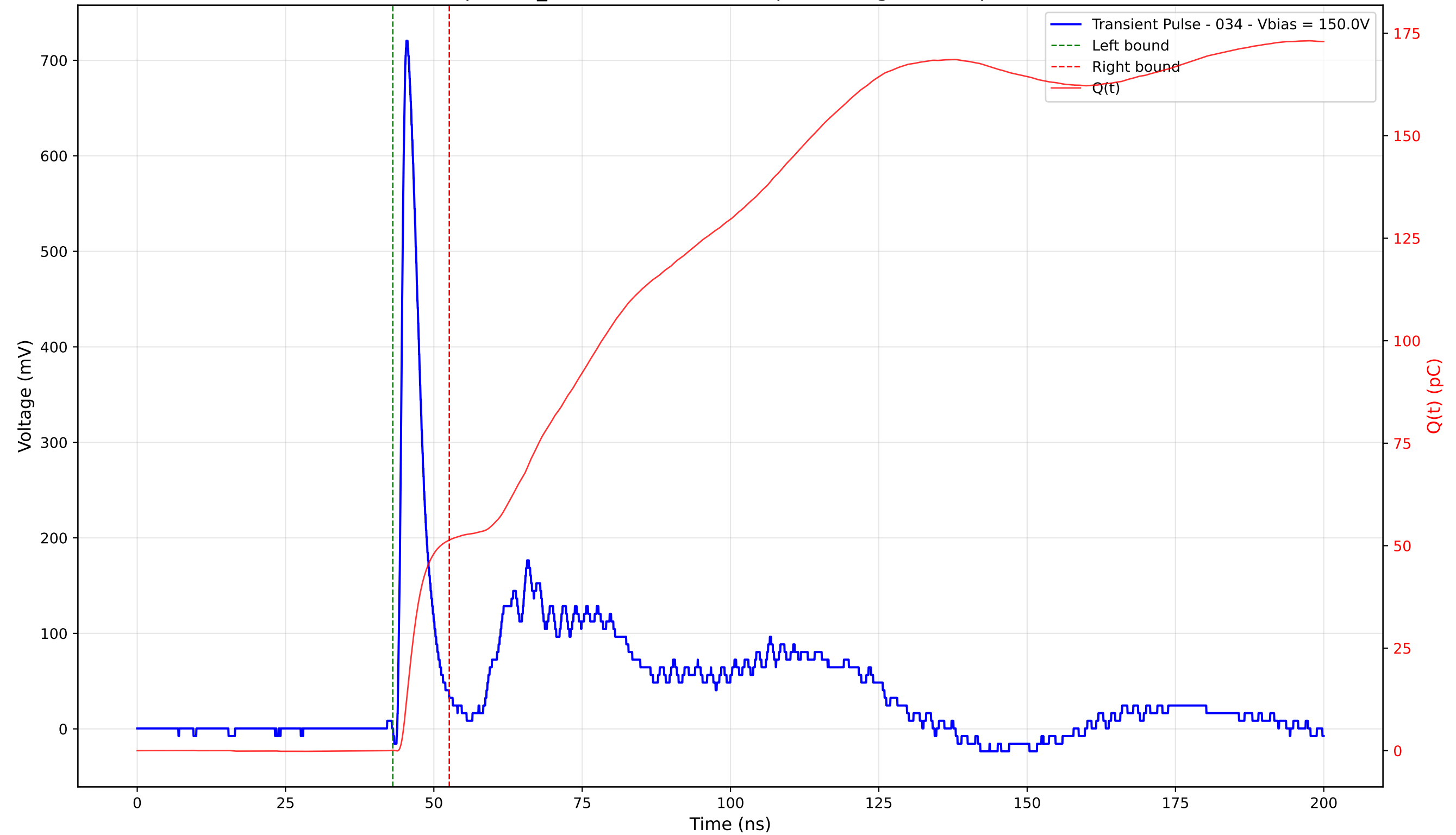
Transient Pulse - Sample: TD_4004 - Position: 170.0 \mu\text{m} - Charge: 51.28 pC - Rise Time: 0.96 ns
