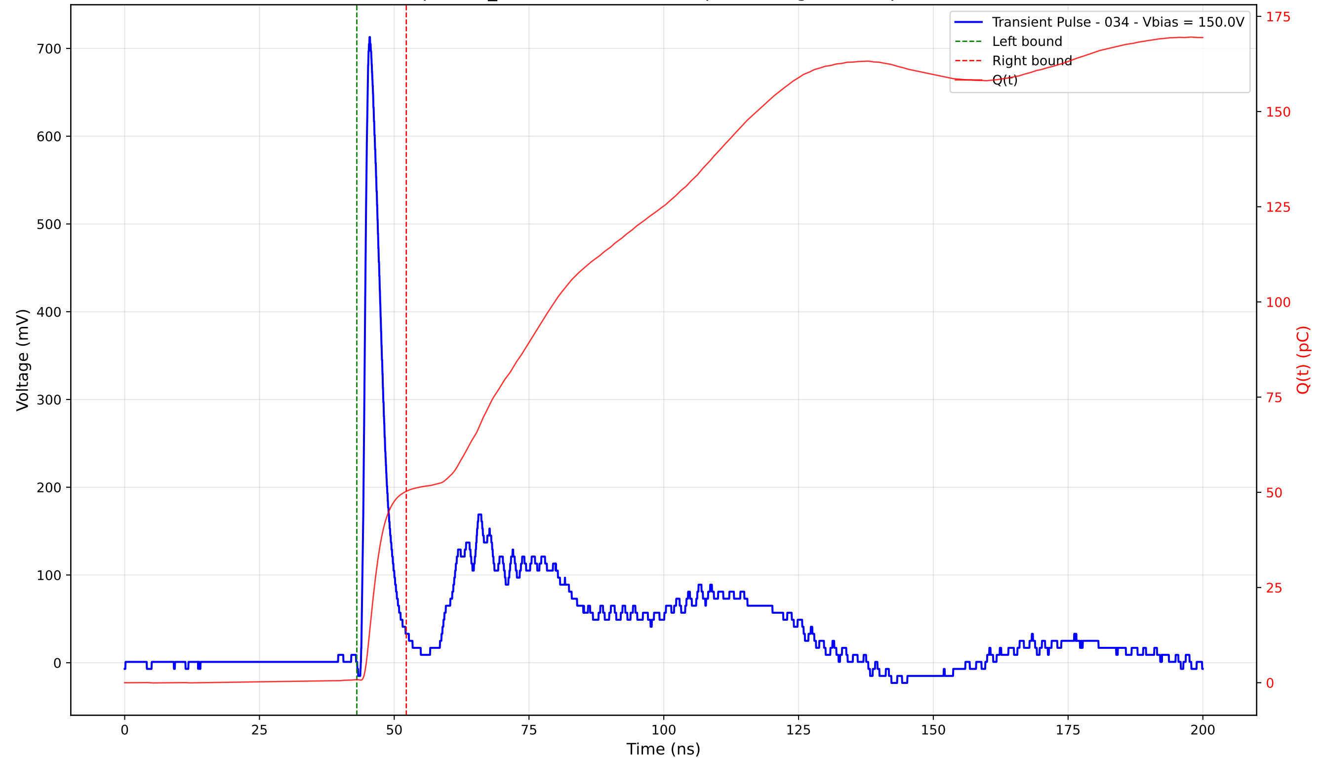
Transient Pulse - Sample: TD_4004 - Position: 220.0 \mu\text{m} - Charge: 49.44 pC - Rise Time: 0.99 ns
