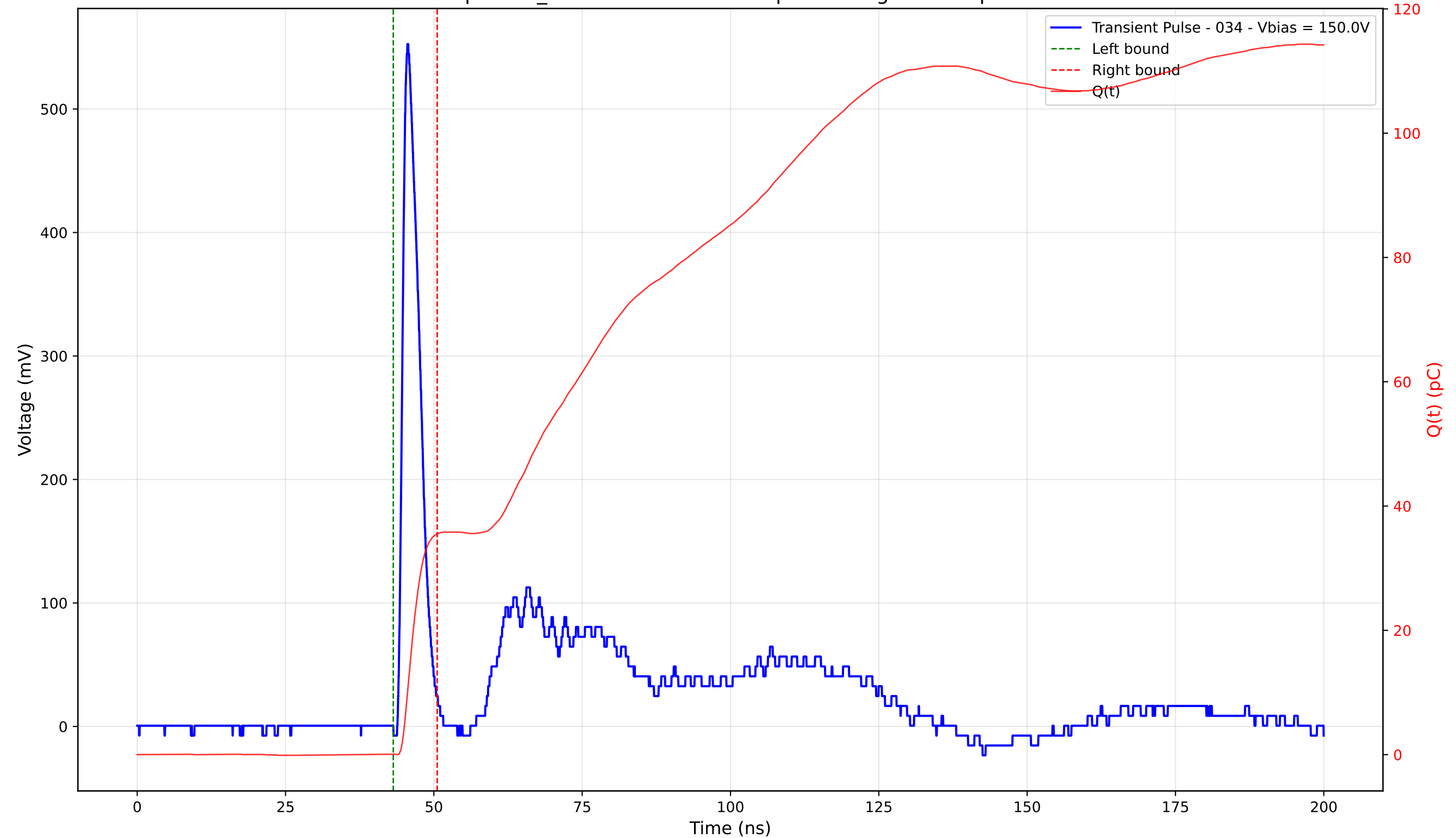
Transient Pulse - Sample: TD_4004 - Position: 295.0 \mu\text{m} - Charge: 35.44 pC - Rise Time: 1.07 ns
