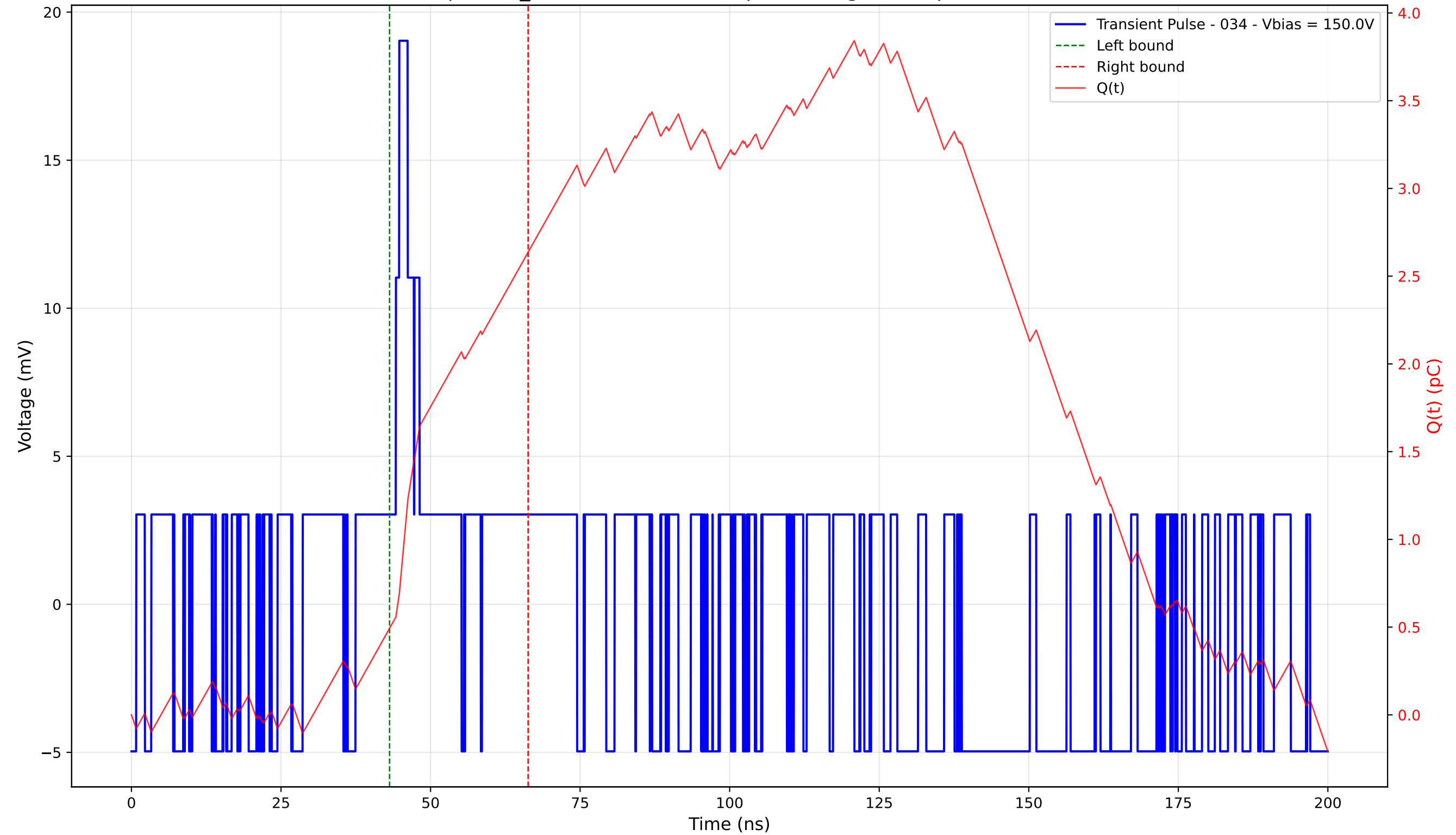
Transient Pulse - Sample: TD_4004 - Position: 30.0 \mu\text{m} - Charge: 2.14 pC - Rise Time: 0.00 ns (N/A)
