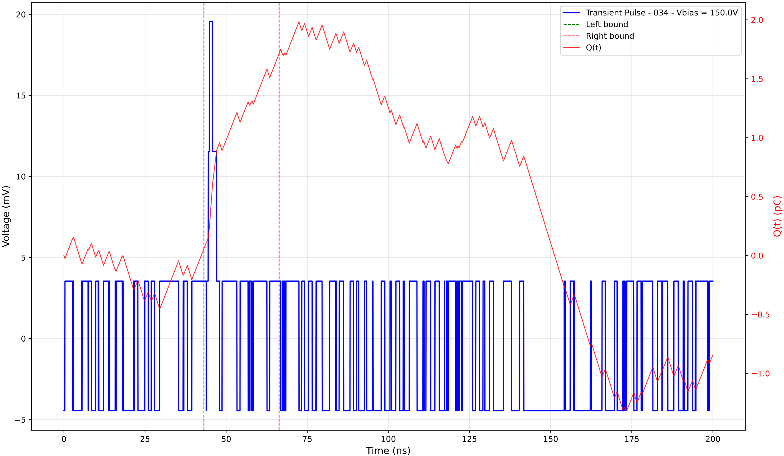
Transient Pulse - Sample: TD_4004 - Position: 25.0 \mu\text{m} - Charge: 1.65 pC - Rise Time: 0.00 ns (N/A)
