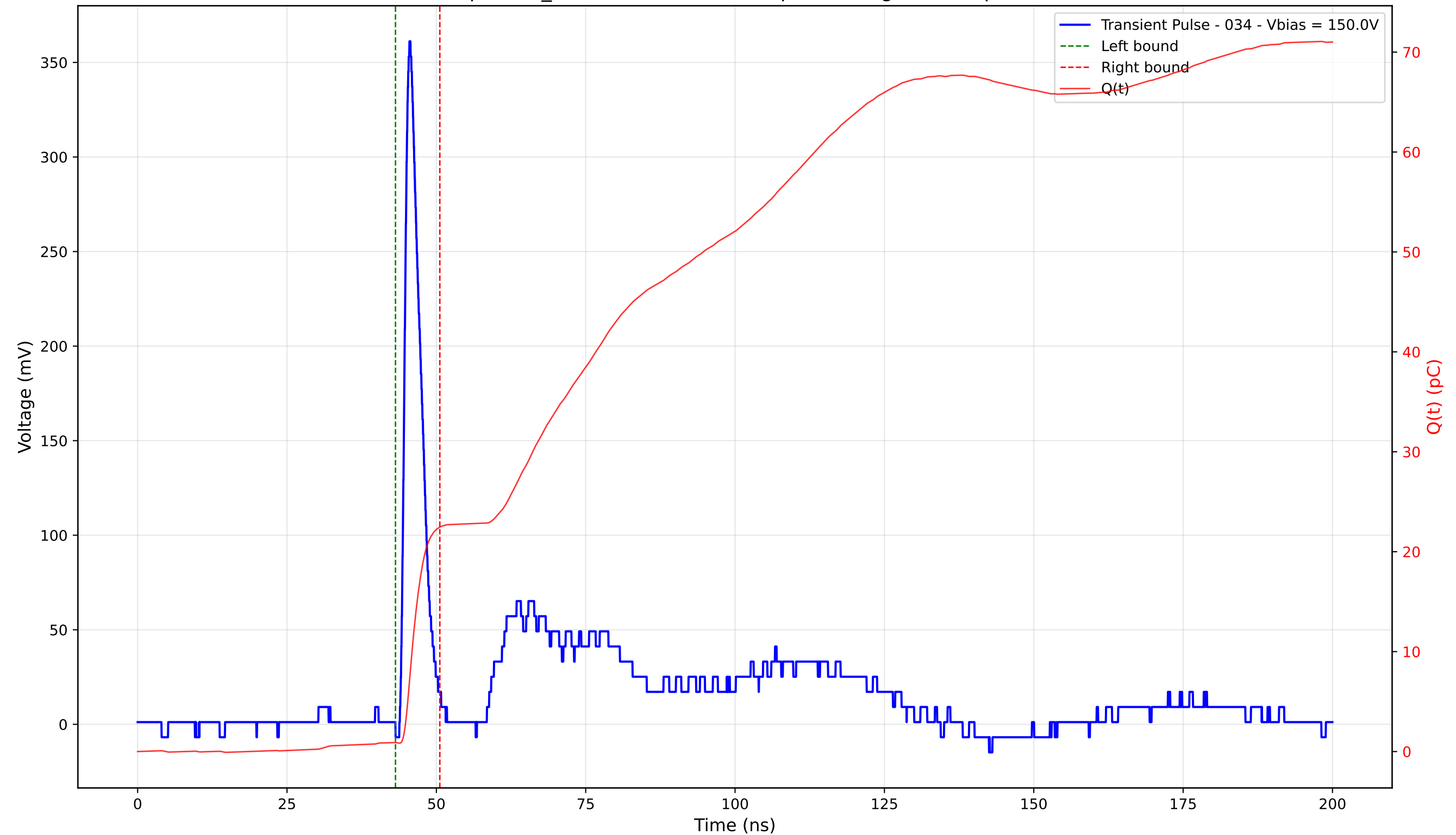
Transient Pulse - Sample: TD_4004 - Position: 350.0 \mu\text{m} - Charge: 21.55 pC - Rise Time: 1.05 ns
