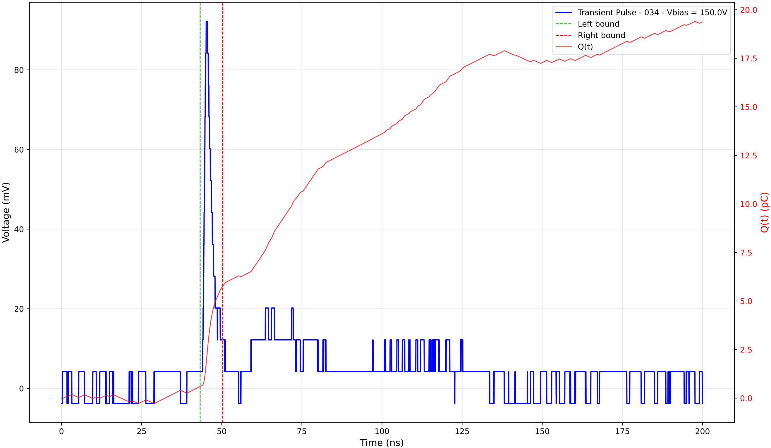
Transient Pulse - Sample: TD_4004 - Position: 50.0 \mu\text{m} - Charge: 5.17 pC - Rise Time: 0.97 ns
