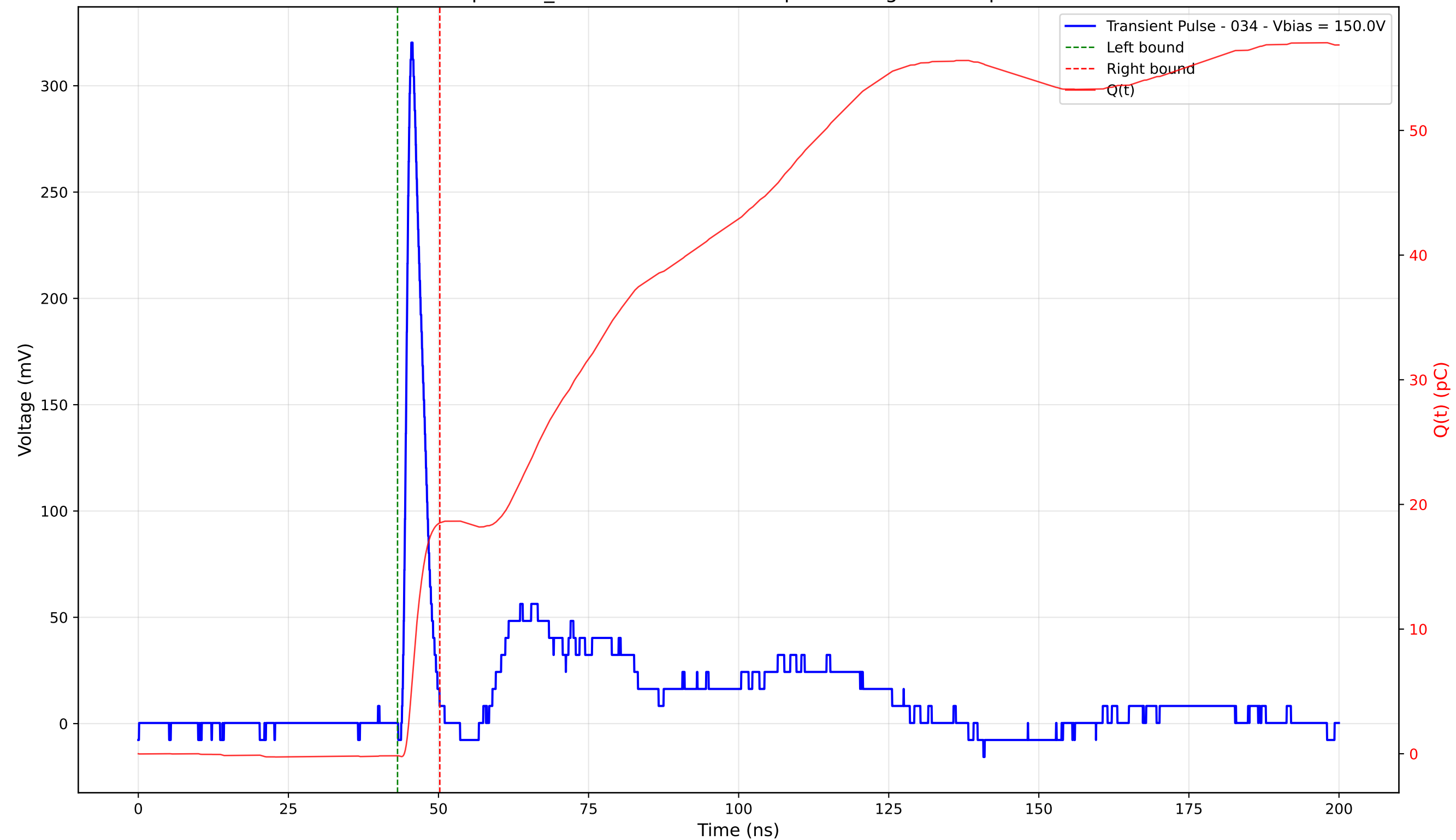
Transient Pulse - Sample: TD_4004 - Position: 380.0 \mu\text{m} - Charge: 18.67 pC - Rise Time: 1.04 ns
