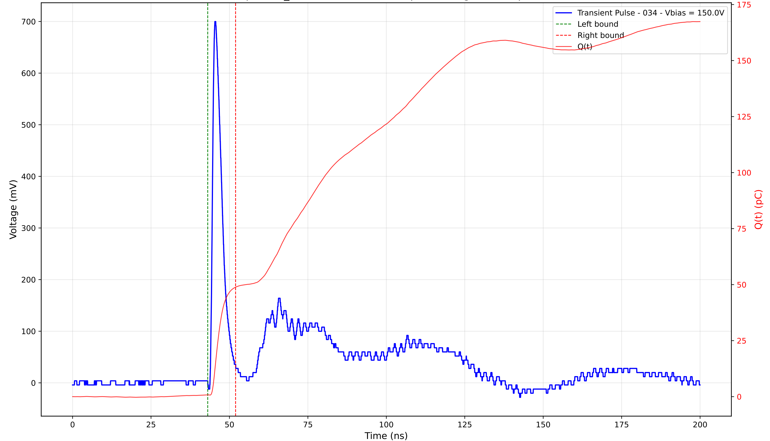
Transient Pulse - Sample: TD_4004 - Position: 225.0 \mu\text{m} - Charge: 48.06 pC - Rise Time: 0.98 ns
