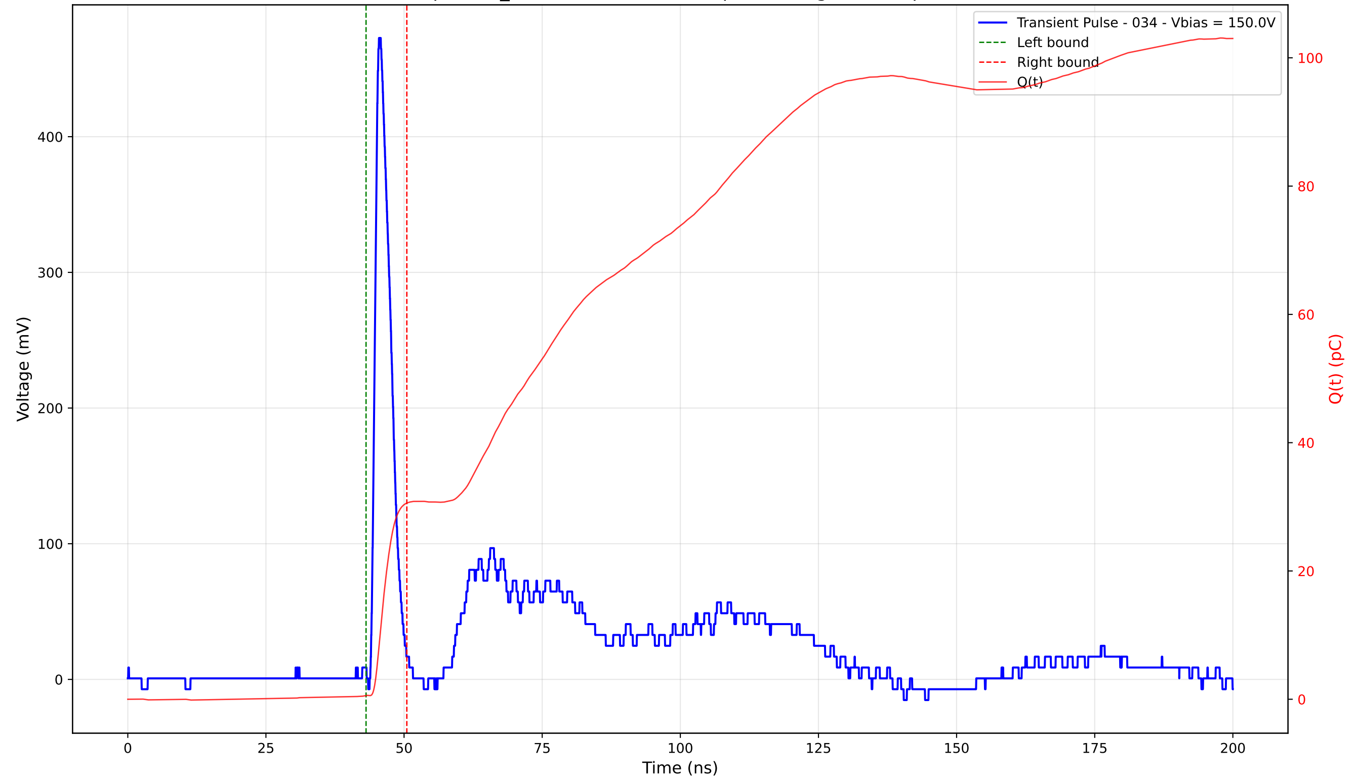
Transient Pulse - Sample: TD_4004 - Position: 315.0 \mu\text{m} - Charge: 30.00 pC - Rise Time: 1.05 ns
