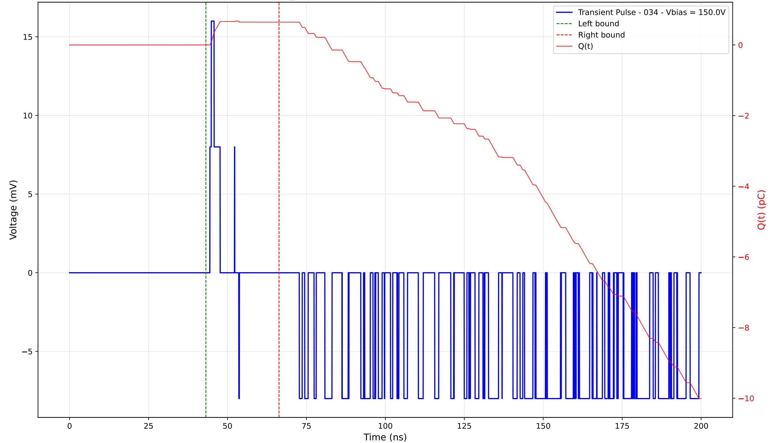
Transient Pulse - Sample: TD_4004 - Position: 20.0 \mu\text{m} - Charge: 0.65 pC - Rise Time: 0.46 ns
