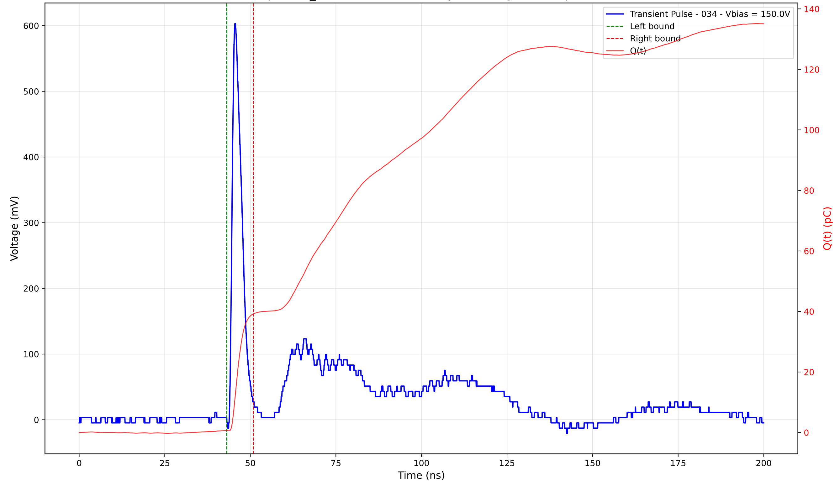
Transient Pulse - Sample: TD_4004 - Position: 260.0 \mu\text{m} - Charge: 38.56 pC - Rise Time: 1.05 ns
