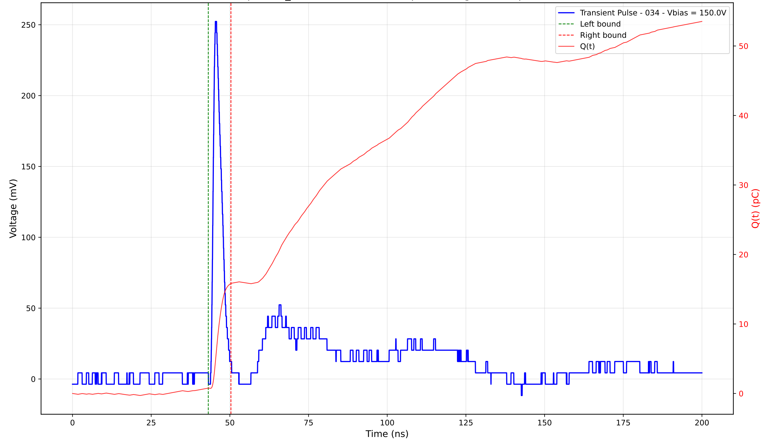
Transient Pulse - Sample: TD_4004 - Position: 390.0 \mu\text{m} - Charge: 15.03 pC - Rise Time: 1.01 ns
