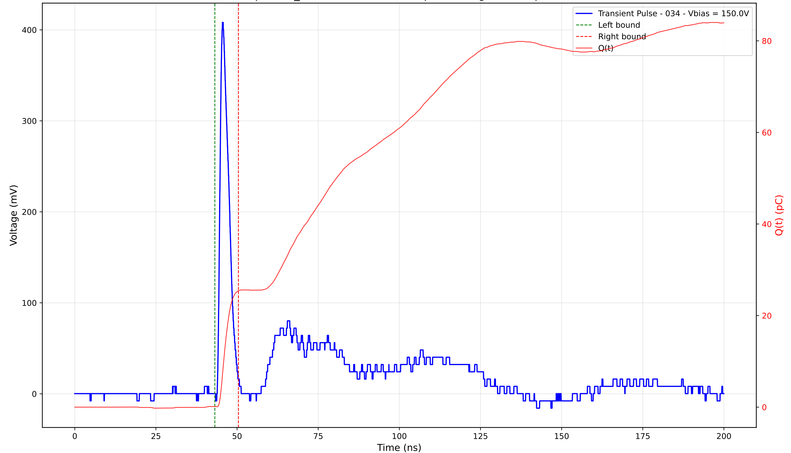
Transient Pulse - Sample: TD_4004 - Position: 330.0 \mu\text{m} - Charge: 25.28 pC - Rise Time: 1.04 ns
