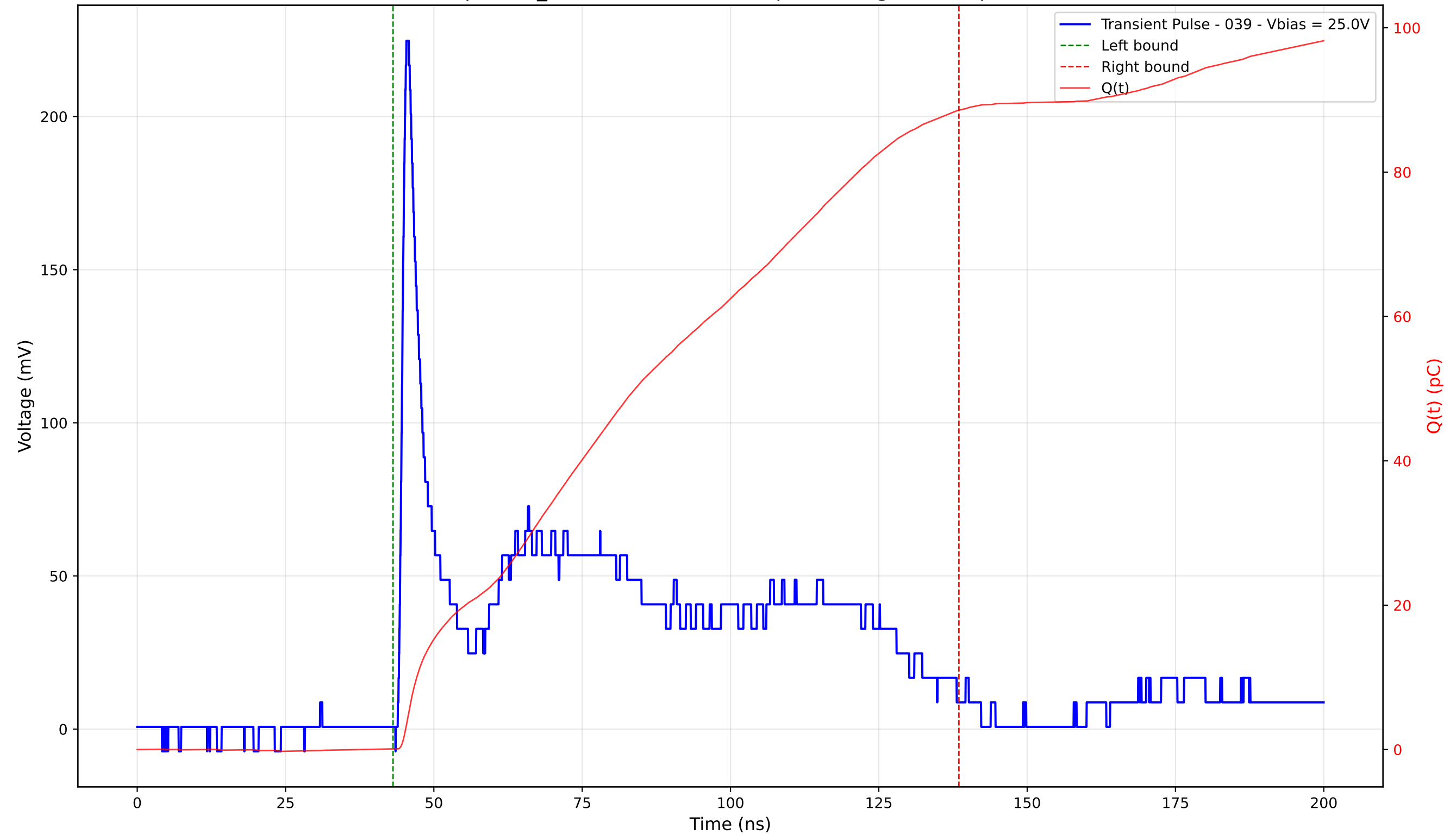
Transient Pulse - Sample: TD_4004 - Position: 205.0 \mu\text{m} - Charge: 88.50 pC - Rise Time: 1.07 ns
