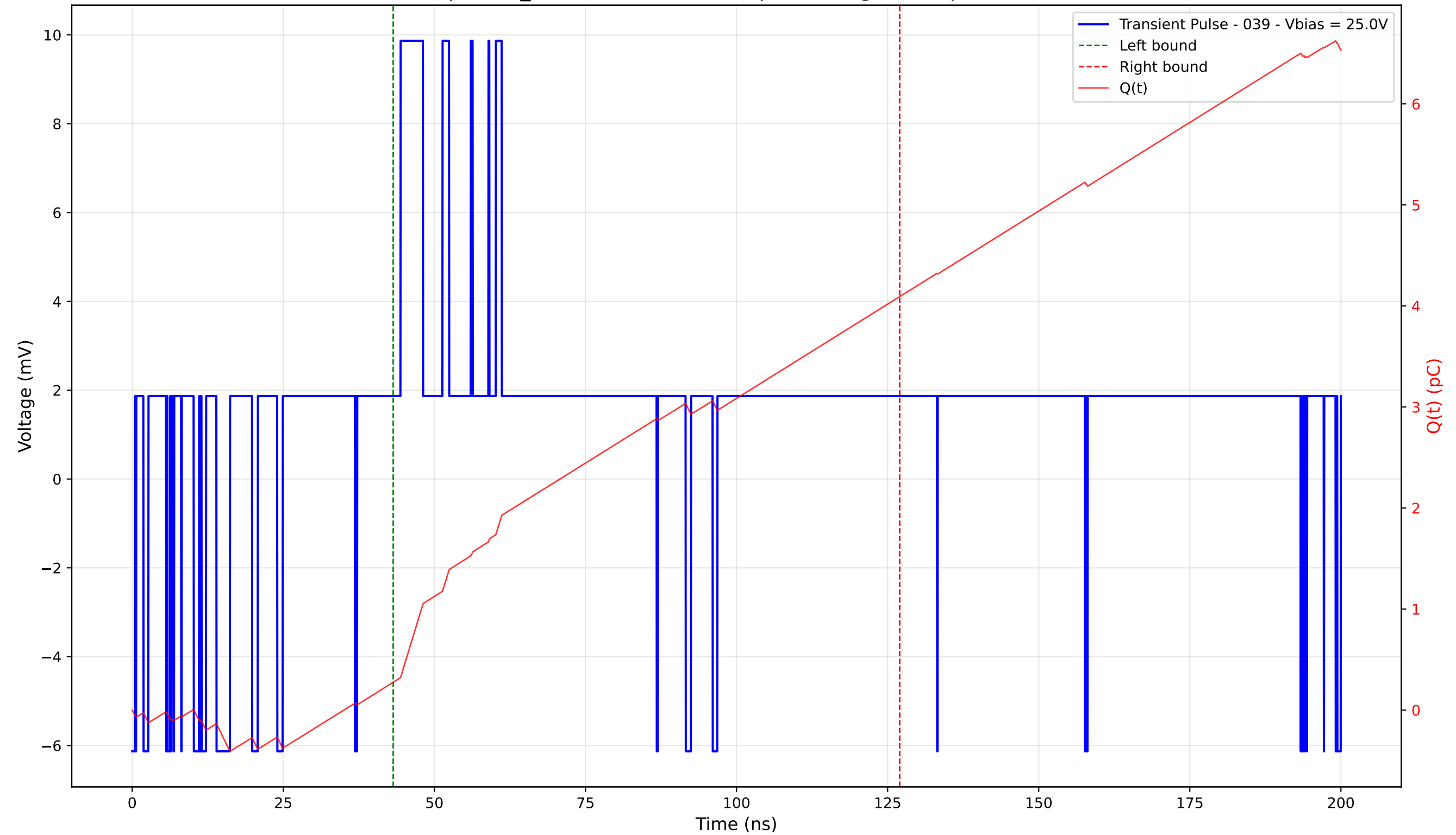
Transient Pulse - Sample: TD_4004 - Position: 430.0 \mu\text{m} - Charge: 3.82 pC - Rise Time: 0.00 ns (N/A)
