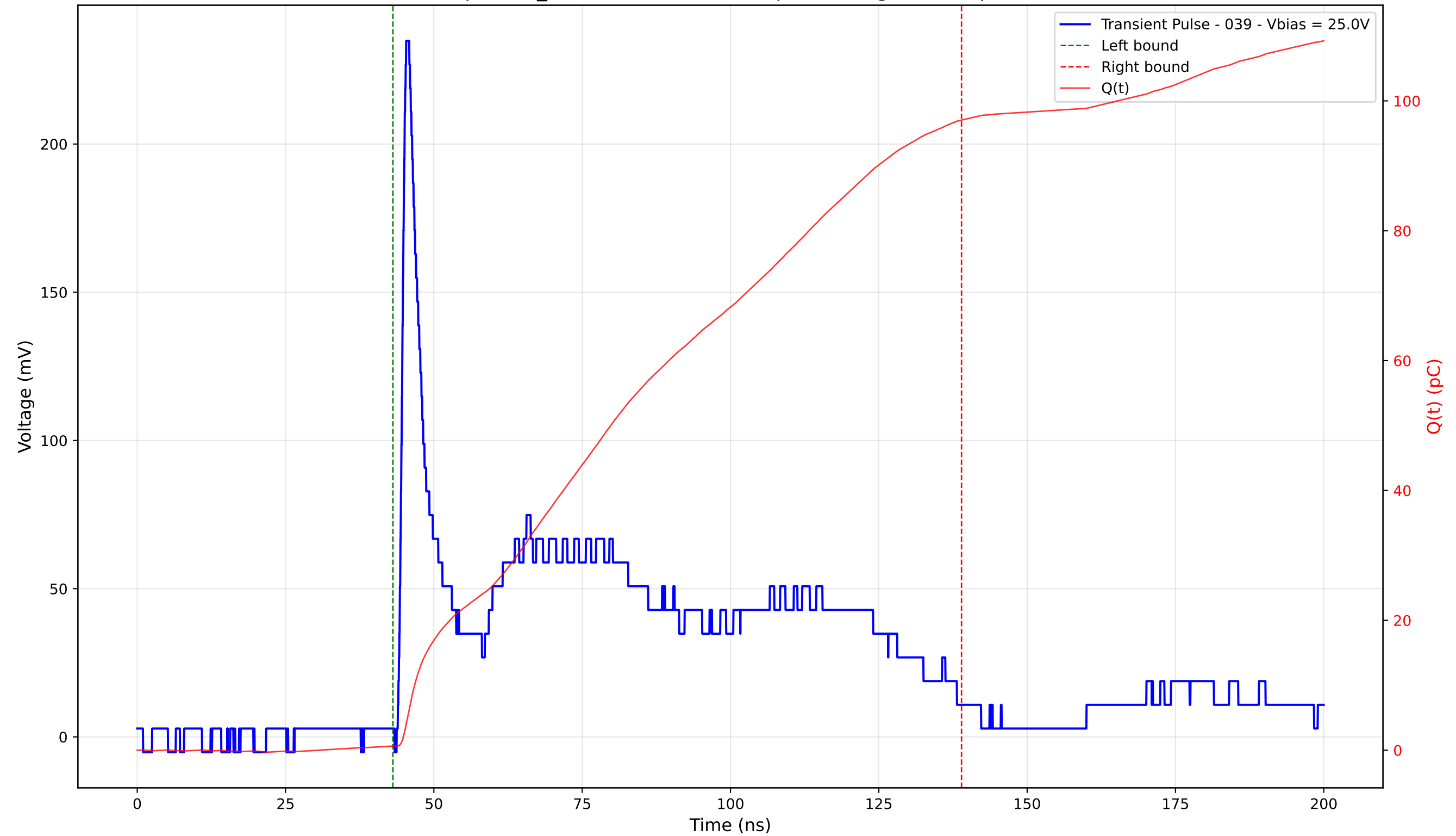
Transient Pulse - Sample: TD_4004 - Position: 200.0 \mu\text{m} - Charge: 96.39 pC - Rise Time: 1.07 ns
