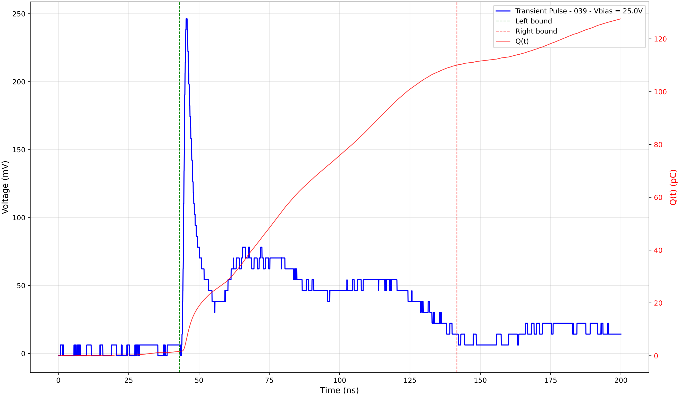
Transient Pulse - Sample: TD_4004 - Position: 195.0 \mu\text{m} - Charge: 108.39 pC - Rise Time: 1.03 ns
