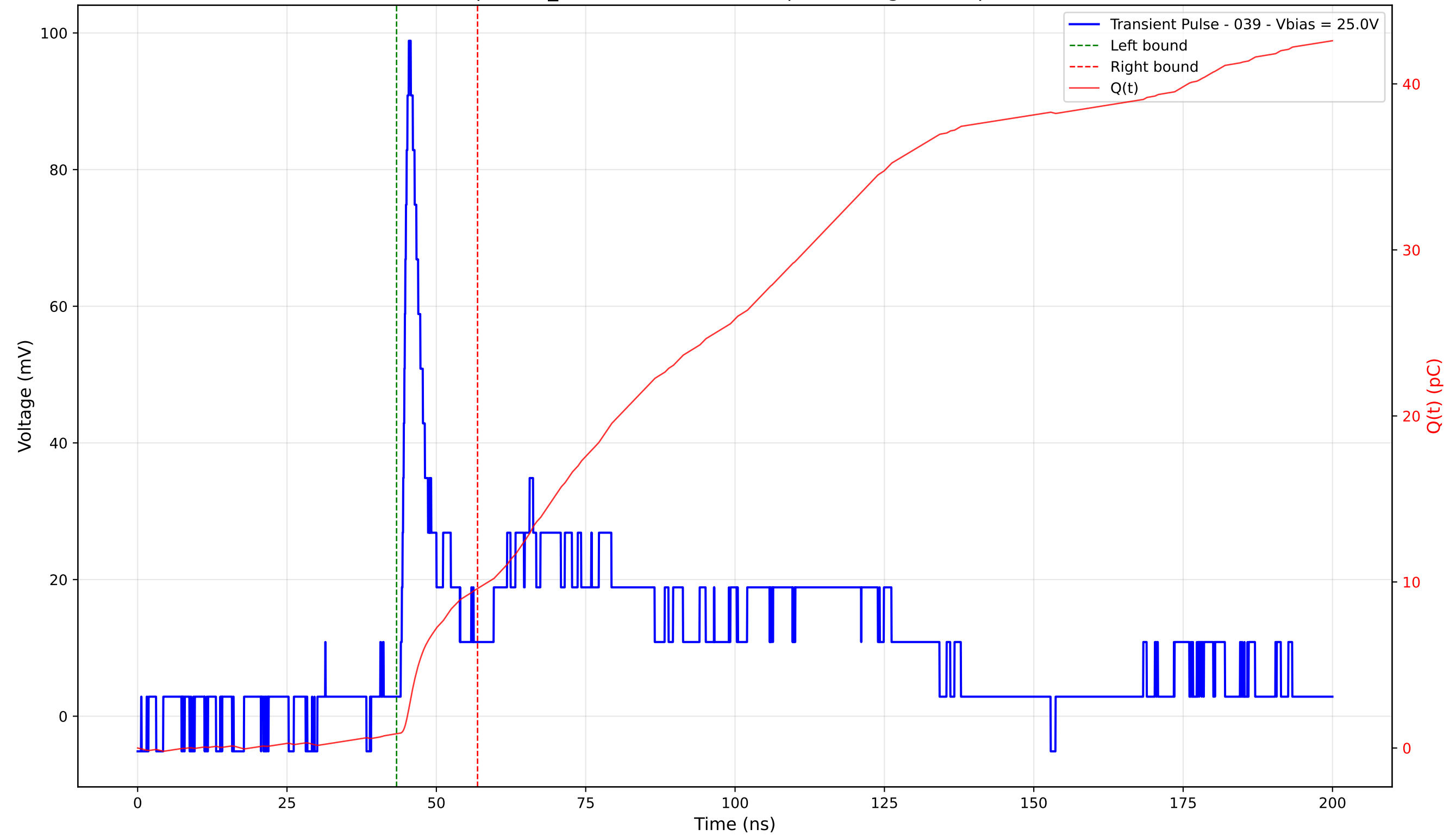
Transient Pulse - Sample: TD_4004 - Position: 300.0 \mu\text{m} - Charge: 8.75 pC - Rise Time: 1.12 ns
