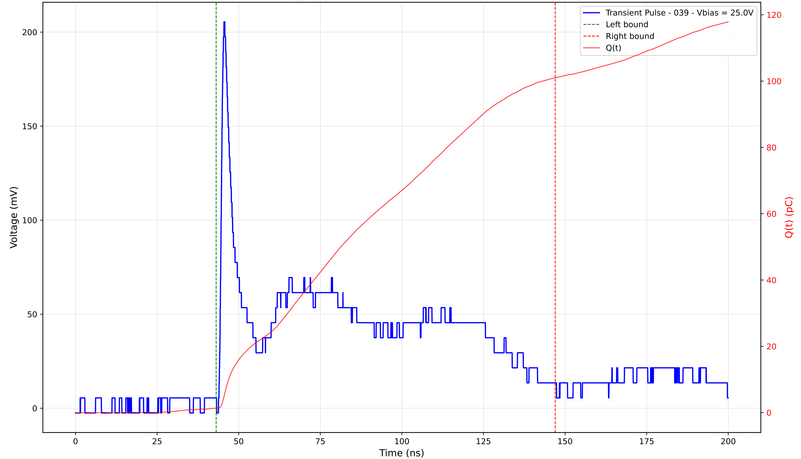
Transient Pulse - Sample: TD_4004 - Position: 175.0 \mu\text{m} - Charge: 99.64 pC - Rise Time: 1.14 ns
