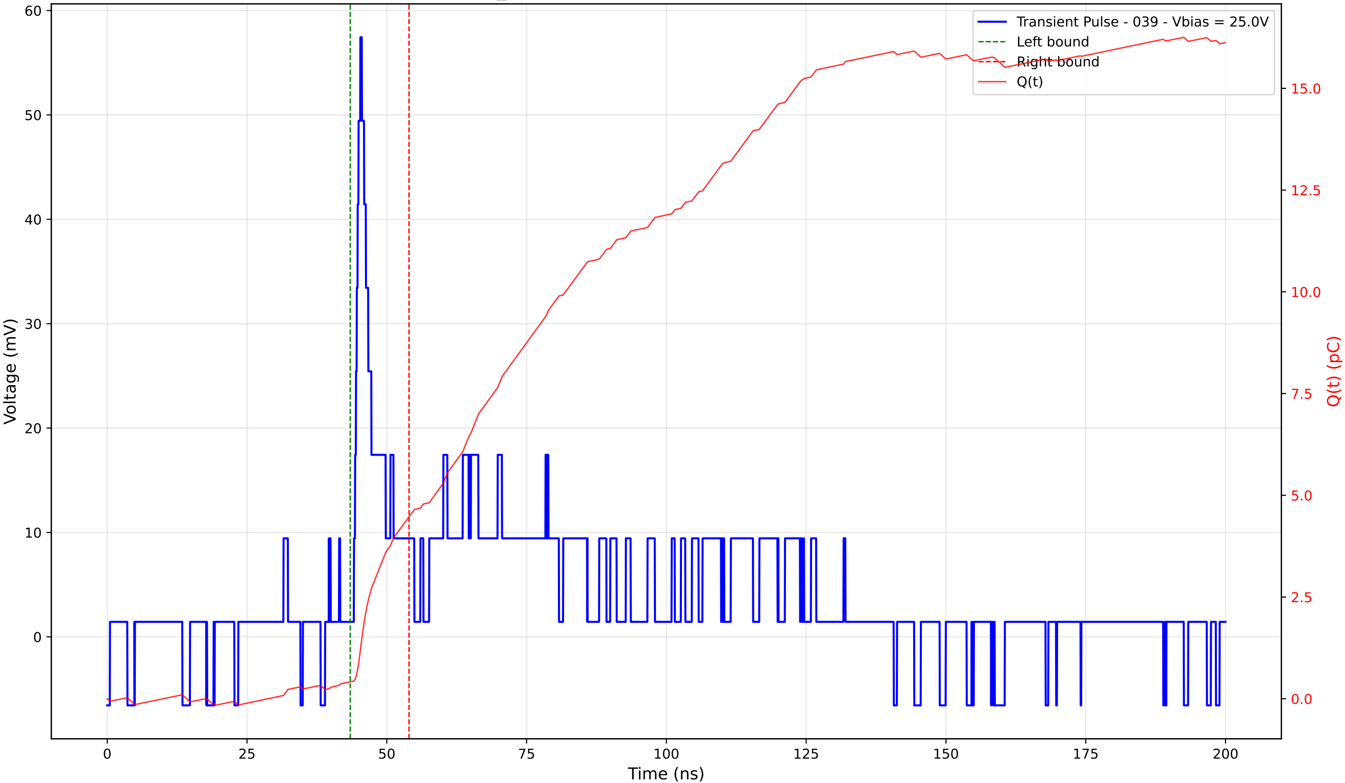
Transient Pulse - Sample: TD_4004 - Position: 55.0 \mu\text{m} - Charge: 4.06 pC - Rise Time: 1.15 ns
