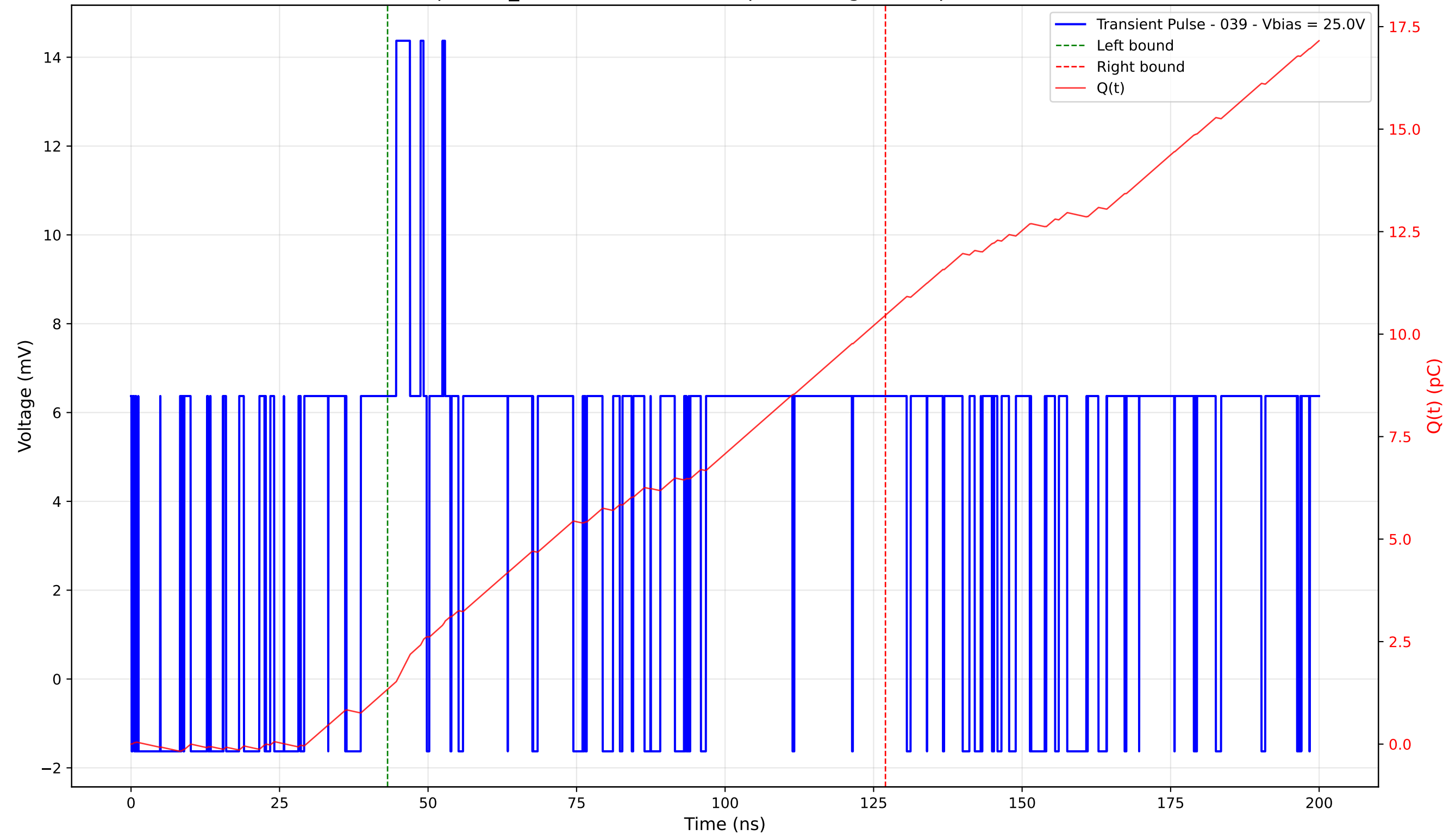
Transient Pulse - Sample: TD_4004 - Position: 425.0 \mu\text{m} - Charge: 9.13 pC - Rise Time: 0.00 ns (N/A)
