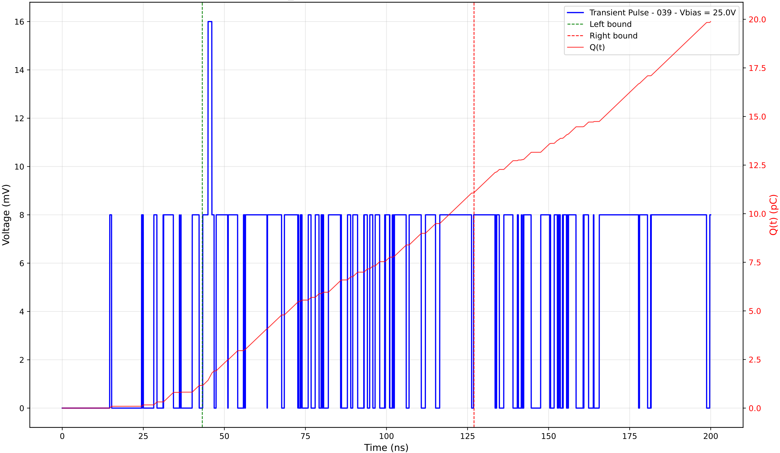
Transient Pulse - Sample: TD_4004 - Position: 35.0 \mu\text{m} - Charge: 9.92 pC - Rise Time: 1.66 ns
