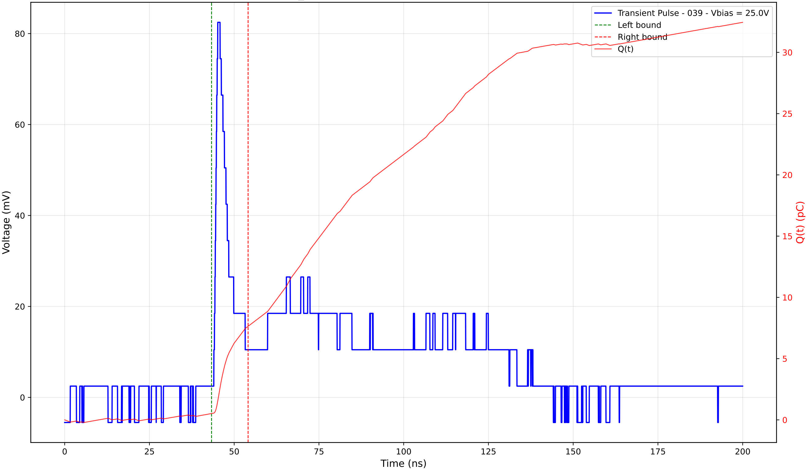
Transient Pulse - Sample: TD_4004 - Position: 315.0 \mu\text{m} - Charge: 7.12 pC - Rise Time: 0.99 ns
