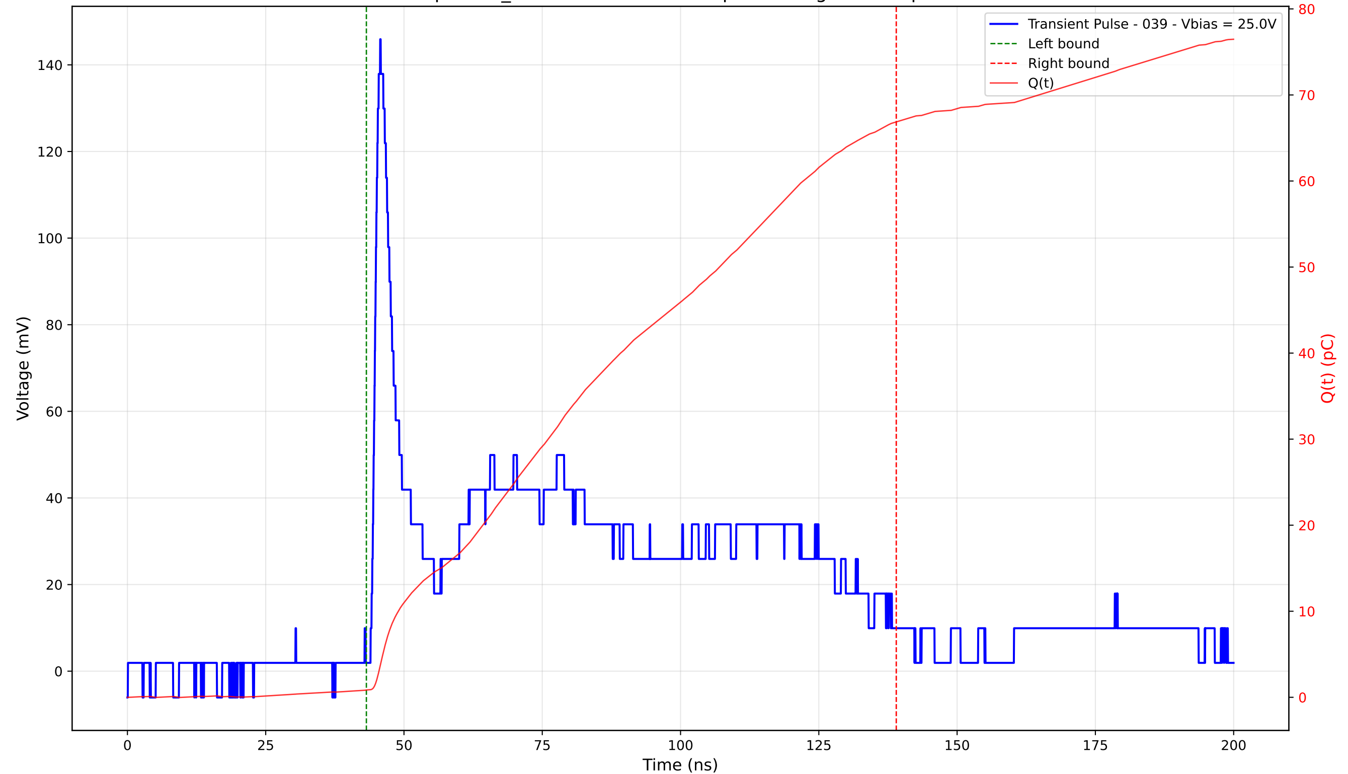
Transient Pulse - Sample: TD_4004 - Position: 145.0 \mu\text{m} - Charge: 66.03 pC - Rise Time: 1.29 ns
