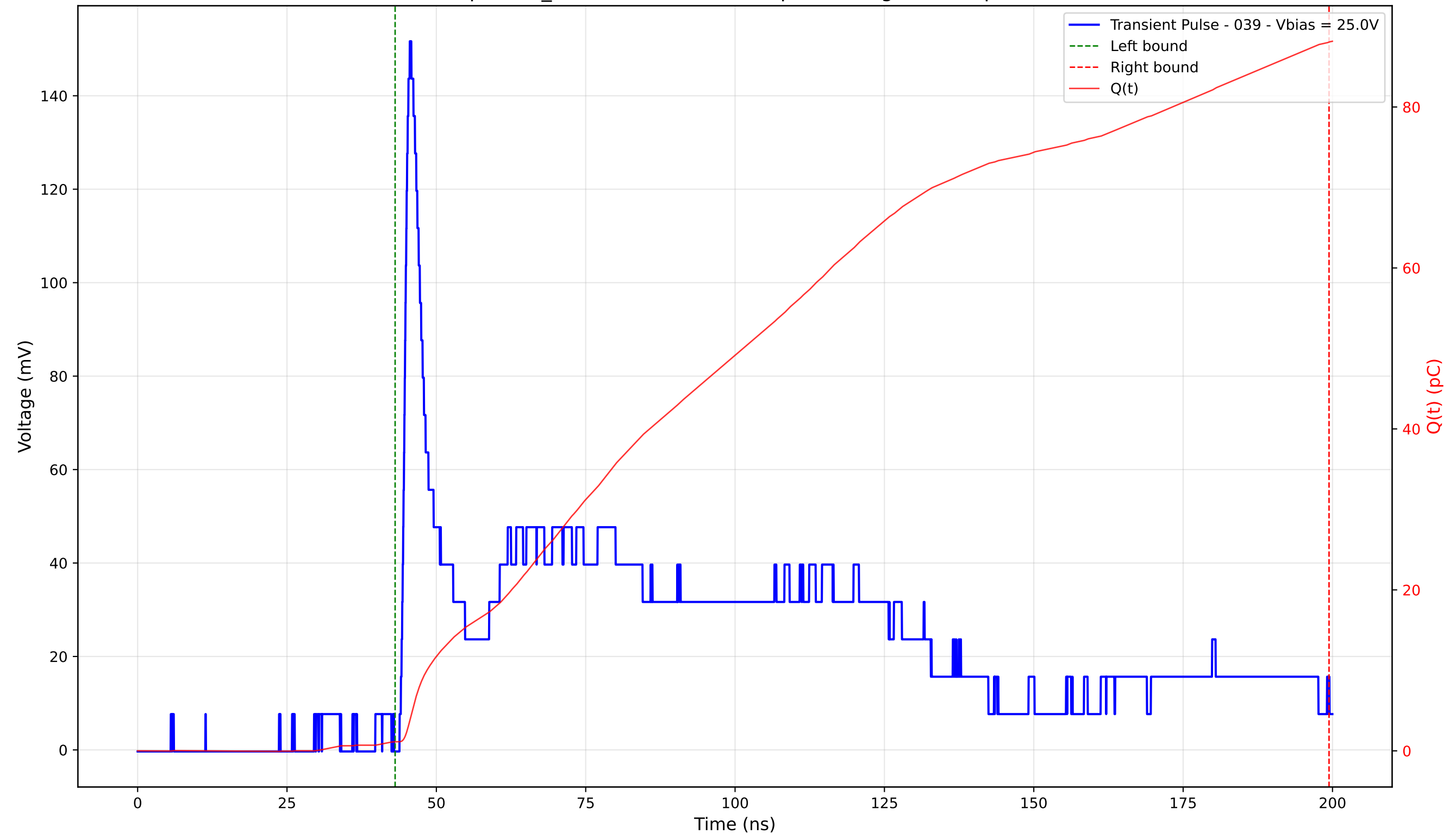
Transient Pulse - Sample: TD_4004 - Position: 150.0 \mu\text{m} - Charge: 86.95 pC - Rise Time: 1.26 ns
