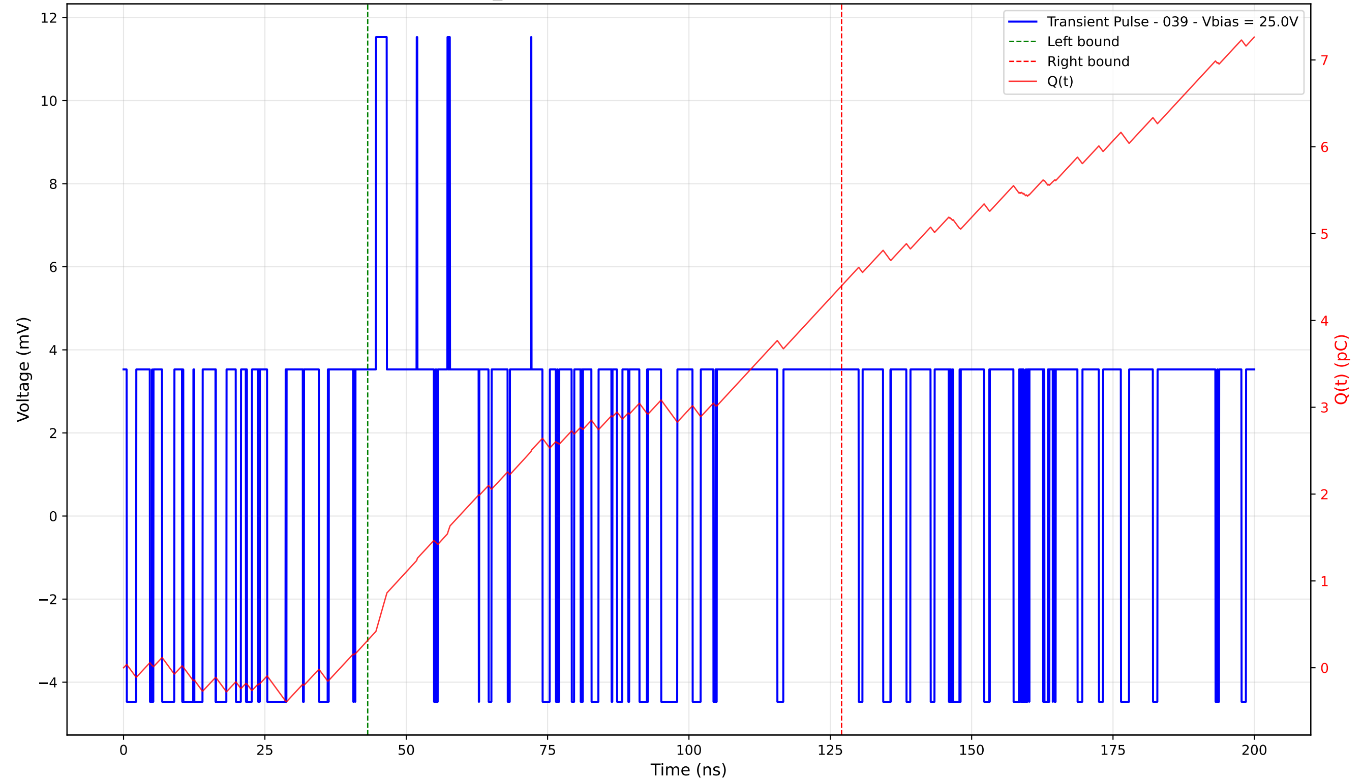
Transient Pulse - Sample: TD_4004 - Position: 40.0 \mu\text{m} - Charge: 4.08 pC - Rise Time: 0.00 ns (N/A)
