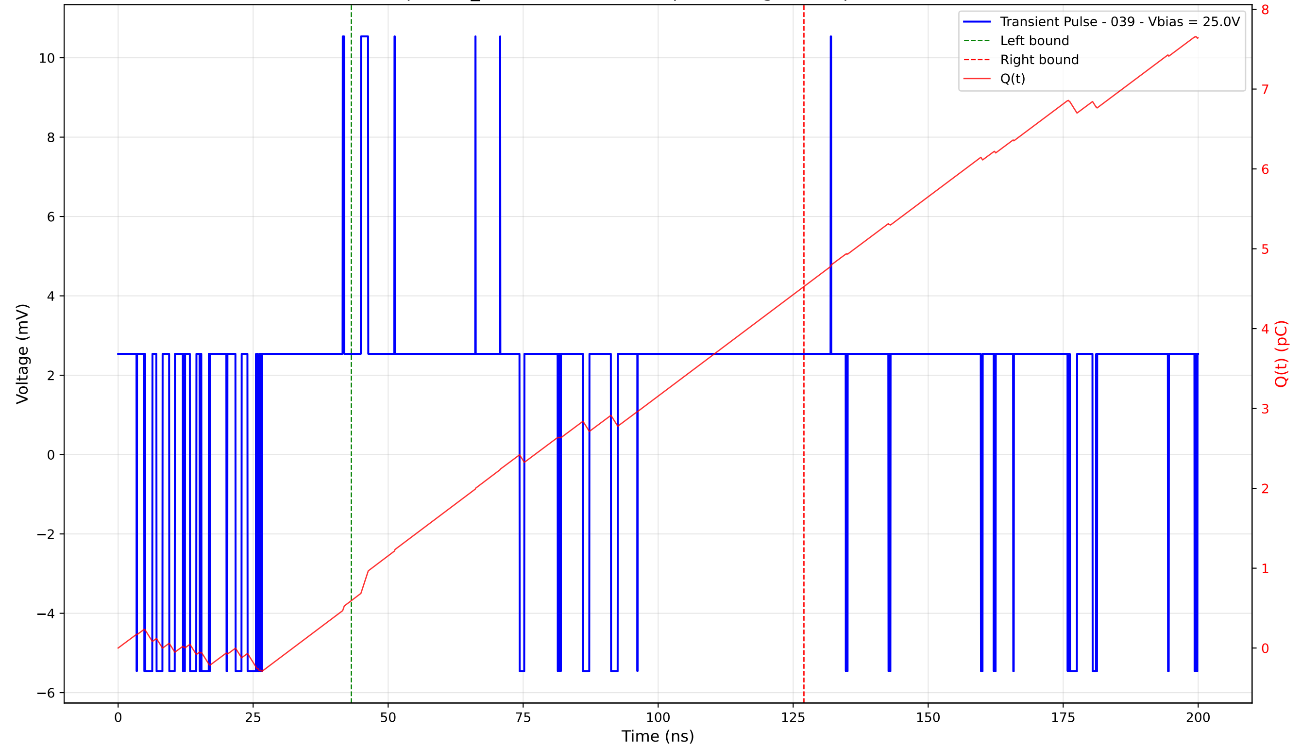
Transient Pulse - Sample: TD_4004 - Position: 30.0 \mu\text{m} - Charge: 3.93 pC - Rise Time: 0.00 ns (N/A)
