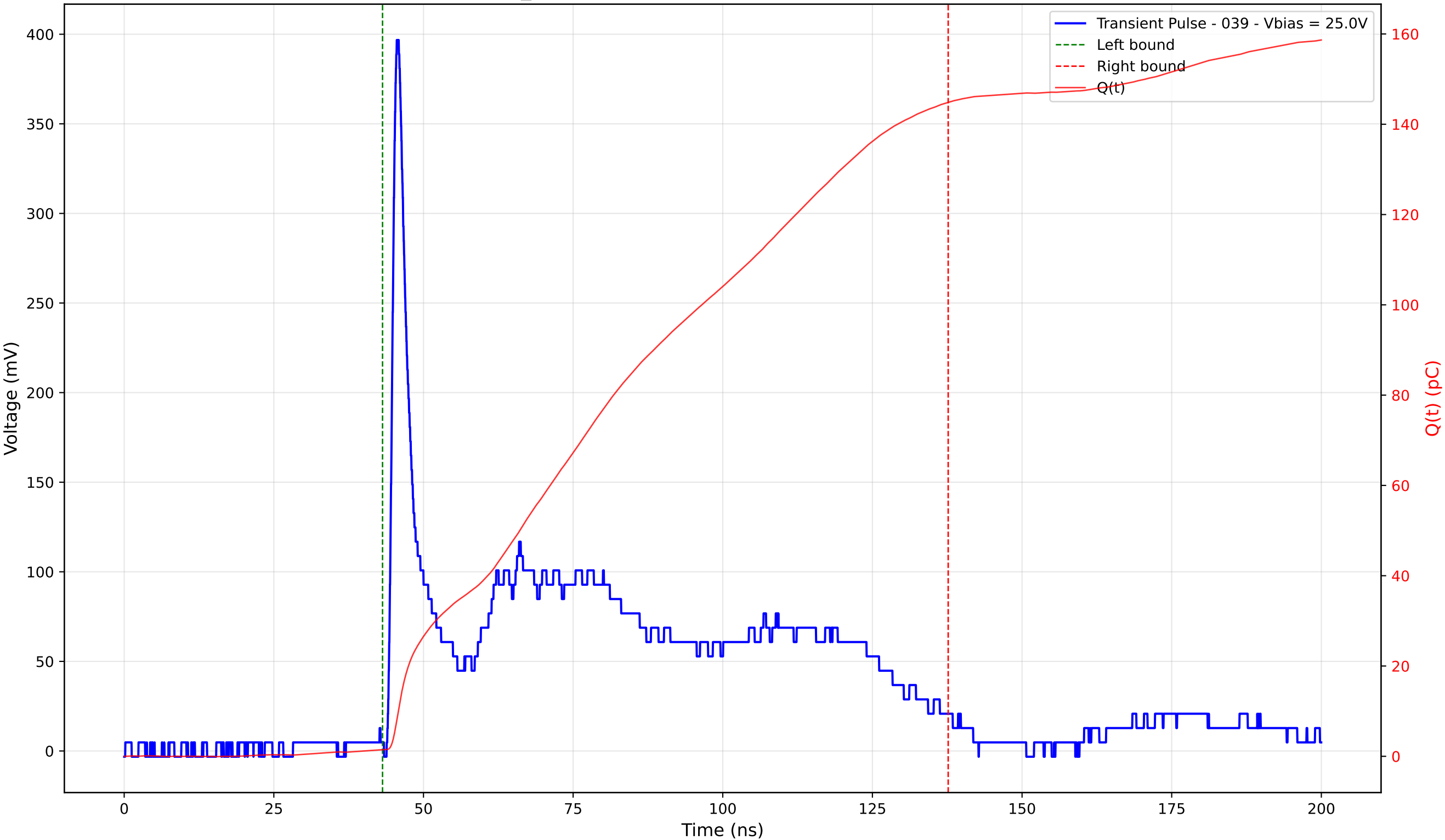
Transient Pulse - Sample: TD_4004 - Position: 115.0 \mu\text{m} - Charge: 143.34 pC - Rise Time: 1.11 ns
