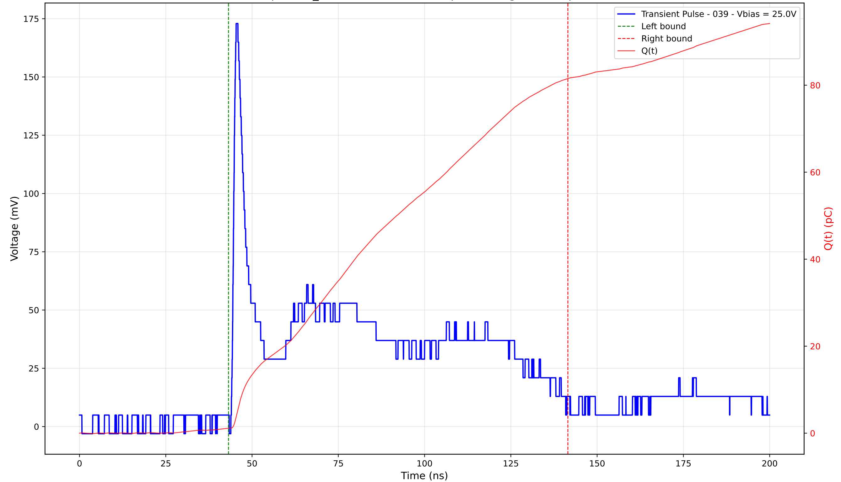
Transient Pulse - Sample: TD_4004 - Position: 165.0 \mu\text{m} - Charge: 80.36 pC - Rise Time: 1.05 ns
