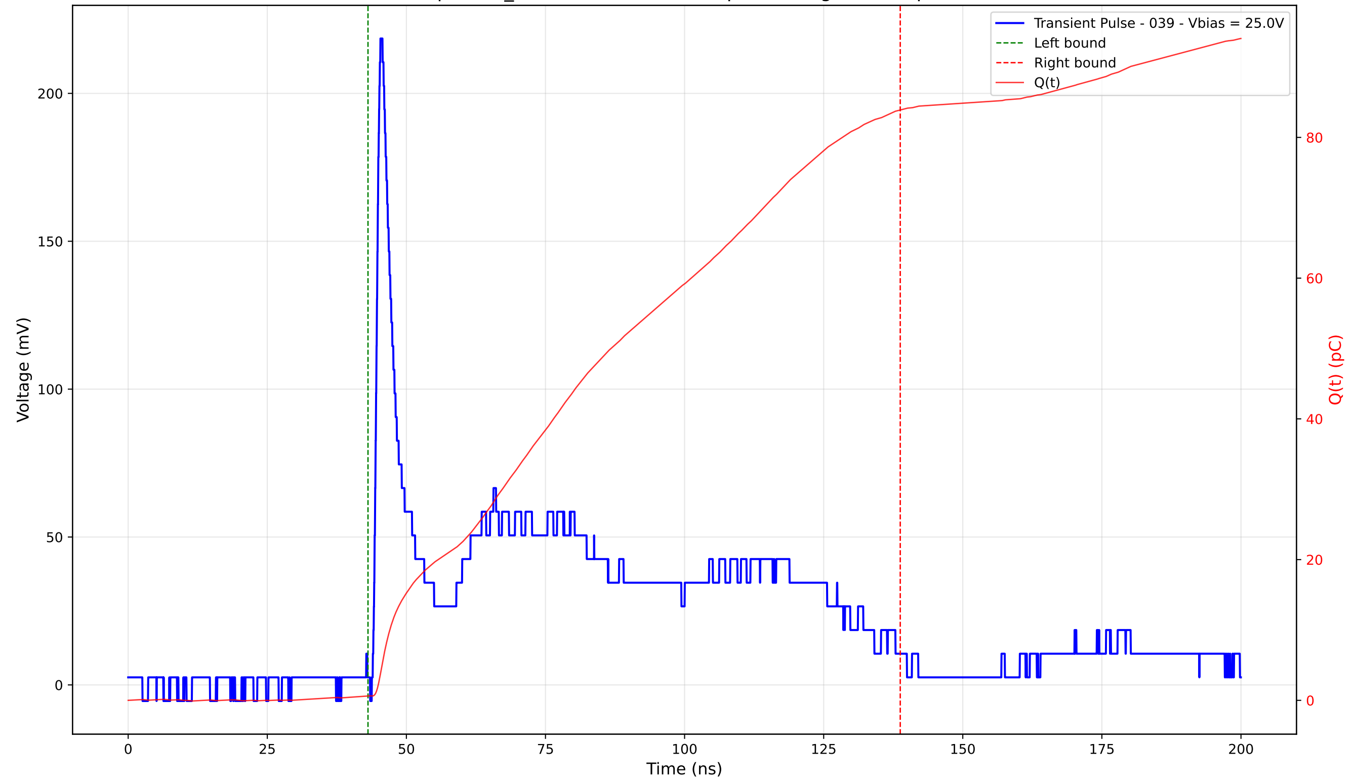
Transient Pulse - Sample: TD_4004 - Position: 220.0 \mu\text{m} - Charge: 83.27 pC - Rise Time: 1.01 ns
