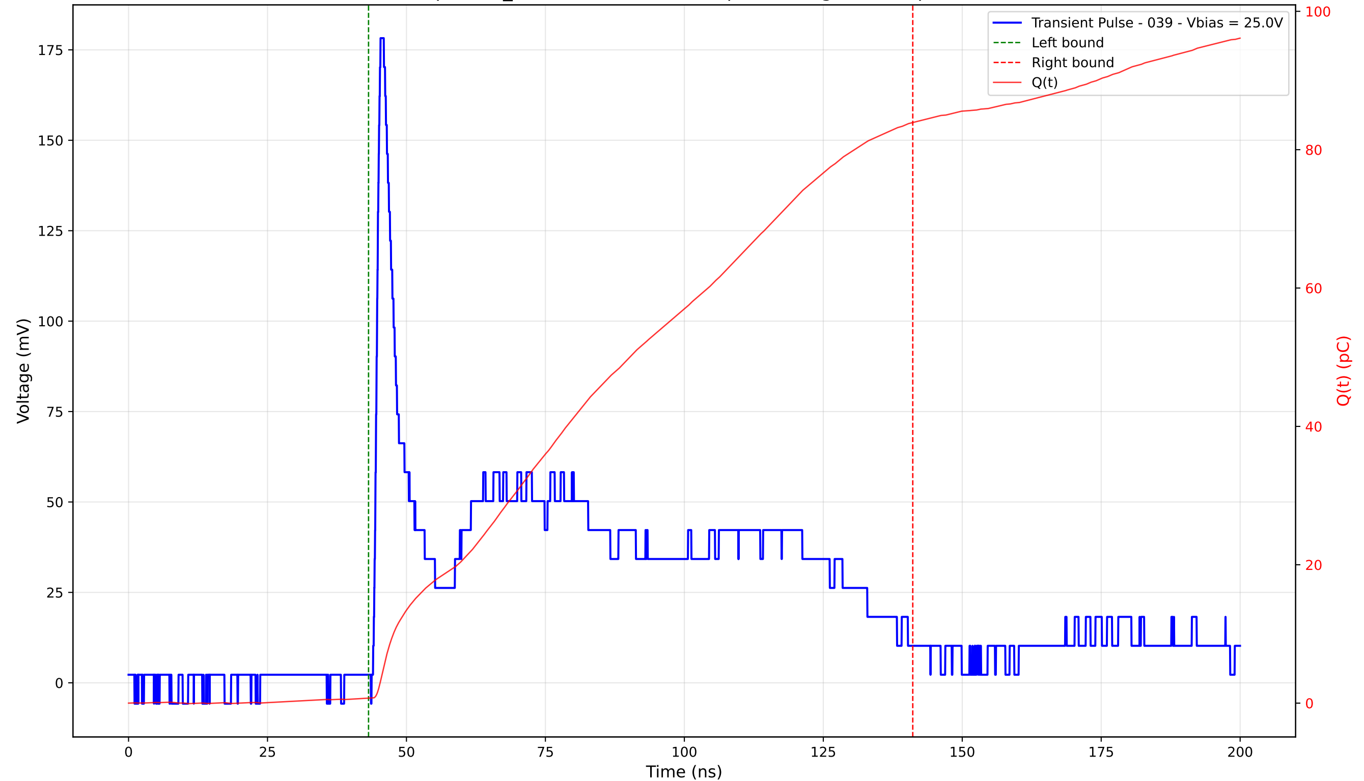
Transient Pulse - Sample: TD_4004 - Position: 170.0 \mu\text{m} - Charge: 83.22 pC - Rise Time: 1.02 ns
