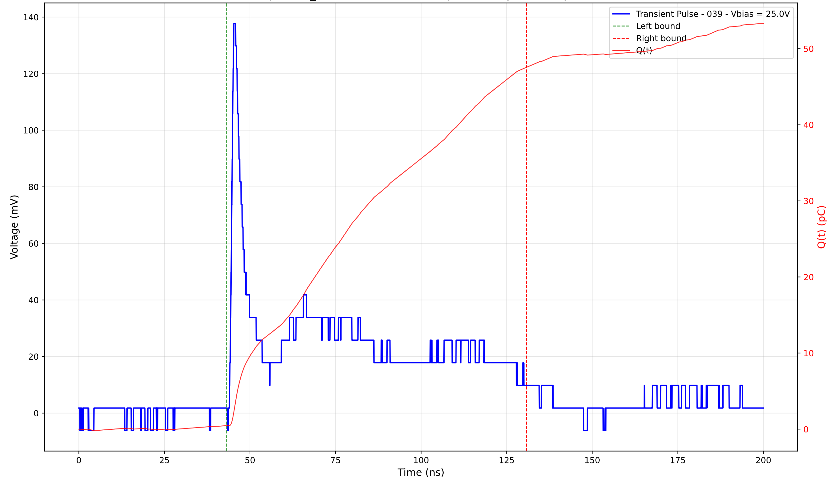
Transient Pulse - Sample: TD_4004 - Position: 255.0 \mu\text{m} - Charge: 47.10 pC - Rise Time: 1.05 ns
