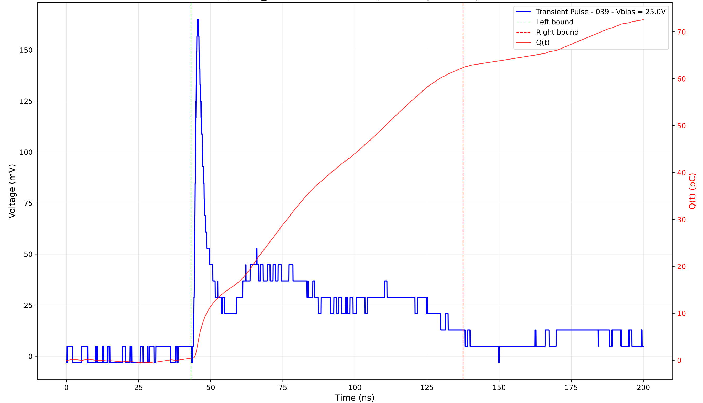
Transient Pulse - Sample: TD_4004 - Position: 235.0 \mu\text{m} - Charge: 61.93 pC - Rise Time: 1.03 ns
