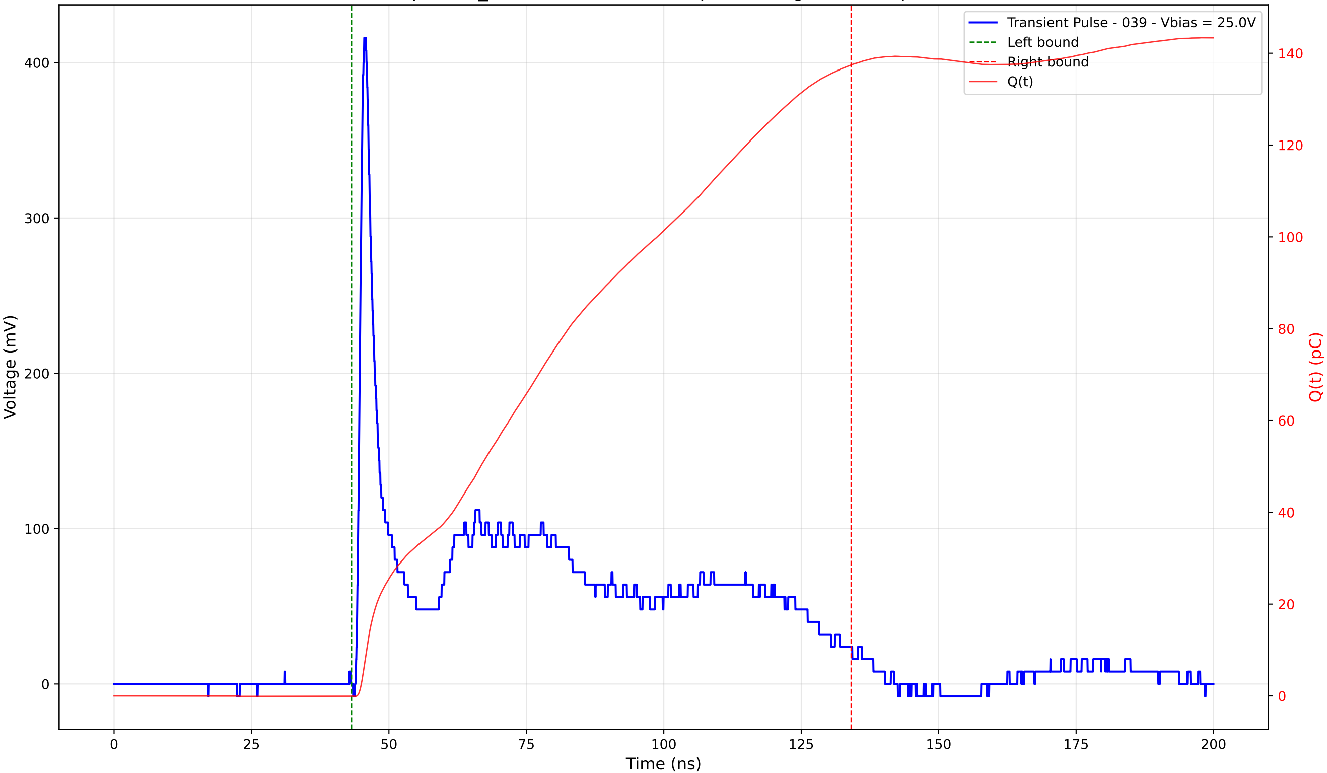
Transient Pulse - Sample: TD_4004 - Position: 110.0 \mu\text{m} - Charge: 137.51 pC - Rise Time: 1.02 ns
