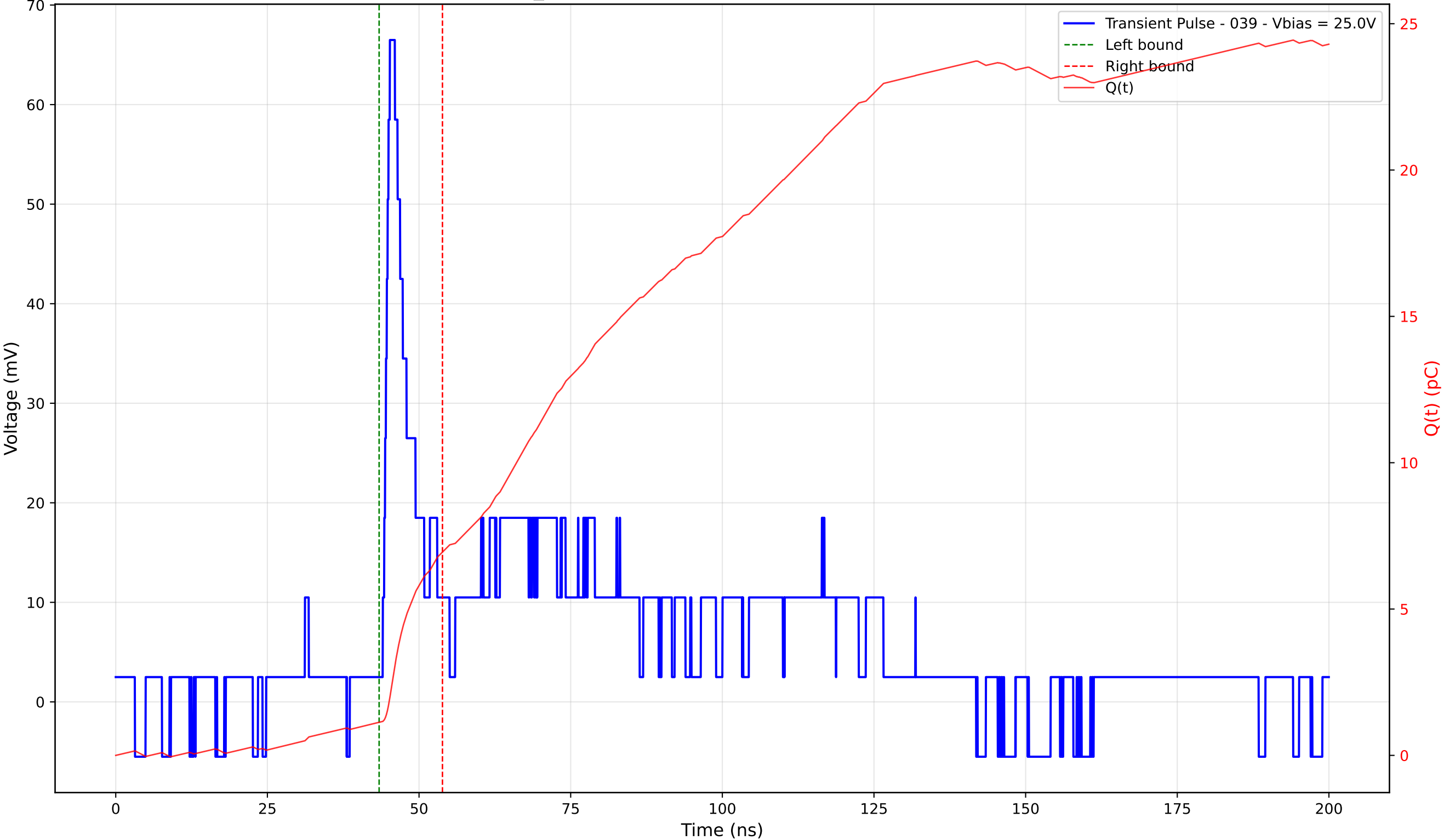
Transient Pulse - Sample: TD_4004 - Position: 365.0 \mu\text{m} - Charge: 5.82 pC - Rise Time: 1.17 ns
