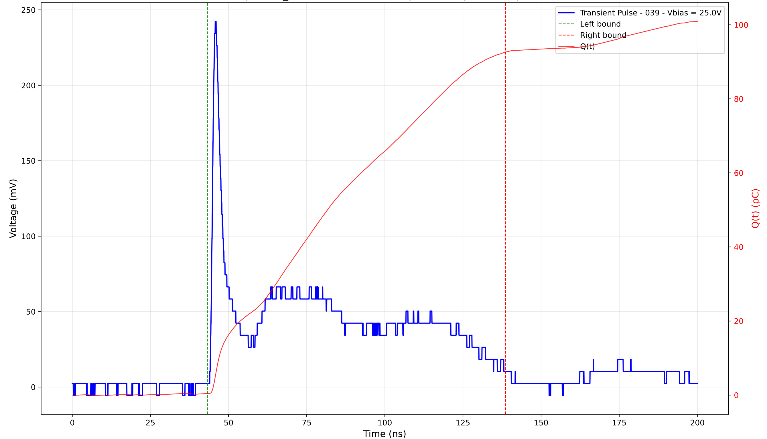
Transient Pulse - Sample: TD_4004 - Position: 130.0 \mu\text{m} - Charge: 92.23 pC - Rise Time: 1.17 ns
