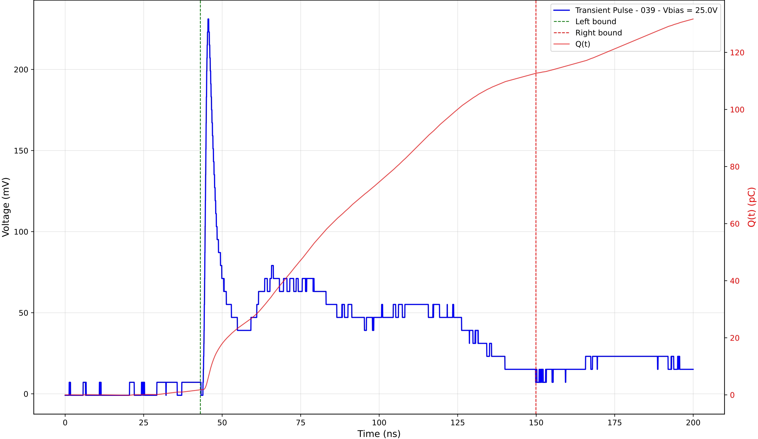
Transient Pulse - Sample: TD_4004 - Position: 185.0 \mu\text{m} - Charge: 110.90 pC - Rise Time: 1.08 ns
