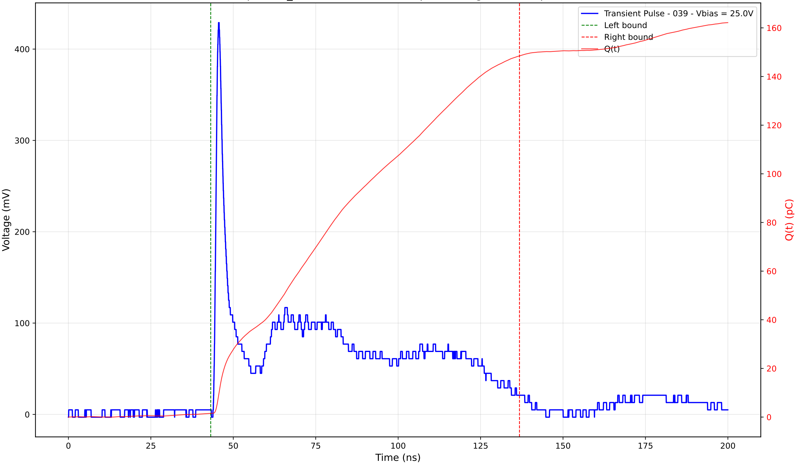
Transient Pulse - Sample: TD_4004 - Position: 105.0 \mu\text{m} - Charge: 146.93 pC - Rise Time: 1.07 ns
