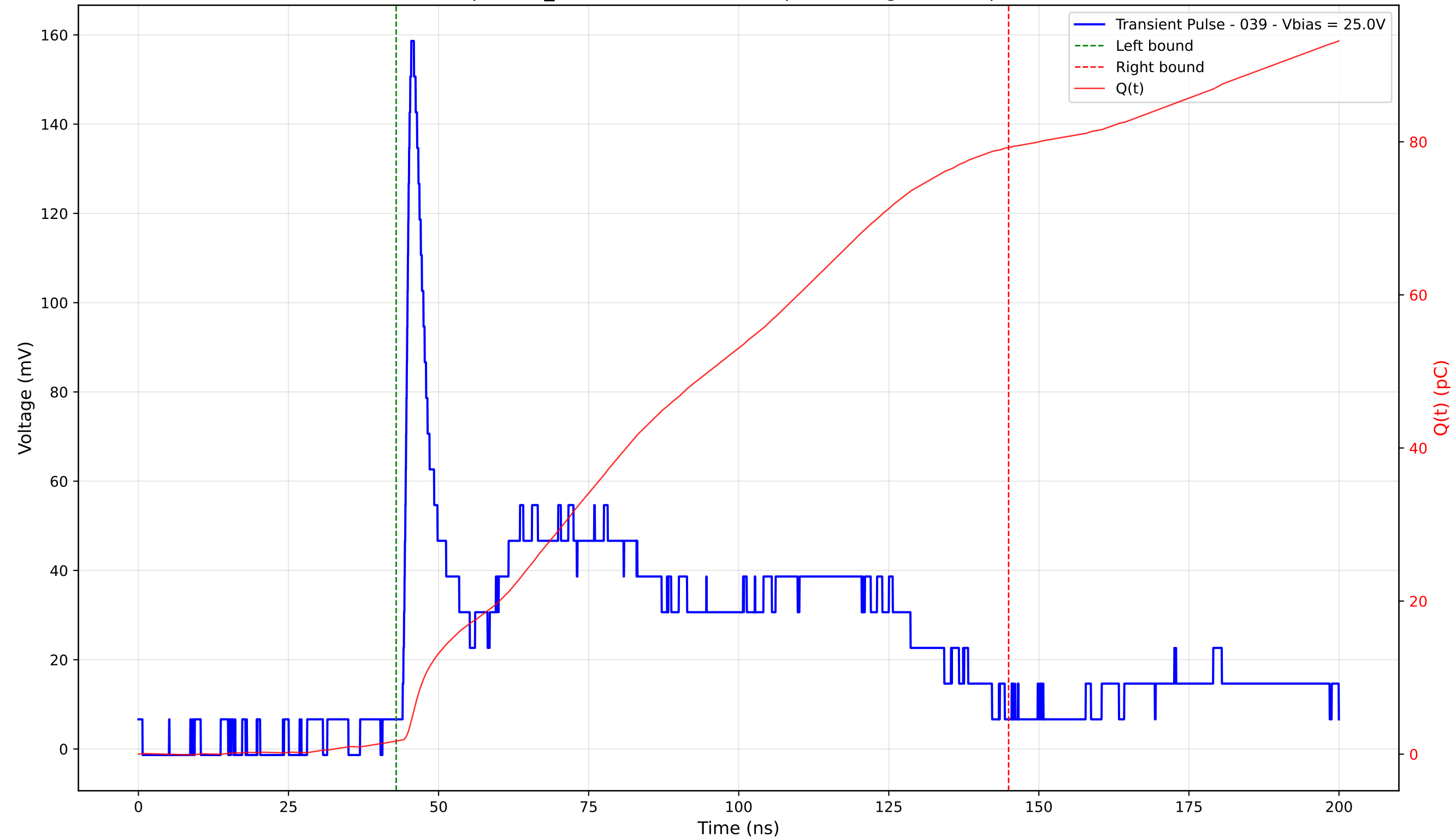
Transient Pulse - Sample: TD_4004 - Position: 155.0 \mu\text{m} - Charge: 77.55 pC - Rise Time: 1.16 ns
