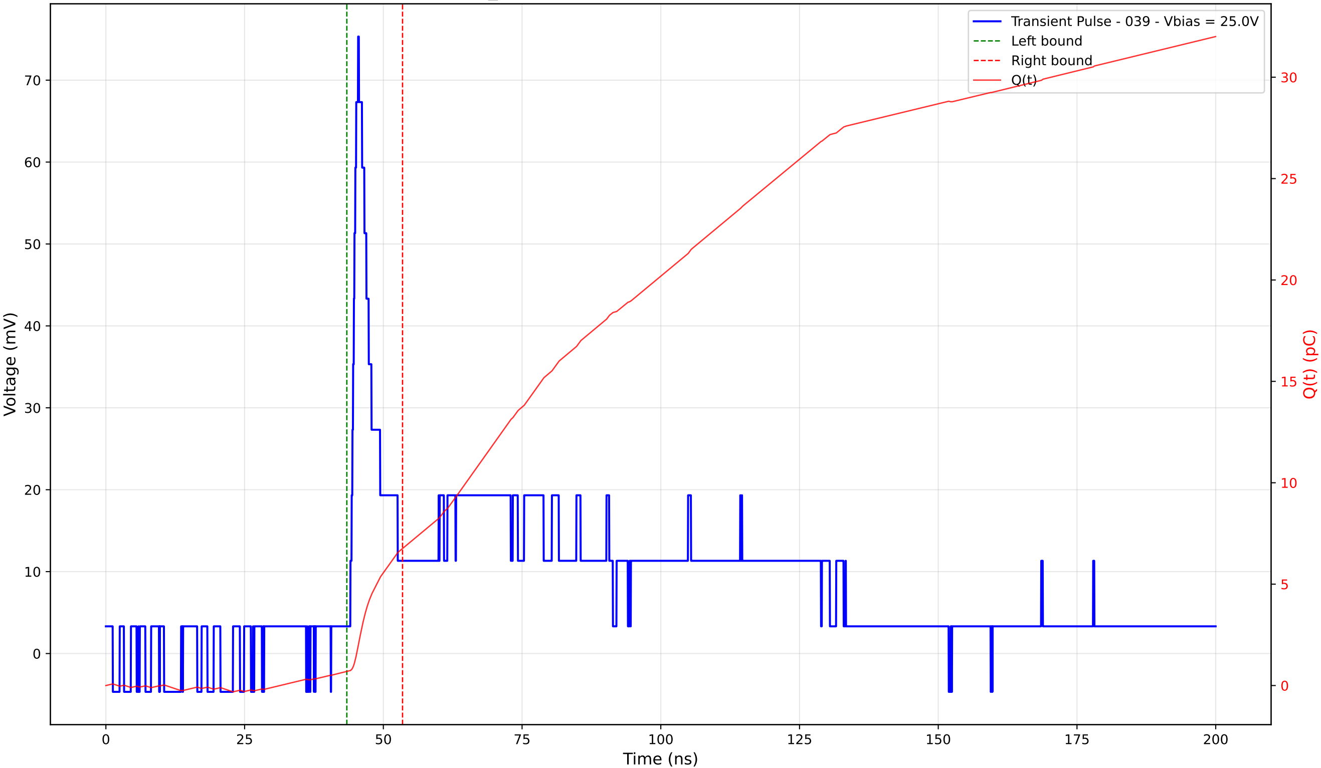
Transient Pulse - Sample: TD_4004 - Position: 335.0 \mu\text{m} - Charge: 6.06 pC - Rise Time: 1.39 ns
