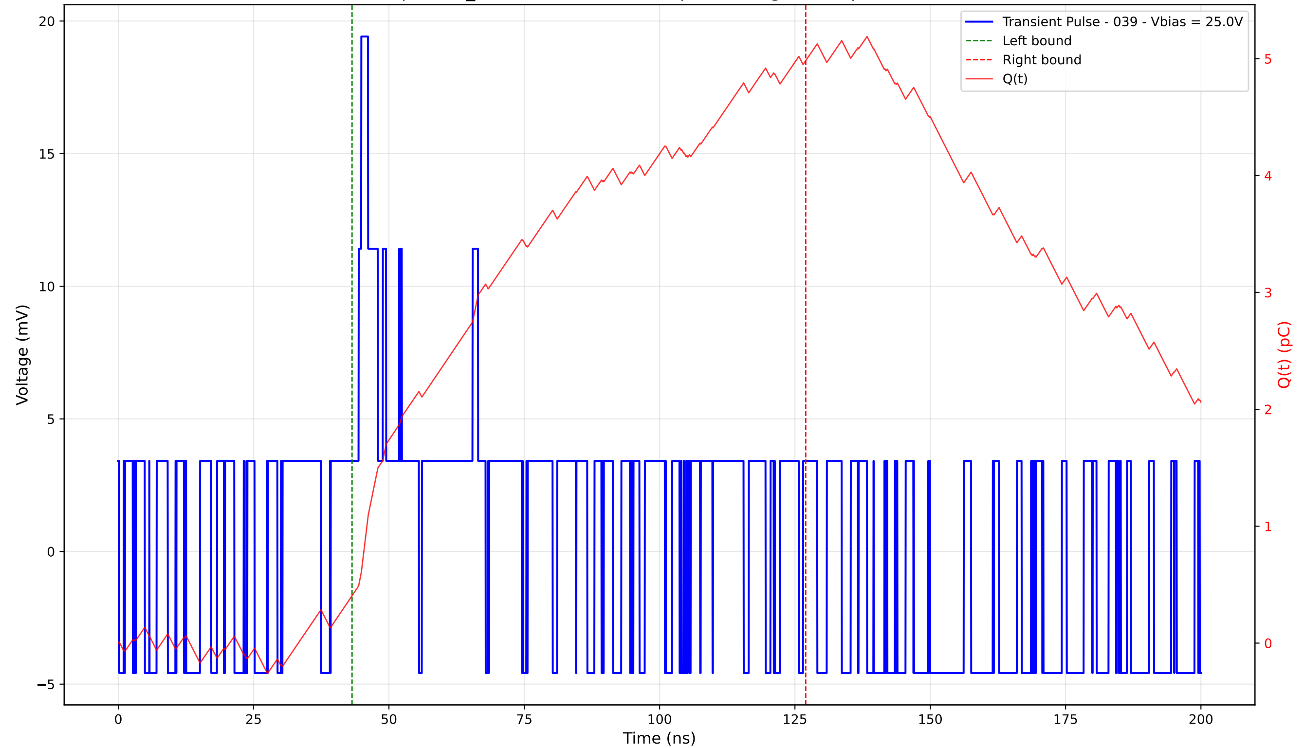
Transient Pulse - Sample: TD_4004 - Position: 420.0 \mu\text{m} - Charge: 4.58 pC - Rise Time: 0.00 ns (N/A)
