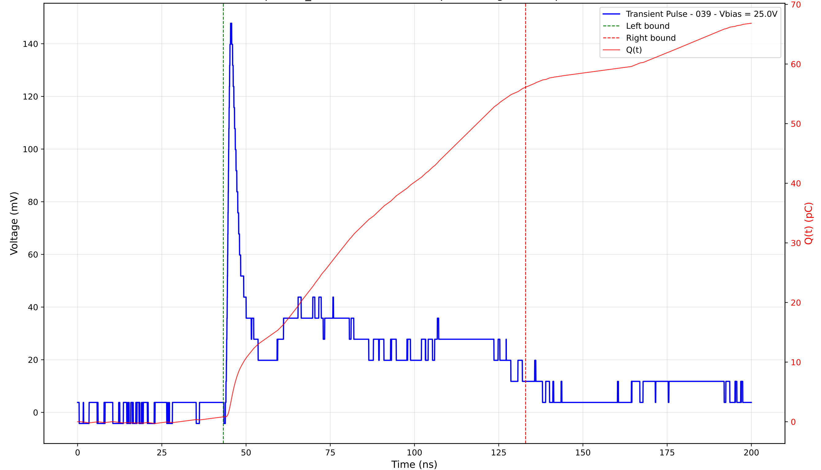
Transient Pulse - Sample: TD_4004 - Position: 240.0 \mu\text{m} - Charge: 55.27 pC - Rise Time: 1.07 ns
