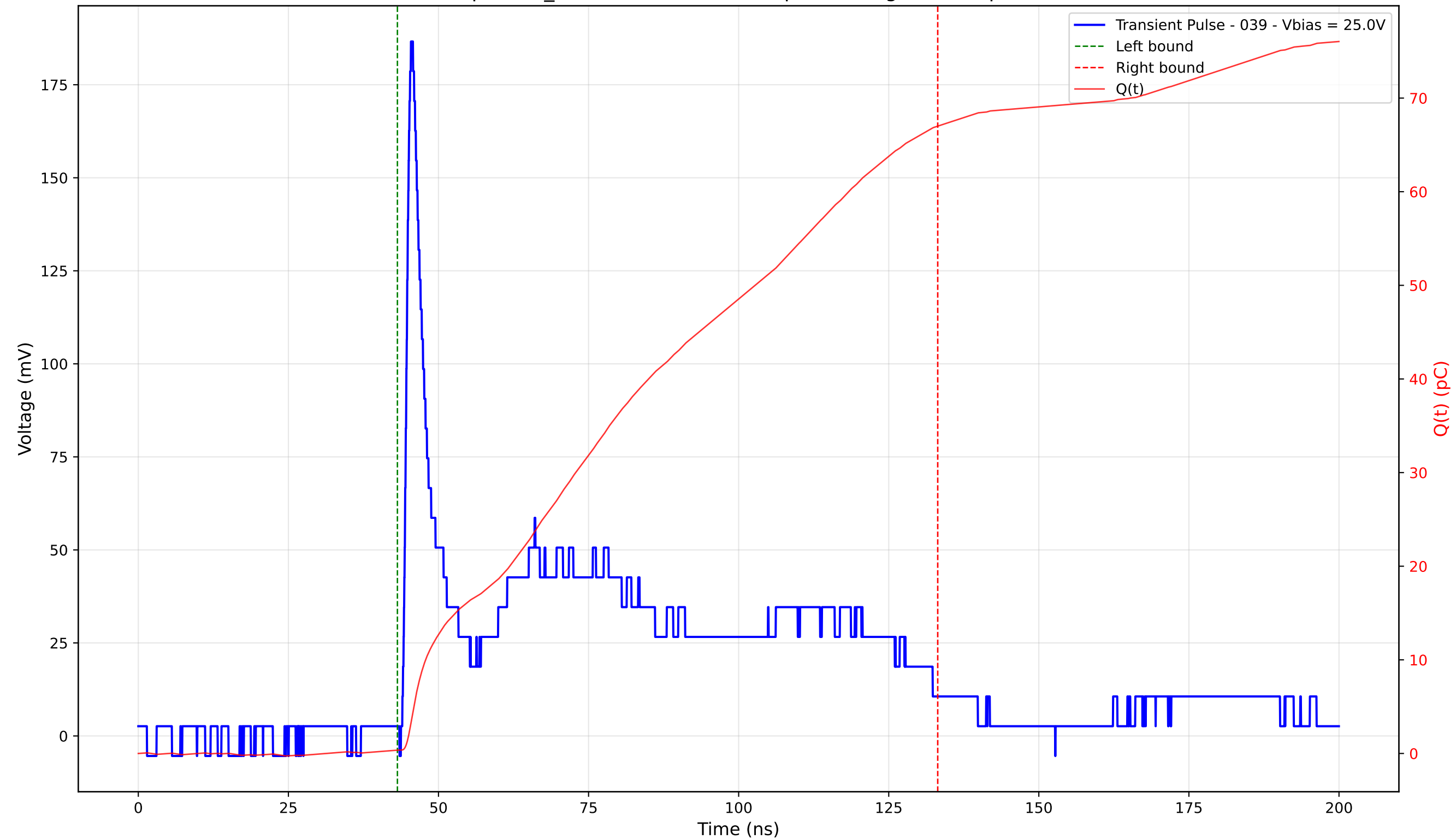
Transient Pulse - Sample: TD_4004 - Position: 230.0 \mu\text{m} - Charge: 66.64 pC - Rise Time: 1.00 ns
