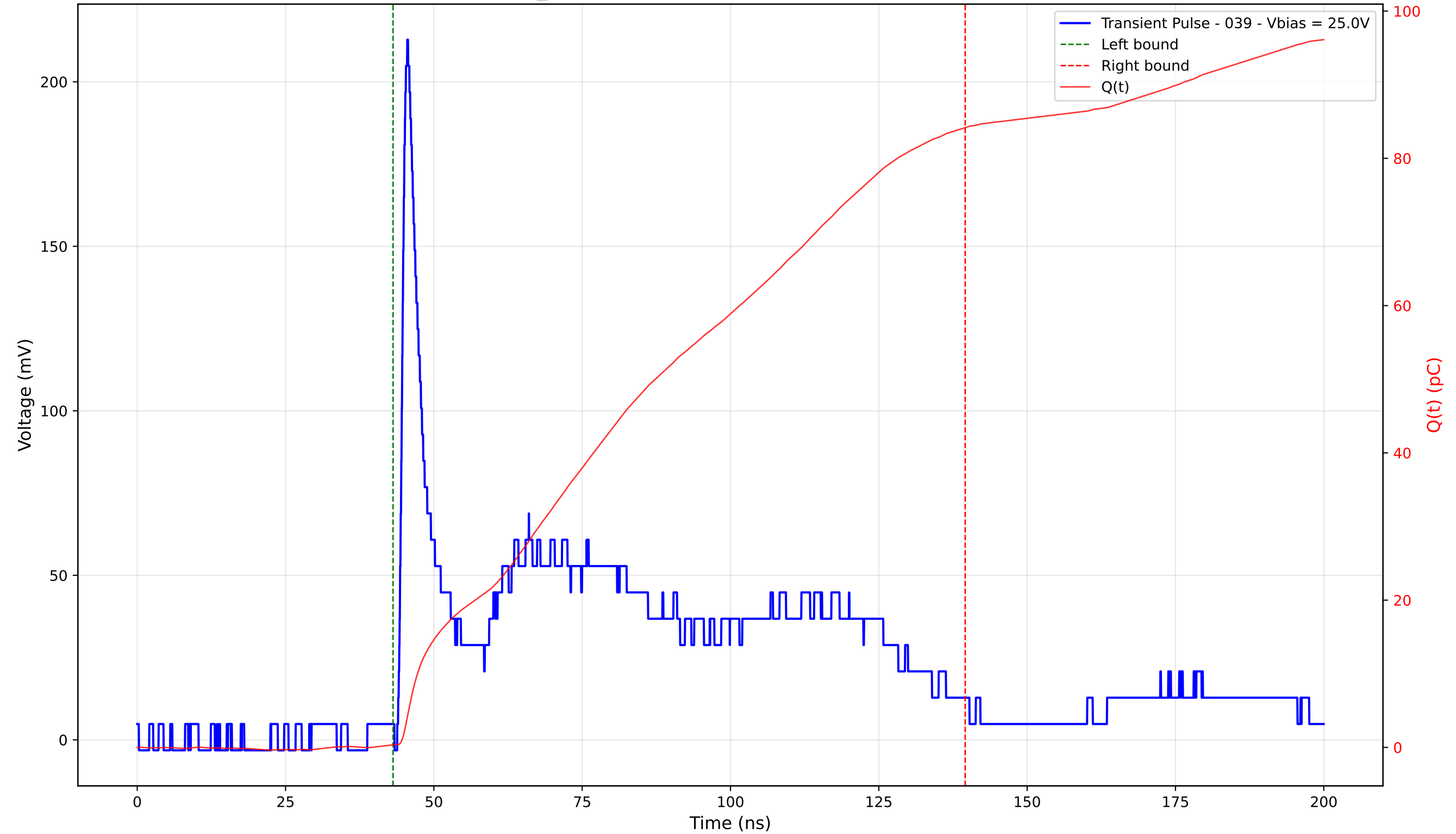
Transient Pulse - Sample: TD_4004 - Position: 215.0 \mu\text{m} - Charge: 83.83 pC - Rise Time: 1.04 ns
