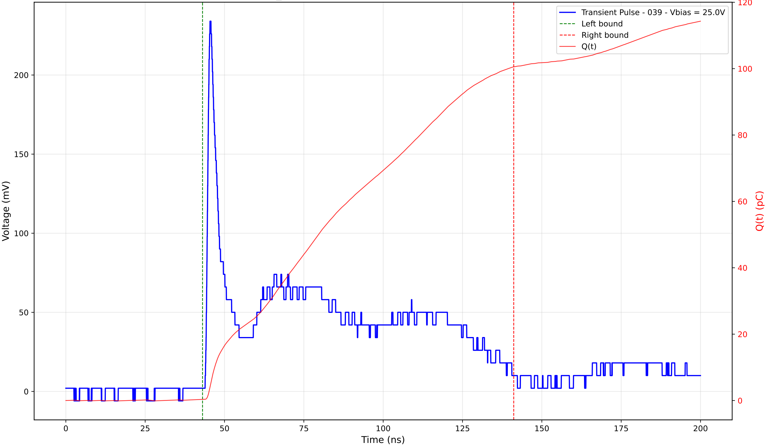
Transient Pulse - Sample: TD_4004 - Position: 190.0 \mu\text{m} - Charge: 100.21 pC - Rise Time: 1.13 ns
