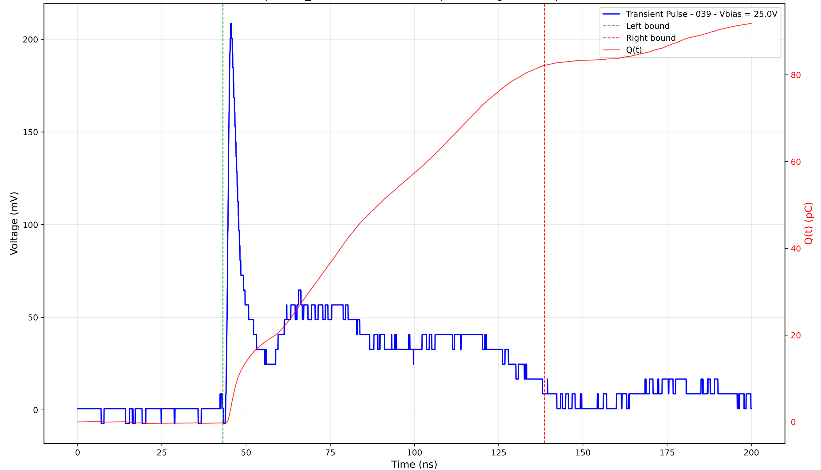
Transient Pulse - Sample: TD_4004 - Position: 210.0 \mu\text{m} - Charge: 82.35 pC - Rise Time: 1.05 ns
