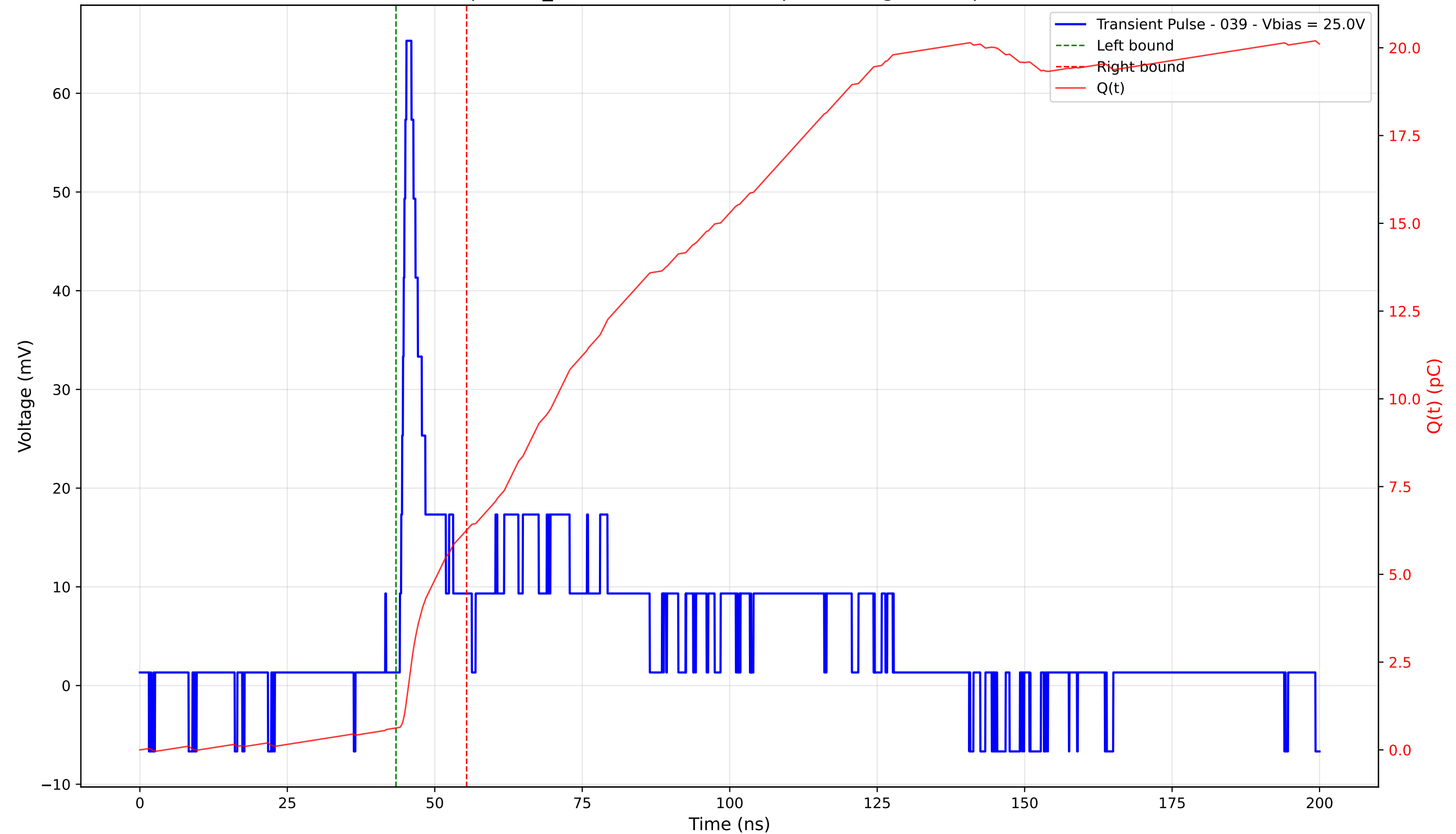
Transient Pulse - Sample: TD_4004 - Position: 375.0 \mu\text{m} - Charge: 5.64 pC - Rise Time: 1.11 ns
