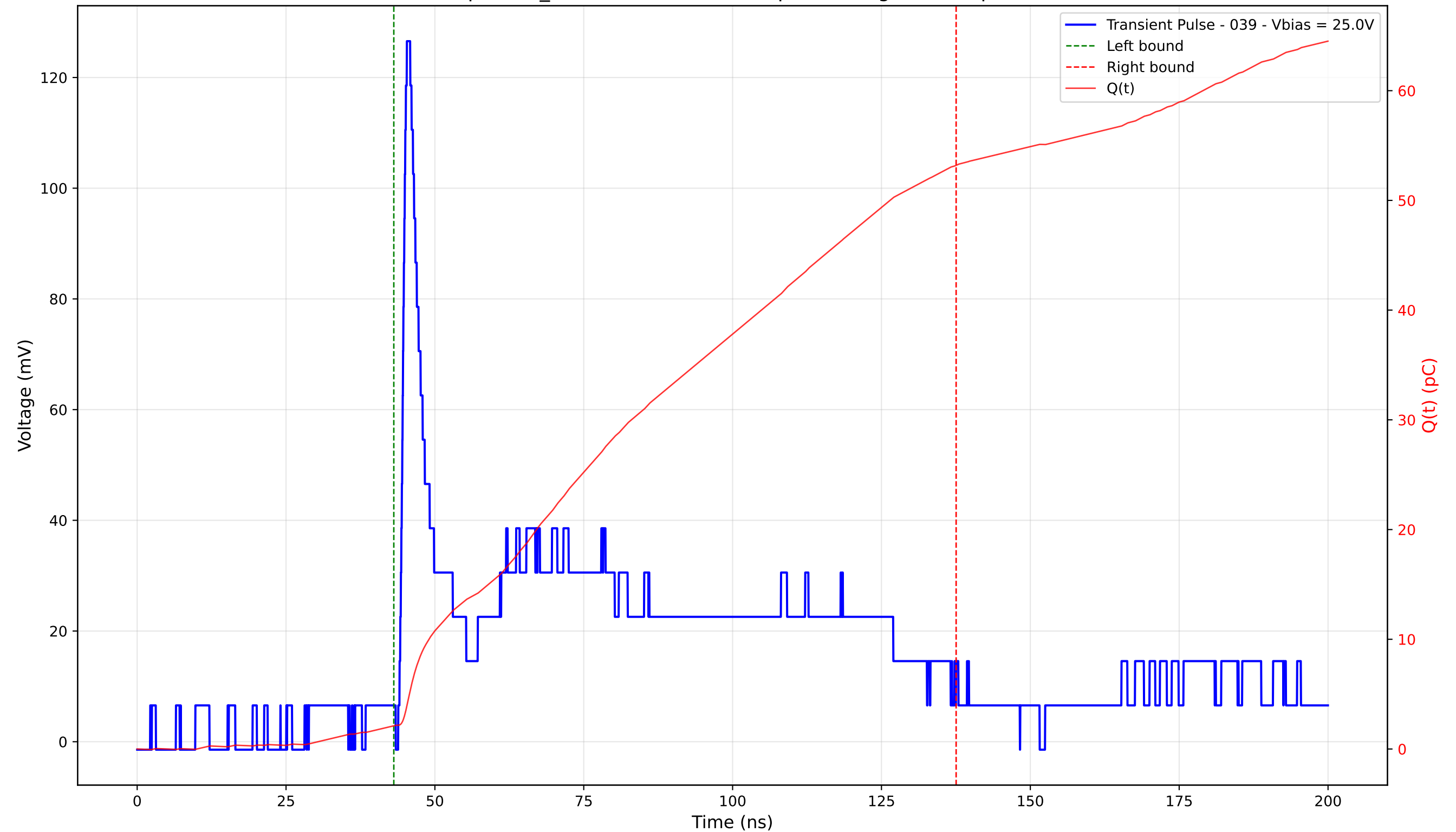
Transient Pulse - Sample: TD_4004 - Position: 285.0 \mu\text{m} - Charge: 51.06 pC - Rise Time: 1.06 ns
