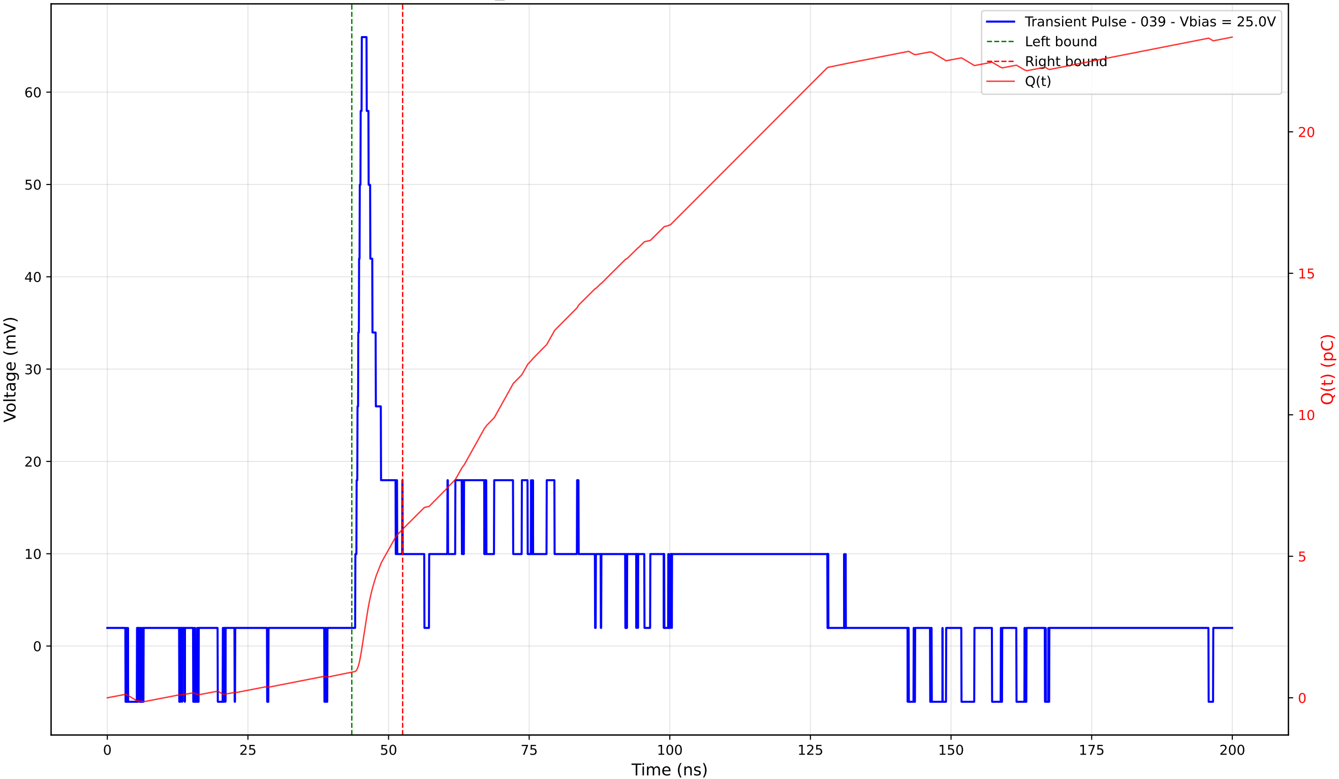
Transient Pulse - Sample: TD_4004 - Position: 385.0 \mu\text{m} - Charge: 5.06 pC - Rise Time: 1.15 ns
