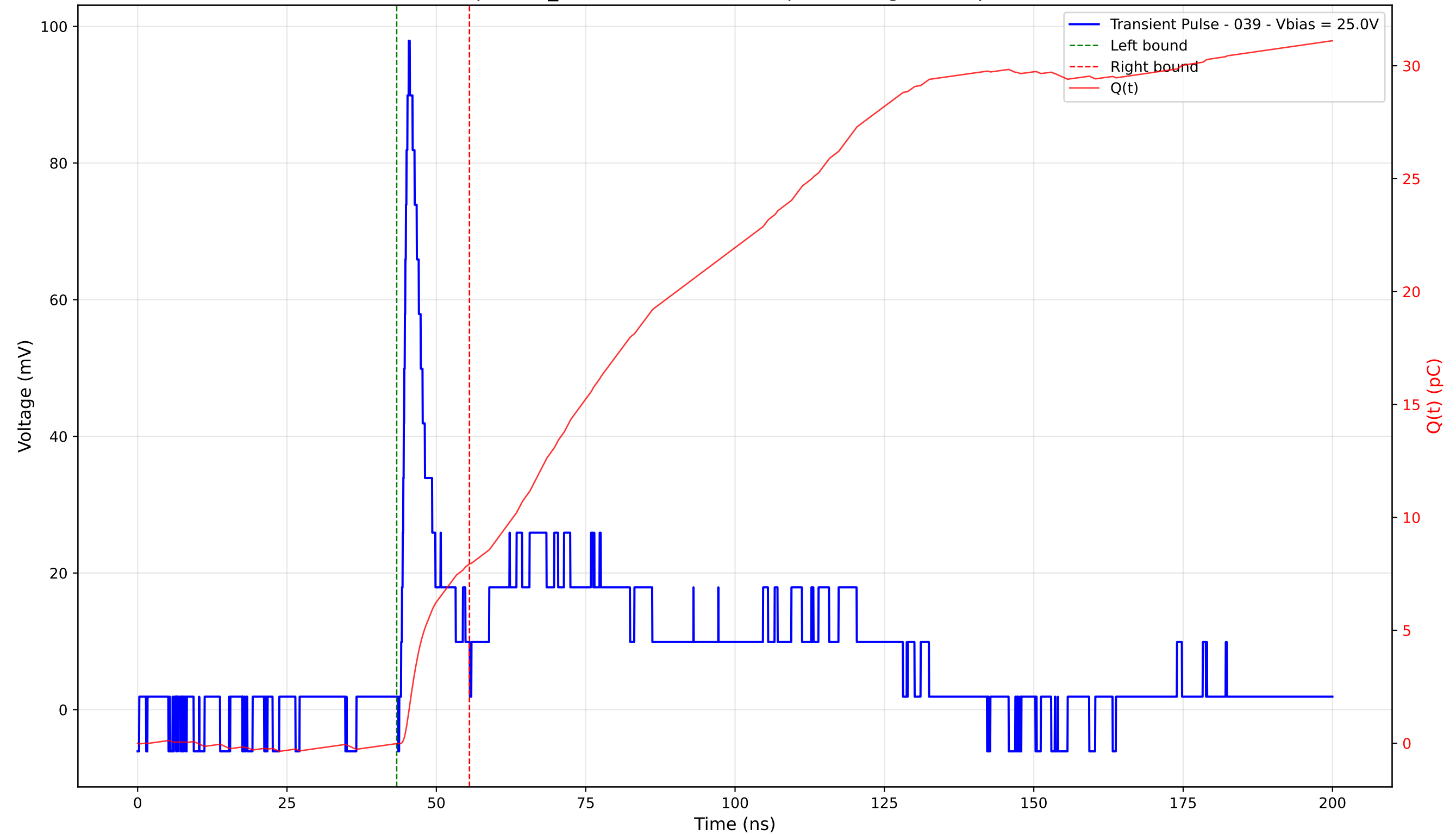
Transient Pulse - Sample: TD_4004 - Position: 305.0 \mu\text{m} - Charge: 7.96 pC - Rise Time: 1.06 ns
