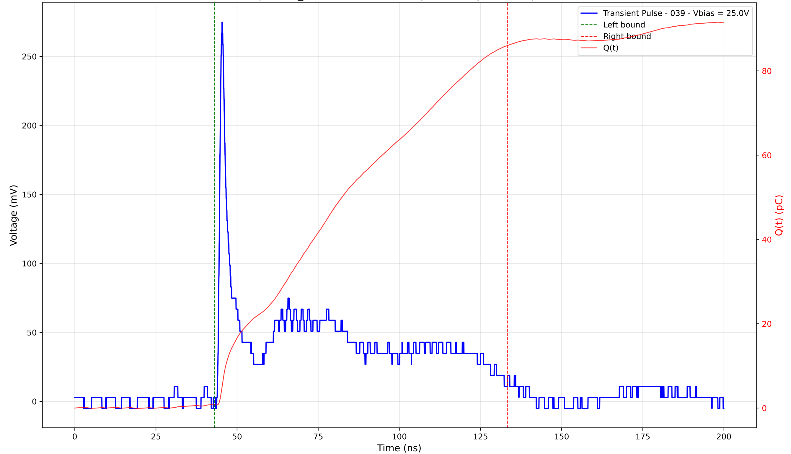
Transient Pulse - Sample: TD_4004 - Position: 75.0 \mu\text{m} - Charge: 85.22 pC - Rise Time: 0.98 ns
