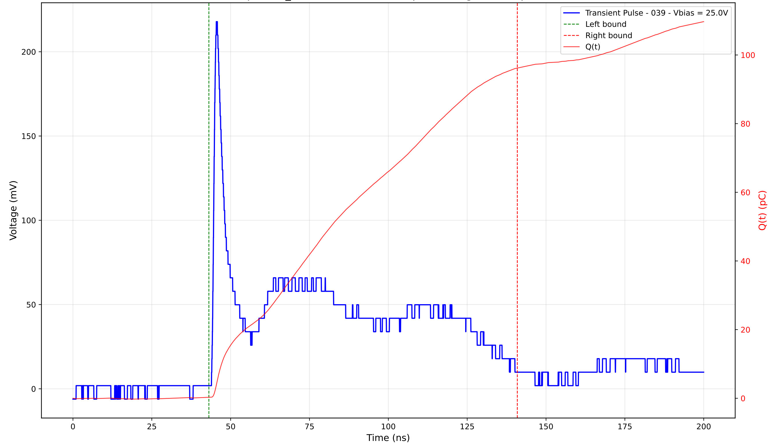
Transient Pulse - Sample: TD_4004 - Position: 180.0 \mu\text{m} - Charge: 95.92 pC - Rise Time: 1.09 ns
