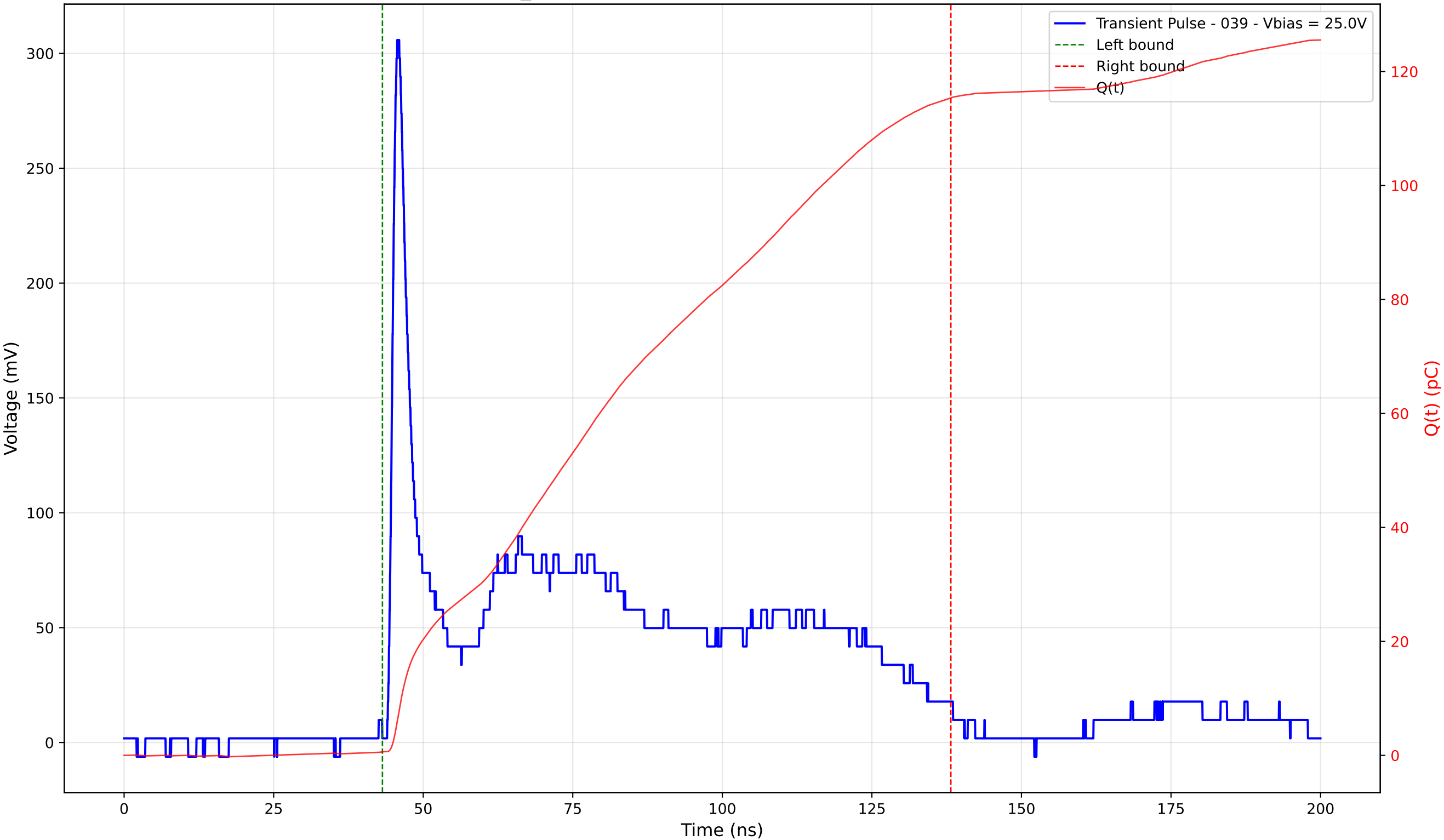
Transient Pulse - Sample: TD_4004 - Position: 125.0 \mu\text{m} - Charge: 114.76 pC - Rise Time: 1.15 ns
