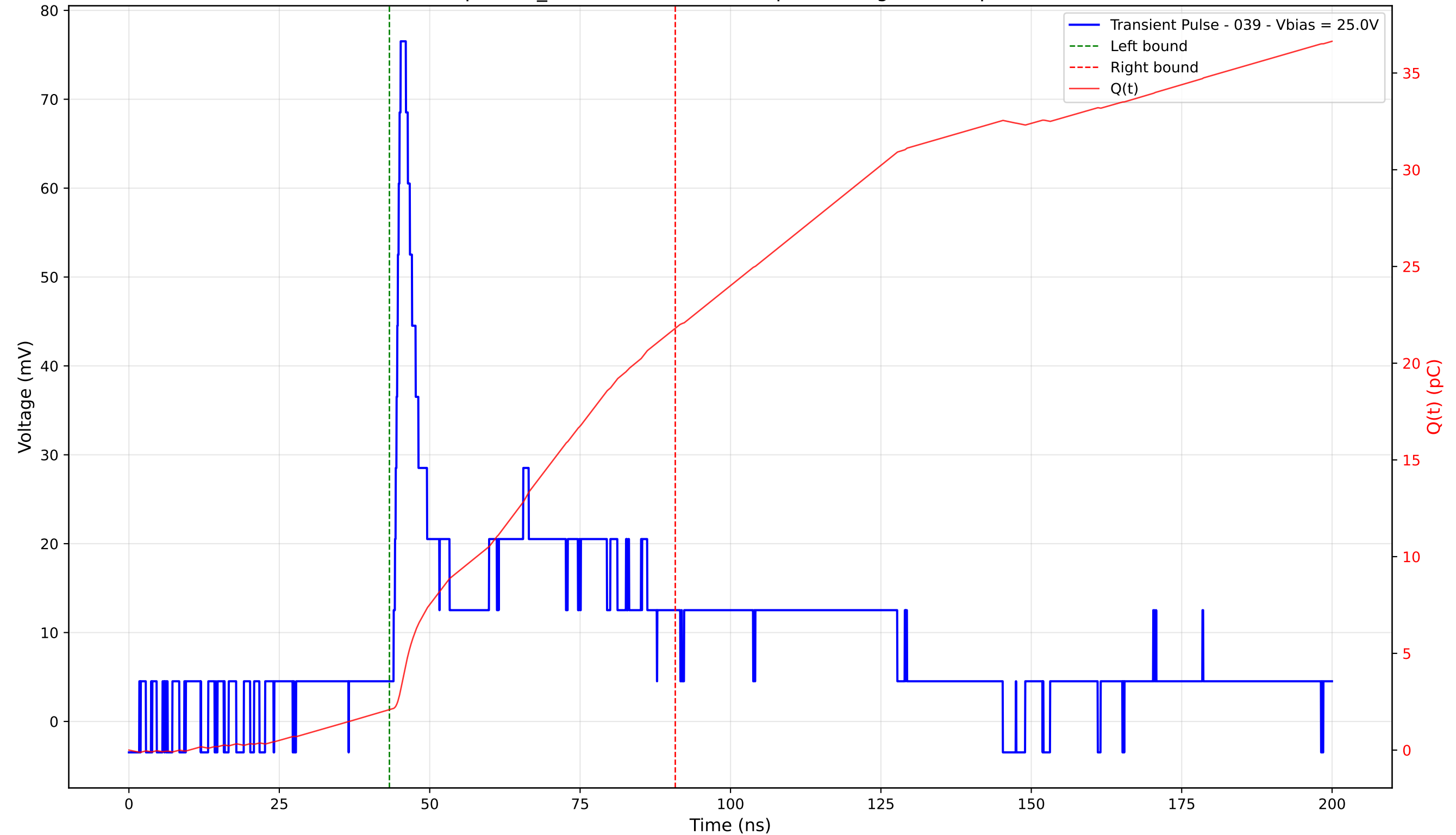
Transient Pulse - Sample: TD_4004 - Position: 355.0 \mu\text{m} - Charge: 19.72 pC - Rise Time: 1.17 ns
