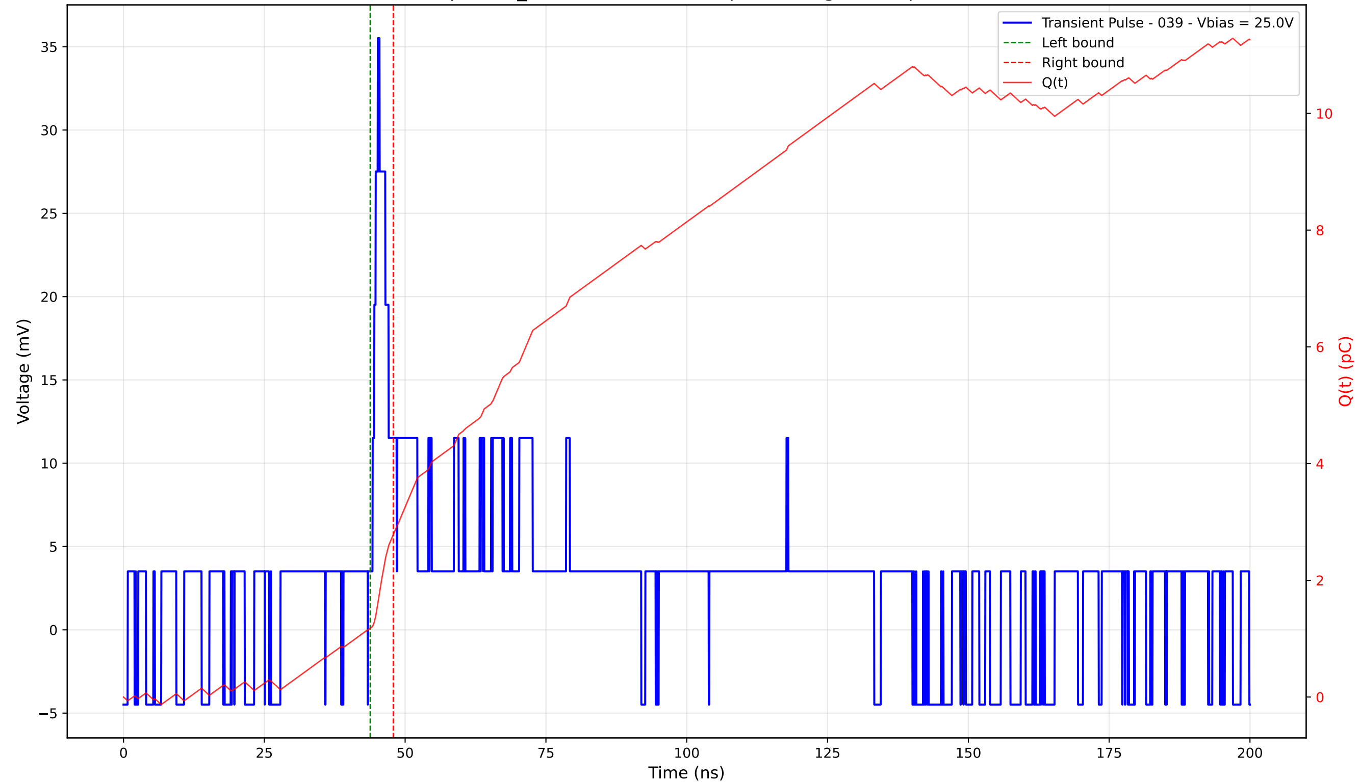
Transient Pulse - Sample: TD_4004 - Position: 50.0 \mu\text{m} - Charge: 1.61 pC - Rise Time: 0.94 ns
