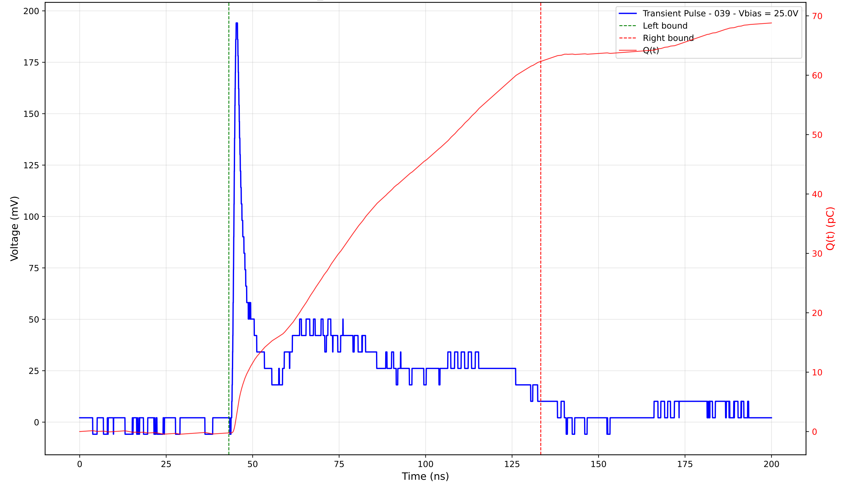
Transient Pulse - Sample: TD_4004 - Position: 70.0 \mu\text{m} - Charge: 62.54 pC - Rise Time: 0.92 ns
