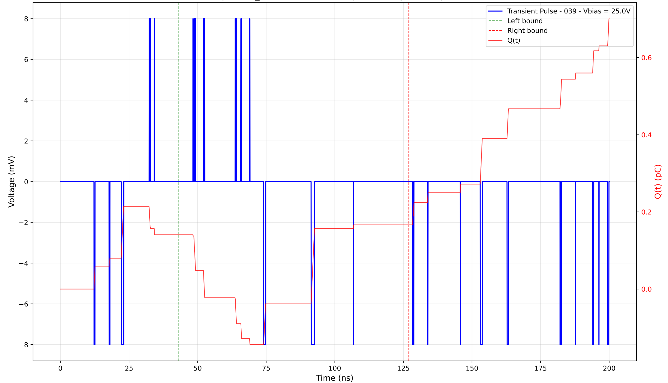
Transient Pulse - Sample: TD_4004 - Position: 5.0 \mu\text{m} - Charge: 0.03 pC - Rise Time: 0.02 ns
