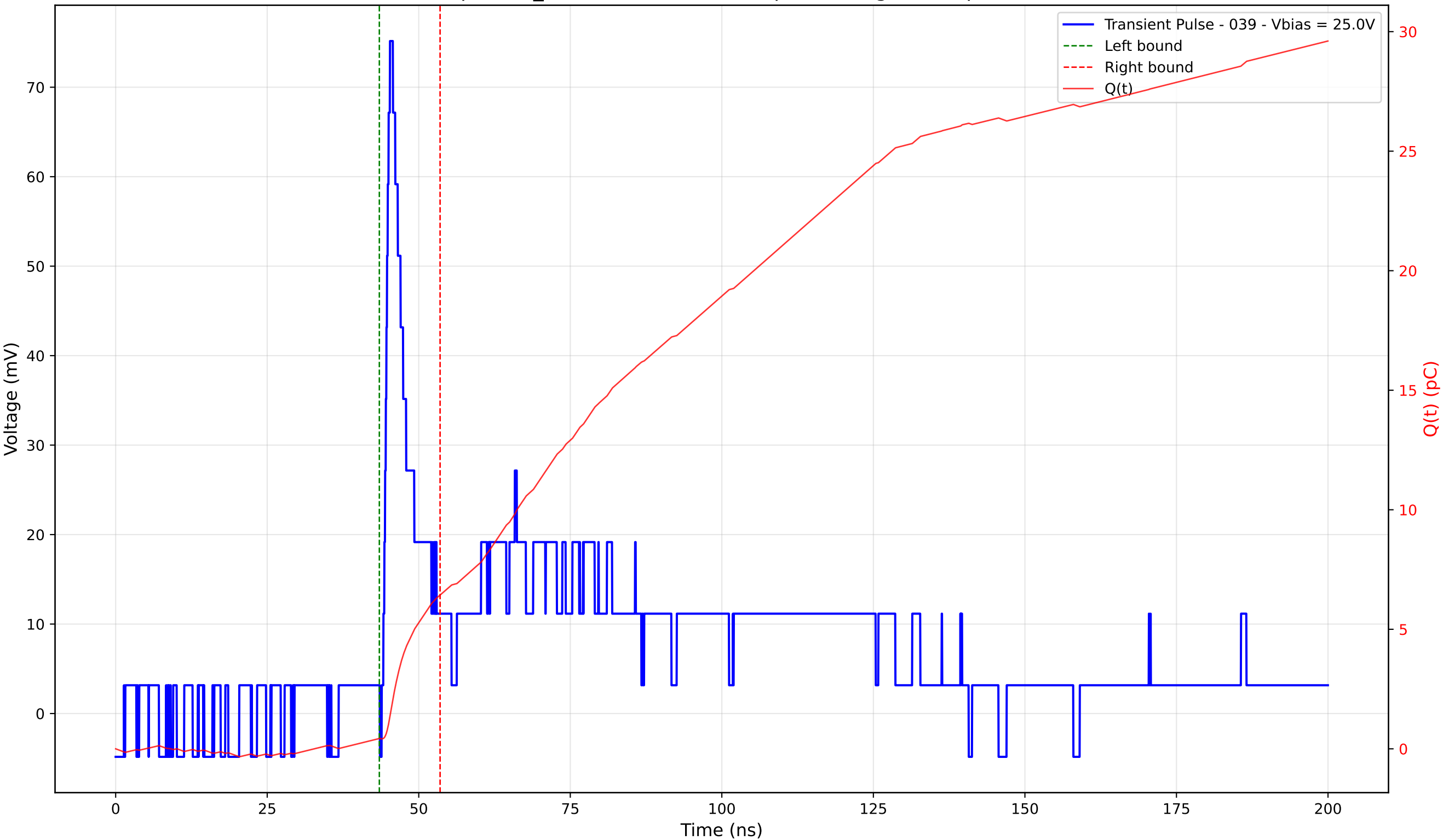
Transient Pulse - Sample: TD_4004 - Position: 340.0 \mu\text{m} - Charge: 6.00 pC - Rise Time: 1.09 ns
