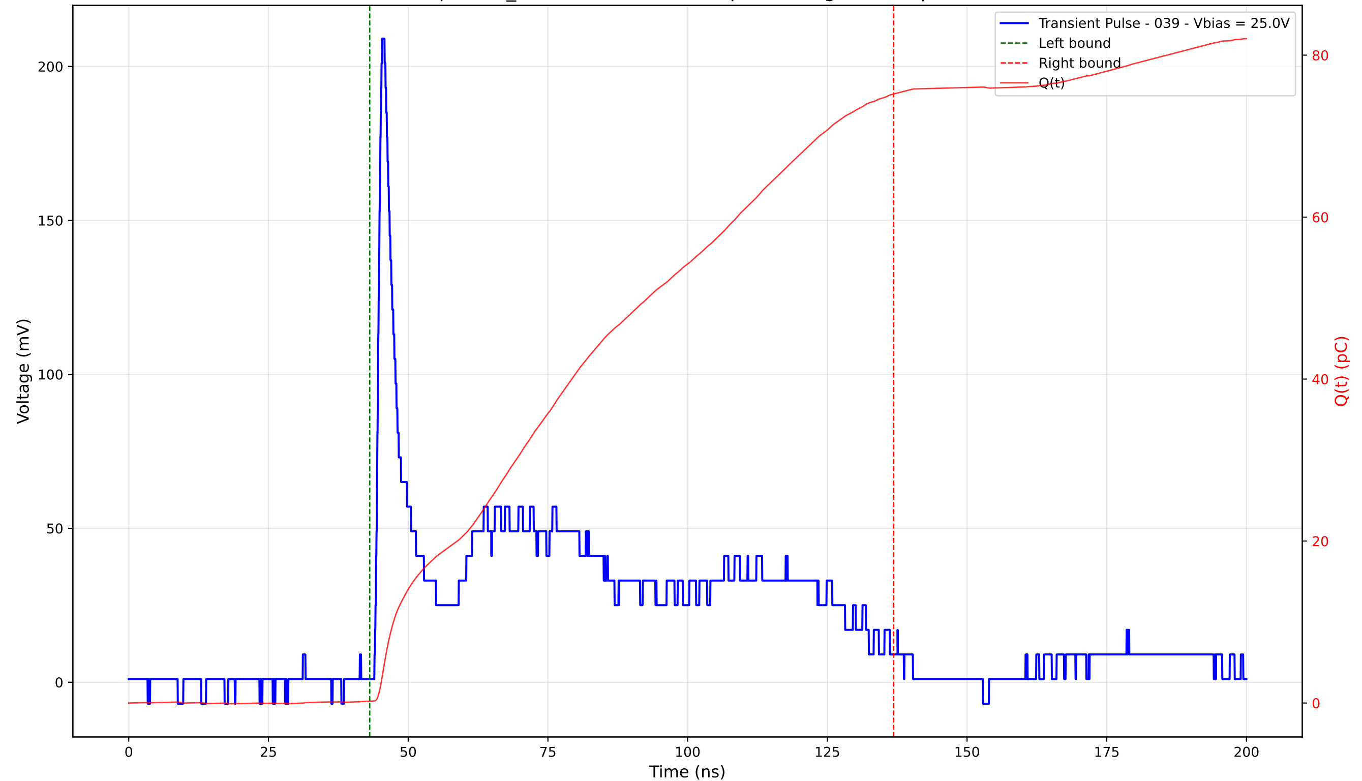
Transient Pulse - Sample: TD_4004 - Position: 225.0 \mu\text{m} - Charge: 74.99 pC - Rise Time: 1.03 ns
