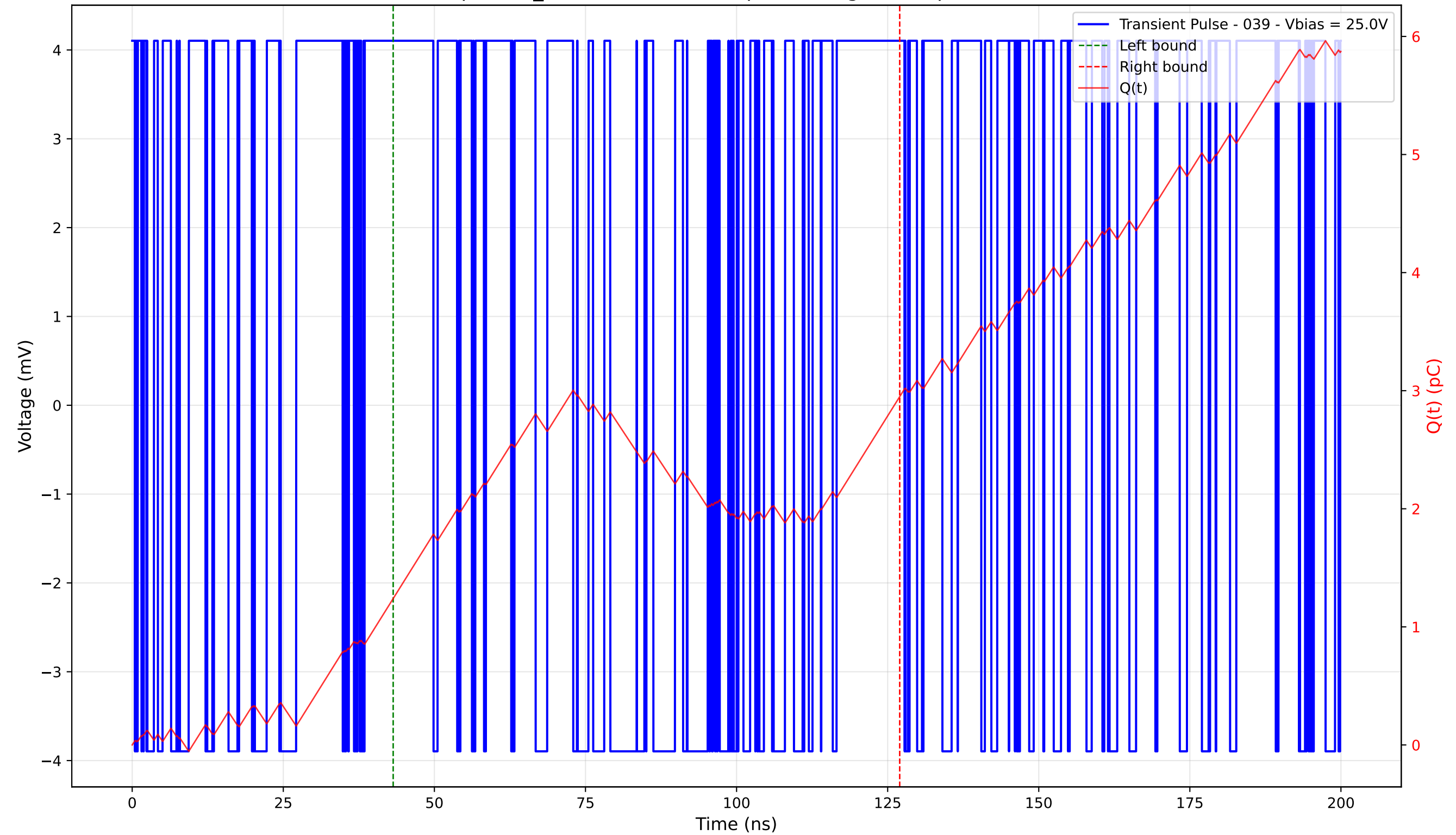
Transient Pulse - Sample: TD_4004 - Position: 0.0 \mu m - Charge: 1.71 pC - Rise Time: 0.00 ns (N/A)
