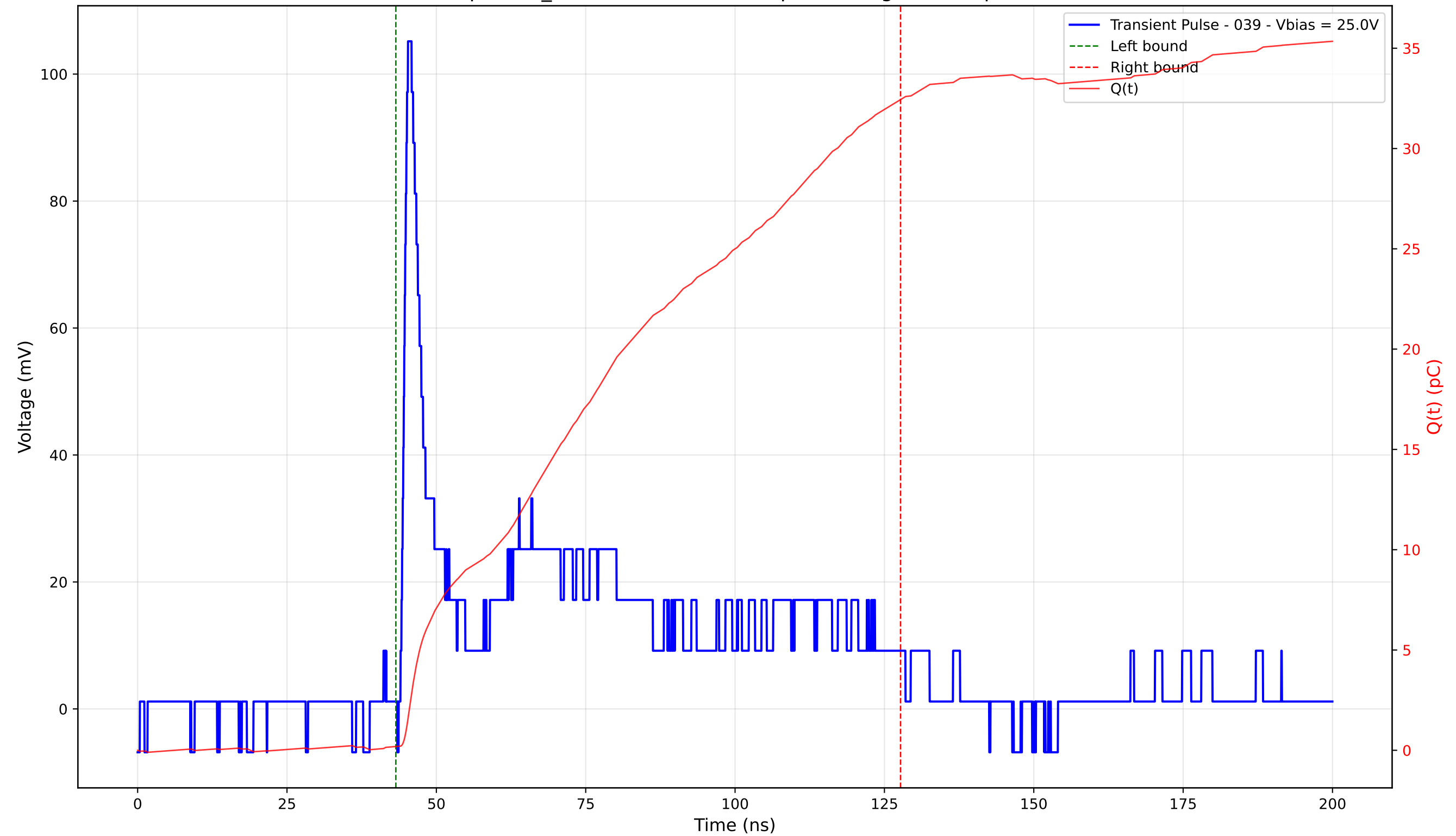
Transient Pulse - Sample: TD_4004 - Position: 290.0 \mu\text{m} - Charge: 32.26 pC - Rise Time: 0.94 ns
