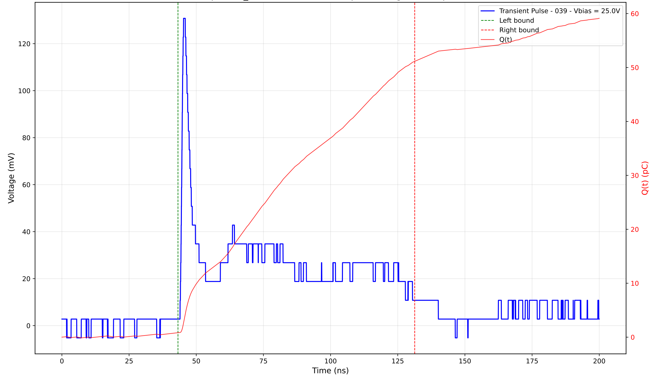
Transient Pulse - Sample: TD_4004 - Position: 250.0 \mu\text{m} - Charge: 50.34 pC - Rise Time: 1.01 ns
