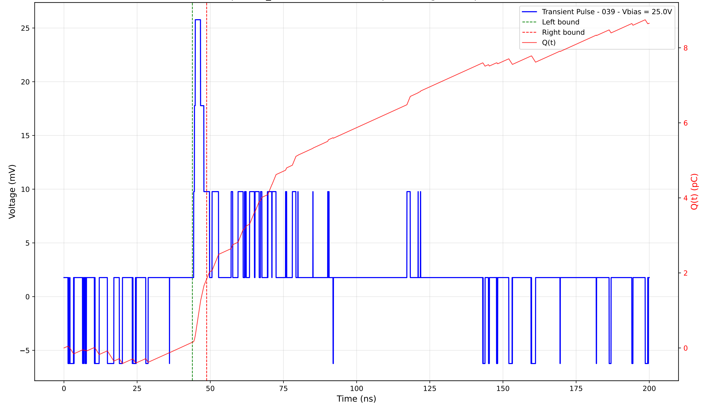
Transient Pulse - Sample: TD_4004 - Position: 410.0 \mu\text{m} - Charge: 1.69 pC - Rise Time: 0.56 ns
