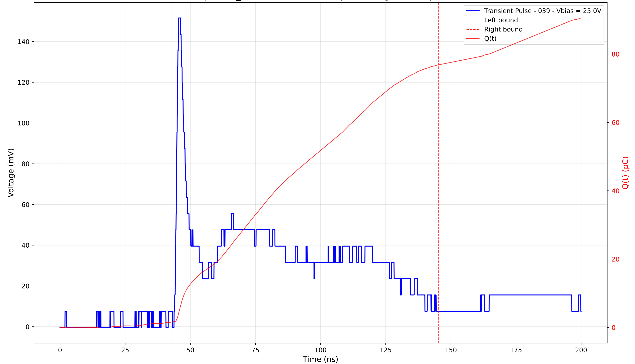
Transient Pulse - Sample: TD_4004 - Position: 140.0 \mu\text{m} - Charge: 75.22 pC - Rise Time: 1.34 ns
