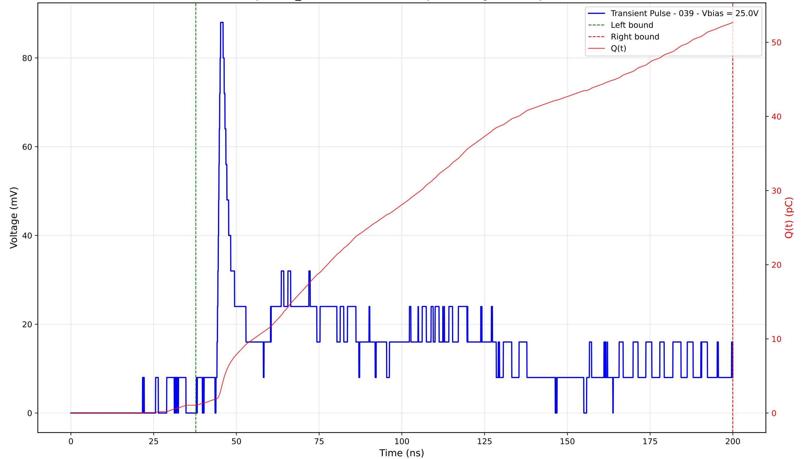
Transient Pulse - Sample: TD_4004 - Position: 325.0 \mu\text{m} - Charge: 51.64 pC - Rise Time: 0.96 ns
