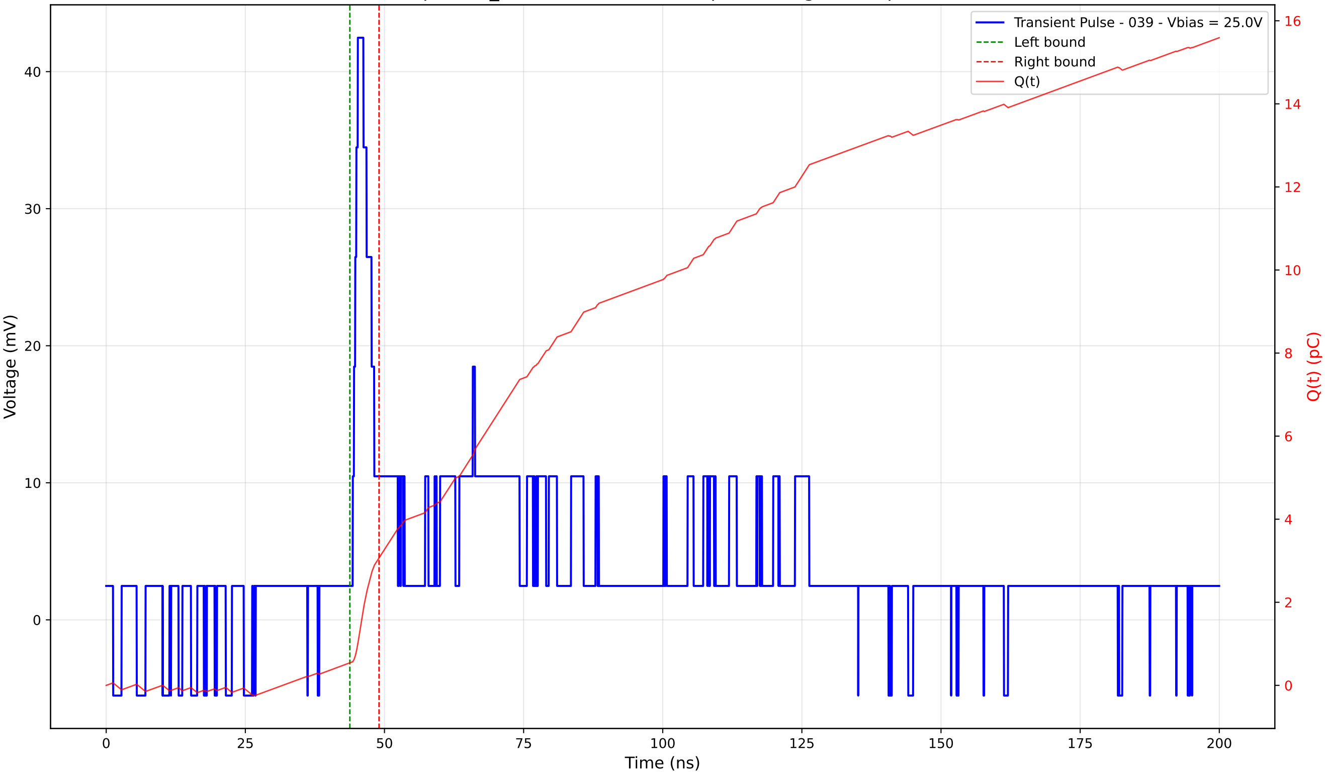
Transient Pulse - Sample: TD_4004 - Position: 400.0 \mu\text{m} - Charge: 2.53 pC - Rise Time: 0.92 ns
