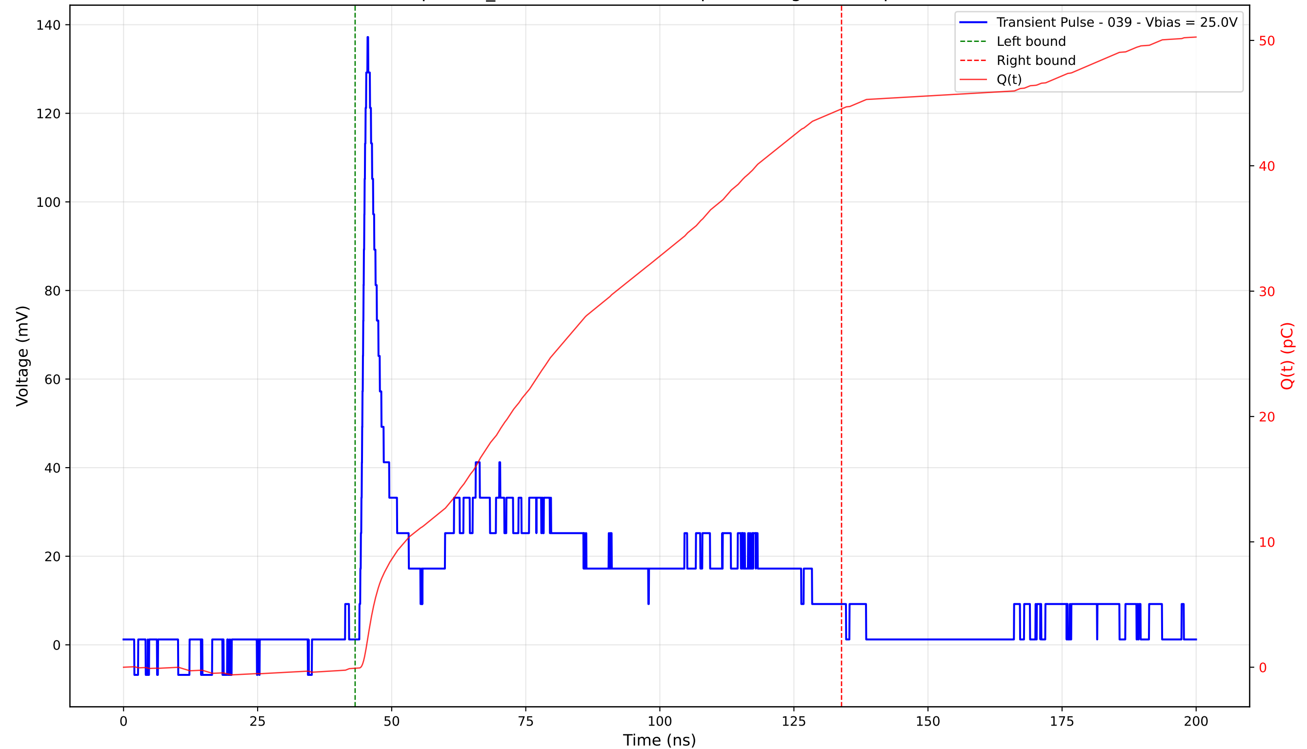
Transient Pulse - Sample: TD_4004 - Position: 280.0 \mu\text{m} - Charge: 44.64 pC - Rise Time: 1.11 ns
