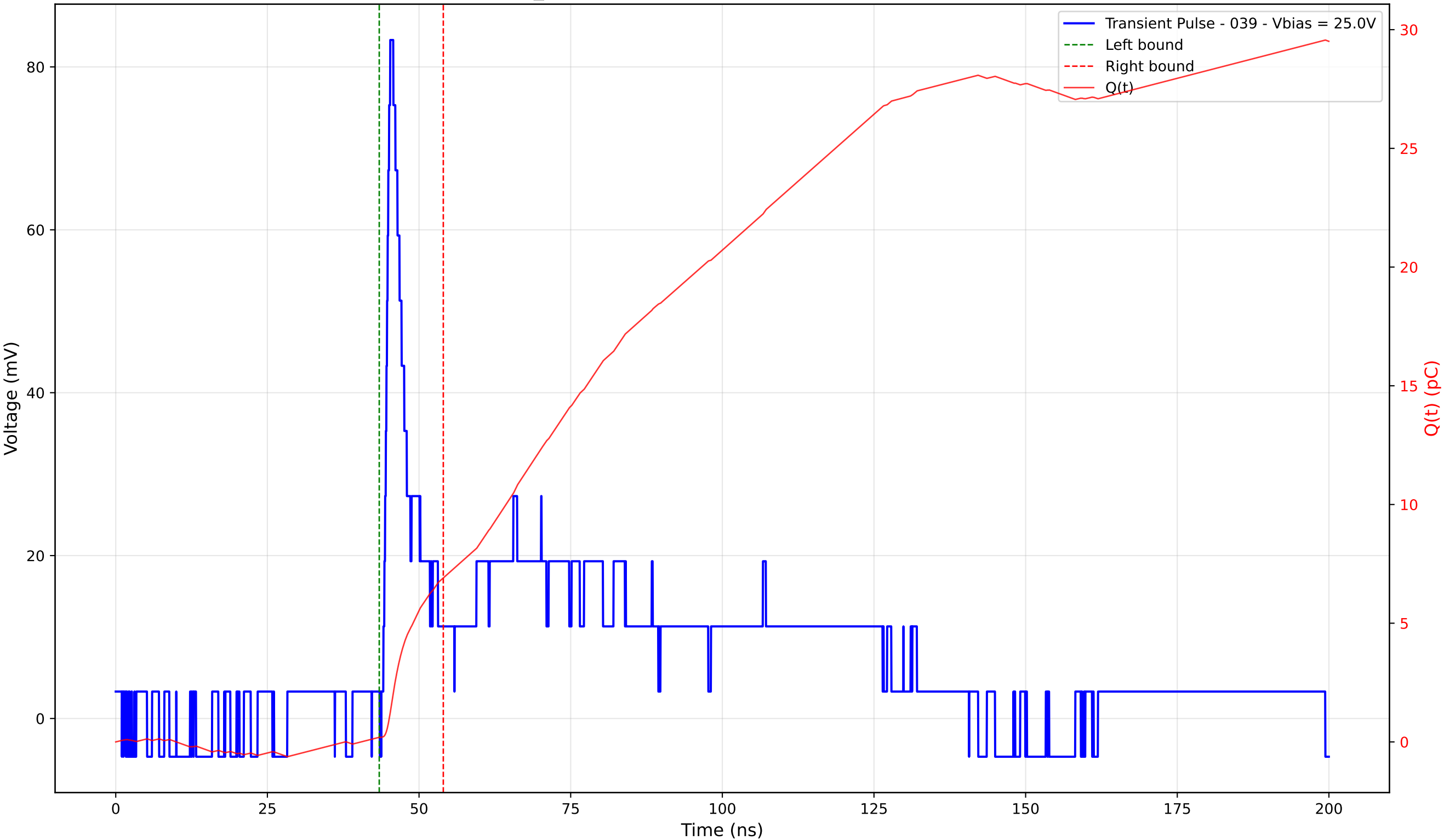
Transient Pulse - Sample: TD_4004 - Position: 345.0 \mu\text{m} - Charge: 6.71 pC - Rise Time: 0.95 ns
