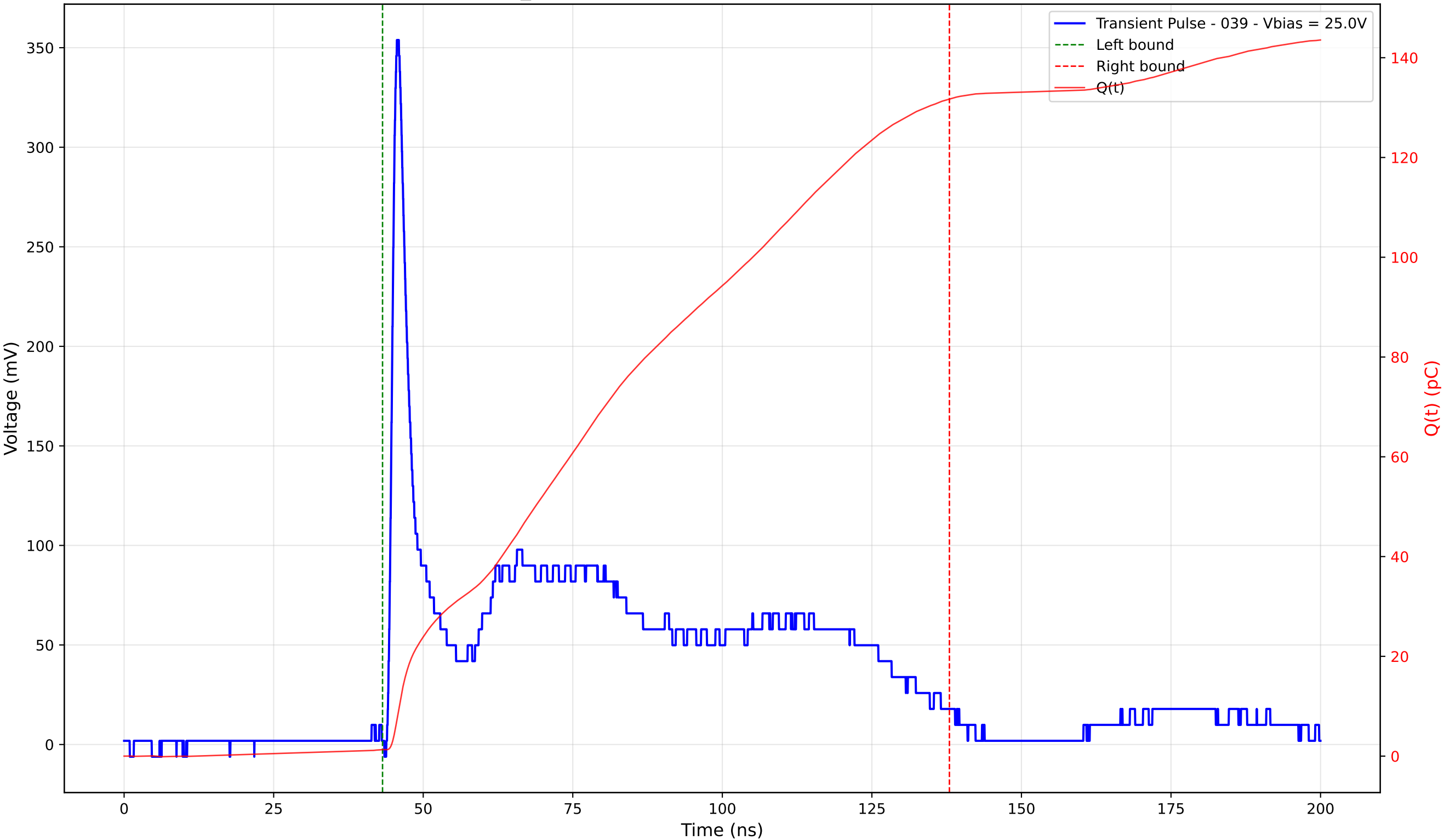
Transient Pulse - Sample: TD_4004 - Position: 120.0 \mu\text{m} - Charge: 130.40 pC - Rise Time: 1.12 ns
