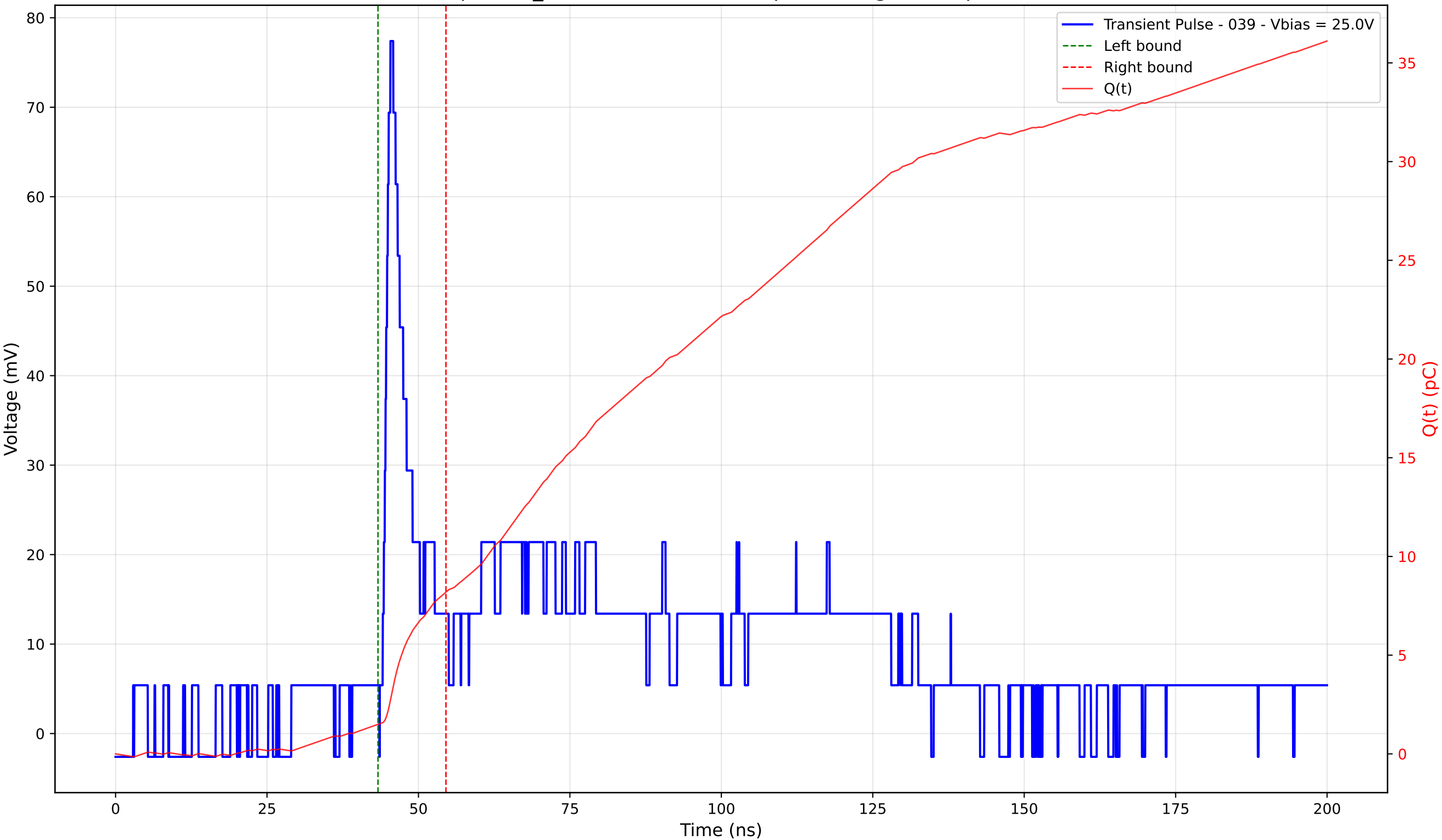
Transient Pulse - Sample: TD_4004 - Position: 360.0 \mu\text{m} - Charge: 6.71 pC - Rise Time: 1.27 ns
