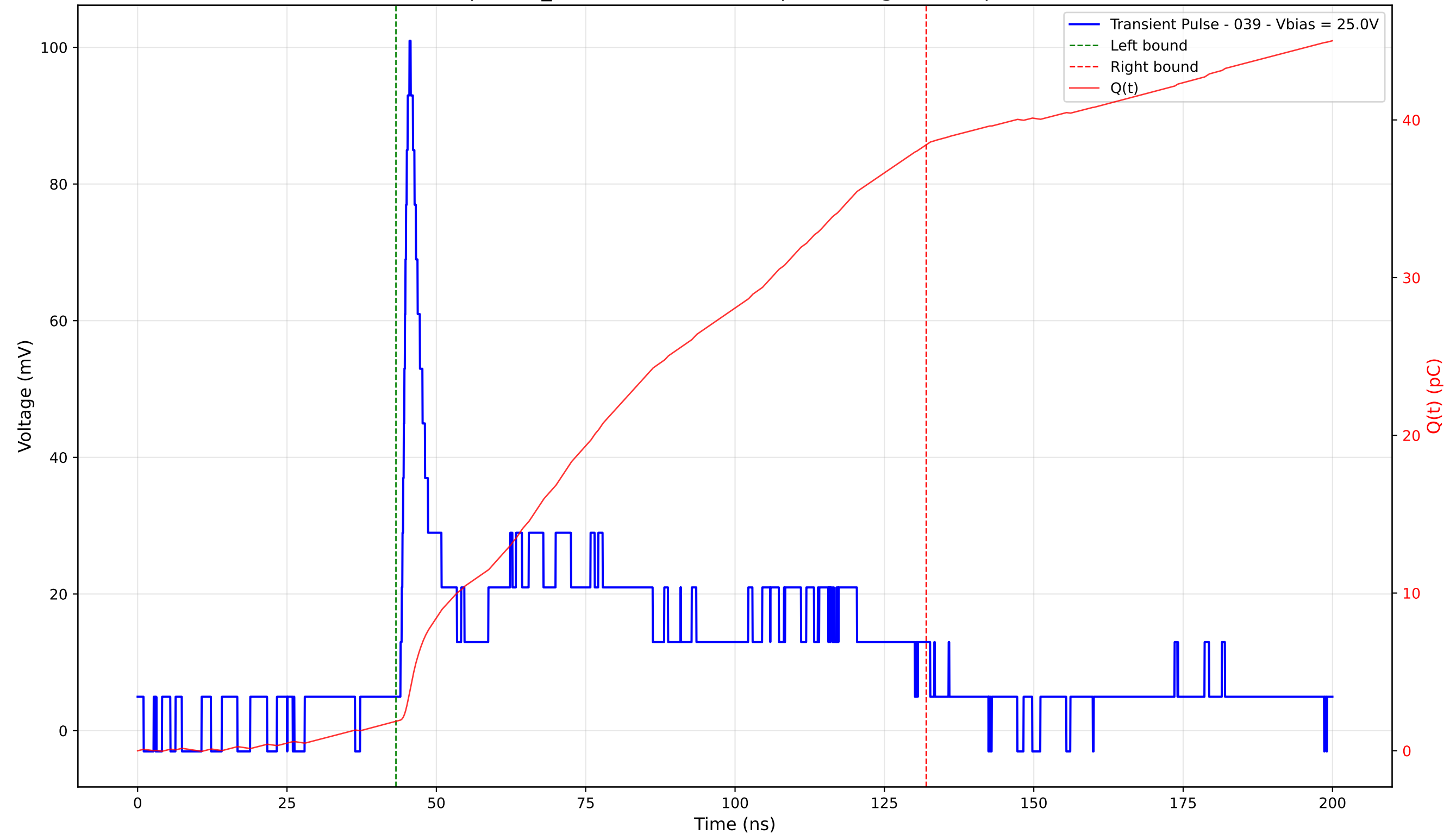
Transient Pulse - Sample: TD_4004 - Position: 295.0 \mu\text{m} - Charge: 36.56 pC - Rise Time: 1.21 ns
