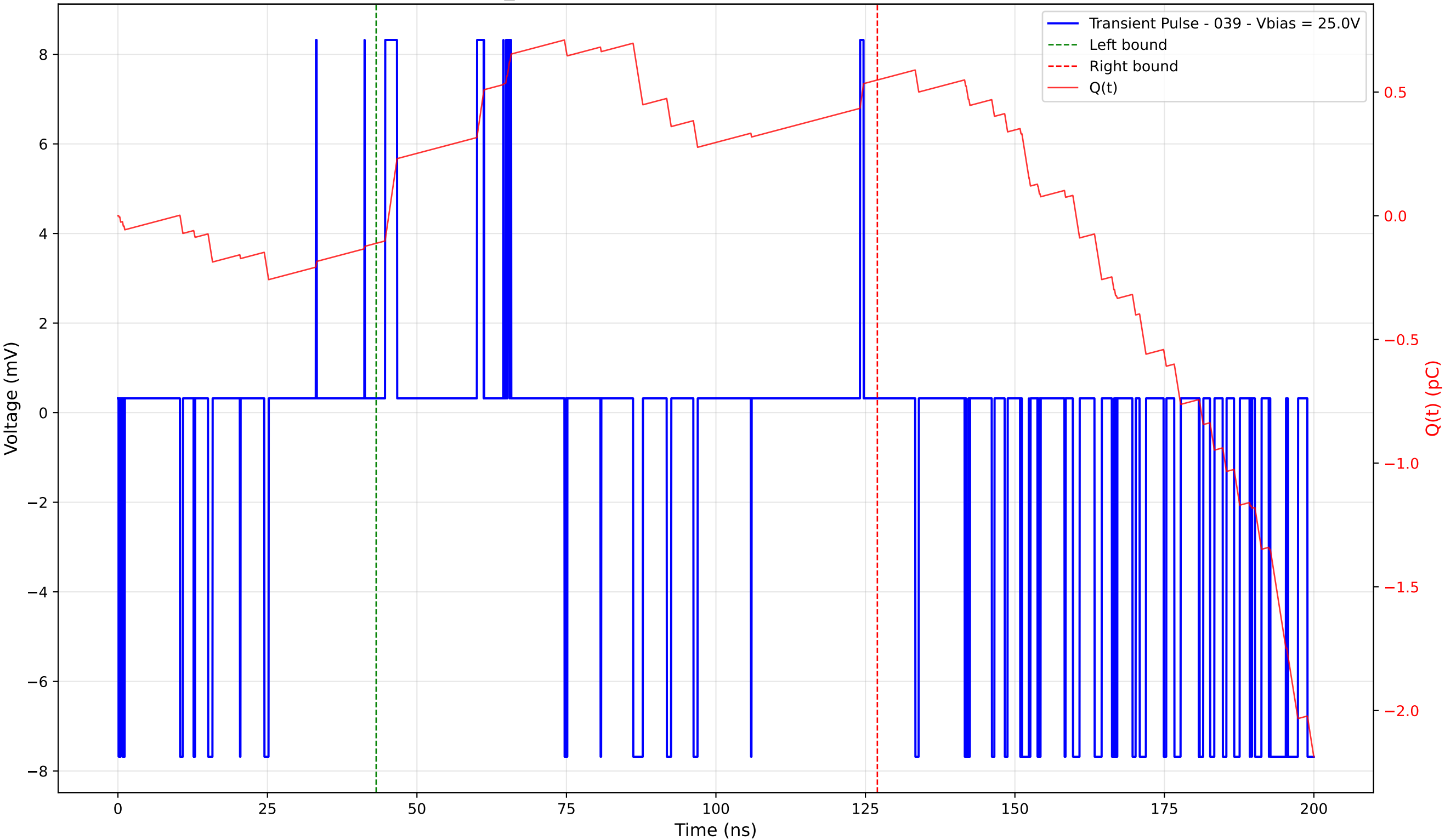
Transient Pulse - Sample: TD_4004 - Position: 20.0 \mu\text{m} - Charge: 0.66 pC - Rise Time: 0.00 ns (N/A)
