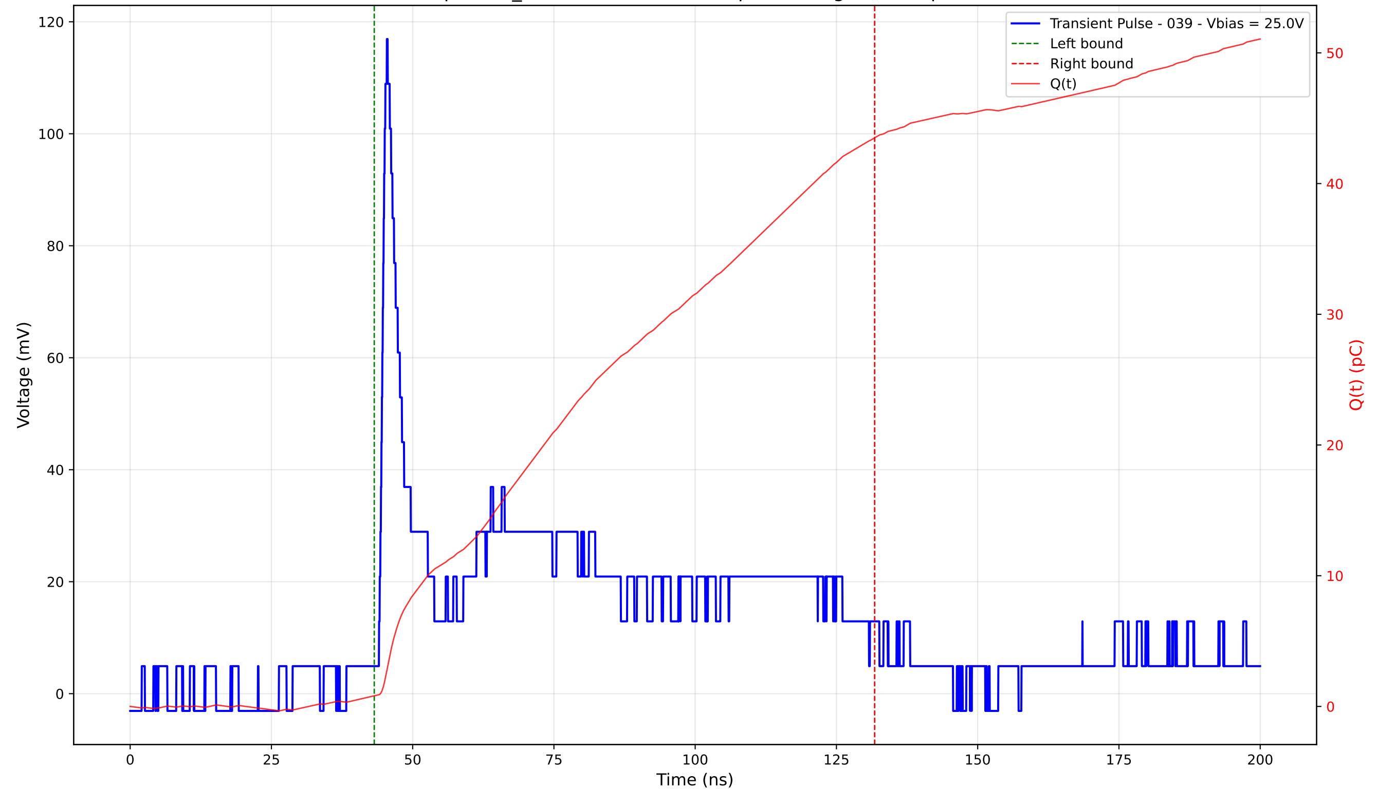
Transient Pulse - Sample: TD_4004 - Position: 270.0 \mu\text{m} - Charge: 42.70 pC - Rise Time: 1.12 ns
