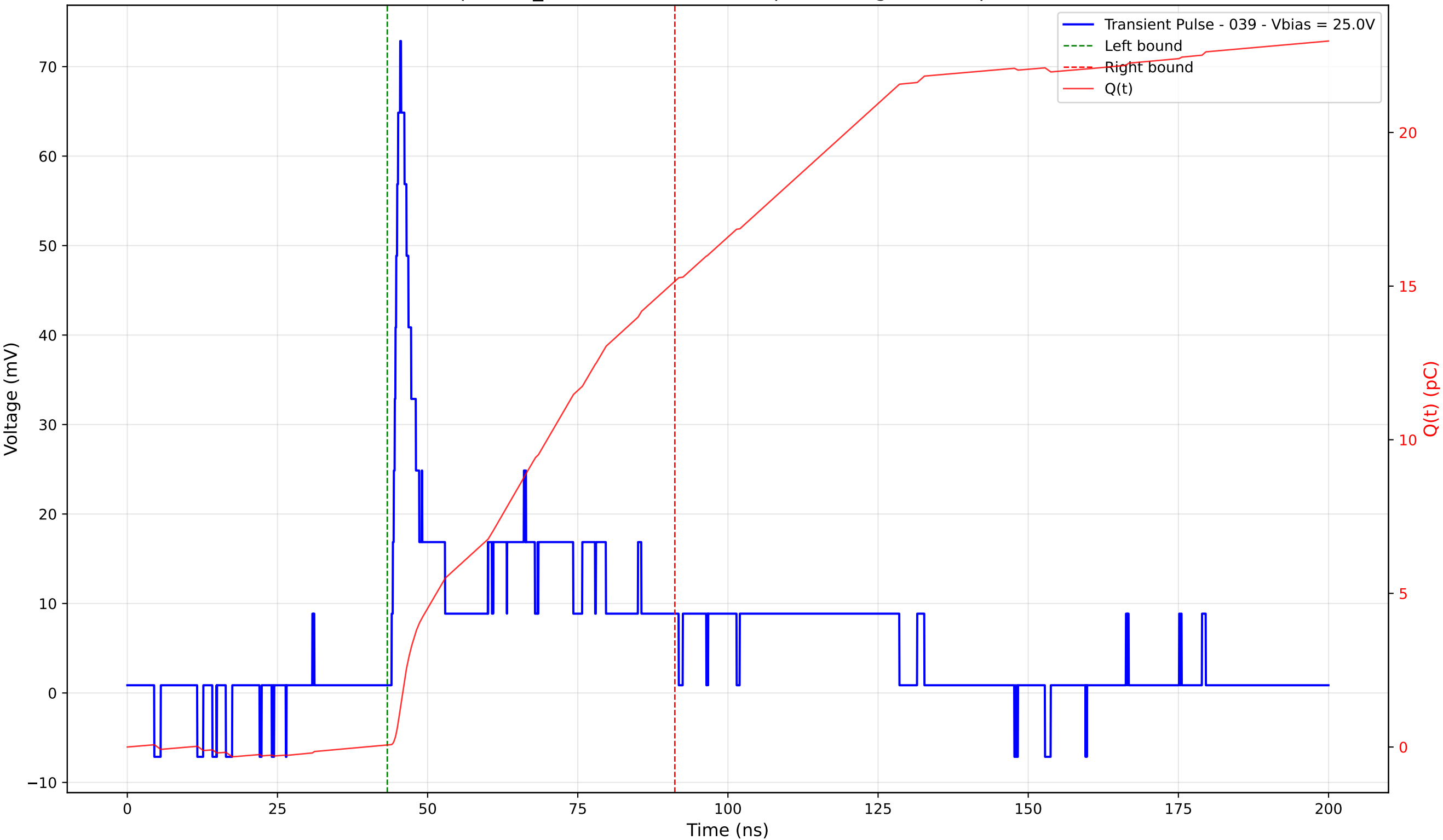
Transient Pulse - Sample: TD_4004 - Position: 380.0 \mu\text{m} - Charge: 15.10 pC - Rise Time: 1.42 ns
