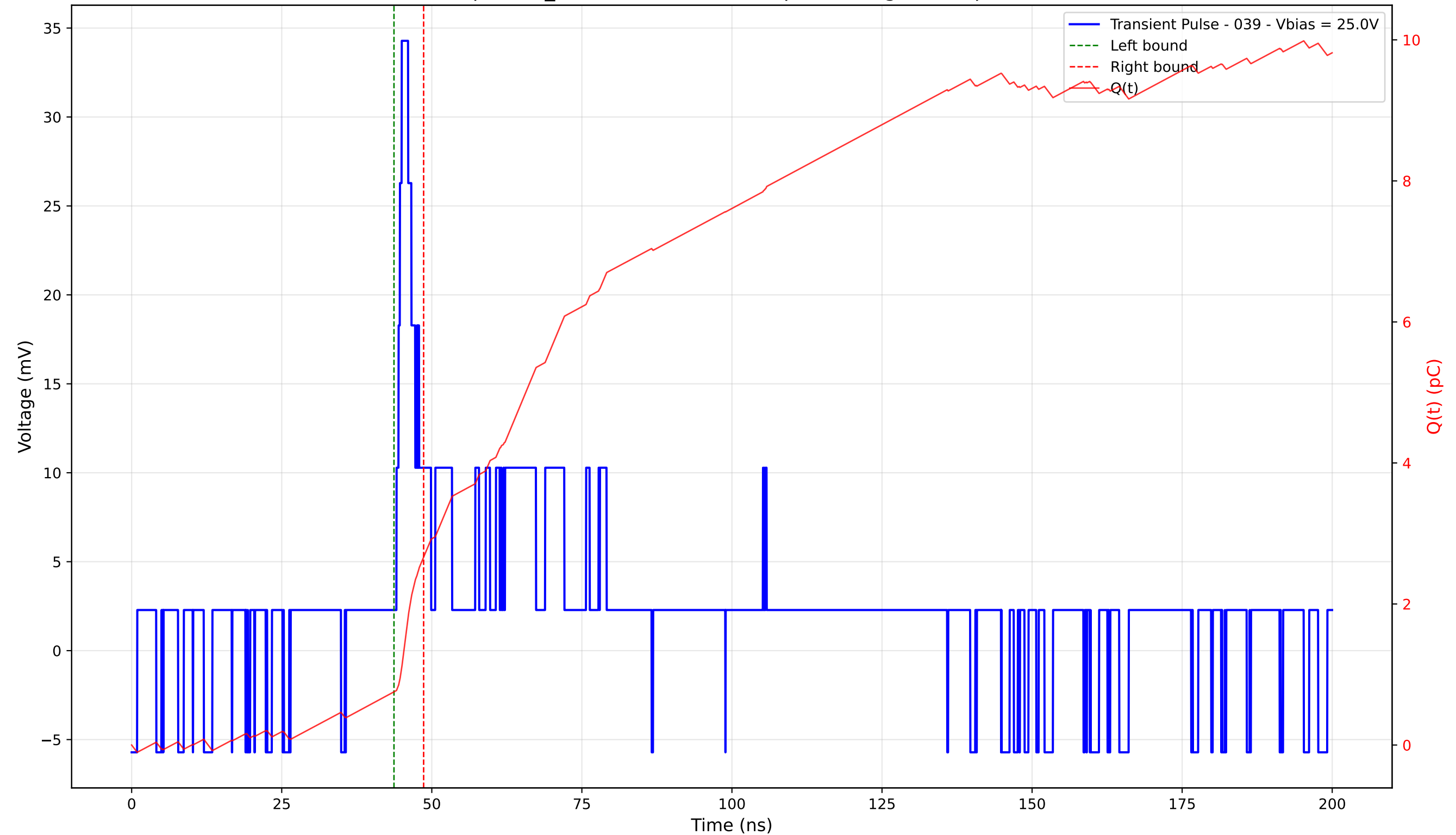
Transient Pulse - Sample: TD_4004 - Position: 405.0 \mu\text{m} - Charge: 1.91 pC - Rise Time: 0.88 ns
