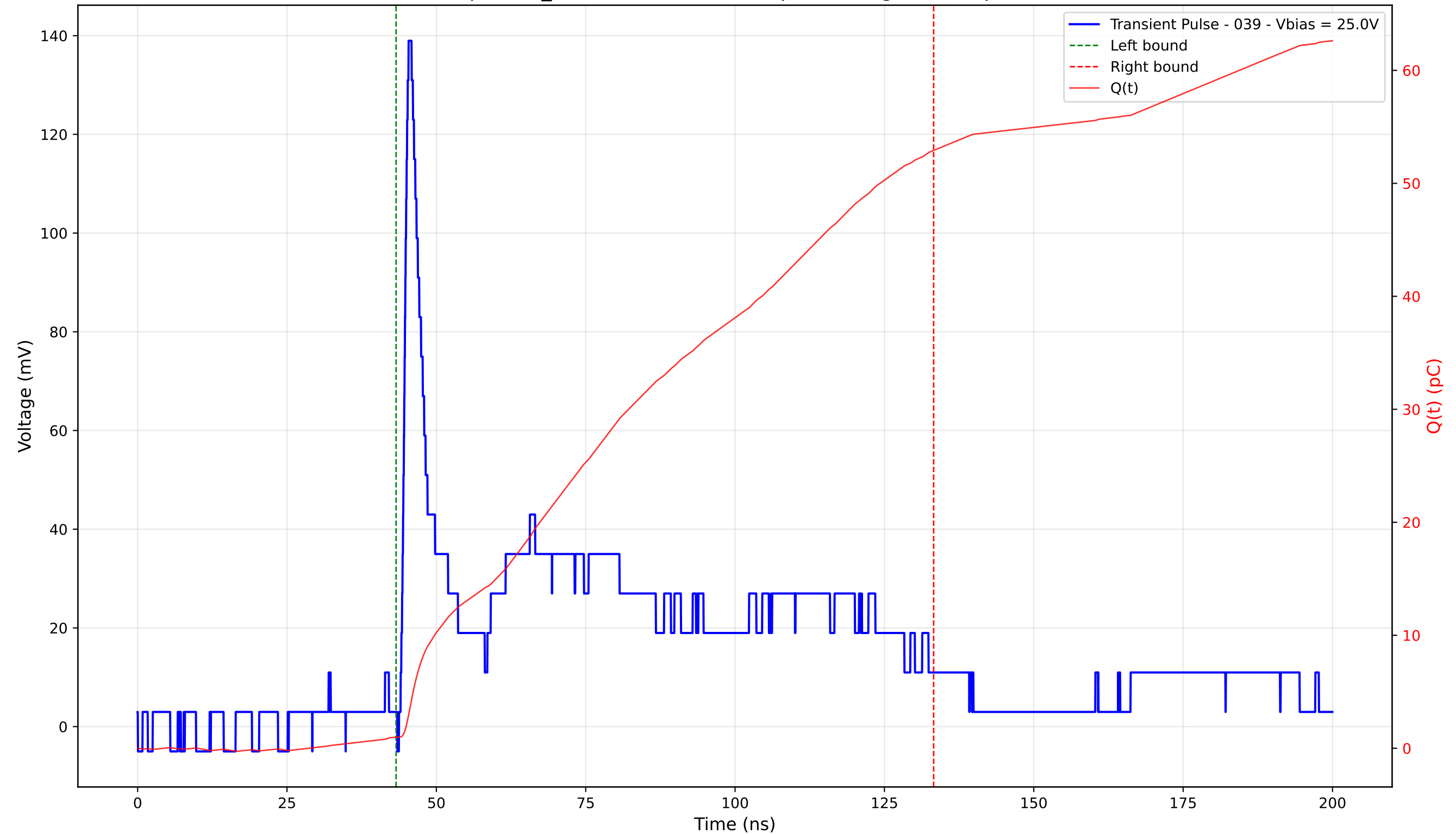
Transient Pulse - Sample: TD_4004 - Position: 245.0 \mu\text{m} - Charge: 51.92 pC - Rise Time: 1.07 ns
