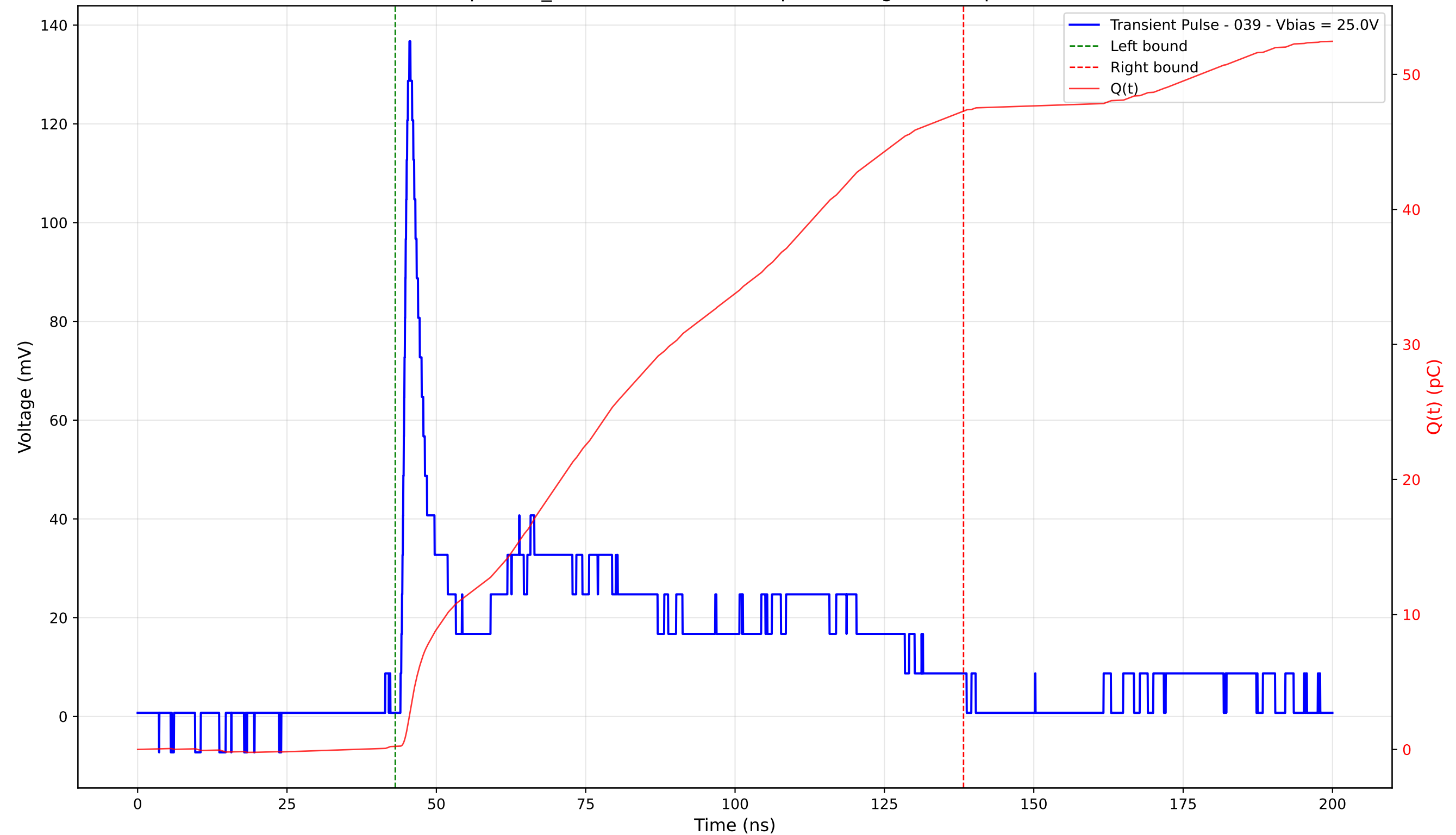
Transient Pulse - Sample: TD_4004 - Position: 260.0 \mu\text{m} - Charge: 47.07 pC - Rise Time: 1.11 ns
