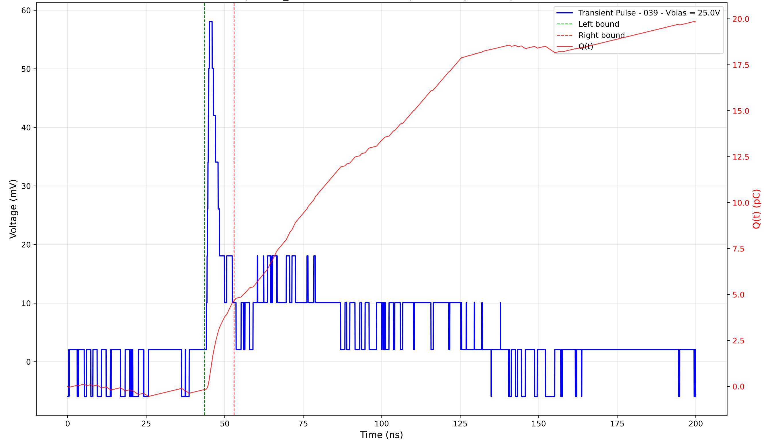
Transient Pulse - Sample: TD_4004 - Position: 370.0 \mu\text{m} - Charge: 4.83 pC - Rise Time: 0.93 ns
