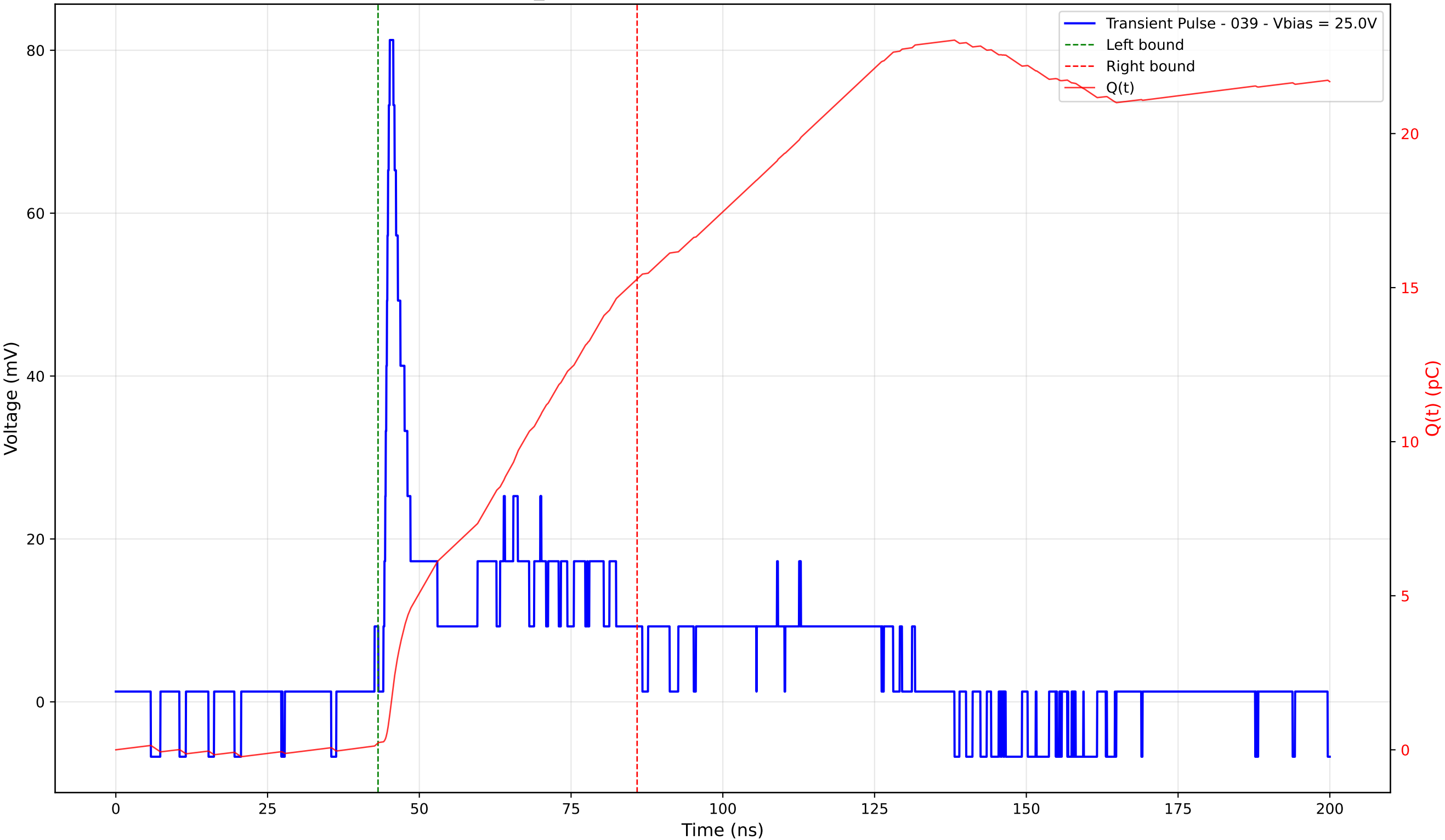
Transient Pulse - Sample: TD_4004 - Position: 60.0 \mu\text{m} - Charge: 15.05 pC - Rise Time: 0.88 ns
