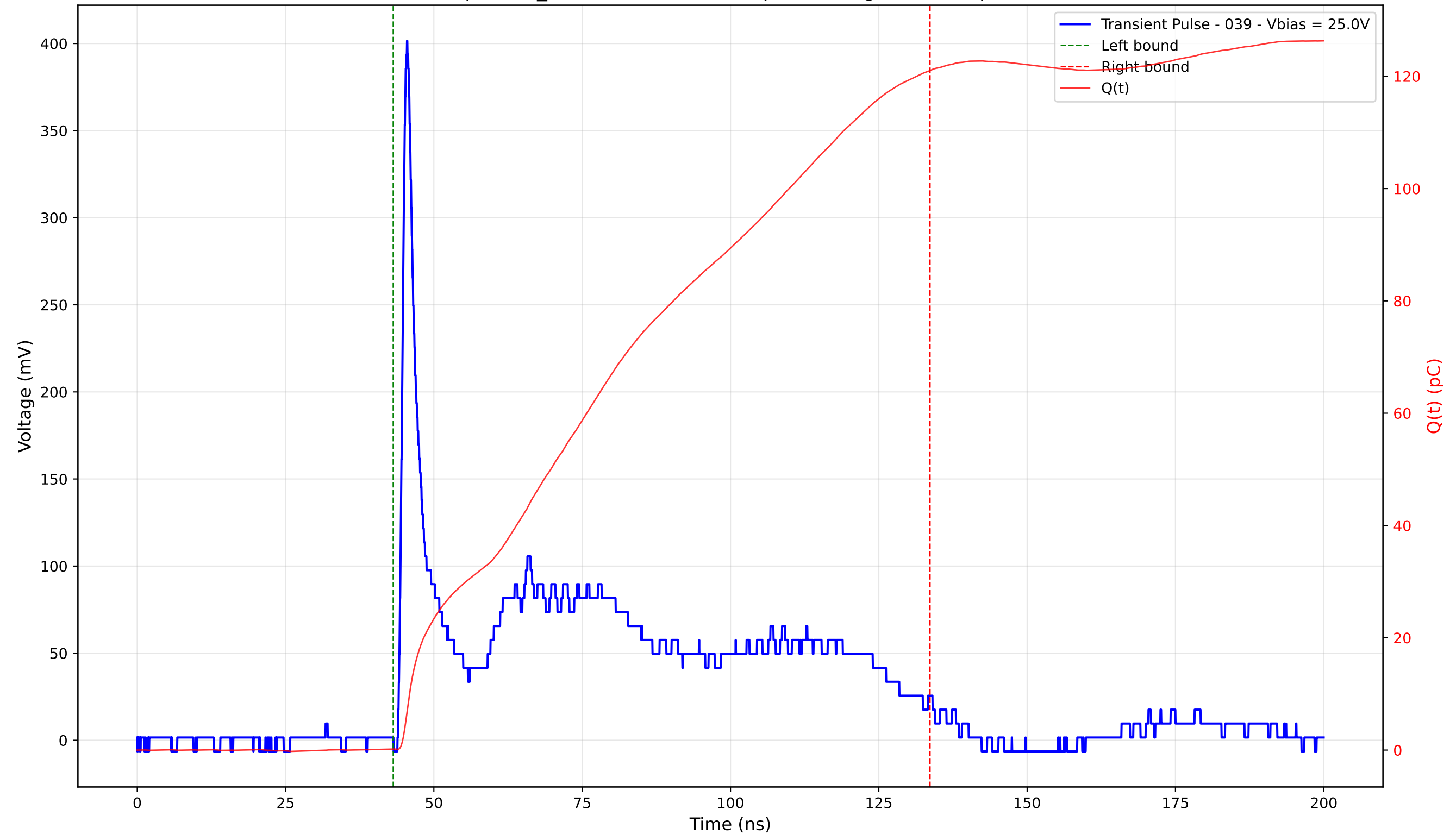
Transient Pulse - Sample: TD_4004 - Position: 90.0 \mu\text{m} - Charge: 120.82 pC - Rise Time: 1.00 ns
