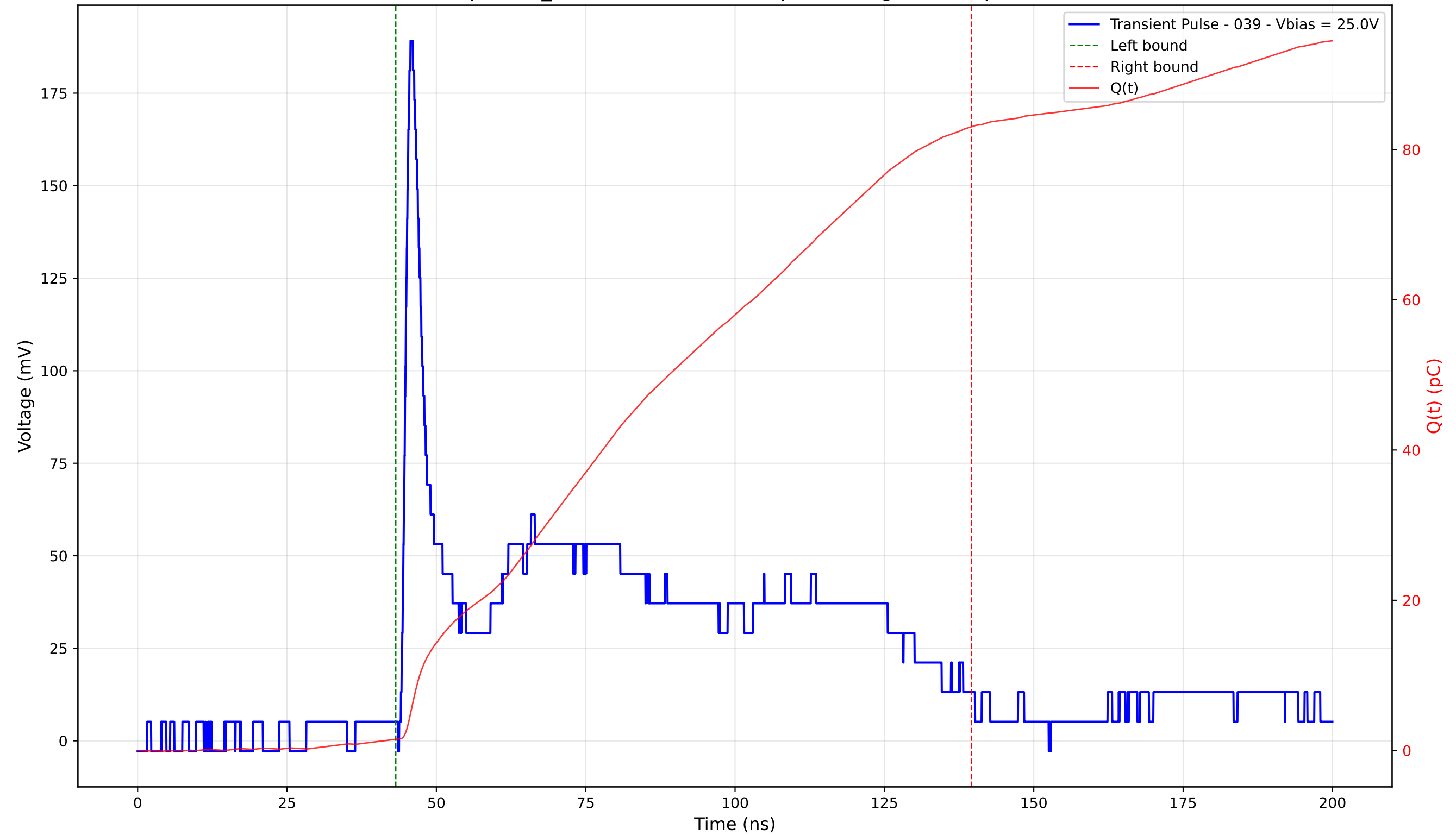
Transient Pulse - Sample: TD_4004 - Position: 135.0 \mu\text{m} - Charge: 81.53 pC - Rise Time: 1.21 ns
