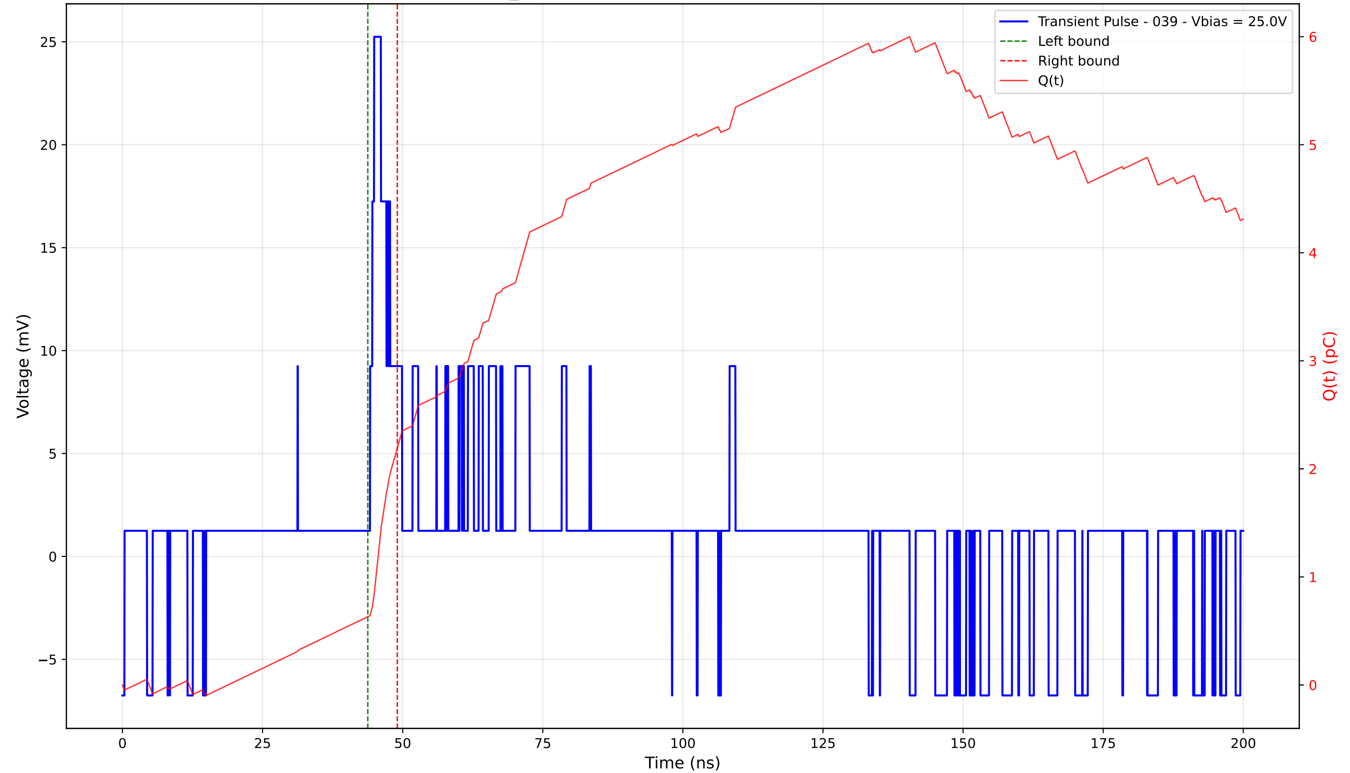
Transient Pulse - Sample: TD_4004 - Position: 415.0 \mu\text{m} - Charge: 1.56 pC - Rise Time: 0.74 ns
