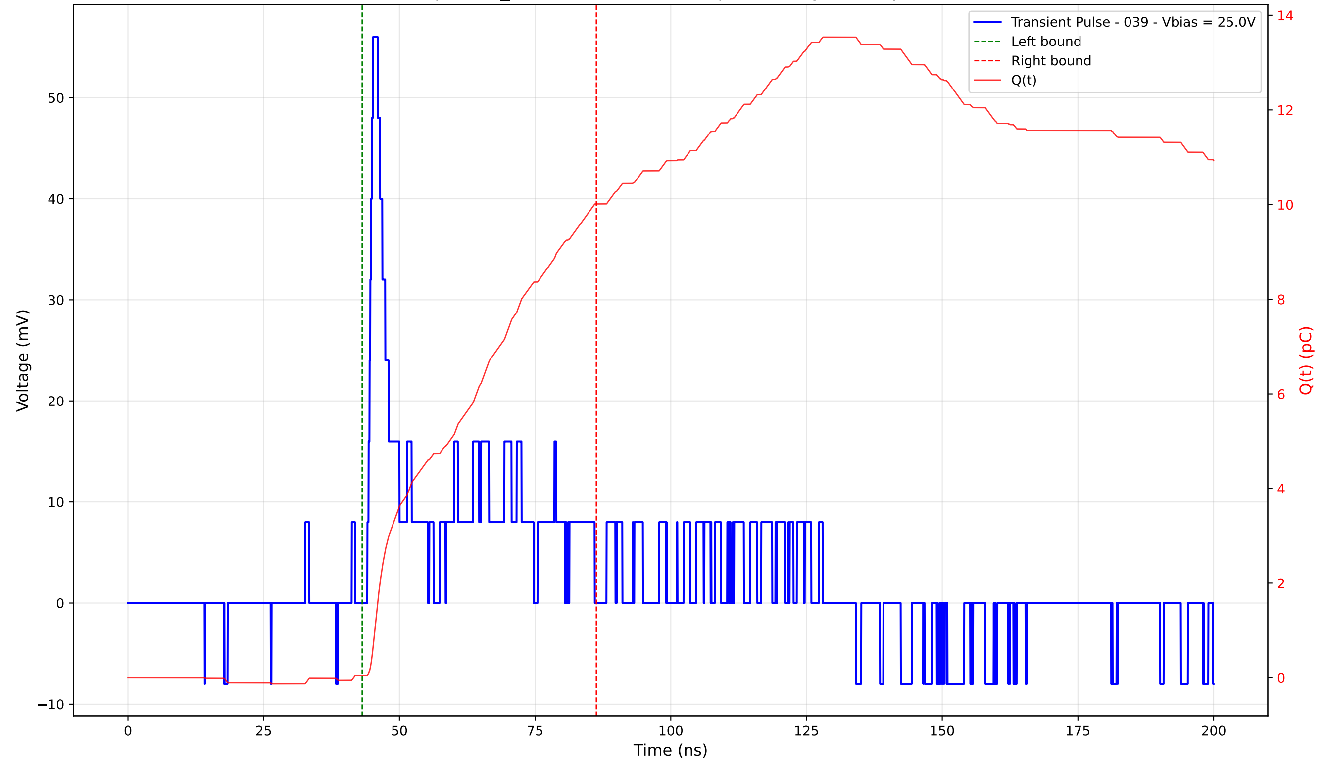
Transient Pulse - Sample: TD_4004 - Position: 390.0 \mu\text{m} - Charge: 9.97 pC - Rise Time: 1.03 ns
