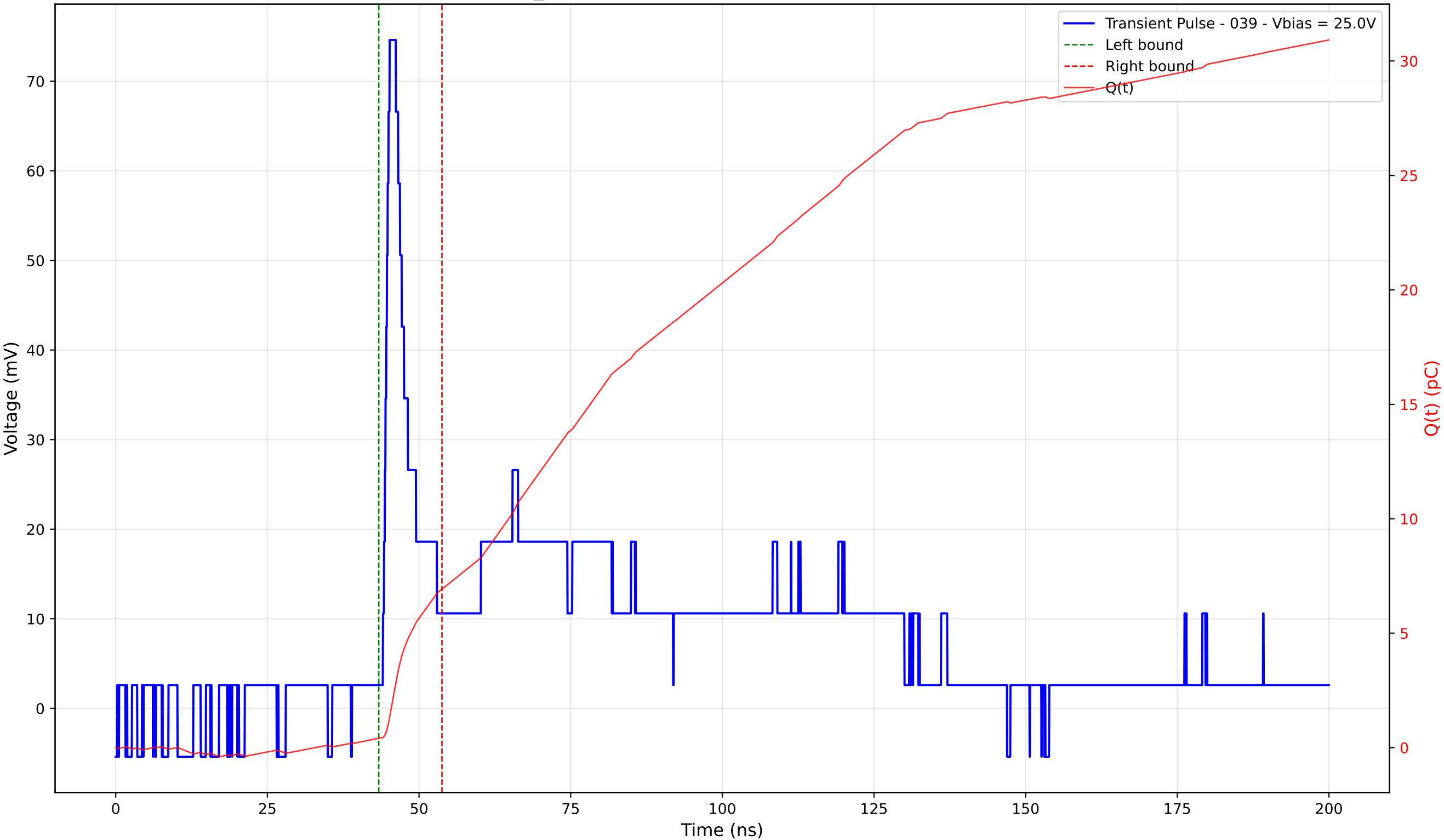
Transient Pulse - Sample: TD_4004 - Position: 330.0 \mu\text{m} - Charge: 6.52 pC - Rise Time: 1.11 ns
