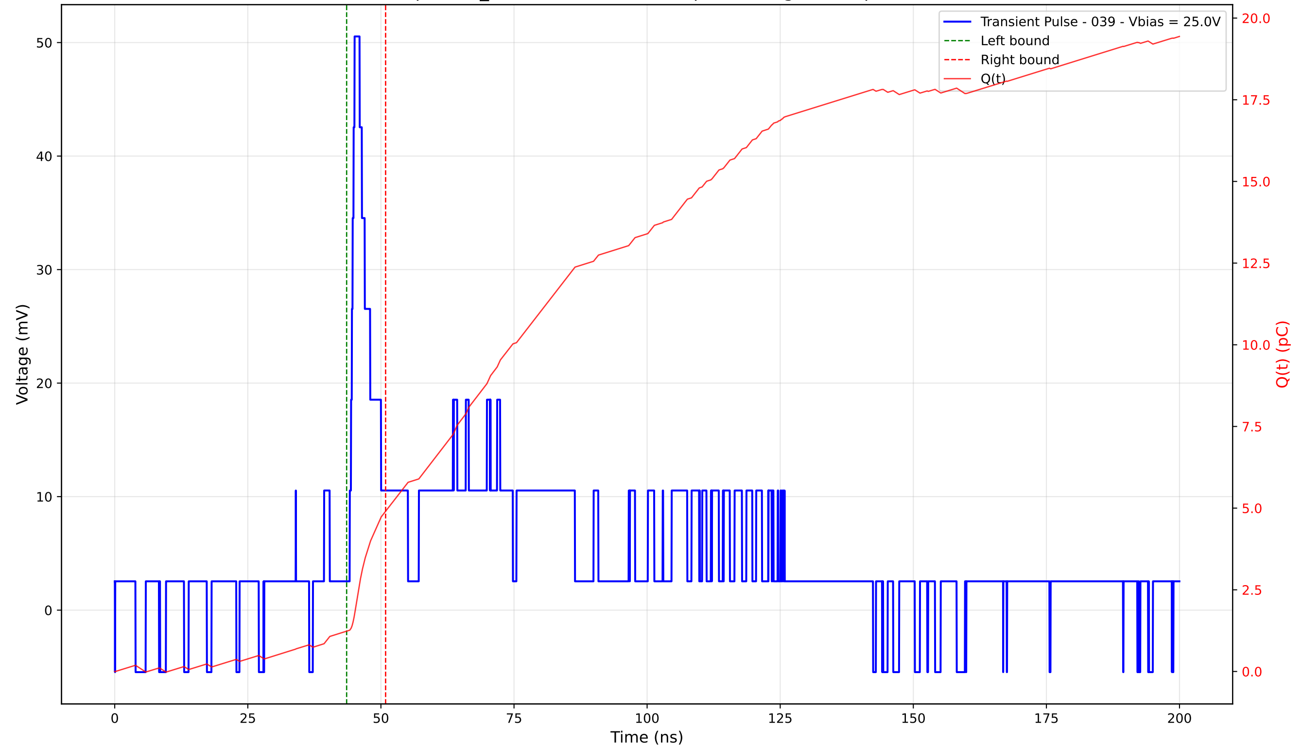
Transient Pulse - Sample: TD_4004 - Position: 395.0 \mu\text{m} - Charge: 3.67 pC - Rise Time: 0.91 ns
