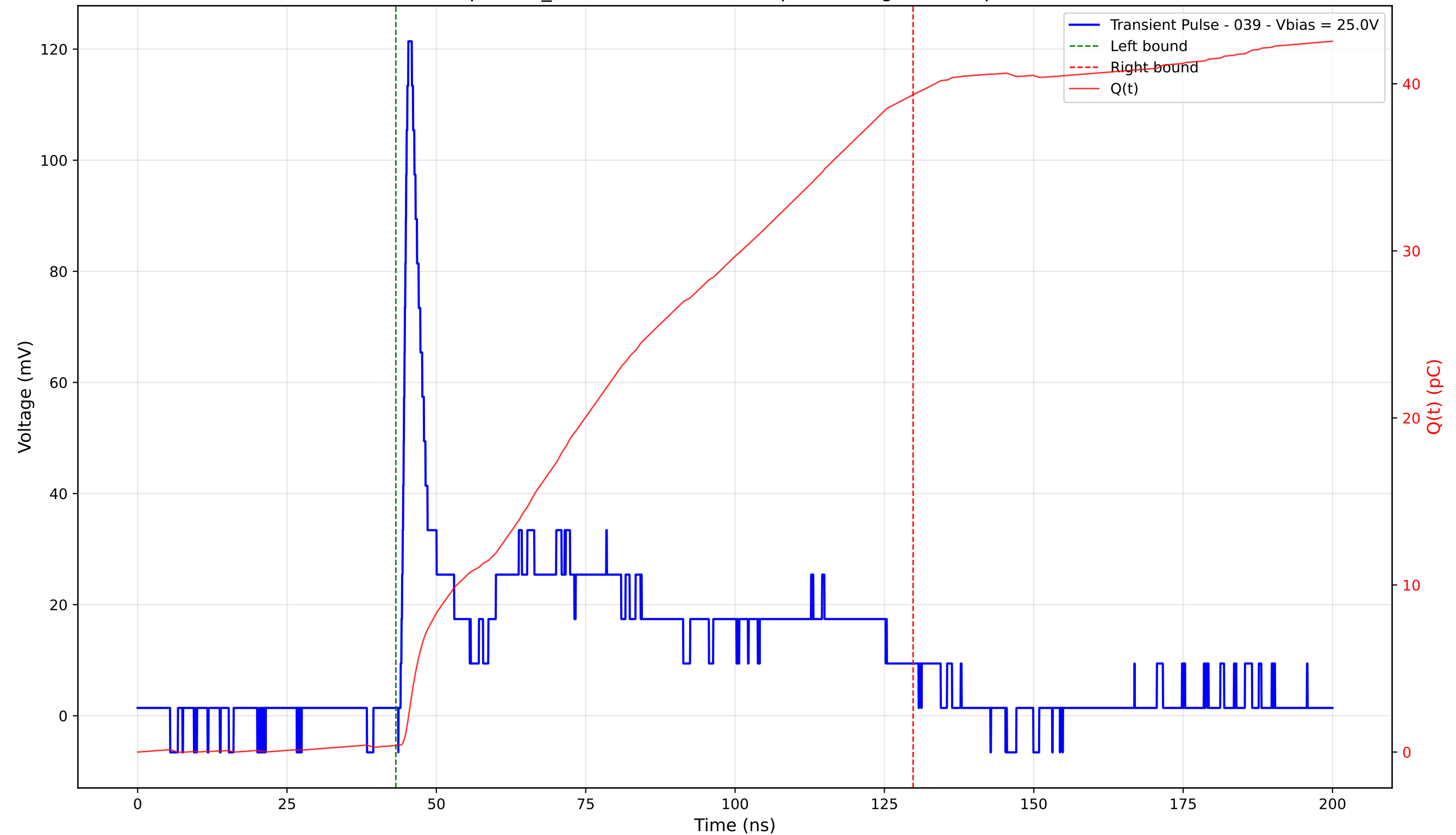
Transient Pulse - Sample: TD_4004 - Position: 275.0 \mu\text{m} - Charge: 38.96 pC - Rise Time: 0.99 ns
