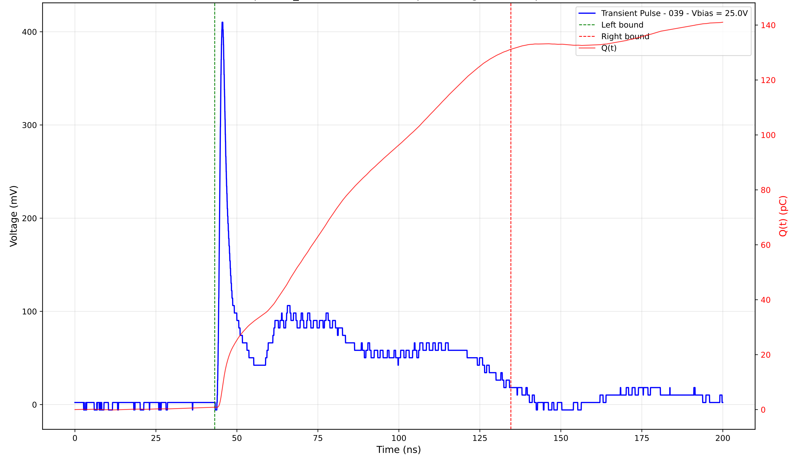
Transient Pulse - Sample: TD_4004 - Position: 95.0 \mu\text{m} - Charge: 130.31 pC - Rise Time: 1.02 ns
