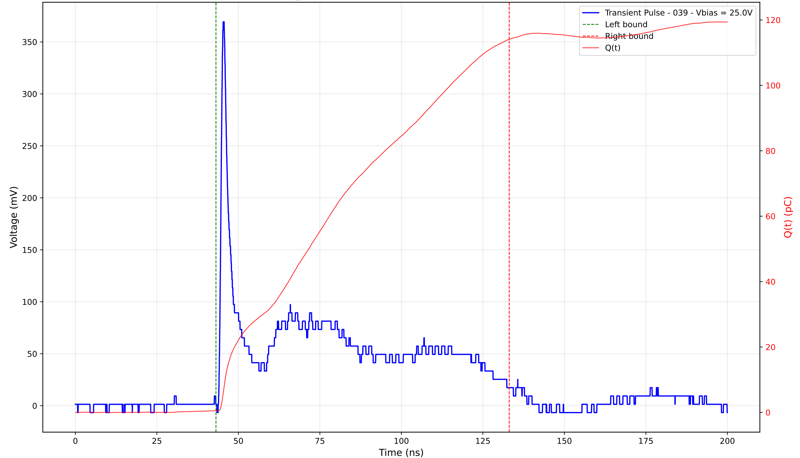
Transient Pulse - Sample: TD_4004 - Position: 85.0 \mu\text{m} - Charge: 113.52 pC - Rise Time: 0.97 ns
