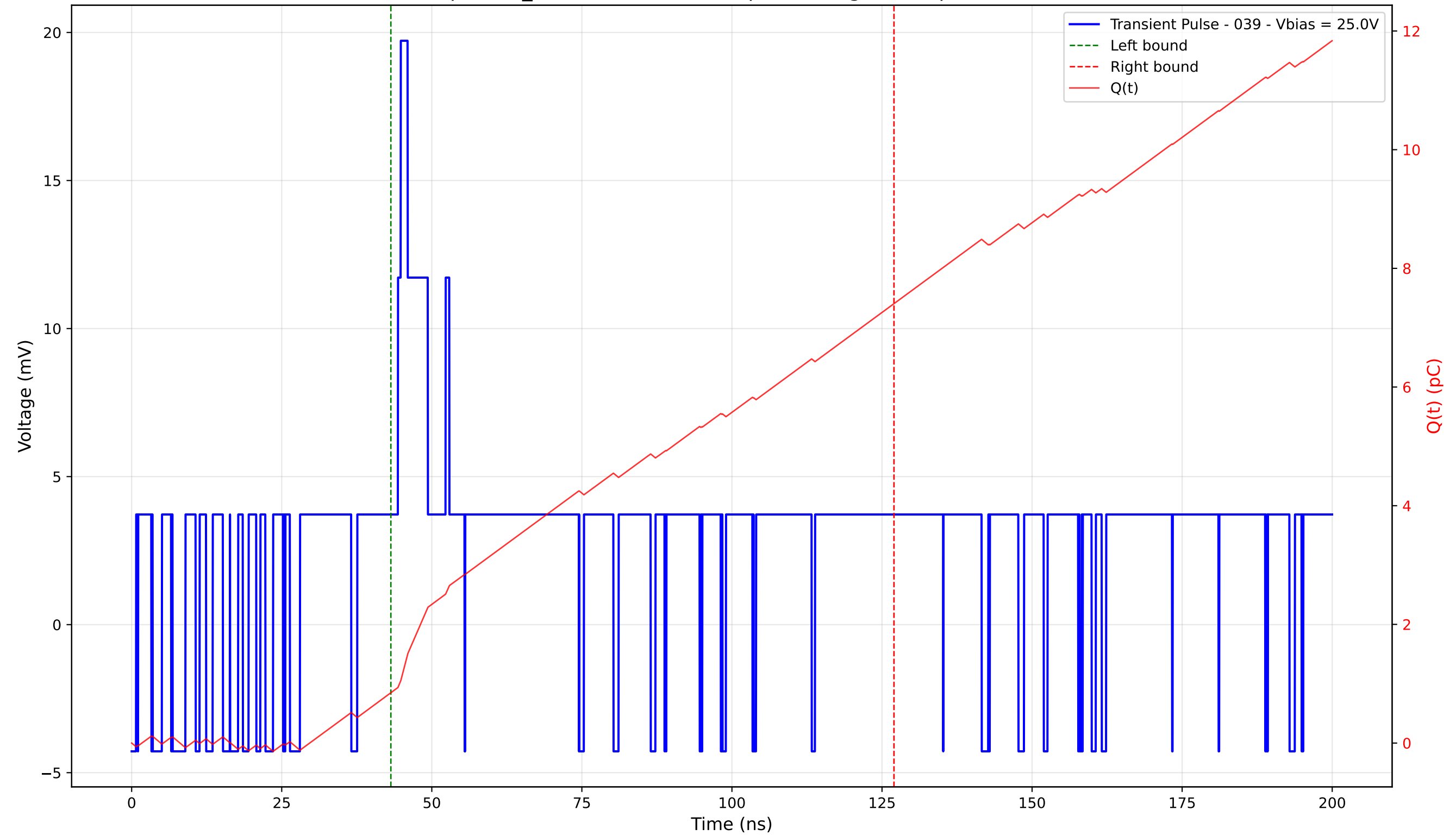
Transient Pulse - Sample: TD_4004 - Position: 45.0 \mu\text{m} - Charge: 6.56 pC - Rise Time: 0.00 ns (N/A)
