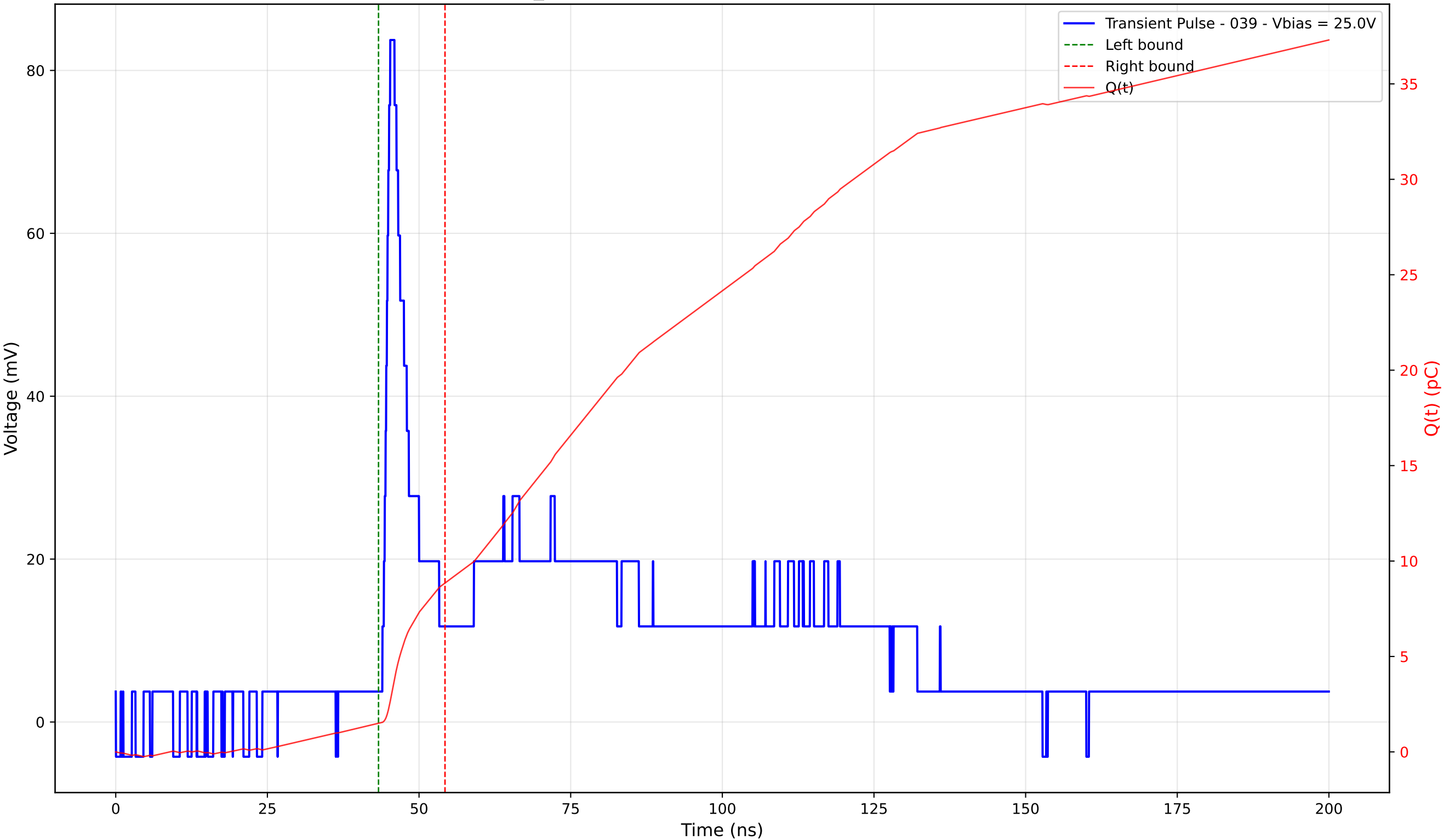
Transient Pulse - Sample: TD_4004 - Position: 320.0 \mu\text{m} - Charge: 7.35 pC - Rise Time: 1.11 ns
