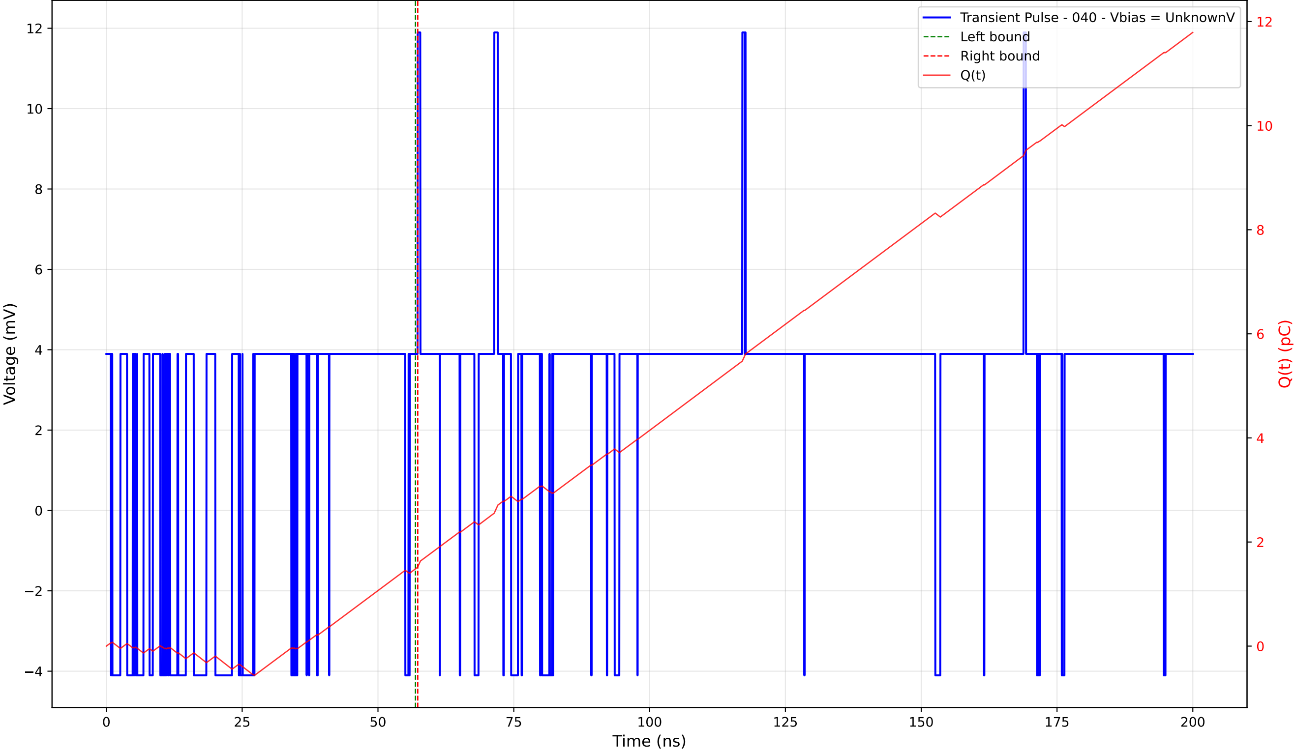
Transient Pulse - Sample: TD_4004 - Position: 250.0 \mu\text{m} - Charge: 0.04 pC - Rise Time: 0.00 ns (N/A)
