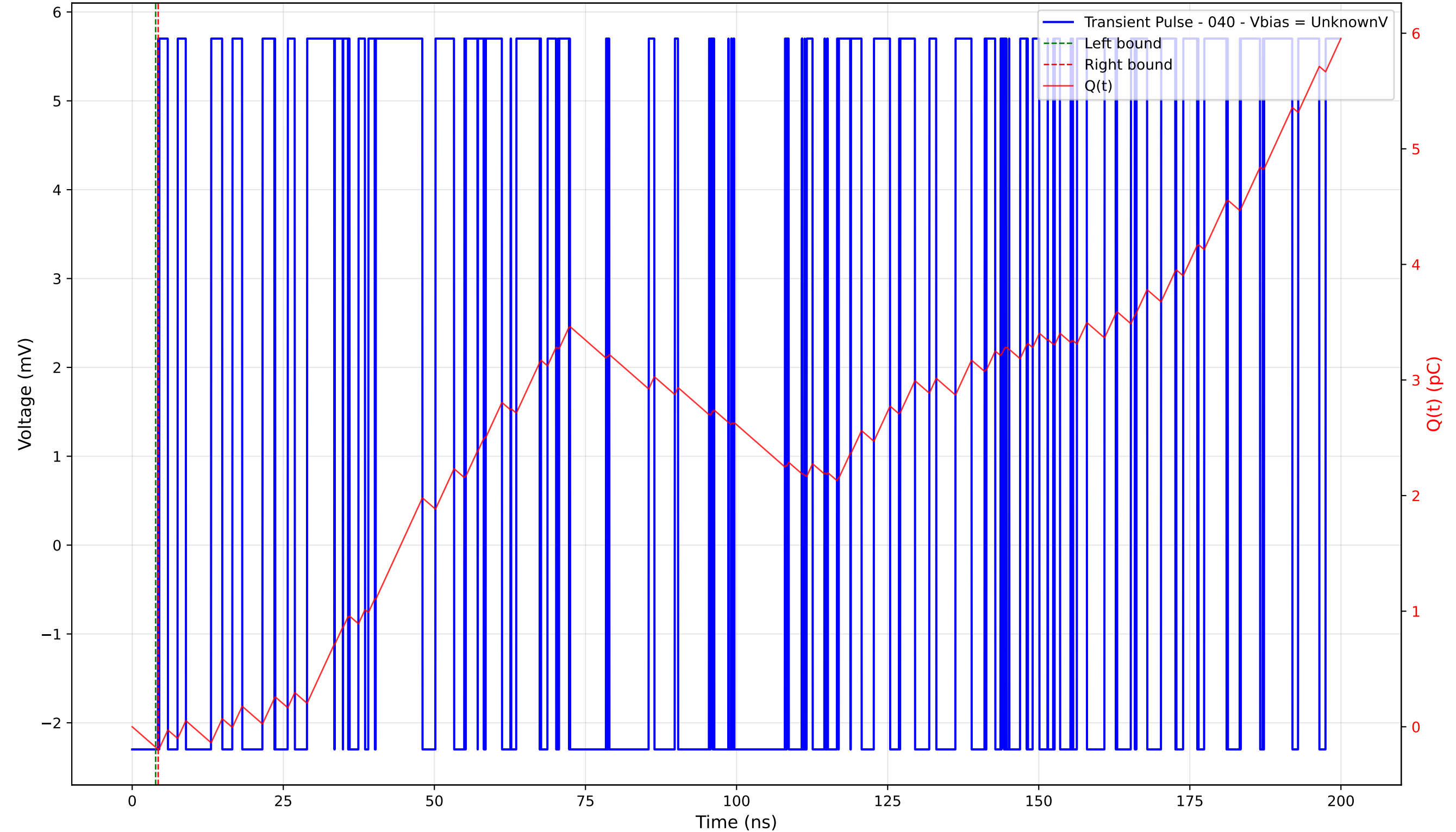
Transient Pulse - Sample: TD_4004 - Position: 55.0 \mu\text{m} - Charge: 0.01 pC - Rise Time: 0.00 ns (N/A)
