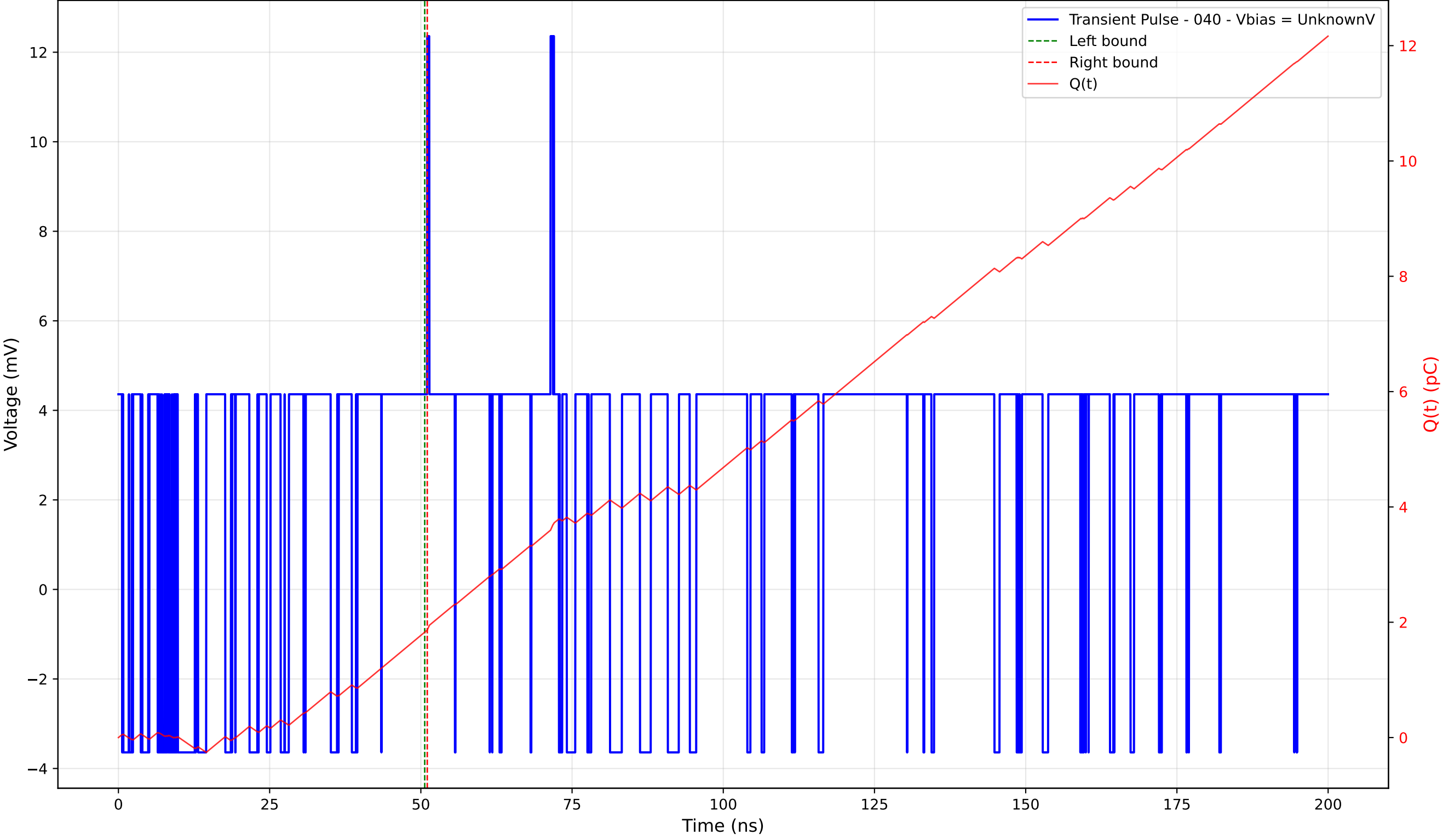
Transient Pulse - Sample: TD_4004 - Position: 300.0 \mu\text{m} - Charge: 0.04 pC - Rise Time: 0.00 ns (N/A)
