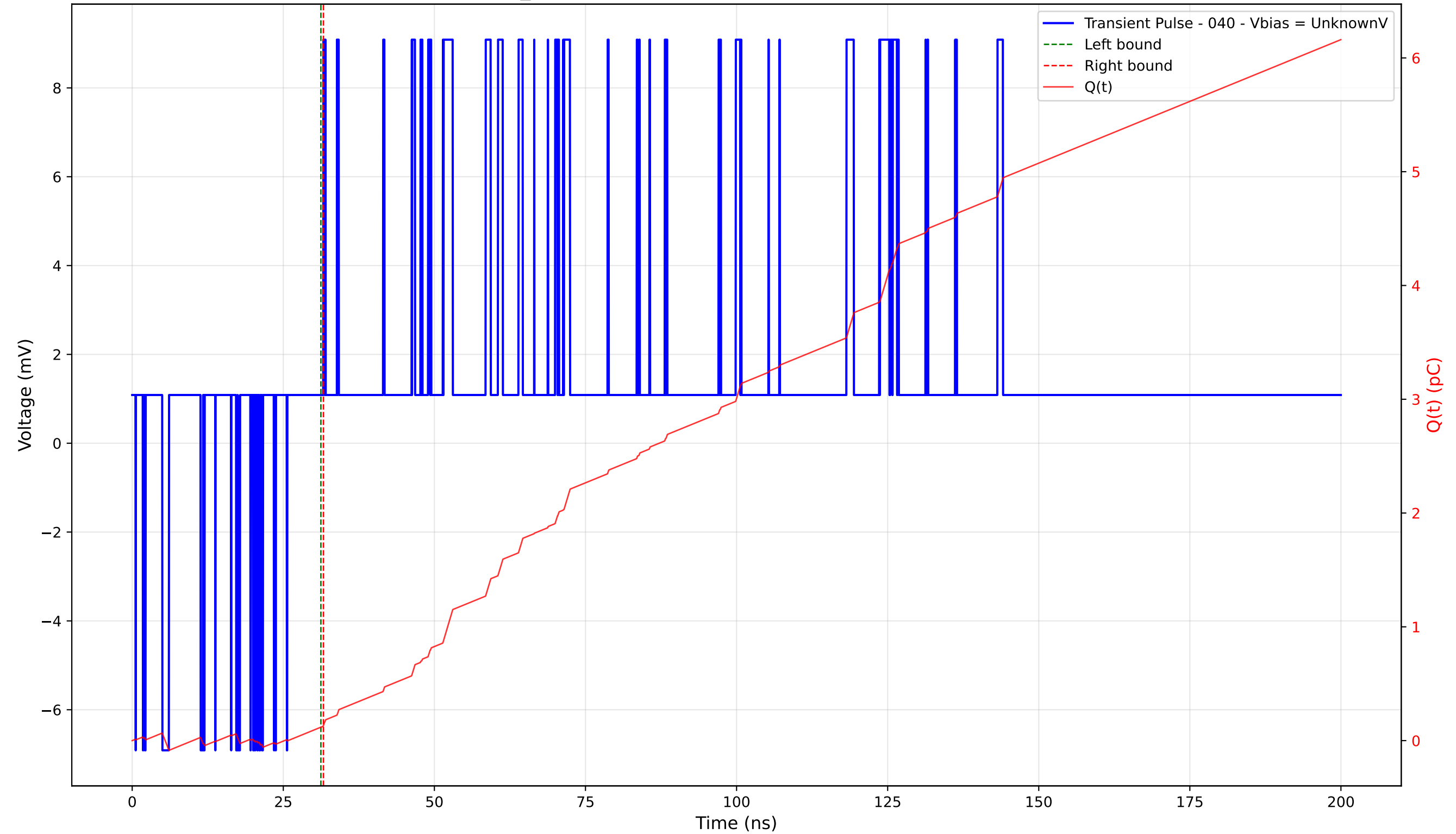
Transient Pulse - Sample: TD_4004 - Position: 245.0 \mu\text{m} - Charge: 0.01 pC - Rise Time: 0.00 ns (N/A)
