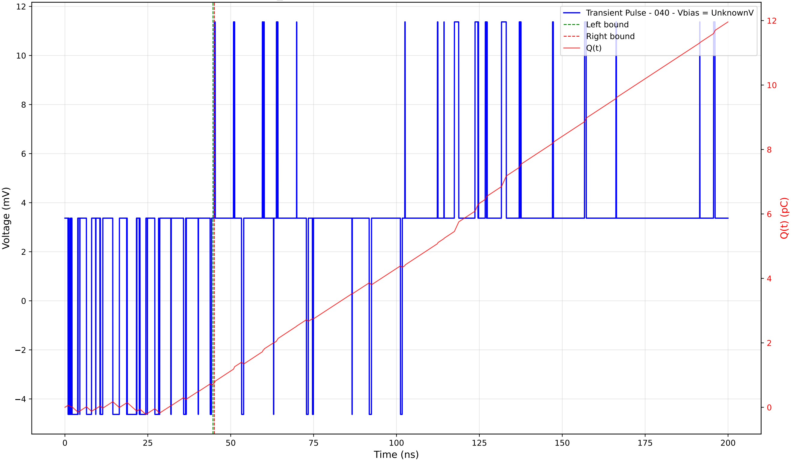
Transient Pulse - Sample: TD_4004 - Position: 175.0 \mu\text{m} - Charge: 0.03 pC - Rise Time: 0.00 ns (N/A)
