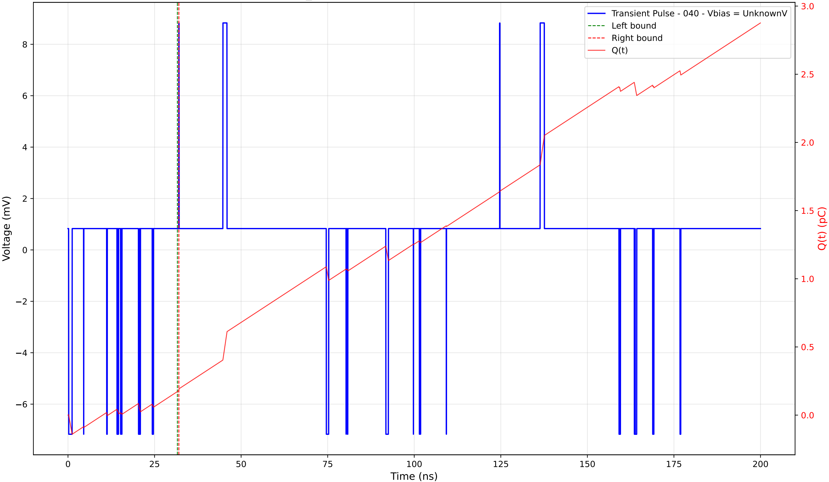
Transient Pulse - Sample: TD_4004 - Position: 355.0 \mu\text{m} - Charge: 0.01 pC - Rise Time: 0.02 ns
