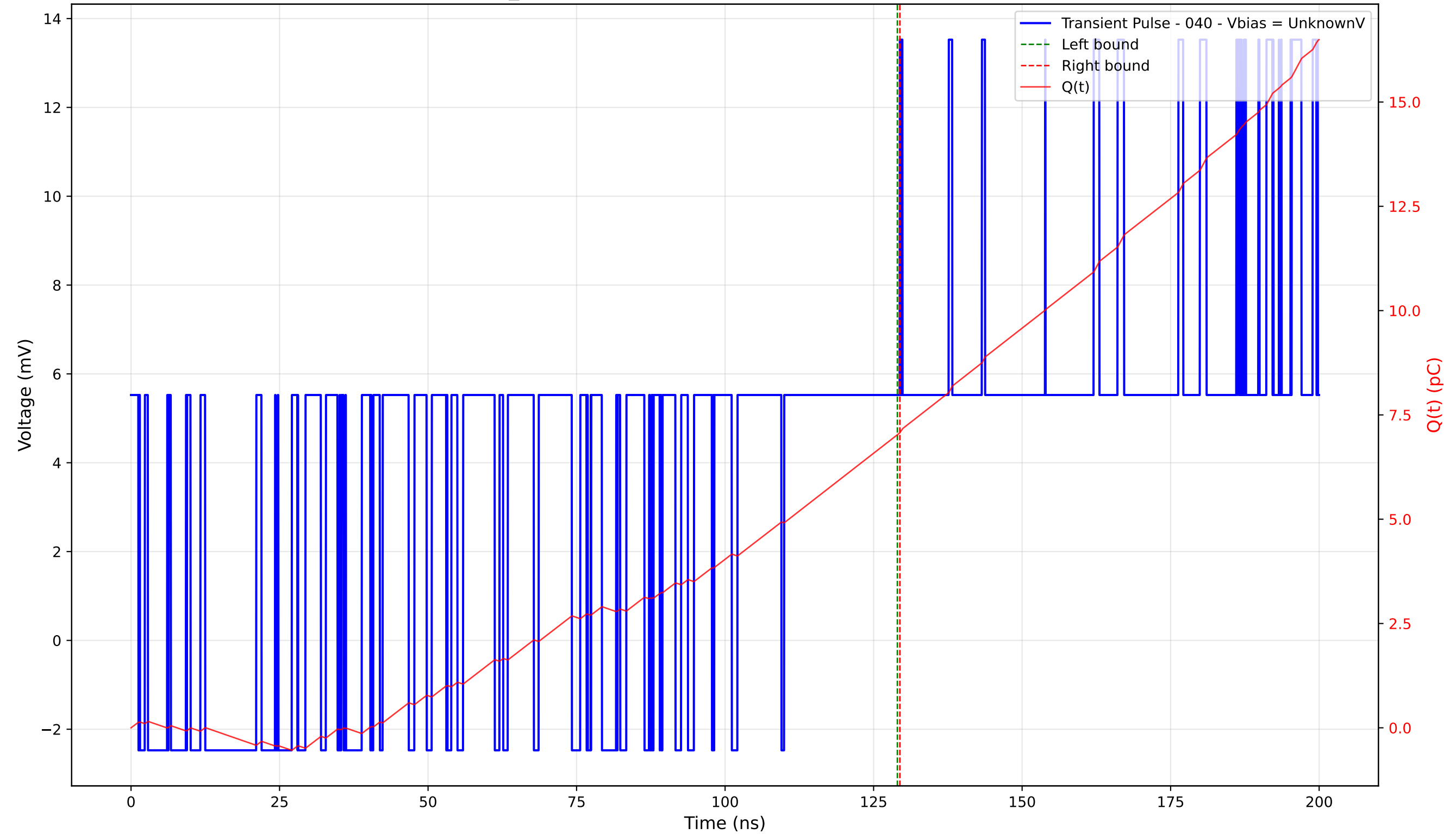
Transient Pulse - Sample: TD_4004 - Position: 110.0 \mu\text{m} - Charge: 0.05 pC - Rise Time: 0.00 ns (N/A)
