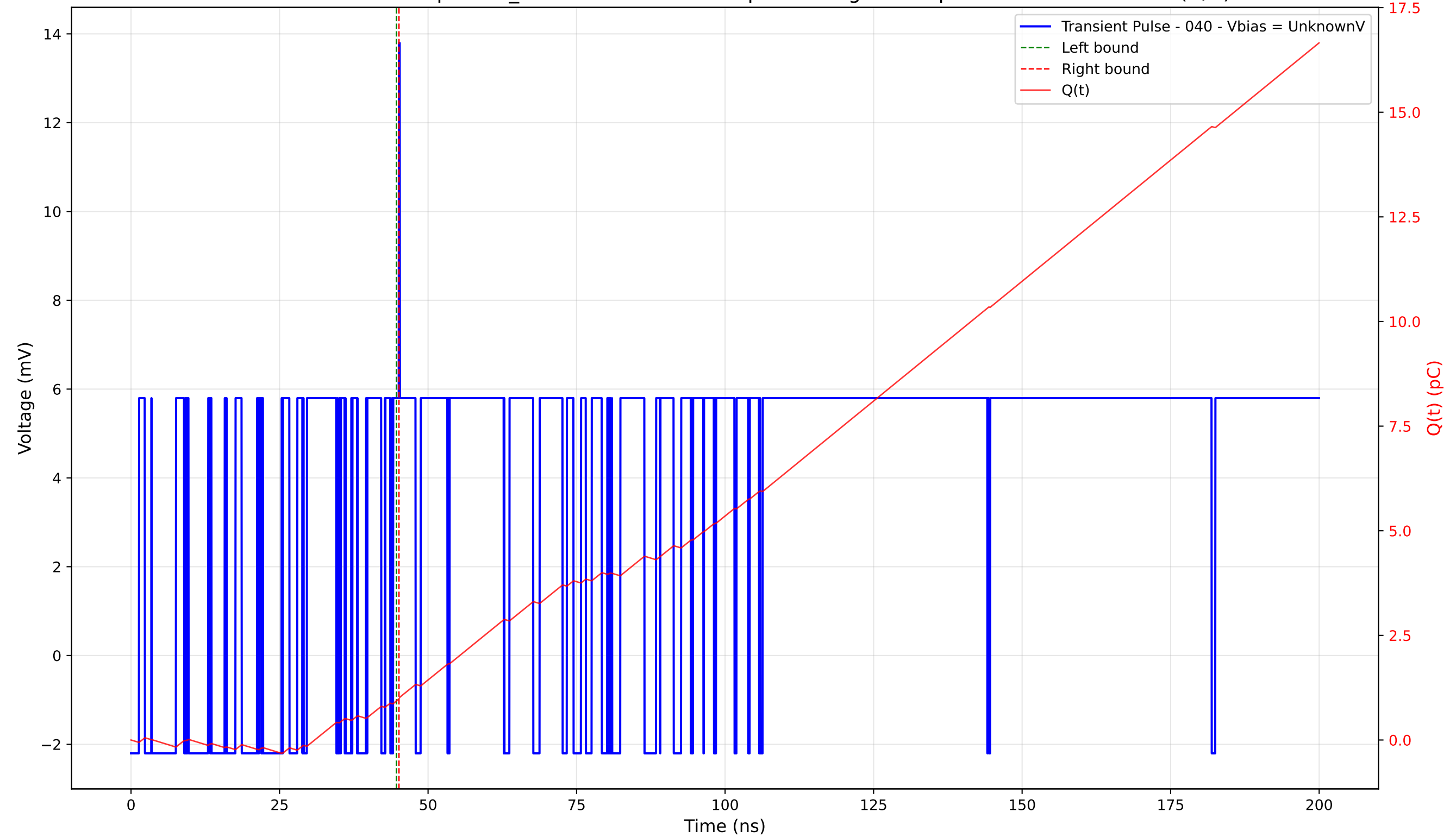
Transient Pulse - Sample: TD_4004 - Position: 145.0 \mu\text{m} - Charge: 0.05 pC - Rise Time: 0.00 ns (N/A)
