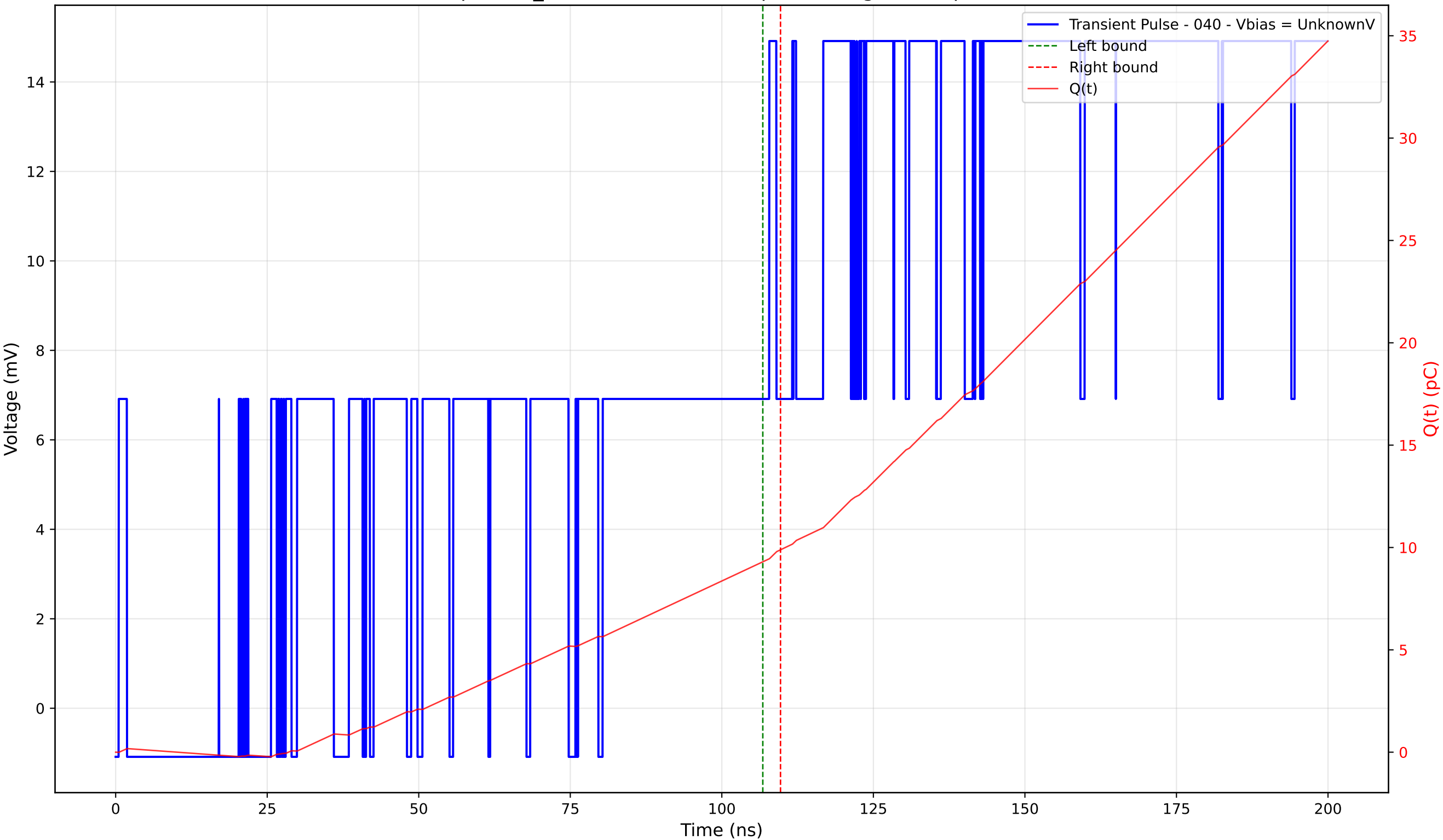
Transient Pulse - Sample: TD_4004 - Position: 75.0 \mu\text{m} - Charge: 0.59 pC - Rise Time: 27.50 ns
