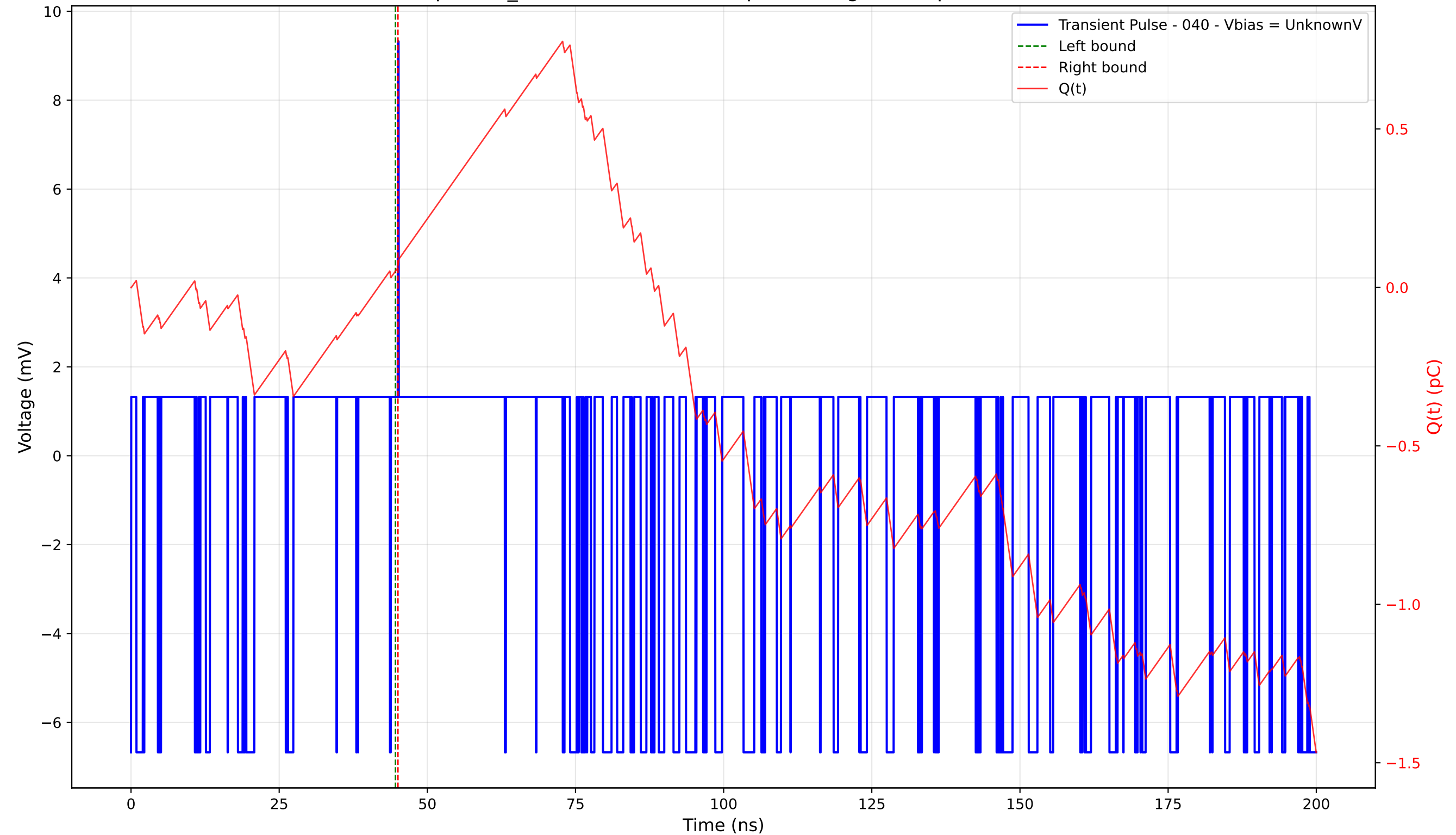
Transient Pulse - Sample: TD_4004 - Position: 290.0 \mu\text{m} - Charge: 0.02 pC - Rise Time: 0.00 ns (N/A)
