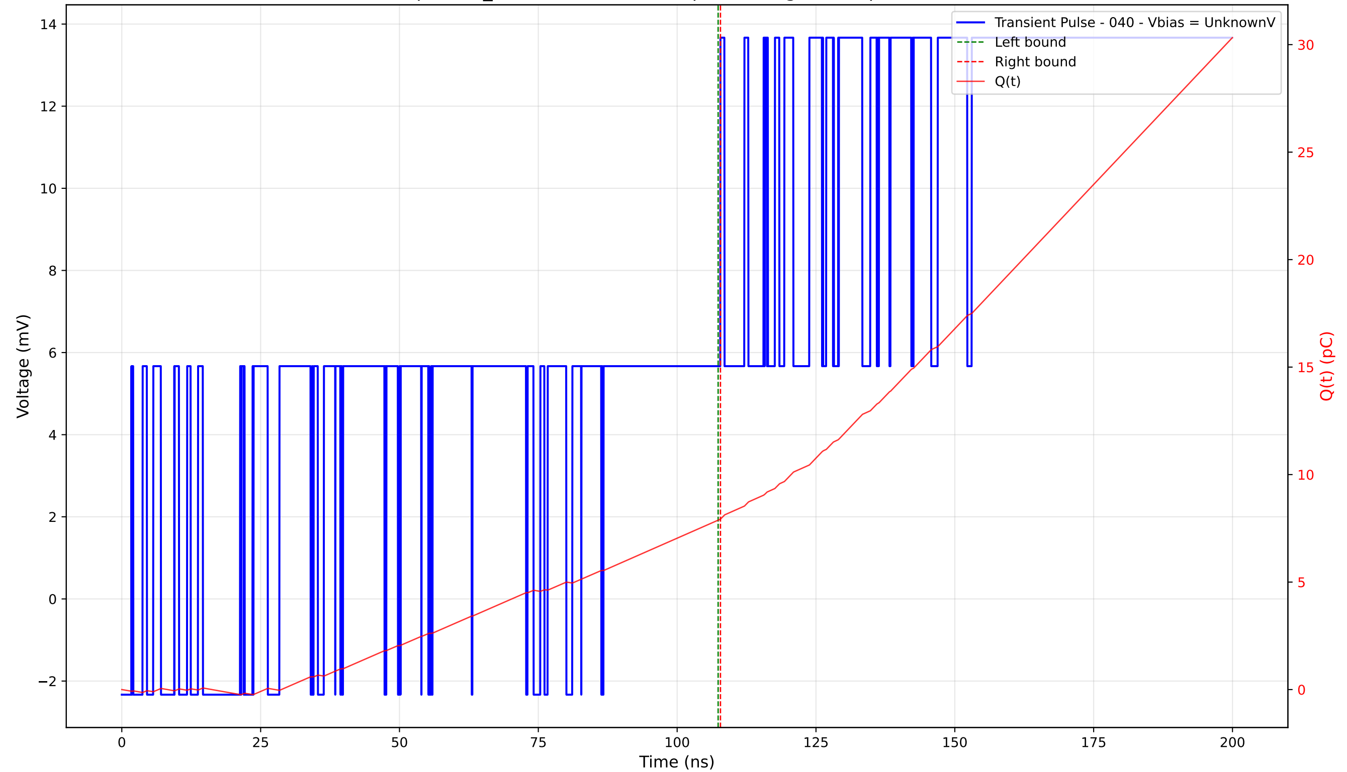
Transient Pulse - Sample: TD_4004 - Position: 90.0 \mu\text{m} - Charge: 0.05 pC - Rise Time: 0.00 ns (N/A)
