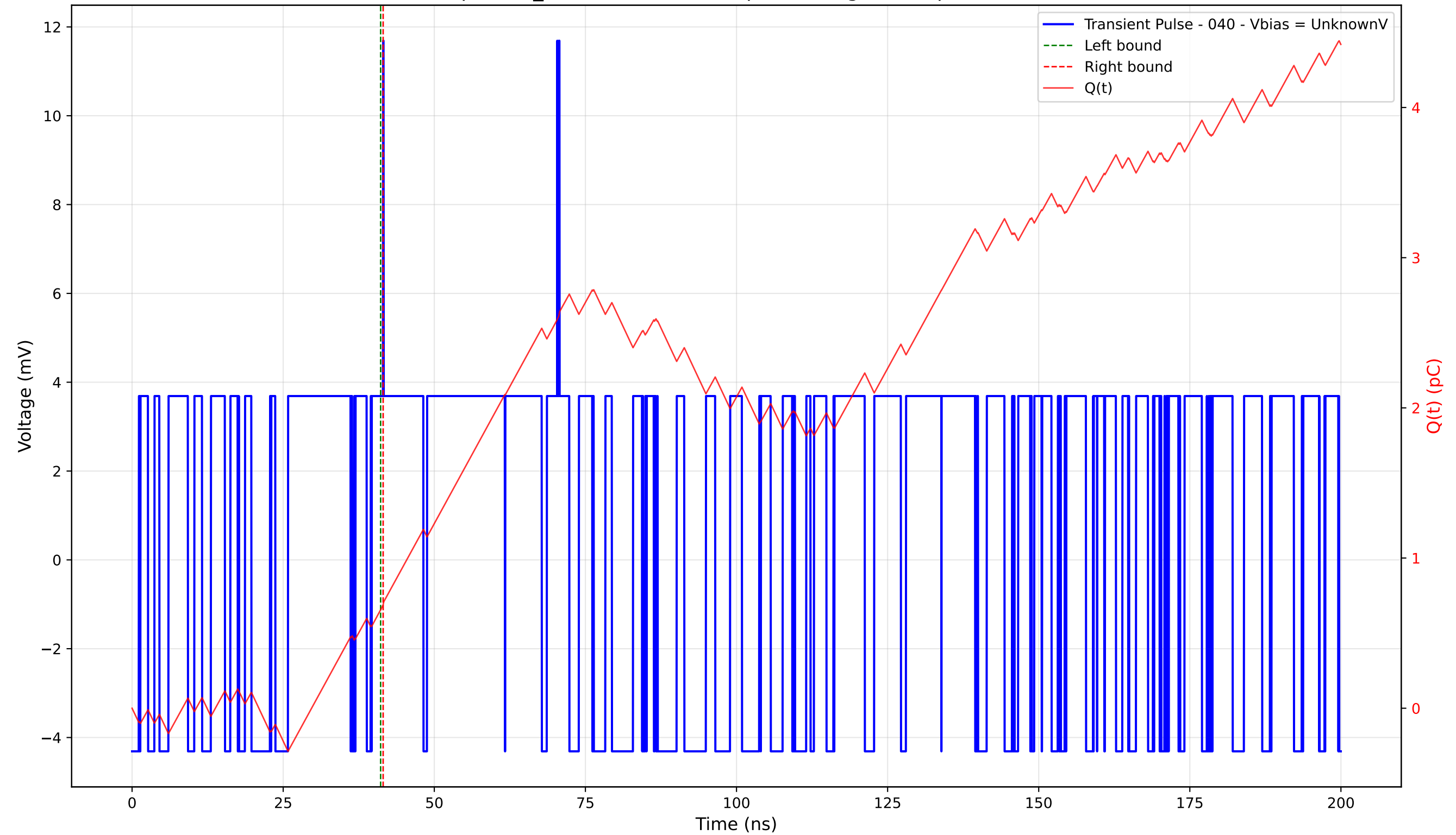
Transient Pulse - Sample: TD_4004 - Position: 5.0 \mu m - Charge: 0.04 pC - Rise Time: 0.00 ns (N/A)
