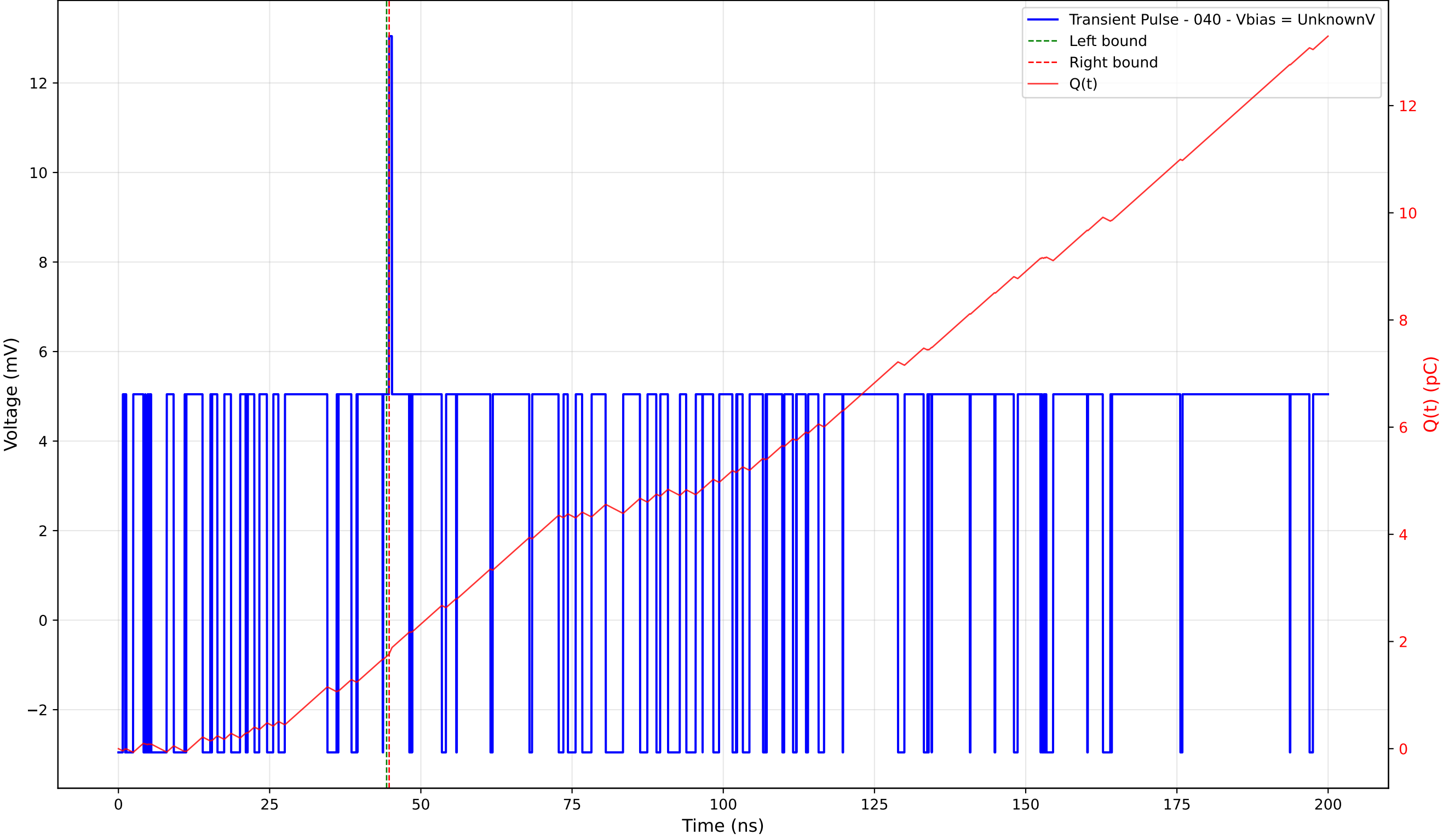
Transient Pulse - Sample: TD_4004 - Position: 140.0 \mu\text{m} - Charge: 0.05 pC - Rise Time: 0.00 ns (N/A)
