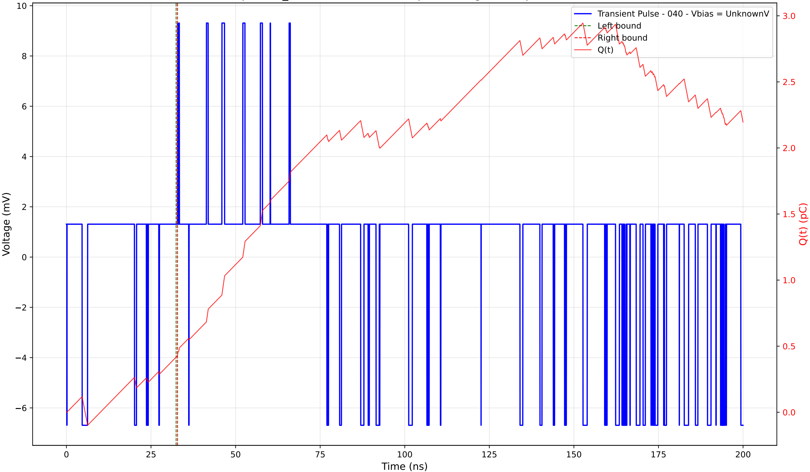
Transient Pulse - Sample: TD_4004 - Position: 405.0 \mu\text{m} - Charge: 0.02 pC - Rise Time: 0.00 ns (N/A)
