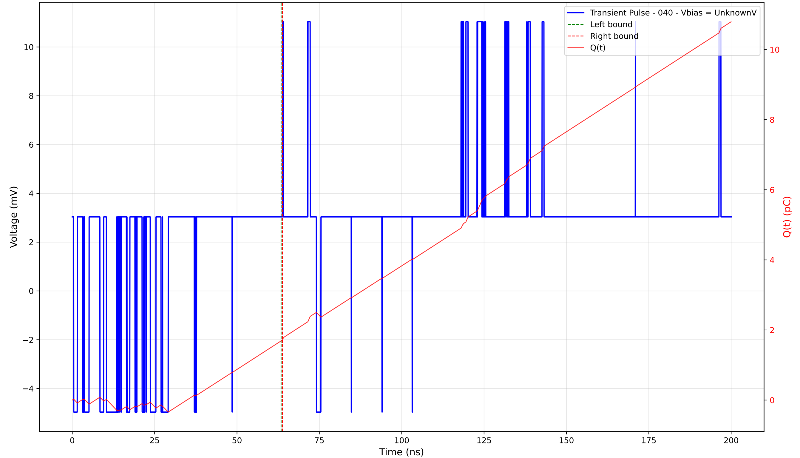
Transient Pulse - Sample: TD_4004 - Position: 70.0 \mu\text{m} - Charge: 0.03 pC - Rise Time: 0.00 ns (N/A)
