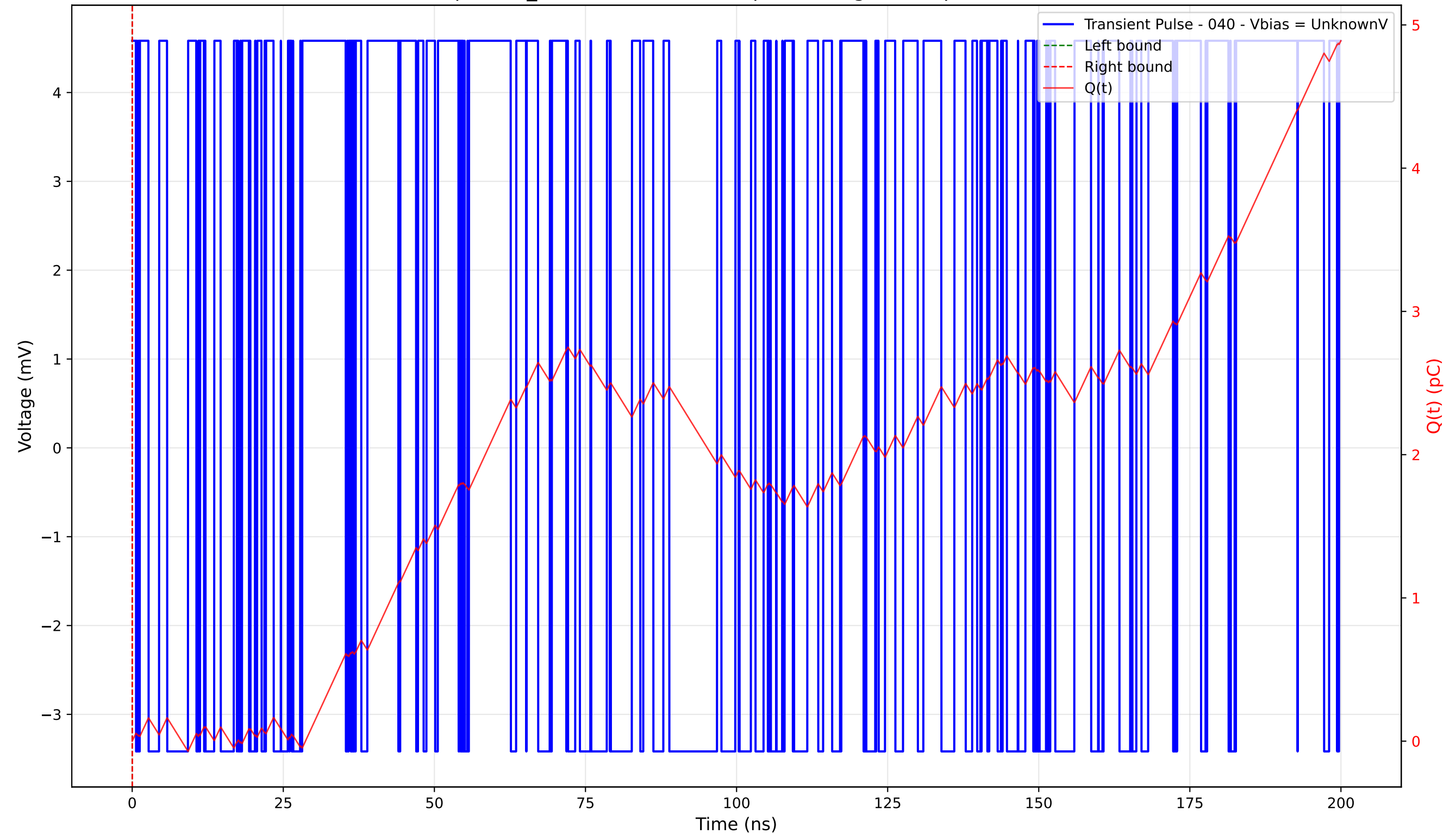
Transient Pulse - Sample: TD_4004 - Position: 50.0 \mu\text{m} - Charge: 0.00 pC - Rise Time: 0.00 ns (N/A)
