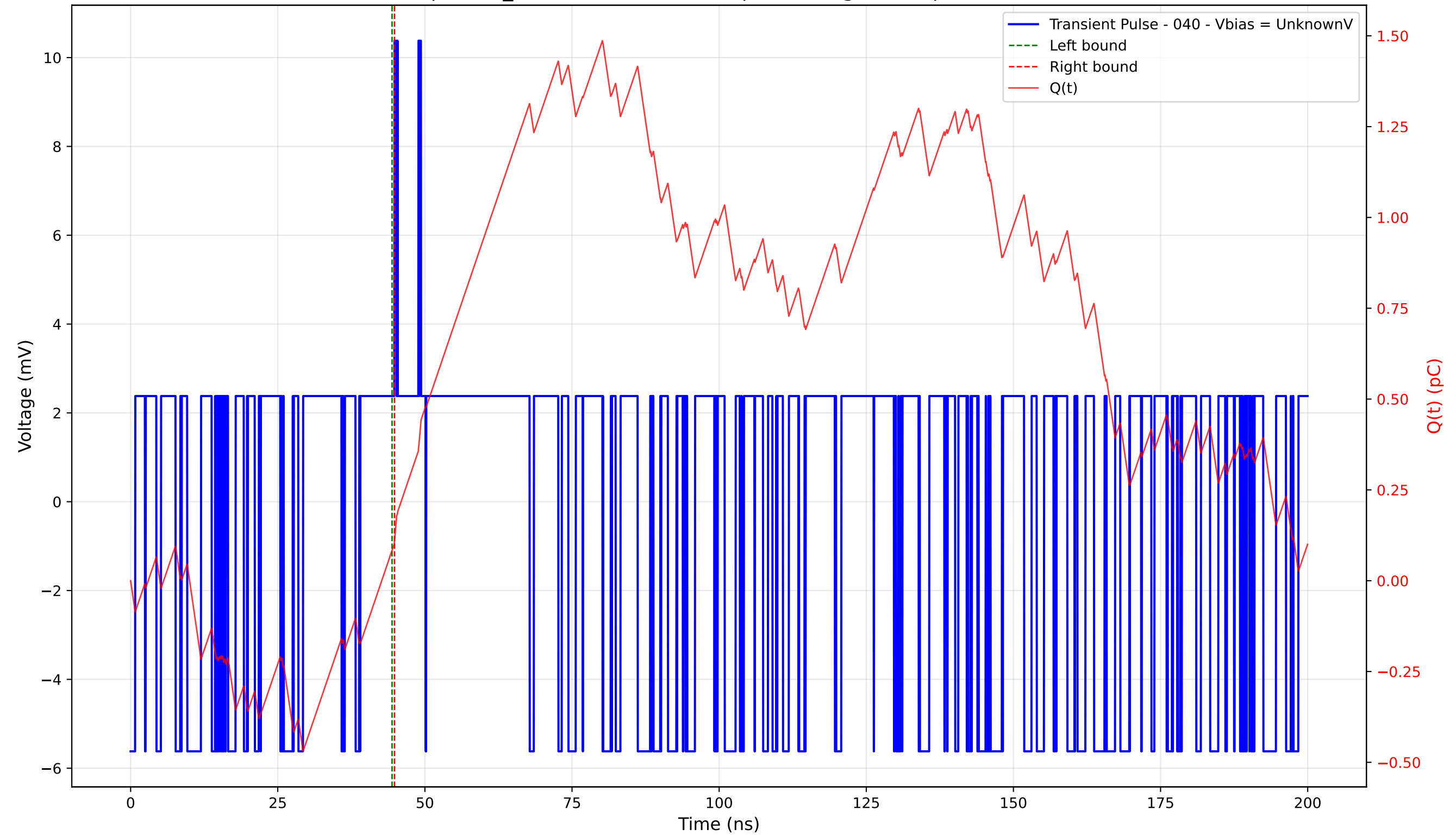
Transient Pulse - Sample: TD_4004 - Position: 370.0 \mu\text{m} - Charge: 0.02 pC - Rise Time: 0.00 ns (N/A)
