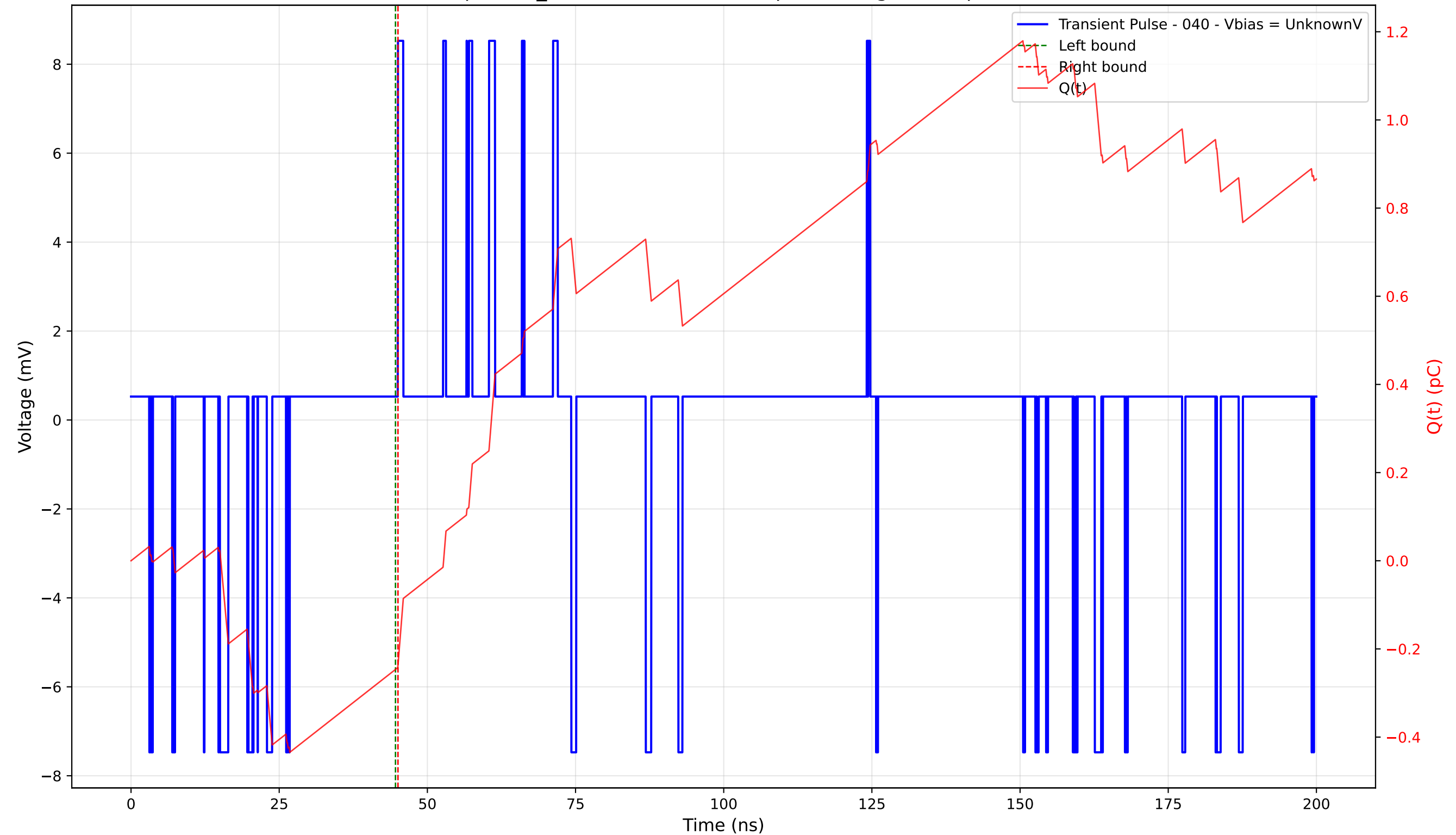
Transient Pulse - Sample: TD_4004 - Position: 375.0 \mu\text{m} - Charge: 0.01 pC - Rise Time: 0.02 ns
