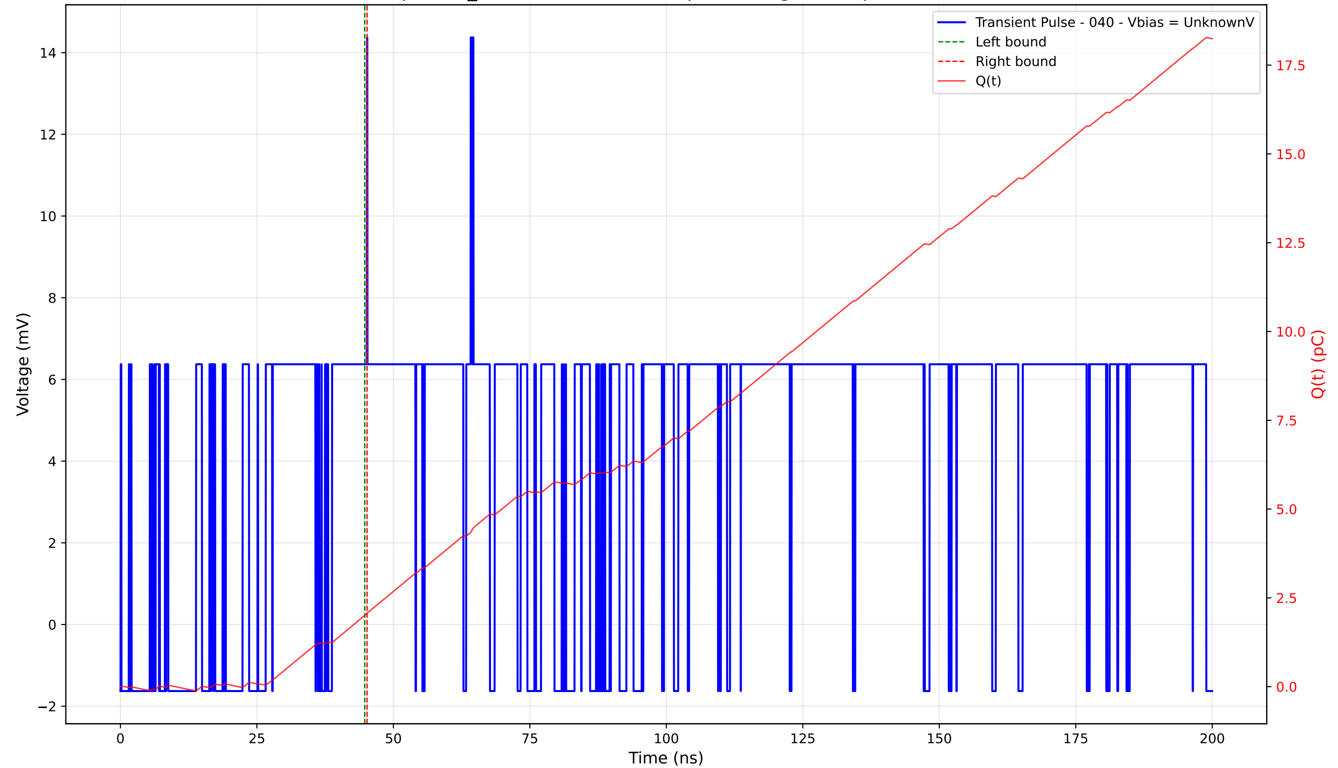
Transient Pulse - Sample: TD_4004 - Position: 330.0 \mu\text{m} - Charge: 0.06 pC - Rise Time: 0.00 ns (N/A)
