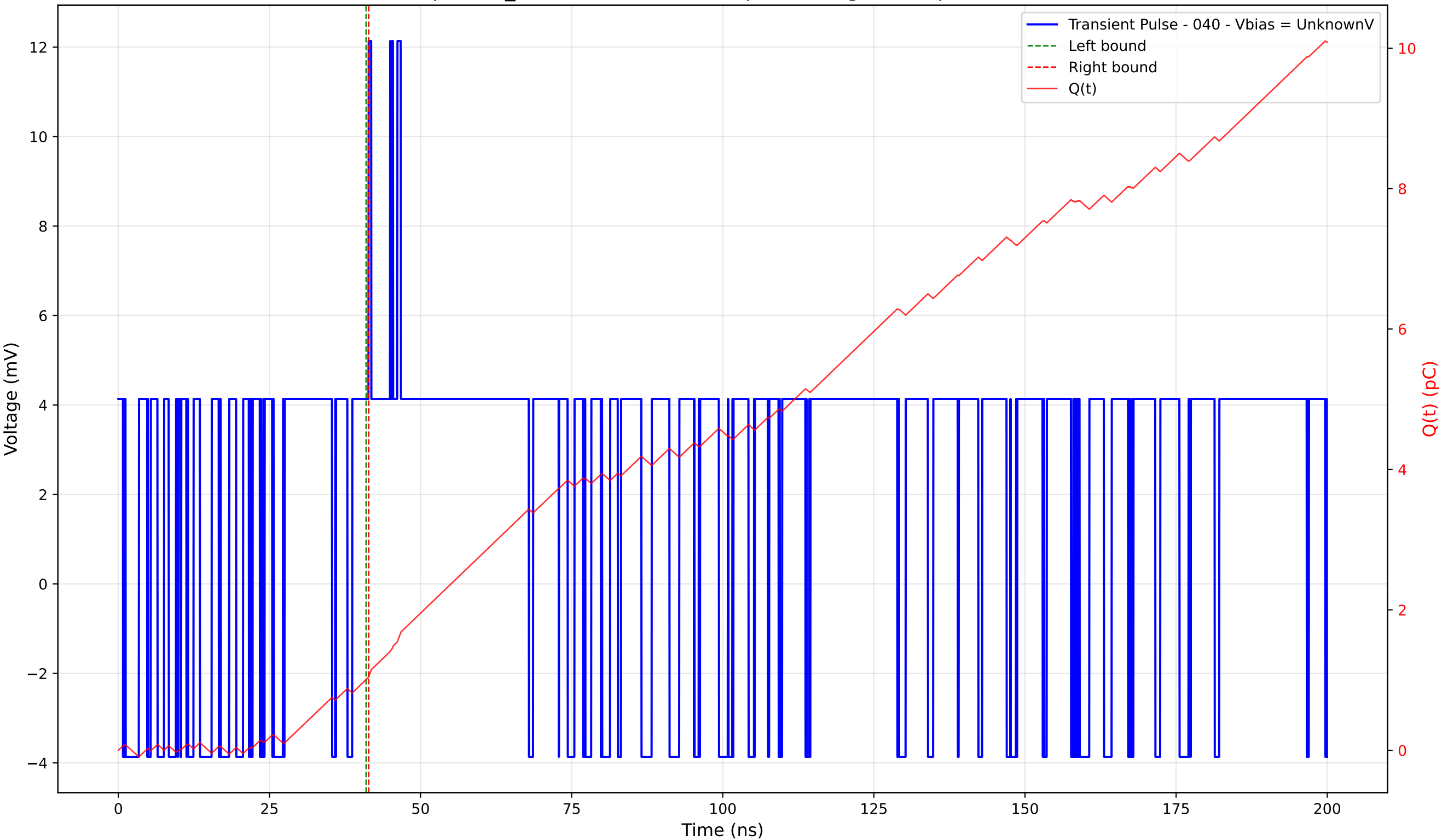
Transient Pulse - Sample: TD_4004 - Position: 365.0 \mu\text{m} - Charge: 0.04 pC - Rise Time: 0.00 ns (N/A)
