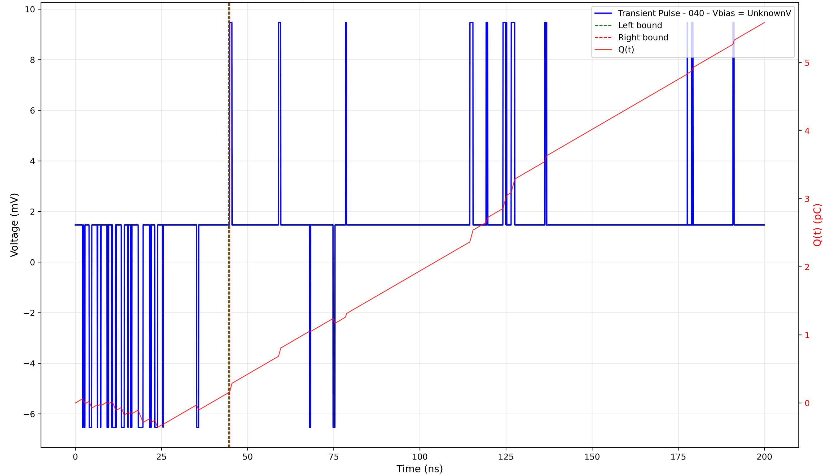
Transient Pulse - Sample: TD_4004 - Position: 205.0 \mu\text{m} - Charge: 0.02 pC - Rise Time: 0.00 ns (N/A)
