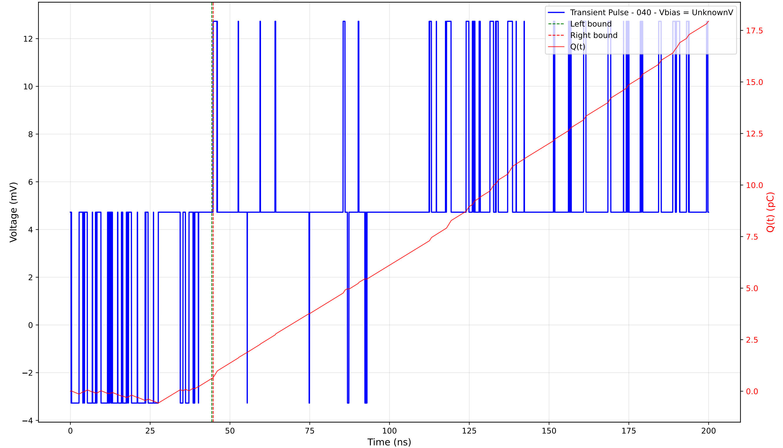
Transient Pulse - Sample: TD_4004 - Position: 190.0 \mu\text{m} - Charge: 0.04 pC - Rise Time: 0.00 ns (N/A)
