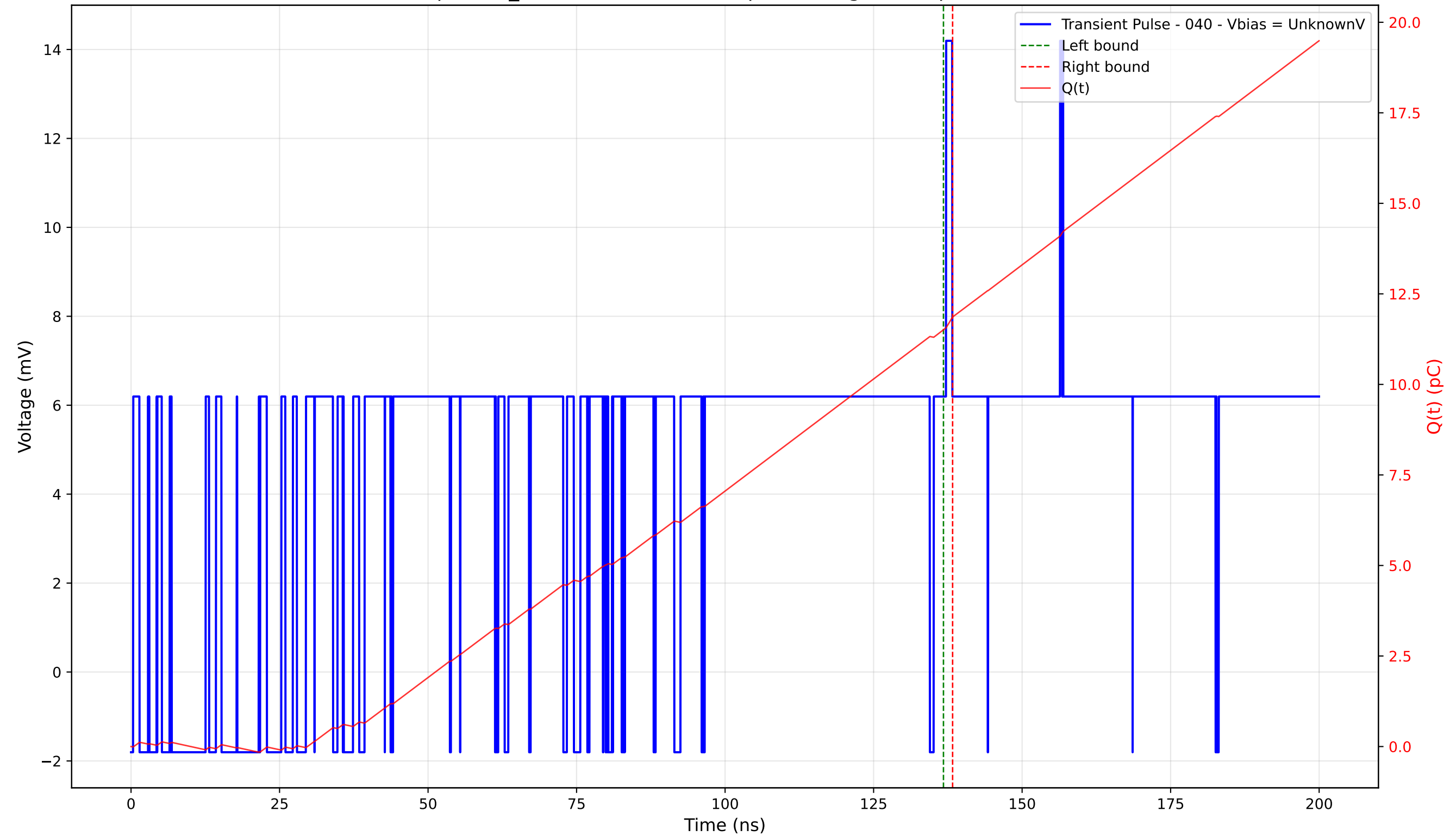
Transient Pulse - Sample: TD_4004 - Position: 255.0 \mu\text{m} - Charge: 0.36 pC - Rise Time: 0.00 ns (N/A)
