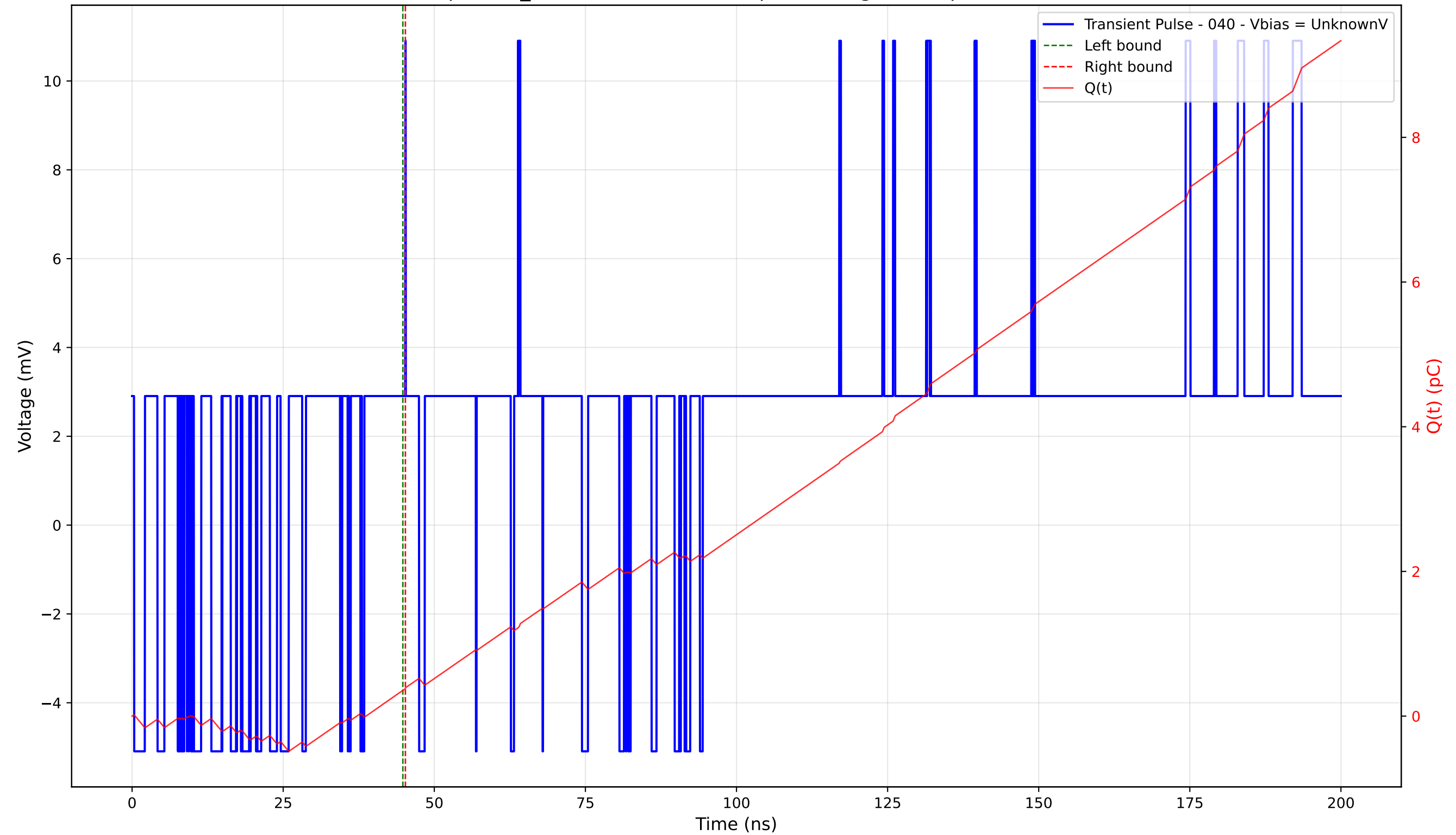
Transient Pulse - Sample: TD_4004 - Position: 165.0 \mu\text{m} - Charge: 0.03 pC - Rise Time: 0.00 ns (N/A)
