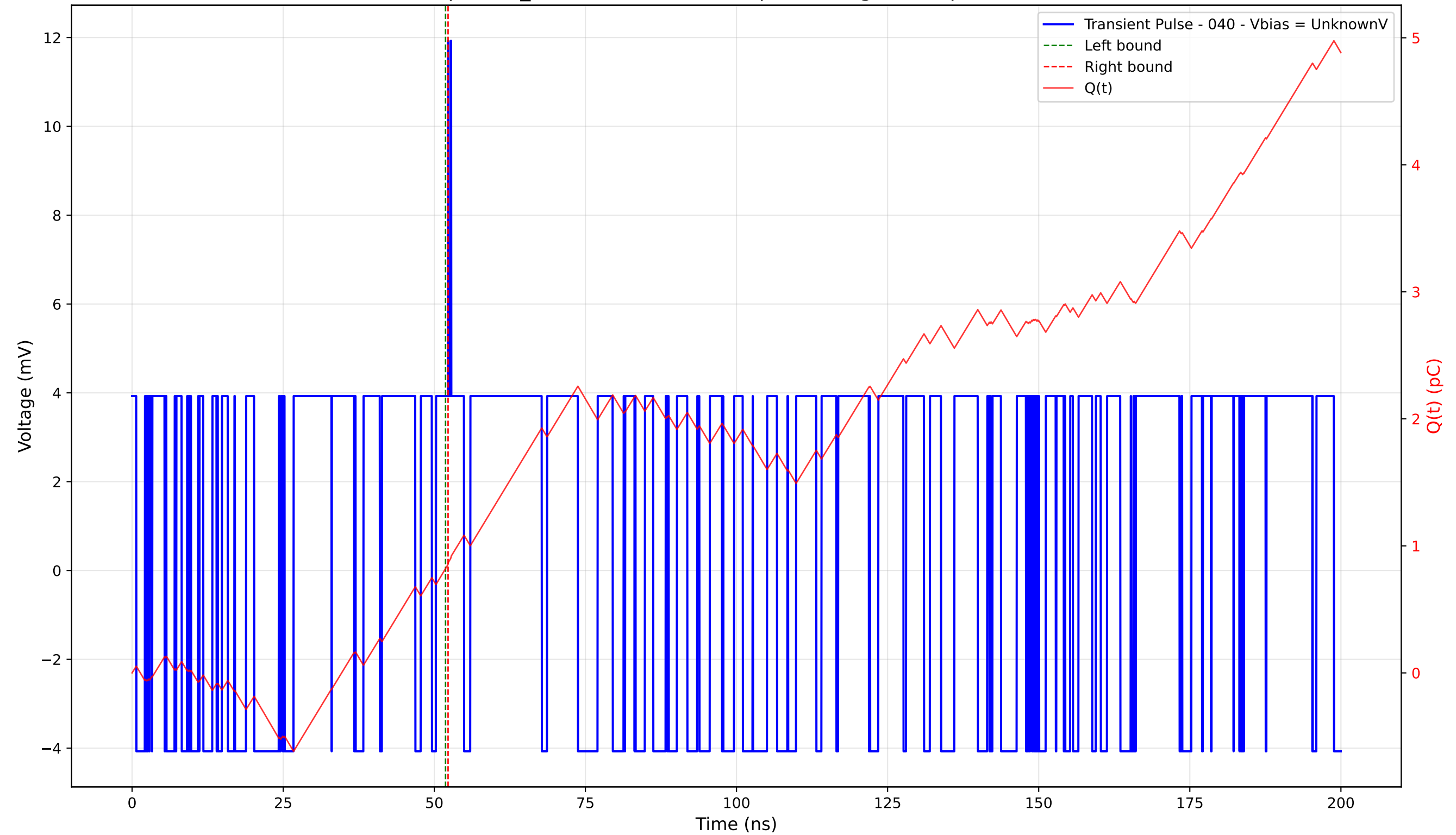
Transient Pulse - Sample: TD_4004 - Position: 345.0 \mu\text{m} - Charge: 0.04 pC - Rise Time: 0.00 ns (N/A)
