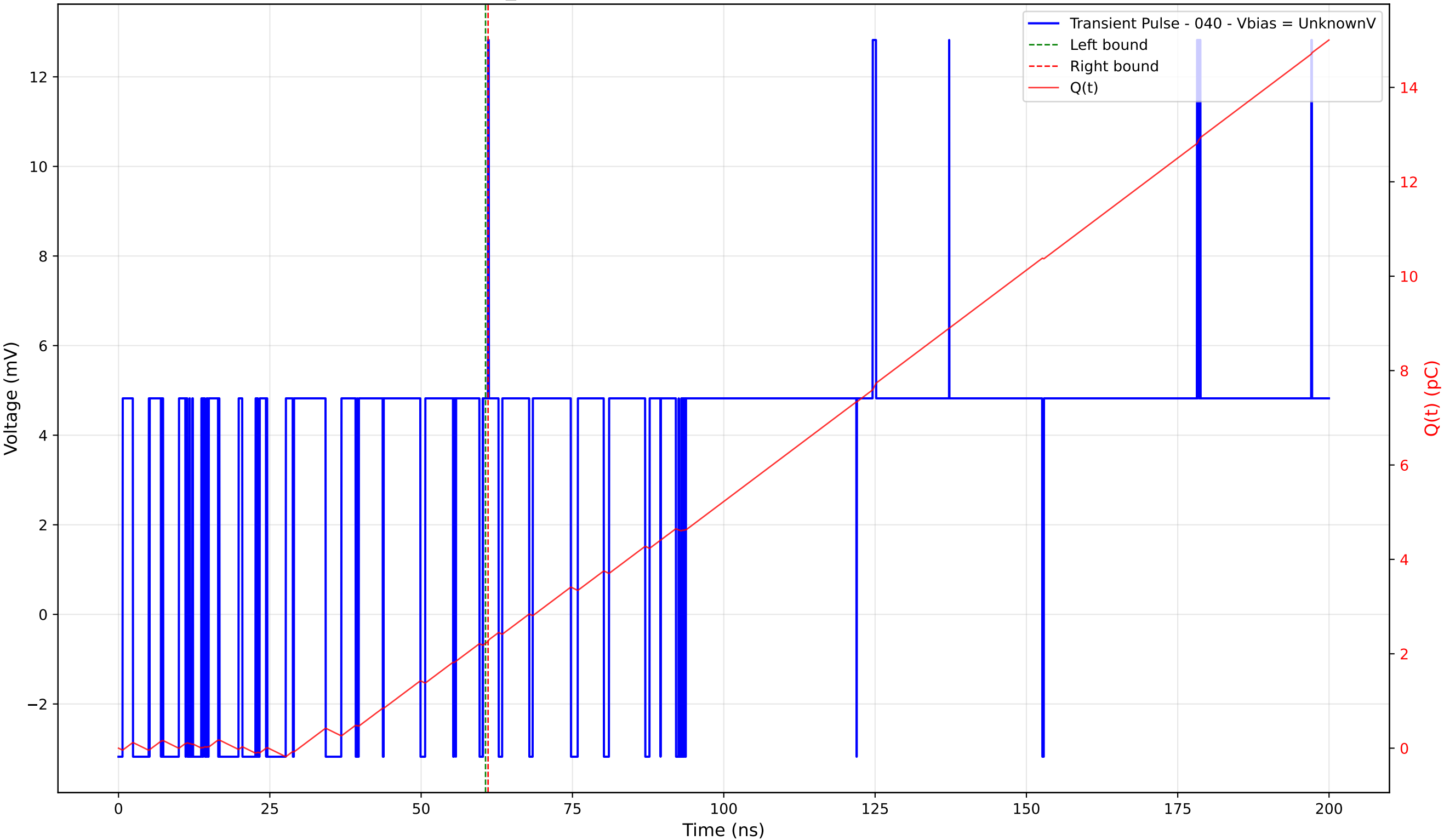
Transient Pulse - Sample: TD_4004 - Position: 180.0 \mu\text{m} - Charge: 0.05 pC - Rise Time: 0.00 ns (N/A)
