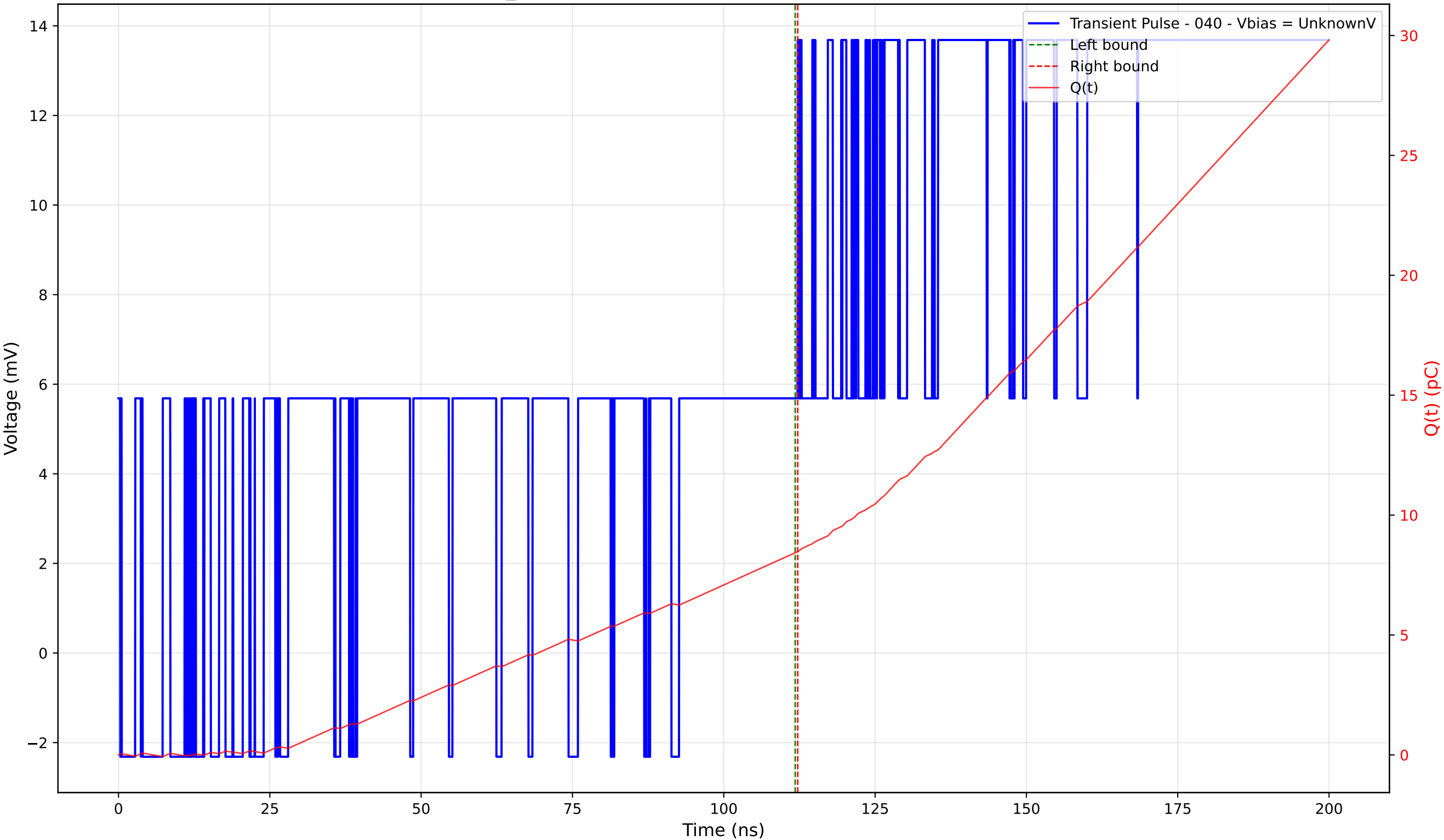
Transient Pulse - Sample: TD_4004 - Position: 100.0 \mu\text{m} - Charge: 0.05 pC - Rise Time: 0.00 ns (N/A)
