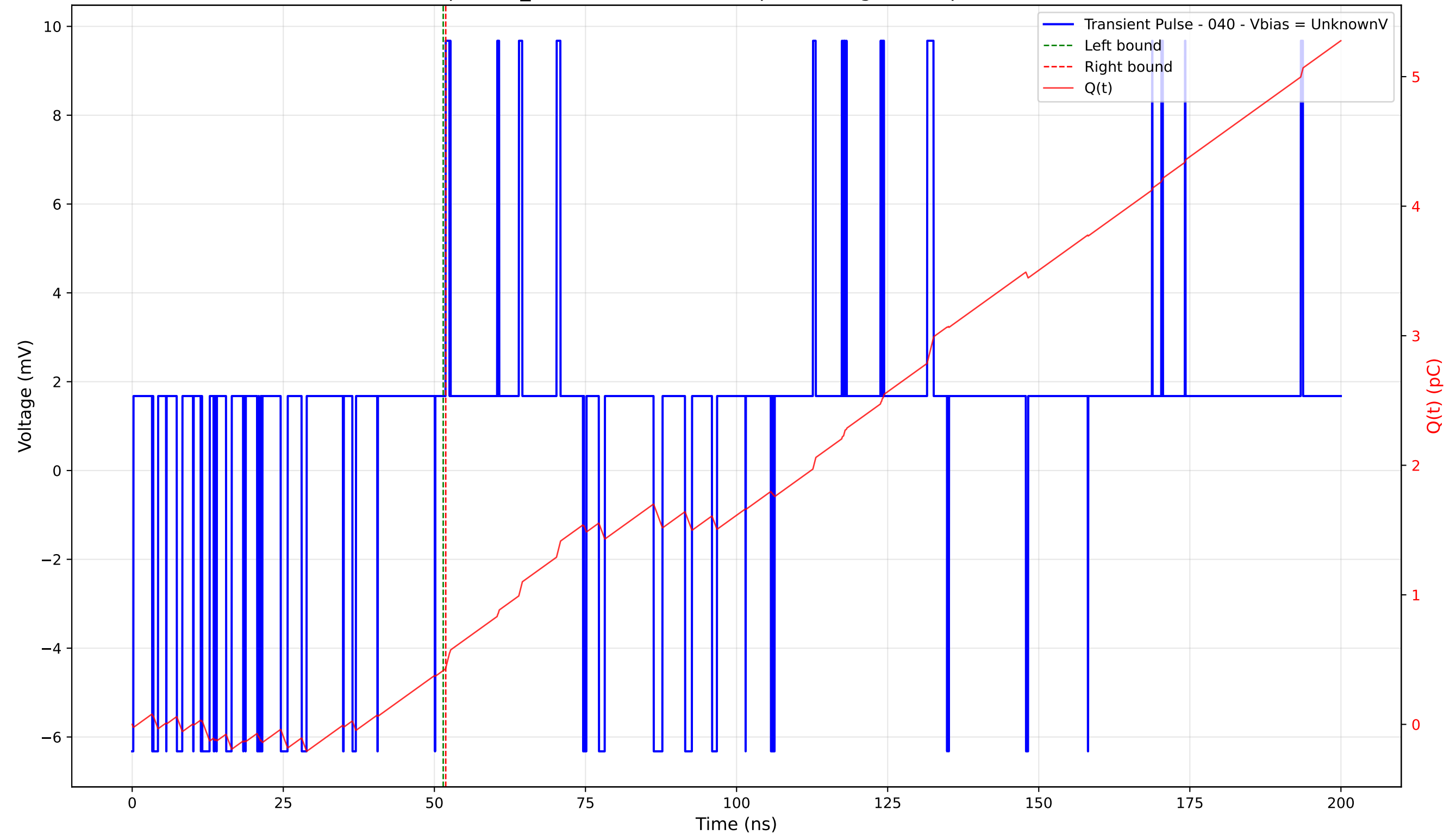
Transient Pulse - Sample: TD_4004 - Position: 270.0 \mu\text{m} - Charge: 0.02 pC - Rise Time: 0.00 ns (N/A)
