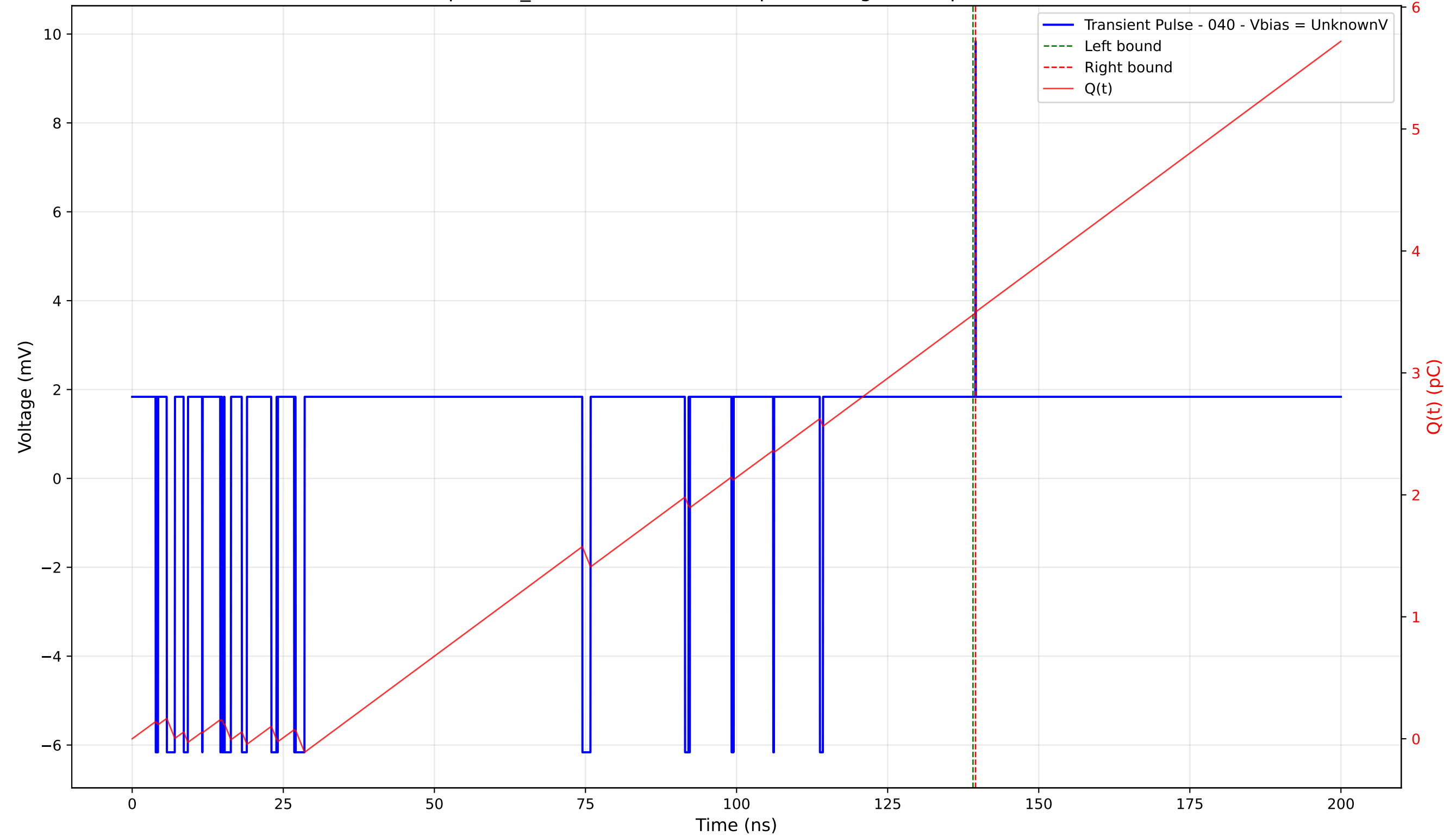
Transient Pulse - Sample: TD_4004 - Position: 150.0 \mu\text{m} - Charge: 0.02 pC - Rise Time: 0.00 ns (N/A)
