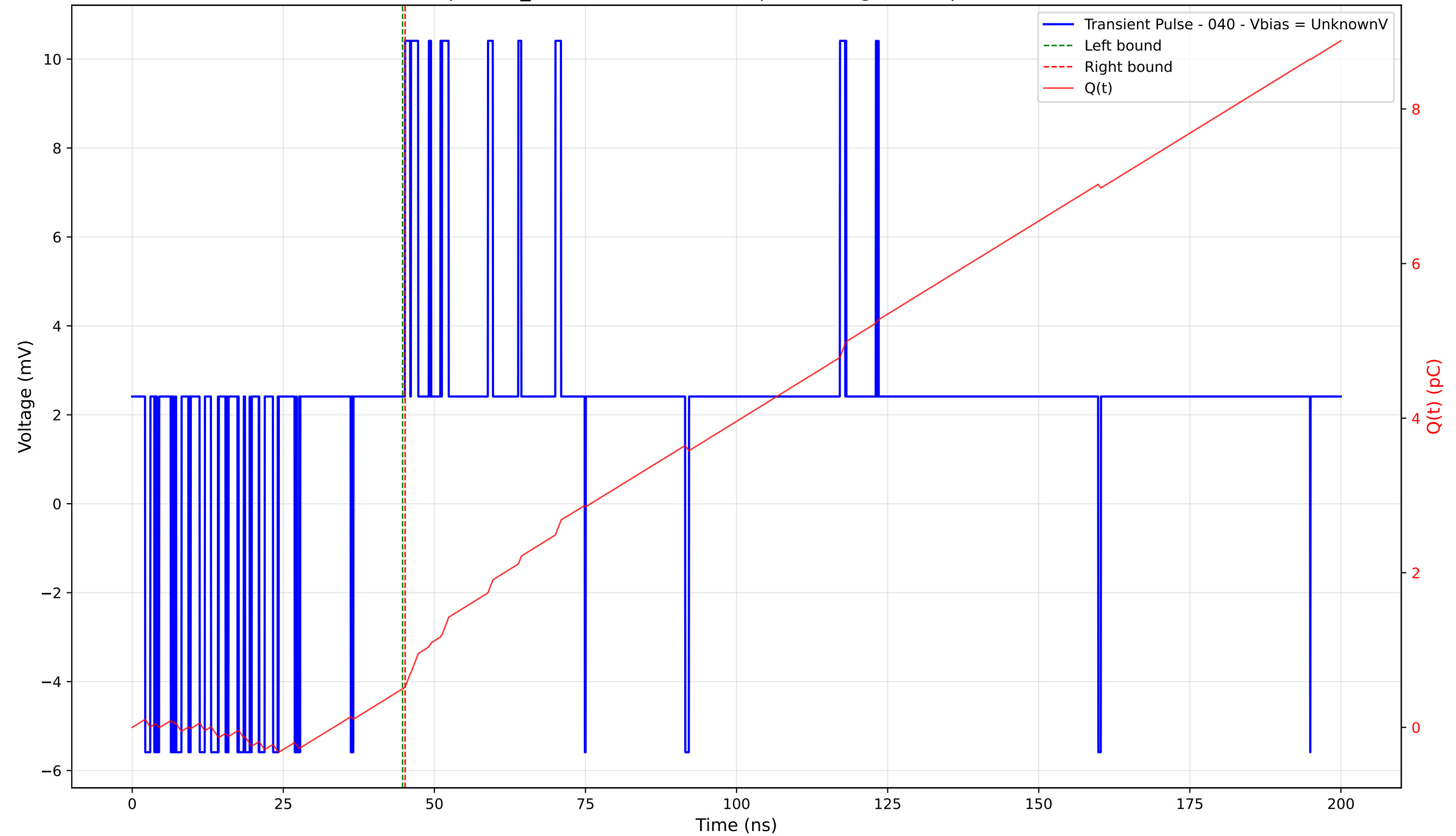
Transient Pulse - Sample: TD_4004 - Position: 385.0 \mu\text{m} - Charge: 0.03 pC - Rise Time: 0.00 ns (N/A)
