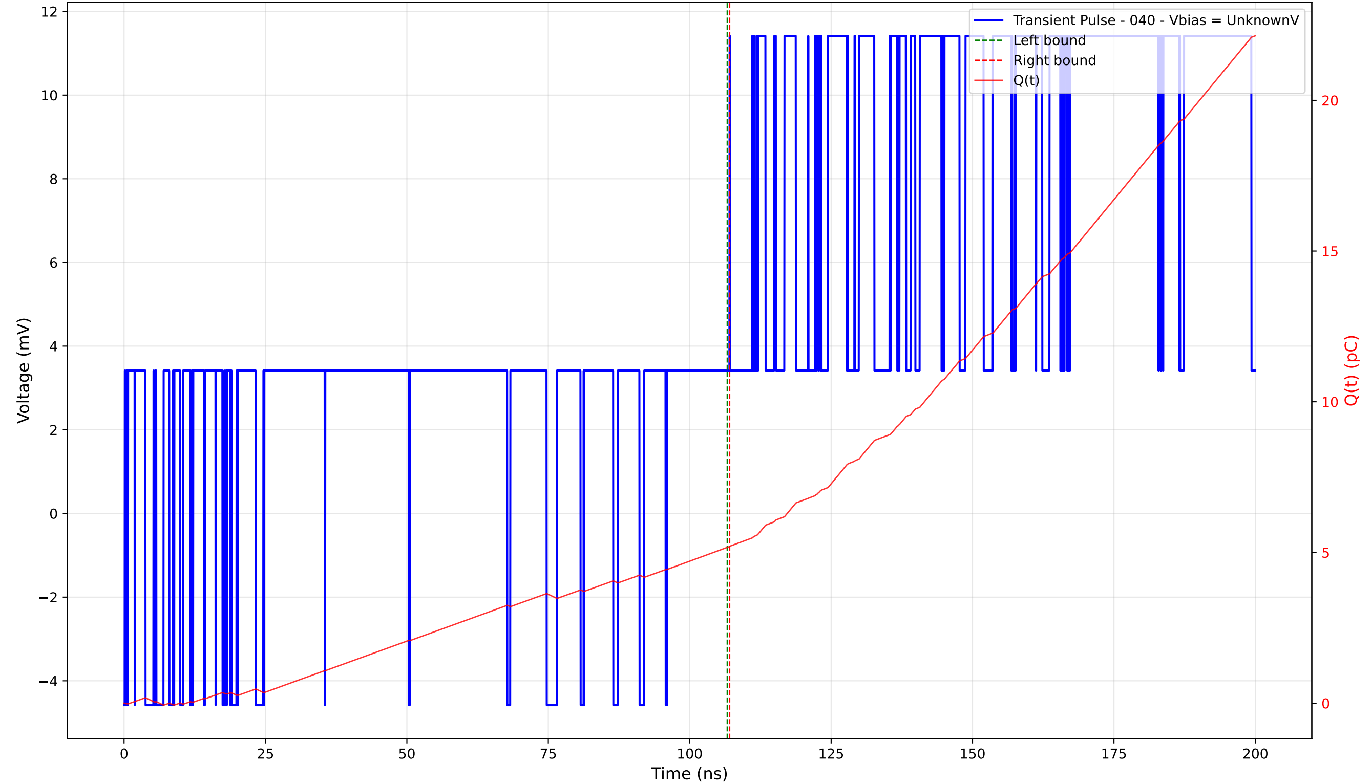
Transient Pulse - Sample: TD_4004 - Position: 105.0 \mu\text{m} - Charge: 0.03 pC - Rise Time: 0.00 ns (N/A)
