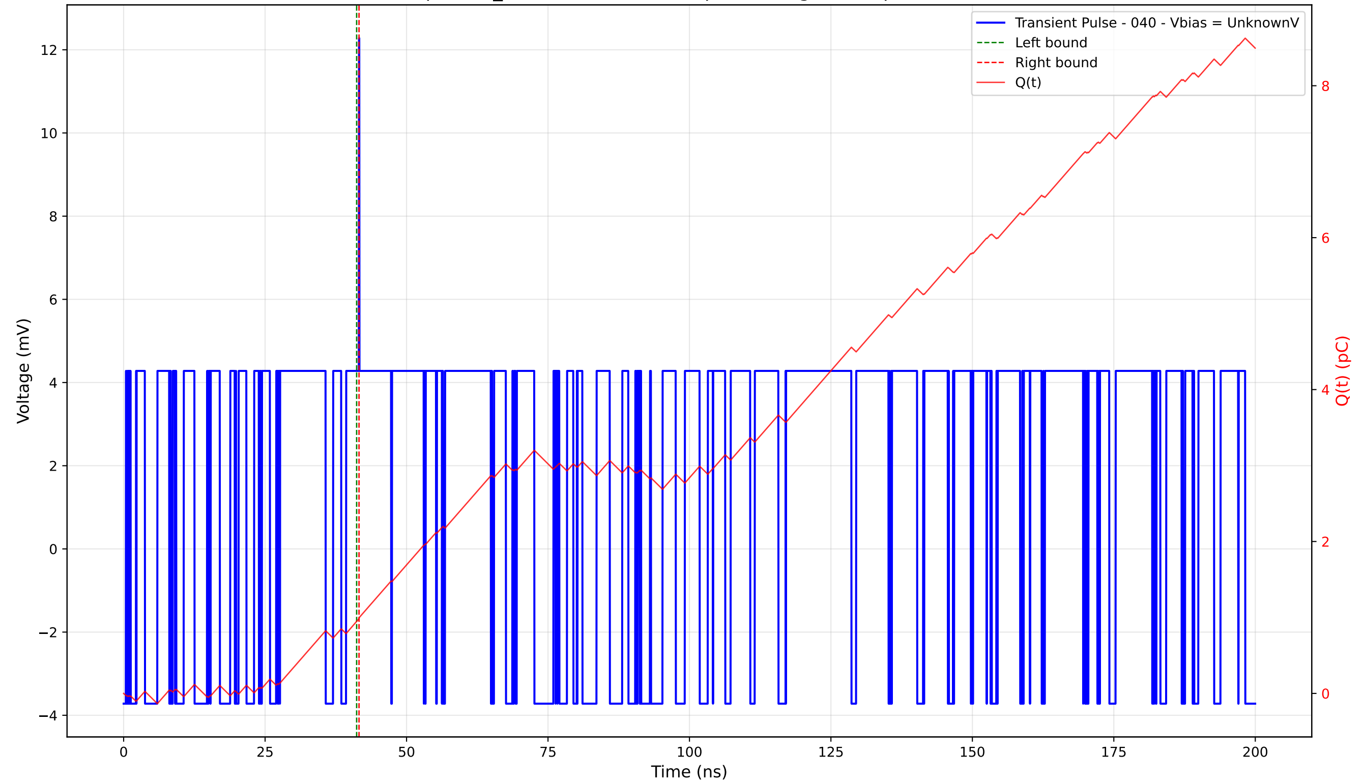
Transient Pulse - Sample: TD_4004 - Position: 45.0 \mu\text{m} - Charge: 0.04 pC - Rise Time: 0.00 ns (N/A)
