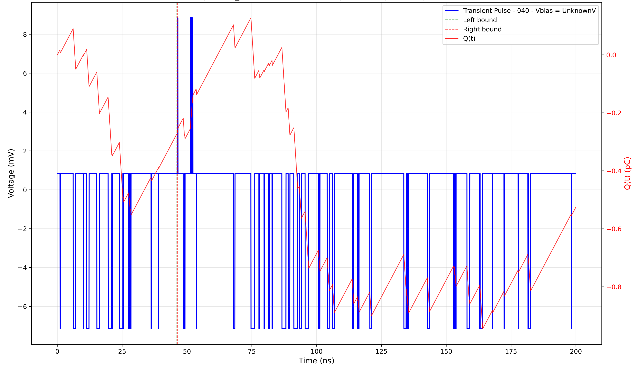
Transient Pulse - Sample: TD_4004 - Position: 325.0 \mu\text{m} - Charge: 0.01 pC - Rise Time: 0.02 ns
