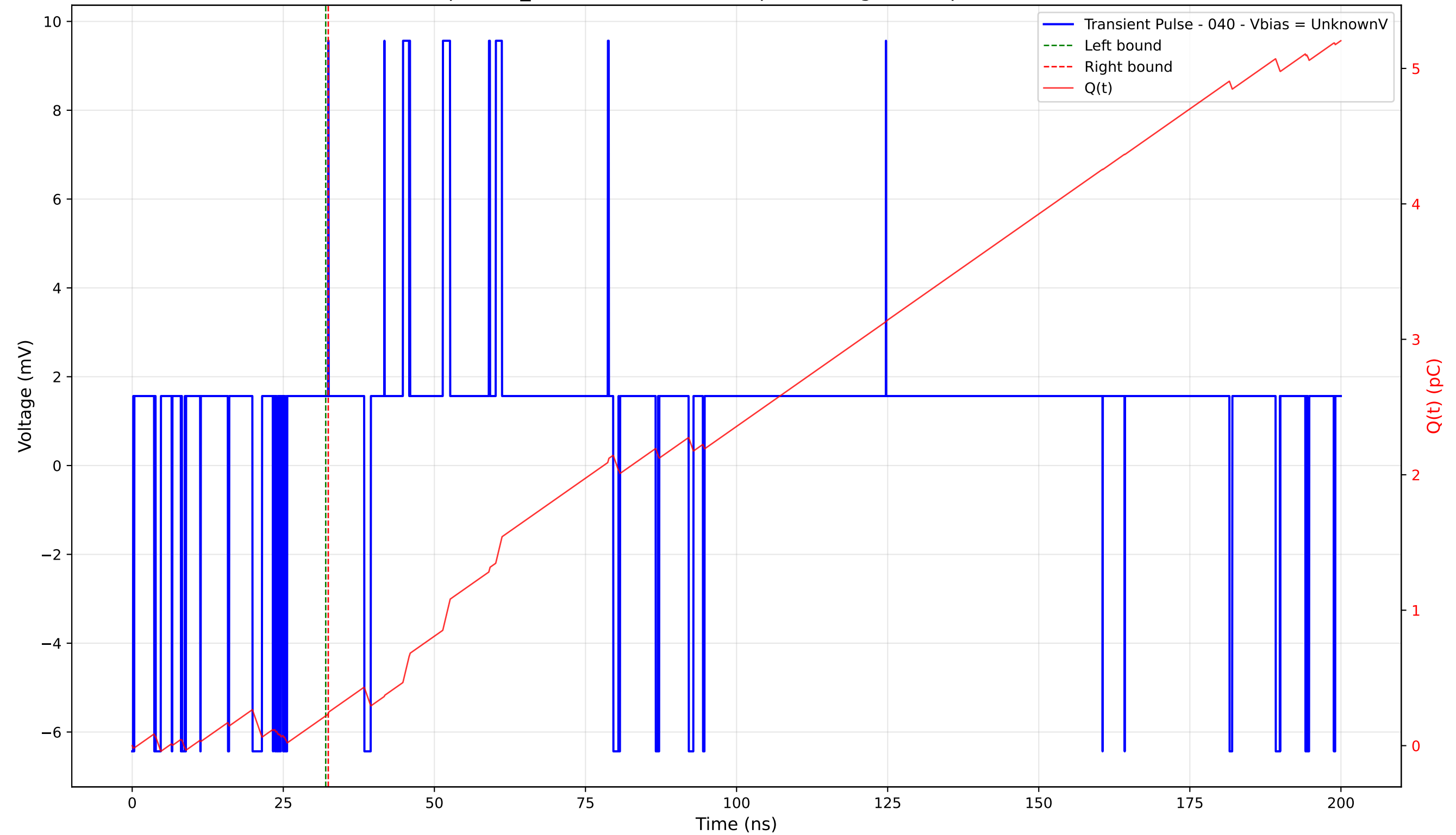
Transient Pulse - Sample: TD_4004 - Position: 315.0 \mu\text{m} - Charge: 0.02 pC - Rise Time: 0.00 ns (N/A)
