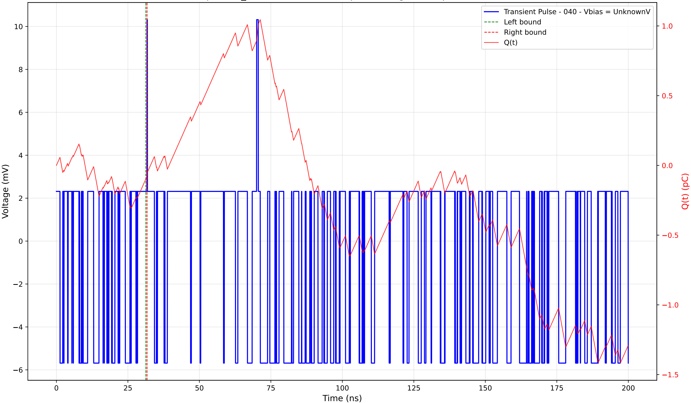
Transient Pulse - Sample: TD_4004 - Position: 40.0 \mu\text{m} - Charge: 0.02 pC - Rise Time: 0.00 ns (N/A)
