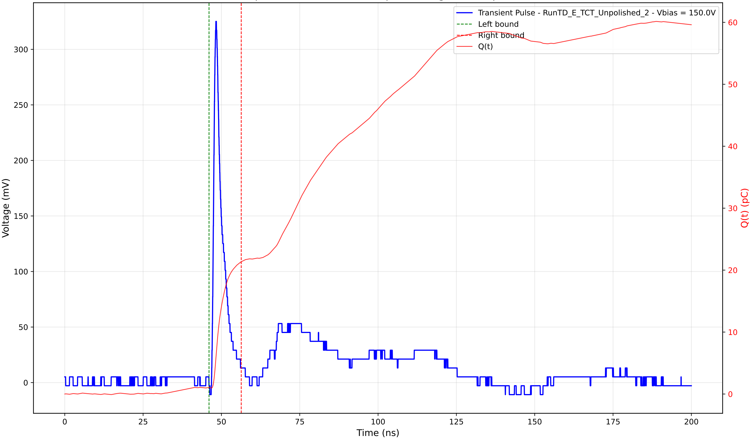
Transient Pulse - Sample: TD - Position: 135.0 \mu\text{m} - Charge: 20.28 pC - Rise Time: 0.91 ns
