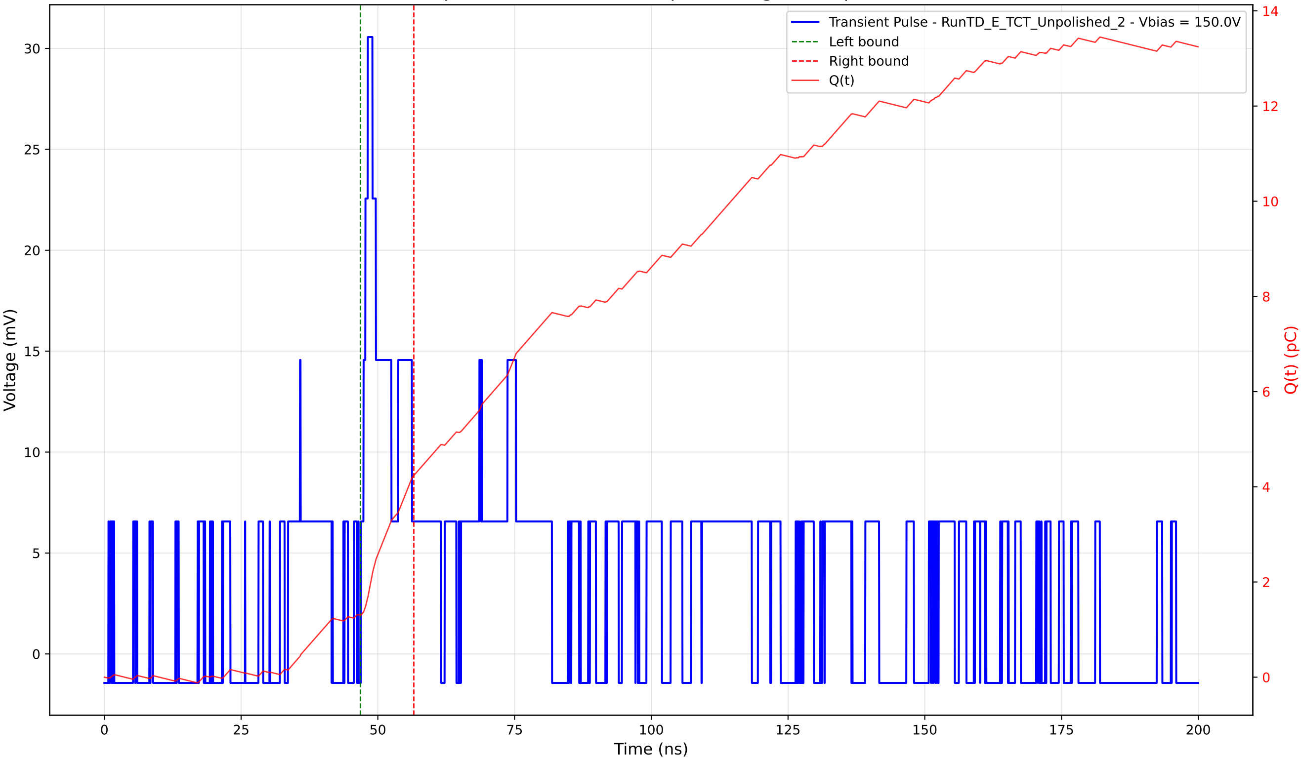
Transient Pulse - Sample: TD - Position: 365.0 \mu\text{m} - Charge: 2.93 pC - Rise Time: 1.27 ns
