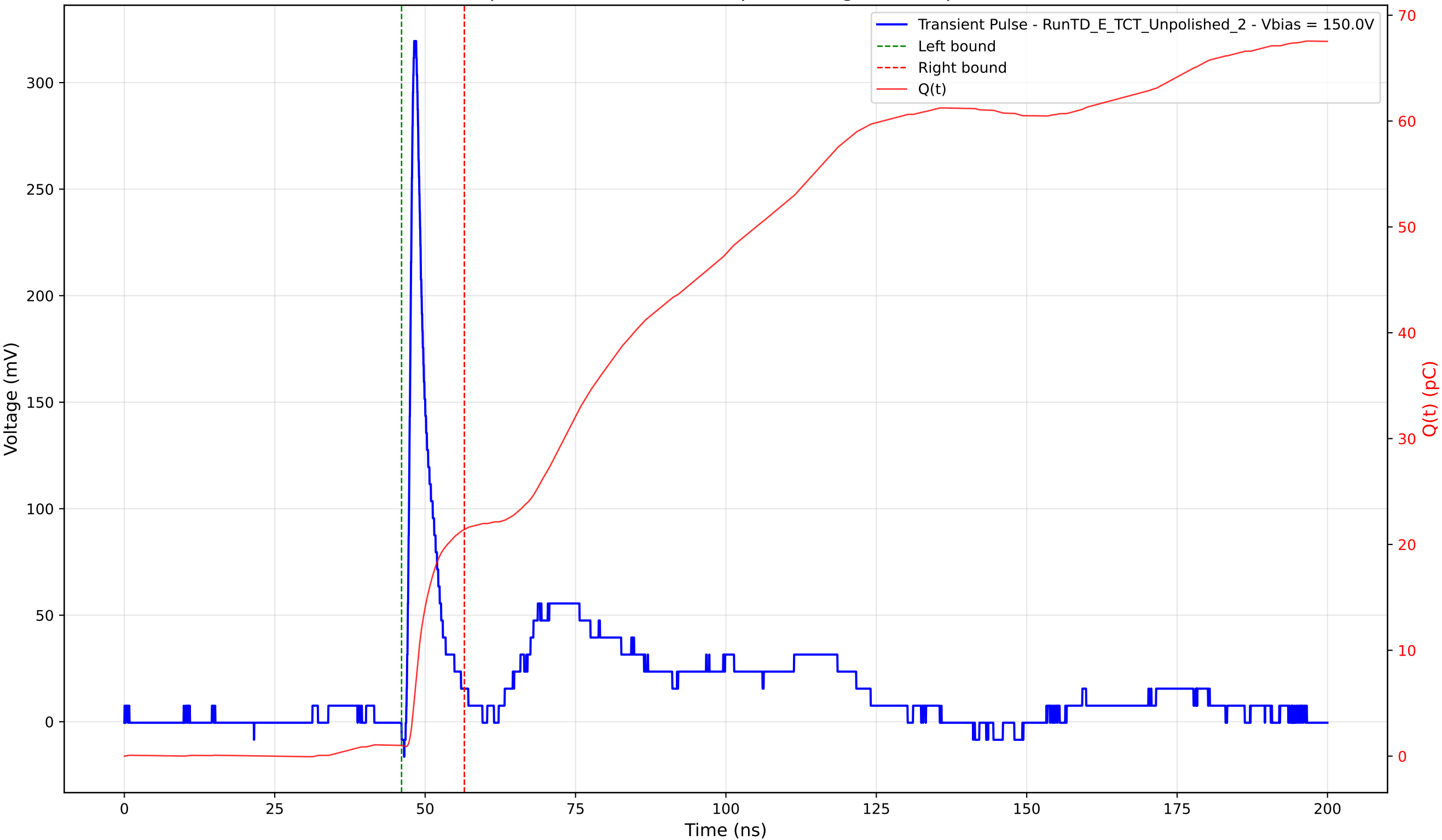
Transient Pulse - Sample: TD - Position: 130.0 \mu\text{m} - Charge: 20.39 pC - Rise Time: 0.92 ns
