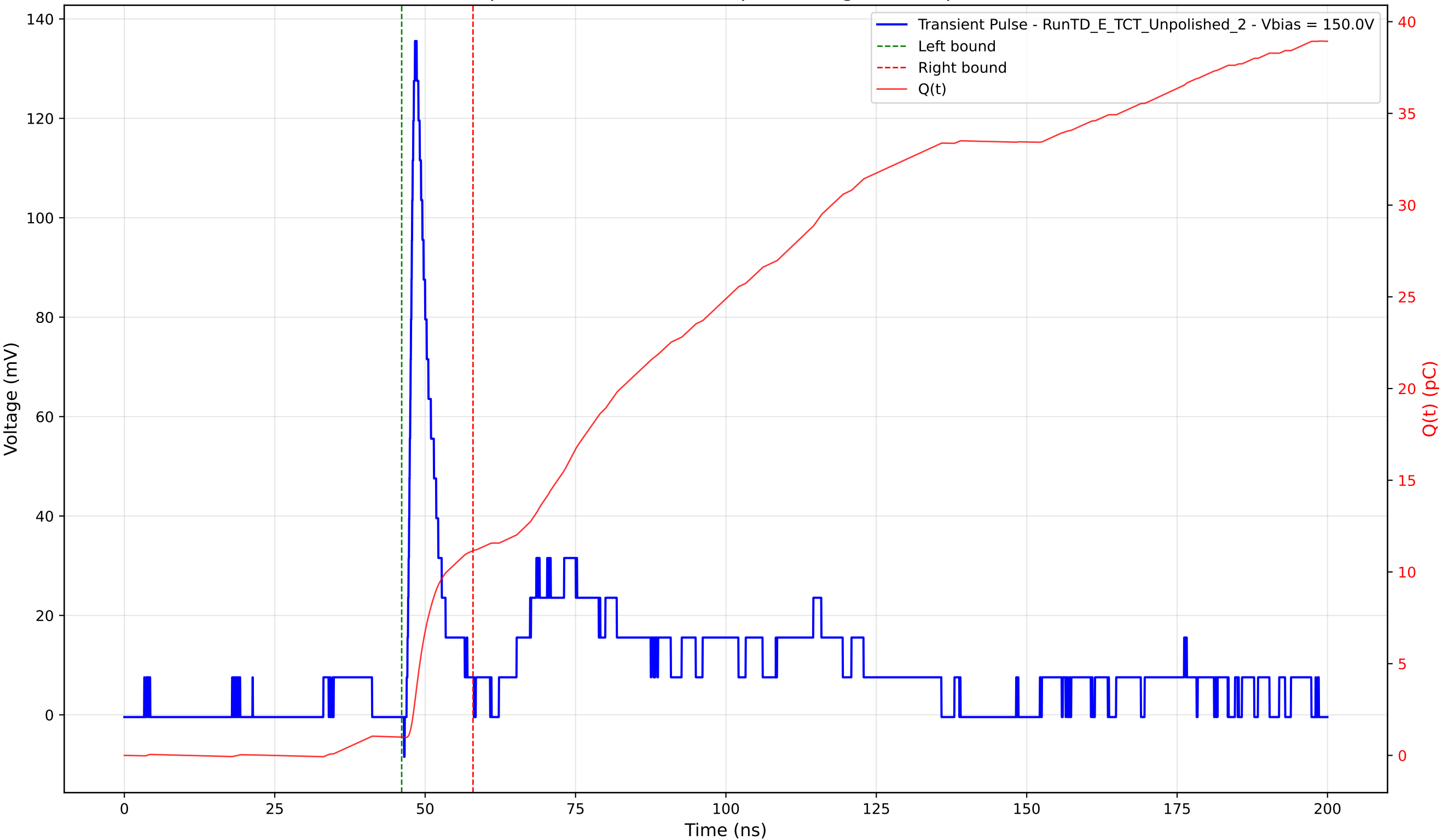
Transient Pulse - Sample: TD - Position: 245.0 \mu\text{m} - Charge: 10.16 pC - Rise Time: 1.06 ns
