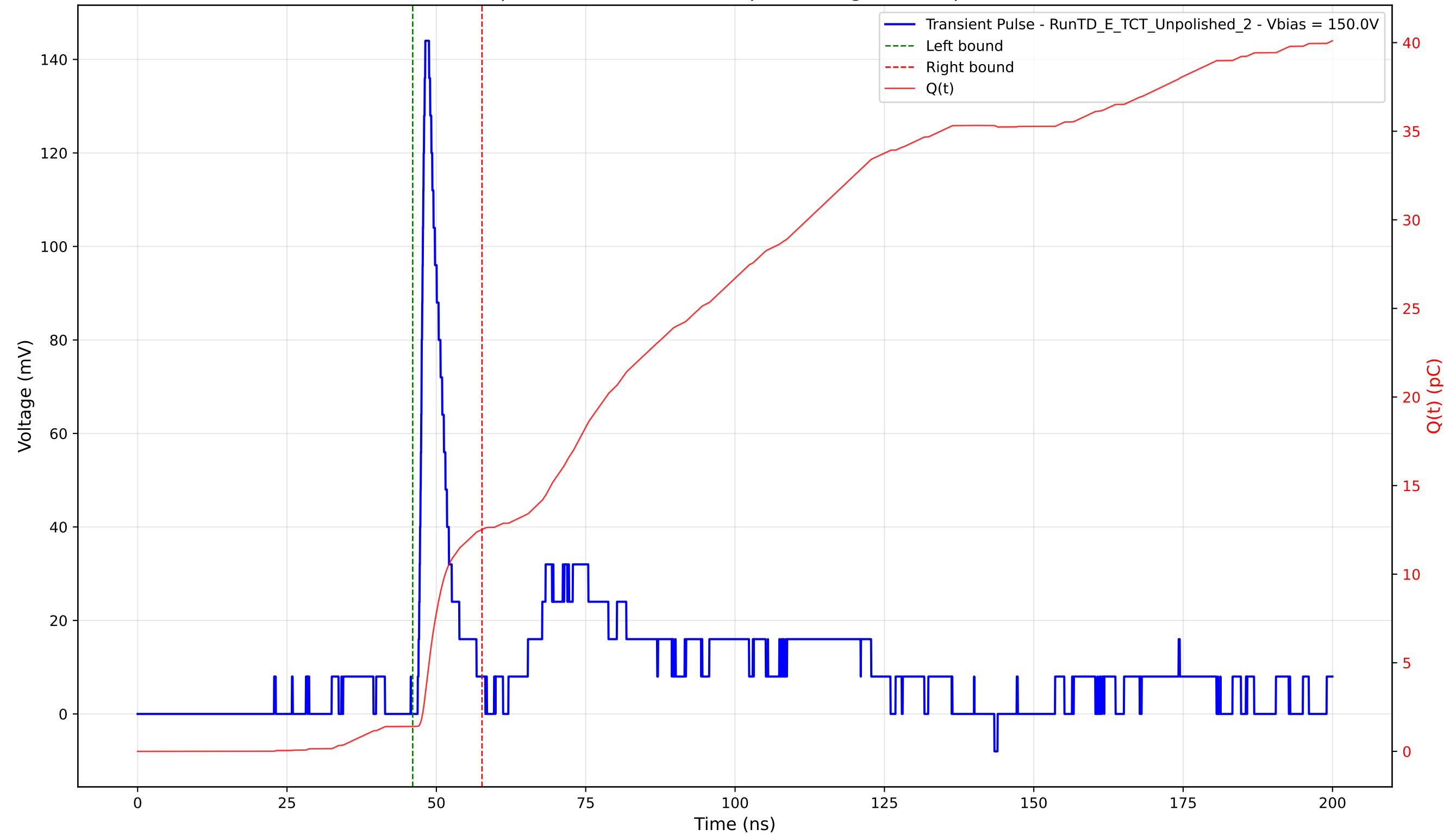
Transient Pulse - Sample: TD - Position: 280.0 \mu\text{m} - Charge: 11.12 pC - Rise Time: 1.02 ns
