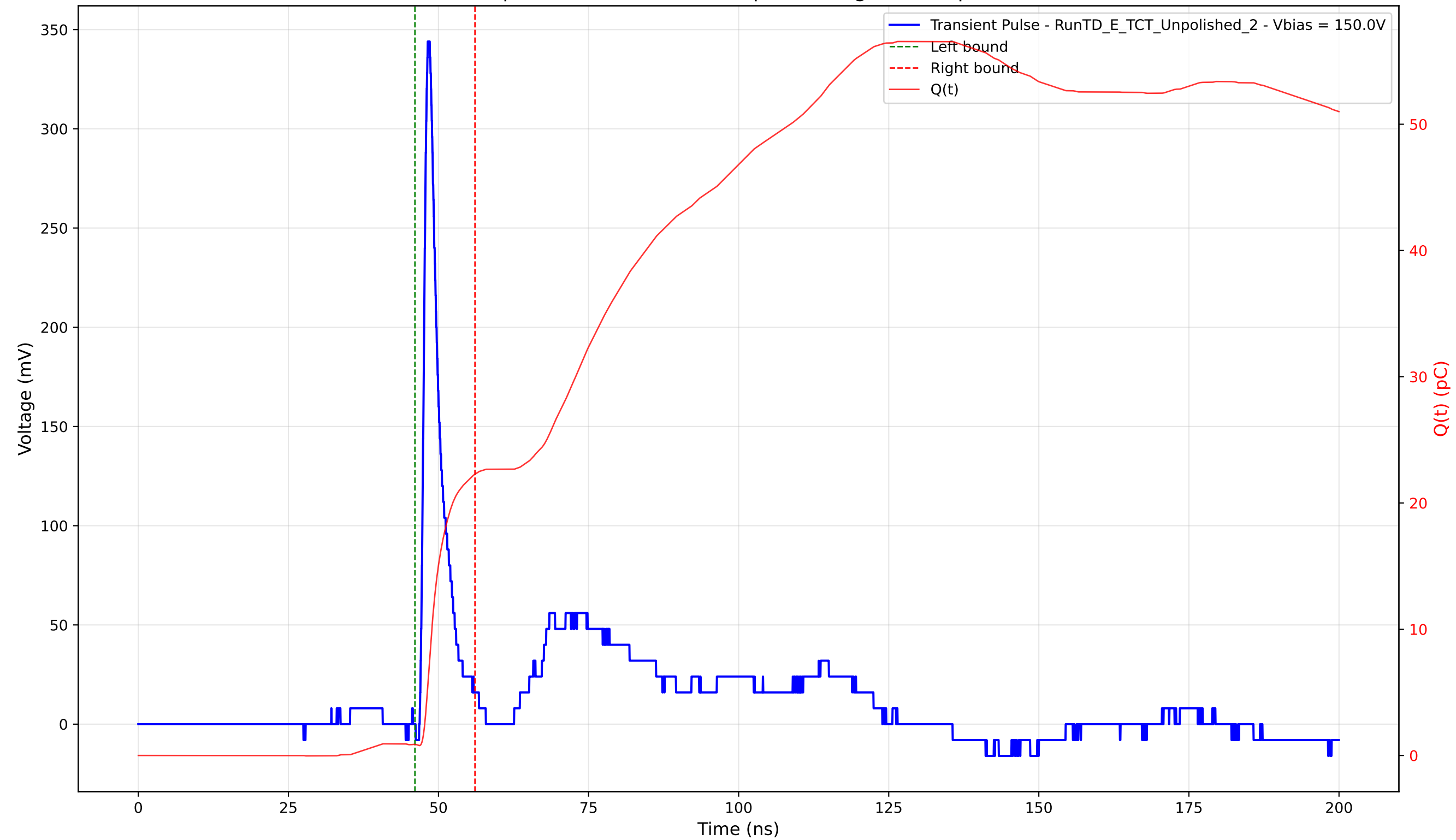
Transient Pulse - Sample: TD - Position: 165.0 \mu\text{m} - Charge: 21.40 pC - Rise Time: 0.93 ns
