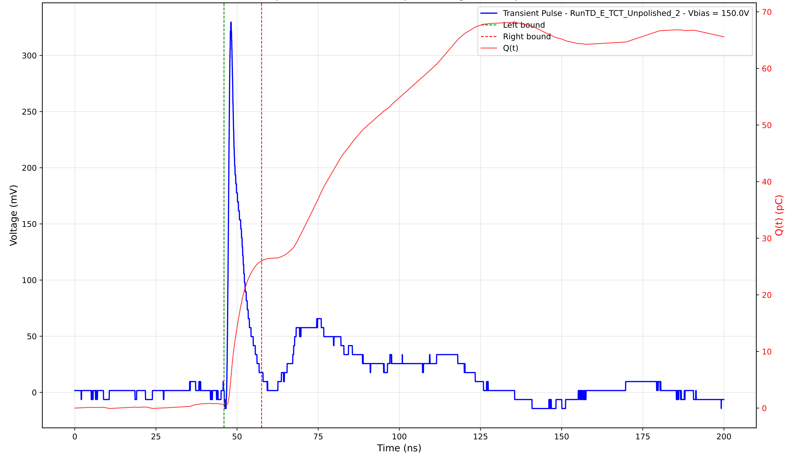
Transient Pulse - Sample: TD - Position: 75.0 \mu\text{m} - Charge: 25.28 pC - Rise Time: 0.84 ns
