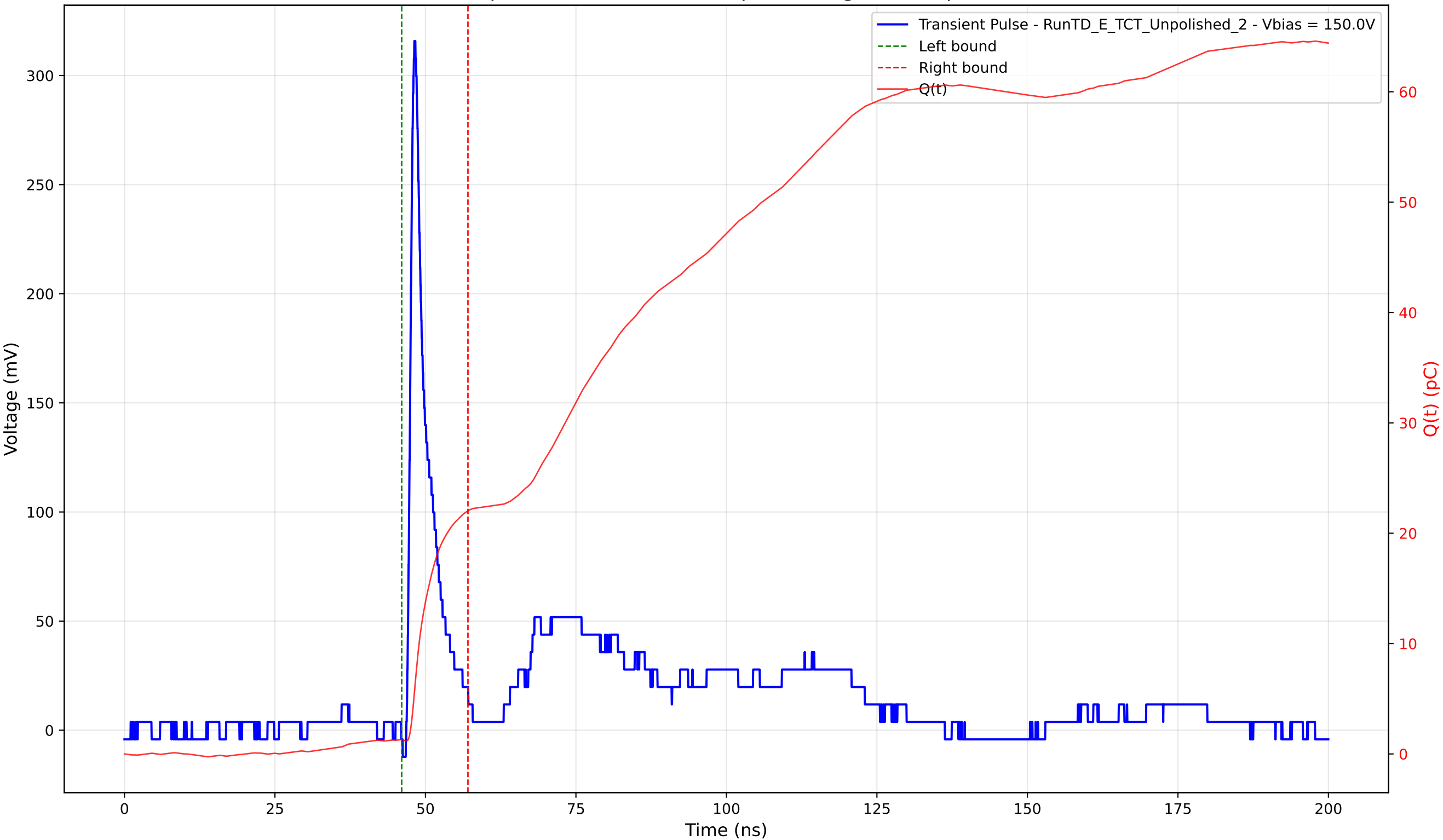
Transient Pulse - Sample: TD - Position: 100.0 \mu\text{m} - Charge: 20.74 pC - Rise Time: 0.91 ns
