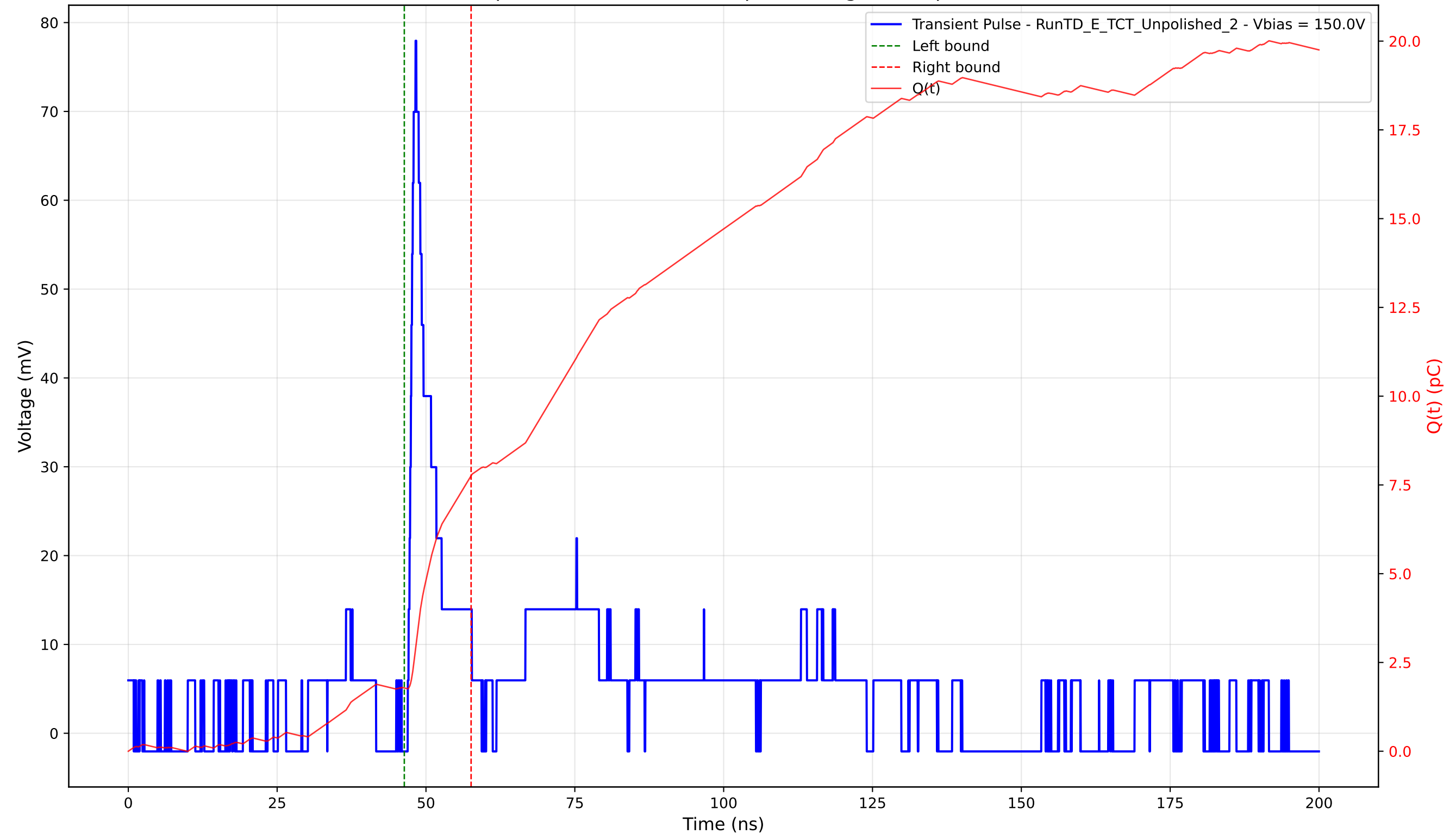
Transient Pulse - Sample: TD - Position: 375.0 \mu\text{m} - Charge: 5.99 pC - Rise Time: 1.18 ns
