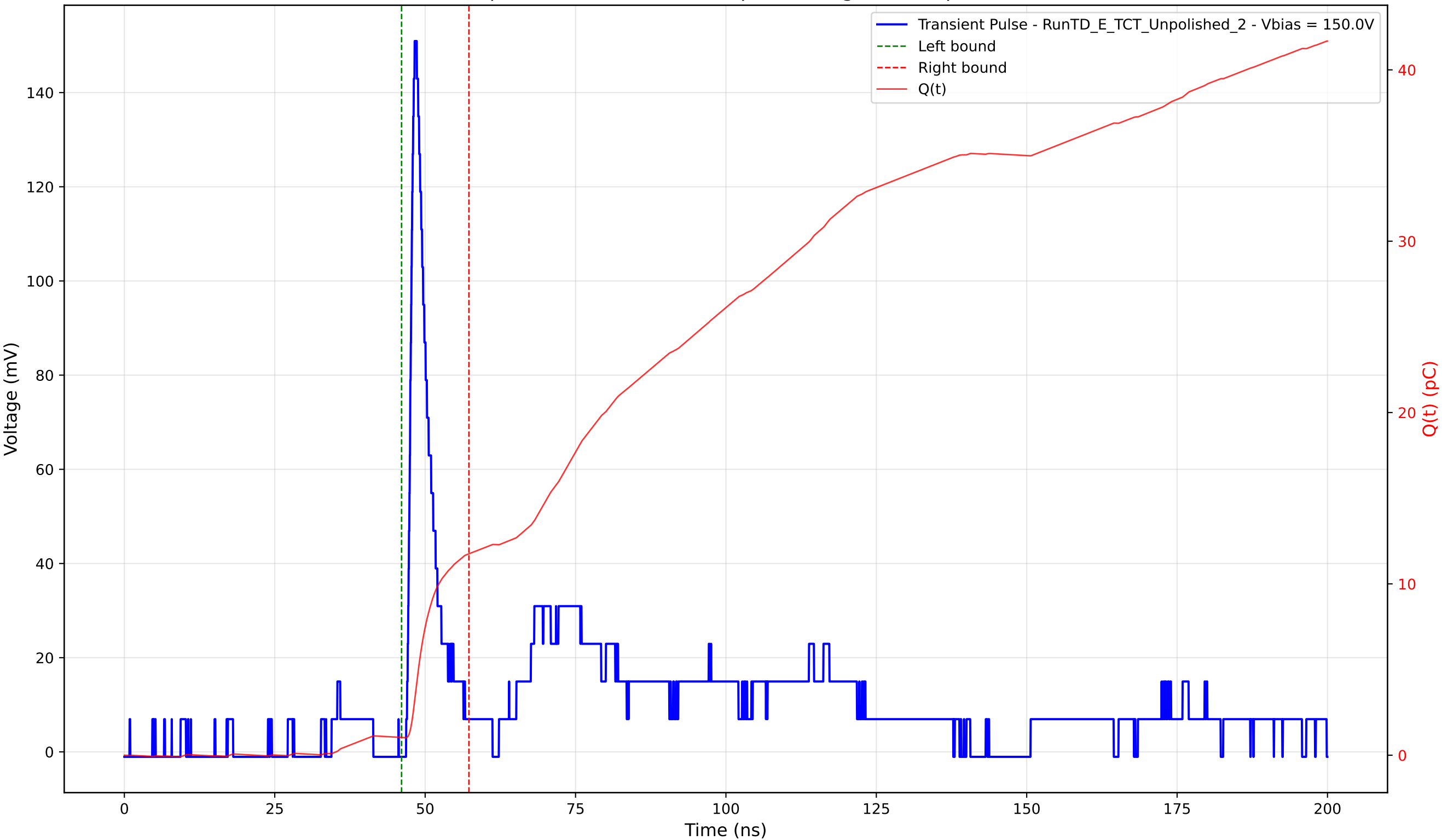
Transient Pulse - Sample: TD - Position: 255.0 \mu\text{m} - Charge: 10.72 pC - Rise Time: 1.02 ns
