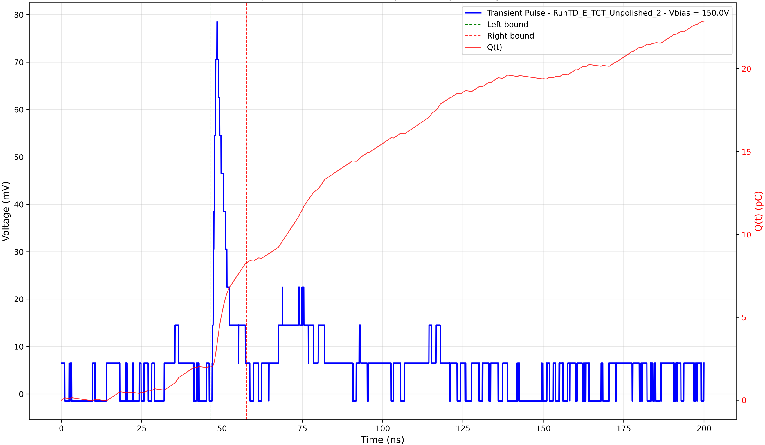
Transient Pulse - Sample: TD - Position: 325.0 \mu\text{m} - Charge: 6.22 pC - Rise Time: 1.32 ns
