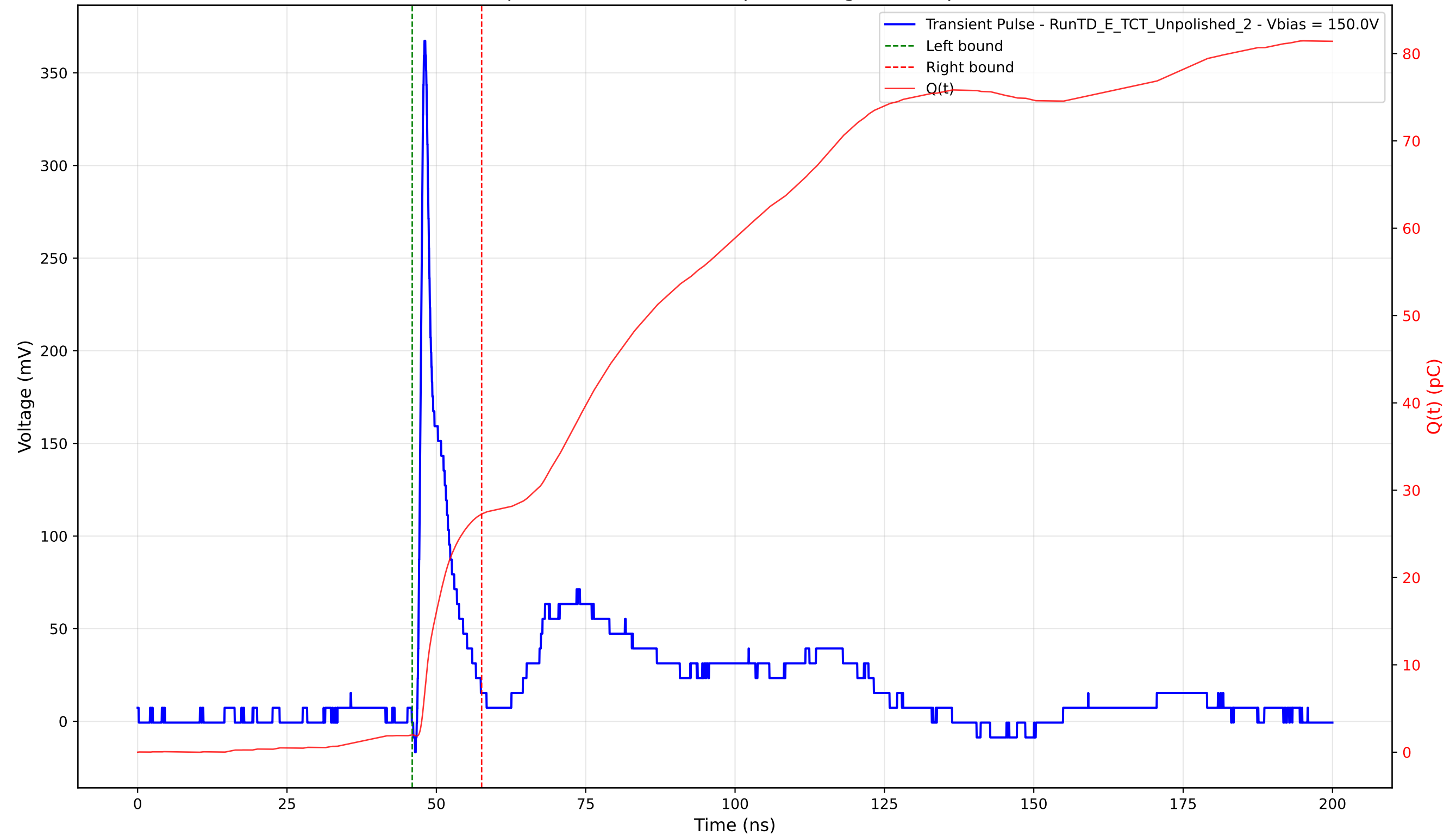
Transient Pulse - Sample: TD - Position: 45.0 \mu\text{m} - Charge: 25.29 pC - Rise Time: 0.85 ns
