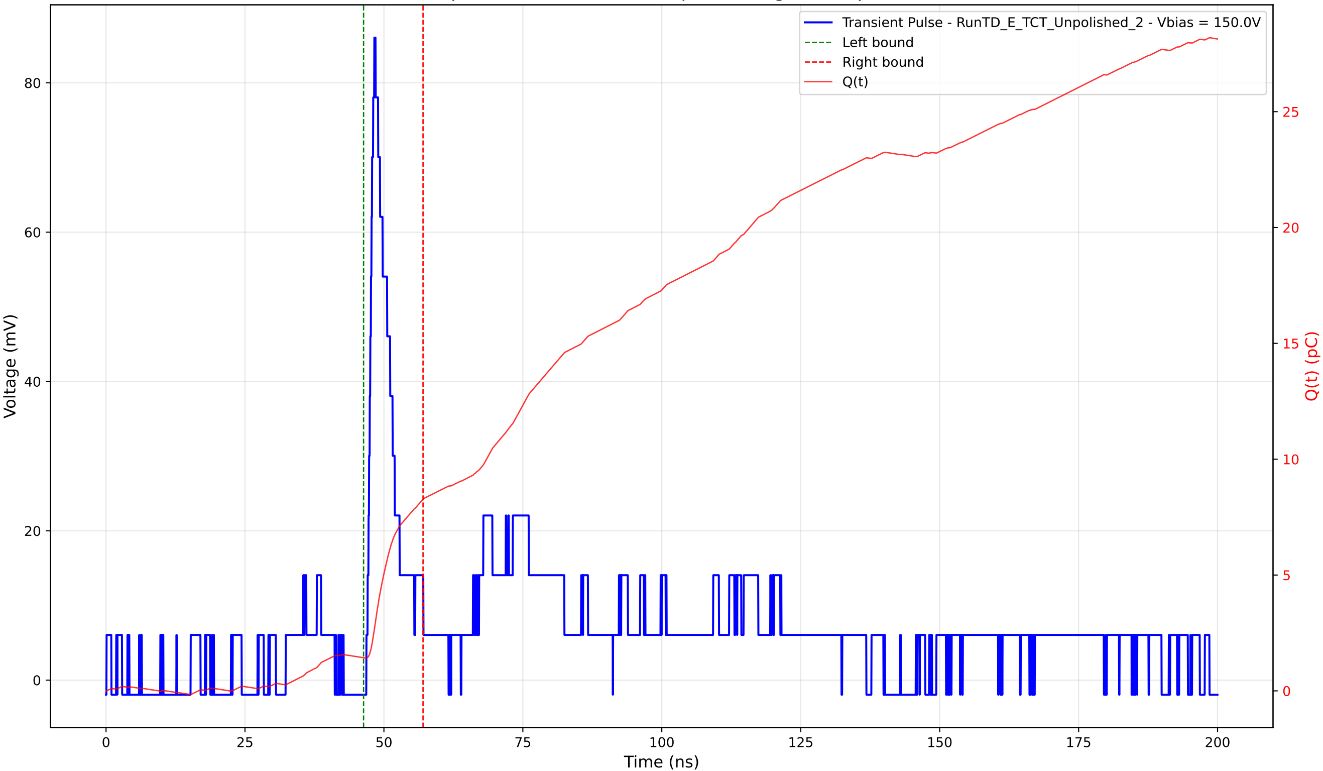
Transient Pulse - Sample: TD - Position: 295.0 \mu\text{m} - Charge: 6.85 pC - Rise Time: 1.01 ns
