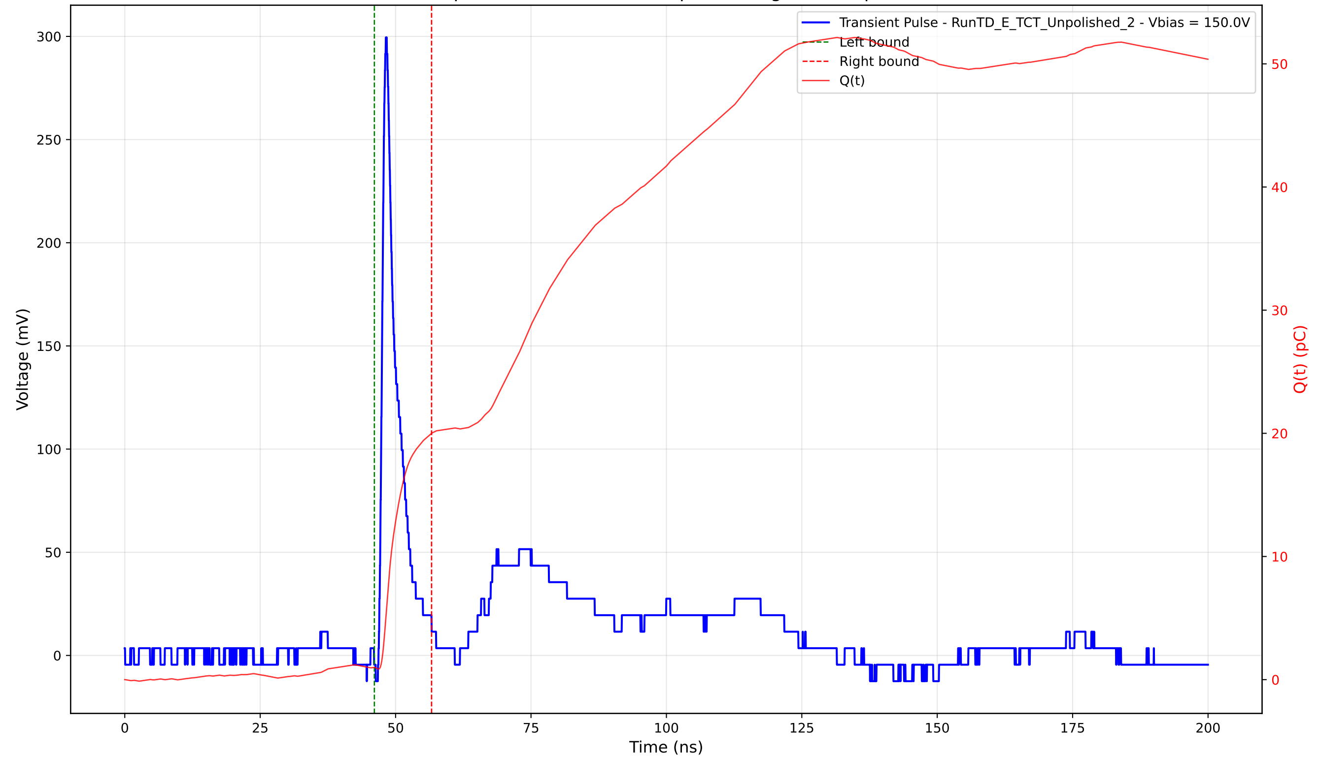
Transient Pulse - Sample: TD - Position: 140.0 \mu\text{m} - Charge: 19.02 pC - Rise Time: 0.89 ns
