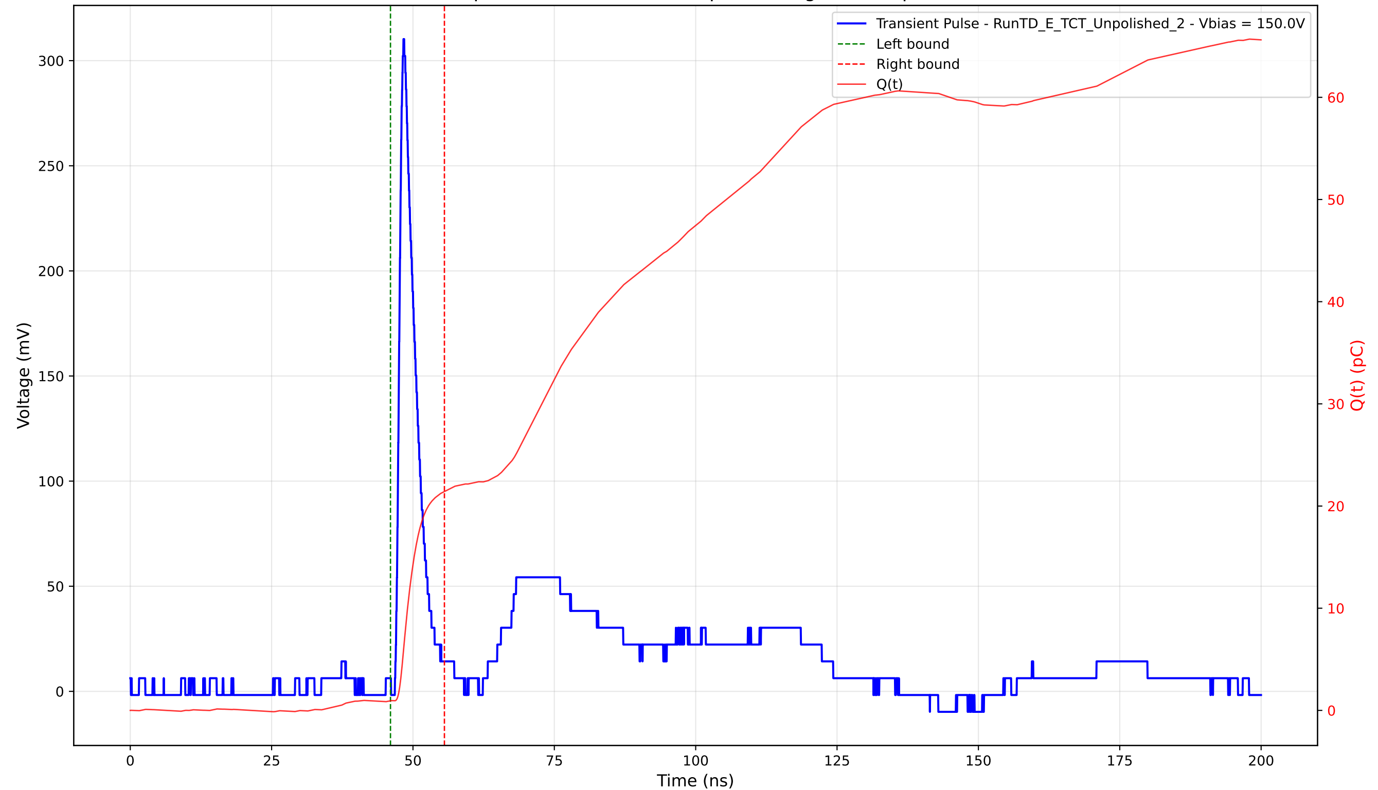
Transient Pulse - Sample: TD - Position: 205.0 \mu\text{m} - Charge: 20.48 pC - Rise Time: 1.02 ns
