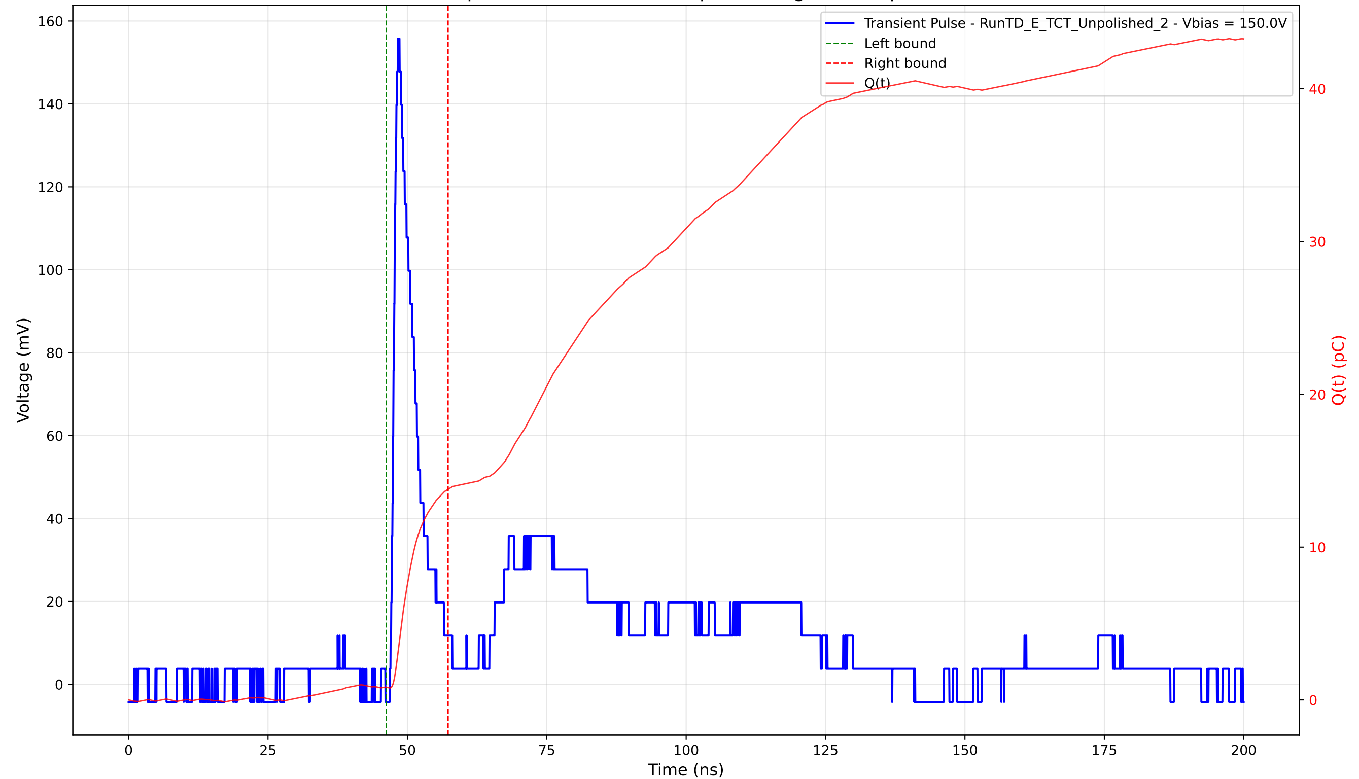
Transient Pulse - Sample: TD - Position: 155.0 \mu\text{m} - Charge: 12.96 pC - Rise Time: 1.05 ns
