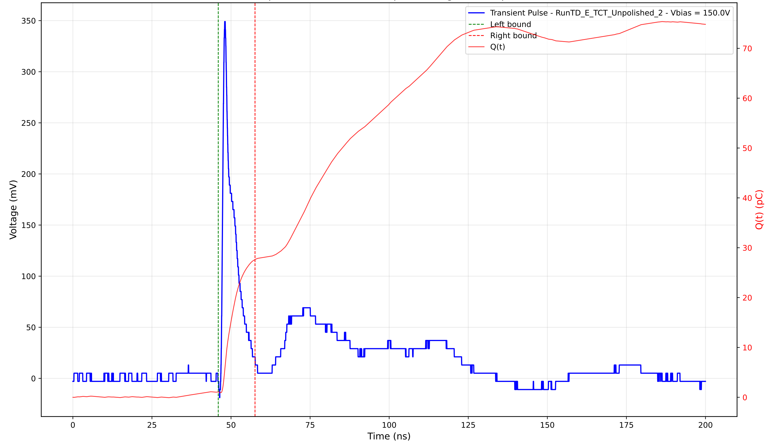
Transient Pulse - Sample: TD - Position: 70.0 \mu\text{m} - Charge: 26.58 pC - Rise Time: 0.82 ns
