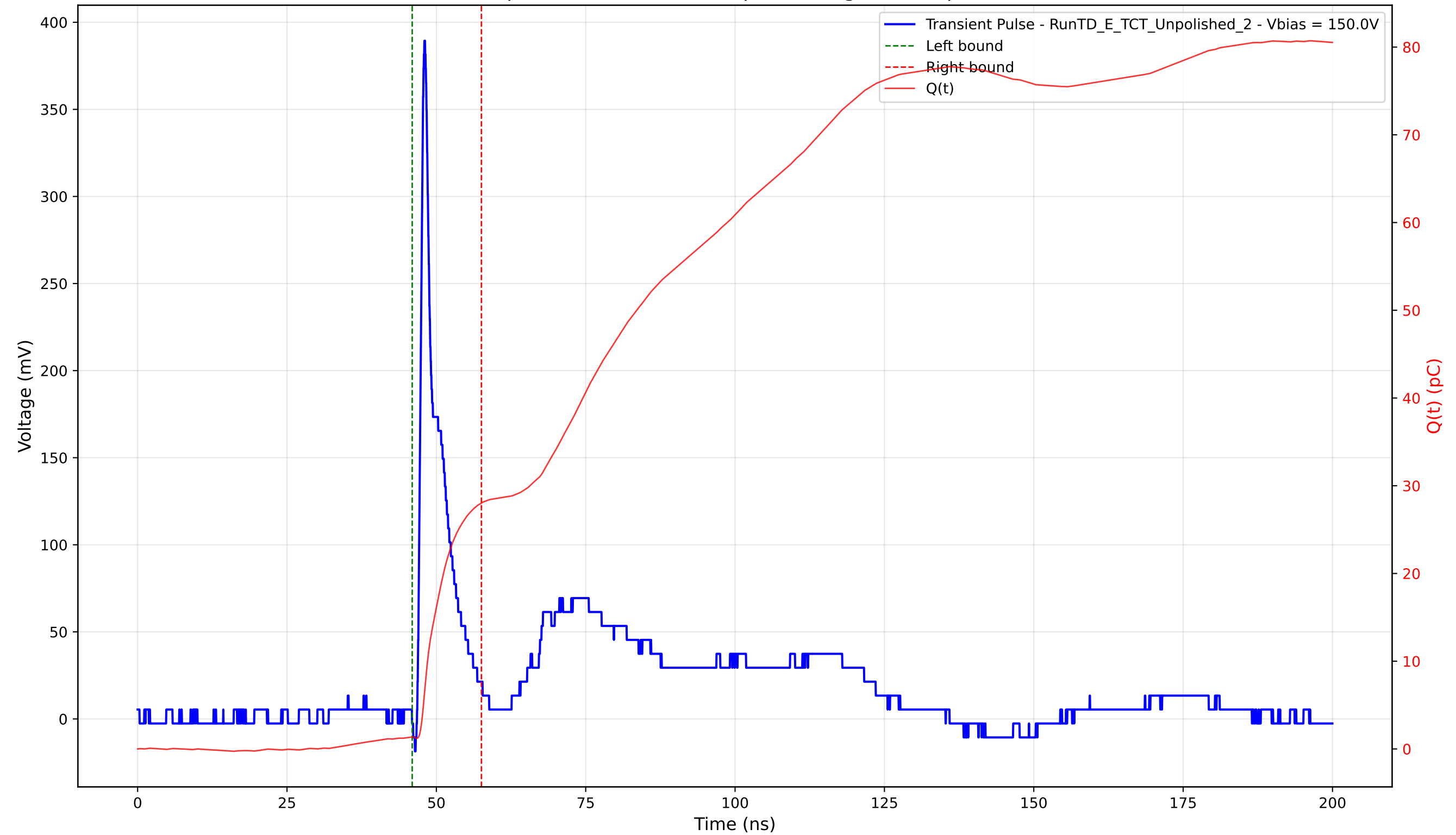
Transient Pulse - Sample: TD - Position: 55.0 \mu\text{m} - Charge: 26.67 pC - Rise Time: 0.84 ns
