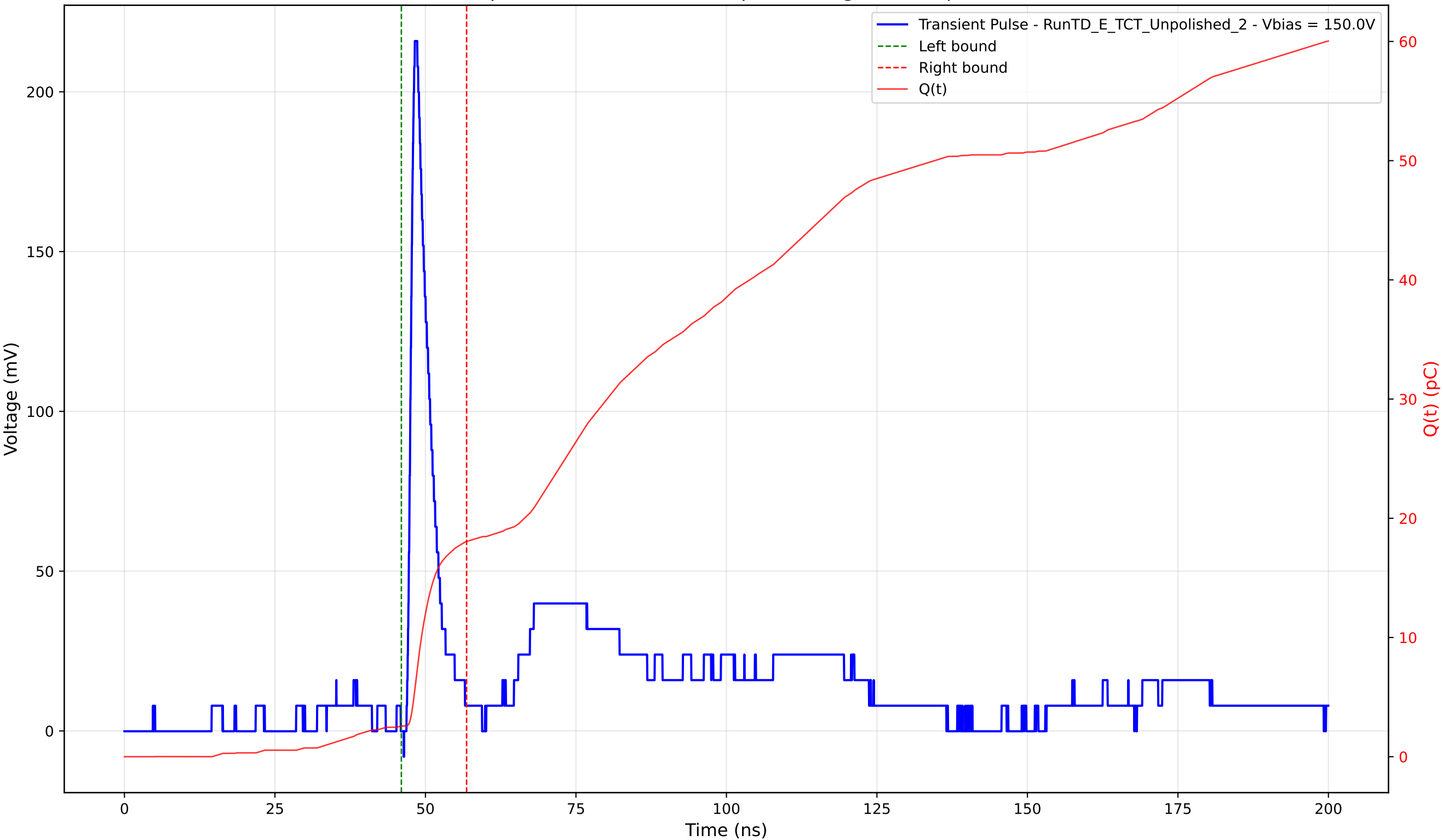
Transient Pulse - Sample: TD - Position: 225.0 \mu\text{m} - Charge: 15.48 pC - Rise Time: 1.01 ns
