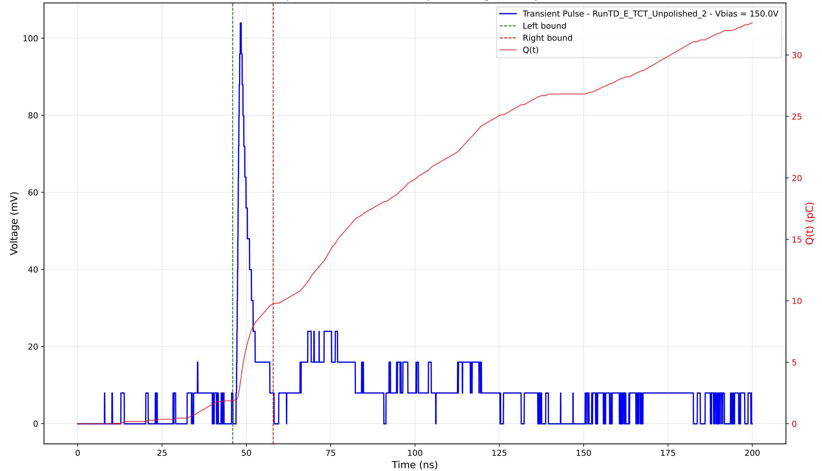
Transient Pulse - Sample: TD - Position: 340.0 \mu\text{m} - Charge: 7.85 pC - Rise Time: 0.93 ns
