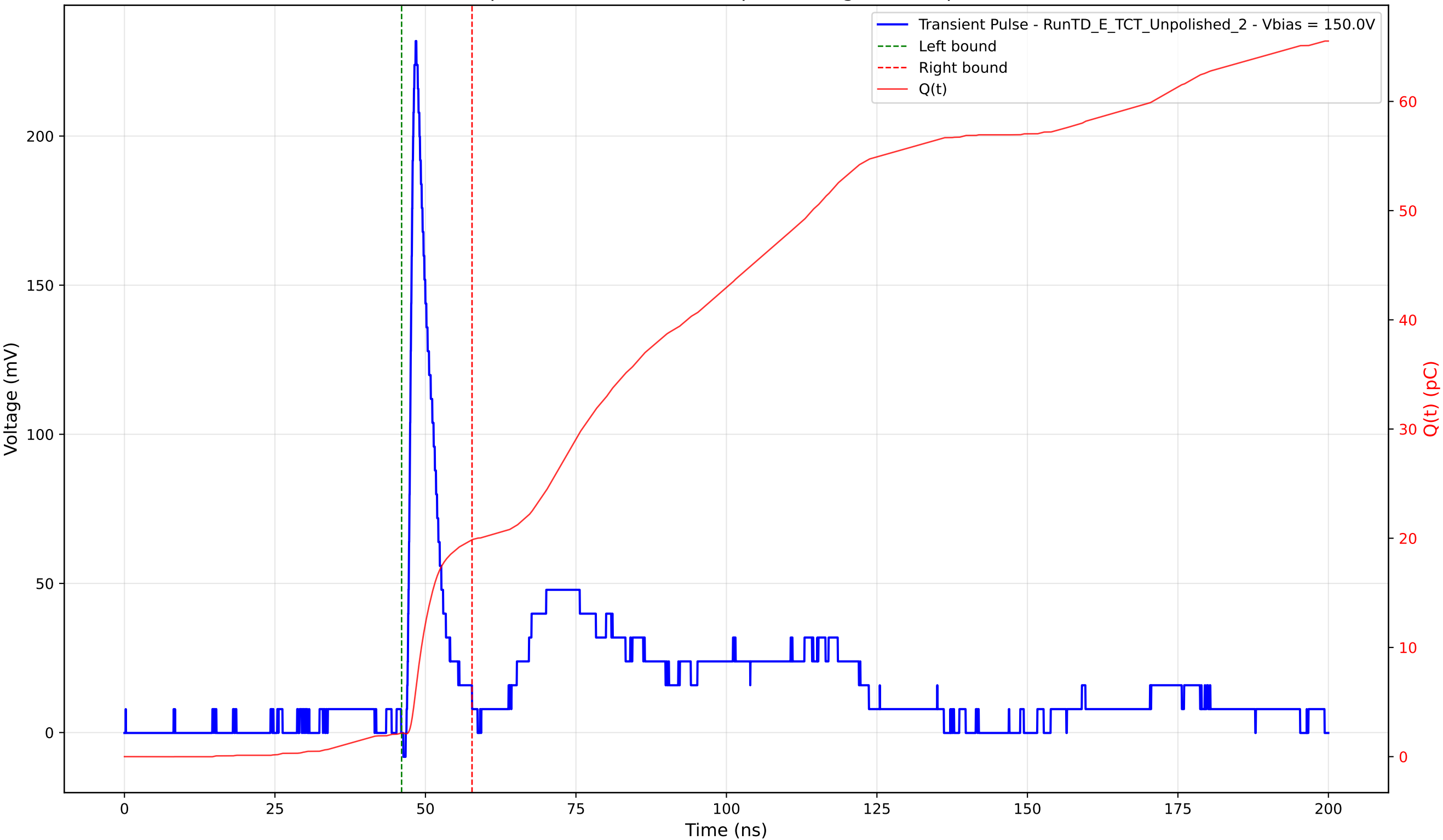
Transient Pulse - Sample: TD - Position: 195.0 \mu\text{m} - Charge: 17.71 pC - Rise Time: 1.04 ns
