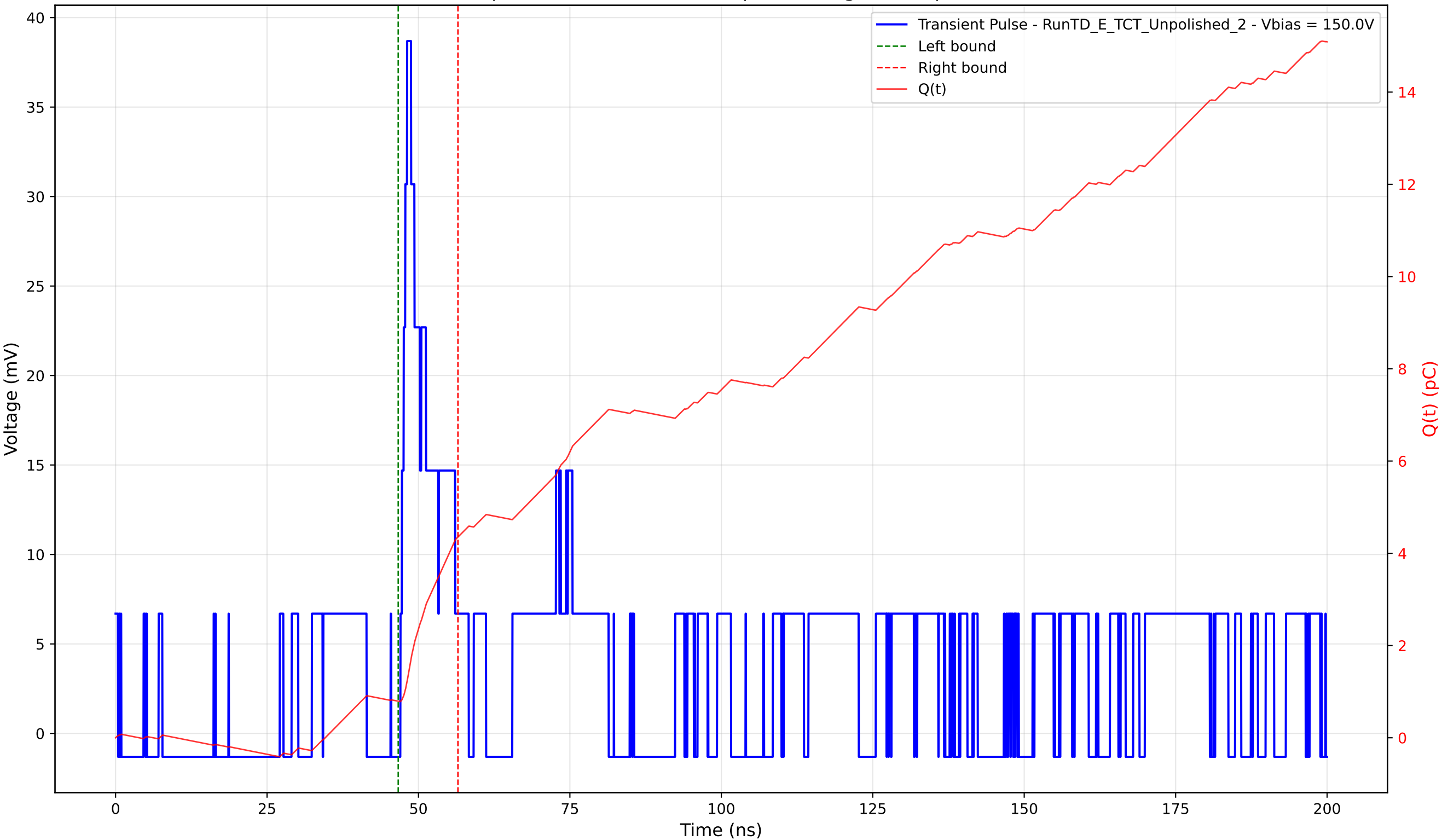
Transient Pulse - Sample: TD - Position: 350.0 \mu\text{m} - Charge: 3.56 pC - Rise Time: 1.11 ns
