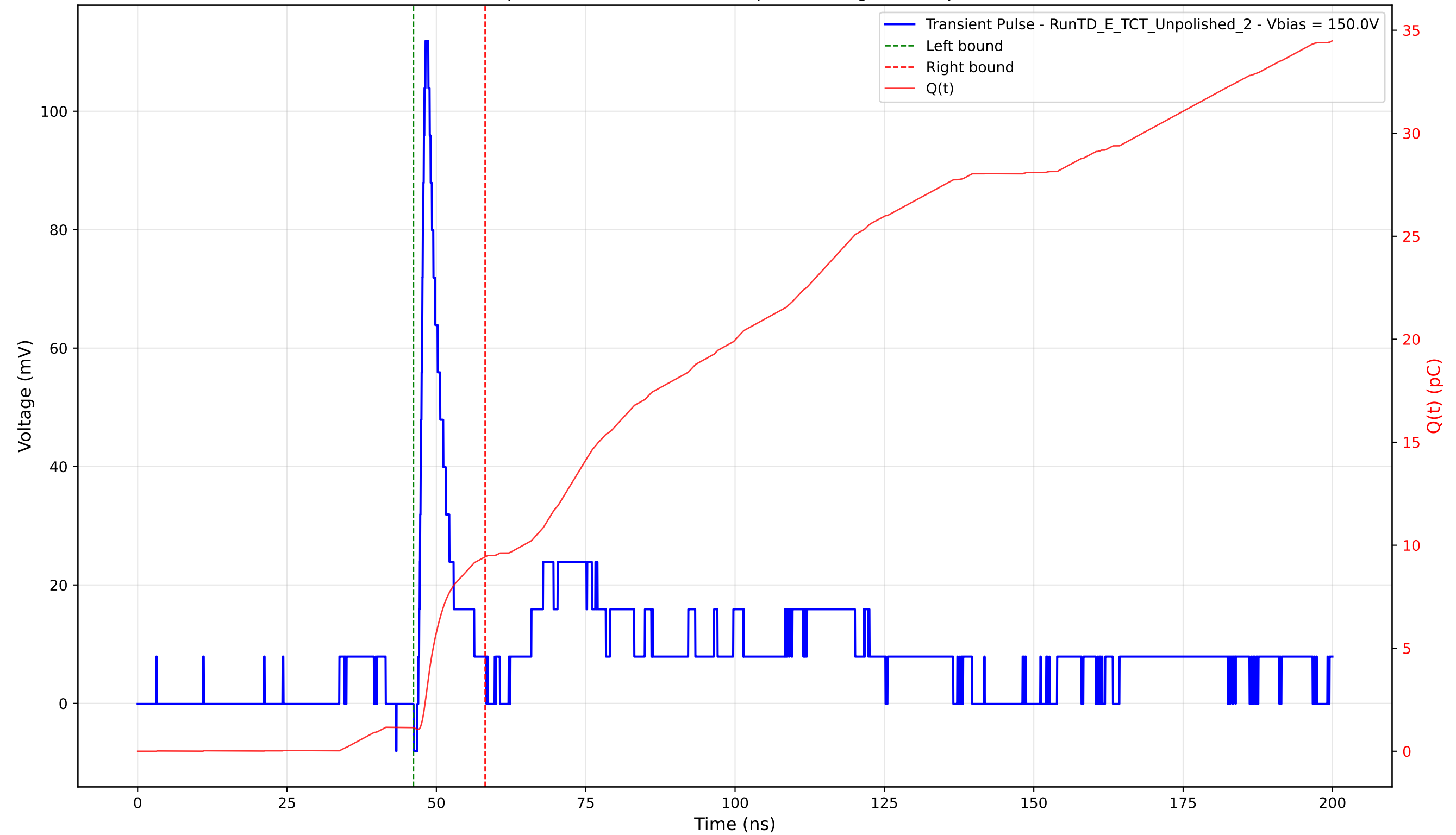
Transient Pulse - Sample: TD - Position: 310.0 \mu\text{m} - Charge: 8.29 pC - Rise Time: 0.89 ns
