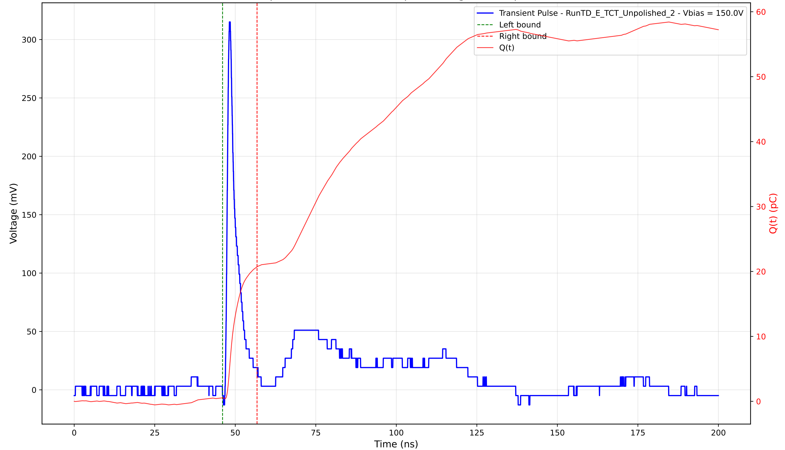
Transient Pulse - Sample: TD - Position: 125.0 \mu\text{m} - Charge: 20.19 pC - Rise Time: 0.93 ns
