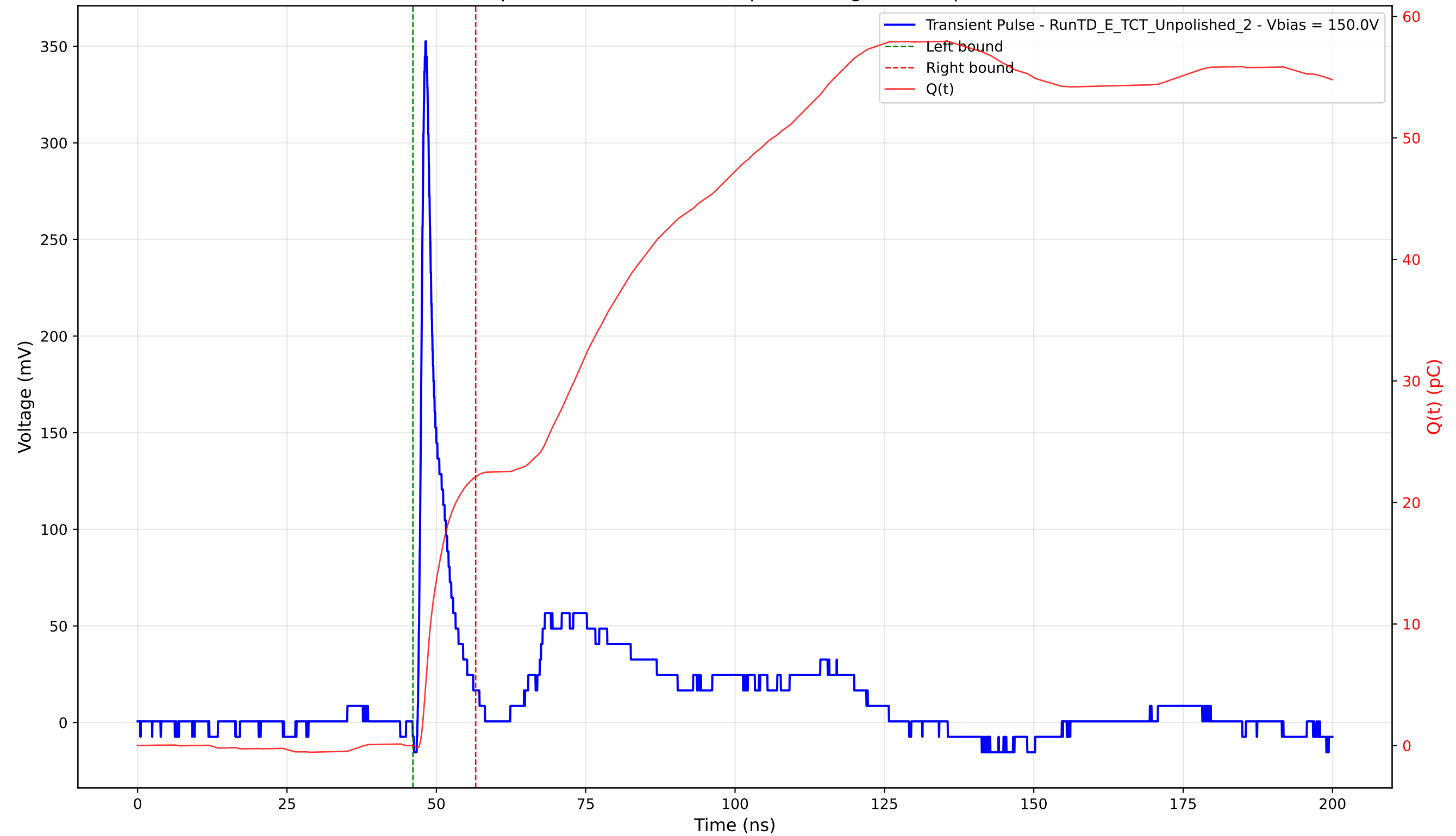
Transient Pulse - Sample: TD - Position: 105.0 \mu\text{m} - Charge: 22.12 pC - Rise Time: 0.87 ns
