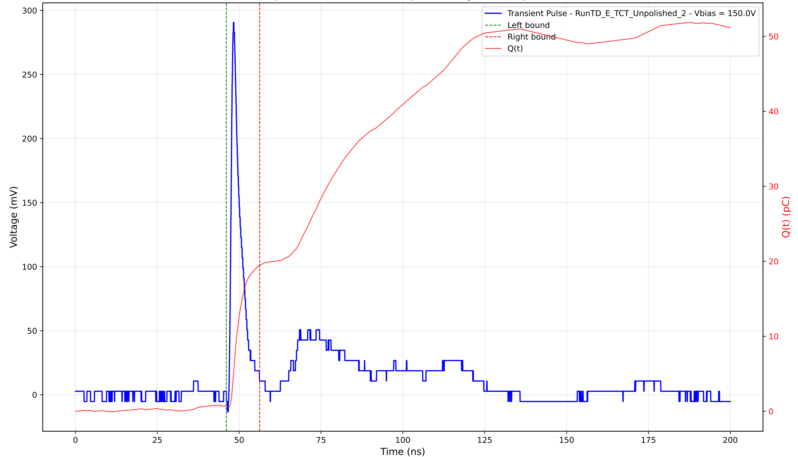
Transient Pulse - Sample: TD - Position: 200.0 \mu\text{m} - Charge: 18.76 pC - Rise Time: 0.93 ns
