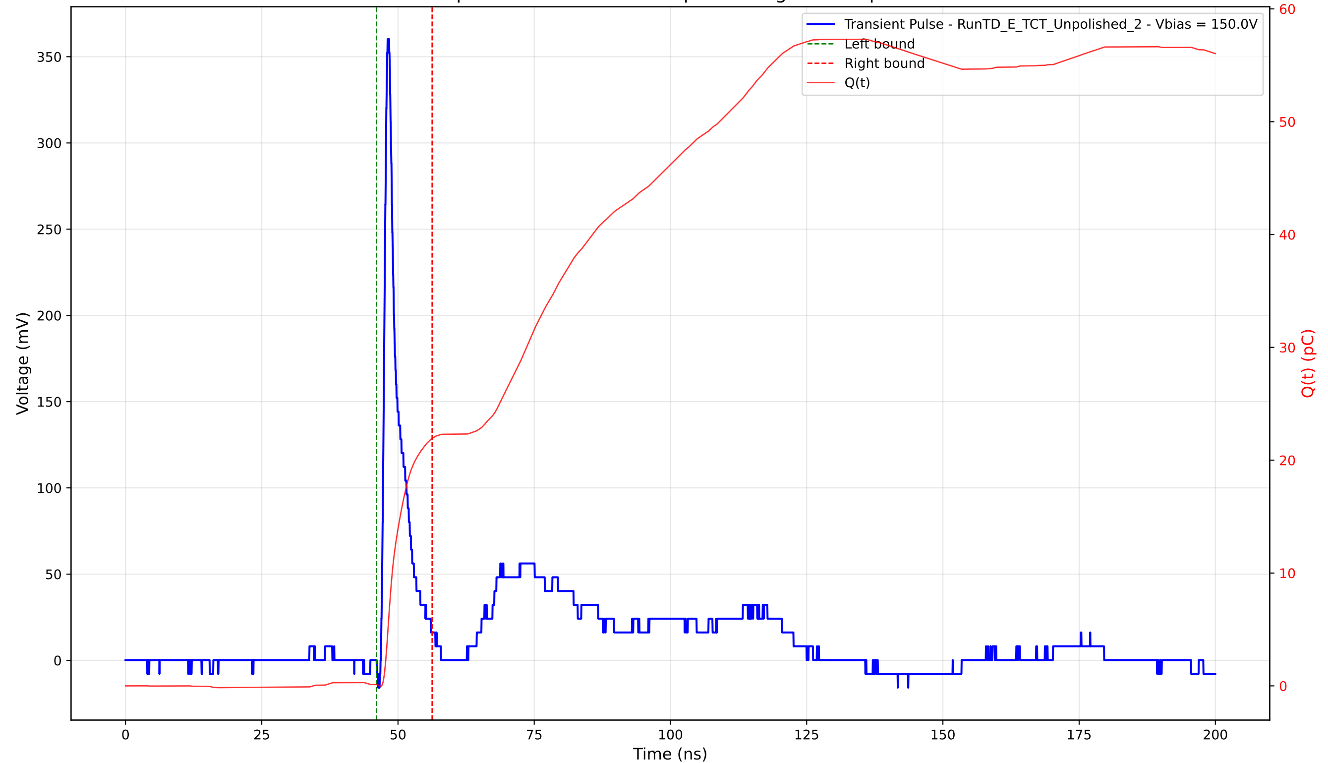
Transient Pulse - Sample: TD - Position: 115.0 \mu\text{m} - Charge: 21.81 pC - Rise Time: 0.87 ns
