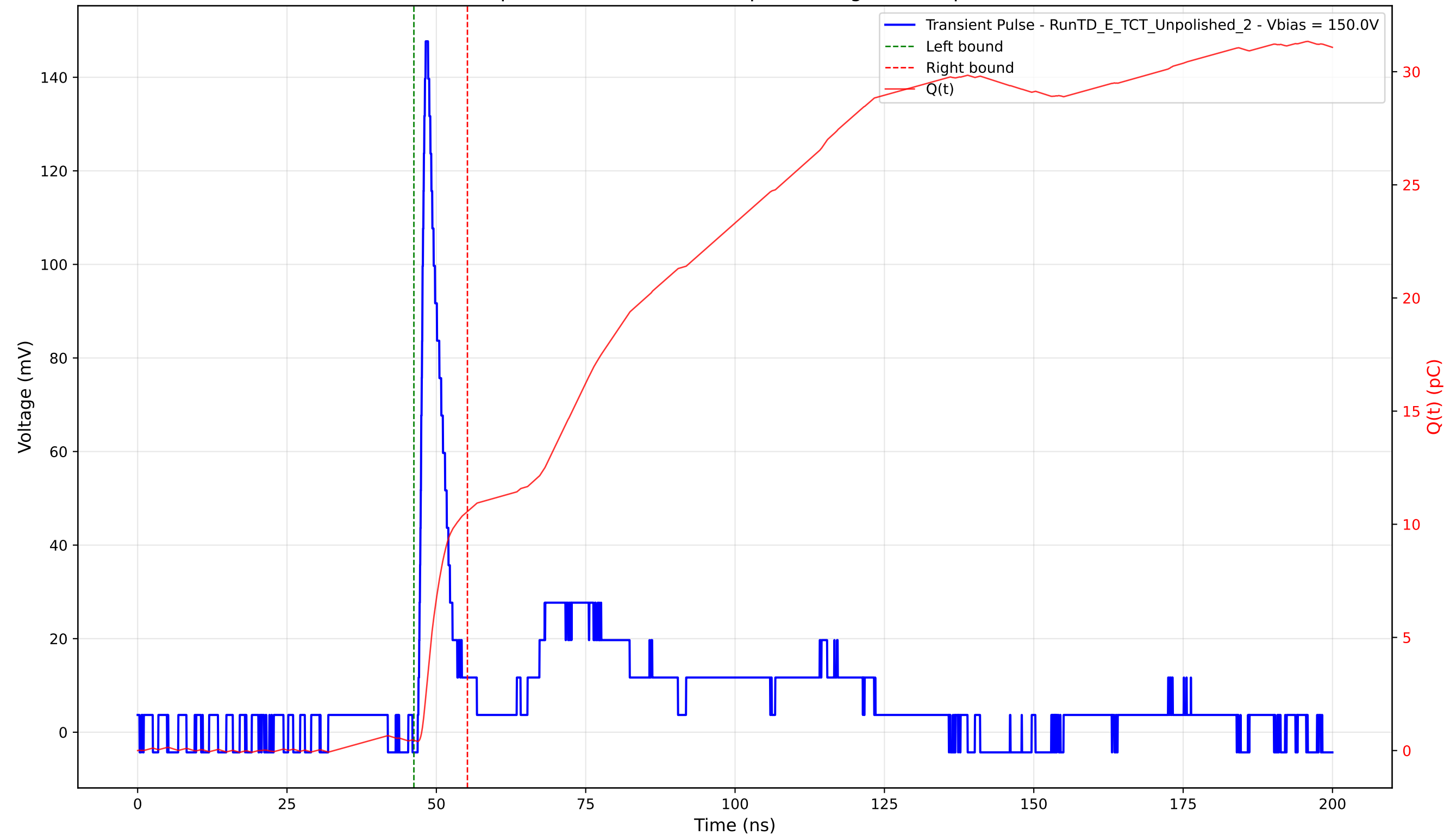
Transient Pulse - Sample: TD - Position: 270.0 \mu\text{m} - Charge: 10.11 pC - Rise Time: 0.97 ns
