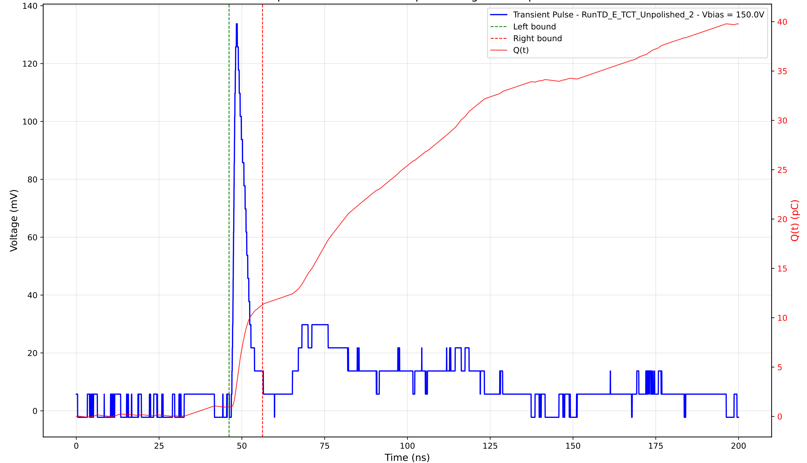
Transient Pulse - Sample: TD - Position: 265.0 \mu\text{m} - Charge: 10.35 pC - Rise Time: 1.12 ns
