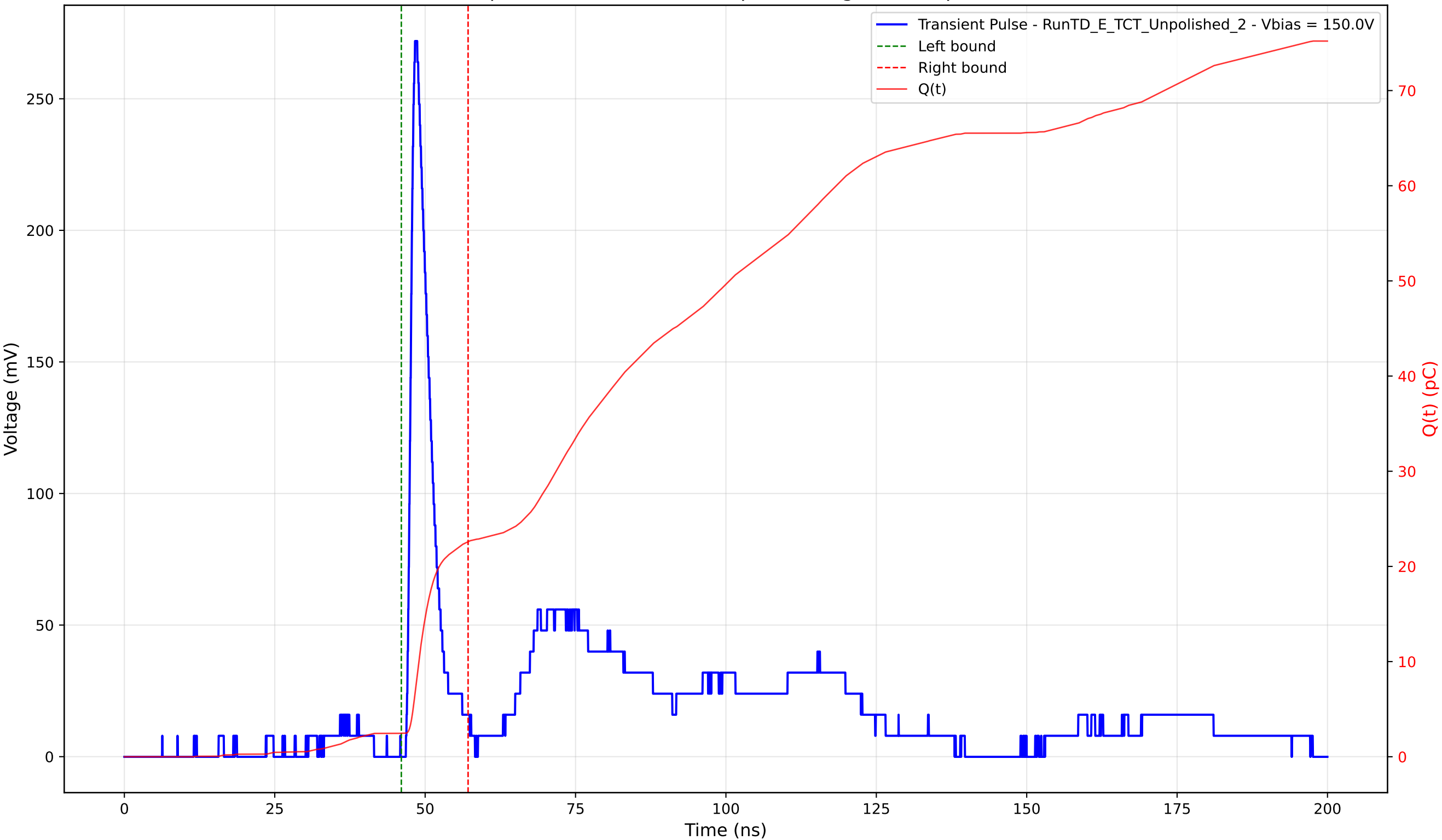
Transient Pulse - Sample: TD - Position: 185.0 \mu\text{m} - Charge: 20.14 pC - Rise Time: 1.01 ns
