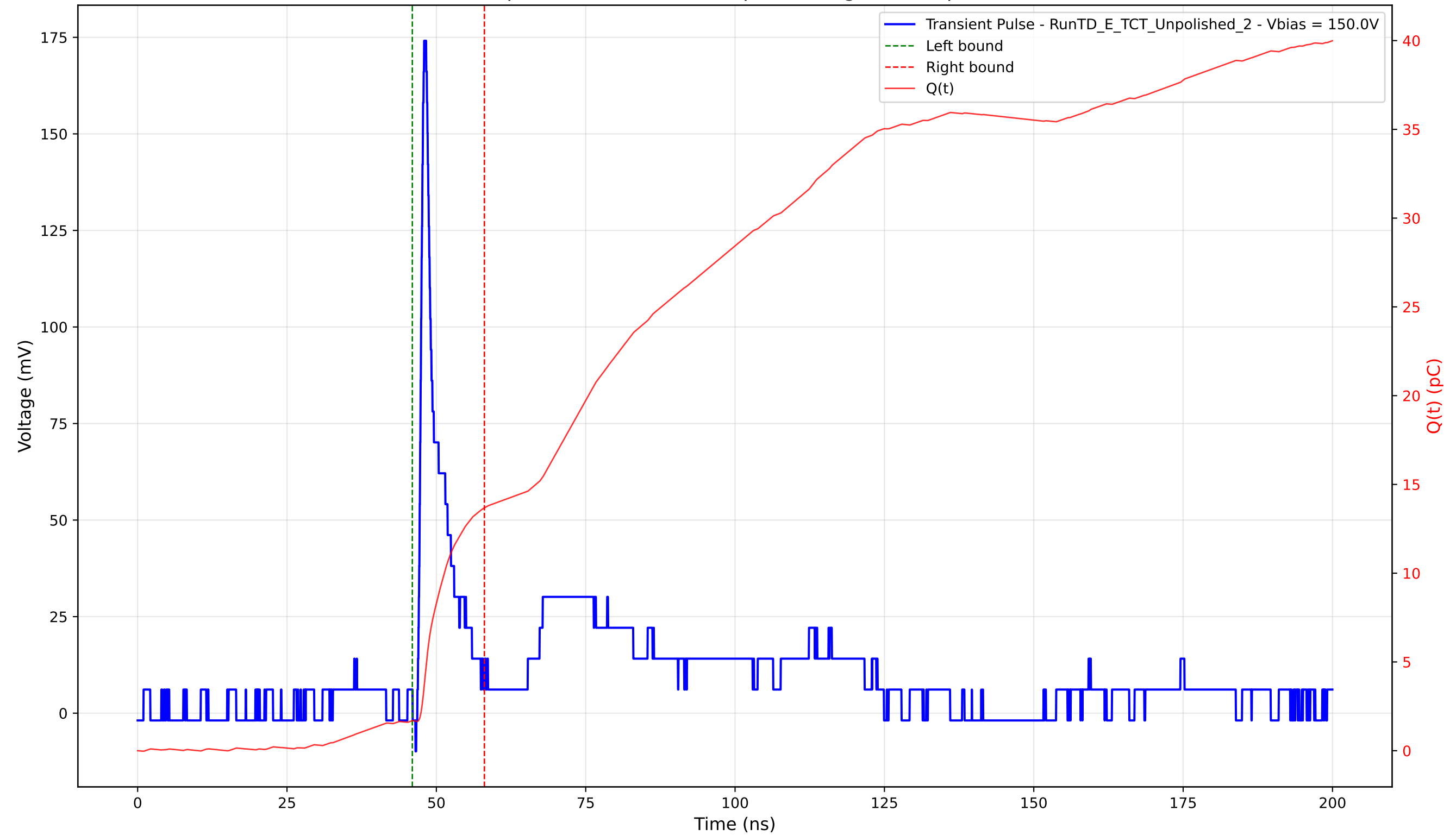
Transient Pulse - Sample: TD - Position: 35.0 \mu\text{m} - Charge: 11.97 pC - Rise Time: 0.79 ns
