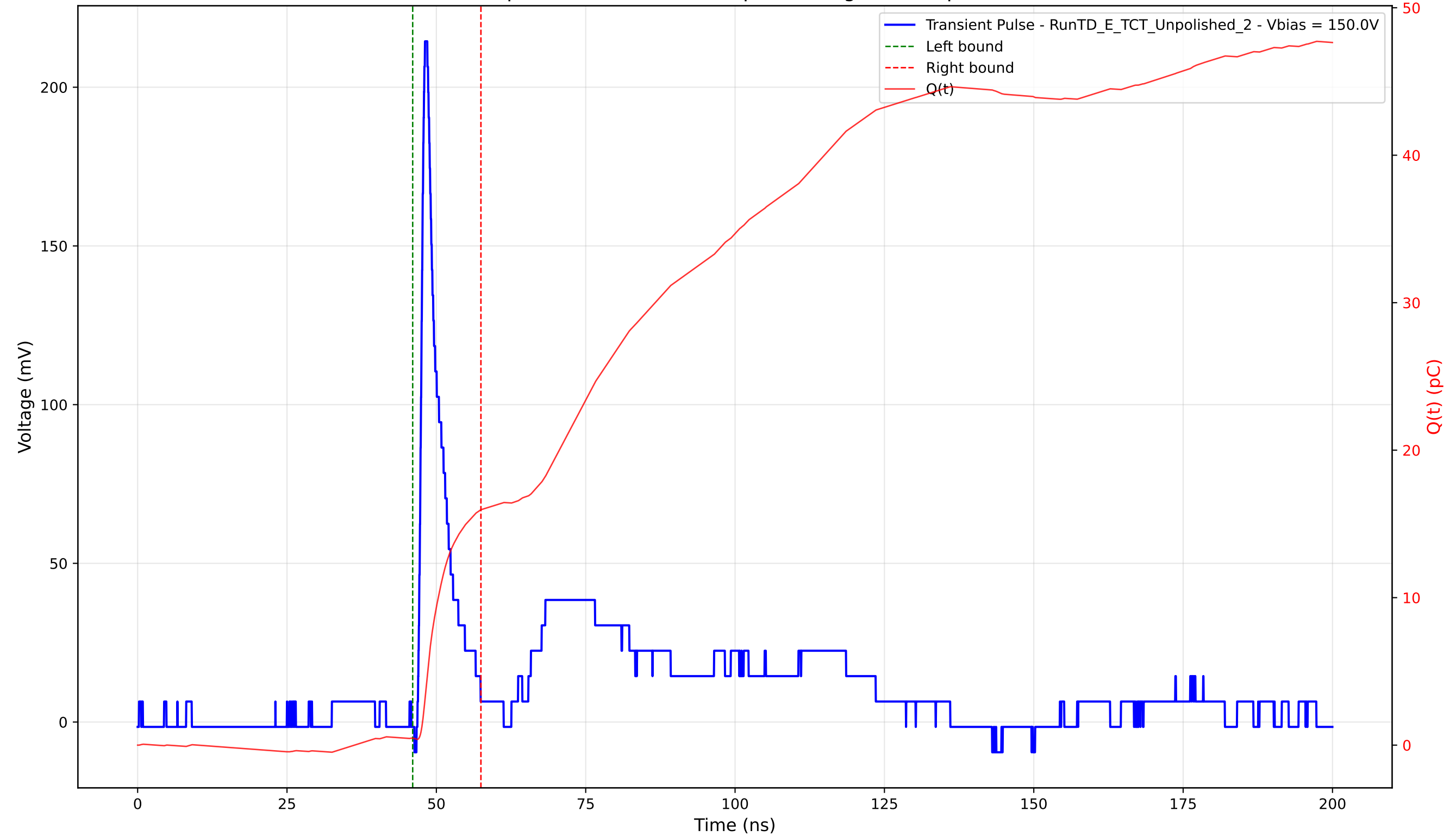
Transient Pulse - Sample: TD - Position: 90.0 \mu\text{m} - Charge: 15.49 pC - Rise Time: 0.92 ns
