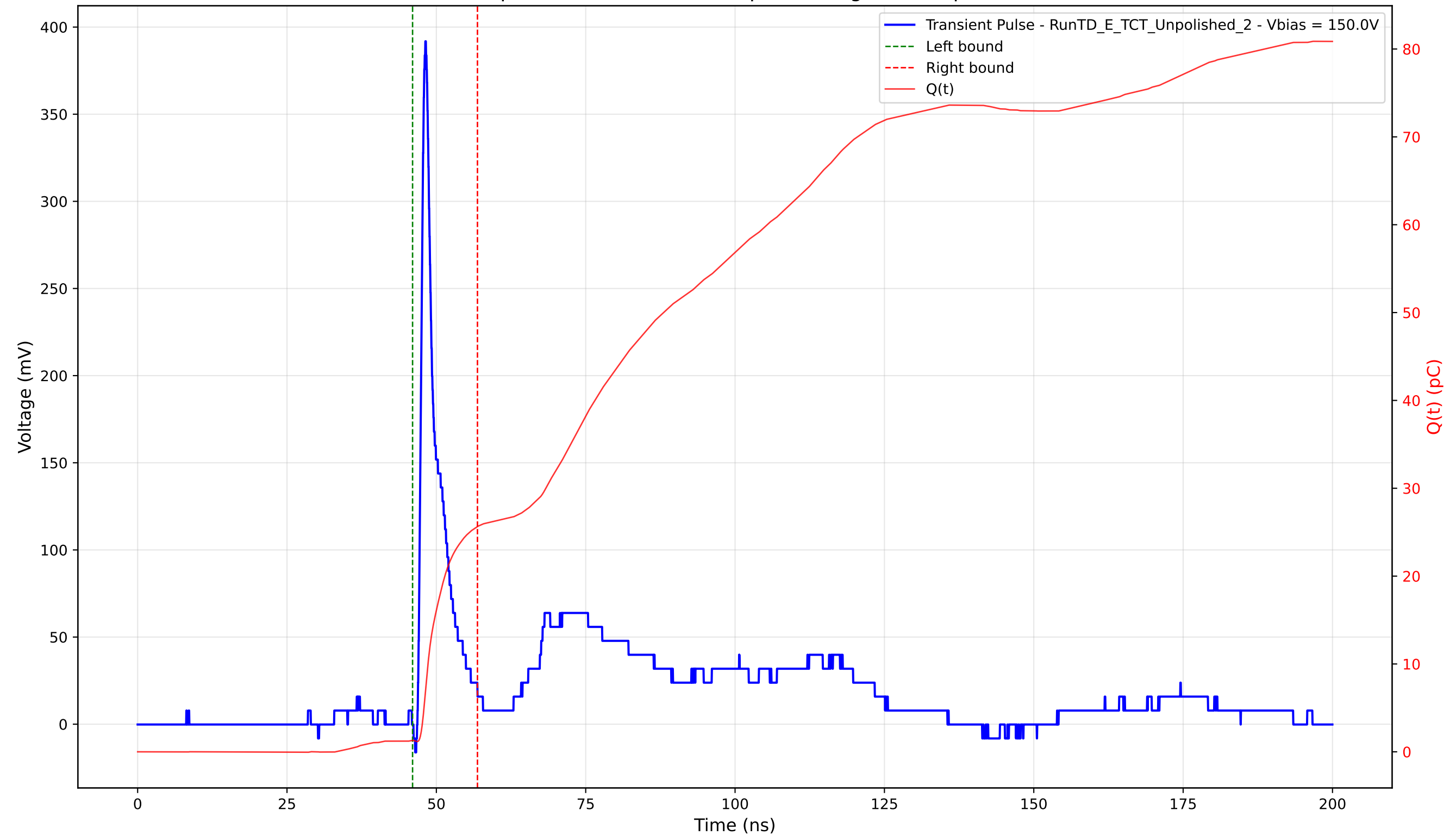
Transient Pulse - Sample: TD - Position: 110.0 \mu\text{m} - Charge: 24.36 pC - Rise Time: 0.88 ns
