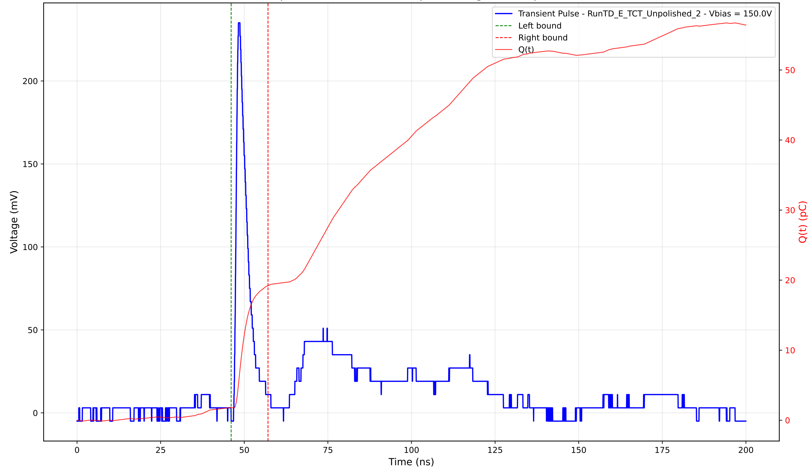
Transient Pulse - Sample: TD - Position: 180.0 \mu\text{m} - Charge: 17.40 pC - Rise Time: 0.99 ns
