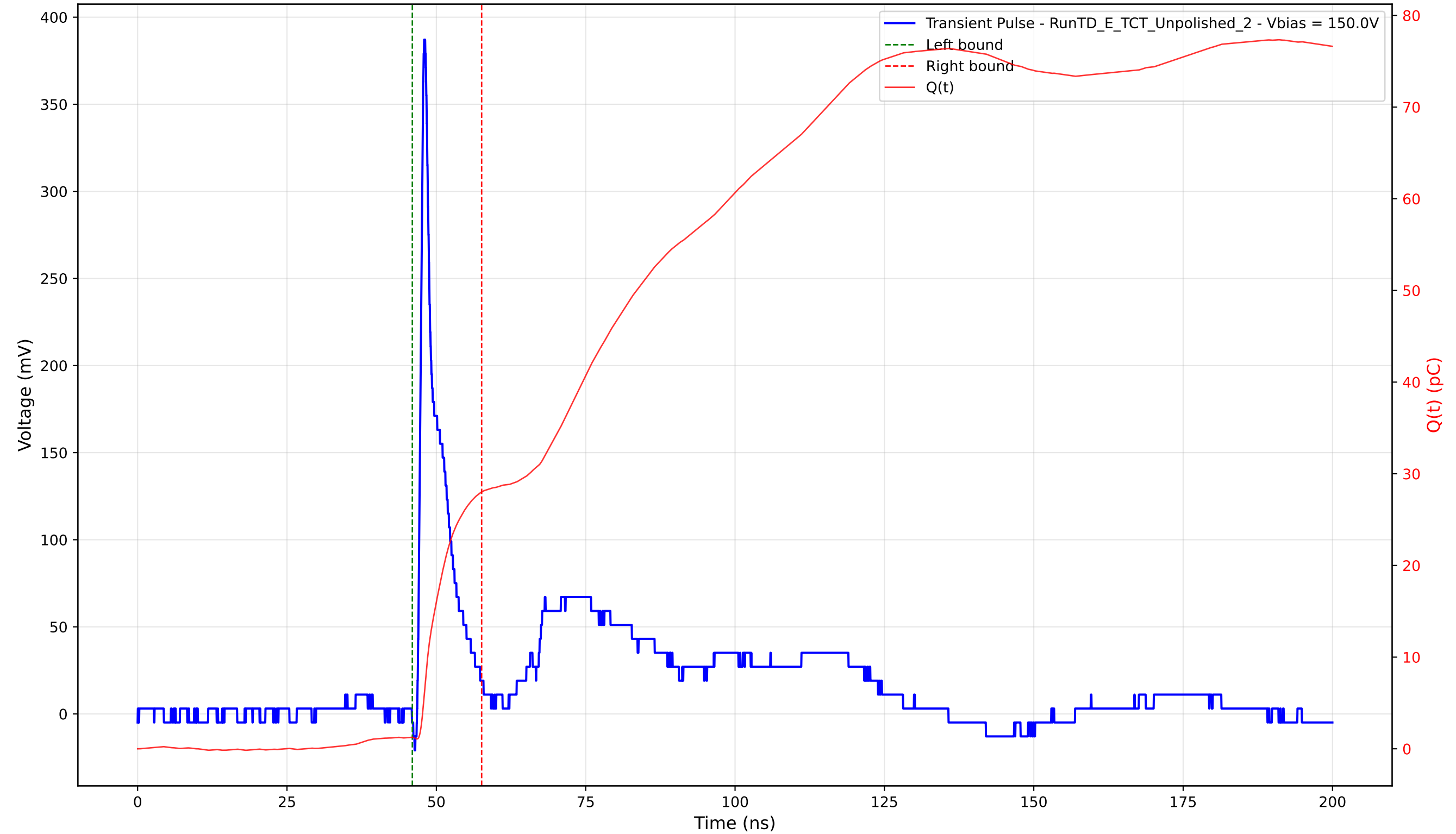
Transient Pulse - Sample: TD - Position: 60.0 \mu\text{m} - Charge: 26.76 pC - Rise Time: 0.81 ns
