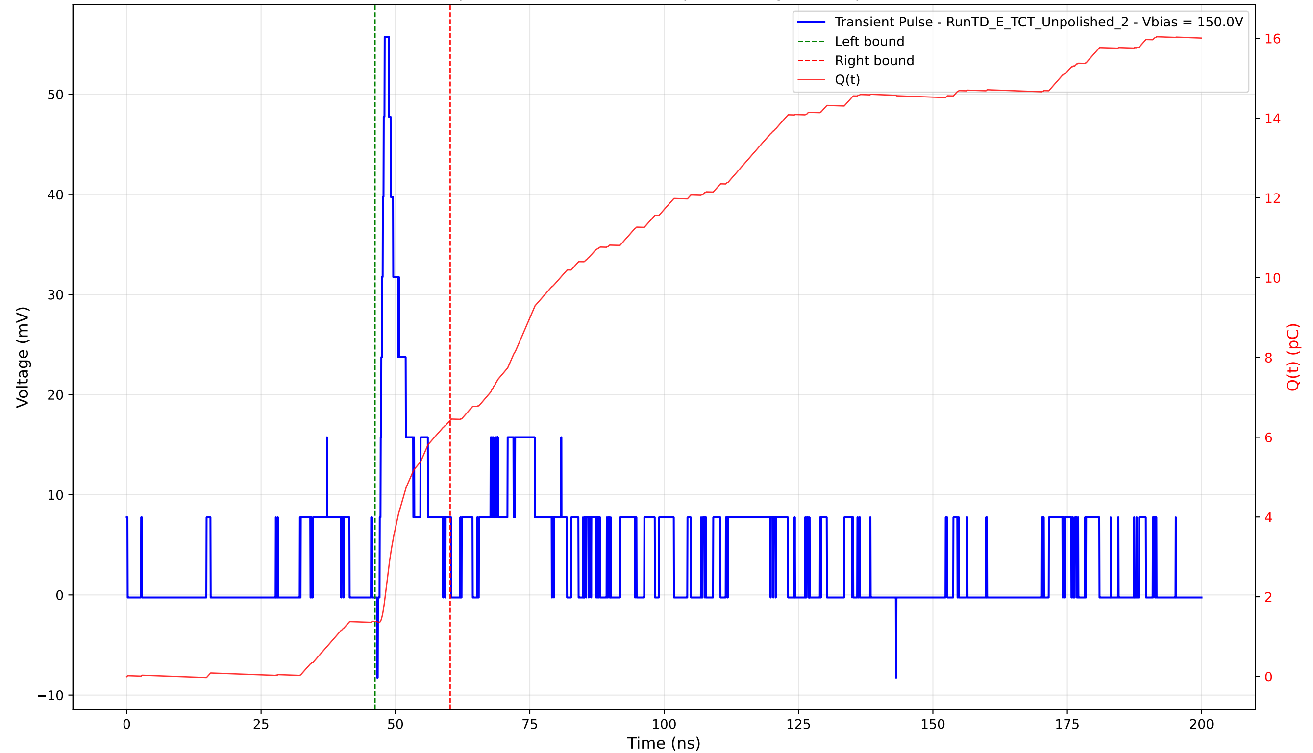
Transient Pulse - Sample: TD - Position: 395.0 \mu\text{m} - Charge: 5.04 pC - Rise Time: 0.93 ns
