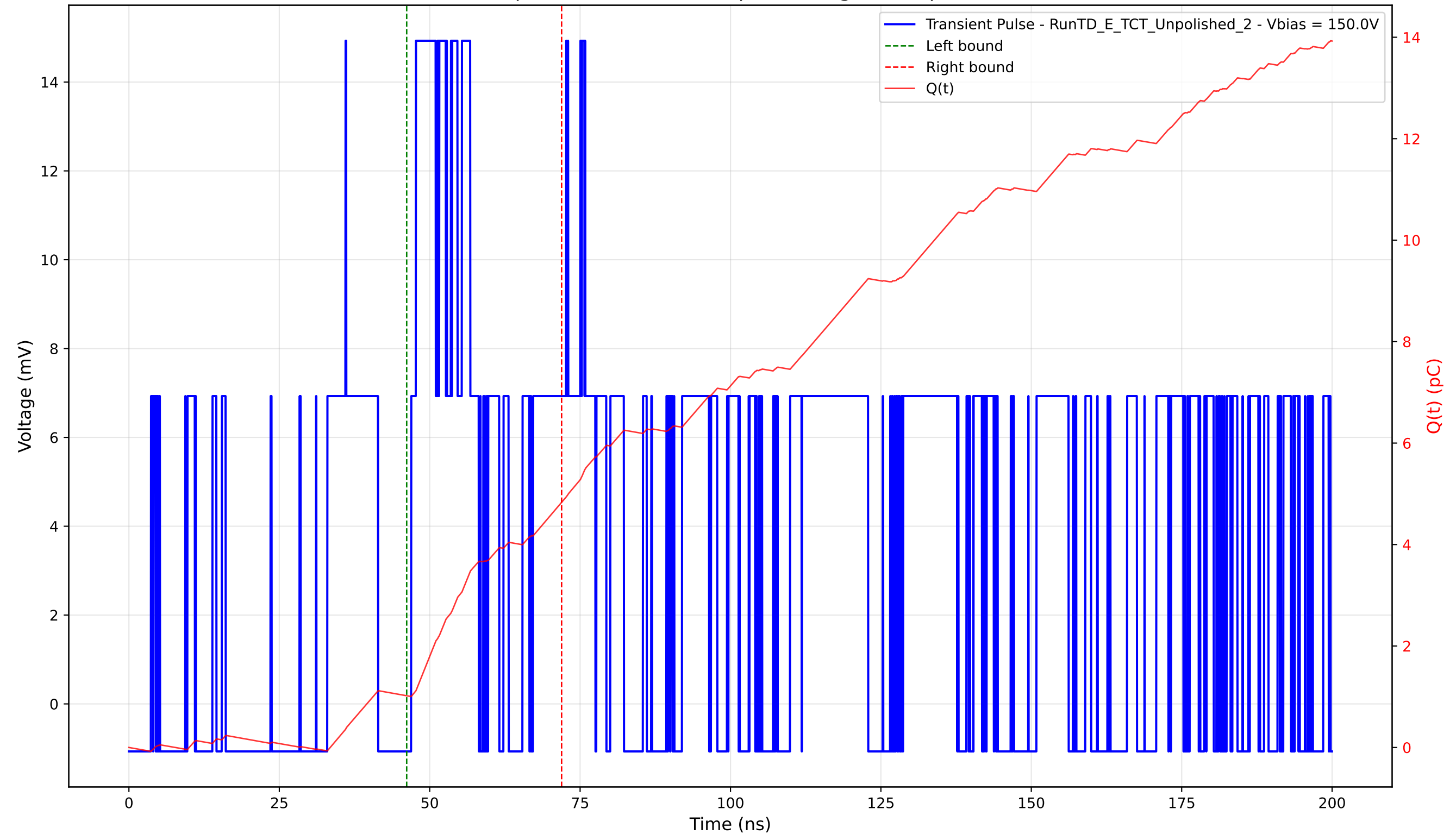
Transient Pulse - Sample: TD - Position: 5.0 \mu\text{m} - Charge: 3.81 pC - Rise Time: 3.04 ns
