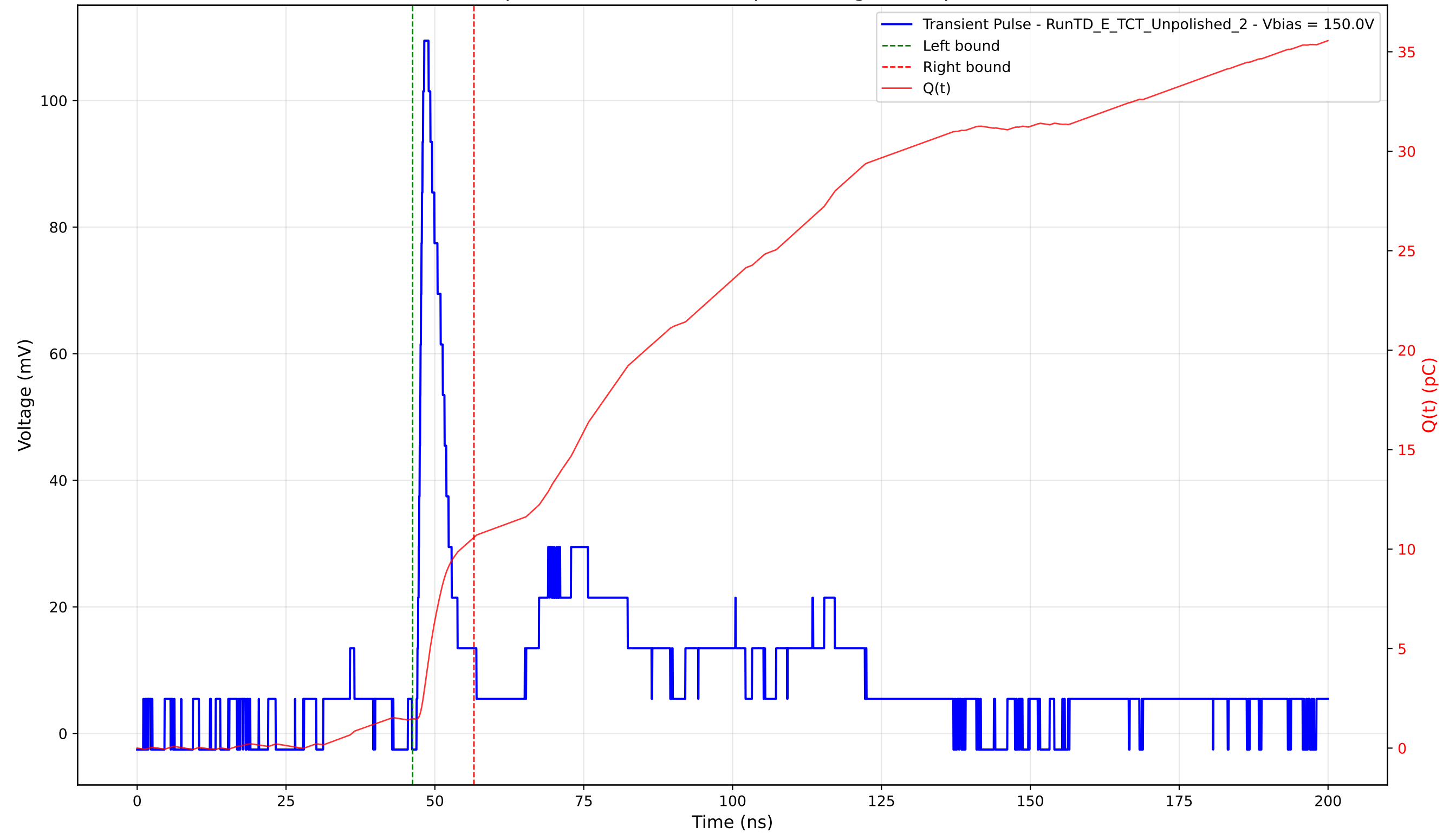
Transient Pulse - Sample: TD - Position: 260.0 \mu\text{m} - Charge: 9.12 pC - Rise Time: 0.97 ns
