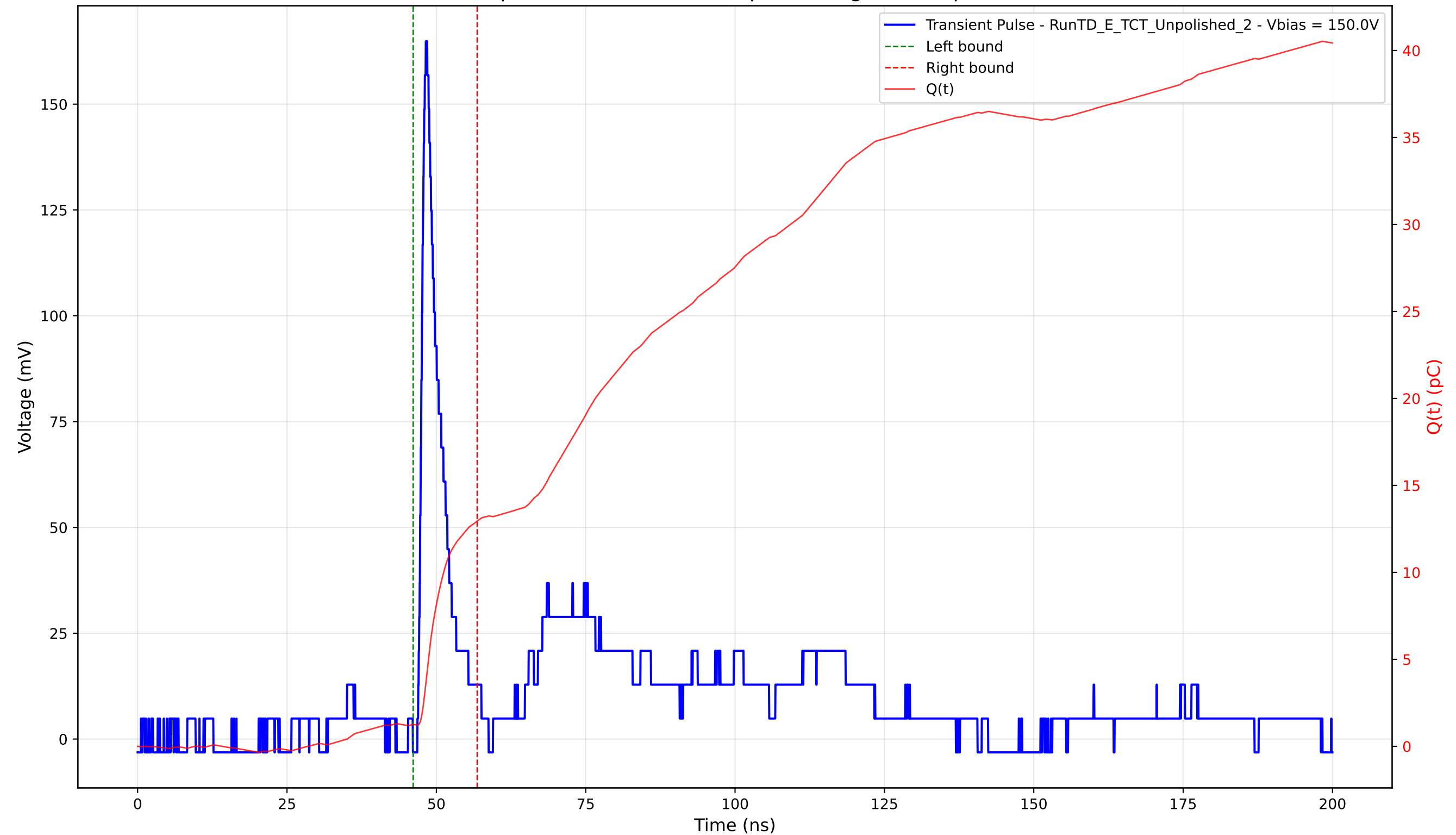
Transient Pulse - Sample: TD - Position: 235.0 \mu\text{m} - Charge: 11.69 pC - Rise Time: 0.93 ns
