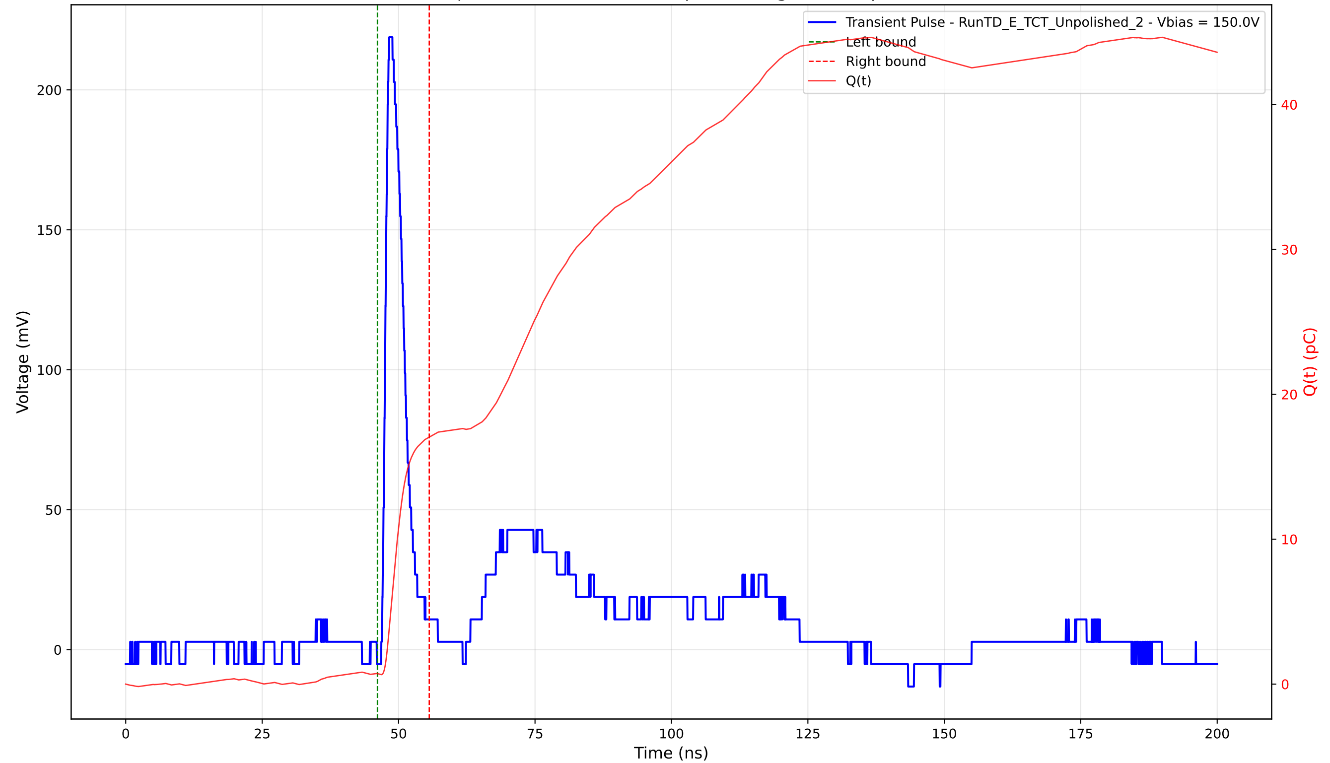
Transient Pulse - Sample: TD - Position: 210.0 \mu\text{m} - Charge: 16.33 pC - Rise Time: 0.99 ns
