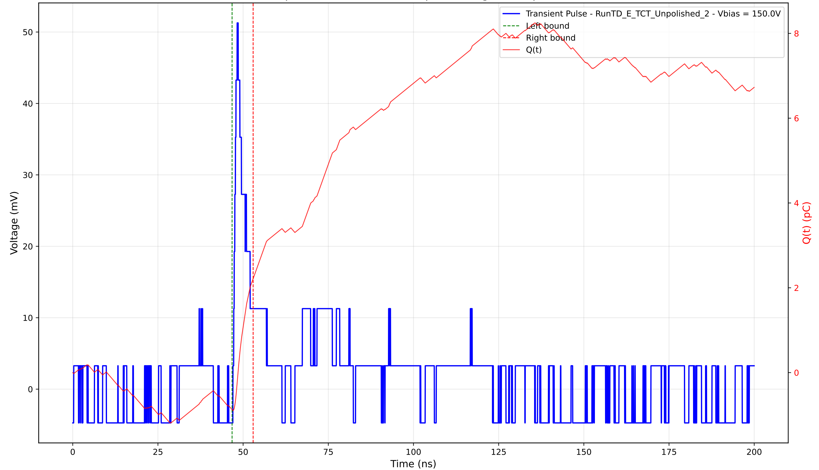
Transient Pulse - Sample: TD - Position: 405.0 \mu\text{m} - Charge: 3.09 pC - Rise Time: 1.02 ns
