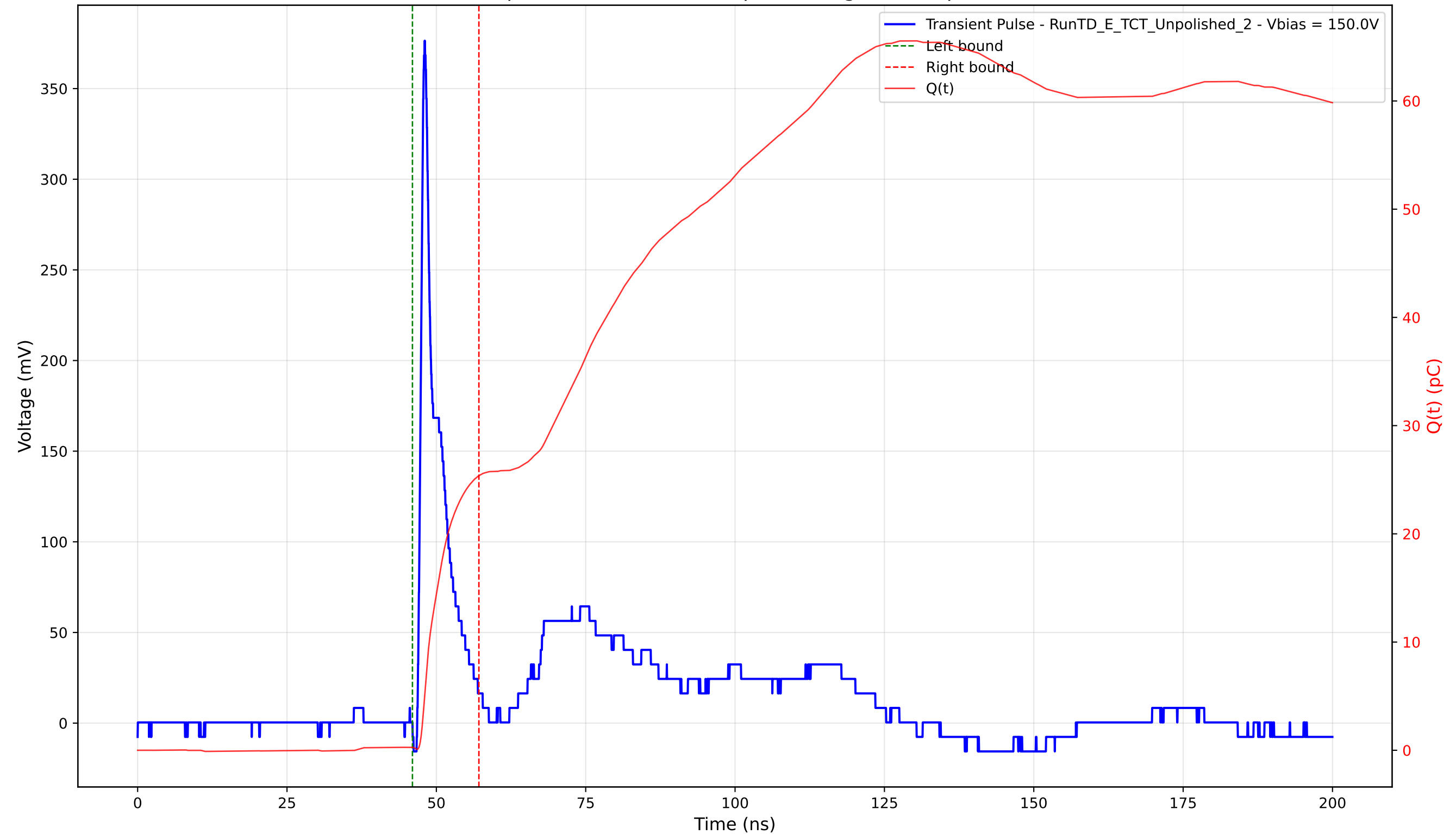
Transient Pulse - Sample: TD - Position: 50.0 \mu\text{m} - Charge: 25.08 pC - Rise Time: 0.83 ns
