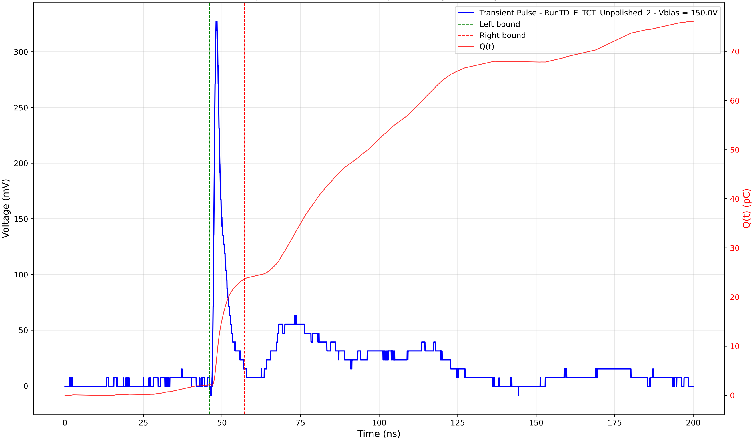
Transient Pulse - Sample: TD - Position: 120.0 \mu\text{m} - Charge: 21.55 pC - Rise Time: 0.88 ns
