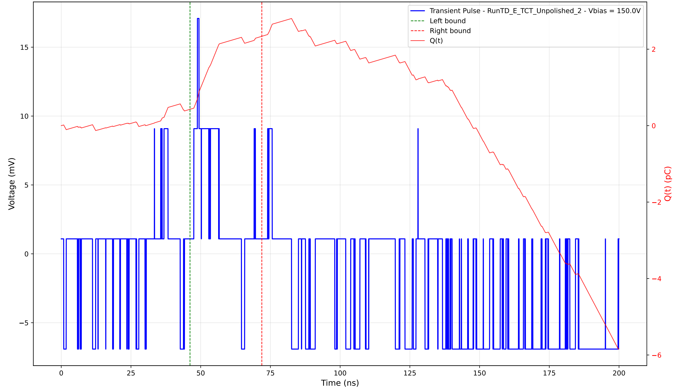
Transient Pulse - Sample: TD - Position: 0.0 \mu\text{m} - Charge: 1.91 pC - Rise Time: 1.30 ns
