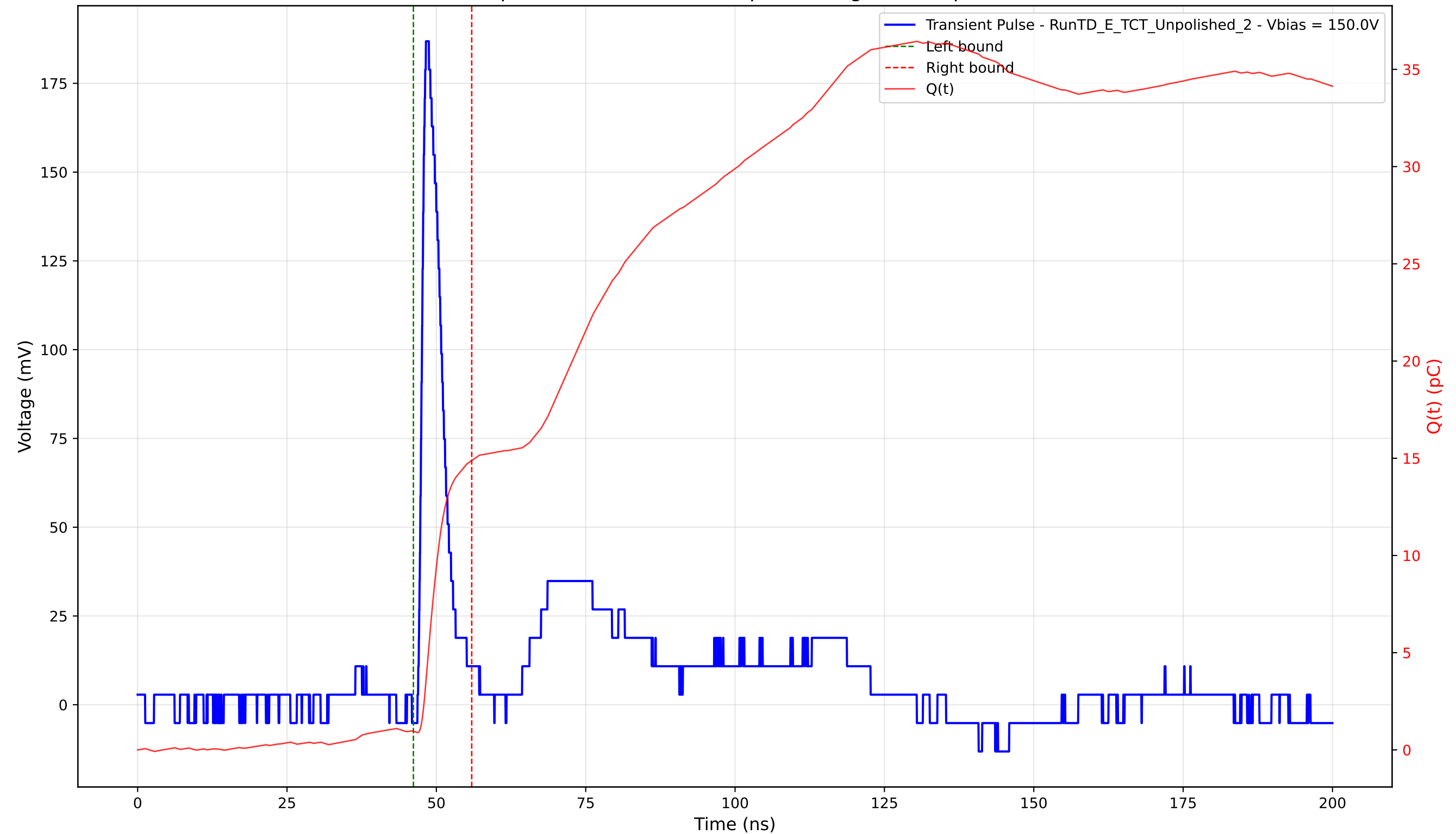
Transient Pulse - Sample: TD - Position: 215.0 \mu\text{m} - Charge: 13.93 pC - Rise Time: 0.98 ns
