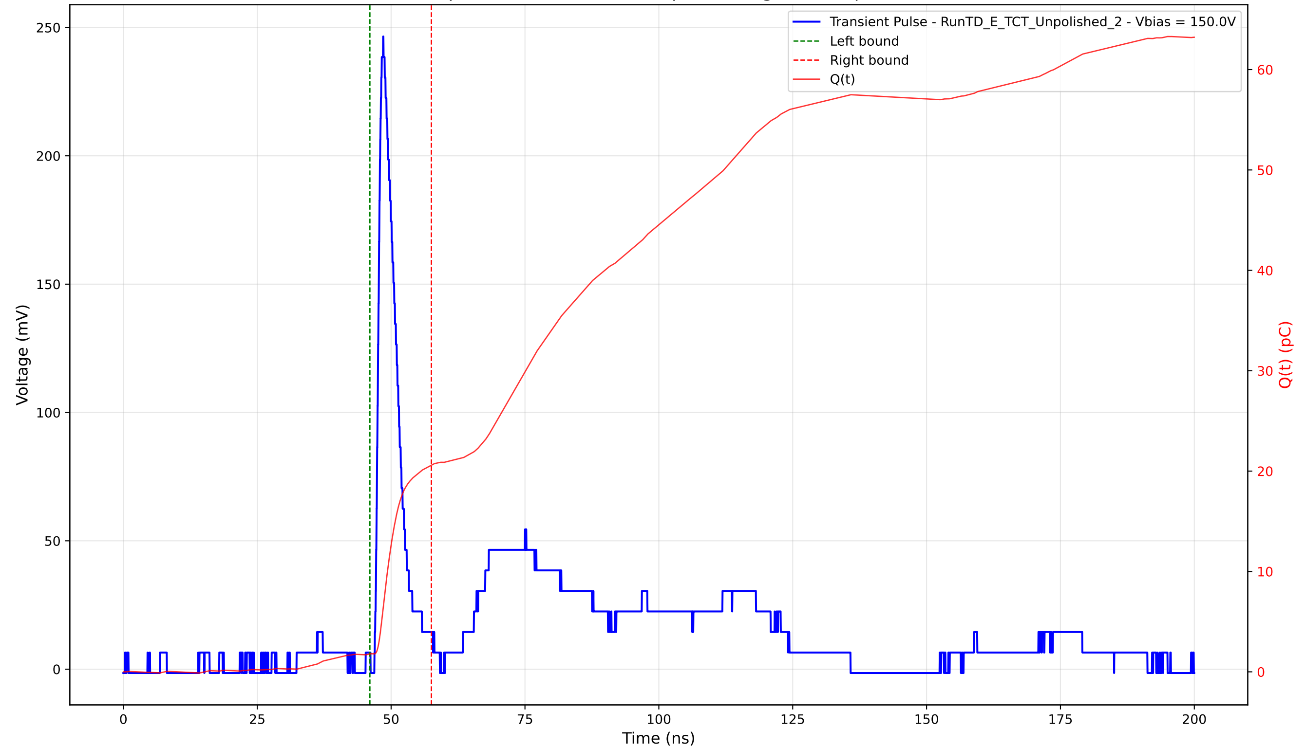
Transient Pulse - Sample: TD - Position: 190.0 \mu\text{m} - Charge: 18.80 pC - Rise Time: 0.97 ns
