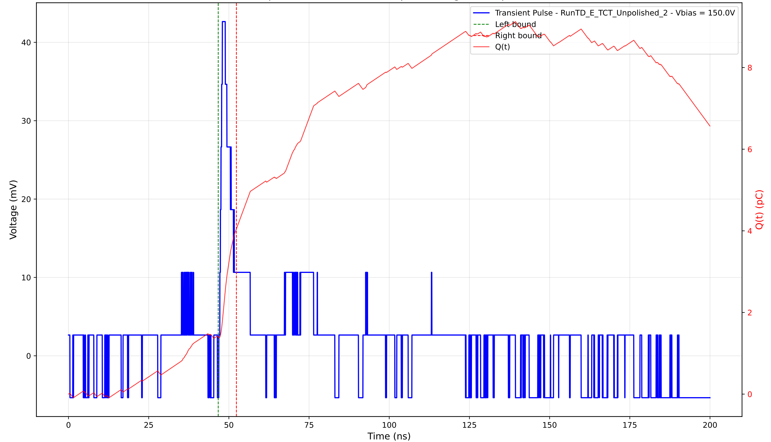
Transient Pulse - Sample: TD - Position: 410.0 \mu\text{m} - Charge: 2.65 pC - Rise Time: 0.80 ns
