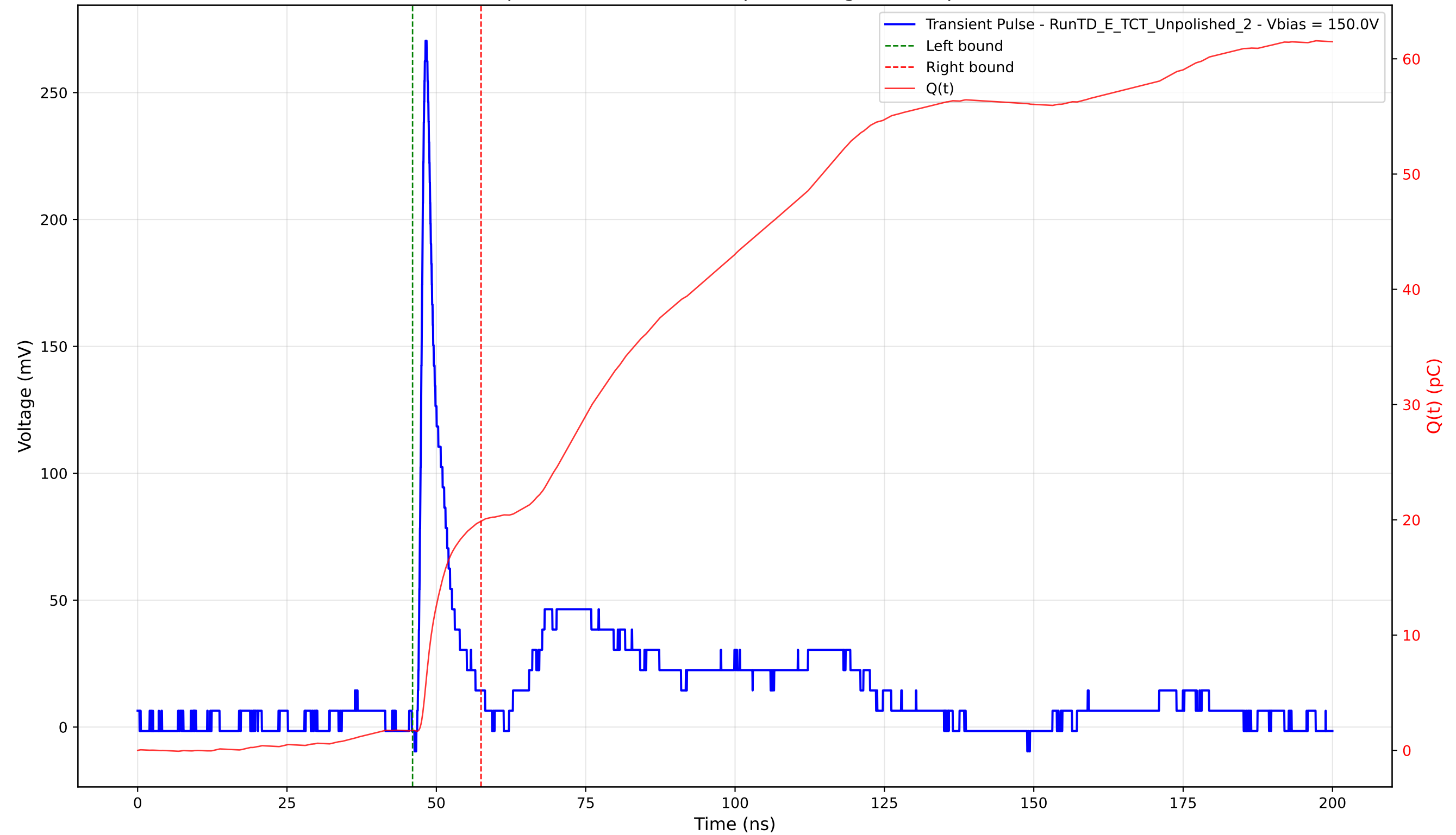
Transient Pulse - Sample: TD - Position: 95.0 \mu\text{m} - Charge: 18.15 pC - Rise Time: 0.91 ns
