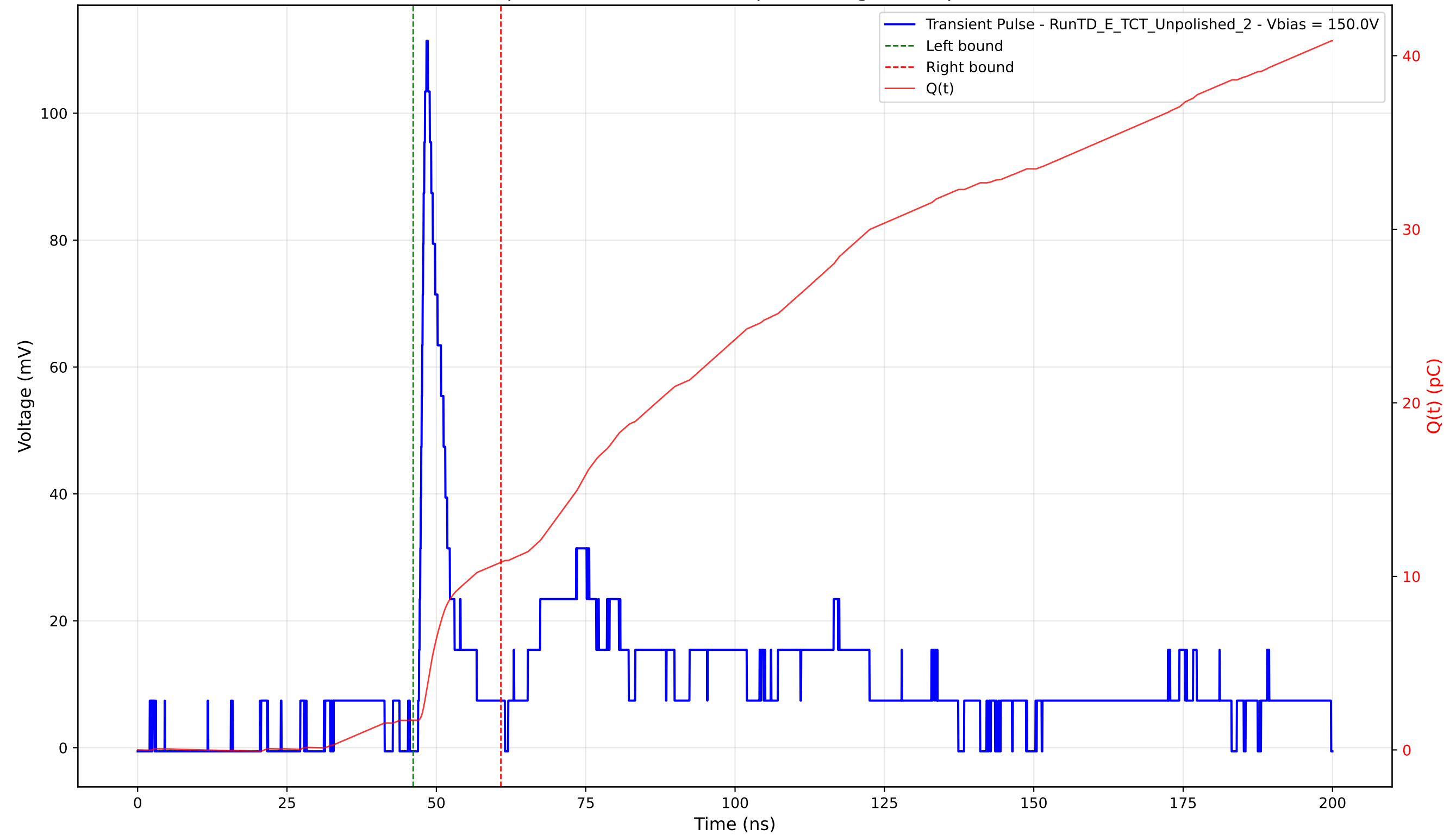
Transient Pulse - Sample: TD - Position: 285.0 \mu\text{m} - Charge: 9.11 pC - Rise Time: 1.01 ns
