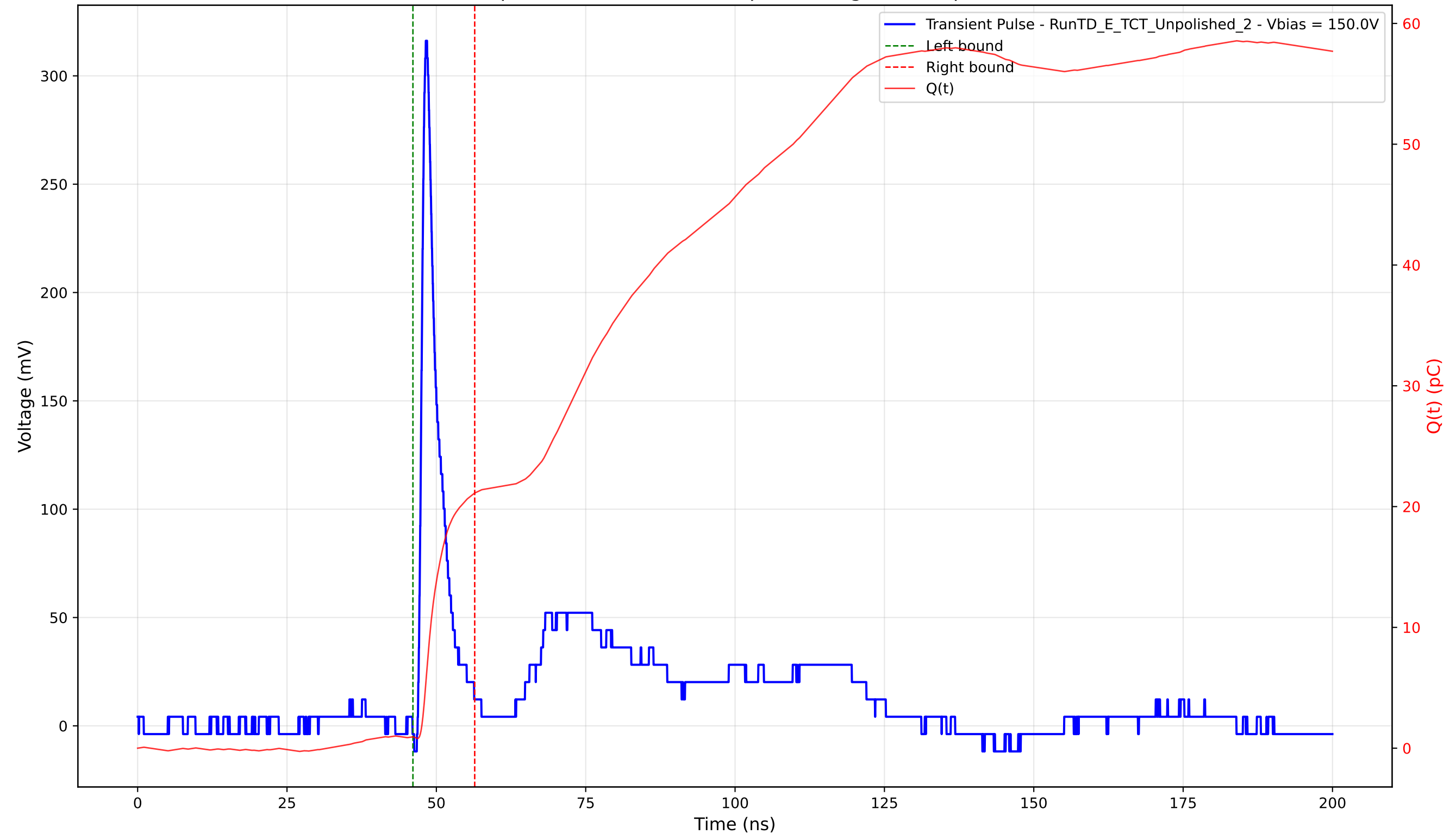
Transient Pulse - Sample: TD - Position: 170.0 \mu\text{m} - Charge: 20.19 pC - Rise Time: 0.93 ns
