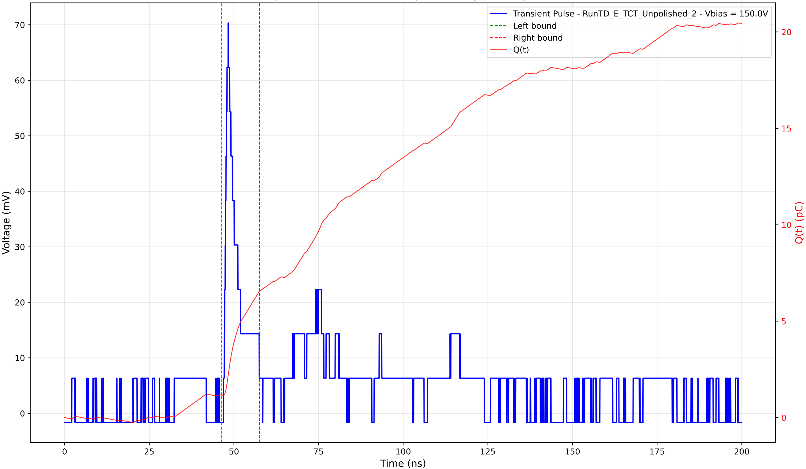
Transient Pulse - Sample: TD - Position: 390.0 \mu\text{m} - Charge: 5.40 pC - Rise Time: 1.18 ns
