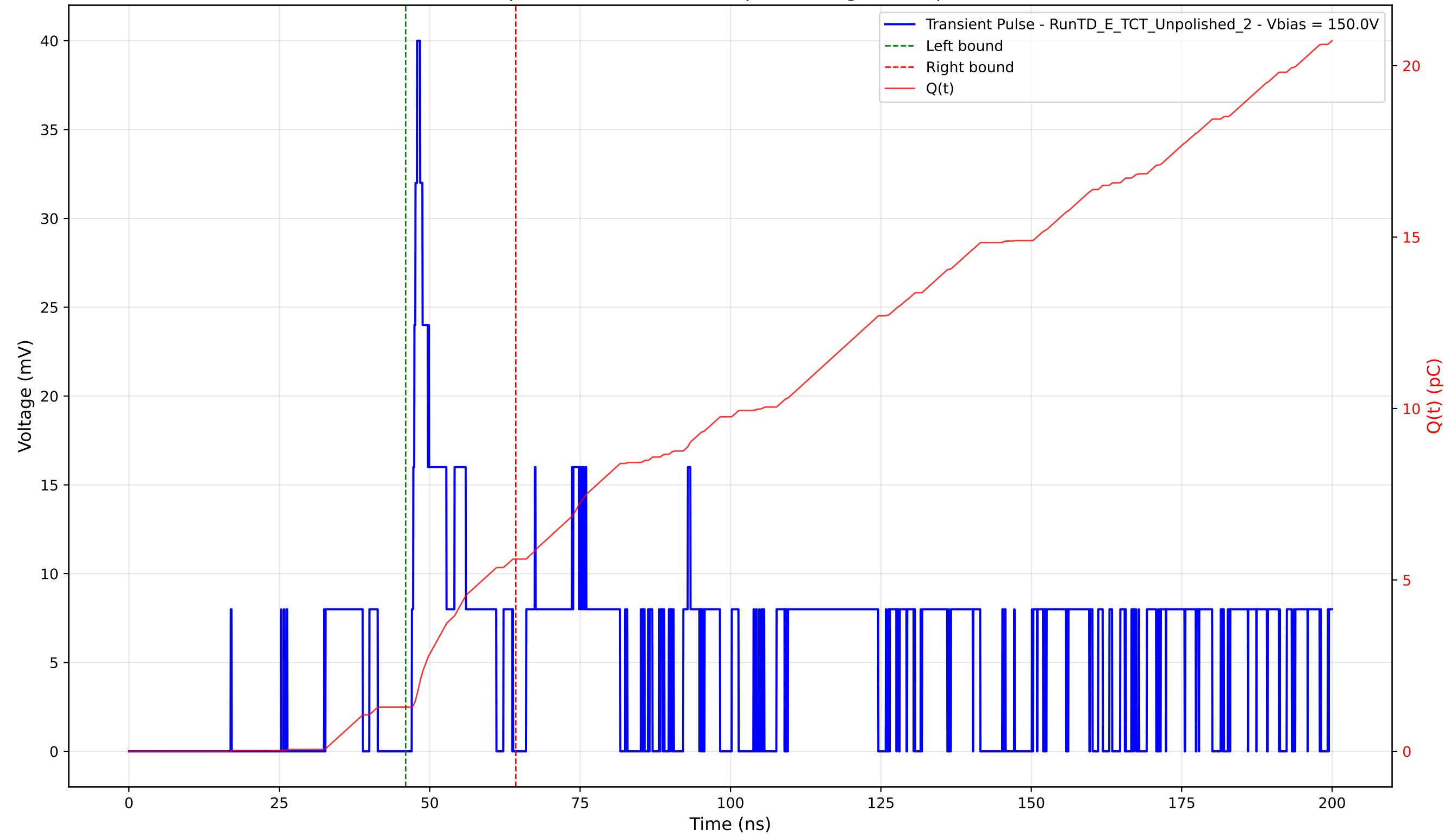
Transient Pulse - Sample: TD - Position: 25.0 \mu\text{m} - Charge: 4.32 pC - Rise Time: 0.89 ns
