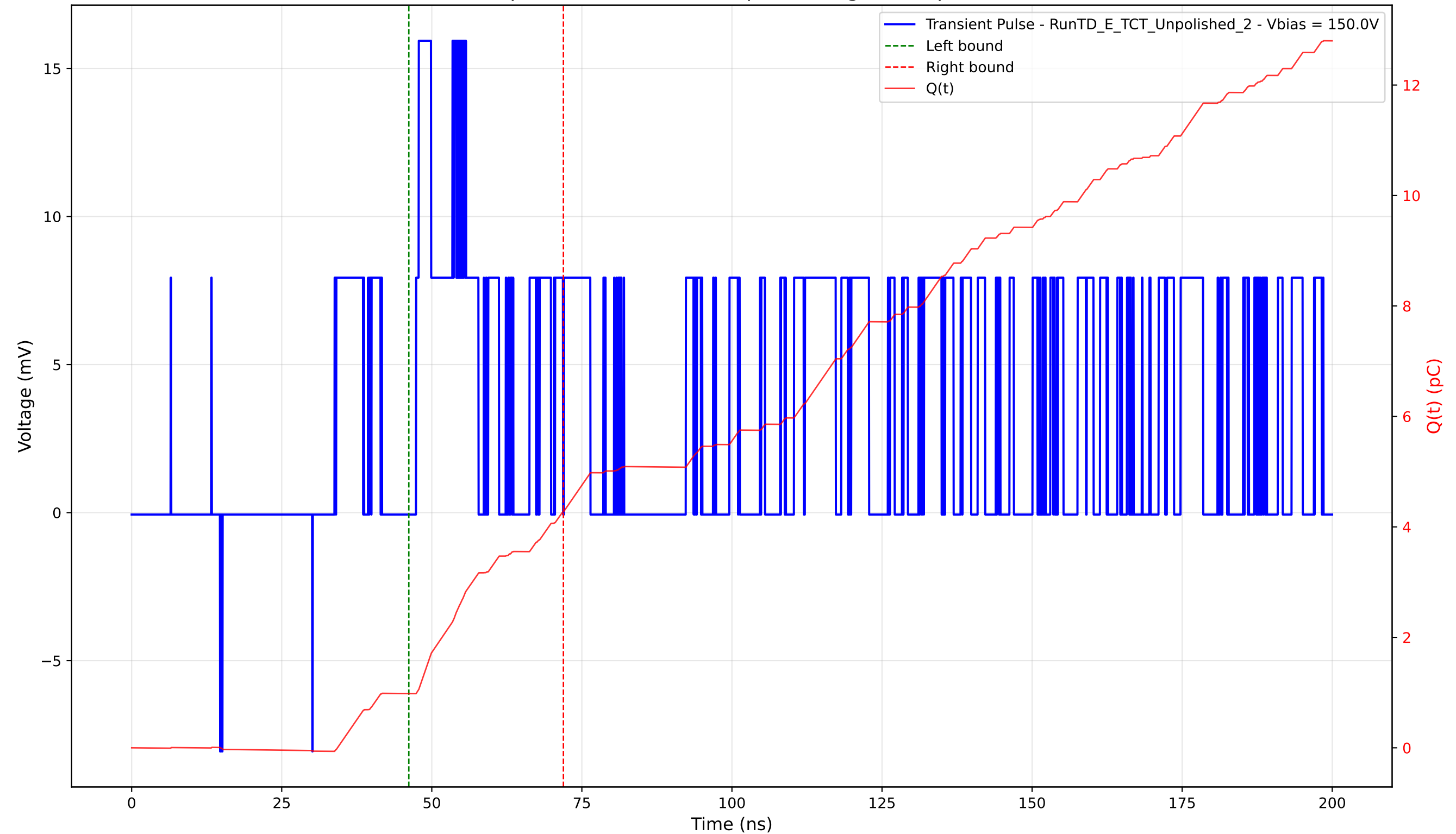
Transient Pulse - Sample: TD - Position: 10.0 \mu m - Charge: 3.30 pC - Rise Time: 0.46 ns
