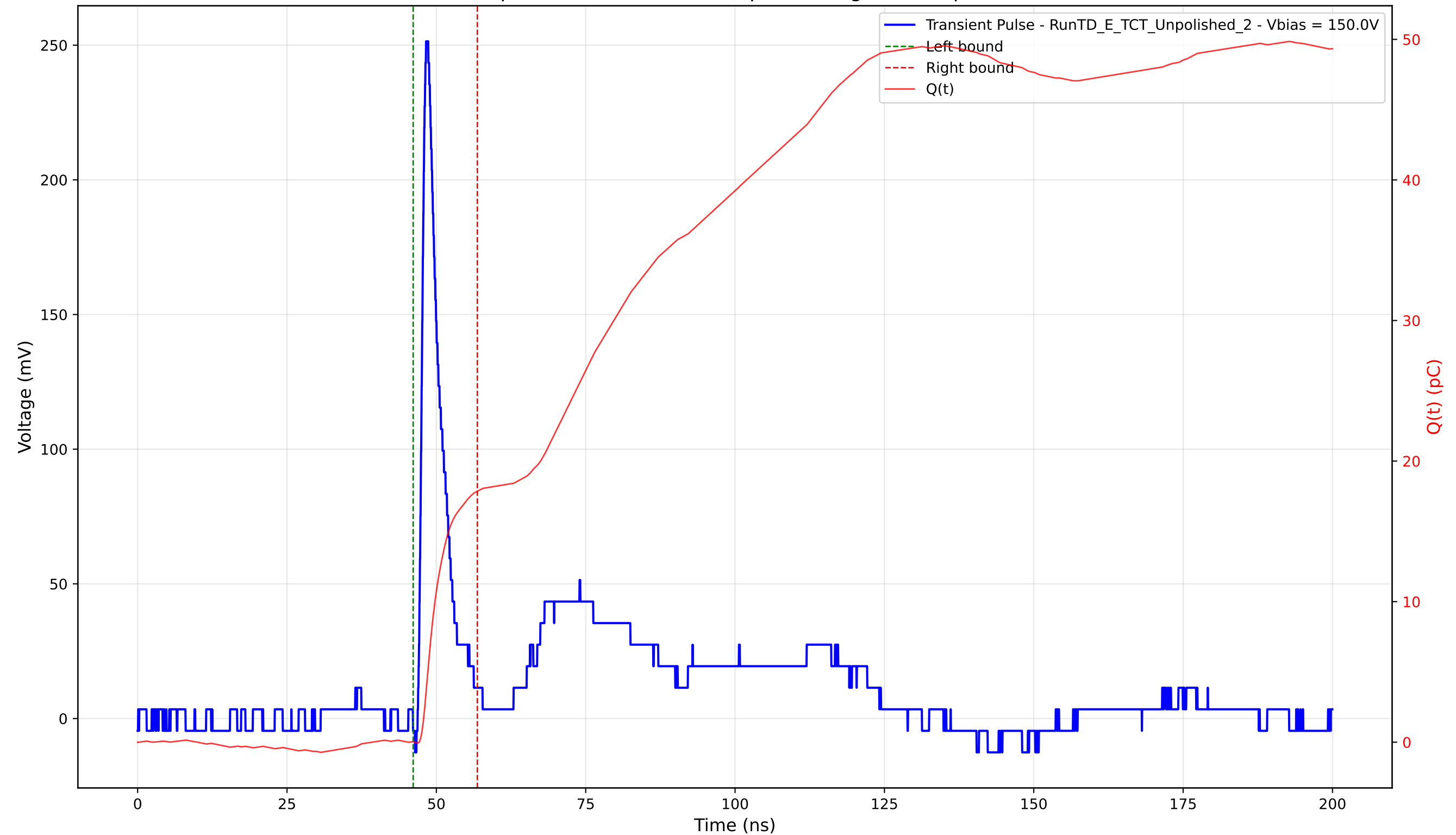
Transient Pulse - Sample: TD - Position: 160.0 \mu\text{m} - Charge: 17.82 pC - Rise Time: 0.95 ns
