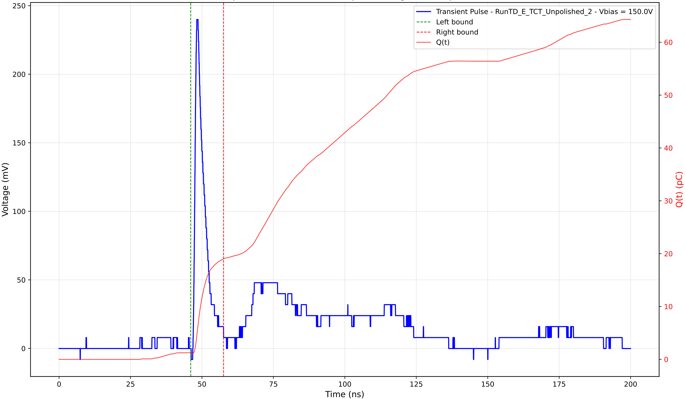
Transient Pulse - Sample: TD - Position: 175.0 \mu\text{m} - Charge: 17.79 pC - Rise Time: 0.96 ns
