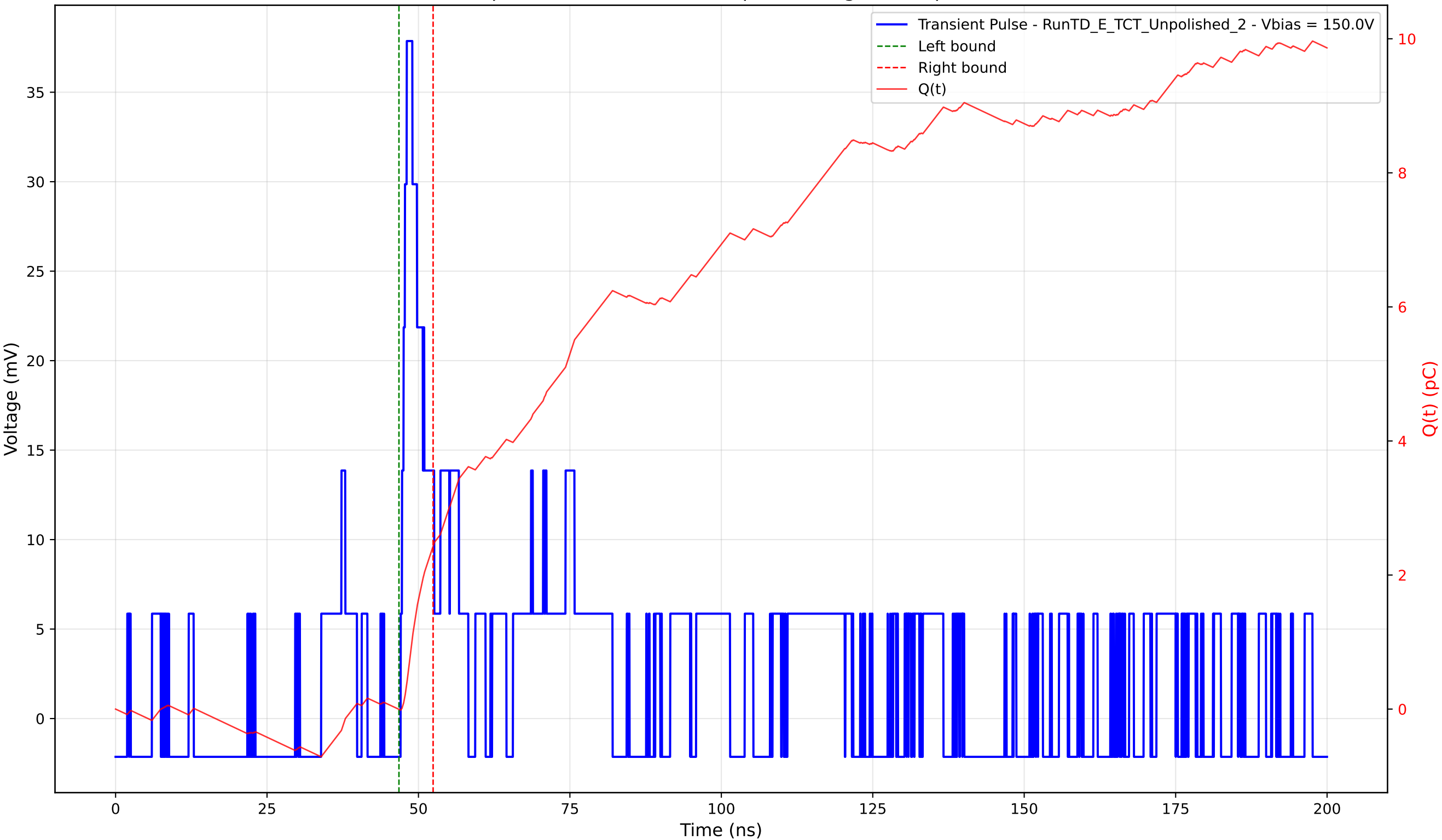
Transient Pulse - Sample: TD - Position: 415.0 \mu\text{m} - Charge: 2.44 pC - Rise Time: 1.01 ns
