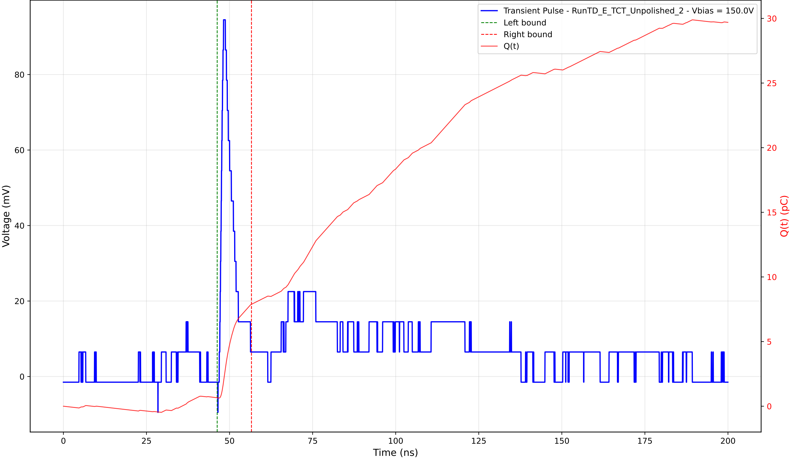
Transient Pulse - Sample: TD - Position: 300.0 \mu\text{m} - Charge: 7.22 pC - Rise Time: 0.95 ns
