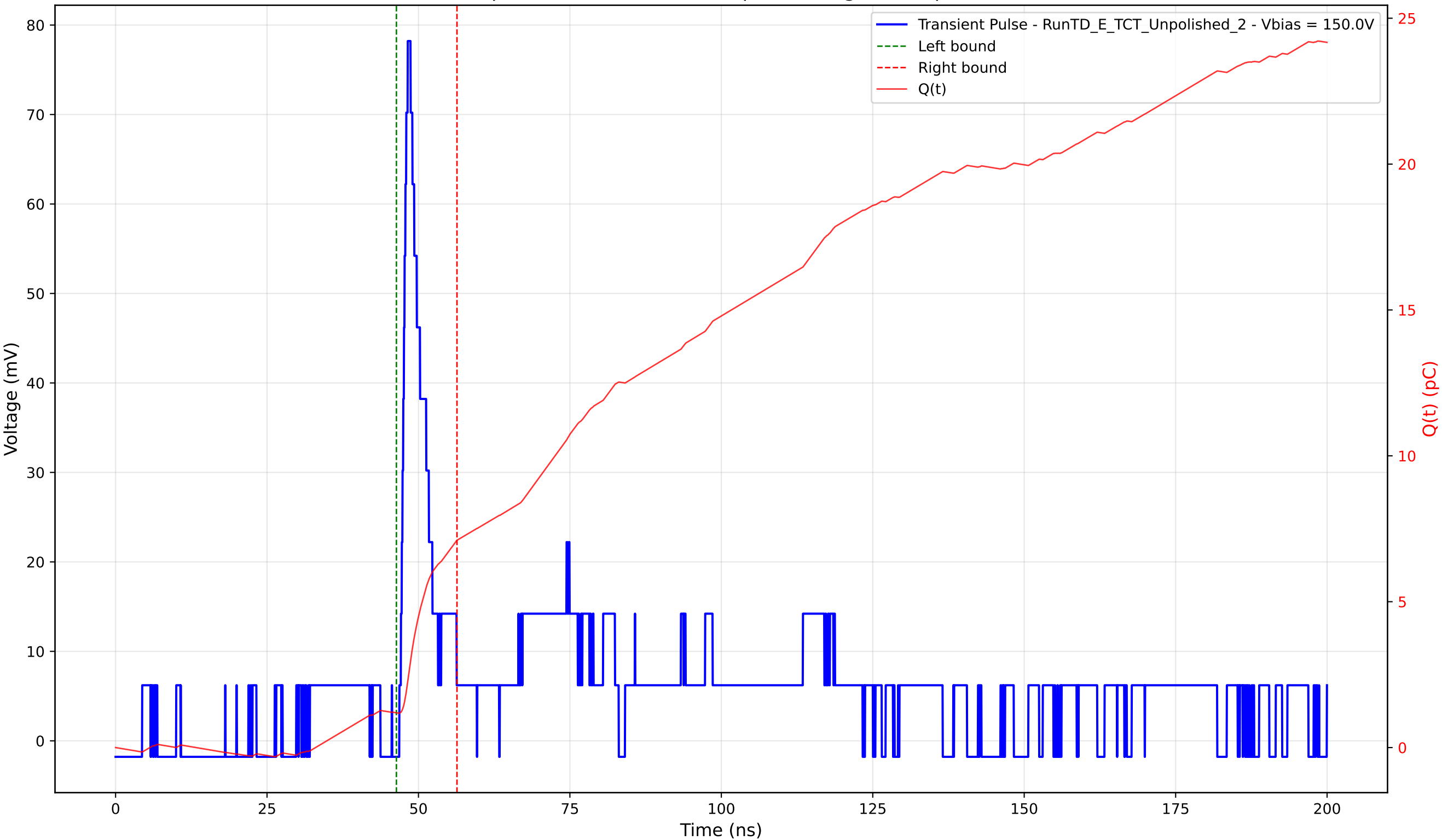
Transient Pulse - Sample: TD - Position: 330.0 \mu\text{m} - Charge: 5.92 pC - Rise Time: 1.14 ns
