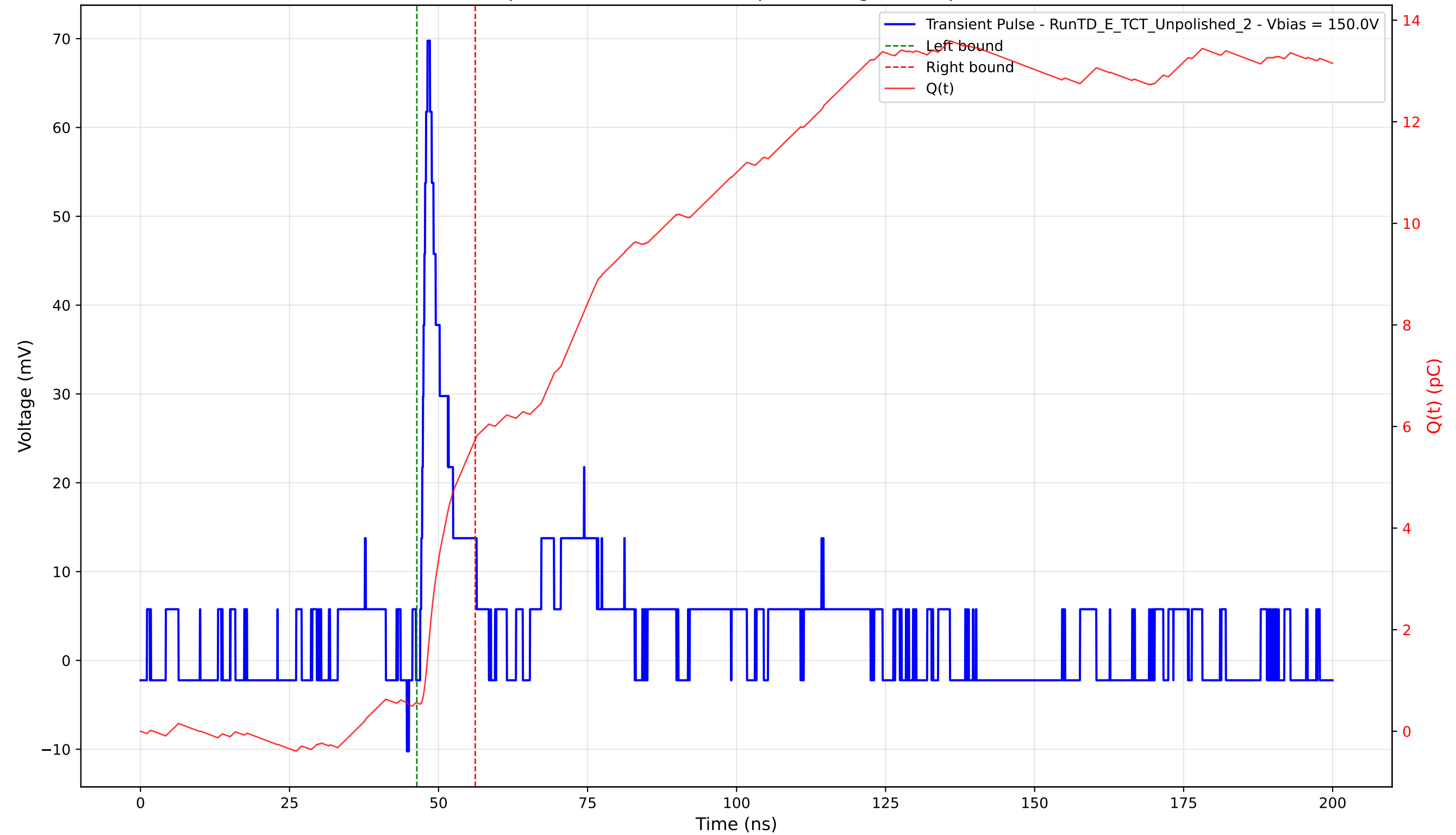
Transient Pulse - Sample: TD - Position: 345.0 \mu\text{m} - Charge: 5.19 pC - Rise Time: 1.06 ns
