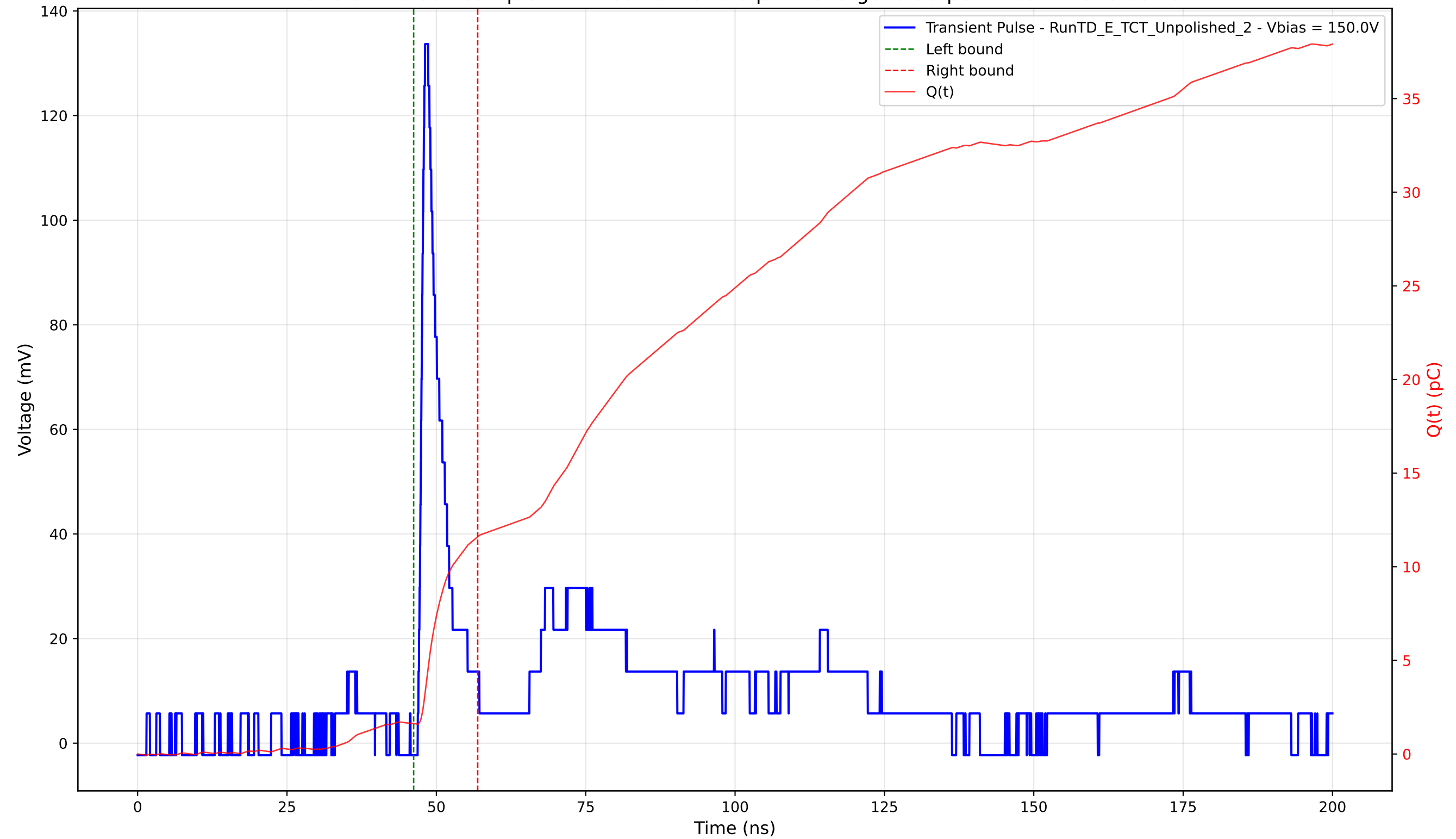
Transient Pulse - Sample: TD - Position: 315.0 \mu\text{m} - Charge: 9.99 pC - Rise Time: 0.98 ns
