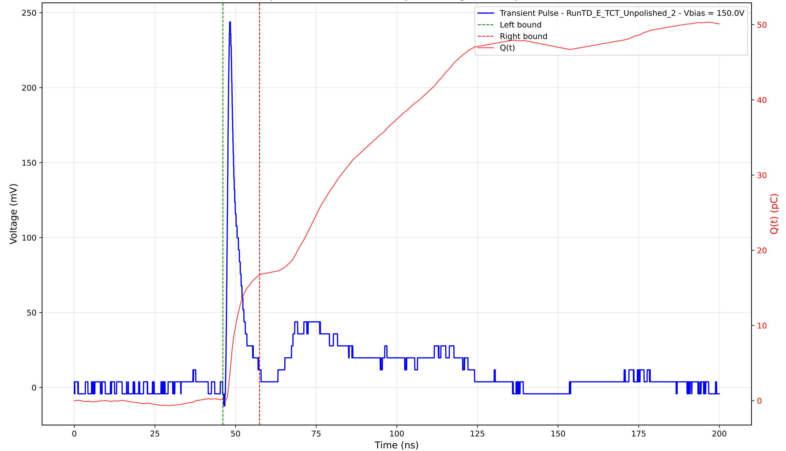
Transient Pulse - Sample: TD - Position: 145.0 \mu\text{m} - Charge: 16.56 pC - Rise Time: 0.89 ns
