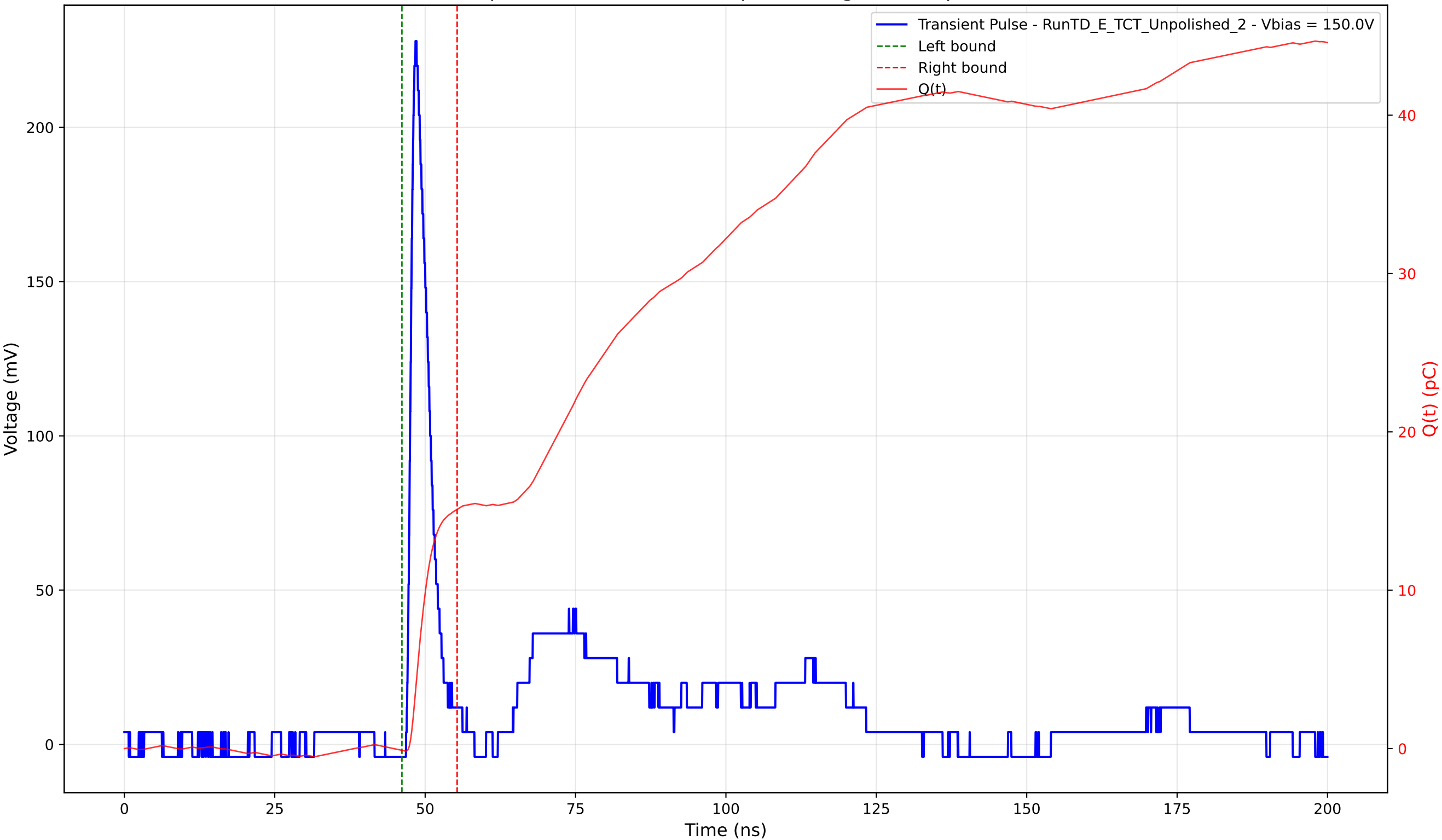
Transient Pulse - Sample: TD - Position: 220.0 \mu\text{m} - Charge: 15.22 pC - Rise Time: 1.03 ns
