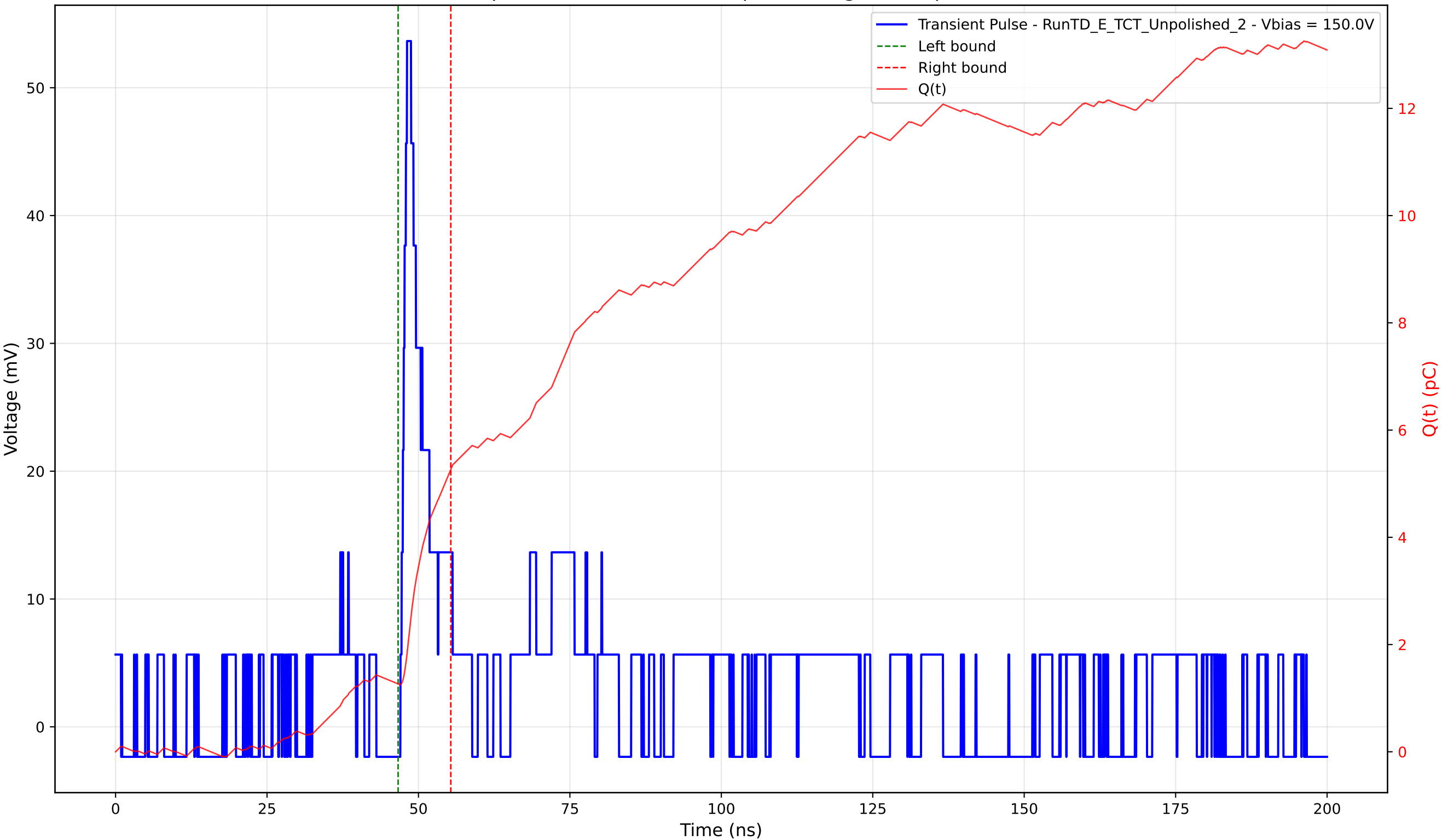
Transient Pulse - Sample: TD - Position: 400.0 \mu\text{m} - Charge: 4.00 pC - Rise Time: 1.08 ns
