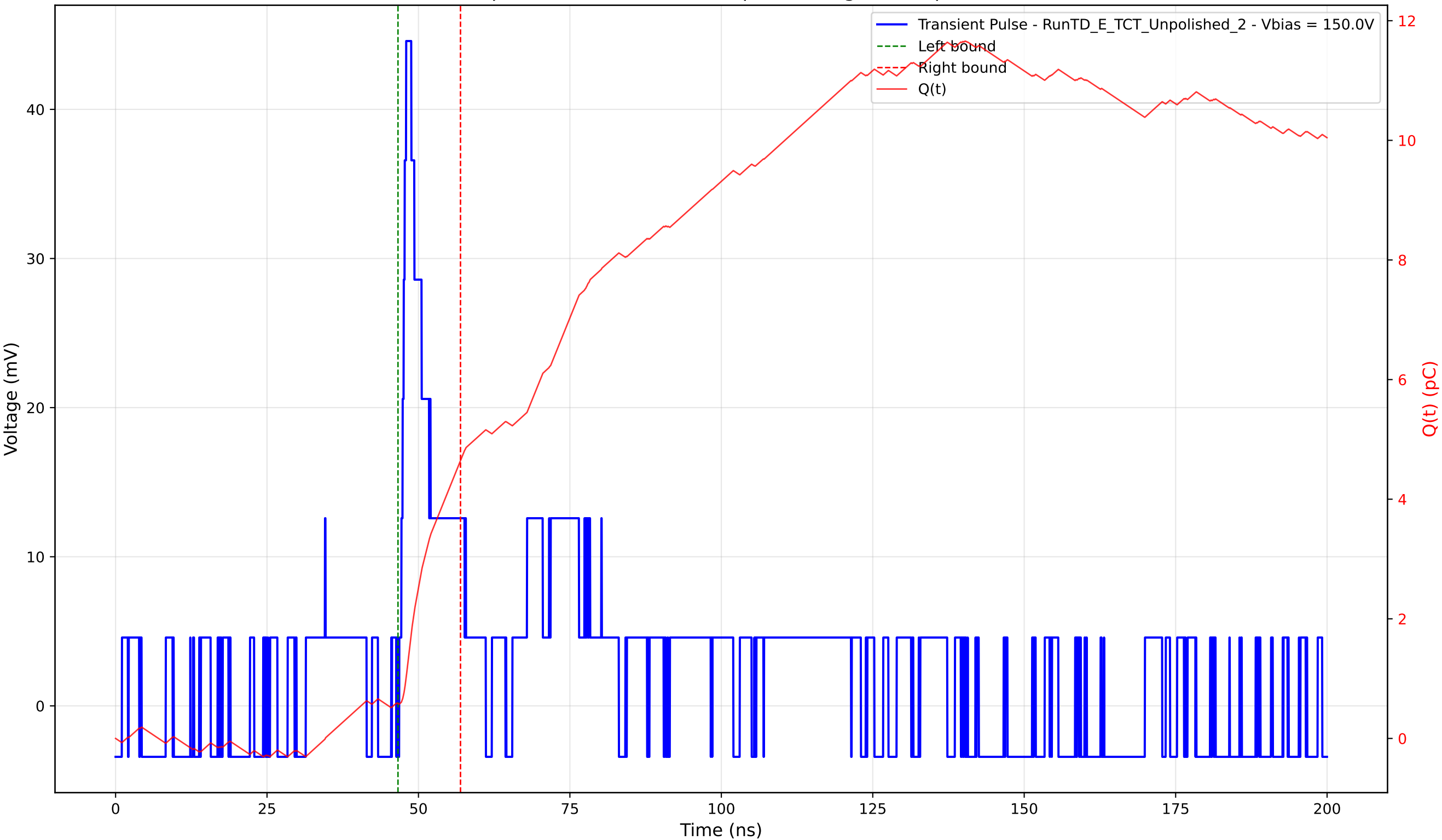
Transient Pulse - Sample: TD - Position: 370.0 \mu\text{m} - Charge: 4.07 pC - Rise Time: 1.14 ns
