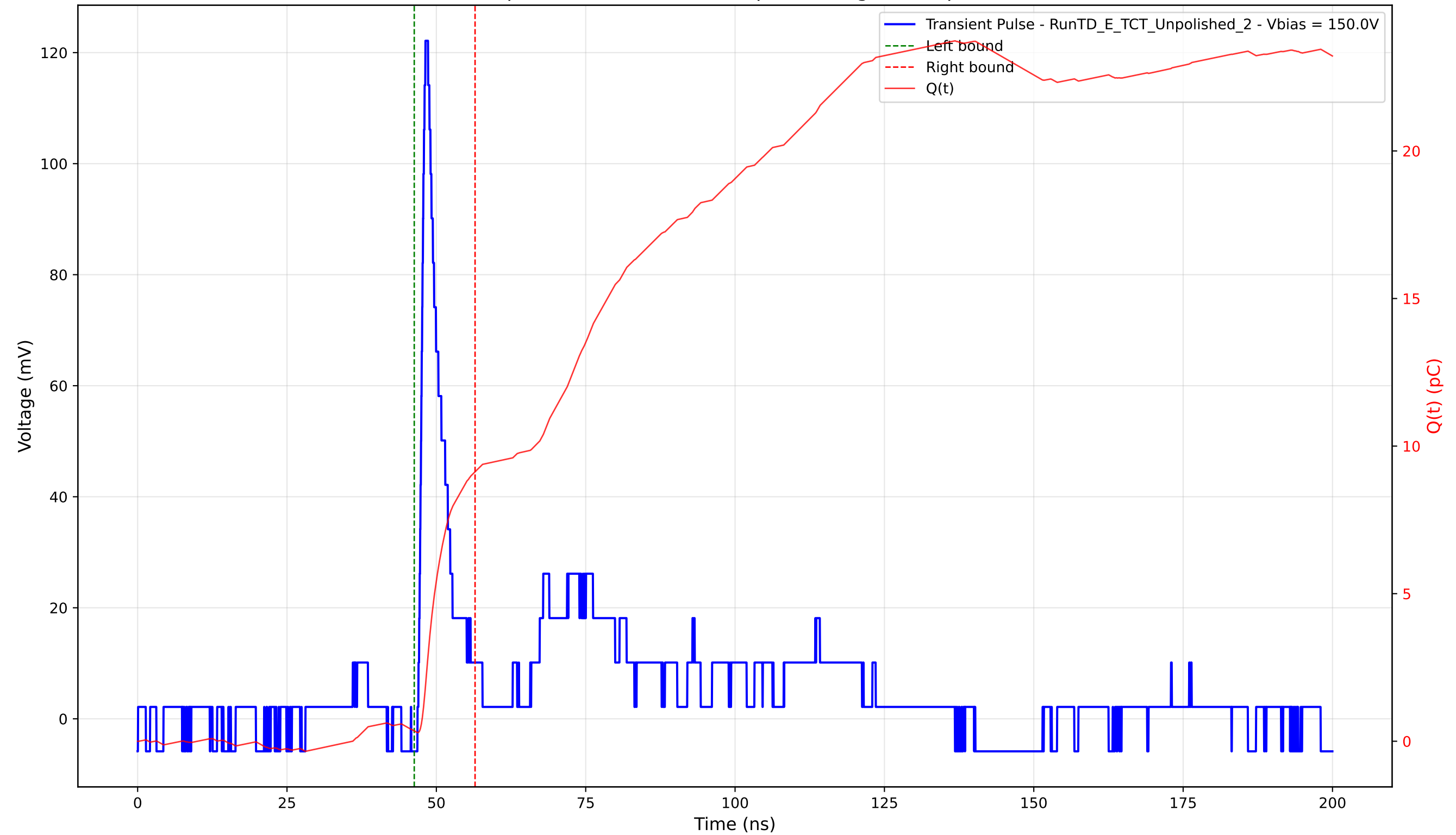
Transient Pulse - Sample: TD - Position: 240.0 \mu\text{m} - Charge: 8.78 pC - Rise Time: 0.91 ns
