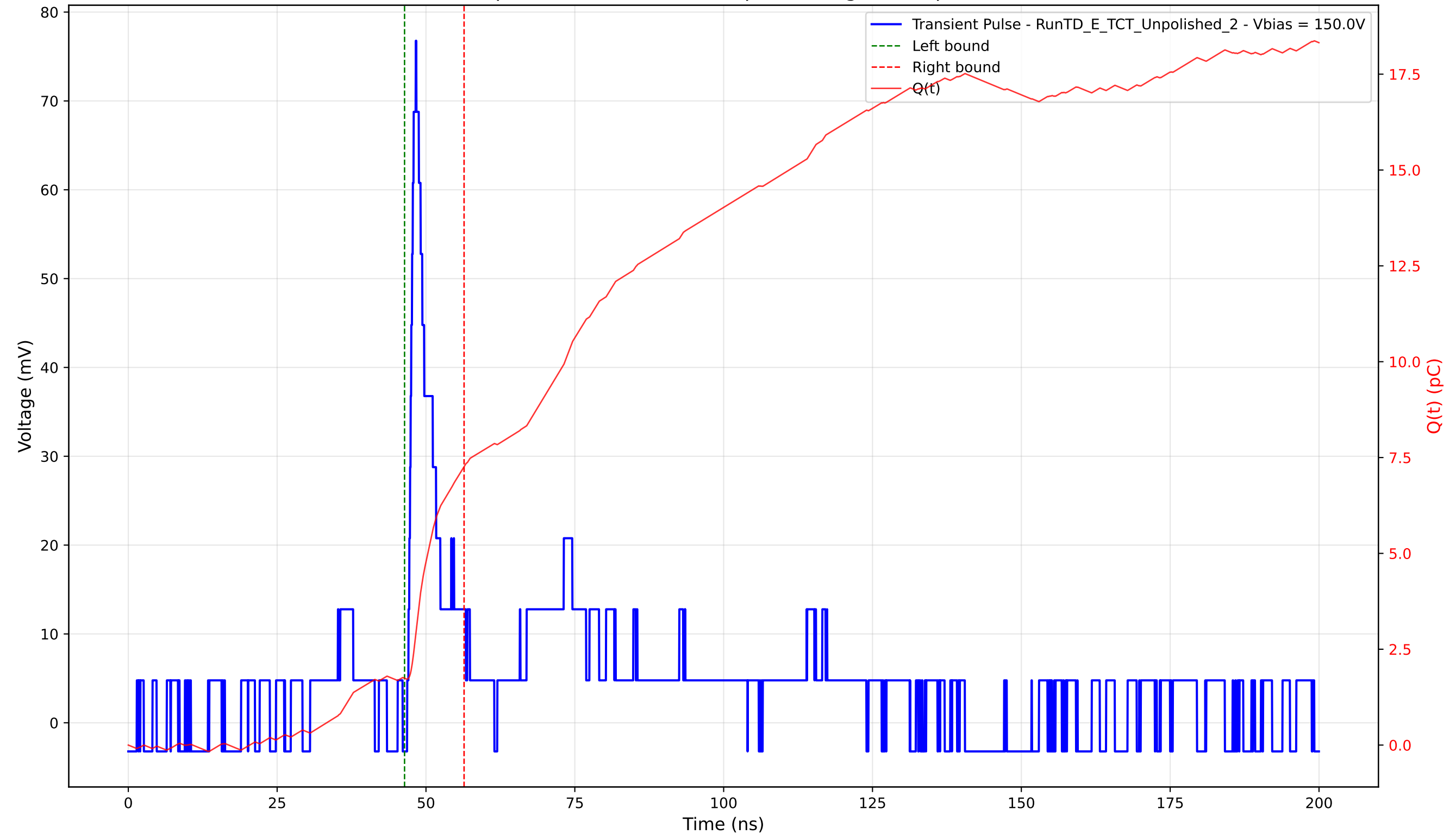
Transient Pulse - Sample: TD - Position: 385.0 \mu\text{m} - Charge: 5.52 pC - Rise Time: 1.23 ns
