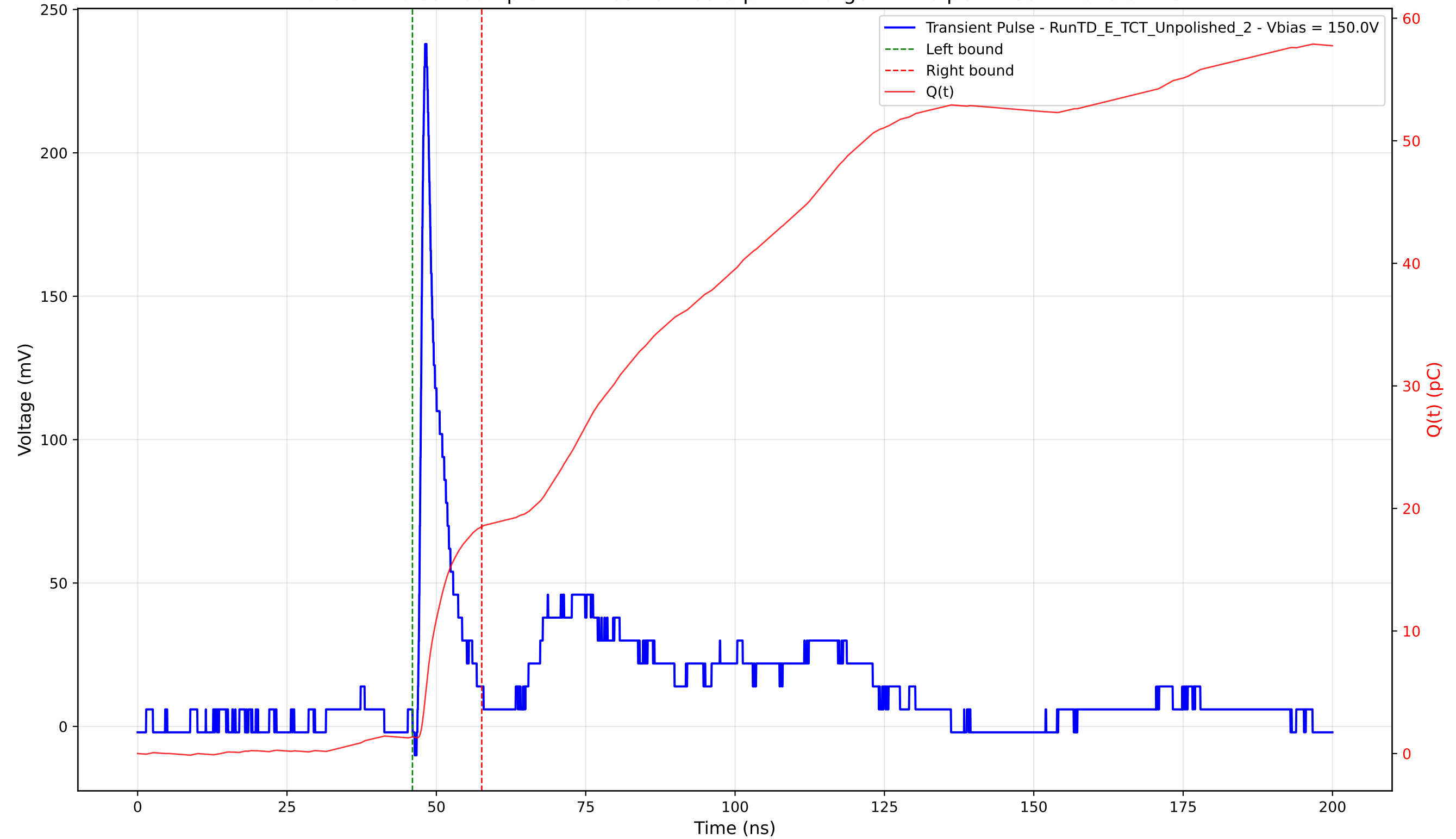
Transient Pulse - Sample: TD - Position: 85.0 \mu\text{m} - Charge: 17.16 pC - Rise Time: 0.92 ns
