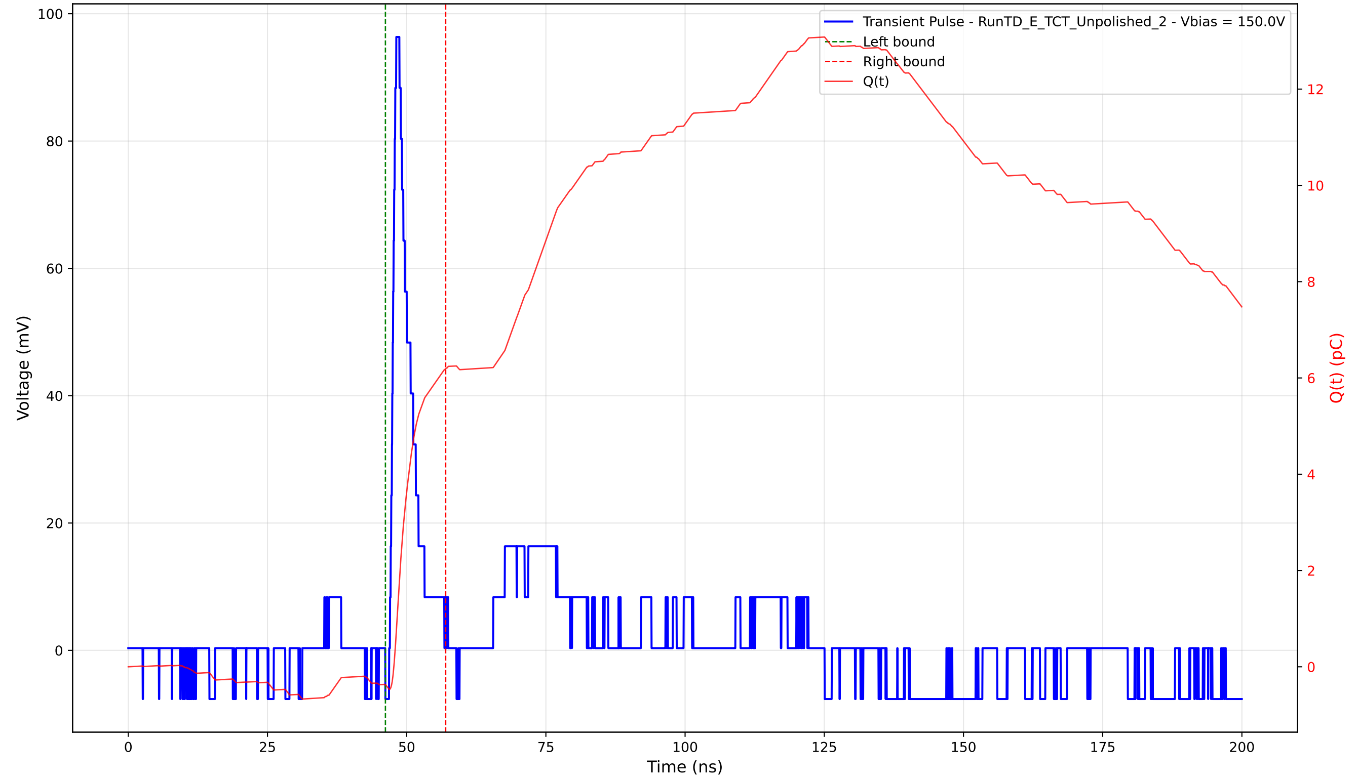
Transient Pulse - Sample: TD - Position: 335.0 \mu\text{m} - Charge: 6.56 pC - Rise Time: 0.84 ns
