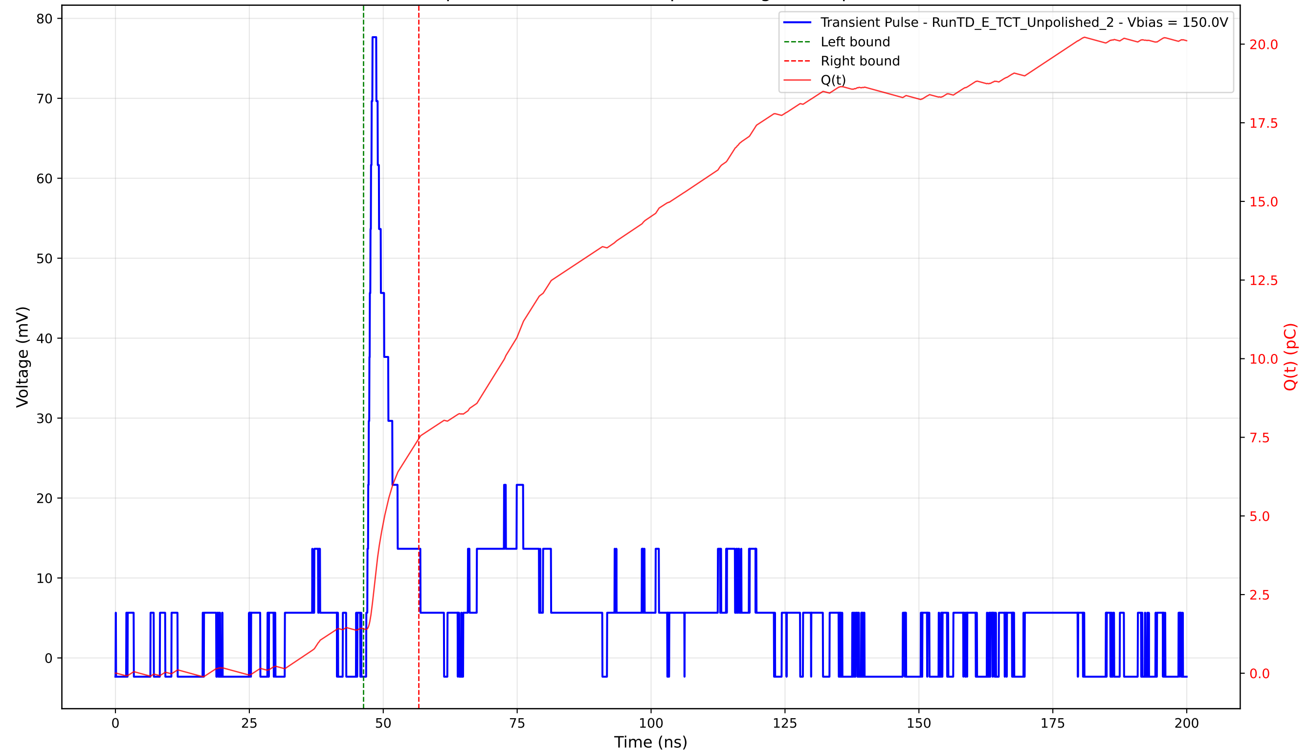
Transient Pulse - Sample: TD - Position: 380.0 \mu\text{m} - Charge: 6.06 pC - Rise Time: 0.95 ns
