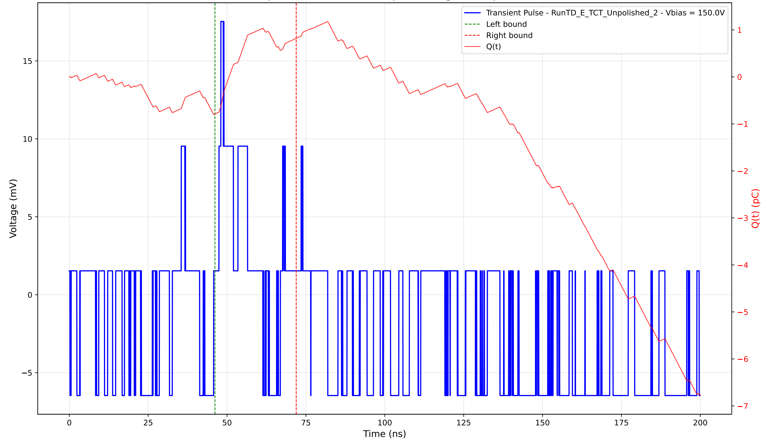
Transient Pulse - Sample: TD - Position: 15.0 \mu\text{m} - Charge: 1.61 pC - Rise Time: 0.62 ns
