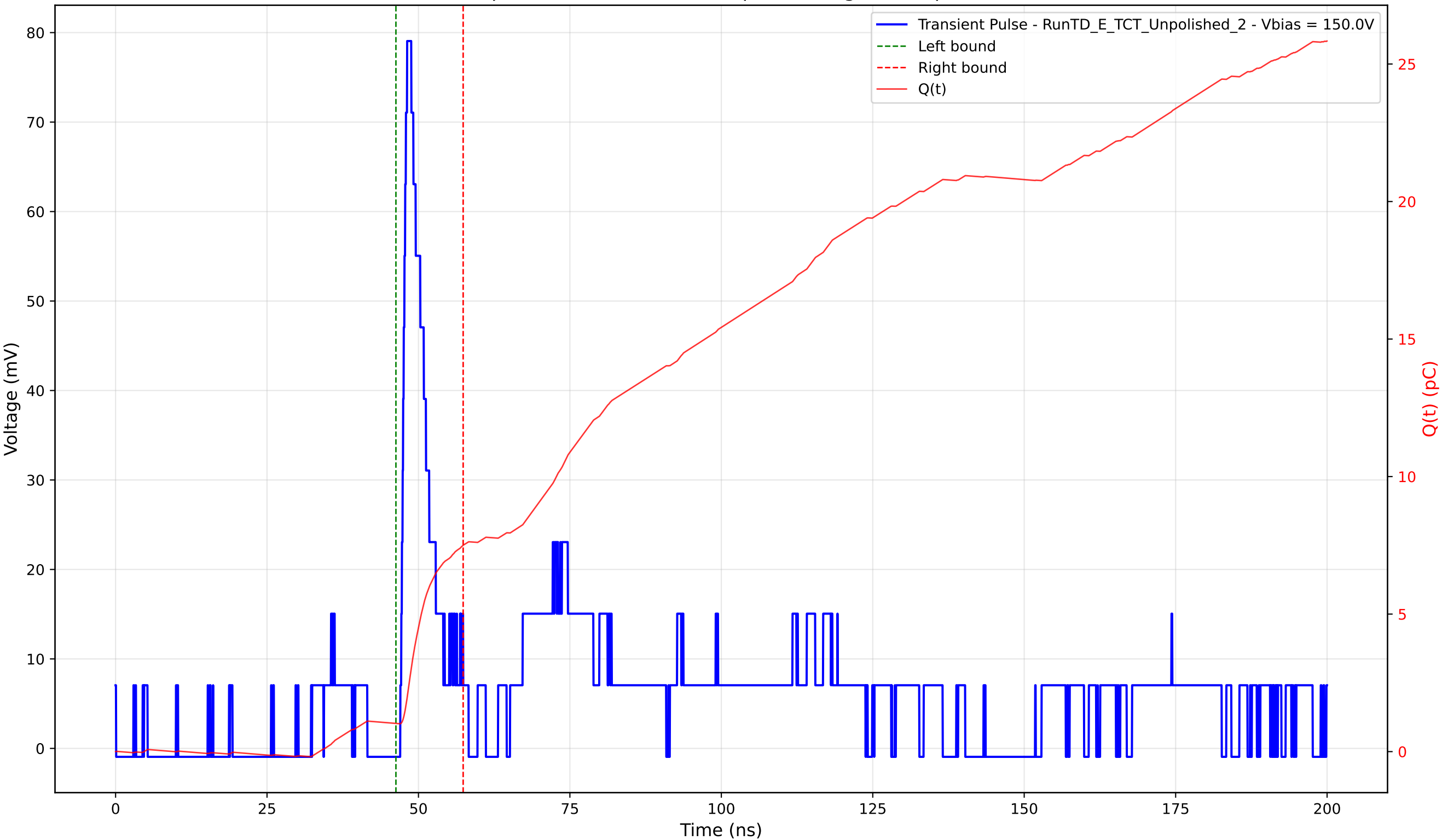
Transient Pulse - Sample: TD - Position: 290.0 \mu\text{m} - Charge: 6.48 pC - Rise Time: 0.98 ns
