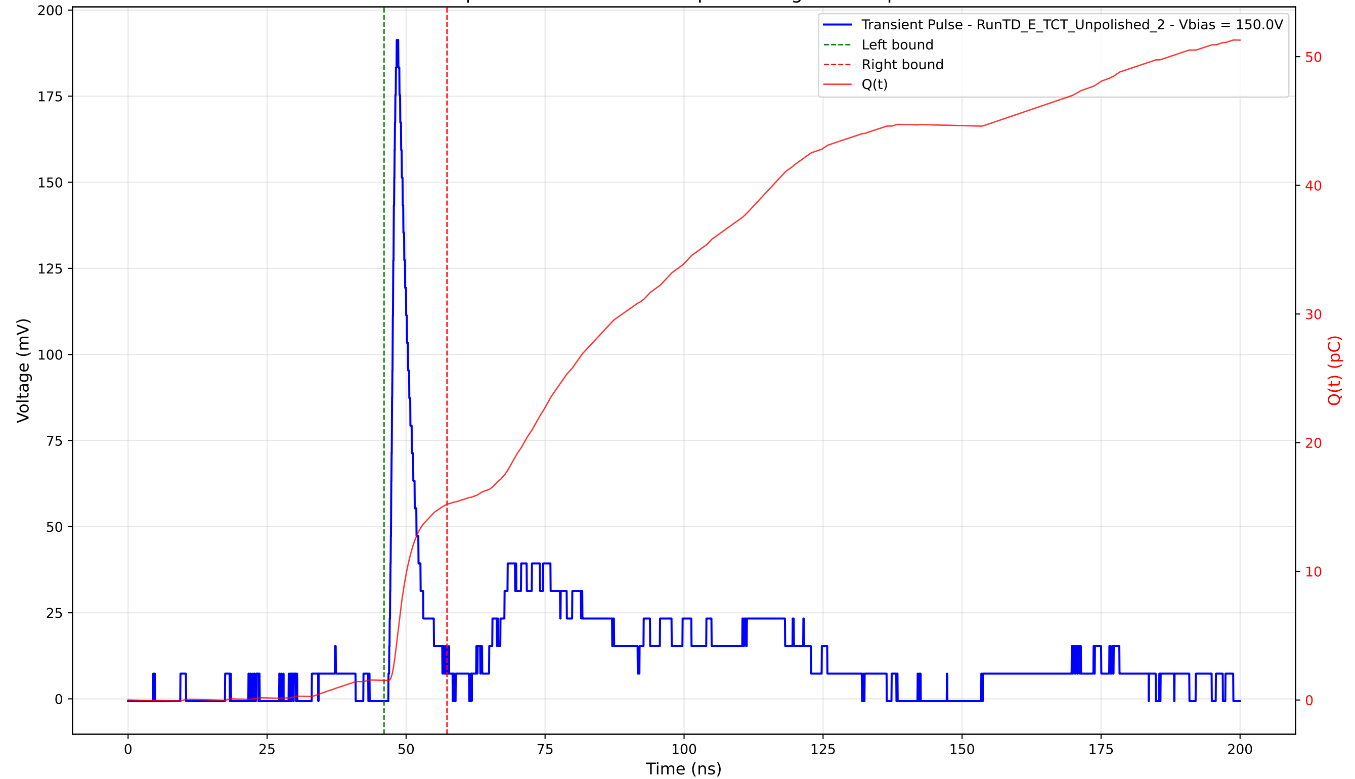
Transient Pulse - Sample: TD - Position: 250.0 \mu\text{m} - Charge: 13.68 pC - Rise Time: 1.03 ns
