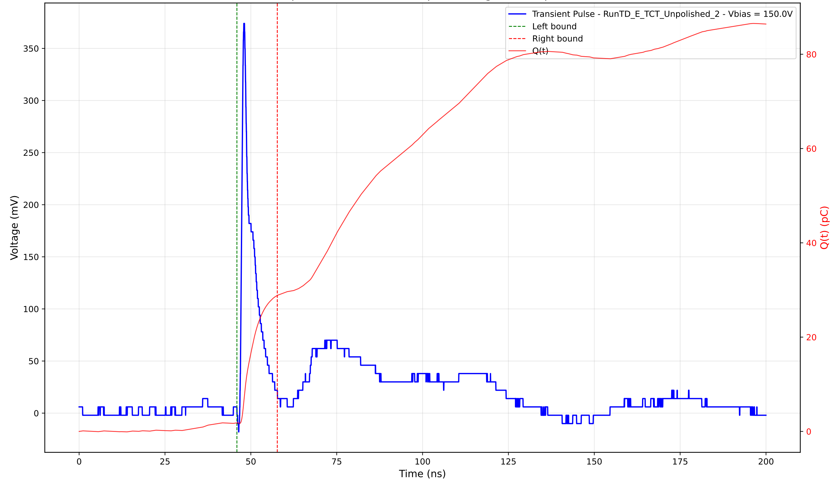
Transient Pulse - Sample: TD - Position: 65.0 \mu\text{m} - Charge: 27.02 pC - Rise Time: 0.81 ns
