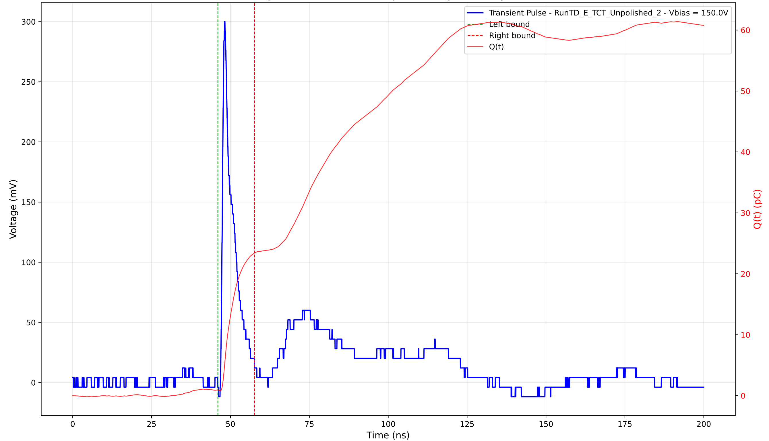
Transient Pulse - Sample: TD - Position: 80.0 \mu\text{m} - Charge: 22.48 pC - Rise Time: 0.90 ns
