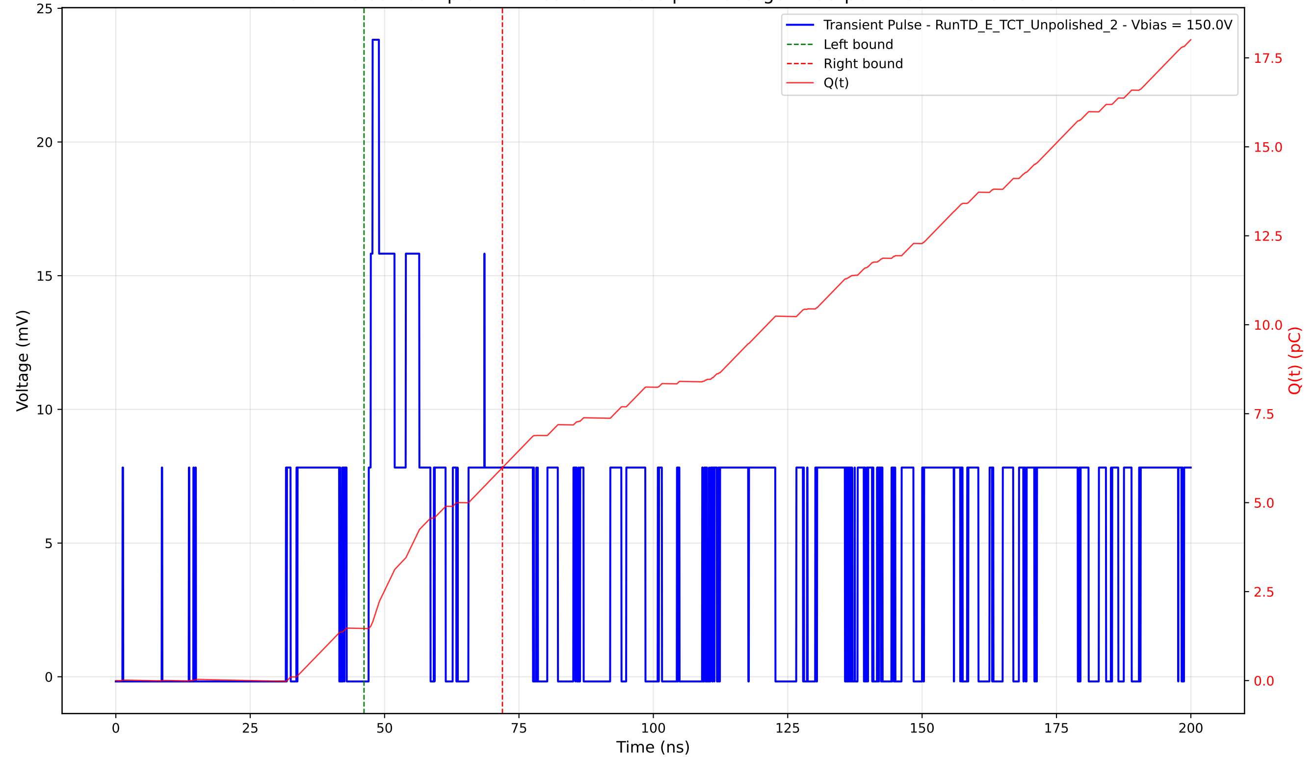
Transient Pulse - Sample: TD - Position: 355.0 \mu\text{m} - Charge: 4.53 pC - Rise Time: 0.73 ns
