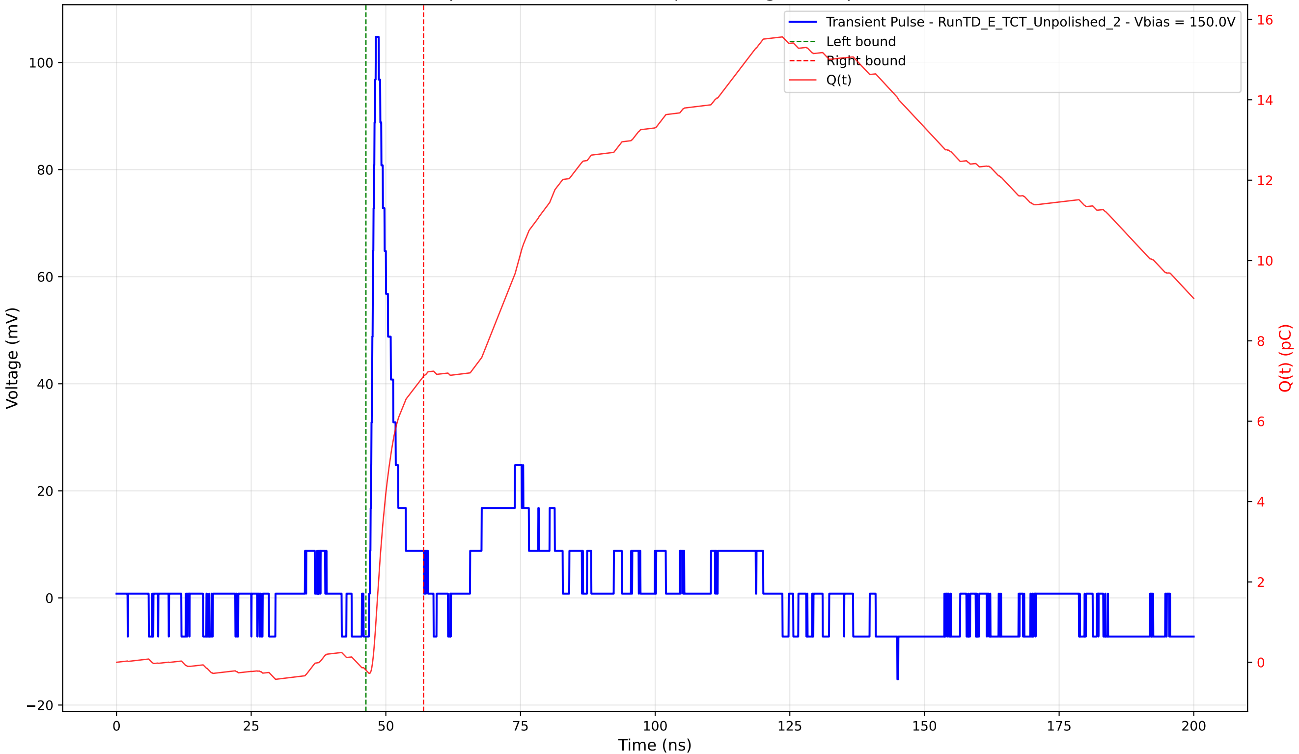
Transient Pulse - Sample: TD - Position: 320.0 \mu\text{m} - Charge: 7.32 pC - Rise Time: 0.86 ns
