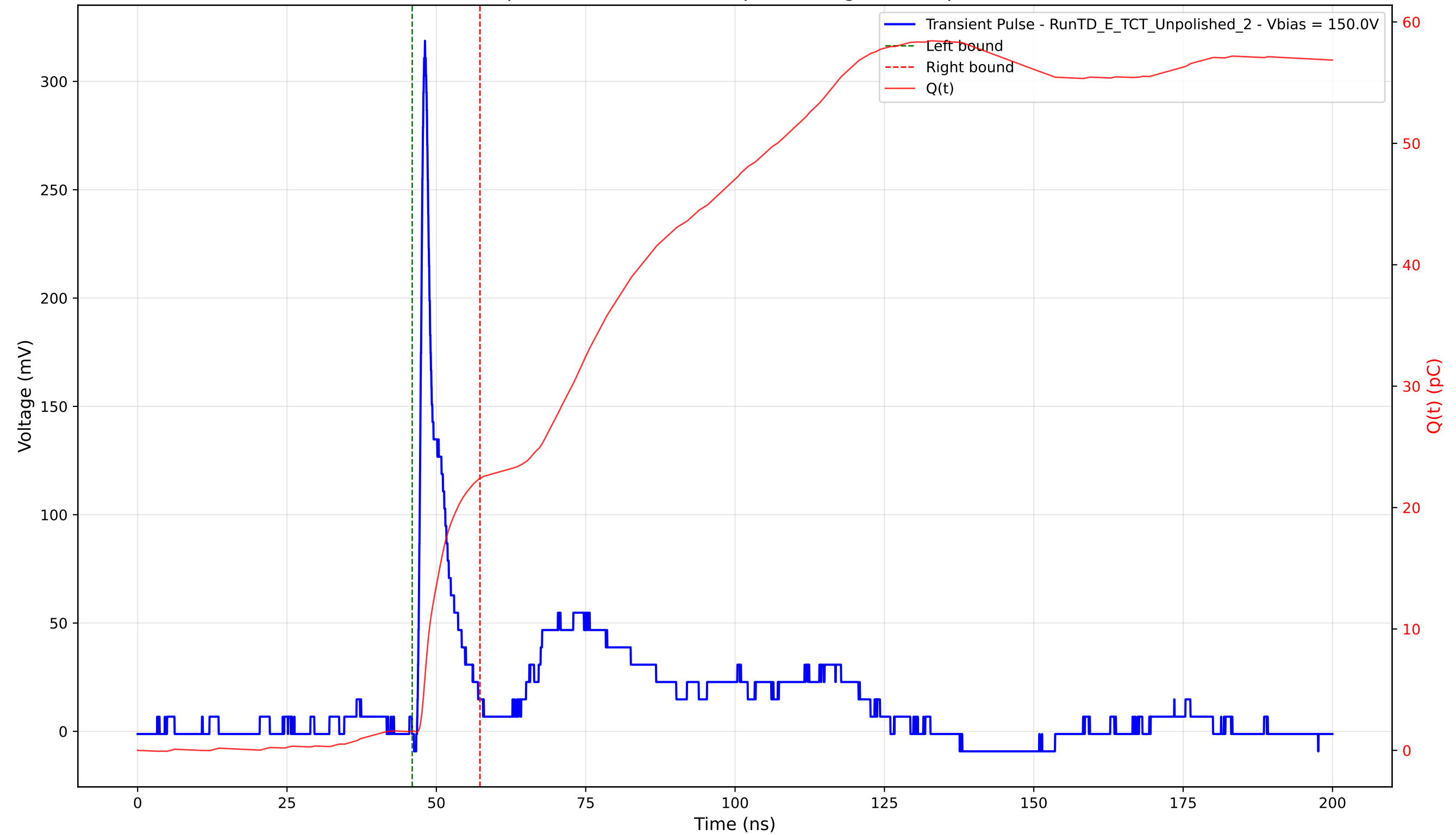
Transient Pulse - Sample: TD - Position: 40.0 \mu\text{m} - Charge: 20.80 pC - Rise Time: 0.88 ns
