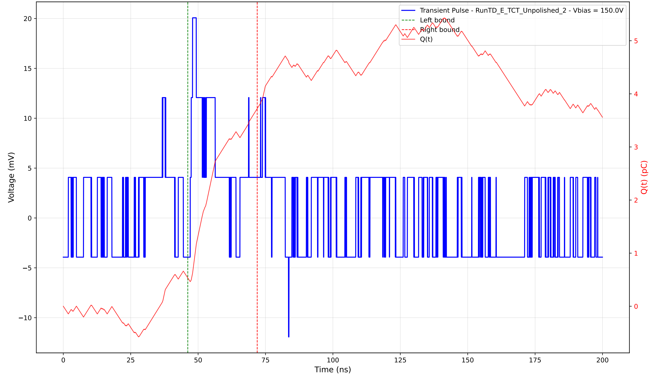
Transient Pulse - Sample: TD - Position: 360.0 \mu\text{m} - Charge: 3.19 pC - Rise Time: 0.00 ns (N/A)
