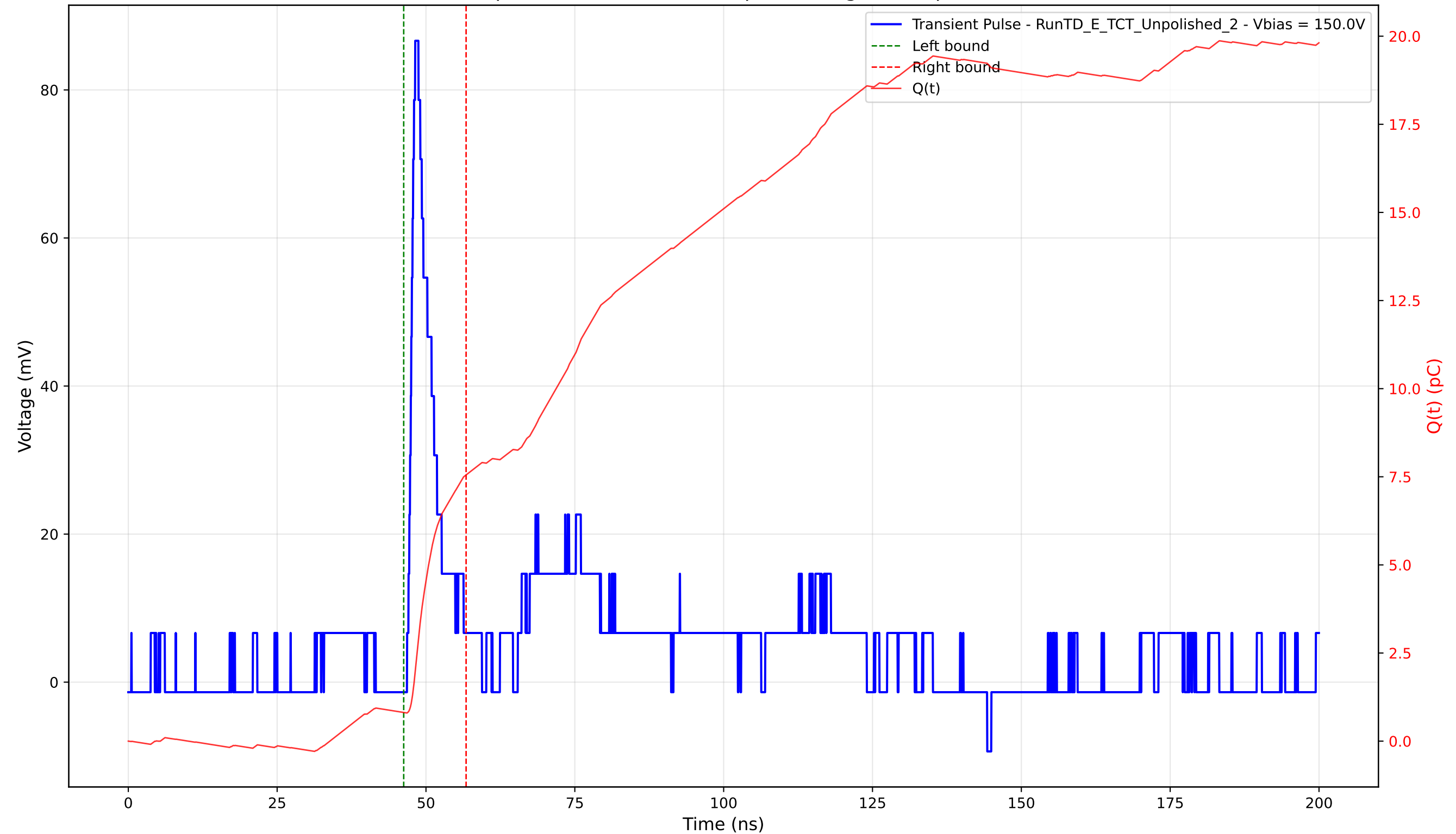
Transient Pulse - Sample: TD - Position: 305.0 \mu\text{m} - Charge: 6.74 pC - Rise Time: 0.93 ns
