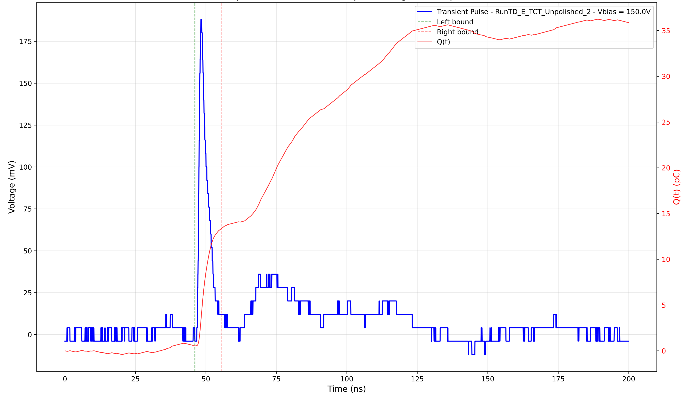
Transient Pulse - Sample: TD - Position: 230.0 \mu\text{m} - Charge: 12.77 pC - Rise Time: 0.98 ns
