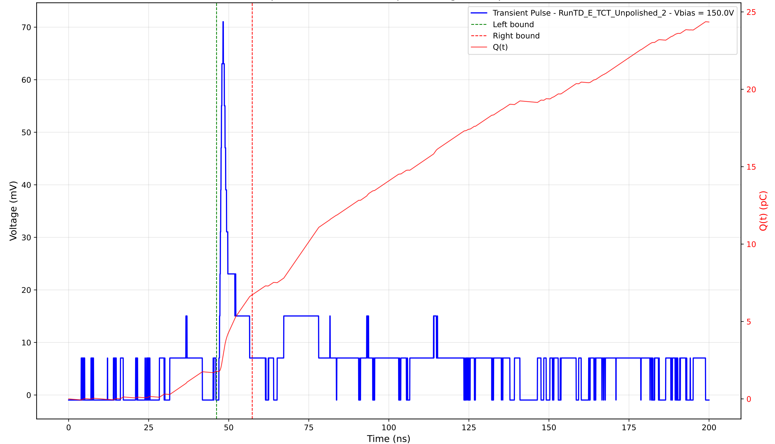
Transient Pulse - Sample: TD - Position: 30.0 \mu\text{m} - Charge: 4.95 pC - Rise Time: 1.10 ns
