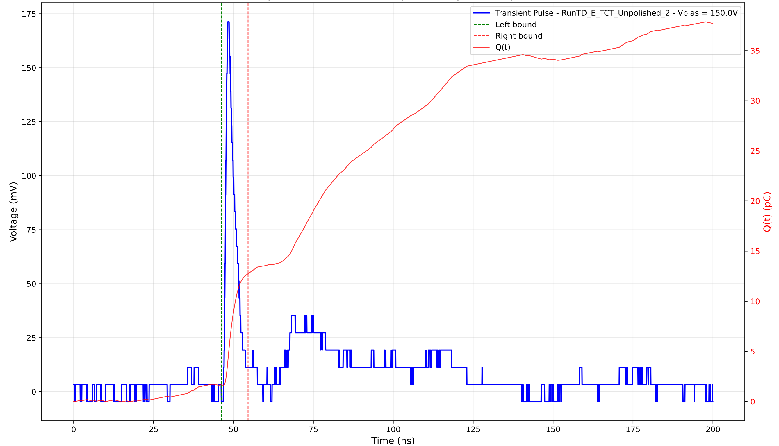
Transient Pulse - Sample: TD - Position: 275.0 \mu\text{m} - Charge: 11.08 pC - Rise Time: 0.95 ns
