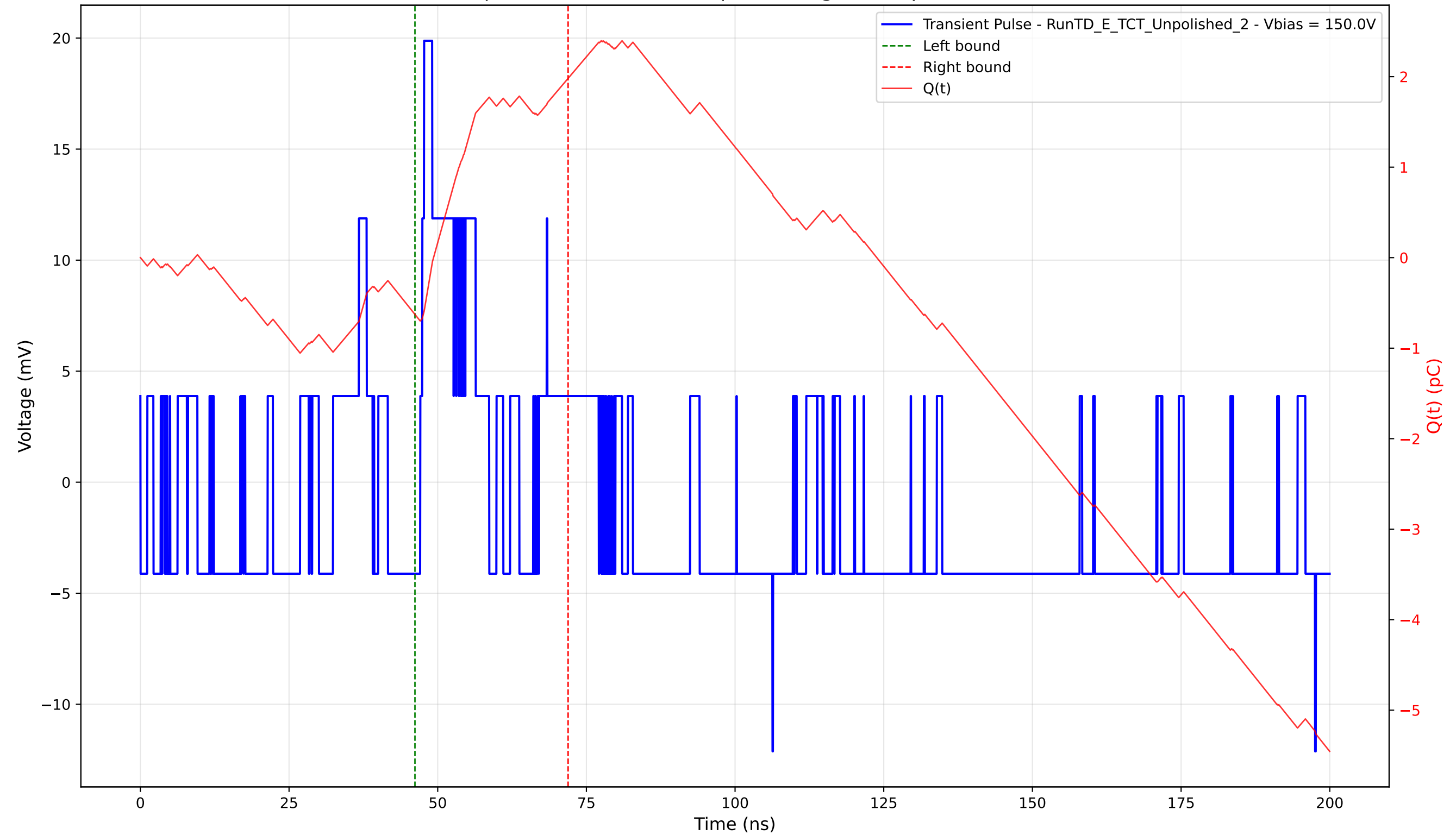
Transient Pulse - Sample: TD - Position: 20.0 \mu\text{m} - Charge: 2.61 pC - Rise Time: 0.00 ns (N/A)
