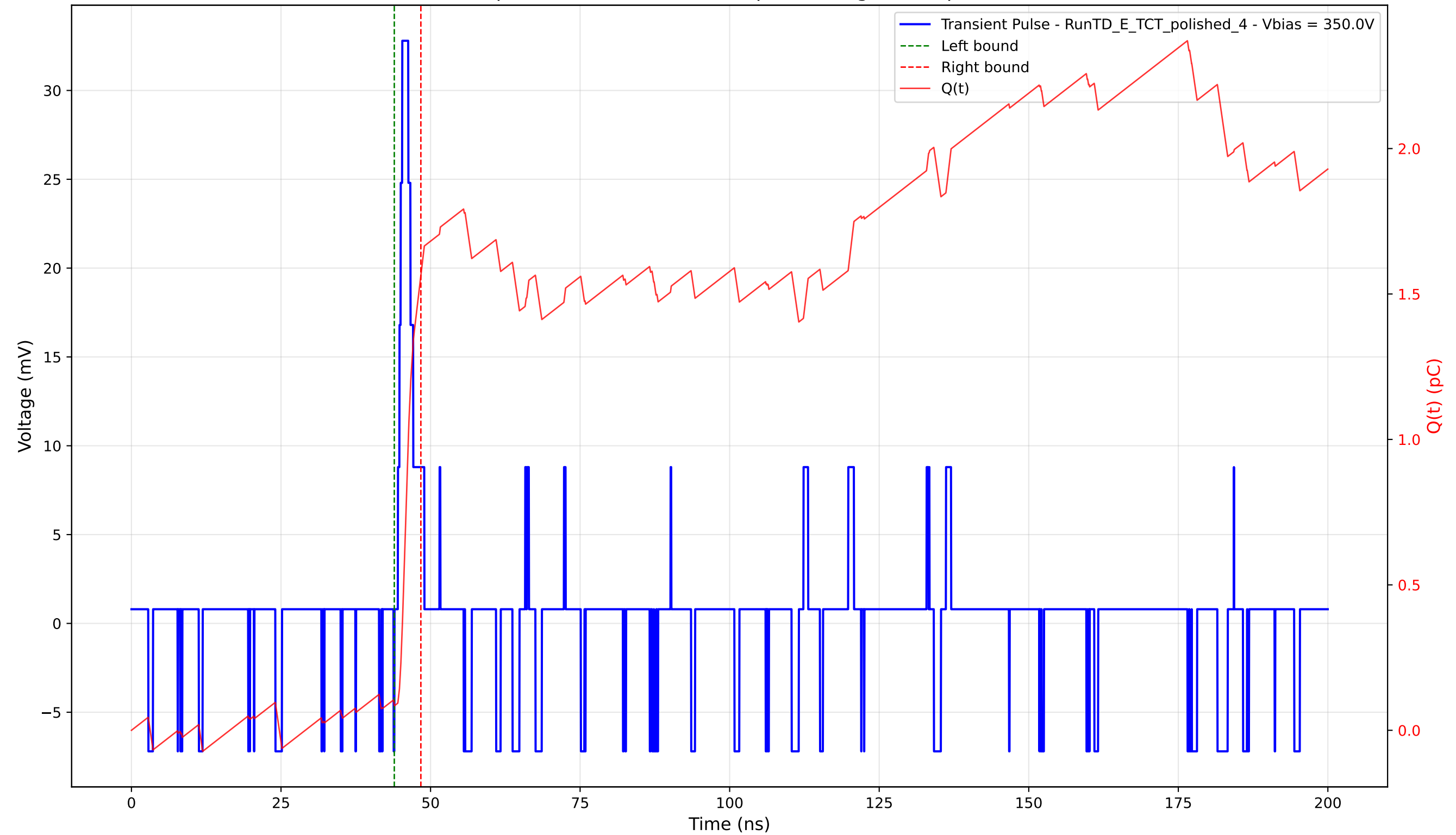
Transient Pulse - Sample: 4003 - Position: 35.0 \mu\text{m} - Charge: 1.48 pC - Rise Time: 0.73 ns
