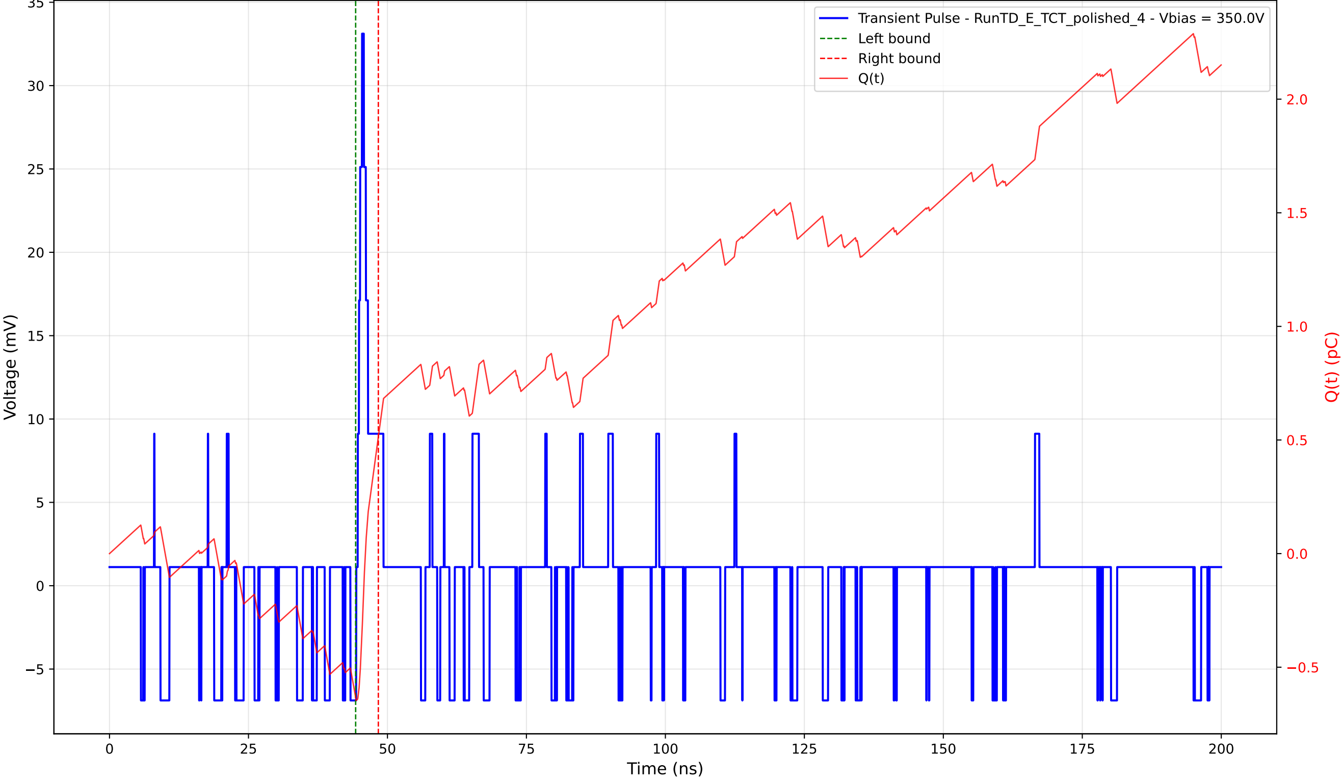
Transient Pulse - Sample: 4003 - Position: 15.0 \mu\text{m} - Charge: 1.15 pC - Rise Time: 0.77 ns
