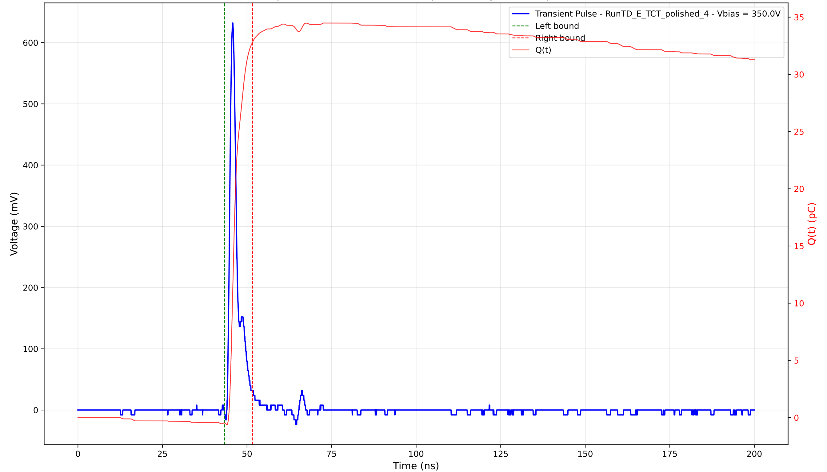
Transient Pulse - Sample: 4003 - Position: 210.0 \mu\text{m} - Charge: 33.26 pC - Rise Time: 1.06 ns
