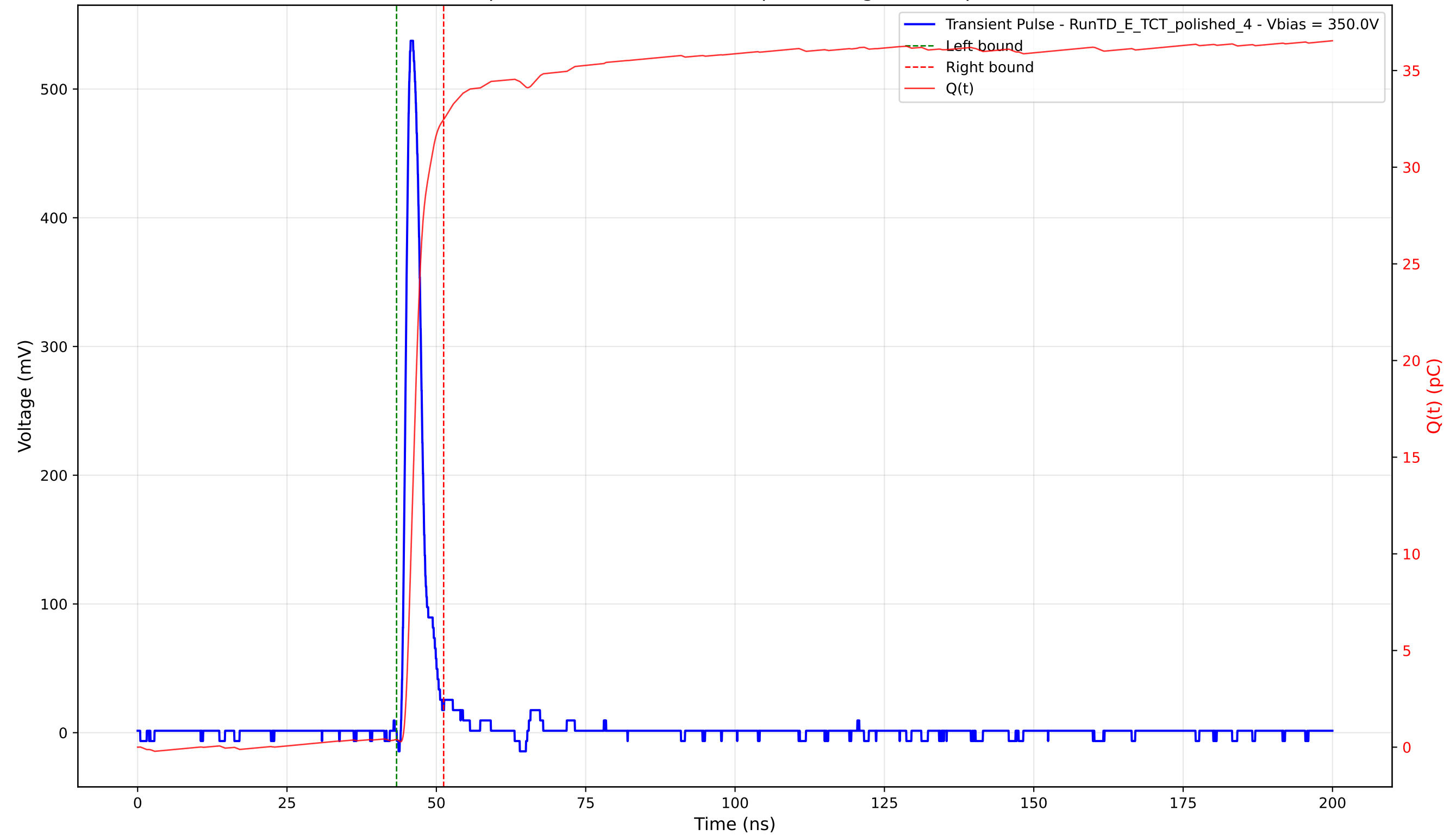
Transient Pulse - Sample: 4003 - Position: 265.0 \mu\text{m} - Charge: 32.07 pC - Rise Time: 1.08 ns
