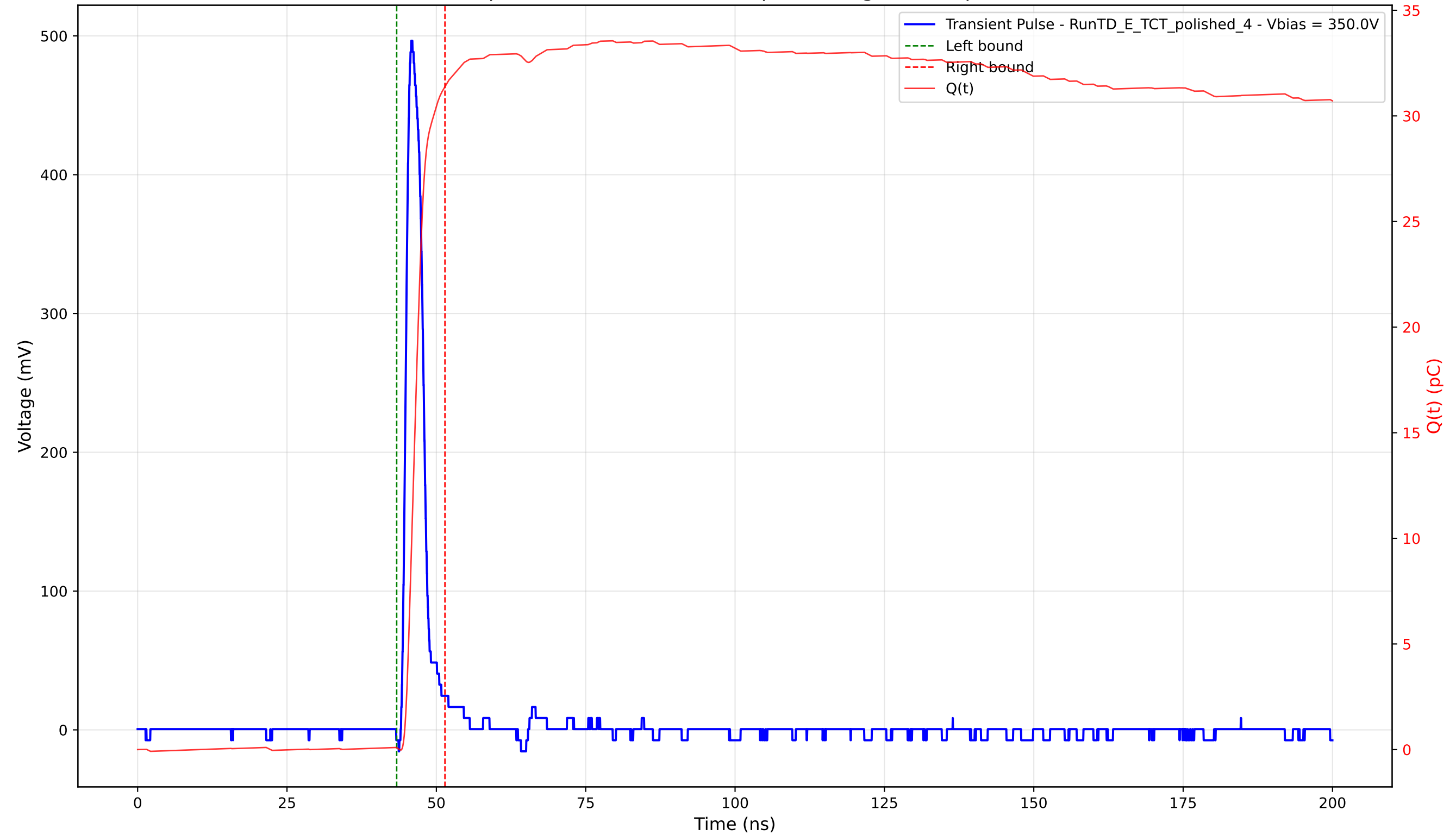
Transient Pulse - Sample: 4003 - Position: 290.0 \mu\text{m} - Charge: 31.29 pC - Rise Time: 1.09 ns
