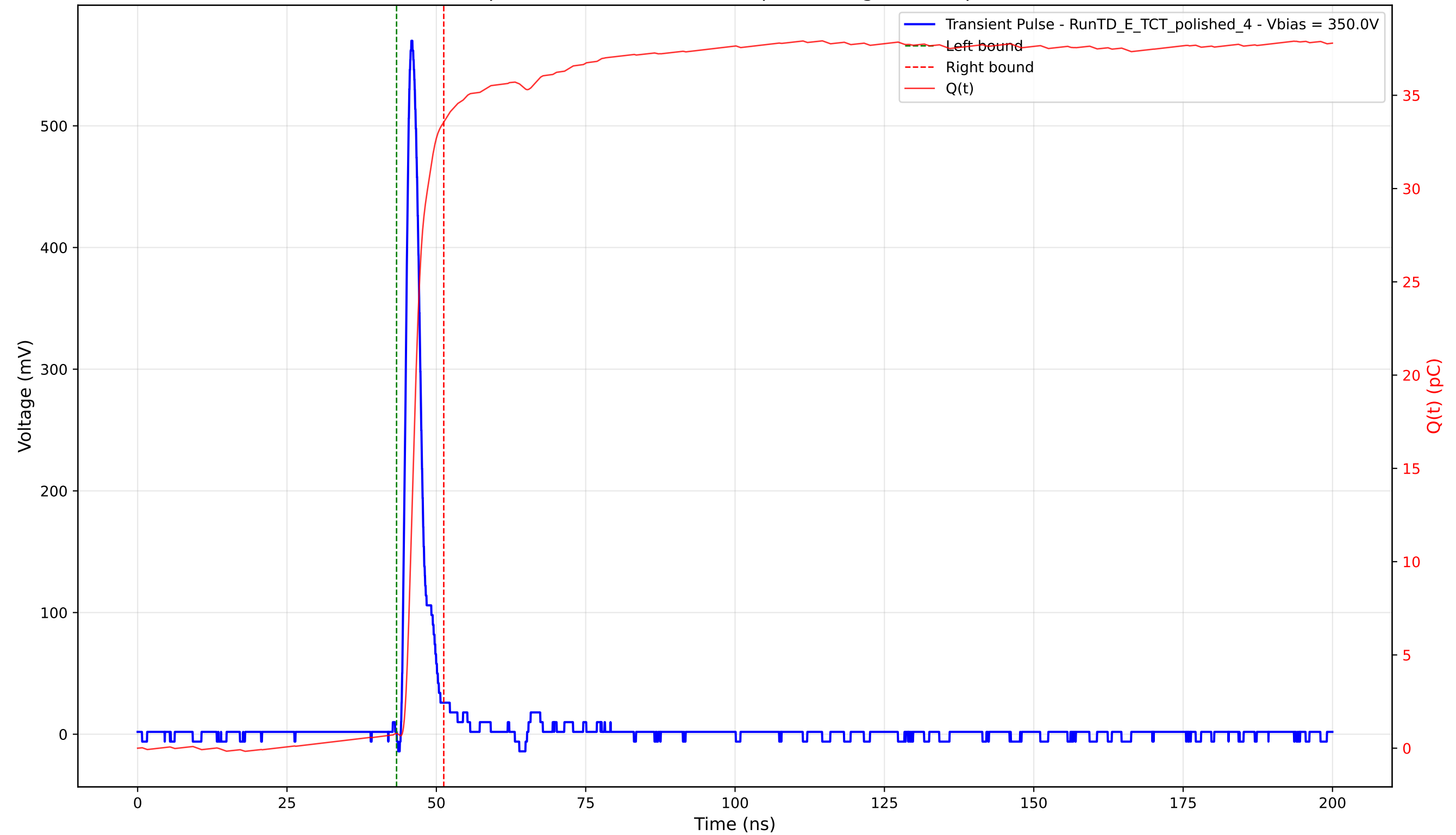
Transient Pulse - Sample: 4003 - Position: 255.0 \mu\text{m} - Charge: 32.78 pC - Rise Time: 1.10 ns
