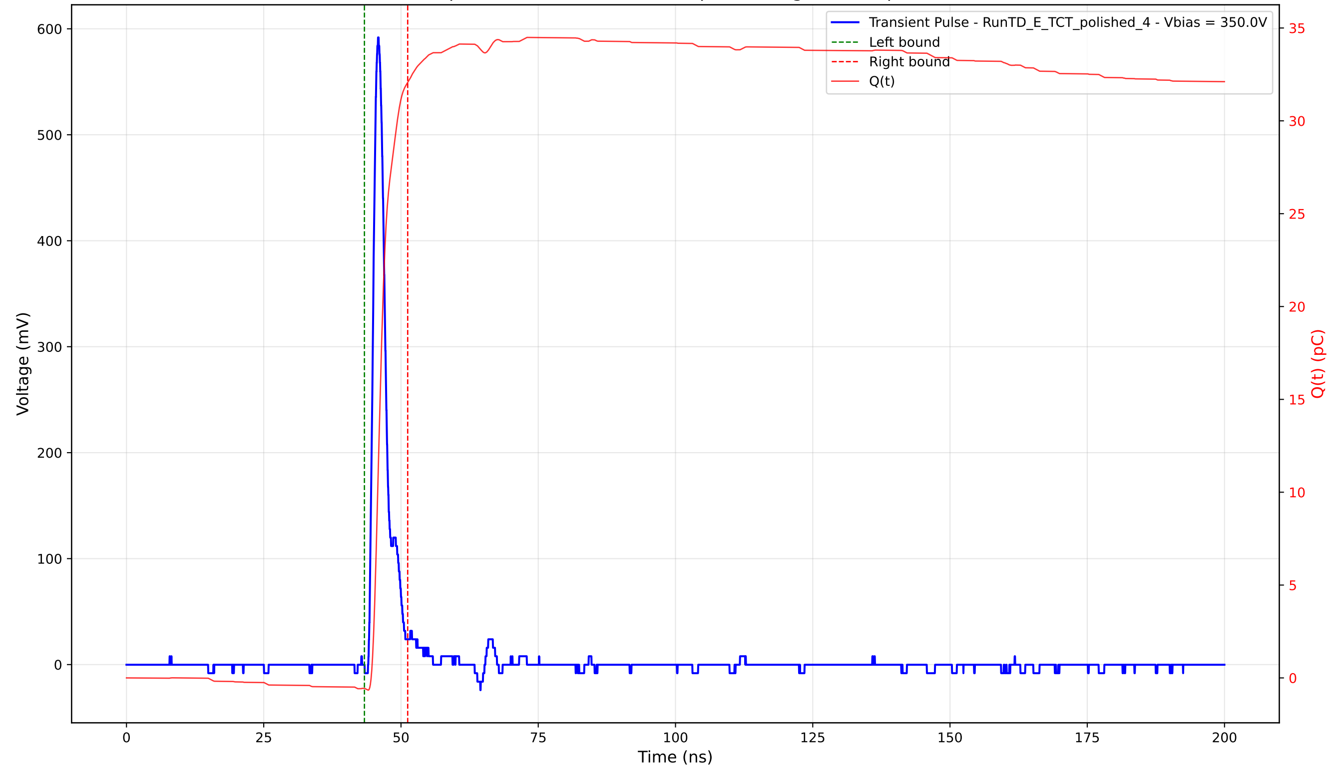
Transient Pulse - Sample: 4003 - Position: 240.0 \mu\text{m} - Charge: 32.62 pC - Rise Time: 1.11 ns
