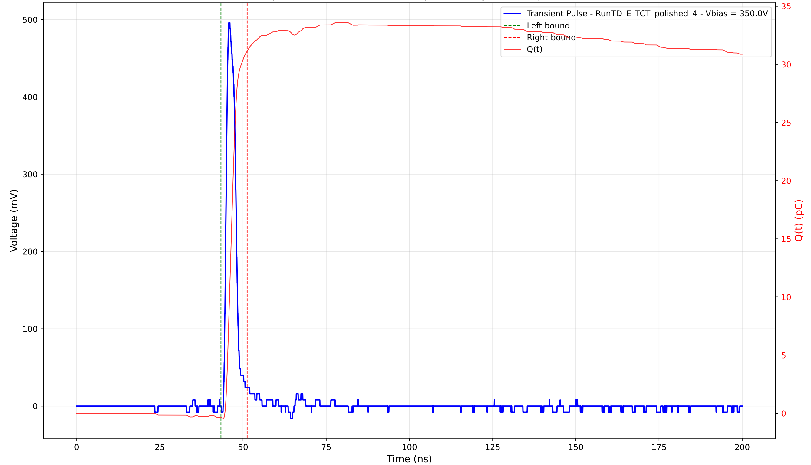
Transient Pulse - Sample: 4003 - Position: 295.0 \mu\text{m} - Charge: 31.49 pC - Rise Time: 1.08 ns
