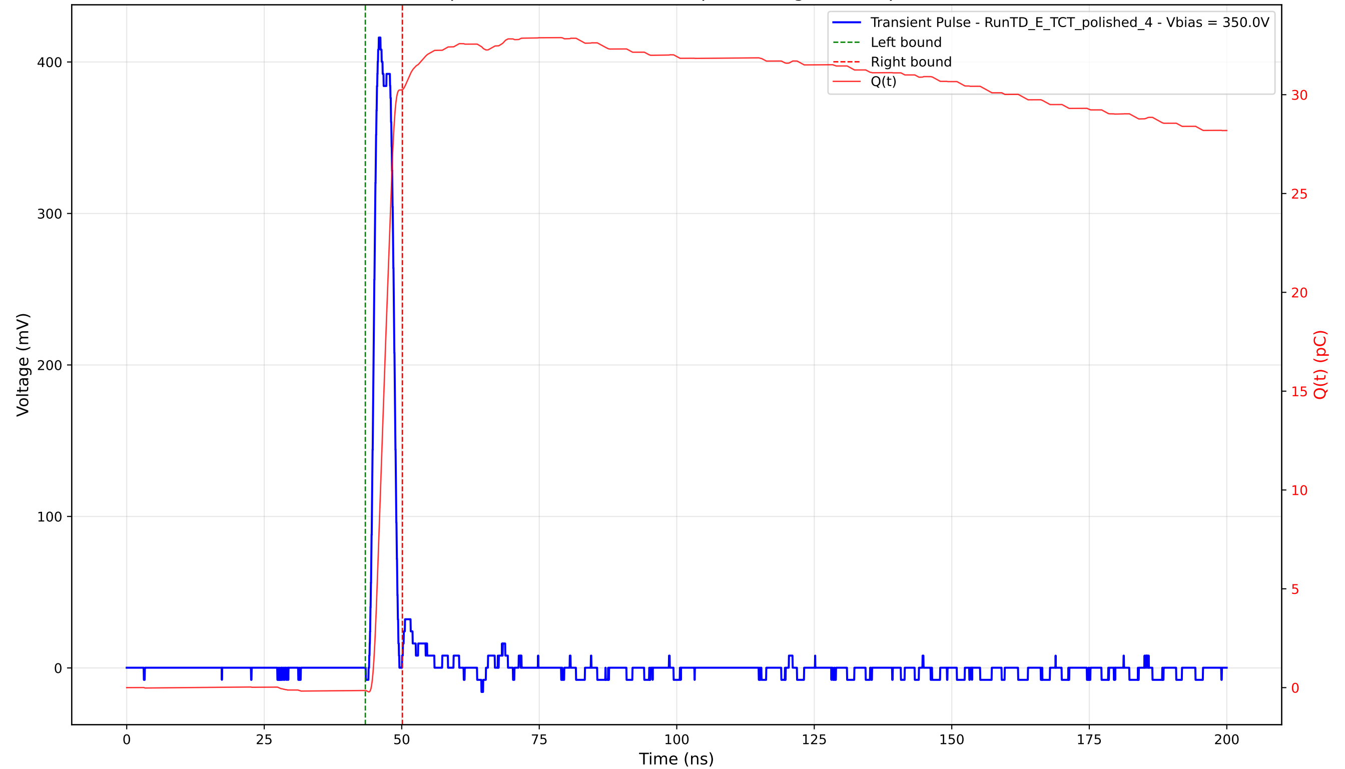
Transient Pulse - Sample: 4003 - Position: 345.0 \mu\text{m} - Charge: 30.39 pC - Rise Time: 1.12 ns
