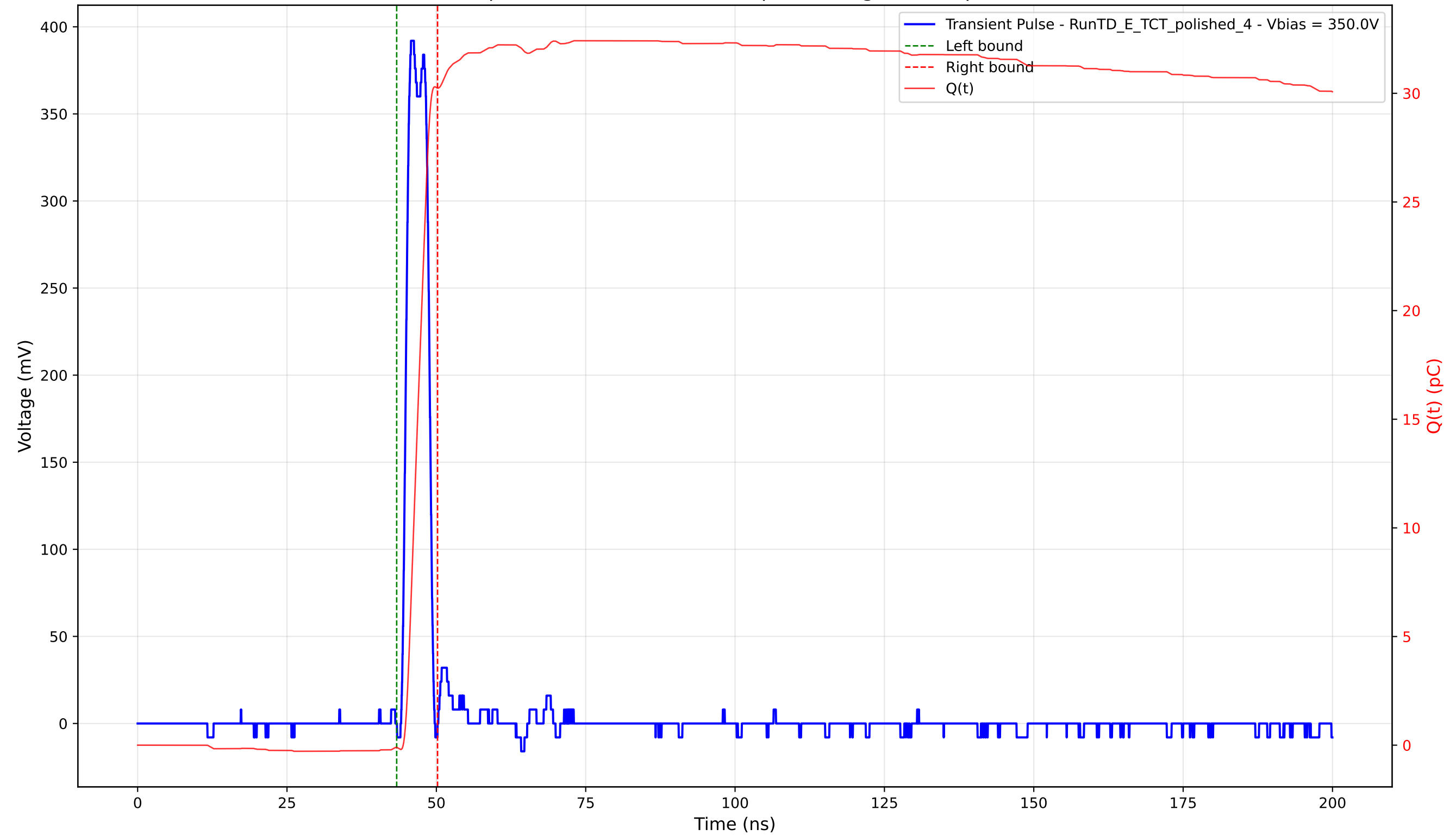
Transient Pulse - Sample: 4003 - Position: 355.0 \mu\text{m} - Charge: 30.34 pC - Rise Time: 1.12 ns
