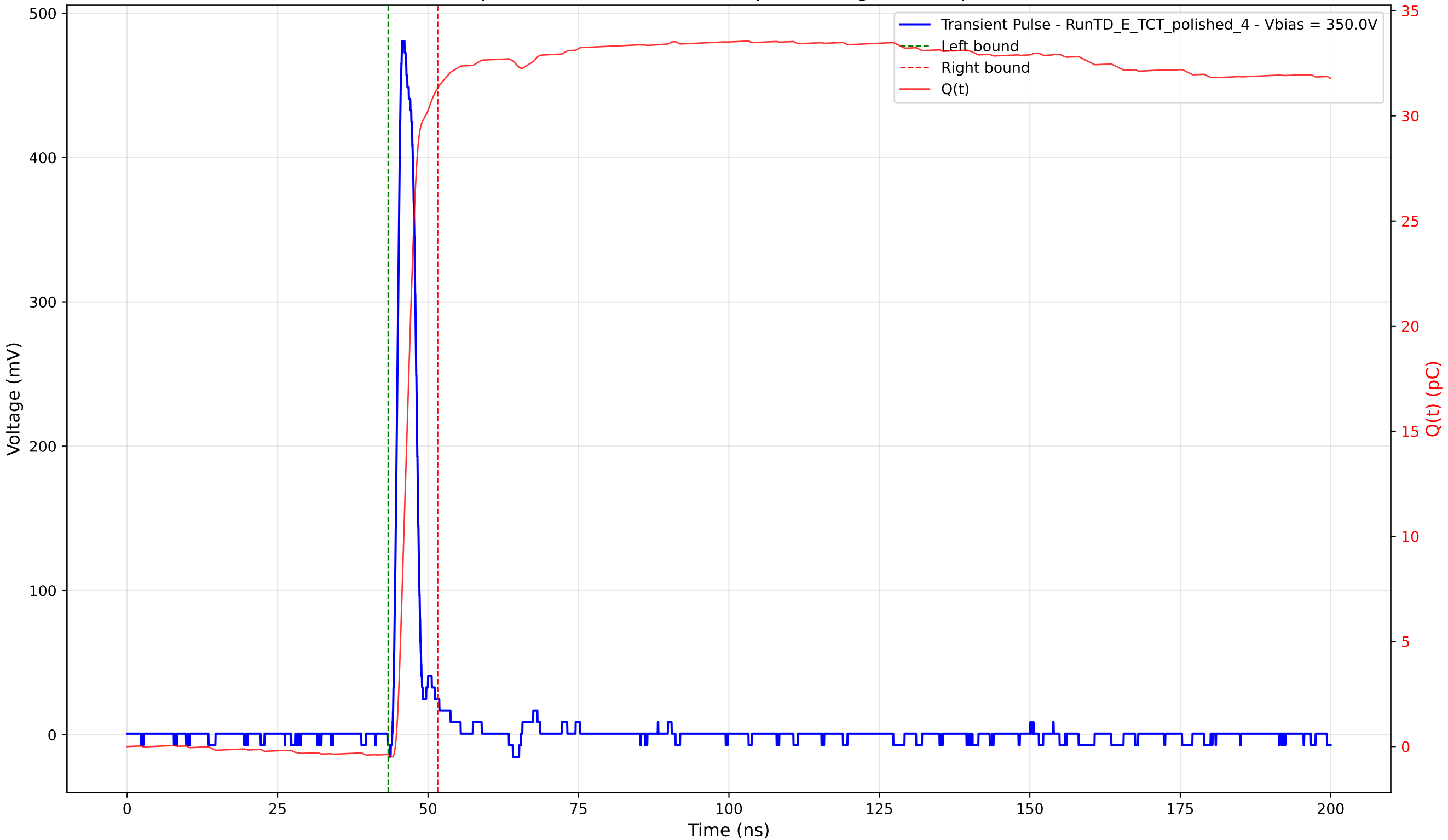
Transient Pulse - Sample: 4003 - Position: 305.0 \mu\text{m} - Charge: 31.70 pC - Rise Time: 1.06 ns
