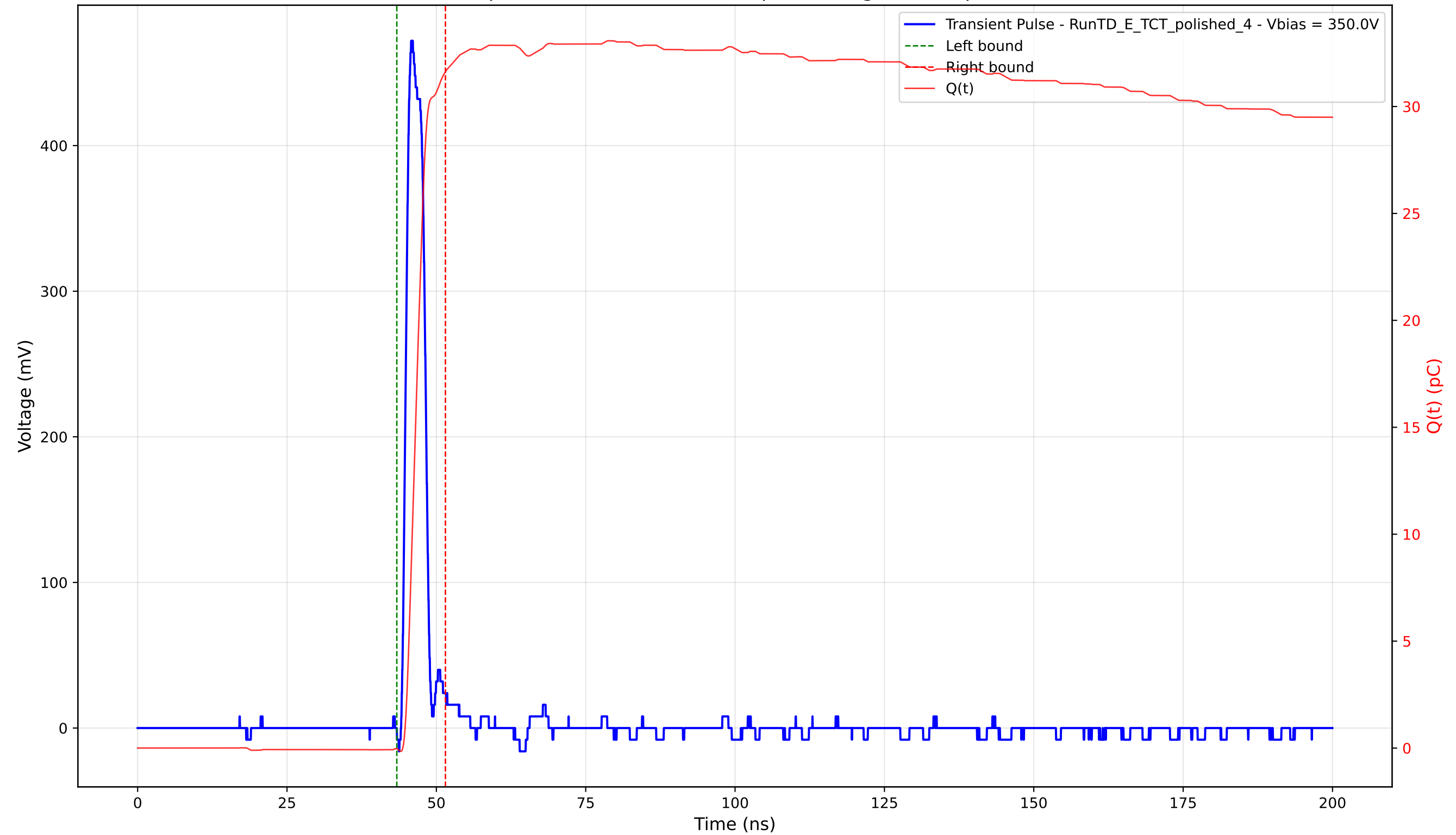
Transient Pulse - Sample: 4003 - Position: 315.0 \mu\text{m} - Charge: 31.66 pC - Rise Time: 1.10 ns
