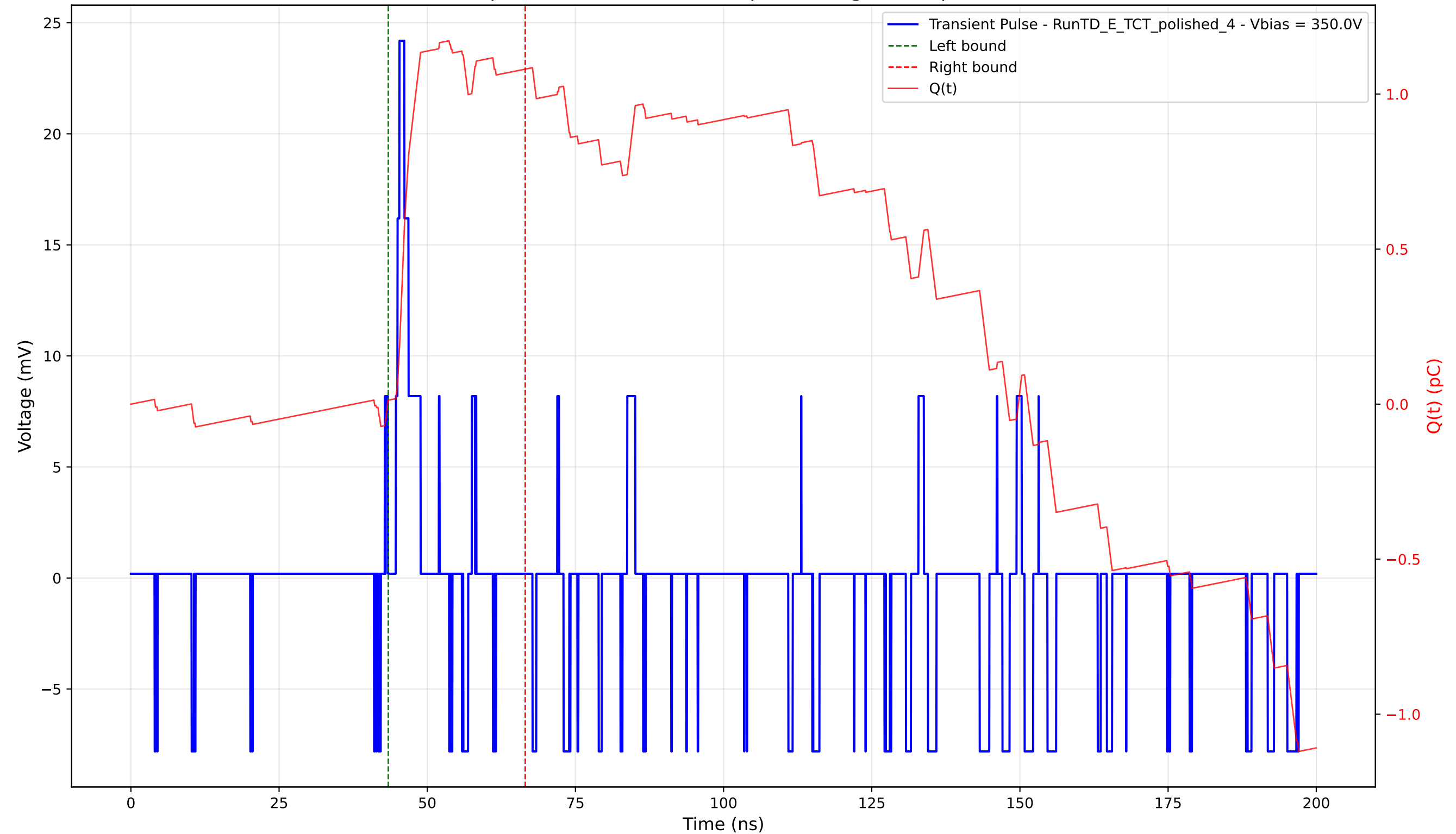
Transient Pulse - Sample: 4003 - Position: 65.0 \mu\text{m} - Charge: 1.07 pC - Rise Time: 0.61 ns
