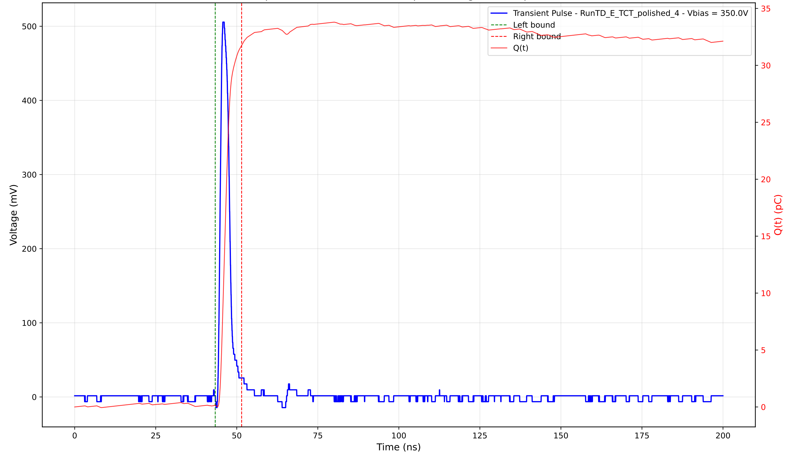
Transient Pulse - Sample: 4003 - Position: 285.0 \mu\text{m} - Charge: 31.60 pC - Rise Time: 1.06 ns
