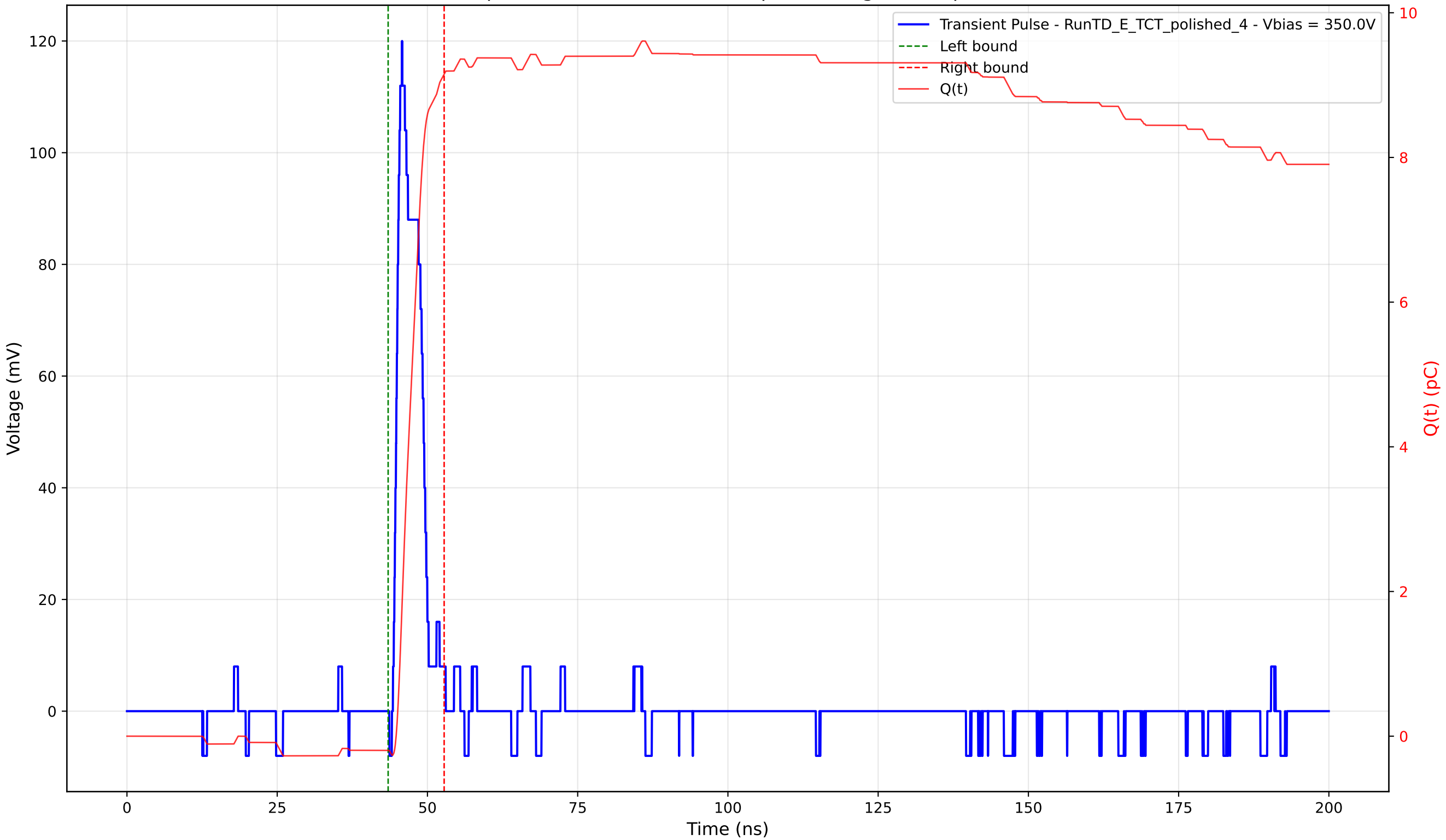
Transient Pulse - Sample: 4003 - Position: 405.0 \mu\text{m} - Charge: 9.35 pC - Rise Time: 1.07 ns
