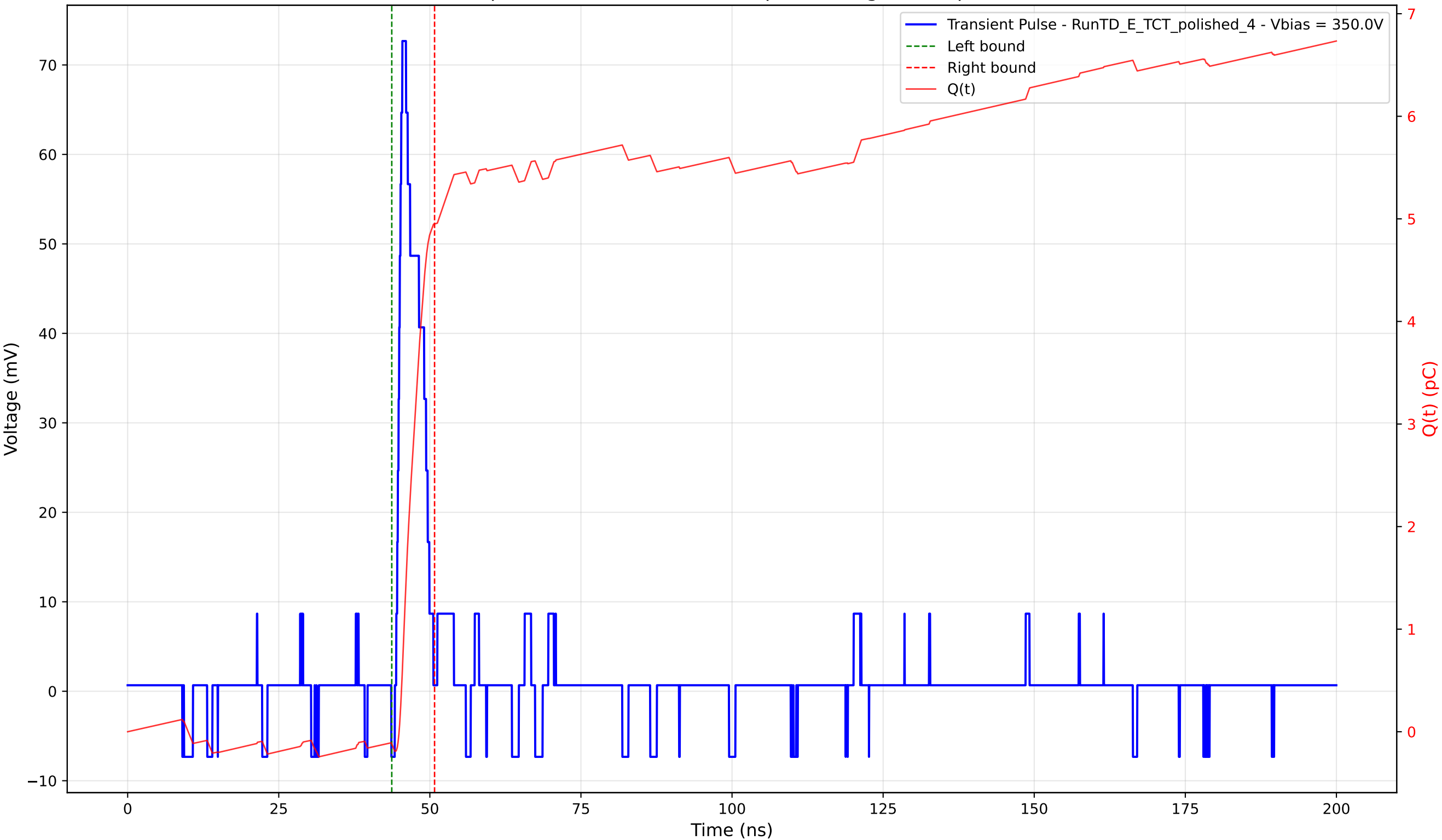
Transient Pulse - Sample: 4003 - Position: 410.0 \mu\text{m} - Charge: 5.07 pC - Rise Time: 1.00 ns
