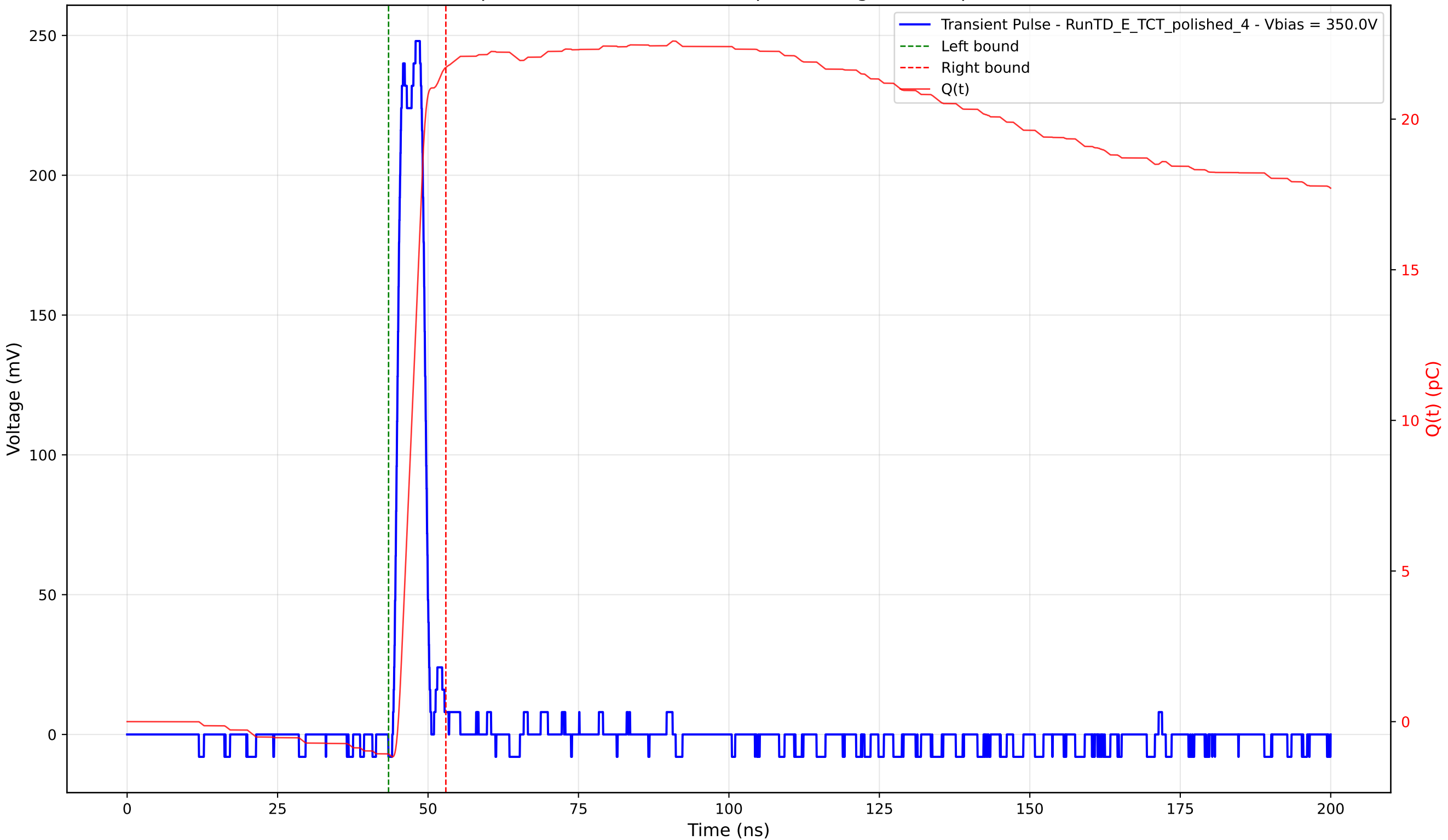
Transient Pulse - Sample: 4003 - Position: 390.0 \mu\text{m} - Charge: 22.79 pC - Rise Time: 1.12 ns
