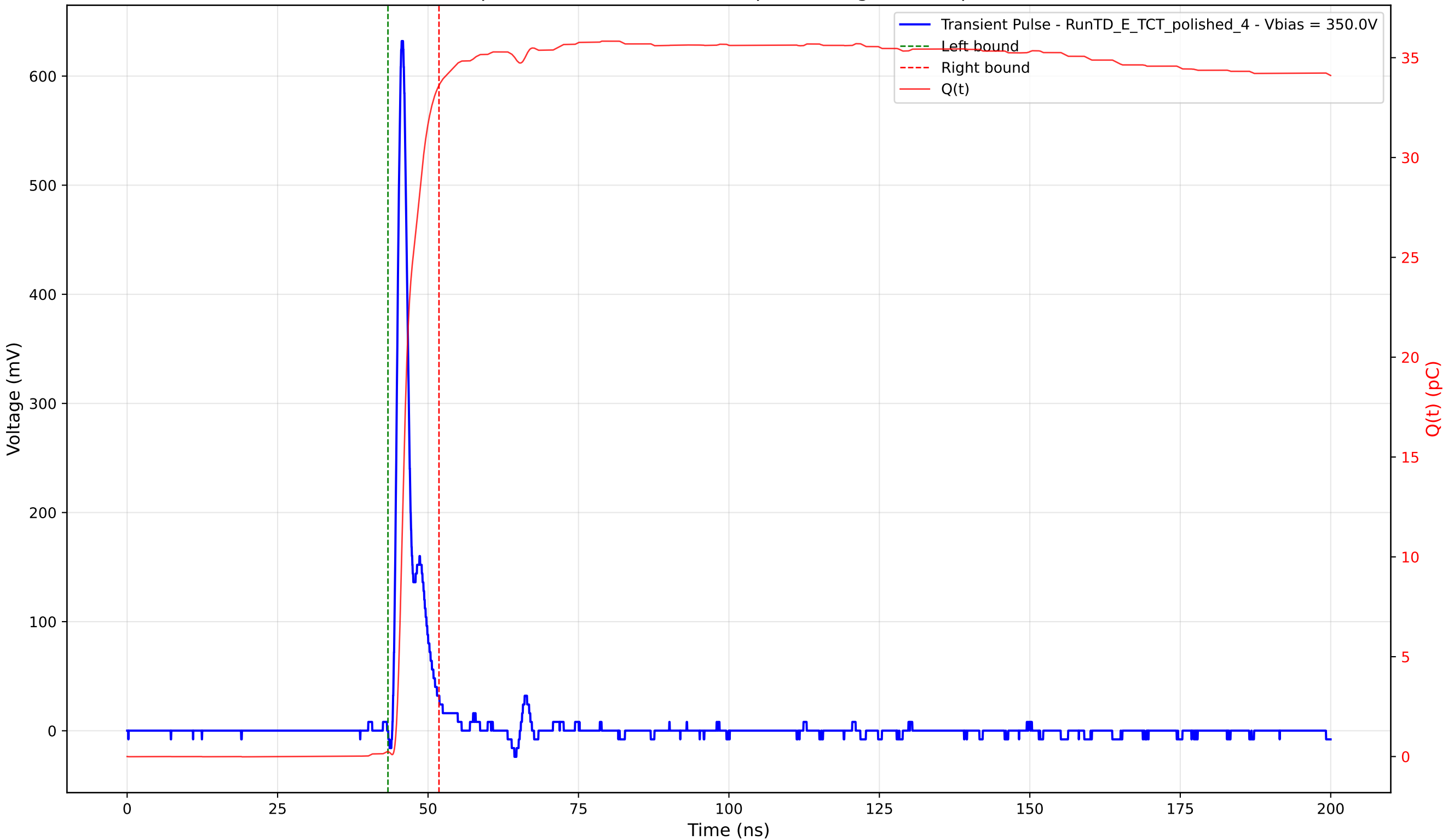
Transient Pulse - Sample: 4003 - Position: 200.0 \mu\text{m} - Charge: 33.37 pC - Rise Time: 1.02 ns
