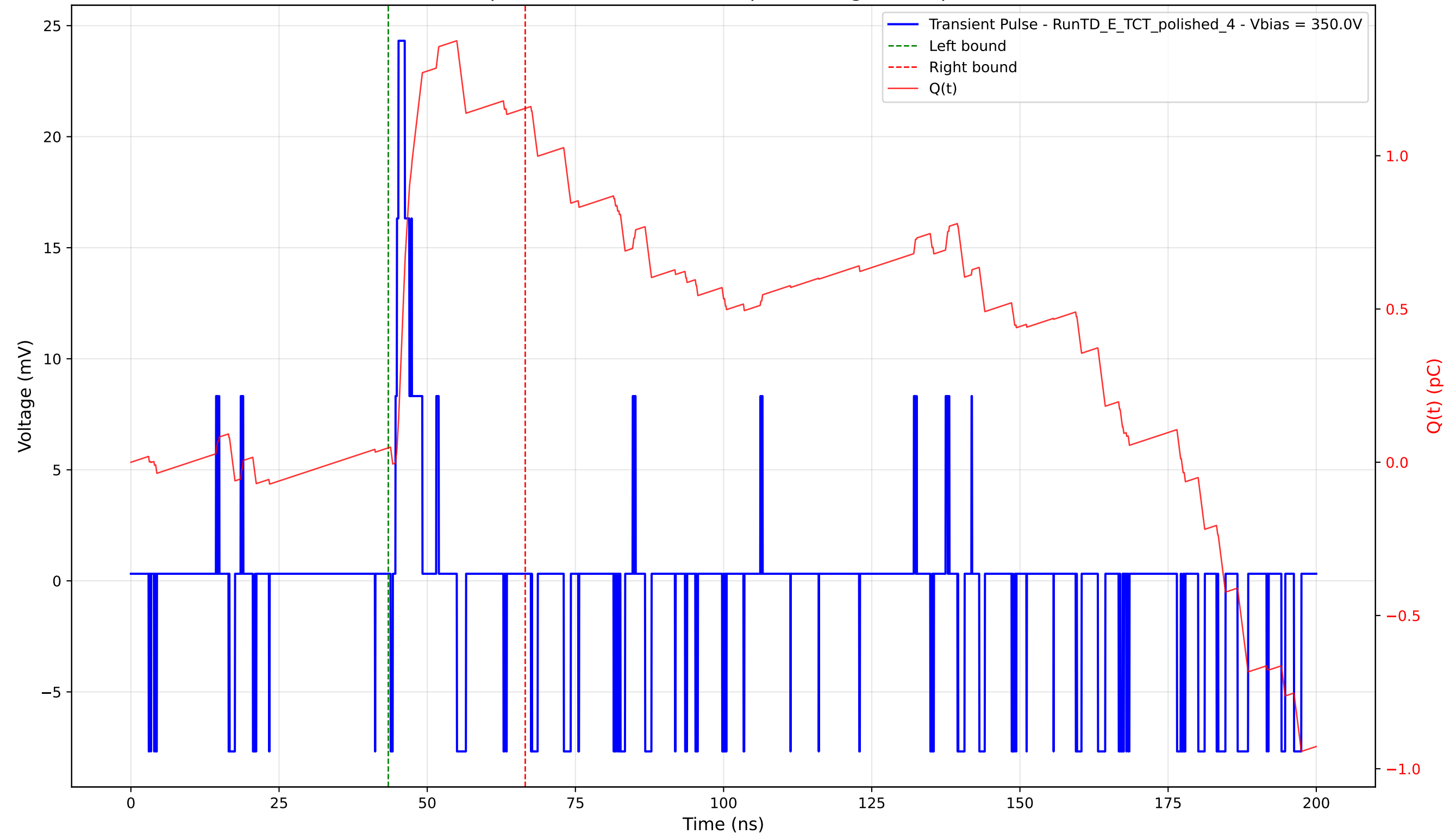
Transient Pulse - Sample: 4003 - Position: 75.0 \mu\text{m} - Charge: 1.11 pC - Rise Time: 0.51 ns
