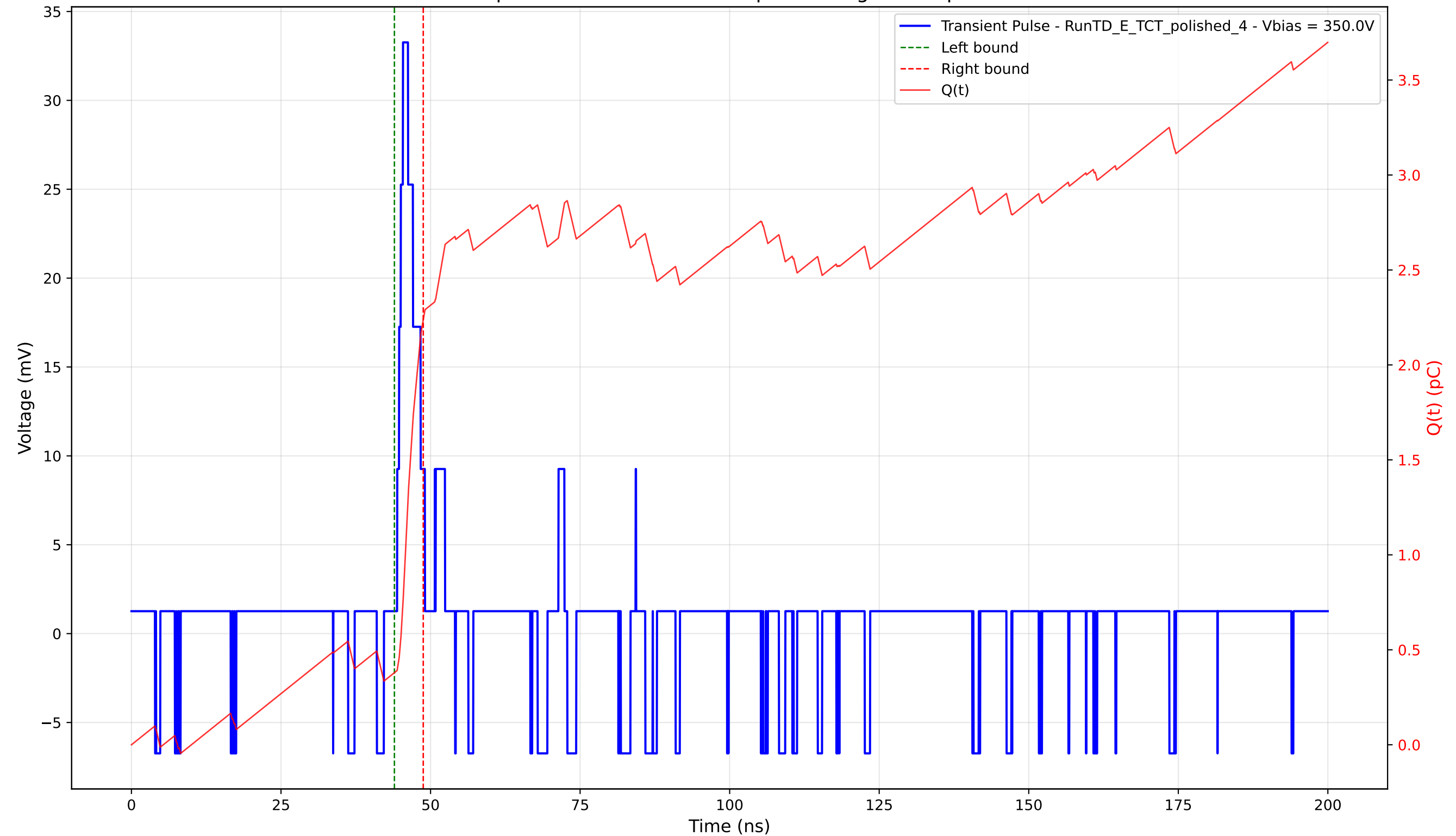
Transient Pulse - Sample: 4003 - Position: 25.0 \mu\text{m} - Charge: 1.86 pC - Rise Time: 0.97 ns
