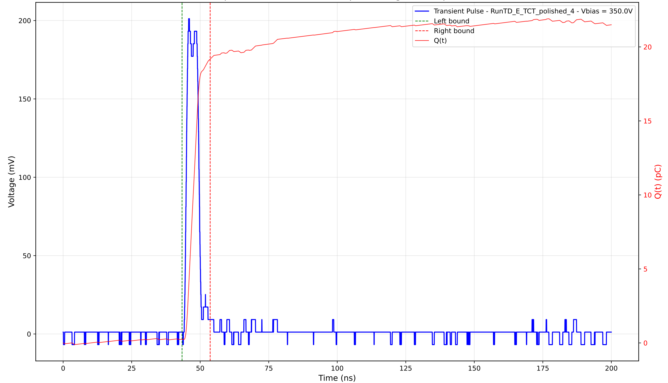
Transient Pulse - Sample: 4003 - Position: 395.0 \mu\text{m} - Charge: 18.92 pC - Rise Time: 1.11 ns
