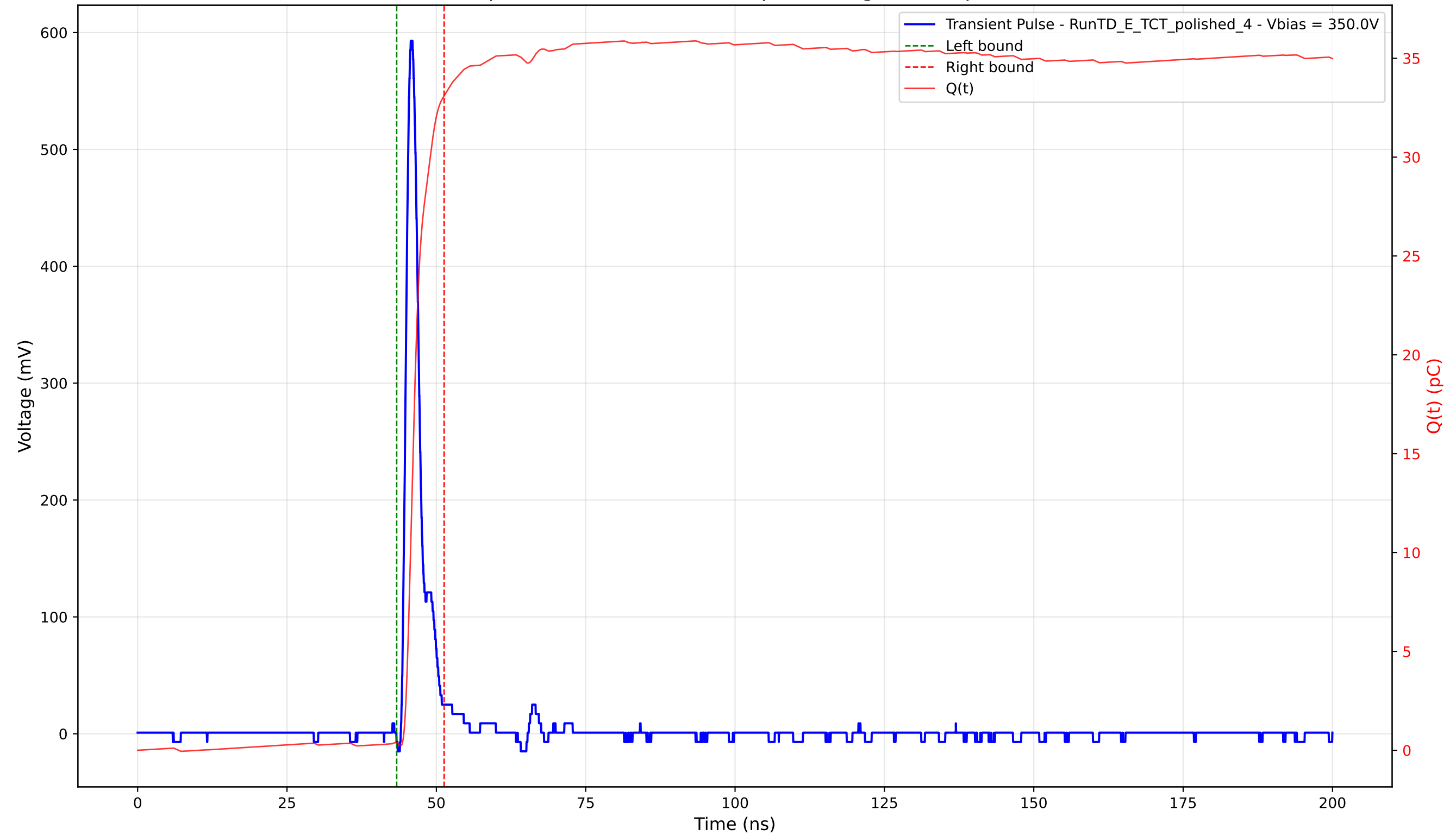
Transient Pulse - Sample: 4003 - Position: 235.0 \mu\text{m} - Charge: 32.72 pC - Rise Time: 1.07 ns
