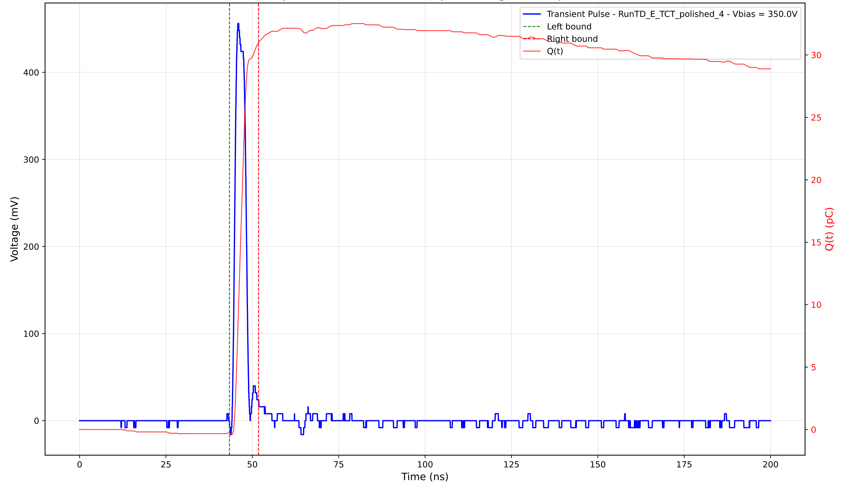
Transient Pulse - Sample: 4003 - Position: 320.0 \mu\text{m} - Charge: 31.25 pC - Rise Time: 1.09 ns
