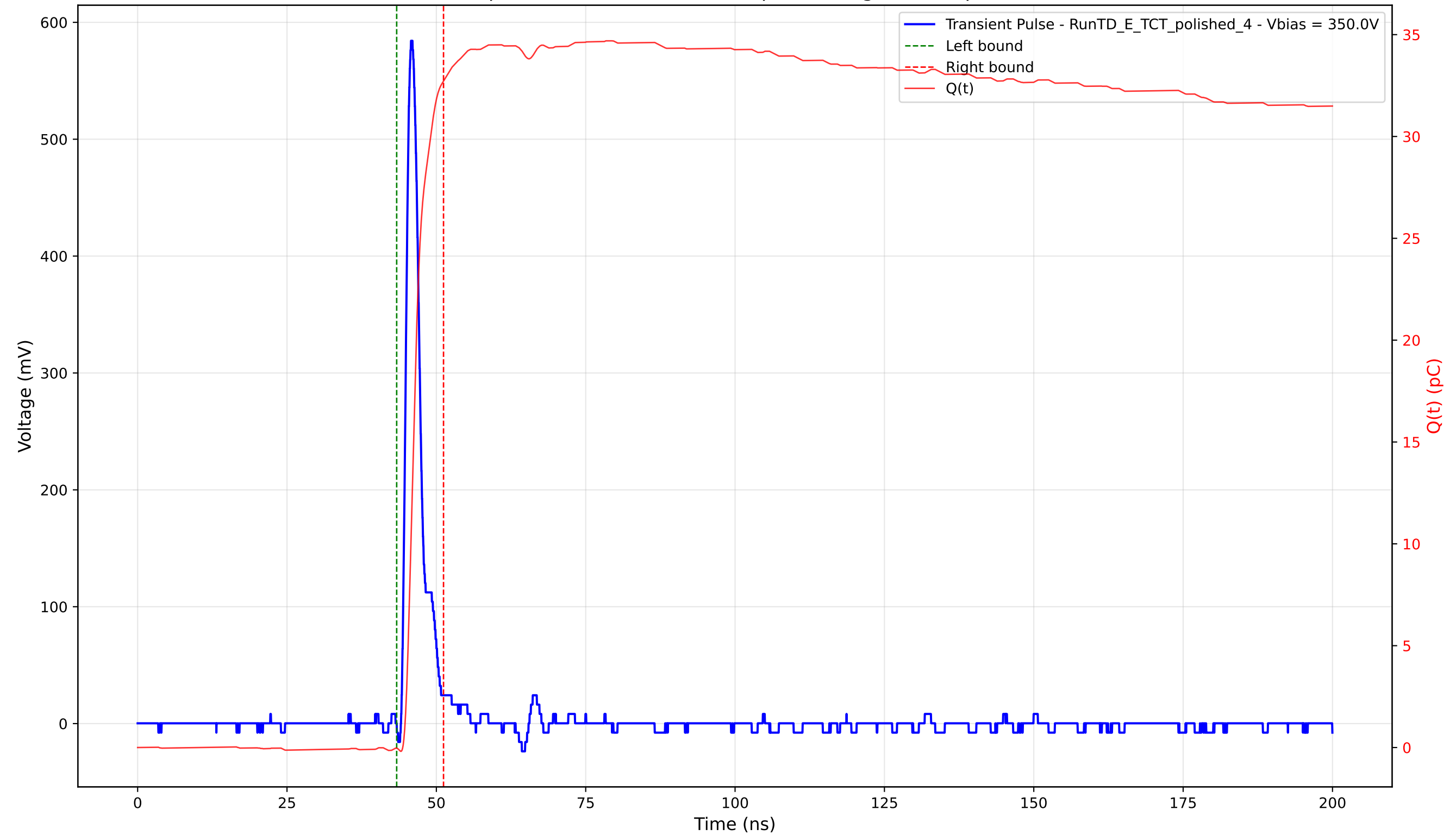
Transient Pulse - Sample: 4003 - Position: 245.0 \mu\text{m} - Charge: 32.75 pC - Rise Time: 1.07 ns
