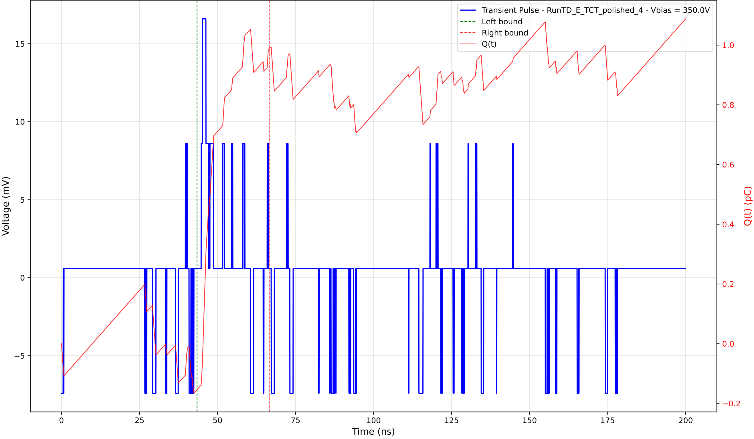
Transient Pulse - Sample: 4003 - Position: 10.0 \mu\text{m} - Charge: 1.14 pC - Rise Time: 0.40 ns
