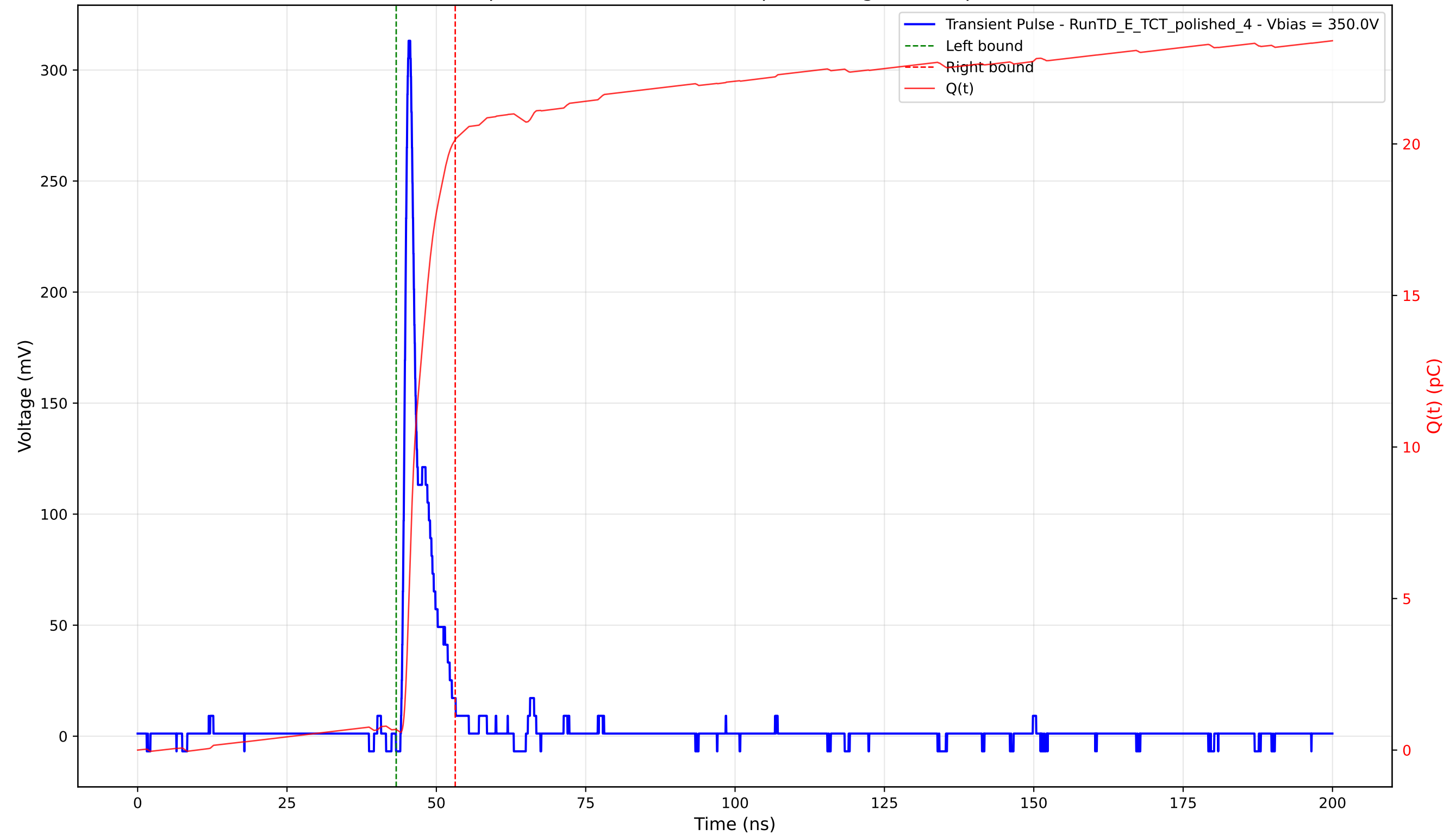
Transient Pulse - Sample: 4003 - Position: 100.0 \mu\text{m} - Charge: 19.47 pC - Rise Time: 0.90 ns
