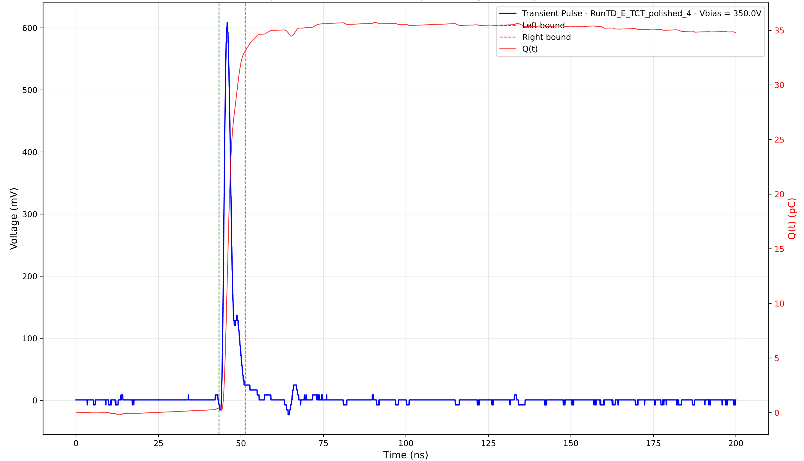
Transient Pulse - Sample: 4003 - Position: 230.0 \mu\text{m} - Charge: 32.69 pC - Rise Time: 1.09 ns
