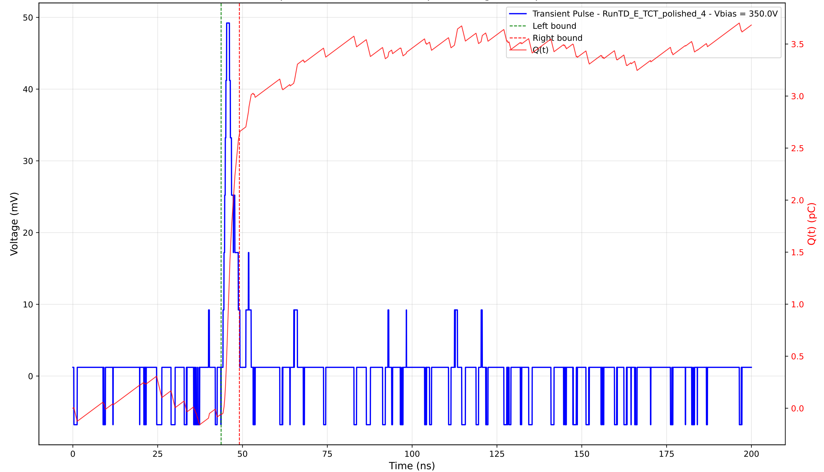
Transient Pulse - Sample: 4003 - Position: 45.0 \mu\text{m} - Charge: 2.70 pC - Rise Time: 1.07 ns
