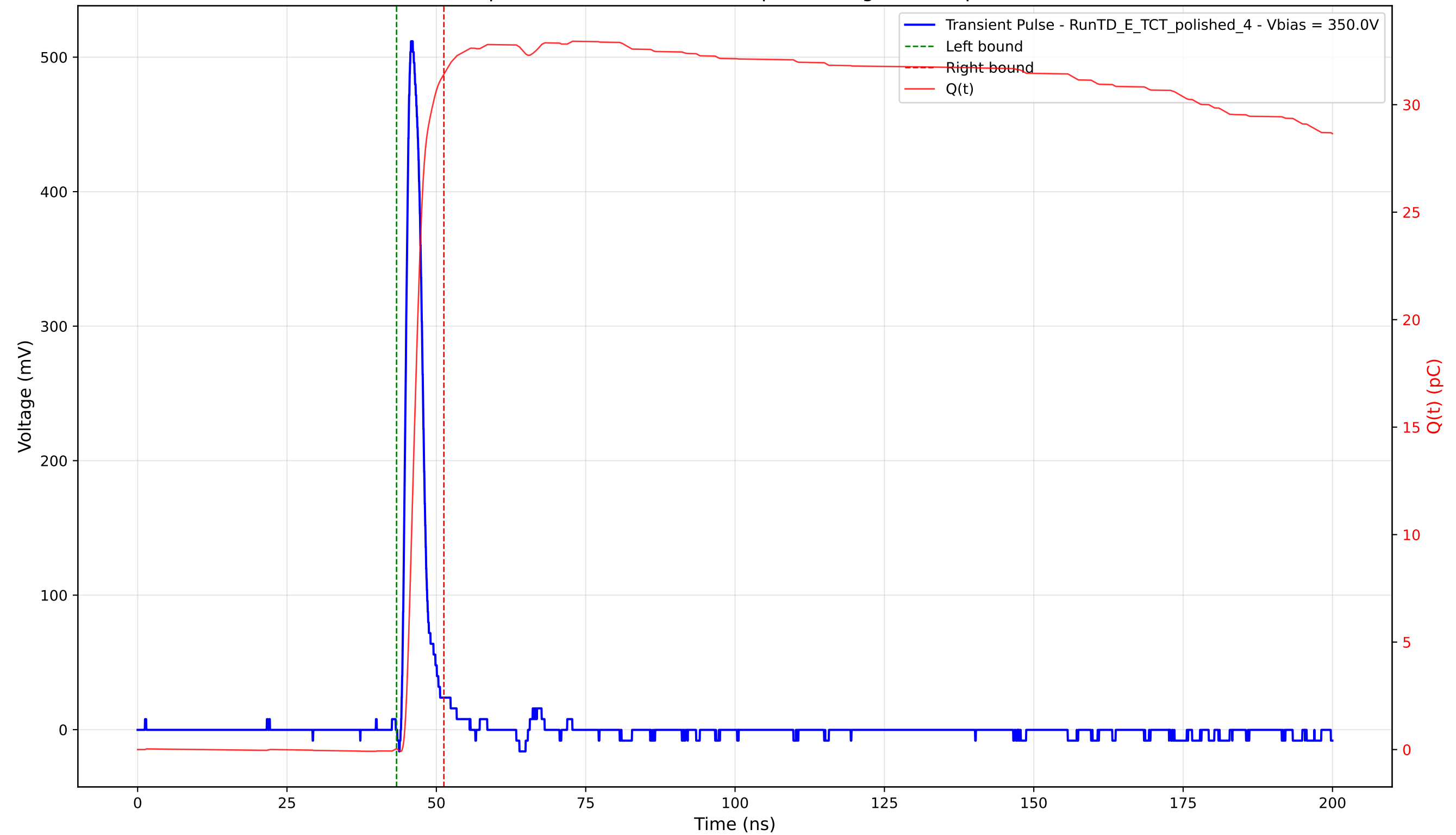
Transient Pulse - Sample: 4003 - Position: 280.0 \mu\text{m} - Charge: 31.39 pC - Rise Time: 1.08 ns
