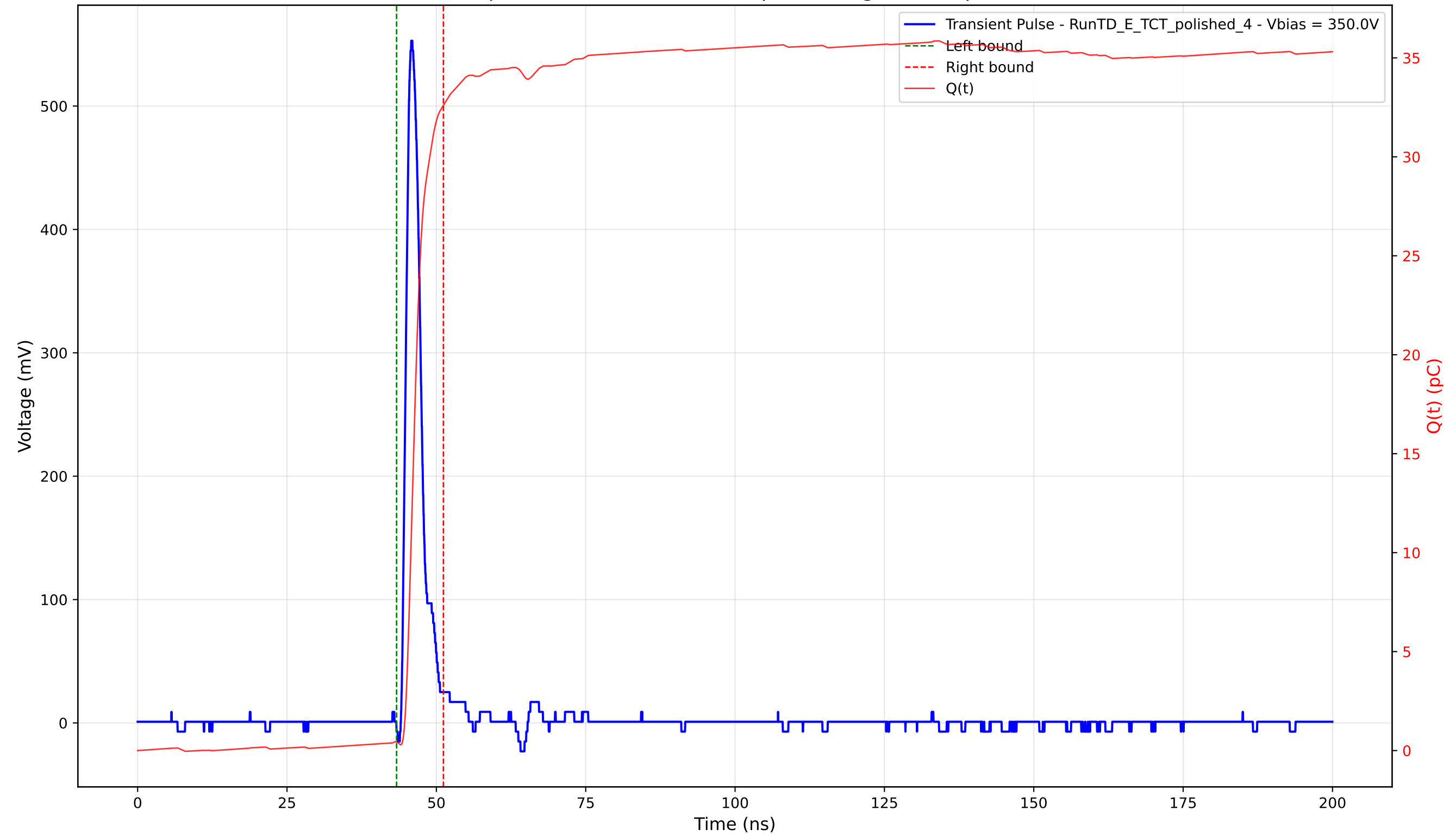
Transient Pulse - Sample: 4003 - Position: 260.0 \mu\text{m} - Charge: 32.16 pC - Rise Time: 1.10 ns
