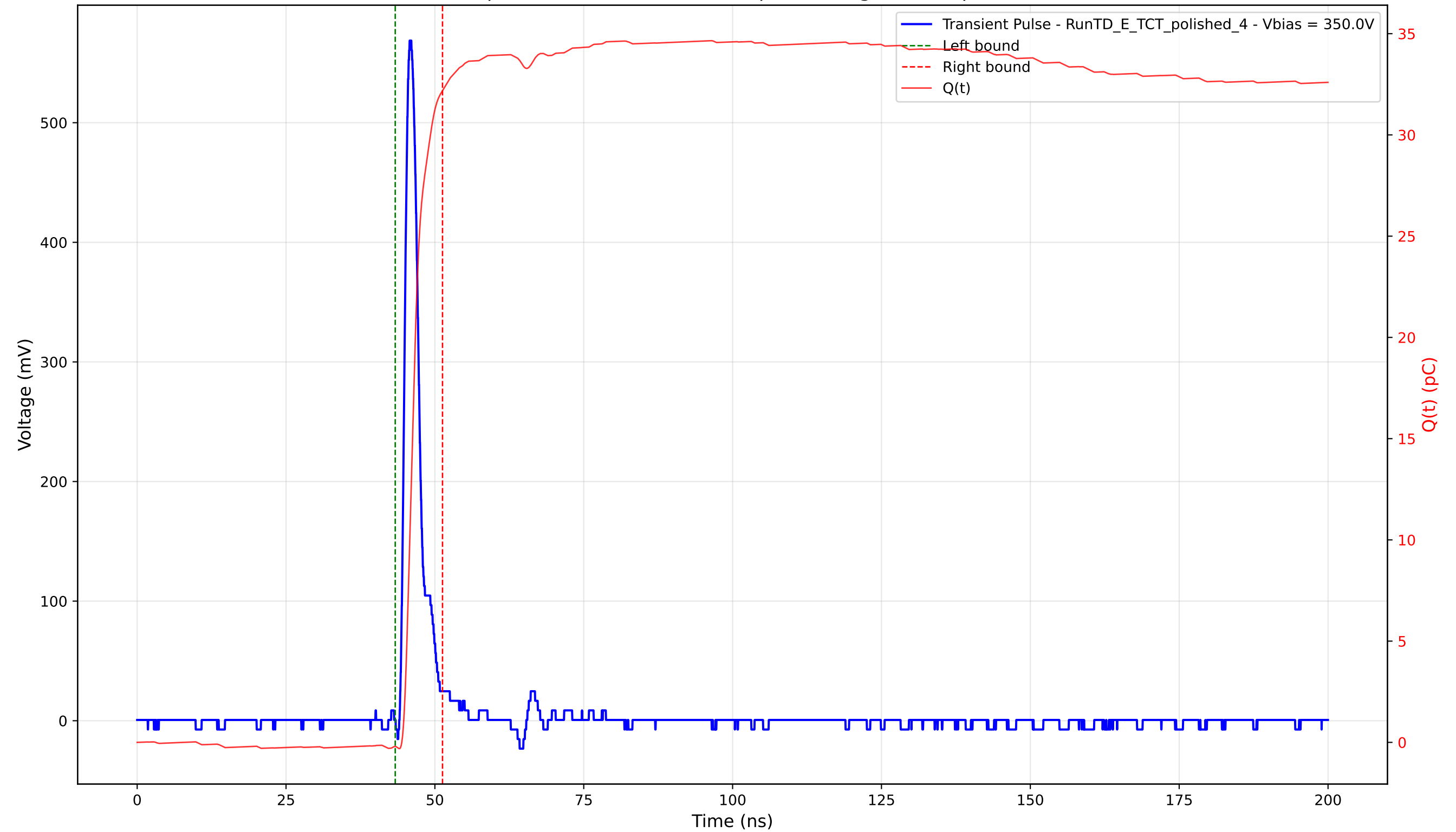
Transient Pulse - Sample: 4003 - Position: 250.0 \mu\text{m} - Charge: 32.39 pC - Rise Time: 1.10 ns
