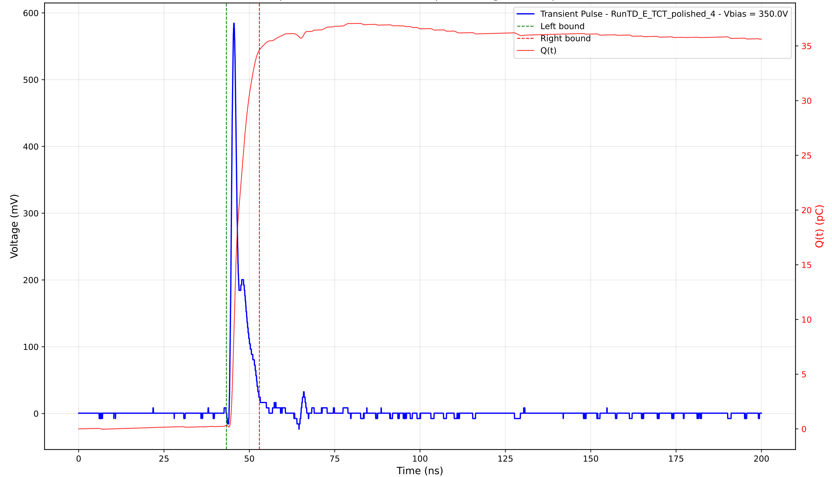
Transient Pulse - Sample: 4003 - Position: 130.0 \mu\text{m} - Charge: 34.29 pC - Rise Time: 0.89 ns
