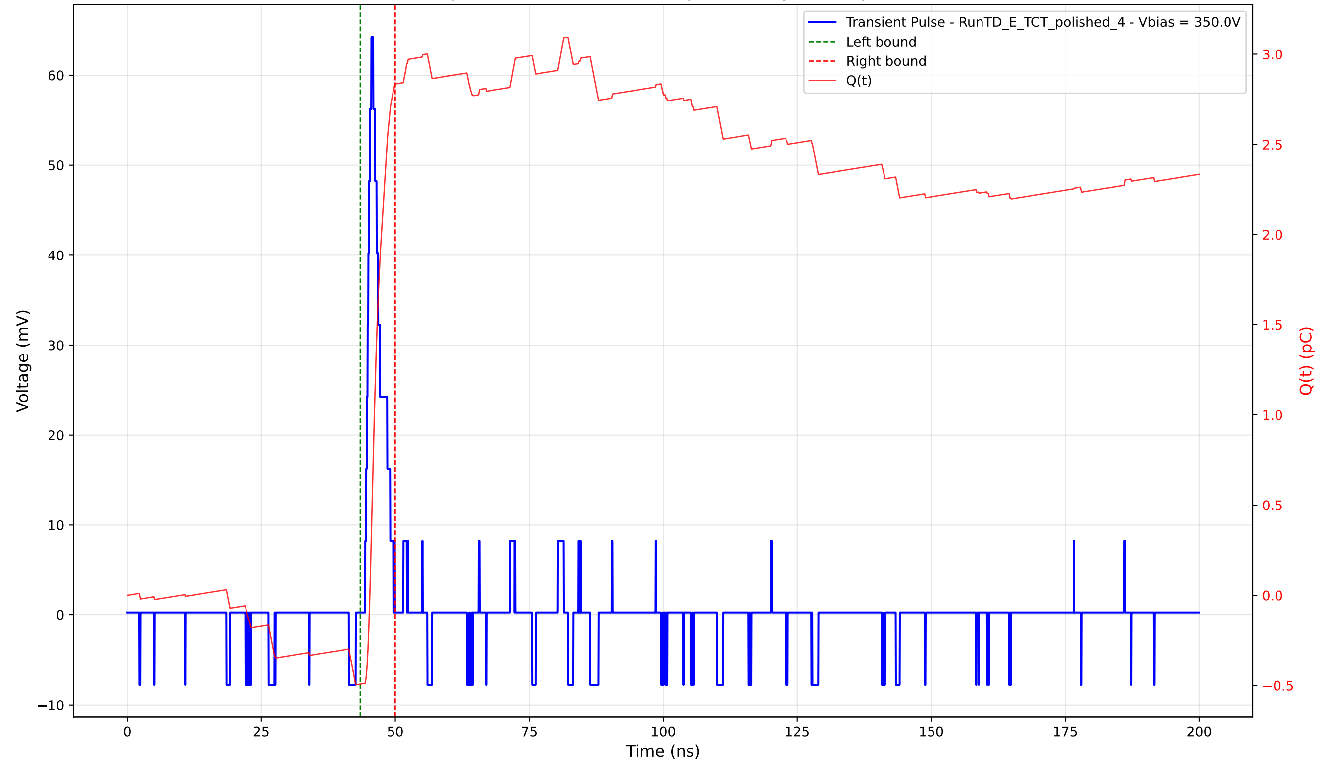
Transient Pulse - Sample: 4003 - Position: 50.0 \mu\text{m} - Charge: 3.33 pC - Rise Time: 1.14 ns
