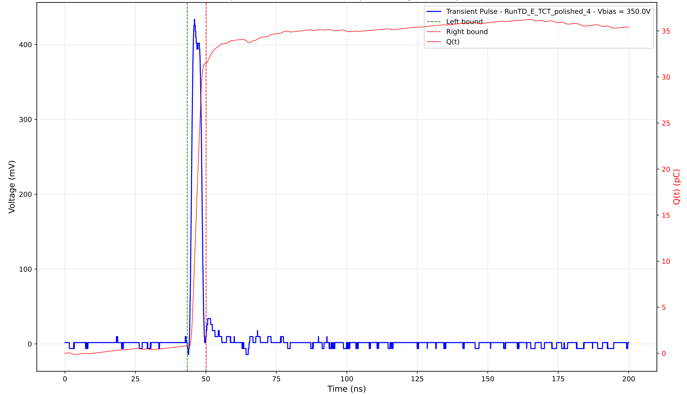
Transient Pulse - Sample: 4003 - Position: 340.0 \mu\text{m} - Charge: 30.63 pC - Rise Time: 1.12 ns
