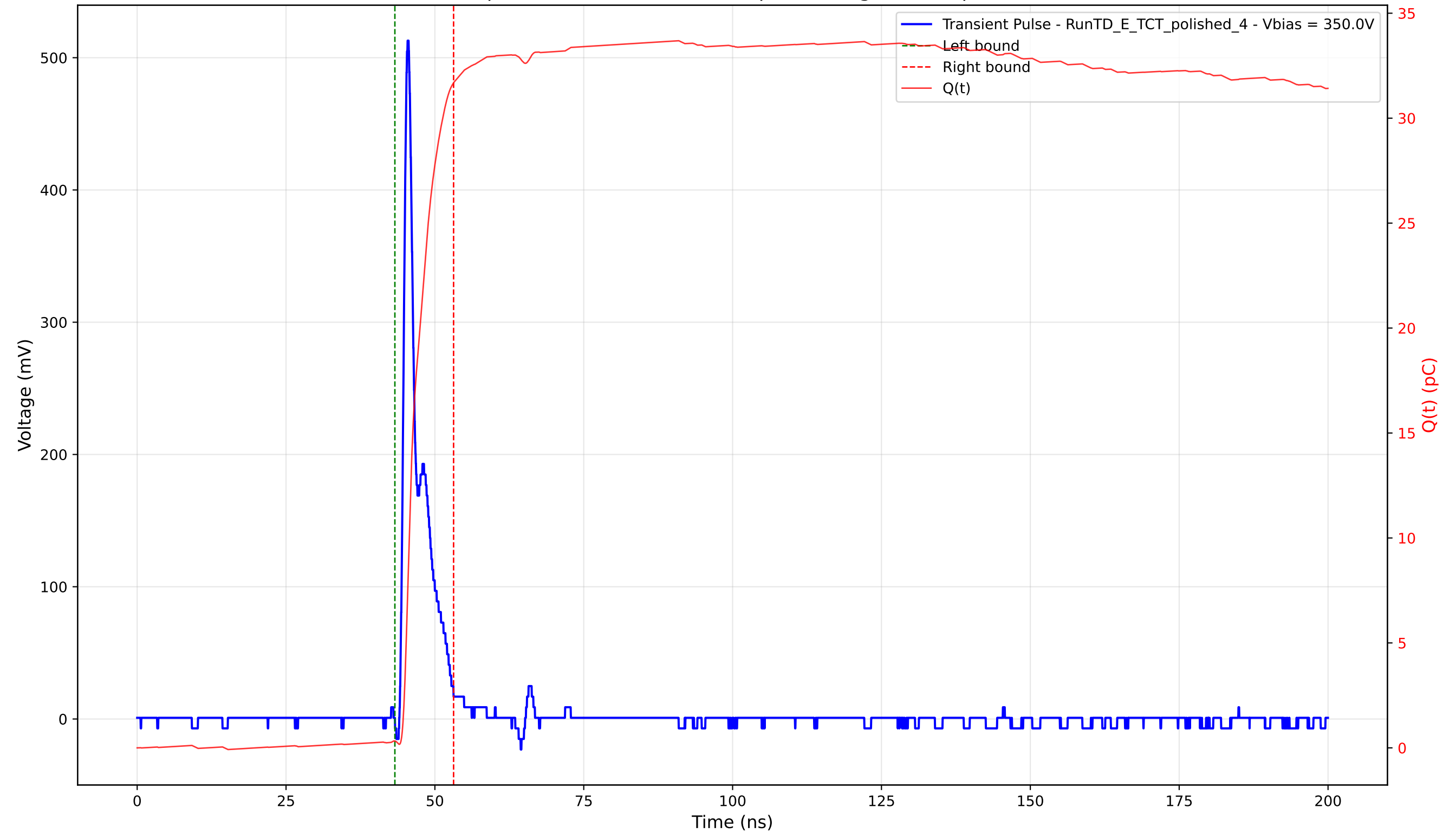
Transient Pulse - Sample: 4003 - Position: 115.0 \mu\text{m} - Charge: 31.36 pC - Rise Time: 0.89 ns
