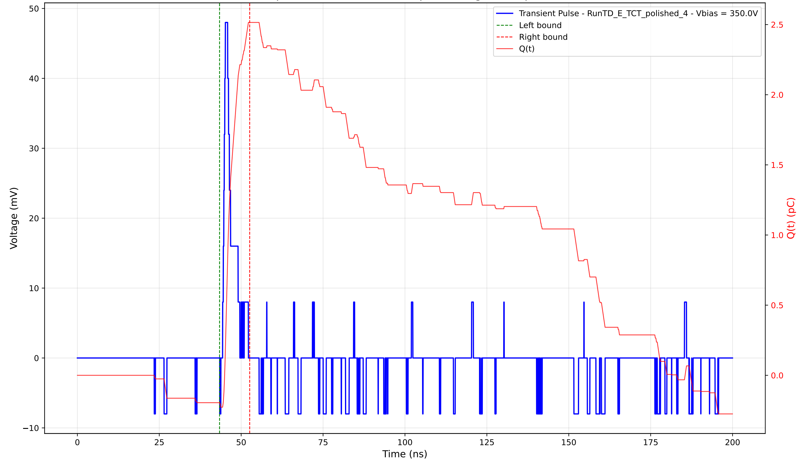
Transient Pulse - Sample: 4003 - Position: 80.0 \mu\text{m} - Charge: 2.71 pC - Rise Time: 0.83 ns
