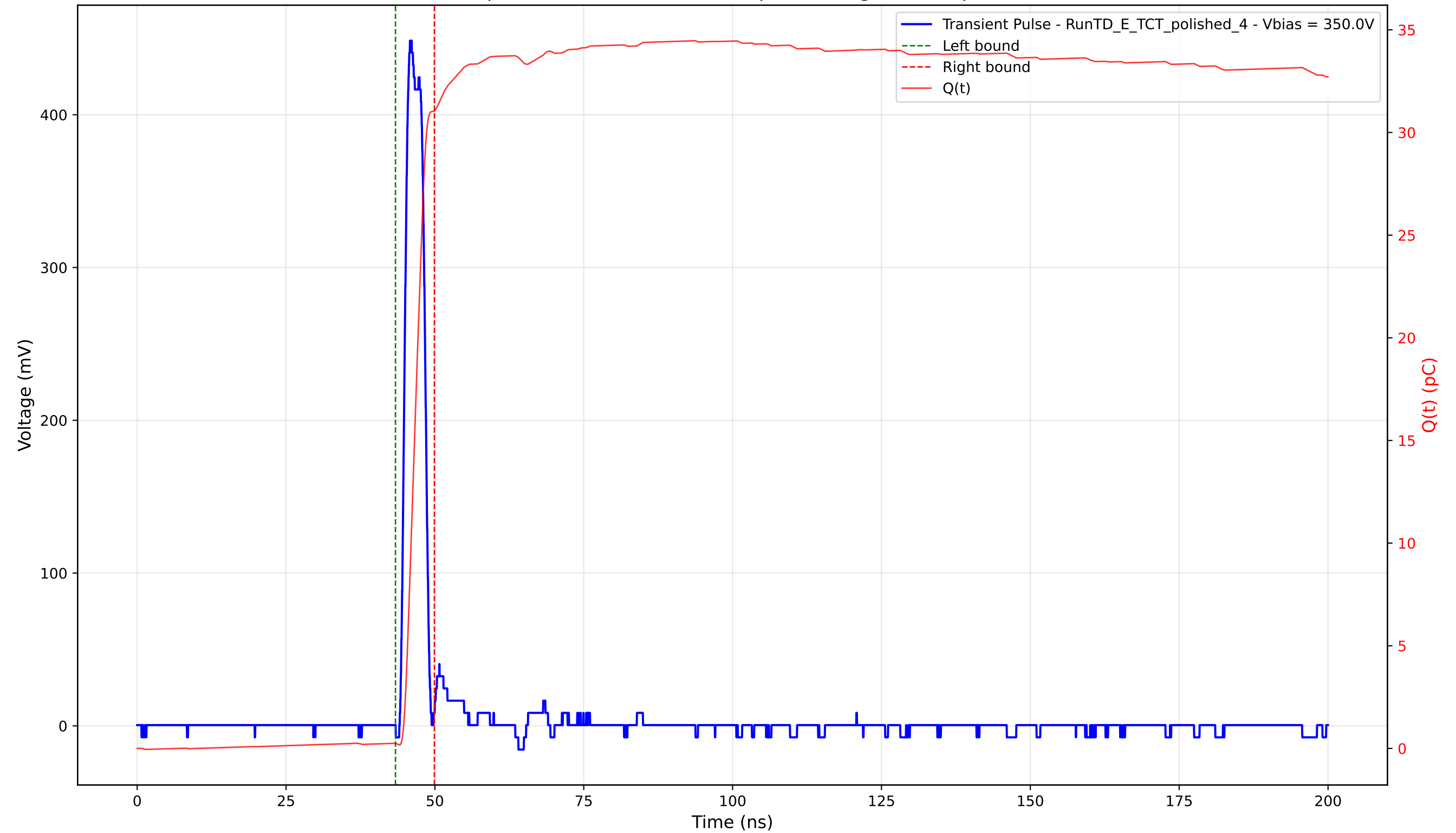
Transient Pulse - Sample: 4003 - Position: 330.0 \mu\text{m} - Charge: 30.80 pC - Rise Time: 1.11 ns
