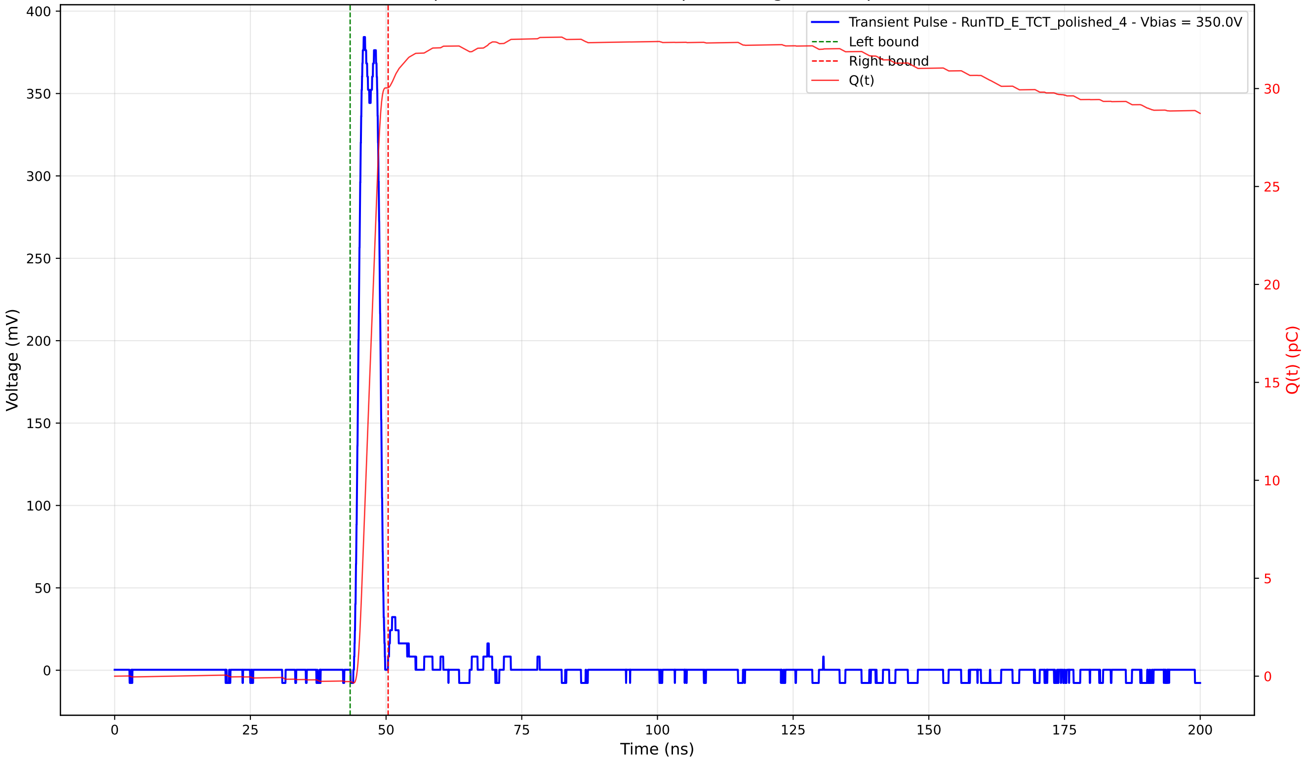
Transient Pulse - Sample: 4003 - Position: 360.0 \mu\text{m} - Charge: 30.31 pC - Rise Time: 1.16 ns
