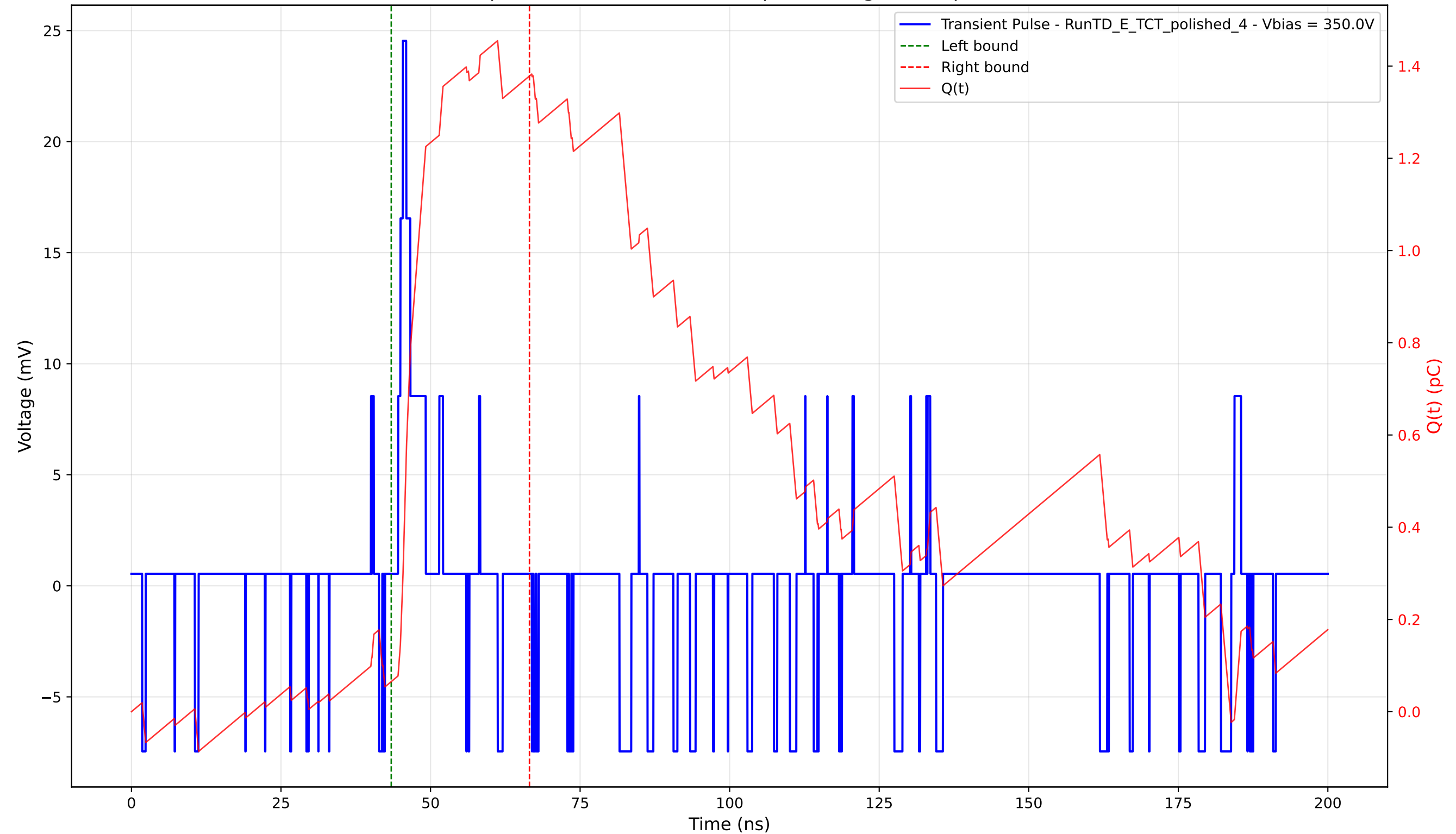
Transient Pulse - Sample: 4003 - Position: 425.0 \mu\text{m} - Charge: 1.31 pC - Rise Time: 0.80 ns
