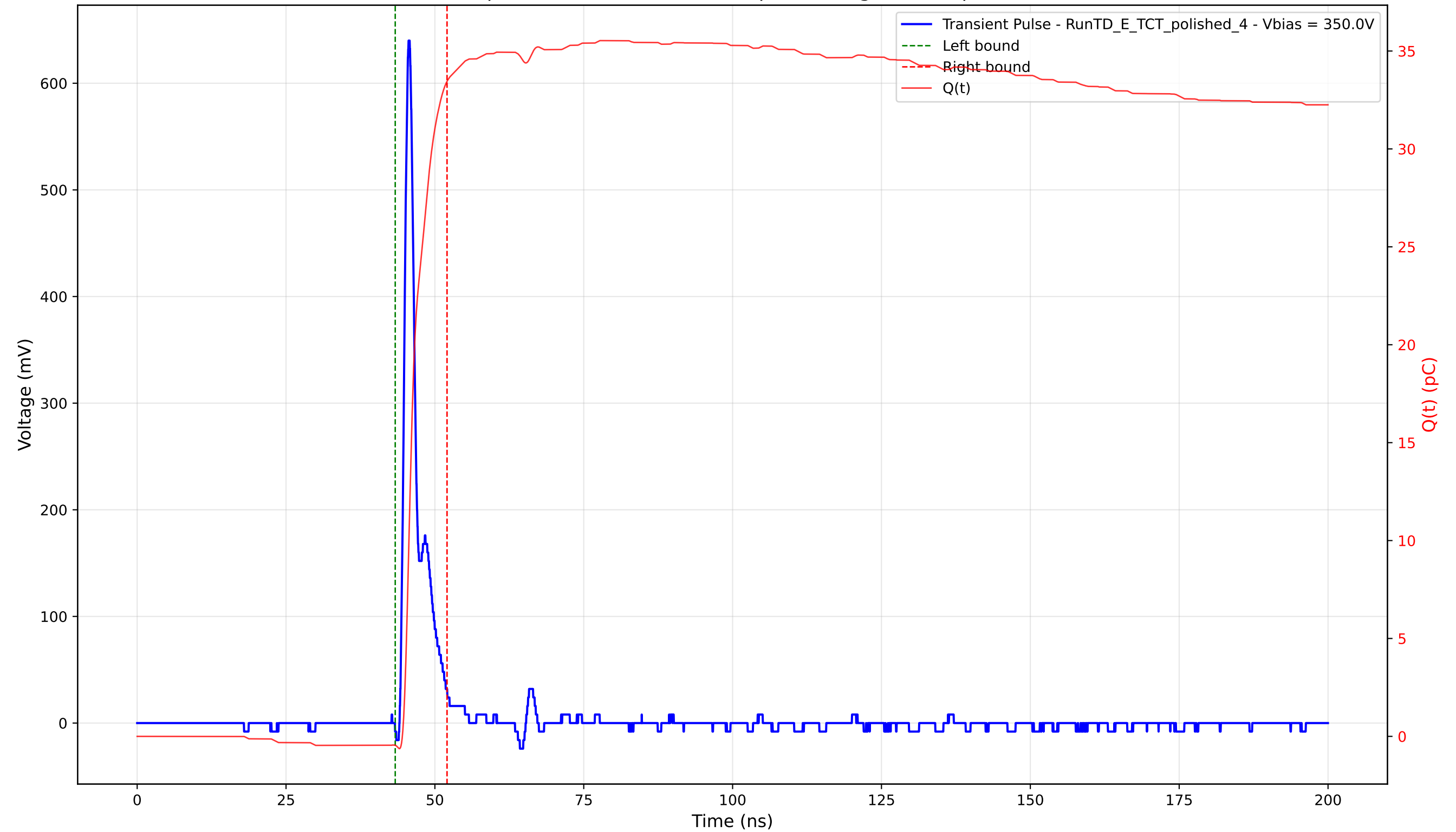
Transient Pulse - Sample: 4003 - Position: 185.0 \mu\text{m} - Charge: 33.91 pC - Rise Time: 0.98 ns
