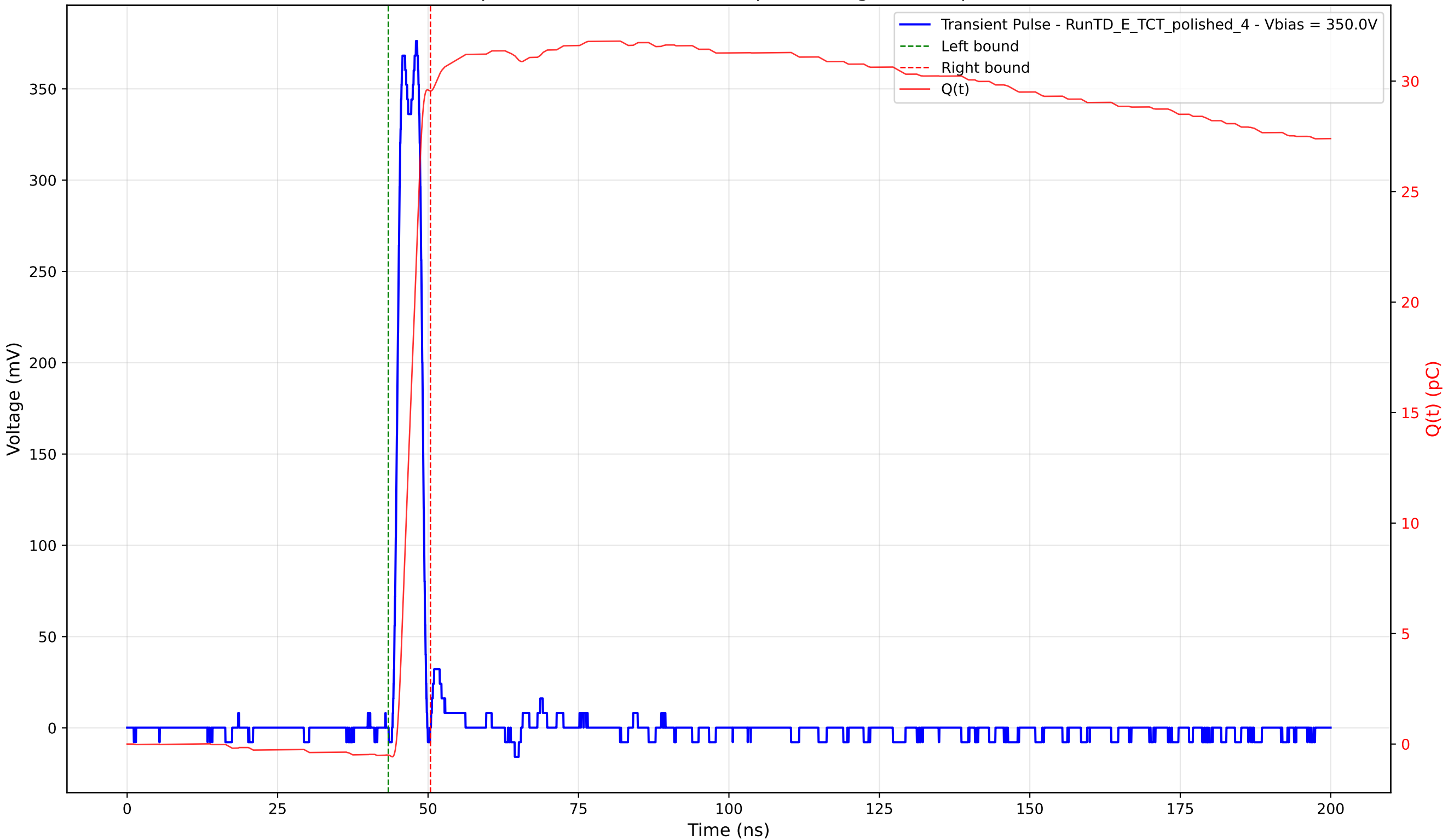
Transient Pulse - Sample: 4003 - Position: 365.0 \mu\text{m} - Charge: 30.04 pC - Rise Time: 1.15 ns
