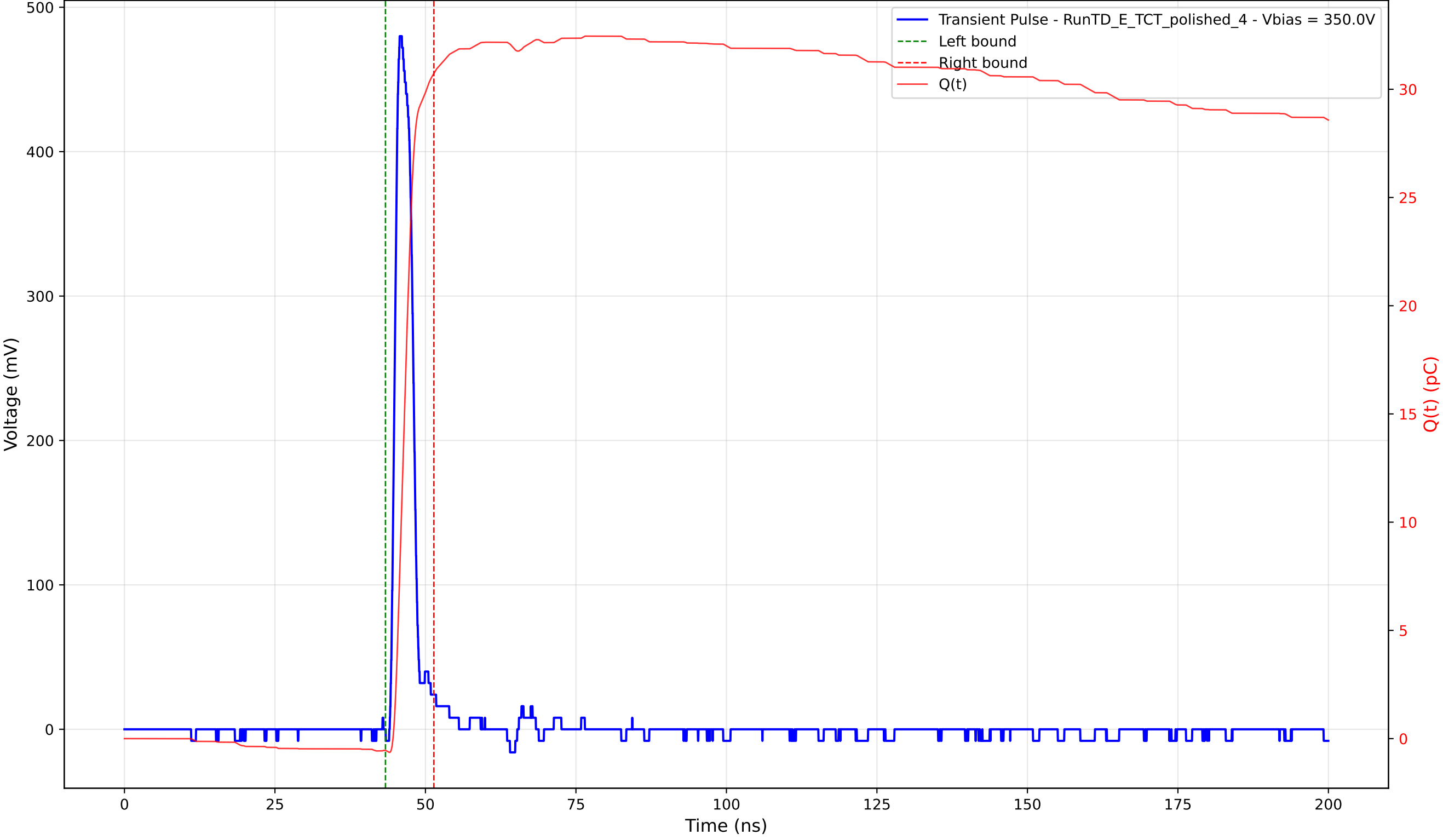
Transient Pulse - Sample: 4003 - Position: 300.0 \mu\text{m} - Charge: 31.28 pC - Rise Time: 1.06 ns
