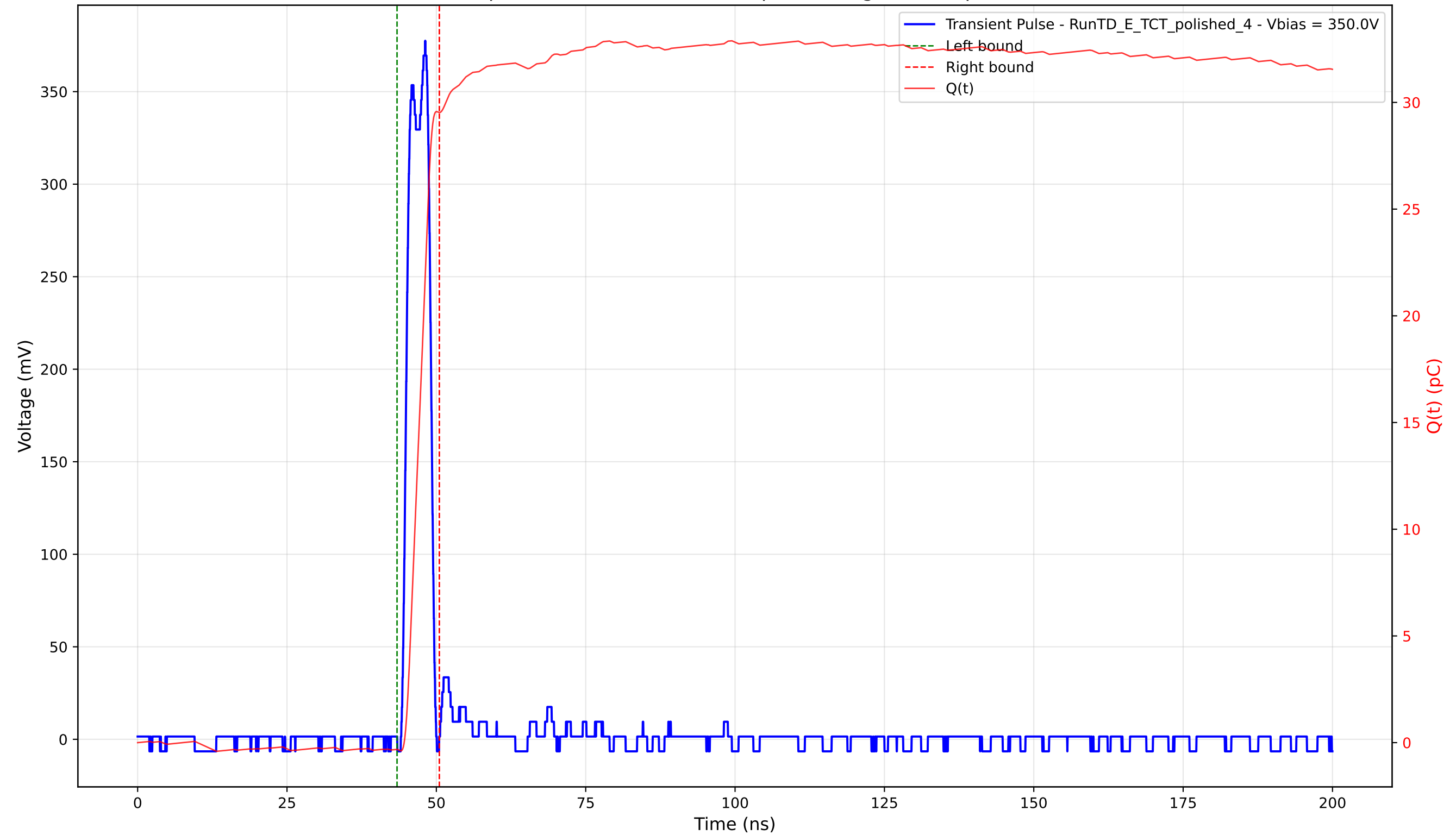
Transient Pulse - Sample: 4003 - Position: 370.0 \mu\text{m} - Charge: 29.83 pC - Rise Time: 1.29 ns
