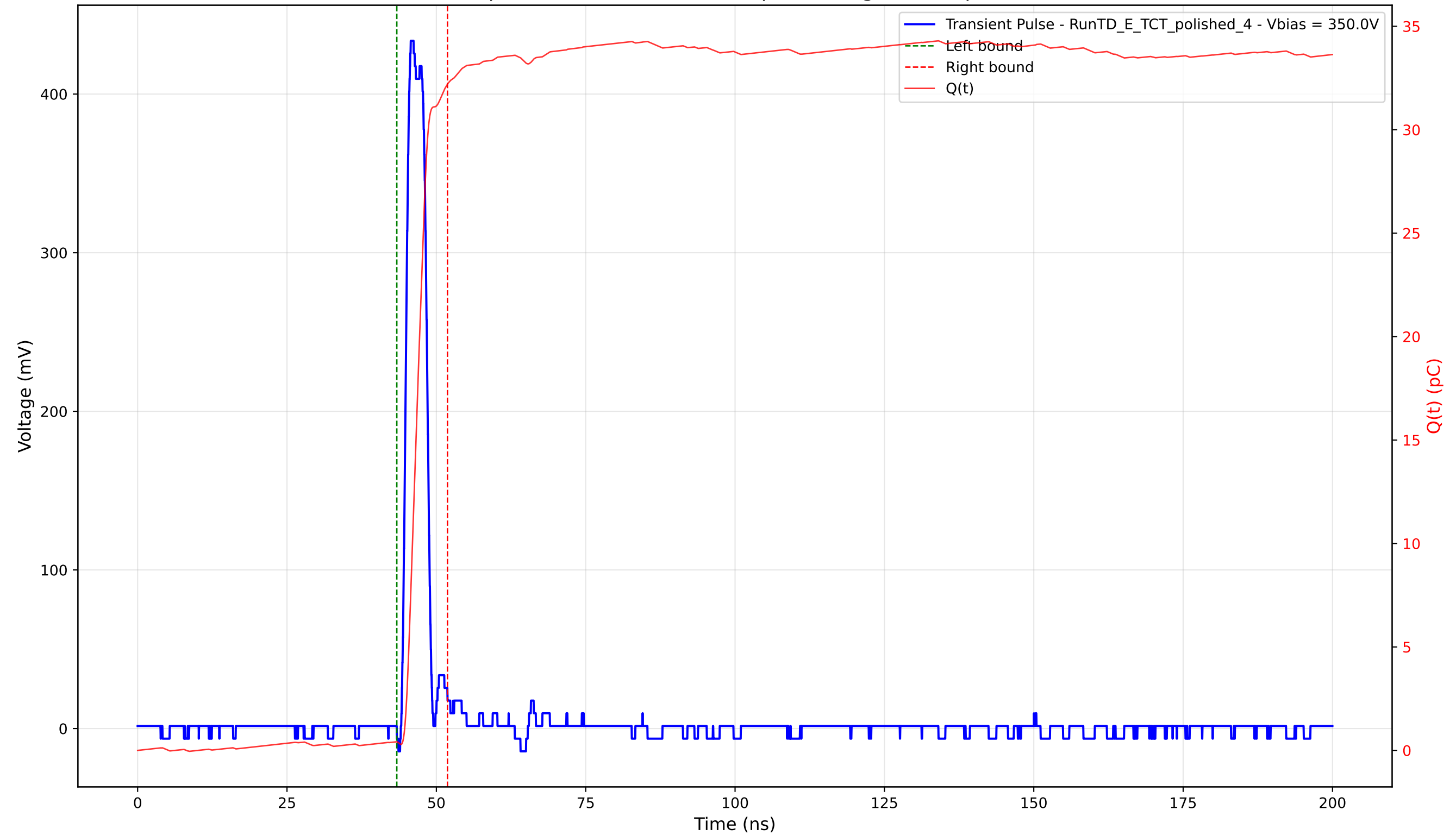
Transient Pulse - Sample: 4003 - Position: 335.0 \mu\text{m} - Charge: 31.79 pC - Rise Time: 1.08 ns
