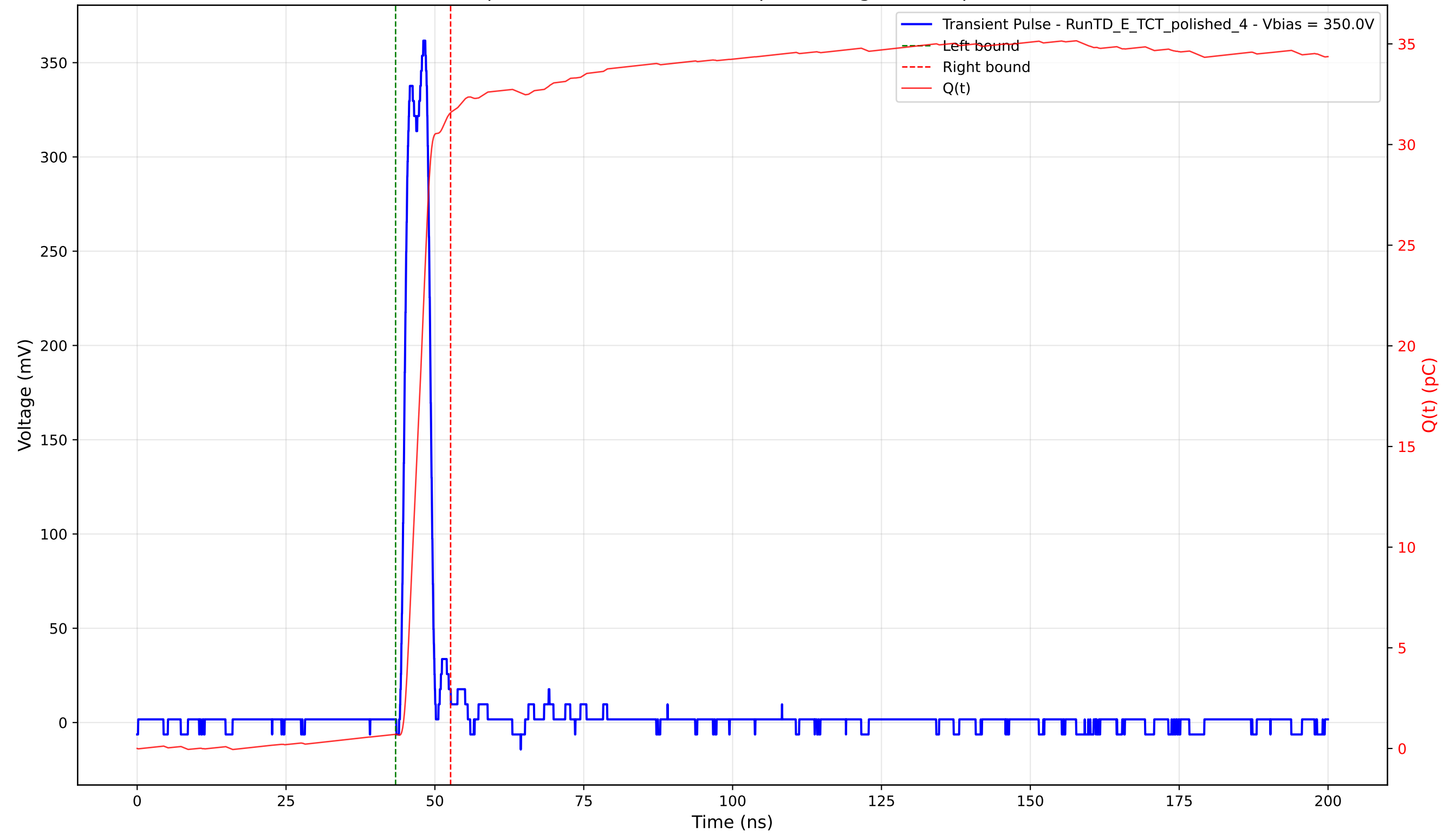
Transient Pulse - Sample: 4003 - Position: 375.0 \mu\text{m} - Charge: 30.88 pC - Rise Time: 1.29 ns
