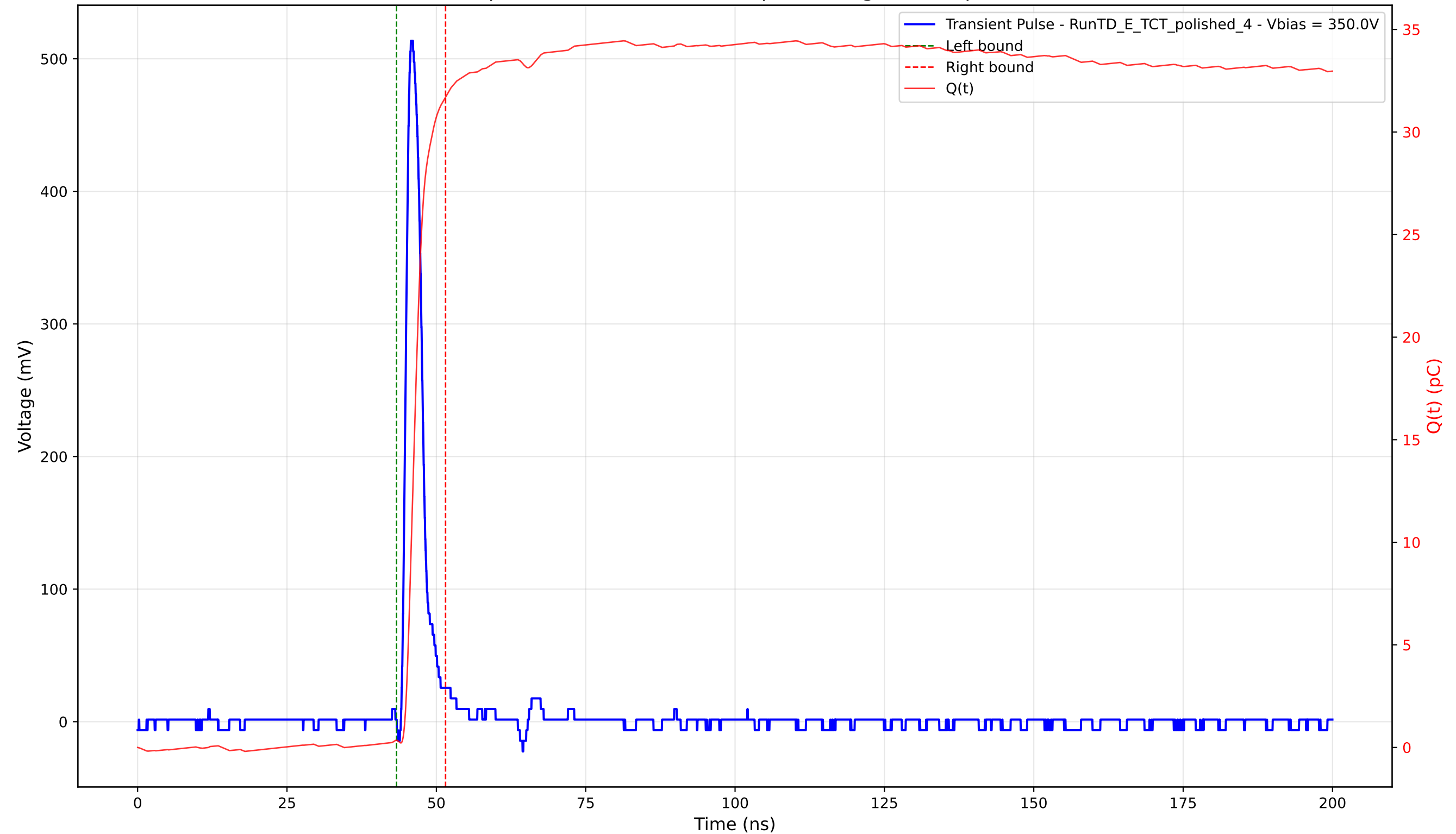
Transient Pulse - Sample: 4003 - Position: 275.0 \mu\text{m} - Charge: 31.35 pC - Rise Time: 1.08 ns
