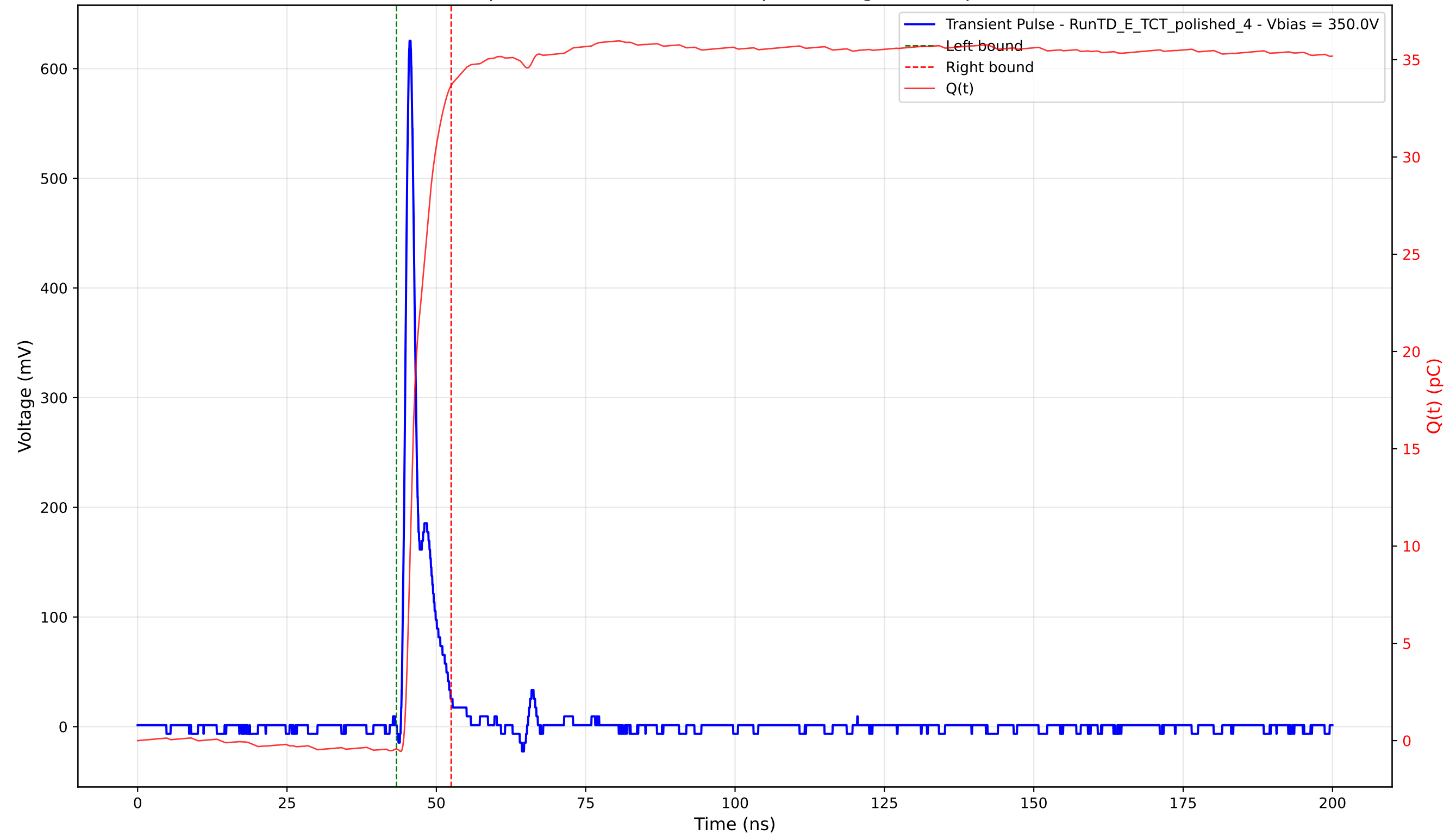
Transient Pulse - Sample: 4003 - Position: 165.0 \mu\text{m} - Charge: 34.11 pC - Rise Time: 0.97 ns
