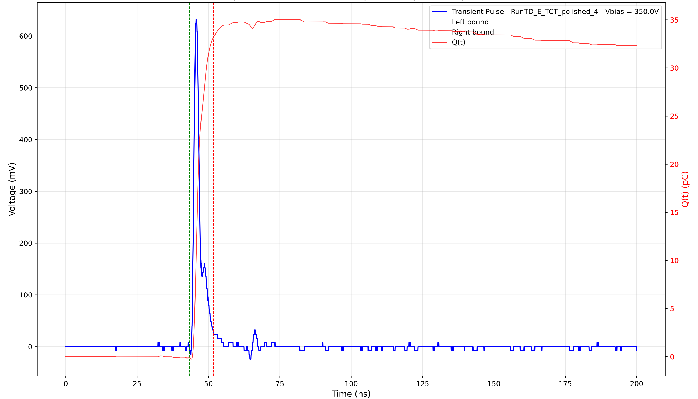
Transient Pulse - Sample: 4003 - Position: 205.0 \mu\text{m} - Charge: 33.31 pC - Rise Time: 1.04 ns
