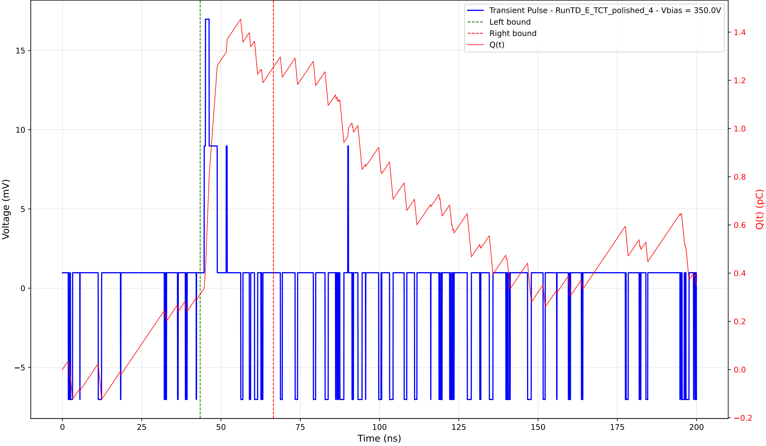
Transient Pulse - Sample: 4003 - Position: 70.0 \mu\text{m} - Charge: 0.94 pC - Rise Time: 0.42 ns
