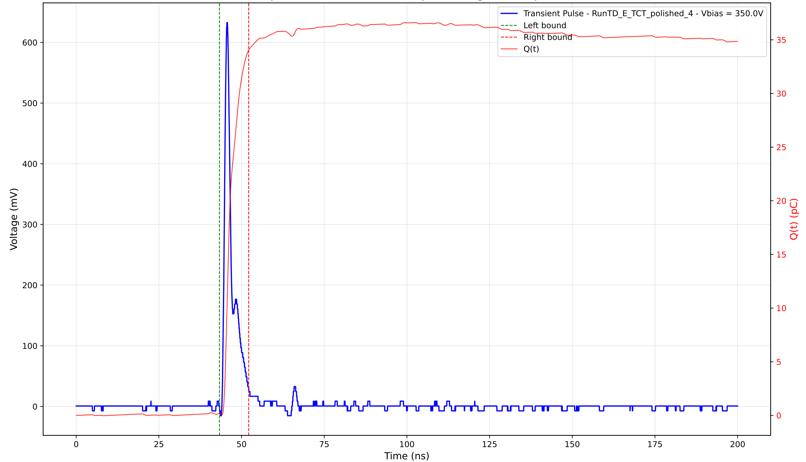
Transient Pulse - Sample: 4003 - Position: 180.0 \mu\text{m} - Charge: 33.87 pC - Rise Time: 0.99 ns
