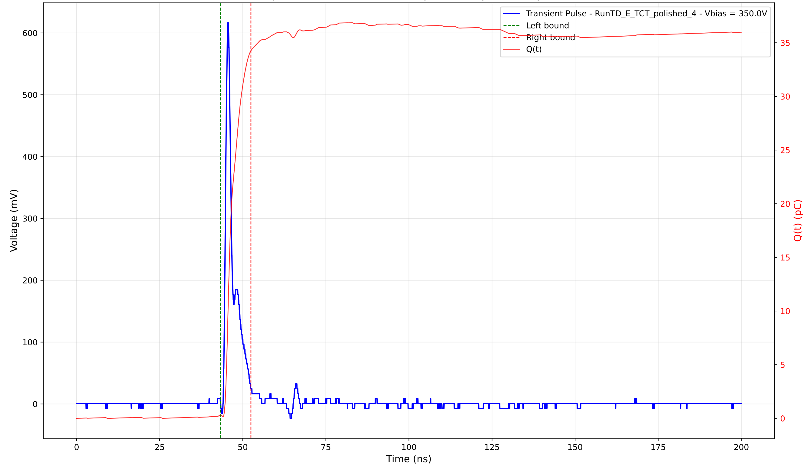
Transient Pulse - Sample: 4003 - Position: 160.0 \mu\text{m} - Charge: 33.95 pC - Rise Time: 0.93 ns
