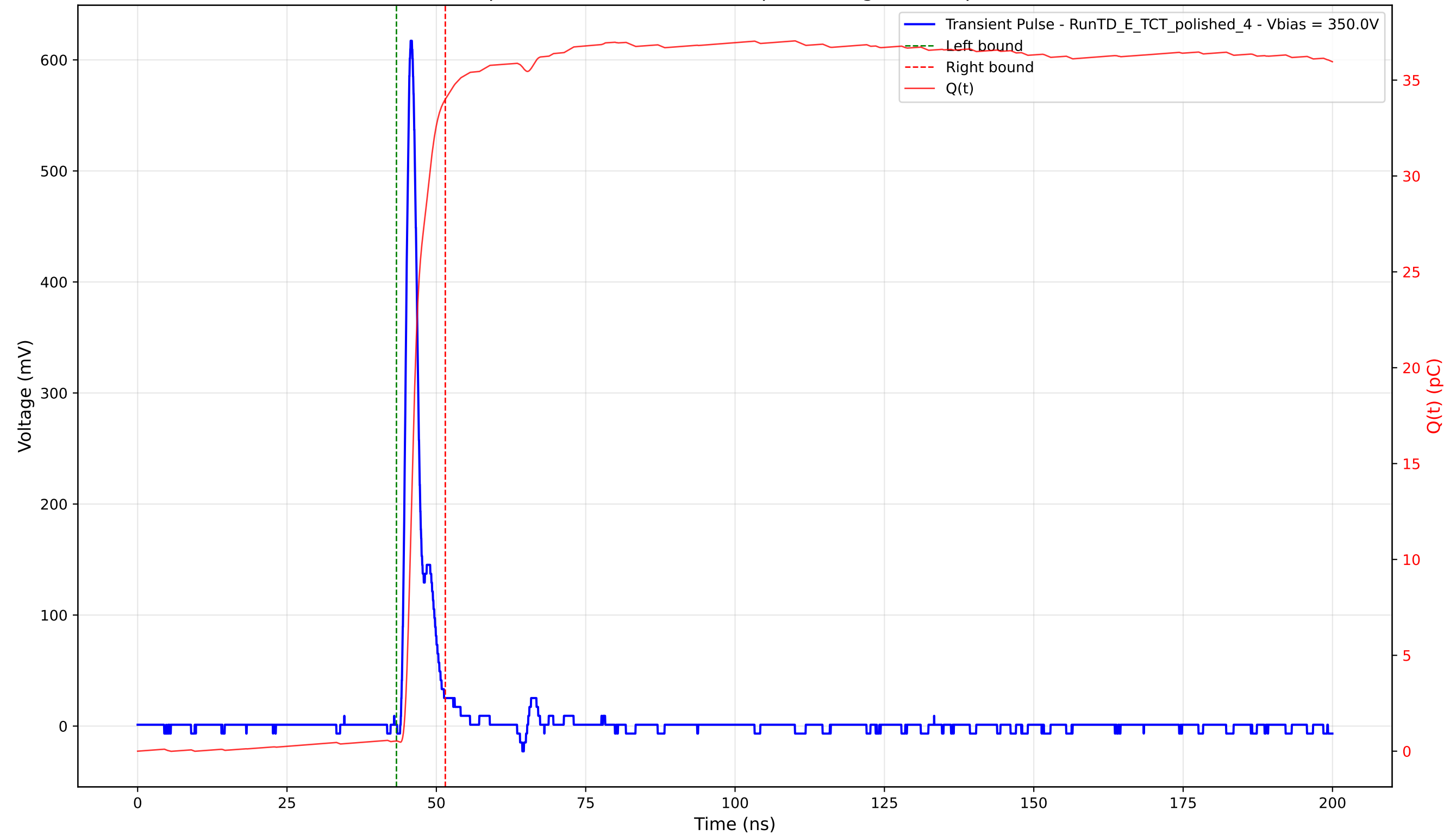
Transient Pulse - Sample: 4003 - Position: 220.0 \mu\text{m} - Charge: 33.47 pC - Rise Time: 1.07 ns
