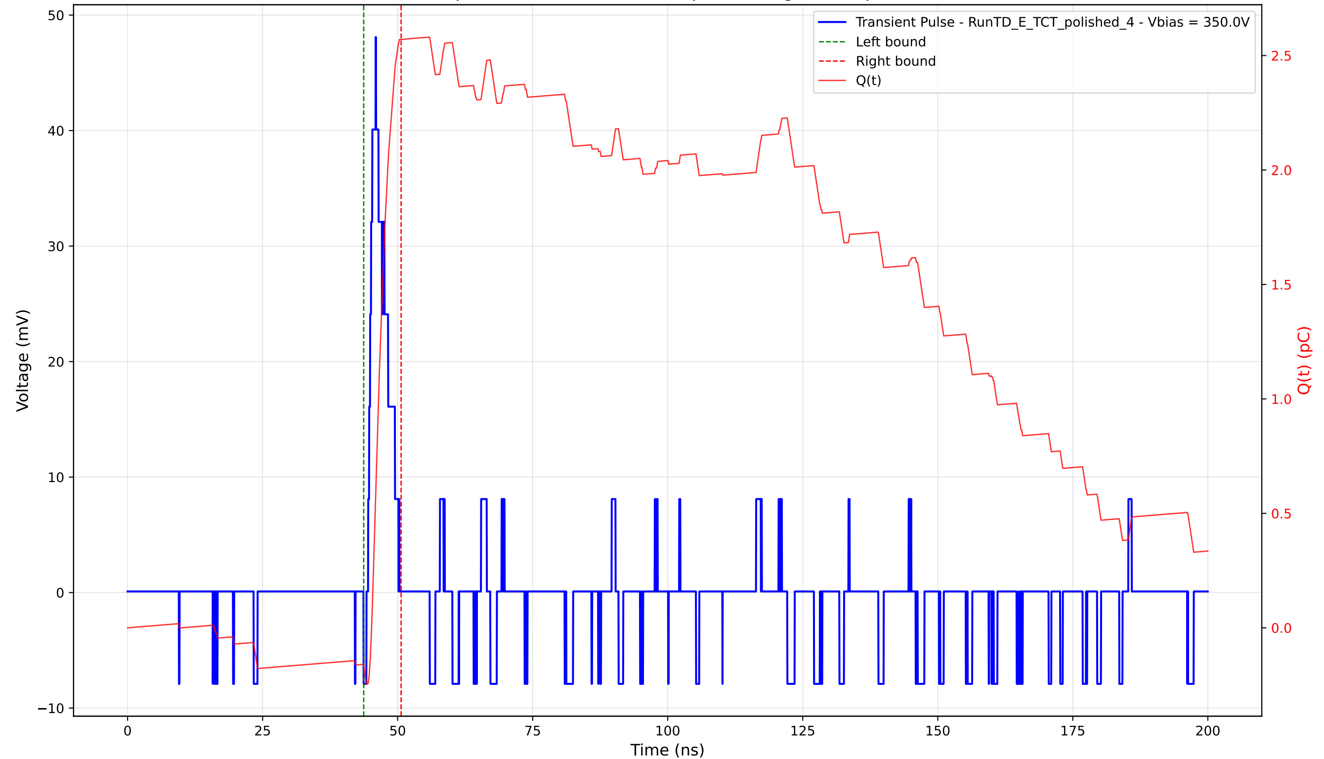
Transient Pulse - Sample: 4003 - Position: 60.0 \mu\text{m} - Charge: 2.74 pC - Rise Time: 1.39 ns
