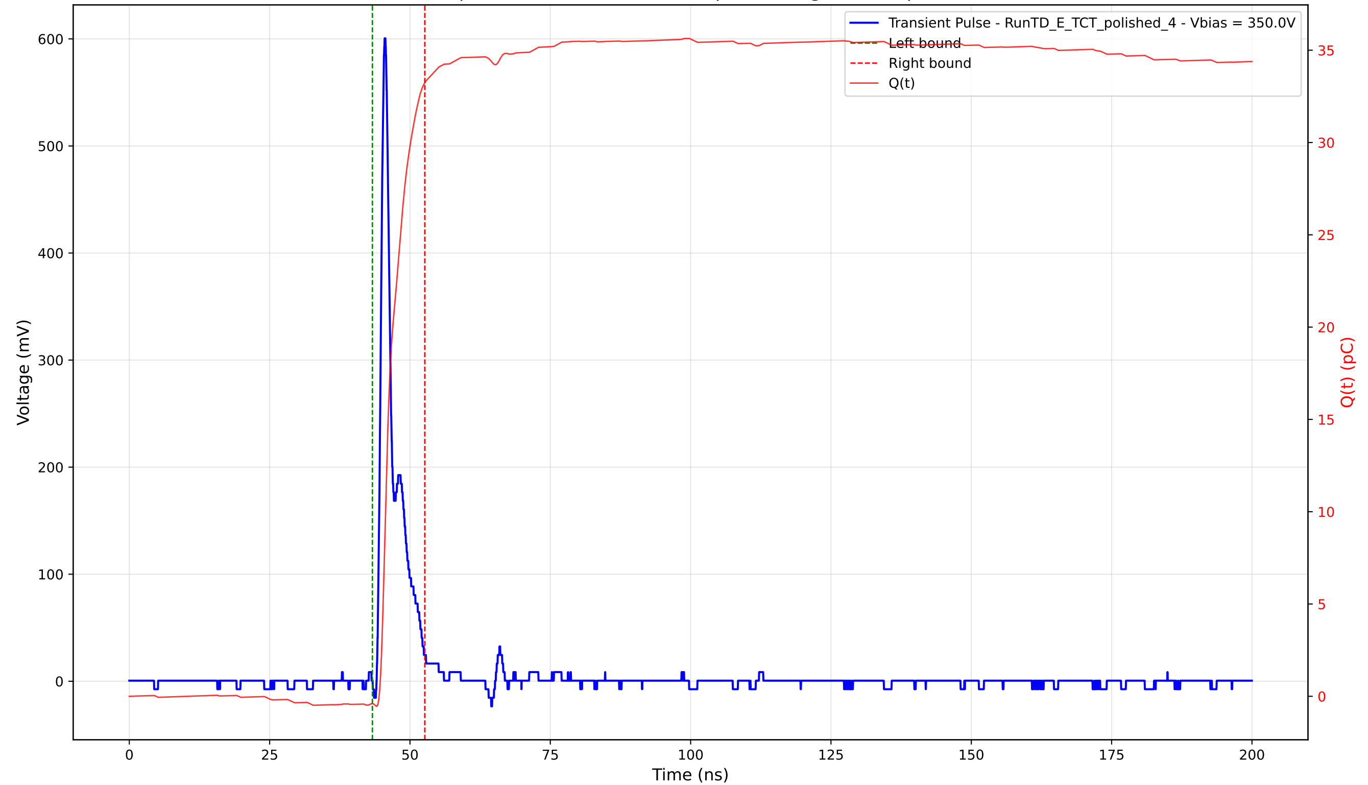
Transient Pulse - Sample: 4003 - Position: 150.0 \mu\text{m} - Charge: 33.63 pC - Rise Time: 0.93 ns
