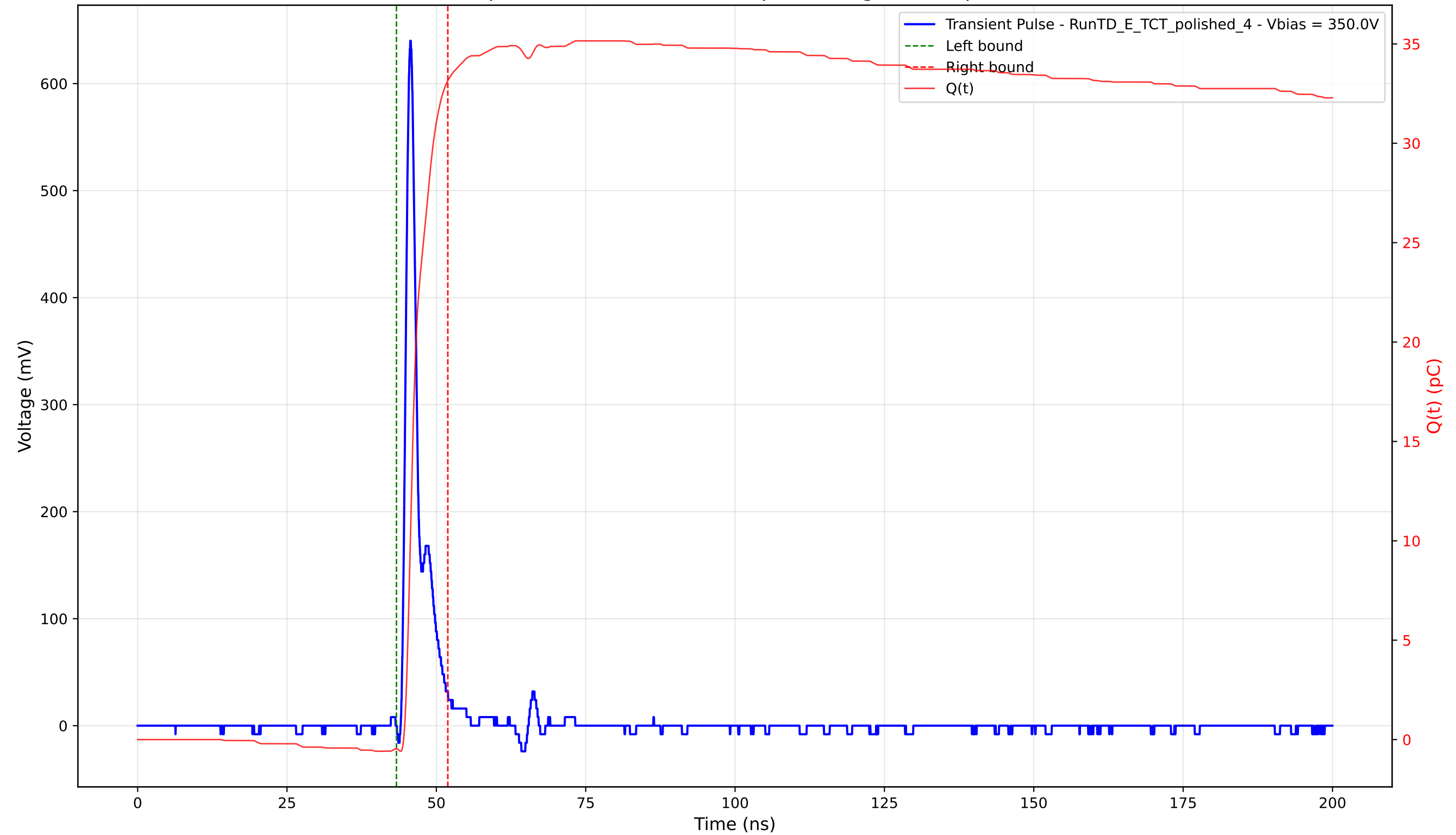
Transient Pulse - Sample: 4003 - Position: 190.0 \mu\text{m} - Charge: 33.62 pC - Rise Time: 1.02 ns
