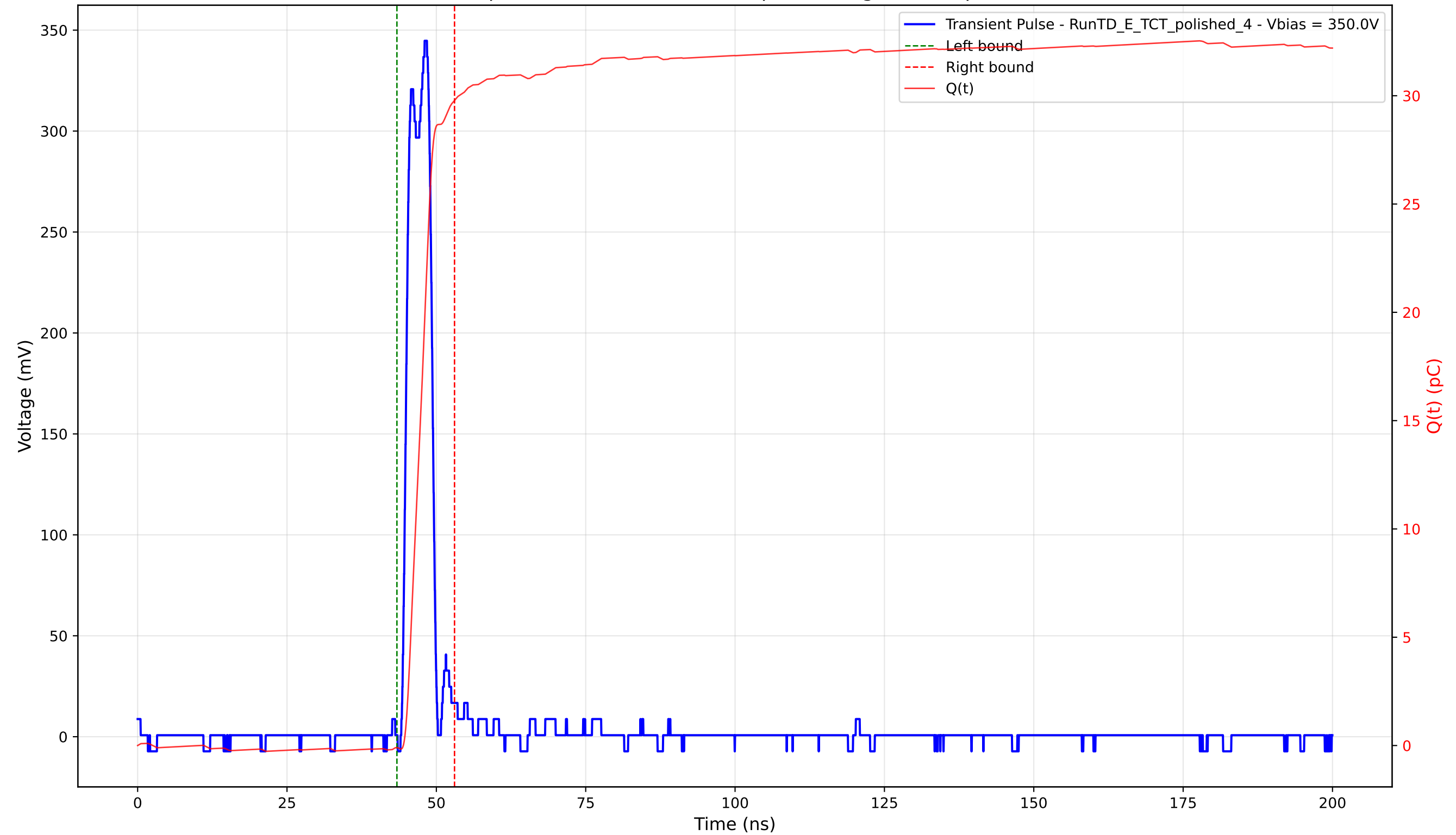
Transient Pulse - Sample: 4003 - Position: 380.0 \mu\text{m} - Charge: 29.88 pC - Rise Time: 1.24 ns
