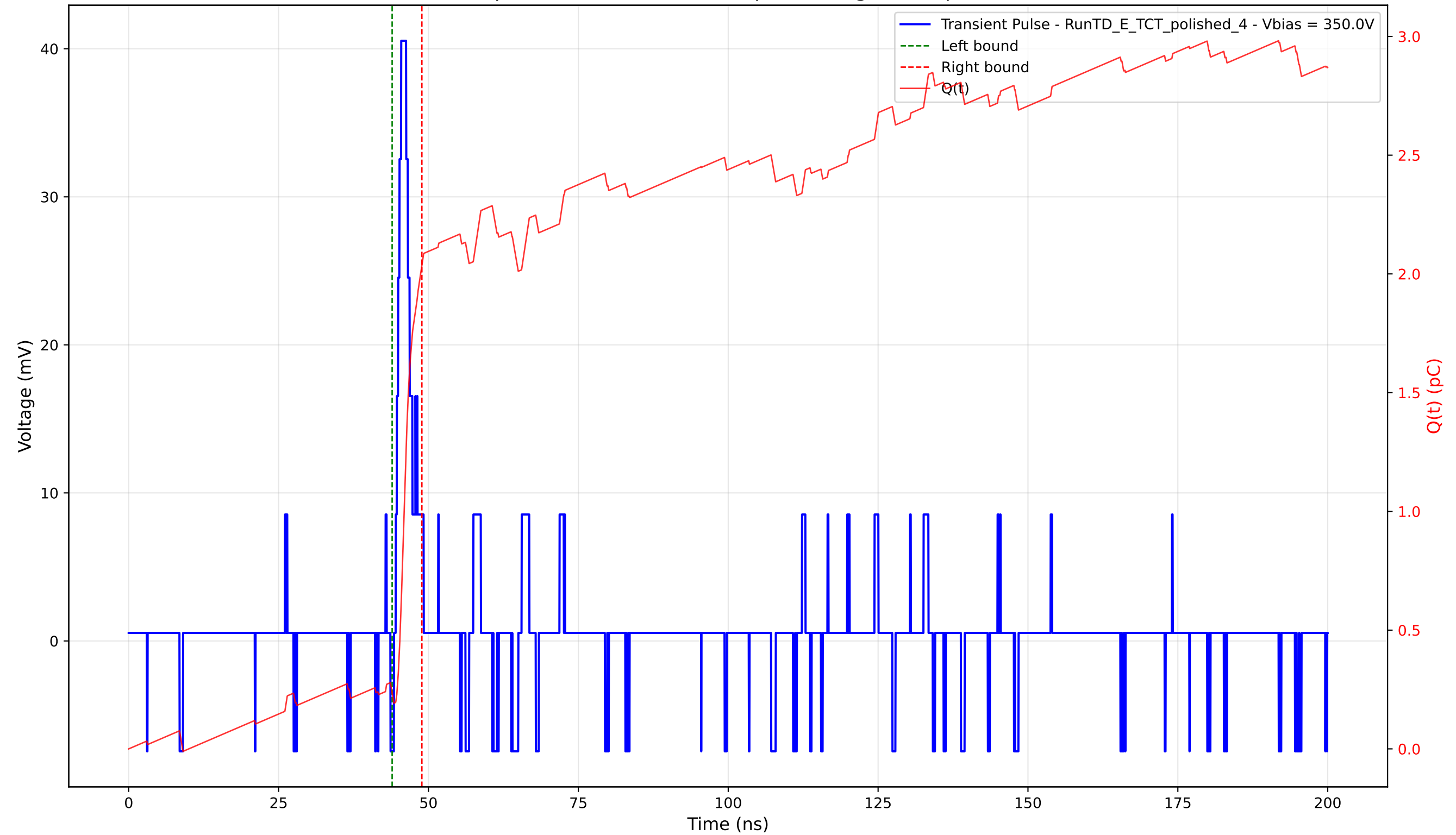
Transient Pulse - Sample: 4003 - Position: 40.0 \mu\text{m} - Charge: 1.80 pC - Rise Time: 0.91 ns
