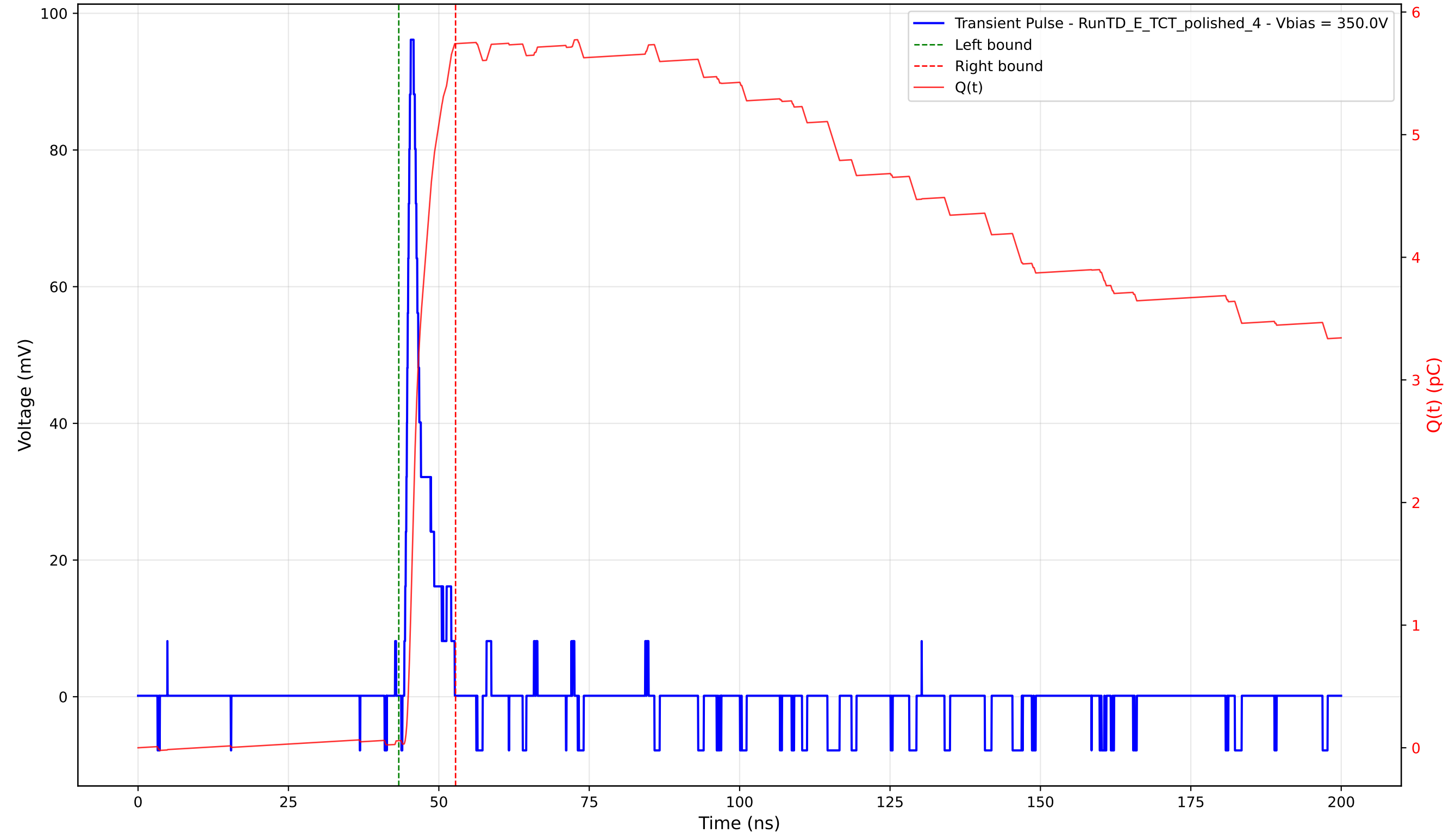
Transient Pulse - Sample: 4003 - Position: 85.0 \mu\text{m} - Charge: 5.68 pC - Rise Time: 0.80 ns
