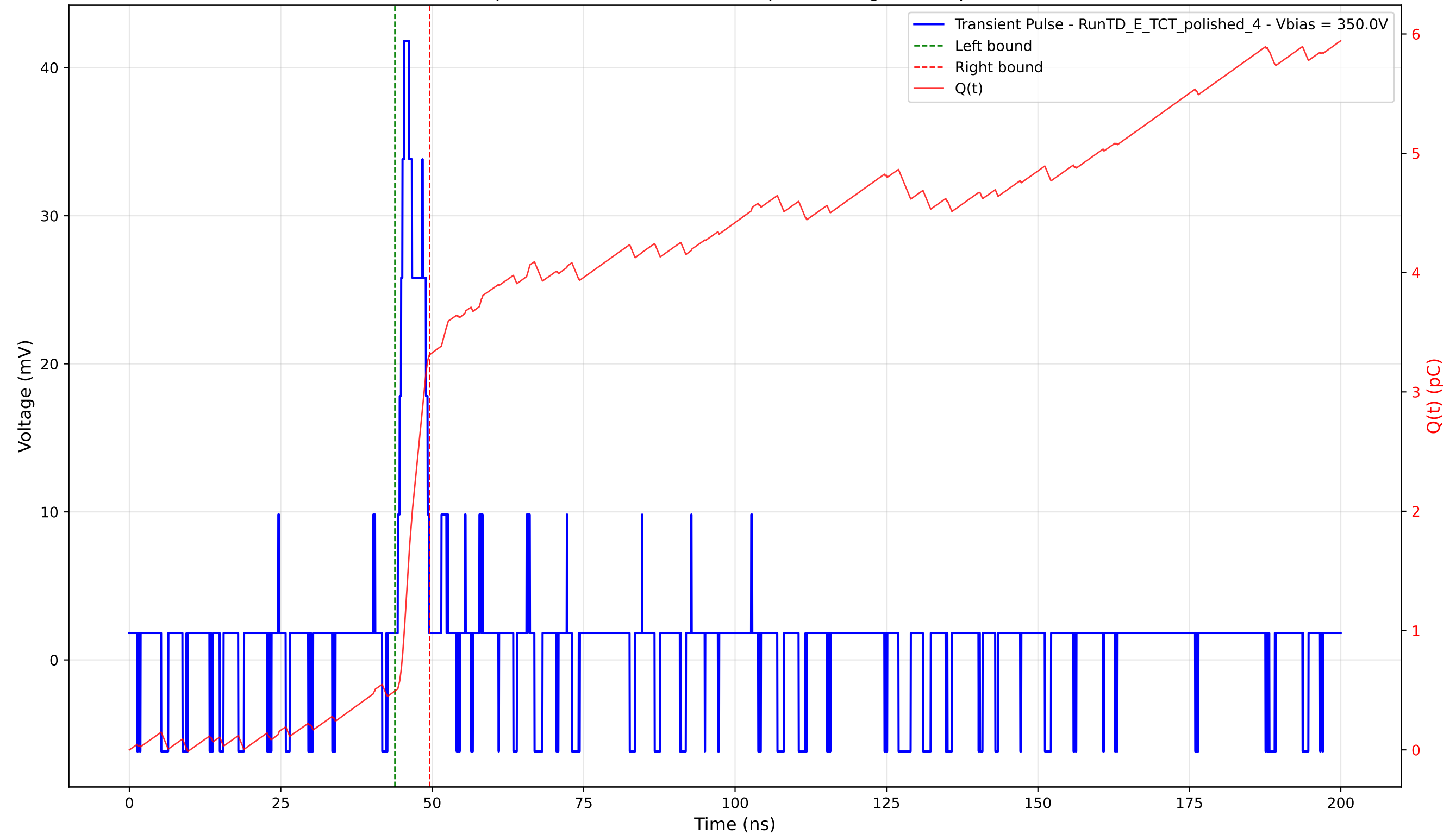
Transient Pulse - Sample: 4003 - Position: 415.0 \mu\text{m} - Charge: 2.82 pC - Rise Time: 1.05 ns
