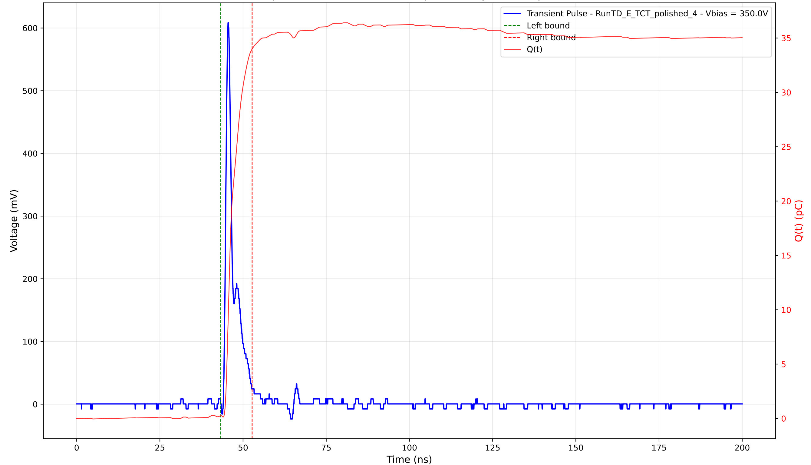
Transient Pulse - Sample: 4003 - Position: 155.0 \mu\text{m} - Charge: 33.73 pC - Rise Time: 0.95 ns
