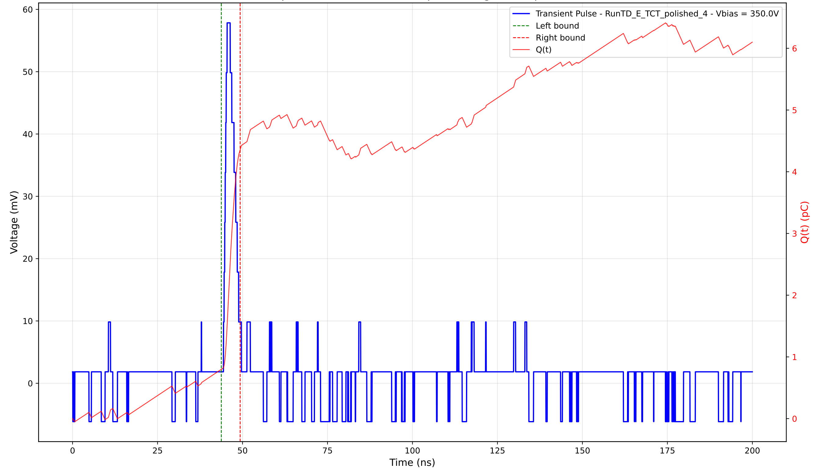
Transient Pulse - Sample: 4003 - Position: 55.0 \mu\text{m} - Charge: 3.56 pC - Rise Time: 1.07 ns
