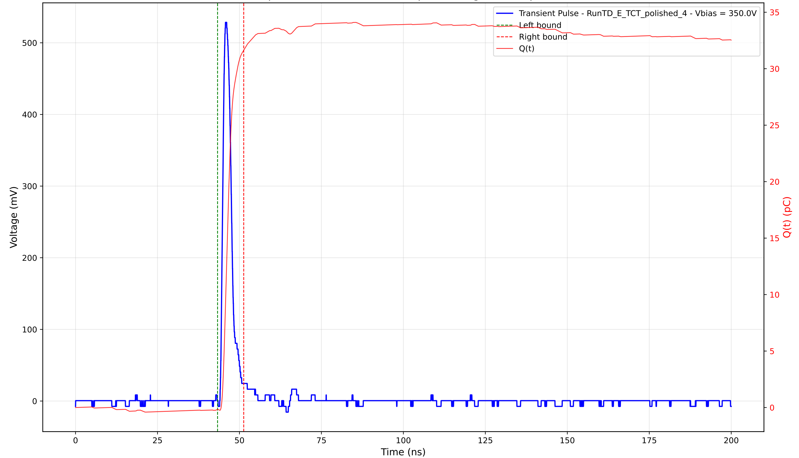
Transient Pulse - Sample: 4003 - Position: 270.0 \mu\text{m} - Charge: 31.81 pC - Rise Time: 1.11 ns
