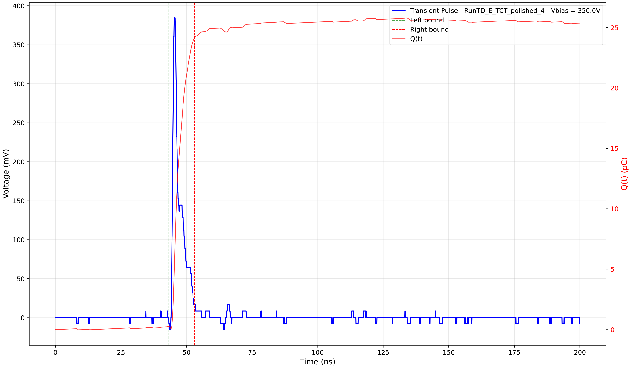
Transient Pulse - Sample: 4003 - Position: 105.0 \mu\text{m} - Charge: 23.87 pC - Rise Time: 0.91 ns
