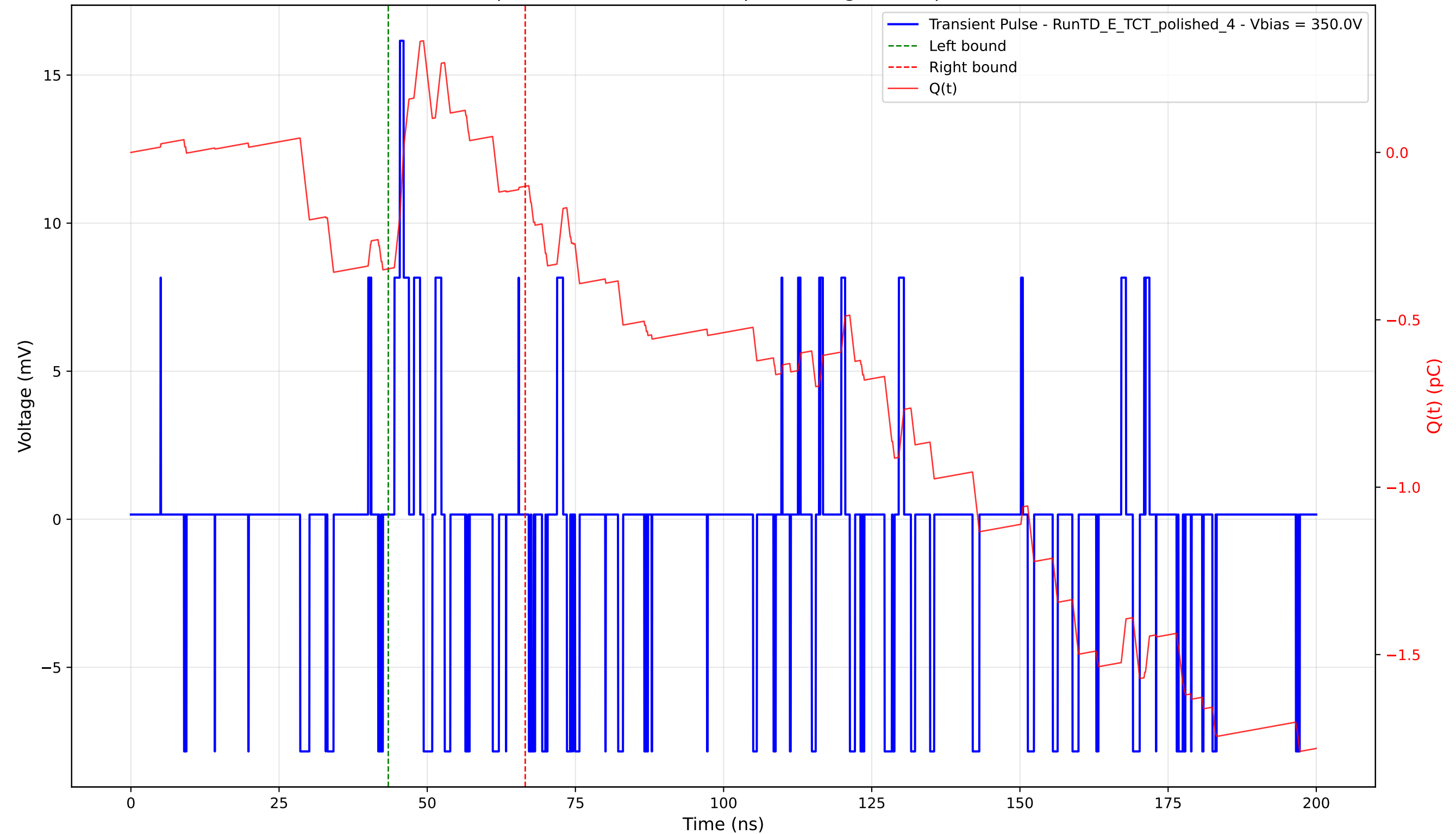
Transient Pulse - Sample: 4003 - Position: 5.0 \mu\text{m} - Charge: 0.25 pC - Rise Time: 0.94 ns
