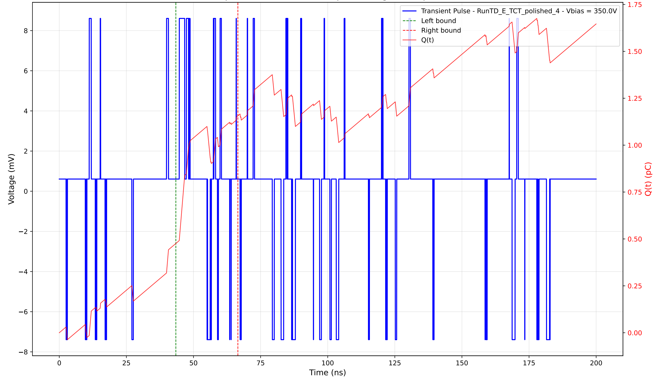
Transient Pulse - Sample: 4003 - Position: 0.0 \mu\text{m} - Charge: 0.68 pC - Rise Time: 0.02 ns
