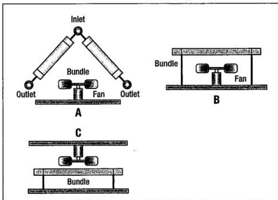
Fig. 1. Types of ACHEs: (a) A-frame configuration with forced draft; (b) horizontal with forced draft and (c) horizontal with induced draft.
