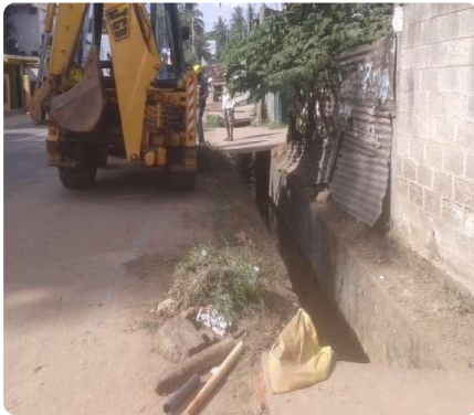
Greater Kurunegala Water Supply — trenching
