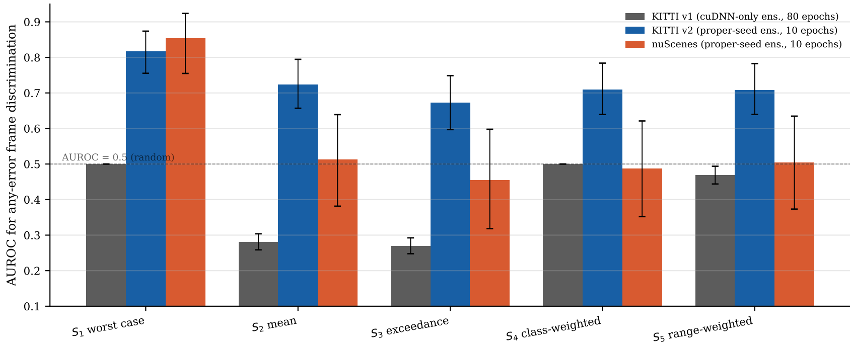
Deep-ensemble runtime monitor AUROC across diversity and dataset regimes
