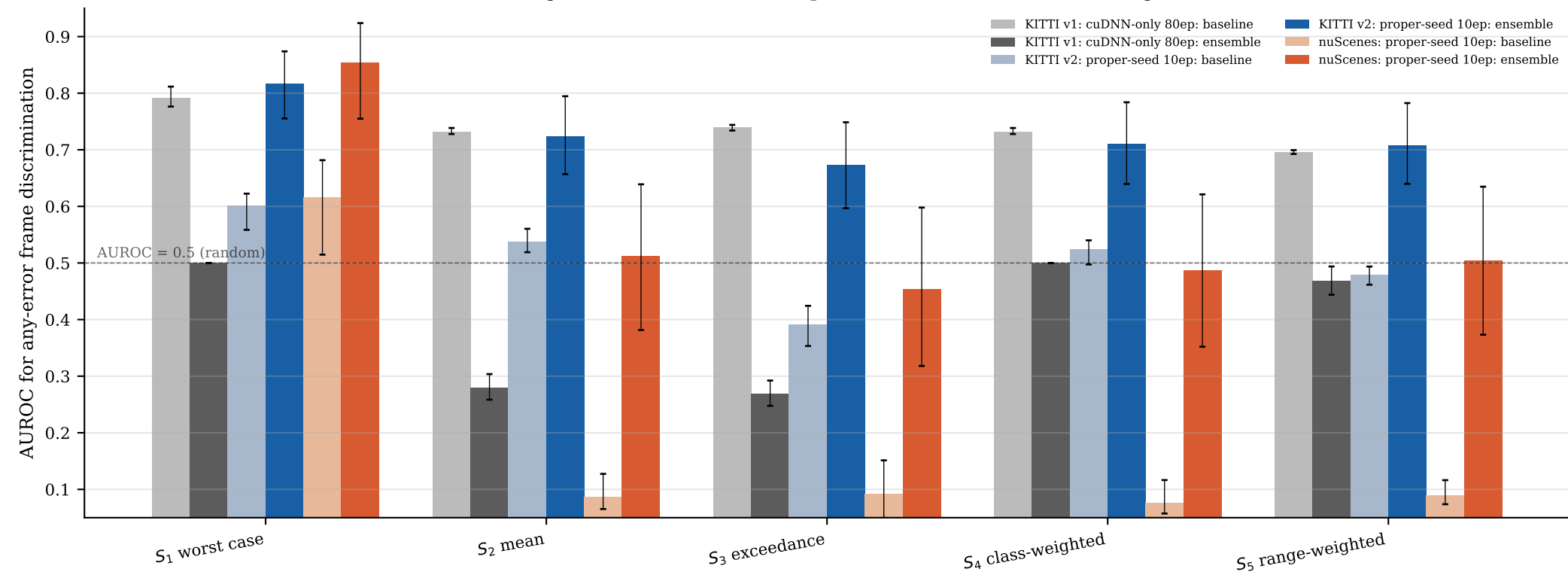
Baseline (single-model softmax) vs deep-ensemble monitor across configurations
