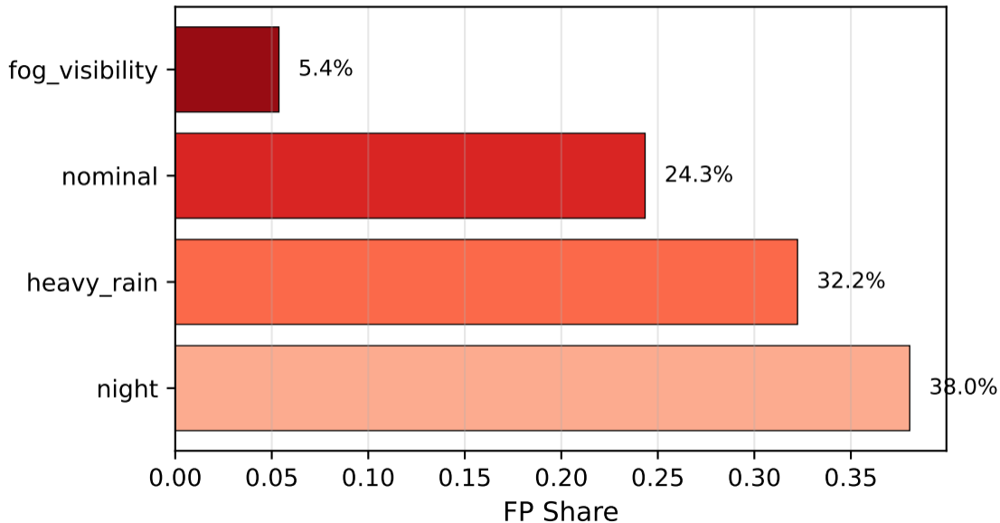
Triggering Condition Ranking (ISO 21448, Clause 7)
