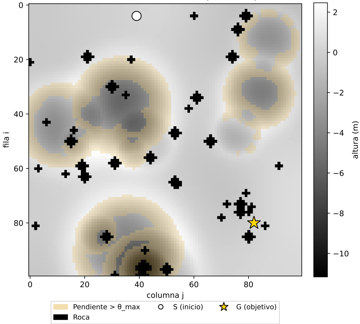
Terreno sintético 100x100 (semilla 0)
