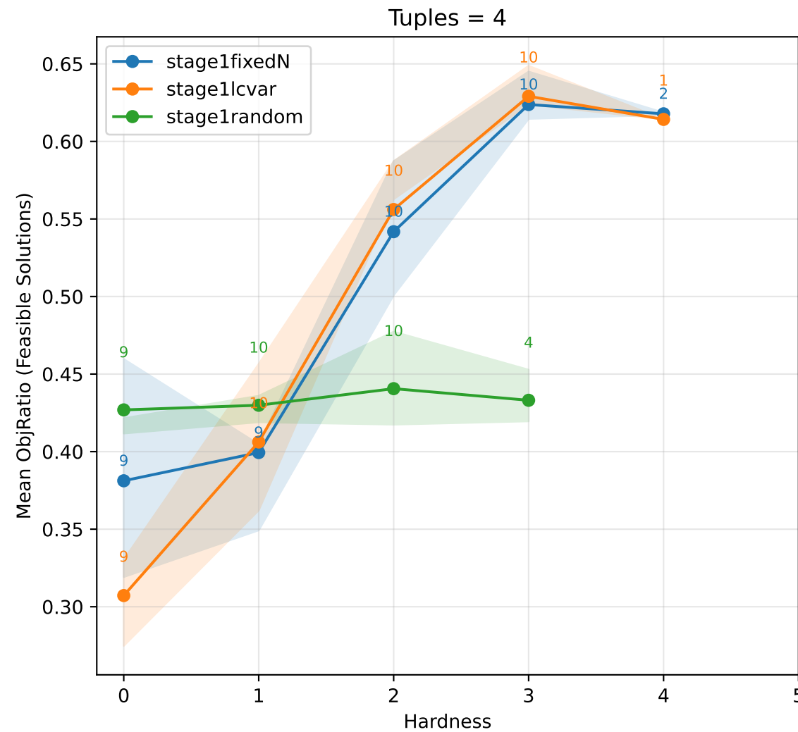
Mean Objective Ratio by Hardness
