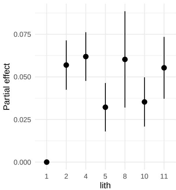
lith
