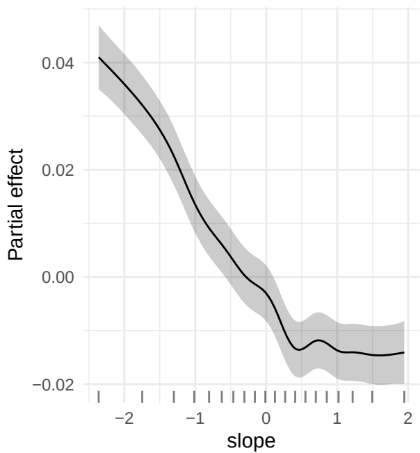
s(slope)
