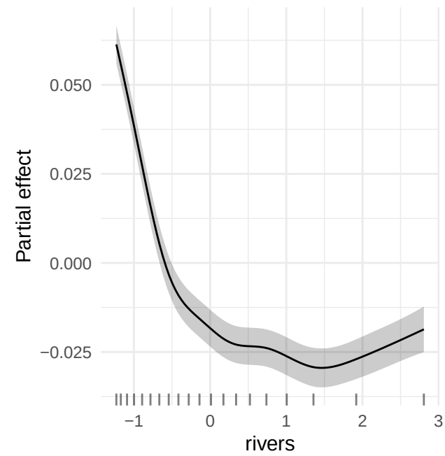
s(rivers)
