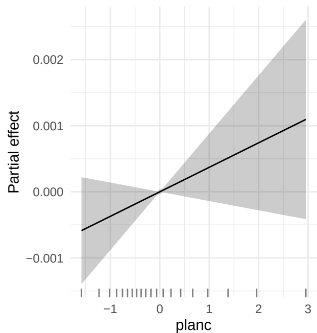
planc
