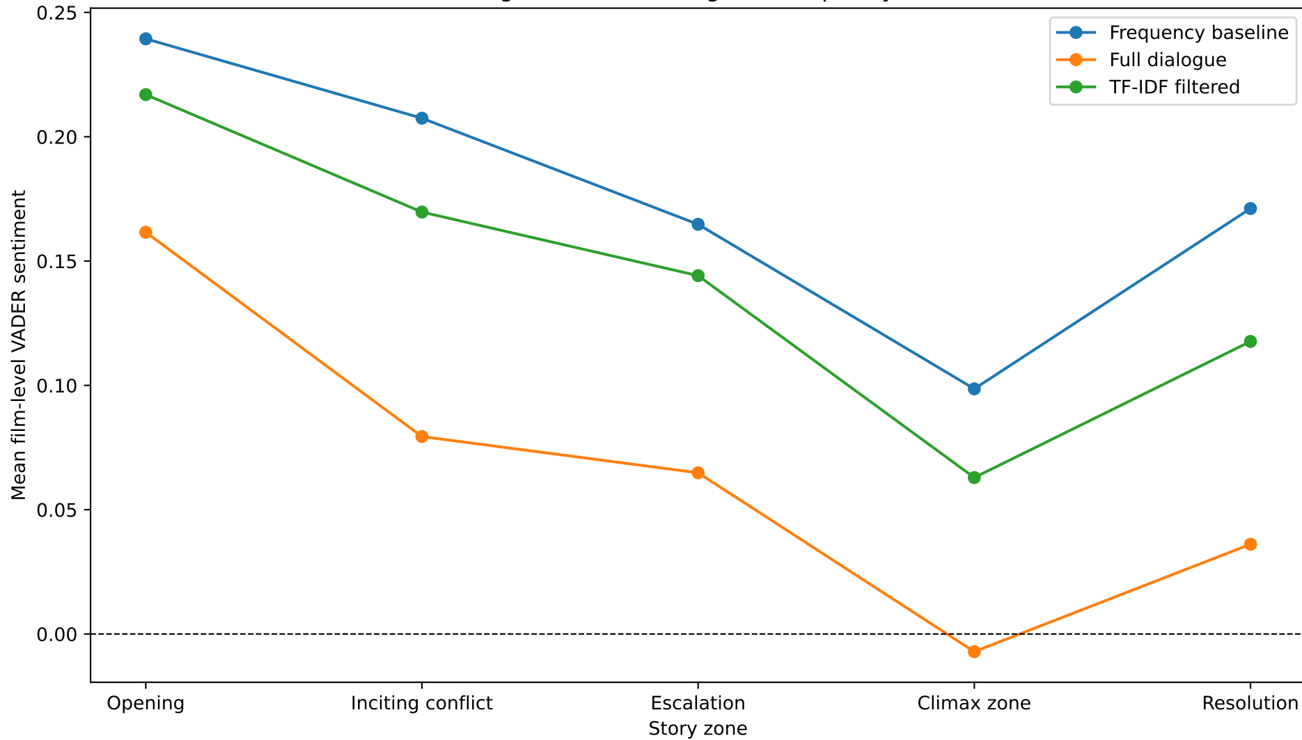
Full dialogue, TF-IDF filtering, and frequency baseline
