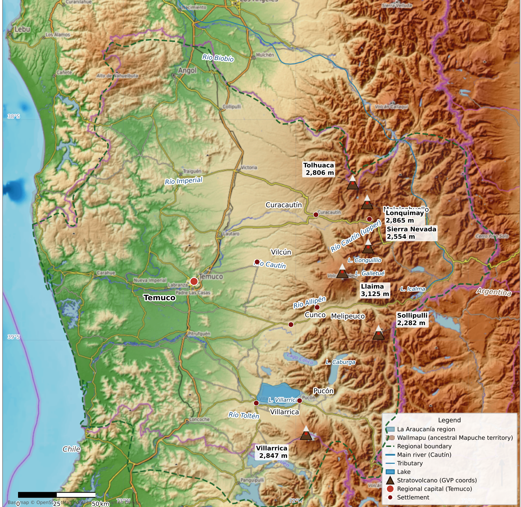
B — La Araucanía: physiography, volcanic arc & settlements
