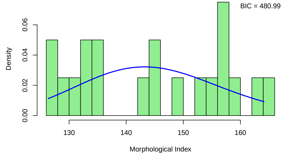
Gaussian Mixture Model Fit
