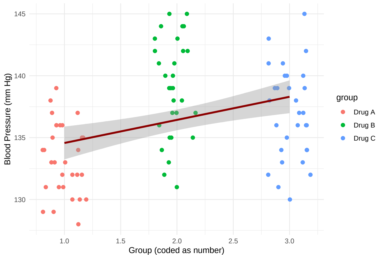
Linear Regression: Blood Pressure vs Group (numeric code)
