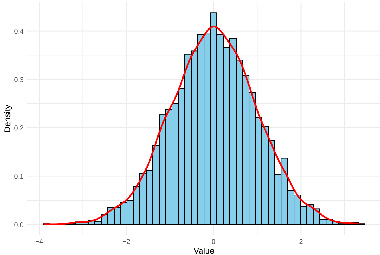
Histogram of generated data with density line
