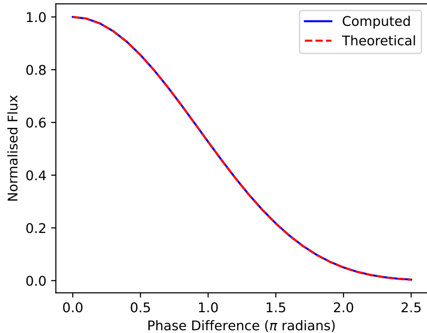
Centre Flux
