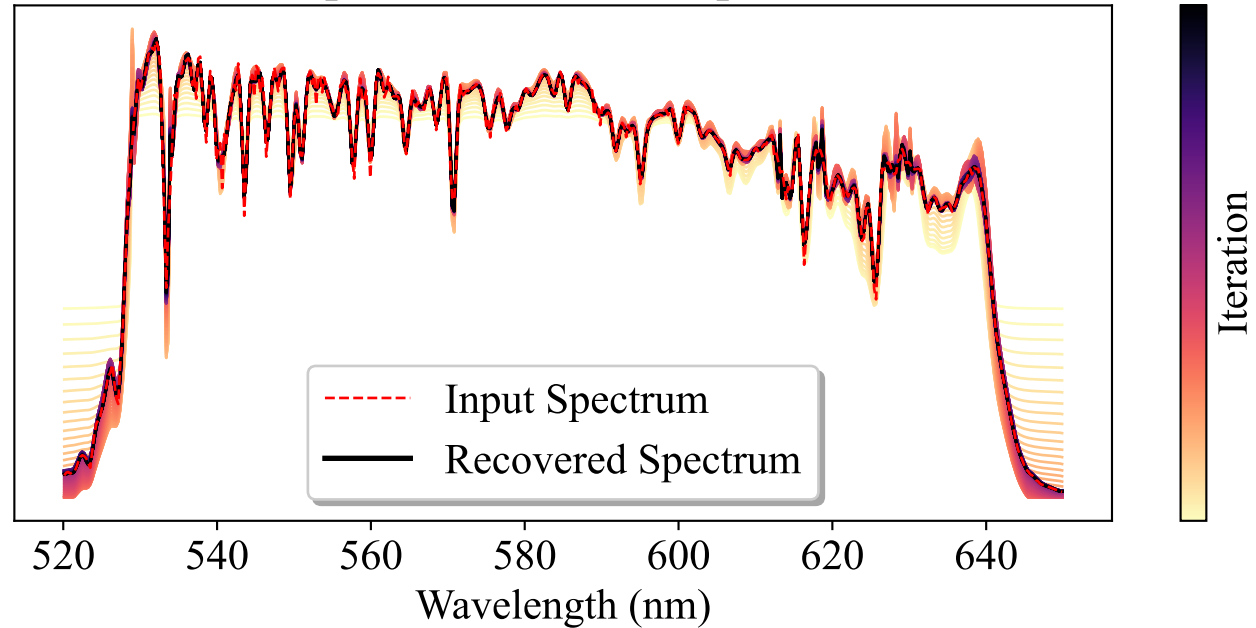
Input & Recovered Spectra
