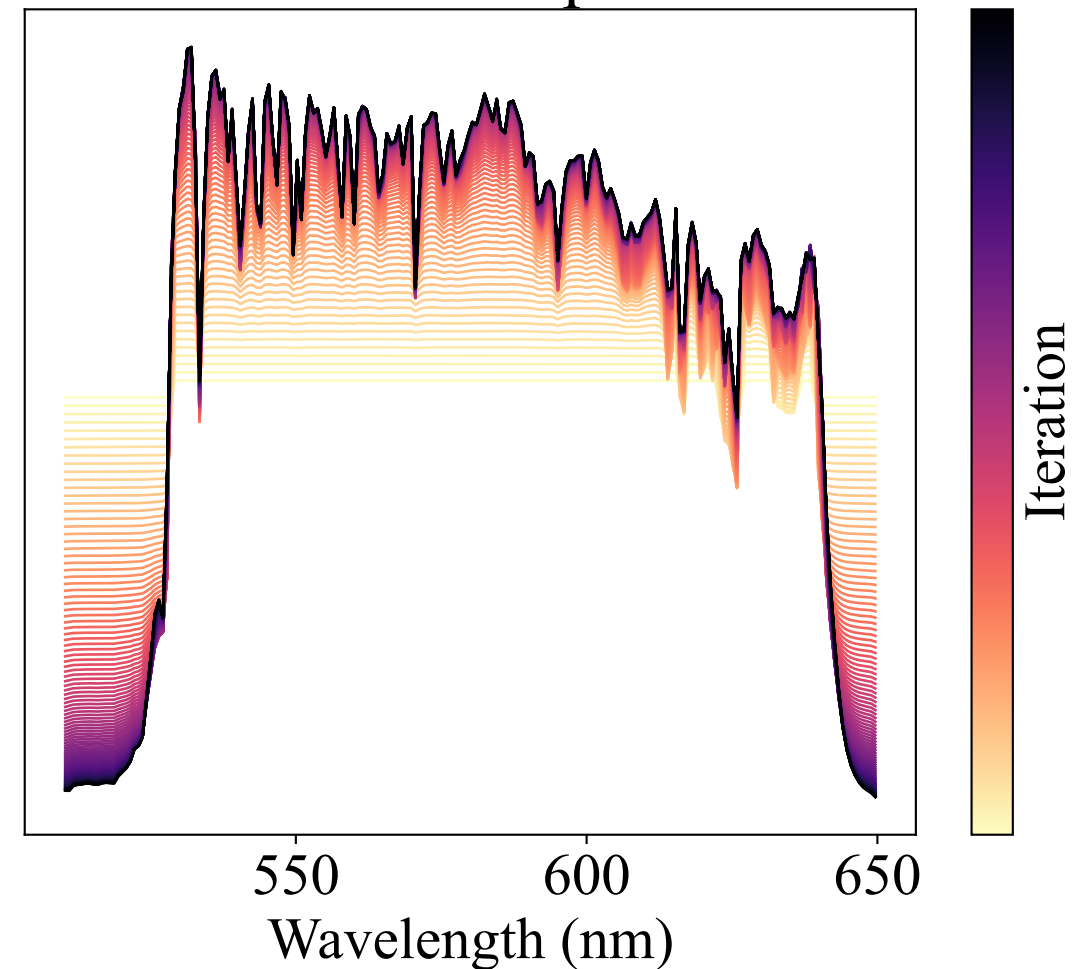
Recovered Spectra
