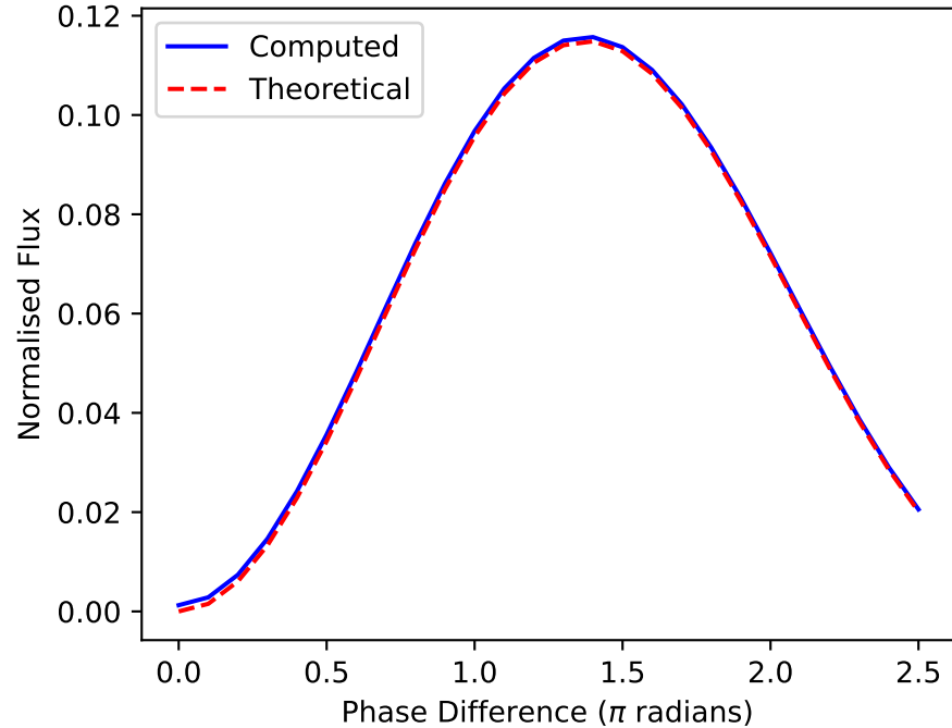
Sidelobe Flux
