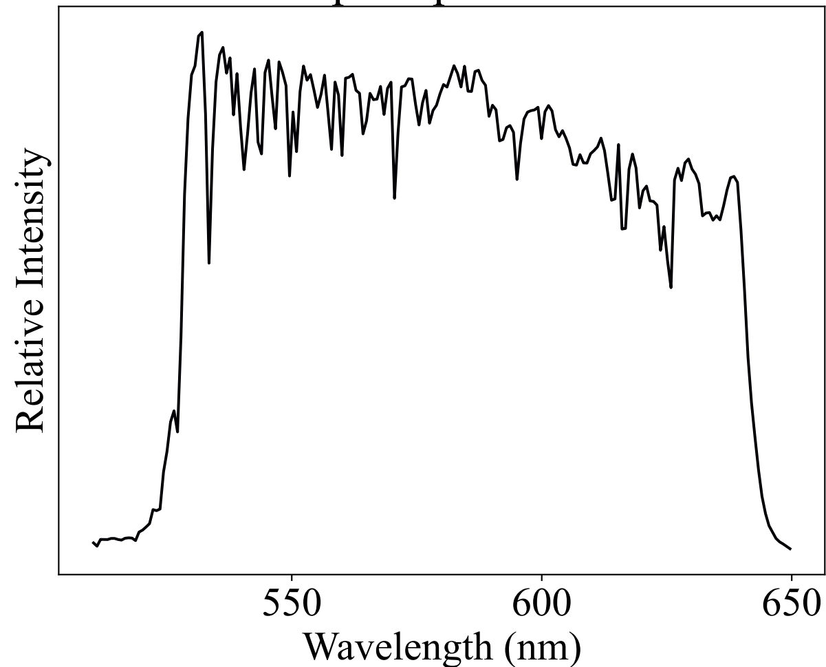
Input Spectrum
