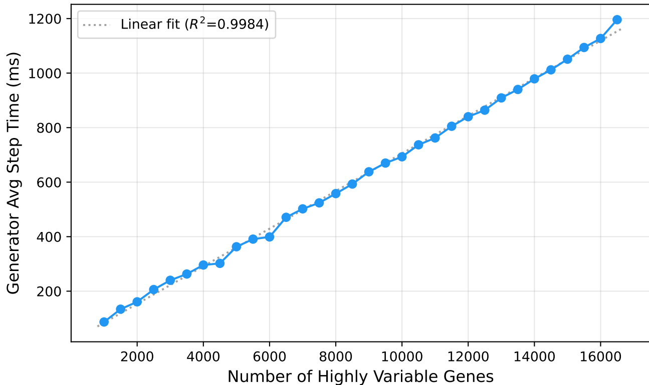
Generator Step Time vs. HVG Count
