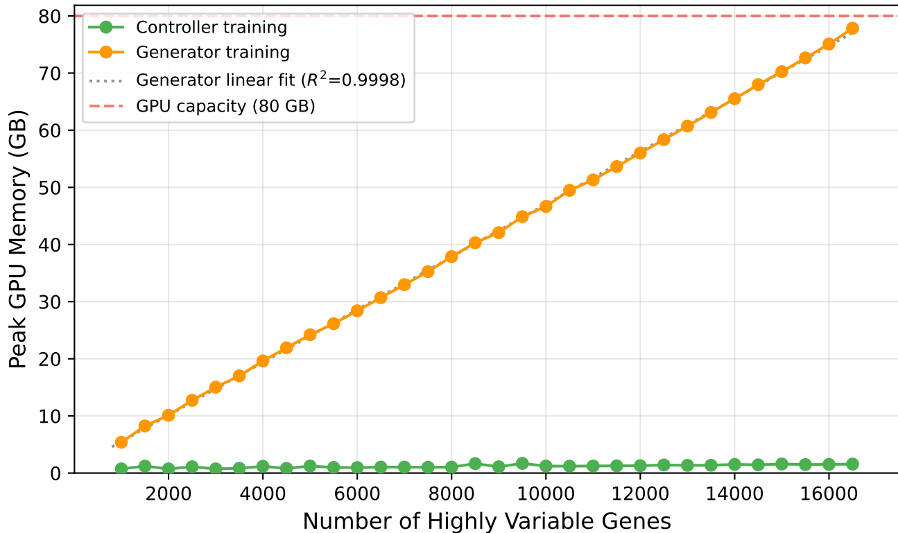
GPU Memory Requirement vs. HVG Count
