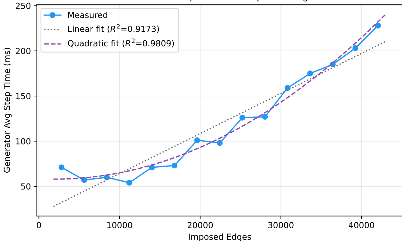
Generator Step Time vs. Imposed Edges
