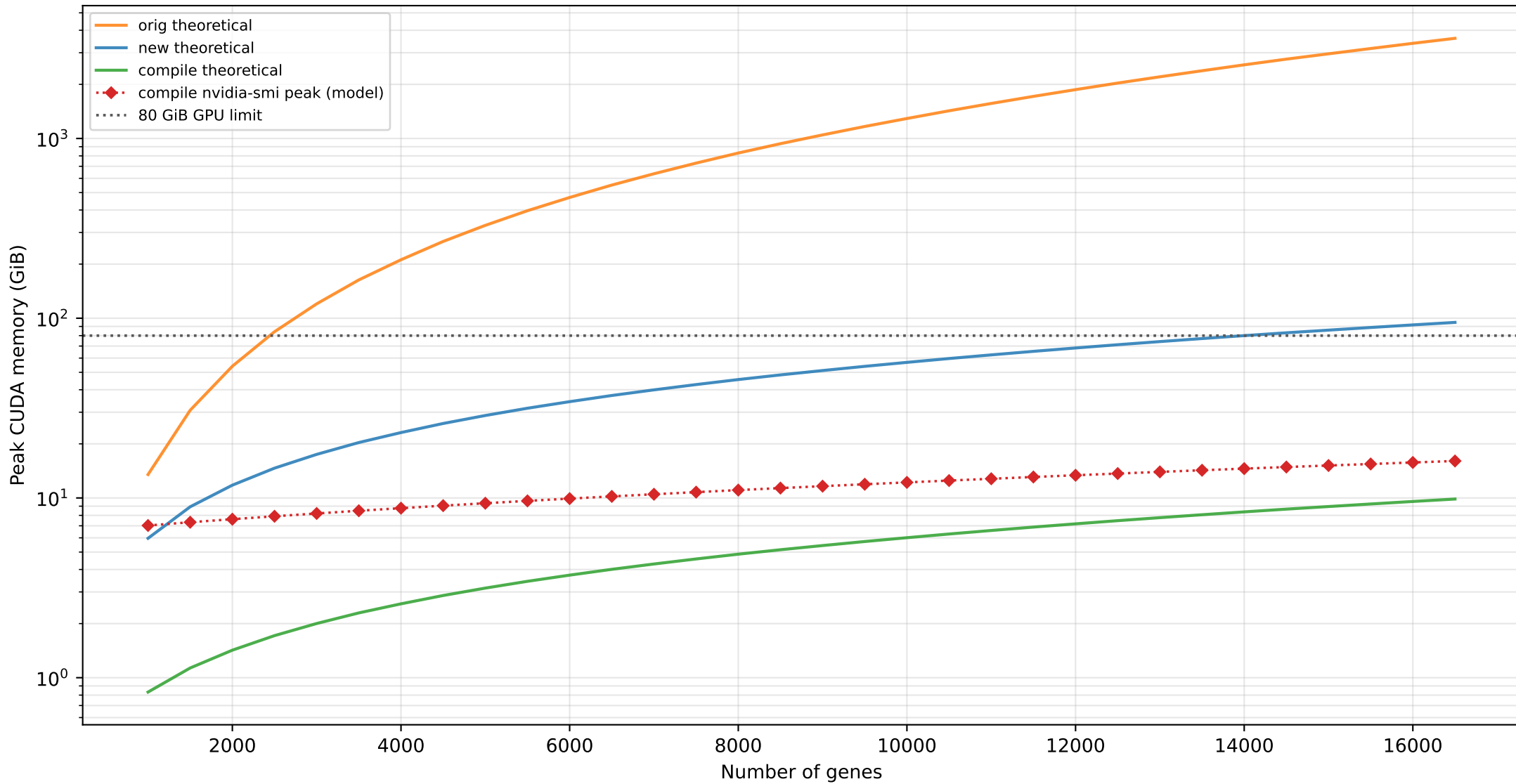
Analytic memory estimate lines = gpu_memory_model.py, no measurements
