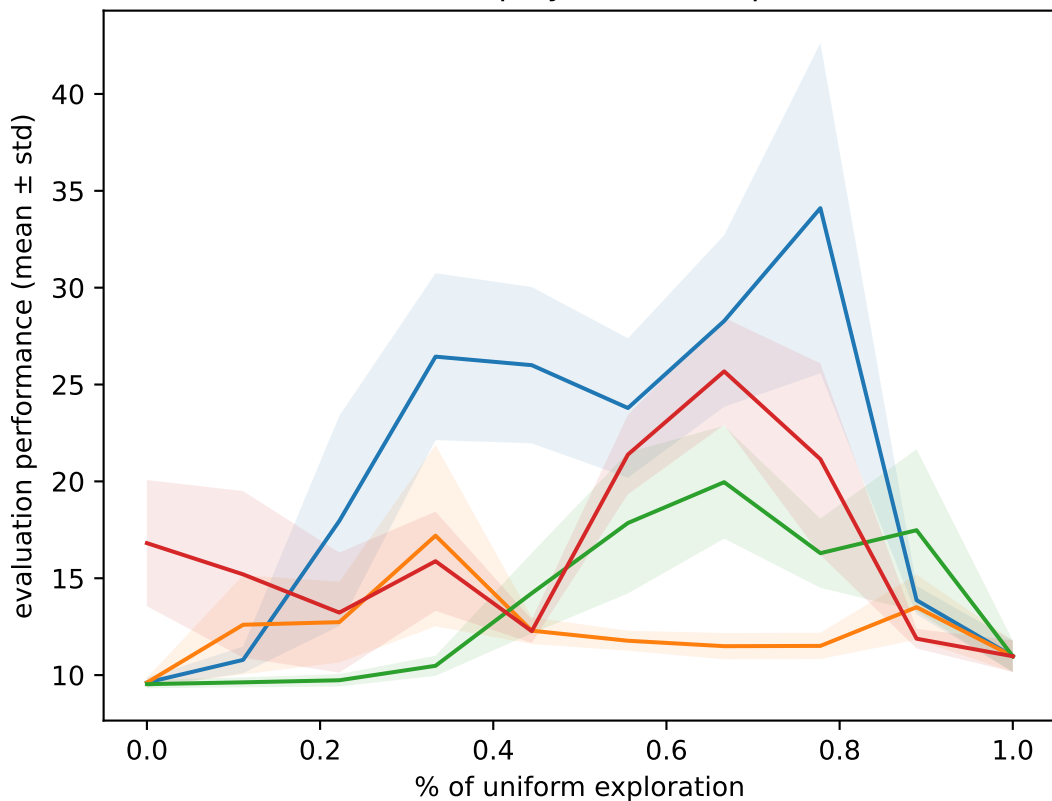
Offline learning performance for different replay buffer compositions
