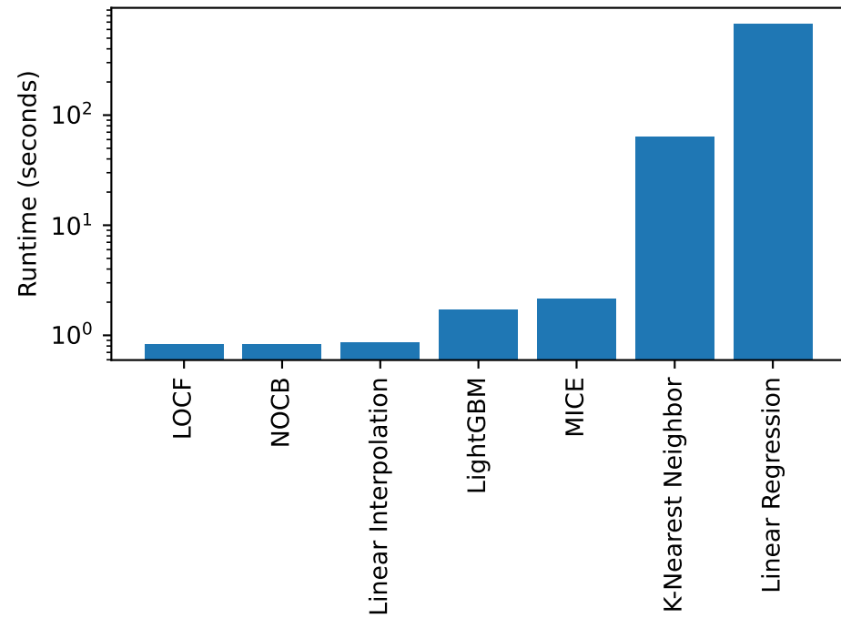
Runtime (s)
