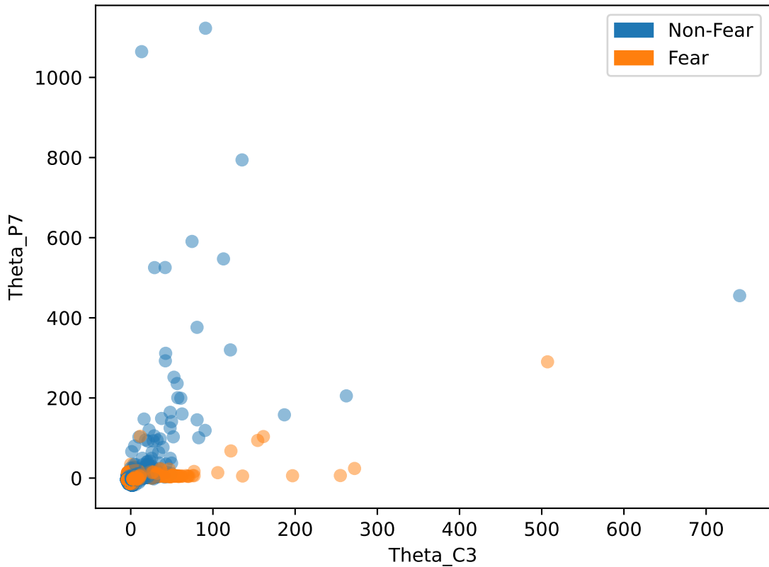
Best features visualization on binary-scene classification EEG
