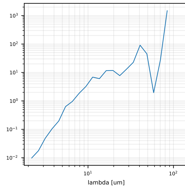
I radial PSD (DCT bins)
