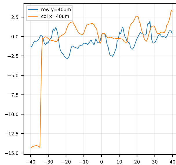
H central profiles [um]
