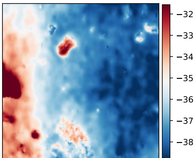
A absolute height [um]
