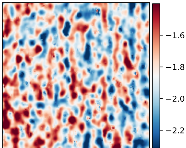
A absolute height [um]
