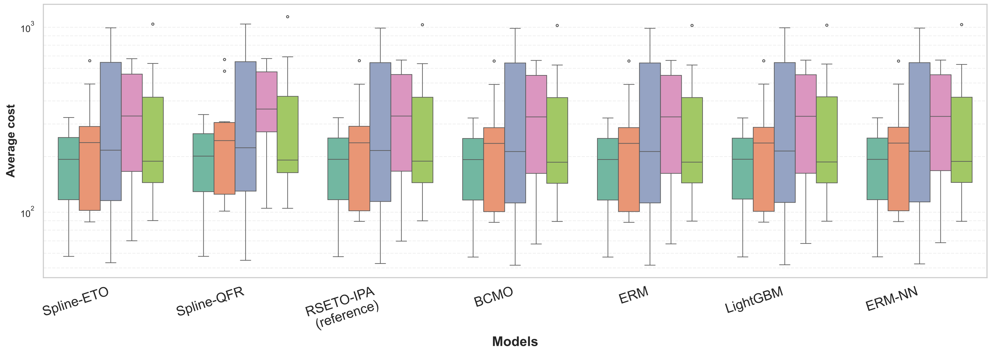
METRIC1
