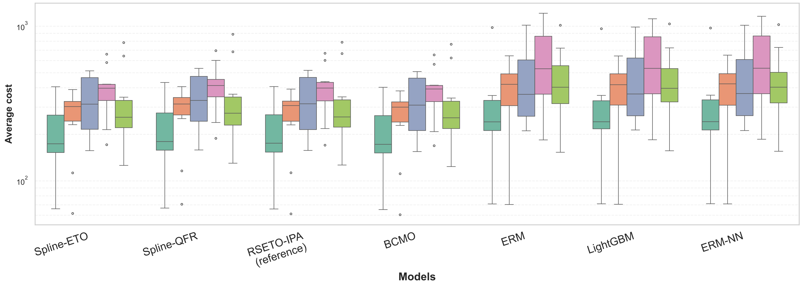
METRIC2
