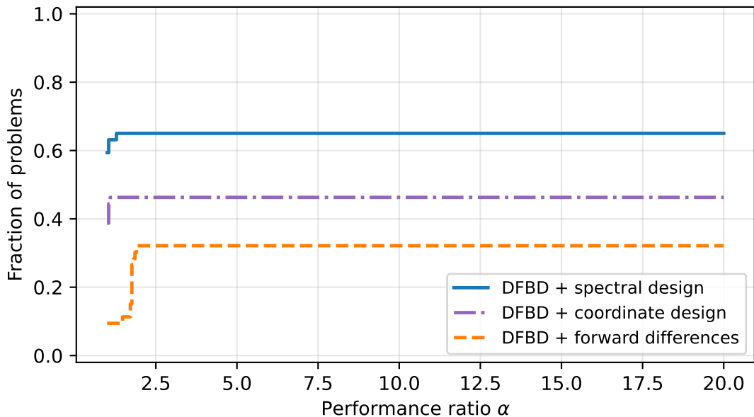
Performance profile, \tau = 1e-07 ( \sigma = 0.1 )
