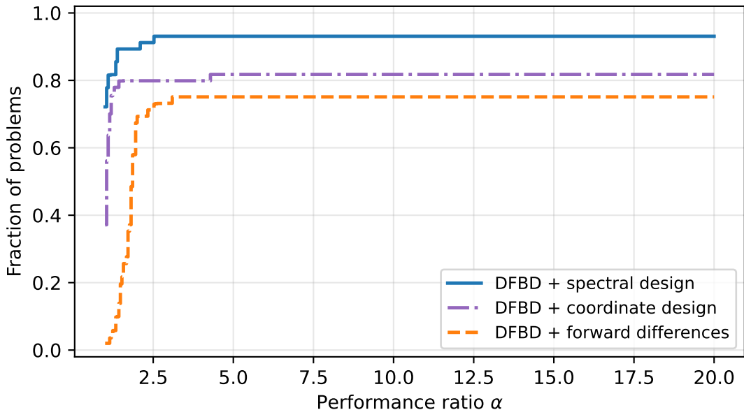
Performance profile, \tau = 0.01 ( \sigma = 0.0001 )
