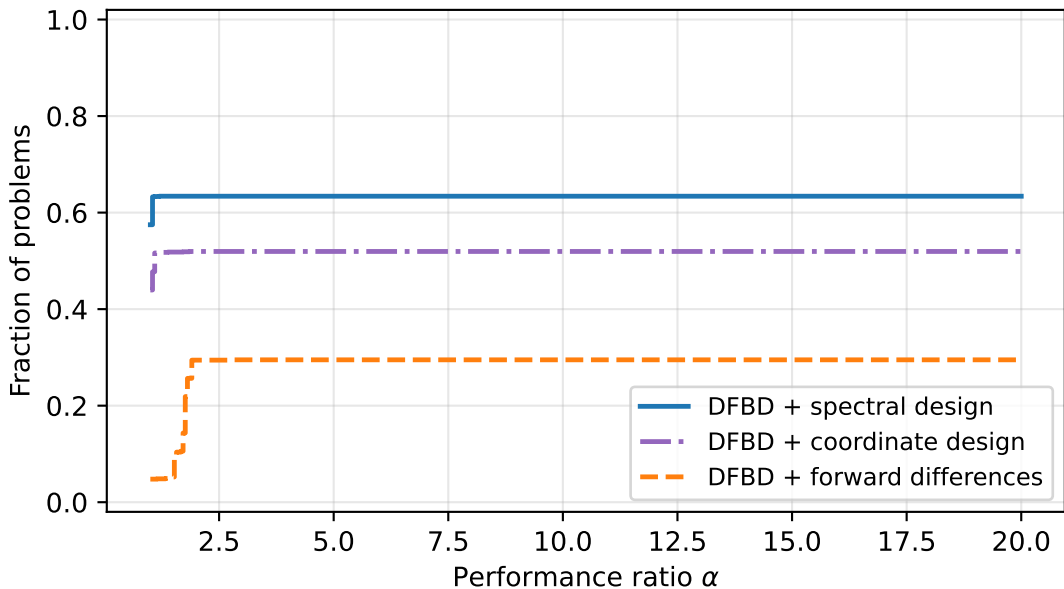
Performance profile, \tau = 1e - 07 ( \sigma = 0.0001 )
