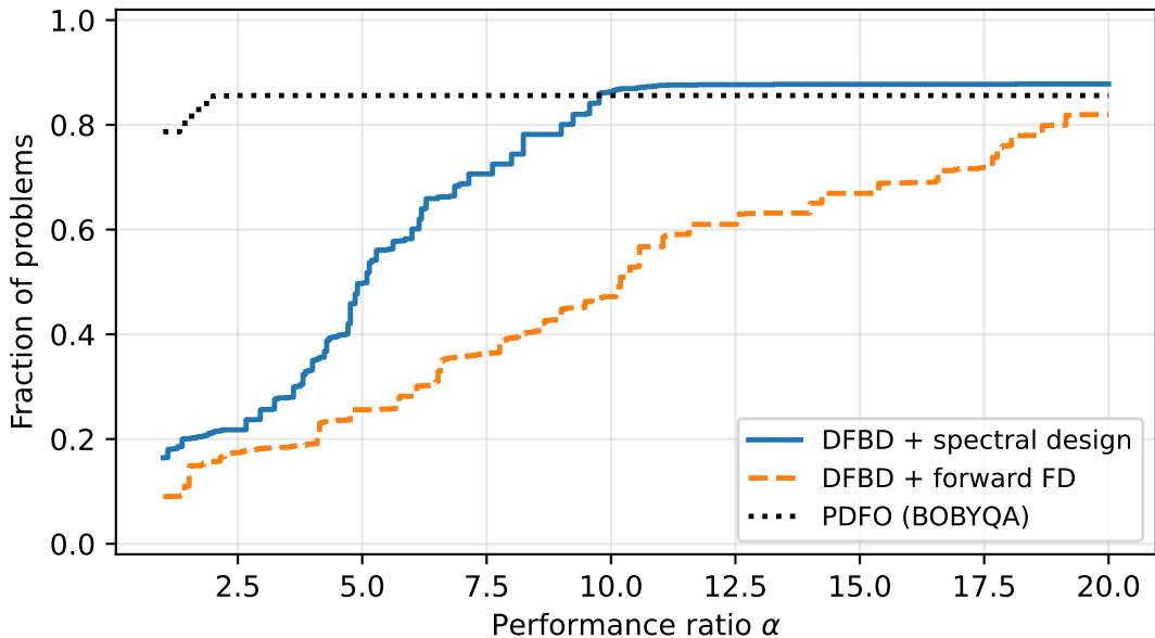
Performance profile, \tau = 0.1 ( \sigma = 0.1 )
