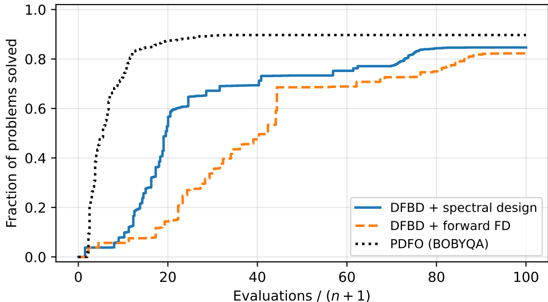
Data profile, \tau = 0.01 ( \sigma = 0.0001 )
