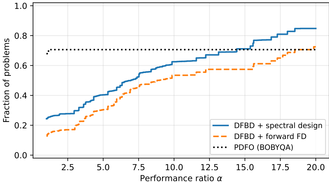
Performance profile, \tau = 0.01 ( \sigma = 0.1 )
